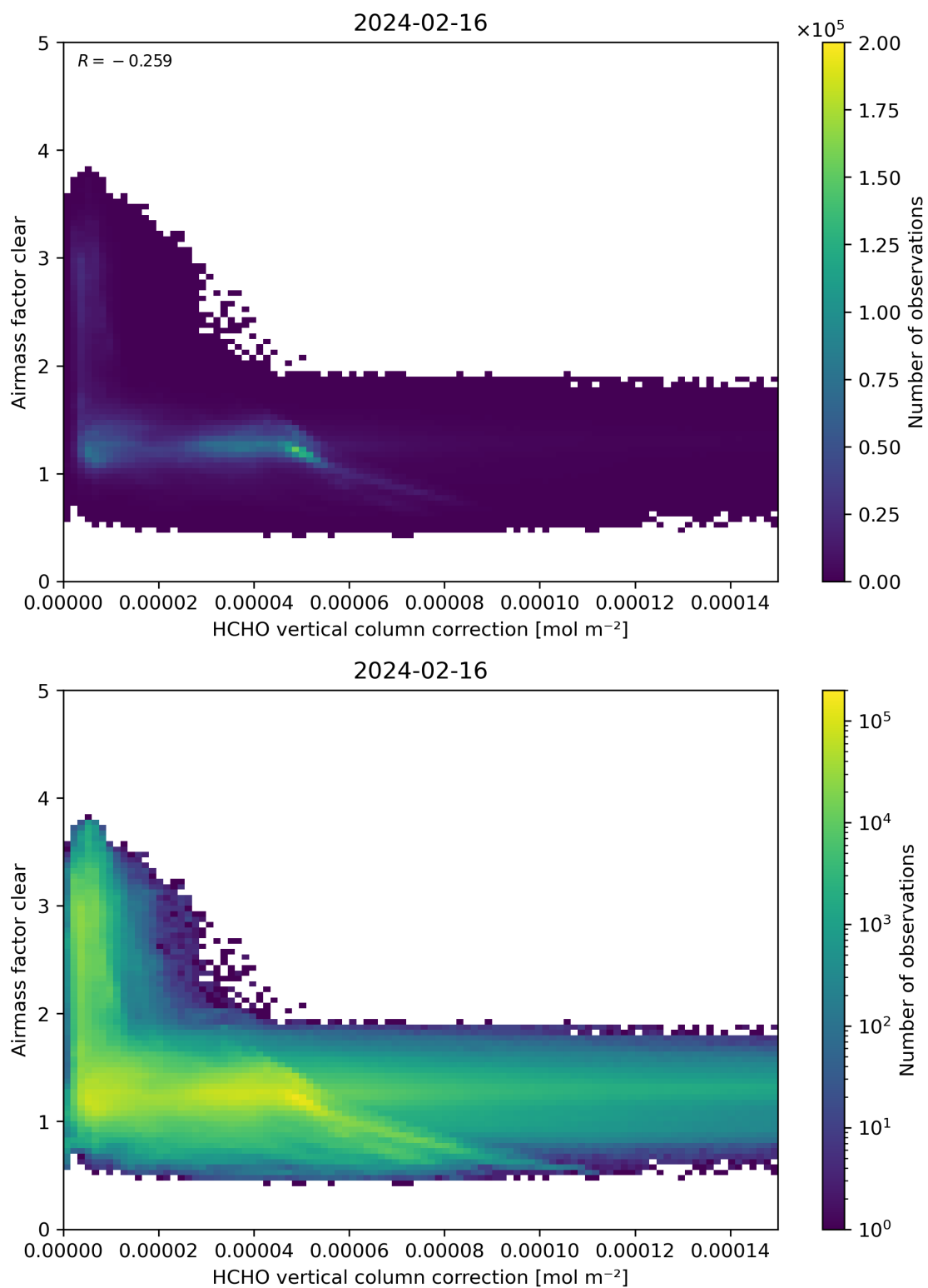
Figure 115: Scatter density plot of “HCHO vertical column correction” against “Airmass factor clear” for 2024-02-16 to 2024-02-17.
