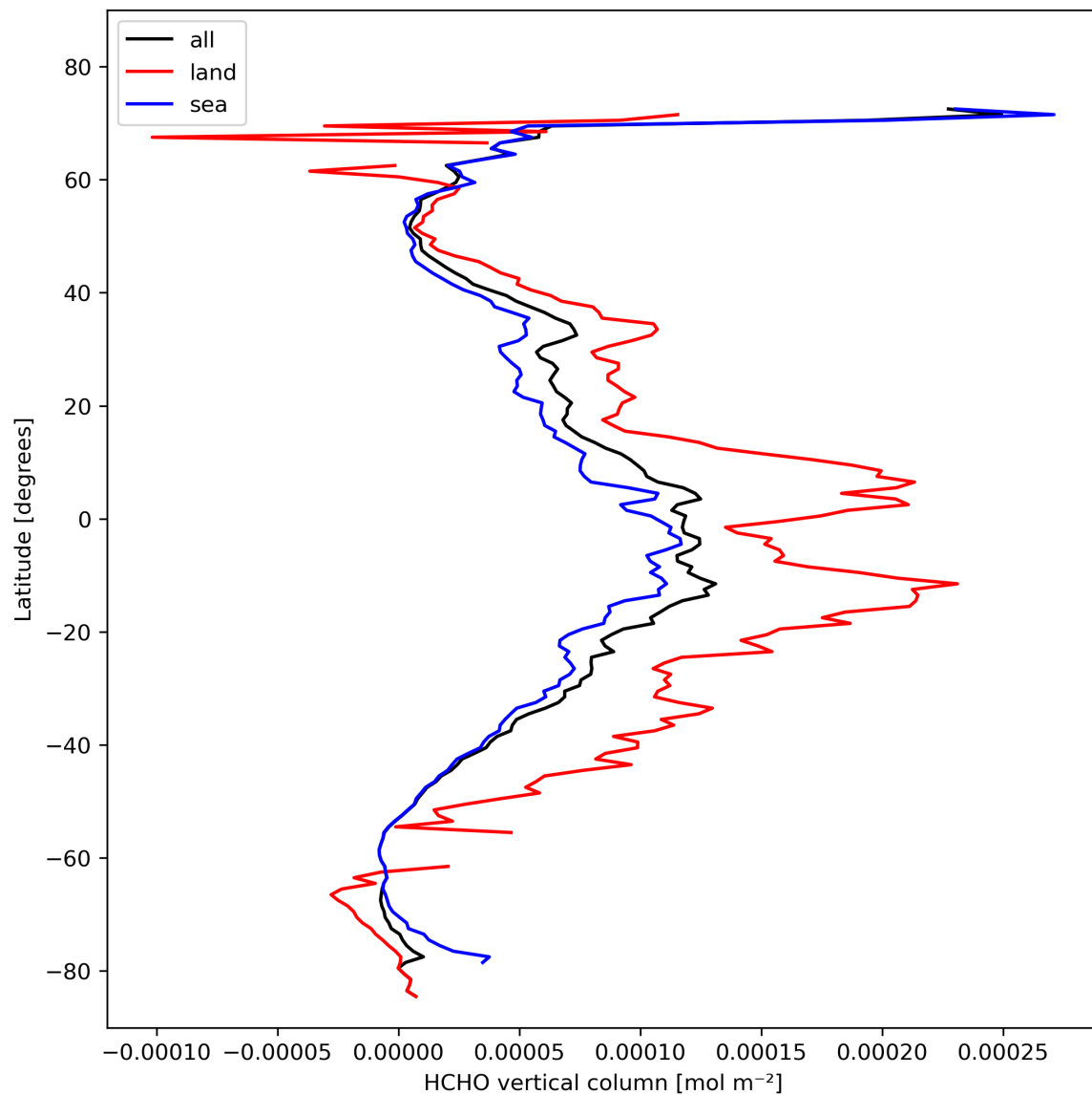
Figure 21: Zonal average of “HCHO vertical column” for 2024-02-16 to 2024-02-17.
