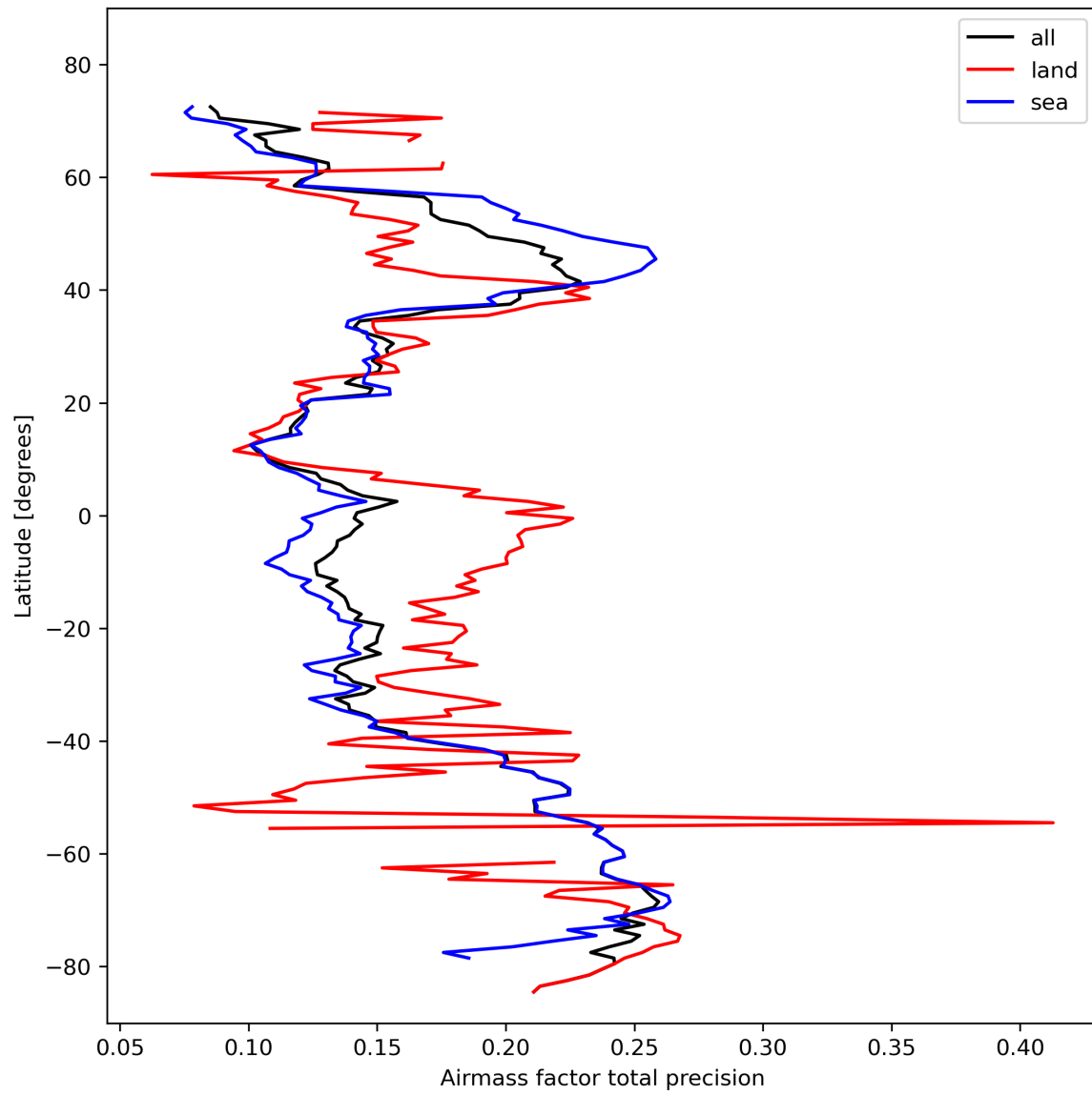
Figure 27: Zonal average of “Airmass factor total precision” for 2024-02-16 to 2024-02-17.
