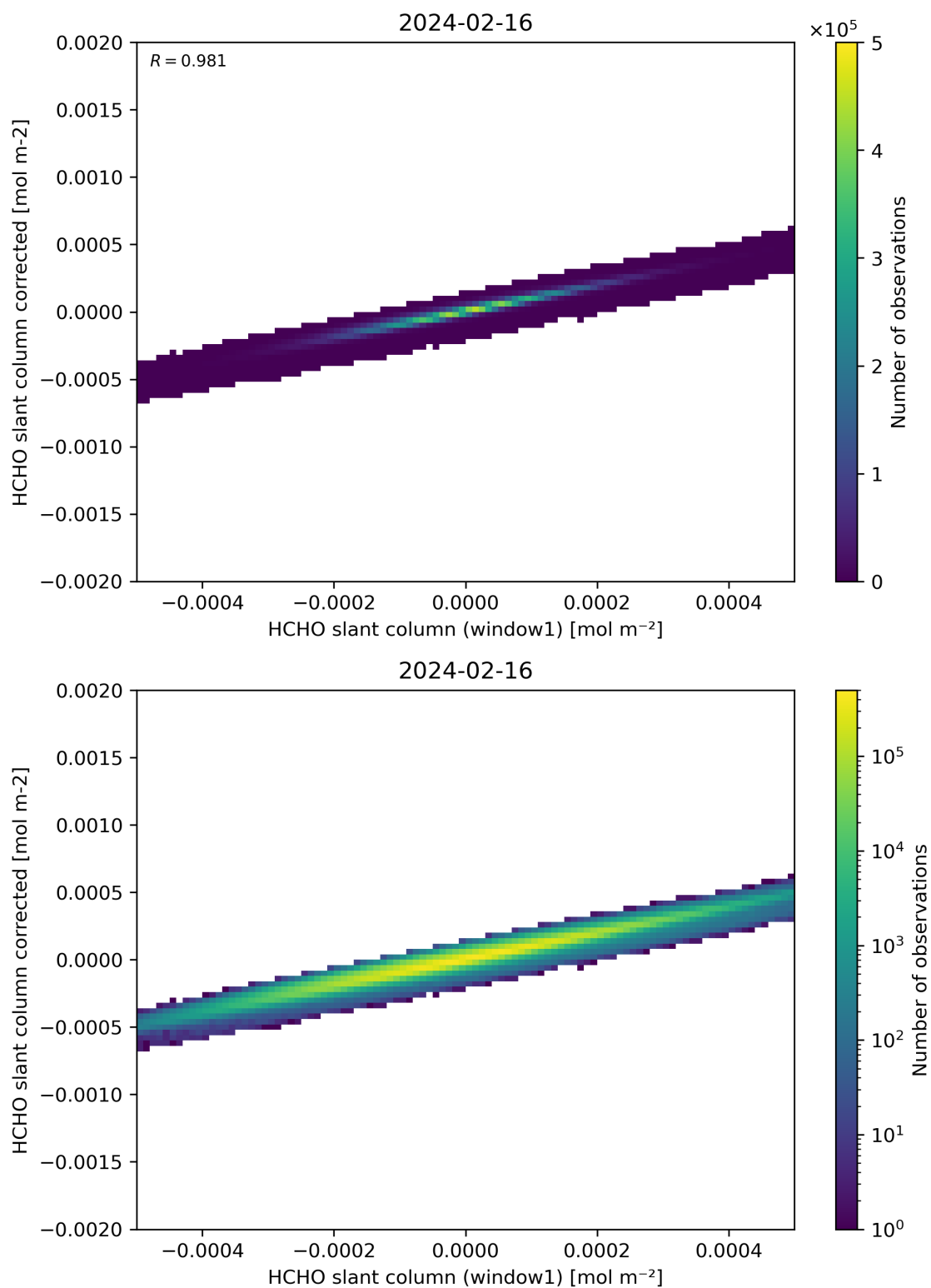
Figure 82: Scatter density plot of “HCHO slant column (window1)” against “HCHO slant column corrected” for 2024-02-16 to 2024-02-17.
