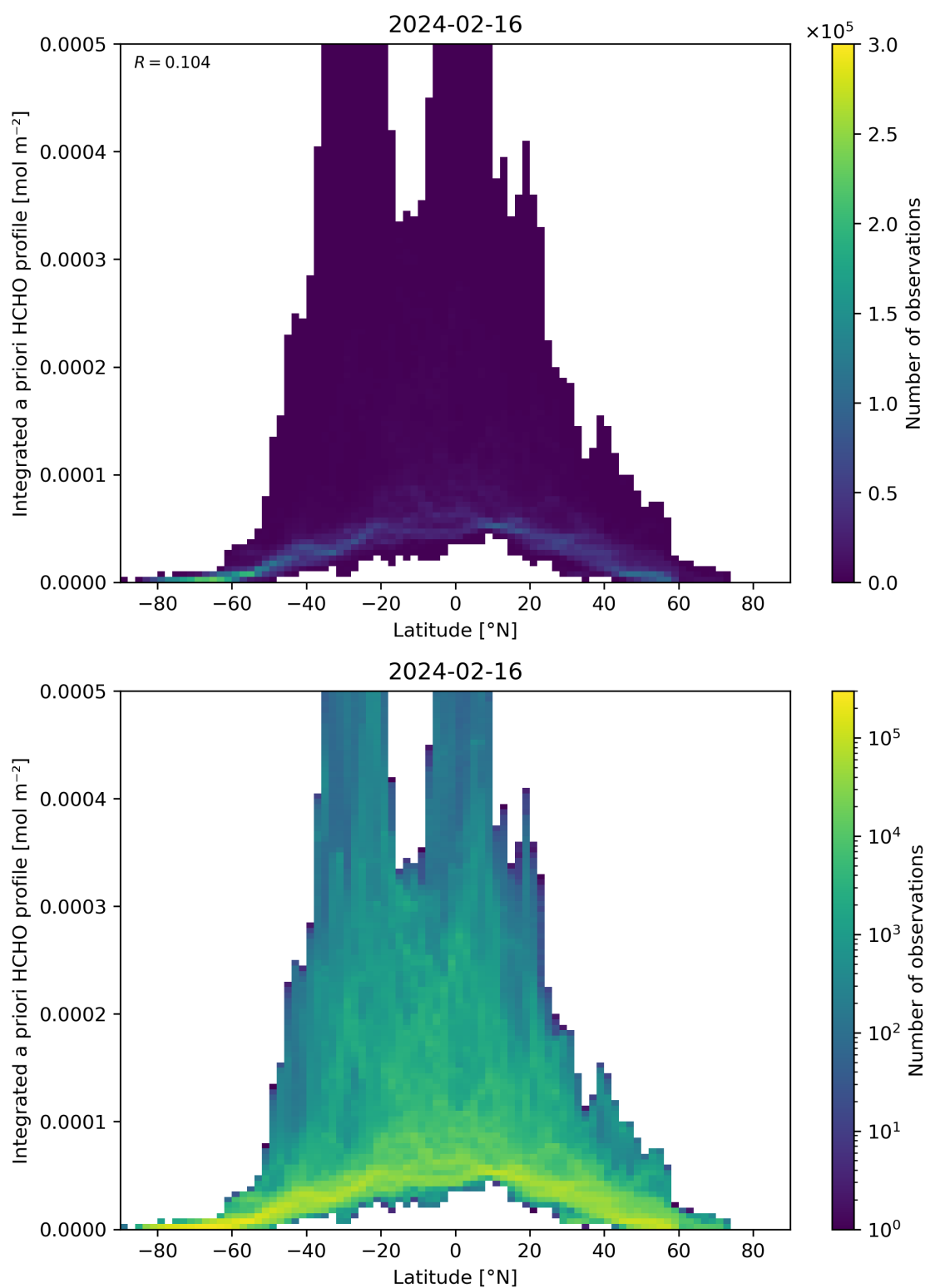
Figure 166: Scatter density plot of “Latitude” against “Integrated a priori HCHO profile” for 2024-02-16 to 2024-02-17.
