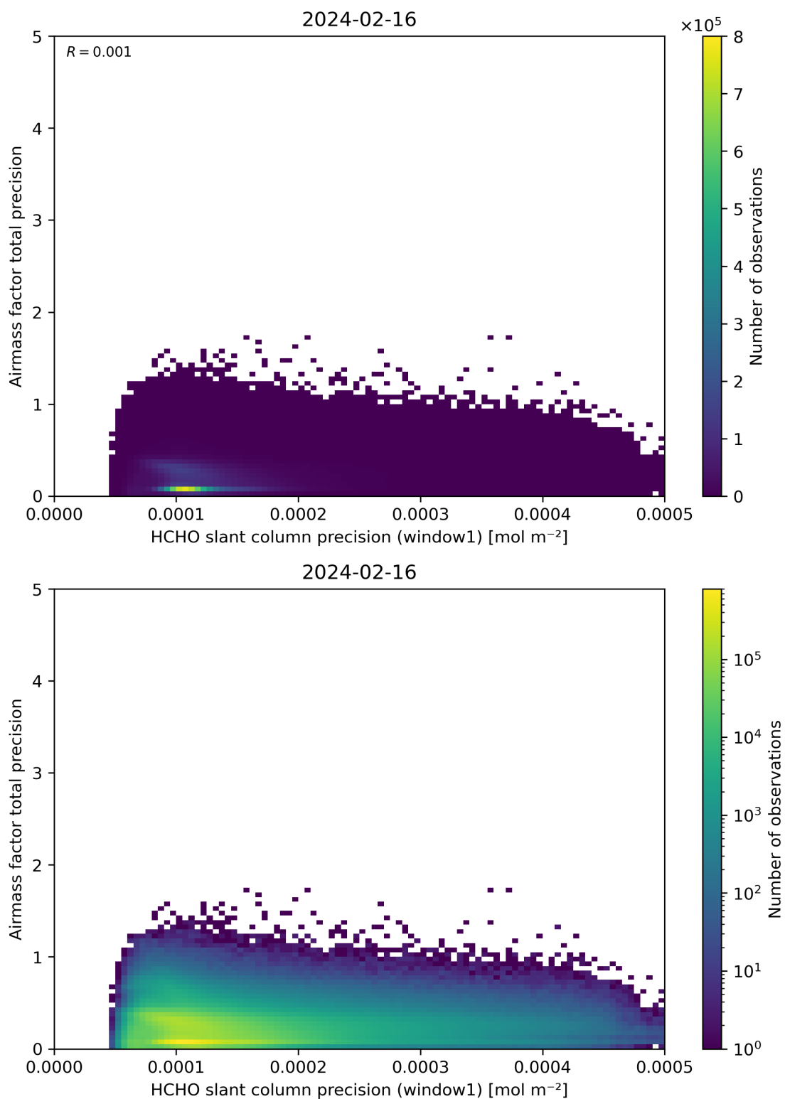
Figure 95: Scatter density plot of “HCHO slant column precision (window1)” against “Airmass factor total precision” for 2024-02-16 to 2024-02-17.
