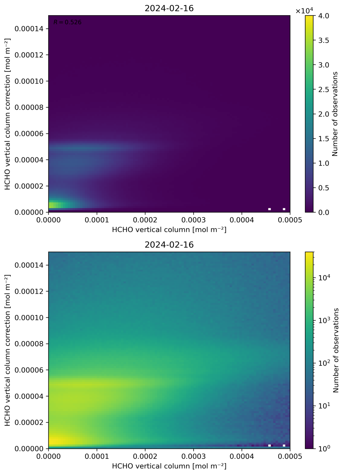
Figure 133: Scatter density plot of “HCHO vertical column” against “HCHO vertical column correction” for 2024-02-16 to 2024-02-17.
