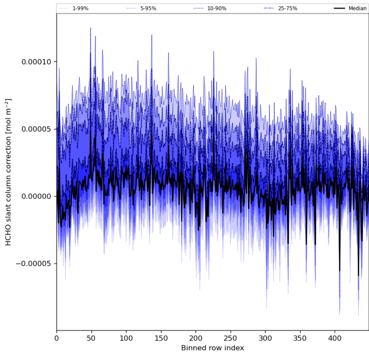
Figure 61: Along track statistics of “HCHO slant column correction” for 2024-02-16 to 2024-02-17
