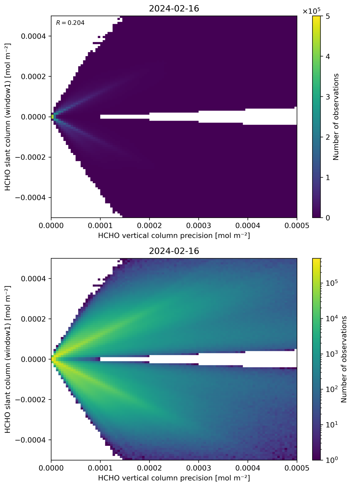
Figure 142: Scatter density plot of “HCHO vertical column precision” against “HCHO slant column (window1)” for 2024-02-16 to 2024-02-17.
