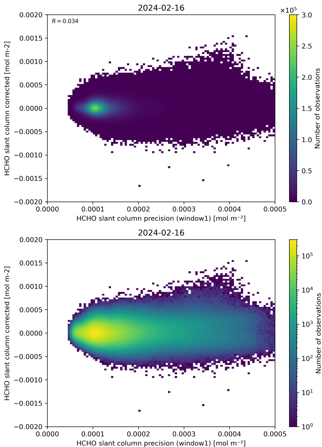
Figure 92: Scatter density plot of “HCHO slant column precision (window1)” against “HCHO slant column corrected” for 2024-02-16 to 2024-02-17.
