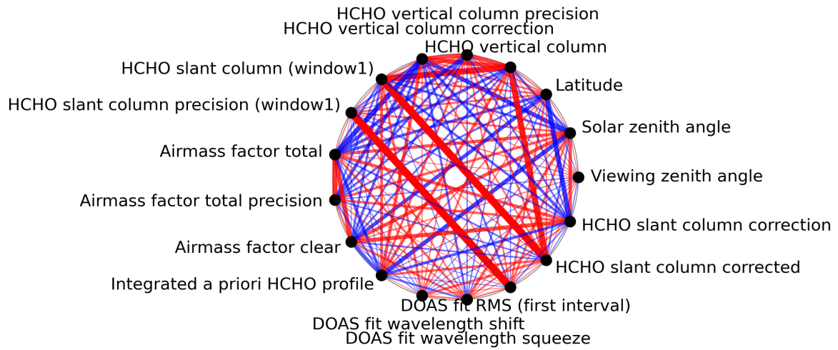
Figure 1: Map of correlation graph for 2024-02-16 to 2024-02-17.
