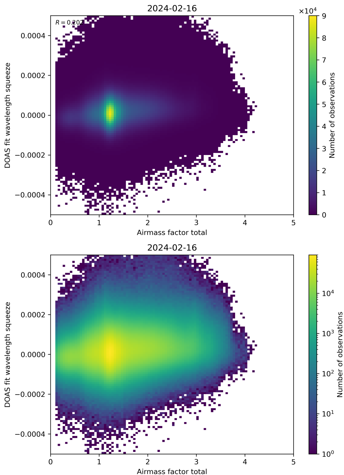
Figure 99: Scatter density plot of “Airmass factor total” against “DOAS fit wavelength squeeze” for 2024-02-16 to 2024-02-17.
