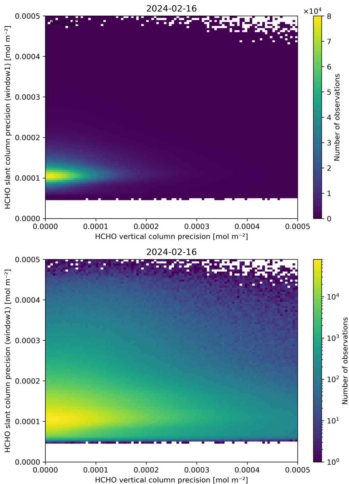
Figure 143: Scatter density plot of “HCHO vertical column precision” against “HCHO slant column precision (window1)” for 2024-02-16 to 2024-02-17.
