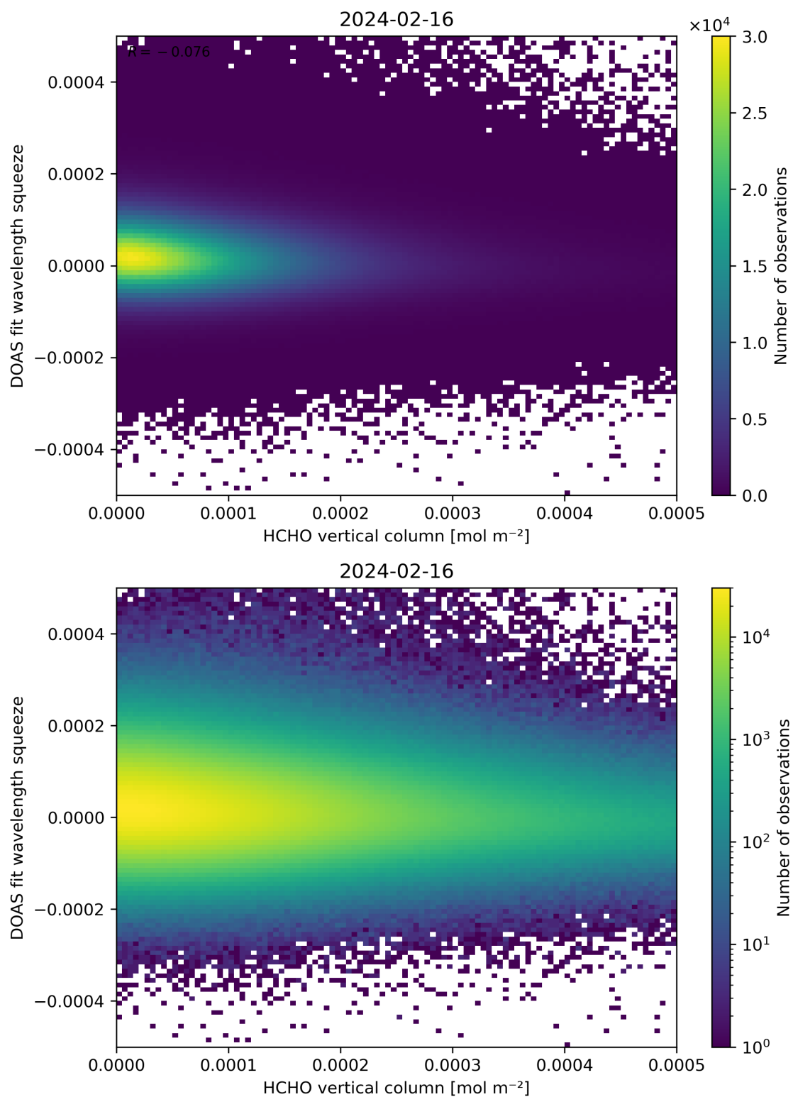
Figure 125: Scatter density plot of “HCHO vertical column” against “DOAS fit wavelength squeeze” for 2024-02-16 to 2024-02-17.
