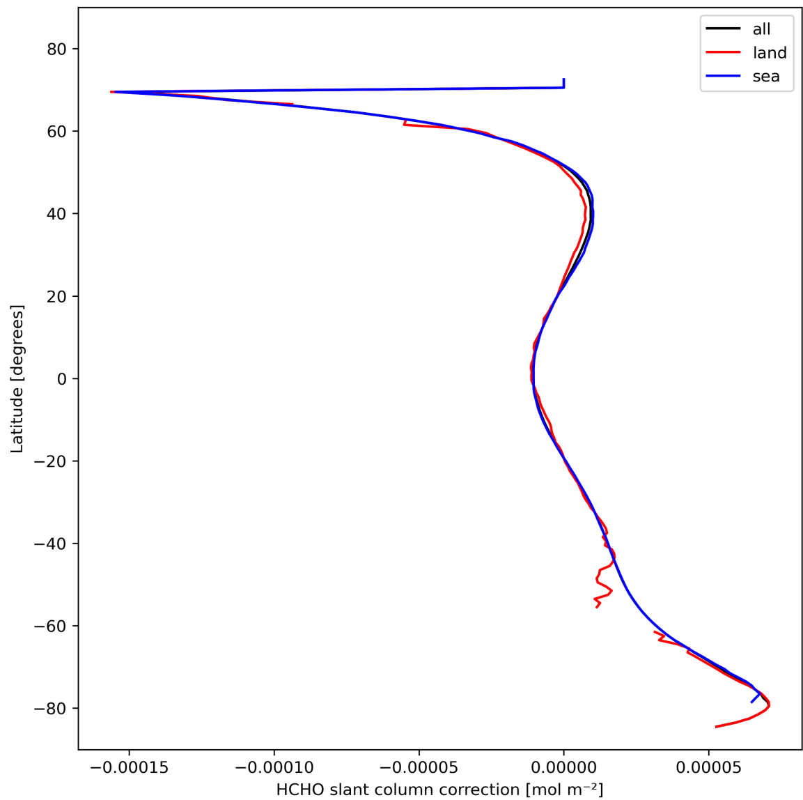
Figure 33: Zonal average of “HCHO slant column correction” for 2024-02-16 to 2024-02-17.
