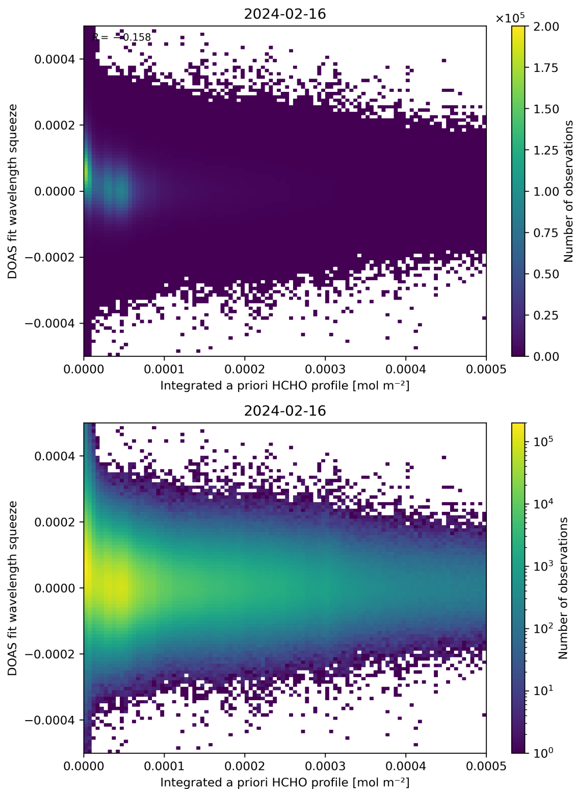
Figure 150: Scatter density plot of “Integrated a priori HCHO profile” against “DOAS fit wavelength squeeze” for 2024-02-16 to 2024-02-17.
