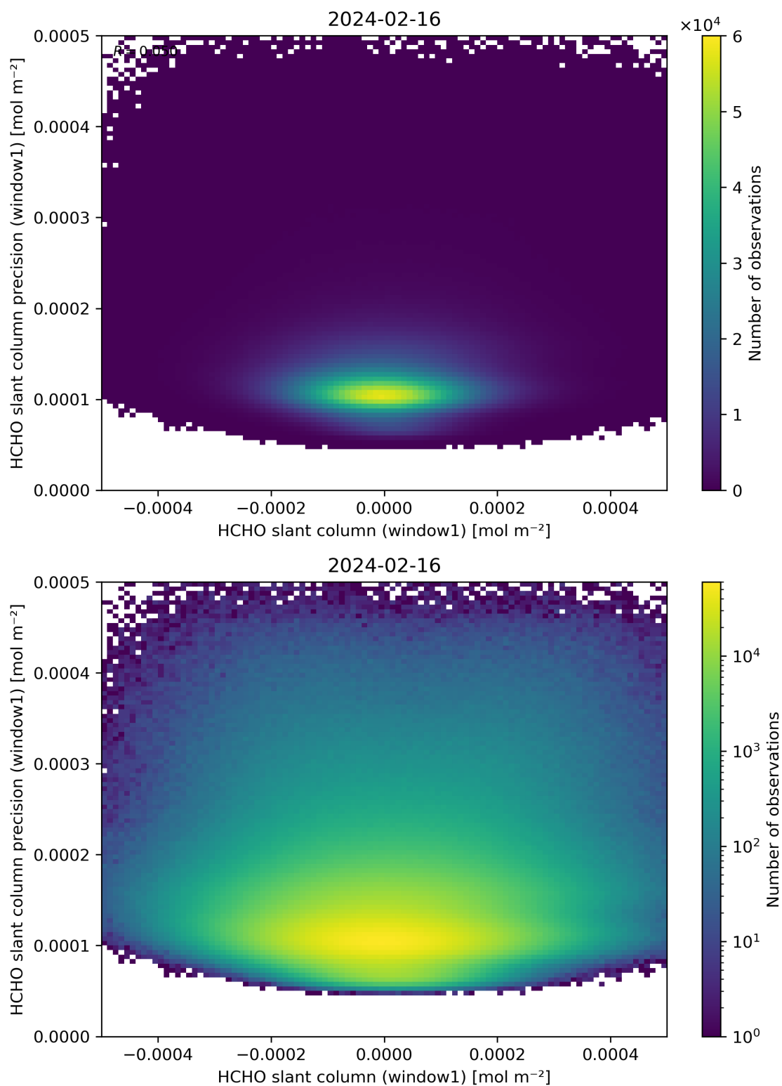
Figure 84: Scatter density plot of “HCHO slant column (window1)” against “HCHO slant column precision (window1)” for 2024-02-16 to 2024-02-17.
