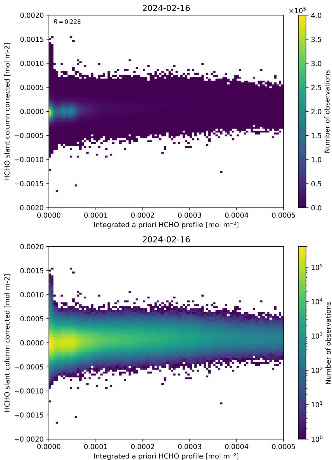
Figure 151: Scatter density plot of “Integrated a priori HCHO profile” against “HCHO slant column corrected” for 2024-02-16 to 2024-02-17.
