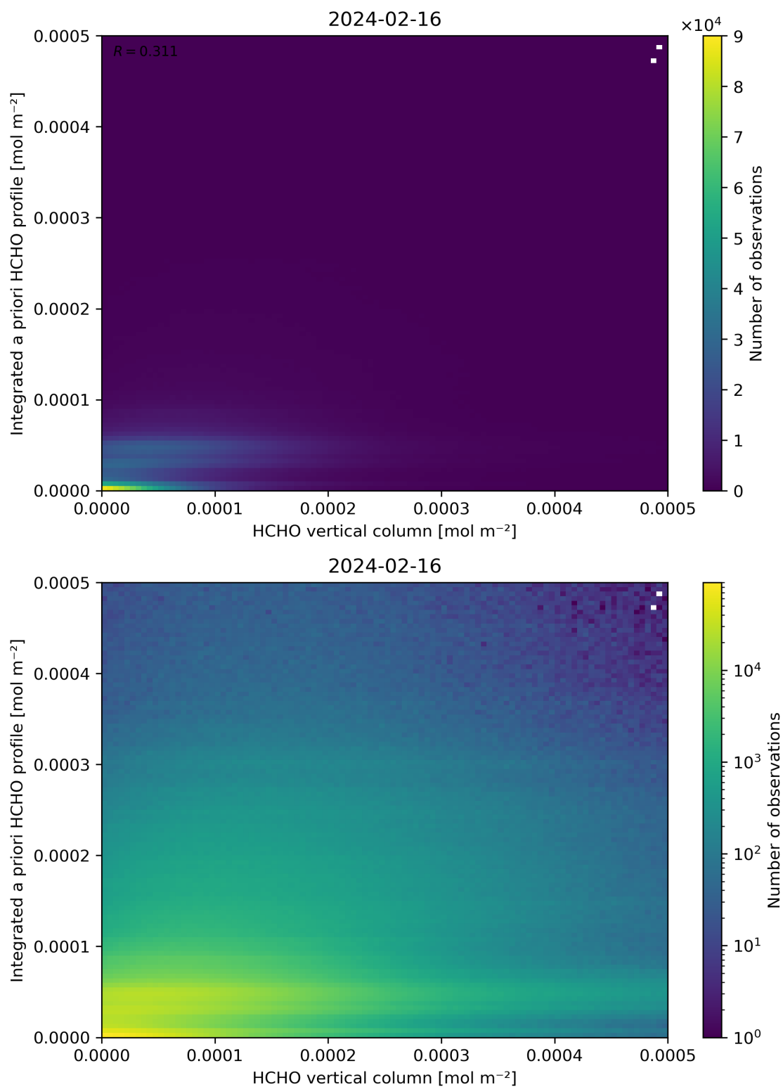
Figure 135: Scatter density plot of “HCHO vertical column” against “Integrated a priori HCHO profile” for 2024-02-16 to 2024-02-17.
