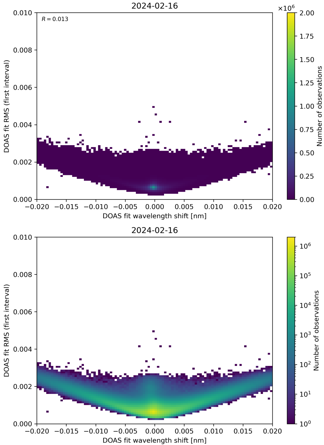
Figure 64: Scatter density plot of “DOAS fit wavelength shift” against “DOAS fit RMS (first interval)” for 2024-02-16 to 2024-02-17.
