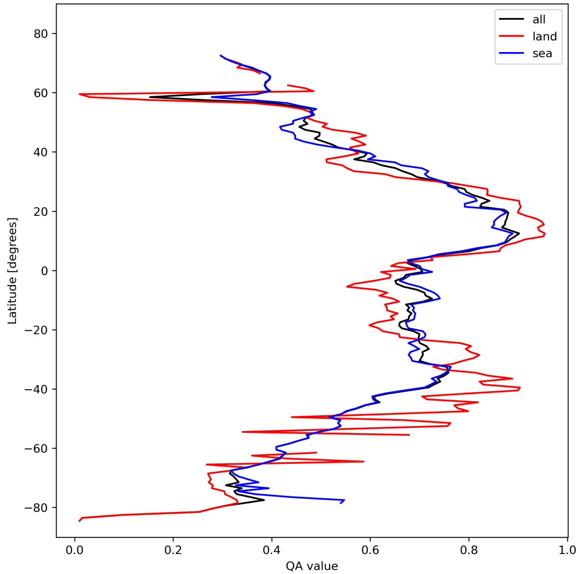
Figure 20: Zonal average of “QA value” for 2024-02-16 to 2024-02-17.
