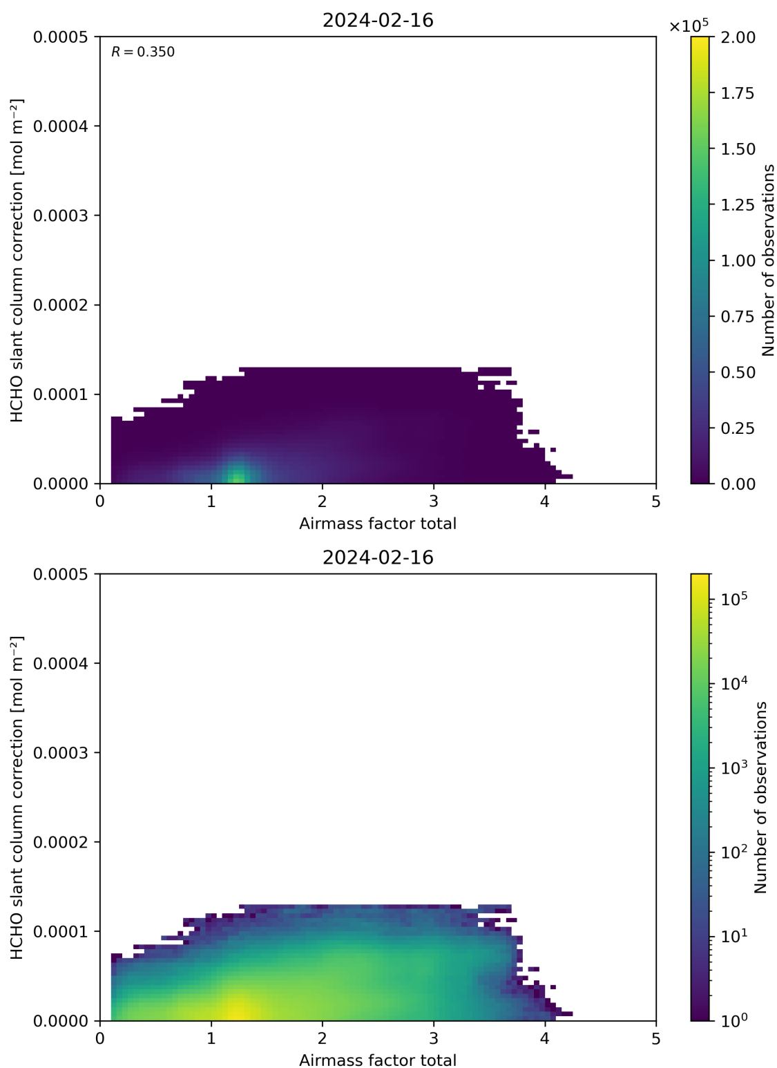
Figure 102: Scatter density plot of “Airmass factor total” against “HCHO slant column correction” for 2024-02-16 to 2024-02-17.
