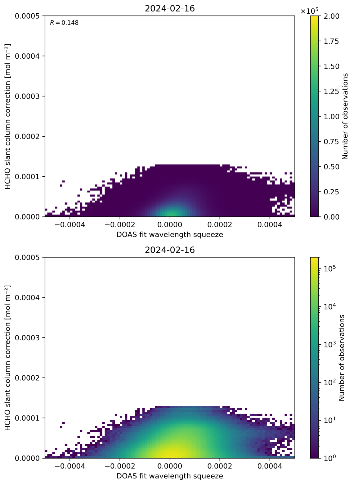
Figure 70: Scatter density plot of “DOAS fit wavelength squeeze” against “HCHO slant column correction” for 2024-02-16 to 2024-02-17.
