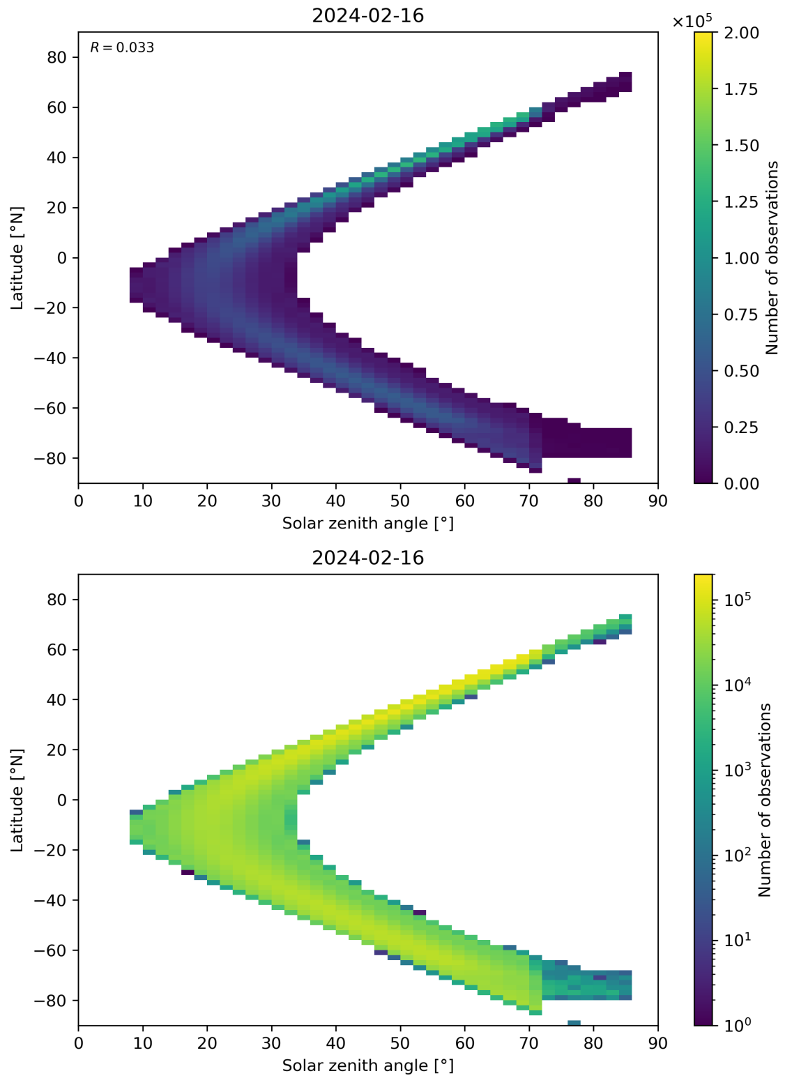
Figure 181: Scatter density plot of “Solar zenith angle” against “Latitude” for 2024-02-16 to 2024-02-17.
