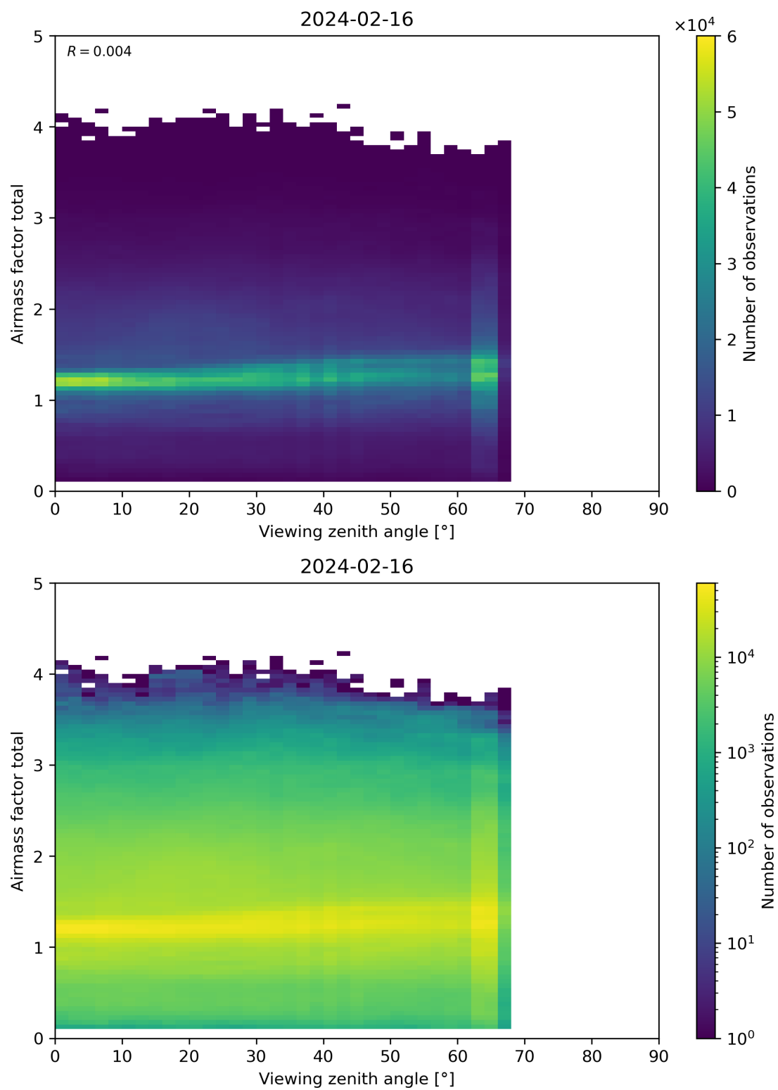
Figure 190: Scatter density plot of “Viewing zenith angle” against “Airmass factor total” for 2024-02-16 to 2024-02-17.
