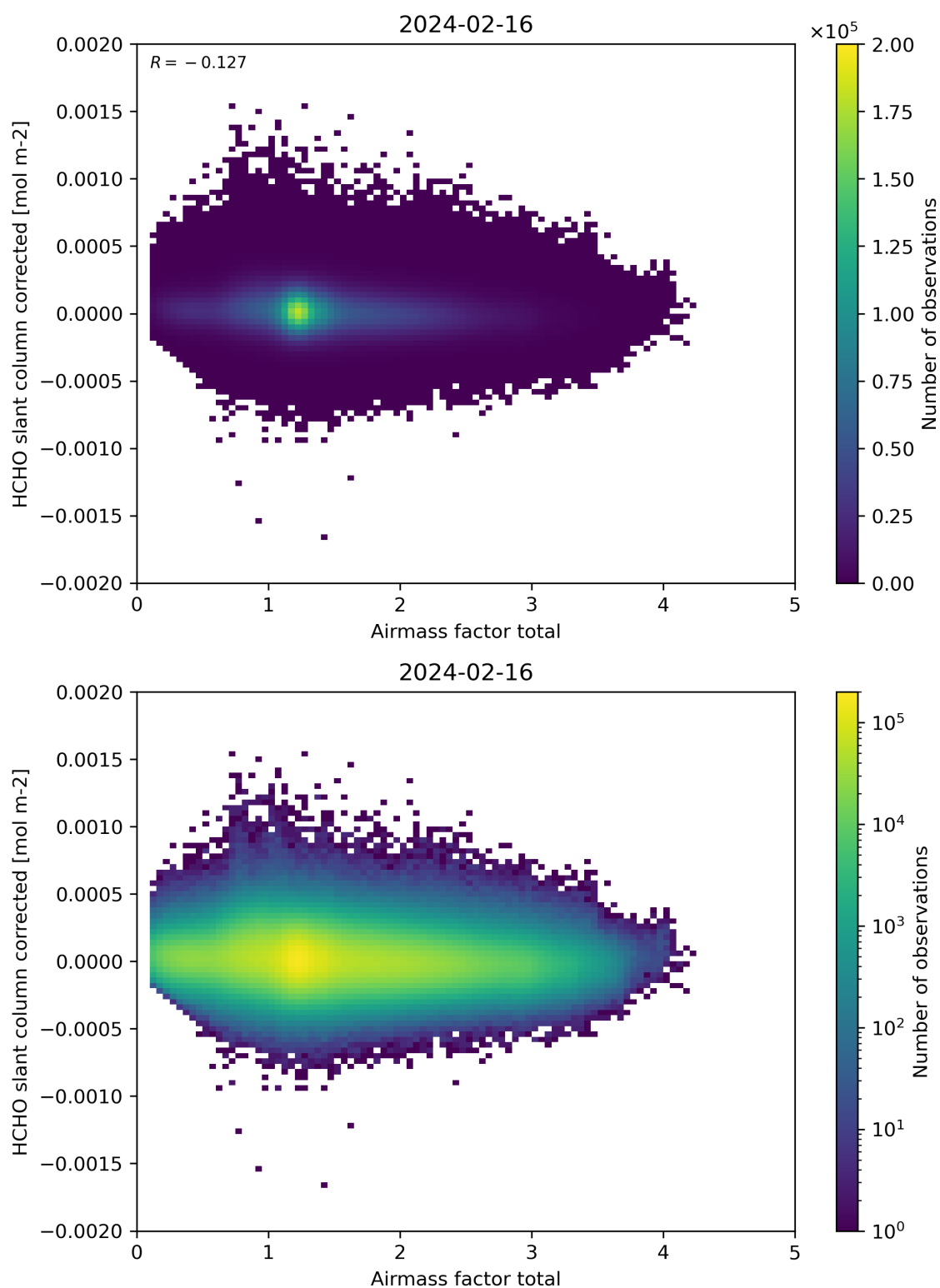
Figure 101: Scatter density plot of “Airmass factor total” against “HCHO slant column corrected” for 2024-02-16 to 2024-02-17.
