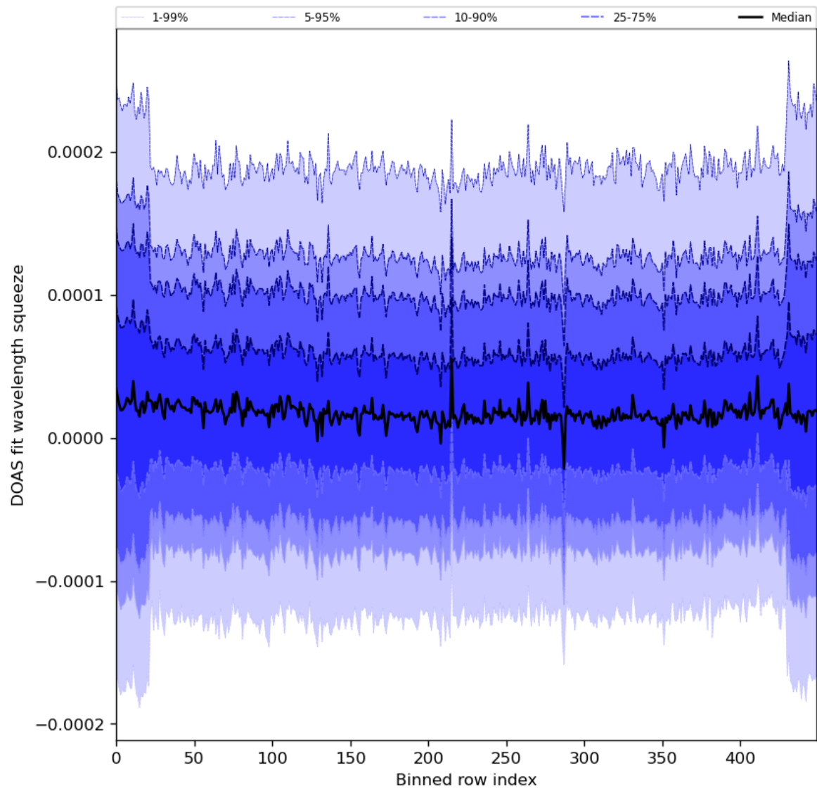
Figure 59: Along track statistics of “DOAS fit wavelength squeeze” for 2024-02-16 to 2024-02-17
