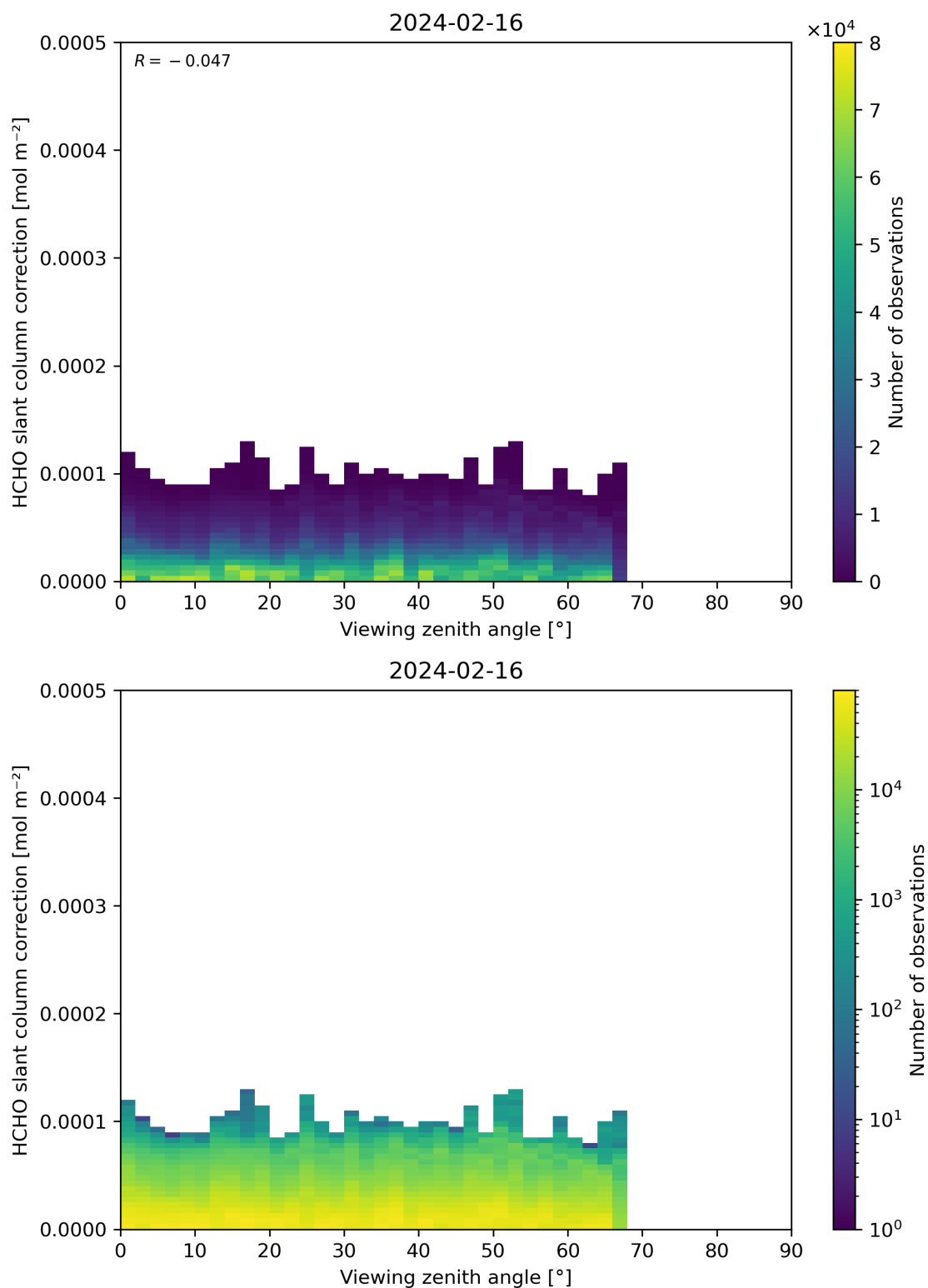
Figure 187: Scatter density plot of “Viewing zenith angle” against “HCHO slant column correction” for 2024-02-16 to 2024-02-17.
