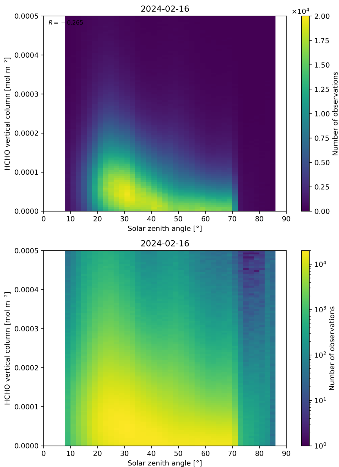
Figure 177: Scatter density plot of “Solar zenith angle” against “HCHO vertical column” for 2024-02-16 to 2024-02-17.
