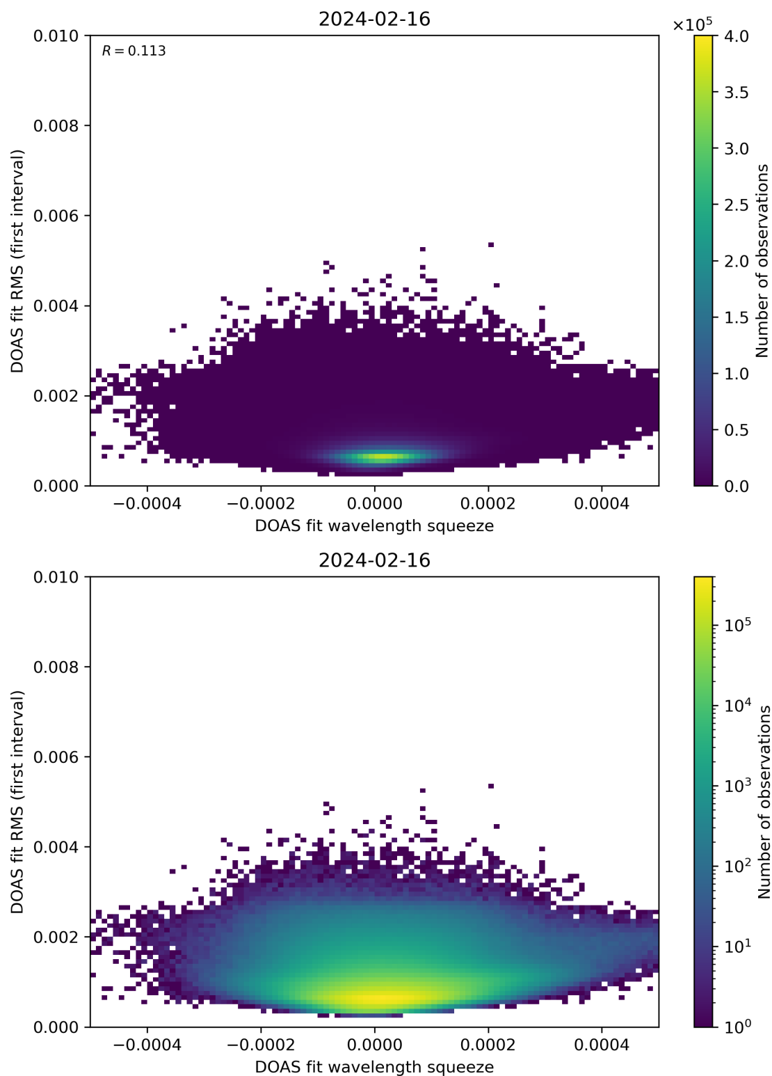
Figure 68: Scatter density plot of “DOAS fit wavelength squeeze” against “DOAS fit RMS (first interval)” for 2024-02-16 to 2024-02-17.
