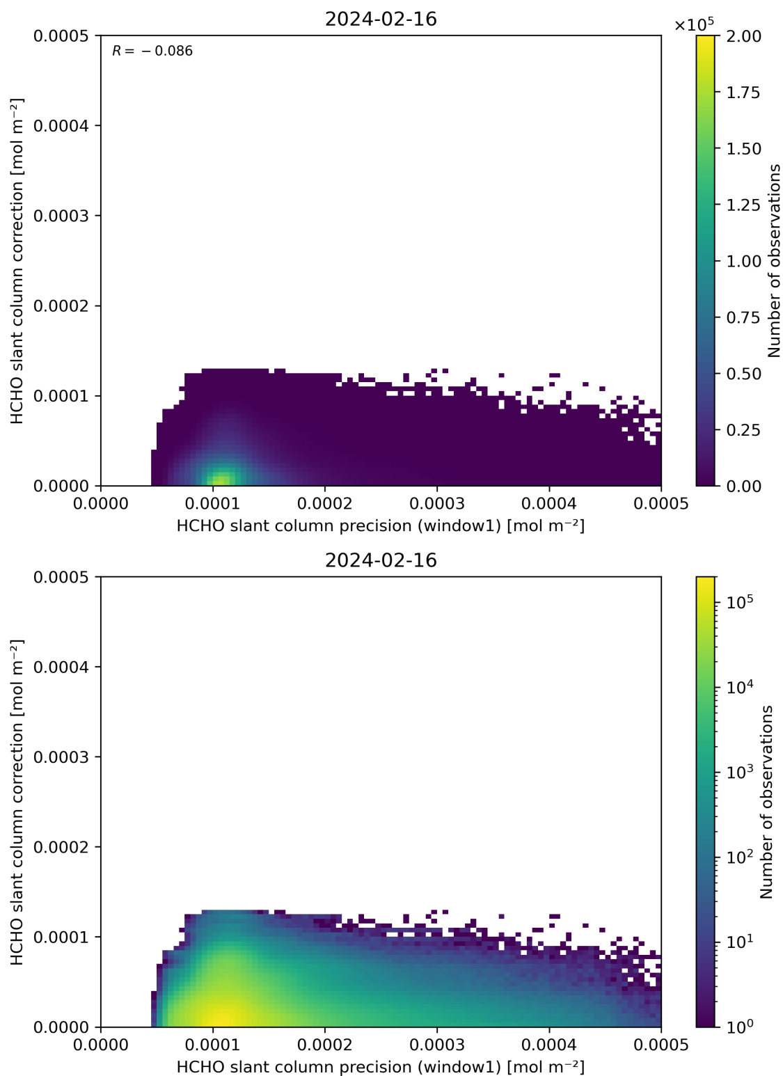
Figure 93: Scatter density plot of “HCHO slant column precision (window1)” against “HCHO slant column correction” for 2024-02-16 to 2024-02-17.
