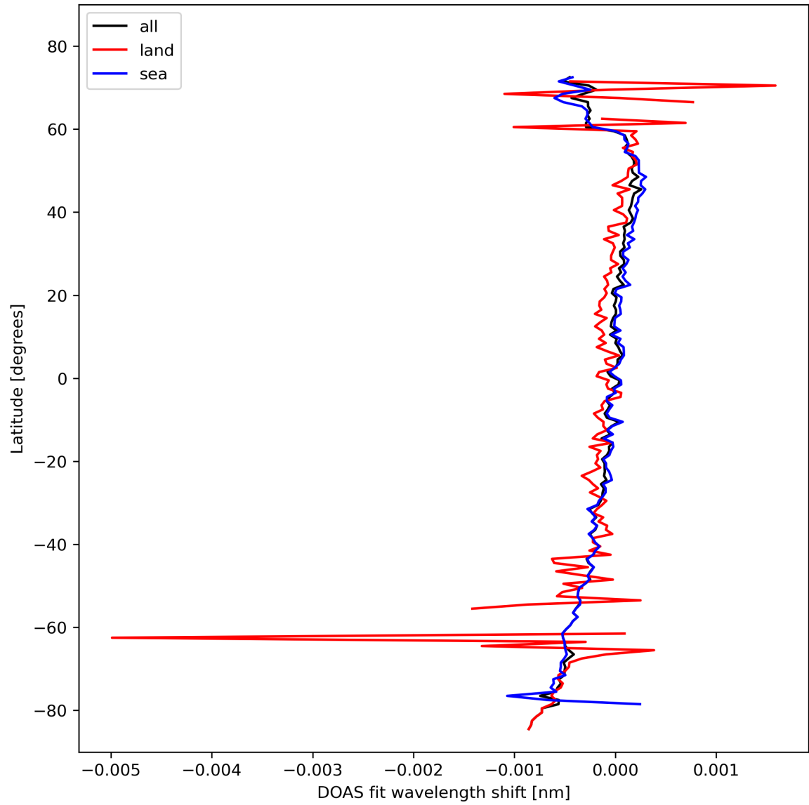
Figure 30: Zonal average of "DOAS fit wavelength shift" for 2024-02-16 to 2024-02-17.
