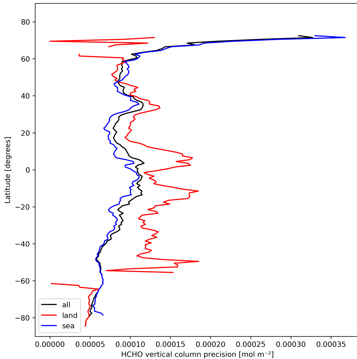
Figure 22: Zonal average of “HCHO vertical column precision” for 2024-02-16 to 2024-02-17.
