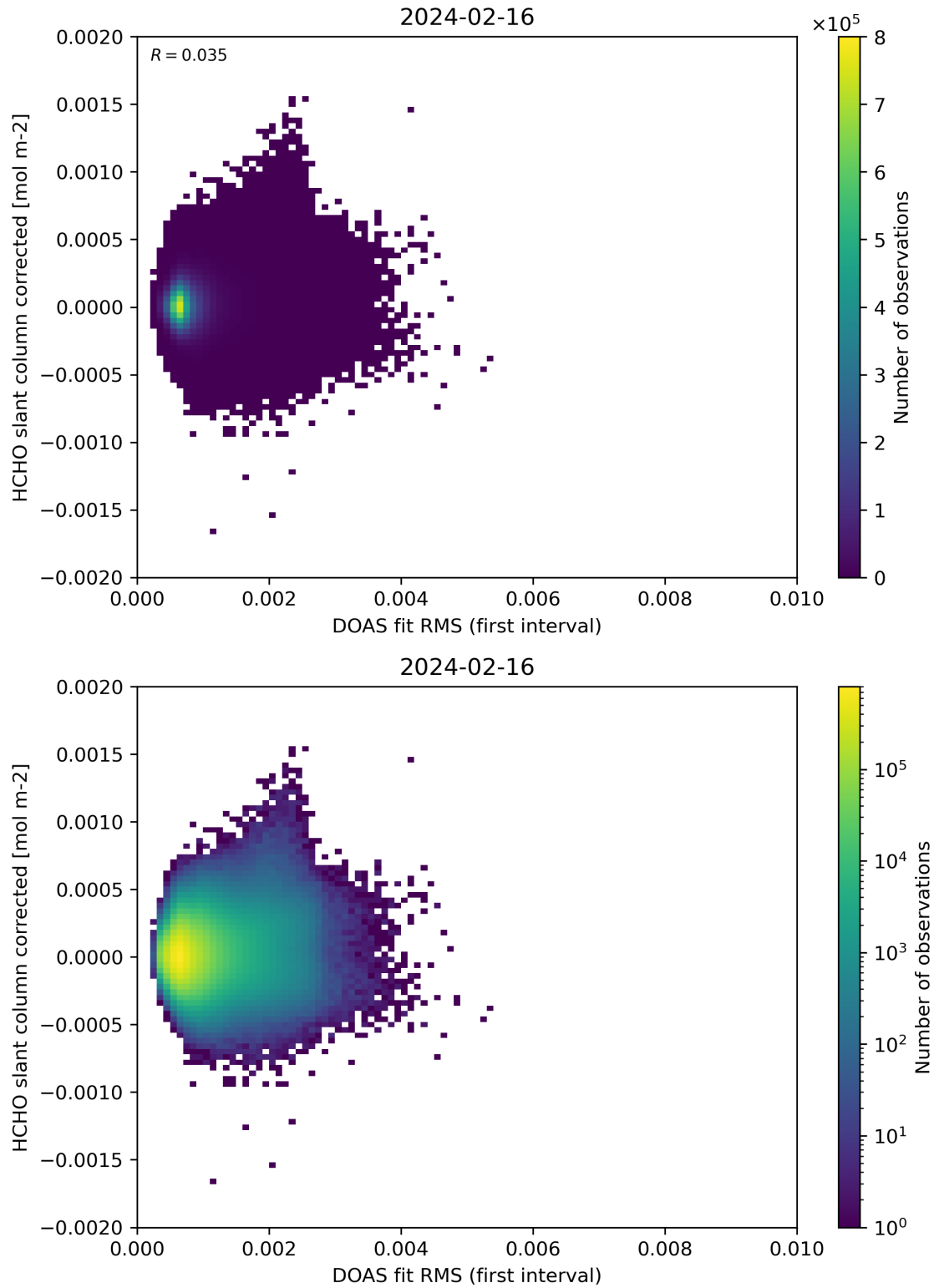
Figure 62: Scatter density plot of “DOAS fit RMS (first interval)” against “HCHO slant column corrected” for 2024-02-16 to 2024-02-17.
