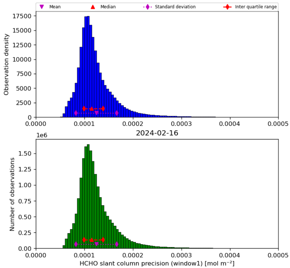
Figure 39: Histogram of “HCHO slant column precision (window1)” for 2024-02-16 to 2024-02-17
