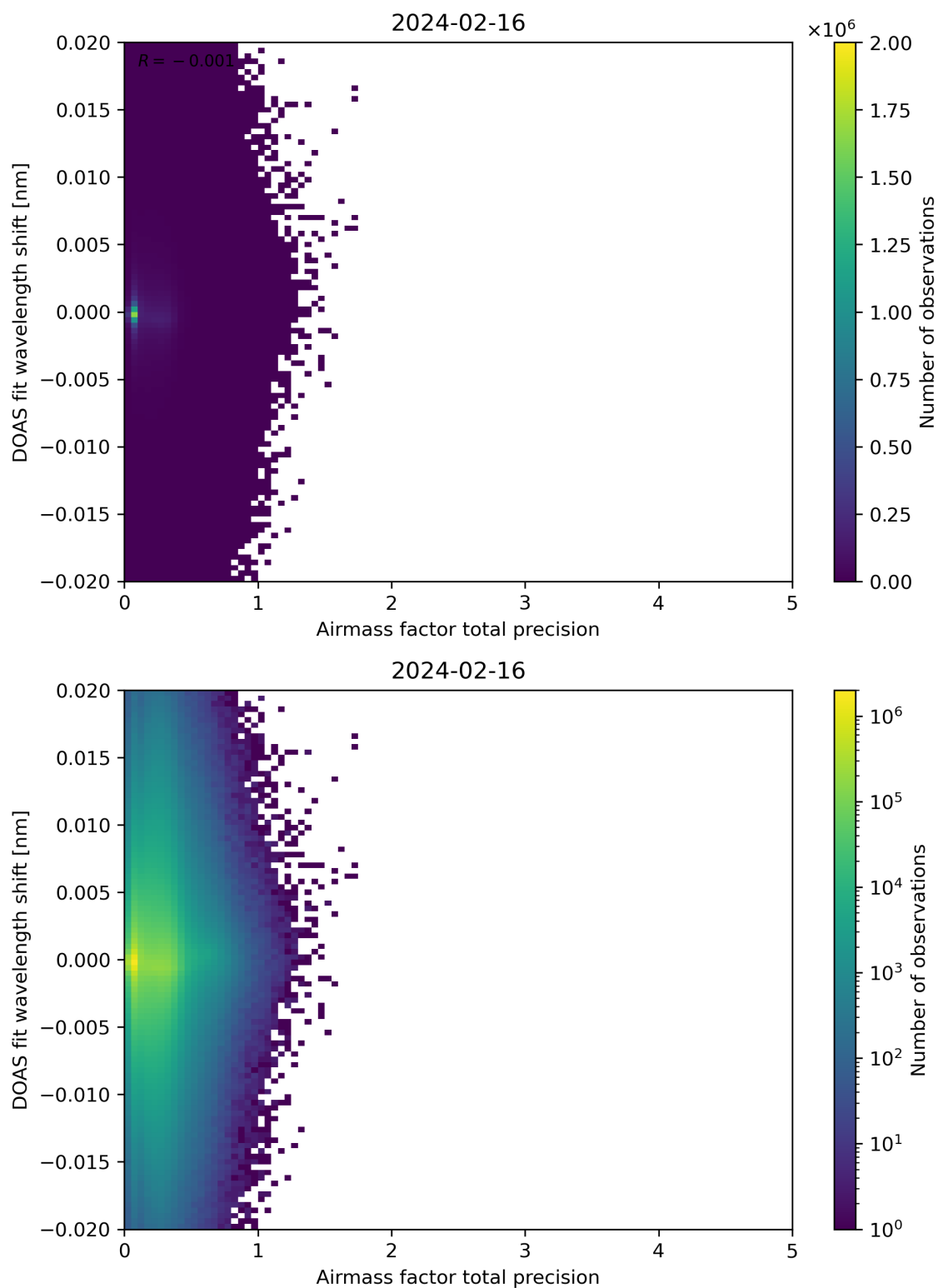
Figure 106: Scatter density plot of “Airmass factor total precision” against “DOAS fit wavelength shift” for 2024-02-16 to 2024-02-17.
