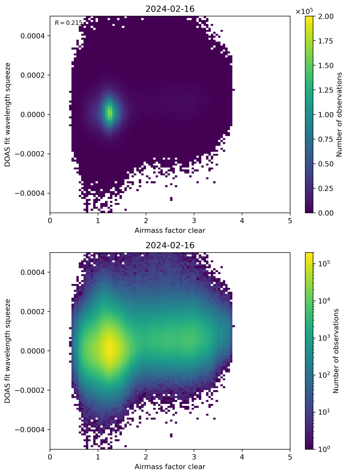
Figure 73: Scatter density plot of “Airmass factor clear” against “DOAS fit wavelength squeeze” for 2024-02-16 to 2024-02-17.
