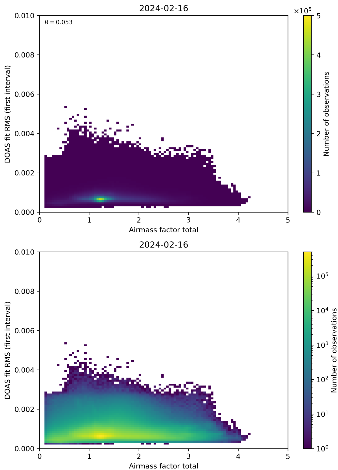
Figure 97: Scatter density plot of “Airmass factor total” against “DOAS fit RMS (first interval)” for 2024-02-16 to 2024-02-17.
