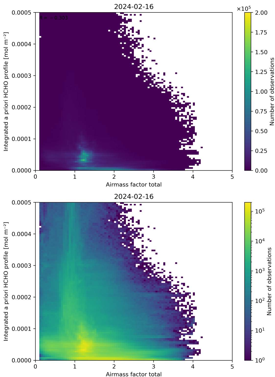
Figure 104: Scatter density plot of “Airmass factor total” against “Integrated a priori HCHO profile” for 2024-02-16 to 2024-02-17.
