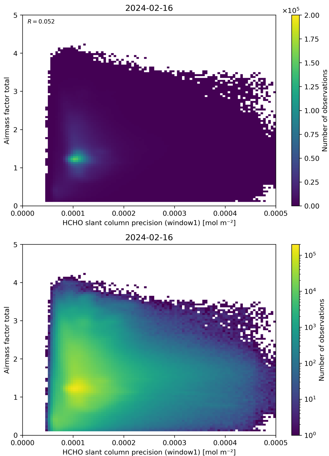
Figure 94: Scatter density plot of “HCHO slant column precision (window1)” against “Airmass factor total” for 2024-02-16 to 2024-02-17.
