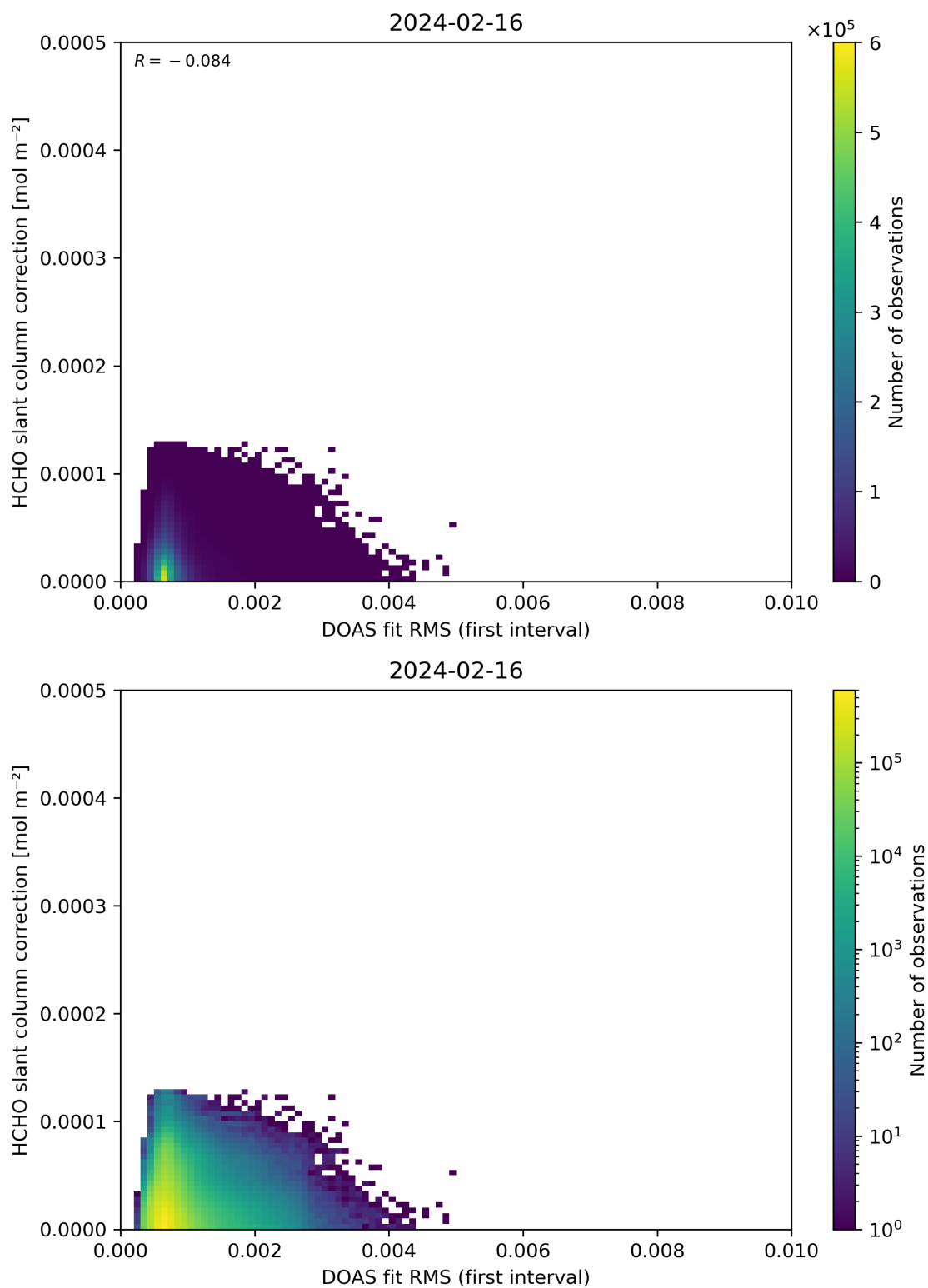
Figure 63: Scatter density plot of “DOAS fit RMS (first interval)” against “HCHO slant column correction” for 2024-02-16 to 2024-02-17.
