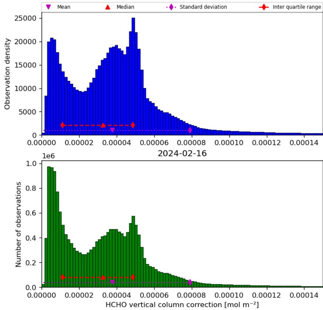
Figure 37: Histogram of “HCHO vertical column correction” for 2024-02-16 to 2024-02-17
