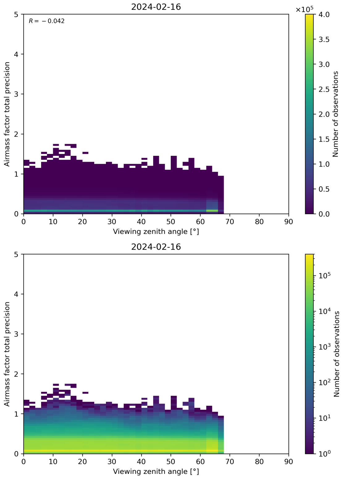
Figure 191: Scatter density plot of “Viewing zenith angle” against “Airmass factor total precision” for 2024-02-16 to 2024-02-17.
