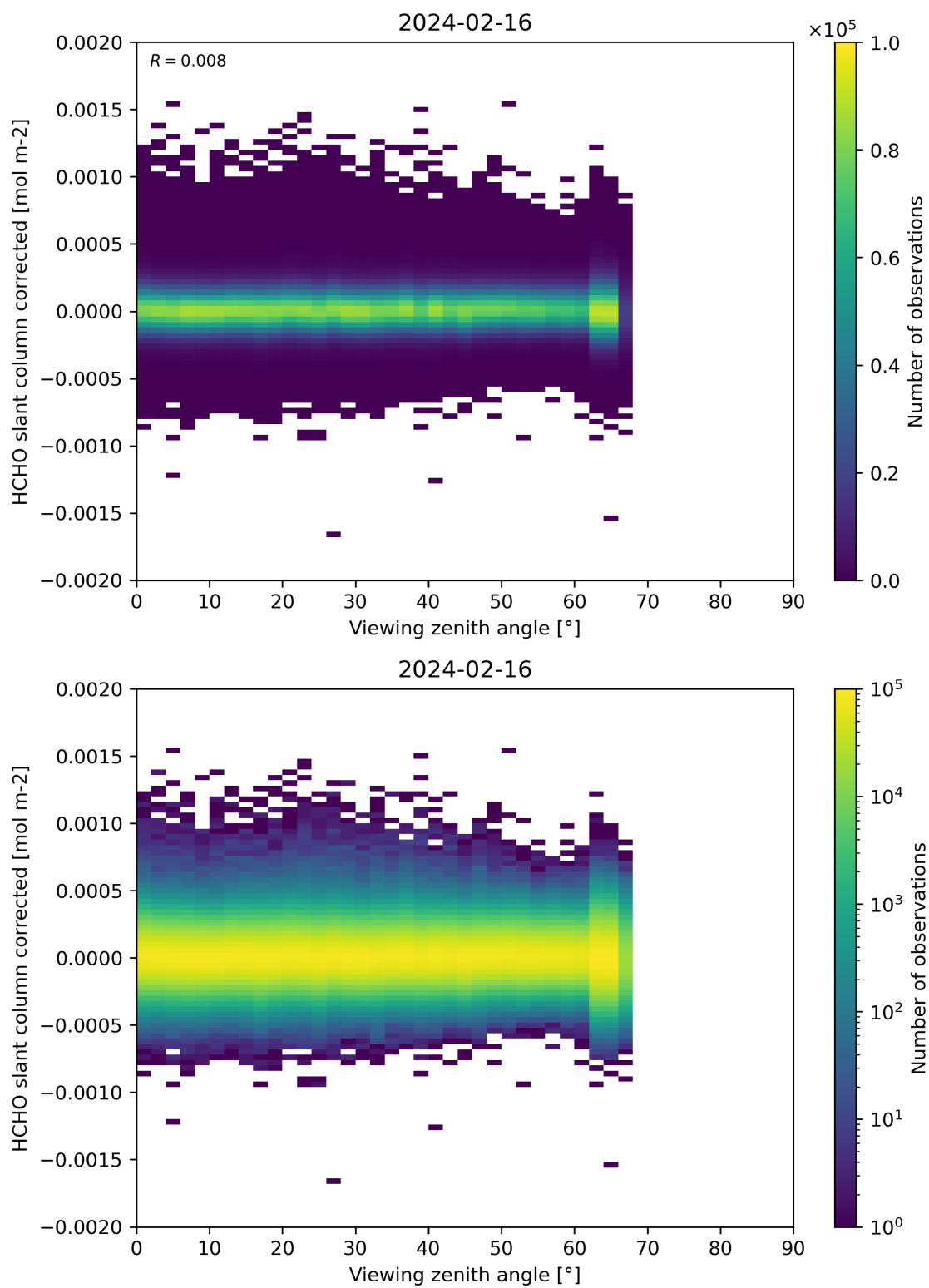
Figure 186: Scatter density plot of “Viewing zenith angle” against “HCHO slant column corrected” for 2024-02-16 to 2024-02-17.
