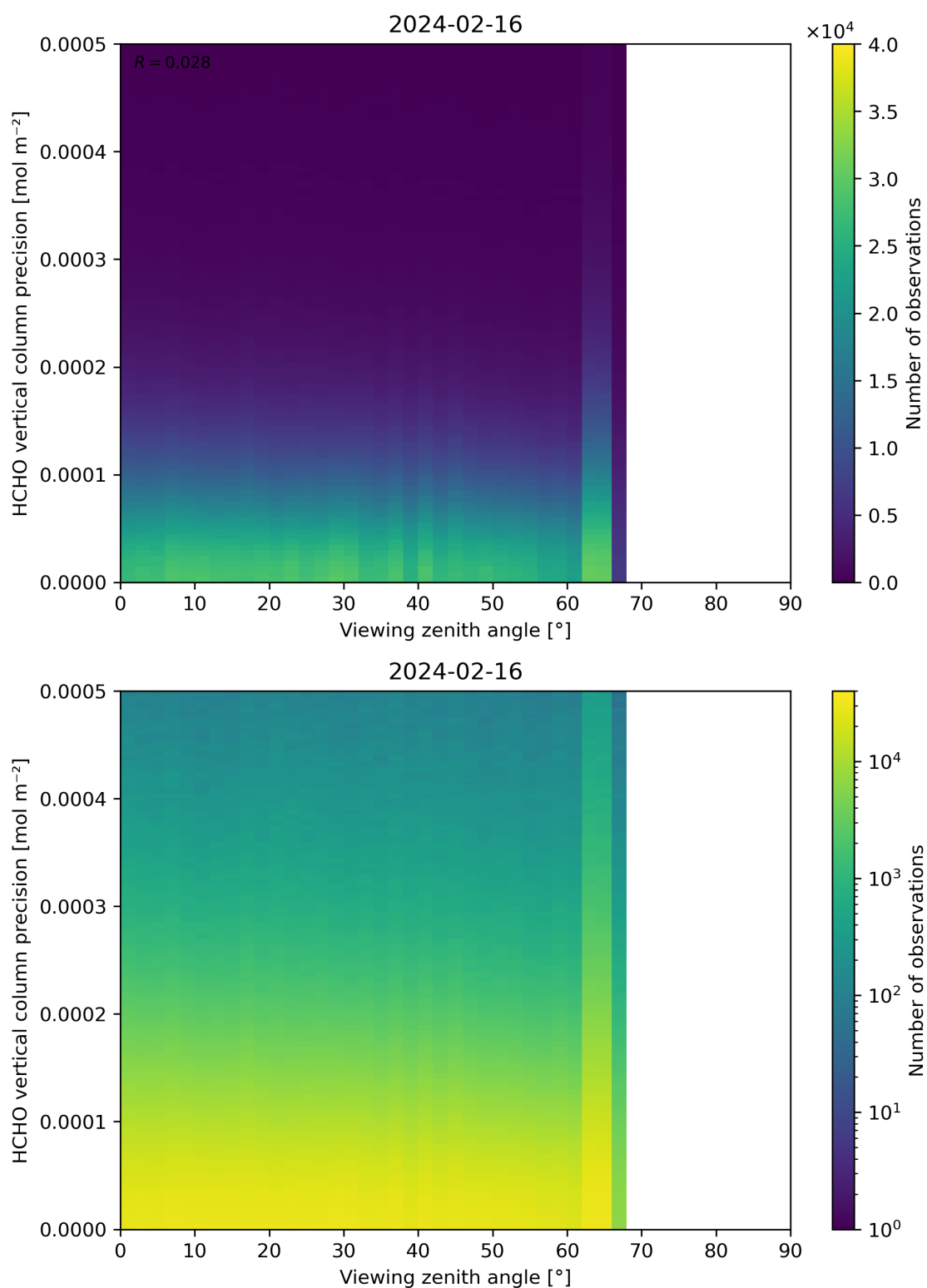
Figure 194: Scatter density plot of “Viewing zenith angle” against “HCHO vertical column precision” for 2024-02-16 to 2024-02-17.
