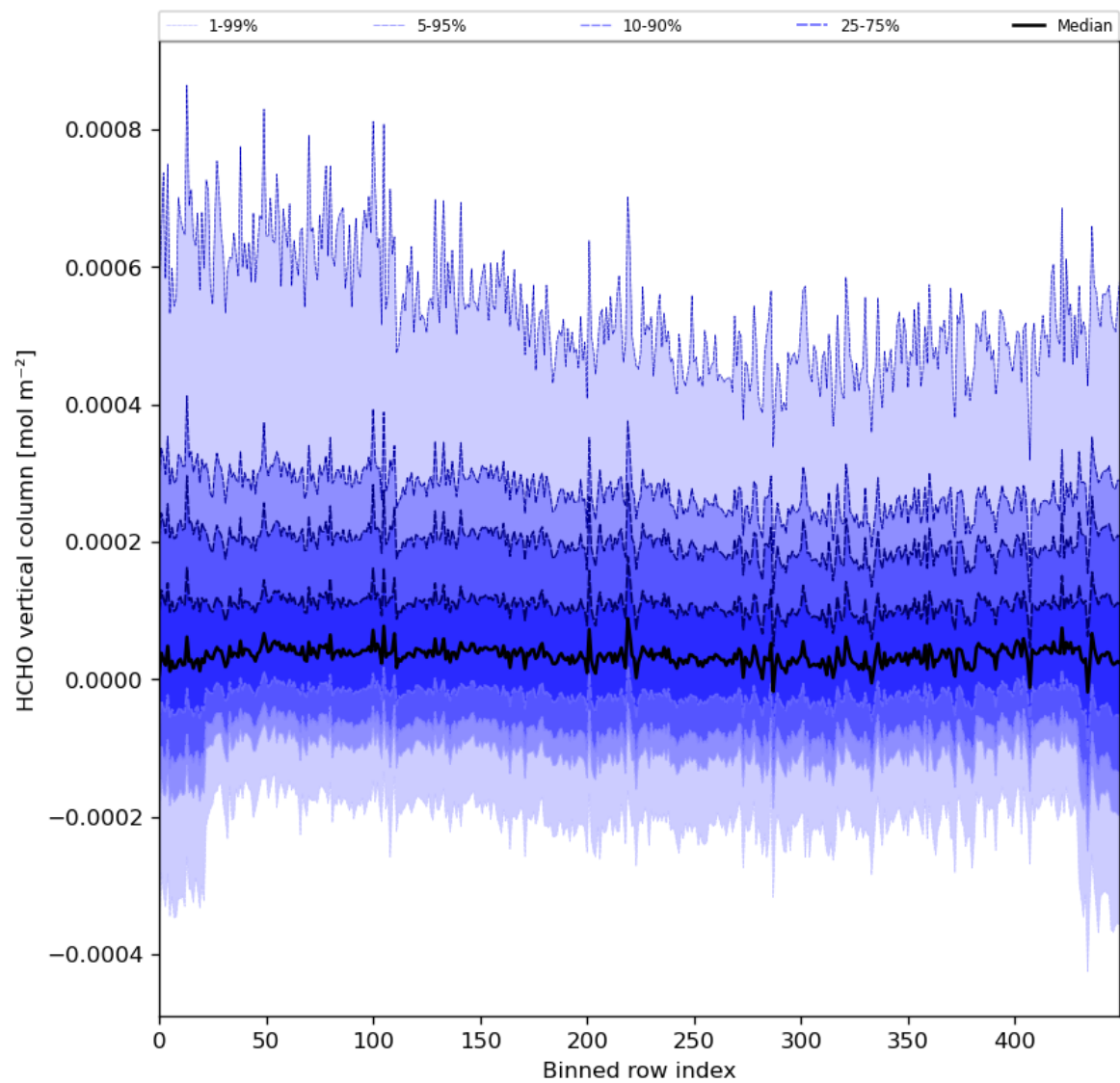
Figure 49: Along track statistics of “HCHO vertical column” for 2024-02-16 to 2024-02-17
