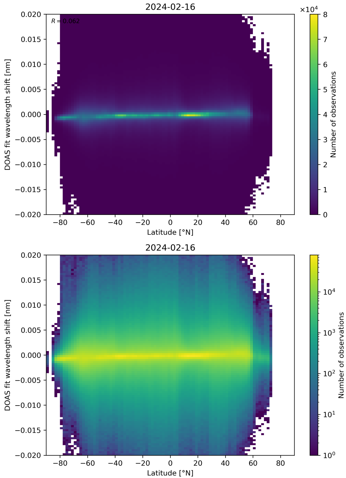
Figure 154: Scatter density plot of “Latitude” against “DOAS fit wavelength shift” for 2024-02-16 to 2024-02-17.
