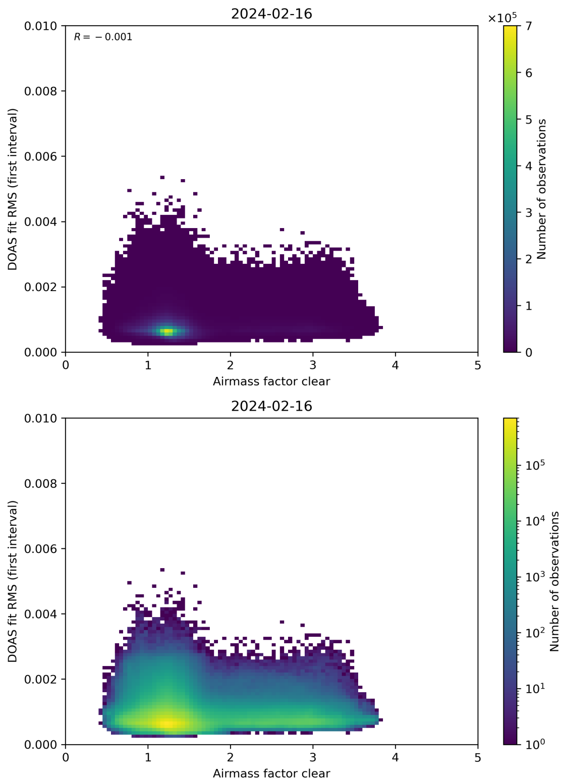
Figure 71: Scatter density plot of “Airmass factor clear” against “DOAS fit RMS (first interval)” for 2024-02-16 to 2024-02-17.
