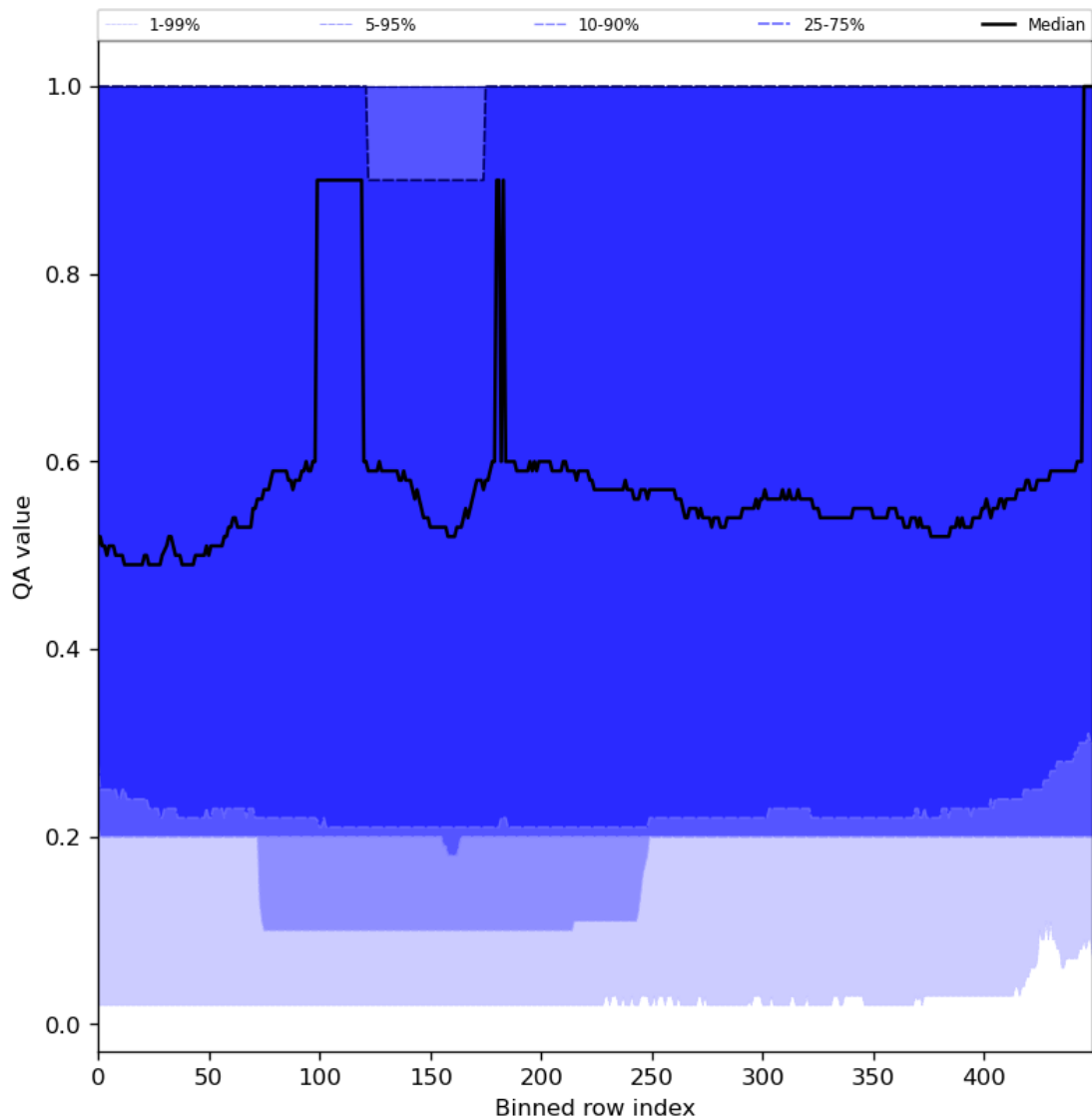
Figure 48: Along track statistics of “QA value” for 2024-02-16 to 2024-02-17
