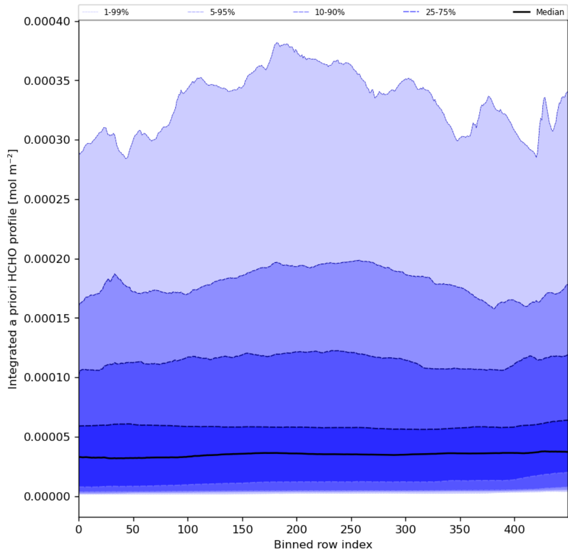
Figure 57: Along track statistics of "Integrated a priori HCHO profile" for 2024-02-16 to 2024-02-17
