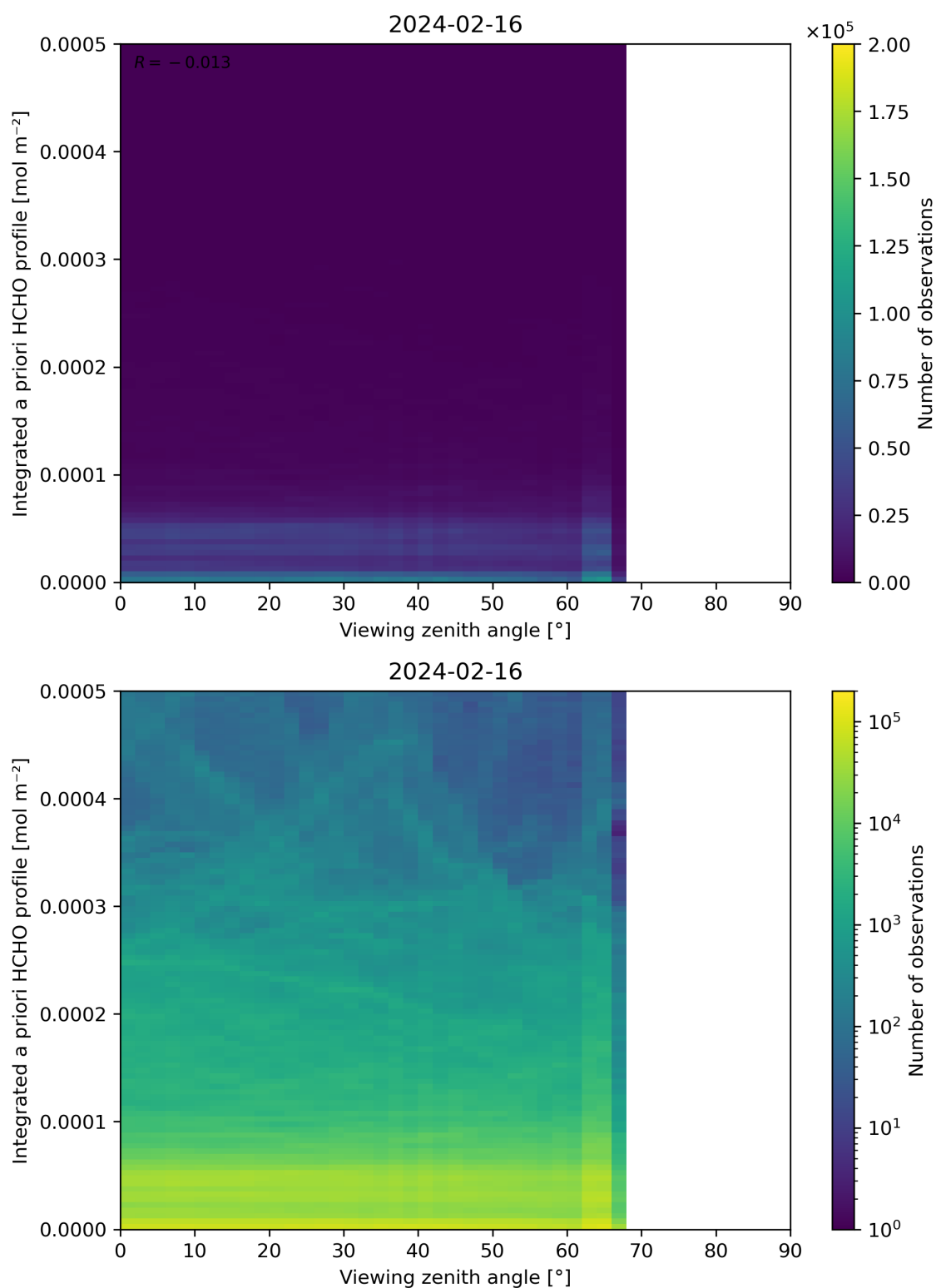
Figure 195: Scatter density plot of “Viewing zenith angle” against “Integrated a priori HCHO profile” for 2024-02-16 to 2024-02-17.
