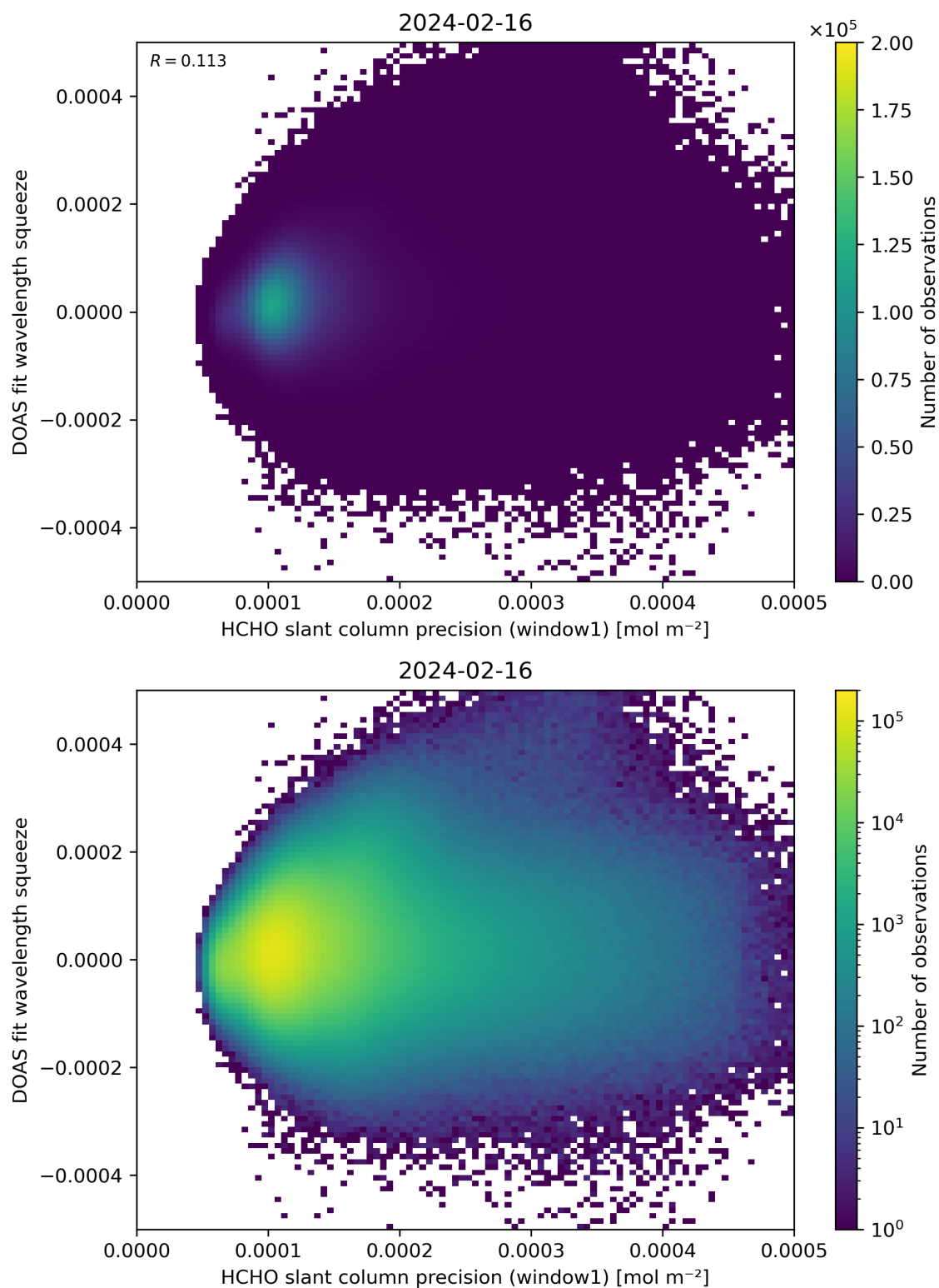
Figure 90: Scatter density plot of “HCHO slant column precision (window1)” against “DOAS fit wavelength squeeze” for 2024-02-16 to 2024-02-17.
