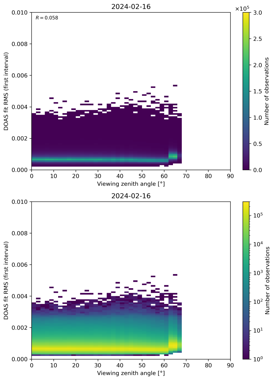
Figure 182: Scatter density plot of “Viewing zenith angle” against “DOAS fit RMS (first interval)” for 2024-02-16 to 2024-02-17.
