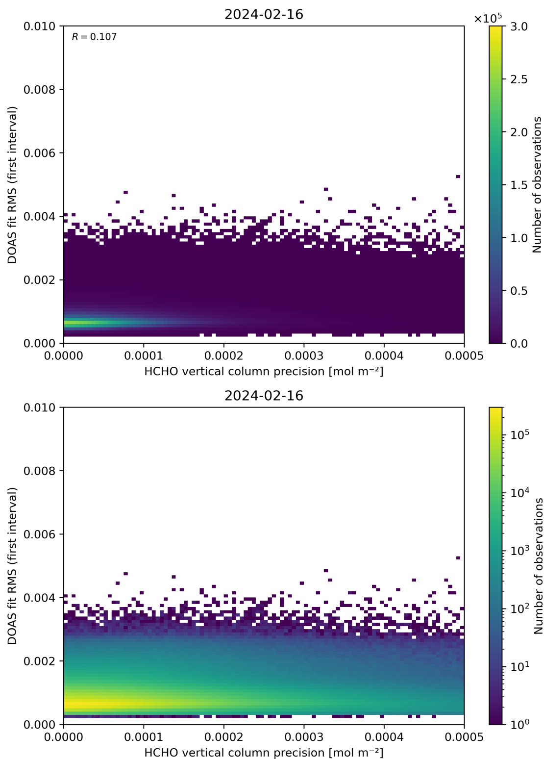
Figure 136: Scatter density plot of “HCHO vertical column precision” against “DOAS fit RMS (first interval)” for 2024-02-16 to 2024-02-17.
