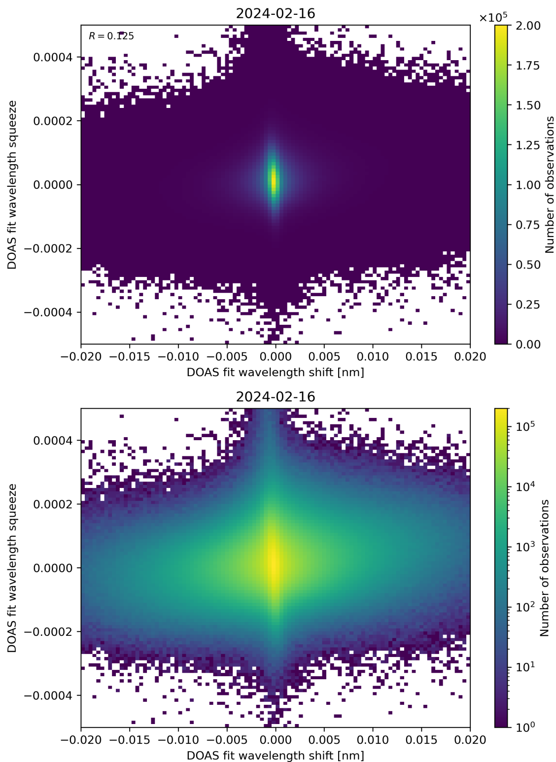
Figure 65: Scatter density plot of “DOAS fit wavelength shift” against “DOAS fit wavelength squeeze” for 2024-02-16 to 2024-02-17.
