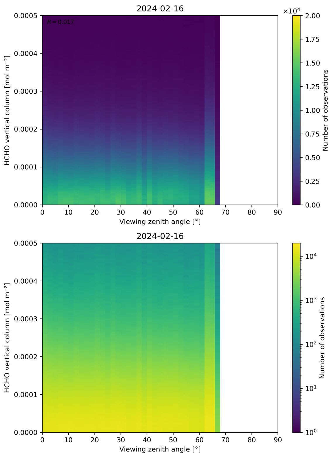
Figure 192: Scatter density plot of “Viewing zenith angle” against “HCHO vertical column” for 2024-02-16 to 2024-02-17.
