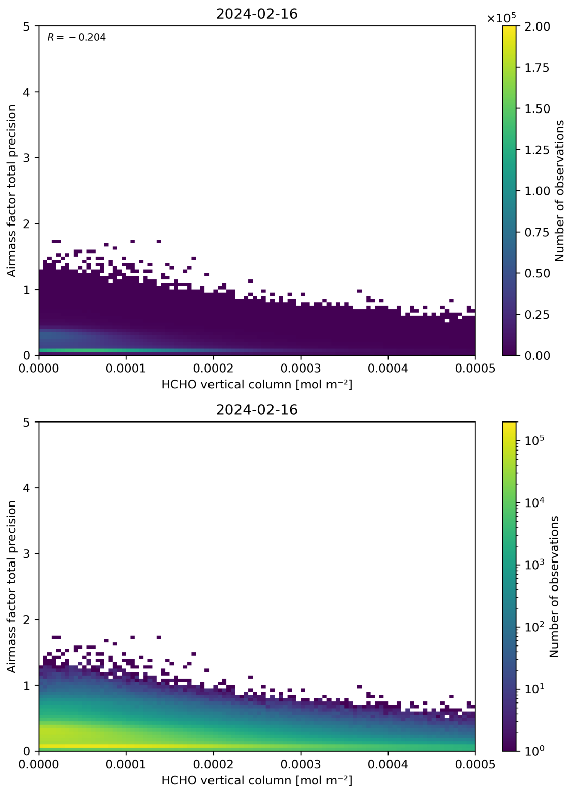
Figure 132: Scatter density plot of “HCHO vertical column” against “Airmass factor total precision” for 2024-02-16 to 2024-02-17.
