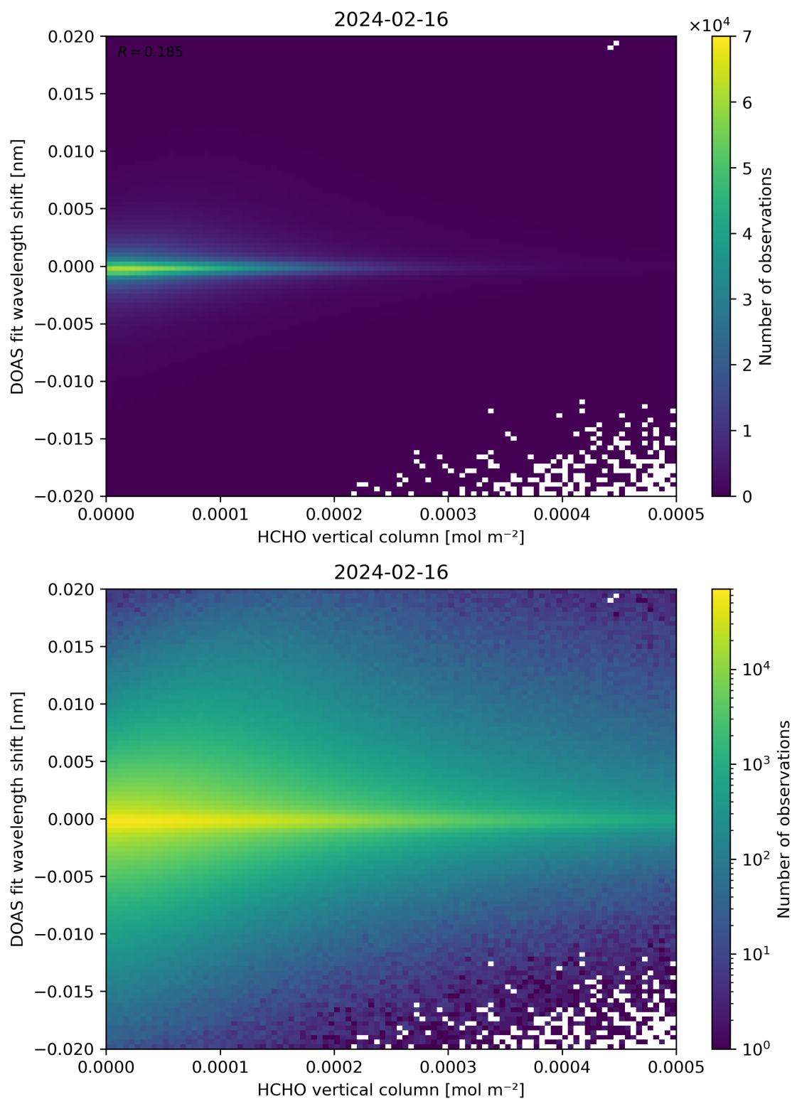
Figure 124: Scatter density plot of “HCHO vertical column” against “DOAS fit wavelength shift” for 2024-02-16 to 2024-02-17.
