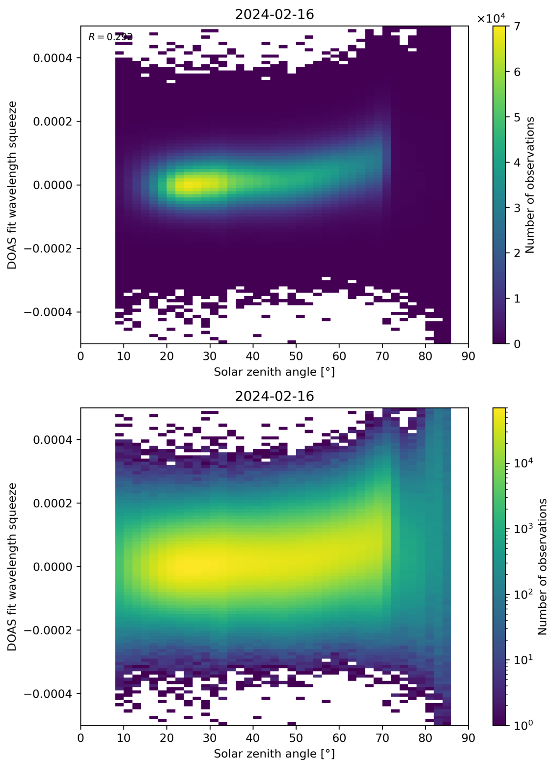
Figure 169: Scatter density plot of “Solar zenith angle” against “DOAS fit wavelength squeeze” for 2024-02-16 to 2024-02-17.
