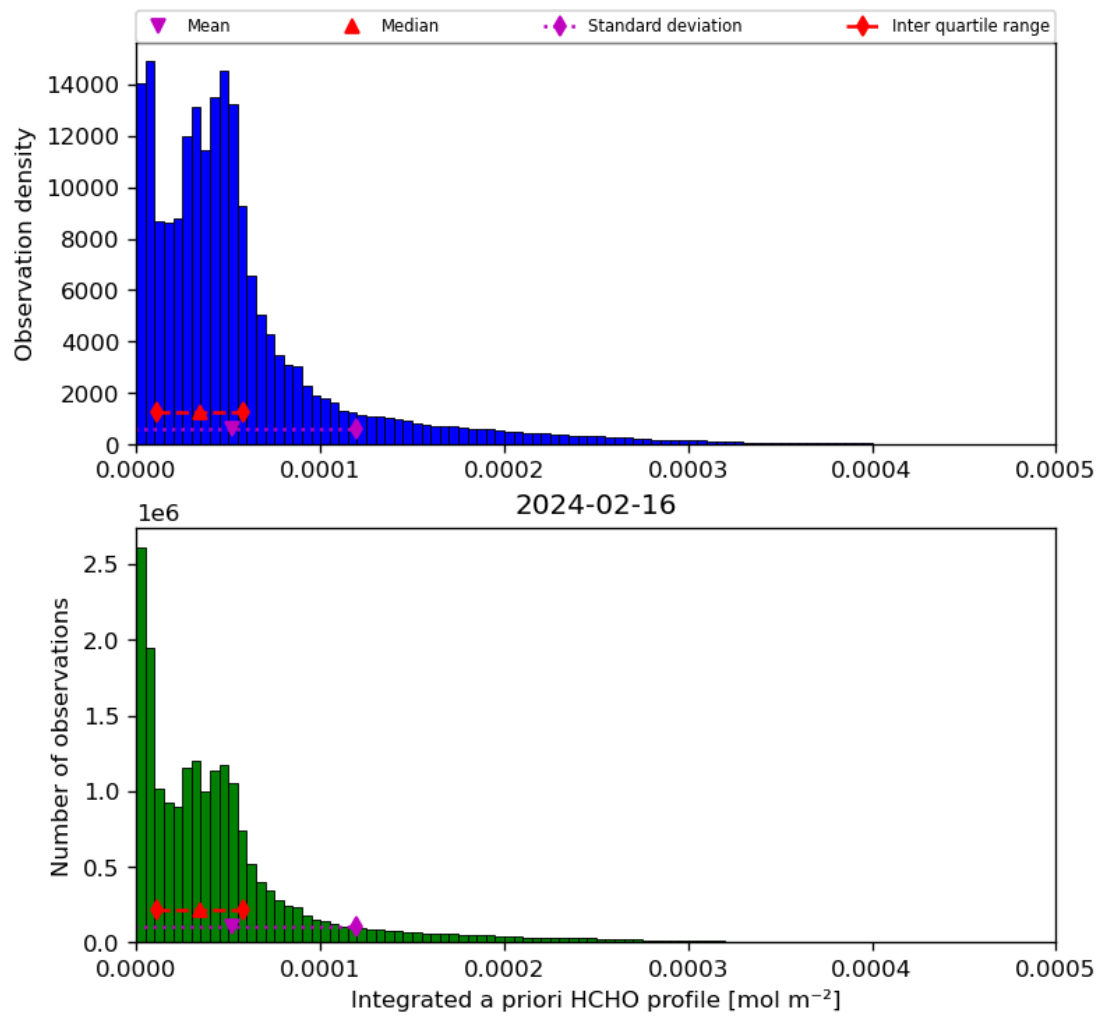
Figure 43: Histogram of “Integrated a priori HCHO profile” for 2024-02-16 to 2024-02-17
