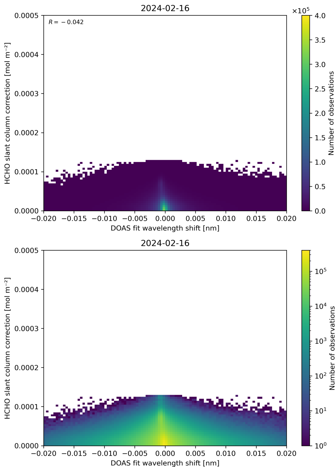
Figure 67: Scatter density plot of “DOAS fit wavelength shift” against “HCHO slant column correction” for 2024-02-16 to 2024-02-17.
