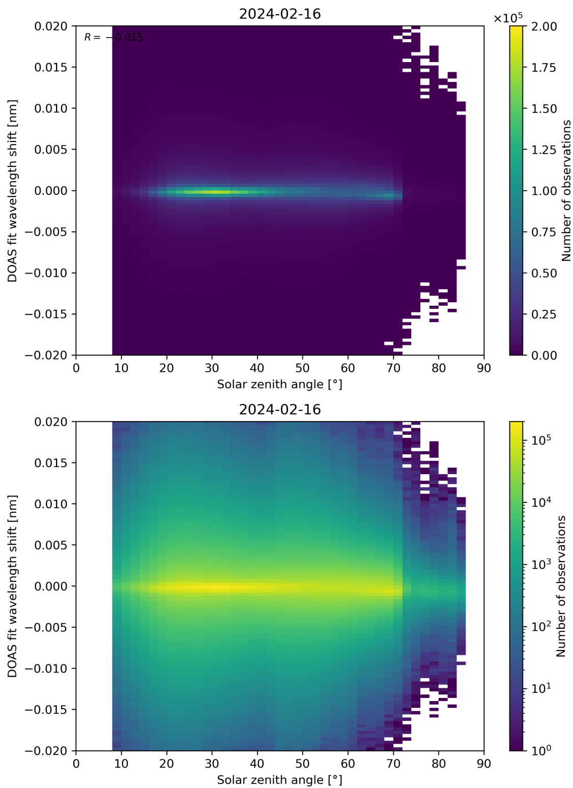
Figure 168: Scatter density plot of “Solar zenith angle” against “DOAS fit wavelength shift” for 2024-02-16 to 2024-02-17.
