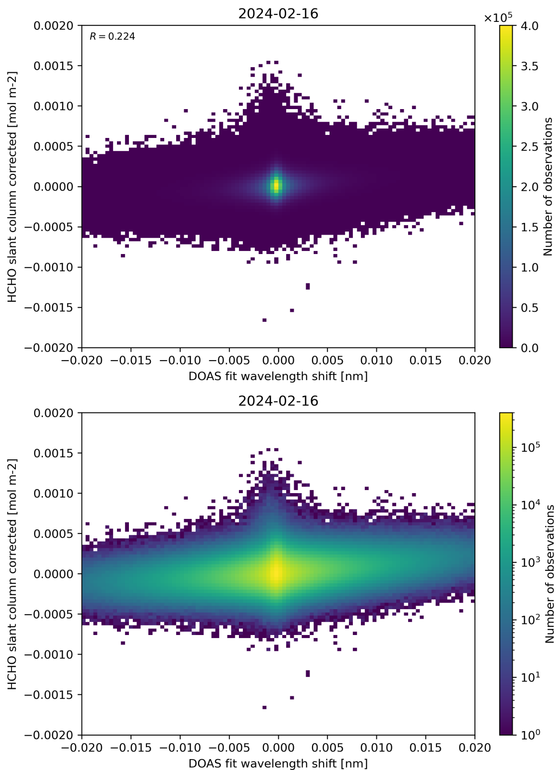
Figure 66: Scatter density plot of “DOAS fit wavelength shift” against “HCHO slant column corrected” for 2024-02-16 to 2024-02-17.
