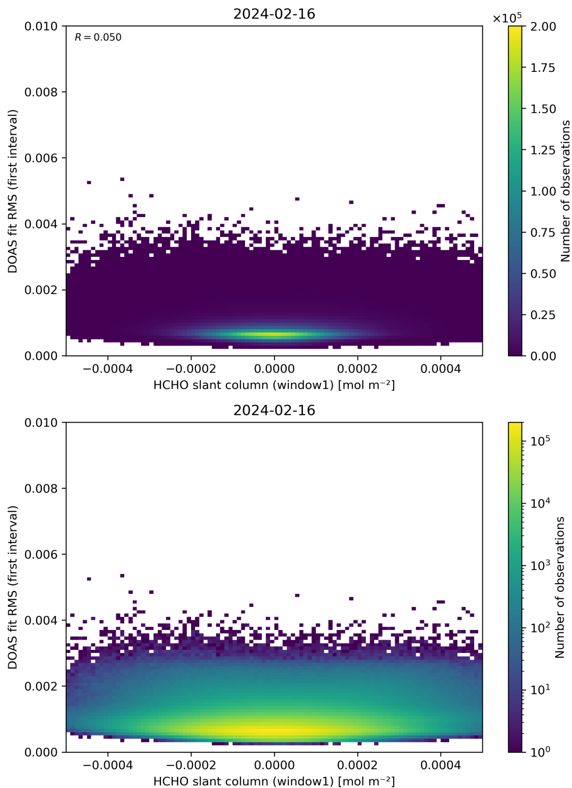
Figure 78: Scatter density plot of “HCHO slant column (window1)” against “DOAS fit RMS (first interval)” for 2024-02-16 to 2024-02-17.
