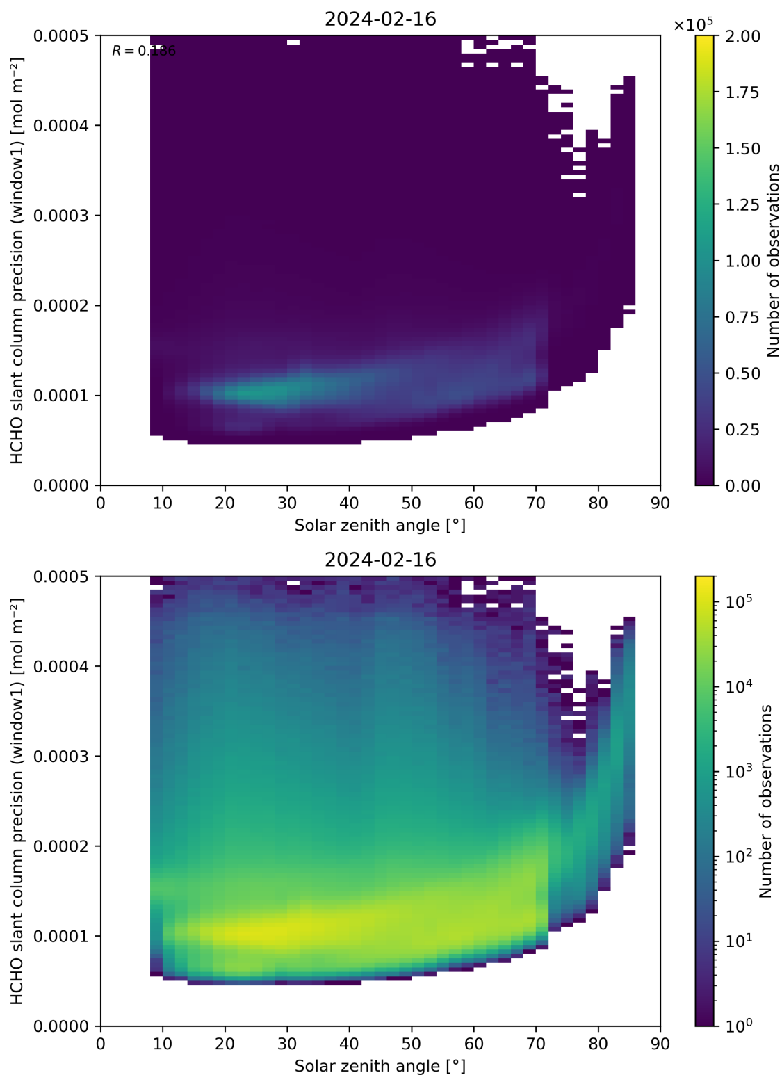
Figure 174: Scatter density plot of “Solar zenith angle” against “HCHO slant column precision (window1)” for 2024-02-16 to 2024-02-17.
