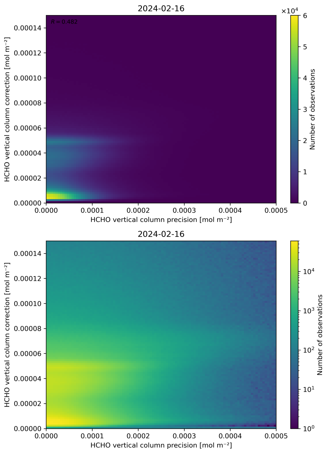
Figure 146: Scatter density plot of “HCHO vertical column precision” against “HCHO vertical column correction” for 2024-02-16 to 2024-02-17.
