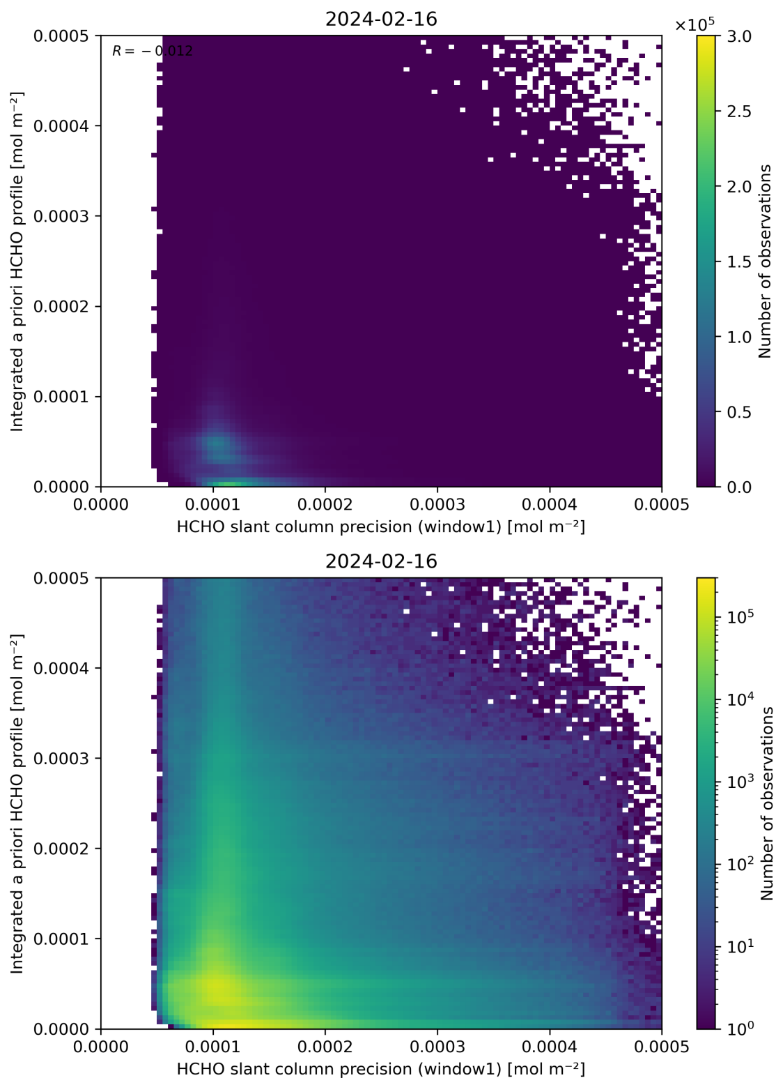
Figure 96: Scatter density plot of “HCHO slant column precision (window1)” against “Integrated a priori HCHO profile” for 2024-02-16 to 2024-02-17.
