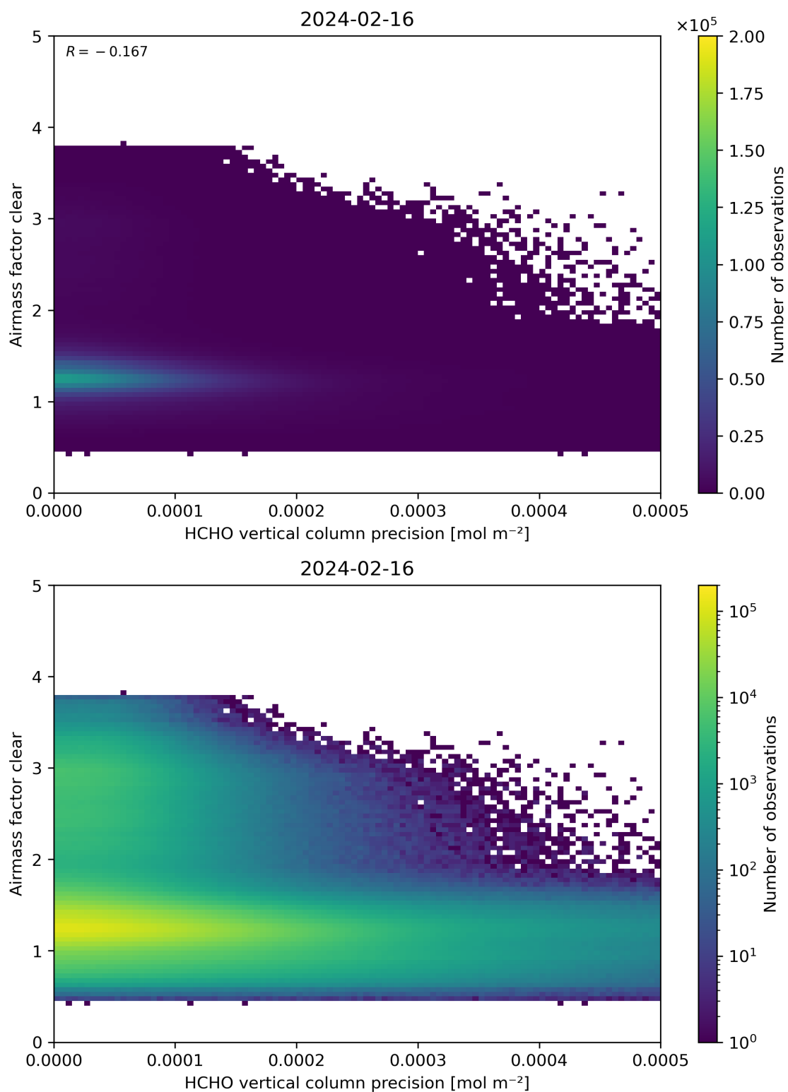
Figure 139: Scatter density plot of “HCHO vertical column precision” against “Airmass factor clear” for 2024-02-16 to 2024-02-17.
