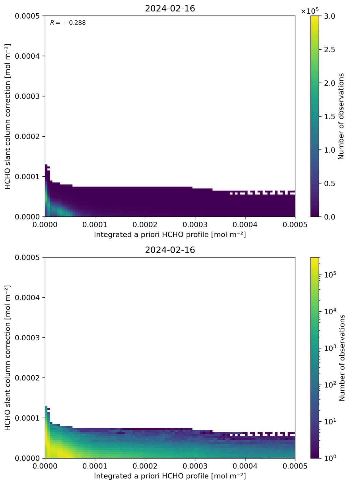
Figure 152: Scatter density plot of “Integrated a priori HCHO profile” against “HCHO slant column correction” for 2024-02-16 to 2024-02-17.
