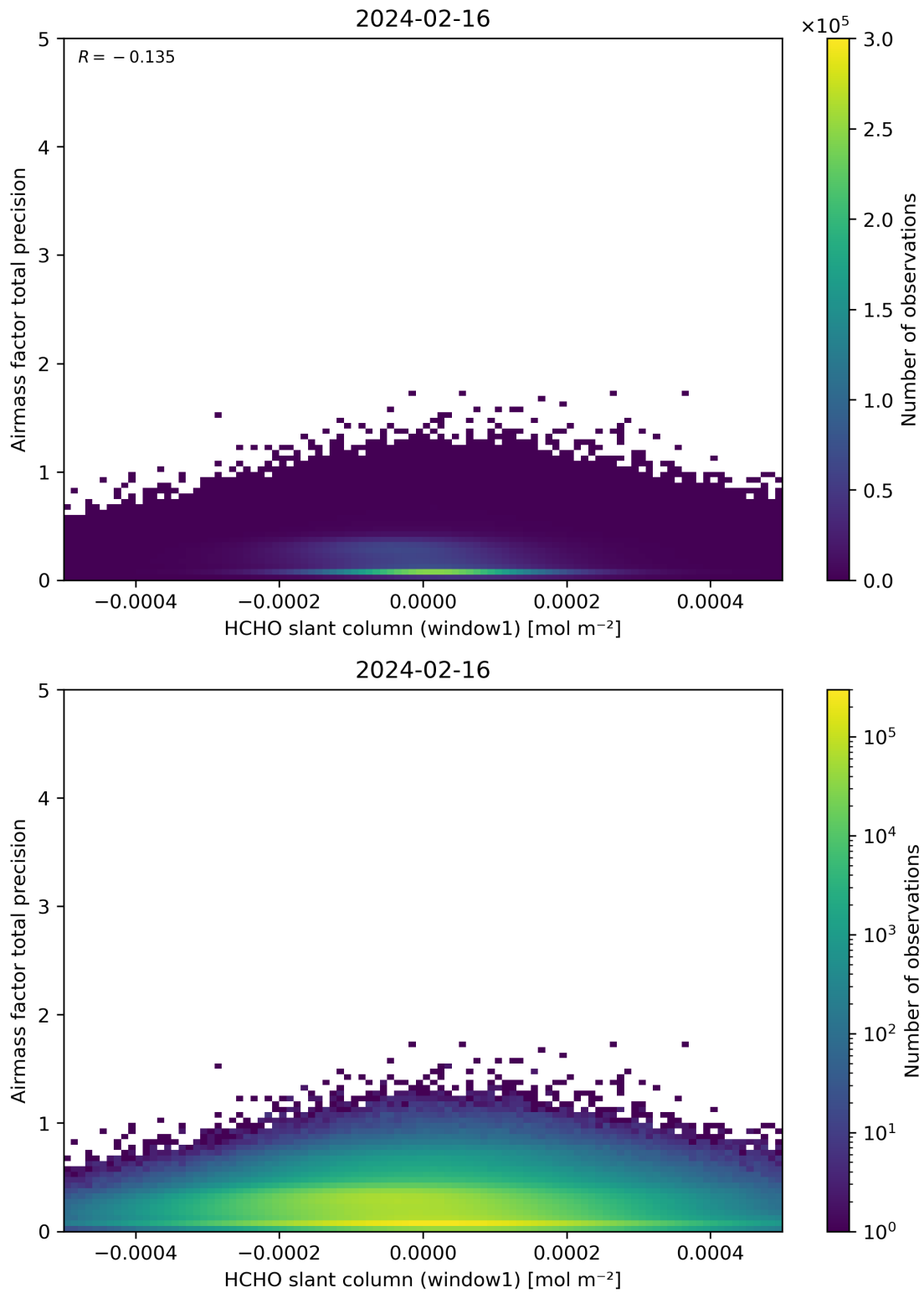
Figure 86: Scatter density plot of “HCHO slant column (window1)” against “Airmass factor total precision” for 2024-02-16 to 2024-02-17.
