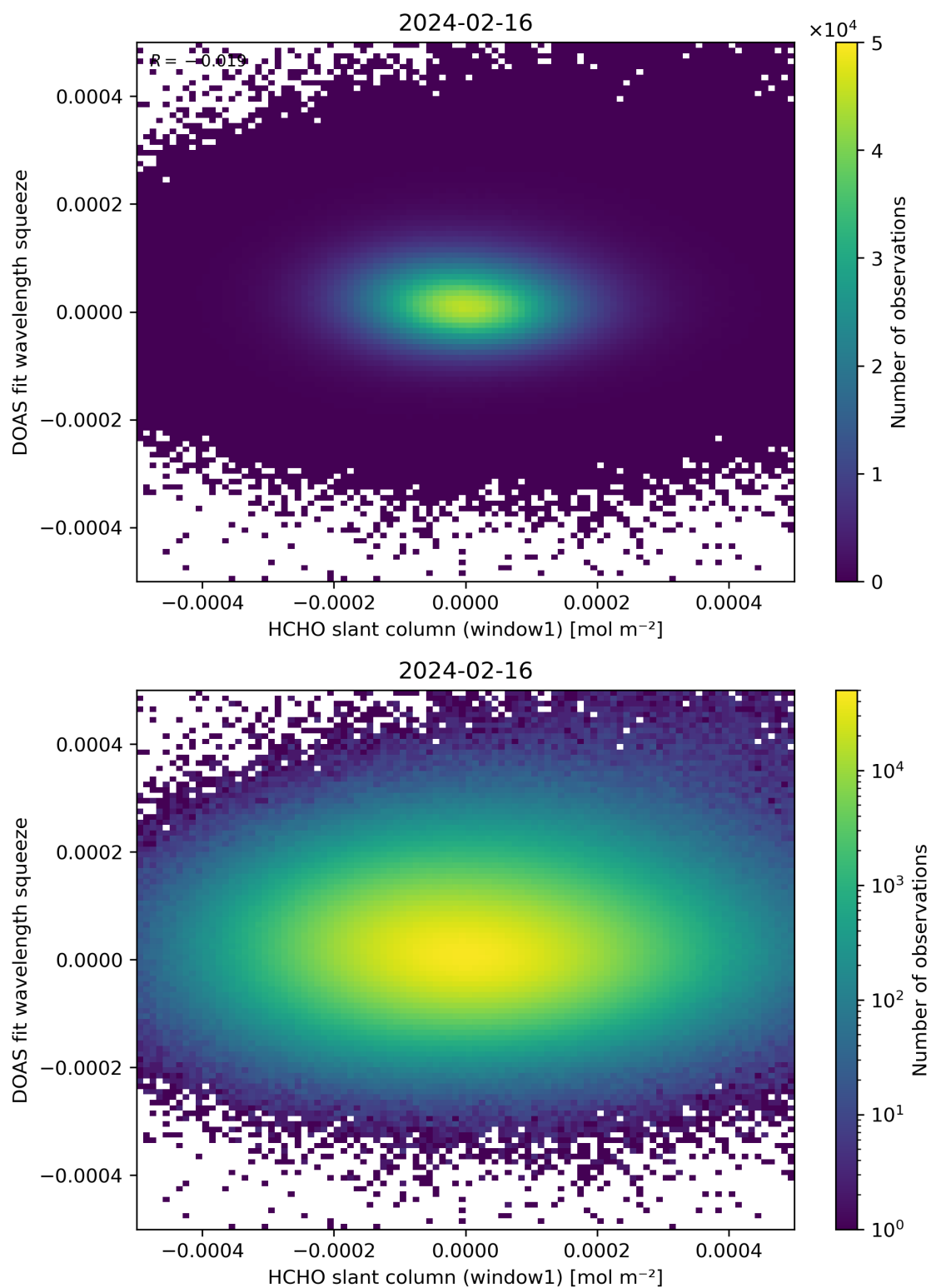
Figure 80: Scatter density plot of “HCHO slant column (window1)” against “DOAS fit wavelength squeeze” for 2024-02-16 to 2024-02-17.
