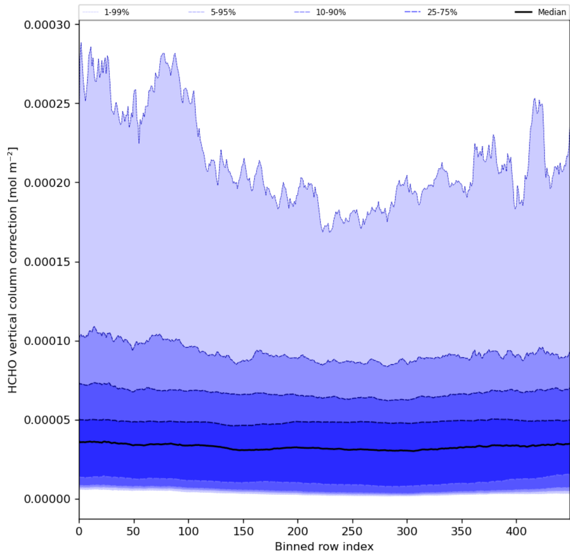
Figure 51: Along track statistics of “HCHO vertical column correction” for 2024-02-16 to 2024-02-17
