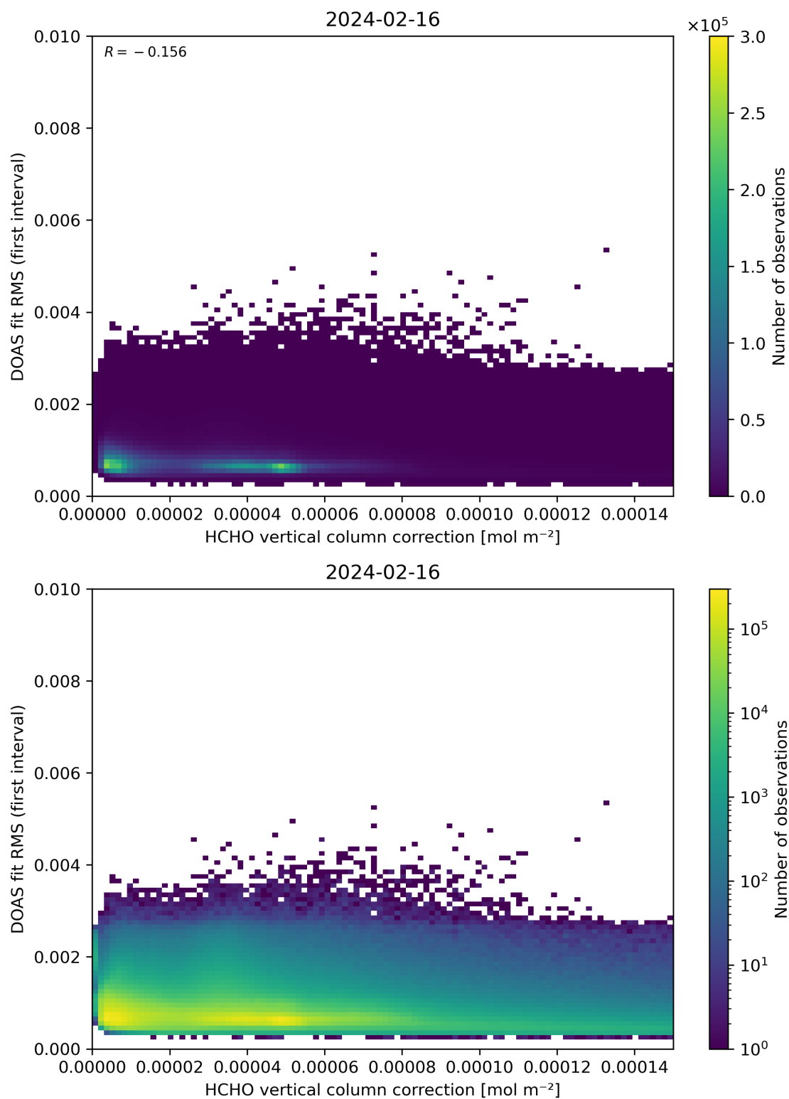
Figure 112: Scatter density plot of “HCHO vertical column correction” against “DOAS fit RMS (first interval)” for 2024-02-16 to 2024-02-17.
