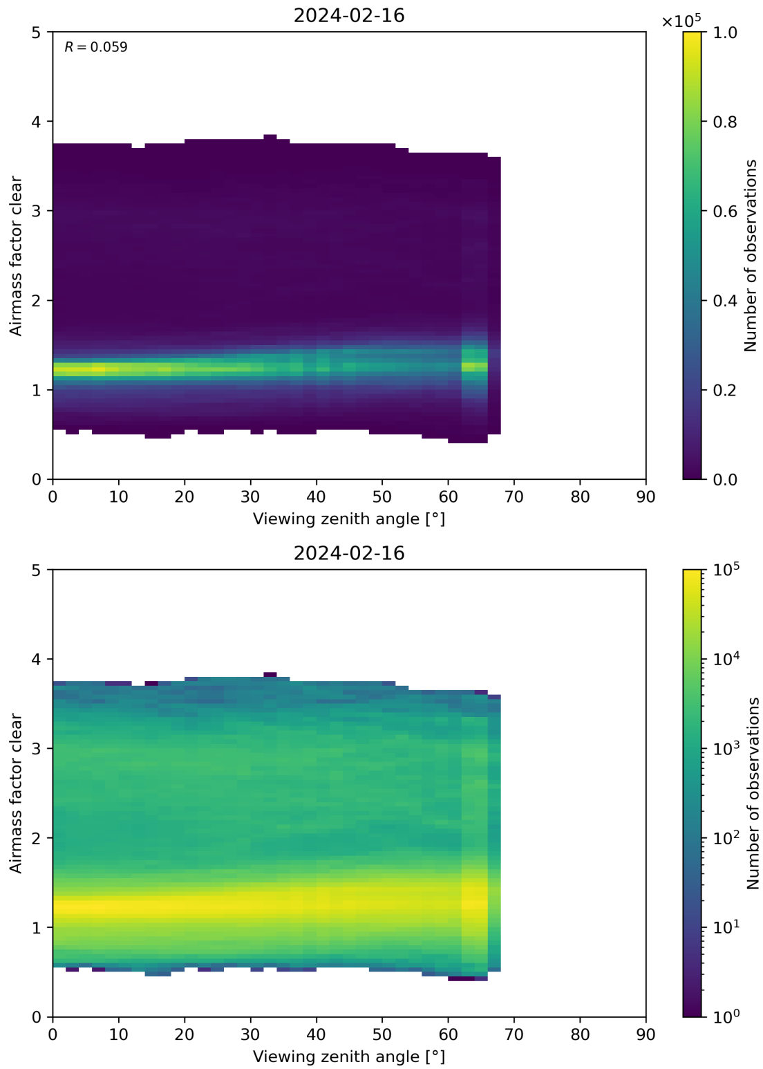
Figure 185: Scatter density plot of “Viewing zenith angle” against “Airmass factor clear” for 2024-02-16 to 2024-02-17.
