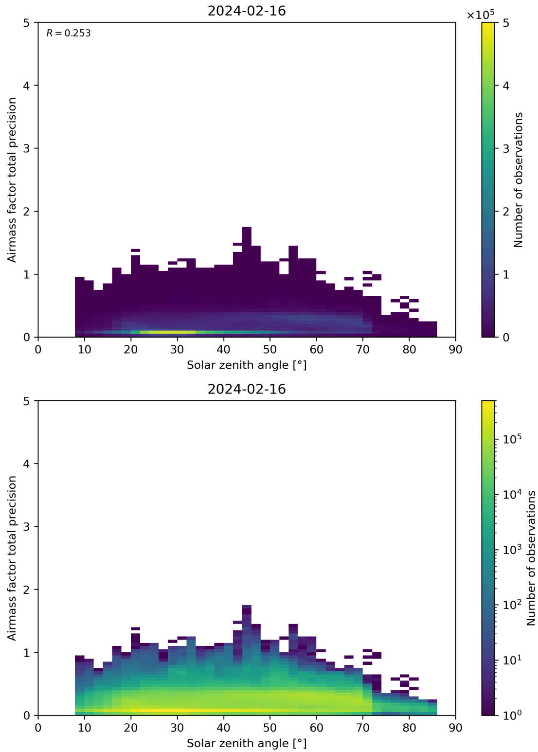
Figure 176: Scatter density plot of “Solar zenith angle” against “Airmass factor total precision” for 2024-02-16 to 2024-02-17.
