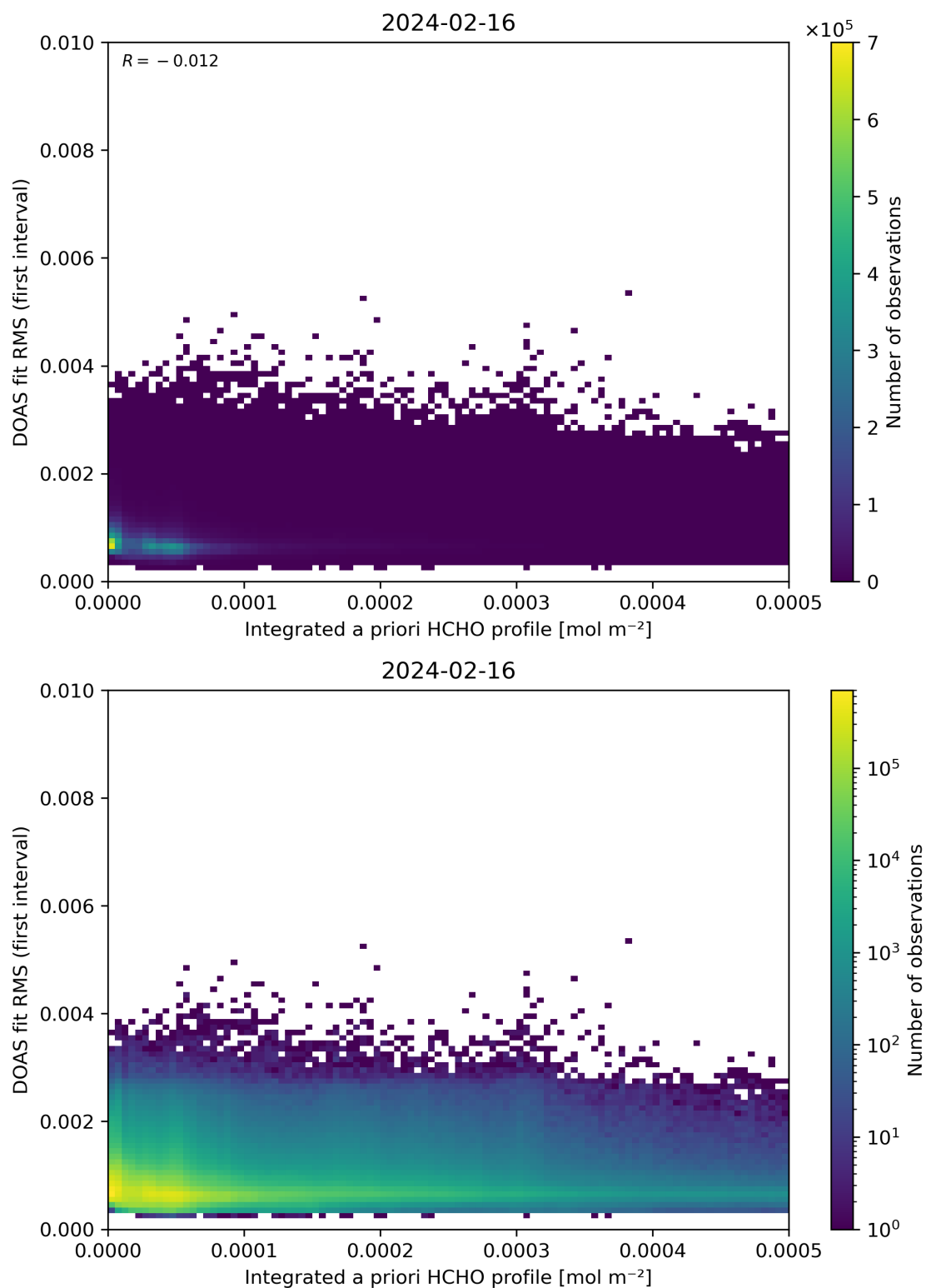
Figure 148: Scatter density plot of “Integrated a priori HCHO profile” against “DOAS fit RMS (first interval)” for 2024-02-16 to 2024-02-17.
