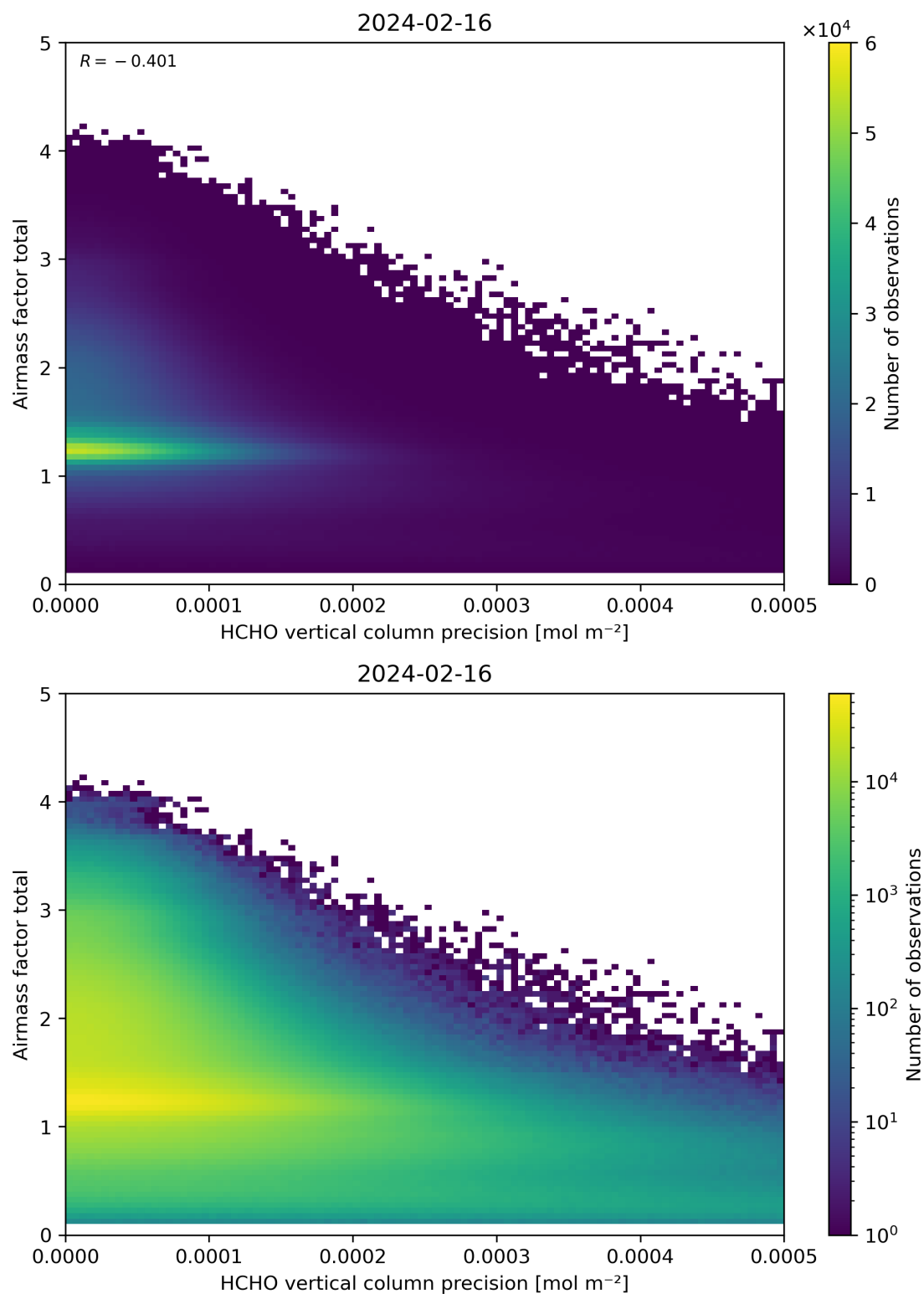
Figure 144: Scatter density plot of “HCHO vertical column precision” against “Airmass factor total” for 2024-02-16 to 2024-02-17.
