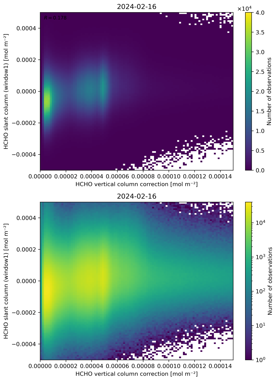
Figure 118: Scatter density plot of “HCHO vertical column correction” against “HCHO slant column (window1)” for 2024-02-16 to 2024-02-17.
