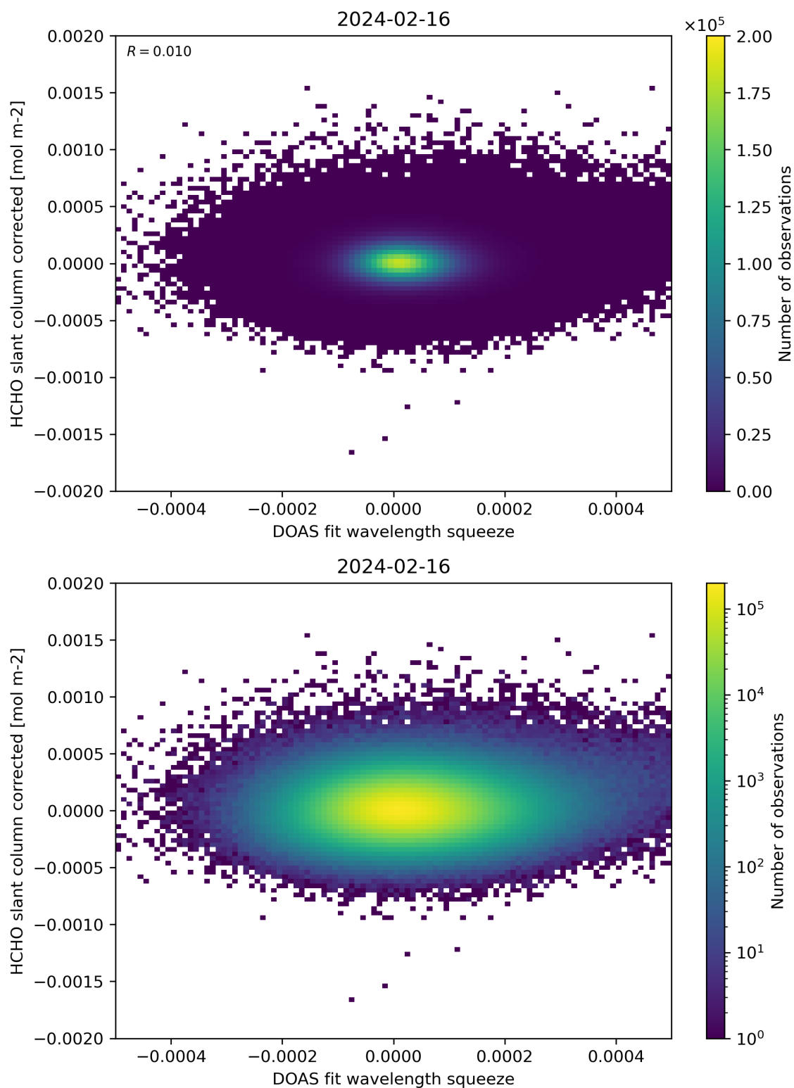
Figure 69: Scatter density plot of “DOAS fit wavelength squeeze” against “HCHO slant column corrected” for 2024-02-16 to 2024-02-17.
