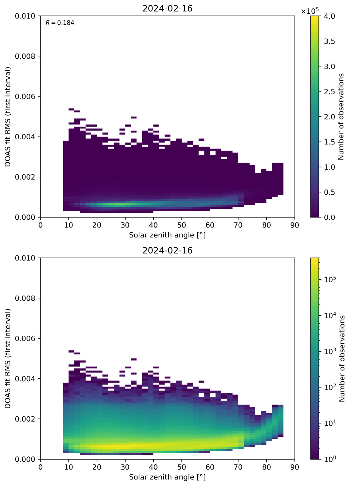
Figure 167: Scatter density plot of “Solar zenith angle” against “DOAS fit RMS (first interval)” for 2024-02-16 to 2024-02-17.
