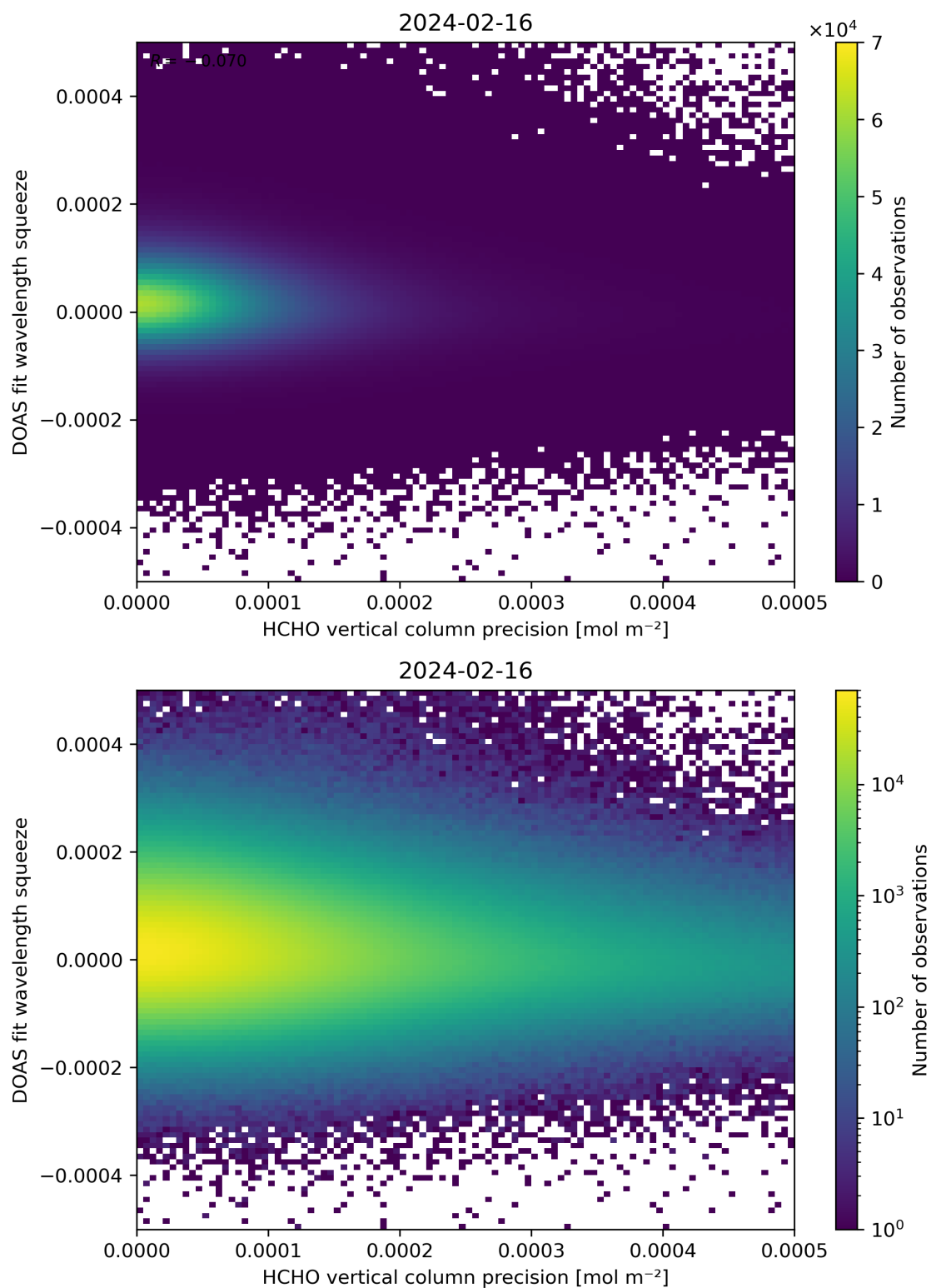
Figure 138: Scatter density plot of “HCHO vertical column precision” against “DOAS fit wavelength squeeze” for 2024-02-16 to 2024-02-17.
