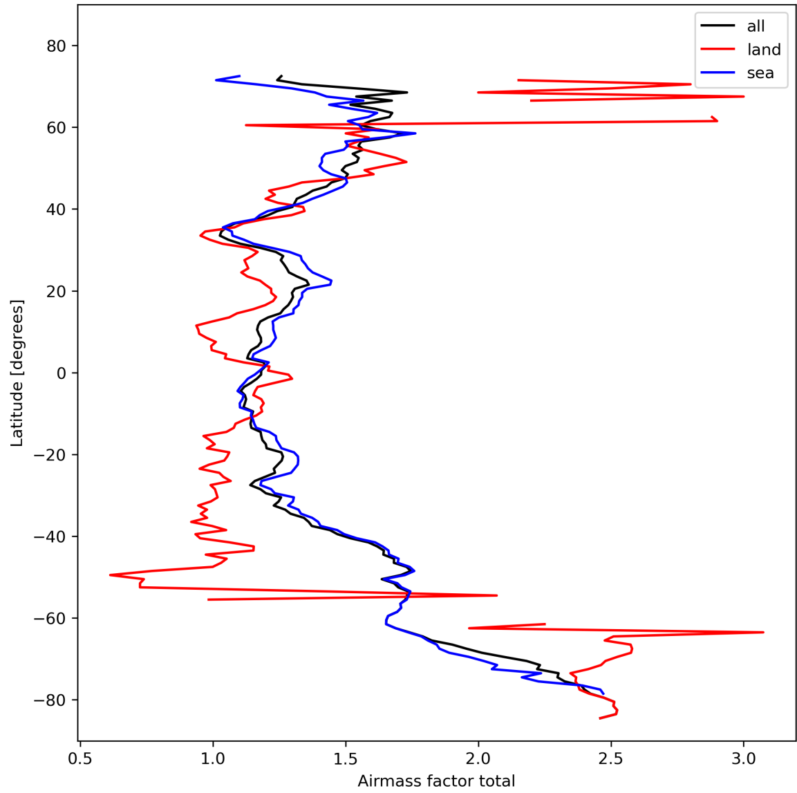
Figure 26: Zonal average of “Airmass factor total” for 2024-02-16 to 2024-02-17.
