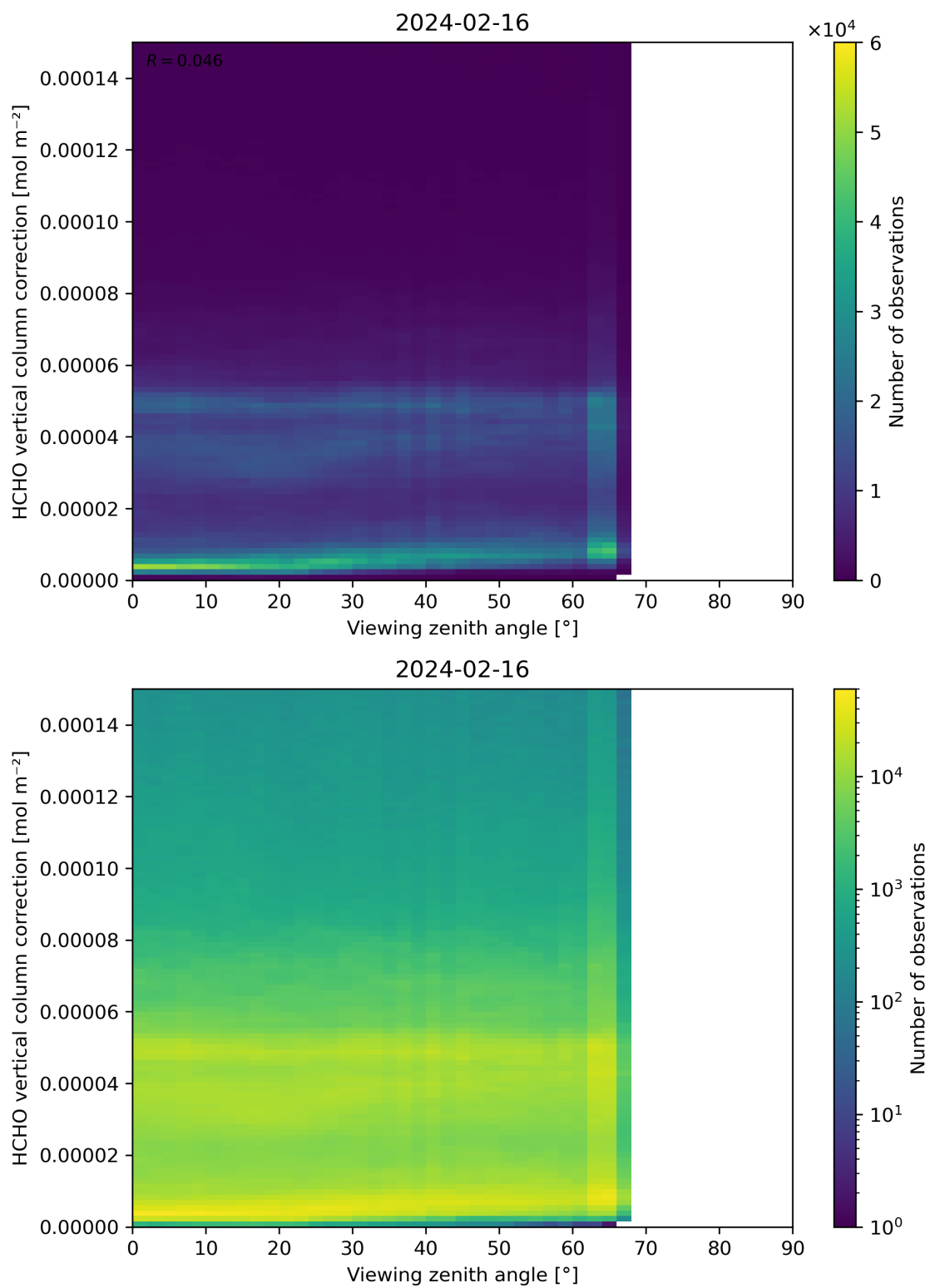
Figure 193: Scatter density plot of “Viewing zenith angle” against “HCHO vertical column correction” for 2024-02-16 to 2024-02-17.
