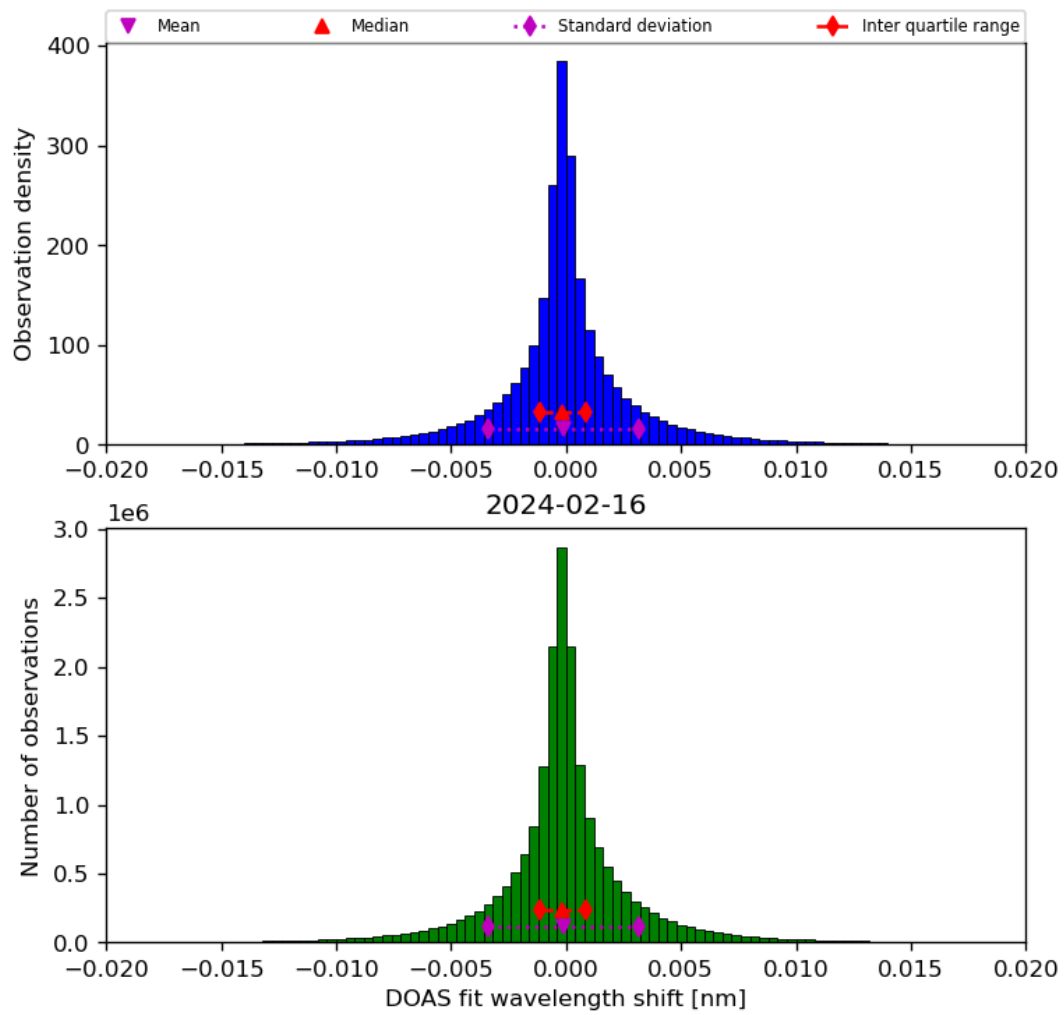
Figure 44: Histogram of “DOAS fit wavelength shift” for 2024-02-16 to 2024-02-17
