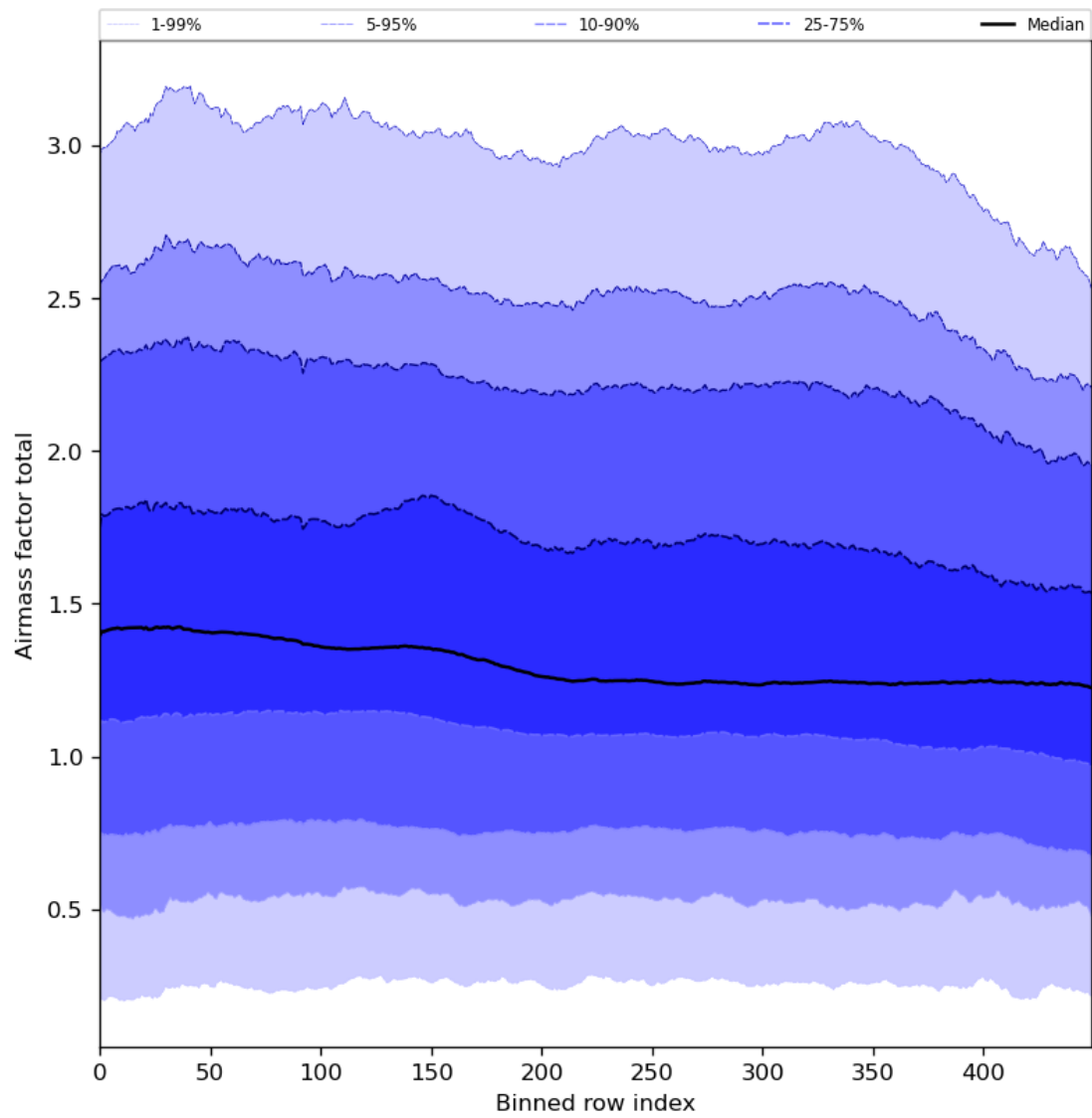
Figure 54: Along track statistics of “Airmass factor total” for 2024-02-16 to 2024-02-17
