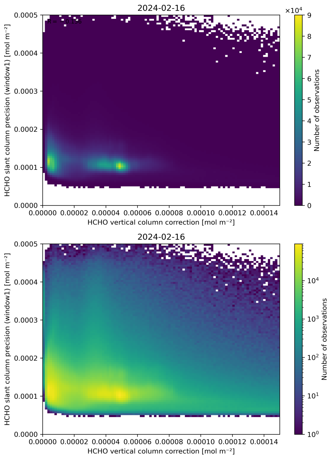
Figure 119: Scatter density plot of “HCHO vertical column correction” against “HCHO slant column precision (window1)” for 2024-02-16 to 2024-02-17.
