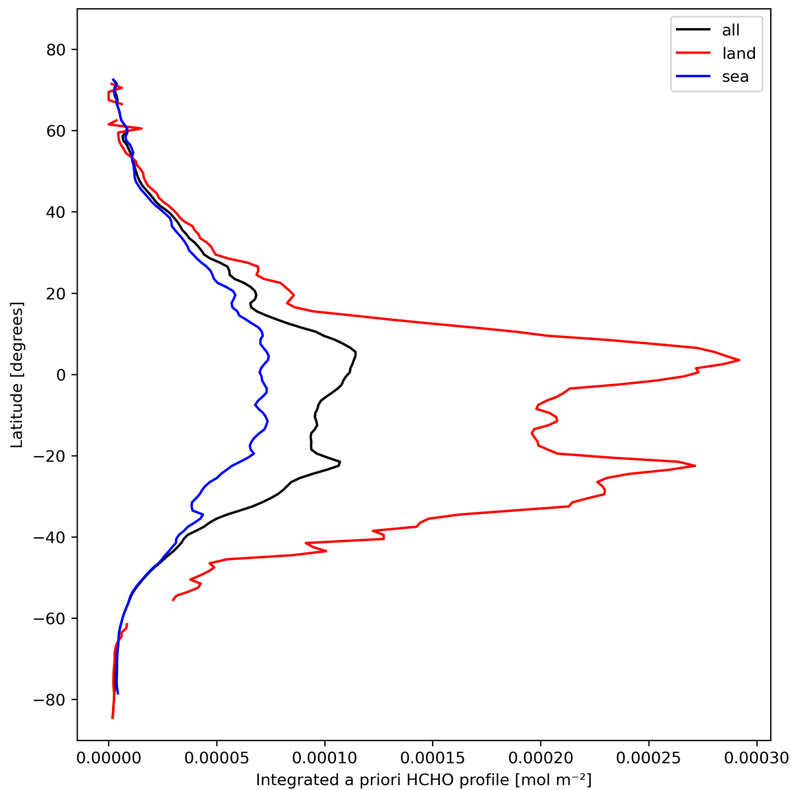
Figure 29: Zonal average of “Integrated a priori HCHO profile” for 2024-02-16 to 2024-02-17.
