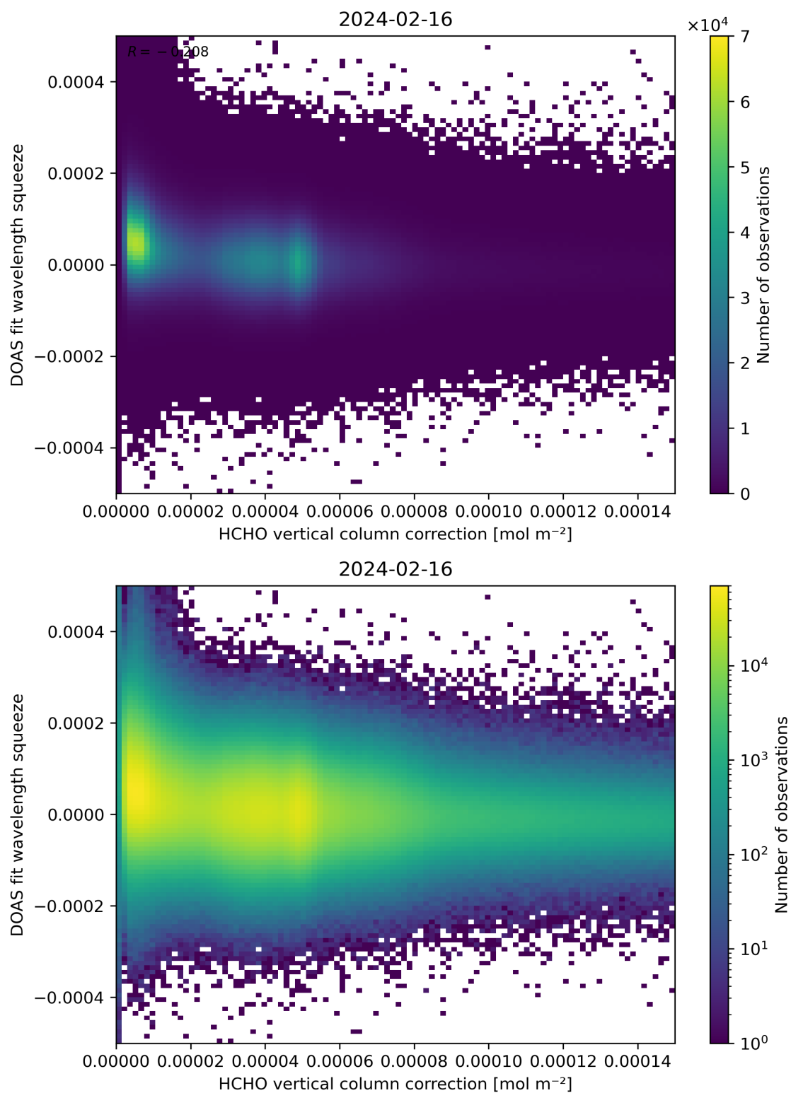
Figure 114: Scatter density plot of “HCHO vertical column correction” against “DOAS fit wavelength squeeze” for 2024-02-16 to 2024-02-17.
