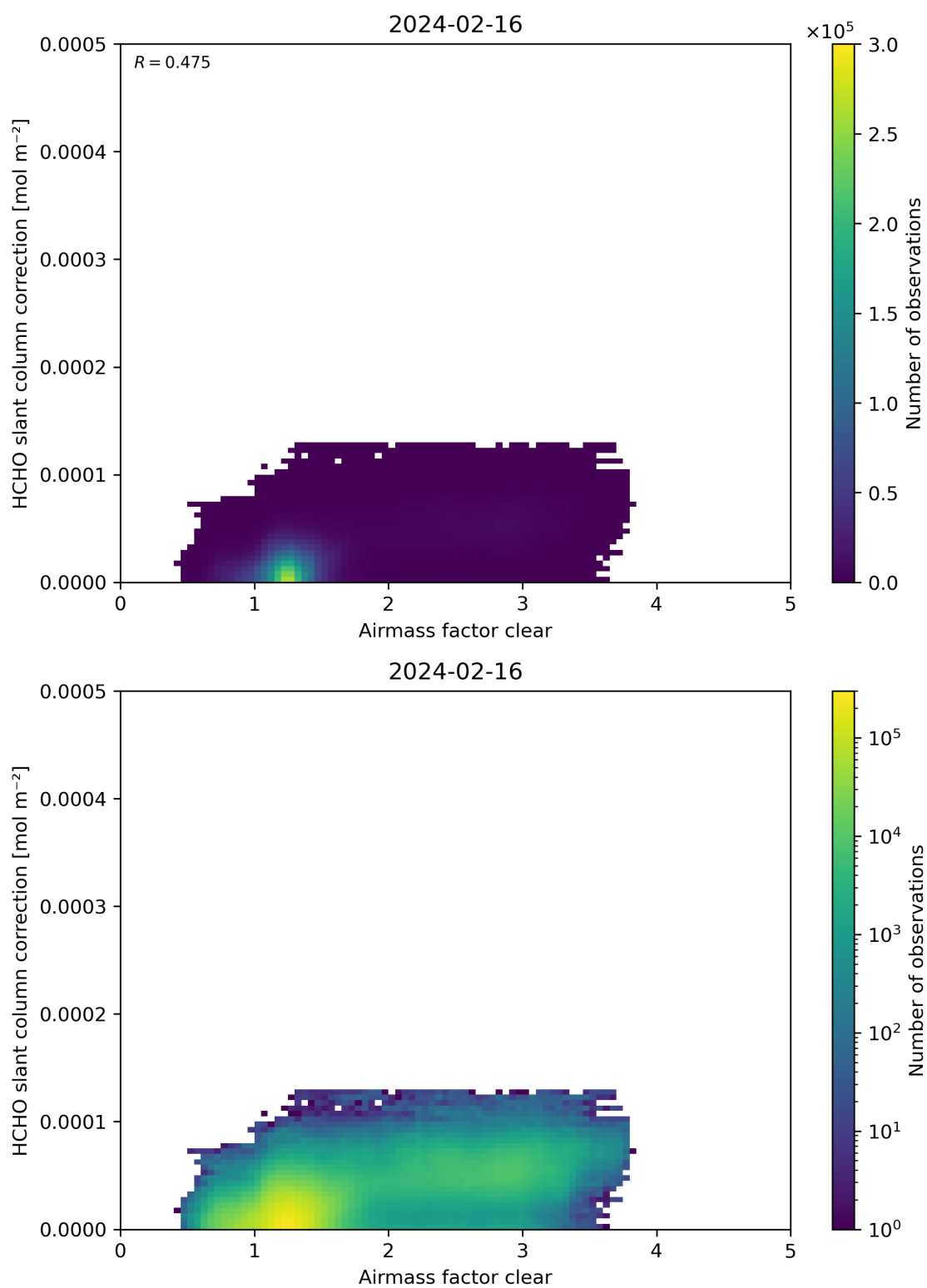
Figure 75: Scatter density plot of “Airmass factor clear” against “HCHO slant column correction” for 2024-02-16 to 2024-02-17.
