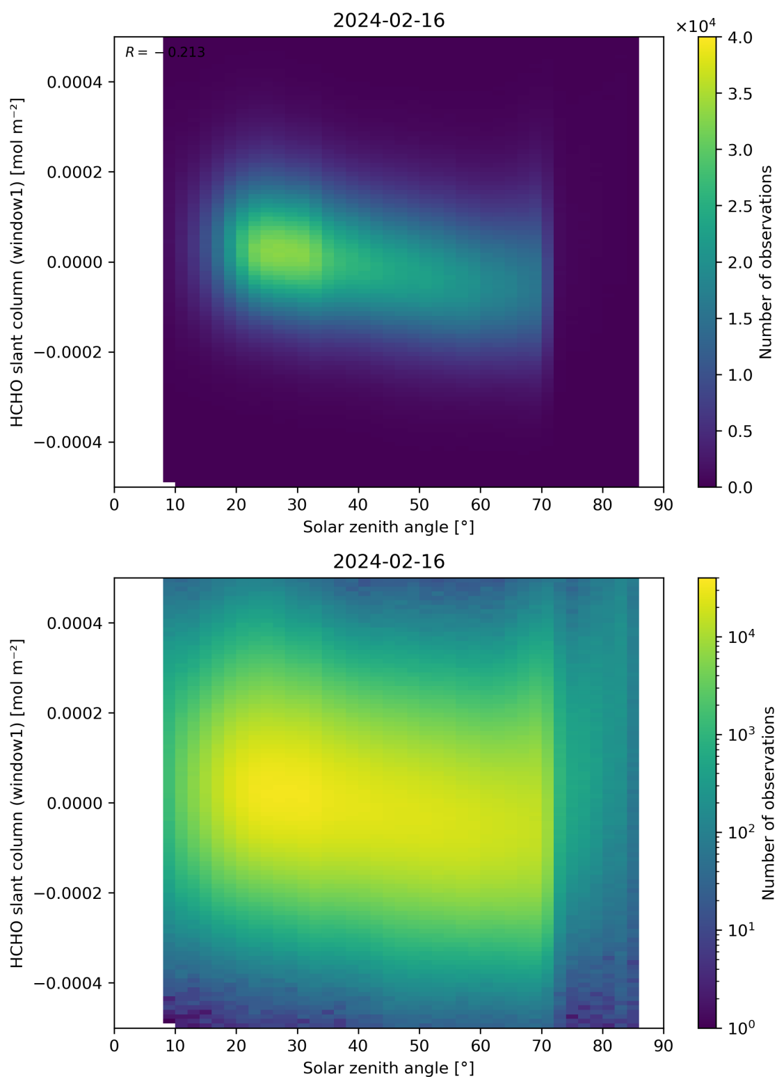
Figure 173: Scatter density plot of “Solar zenith angle” against “HCHO slant column (window1)” for 2024-02-16 to 2024-02-17.
