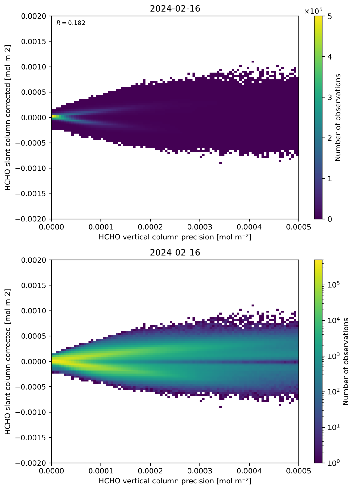
Figure 140: Scatter density plot of “HCHO vertical column precision” against “HCHO slant column corrected” for 2024-02-16 to 2024-02-17.
