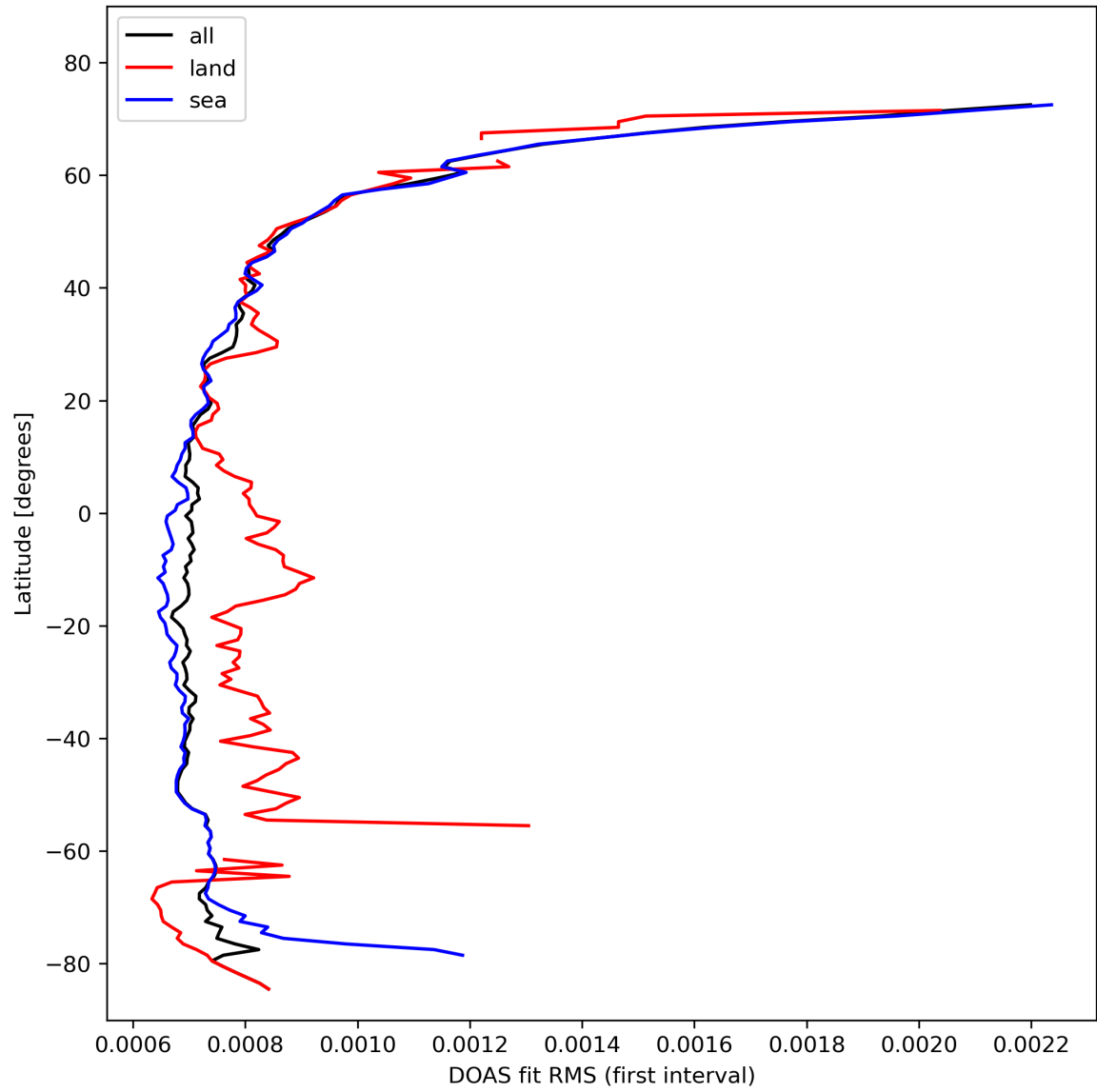
Figure 32: Zonal average of “DOAS fit RMS (first interval)” for 2024-02-16 to 2024-02-17.
