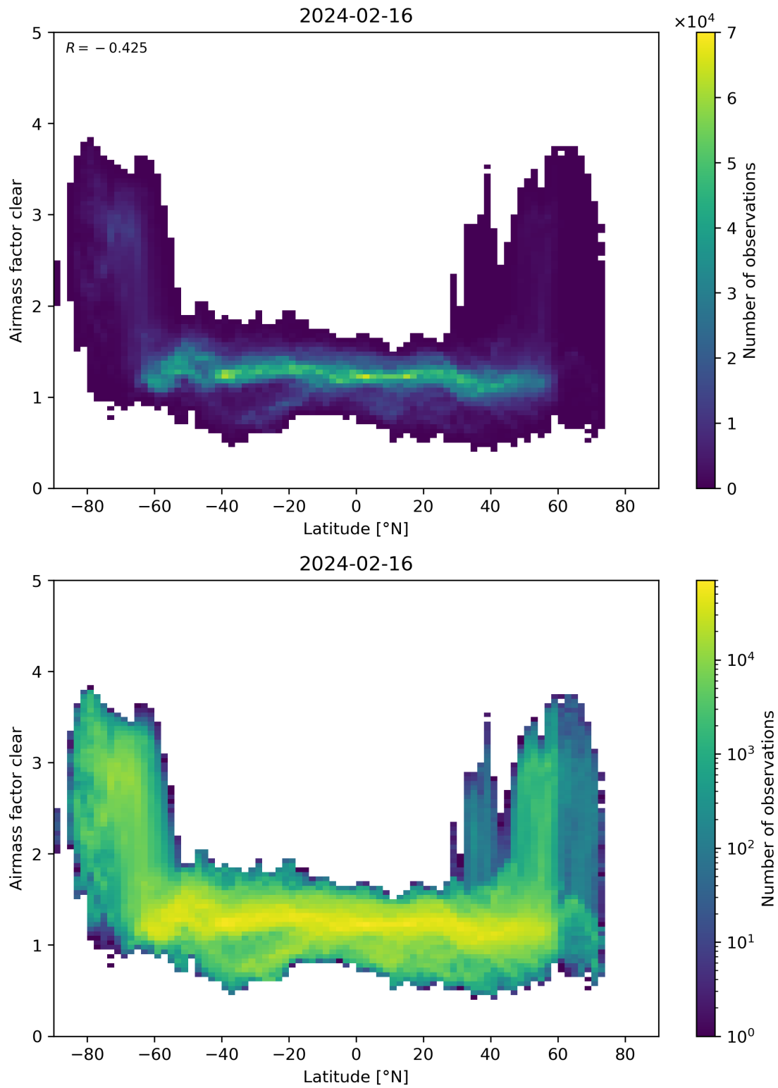
Figure 156: Scatter density plot of “Latitude” against “Airmass factor clear” for 2024-02-16 to 2024-02-17.
