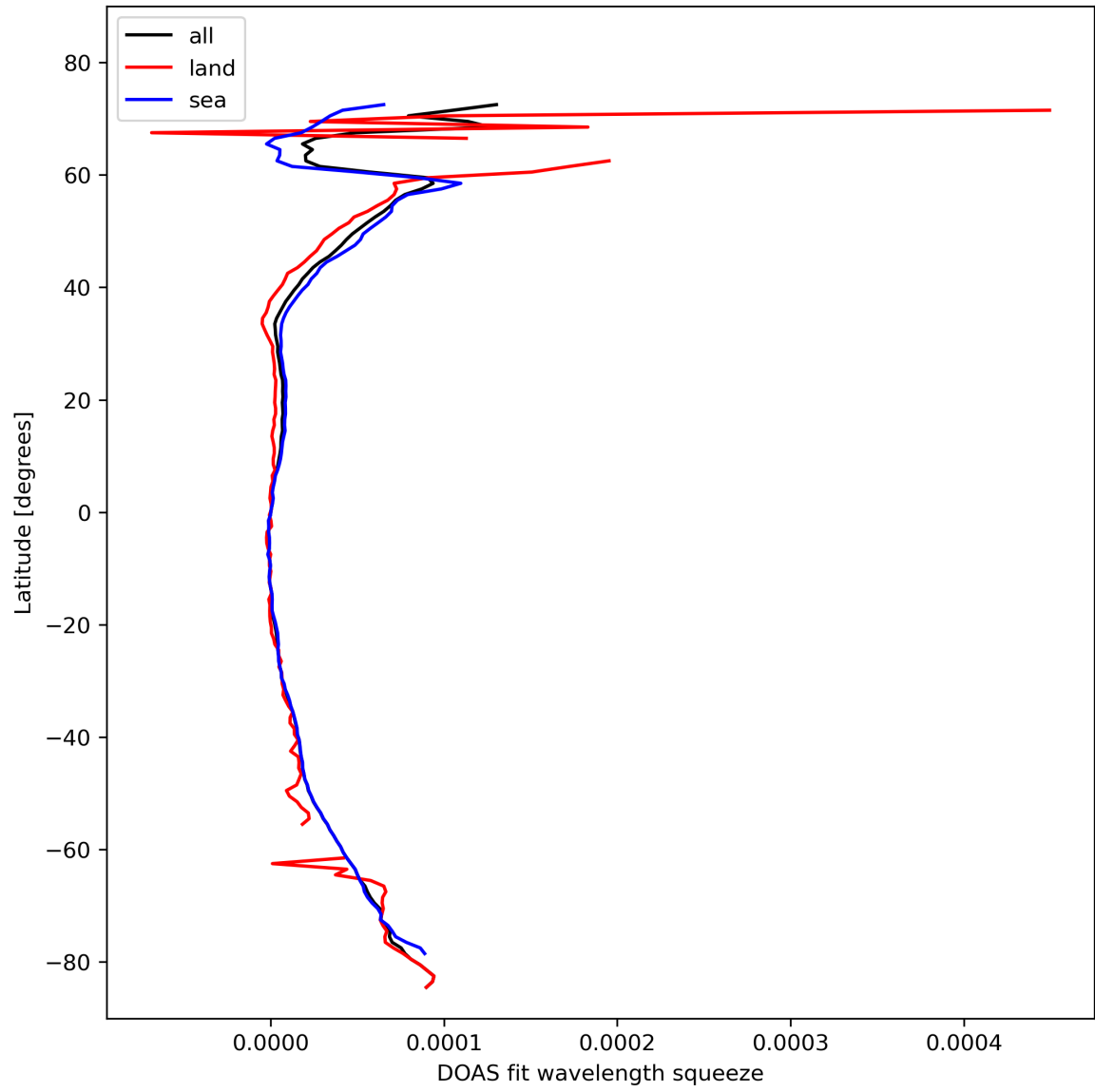
Figure 31: Zonal average of “DOAS fit wavelength squeeze” for 2024-02-16 to 2024-02-17.
