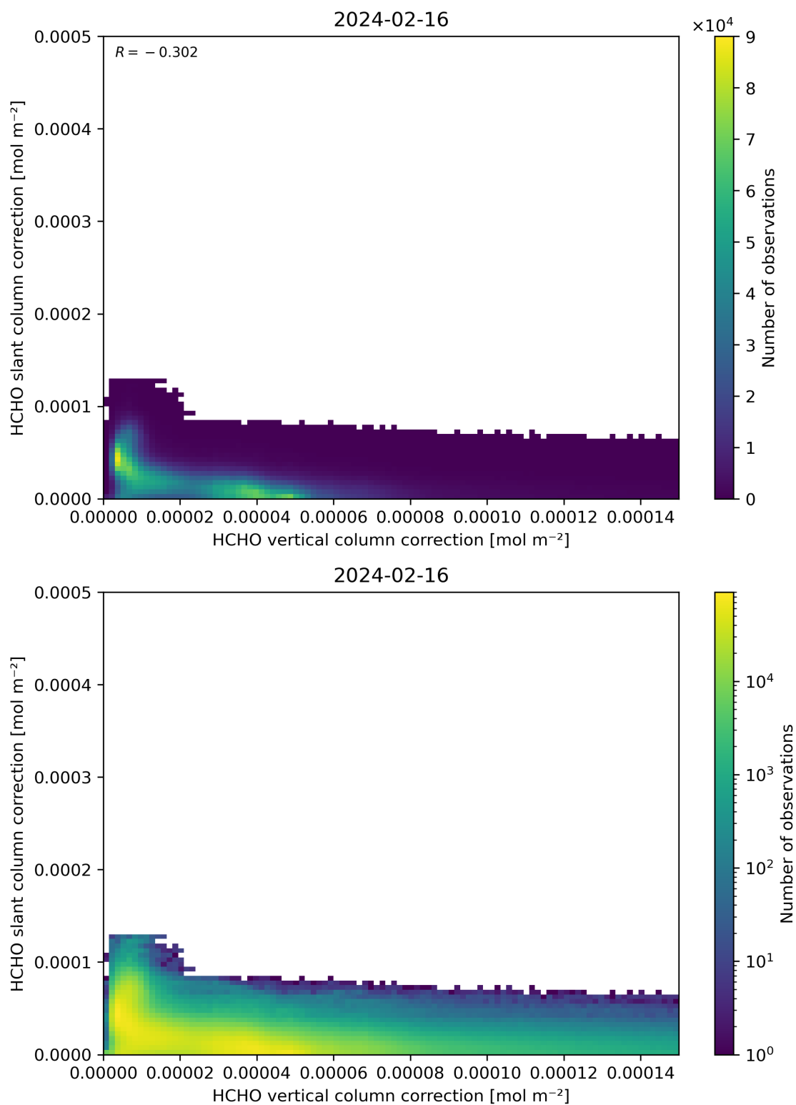
Figure 117: Scatter density plot of “HCHO vertical column correction” against “HCHO slant column correction” for 2024-02-16 to 2024-02-17.
