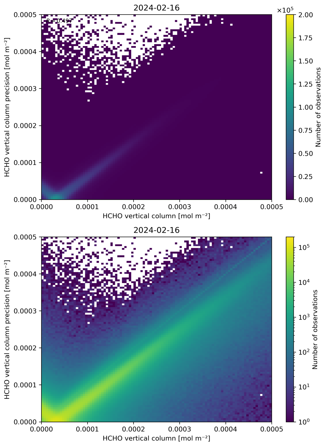
Figure 134: Scatter density plot of “HCHO vertical column” against “HCHO vertical column precision” for 2024-02-16 to 2024-02-17.
