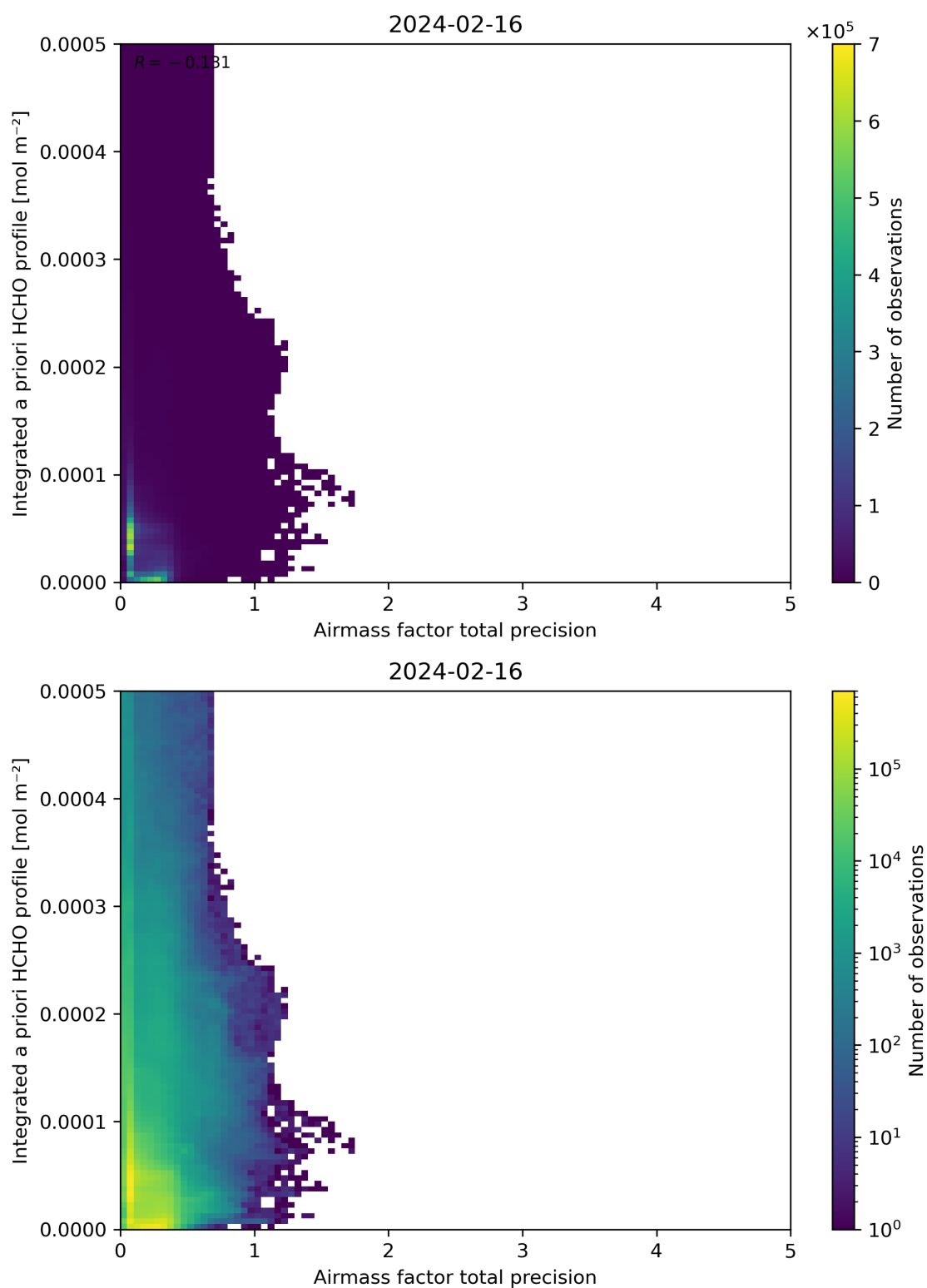
Figure 111: Scatter density plot of “Airmass factor total precision” against “Integrated a priori HCHO profile” for 2024-02-16 to 2024-02-17.
