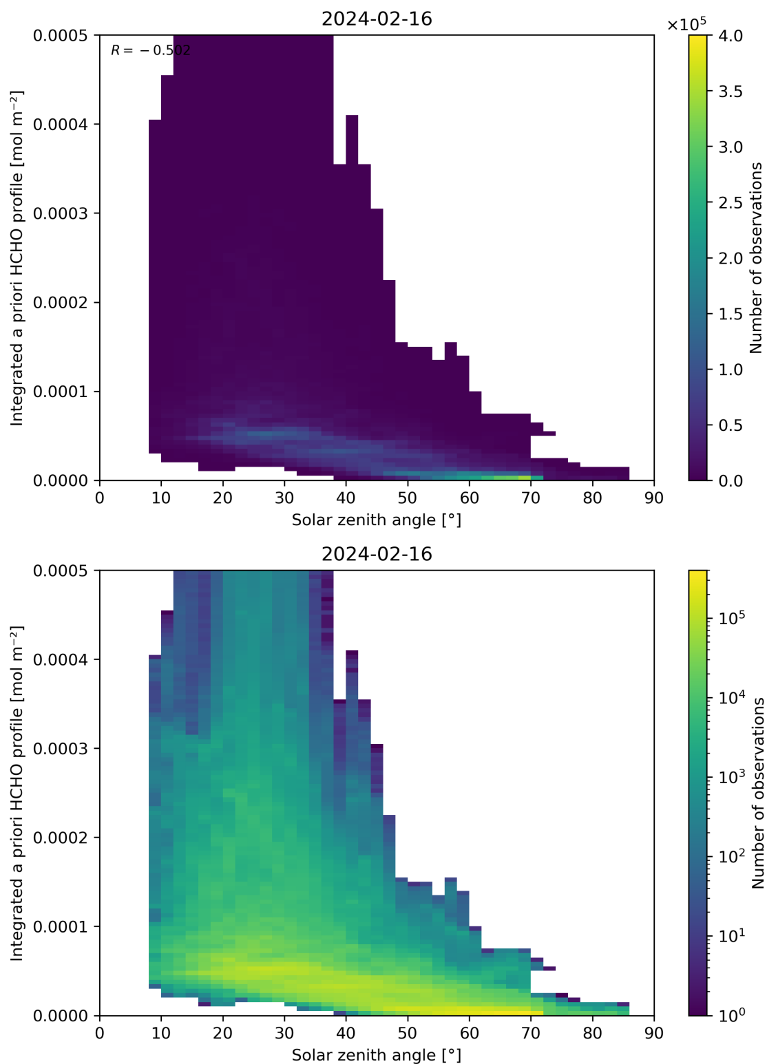
Figure 180: Scatter density plot of “Solar zenith angle” against “Integrated a priori HCHO profile” for 2024-02-16 to 2024-02-17.
