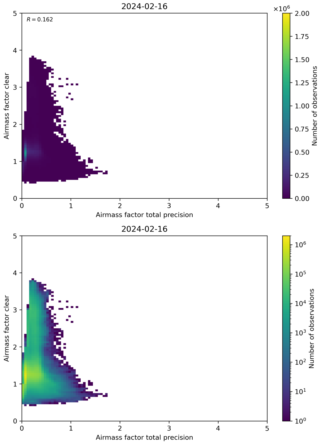
Figure 108: Scatter density plot of “Airmass factor total precision” against “Airmass factor clear” for 2024-02-16 to 2024-02-17.
