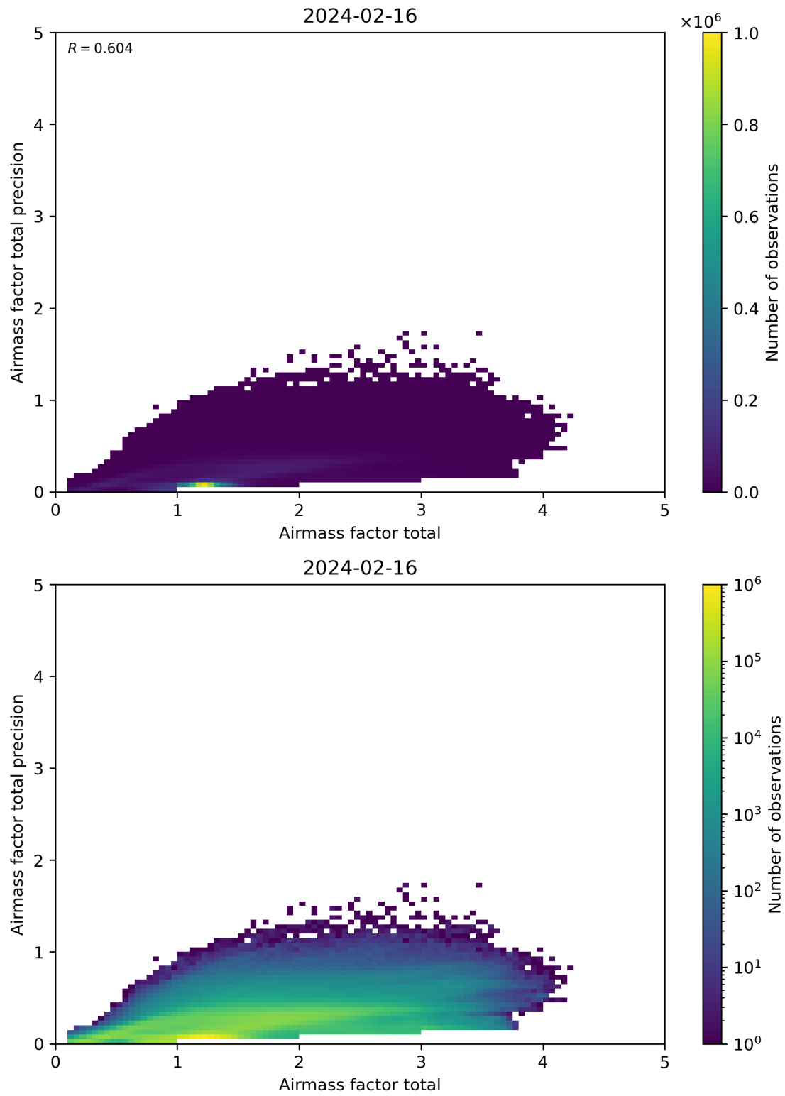
Figure 103: Scatter density plot of “Airmass factor total” against “Airmass factor total precision” for 2024-02-16 to 2024-02-17.
