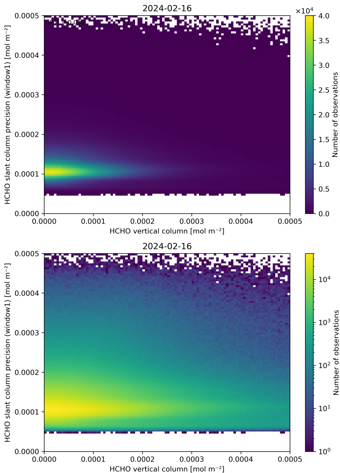
Figure 130: Scatter density plot of “HCHO vertical column” against “HCHO slant column precision (window1)” for 2024-02-16 to 2024-02-17.
