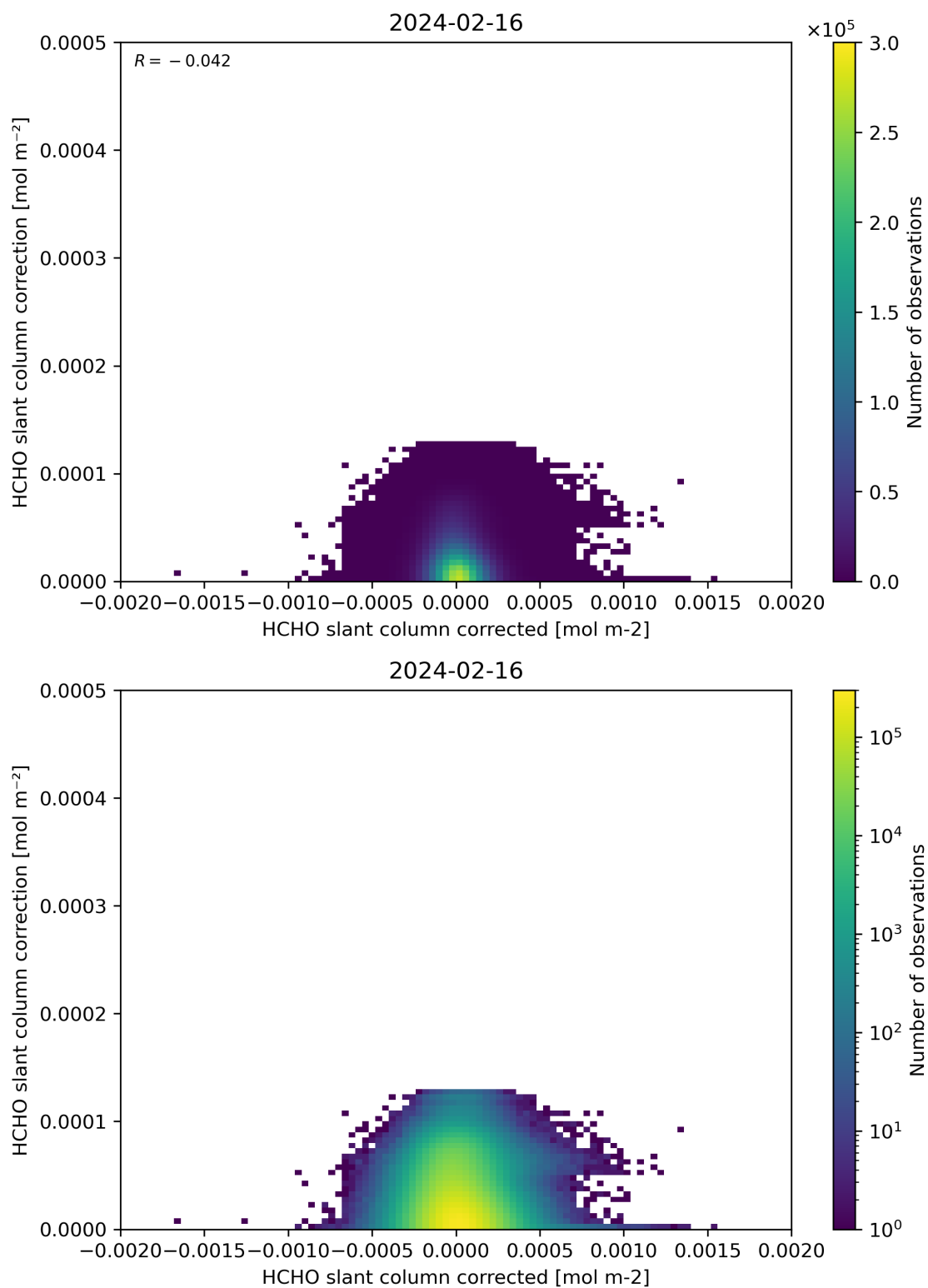
Figure 77: Scatter density plot of “HCHO slant column corrected” against “HCHO slant column correction” for 2024-02-16 to 2024-02-17.
