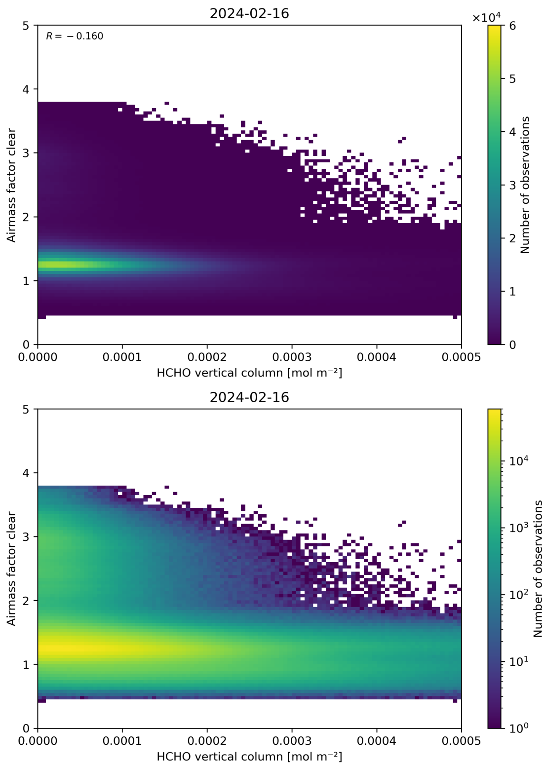
Figure 126: Scatter density plot of “HCHO vertical column” against “Airmass factor clear” for 2024-02-16 to 2024-02-17.
