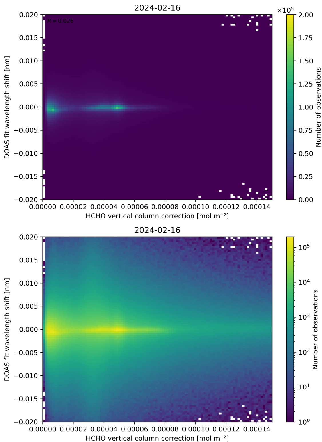
Figure 113: Scatter density plot of “HCHO vertical column correction” against “DOAS fit wavelength shift” for 2024-02-16 to 2024-02-17.
