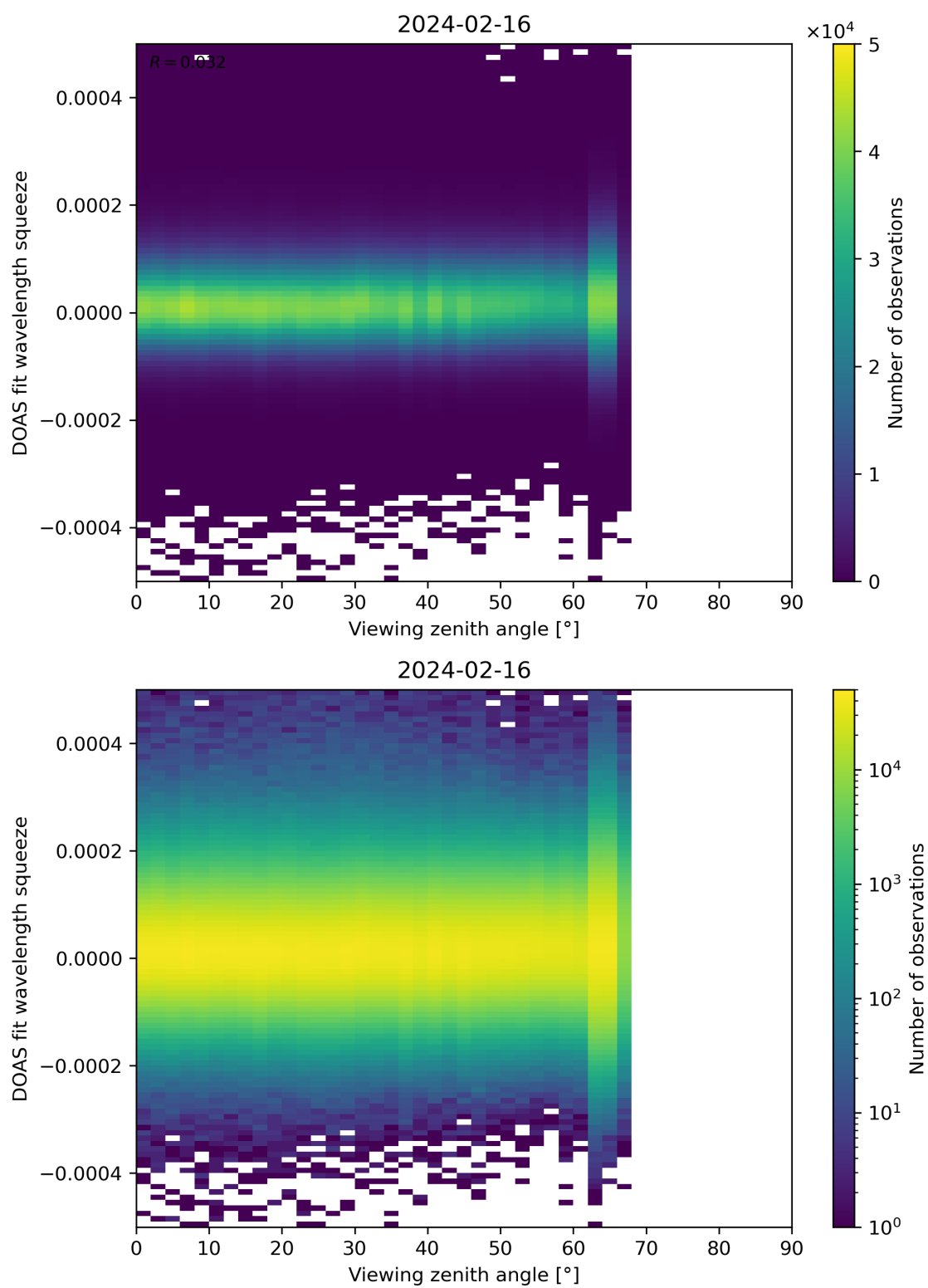
Figure 184: Scatter density plot of “Viewing zenith angle” against “DOAS fit wavelength squeeze” for 2024-02-16 to 2024-02-17.
