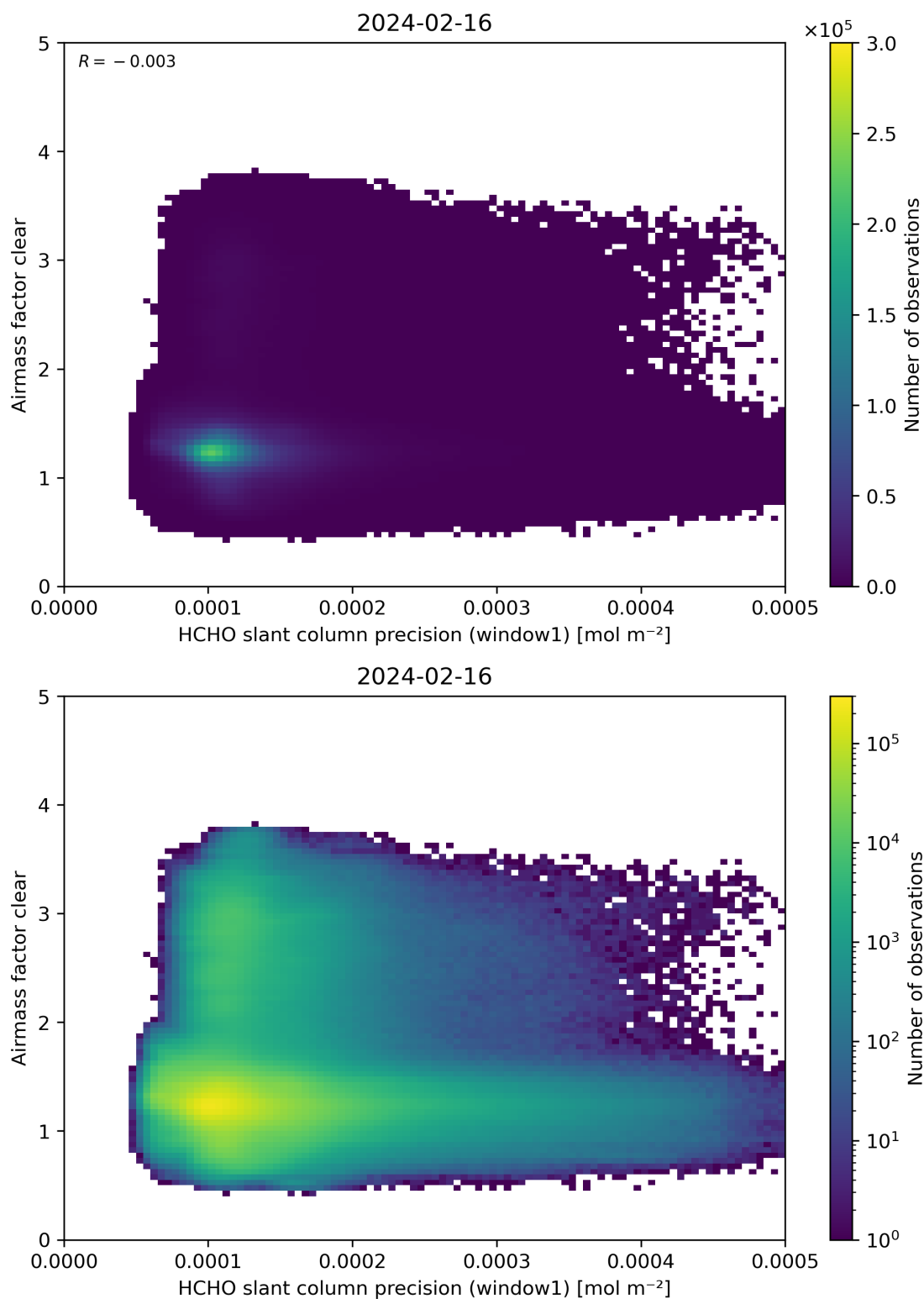
Figure 91: Scatter density plot of “HCHO slant column precision (window1)” against “Airmass factor clear” for 2024-02-16 to 2024-02-17.
