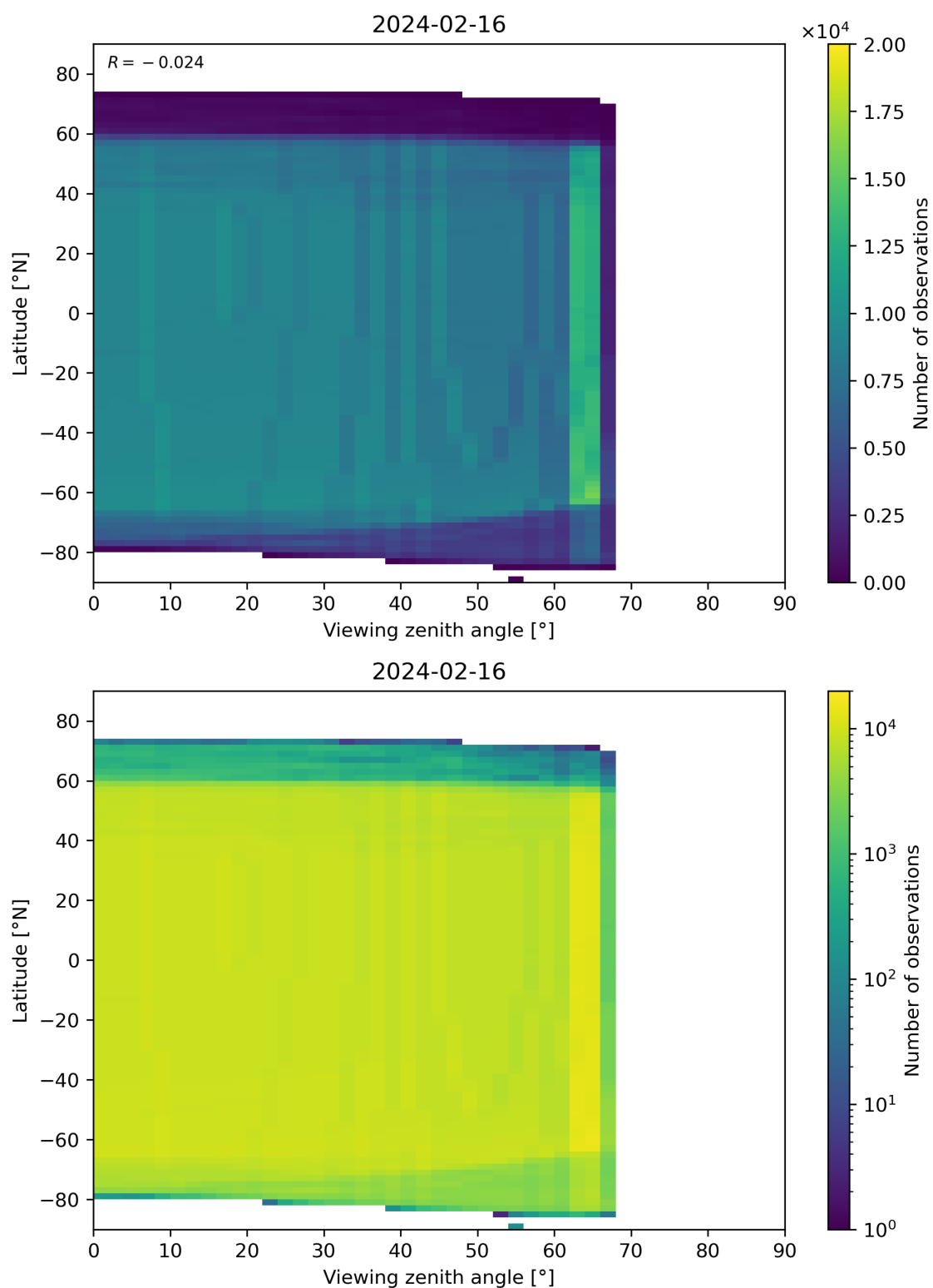
Figure 196: Scatter density plot of “Viewing zenith angle” against “Latitude” for 2024-02-16 to 2024-02-17.
