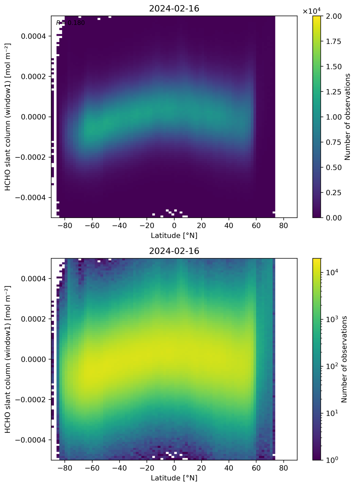
Figure 159: Scatter density plot of “Latitude” against “HCHO slant column (window1)” for 2024-02-16 to 2024-02-17.
