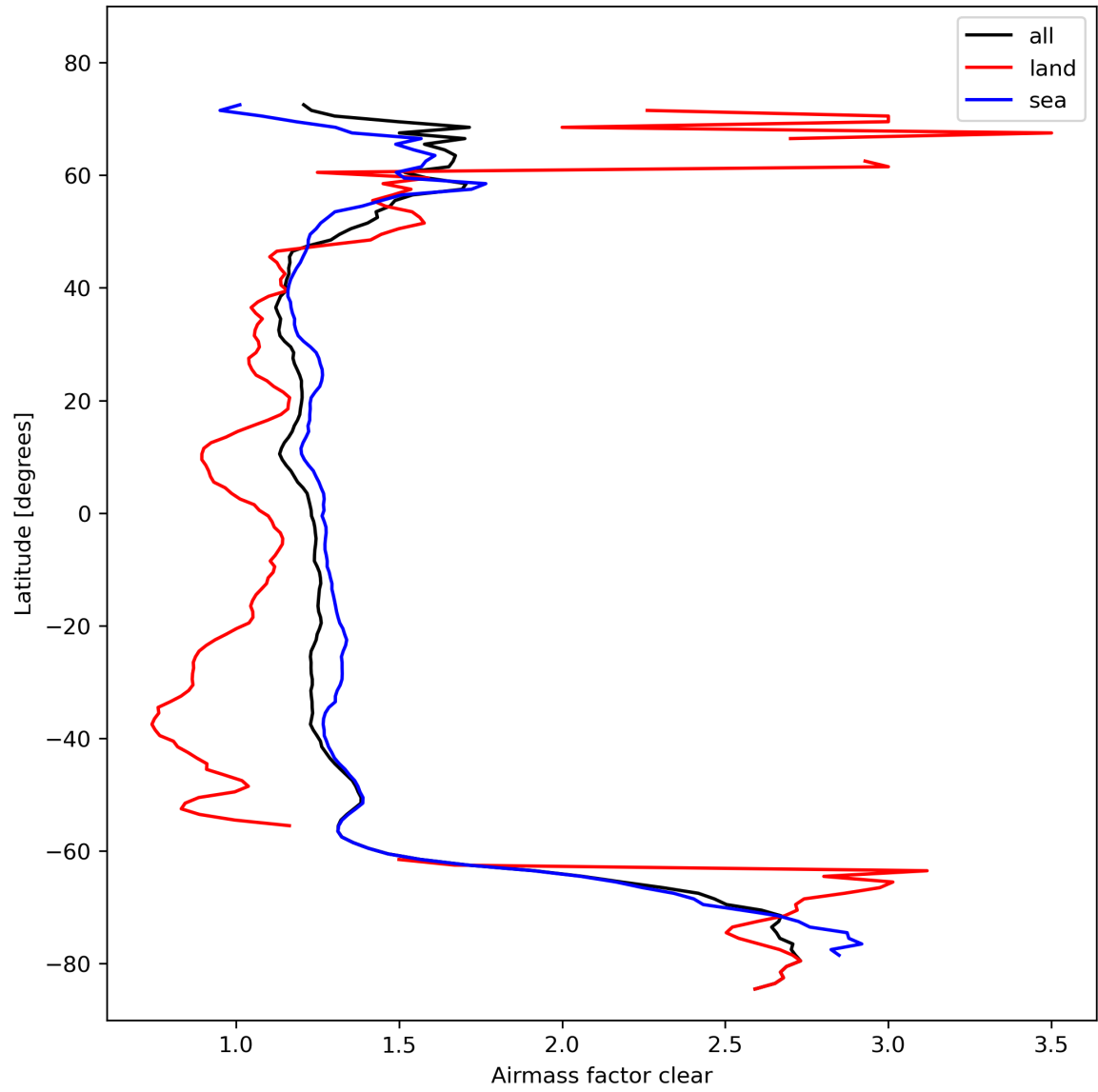
Figure 28: Zonal average of “Airmass factor clear” for 2024-02-16 to 2024-02-17.
