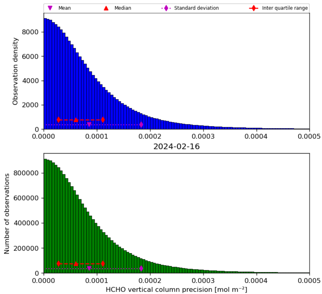
Figure 36: Histogram of “HCHO vertical column precision” for 2024-02-16 to 2024-02-17
