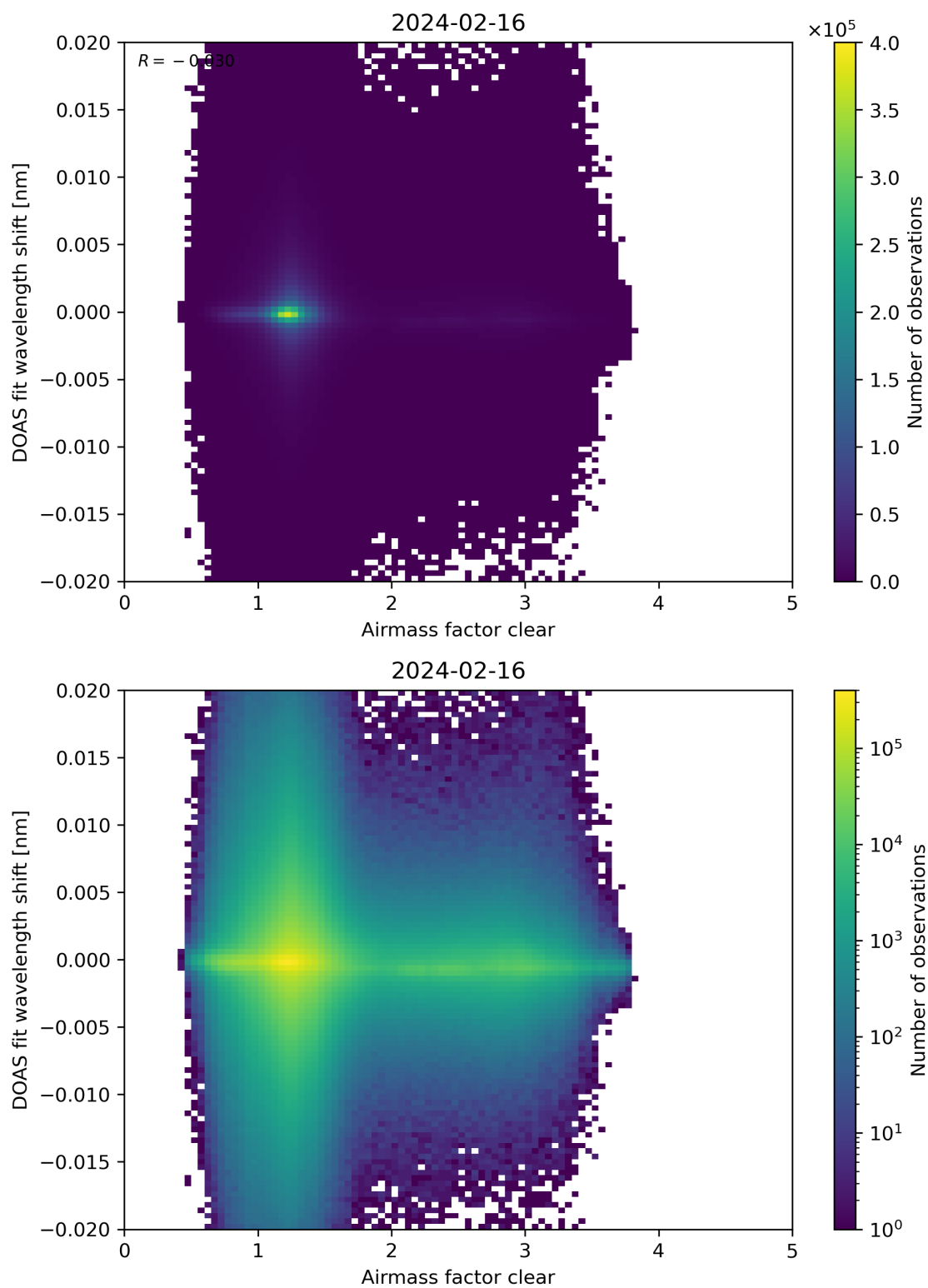
Figure 72: Scatter density plot of “Airmass factor clear” against “DOAS fit wavelength shift” for 2024-02-16 to 2024-02-17.
