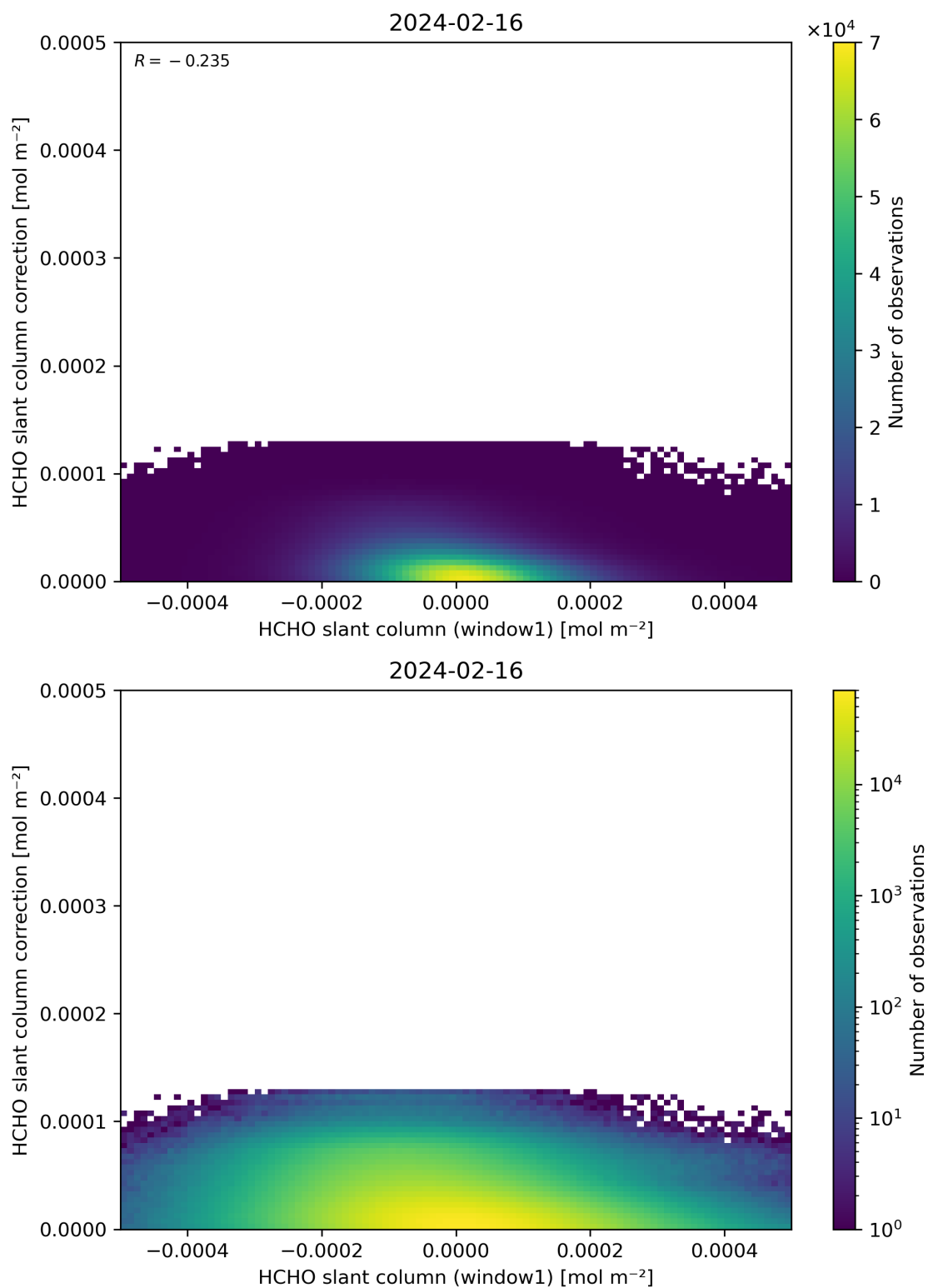
Figure 83: Scatter density plot of “HCHO slant column (window1)” against “HCHO slant column correction” for 2024-02-16 to 2024-02-17.
