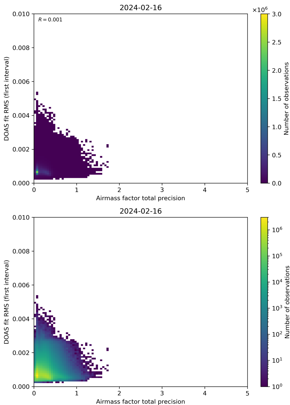
Figure 105: Scatter density plot of “Airmass factor total precision” against “DOAS fit RMS (first interval)” for 2024-02-16 to 2024-02-17.
