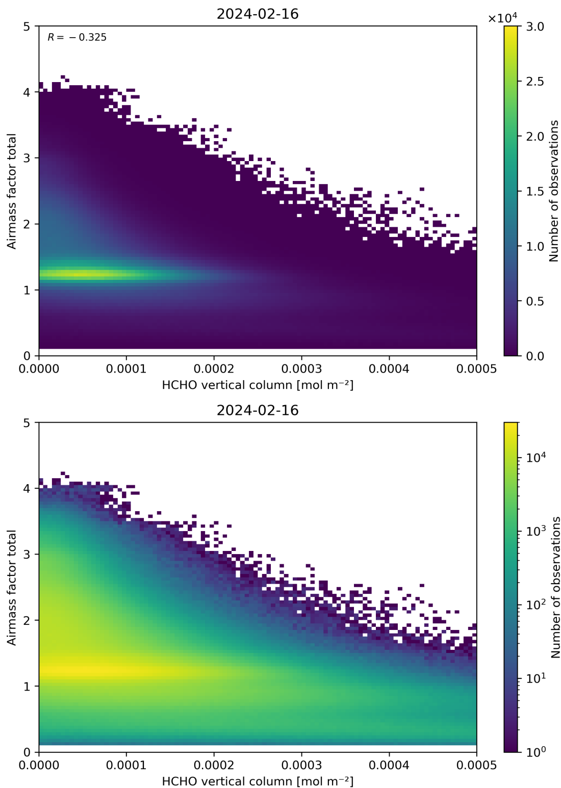
Figure 131: Scatter density plot of “HCHO vertical column” against “Airmass factor total” for 2024-02-16 to 2024-02-17.
