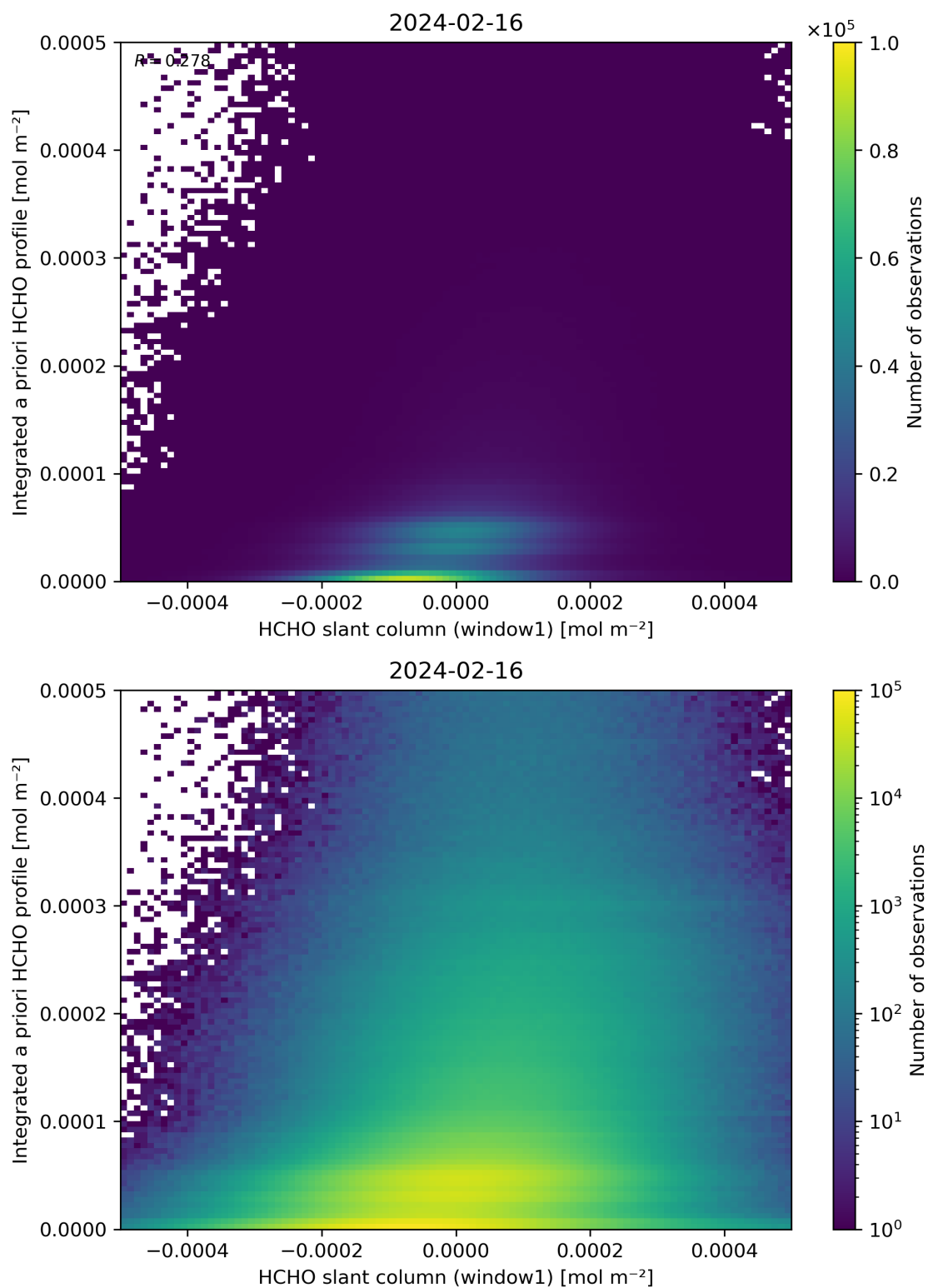
Figure 87: Scatter density plot of “HCHO slant column (window1)” against “Integrated a priori HCHO profile” for 2024-02-16 to 2024-02-17.
