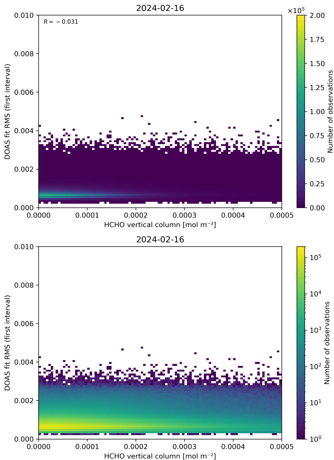
Figure 123: Scatter density plot of “HCHO vertical column” against “DOAS fit RMS (first interval)” for 2024-02-16 to 2024-02-17.
