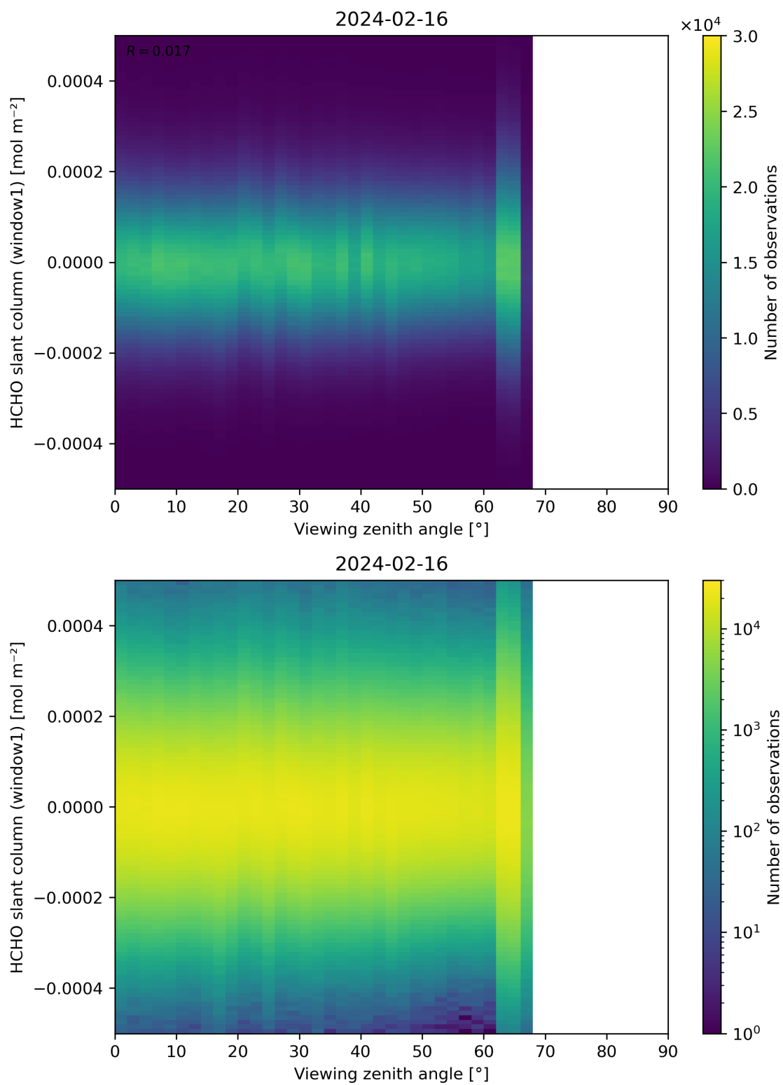
Figure 188: Scatter density plot of “Viewing zenith angle” against “HCHO slant column (window1)” for 2024-02-16 to 2024-02-17.
