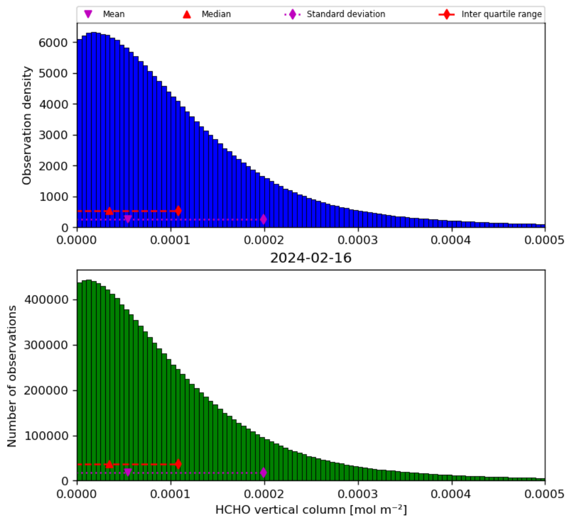
Figure 35: Histogram of “HCHO vertical column” for 2024-02-16 to 2024-02-17
