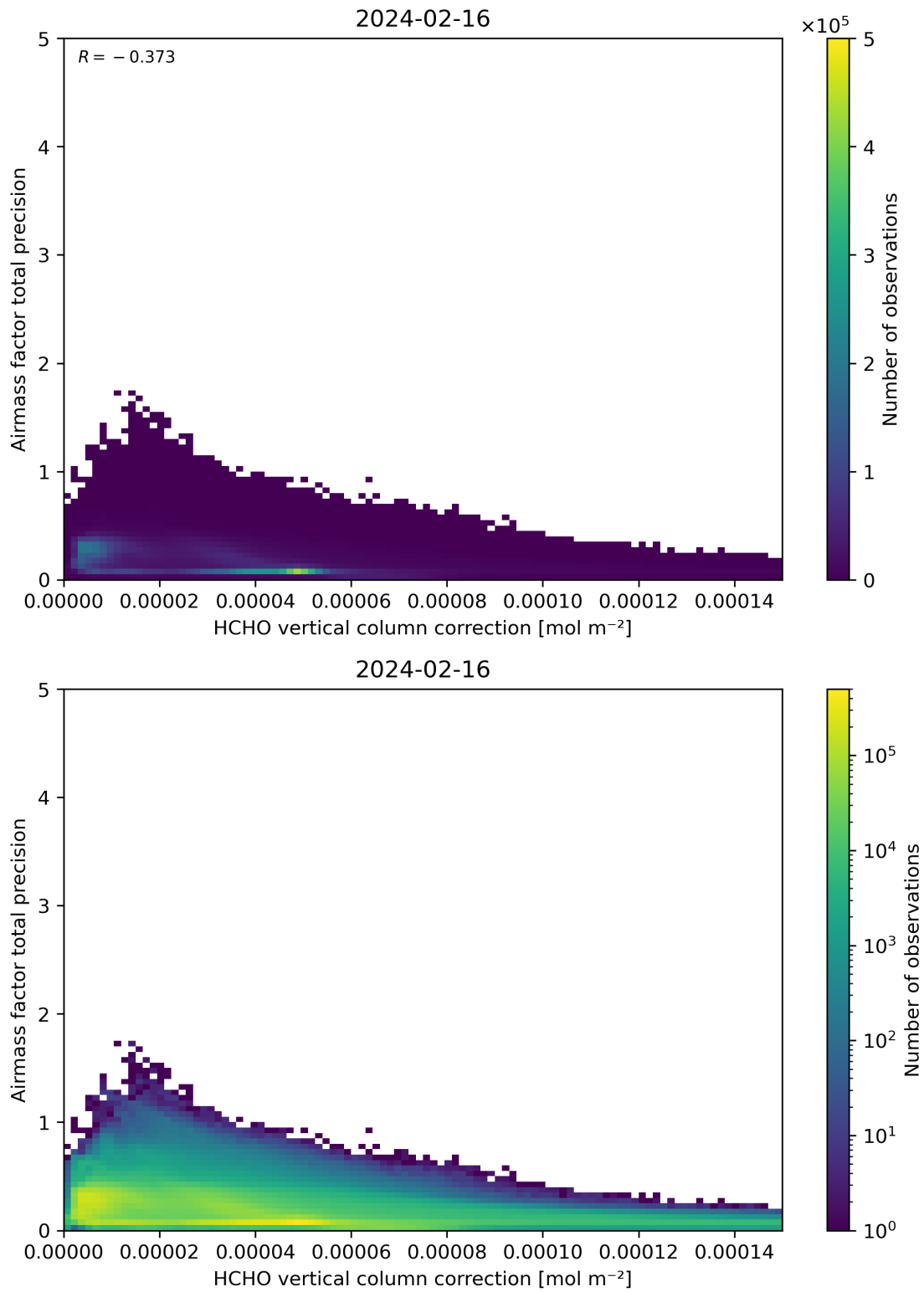
Figure 121: Scatter density plot of “HCHO vertical column correction” against “Airmass factor total precision” for 2024-02-16 to 2024-02-17.
