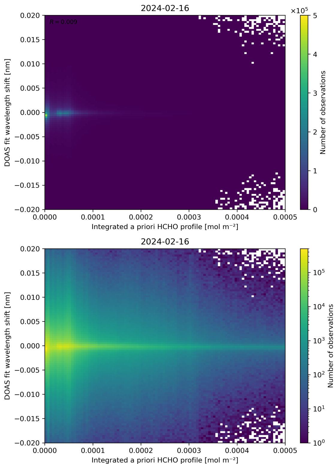
Figure 149: Scatter density plot of “Integrated a priori HCHO profile” against “DOAS fit wavelength shift” for 2024-02-16 to 2024-02-17.
