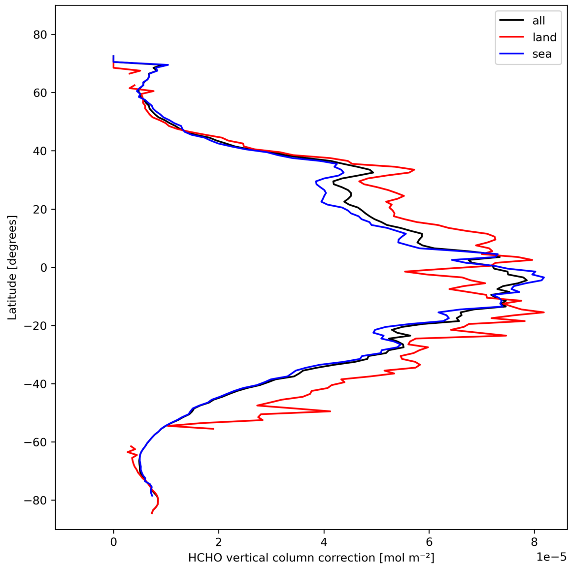
Figure 23: Zonal average of “HCHO vertical column correction” for 2024-02-16 to 2024-02-17.
