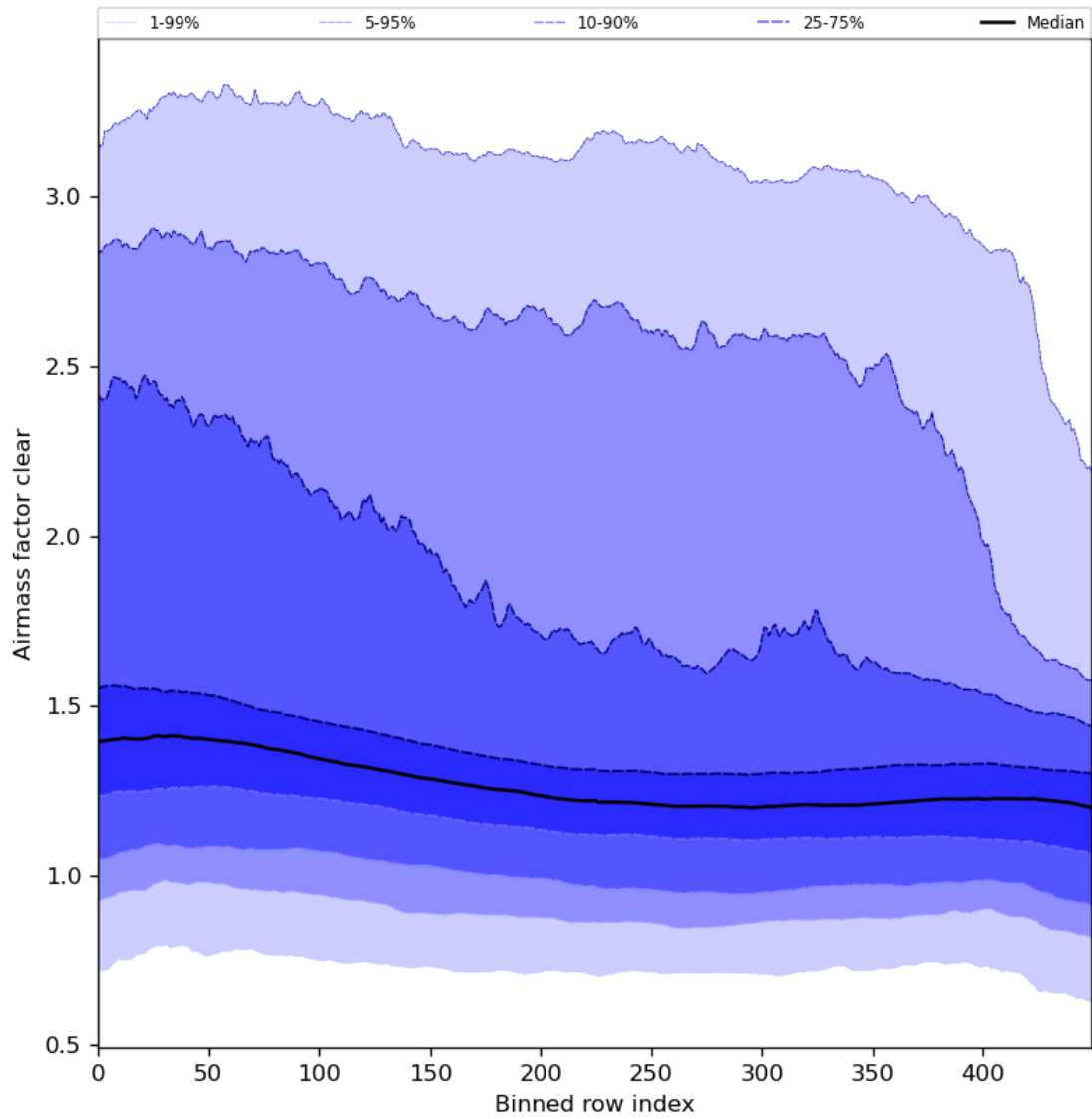
Figure 56: Along track statistics of “Airmass factor clear” for 2024-02-16 to 2024-02-17
