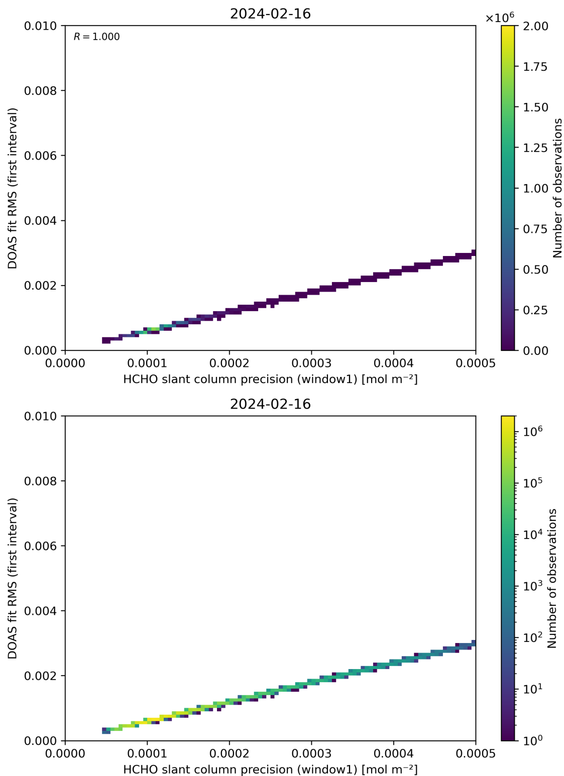
Figure 88: Scatter density plot of “HCHO slant column precision (window1)” against “DOAS fit RMS (first interval)” for 2024-02-16 to 2024-02-17.
