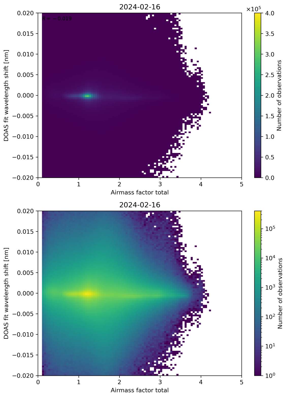
Figure 98: Scatter density plot of “Airmass factor total” against “DOAS fit wavelength shift” for 2024-02-16 to 2024-02-17.
