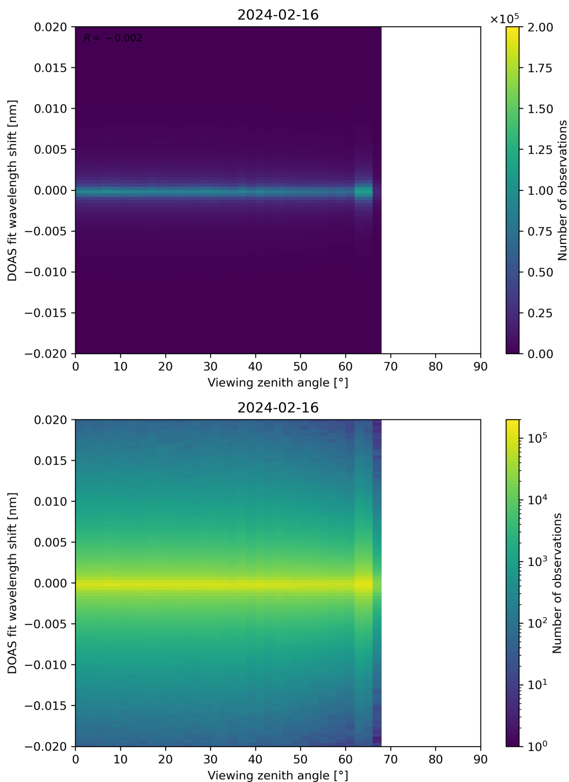
Figure 183: Scatter density plot of “Viewing zenith angle” against “DOAS fit wavelength shift” for 2024-02-16 to 2024-02-17.
