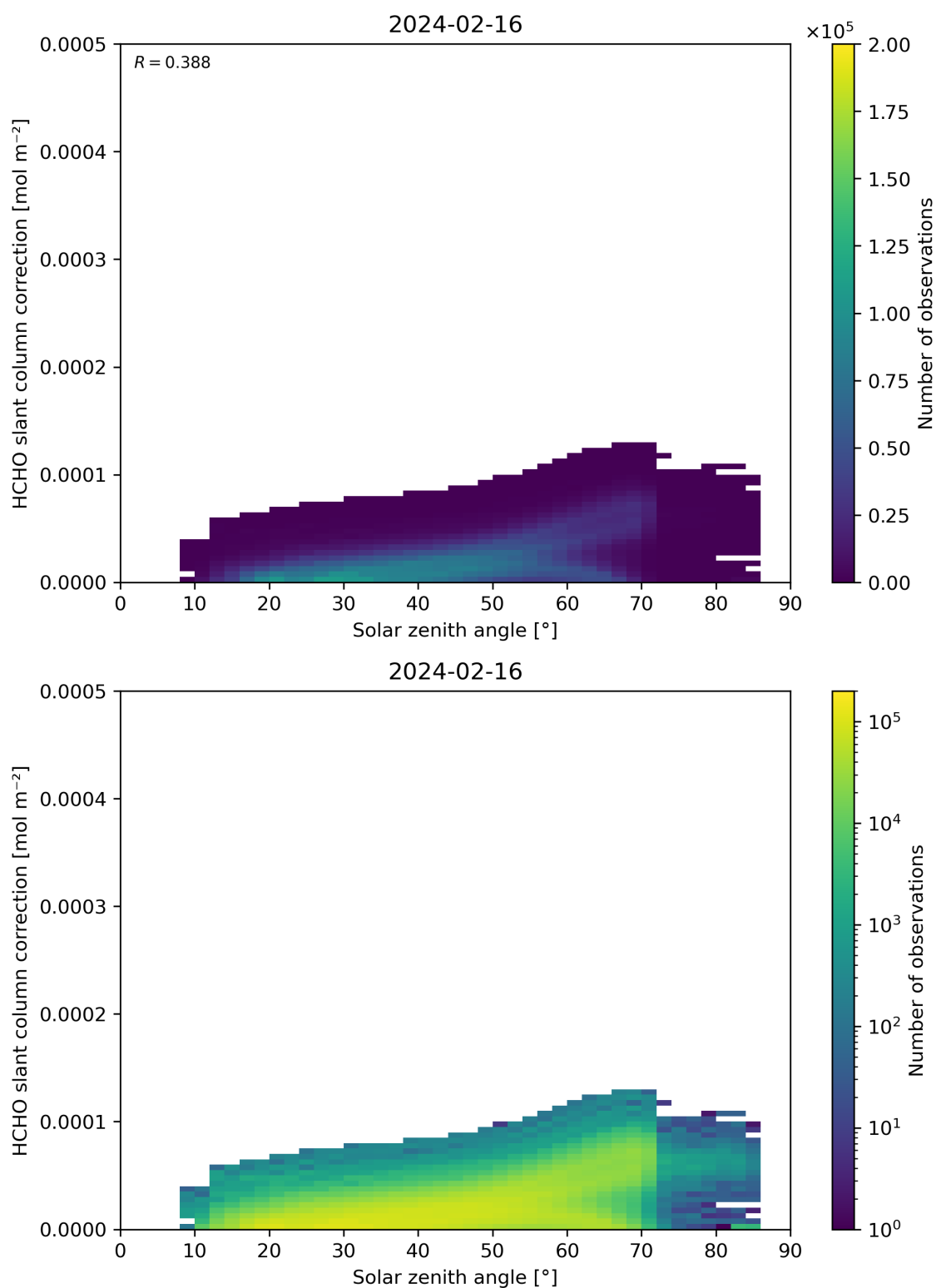
Figure 172: Scatter density plot of “Solar zenith angle” against “HCHO slant column correction” for 2024-02-16 to 2024-02-17.
