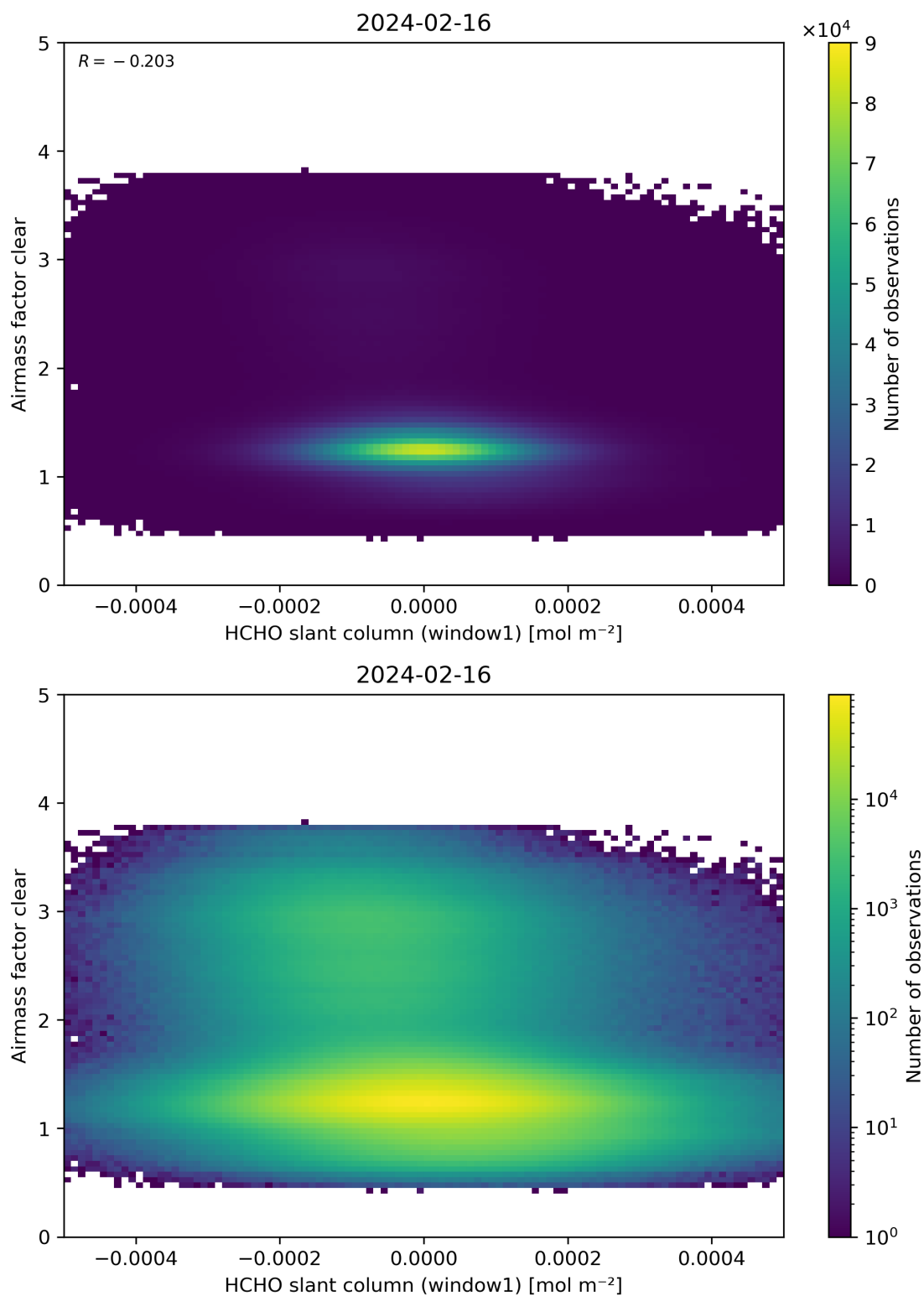
Figure 81: Scatter density plot of “HCHO slant column (window1)” against “Airmass factor clear” for 2024-02-16 to 2024-02-17.
