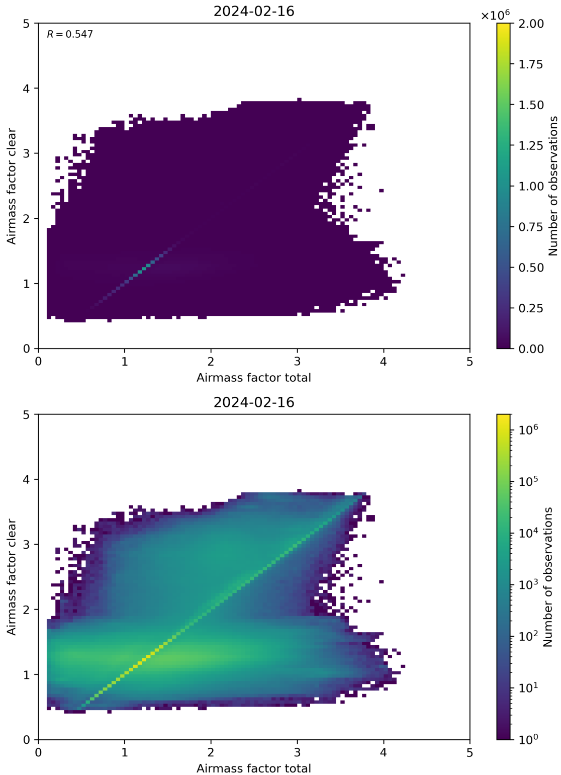
Figure 100: Scatter density plot of “Airmass factor total” against “Airmass factor clear” for 2024-02-16 to 2024-02-17.
