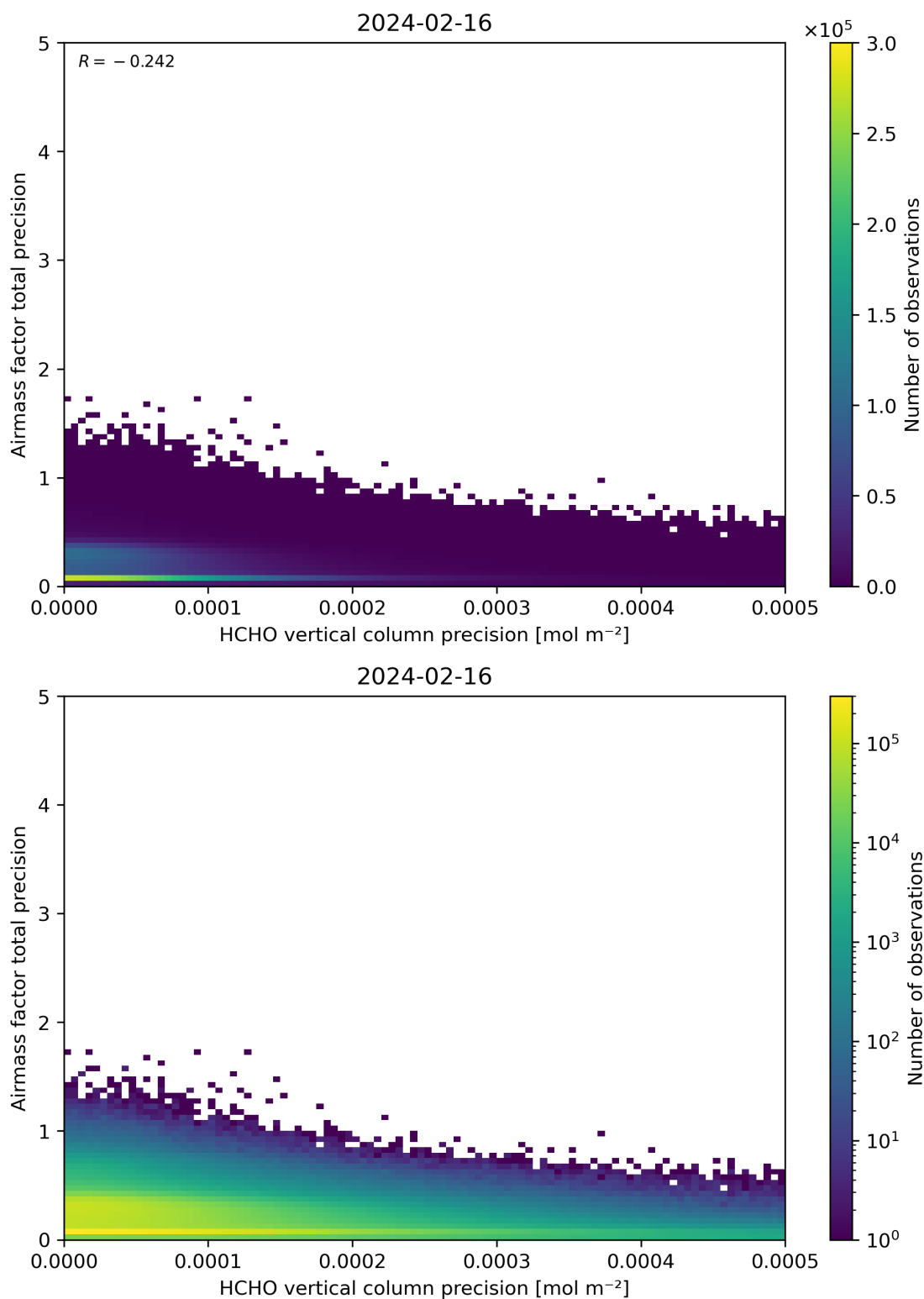
Figure 145: Scatter density plot of “HCHO vertical column precision” against “Airmass factor total precision” for 2024-02-16 to 2024-02-17.
