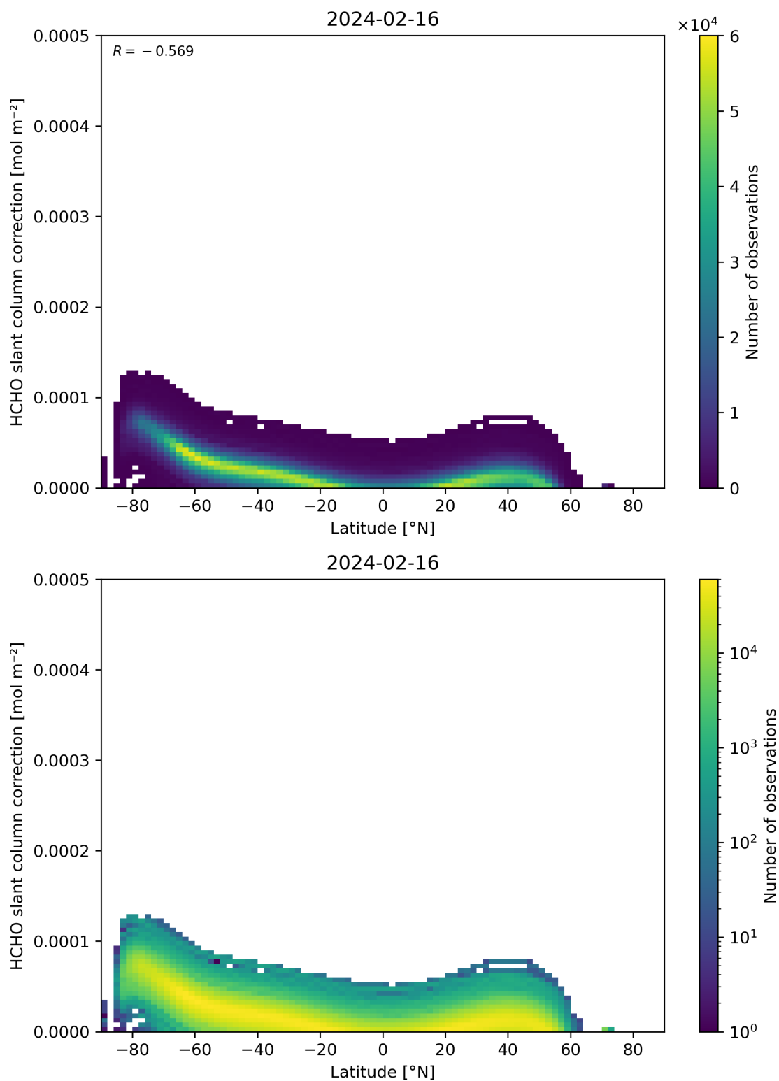
Figure 158: Scatter density plot of “Latitude” against “HCHO slant column correction” for 2024-02-16 to 2024-02-17.
