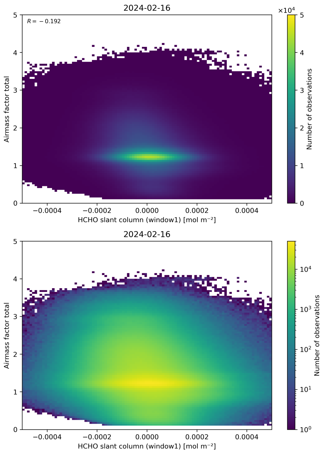
Figure 85: Scatter density plot of “HCHO slant column (window1)” against “Airmass factor total” for 2024-02-16 to 2024-02-17.
