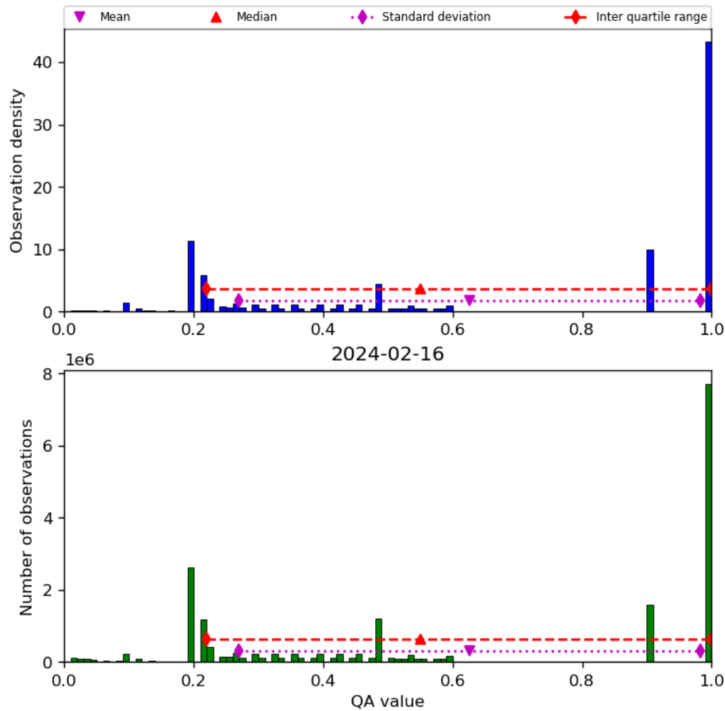
Figure 34: Histogram of “QA value” for 2024-02-16 to 2024-02-17
