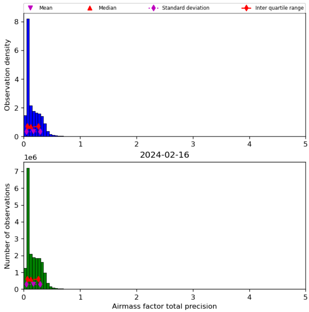
Figure 41: Histogram of “Airmass factor total precision” for 2024-02-16 to 2024-02-17
