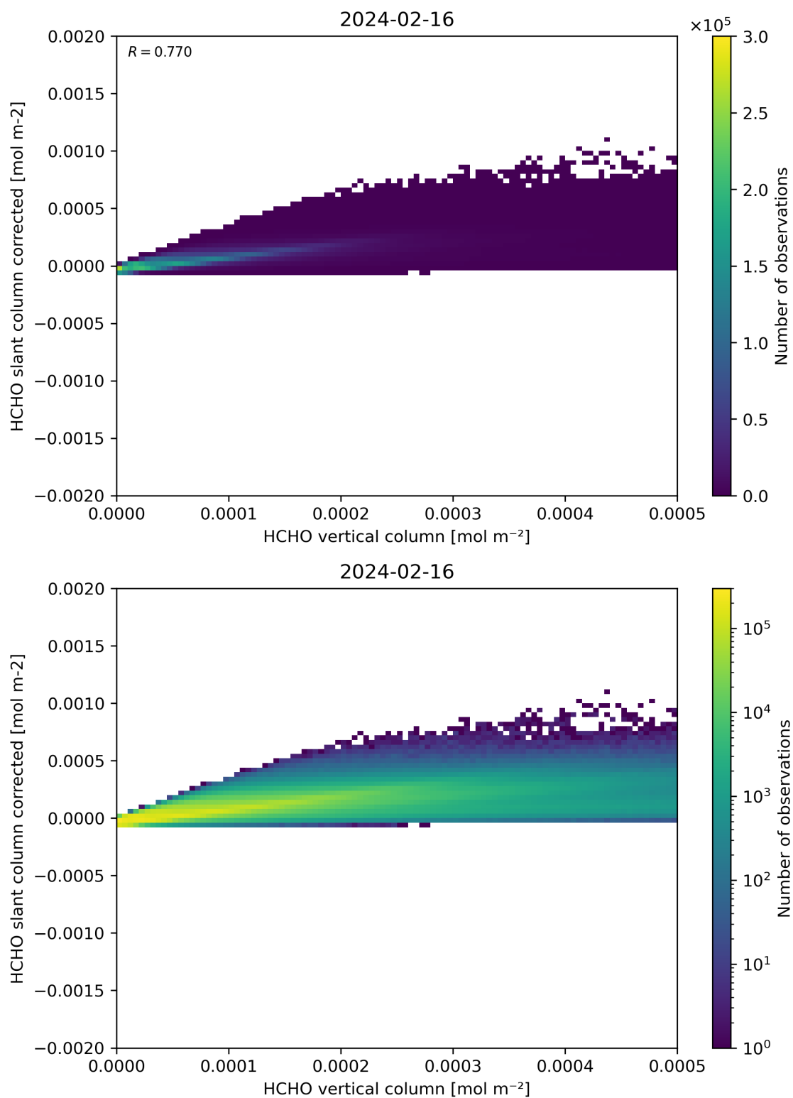
Figure 127: Scatter density plot of “HCHO vertical column” against “HCHO slant column corrected” for 2024-02-16 to 2024-02-17.
