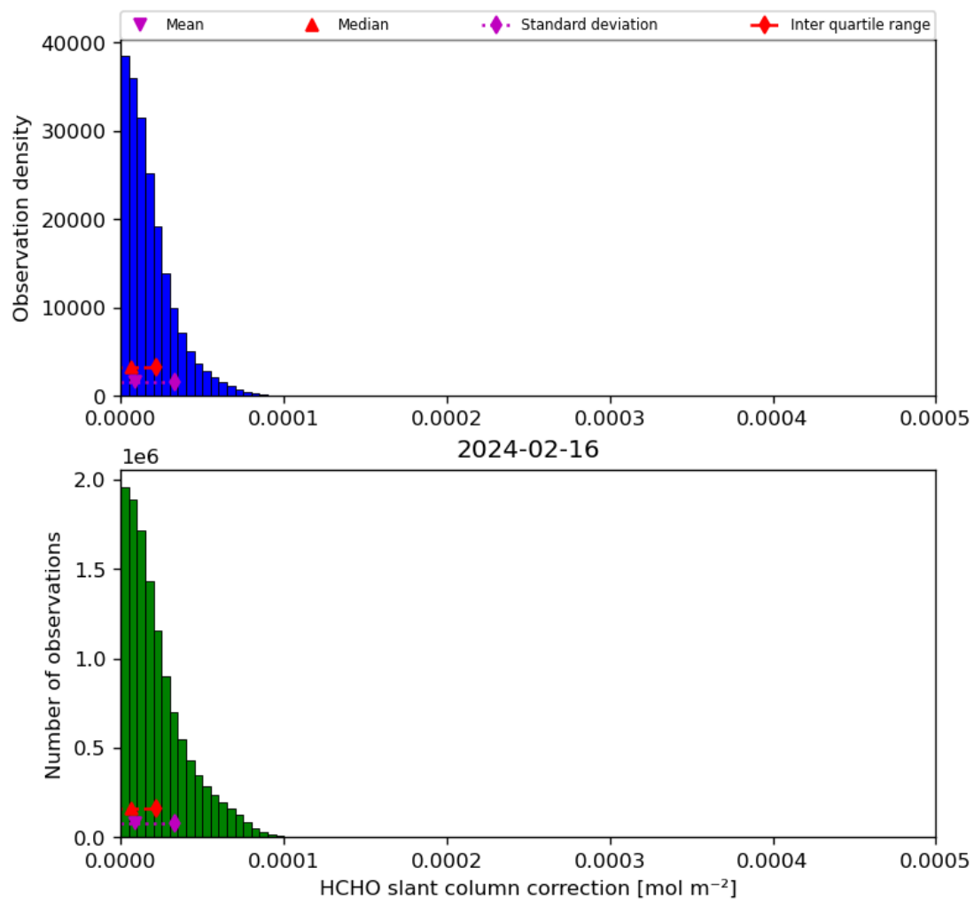
Figure 47: Histogram of “HCHO slant column correction” for 2024-02-16 to 2024-02-17
