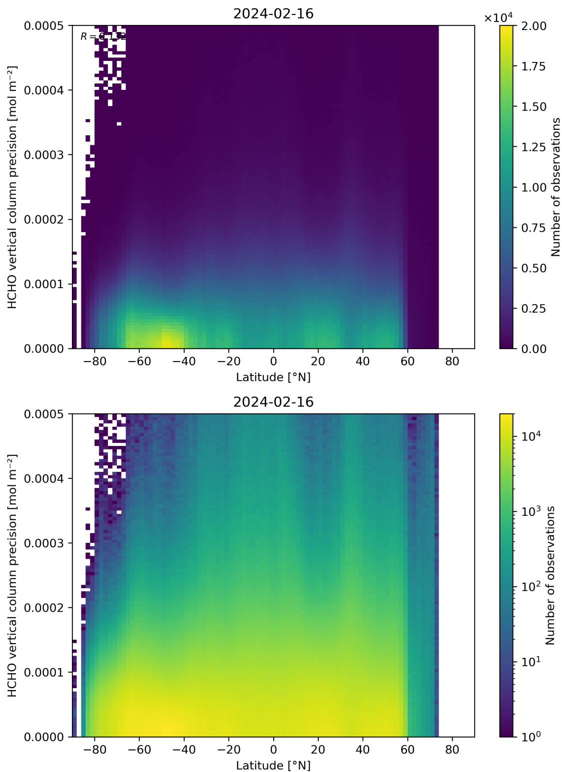
Figure 165: Scatter density plot of “Latitude” against “HCHO vertical column precision” for 2024-02-16 to 2024-02-17.
