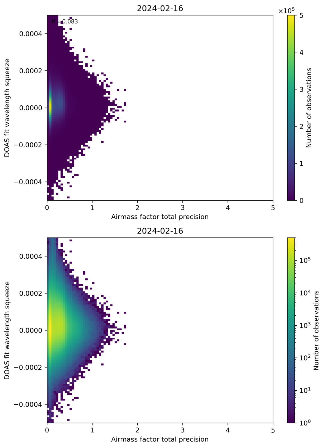
Figure 107: Scatter density plot of “Airmass factor total precision” against “DOAS fit wavelength squeeze” for 2024-02-16 to 2024-02-17.
