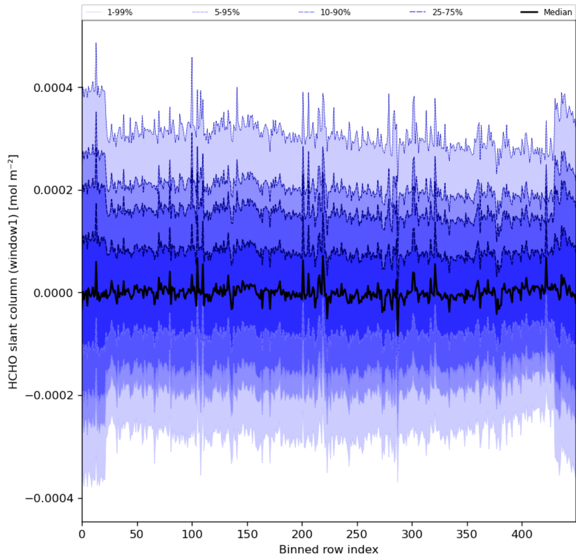
Figure 52: Along track statistics of “HCHO slant column (window1)” for 2024-02-16 to 2024-02-17
