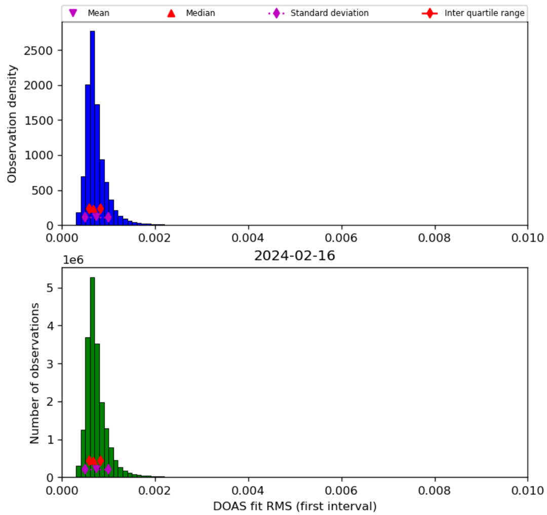
Figure 46: Histogram of “DOAS fit RMS (first interval)” for 2024-02-16 to 2024-02-17
