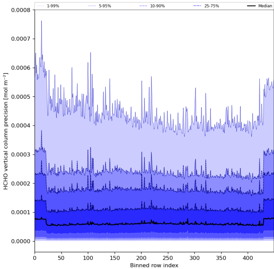
Figure 50: Along track statistics of “HCHO vertical column precision” for 2024-02-16 to 2024-02-17
