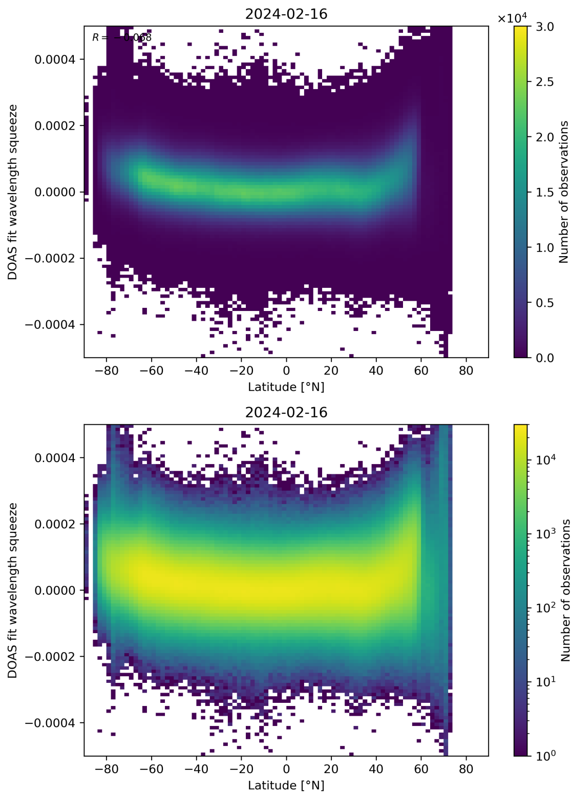
Figure 155: Scatter density plot of “Latitude” against “DOAS fit wavelength squeeze” for 2024-02-16 to 2024-02-17.
