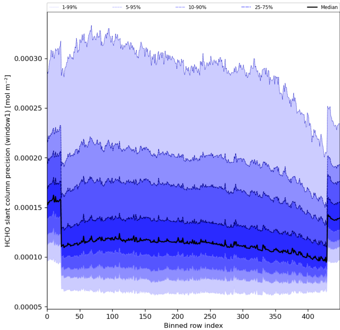
Figure 53: Along track statistics of “HCHO slant column precision (window1)” for 2024-02-16 to 2024-02-17
