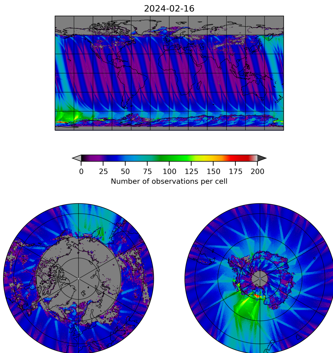
Figure 19: Map of the number of observations for 2024-02-16 to 2024-02-17
