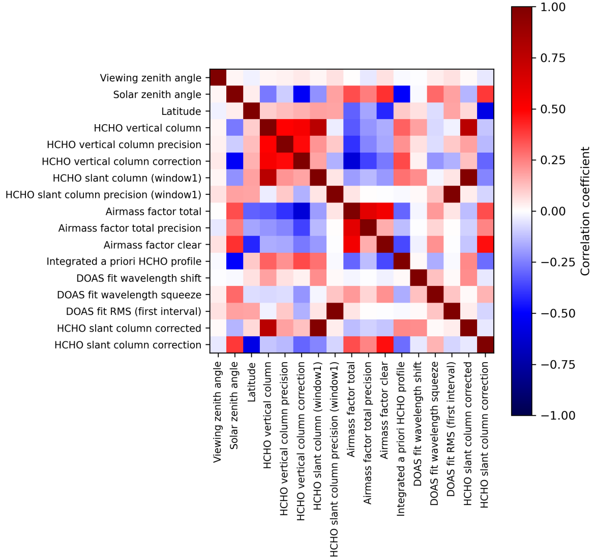
Figure 2: Map of correlation matrix for 2024-02-16 to 2024-02-17.
