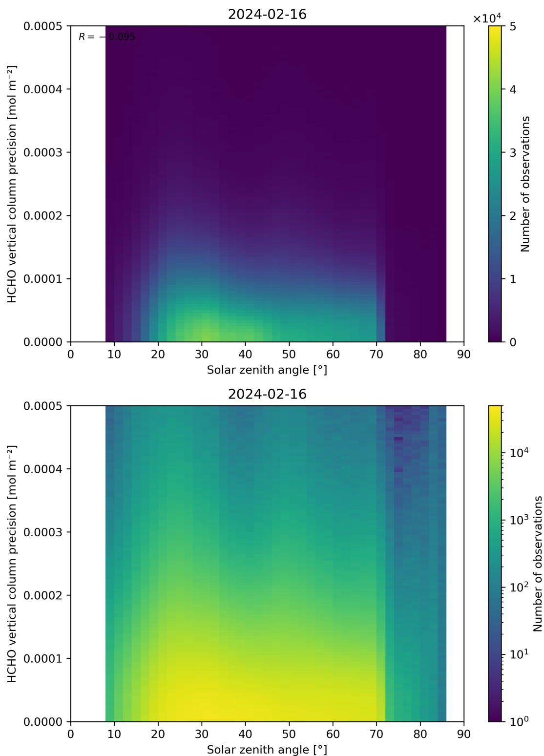
Figure 179: Scatter density plot of “Solar zenith angle” against “HCHO vertical column precision” for 2024-02-16 to 2024-02-17.
