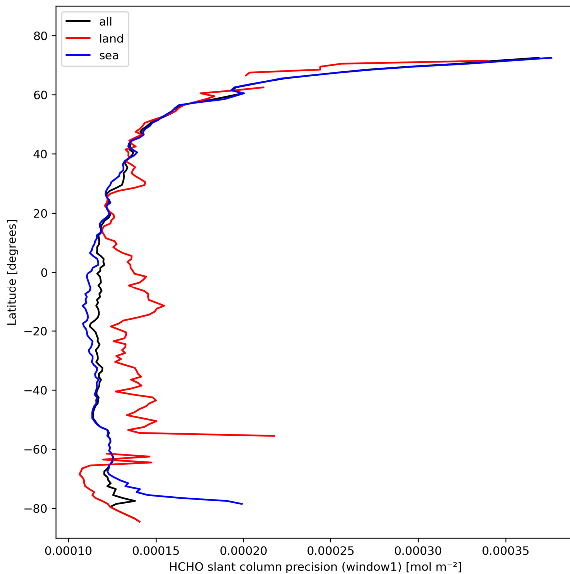
Figure 25: Zonal average of “HCHO slant column precision (window1)” for 2024-02-16 to 2024-02-17.
