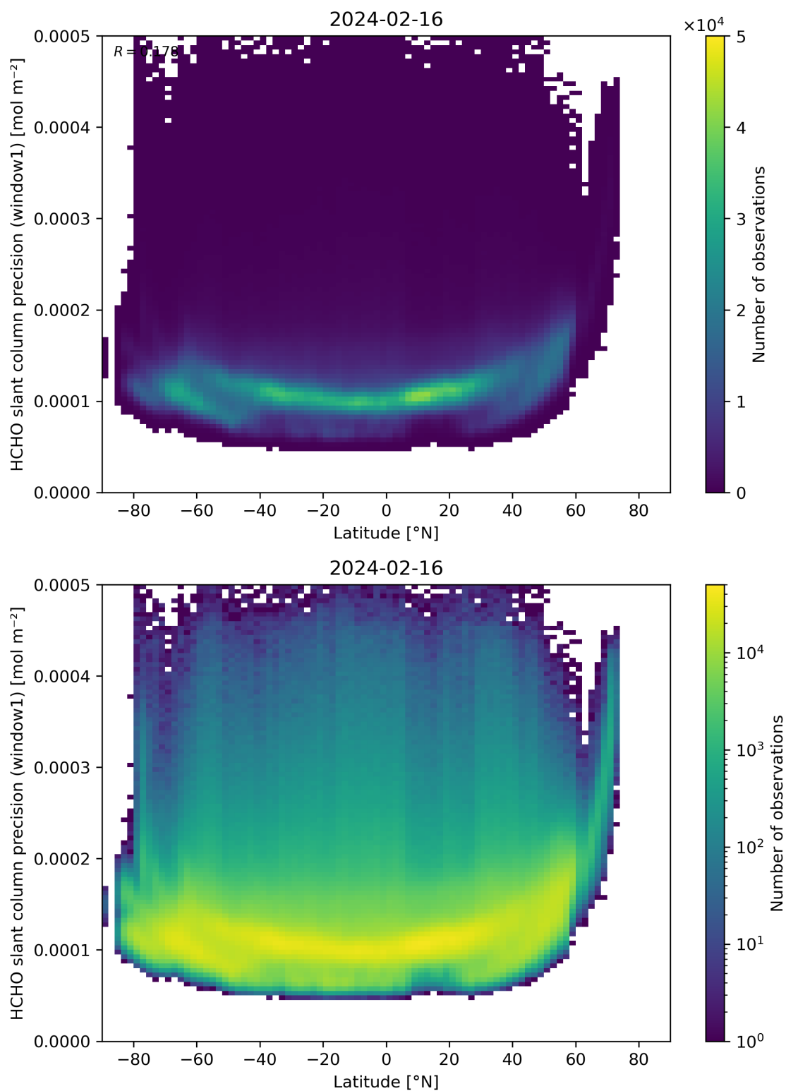
Figure 160: Scatter density plot of “Latitude” against “HCHO slant column precision (window1)” for 2024-02-16 to 2024-02-17.
