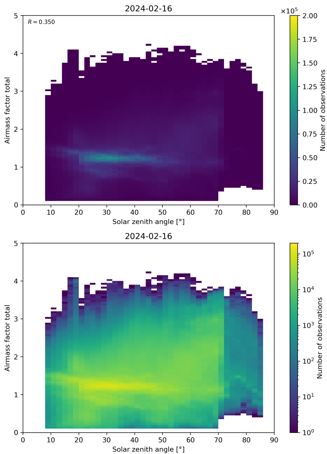
Figure 175: Scatter density plot of “Solar zenith angle” against “Airmass factor total” for 2024-02-16 to 2024-02-17.
