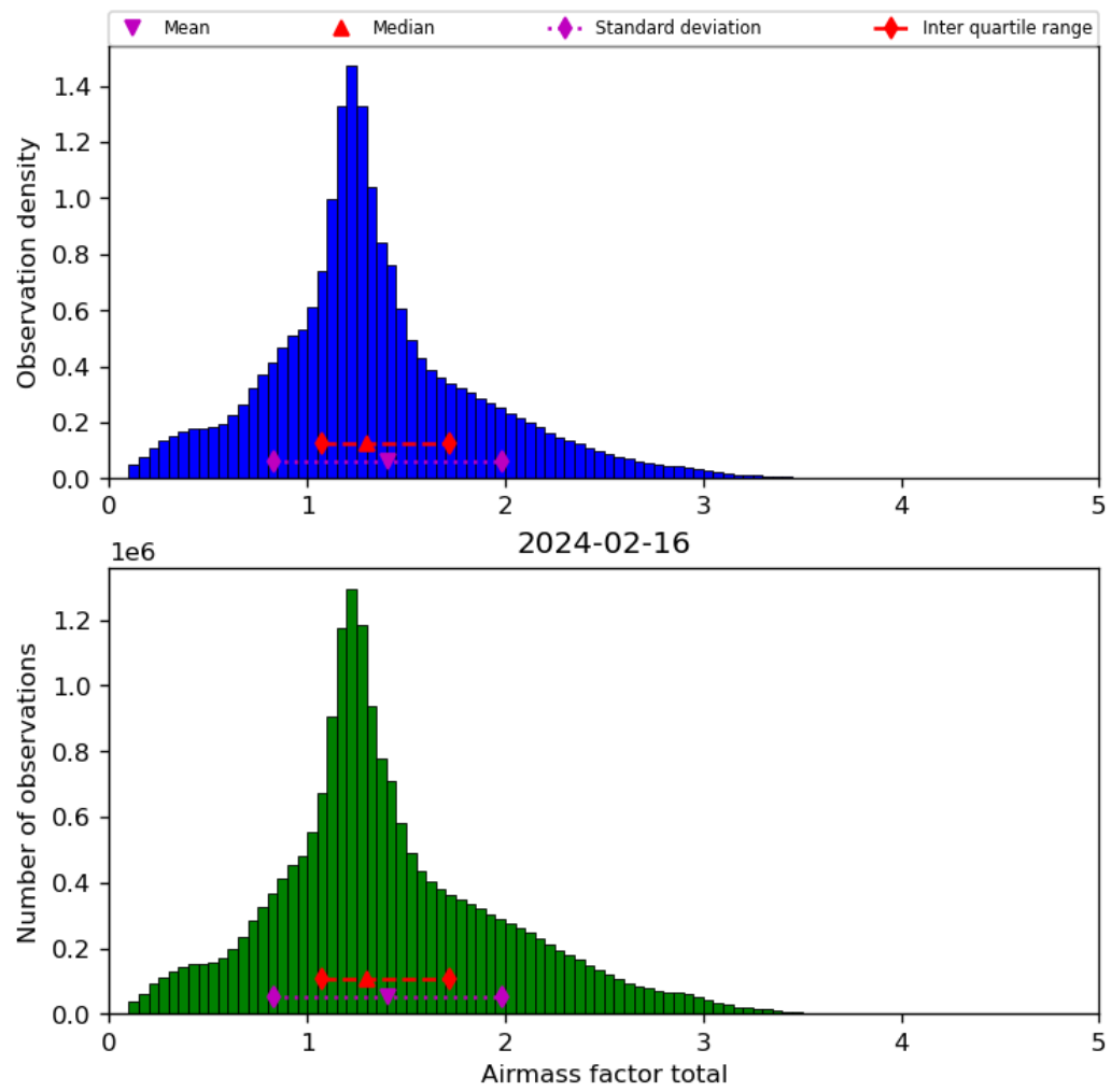
Figure 40: Histogram of “Airmass factor total” for 2024-02-16 to 2024-02-17
