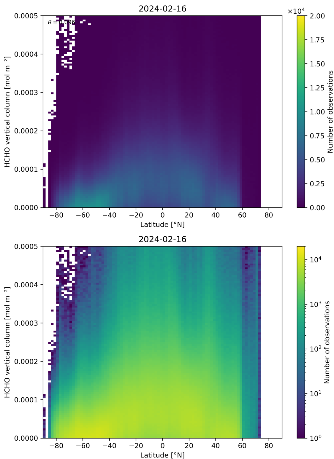
Figure 163: Scatter density plot of “Latitude” against “HCHO vertical column” for 2024-02-16 to 2024-02-17.
