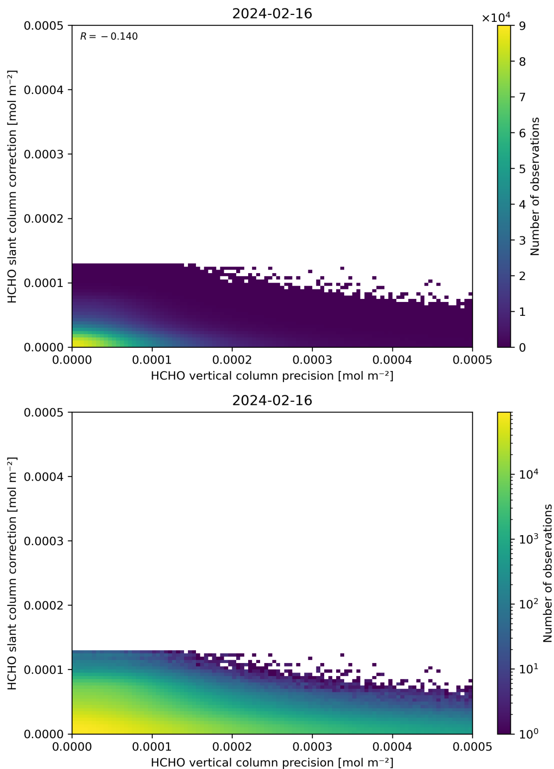
Figure 141: Scatter density plot of “HCHO vertical column precision” against “HCHO slant column correction” for 2024-02-16 to 2024-02-17.
