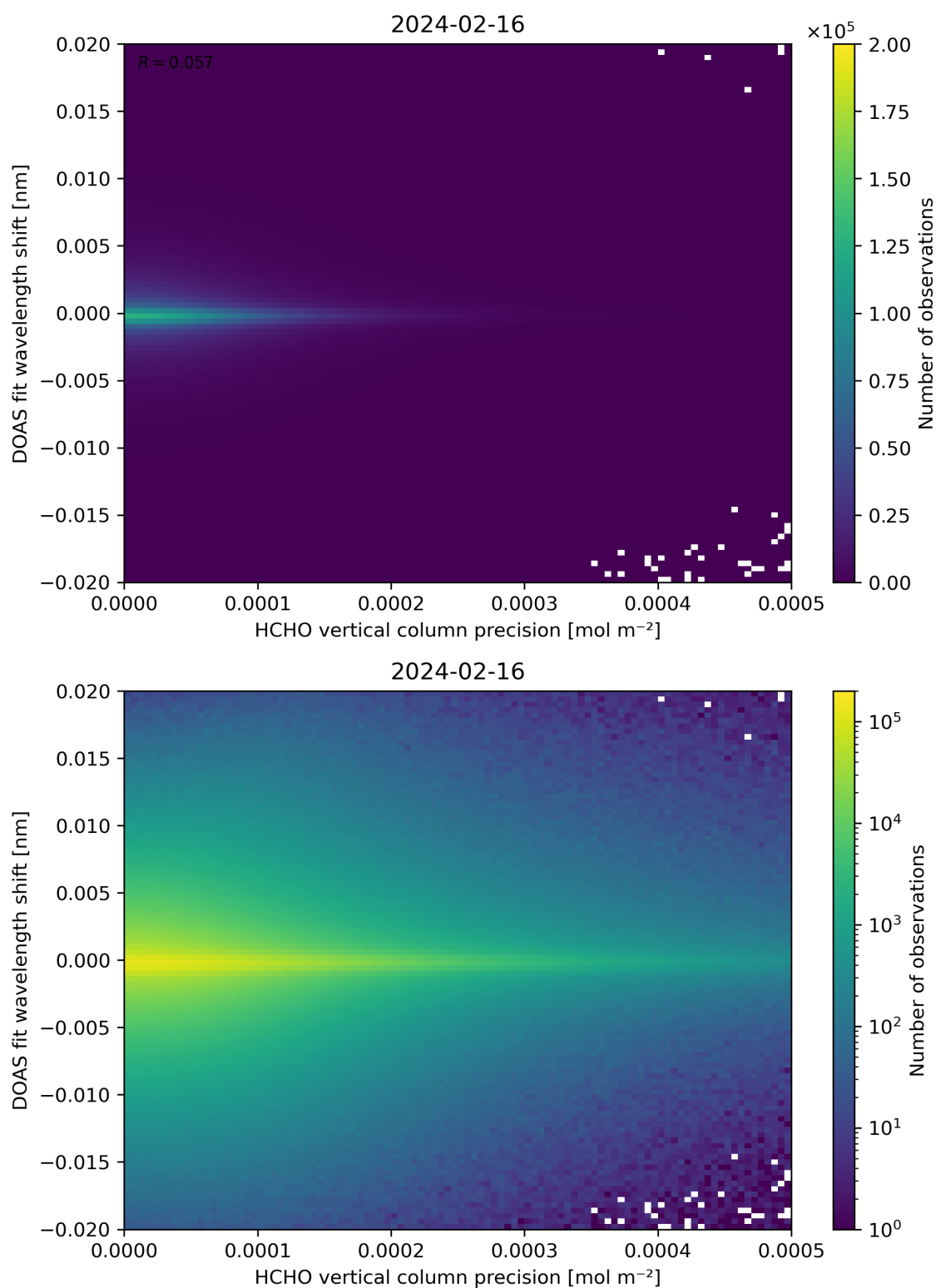
Figure 137: Scatter density plot of “HCHO vertical column precision” against “DOAS fit wavelength shift” for 2024-02-16 to 2024-02-17.
