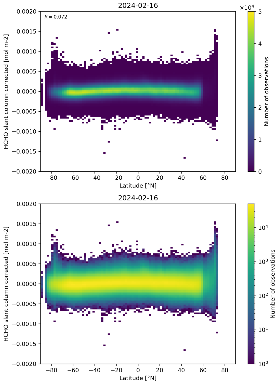
Figure 157: Scatter density plot of “Latitude” against “HCHO slant column corrected” for 2024-02-16 to 2024-02-17.
