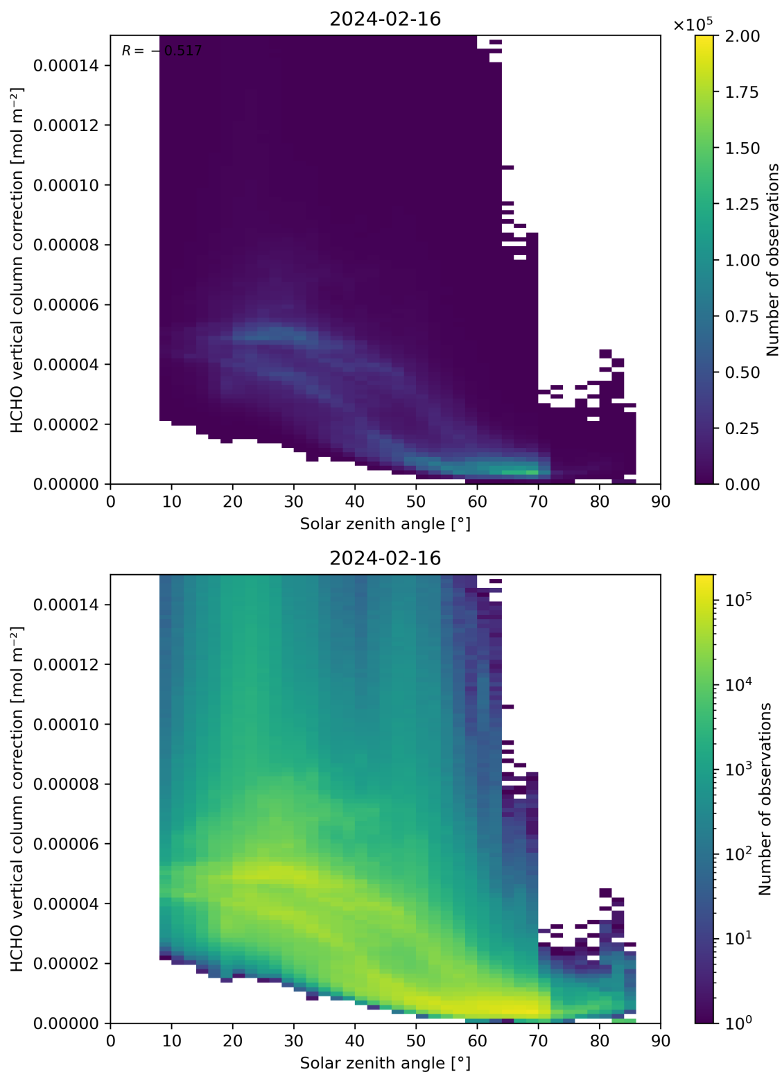
Figure 178: Scatter density plot of “Solar zenith angle” against “HCHO vertical column correction” for 2024-02-16 to 2024-02-17.
