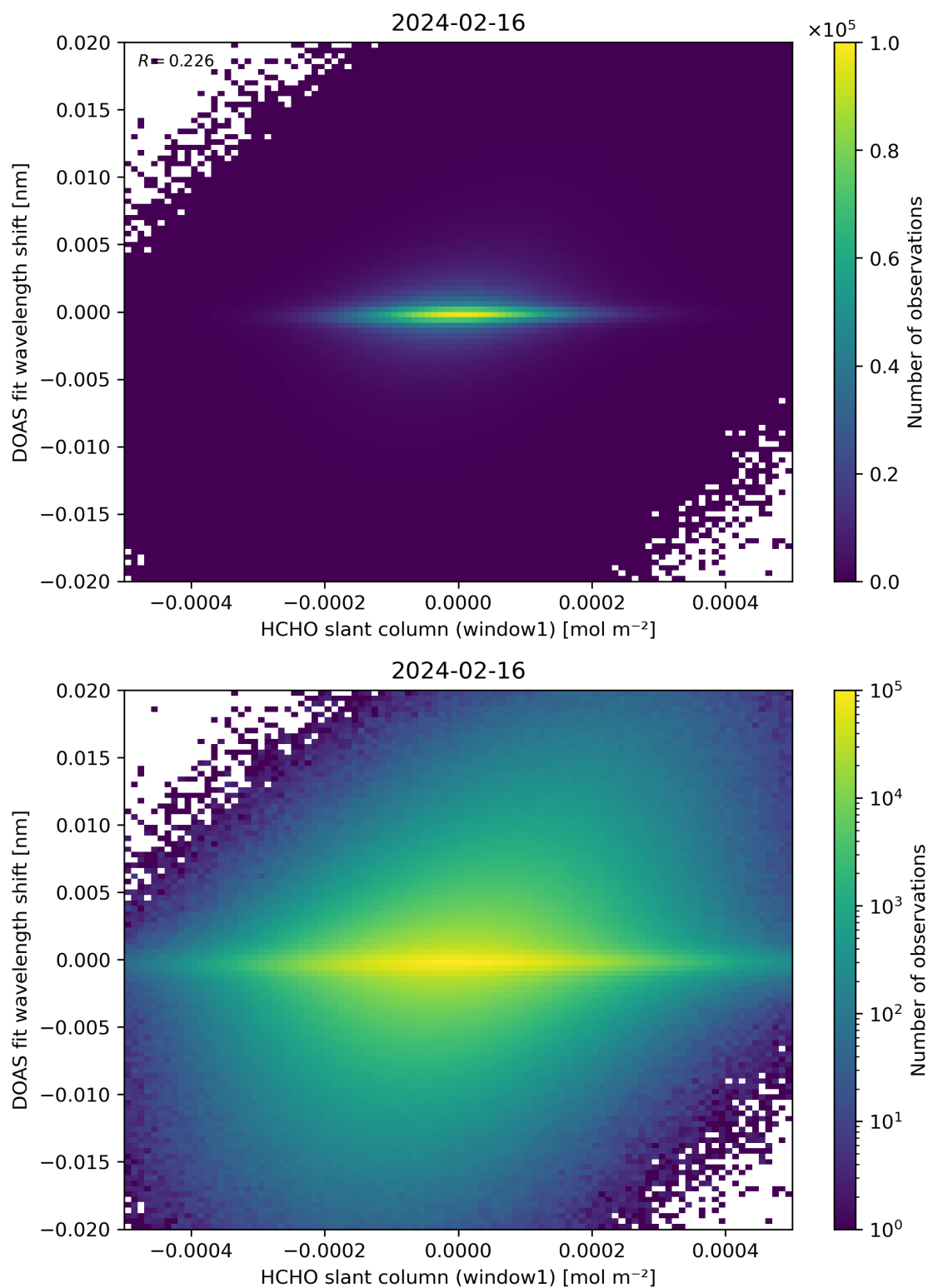
Figure 79: Scatter density plot of “HCHO slant column (window1)” against “DOAS fit wavelength shift” for 2024-02-16 to 2024-02-17.
