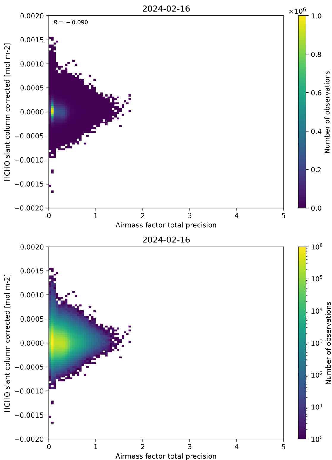
Figure 109: Scatter density plot of “Airmass factor total precision” against “HCHO slant column corrected” for 2024-02-16 to 2024-02-17.
