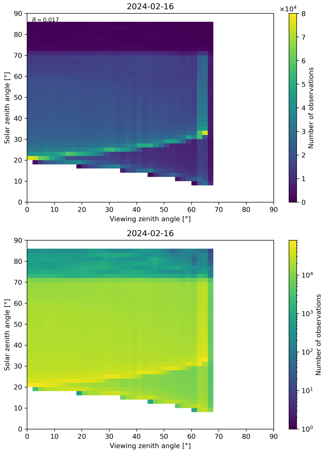
Figure 197: Scatter density plot of “Viewing zenith angle” against “Solar zenith angle” for 2024-02-16 to 2024-02-17.
