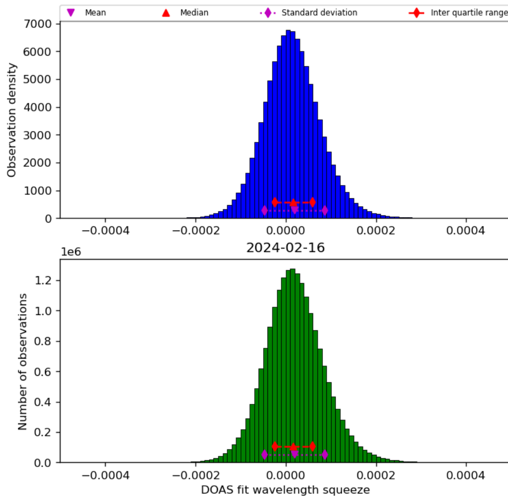
Figure 45: Histogram of “DOAS fit wavelength squeeze” for 2024-02-16 to 2024-02-17
