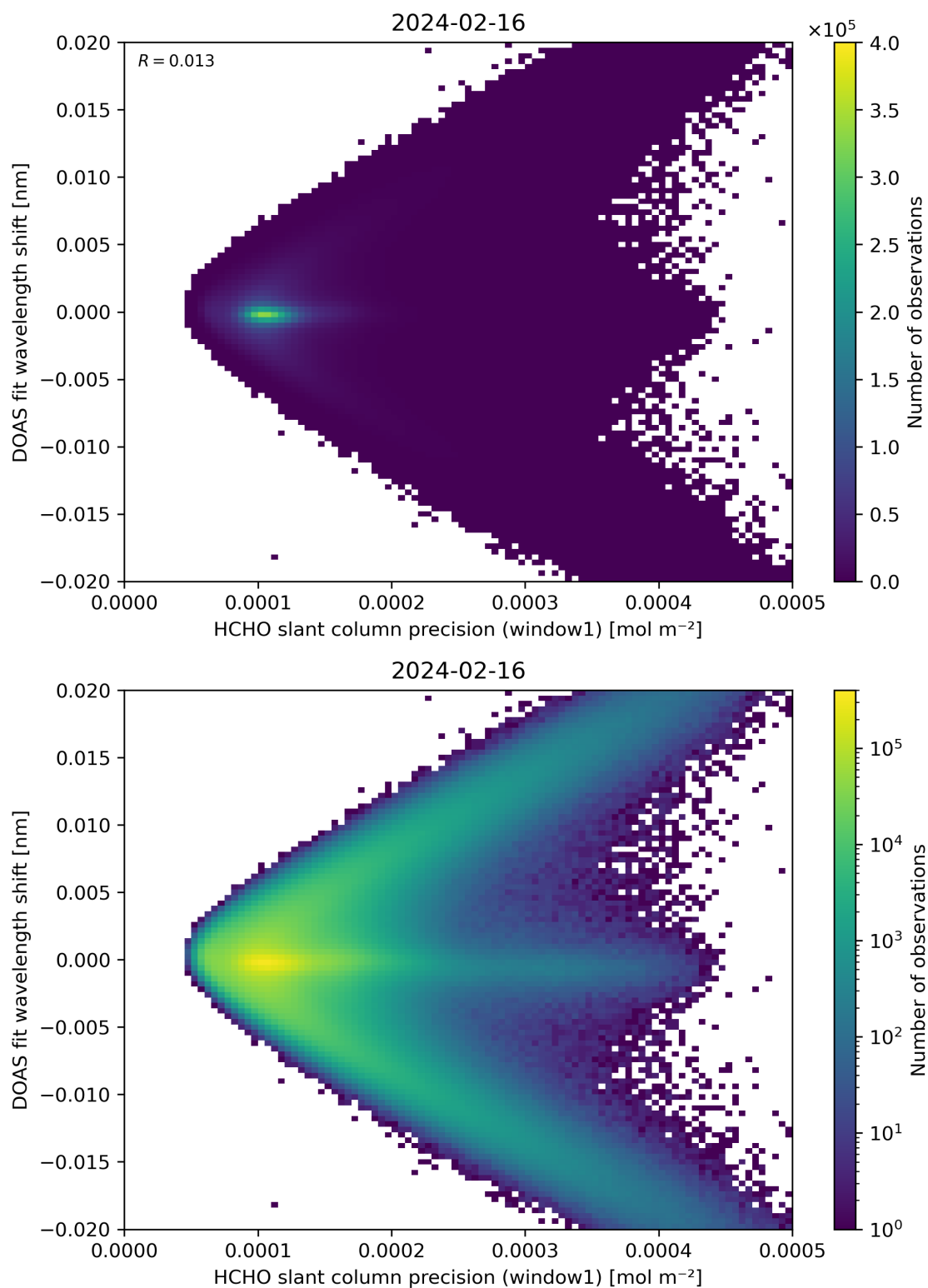
Figure 89: Scatter density plot of “HCHO slant column precision (window1)” against “DOAS fit wavelength shift” for 2024-02-16 to 2024-02-17.
