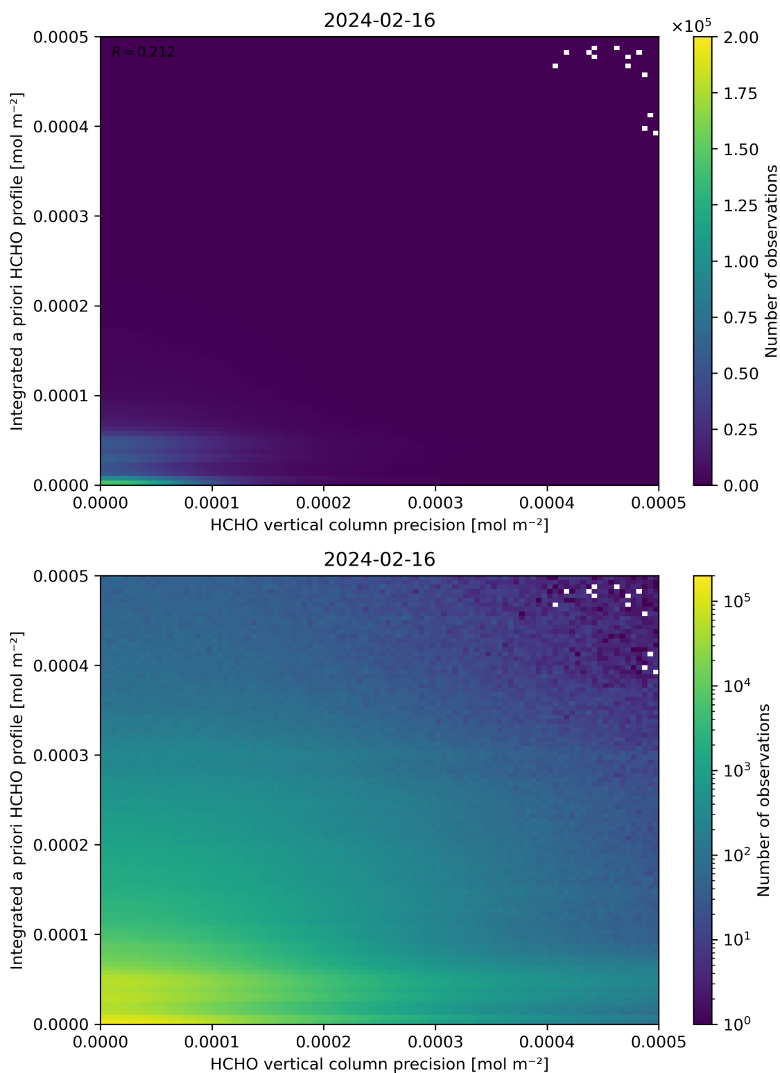
Figure 147: Scatter density plot of “HCHO vertical column precision” against “Integrated a priori HCHO profile” for 2024-02-16 to 2024-02-17.
