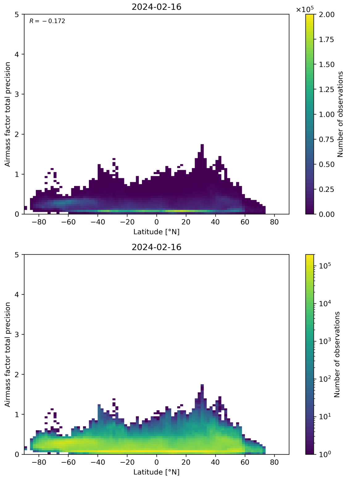
Figure 162: Scatter density plot of “Latitude” against “Airmass factor total precision” for 2024-02-16 to 2024-02-17.
