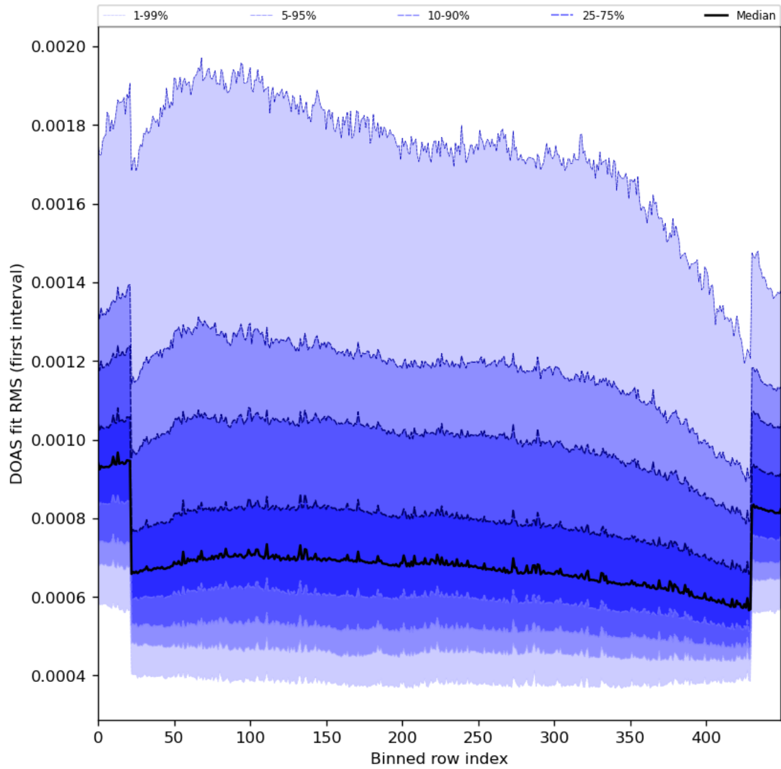
Figure 60: Along track statistics of “DOAS fit RMS (first interval)” for 2024-02-16 to 2024-02-17
