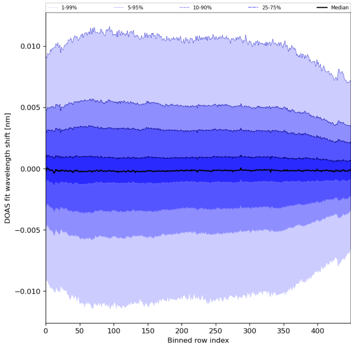
Figure 58: Along track statistics of “DOAS fit wavelength shift” for 2024-02-16 to 2024-02-17
