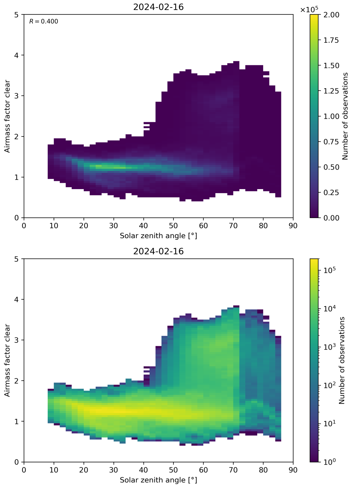
Figure 170: Scatter density plot of “Solar zenith angle” against “Airmass factor clear” for 2024-02-16 to 2024-02-17.
