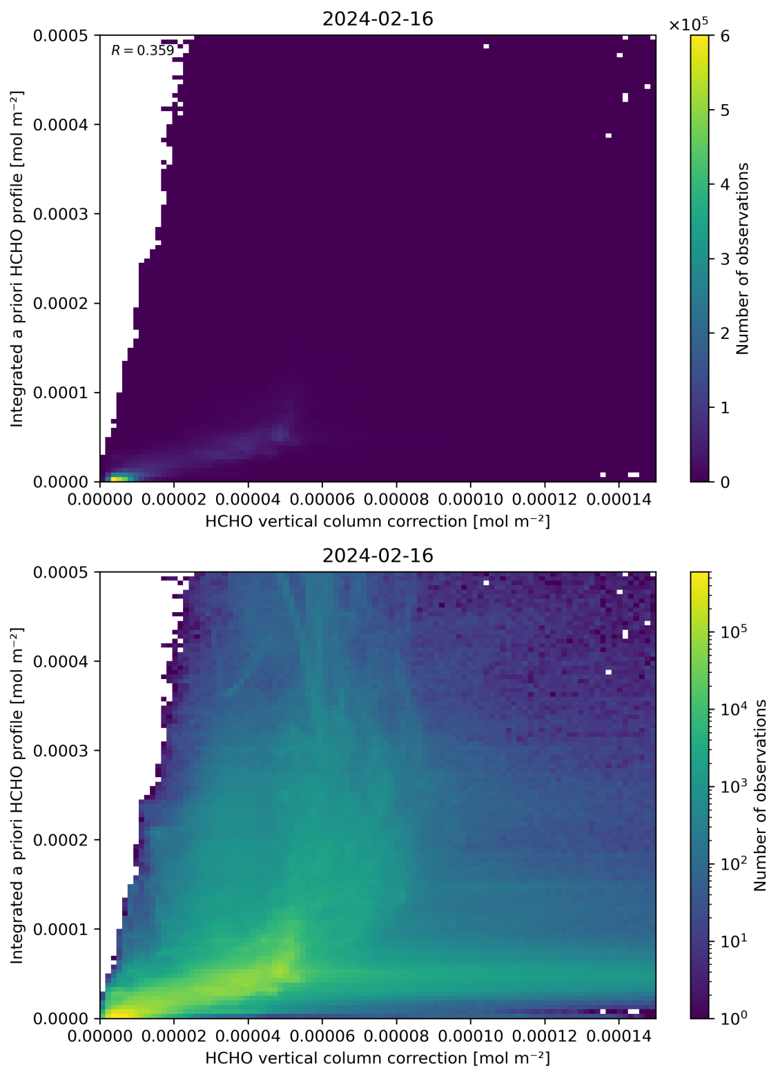
Figure 122: Scatter density plot of “HCHO vertical column correction” against “Integrated a priori HCHO profile” for 2024-02-16 to 2024-02-17.
