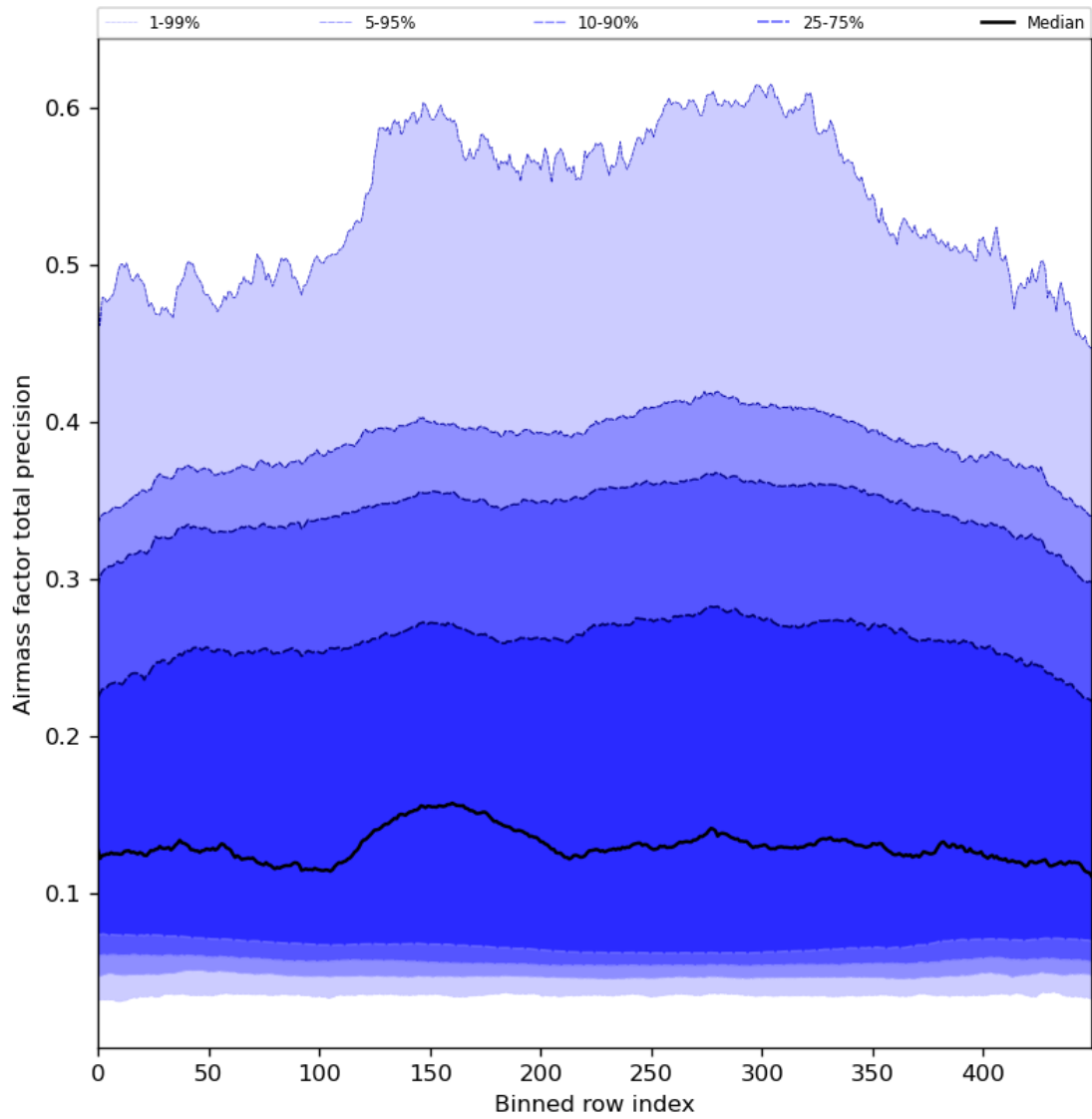
Figure 55: Along track statistics of “Airmass factor total precision” for 2024-02-16 to 2024-02-17
