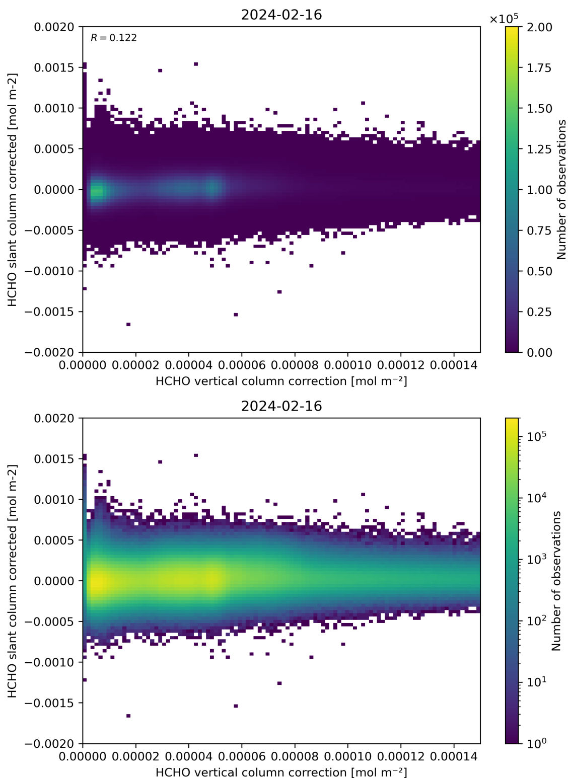
Figure 116: Scatter density plot of “HCHO vertical column correction” against “HCHO slant column corrected” for 2024-02-16 to 2024-02-17.
