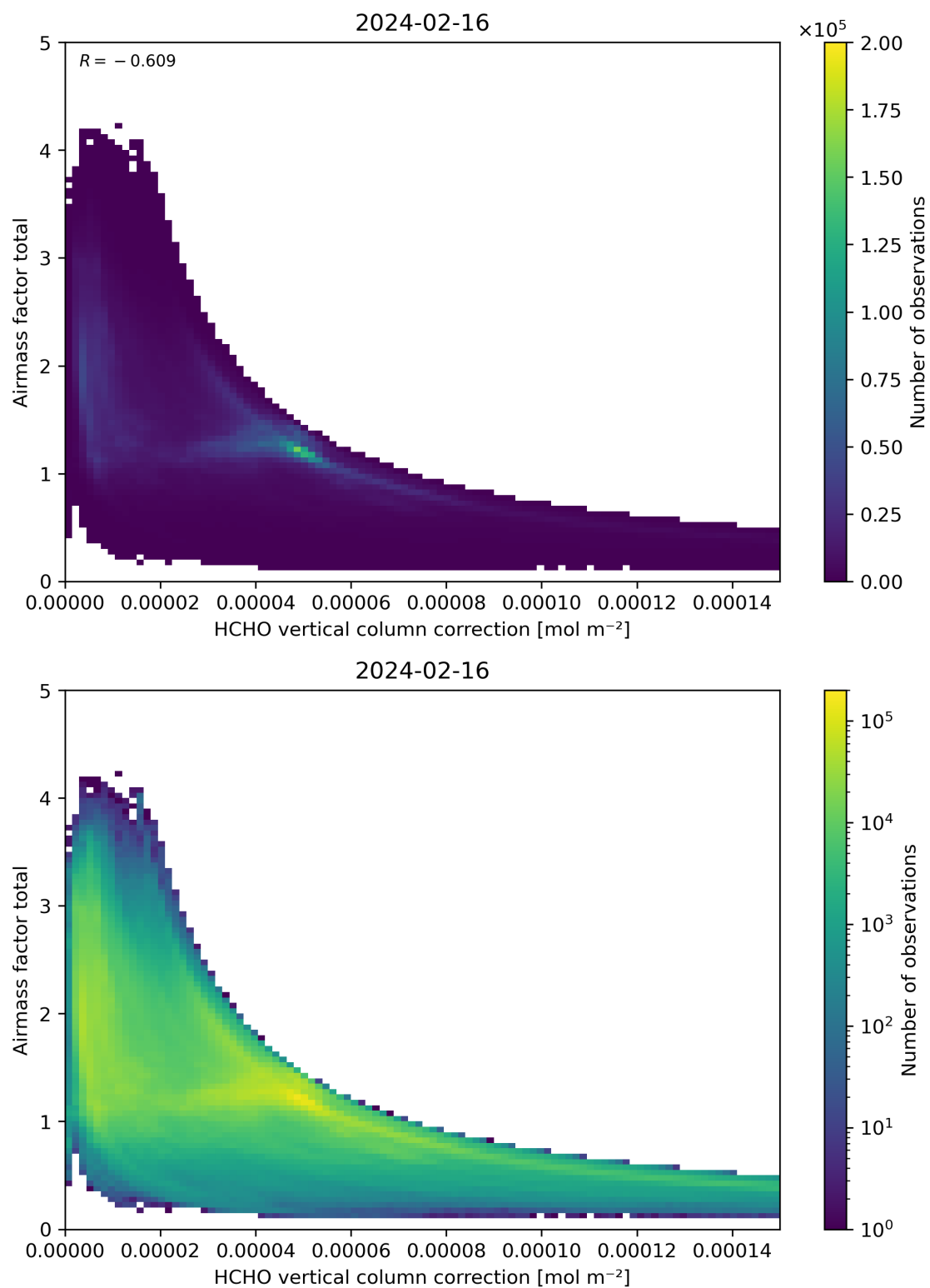
Figure 120: Scatter density plot of “HCHO vertical column correction” against “Airmass factor total” for 2024-02-16 to 2024-02-17.
