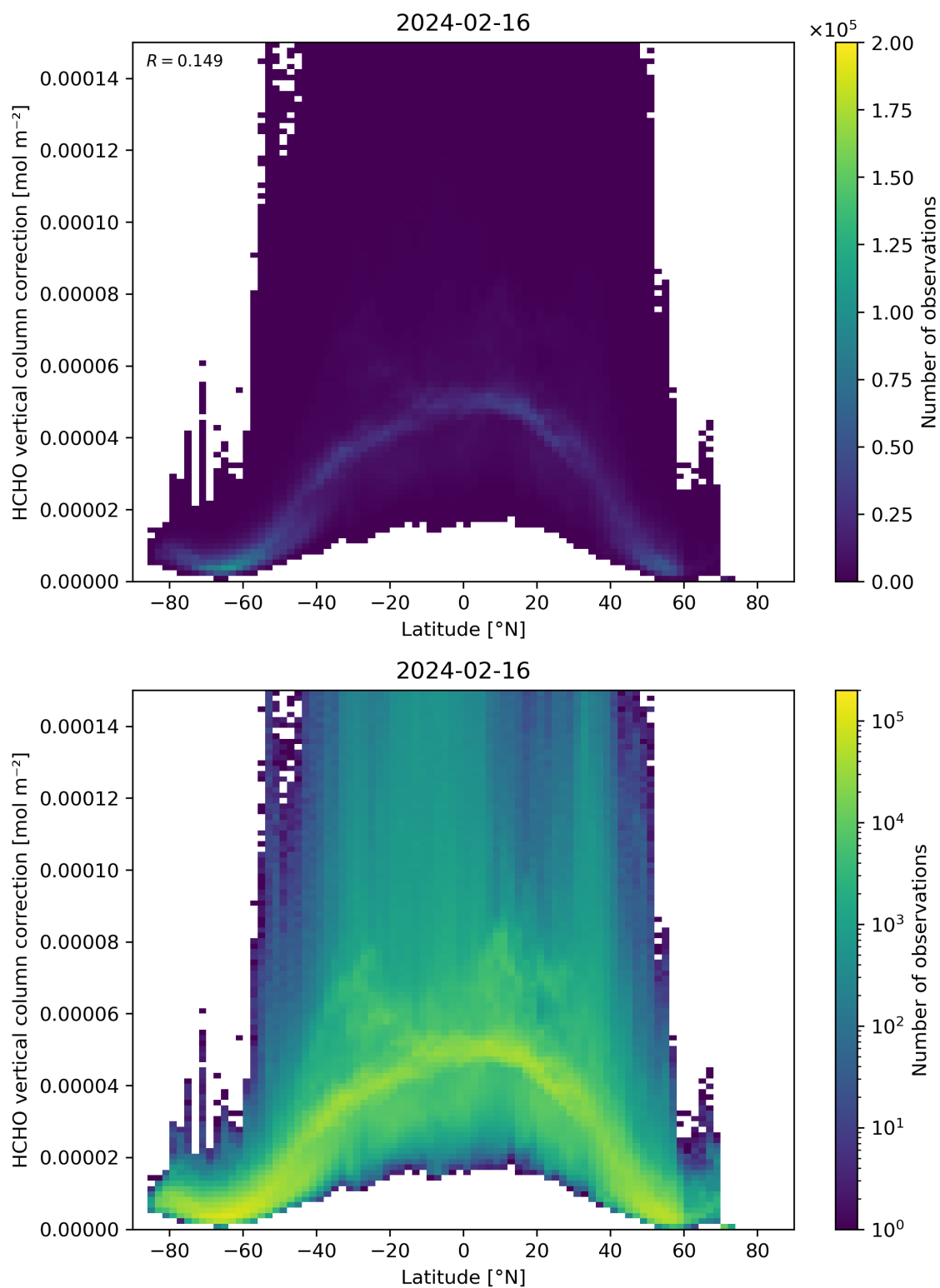
Figure 164: Scatter density plot of “Latitude” against “HCHO vertical column correction” for 2024-02-16 to 2024-02-17.
