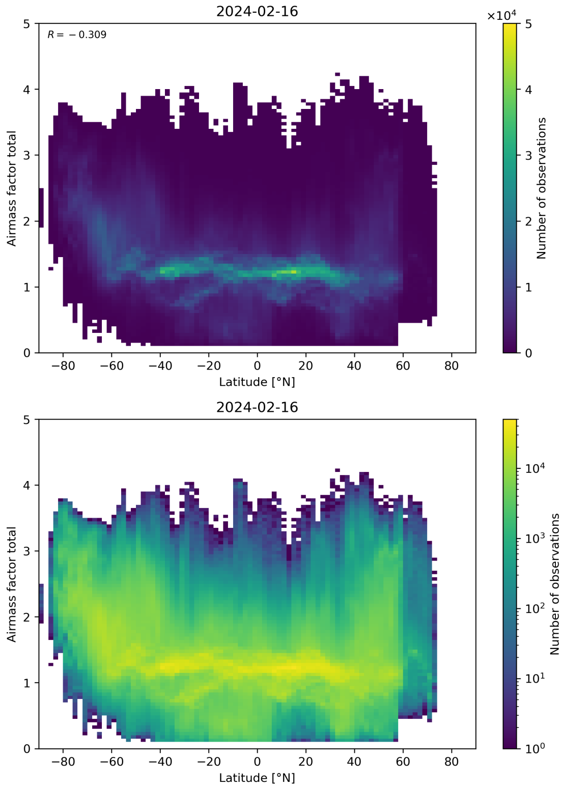
Figure 161: Scatter density plot of “Latitude” against “Airmass factor total” for 2024-02-16 to 2024-02-17.
