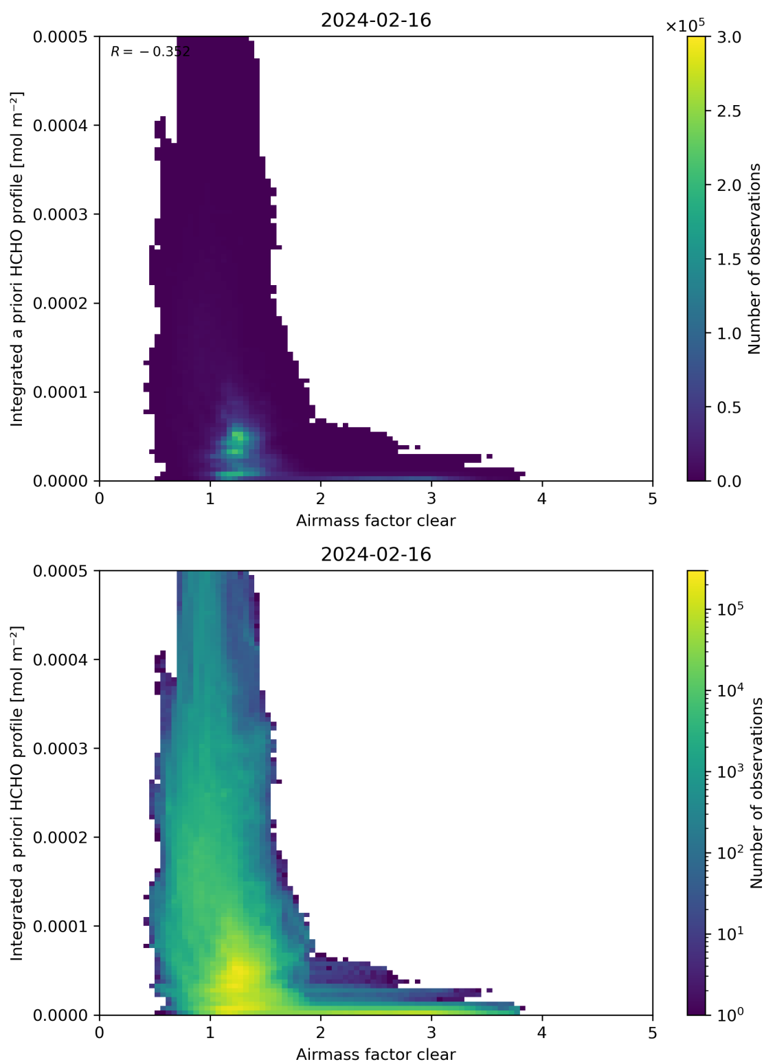
Figure 76: Scatter density plot of “Airmass factor clear” against “Integrated a priori HCHO profile” for 2024-02-16 to 2024-02-17.
