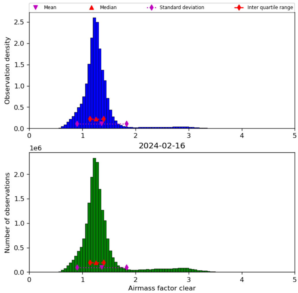
Figure 42: Histogram of “Airmass factor clear” for 2024-02-16 to 2024-02-17
