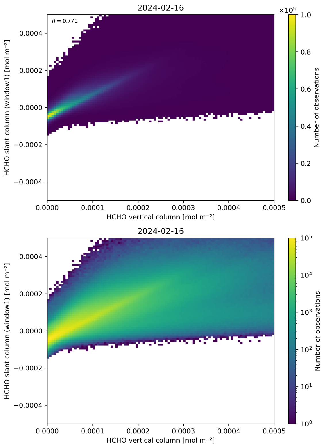
Figure 129: Scatter density plot of “HCHO vertical column” against “HCHO slant column (window1)” for 2024-02-16 to 2024-02-17.
