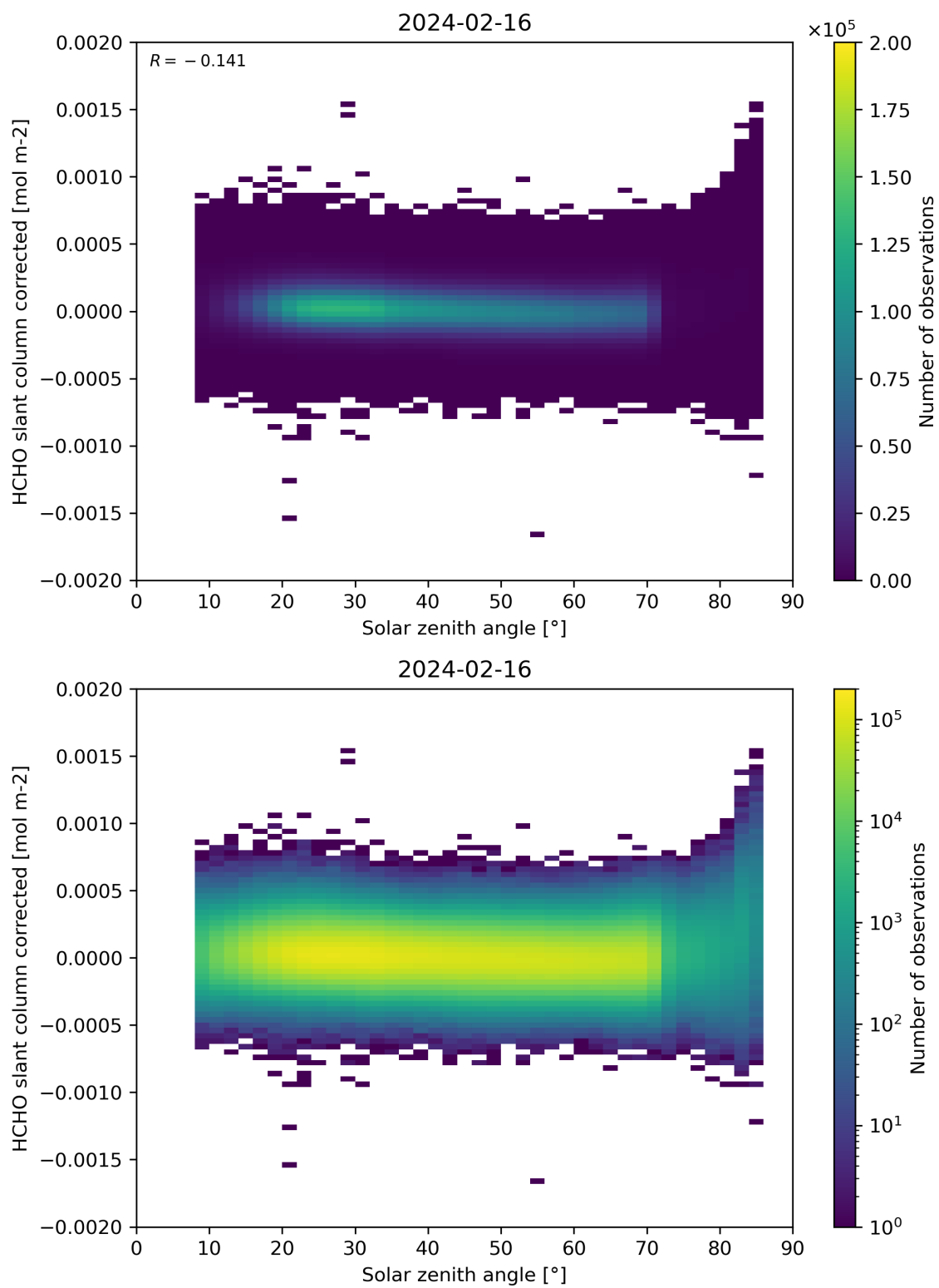
Figure 171: Scatter density plot of “Solar zenith angle” against “HCHO slant column corrected” for 2024-02-16 to 2024-02-17.
