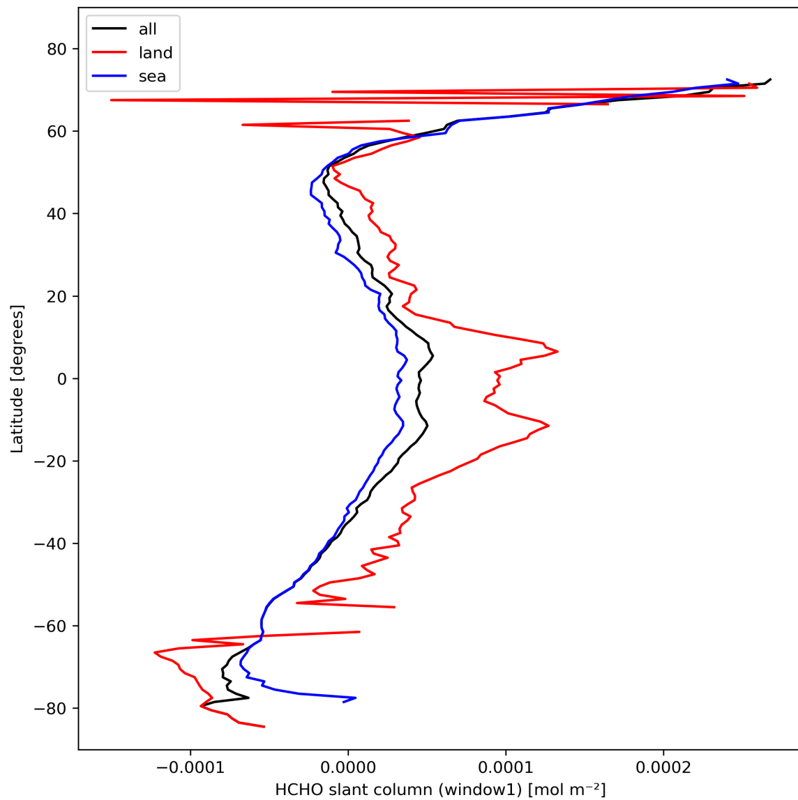
Figure 24: Zonal average of “HCHO slant column (window1)” for 2024-02-16 to 2024-02-17.
