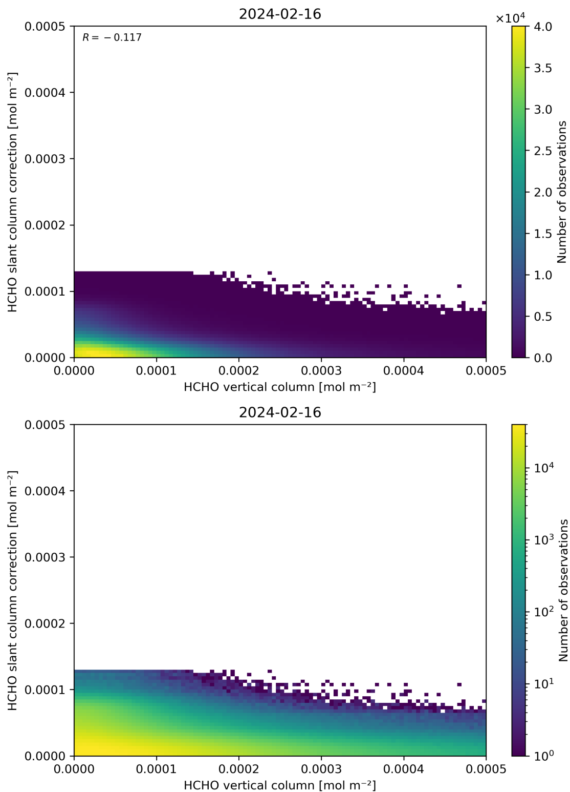
Figure 128: Scatter density plot of “HCHO vertical column” against “HCHO slant column correction” for 2024-02-16 to 2024-02-17.
