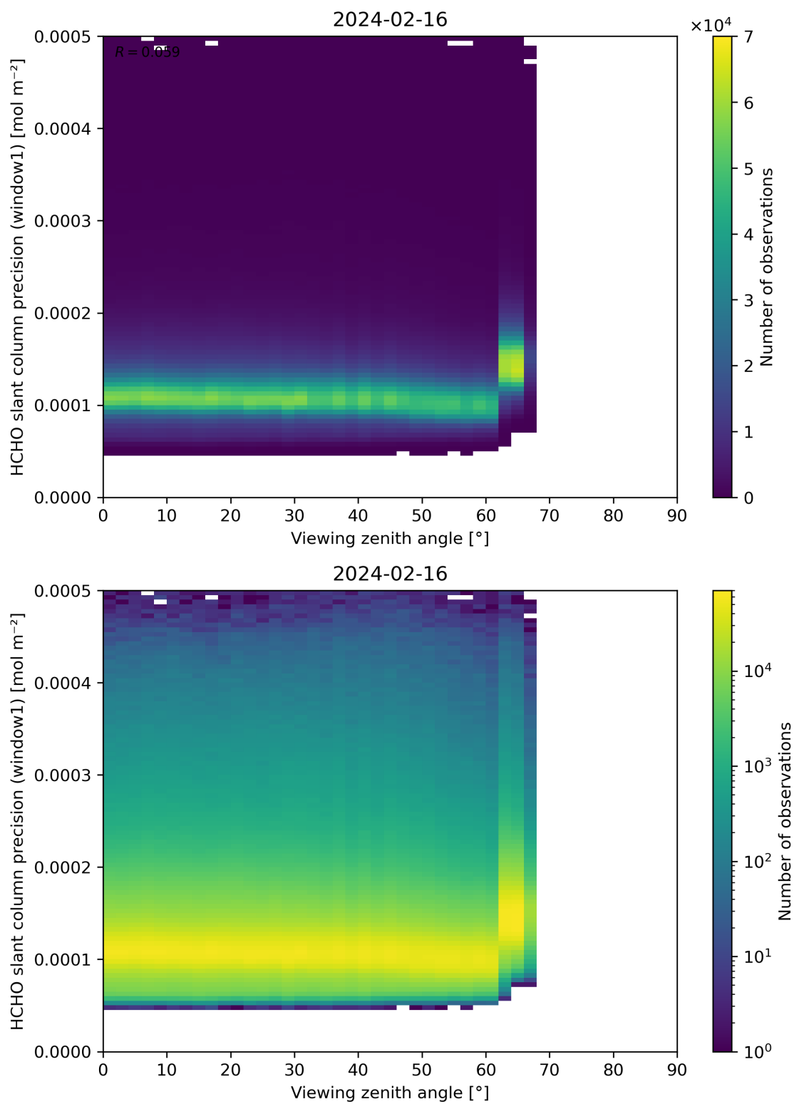
Figure 189: Scatter density plot of “Viewing zenith angle” against “HCHO slant column precision (window1)” for 2024-02-16 to 2024-02-17.
