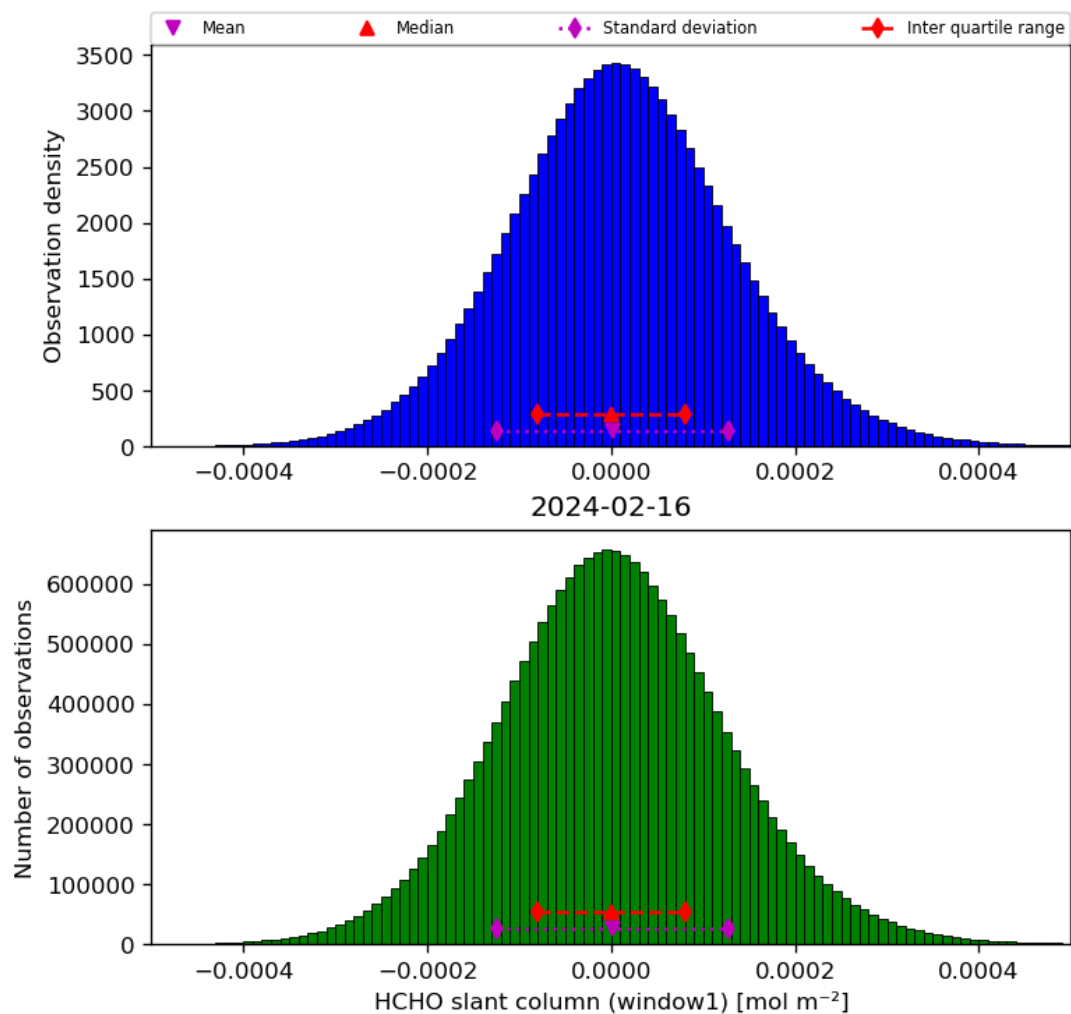
Figure 38: Histogram of “HCHO slant column (window1)” for 2024-02-16 to 2024-02-17
