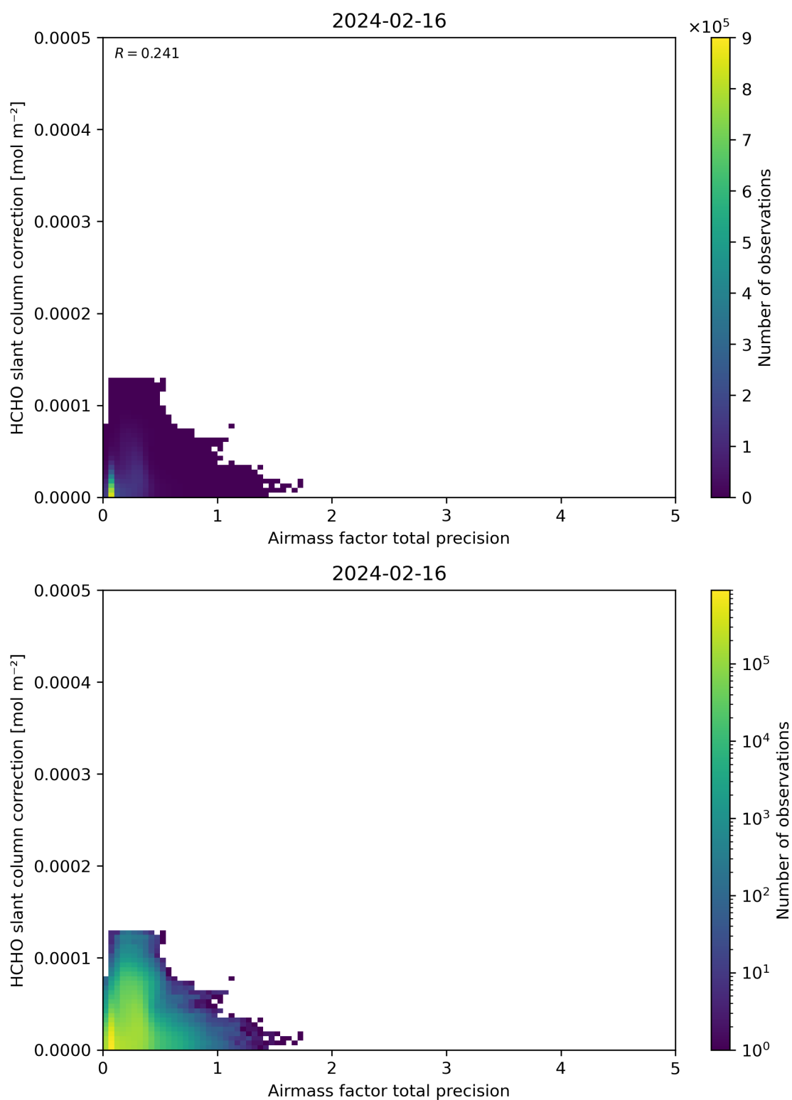
Figure 110: Scatter density plot of “Airmass factor total precision” against “HCHO slant column correction” for 2024-02-16 to 2024-02-17.
