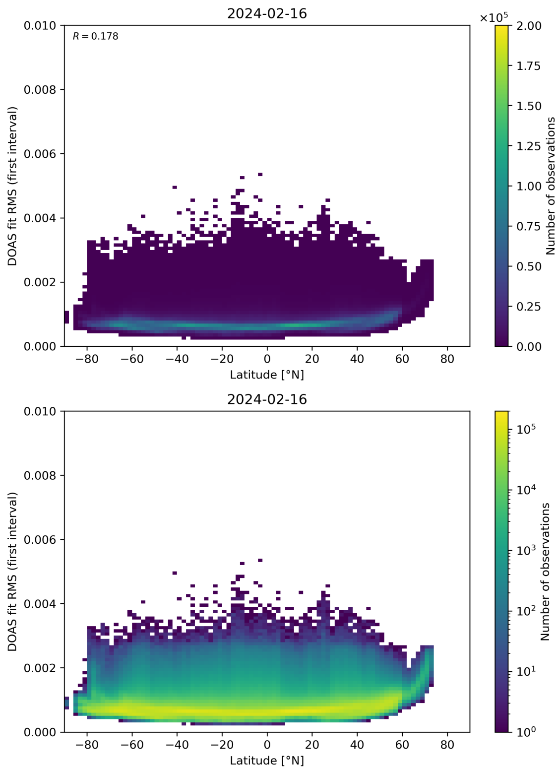
Figure 153: Scatter density plot of “Latitude” against “DOAS fit RMS (first interval)” for 2024-02-16 to 2024-02-17.
