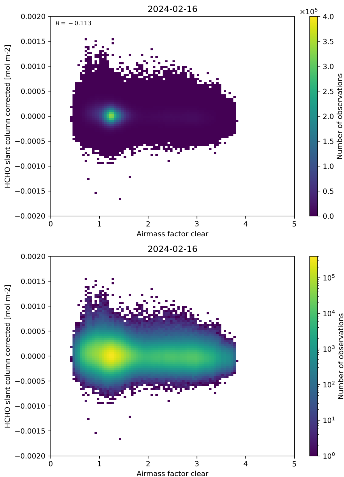
Figure 74: Scatter density plot of “Airmass factor clear” against “HCHO slant column corrected” for 2024-02-16 to 2024-02-17.
