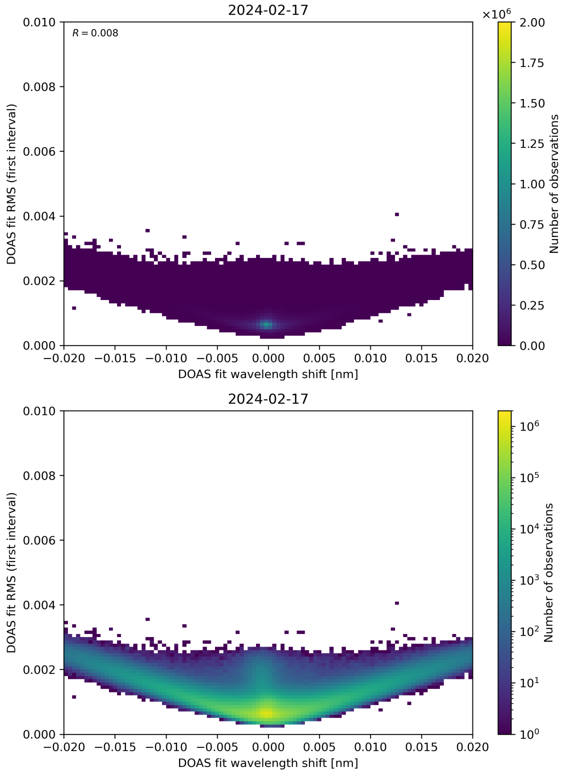
Figure 64: Scatter density plot of “DOAS fit wavelength shift” against “DOAS fit RMS (first interval)” for 2024-02-17 to 2024-02-18.
