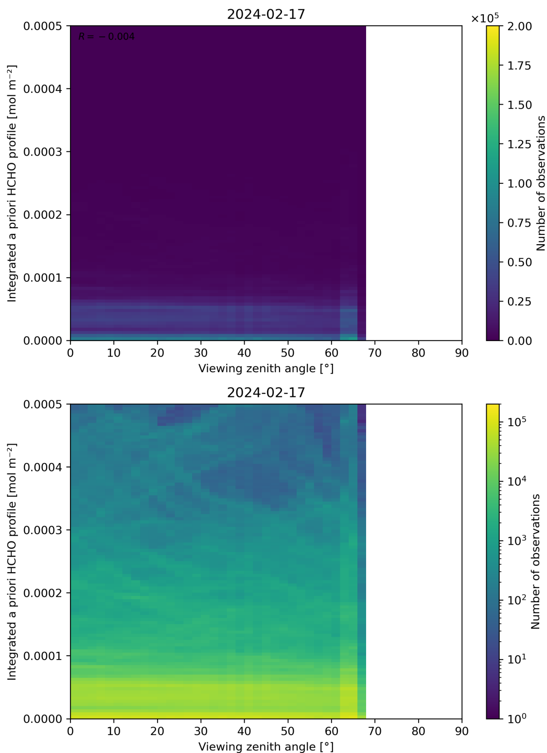
Figure 195: Scatter density plot of “Viewing zenith angle” against “Integrated a priori HCHO profile” for 2024-02-17 to 2024-02-18.
