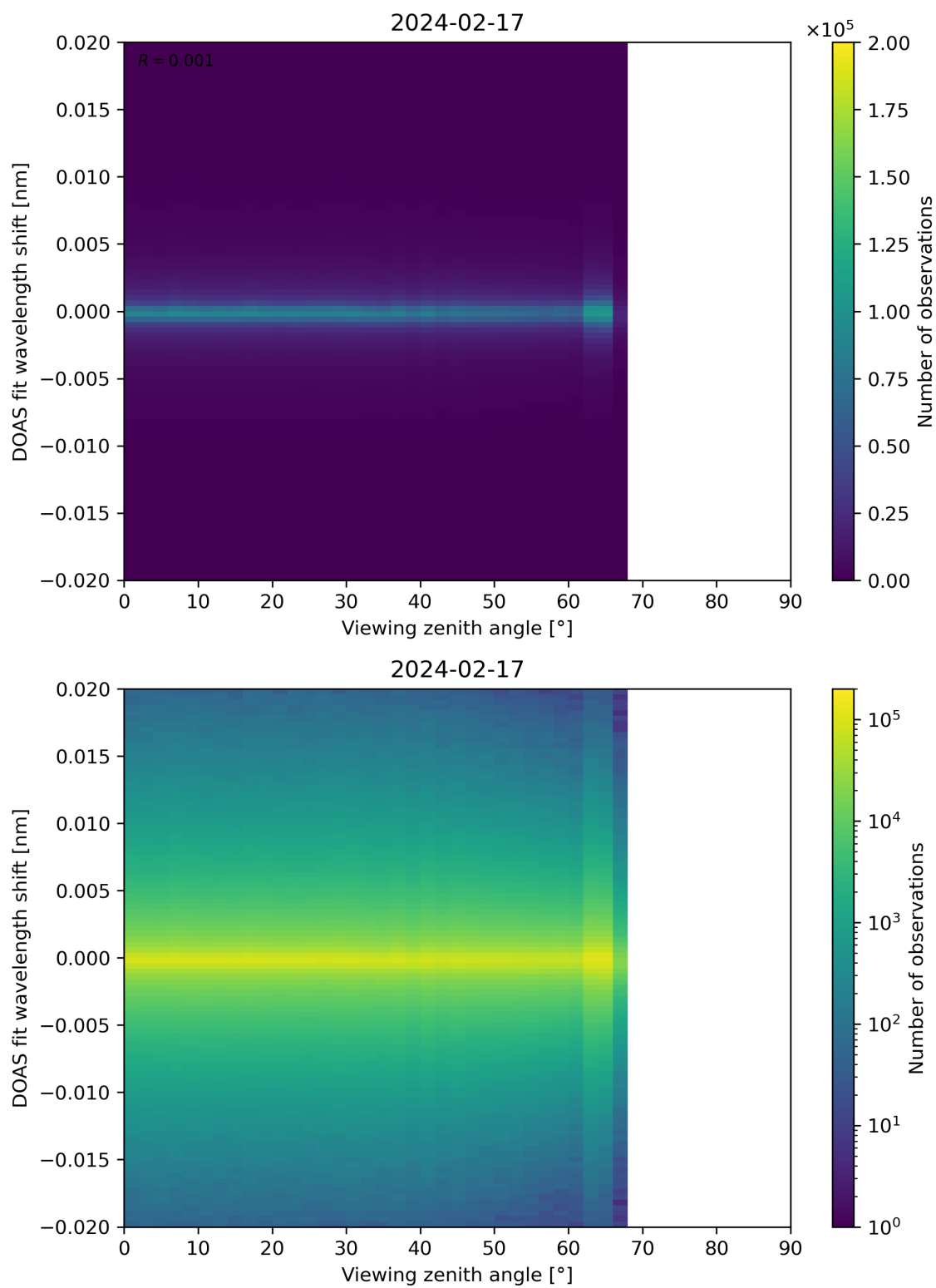
Figure 183: Scatter density plot of “Viewing zenith angle” against “DOAS fit wavelength shift” for 2024-02-17 to 2024-02-18.
