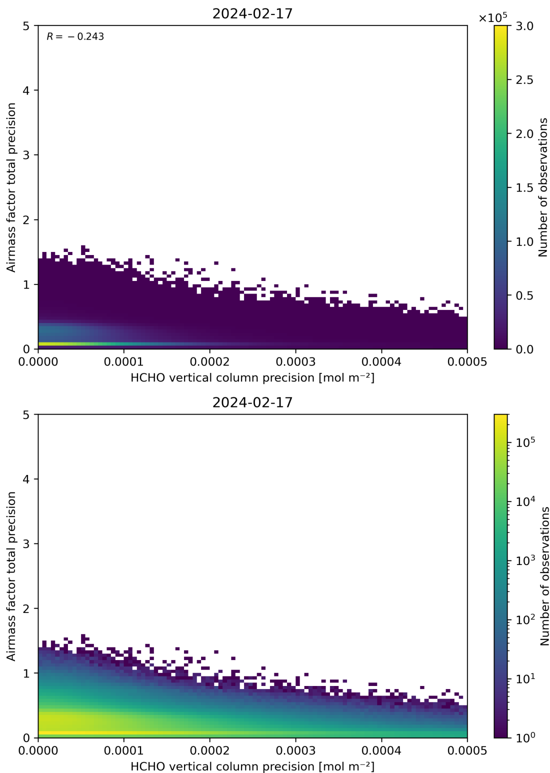
Figure 145: Scatter density plot of “HCHO vertical column precision” against “Airmass factor total precision” for 2024-02-17 to 2024-02-18.
