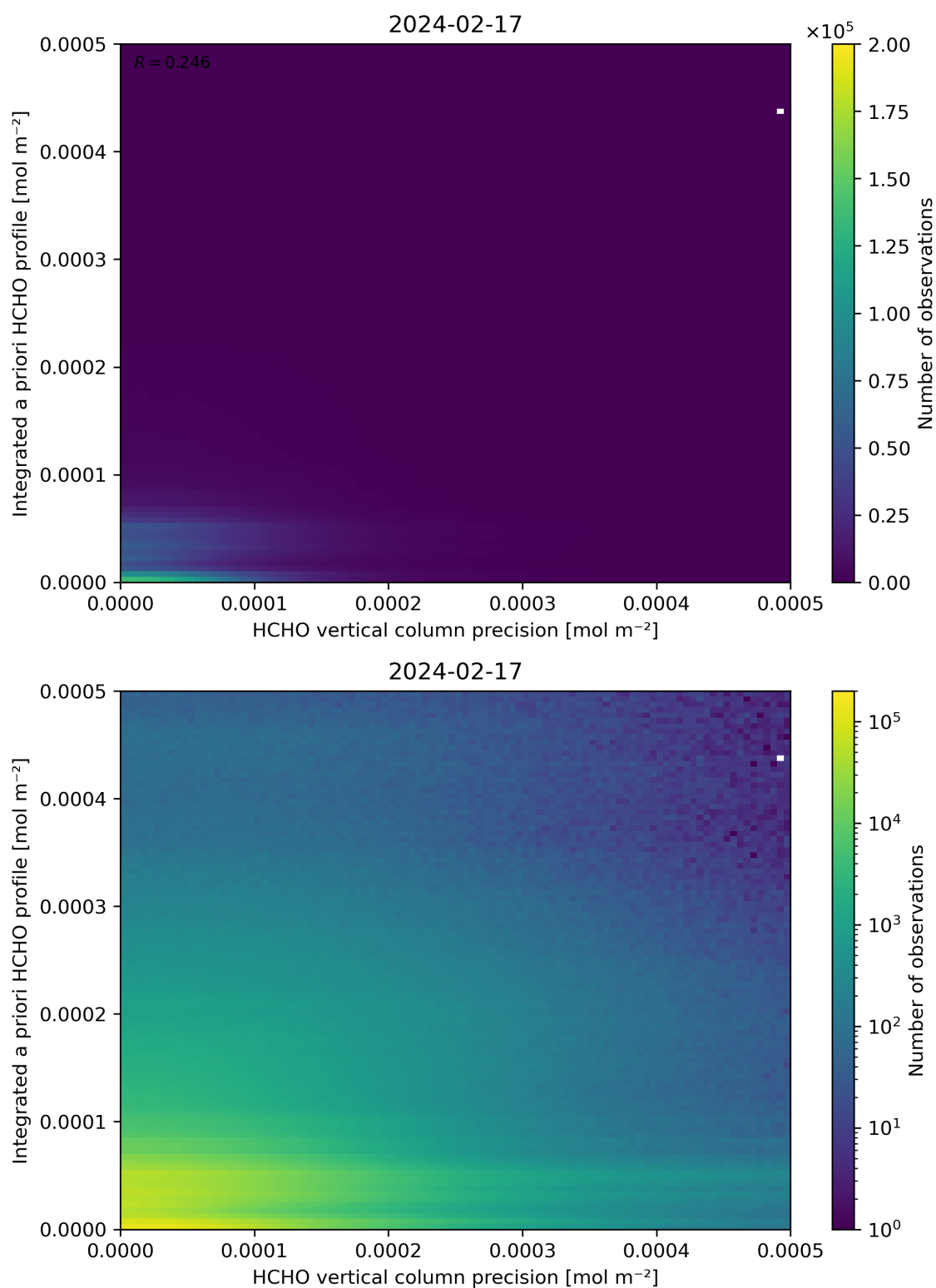
Figure 147: Scatter density plot of “HCHO vertical column precision” against “Integrated a priori HCHO profile” for 2024-02-17 to 2024-02-18.
