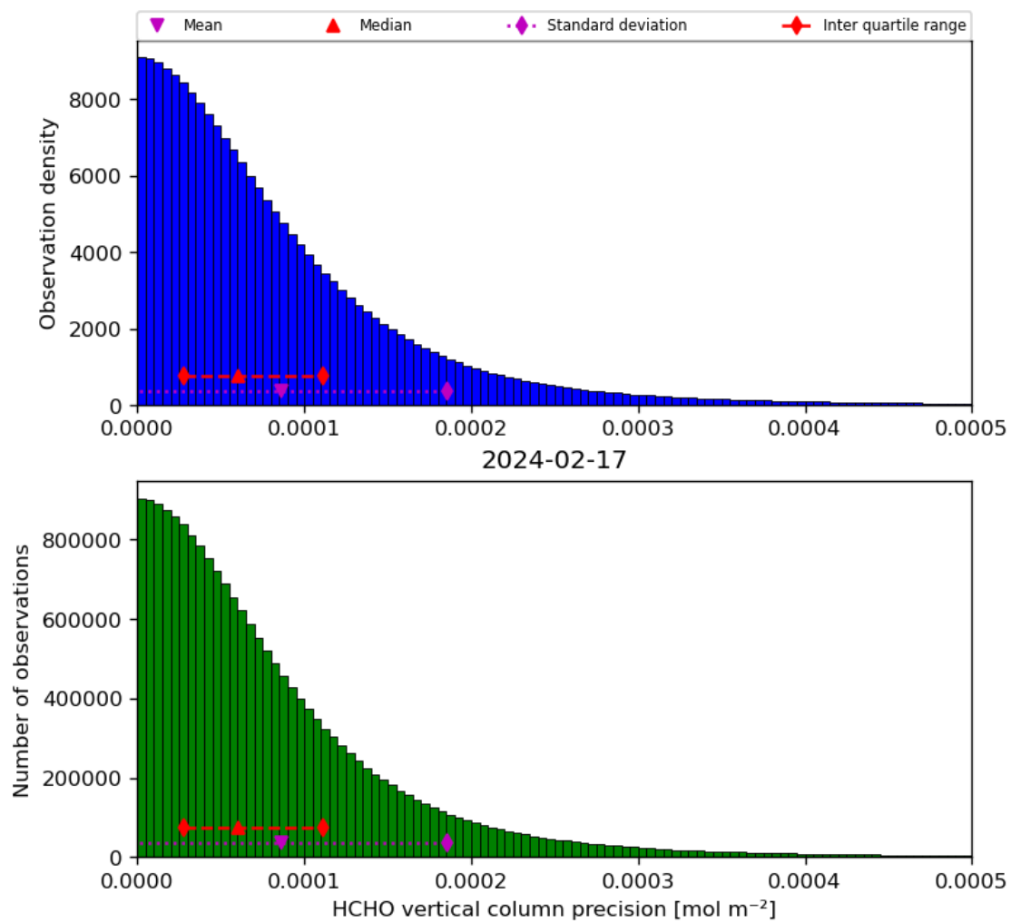
Figure 36: Histogram of “HCHO vertical column precision” for 2024-02-17 to 2024-02-18
