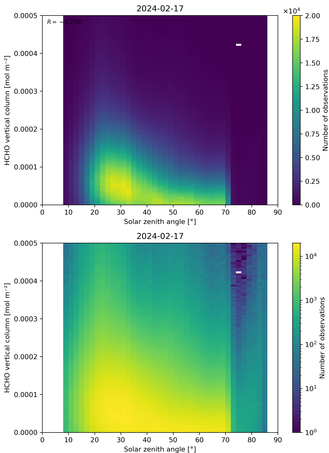
Figure 177: Scatter density plot of “Solar zenith angle” against “HCHO vertical column” for 2024-02-17 to 2024-02-18.
