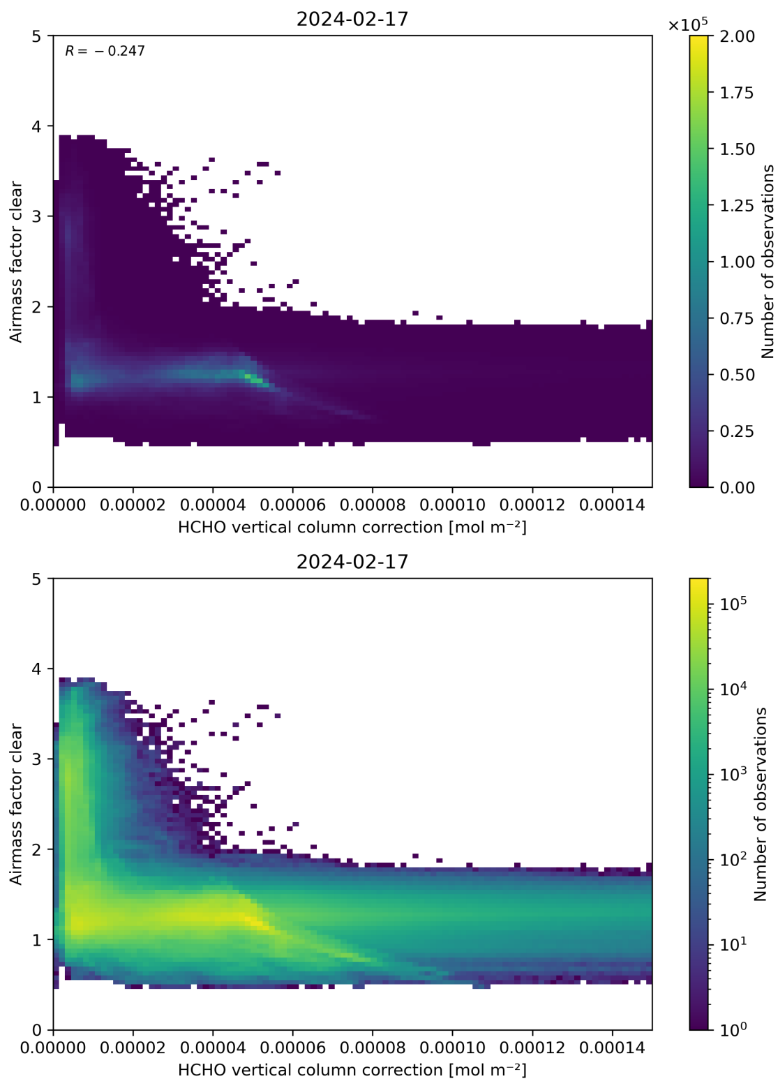
Figure 115: Scatter density plot of “HCHO vertical column correction” against “Airmass factor clear” for 2024-02-17 to 2024-02-18.
