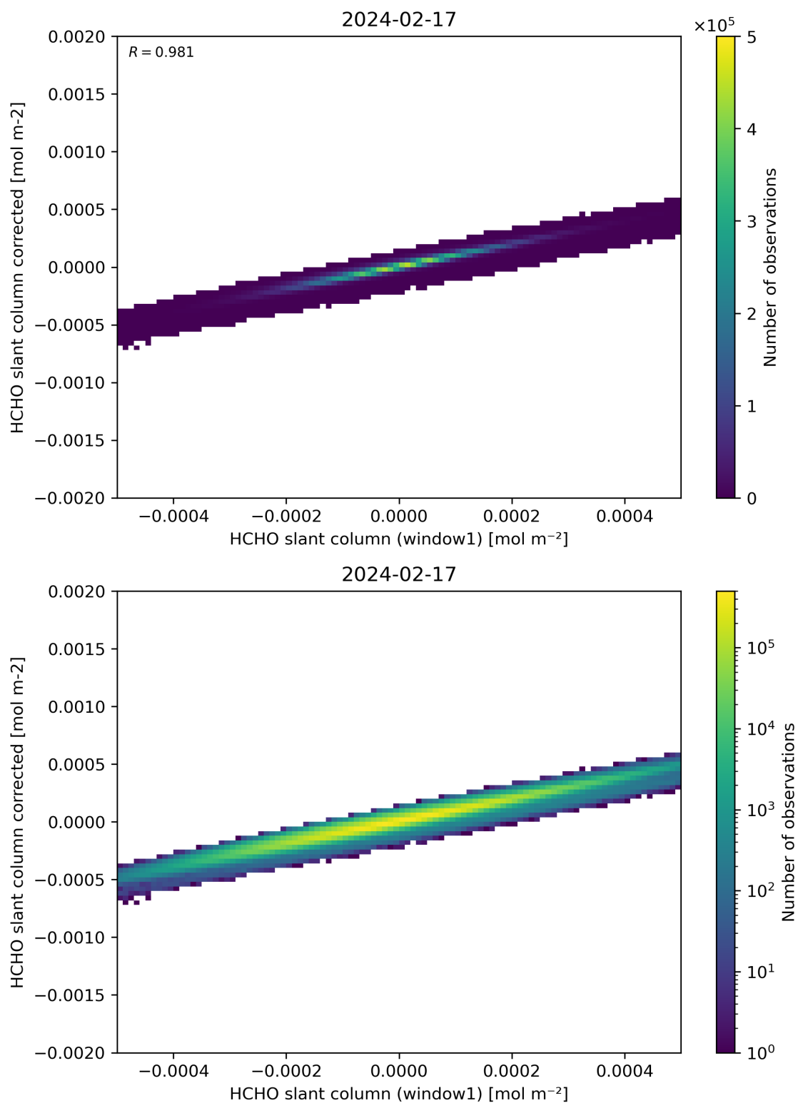
Figure 82: Scatter density plot of “HCHO slant column (window1)” against “HCHO slant column corrected” for 2024-02-17 to 2024-02-18.
