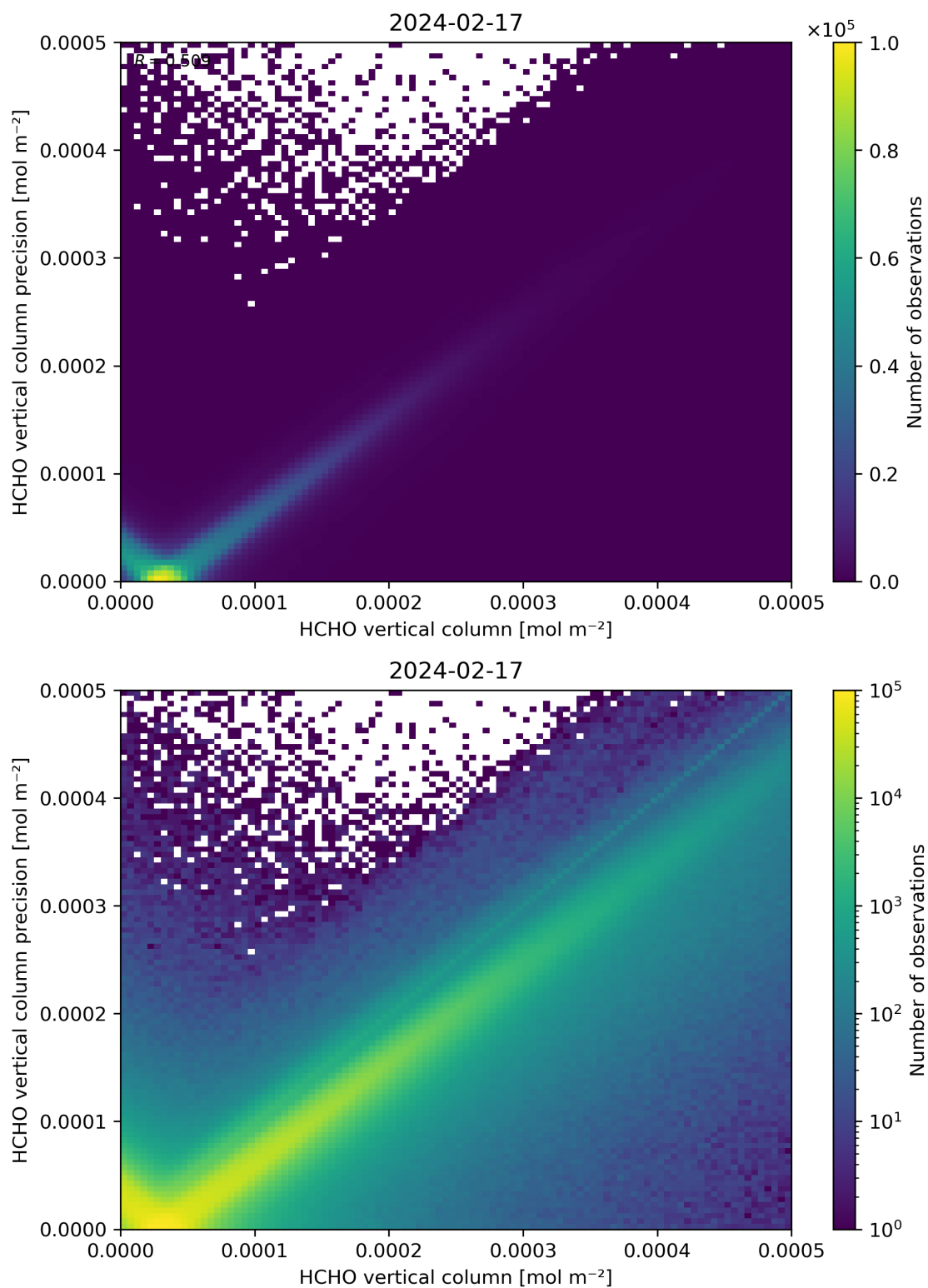
Figure 134: Scatter density plot of “HCHO vertical column” against “HCHO vertical column precision” for 2024-02-17 to 2024-02-18.
