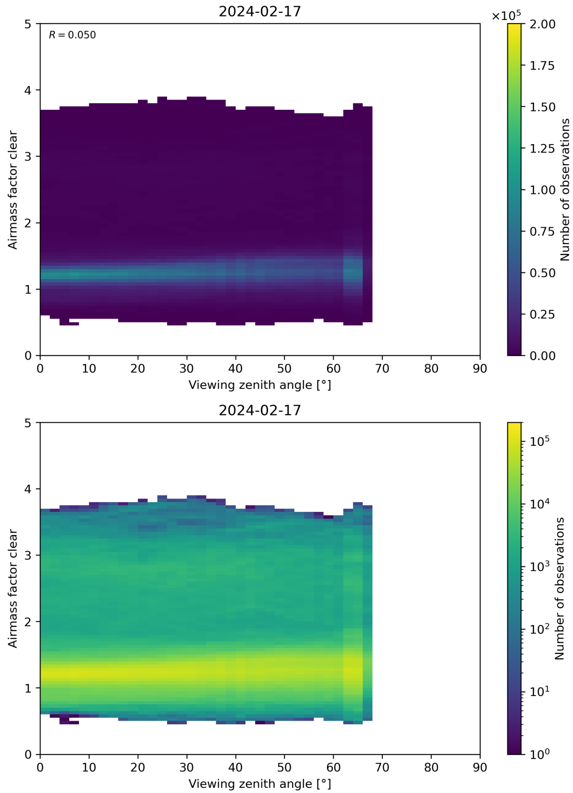
Figure 185: Scatter density plot of “Viewing zenith angle” against “Airmass factor clear” for 2024-02-17 to 2024-02-18.
