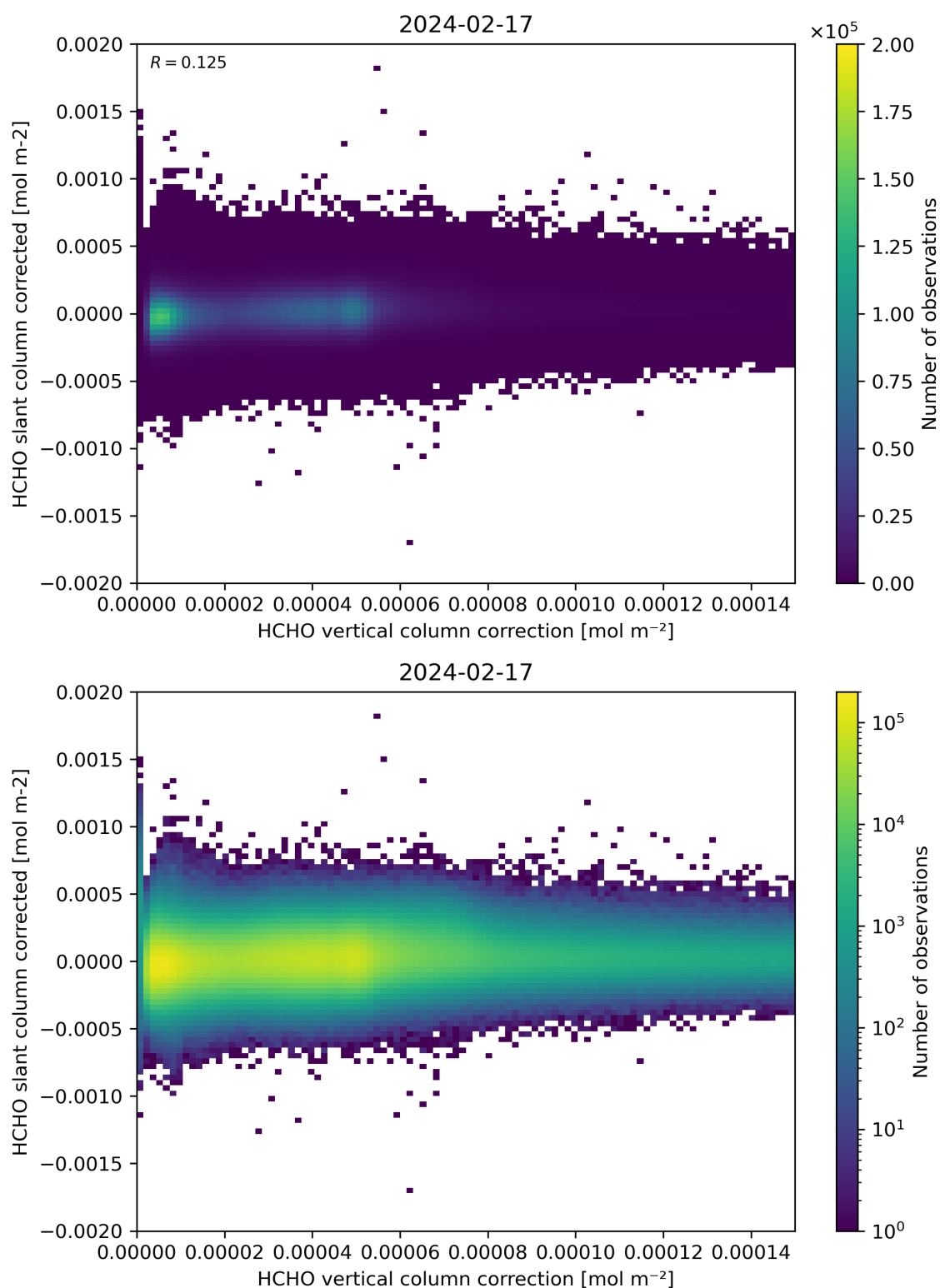
Figure 116: Scatter density plot of “HCHO vertical column correction” against “HCHO slant column corrected” for 2024-02-17 to 2024-02-18.
