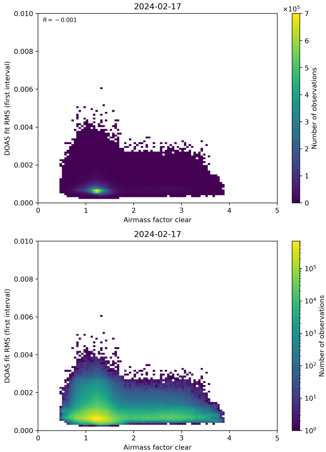
Figure 71: Scatter density plot of “Airmass factor clear” against “DOAS fit RMS (first interval)” for 2024-02-17 to 2024-02-18.
