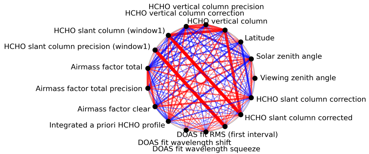
Figure 1: Map of correlation graph for 2024-02-17 to 2024-02-18.
