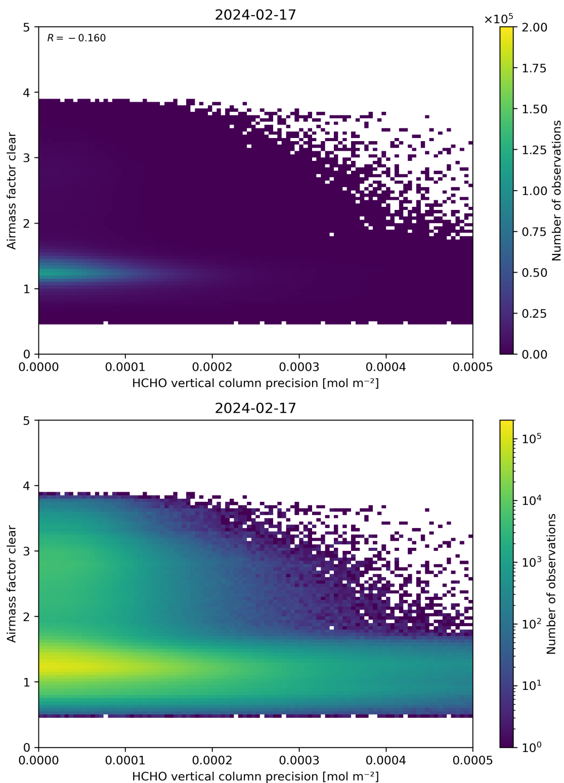
Figure 139: Scatter density plot of “HCHO vertical column precision” against “Airmass factor clear” for 2024-02-17 to 2024-02-18.
