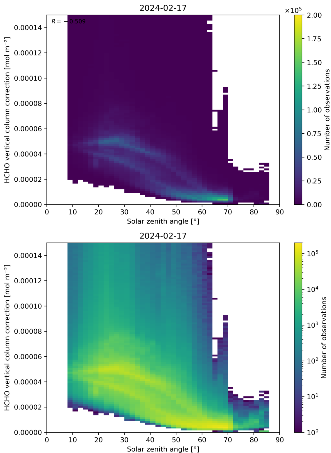
Figure 178: Scatter density plot of “Solar zenith angle” against “HCHO vertical column correction” for 2024-02-17 to 2024-02-18.
