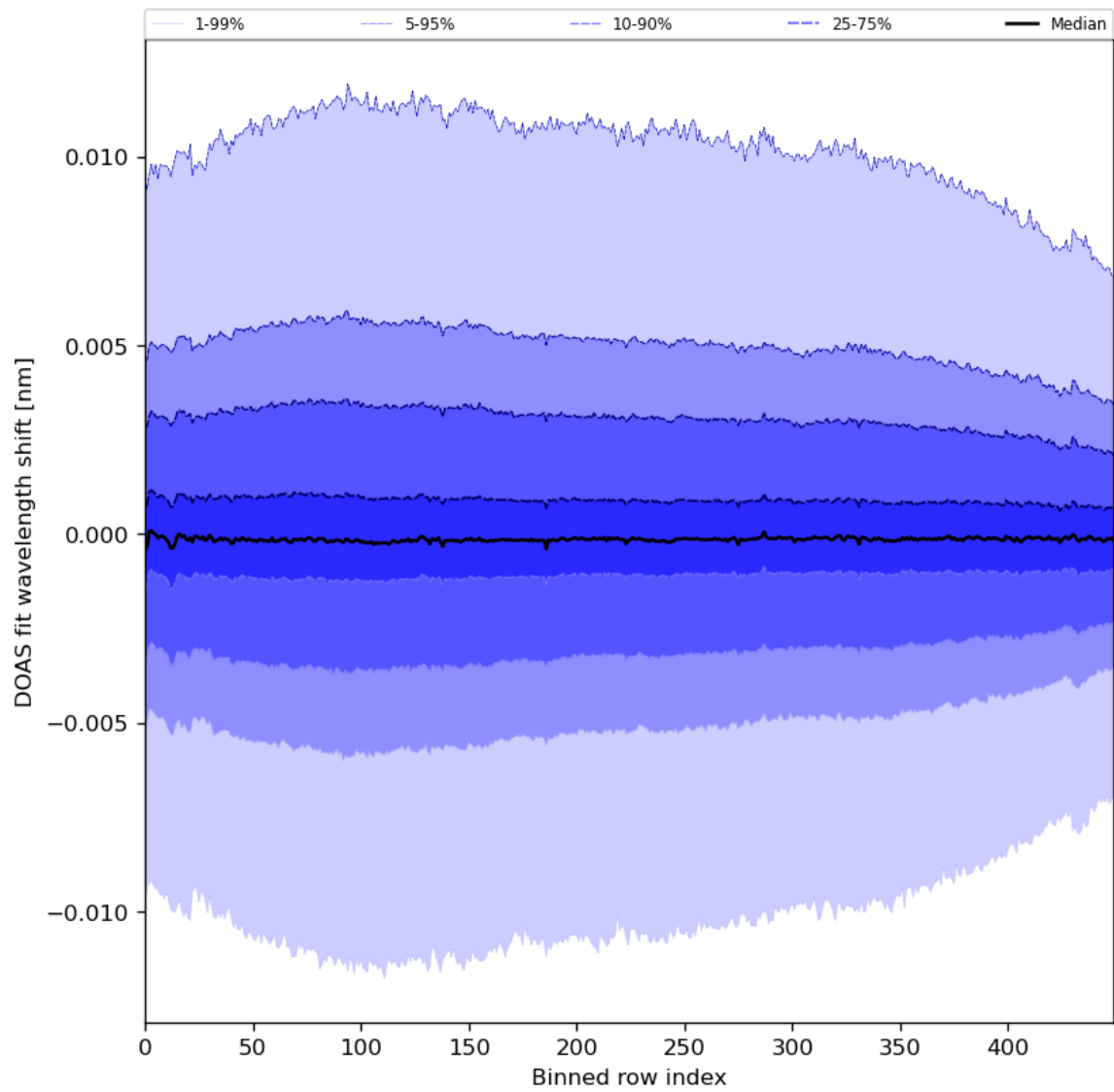
Figure 58: Along track statistics of “DOAS fit wavelength shift” for 2024-02-17 to 2024-02-18
