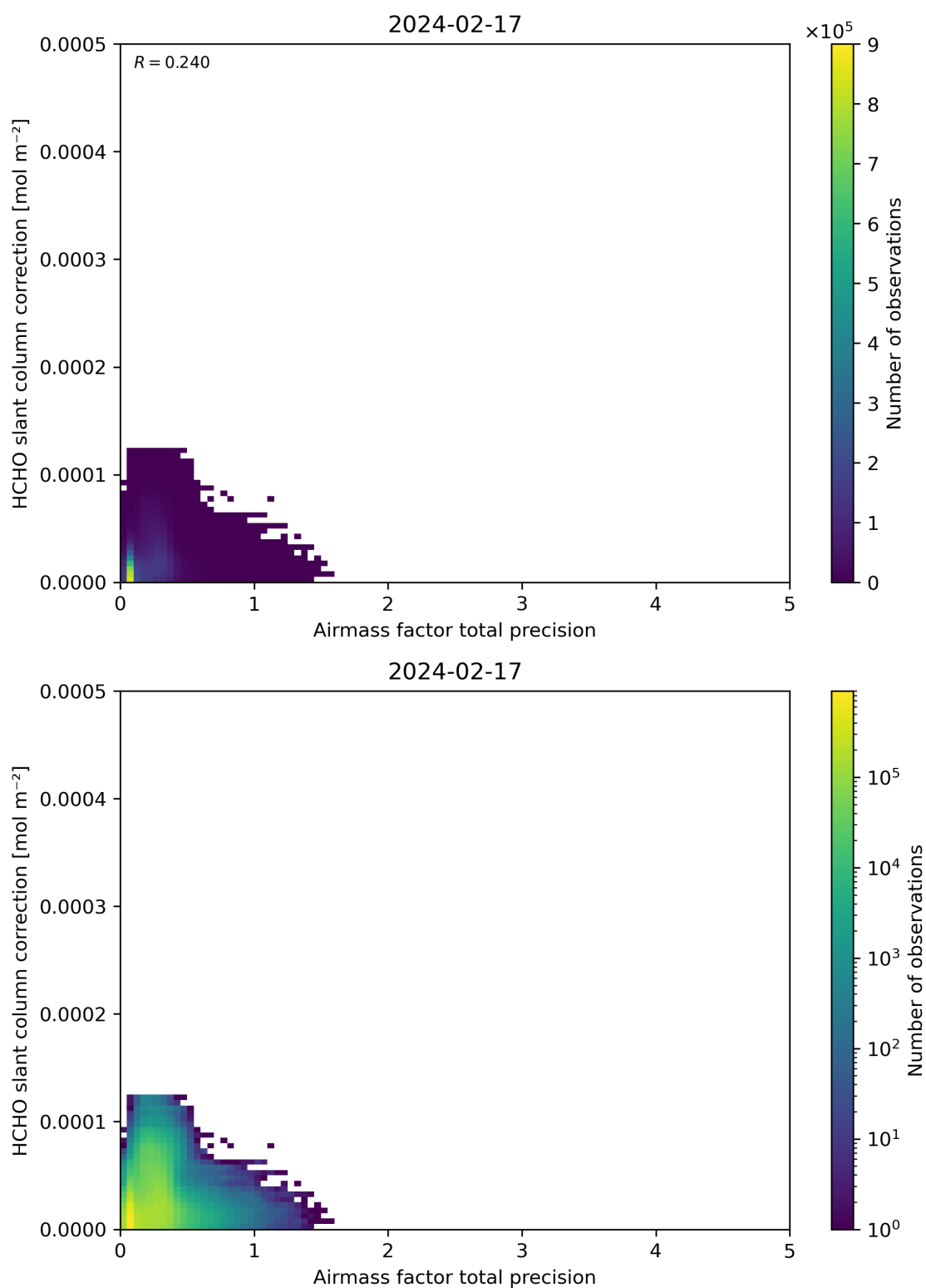
Figure 110: Scatter density plot of “Airmass factor total precision” against “HCHO slant column correction” for 2024-02-17 to 2024-02-18.
