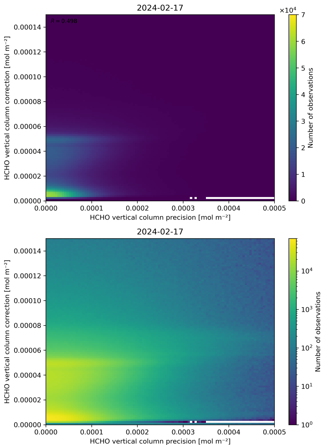
Figure 146: Scatter density plot of “HCHO vertical column precision” against “HCHO vertical column correction” for 2024-02-17 to 2024-02-18.
