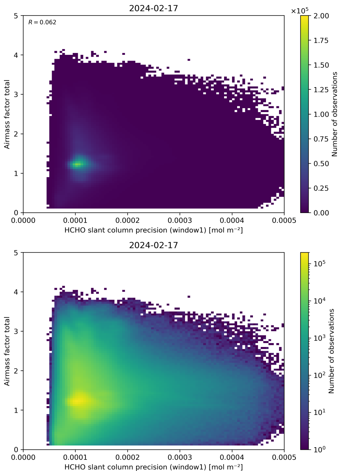
Figure 94: Scatter density plot of “HCHO slant column precision (window1)” against “Airmass factor total” for 2024-02-17 to 2024-02-18.
