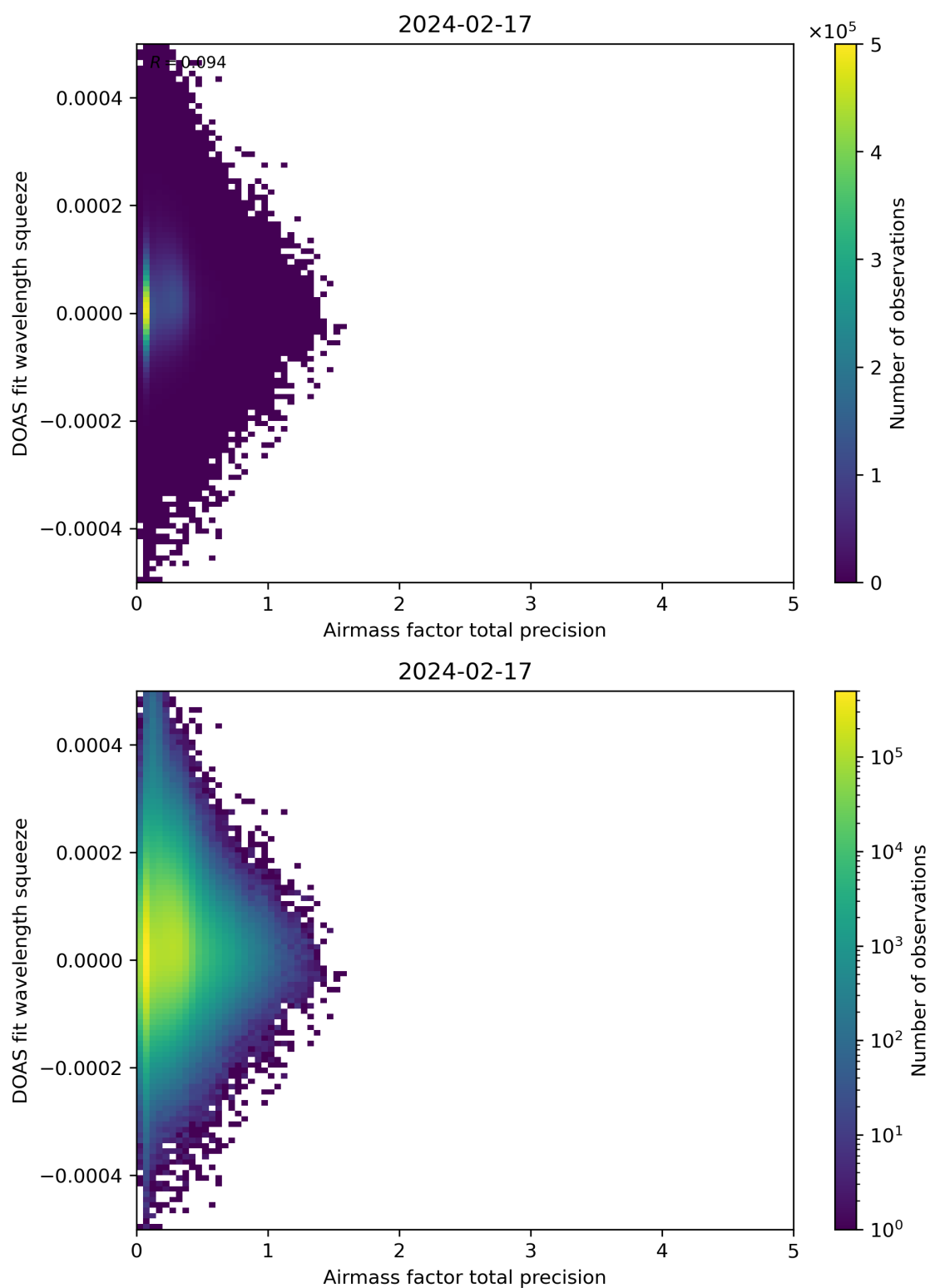
Figure 107: Scatter density plot of “Airmass factor total precision” against “DOAS fit wavelength squeeze” for 2024-02-17 to 2024-02-18.
