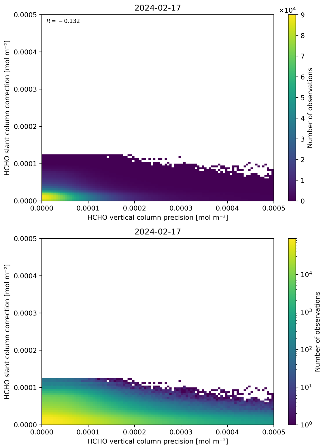
Figure 141: Scatter density plot of “HCHO vertical column precision” against “HCHO slant column correction” for 2024-02-17 to 2024-02-18.
