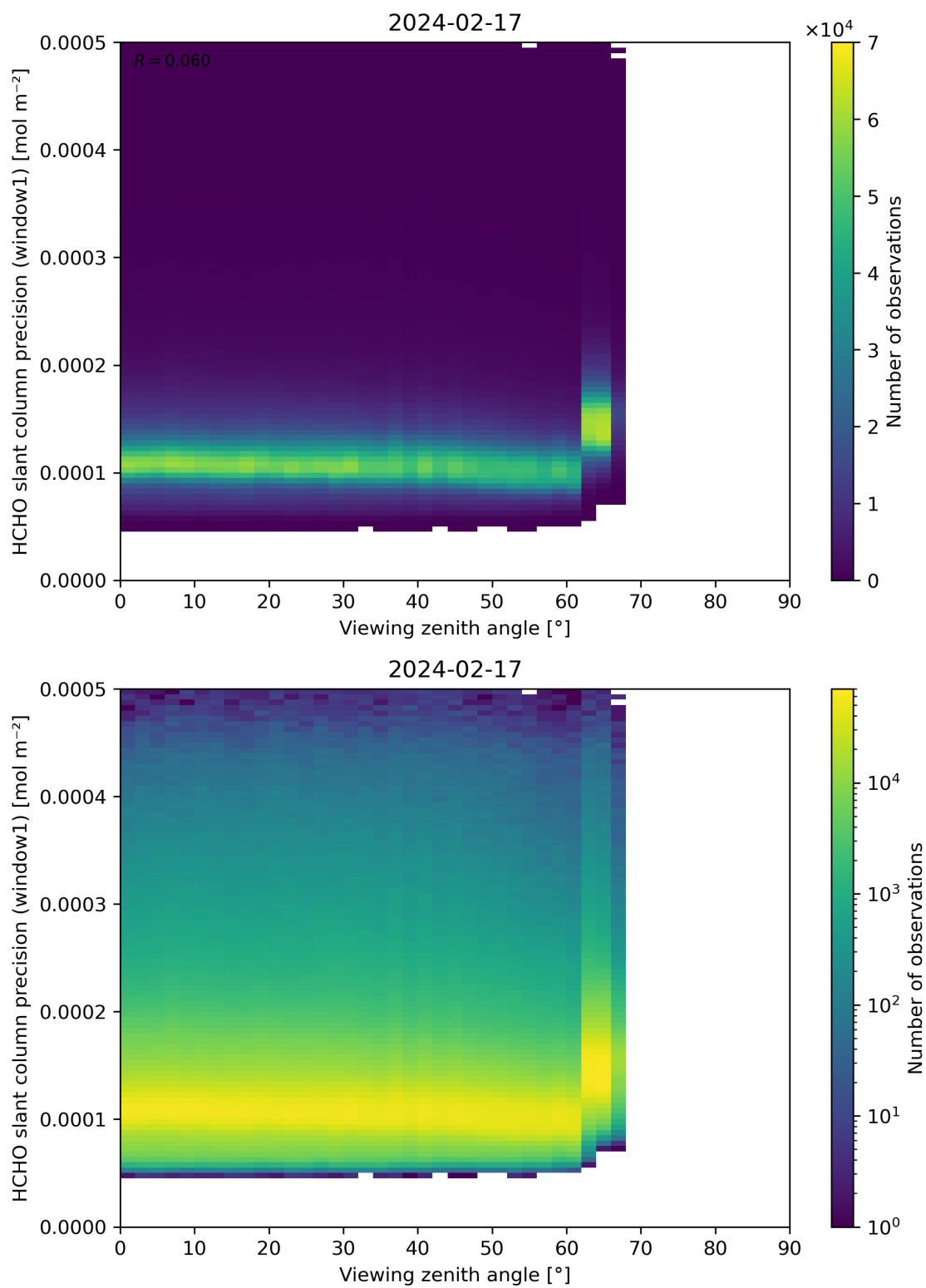
Figure 189: Scatter density plot of “Viewing zenith angle” against “HCHO slant column precision (window1)” for 2024-02-17 to 2024-02-18.
