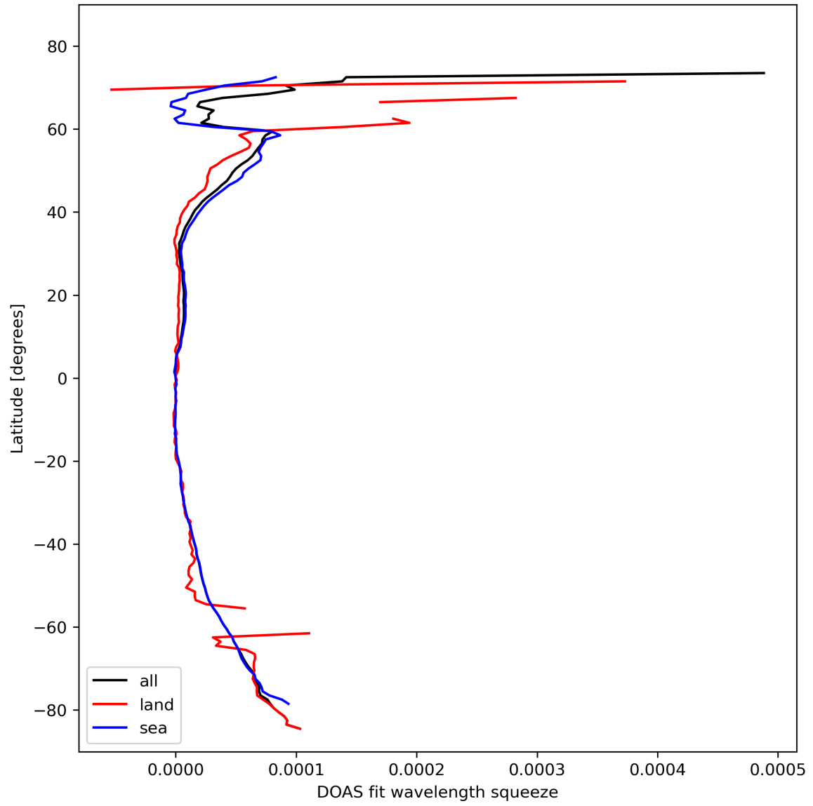
Figure 31: Zonal average of “DOAS fit wavelength squeeze” for 2024-02-17 to 2024-02-18.
