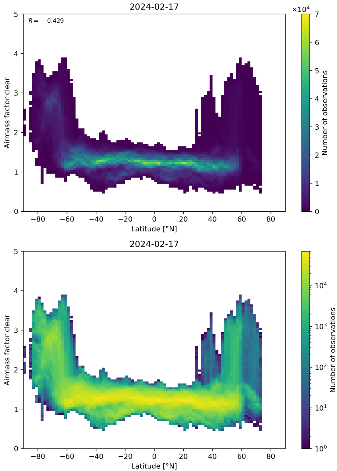
Figure 156: Scatter density plot of “Latitude” against “Airmass factor clear” for 2024-02-17 to 2024-02-18.
