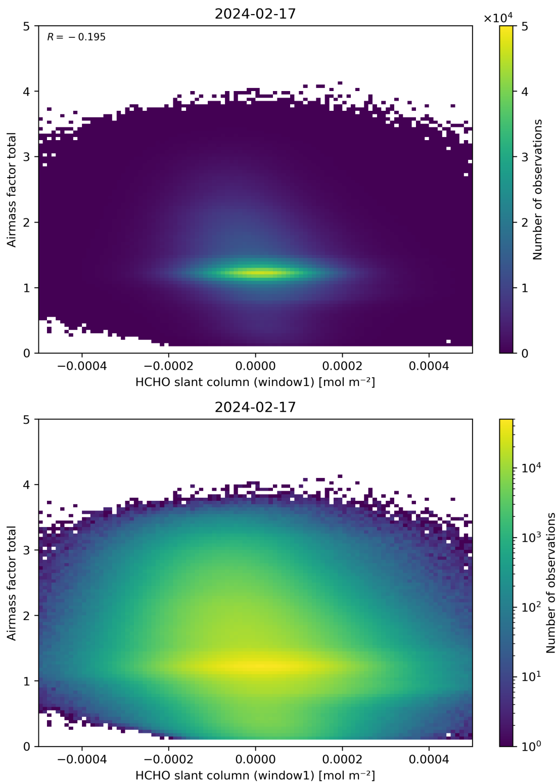
Figure 85: Scatter density plot of “HCHO slant column (window1)” against “Airmass factor total” for 2024-02-17 to 2024-02-18.
