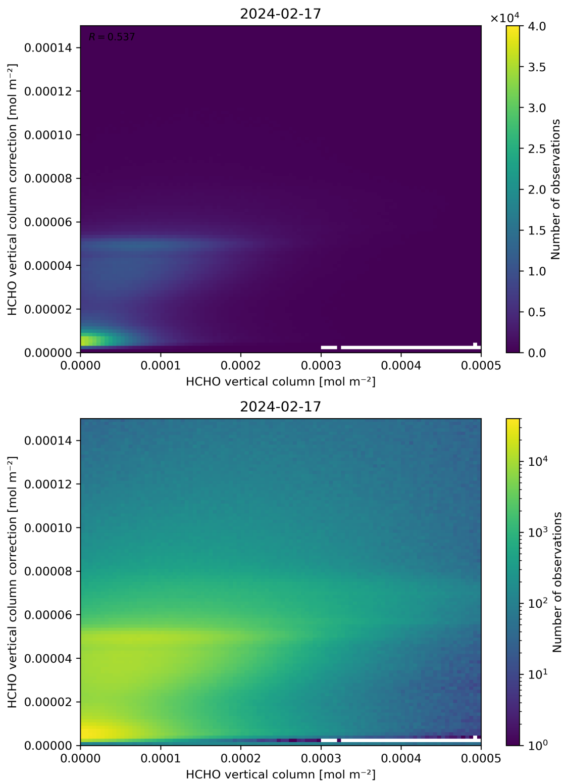
Figure 133: Scatter density plot of “HCHO vertical column” against “HCHO vertical column correction” for 2024-02-17 to 2024-02-18.
