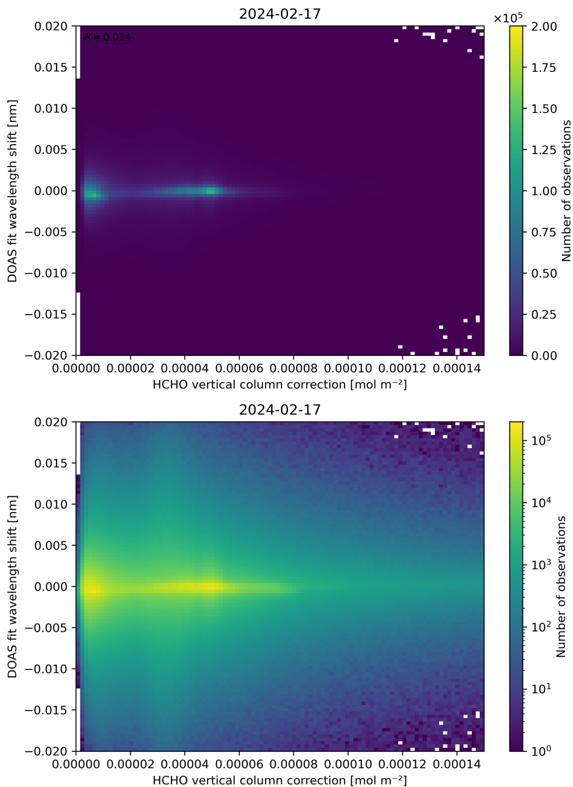
Figure 113: Scatter density plot of “HCHO vertical column correction” against “DOAS fit wavelength shift” for 2024-02-17 to 2024-02-18.
