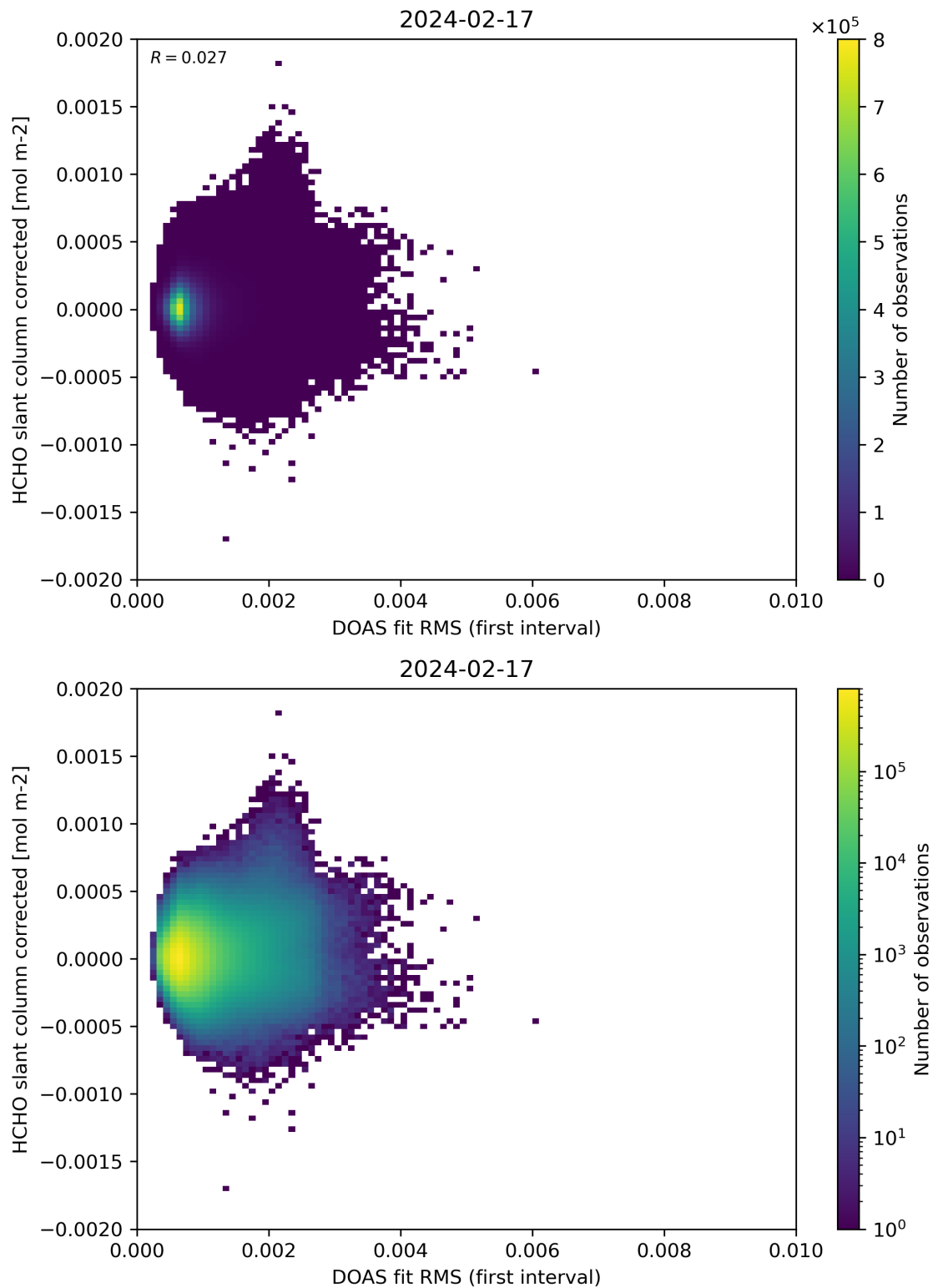
Figure 62: Scatter density plot of “DOAS fit RMS (first interval)” against “HCHO slant column corrected” for 2024-02-17 to 2024-02-18.
