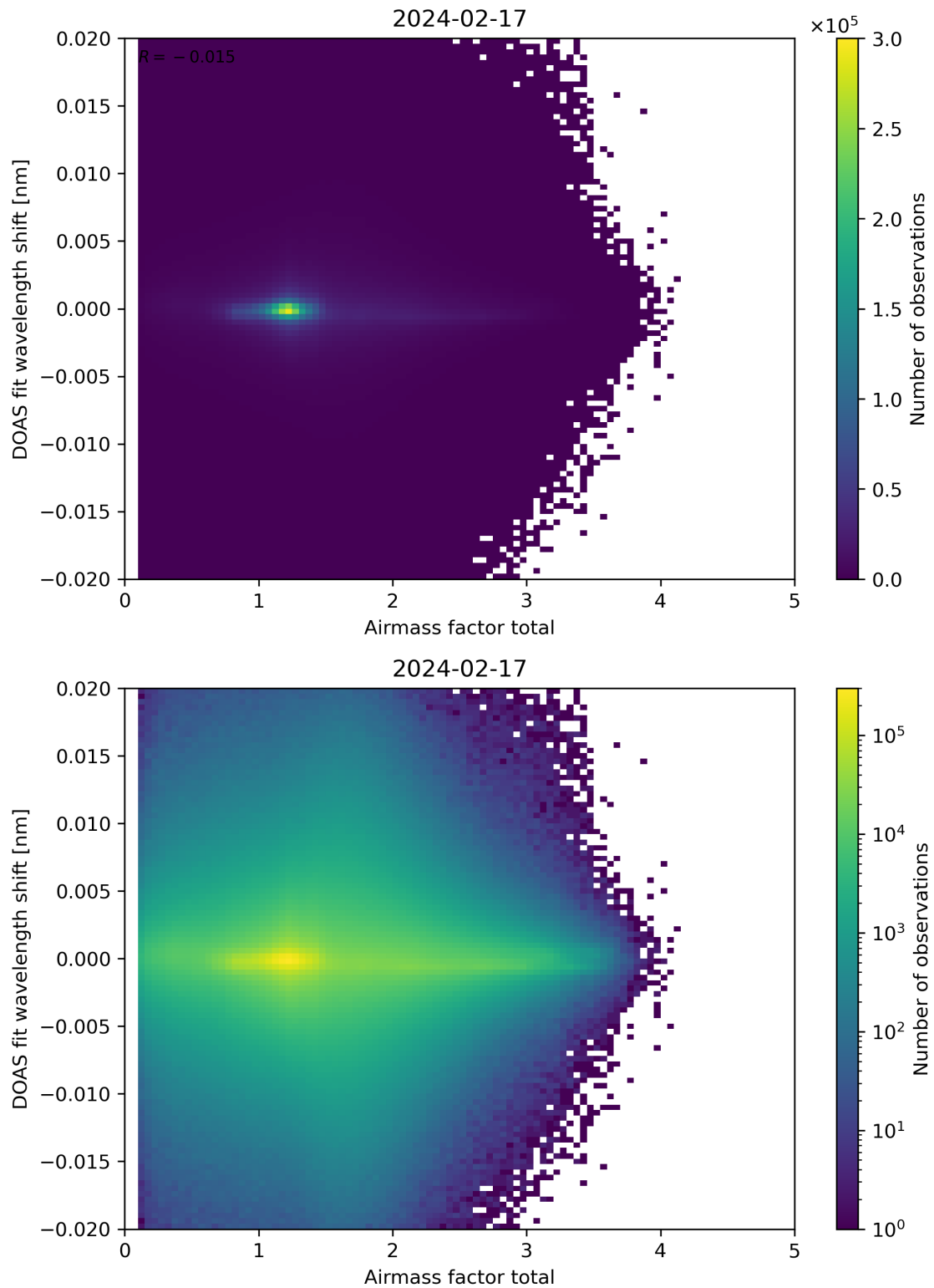
Figure 98: Scatter density plot of “Airmass factor total” against “DOAS fit wavelength shift” for 2024-02-17 to 2024-02-18.
