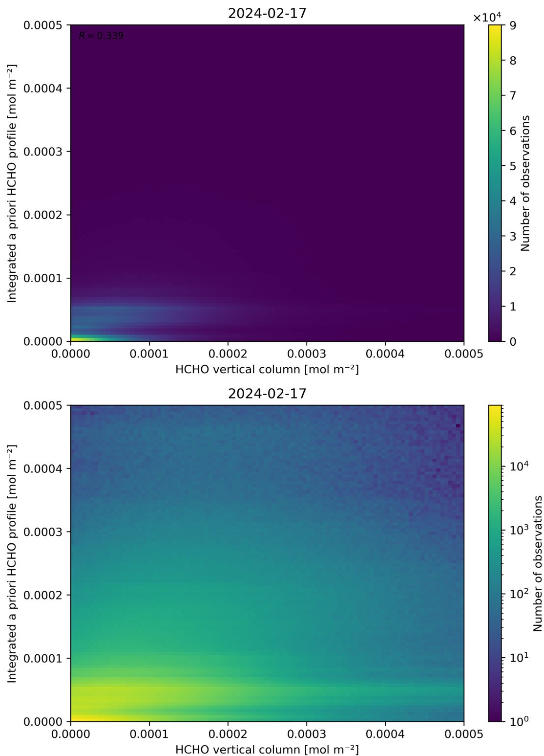
Figure 135: Scatter density plot of “HCHO vertical column” against “Integrated a priori HCHO profile” for 2024-02-17 to 2024-02-18.
