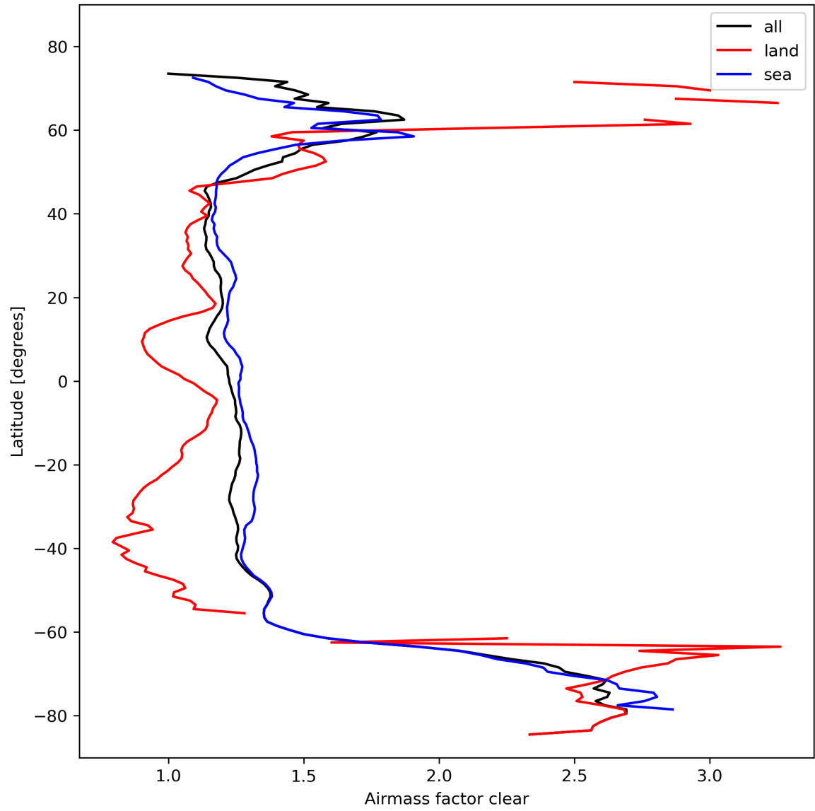
Figure 28: Zonal average of “Airmass factor clear” for 2024-02-17 to 2024-02-18.
