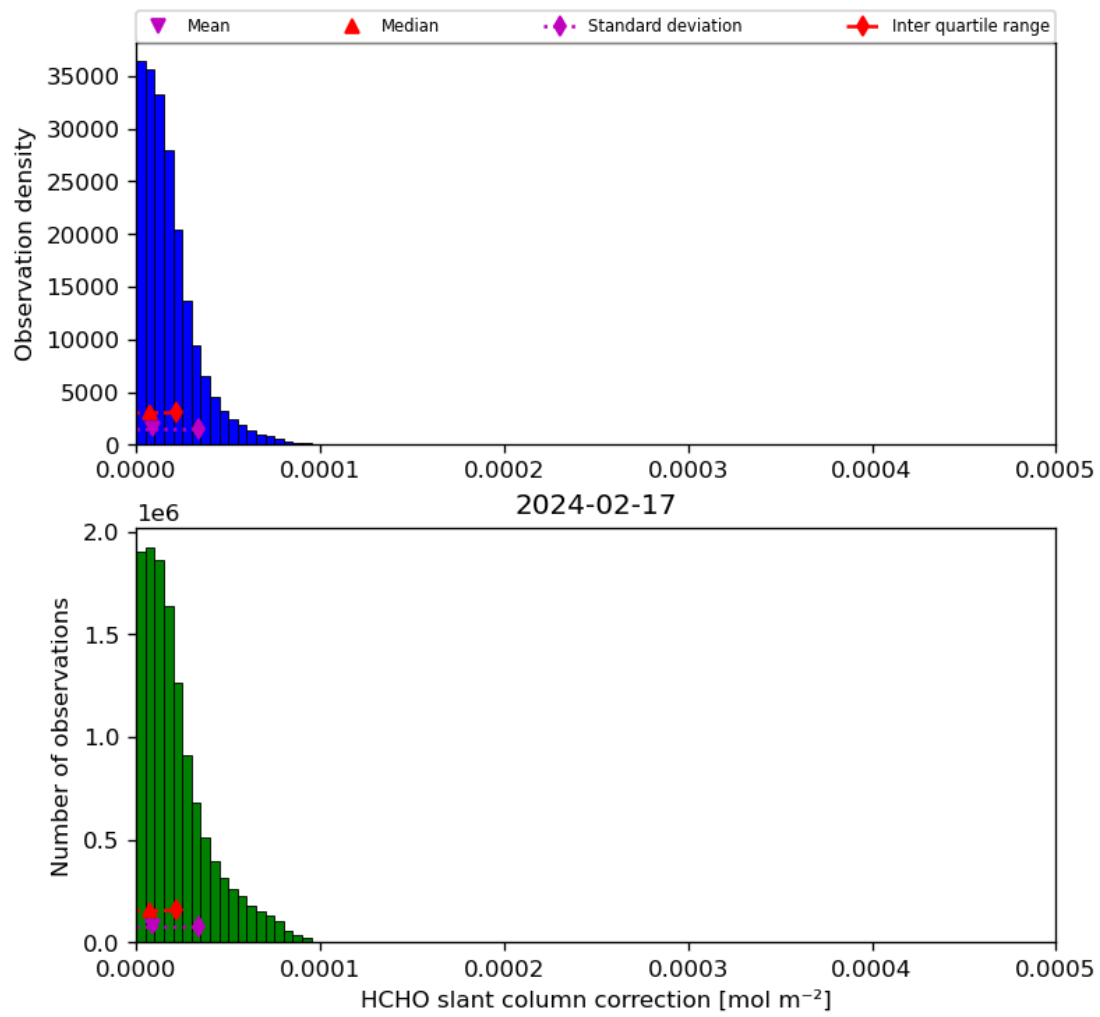
Figure 47: Histogram of “HCHO slant column correction” for 2024-02-17 to 2024-02-18
