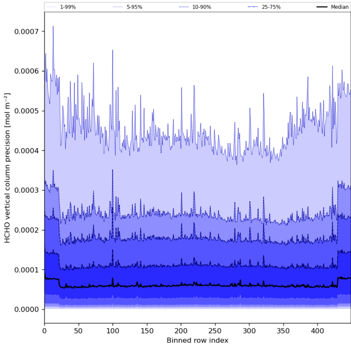
Figure 50: Along track statistics of “HCHO vertical column precision” for 2024-02-17 to 2024-02-18
