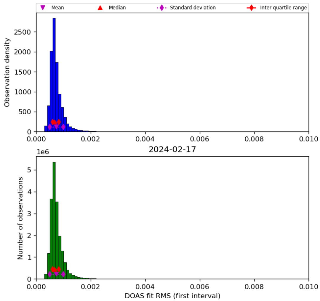
Figure 46: Histogram of “DOAS fit RMS (first interval)” for 2024-02-17 to 2024-02-18
