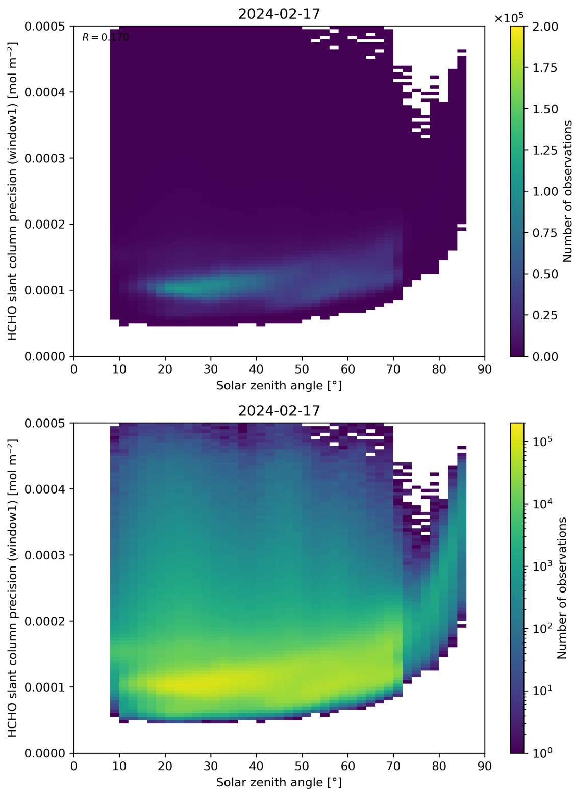
Figure 174: Scatter density plot of “Solar zenith angle” against “HCHO slant column precision (window1)” for 2024-02-17 to 2024-02-18.
