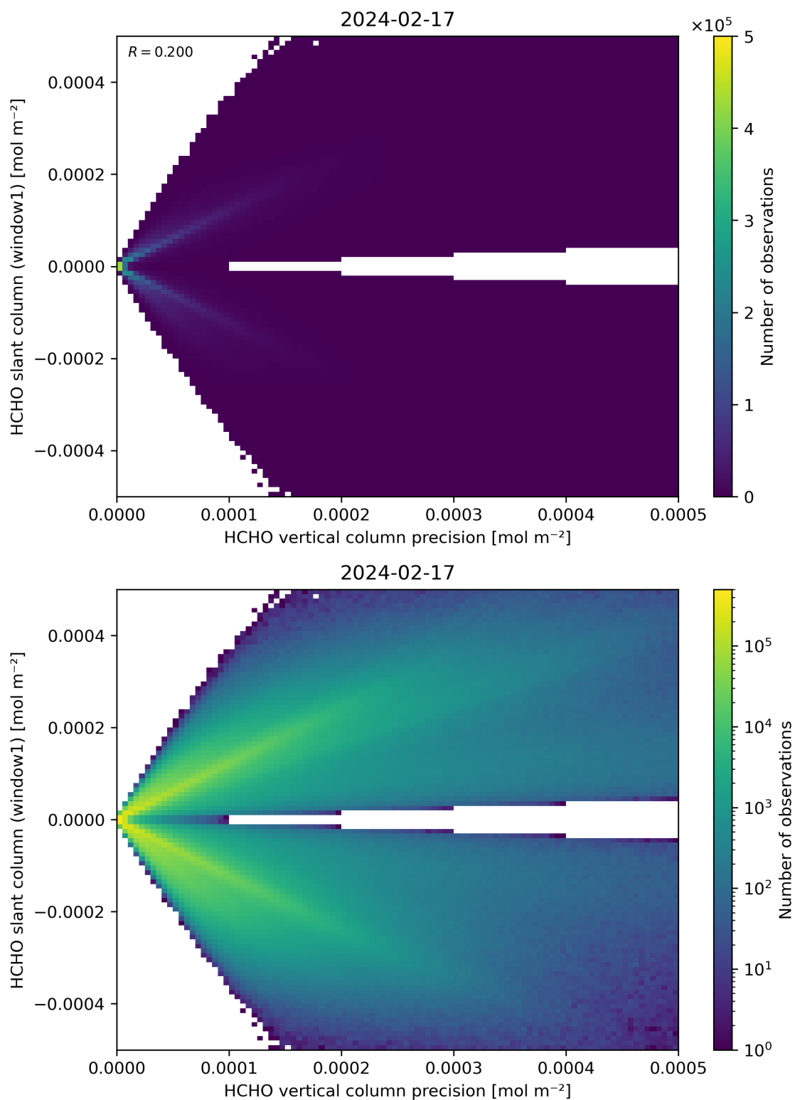
Figure 142: Scatter density plot of “HCHO vertical column precision” against “HCHO slant column (window1)” for 2024-02-17 to 2024-02-18.
