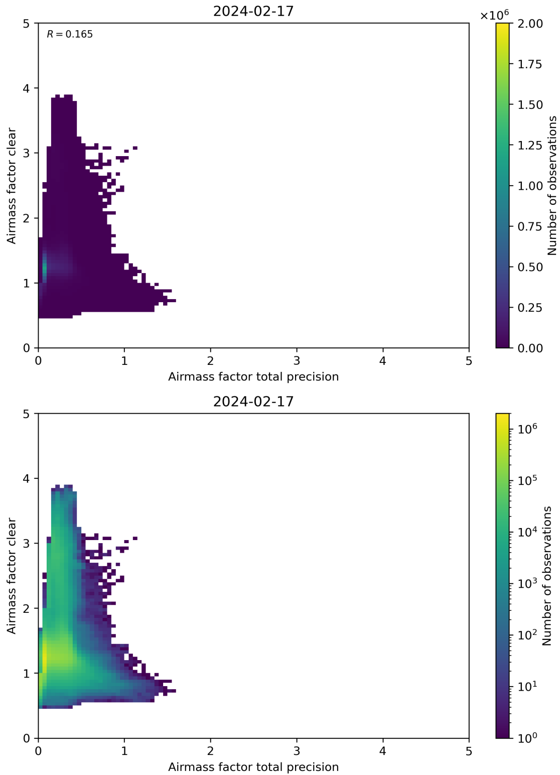
Figure 108: Scatter density plot of “Airmass factor total precision” against “Airmass factor clear” for 2024-02-17 to 2024-02-18.
