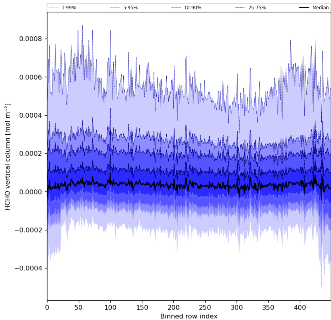
Figure 49: Along track statistics of “HCHO vertical column” for 2024-02-17 to 2024-02-18
