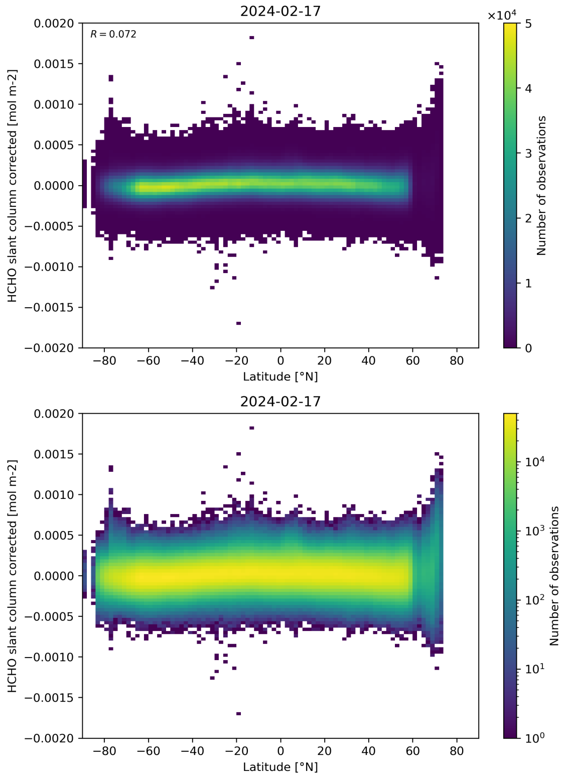
Figure 157: Scatter density plot of “Latitude” against “HCHO slant column corrected” for 2024-02-17 to 2024-02-18.
