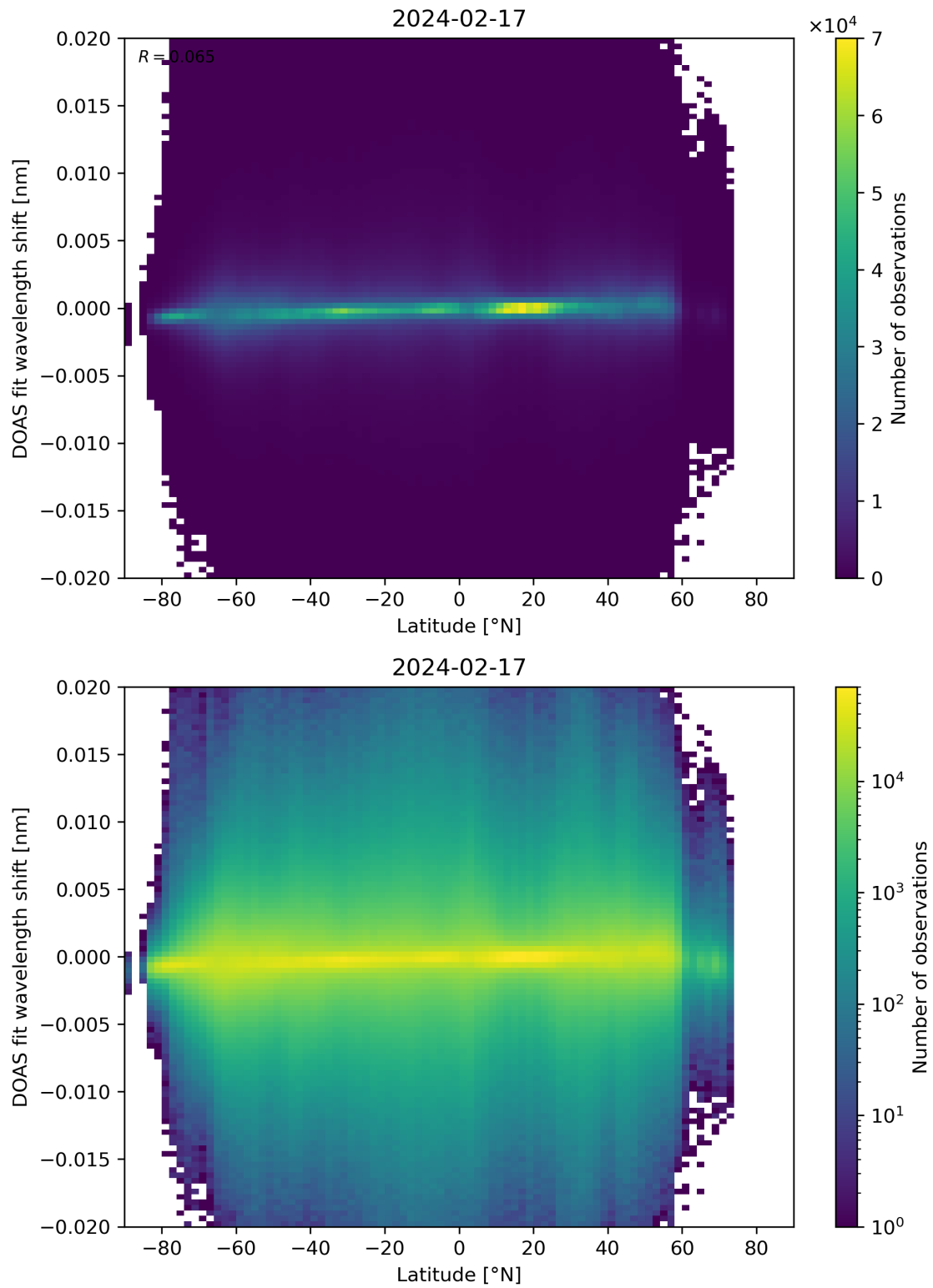
Figure 154: Scatter density plot of “Latitude” against “DOAS fit wavelength shift” for 2024-02-17 to 2024-02-18.
