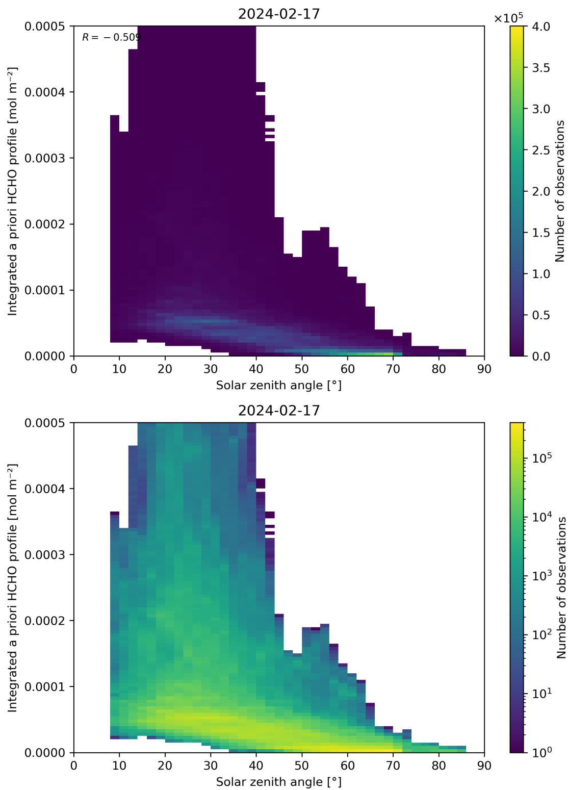
Figure 180: Scatter density plot of “Solar zenith angle” against “Integrated a priori HCHO profile” for 2024-02-17 to 2024-02-18.
