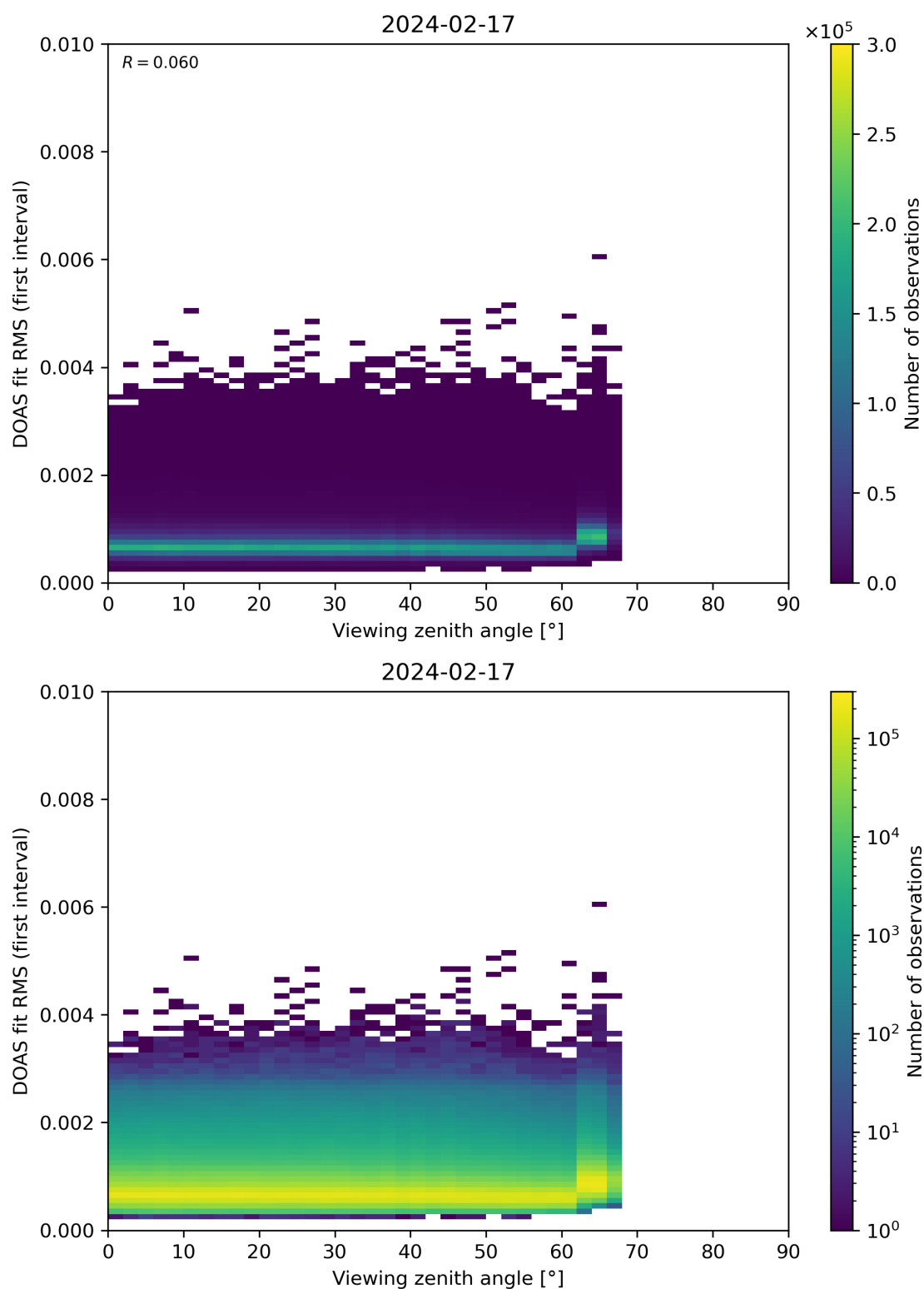
Figure 182: Scatter density plot of “Viewing zenith angle” against “DOAS fit RMS (first interval)” for 2024-02-17 to 2024-02-18.
