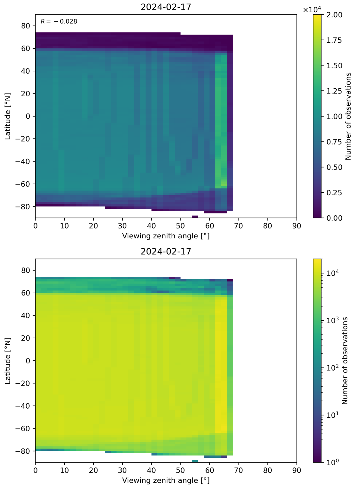
Figure 196: Scatter density plot of “Viewing zenith angle” against “Latitude” for 2024-02-17 to 2024-02-18.
