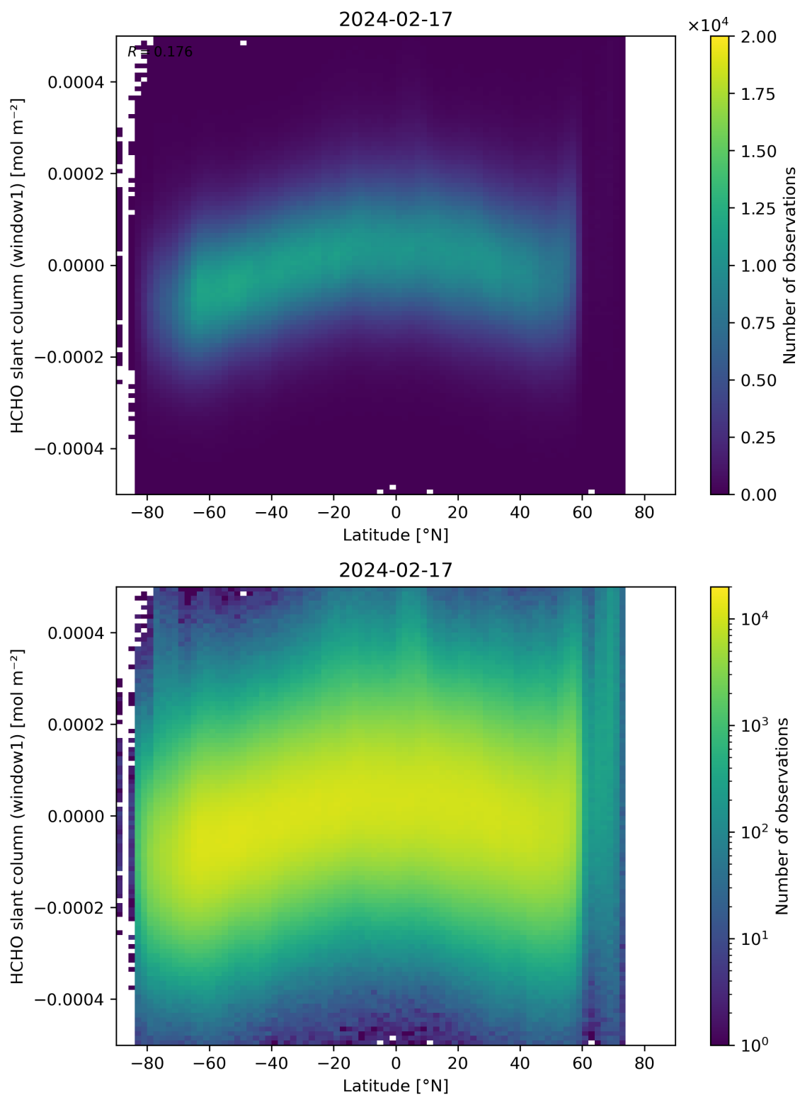
Figure 159: Scatter density plot of “Latitude” against “HCHO slant column (window1)” for 2024-02-17 to 2024-02-18.
