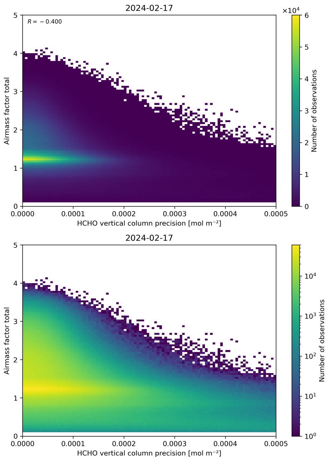
Figure 144: Scatter density plot of “HCHO vertical column precision” against “Airmass factor total” for 2024-02-17 to 2024-02-18.
