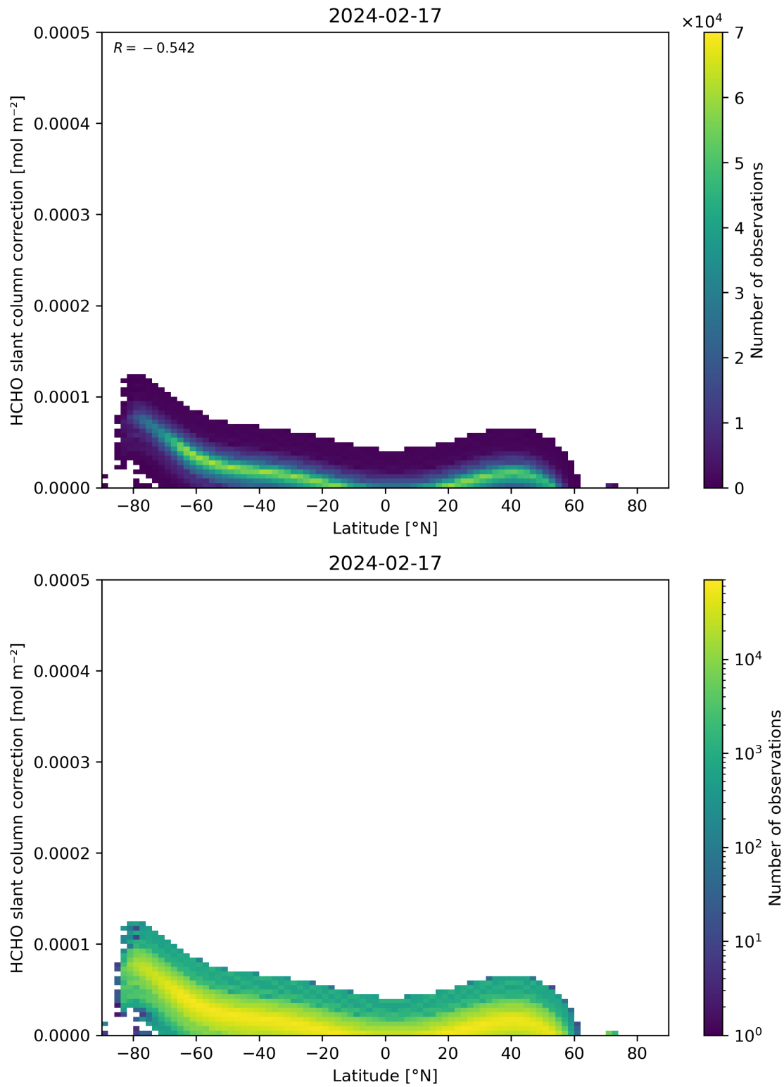
Figure 158: Scatter density plot of “Latitude” against “HCHO slant column correction” for 2024-02-17 to 2024-02-18.
