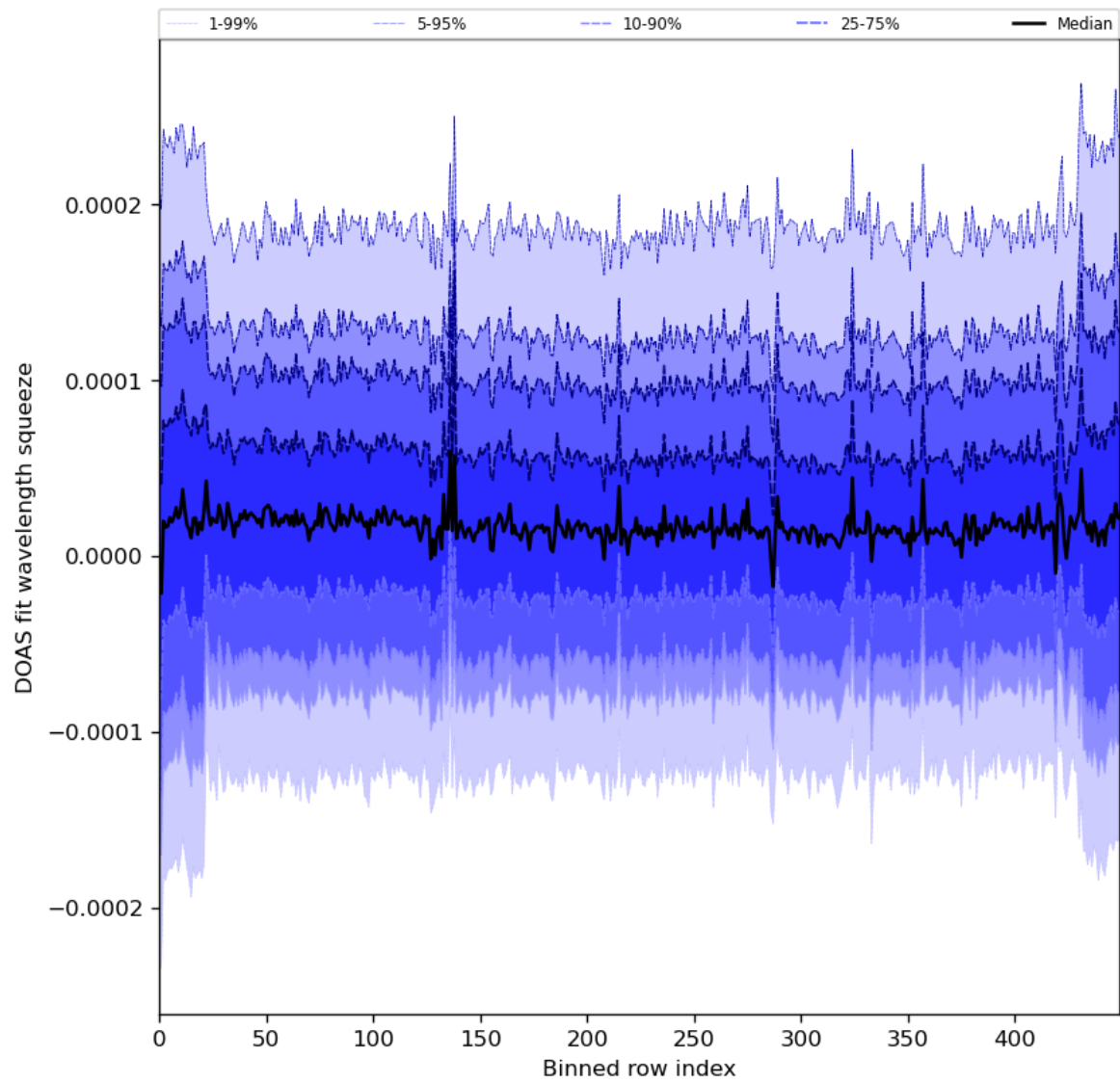
Figure 59: Along track statistics of “DOAS fit wavelength squeeze” for 2024-02-17 to 2024-02-18
