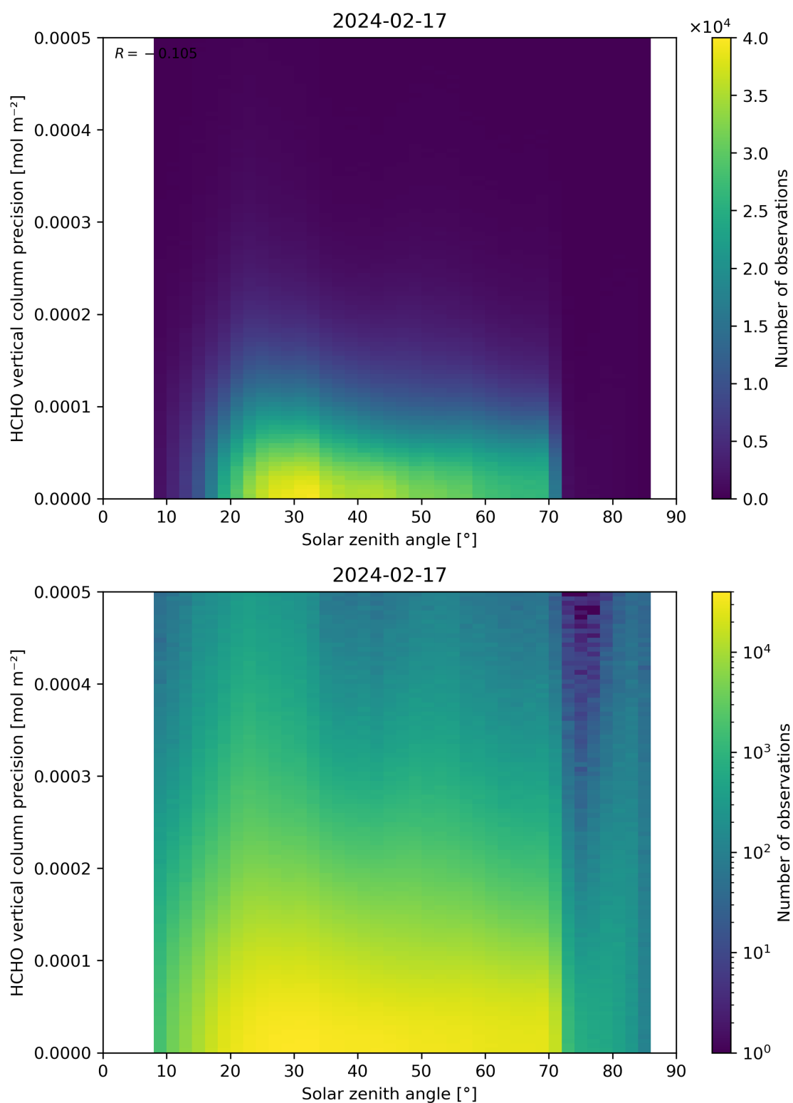
Figure 179: Scatter density plot of “Solar zenith angle” against “HCHO vertical column precision” for 2024-02-17 to 2024-02-18.
