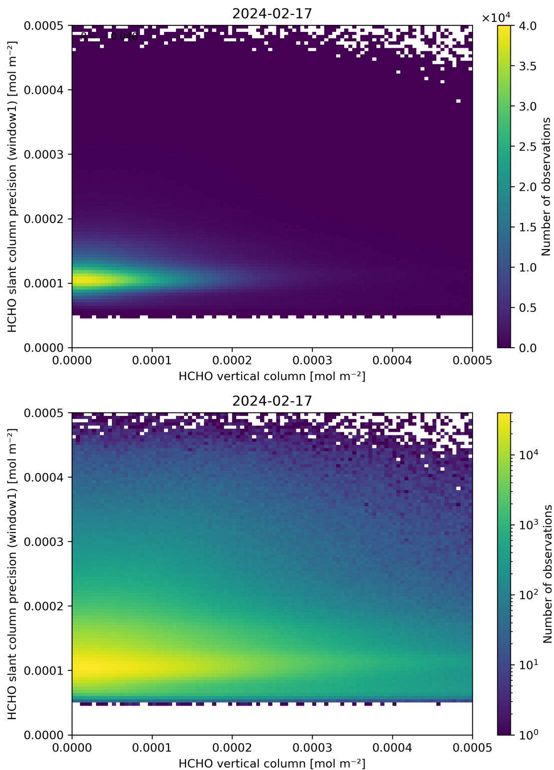
Figure 130: Scatter density plot of “HCHO vertical column” against “HCHO slant column precision (window1)” for 2024-02-17 to 2024-02-18.
