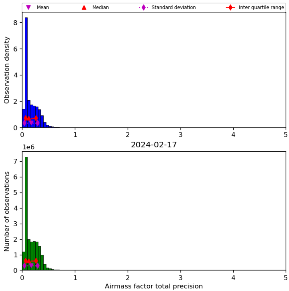
Figure 41: Histogram of “Airmass factor total precision” for 2024-02-17 to 2024-02-18
