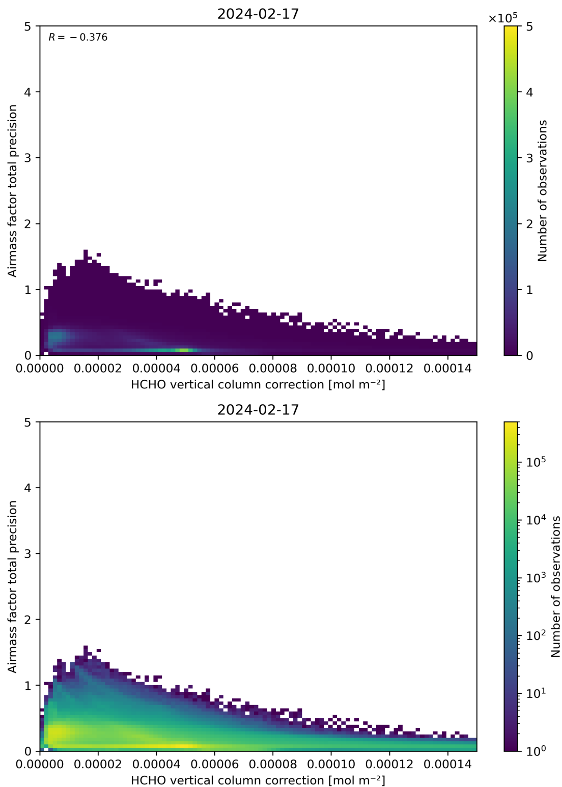
Figure 121: Scatter density plot of “HCHO vertical column correction” against “Airmass factor total precision” for 2024-02-17 to 2024-02-18.
