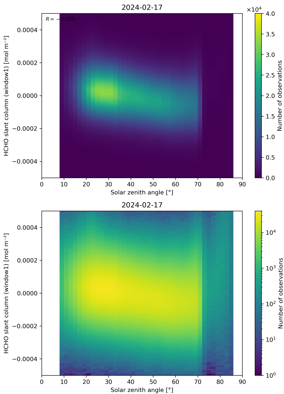
Figure 173: Scatter density plot of “Solar zenith angle” against “HCHO slant column (window1)” for 2024-02-17 to 2024-02-18.
