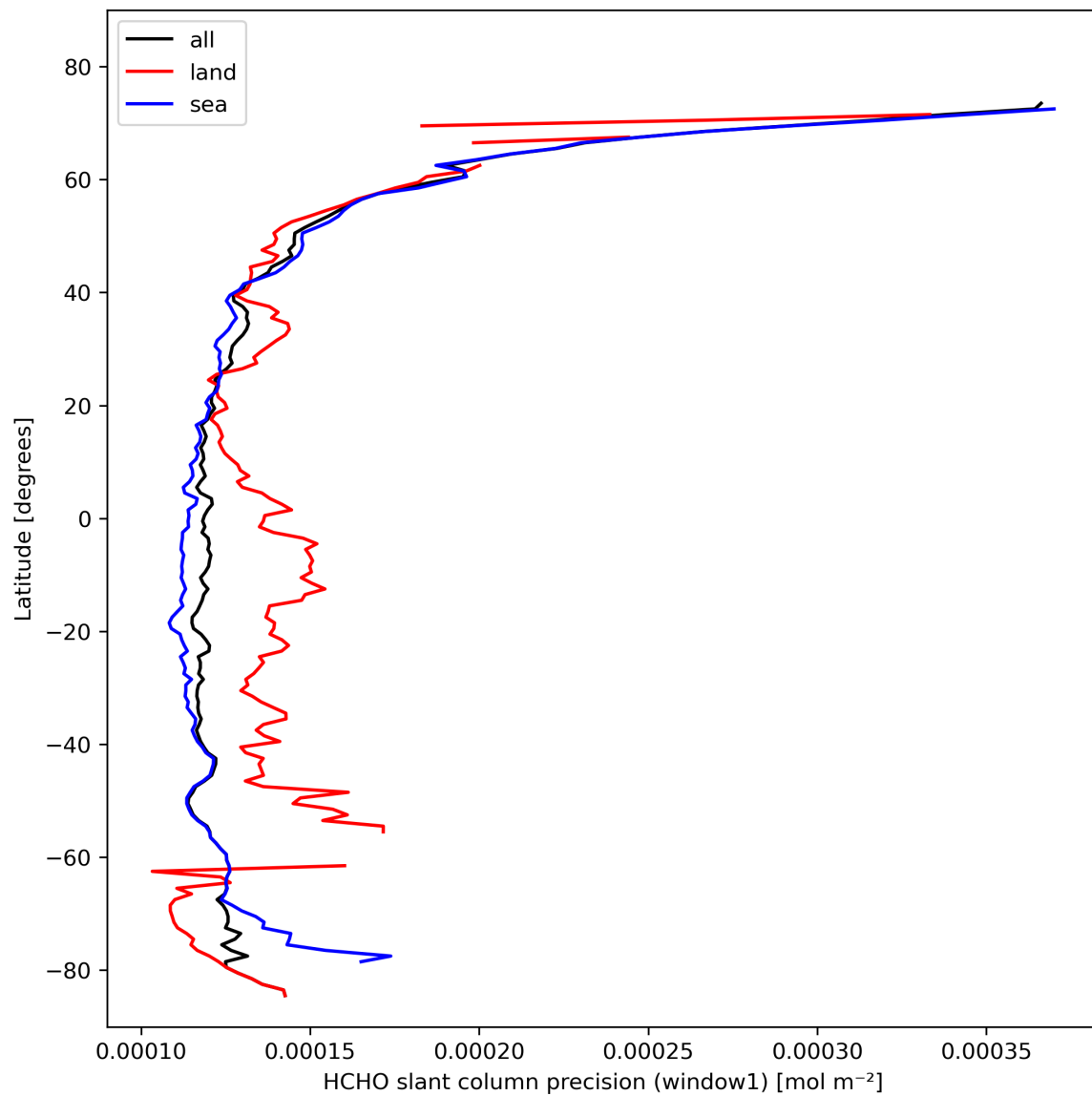
Figure 25: Zonal average of “HCHO slant column precision (window1)” for 2024-02-17 to 2024-02-18.
