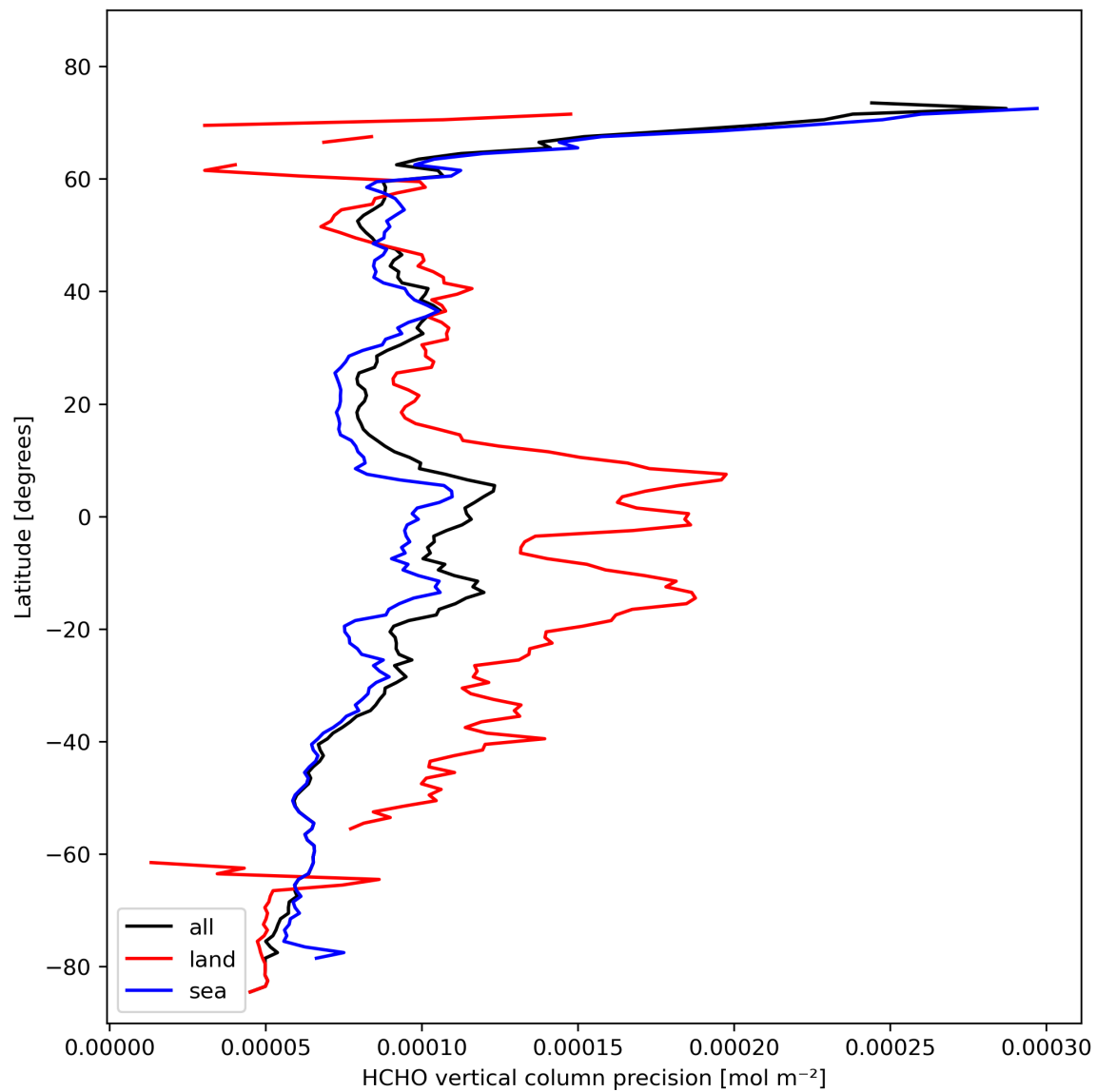
Figure 22: Zonal average of “HCHO vertical column precision” for 2024-02-17 to 2024-02-18.
