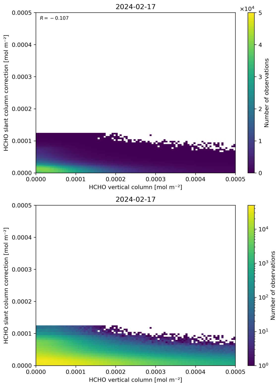
Figure 128: Scatter density plot of “HCHO vertical column” against “HCHO slant column correction” for 2024-02-17 to 2024-02-18.
