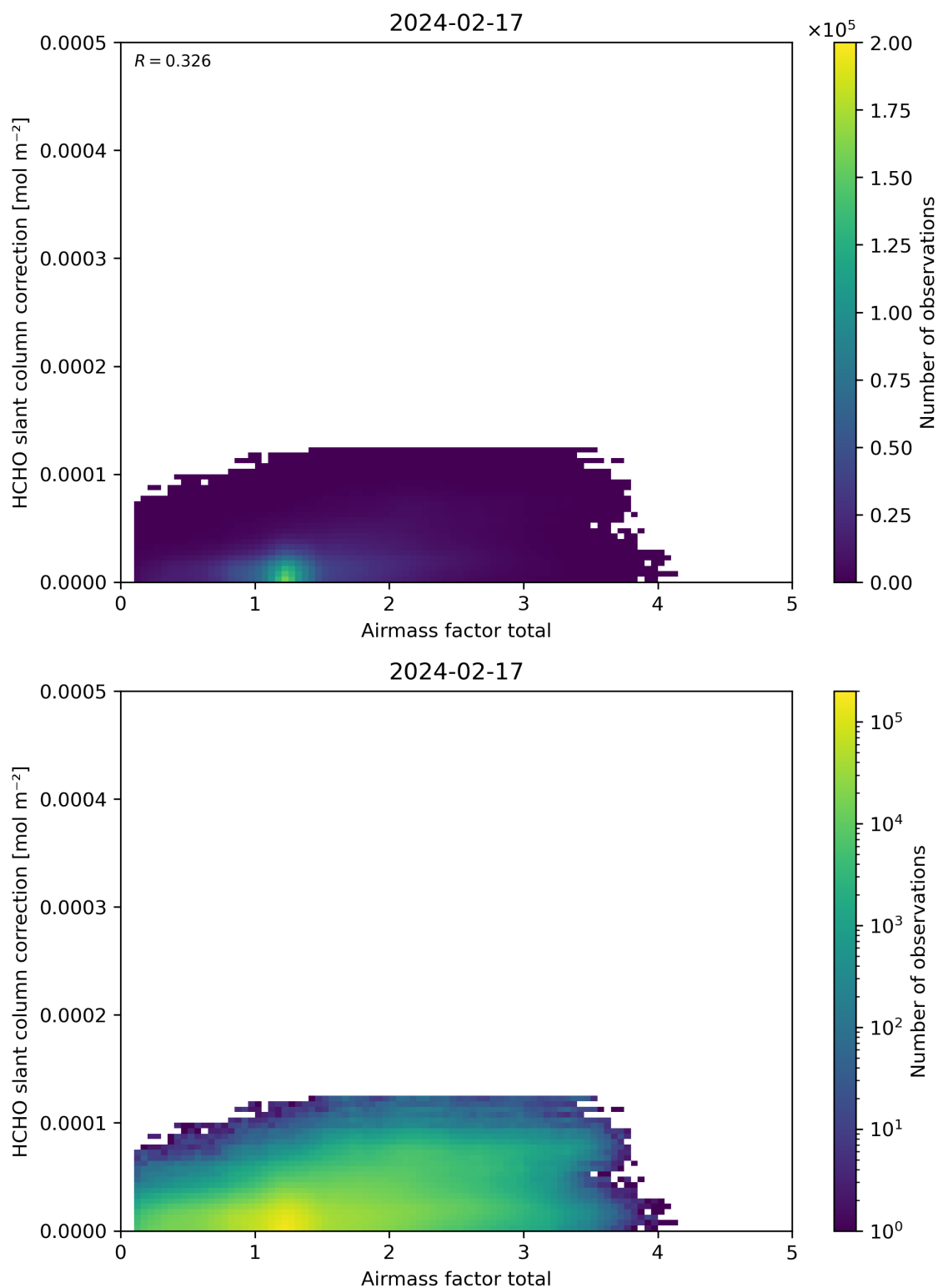
Figure 102: Scatter density plot of “Airmass factor total” against “HCHO slant column correction” for 2024-02-17 to 2024-02-18.
