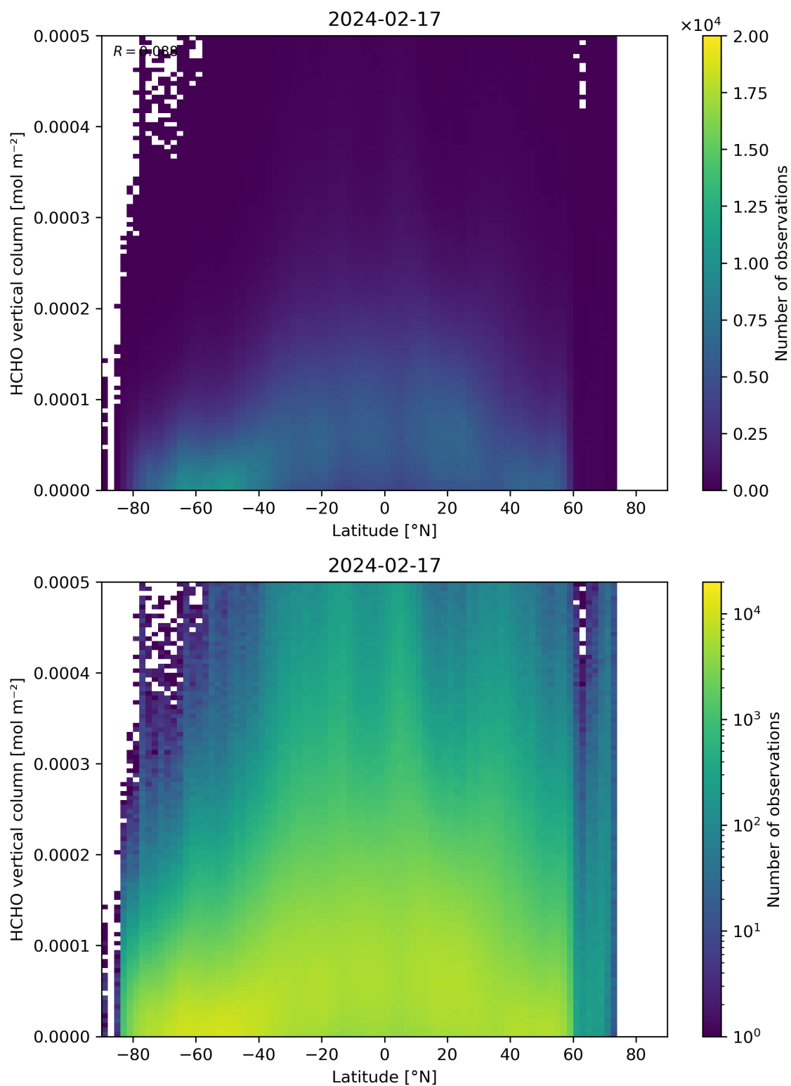
Figure 163: Scatter density plot of “Latitude” against “HCHO vertical column” for 2024-02-17 to 2024-02-18.
