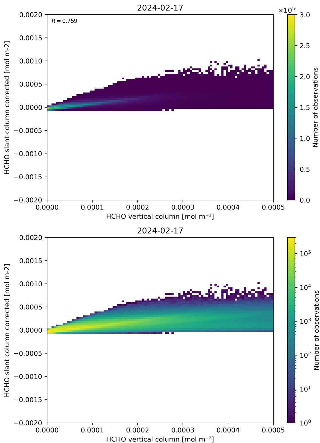
Figure 127: Scatter density plot of “HCHO vertical column” against “HCHO slant column corrected” for 2024-02-17 to 2024-02-18.
