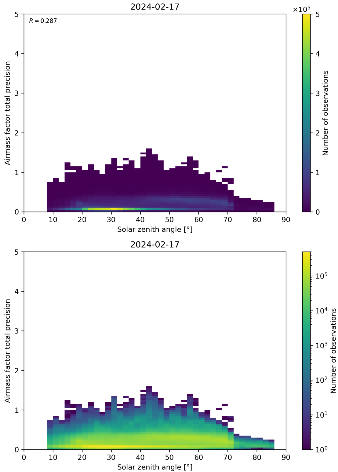
Figure 176: Scatter density plot of “Solar zenith angle” against “Airmass factor total precision” for 2024-02-17 to 2024-02-18.
