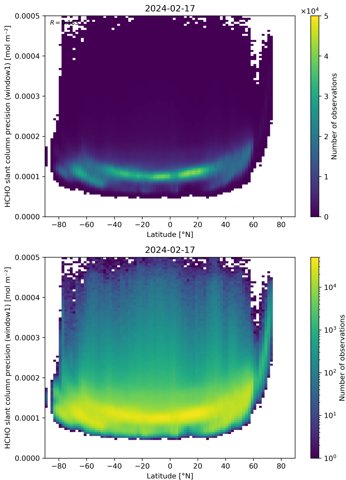
Figure 160: Scatter density plot of “Latitude” against “HCHO slant column precision (window1)” for 2024-02-17 to 2024-02-18.
