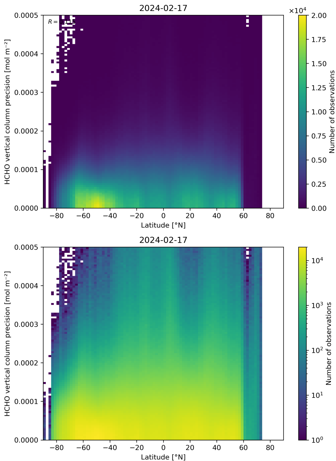
Figure 165: Scatter density plot of “Latitude” against “HCHO vertical column precision” for 2024-02-17 to 2024-02-18.
