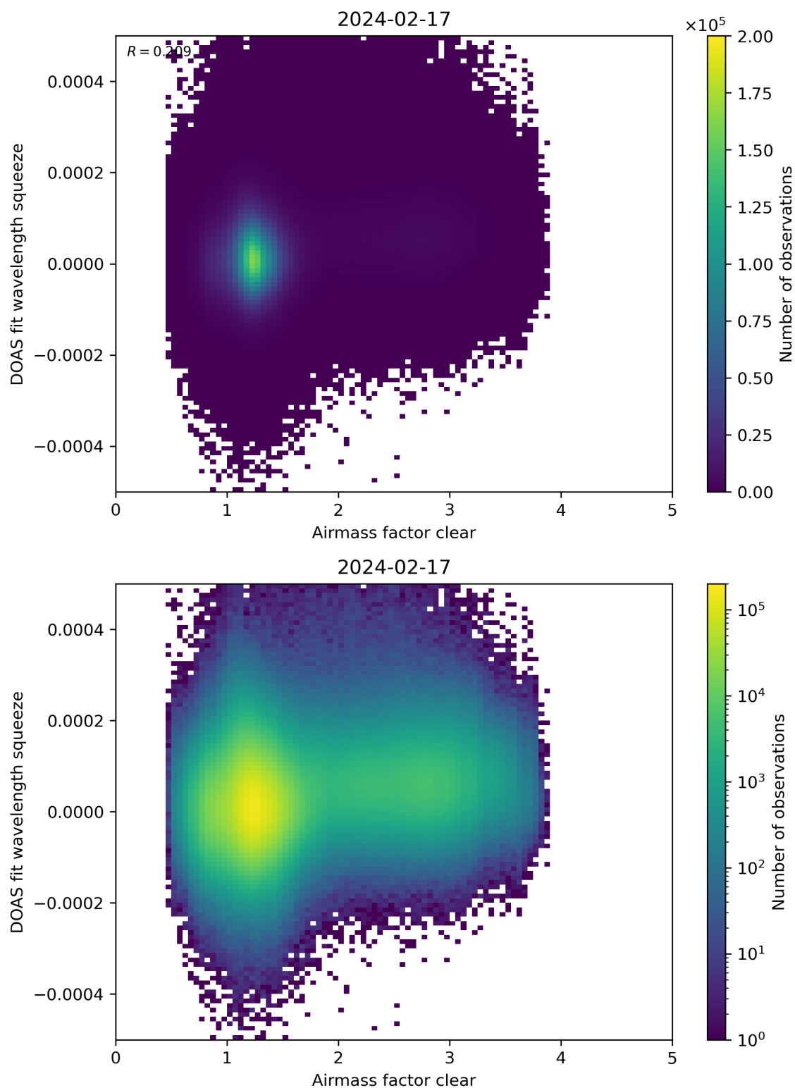
Figure 73: Scatter density plot of “Airmass factor clear” against “DOAS fit wavelength squeeze” for 2024-02-17 to 2024-02-18.
