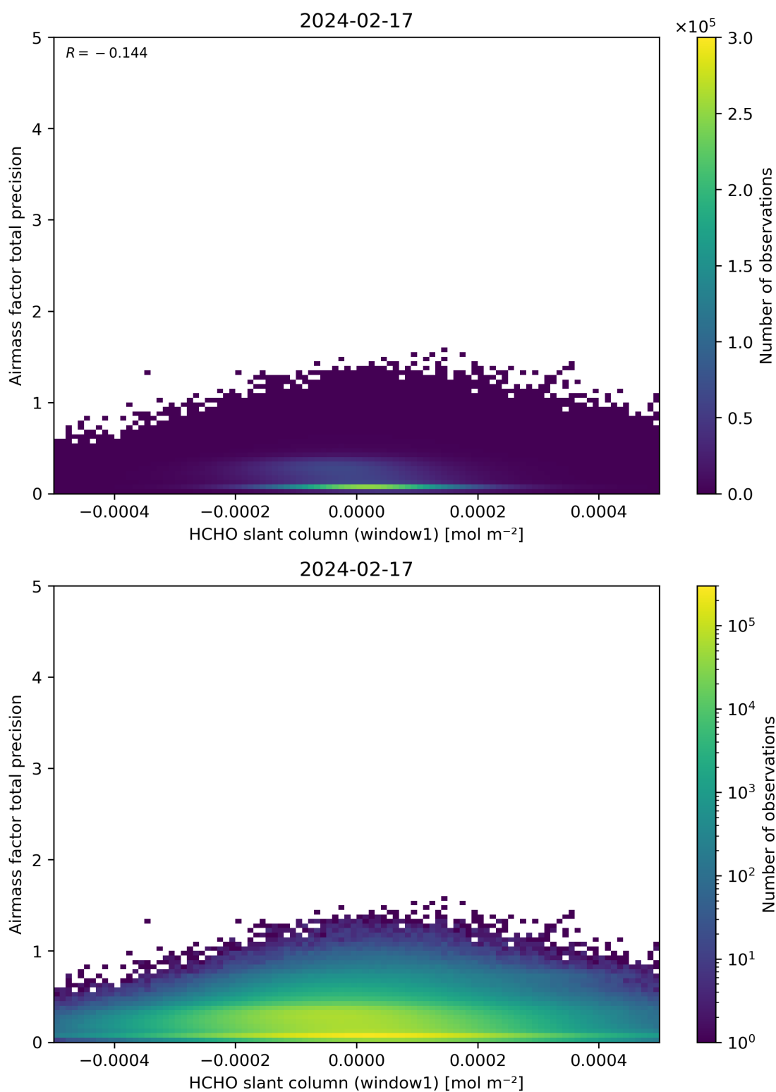
Figure 86: Scatter density plot of “HCHO slant column (window1)” against “Airmass factor total precision” for 2024-02-17 to 2024-02-18.
