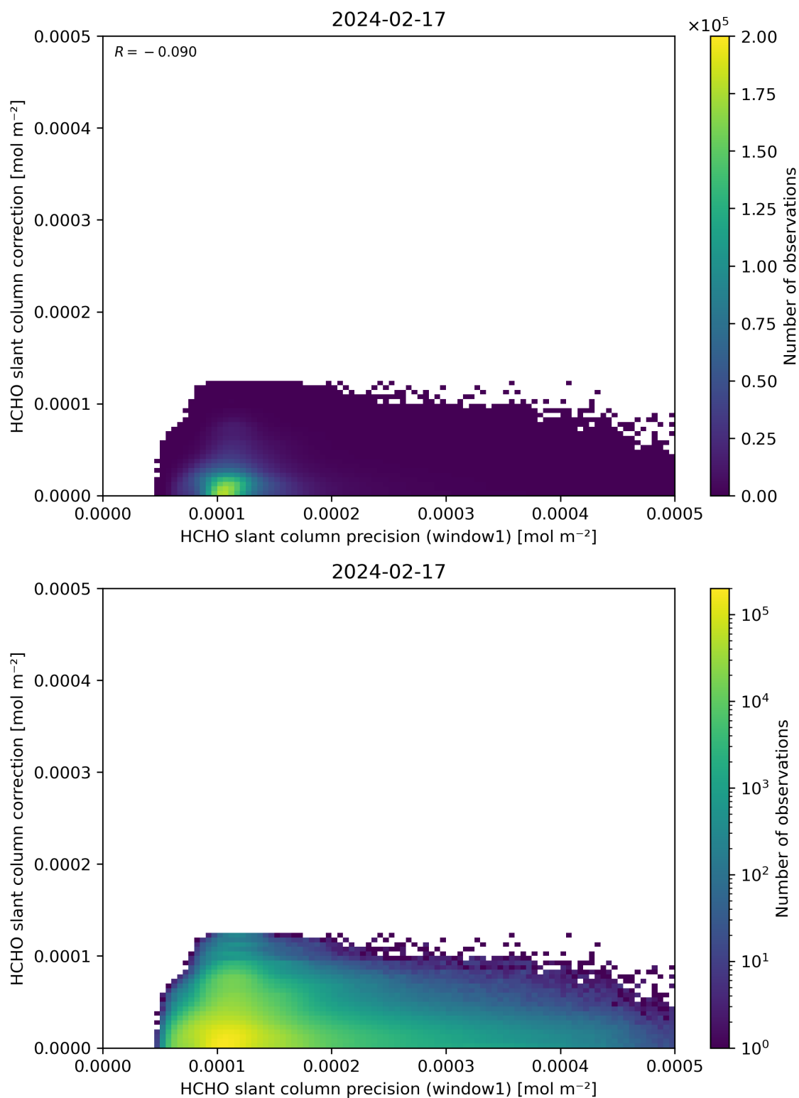
Figure 93: Scatter density plot of “HCHO slant column precision (window1)” against “HCHO slant column correction” for 2024-02-17 to 2024-02-18.
