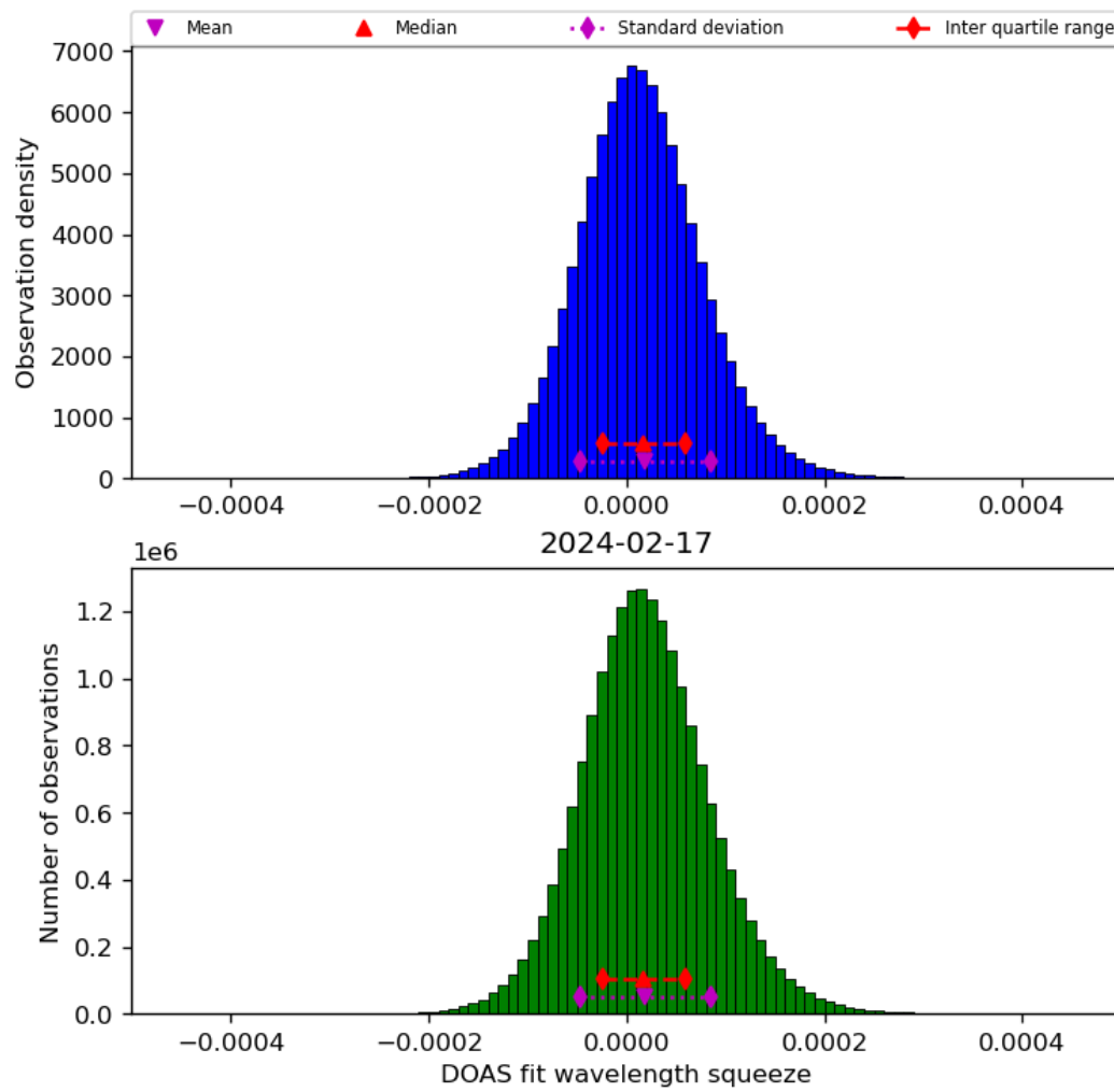
Figure 45: Histogram of “DOAS fit wavelength squeeze” for 2024-02-17 to 2024-02-18
