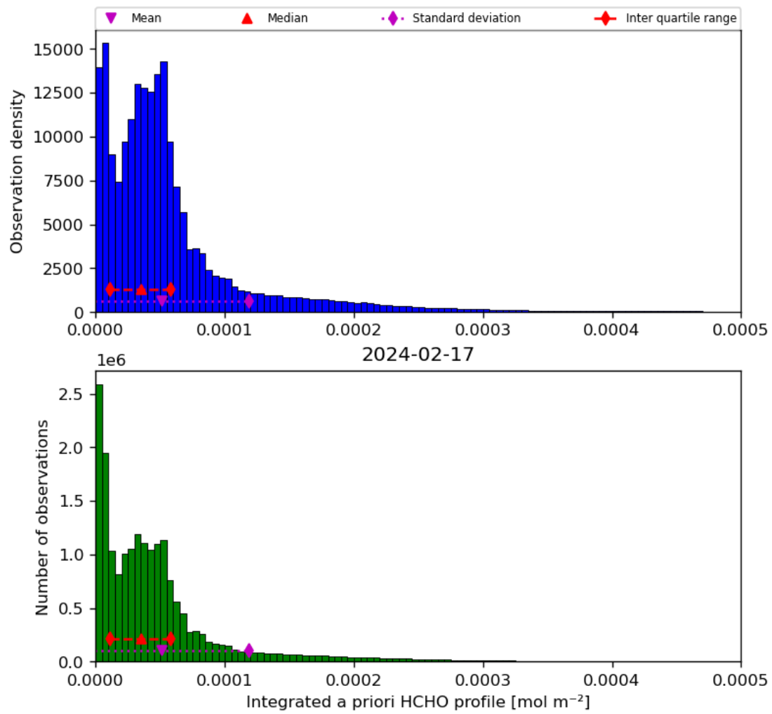
Figure 43: Histogram of “Integrated a priori HCHO profile” for 2024-02-17 to 2024-02-18
