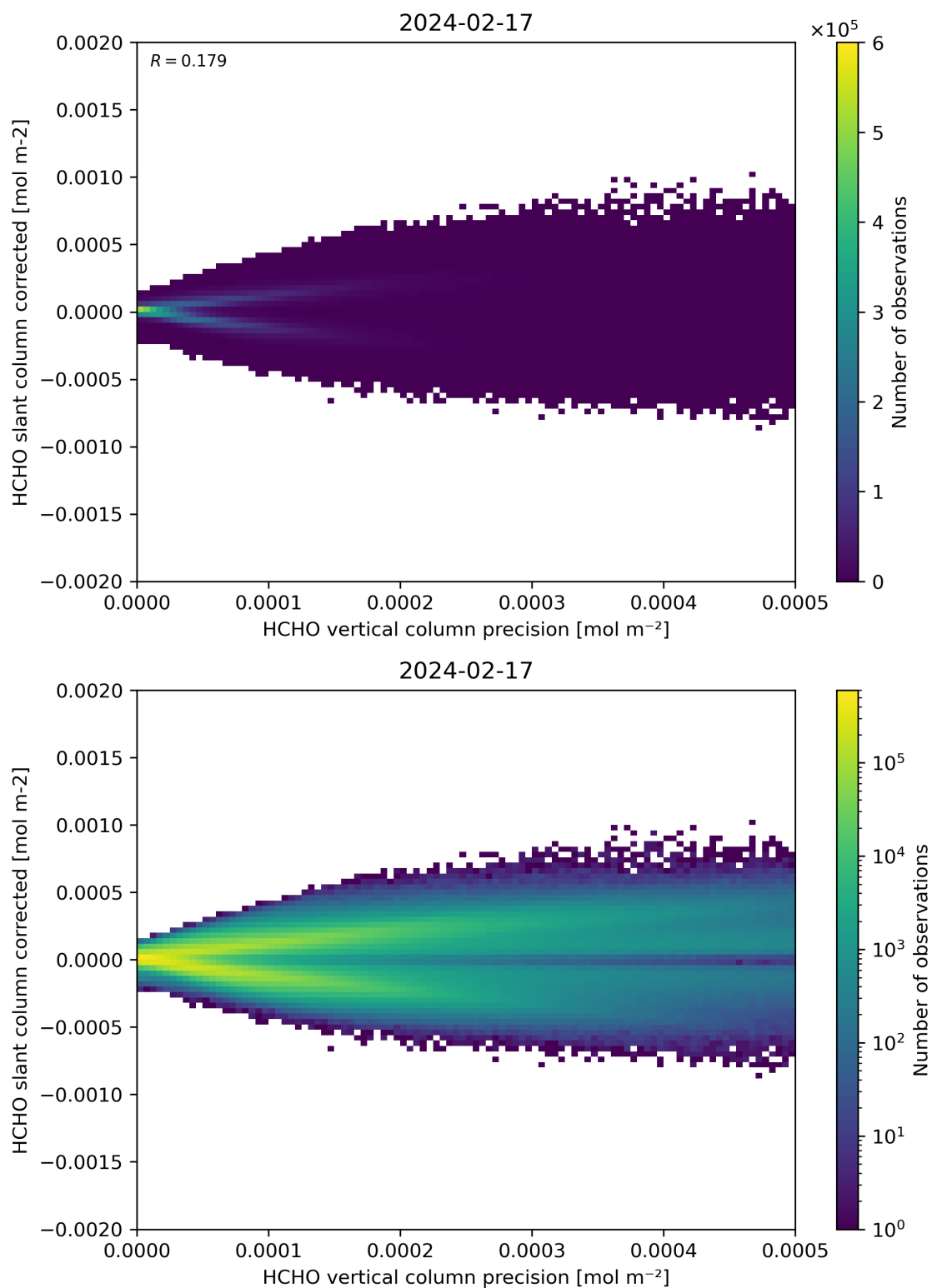
Figure 140: Scatter density plot of “HCHO vertical column precision” against “HCHO slant column corrected” for 2024-02-17 to 2024-02-18.
