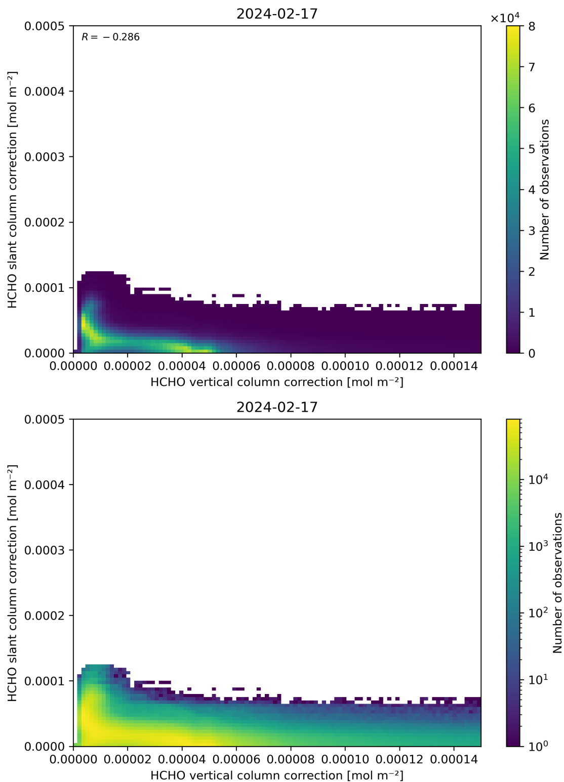
Figure 117: Scatter density plot of “HCHO vertical column correction” against “HCHO slant column correction” for 2024-02-17 to 2024-02-18.
