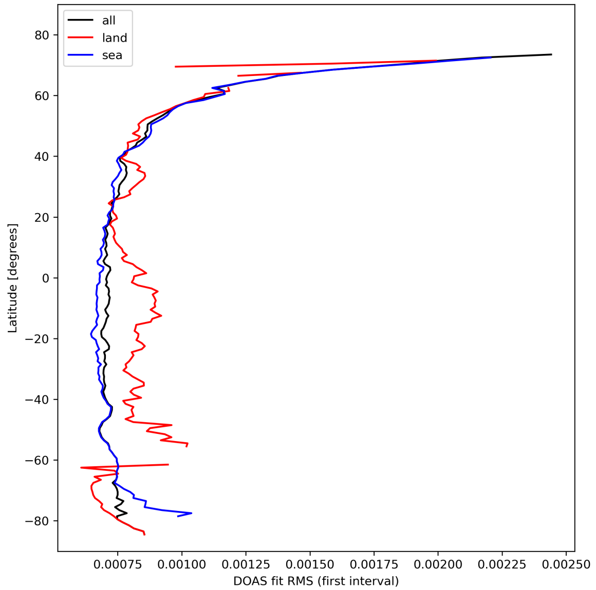
Figure 32: Zonal average of “DOAS fit RMS (first interval)” for 2024-02-17 to 2024-02-18.
