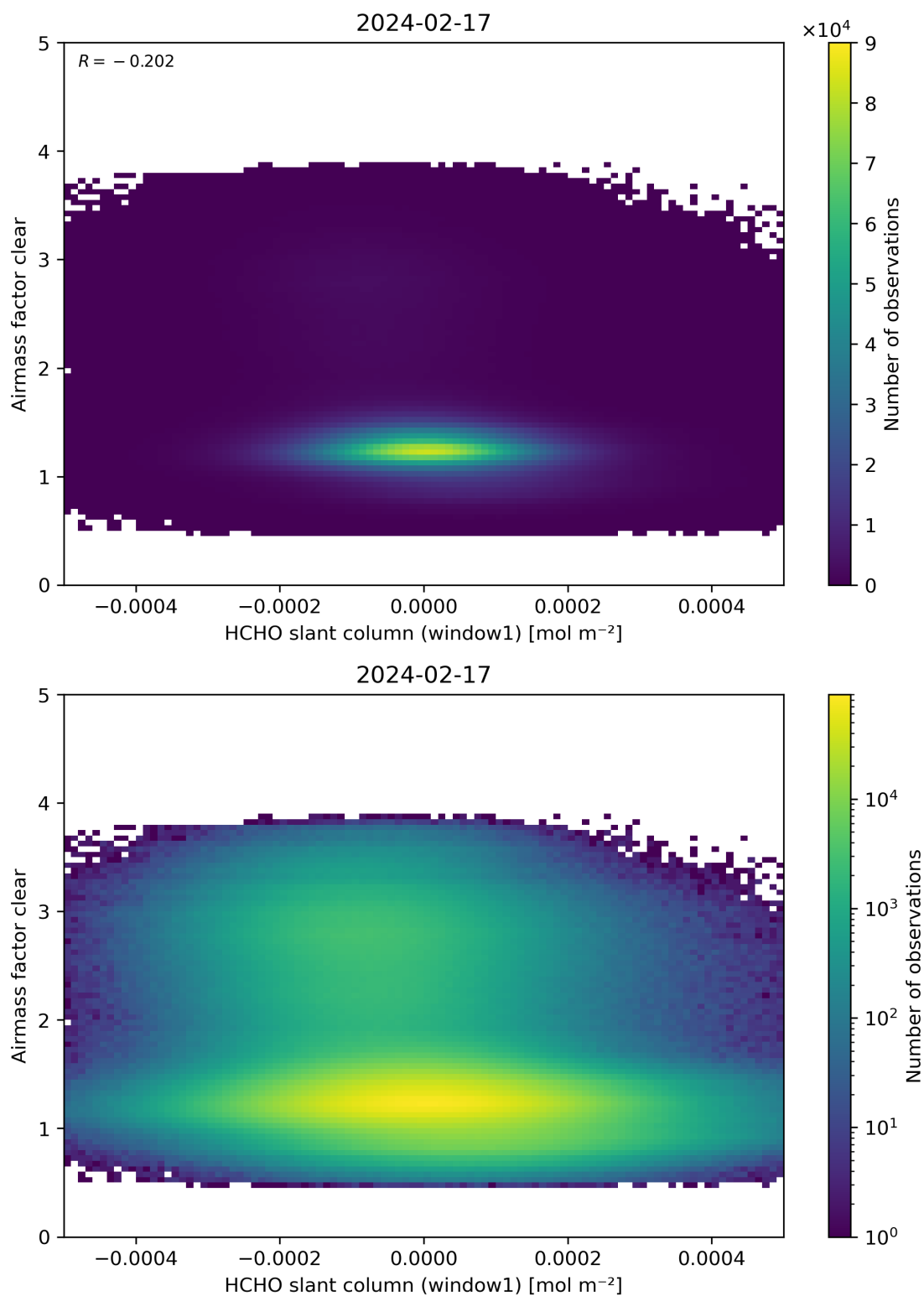
Figure 81: Scatter density plot of “HCHO slant column (window1)” against “Airmass factor clear” for 2024-02-17 to 2024-02-18.
