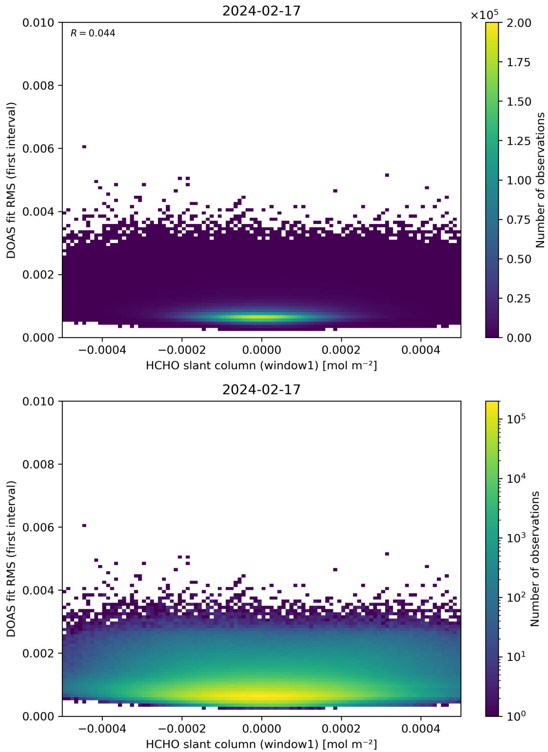
Figure 78: Scatter density plot of “HCHO slant column (window1)” against “DOAS fit RMS (first interval)” for 2024-02-17 to 2024-02-18.
