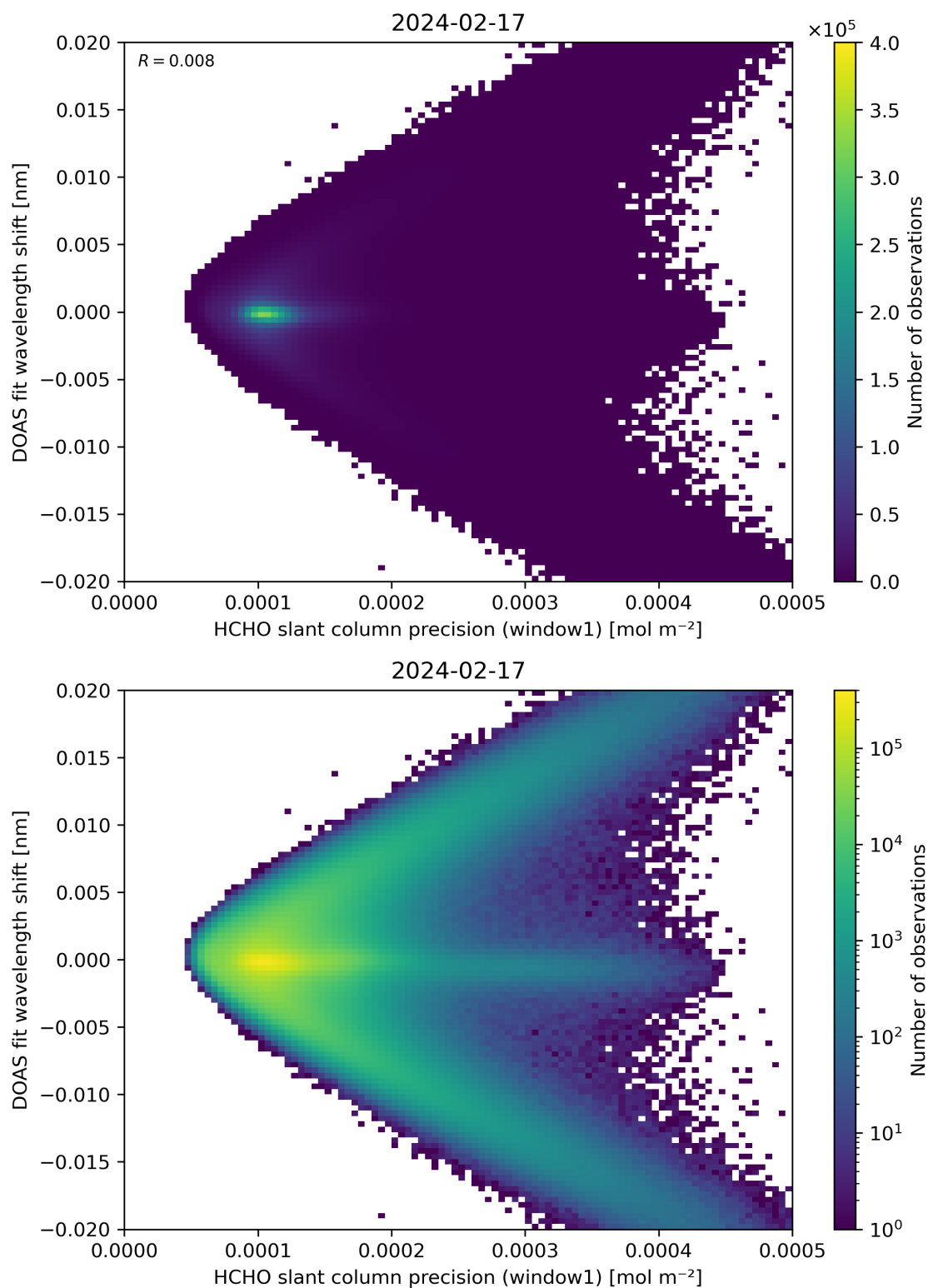
Figure 89: Scatter density plot of “HCHO slant column precision (window1)” against “DOAS fit wavelength shift” for 2024-02-17 to 2024-02-18.
