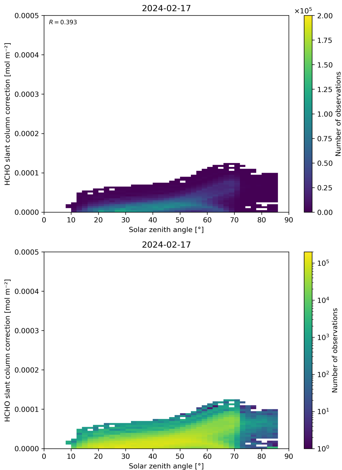
Figure 172: Scatter density plot of “Solar zenith angle” against “HCHO slant column correction” for 2024-02-17 to 2024-02-18.
