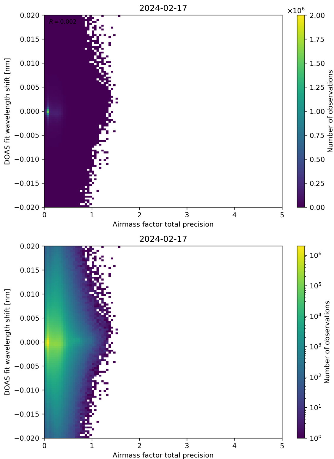
Figure 106: Scatter density plot of “Airmass factor total precision” against “DOAS fit wavelength shift” for 2024-02-17 to 2024-02-18.
