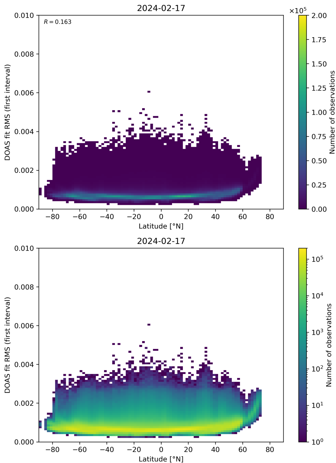
Figure 153: Scatter density plot of “Latitude” against “DOAS fit RMS (first interval)” for 2024-02-17 to 2024-02-18.
