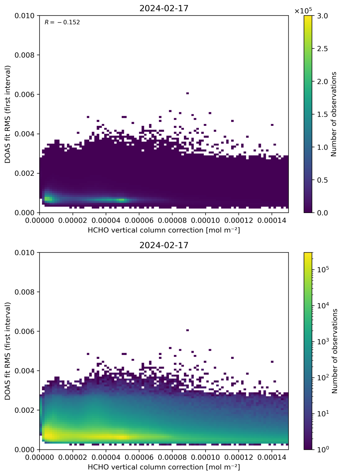
Figure 112: Scatter density plot of “HCHO vertical column correction” against “DOAS fit RMS (first interval)” for 2024-02-17 to 2024-02-18.
