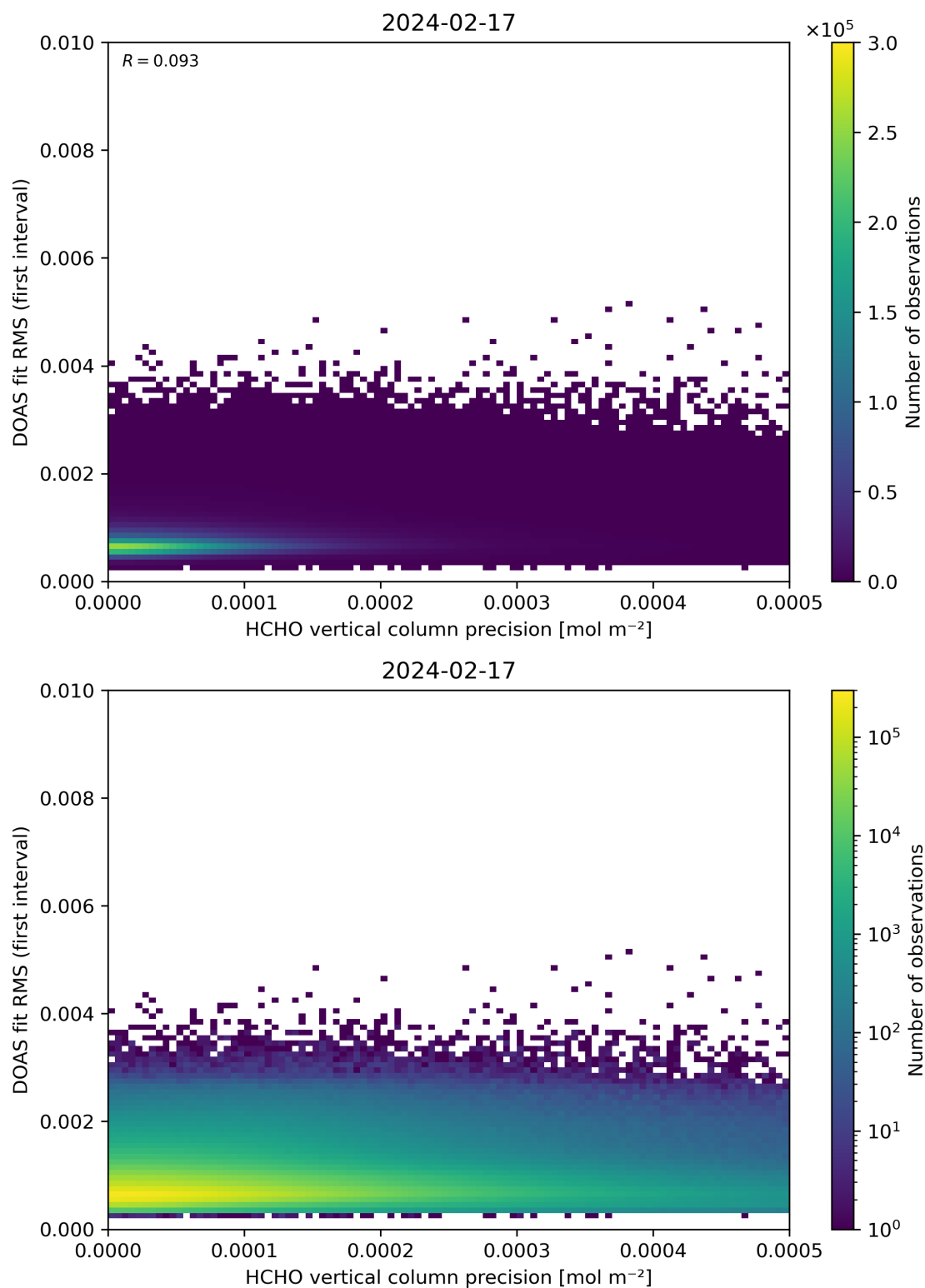
Figure 136: Scatter density plot of “HCHO vertical column precision” against “DOAS fit RMS (first interval)” for 2024-02-17 to 2024-02-18.
