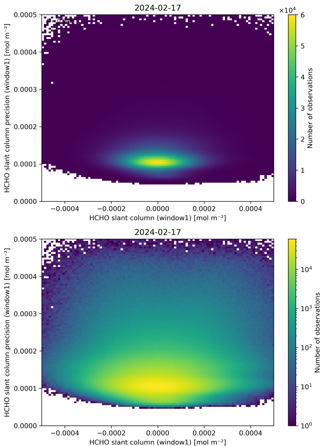
Figure 84: Scatter density plot of “HCHO slant column (window1)” against “HCHO slant column precision (window1)” for 2024-02-17 to 2024-02-18.
