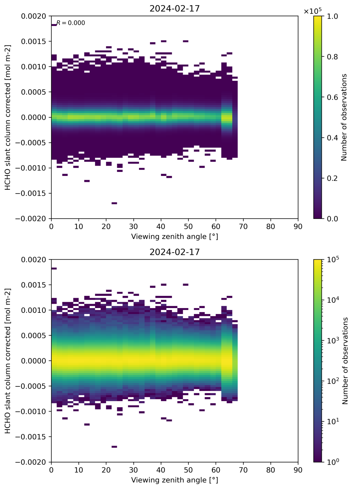
Figure 186: Scatter density plot of “Viewing zenith angle” against “HCHO slant column corrected” for 2024-02-17 to 2024-02-18.
