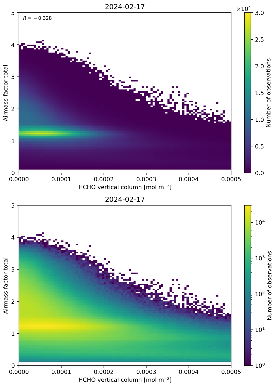
Figure 131: Scatter density plot of “HCHO vertical column” against “Airmass factor total” for 2024-02-17 to 2024-02-18.
