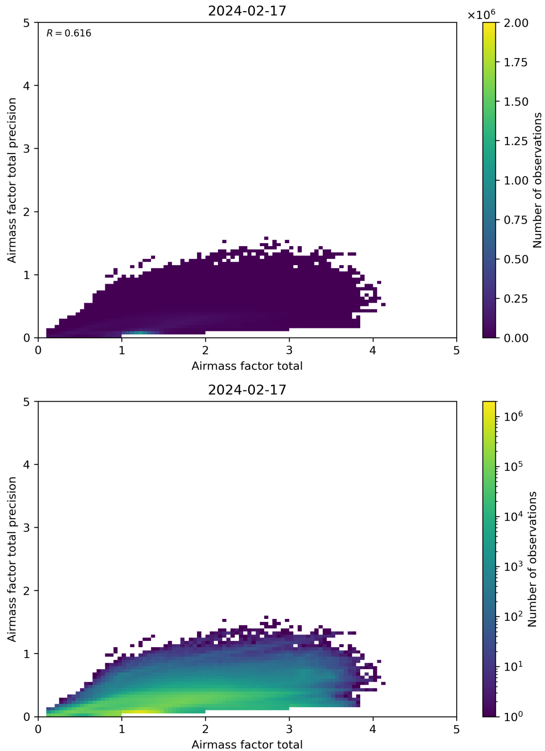
Figure 103: Scatter density plot of “Airmass factor total” against “Airmass factor total precision” for 2024-02-17 to 2024-02-18.
