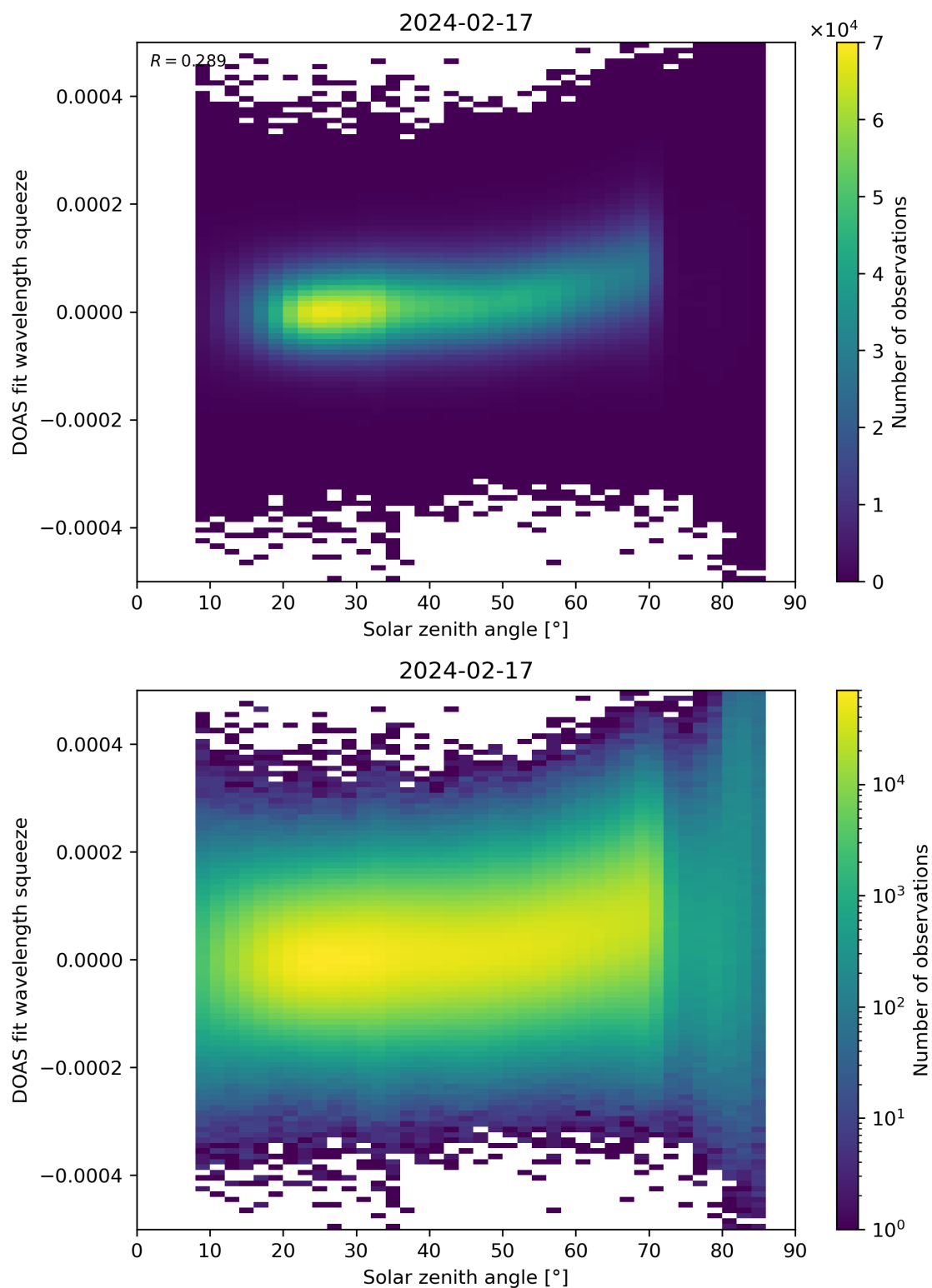
Figure 169: Scatter density plot of “Solar zenith angle” against “DOAS fit wavelength squeeze” for 2024-02-17 to 2024-02-18.
