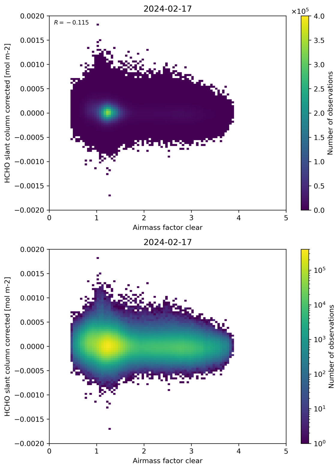
Figure 74: Scatter density plot of “Airmass factor clear” against “HCHO slant column corrected” for 2024-02-17 to 2024-02-18.
