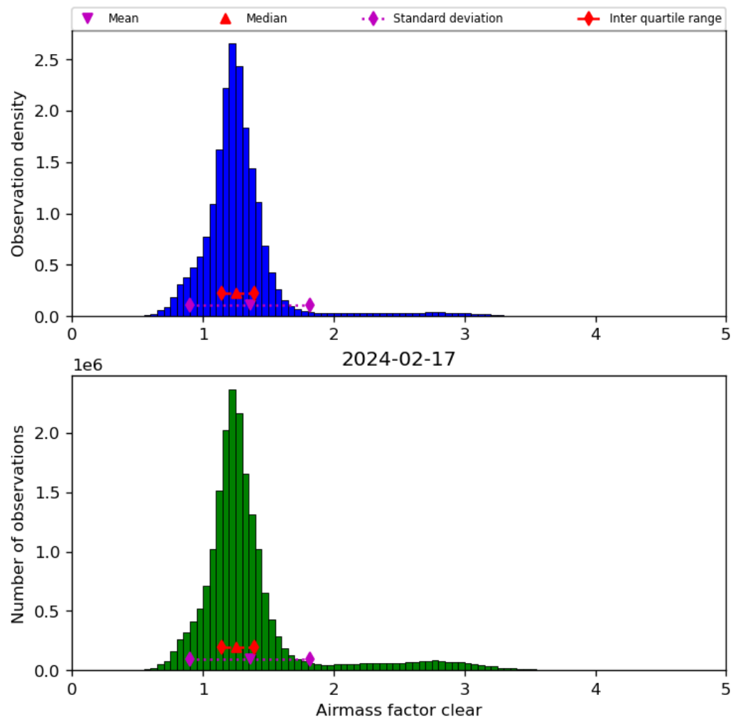
Figure 42: Histogram of “Airmass factor clear” for 2024-02-17 to 2024-02-18
