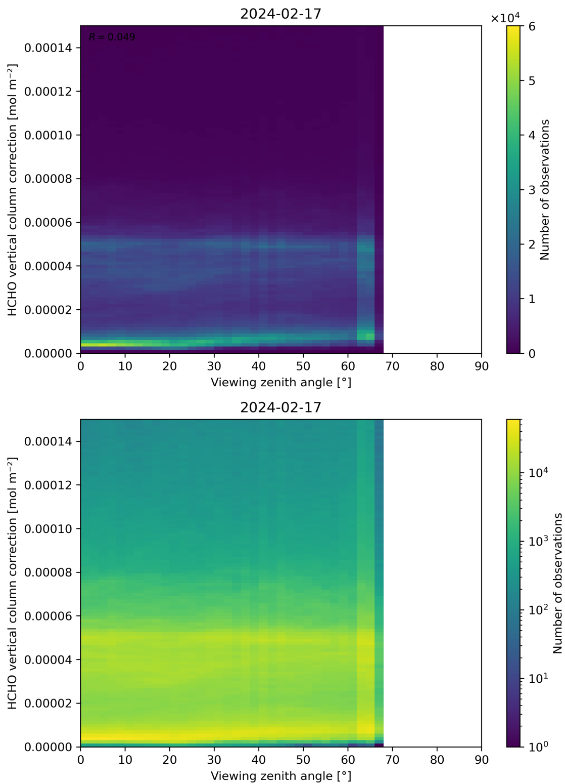
Figure 193: Scatter density plot of “Viewing zenith angle” against “HCHO vertical column correction” for 2024-02-17 to 2024-02-18.
