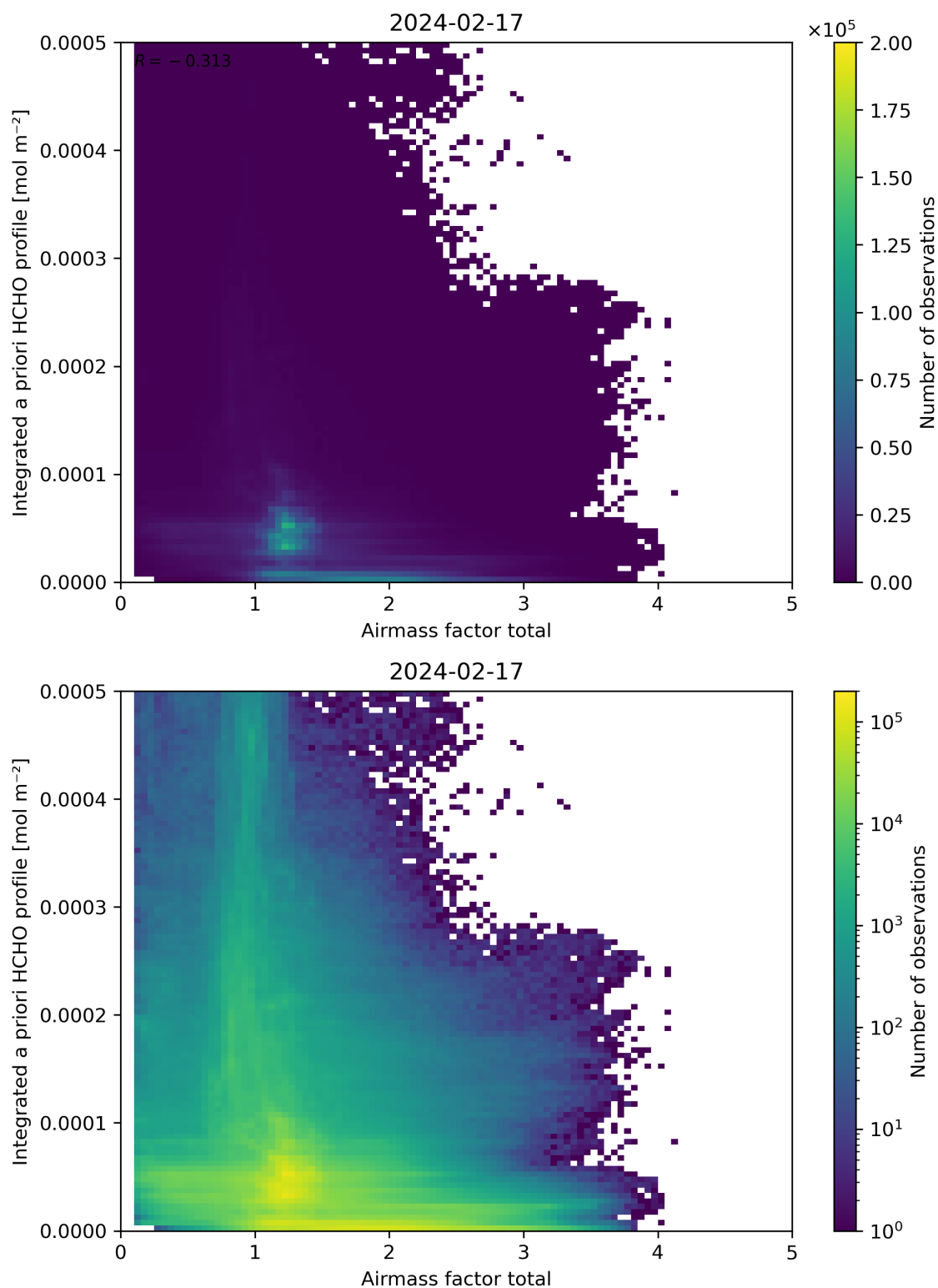
Figure 104: Scatter density plot of “Airmass factor total” against “Integrated a priori HCHO profile” for 2024-02-17 to 2024-02-18.
