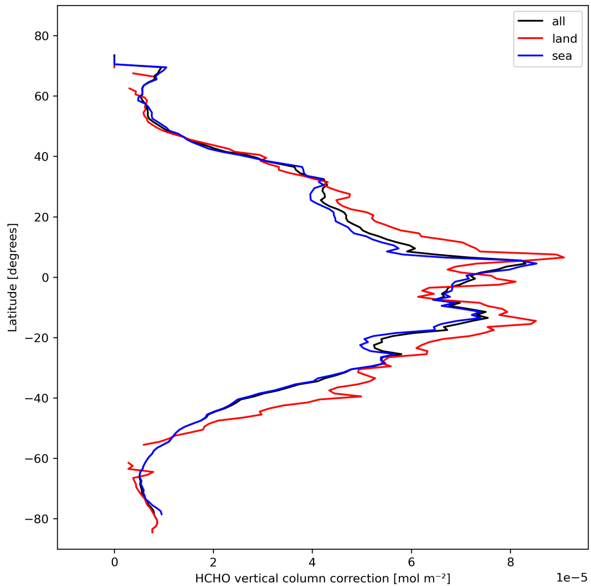
Figure 23: Zonal average of “HCHO vertical column correction” for 2024-02-17 to 2024-02-18.
