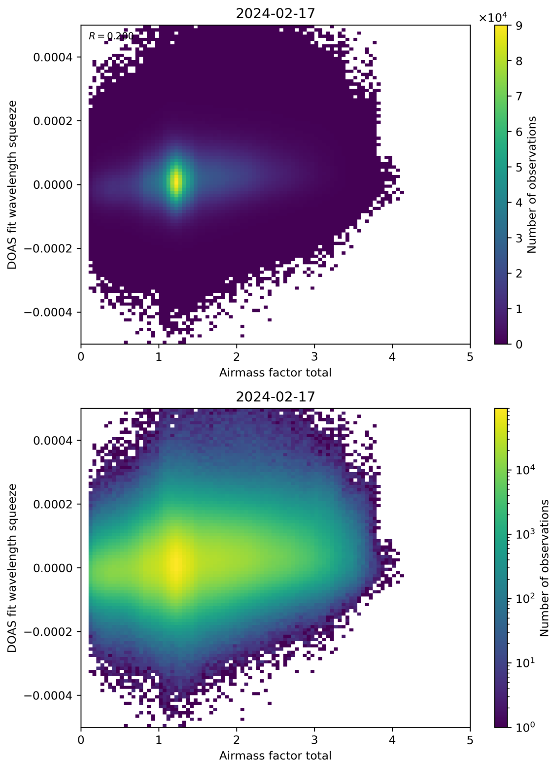
Figure 99: Scatter density plot of “Airmass factor total” against “DOAS fit wavelength squeeze” for 2024-02-17 to 2024-02-18.
