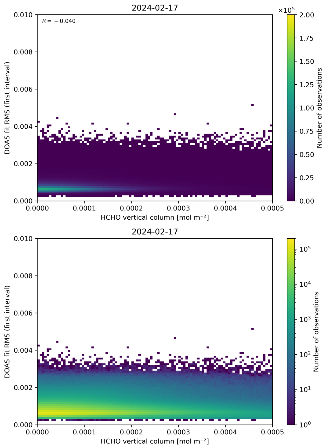
Figure 123: Scatter density plot of “HCHO vertical column” against “DOAS fit RMS (first interval)” for 2024-02-17 to 2024-02-18.
