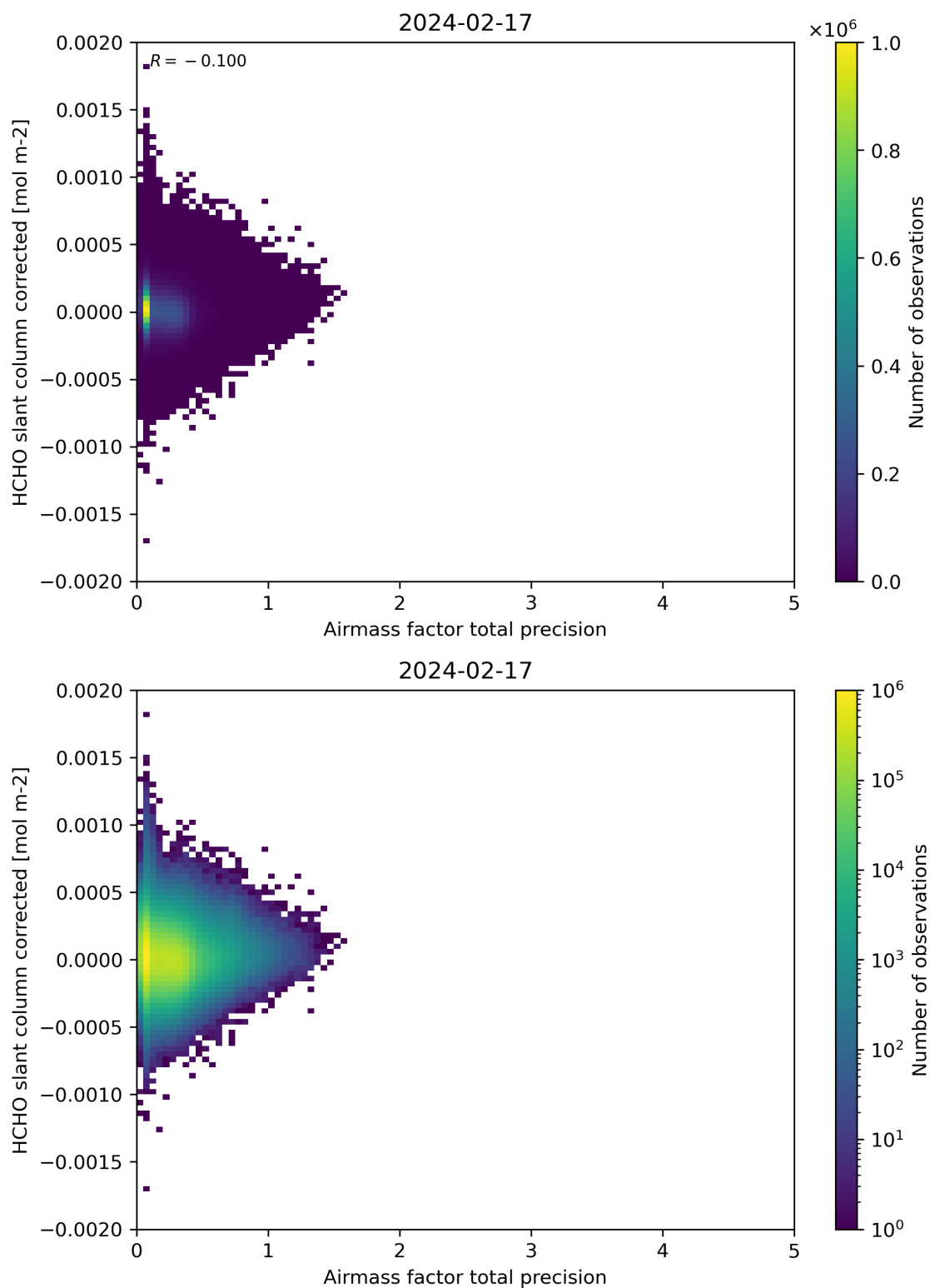
Figure 109: Scatter density plot of “Airmass factor total precision” against “HCHO slant column corrected” for 2024-02-17 to 2024-02-18.
