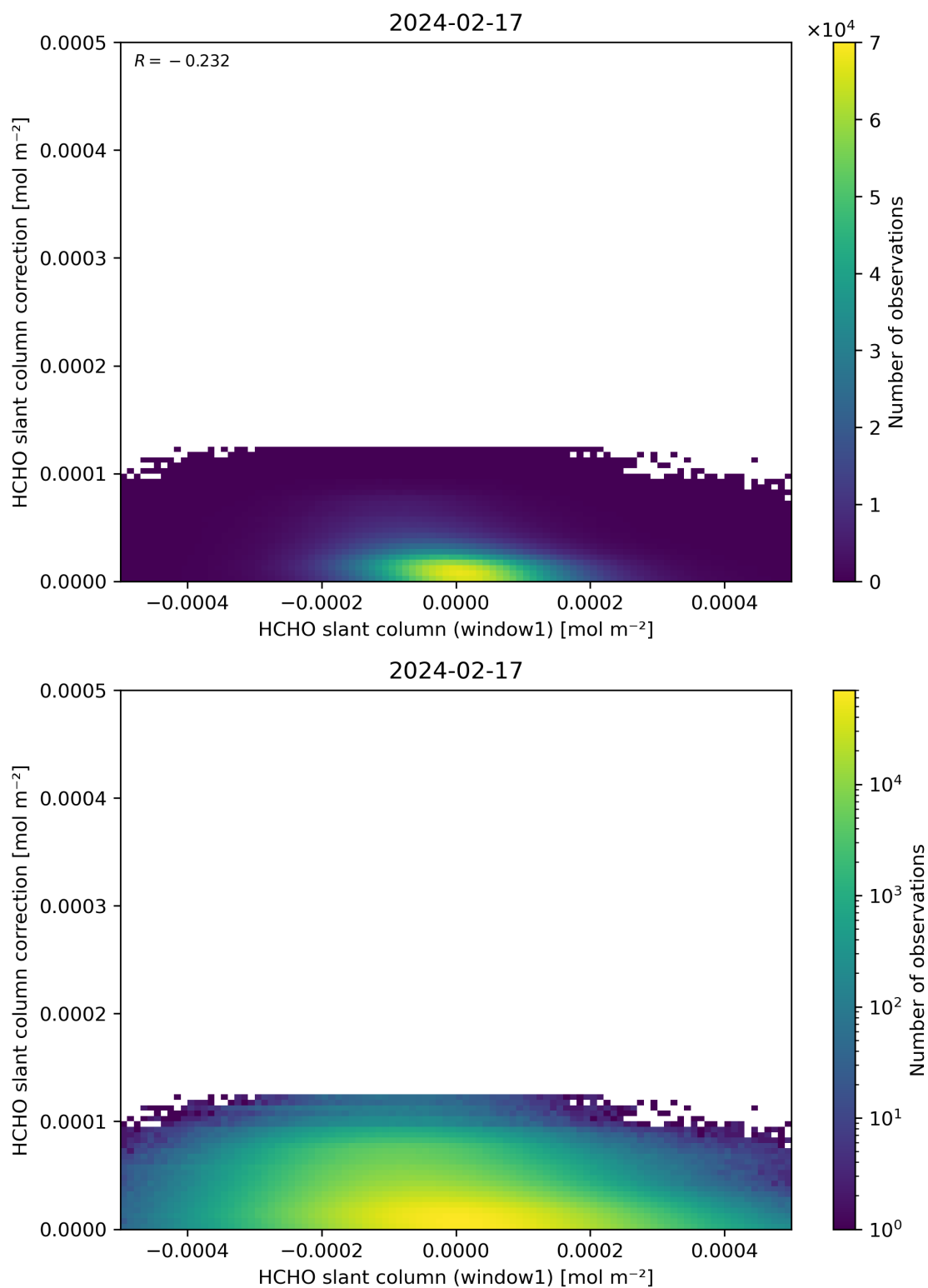
Figure 83: Scatter density plot of “HCHO slant column (window1)” against “HCHO slant column correction” for 2024-02-17 to 2024-02-18.
