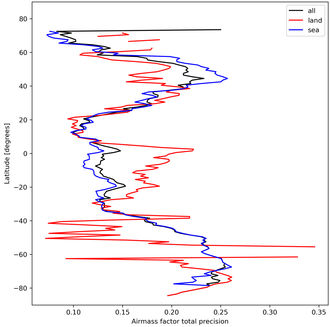
Figure 27: Zonal average of “Airmass factor total precision” for 2024-02-17 to 2024-02-18.
