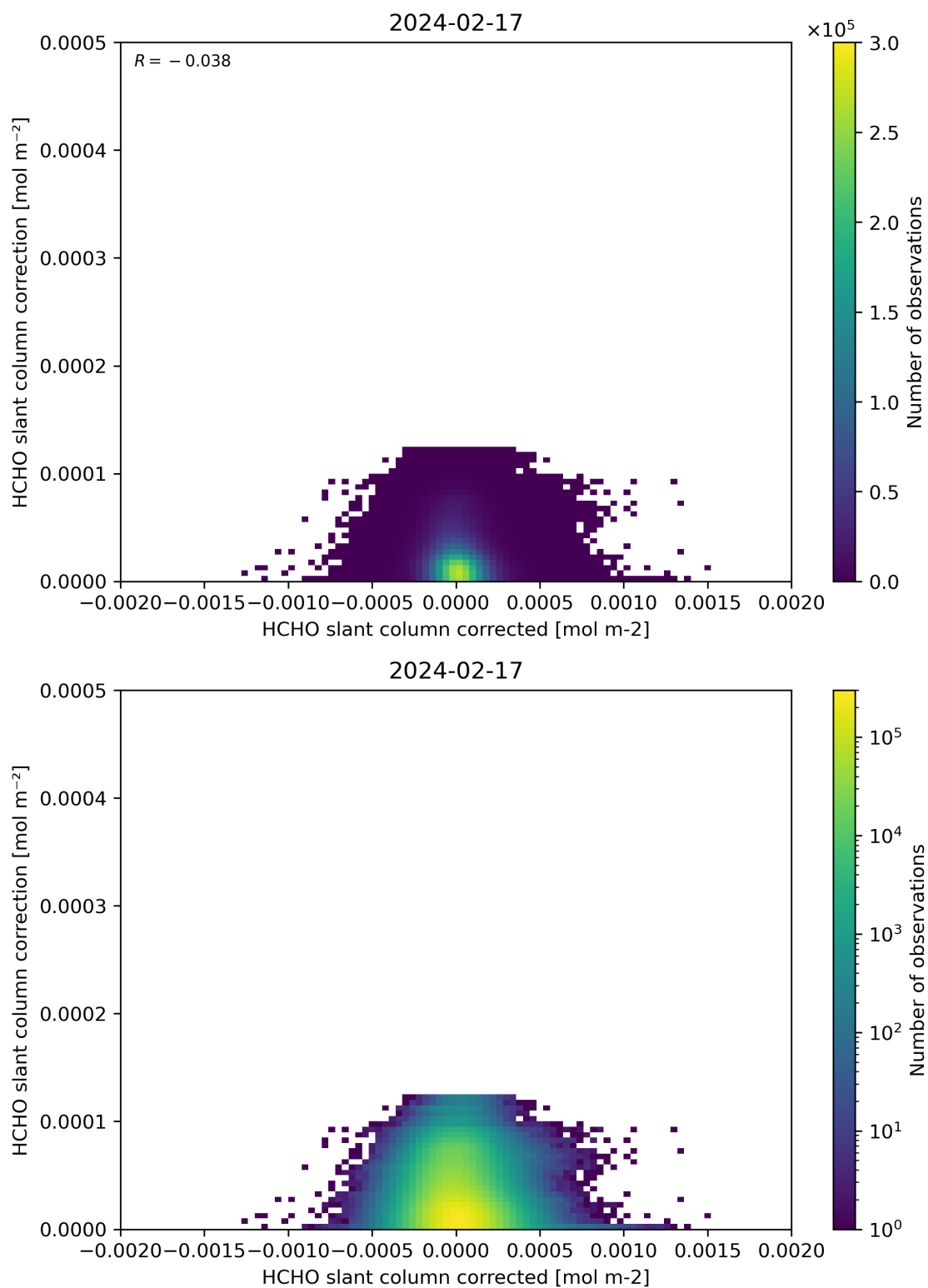
Figure 77: Scatter density plot of “HCHO slant column corrected” against “HCHO slant column correction” for 2024-02-17 to 2024-02-18.
