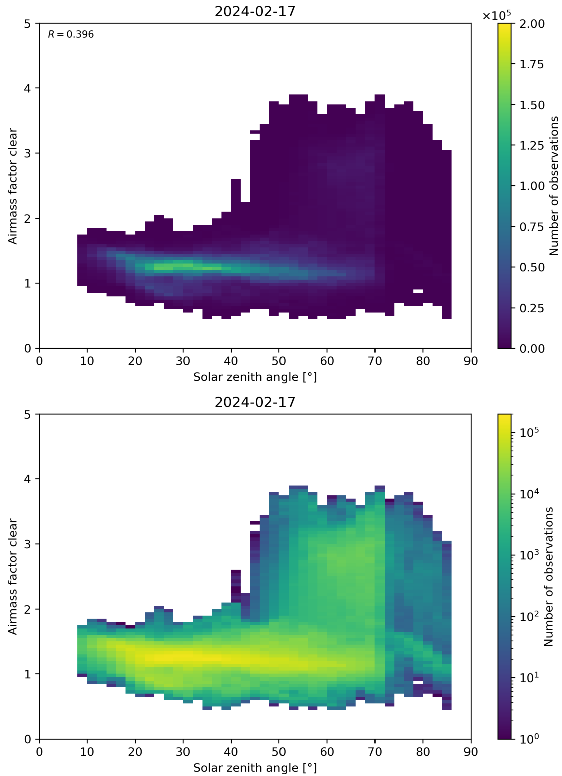
Figure 170: Scatter density plot of “Solar zenith angle” against “Airmass factor clear” for 2024-02-17 to 2024-02-18.
