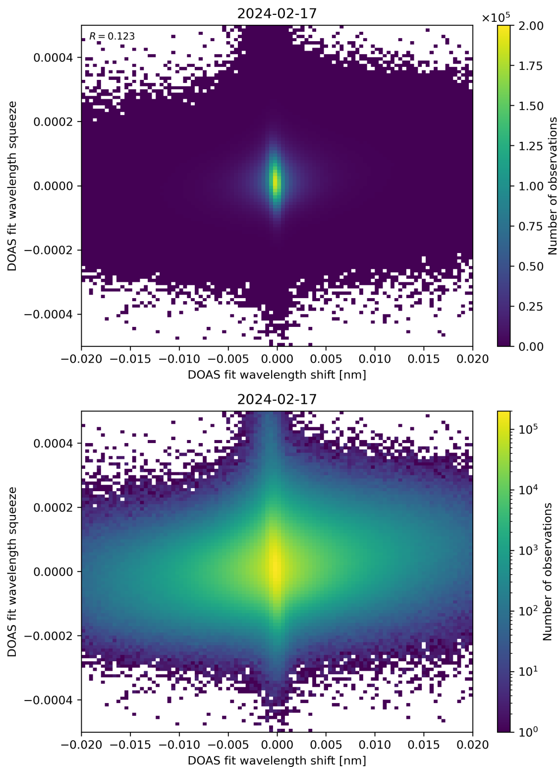
Figure 65: Scatter density plot of “DOAS fit wavelength shift” against “DOAS fit wavelength squeeze” for 2024-02-17 to 2024-02-18.
