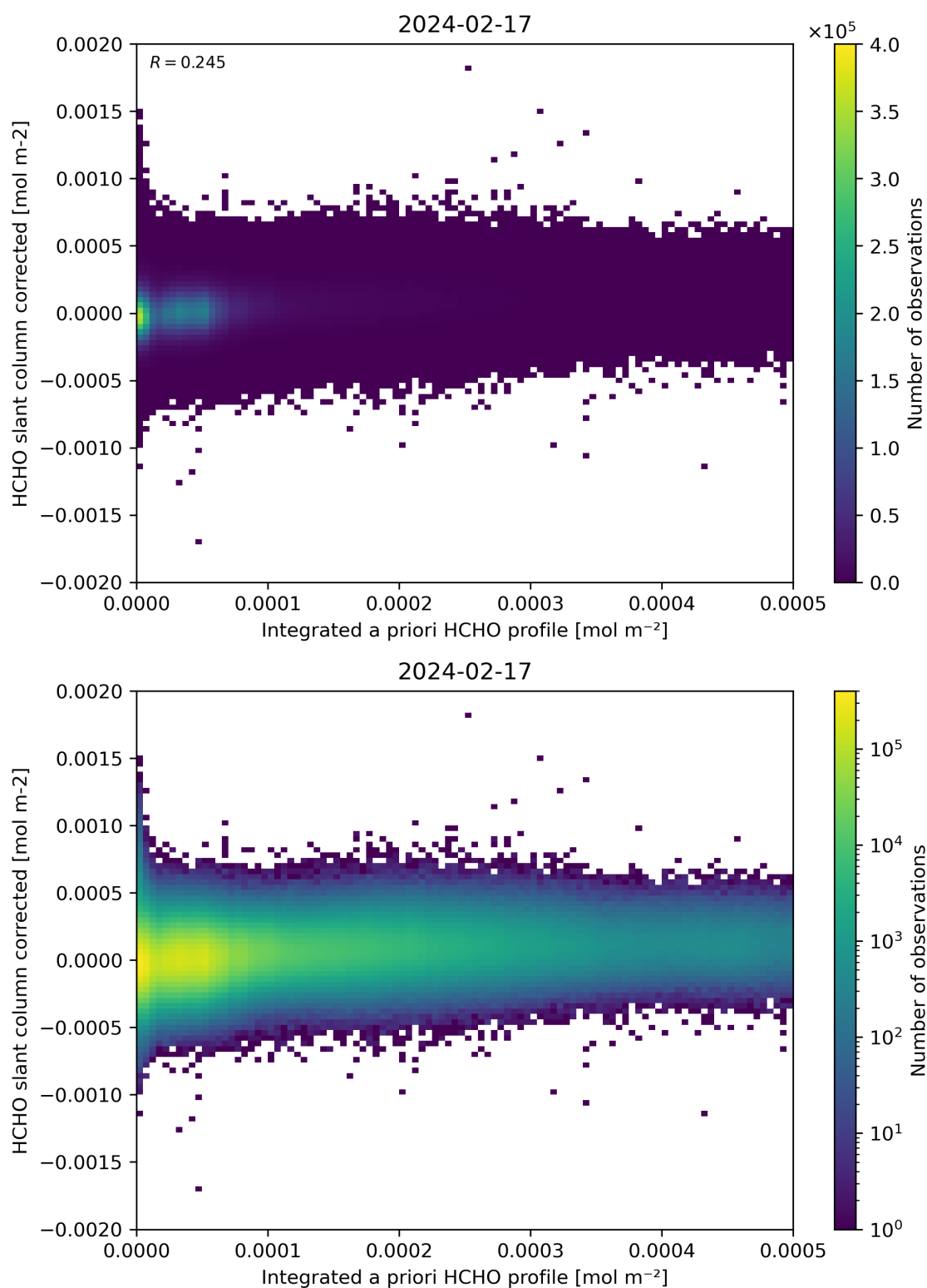
Figure 151: Scatter density plot of “Integrated a priori HCHO profile” against “HCHO slant column corrected” for 2024-02-17 to 2024-02-18.
