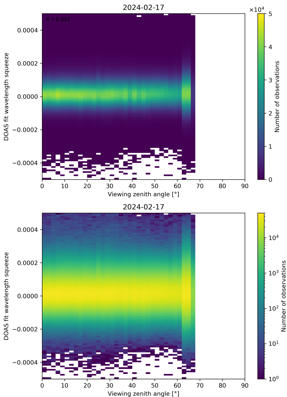
Figure 184: Scatter density plot of “Viewing zenith angle” against “DOAS fit wavelength squeeze” for 2024-02-17 to 2024-02-18.
