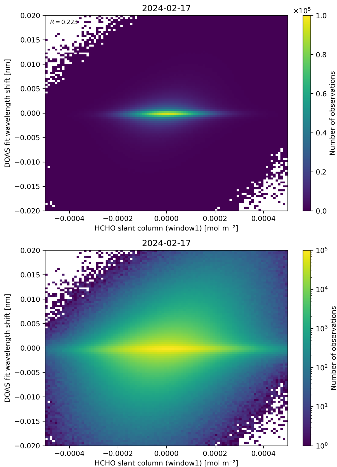
Figure 79: Scatter density plot of “HCHO slant column (window1)” against “DOAS fit wavelength shift” for 2024-02-17 to 2024-02-18.
