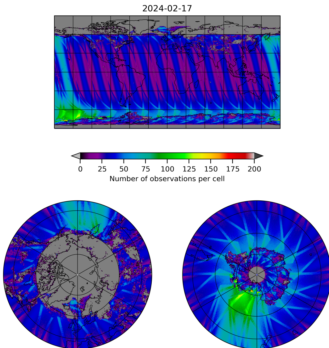
Figure 19: Map of the number of observations for 2024-02-17 to 2024-02-18
