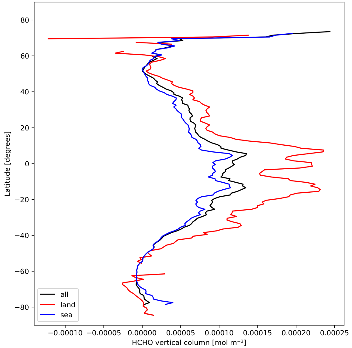
Figure 21: Zonal average of “HCHO vertical column” for 2024-02-17 to 2024-02-18.
