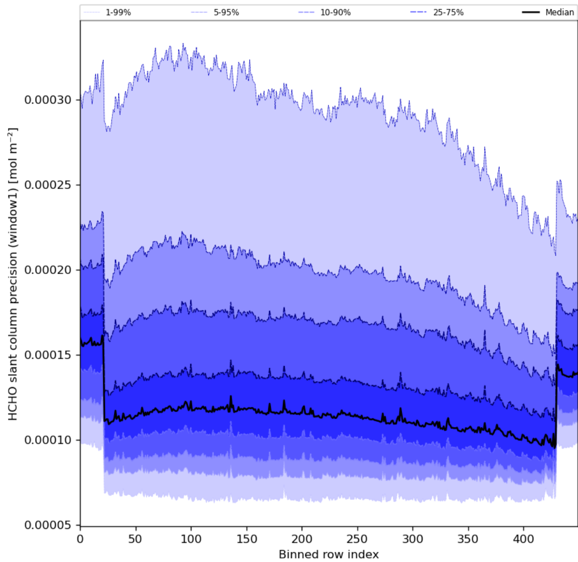
Figure 53: Along track statistics of “HCHO slant column precision (window1)” for 2024-02-17 to 2024-02-18
