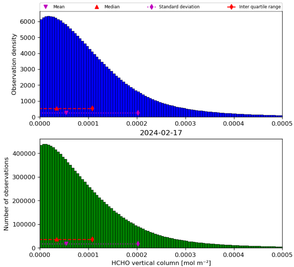
Figure 35: Histogram of “HCHO vertical column” for 2024-02-17 to 2024-02-18
