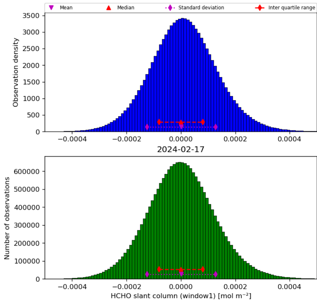
Figure 38: Histogram of “HCHO slant column (window1)” for 2024-02-17 to 2024-02-18
