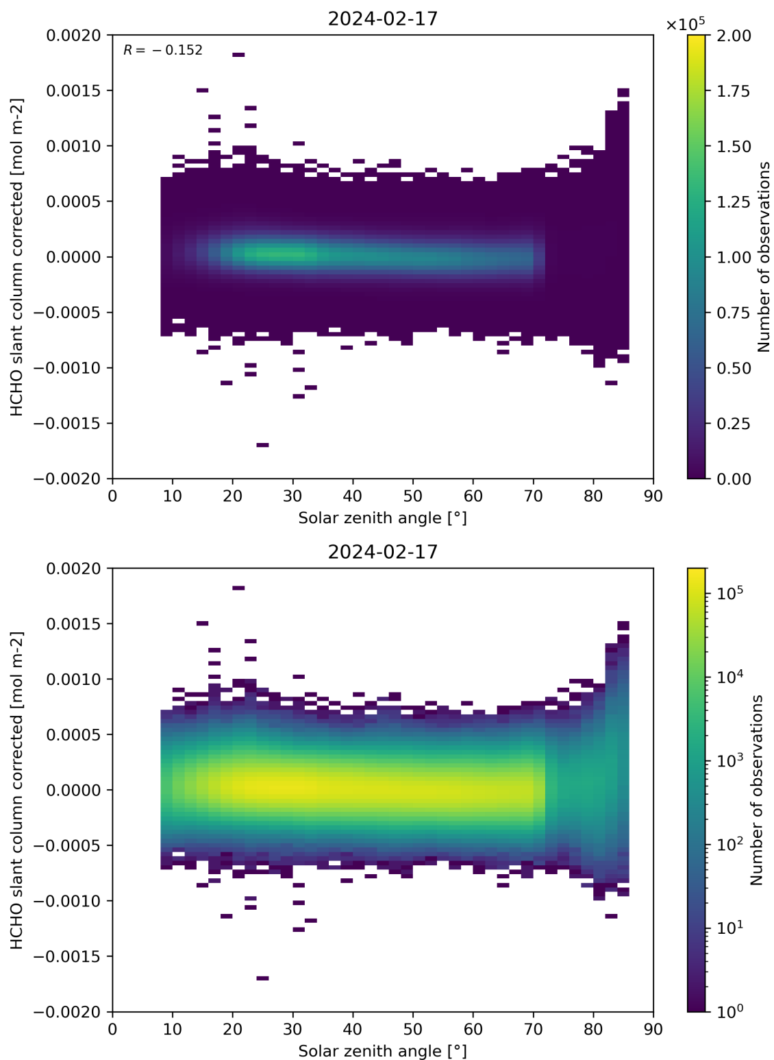
Figure 171: Scatter density plot of “Solar zenith angle” against “HCHO slant column corrected” for 2024-02-17 to 2024-02-18.
