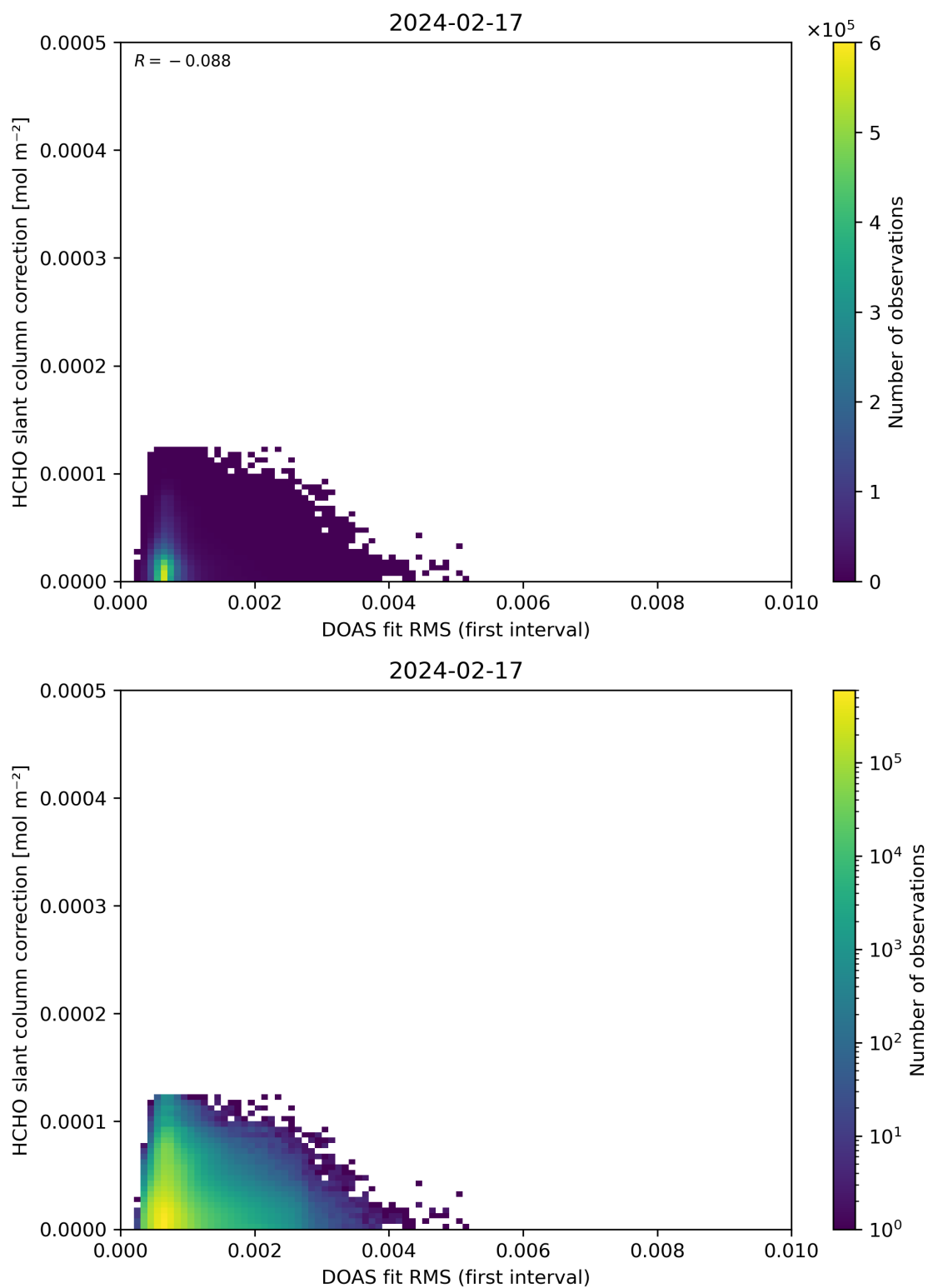
Figure 63: Scatter density plot of “DOAS fit RMS (first interval)” against “HCHO slant column correction” for 2024-02-17 to 2024-02-18.
