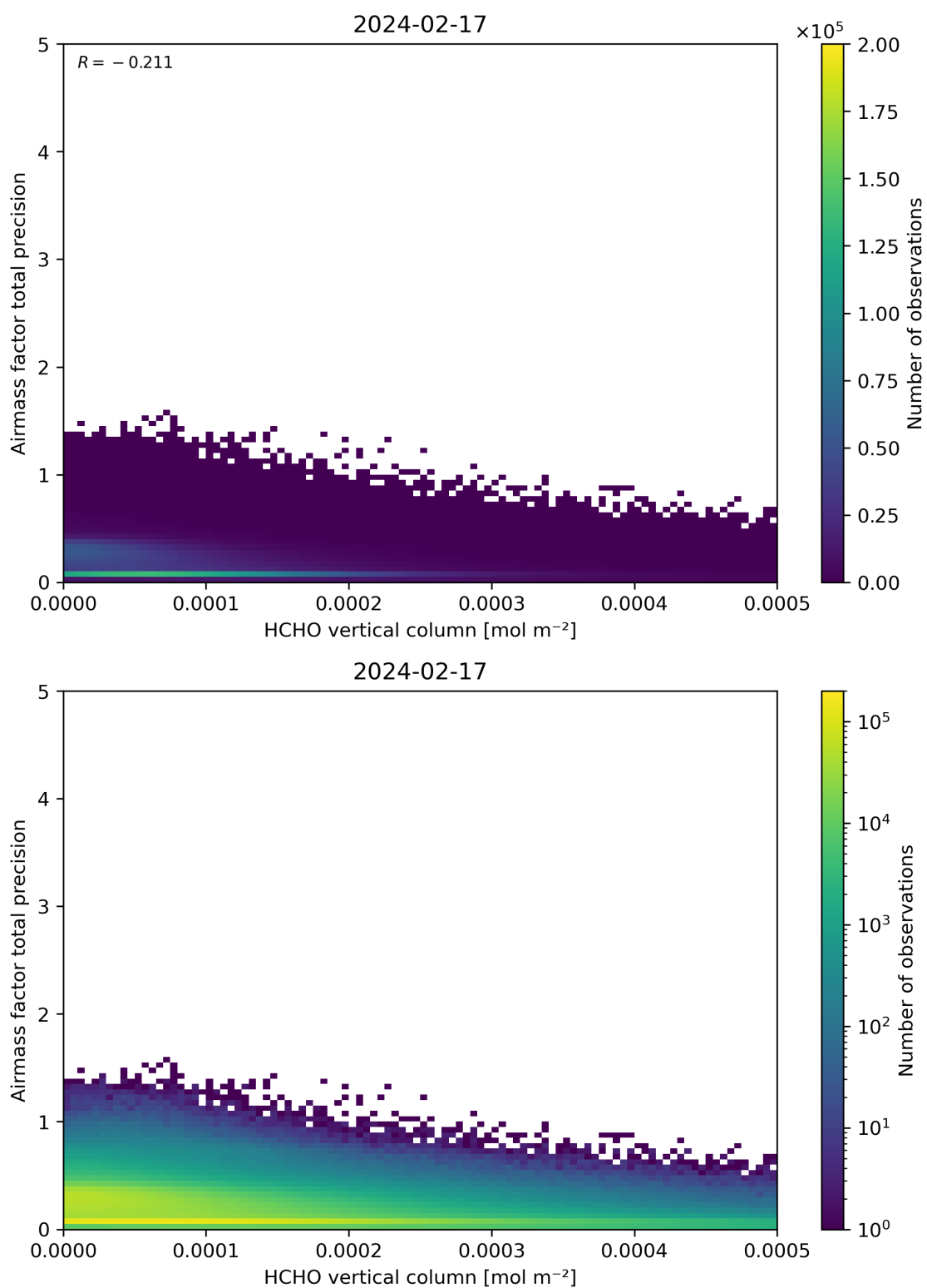
Figure 132: Scatter density plot of “HCHO vertical column” against “Airmass factor total precision” for 2024-02-17 to 2024-02-18.
