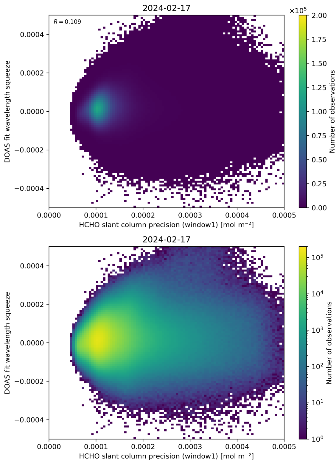
Figure 90: Scatter density plot of “HCHO slant column precision (window1)” against “DOAS fit wavelength squeeze” for 2024-02-17 to 2024-02-18.
