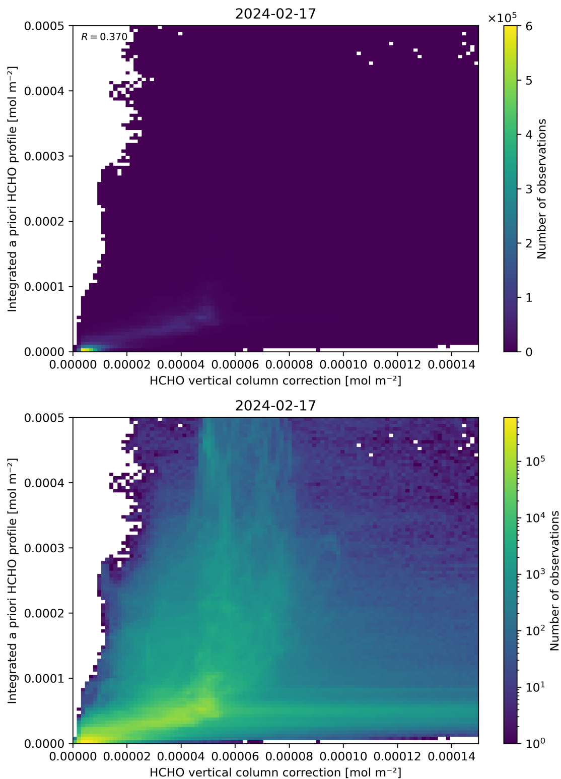
Figure 122: Scatter density plot of “HCHO vertical column correction” against “Integrated a priori HCHO profile” for 2024-02-17 to 2024-02-18.
