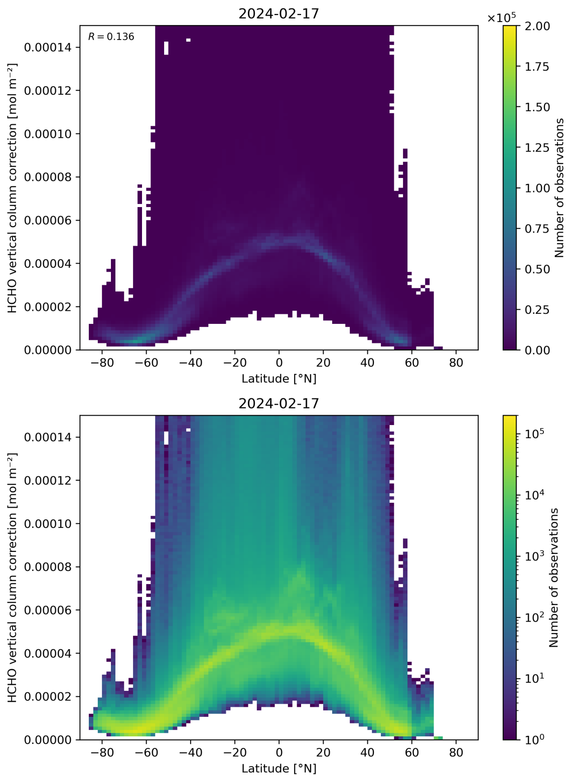
Figure 164: Scatter density plot of “Latitude” against “HCHO vertical column correction” for 2024-02-17 to 2024-02-18.
