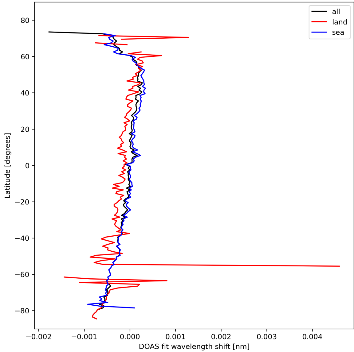
Figure 30: Zonal average of "DOAS fit wavelength shift" for 2024-02-17 to 2024-02-18.
