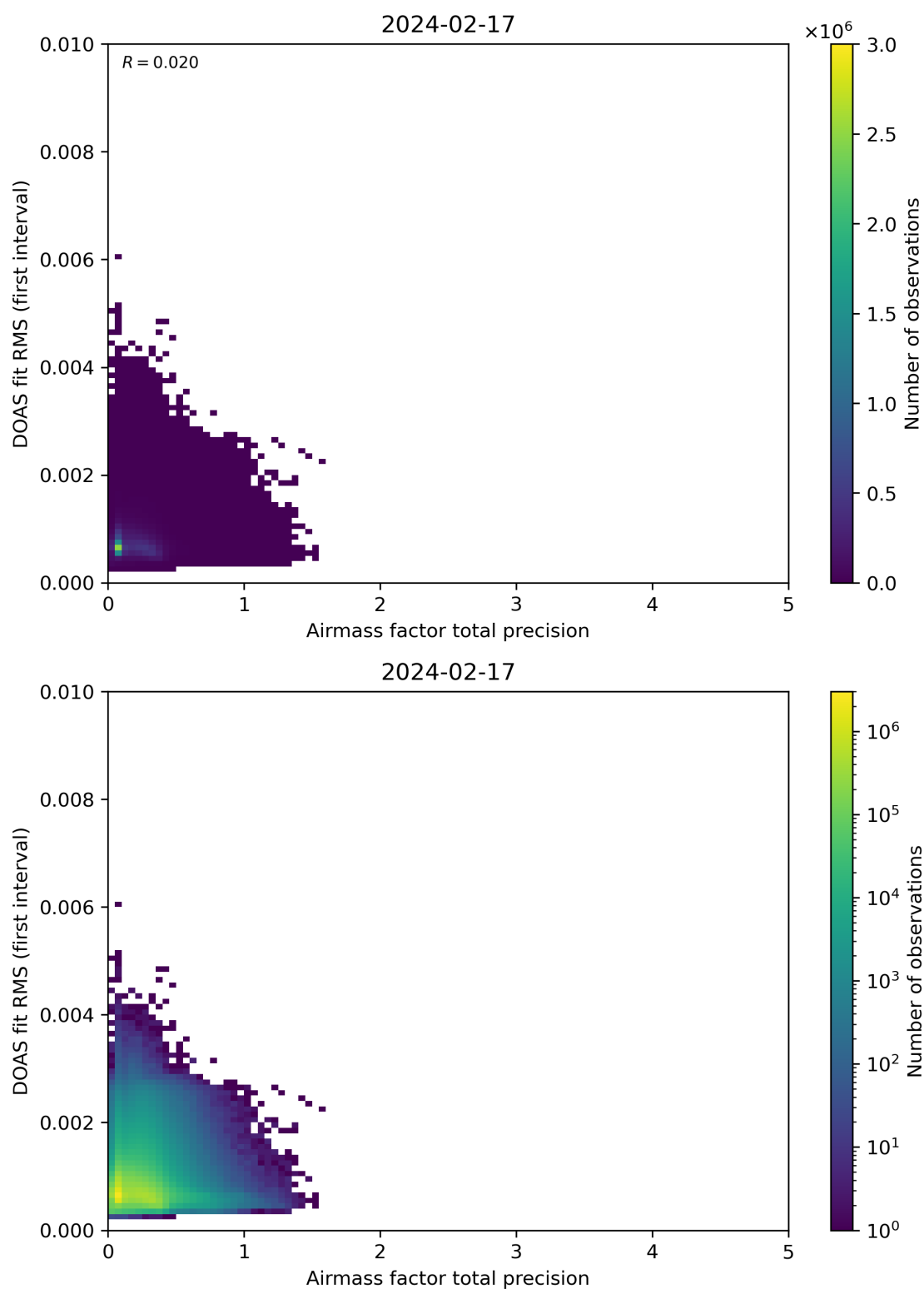
Figure 105: Scatter density plot of “Airmass factor total precision” against “DOAS fit RMS (first interval)” for 2024-02-17 to 2024-02-18.
