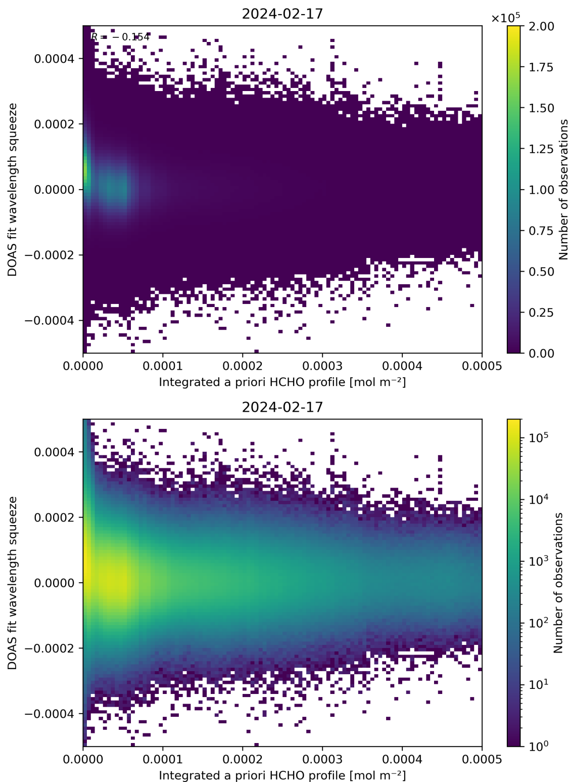
Figure 150: Scatter density plot of “Integrated a priori HCHO profile” against “DOAS fit wavelength squeeze” for 2024-02-17 to 2024-02-18.
