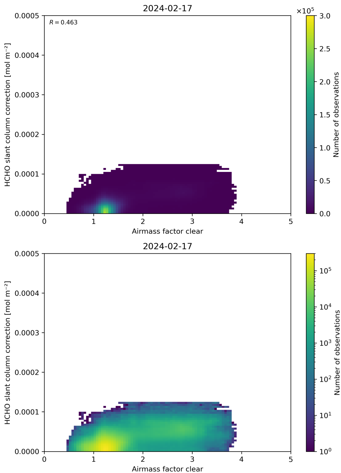
Figure 75: Scatter density plot of “Airmass factor clear” against “HCHO slant column correction” for 2024-02-17 to 2024-02-18.
