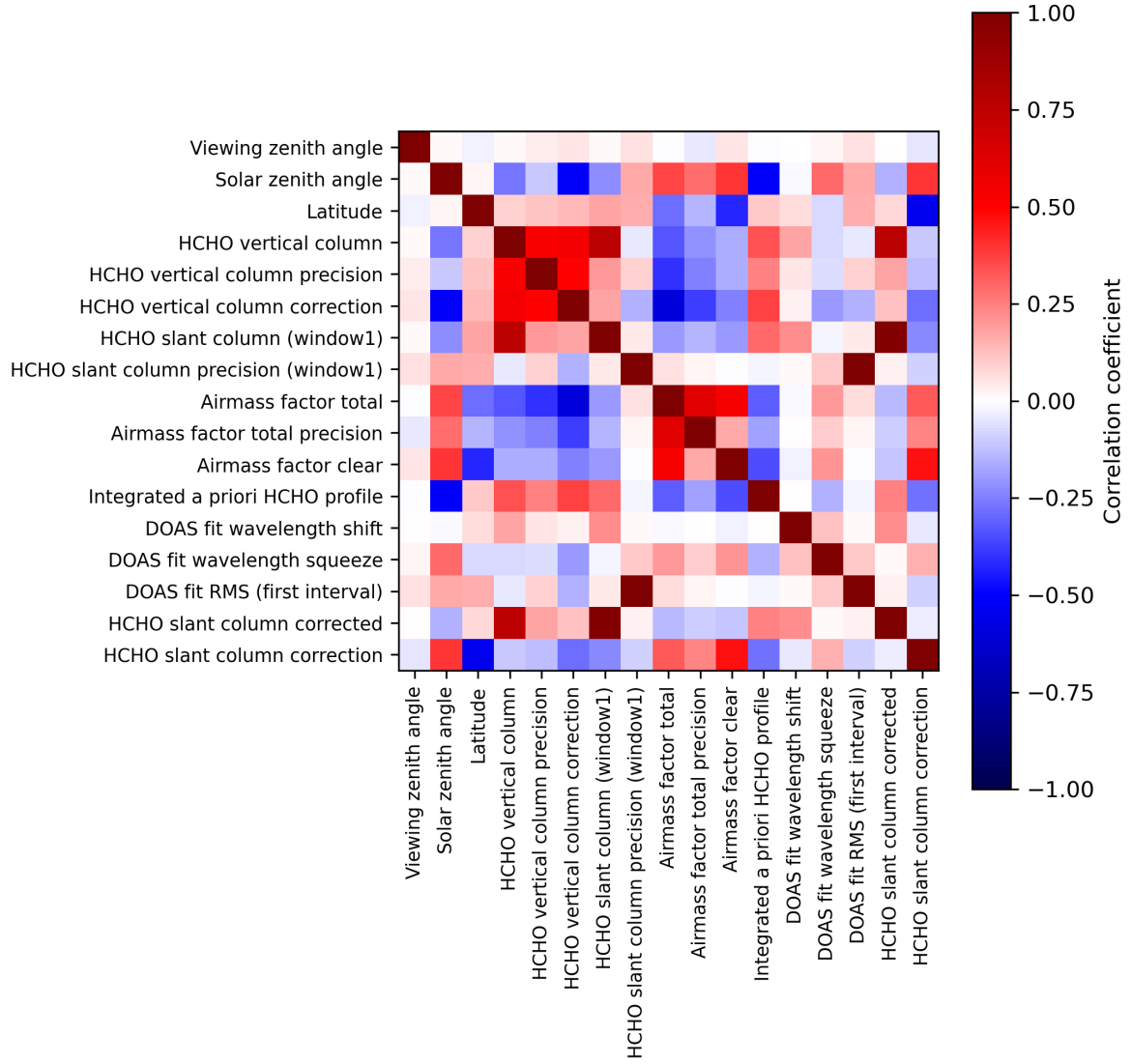
Figure 2: Map of correlation matrix for 2024-02-17 to 2024-02-18.
