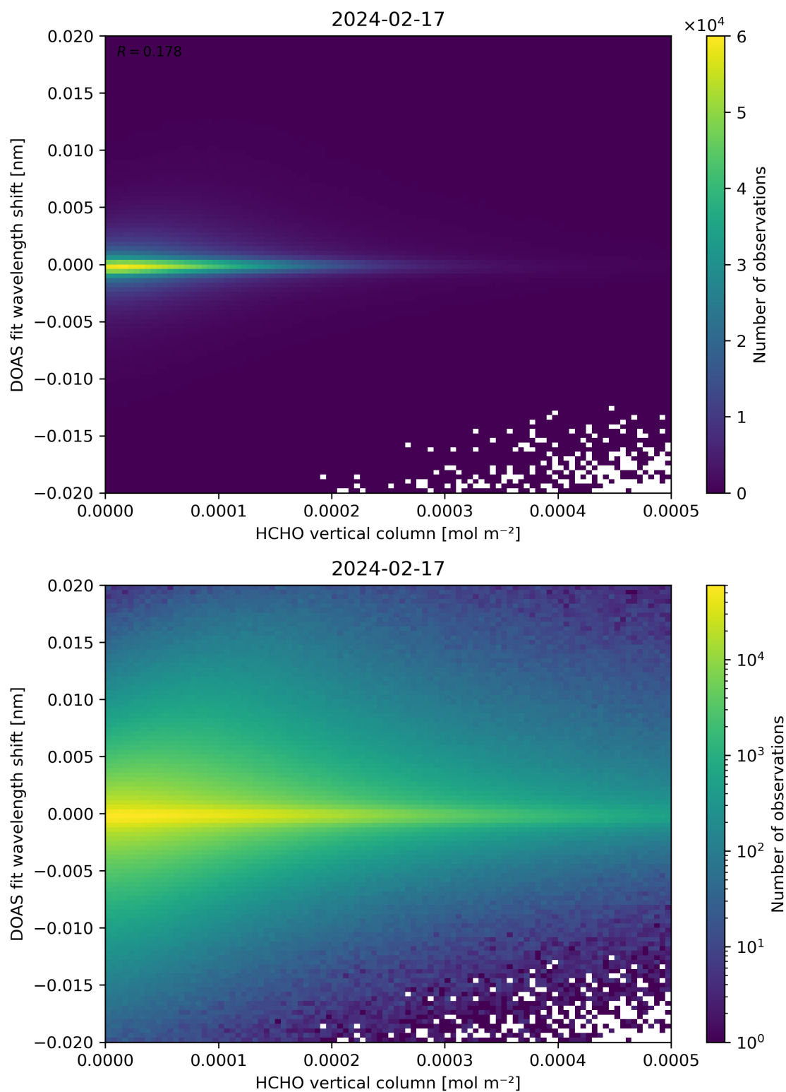
Figure 124: Scatter density plot of “HCHO vertical column” against “DOAS fit wavelength shift” for 2024-02-17 to 2024-02-18.
