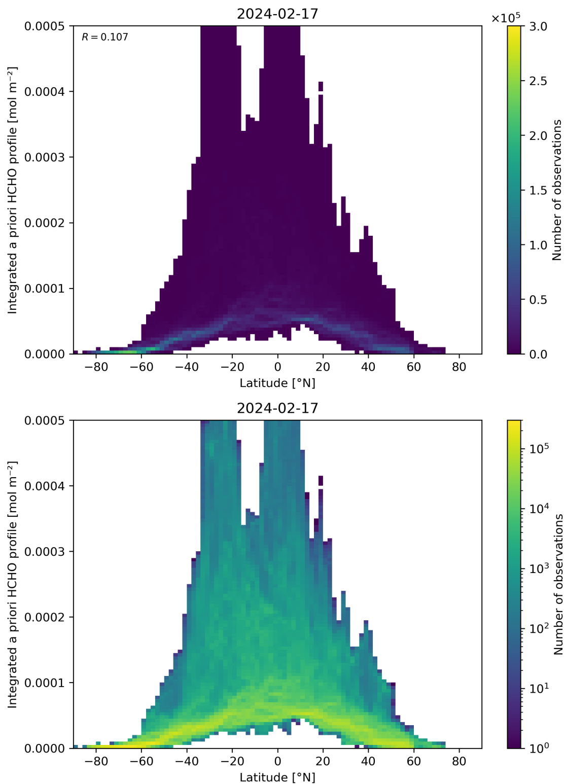
Figure 166: Scatter density plot of “Latitude” against “Integrated a priori HCHO profile” for 2024-02-17 to 2024-02-18.
