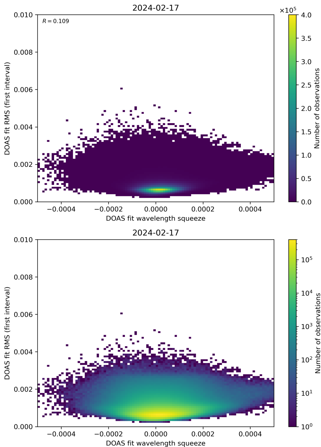
Figure 68: Scatter density plot of “DOAS fit wavelength squeeze” against “DOAS fit RMS (first interval)” for 2024-02-17 to 2024-02-18.
