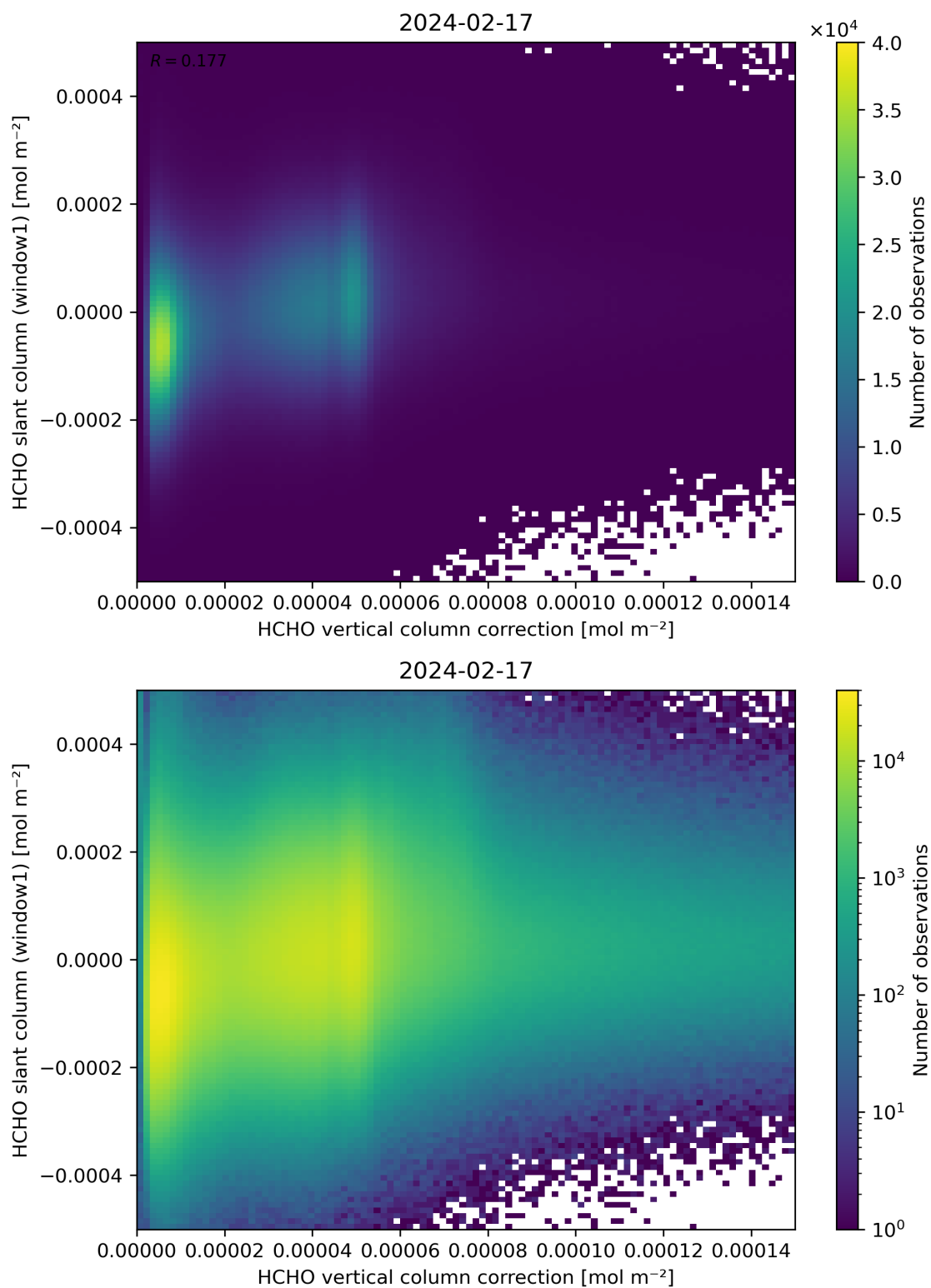
Figure 118: Scatter density plot of “HCHO vertical column correction” against “HCHO slant column (window1)” for 2024-02-17 to 2024-02-18.
