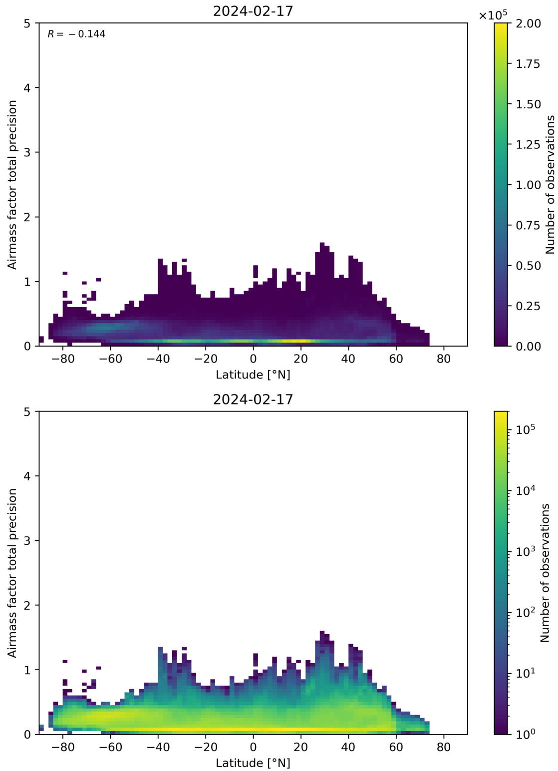
Figure 162: Scatter density plot of “Latitude” against “Airmass factor total precision” for 2024-02-17 to 2024-02-18.
