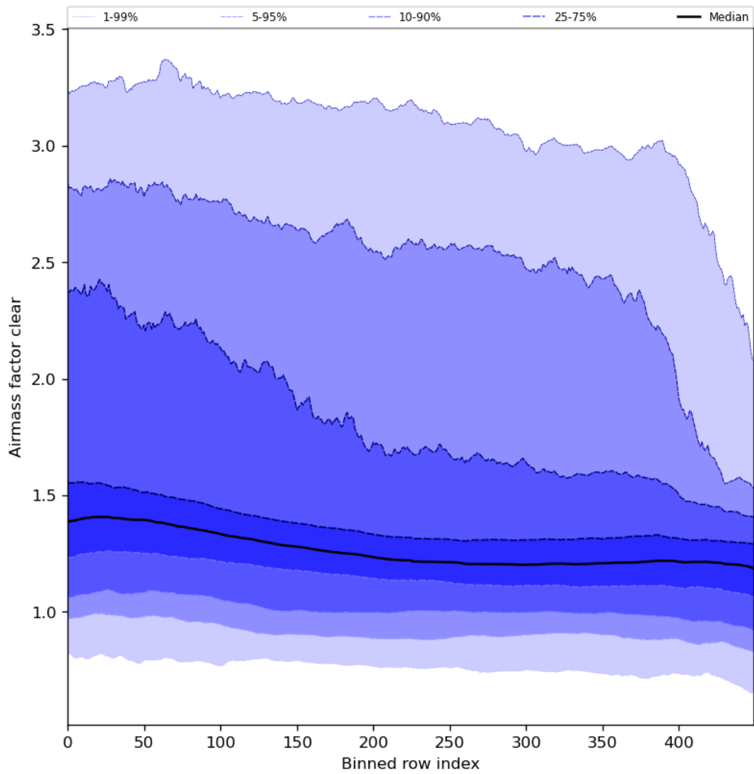
Figure 56: Along track statistics of “Air mass factor clear” for 2024-02-17 to 2024-02-18
