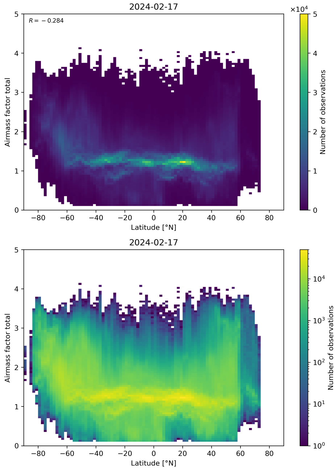
Figure 161: Scatter density plot of “Latitude” against “Airmass factor total” for 2024-02-17 to 2024-02-18.
