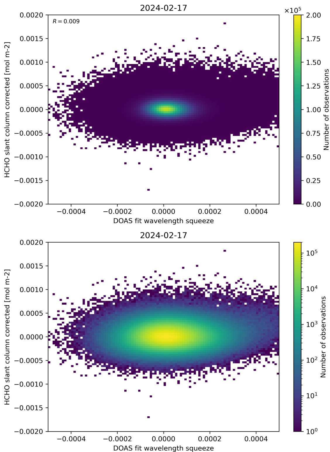
Figure 69: Scatter density plot of “DOAS fit wavelength squeeze” against “HCHO slant column corrected” for 2024-02-17 to 2024-02-18.
