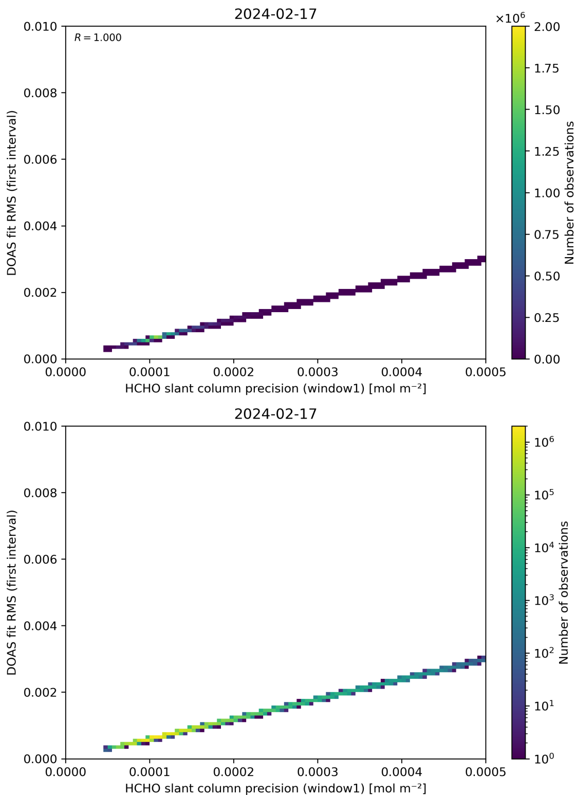
Figure 88: Scatter density plot of “HCHO slant column precision (window1)” against “DOAS fit RMS (first interval)” for 2024-02-17 to 2024-02-18.
