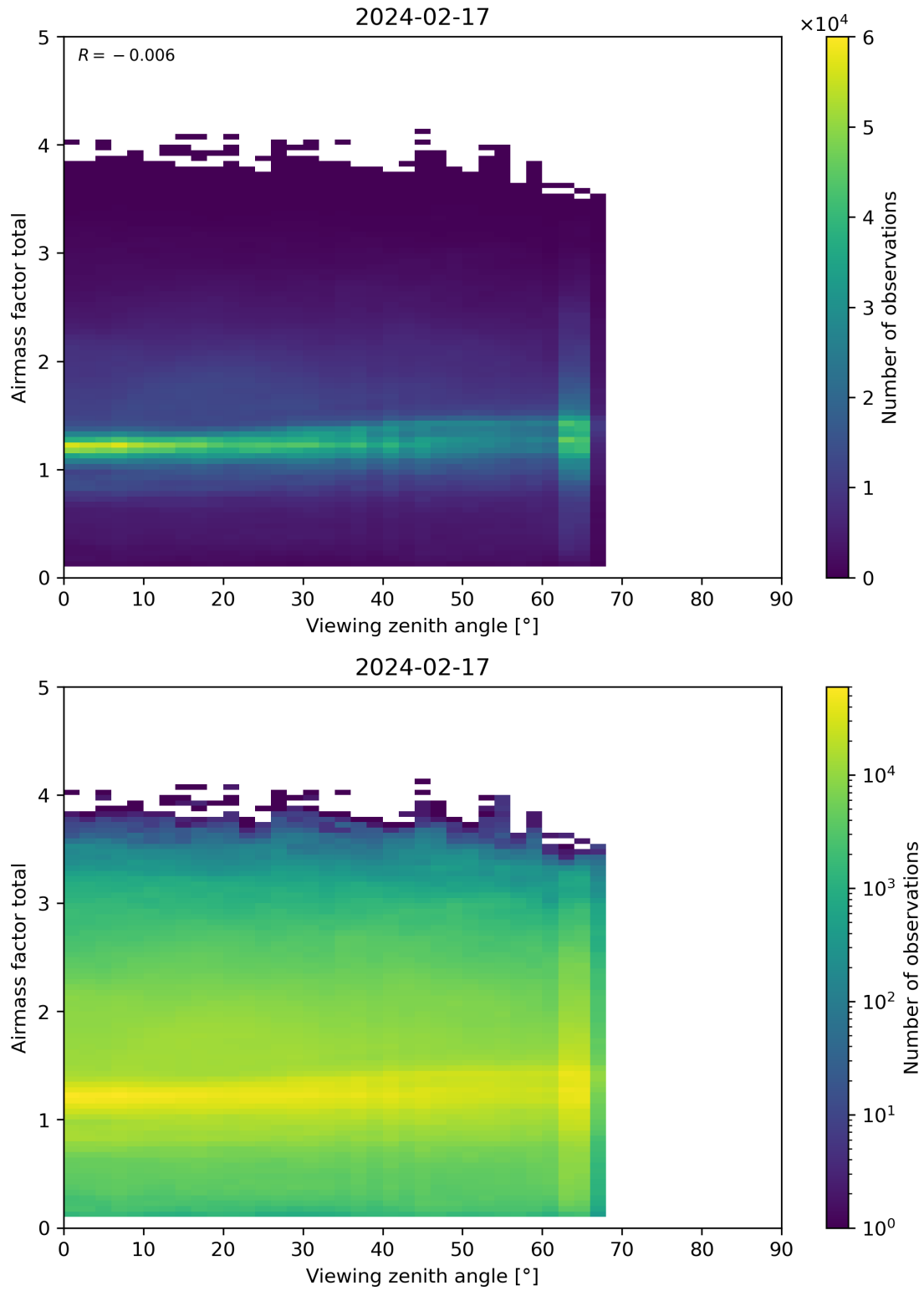
Figure 190: Scatter density plot of “Viewing zenith angle” against “Airmass factor total” for 2024-02-17 to 2024-02-18.
