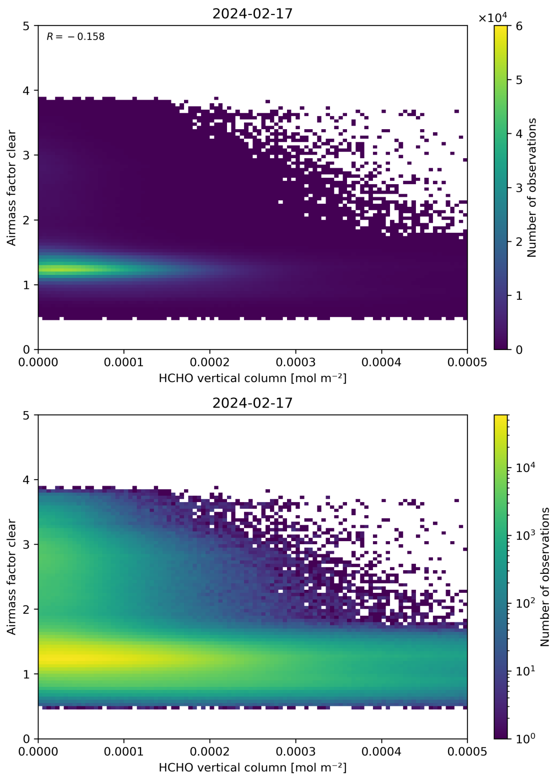
Figure 126: Scatter density plot of “HCHO vertical column” against “Airmass factor clear” for 2024-02-17 to 2024-02-18.
