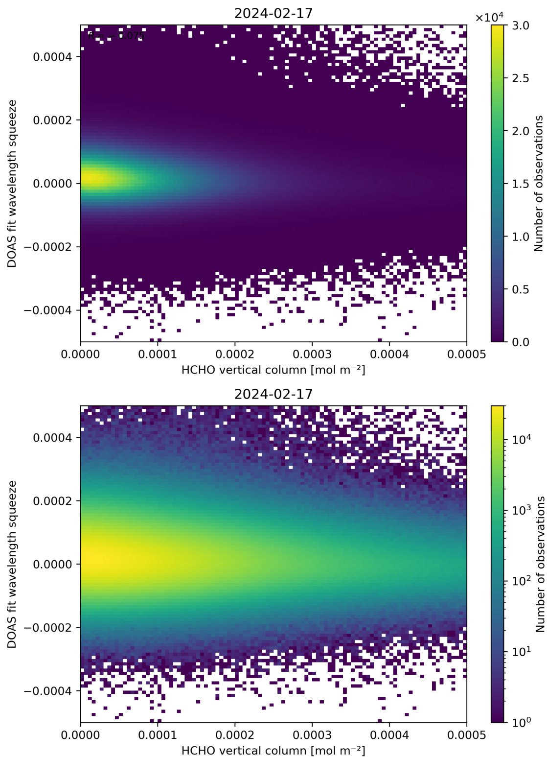
Figure 125: Scatter density plot of “HCHO vertical column” against “DOAS fit wavelength squeeze” for 2024-02-17 to 2024-02-18.
