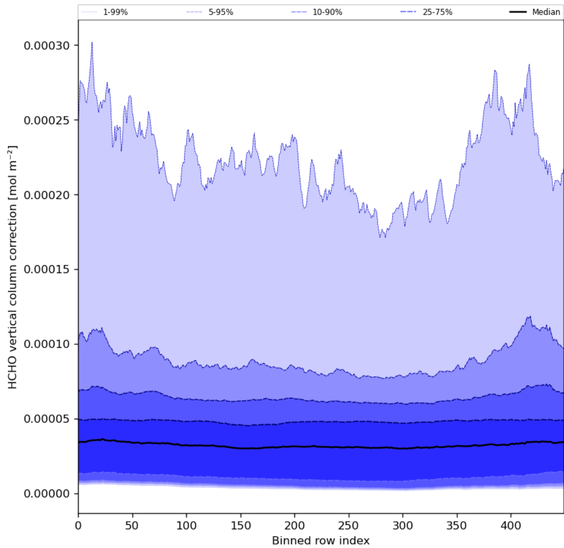
Figure 51: Along track statistics of “HCHO vertical column correction” for 2024-02-17 to 2024-02-18
