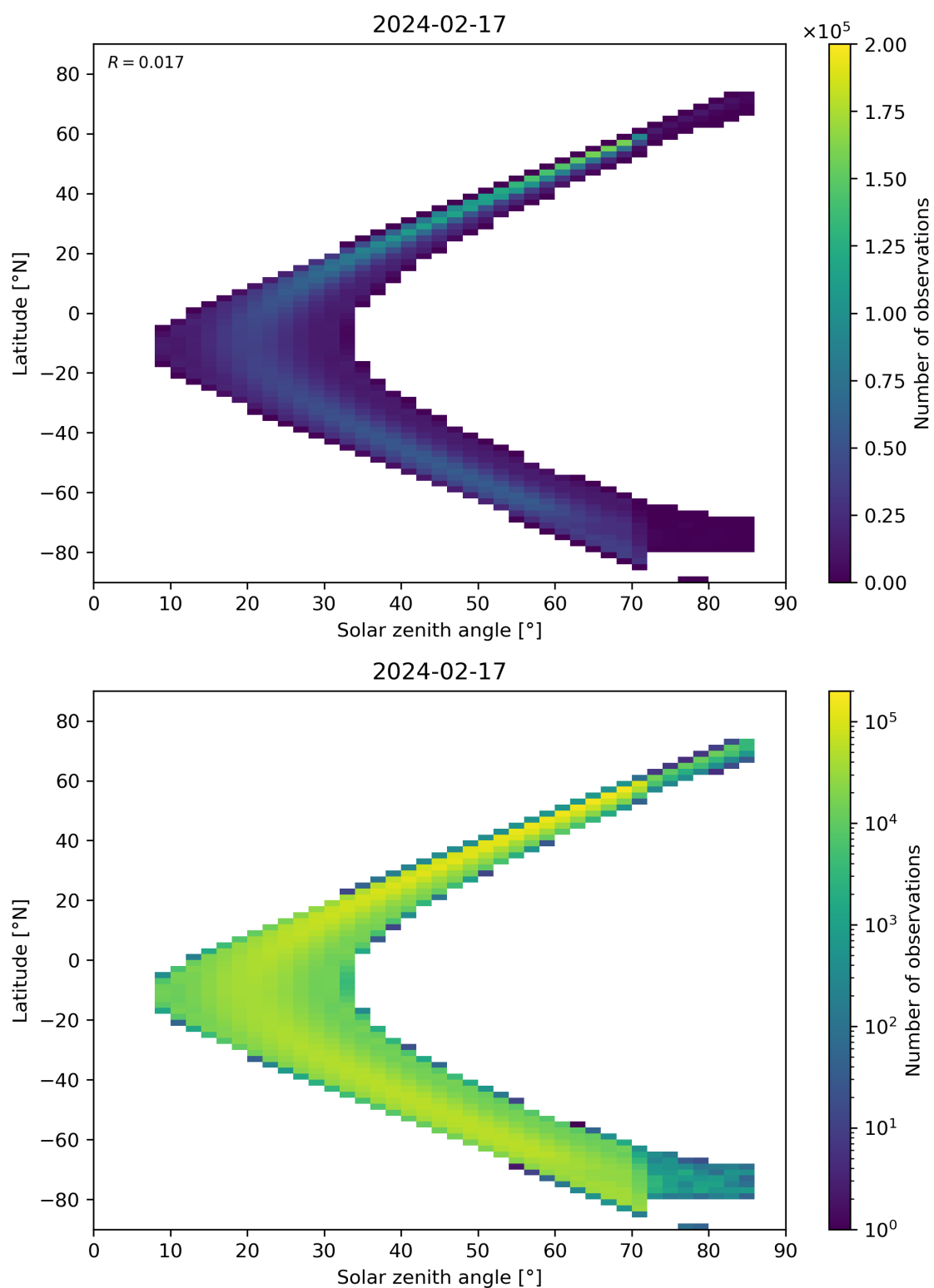
Figure 181: Scatter density plot of “Solar zenith angle” against “Latitude” for 2024-02-17 to 2024-02-18.
