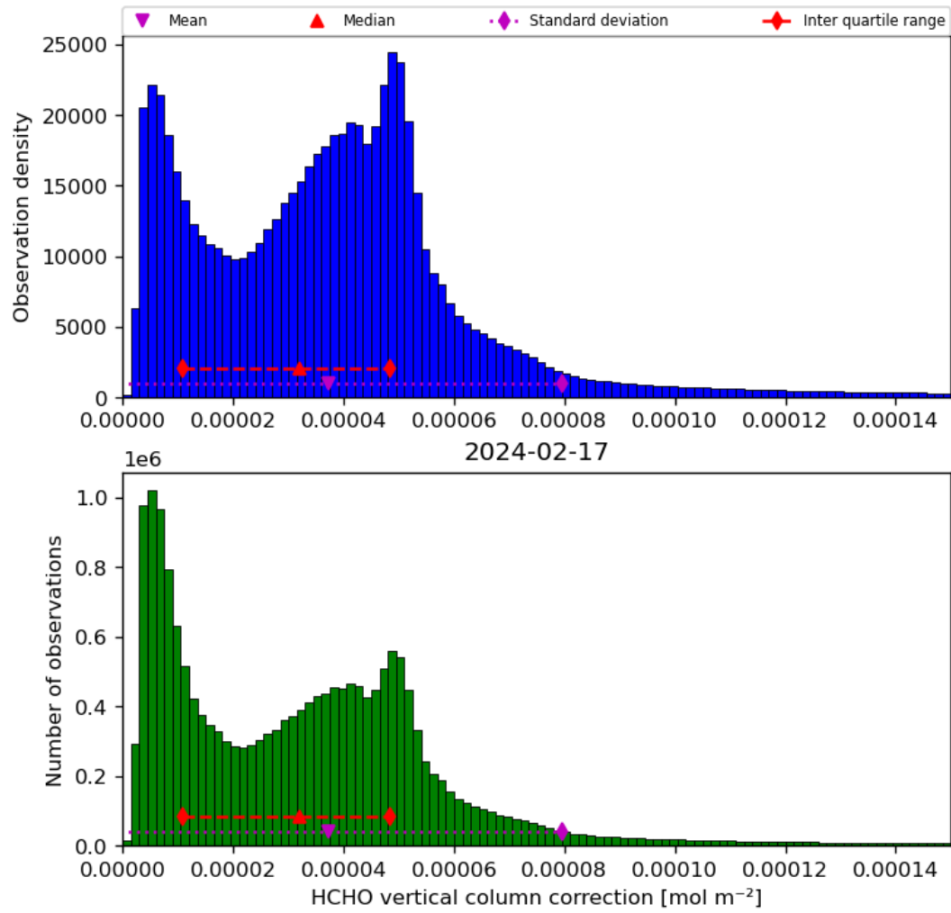
Figure 37: Histogram of “HCHO vertical column correction” for 2024-02-17 to 2024-02-18
