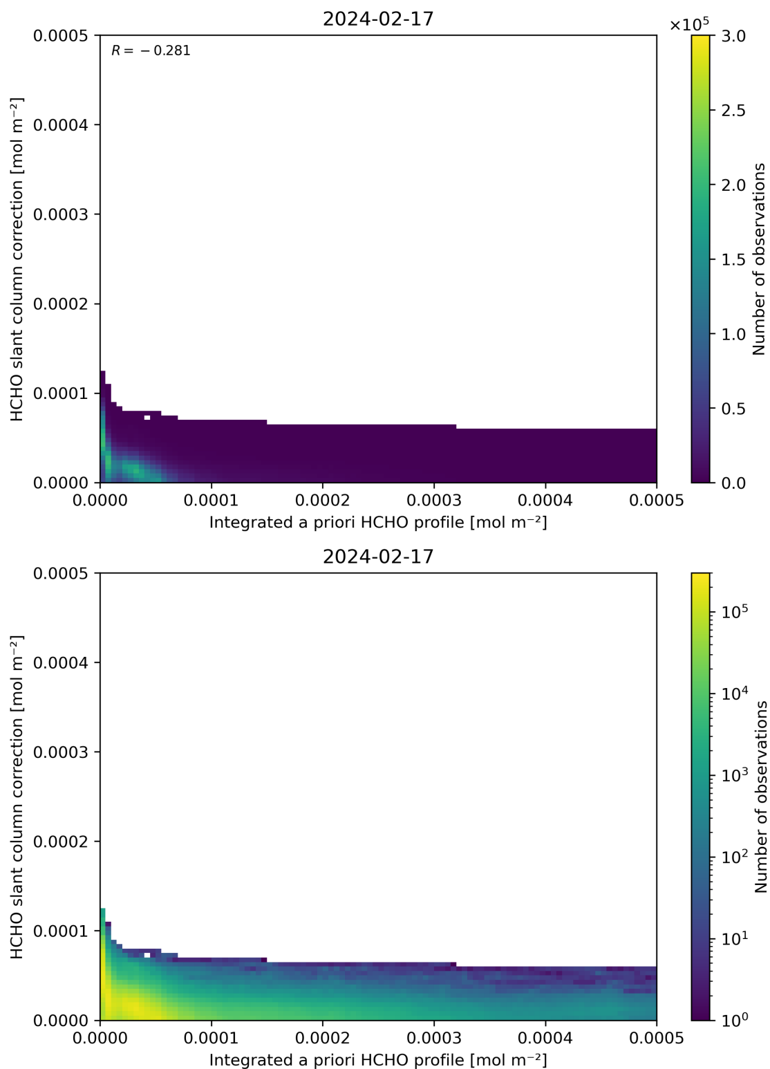
Figure 152: Scatter density plot of “Integrated a priori HCHO profile” against “HCHO slant column correction” for 2024-02-17 to 2024-02-18.
