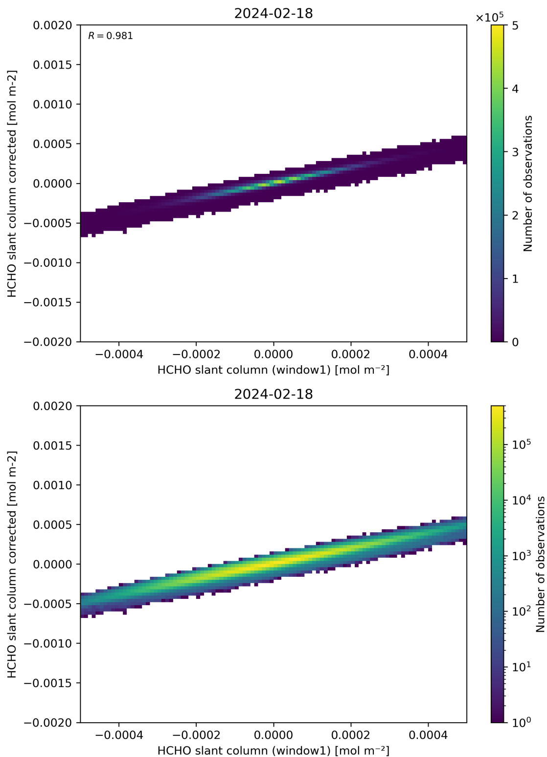
Figure 82: Scatter density plot of “HCHO slant column (window1)” against “HCHO slant column corrected” for 2024-02-17 to 2024-02-19.
