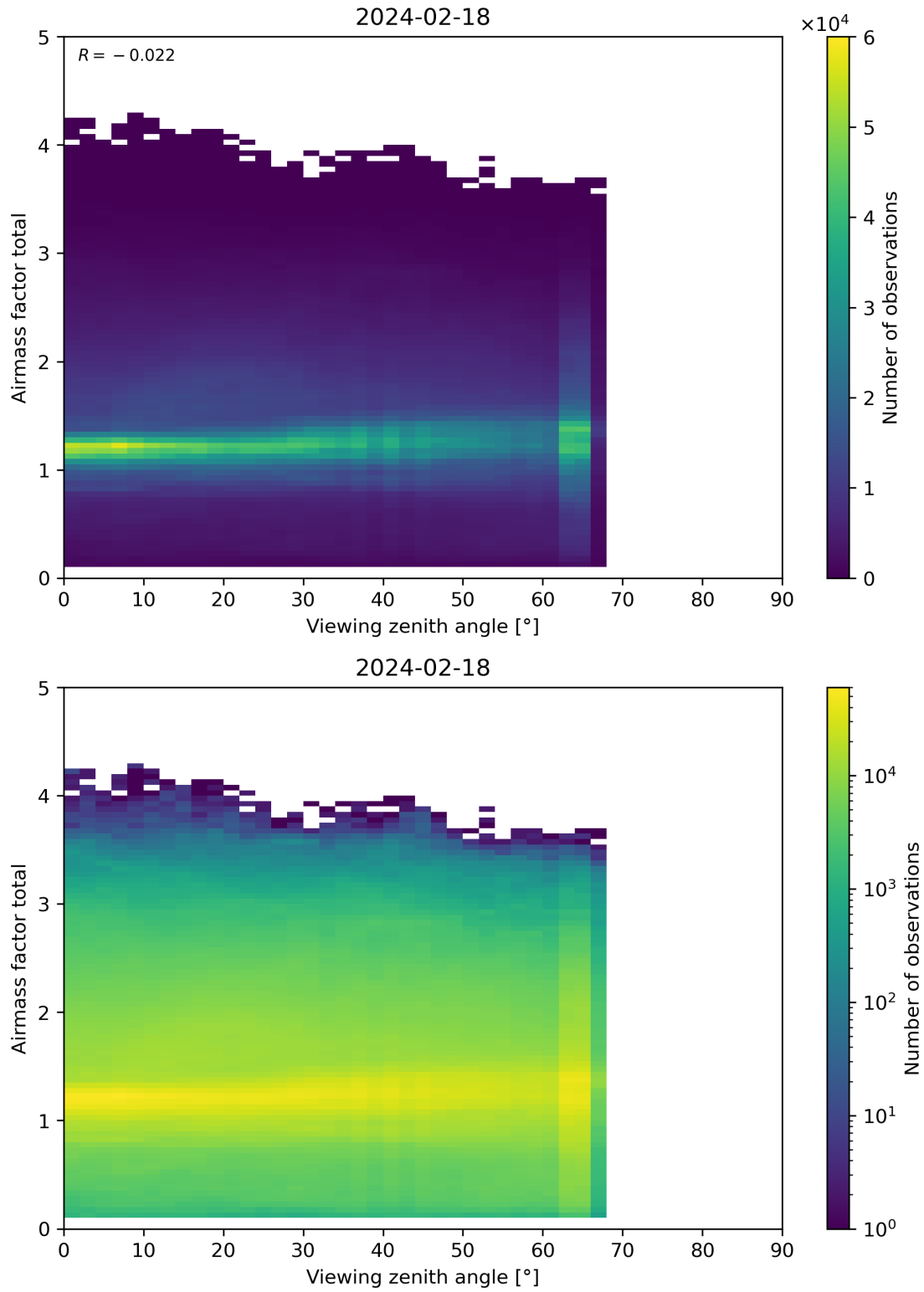
Figure 190: Scatter density plot of “Viewing zenith angle” against “Airmass factor total” for 2024-02-17 to 2024-02-19.
