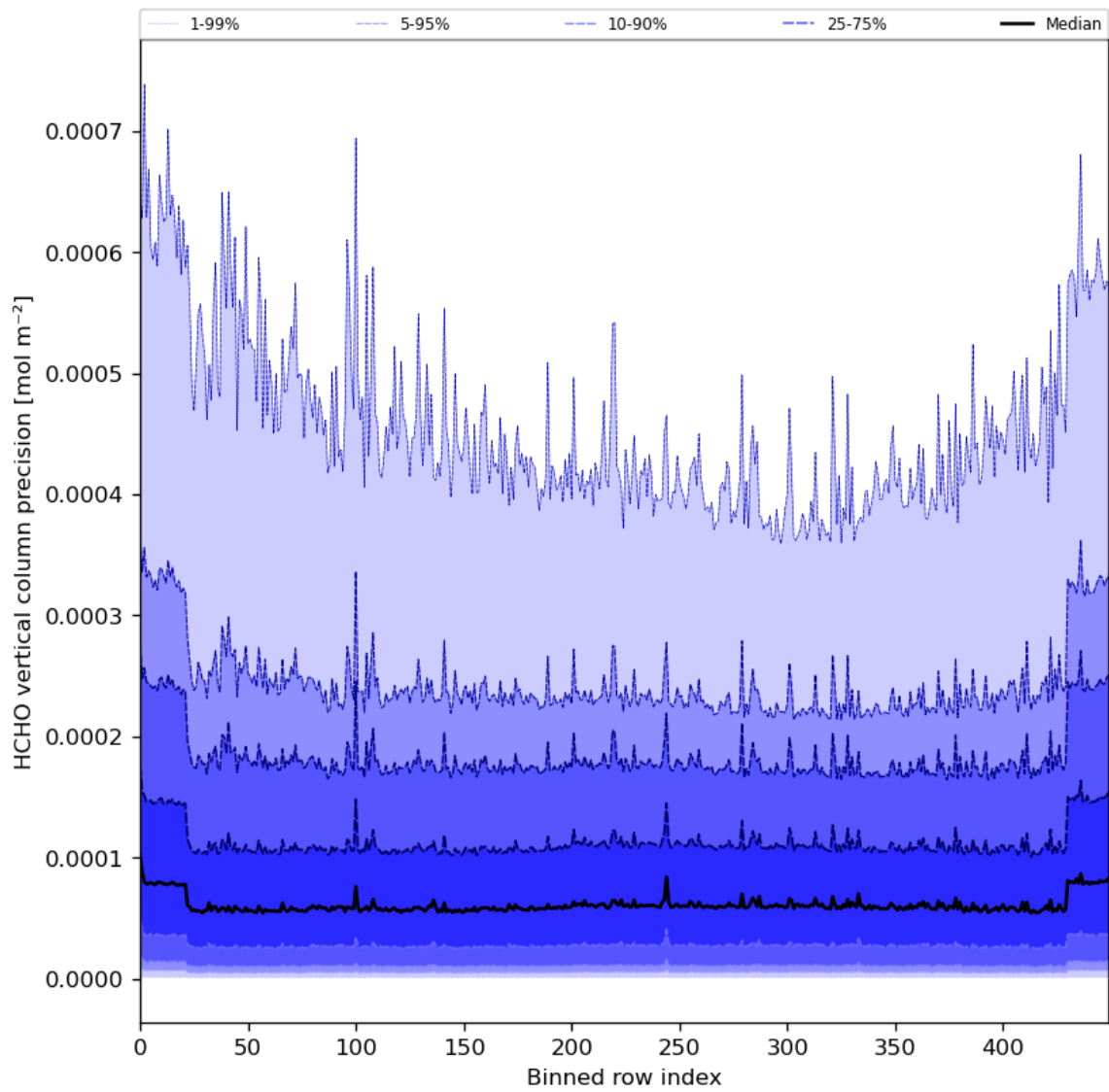
Figure 50: Along track statistics of “HCHO vertical column precision” for 2024-02-17 to 2024-02-19
