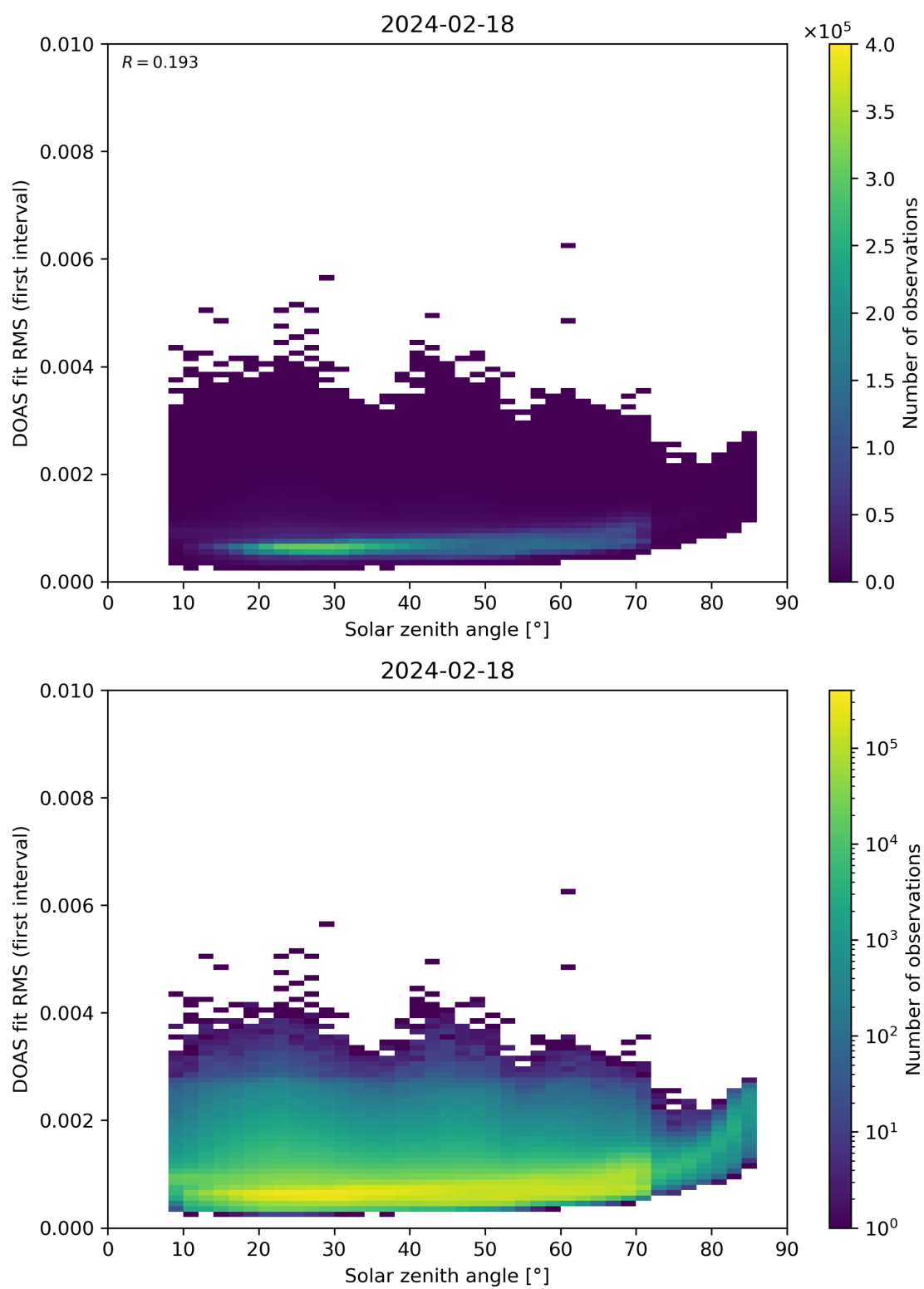
Figure 167: Scatter density plot of “Solar zenith angle” against “DOAS fit RMS (first interval)” for 2024-02-17 to 2024-02-19.
