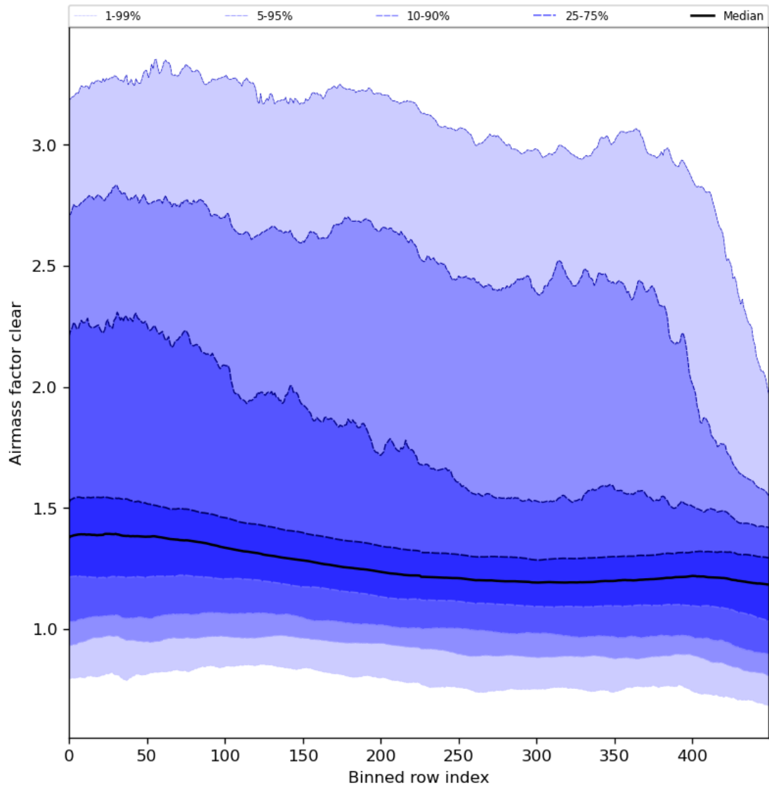
Figure 56: Along track statistics of “Airmass factor clear” for 2024-02-17 to 2024-02-19
