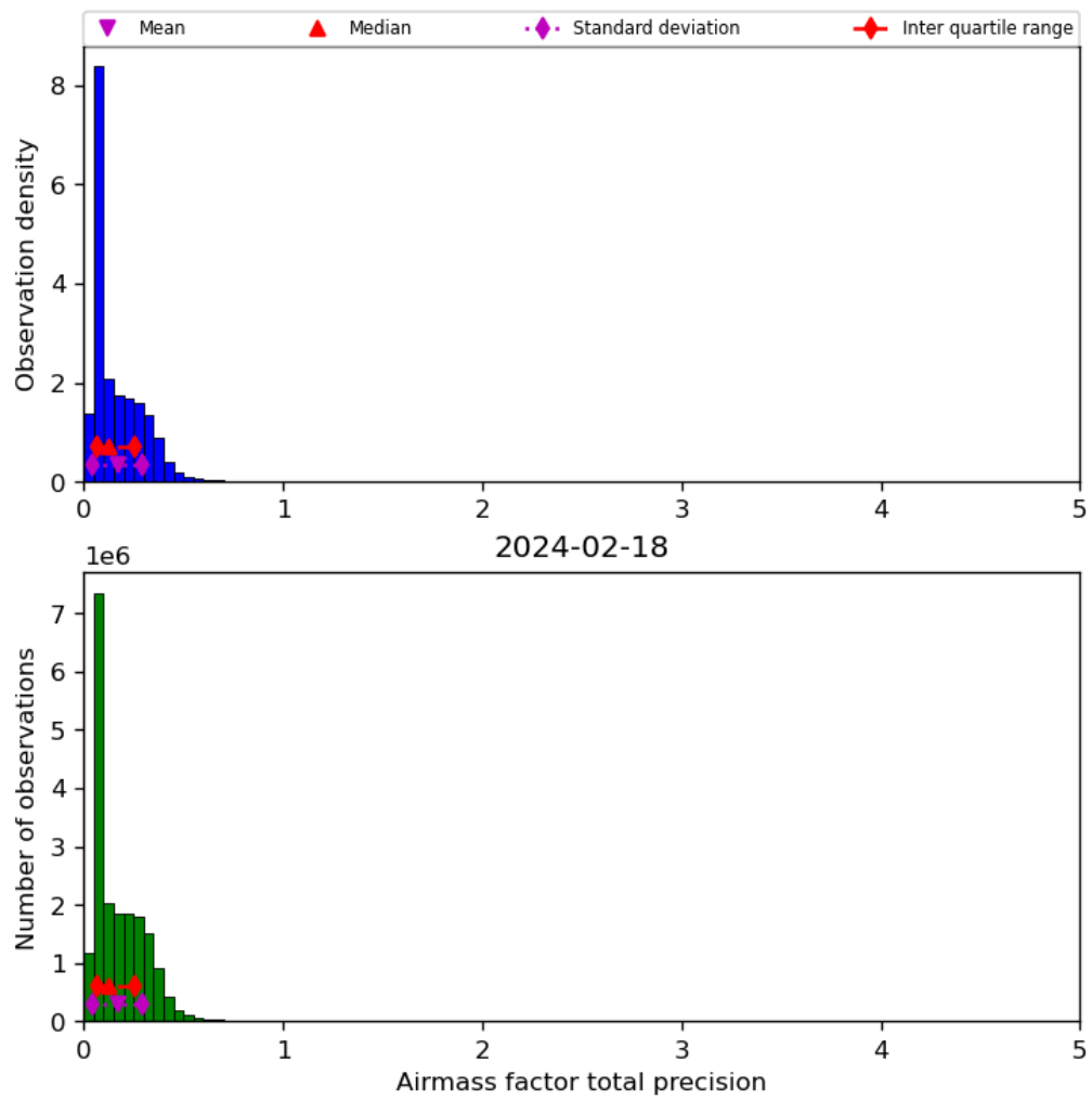
Figure 41: Histogram of “Airmass factor total precision” for 2024-02-17 to 2024-02-19
