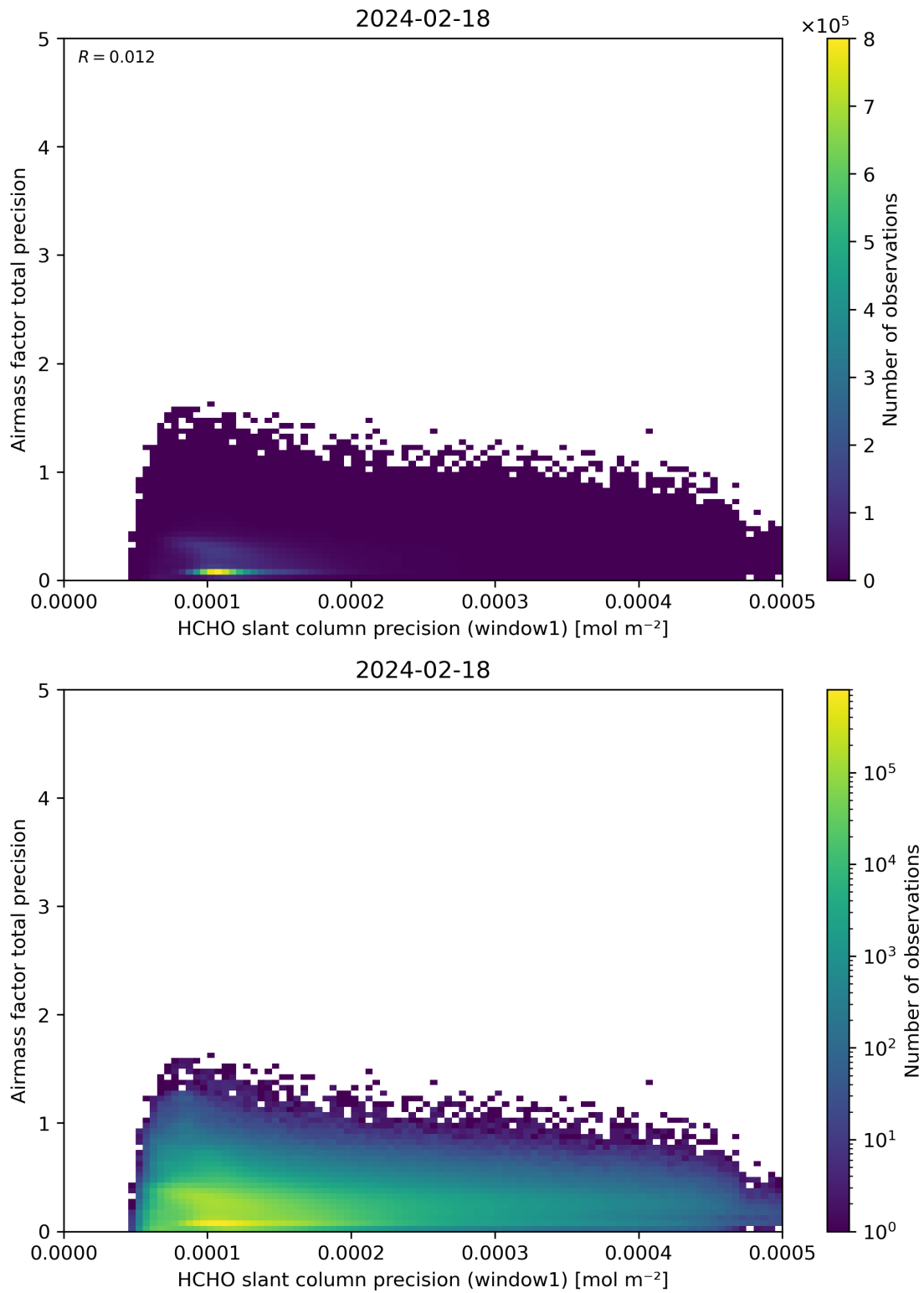
Figure 95: Scatter density plot of “HCHO slant column precision (window1)” against “Airmass factor total precision” for 2024-02-17 to 2024-02-19.
