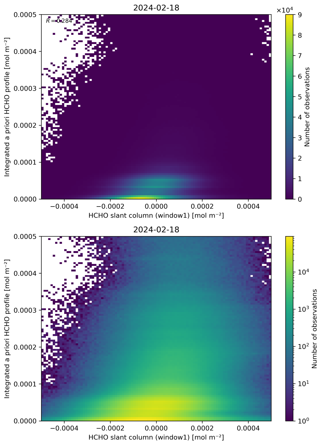
Figure 87: Scatter density plot of “HCHO slant column (window1)” against “Integrated a priori HCHO profile” for 2024-02-17 to 2024-02-19.
