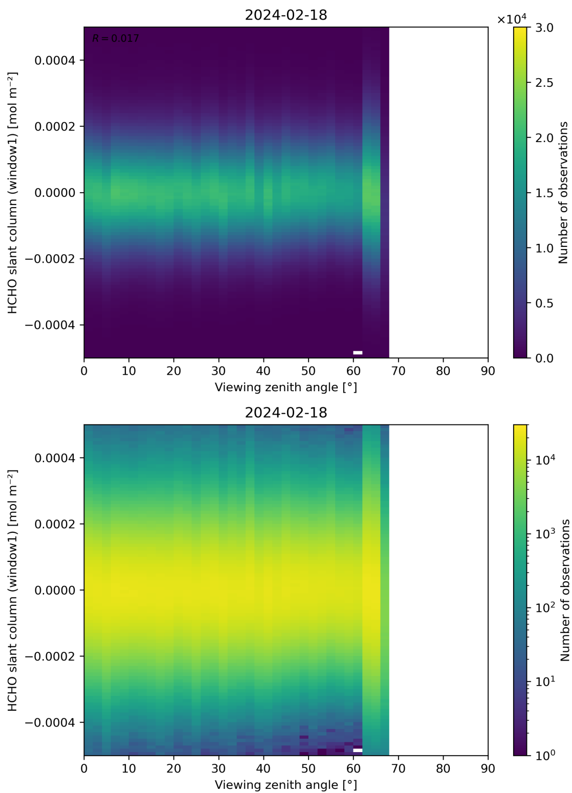
Figure 188: Scatter density plot of “Viewing zenith angle” against “HCHO slant column (window1)” for 2024-02-17 to 2024-02-19.
