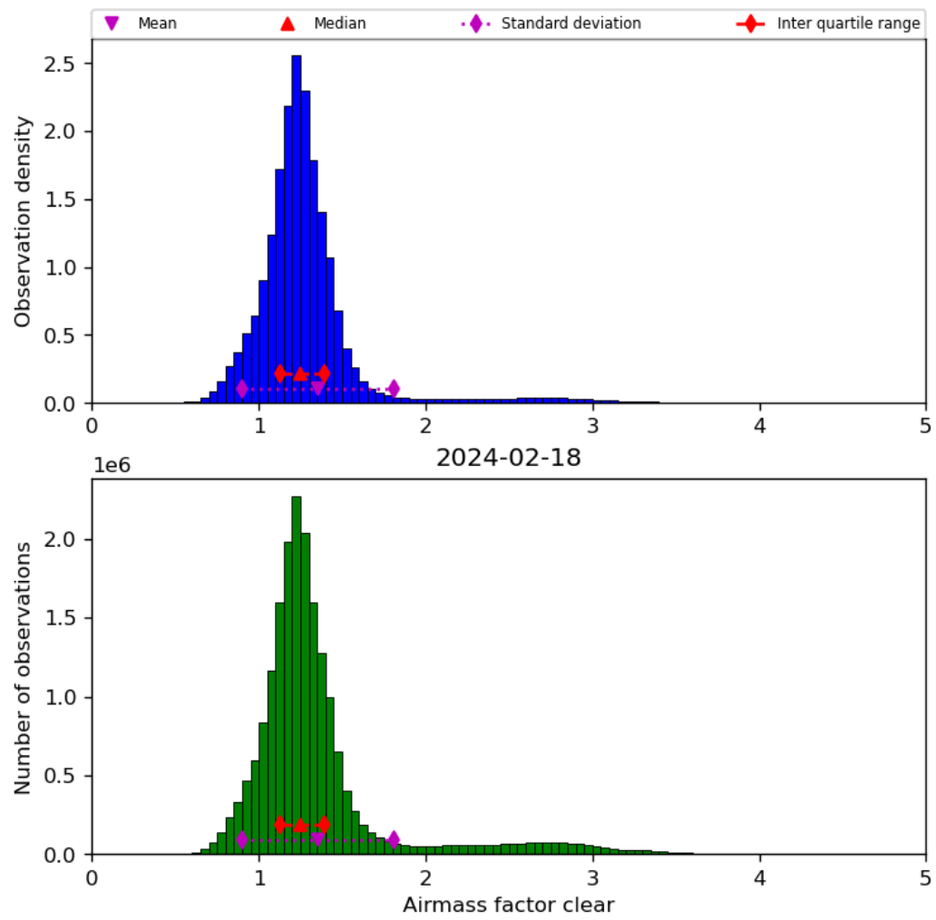
Figure 42: Histogram of “Airmass factor clear” for 2024-02-17 to 2024-02-19
