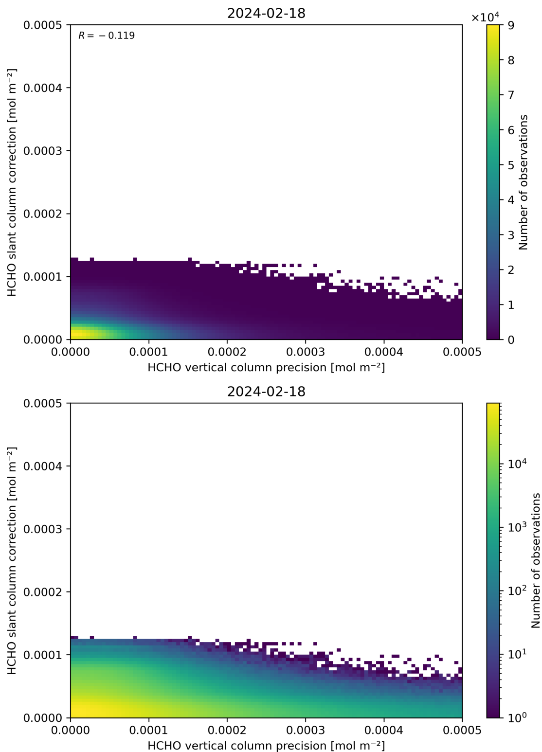
Figure 141: Scatter density plot of “HCHO vertical column precision” against “HCHO slant column correction” for 2024-02-17 to 2024-02-19.
