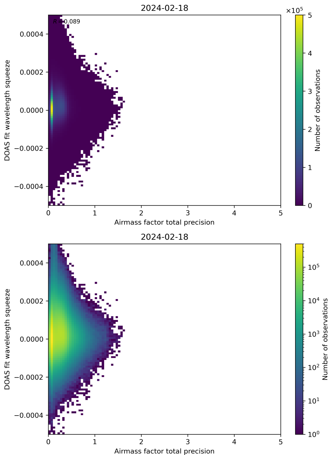
Figure 107: Scatter density plot of “Airmass factor total precision” against “DOAS fit wavelength squeeze” for 2024-02-17 to 2024-02-19.
