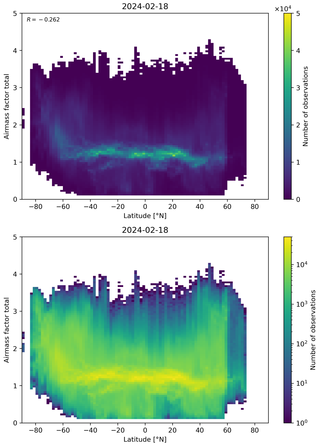
Figure 161: Scatter density plot of “Latitude” against “Airmass factor total” for 2024-02-17 to 2024-02-19.
