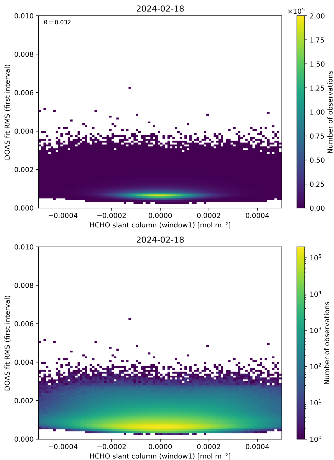
Figure 78: Scatter density plot of “HCHO slant column (window1)” against “DOAS fit RMS (first interval)” for 2024-02-17 to 2024-02-19.
