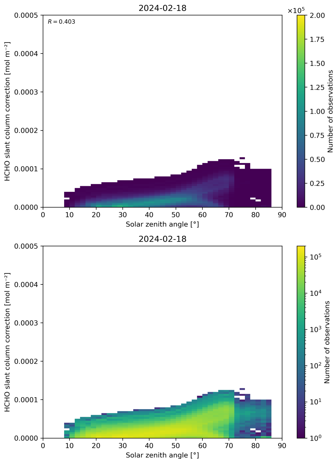
Figure 172: Scatter density plot of “Solar zenith angle” against “HCHO slant column correction” for 2024-02-17 to 2024-02-19.
