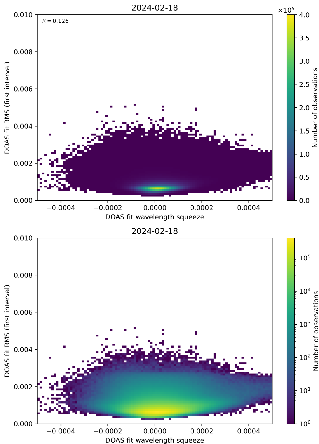
Figure 68: Scatter density plot of “DOAS fit wavelength squeeze” against “DOAS fit RMS (first interval)” for 2024-02-17 to 2024-02-19.
