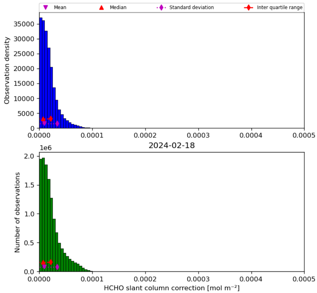
Figure 47: Histogram of “HCHO slant column correction” for 2024-02-17 to 2024-02-19
