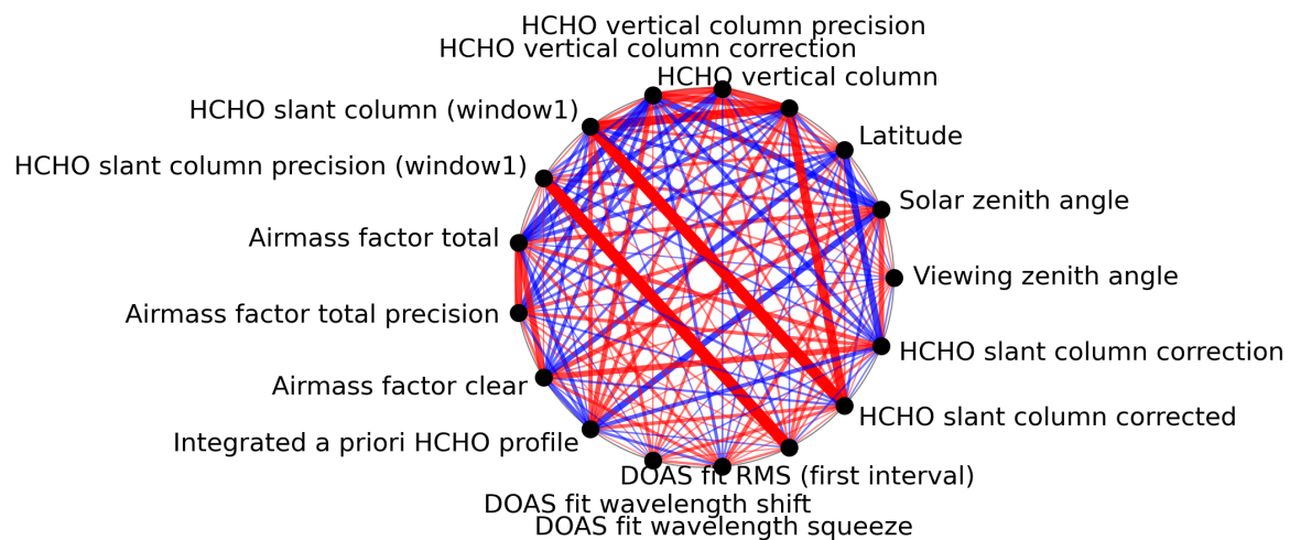
Figure 1: Map of correlation graph for 2024-02-17 to 2024-02-19.
