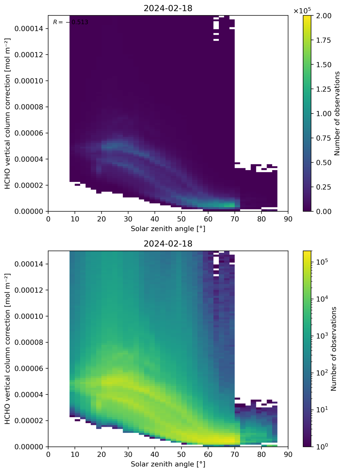
Figure 178: Scatter density plot of “Solar zenith angle” against “HCHO vertical column correction” for 2024-02-17 to 2024-02-19.
