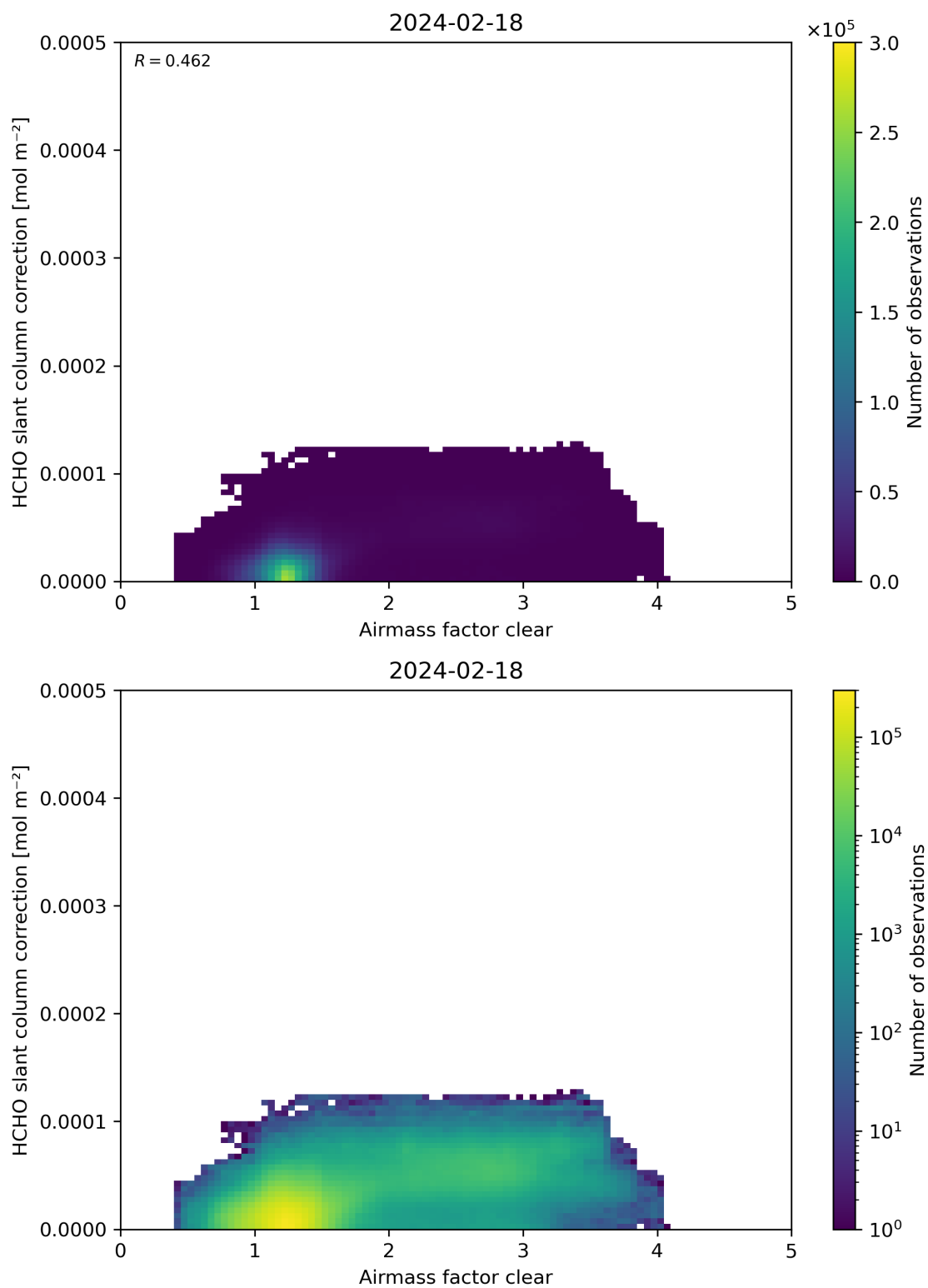
Figure 75: Scatter density plot of “Airmass factor clear” against “HCHO slant column correction” for 2024-02-17 to 2024-02-19.
