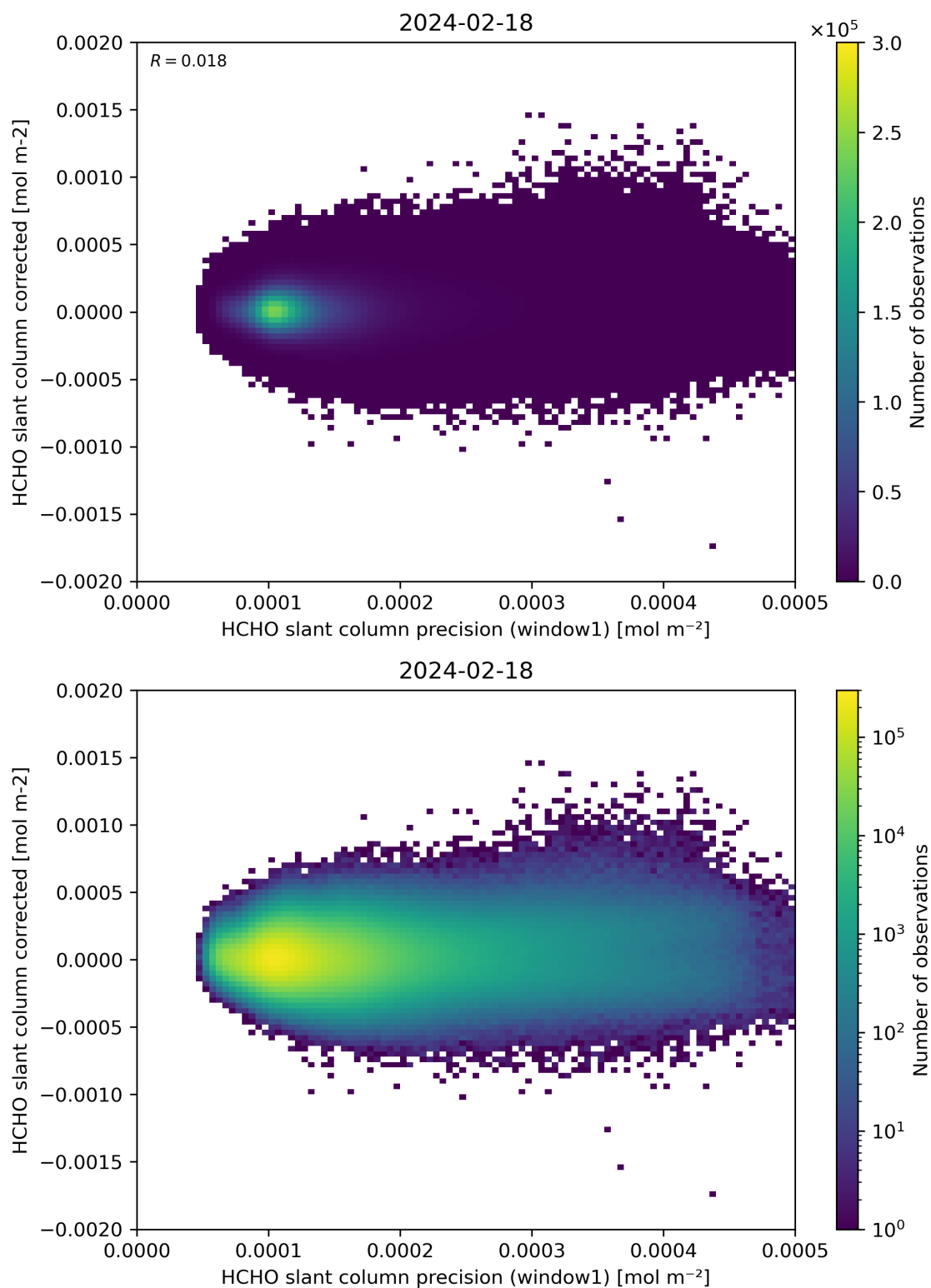
Figure 92: Scatter density plot of “HCHO slant column precision (window1)” against “HCHO slant column corrected” for 2024-02-17 to 2024-02-19.
