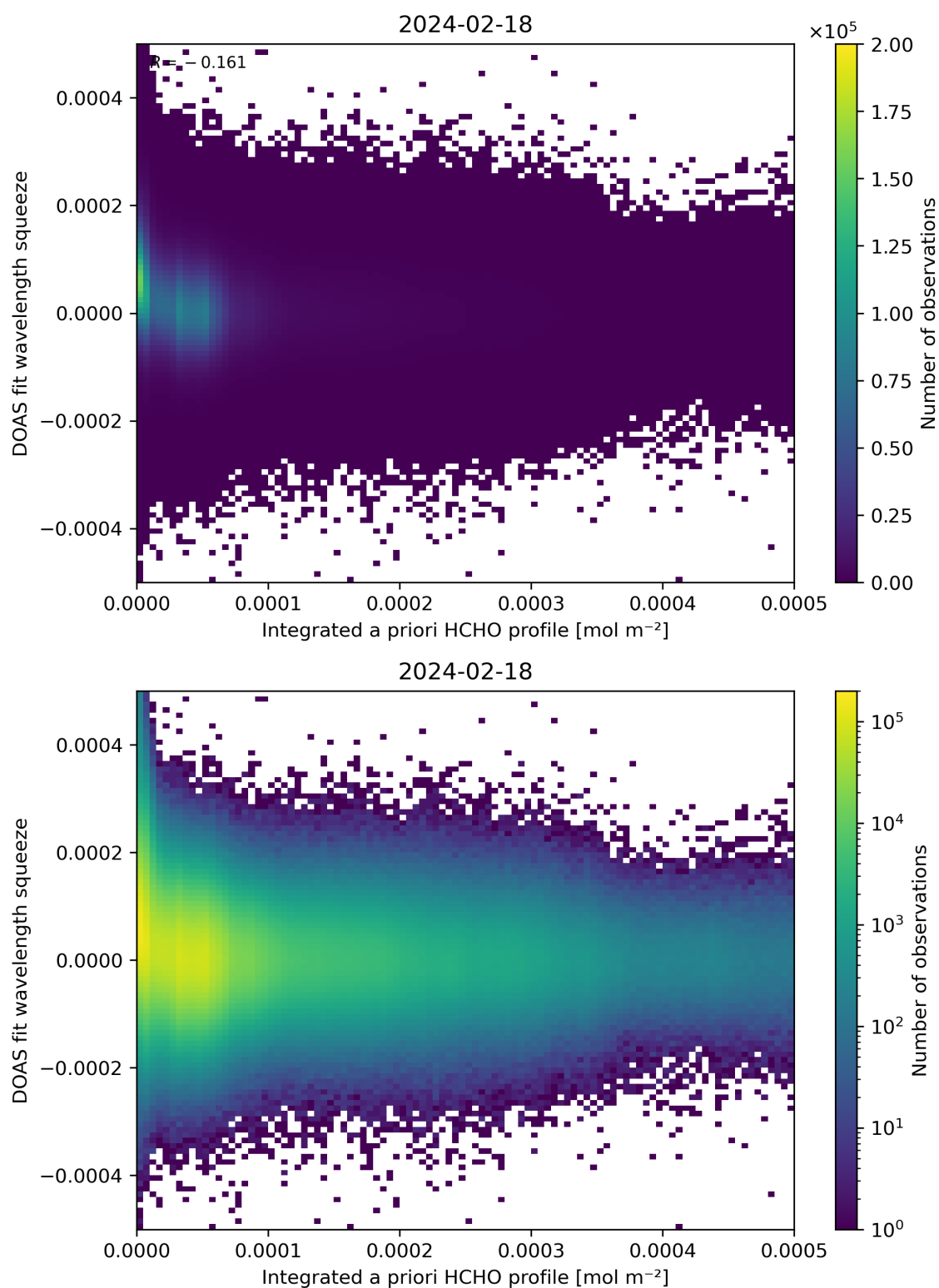
Figure 150: Scatter density plot of “Integrated a priori HCHO profile” against “DOAS fit wavelength squeeze” for 2024-02-17 to 2024-02-19.
