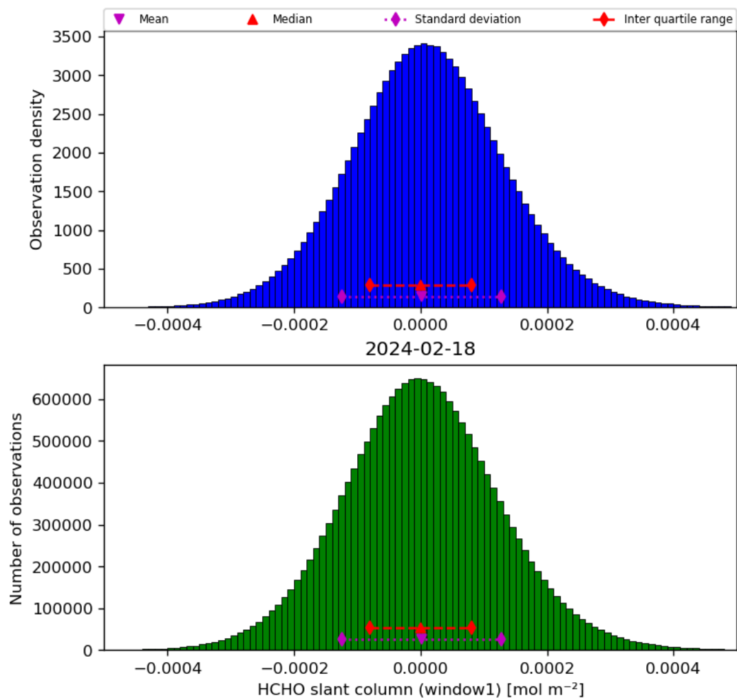
Figure 38: Histogram of “HCHO slant column (window1)” for 2024-02-17 to 2024-02-19
