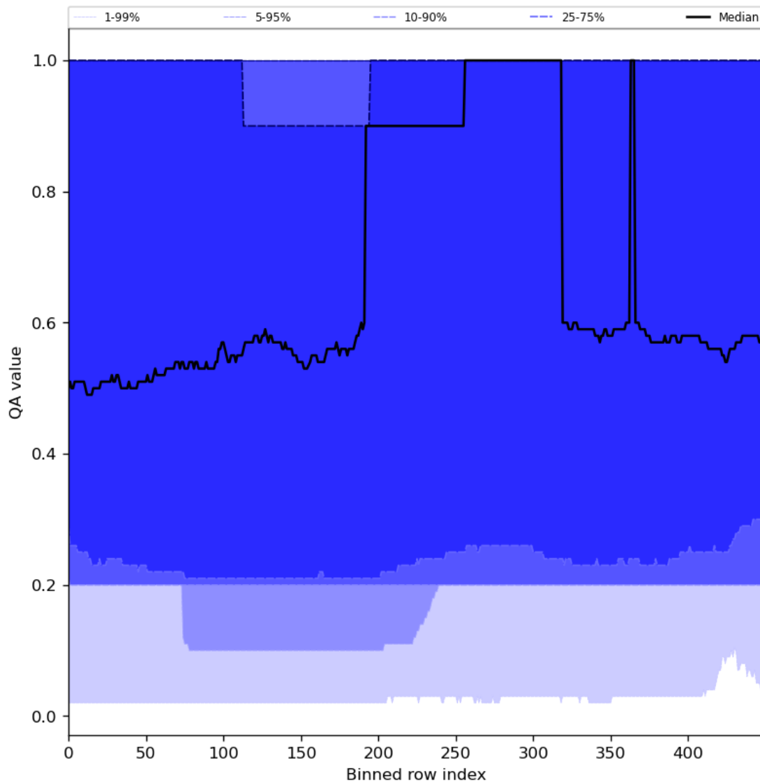
Figure 48: Along track statistics of “QA value” for 2024-02-17 to 2024-02-19
