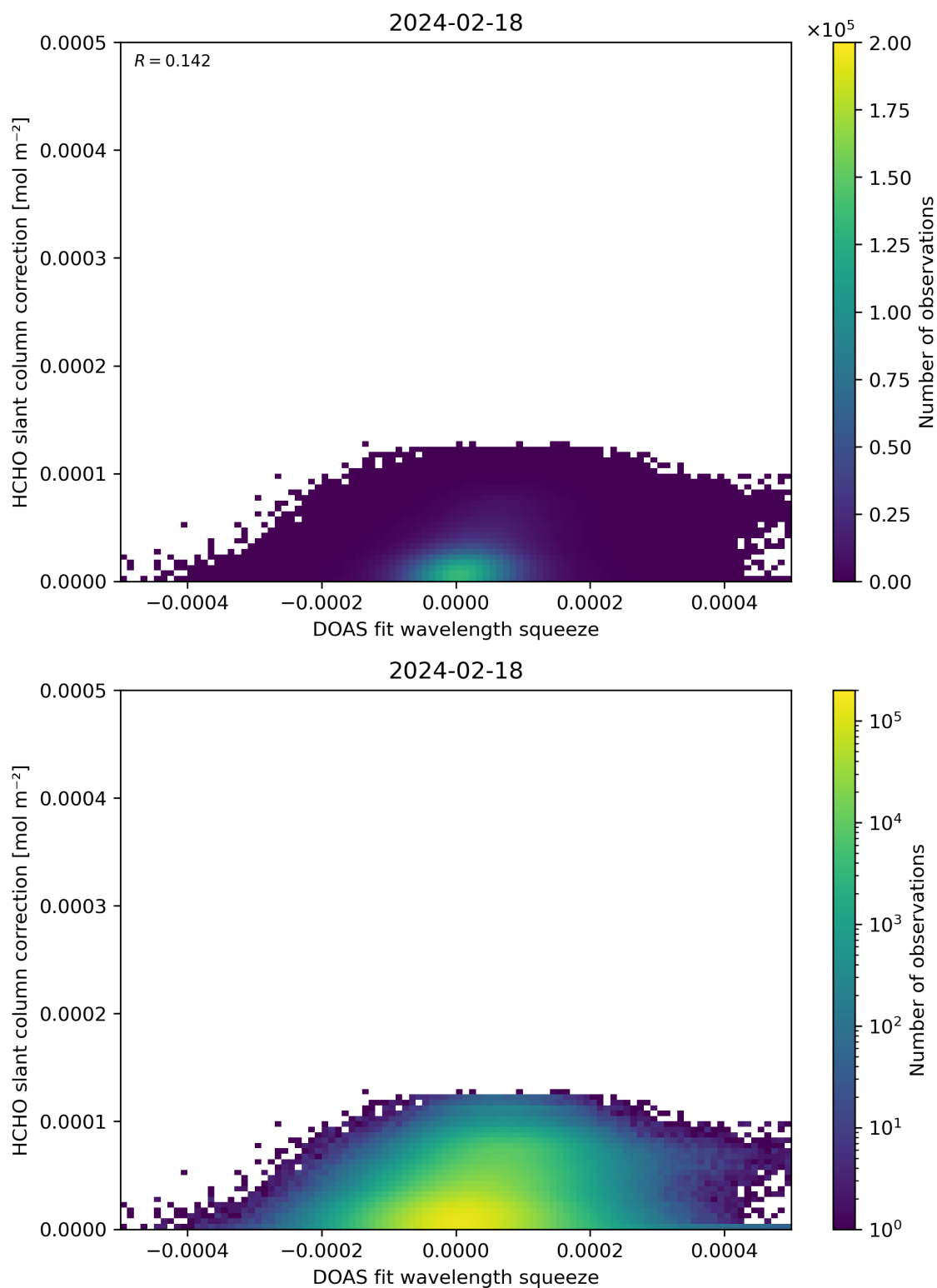
Figure 70: Scatter density plot of “DOAS fit wavelength squeeze” against “HCHO slant column correction” for 2024-02-17 to 2024-02-19.
