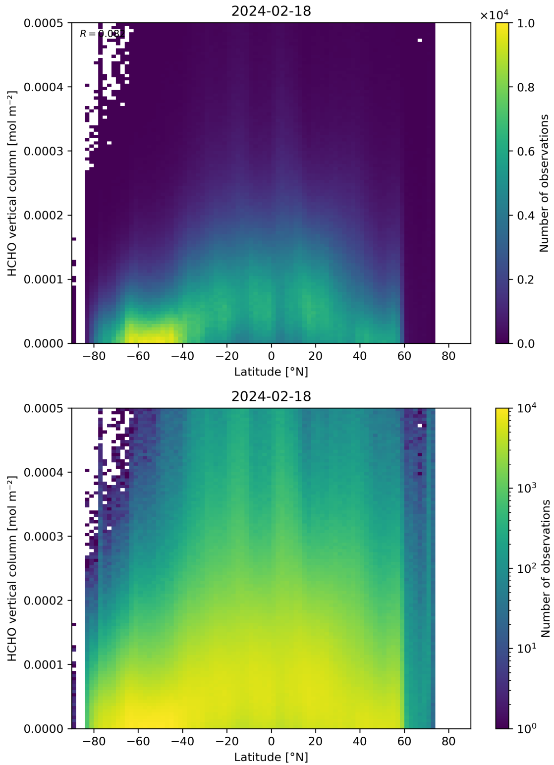
Figure 163: Scatter density plot of “Latitude” against “HCHO vertical column” for 2024-02-17 to 2024-02-19.
