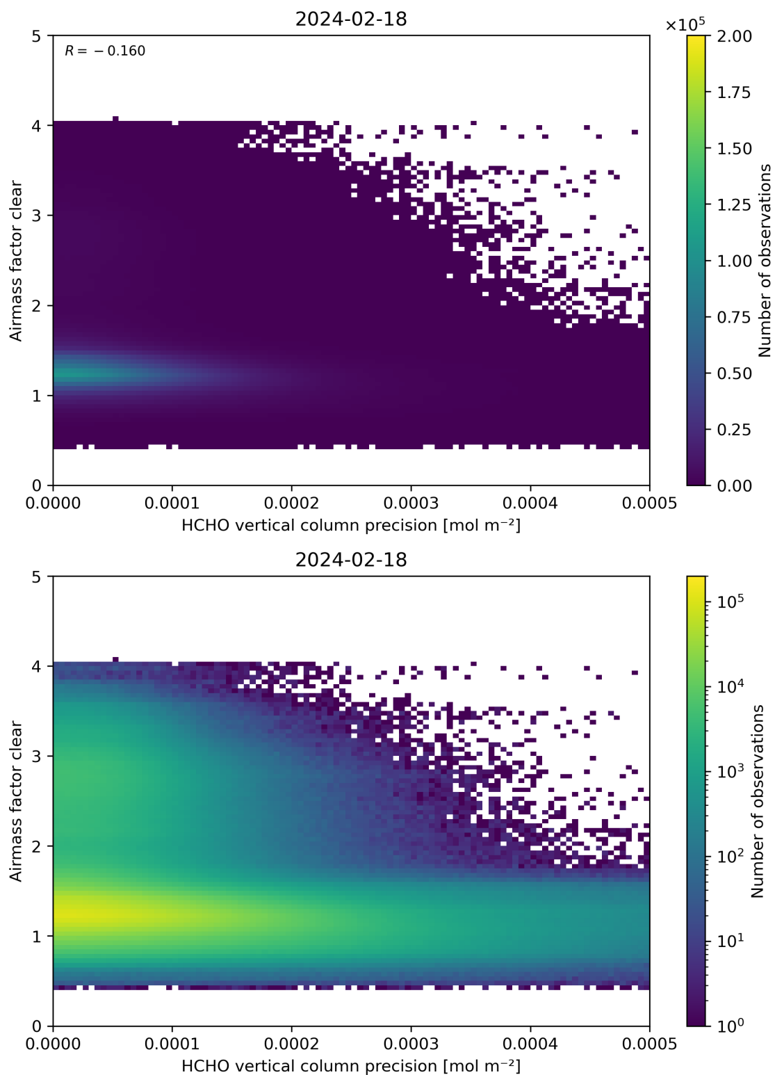
Figure 139: Scatter density plot of “HCHO vertical column precision” against “Airmass factor clear” for 2024-02-17 to 2024-02-19.
