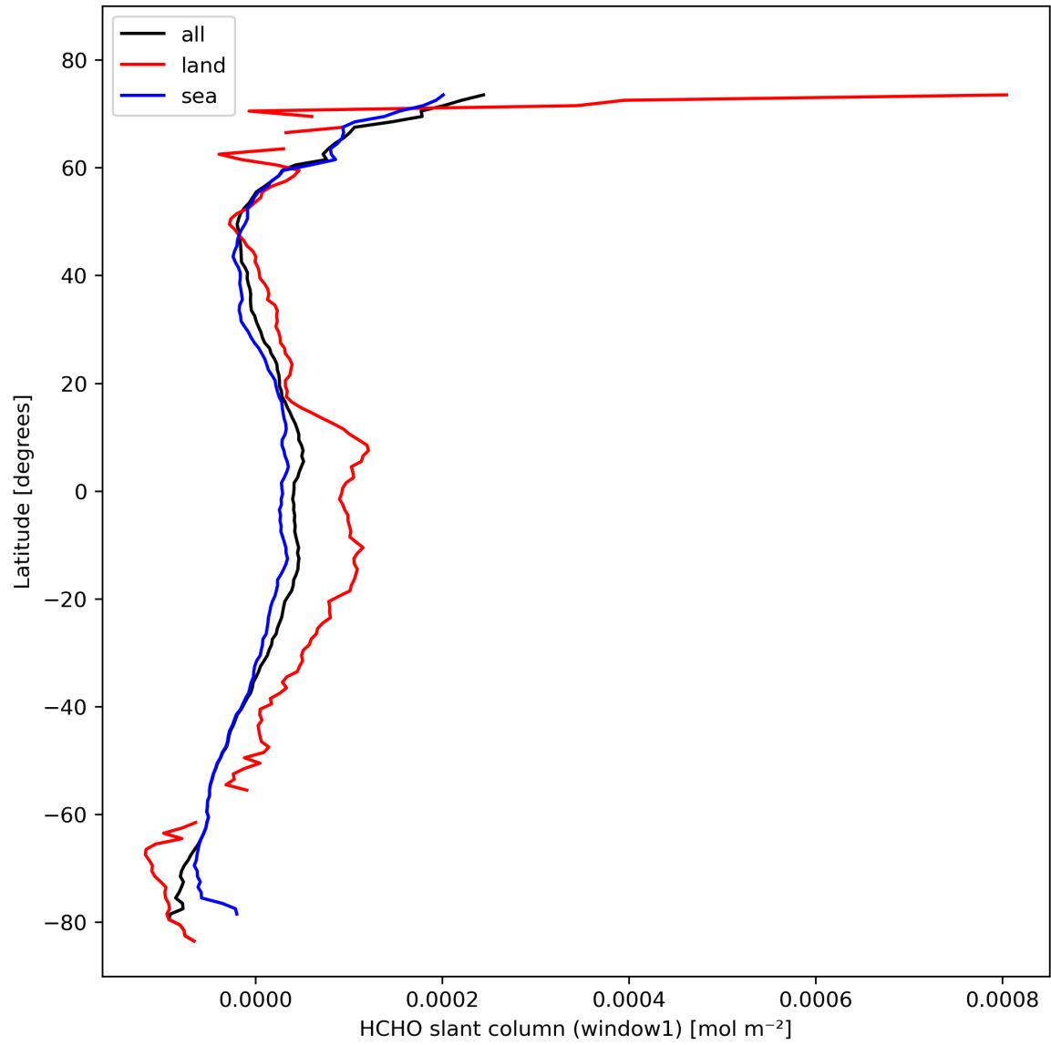
Figure 24: Zonal average of “HCHO slant column (window1)” for 2024-02-17 to 2024-02-19.
