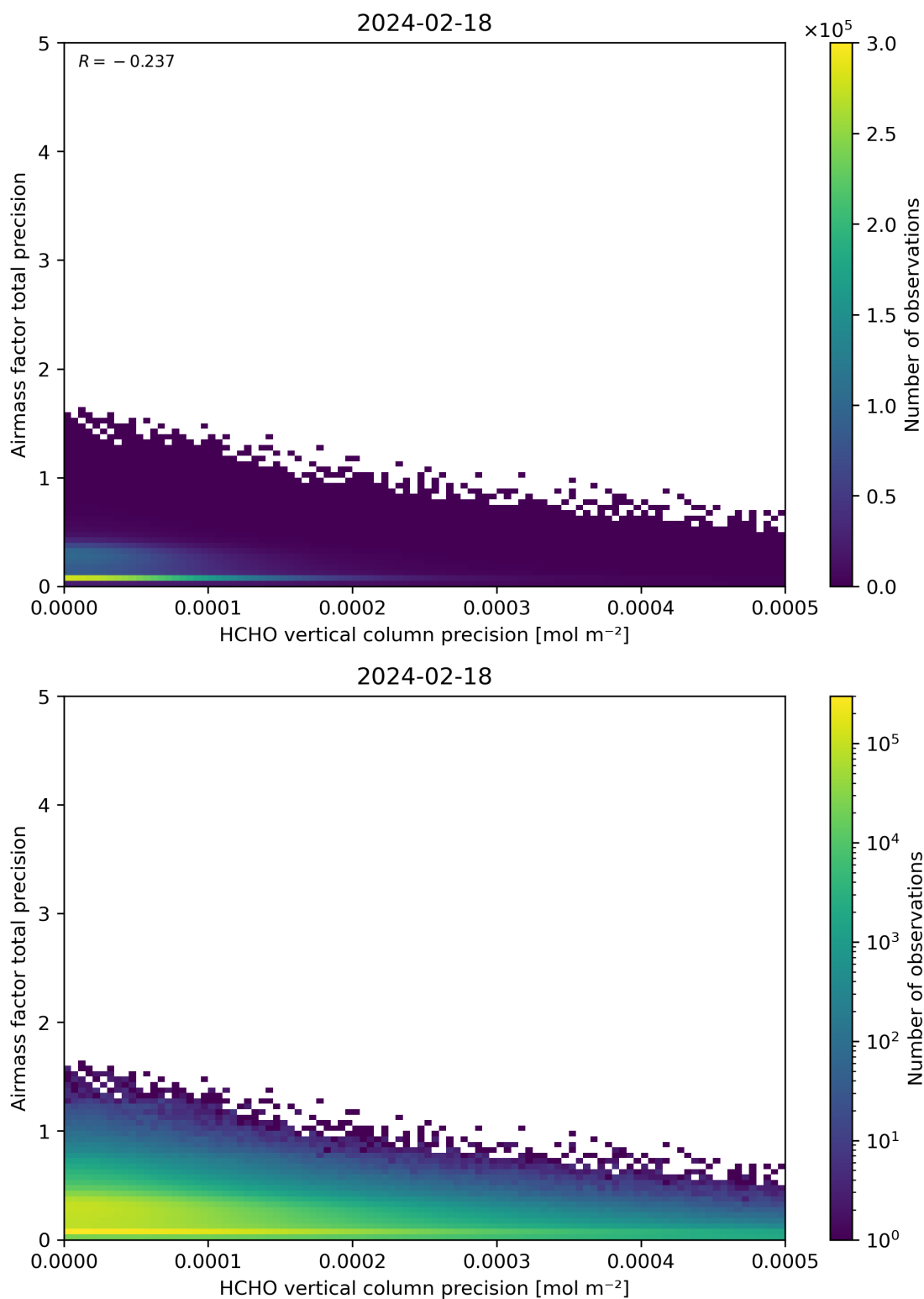
Figure 145: Scatter density plot of “HCHO vertical column precision” against “Airmass factor total precision” for 2024-02-17 to 2024-02-19.
