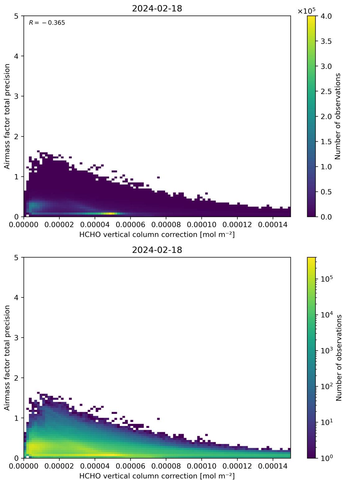
Figure 121: Scatter density plot of “HCHO vertical column correction” against “Airmass factor total precision” for 2024-02-17 to 2024-02-19.
