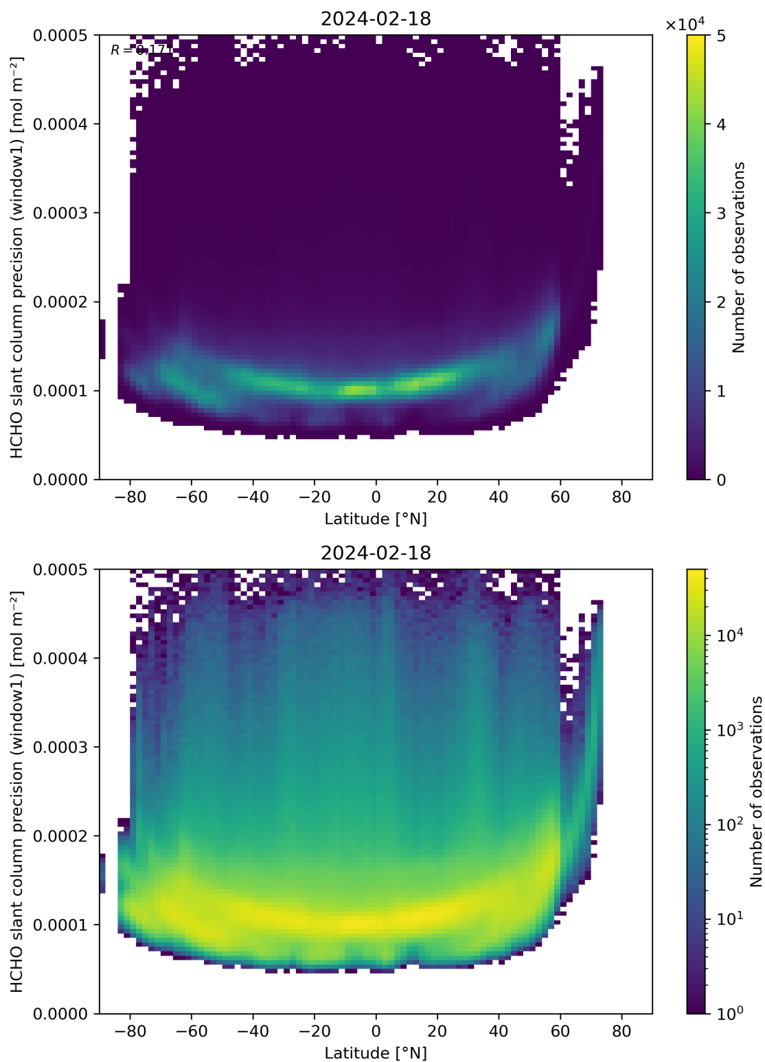
Figure 160: Scatter density plot of “Latitude” against “HCHO slant column precision (window1)” for 2024-02-17 to 2024-02-19.
