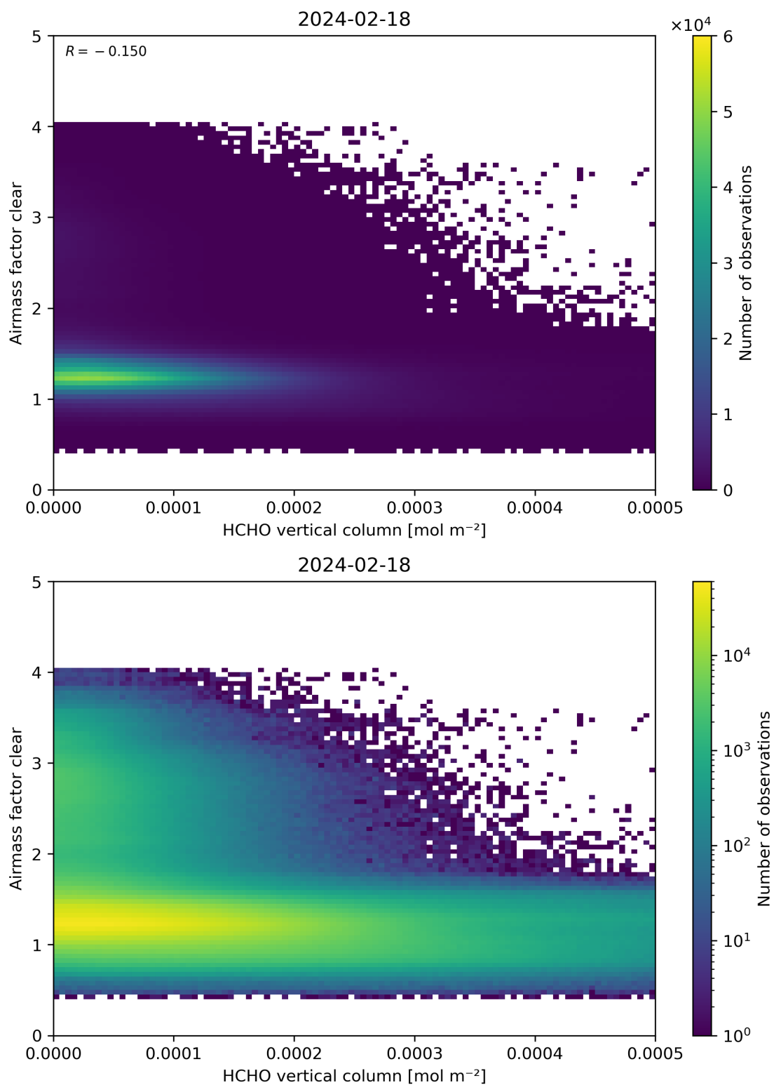
Figure 126: Scatter density plot of “HCHO vertical column” against “Airmass factor clear” for 2024-02-17 to 2024-02-19.
