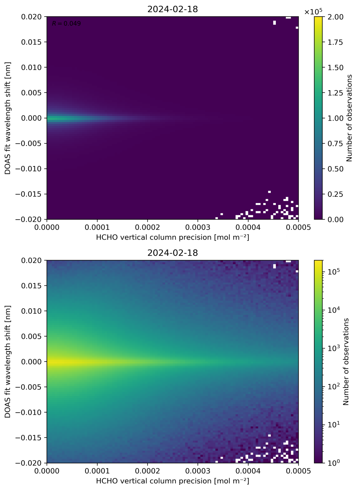
Figure 137: Scatter density plot of “HCHO vertical column precision” against “DOAS fit wavelength shift” for 2024-02-17 to 2024-02-19.
