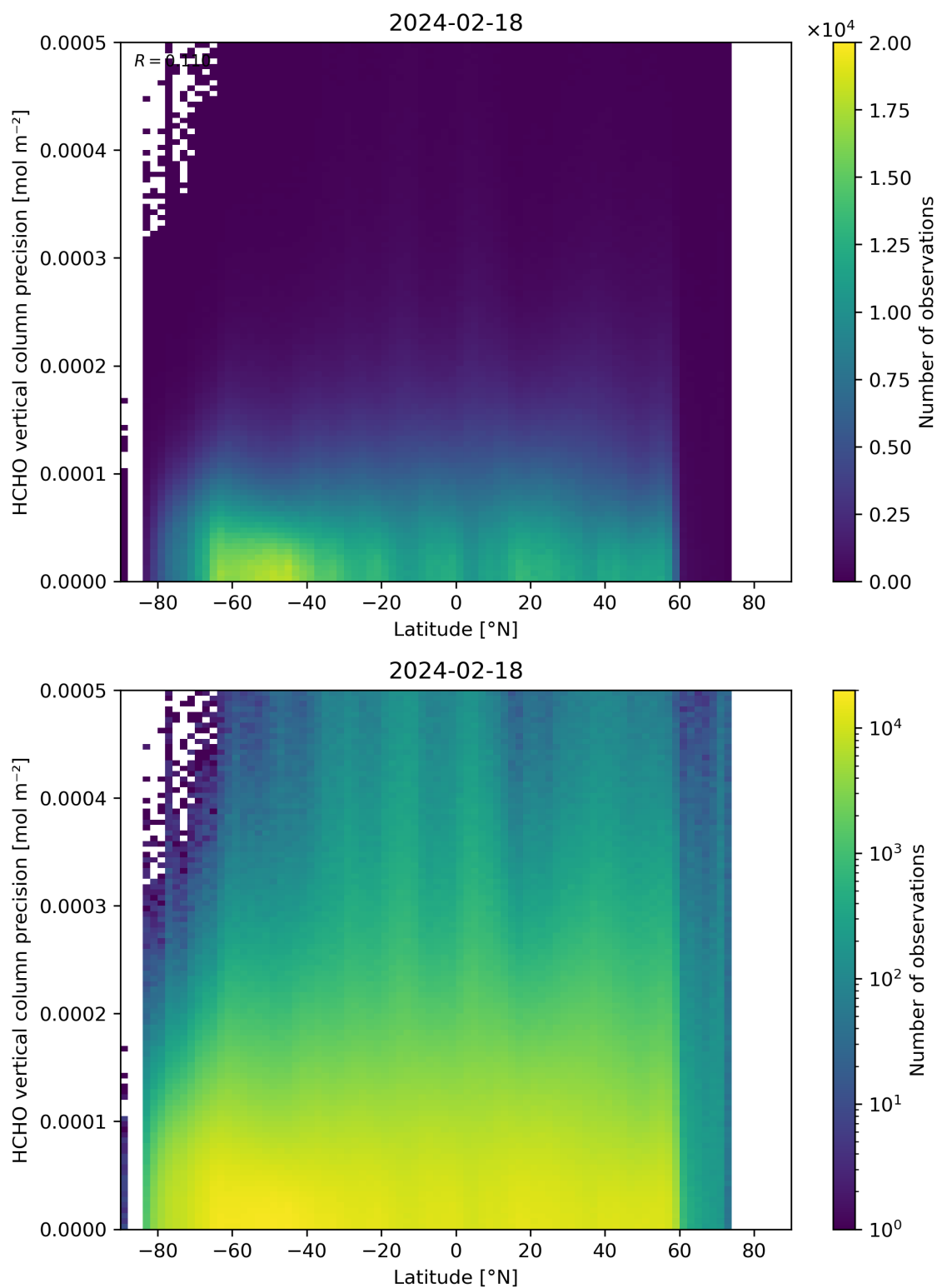
Figure 165: Scatter density plot of “Latitude” against “HCHO vertical column precision” for 2024-02-17 to 2024-02-19.
