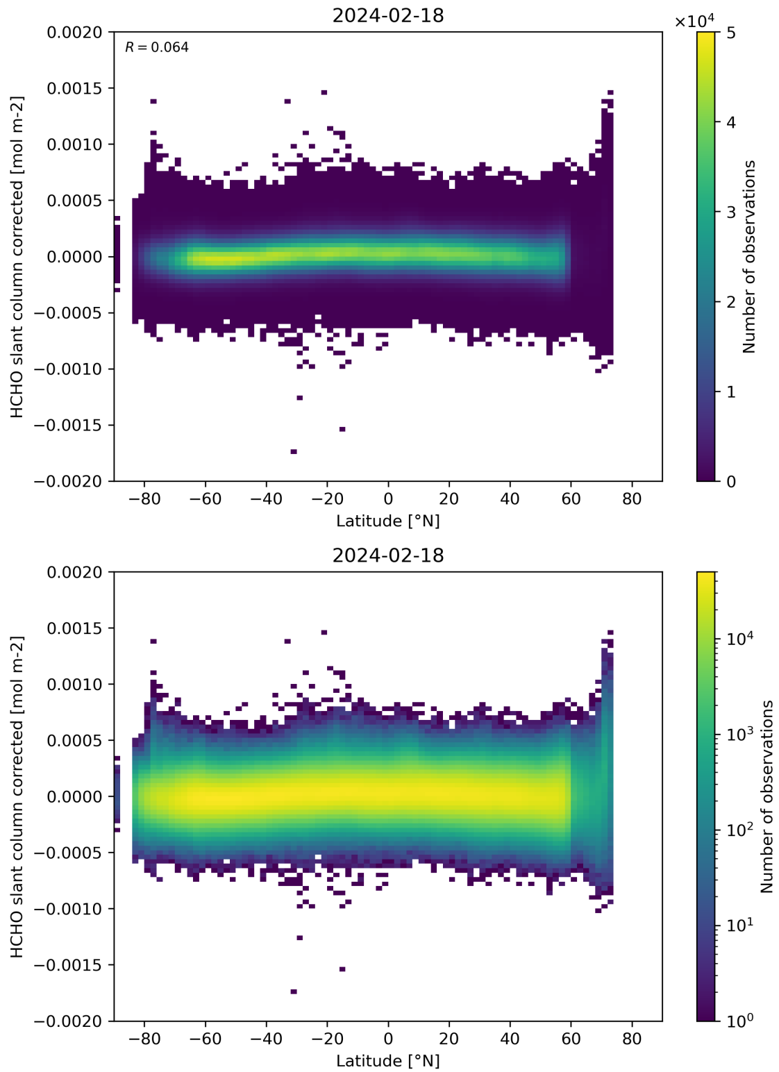
Figure 157: Scatter density plot of “Latitude” against “HCHO slant column corrected” for 2024-02-17 to 2024-02-19.
