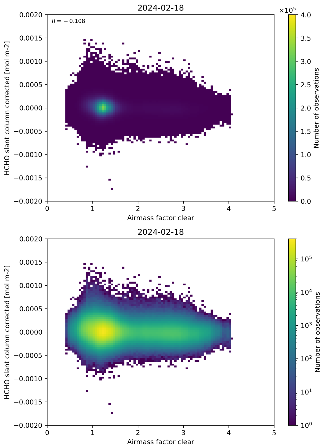
Figure 74: Scatter density plot of “Airmass factor clear” against “HCHO slant column corrected” for 2024-02-17 to 2024-02-19.
