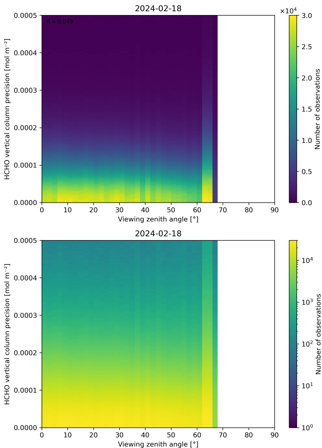
Figure 194: Scatter density plot of “Viewing zenith angle” against “HCHO vertical column precision” for 2024-02-17 to 2024-02-19.
