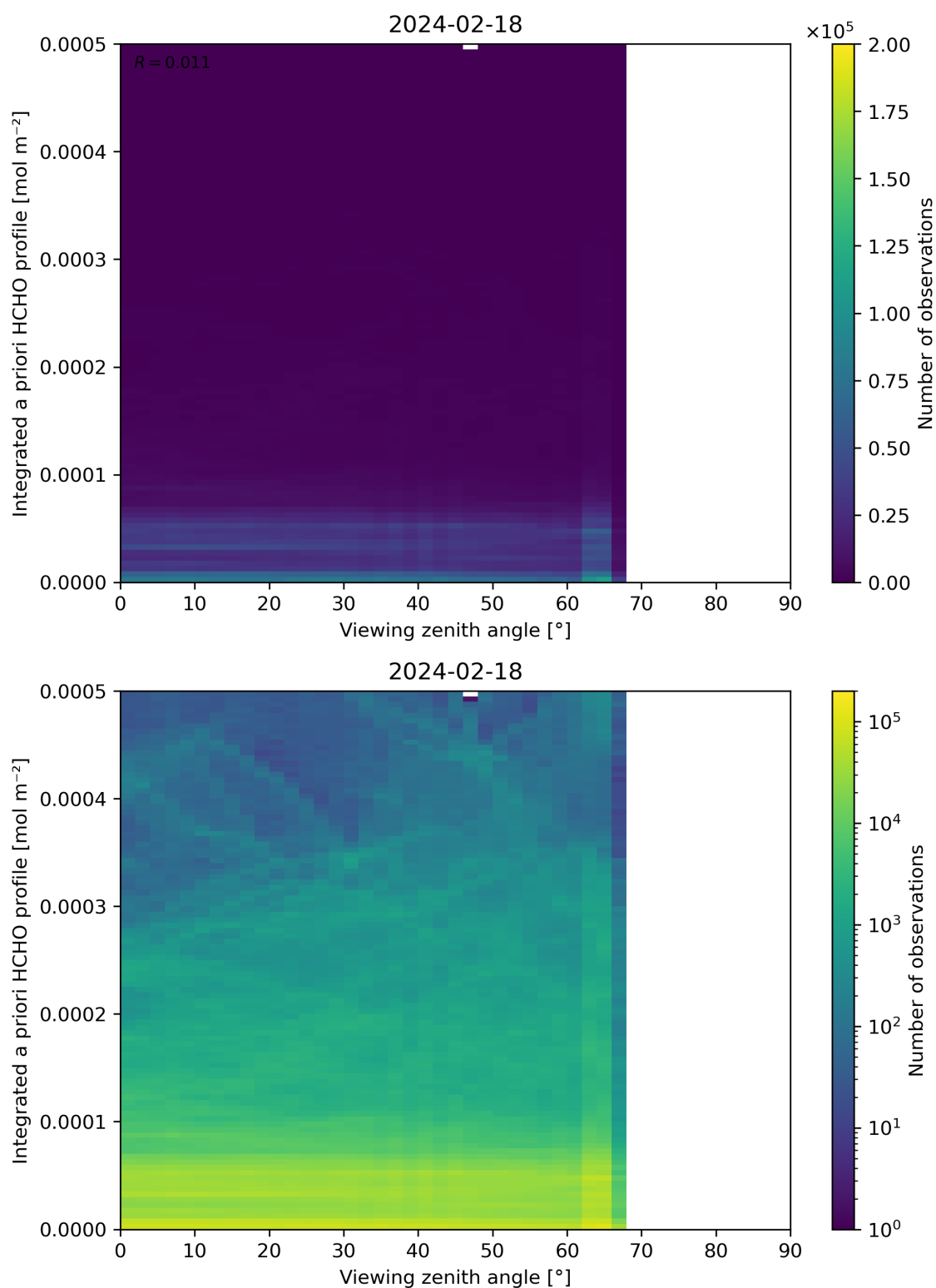
Figure 195: Scatter density plot of “Viewing zenith angle” against “Integrated a priori HCHO profile” for 2024-02-17 to 2024-02-19.
