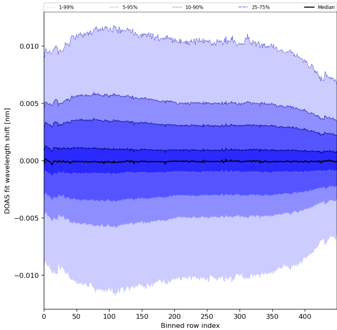
Figure 58: Along track statistics of “DOAS fit wavelength shift” for 2024-02-17 to 2024-02-19
