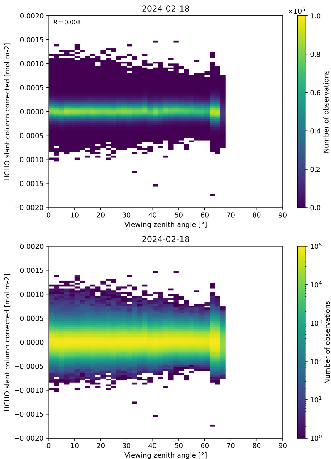
Figure 186: Scatter density plot of “Viewing zenith angle” against “HCHO slant column corrected” for 2024-02-17 to 2024-02-19.
