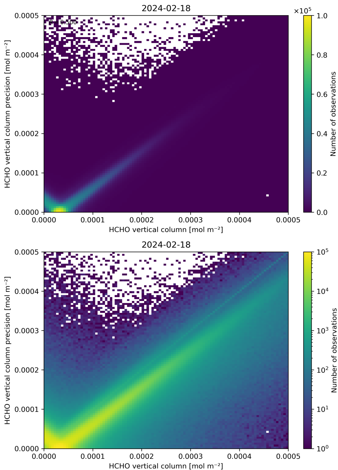
Figure 134: Scatter density plot of “HCHO vertical column” against “HCHO vertical column precision” for 2024-02-17 to 2024-02-19.
