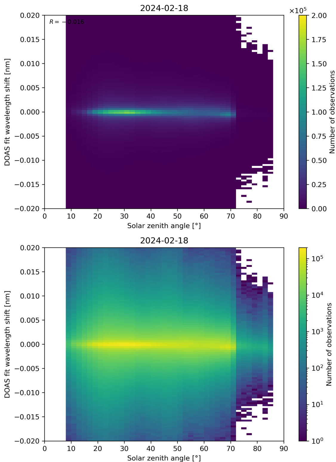
Figure 168: Scatter density plot of “Solar zenith angle” against “DOAS fit wavelength shift” for 2024-02-17 to 2024-02-19.
