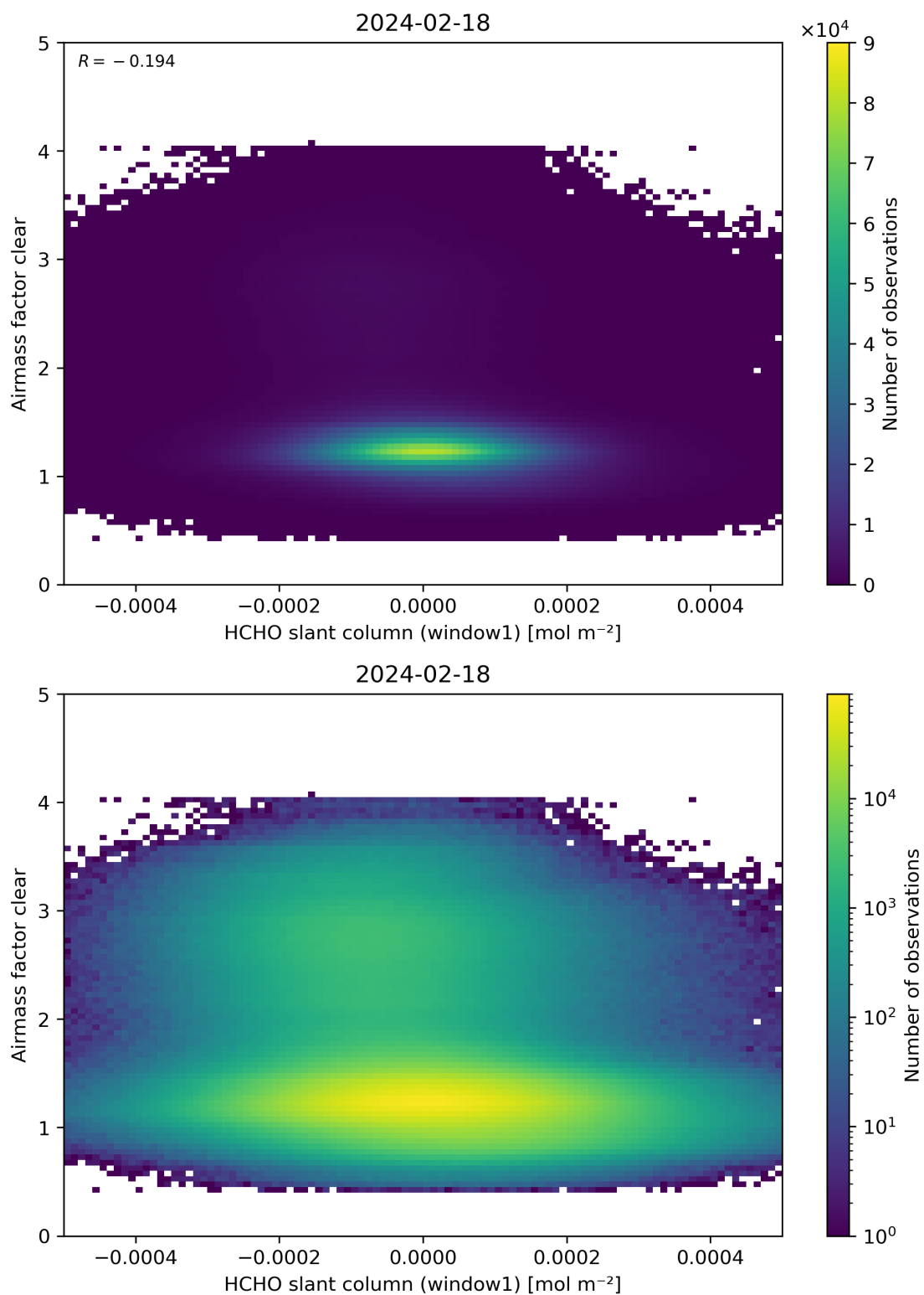
Figure 81: Scatter density plot of “HCHO slant column (window1)” against “Airmass factor clear” for 2024-02-17 to 2024-02-19.
