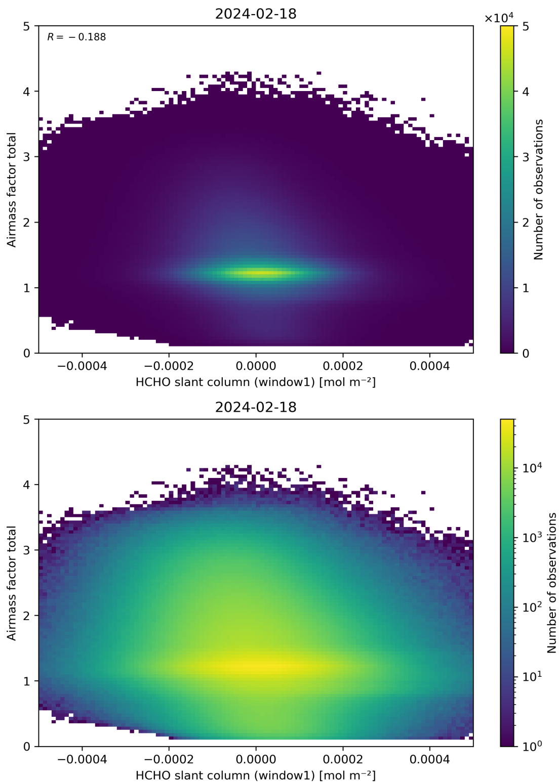
Figure 85: Scatter density plot of “HCHO slant column (window1)” against “Airmass factor total” for 2024-02-17 to 2024-02-19.
