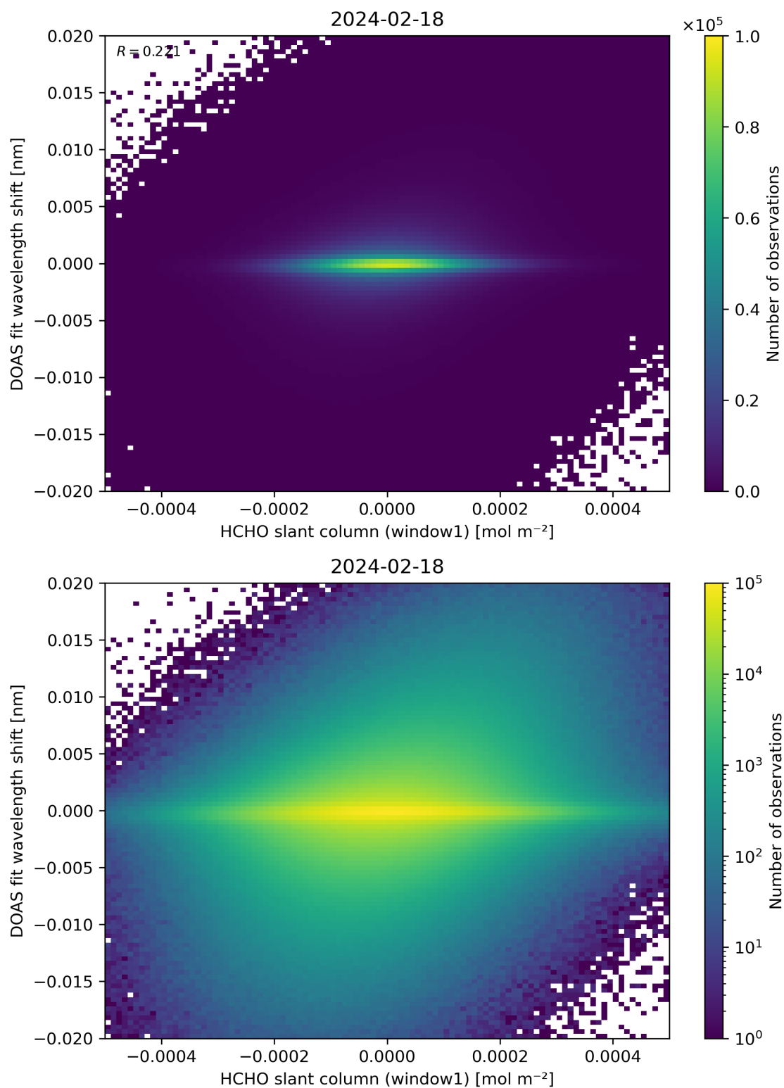
Figure 79: Scatter density plot of “HCHO slant column (window1)” against “DOAS fit wavelength shift” for 2024-02-17 to 2024-02-19.
