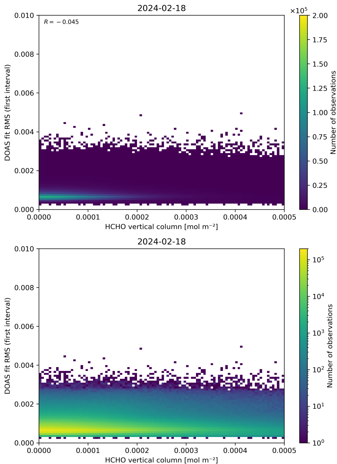
Figure 123: Scatter density plot of “HCHO vertical column” against “DOAS fit RMS (first interval)” for 2024-02-17 to 2024-02-19.
