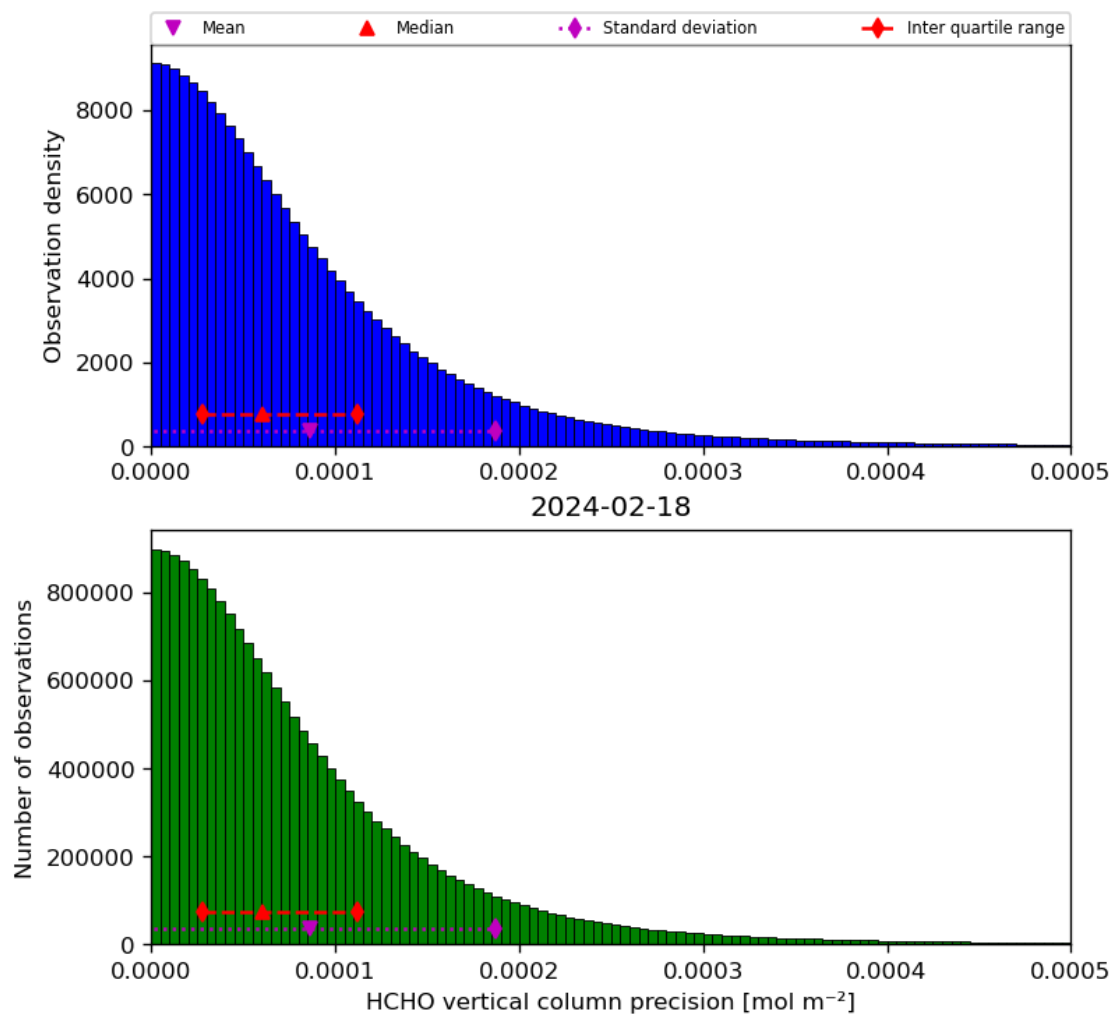
Figure 36: Histogram of “HCHO vertical column precision” for 2024-02-17 to 2024-02-19
