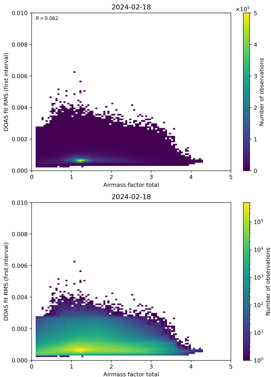
Figure 97: Scatter density plot of “Airmass factor total” against “DOAS fit RMS (first interval)” for 2024-02-17 to 2024-02-19.
