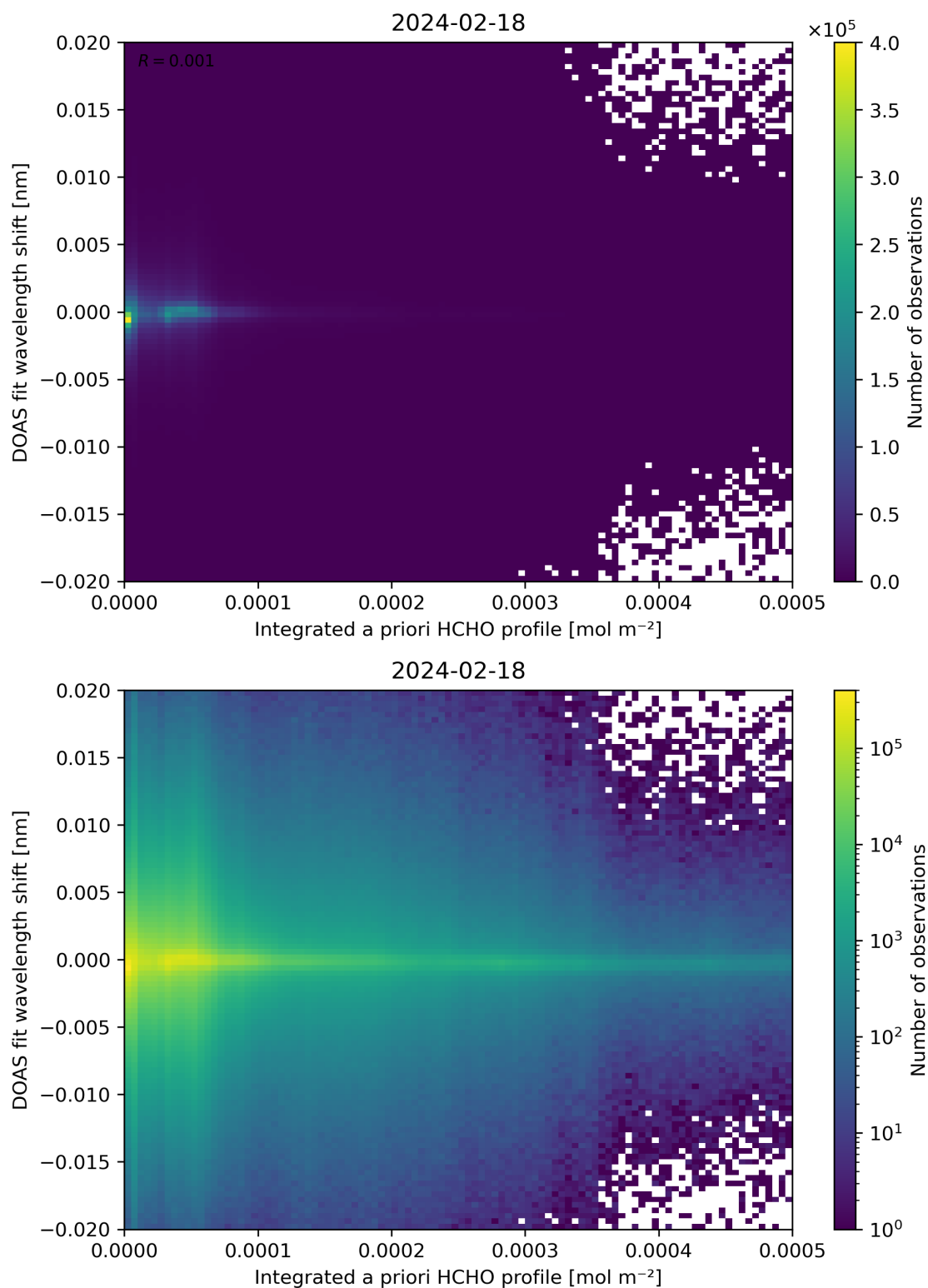
Figure 149: Scatter density plot of “Integrated a priori HCHO profile” against “DOAS fit wavelength shift” for 2024-02-17 to 2024-02-19.
