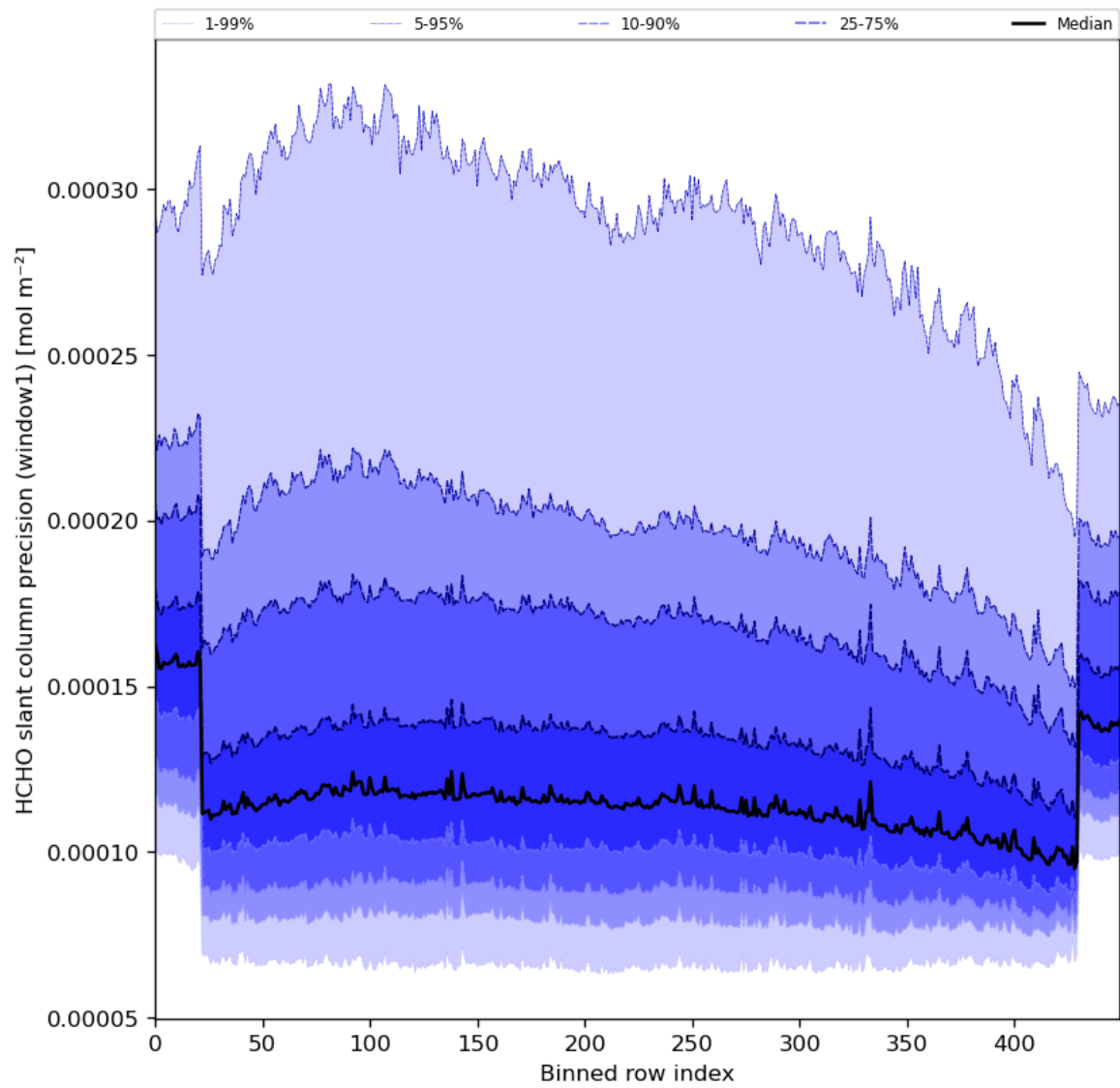
Figure 53: Along track statistics of “HCHO slant column precision (window1)” for 2024-02-17 to 2024-02-19
