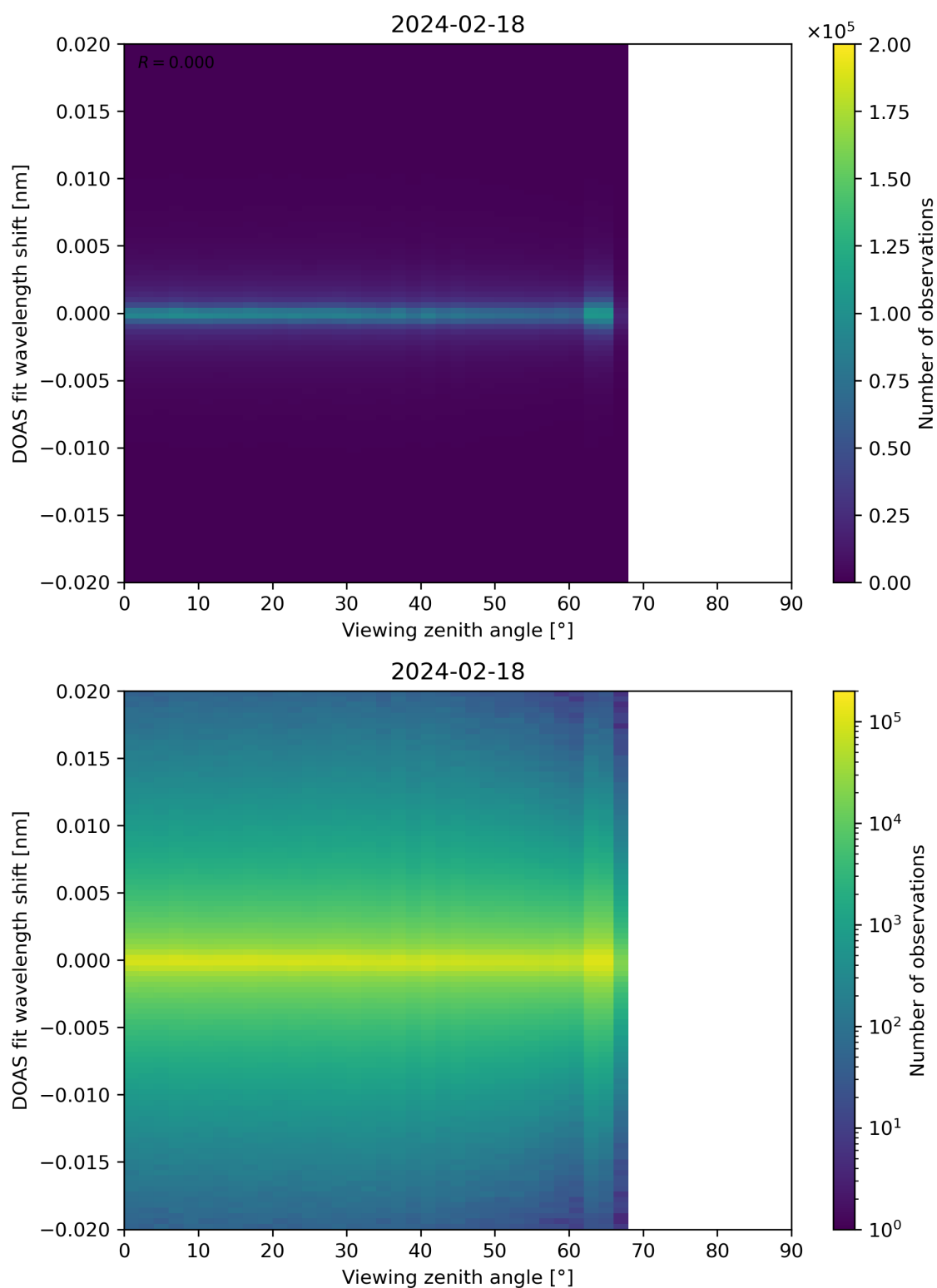
Figure 183: Scatter density plot of “Viewing zenith angle” against “DOAS fit wavelength shift” for 2024-02-17 to 2024-02-19.
