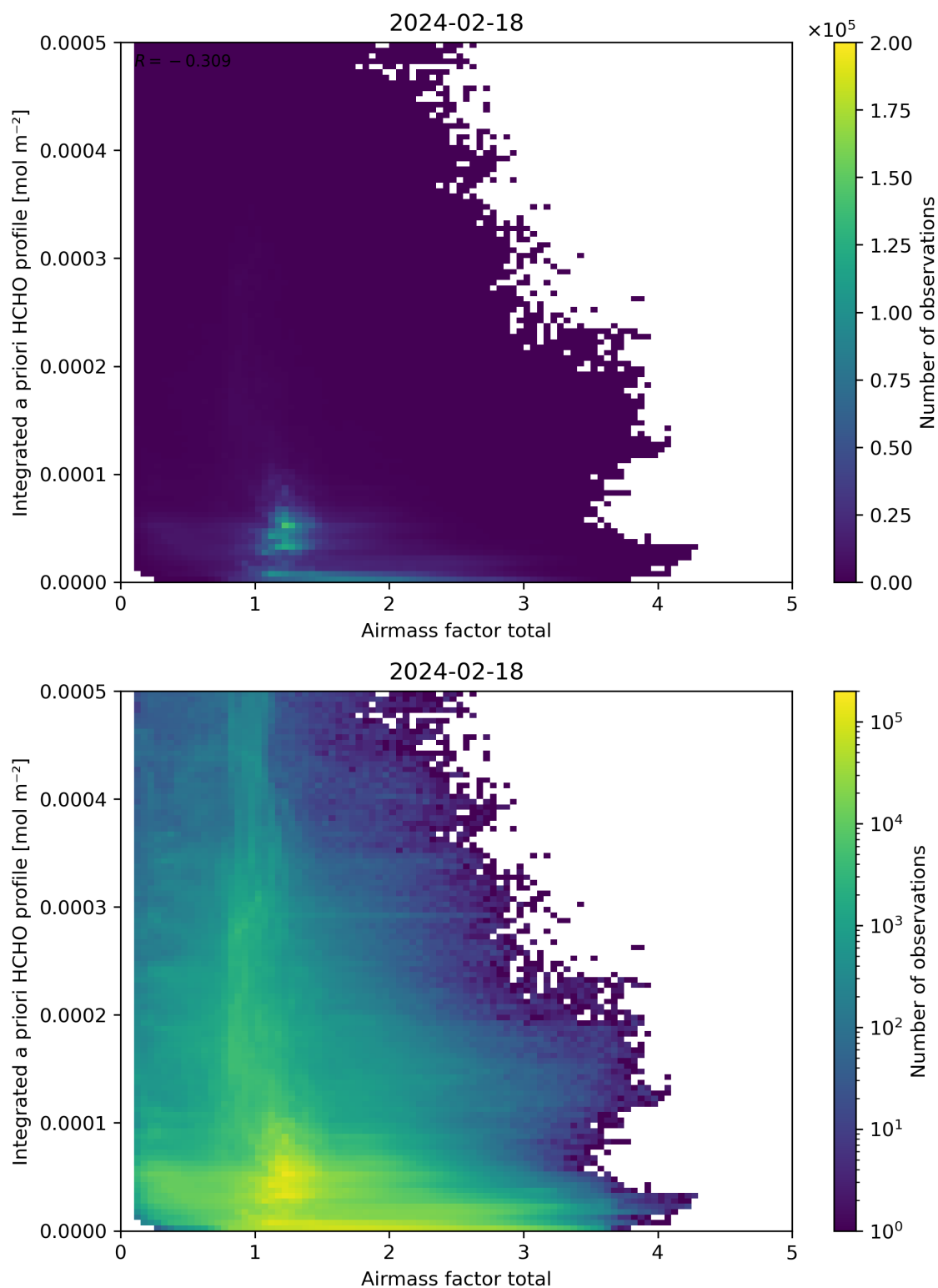
Figure 104: Scatter density plot of “Airmass factor total” against “Integrated a priori HCHO profile” for 2024-02-17 to 2024-02-19.
