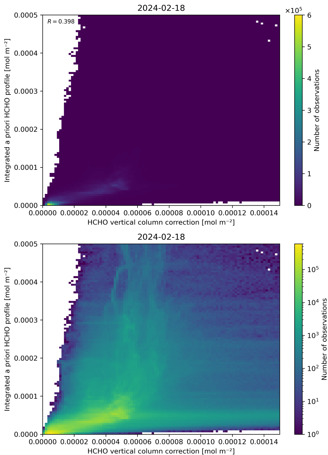
Figure 122: Scatter density plot of “HCHO vertical column correction” against “Integrated a priori HCHO profile” for 2024-02-17 to 2024-02-19.
