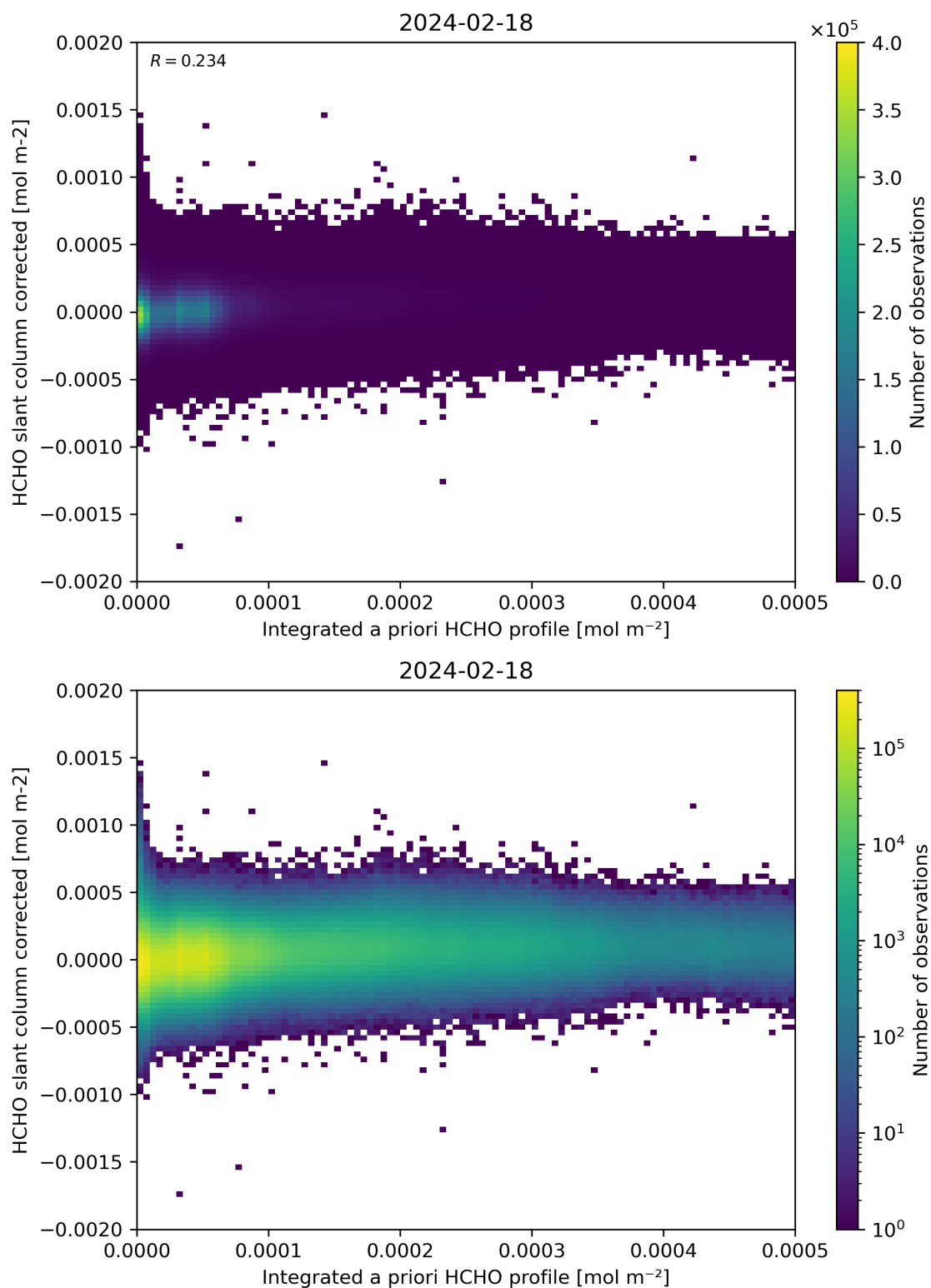
Figure 151: Scatter density plot of “Integrated a priori HCHO profile” against “HCHO slant column corrected” for 2024-02-17 to 2024-02-19.
