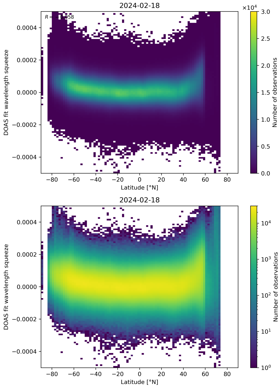
Figure 155: Scatter density plot of “Latitude” against “DOAS fit wavelength squeeze” for 2024-02-17 to 2024-02-19.
