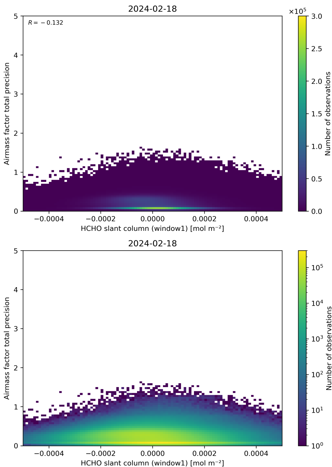
Figure 86: Scatter density plot of “HCHO slant column (window1)” against “Airmass factor total precision” for 2024-02-17 to 2024-02-19.
