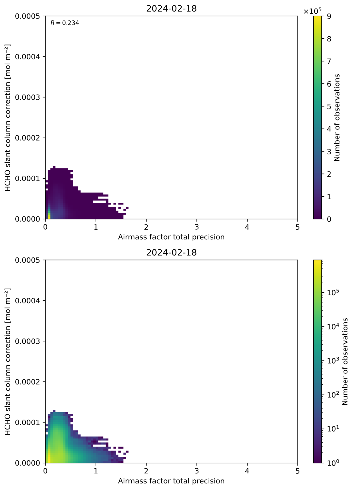
Figure 110: Scatter density plot of “Airmass factor total precision” against “HCHO slant column correction” for 2024-02-17 to 2024-02-19.
