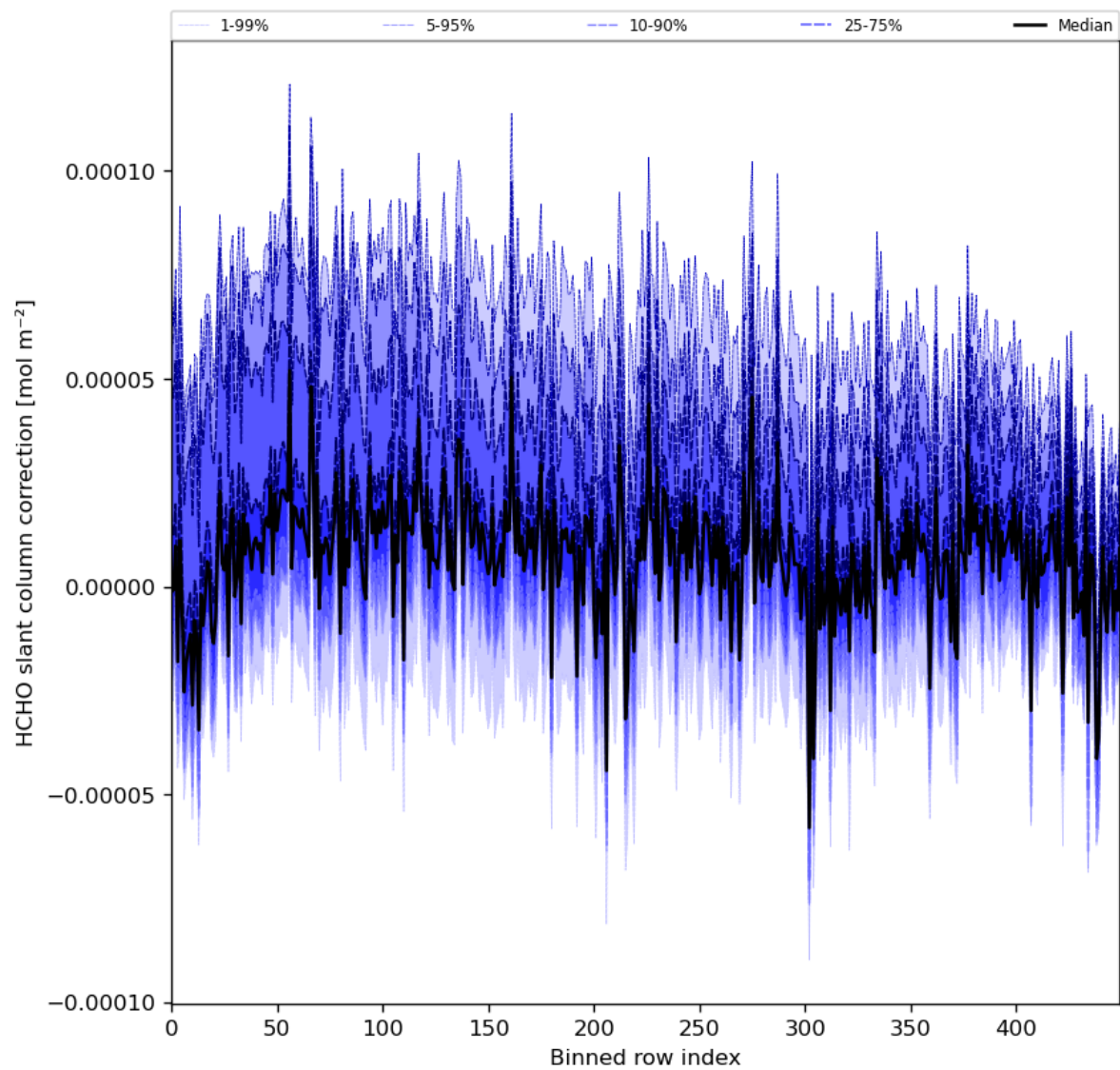
Figure 61: Along track statistics of “HCHO slant column correction” for 2024-02-17 to 2024-02-19
