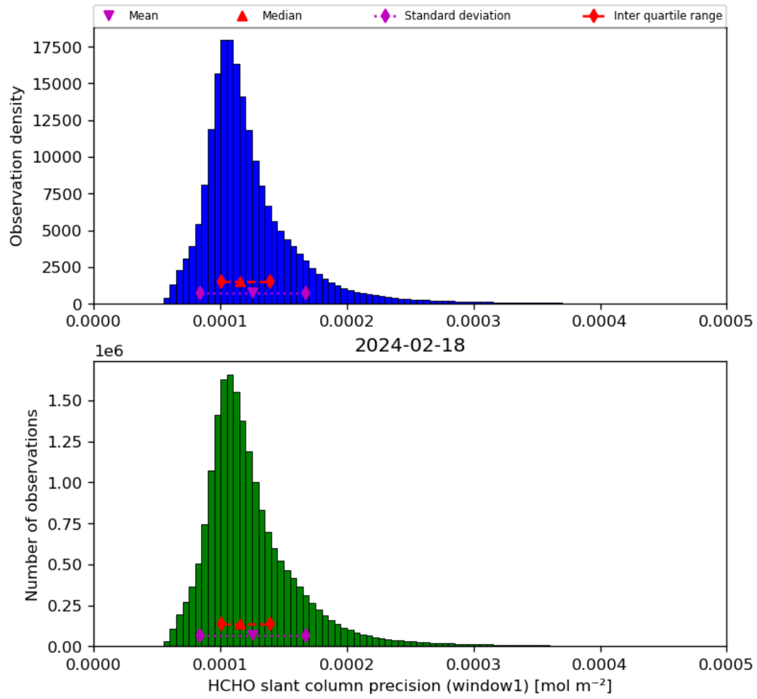
Figure 39: Histogram of “HCHO slant column precision (window1)” for 2024-02-17 to 2024-02-19
