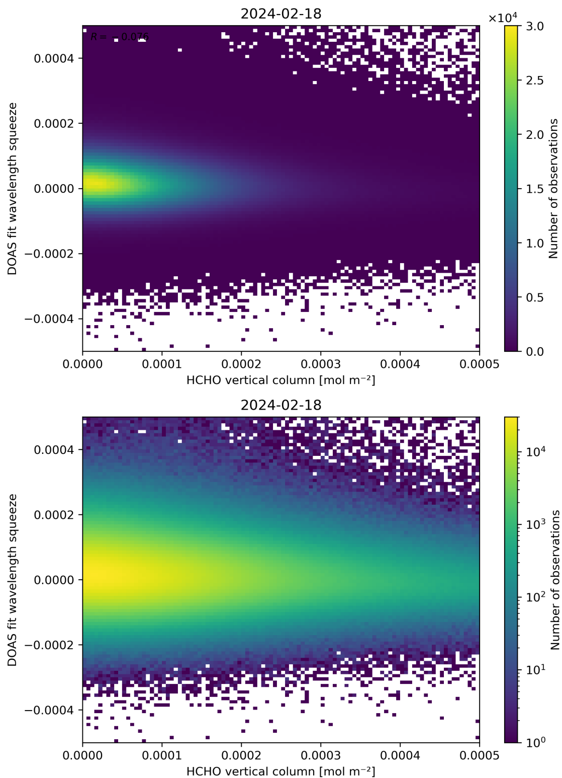
Figure 125: Scatter density plot of “HCHO vertical column” against “DOAS fit wavelength squeeze” for 2024-02-17 to 2024-02-19.
