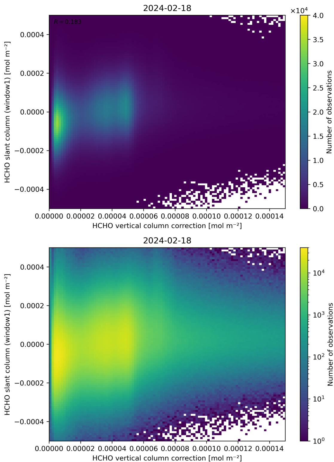
Figure 118: Scatter density plot of “HCHO vertical column correction” against “HCHO slant column (window1)” for 2024-02-17 to 2024-02-19.
