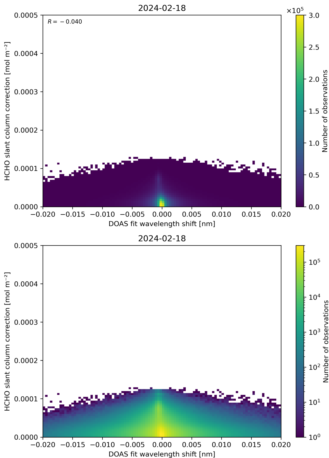
Figure 67: Scatter density plot of “DOAS fit wavelength shift” against “HCHO slant column correction” for 2024-02-17 to 2024-02-19.
