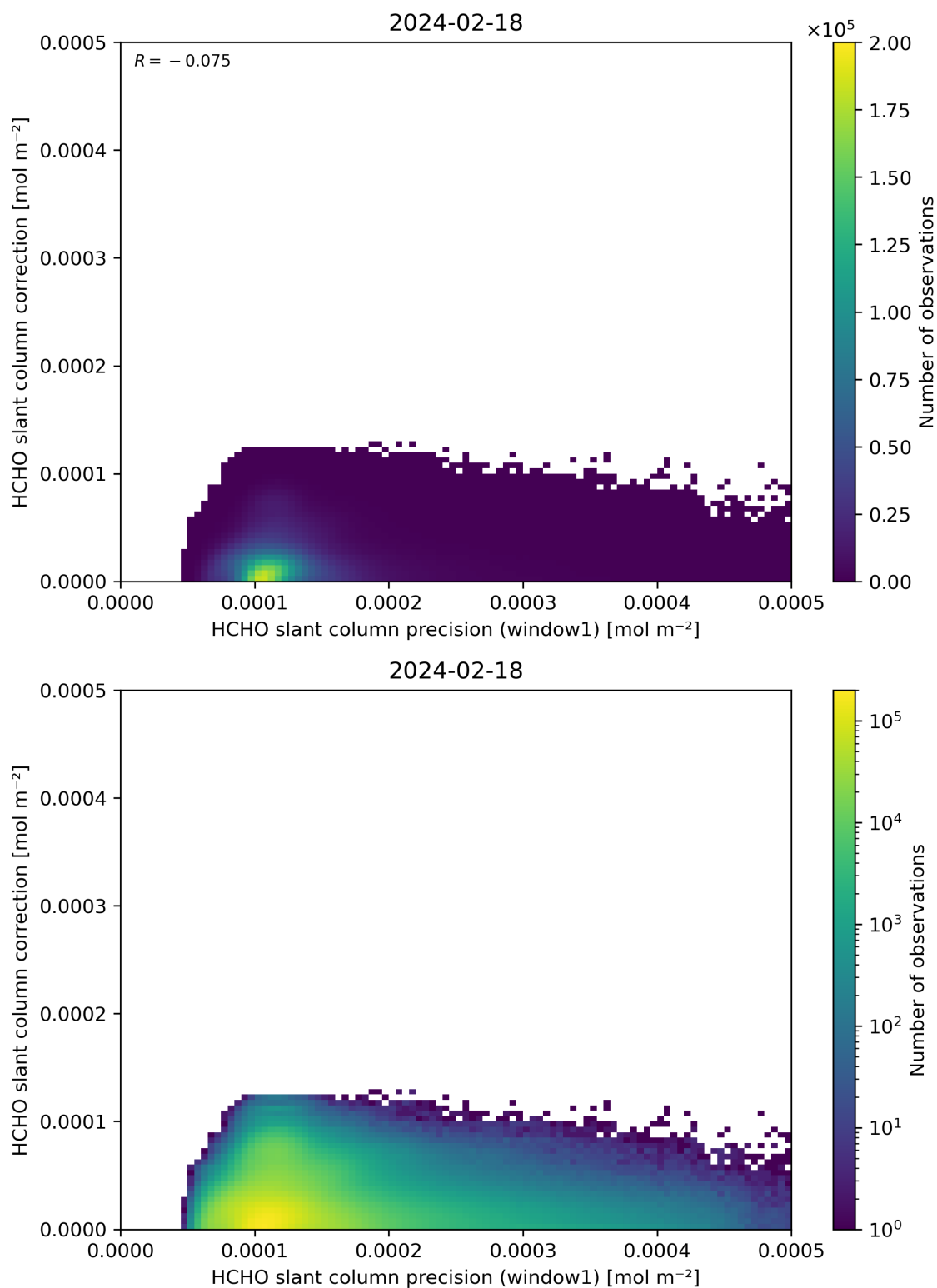
Figure 93: Scatter density plot of “HCHO slant column precision (window1)” against “HCHO slant column correction” for 2024-02-17 to 2024-02-19.
