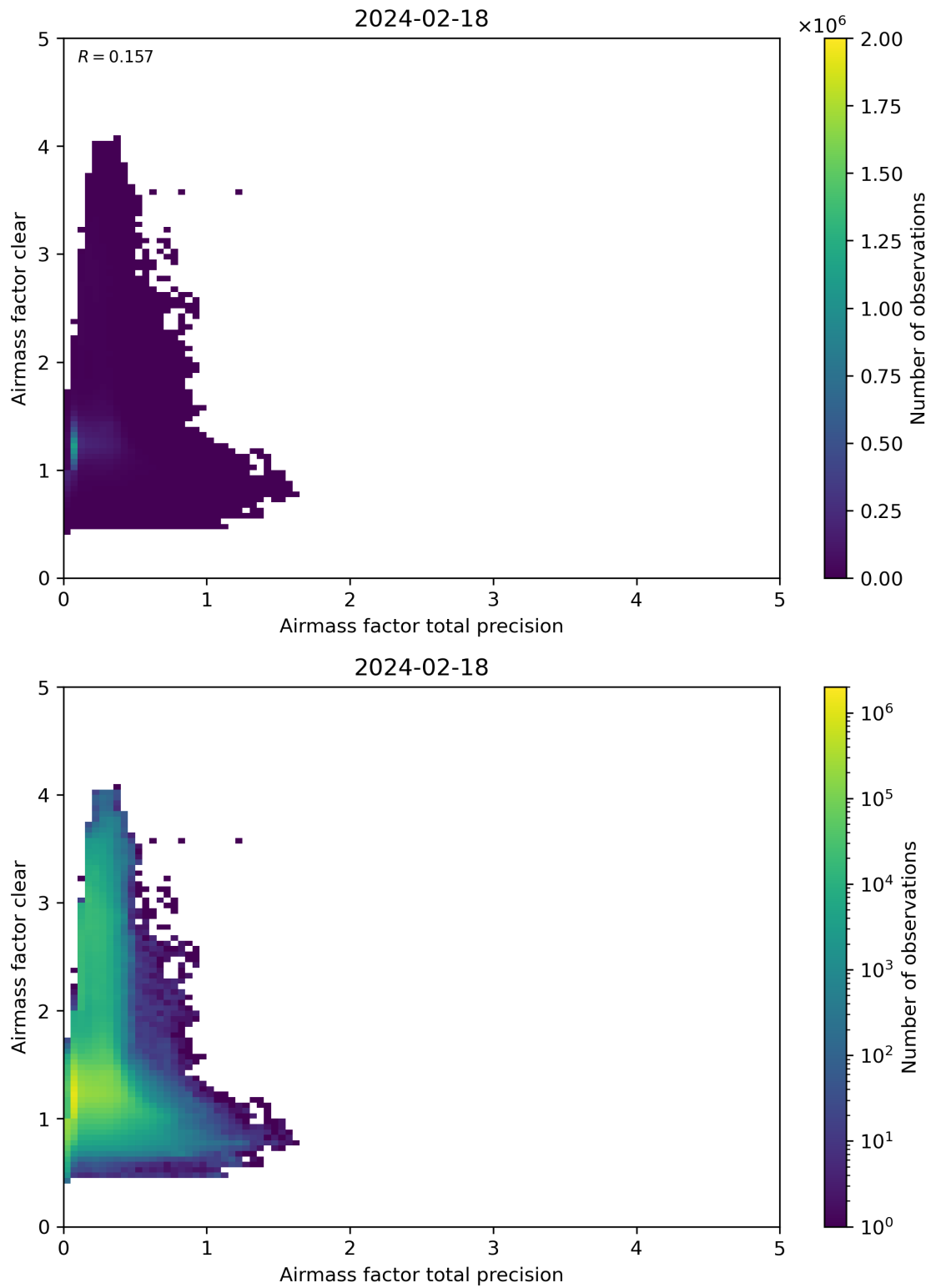
Figure 108: Scatter density plot of “Airmass factor total precision” against “Airmass factor clear” for 2024-02-17 to 2024-02-19.
