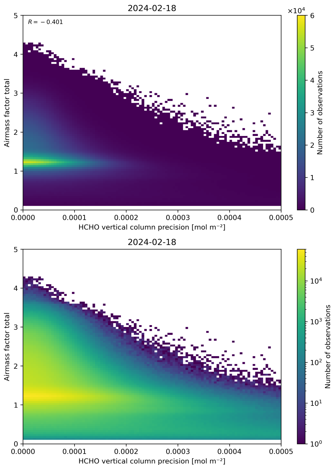
Figure 144: Scatter density plot of “HCHO vertical column precision” against “Airmass factor total” for 2024-02-17 to 2024-02-19.
