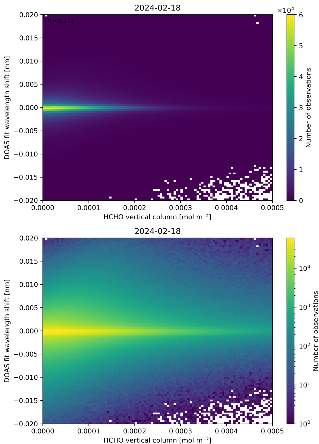
Figure 124: Scatter density plot of “HCHO vertical column” against “DOAS fit wavelength shift” for 2024-02-17 to 2024-02-19.
