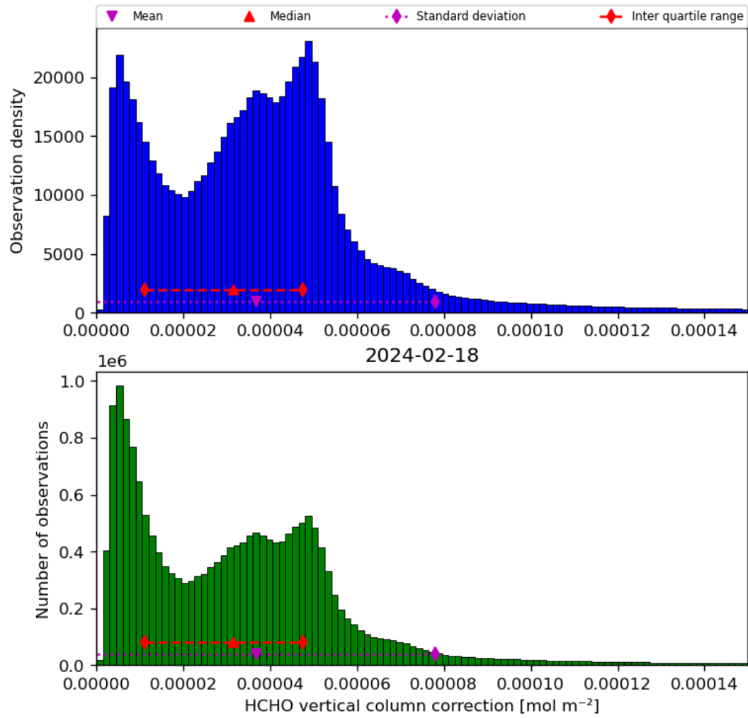
Figure 37: Histogram of “HCHO vertical column correction” for 2024-02-17 to 2024-02-19
