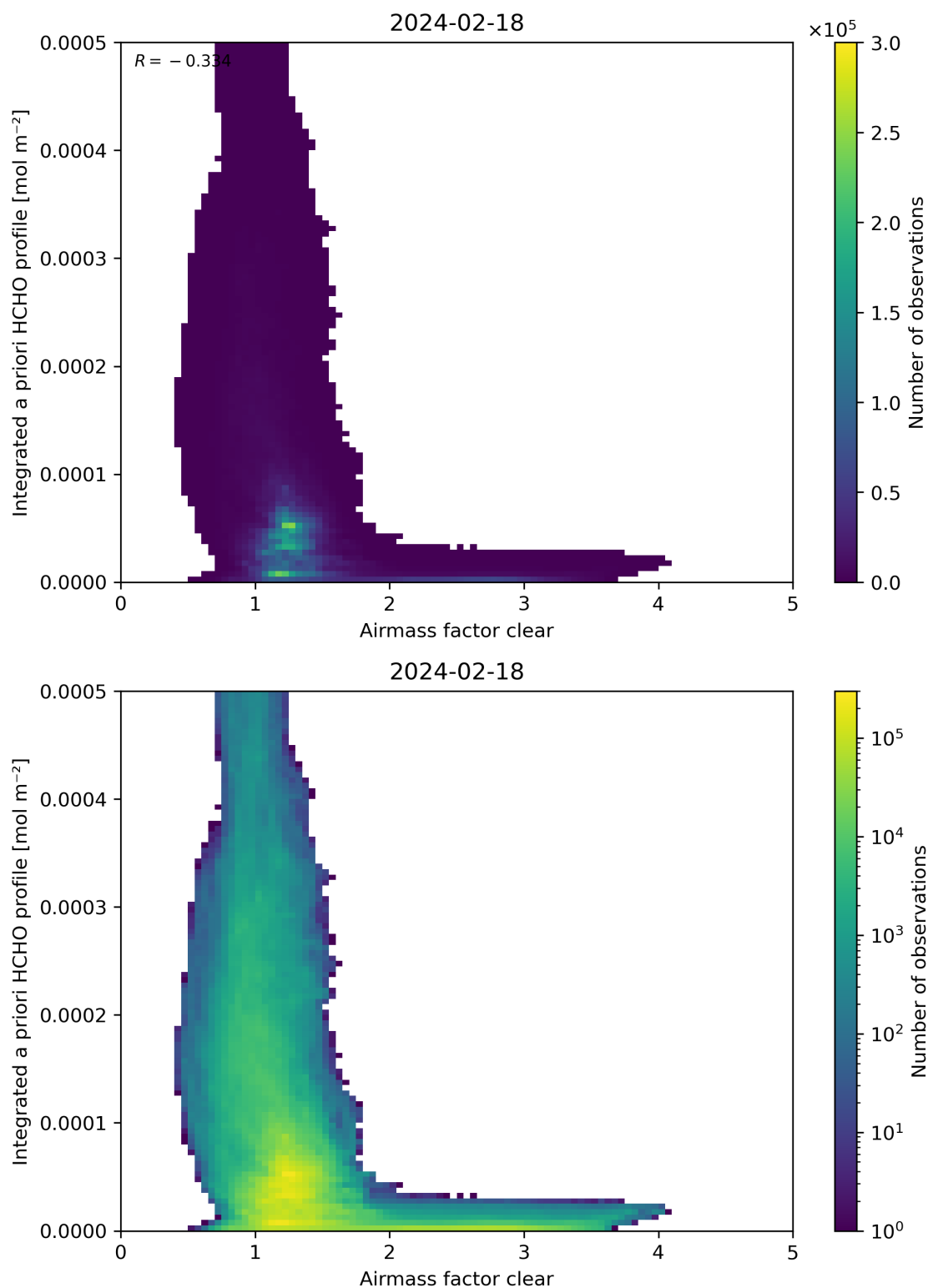
Figure 76: Scatter density plot of “Airmass factor clear” against “Integrated a priori HCHO profile” for 2024-02-17 to 2024-02-19.
