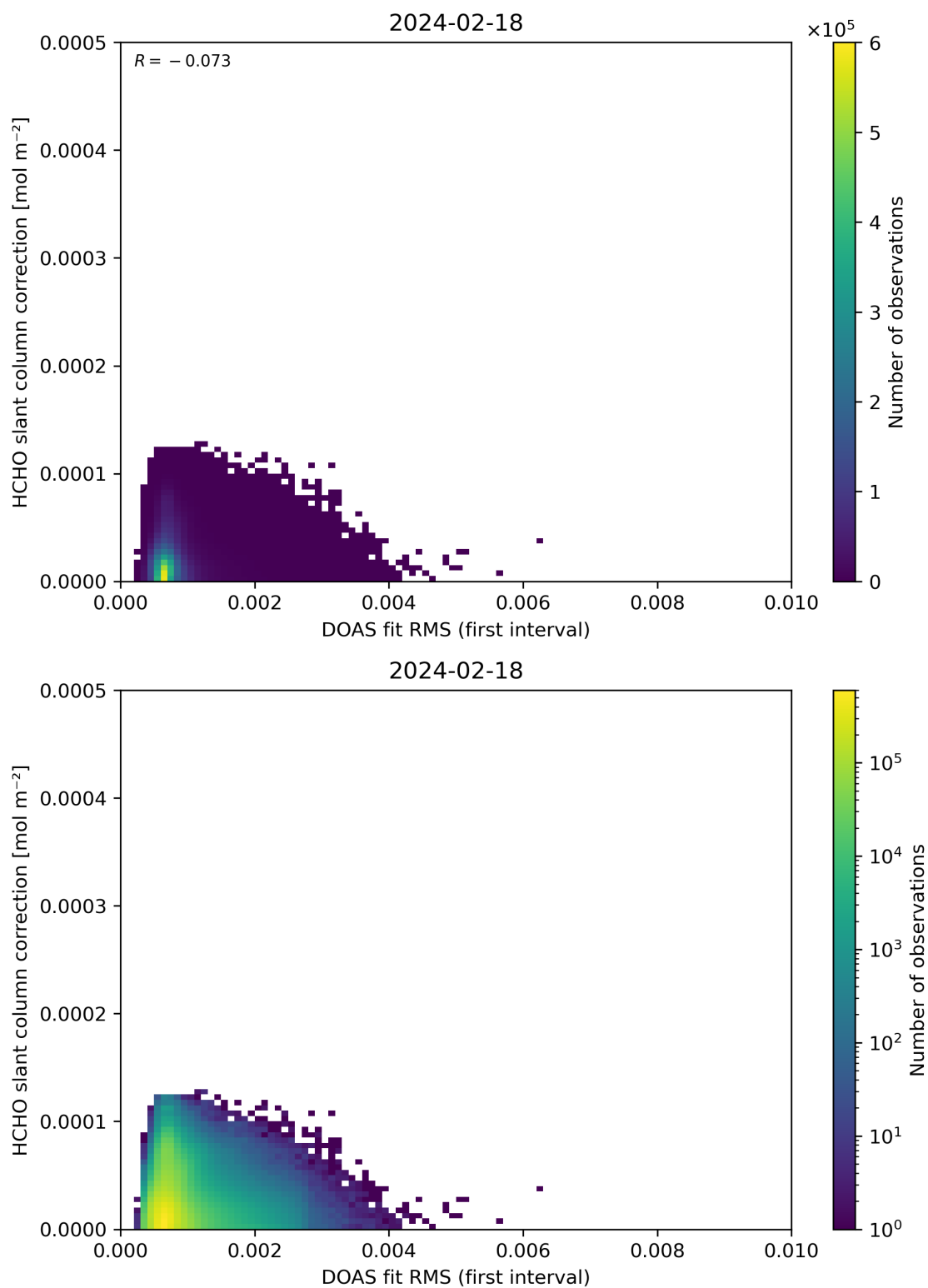
Figure 63: Scatter density plot of “DOAS fit RMS (first interval)” against “HCHO slant column correction” for 2024-02-17 to 2024-02-19.
