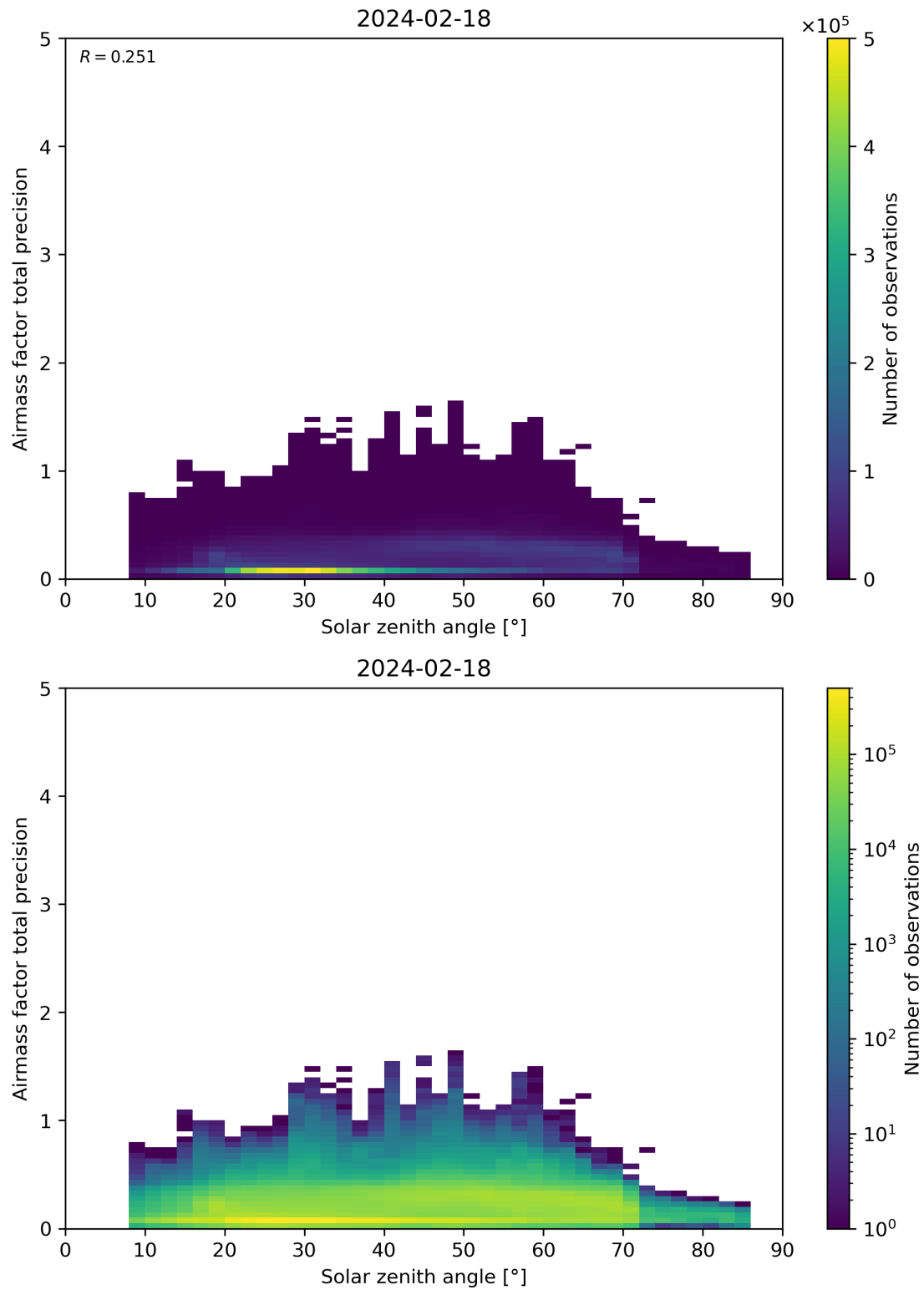
Figure 176: Scatter density plot of “Solar zenith angle” against “Airmass factor total precision” for 2024-02-17 to 2024-02-19.
