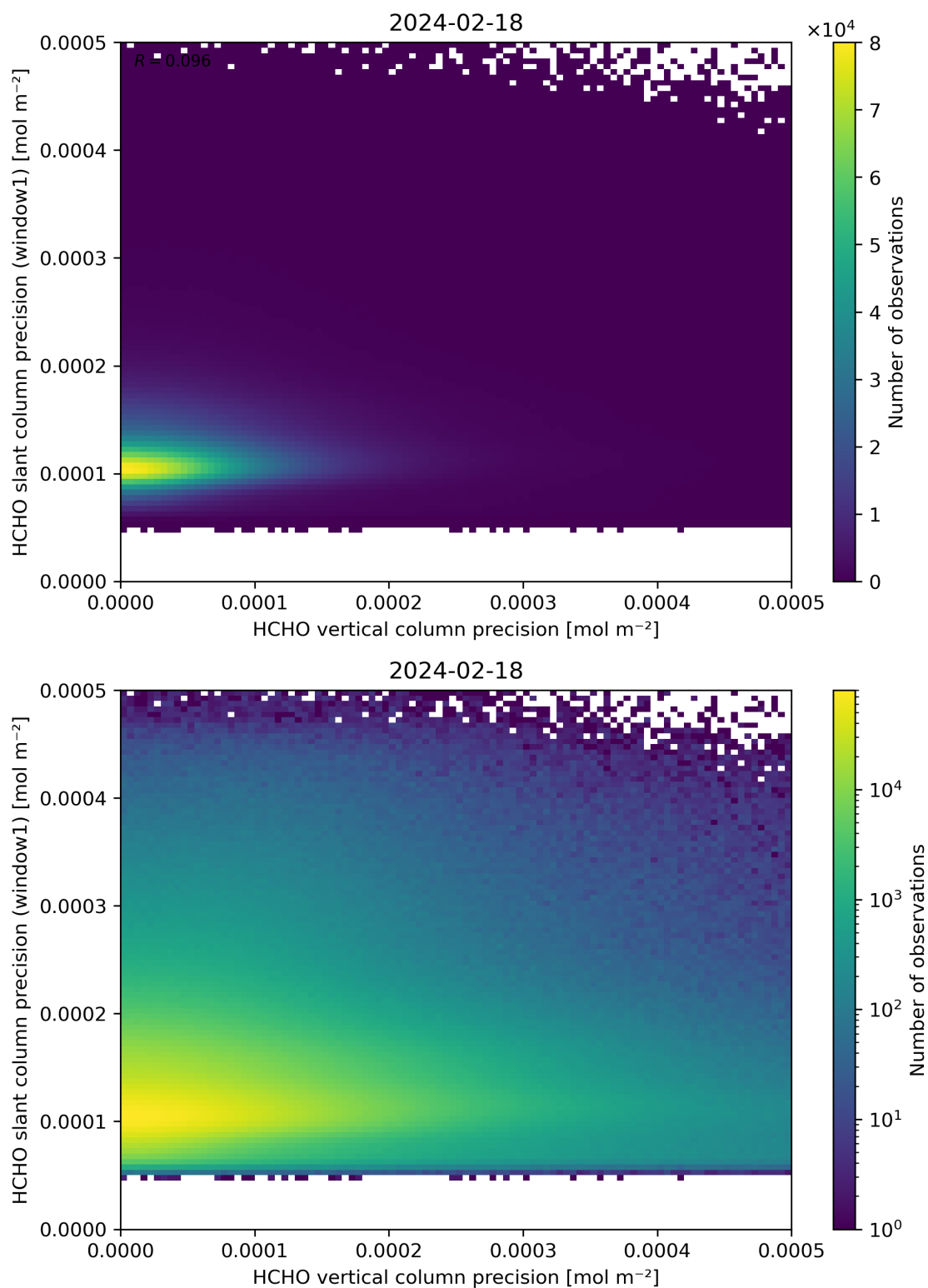
Figure 143: Scatter density plot of “HCHO vertical column precision” against “HCHO slant column precision (window1)” for 2024-02-17 to 2024-02-19.
