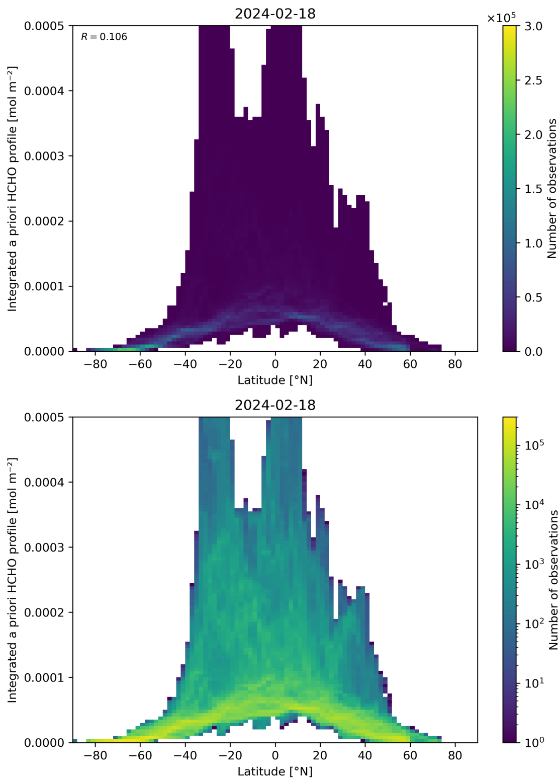
Figure 166: Scatter density plot of “Latitude” against “Integrated a priori HCHO profile” for 2024-02-17 to 2024-02-19.
