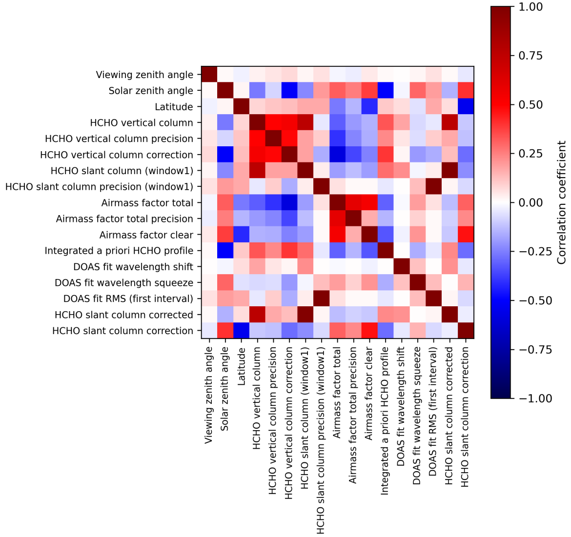
Figure 2: Map of correlation matrix for 2024-02-17 to 2024-02-19.
