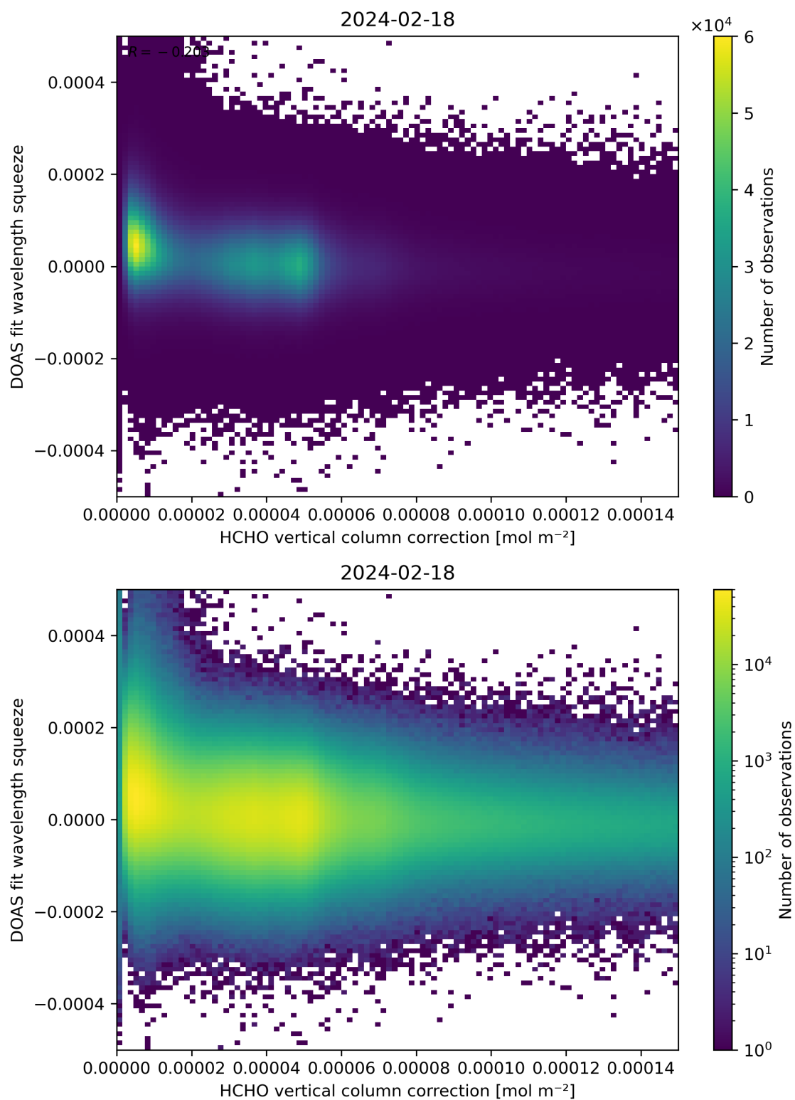
Figure 114: Scatter density plot of “HCHO vertical column correction” against “DOAS fit wavelength squeeze” for 2024-02-17 to 2024-02-19.
