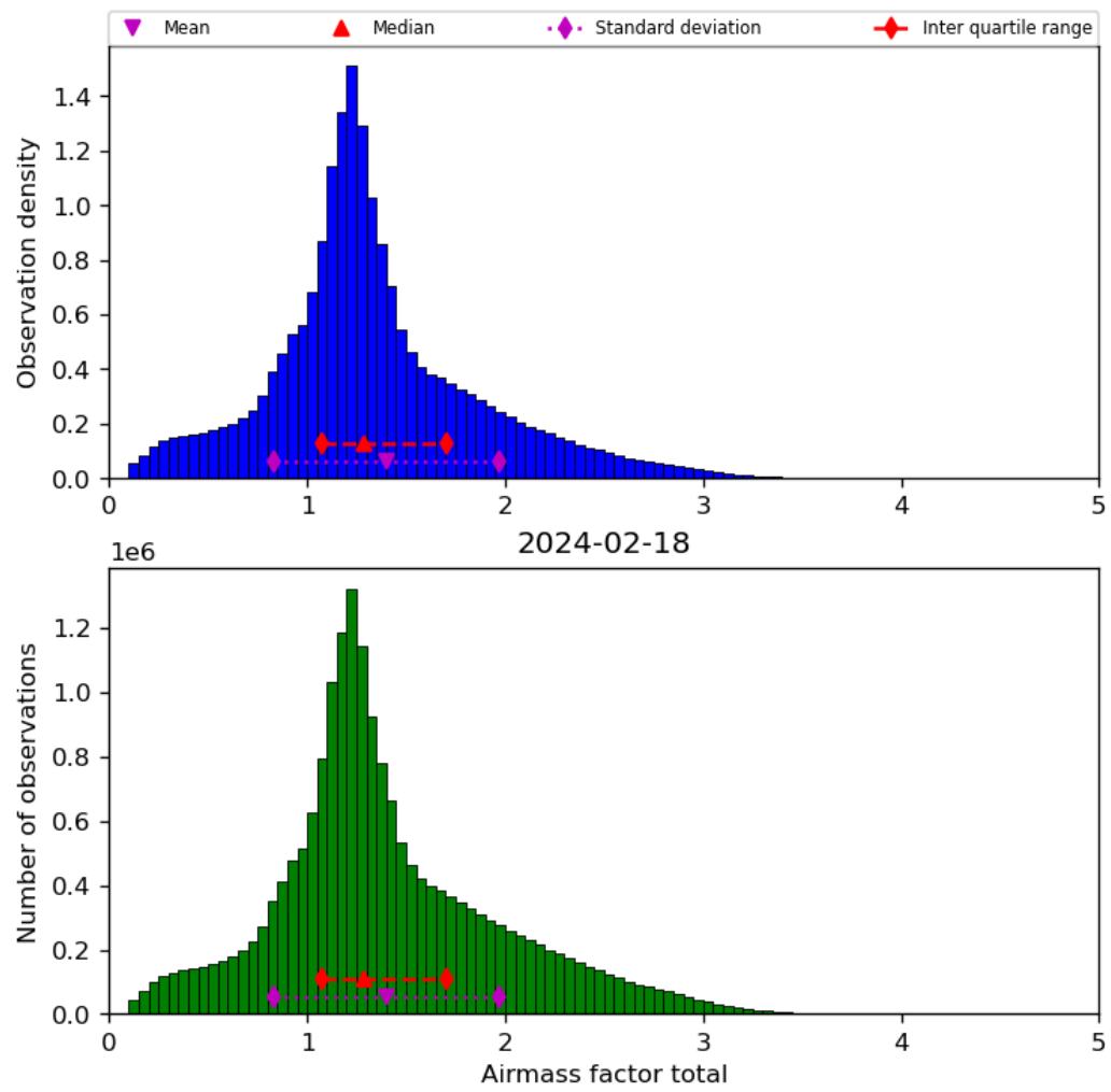
Figure 40: Histogram of “Airmass factor total” for 2024-02-17 to 2024-02-19
