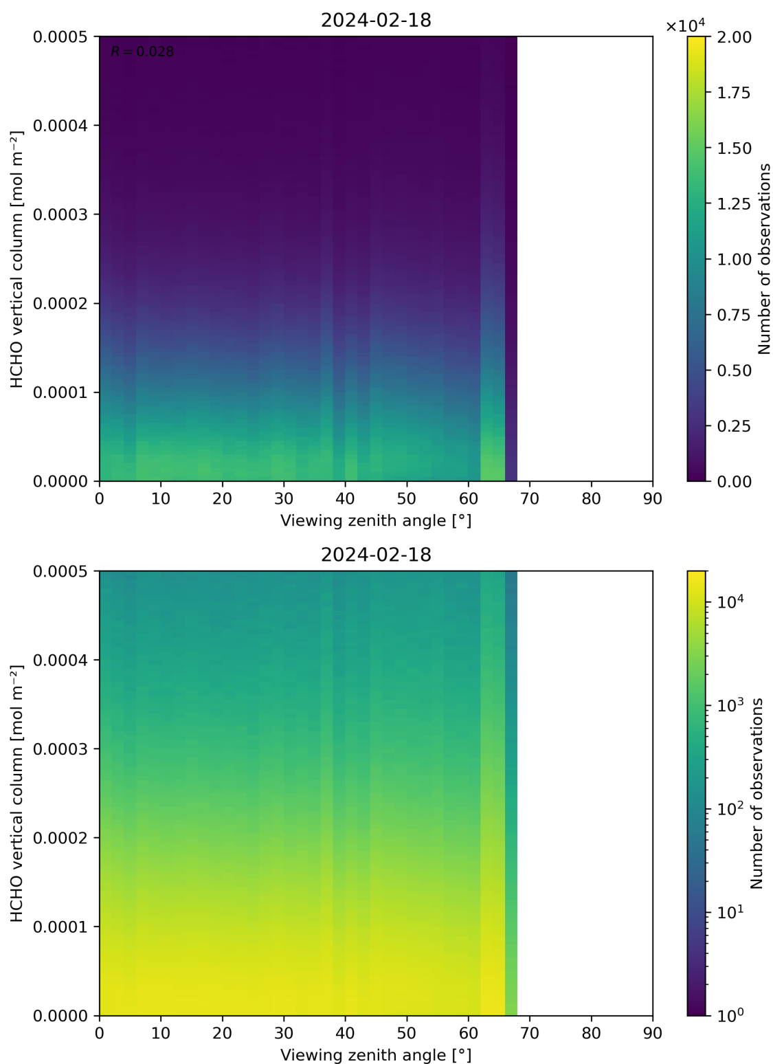
Figure 192: Scatter density plot of “Viewing zenith angle” against “HCHO vertical column” for 2024-02-17 to 2024-02-19.
