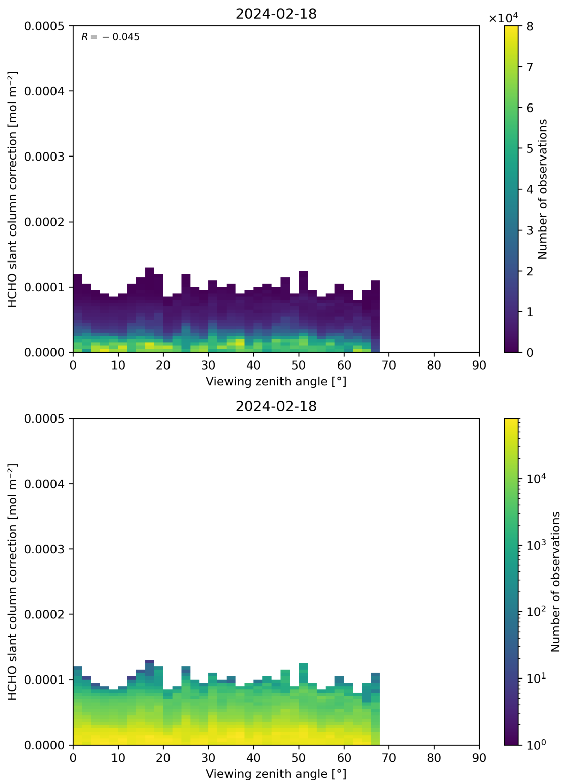
Figure 187: Scatter density plot of “Viewing zenith angle” against “HCHO slant column correction” for 2024-02-17 to 2024-02-19.
