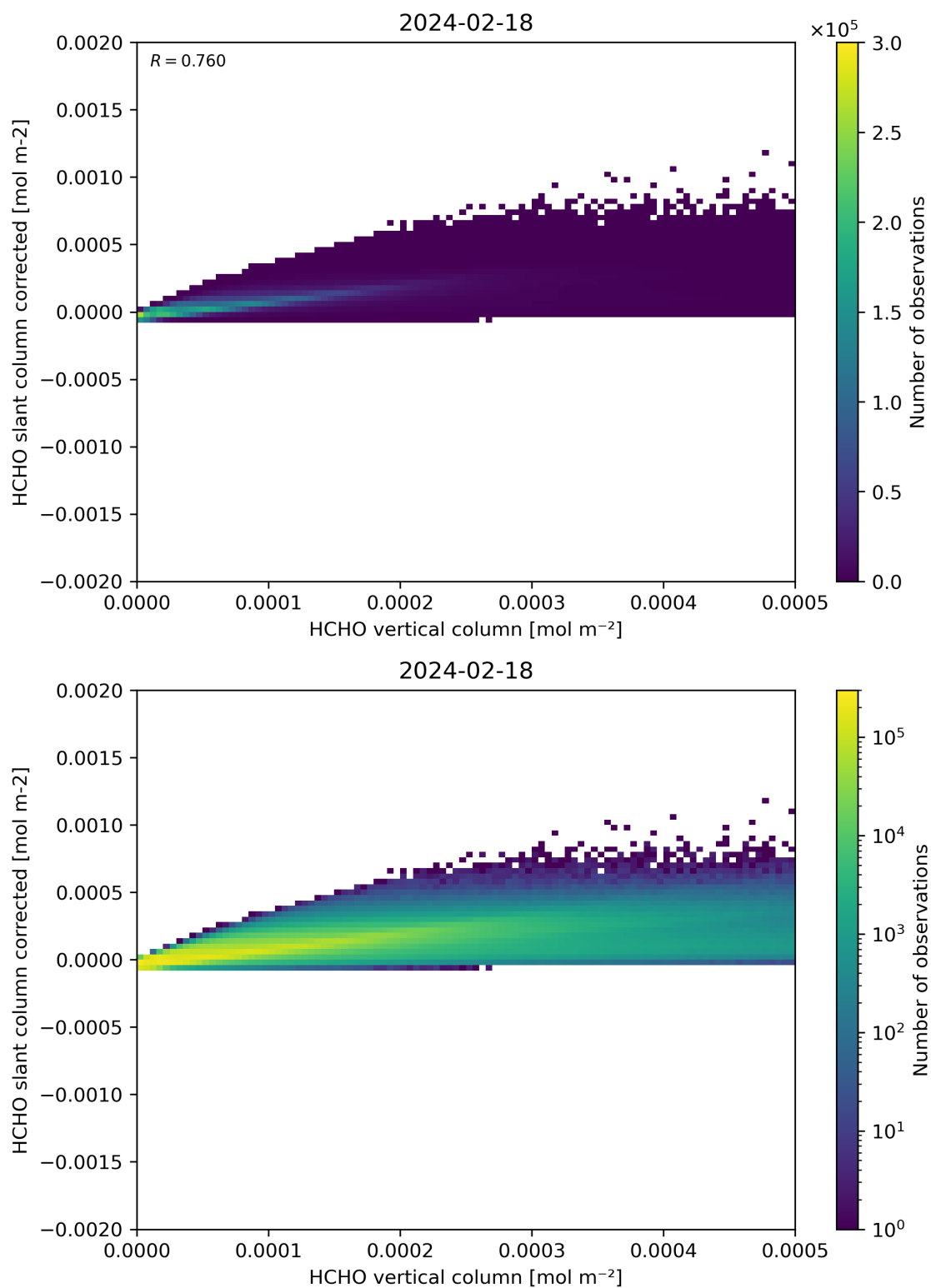
Figure 127: Scatter density plot of “HCHO vertical column” against “HCHO slant column corrected” for 2024-02-17 to 2024-02-19.
