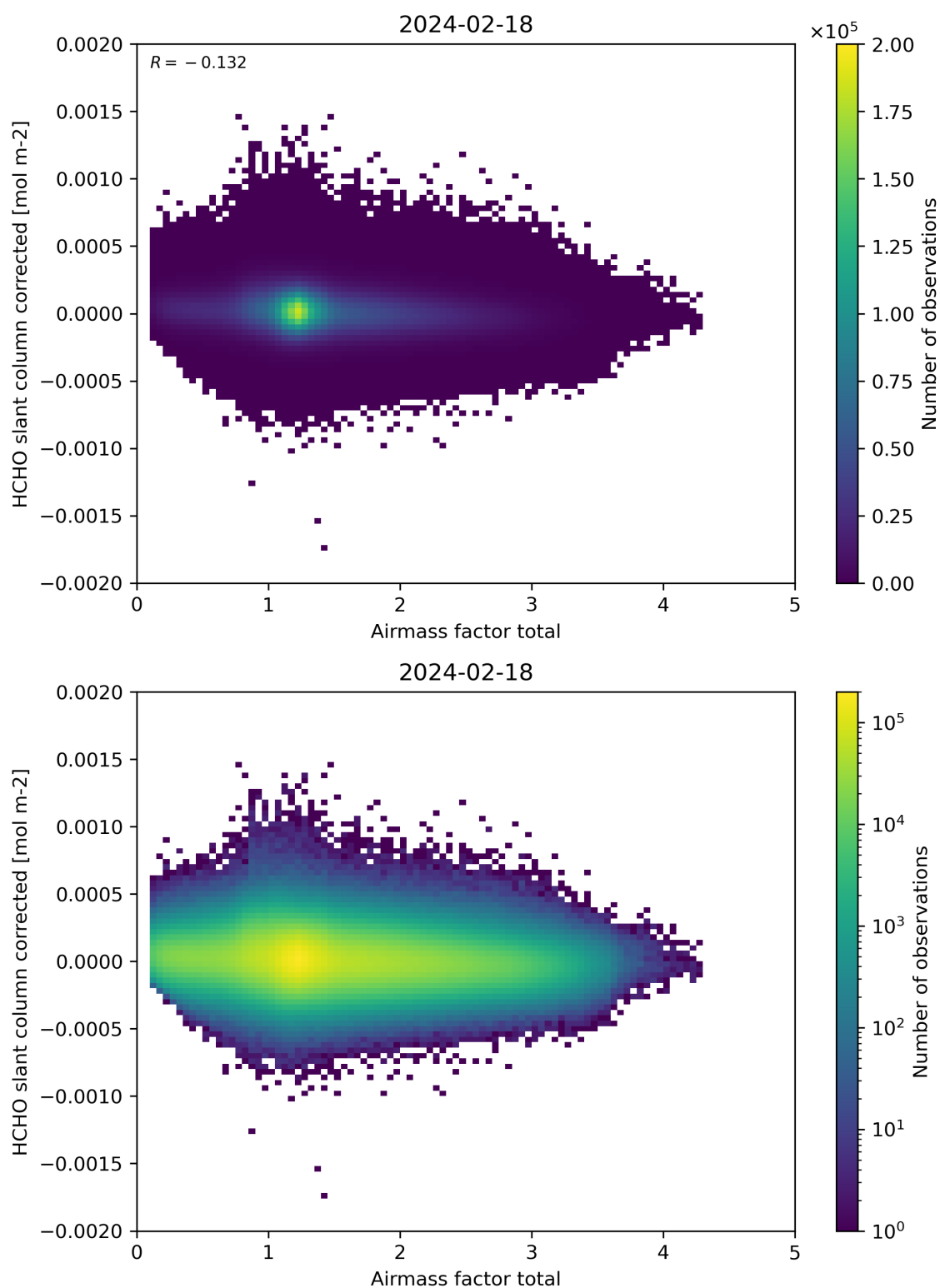
Figure 101: Scatter density plot of “Airmass factor total” against “HCHO slant column corrected” for 2024-02-17 to 2024-02-19.
