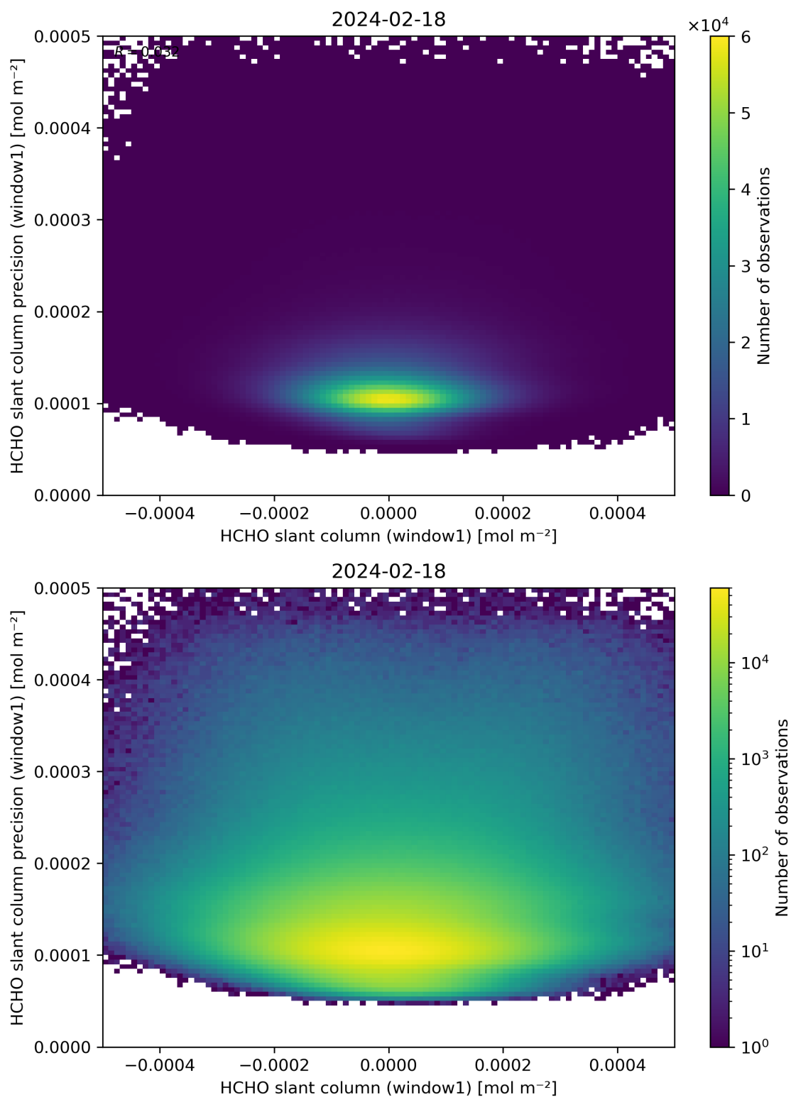
Figure 84: Scatter density plot of “HCHO slant column (window1)” against “HCHO slant column precision (window1)” for 2024-02-17 to 2024-02-19.
