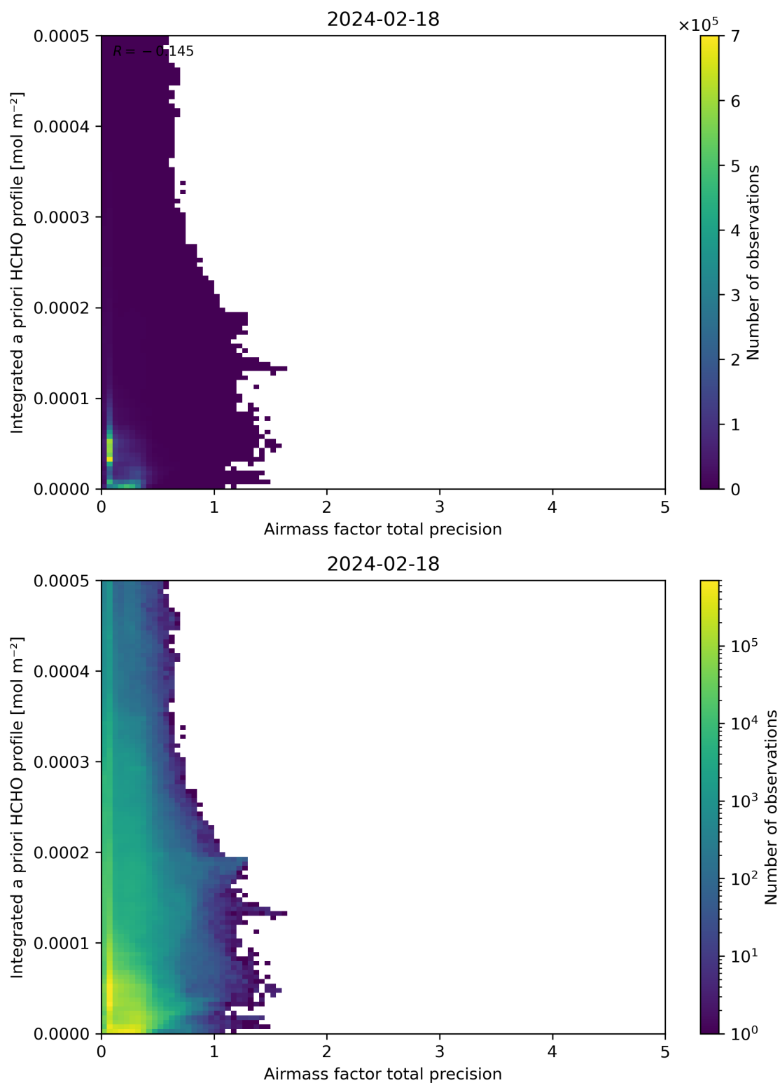
Figure 111: Scatter density plot of “Airmass factor total precision” against “Integrated a priori HCHO profile” for 2024-02-17 to 2024-02-19.
