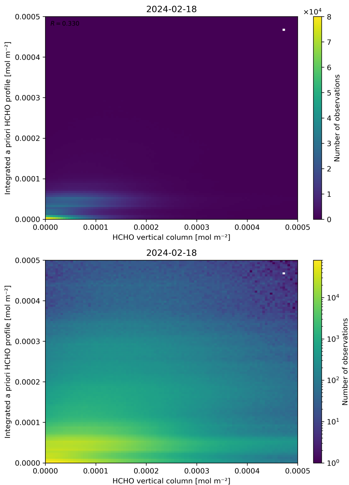
Figure 135: Scatter density plot of “HCHO vertical column” against “Integrated a priori HCHO profile” for 2024-02-17 to 2024-02-19.
