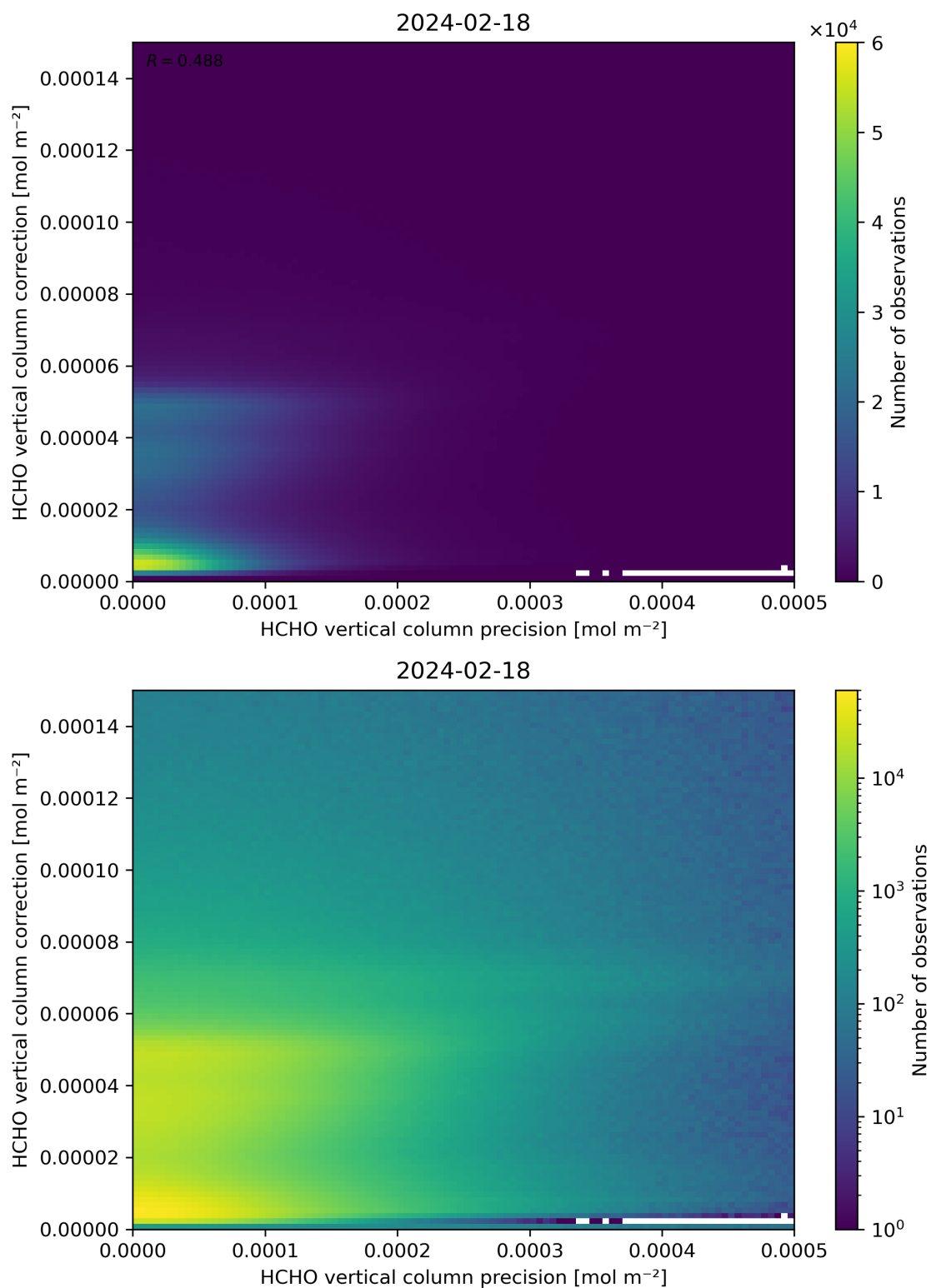
Figure 146: Scatter density plot of “HCHO vertical column precision” against “HCHO vertical column correction” for 2024-02-17 to 2024-02-19.
