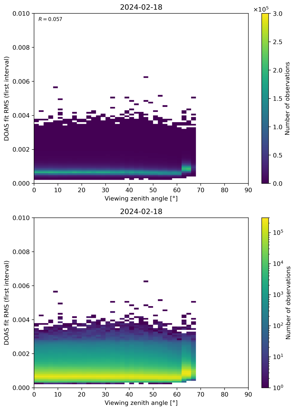
Figure 182: Scatter density plot of “Viewing zenith angle” against “DOAS fit RMS (first interval)” for 2024-02-17 to 2024-02-19.
