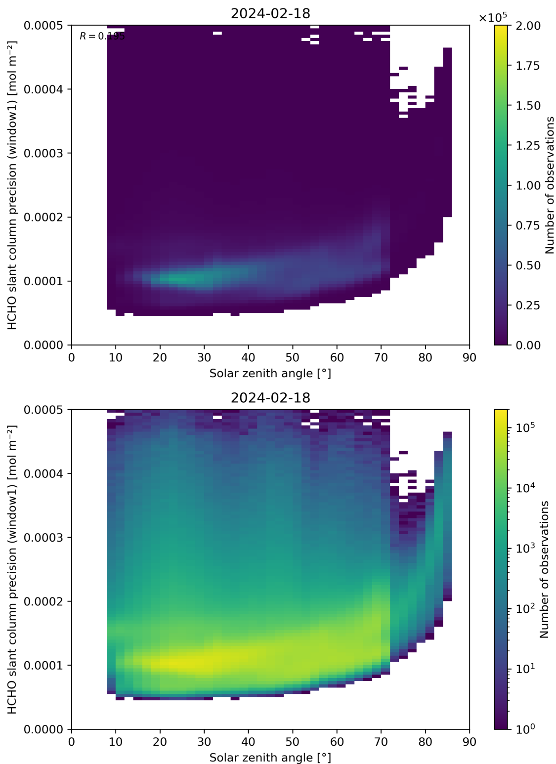
Figure 174: Scatter density plot of “Solar zenith angle” against “HCHO slant column precision (window1)” for 2024-02-17 to 2024-02-19.
