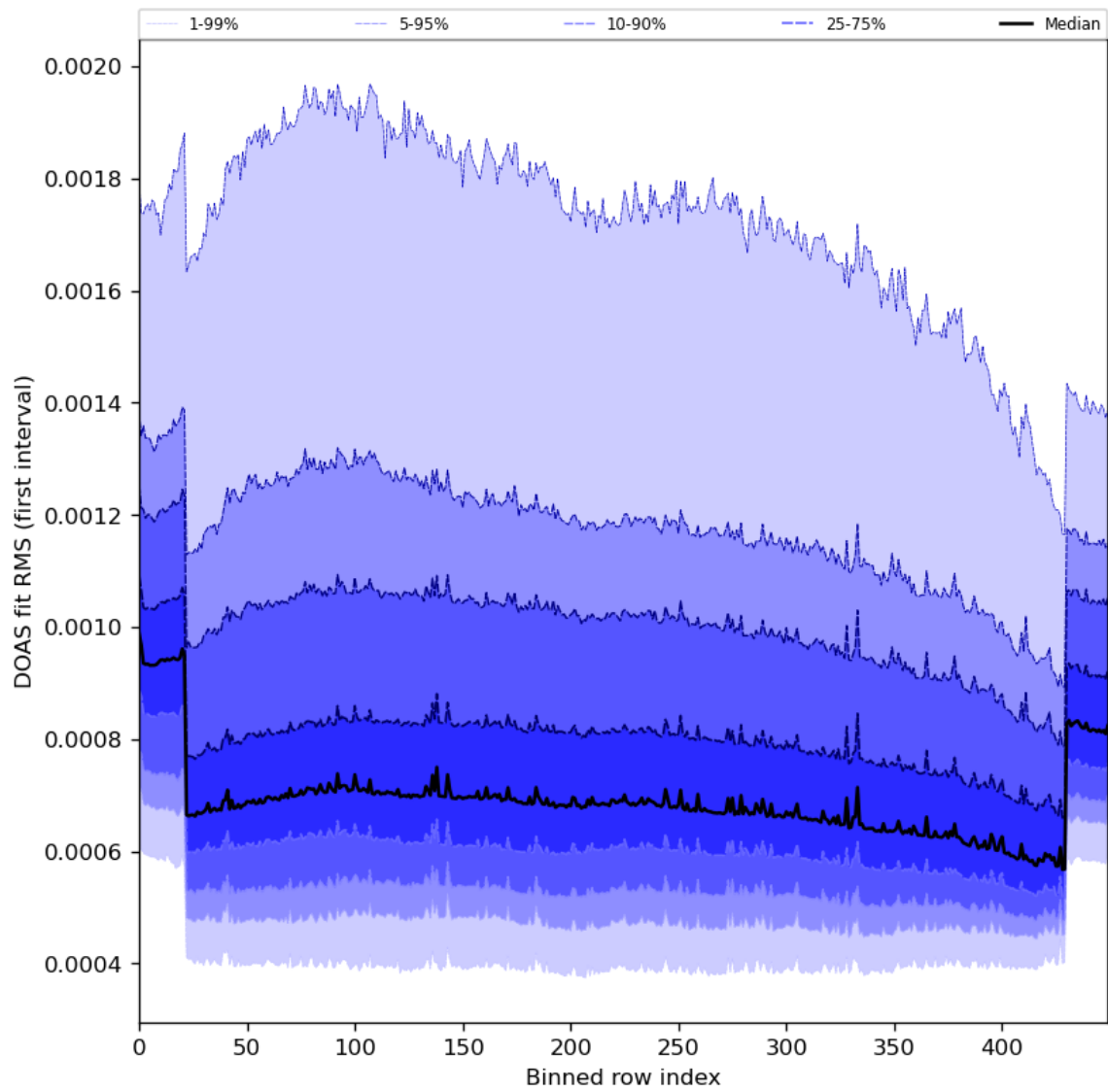
Figure 60: Along track statistics of “DOAS fit RMS (first interval)” for 2024-02-17 to 2024-02-19
