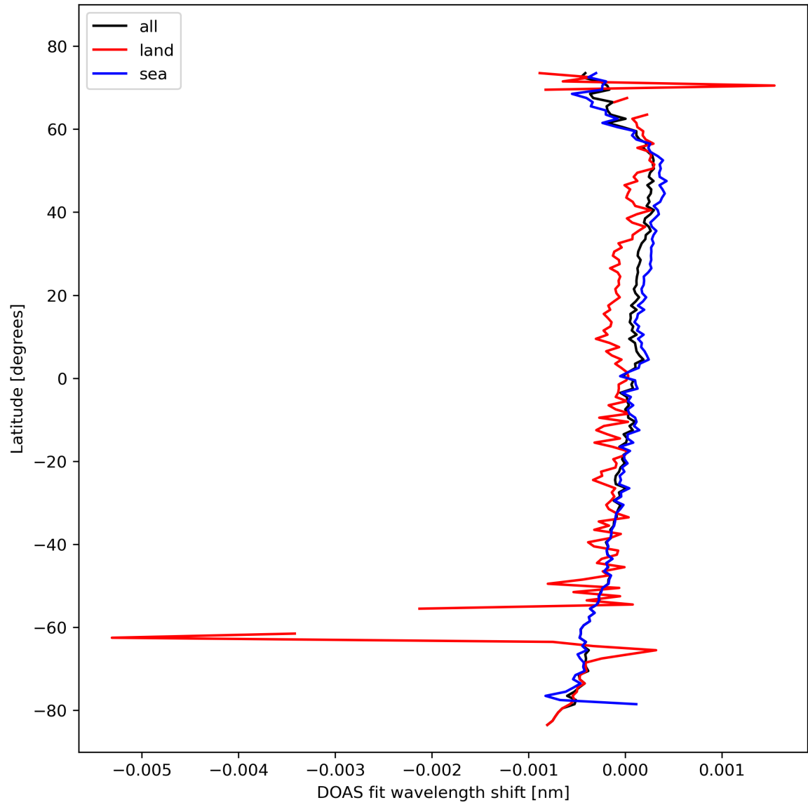
Figure 30: Zonal average of “DOAS fit wavelength shift” for 2024-02-17 to 2024-02-19.
