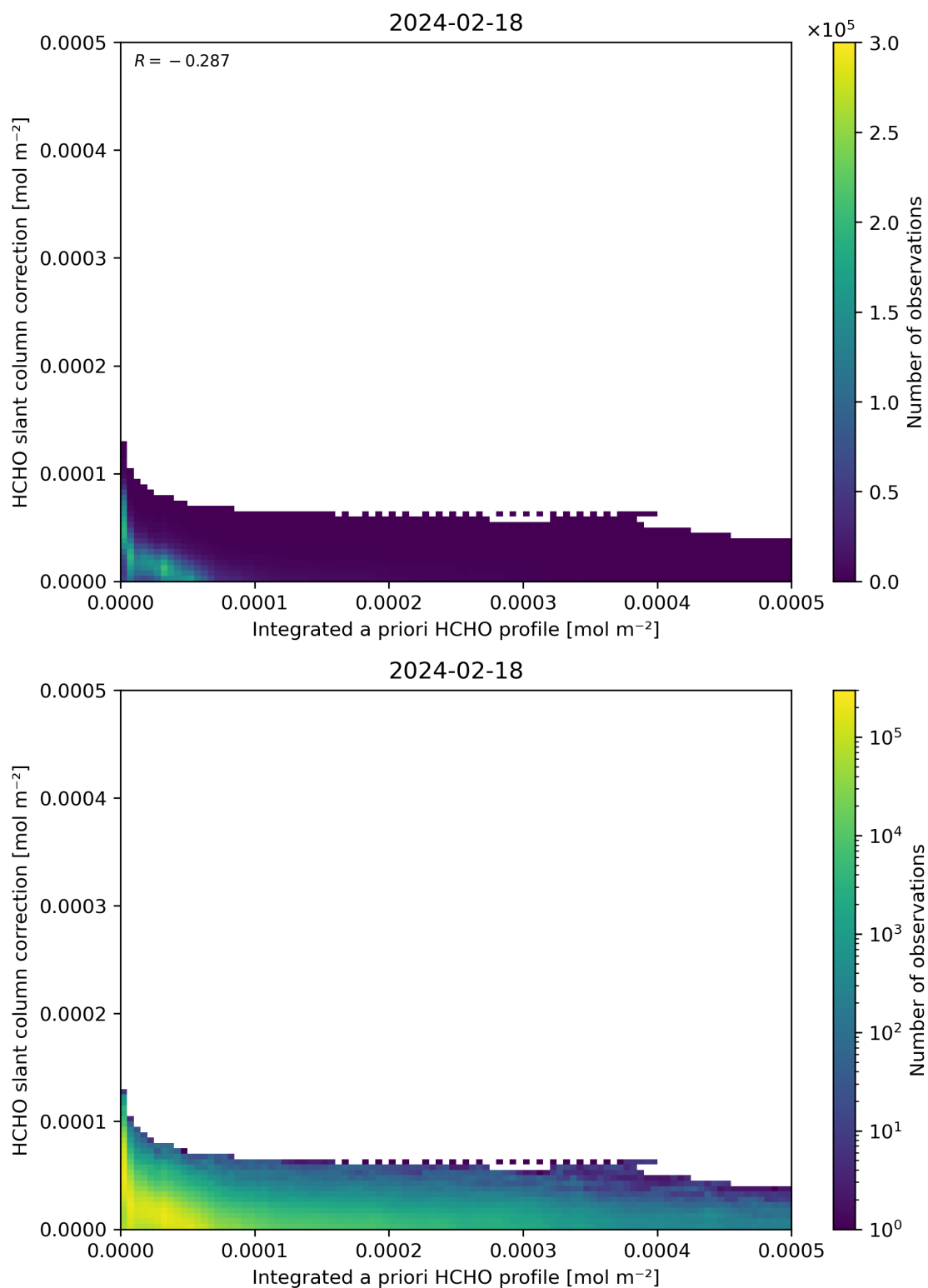
Figure 152: Scatter density plot of “Integrated a priori HCHO profile” against “HCHO slant column correction” for 2024-02-17 to 2024-02-19.
