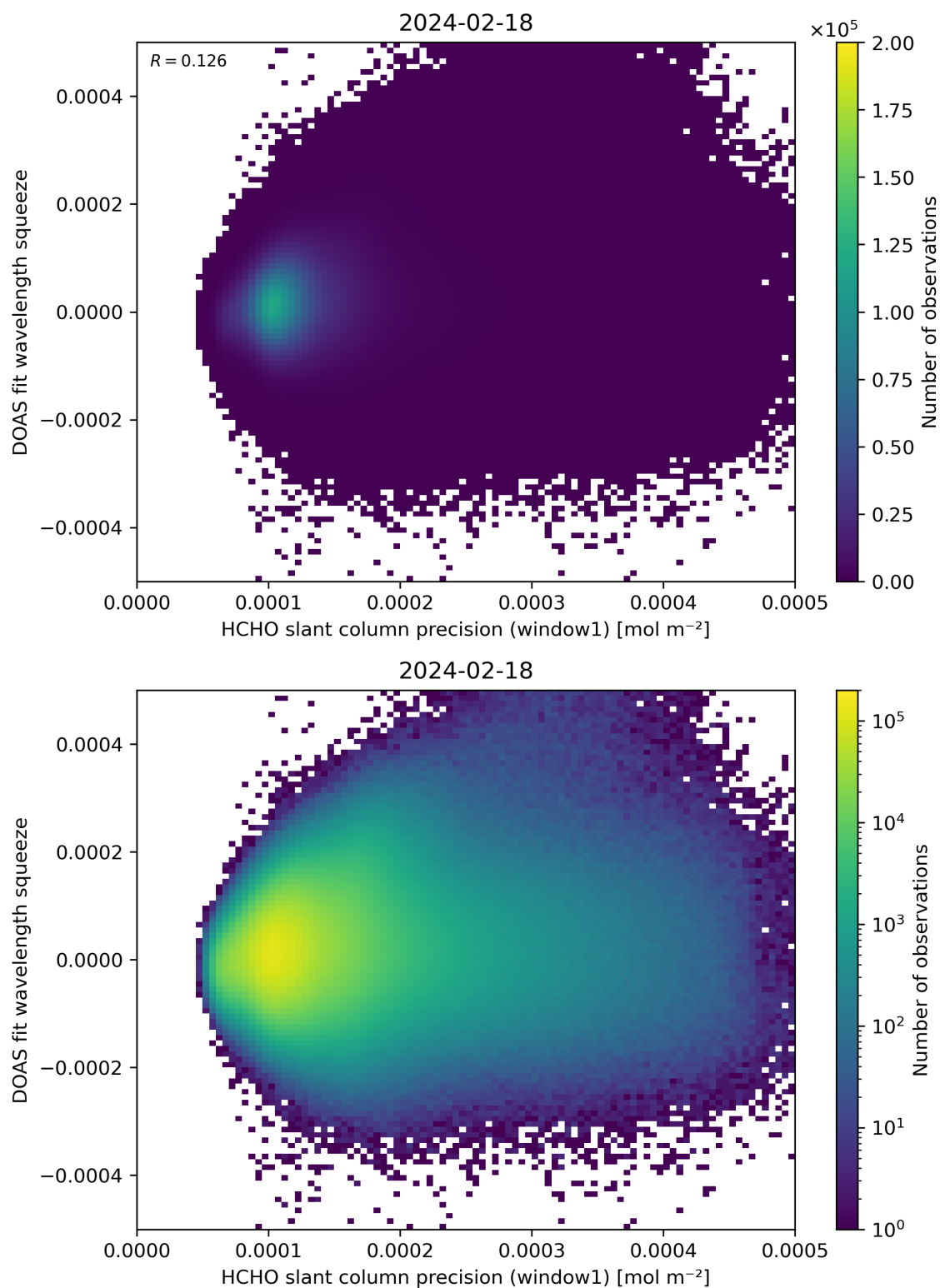
Figure 90: Scatter density plot of “HCHO slant column precision (window1)” against “DOAS fit wavelength squeeze” for 2024-02-17 to 2024-02-19.
