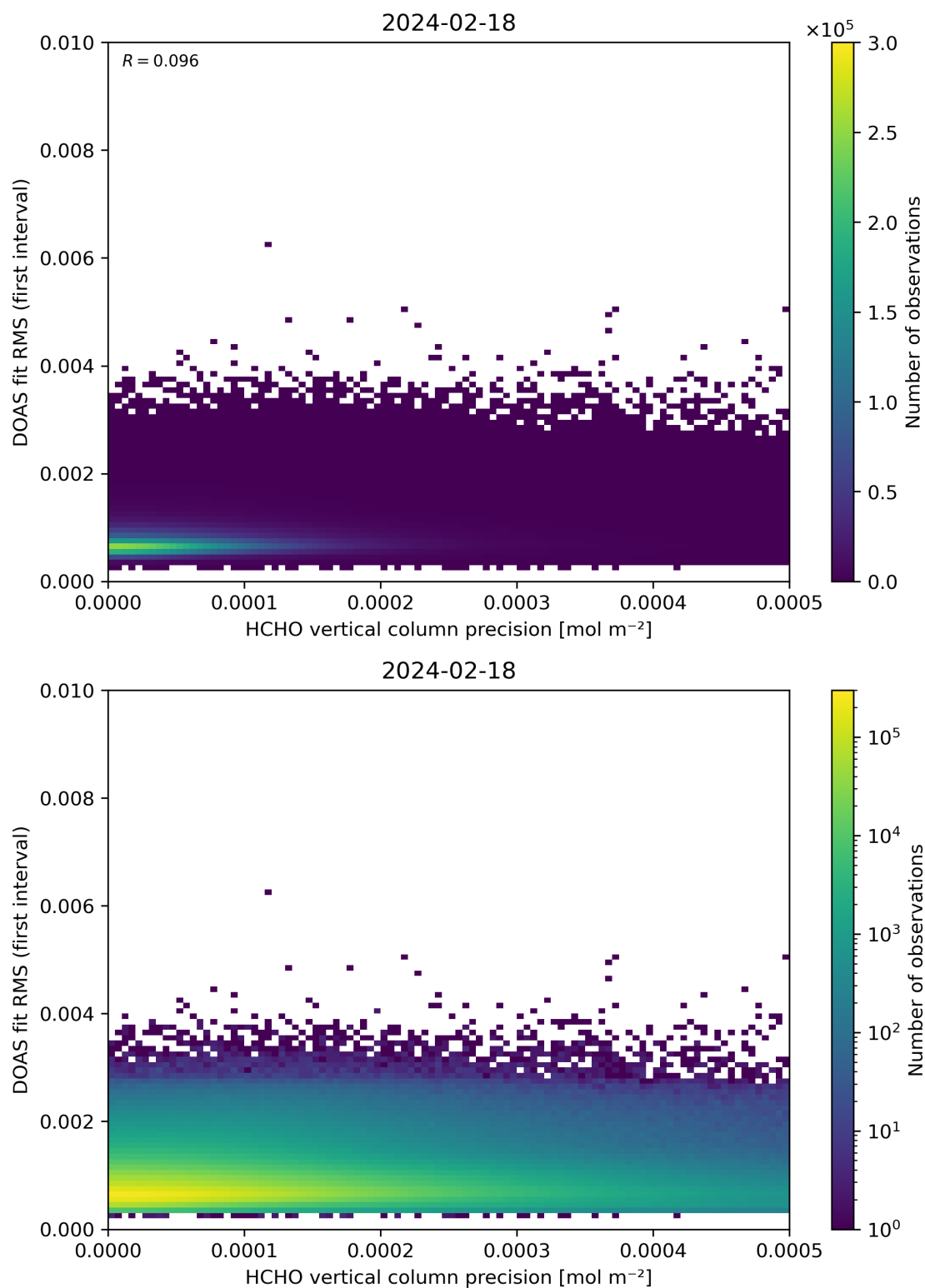
Figure 136: Scatter density plot of “HCHO vertical column precision” against “DOAS fit RMS (first interval)” for 2024-02-17 to 2024-02-19.
