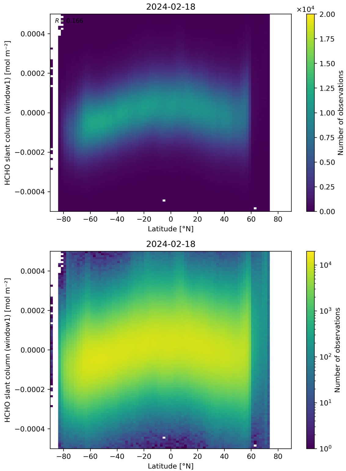
Figure 159: Scatter density plot of “Latitude” against “HCHO slant column (window1)” for 2024-02-17 to 2024-02-19.
