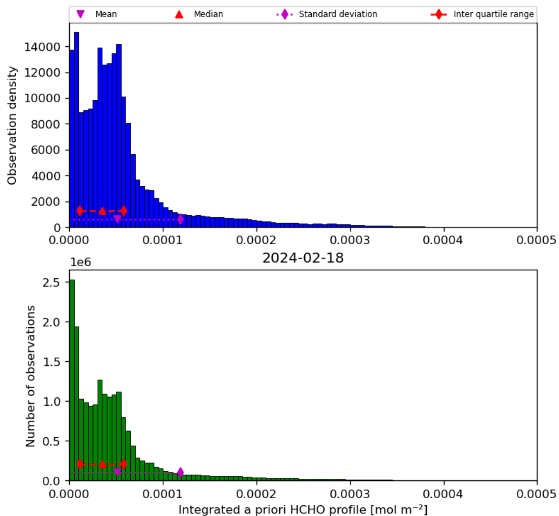
Figure 43: Histogram of “Integrated a priori HCHO profile” for 2024-02-17 to 2024-02-19
