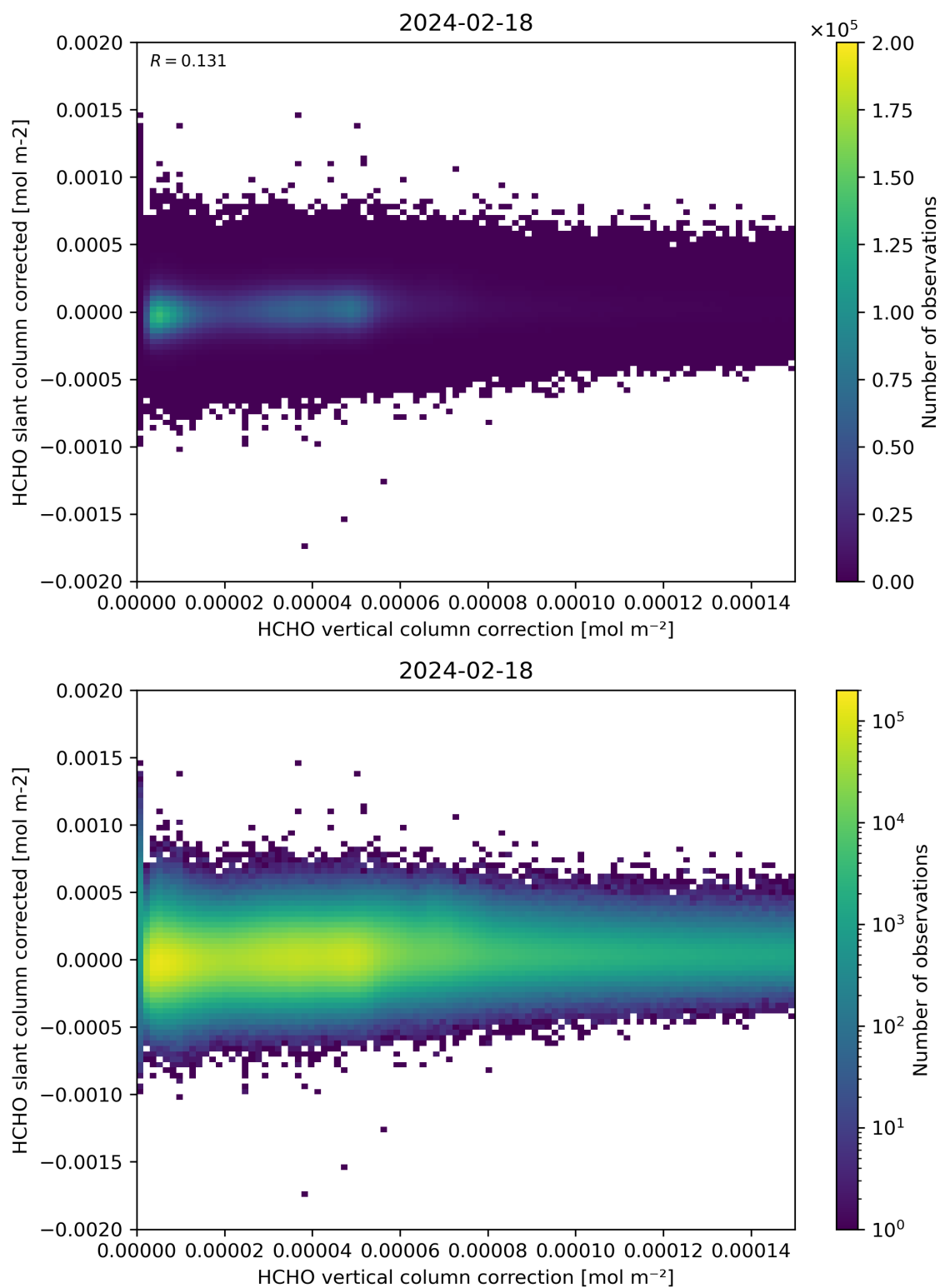
Figure 116: Scatter density plot of “HCHO vertical column correction” against “HCHO slant column corrected” for 2024-02-17 to 2024-02-19.
