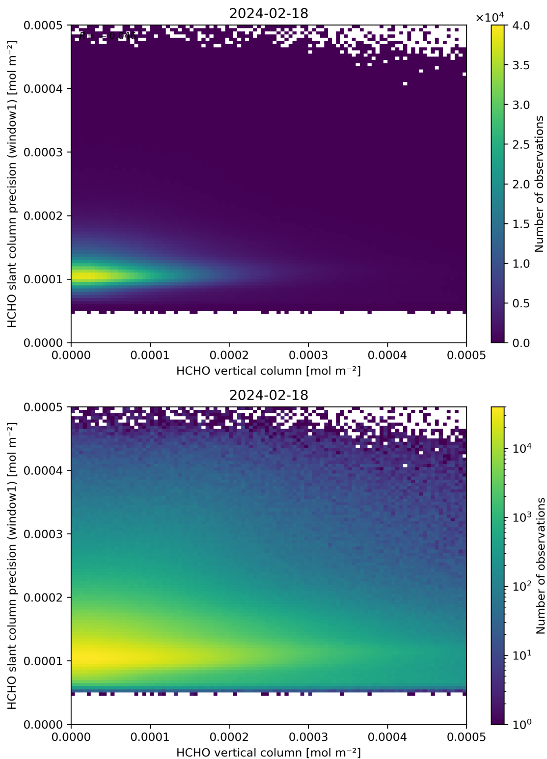
Figure 130: Scatter density plot of “HCHO vertical column” against “HCHO slant column precision (window1)” for 2024-02-17 to 2024-02-19.
