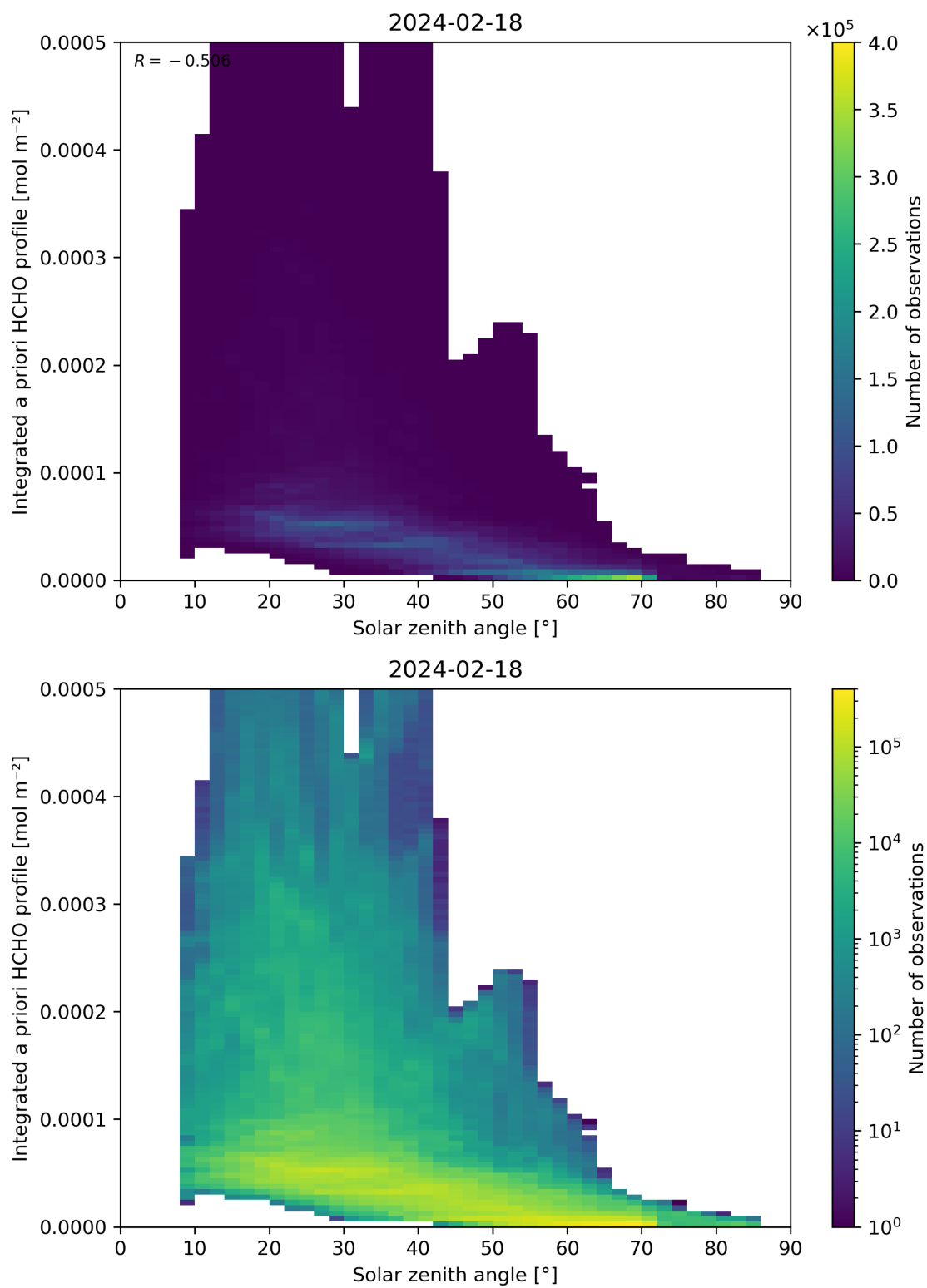
Figure 180: Scatter density plot of “Solar zenith angle” against “Integrated a priori HCHO profile” for 2024-02-17 to 2024-02-19.
