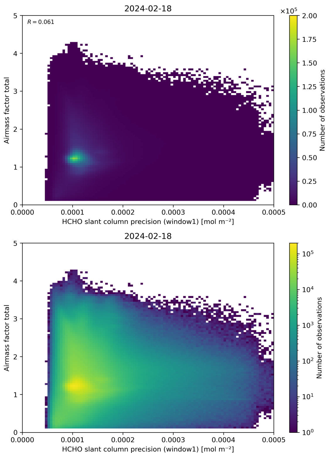
Figure 94: Scatter density plot of “HCHO slant column precision (window1)” against “Airmass factor total” for 2024-02-17 to 2024-02-19.
