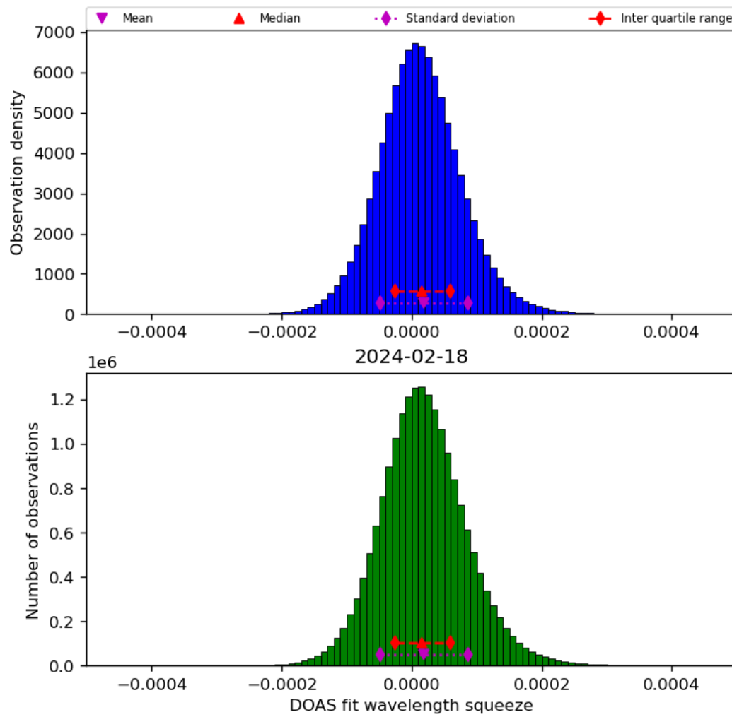
Figure 45: Histogram of “DOAS fit wavelength squeeze” for 2024-02-17 to 2024-02-19
