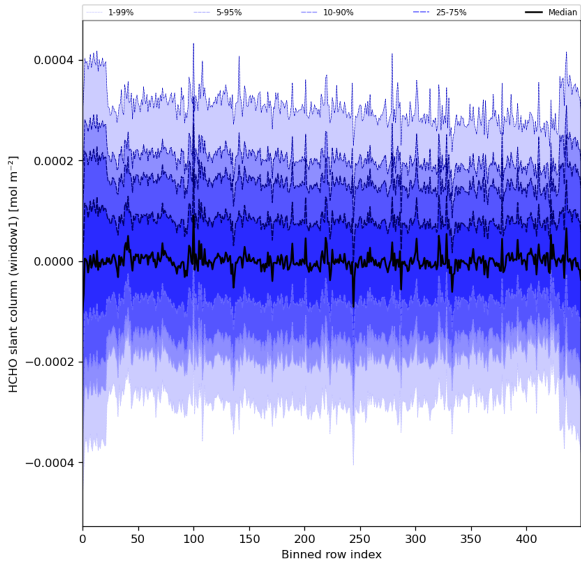
Figure 52: Along track statistics of “HCHO slant column (window1)” for 2024-02-17 to 2024-02-19
