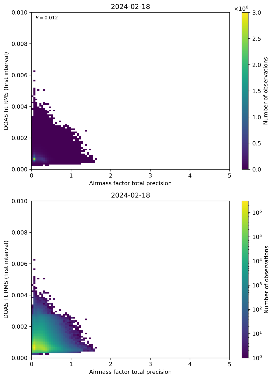
Figure 105: Scatter density plot of “Airmass factor total precision” against “DOAS fit RMS (first interval)” for 2024-02-17 to 2024-02-19.
