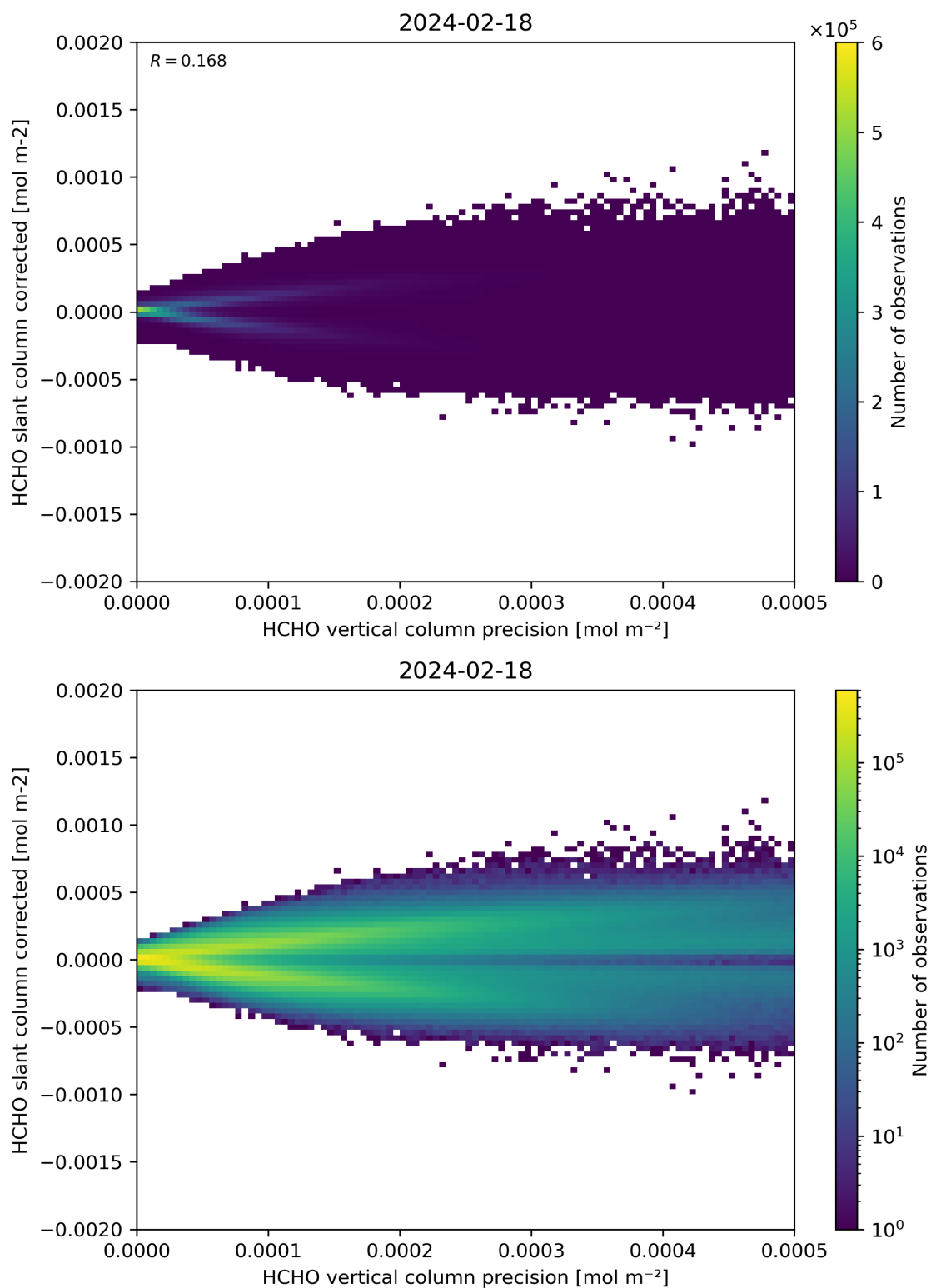
Figure 140: Scatter density plot of “HCHO vertical column precision” against “HCHO slant column corrected” for 2024-02-17 to 2024-02-19.
