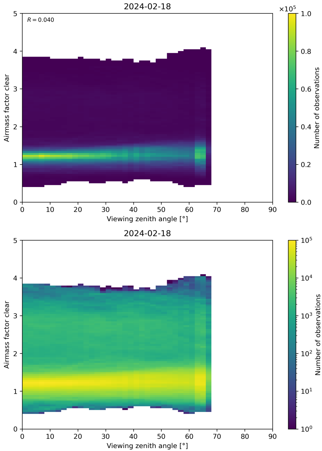
Figure 185: Scatter density plot of “Viewing zenith angle” against “Airmass factor clear” for 2024-02-17 to 2024-02-19.
