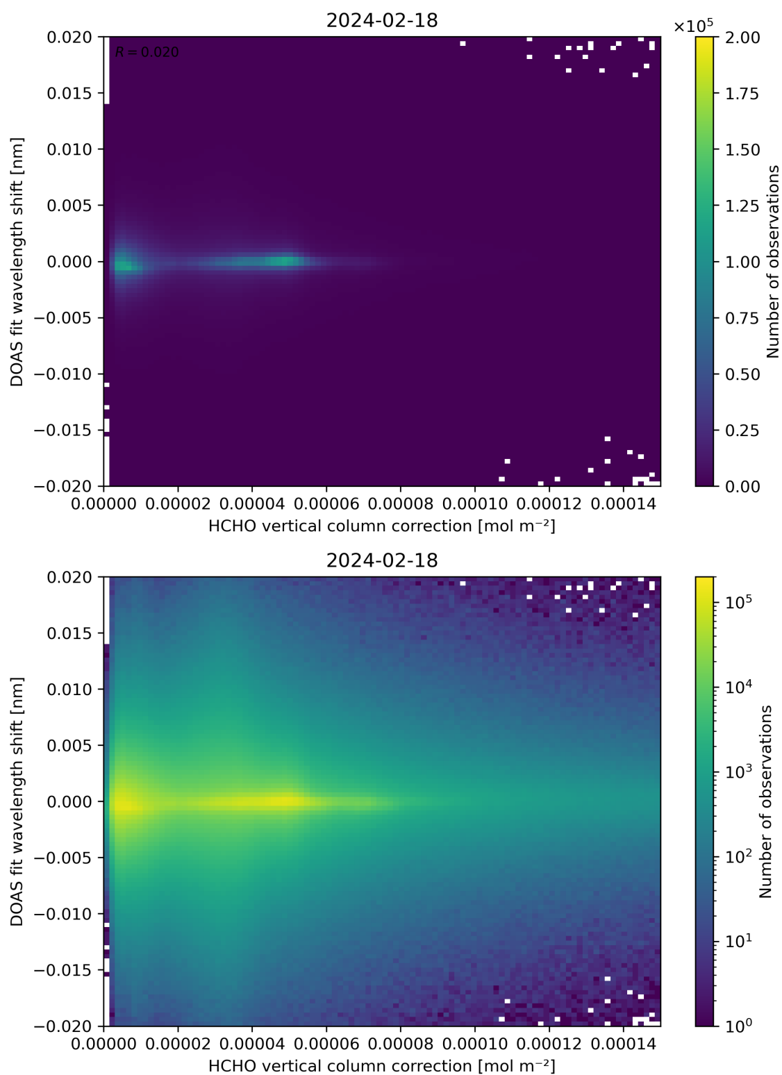
Figure 113: Scatter density plot of “HCHO vertical column correction” against “DOAS fit wavelength shift” for 2024-02-17 to 2024-02-19.
