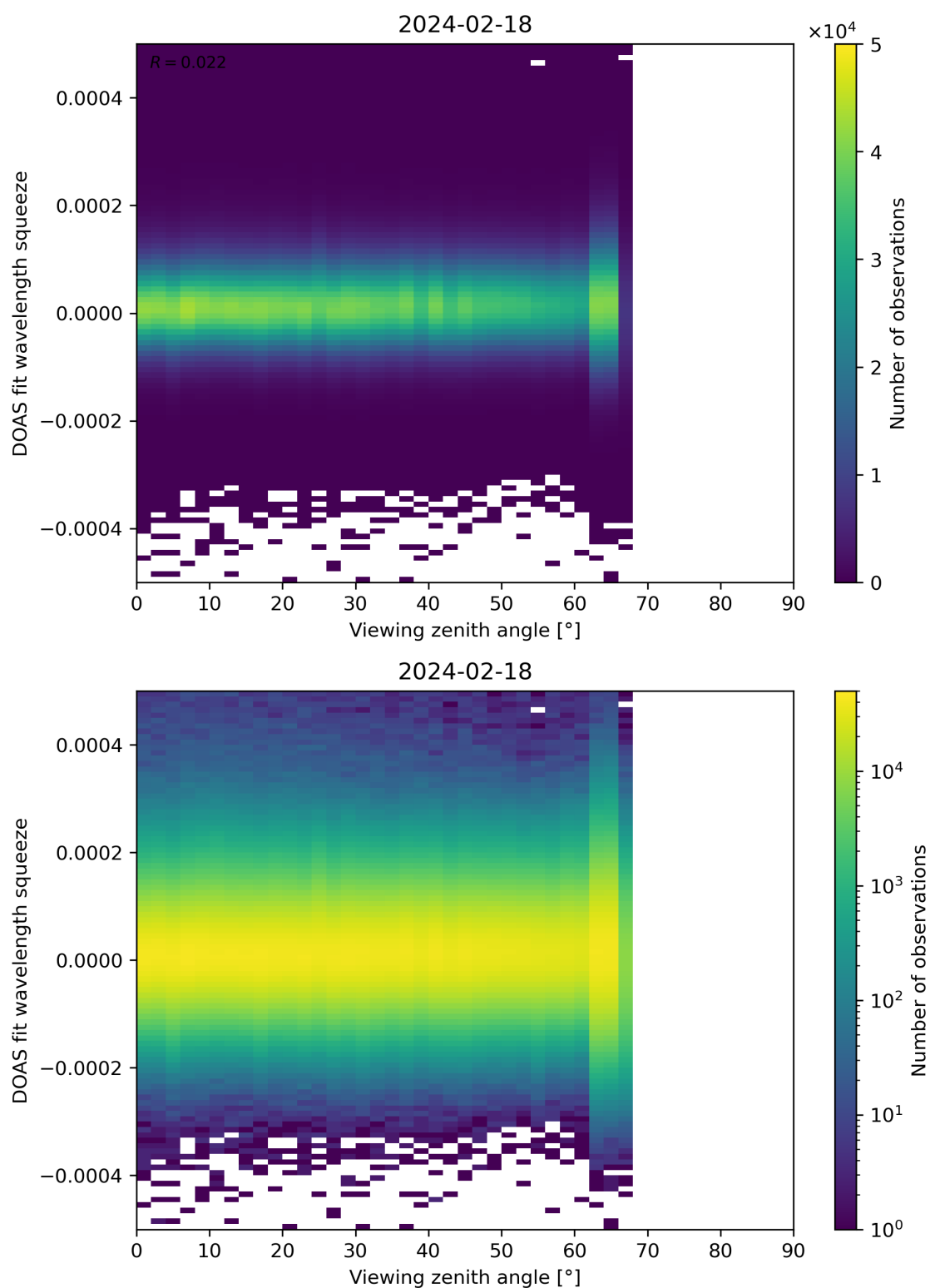
Figure 184: Scatter density plot of “Viewing zenith angle” against “DOAS fit wavelength squeeze” for 2024-02-17 to 2024-02-19.
