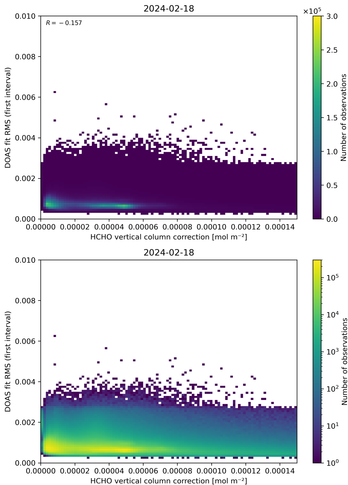
Figure 112: Scatter density plot of “HCHO vertical column correction” against “DOAS fit RMS (first interval)” for 2024-02-17 to 2024-02-19.
