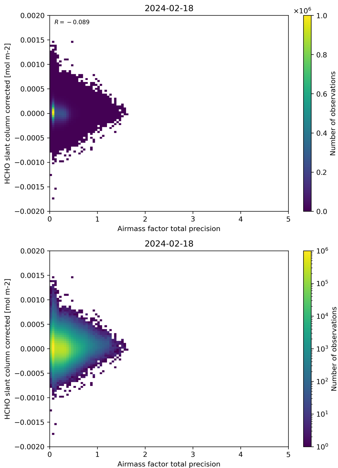
Figure 109: Scatter density plot of “Airmass factor total precision” against “HCHO slant column corrected” for 2024-02-17 to 2024-02-19.
