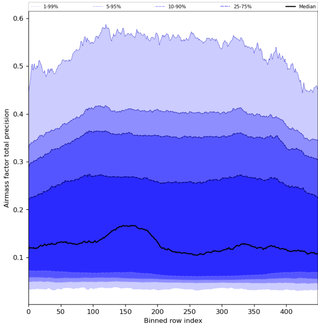
Figure 55: Along track statistics of “Airmass factor total precision” for 2024-02-17 to 2024-02-19
