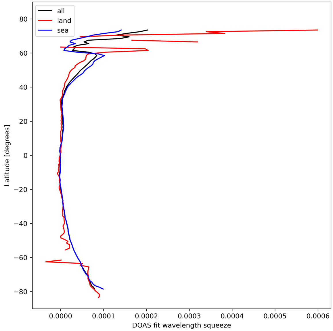
Figure 31: Zonal average of “DOAS fit wavelength squeeze” for 2024-02-17 to 2024-02-19.
