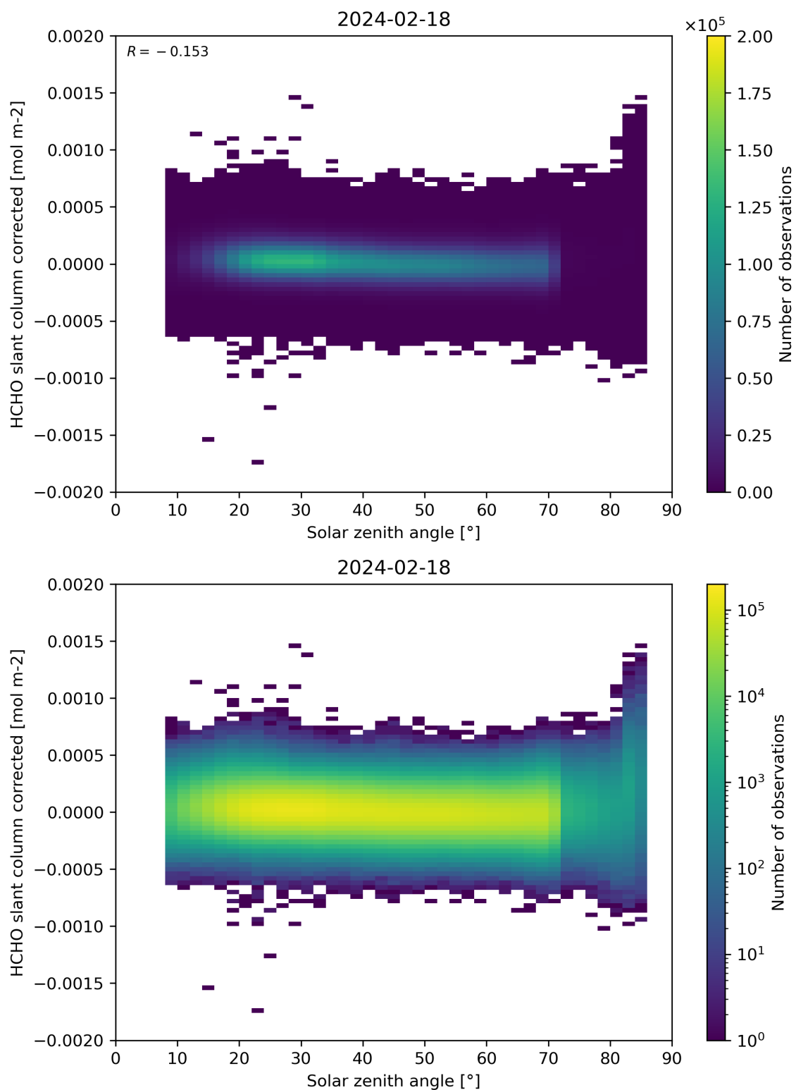
Figure 171: Scatter density plot of “Solar zenith angle” against “HCHO slant column corrected” for 2024-02-17 to 2024-02-19.
