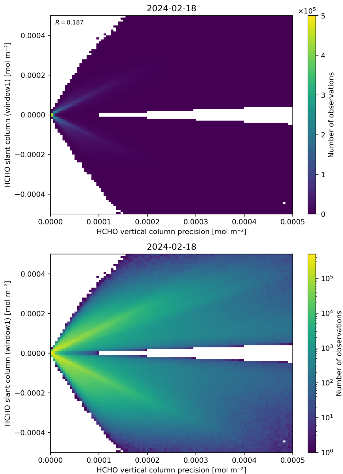
Figure 142: Scatter density plot of “HCHO vertical column precision” against “HCHO slant column (window1)” for 2024-02-17 to 2024-02-19.
