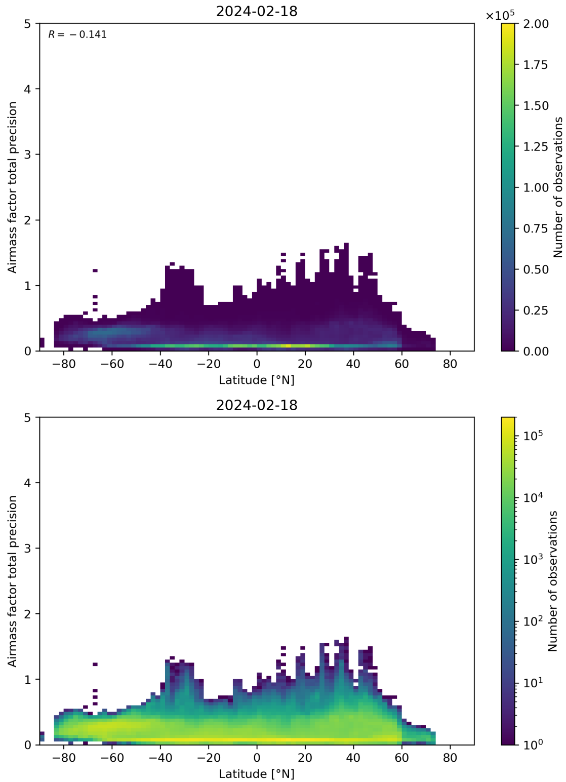
Figure 162: Scatter density plot of “Latitude” against “Airmass factor total precision” for 2024-02-17 to 2024-02-19.
