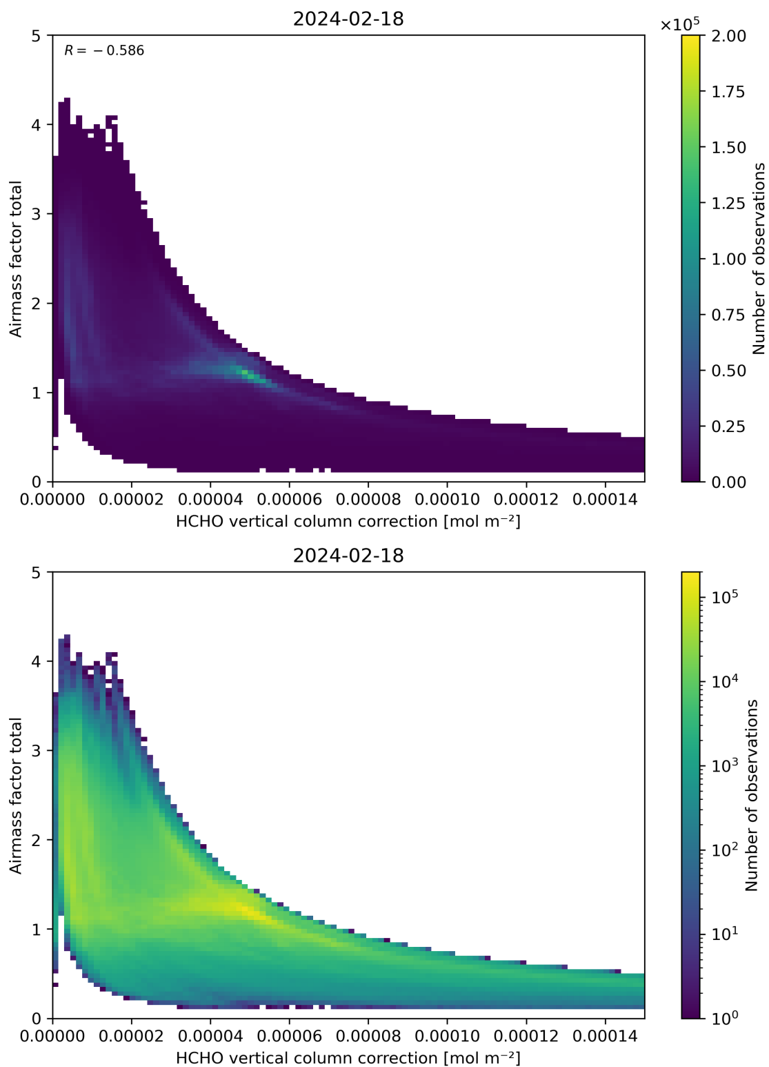
Figure 120: Scatter density plot of “HCHO vertical column correction” against “Airmass factor total” for 2024-02-17 to 2024-02-19.
