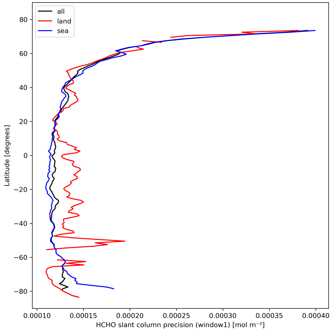
Figure 25: Zonal average of “HCHO slant column precision (window1)” for 2024-02-17 to 2024-02-19.
