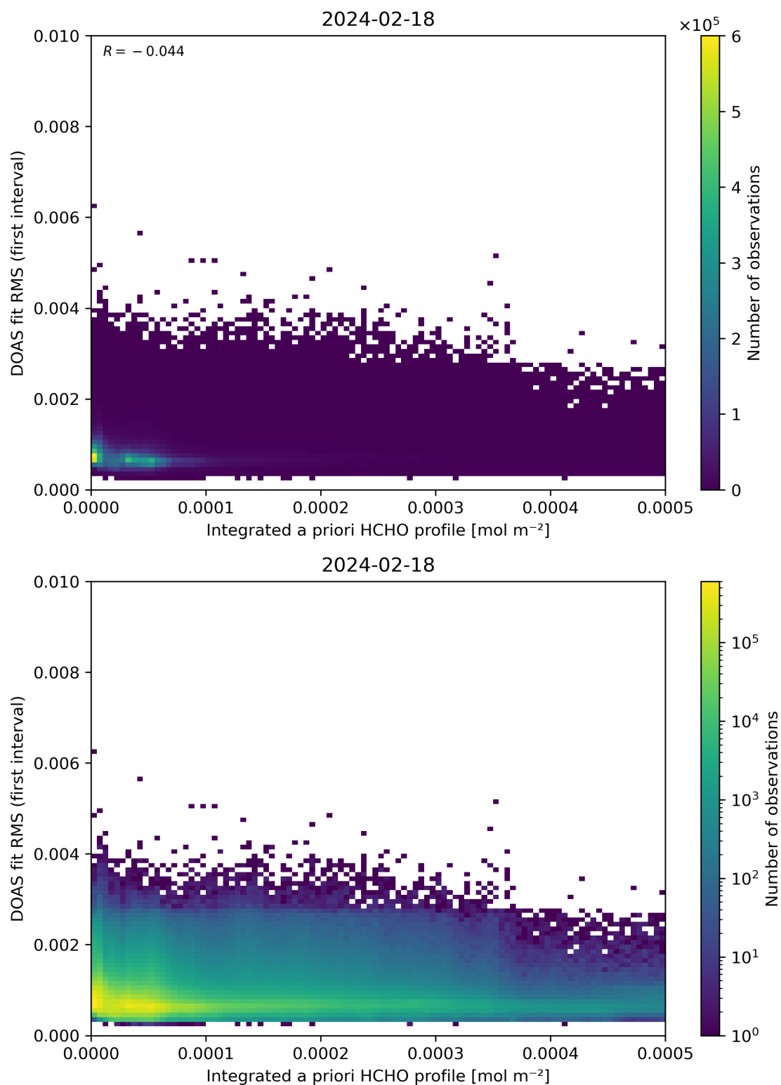
Figure 148: Scatter density plot of “Integrated a priori HCHO profile” against “DOAS fit RMS (first interval)” for 2024-02-17 to 2024-02-19.
