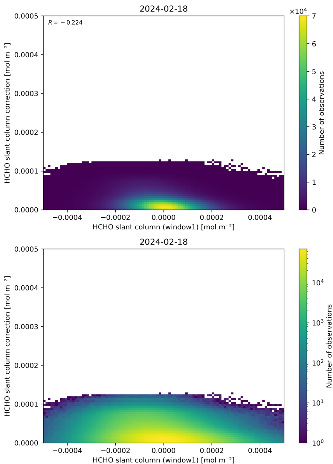
Figure 83: Scatter density plot of “HCHO slant column (window1)” against “HCHO slant column correction” for 2024-02-17 to 2024-02-19.
