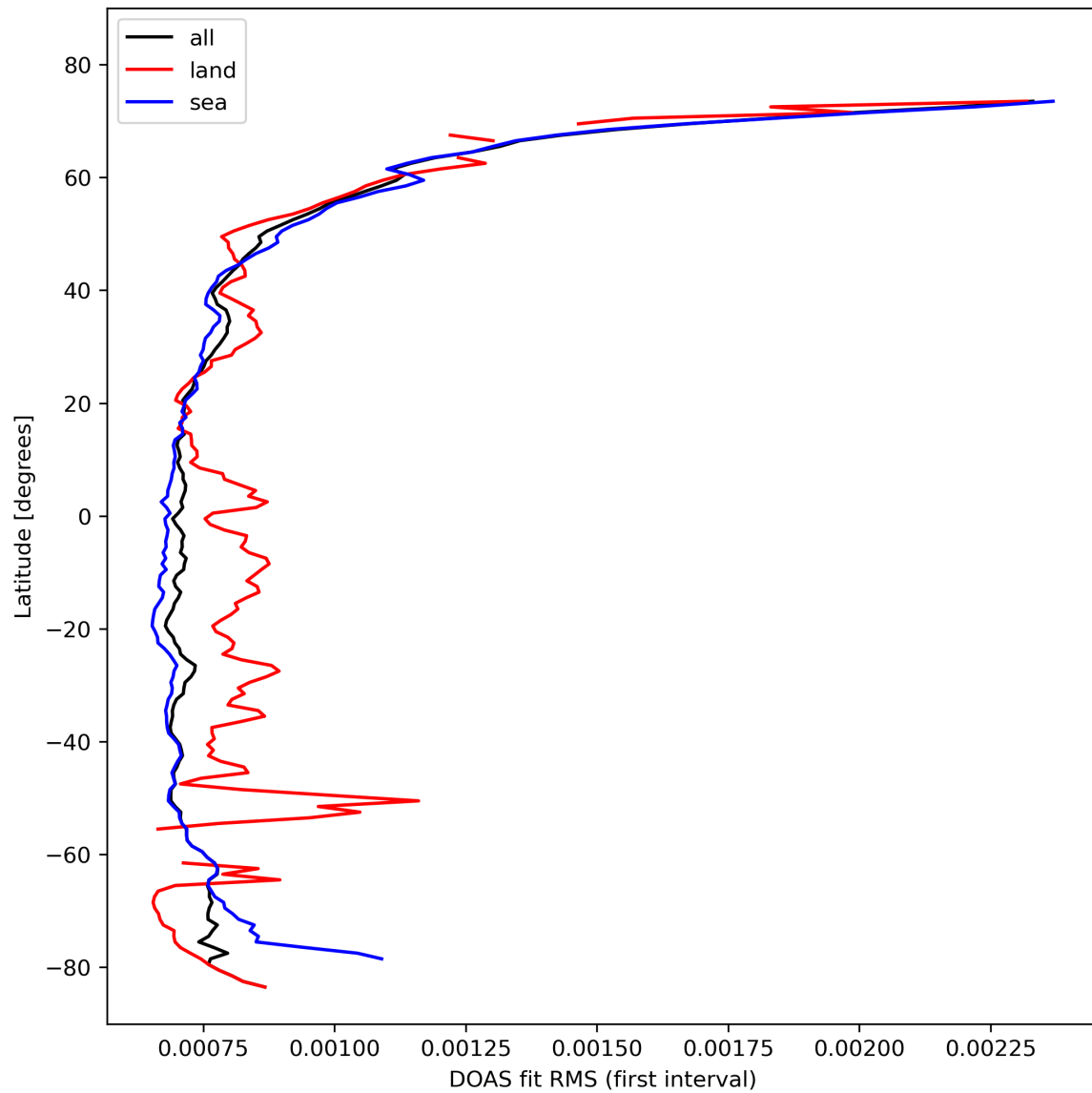
Figure 32: Zonal average of “DOAS fit RMS (first interval)” for 2024-02-17 to 2024-02-19.
