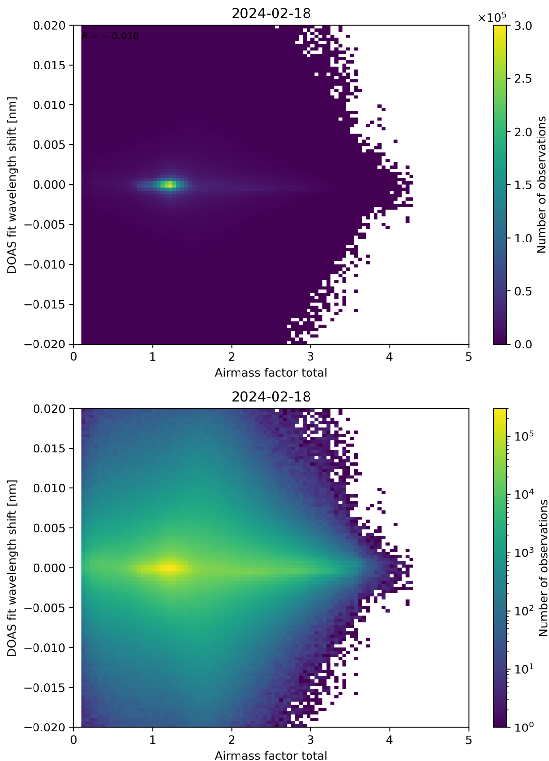
Figure 98: Scatter density plot of “Airmass factor total” against “DOAS fit wavelength shift” for 2024-02-17 to 2024-02-19.
