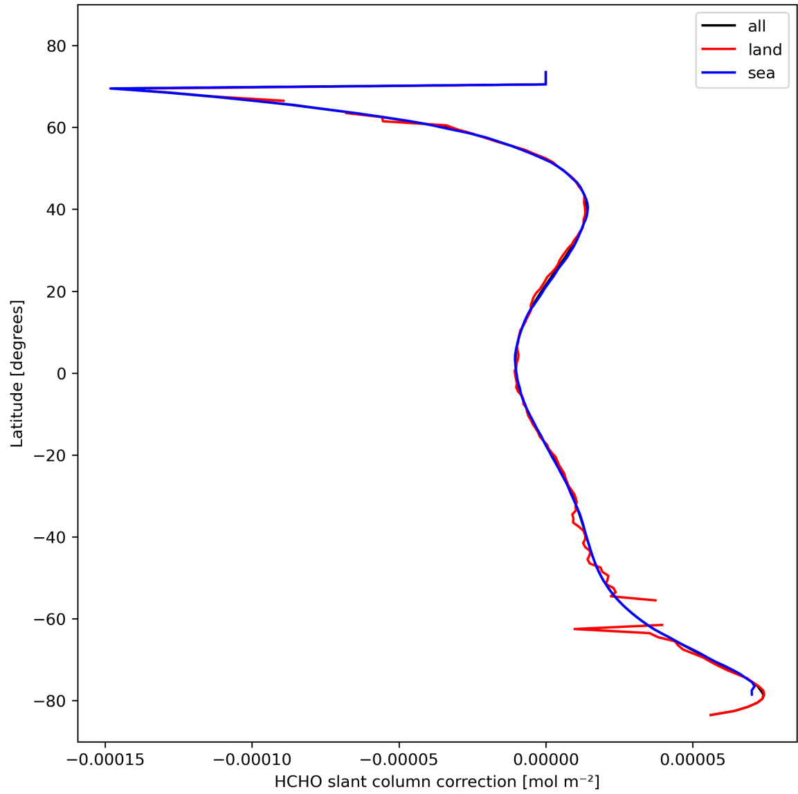
Figure 33: Zonal average of "HCHO slant column correction" for 2024-02-17 to 2024-02-19.
