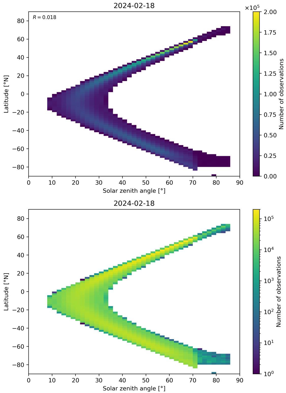
Figure 181: Scatter density plot of “Solar zenith angle” against “Latitude” for 2024-02-17 to 2024-02-19.
