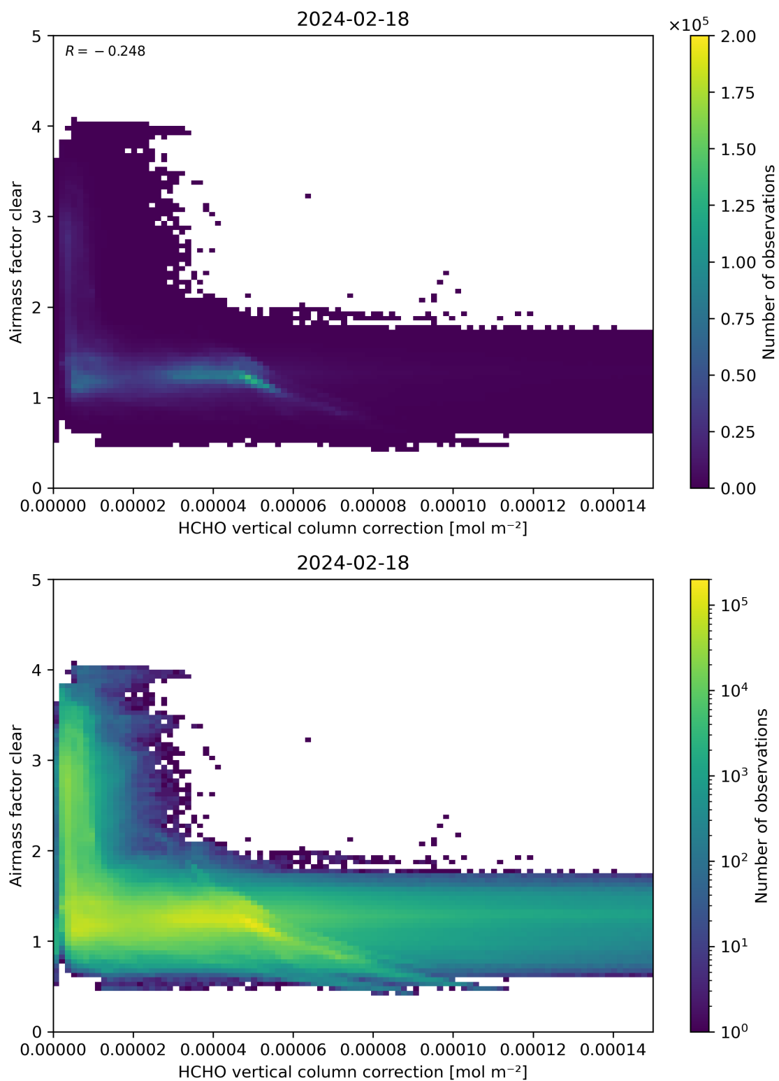
Figure 115: Scatter density plot of “HCHO vertical column correction” against “Airmass factor clear” for 2024-02-17 to 2024-02-19.
