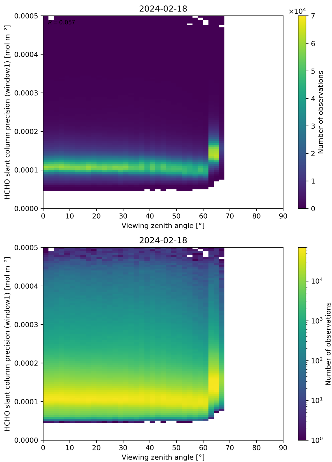
Figure 189: Scatter density plot of “Viewing zenith angle” against “HCHO slant column precision (window1)” for 2024-02-17 to 2024-02-19.
