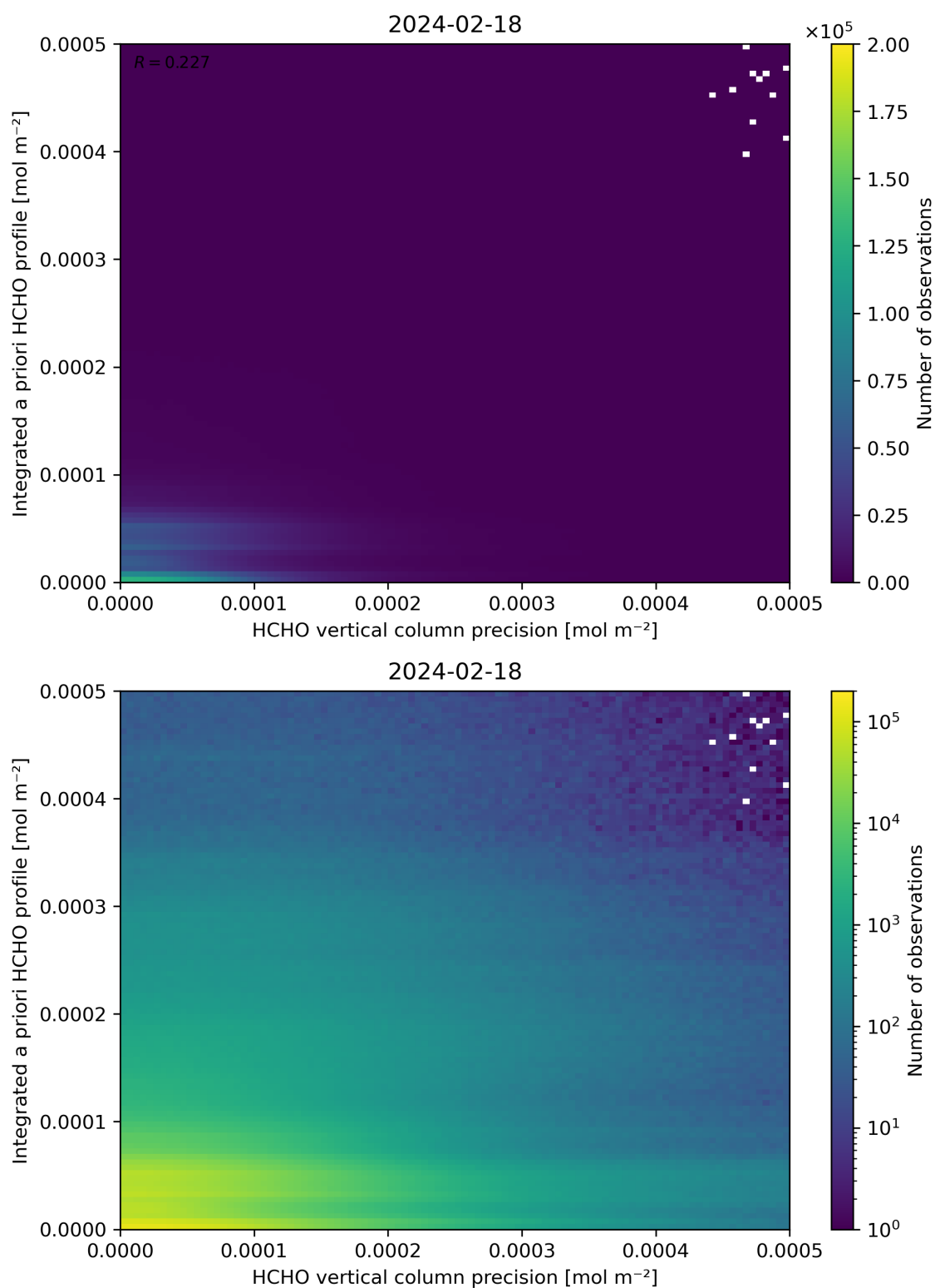
Figure 147: Scatter density plot of “HCHO vertical column precision” against “Integrated a priori HCHO profile” for 2024-02-17 to 2024-02-19.
