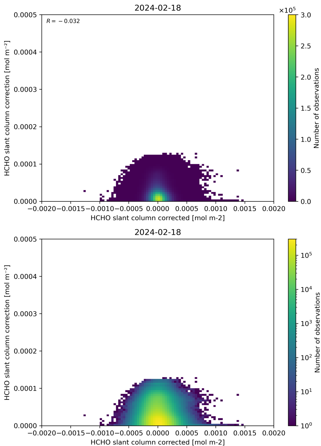
Figure 77: Scatter density plot of “HCHO slant column corrected” against “HCHO slant column correction” for 2024-02-17 to 2024-02-19.
