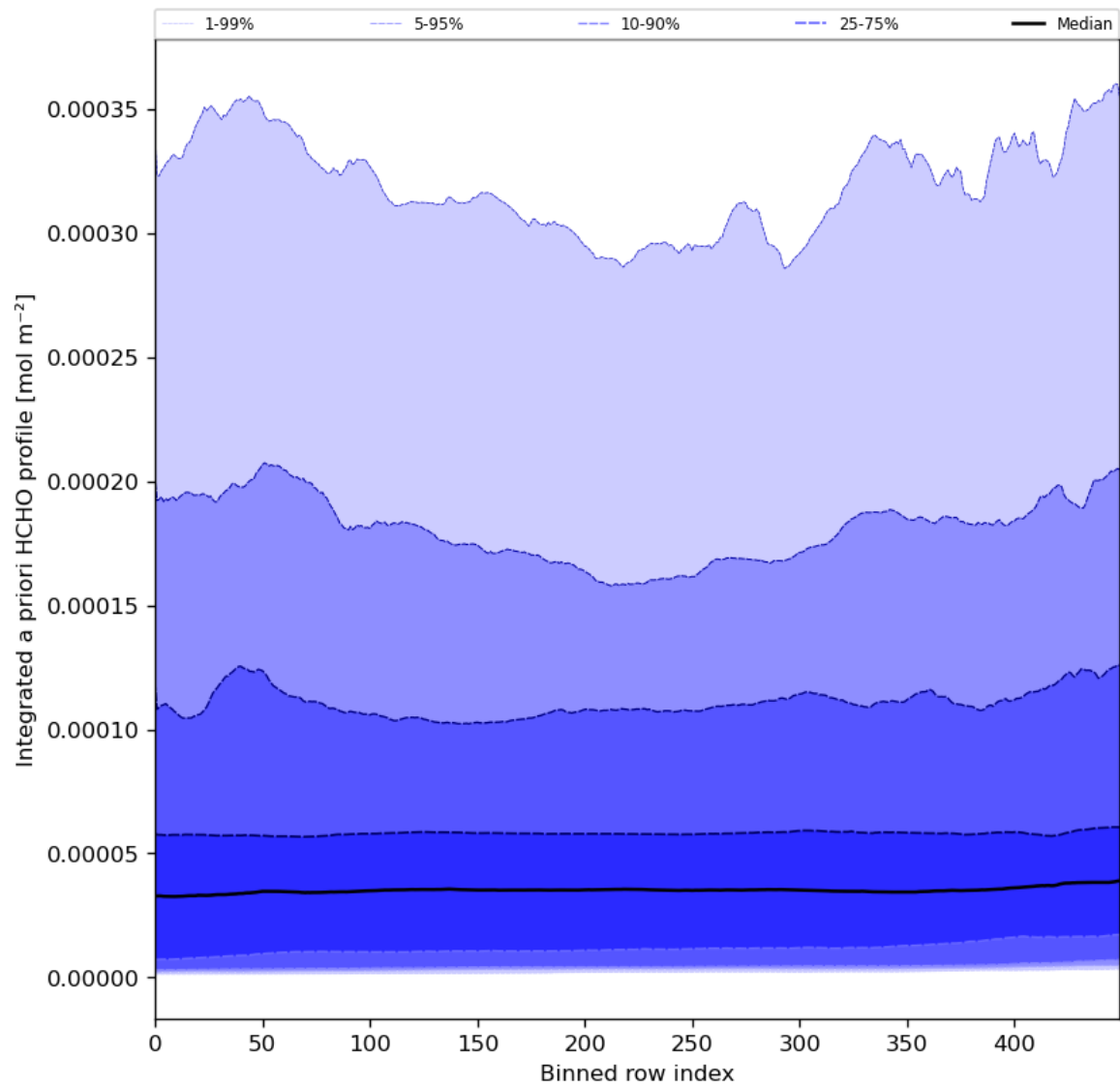
Figure 57: Along track statistics of “Integrated a priori HCHO profile” for 2024-02-17 to 2024-02-19
