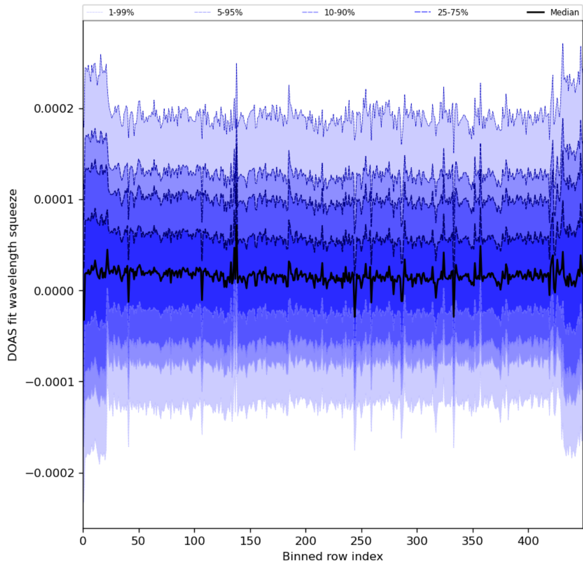
Figure 59: Along track statistics of “DOAS fit wavelength squeeze” for 2024-02-17 to 2024-02-19
