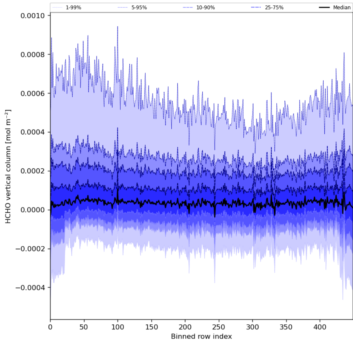
Figure 49: Along track statistics of “HCHO vertical column” for 2024-02-17 to 2024-02-19
