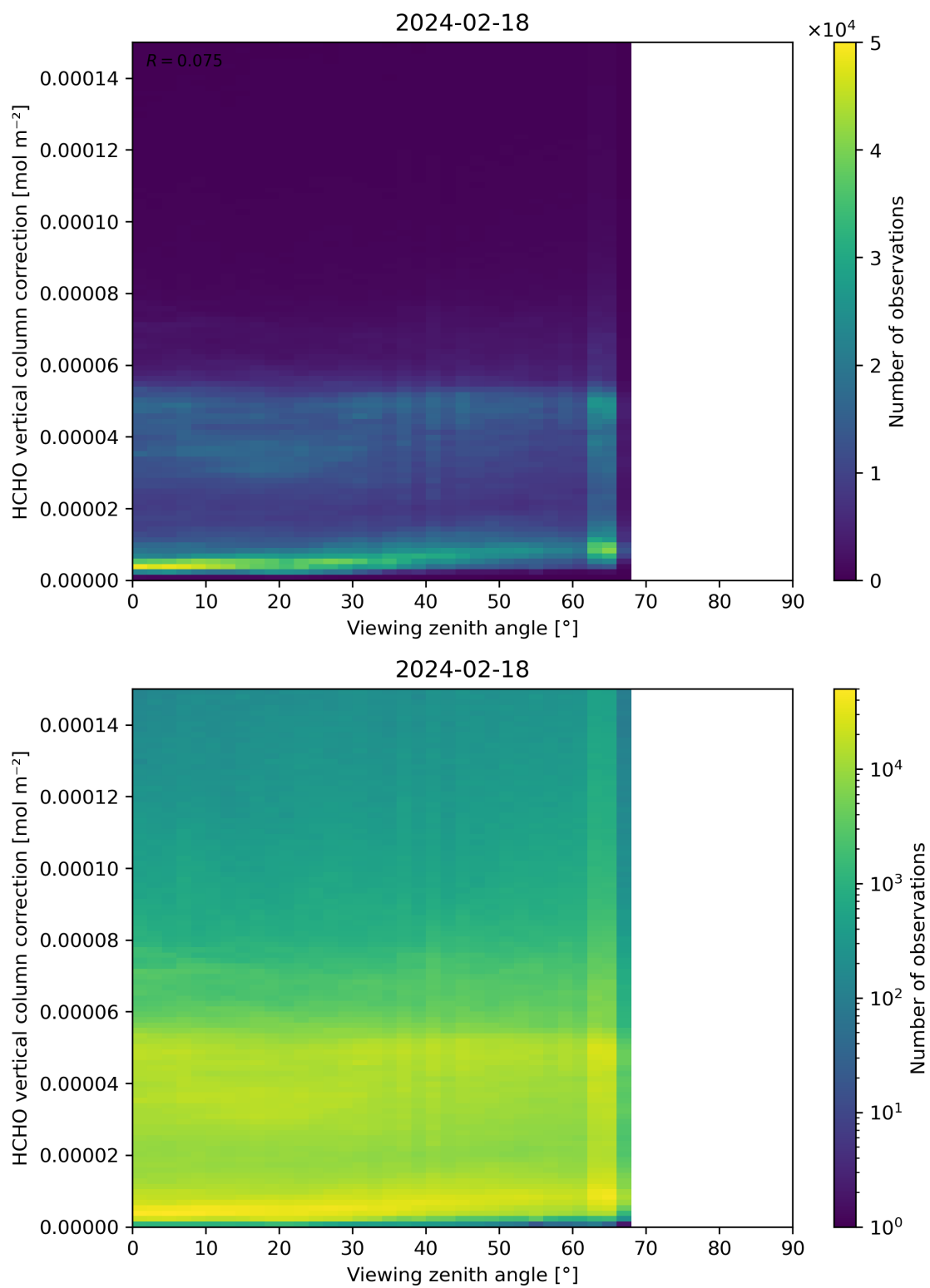
Figure 193: Scatter density plot of “Viewing zenith angle” against “HCHO vertical column correction” for 2024-02-17 to 2024-02-19.
