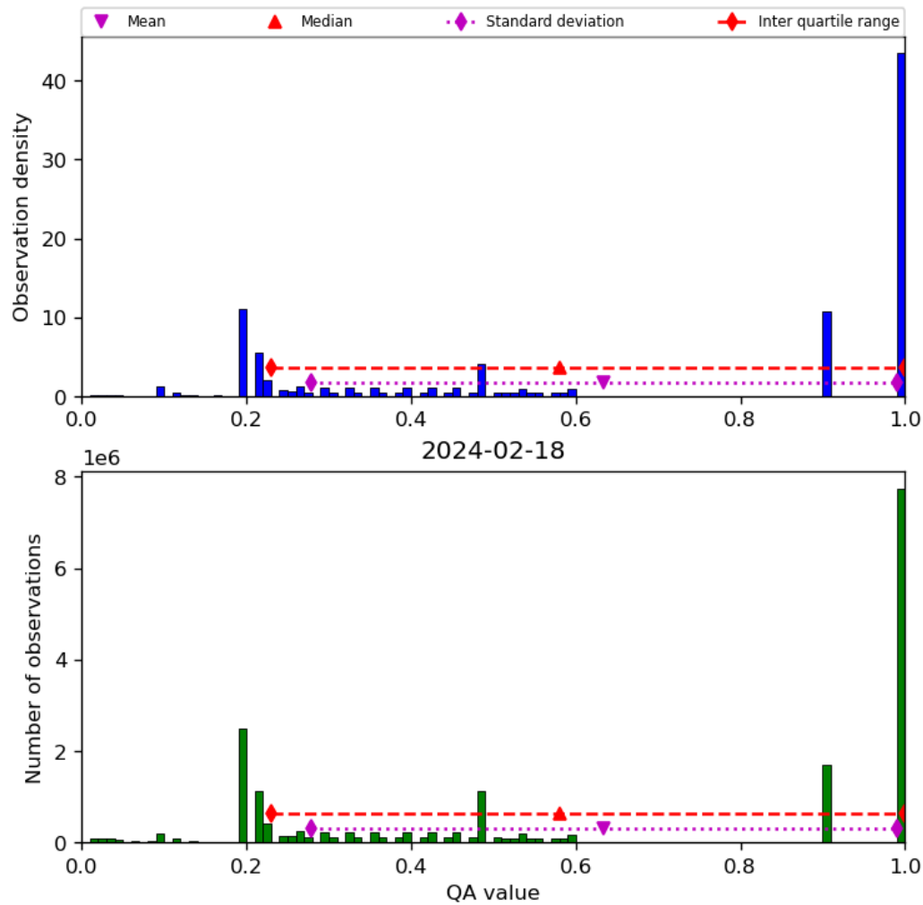
Figure 34: Histogram of “QA value” for 2024-02-17 to 2024-02-19
