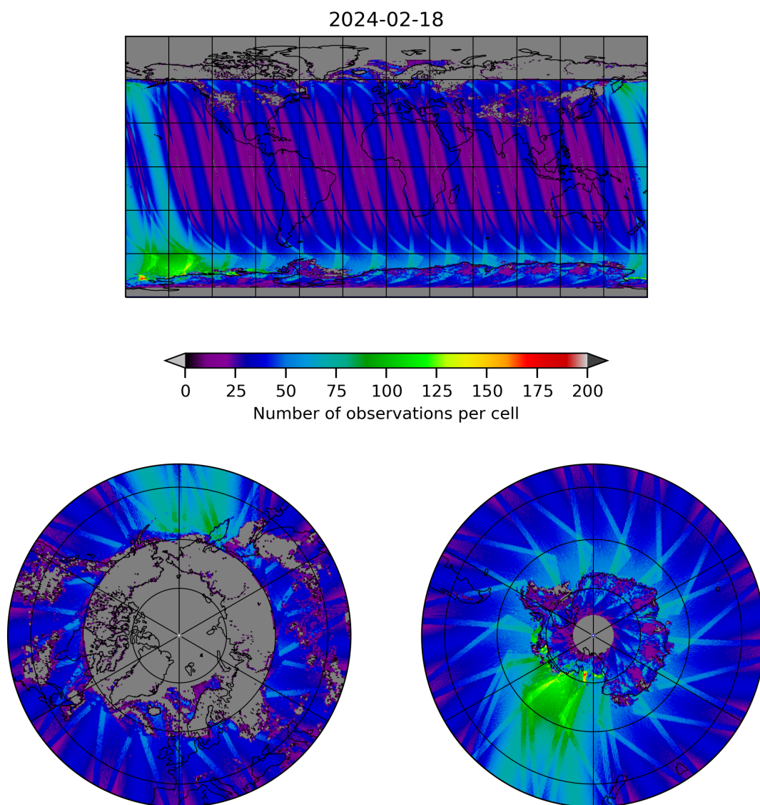
Figure 19: Map of the number of observations for 2024-02-17 to 2024-02-19
