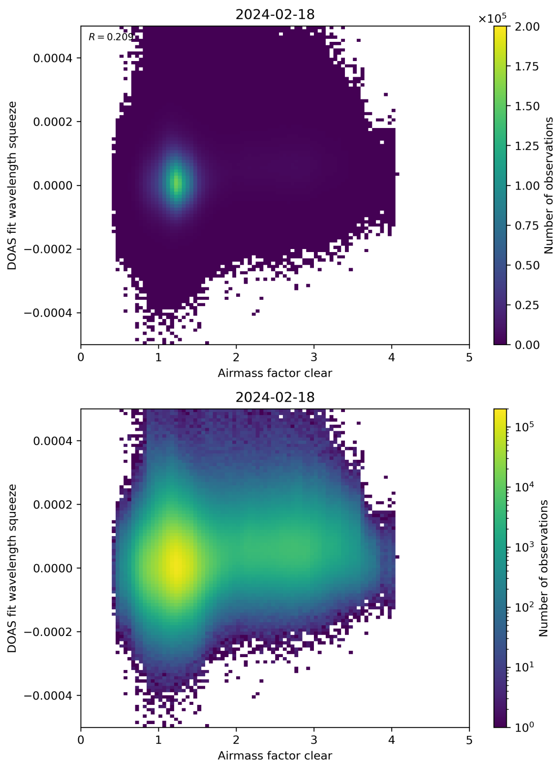
Figure 73: Scatter density plot of “Airmass factor clear” against “DOAS fit wavelength squeeze” for 2024-02-17 to 2024-02-19.
