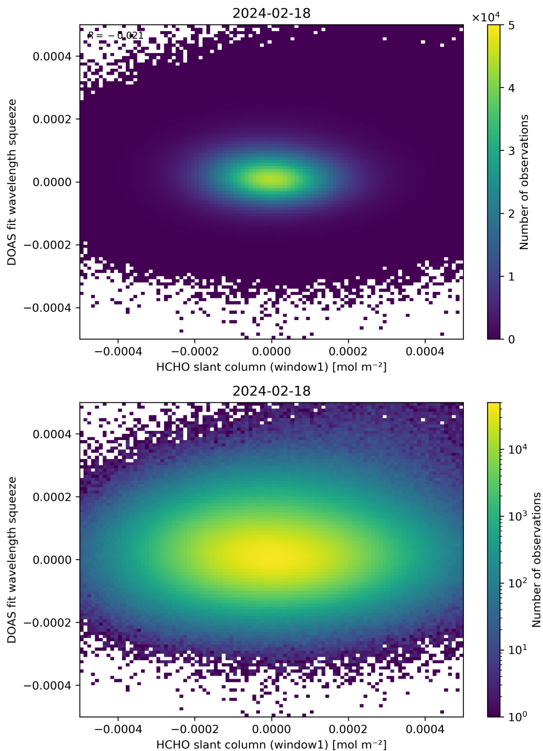
Figure 80: Scatter density plot of “HCHO slant column (window1)” against “DOAS fit wavelength squeeze” for 2024-02-17 to 2024-02-19.
