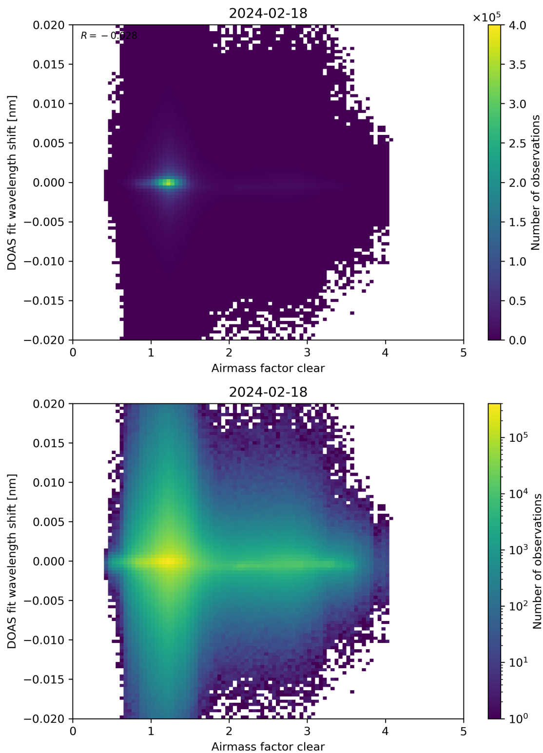
Figure 72: Scatter density plot of “Airmass factor clear” against “DOAS fit wavelength shift” for 2024-02-17 to 2024-02-19.
