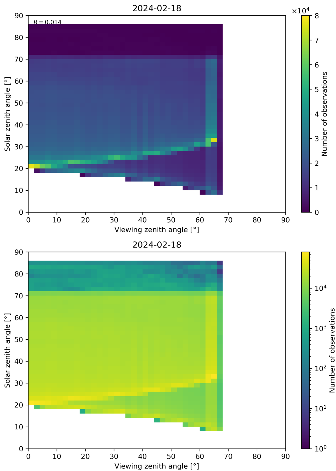
Figure 197: Scatter density plot of “Viewing zenith angle” against “Solar zenith angle” for 2024-02-17 to 2024-02-19.
