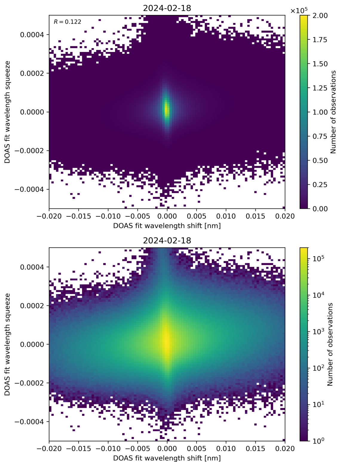
Figure 65: Scatter density plot of “DOAS fit wavelength shift” against “DOAS fit wavelength squeeze” for 2024-02-17 to 2024-02-19.
