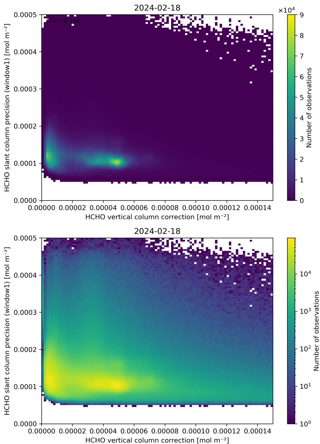
Figure 119: Scatter density plot of “HCHO vertical column correction” against “HCHO slant column precision (window1)” for 2024-02-17 to 2024-02-19.
