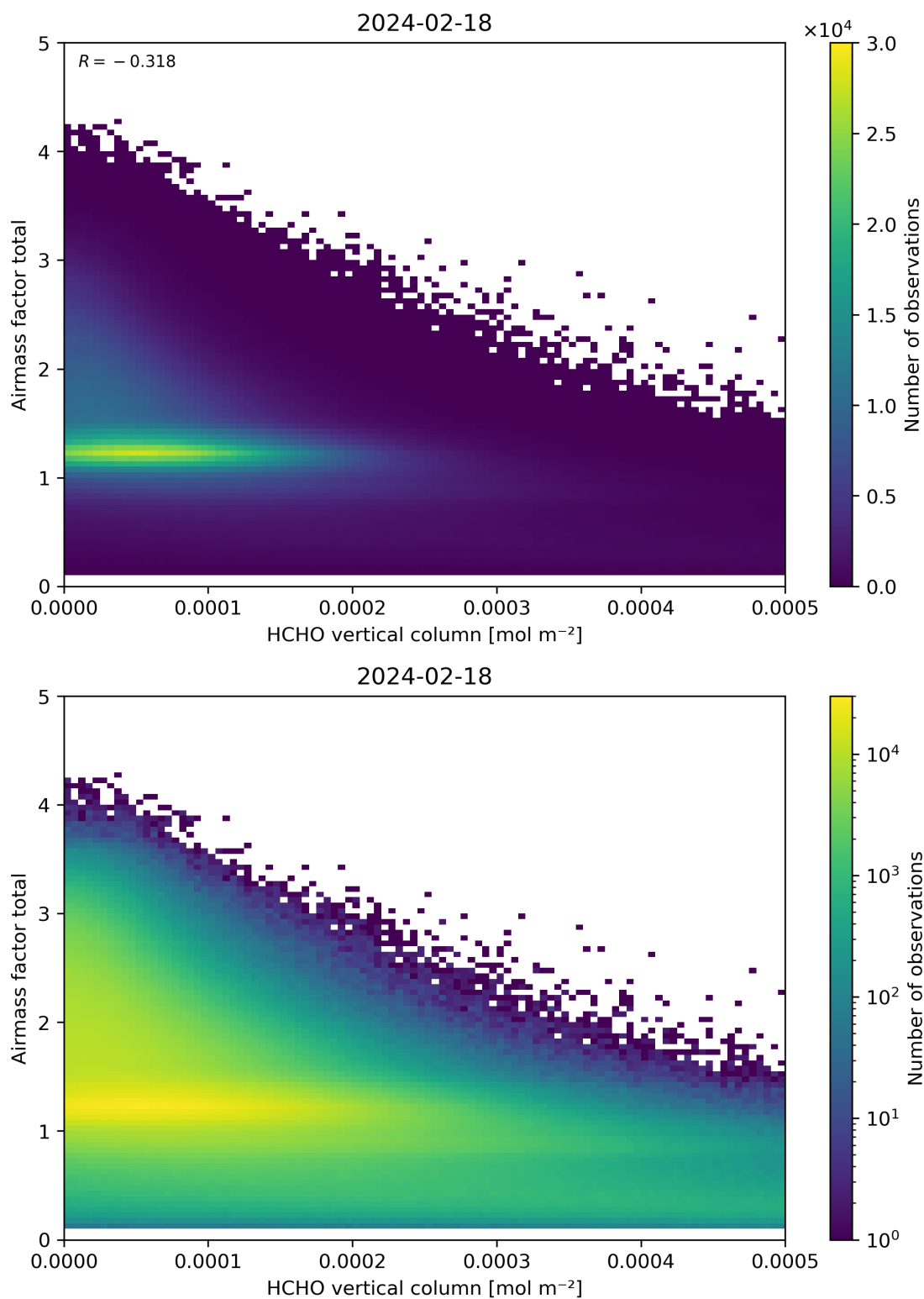
Figure 131: Scatter density plot of “HCHO vertical column” against “Airmass factor total” for 2024-02-17 to 2024-02-19.
