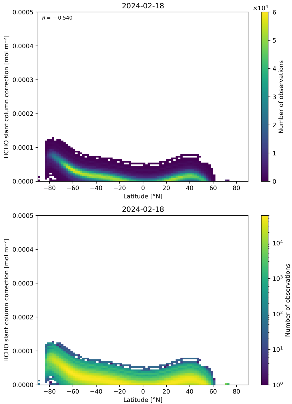
Figure 158: Scatter density plot of “Latitude” against “HCHO slant column correction” for 2024-02-17 to 2024-02-19.
