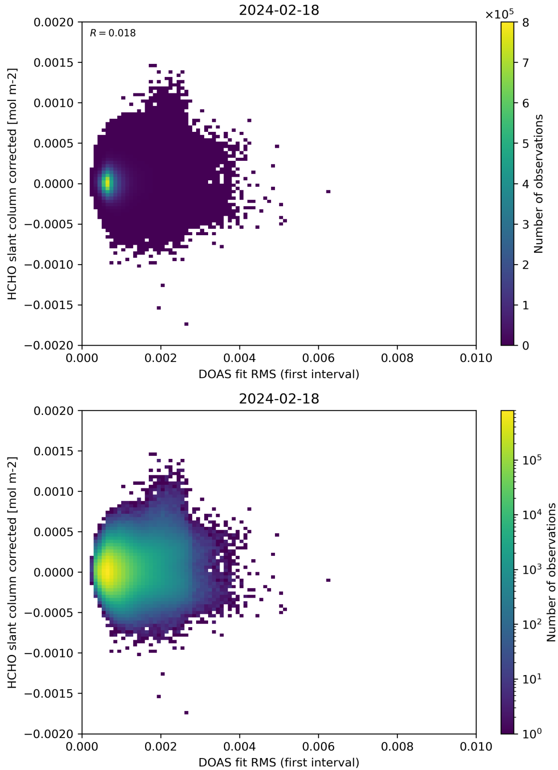
Figure 62: Scatter density plot of “DOAS fit RMS (first interval)” against “HCHO slant column corrected” for 2024-02-17 to 2024-02-19.
