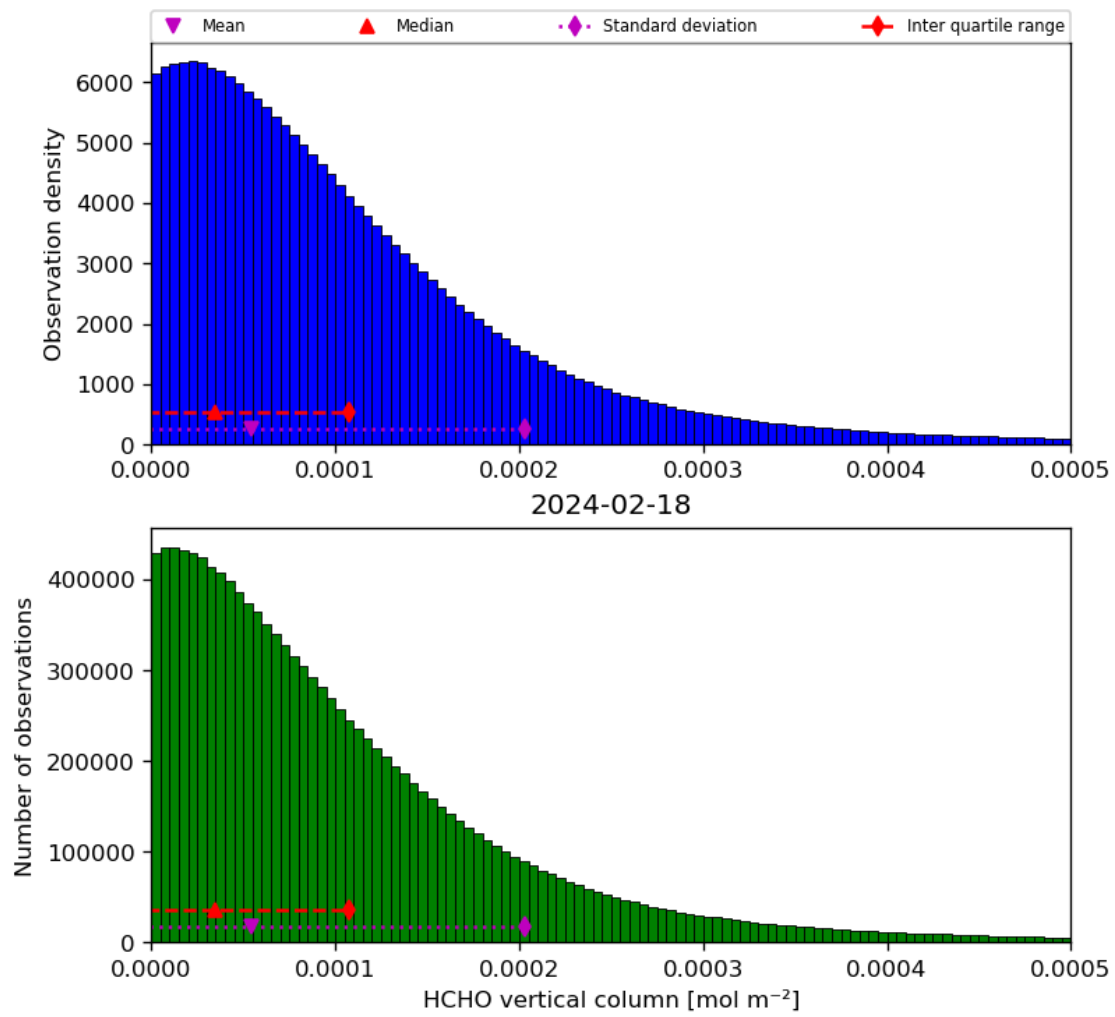
Figure 35: Histogram of “HCHO vertical column” for 2024-02-17 to 2024-02-19
