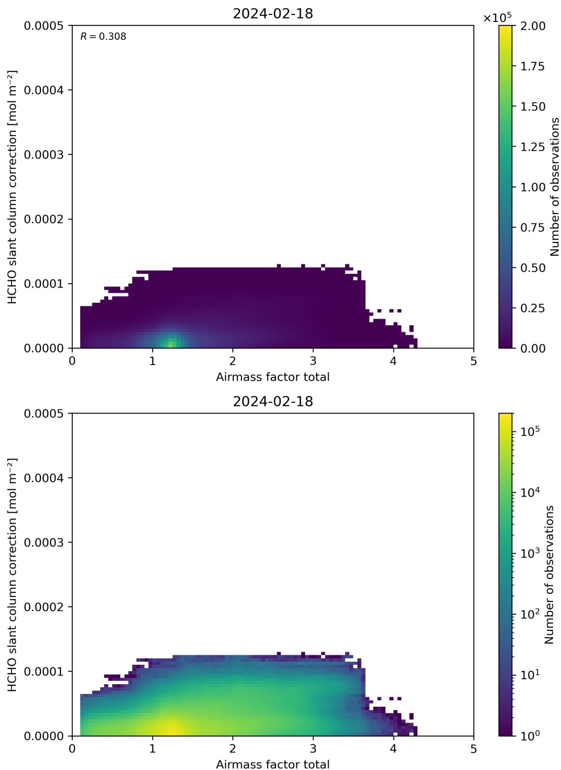
Figure 102: Scatter density plot of “Airmass factor total” against “HCHO slant column correction” for 2024-02-17 to 2024-02-19.
