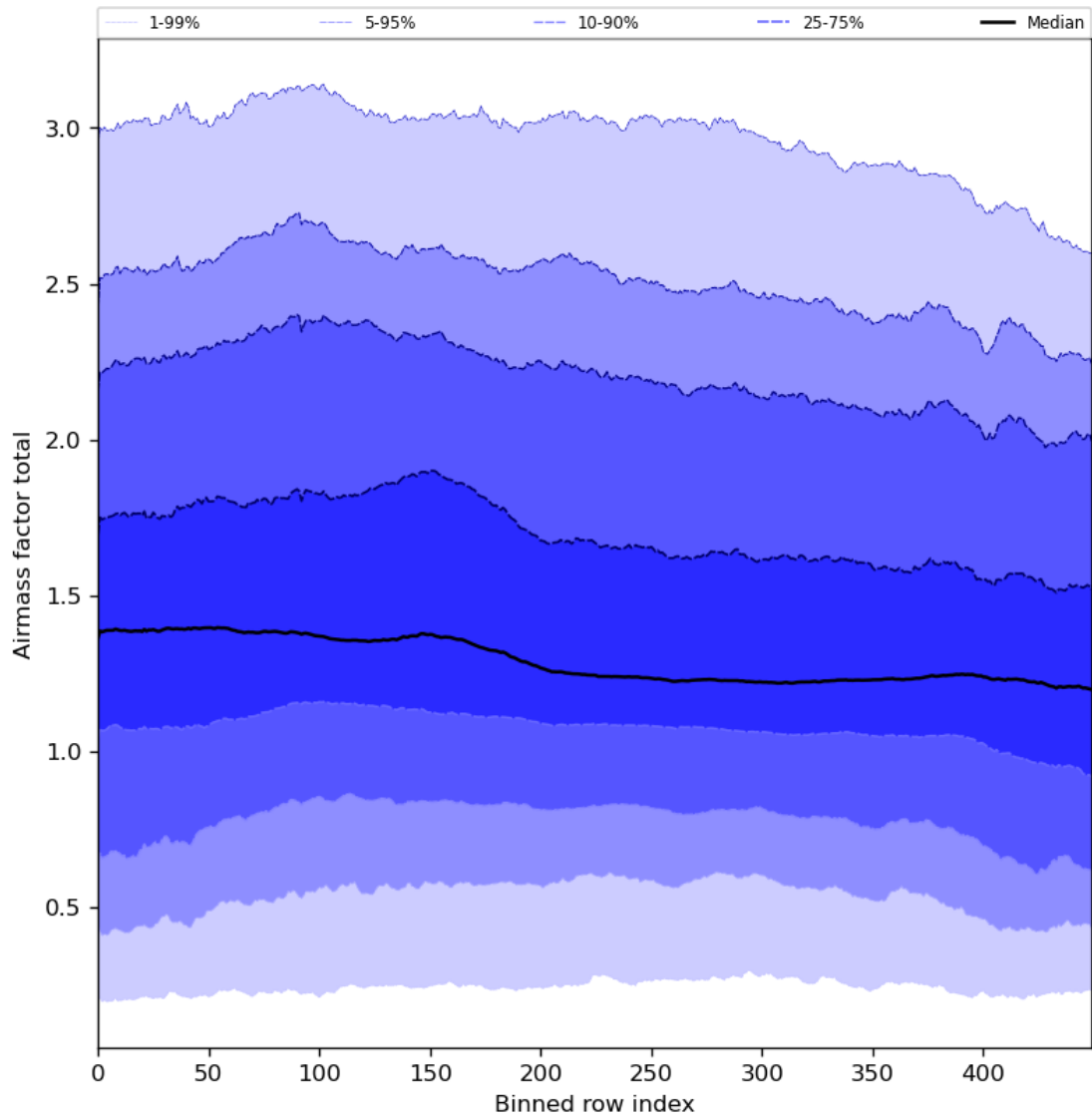
Figure 54: Along track statistics of “Airmass factor total” for 2024-02-17 to 2024-02-19
