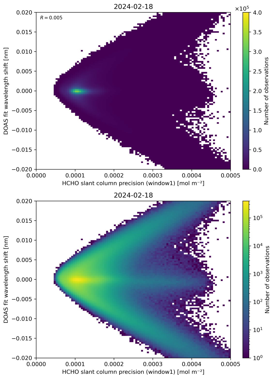
Figure 89: Scatter density plot of “HCHO slant column precision (window1)” against “DOAS fit wavelength shift” for 2024-02-17 to 2024-02-19.
