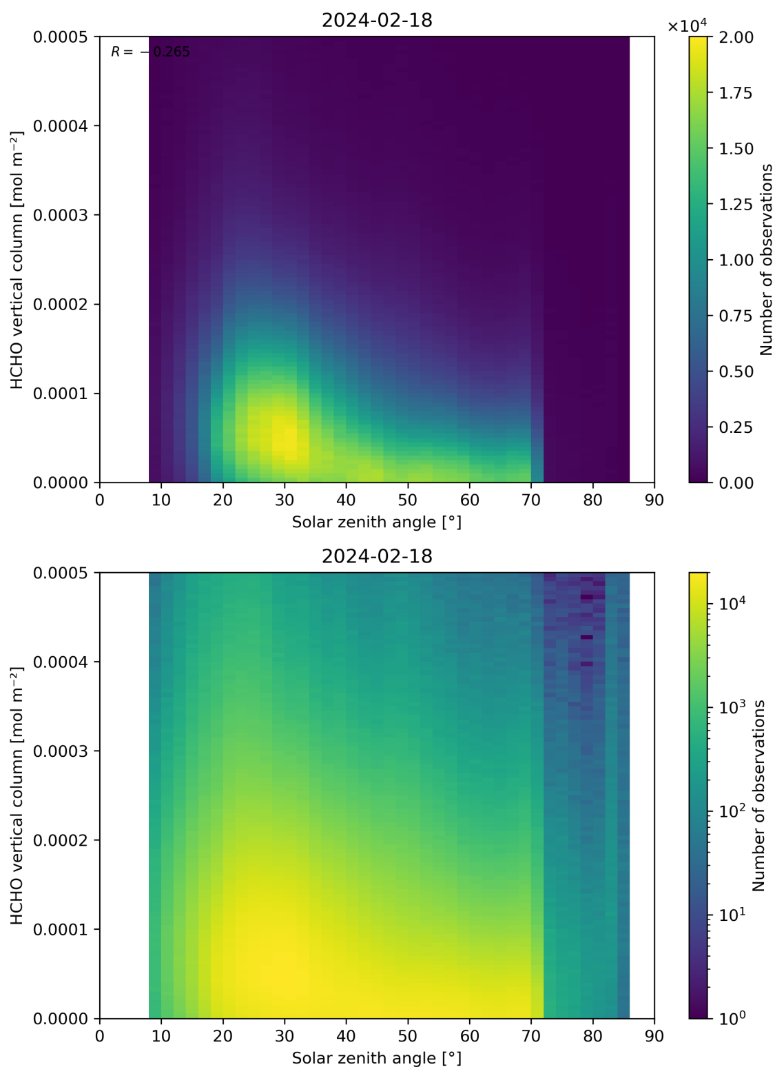
Figure 177: Scatter density plot of “Solar zenith angle” against “HCHO vertical column” for 2024-02-17 to 2024-02-19.
