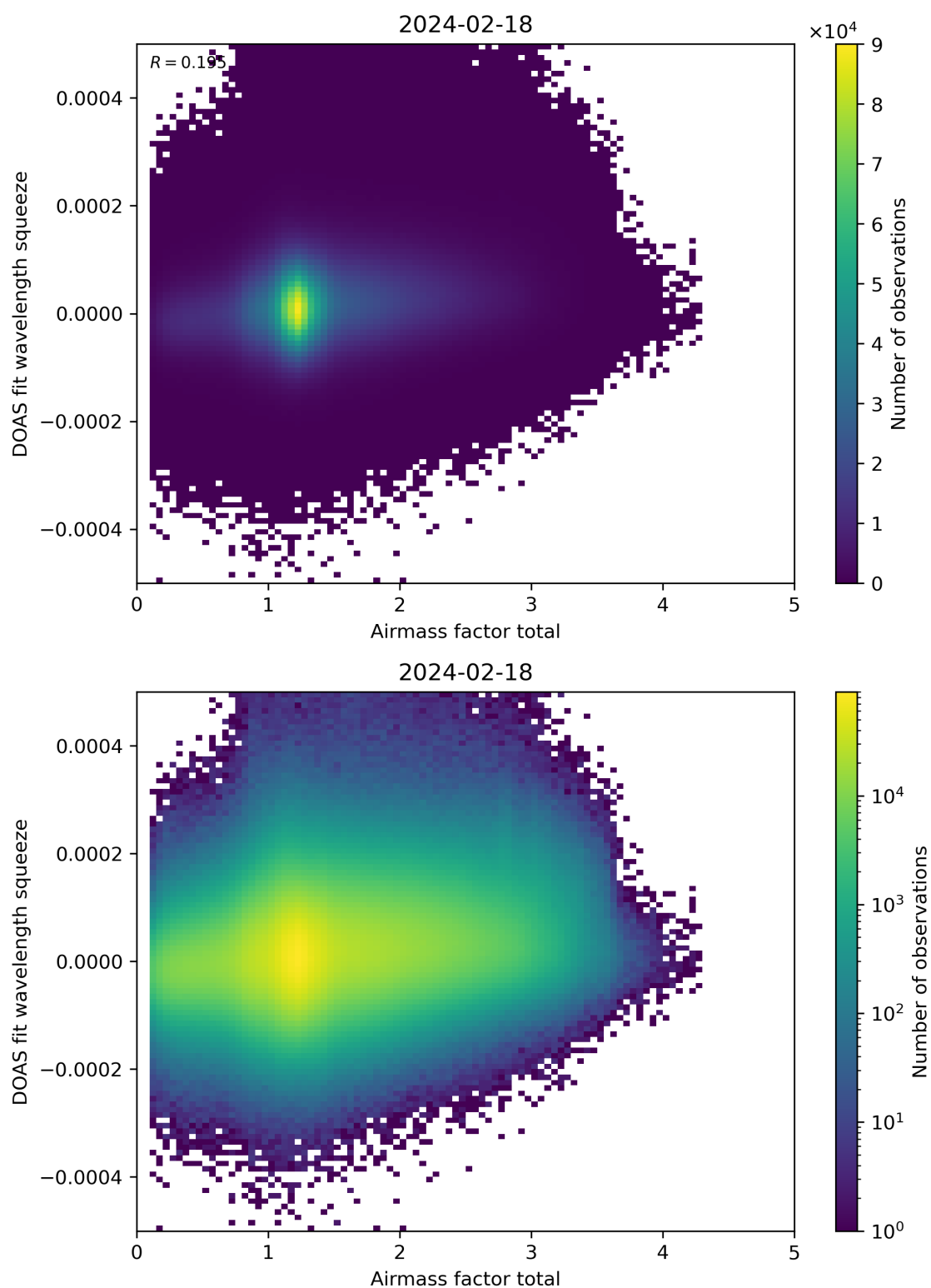
Figure 99: Scatter density plot of “Airmass factor total” against “DOAS fit wavelength squeeze” for 2024-02-17 to 2024-02-19.
