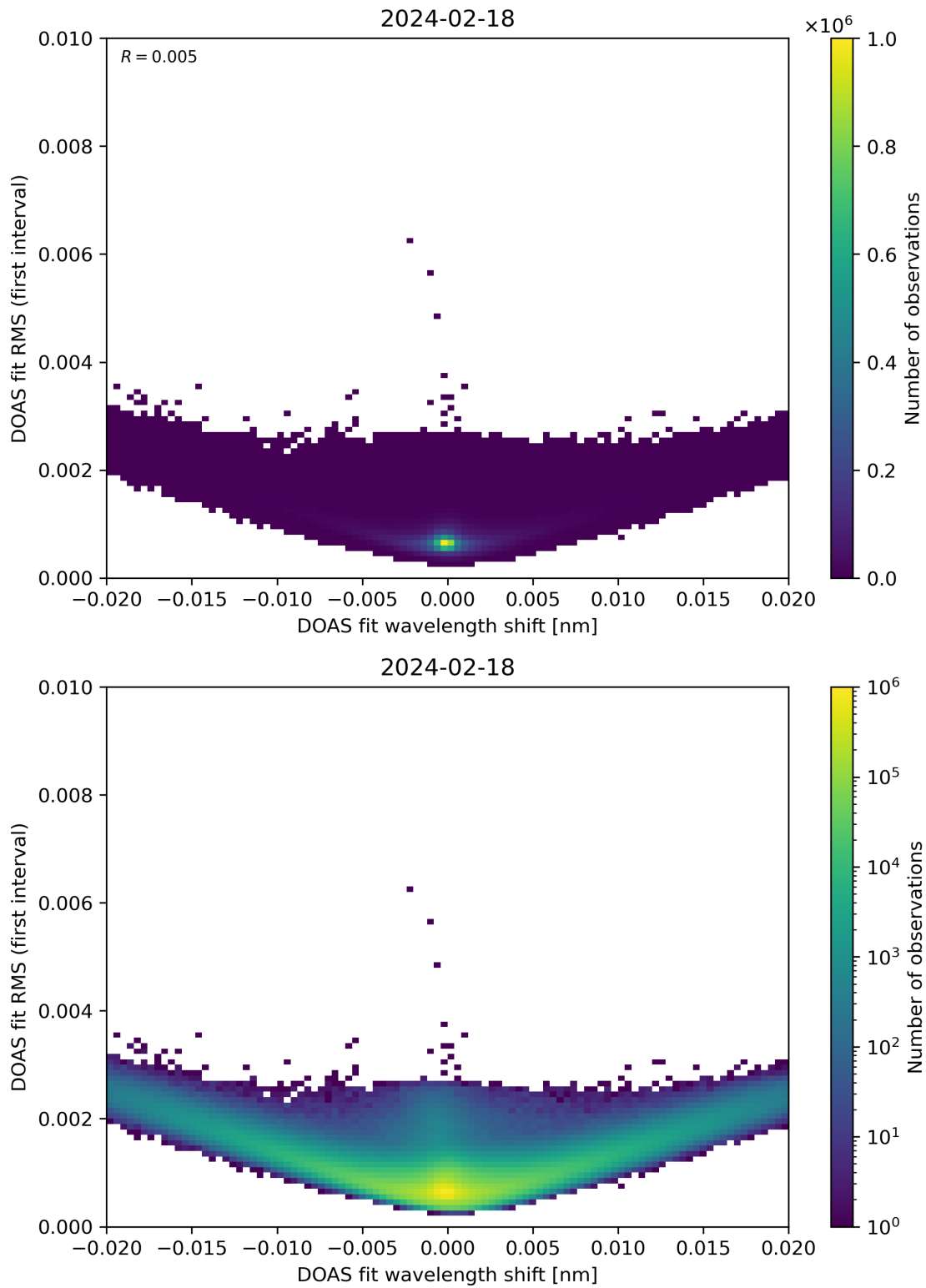
Figure 64: Scatter density plot of “DOAS fit wavelength shift” against “DOAS fit RMS (first interval)” for 2024-02-17 to 2024-02-19.
