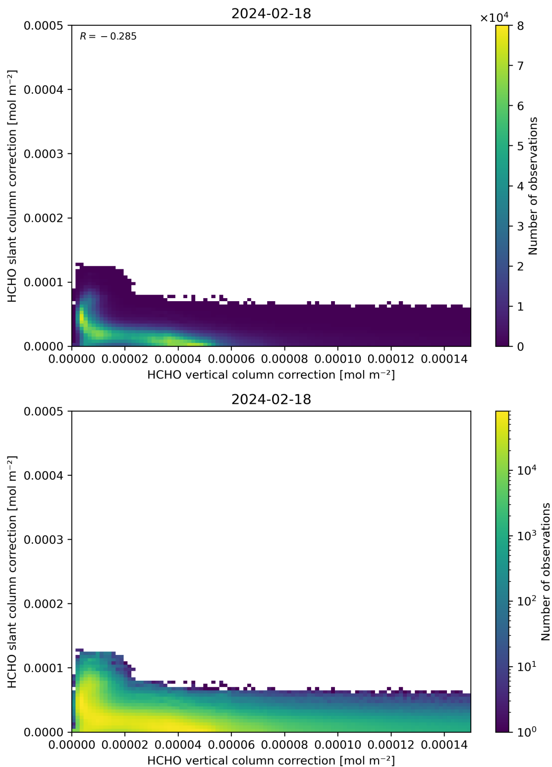
Figure 117: Scatter density plot of “HCHO vertical column correction” against “HCHO slant column correction” for 2024-02-17 to 2024-02-19.
