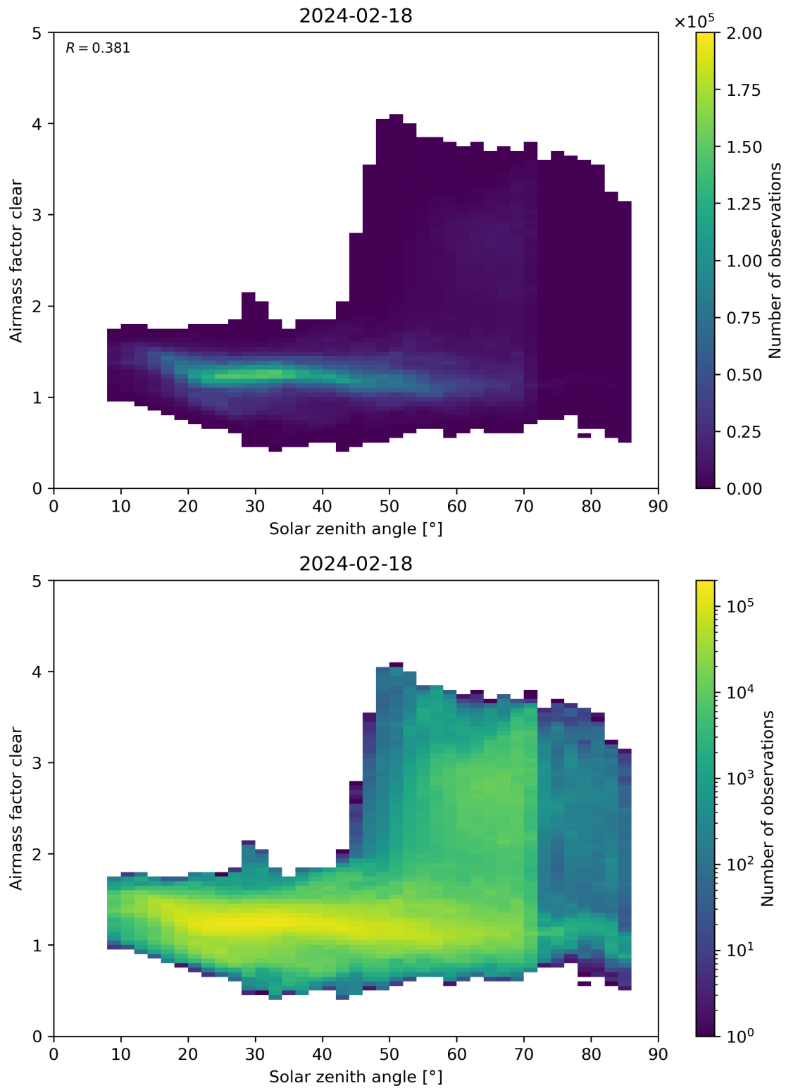
Figure 170: Scatter density plot of “Solar zenith angle” against “Airmass factor clear” for 2024-02-17 to 2024-02-19.
