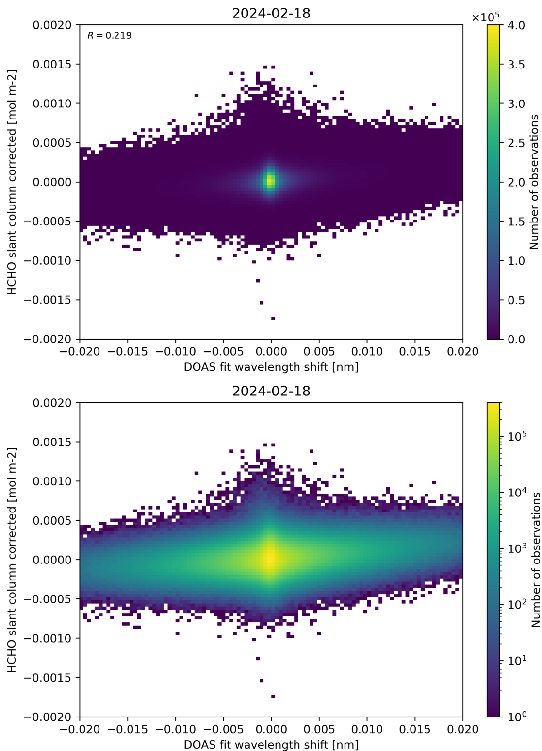
Figure 66: Scatter density plot of “DOAS fit wavelength shift” against “HCHO slant column corrected” for 2024-02-17 to 2024-02-19.
