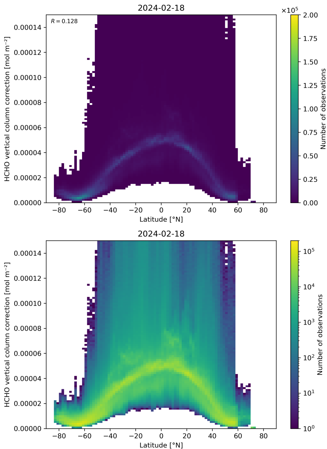
Figure 164: Scatter density plot of “Latitude” against “HCHO vertical column correction” for 2024-02-17 to 2024-02-19.
