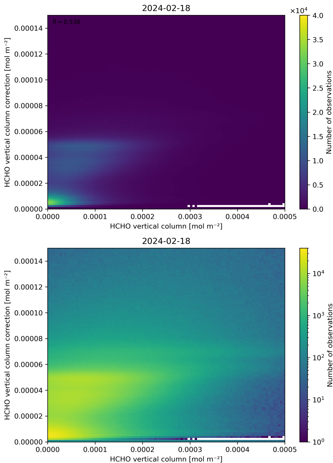
Figure 133: Scatter density plot of “HCHO vertical column” against “HCHO vertical column correction” for 2024-02-17 to 2024-02-19.
