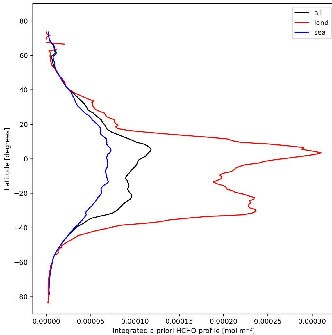
Figure 29: Zonal average of “Integrated a priori HCHO profile” for 2024-02-17 to 2024-02-19.
