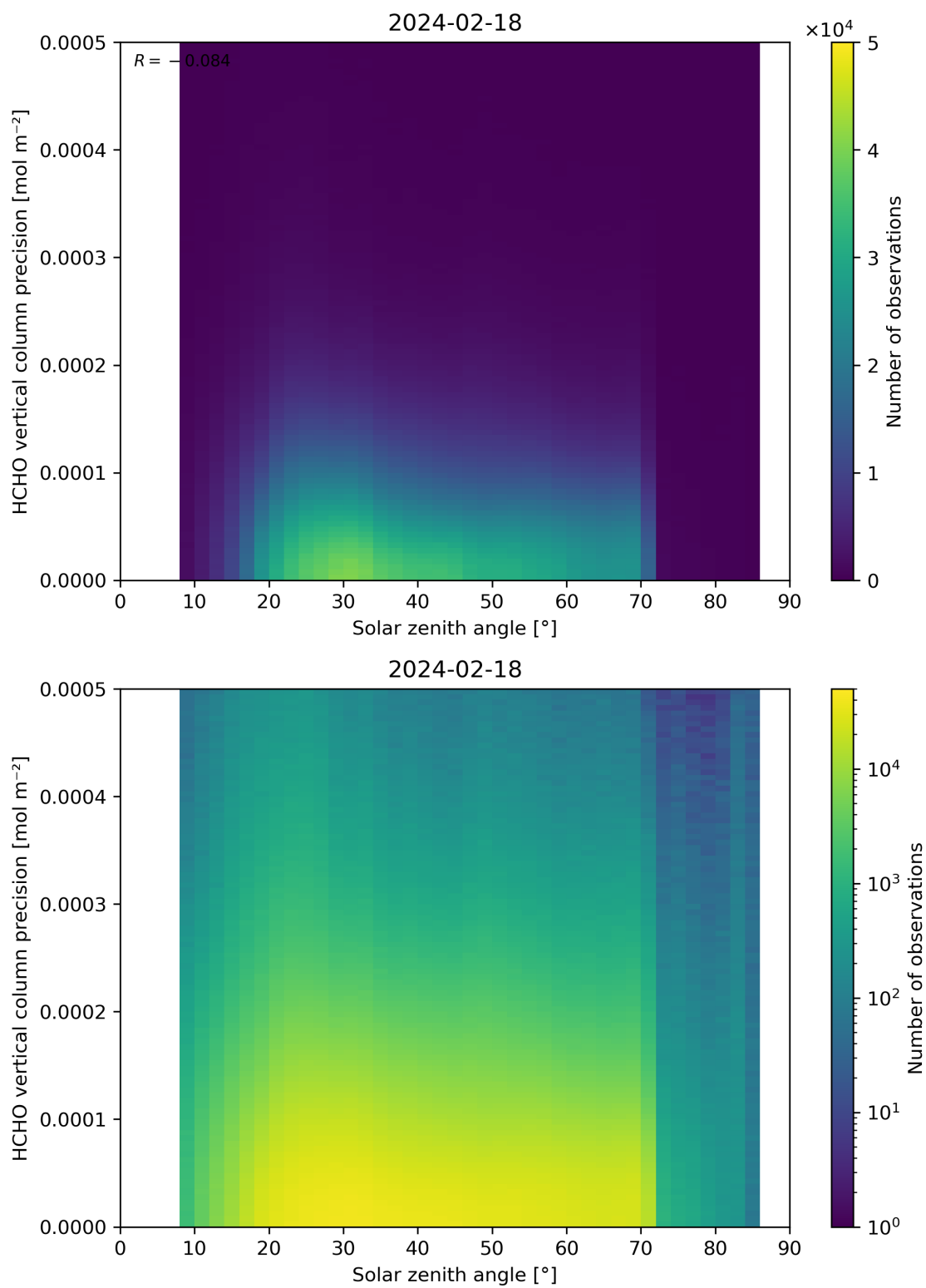
Figure 179: Scatter density plot of “Solar zenith angle” against “HCHO vertical column precision” for 2024-02-17 to 2024-02-19.
