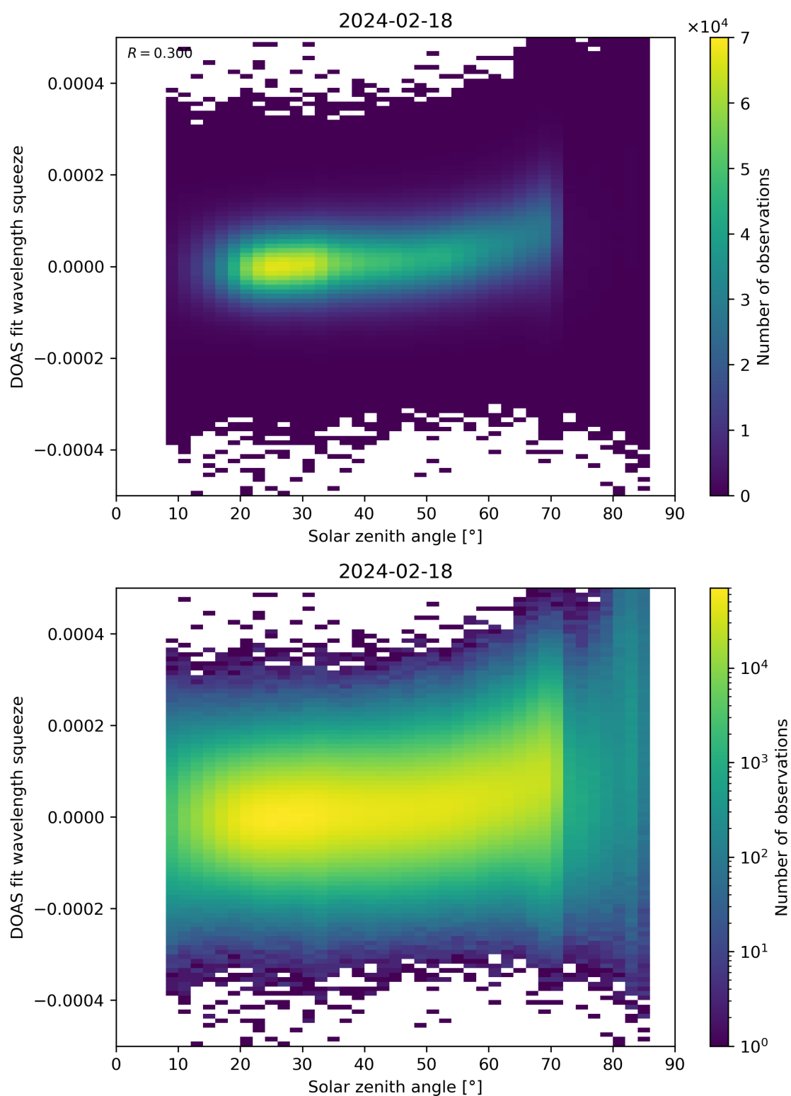
Figure 169: Scatter density plot of “Solar zenith angle” against “DOAS fit wavelength squeeze” for 2024-02-17 to 2024-02-19.
