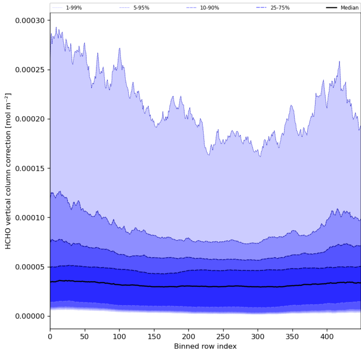
Figure 51: Along track statistics of “HCHO vertical column correction” for 2024-02-17 to 2024-02-19
