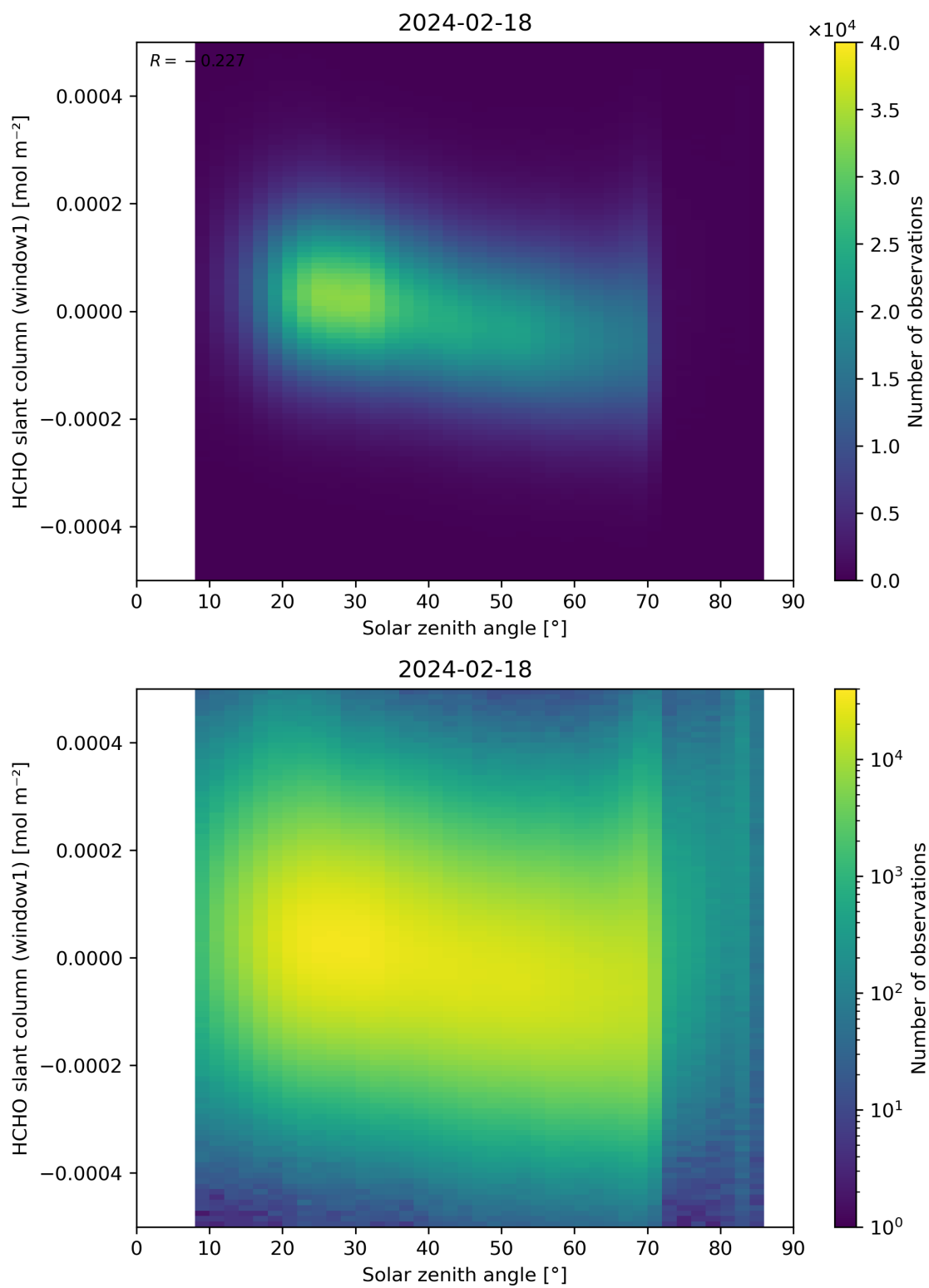
Figure 173: Scatter density plot of “Solar zenith angle” against “HCHO slant column (window1)” for 2024-02-17 to 2024-02-19.
