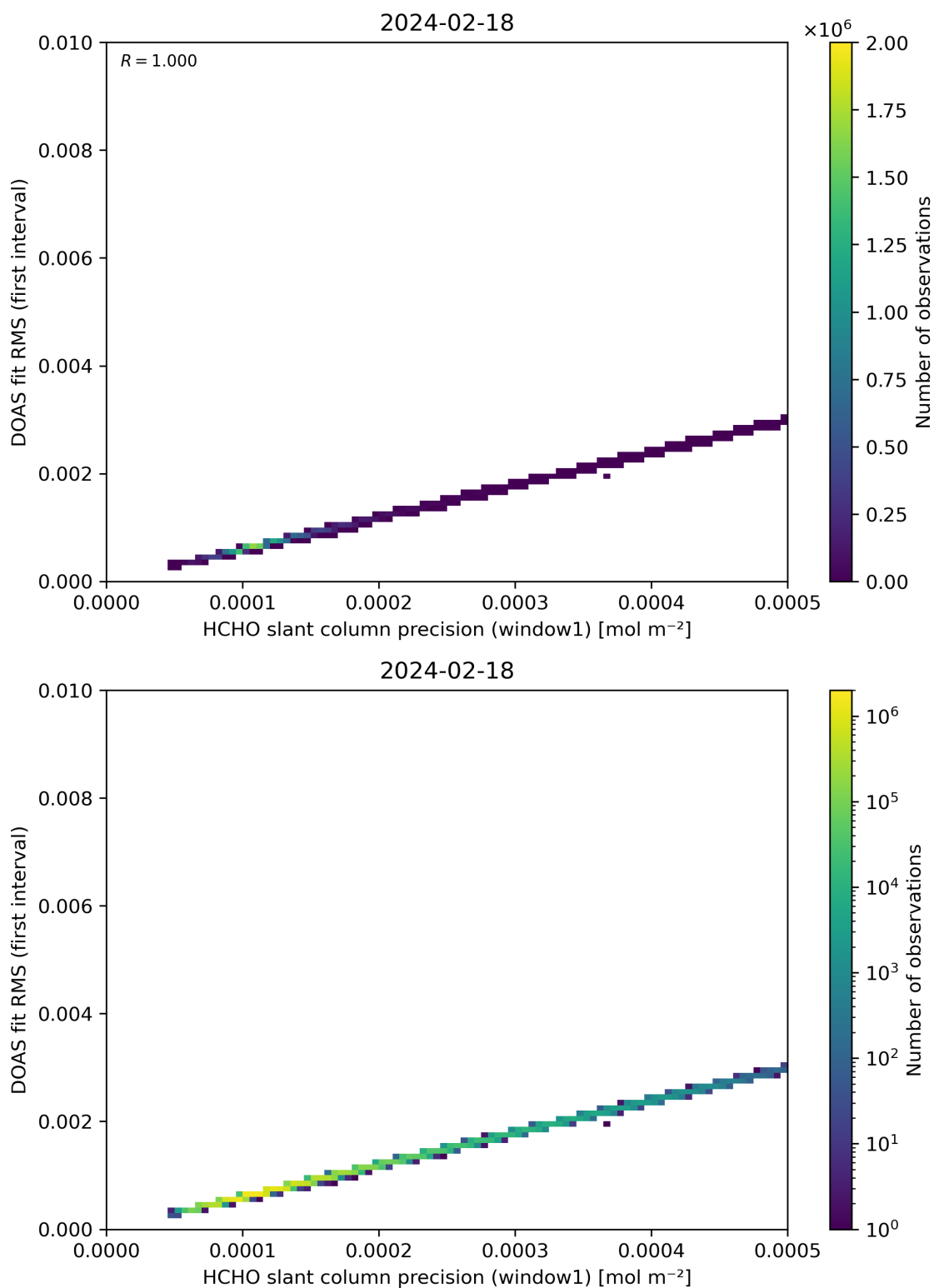
Figure 88: Scatter density plot of “HCHO slant column precision (window1)” against “DOAS fit RMS (first interval)” for 2024-02-17 to 2024-02-19.
