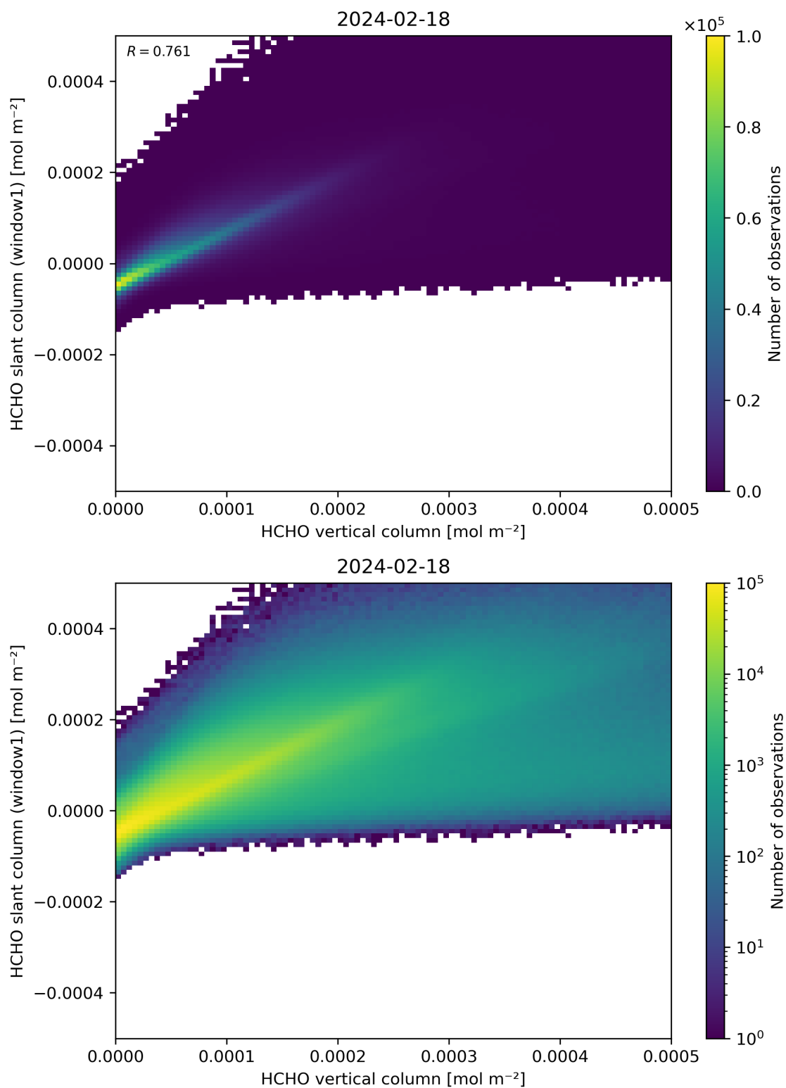
Figure 129: Scatter density plot of “HCHO vertical column” against “HCHO slant column (window1)” for 2024-02-17 to 2024-02-19.
