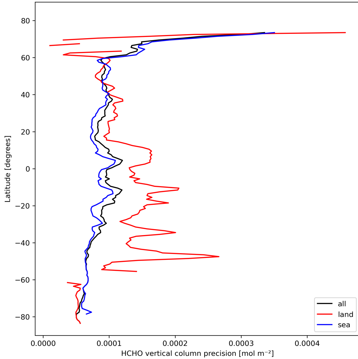
Figure 22: Zonal average of “HCHO vertical column precision” for 2024-02-17 to 2024-02-19.
