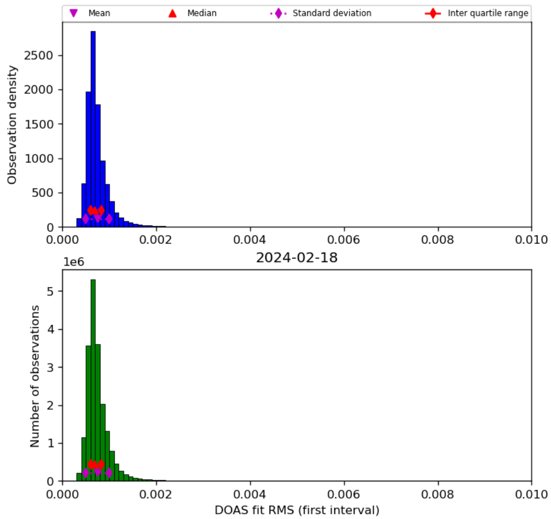
Figure 46: Histogram of “DOAS fit RMS (first interval)” for 2024-02-17 to 2024-02-19
