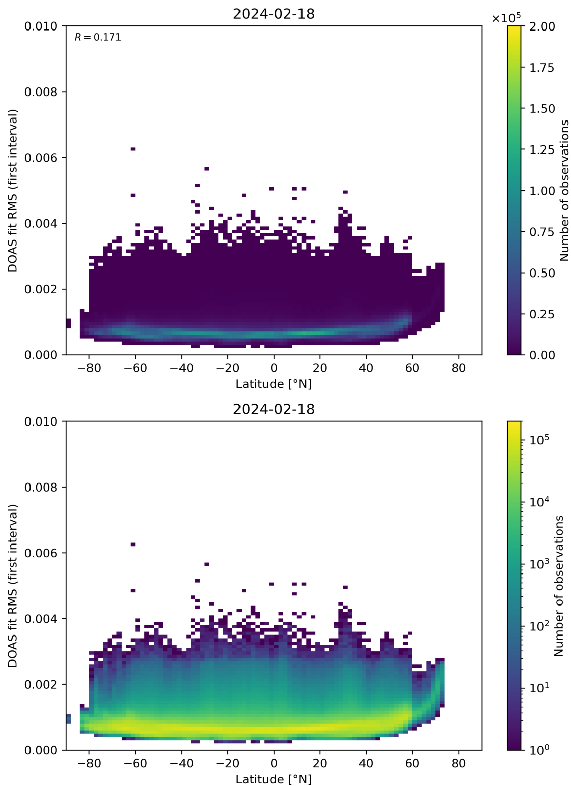
Figure 153: Scatter density plot of “Latitude” against “DOAS fit RMS (first interval)” for 2024-02-17 to 2024-02-19.
