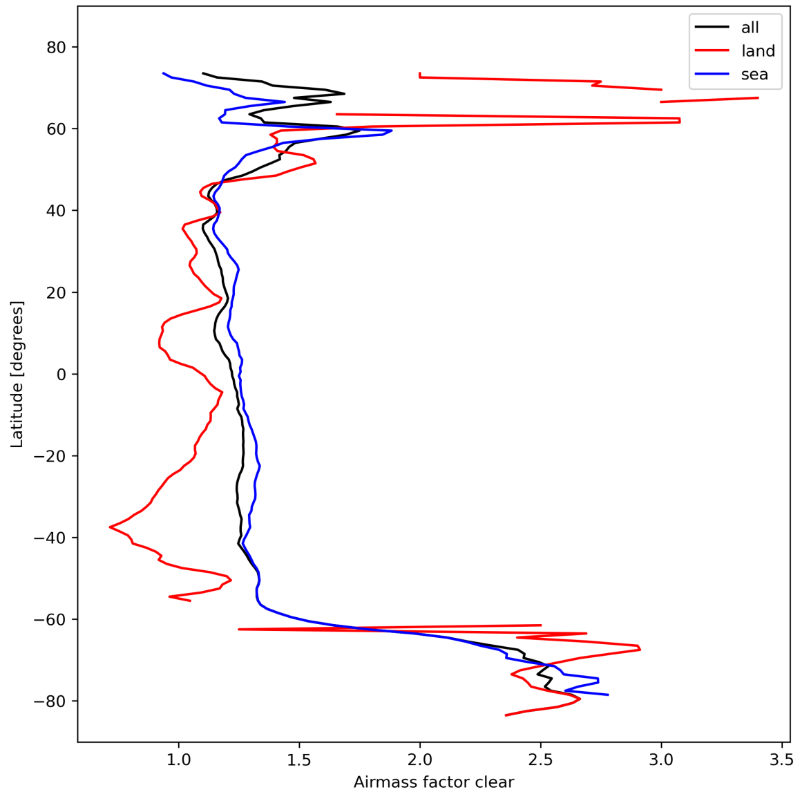
Figure 28: Zonal average of “Airmass factor clear” for 2024-02-17 to 2024-02-19.
