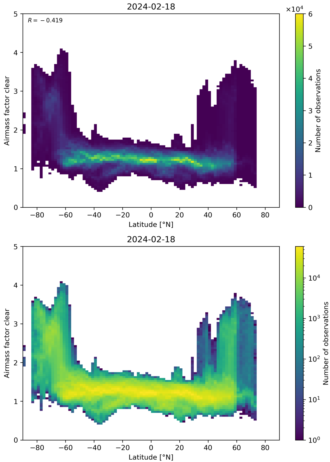
Figure 156: Scatter density plot of “Latitude” against “Airmass factor clear” for 2024-02-17 to 2024-02-19.
