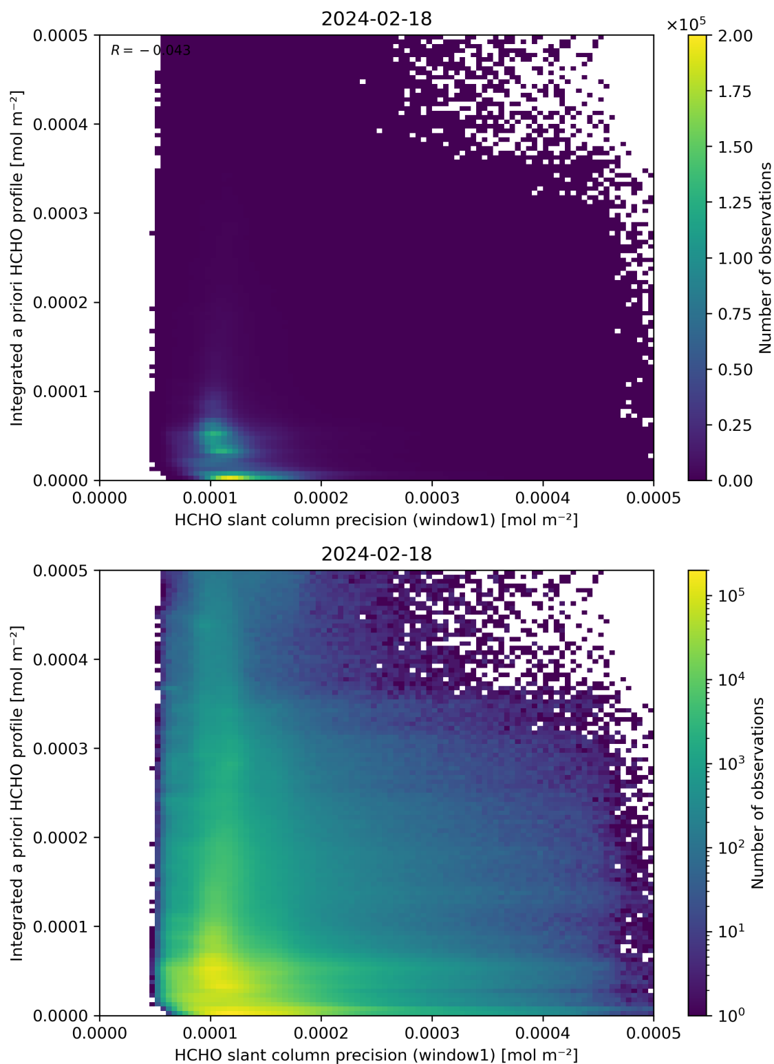
Figure 96: Scatter density plot of “HCHO slant column precision (window1)” against “Integrated a priori HCHO profile” for 2024-02-17 to 2024-02-19.
