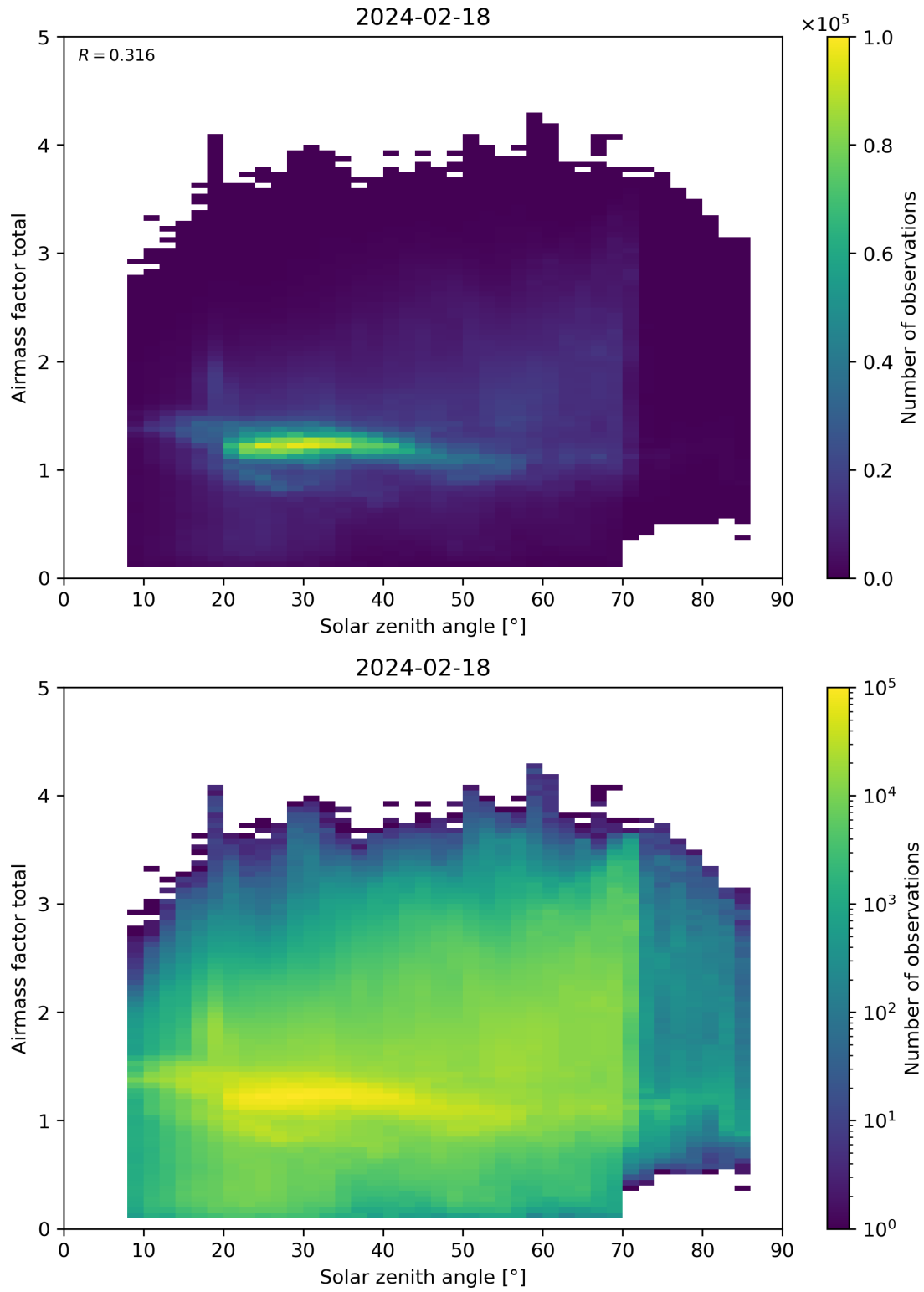
Figure 175: Scatter density plot of “Solar zenith angle” against “Airmass factor total” for 2024-02-17 to 2024-02-19.
