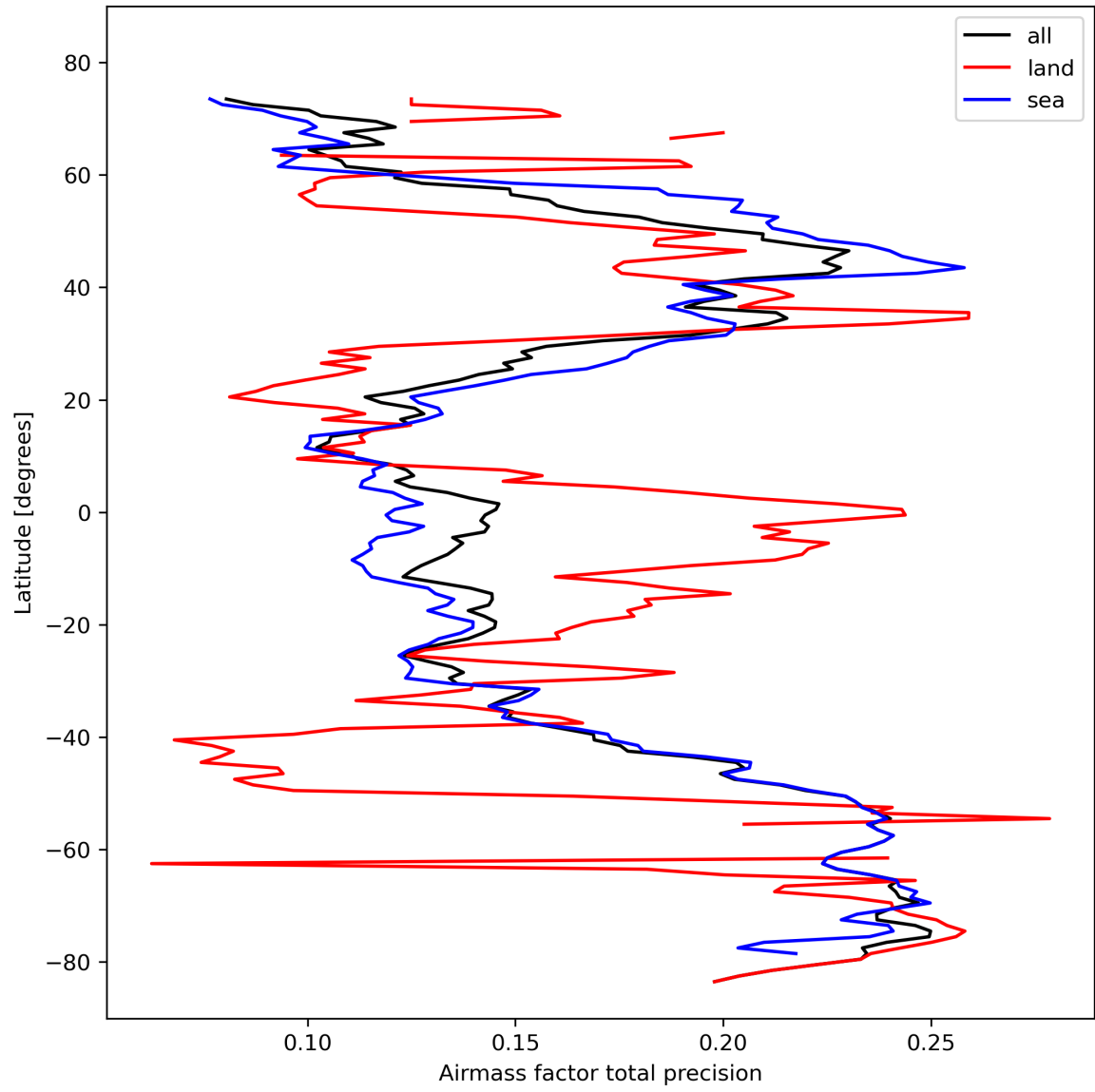
Figure 27: Zonal average of “Airmass factor total precision” for 2024-02-17 to 2024-02-19.
