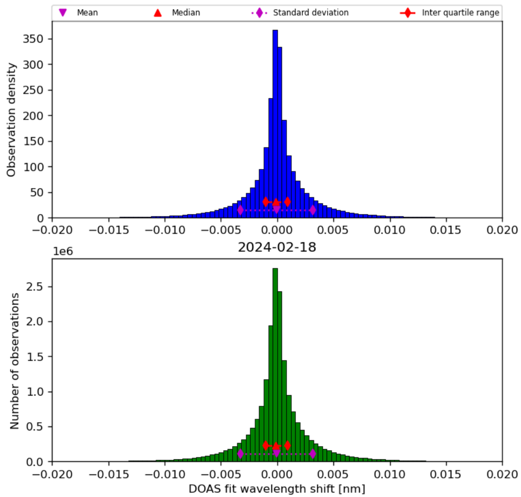
Figure 44: Histogram of “DOAS fit wavelength shift” for 2024-02-17 to 2024-02-19
