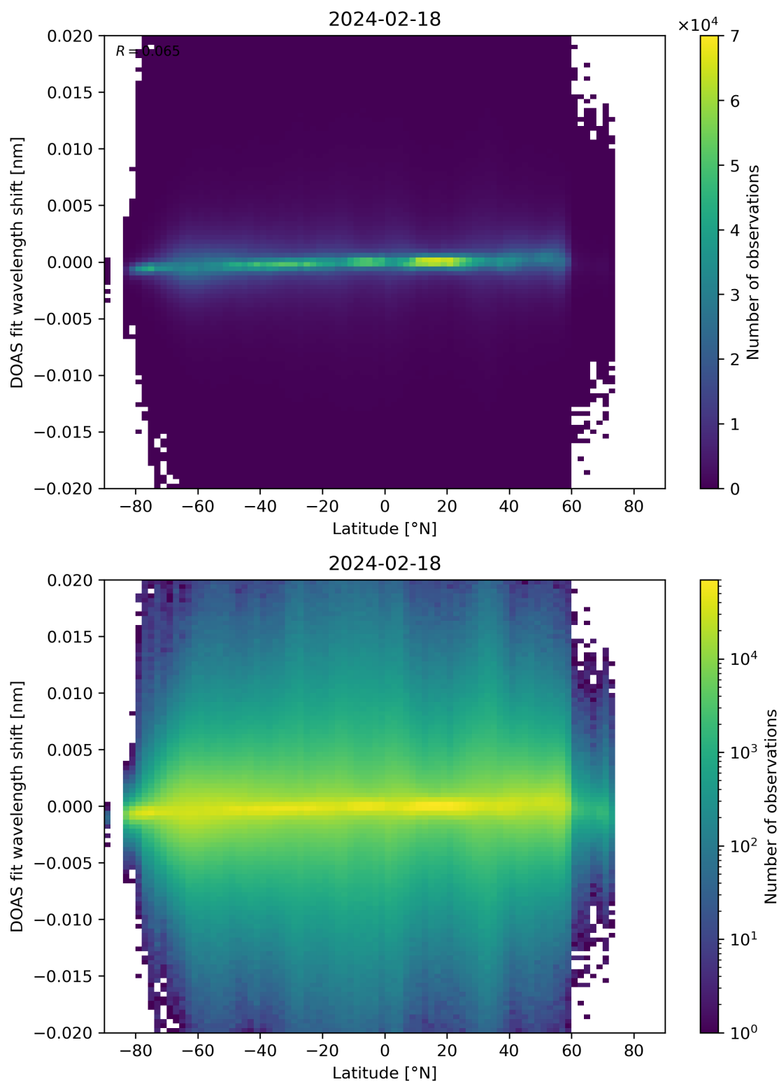
Figure 154: Scatter density plot of “Latitude” against “DOAS fit wavelength shift” for 2024-02-17 to 2024-02-19.
