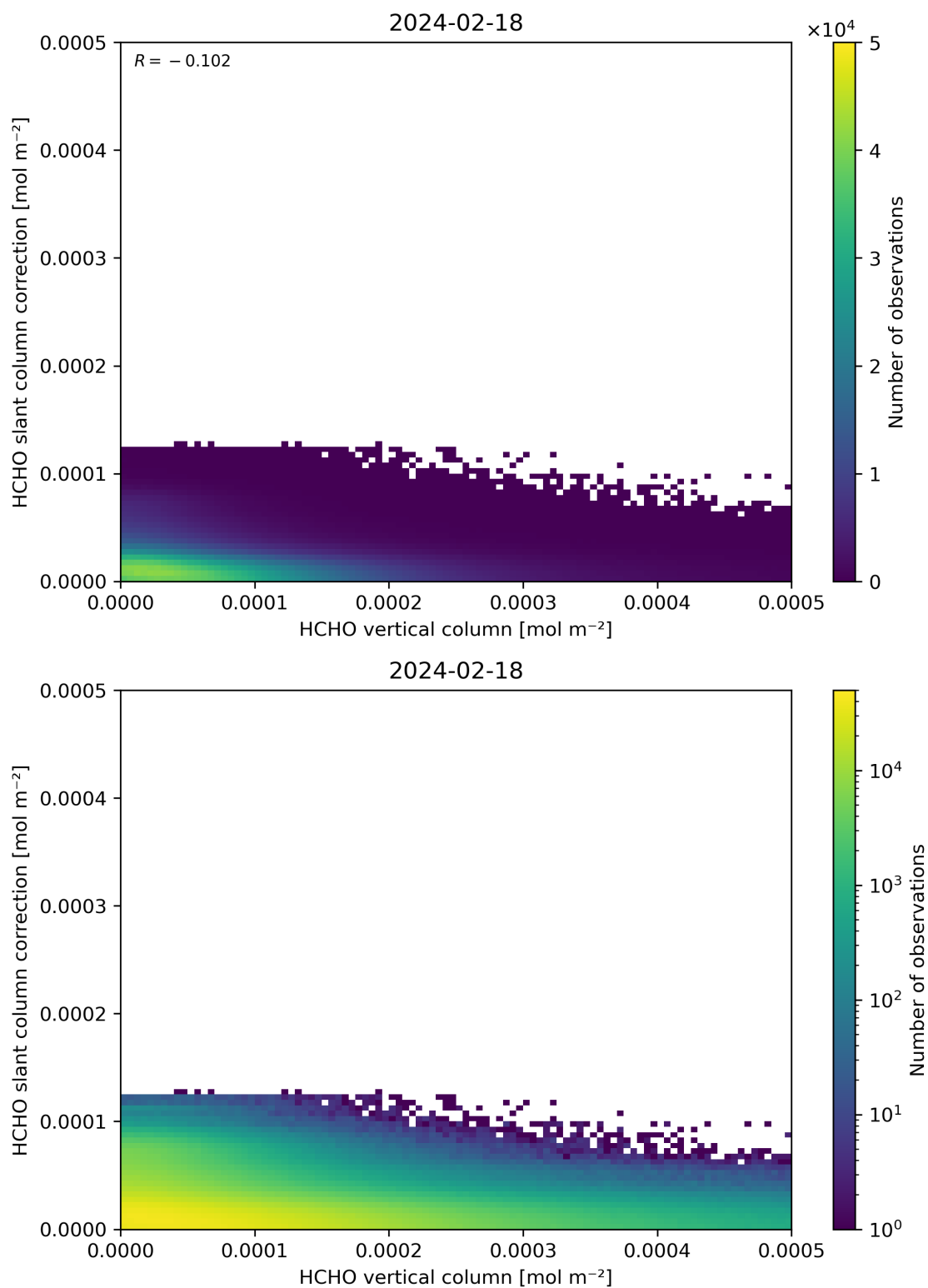
Figure 128: Scatter density plot of “HCHO vertical column” against “HCHO slant column correction” for 2024-02-17 to 2024-02-19.
