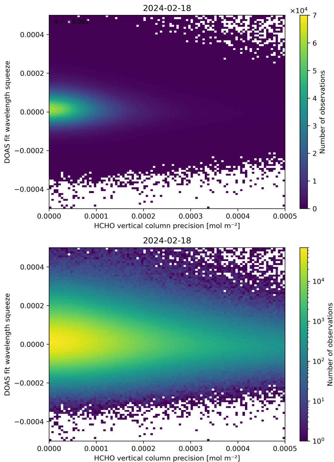
Figure 138: Scatter density plot of “HCHO vertical column precision” against “DOAS fit wavelength squeeze” for 2024-02-17 to 2024-02-19.
