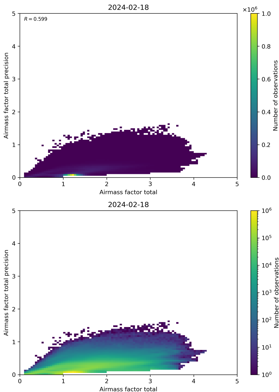
Figure 103: Scatter density plot of “Airmass factor total” against “Airmass factor total precision” for 2024-02-17 to 2024-02-19.
