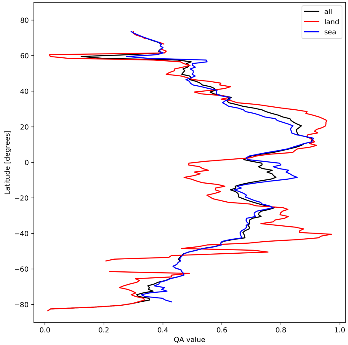
Figure 20: Zonal average of “QA value” for 2024-02-17 to 2024-02-19.
