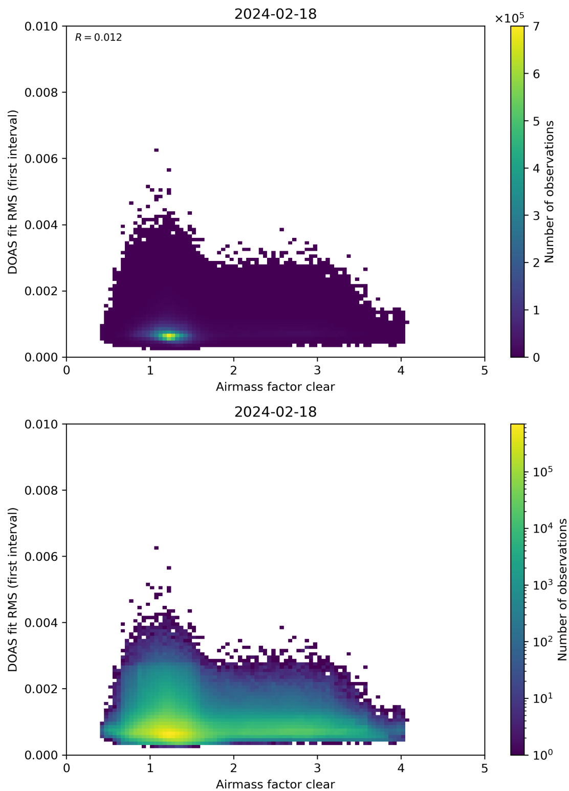
Figure 71: Scatter density plot of “Airmass factor clear” against “DOAS fit RMS (first interval)” for 2024-02-17 to 2024-02-19.
