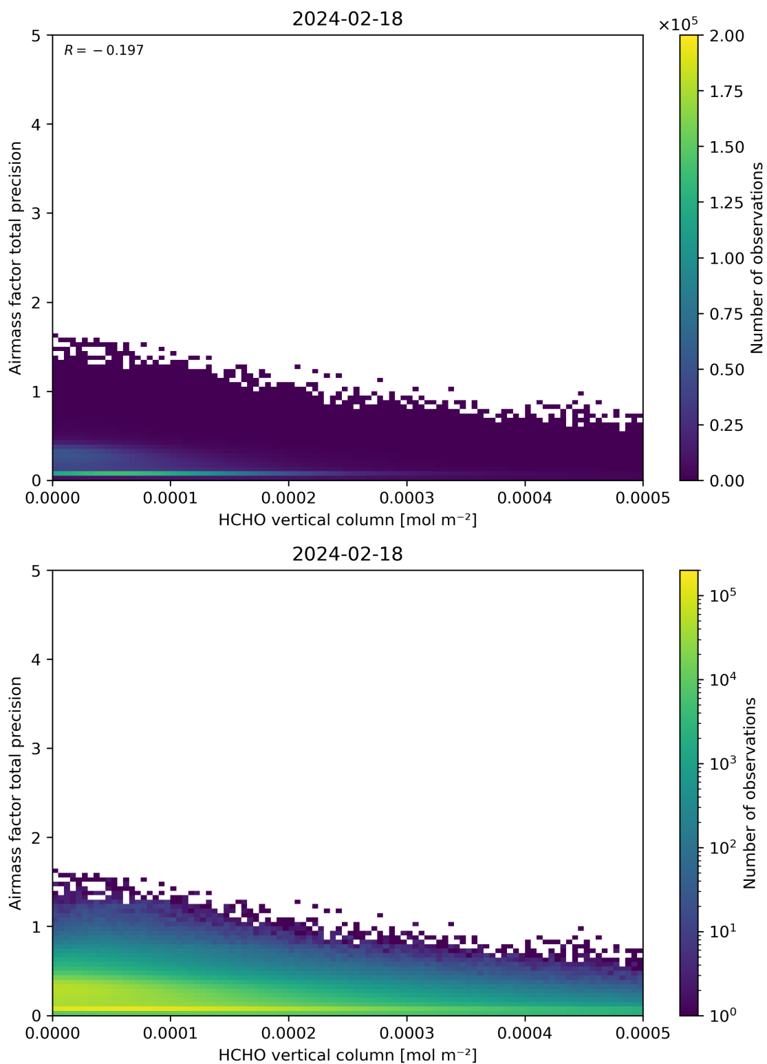
Figure 132: Scatter density plot of “HCHO vertical column” against “Airmass factor total precision” for 2024-02-17 to 2024-02-19.
