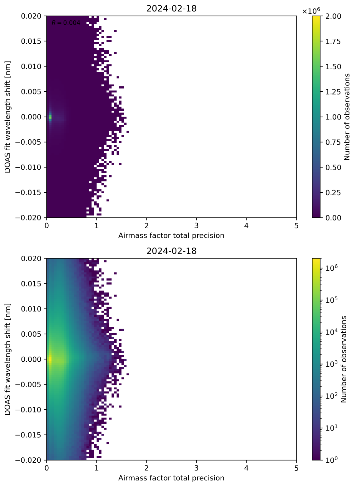
Figure 106: Scatter density plot of “Airmass factor total precision” against “DOAS fit wavelength shift” for 2024-02-17 to 2024-02-19.
