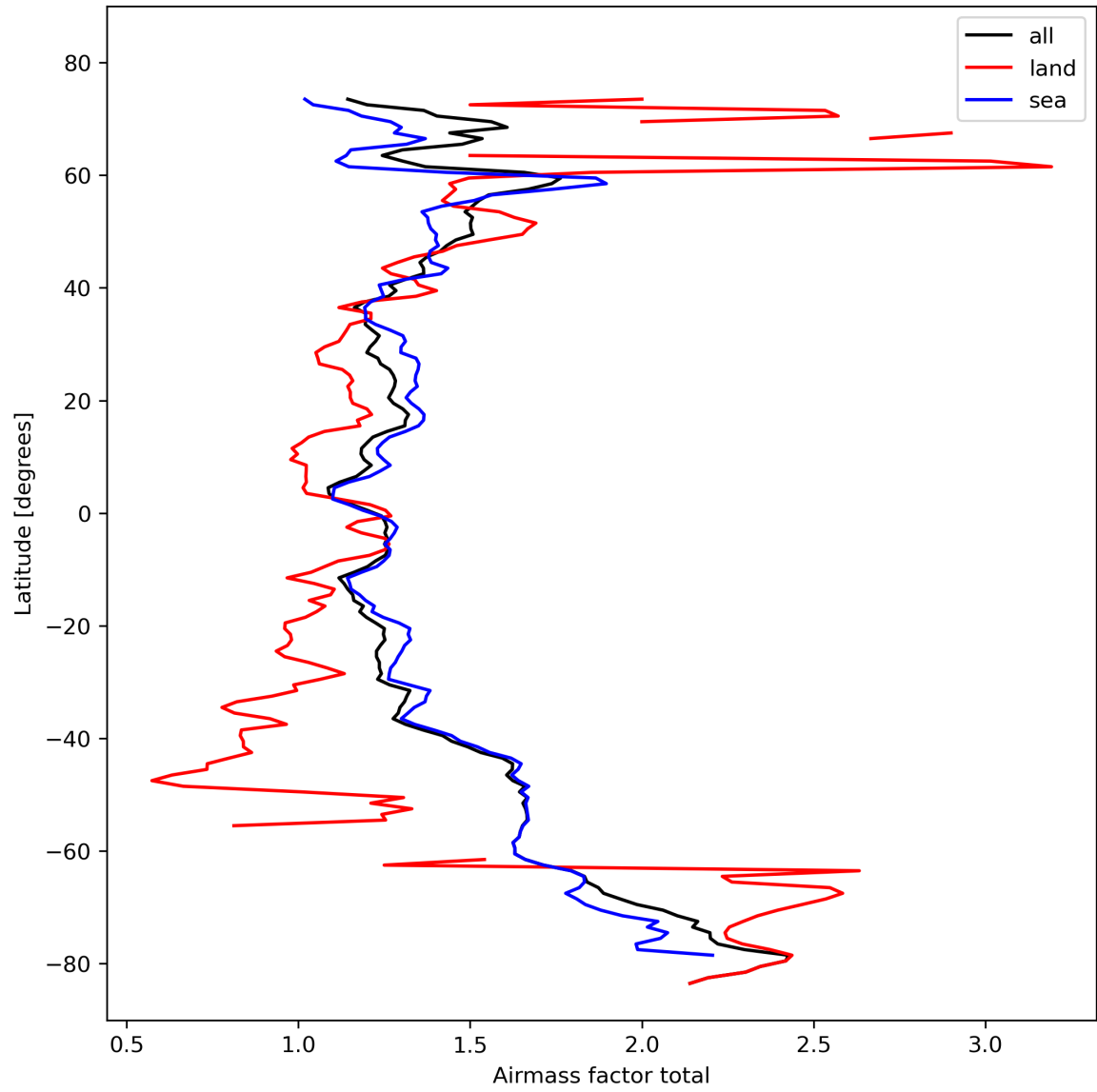
Figure 26: Zonal average of “Airmass factor total” for 2024-02-17 to 2024-02-19.
