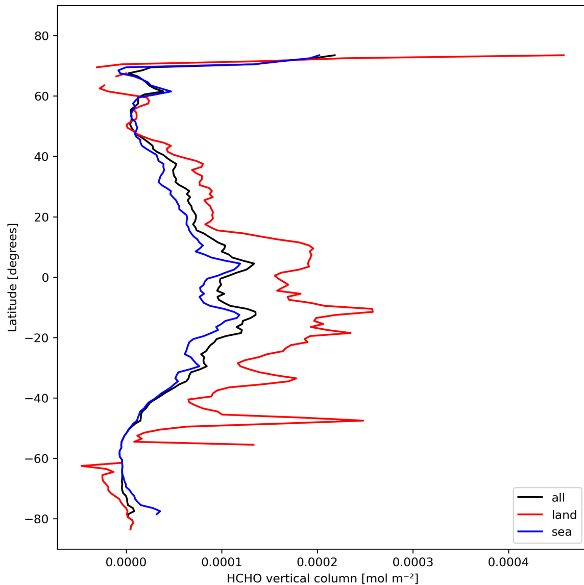
Figure 21: Zonal average of “HCHO vertical column” for 2024-02-17 to 2024-02-19.
