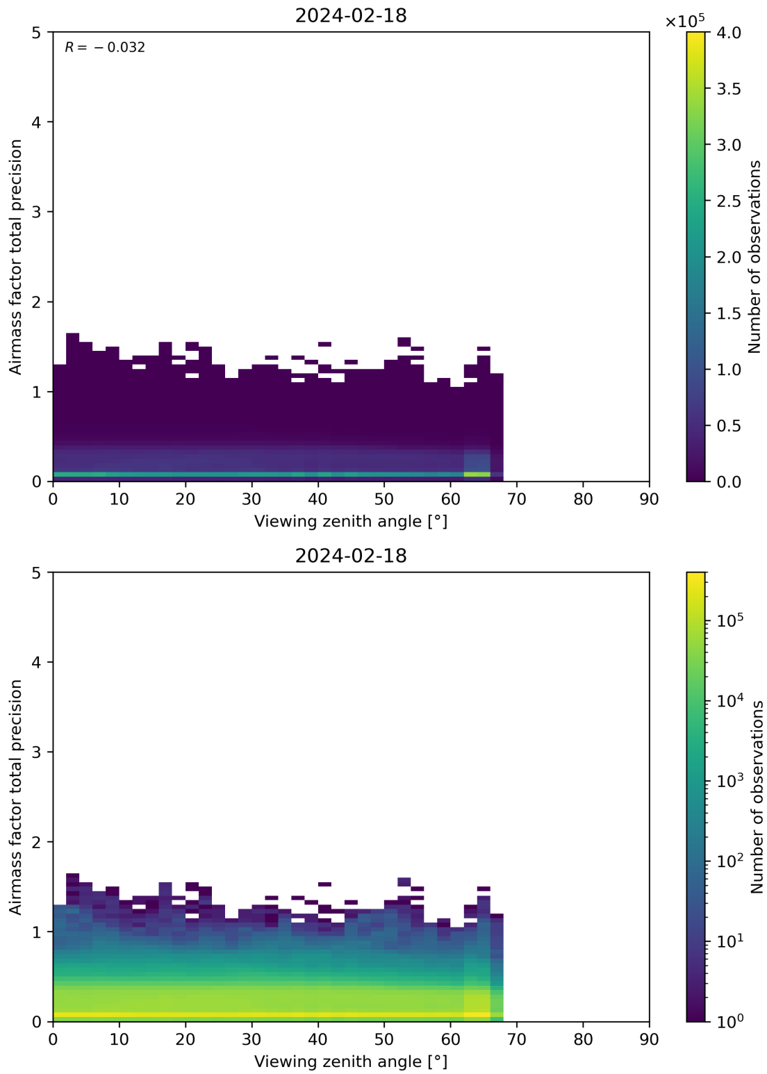
Figure 191: Scatter density plot of “Viewing zenith angle” against “Airmass factor total precision” for 2024-02-17 to 2024-02-19.
