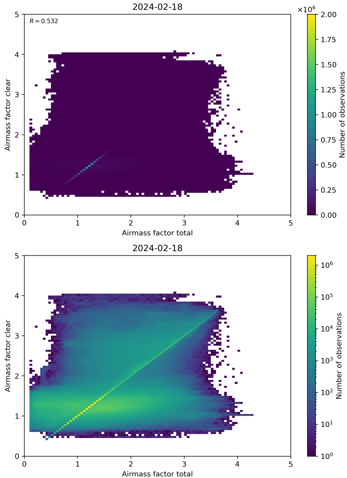
Figure 100: Scatter density plot of “Airmass factor total” against “Airmass factor clear” for 2024-02-17 to 2024-02-19.
