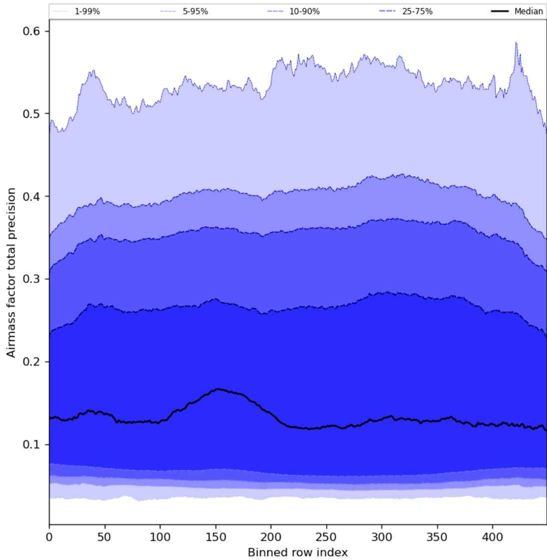
Figure 55: Along track statistics of “Airmass factor total precision” for 2024-02-19 to 2024-02-21
