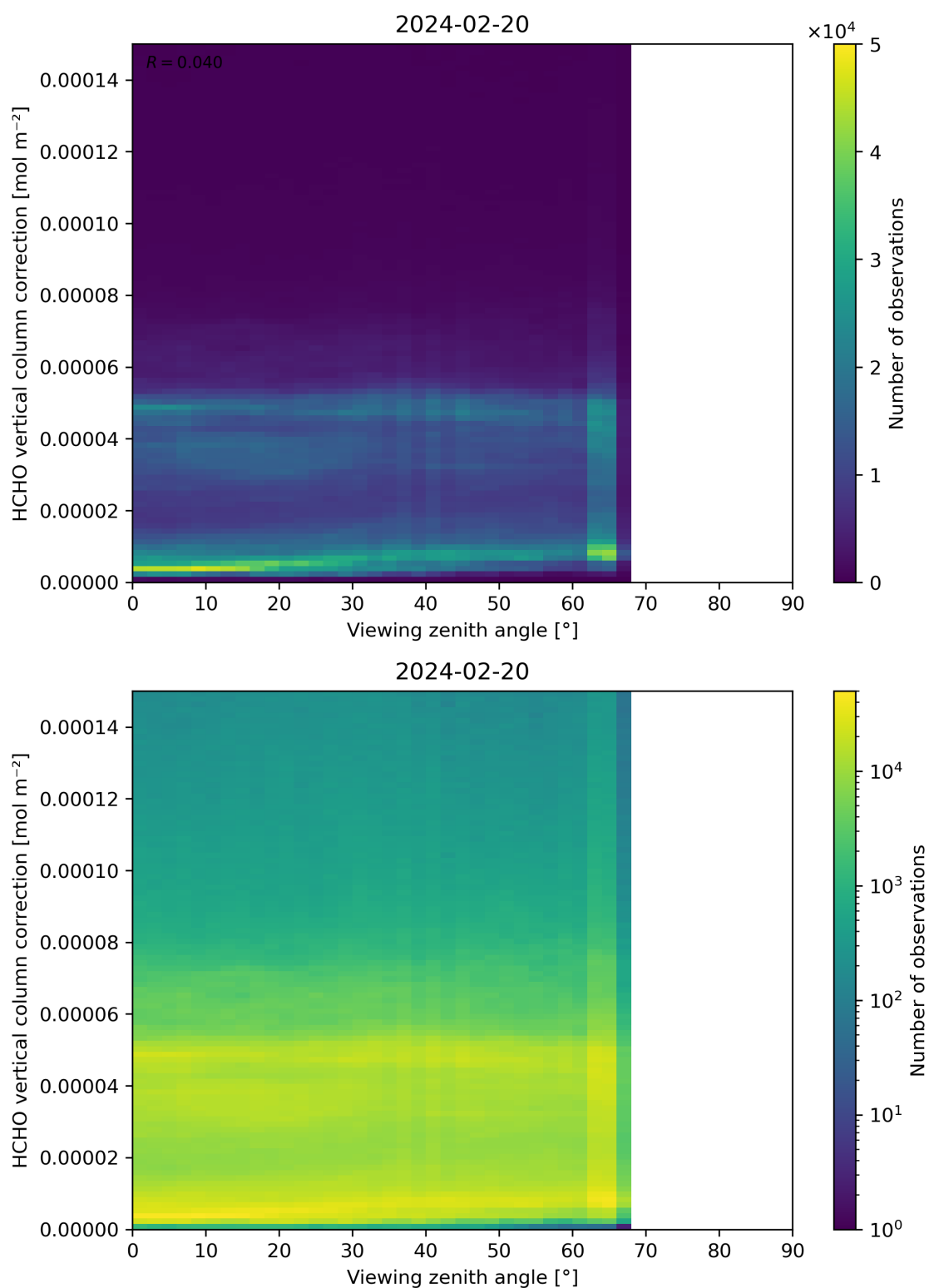
Figure 193: Scatter density plot of “Viewing zenith angle” against “HCHO vertical column correction” for 2024-02-19 to 2024-02-21.
