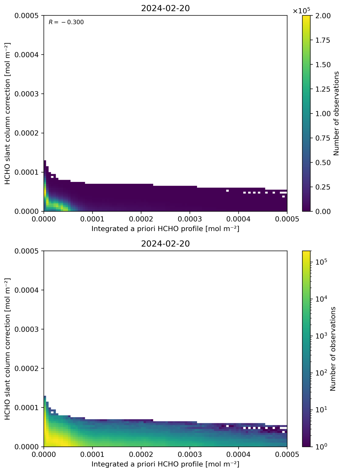
Figure 152: Scatter density plot of “Integrated a priori HCHO profile” against “HCHO slant column correction” for 2024-02-19 to 2024-02-21.
