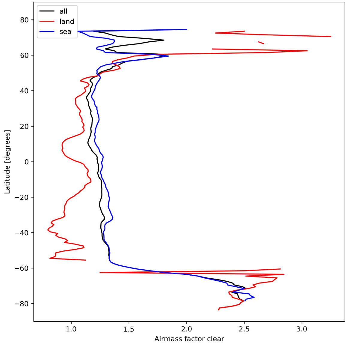
Figure 28: Zonal average of “Airmass factor clear” for 2024-02-19 to 2024-02-21.
