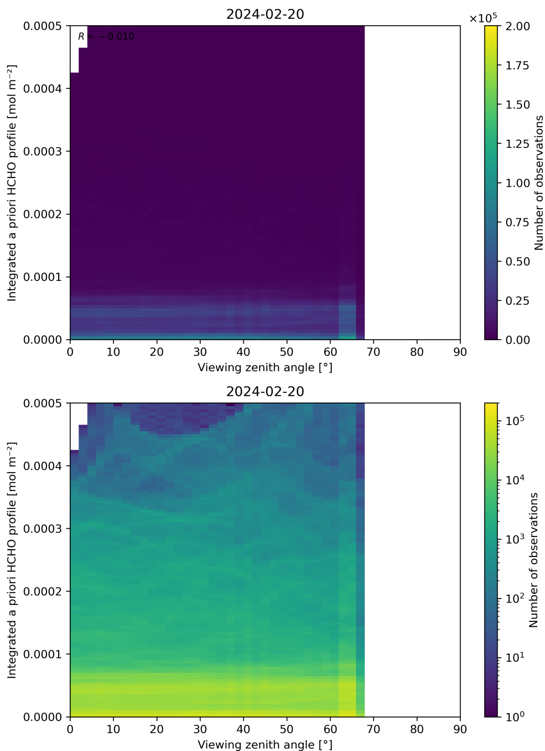
Figure 195: Scatter density plot of “Viewing zenith angle” against “Integrated a priori HCHO profile” for 2024-02-19 to 2024-02-21.
