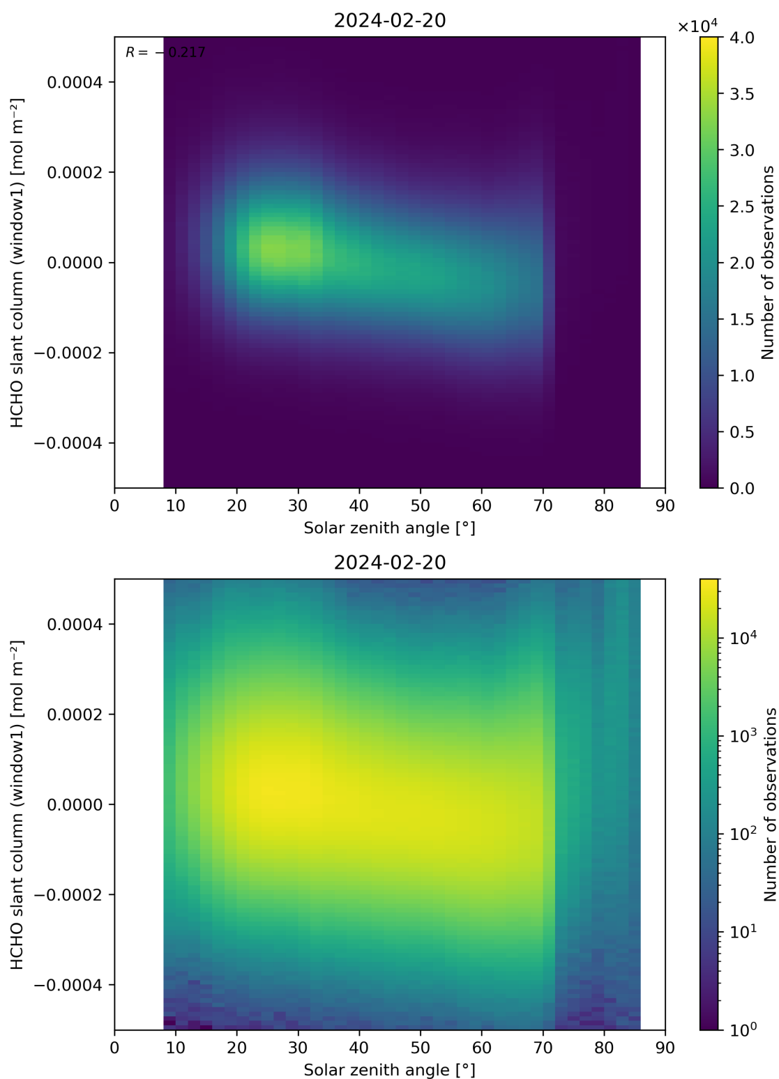
Figure 173: Scatter density plot of “Solar zenith angle” against “HCHO slant column (window1)” for 2024-02-19 to 2024-02-21.
