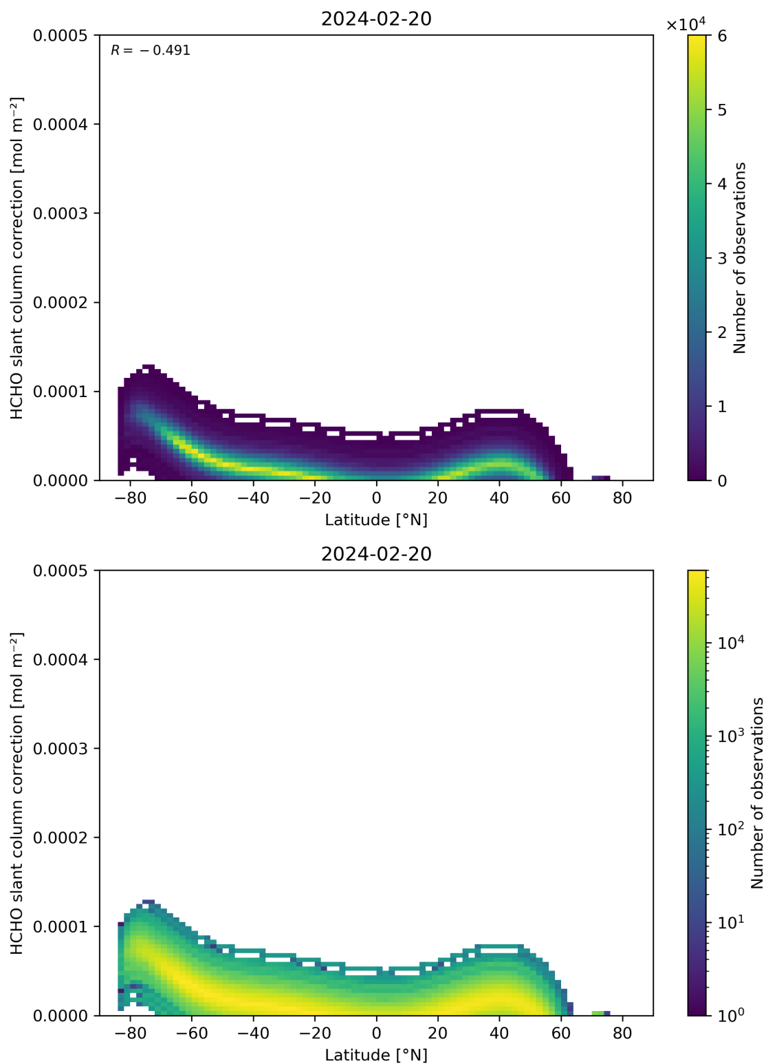
Figure 158: Scatter density plot of “Latitude” against “HCHO slant column correction” for 2024-02-19 to 2024-02-21.
