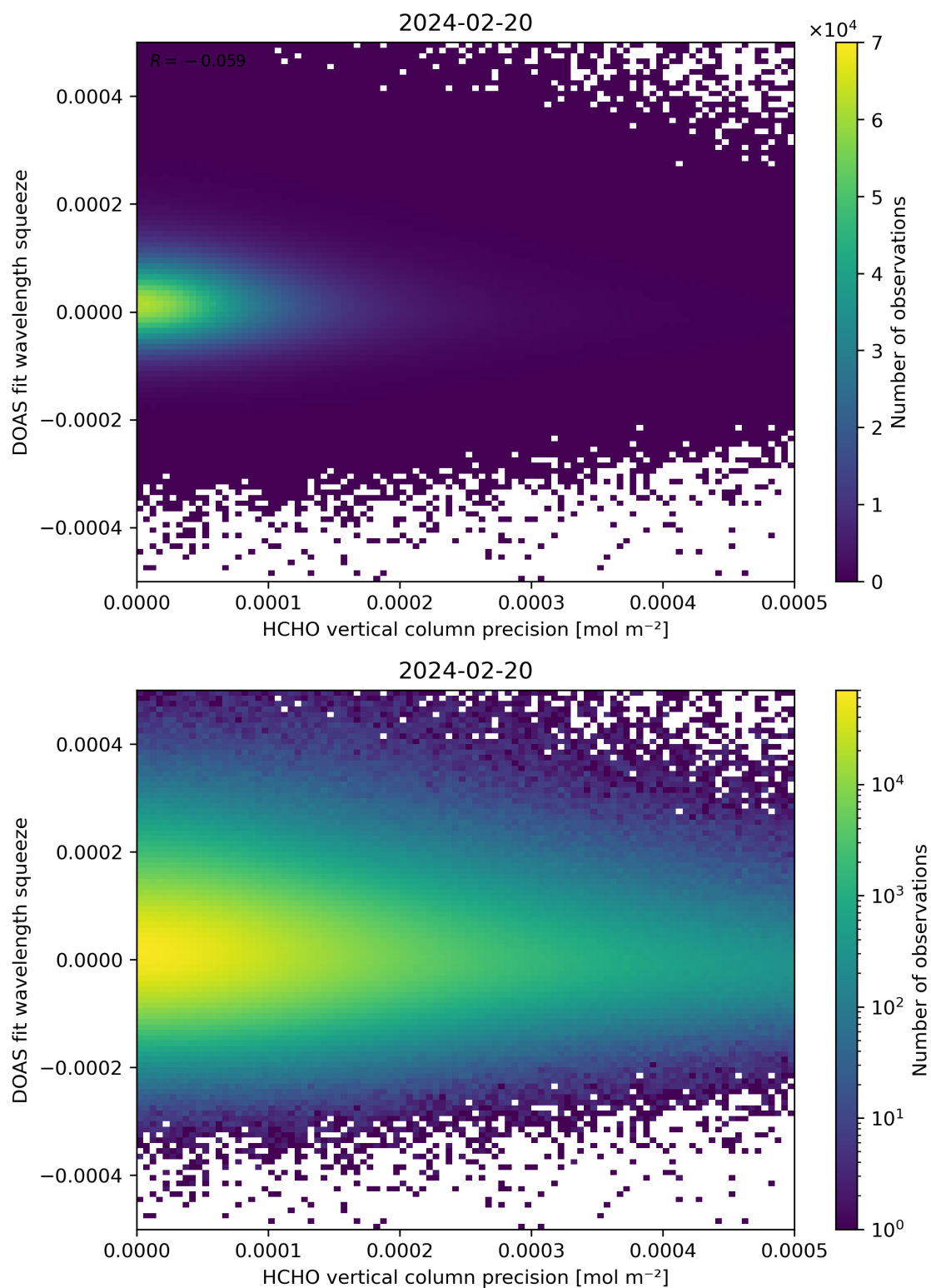
Figure 138: Scatter density plot of “HCHO vertical column precision” against “DOAS fit wavelength squeeze” for 2024-02-19 to 2024-02-21.
