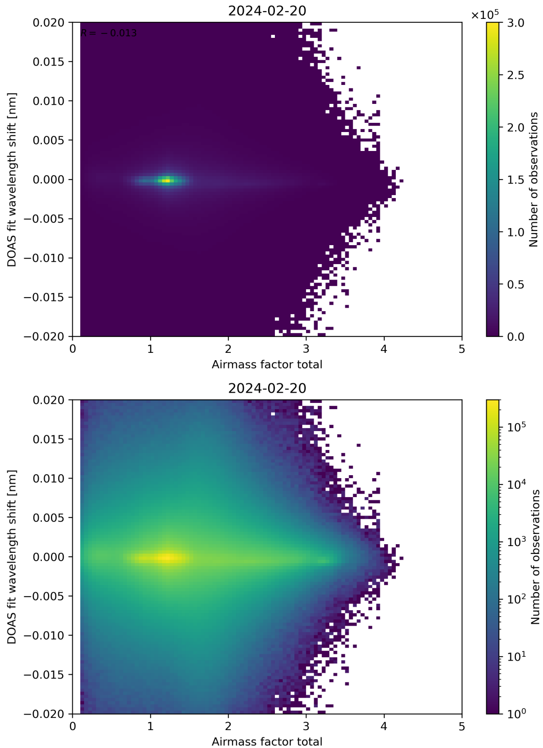
Figure 98: Scatter density plot of “Airmass factor total” against “DOAS fit wavelength shift” for 2024-02-19 to 2024-02-21.
