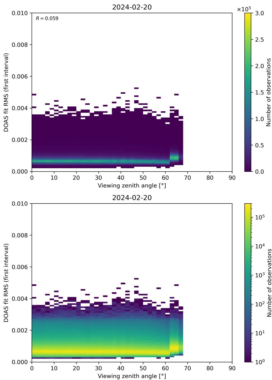
Figure 182: Scatter density plot of “Viewing zenith angle” against “DOAS fit RMS (first interval)” for 2024-02-19 to 2024-02-21.
