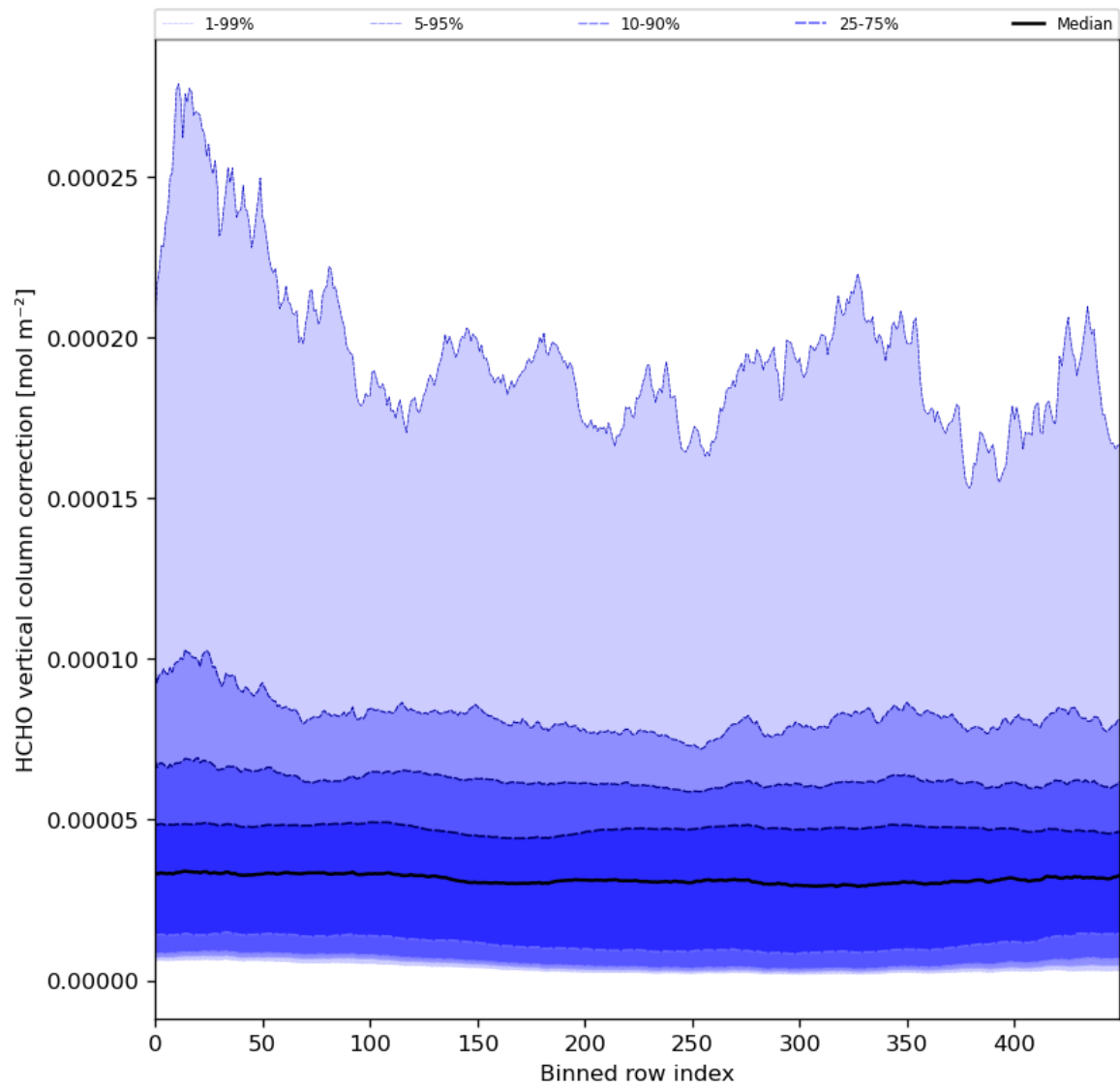
Figure 51: Along track statistics of “HCHO vertical column correction” for 2024-02-19 to 2024-02-21
