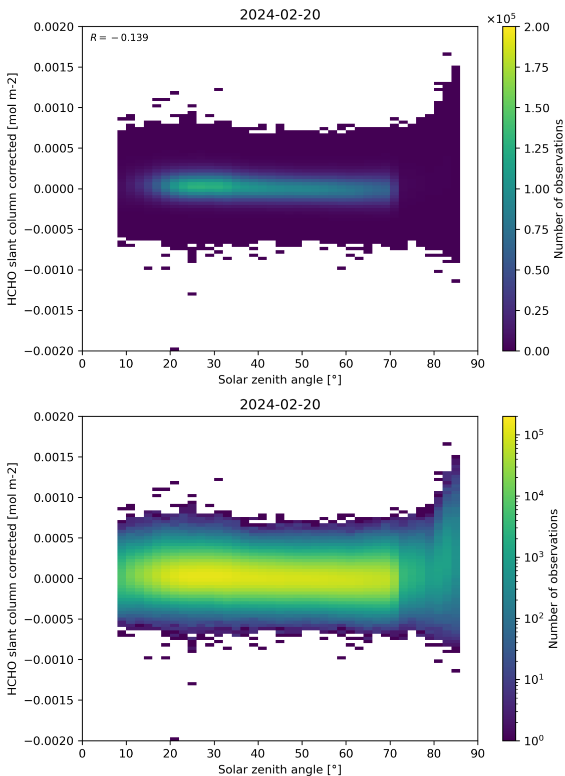
Figure 171: Scatter density plot of “Solar zenith angle” against “HCHO slant column corrected” for 2024-02-19 to 2024-02-21.
