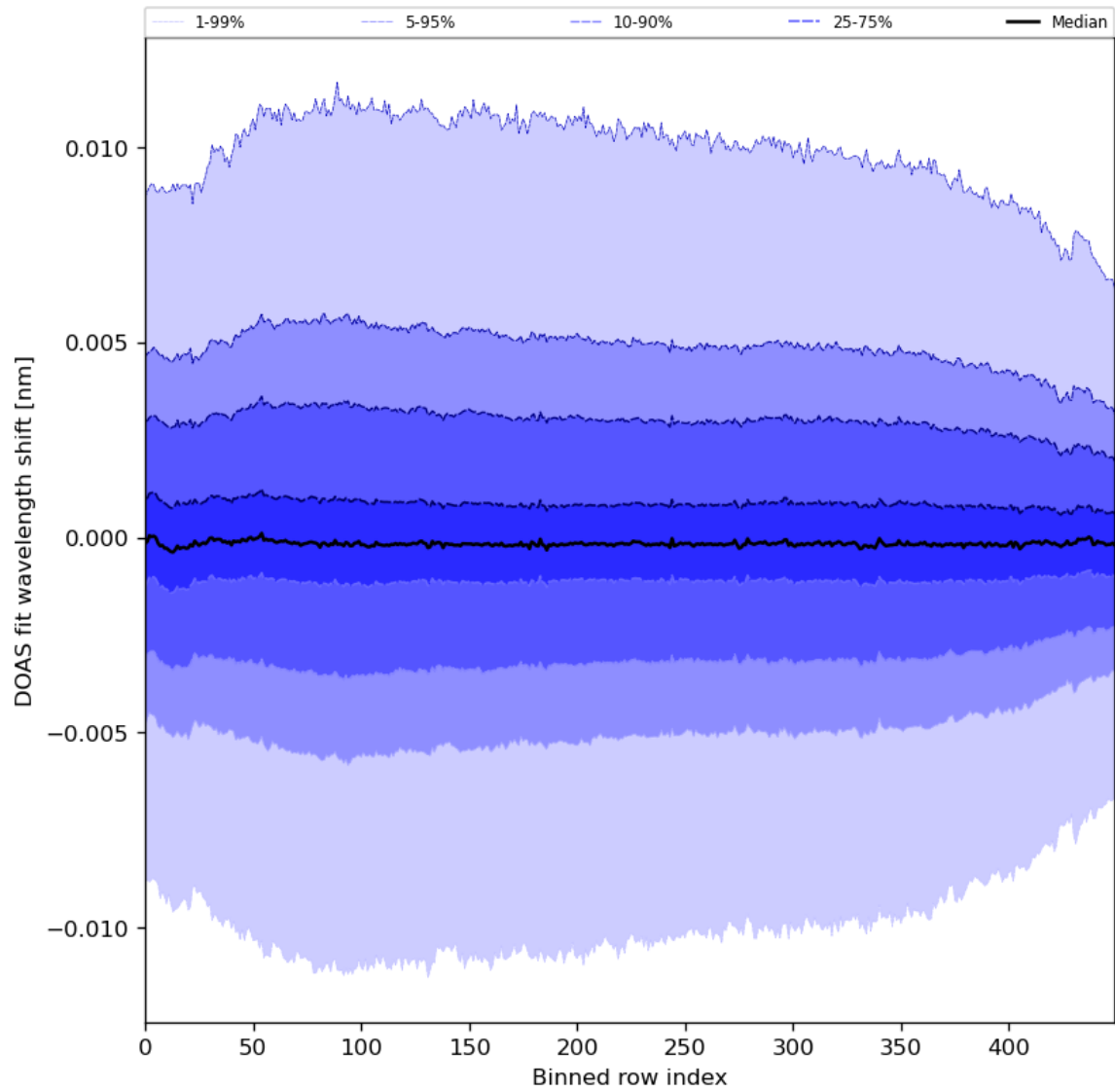
Figure 58: Along track statistics of “DOAS fit wavelength shift” for 2024-02-19 to 2024-02-21
