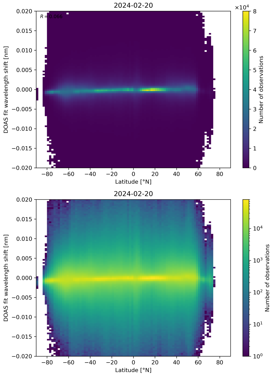
Figure 154: Scatter density plot of “Latitude” against “DOAS fit wavelength shift” for 2024-02-19 to 2024-02-21.
