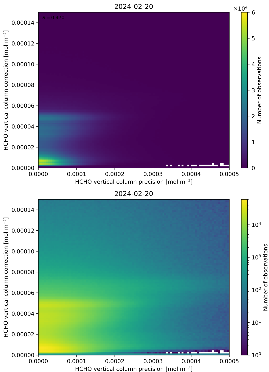
Figure 146: Scatter density plot of “HCHO vertical column precision” against “HCHO vertical column correction” for 2024-02-19 to 2024-02-21.
