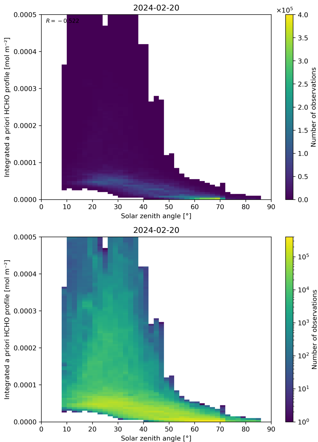
Figure 180: Scatter density plot of “Solar zenith angle” against “Integrated a priori HCHO profile” for 2024-02-19 to 2024-02-21.
