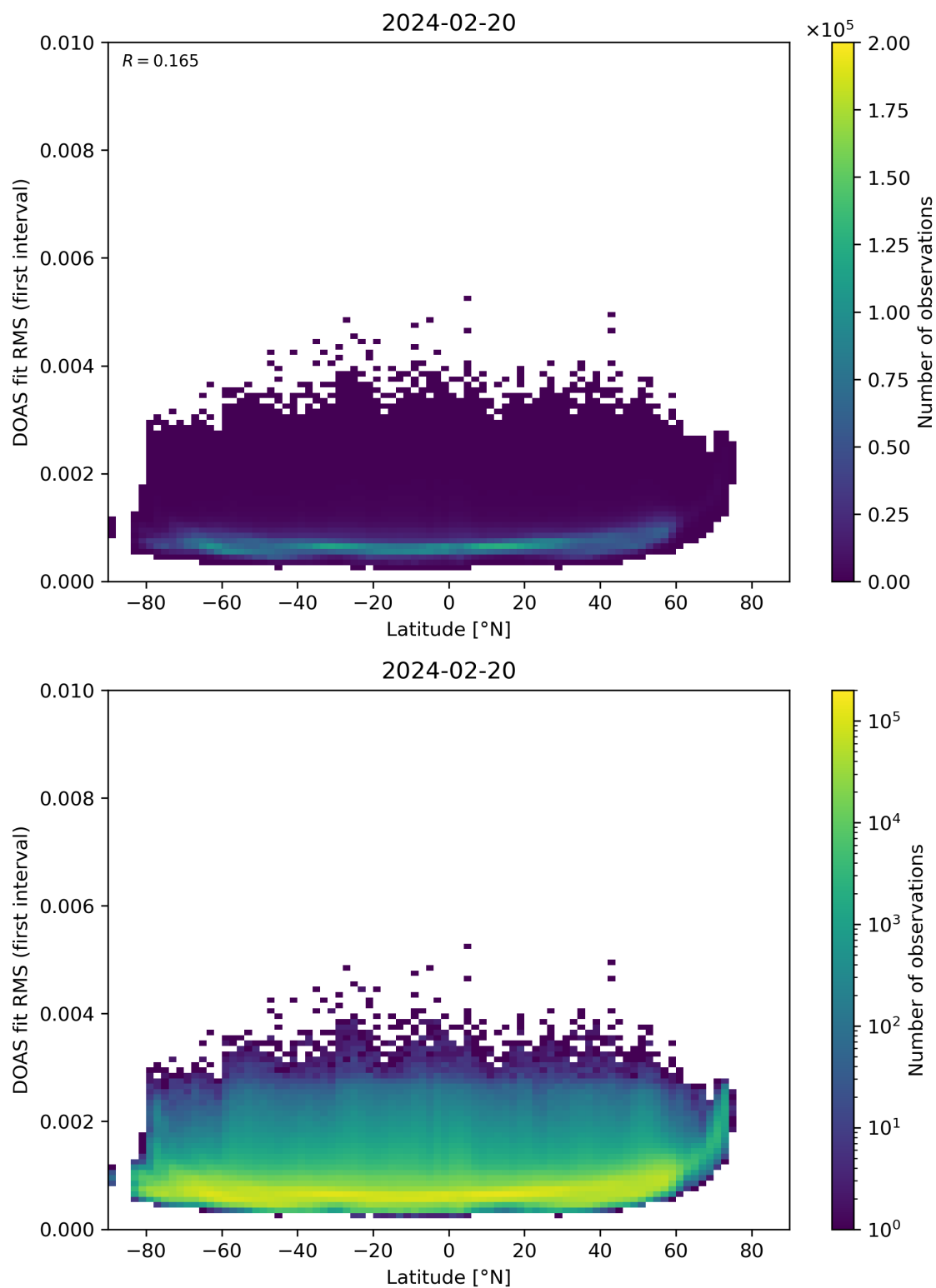
Figure 153: Scatter density plot of “Latitude” against “DOAS fit RMS (first interval)” for 2024-02-19 to 2024-02-21.
