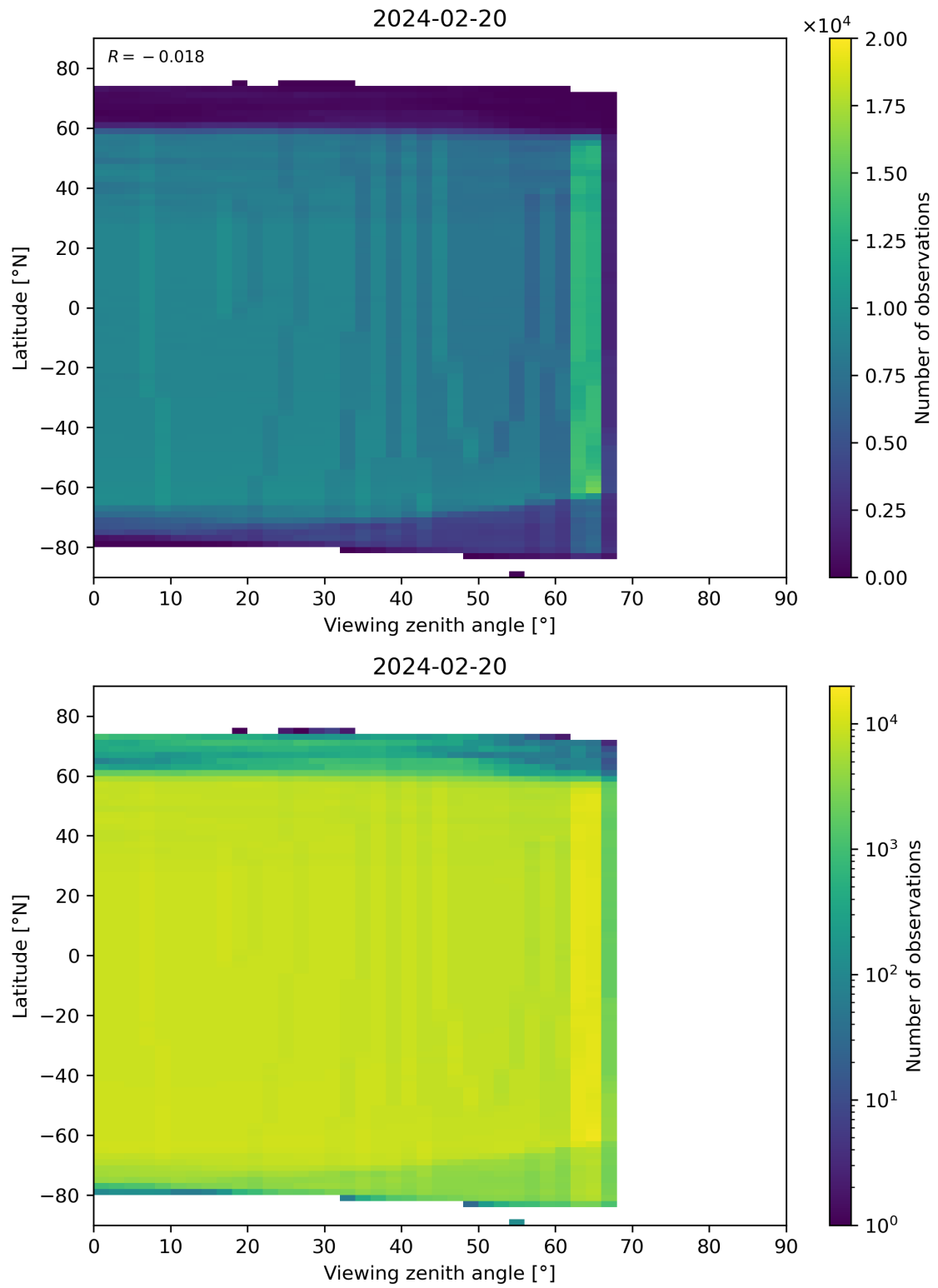
Figure 196: Scatter density plot of “Viewing zenith angle” against “Latitude” for 2024-02-19 to 2024-02-21.
