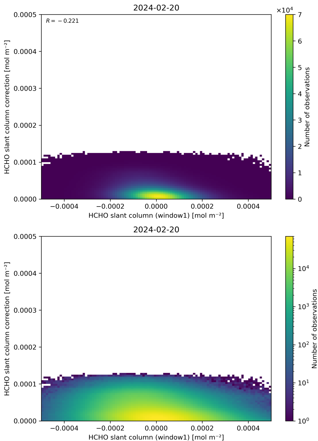
Figure 83: Scatter density plot of “HCHO slant column (window1)” against “HCHO slant column correction” for 2024-02-19 to 2024-02-21.
