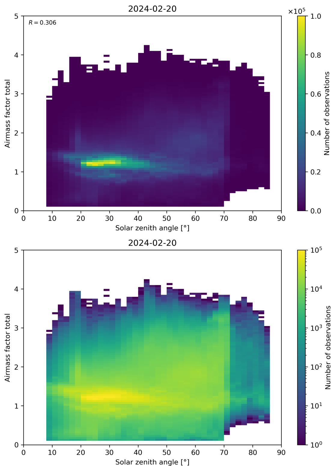
Figure 175: Scatter density plot of “Solar zenith angle” against “Airmass factor total” for 2024-02-19 to 2024-02-21.
