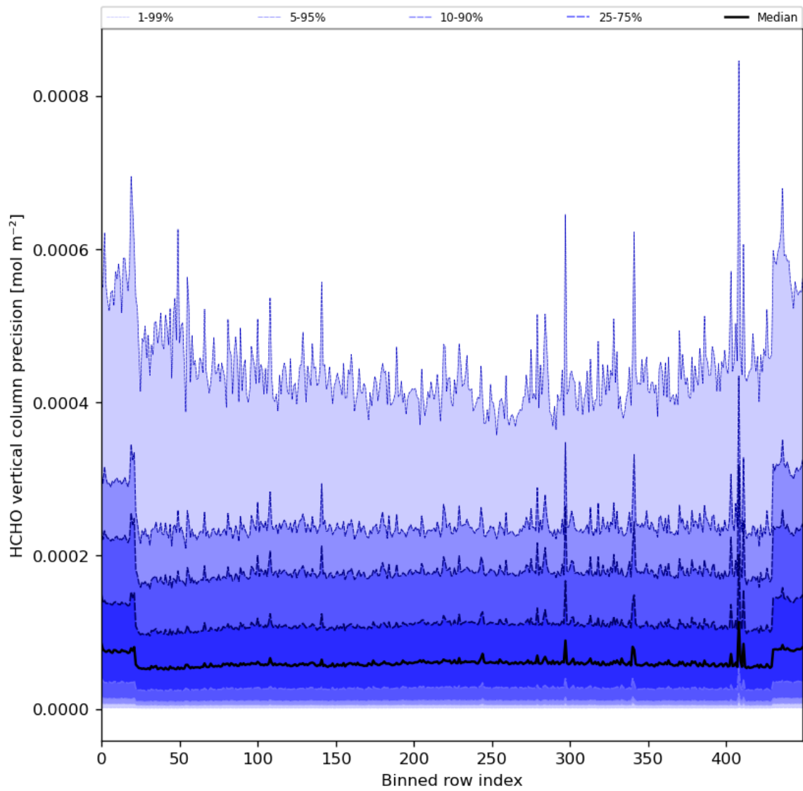
Figure 50: Along track statistics of “HCHO vertical column precision” for 2024-02-19 to 2024-02-21
