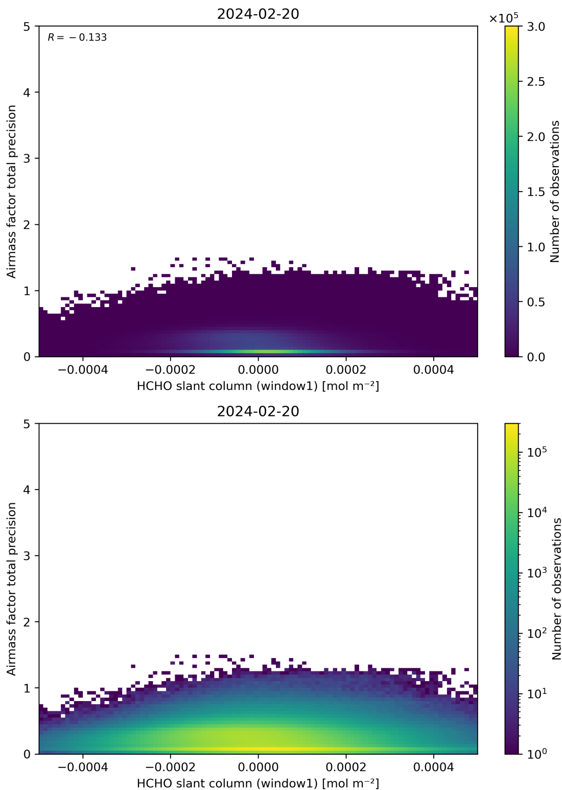
Figure 86: Scatter density plot of “HCHO slant column (window1)” against “Airmass factor total precision” for 2024-02-19 to 2024-02-21.
