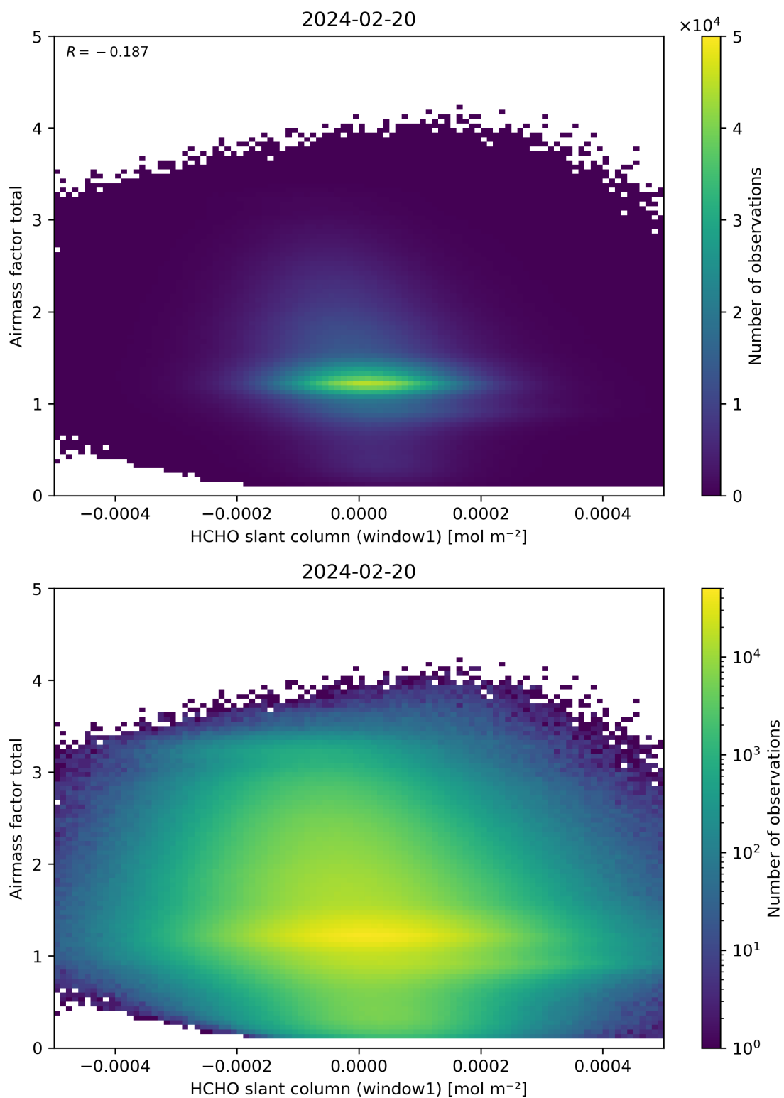
Figure 85: Scatter density plot of “HCHO slant column (window1)” against “Airmass factor total” for 2024-02-19 to 2024-02-21.
