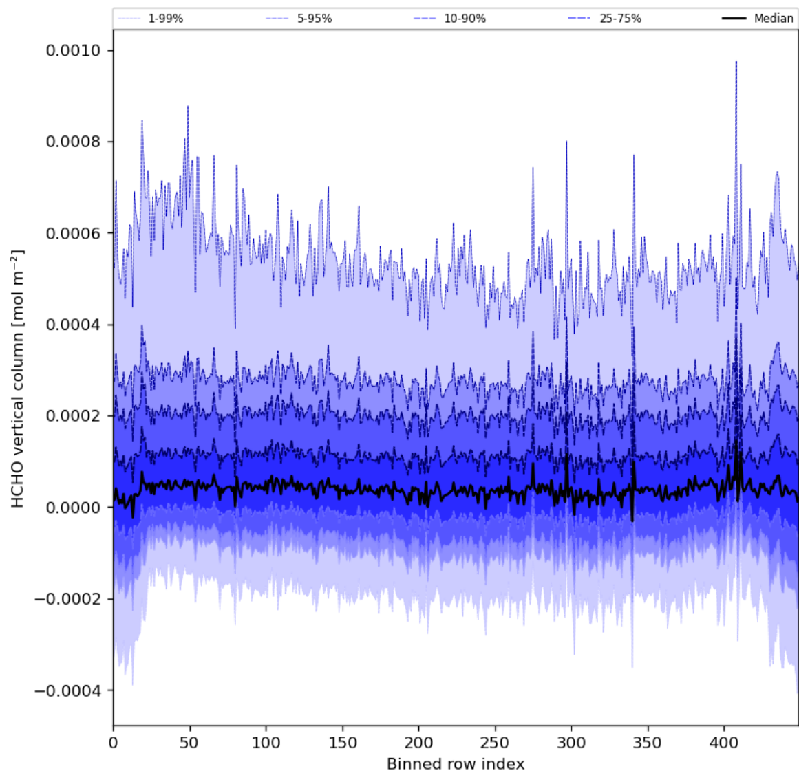
Figure 49: Along track statistics of “HCHO vertical column” for 2024-02-19 to 2024-02-21
