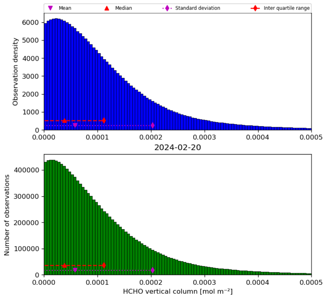
Figure 35: Histogram of “HCHO vertical column” for 2024-02-19 to 2024-02-21
