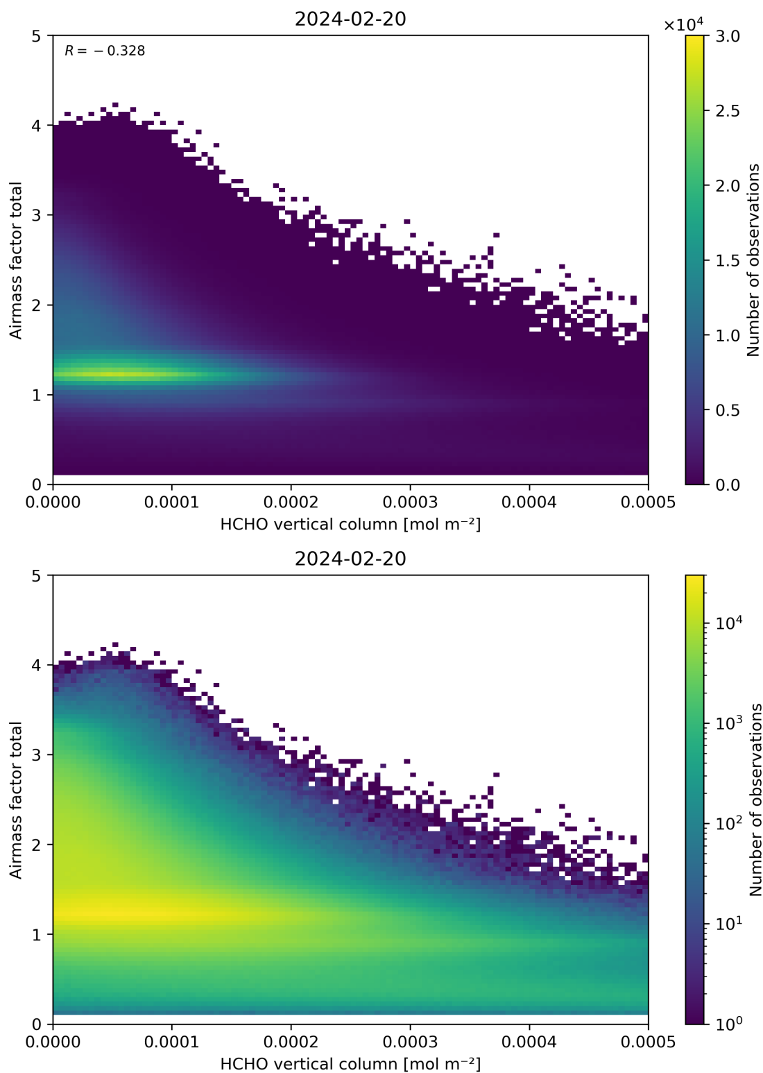
Figure 131: Scatter density plot of “HCHO vertical column” against “Airmass factor total” for 2024-02-19 to 2024-02-21.
