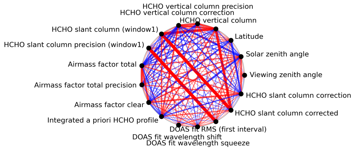
Figure 1: Map of correlation graph for 2024-02-19 to 2024-02-21.
