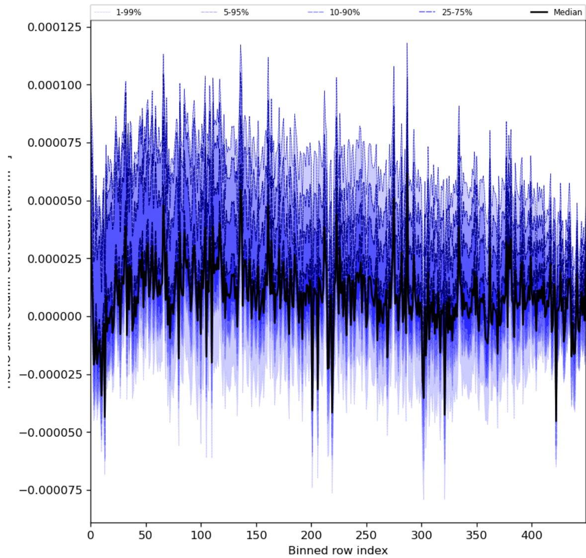
Figure 61: Along track statistics of “HCHO slant column correction” for 2024-02-19 to 2024-02-21
