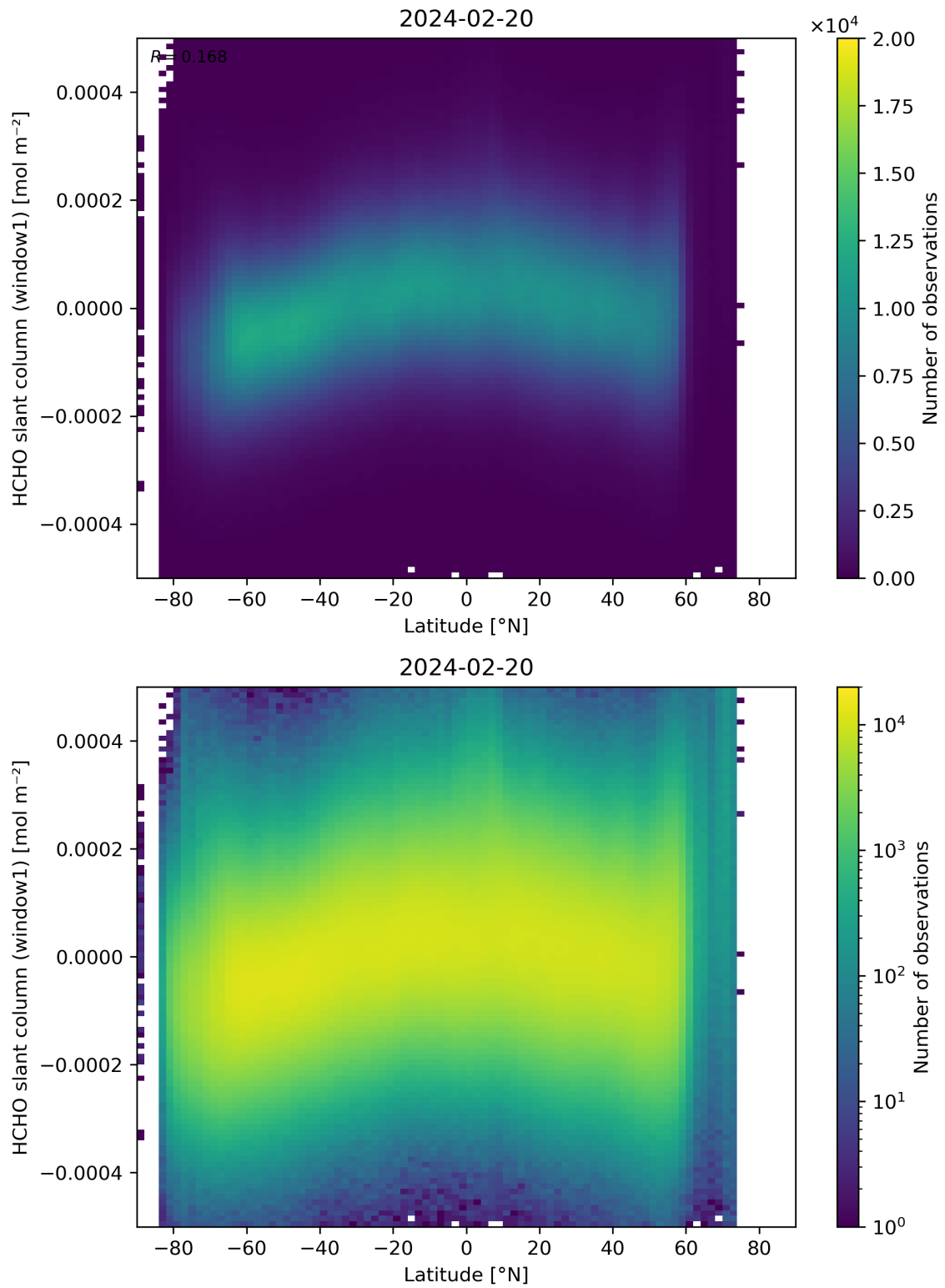
Figure 159: Scatter density plot of “Latitude” against “HCHO slant column (window1)” for 2024-02-19 to 2024-02-21.
