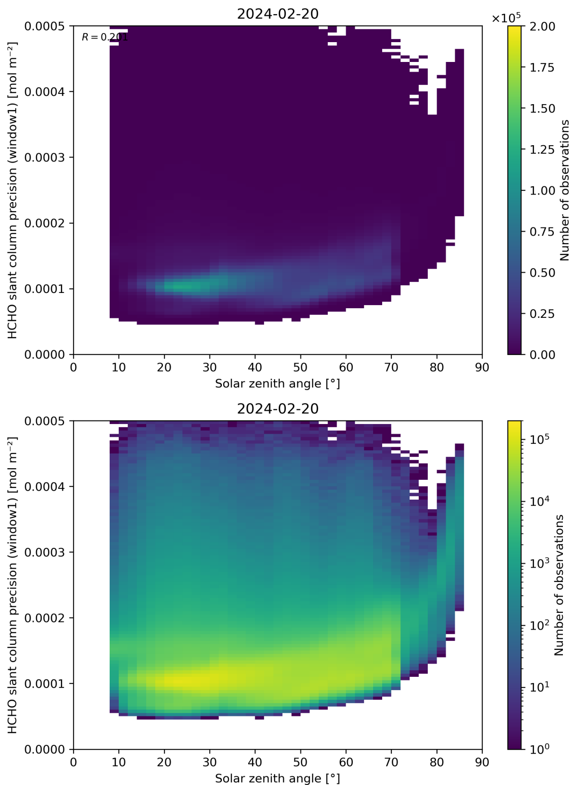
Figure 174: Scatter density plot of “Solar zenith angle” against “HCHO slant column precision (window1)” for 2024-02-19 to 2024-02-21.
