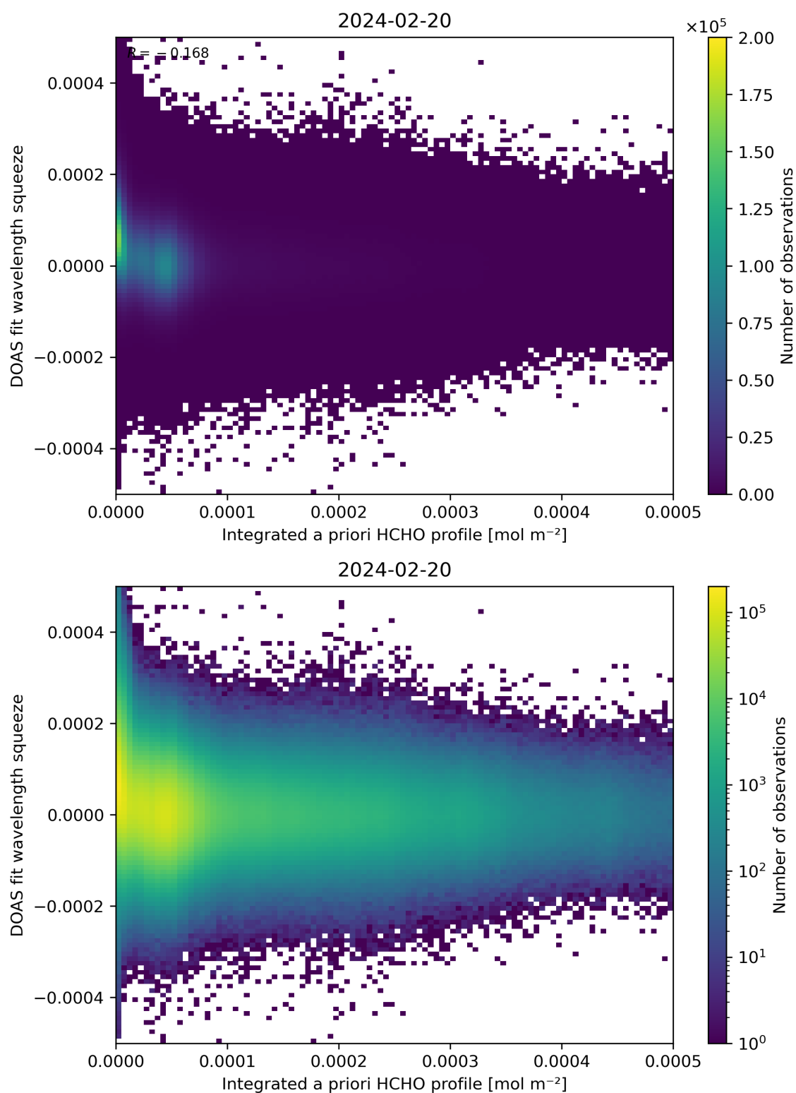
Figure 150: Scatter density plot of “Integrated a priori HCHO profile” against “DOAS fit wavelength squeeze” for 2024-02-19 to 2024-02-21.
