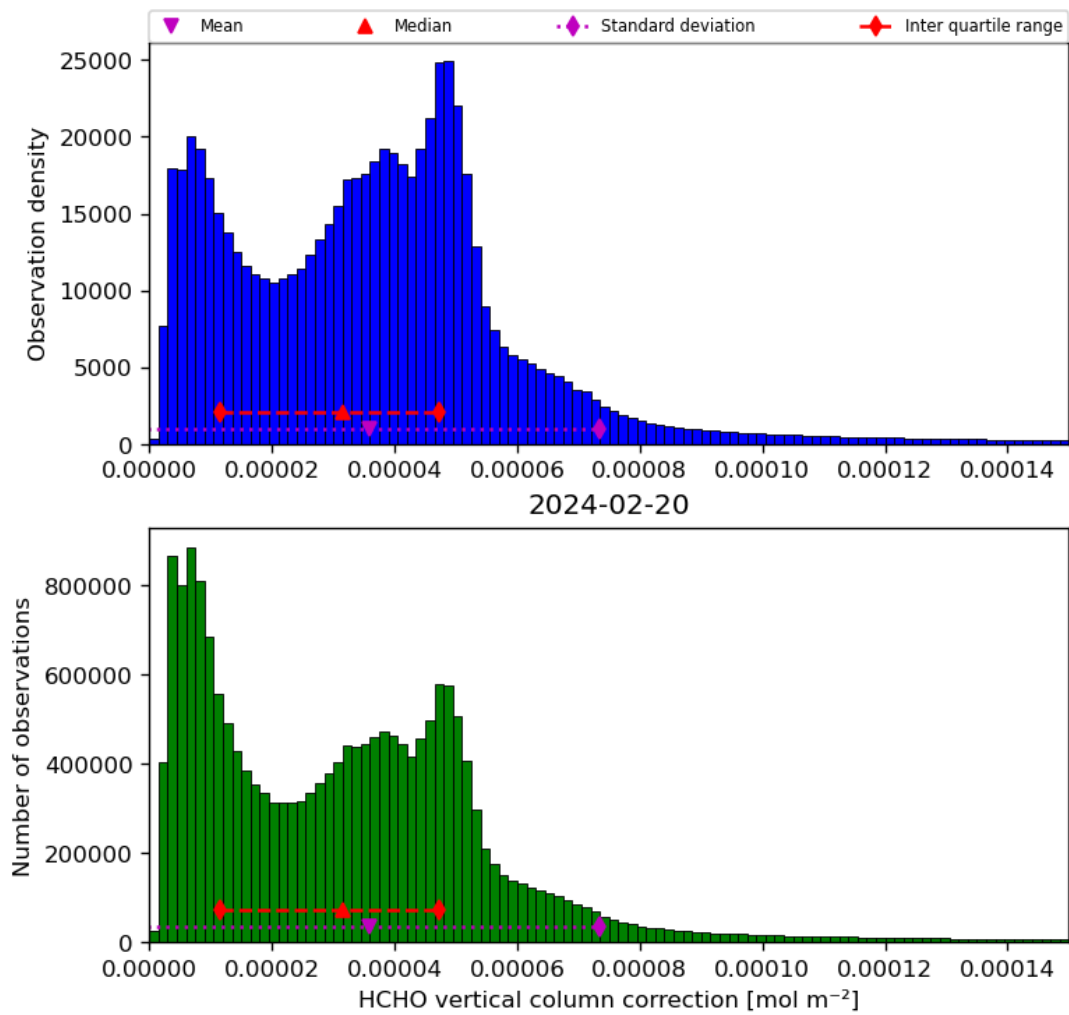
Figure 37: Histogram of “HCHO vertical column correction” for 2024-02-19 to 2024-02-21
