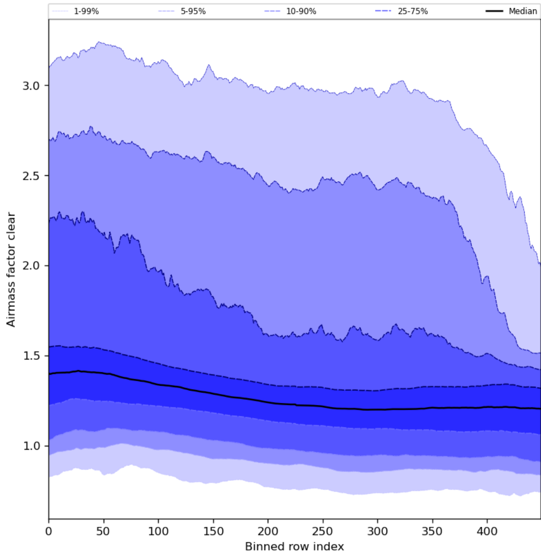
Figure 56: Along track statistics of “Airmass factor clear” for 2024-02-19 to 2024-02-21
