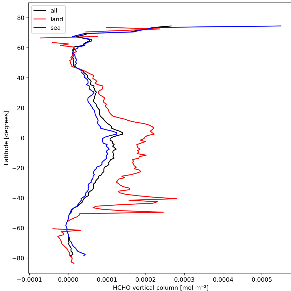
Figure 21: Zonal average of “HCHO vertical column” for 2024-02-19 to 2024-02-21.
