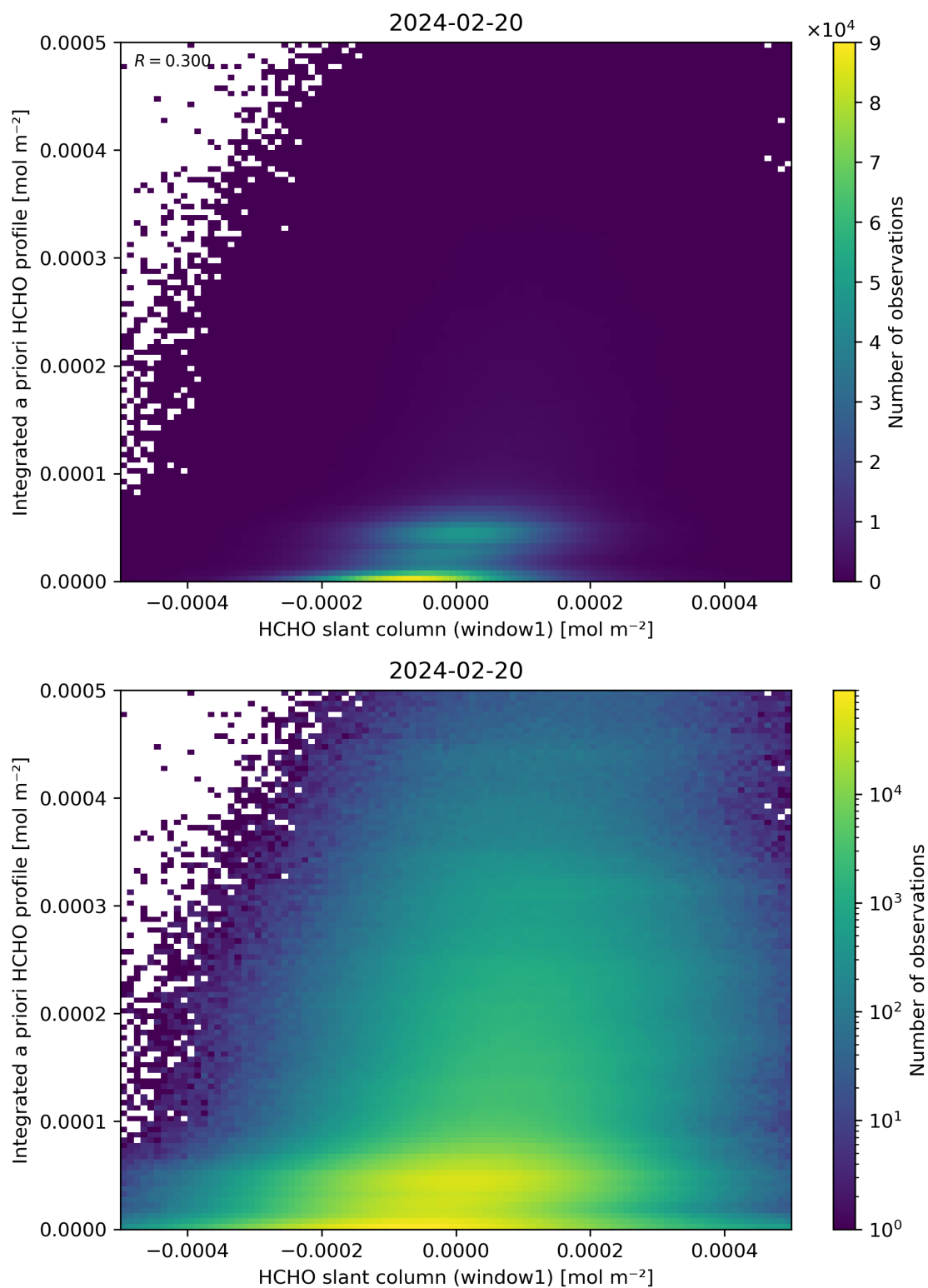
Figure 87: Scatter density plot of “HCHO slant column (window1)” against “Integrated a priori HCHO profile” for 2024-02-19 to 2024-02-21.
