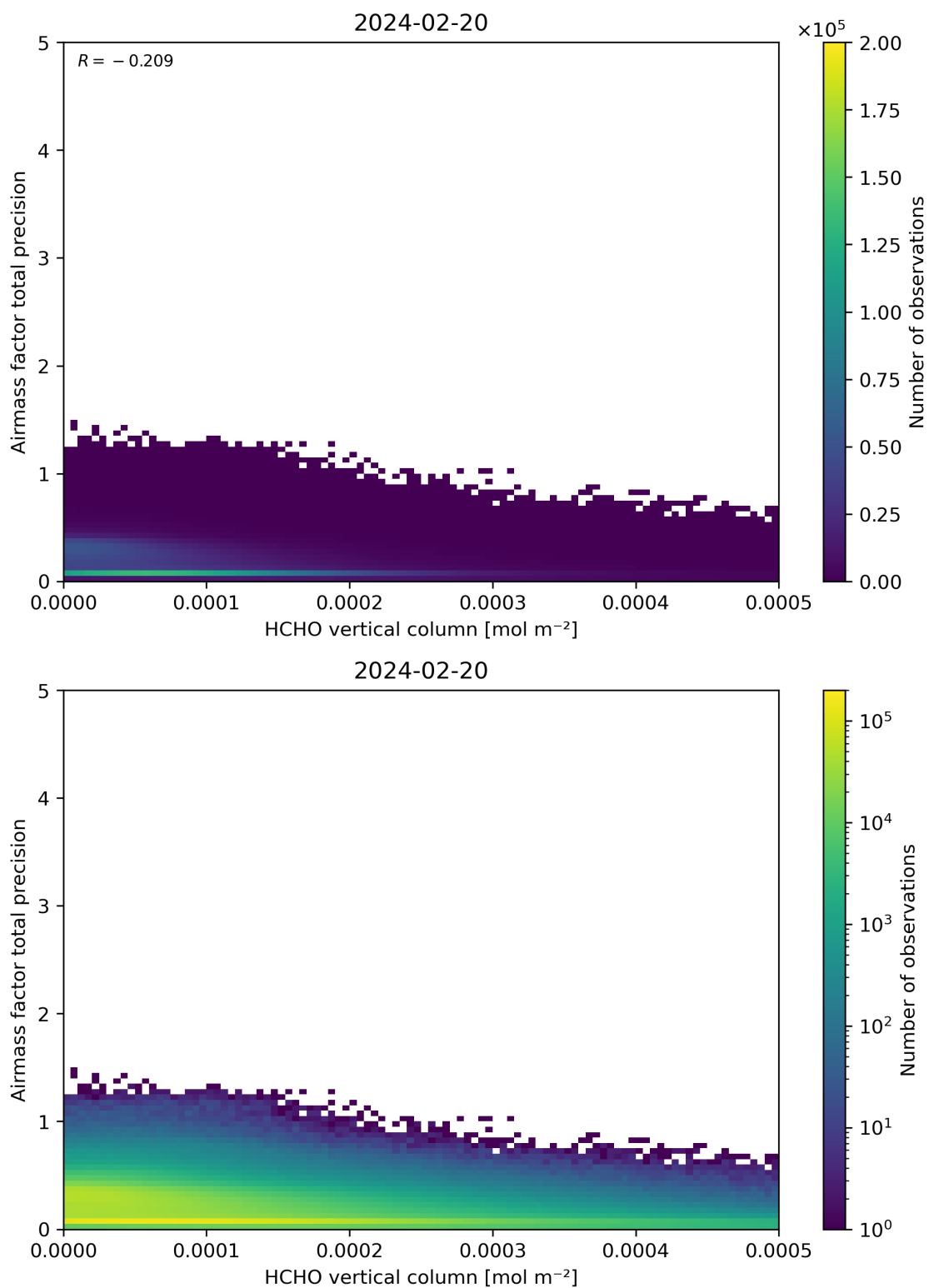
Figure 132: Scatter density plot of “HCHO vertical column” against “Airmass factor total precision” for 2024-02-19 to 2024-02-21.
