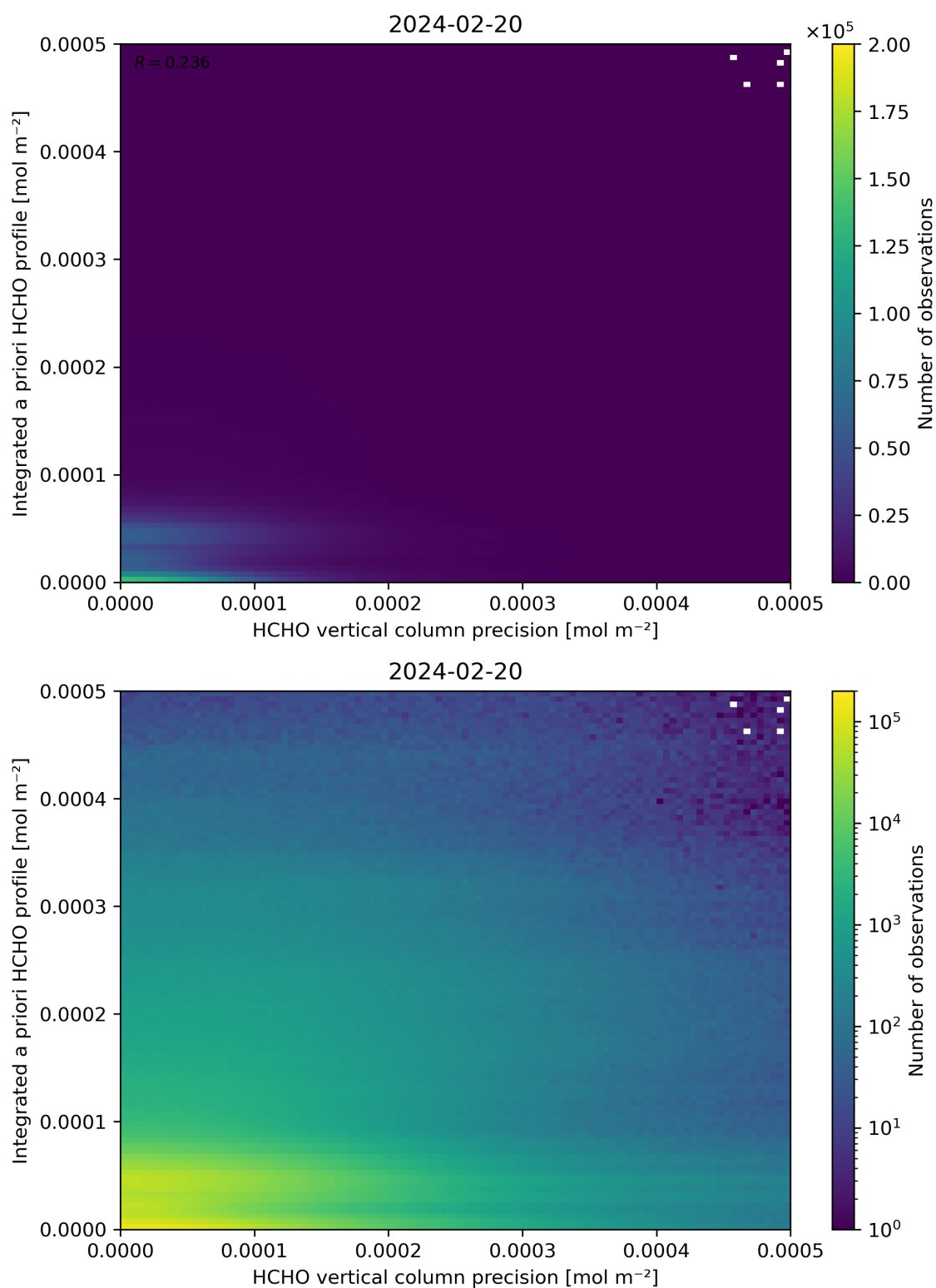
Figure 147: Scatter density plot of “HCHO vertical column precision” against “Integrated a priori HCHO profile” for 2024-02-19 to 2024-02-21.
