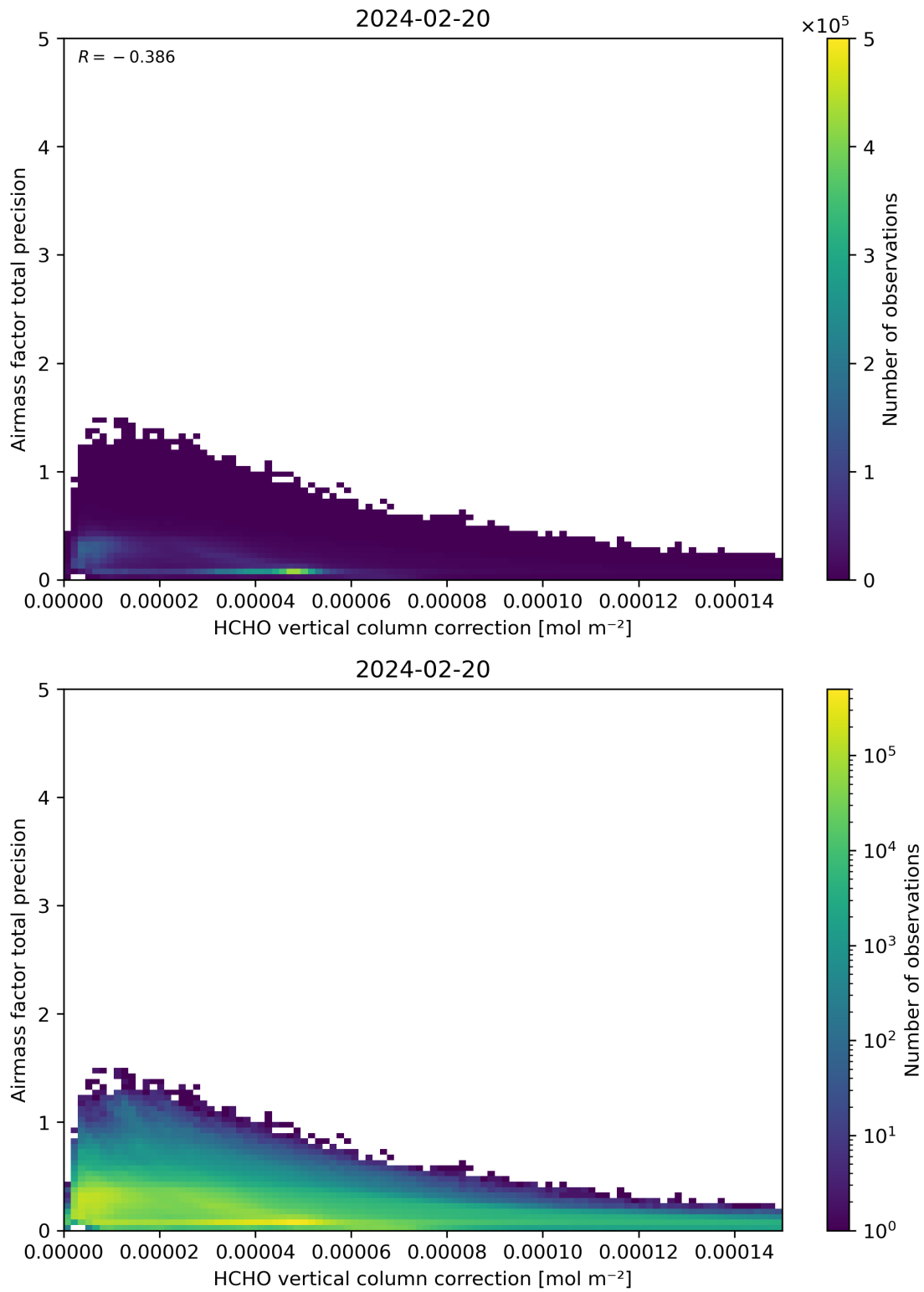
Figure 121: Scatter density plot of “HCHO vertical column correction” against “Airmass factor total precision” for 2024-02-19 to 2024-02-21.
