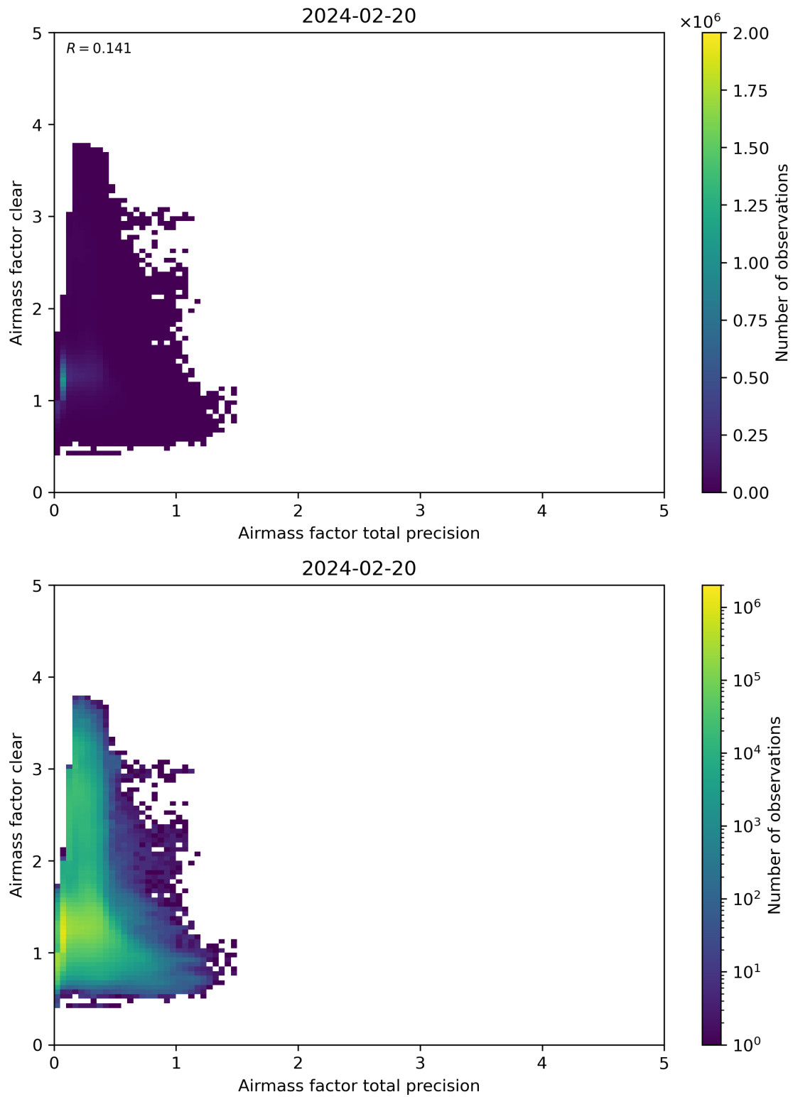
Figure 108: Scatter density plot of “Airmass factor total precision” against “Airmass factor clear” for 2024-02-19 to 2024-02-21.
