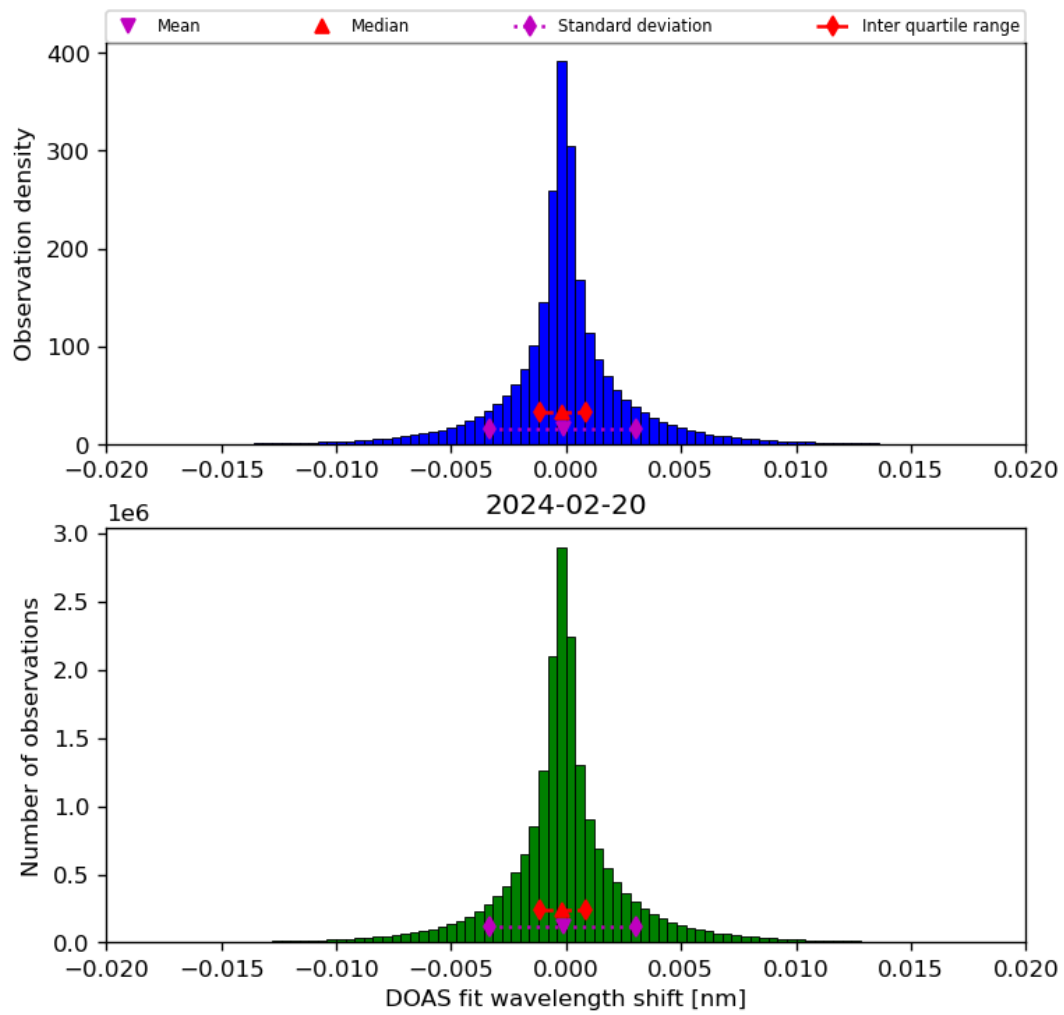
Figure 44: Histogram of “DOAS fit wavelength shift” for 2024-02-19 to 2024-02-21
