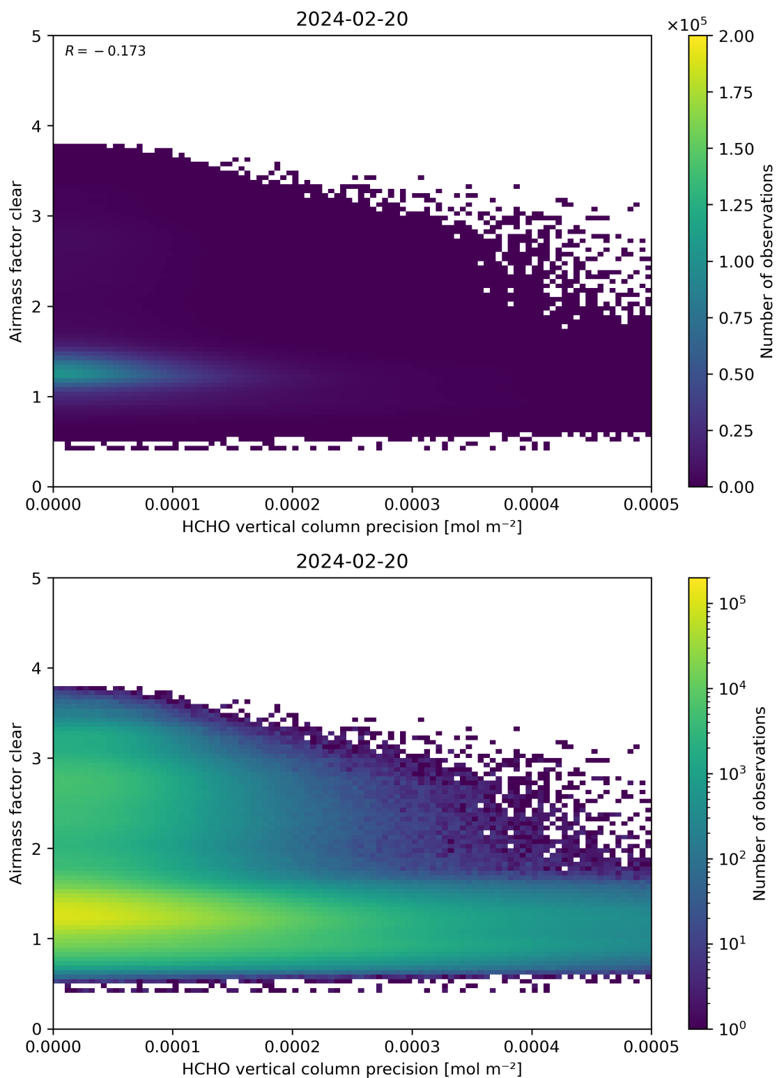
Figure 139: Scatter density plot of “HCHO vertical column precision” against “Airmass factor clear” for 2024-02-19 to 2024-02-21.
