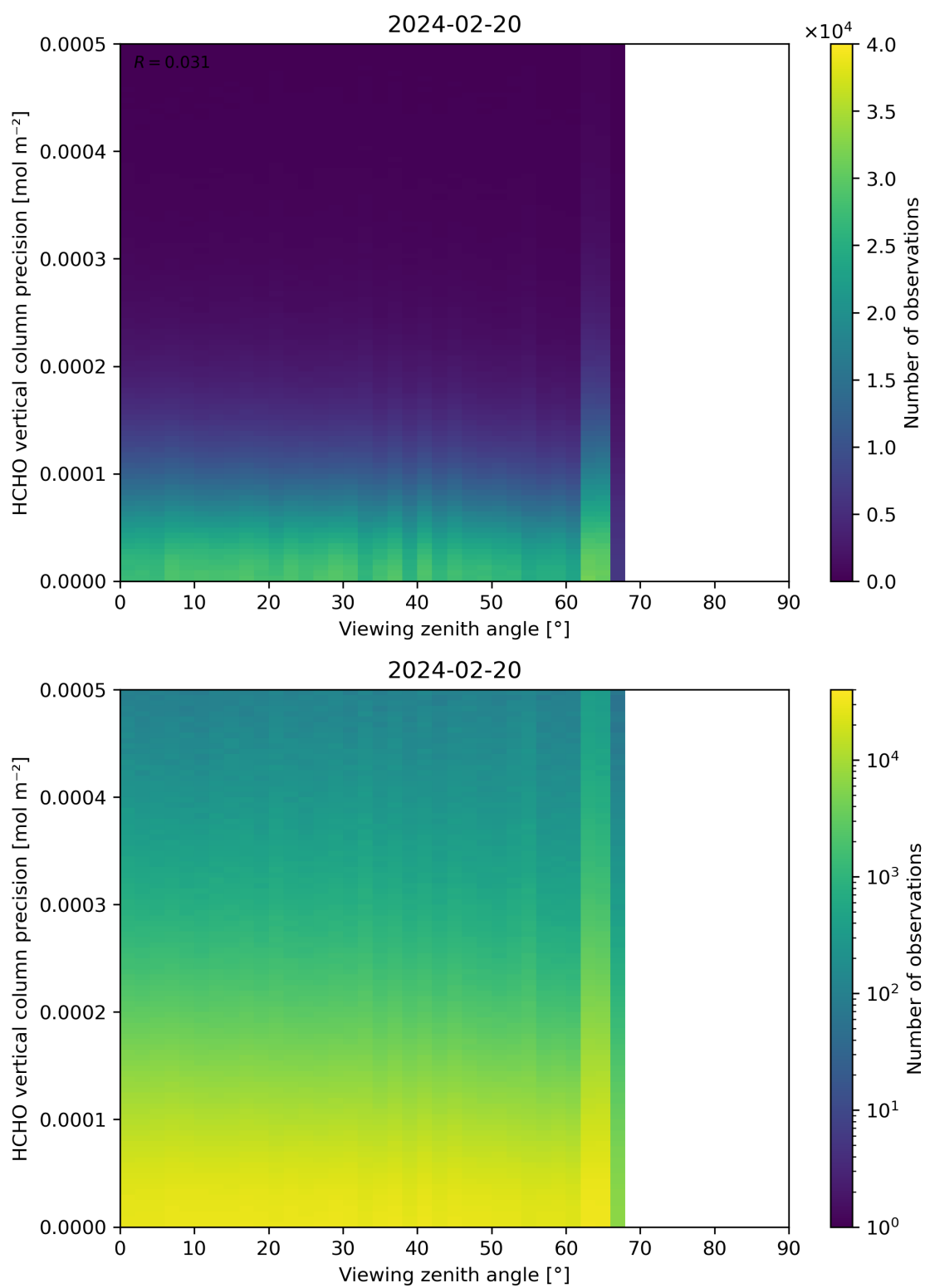
Figure 194: Scatter density plot of “Viewing zenith angle” against “HCHO vertical column precision” for 2024-02-19 to 2024-02-21.
