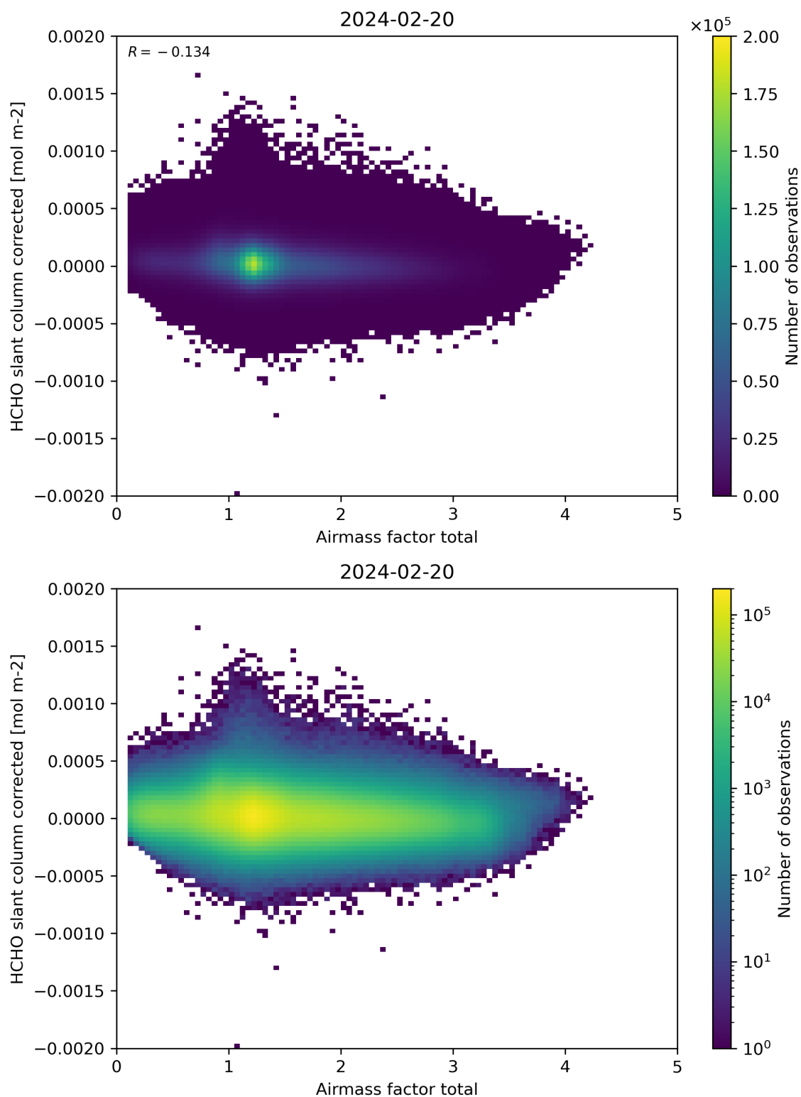
Figure 101: Scatter density plot of “Airmass factor total” against “HCHO slant column corrected” for 2024-02-19 to 2024-02-21.
