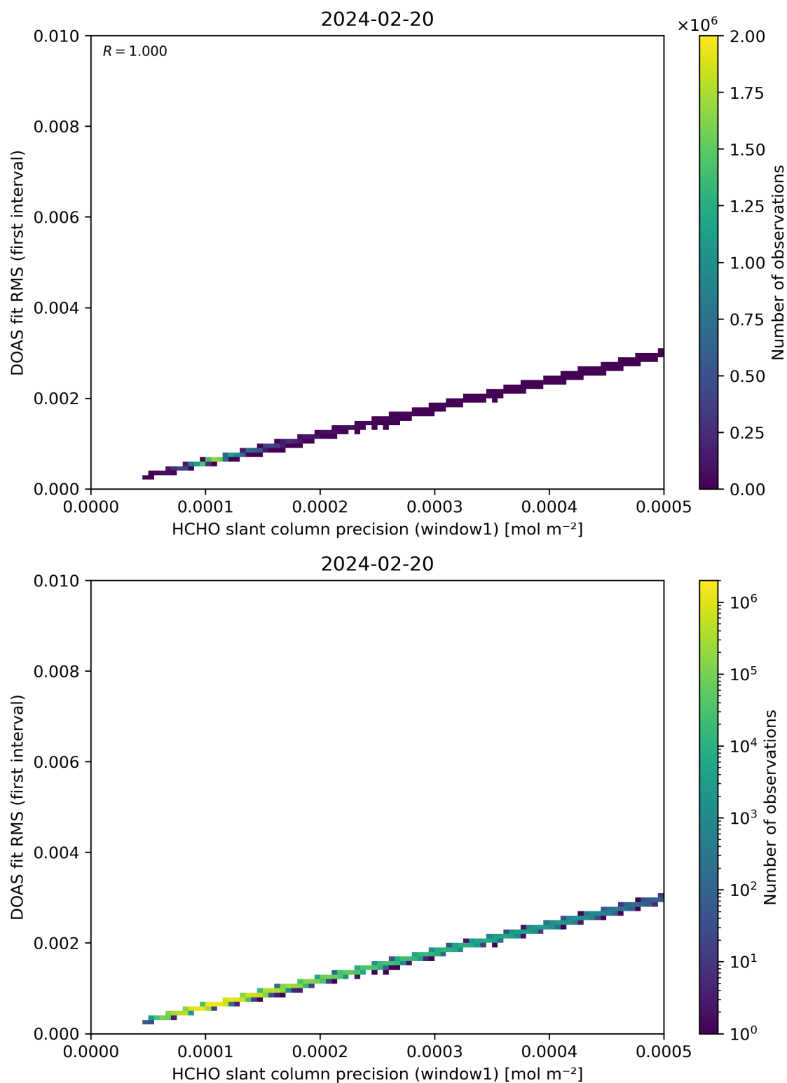
Figure 88: Scatter density plot of “HCHO slant column precision (window1)” against “DOAS fit RMS (first interval)” for 2024-02-19 to 2024-02-21.
