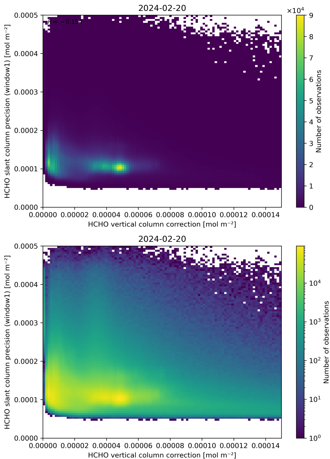
Figure 119: Scatter density plot of “HCHO vertical column correction” against “HCHO slant column precision (window1)” for 2024-02-19 to 2024-02-21.
