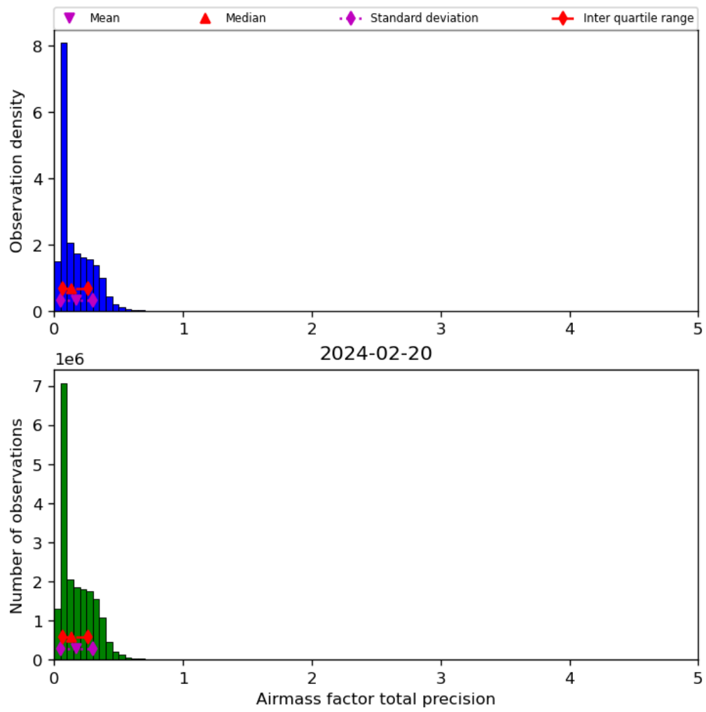
Figure 41: Histogram of “Airmass factor total precision” for 2024-02-19 to 2024-02-21
