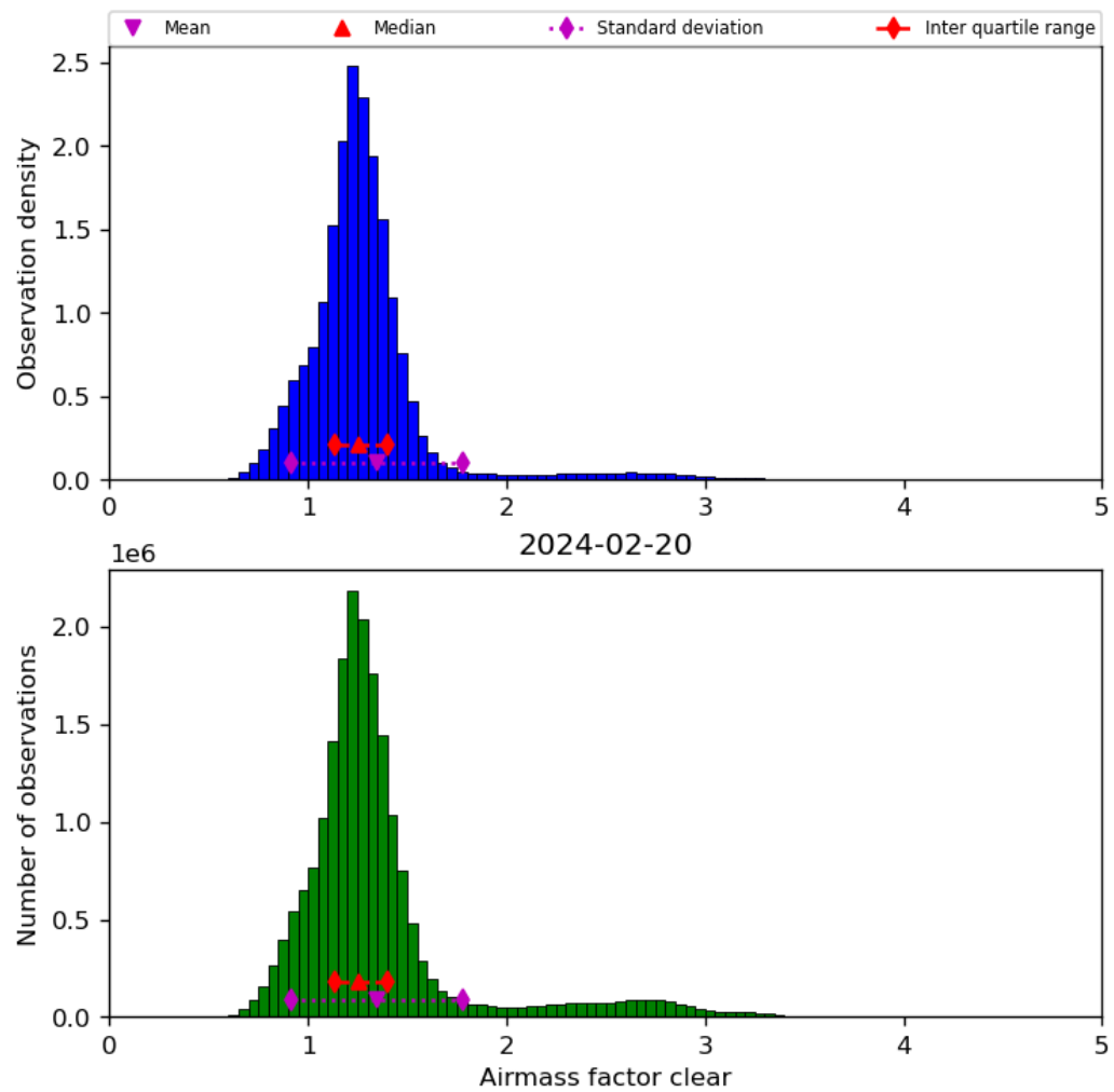
Figure 42: Histogram of “Airmass factor clear” for 2024-02-19 to 2024-02-21
