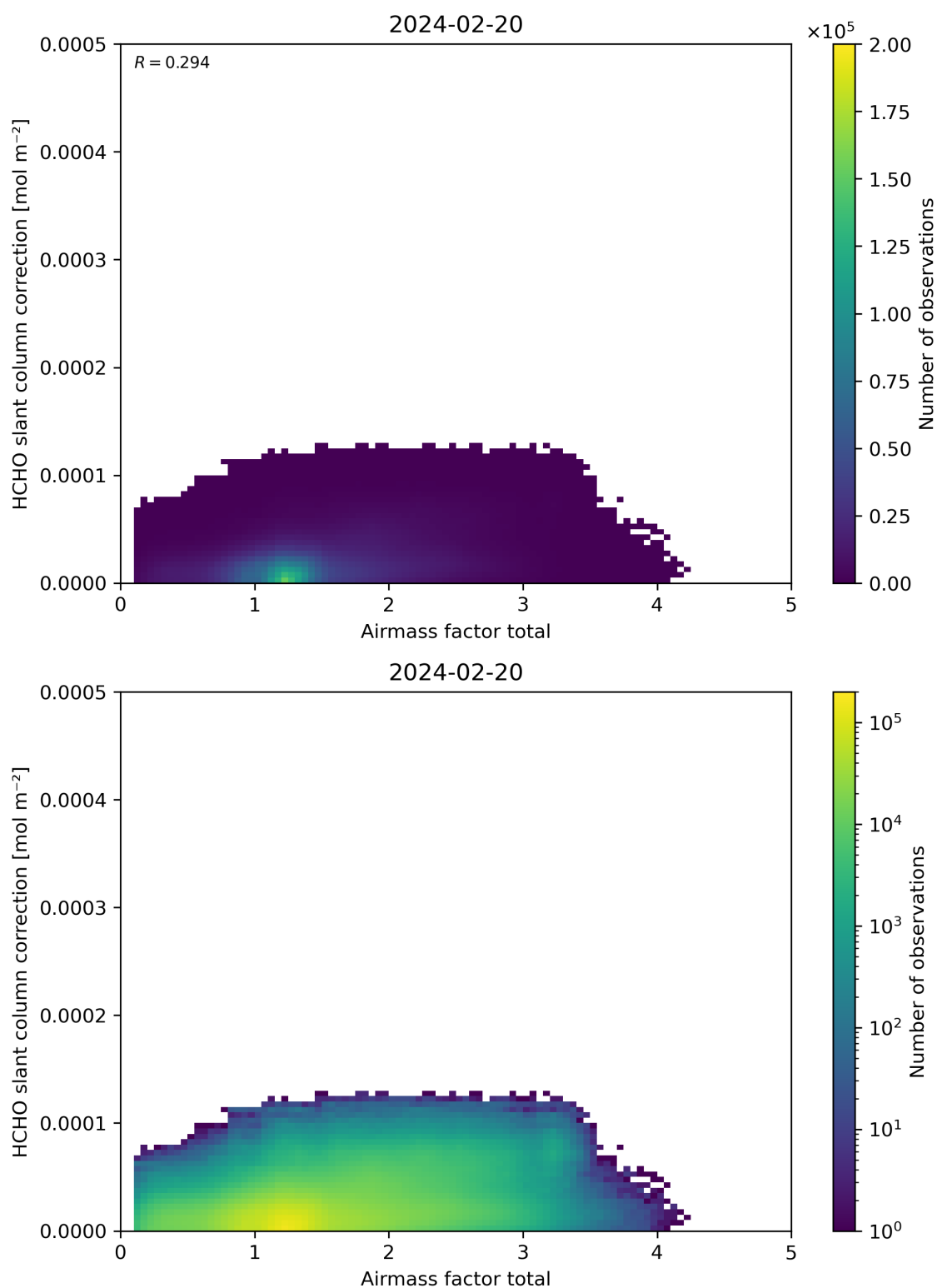
Figure 102: Scatter density plot of “Airmass factor total” against “HCHO slant column correction” for 2024-02-19 to 2024-02-21.
