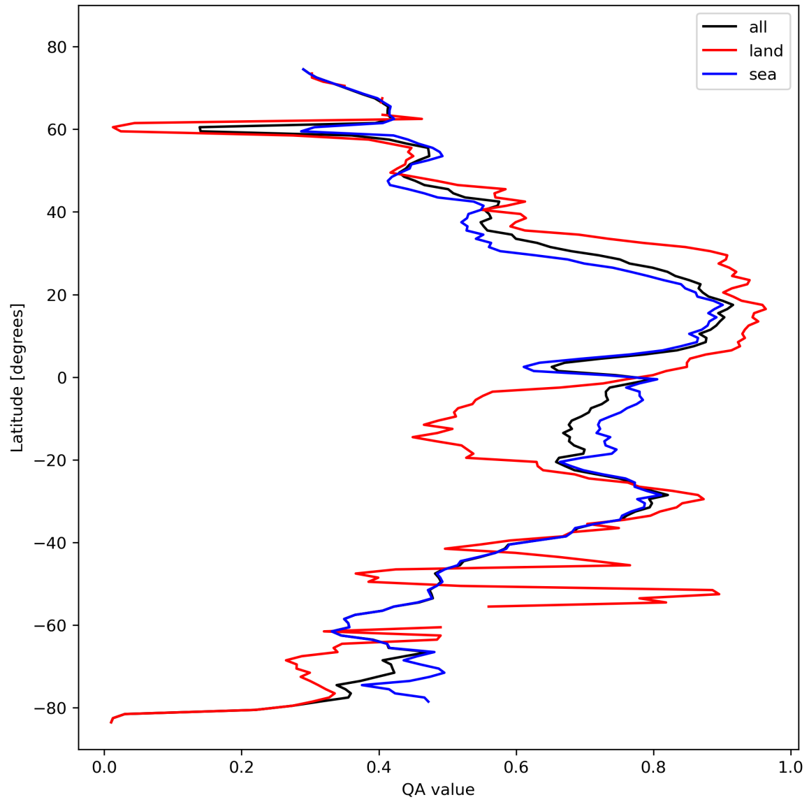
Figure 20: Zonal average of “QA value” for 2024-02-19 to 2024-02-21.
