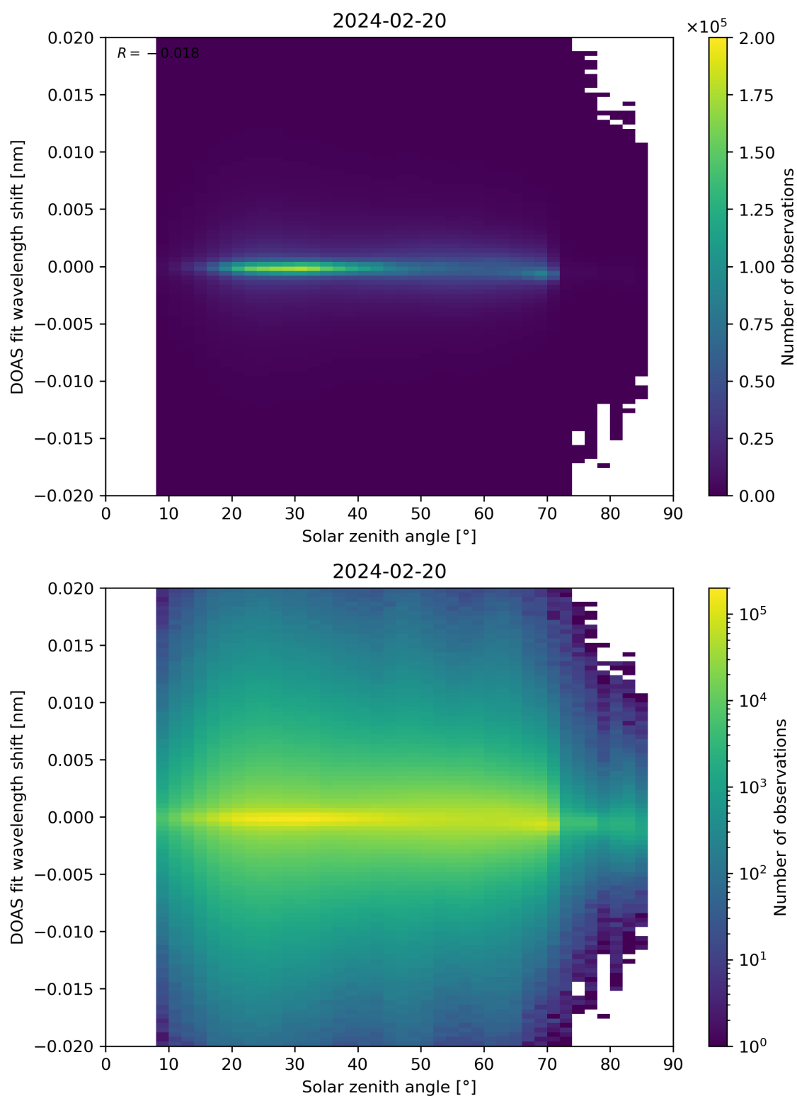
Figure 168: Scatter density plot of “Solar zenith angle” against “DOAS fit wavelength shift” for 2024-02-19 to 2024-02-21.
