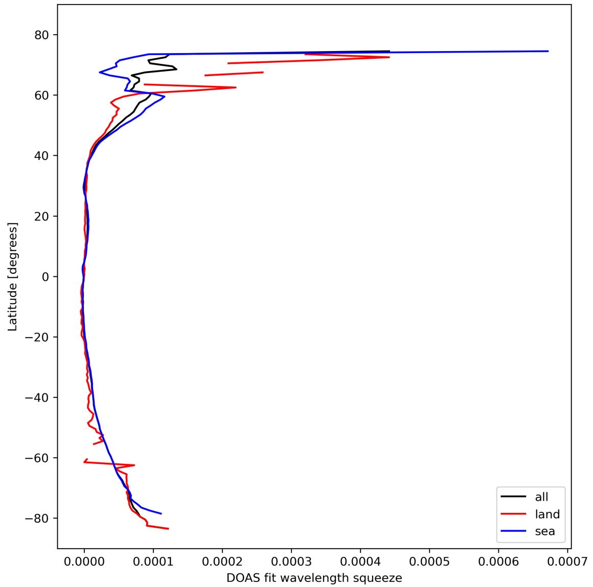
Figure 31: Zonal average of “DOAS fit wavelength squeeze” for 2024-02-19 to 2024-02-21.
