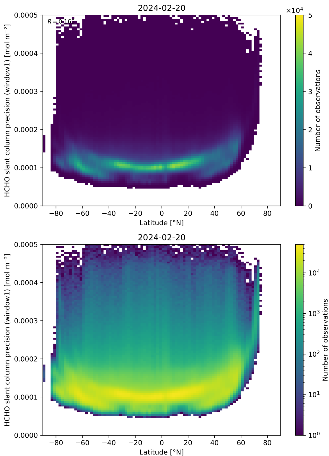
Figure 160: Scatter density plot of “Latitude” against “HCHO slant column precision (window1)” for 2024-02-19 to 2024-02-21.
