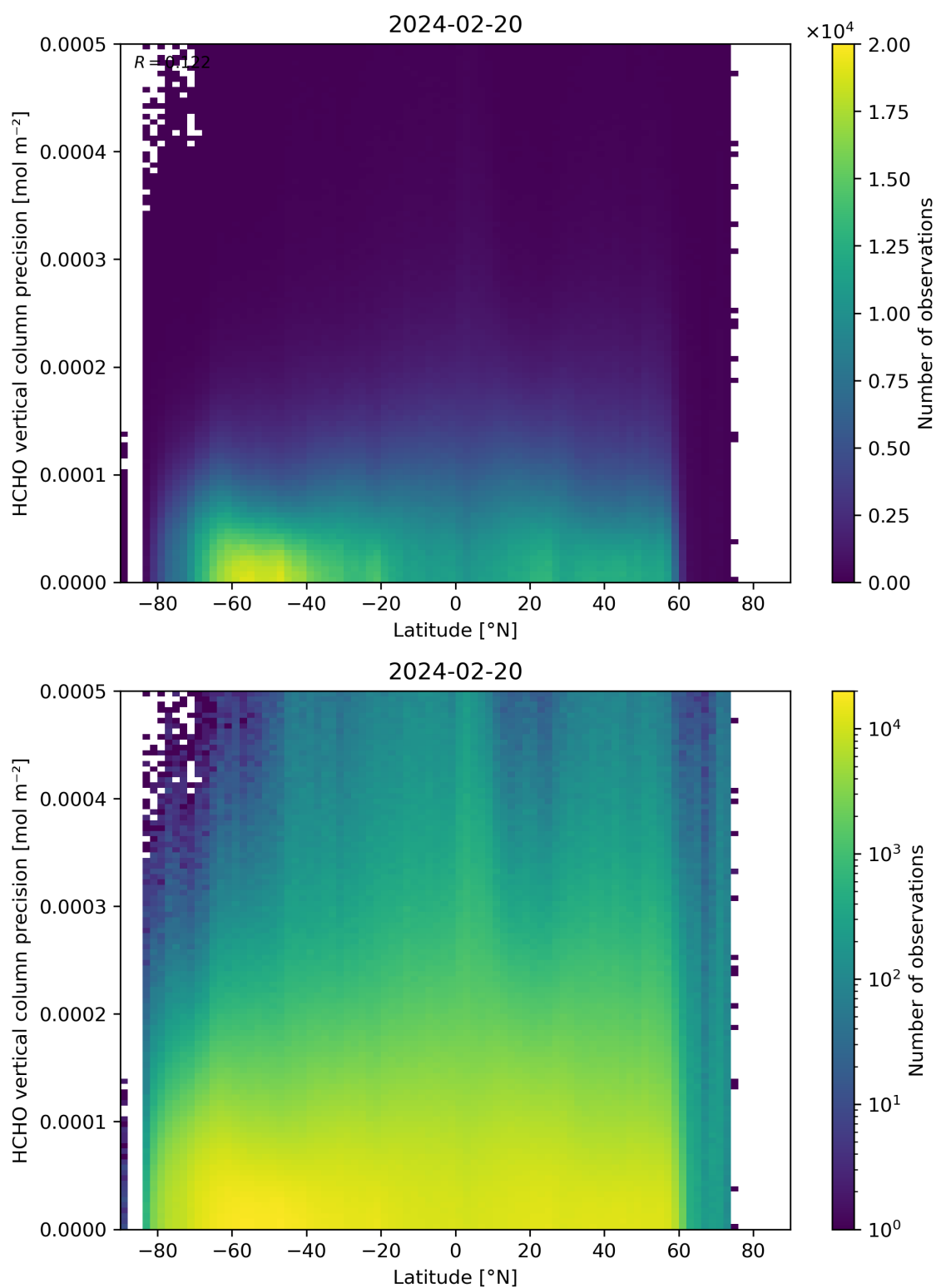
Figure 165: Scatter density plot of “Latitude” against “HCHO vertical column precision” for 2024-02-19 to 2024-02-21.
