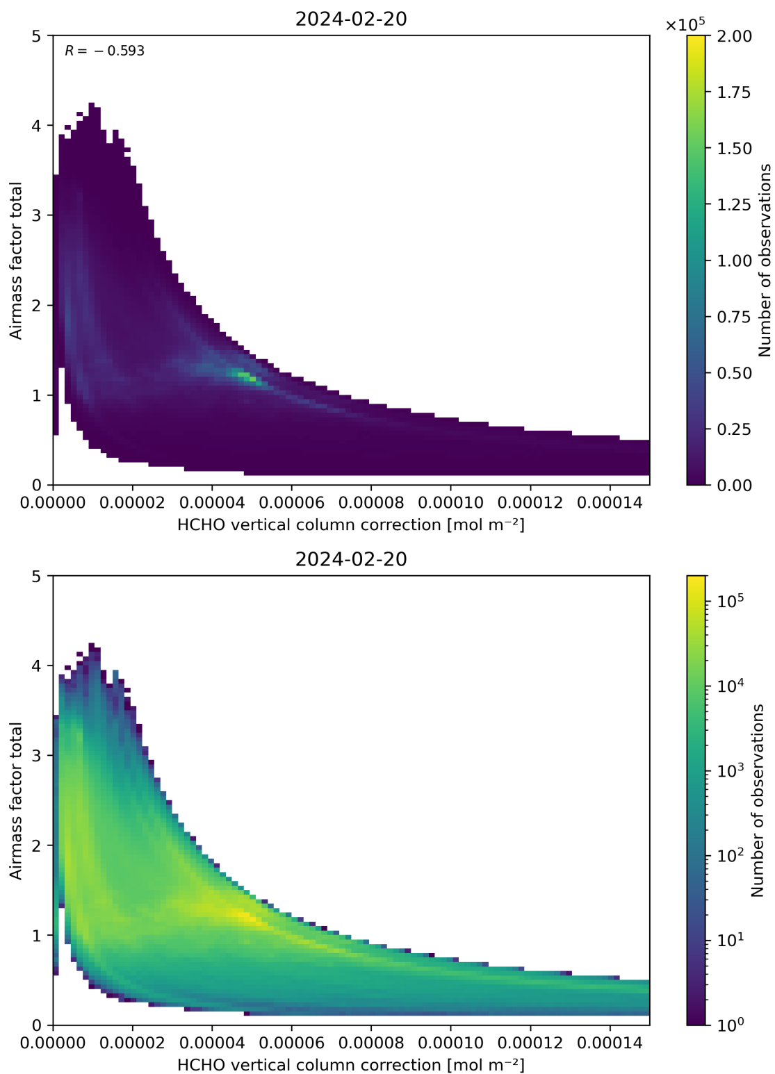
Figure 120: Scatter density plot of “HCHO vertical column correction” against “Airmass factor total” for 2024-02-19 to 2024-02-21.
