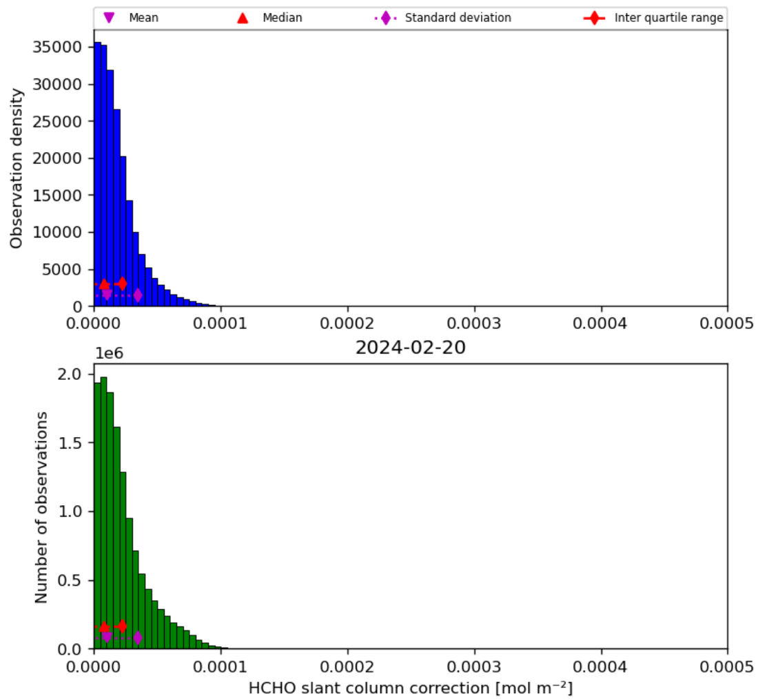
Figure 47: Histogram of “HCHO slant column correction” for 2024-02-19 to 2024-02-21
