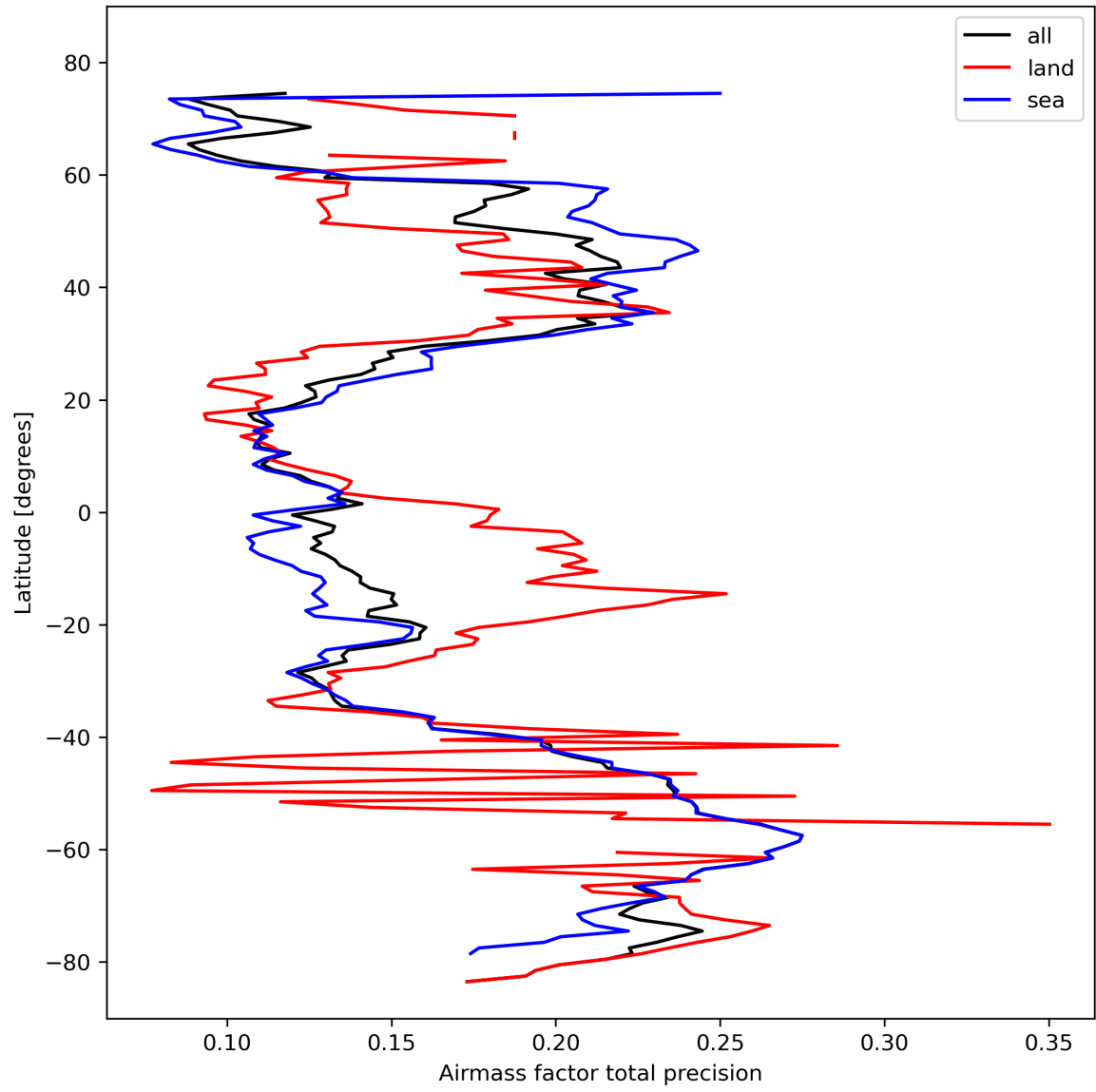
Figure 27: Zonal average of “Airmass factor total precision” for 2024-02-19 to 2024-02-21.
