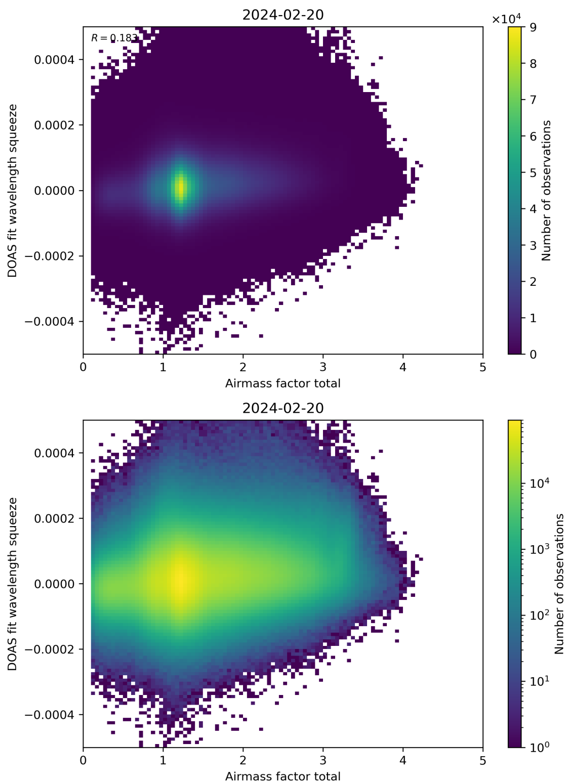
Figure 99: Scatter density plot of “Airmass factor total” against “DOAS fit wavelength squeeze” for 2024-02-19 to 2024-02-21.
