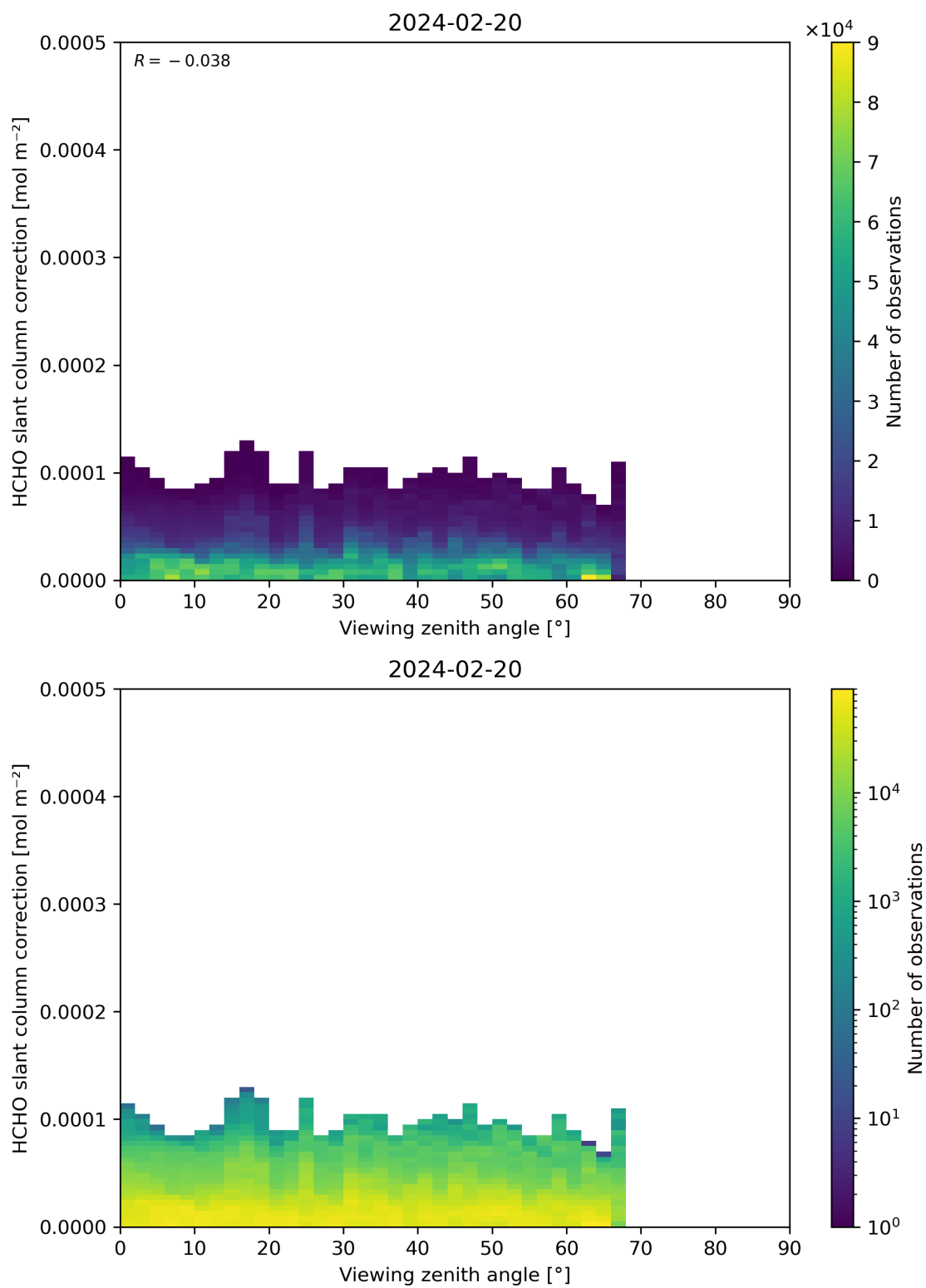
Figure 187: Scatter density plot of “Viewing zenith angle” against “HCHO slant column correction” for 2024-02-19 to 2024-02-21.
