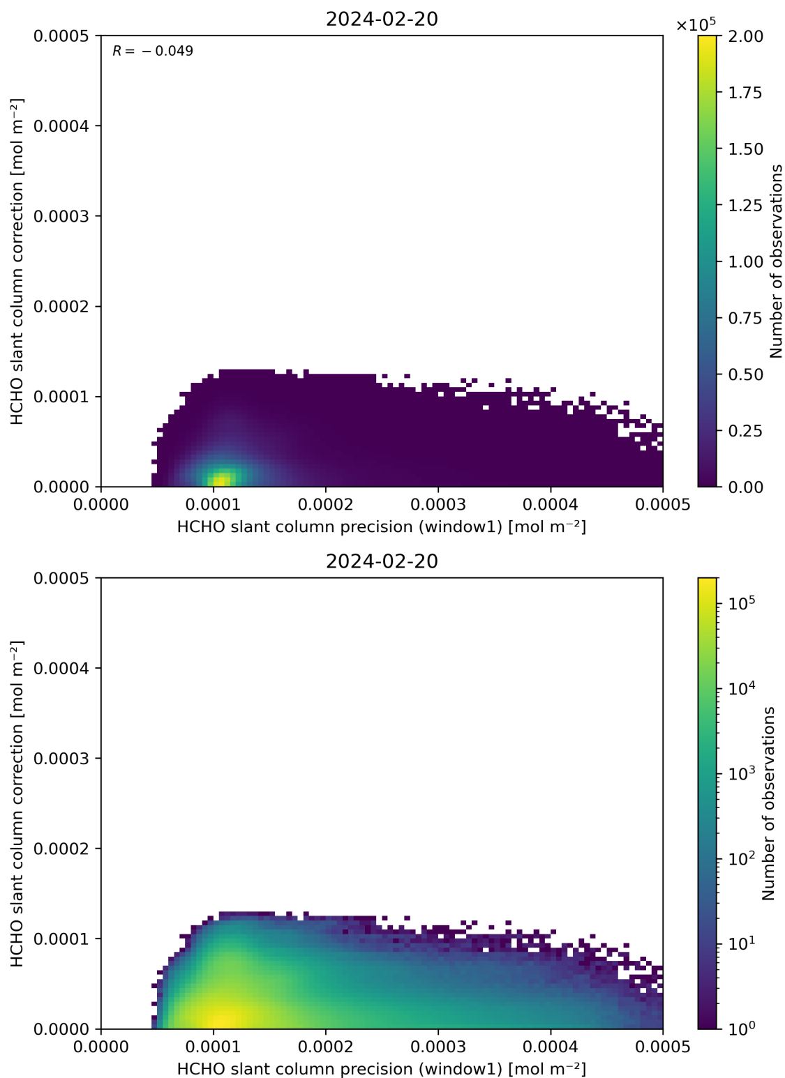
Figure 93: Scatter density plot of “HCHO slant column precision (window1)” against “HCHO slant column correction” for 2024-02-19 to 2024-02-21.
