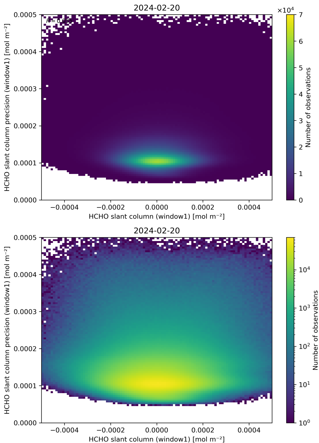
Figure 84: Scatter density plot of “HCHO slant column (window1)” against “HCHO slant column precision (window1)” for 2024-02-19 to 2024-02-21.
