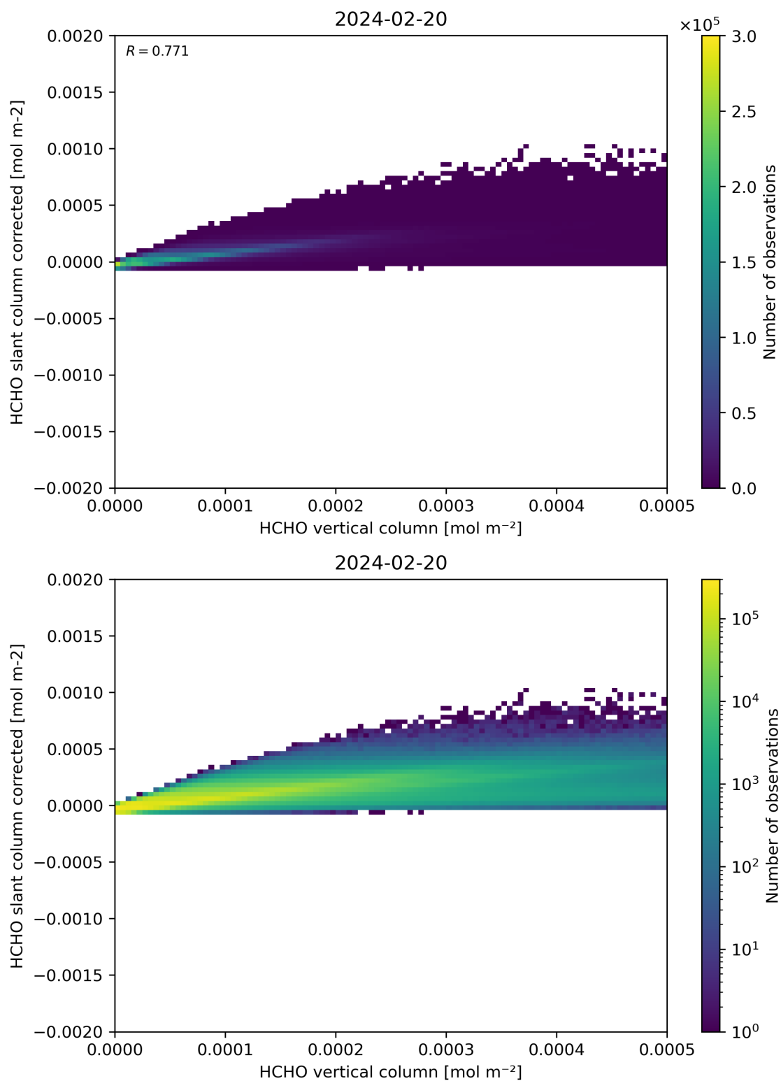
Figure 127: Scatter density plot of “HCHO vertical column” against “HCHO slant column corrected” for 2024-02-19 to 2024-02-21.
