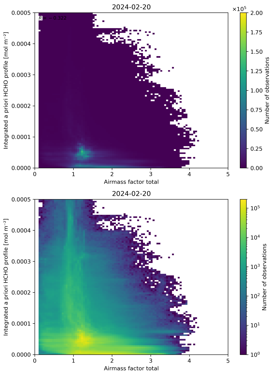
Figure 104: Scatter density plot of “Airmass factor total” against “Integrated a priori HCHO profile” for 2024-02-19 to 2024-02-21.
