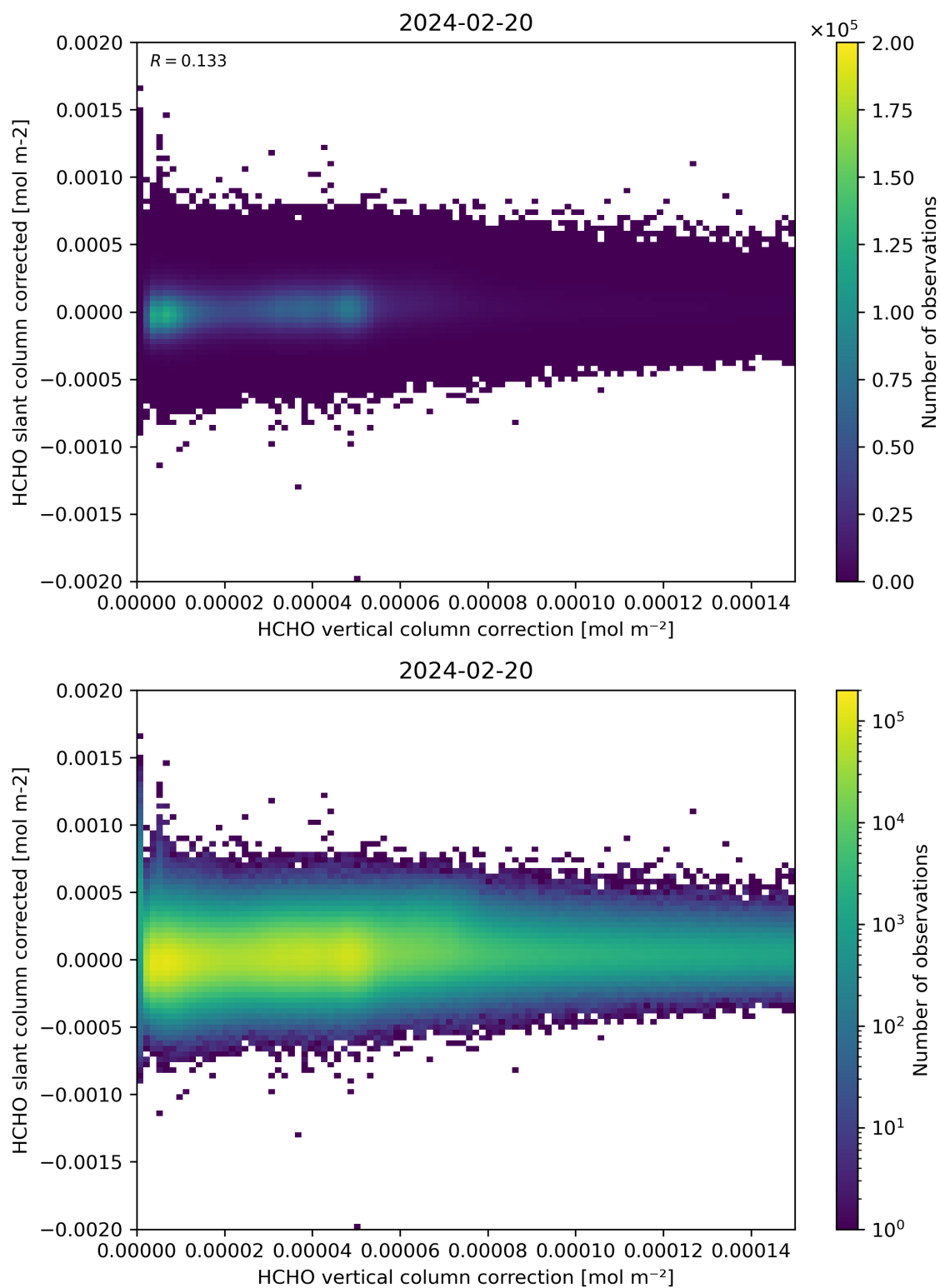
Figure 116: Scatter density plot of “HCHO vertical column correction” against “HCHO slant column corrected” for 2024-02-19 to 2024-02-21.
