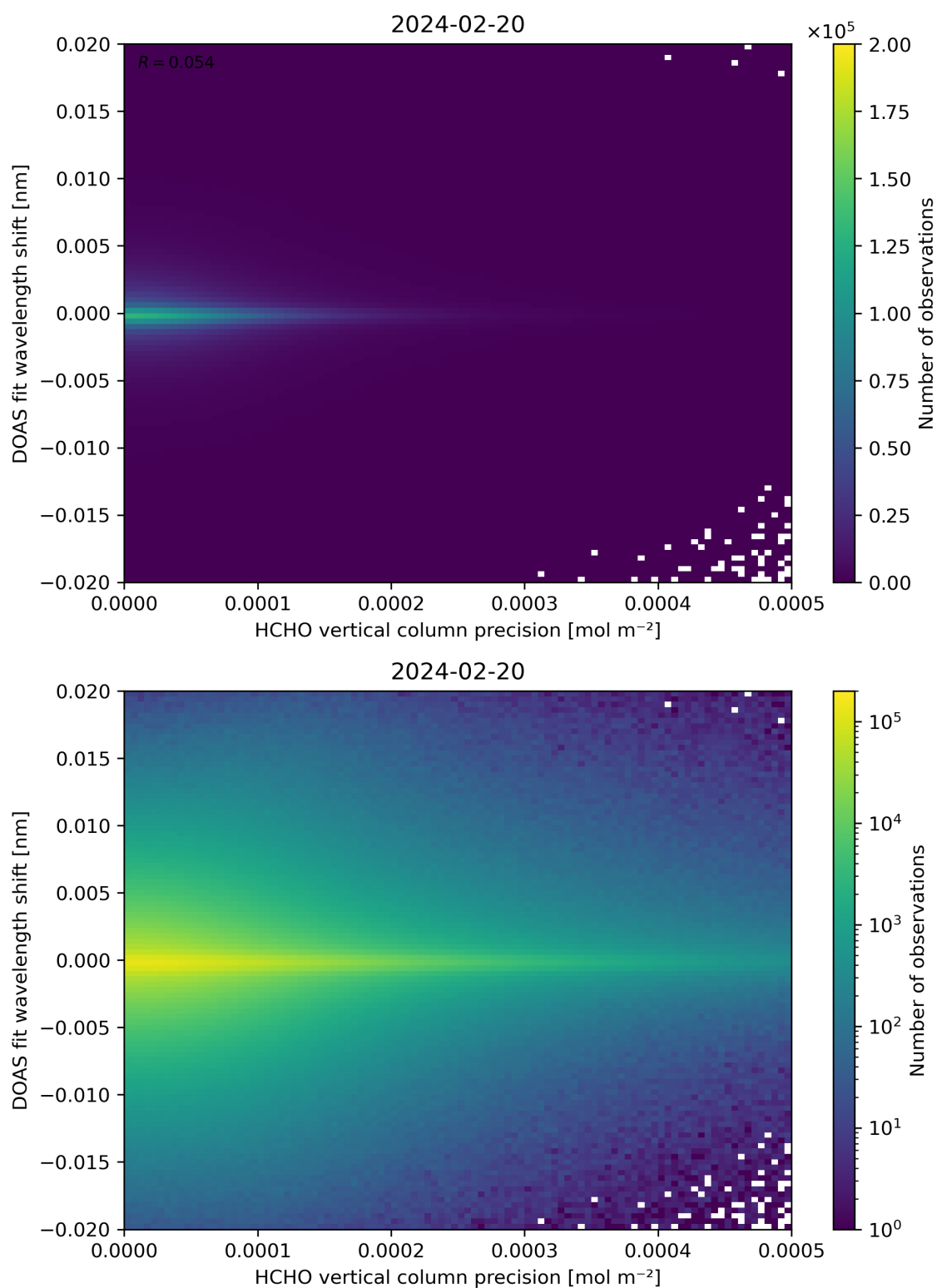
Figure 137: Scatter density plot of “HCHO vertical column precision” against “DOAS fit wavelength shift” for 2024-02-19 to 2024-02-21.
