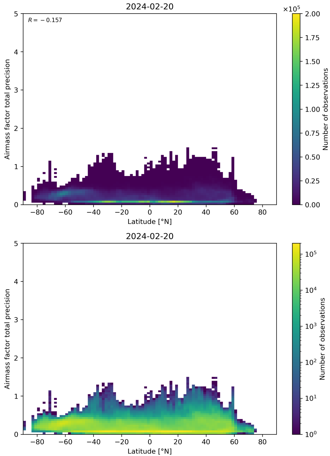
Figure 162: Scatter density plot of “Latitude” against “Airmass factor total precision” for 2024-02-19 to 2024-02-21.
