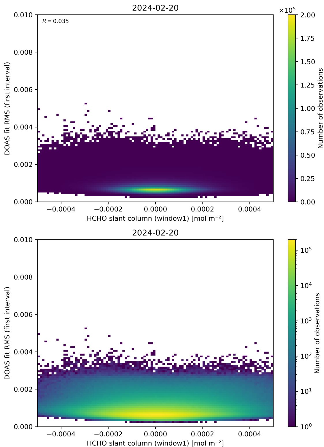
Figure 78: Scatter density plot of “HCHO slant column (window1)” against “DOAS fit RMS (first interval)” for 2024-02-19 to 2024-02-21.
