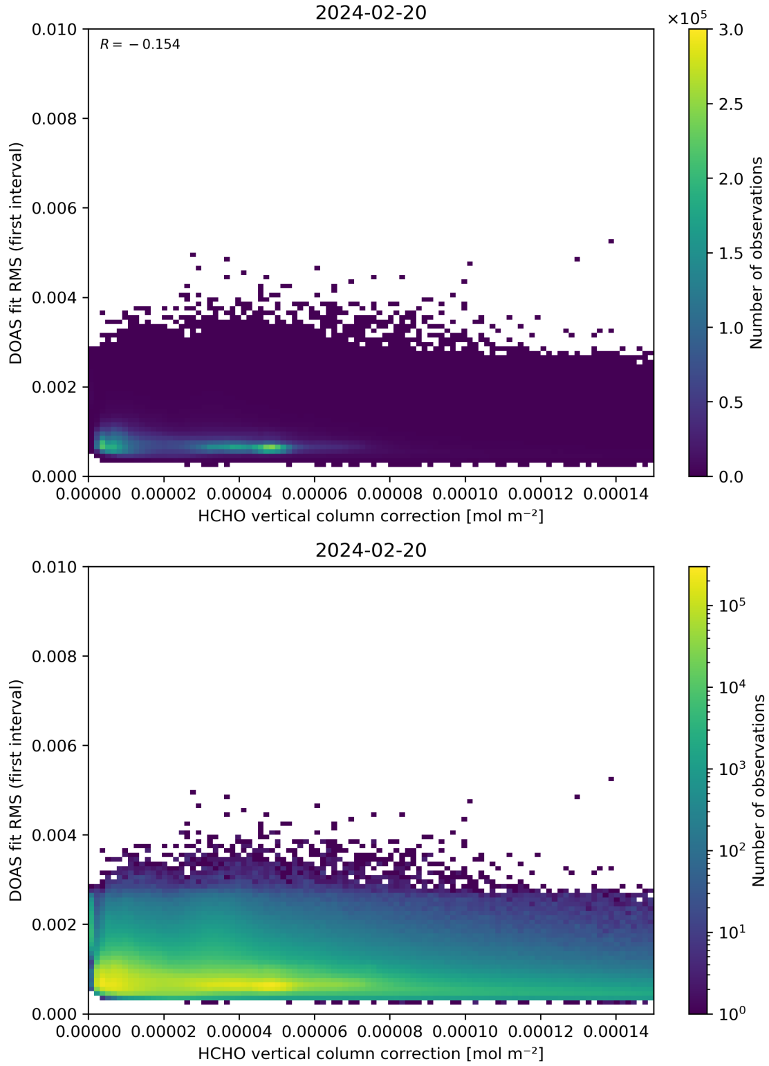
Figure 112: Scatter density plot of “HCHO vertical column correction” against “DOAS fit RMS (first interval)” for 2024-02-19 to 2024-02-21.
