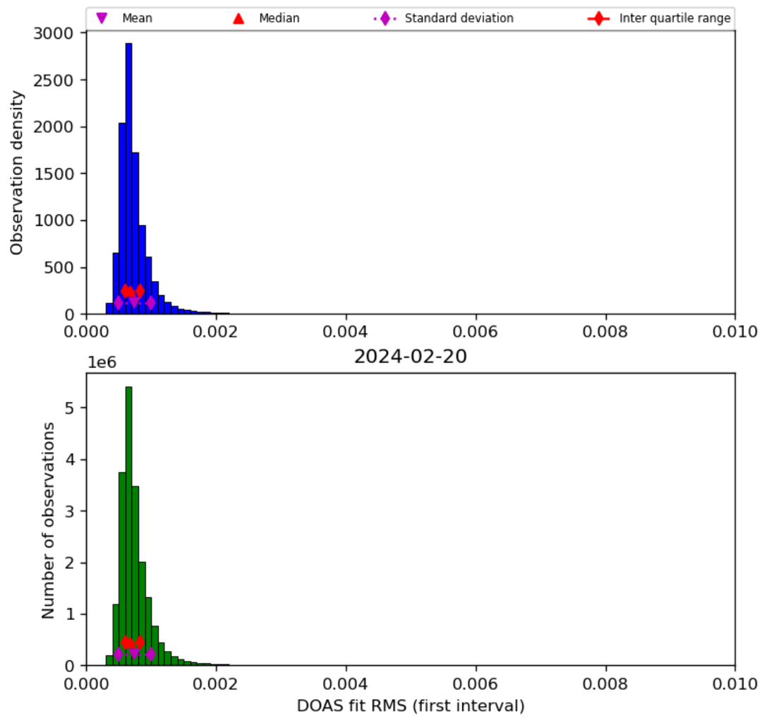
Figure 46: Histogram of “DOAS fit RMS (first interval)” for 2024-02-19 to 2024-02-21
