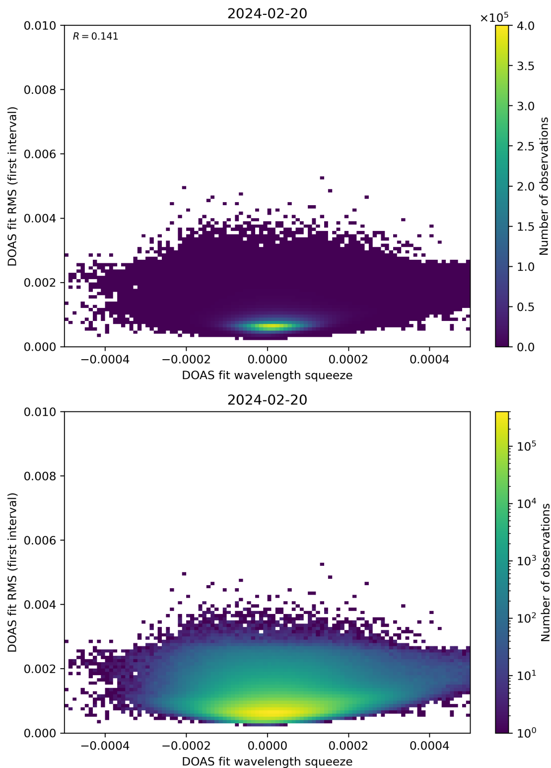
Figure 68: Scatter density plot of “DOAS fit wavelength squeeze” against “DOAS fit RMS (first interval)” for 2024-02-19 to 2024-02-21.
