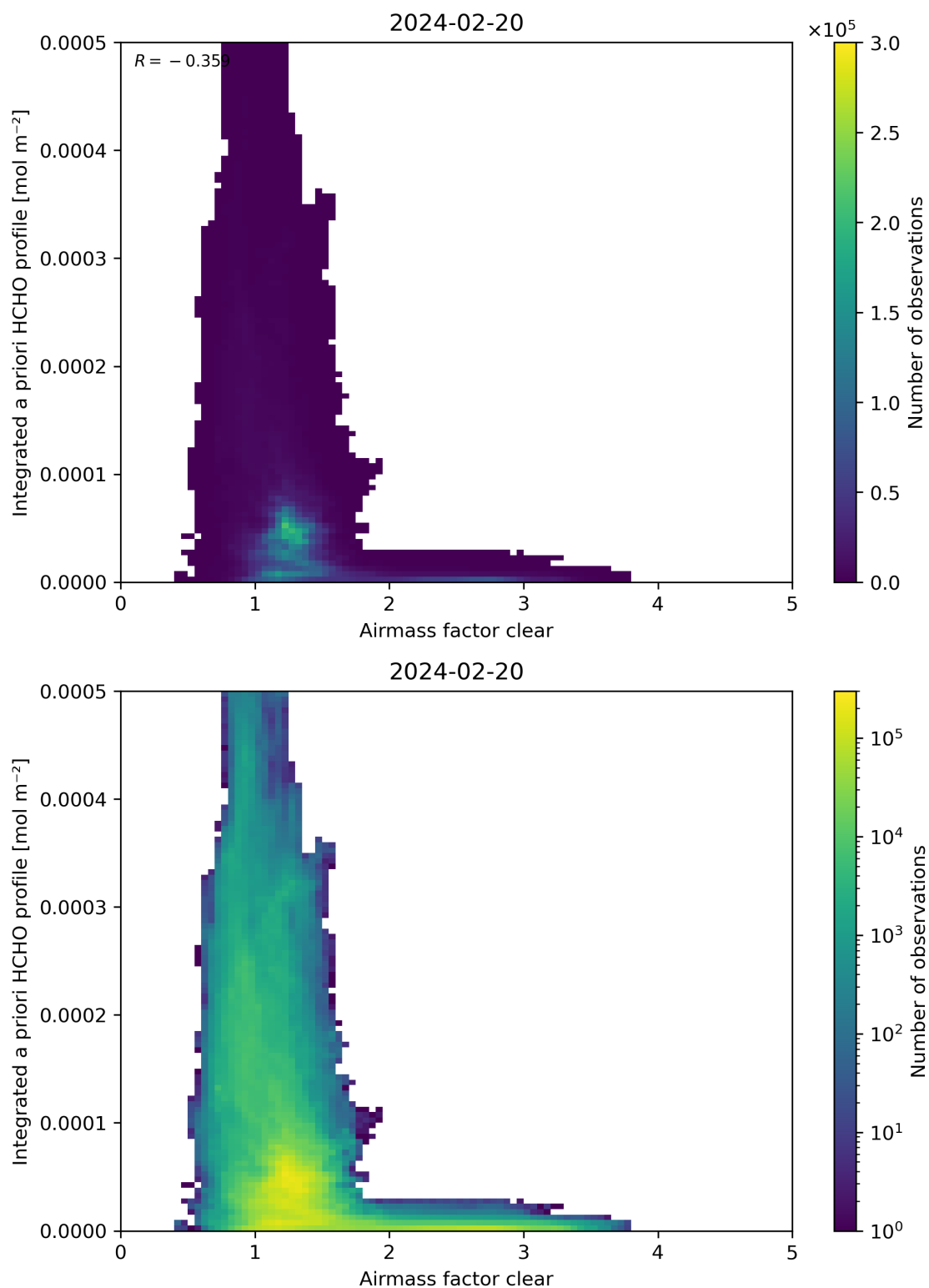
Figure 76: Scatter density plot of “Airmass factor clear” against “Integrated a priori HCHO profile” for 2024-02-19 to 2024-02-21.
