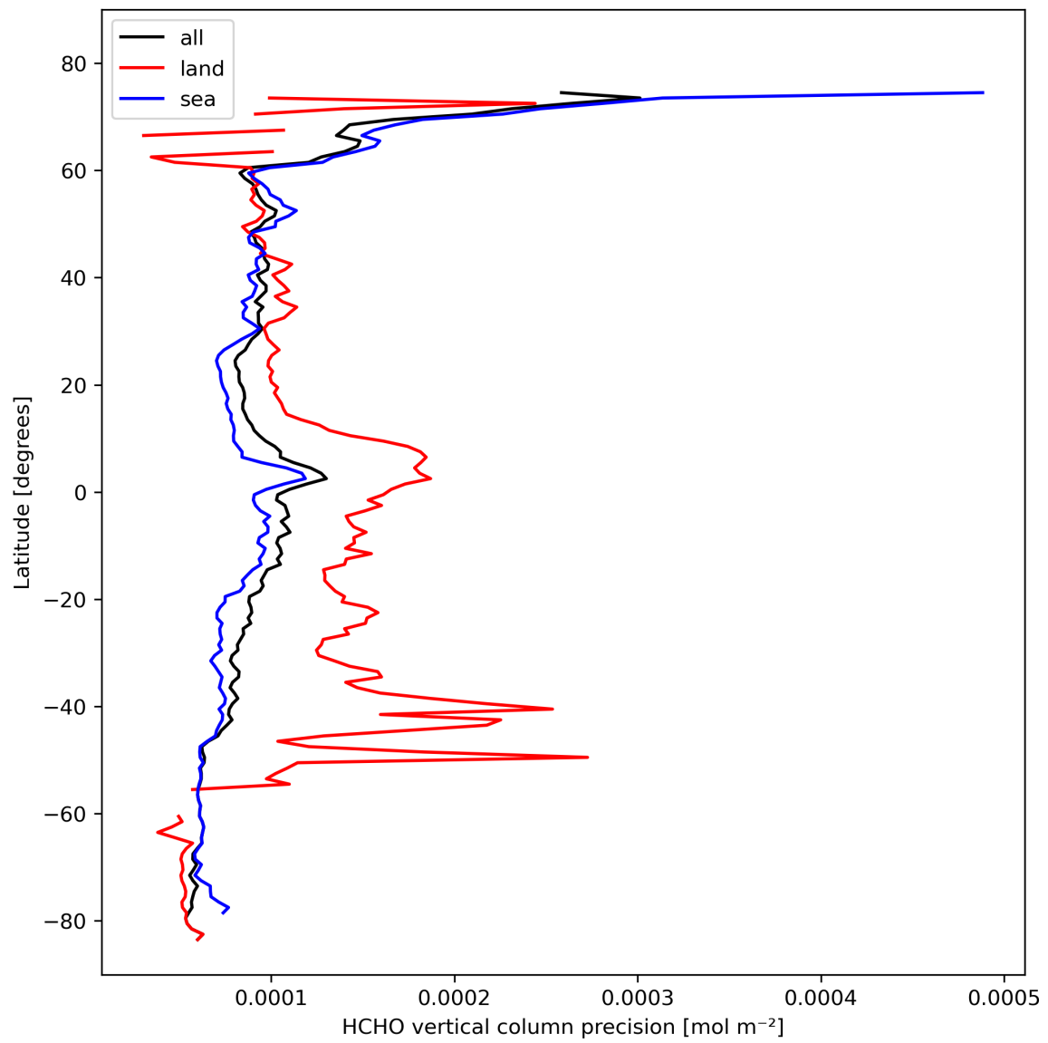
Figure 22: Zonal average of “HCHO vertical column precision” for 2024-02-19 to 2024-02-21.
