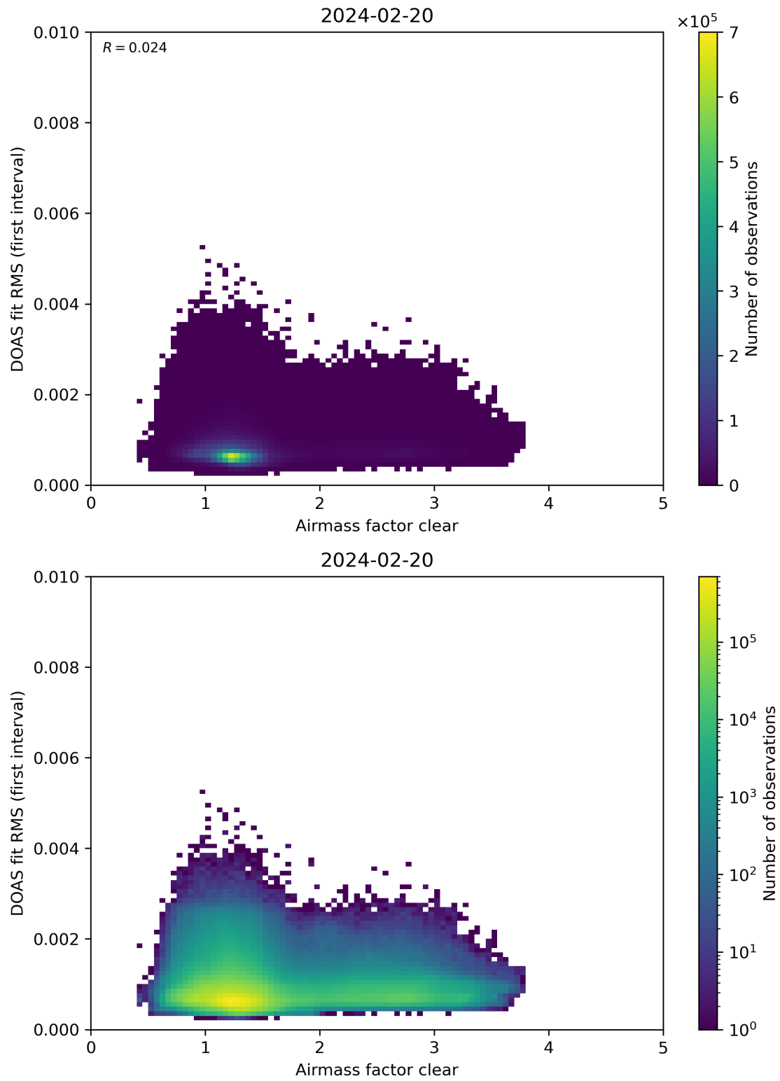
Figure 71: Scatter density plot of “Airmass factor clear” against “DOAS fit RMS (first interval)” for 2024-02-19 to 2024-02-21.
