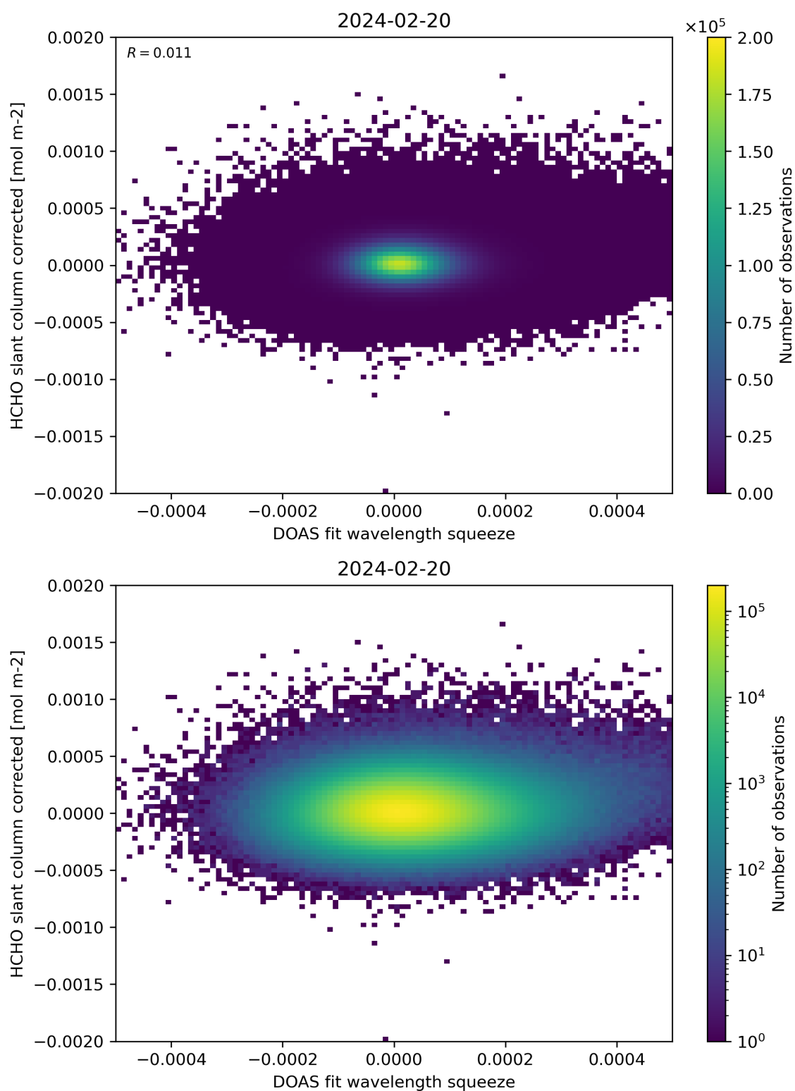
Figure 69: Scatter density plot of “DOAS fit wavelength squeeze” against “HCHO slant column corrected” for 2024-02-19 to 2024-02-21.
