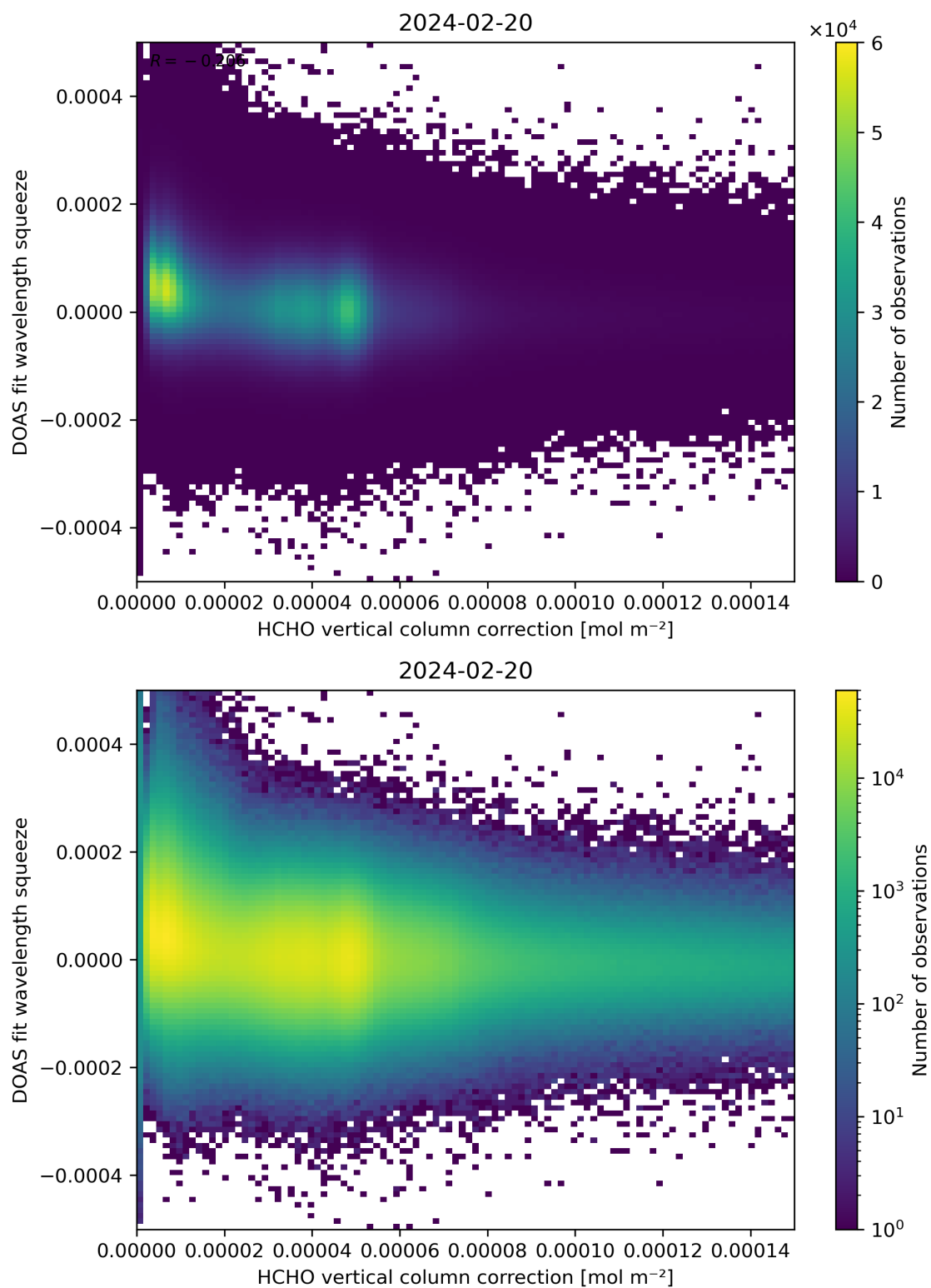
Figure 114: Scatter density plot of “HCHO vertical column correction” against “DOAS fit wavelength squeeze” for 2024-02-19 to 2024-02-21.
