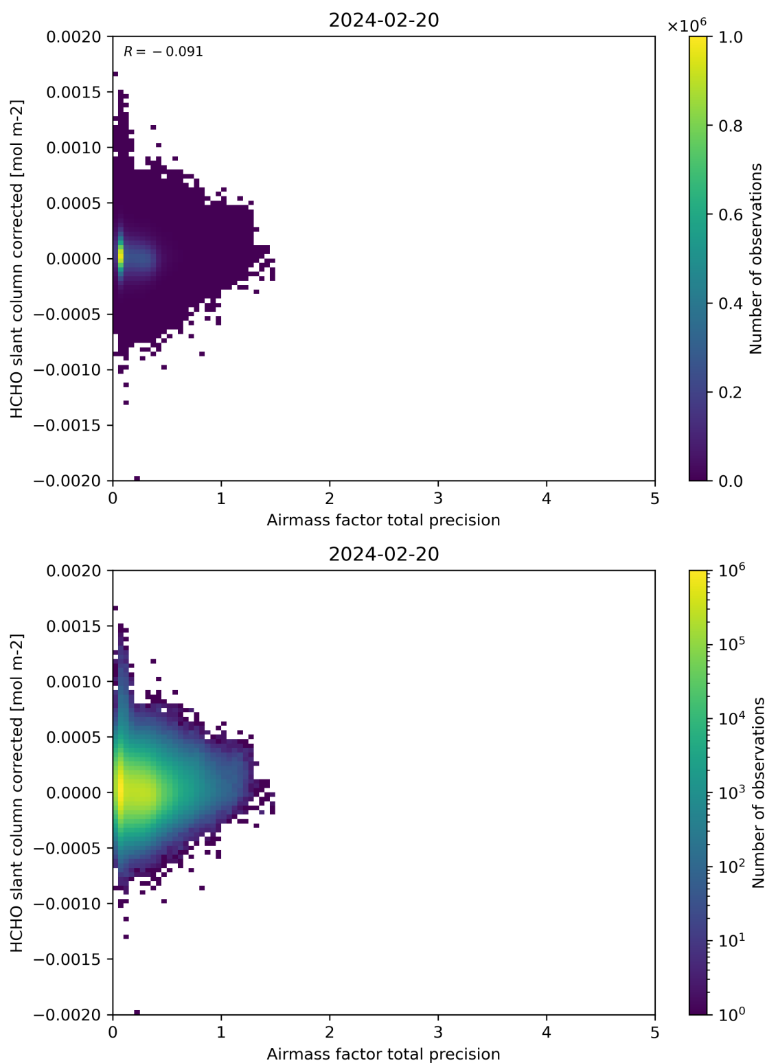
Figure 109: Scatter density plot of “Airmass factor total precision” against “HCHO slant column corrected” for 2024-02-19 to 2024-02-21.
