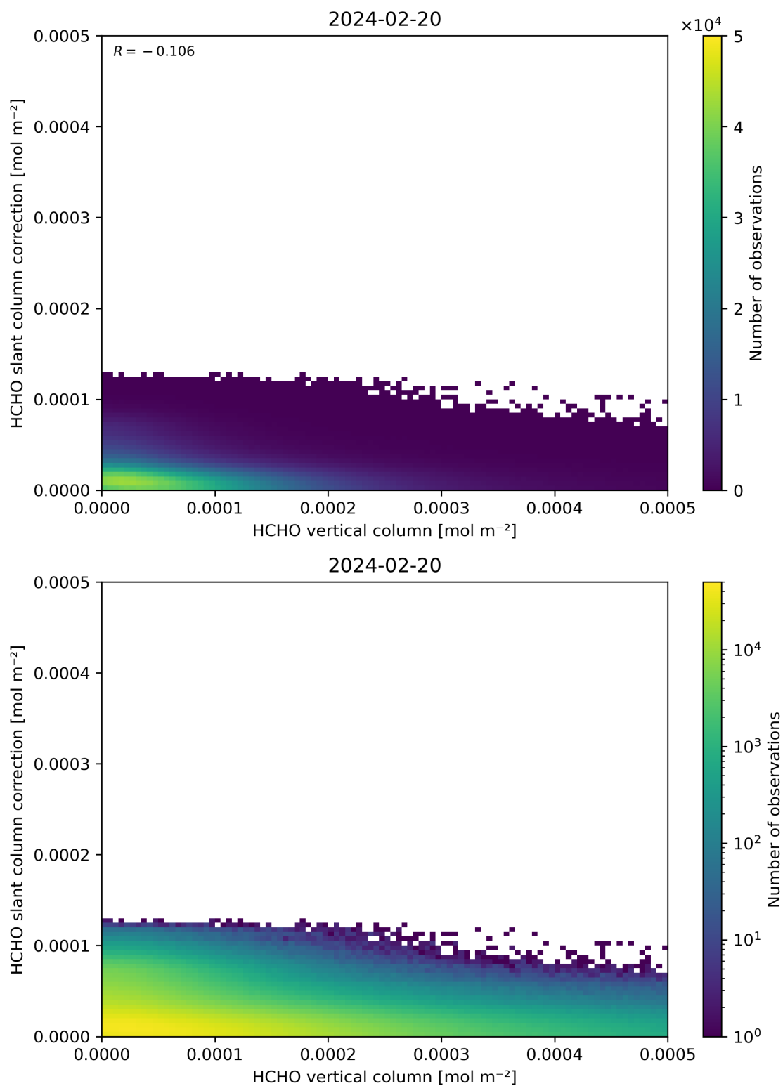
Figure 128: Scatter density plot of “HCHO vertical column” against “HCHO slant column correction” for 2024-02-19 to 2024-02-21.
