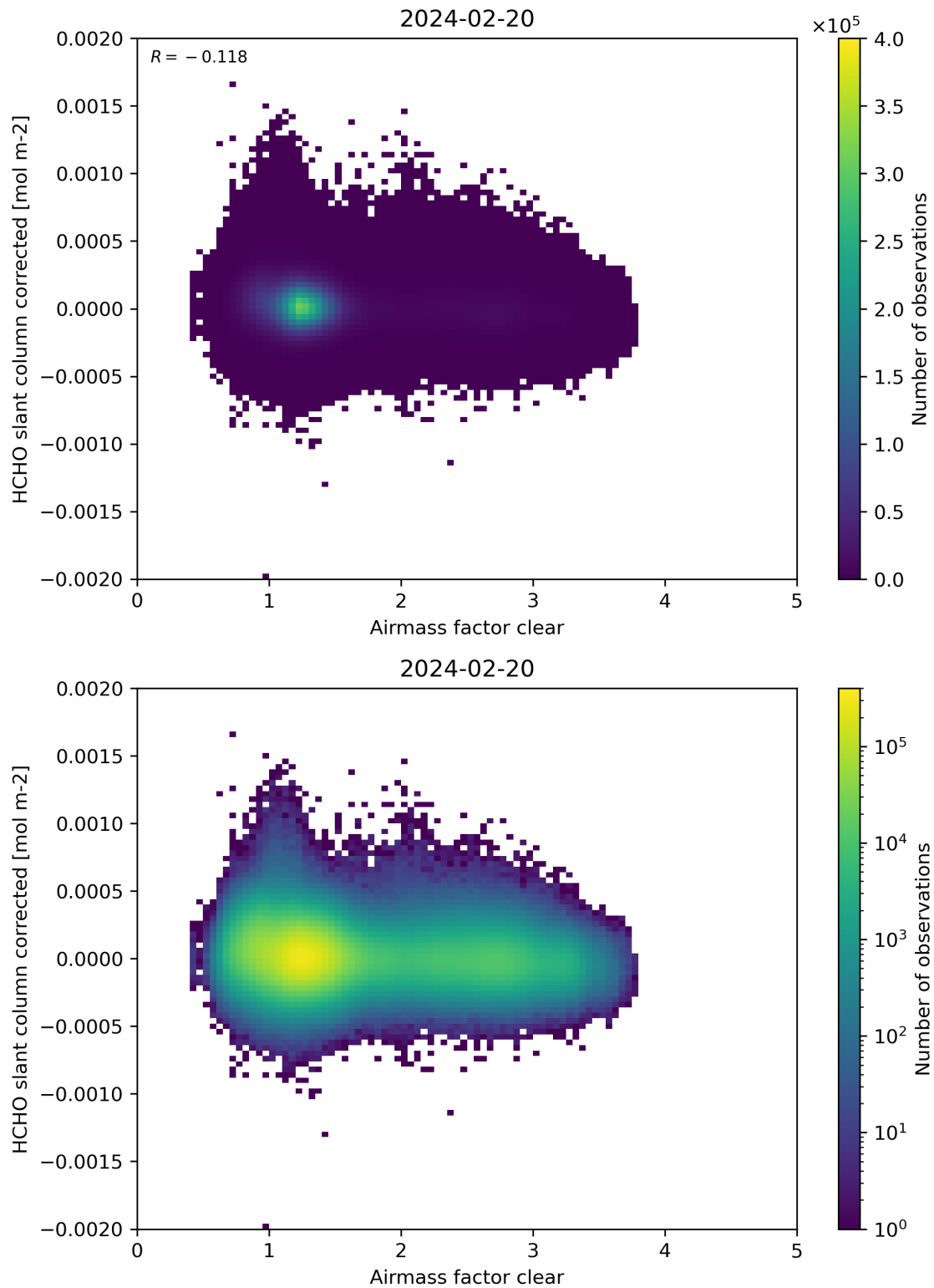
Figure 74: Scatter density plot of “Airmass factor clear” against “HCHO slant column corrected” for 2024-02-19 to 2024-02-21.
