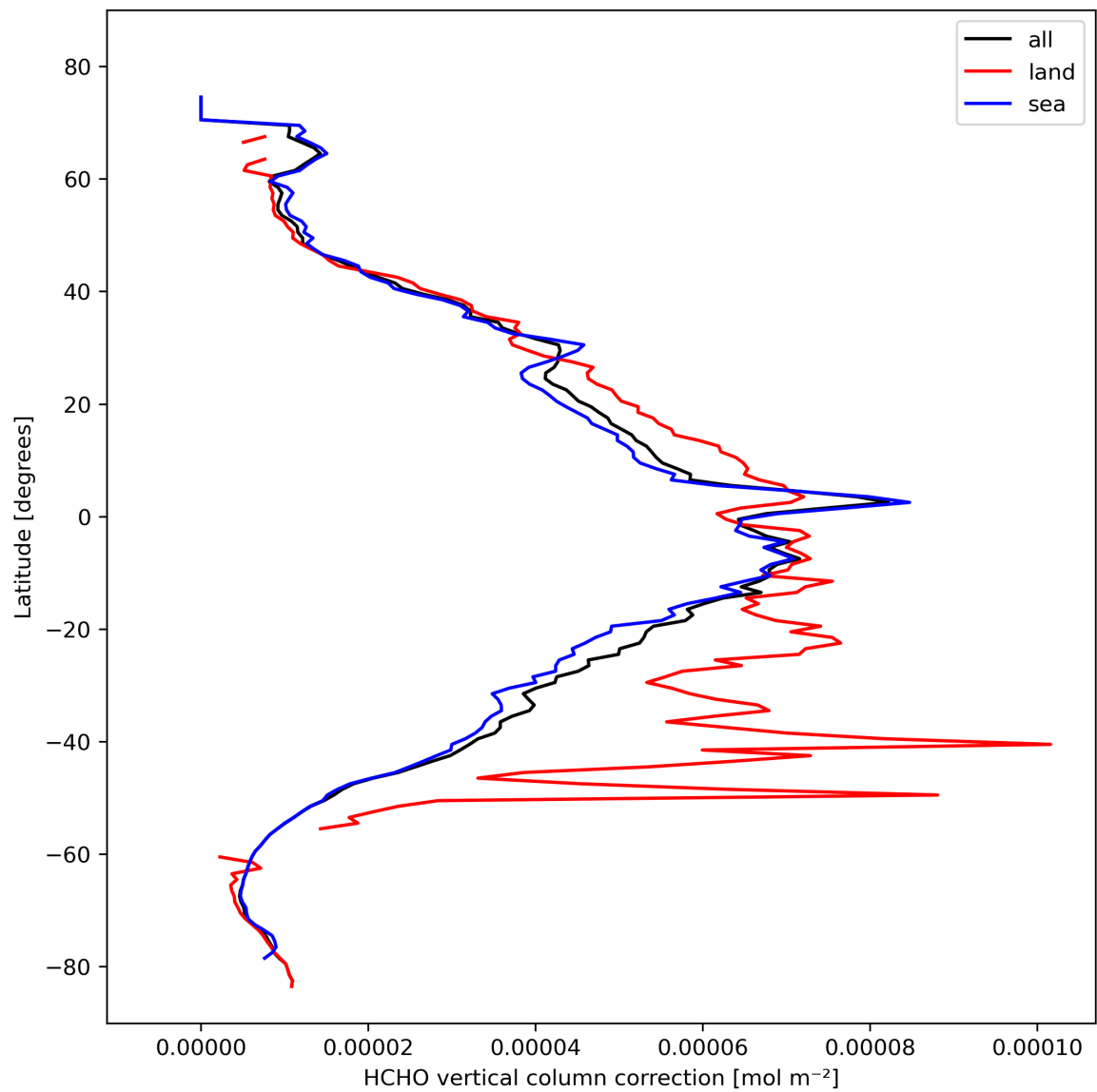
Figure 23: Zonal average of “HCHO vertical column correction” for 2024-02-19 to 2024-02-21.
