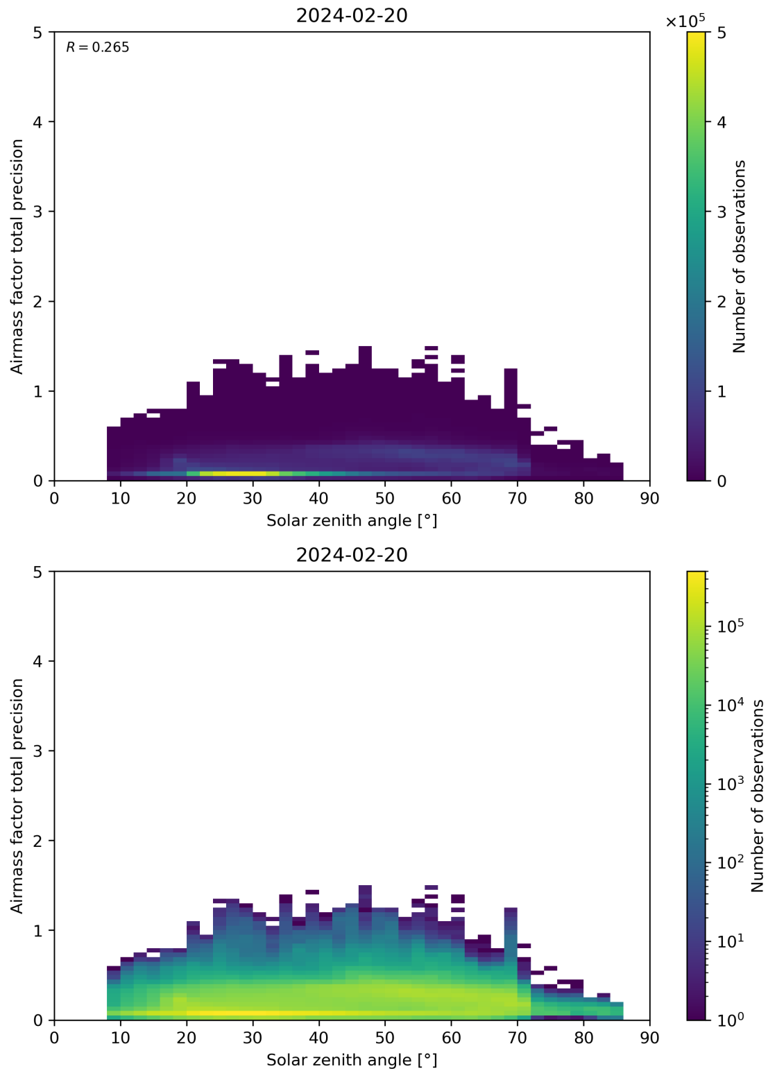
Figure 176: Scatter density plot of “Solar zenith angle” against “Airmass factor total precision” for 2024-02-19 to 2024-02-21.
