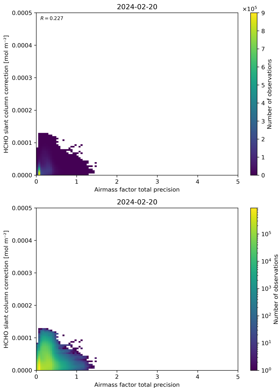
Figure 110: Scatter density plot of “Airmass factor total precision” against “HCHO slant column correction” for 2024-02-19 to 2024-02-21.
