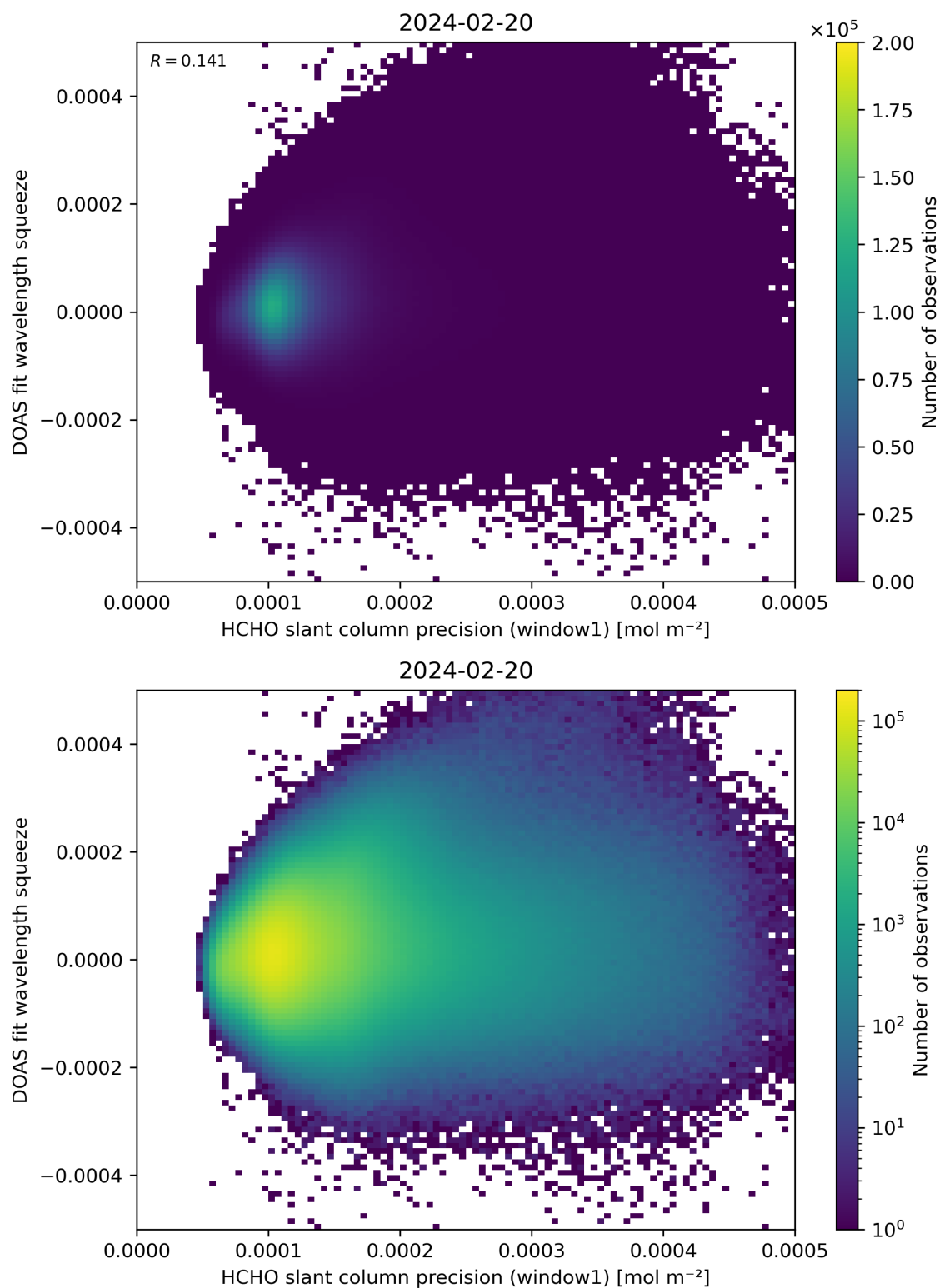
Figure 90: Scatter density plot of “HCHO slant column precision (window1)” against “DOAS fit wavelength squeeze” for 2024-02-19 to 2024-02-21.
