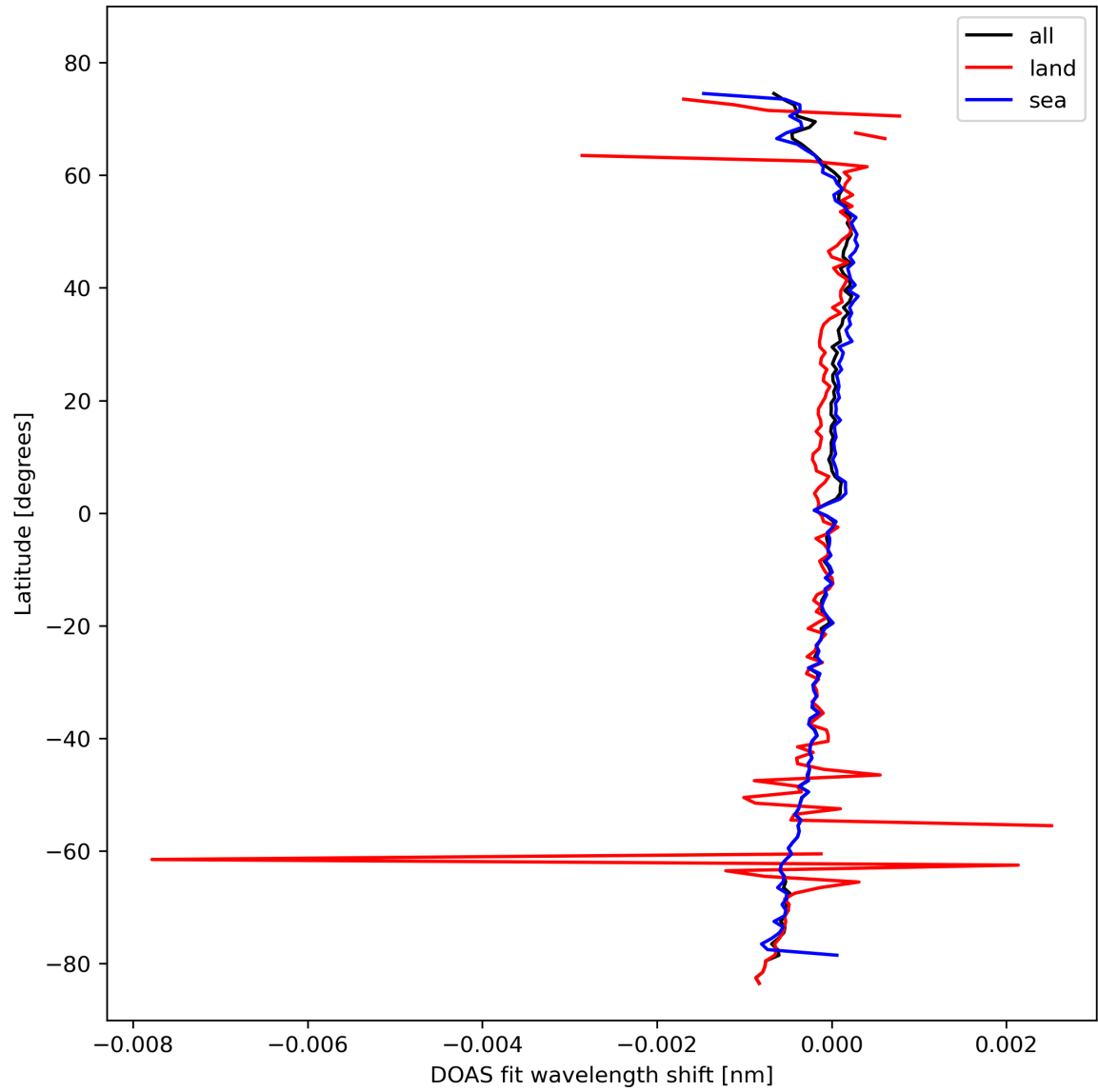
Figure 30: Zonal average of "DOAS fit wavelength shift" for 2024-02-19 to 2024-02-21.
