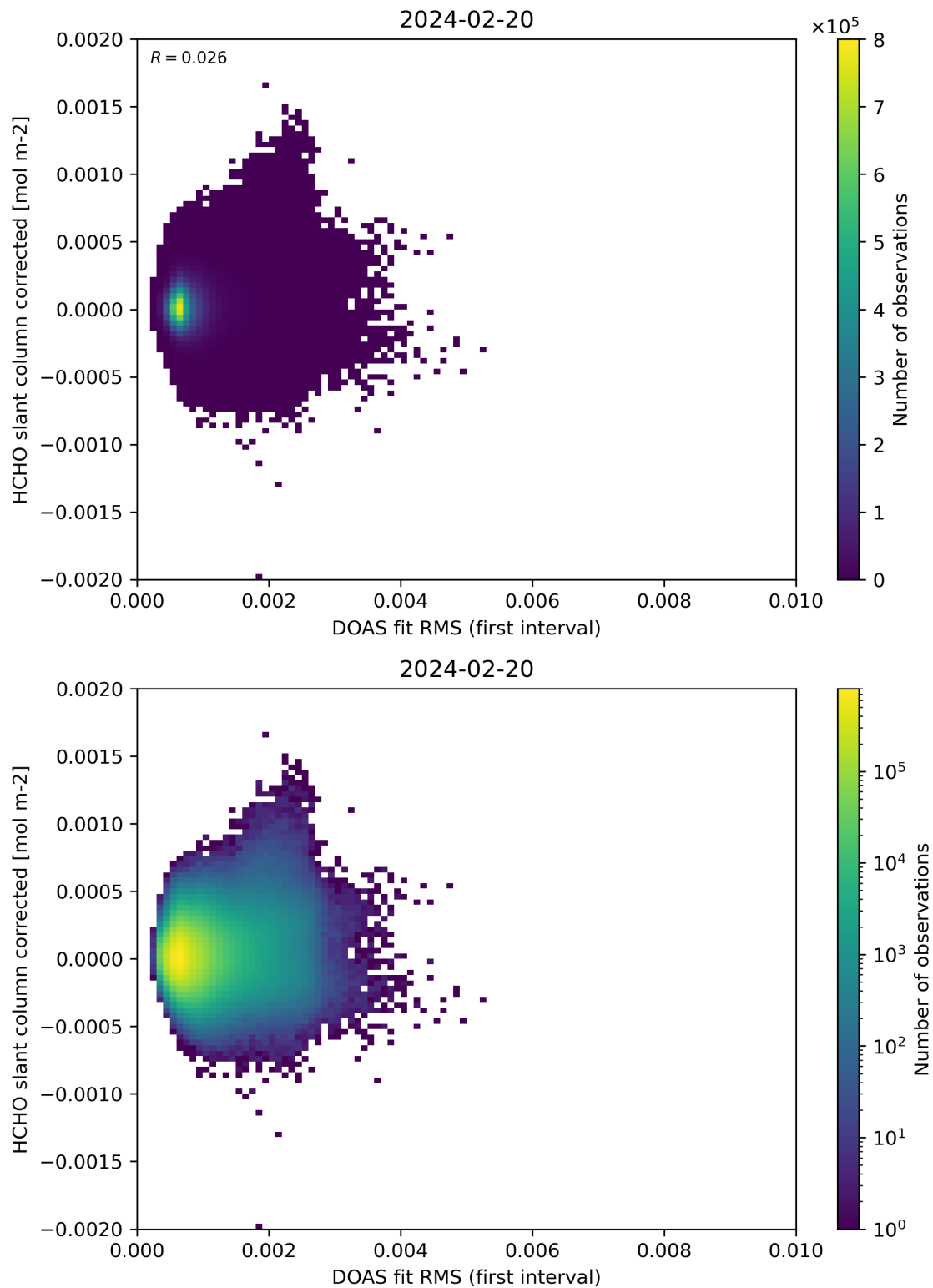
Figure 62: Scatter density plot of “DOAS fit RMS (first interval)” against “HCHO slant column corrected” for 2024-02-19 to 2024-02-21.
