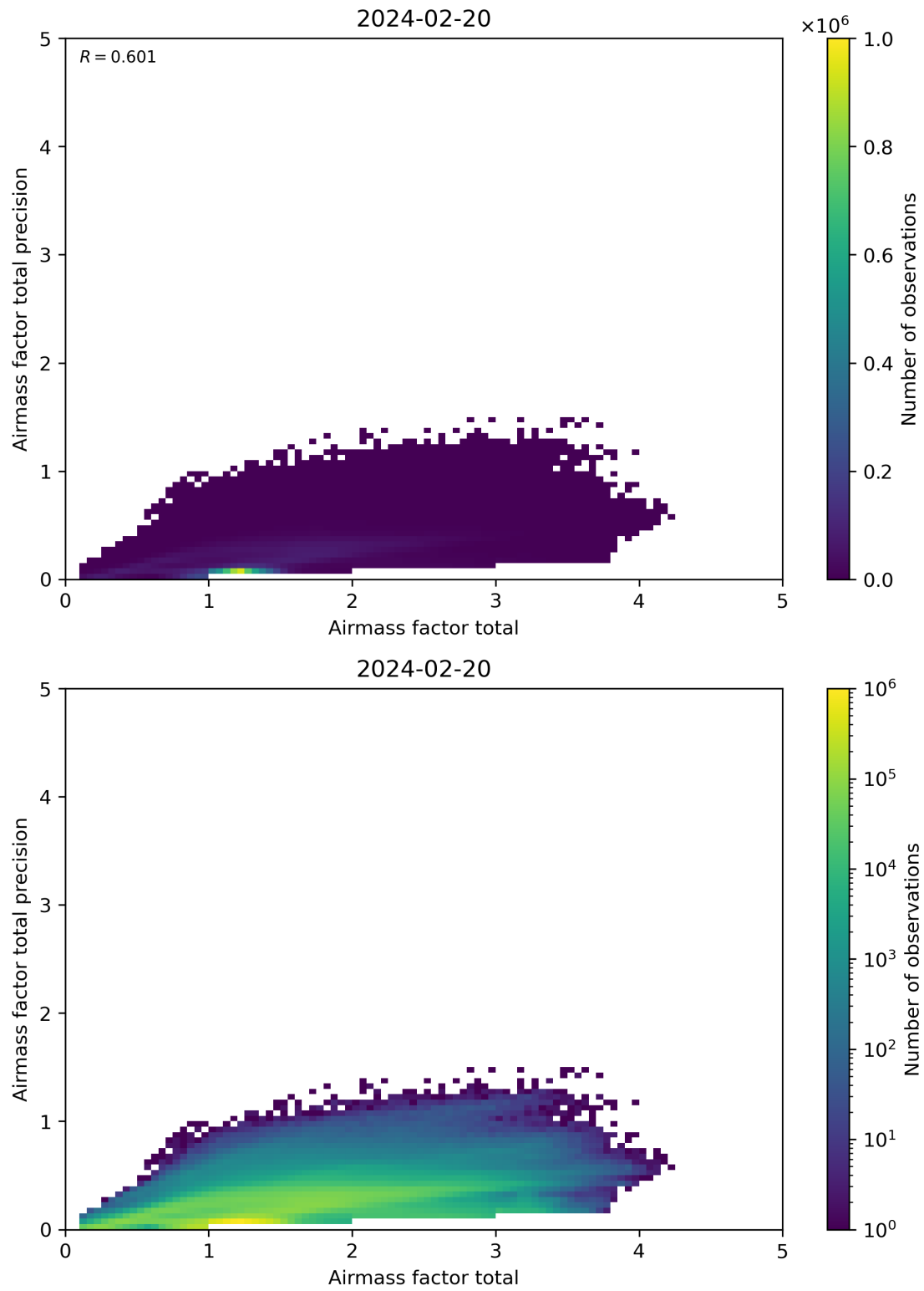
Figure 103: Scatter density plot of “Airmass factor total” against “Airmass factor total precision” for 2024-02-19 to 2024-02-21.
