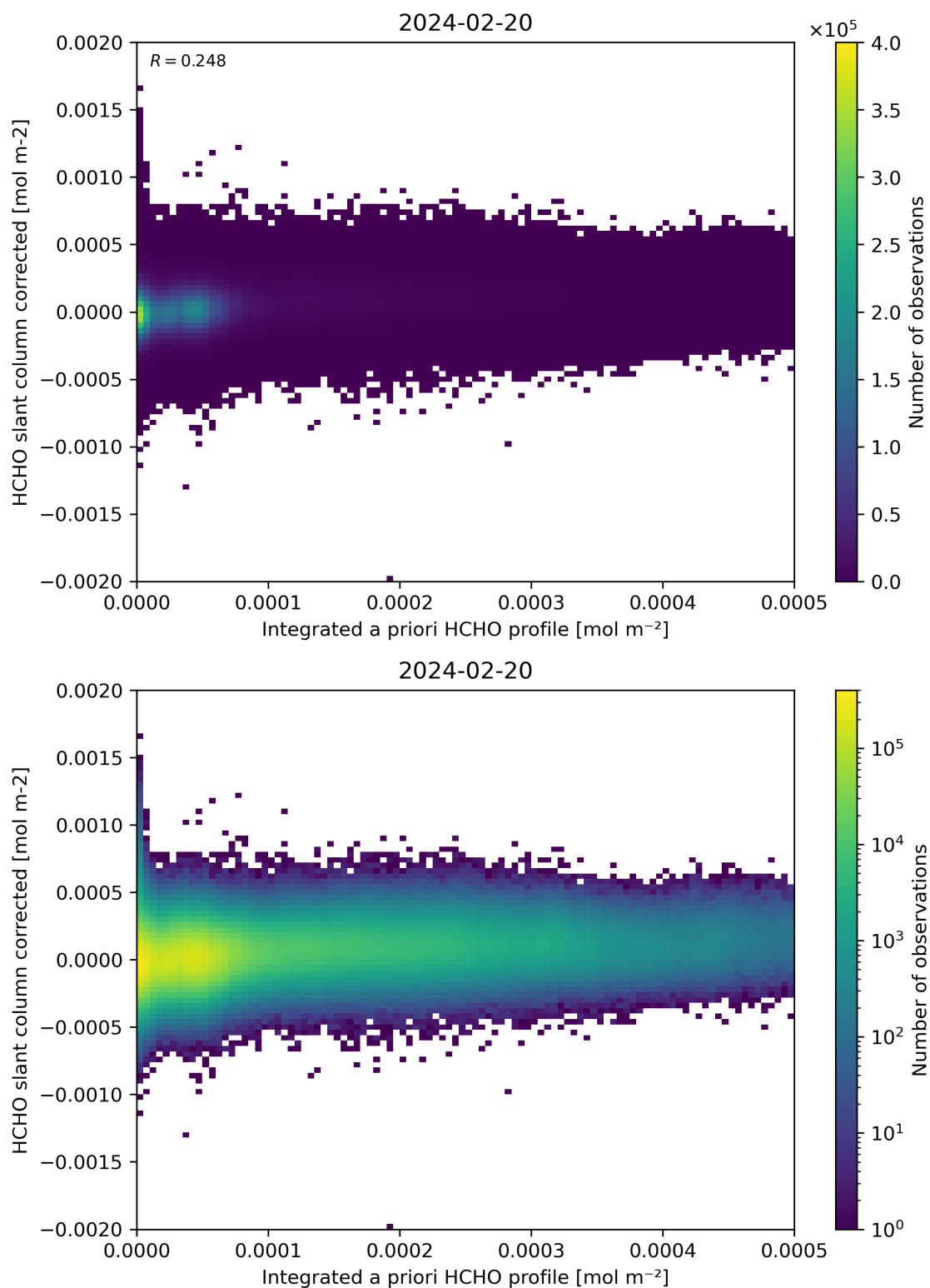
Figure 151: Scatter density plot of “Integrated a priori HCHO profile” against “HCHO slant column corrected” for 2024-02-19 to 2024-02-21.
