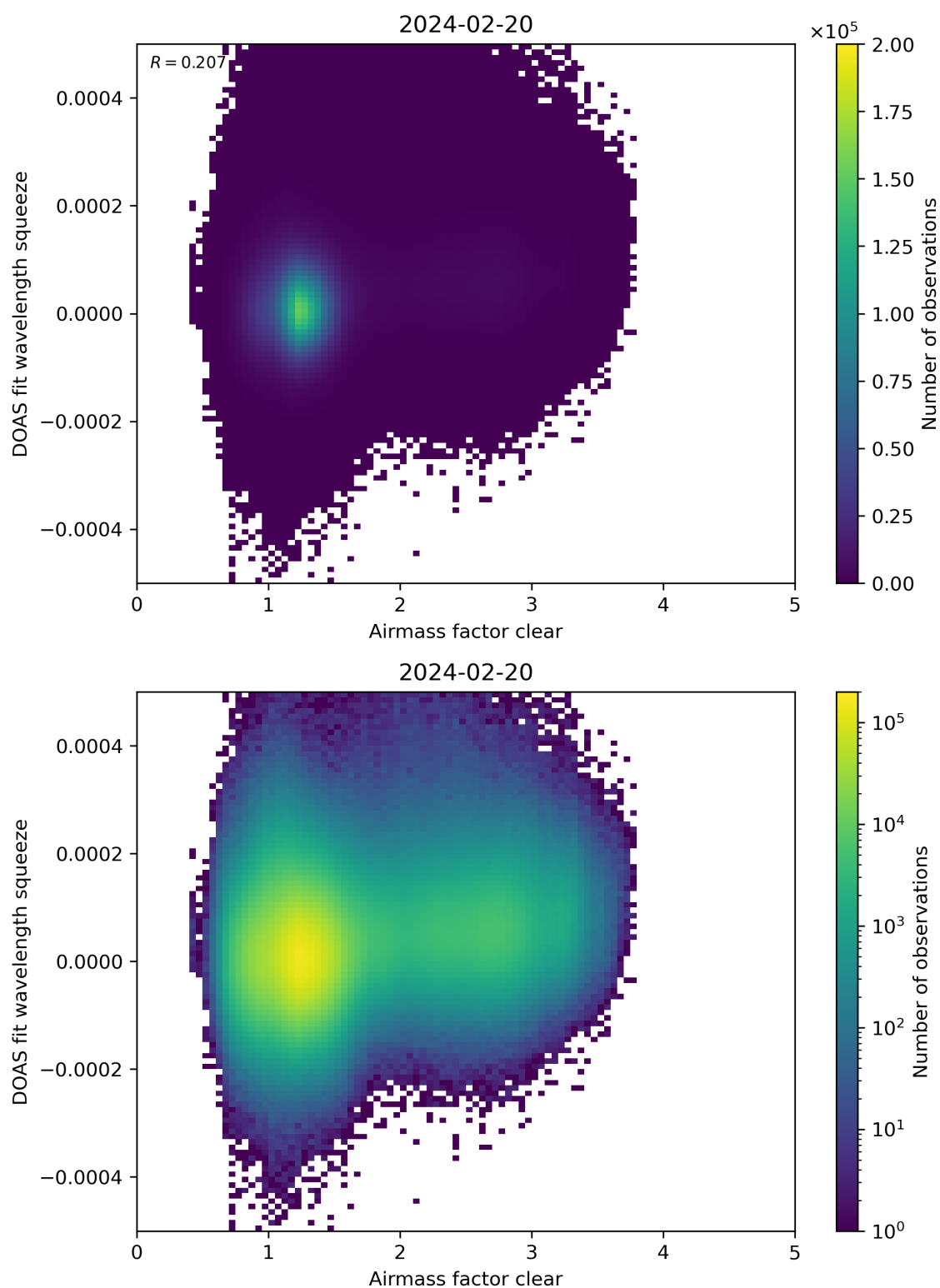
Figure 73: Scatter density plot of “Airmass factor clear” against “DOAS fit wavelength squeeze” for 2024-02-19 to 2024-02-21.
