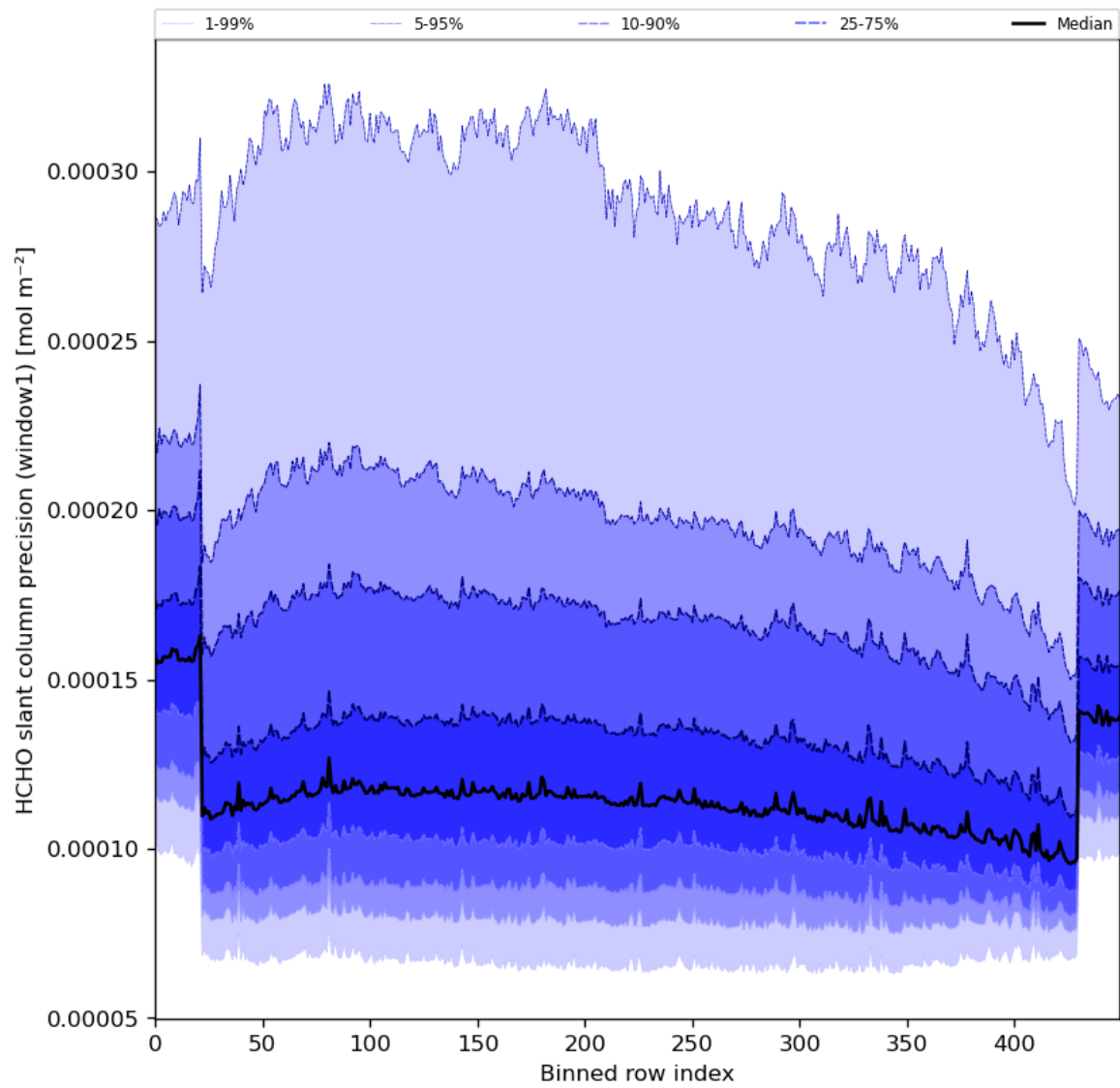
Figure 53: Along track statistics of “HCHO slant column precision (window1)” for 2024-02-19 to 2024-02-21
