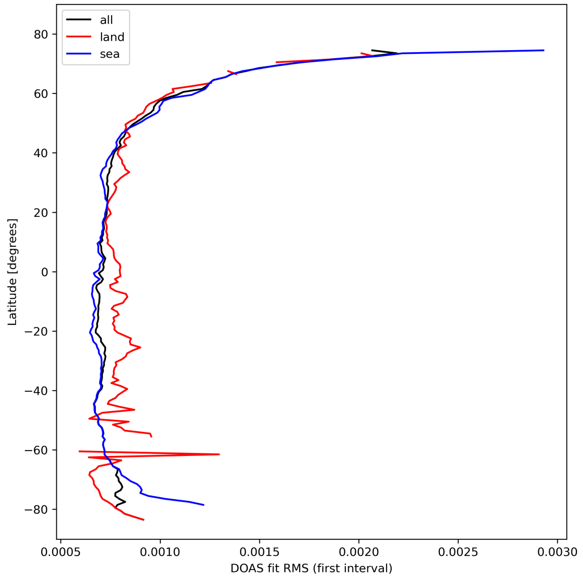
Figure 32: Zonal average of “DOAS fit RMS (first interval)” for 2024-02-19 to 2024-02-21.
