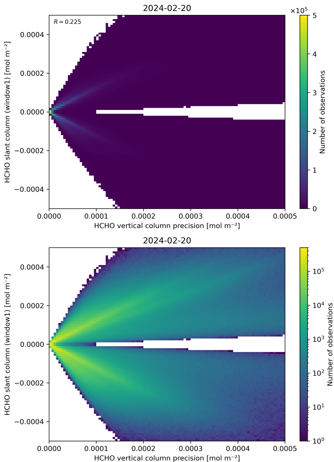
Figure 142: Scatter density plot of “HCHO vertical column precision” against “HCHO slant column (window1)” for 2024-02-19 to 2024-02-21.
