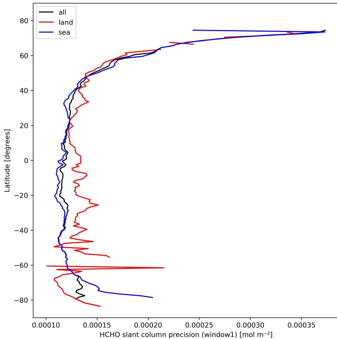
Figure 25: Zonal average of “HCHO slant column precision (window1)” for 2024-02-19 to 2024-02-21.
