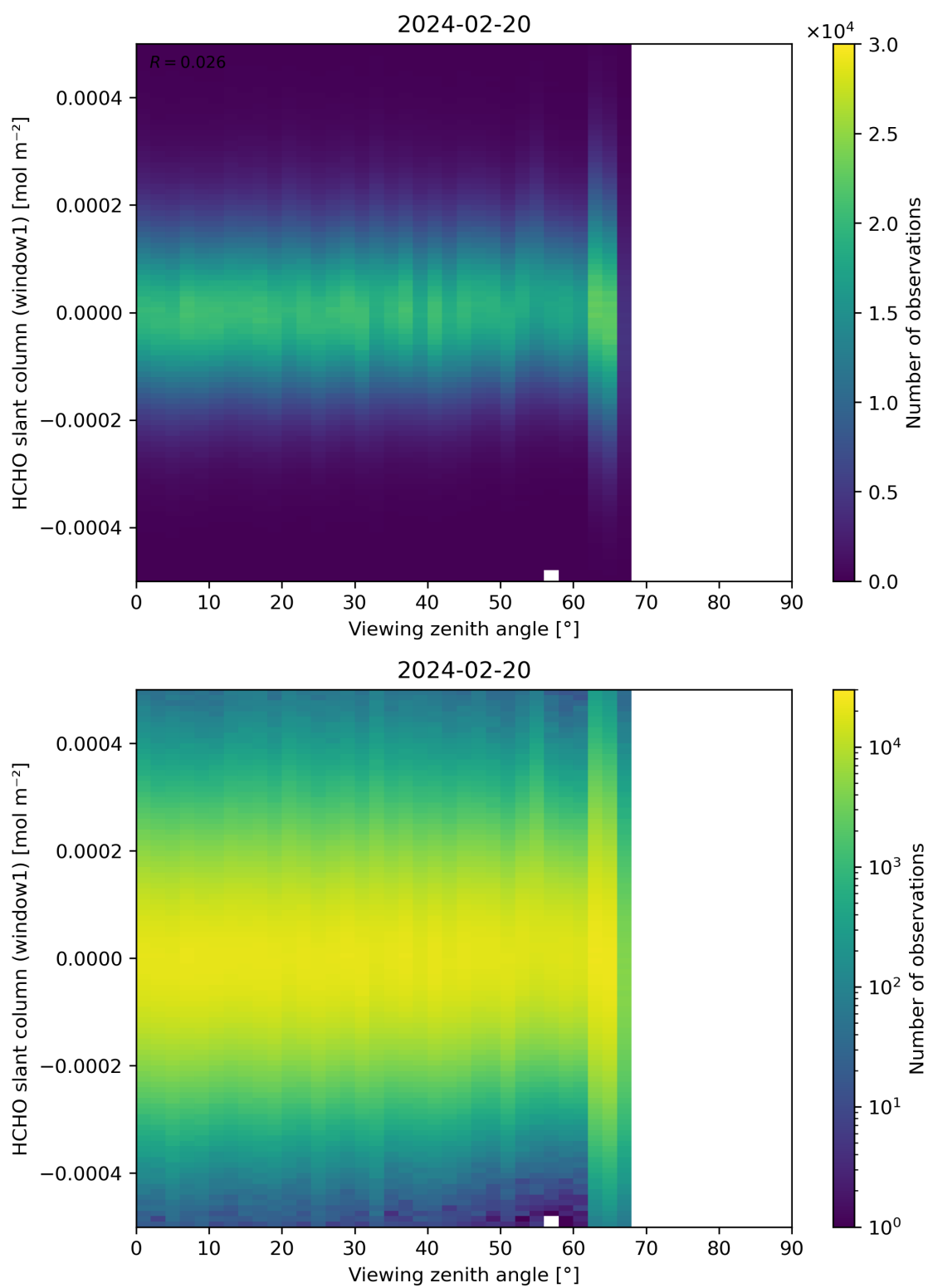
Figure 188: Scatter density plot of “Viewing zenith angle” against “HCHO slant column (window1)” for 2024-02-19 to 2024-02-21.
