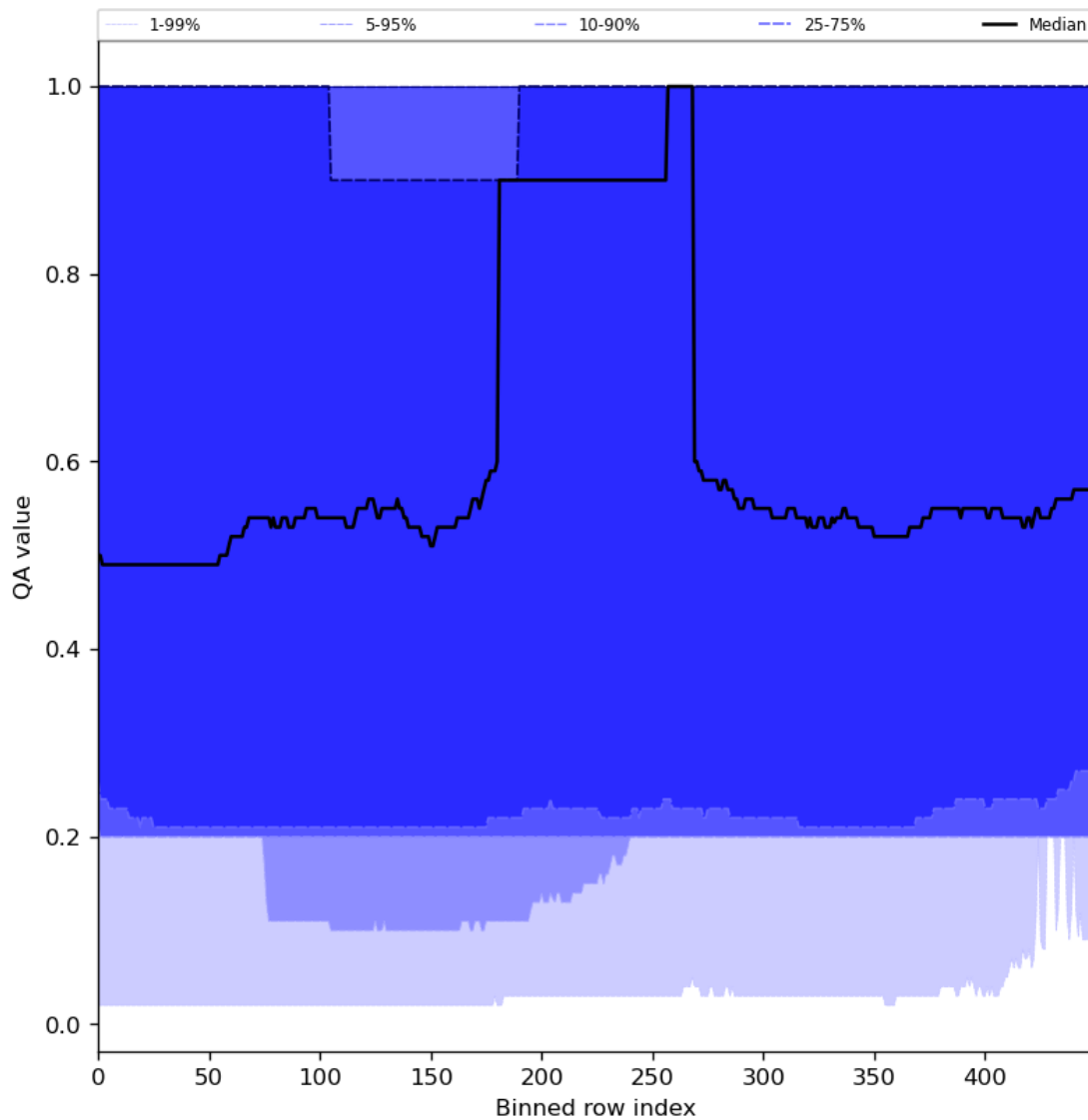
Figure 48: Along track statistics of “QA value” for 2024-02-19 to 2024-02-21
