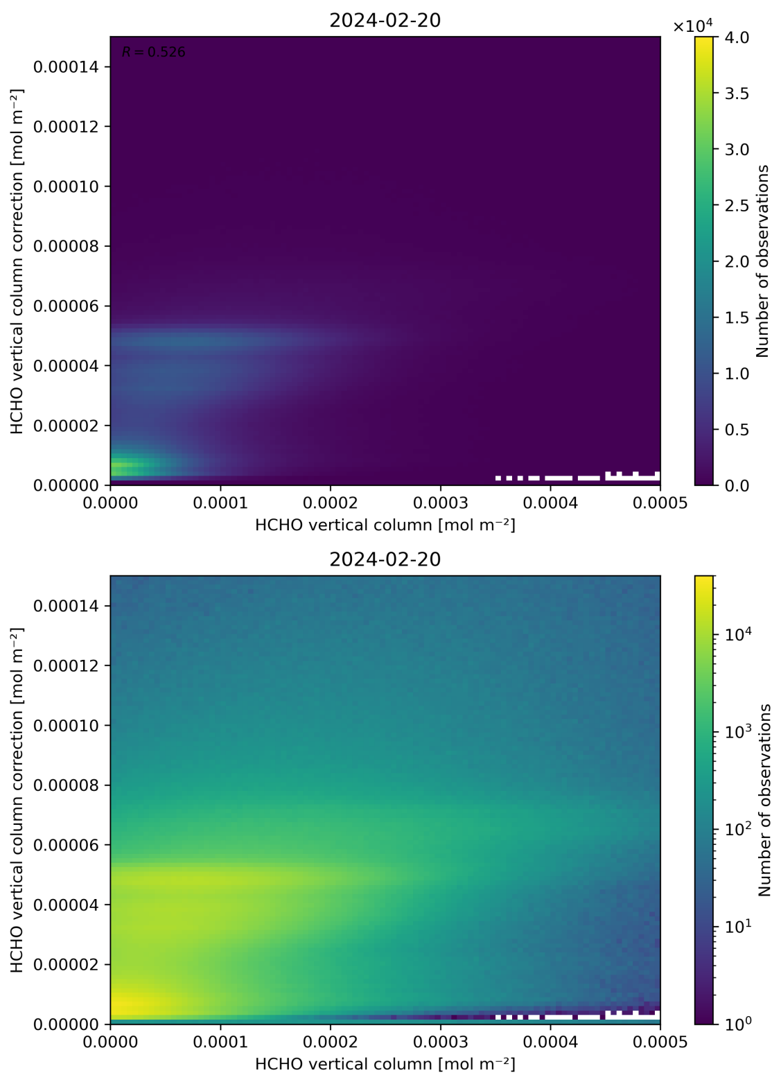
Figure 133: Scatter density plot of “HCHO vertical column” against “HCHO vertical column correction” for 2024-02-19 to 2024-02-21.
