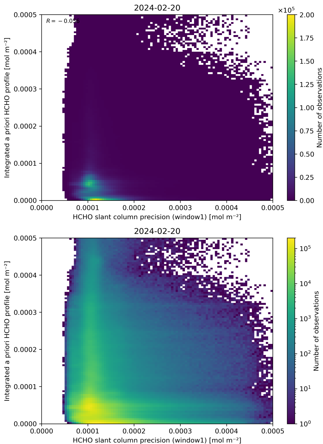
Figure 96: Scatter density plot of “HCHO slant column precision (window1)” against “Integrated a priori HCHO profile” for 2024-02-19 to 2024-02-21.
