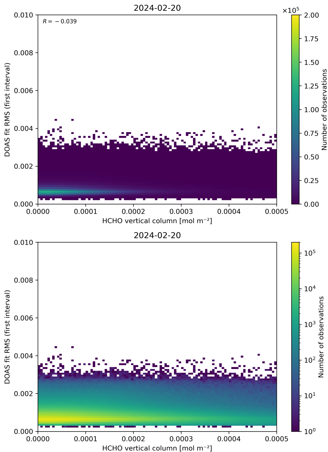
Figure 123: Scatter density plot of “HCHO vertical column” against “DOAS fit RMS (first interval)” for 2024-02-19 to 2024-02-21.
