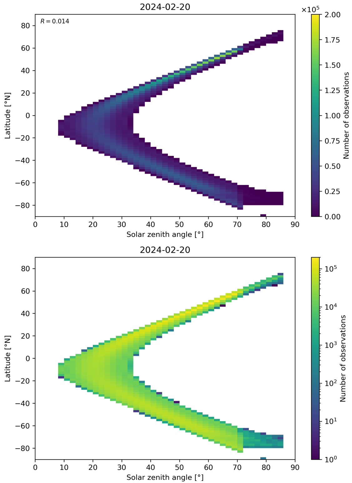
Figure 181: Scatter density plot of “Solar zenith angle” against “Latitude” for 2024-02-19 to 2024-02-21.
