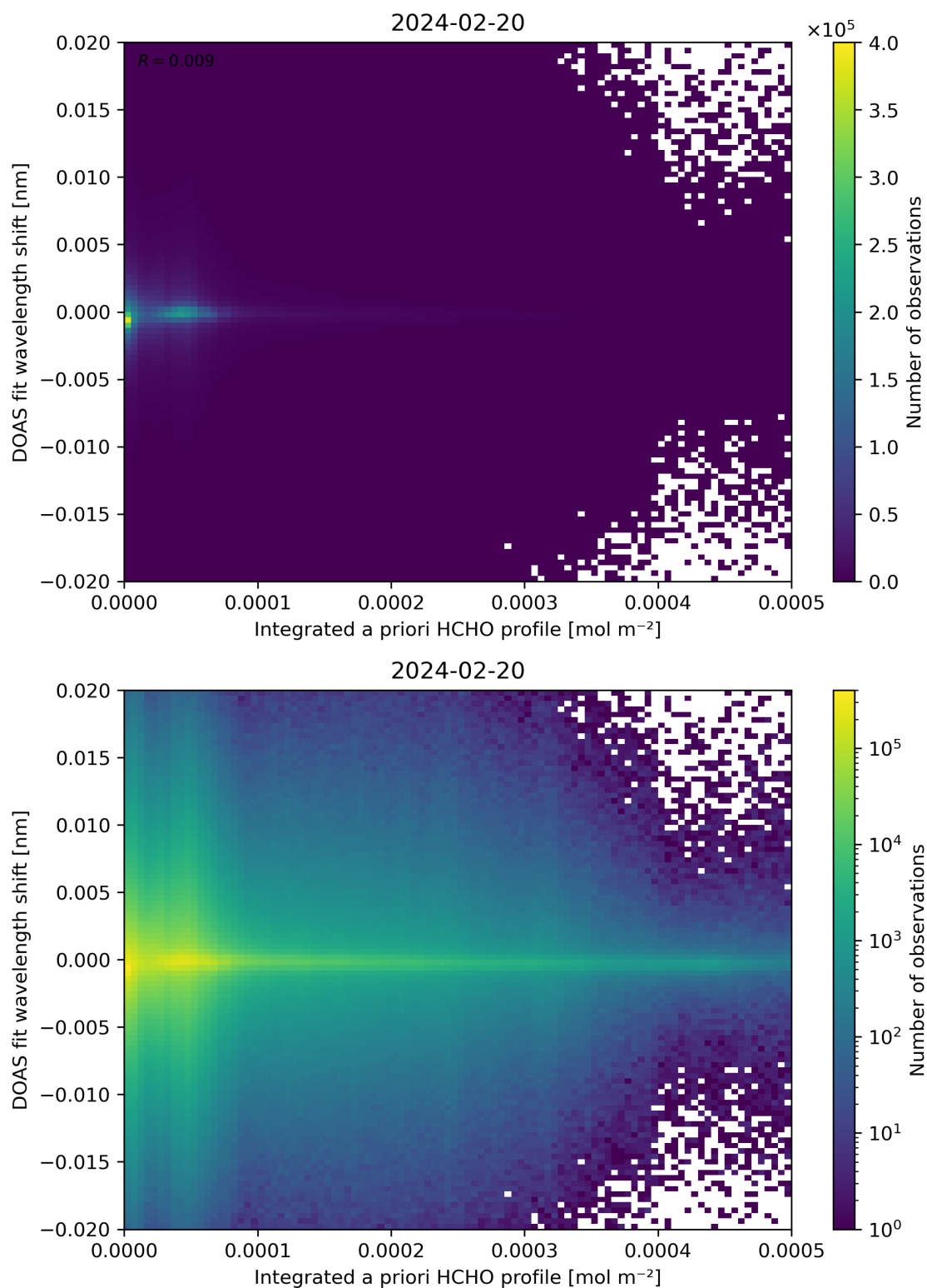
Figure 149: Scatter density plot of “Integrated a priori HCHO profile” against “DOAS fit wavelength shift” for 2024-02-19 to 2024-02-21.
