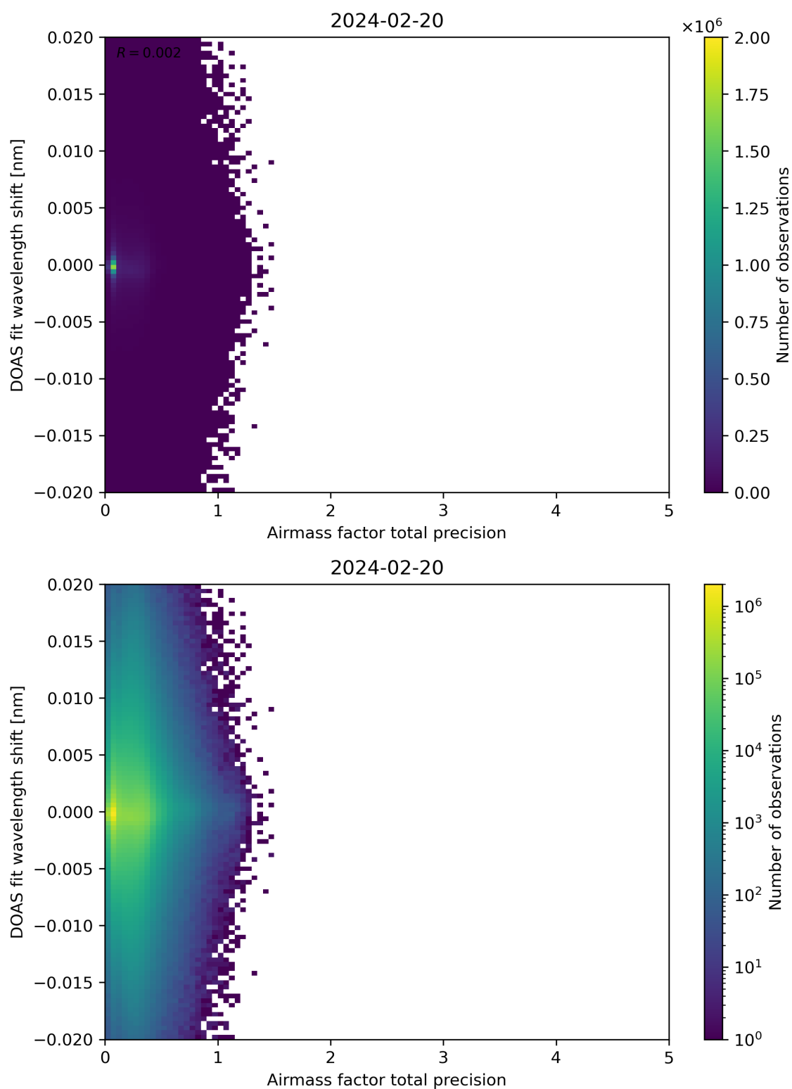
Figure 106: Scatter density plot of “Airmass factor total precision” against “DOAS fit wavelength shift” for 2024-02-19 to 2024-02-21.
