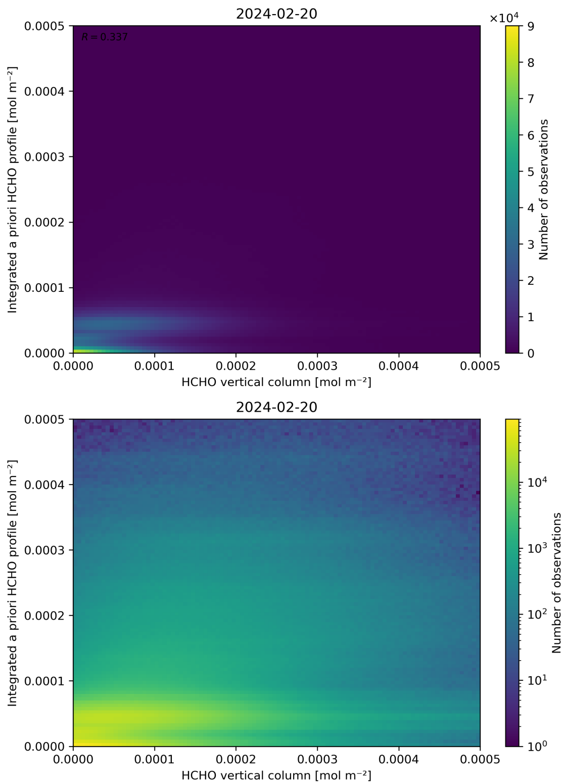
Figure 135: Scatter density plot of “HCHO vertical column” against “Integrated a priori HCHO profile” for 2024-02-19 to 2024-02-21.
