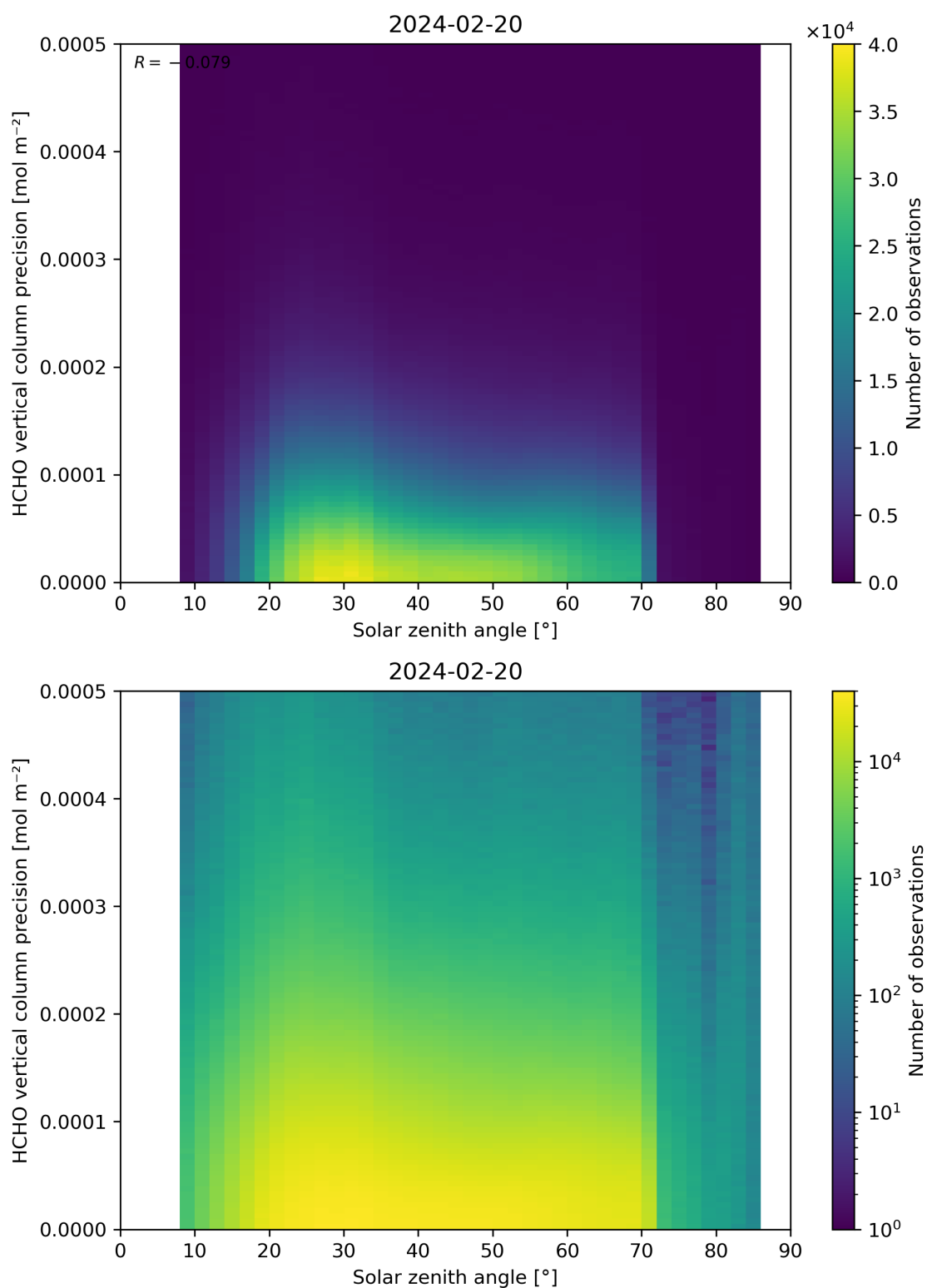
Figure 179: Scatter density plot of “Solar zenith angle” against “HCHO vertical column precision” for 2024-02-19 to 2024-02-21.
