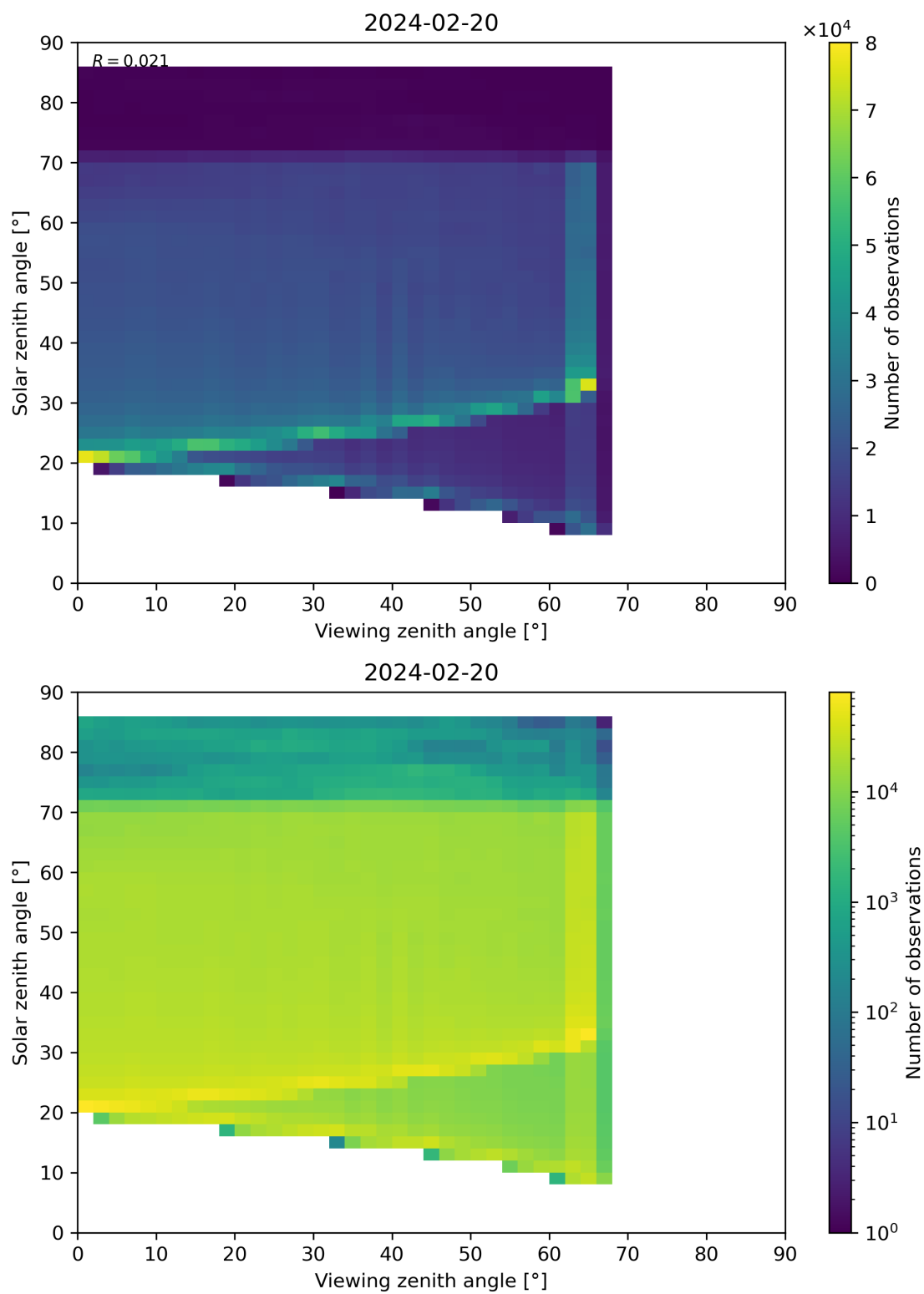
Figure 197: Scatter density plot of “Viewing zenith angle” against “Solar zenith angle” for 2024-02-19 to 2024-02-21.
