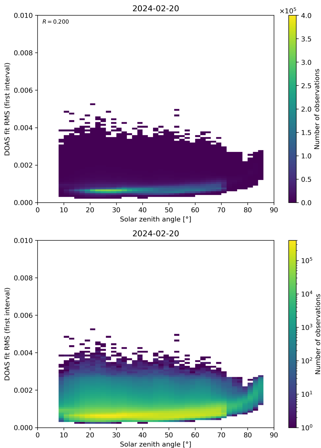
Figure 167: Scatter density plot of “Solar zenith angle” against “DOAS fit RMS (first interval)” for 2024-02-19 to 2024-02-21.
