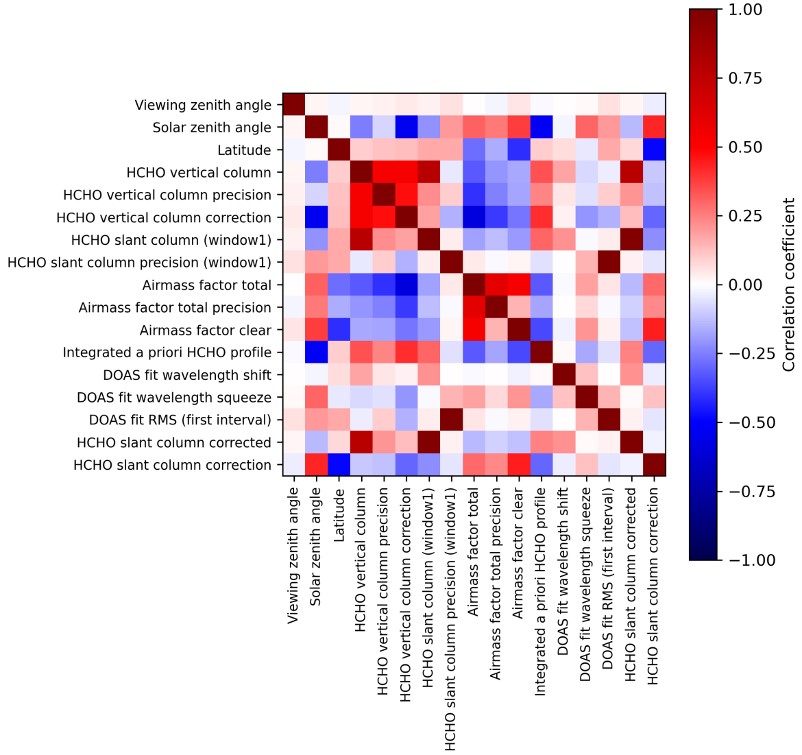
Figure 2: Map of correlation matrix for 2024-02-19 to 2024-02-21.
