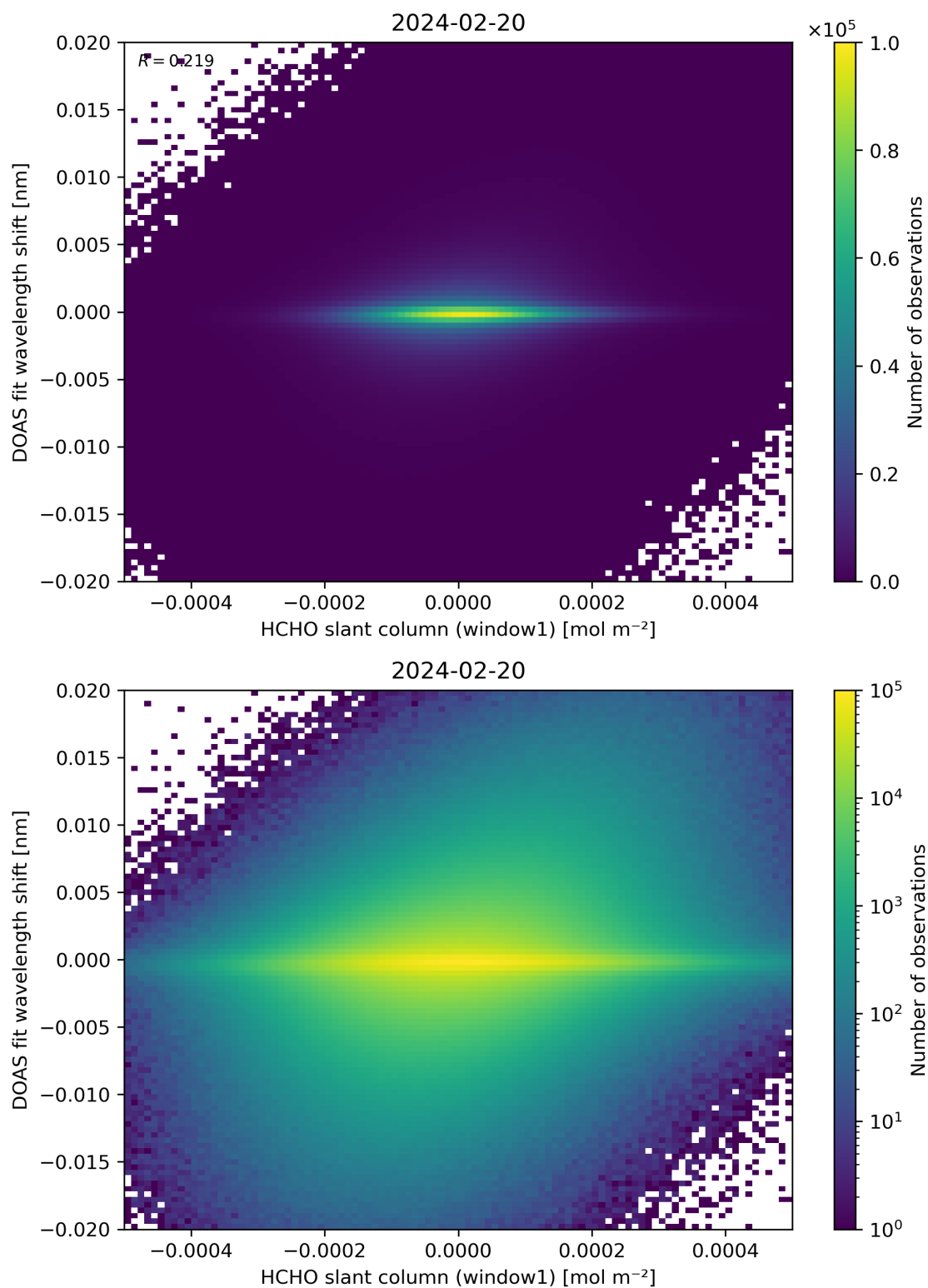
Figure 79: Scatter density plot of “HCHO slant column (window1)” against “DOAS fit wavelength shift” for 2024-02-19 to 2024-02-21.
