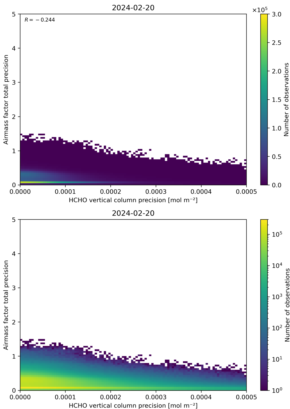
Figure 145: Scatter density plot of “HCHO vertical column precision” against “Airmass factor total precision” for 2024-02-19 to 2024-02-21.
