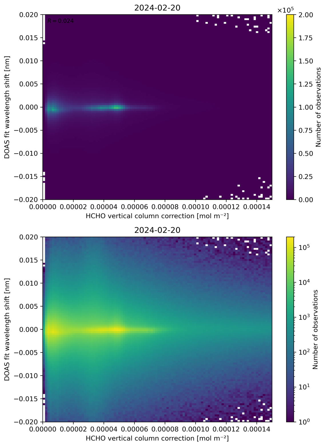
Figure 113: Scatter density plot of “HCHO vertical column correction” against “DOAS fit wavelength shift” for 2024-02-19 to 2024-02-21.
