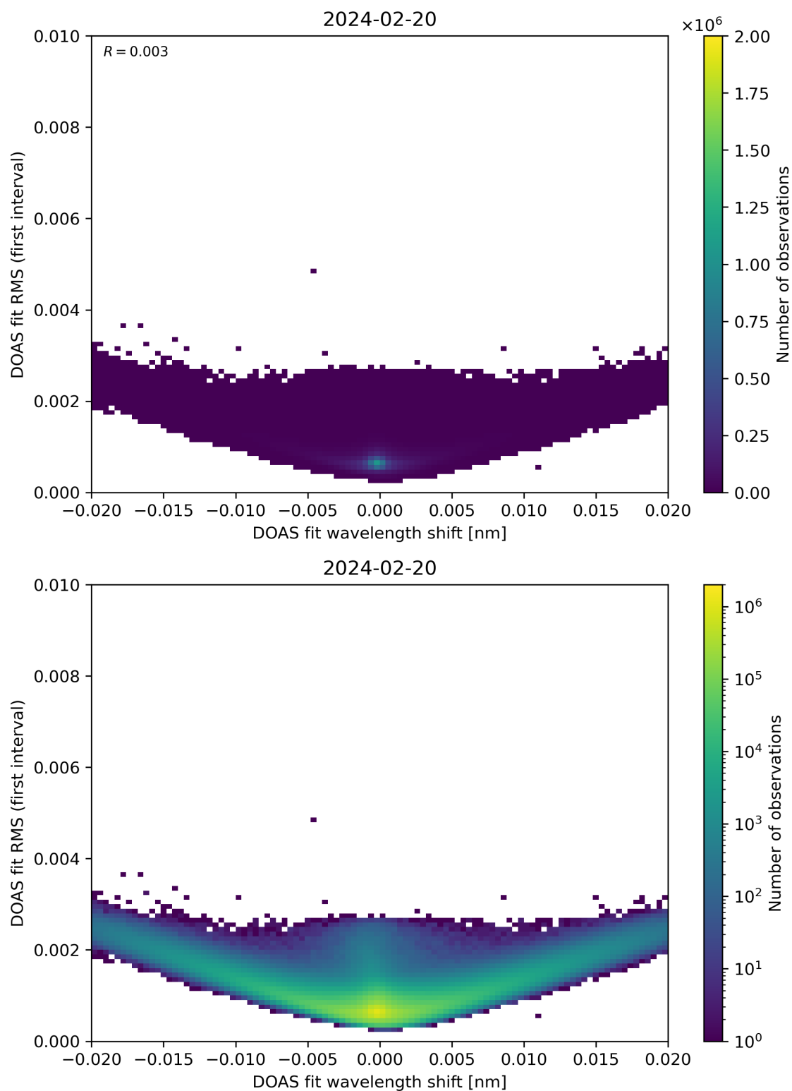
Figure 64: Scatter density plot of “DOAS fit wavelength shift” against “DOAS fit RMS (first interval)” for 2024-02-19 to 2024-02-21.
