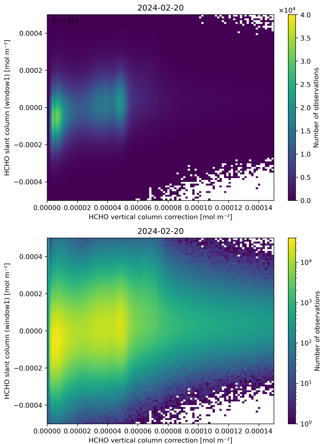
Figure 118: Scatter density plot of “HCHO vertical column correction” against “HCHO slant column (window1)” for 2024-02-19 to 2024-02-21.
