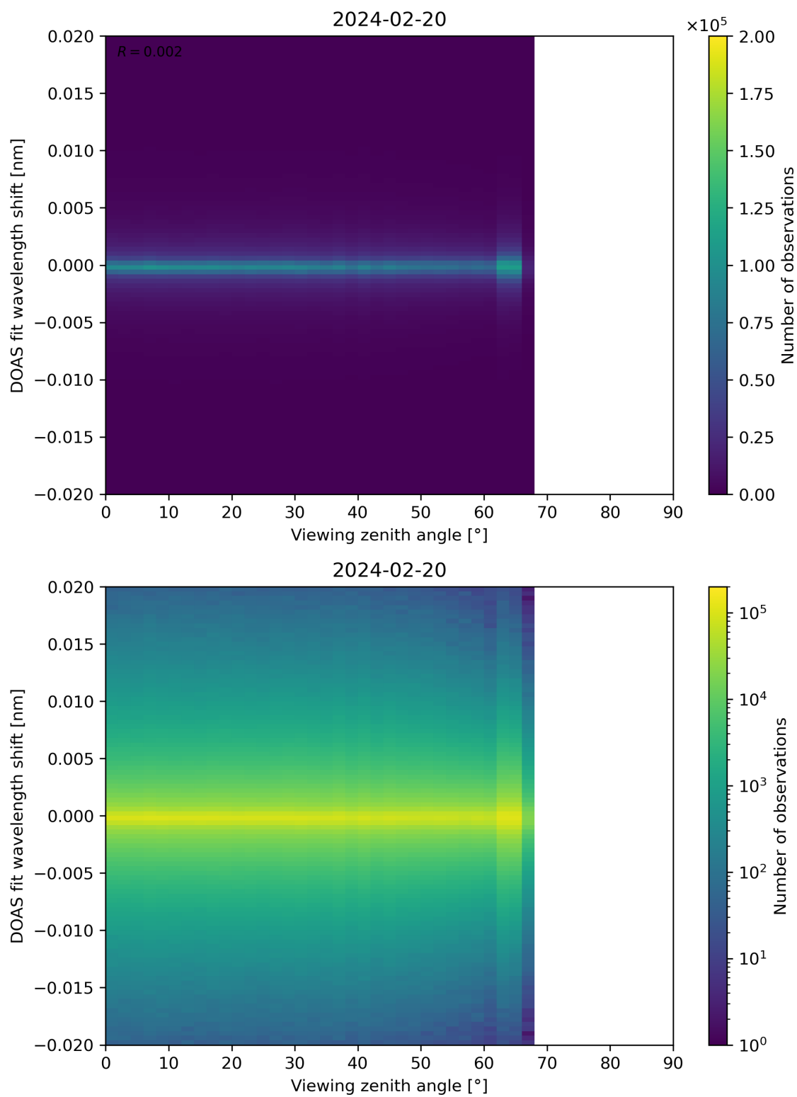
Figure 183: Scatter density plot of “Viewing zenith angle” against “DOAS fit wavelength shift” for 2024-02-19 to 2024-02-21.
