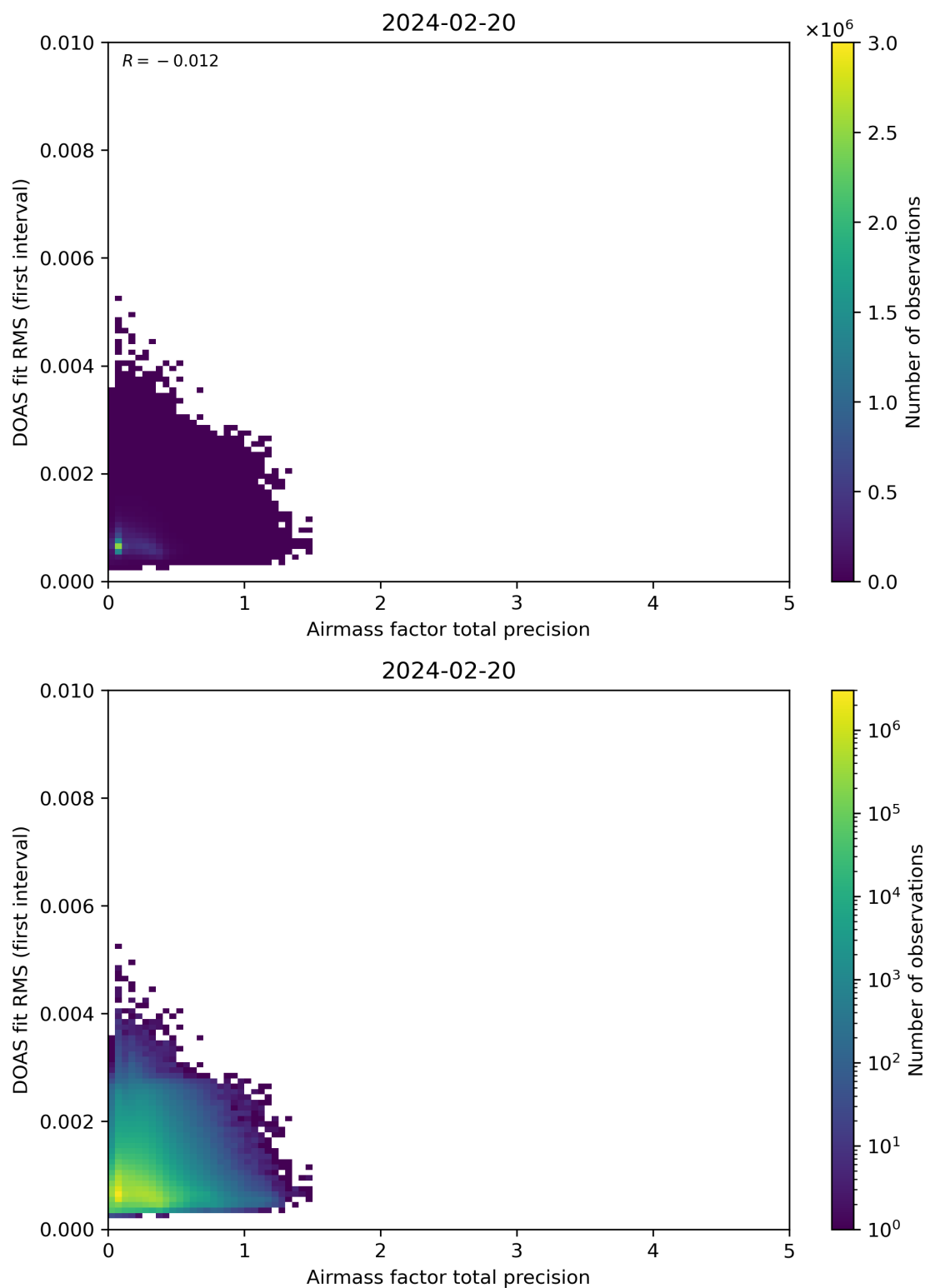
Figure 105: Scatter density plot of “Airmass factor total precision” against “DOAS fit RMS (first interval)” for 2024-02-19 to 2024-02-21.
