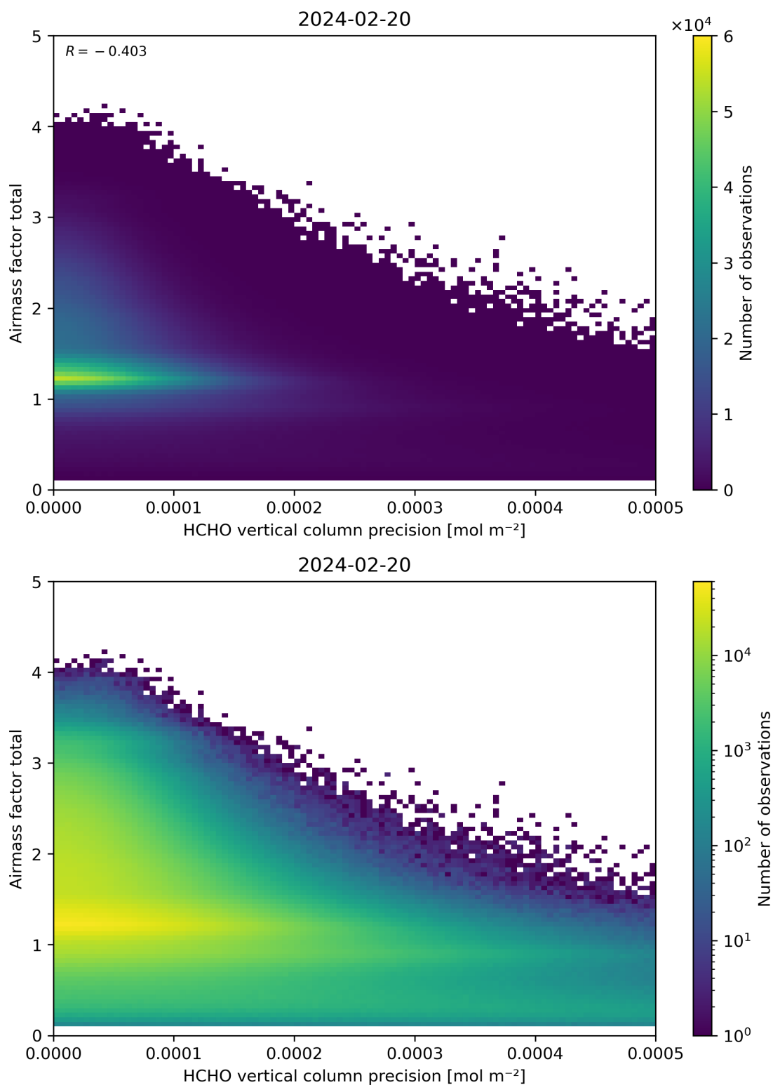
Figure 144: Scatter density plot of “HCHO vertical column precision” against “Airmass factor total” for 2024-02-19 to 2024-02-21.
