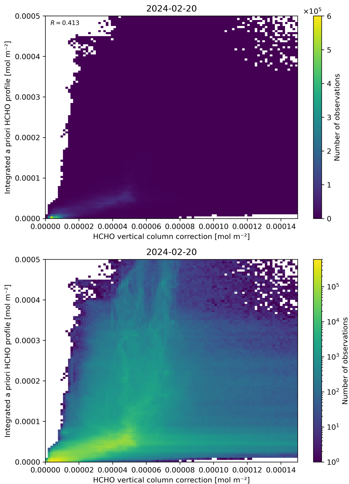
Figure 122: Scatter density plot of “HCHO vertical column correction” against “Integrated a priori HCHO profile” for 2024-02-19 to 2024-02-21.
