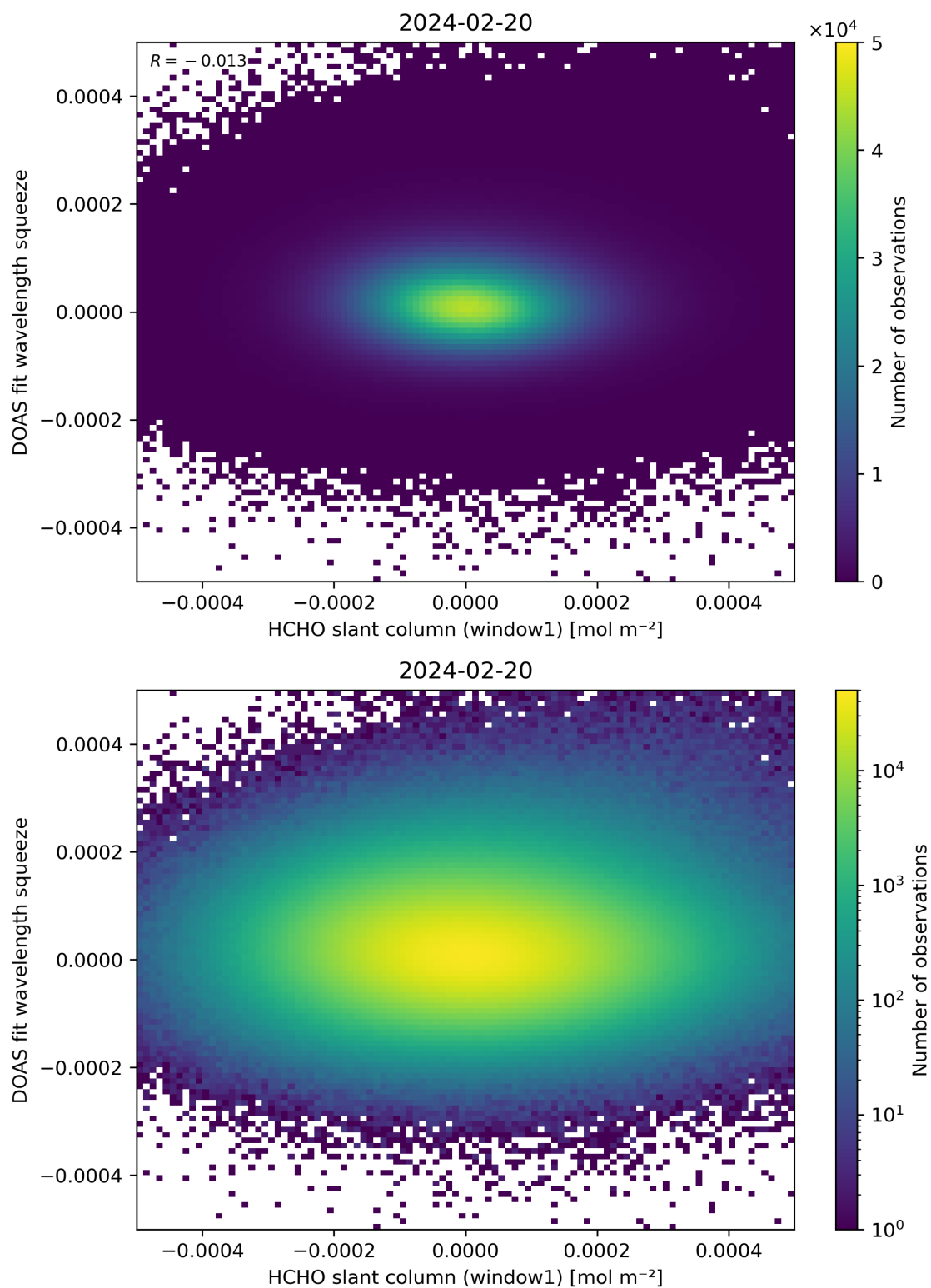
Figure 80: Scatter density plot of “HCHO slant column (window1)” against “DOAS fit wavelength squeeze” for 2024-02-19 to 2024-02-21.
