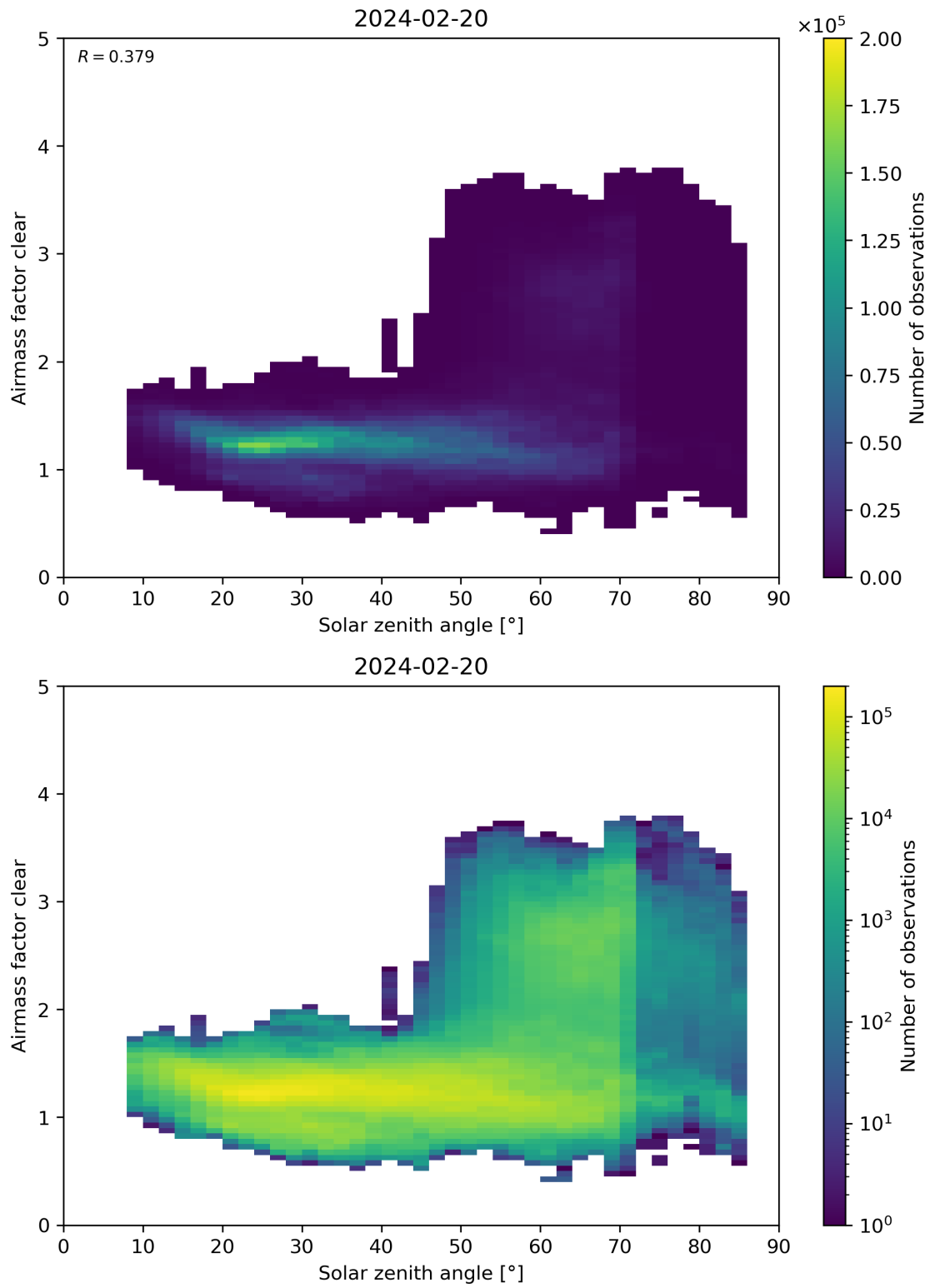
Figure 170: Scatter density plot of “Solar zenith angle” against “Airmass factor clear” for 2024-02-19 to 2024-02-21.
