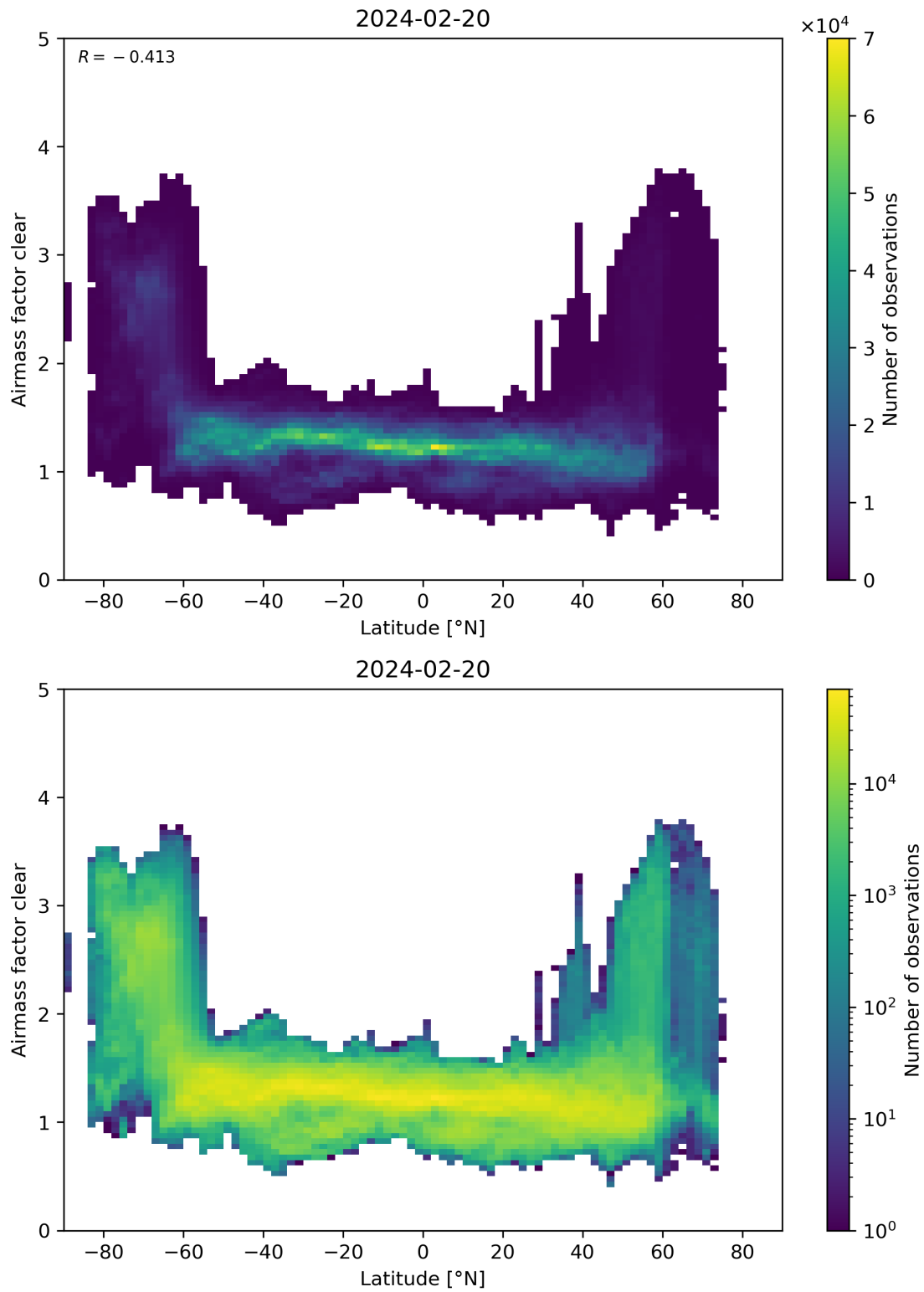
Figure 156: Scatter density plot of “Latitude” against “Airmass factor clear” for 2024-02-19 to 2024-02-21.
