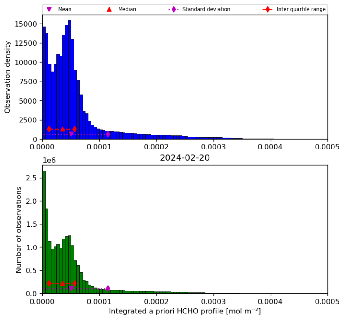
Figure 43: Histogram of “Integrated a priori HCHO profile” for 2024-02-19 to 2024-02-21
