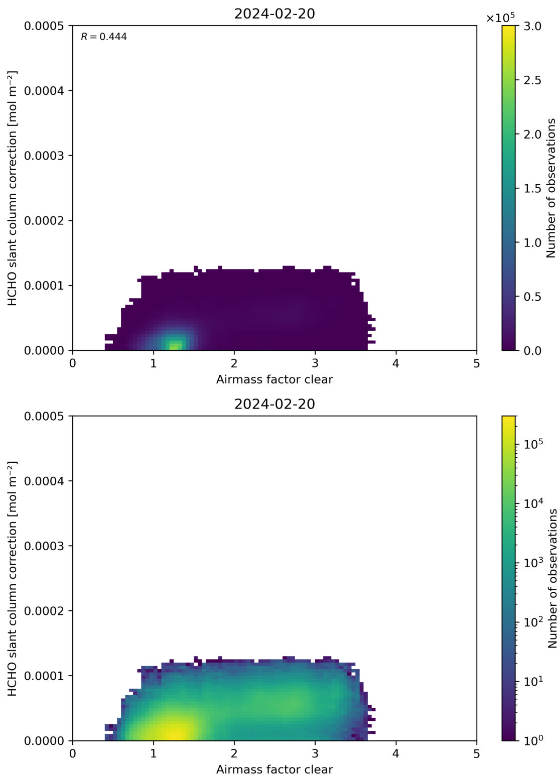
Figure 75: Scatter density plot of “Airmass factor clear” against “HCHO slant column correction” for 2024-02-19 to 2024-02-21.
