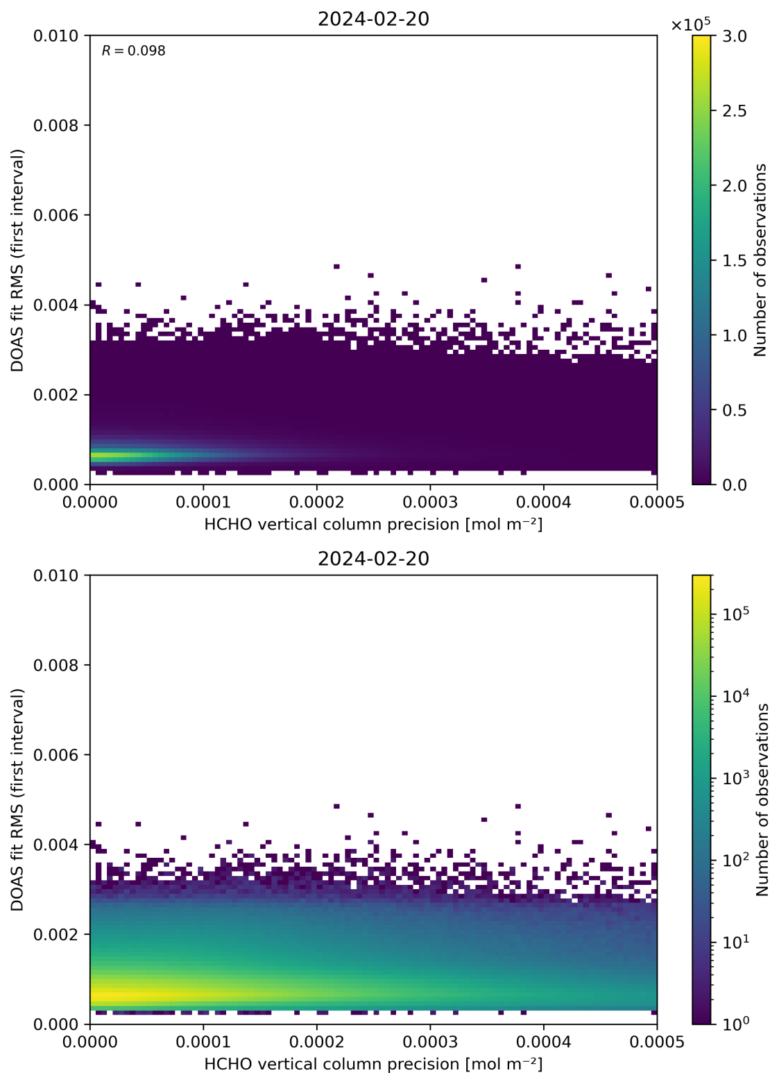
Figure 136: Scatter density plot of “HCHO vertical column precision” against “DOAS fit RMS (first interval)” for 2024-02-19 to 2024-02-21.
