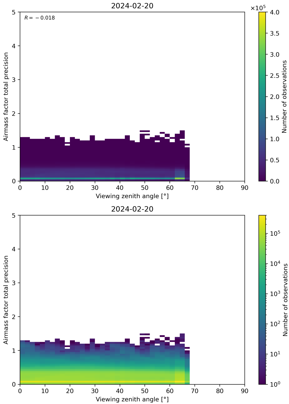
Figure 191: Scatter density plot of “Viewing zenith angle” against “Airmass factor total precision” for 2024-02-19 to 2024-02-21.
