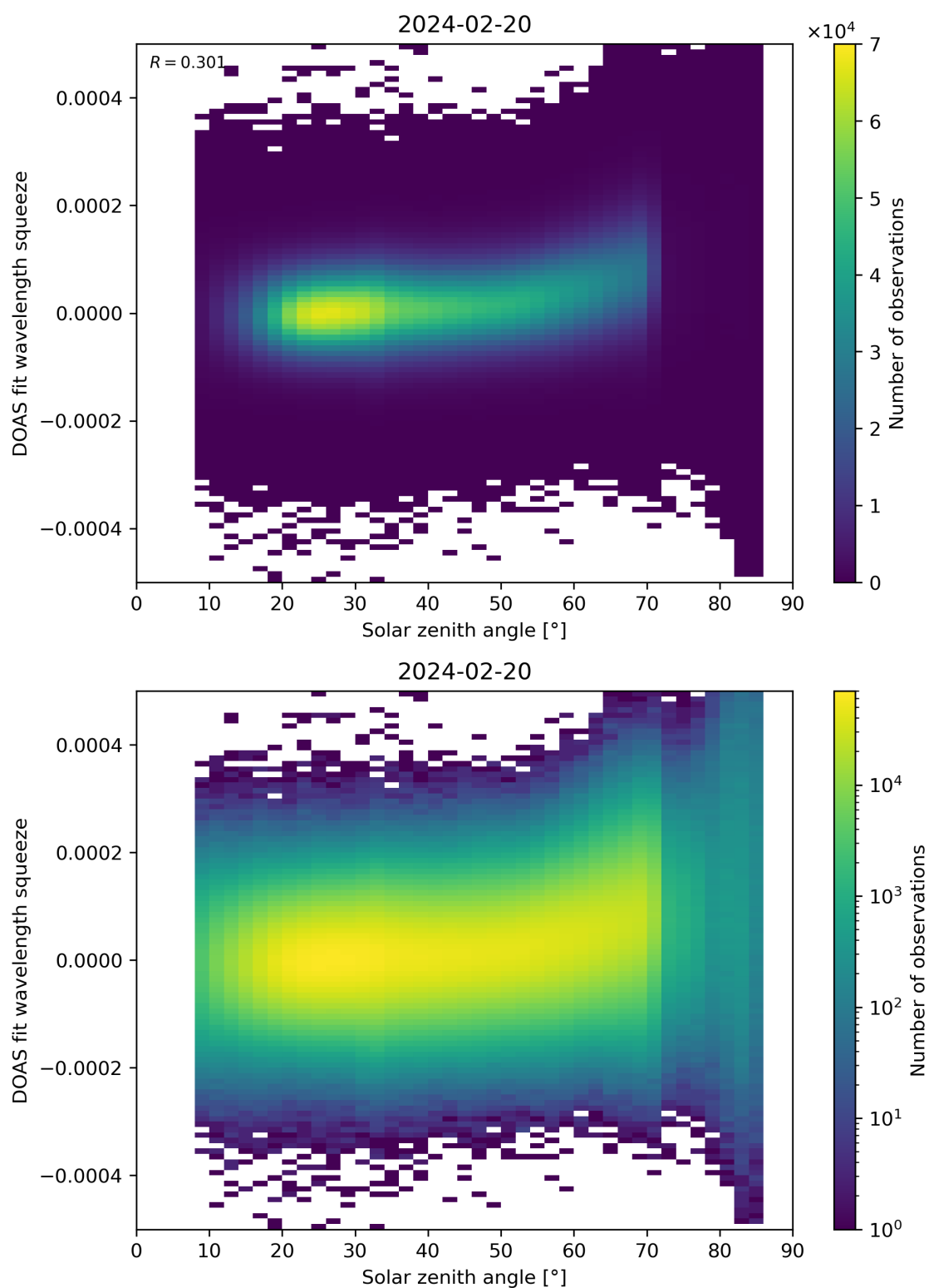
Figure 169: Scatter density plot of “Solar zenith angle” against “DOAS fit wavelength squeeze” for 2024-02-19 to 2024-02-21.
