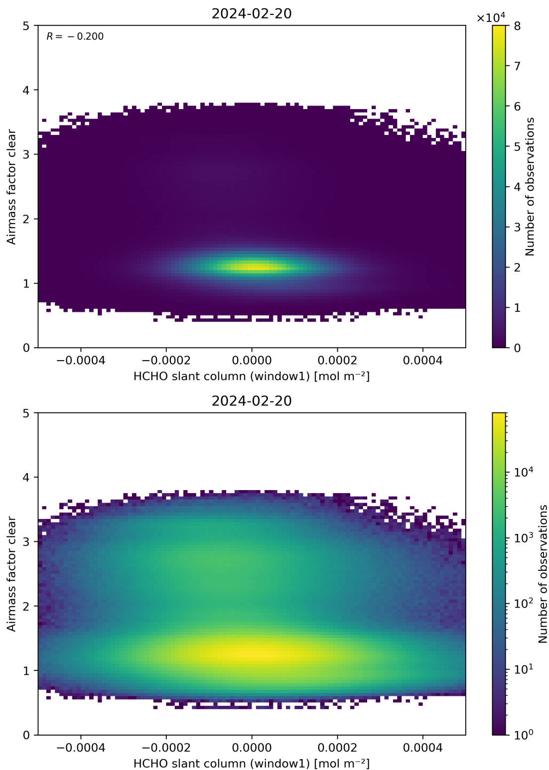
Figure 81: Scatter density plot of “HCHO slant column (window1)” against “Airmass factor clear” for 2024-02-19 to 2024-02-21.
