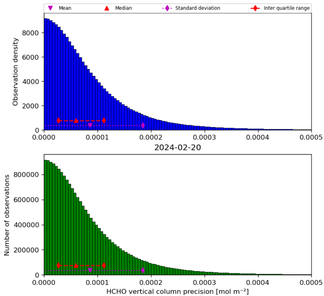
Figure 36: Histogram of “HCHO vertical column precision” for 2024-02-19 to 2024-02-21
