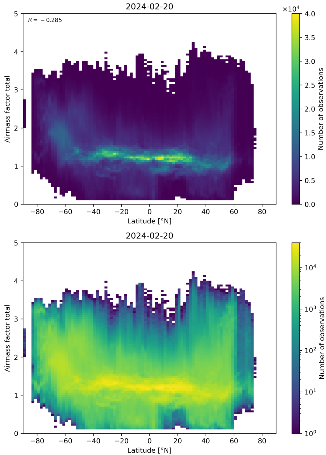
Figure 161: Scatter density plot of “Latitude” against “Airmass factor total” for 2024-02-19 to 2024-02-21.
