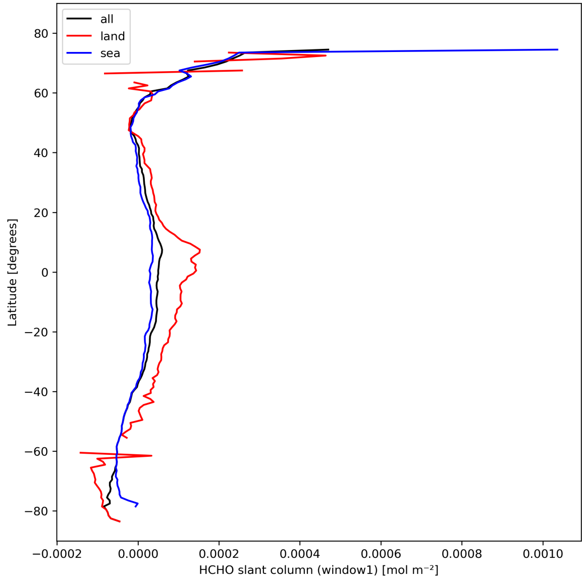
Figure 24: Zonal average of “HCHO slant column (window1)” for 2024-02-19 to 2024-02-21.
