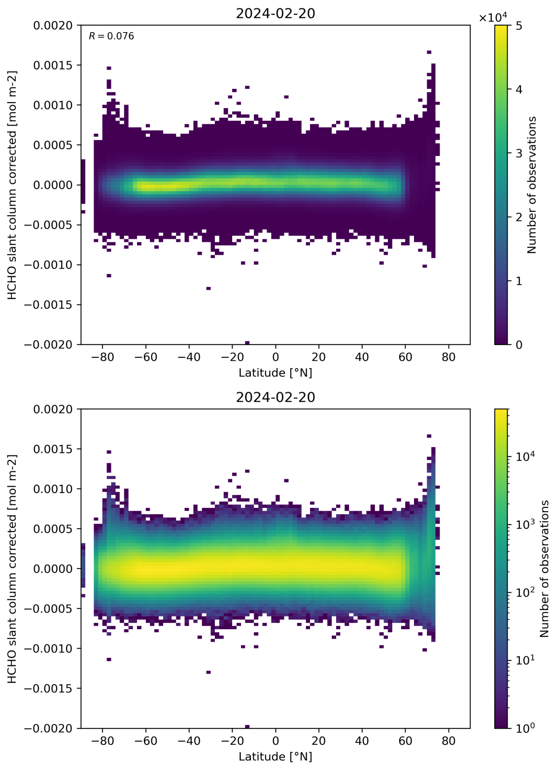
Figure 157: Scatter density plot of “Latitude” against “HCHO slant column corrected” for 2024-02-19 to 2024-02-21.
