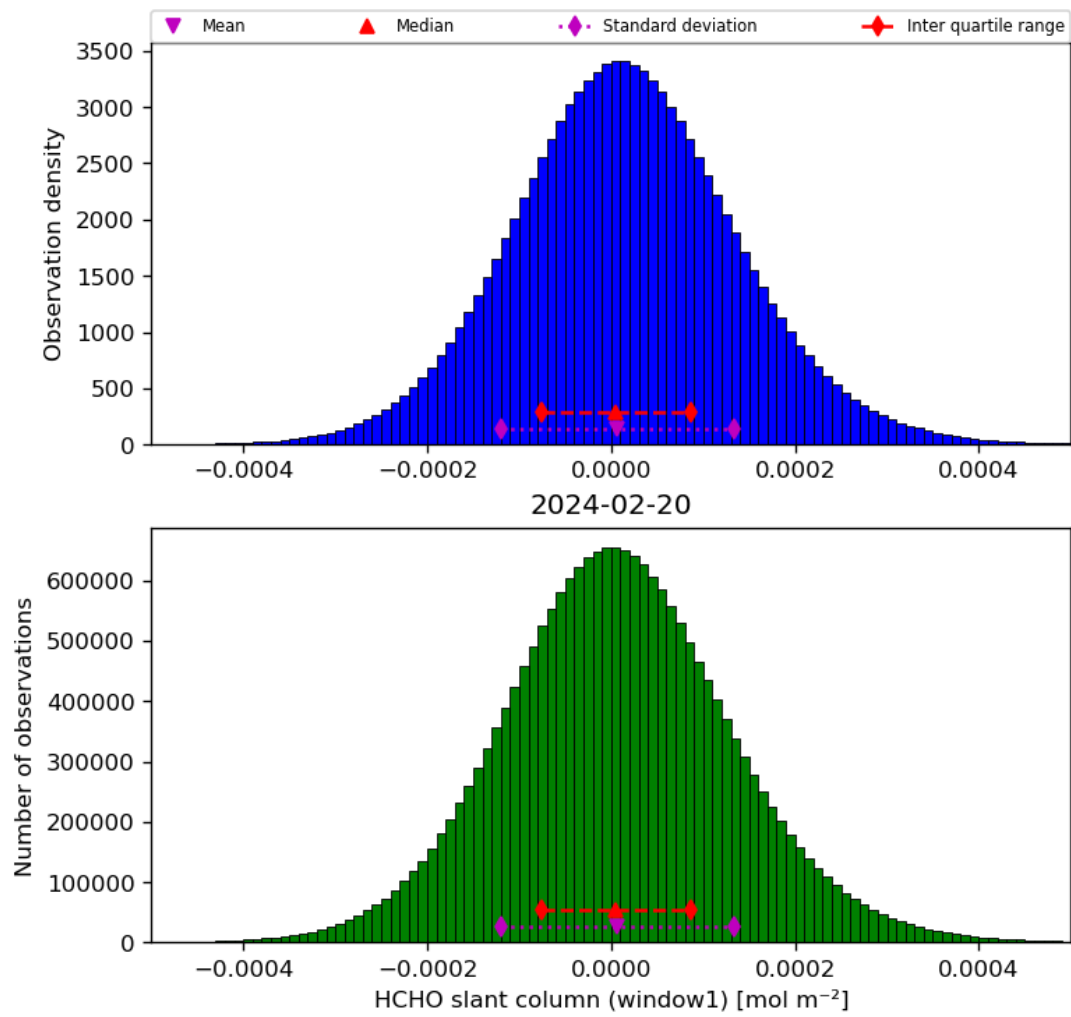
Figure 38: Histogram of “HCHO slant column (window1)” for 2024-02-19 to 2024-02-21
