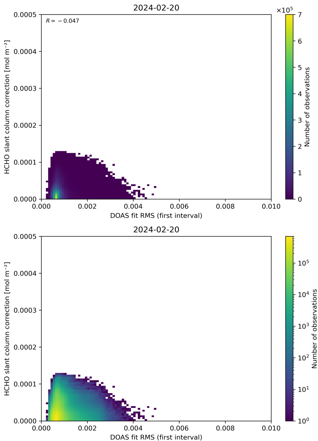
Figure 63: Scatter density plot of “DOAS fit RMS (first interval)” against “HCHO slant column correction” for 2024-02-19 to 2024-02-21.
