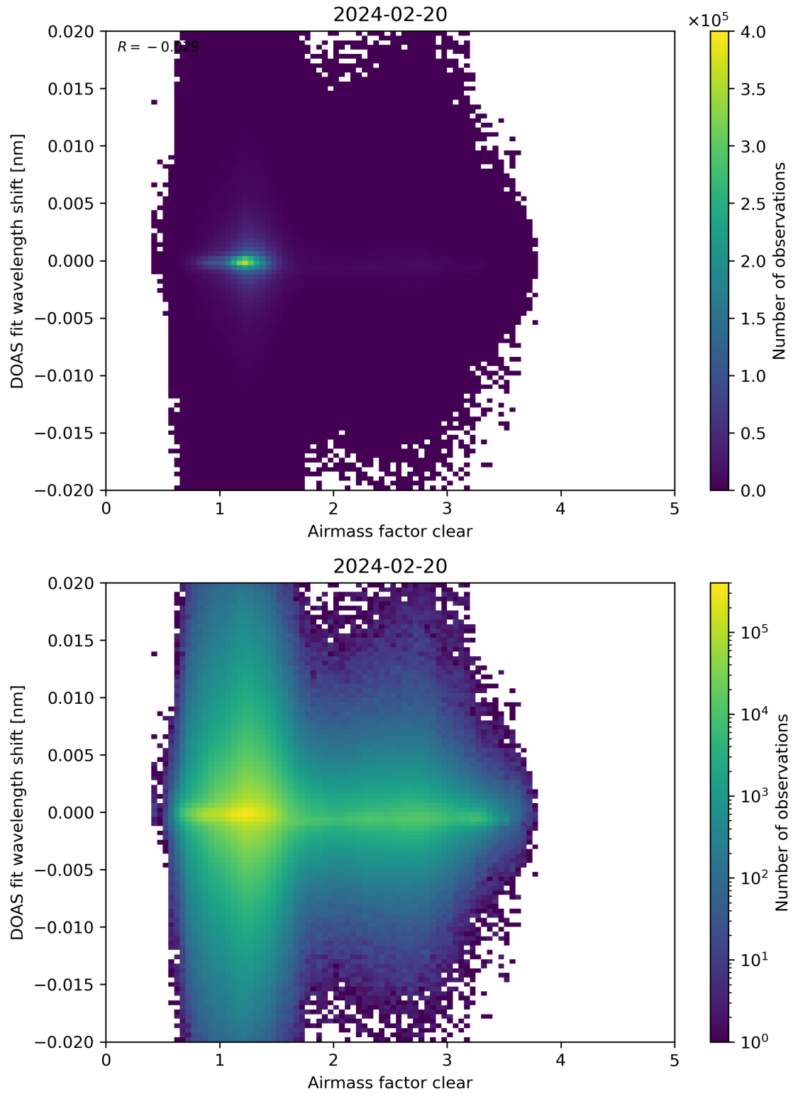
Figure 72: Scatter density plot of “Airmass factor clear” against “DOAS fit wavelength shift” for 2024-02-19 to 2024-02-21.
