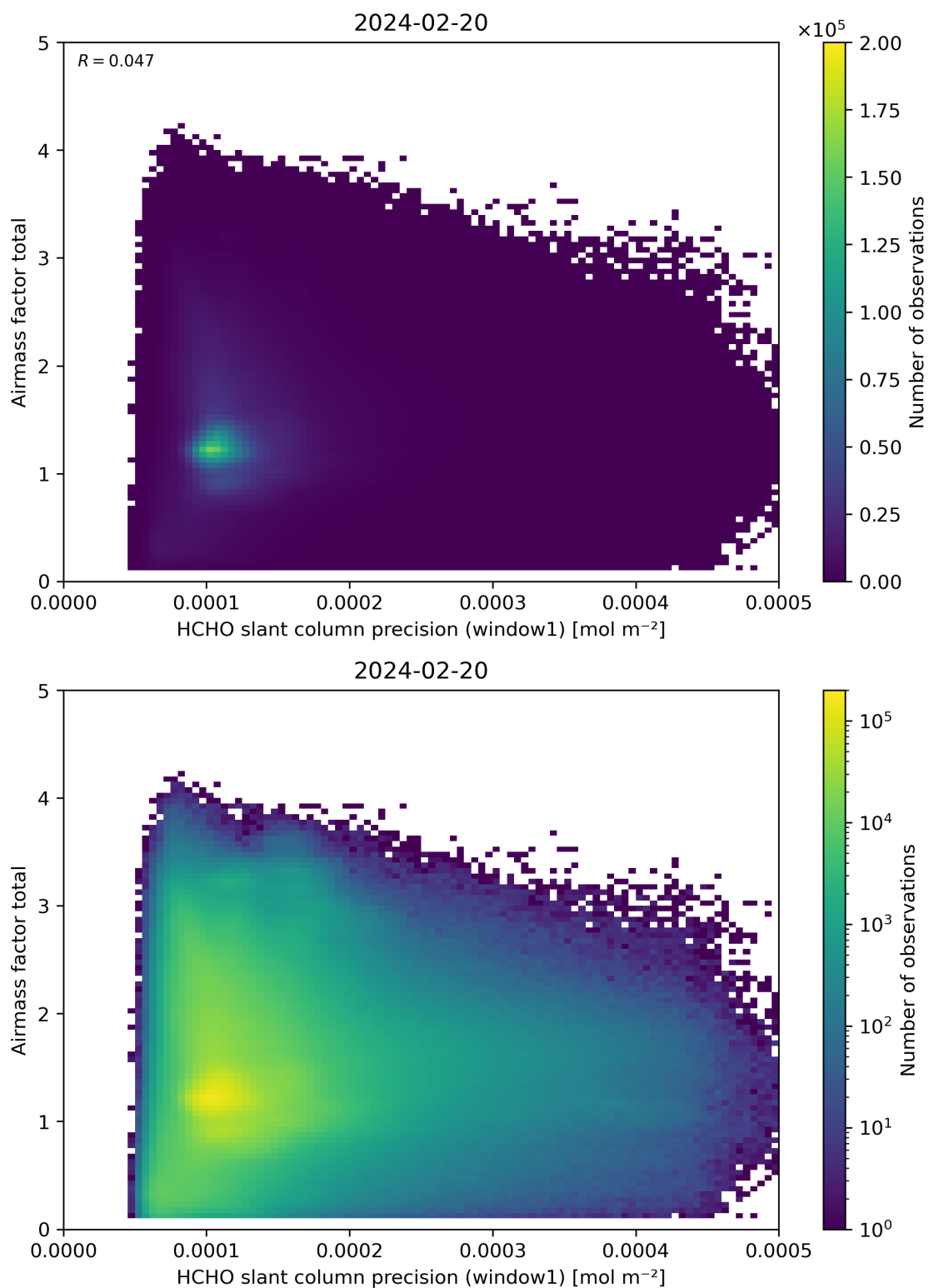
Figure 94: Scatter density plot of “HCHO slant column precision (window1)” against “Airmass factor total” for 2024-02-19 to 2024-02-21.
