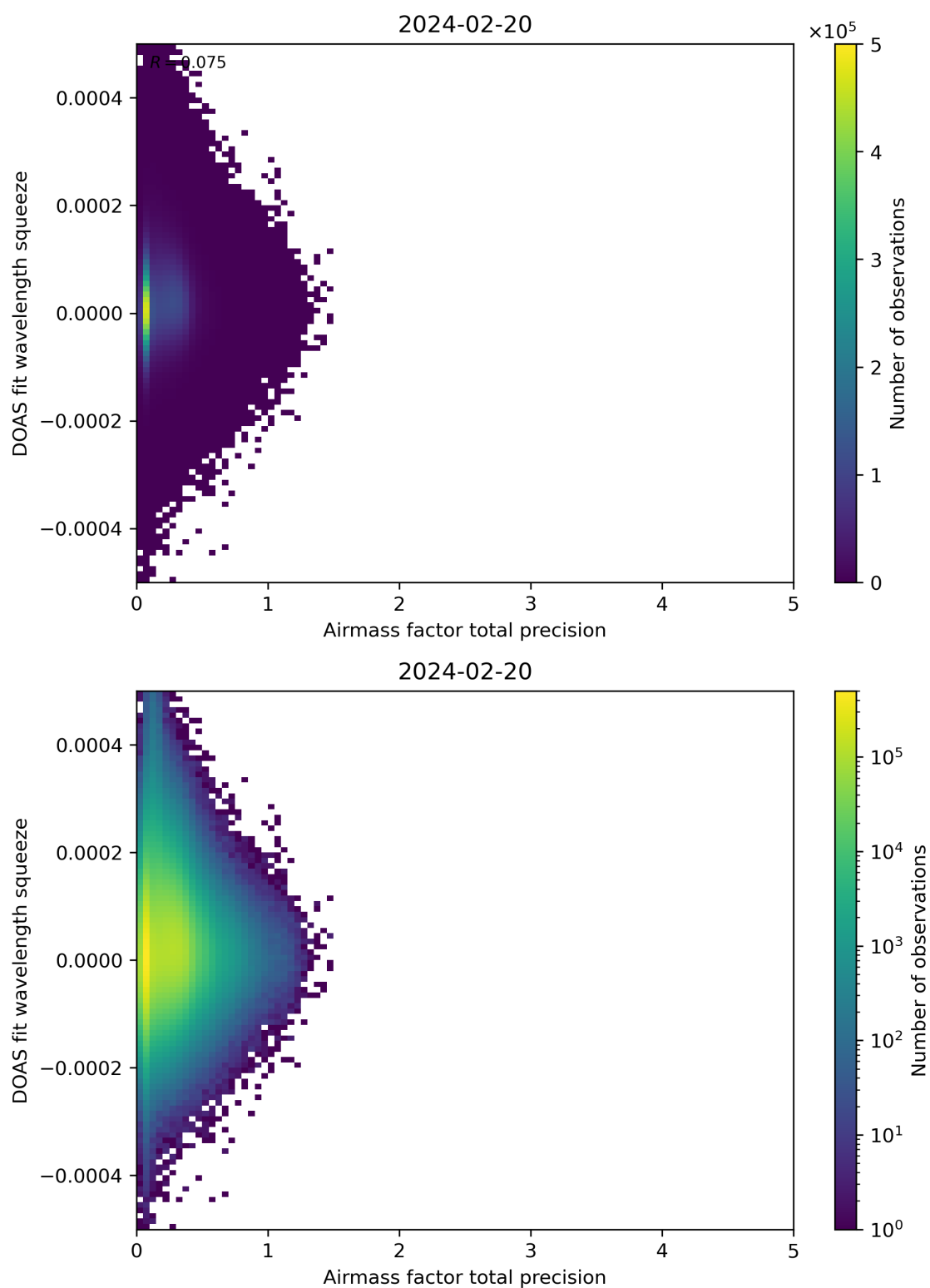
Figure 107: Scatter density plot of “Airmass factor total precision” against “DOAS fit wavelength squeeze” for 2024-02-19 to 2024-02-21.
