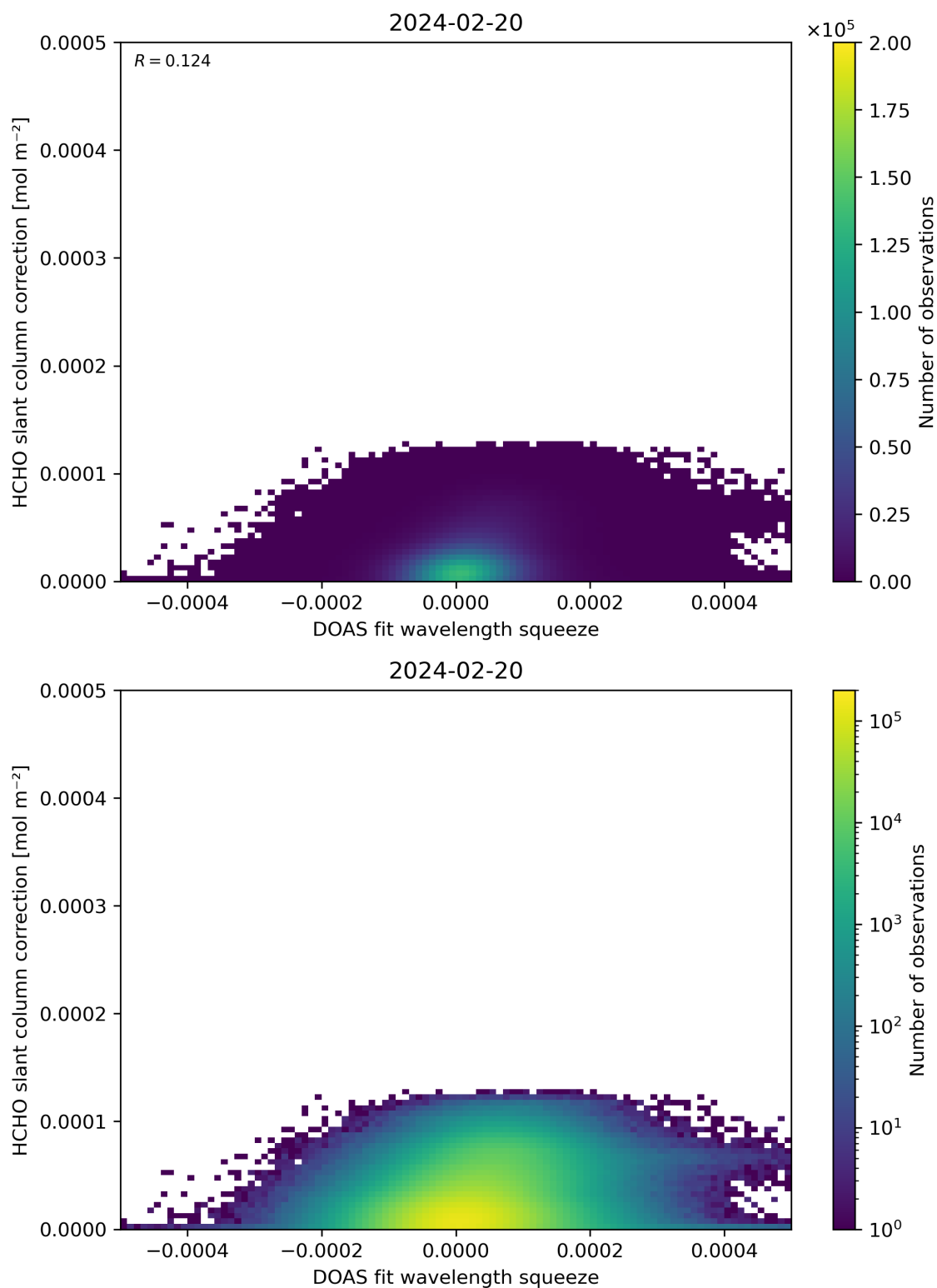
Figure 70: Scatter density plot of “DOAS fit wavelength squeeze” against “HCHO slant column correction” for 2024-02-19 to 2024-02-21.
