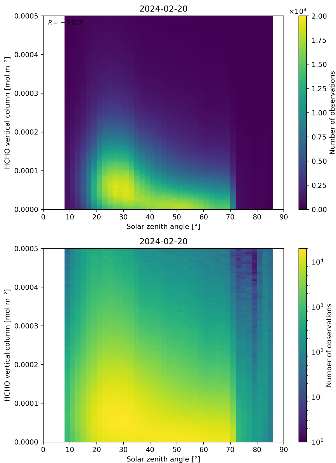
Figure 177: Scatter density plot of “Solar zenith angle” against “HCHO vertical column” for 2024-02-19 to 2024-02-21.
