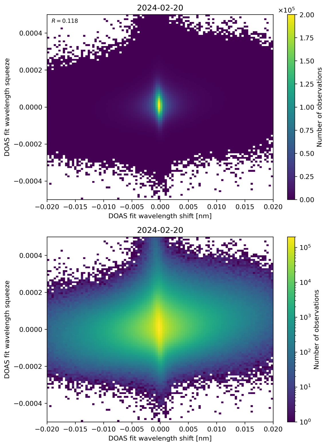
Figure 65: Scatter density plot of “DOAS fit wavelength shift” against “DOAS fit wavelength squeeze” for 2024-02-19 to 2024-02-21.
