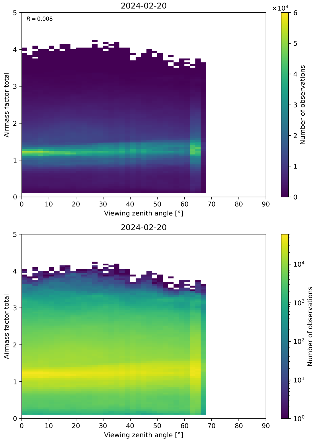
Figure 190: Scatter density plot of “Viewing zenith angle” against “Airmass factor total” for 2024-02-19 to 2024-02-21.
