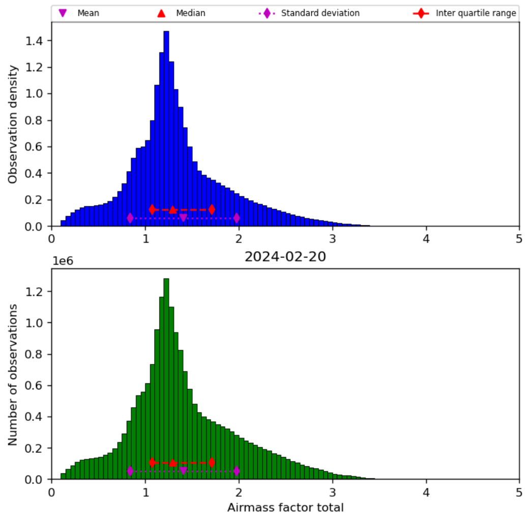
Figure 40: Histogram of “Airmass factor total” for 2024-02-19 to 2024-02-21
