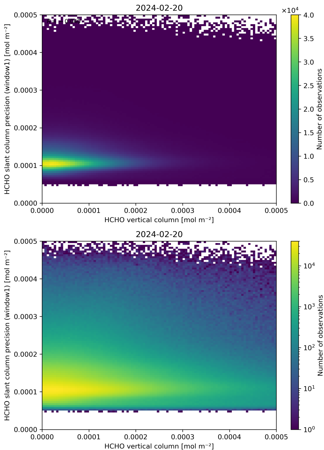
Figure 130: Scatter density plot of “HCHO vertical column” against “HCHO slant column precision (window1)” for 2024-02-19 to 2024-02-21.
