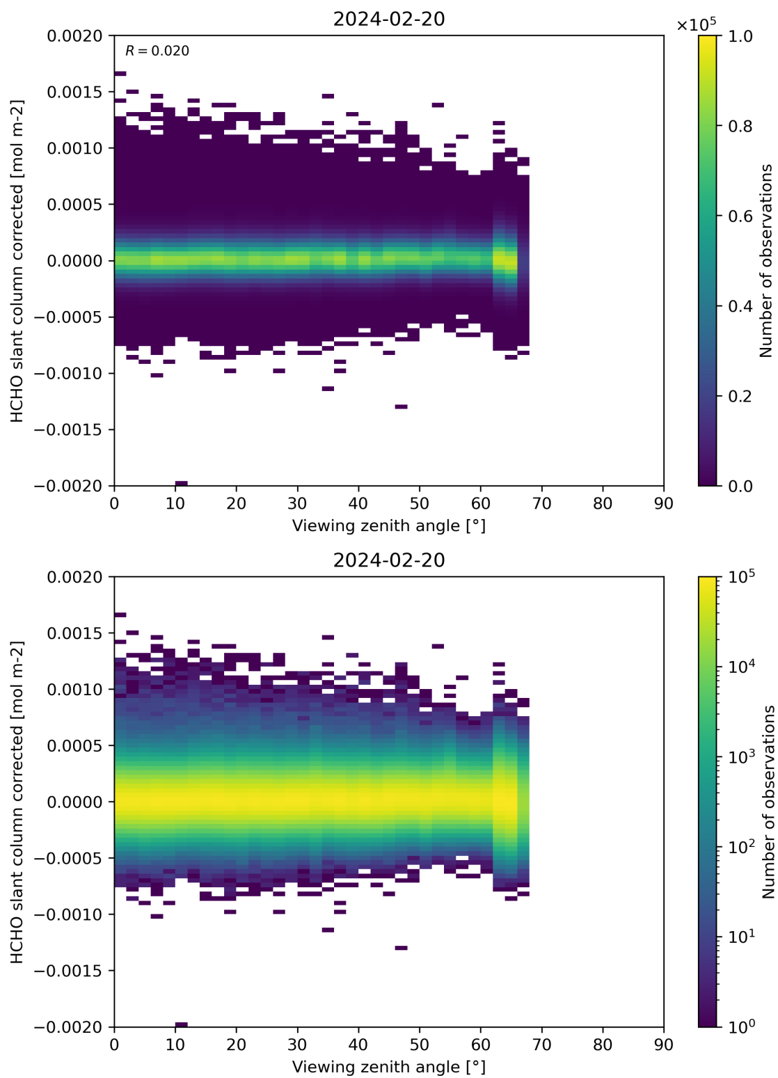
Figure 186: Scatter density plot of “Viewing zenith angle” against “HCHO slant column corrected” for 2024-02-19 to 2024-02-21.
