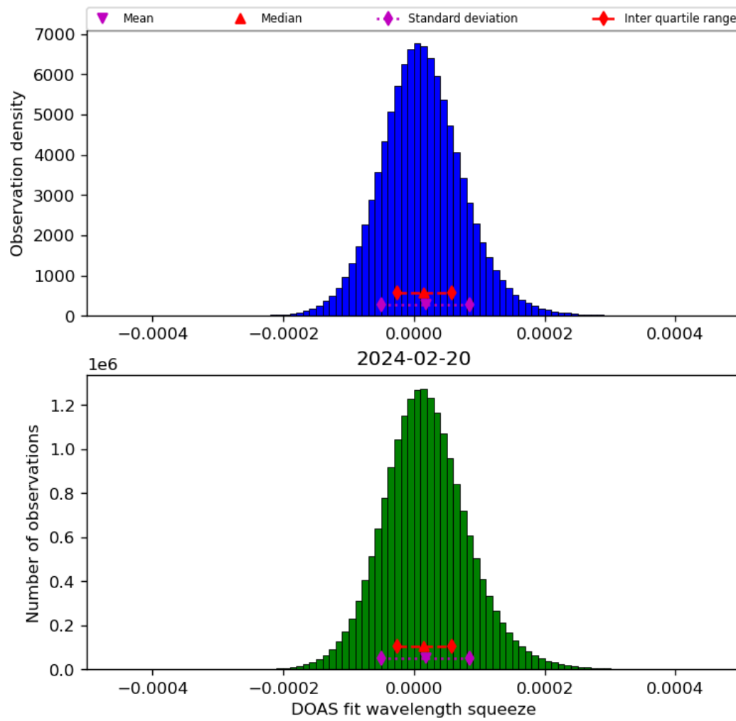
Figure 45: Histogram of “DOAS fit wavelength squeeze” for 2024-02-19 to 2024-02-21
