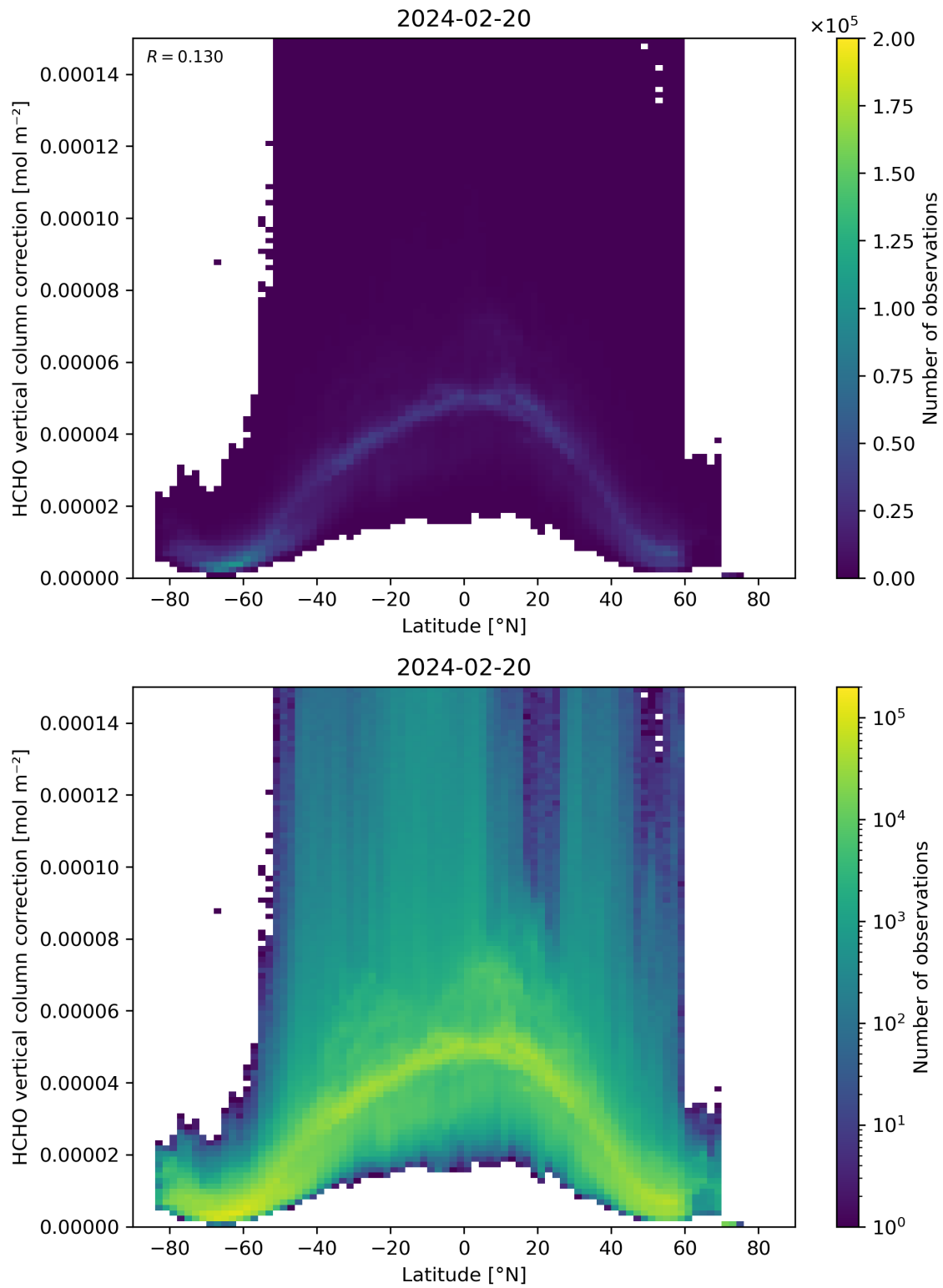
Figure 164: Scatter density plot of “Latitude” against “HCHO vertical column correction” for 2024-02-19 to 2024-02-21.
