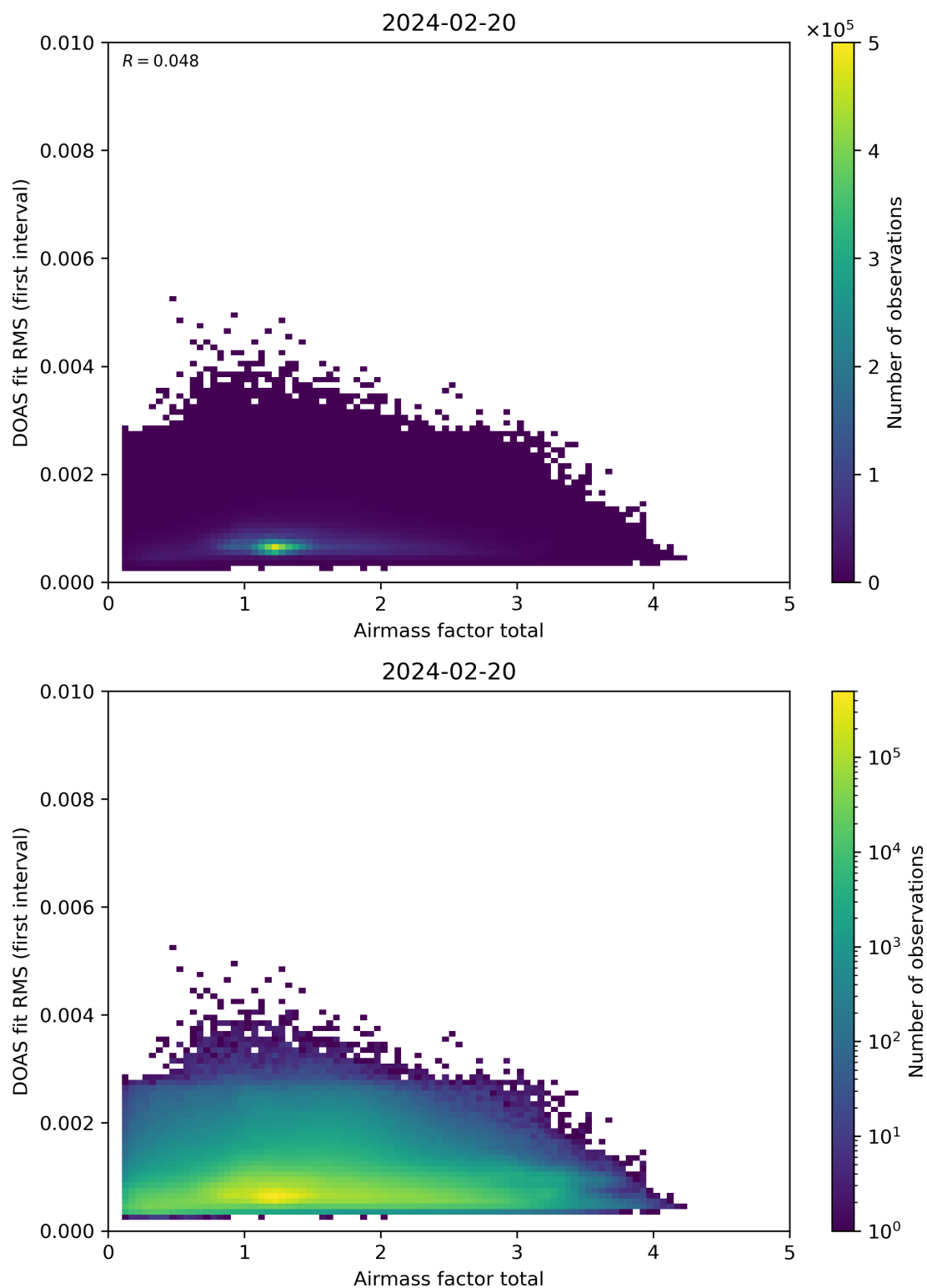
Figure 97: Scatter density plot of “Airmass factor total” against “DOAS fit RMS (first interval)” for 2024-02-19 to 2024-02-21.
