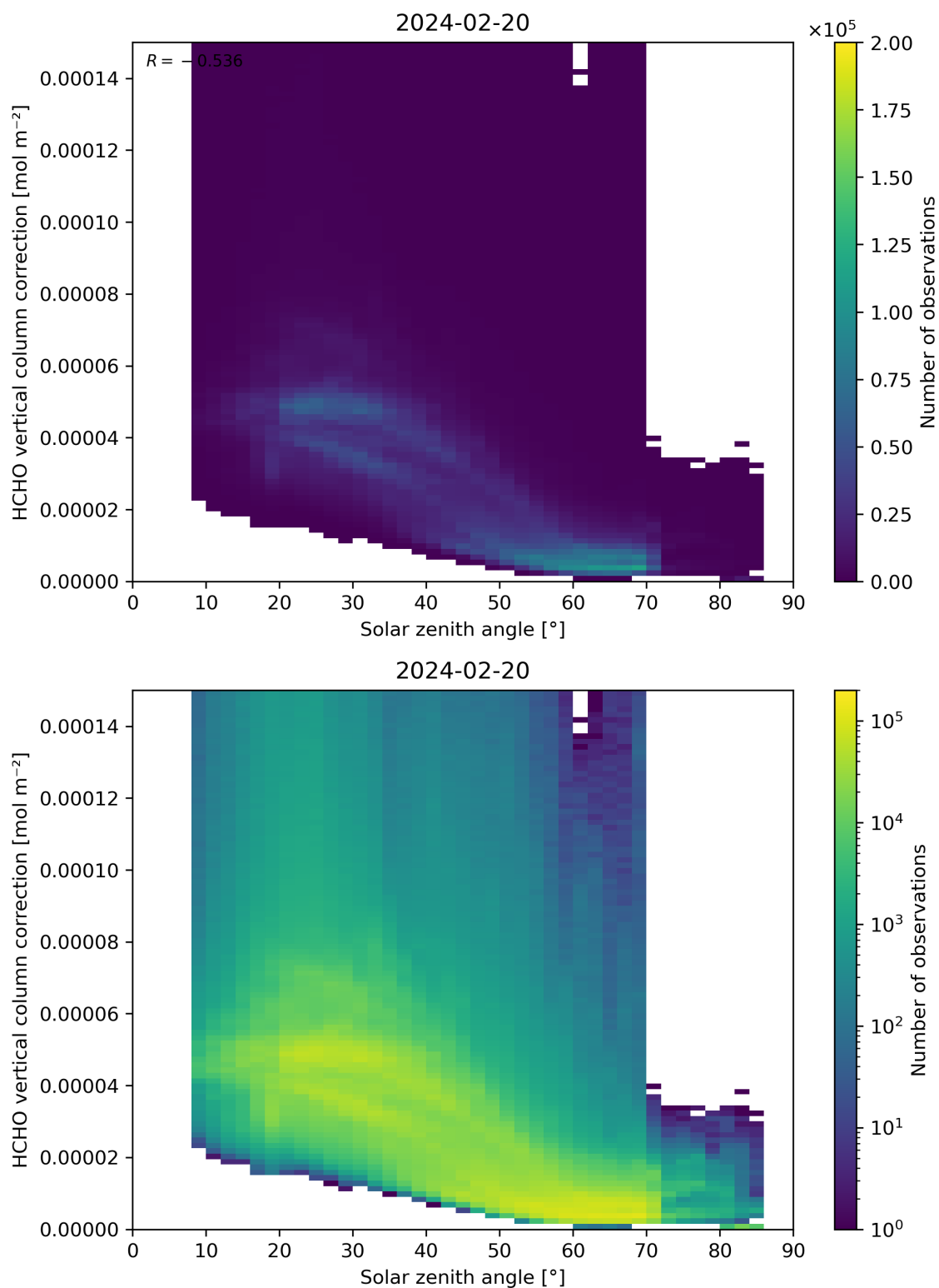
Figure 178: Scatter density plot of “Solar zenith angle” against “HCHO vertical column correction” for 2024-02-19 to 2024-02-21.
