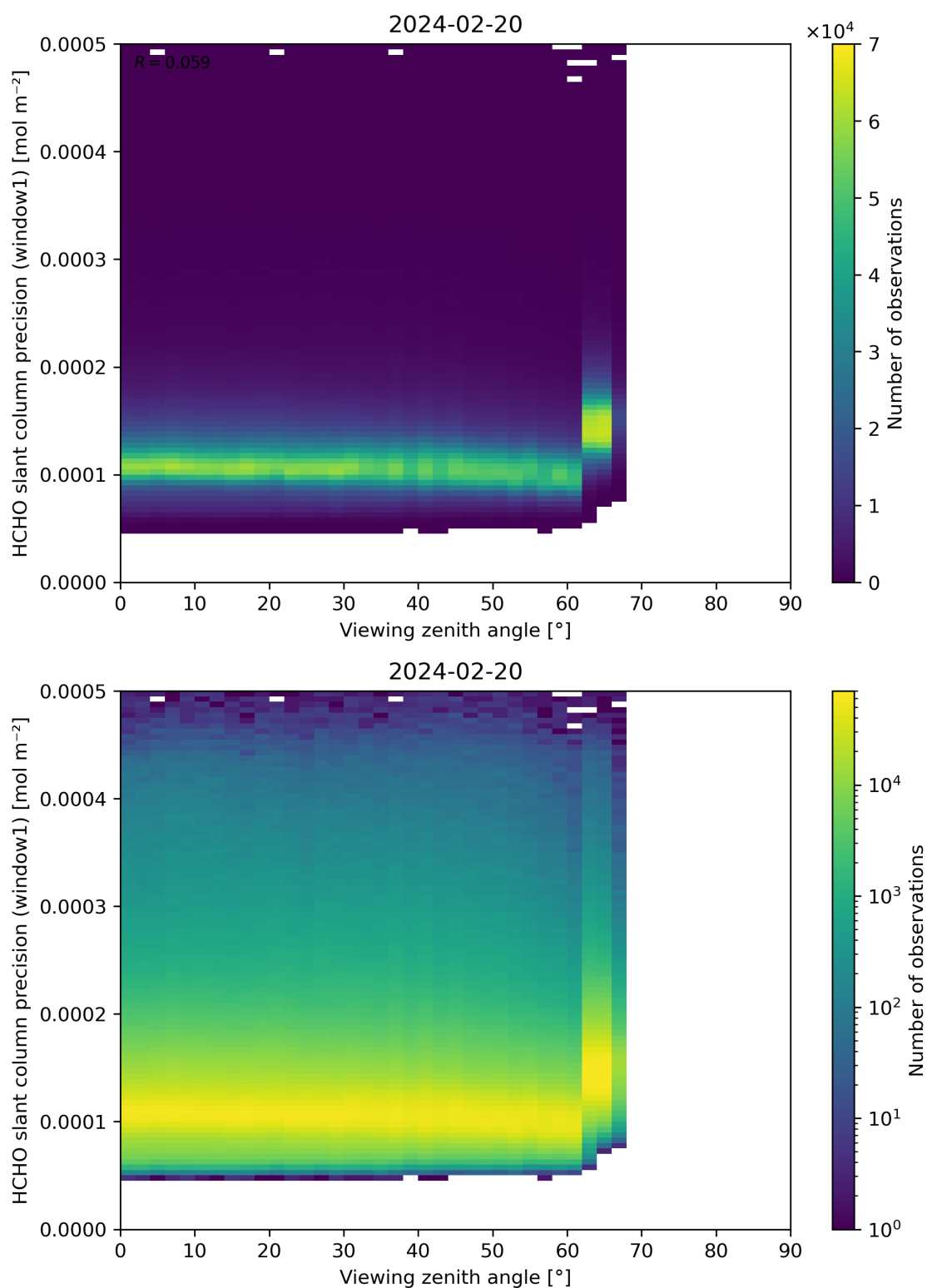
Figure 189: Scatter density plot of “Viewing zenith angle” against “HCHO slant column precision (window1)” for 2024-02-19 to 2024-02-21.
