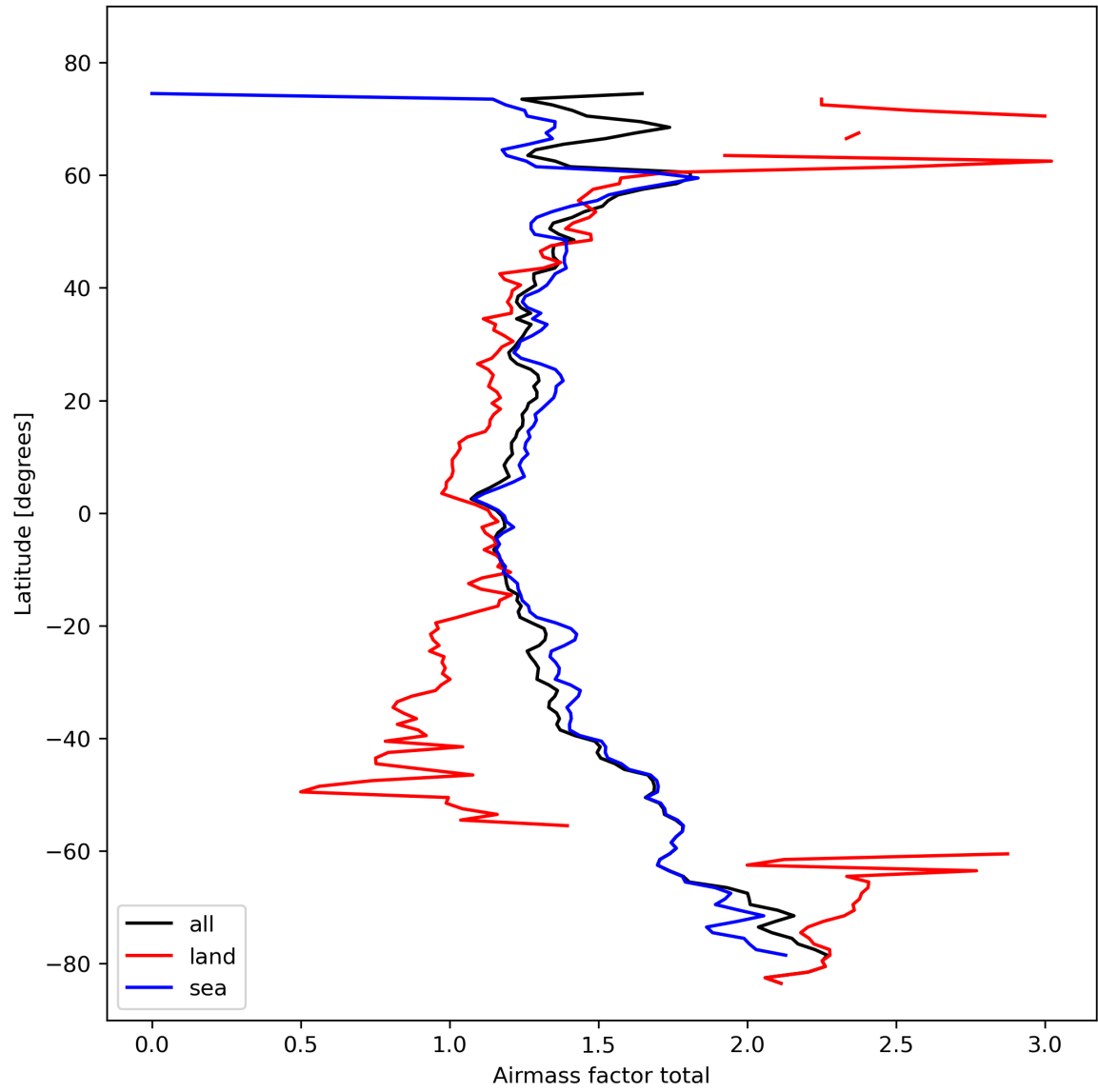
Figure 26: Zonal average of “Airmass factor total” for 2024-02-19 to 2024-02-21.
