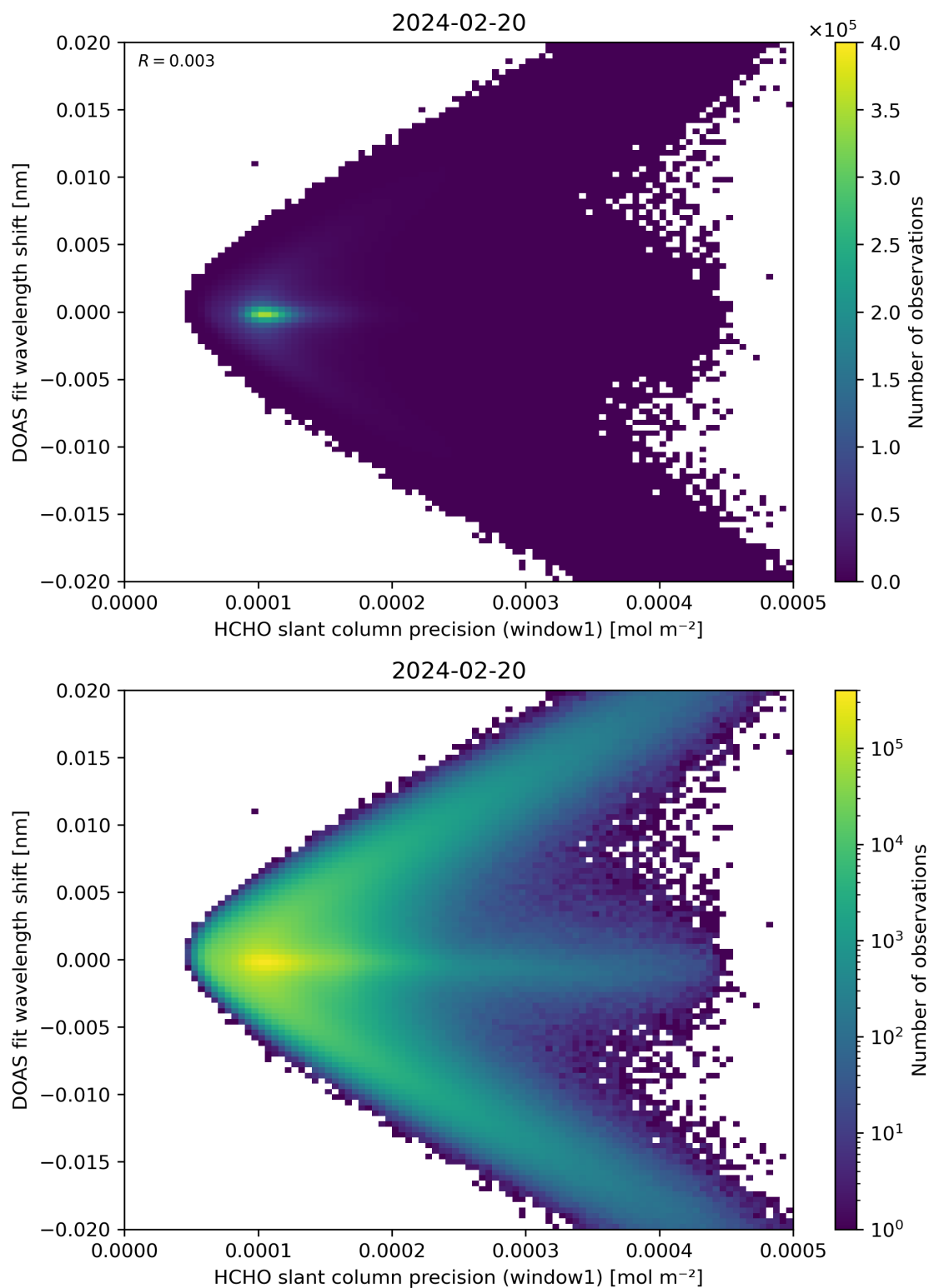
Figure 89: Scatter density plot of “HCHO slant column precision (window1)” against “DOAS fit wavelength shift” for 2024-02-19 to 2024-02-21.
