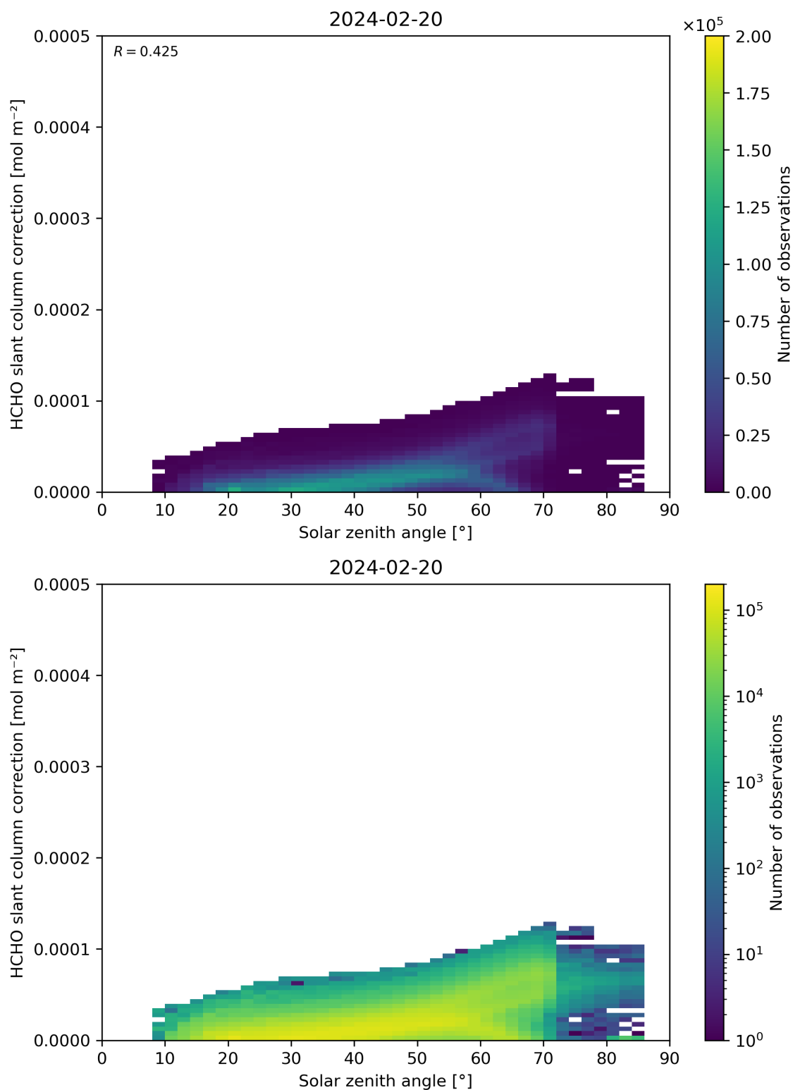
Figure 172: Scatter density plot of “Solar zenith angle” against “HCHO slant column correction” for 2024-02-19 to 2024-02-21.
