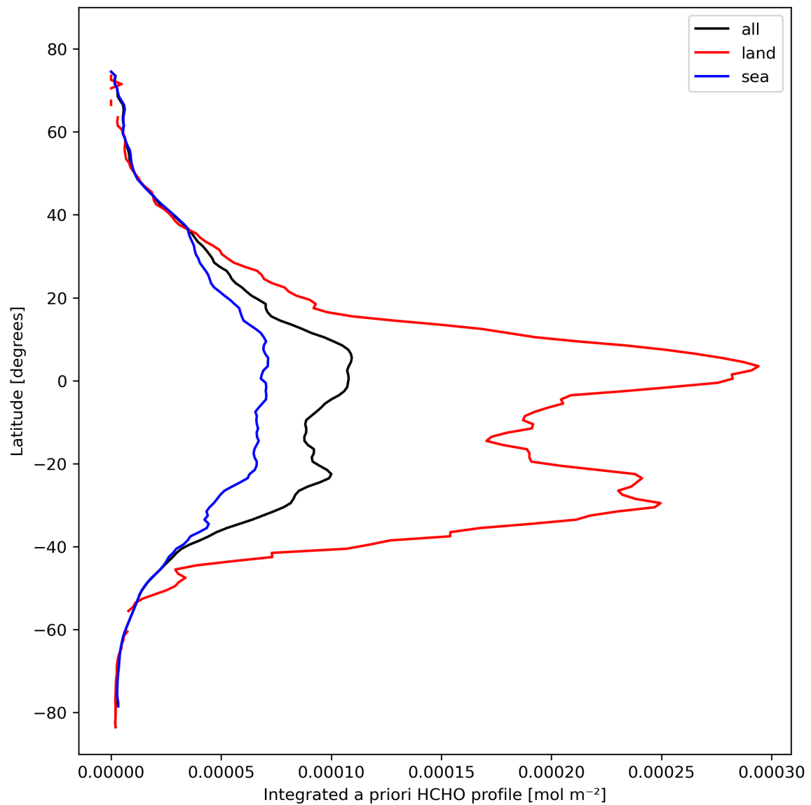
Figure 29: Zonal average of “Integrated a priori HCHO profile” for 2024-02-19 to 2024-02-21.
