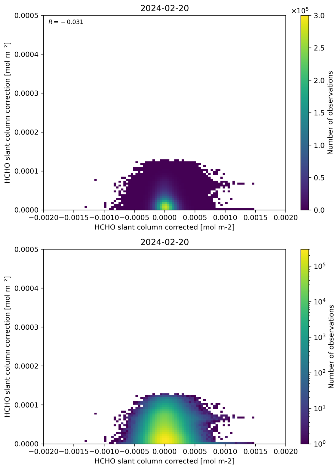
Figure 77: Scatter density plot of “HCHO slant column corrected” against “HCHO slant column correction” for 2024-02-19 to 2024-02-21.
