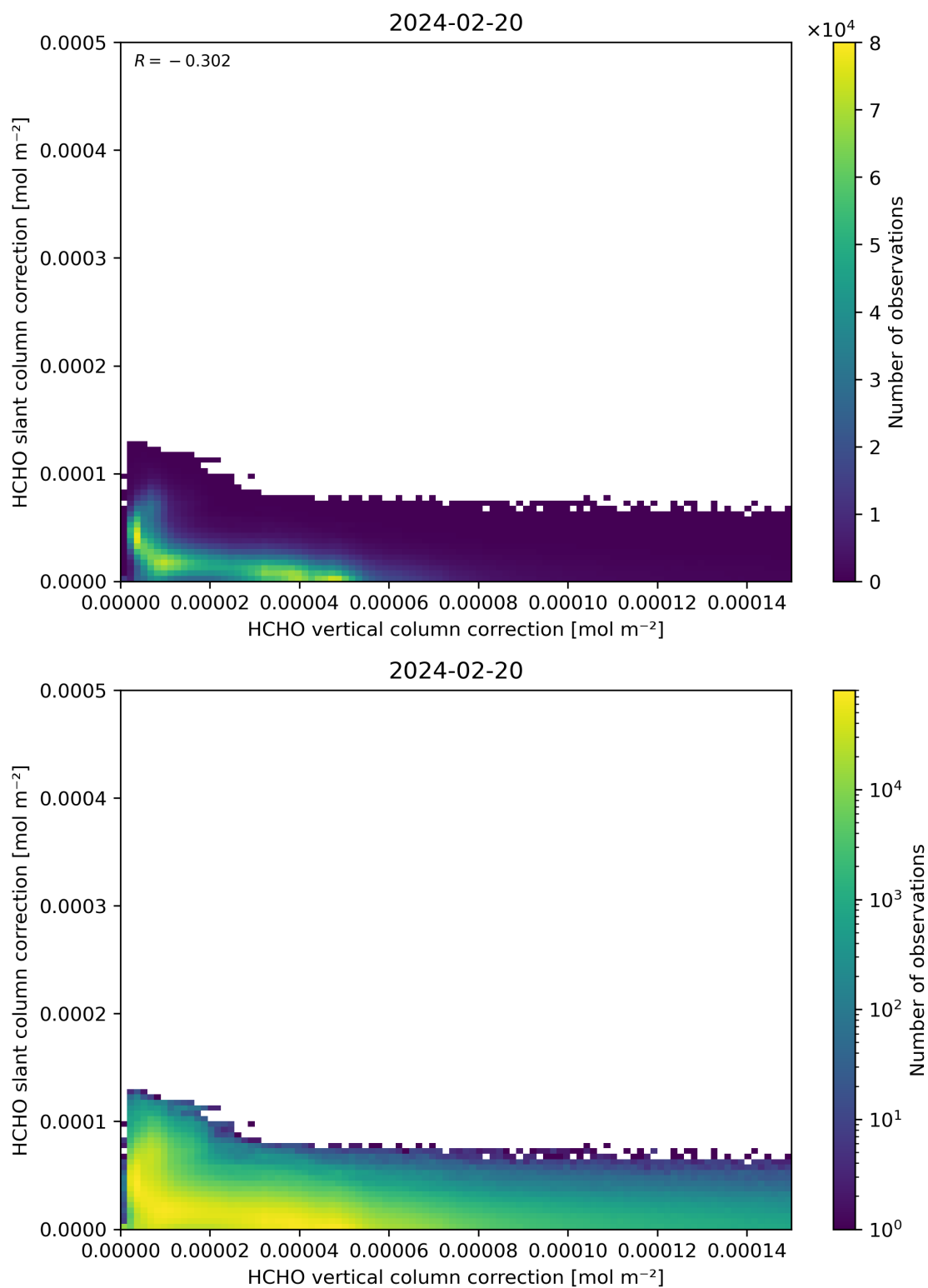
Figure 117: Scatter density plot of “HCHO vertical column correction” against “HCHO slant column correction” for 2024-02-19 to 2024-02-21.
