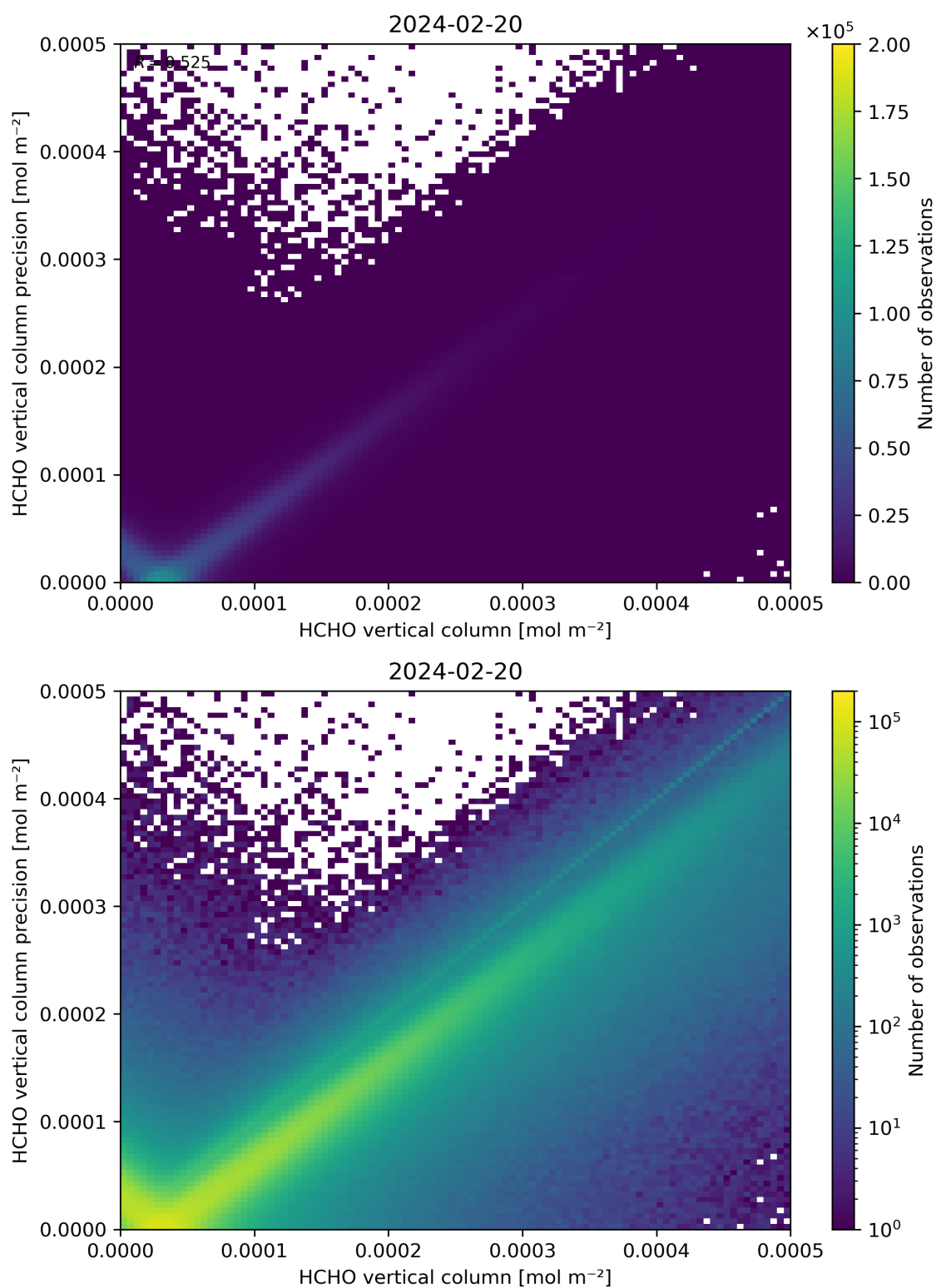
Figure 134: Scatter density plot of “HCHO vertical column” against “HCHO vertical column precision” for 2024-02-19 to 2024-02-21.
