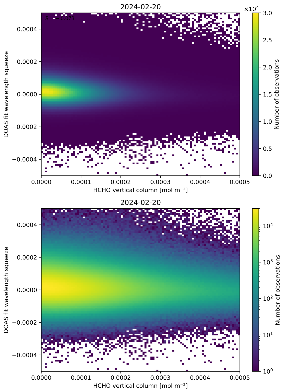
Figure 125: Scatter density plot of “HCHO vertical column” against “DOAS fit wavelength squeeze” for 2024-02-19 to 2024-02-21.
