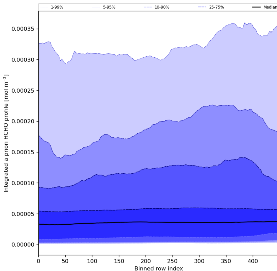
Figure 57: Along track statistics of “Integrated a priori HCHO profile” for 2024-02-19 to 2024-02-21
