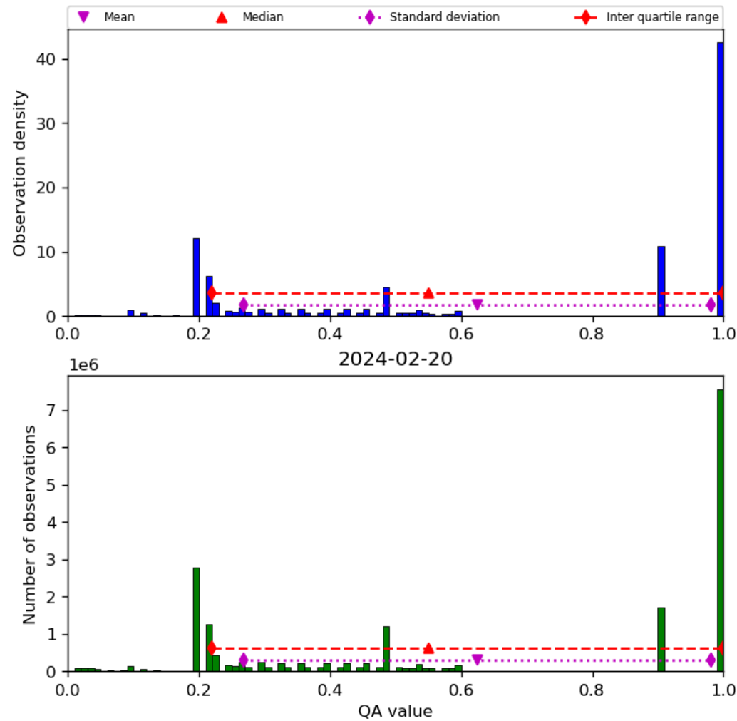
Figure 34: Histogram of “QA value” for 2024-02-19 to 2024-02-21
