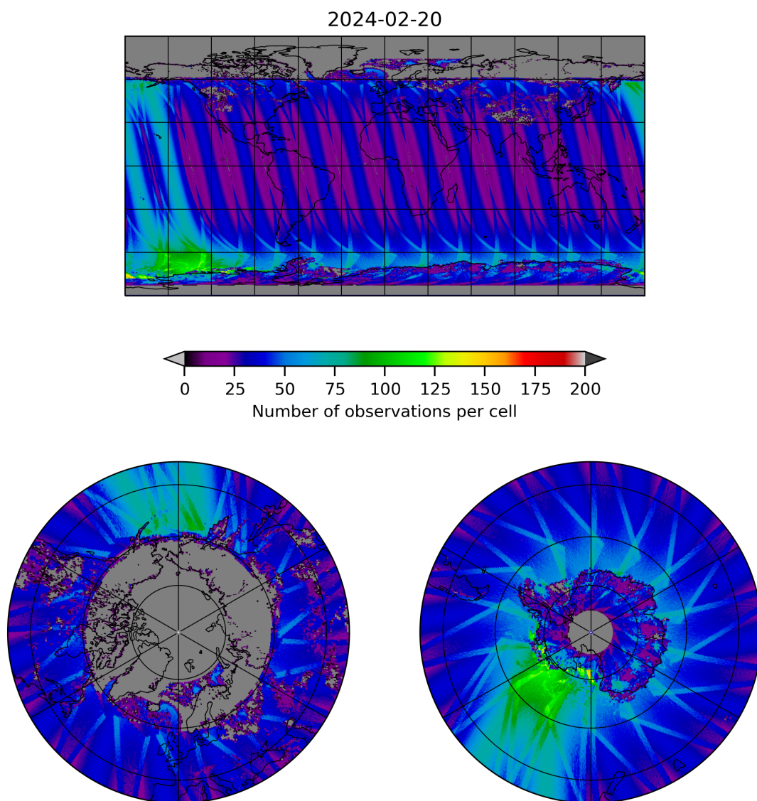
Figure 19: Map of the number of observations for 2024-02-19 to 2024-02-21
