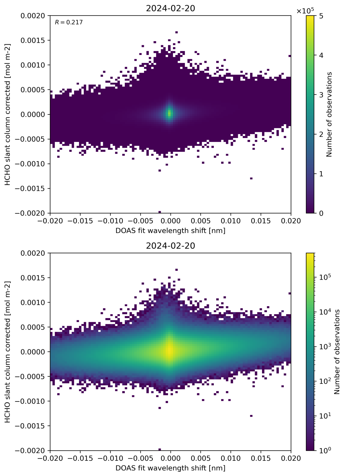
Figure 66: Scatter density plot of “DOAS fit wavelength shift” against “HCHO slant column corrected” for 2024-02-19 to 2024-02-21.
