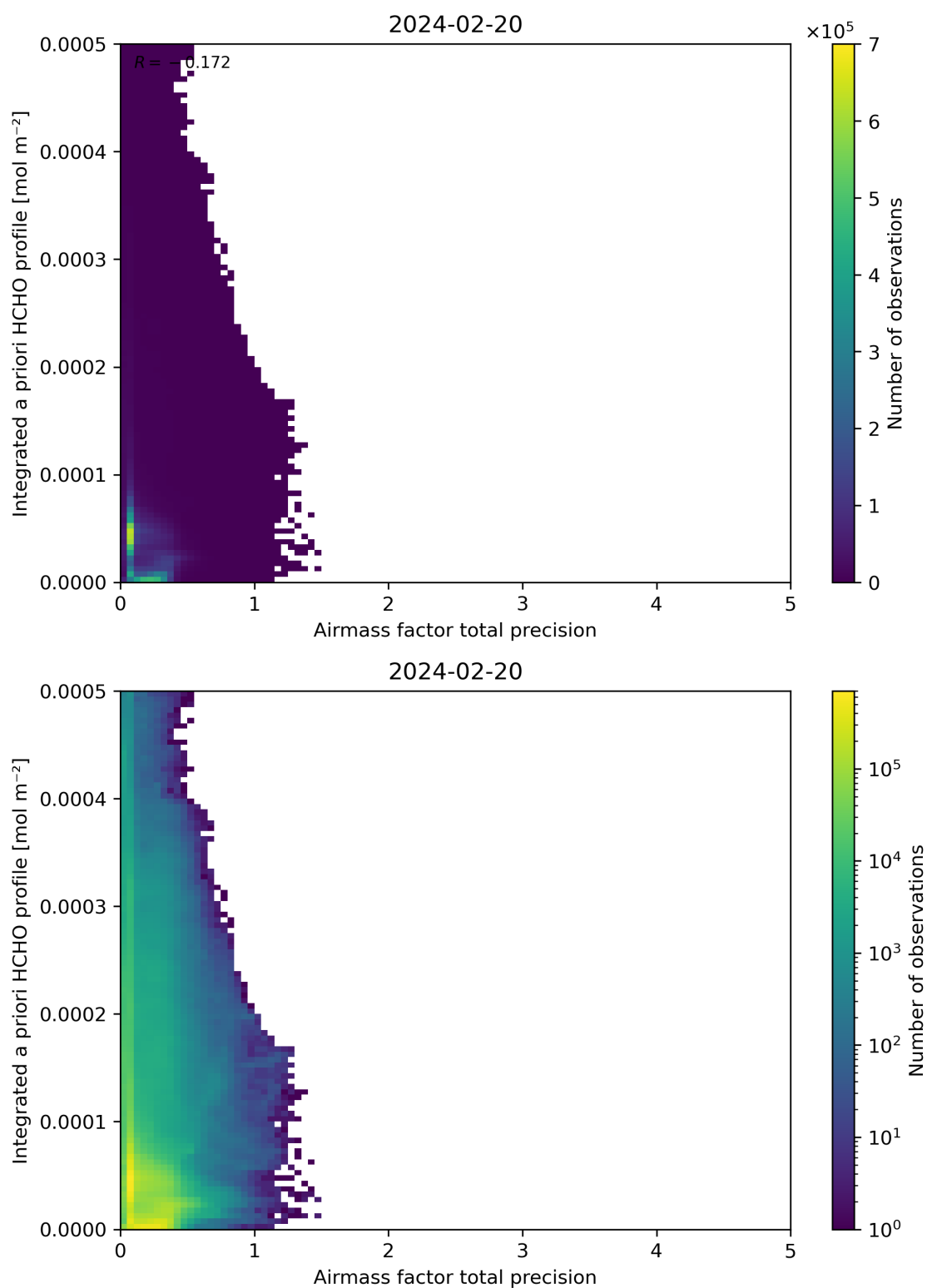
Figure 111: Scatter density plot of “Airmass factor total precision” against “Integrated a priori HCHO profile” for 2024-02-19 to 2024-02-21.
