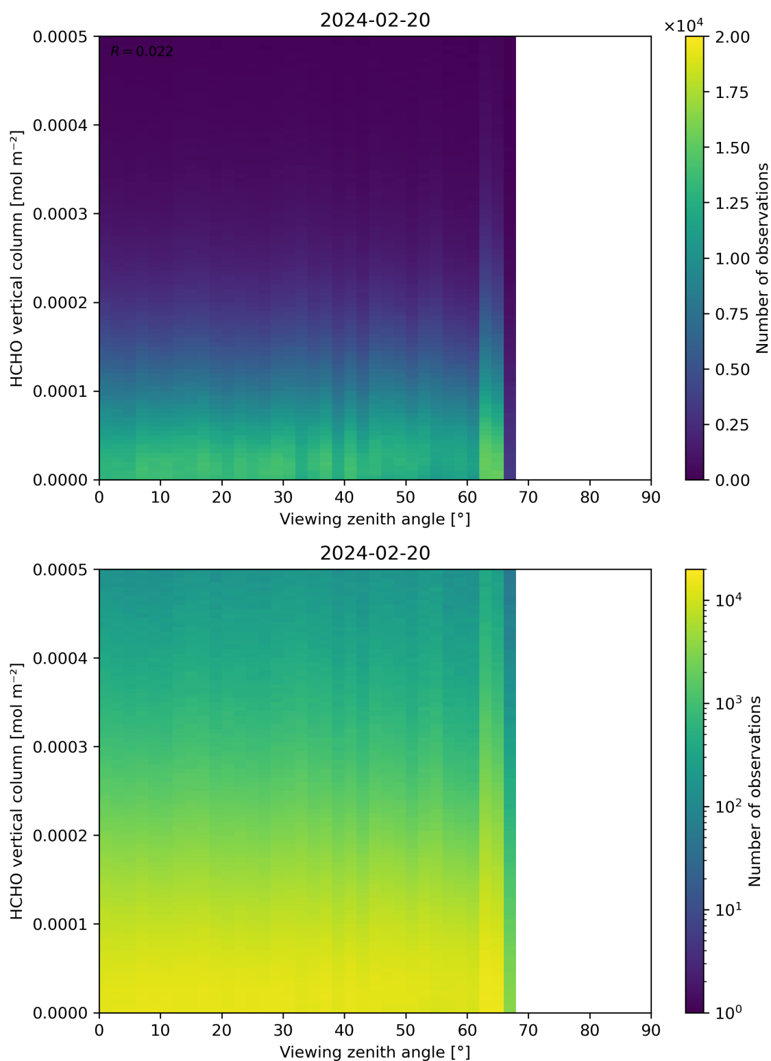
Figure 192: Scatter density plot of “Viewing zenith angle” against “HCHO vertical column” for 2024-02-19 to 2024-02-21.
