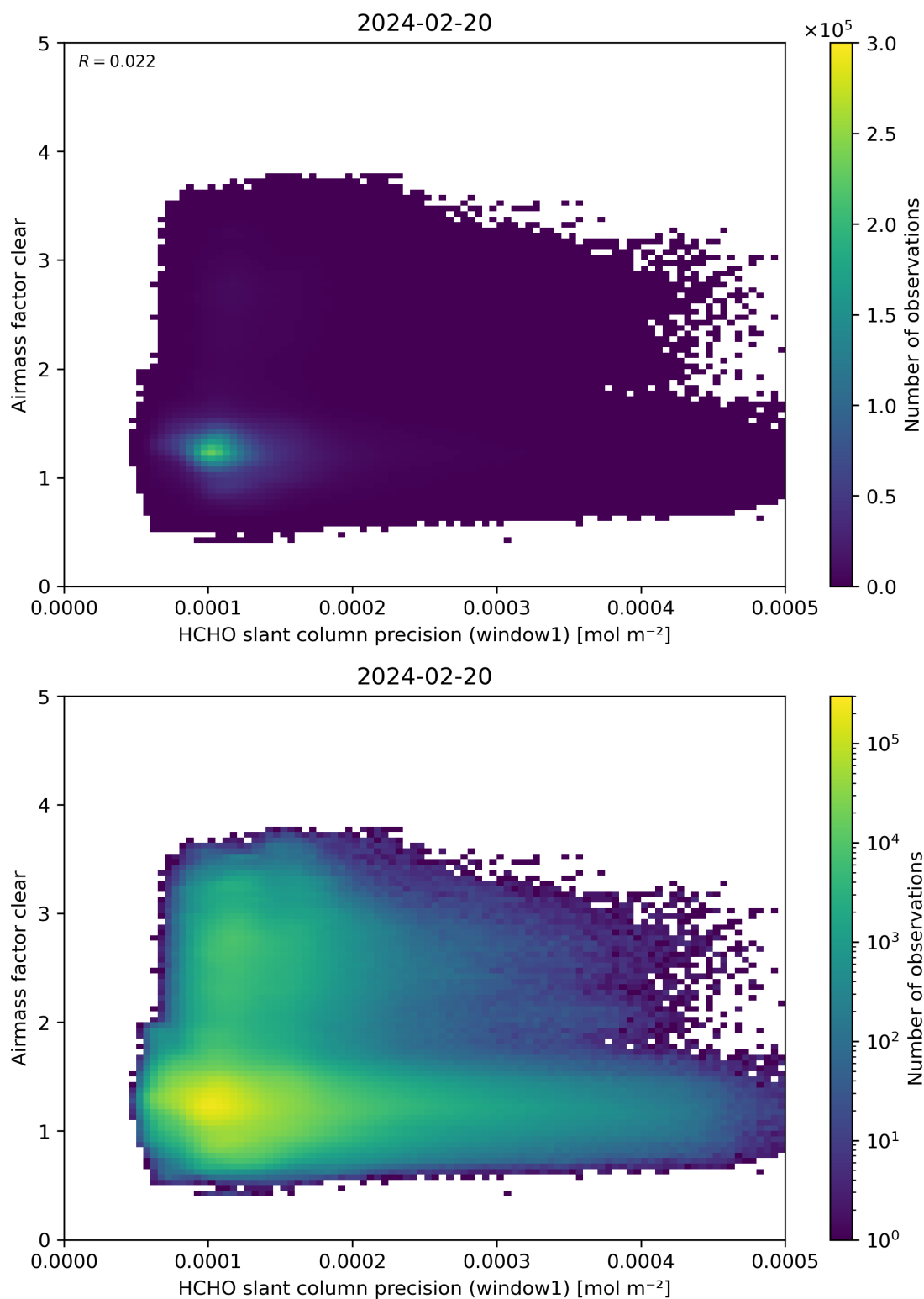
Figure 91: Scatter density plot of “HCHO slant column precision (window1)” against “Airmass factor clear” for 2024-02-19 to 2024-02-21.
