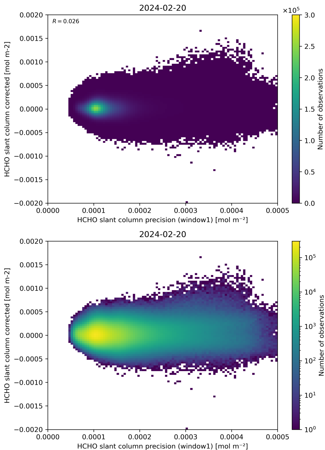
Figure 92: Scatter density plot of “HCHO slant column precision (window1)” against “HCHO slant column corrected” for 2024-02-19 to 2024-02-21.
