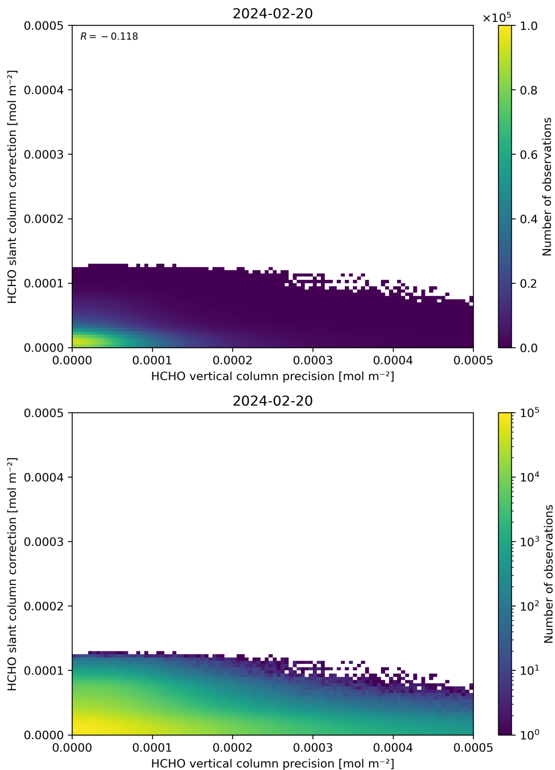
Figure 141: Scatter density plot of “HCHO vertical column precision” against “HCHO slant column correction” for 2024-02-19 to 2024-02-21.
