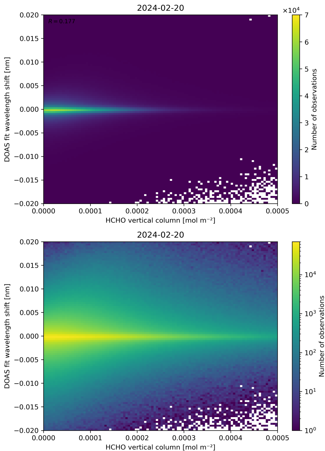
Figure 124: Scatter density plot of “HCHO vertical column” against “DOAS fit wavelength shift” for 2024-02-19 to 2024-02-21.
