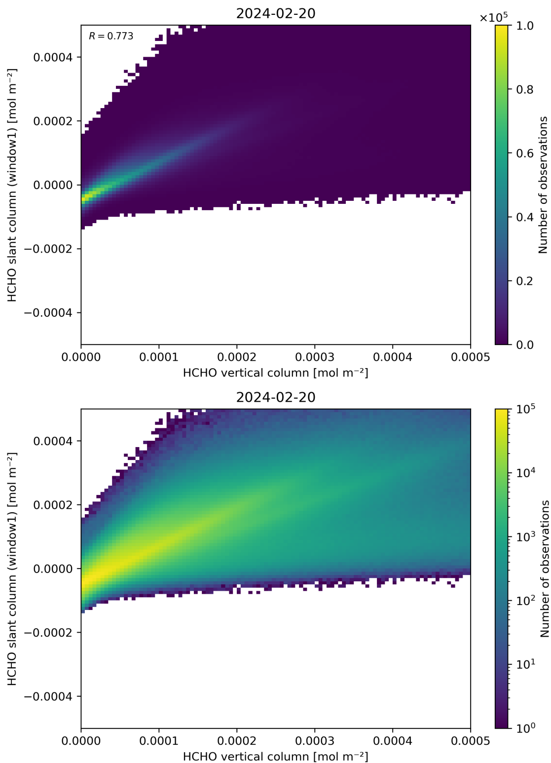
Figure 129: Scatter density plot of “HCHO vertical column” against “HCHO slant column (window1)” for 2024-02-19 to 2024-02-21.
