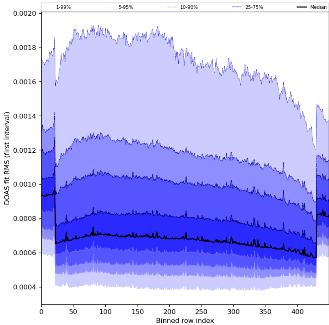
Figure 60: Along track statistics of “DOAS fit RMS (first interval)” for 2024-02-19 to 2024-02-21
