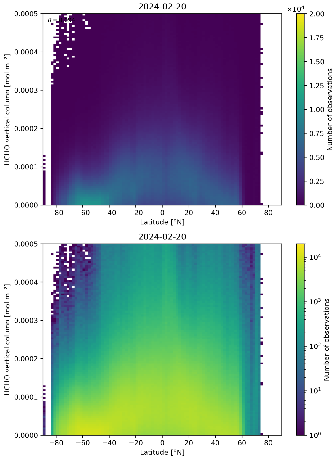
Figure 163: Scatter density plot of “Latitude” against “HCHO vertical column” for 2024-02-19 to 2024-02-21.
