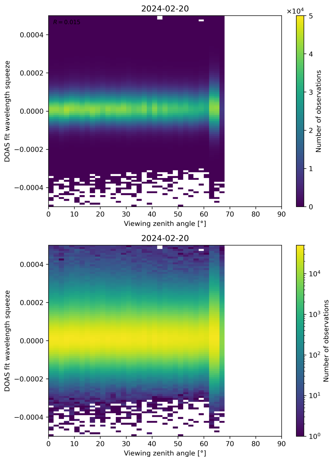
Figure 184: Scatter density plot of “Viewing zenith angle” against “DOAS fit wavelength squeeze” for 2024-02-19 to 2024-02-21.
