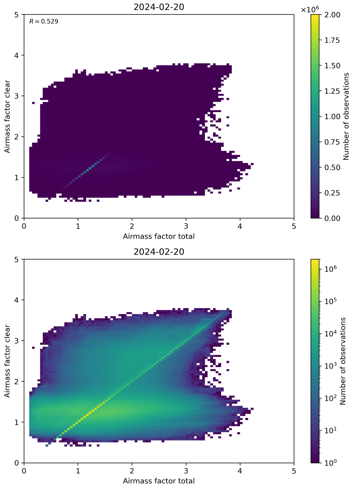
Figure 100: Scatter density plot of “Airmass factor total” against “Airmass factor clear” for 2024-02-19 to 2024-02-21.
