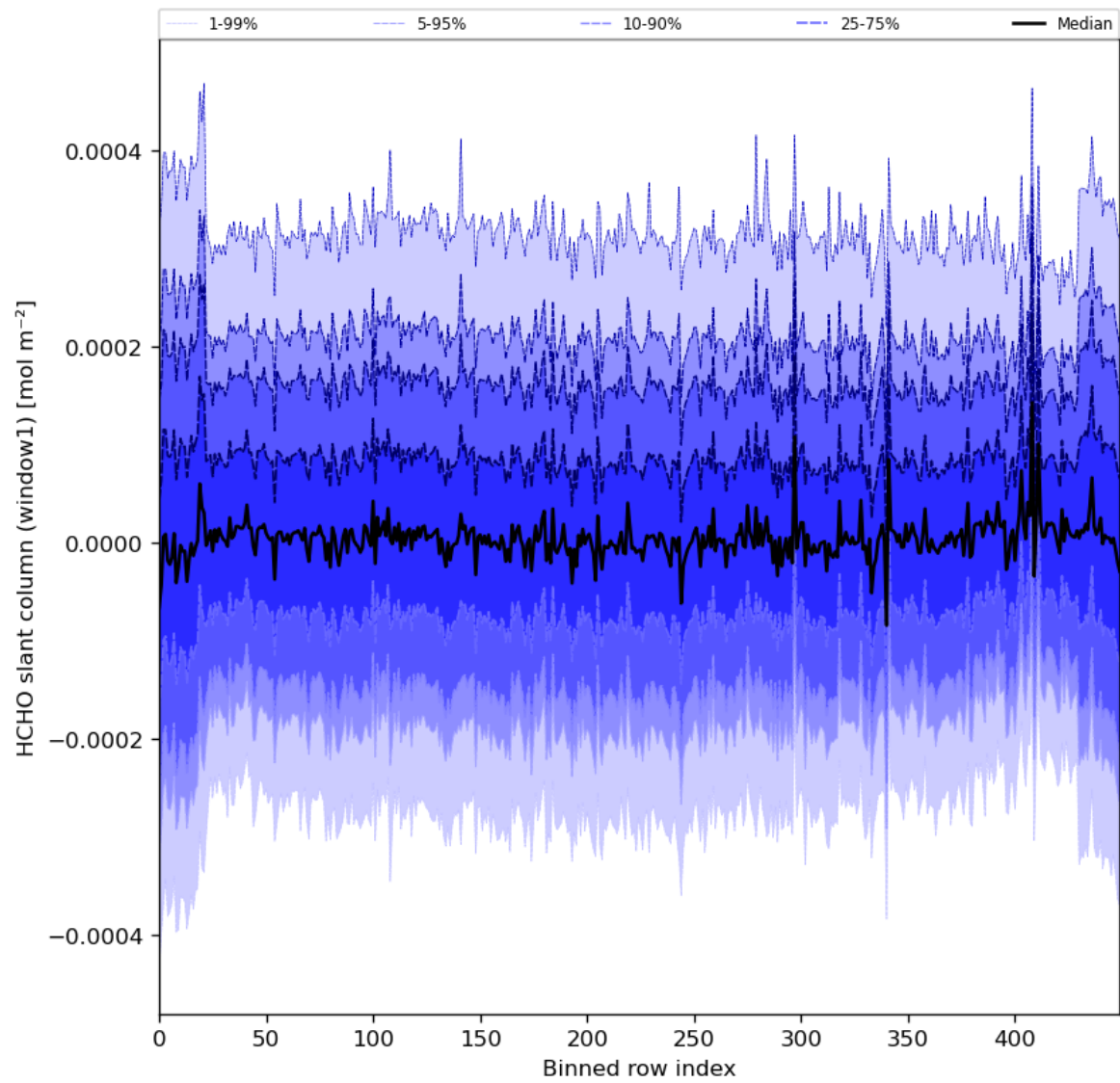
Figure 52: Along track statistics of “HCHO slant column (window1)” for 2024-02-19 to 2024-02-21
