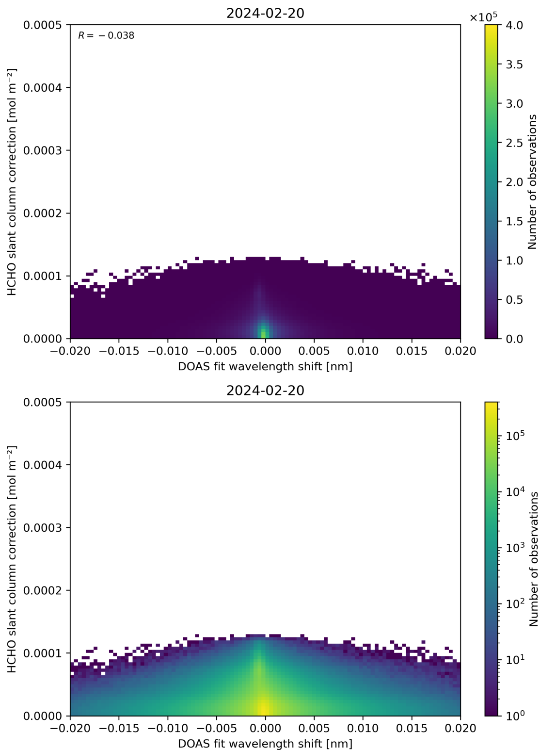
Figure 67: Scatter density plot of “DOAS fit wavelength shift” against “HCHO slant column correction” for 2024-02-19 to 2024-02-21.
