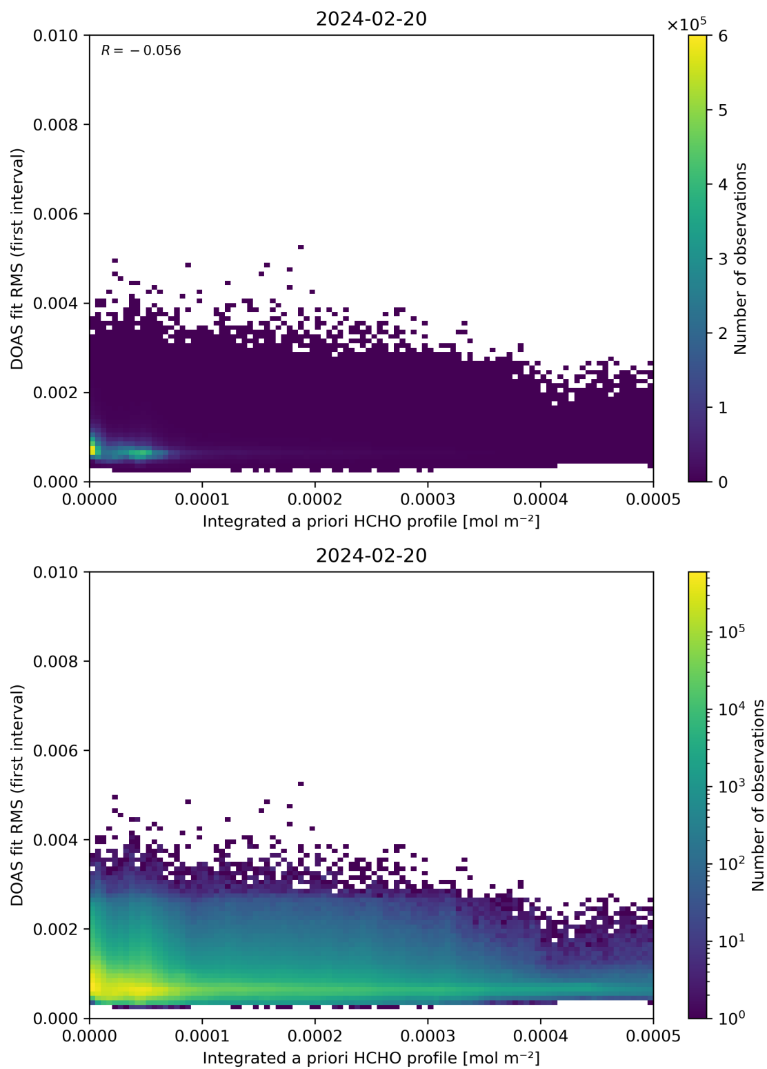
Figure 148: Scatter density plot of “Integrated a priori HCHO profile” against “DOAS fit RMS (first interval)” for 2024-02-19 to 2024-02-21.
