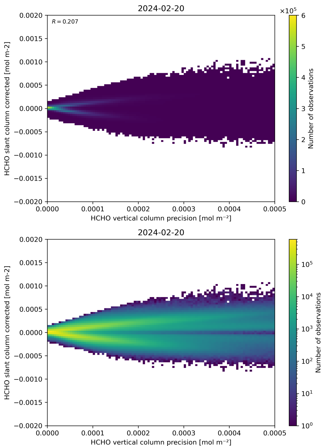
Figure 140: Scatter density plot of “HCHO vertical column precision” against “HCHO slant column corrected” for 2024-02-19 to 2024-02-21.
