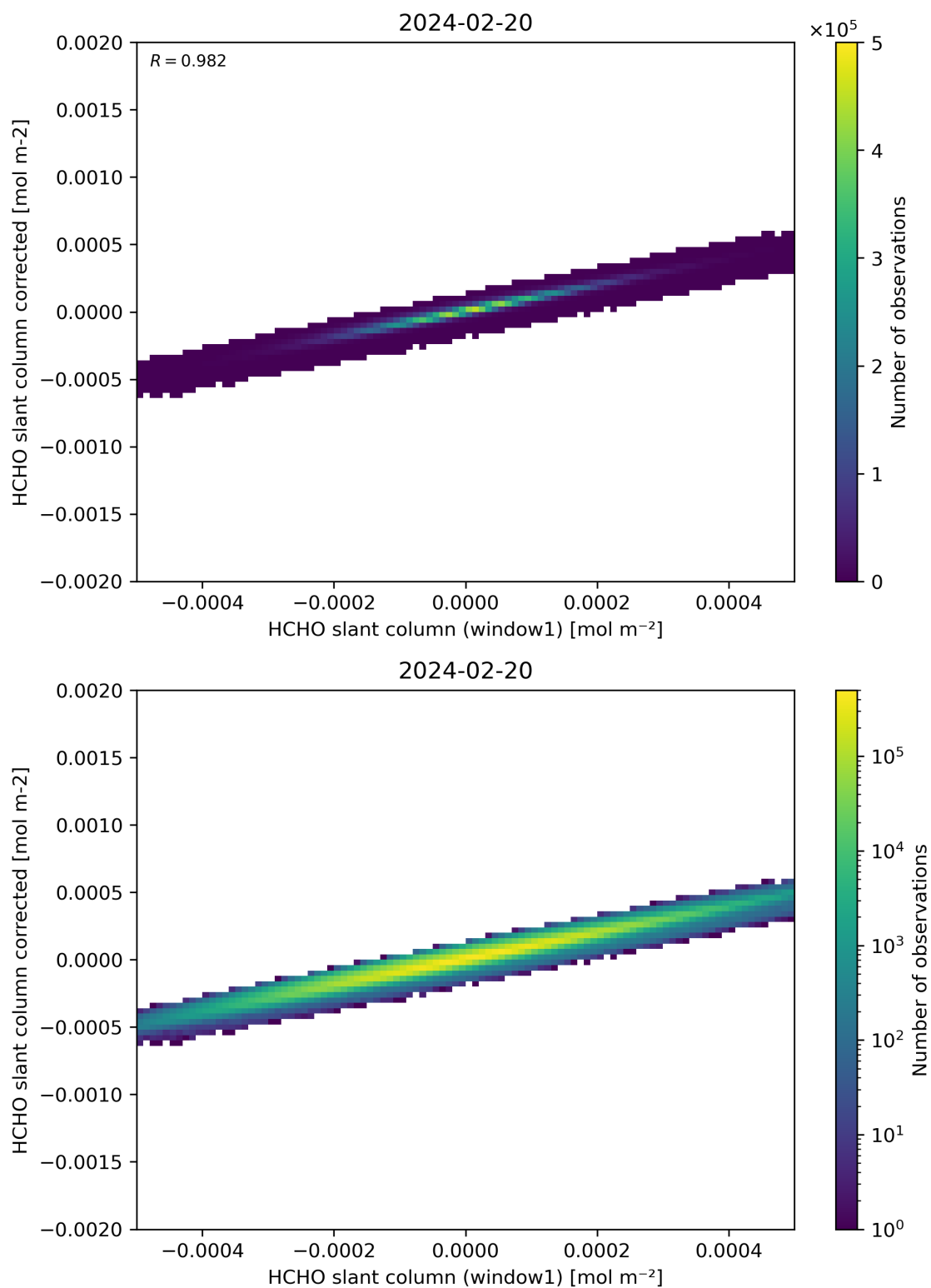
Figure 82: Scatter density plot of “HCHO slant column (window1)” against “HCHO slant column corrected” for 2024-02-19 to 2024-02-21.
