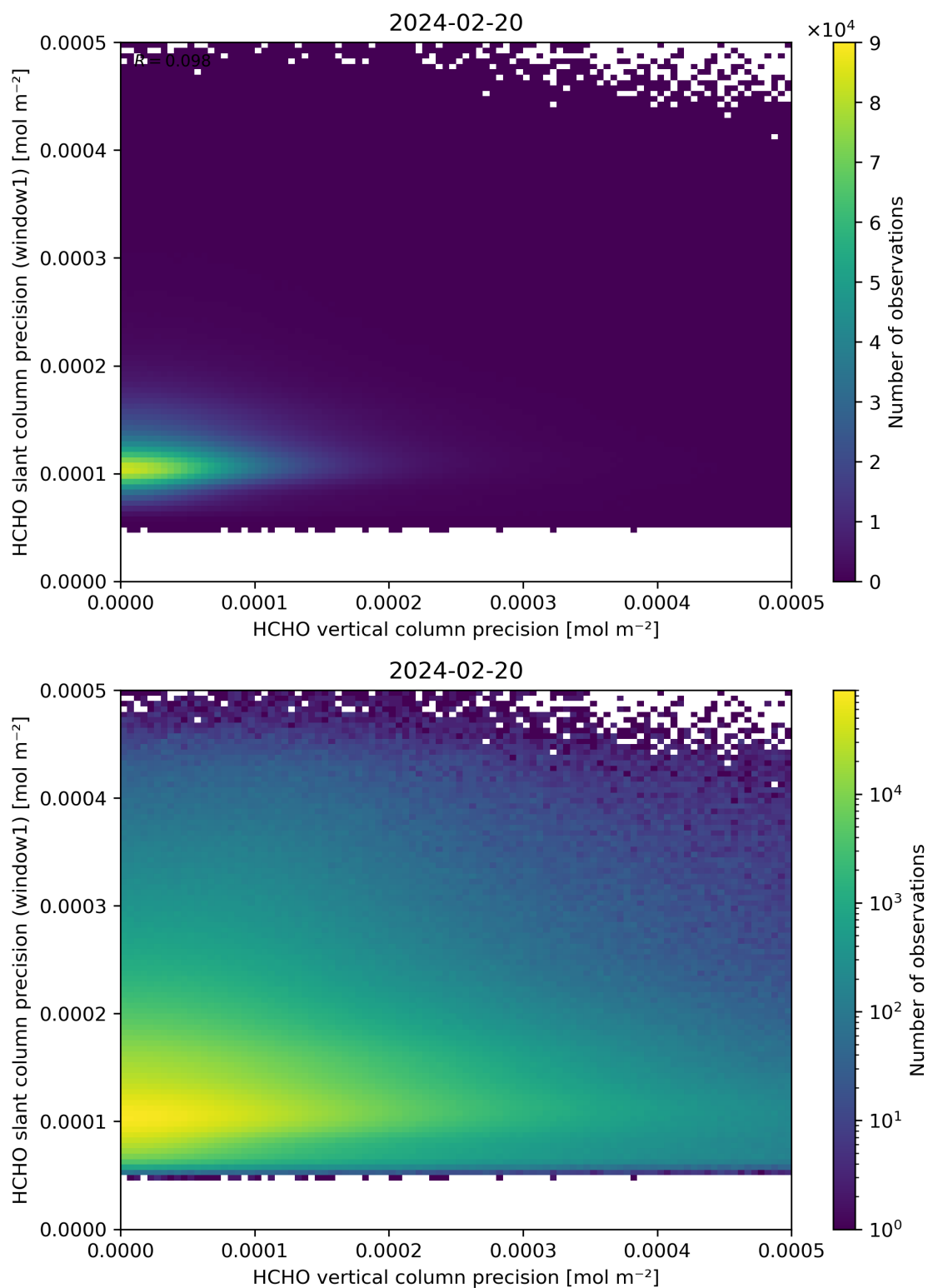
Figure 143: Scatter density plot of “HCHO vertical column precision” against “HCHO slant column precision (window1)” for 2024-02-19 to 2024-02-21.
