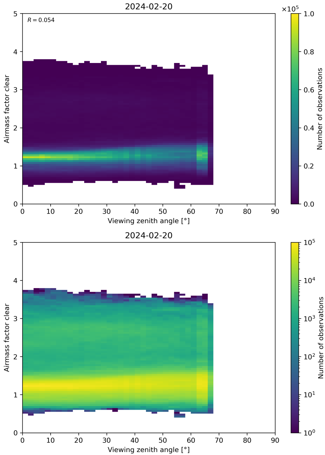
Figure 185: Scatter density plot of “Viewing zenith angle” against “Airmass factor clear” for 2024-02-19 to 2024-02-21.
