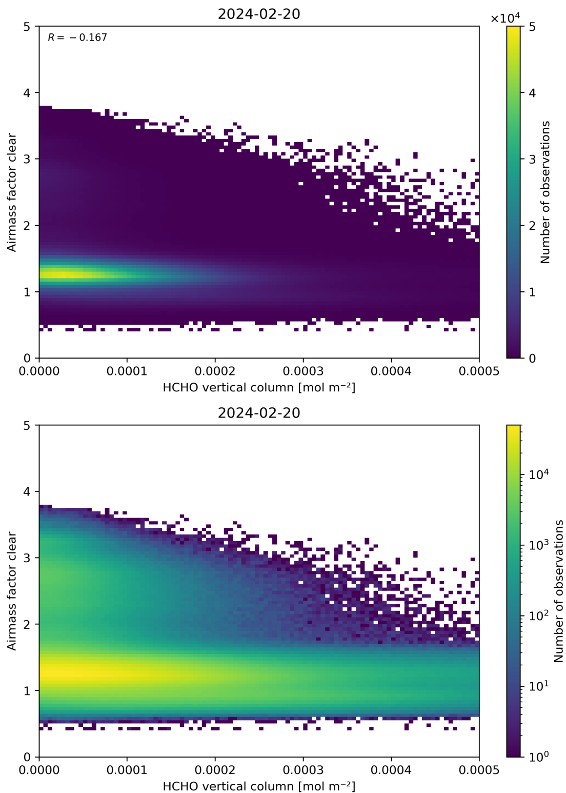
Figure 126: Scatter density plot of “HCHO vertical column” against “Airmass factor clear” for 2024-02-19 to 2024-02-21.
