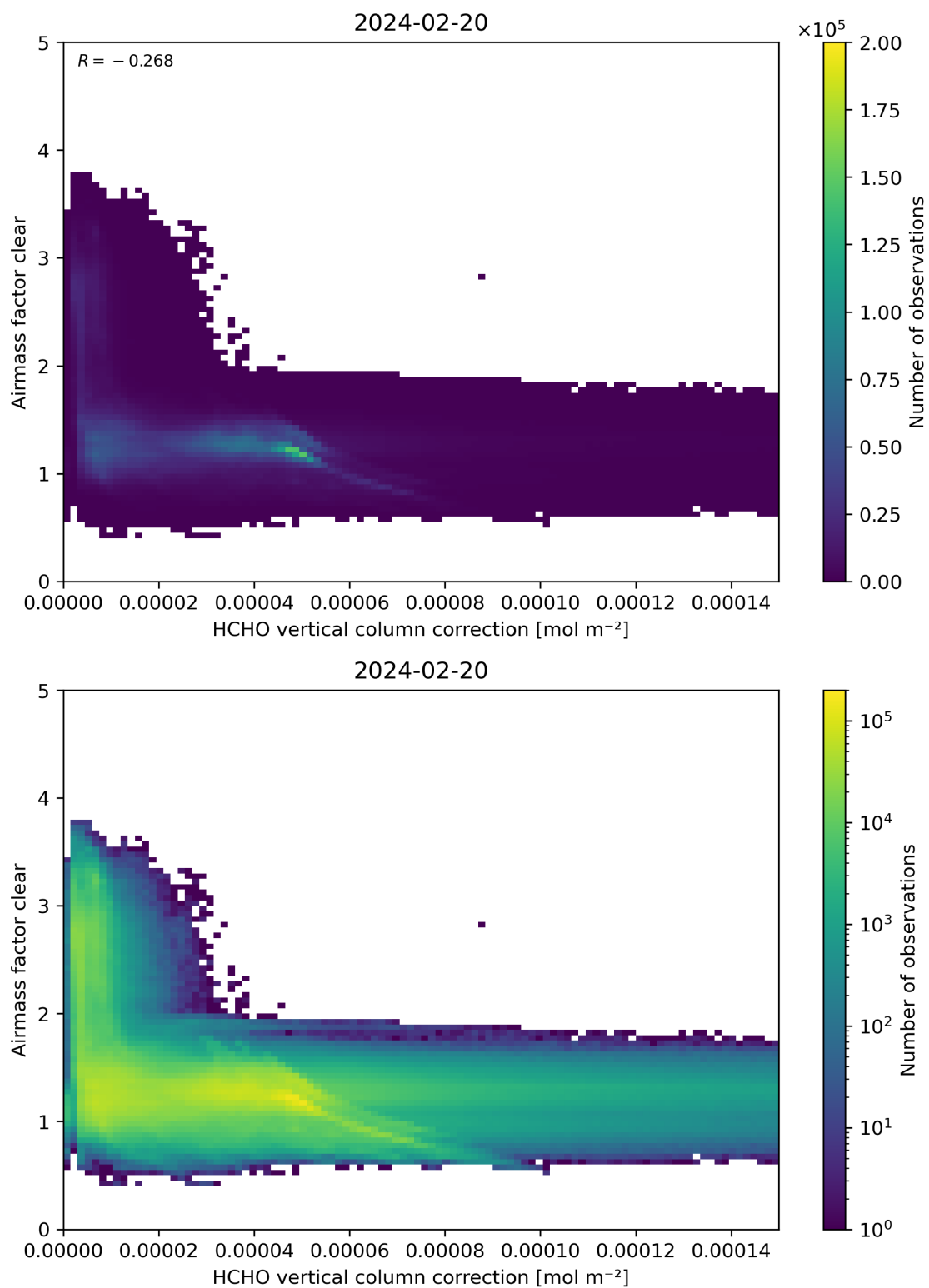
Figure 115: Scatter density plot of “HCHO vertical column correction” against “Airmass factor clear” for 2024-02-19 to 2024-02-21.
