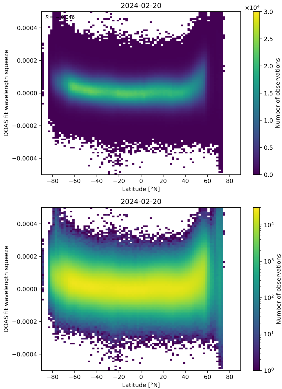
Figure 155: Scatter density plot of “Latitude” against “DOAS fit wavelength squeeze” for 2024-02-19 to 2024-02-21.
