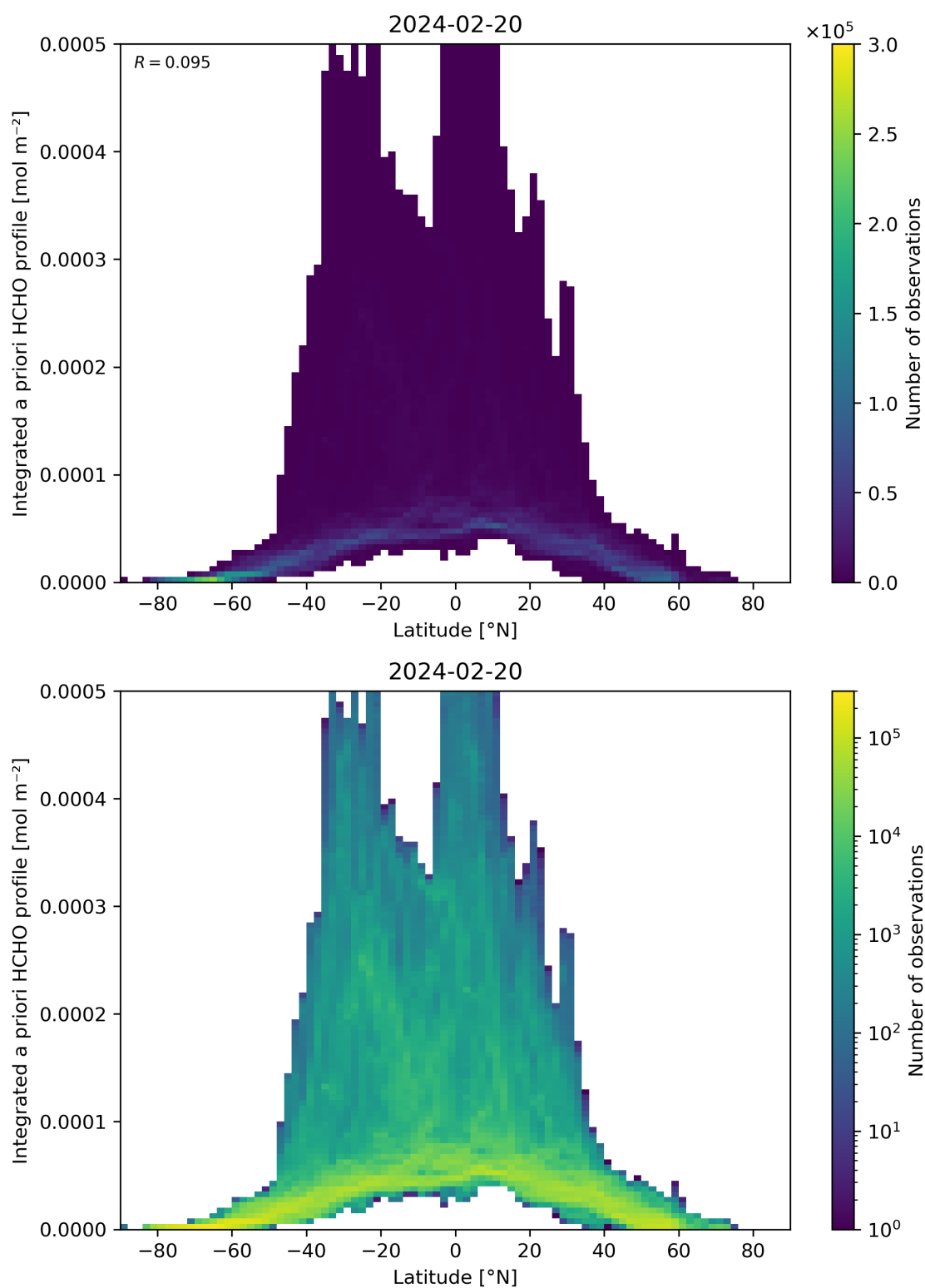
Figure 166: Scatter density plot of “Latitude” against “Integrated a priori HCHO profile” for 2024-02-19 to 2024-02-21.
