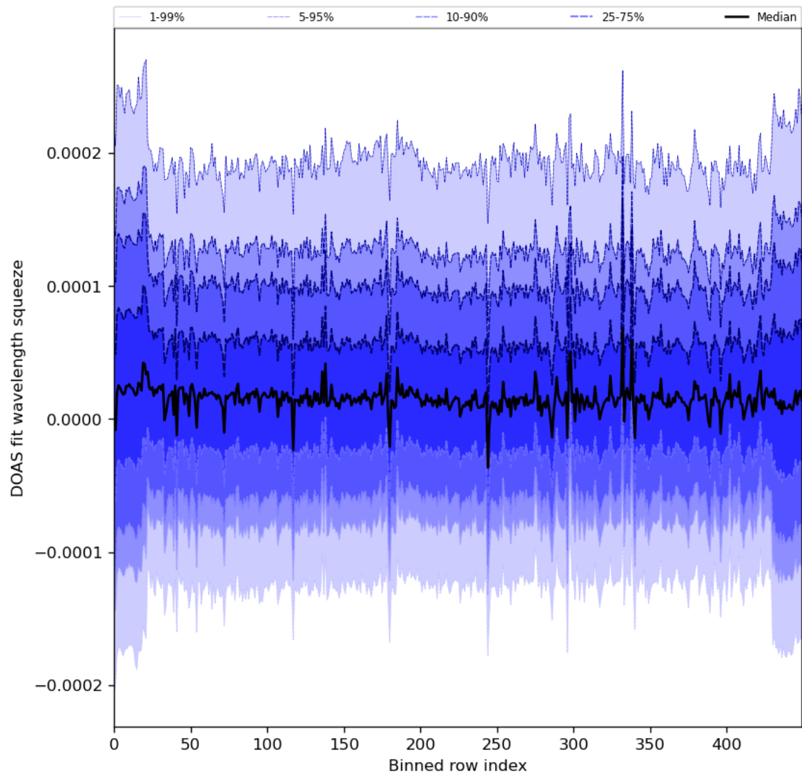
Figure 59: Along track statistics of “DOAS fit wavelength squeeze” for 2024-02-19 to 2024-02-21
