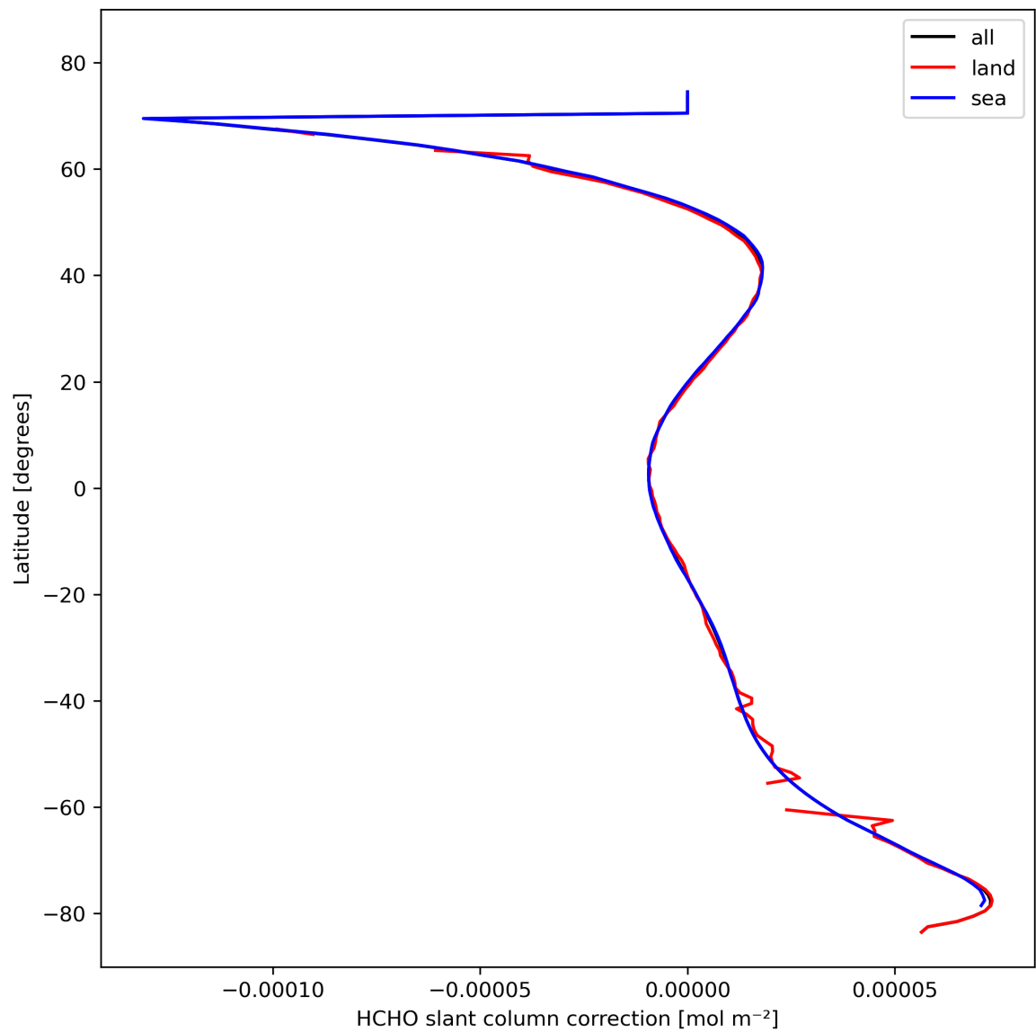
Figure 33: Zonal average of “HCHO slant column correction” for 2024-02-19 to 2024-02-21.
