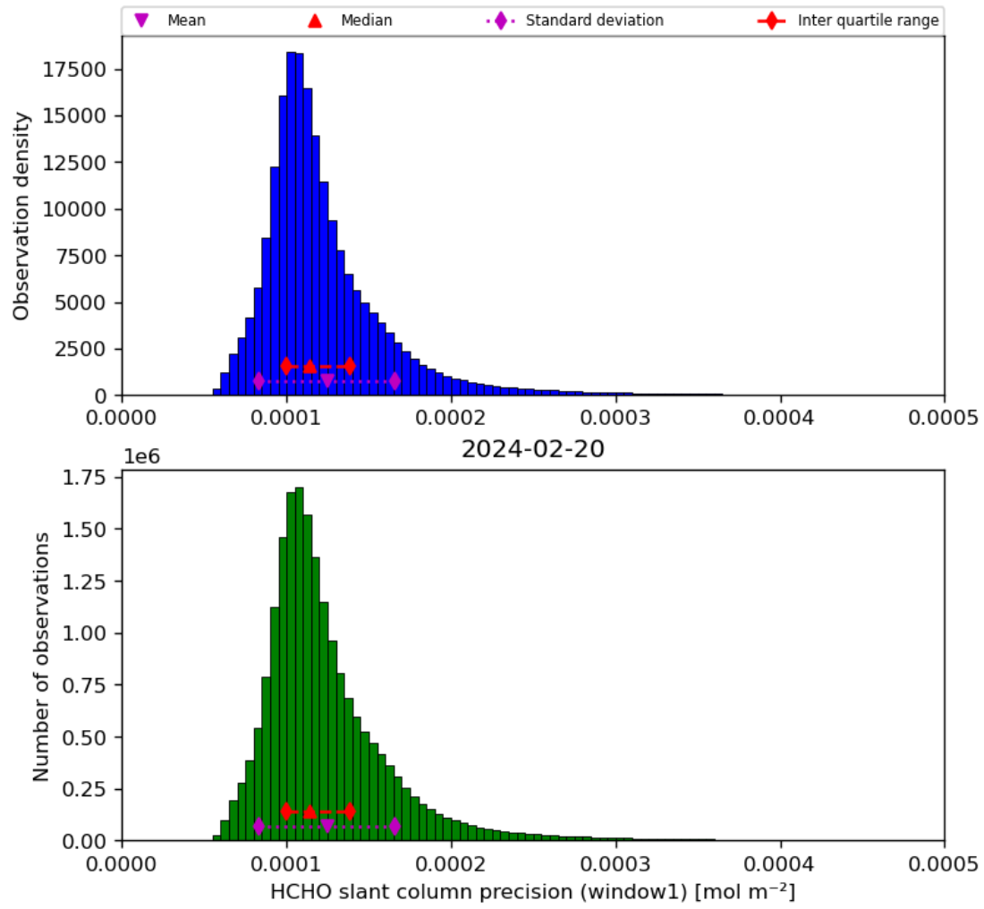
Figure 39: Histogram of “HCHO slant column precision (window1)” for 2024-02-19 to 2024-02-21
