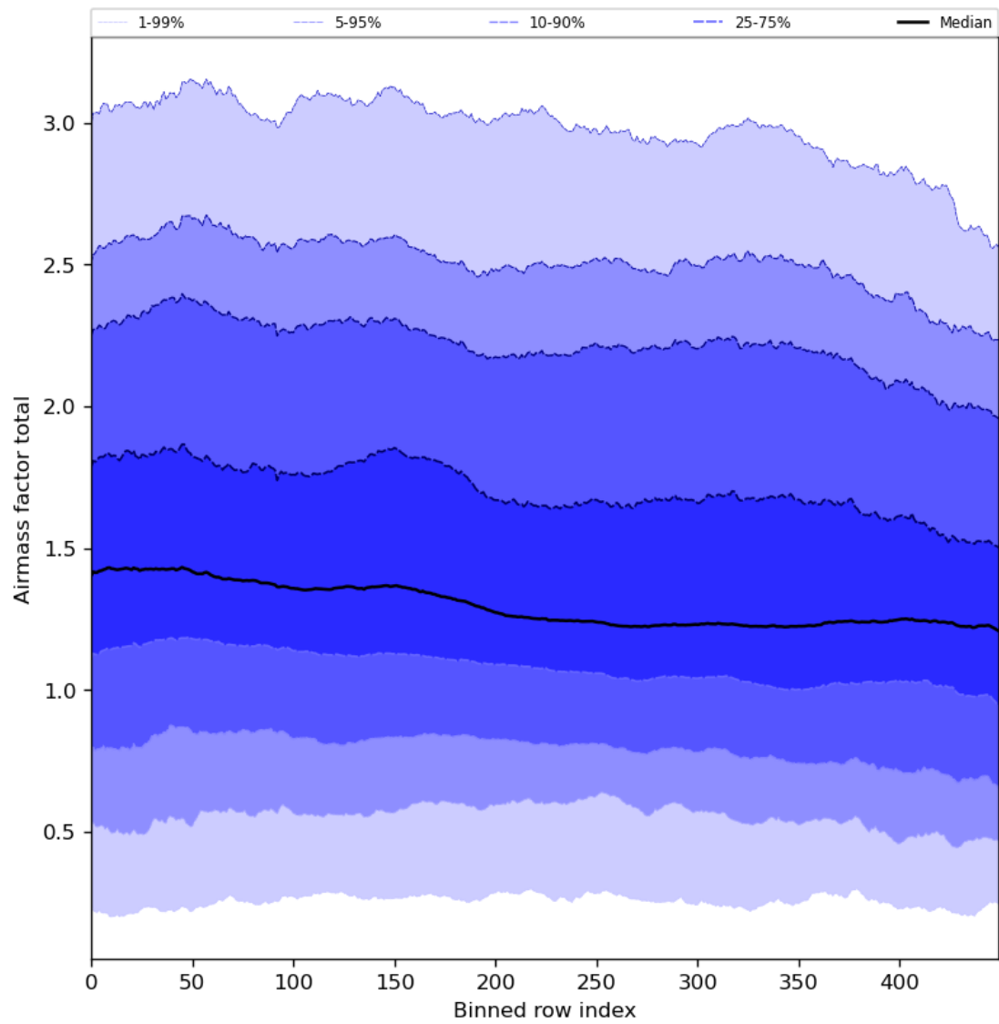
Figure 54: Along track statistics of “Airmass factor total” for 2024-02-19 to 2024-02-21
