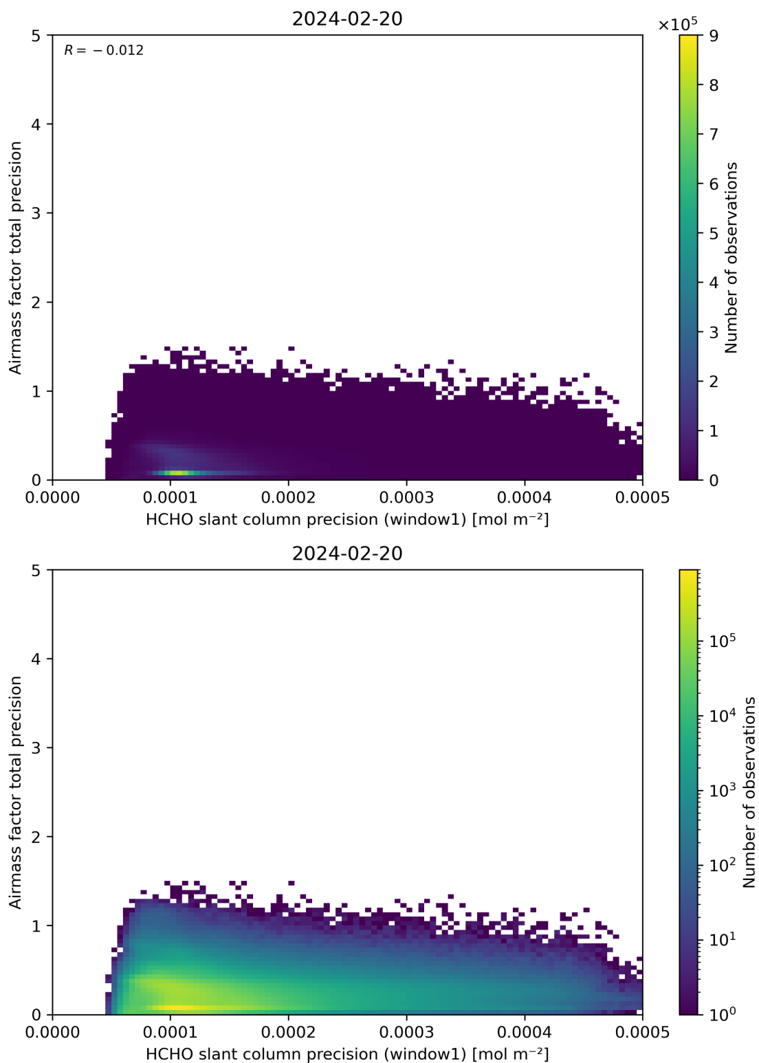
Figure 95: Scatter density plot of “HCHO slant column precision (window1)” against “Airmass factor total precision” for 2024-02-19 to 2024-02-21.
