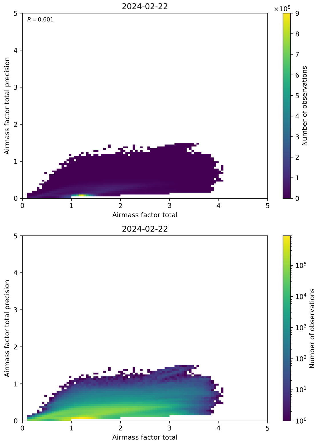
Figure 103: Scatter density plot of “Airmass factor total” against “Airmass factor total precision” for 2024-02-22 to 2024-02-23.
