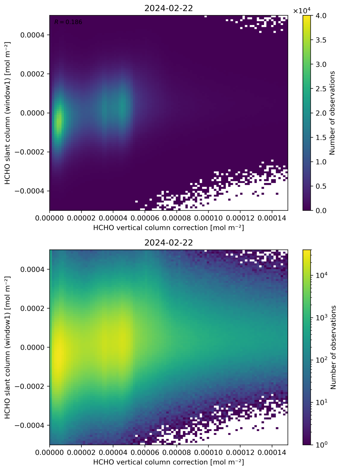
Figure 118: Scatter density plot of “HCHO vertical column correction” against “HCHO slant column (window1)” for 2024-02-22 to 2024-02-23.
