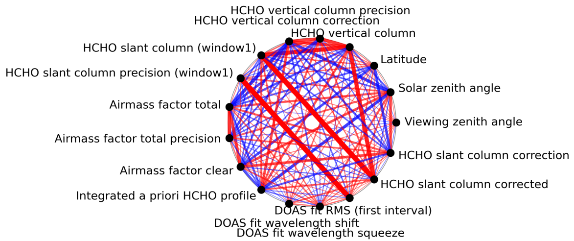
Figure 1: Map of correlation graph for 2024-02-22 to 2024-02-23.
