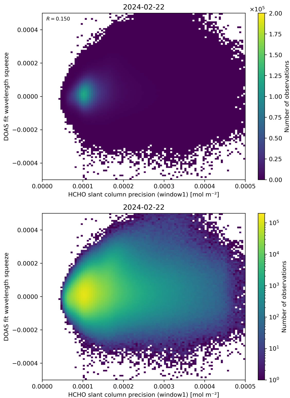
Figure 90: Scatter density plot of “HCHO slant column precision (window1)” against “DOAS fit wavelength squeeze” for 2024-02-22 to 2024-02-23.
