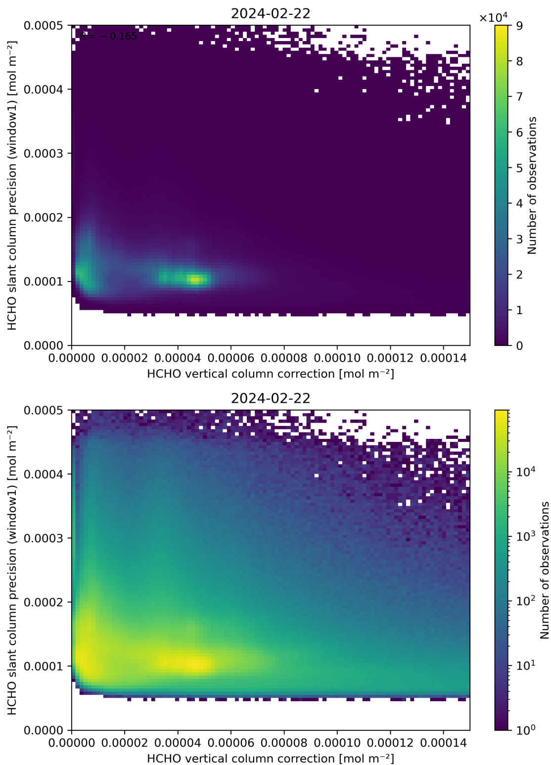
Figure 119: Scatter density plot of “HCHO vertical column correction” against “HCHO slant column precision (window1)” for 2024-02-22 to 2024-02-23.
