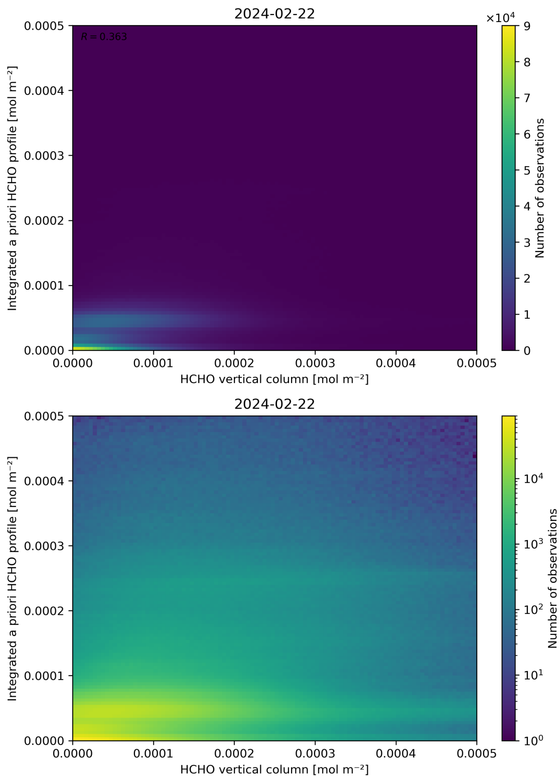
Figure 135: Scatter density plot of “HCHO vertical column” against “Integrated a priori HCHO profile” for 2024-02-22 to 2024-02-23.
