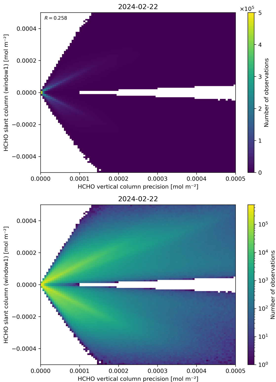
Figure 142: Scatter density plot of “HCHO vertical column precision” against “HCHO slant column (window1)” for 2024-02-22 to 2024-02-23.
