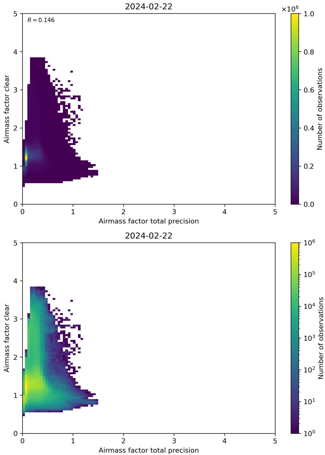
Figure 108: Scatter density plot of “Airmass factor total precision” against “Airmass factor clear” for 2024-02-22 to 2024-02-23.
