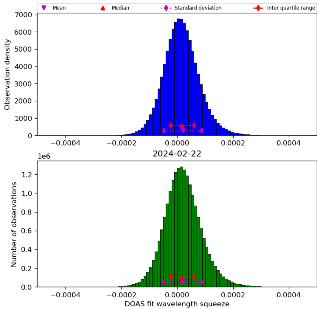
Figure 45: Histogram of “DOAS fit wavelength squeeze” for 2024-02-22 to 2024-02-23
