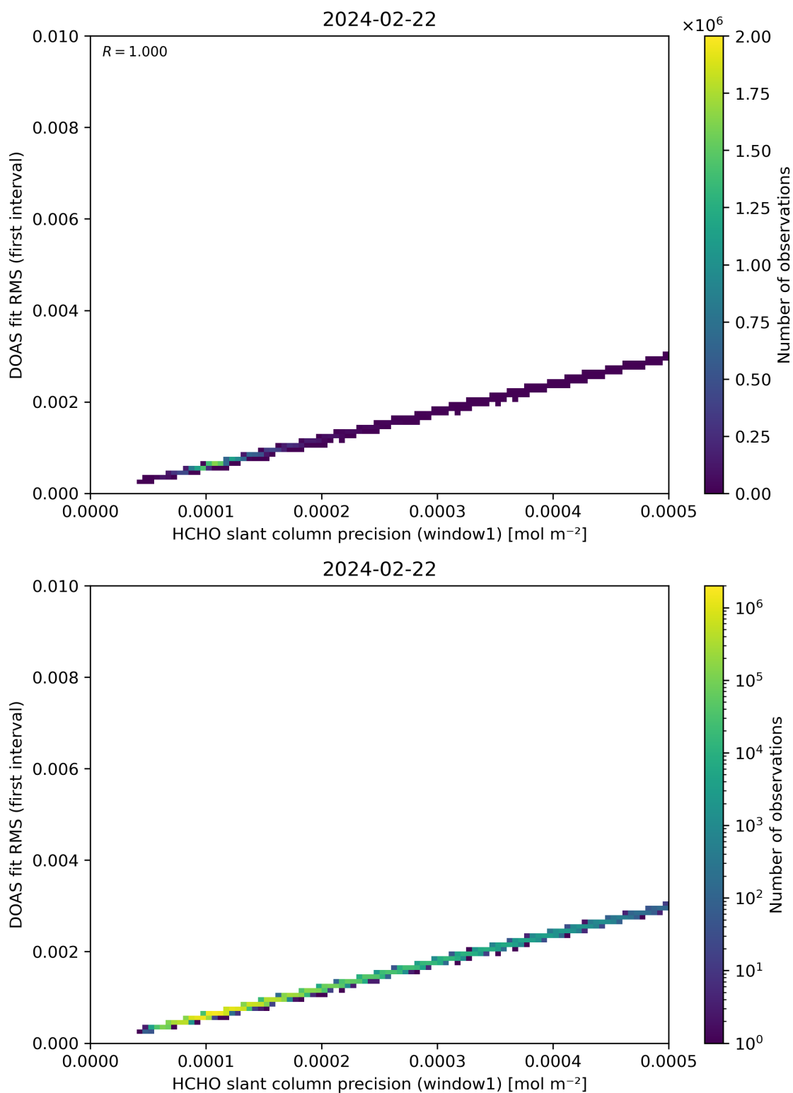
Figure 88: Scatter density plot of “HCHO slant column precision (window1)” against “DOAS fit RMS (first interval)” for 2024-02-22 to 2024-02-23.
