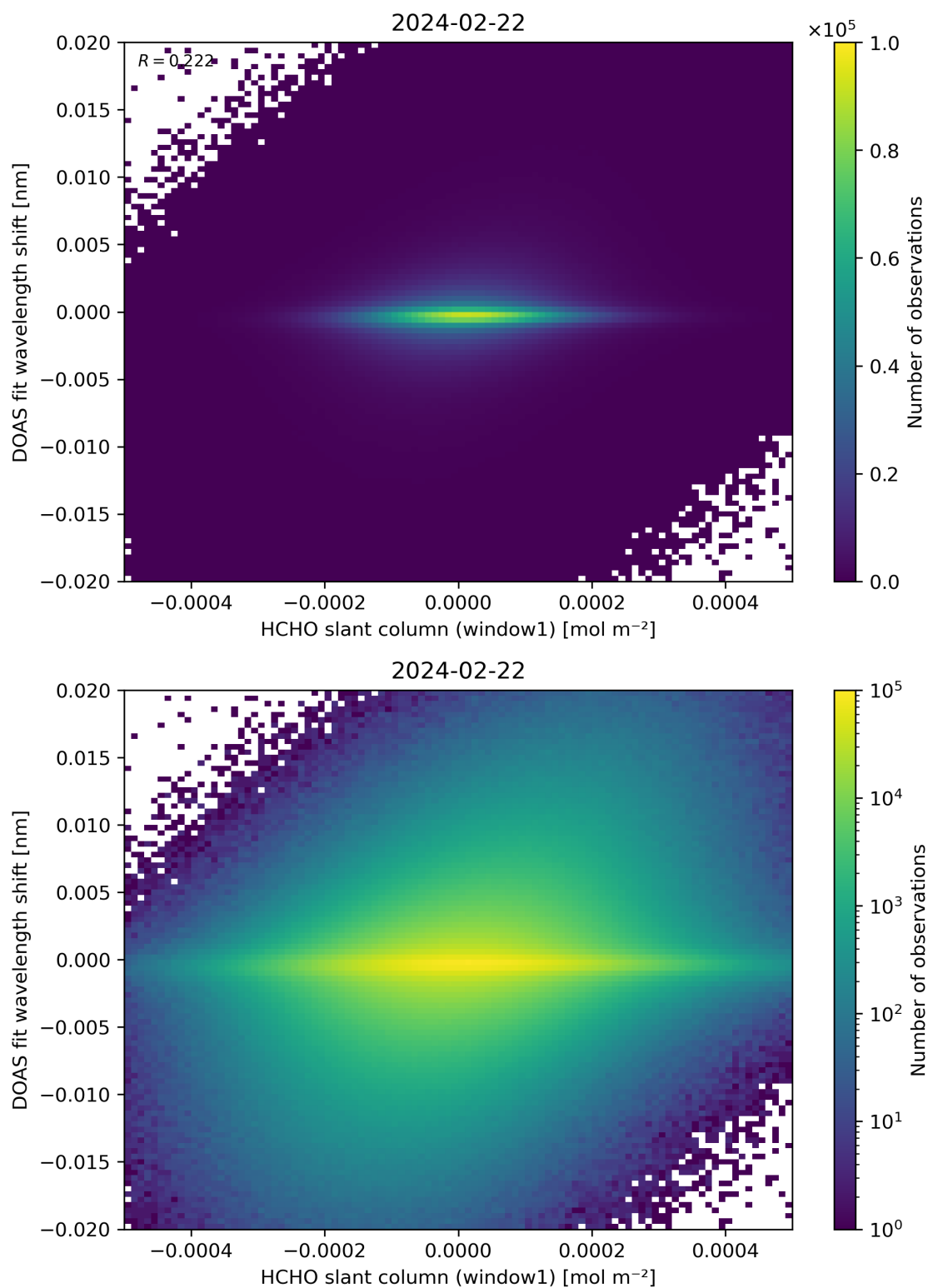
Figure 79: Scatter density plot of “HCHO slant column (window1)” against “DOAS fit wavelength shift” for 2024-02-22 to 2024-02-23.
