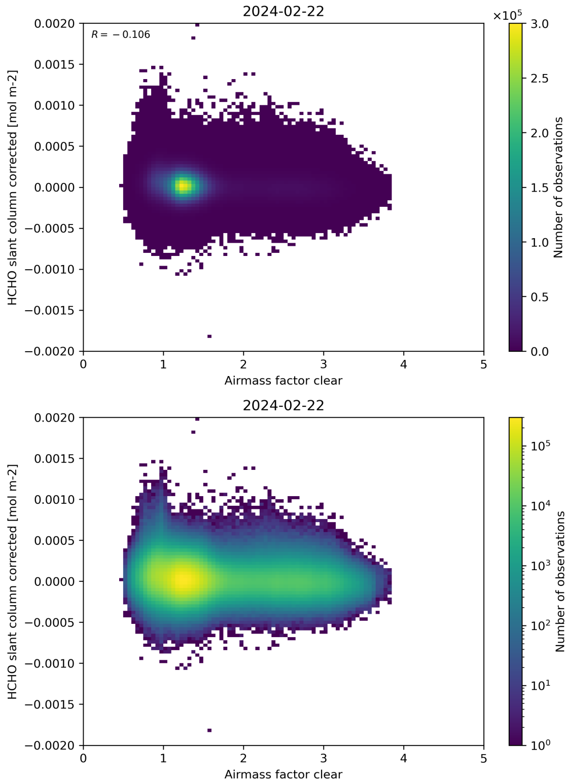
Figure 74: Scatter density plot of “Airmass factor clear” against “HCHO slant column corrected” for 2024-02-22 to 2024-02-23.
