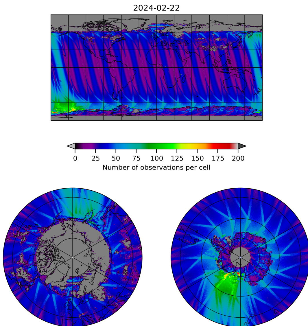
Figure 19: Map of the number of observations for 2024-02-22 to 2024-02-23
