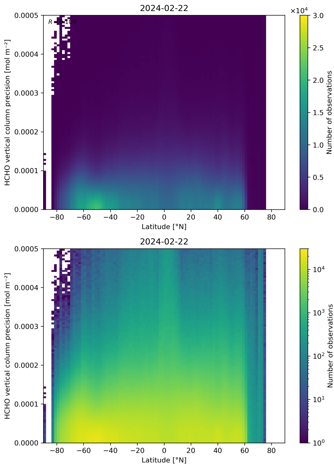
Figure 165: Scatter density plot of “Latitude” against “HCHO vertical column precision” for 2024-02-22 to 2024-02-23.
