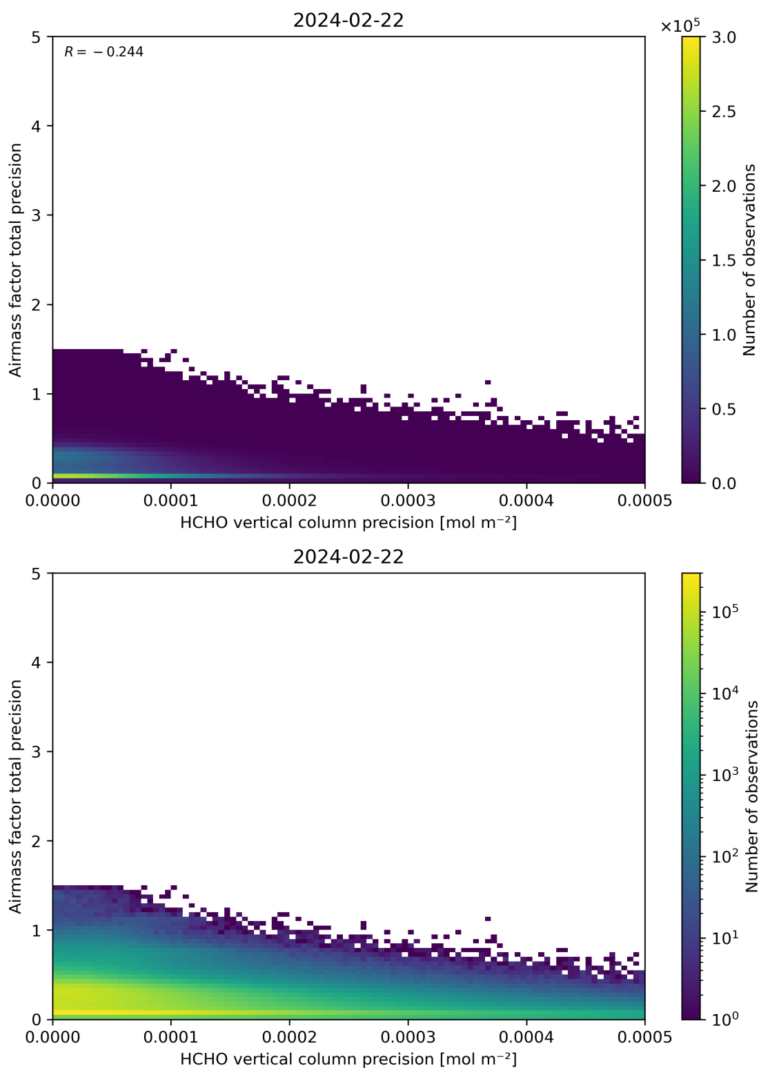
Figure 145: Scatter density plot of “HCHO vertical column precision” against “Airmass factor total precision” for 2024-02-22 to 2024-02-23.
