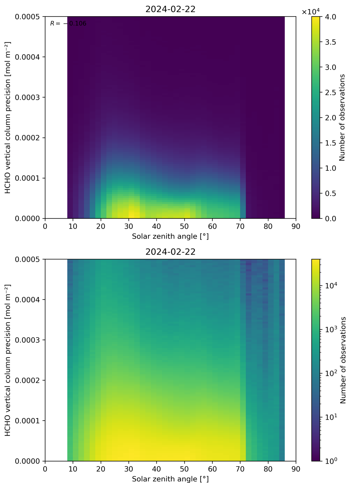
Figure 179: Scatter density plot of “Solar zenith angle” against “HCHO vertical column precision” for 2024-02-22 to 2024-02-23.
