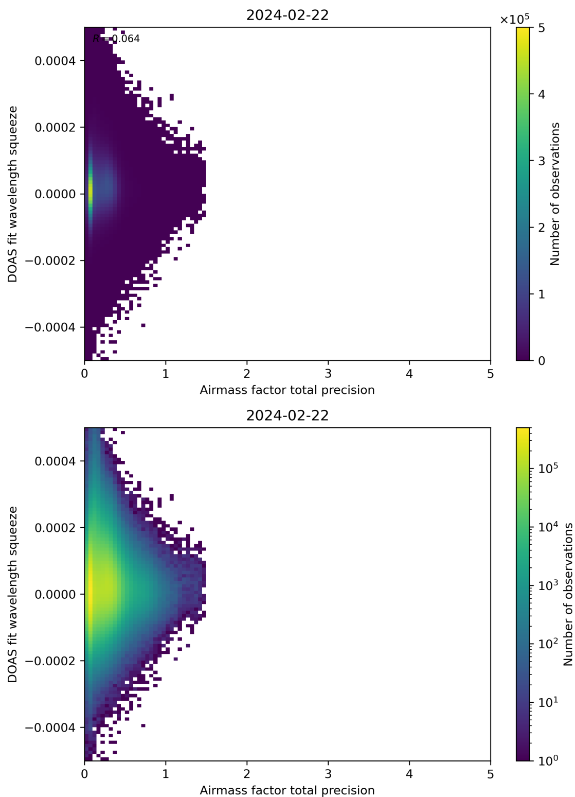
Figure 107: Scatter density plot of “Airmass factor total precision” against “DOAS fit wavelength squeeze” for 2024-02-22 to 2024-02-23.
