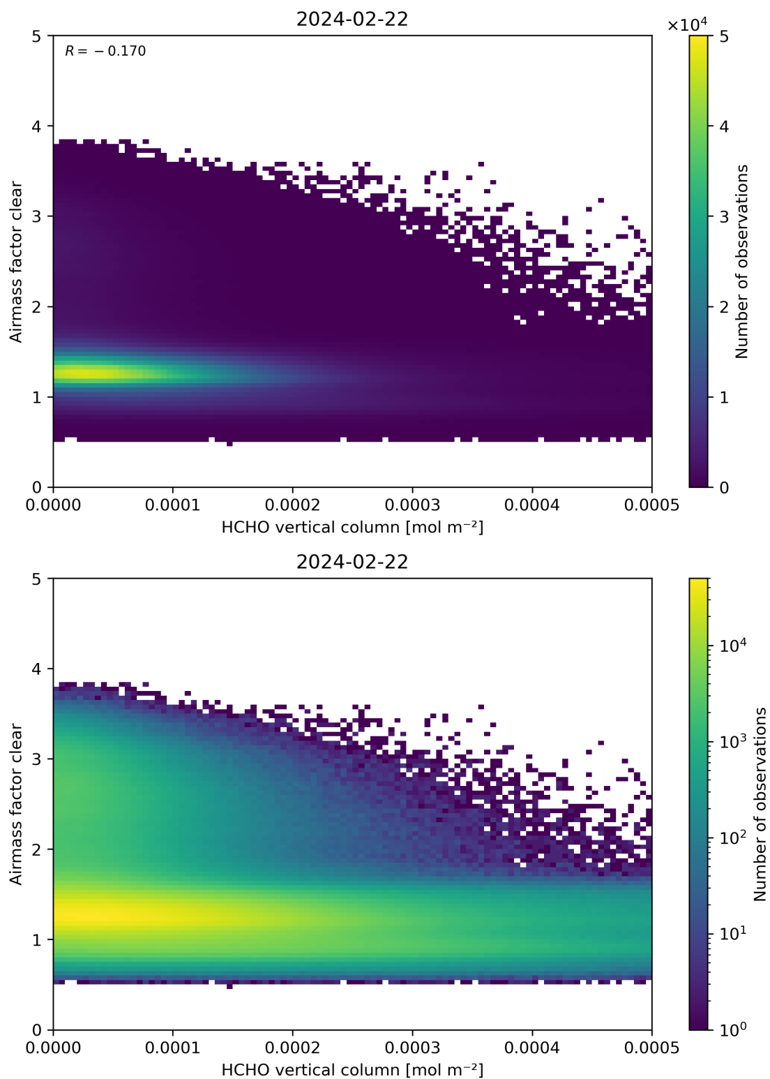
Figure 126: Scatter density plot of “HCHO vertical column” against “Airmass factor clear” for 2024-02-22 to 2024-02-23.
