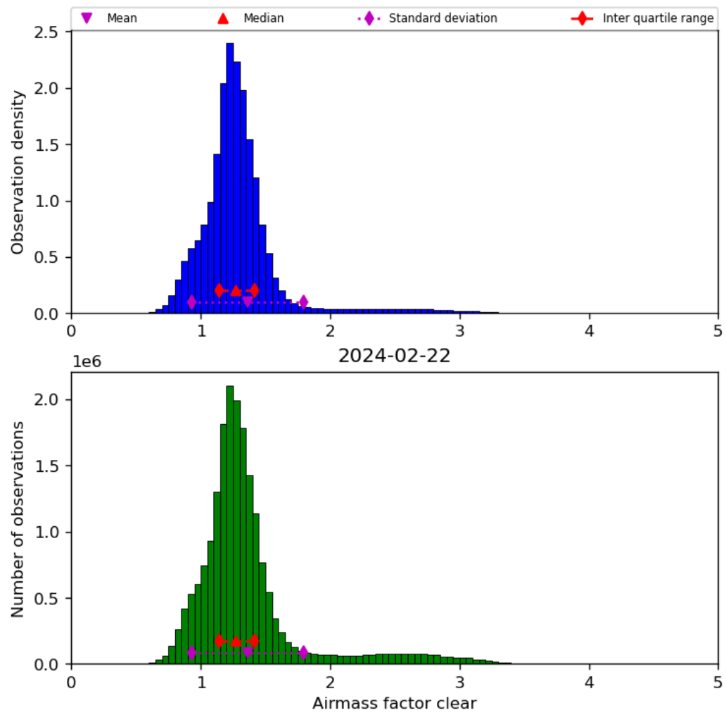
Figure 42: Histogram of “Airmass factor clear” for 2024-02-22 to 2024-02-23
