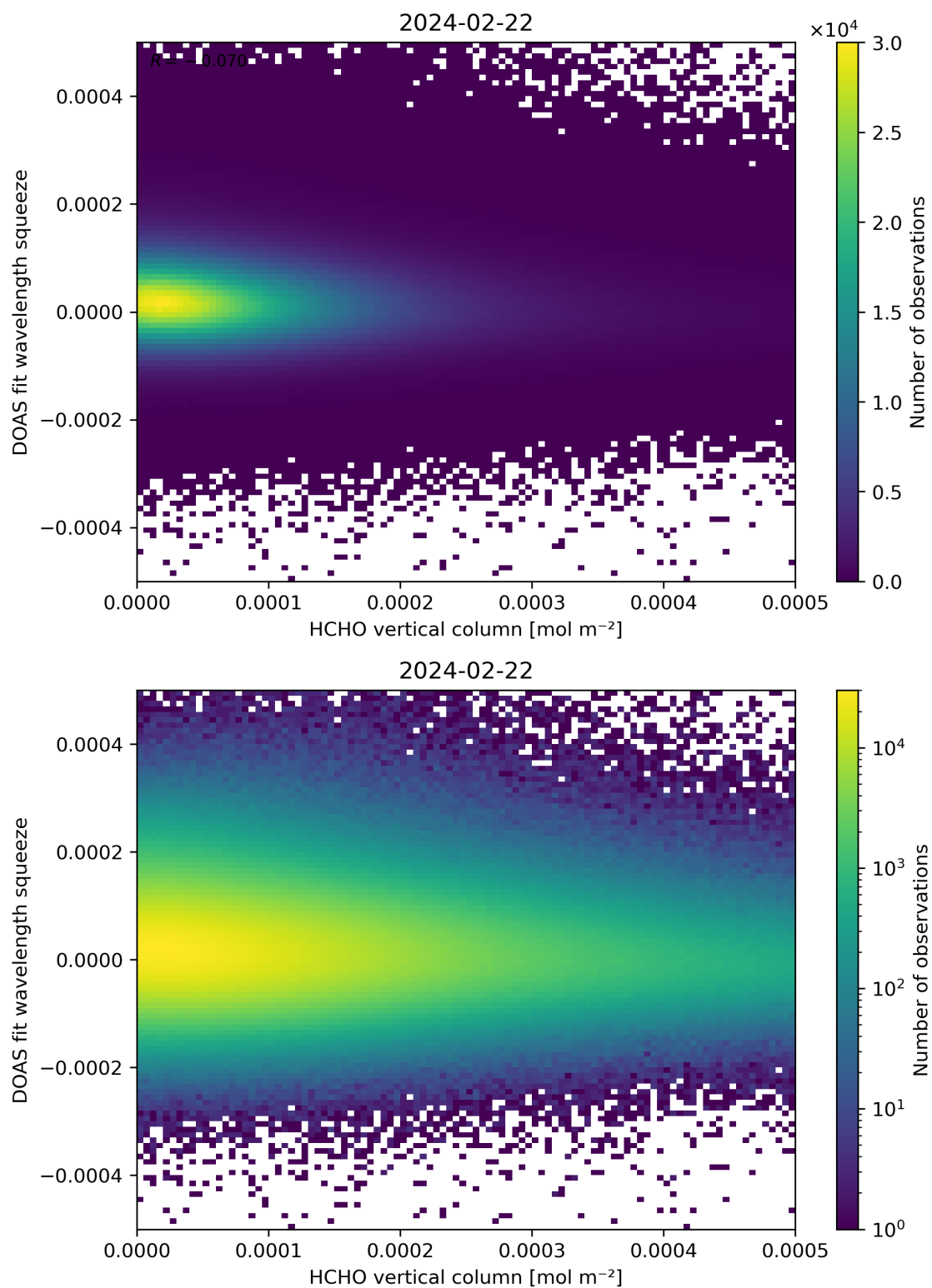
Figure 125: Scatter density plot of “HCHO vertical column” against “DOAS fit wavelength squeeze” for 2024-02-22 to 2024-02-23.
