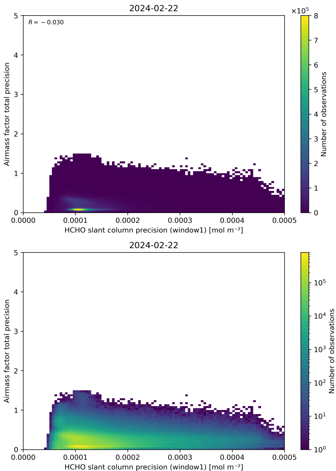
Figure 95: Scatter density plot of “HCHO slant column precision (window1)” against “Airmass factor total precision” for 2024-02-22 to 2024-02-23.
