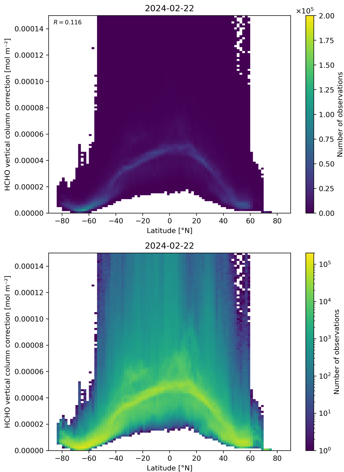
Figure 164: Scatter density plot of “Latitude” against “HCHO vertical column correction” for 2024-02-22 to 2024-02-23.
