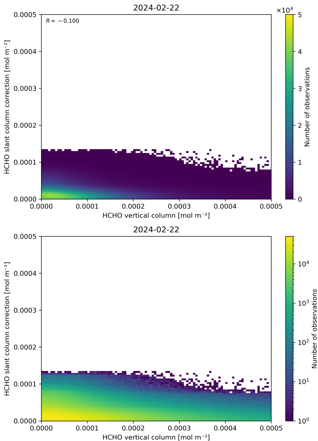
Figure 128: Scatter density plot of “HCHO vertical column” against “HCHO slant column correction” for 2024-02-22 to 2024-02-23.
