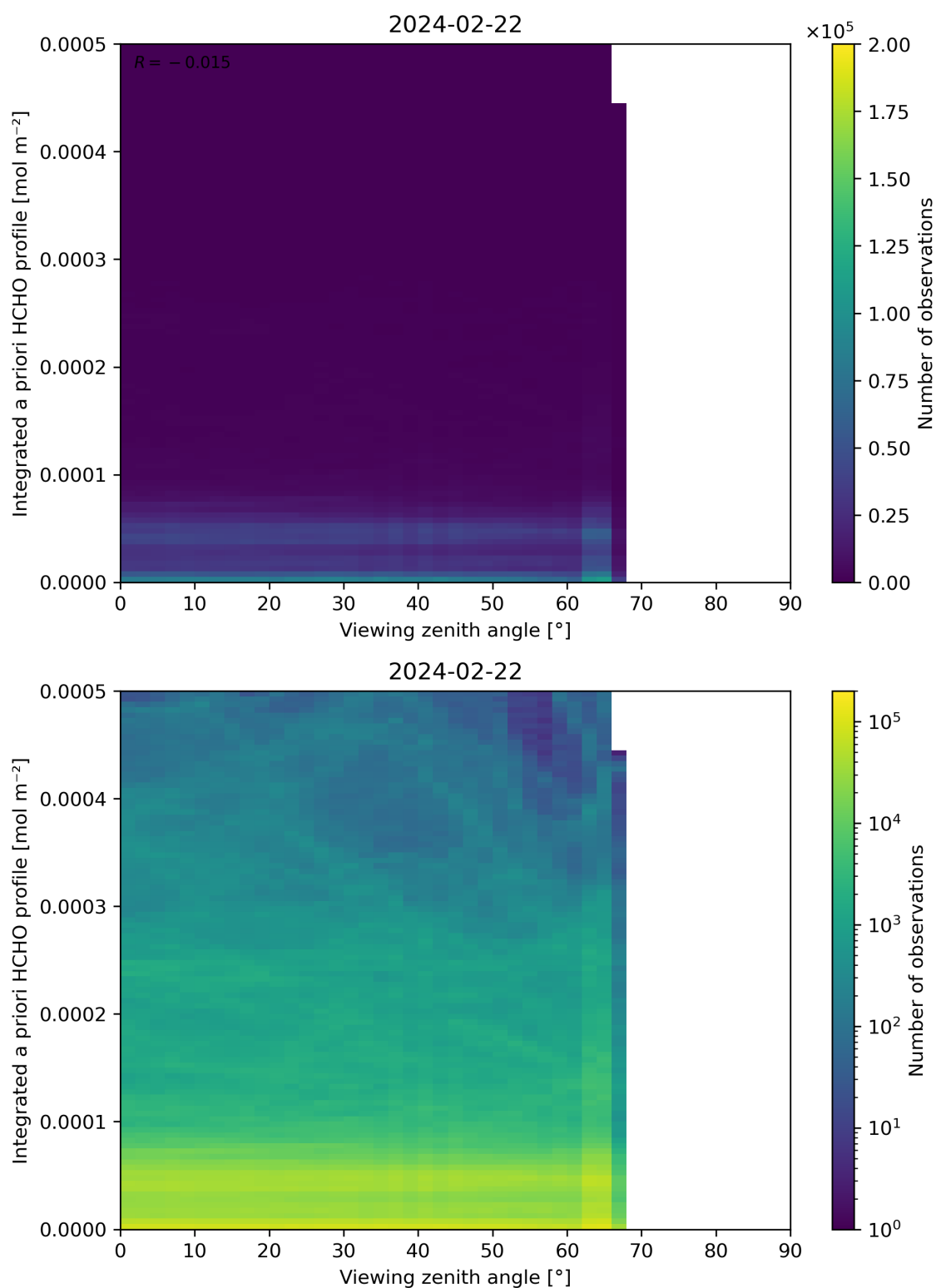
Figure 195: Scatter density plot of “Viewing zenith angle” against “Integrated a priori HCHO profile” for 2024-02-22 to 2024-02-23.
