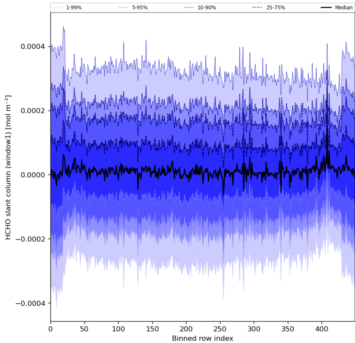
Figure 52: Along track statistics of “HCHO slant column (window1)” for 2024-02-22 to 2024-02-23
