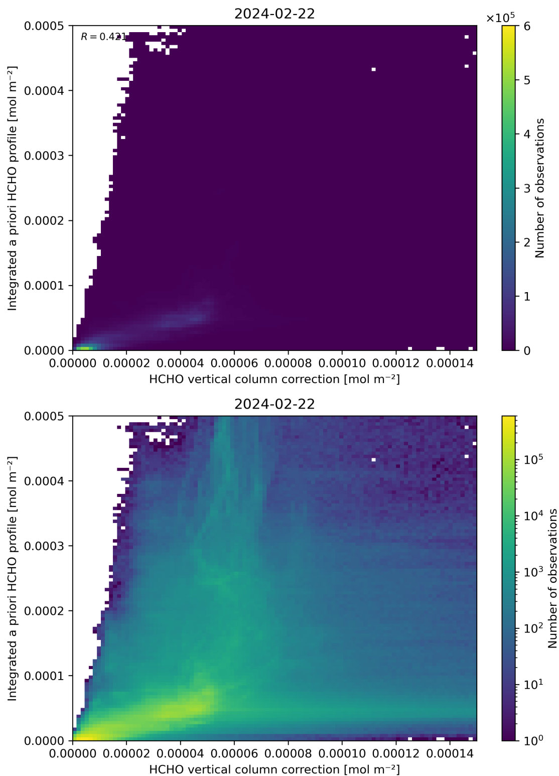
Figure 122: Scatter density plot of “HCHO vertical column correction” against “Integrated a priori HCHO profile” for 2024-02-22 to 2024-02-23.
