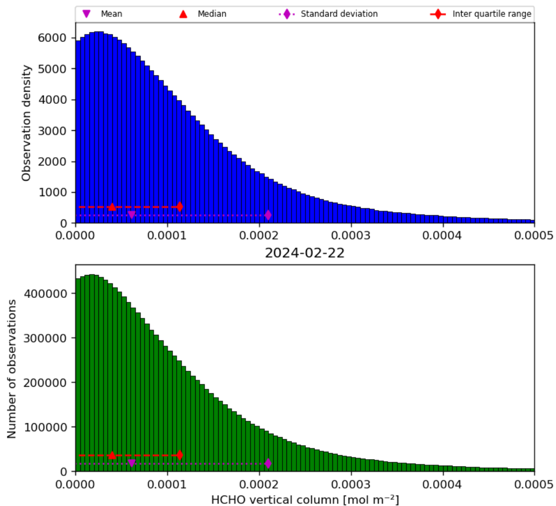
Figure 35: Histogram of “HCHO vertical column” for 2024-02-22 to 2024-02-23
