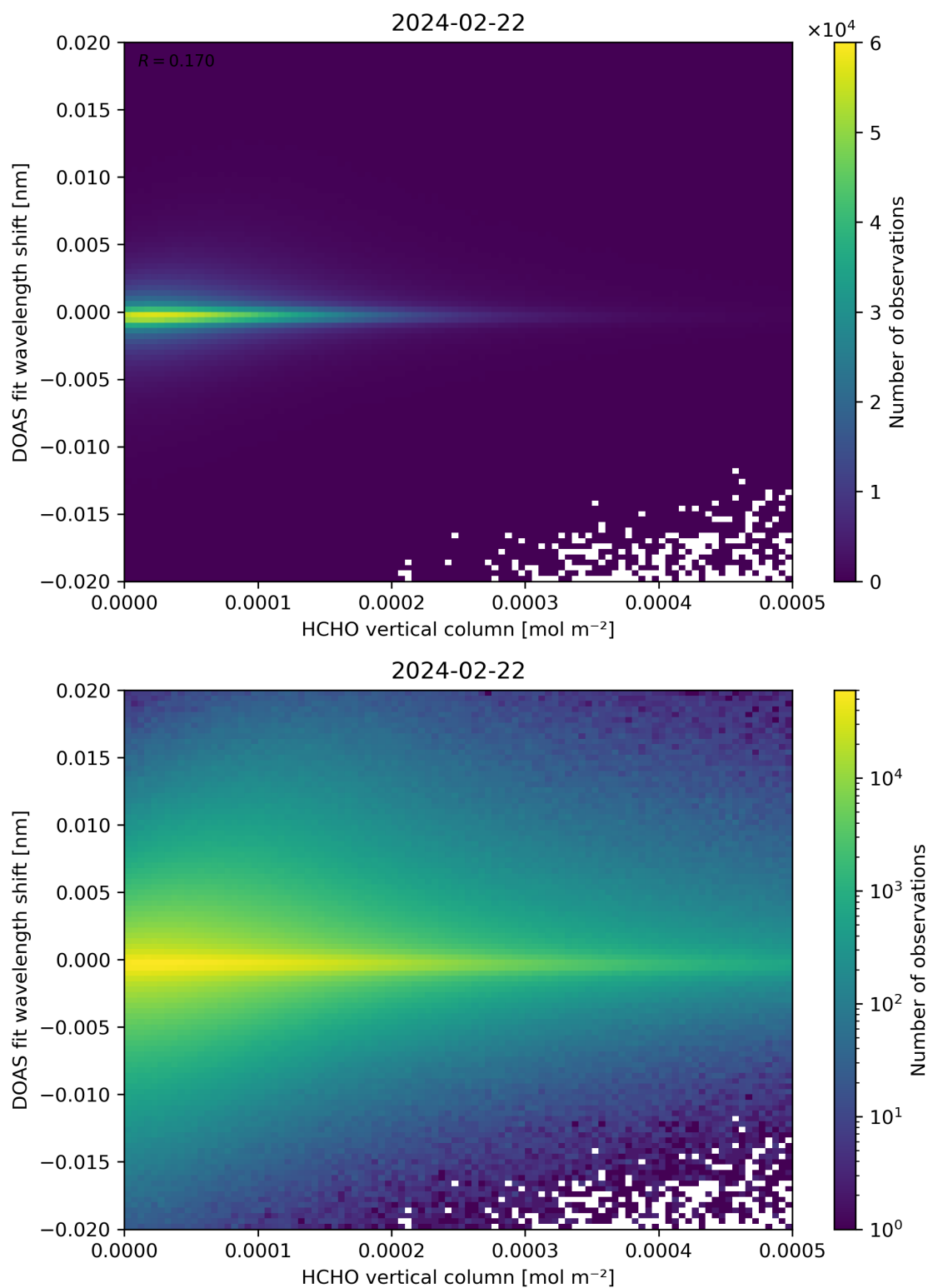
Figure 124: Scatter density plot of “HCHO vertical column” against “DOAS fit wavelength shift” for 2024-02-22 to 2024-02-23.
