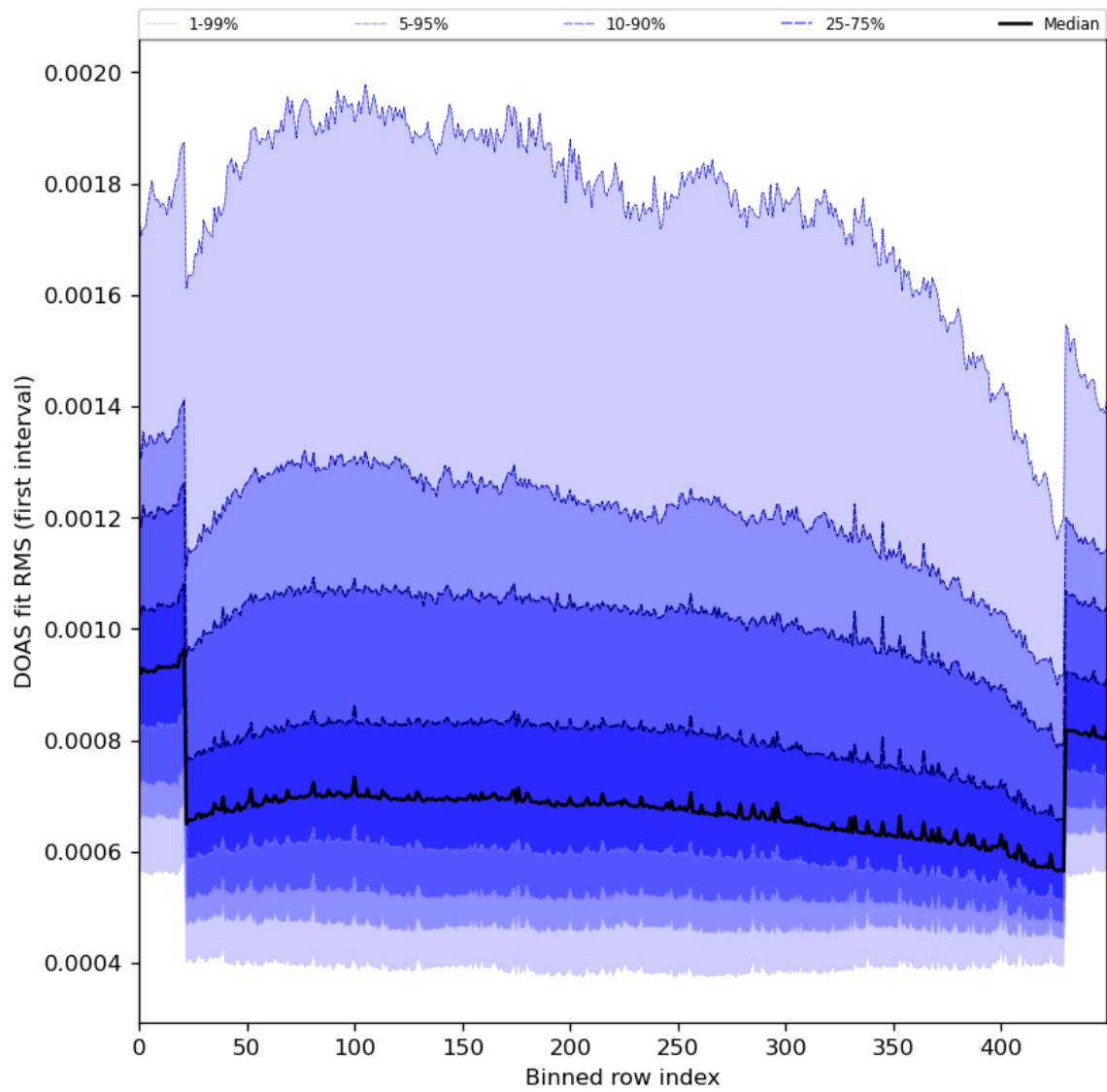
Figure 60: Along track statistics of “DOAS fit RMS (first interval)” for 2024-02-22 to 2024-02-23
