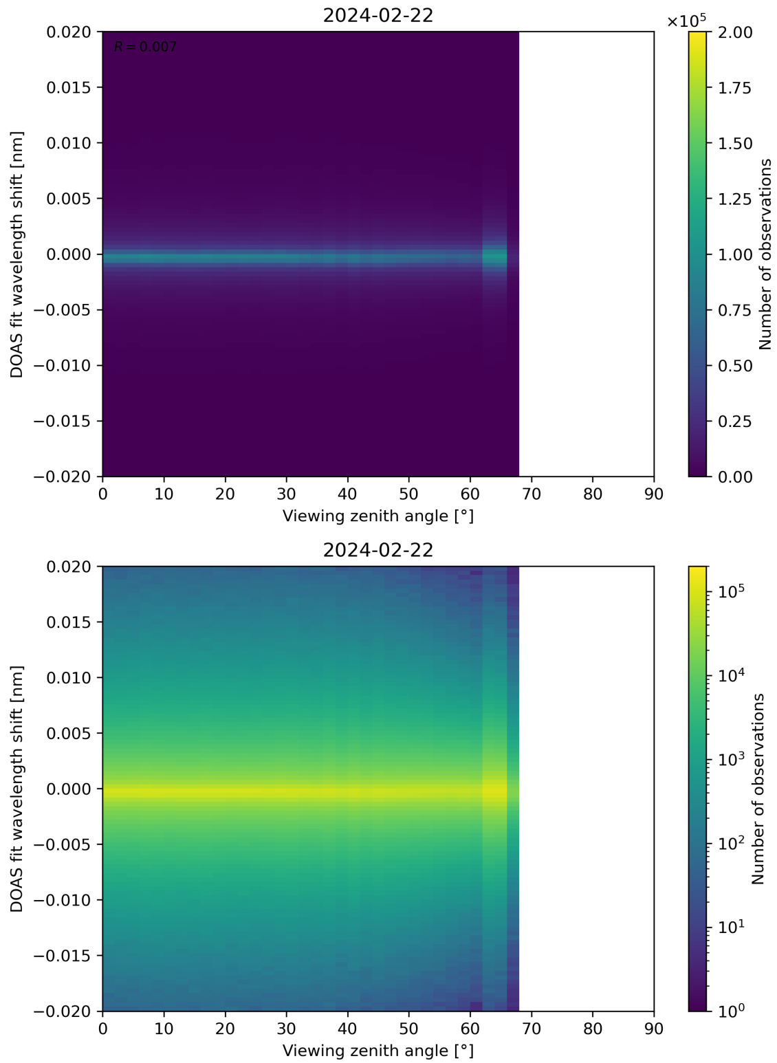
Figure 183: Scatter density plot of “Viewing zenith angle” against “DOAS fit wavelength shift” for 2024-02-22 to 2024-02-23.
