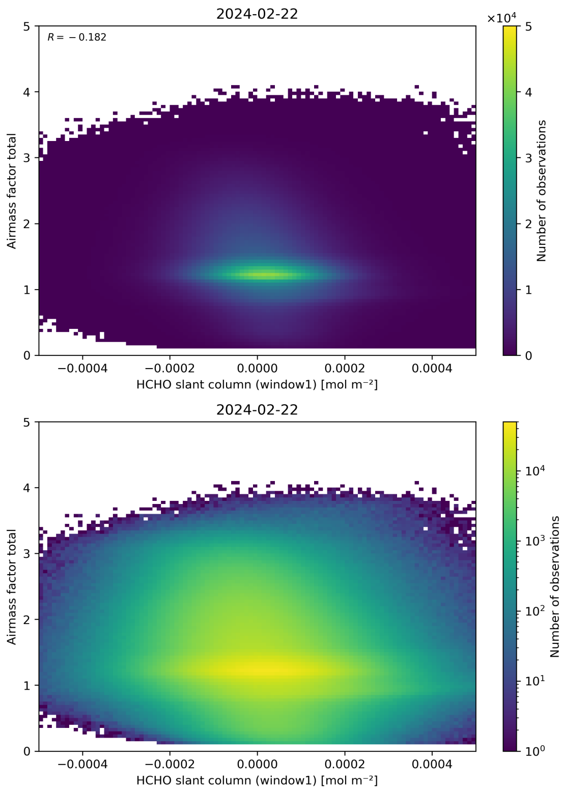
Figure 85: Scatter density plot of “HCHO slant column (window1)” against “Airmass factor total” for 2024-02-22 to 2024-02-23.
