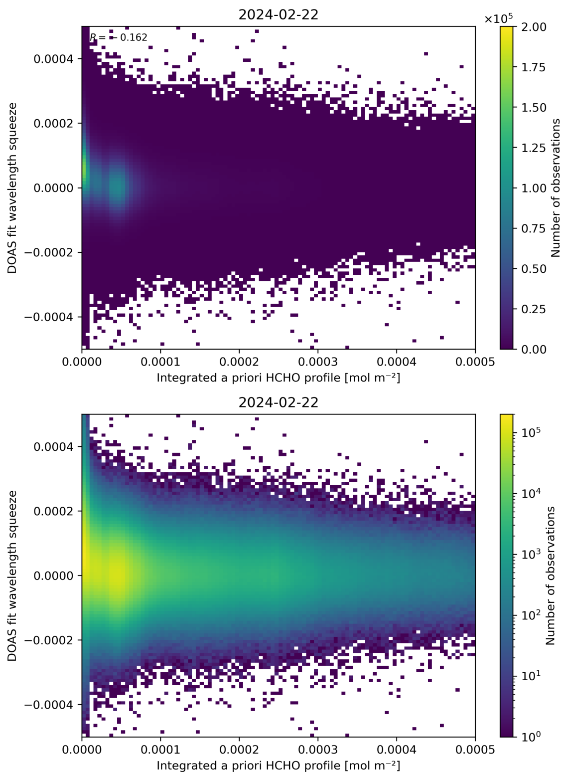
Figure 150: Scatter density plot of “Integrated a priori HCHO profile” against “DOAS fit wavelength squeeze” for 2024-02-22 to 2024-02-23.
