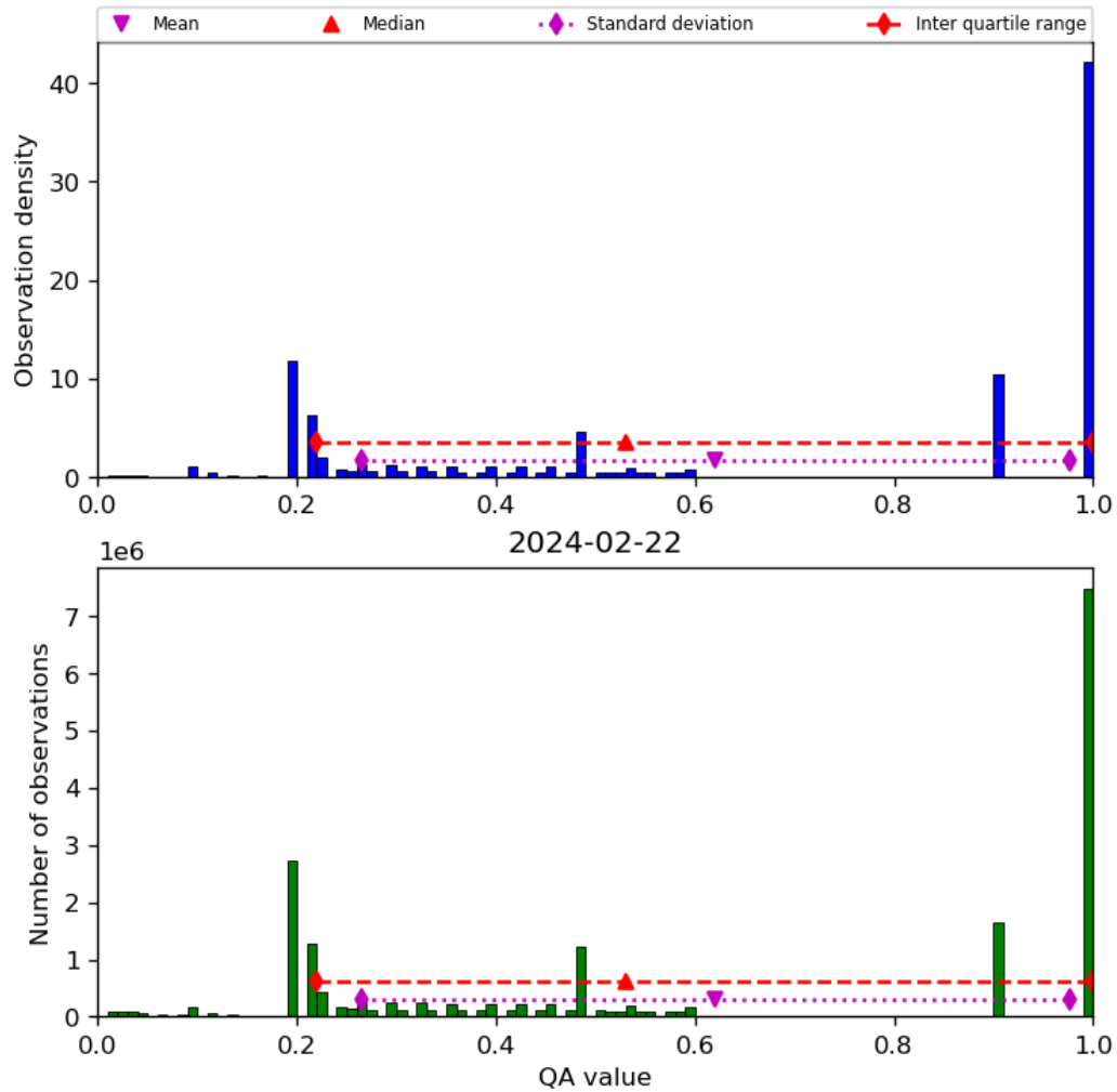
Figure 34: Histogram of “QA value” for 2024-02-22 to 2024-02-23
