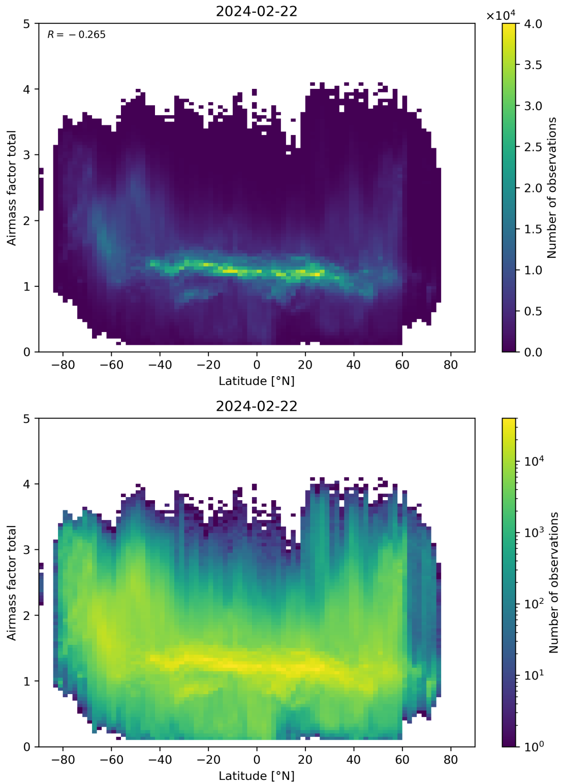
Figure 161: Scatter density plot of “Latitude” against “Airmass factor total” for 2024-02-22 to 2024-02-23.
