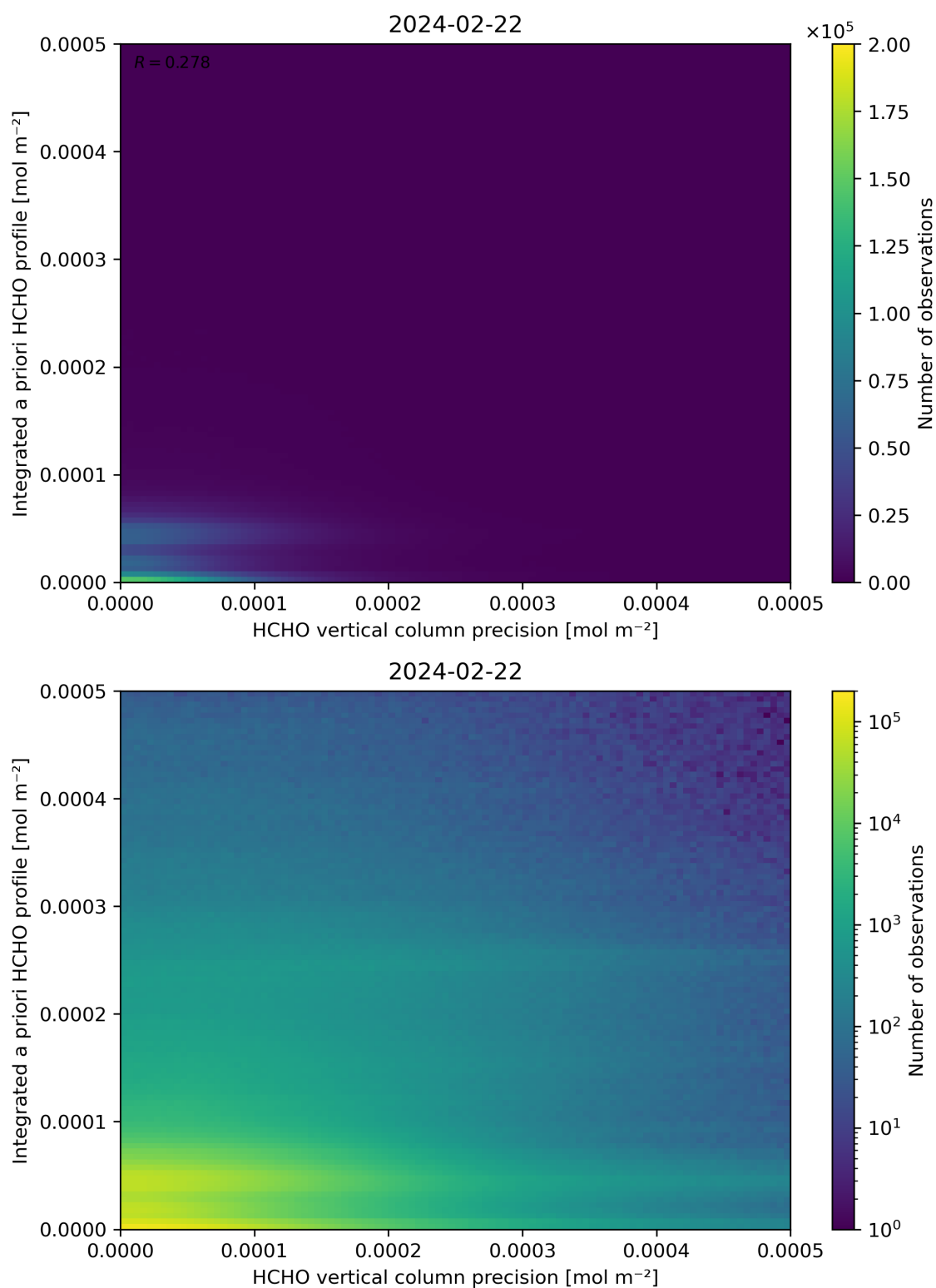
Figure 147: Scatter density plot of “HCHO vertical column precision” against “Integrated a priori HCHO profile” for 2024-02-22 to 2024-02-23.
