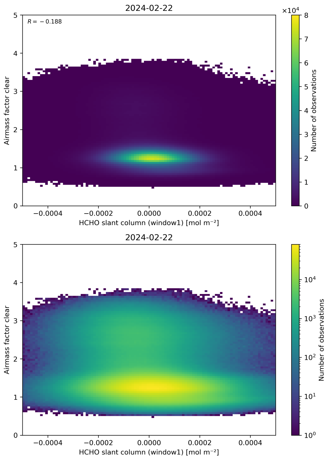
Figure 81: Scatter density plot of “HCHO slant column (window1)” against “Airmass factor clear” for 2024-02-22 to 2024-02-23.
