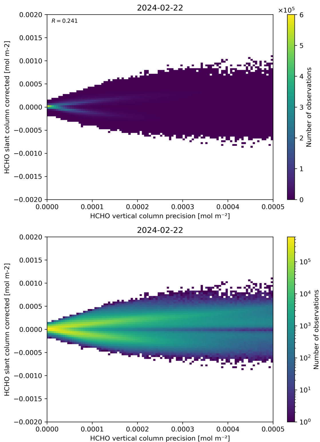
Figure 140: Scatter density plot of “HCHO vertical column precision” against “HCHO slant column corrected” for 2024-02-22 to 2024-02-23.
