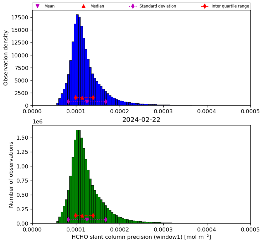
Figure 39: Histogram of “HCHO slant column precision (window1)” for 2024-02-22 to 2024-02-23
