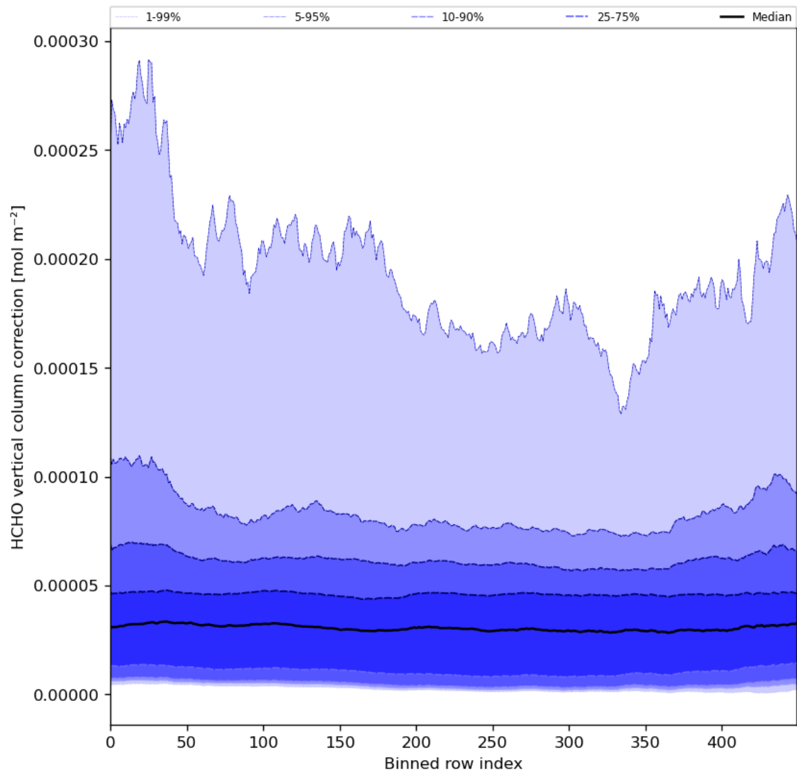
Figure 51: Along track statistics of “HCHO vertical column correction” for 2024-02-22 to 2024-02-23
