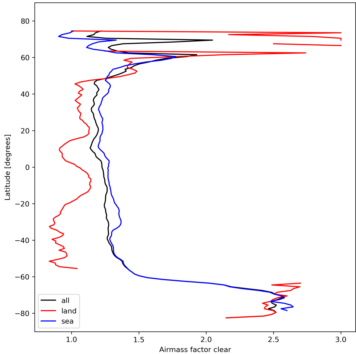
Figure 28: Zonal average of “Airmass factor clear” for 2024-02-22 to 2024-02-23.
