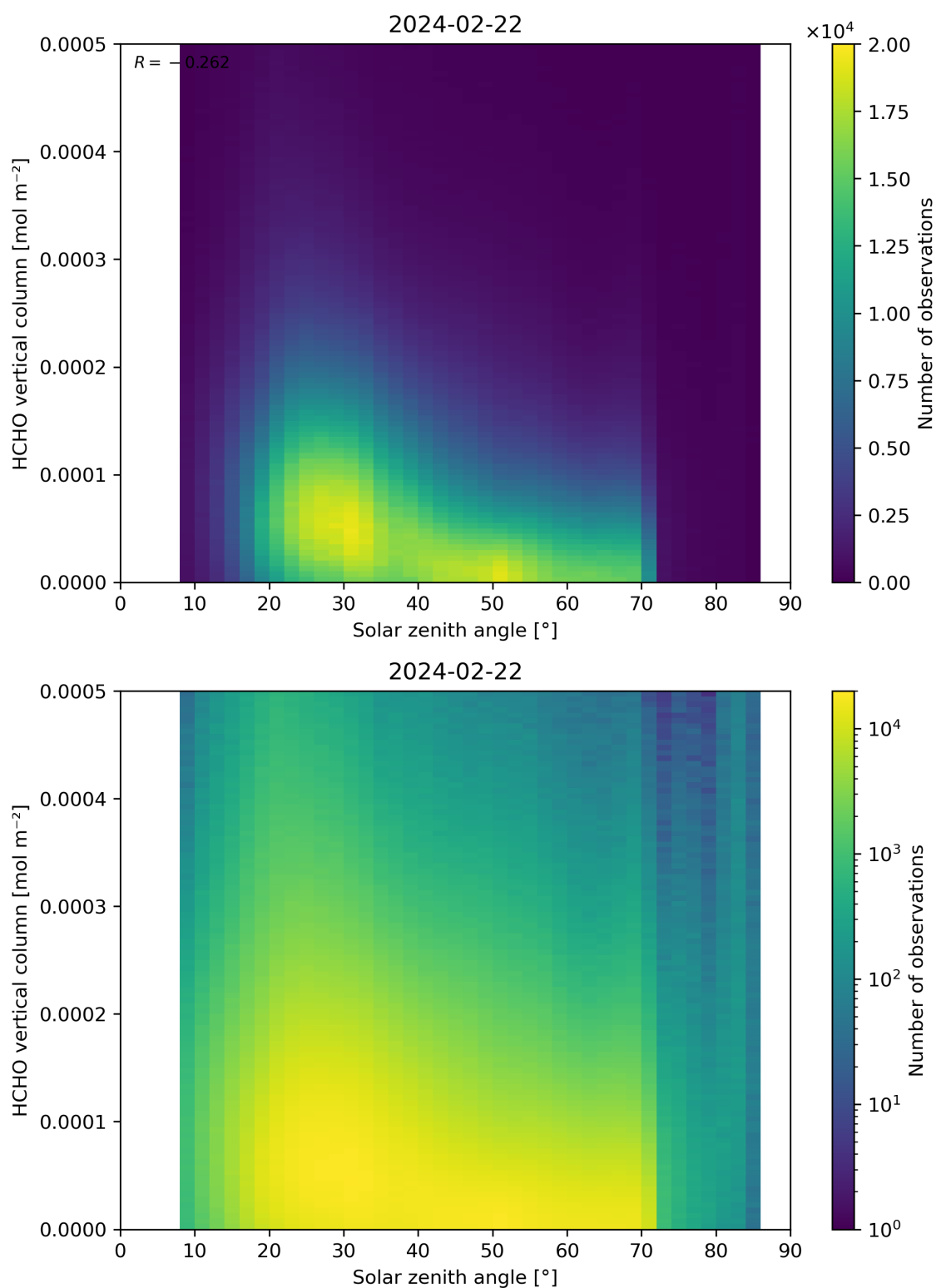
Figure 177: Scatter density plot of “Solar zenith angle” against “HCHO vertical column” for 2024-02-22 to 2024-02-23.
