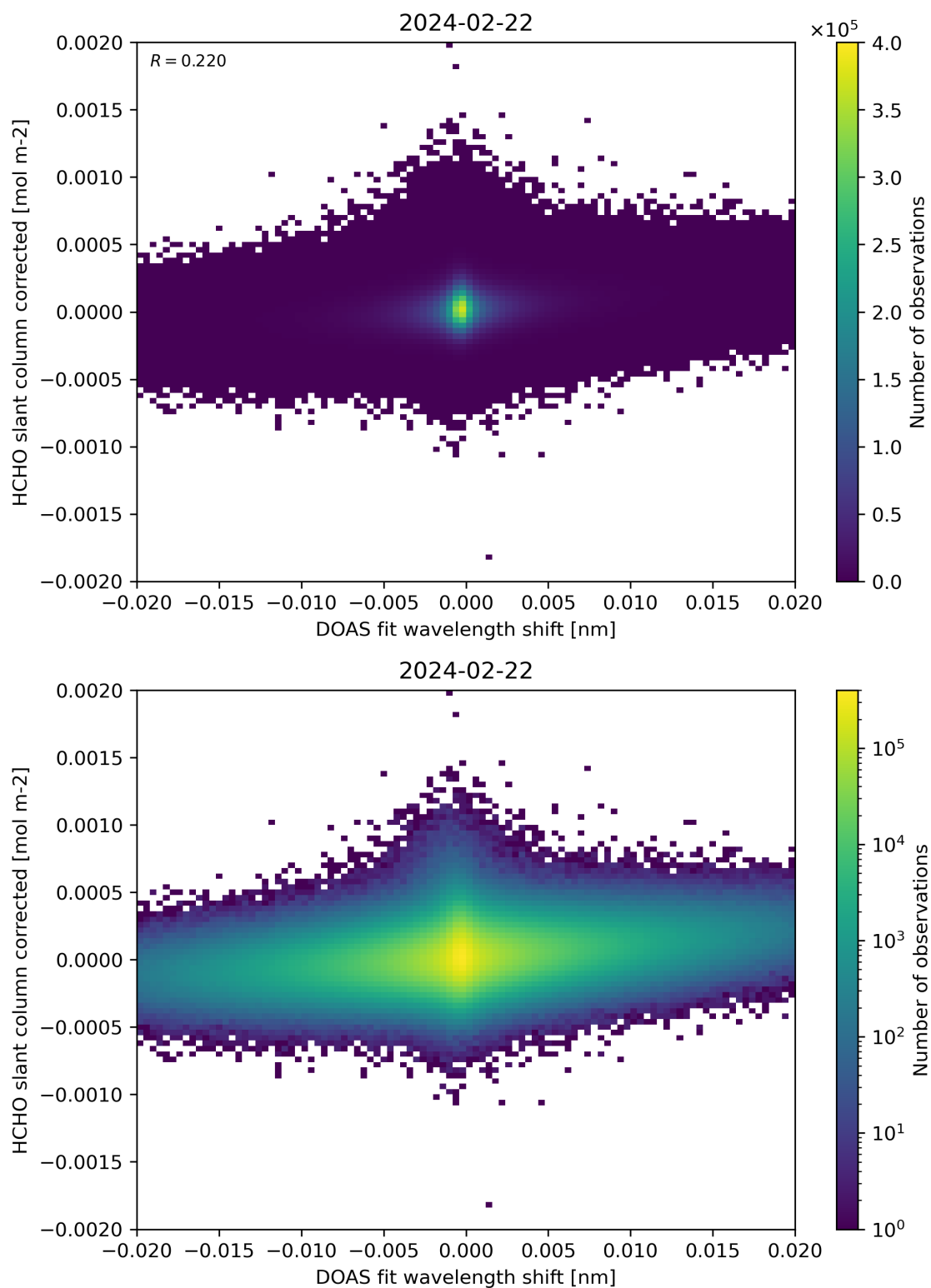
Figure 66: Scatter density plot of “DOAS fit wavelength shift” against “HCHO slant column corrected” for 2024-02-22 to 2024-02-23.
