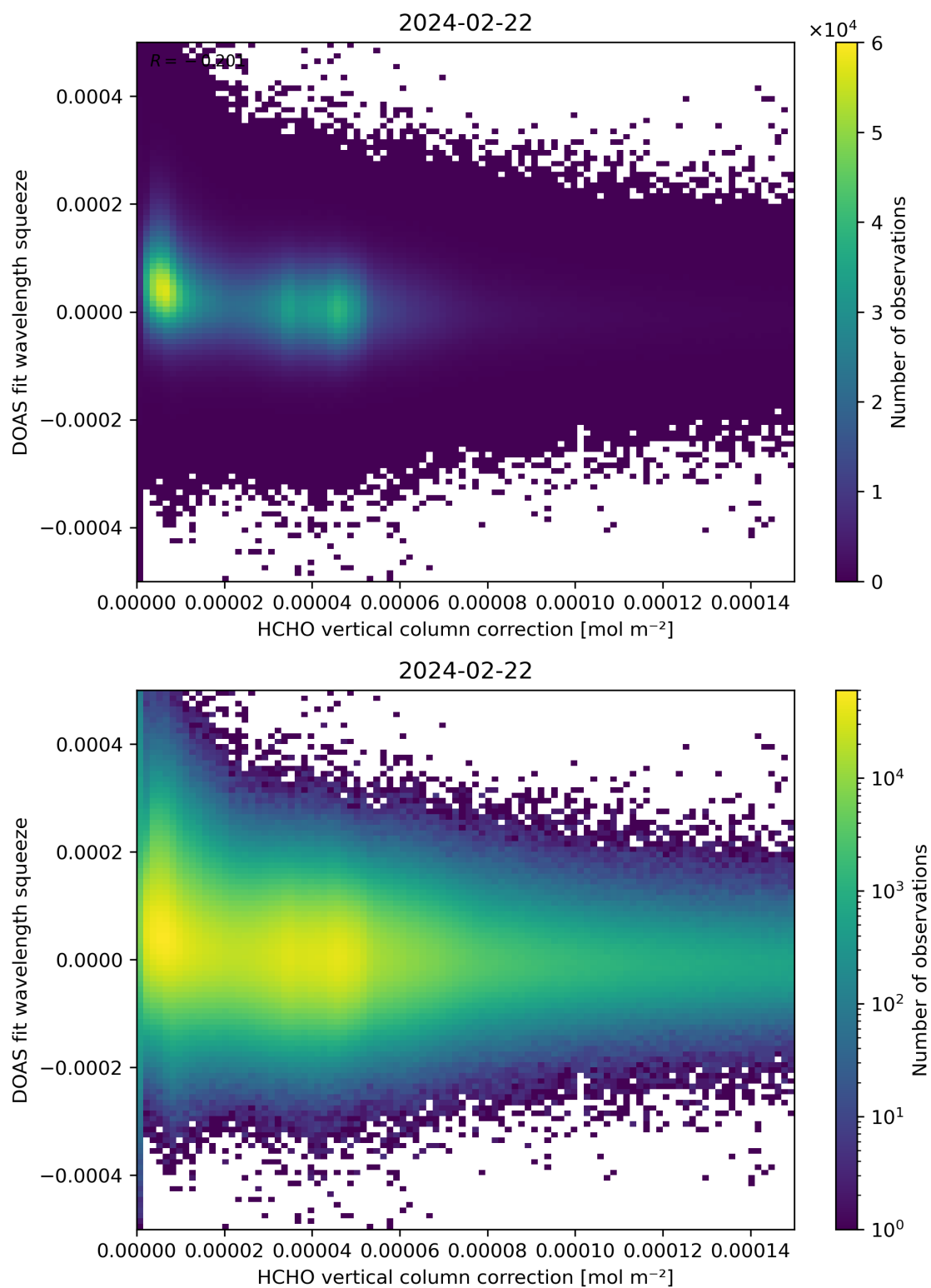
Figure 114: Scatter density plot of “HCHO vertical column correction” against “DOAS fit wavelength squeeze” for 2024-02-22 to 2024-02-23.
