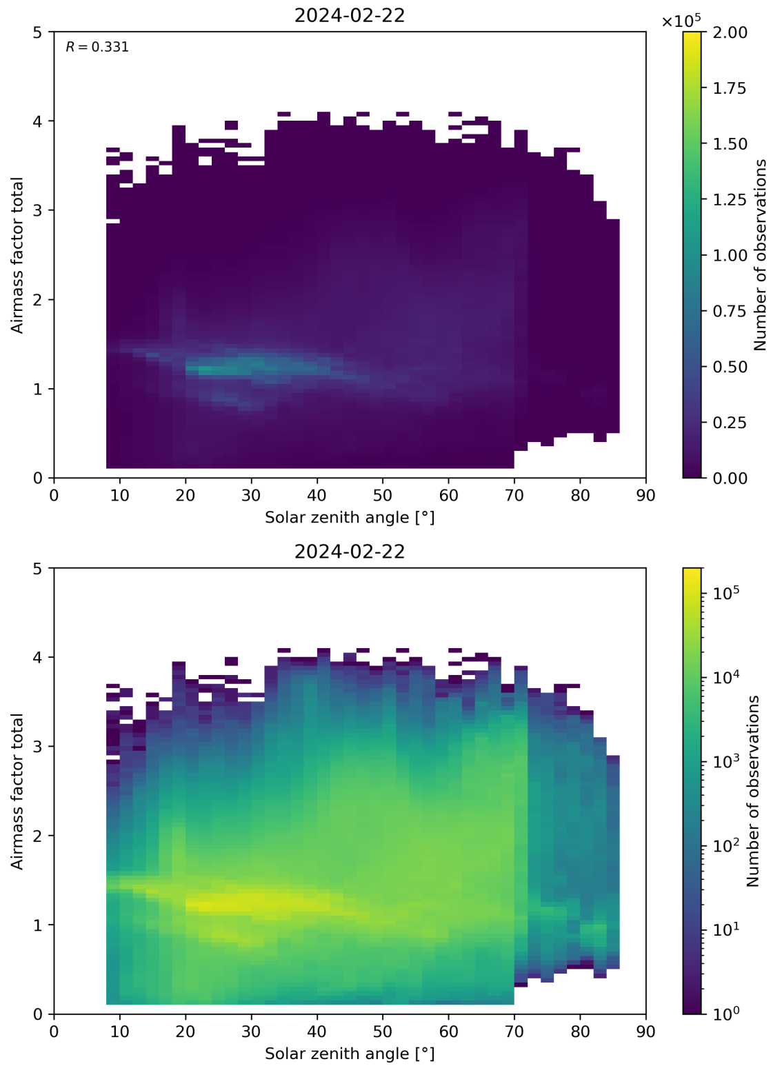
Figure 175: Scatter density plot of “Solar zenith angle” against “Airmass factor total” for 2024-02-22 to 2024-02-23.
