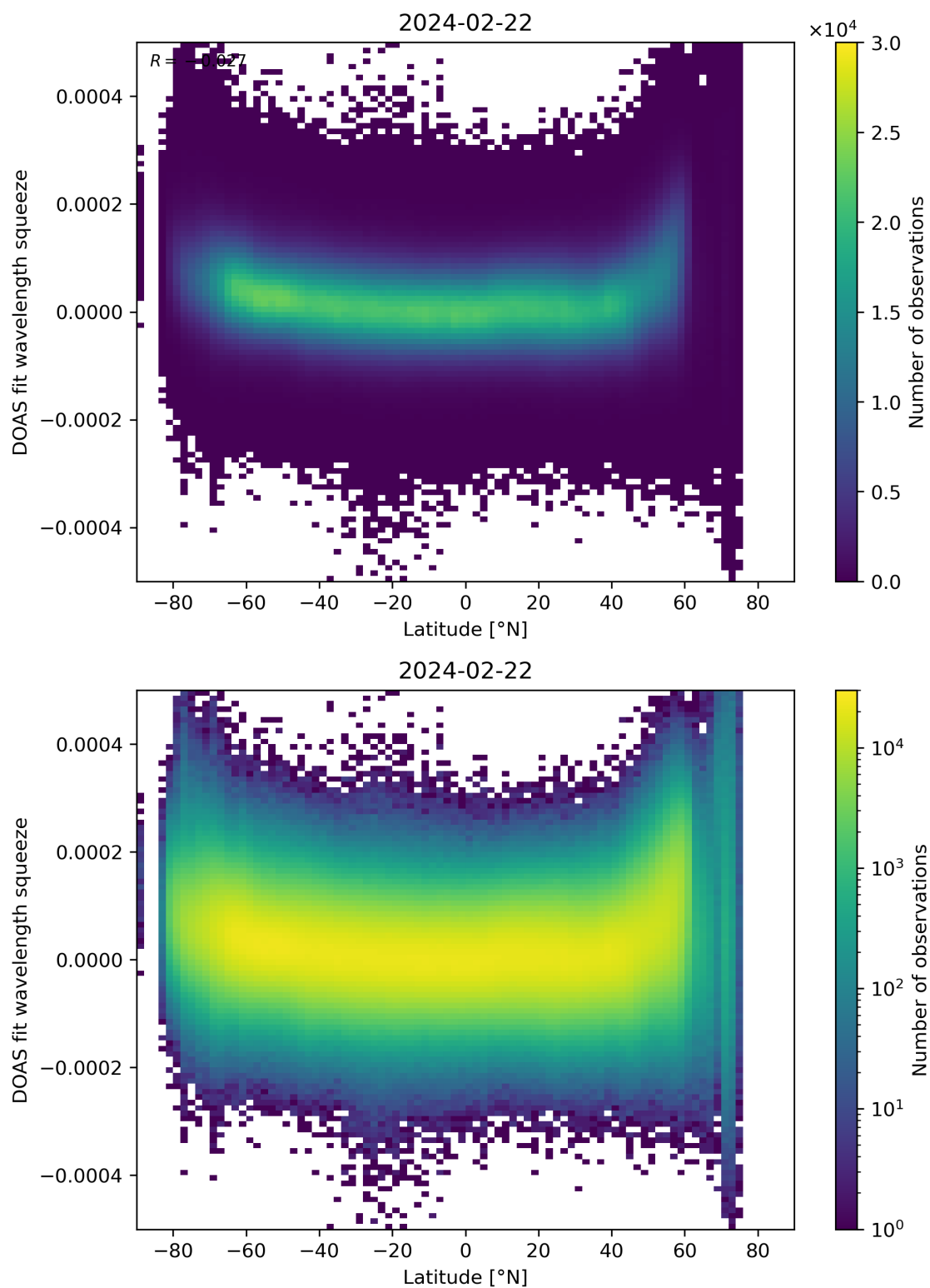
Figure 155: Scatter density plot of “Latitude” against “DOAS fit wavelength squeeze” for 2024-02-22 to 2024-02-23.
