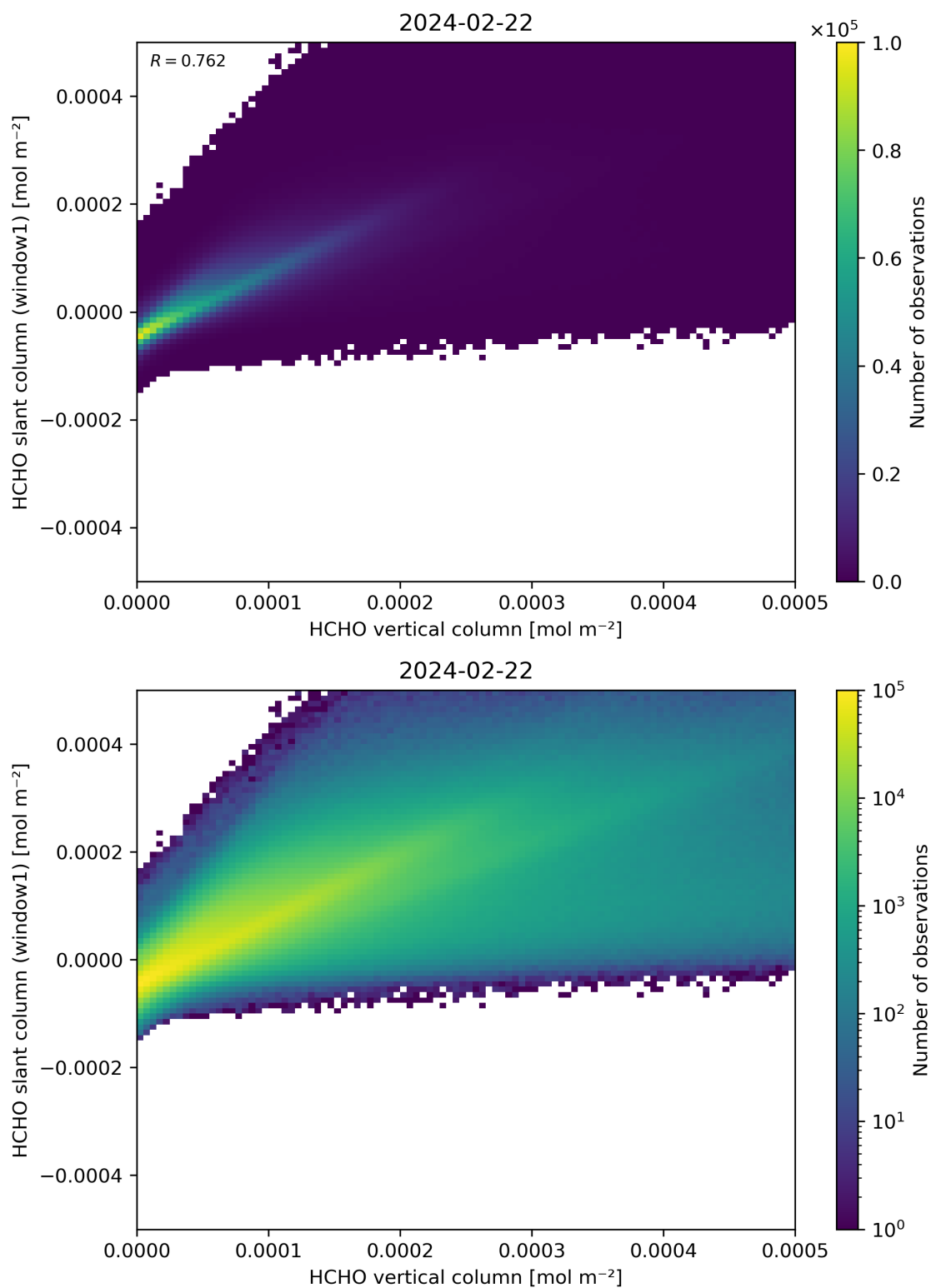
Figure 129: Scatter density plot of “HCHO vertical column” against “HCHO slant column (window1)” for 2024-02-22 to 2024-02-23.
