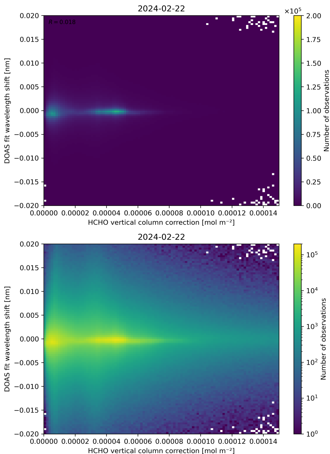
Figure 113: Scatter density plot of “HCHO vertical column correction” against “DOAS fit wavelength shift” for 2024-02-22 to 2024-02-23.
