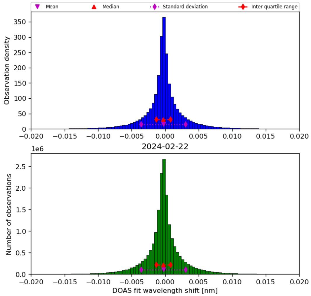
Figure 44: Histogram of “DOAS fit wavelength shift” for 2024-02-22 to 2024-02-23
