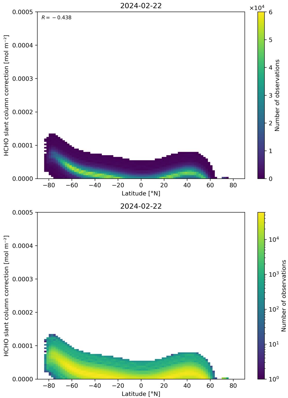
Figure 158: Scatter density plot of “Latitude” against “HCHO slant column correction” for 2024-02-22 to 2024-02-23.
