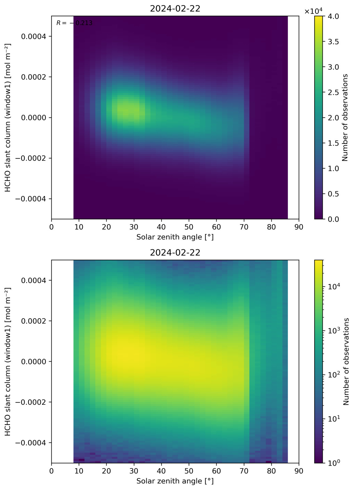
Figure 173: Scatter density plot of “Solar zenith angle” against “HCHO slant column (window1)” for 2024-02-22 to 2024-02-23.
