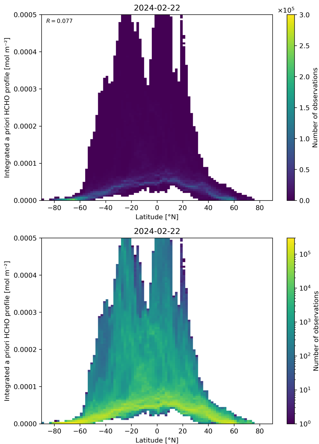
Figure 166: Scatter density plot of “Latitude” against “Integrated a priori HCHO profile” for 2024-02-22 to 2024-02-23.
