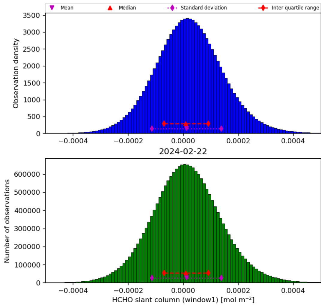
Figure 38: Histogram of “HCHO slant column (window1)” for 2024-02-22 to 2024-02-23
