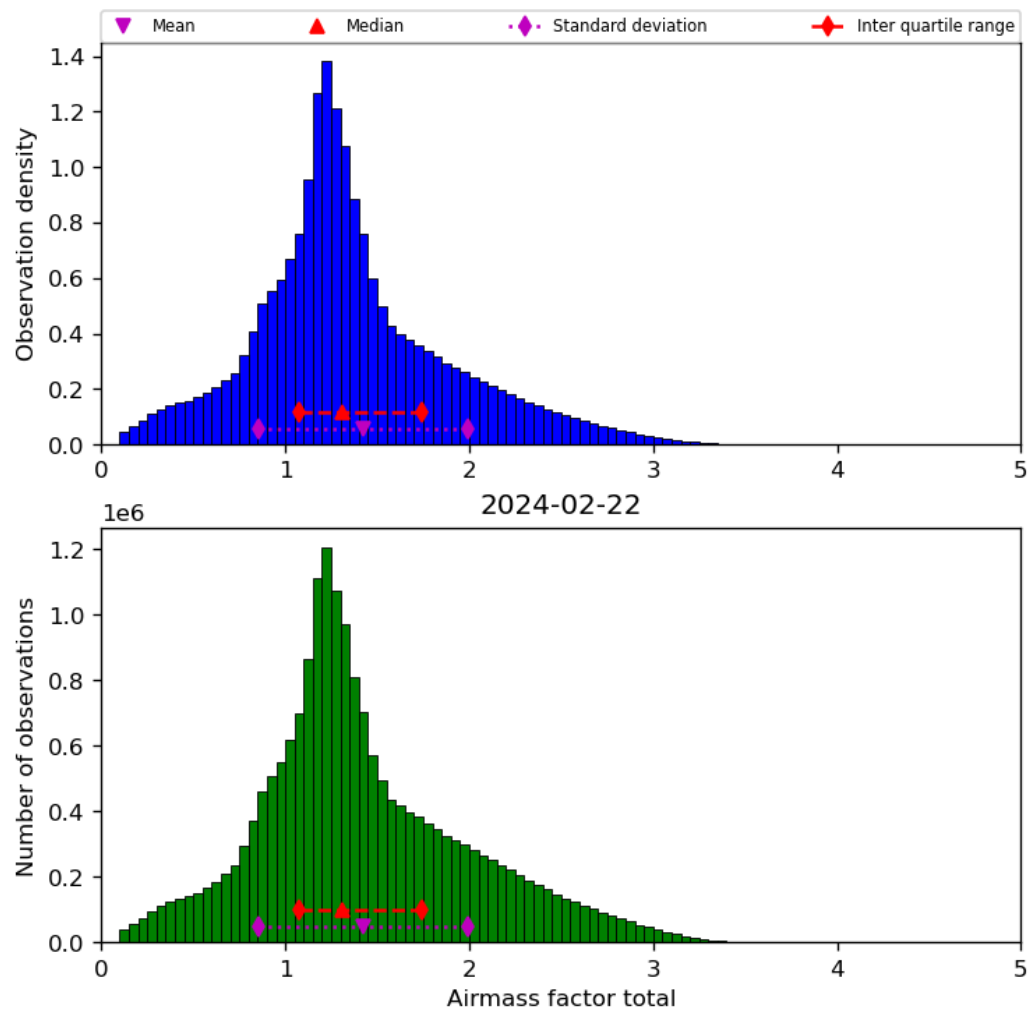
Figure 40: Histogram of “Airmass factor total” for 2024-02-22 to 2024-02-23
