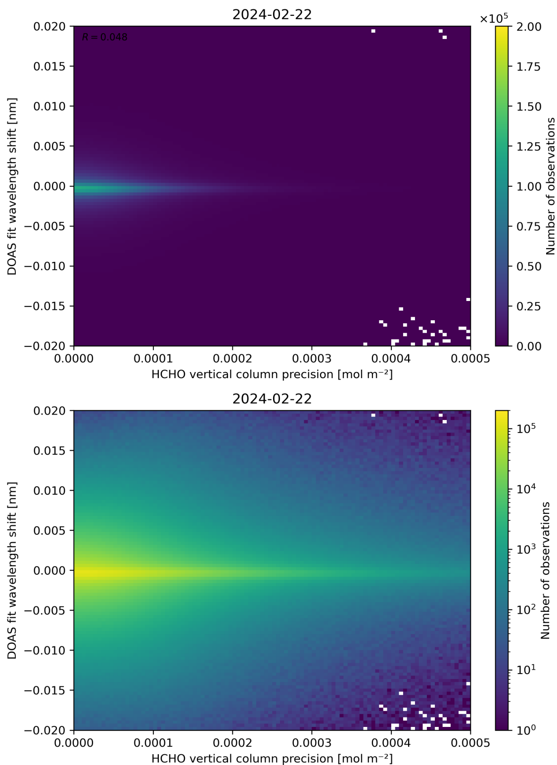
Figure 137: Scatter density plot of “HCHO vertical column precision” against “DOAS fit wavelength shift” for 2024-02-22 to 2024-02-23.
