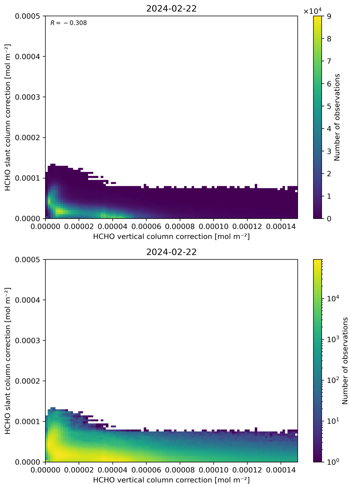
Figure 117: Scatter density plot of “HCHO vertical column correction” against “HCHO slant column correction” for 2024-02-22 to 2024-02-23.
