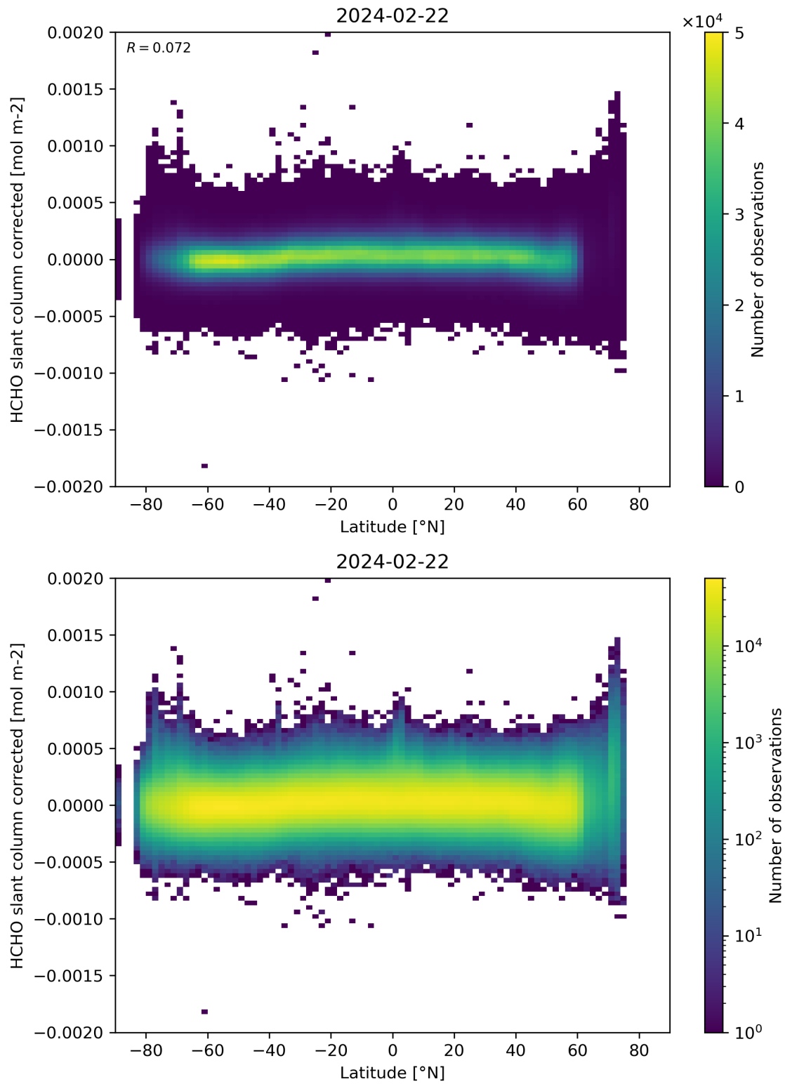
Figure 157: Scatter density plot of “Latitude” against “HCHO slant column corrected” for 2024-02-22 to 2024-02-23.
