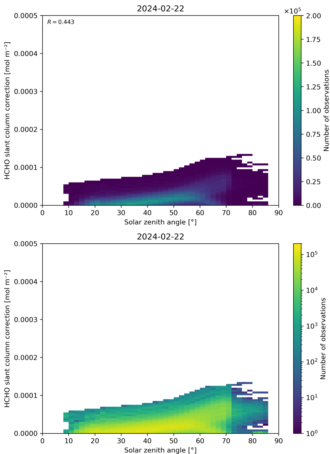
Figure 172: Scatter density plot of “Solar zenith angle” against “HCHO slant column correction” for 2024-02-22 to 2024-02-23.
