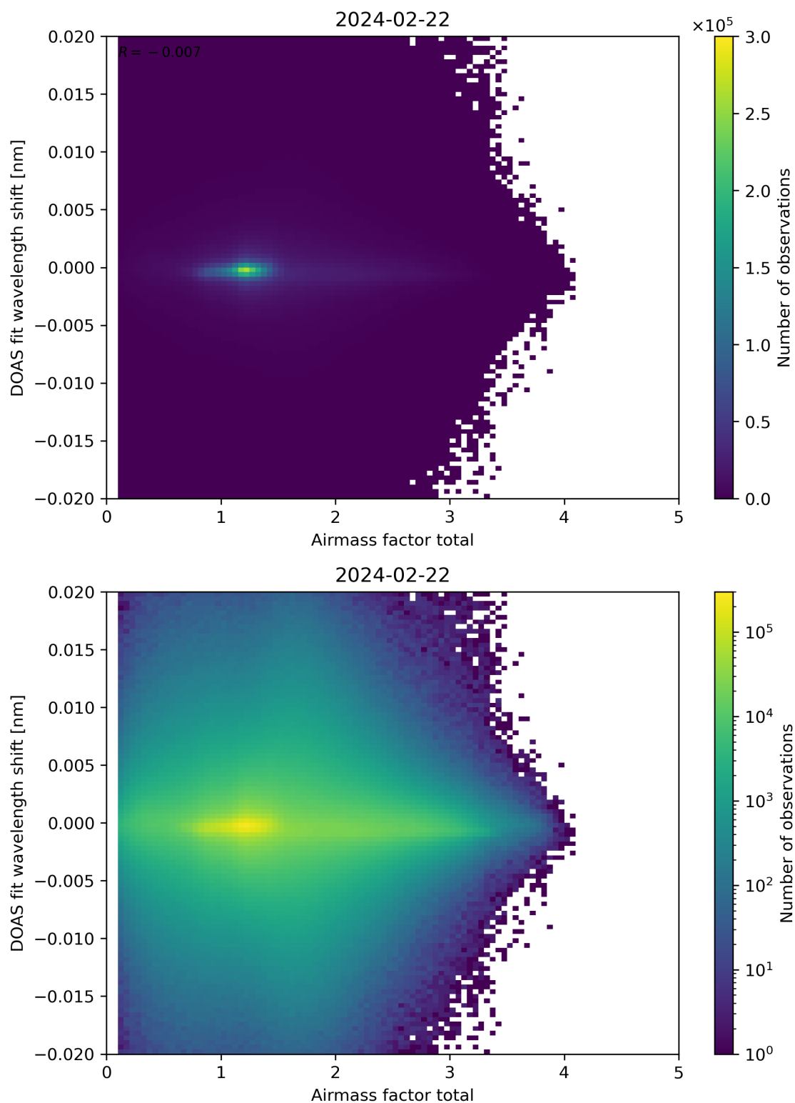
Figure 98: Scatter density plot of “Airmass factor total” against “DOAS fit wavelength shift” for 2024-02-22 to 2024-02-23.
