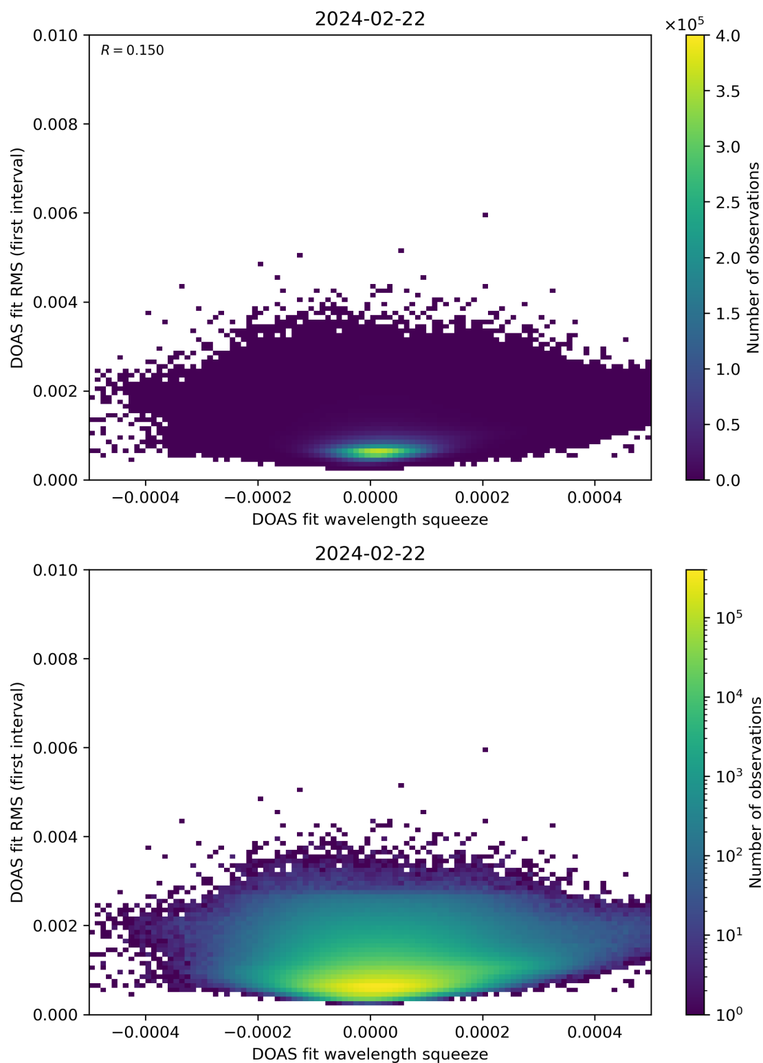
Figure 68: Scatter density plot of “DOAS fit wavelength squeeze” against “DOAS fit RMS (first interval)” for 2024-02-22 to 2024-02-23.
