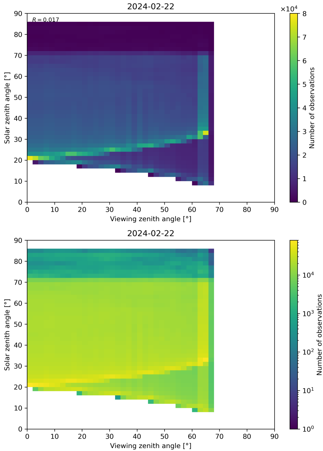
Figure 197: Scatter density plot of “Viewing zenith angle” against “Solar zenith angle” for 2024-02-22 to 2024-02-23.
