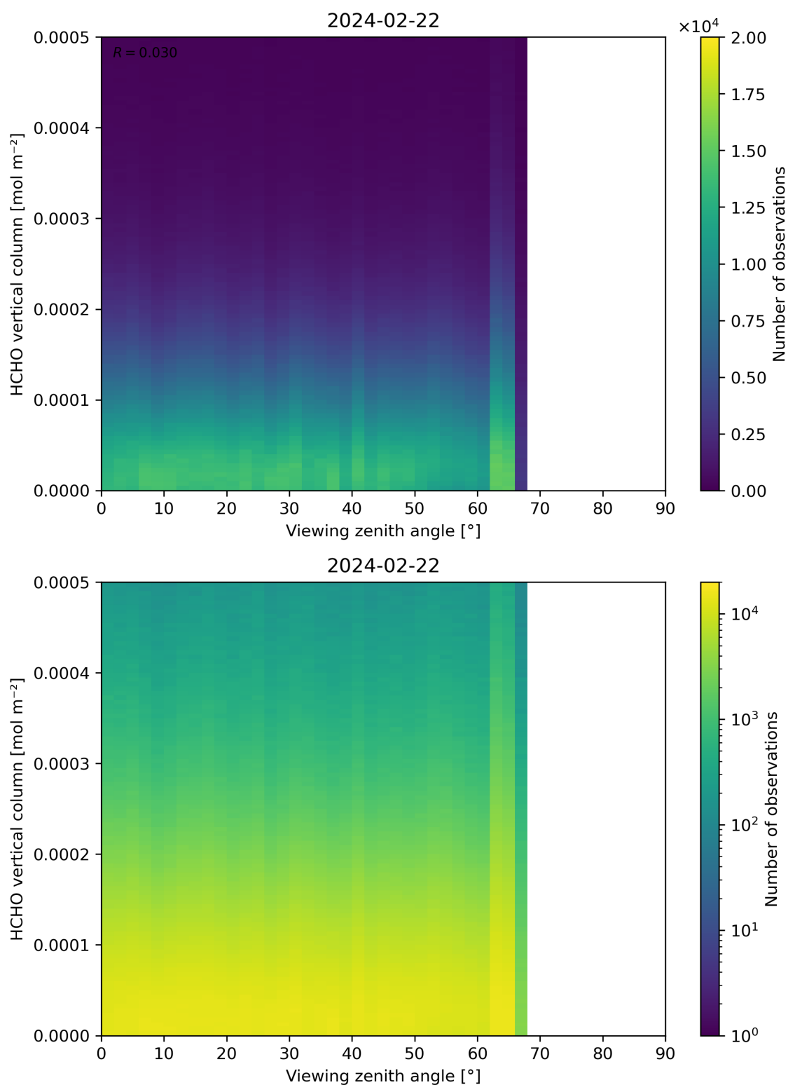
Figure 192: Scatter density plot of “Viewing zenith angle” against “HCHO vertical column” for 2024-02-22 to 2024-02-23.
