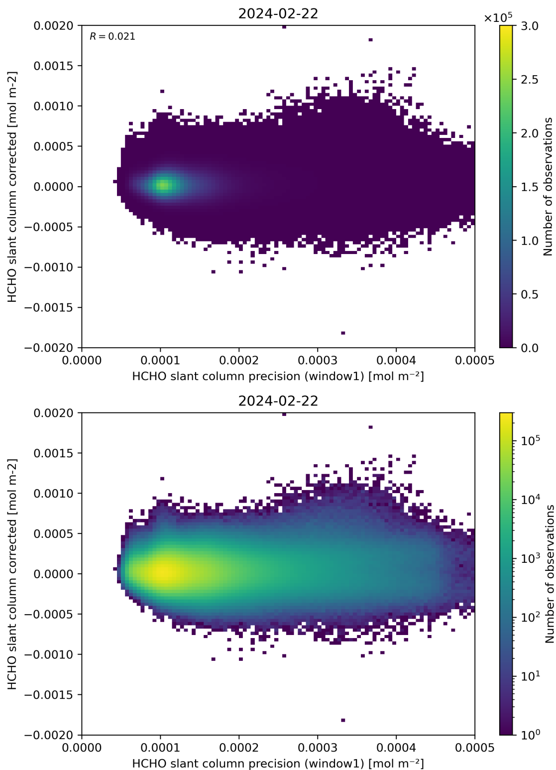
Figure 92: Scatter density plot of “HCHO slant column precision (window1)” against “HCHO slant column corrected” for 2024-02-22 to 2024-02-23.
