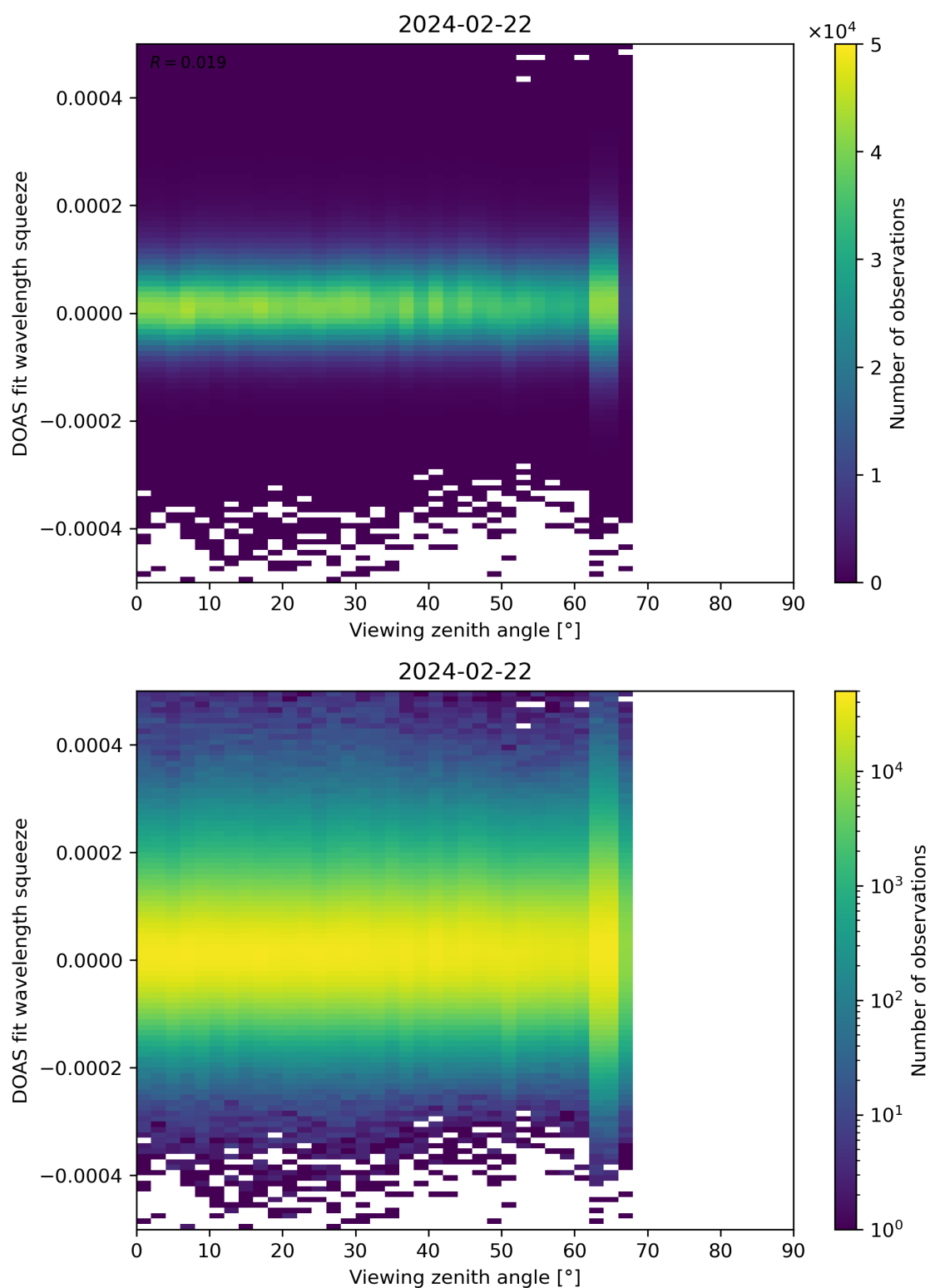
Figure 184: Scatter density plot of “Viewing zenith angle” against “DOAS fit wavelength squeeze” for 2024-02-22 to 2024-02-23.
