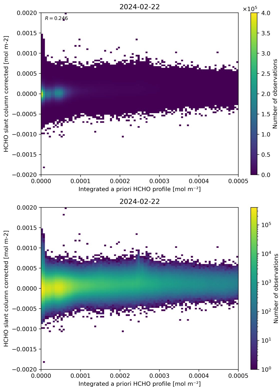
Figure 151: Scatter density plot of “Integrated a priori HCHO profile” against “HCHO slant column corrected” for 2024-02-22 to 2024-02-23.
