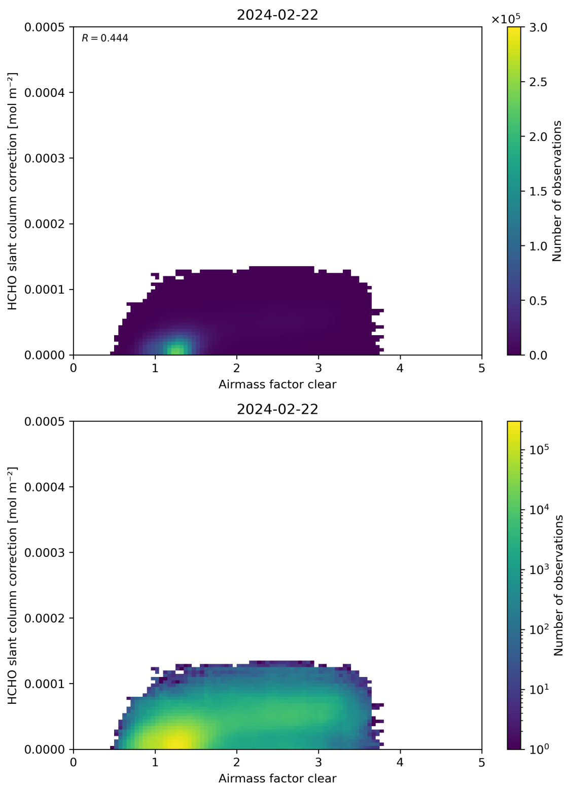
Figure 75: Scatter density plot of “Airmass factor clear” against “HCHO slant column correction” for 2024-02-22 to 2024-02-23.
