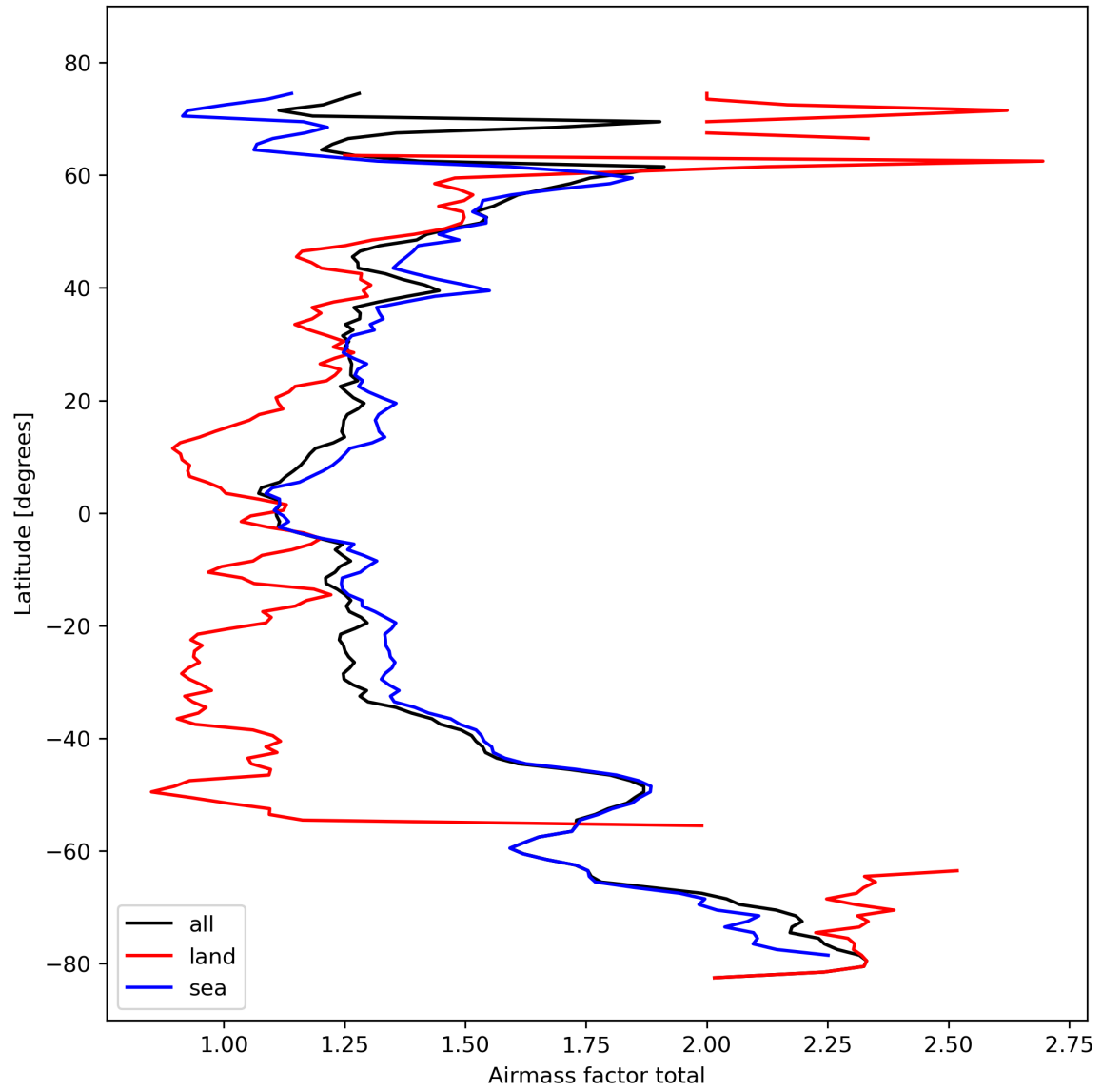
Figure 26: Zonal average of “Airmass factor total” for 2024-02-22 to 2024-02-23.
