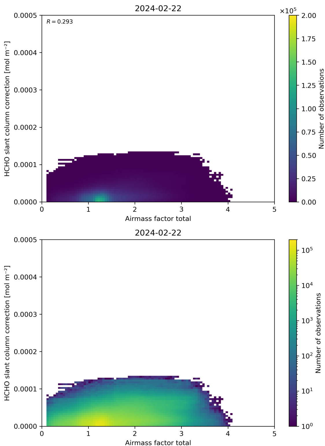
Figure 102: Scatter density plot of “Airmass factor total” against “HCHO slant column correction” for 2024-02-22 to 2024-02-23.
