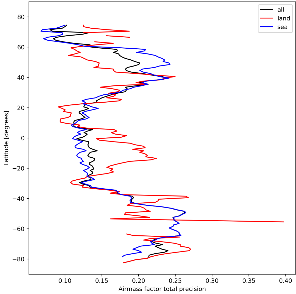
Figure 27: Zonal average of “Airmass factor total precision” for 2024-02-22 to 2024-02-23.
