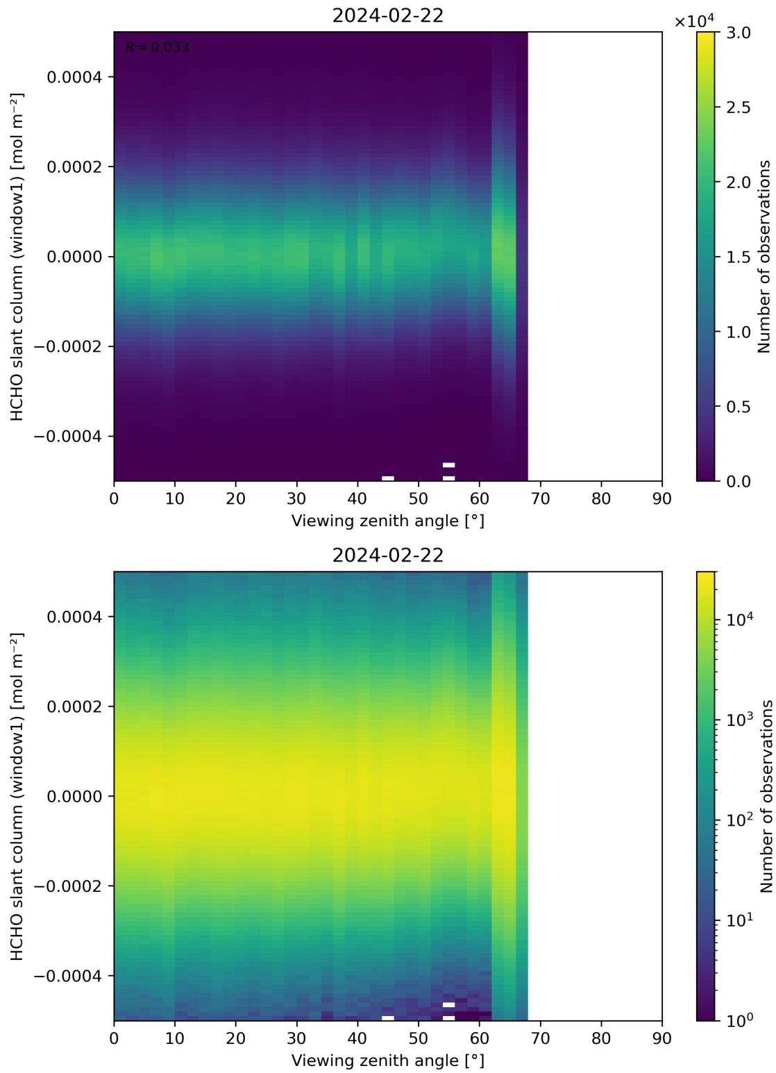
Figure 188: Scatter density plot of “Viewing zenith angle” against “HCHO slant column (window1)” for 2024-02-22 to 2024-02-23.
