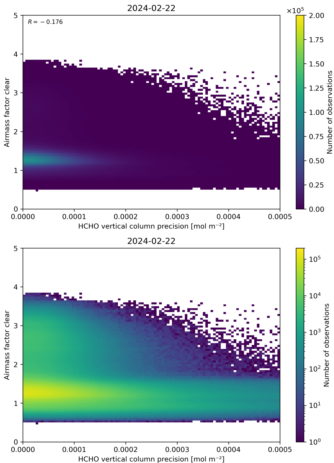
Figure 139: Scatter density plot of “HCHO vertical column precision” against “Airmass factor clear” for 2024-02-22 to 2024-02-23.
