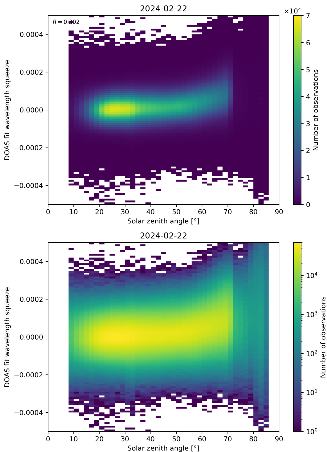
Figure 169: Scatter density plot of “Solar zenith angle” against “DOAS fit wavelength squeeze” for 2024-02-22 to 2024-02-23.
