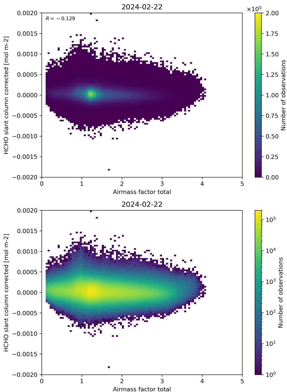
Figure 101: Scatter density plot of “Airmass factor total” against “HCHO slant column corrected” for 2024-02-22 to 2024-02-23.
