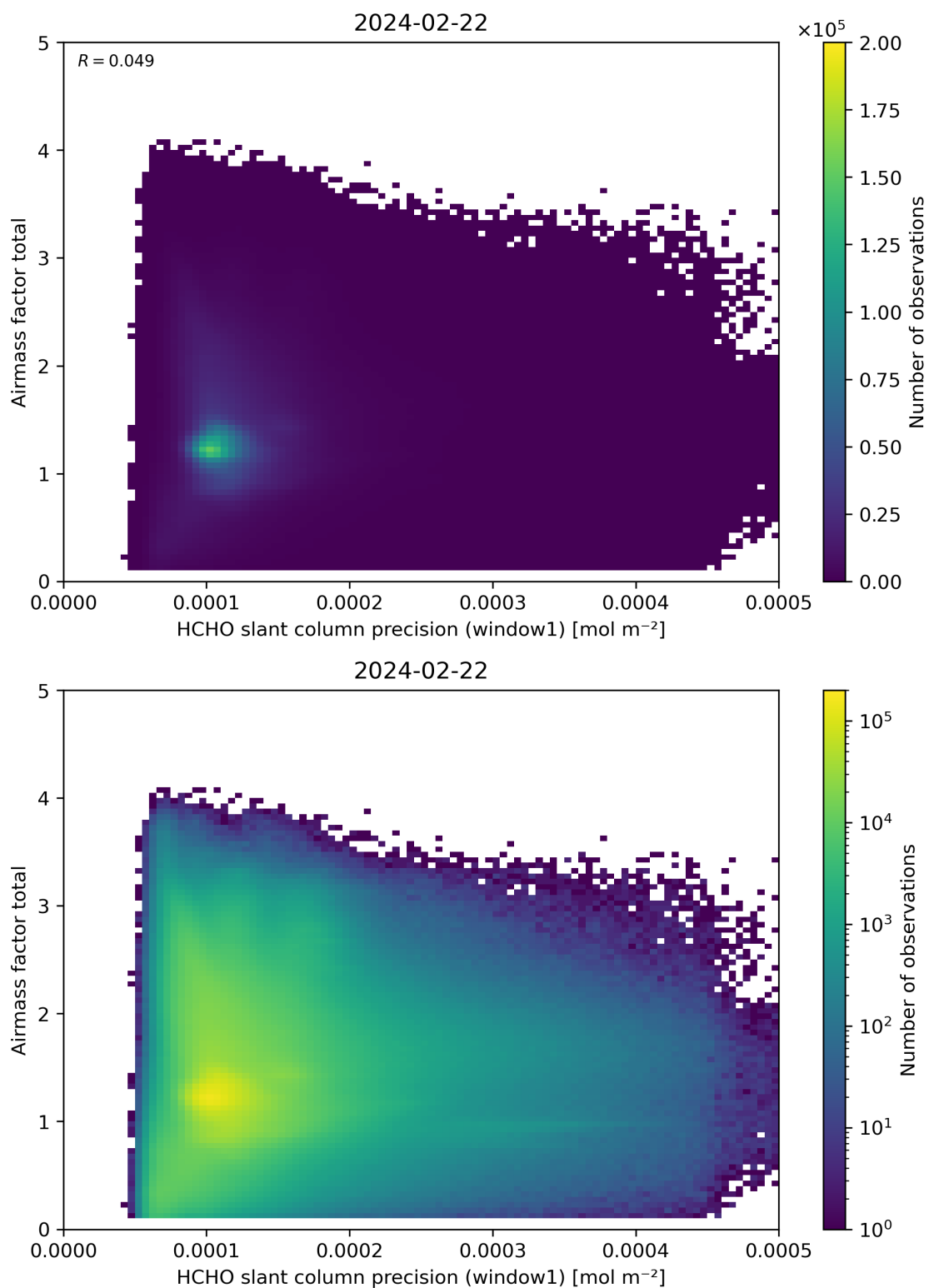
Figure 94: Scatter density plot of “HCHO slant column precision (window1)” against “Airmass factor total” for 2024-02-22 to 2024-02-23.
