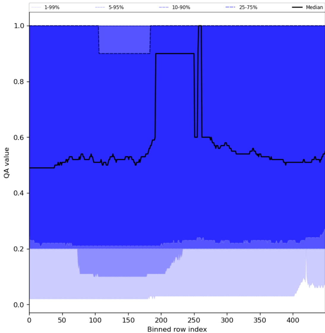
Figure 48: Along track statistics of “QA value” for 2024-02-22 to 2024-02-23
