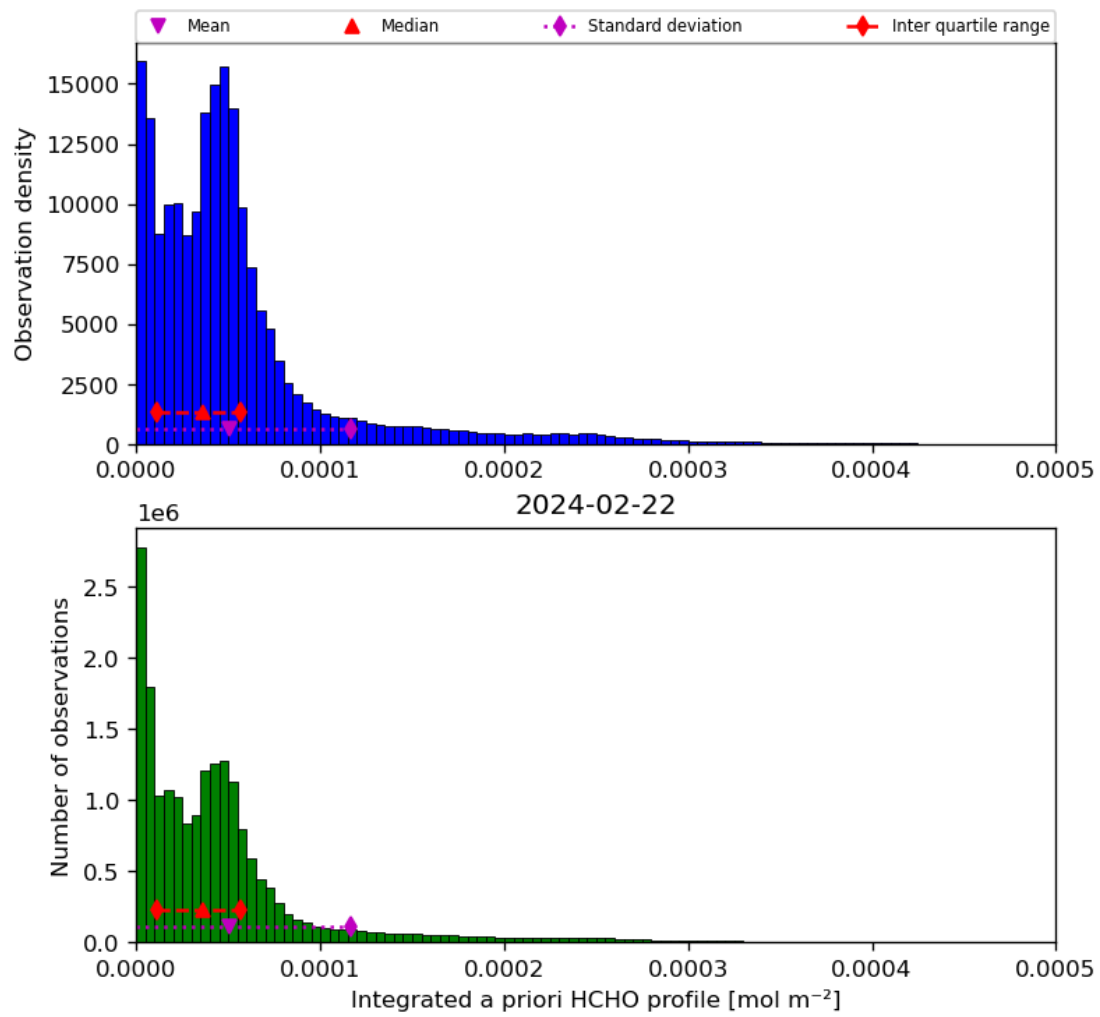
Figure 43: Histogram of “Integrated a priori HCHO profile” for 2024-02-22 to 2024-02-23
