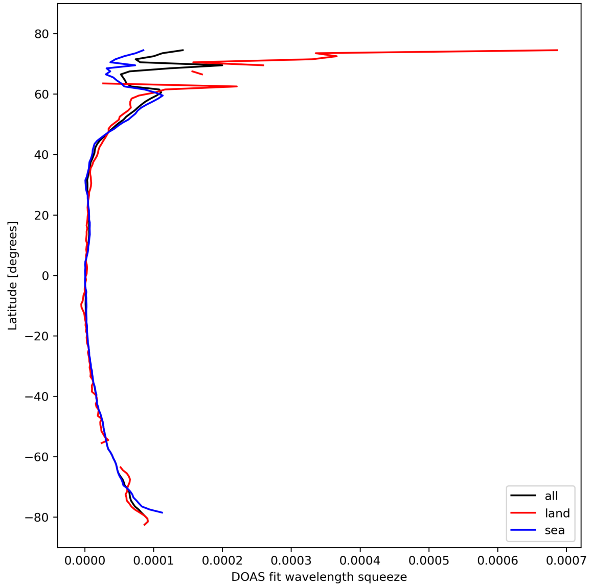
Figure 31: Zonal average of “DOAS fit wavelength squeeze” for 2024-02-22 to 2024-02-23.
