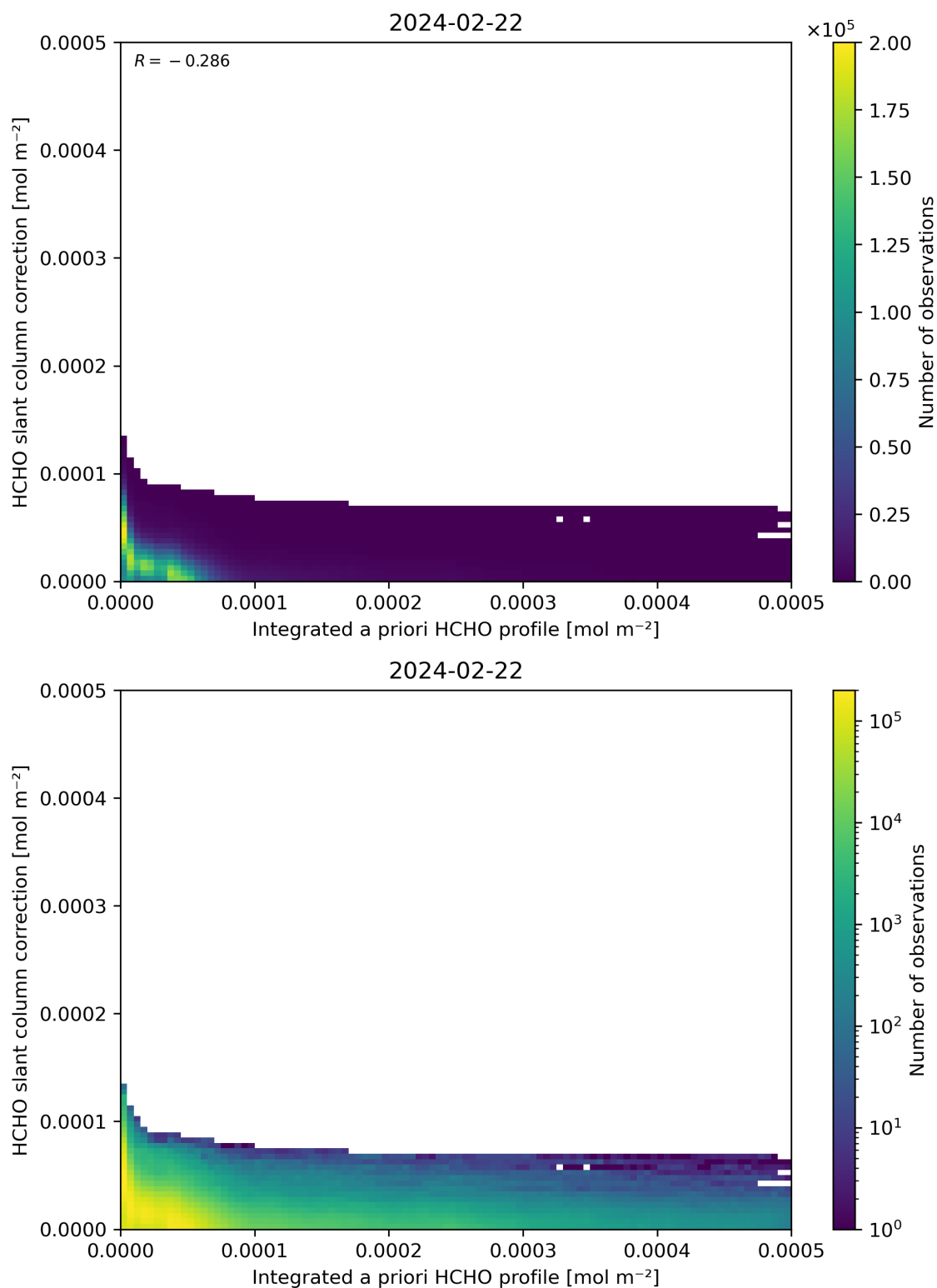
Figure 152: Scatter density plot of “Integrated a priori HCHO profile” against “HCHO slant column correction” for 2024-02-22 to 2024-02-23.
