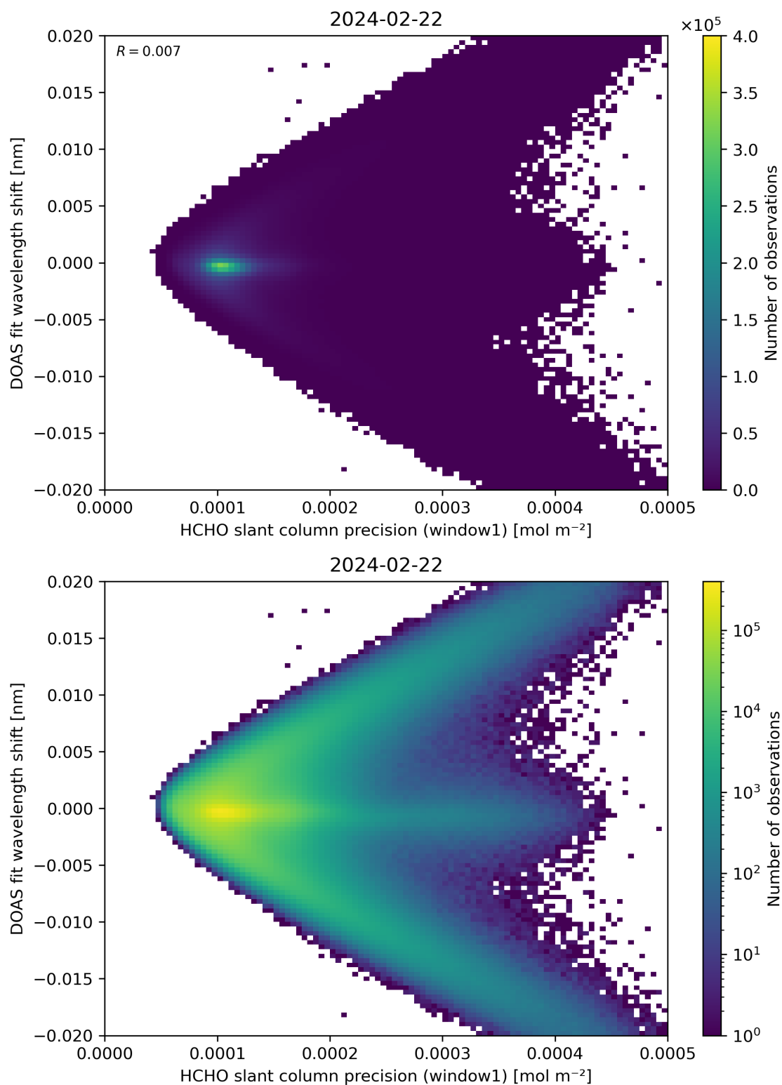
Figure 89: Scatter density plot of “HCHO slant column precision (window1)” against “DOAS fit wavelength shift” for 2024-02-22 to 2024-02-23.
