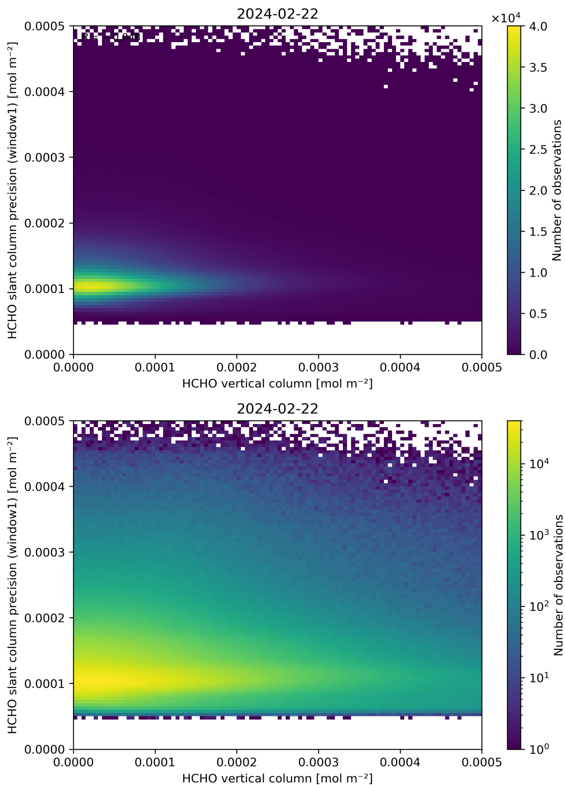
Figure 130: Scatter density plot of “HCHO vertical column” against “HCHO slant column precision (window1)” for 2024-02-22 to 2024-02-23.
