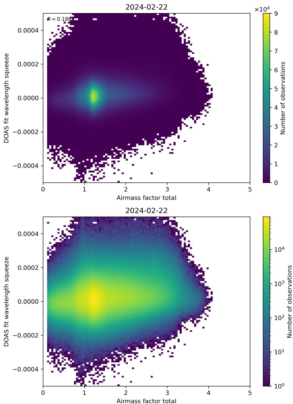
Figure 99: Scatter density plot of “Airmass factor total” against “DOAS fit wavelength squeeze” for 2024-02-22 to 2024-02-23.
