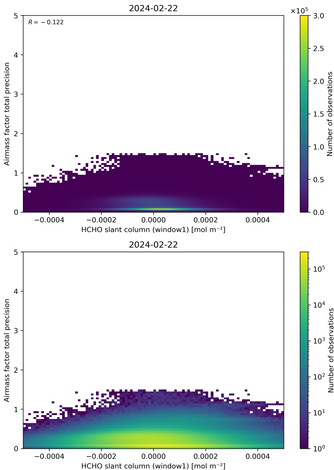
Figure 86: Scatter density plot of “HCHO slant column (window1)” against “Airmass factor total precision” for 2024-02-22 to 2024-02-23.
