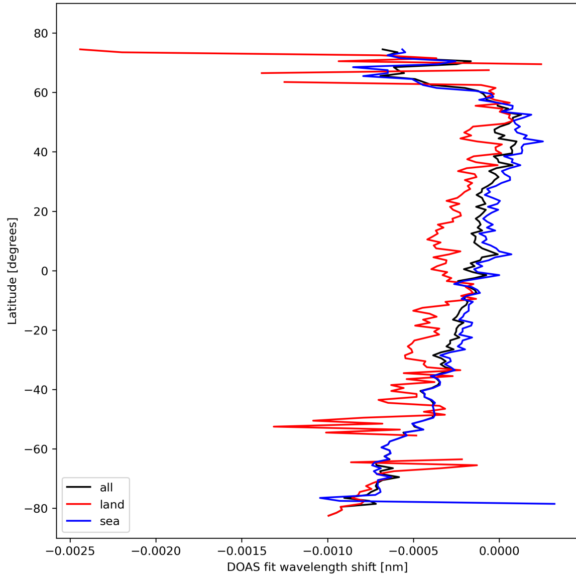
Figure 30: Zonal average of “DOAS fit wavelength shift” for 2024-02-22 to 2024-02-23.
