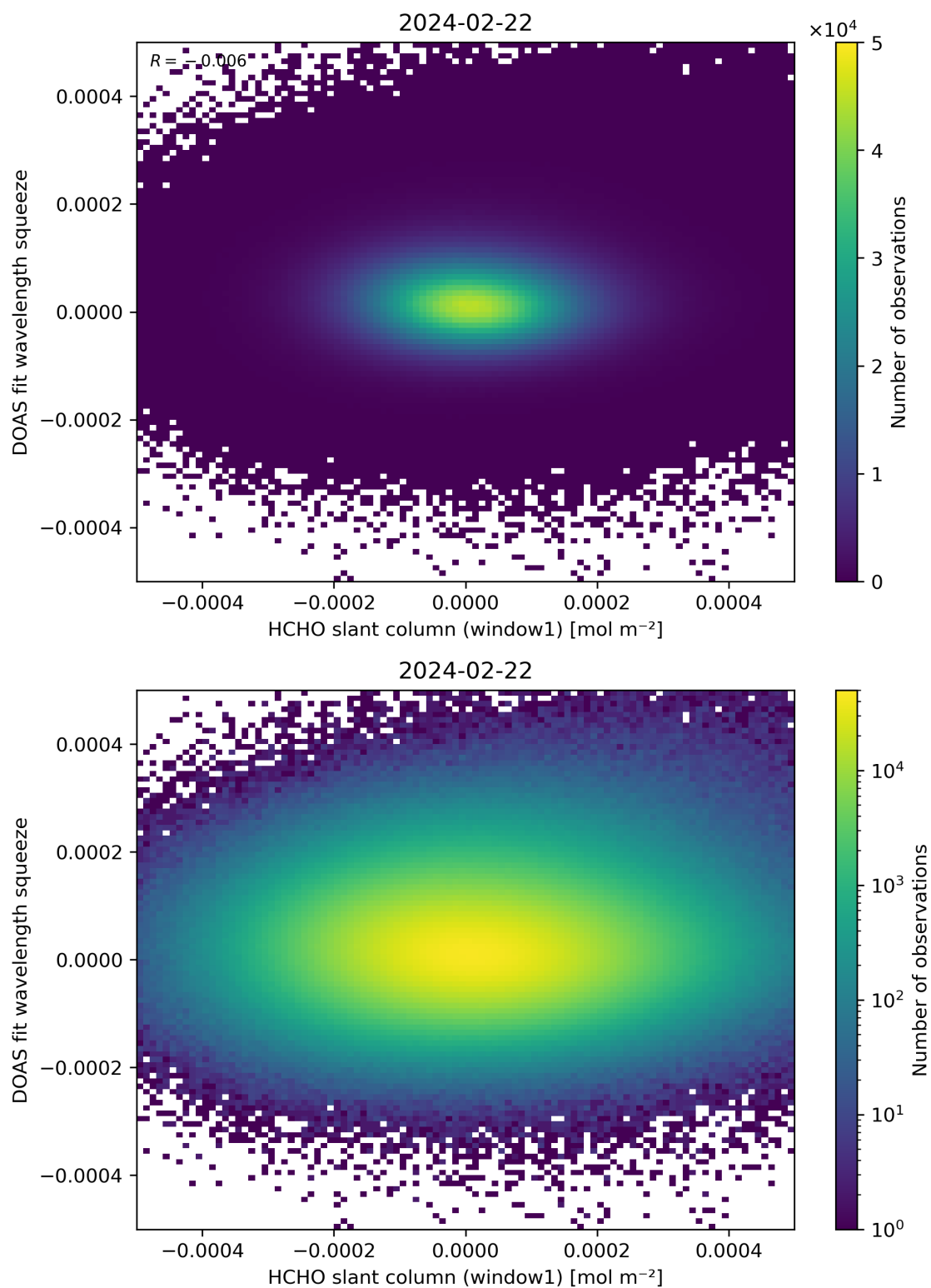
Figure 80: Scatter density plot of “HCHO slant column (window1)” against “DOAS fit wavelength squeeze” for 2024-02-22 to 2024-02-23.
