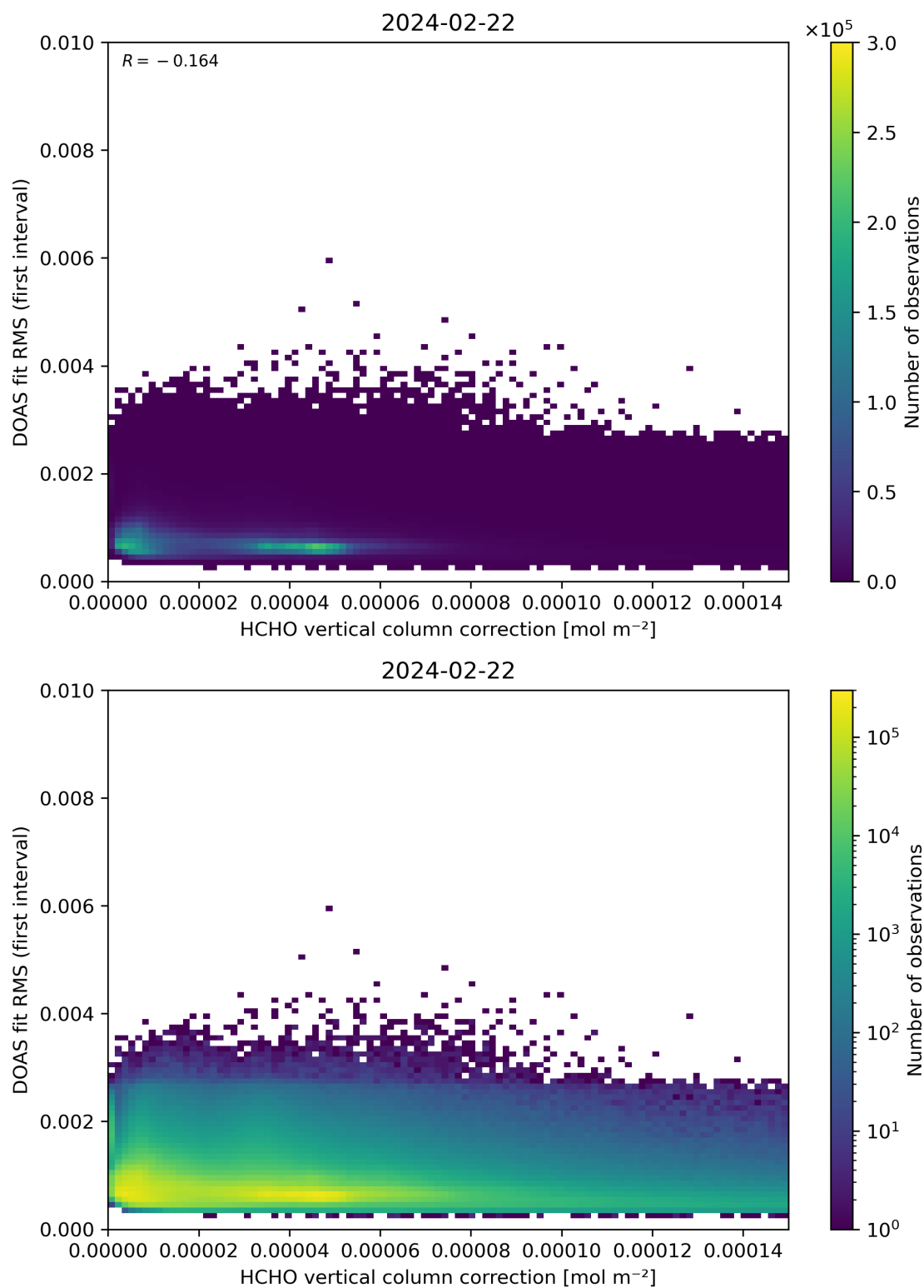
Figure 112: Scatter density plot of “HCHO vertical column correction” against “DOAS fit RMS (first interval)” for 2024-02-22 to 2024-02-23.
