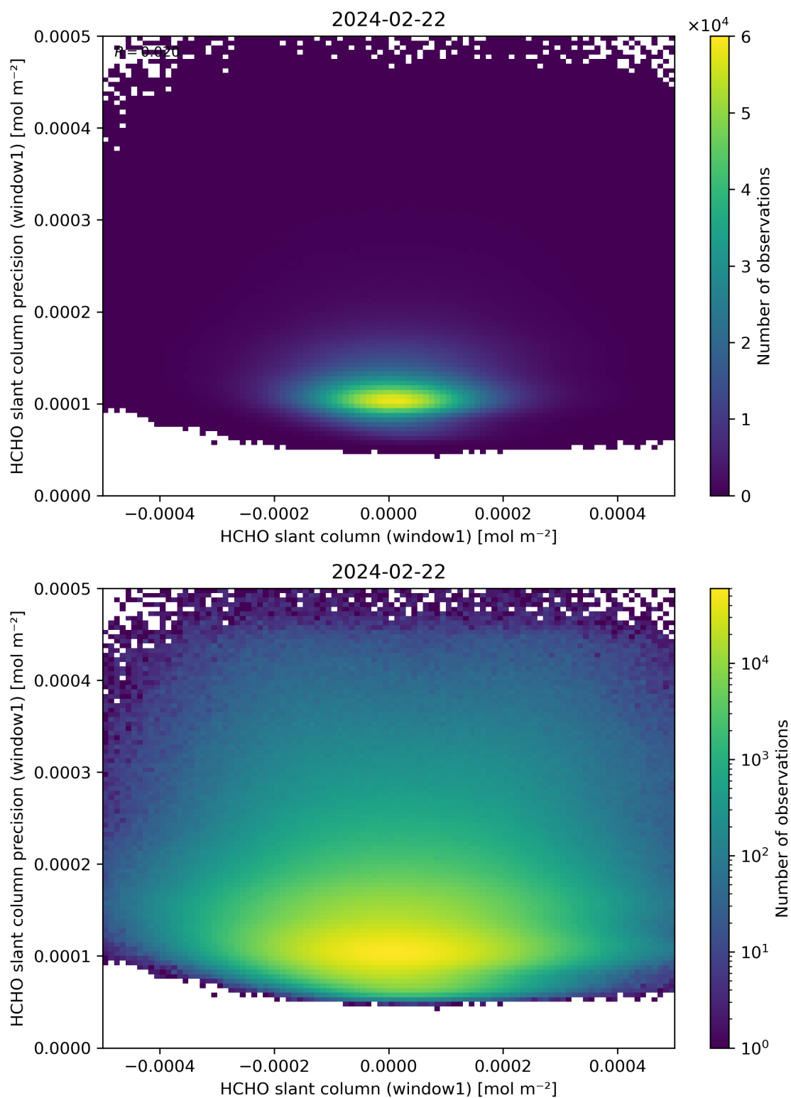
Figure 84: Scatter density plot of “HCHO slant column (window1)” against “HCHO slant column precision (window1)” for 2024-02-22 to 2024-02-23.
