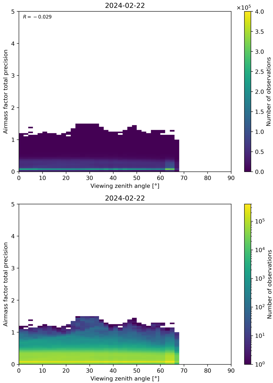
Figure 191: Scatter density plot of “Viewing zenith angle” against “Airmass factor total precision” for 2024-02-22 to 2024-02-23.
