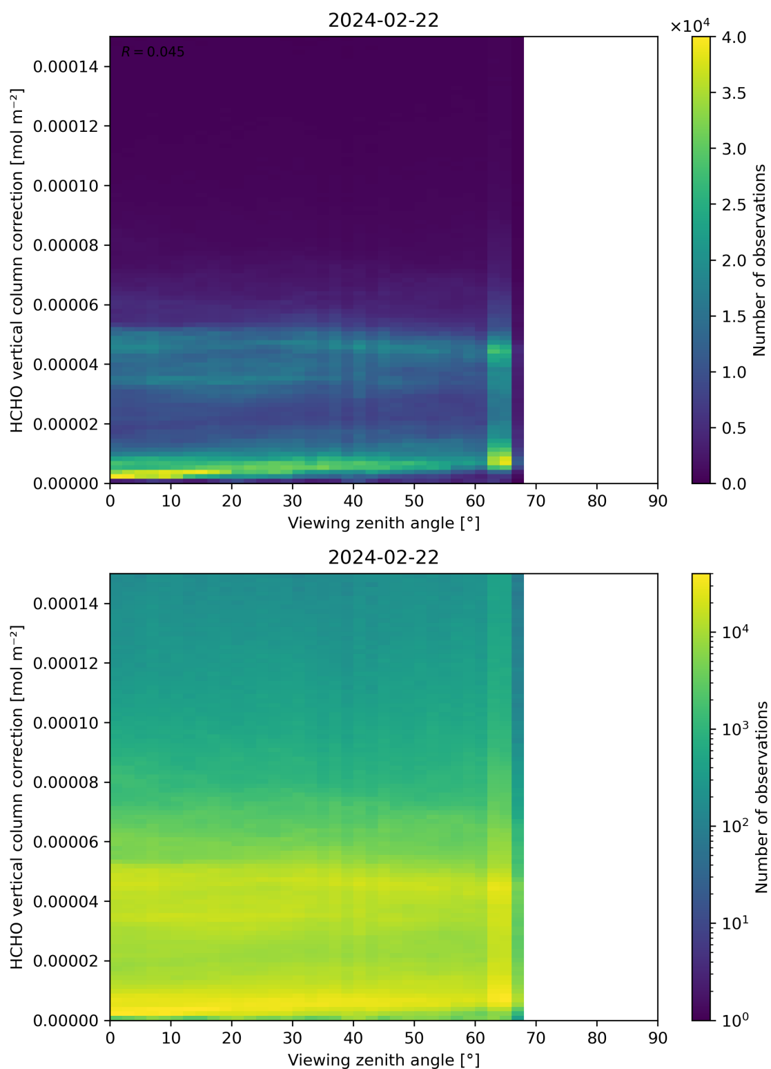
Figure 193: Scatter density plot of “Viewing zenith angle” against “HCHO vertical column correction” for 2024-02-22 to 2024-02-23.
