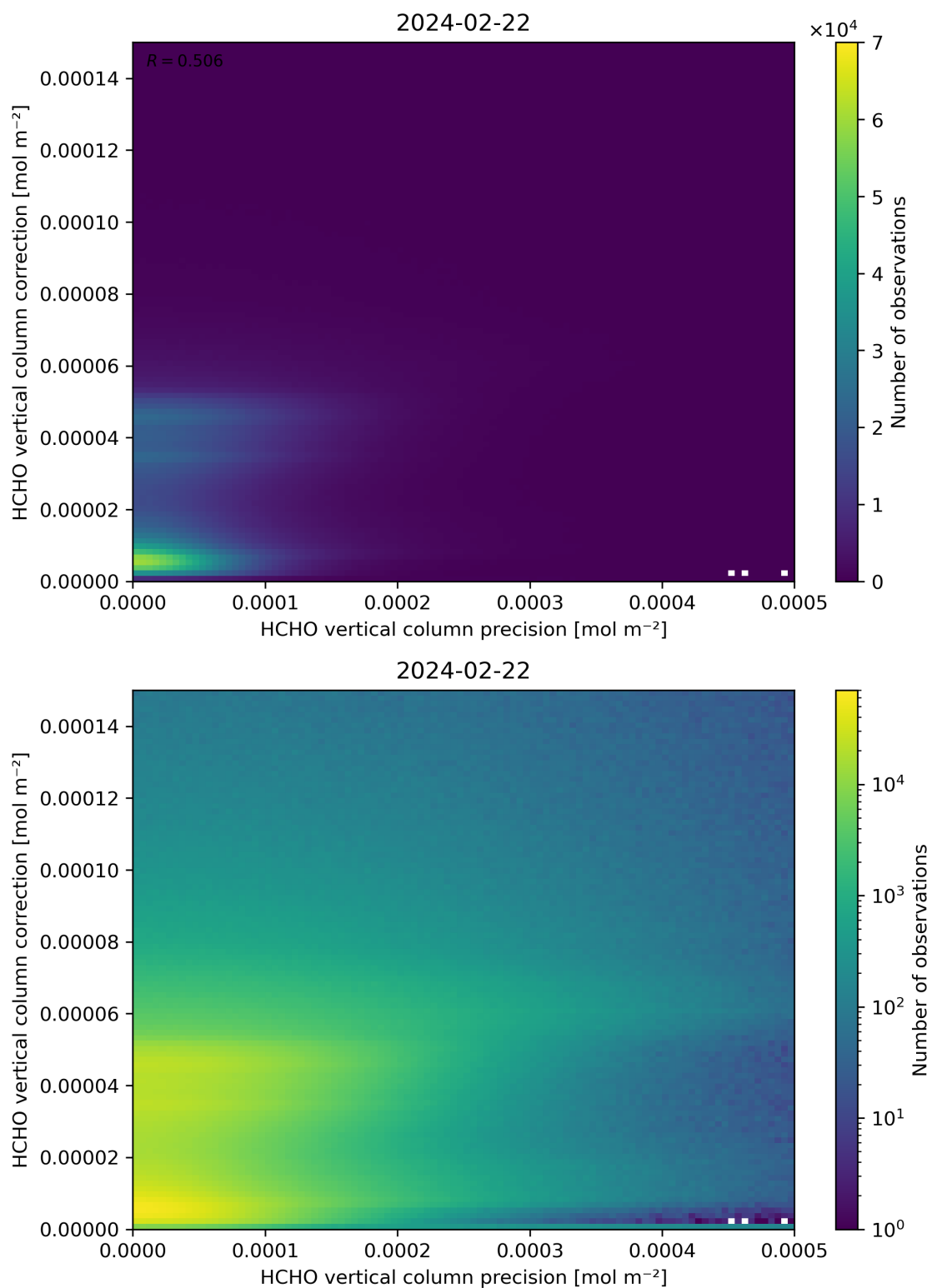
Figure 146: Scatter density plot of “HCHO vertical column precision” against “HCHO vertical column correction” for 2024-02-22 to 2024-02-23.
