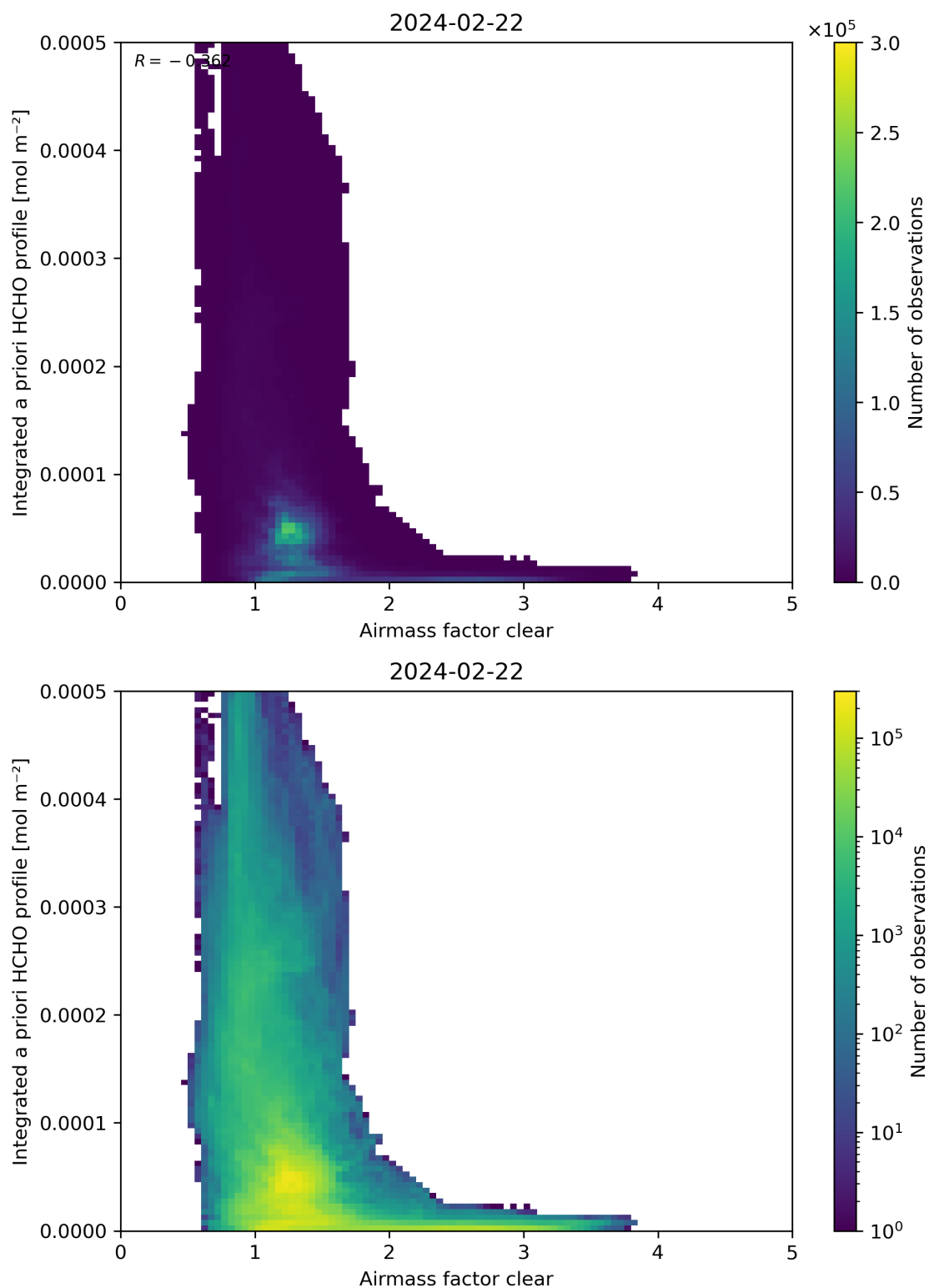
Figure 76: Scatter density plot of “Airmass factor clear” against “Integrated a priori HCHO profile” for 2024-02-22 to 2024-02-23.
