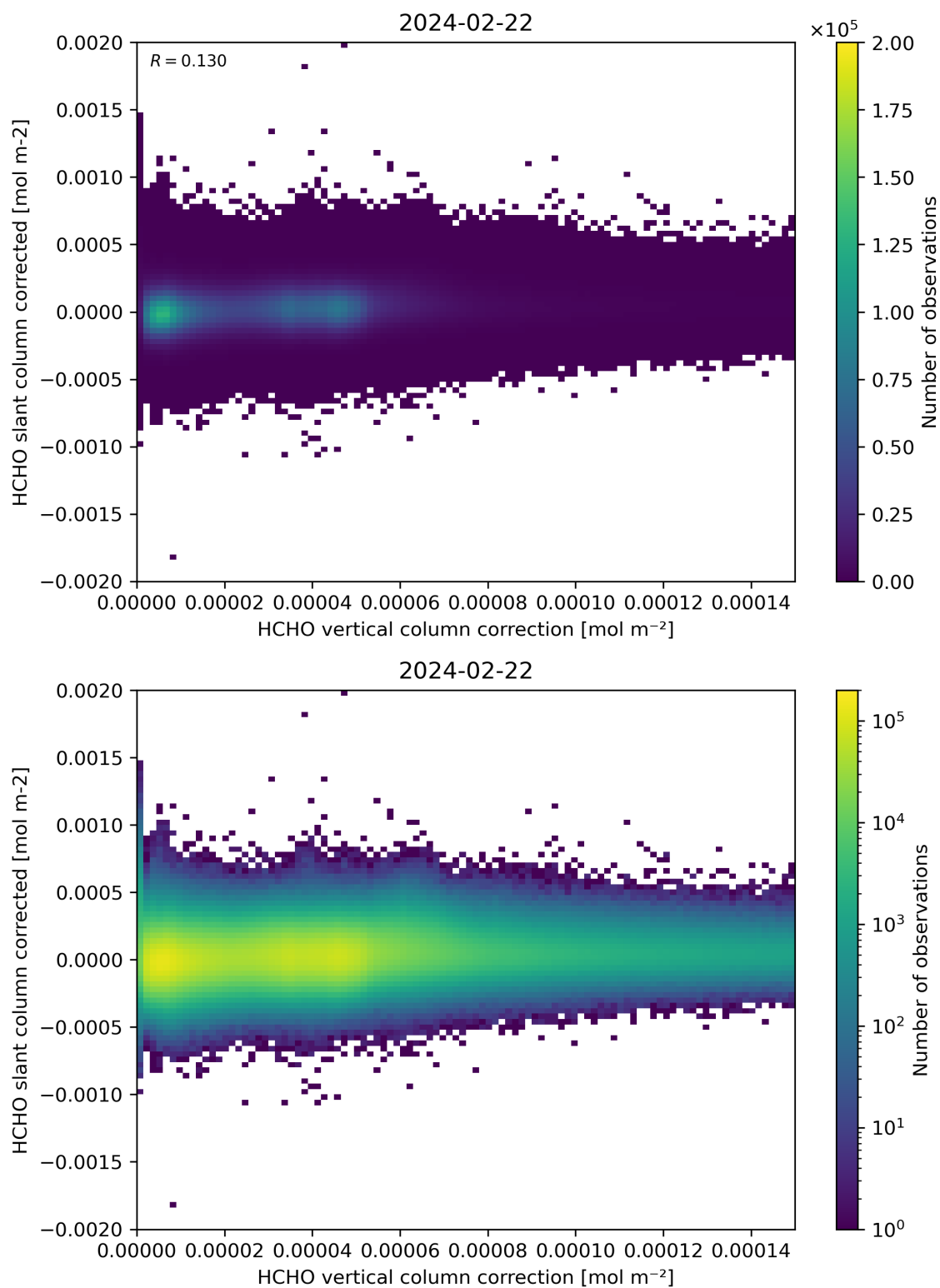
Figure 116: Scatter density plot of “HCHO vertical column correction” against “HCHO slant column corrected” for 2024-02-22 to 2024-02-23.
