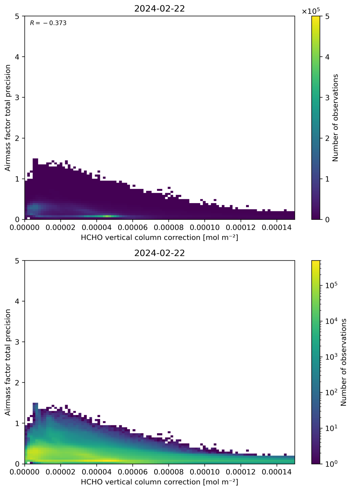
Figure 121: Scatter density plot of “HCHO vertical column correction” against “Airmass factor total precision” for 2024-02-22 to 2024-02-23.
