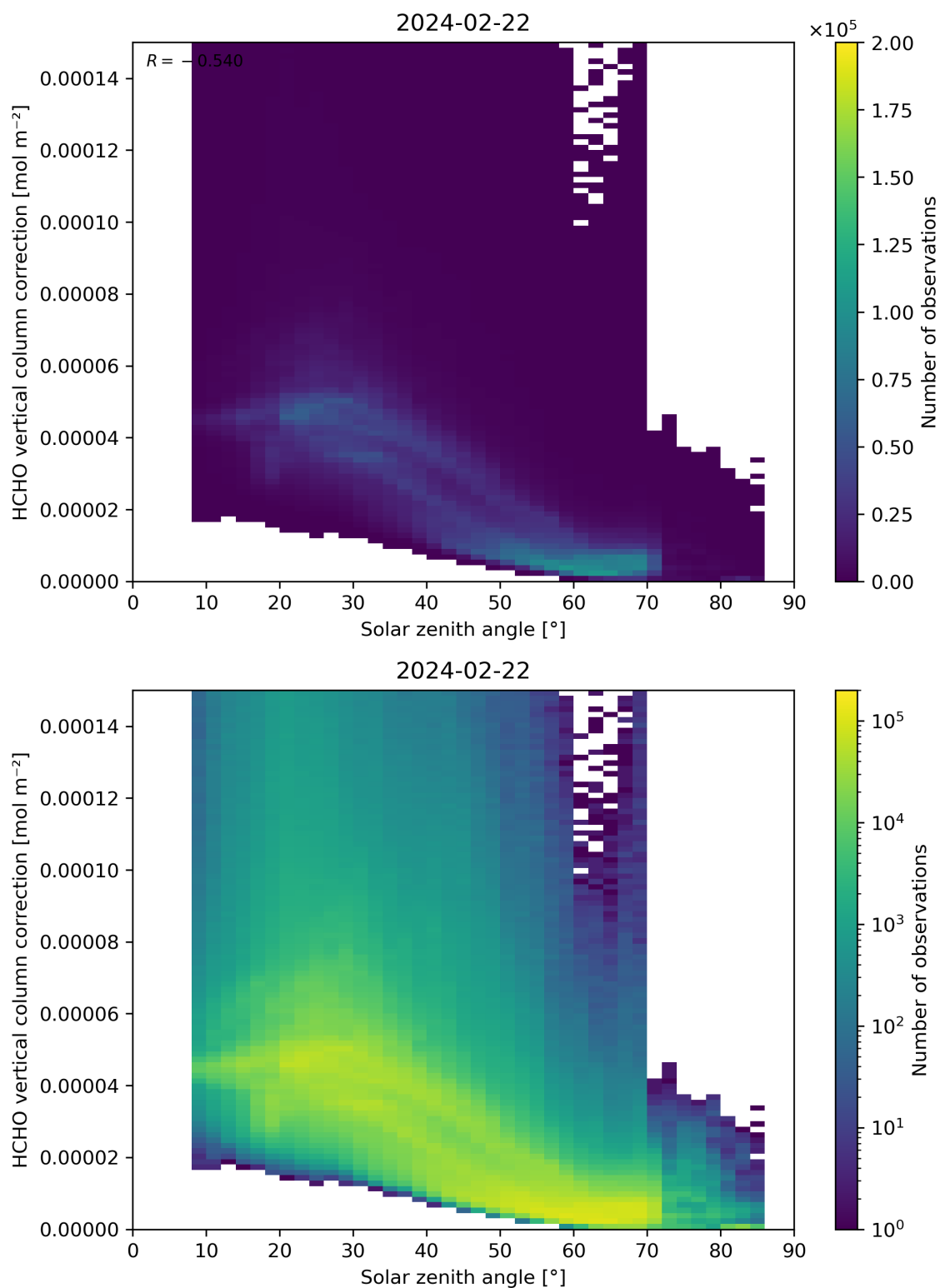
Figure 178: Scatter density plot of “Solar zenith angle” against “HCHO vertical column correction” for 2024-02-22 to 2024-02-23.
