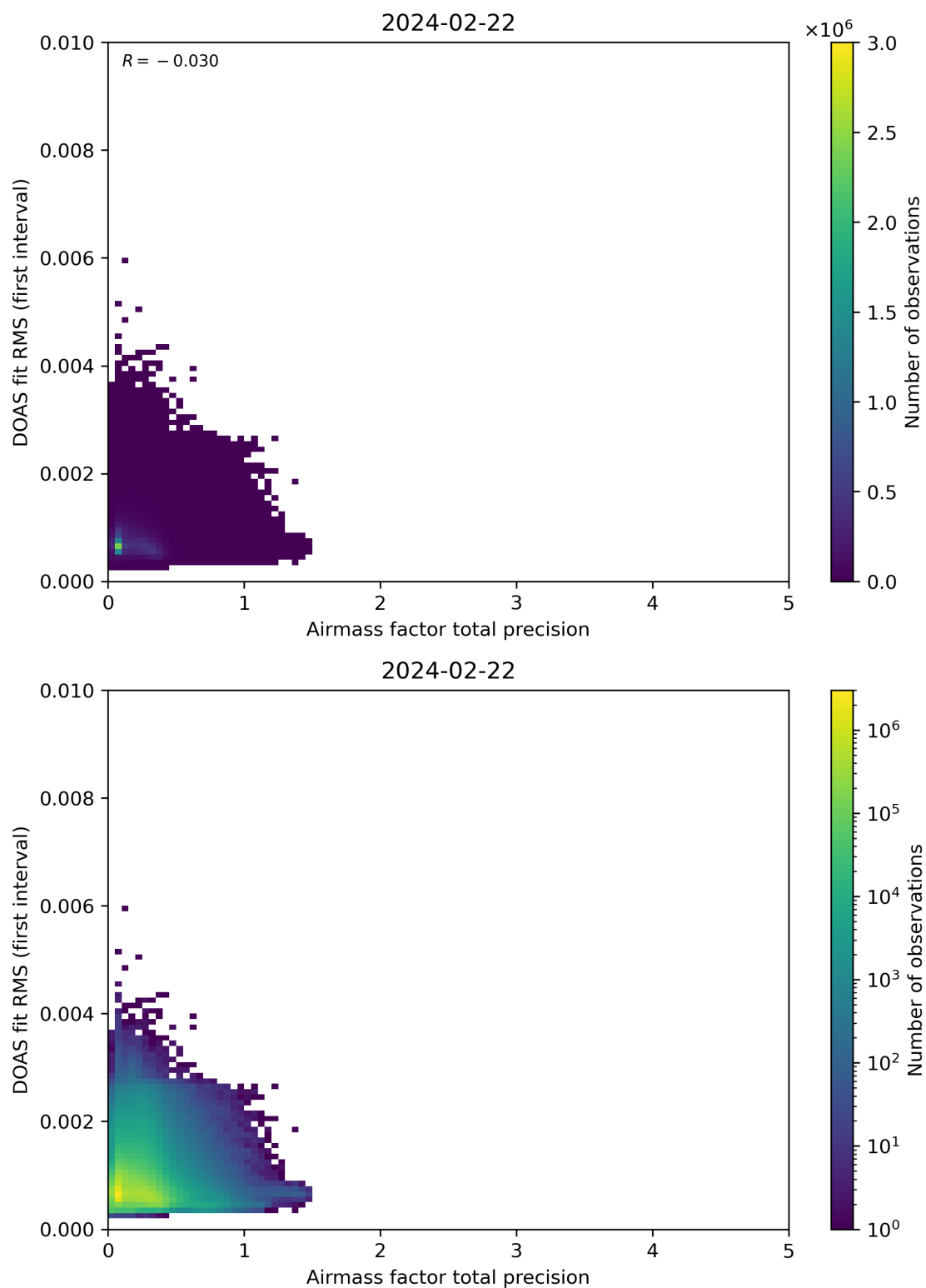
Figure 105: Scatter density plot of “Airmass factor total precision” against “DOAS fit RMS (first interval)” for 2024-02-22 to 2024-02-23.
