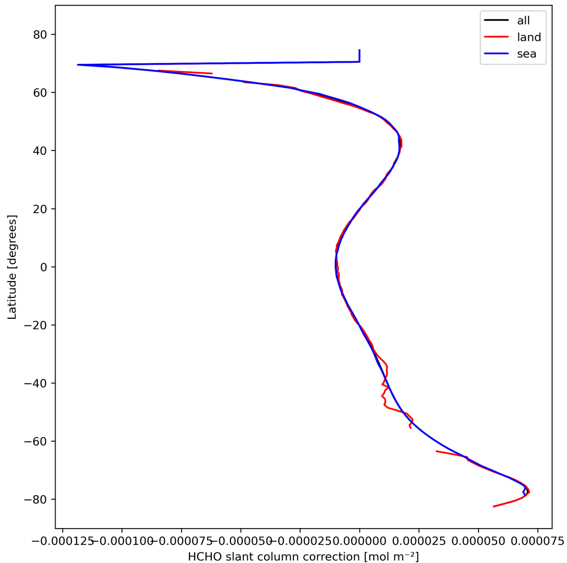
Figure 33: Zonal average of “HCHO slant column correction” for 2024-02-22 to 2024-02-23.
