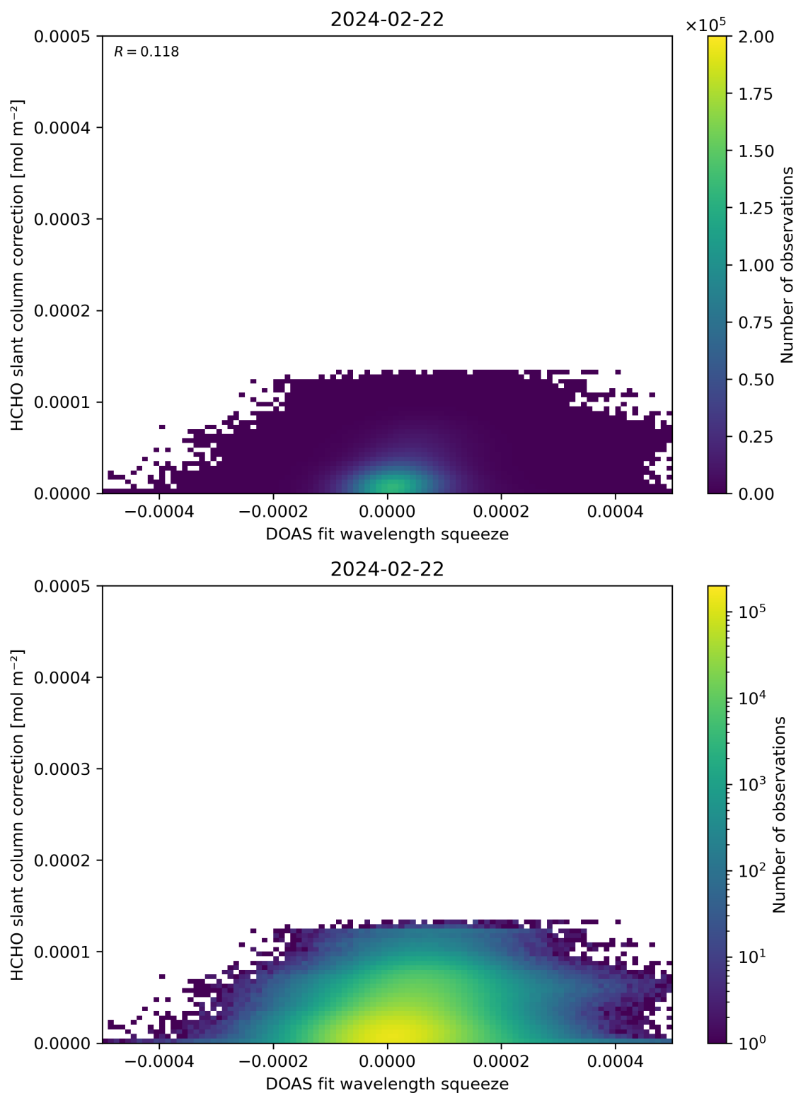
Figure 70: Scatter density plot of “DOAS fit wavelength squeeze” against “HCHO slant column correction” for 2024-02-22 to 2024-02-23.
