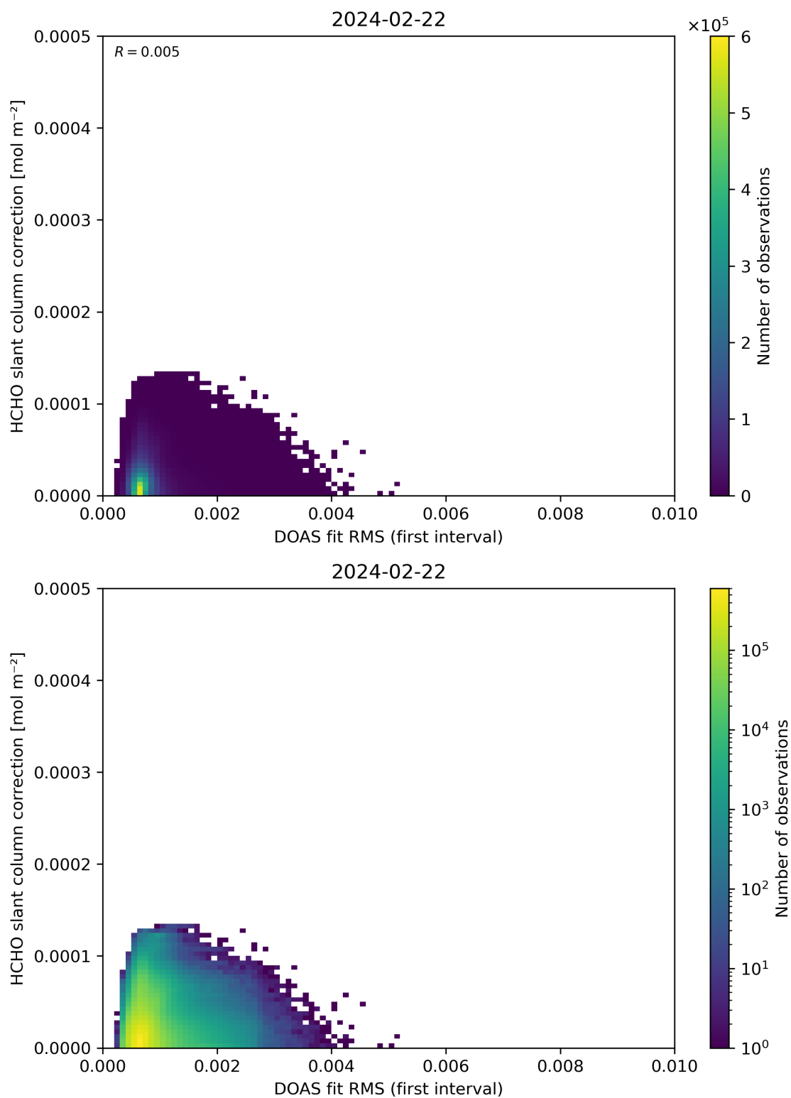
Figure 63: Scatter density plot of “DOAS fit RMS (first interval)” against “HCHO slant column correction” for 2024-02-22 to 2024-02-23.
