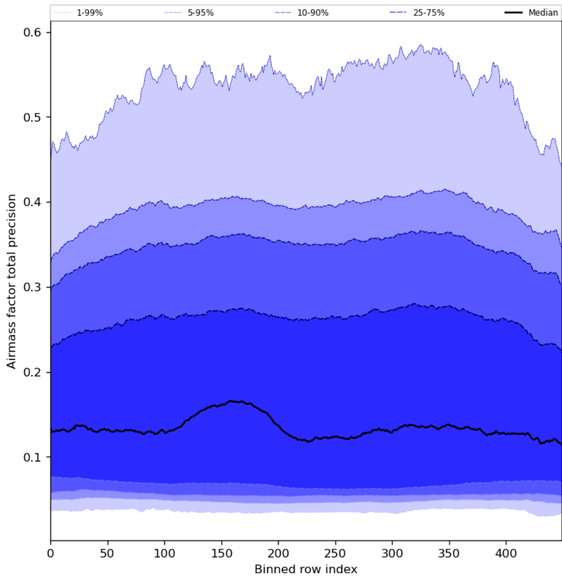
Figure 55: Along track statistics of “Airmass factor total precision” for 2024-02-22 to 2024-02-23
