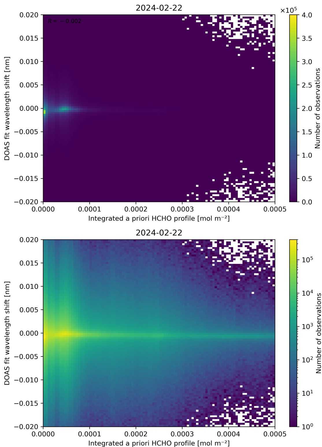
Figure 149: Scatter density plot of “Integrated a priori HCHO profile” against “DOAS fit wavelength shift” for 2024-02-22 to 2024-02-23.
