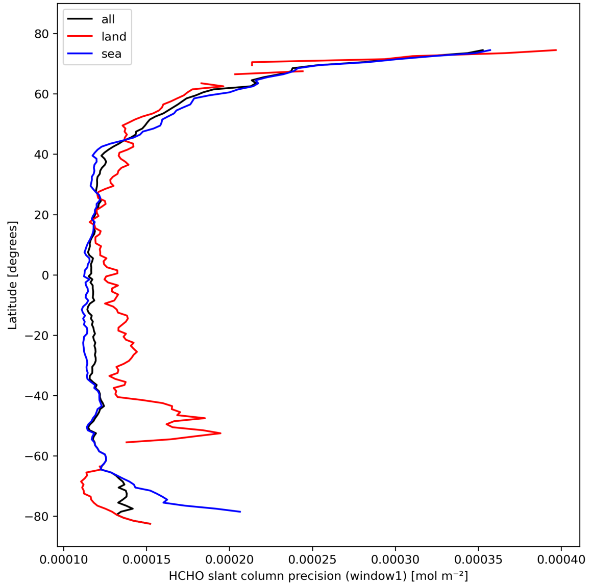
Figure 25: Zonal average of “HCHO slant column precision (window1)” for 2024-02-22 to 2024-02-23.
