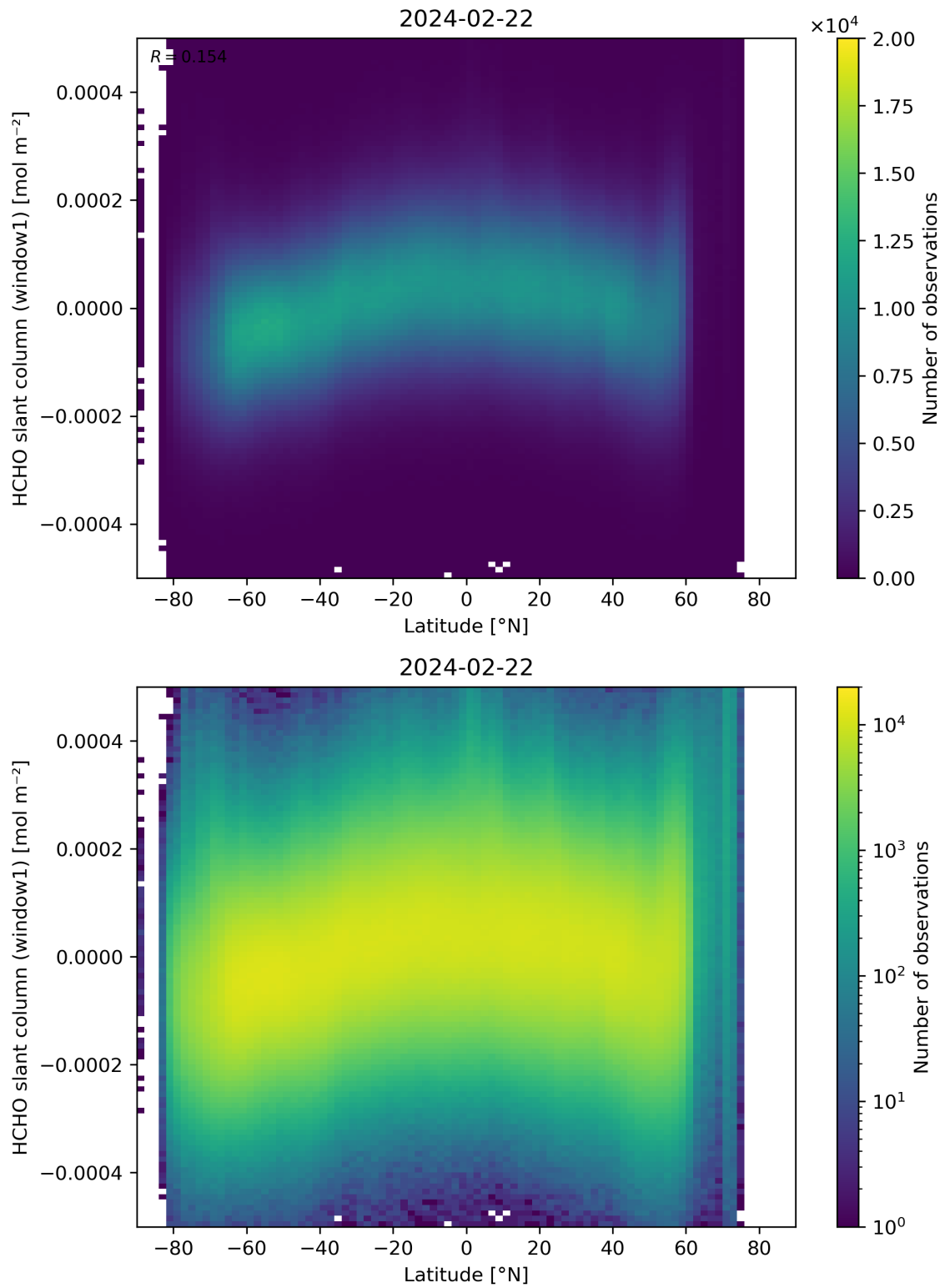
Figure 159: Scatter density plot of “Latitude” against “HCHO slant column (window1)” for 2024-02-22 to 2024-02-23.
