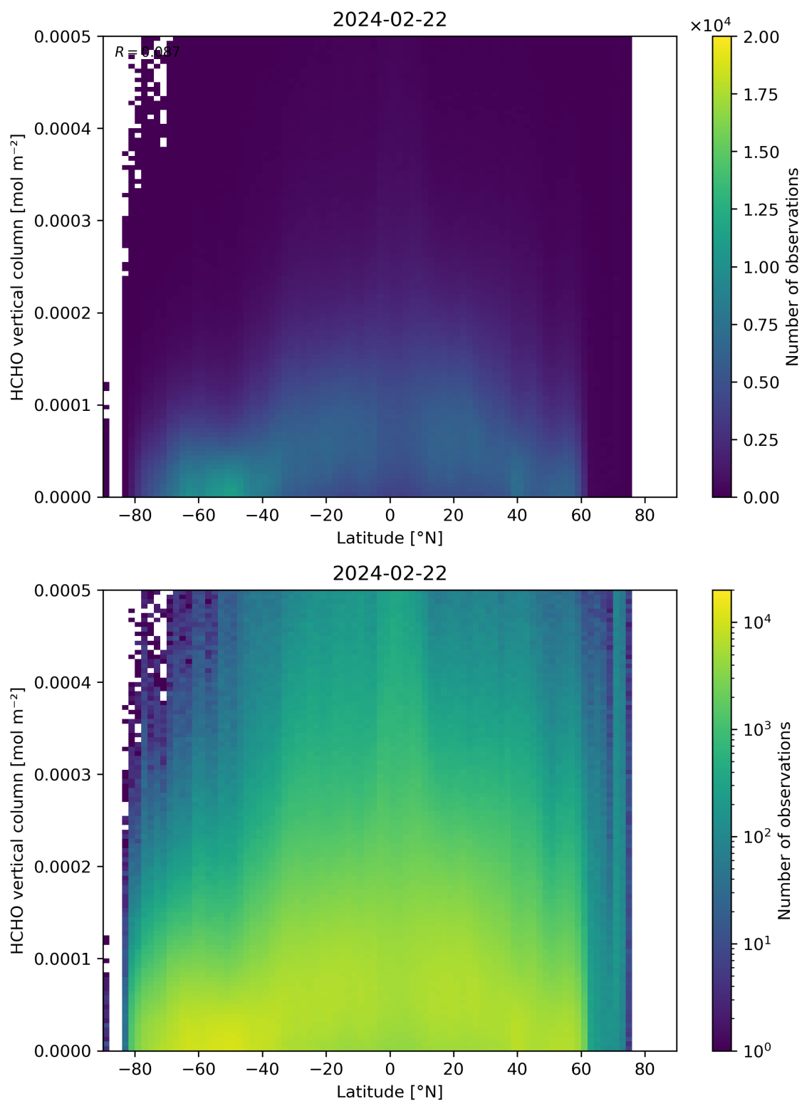
Figure 163: Scatter density plot of “Latitude” against “HCHO vertical column” for 2024-02-22 to 2024-02-23.
