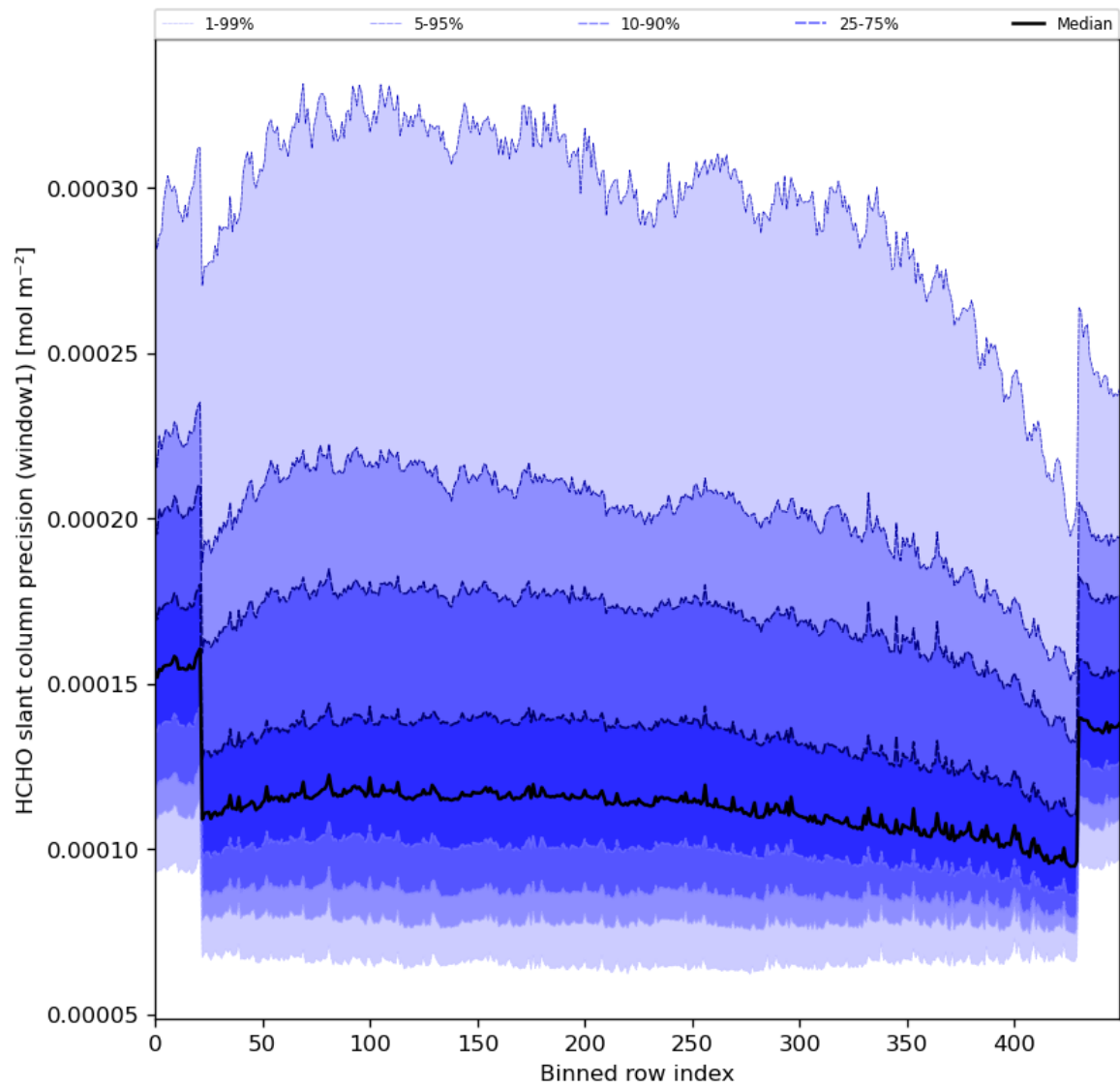
Figure 53: Along track statistics of “HCHO slant column precision (window1)” for 2024-02-22 to 2024-02-23
