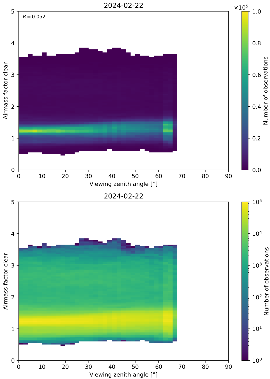
Figure 185: Scatter density plot of “Viewing zenith angle” against “Airmass factor clear” for 2024-02-22 to 2024-02-23.
