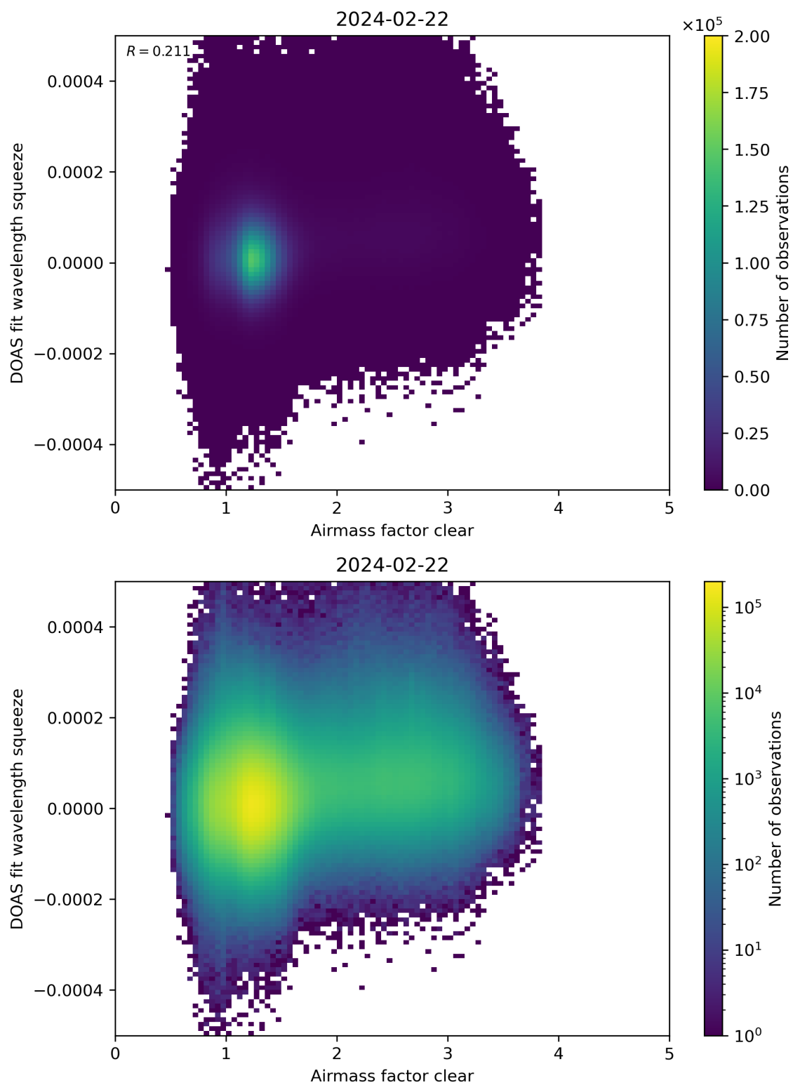
Figure 73: Scatter density plot of “Airmass factor clear” against “DOAS fit wavelength squeeze” for 2024-02-22 to 2024-02-23.
