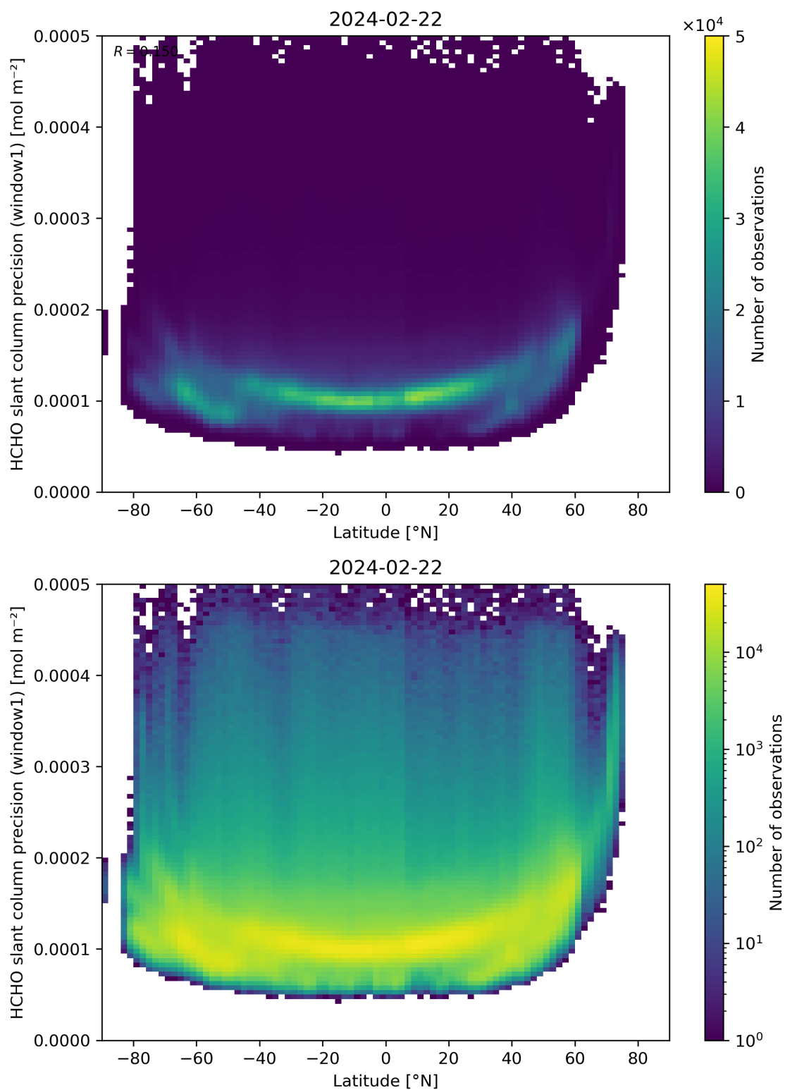
Figure 160: Scatter density plot of “Latitude” against “HCHO slant column precision (window1)” for 2024-02-22 to 2024-02-23.
