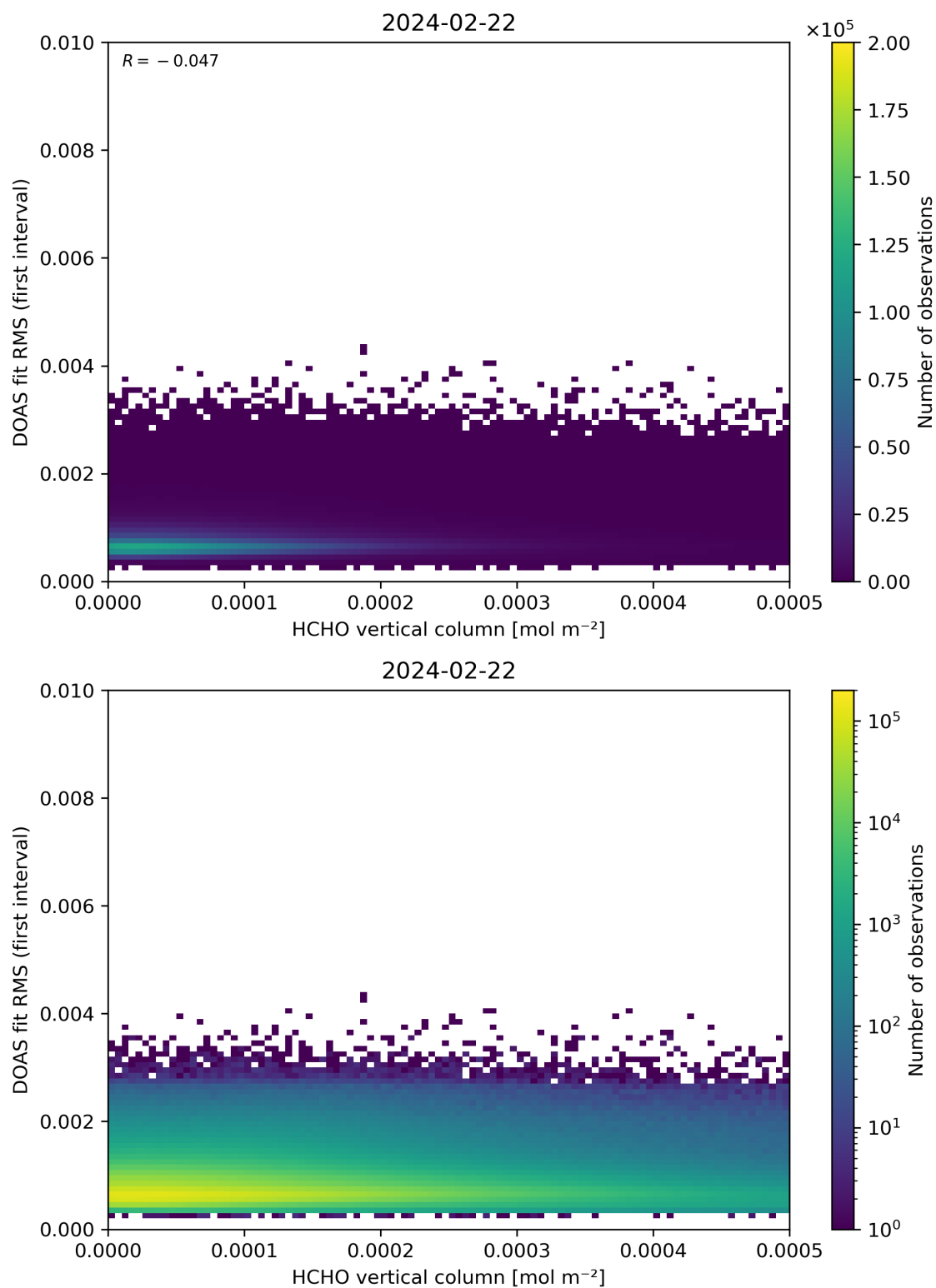
Figure 123: Scatter density plot of “HCHO vertical column” against “DOAS fit RMS (first interval)” for 2024-02-22 to 2024-02-23.
