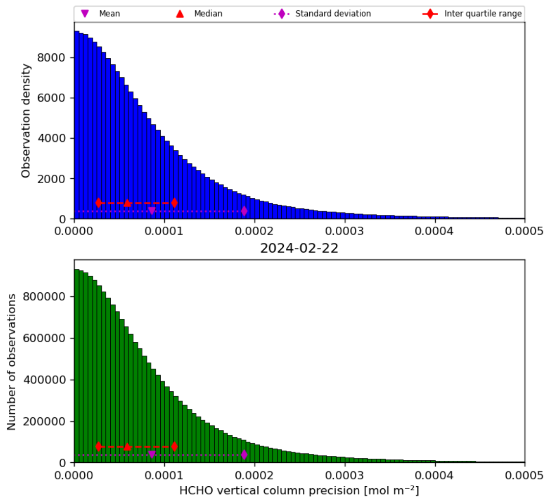
Figure 36: Histogram of “HCHO vertical column precision” for 2024-02-22 to 2024-02-23
