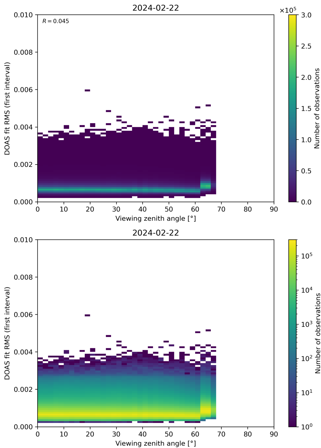
Figure 182: Scatter density plot of “Viewing zenith angle” against “DOAS fit RMS (first interval)” for 2024-02-22 to 2024-02-23.
