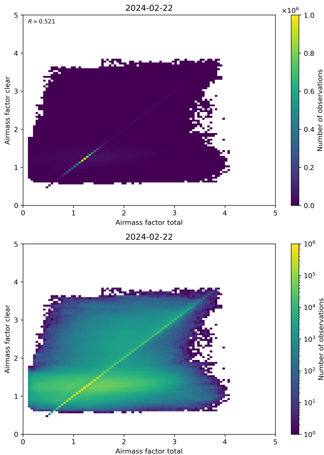
Figure 100: Scatter density plot of “Airmass factor total” against “Airmass factor clear” for 2024-02-22 to 2024-02-23.
