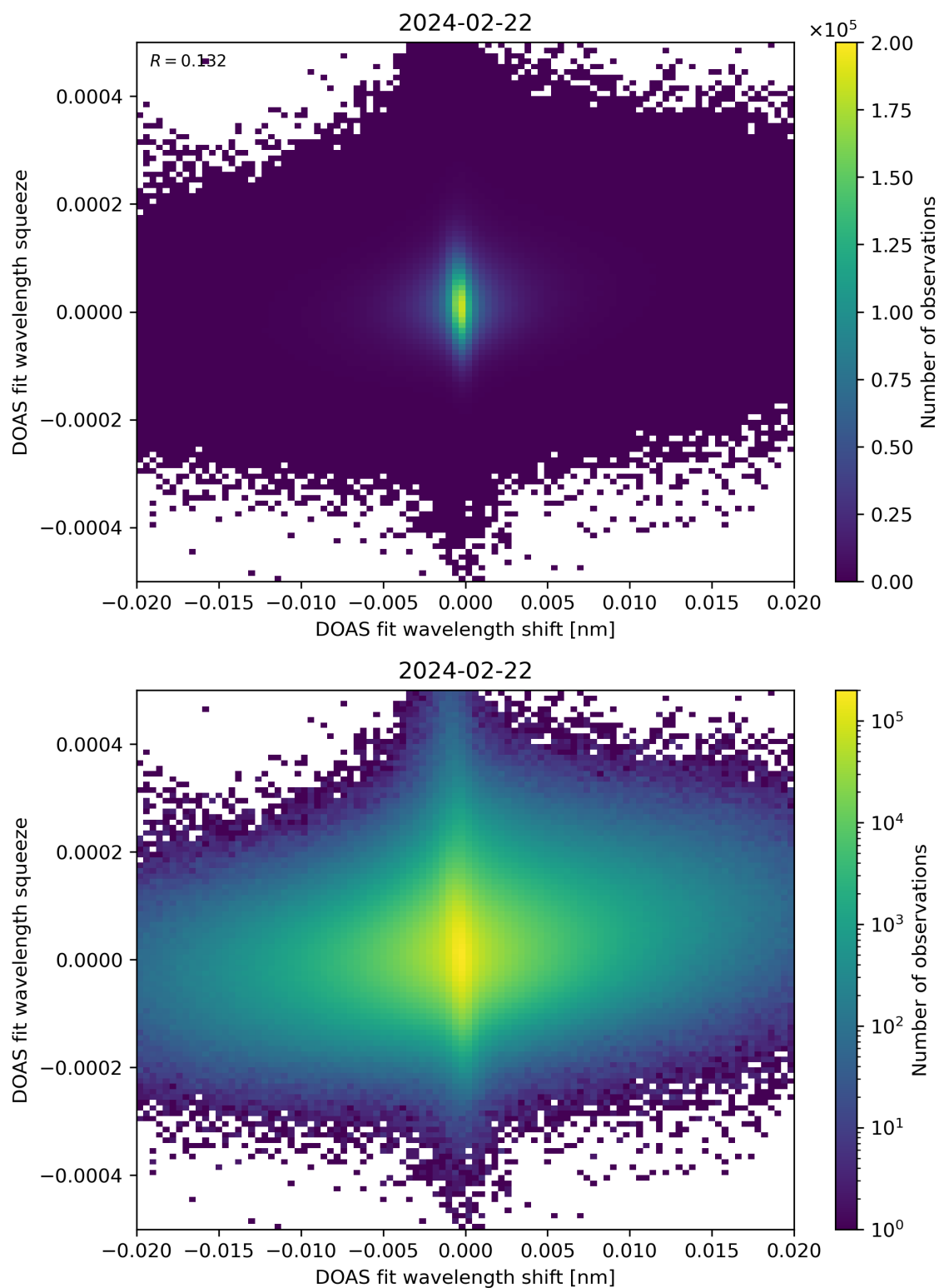
Figure 65: Scatter density plot of “DOAS fit wavelength shift” against “DOAS fit wavelength squeeze” for 2024-02-22 to 2024-02-23.
