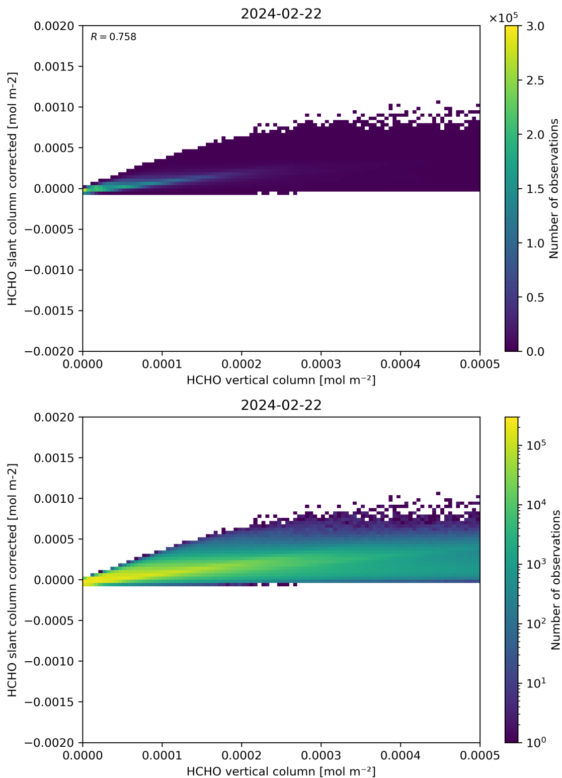
Figure 127: Scatter density plot of “HCHO vertical column” against “HCHO slant column corrected” for 2024-02-22 to 2024-02-23.
