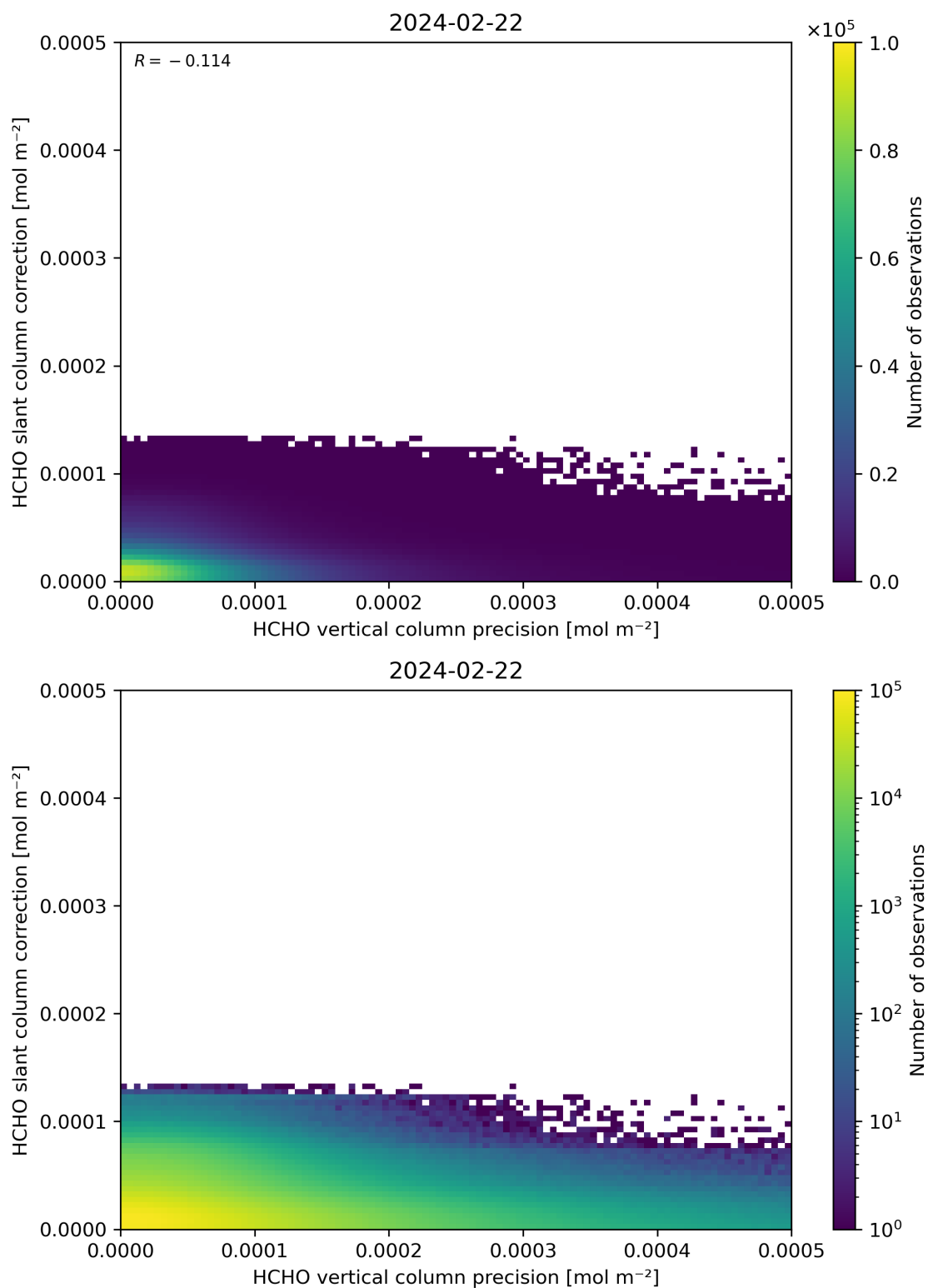
Figure 141: Scatter density plot of “HCHO vertical column precision” against “HCHO slant column correction” for 2024-02-22 to 2024-02-23.
