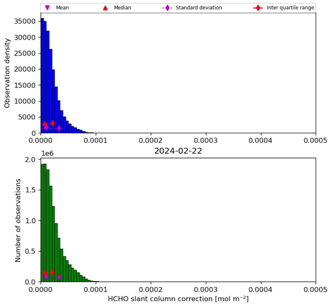
Figure 47: Histogram of “HCHO slant column correction” for 2024-02-22 to 2024-02-23
