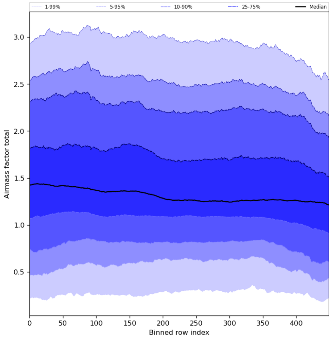
Figure 54: Along track statistics of “Airmass factor total” for 2024-02-22 to 2024-02-23
