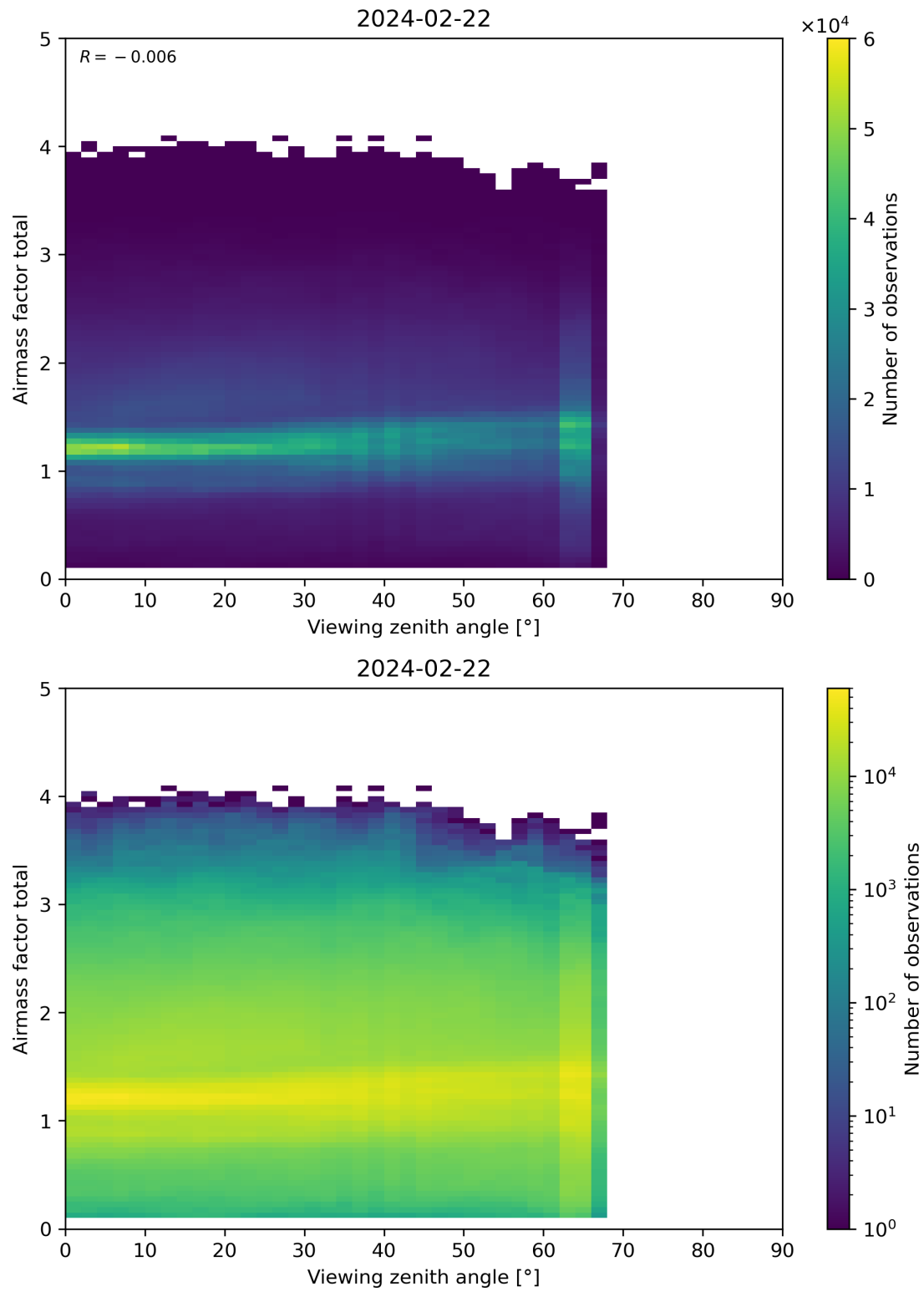
Figure 190: Scatter density plot of “Viewing zenith angle” against “Airmass factor total” for 2024-02-22 to 2024-02-23.
