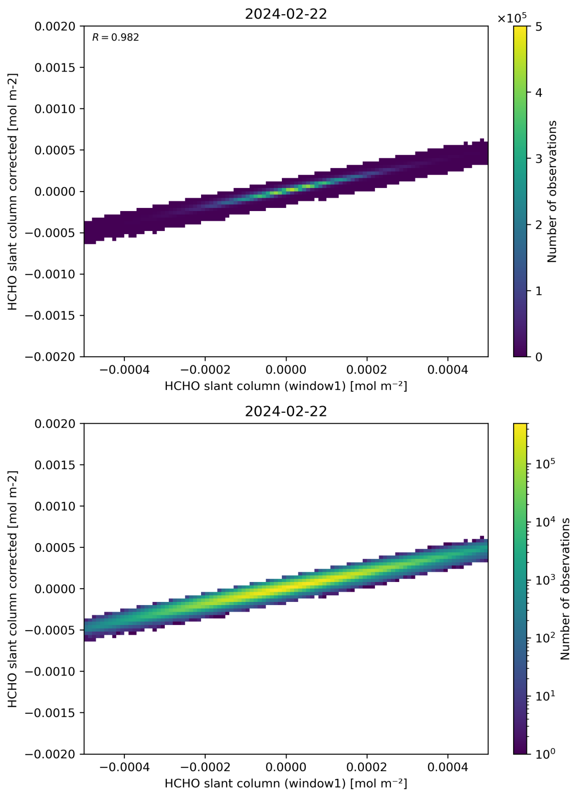
Figure 82: Scatter density plot of “HCHO slant column (window1)” against “HCHO slant column corrected” for 2024-02-22 to 2024-02-23.
