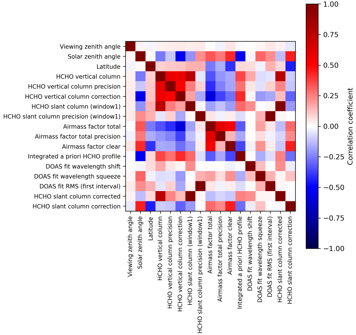
Figure 2: Map of correlation matrix for 2024-02-22 to 2024-02-23.
