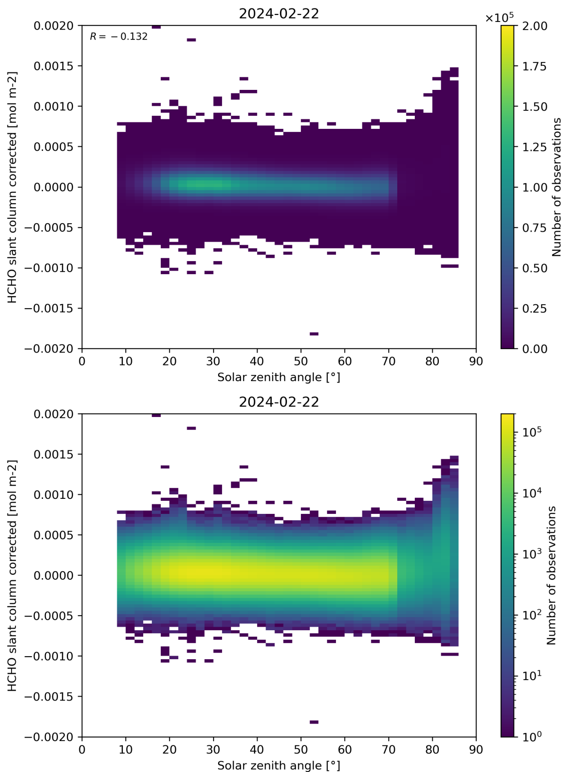
Figure 171: Scatter density plot of “Solar zenith angle” against “HCHO slant column corrected” for 2024-02-22 to 2024-02-23.
