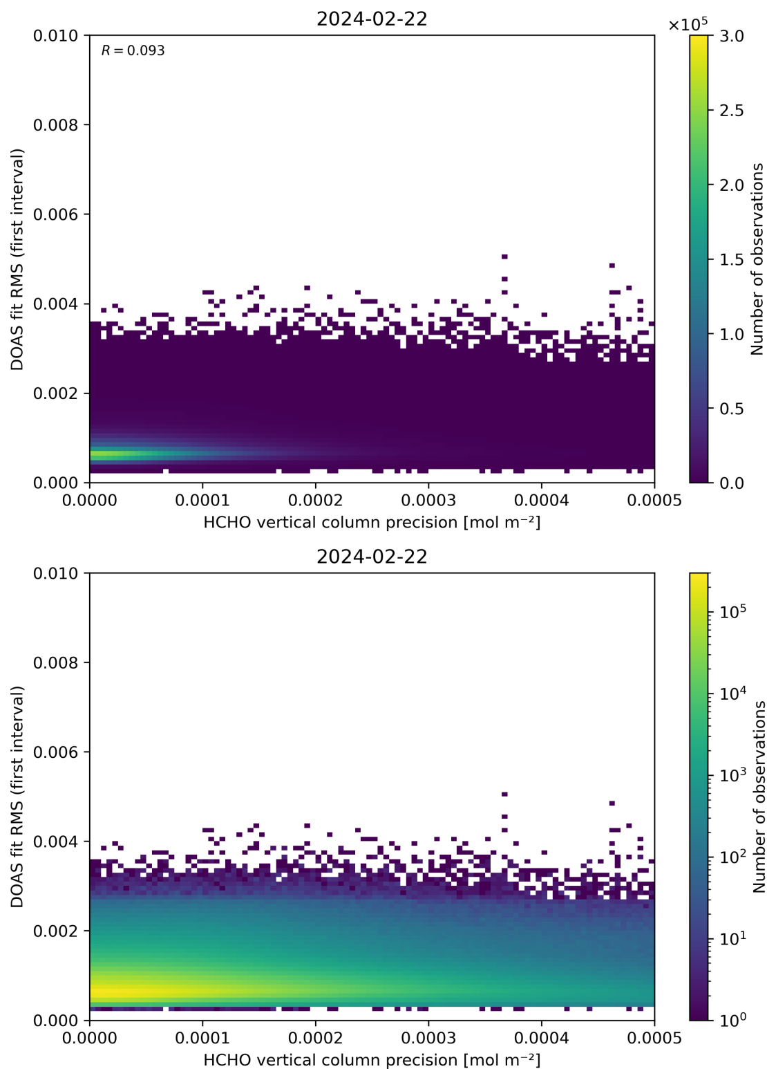
Figure 136: Scatter density plot of “HCHO vertical column precision” against “DOAS fit RMS (first interval)” for 2024-02-22 to 2024-02-23.
