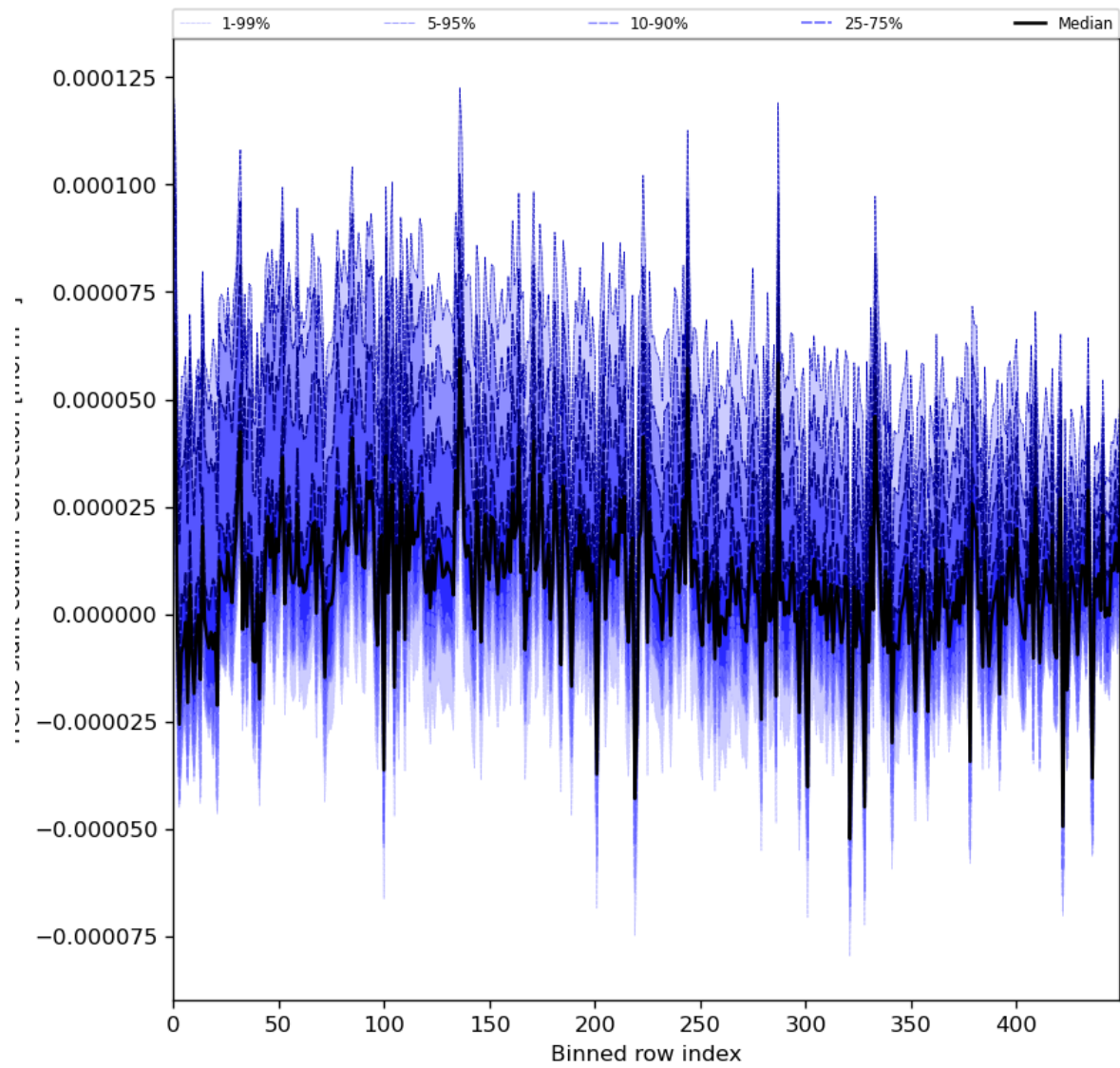
Figure 61: Along track statistics of “HCHO slant column correction” for 2024-02-22 to 2024-02-23
