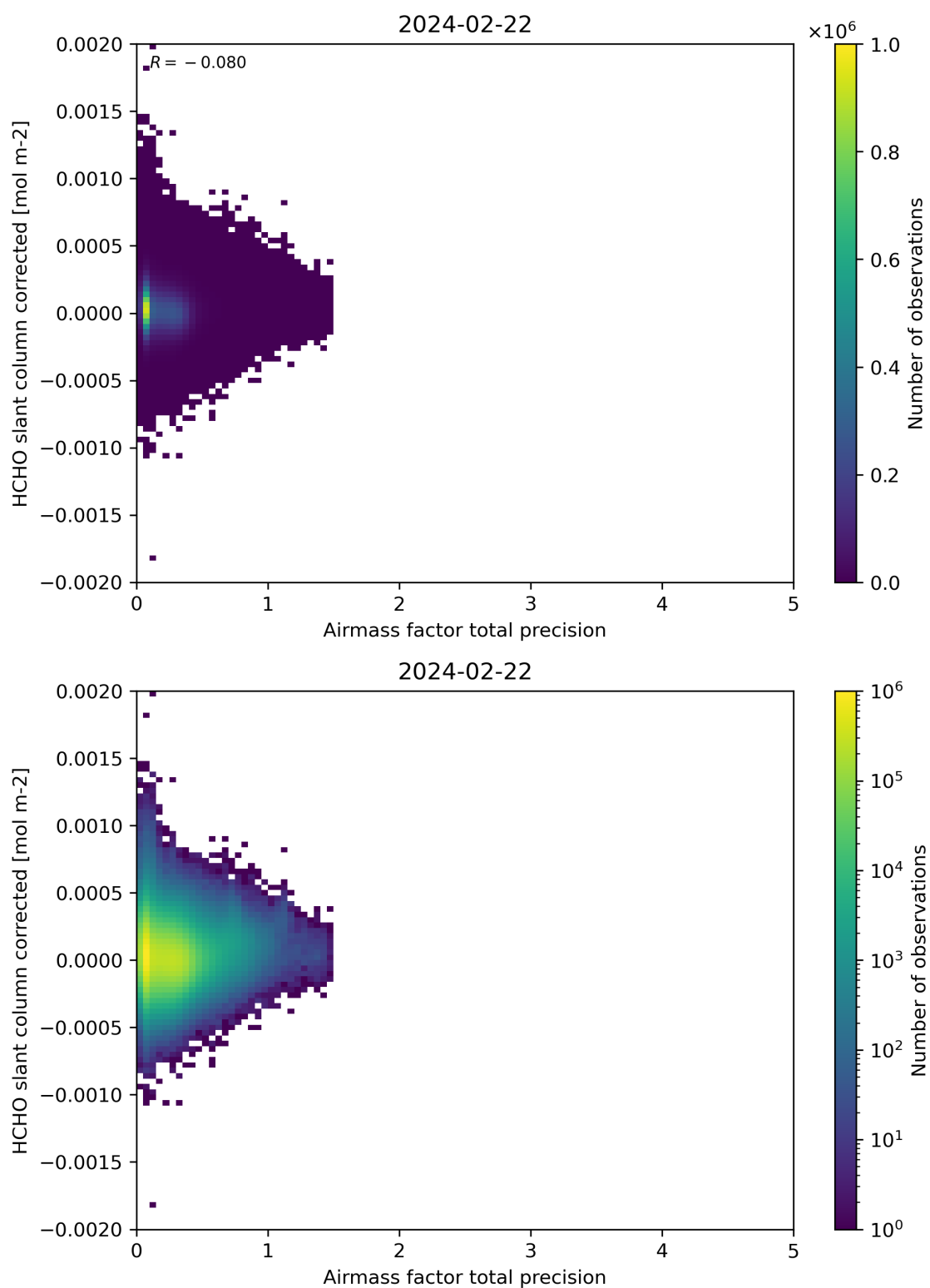
Figure 109: Scatter density plot of “Airmass factor total precision” against “HCHO slant column corrected” for 2024-02-22 to 2024-02-23.
