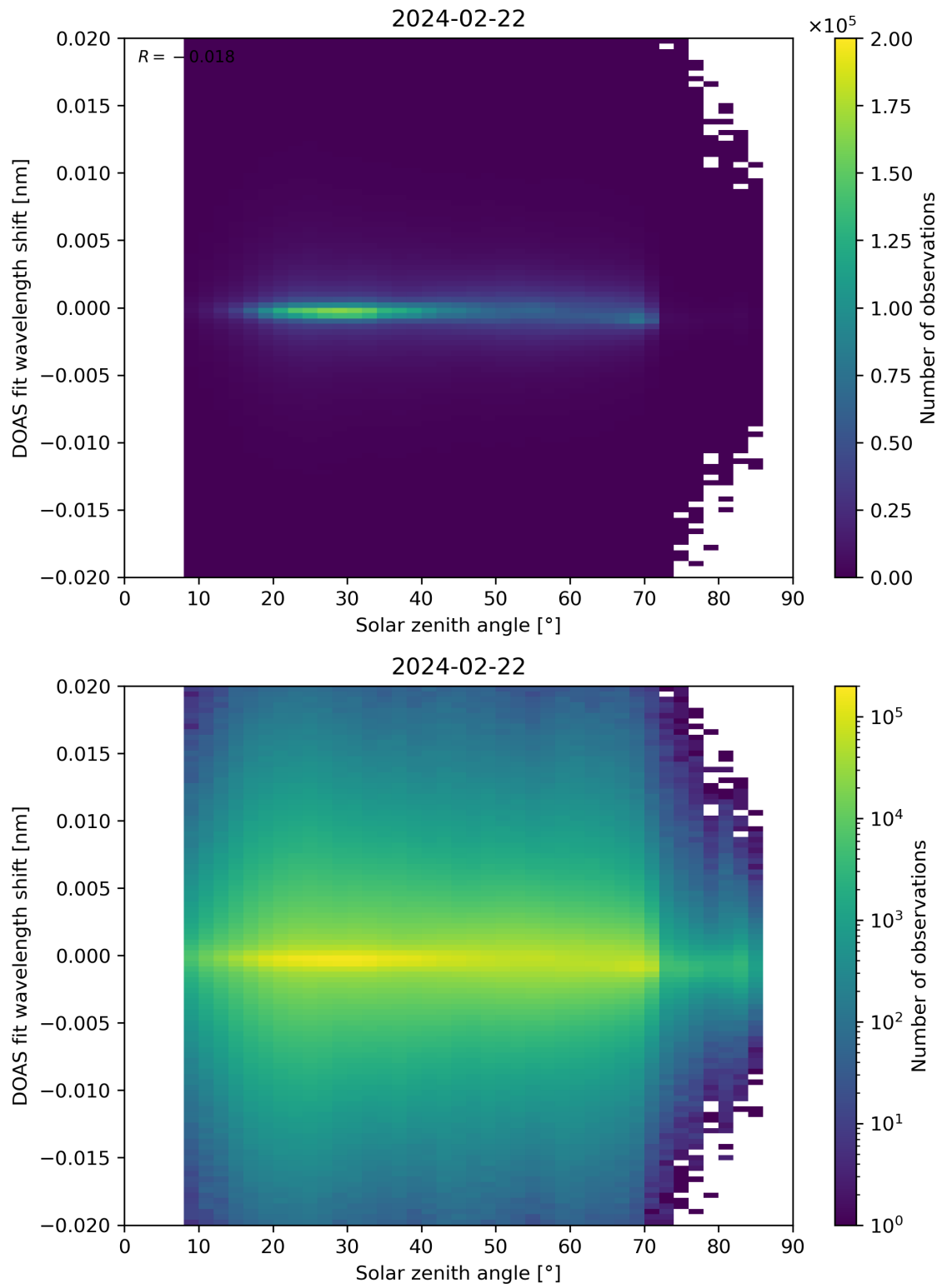
Figure 168: Scatter density plot of “Solar zenith angle” against “DOAS fit wavelength shift” for 2024-02-22 to 2024-02-23.
