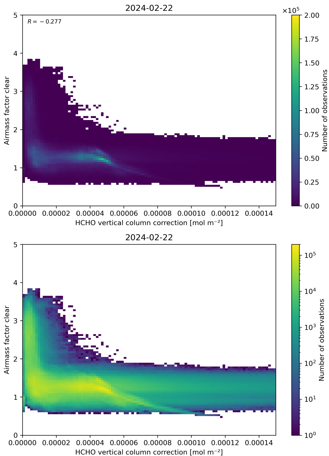
Figure 115: Scatter density plot of “HCHO vertical column correction” against “Airmass factor clear” for 2024-02-22 to 2024-02-23.
