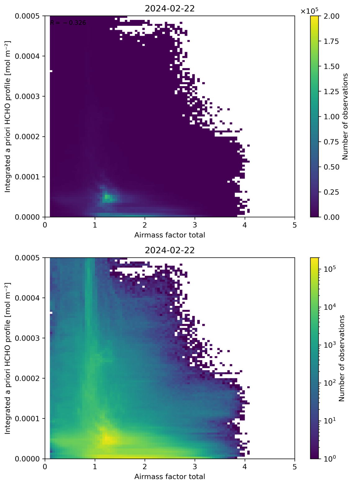
Figure 104: Scatter density plot of “Airmass factor total” against “Integrated a priori HCHO profile” for 2024-02-22 to 2024-02-23.
