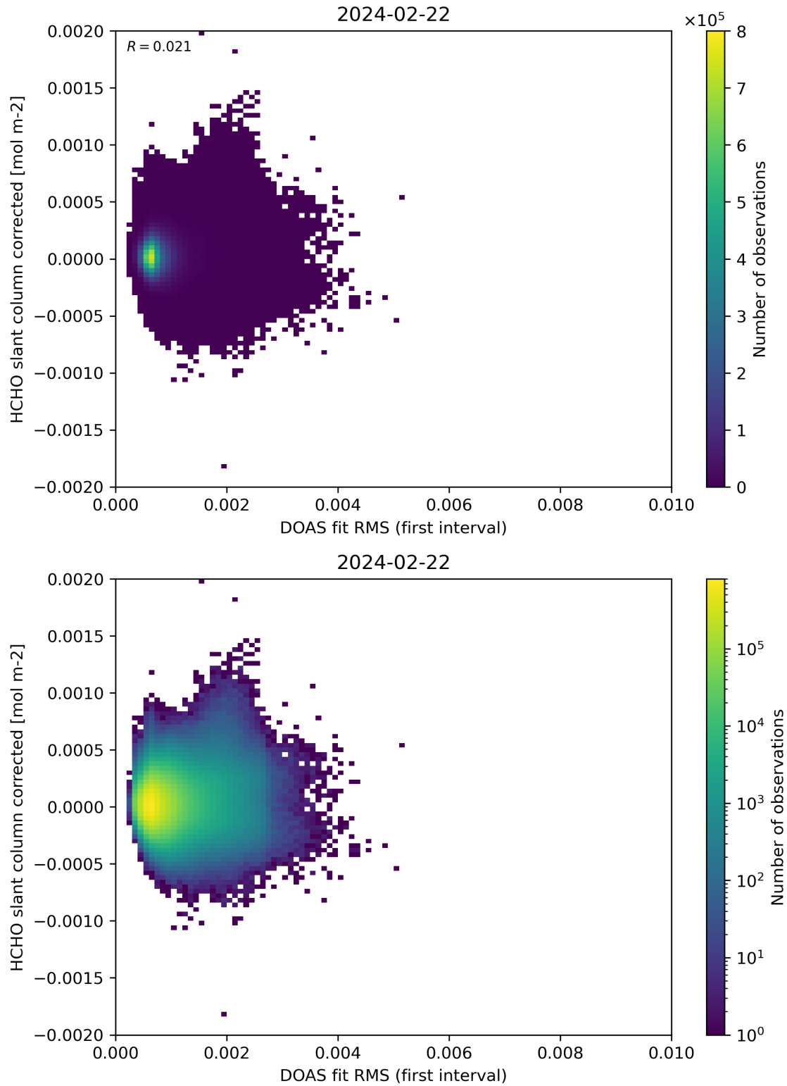
Figure 62: Scatter density plot of “DOAS fit RMS (first interval)” against “HCHO slant column corrected” for 2024-02-22 to 2024-02-23.
