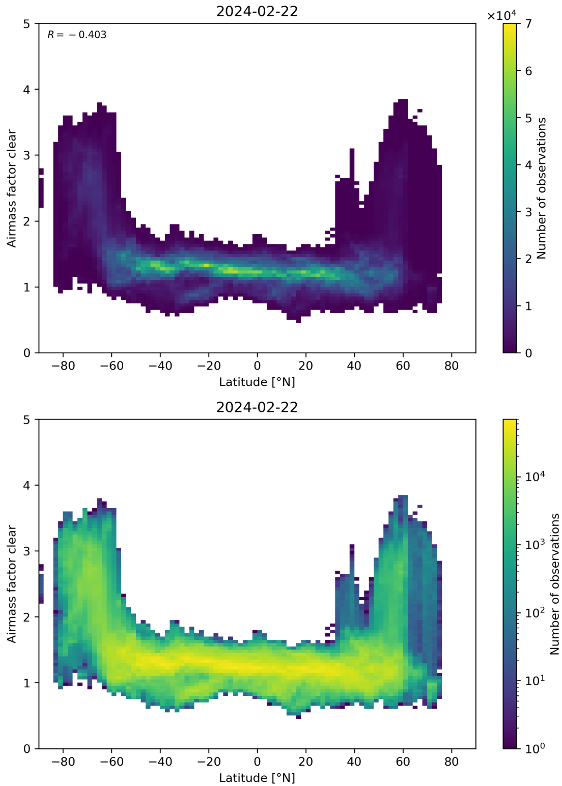
Figure 156: Scatter density plot of “Latitude” against “Airmass factor clear” for 2024-02-22 to 2024-02-23.
