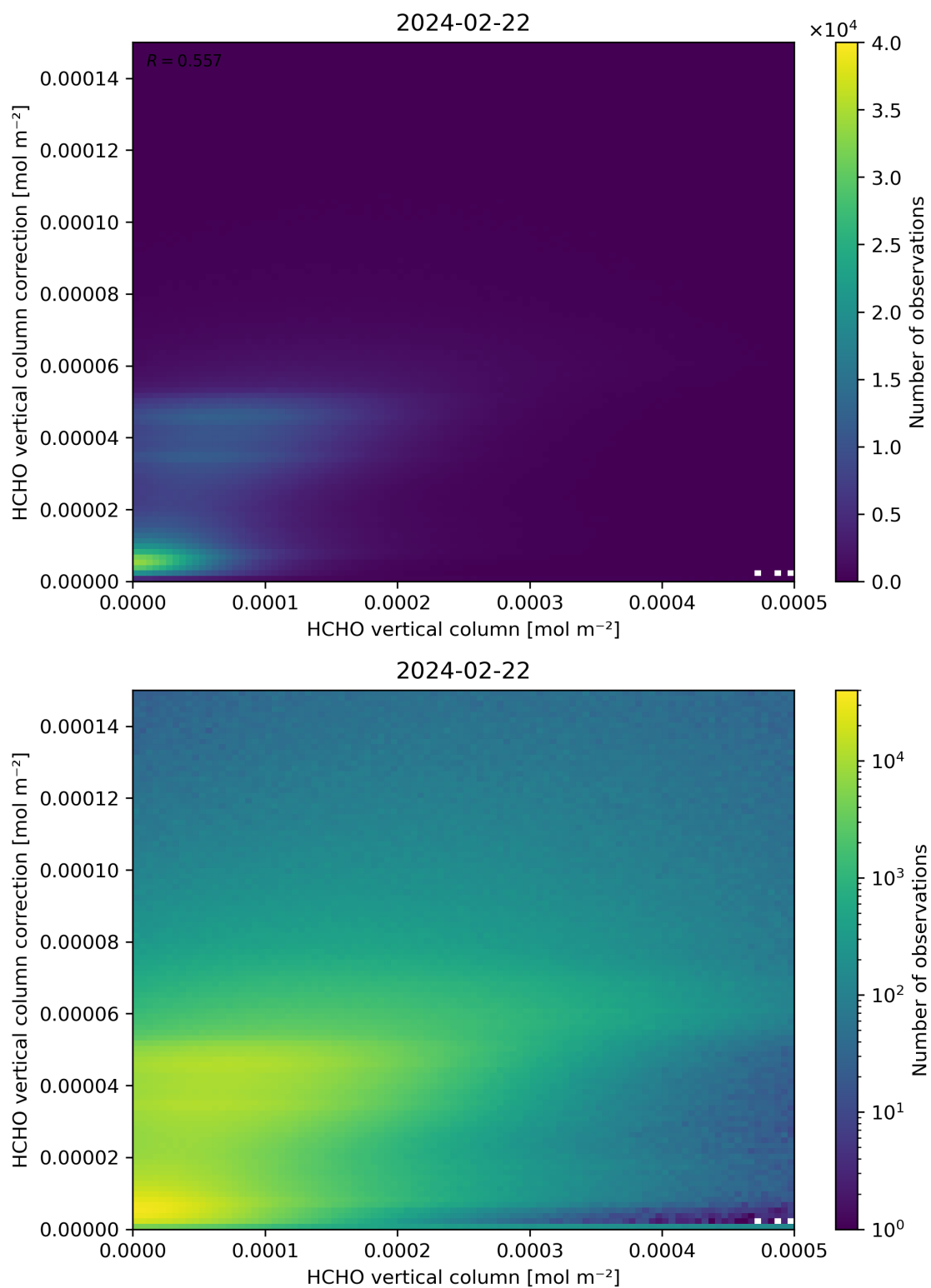
Figure 133: Scatter density plot of “HCHO vertical column” against “HCHO vertical column correction” for 2024-02-22 to 2024-02-23.
