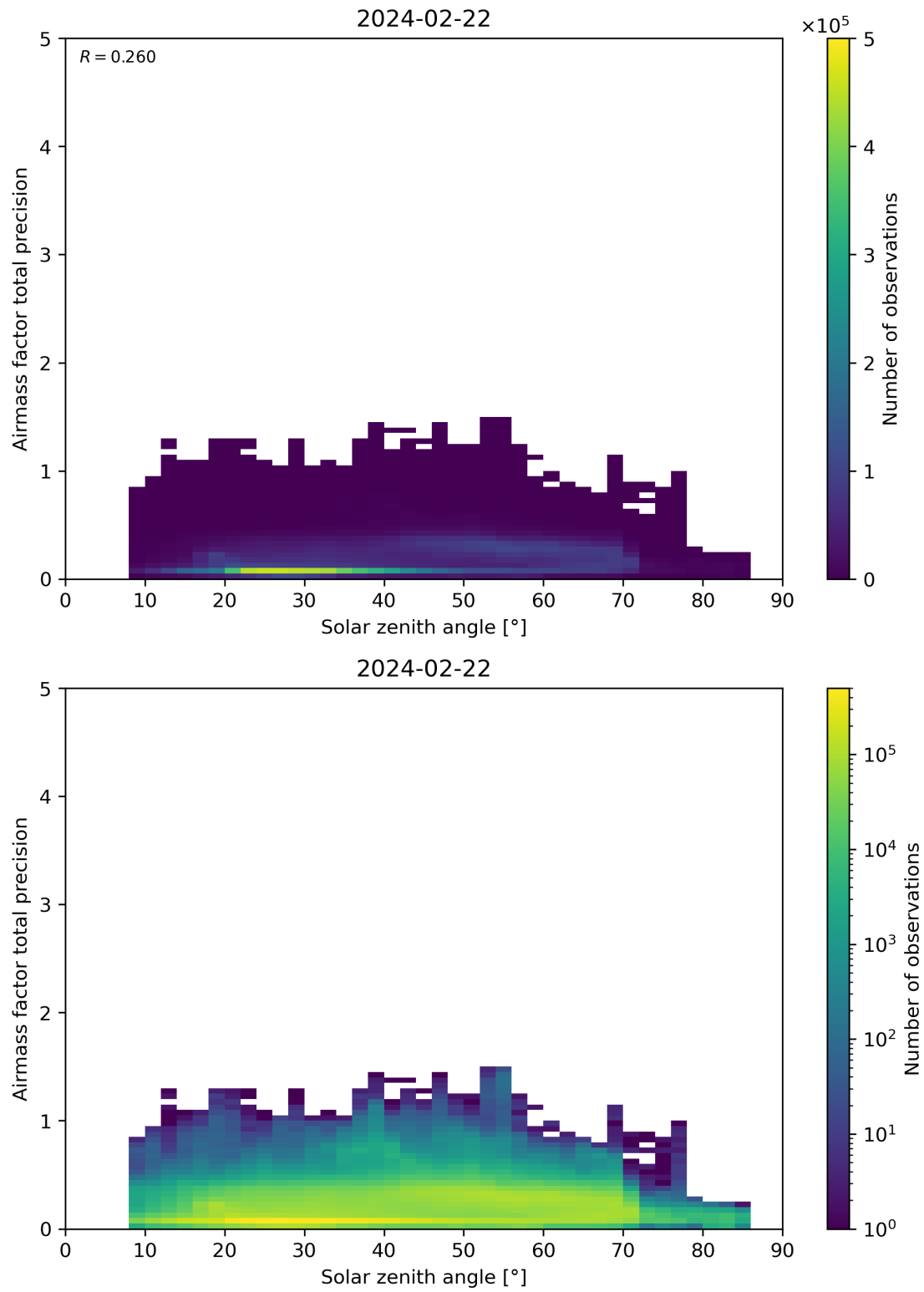
Figure 176: Scatter density plot of “Solar zenith angle” against “Airmass factor total precision” for 2024-02-22 to 2024-02-23.
