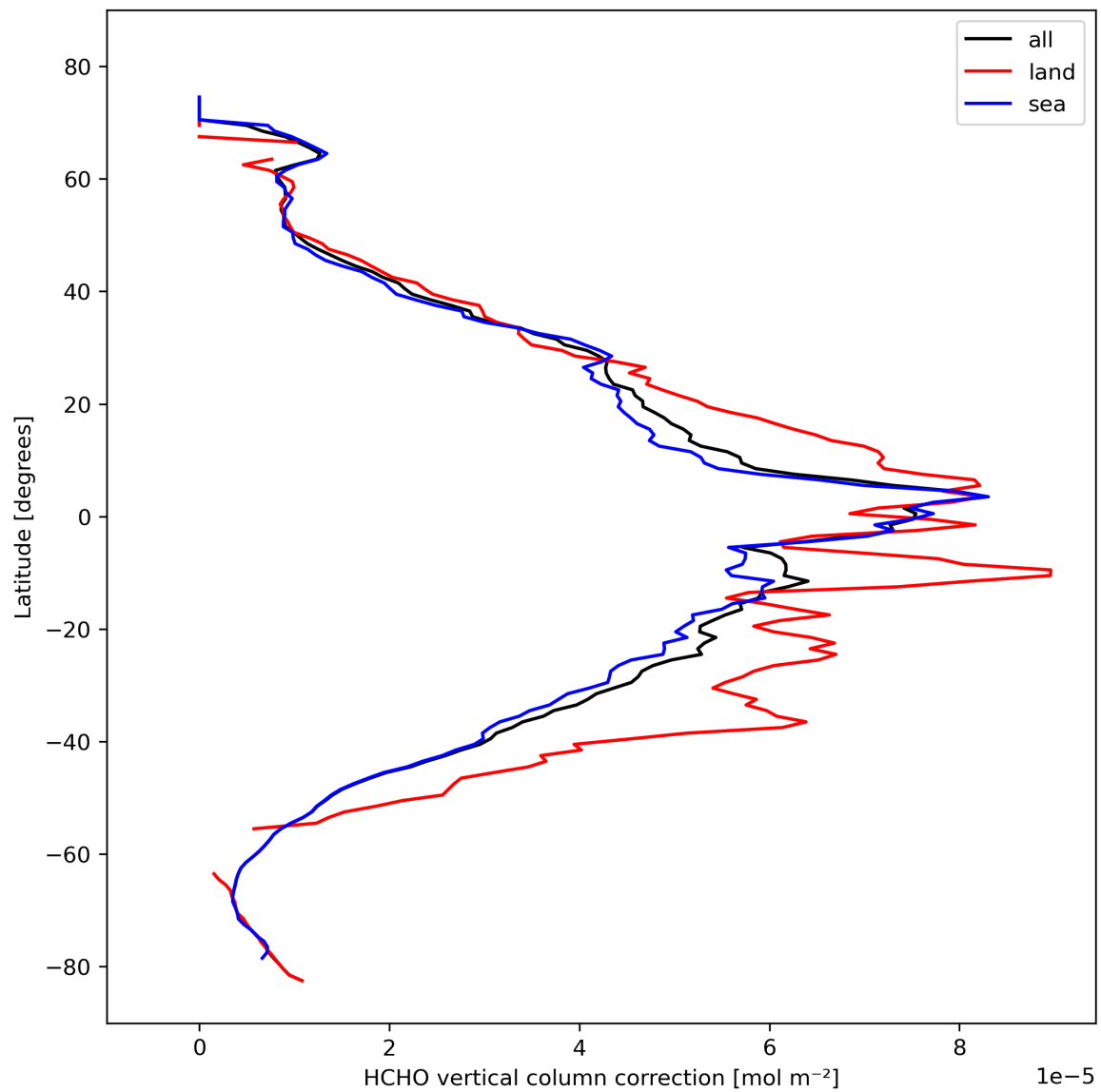
Figure 23: Zonal average of “HCHO vertical column correction” for 2024-02-22 to 2024-02-23.
