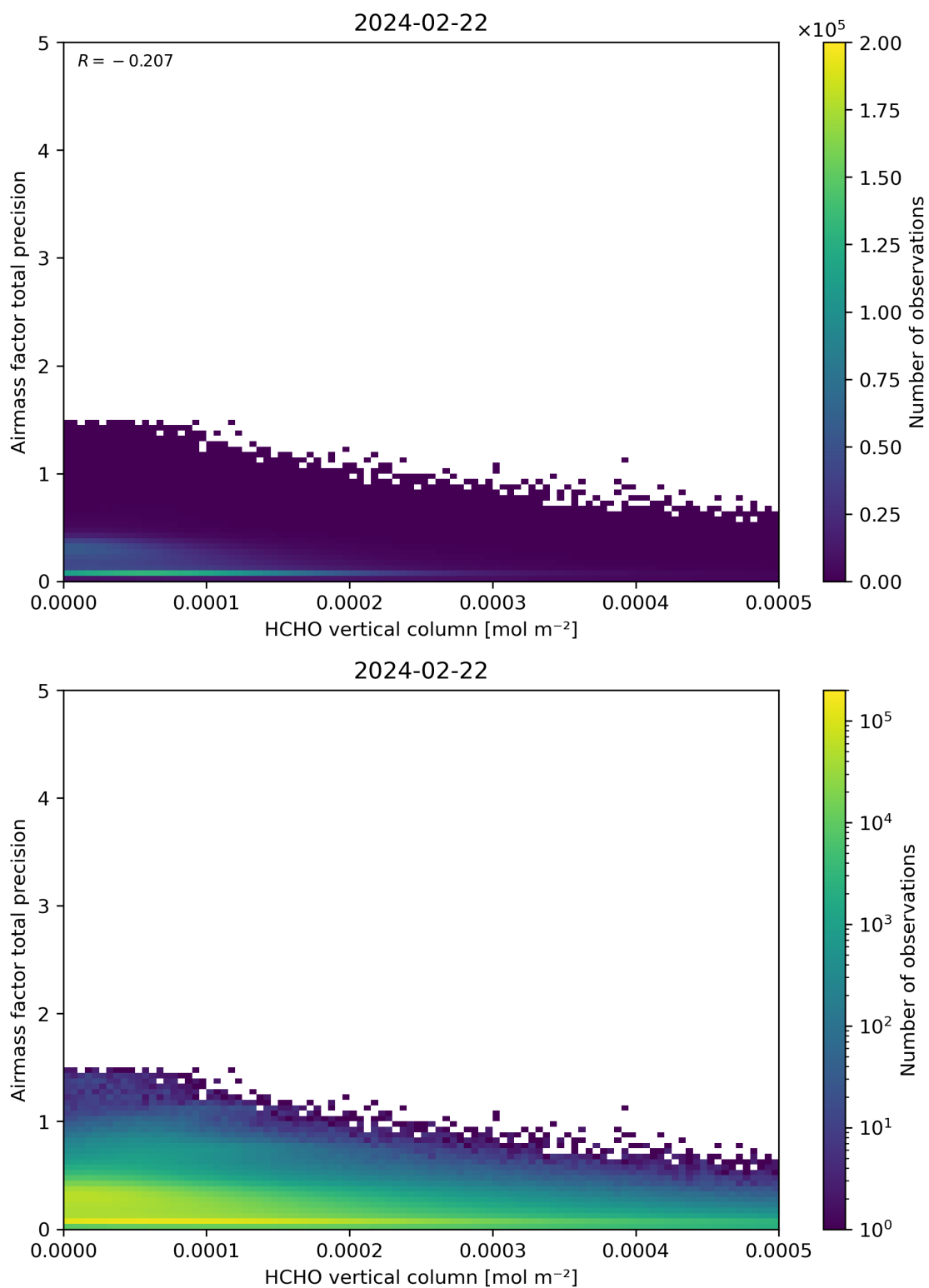
Figure 132: Scatter density plot of “HCHO vertical column” against “Airmass factor total precision” for 2024-02-22 to 2024-02-23.
