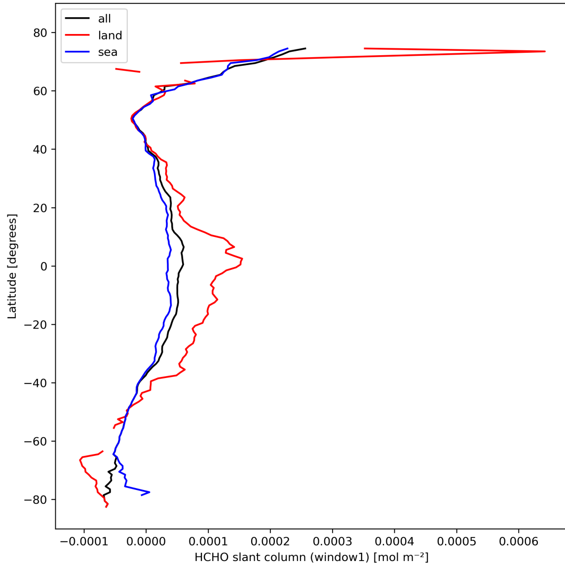
Figure 24: Zonal average of “HCHO slant column (window1)” for 2024-02-22 to 2024-02-23.
