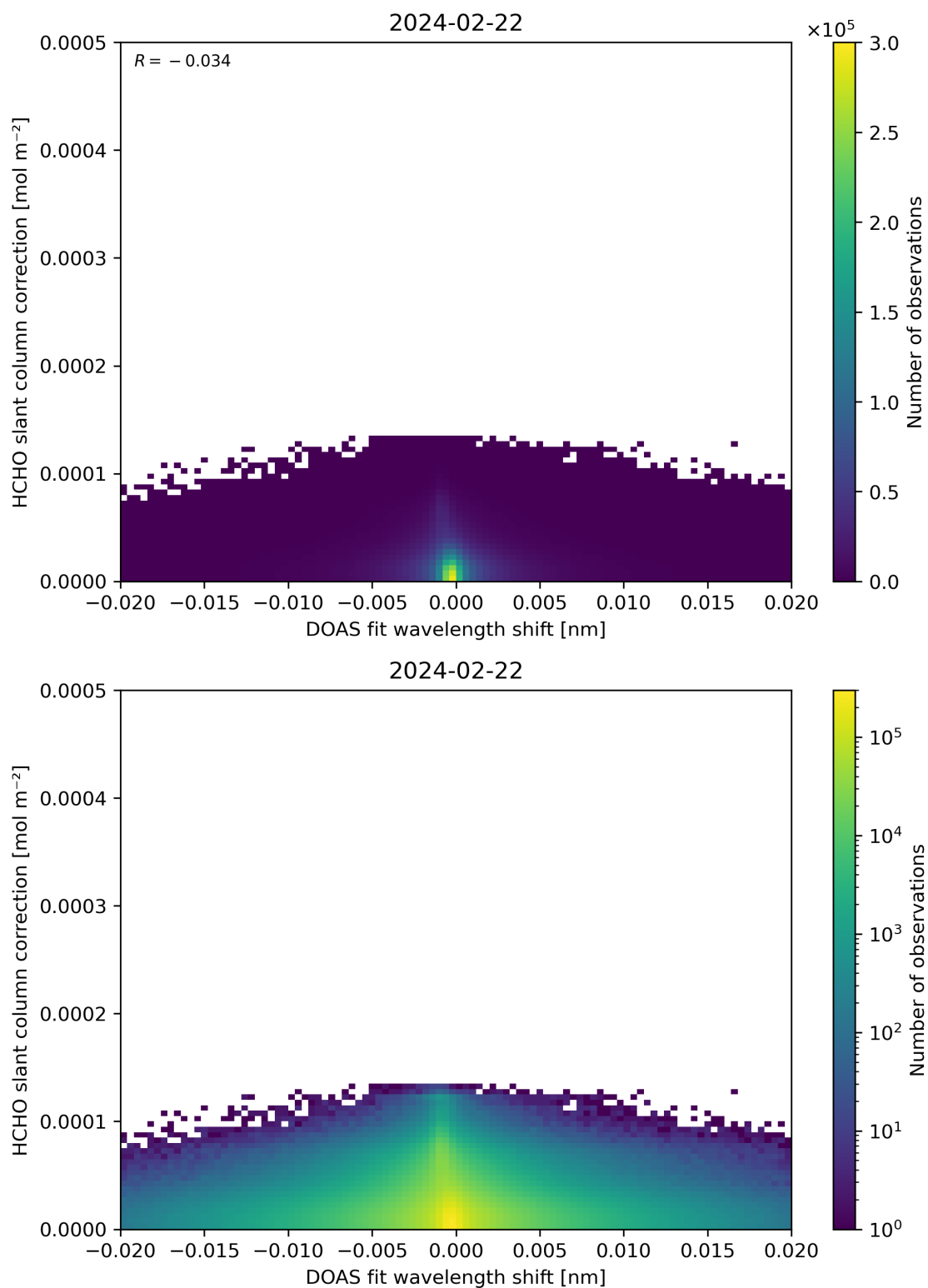
Figure 67: Scatter density plot of “DOAS fit wavelength shift” against “HCHO slant column correction” for 2024-02-22 to 2024-02-23.
