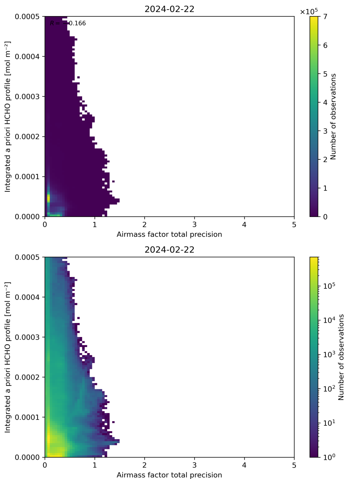
Figure 111: Scatter density plot of “Airmass factor total precision” against “Integrated a priori HCHO profile” for 2024-02-22 to 2024-02-23.
