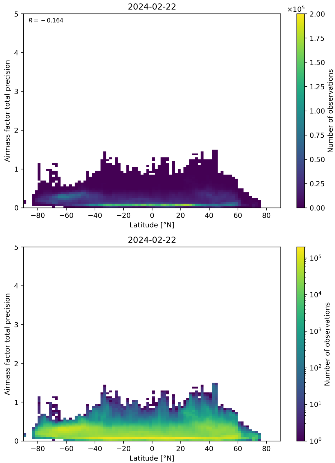
Figure 162: Scatter density plot of “Latitude” against “Airmass factor total precision” for 2024-02-22 to 2024-02-23.
