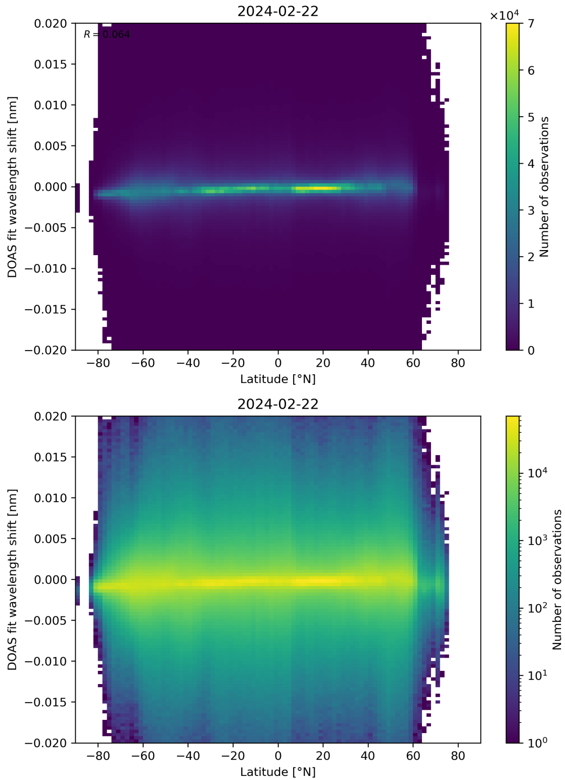
Figure 154: Scatter density plot of “Latitude” against “DOAS fit wavelength shift” for 2024-02-22 to 2024-02-23.
