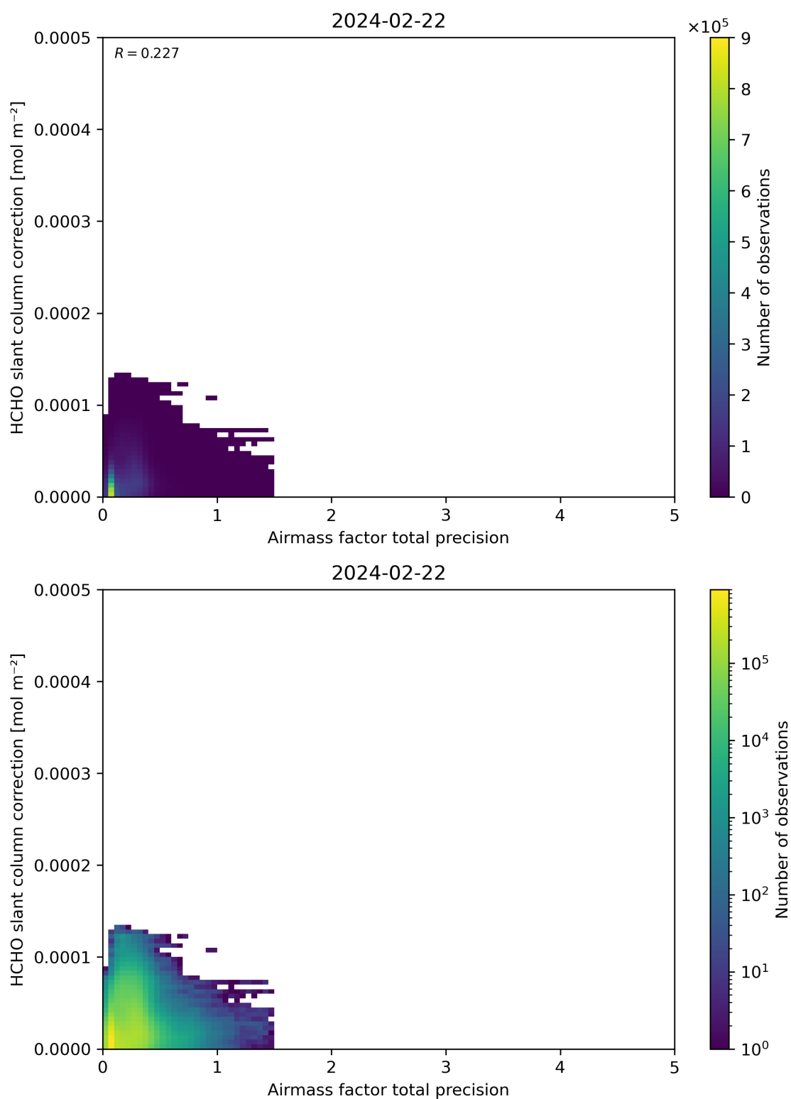
Figure 110: Scatter density plot of “Airmass factor total precision” against “HCHO slant column correction” for 2024-02-22 to 2024-02-23.
