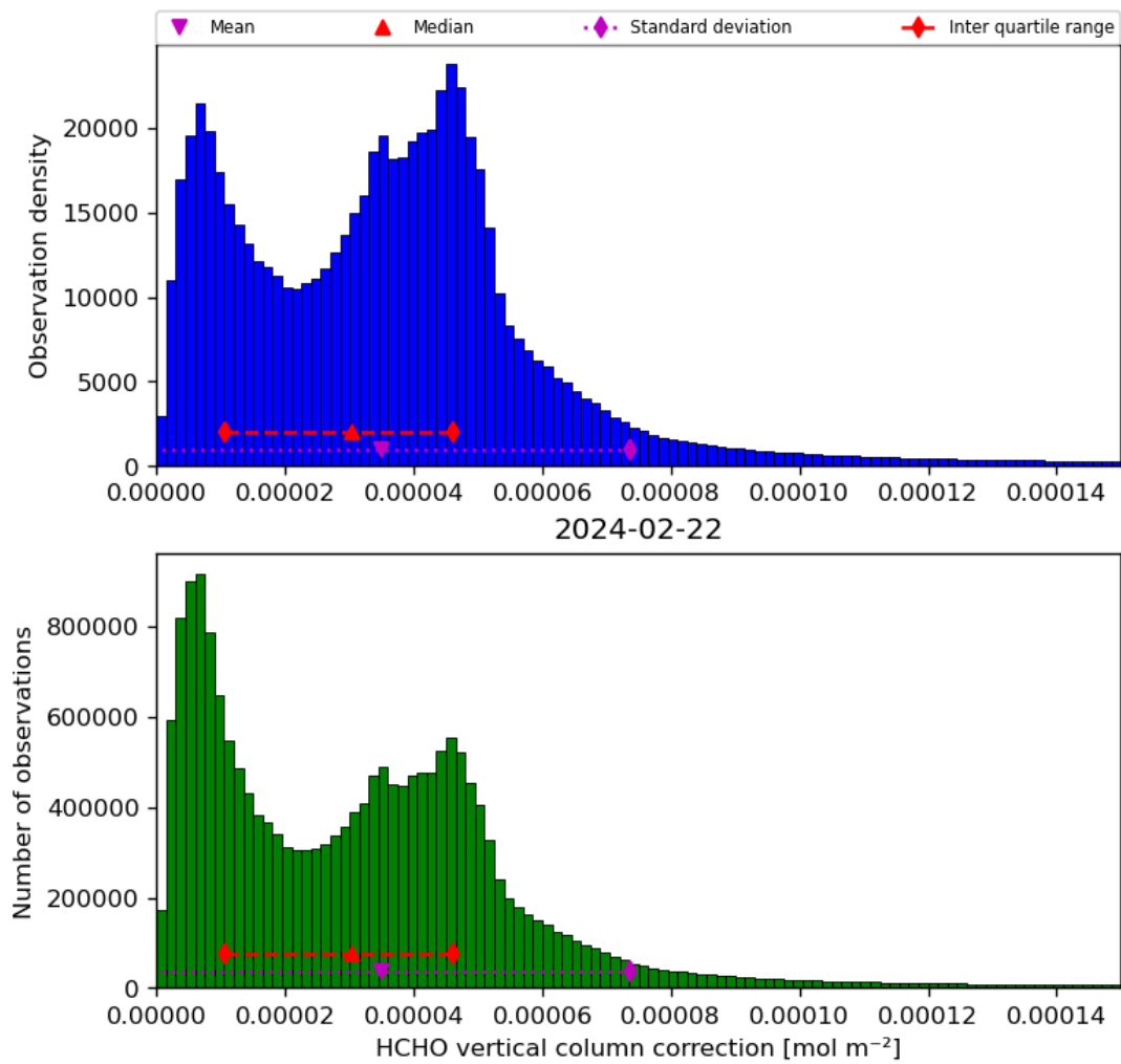
Figure 37: Histogram of “HCHO vertical column correction” for 2024-02-22 to 2024-02-23
