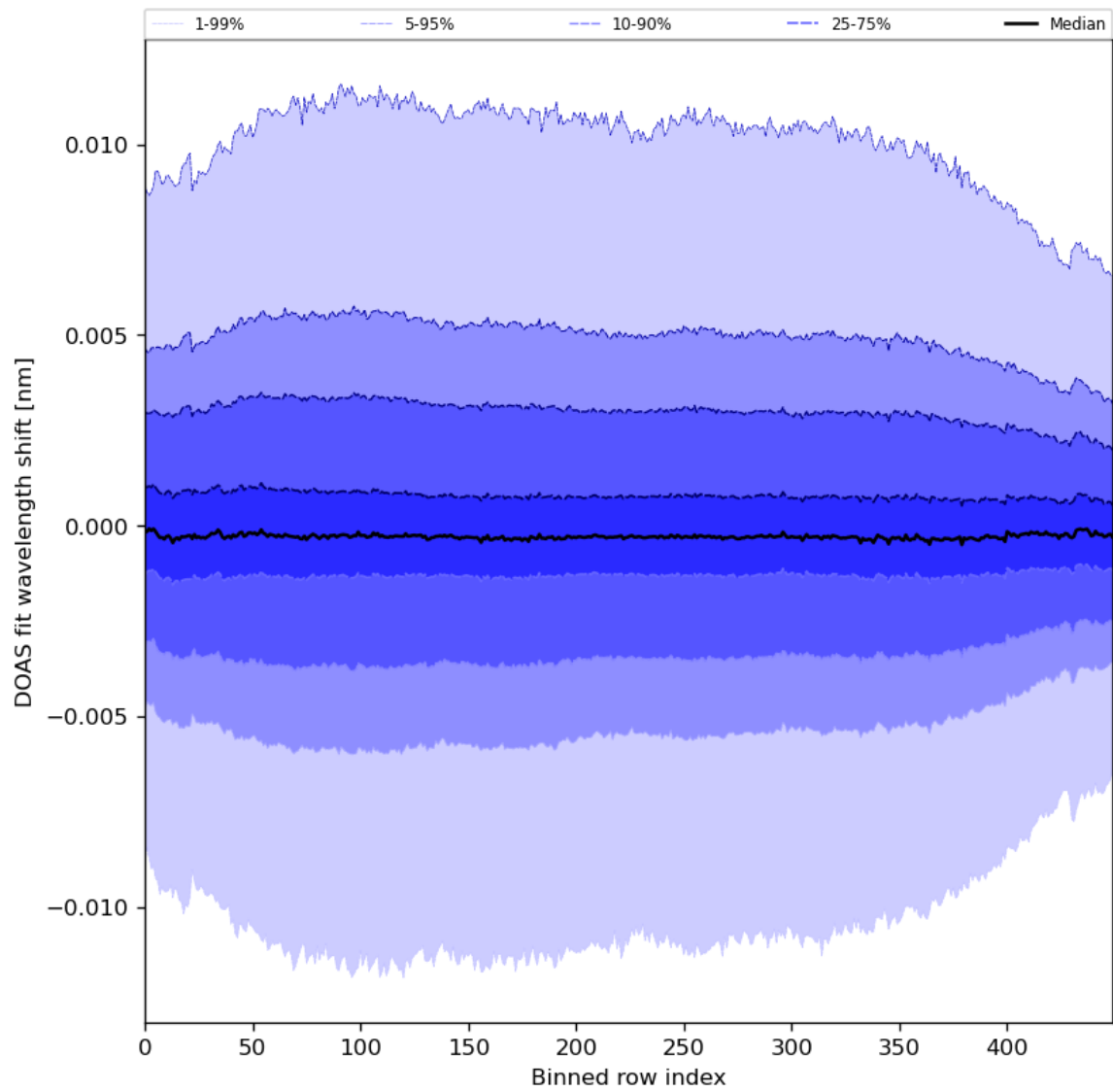
Figure 58: Along track statistics of “DOAS fit wavelength shift” for 2024-02-22 to 2024-02-23
