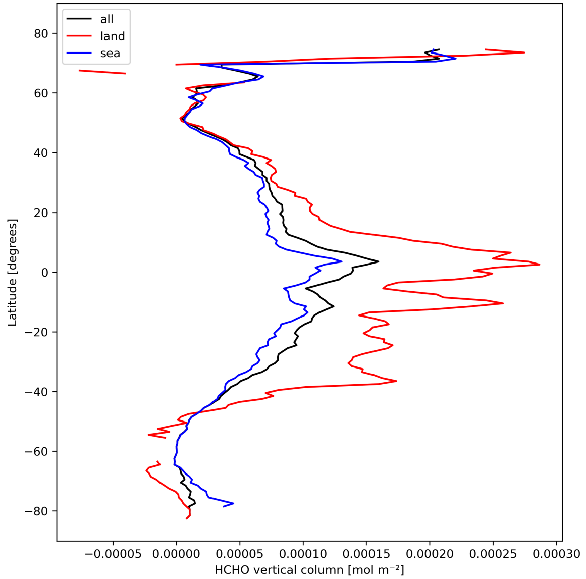
Figure 21: Zonal average of “HCHO vertical column” for 2024-02-22 to 2024-02-23.
