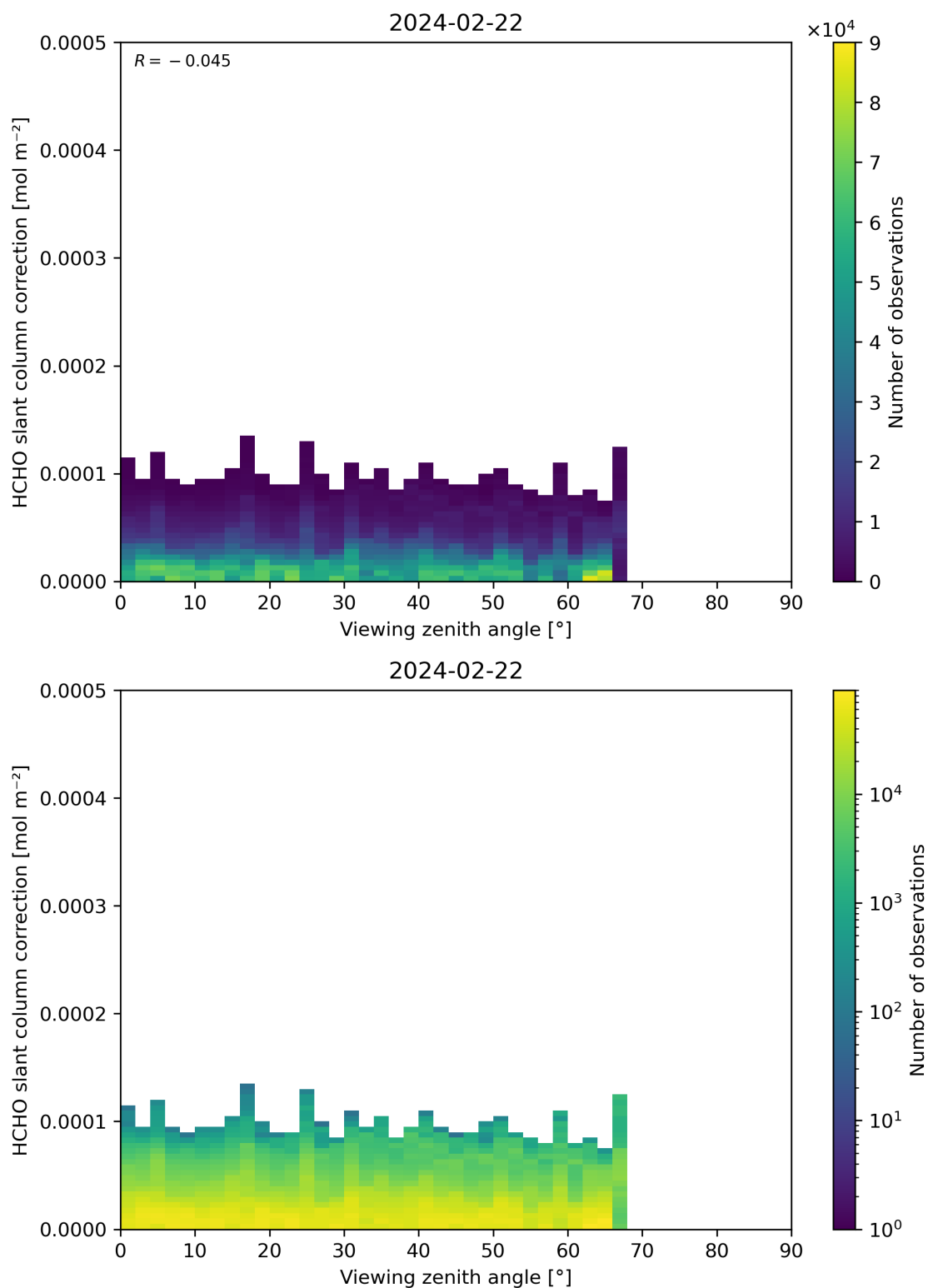
Figure 187: Scatter density plot of “Viewing zenith angle” against “HCHO slant column correction” for 2024-02-22 to 2024-02-23.
