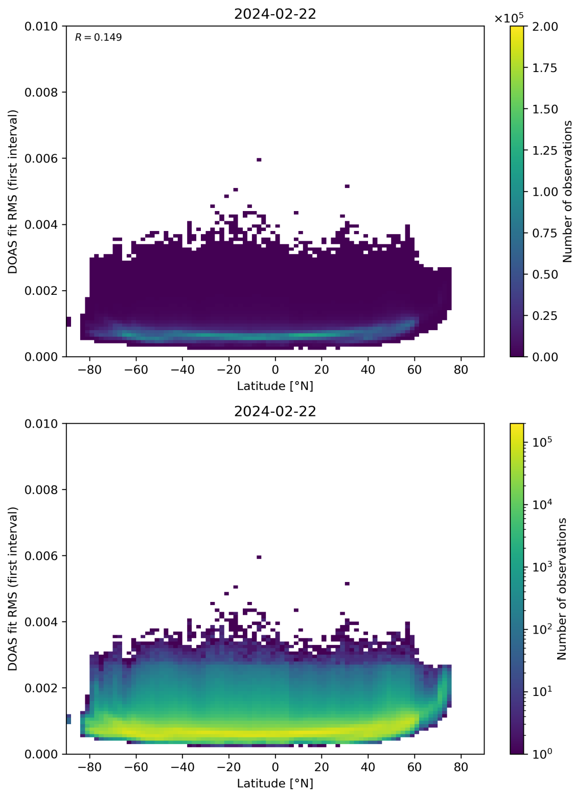
Figure 153: Scatter density plot of “Latitude” against “DOAS fit RMS (first interval)” for 2024-02-22 to 2024-02-23.
