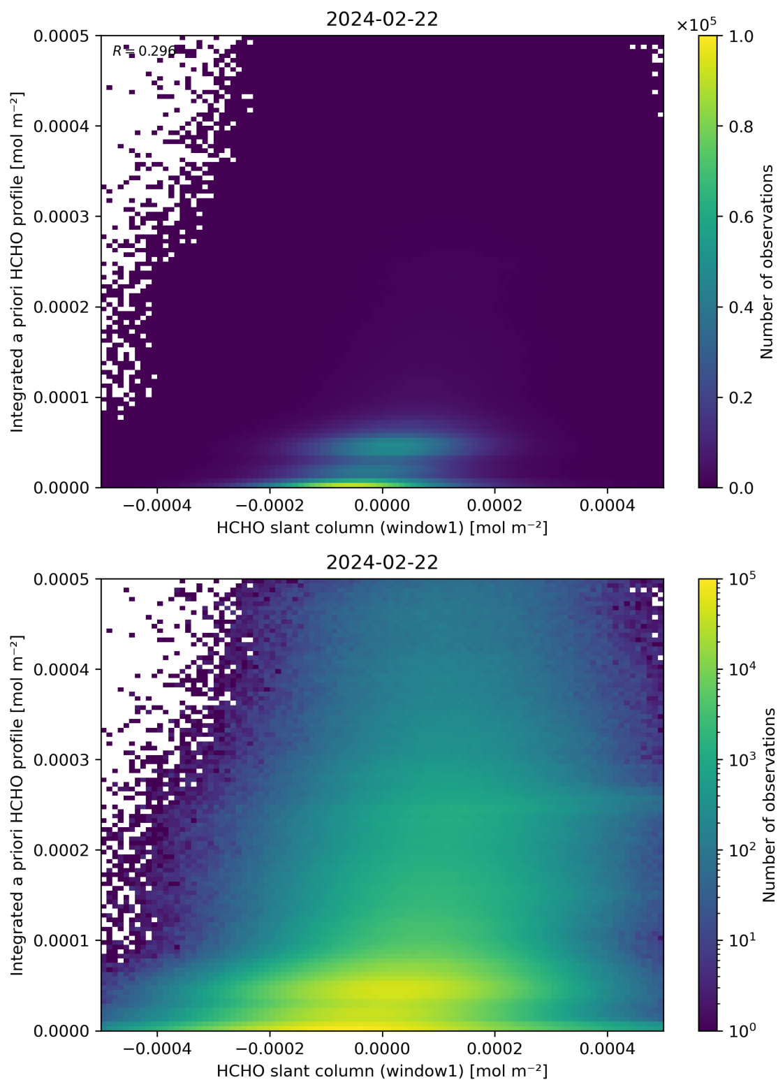
Figure 87: Scatter density plot of “HCHO slant column (window1)” against “Integrated a priori HCHO profile” for 2024-02-22 to 2024-02-23.
