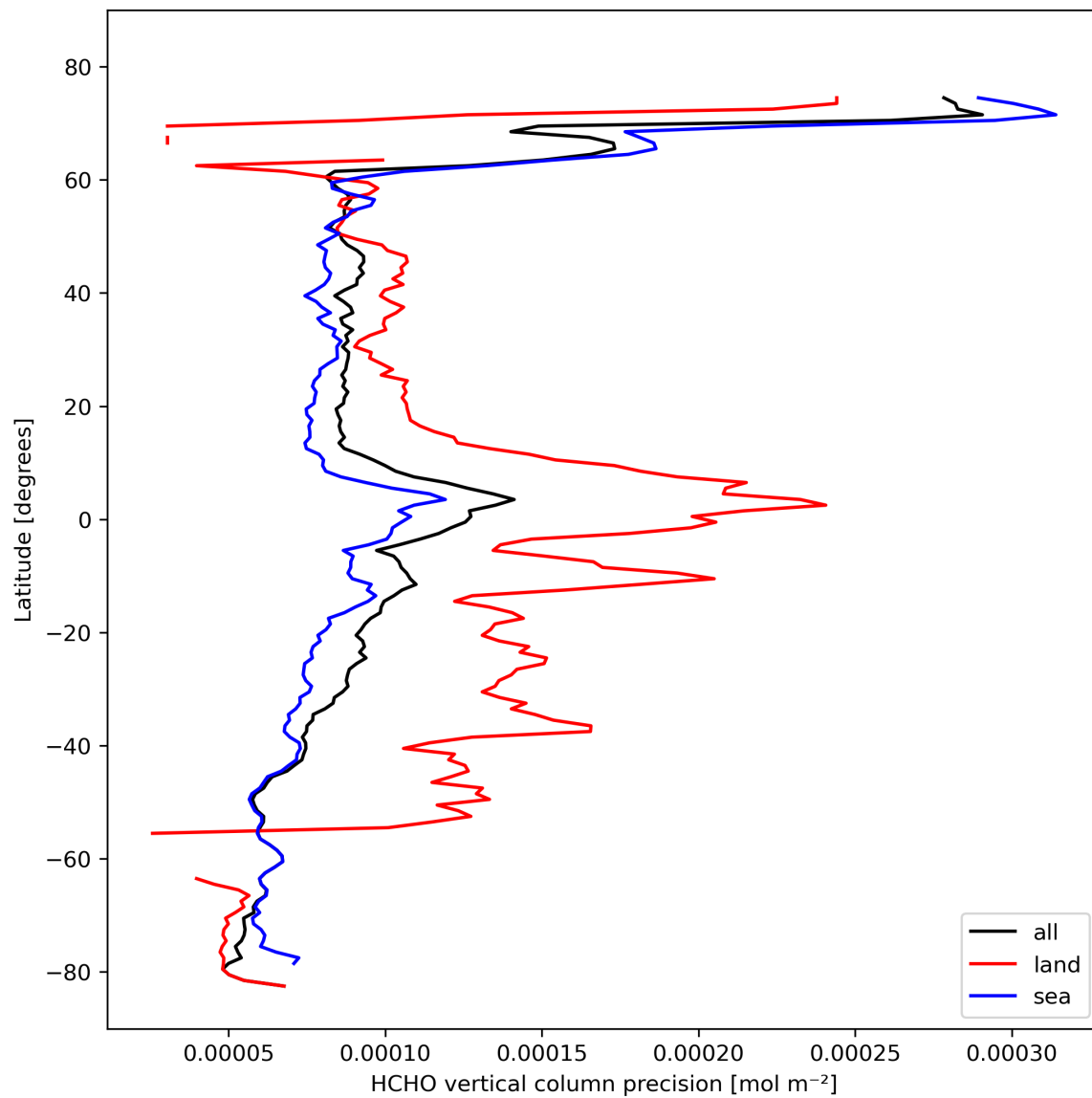
Figure 22: Zonal average of "HCHO vertical column precision" for 2024-02-22 to 2024-02-23.
