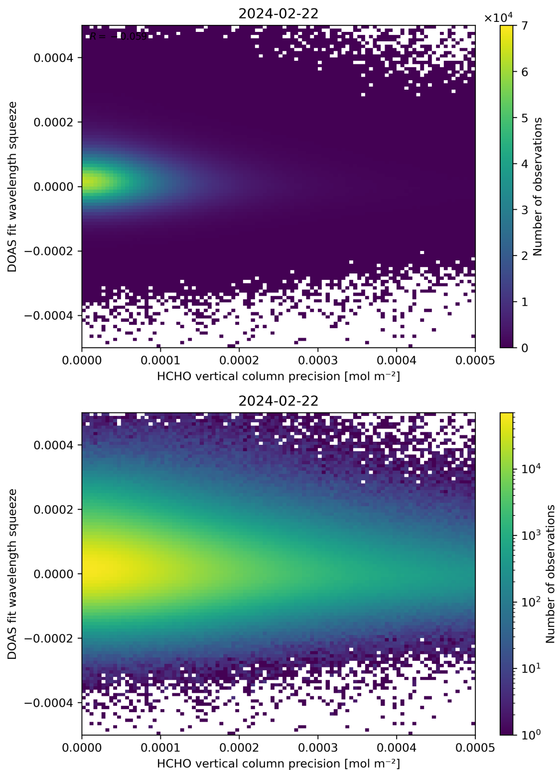
Figure 138: Scatter density plot of “HCHO vertical column precision” against “DOAS fit wavelength squeeze” for 2024-02-22 to 2024-02-23.
