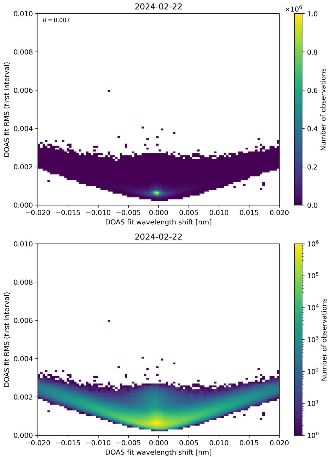
Figure 64: Scatter density plot of “DOAS fit wavelength shift” against “DOAS fit RMS (first interval)” for 2024-02-22 to 2024-02-23.
