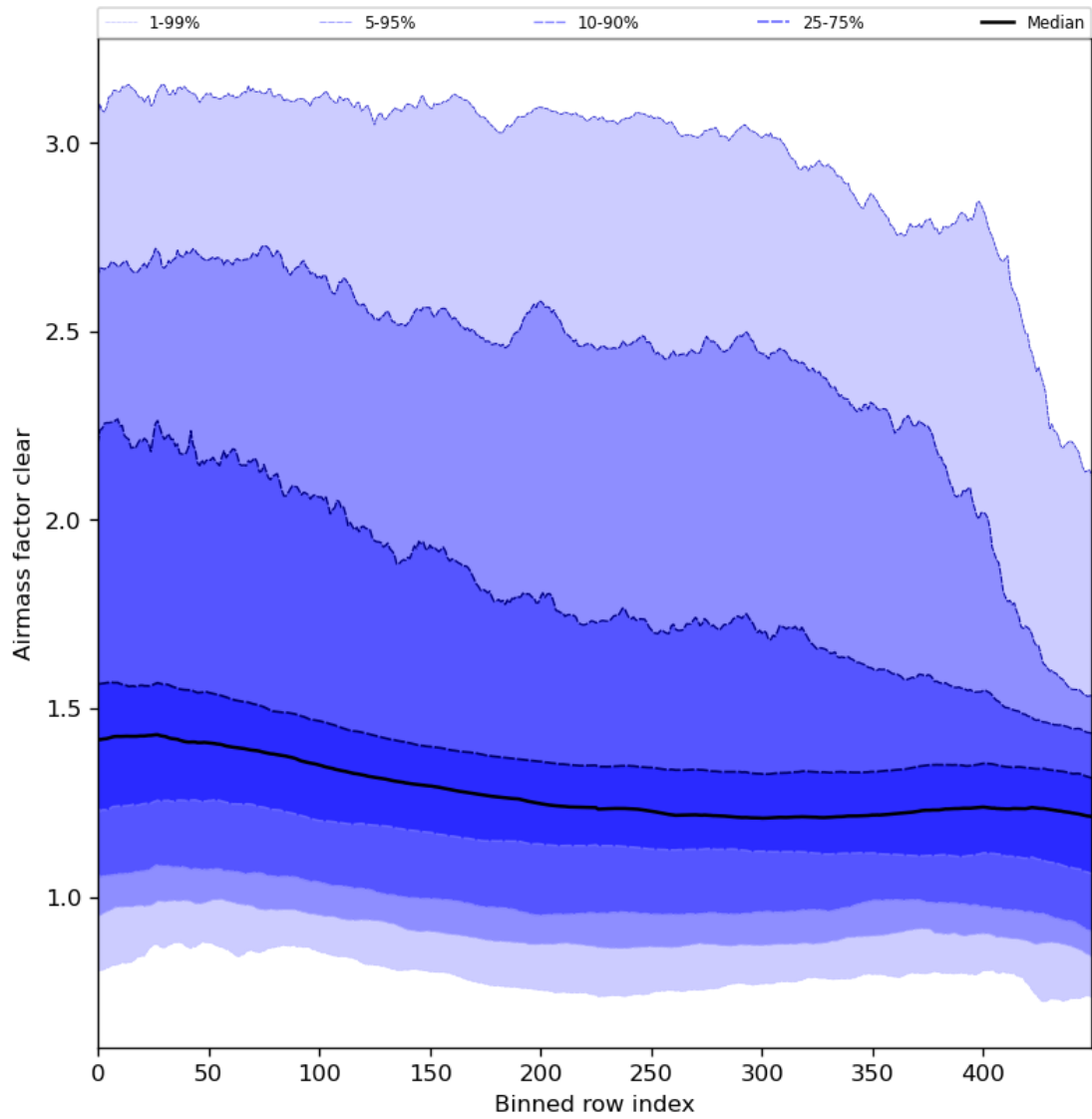
Figure 56: Along track statistics of “Airmass factor clear” for 2024-02-22 to 2024-02-23
