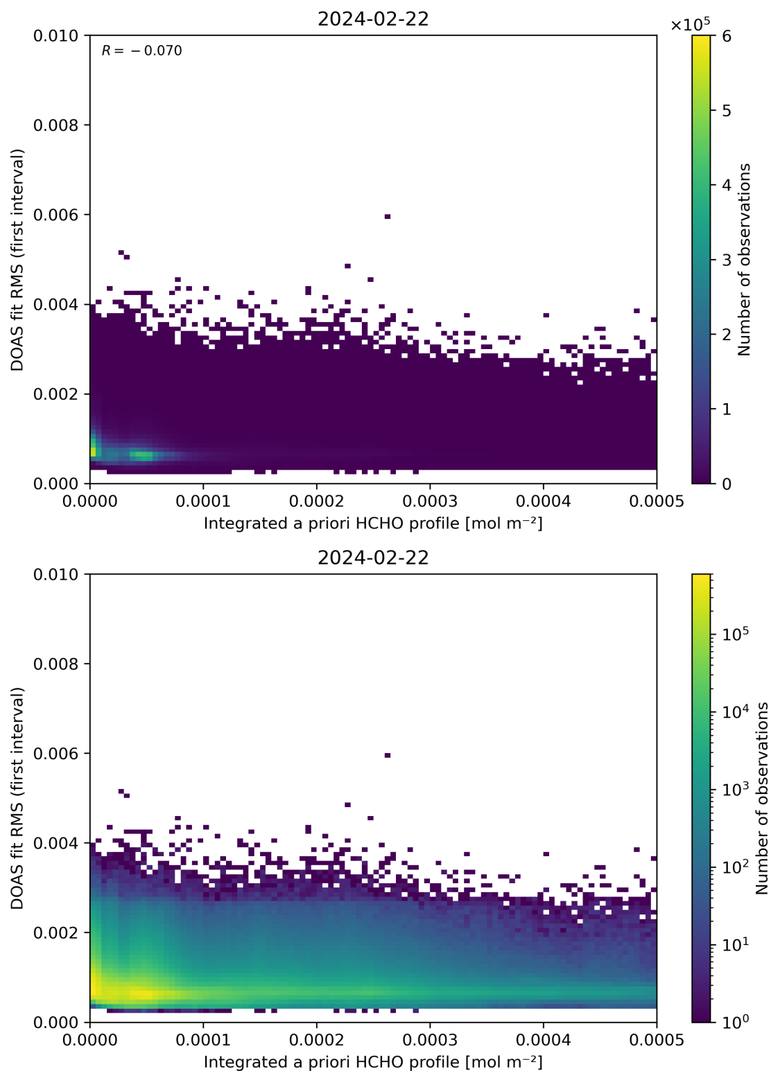
Figure 148: Scatter density plot of “Integrated a priori HCHO profile” against “DOAS fit RMS (first interval)” for 2024-02-22 to 2024-02-23.
