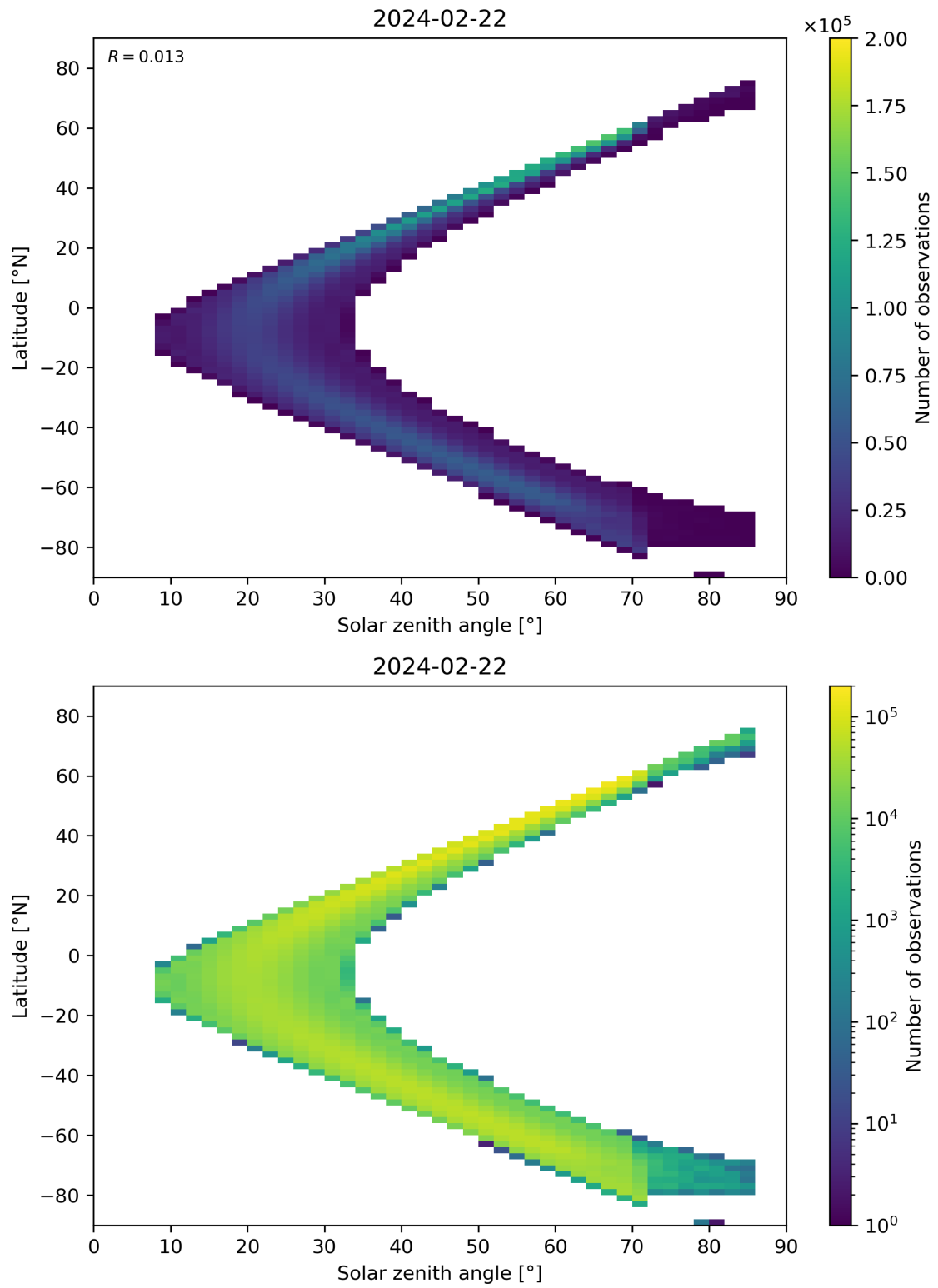
Figure 181: Scatter density plot of “Solar zenith angle” against “Latitude” for 2024-02-22 to 2024-02-23.
