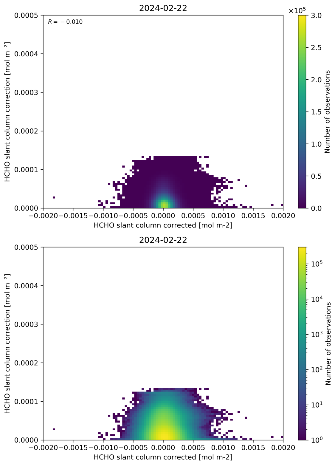
Figure 77: Scatter density plot of “HCHO slant column corrected” against “HCHO slant column correction” for 2024-02-22 to 2024-02-23.
