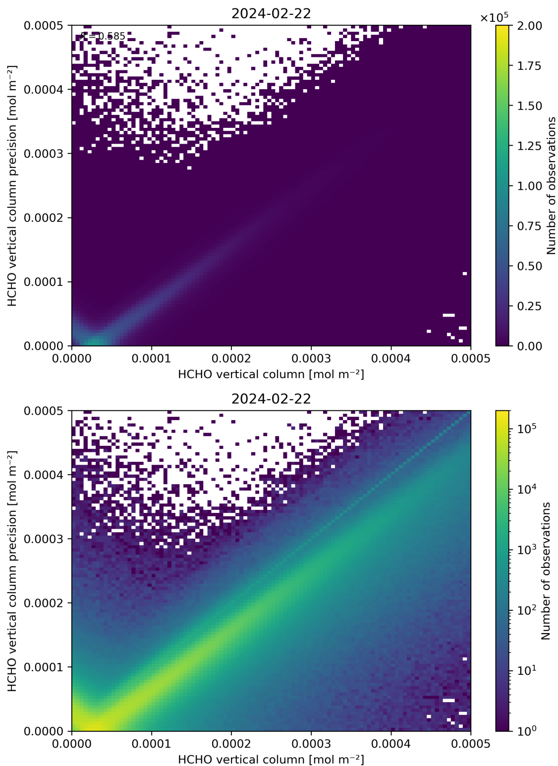
Figure 134: Scatter density plot of “HCHO vertical column” against “HCHO vertical column precision” for 2024-02-22 to 2024-02-23.
