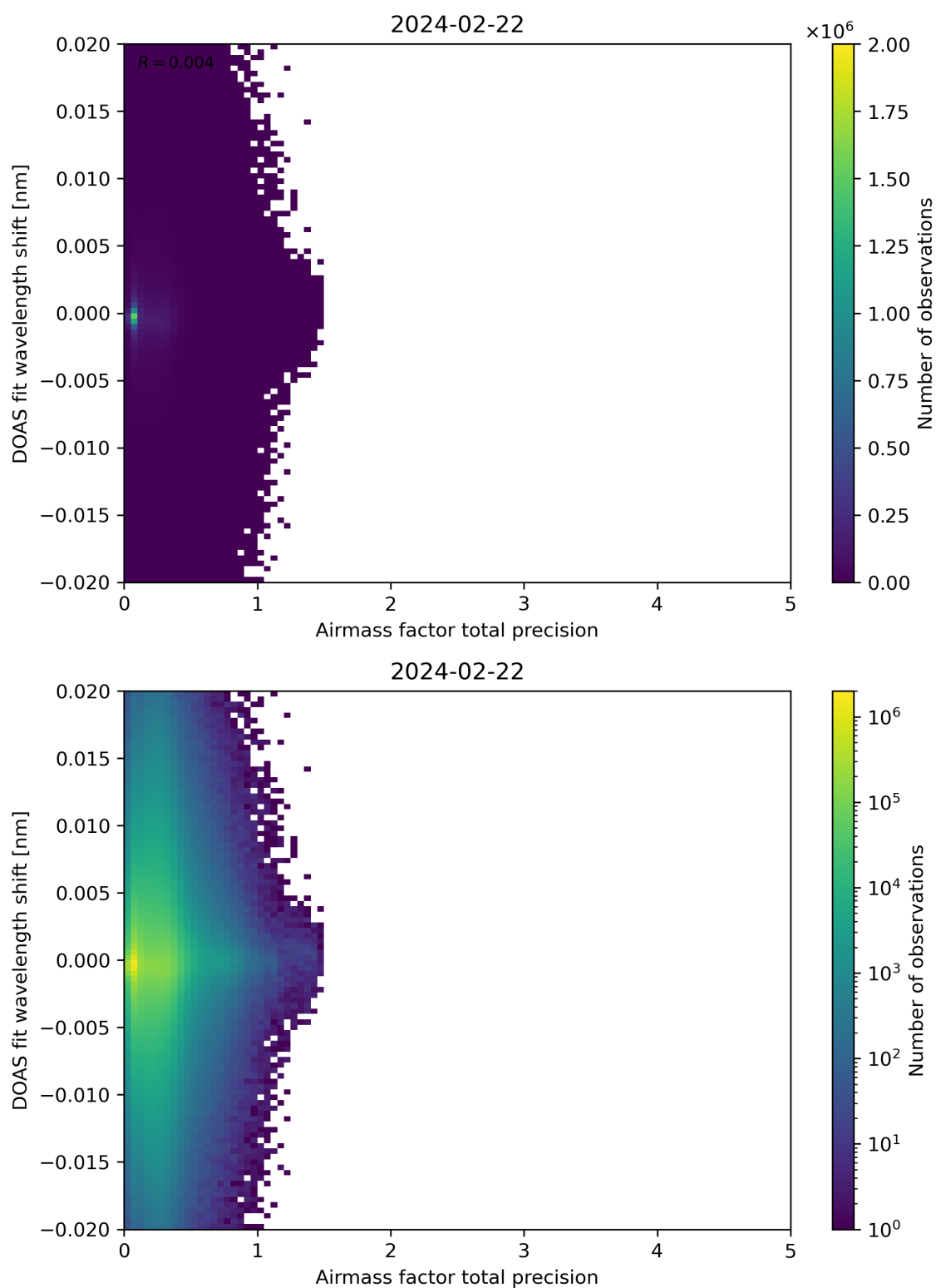
Figure 106: Scatter density plot of “Airmass factor total precision” against “DOAS fit wavelength shift” for 2024-02-22 to 2024-02-23.
