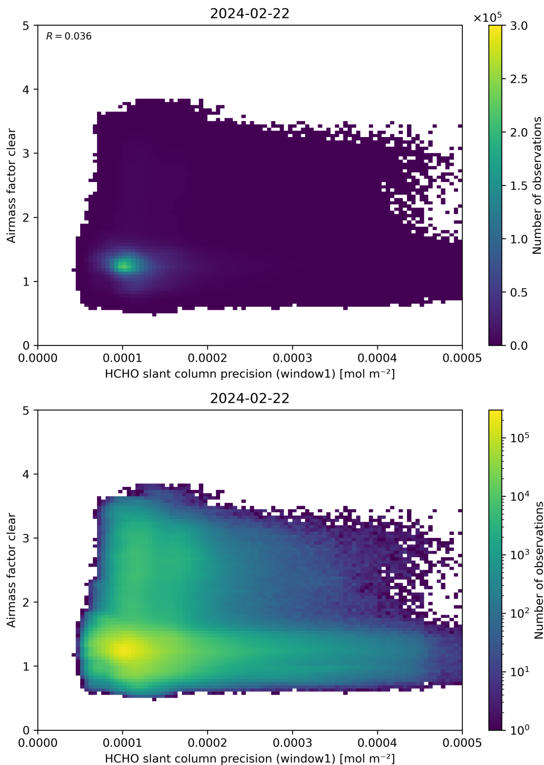
Figure 91: Scatter density plot of “HCHO slant column precision (window1)” against “Airmass factor clear” for 2024-02-22 to 2024-02-23.
