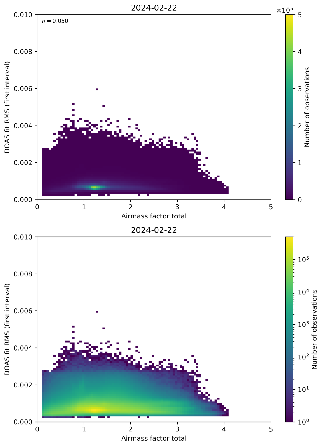
Figure 97: Scatter density plot of “Airmass factor total” against “DOAS fit RMS (first interval)” for 2024-02-22 to 2024-02-23.
