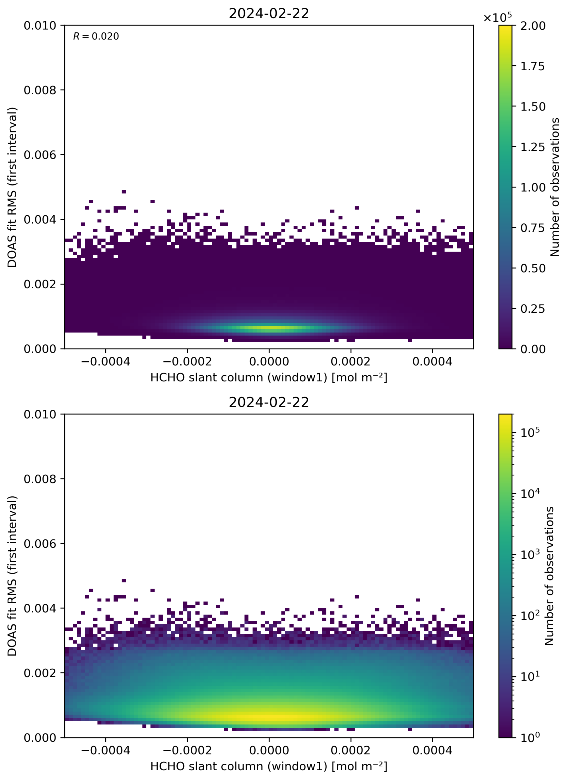
Figure 78: Scatter density plot of “HCHO slant column (window1)” against “DOAS fit RMS (first interval)” for 2024-02-22 to 2024-02-23.
