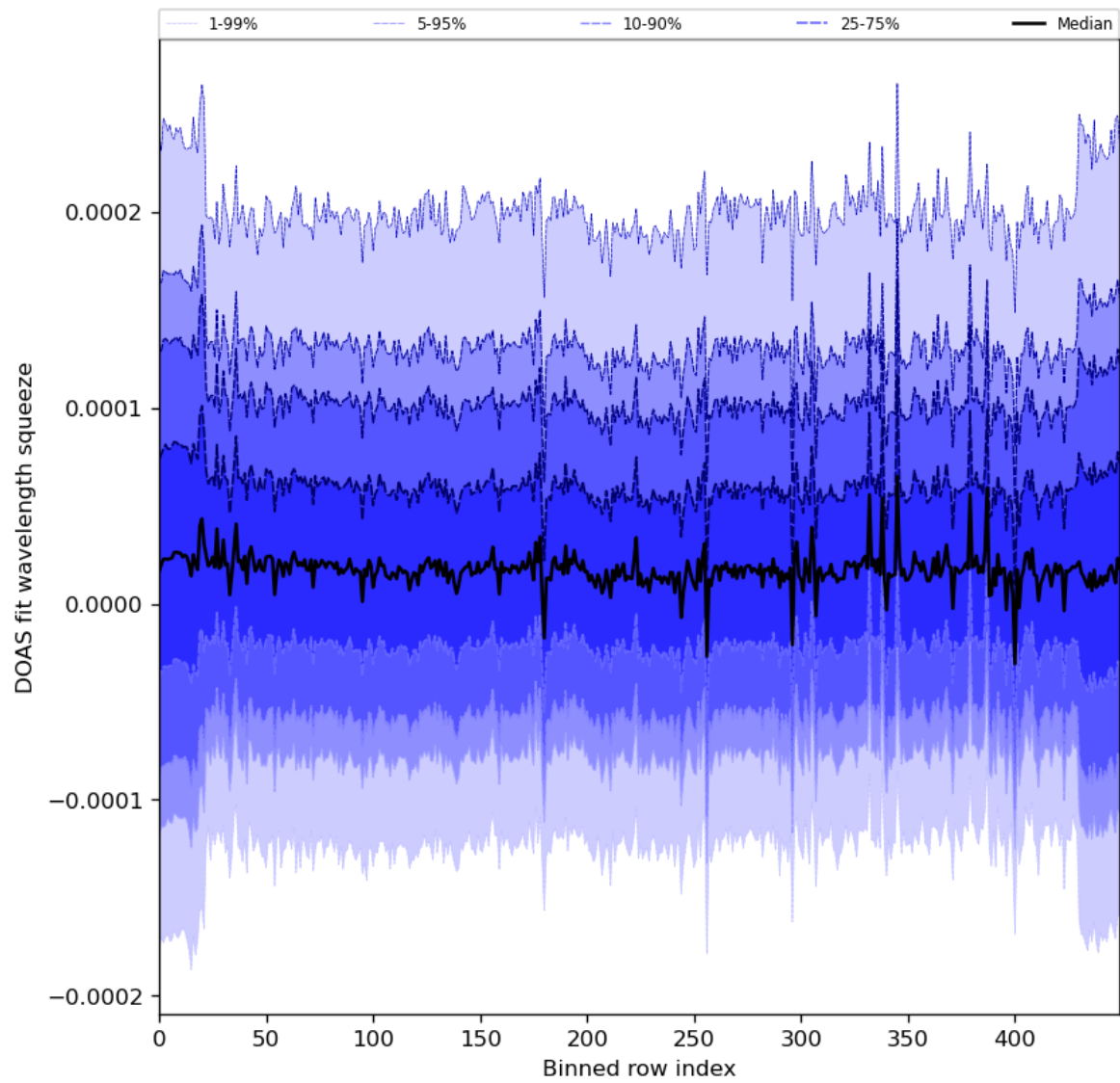
Figure 59: Along track statistics of “DOAS fit wavelength squeeze” for 2024-02-22 to 2024-02-23
