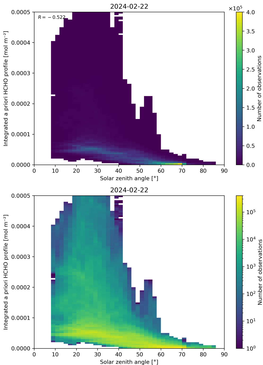
Figure 180: Scatter density plot of “Solar zenith angle” against “Integrated a priori HCHO profile” for 2024-02-22 to 2024-02-23.
