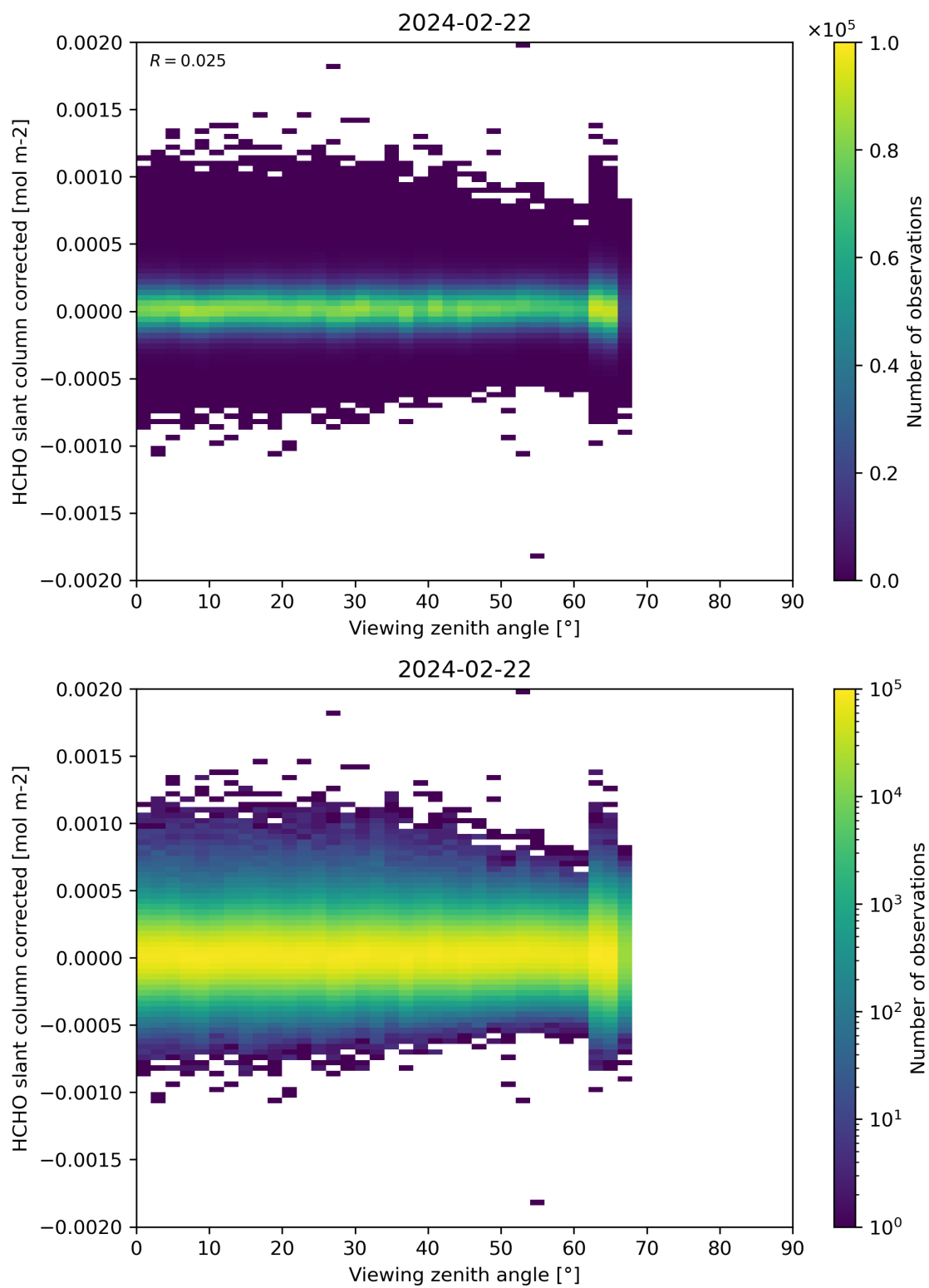
Figure 186: Scatter density plot of “Viewing zenith angle” against “HCHO slant column corrected” for 2024-02-22 to 2024-02-23.
