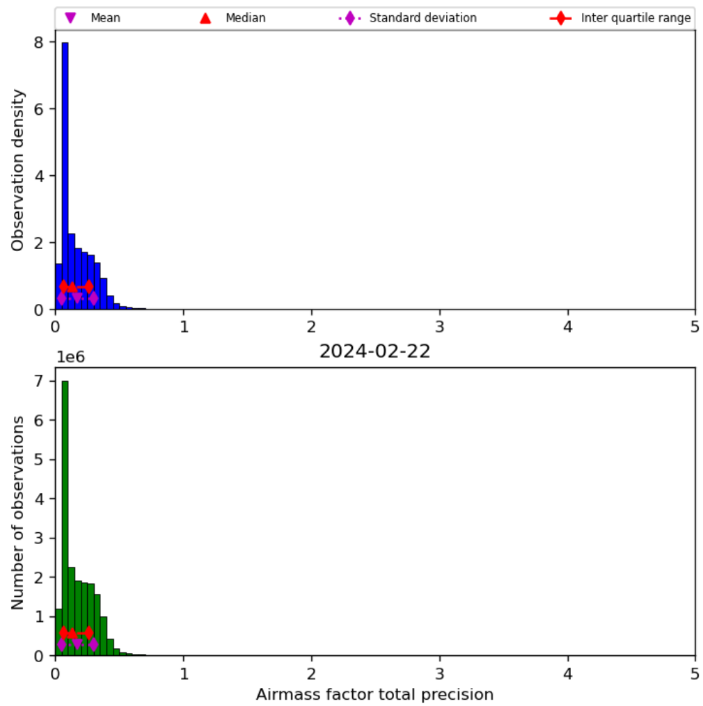
Figure 41: Histogram of “Airmass factor total precision” for 2024-02-22 to 2024-02-23
