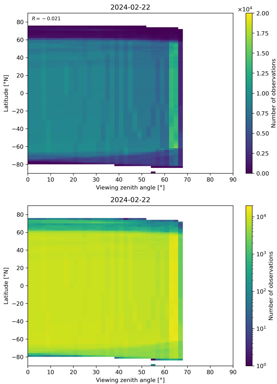
Figure 196: Scatter density plot of “Viewing zenith angle” against “Latitude” for 2024-02-22 to 2024-02-23.
