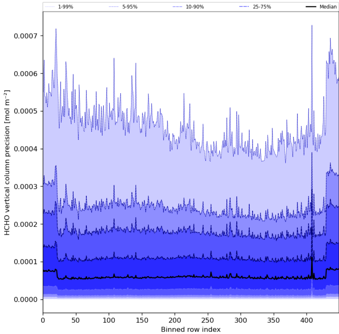
Figure 50: Along track statistics of “HCHO vertical column precision” for 2024-02-22 to 2024-02-23
