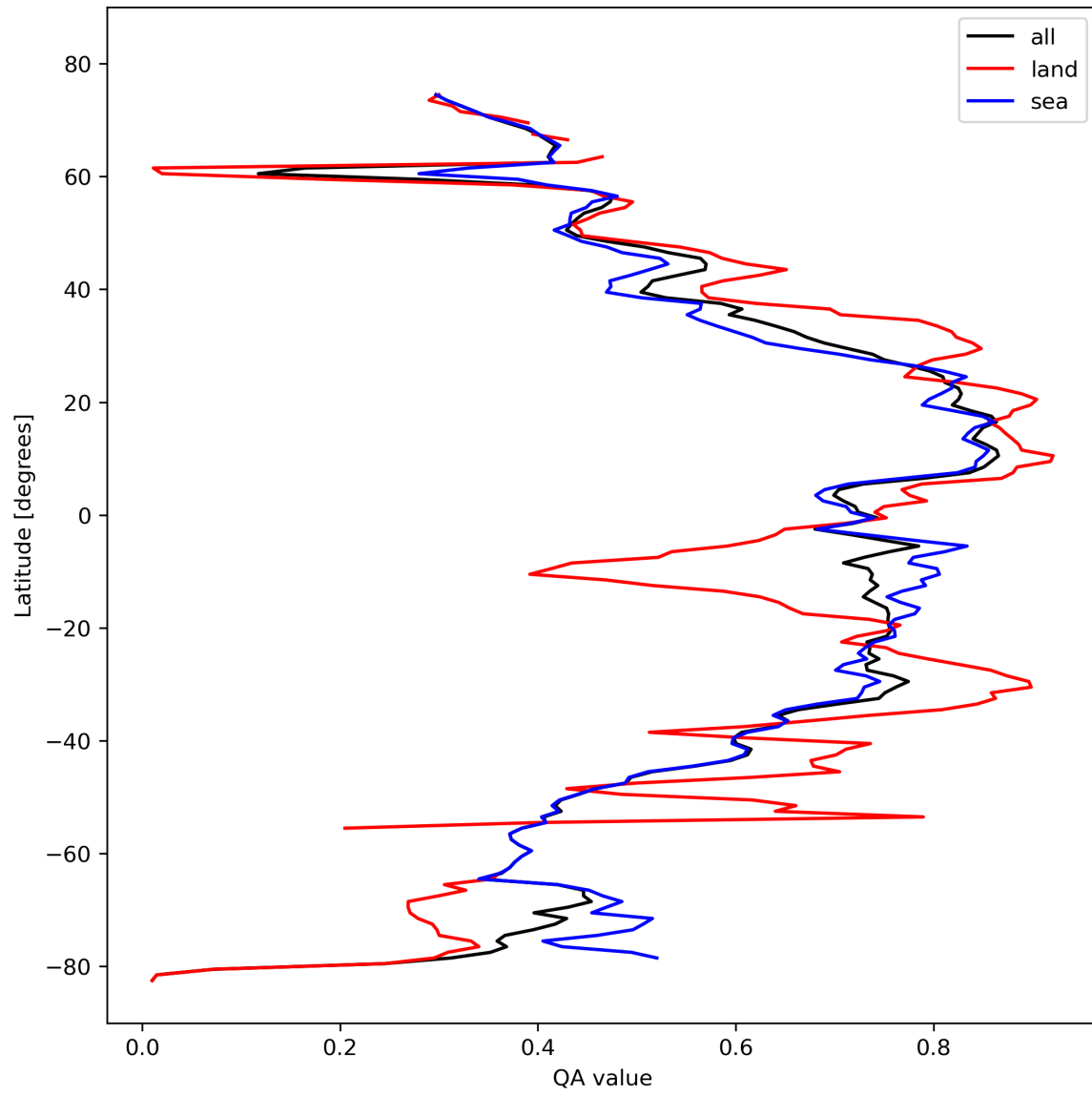
Figure 20: Zonal average of “QA value” for 2024-02-22 to 2024-02-23.
