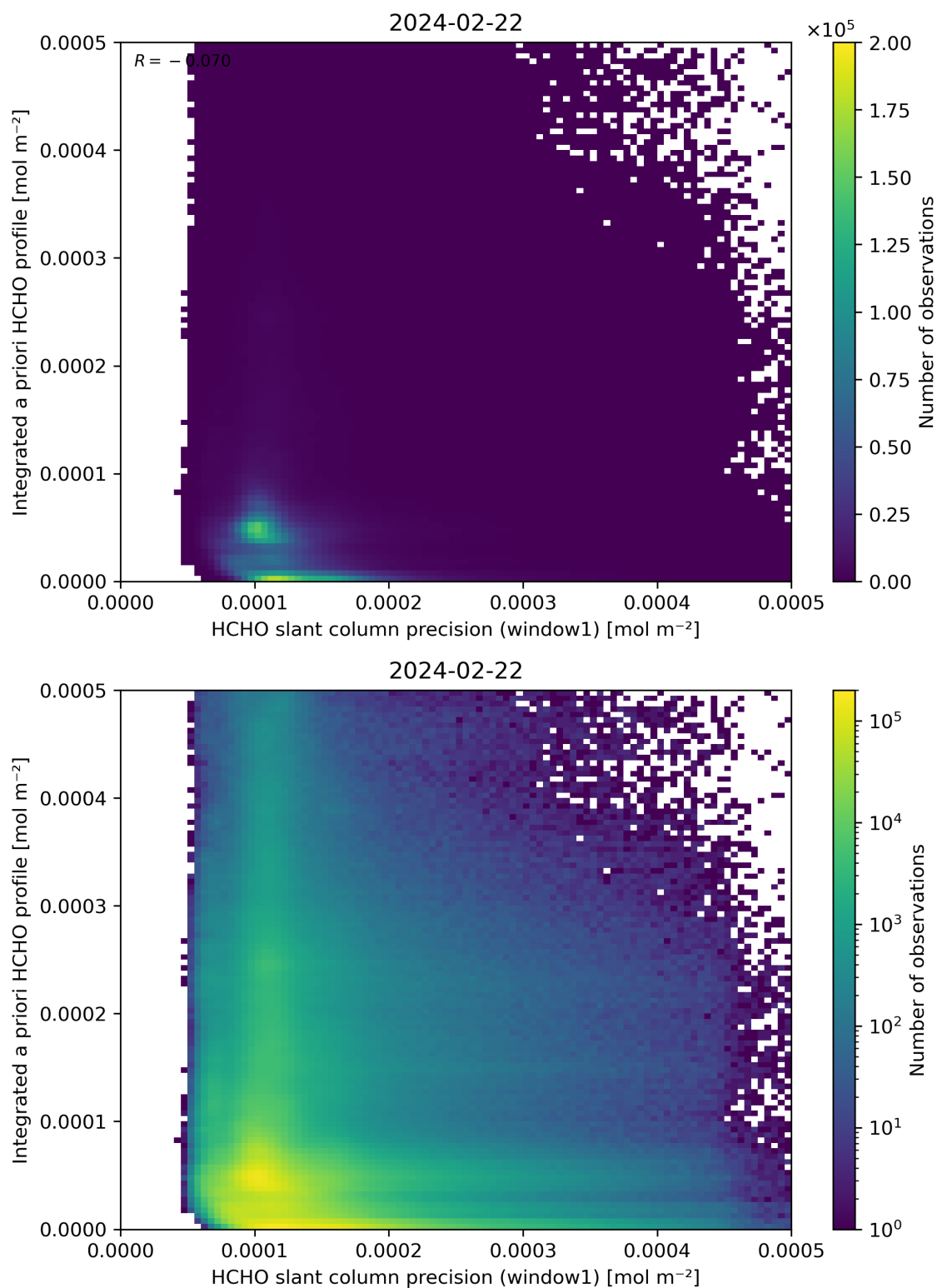
Figure 96: Scatter density plot of “HCHO slant column precision (window1)” against “Integrated a priori HCHO profile” for 2024-02-22 to 2024-02-23.
