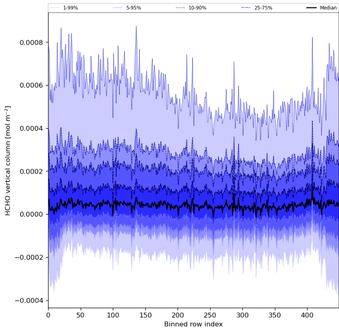
Figure 49: Along track statistics of “HCHO vertical column” for 2024-02-22 to 2024-02-23
