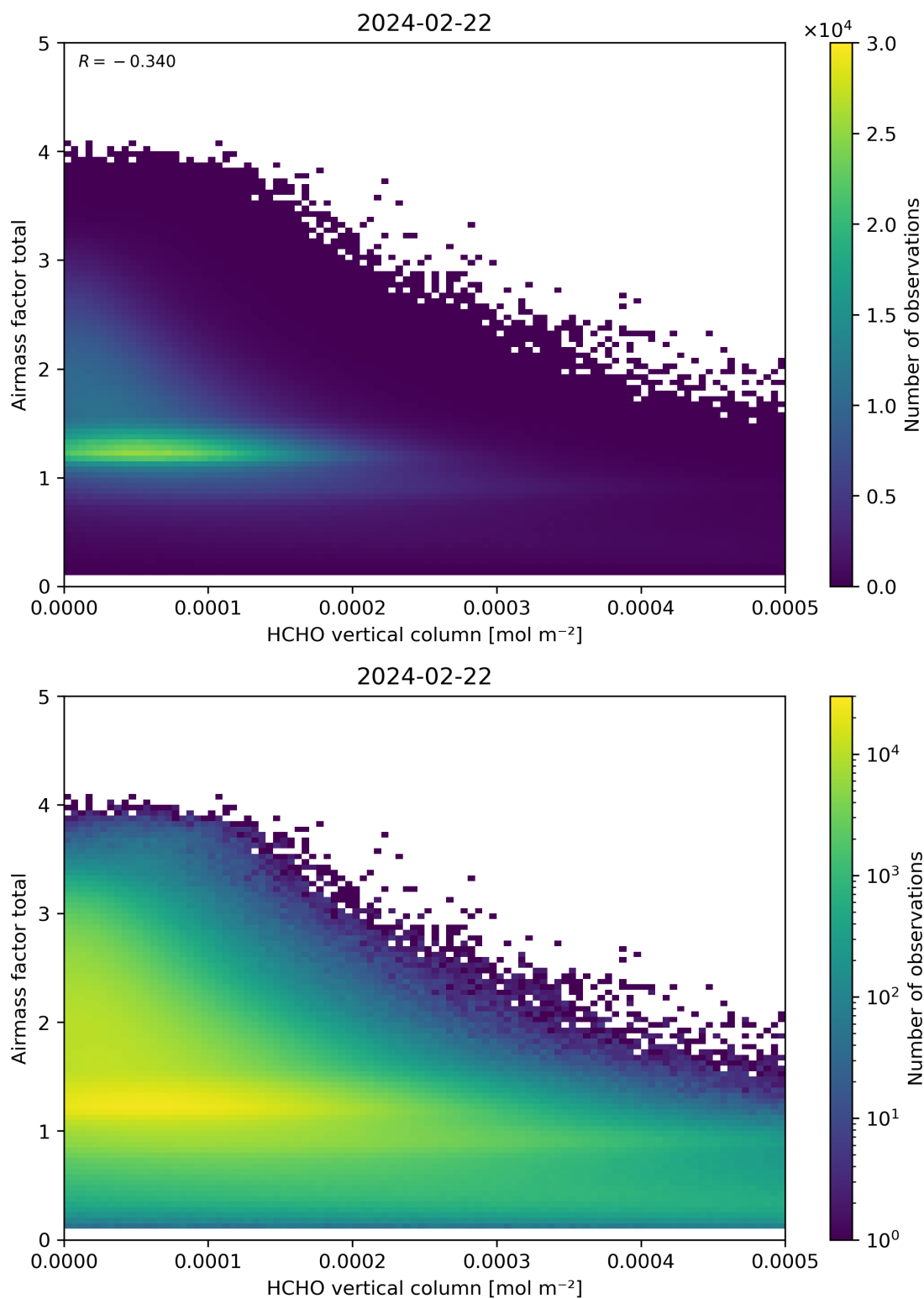
Figure 131: Scatter density plot of “HCHO vertical column” against “Airmass factor total” for 2024-02-22 to 2024-02-23.
