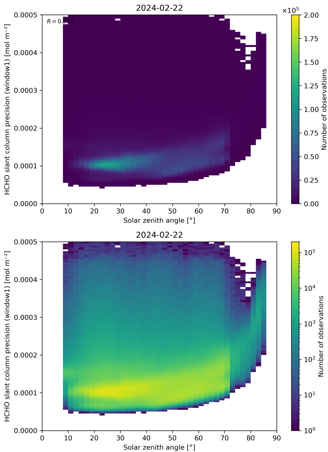
Figure 174: Scatter density plot of “Solar zenith angle” against “HCHO slant column precision (window1)” for 2024-02-22 to 2024-02-23.
