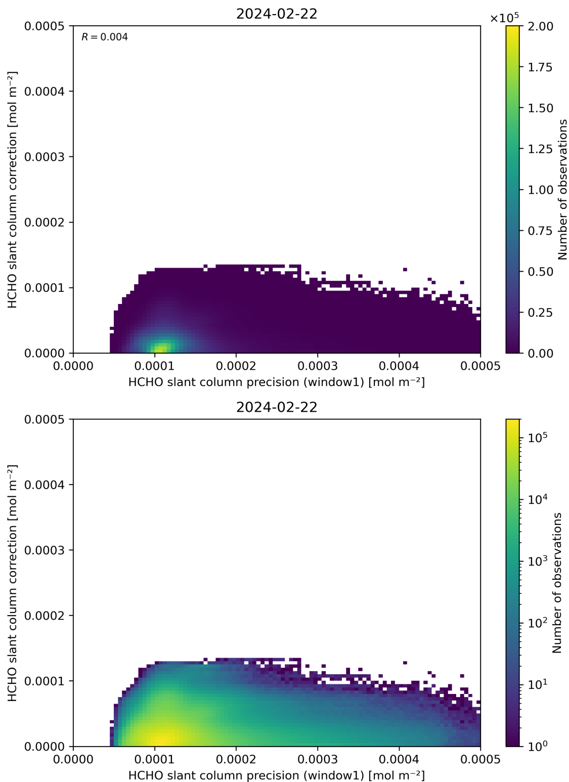
Figure 93: Scatter density plot of “HCHO slant column precision (window1)” against “HCHO slant column correction” for 2024-02-22 to 2024-02-23.
