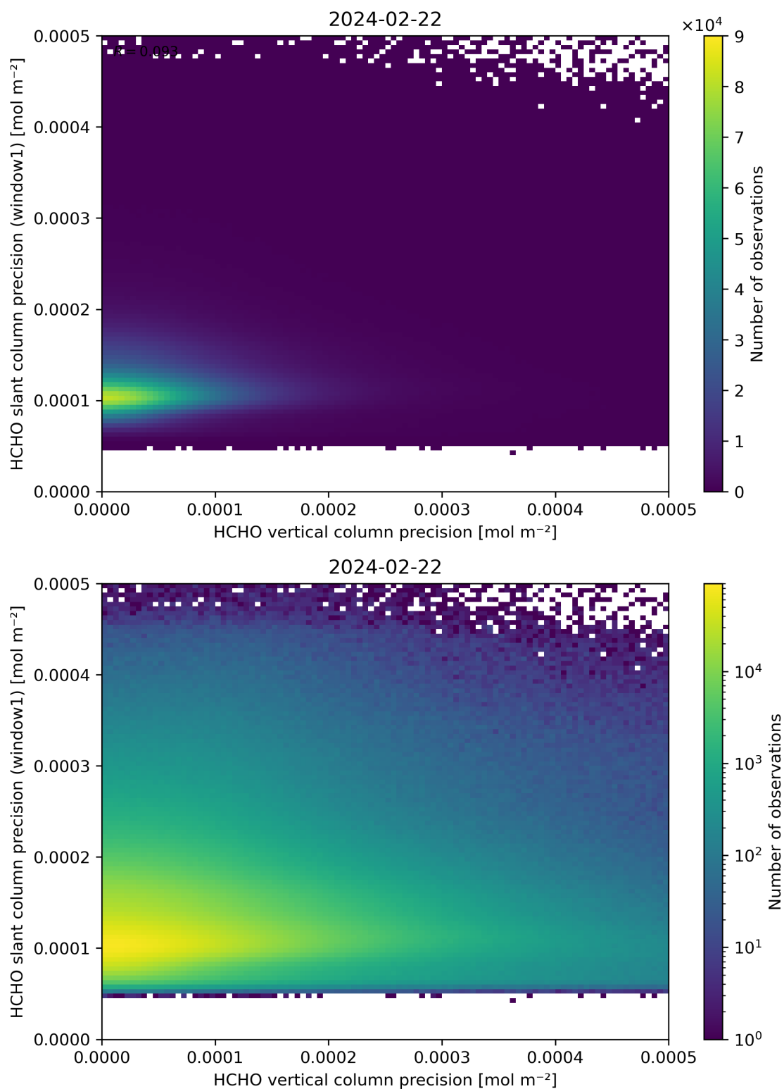
Figure 143: Scatter density plot of “HCHO vertical column precision” against “HCHO slant column precision (window1)” for 2024-02-22 to 2024-02-23.
