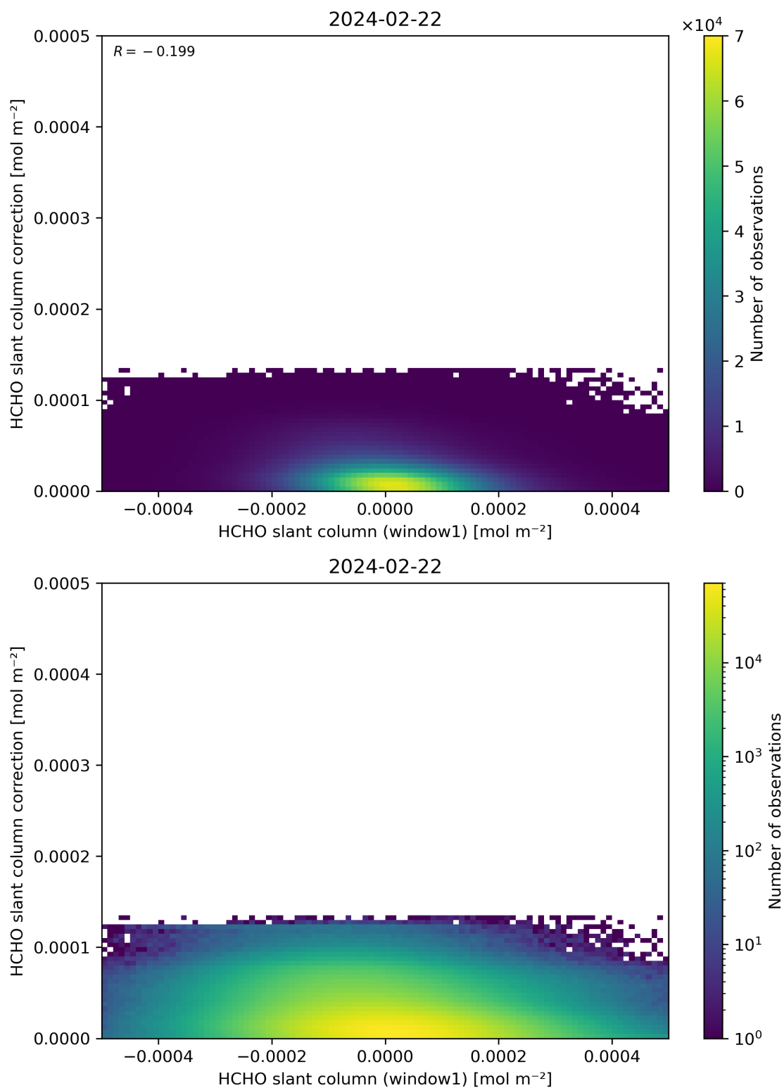
Figure 83: Scatter density plot of “HCHO slant column (window1)” against “HCHO slant column correction” for 2024-02-22 to 2024-02-23.
