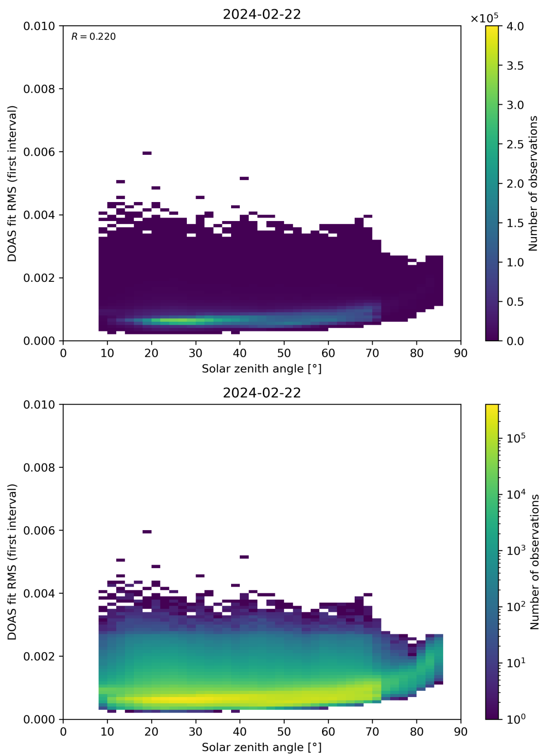
Figure 167: Scatter density plot of “Solar zenith angle” against “DOAS fit RMS (first interval)” for 2024-02-22 to 2024-02-23.
