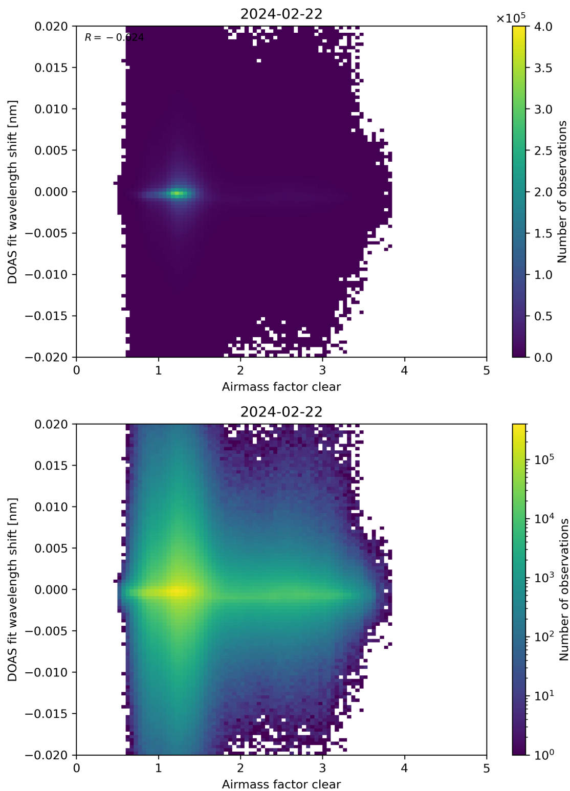
Figure 72: Scatter density plot of “Airmass factor clear” against “DOAS fit wavelength shift” for 2024-02-22 to 2024-02-23.
