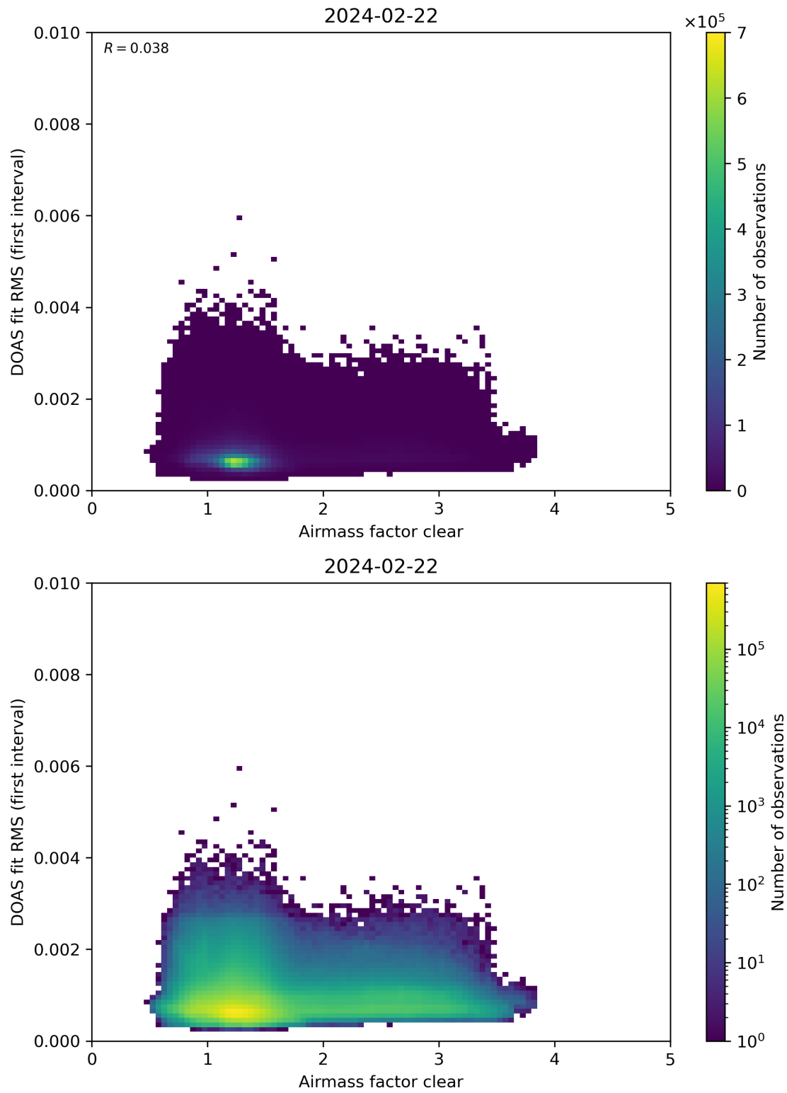
Figure 71: Scatter density plot of “Airmass factor clear” against “DOAS fit RMS (first interval)” for 2024-02-22 to 2024-02-23.
