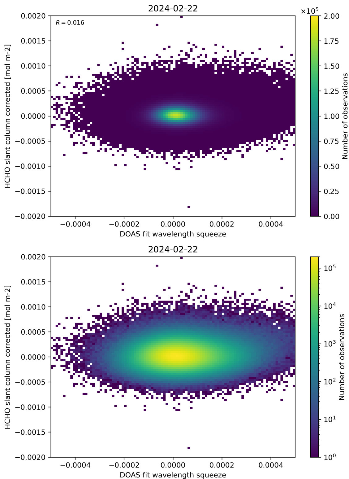
Figure 69: Scatter density plot of “DOAS fit wavelength squeeze” against “HCHO slant column corrected” for 2024-02-22 to 2024-02-23.
