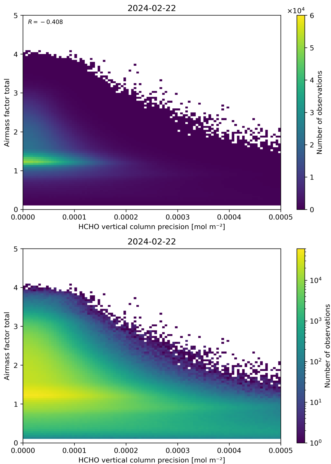
Figure 144: Scatter density plot of “HCHO vertical column precision” against “Airmass factor total” for 2024-02-22 to 2024-02-23.
