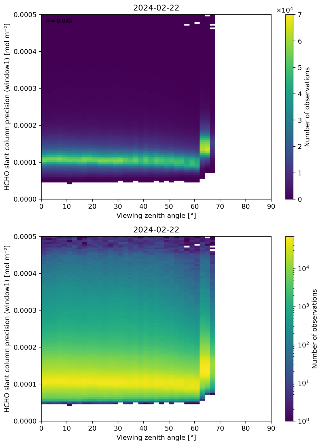
Figure 189: Scatter density plot of “Viewing zenith angle” against “HCHO slant column precision (window1)” for 2024-02-22 to 2024-02-23.
