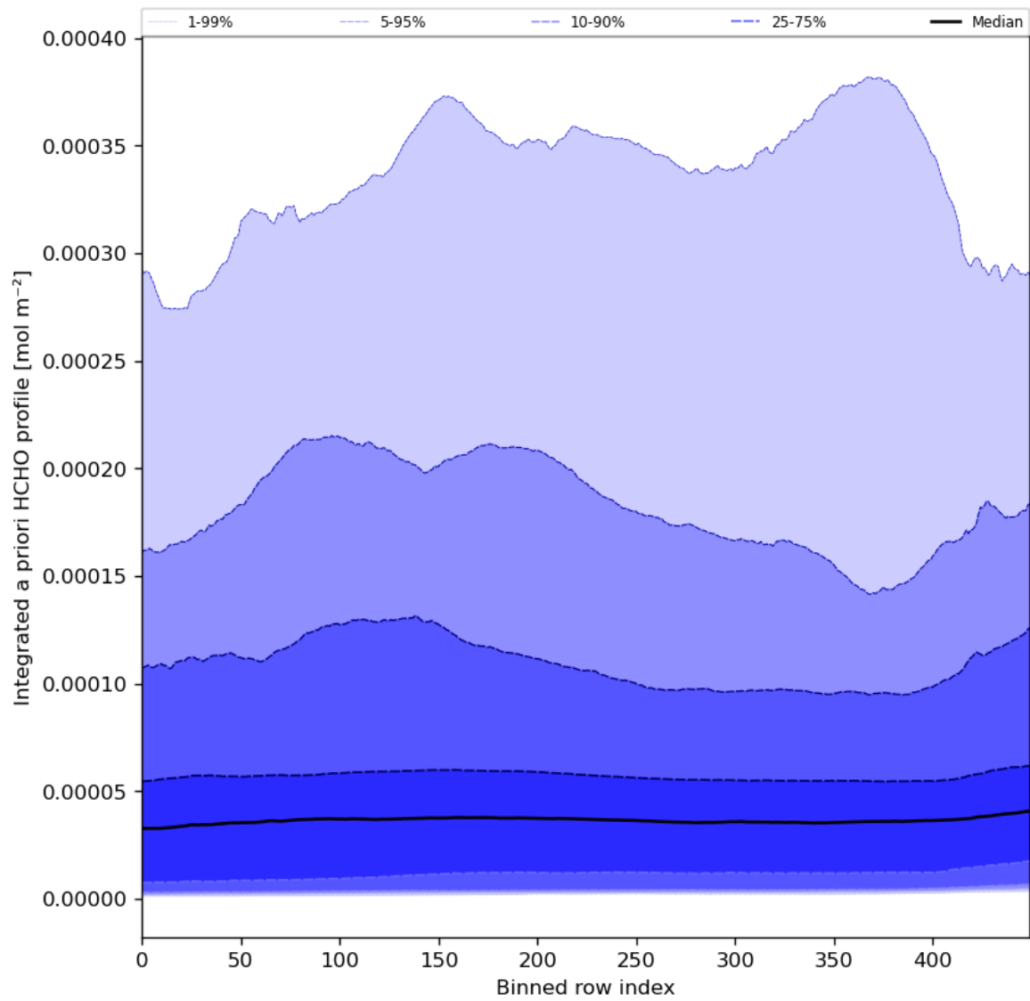
Figure 57: Along track statistics of “Integrated a priori HCHO profile” for 2024-02-22 to 2024-02-23
