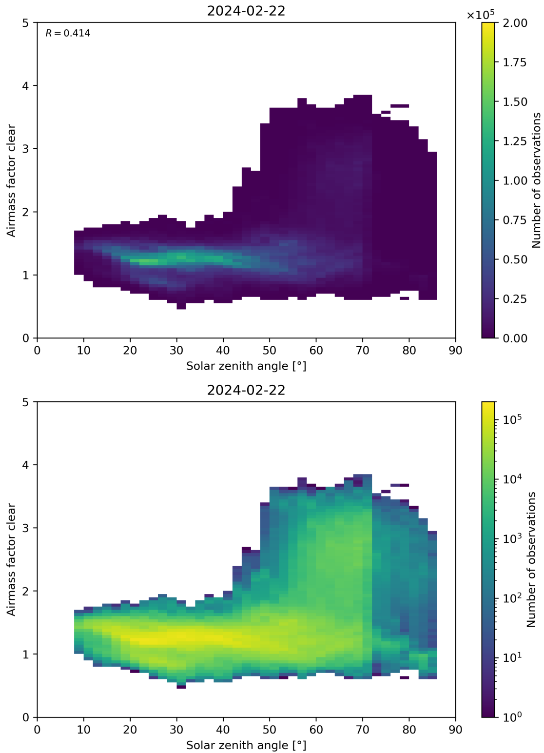
Figure 170: Scatter density plot of “Solar zenith angle” against “Airmass factor clear” for 2024-02-22 to 2024-02-23.
