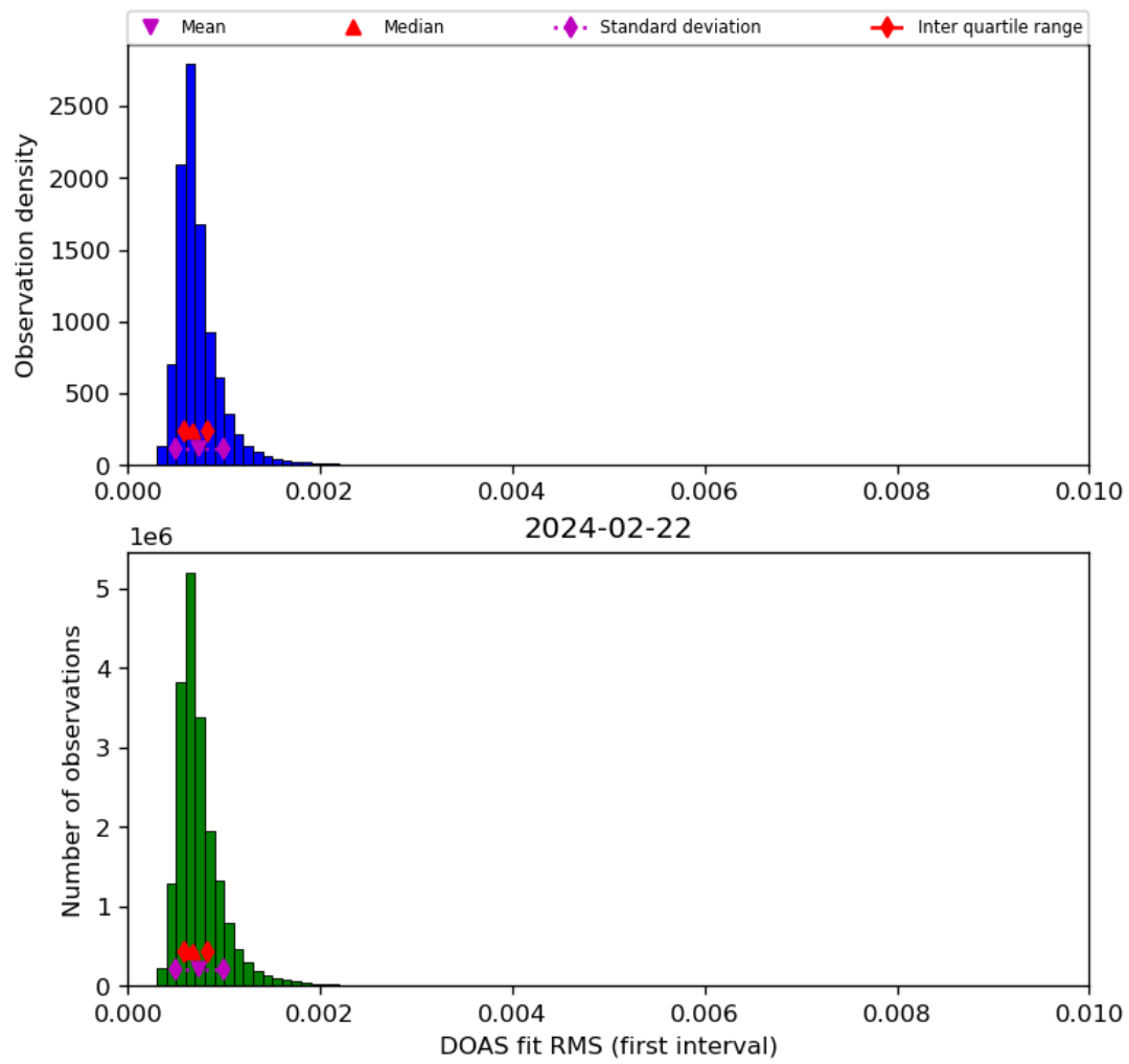
Figure 46: Histogram of “DOAS fit RMS (first interval)” for 2024-02-22 to 2024-02-23
