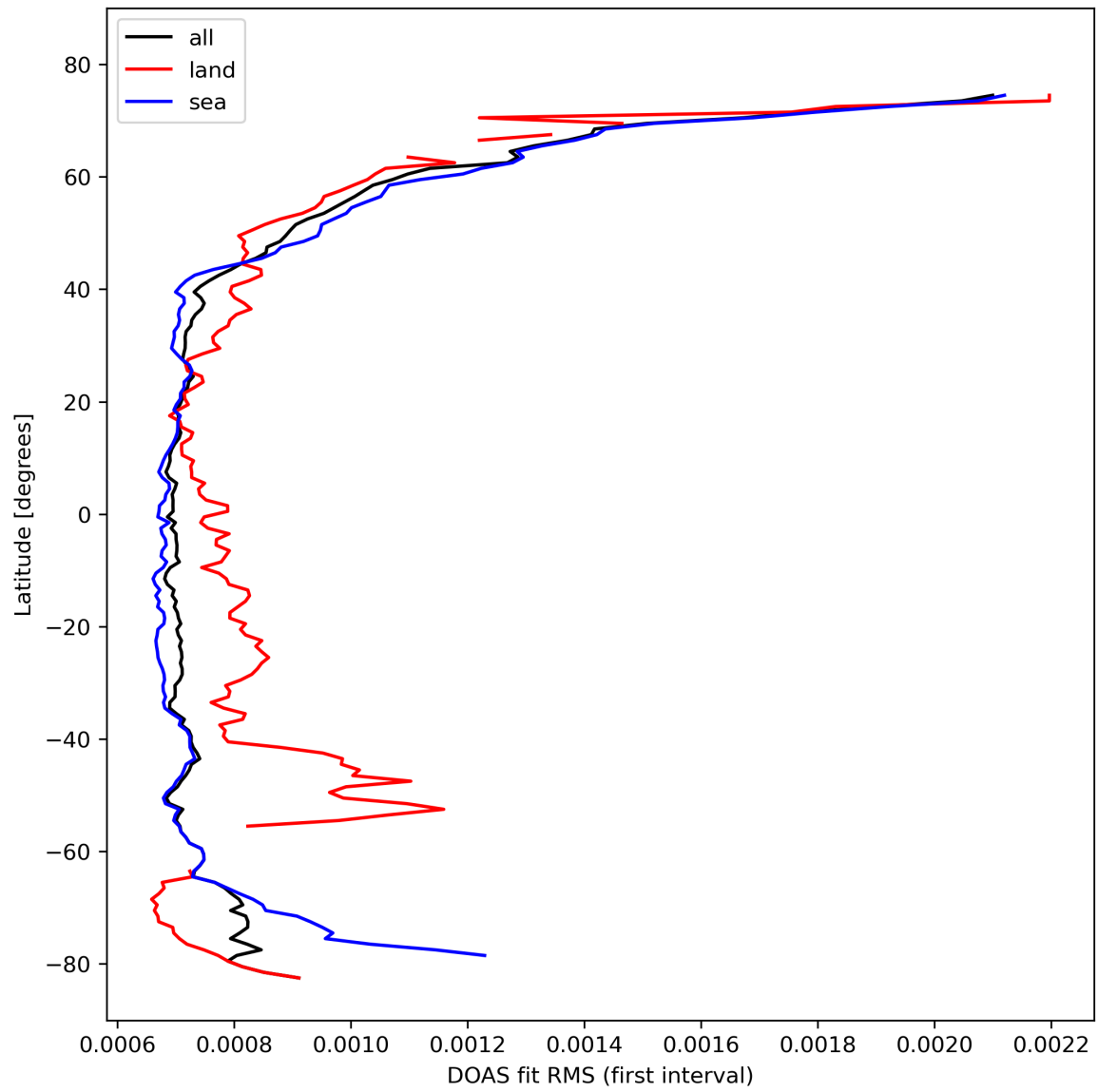
Figure 32: Zonal average of “DOAS fit RMS (first interval)” for 2024-02-22 to 2024-02-23.
