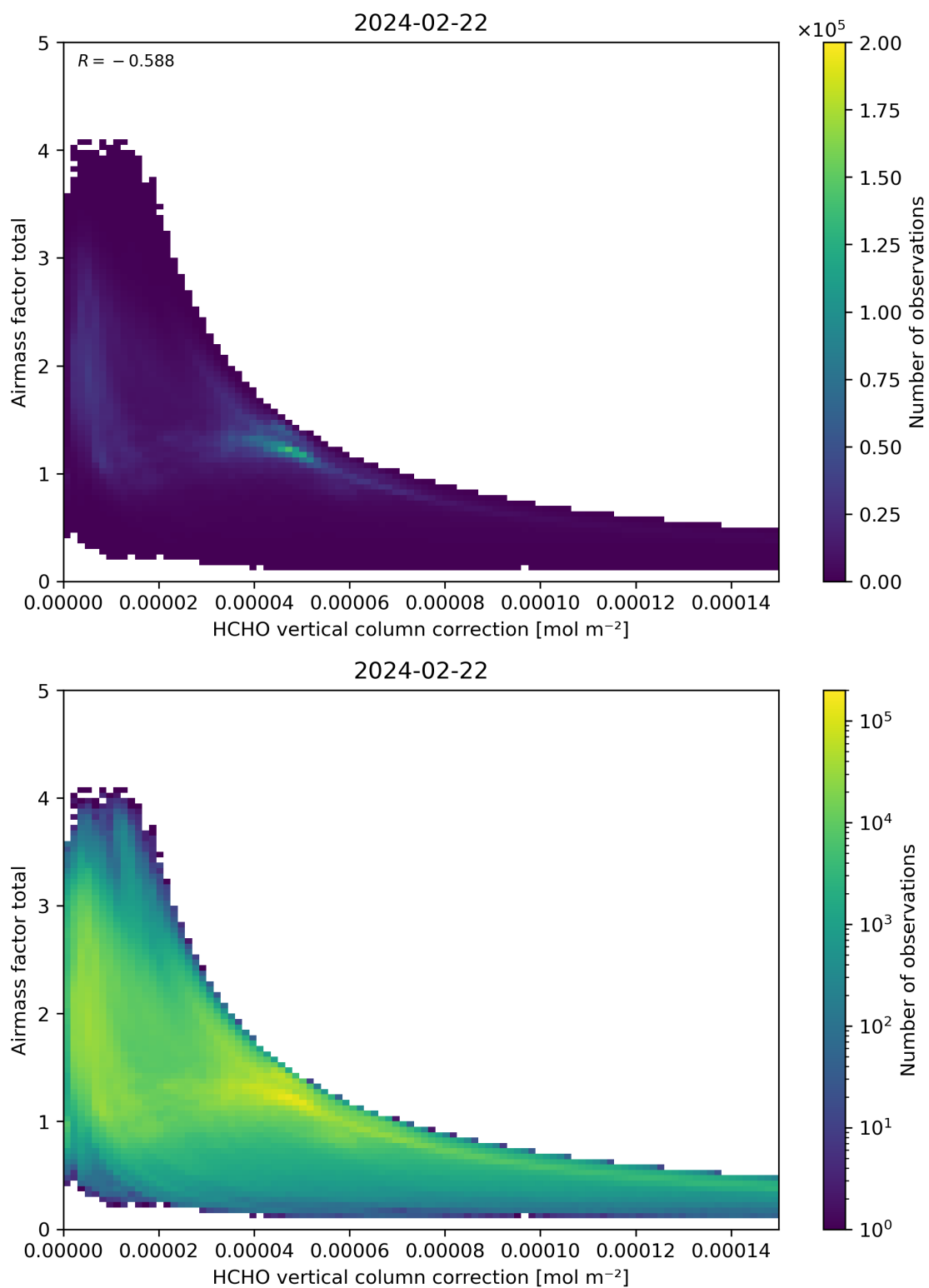
Figure 120: Scatter density plot of “HCHO vertical column correction” against “Airmass factor total” for 2024-02-22 to 2024-02-23.
