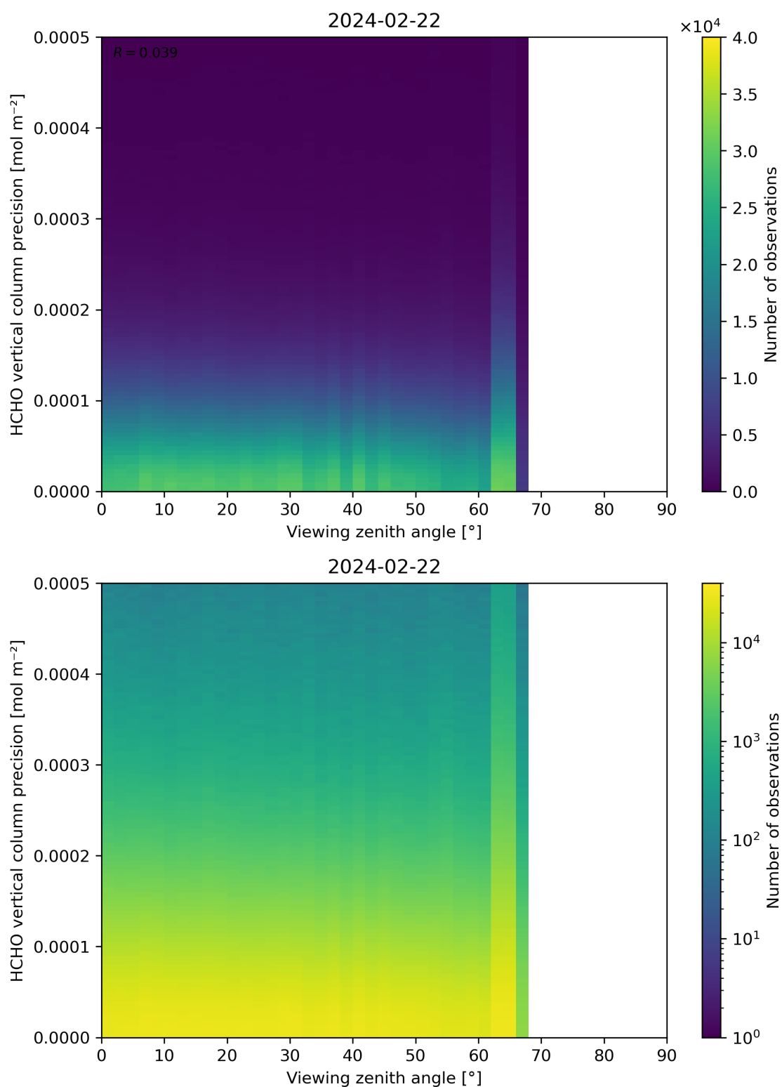
Figure 194: Scatter density plot of “Viewing zenith angle” against “HCHO vertical column precision” for 2024-02-22 to 2024-02-23.
