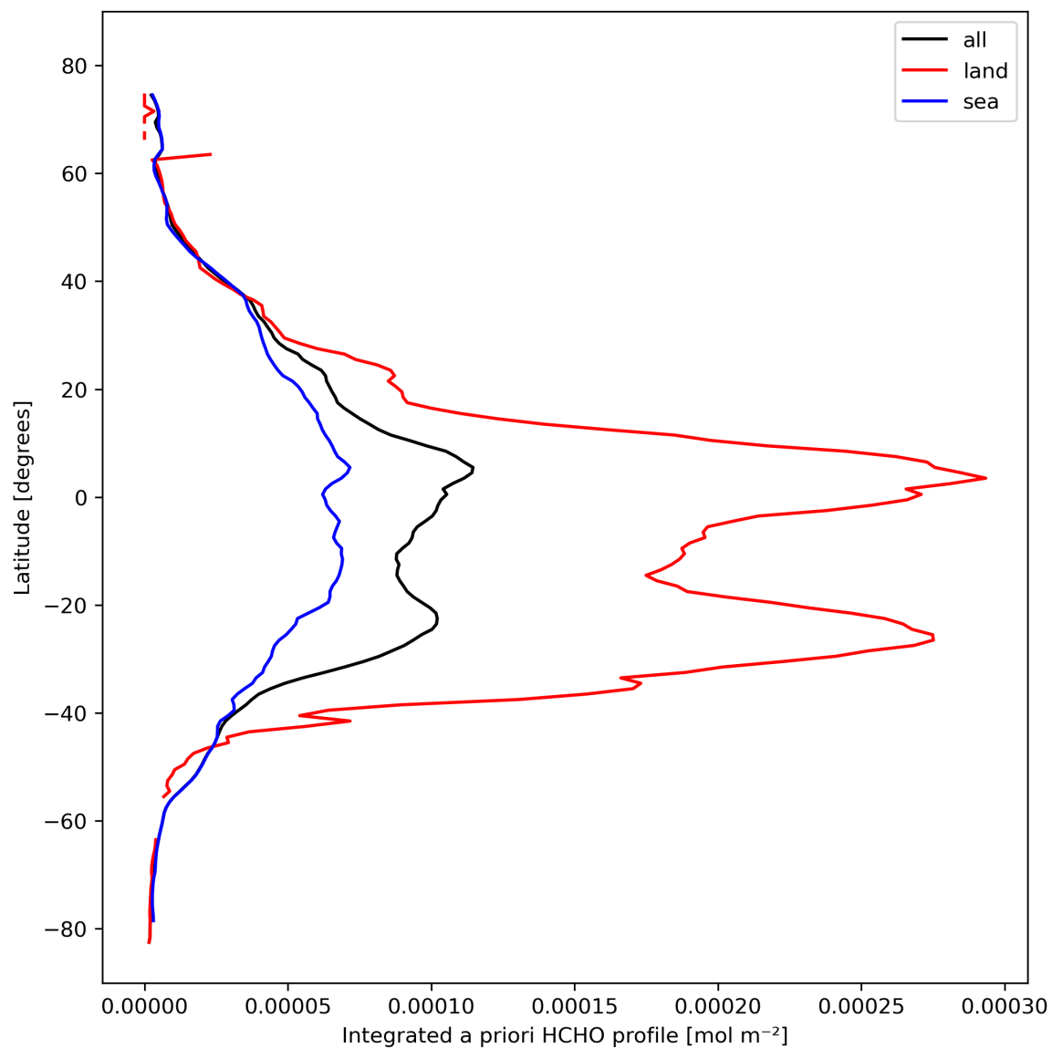
Figure 29: Zonal average of “Integrated a priori HCHO profile” for 2024-02-22 to 2024-02-23.
