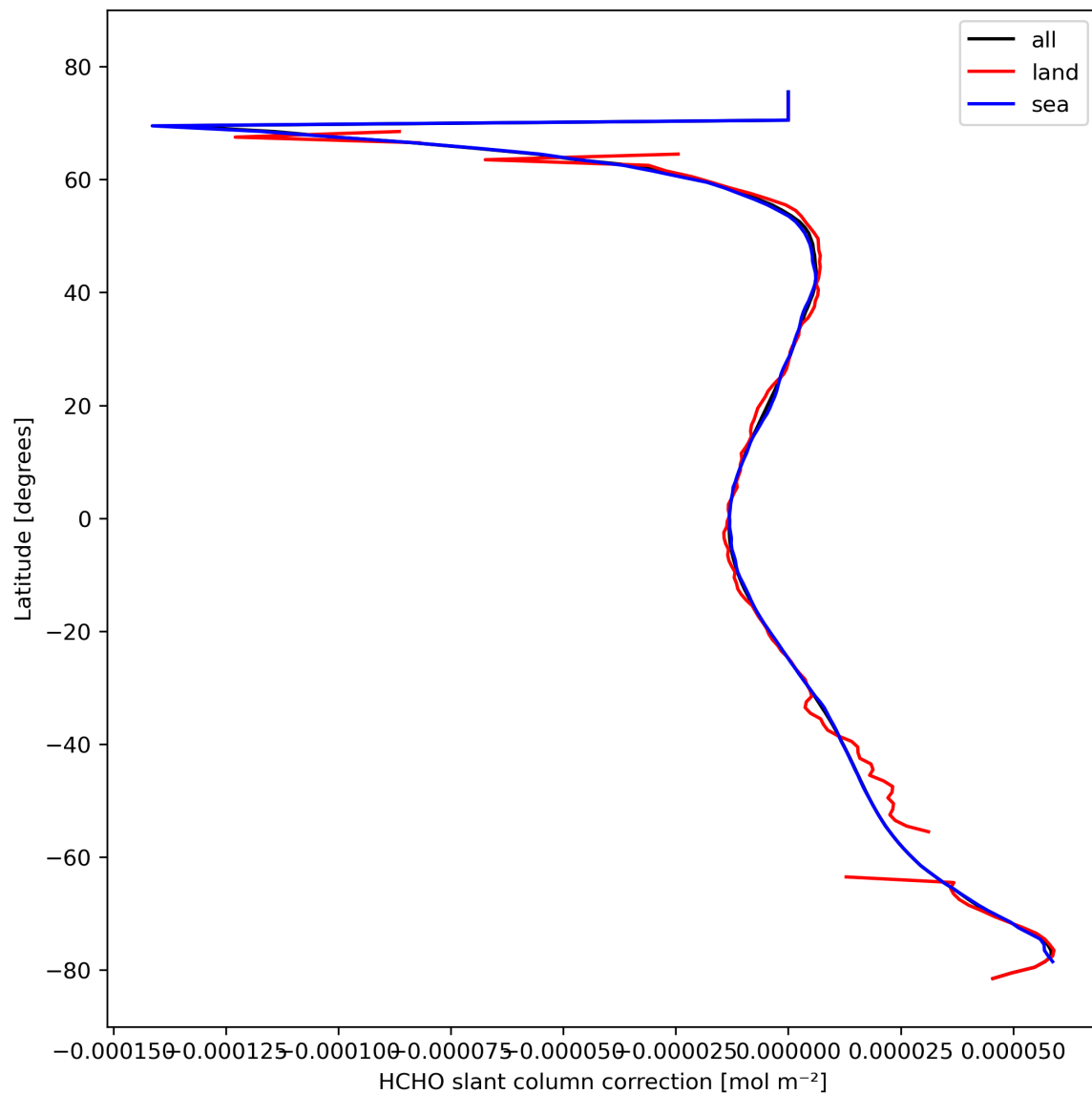
Figure 33: Zonal average of “HCHO slant column correction” for 2024-02-23 to 2024-02-25.
