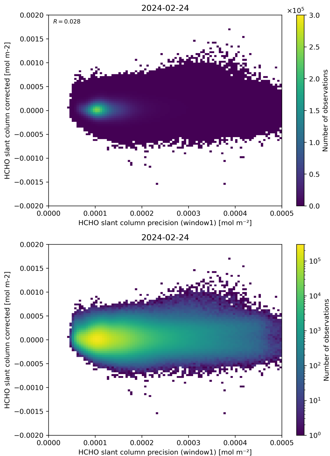
Figure 92: Scatter density plot of “HCHO slant column precision (window1)” against “HCHO slant column corrected” for 2024-02-23 to 2024-02-25.
