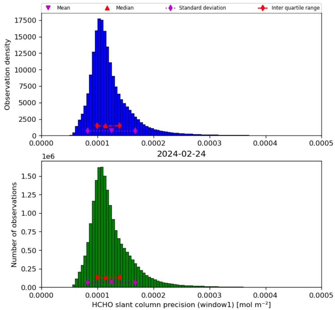
Figure 39: Histogram of “HCHO slant column precision (window1)” for 2024-02-23 to 2024-02-25
