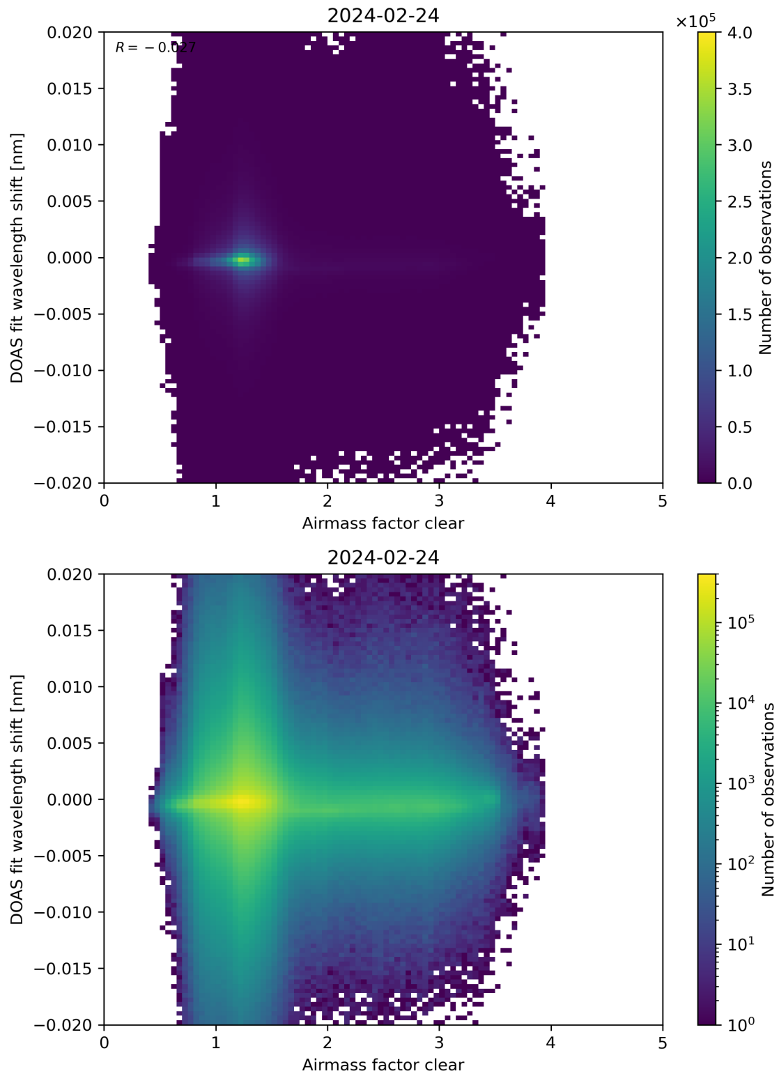
Figure 72: Scatter density plot of “Airmass factor clear” against “DOAS fit wavelength shift” for 2024-02-23 to 2024-02-25.
