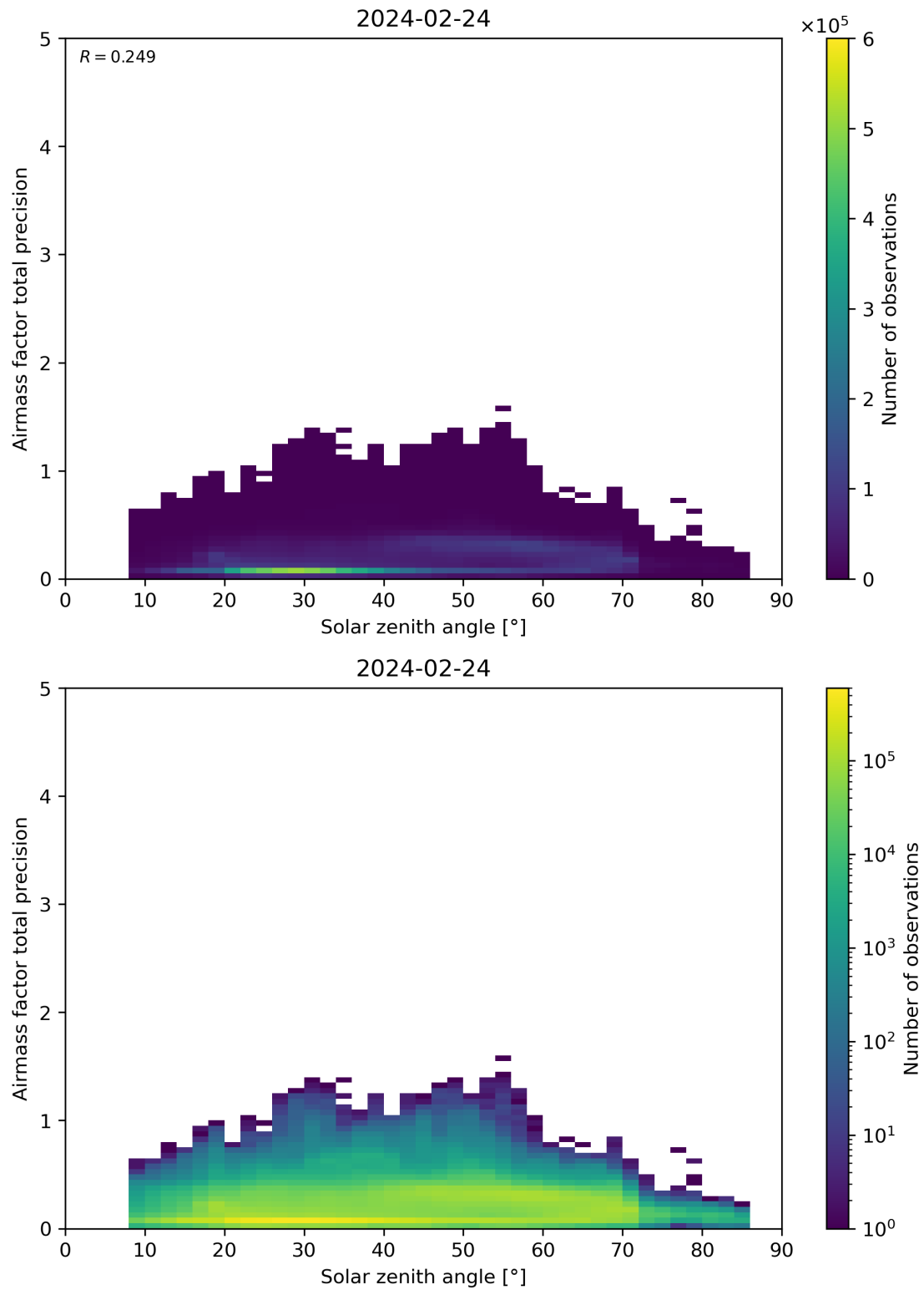
Figure 176: Scatter density plot of “Solar zenith angle” against “Airmass factor total precision” for 2024-02-23 to 2024-02-25.
