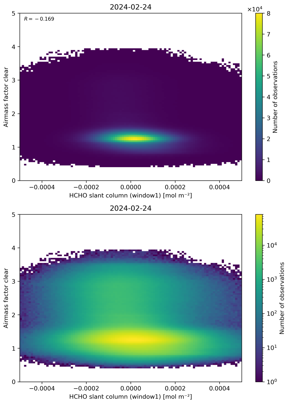
Figure 81: Scatter density plot of “HCHO slant column (window1)” against “Airmass factor clear” for 2024-02-23 to 2024-02-25.
