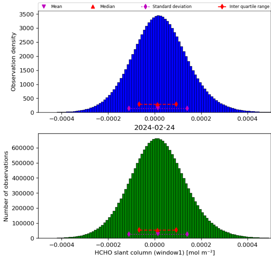
Figure 38: Histogram of “HCHO slant column (window1)” for 2024-02-23 to 2024-02-25
