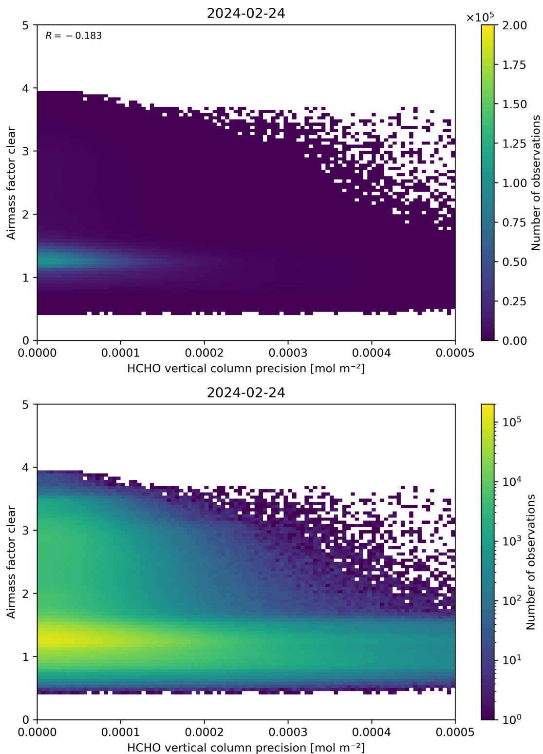
Figure 139: Scatter density plot of “HCHO vertical column precision” against “Airmass factor clear” for 2024-02-23 to 2024-02-25.
