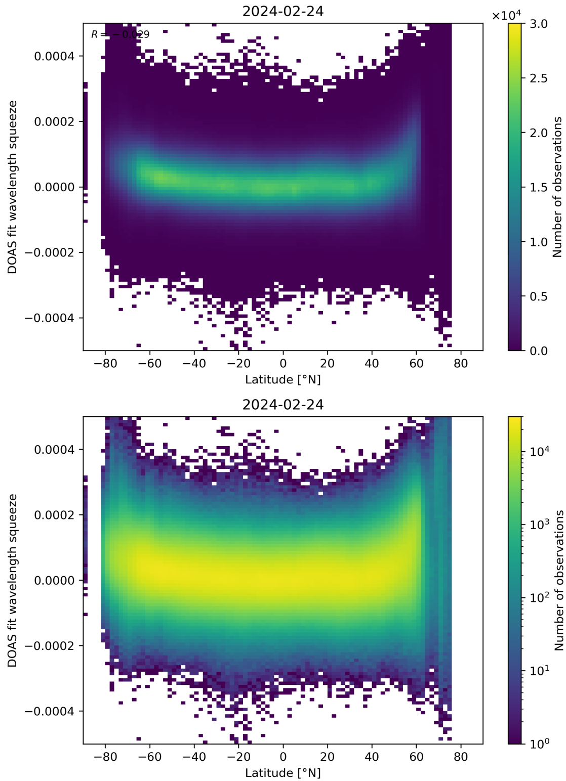
Figure 155: Scatter density plot of “Latitude” against “DOAS fit wavelength squeeze” for 2024-02-23 to 2024-02-25.
