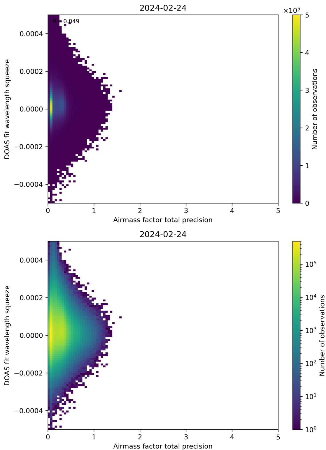
Figure 107: Scatter density plot of “Airmass factor total precision” against “DOAS fit wavelength squeeze” for 2024-02-23 to 2024-02-25.
