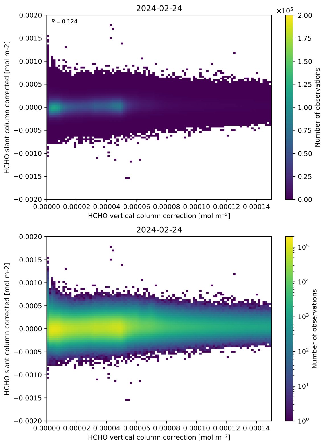
Figure 116: Scatter density plot of “HCHO vertical column correction” against “HCHO slant column corrected” for 2024-02-23 to 2024-02-25.
