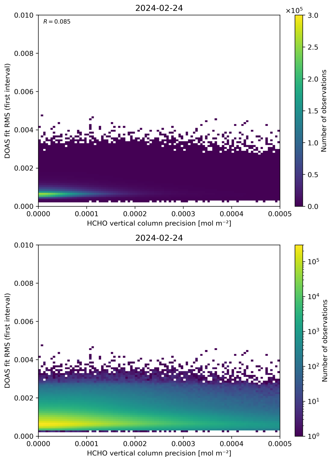
Figure 136: Scatter density plot of “HCHO vertical column precision” against “DOAS fit RMS (first interval)” for 2024-02-23 to 2024-02-25.
