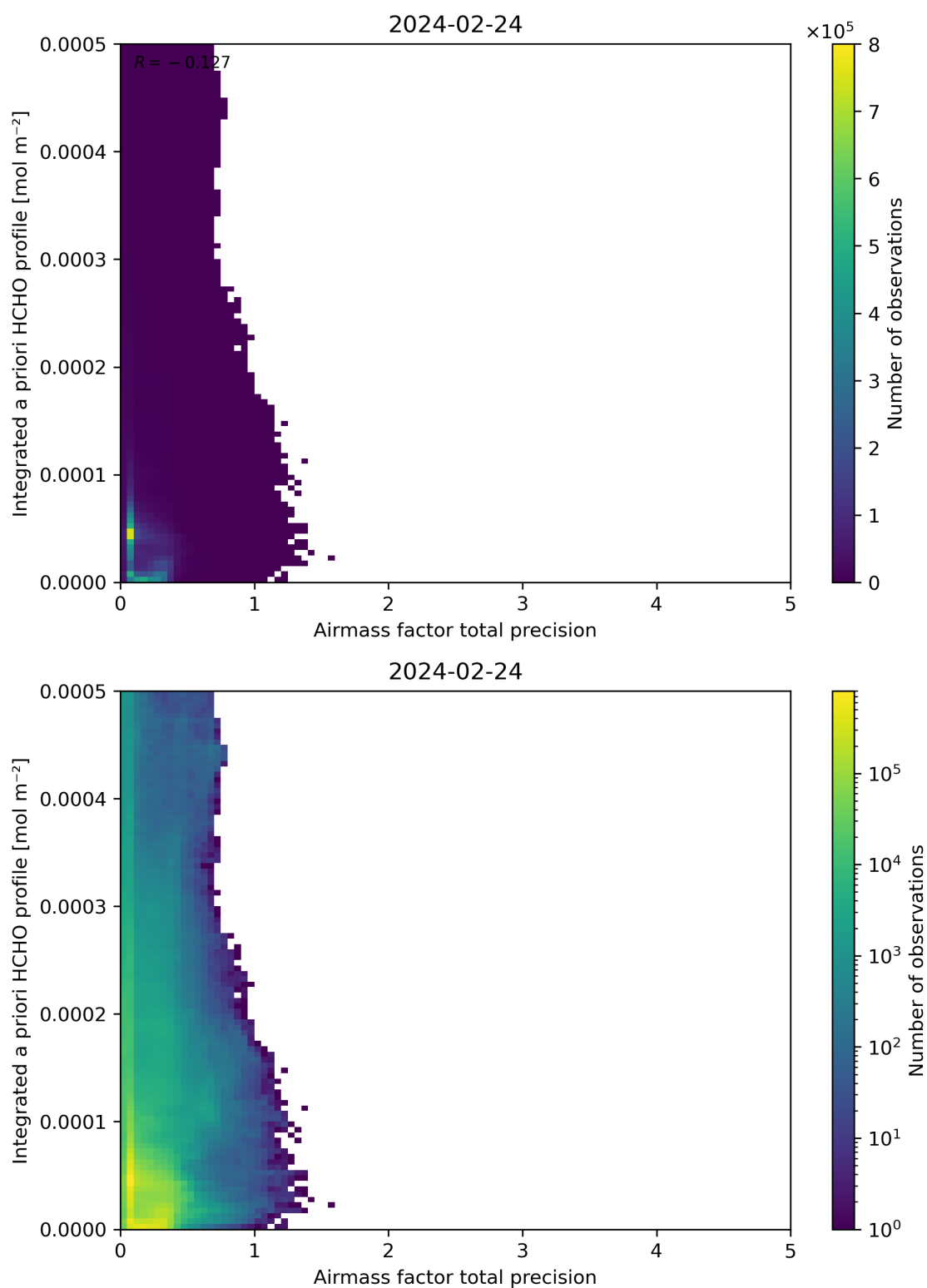
Figure 111: Scatter density plot of “Airmass factor total precision” against “Integrated a priori HCHO profile” for 2024-02-23 to 2024-02-25.
