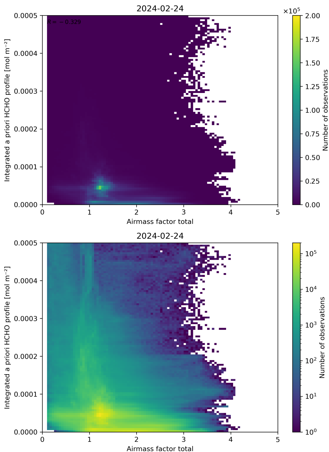
Figure 104: Scatter density plot of “Airmass factor total” against “Integrated a priori HCHO profile” for 2024-02-23 to 2024-02-25.
