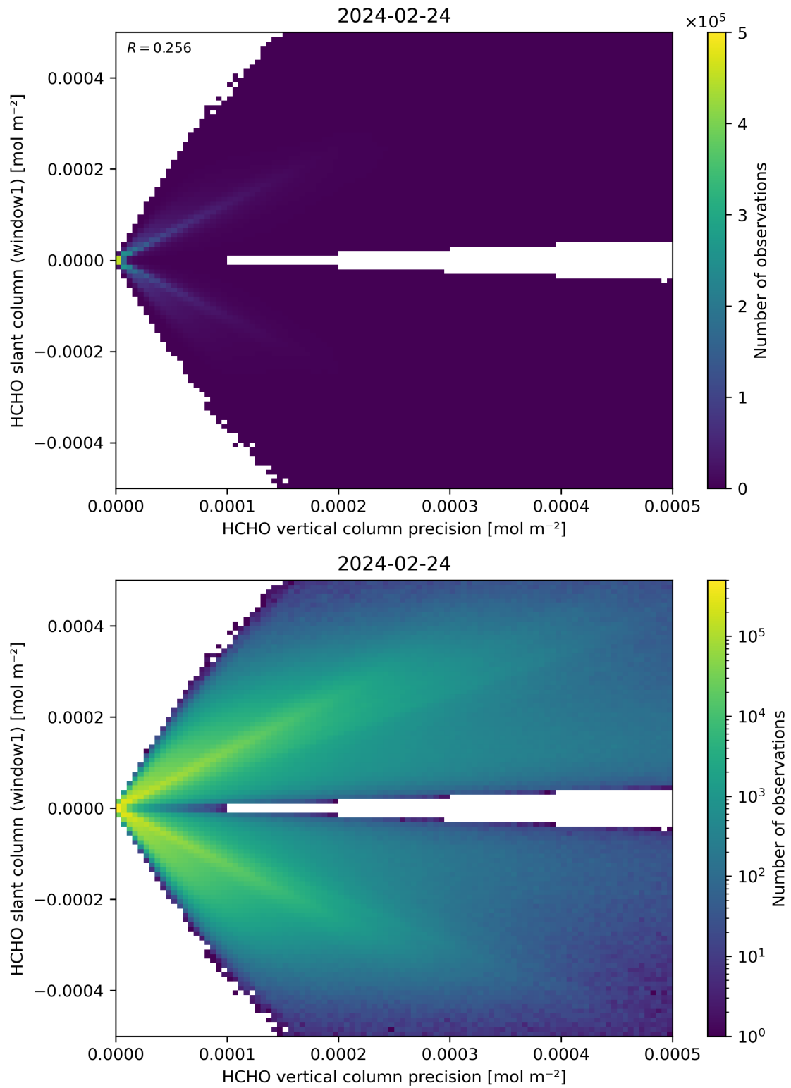
Figure 142: Scatter density plot of “HCHO vertical column precision” against “HCHO slant column (window1)” for 2024-02-23 to 2024-02-25.
