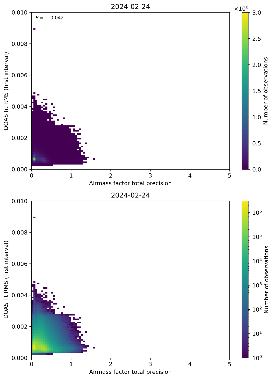
Figure 105: Scatter density plot of “Airmass factor total precision” against “DOAS fit RMS (first interval)” for 2024-02-23 to 2024-02-25.
