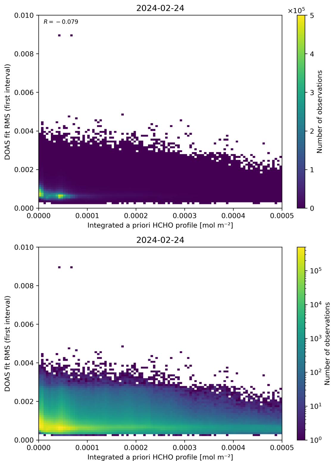
Figure 148: Scatter density plot of “Integrated a priori HCHO profile” against “DOAS fit RMS (first interval)” for 2024-02-23 to 2024-02-25.
