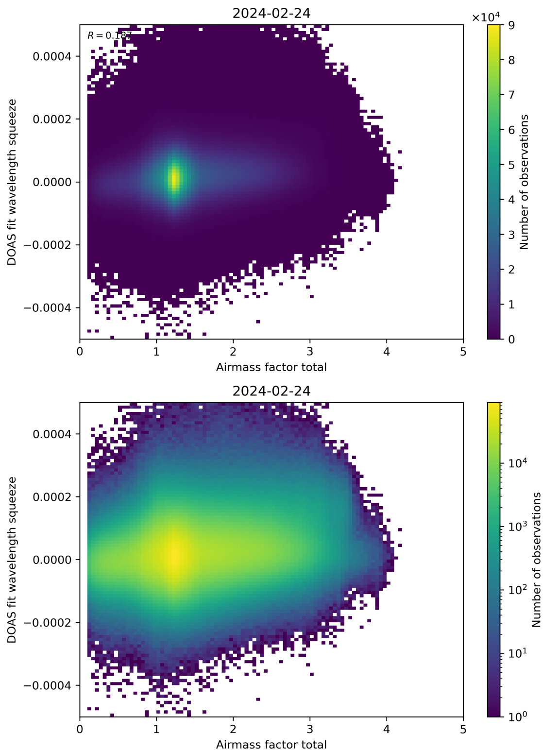
Figure 99: Scatter density plot of “Airmass factor total” against “DOAS fit wavelength squeeze” for 2024-02-23 to 2024-02-25.
