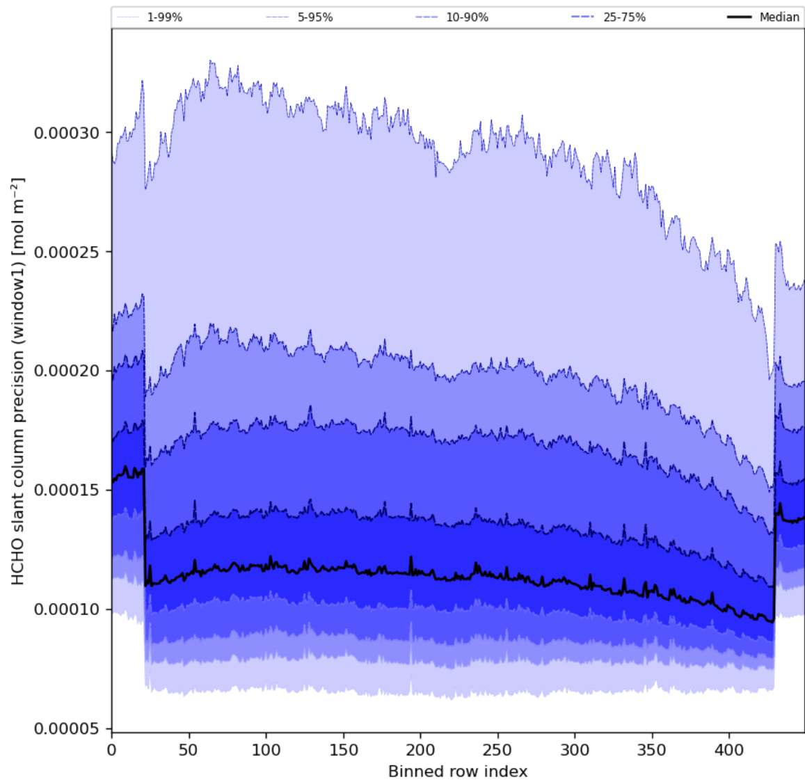
Figure 53: Along track statistics of “HCHO slant column precision (window1)” for 2024-02-23 to 2024-02-25
