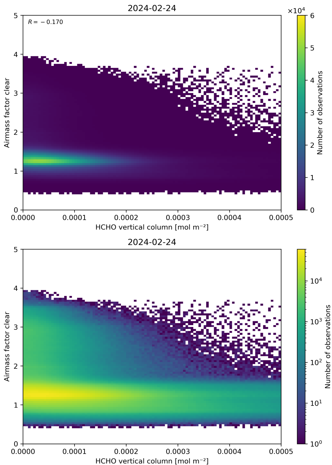
Figure 126: Scatter density plot of “HCHO vertical column” against “Airmass factor clear” for 2024-02-23 to 2024-02-25.
