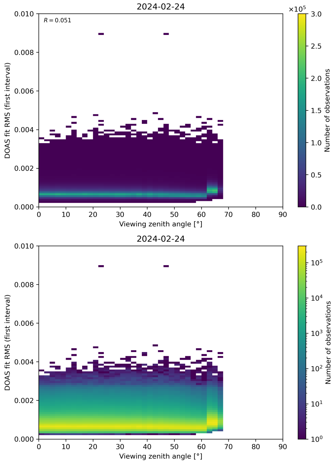
Figure 182: Scatter density plot of “Viewing zenith angle” against “DOAS fit RMS (first interval)” for 2024-02-23 to 2024-02-25.
