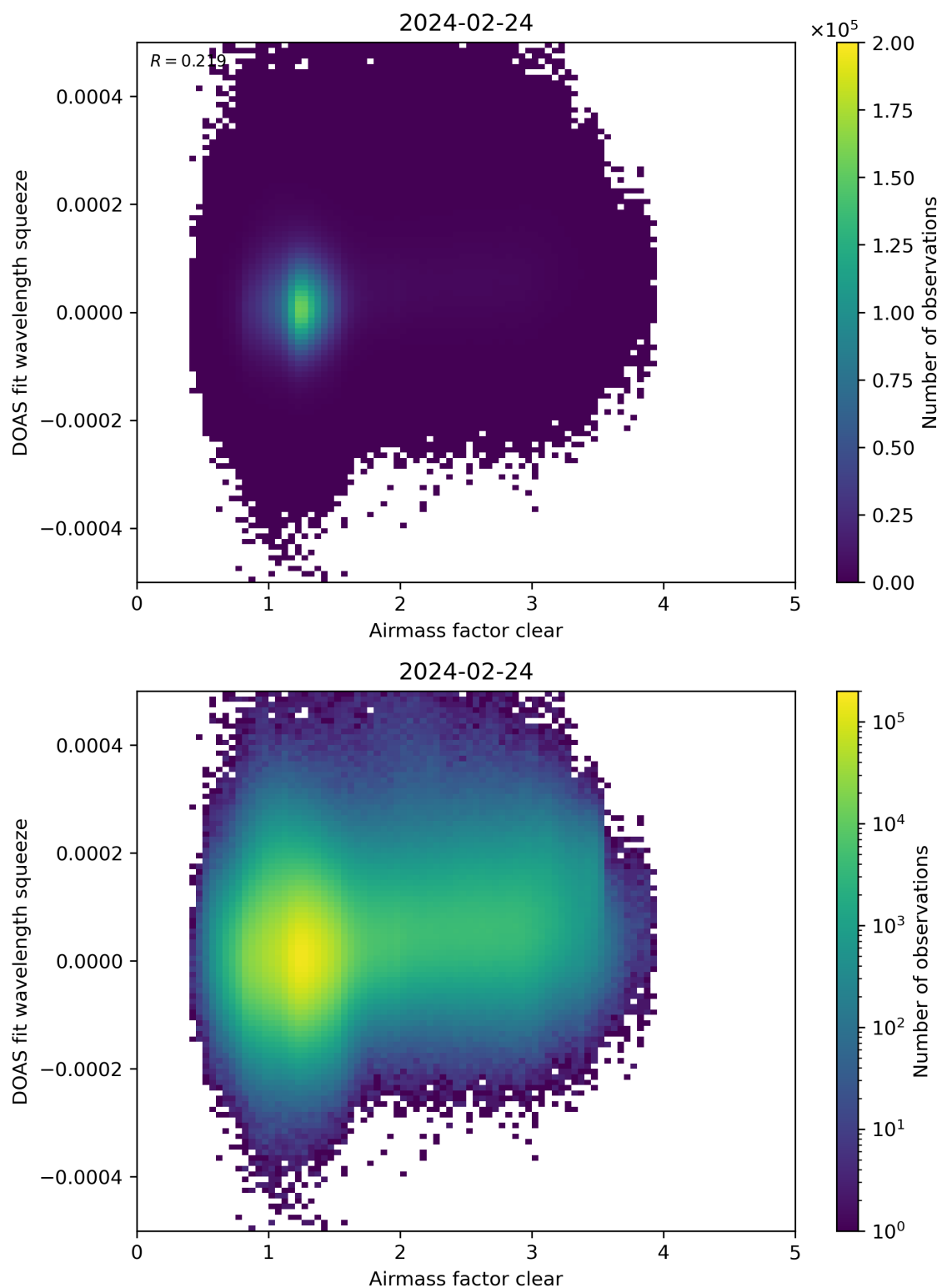
Figure 73: Scatter density plot of “Airmass factor clear” against “DOAS fit wavelength squeeze” for 2024-02-23 to 2024-02-25.
