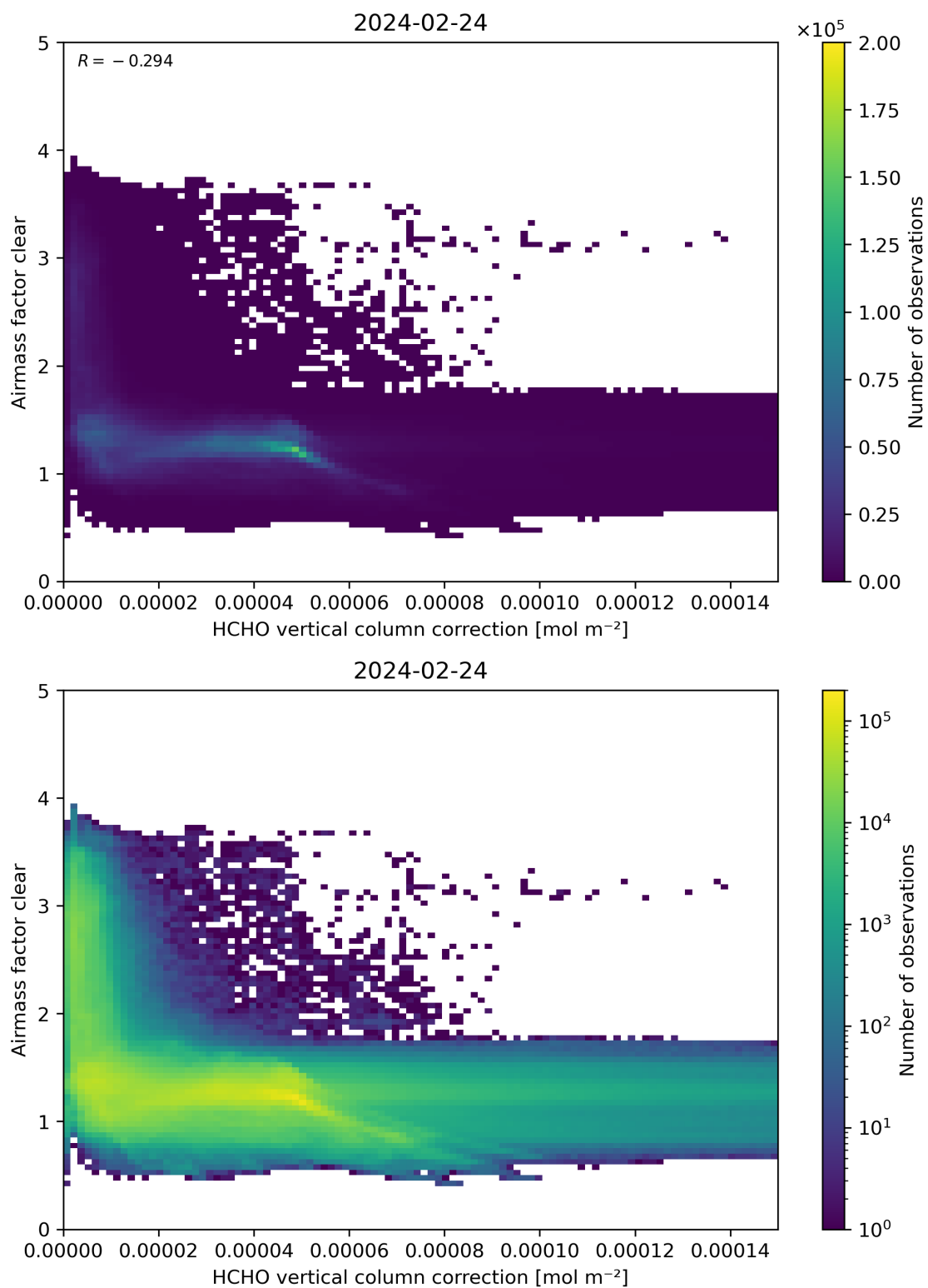
Figure 115: Scatter density plot of “HCHO vertical column correction” against “Airmass factor clear” for 2024-02-23 to 2024-02-25.
