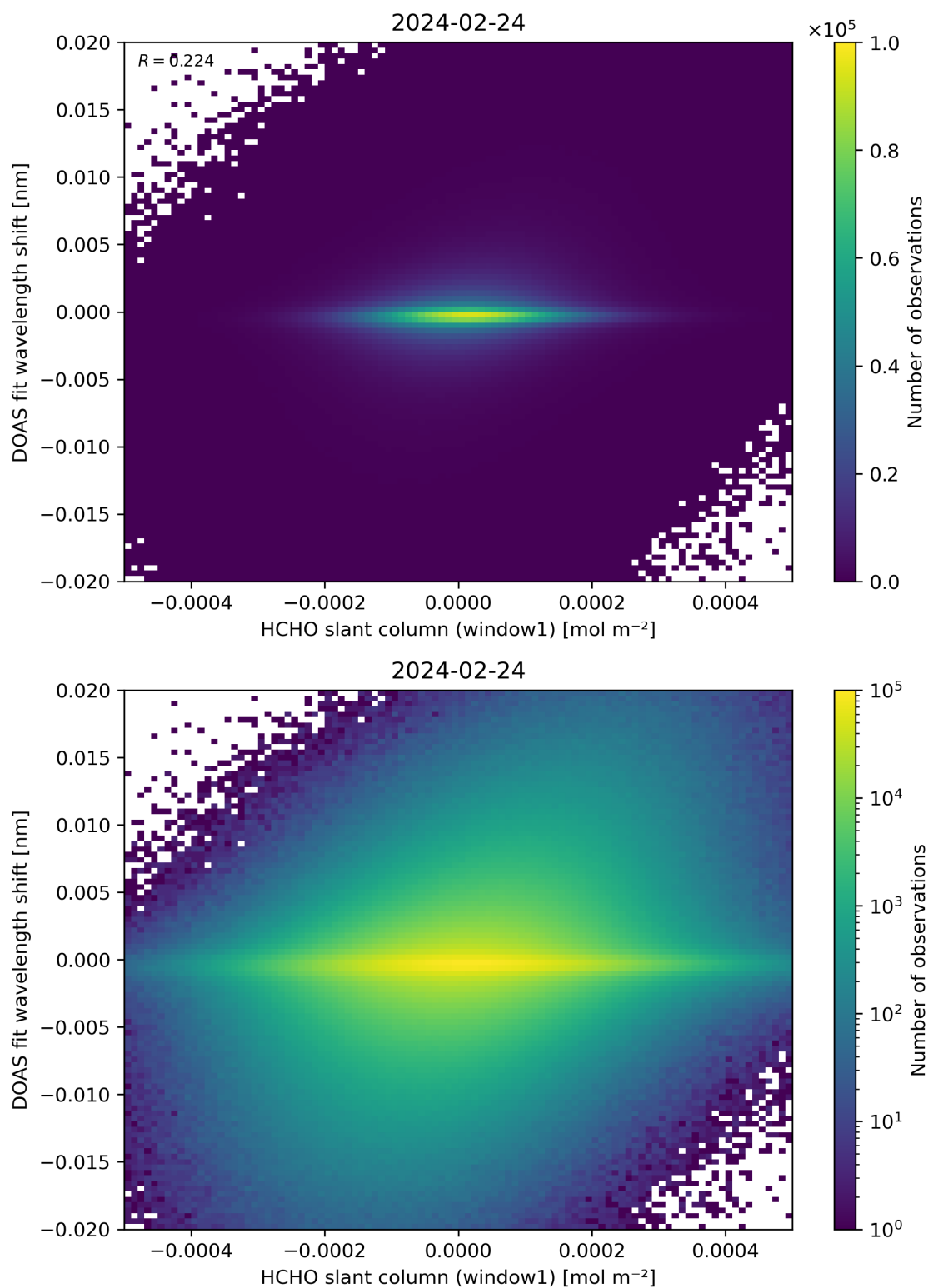
Figure 79: Scatter density plot of “HCHO slant column (window1)” against “DOAS fit wavelength shift” for 2024-02-23 to 2024-02-25.
