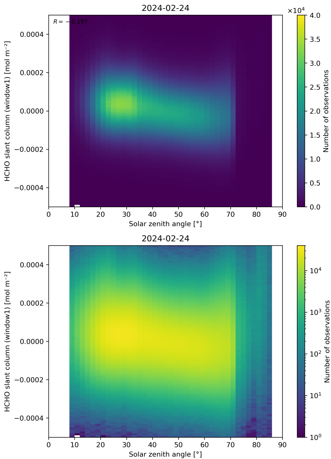
Figure 173: Scatter density plot of “Solar zenith angle” against “HCHO slant column (window1)” for 2024-02-23 to 2024-02-25.
