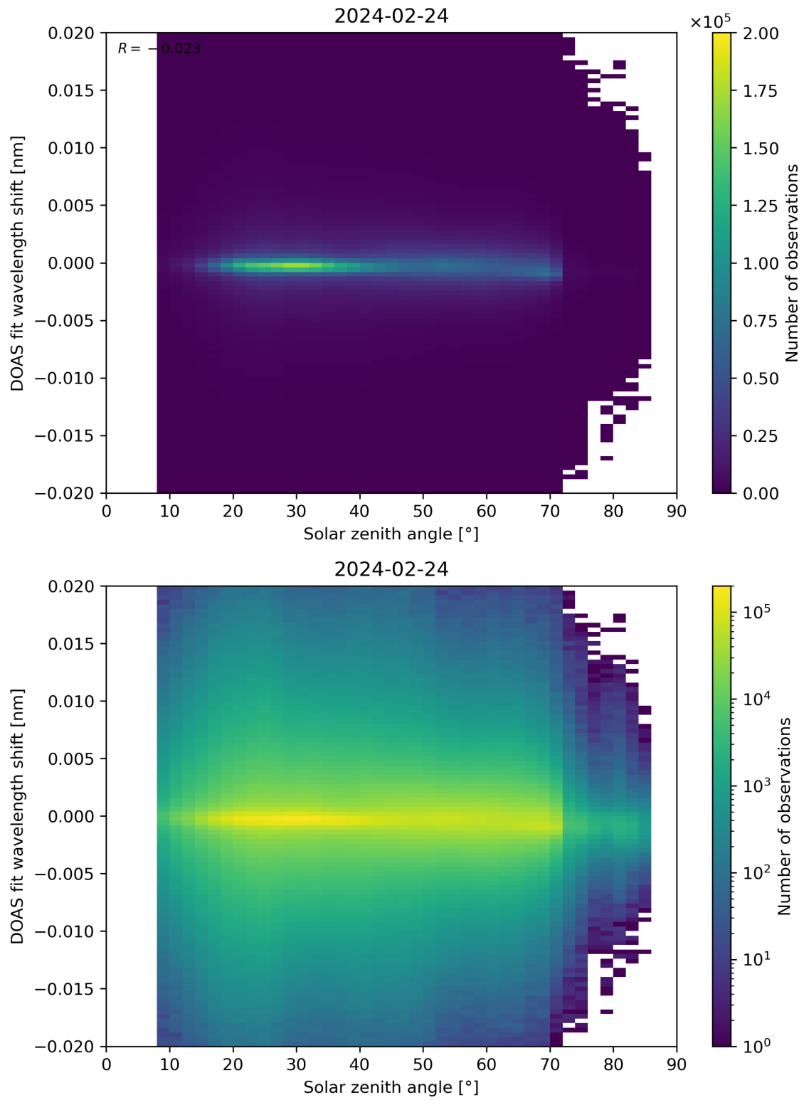
Figure 168: Scatter density plot of “Solar zenith angle” against “DOAS fit wavelength shift” for 2024-02-23 to 2024-02-25.
