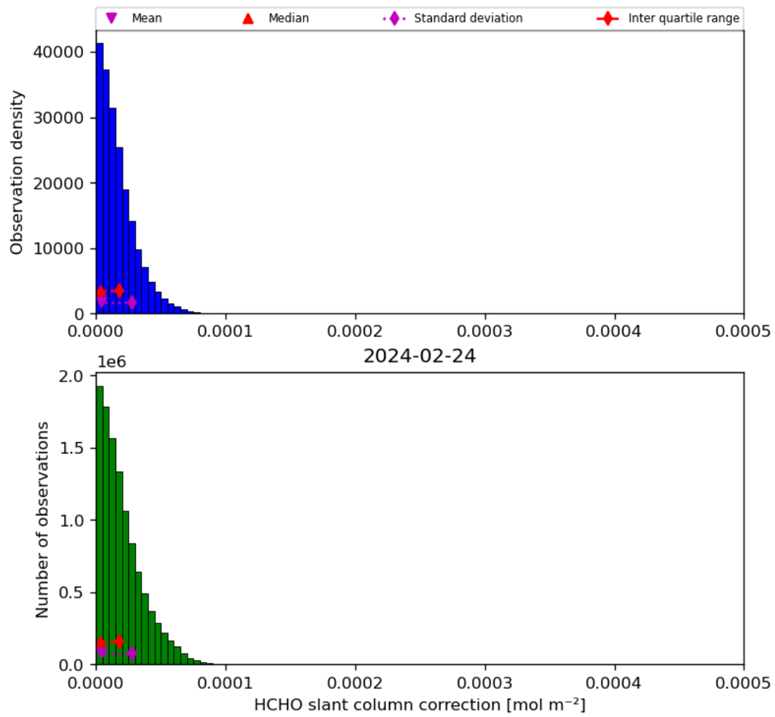
Figure 47: Histogram of “HCHO slant column correction” for 2024-02-23 to 2024-02-25
