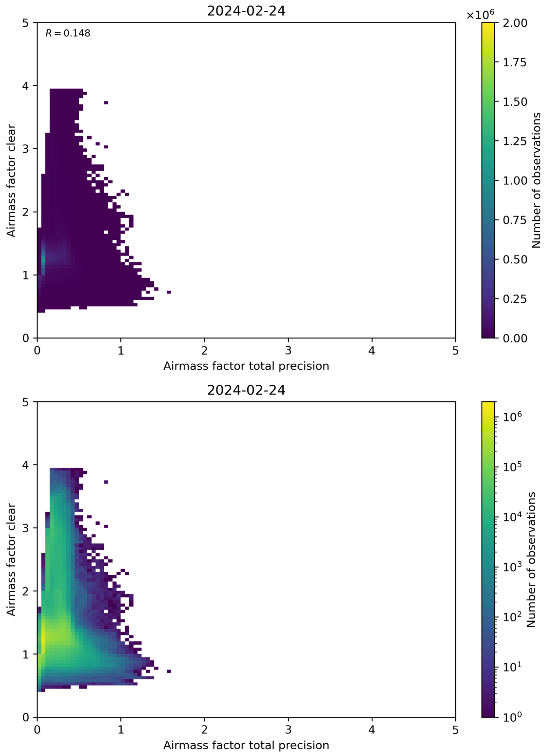
Figure 108: Scatter density plot of “Airmass factor total precision” against “Airmass factor clear” for 2024-02-23 to 2024-02-25.
