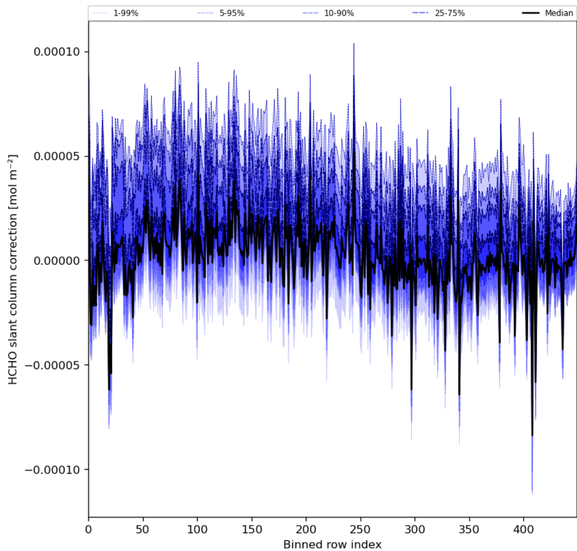
Figure 61: Along track statistics of “HCHO slant column correction” for 2024-02-23 to 2024-02-25
