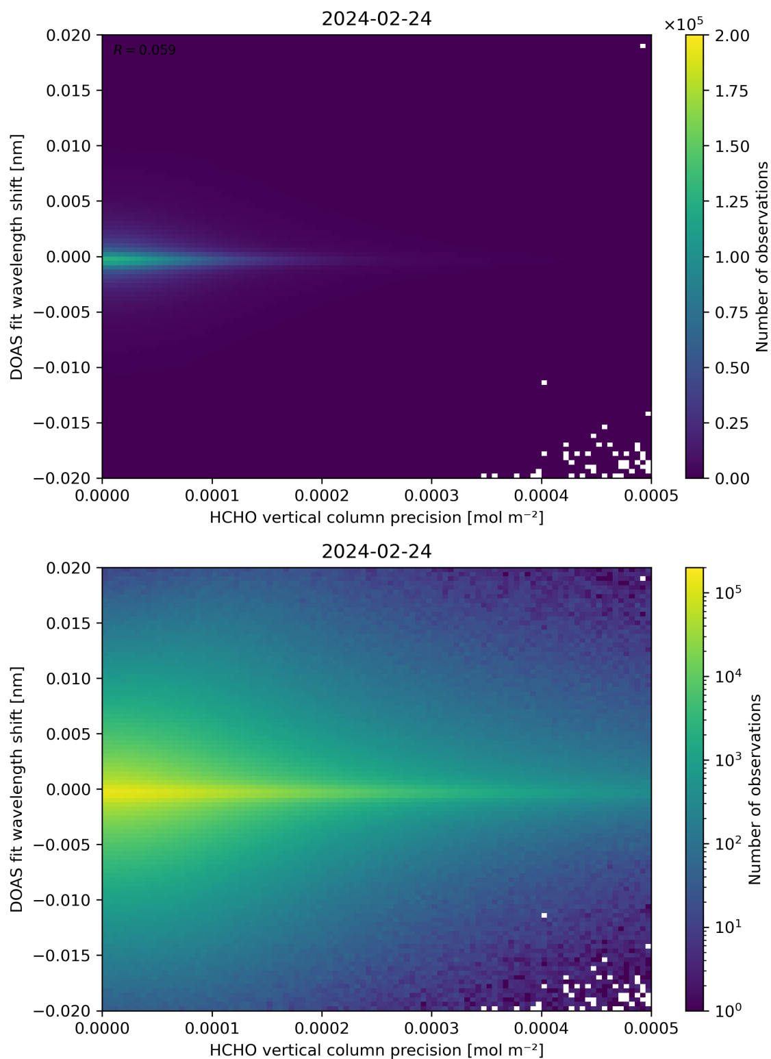
Figure 137: Scatter density plot of “HCHO vertical column precision” against “DOAS fit wavelength shift” for 2024-02-23 to 2024-02-25.
