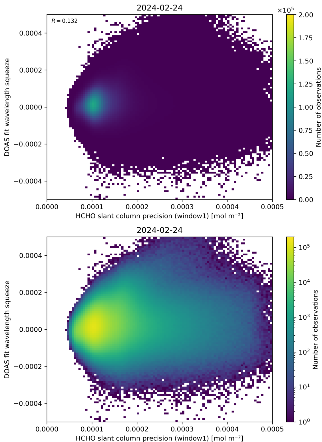
Figure 90: Scatter density plot of “HCHO slant column precision (window1)” against “DOAS fit wavelength squeeze” for 2024-02-23 to 2024-02-25.
