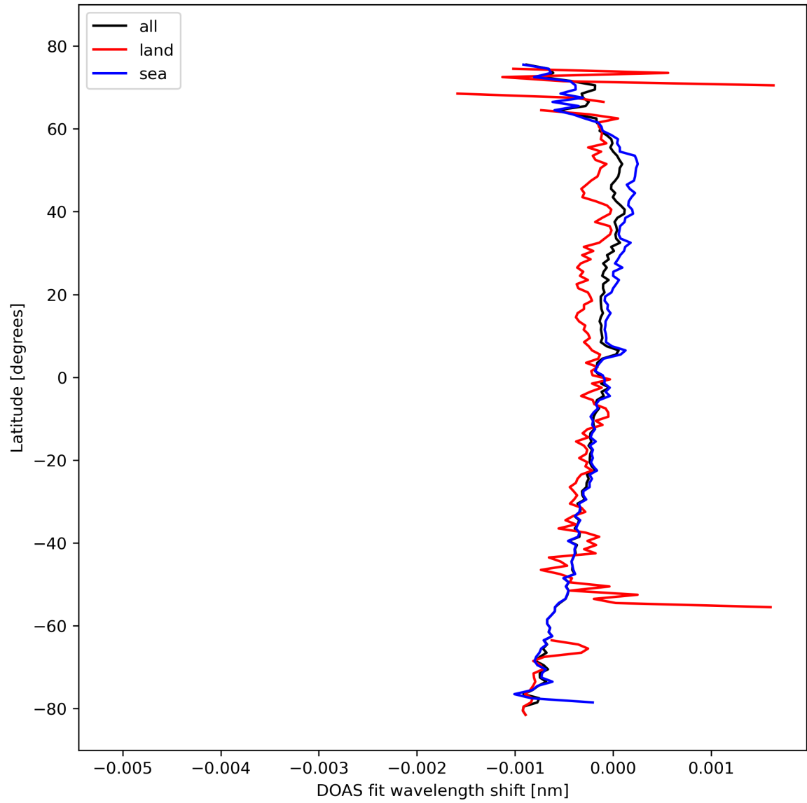
Figure 30: Zonal average of “DOAS fit wavelength shift” for 2024-02-23 to 2024-02-25.
