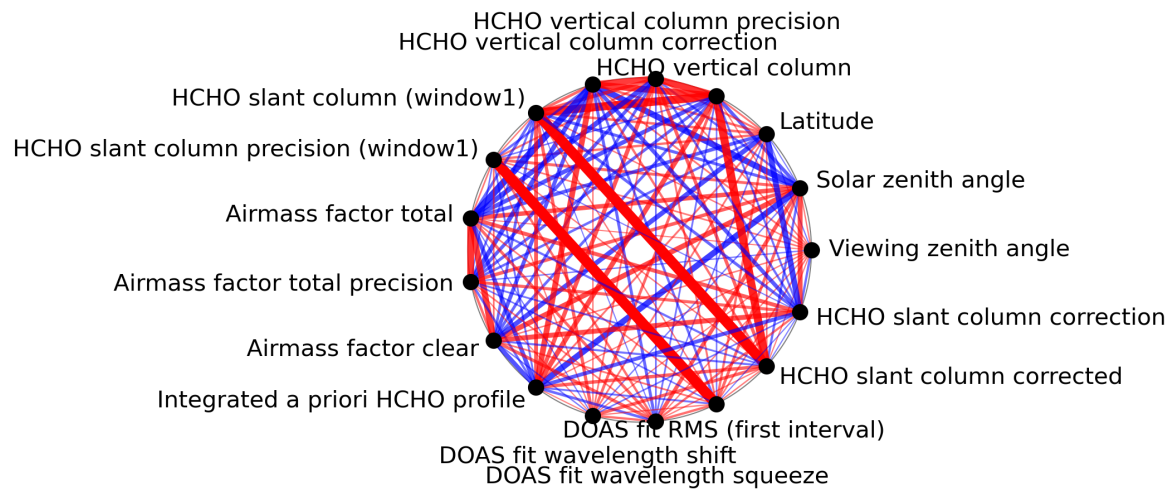
Figure 1: Map of correlation graph for 2024-02-23 to 2024-02-25.
