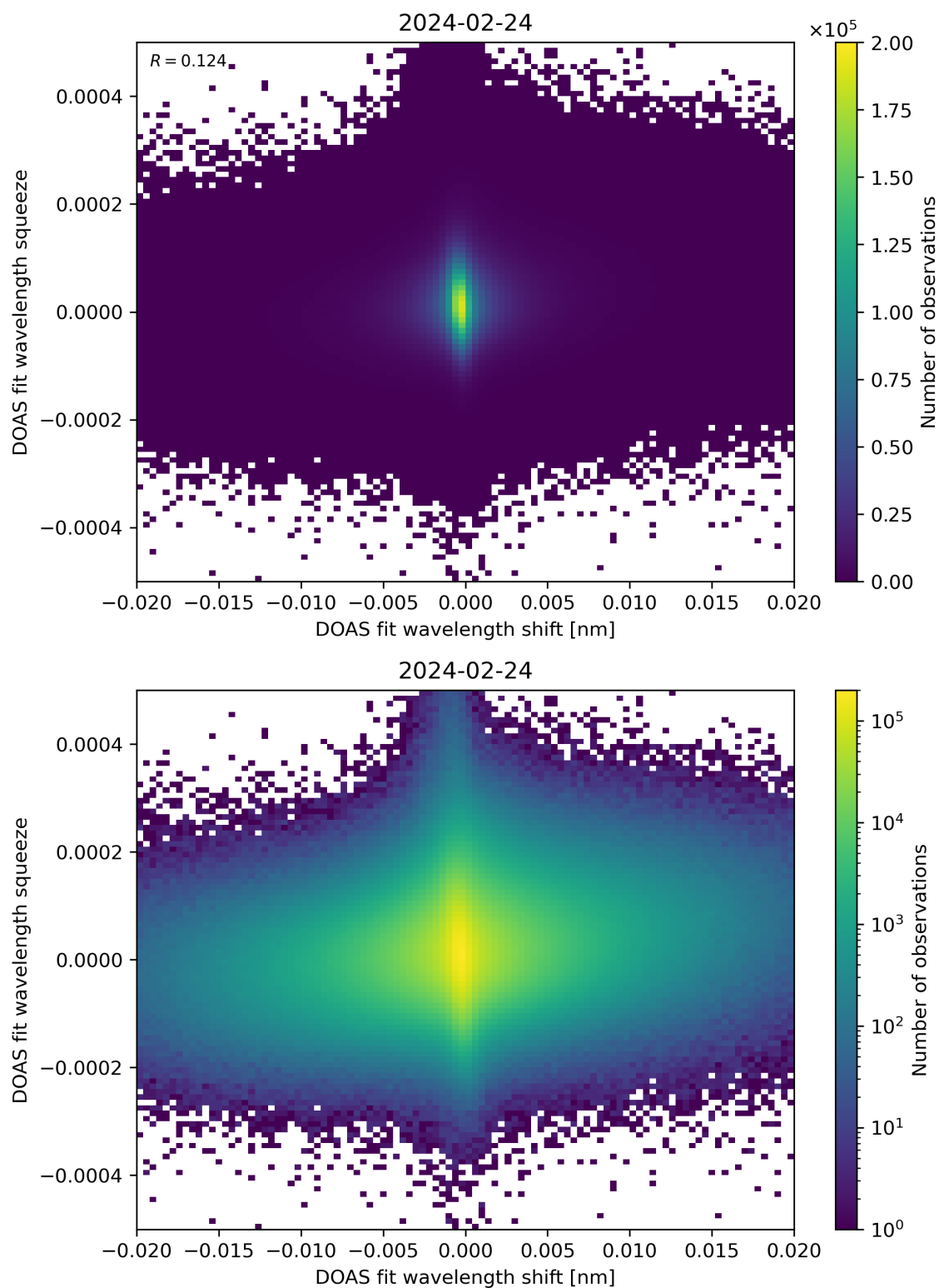
Figure 65: Scatter density plot of “DOAS fit wavelength shift” against “DOAS fit wavelength squeeze” for 2024-02-23 to 2024-02-25.
