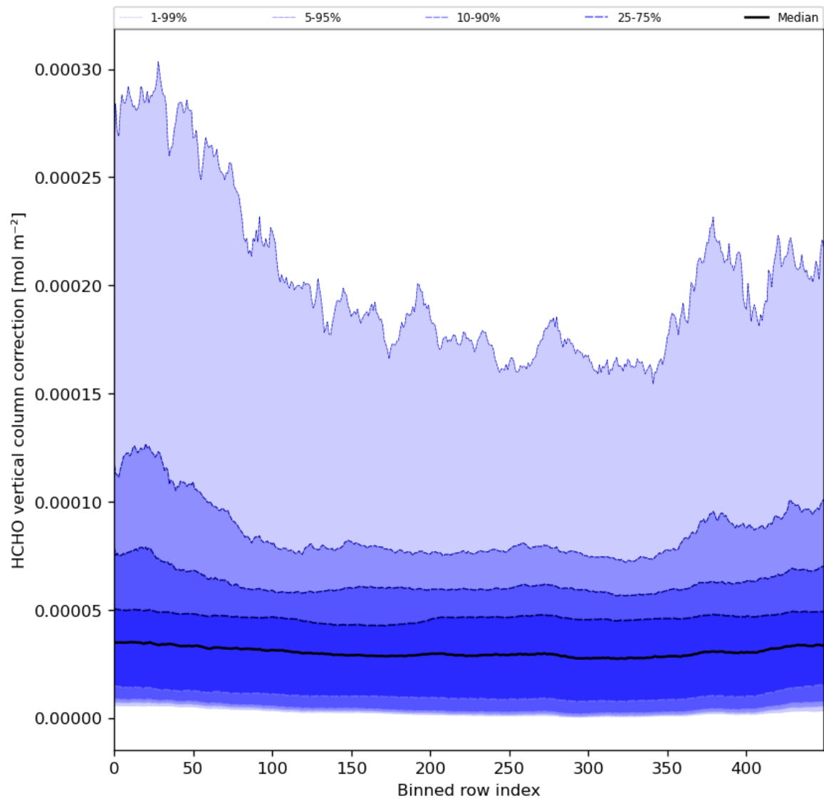
Figure 51: Along track statistics of “HCHO vertical column correction” for 2024-02-23 to 2024-02-25
