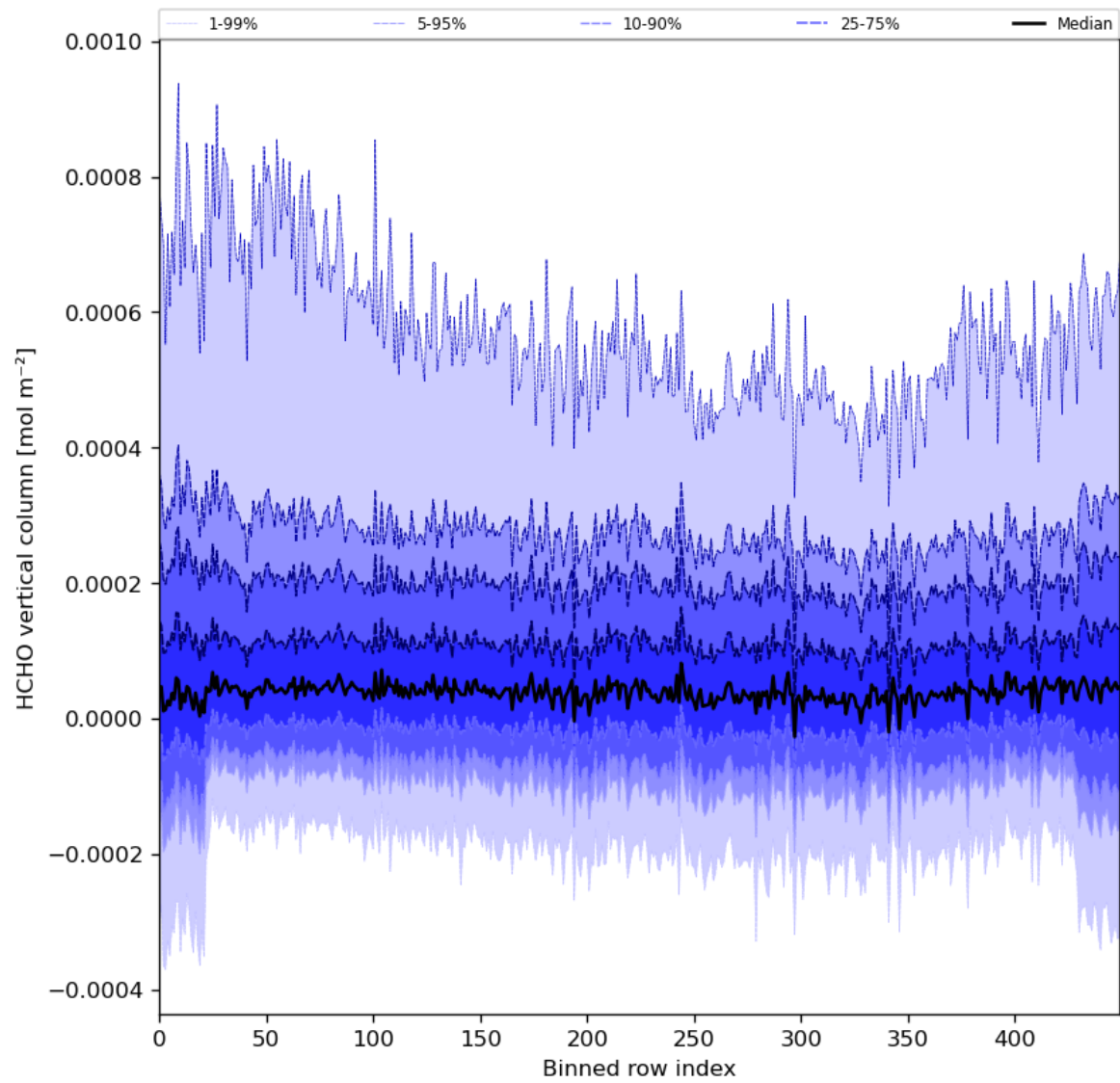
Figure 49: Along track statistics of “HCHO vertical column” for 2024-02-23 to 2024-02-25
