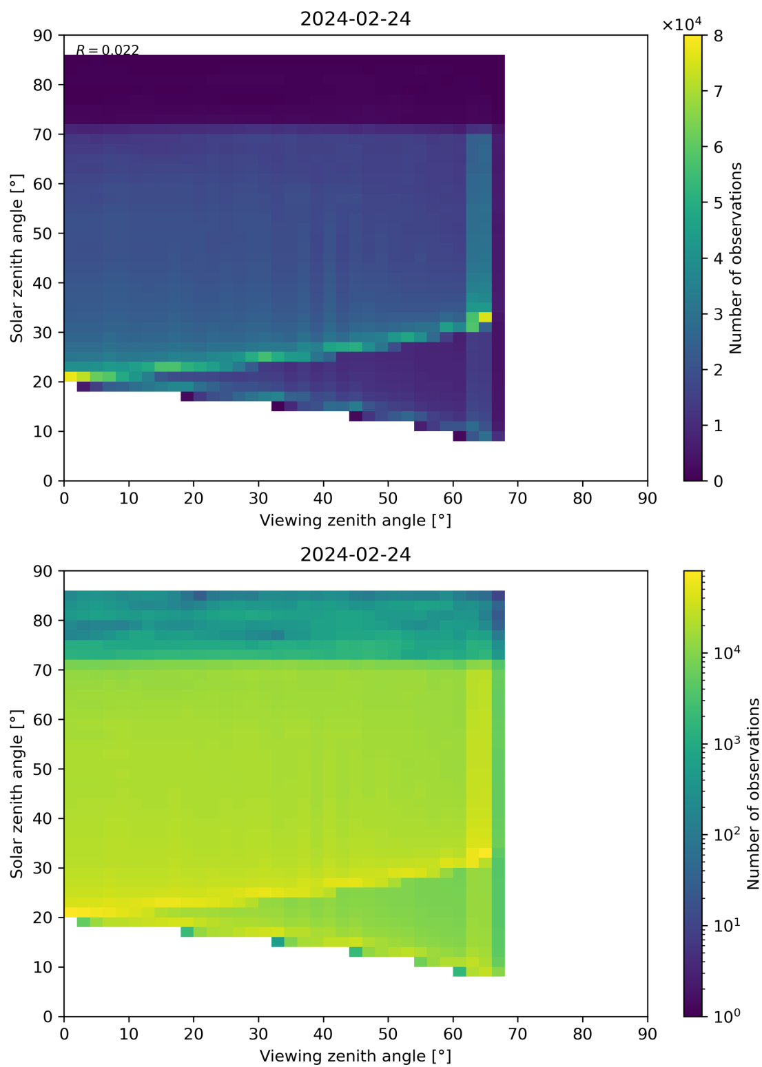
Figure 197: Scatter density plot of “Viewing zenith angle” against “Solar zenith angle” for 2024-02-23 to 2024-02-25.
