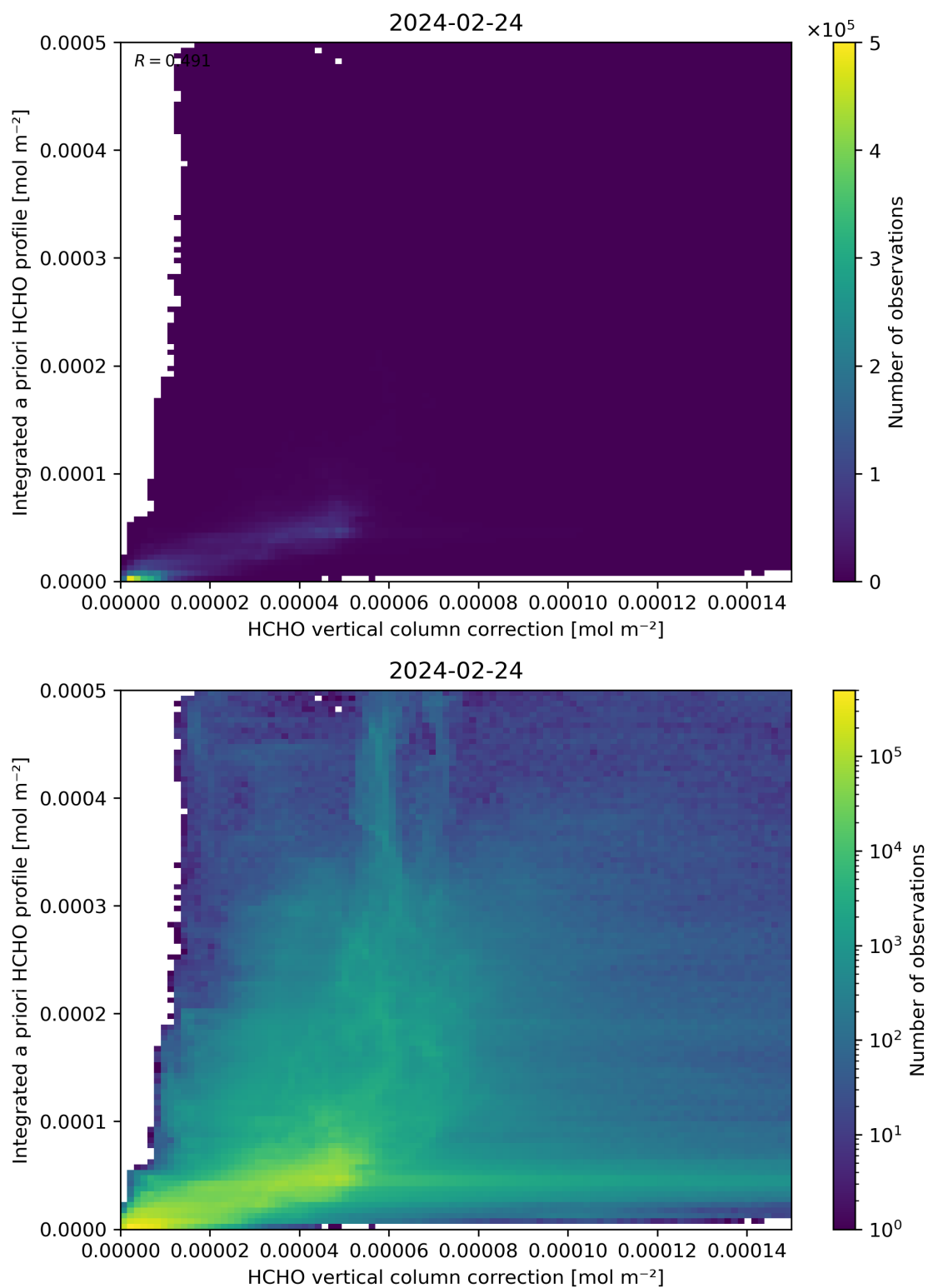
Figure 122: Scatter density plot of “HCHO vertical column correction” against “Integrated a priori HCHO profile” for 2024-02-23 to 2024-02-25.
