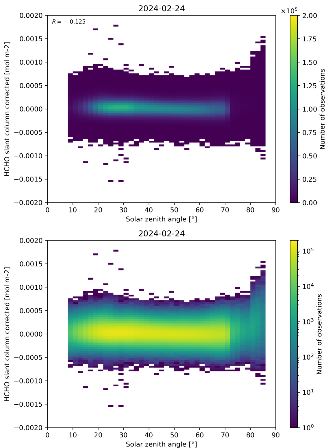
Figure 171: Scatter density plot of “Solar zenith angle” against “HCHO slant column corrected” for 2024-02-23 to 2024-02-25.
