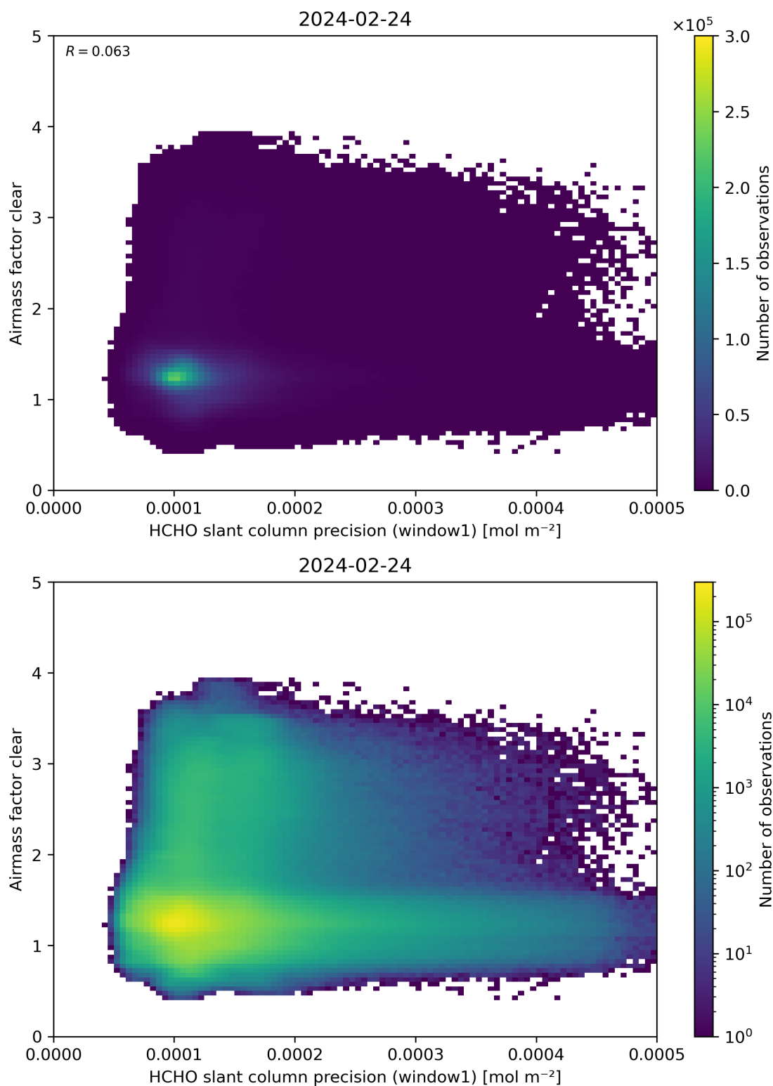
Figure 91: Scatter density plot of “HCHO slant column precision (window1)” against “Airmass factor clear” for 2024-02-23 to 2024-02-25.
