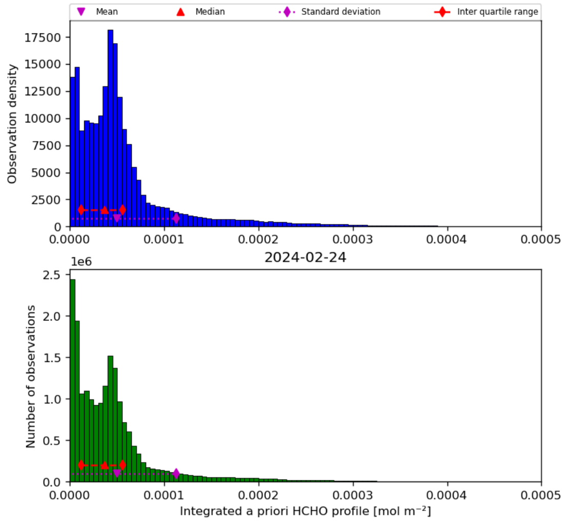
Figure 43: Histogram of “Integrated a priori HCHO profile” for 2024-02-23 to 2024-02-25
