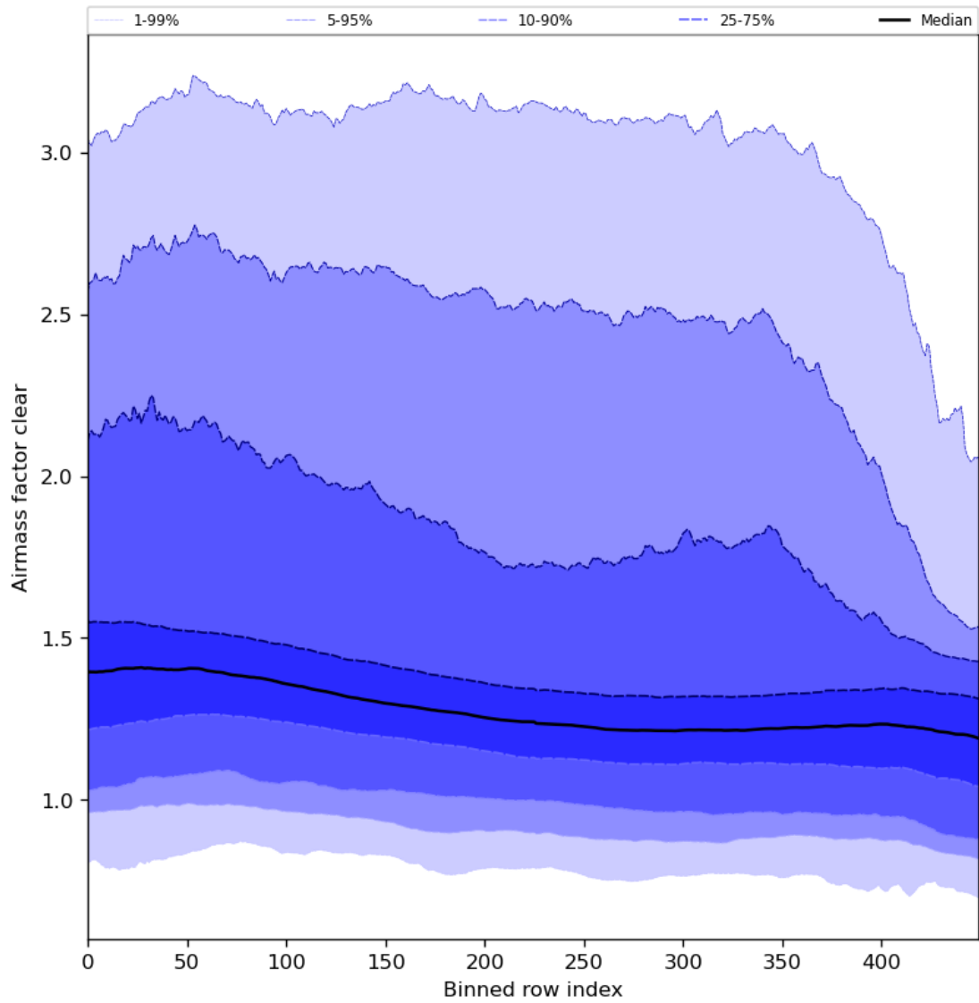
Figure 56: Along track statistics of “Airmass factor clear” for 2024-02-23 to 2024-02-25
