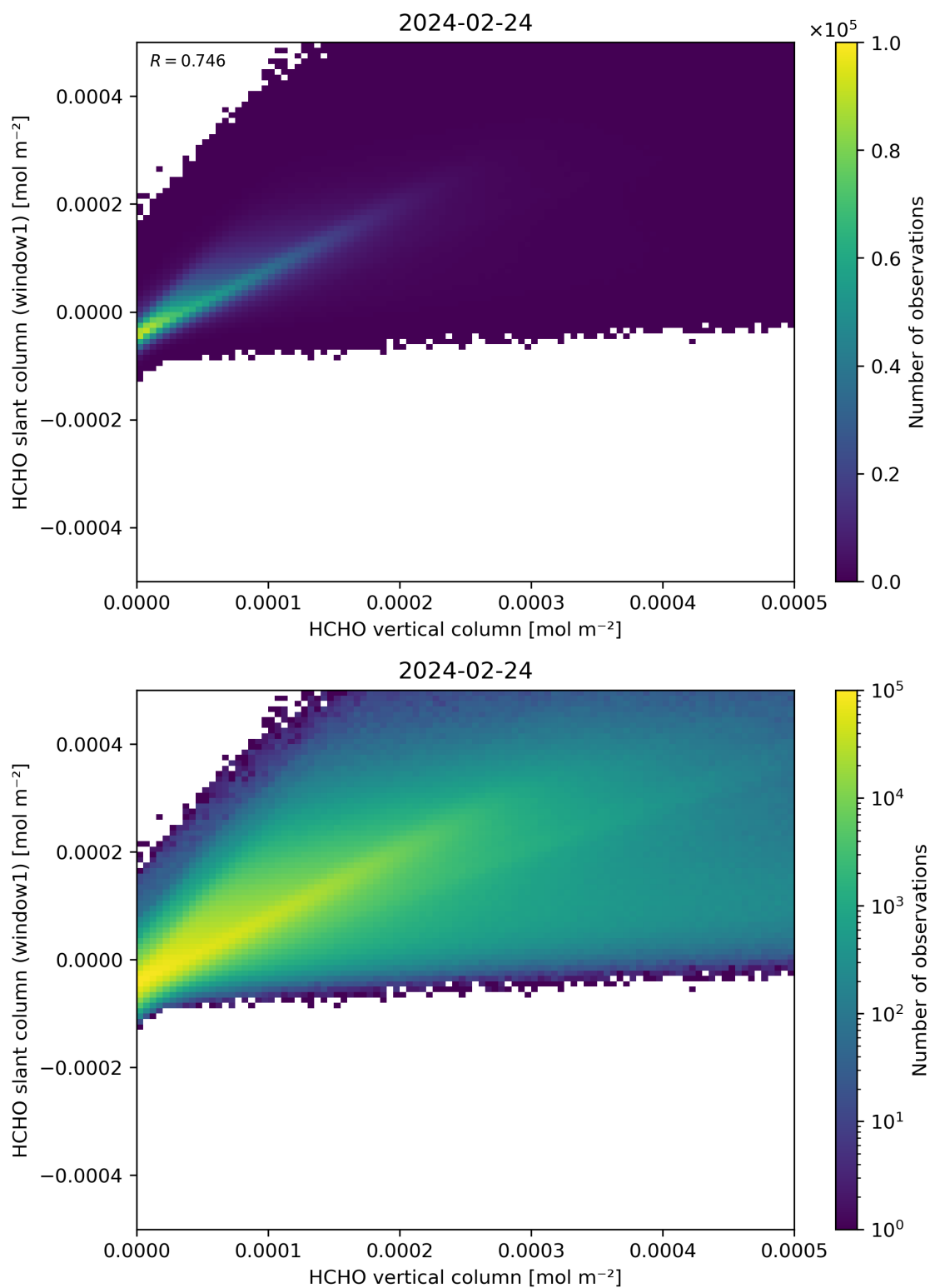
Figure 129: Scatter density plot of “HCHO vertical column” against “HCHO slant column (window1)” for 2024-02-23 to 2024-02-25.
