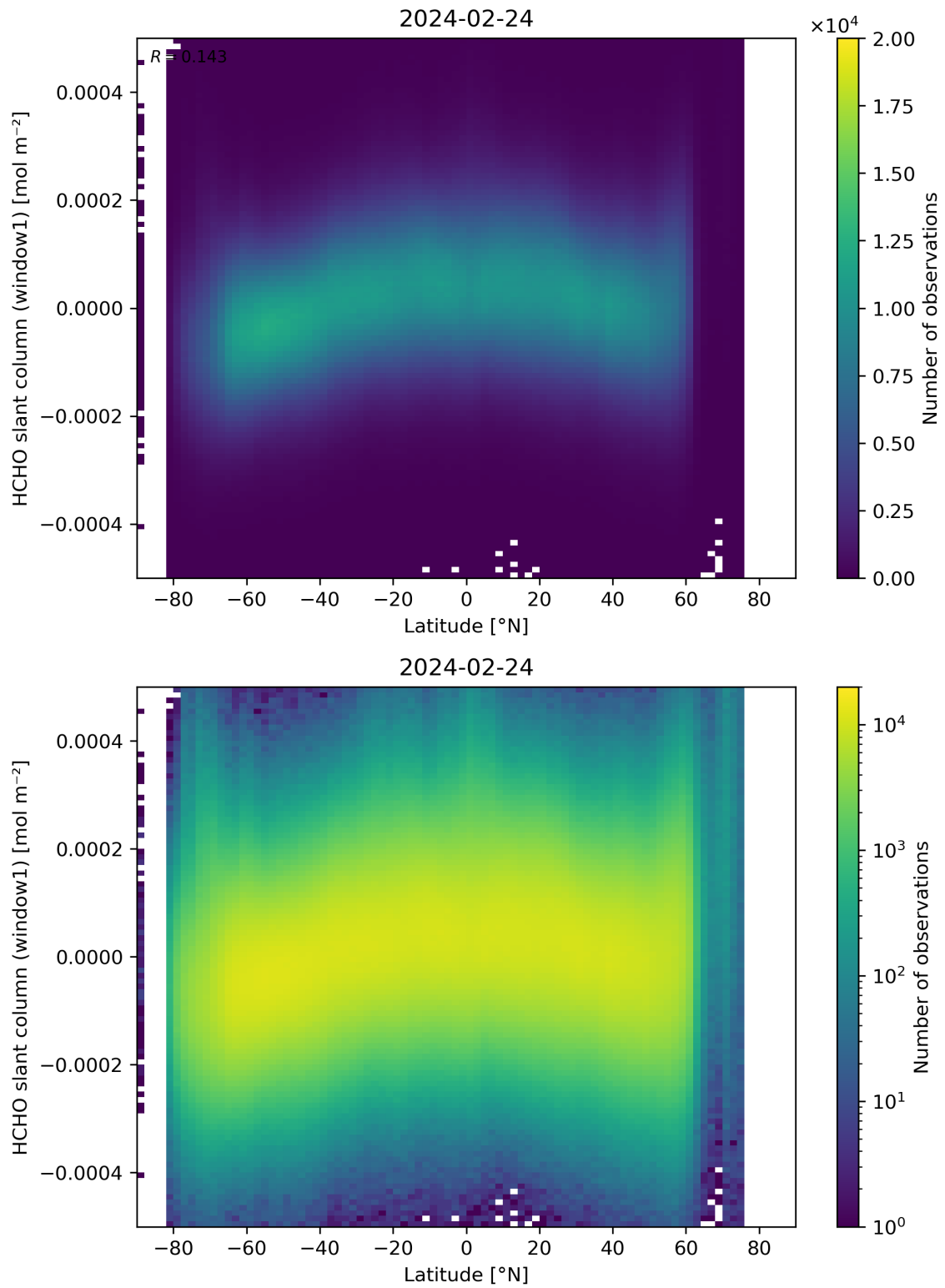
Figure 159: Scatter density plot of “Latitude” against “HCHO slant column (window1)” for 2024-02-23 to 2024-02-25.
