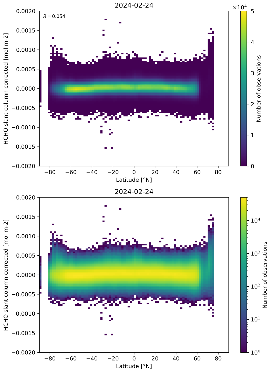
Figure 157: Scatter density plot of “Latitude” against “HCHO slant column corrected” for 2024-02-23 to 2024-02-25.
