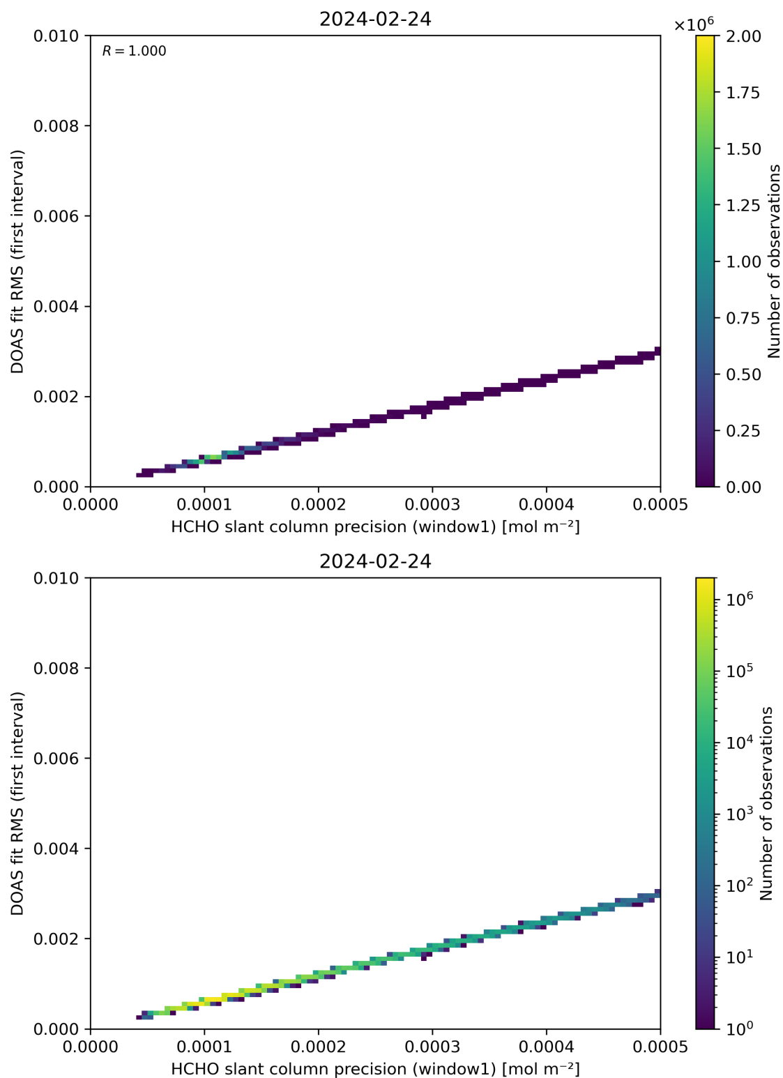
Figure 88: Scatter density plot of “HCHO slant column precision (window1)” against “DOAS fit RMS (first interval)” for 2024-02-23 to 2024-02-25.
