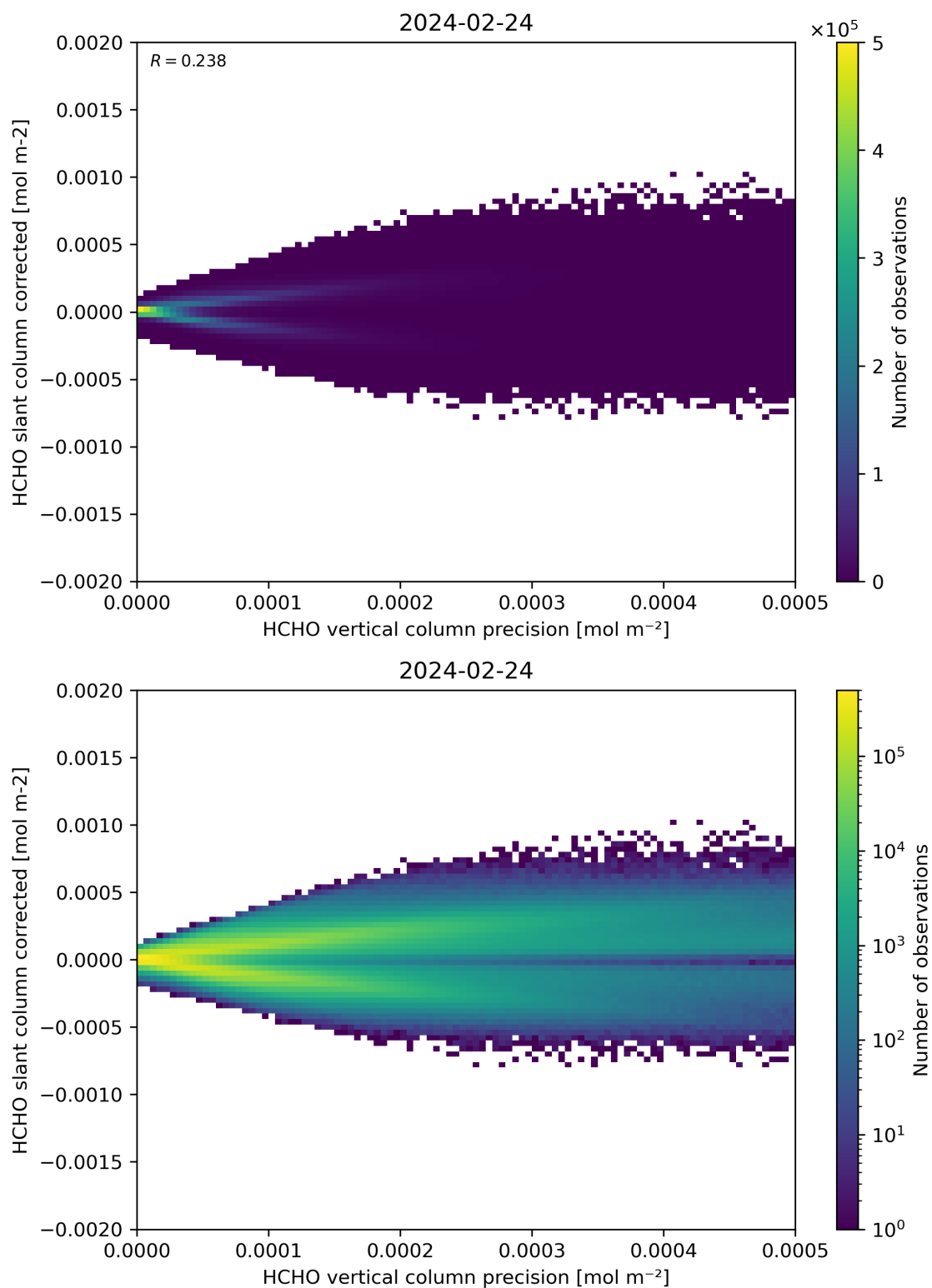
Figure 140: Scatter density plot of “HCHO vertical column precision” against “HCHO slant column corrected” for 2024-02-23 to 2024-02-25.
