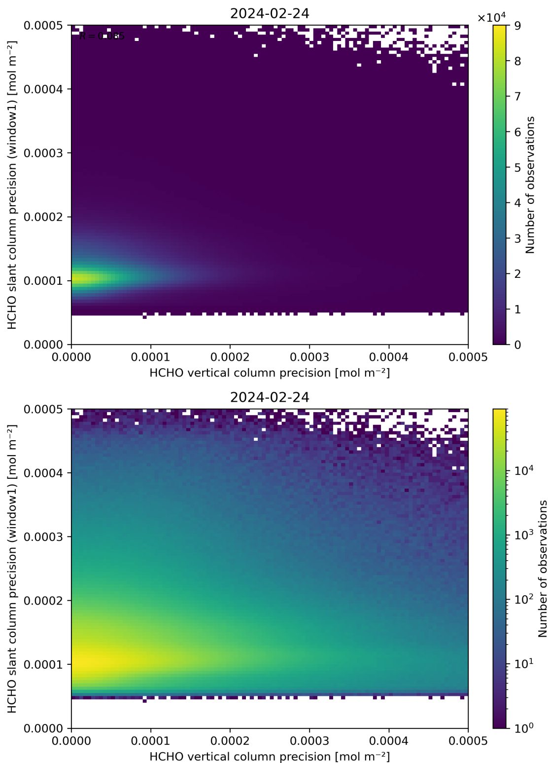
Figure 143: Scatter density plot of “HCHO vertical column precision” against “HCHO slant column precision (window1)” for 2024-02-23 to 2024-02-25.
