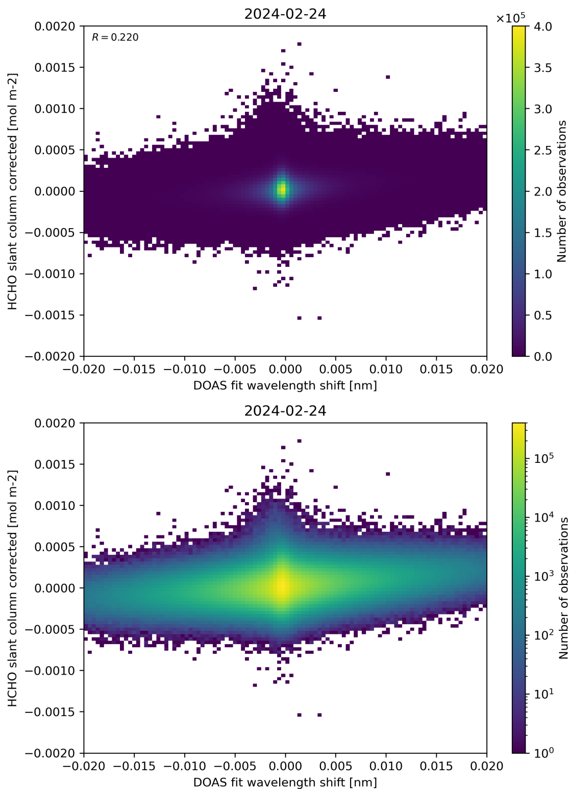
Figure 66: Scatter density plot of “DOAS fit wavelength shift” against “HCHO slant column corrected” for 2024-02-23 to 2024-02-25.
