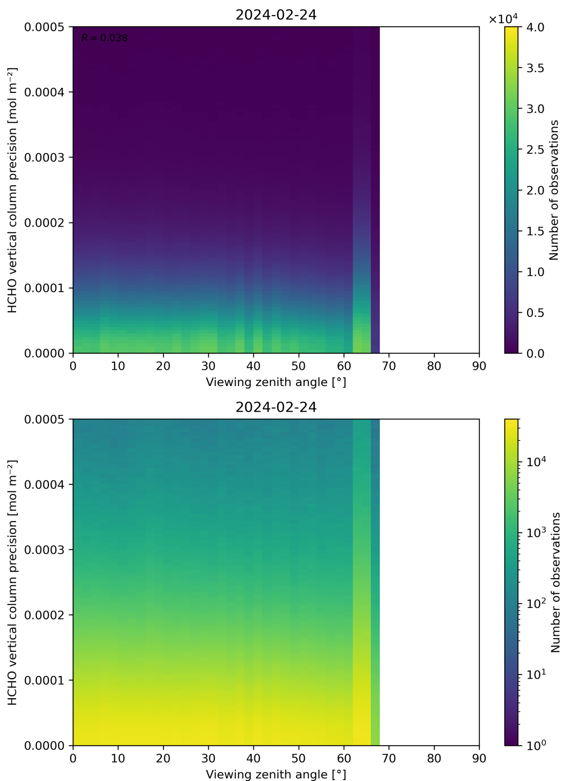
Figure 194: Scatter density plot of “Viewing zenith angle” against “HCHO vertical column precision” for 2024-02-23 to 2024-02-25.
