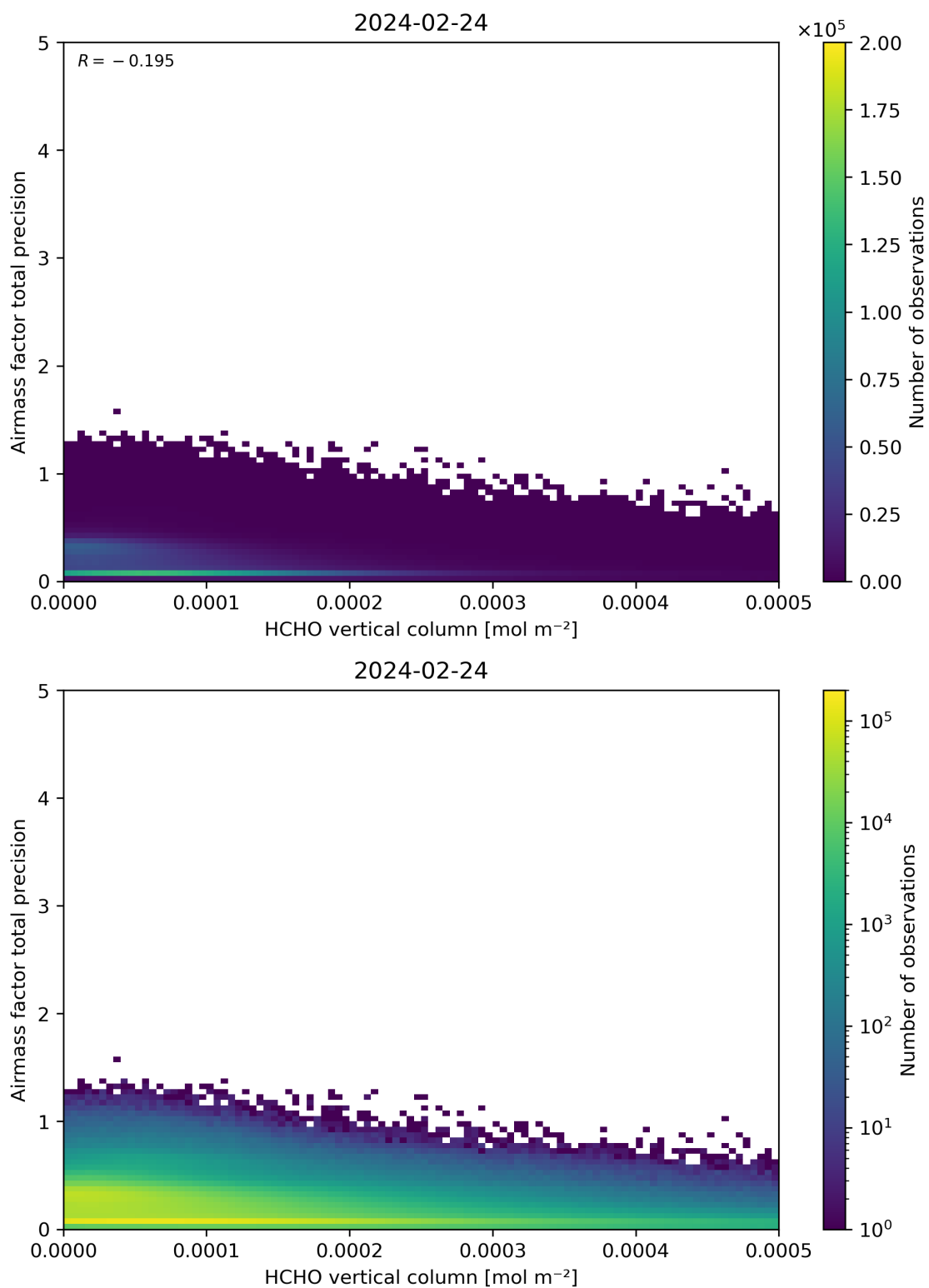
Figure 132: Scatter density plot of “HCHO vertical column” against “Airmass factor total precision” for 2024-02-23 to 2024-02-25.
