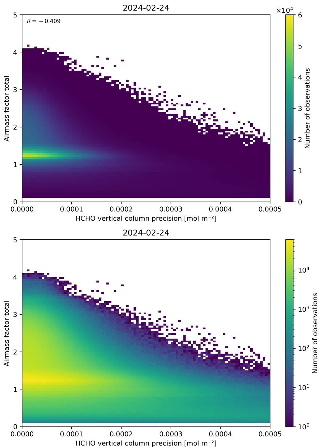
Figure 144: Scatter density plot of “HCHO vertical column precision” against “Airmass factor total” for 2024-02-23 to 2024-02-25.
