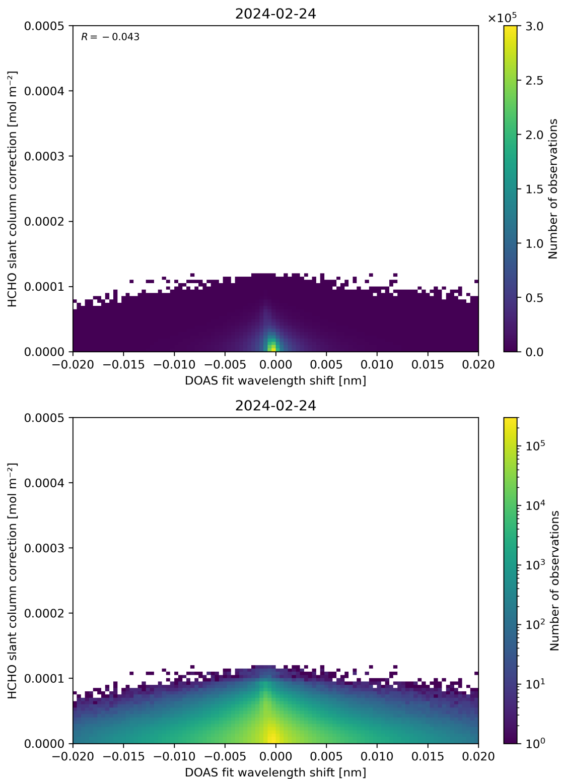
Figure 67: Scatter density plot of “DOAS fit wavelength shift” against “HCHO slant column correction” for 2024-02-23 to 2024-02-25.
