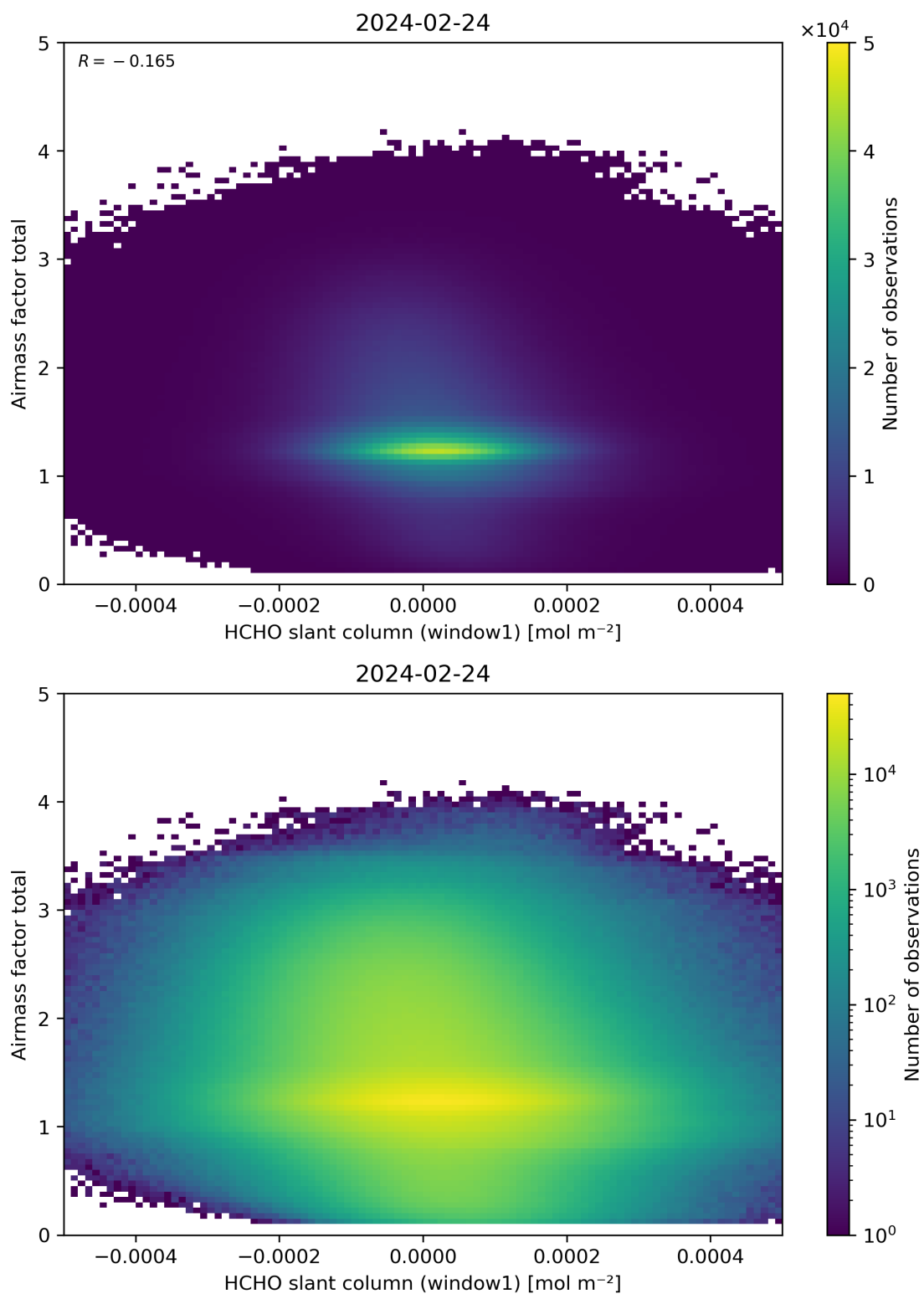
Figure 85: Scatter density plot of “HCHO slant column (window1)” against “Airmass factor total” for 2024-02-23 to 2024-02-25.
