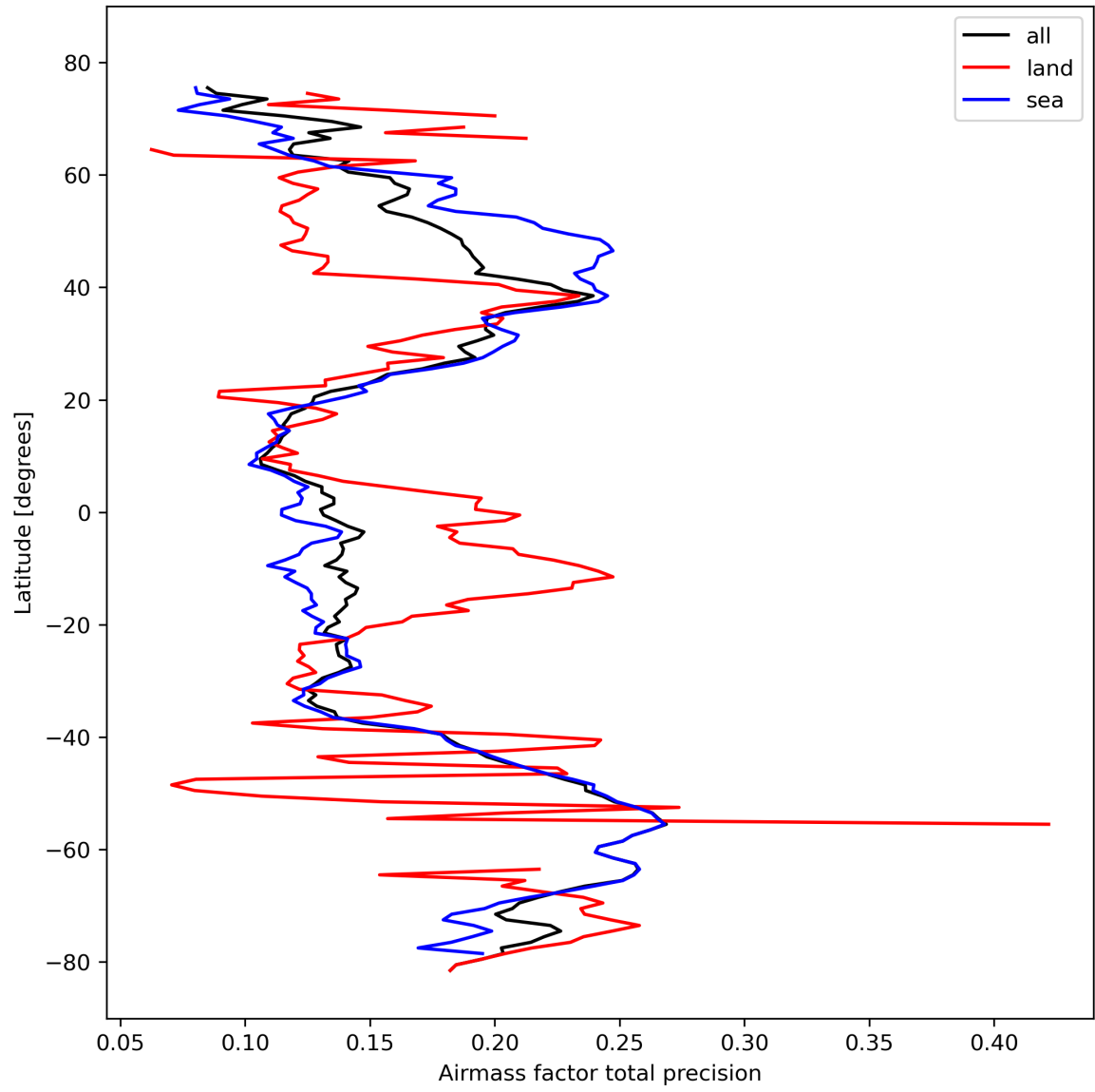
Figure 27: Zonal average of “Airmass factor total precision” for 2024-02-23 to 2024-02-25.
