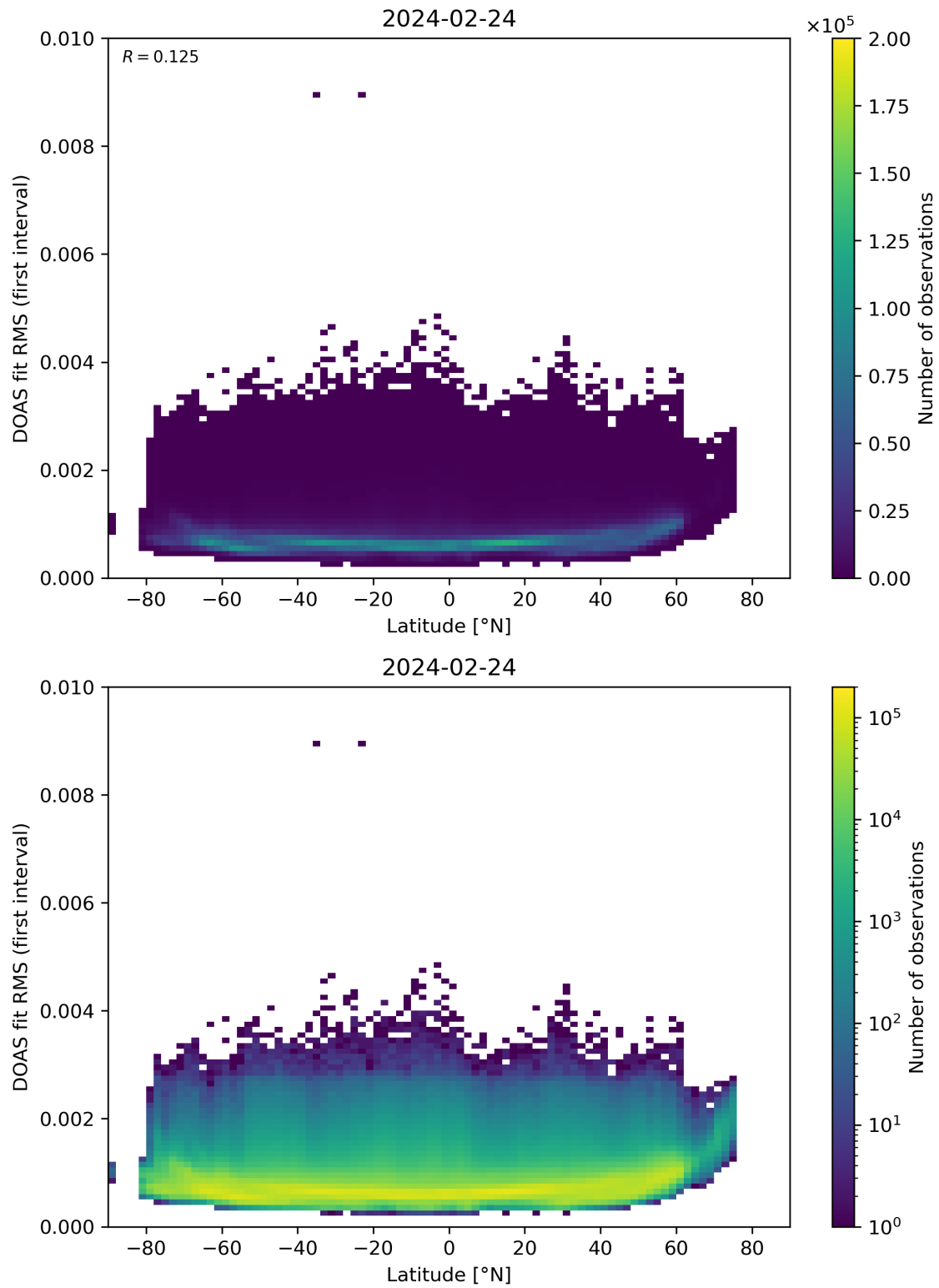
Figure 153: Scatter density plot of “Latitude” against “DOAS fit RMS (first interval)” for 2024-02-23 to 2024-02-25.
