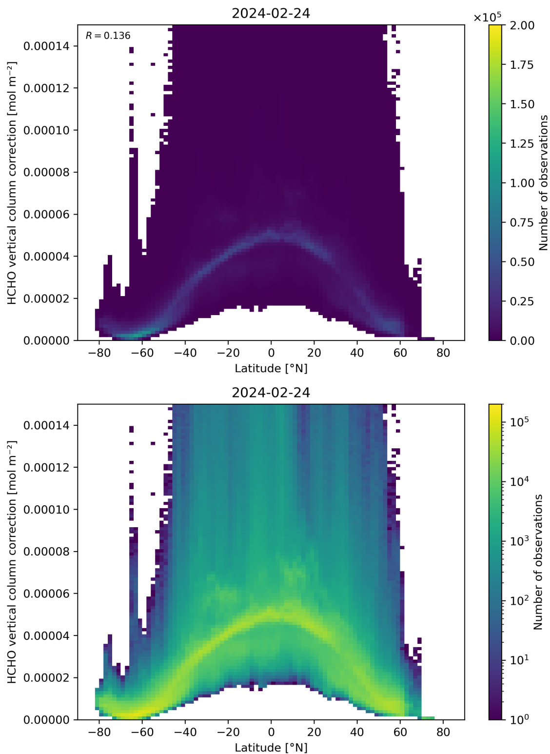
Figure 164: Scatter density plot of “Latitude” against “HCHO vertical column correction” for 2024-02-23 to 2024-02-25.
