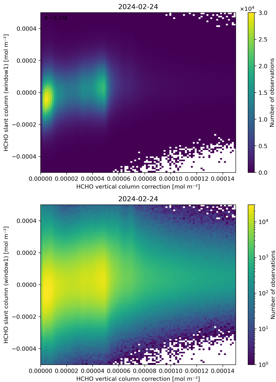
Figure 118: Scatter density plot of “HCHO vertical column correction” against “HCHO slant column (window1)” for 2024-02-23 to 2024-02-25.
