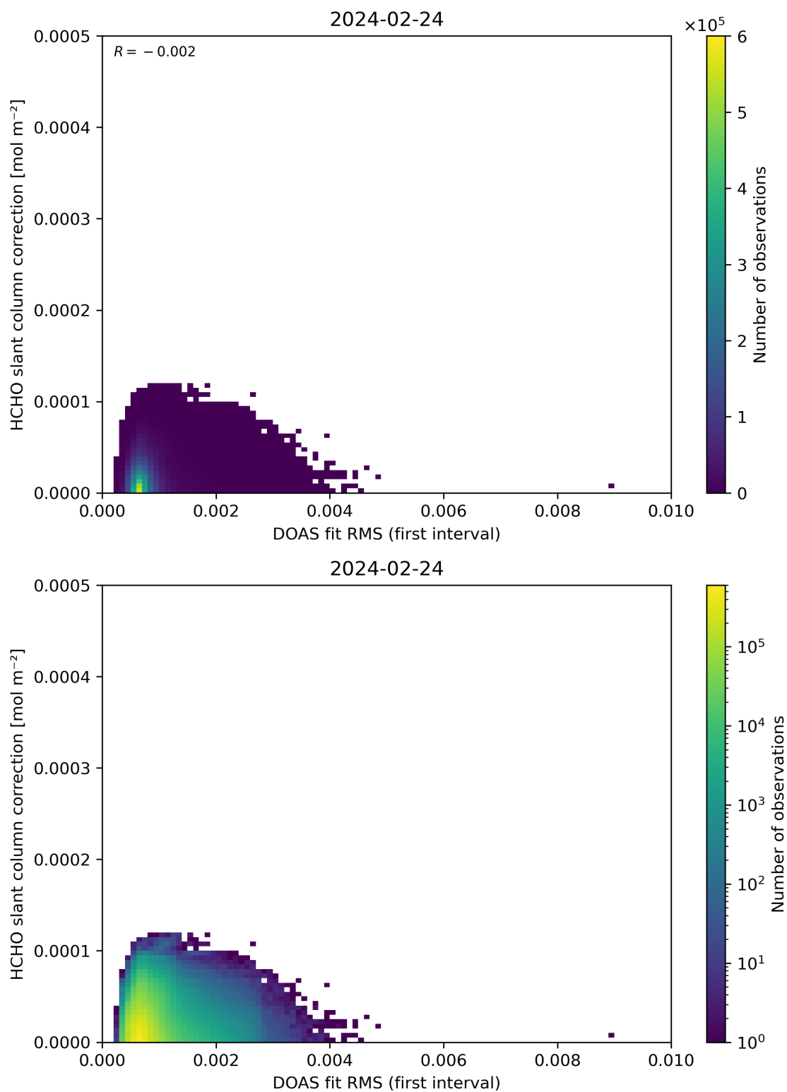
Figure 63: Scatter density plot of “DOAS fit RMS (first interval)” against “HCHO slant column correction” for 2024-02-23 to 2024-02-25.
