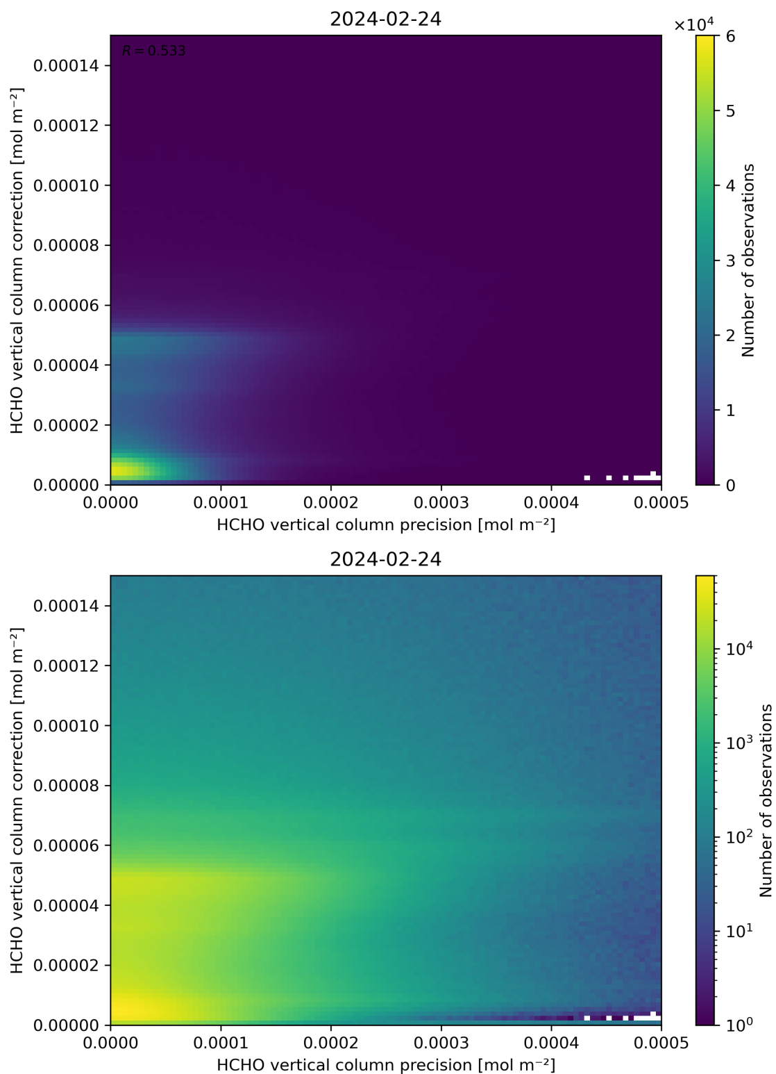
Figure 146: Scatter density plot of “HCHO vertical column precision” against “HCHO vertical column correction” for 2024-02-23 to 2024-02-25.
