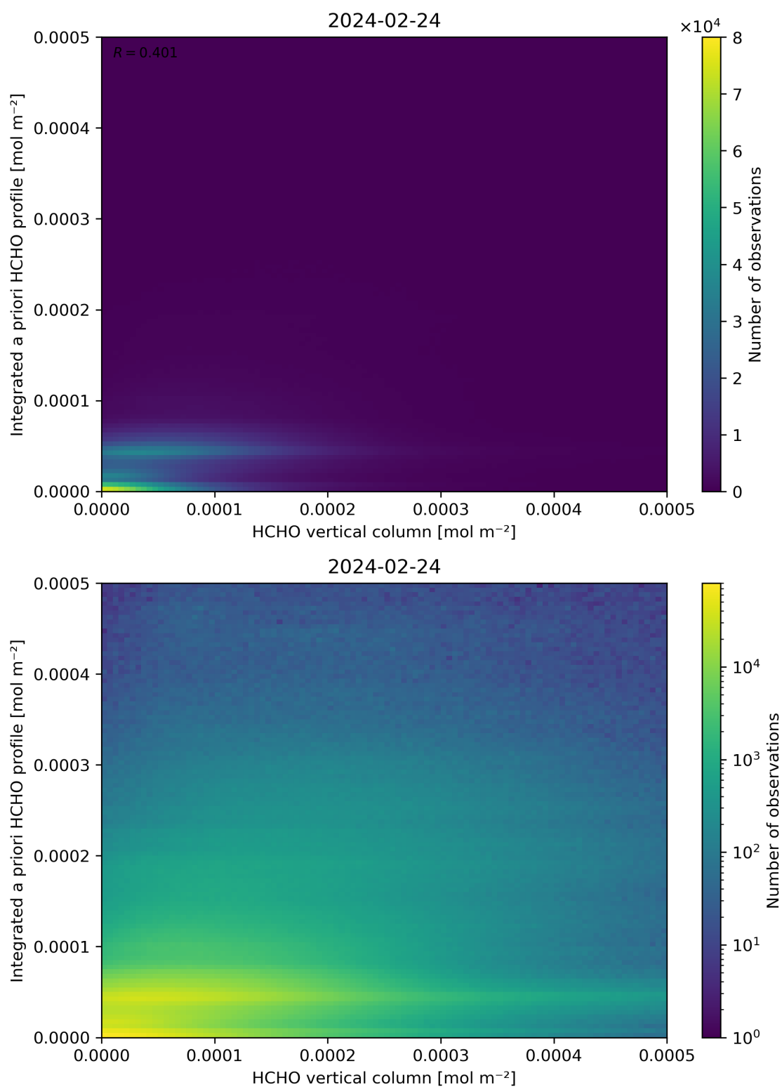
Figure 135: Scatter density plot of “HCHO vertical column” against “Integrated a priori HCHO profile” for 2024-02-23 to 2024-02-25.
