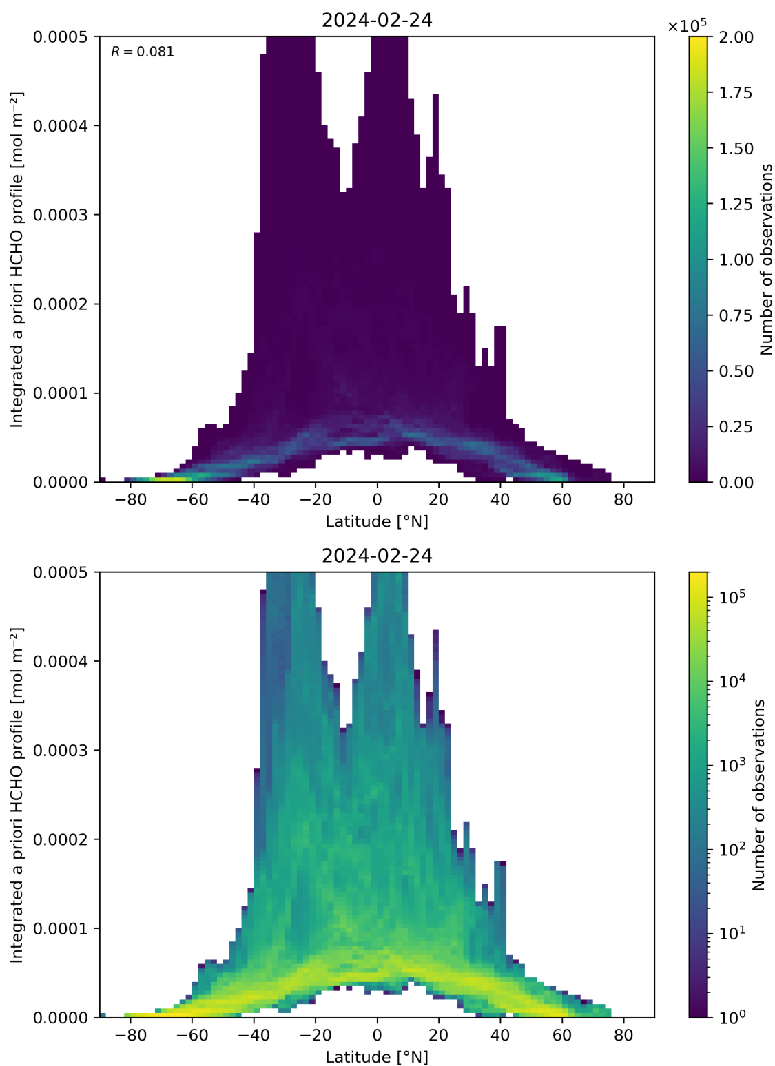
Figure 166: Scatter density plot of “Latitude” against “Integrated a priori HCHO profile” for 2024-02-23 to 2024-02-25.
