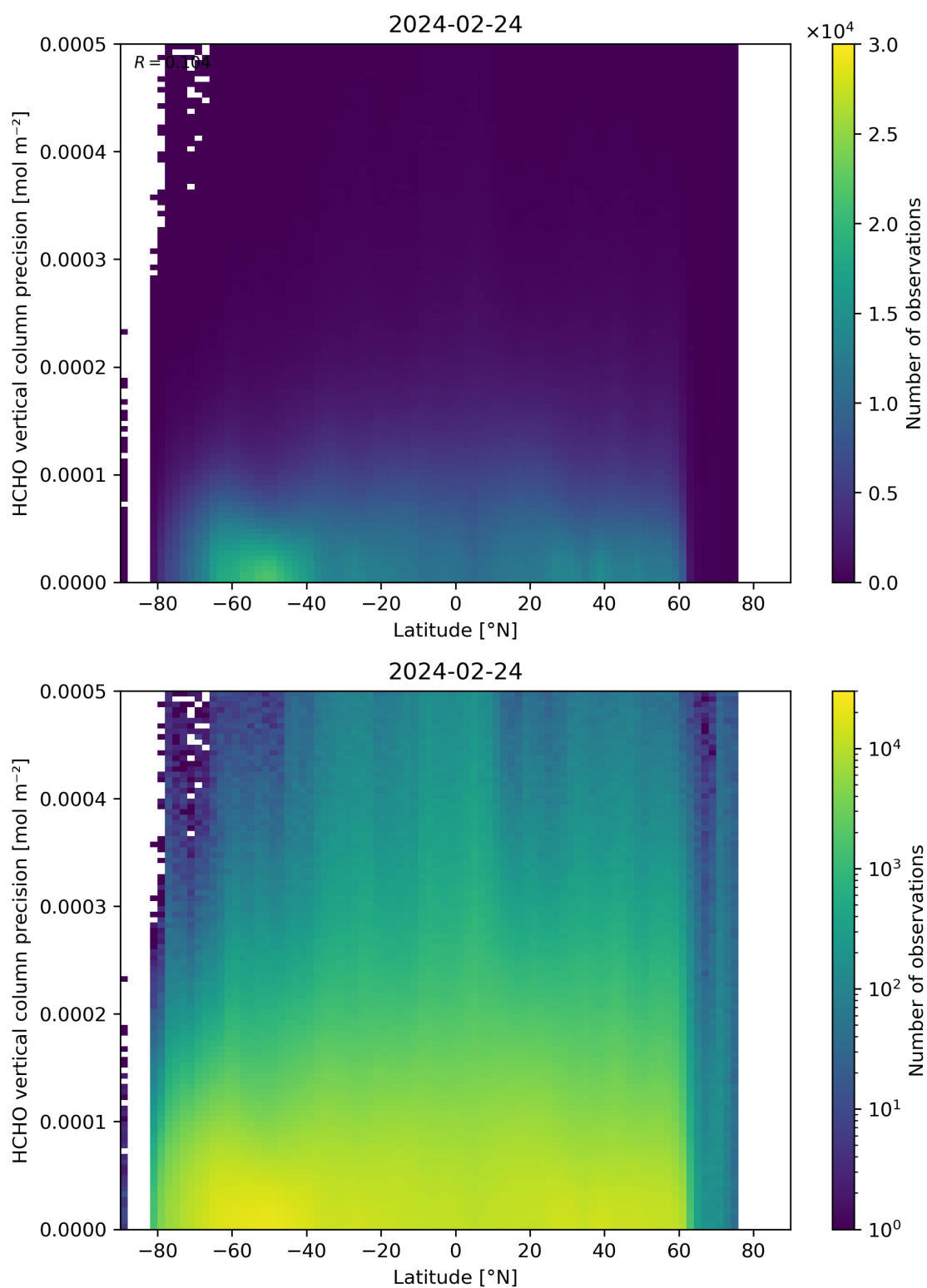
Figure 165: Scatter density plot of “Latitude” against “HCHO vertical column precision” for 2024-02-23 to 2024-02-25.
