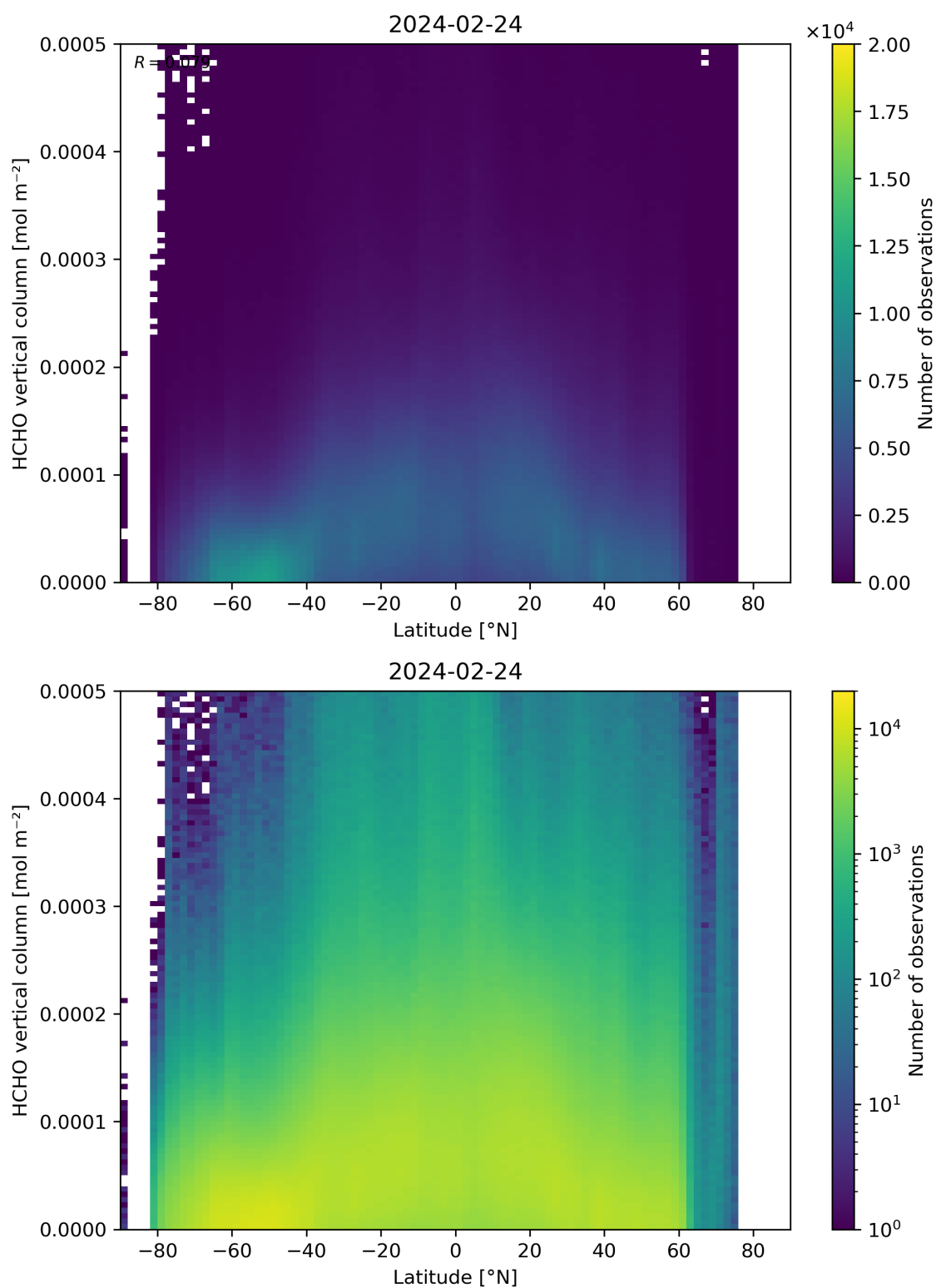
Figure 163: Scatter density plot of “Latitude” against “HCHO vertical column” for 2024-02-23 to 2024-02-25.
