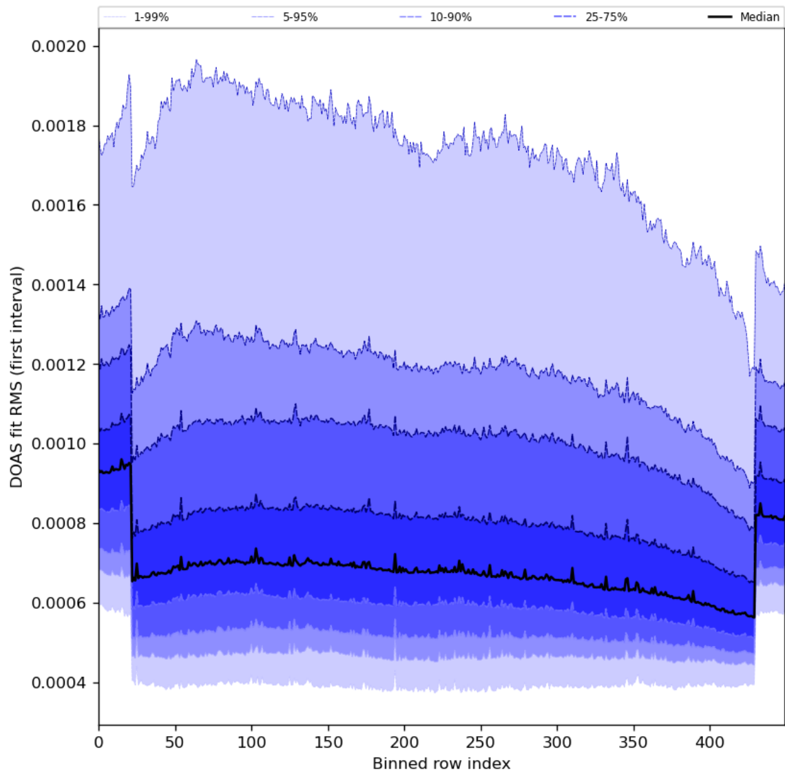
Figure 60: Along track statistics of “DOAS fit RMS (first interval)” for 2024-02-23 to 2024-02-25
