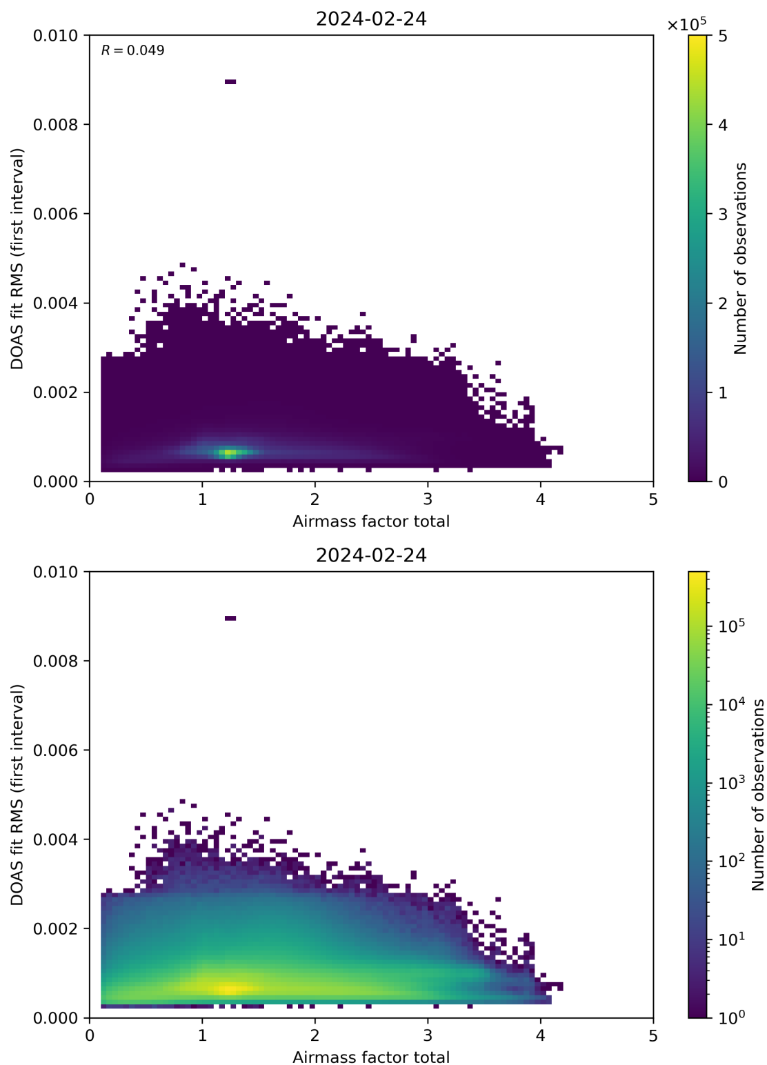
Figure 97: Scatter density plot of “Airmass factor total” against “DOAS fit RMS (first interval)” for 2024-02-23 to 2024-02-25.
