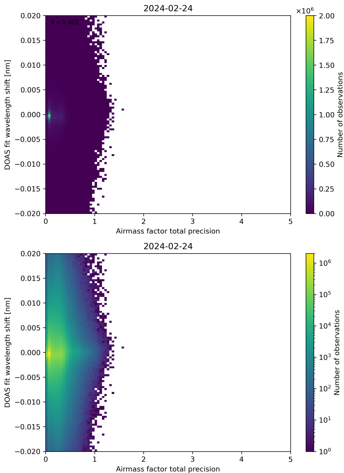
Figure 106: Scatter density plot of “Airmass factor total precision” against “DOAS fit wavelength shift” for 2024-02-23 to 2024-02-25.
