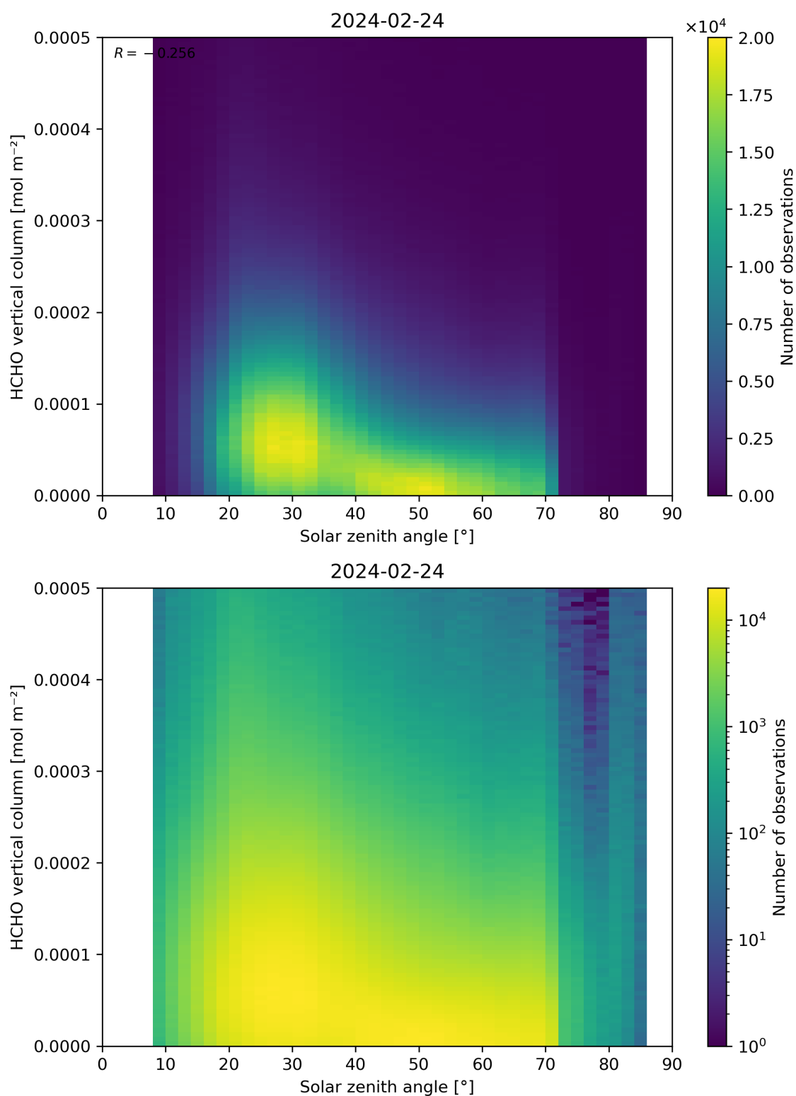
Figure 177: Scatter density plot of “Solar zenith angle” against “HCHO vertical column” for 2024-02-23 to 2024-02-25.
