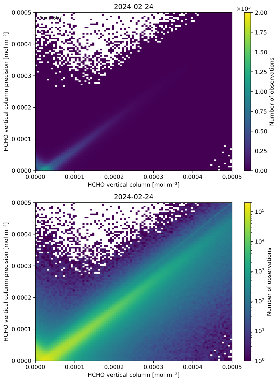
Figure 134: Scatter density plot of “HCHO vertical column” against “HCHO vertical column precision” for 2024-02-23 to 2024-02-25.
