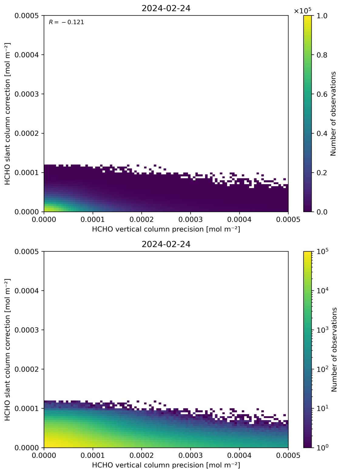
Figure 141: Scatter density plot of “HCHO vertical column precision” against “HCHO slant column correction” for 2024-02-23 to 2024-02-25.
