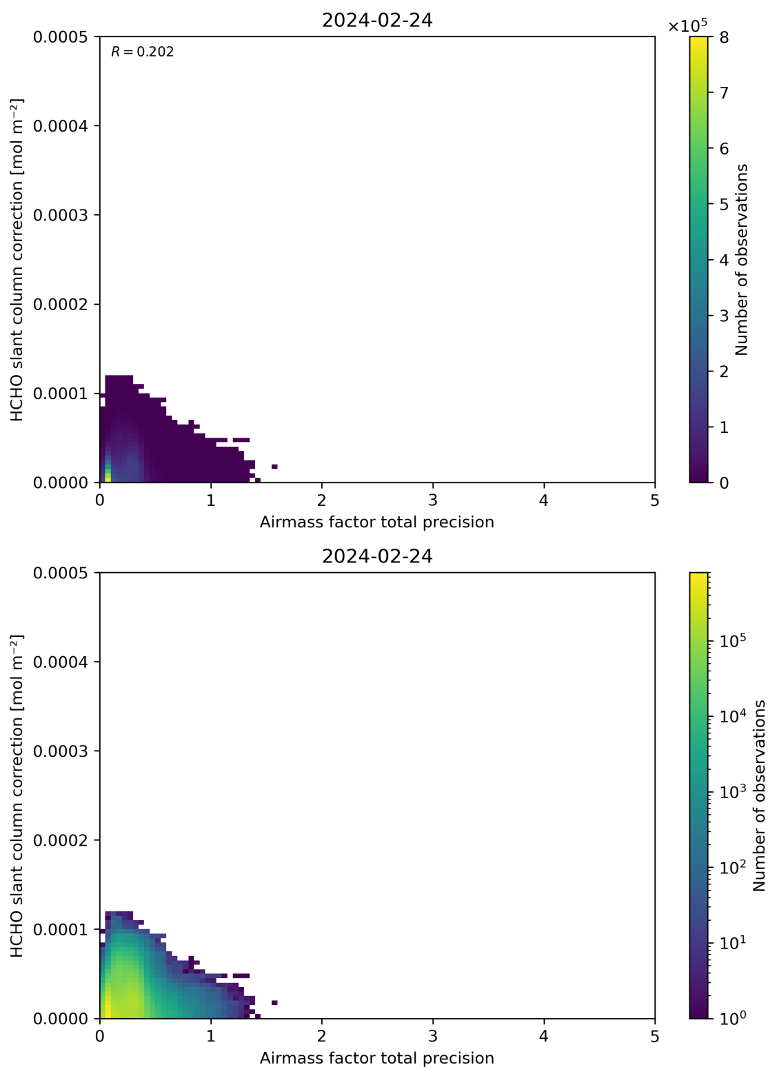
Figure 110: Scatter density plot of “Airmass factor total precision” against “HCHO slant column correction” for 2024-02-23 to 2024-02-25.
