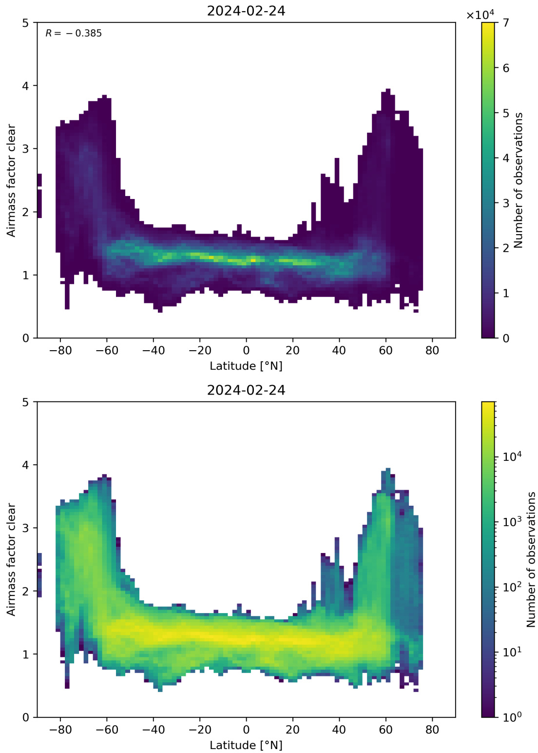
Figure 156: Scatter density plot of “Latitude” against “Airmass factor clear” for 2024-02-23 to 2024-02-25.
