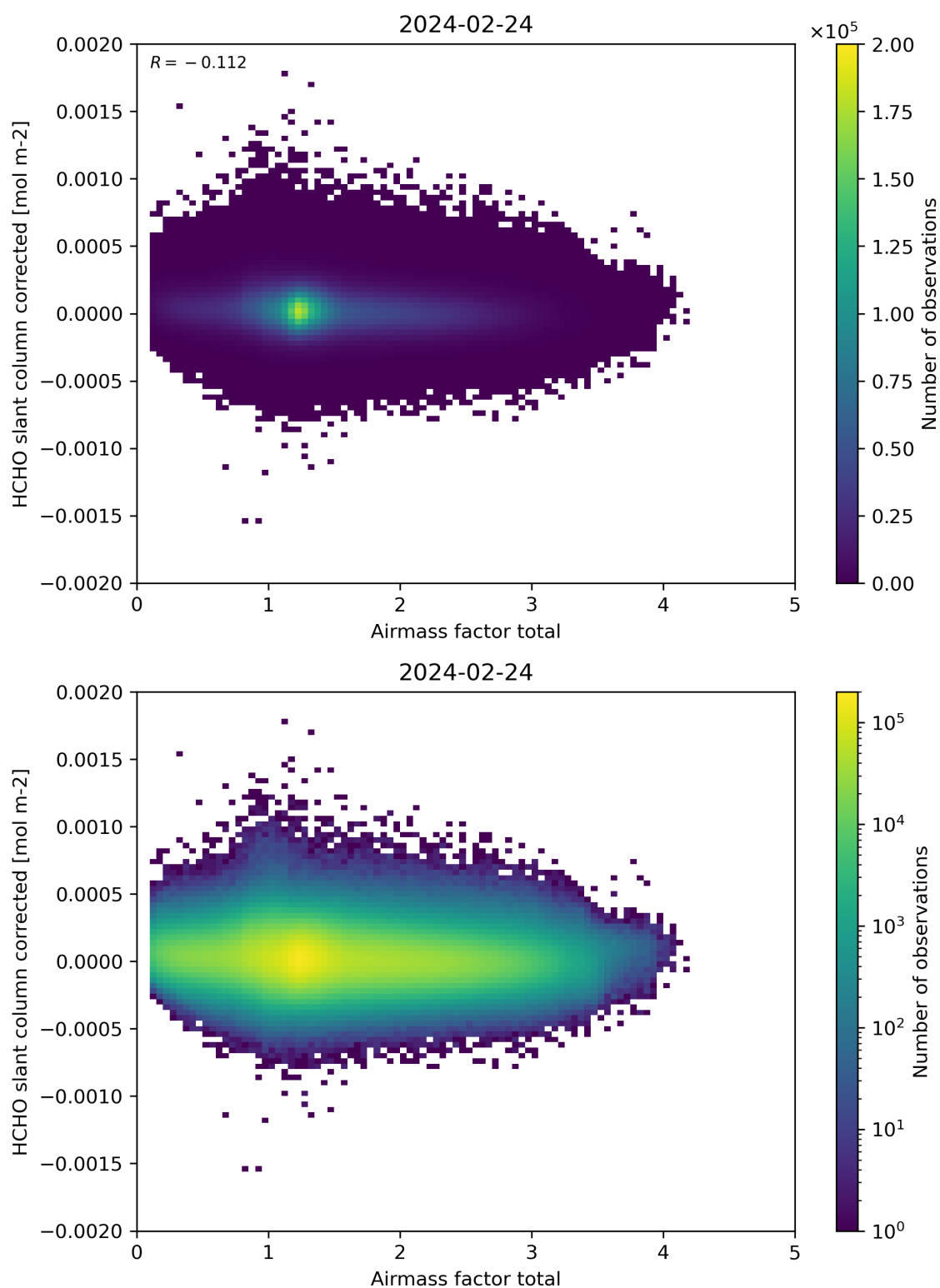
Figure 101: Scatter density plot of “Airmass factor total” against “HCHO slant column corrected” for 2024-02-23 to 2024-02-25.
