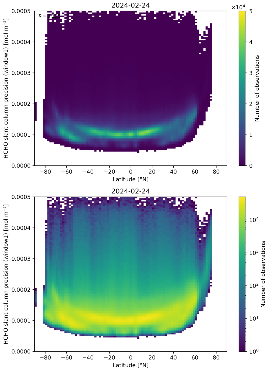
Figure 160: Scatter density plot of “Latitude” against “HCHO slant column precision (window1)” for 2024-02-23 to 2024-02-25.
