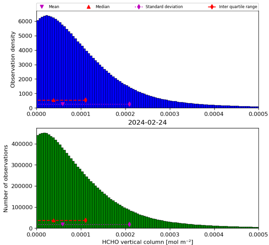
Figure 35: Histogram of “HCHO vertical column” for 2024-02-23 to 2024-02-25
