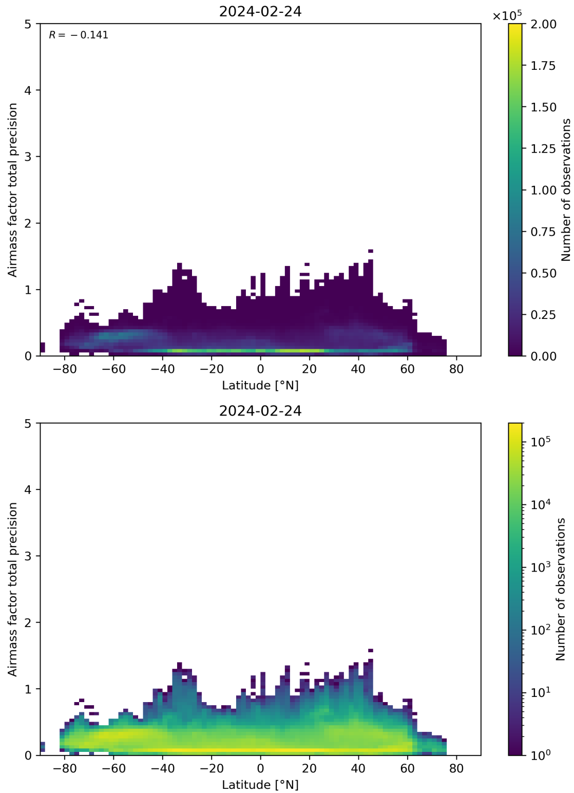
Figure 162: Scatter density plot of “Latitude” against “Airmass factor total precision” for 2024-02-23 to 2024-02-25.
