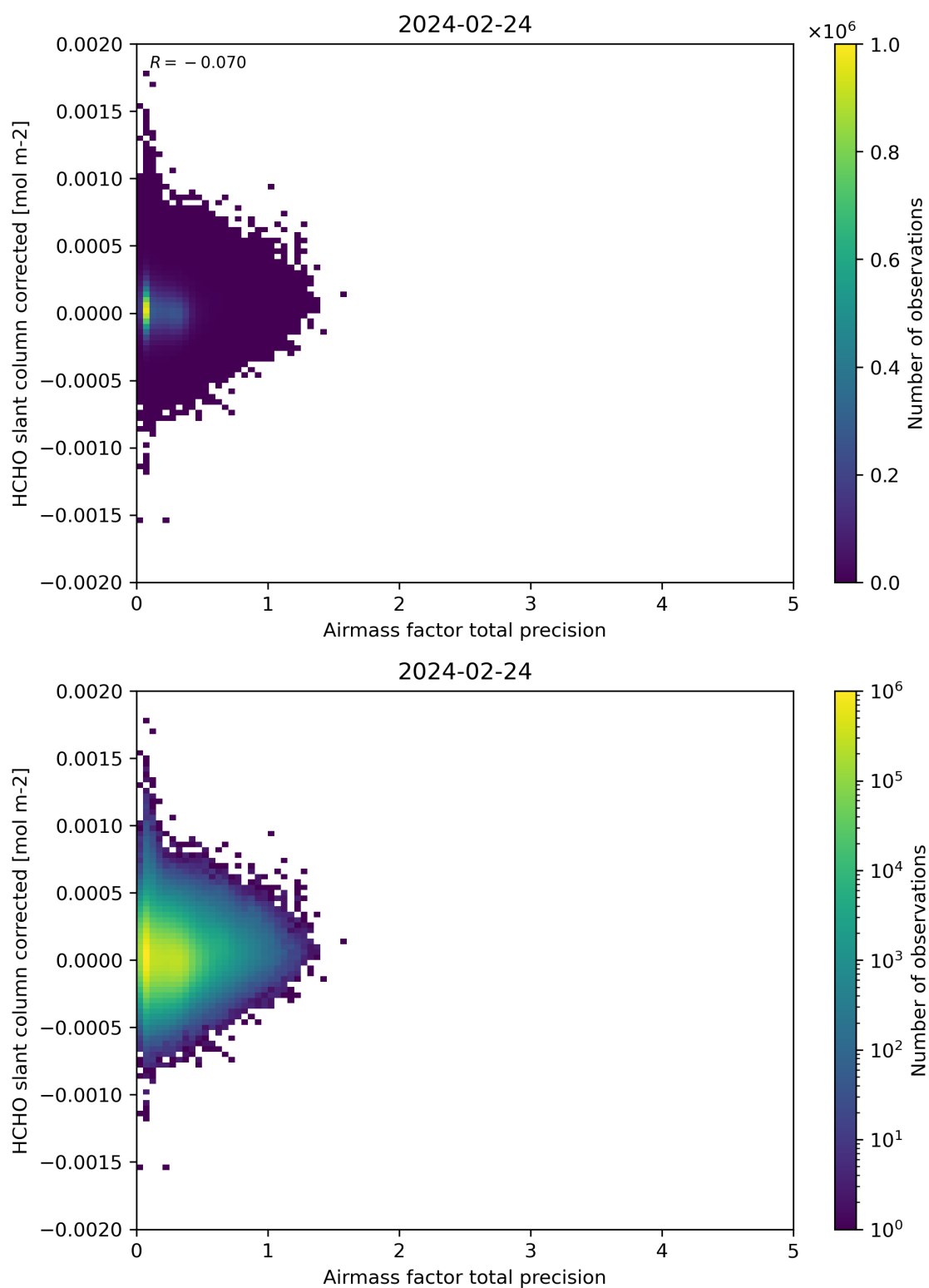
Figure 109: Scatter density plot of “Airmass factor total precision” against “HCHO slant column corrected” for 2024-02-23 to 2024-02-25.
