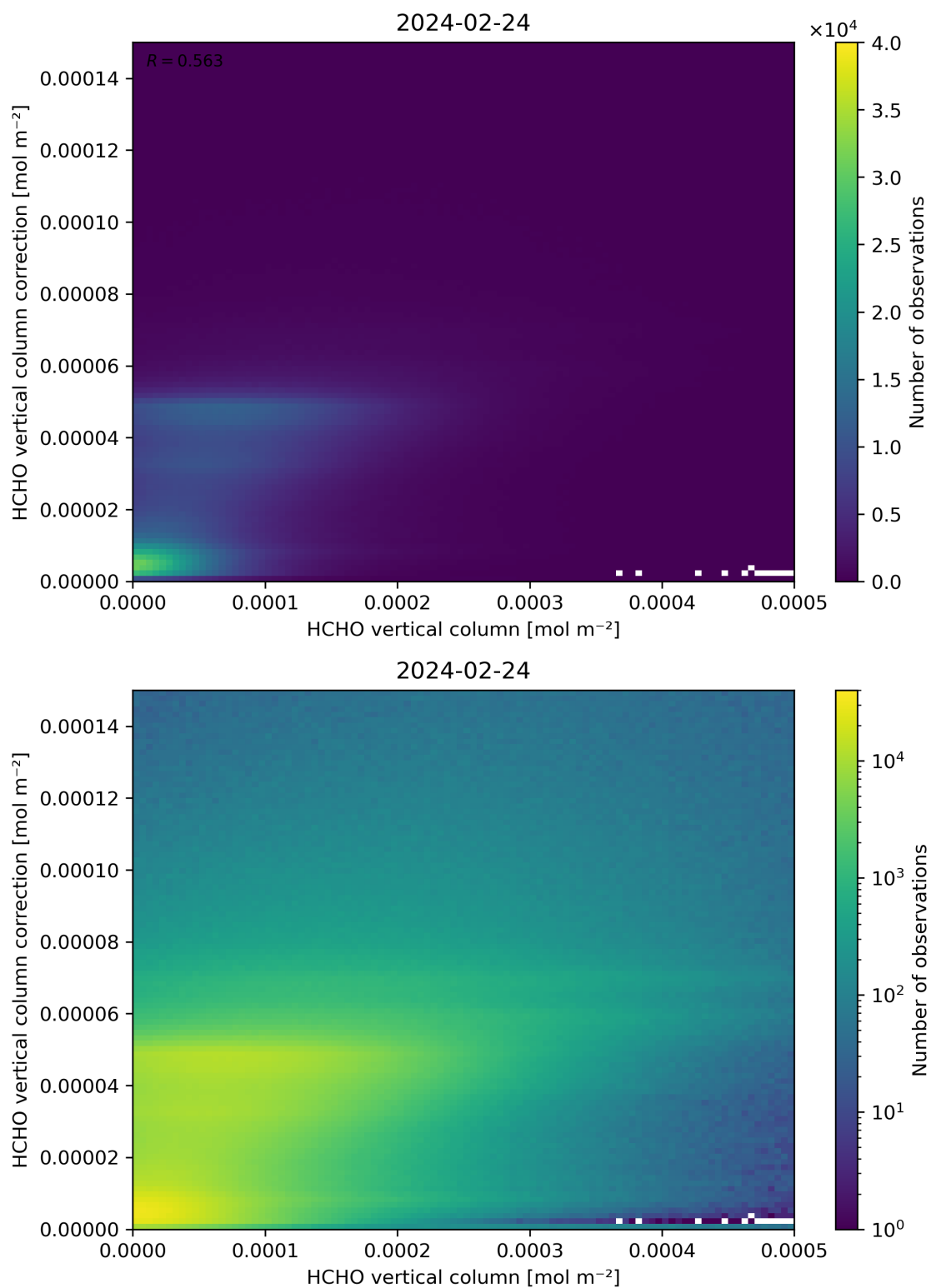
Figure 133: Scatter density plot of “HCHO vertical column” against “HCHO vertical column correction” for 2024-02-23 to 2024-02-25.
