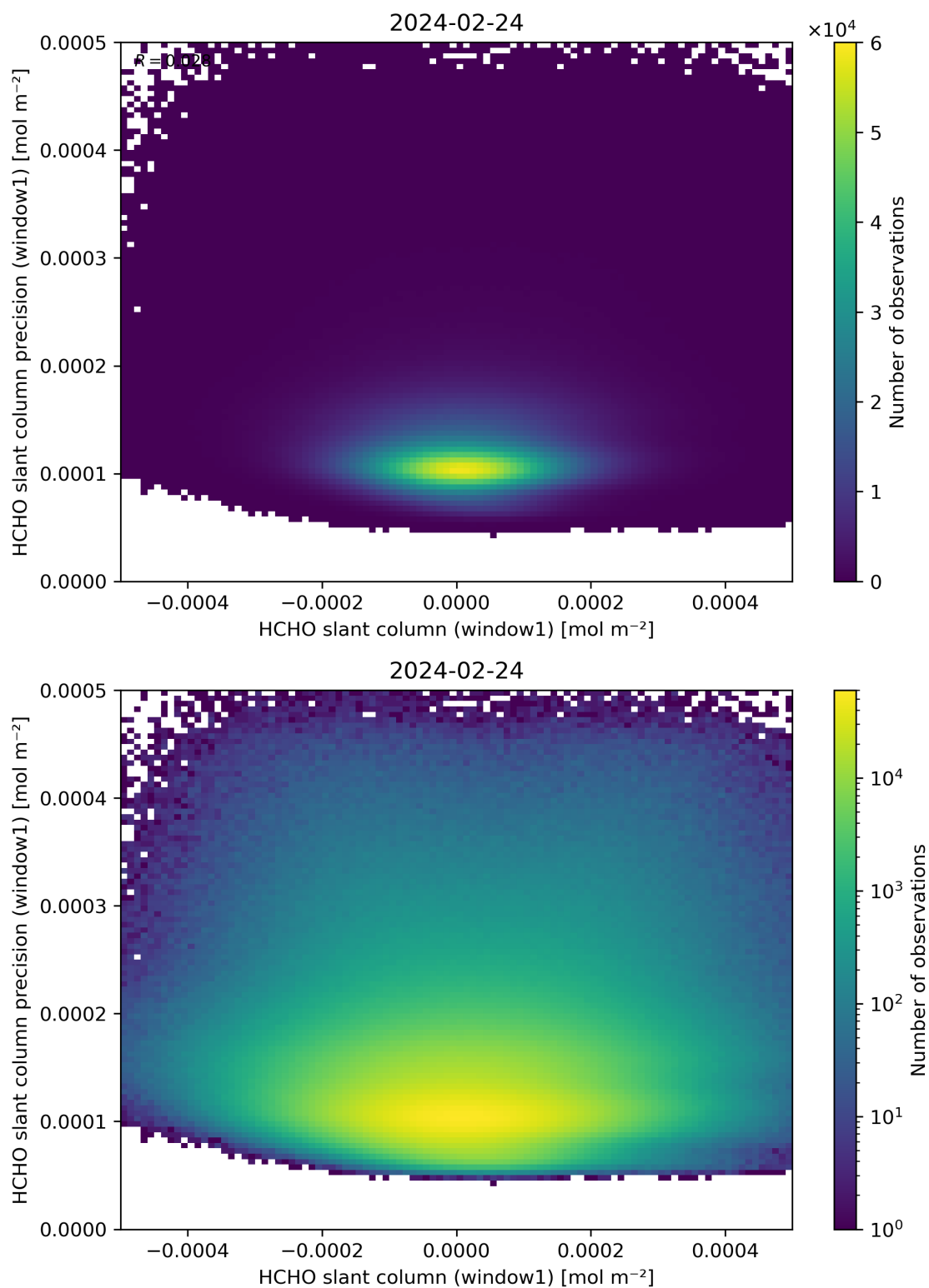
Figure 84: Scatter density plot of “HCHO slant column (window1)” against “HCHO slant column precision (window1)” for 2024-02-23 to 2024-02-25.
