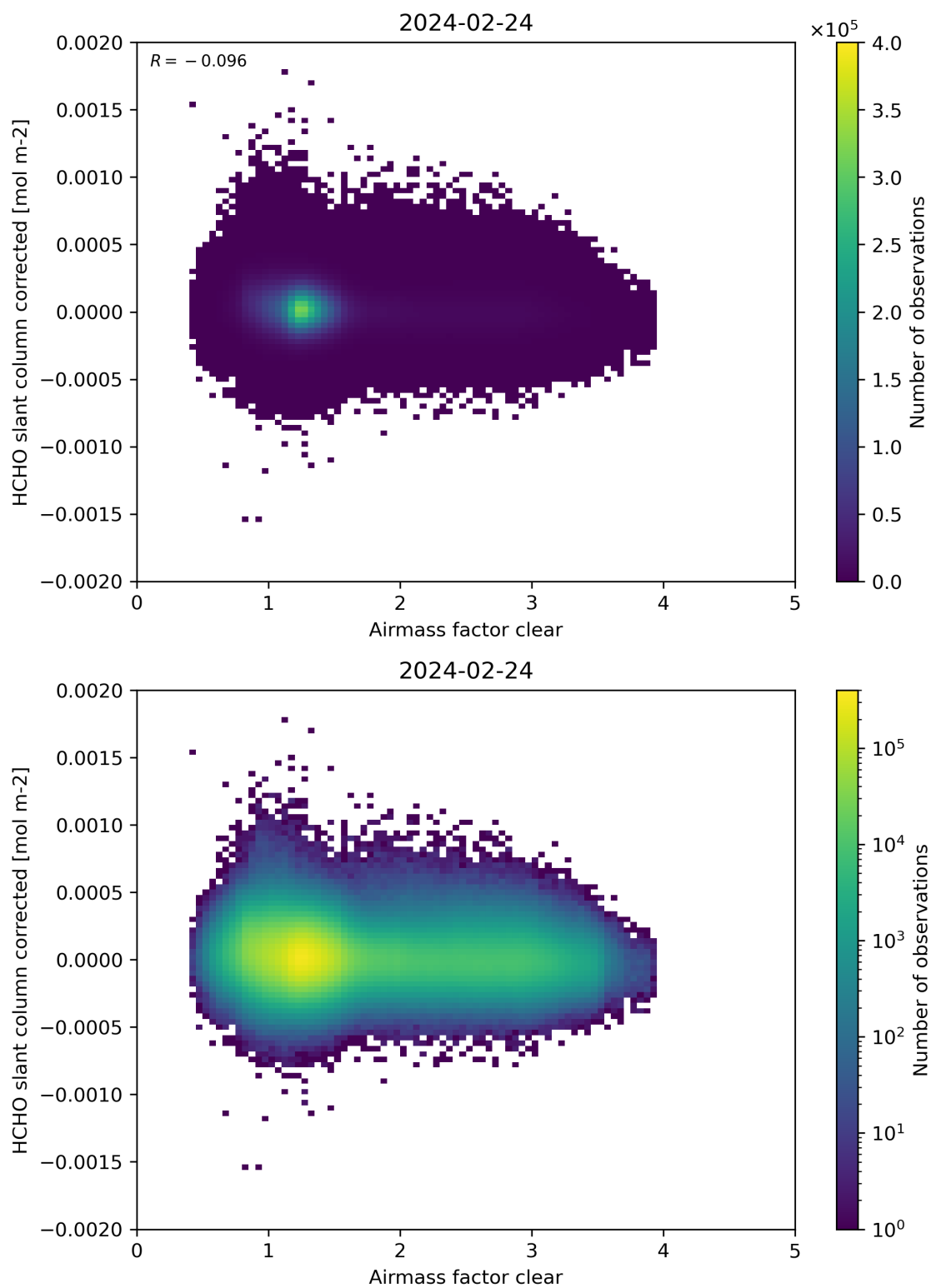
Figure 74: Scatter density plot of “Airmass factor clear” against “HCHO slant column corrected” for 2024-02-23 to 2024-02-25.
