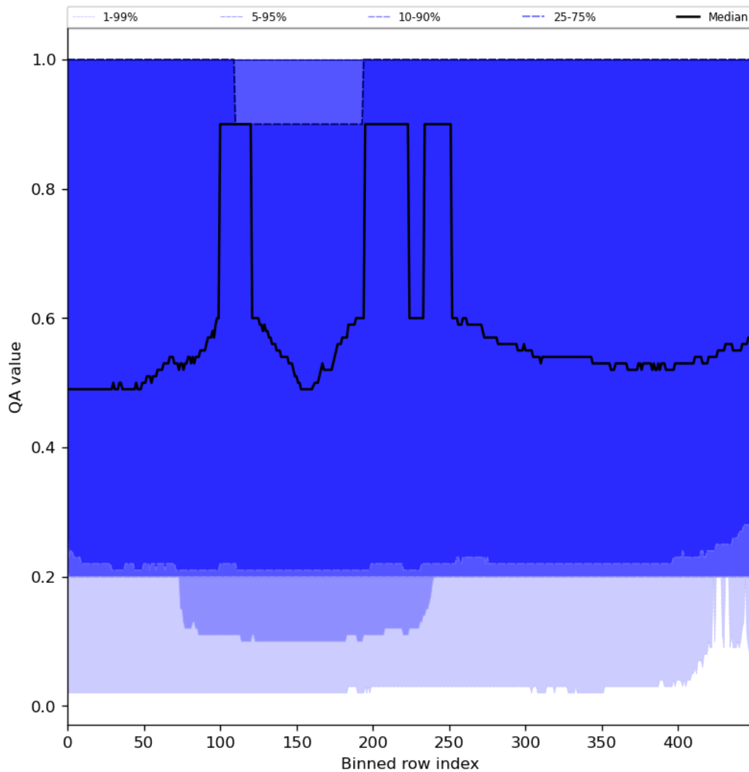
Figure 48: Along track statistics of “QA value” for 2024-02-23 to 2024-02-25
