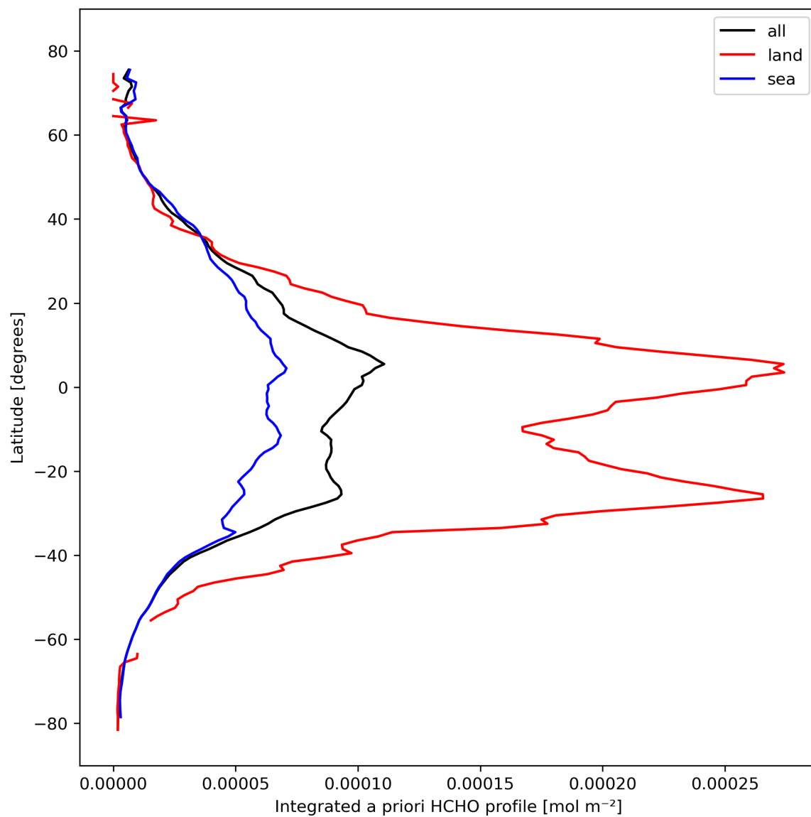
Figure 29: Zonal average of “Integrated a priori HCHO profile” for 2024-02-23 to 2024-02-25.
