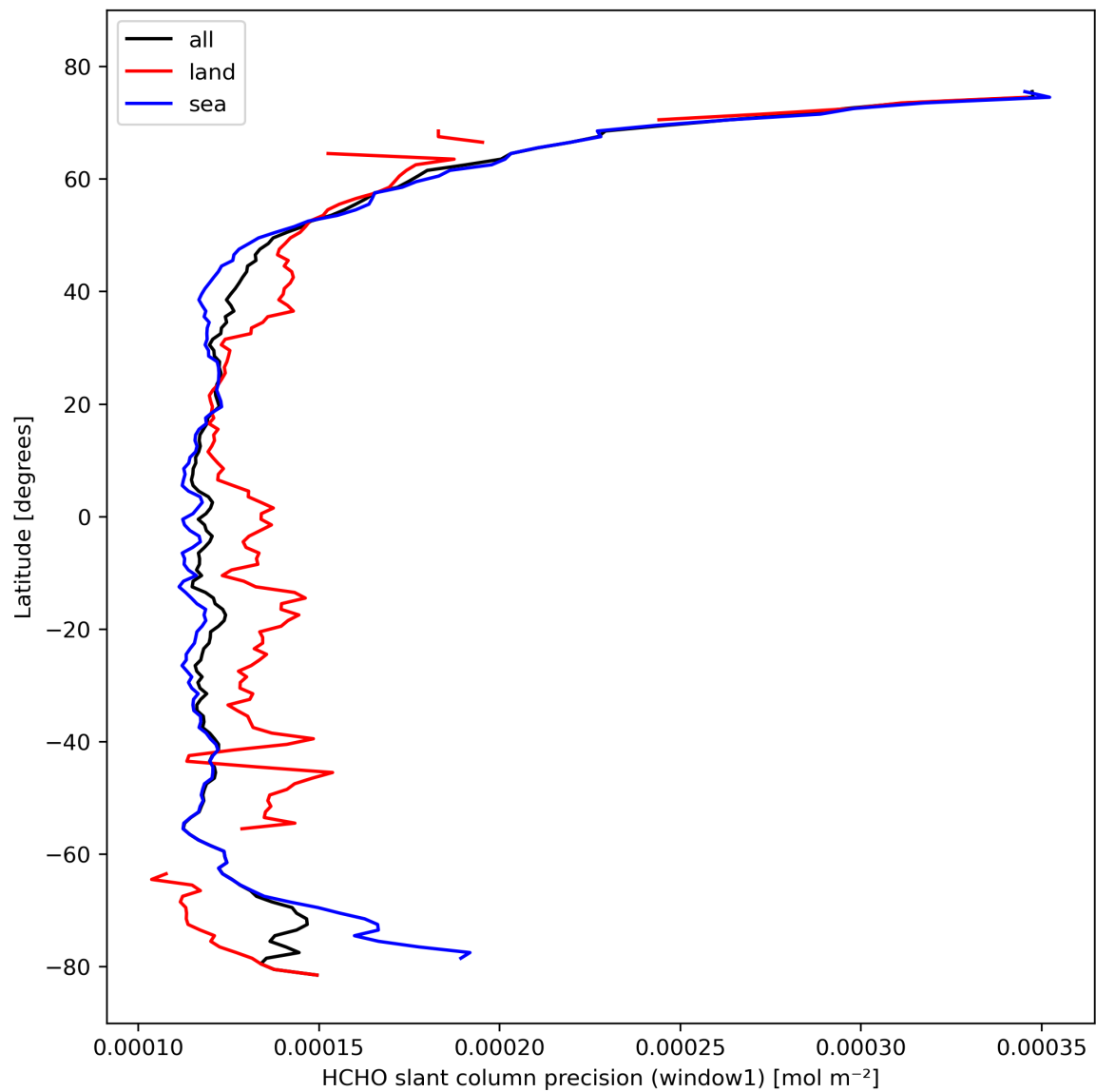
Figure 25: Zonal average of “HCHO slant column precision (window1)” for 2024-02-23 to 2024-02-25.
