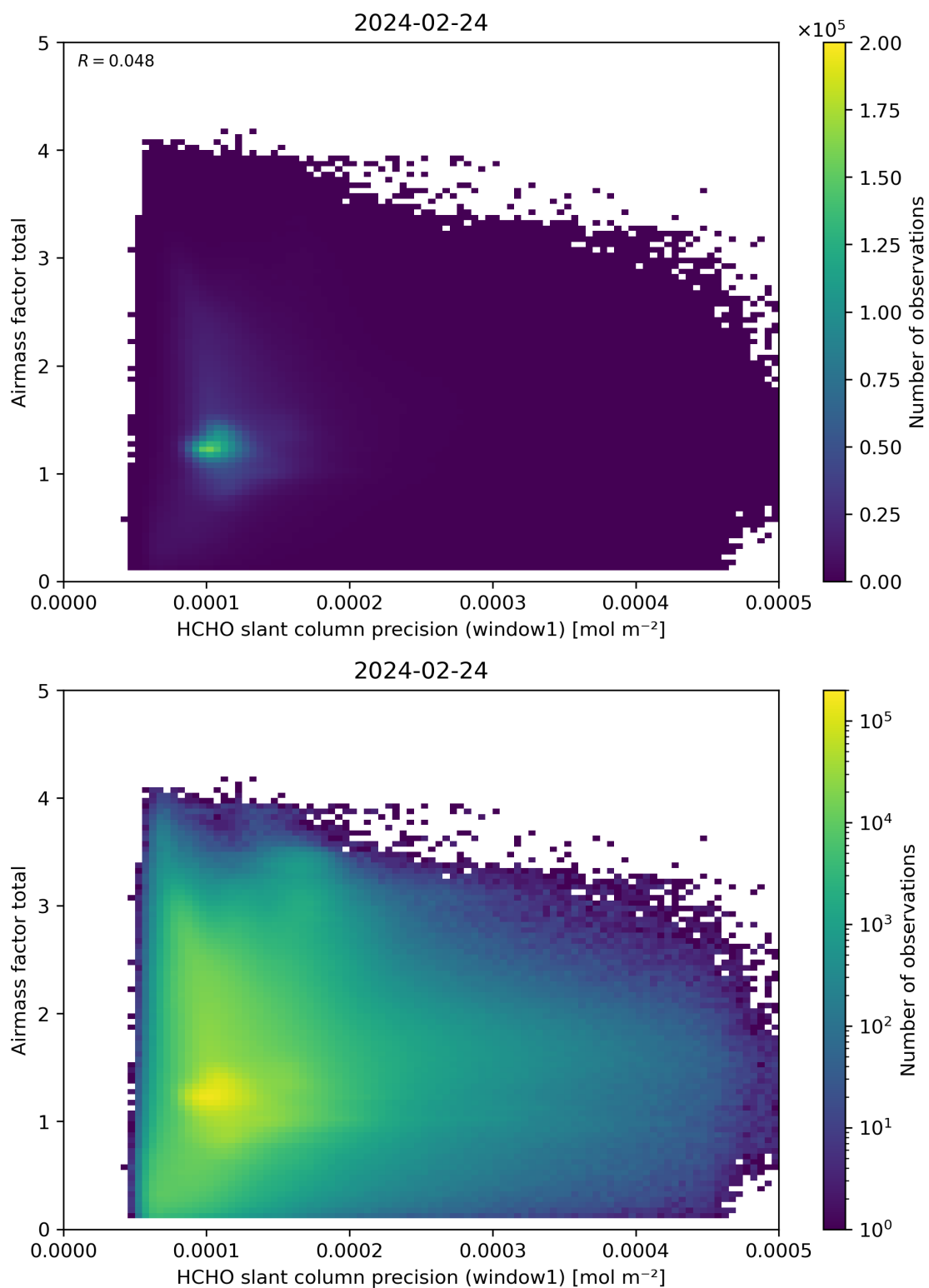
Figure 94: Scatter density plot of “HCHO slant column precision (window1)” against “Airmass factor total” for 2024-02-23 to 2024-02-25.
