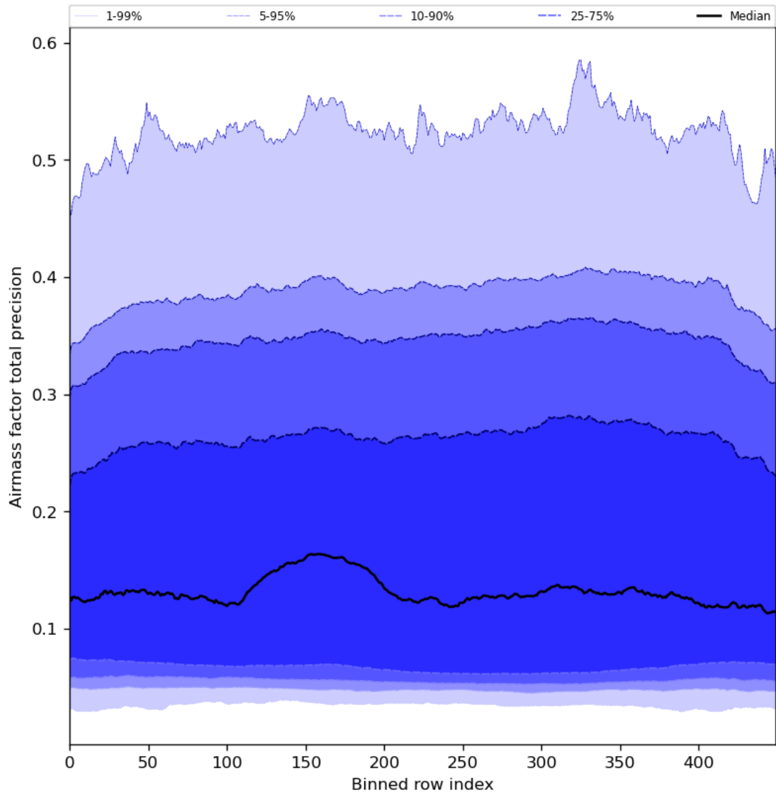
Figure 55: Along track statistics of “Airmass factor total precision” for 2024-02-23 to 2024-02-25
