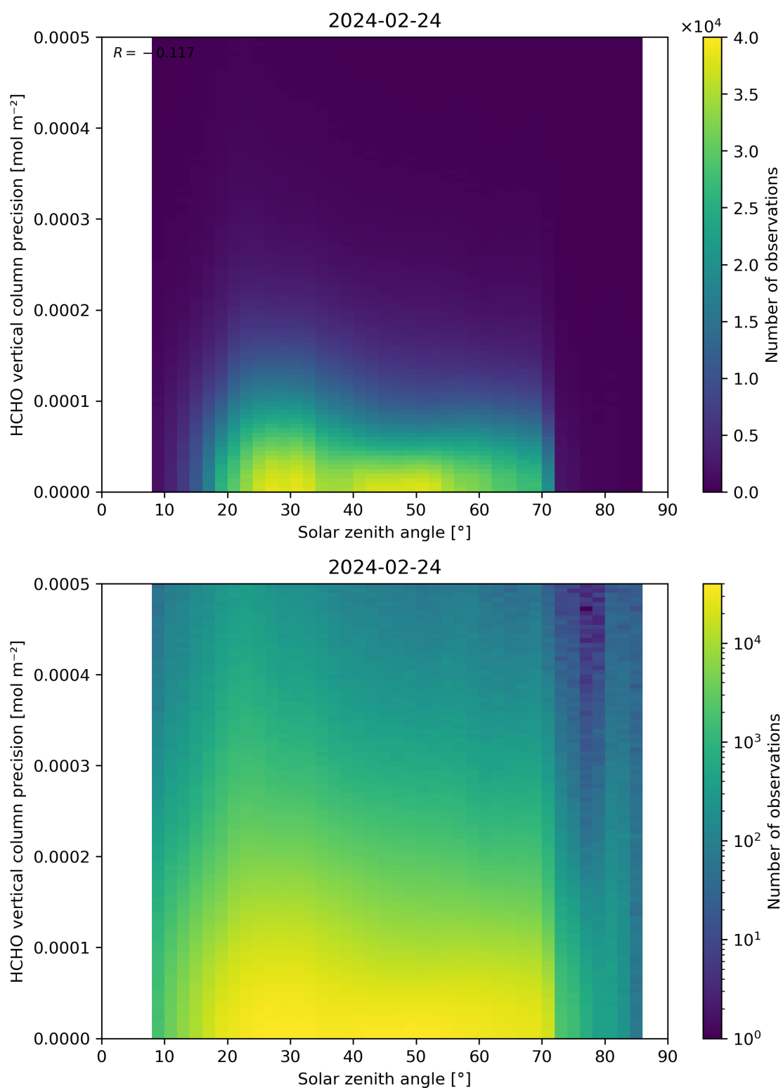
Figure 179: Scatter density plot of “Solar zenith angle” against “HCHO vertical column precision” for 2024-02-23 to 2024-02-25.
