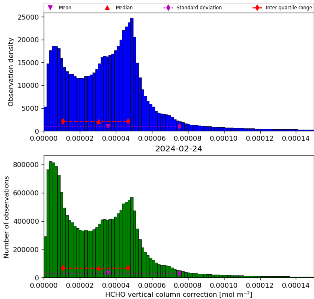
Figure 37: Histogram of “HCHO vertical column correction” for 2024-02-23 to 2024-02-25
