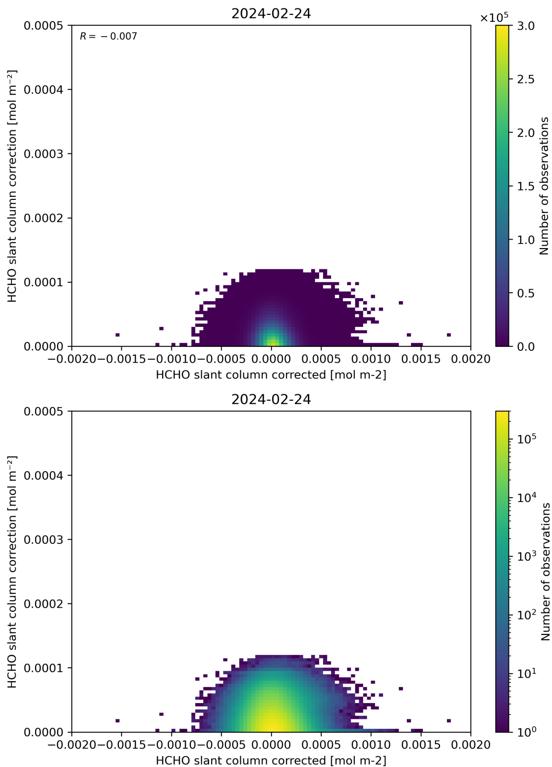
Figure 77: Scatter density plot of “HCHO slant column corrected” against “HCHO slant column correction” for 2024-02-23 to 2024-02-25.
