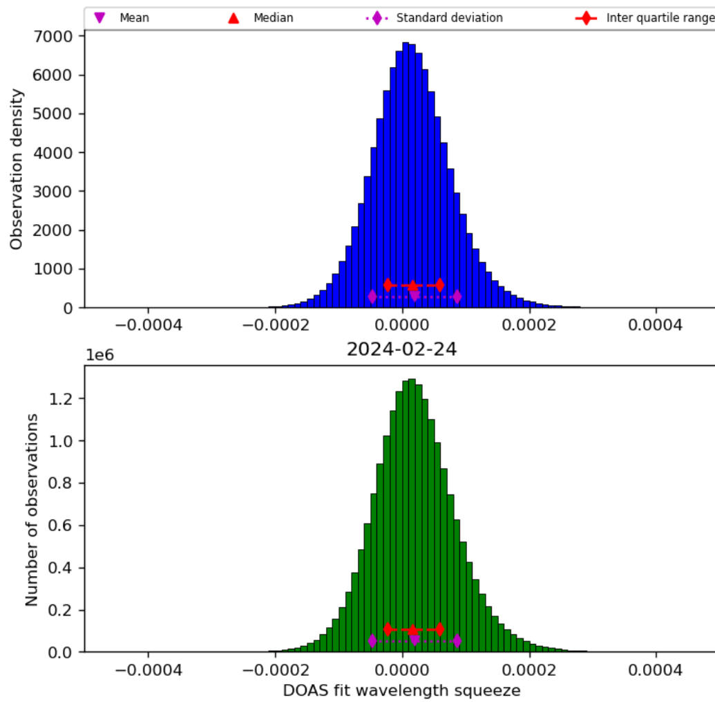
Figure 45: Histogram of “DOAS fit wavelength squeeze” for 2024-02-23 to 2024-02-25
