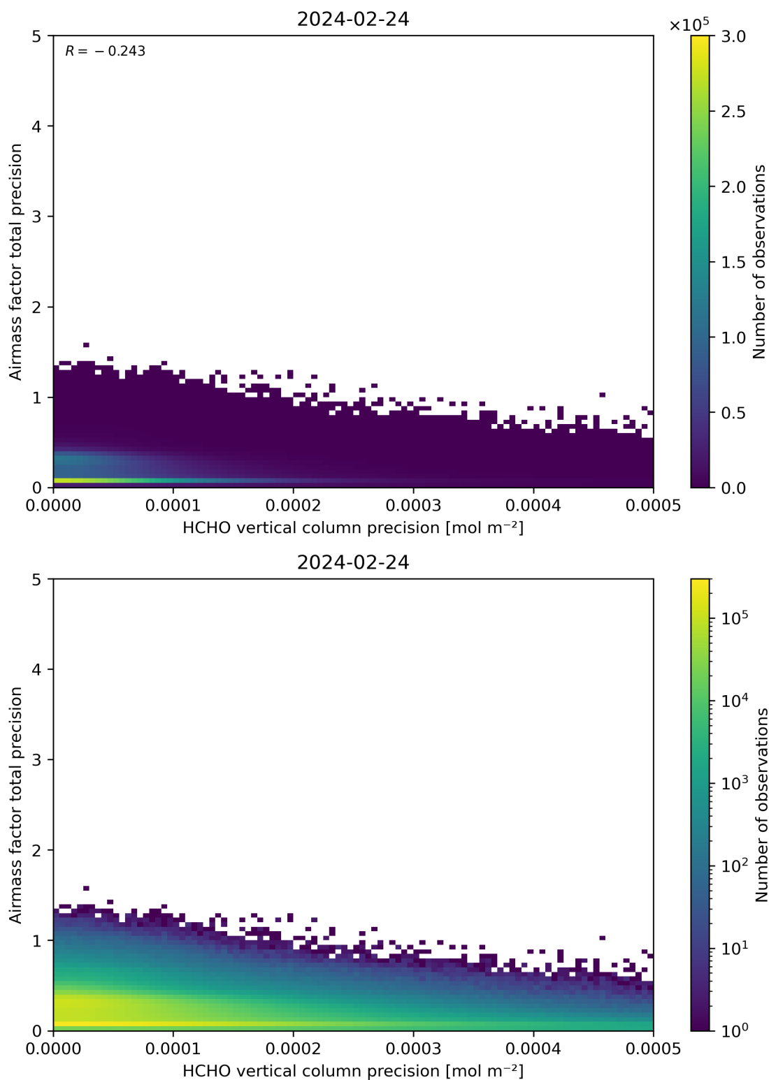
Figure 145: Scatter density plot of “HCHO vertical column precision” against “Airmass factor total precision” for 2024-02-23 to 2024-02-25.
