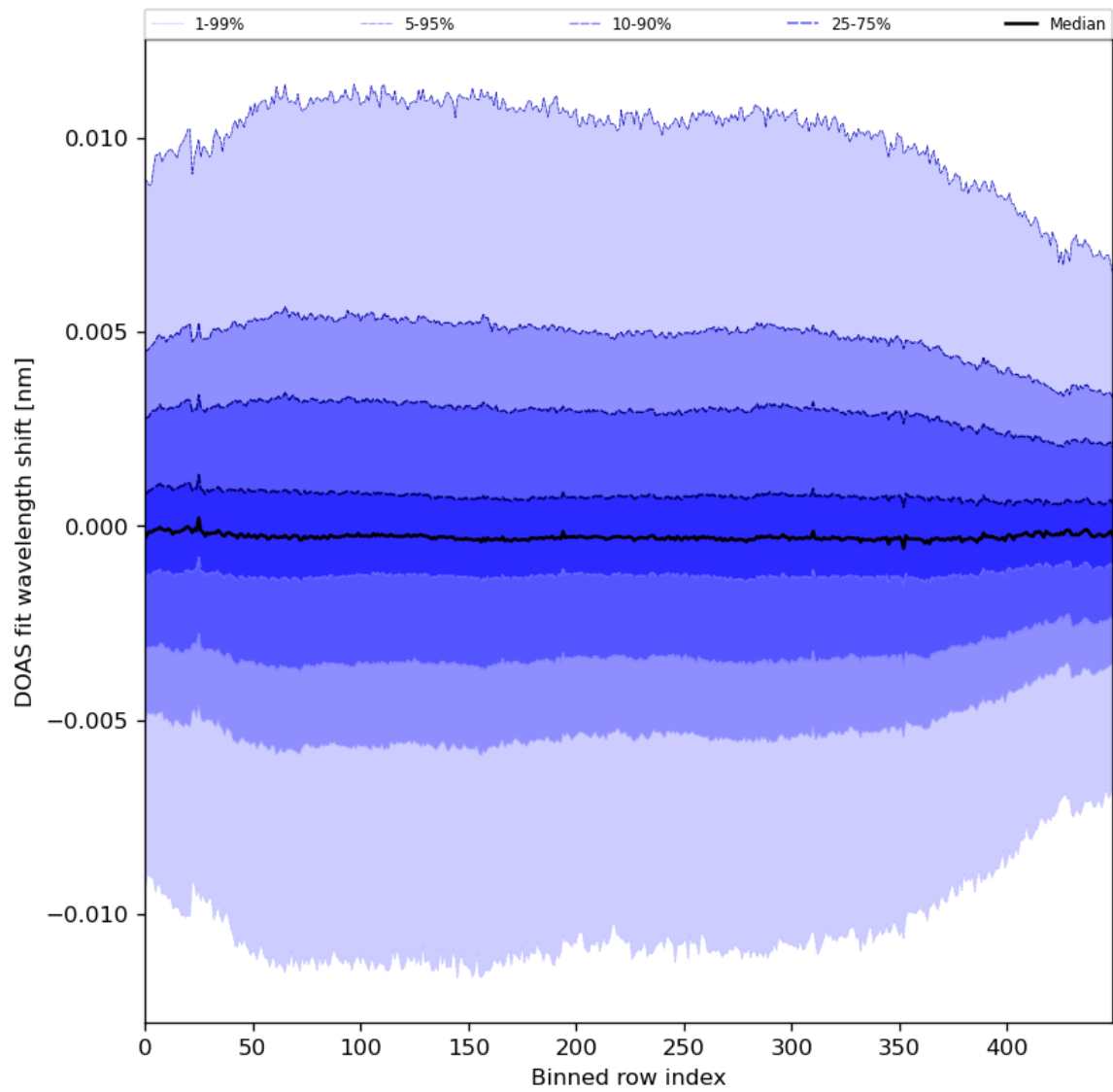
Figure 58: Along track statistics of “DOAS fit wavelength shift” for 2024-02-23 to 2024-02-25
