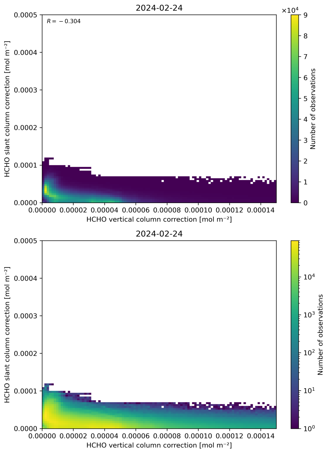
Figure 117: Scatter density plot of “HCHO vertical column correction” against “HCHO slant column correction” for 2024-02-23 to 2024-02-25.
