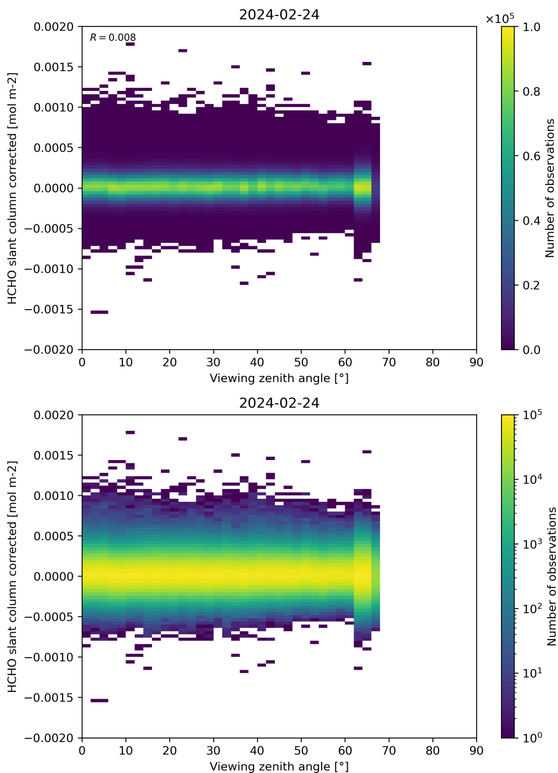
Figure 186: Scatter density plot of “Viewing zenith angle” against “HCHO slant column corrected” for 2024-02-23 to 2024-02-25.
