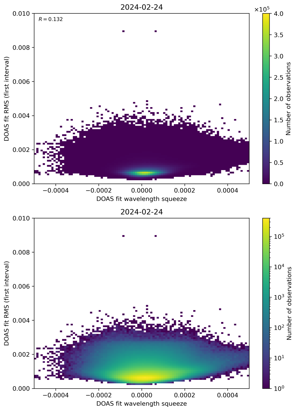
Figure 68: Scatter density plot of “DOAS fit wavelength squeeze” against “DOAS fit RMS (first interval)” for 2024-02-23 to 2024-02-25.
