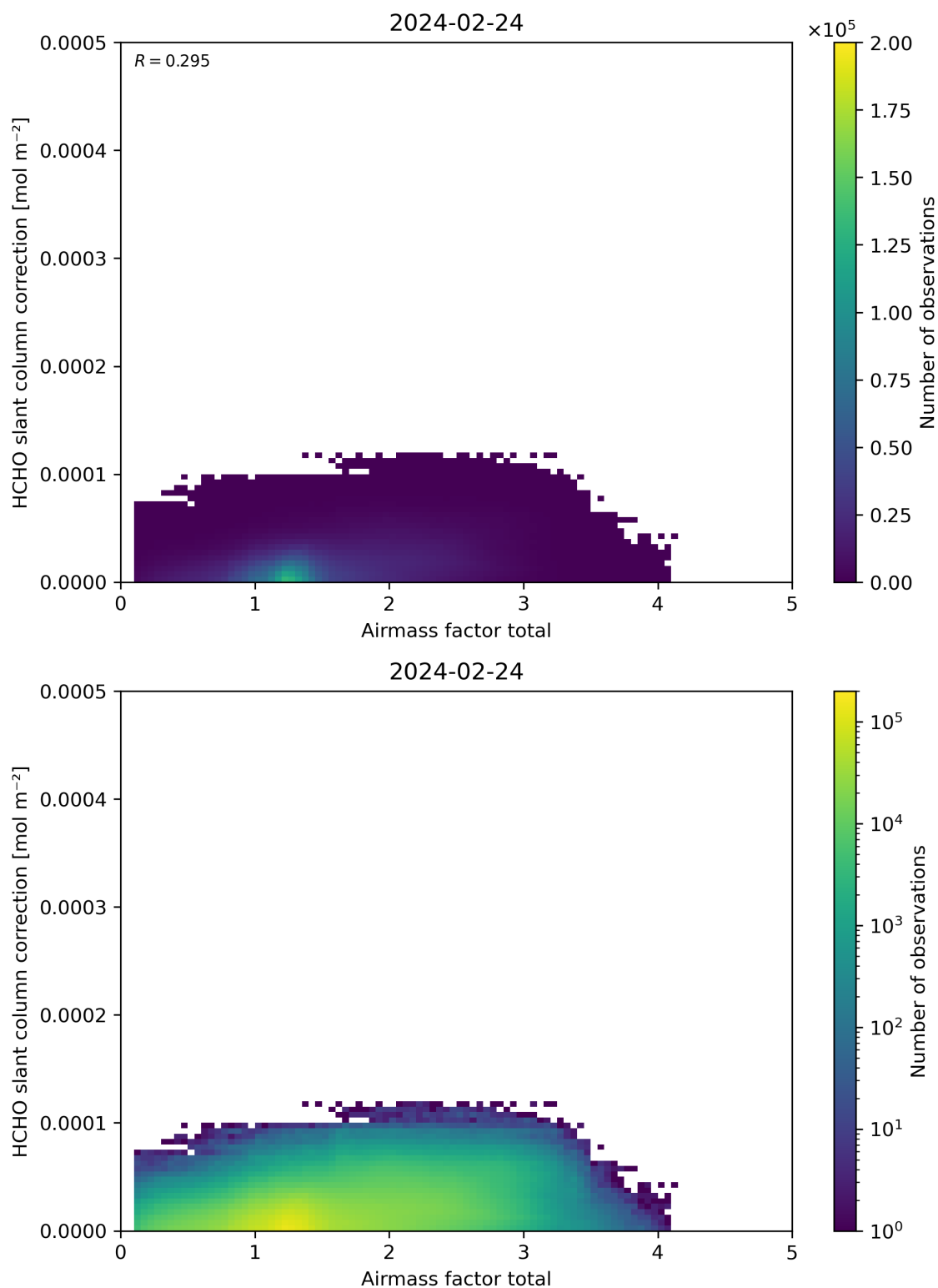
Figure 102: Scatter density plot of “Airmass factor total” against “HCHO slant column correction” for 2024-02-23 to 2024-02-25.
