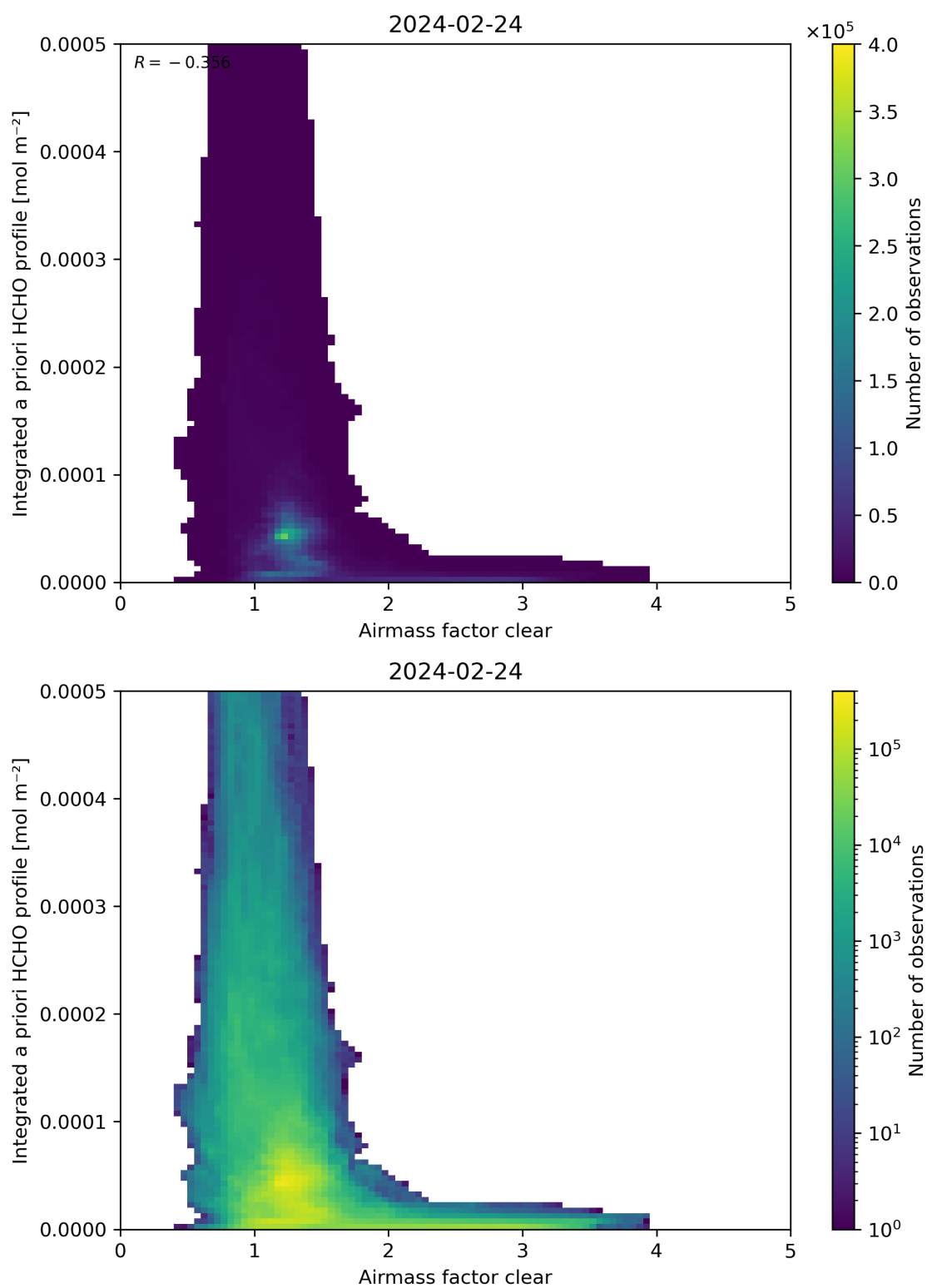
Figure 76: Scatter density plot of “Airmass factor clear” against “Integrated a priori HCHO profile” for 2024-02-23 to 2024-02-25.
