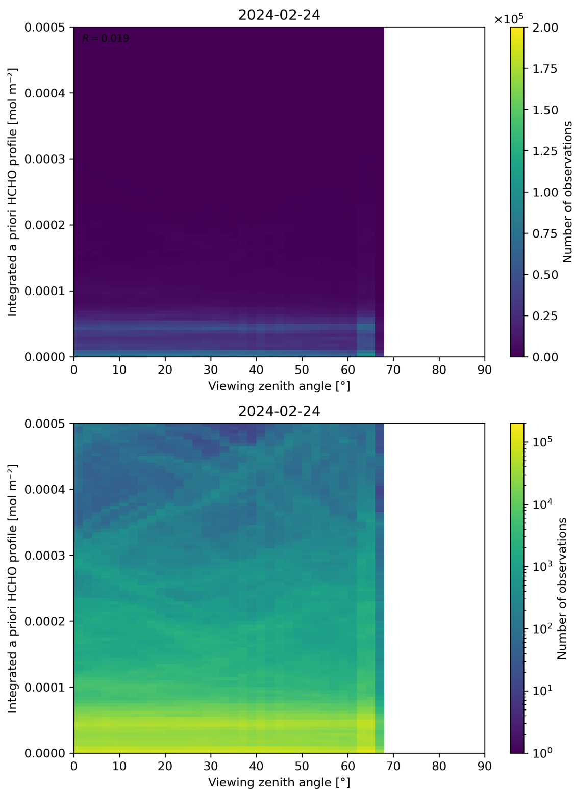
Figure 195: Scatter density plot of “Viewing zenith angle” against “Integrated a priori HCHO profile” for 2024-02-23 to 2024-02-25.
