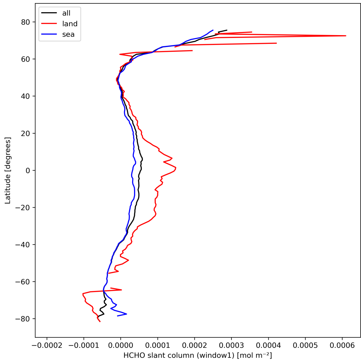
Figure 24: Zonal average of “HCHO slant column (window1)” for 2024-02-23 to 2024-02-25.
