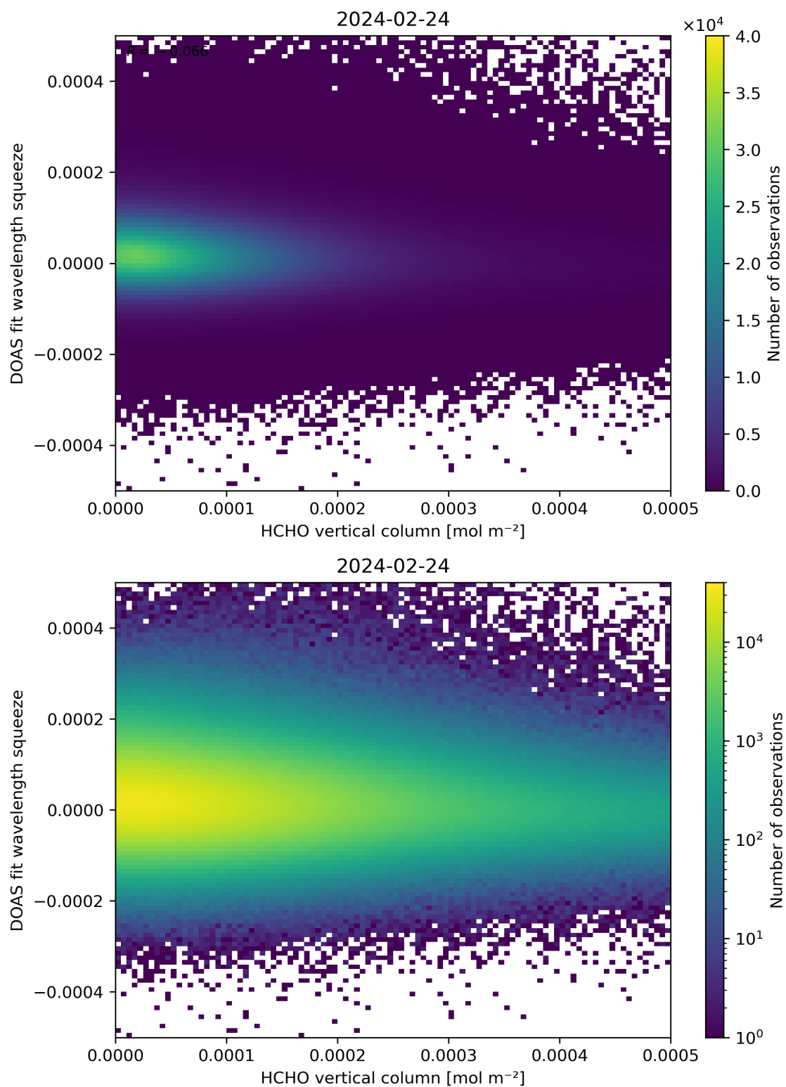
Figure 125: Scatter density plot of “HCHO vertical column” against “DOAS fit wavelength squeeze” for 2024-02-23 to 2024-02-25.
