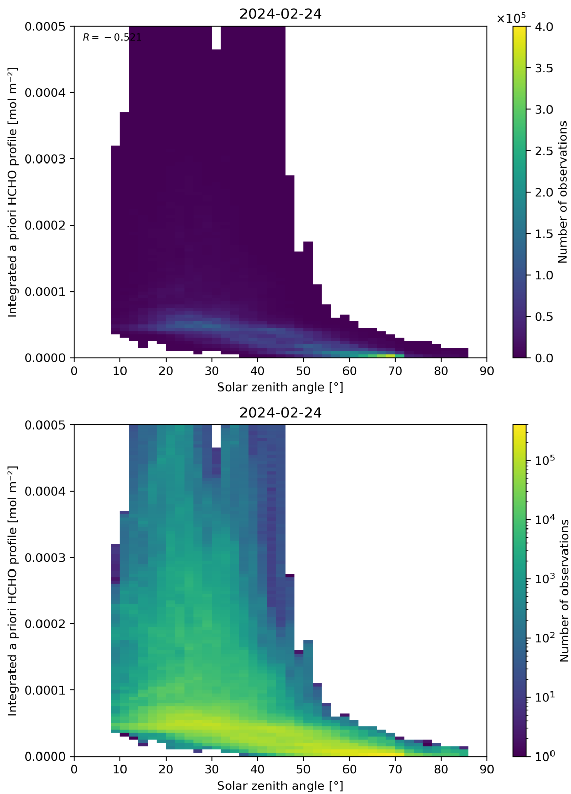
Figure 180: Scatter density plot of “Solar zenith angle” against “Integrated a priori HCHO profile” for 2024-02-23 to 2024-02-25.
