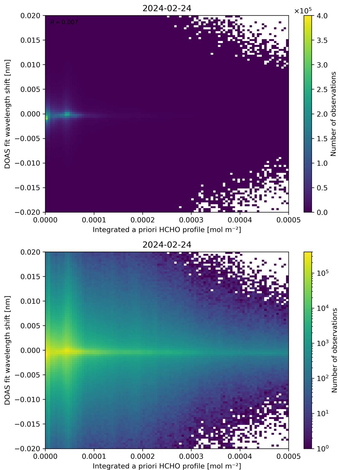
Figure 149: Scatter density plot of “Integrated a priori HCHO profile” against “DOAS fit wavelength shift” for 2024-02-23 to 2024-02-25.
