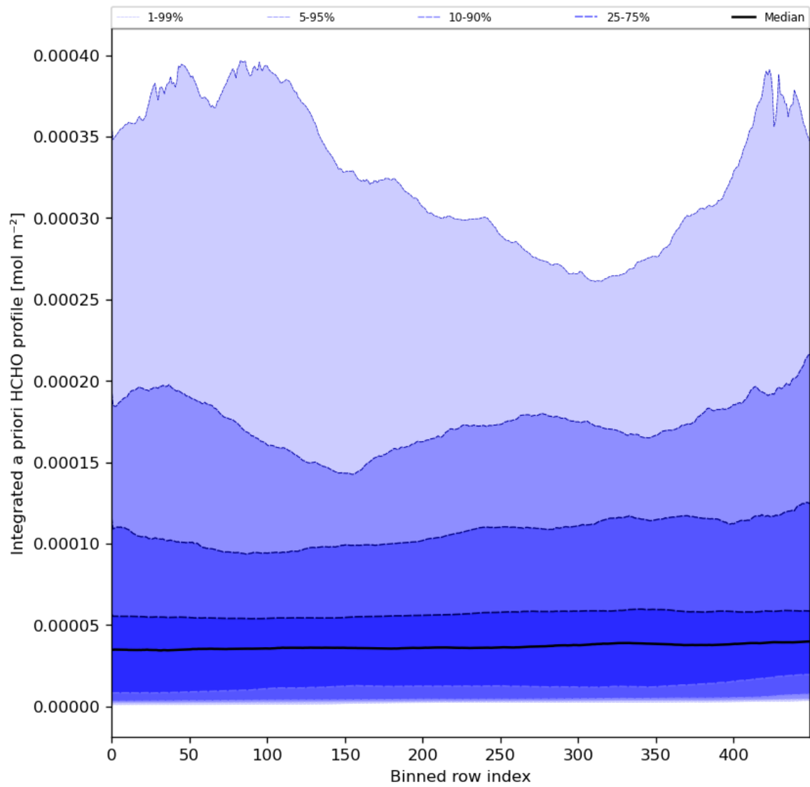
Figure 57: Along track statistics of "Integrated a priori HCHO profile" for 2024-02-23 to 2024-02-25
