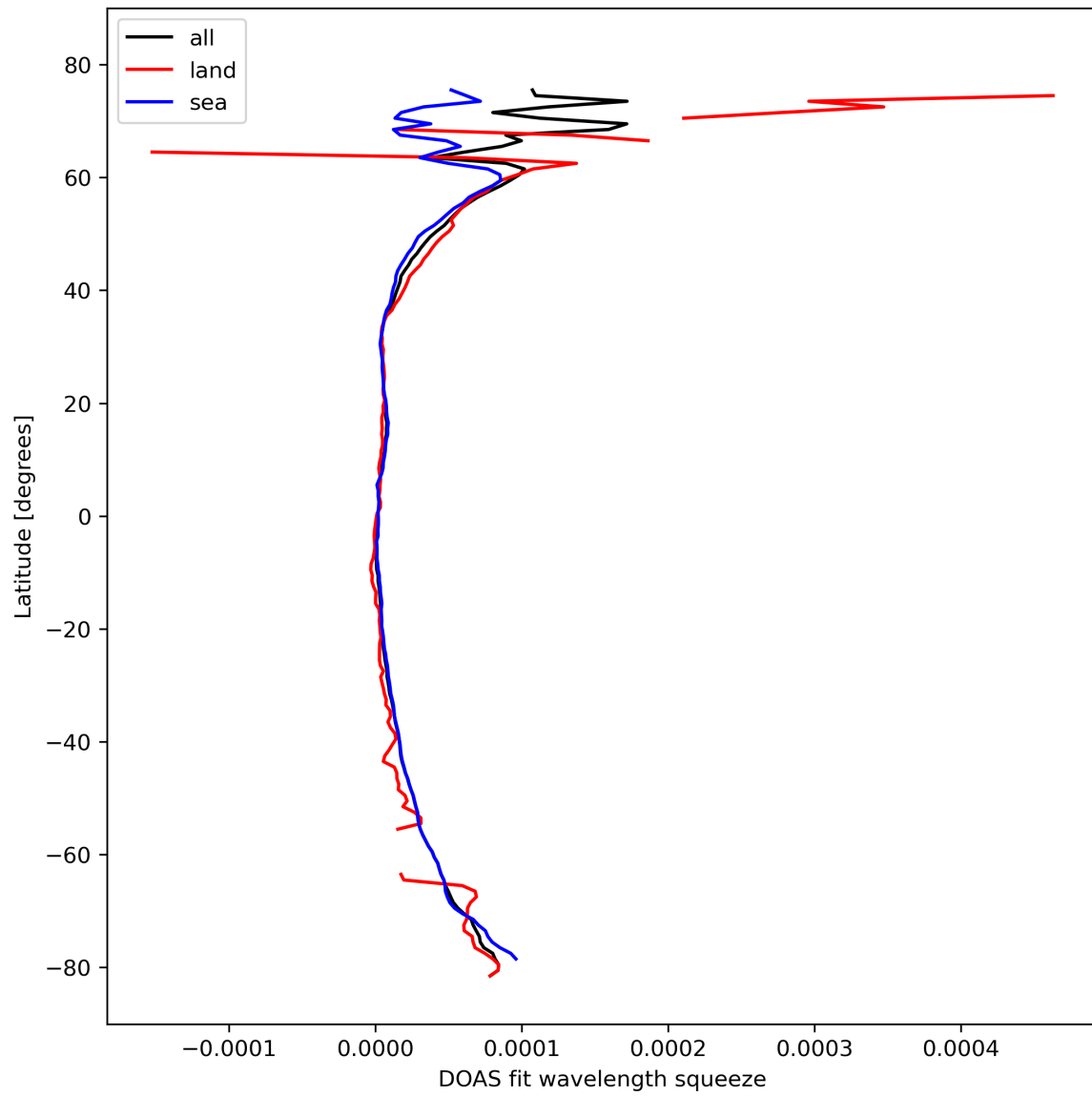
Figure 31: Zonal average of "DOAS fit wavelength squeeze" for 2024-02-23 to 2024-02-25.
