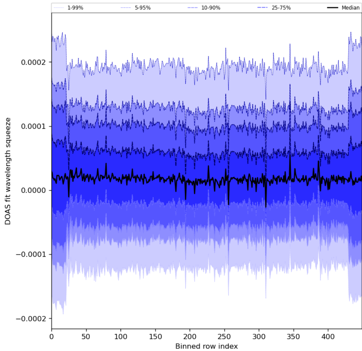
Figure 59: Along track statistics of “DOAS fit wavelength squeeze” for 2024-02-23 to 2024-02-25
