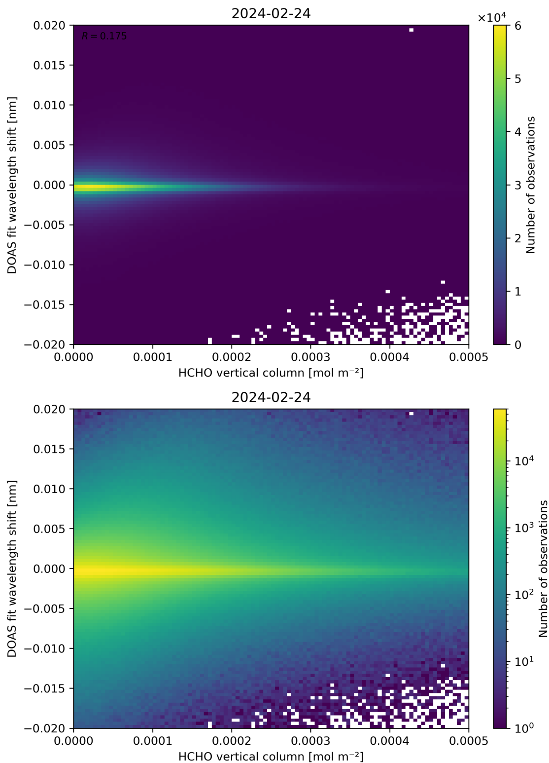
Figure 124: Scatter density plot of “HCHO vertical column” against “DOAS fit wavelength shift” for 2024-02-23 to 2024-02-25.
