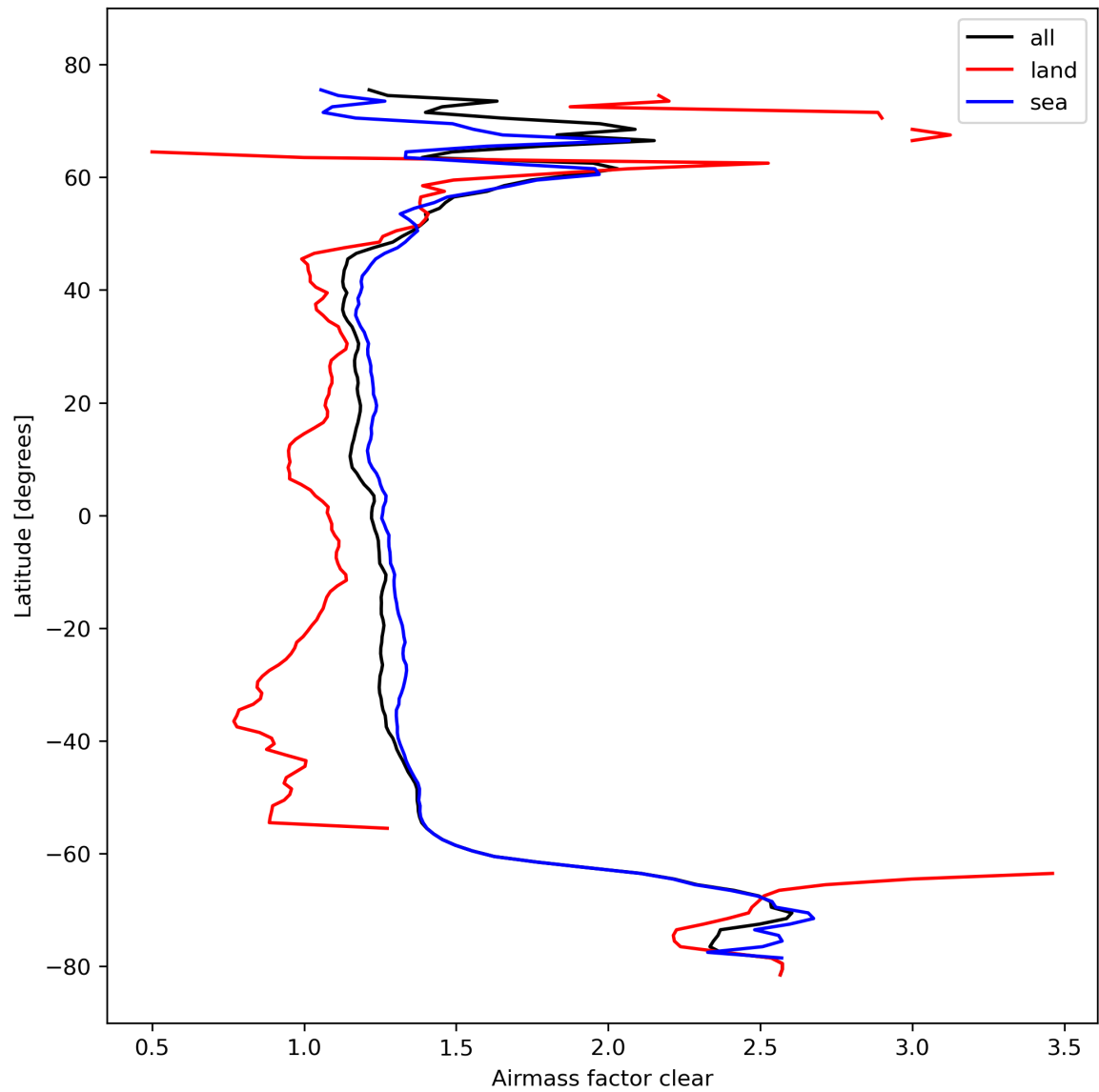
Figure 28: Zonal average of “Airmass factor clear” for 2024-02-23 to 2024-02-25.
