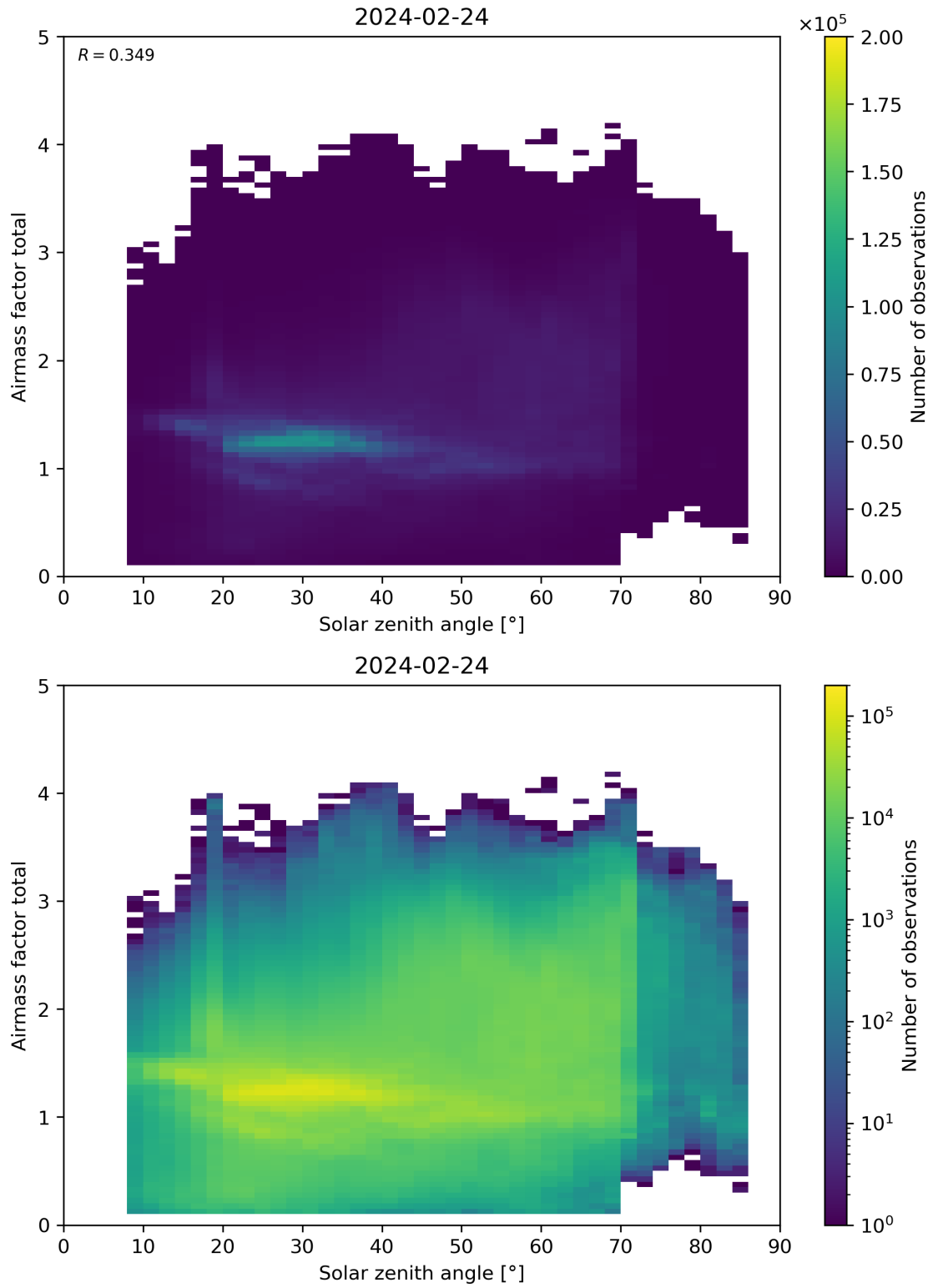
Figure 175: Scatter density plot of “Solar zenith angle” against “Airmass factor total” for 2024-02-23 to 2024-02-25.
