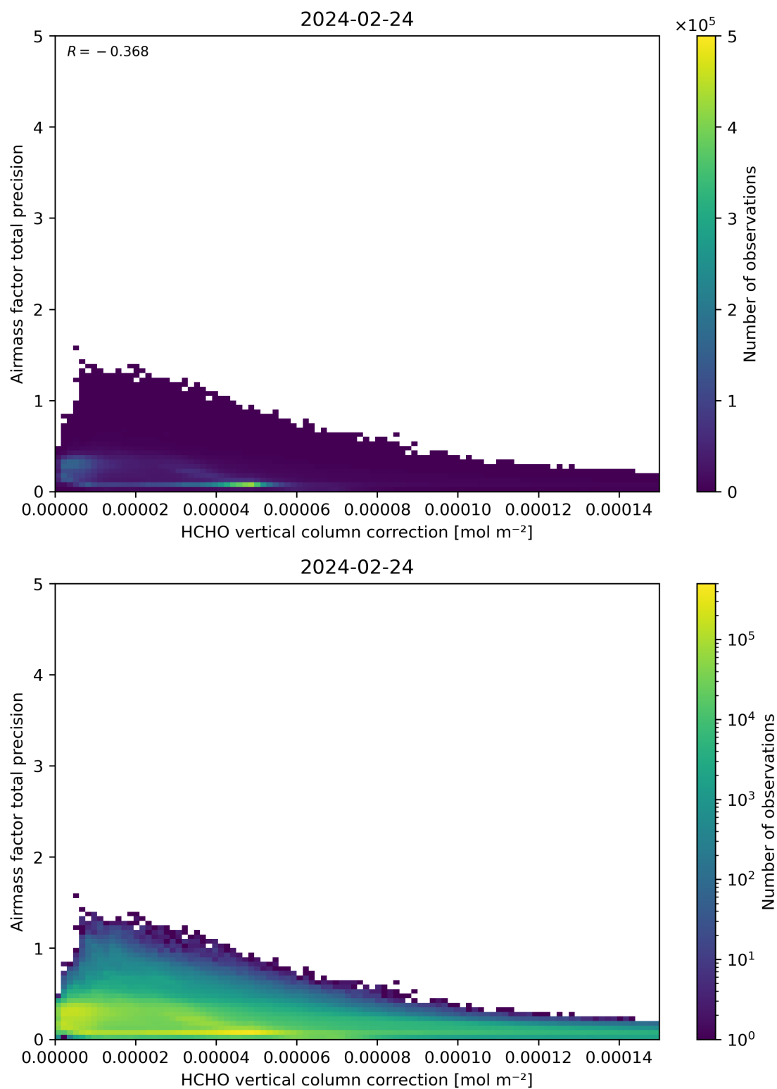
Figure 121: Scatter density plot of “HCHO vertical column correction” against “Airmass factor total precision” for 2024-02-23 to 2024-02-25.
