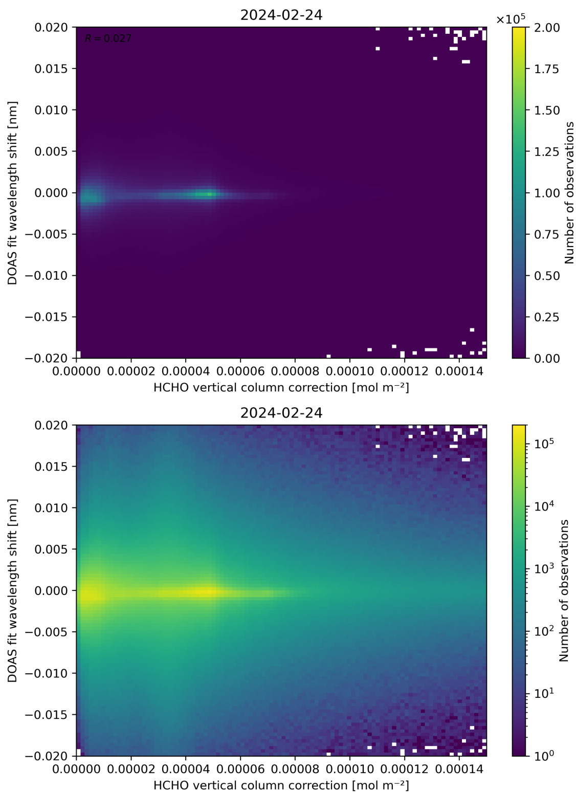
Figure 113: Scatter density plot of “HCHO vertical column correction” against “DOAS fit wavelength shift” for 2024-02-23 to 2024-02-25.
