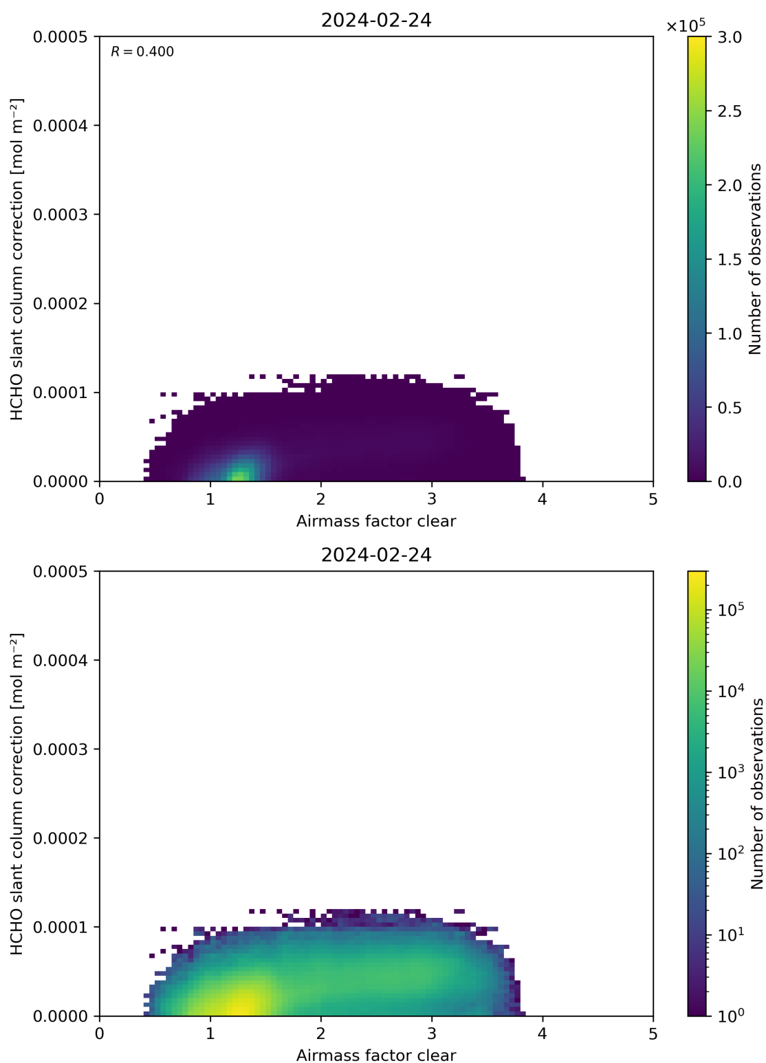
Figure 75: Scatter density plot of “Airmass factor clear” against “HCHO slant column correction” for 2024-02-23 to 2024-02-25.
