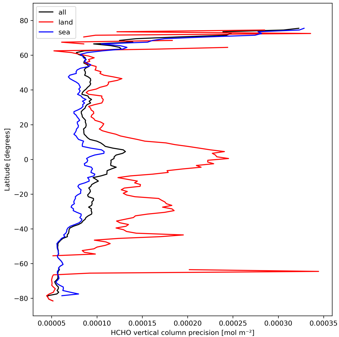
Figure 22: Zonal average of “HCHO vertical column precision” for 2024-02-23 to 2024-02-25.
