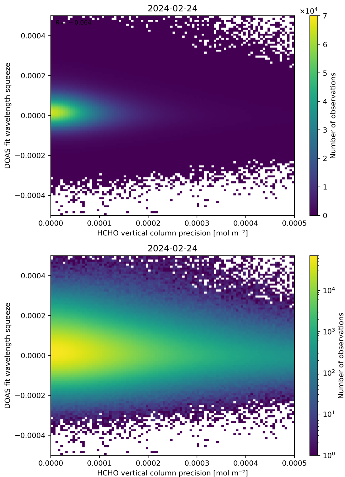
Figure 138: Scatter density plot of “HCHO vertical column precision” against “DOAS fit wavelength squeeze” for 2024-02-23 to 2024-02-25.
