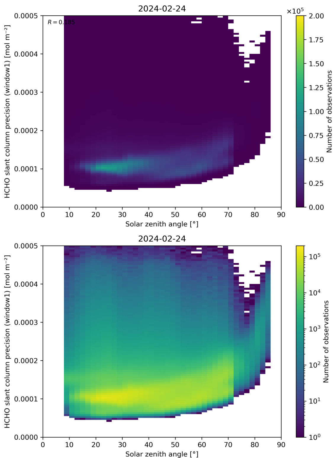
Figure 174: Scatter density plot of “Solar zenith angle” against “HCHO slant column precision (window1)” for 2024-02-23 to 2024-02-25.
