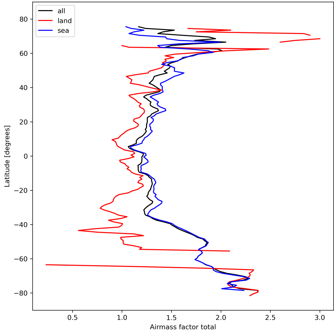
Figure 26: Zonal average of “Airmass factor total” for 2024-02-23 to 2024-02-25.
