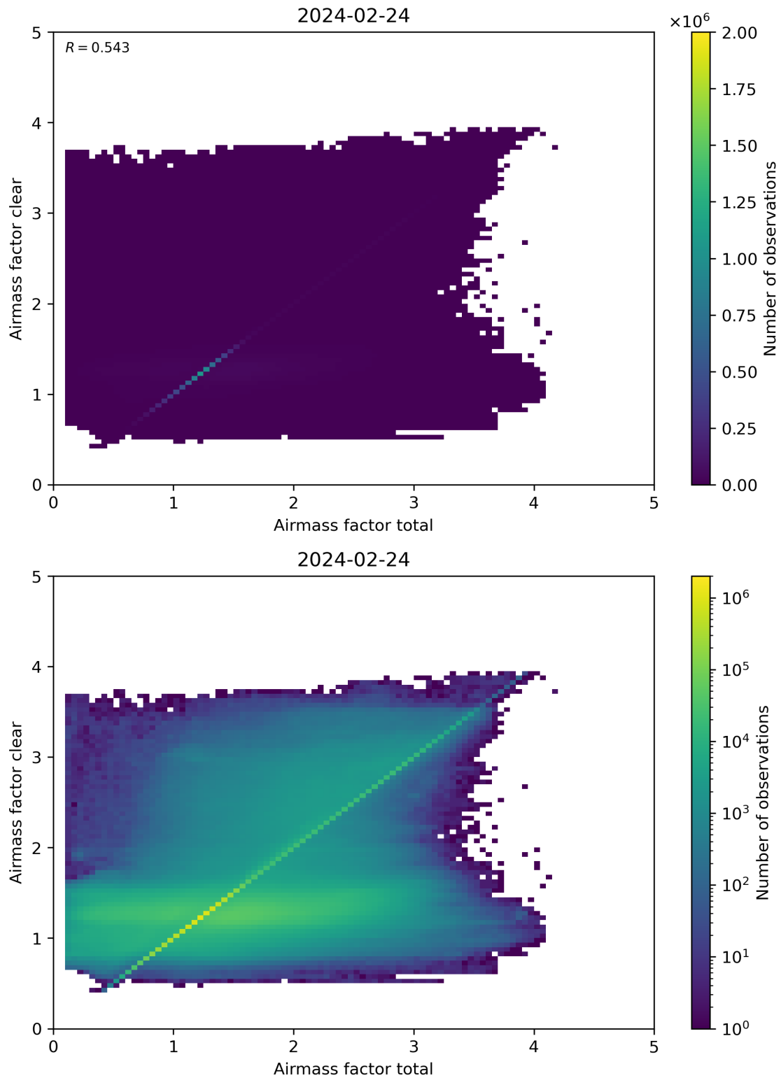
Figure 100: Scatter density plot of “Airmass factor total” against “Airmass factor clear” for 2024-02-23 to 2024-02-25.
