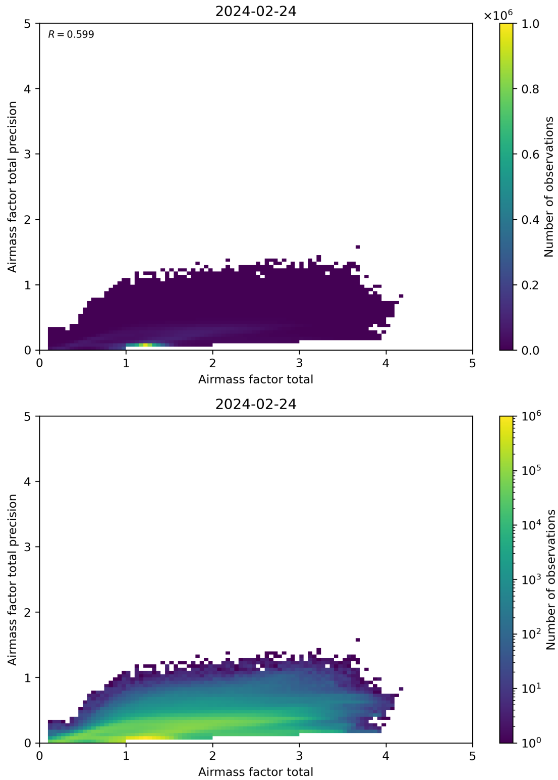
Figure 103: Scatter density plot of “Airmass factor total” against “Airmass factor total precision” for 2024-02-23 to 2024-02-25.
