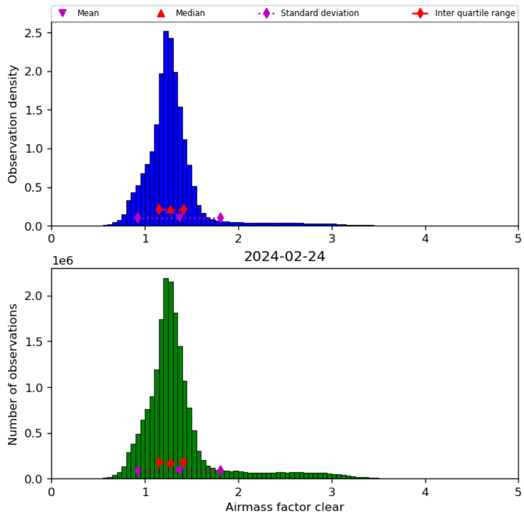
Figure 42: Histogram of “Airmass factor clear” for 2024-02-23 to 2024-02-25
