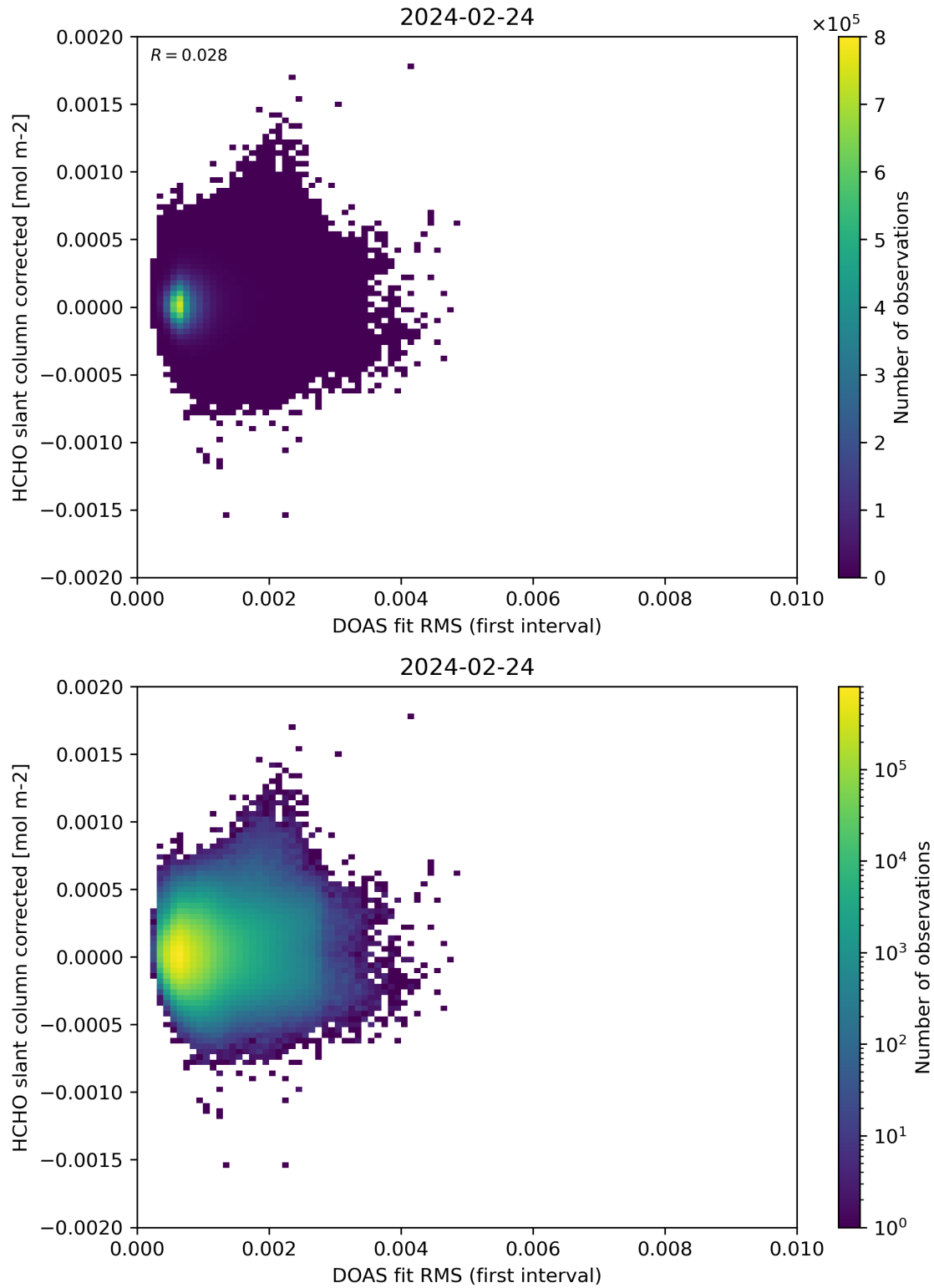
Figure 62: Scatter density plot of “DOAS fit RMS (first interval)” against “HCHO slant column corrected” for 2024-02-23 to 2024-02-25.
