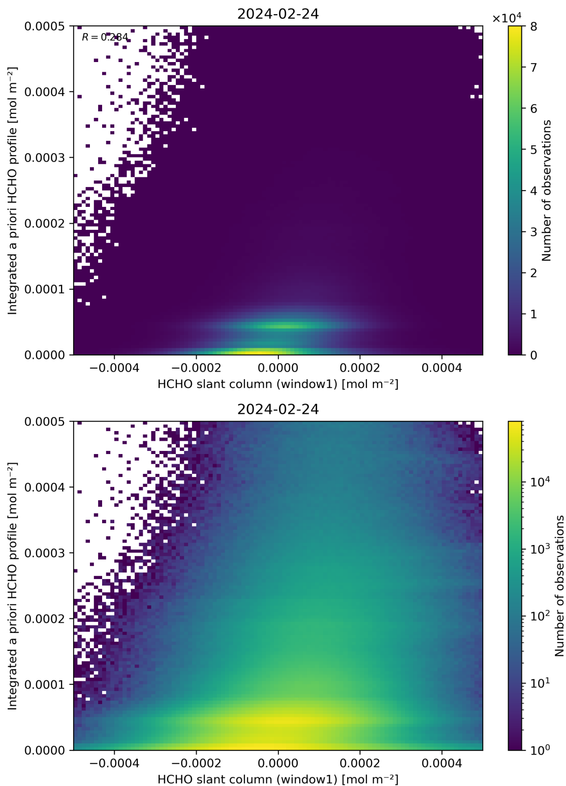
Figure 87: Scatter density plot of “HCHO slant column (window1)” against “Integrated a priori HCHO profile” for 2024-02-23 to 2024-02-25.
