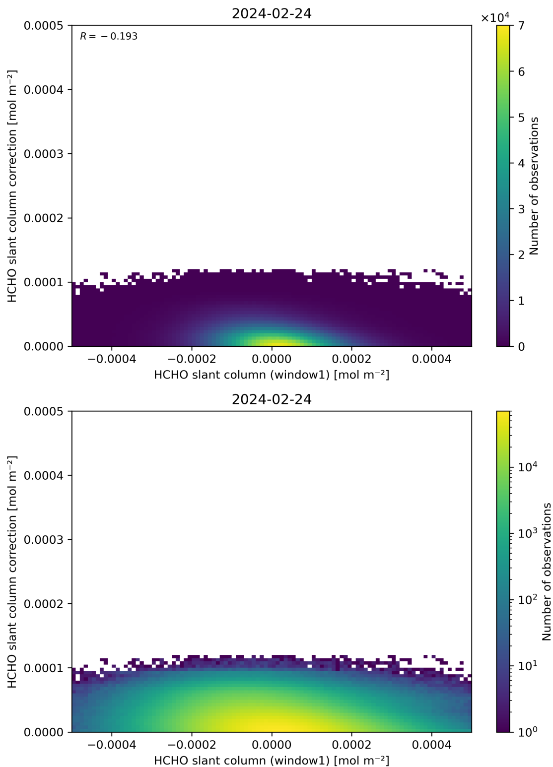
Figure 83: Scatter density plot of “HCHO slant column (window1)” against “HCHO slant column correction” for 2024-02-23 to 2024-02-25.
