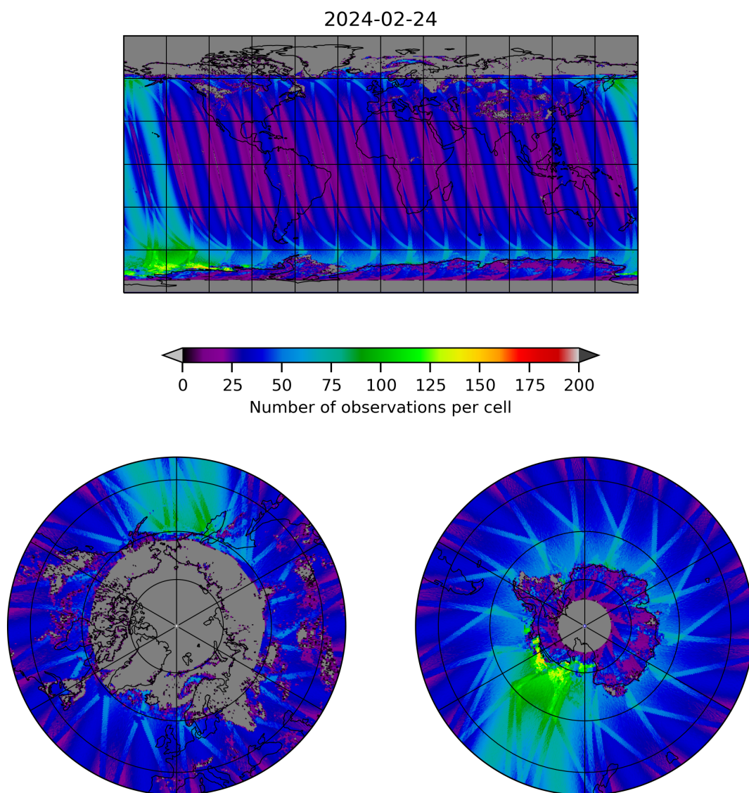
Figure 19: Map of the number of observations for 2024-02-23 to 2024-02-25
