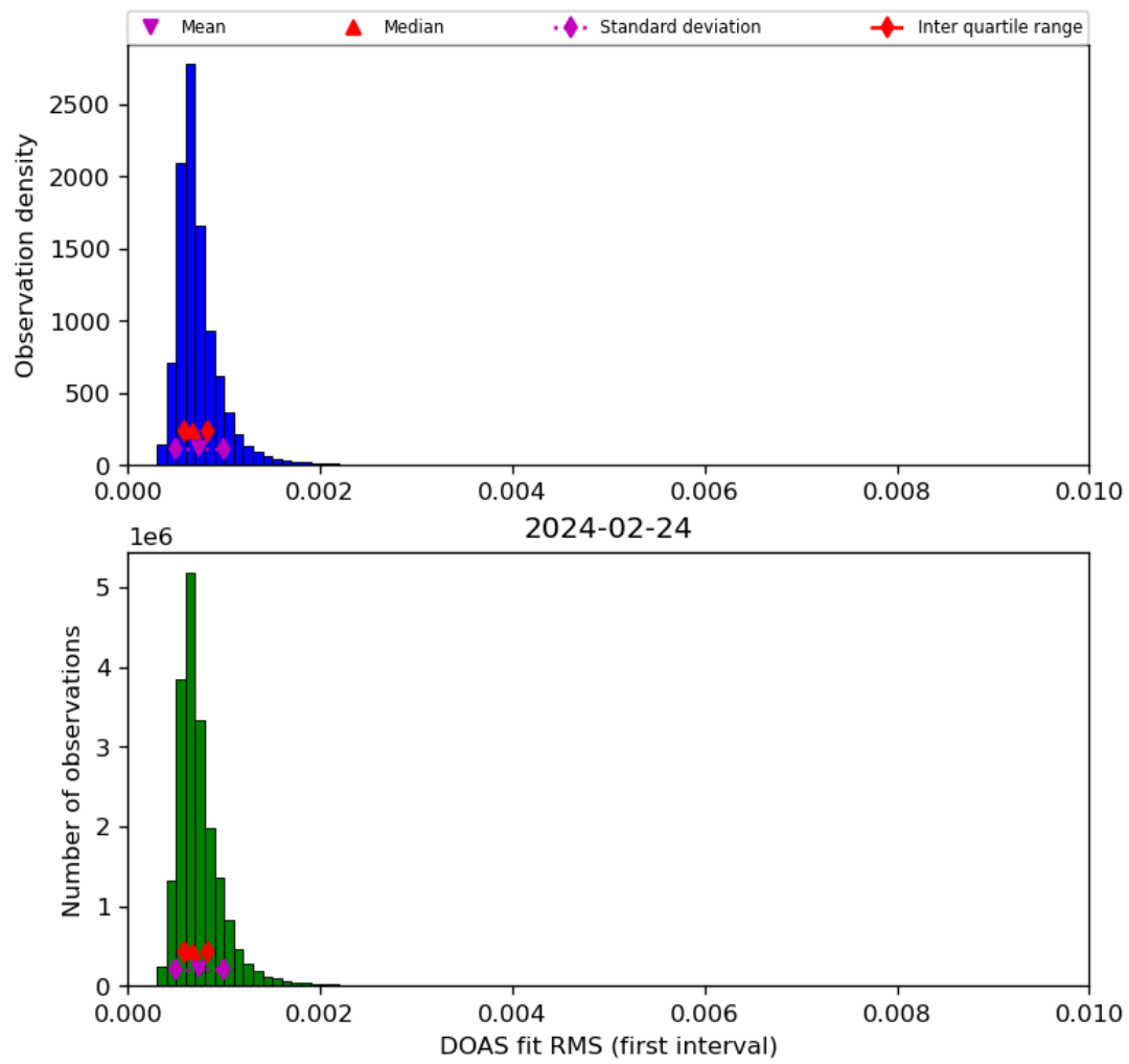
Figure 46: Histogram of “DOAS fit RMS (first interval)” for 2024-02-23 to 2024-02-25
