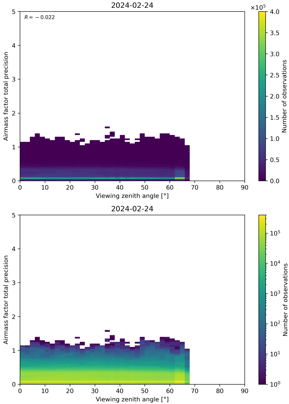
Figure 191: Scatter density plot of “Viewing zenith angle” against “Airmass factor total precision” for 2024-02-23 to 2024-02-25.
