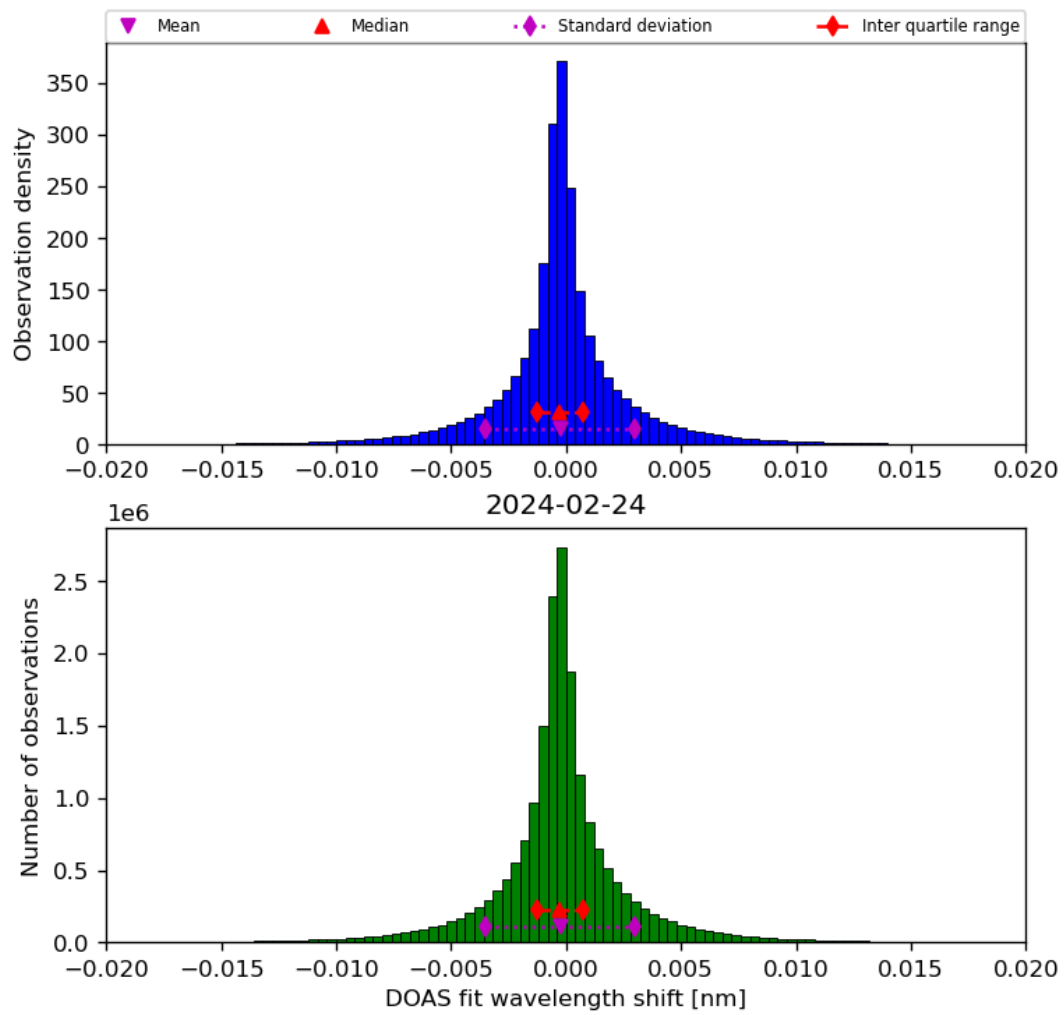
Figure 44: Histogram of “DOAS fit wavelength shift” for 2024-02-23 to 2024-02-25
