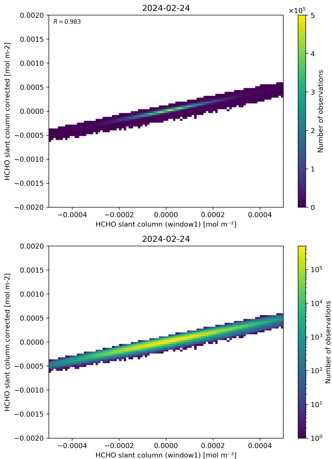
Figure 82: Scatter density plot of “HCHO slant column (window1)” against “HCHO slant column corrected” for 2024-02-23 to 2024-02-25.
