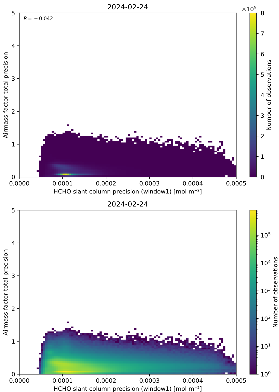
Figure 95: Scatter density plot of “HCHO slant column precision (window1)” against “Airmass factor total precision” for 2024-02-23 to 2024-02-25.
