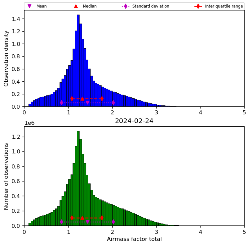
Figure 40: Histogram of “Airmass factor total” for 2024-02-23 to 2024-02-25
