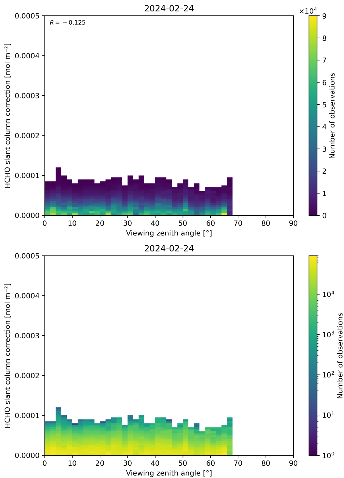
Figure 187: Scatter density plot of “Viewing zenith angle” against “HCHO slant column correction” for 2024-02-23 to 2024-02-25.
