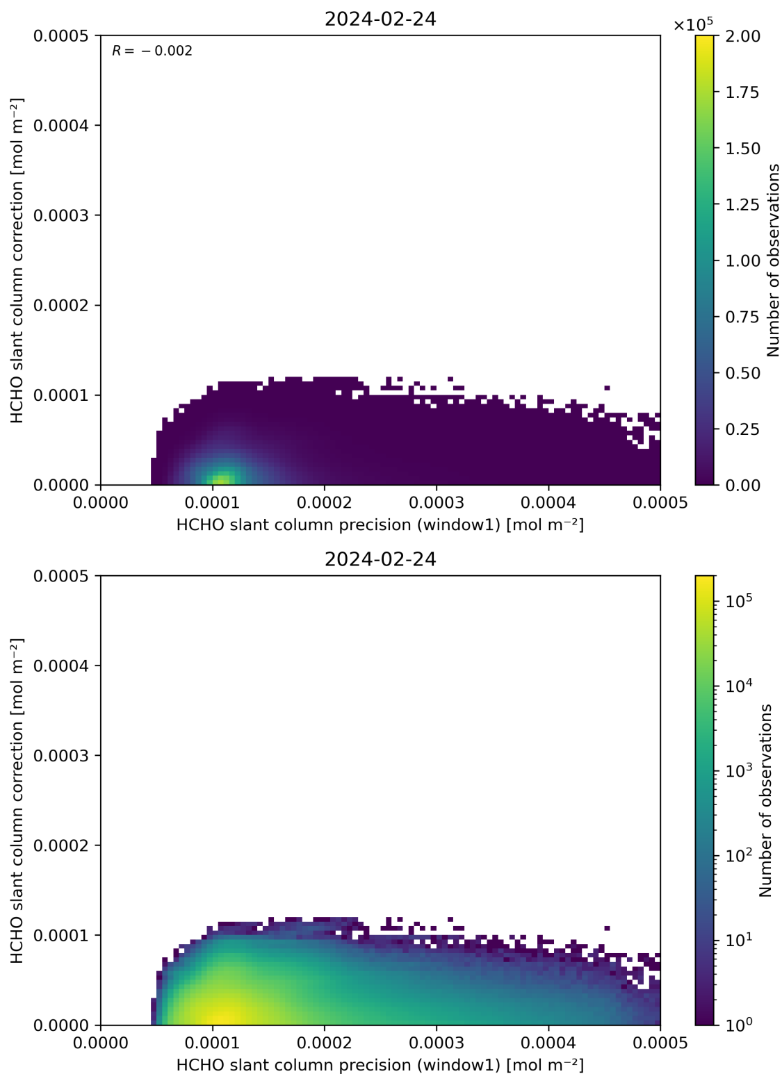
Figure 93: Scatter density plot of “HCHO slant column precision (window1)” against “HCHO slant column correction” for 2024-02-23 to 2024-02-25.
