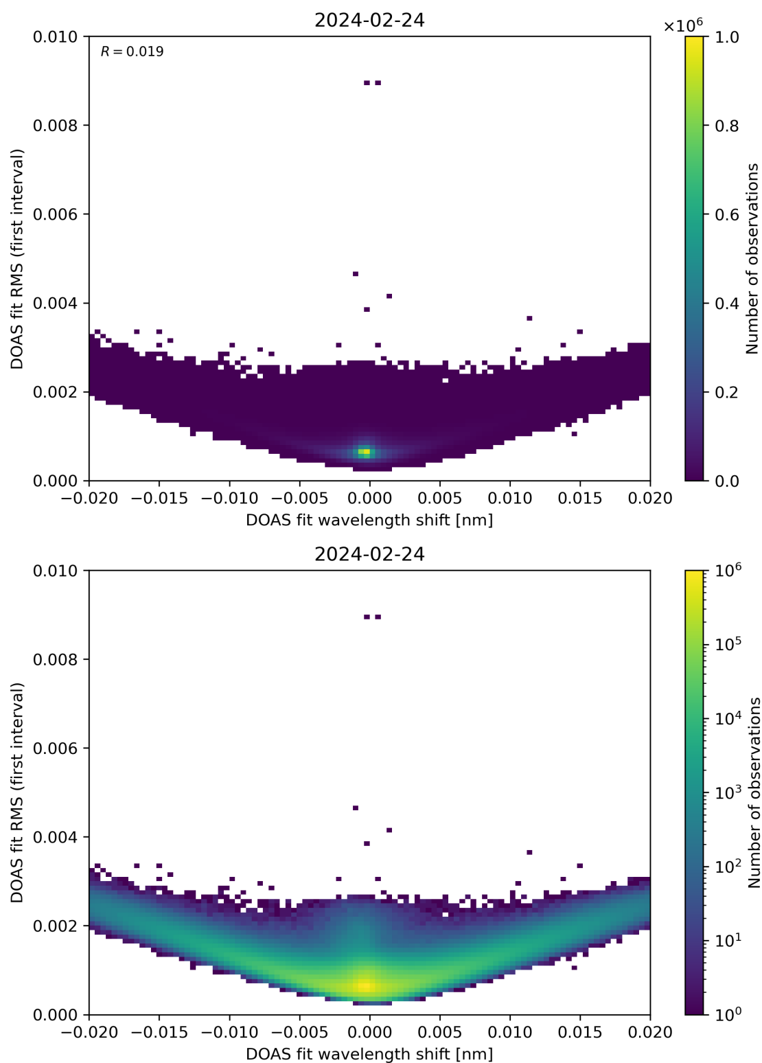
Figure 64: Scatter density plot of “DOAS fit wavelength shift” against “DOAS fit RMS (first interval)” for 2024-02-23 to 2024-02-25.
