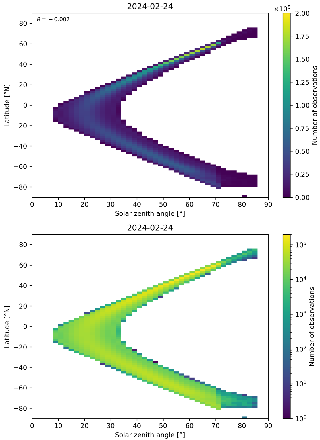
Figure 181: Scatter density plot of “Solar zenith angle” against “Latitude” for 2024-02-23 to 2024-02-25.
