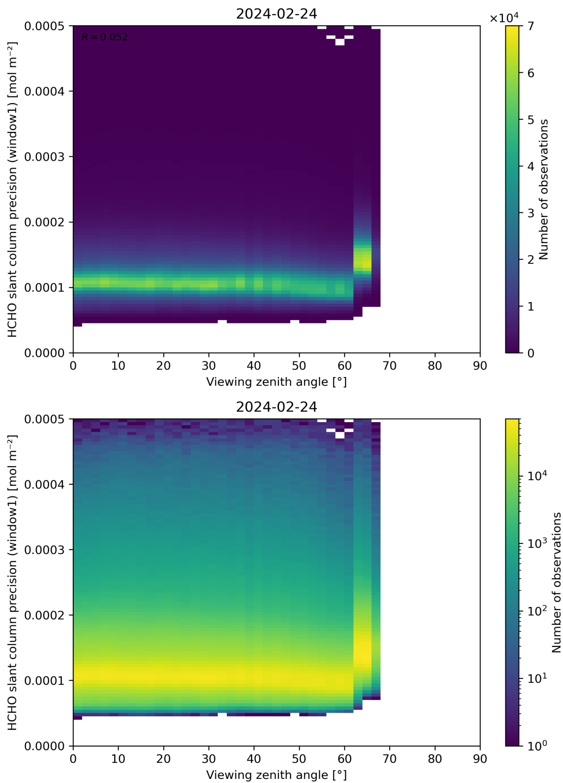
Figure 189: Scatter density plot of “Viewing zenith angle” against “HCHO slant column precision (window1)” for 2024-02-23 to 2024-02-25.
