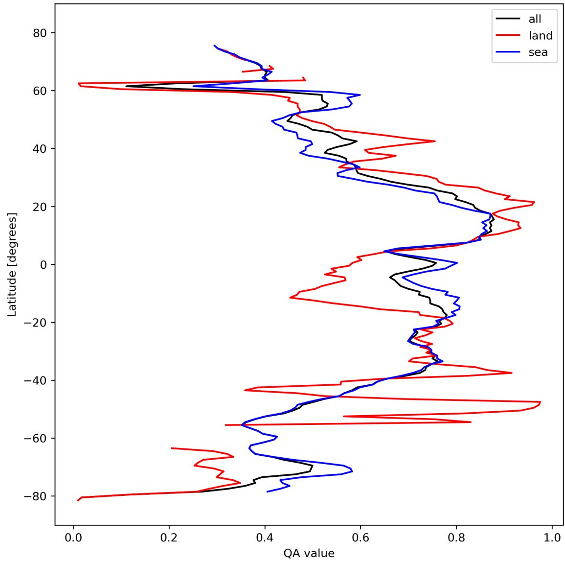
Figure 20: Zonal average of “QA value” for 2024-02-23 to 2024-02-25.
