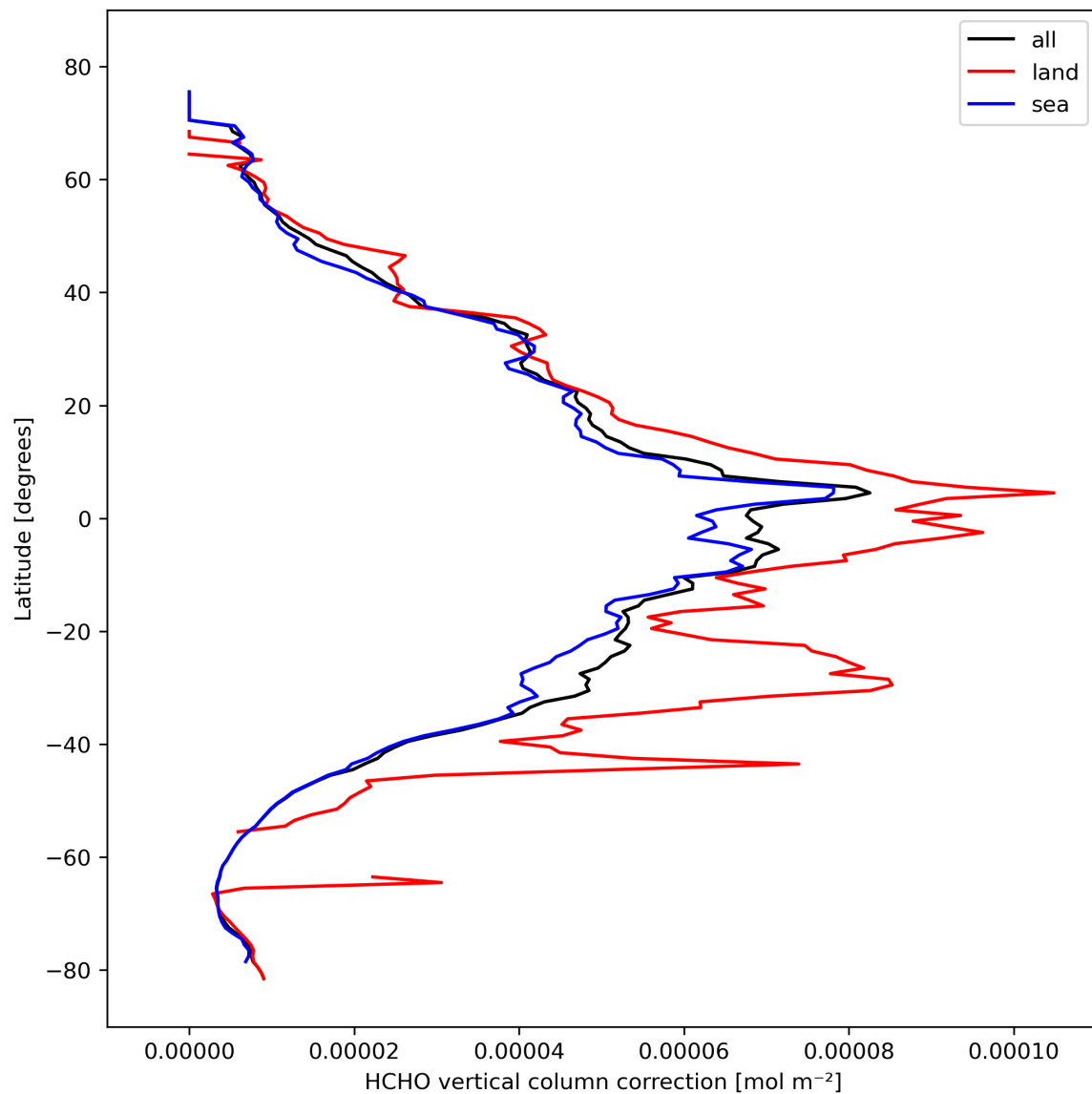
Figure 23: Zonal average of “HCHO vertical column correction” for 2024-02-23 to 2024-02-25.
