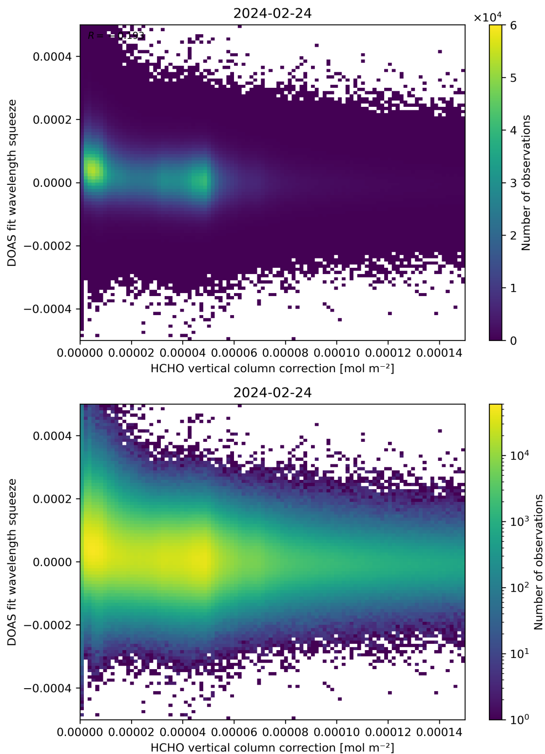
Figure 114: Scatter density plot of “HCHO vertical column correction” against “DOAS fit wavelength squeeze” for 2024-02-23 to 2024-02-25.
