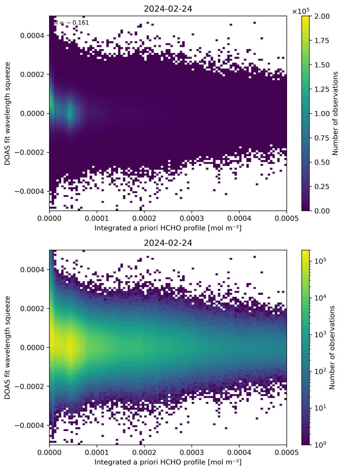
Figure 150: Scatter density plot of “Integrated a priori HCHO profile” against “DOAS fit wavelength squeeze” for 2024-02-23 to 2024-02-25.
