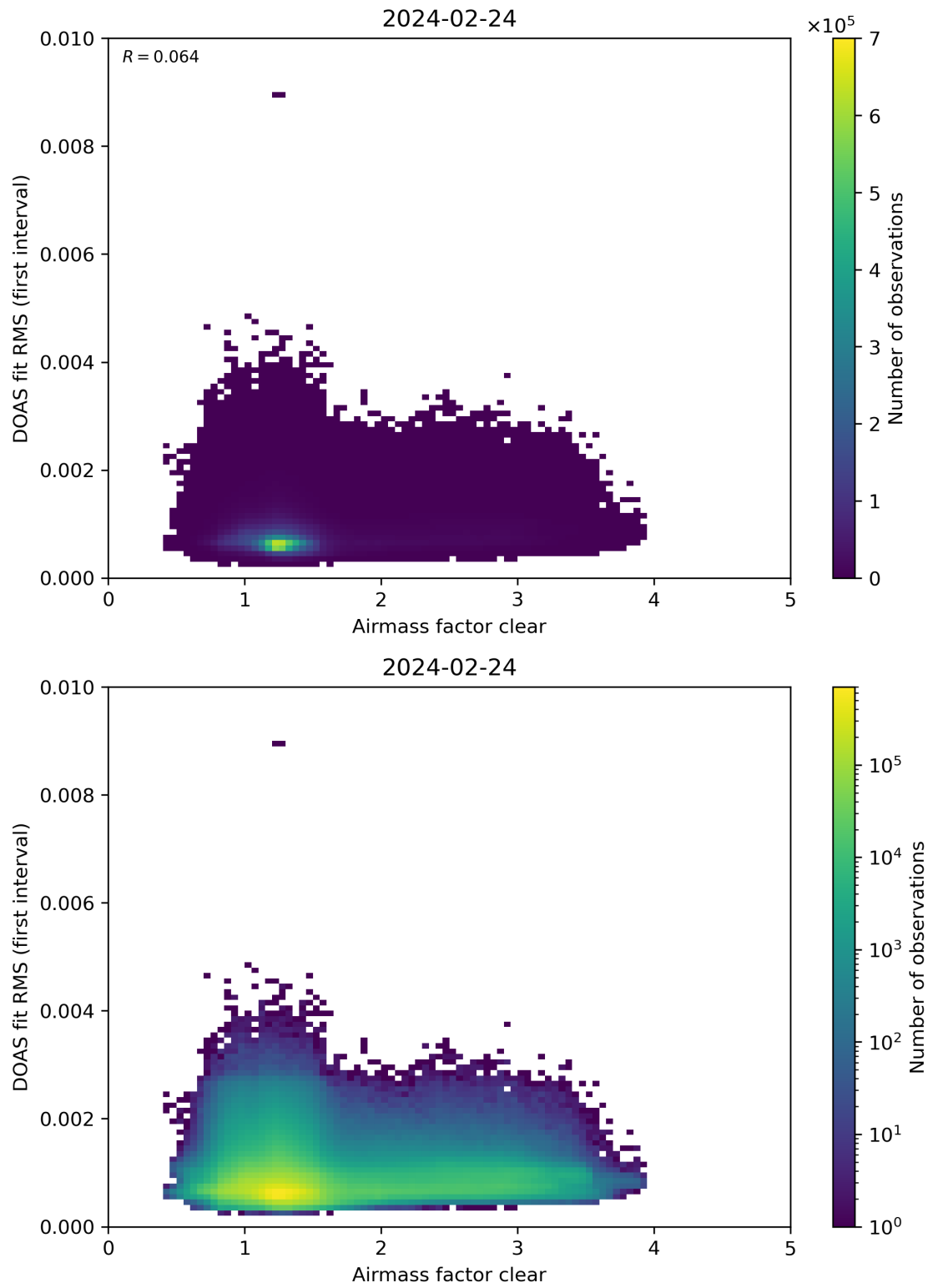
Figure 71: Scatter density plot of “Airmass factor clear” against “DOAS fit RMS (first interval)” for 2024-02-23 to 2024-02-25.
