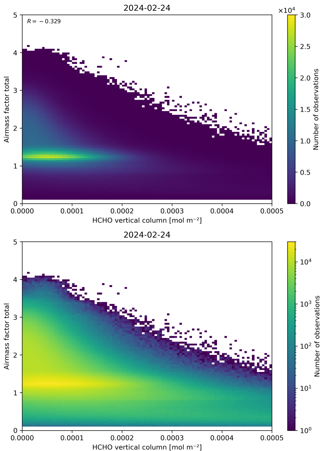
Figure 131: Scatter density plot of “HCHO vertical column” against “Airmass factor total” for 2024-02-23 to 2024-02-25.
