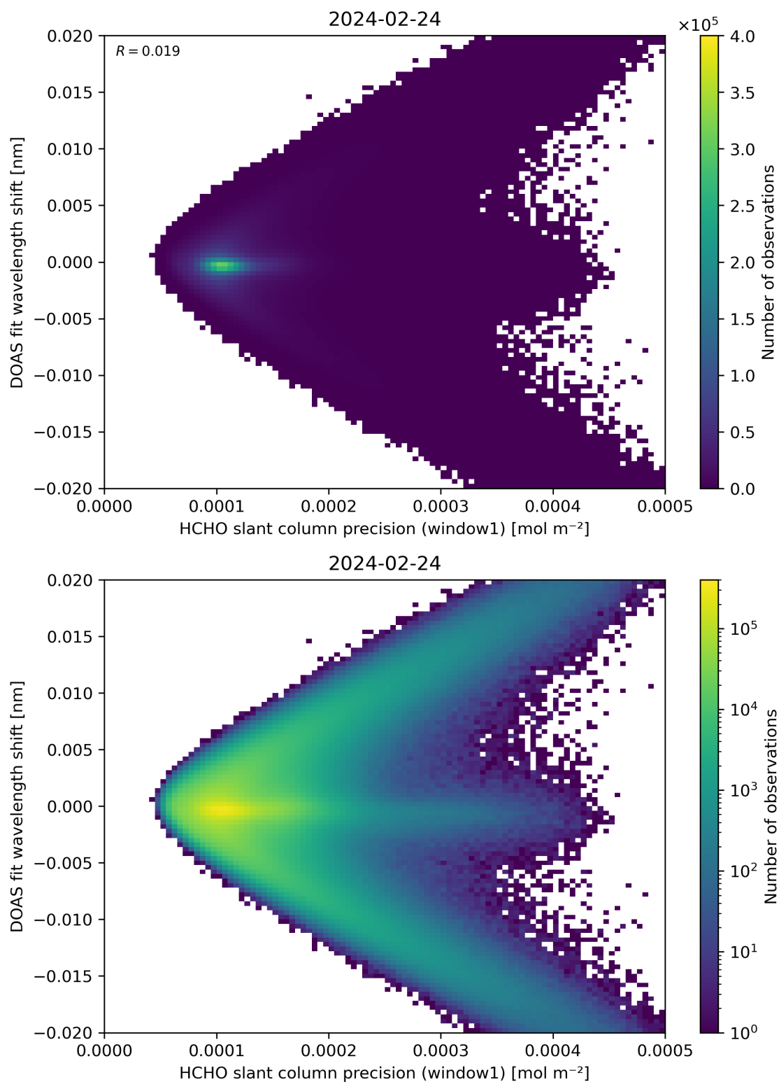
Figure 89: Scatter density plot of “HCHO slant column precision (window1)” against “DOAS fit wavelength shift” for 2024-02-23 to 2024-02-25.
