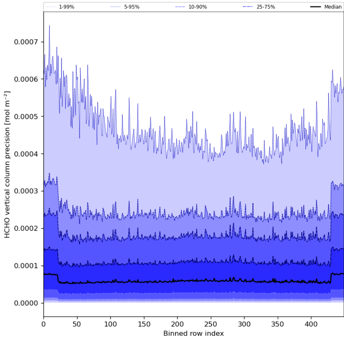
Figure 50: Along track statistics of “HCHO vertical column precision” for 2024-02-23 to 2024-02-25
