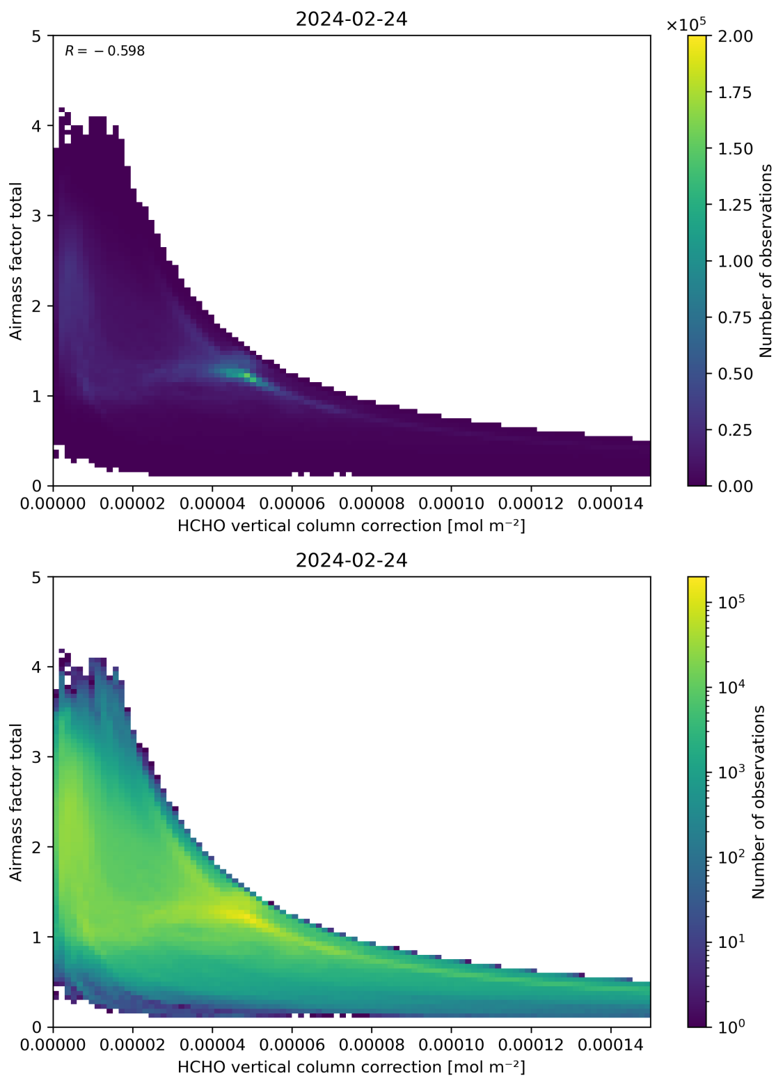
Figure 120: Scatter density plot of “HCHO vertical column correction” against “Airmass factor total” for 2024-02-23 to 2024-02-25.
