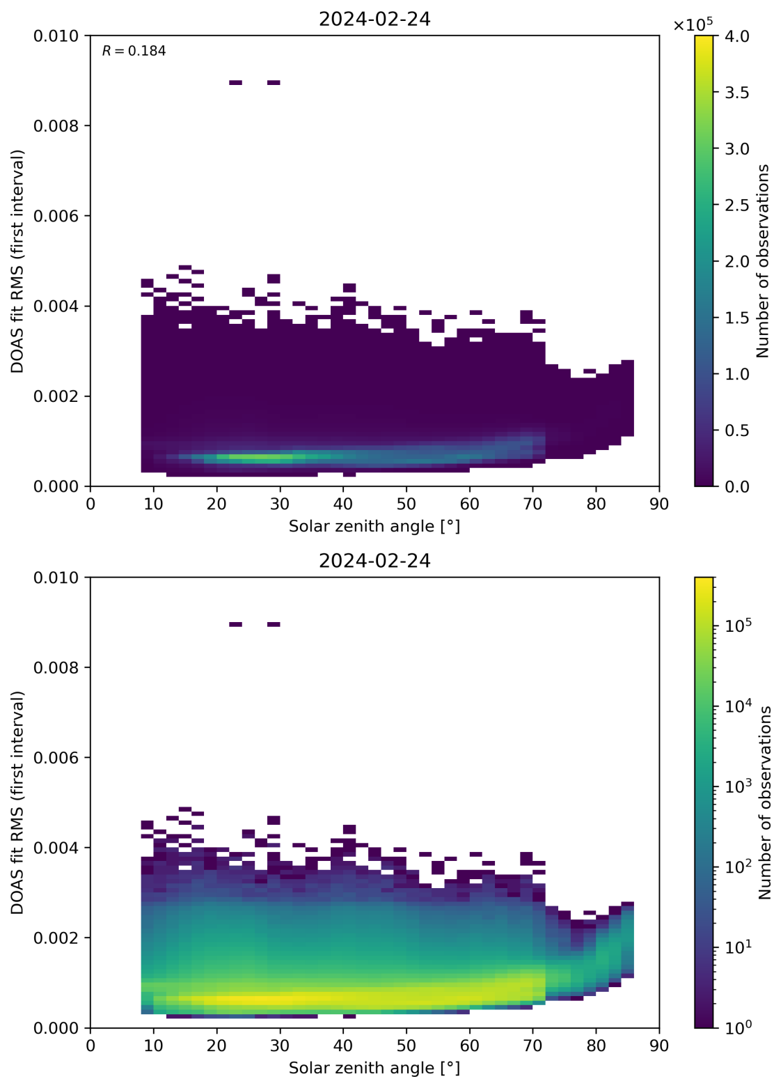
Figure 167: Scatter density plot of “Solar zenith angle” against “DOAS fit RMS (first interval)” for 2024-02-23 to 2024-02-25.
