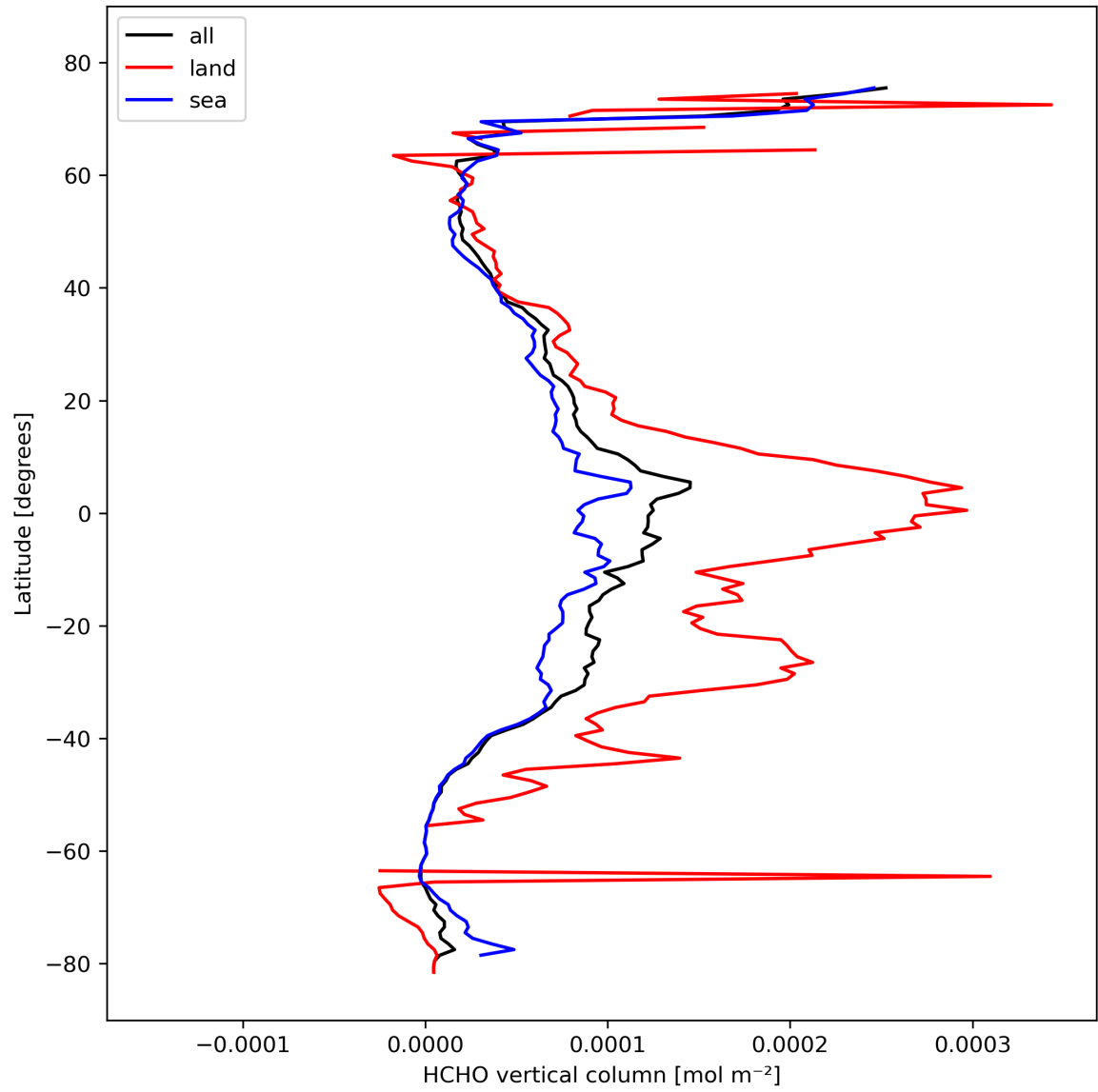
Figure 21: Zonal average of “HCHO vertical column” for 2024-02-23 to 2024-02-25.
