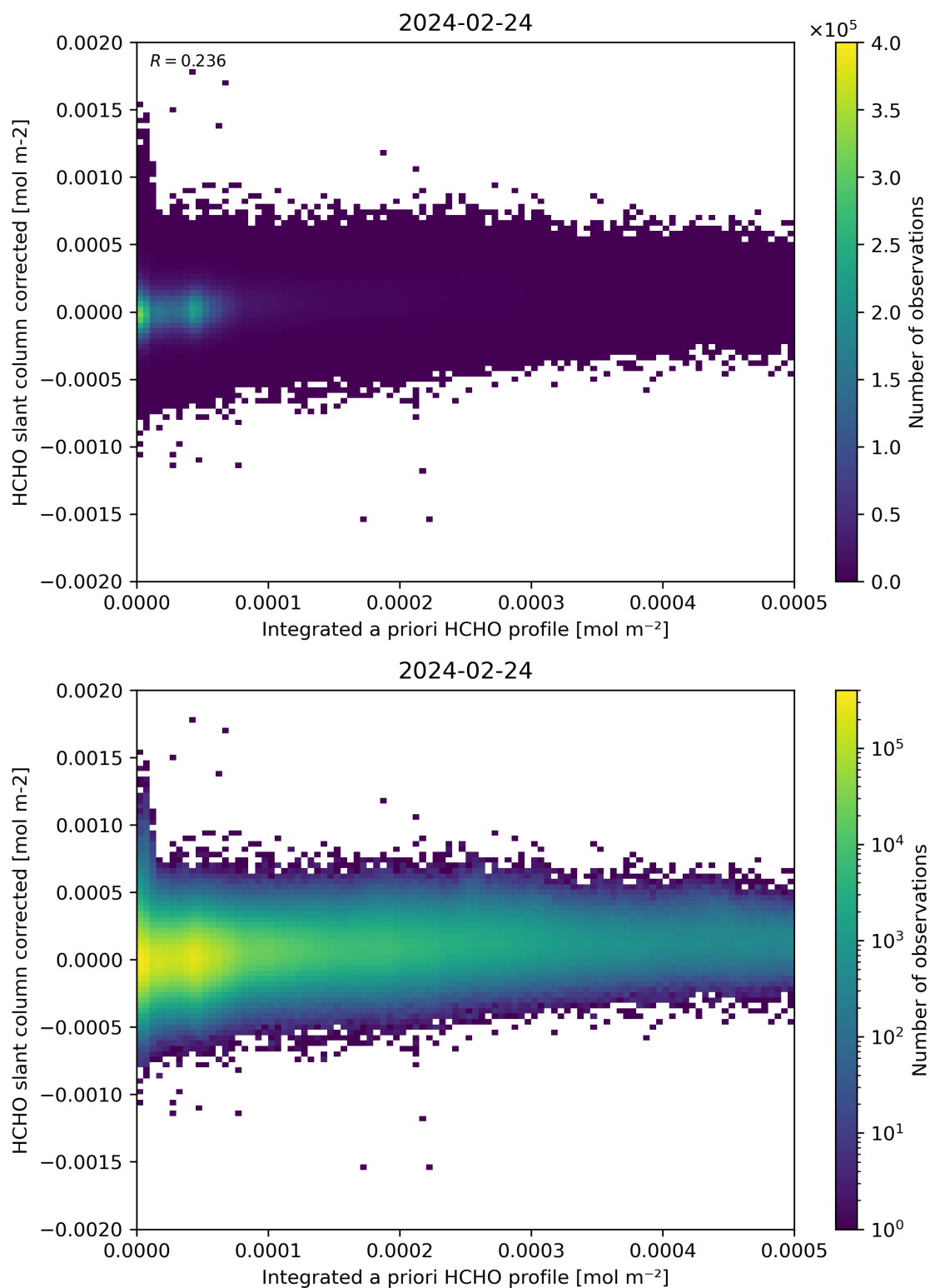
Figure 151: Scatter density plot of “Integrated a priori HCHO profile” against “HCHO slant column corrected” for 2024-02-23 to 2024-02-25.
