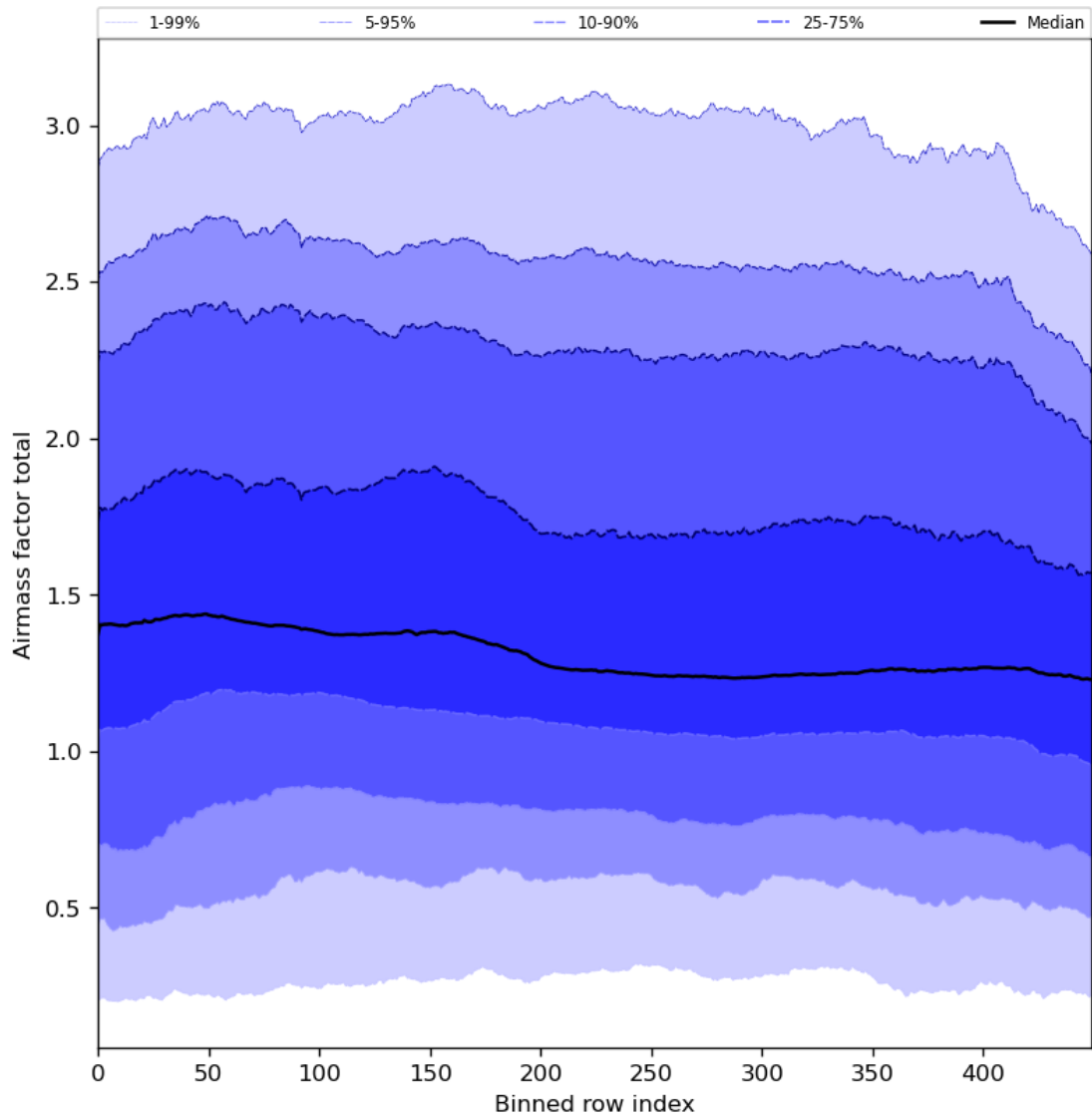
Figure 54: Along track statistics of “Airmass factor total” for 2024-02-23 to 2024-02-25
