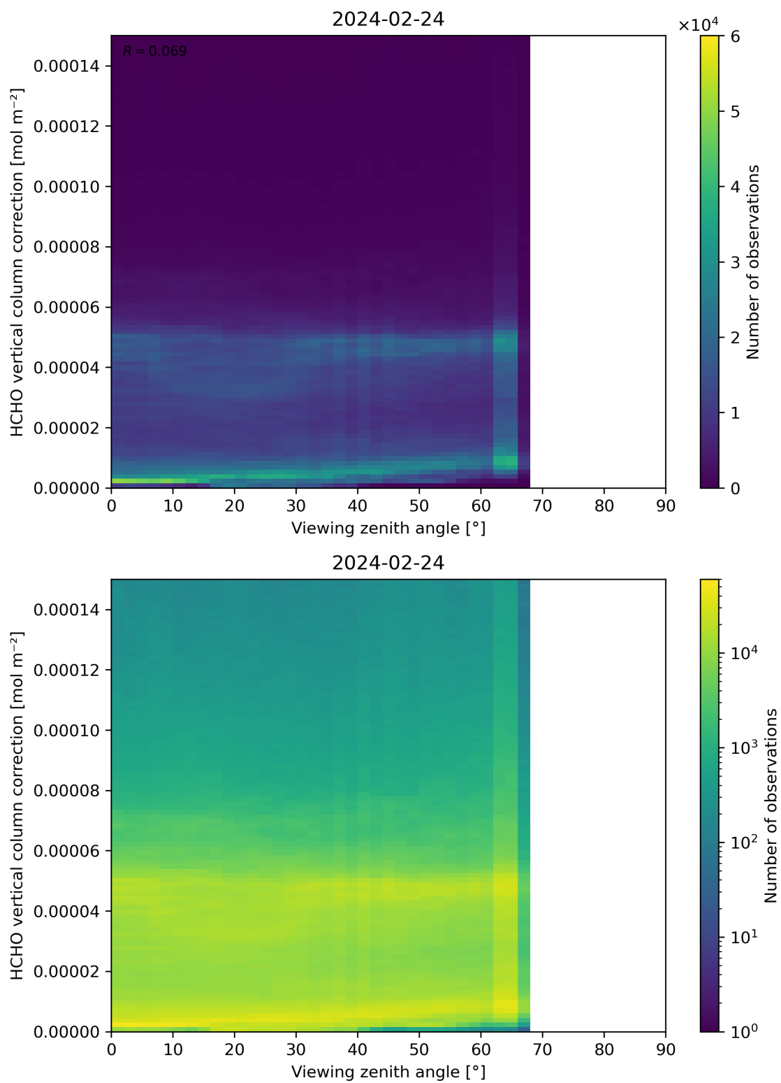
Figure 193: Scatter density plot of “Viewing zenith angle” against “HCHO vertical column correction” for 2024-02-23 to 2024-02-25.
