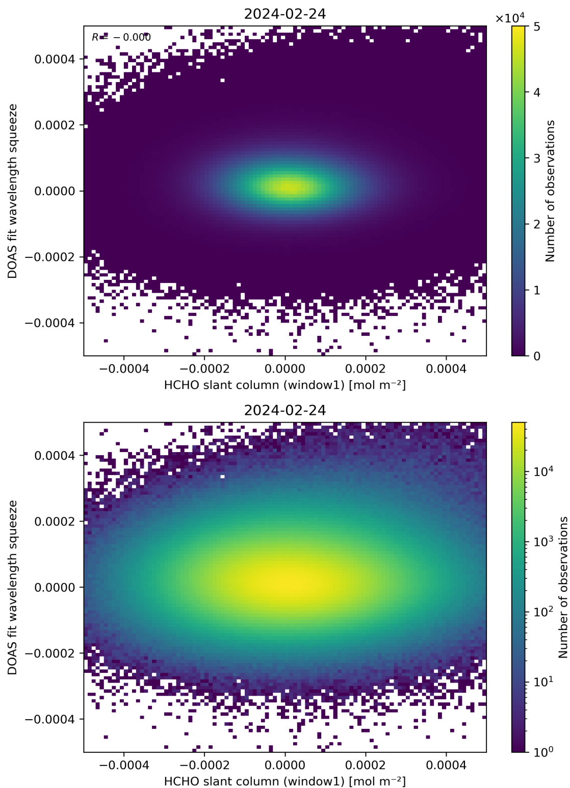
Figure 80: Scatter density plot of “HCHO slant column (window1)” against “DOAS fit wavelength squeeze” for 2024-02-23 to 2024-02-25.
