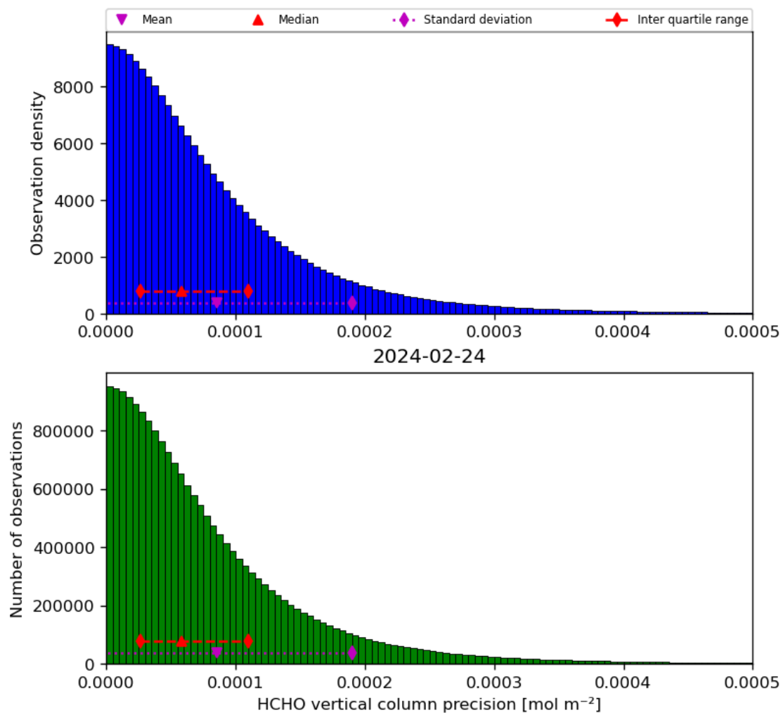
Figure 36: Histogram of “HCHO vertical column precision” for 2024-02-23 to 2024-02-25
