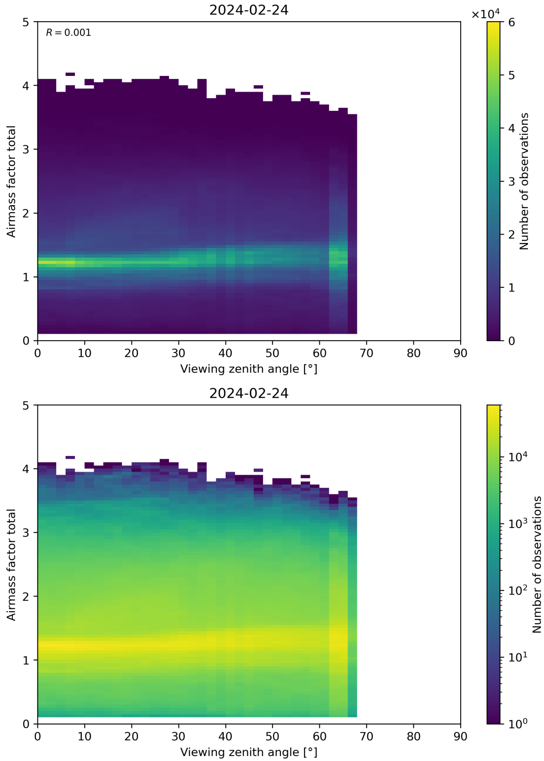
Figure 190: Scatter density plot of “Viewing zenith angle” against “Airmass factor total” for 2024-02-23 to 2024-02-25.
