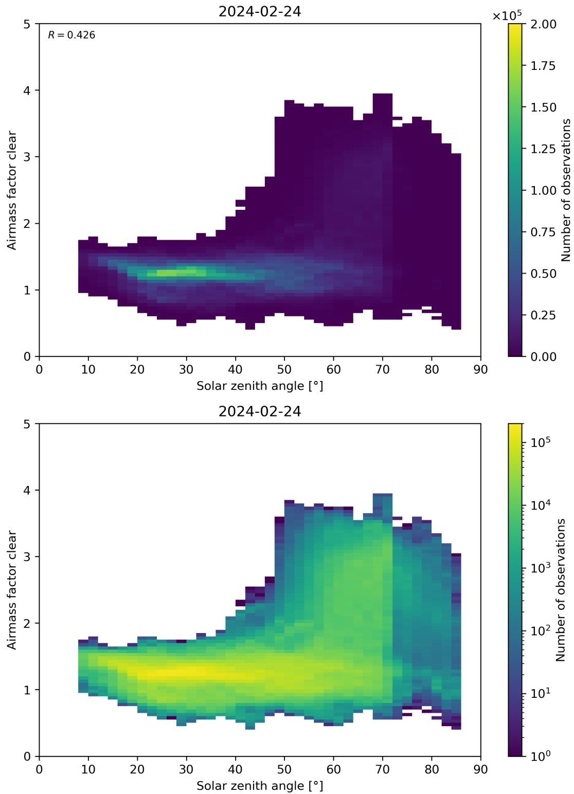
Figure 170: Scatter density plot of “Solar zenith angle” against “Airmass factor clear” for 2024-02-23 to 2024-02-25.
