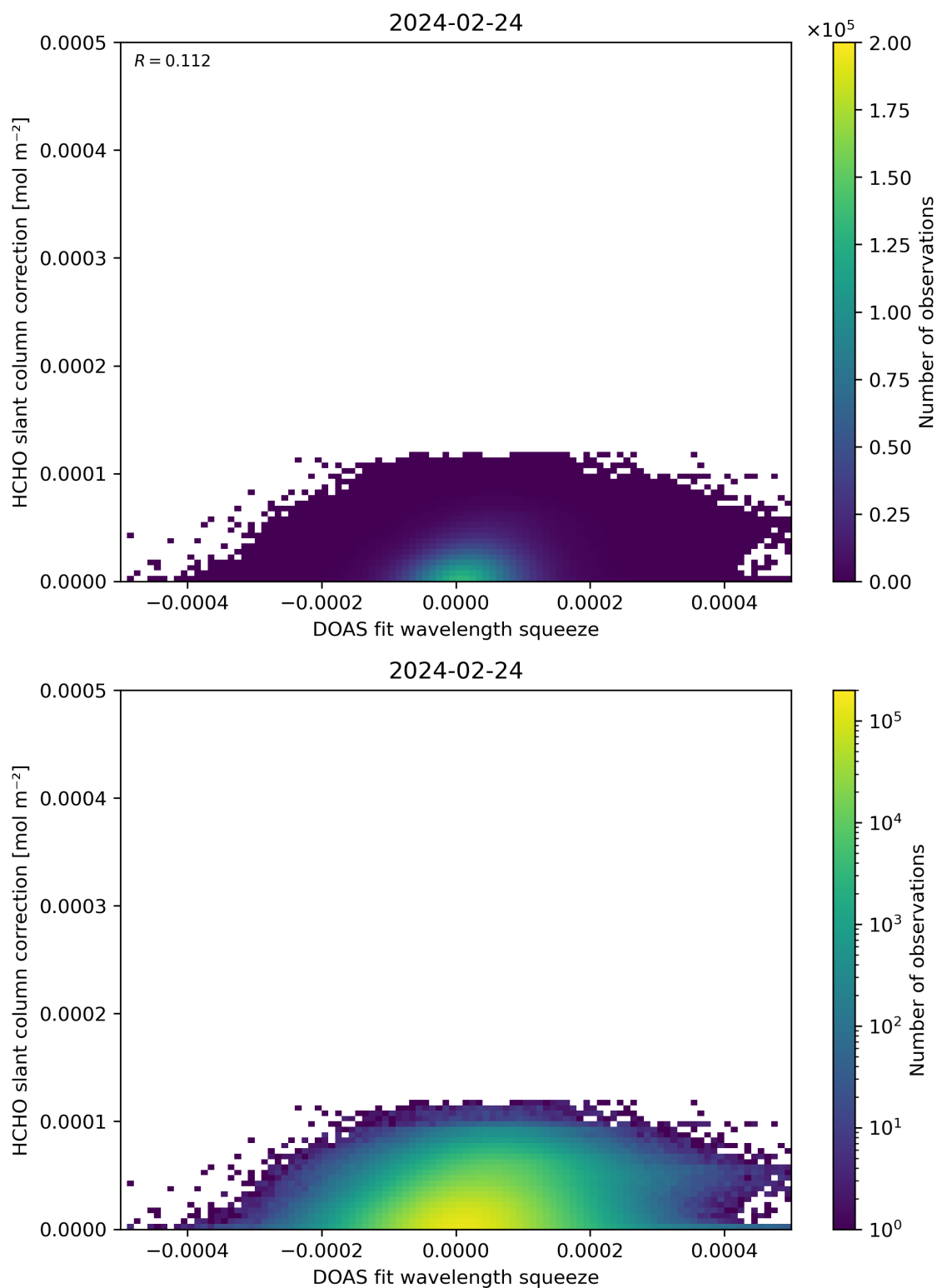
Figure 70: Scatter density plot of “DOAS fit wavelength squeeze” against “HCHO slant column correction” for 2024-02-23 to 2024-02-25.
