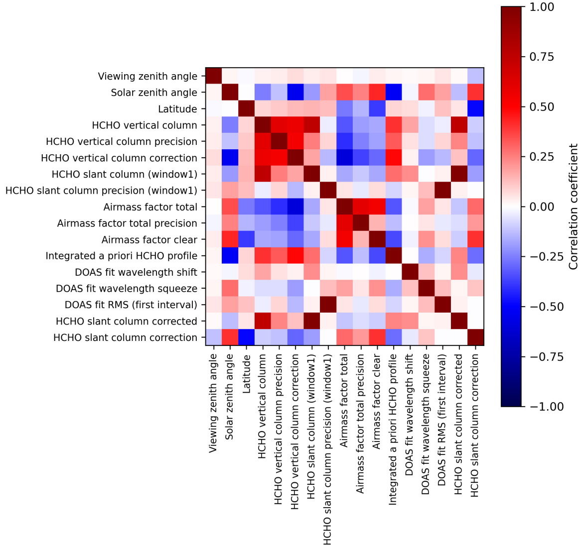
Figure 2: Map of correlation matrix for 2024-02-23 to 2024-02-25.
