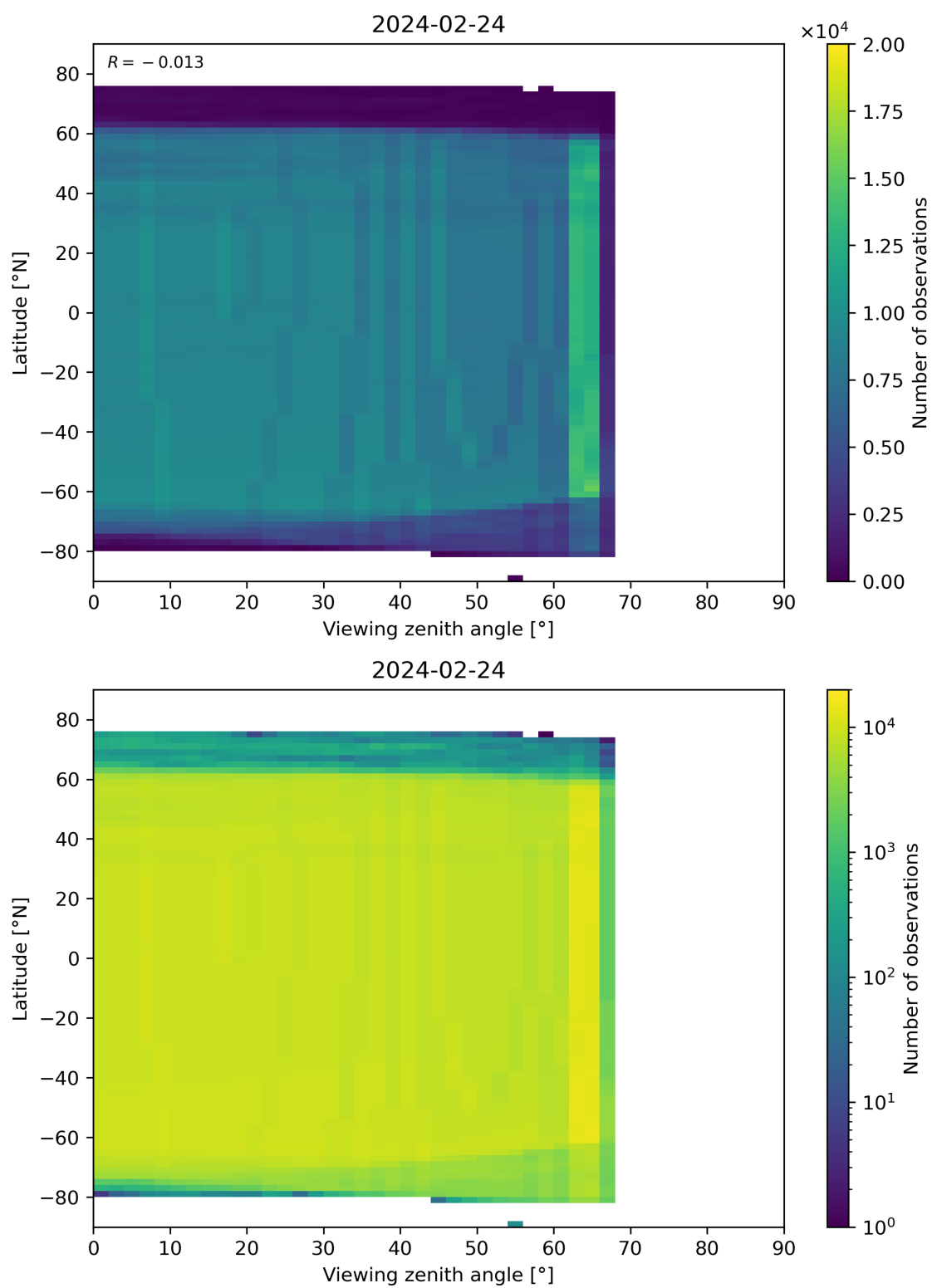
Figure 196: Scatter density plot of “Viewing zenith angle” against “Latitude” for 2024-02-23 to 2024-02-25.
