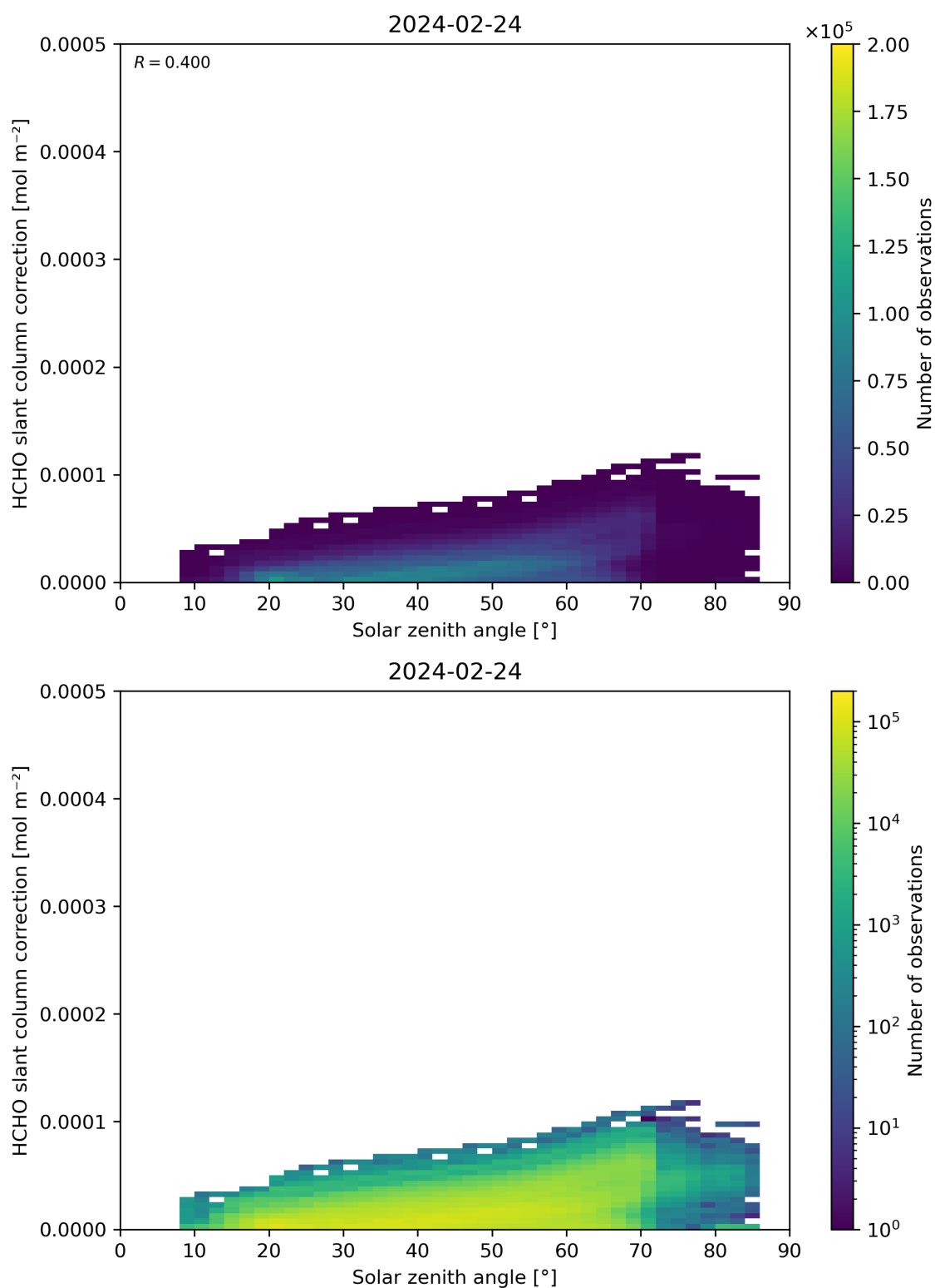
Figure 172: Scatter density plot of “Solar zenith angle” against “HCHO slant column correction” for 2024-02-23 to 2024-02-25.
