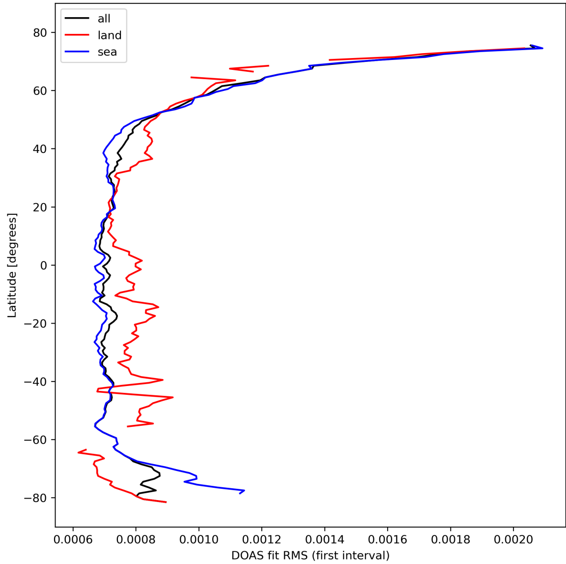
Figure 32: Zonal average of “DOAS fit RMS (first interval)” for 2024-02-23 to 2024-02-25.
