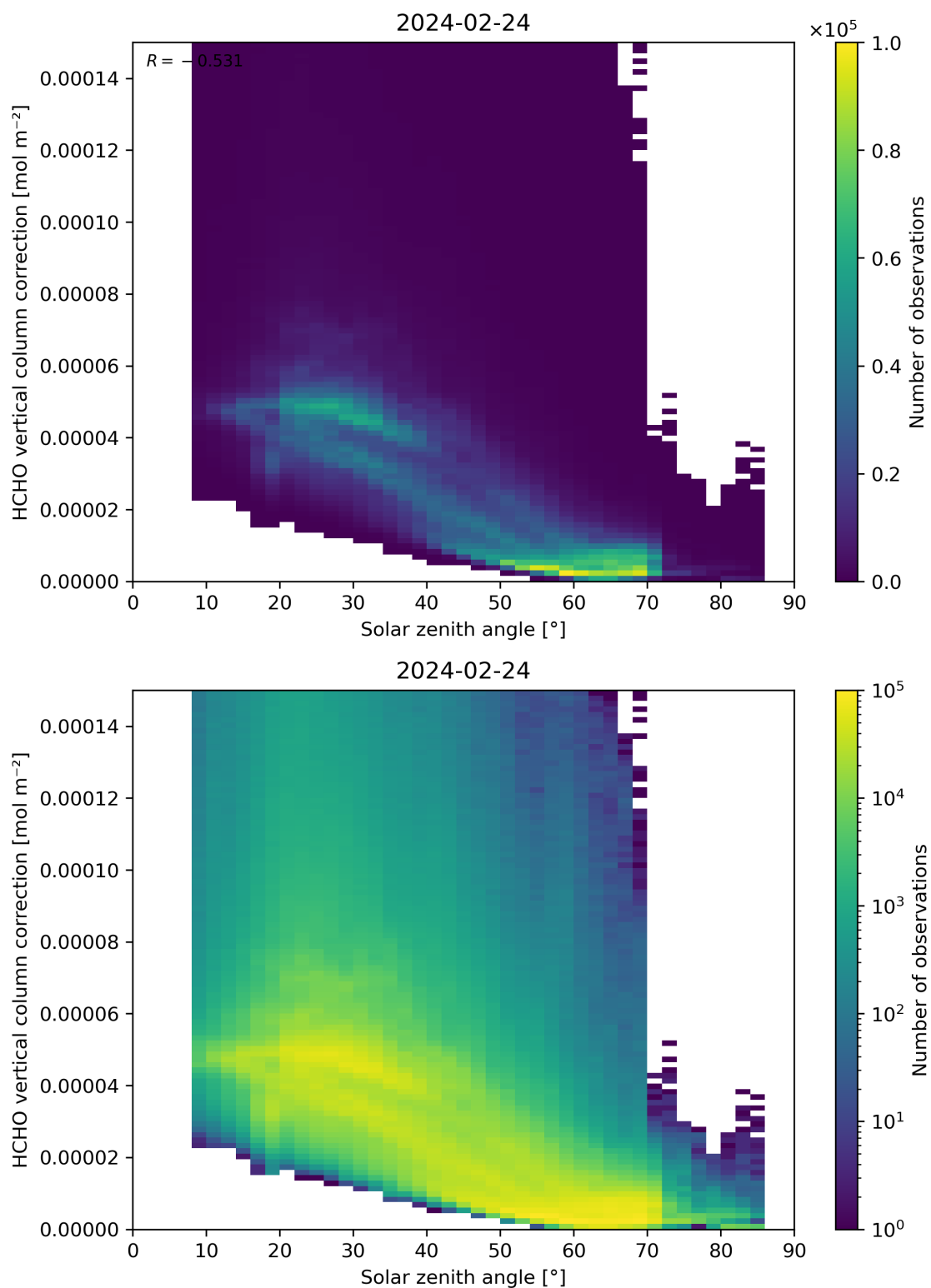
Figure 178: Scatter density plot of “Solar zenith angle” against “HCHO vertical column correction” for 2024-02-23 to 2024-02-25.
