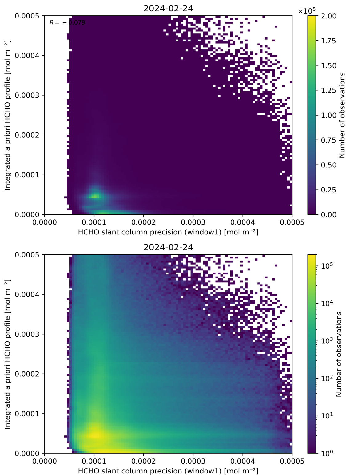
Figure 96: Scatter density plot of “HCHO slant column precision (window1)” against “Integrated a priori HCHO profile” for 2024-02-23 to 2024-02-25.
