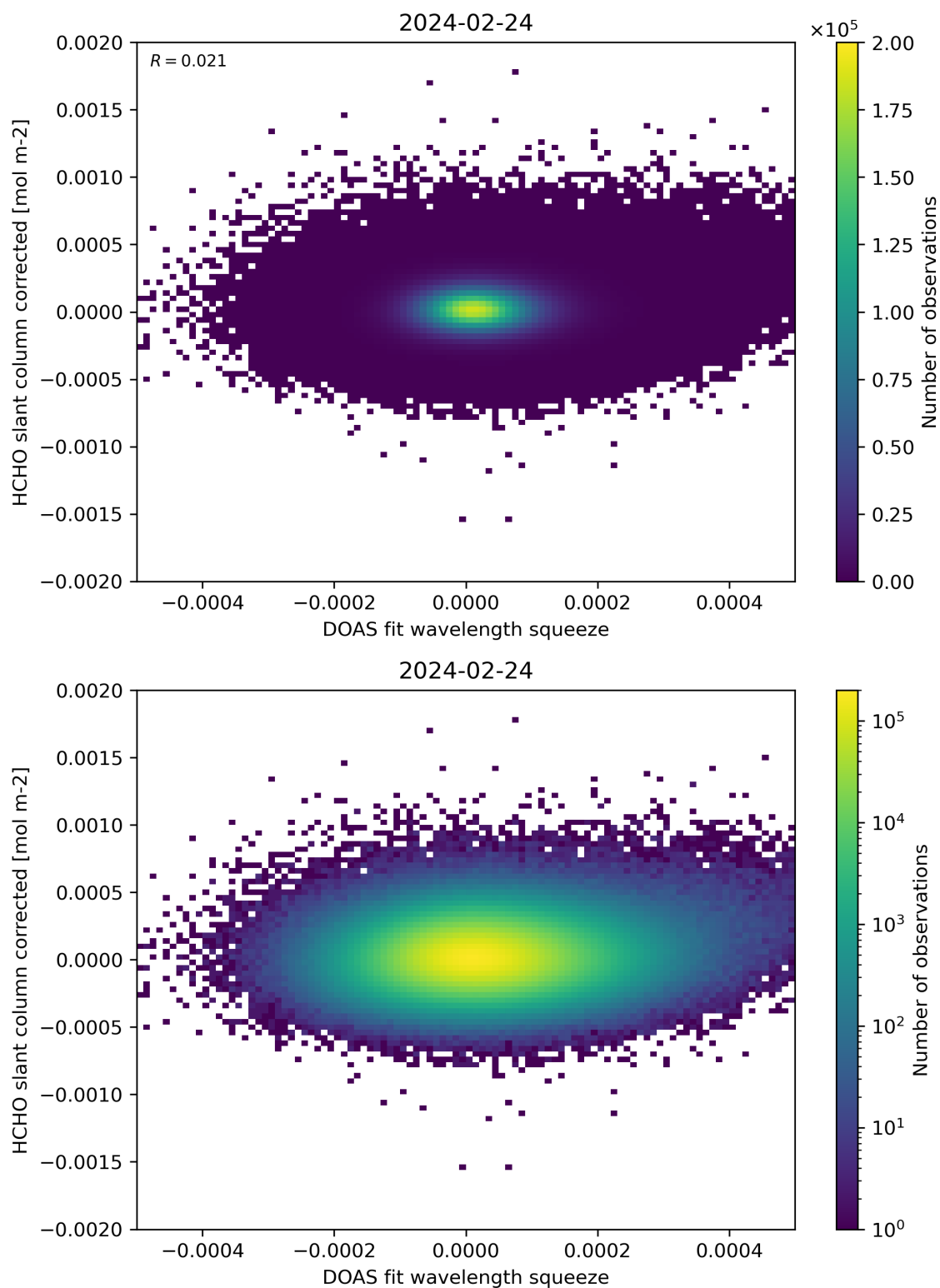
Figure 69: Scatter density plot of “DOAS fit wavelength squeeze” against “HCHO slant column corrected” for 2024-02-23 to 2024-02-25.
