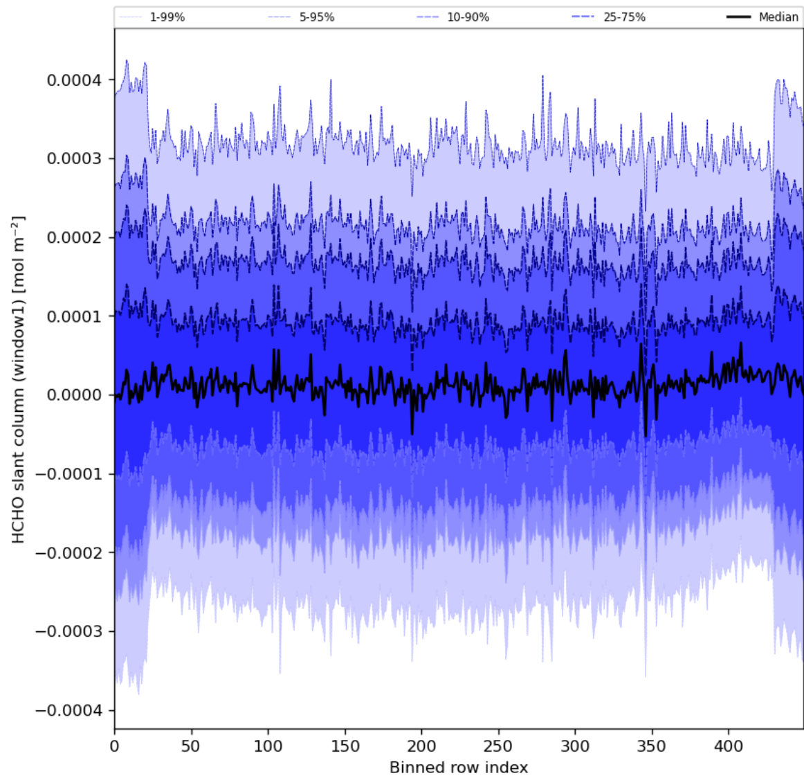
Figure 52: Along track statistics of “HCHO slant column (window1)” for 2024-02-23 to 2024-02-25
