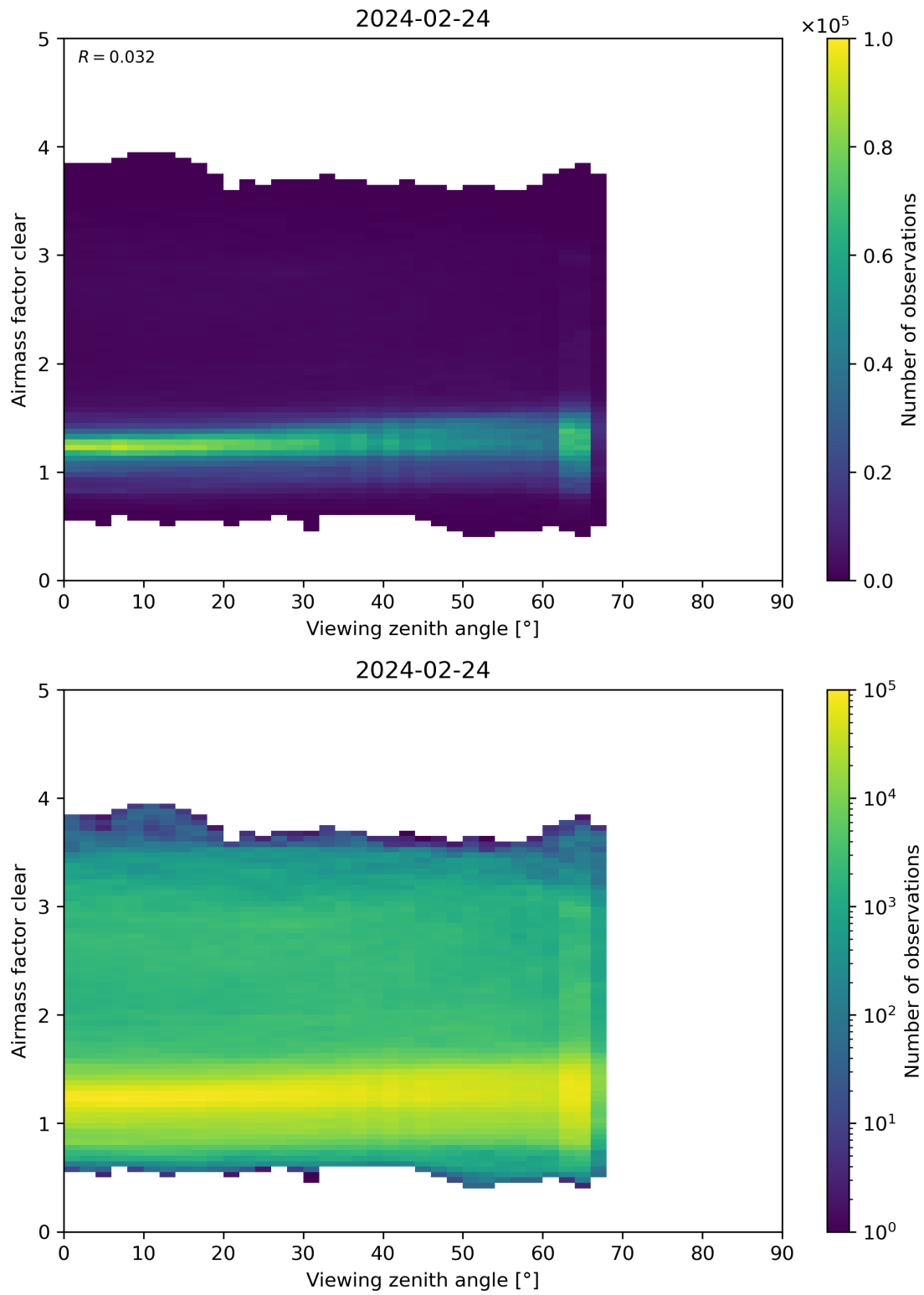
Figure 185: Scatter density plot of “Viewing zenith angle” against “Airmass factor clear” for 2024-02-23 to 2024-02-25.
