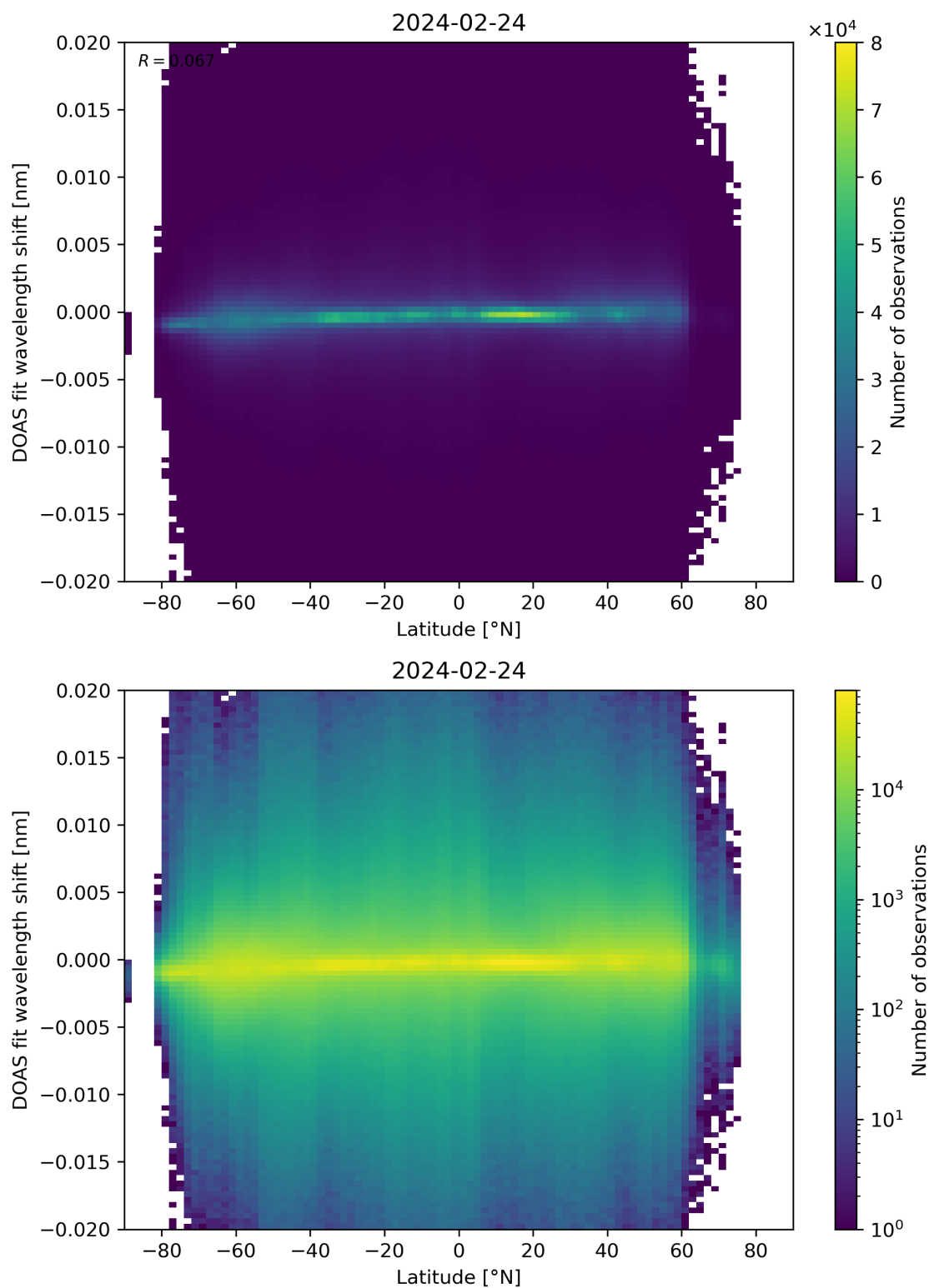
Figure 154: Scatter density plot of “Latitude” against “DOAS fit wavelength shift” for 2024-02-23 to 2024-02-25.
