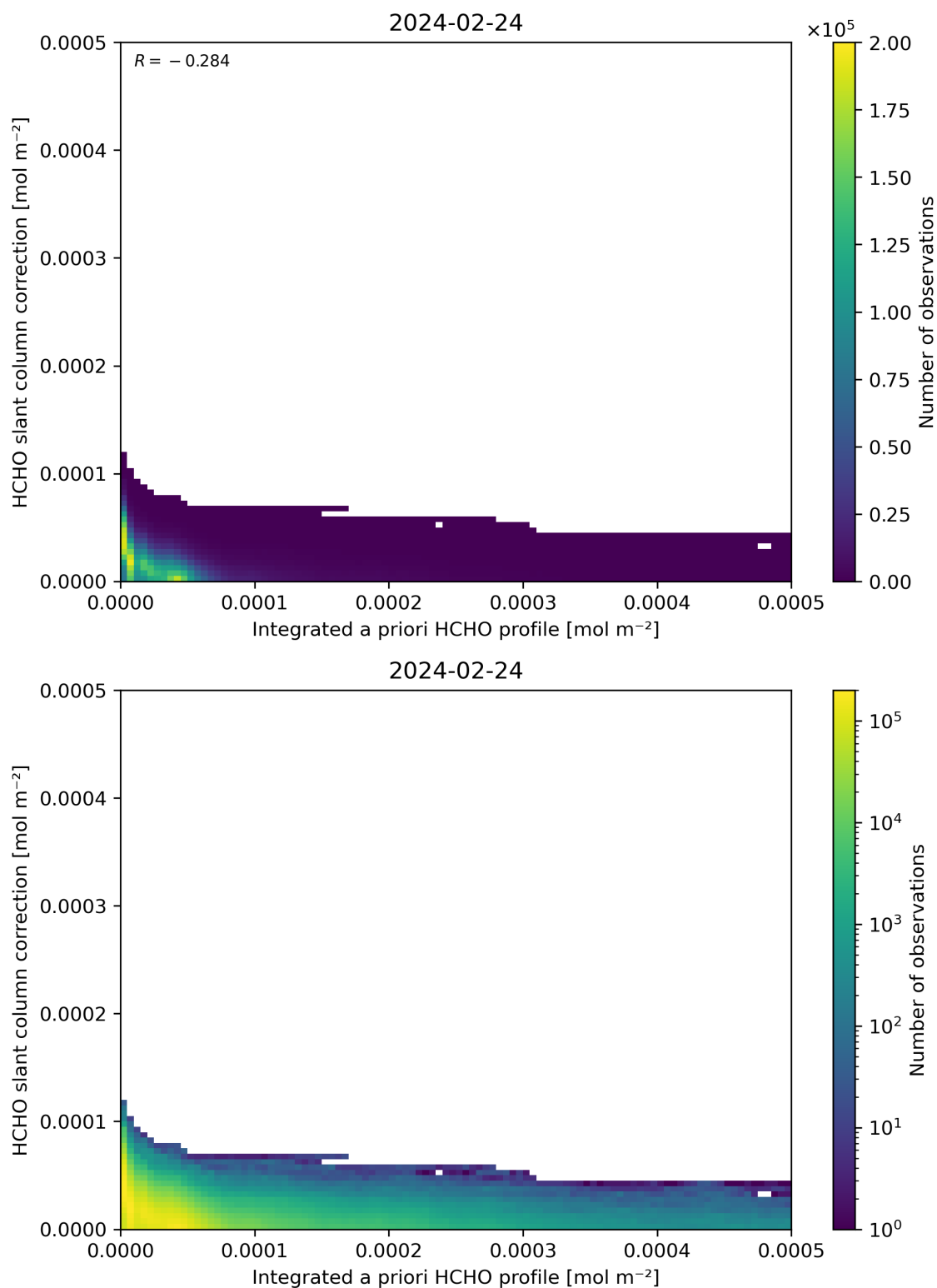
Figure 152: Scatter density plot of “Integrated a priori HCHO profile” against “HCHO slant column correction” for 2024-02-23 to 2024-02-25.
