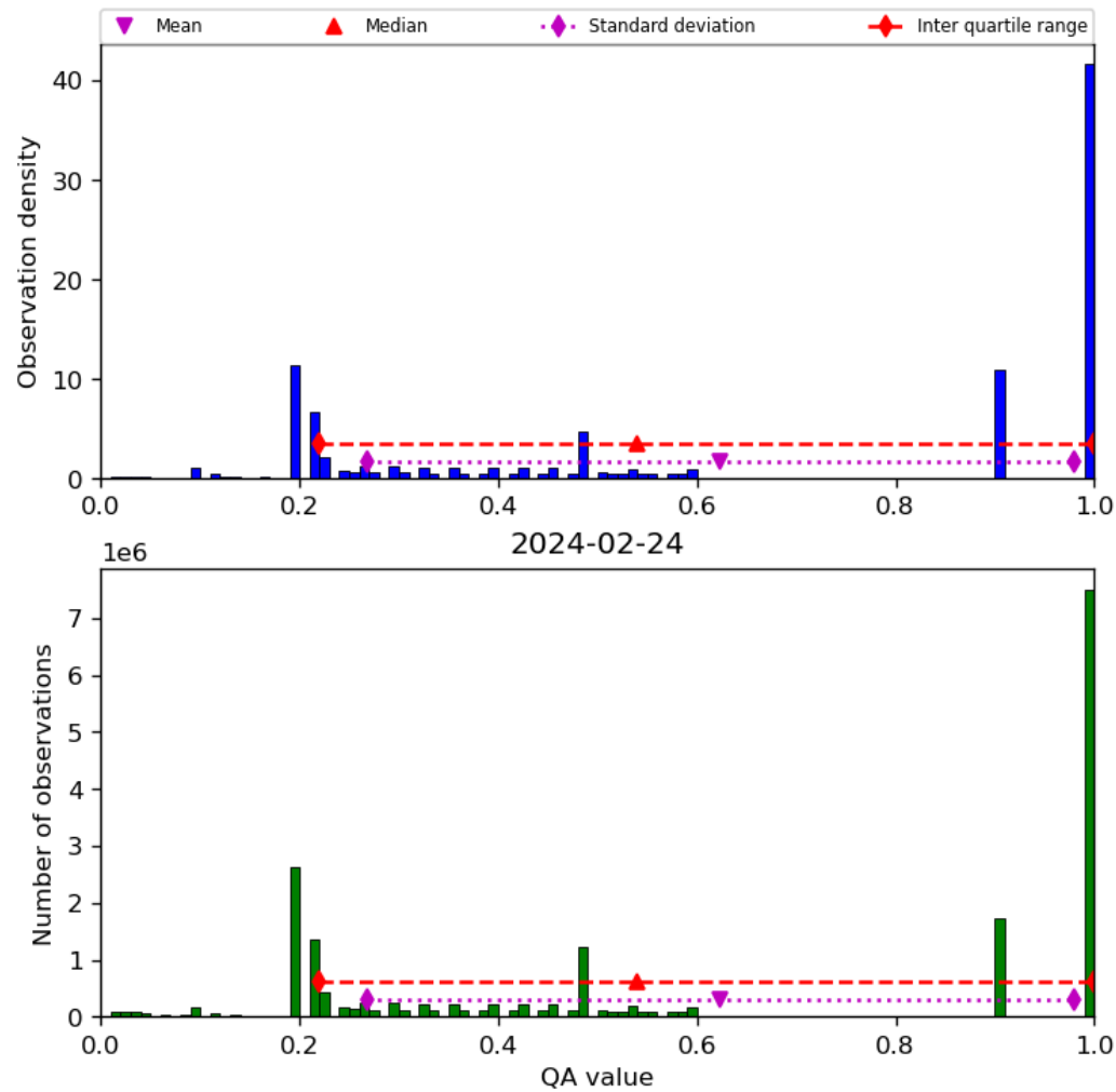
Figure 34: Histogram of “QA value” for 2024-02-23 to 2024-02-25
