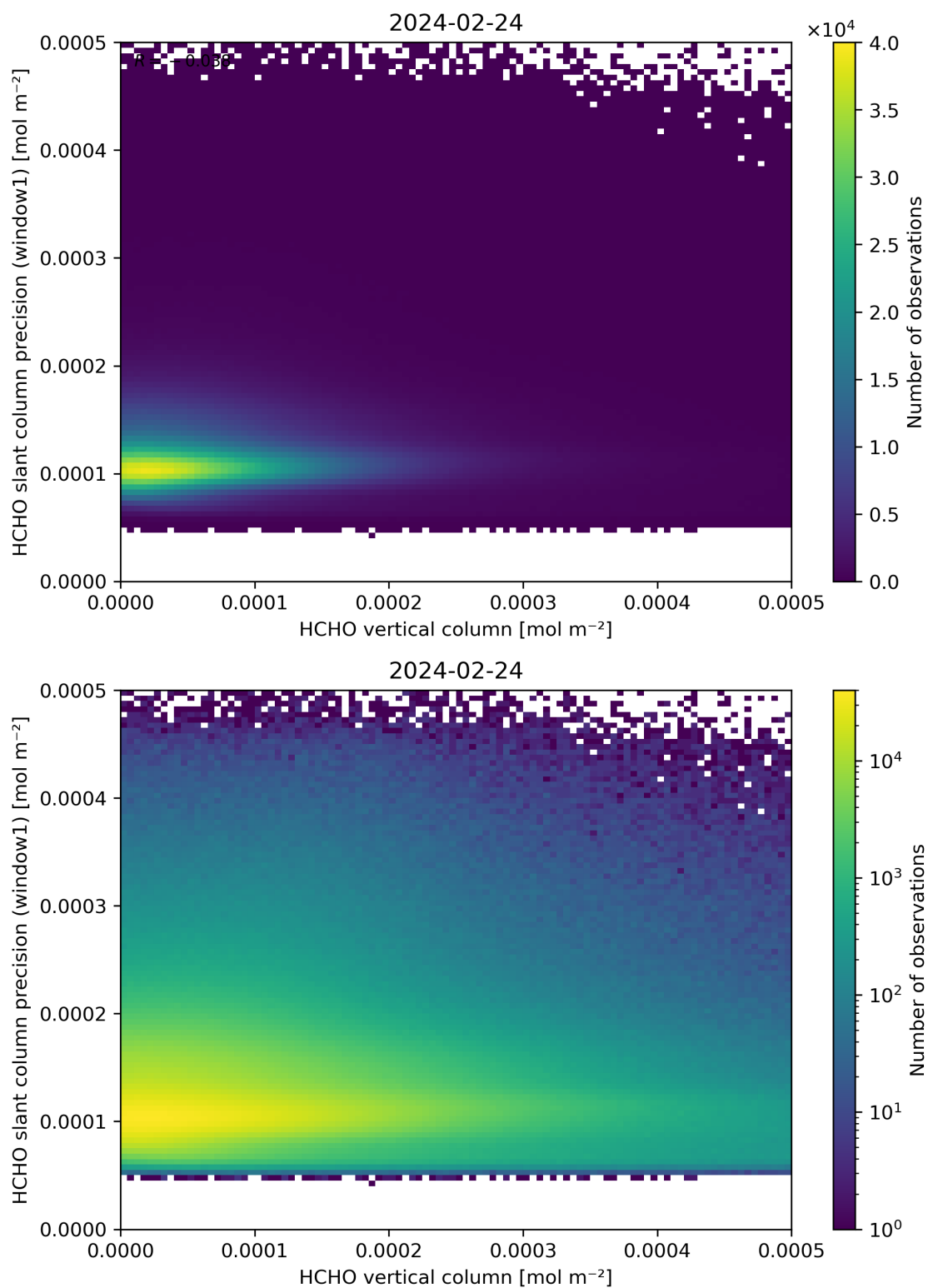
Figure 130: Scatter density plot of “HCHO vertical column” against “HCHO slant column precision (window1)” for 2024-02-23 to 2024-02-25.
