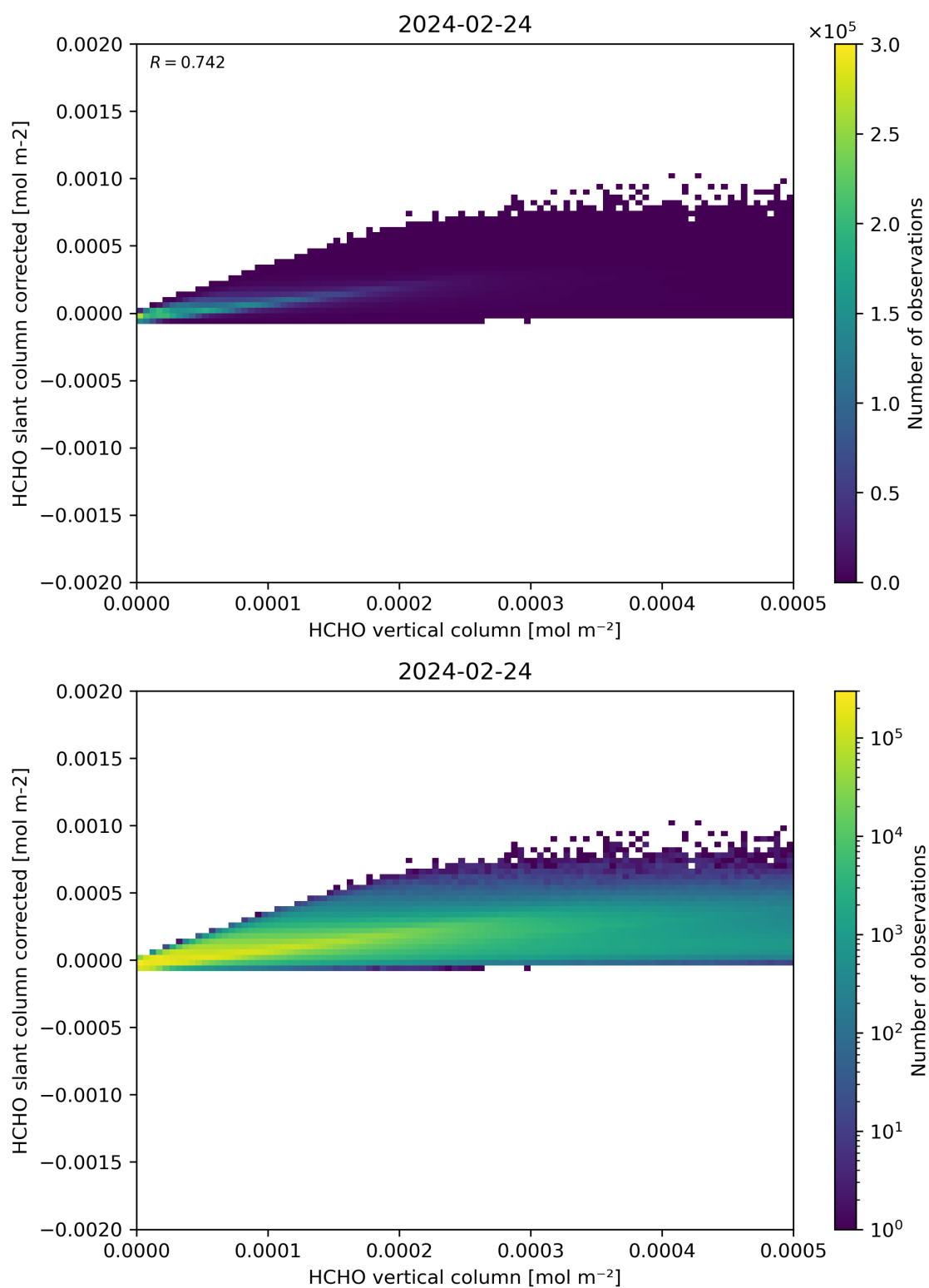
Figure 127: Scatter density plot of “HCHO vertical column” against “HCHO slant column corrected” for 2024-02-23 to 2024-02-25.
