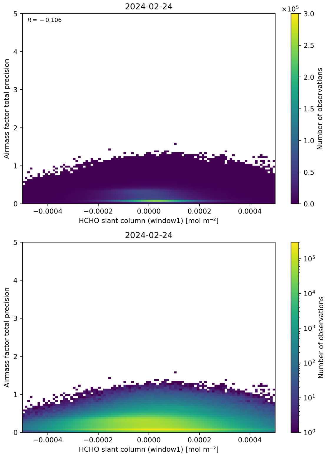
Figure 86: Scatter density plot of “HCHO slant column (window1)” against “Airmass factor total precision” for 2024-02-23 to 2024-02-25.
