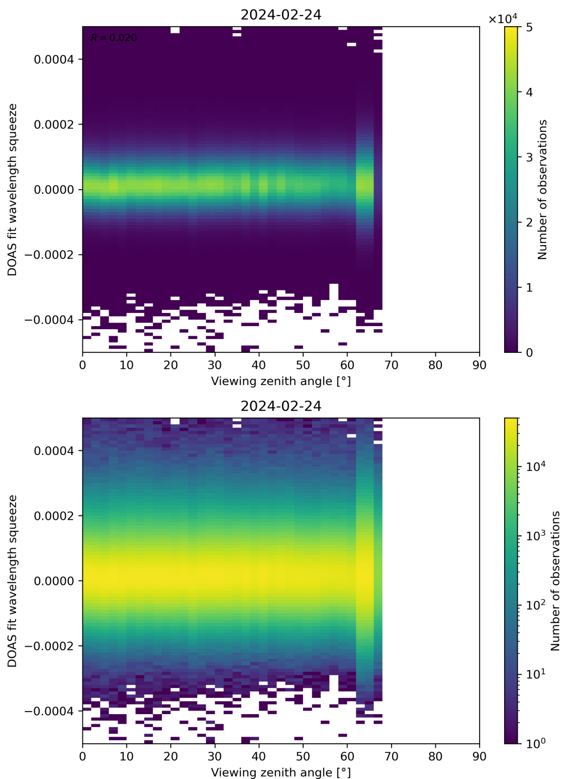
Figure 184: Scatter density plot of “Viewing zenith angle” against “DOAS fit wavelength squeeze” for 2024-02-23 to 2024-02-25.
