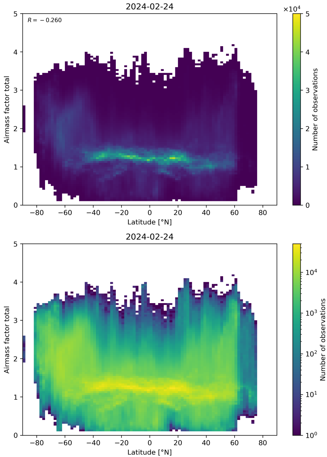
Figure 161: Scatter density plot of “Latitude” against “Airmass factor total” for 2024-02-23 to 2024-02-25.
