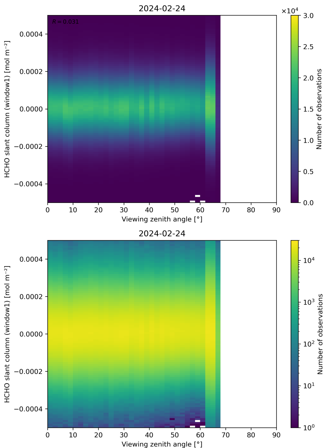
Figure 188: Scatter density plot of “Viewing zenith angle” against “HCHO slant column (window1)” for 2024-02-23 to 2024-02-25.
