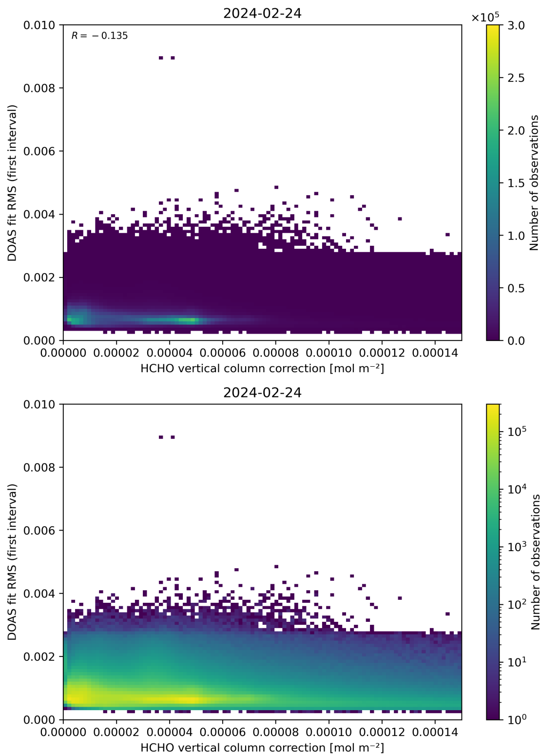
Figure 112: Scatter density plot of “HCHO vertical column correction” against “DOAS fit RMS (first interval)” for 2024-02-23 to 2024-02-25.
