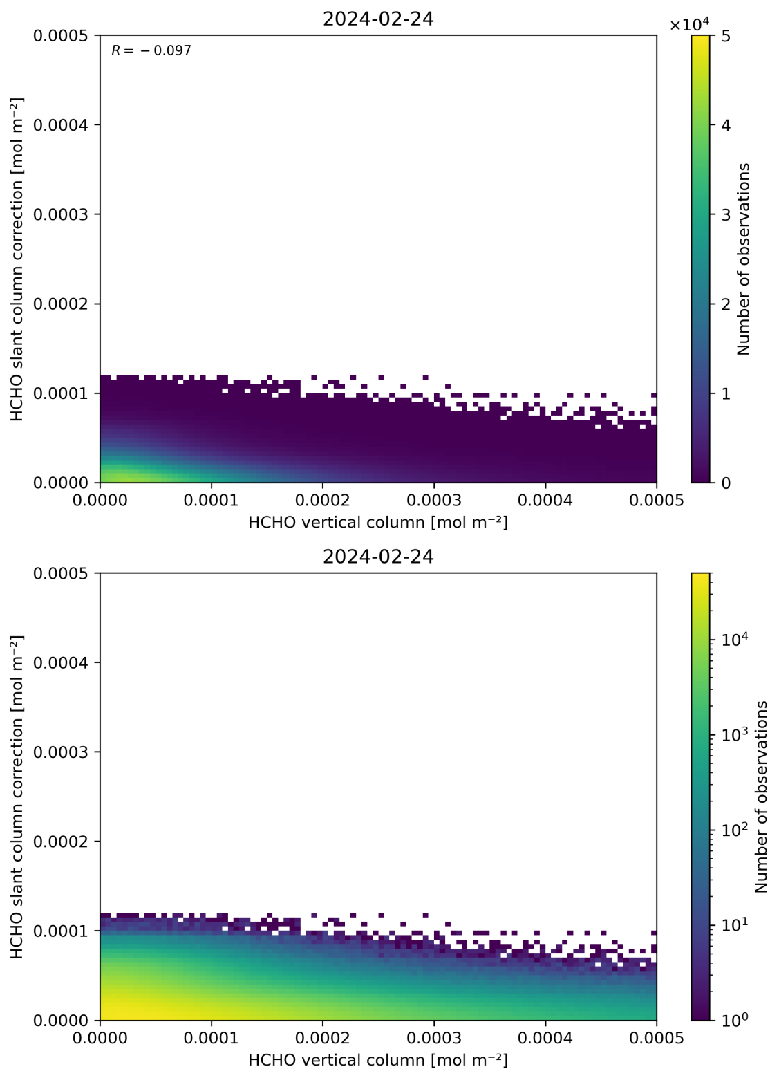
Figure 128: Scatter density plot of “HCHO vertical column” against “HCHO slant column correction” for 2024-02-23 to 2024-02-25.
