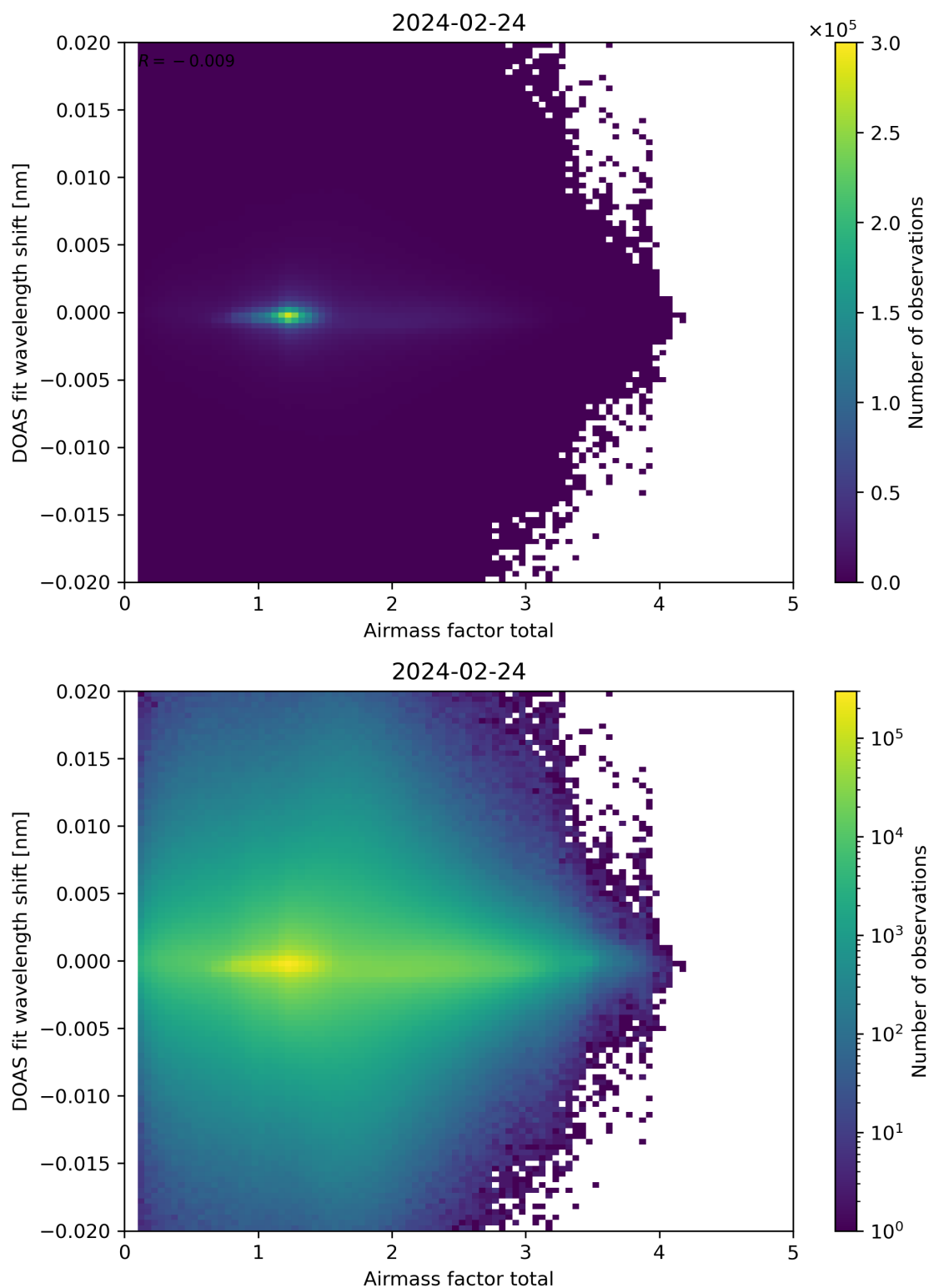
Figure 98: Scatter density plot of “Airmass factor total” against “DOAS fit wavelength shift” for 2024-02-23 to 2024-02-25.
