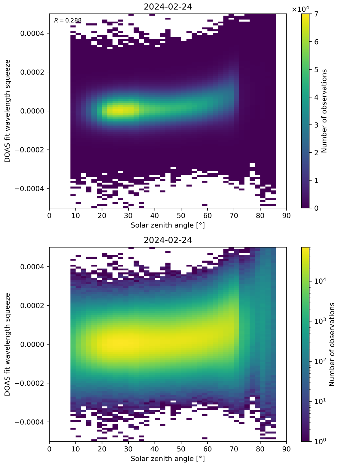
Figure 169: Scatter density plot of “Solar zenith angle” against “DOAS fit wavelength squeeze” for 2024-02-23 to 2024-02-25.
