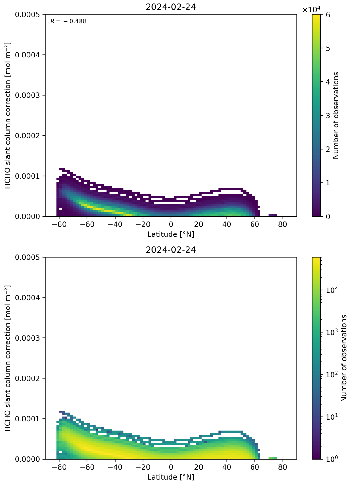
Figure 158: Scatter density plot of “Latitude” against “HCHO slant column correction” for 2024-02-23 to 2024-02-25.
