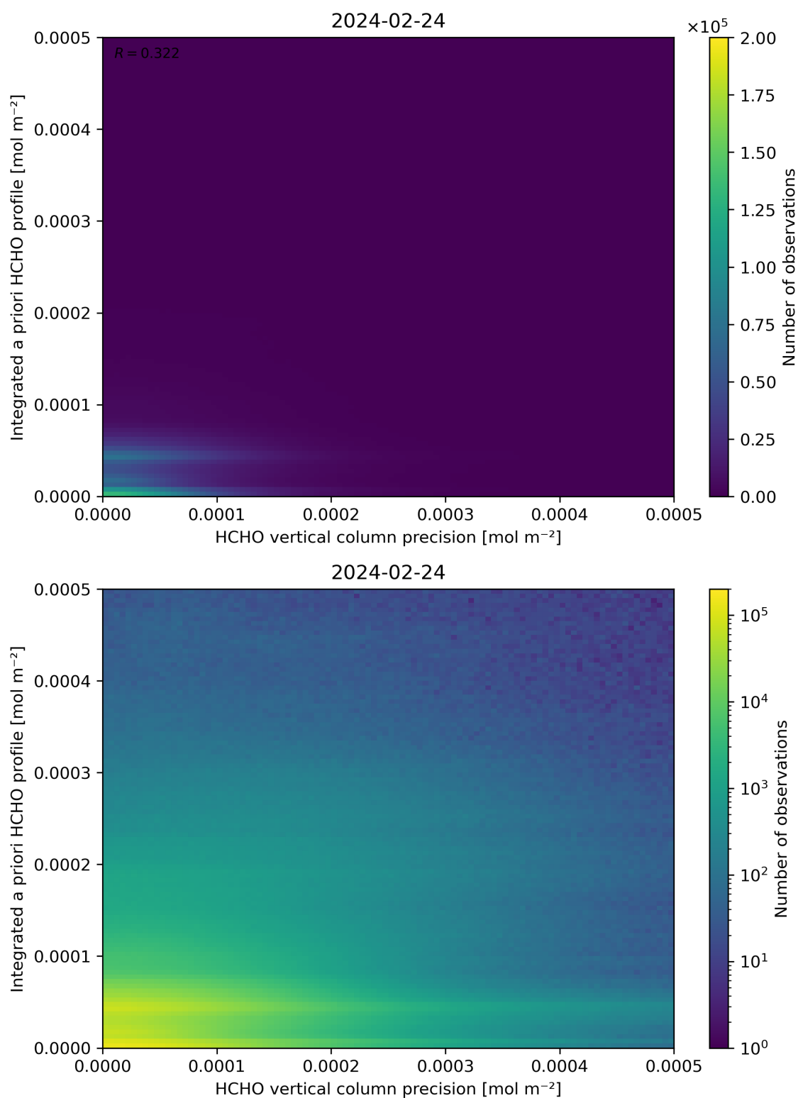
Figure 147: Scatter density plot of “HCHO vertical column precision” against “Integrated a priori HCHO profile” for 2024-02-23 to 2024-02-25.
