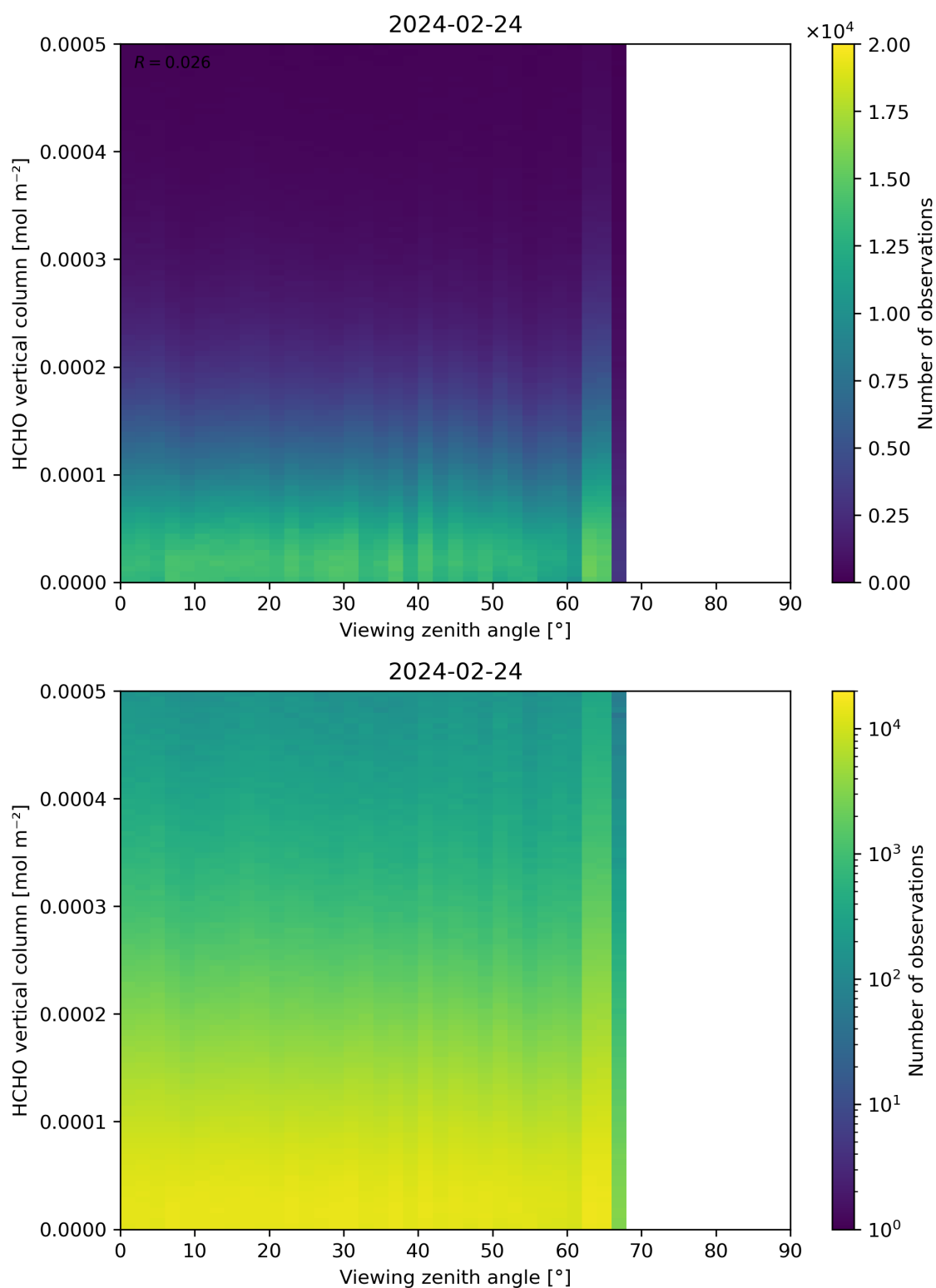
Figure 192: Scatter density plot of “Viewing zenith angle” against “HCHO vertical column” for 2024-02-23 to 2024-02-25.
