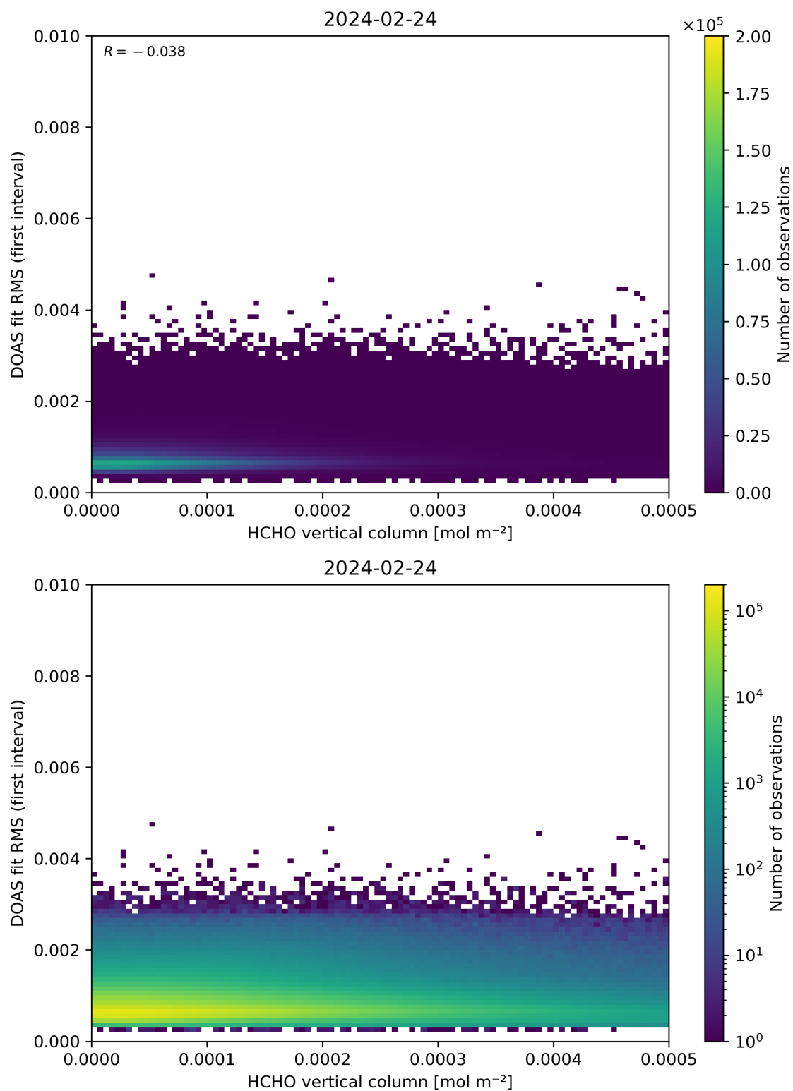
Figure 123: Scatter density plot of “HCHO vertical column” against “DOAS fit RMS (first interval)” for 2024-02-23 to 2024-02-25.
