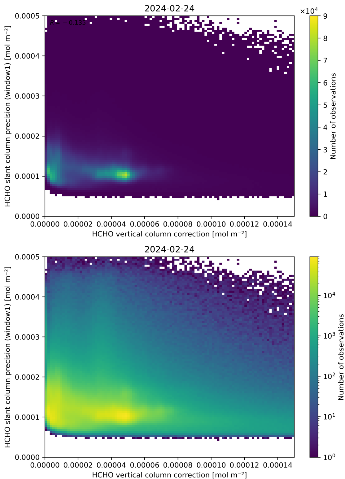
Figure 119: Scatter density plot of “HCHO vertical column correction” against “HCHO slant column precision (window1)” for 2024-02-23 to 2024-02-25.
