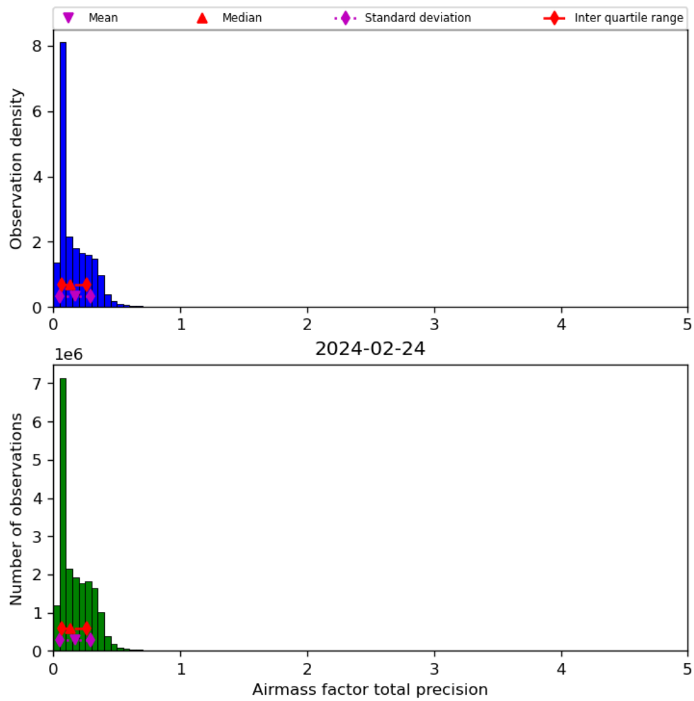
Figure 41: Histogram of “Airmass factor total precision” for 2024-02-23 to 2024-02-25
