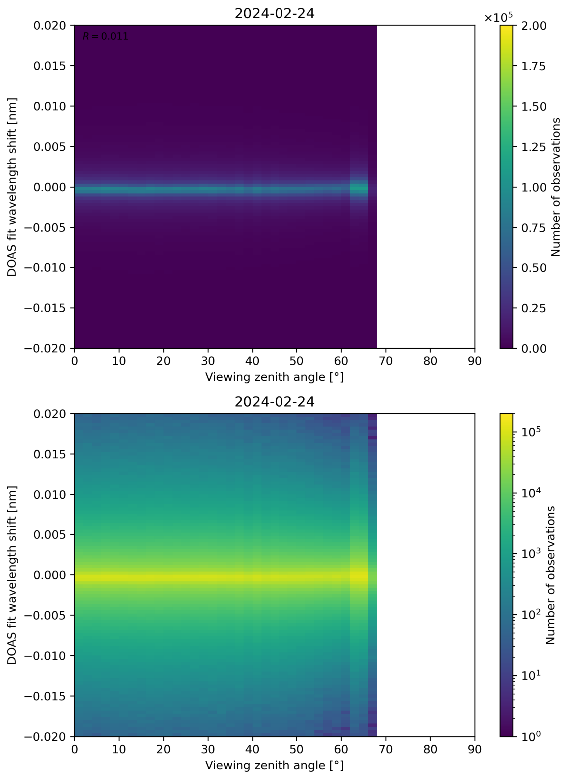
Figure 183: Scatter density plot of “Viewing zenith angle” against “DOAS fit wavelength shift” for 2024-02-23 to 2024-02-25.
