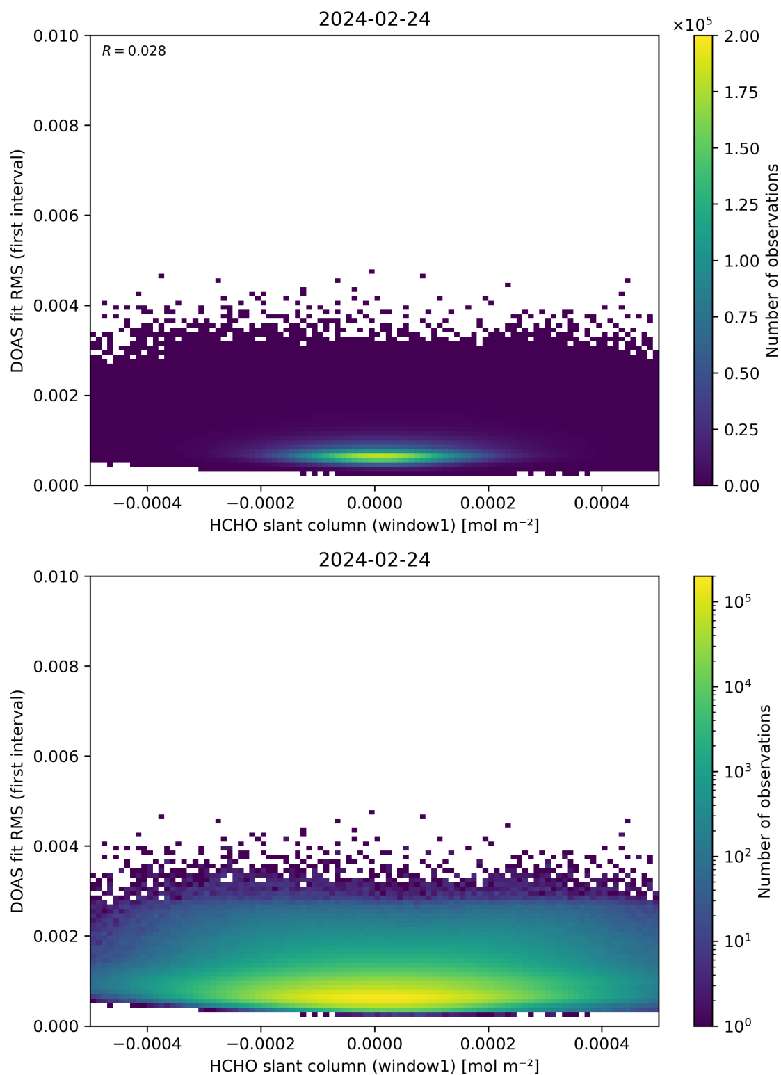
Figure 78: Scatter density plot of “HCHO slant column (window1)” against “DOAS fit RMS (first interval)” for 2024-02-23 to 2024-02-25.
