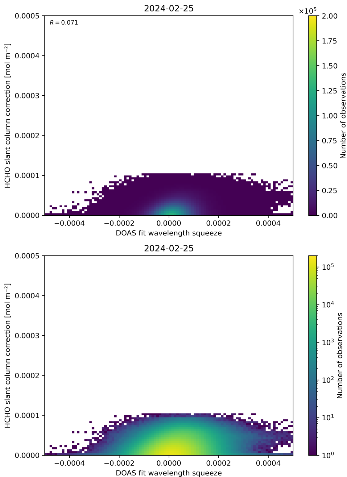
Figure 70: Scatter density plot of “DOAS fit wavelength squeeze” against “HCHO slant column correction” for 2024-02-24 to 2024-02-26.
