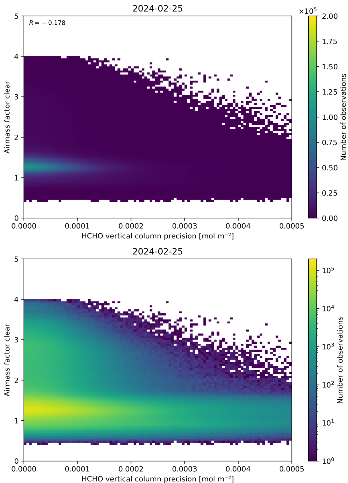
Figure 139: Scatter density plot of “HCHO vertical column precision” against “Airmass factor clear” for 2024-02-24 to 2024-02-26.
