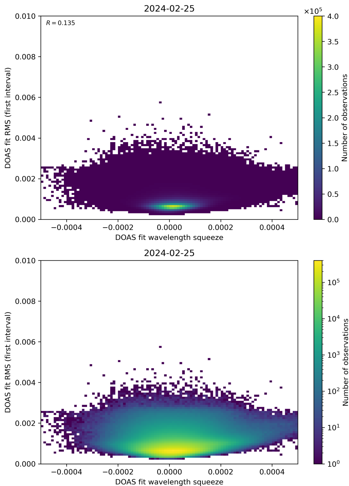
Figure 68: Scatter density plot of “DOAS fit wavelength squeeze” against “DOAS fit RMS (first interval)” for 2024-02-24 to 2024-02-26.
