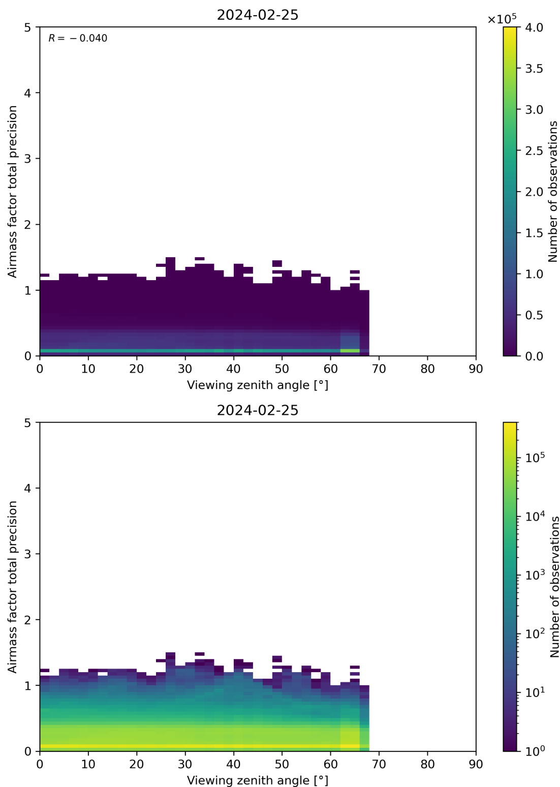
Figure 191: Scatter density plot of “Viewing zenith angle” against “Airmass factor total precision” for 2024-02-24 to 2024-02-26.
