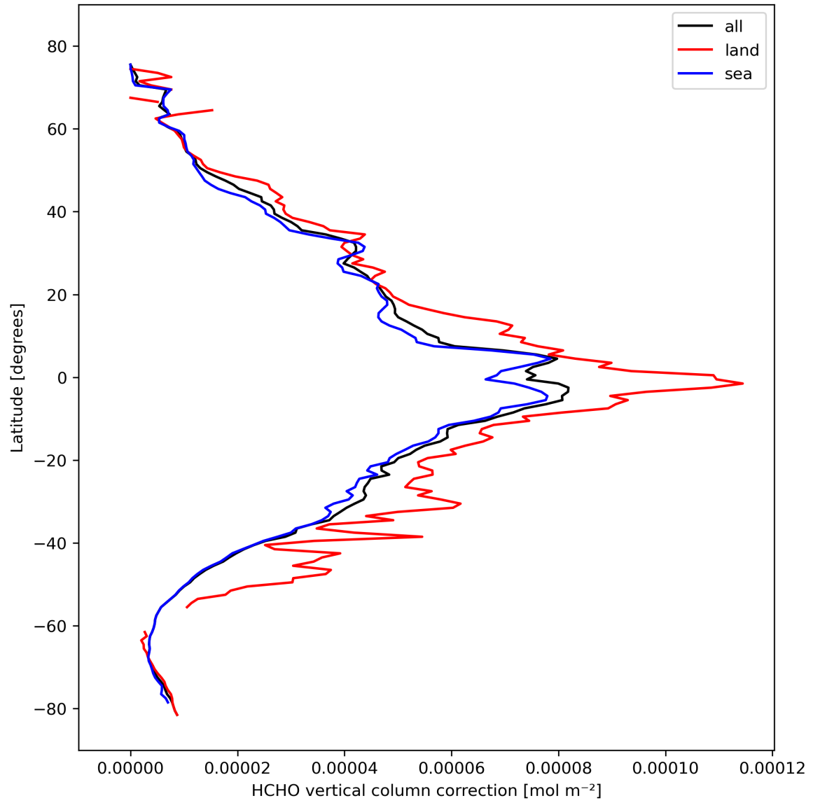
Figure 23: Zonal average of “HCHO vertical column correction” for 2024-02-24 to 2024-02-26.
