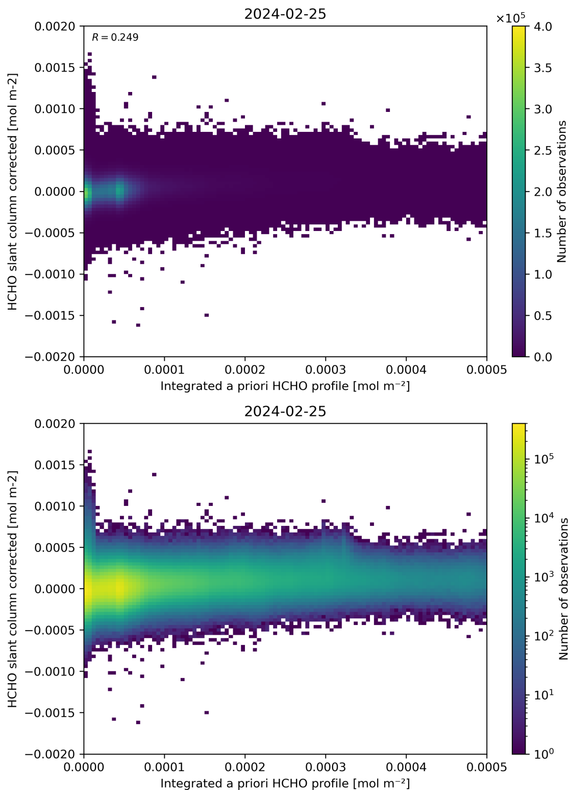
Figure 151: Scatter density plot of “Integrated a priori HCHO profile” against “HCHO slant column corrected” for 2024-02-24 to 2024-02-26.
