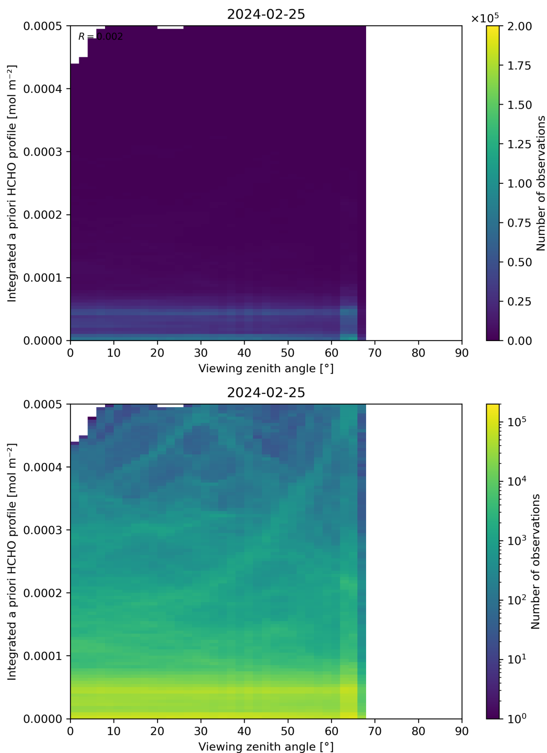
Figure 195: Scatter density plot of “Viewing zenith angle” against “Integrated a priori HCHO profile” for 2024-02-24 to 2024-02-26.
