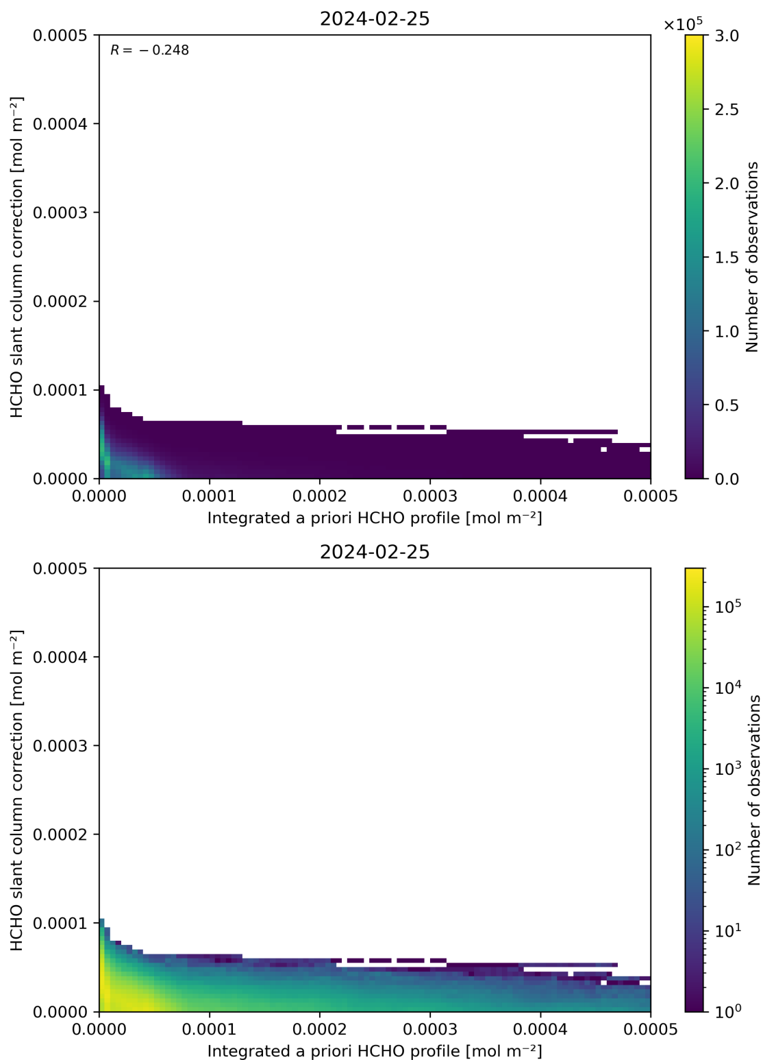
Figure 152: Scatter density plot of “Integrated a priori HCHO profile” against “HCHO slant column correction” for 2024-02-24 to 2024-02-26.
