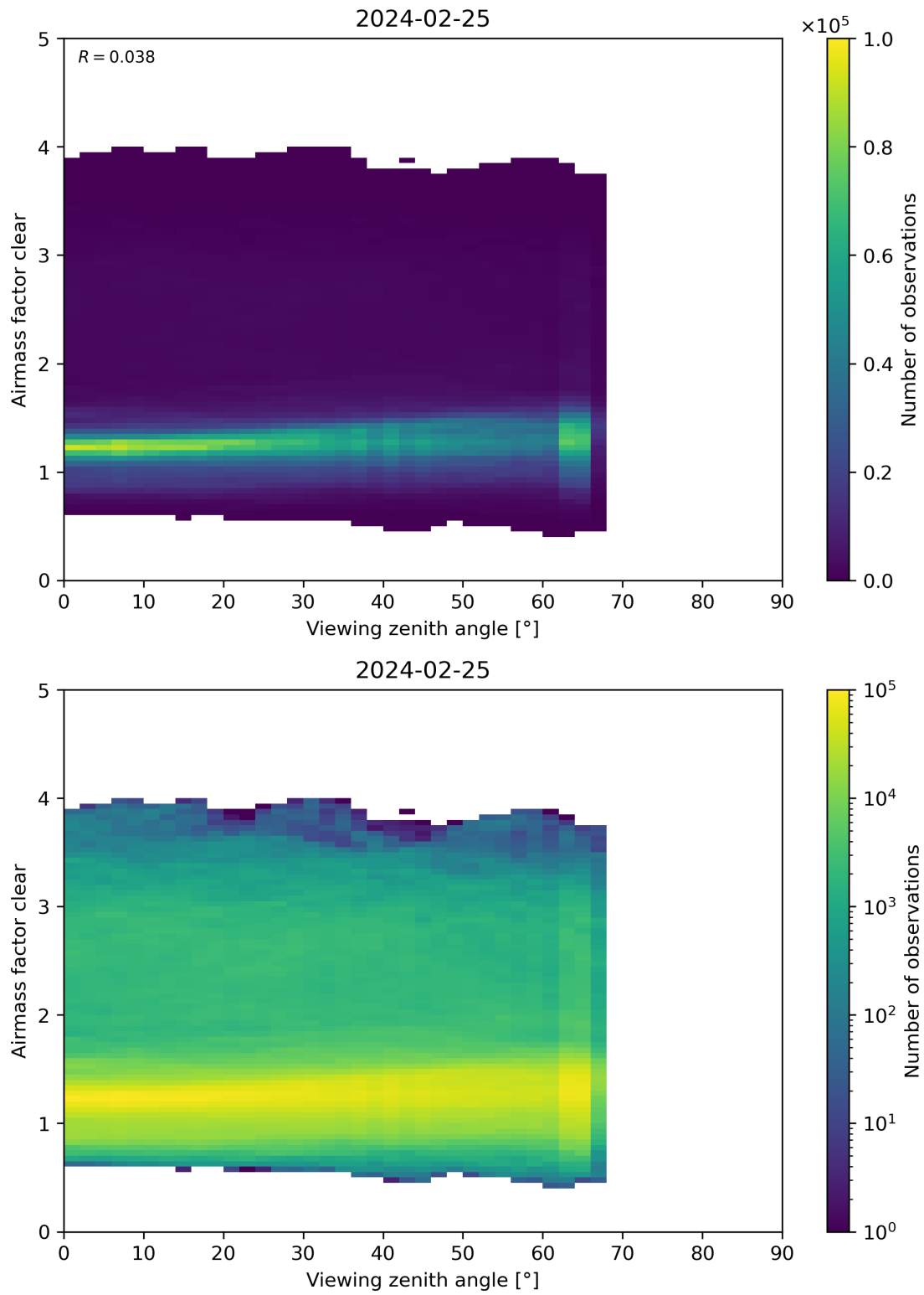
Figure 185: Scatter density plot of “Viewing zenith angle” against “Airmass factor clear” for 2024-02-24 to 2024-02-26.
