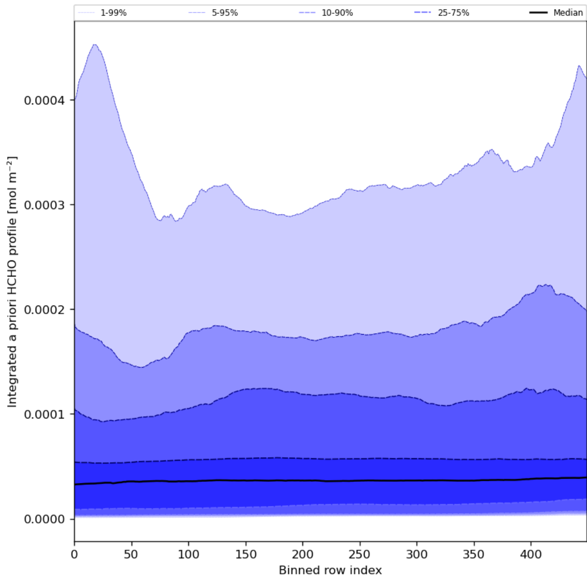
Figure 57: Along track statistics of “Integrated a priori HCHO profile” for 2024-02-24 to 2024-02-26
