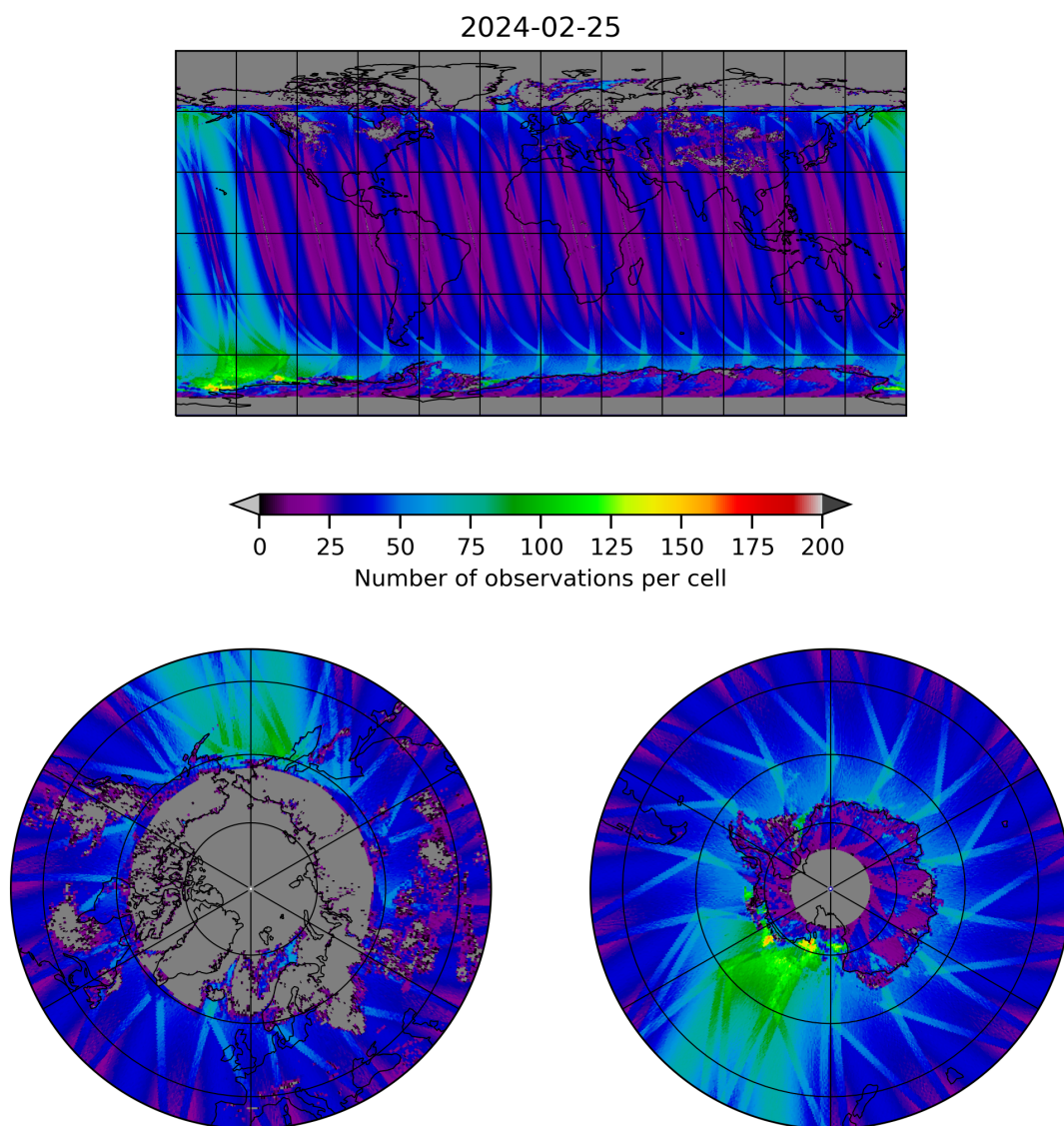
Figure 19: Map of the number of observations for 2024-02-24 to 2024-02-26
