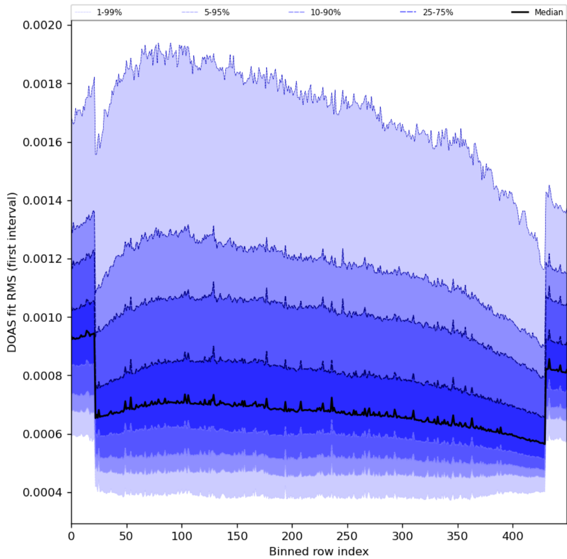
Figure 60: Along track statistics of “DOAS fit RMS (first interval)” for 2024-02-24 to 2024-02-26
