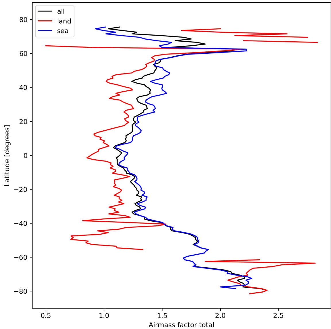
Figure 26: Zonal average of “Airmass factor total” for 2024-02-24 to 2024-02-26.
