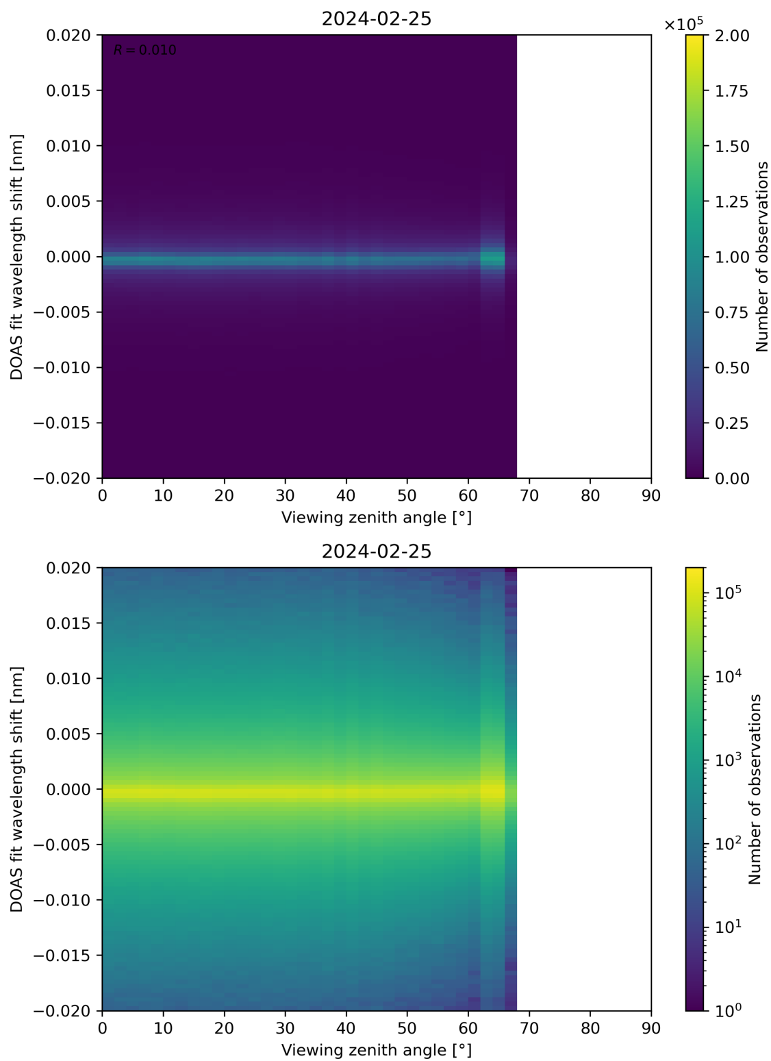
Figure 183: Scatter density plot of “Viewing zenith angle” against “DOAS fit wavelength shift” for 2024-02-24 to 2024-02-26.
