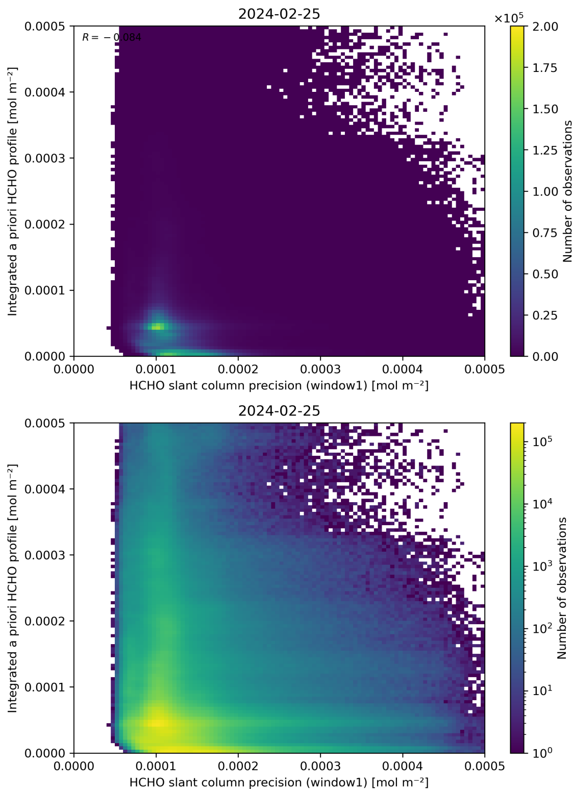
Figure 96: Scatter density plot of “HCHO slant column precision (window1)” against “Integrated a priori HCHO profile” for 2024-02-24 to 2024-02-26.
