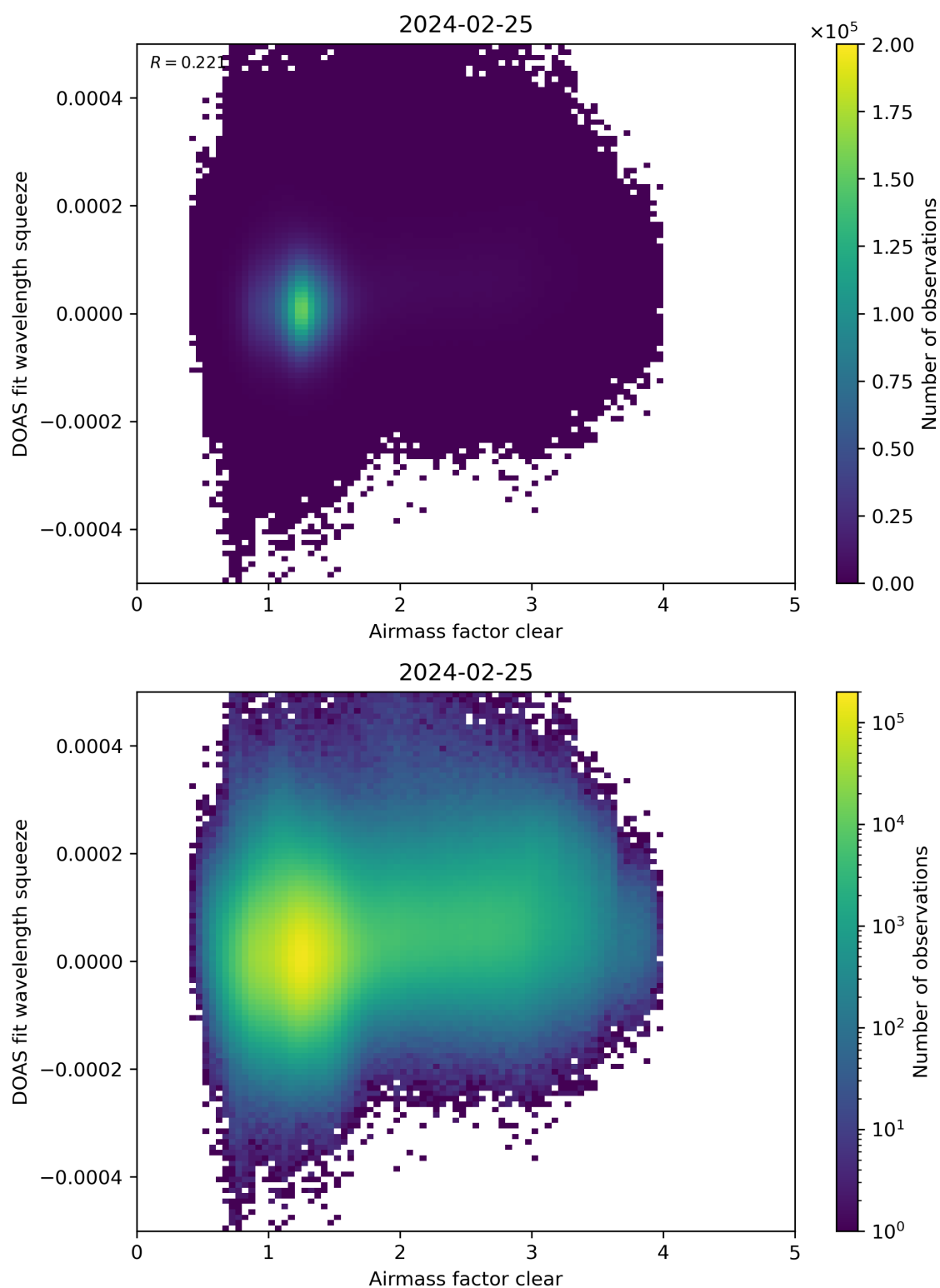
Figure 73: Scatter density plot of “Airmass factor clear” against “DOAS fit wavelength squeeze” for 2024-02-24 to 2024-02-26.
