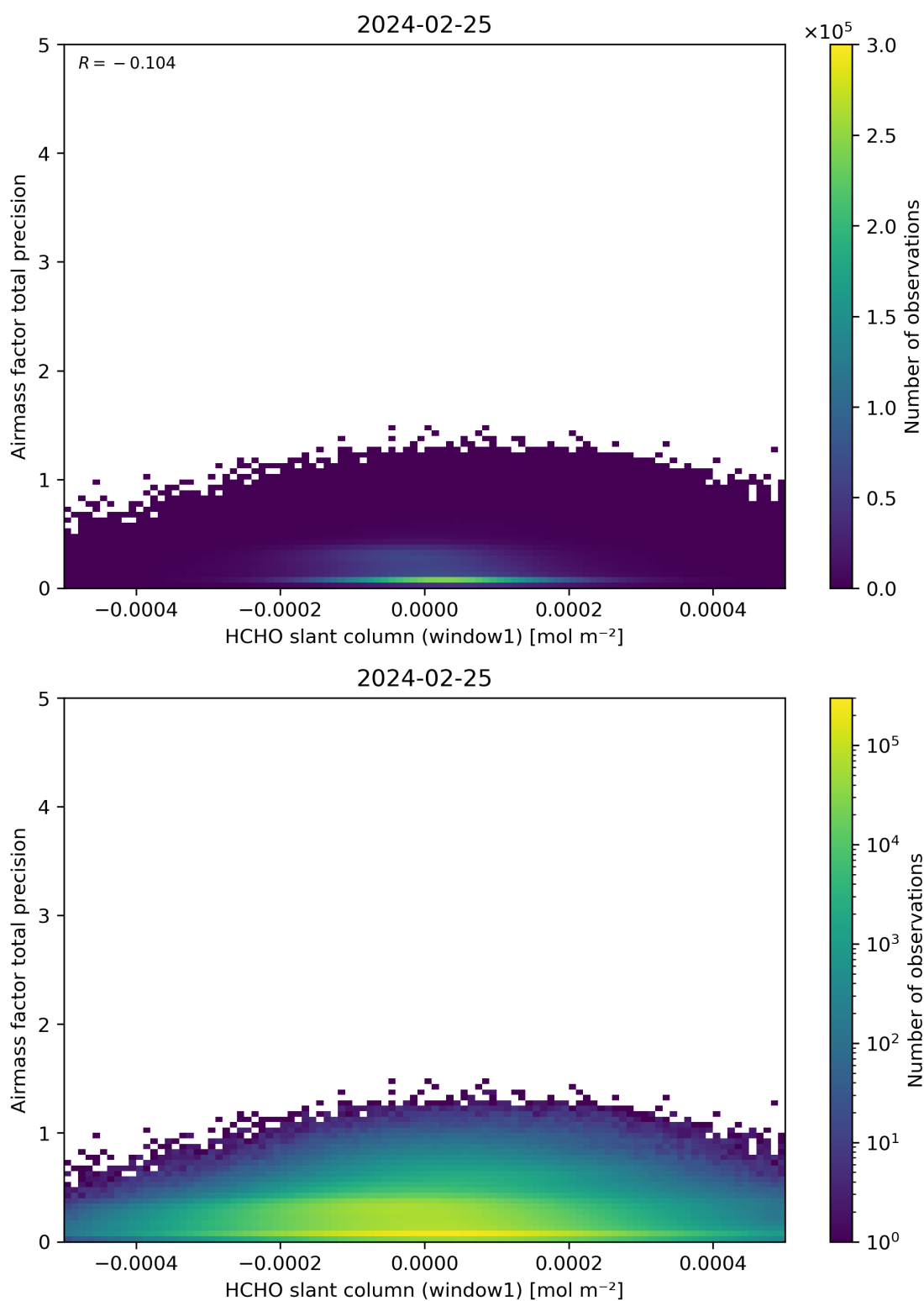
Figure 86: Scatter density plot of “HCHO slant column (window1)” against “Airmass factor total precision” for 2024-02-24 to 2024-02-26.
