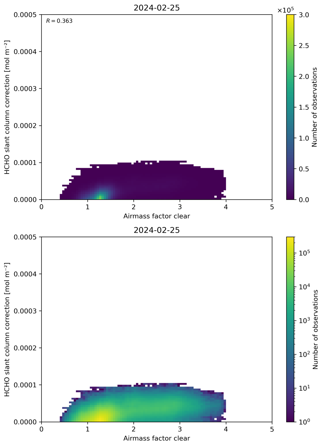
Figure 75: Scatter density plot of “Airmass factor clear” against “HCHO slant column correction” for 2024-02-24 to 2024-02-26.
