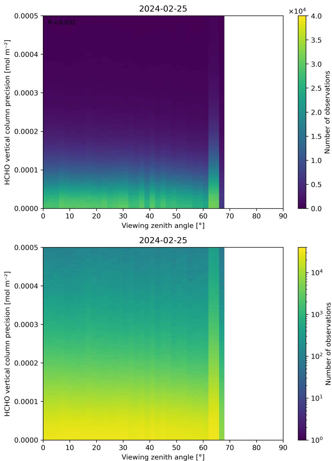
Figure 194: Scatter density plot of “Viewing zenith angle” against “HCHO vertical column precision” for 2024-02-24 to 2024-02-26.
