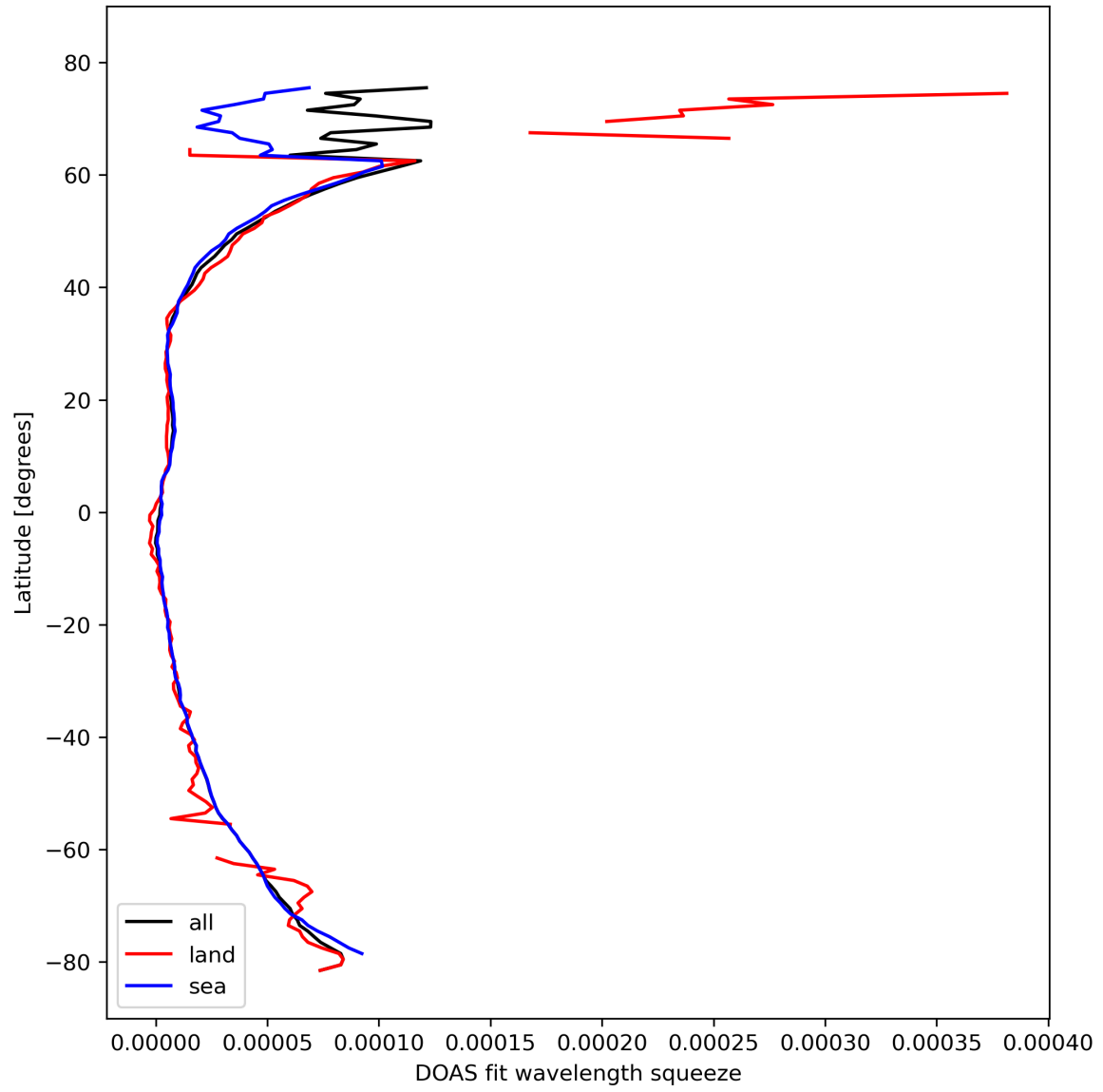
Figure 31: Zonal average of “DOAS fit wavelength squeeze” for 2024-02-24 to 2024-02-26.
