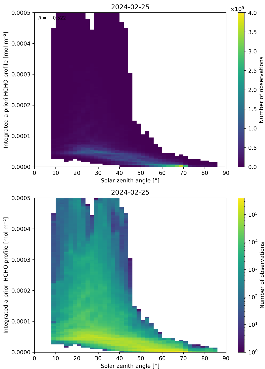
Figure 180: Scatter density plot of “Solar zenith angle” against “Integrated a priori HCHO profile” for 2024-02-24 to 2024-02-26.
