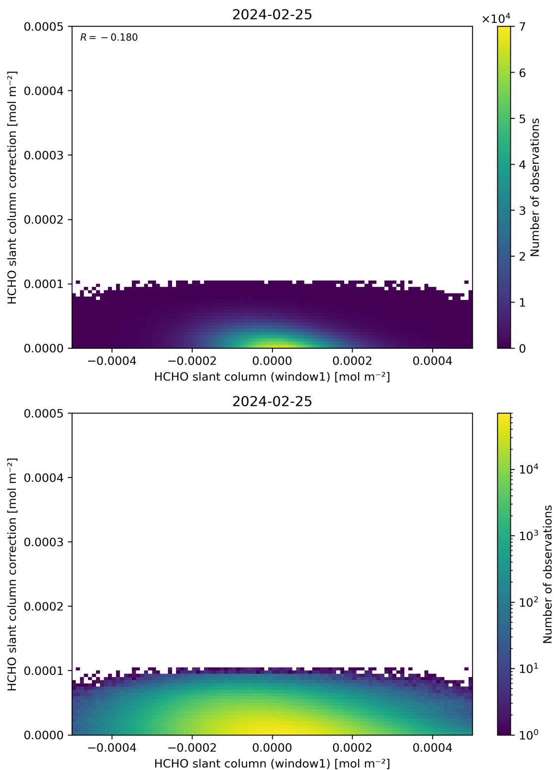
Figure 83: Scatter density plot of “HCHO slant column (window1)” against “HCHO slant column correction” for 2024-02-24 to 2024-02-26.
