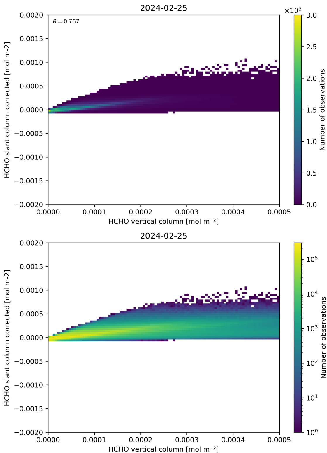
Figure 127: Scatter density plot of “HCHO vertical column” against “HCHO slant column corrected” for 2024-02-24 to 2024-02-26.
