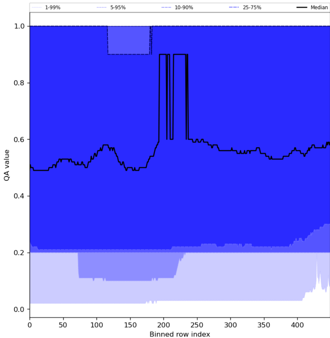
Figure 48: Along track statistics of “QA value” for 2024-02-24 to 2024-02-26
