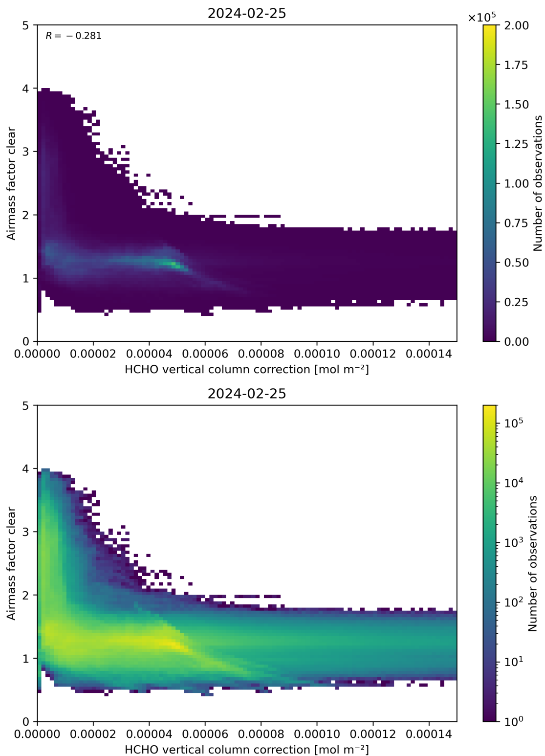
Figure 115: Scatter density plot of “HCHO vertical column correction” against “Airmass factor clear” for 2024-02-24 to 2024-02-26.
