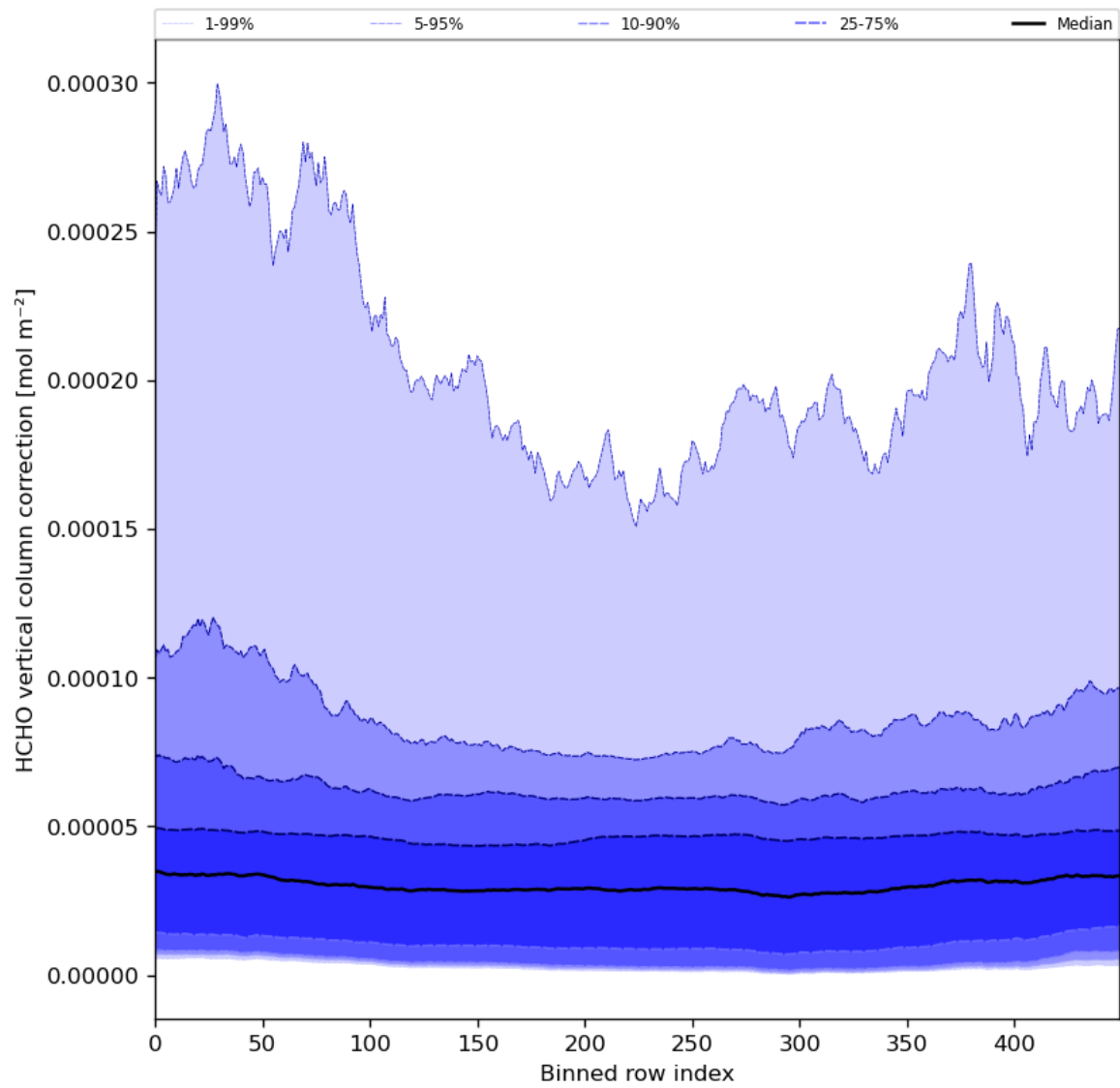
Figure 51: Along track statistics of “HCHO vertical column correction” for 2024-02-24 to 2024-02-26
