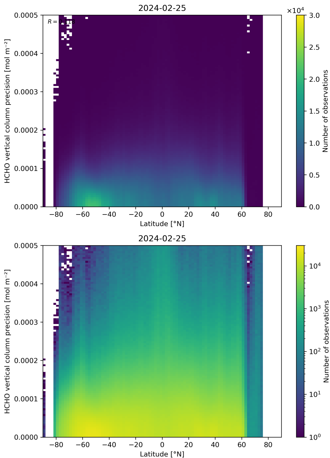
Figure 165: Scatter density plot of “Latitude” against “HCHO vertical column precision” for 2024-02-24 to 2024-02-26.
