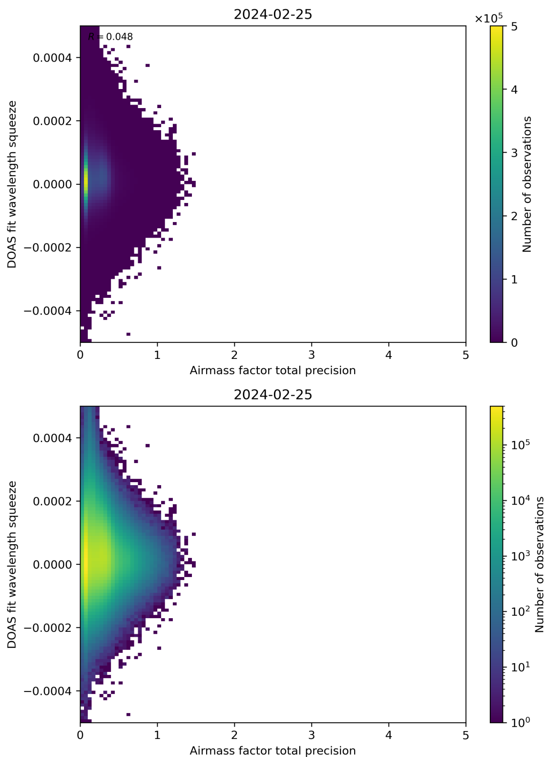
Figure 107: Scatter density plot of “Airmass factor total precision” against “DOAS fit wavelength squeeze” for 2024-02-24 to 2024-02-26.
