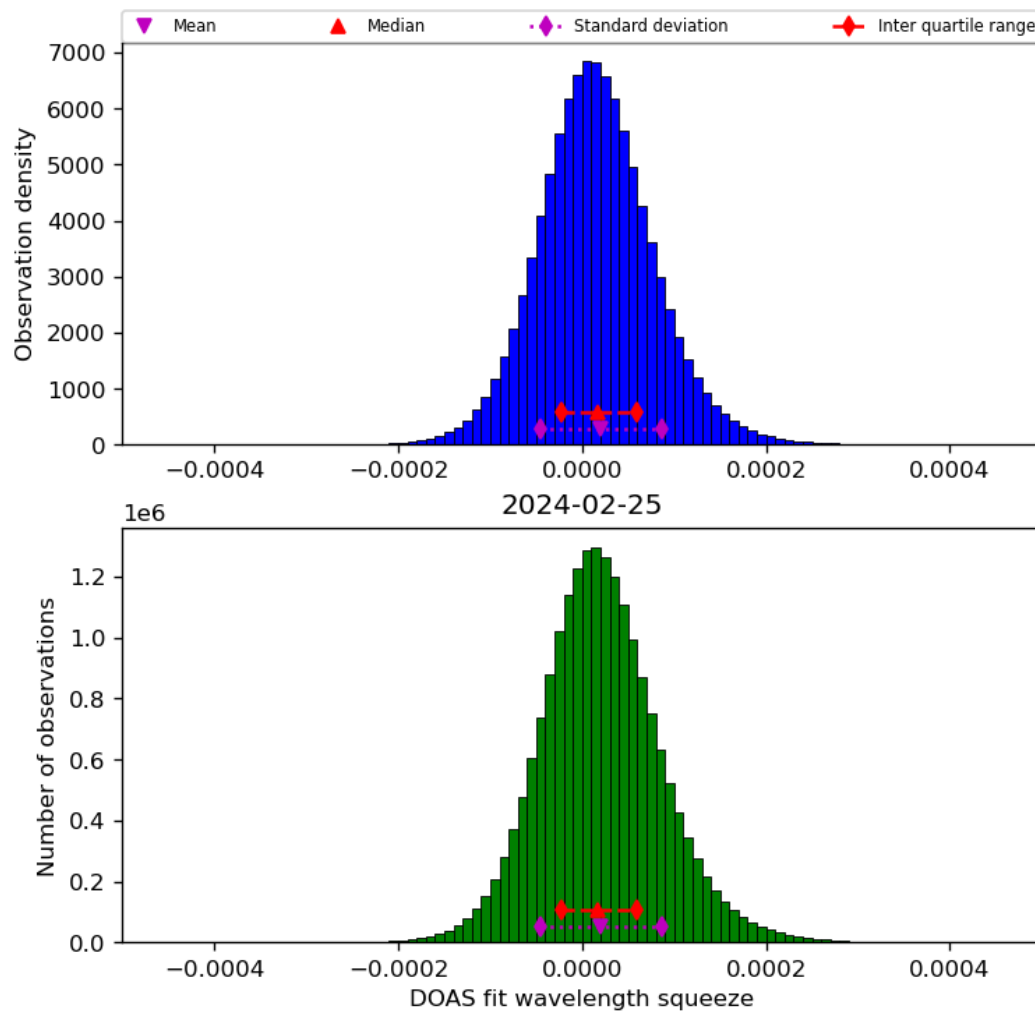
Figure 45: Histogram of “DOAS fit wavelength squeeze” for 2024-02-24 to 2024-02-26
