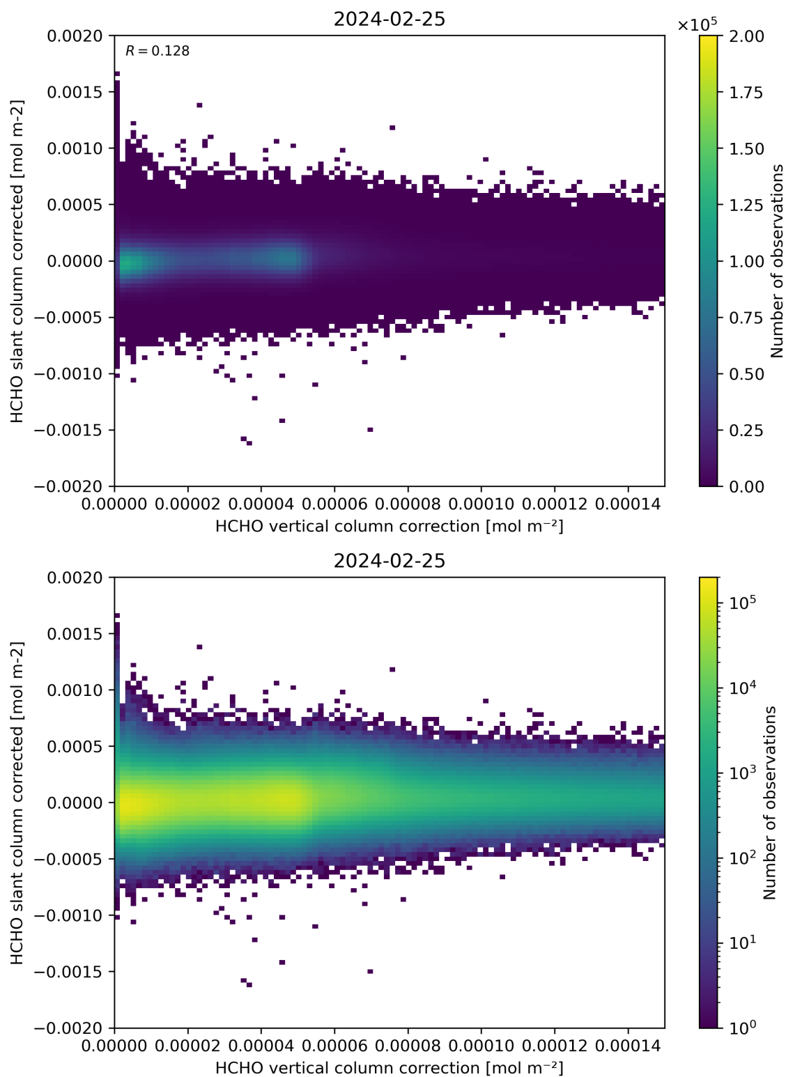
Figure 116: Scatter density plot of “HCHO vertical column correction” against “HCHO slant column corrected” for 2024-02-24 to 2024-02-26.
