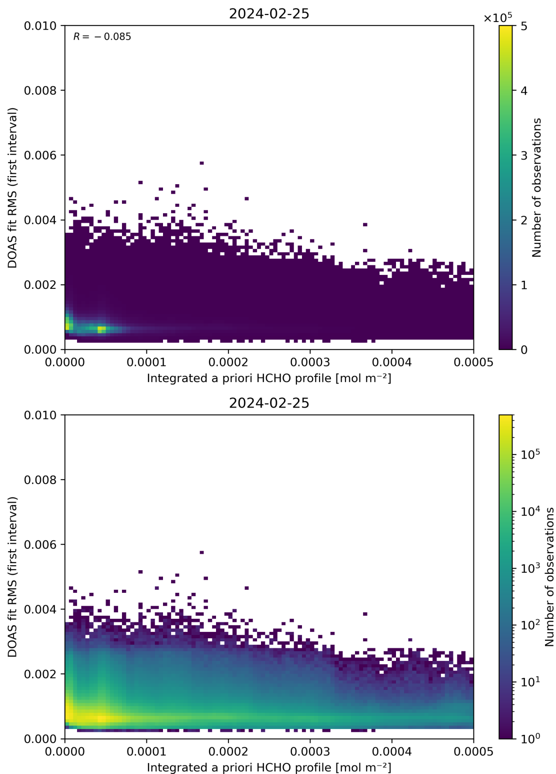
Figure 148: Scatter density plot of “Integrated a priori HCHO profile” against “DOAS fit RMS (first interval)” for 2024-02-24 to 2024-02-26.
