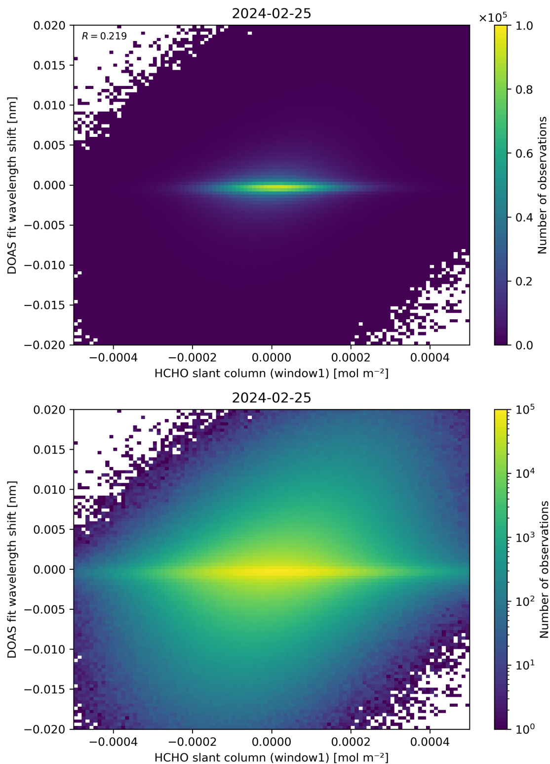
Figure 79: Scatter density plot of “HCHO slant column (window1)” against “DOAS fit wavelength shift” for 2024-02-24 to 2024-02-26.
