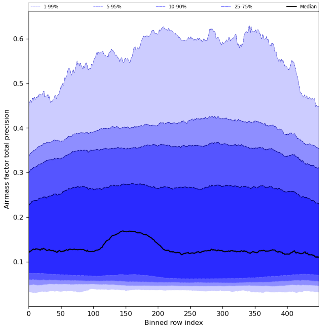
Figure 55: Along track statistics of “Airmass factor total precision” for 2024-02-24 to 2024-02-26
