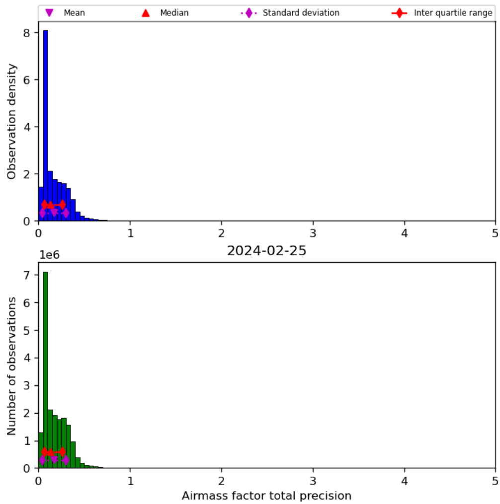
Figure 41: Histogram of “Airmass factor total precision” for 2024-02-24 to 2024-02-26
