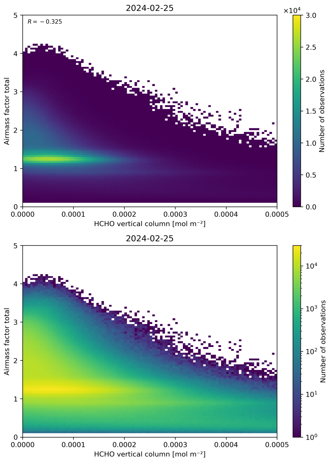
Figure 131: Scatter density plot of “HCHO vertical column” against “Airmass factor total” for 2024-02-24 to 2024-02-26.
