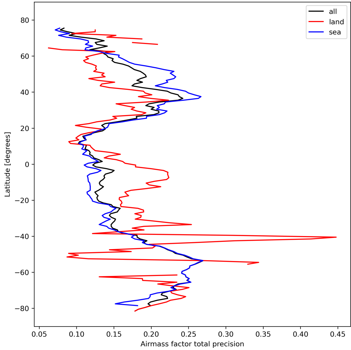
Figure 27: Zonal average of “Airmass factor total precision” for 2024-02-24 to 2024-02-26.
