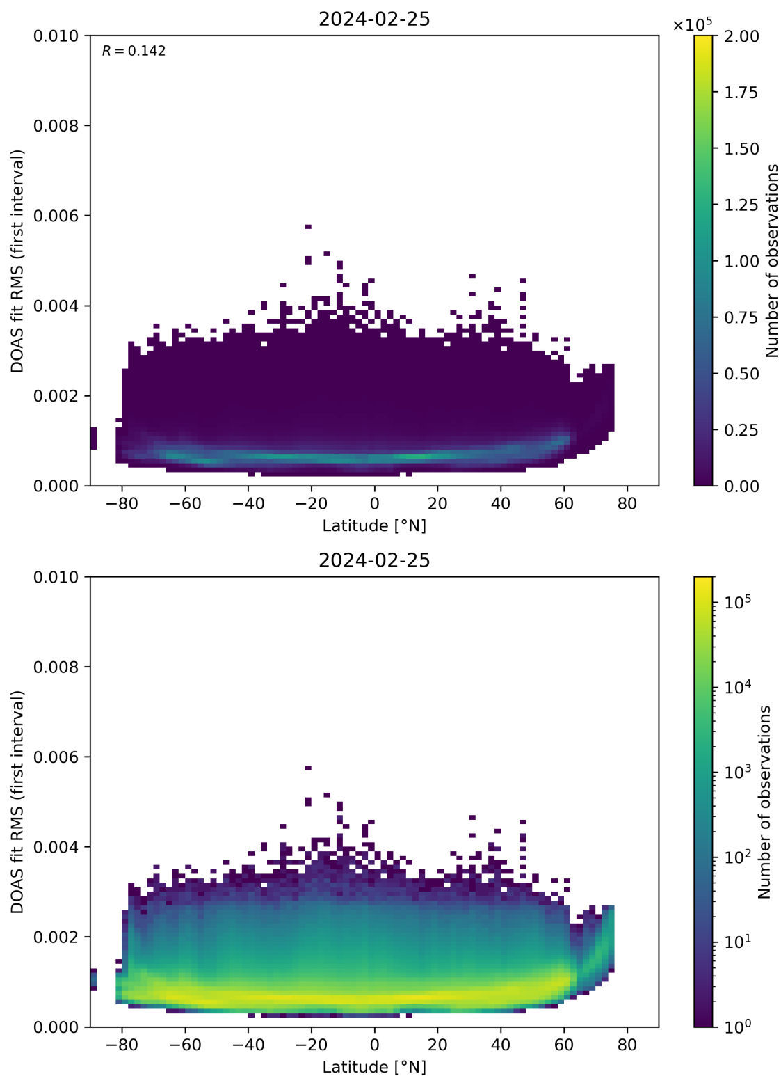
Figure 153: Scatter density plot of “Latitude” against “DOAS fit RMS (first interval)” for 2024-02-24 to 2024-02-26.
