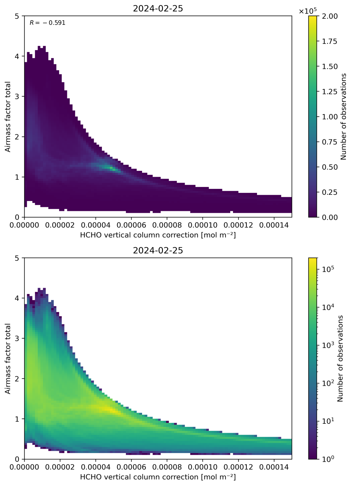
Figure 120: Scatter density plot of “HCHO vertical column correction” against “Airmass factor total” for 2024-02-24 to 2024-02-26.
