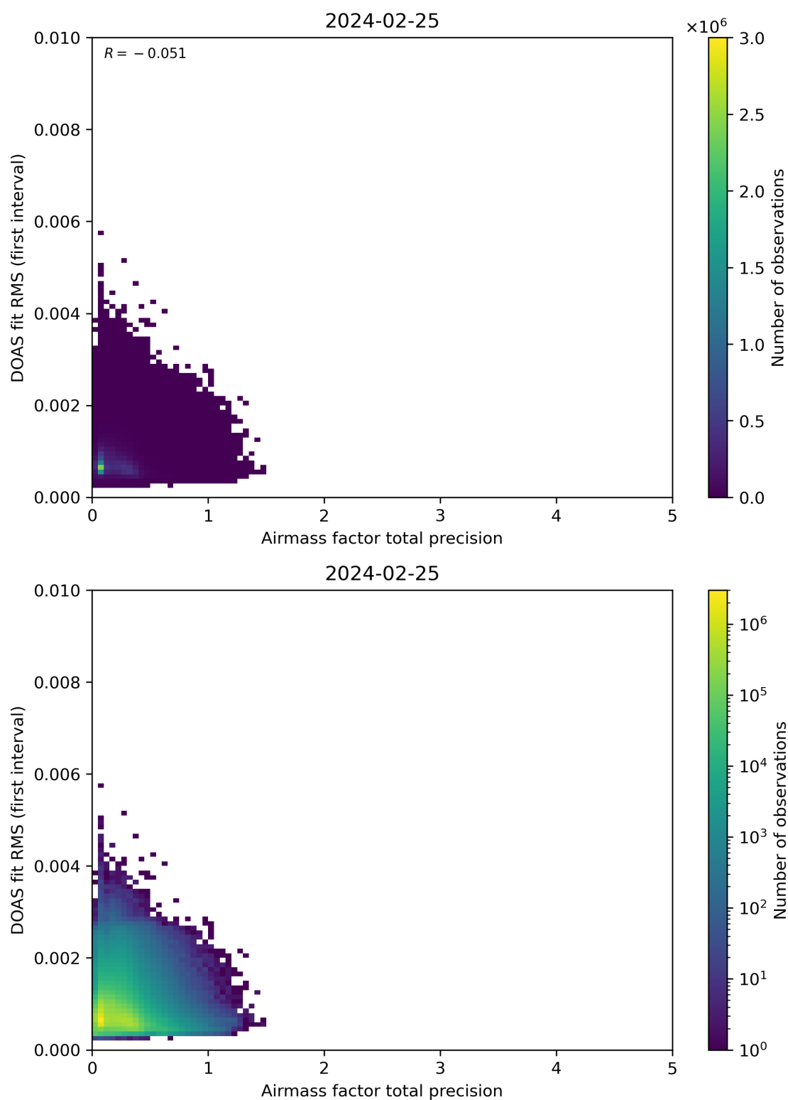
Figure 105: Scatter density plot of “Airmass factor total precision” against “DOAS fit RMS (first interval)” for 2024-02-24 to 2024-02-26.
