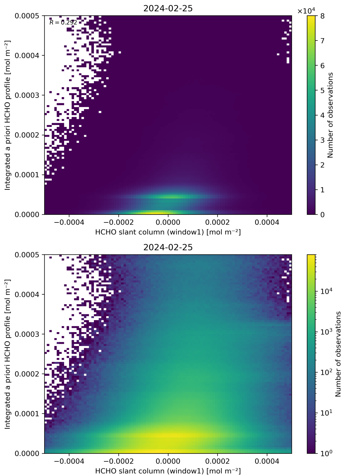
Figure 87: Scatter density plot of “HCHO slant column (window1)” against “Integrated a priori HCHO profile” for 2024-02-24 to 2024-02-26.
