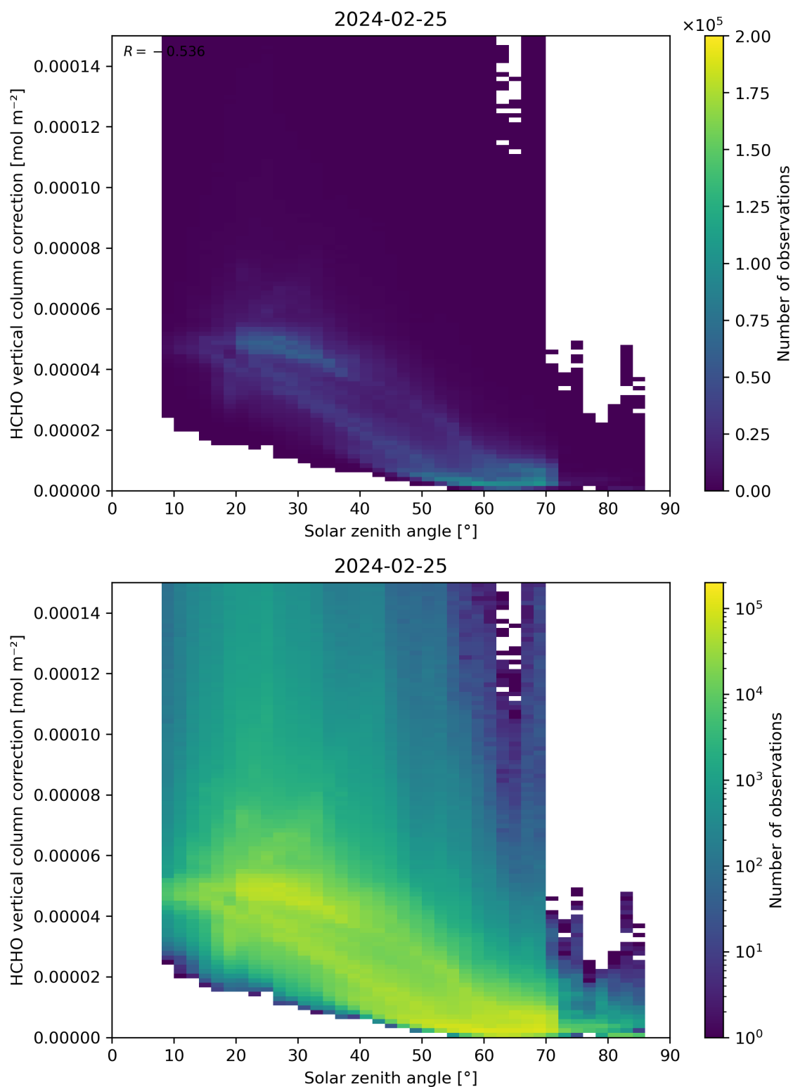
Figure 178: Scatter density plot of “Solar zenith angle” against “HCHO vertical column correction” for 2024-02-24 to 2024-02-26.
