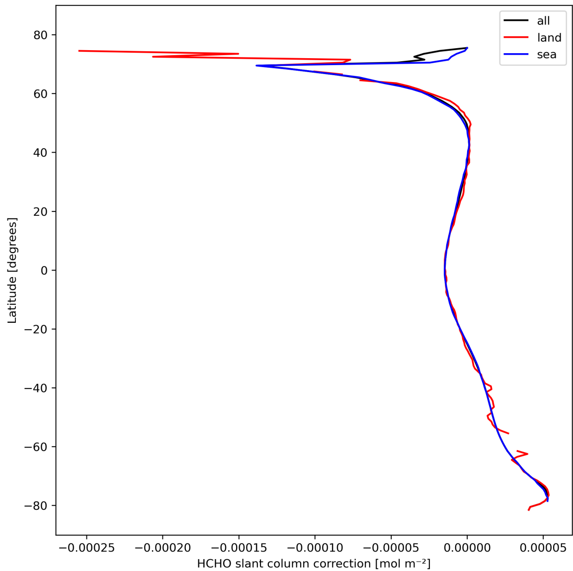
Figure 33: Zonal average of “HCHO slant column correction” for 2024-02-24 to 2024-02-26.
