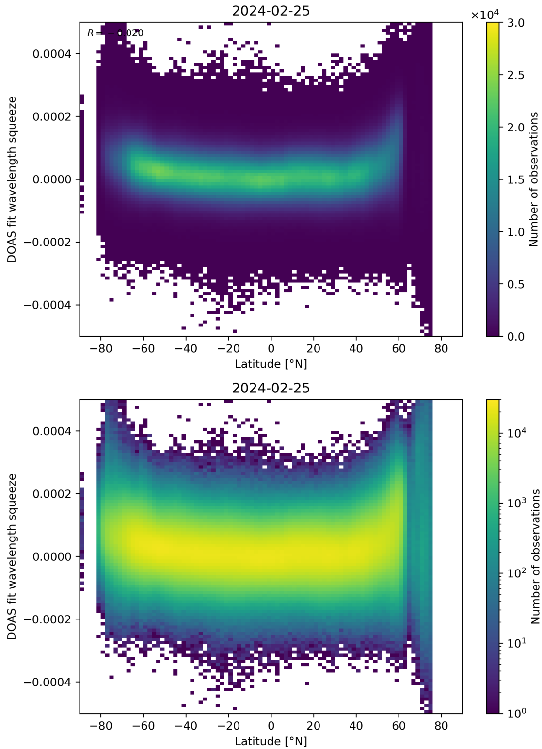
Figure 155: Scatter density plot of “Latitude” against “DOAS fit wavelength squeeze” for 2024-02-24 to 2024-02-26.
