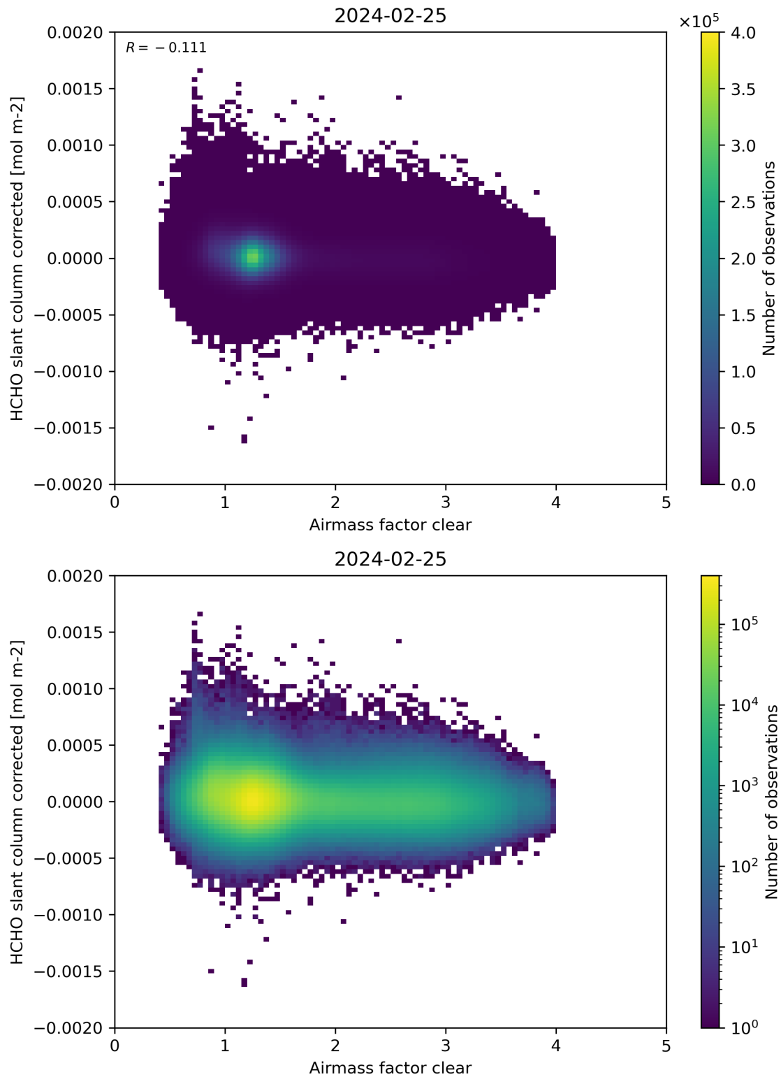
Figure 74: Scatter density plot of “Airmass factor clear” against “HCHO slant column corrected” for 2024-02-24 to 2024-02-26.
