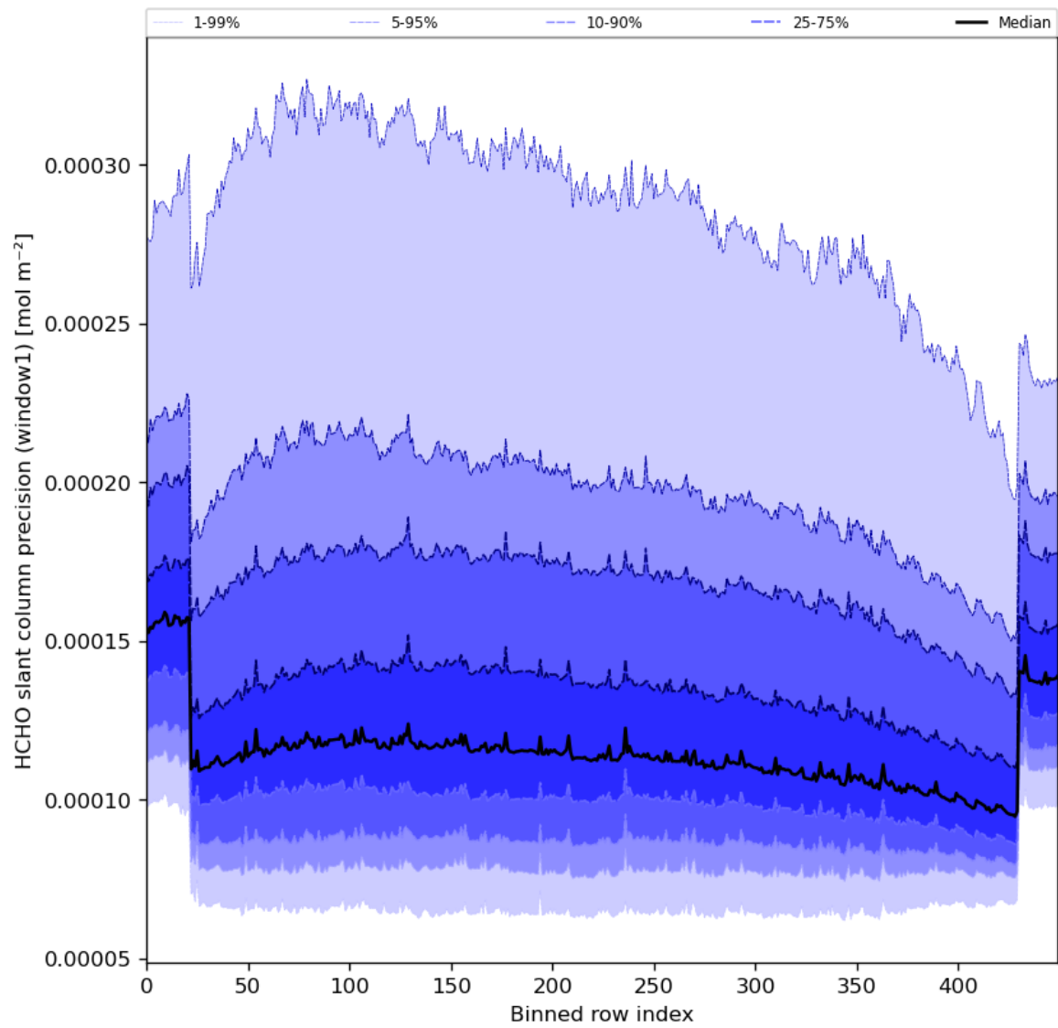
Figure 53: Along track statistics of “HCHO slant column precision (window1)” for 2024-02-24 to 2024-02-26
