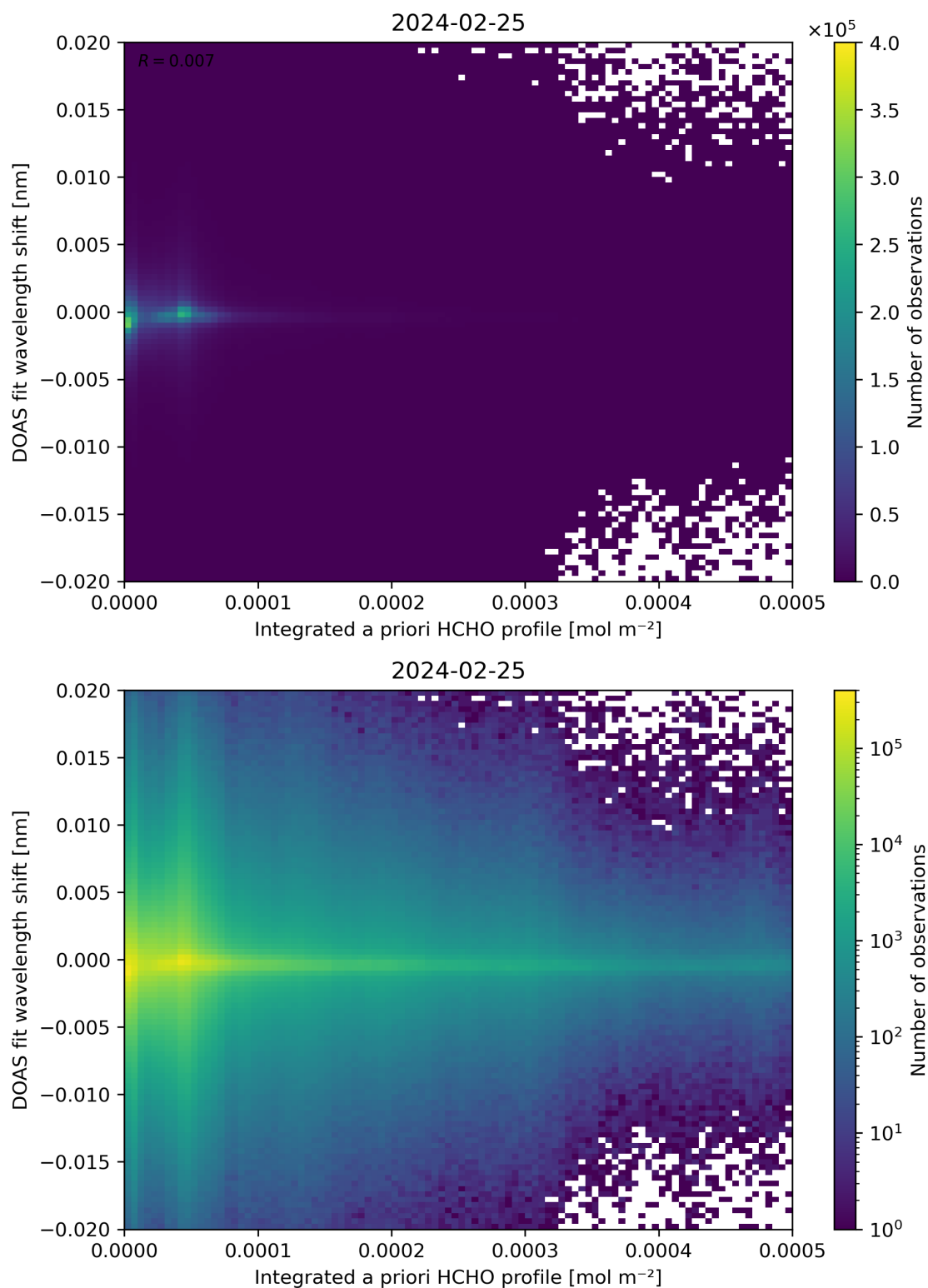
Figure 149: Scatter density plot of “Integrated a priori HCHO profile” against “DOAS fit wavelength shift” for 2024-02-24 to 2024-02-26.
