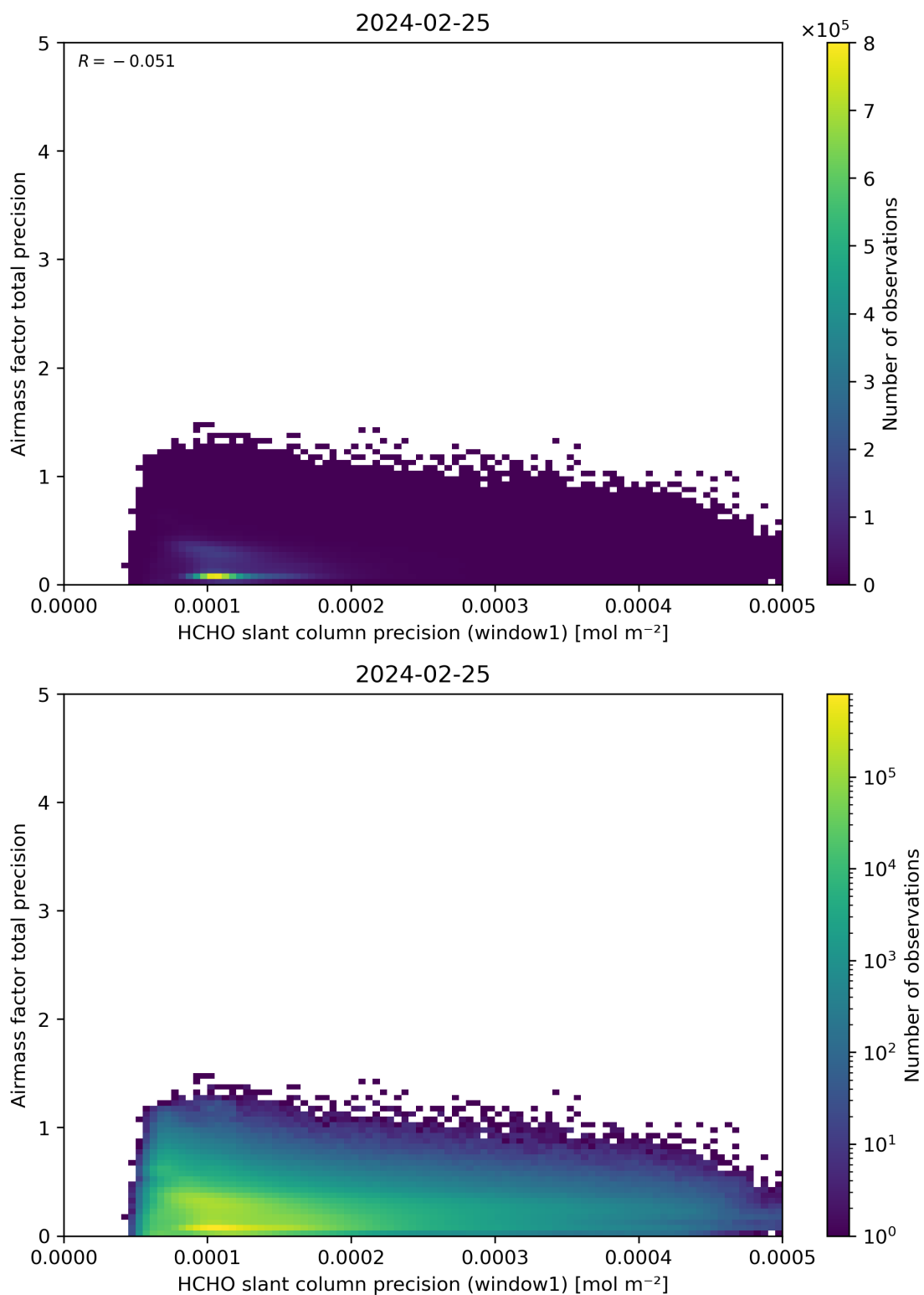
Figure 95: Scatter density plot of “HCHO slant column precision (window1)” against “Airmass factor total precision” for 2024-02-24 to 2024-02-26.
