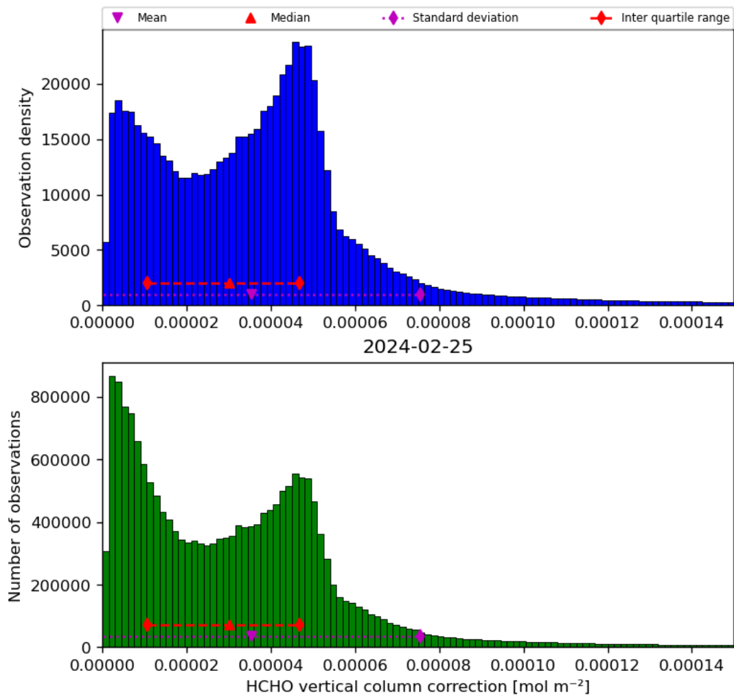
Figure 37: Histogram of “HCHO vertical column correction” for 2024-02-24 to 2024-02-26
