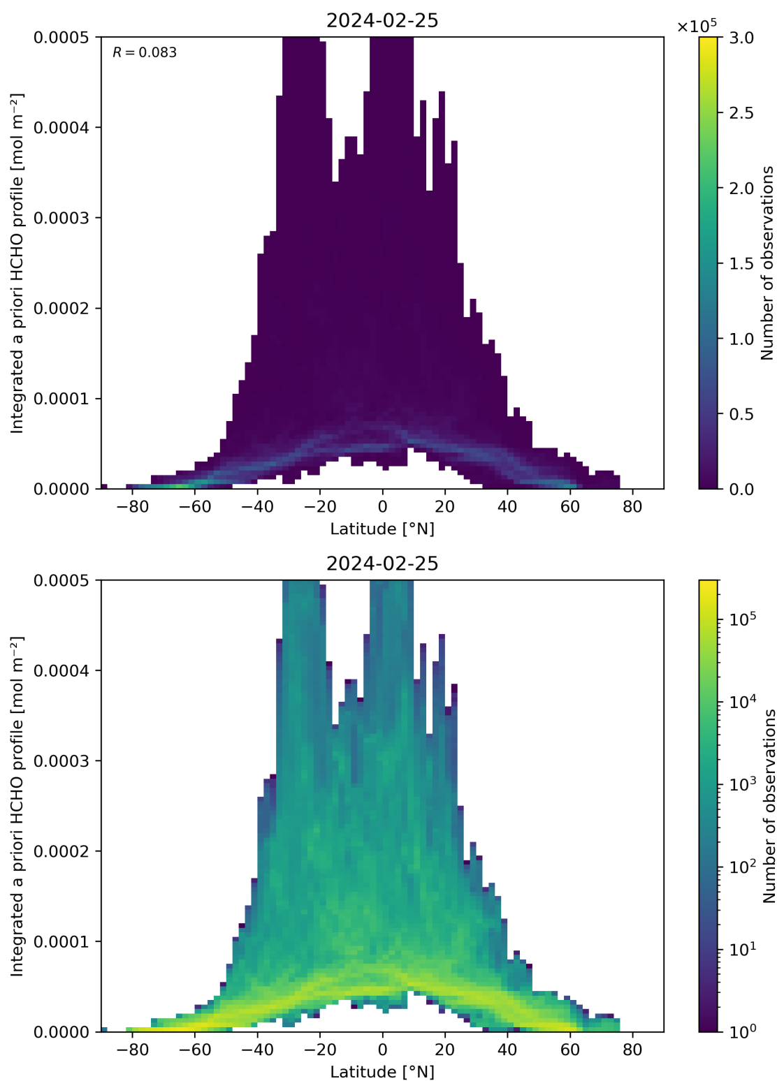
Figure 166: Scatter density plot of “Latitude” against “Integrated a priori HCHO profile” for 2024-02-24 to 2024-02-26.
