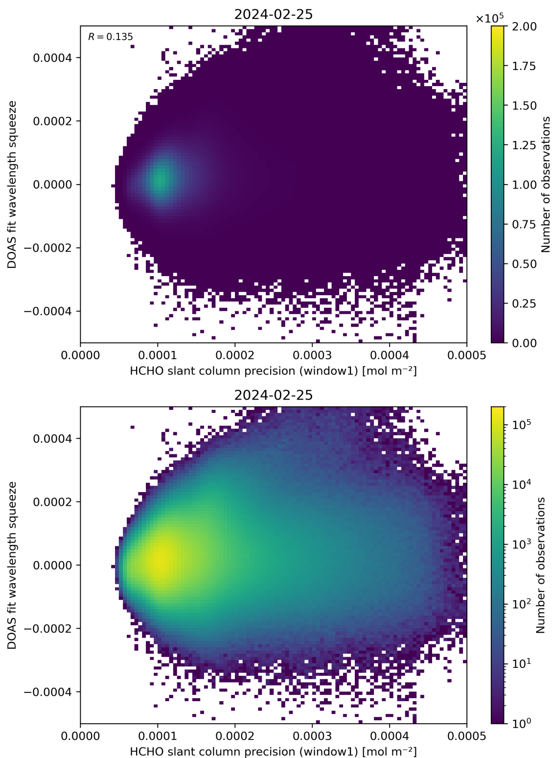
Figure 90: Scatter density plot of “HCHO slant column precision (window1)” against “DOAS fit wavelength squeeze” for 2024-02-24 to 2024-02-26.
