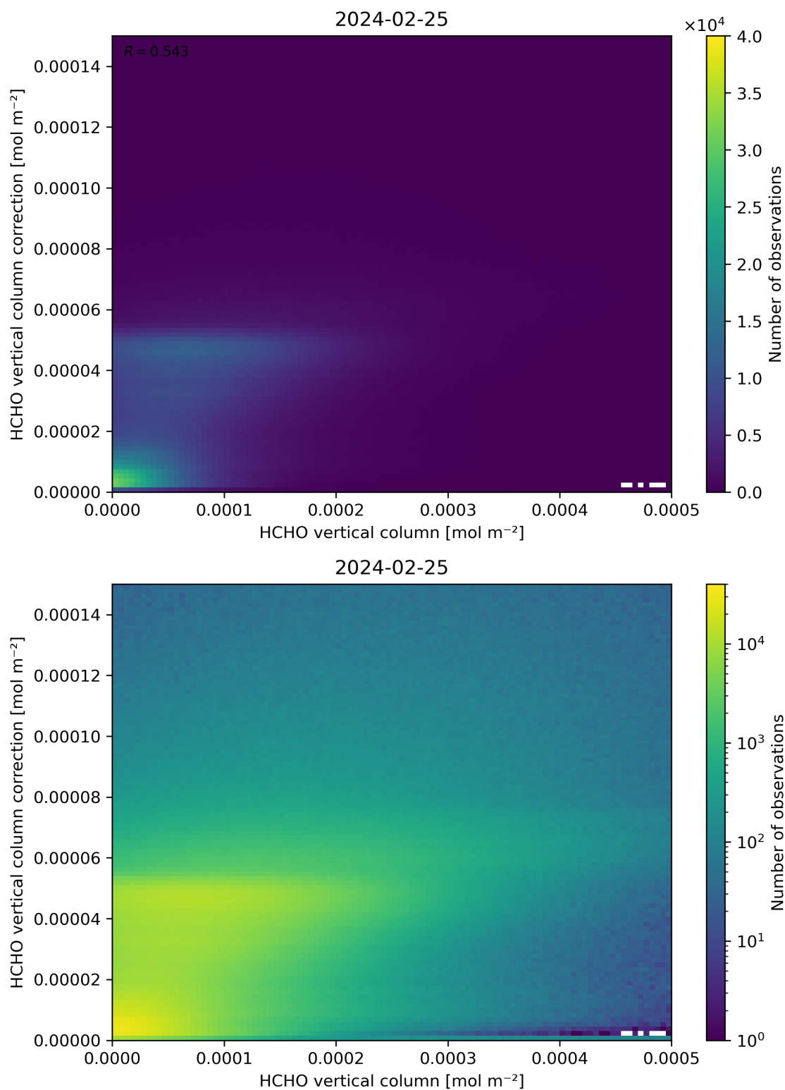
Figure 133: Scatter density plot of “HCHO vertical column” against “HCHO vertical column correction” for 2024-02-24 to 2024-02-26.
