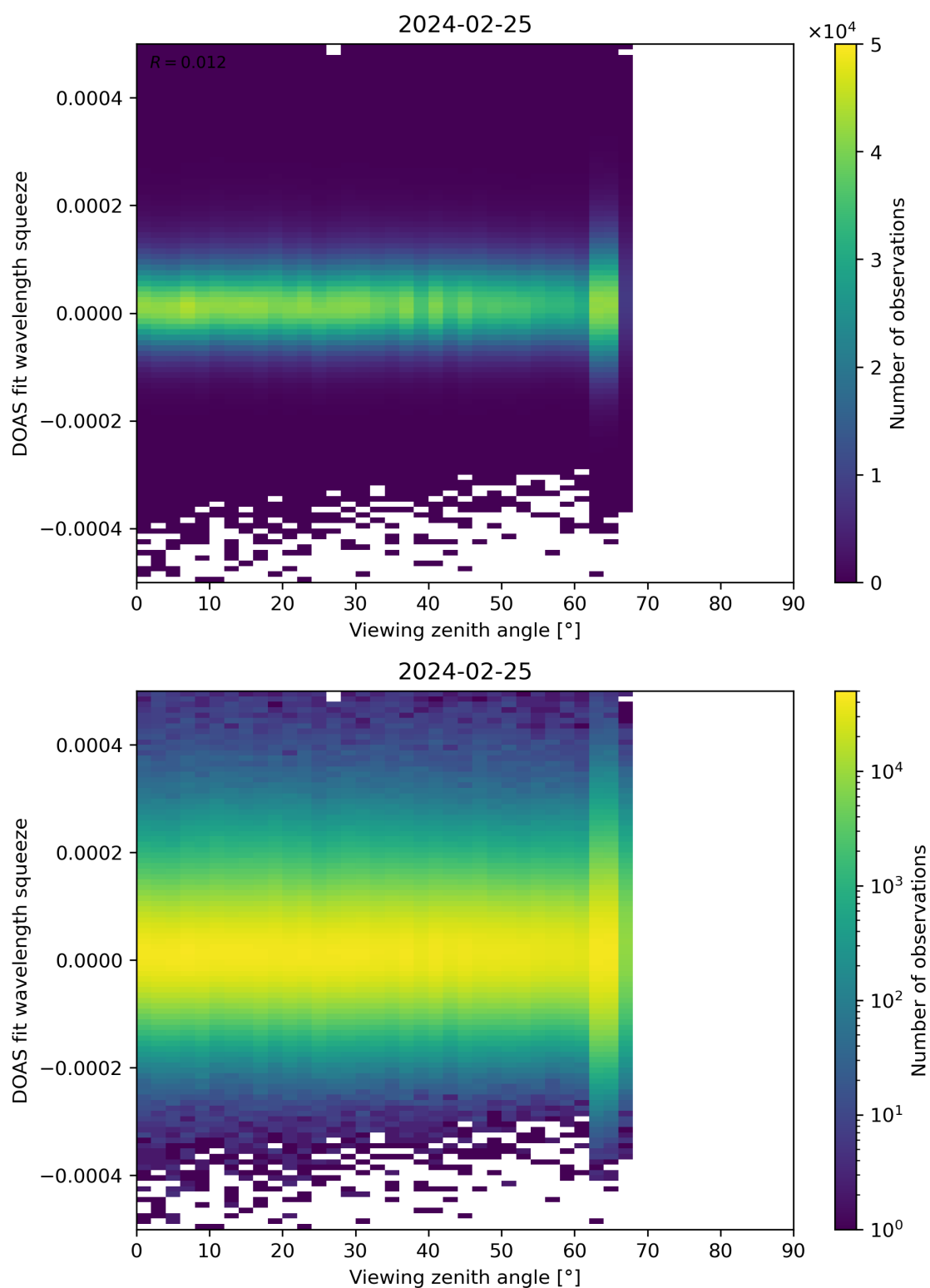
Figure 184: Scatter density plot of “Viewing zenith angle” against “DOAS fit wavelength squeeze” for 2024-02-24 to 2024-02-26.
