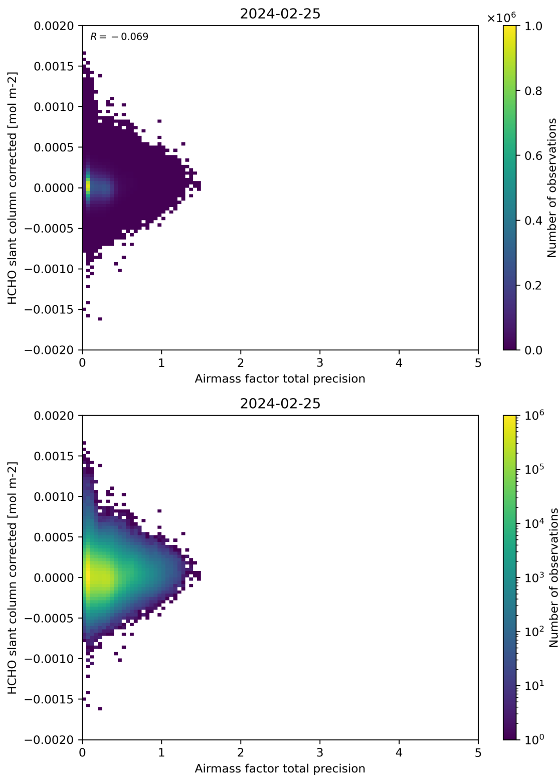
Figure 109: Scatter density plot of “Airmass factor total precision” against “HCHO slant column corrected” for 2024-02-24 to 2024-02-26.
