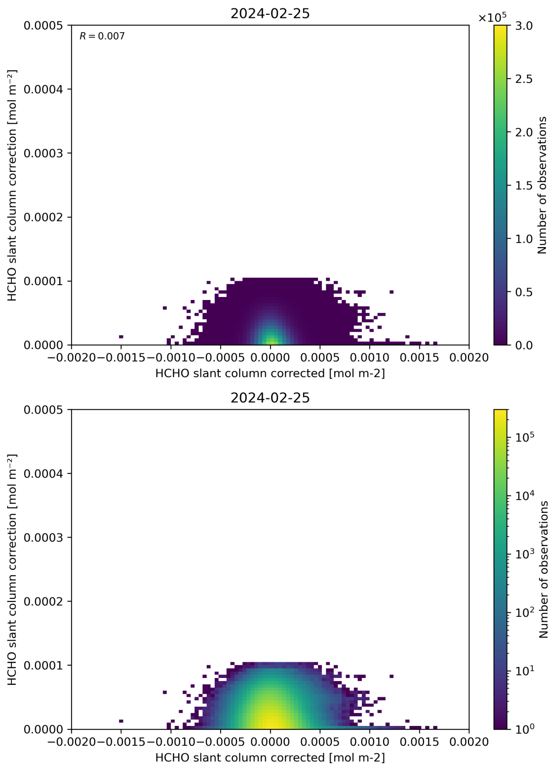
Figure 77: Scatter density plot of “HCHO slant column corrected” against “HCHO slant column correction” for 2024-02-24 to 2024-02-26.
