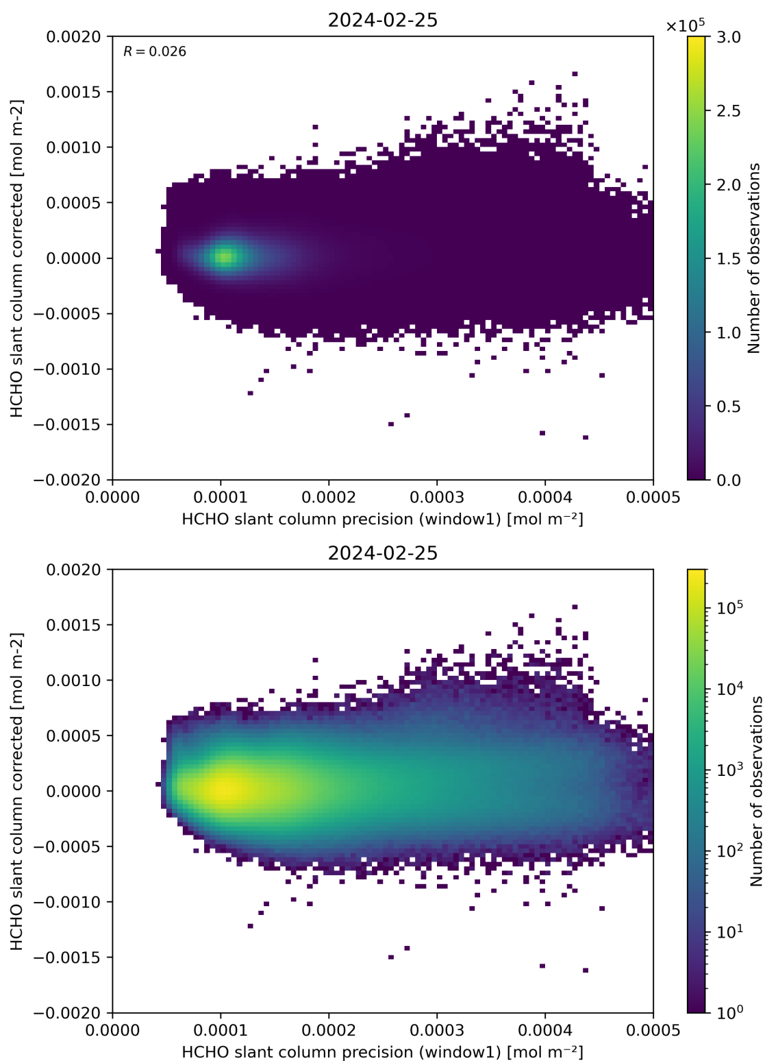
Figure 92: Scatter density plot of “HCHO slant column precision (window1)” against “HCHO slant column corrected” for 2024-02-24 to 2024-02-26.
