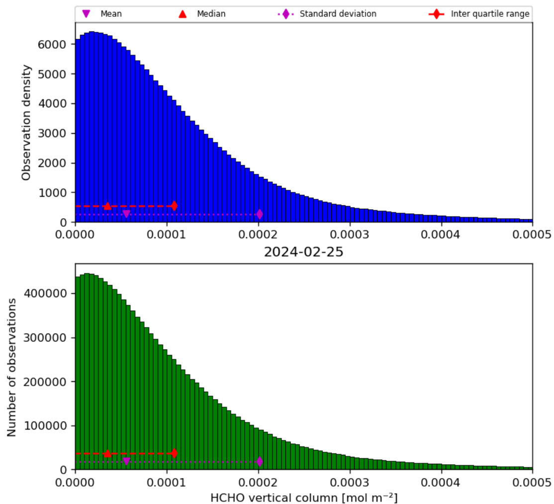
Figure 35: Histogram of “HCHO vertical column” for 2024-02-24 to 2024-02-26
