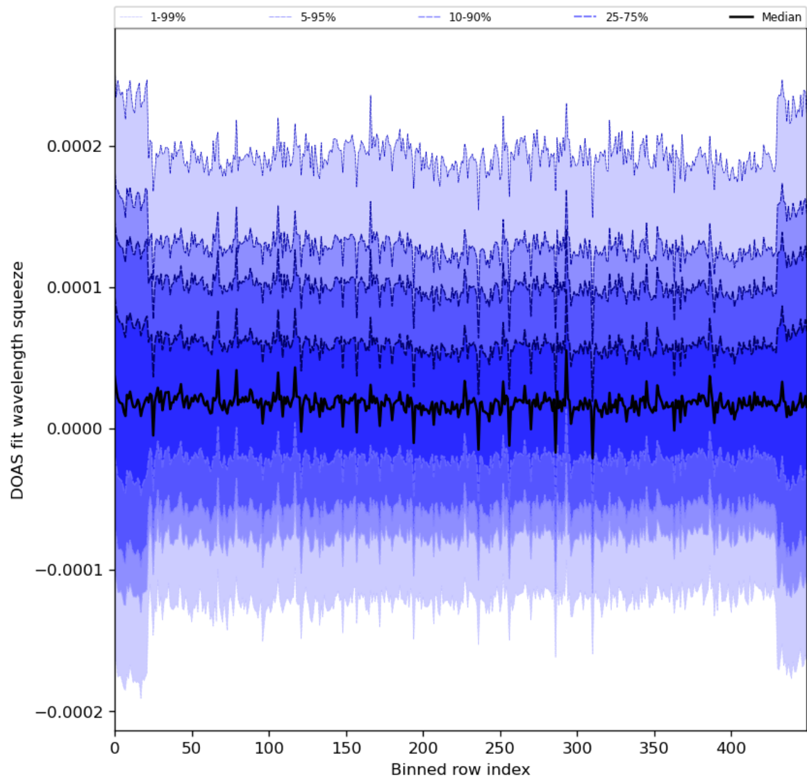
Figure 59: Along track statistics of “DOAS fit wavelength squeeze” for 2024-02-24 to 2024-02-26
