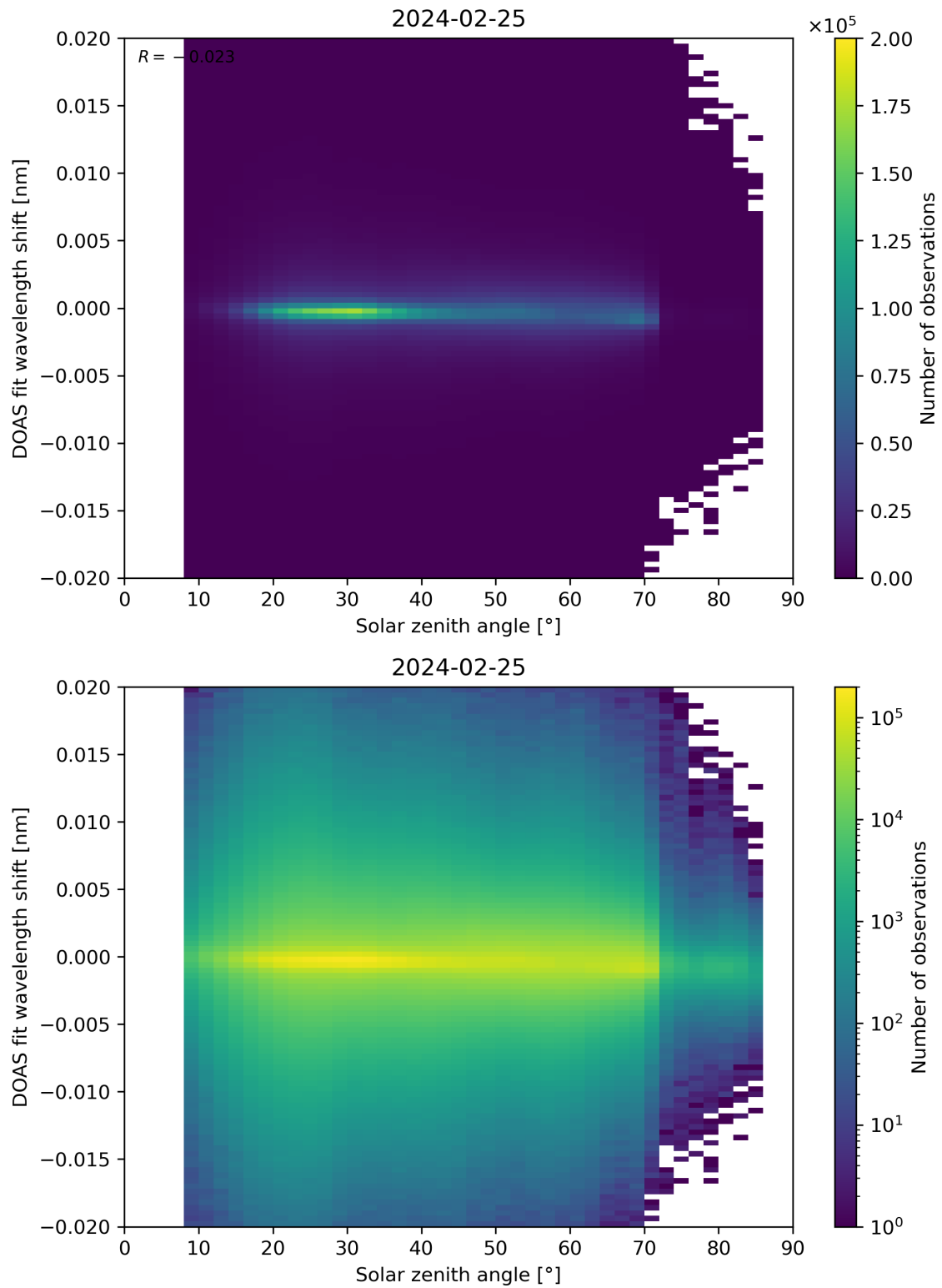
Figure 168: Scatter density plot of “Solar zenith angle” against “DOAS fit wavelength shift” for 2024-02-24 to 2024-02-26.
