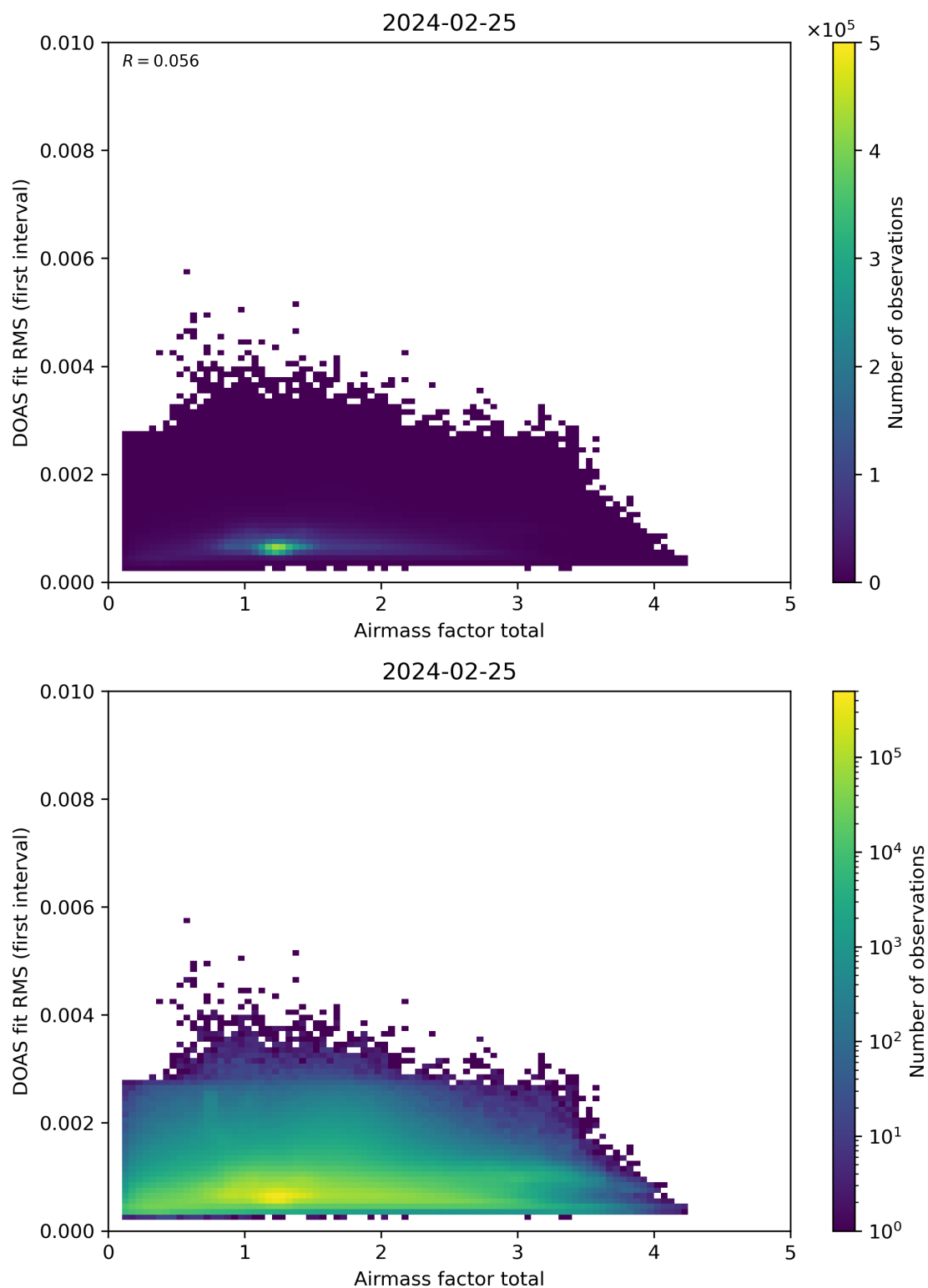
Figure 97: Scatter density plot of “Airmass factor total” against “DOAS fit RMS (first interval)” for 2024-02-24 to 2024-02-26.
