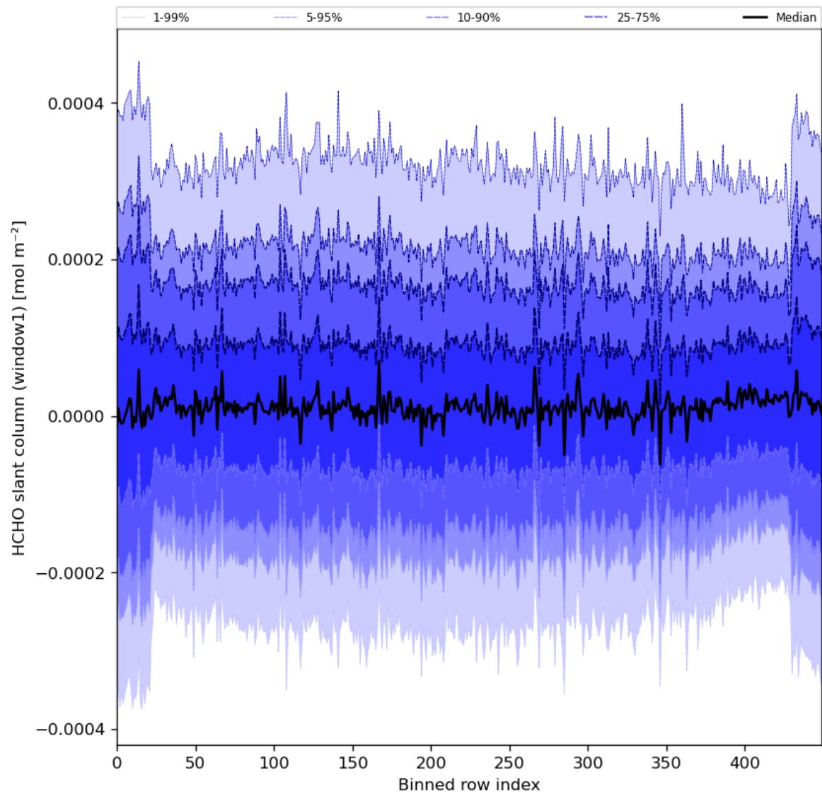
Figure 52: Along track statistics of “HCHO slant column (window1)” for 2024-02-24 to 2024-02-26
