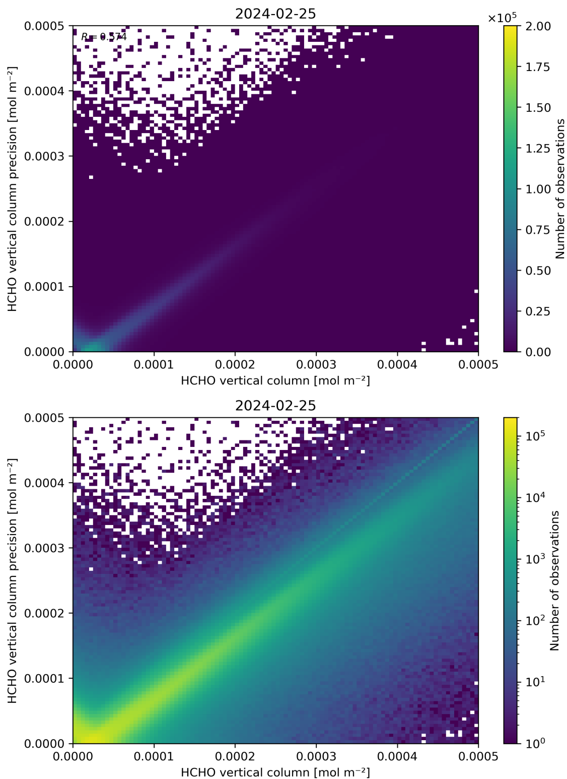
Figure 134: Scatter density plot of “HCHO vertical column” against “HCHO vertical column precision” for 2024-02-24 to 2024-02-26.
