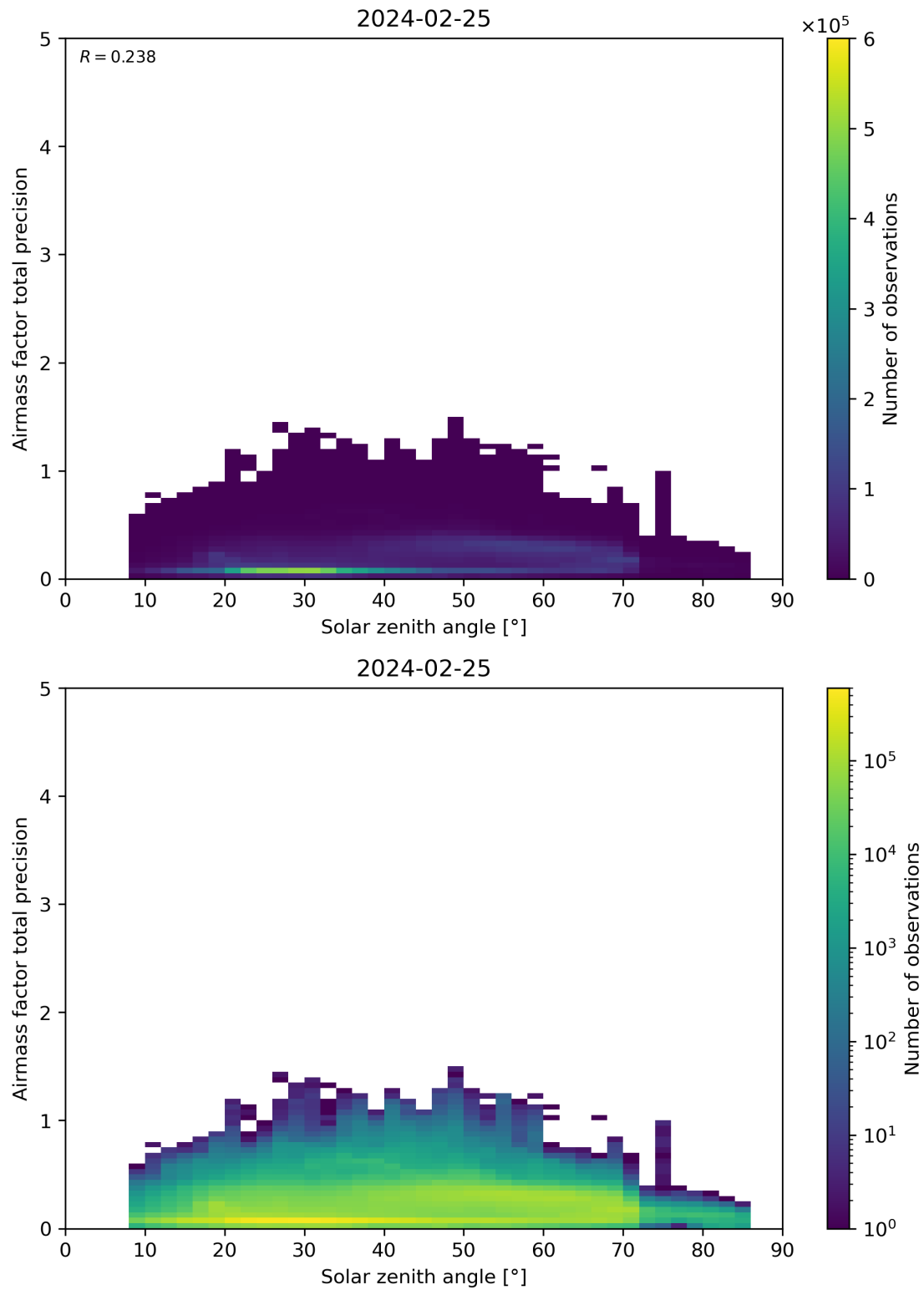
Figure 176: Scatter density plot of “Solar zenith angle” against “Airmass factor total precision” for 2024-02-24 to 2024-02-26.
