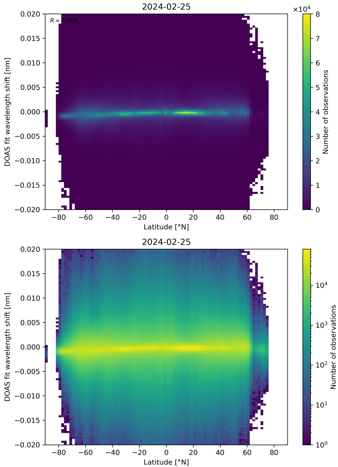
Figure 154: Scatter density plot of “Latitude” against “DOAS fit wavelength shift” for 2024-02-24 to 2024-02-26.
