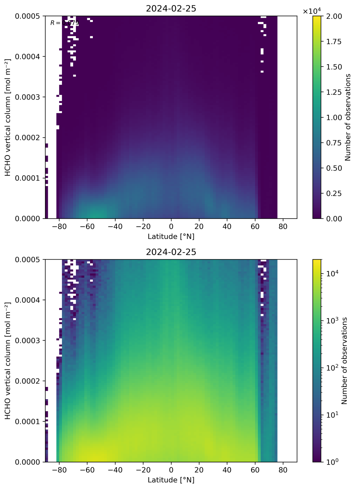
Figure 163: Scatter density plot of “Latitude” against “HCHO vertical column” for 2024-02-24 to 2024-02-26.
