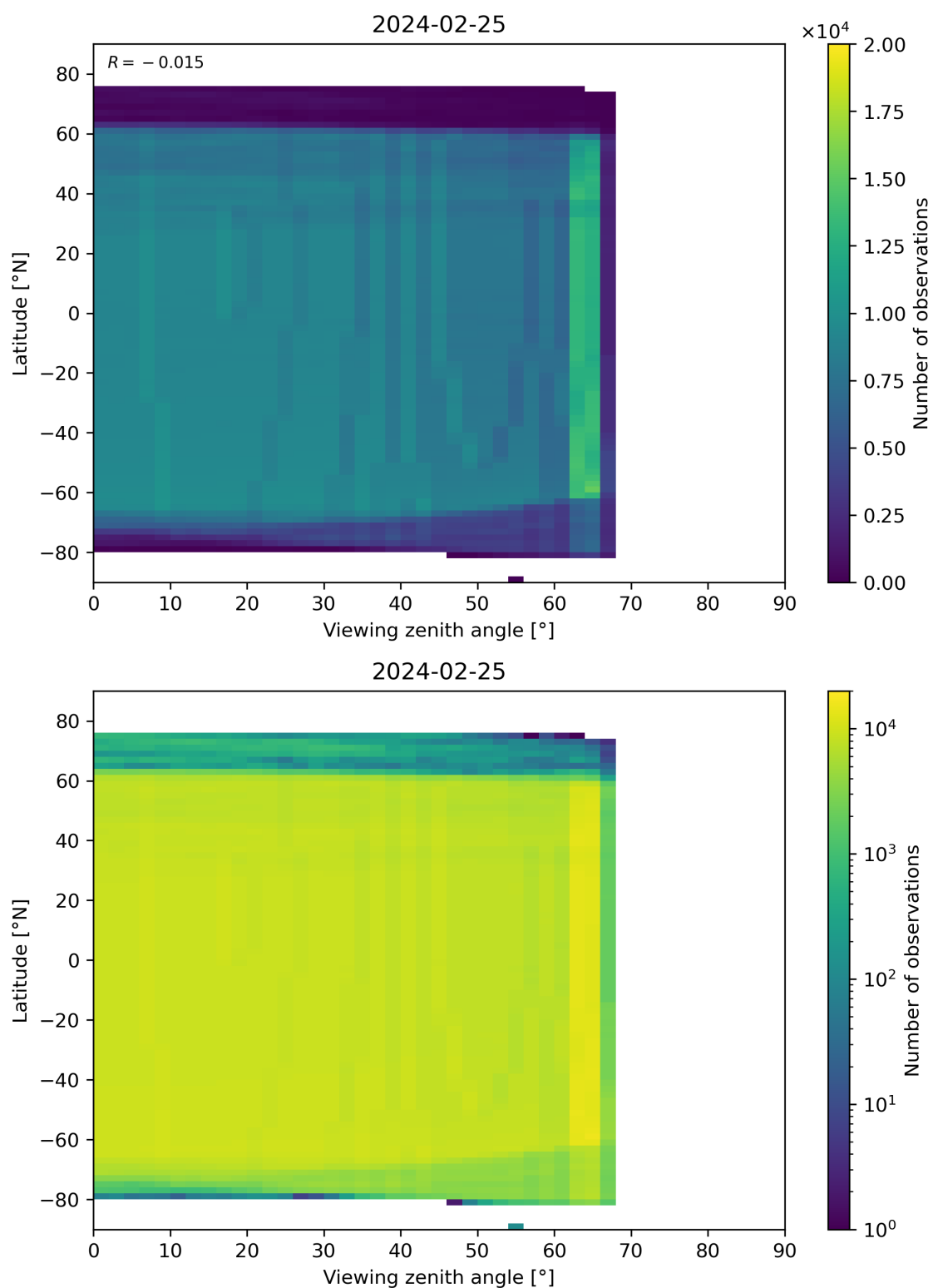
Figure 196: Scatter density plot of “Viewing zenith angle” against “Latitude” for 2024-02-24 to 2024-02-26.
