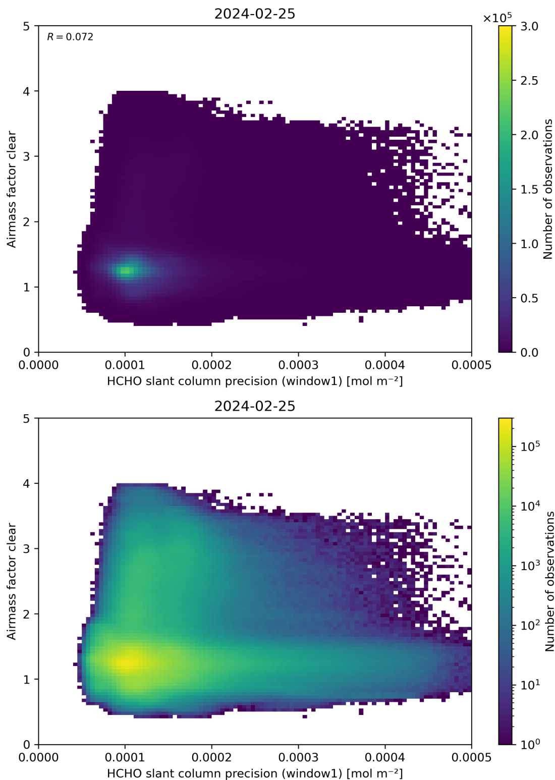
Figure 91: Scatter density plot of “HCHO slant column precision (window1)” against “Airmass factor clear” for 2024-02-24 to 2024-02-26.
