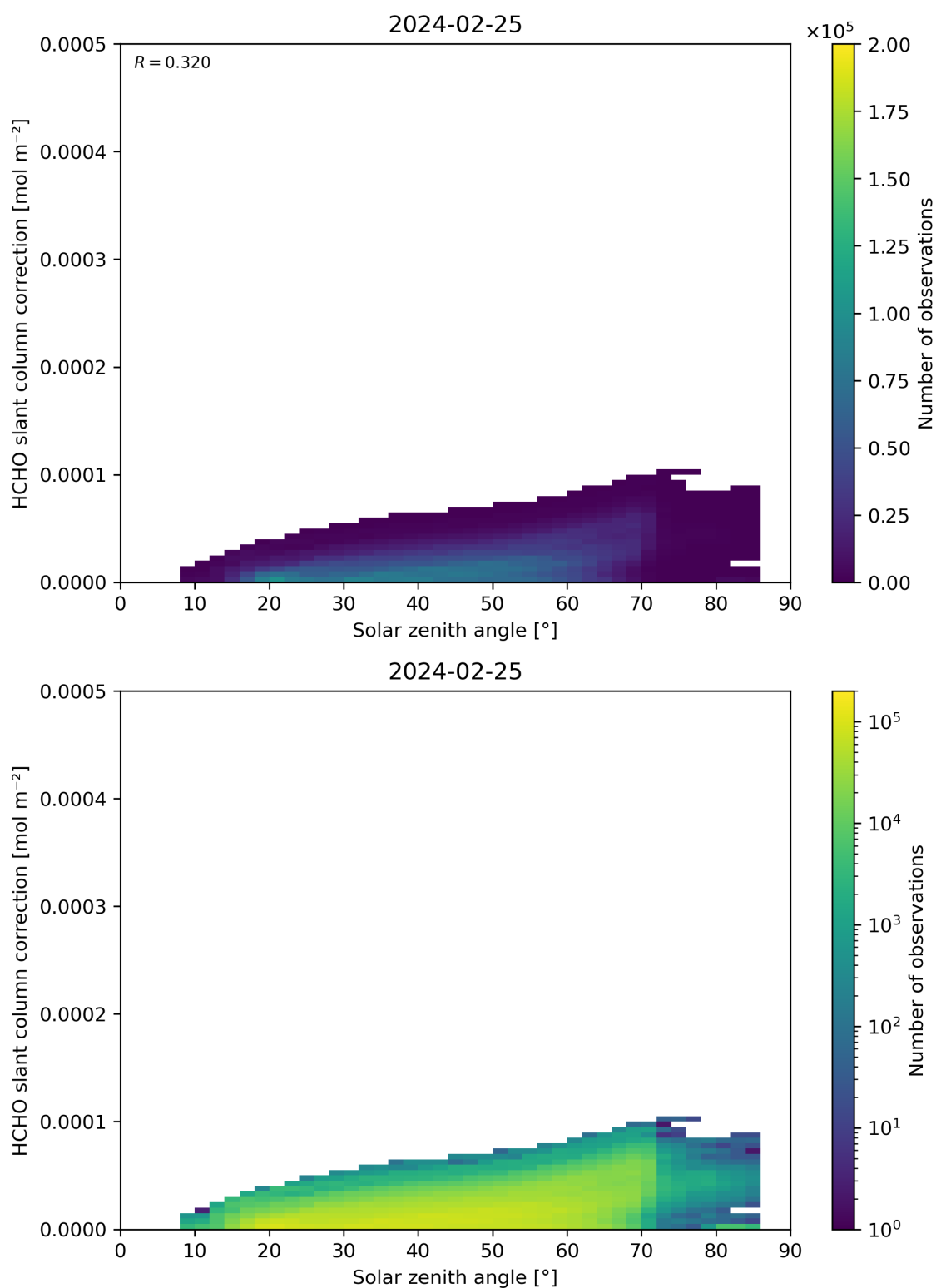
Figure 172: Scatter density plot of “Solar zenith angle” against “HCHO slant column correction” for 2024-02-24 to 2024-02-26.
