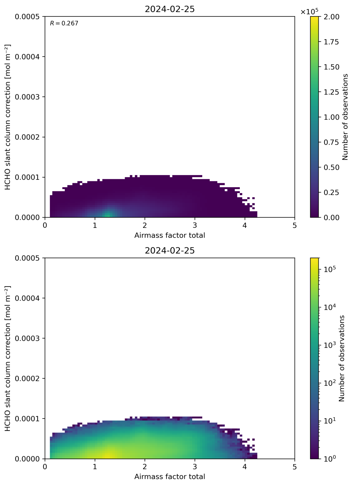
Figure 102: Scatter density plot of “Airmass factor total” against “HCHO slant column correction” for 2024-02-24 to 2024-02-26.
