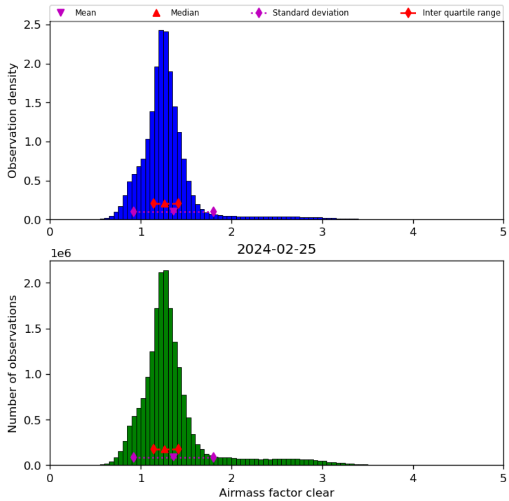
Figure 42: Histogram of “Airmass factor clear” for 2024-02-24 to 2024-02-26
