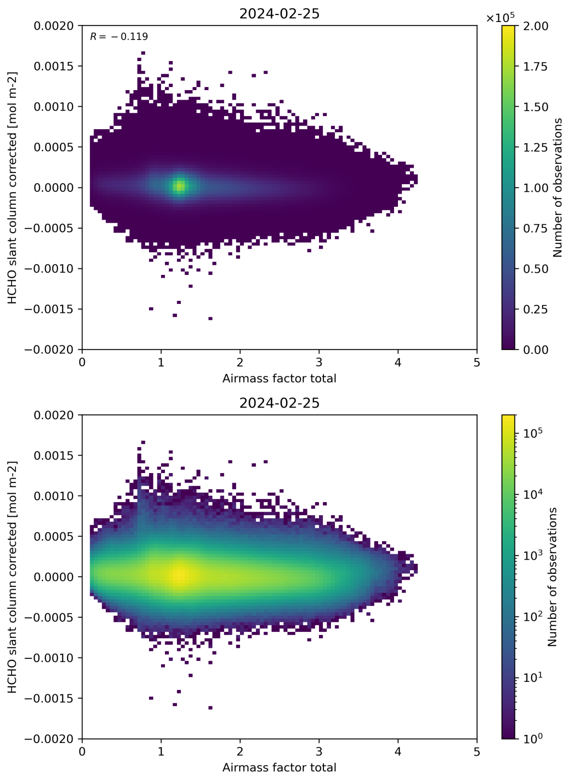
Figure 101: Scatter density plot of “Airmass factor total” against “HCHO slant column corrected” for 2024-02-24 to 2024-02-26.
