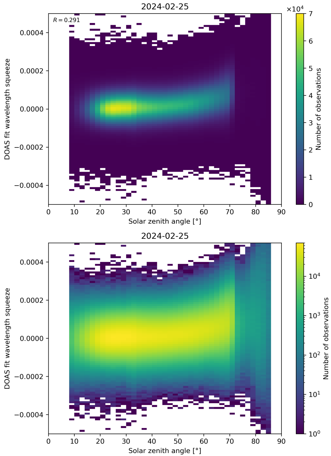
Figure 169: Scatter density plot of “Solar zenith angle” against “DOAS fit wavelength squeeze” for 2024-02-24 to 2024-02-26.
