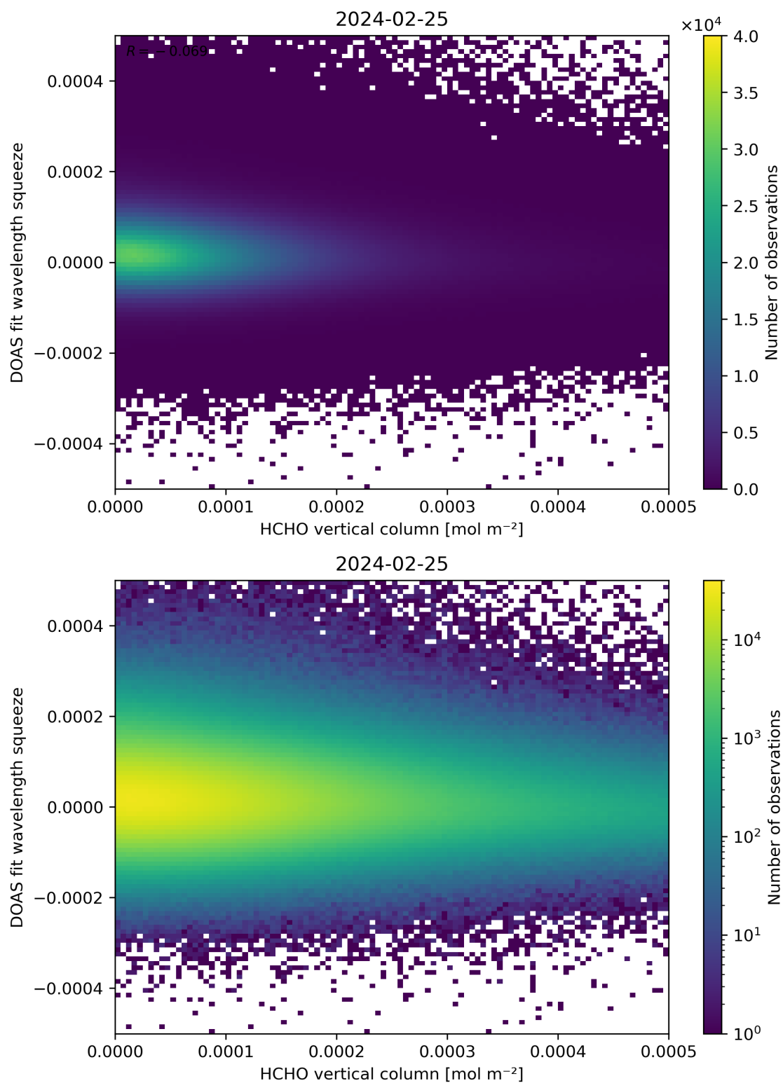
Figure 125: Scatter density plot of “HCHO vertical column” against “DOAS fit wavelength squeeze” for 2024-02-24 to 2024-02-26.
