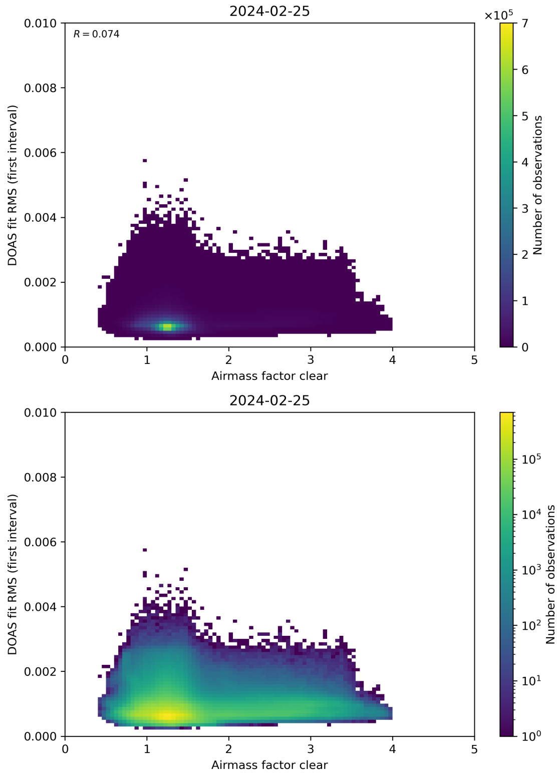
Figure 71: Scatter density plot of “Airmass factor clear” against “DOAS fit RMS (first interval)” for 2024-02-24 to 2024-02-26.
