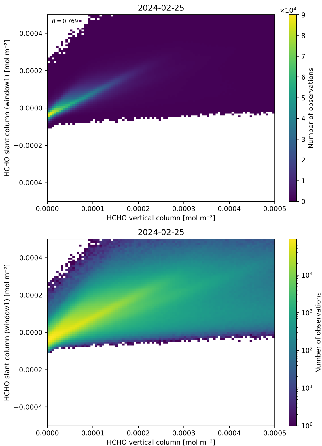
Figure 129: Scatter density plot of “HCHO vertical column” against “HCHO slant column (window1)” for 2024-02-24 to 2024-02-26.
