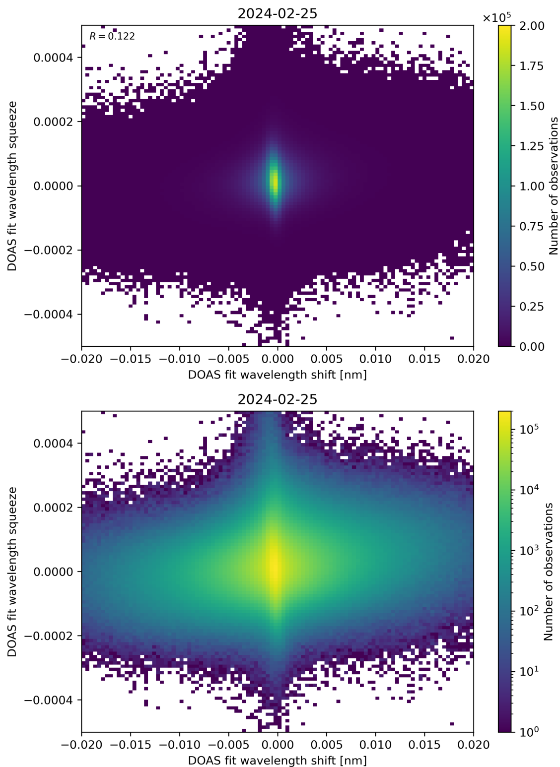
Figure 65: Scatter density plot of “DOAS fit wavelength shift” against “DOAS fit wavelength squeeze” for 2024-02-24 to 2024-02-26.
