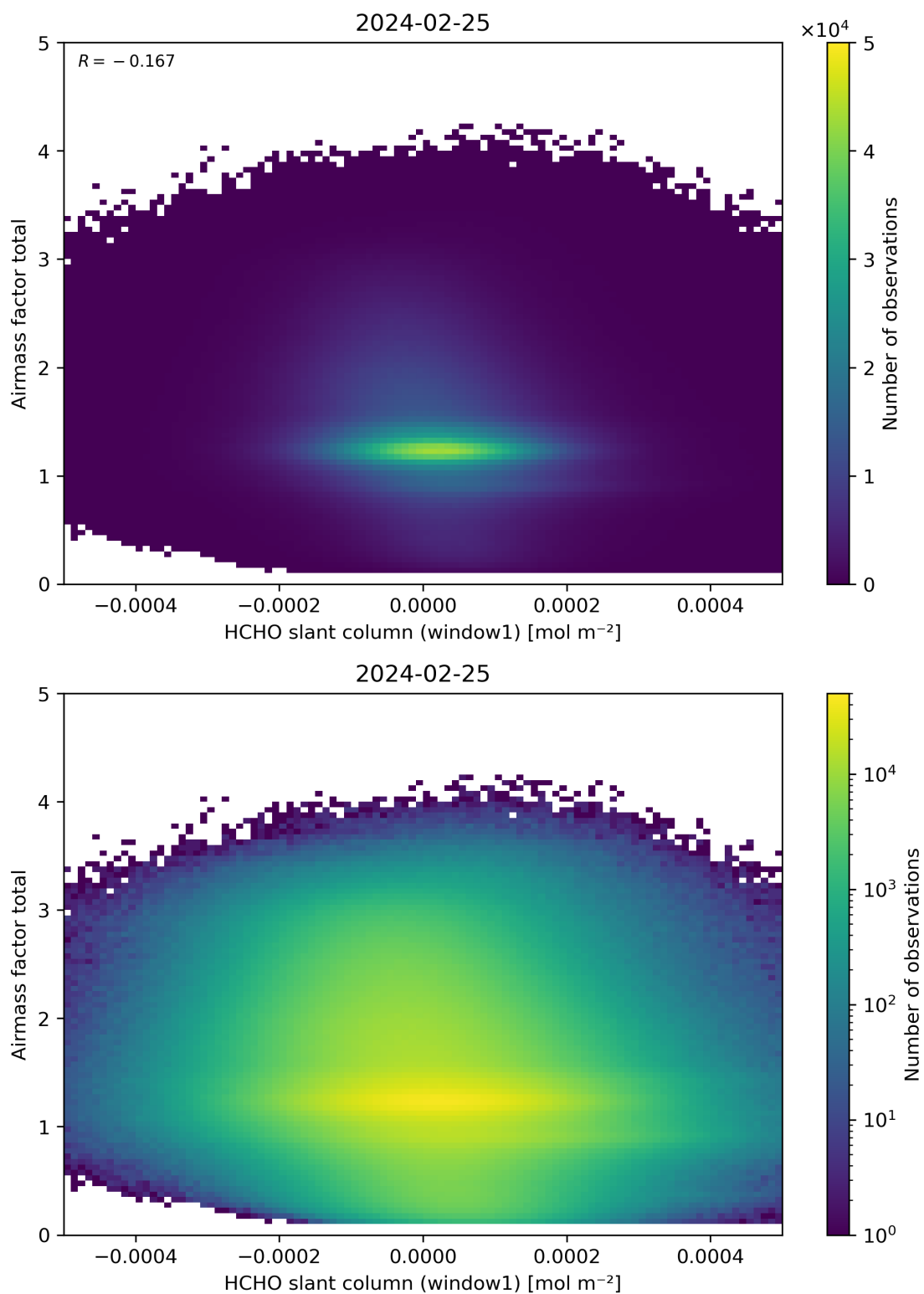
Figure 85: Scatter density plot of “HCHO slant column (window1)” against “Airmass factor total” for 2024-02-24 to 2024-02-26.
