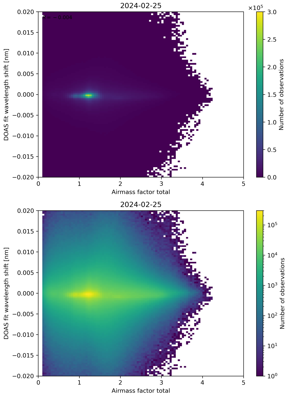
Figure 98: Scatter density plot of “Airmass factor total” against “DOAS fit wavelength shift” for 2024-02-24 to 2024-02-26.
