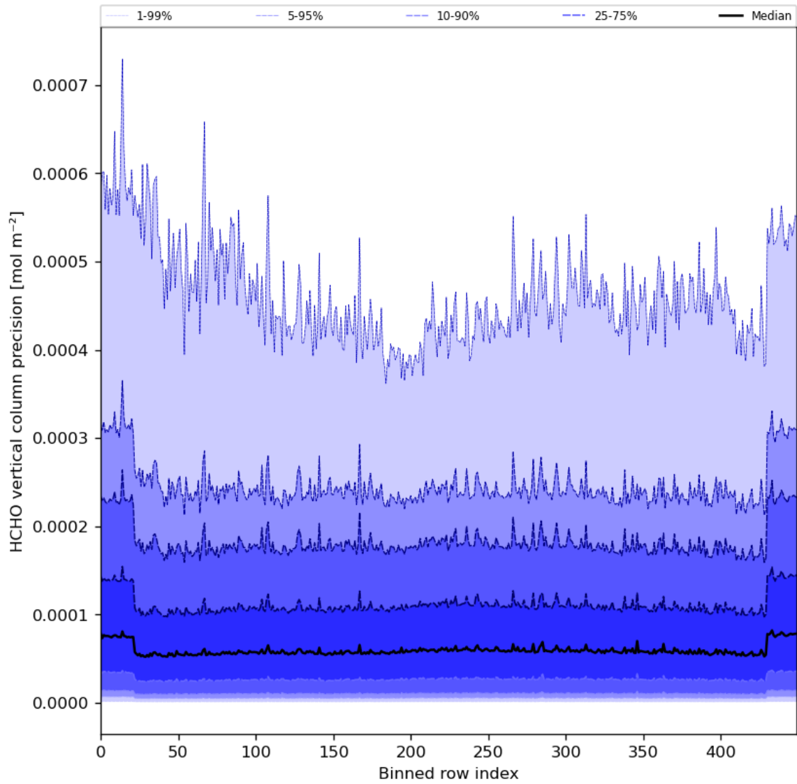
Figure 50: Along track statistics of “HCHO vertical column precision” for 2024-02-24 to 2024-02-26
