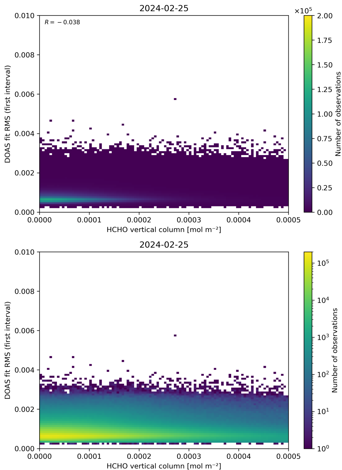
Figure 123: Scatter density plot of “HCHO vertical column” against “DOAS fit RMS (first interval)” for 2024-02-24 to 2024-02-26.
