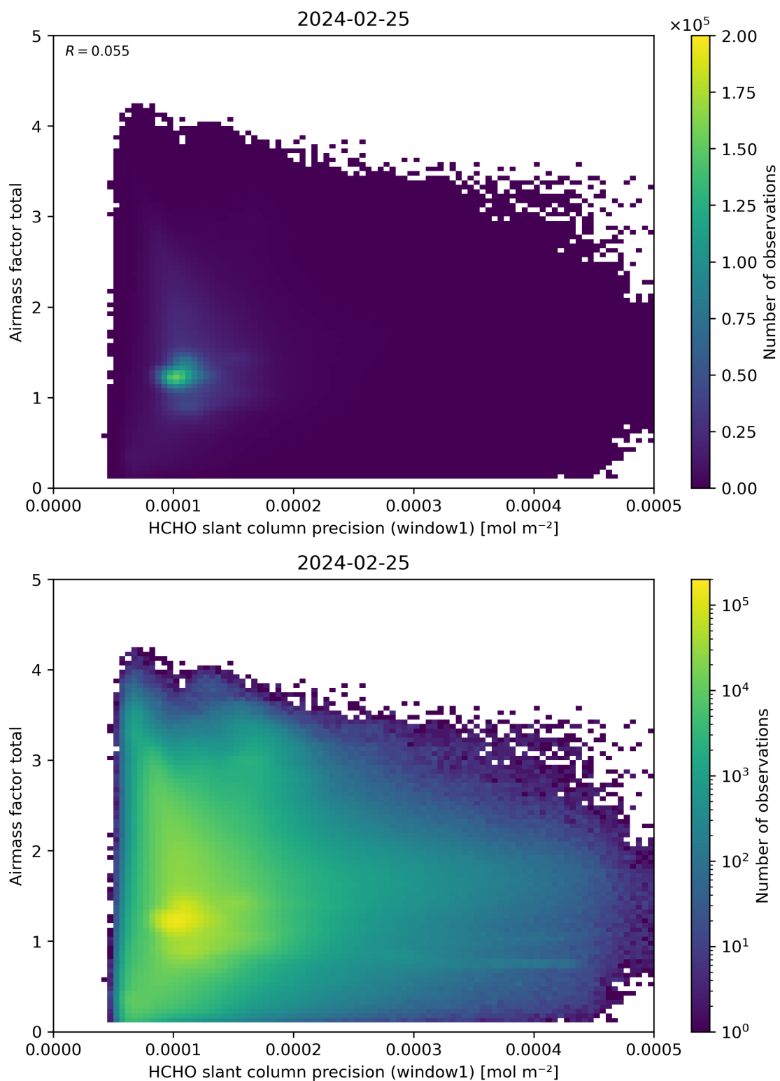
Figure 94: Scatter density plot of “HCHO slant column precision (window1)” against “Airmass factor total” for 2024-02-24 to 2024-02-26.
