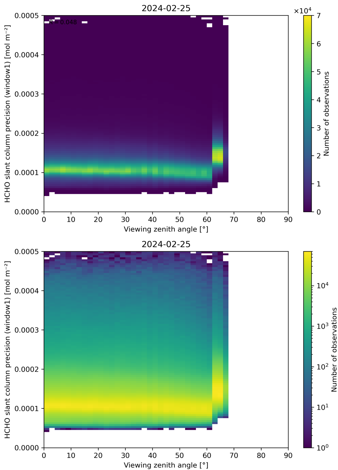
Figure 189: Scatter density plot of “Viewing zenith angle” against “HCHO slant column precision (window1)” for 2024-02-24 to 2024-02-26.
