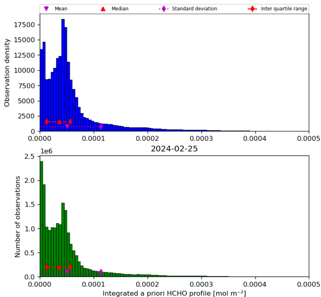
Figure 43: Histogram of “Integrated a priori HCHO profile” for 2024-02-24 to 2024-02-26
