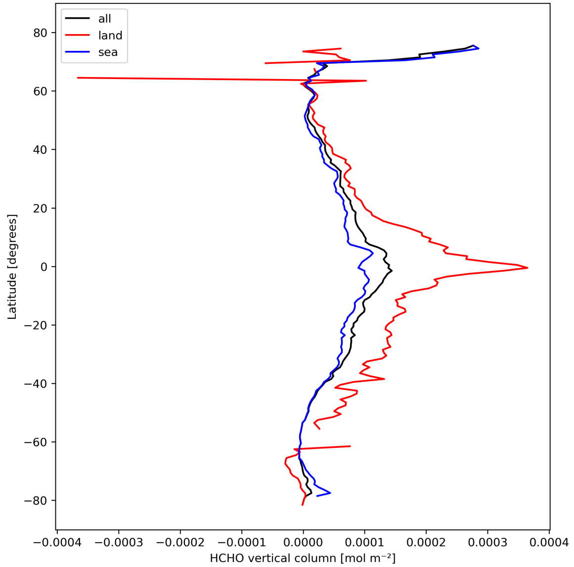
Figure 21: Zonal average of “HCHO vertical column” for 2024-02-24 to 2024-02-26.
