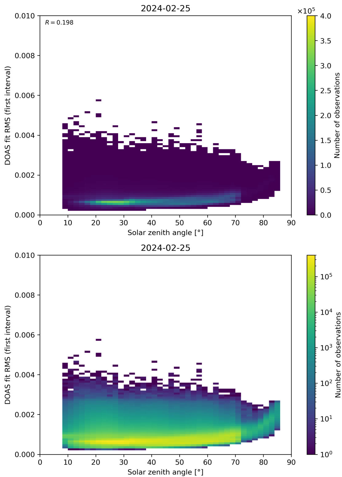
Figure 167: Scatter density plot of “Solar zenith angle” against “DOAS fit RMS (first interval)” for 2024-02-24 to 2024-02-26.
