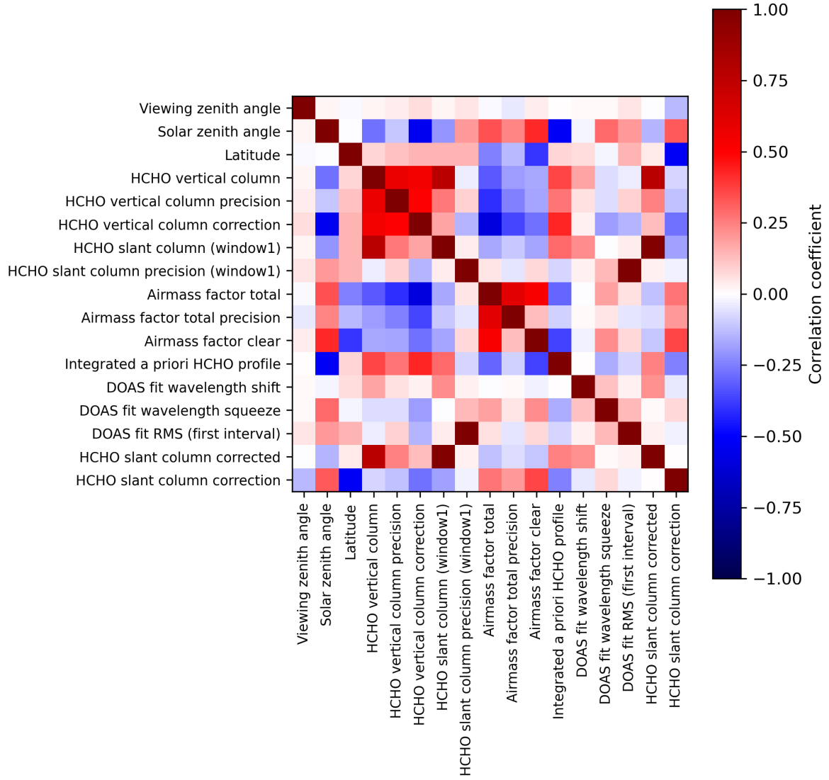
Figure 2: Map of correlation matrix for 2024-02-24 to 2024-02-26.
