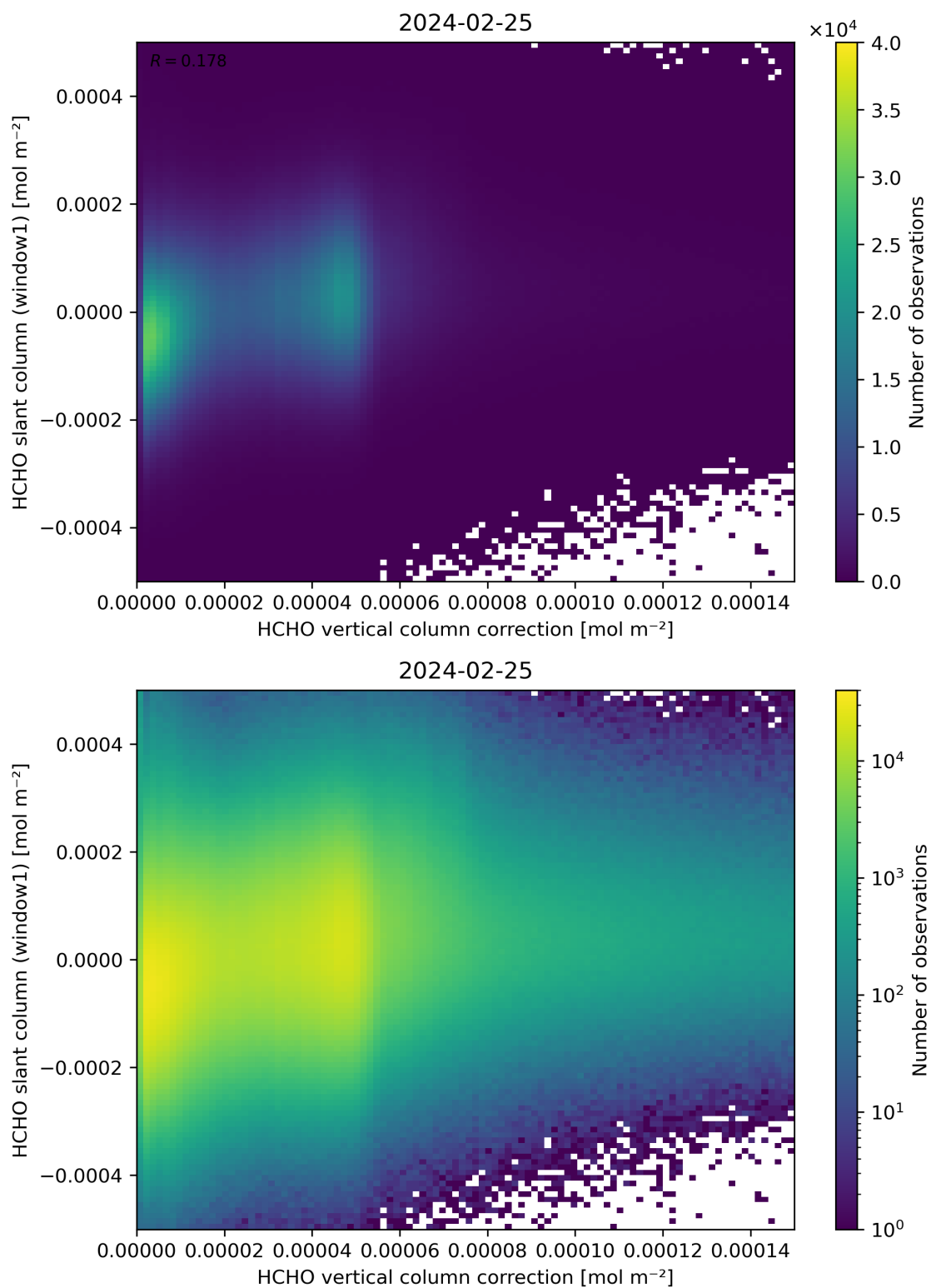
Figure 118: Scatter density plot of “HCHO vertical column correction” against “HCHO slant column (window1)” for 2024-02-24 to 2024-02-26.
