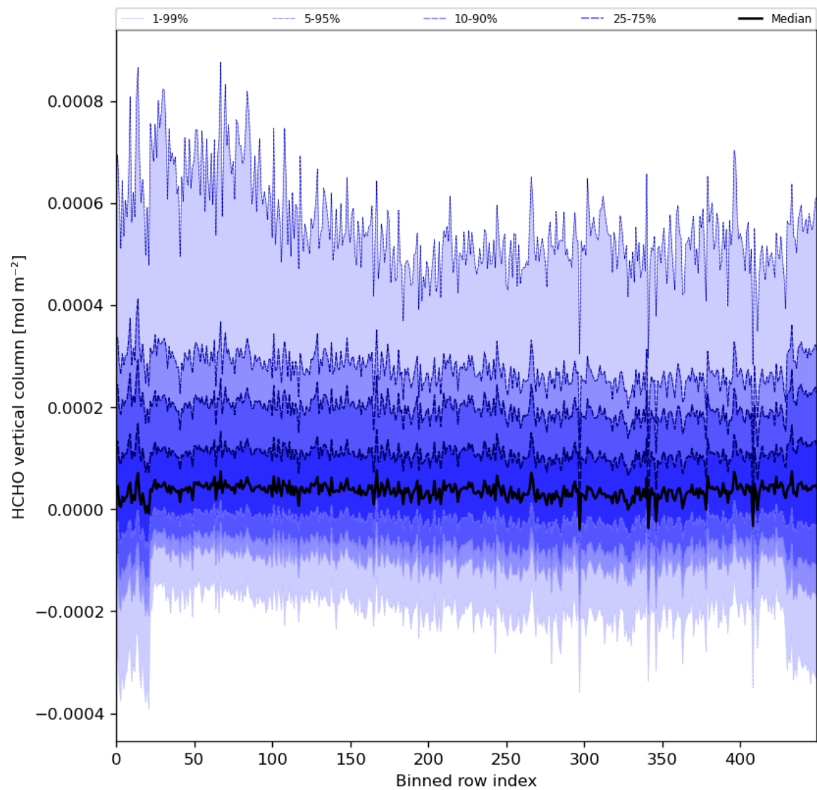
Figure 49: Along track statistics of “HCHO vertical column” for 2024-02-24 to 2024-02-26
