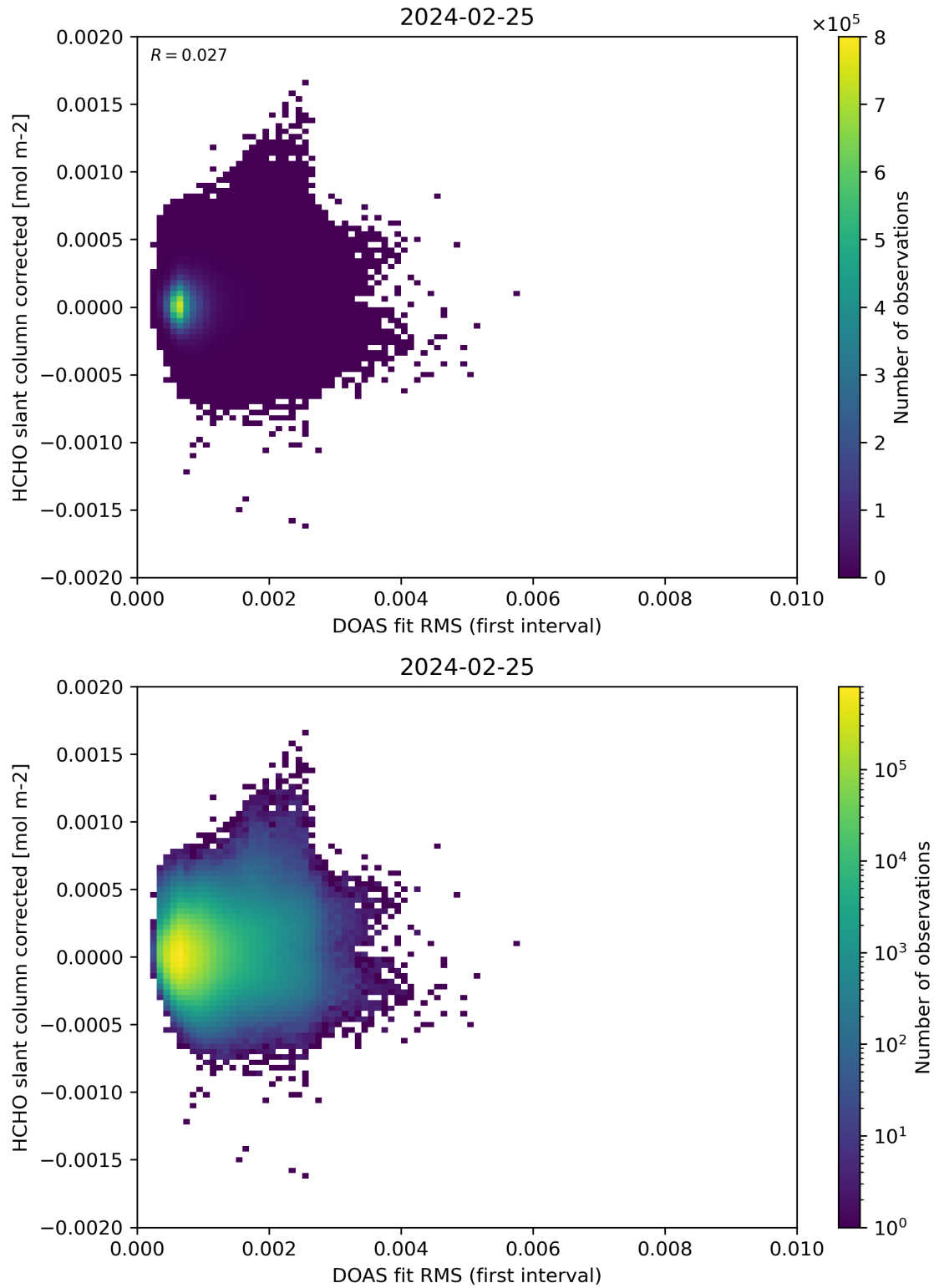
Figure 62: Scatter density plot of “DOAS fit RMS (first interval)” against “HCHO slant column corrected” for 2024-02-24 to 2024-02-26.
