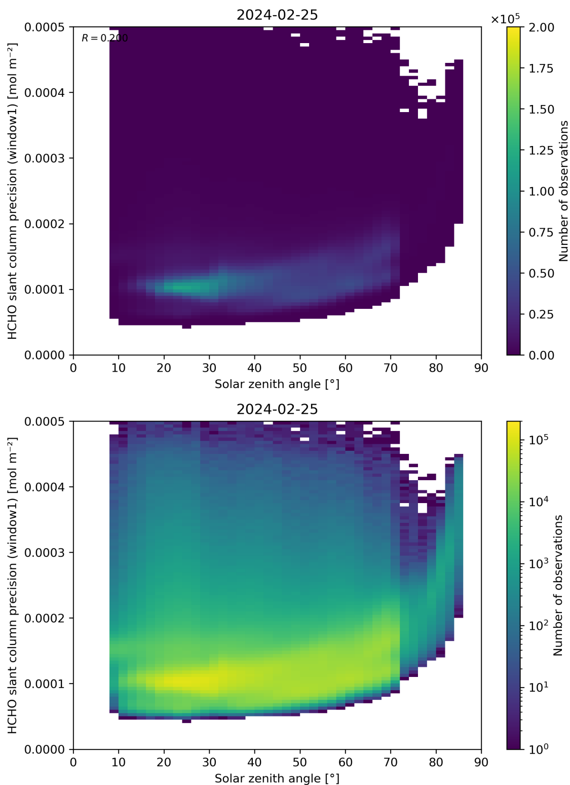
Figure 174: Scatter density plot of “Solar zenith angle” against “HCHO slant column precision (window1)” for 2024-02-24 to 2024-02-26.
