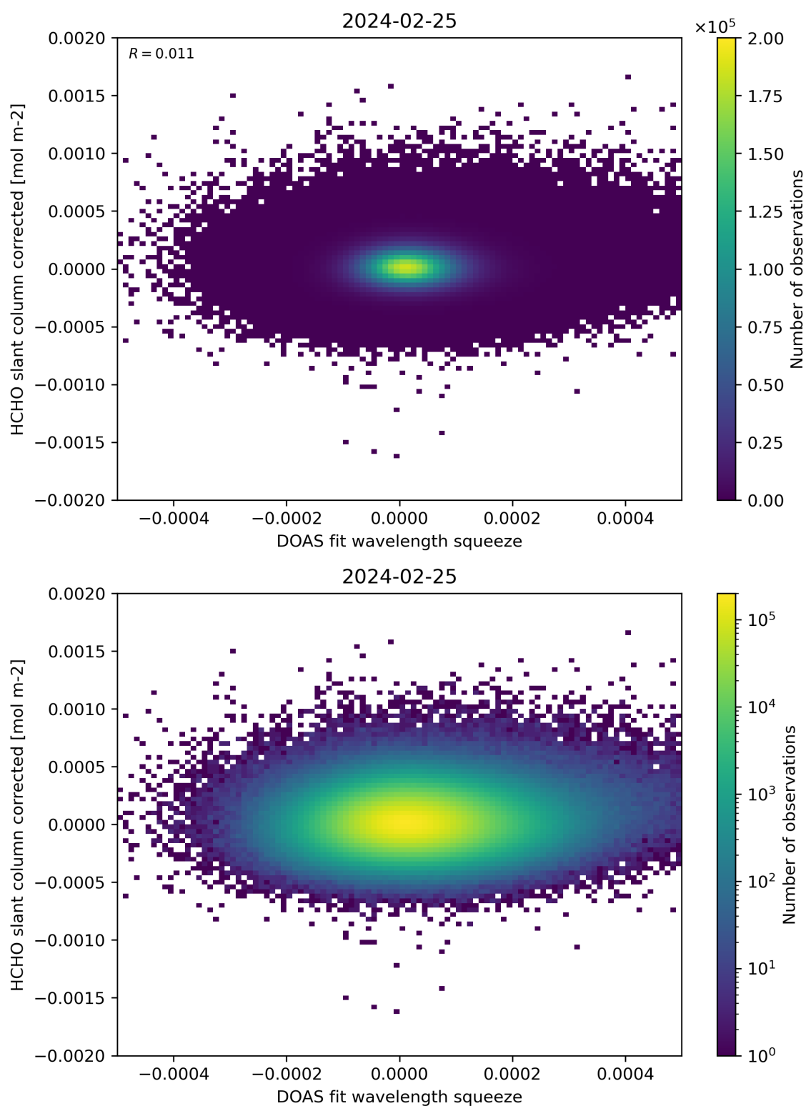
Figure 69: Scatter density plot of “DOAS fit wavelength squeeze” against “HCHO slant column corrected” for 2024-02-24 to 2024-02-26.
