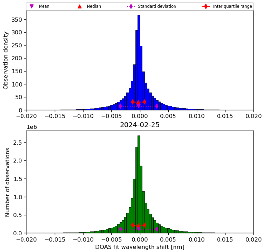
Figure 44: Histogram of “DOAS fit wavelength shift” for 2024-02-24 to 2024-02-26
