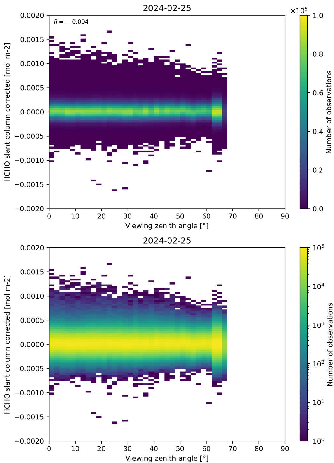
Figure 186: Scatter density plot of “Viewing zenith angle” against “HCHO slant column corrected” for 2024-02-24 to 2024-02-26.
