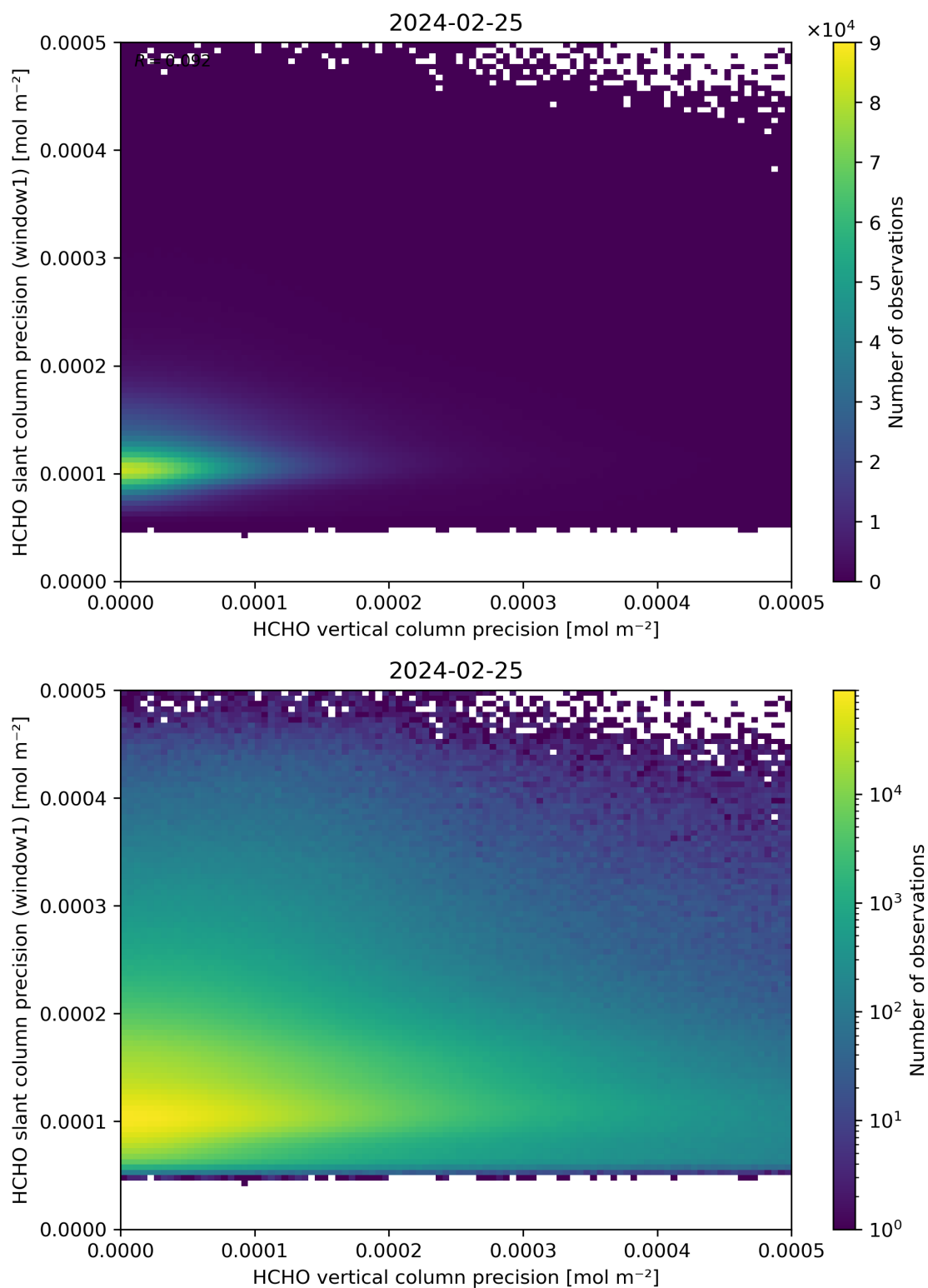
Figure 143: Scatter density plot of “HCHO vertical column precision” against “HCHO slant column precision (window1)” for 2024-02-24 to 2024-02-26.
