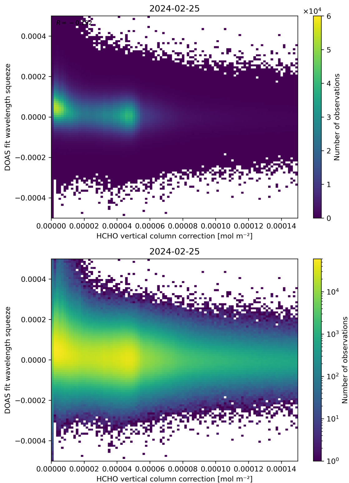
Figure 114: Scatter density plot of “HCHO vertical column correction” against “DOAS fit wavelength squeeze” for 2024-02-24 to 2024-02-26.
