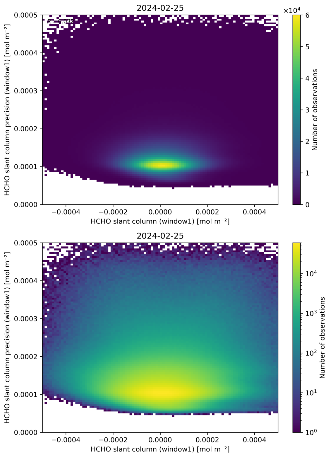
Figure 84: Scatter density plot of “HCHO slant column (window1)” against “HCHO slant column precision (window1)” for 2024-02-24 to 2024-02-26.
