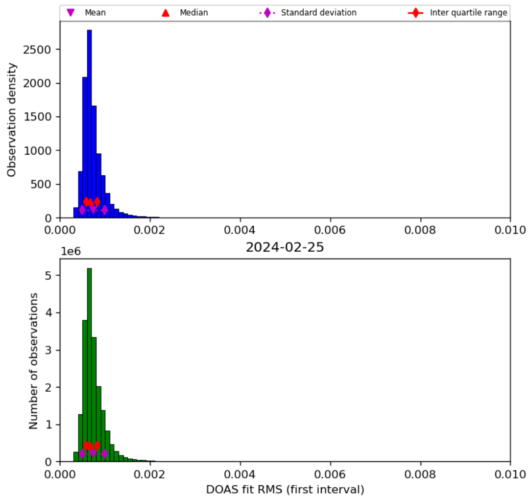
Figure 46: Histogram of “DOAS fit RMS (first interval)” for 2024-02-24 to 2024-02-26
