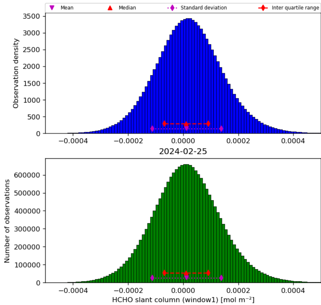
Figure 38: Histogram of “HCHO slant column (window1)” for 2024-02-24 to 2024-02-26
