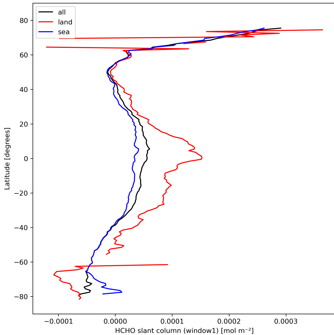
Figure 24: Zonal average of “HCHO slant column (window1)” for 2024-02-24 to 2024-02-26.
