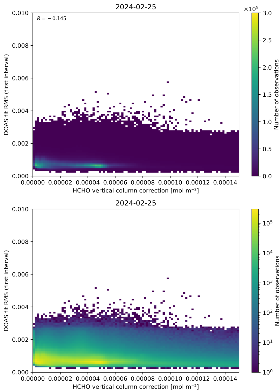
Figure 112: Scatter density plot of “HCHO vertical column correction” against “DOAS fit RMS (first interval)” for 2024-02-24 to 2024-02-26.
