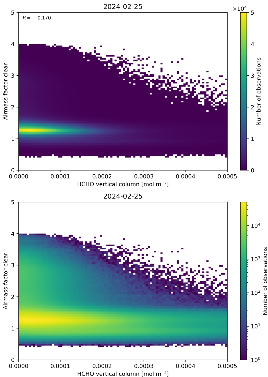
Figure 126: Scatter density plot of “HCHO vertical column” against “Airmass factor clear” for 2024-02-24 to 2024-02-26.
