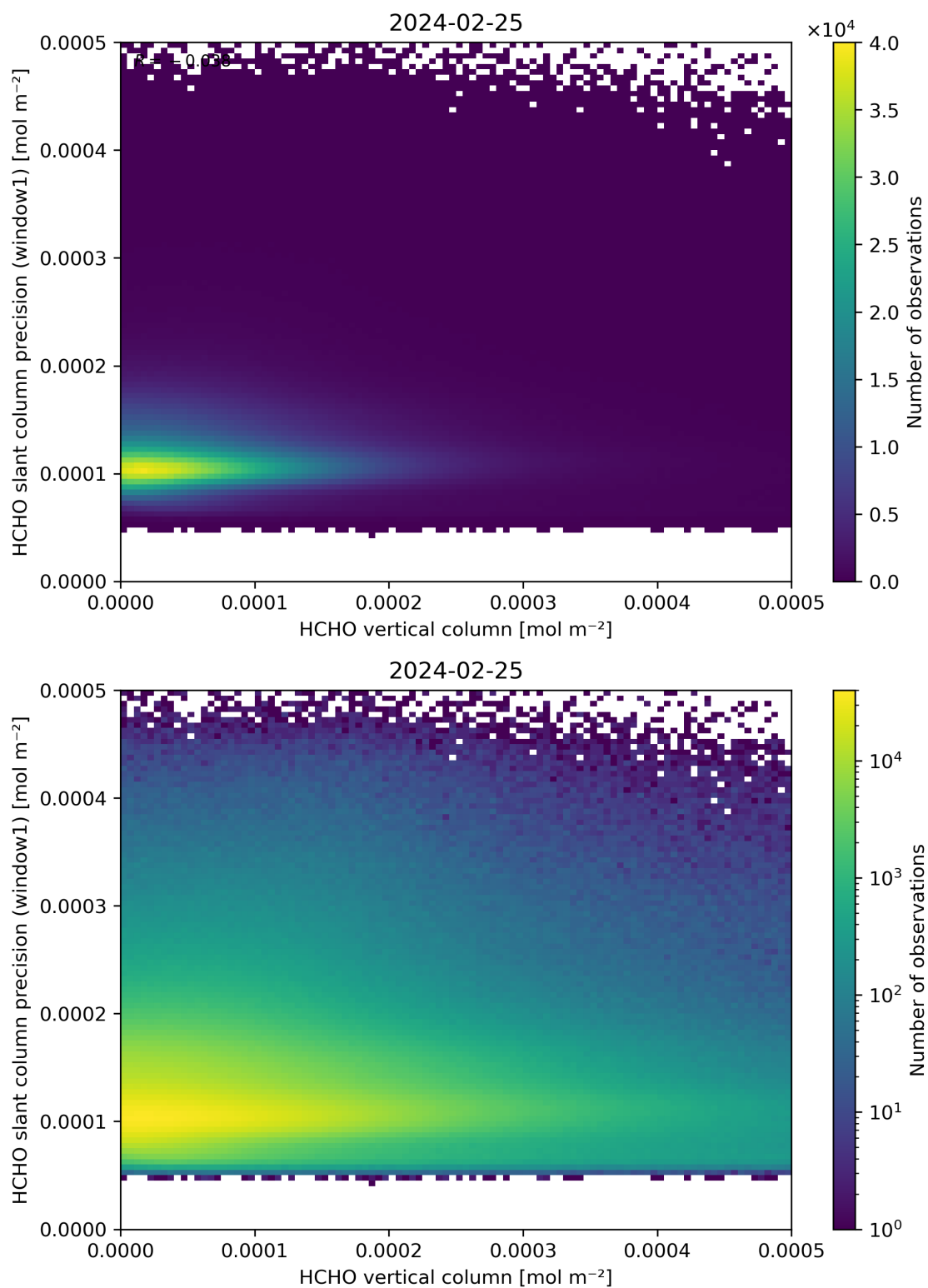
Figure 130: Scatter density plot of “HCHO vertical column” against “HCHO slant column precision (window1)” for 2024-02-24 to 2024-02-26.
