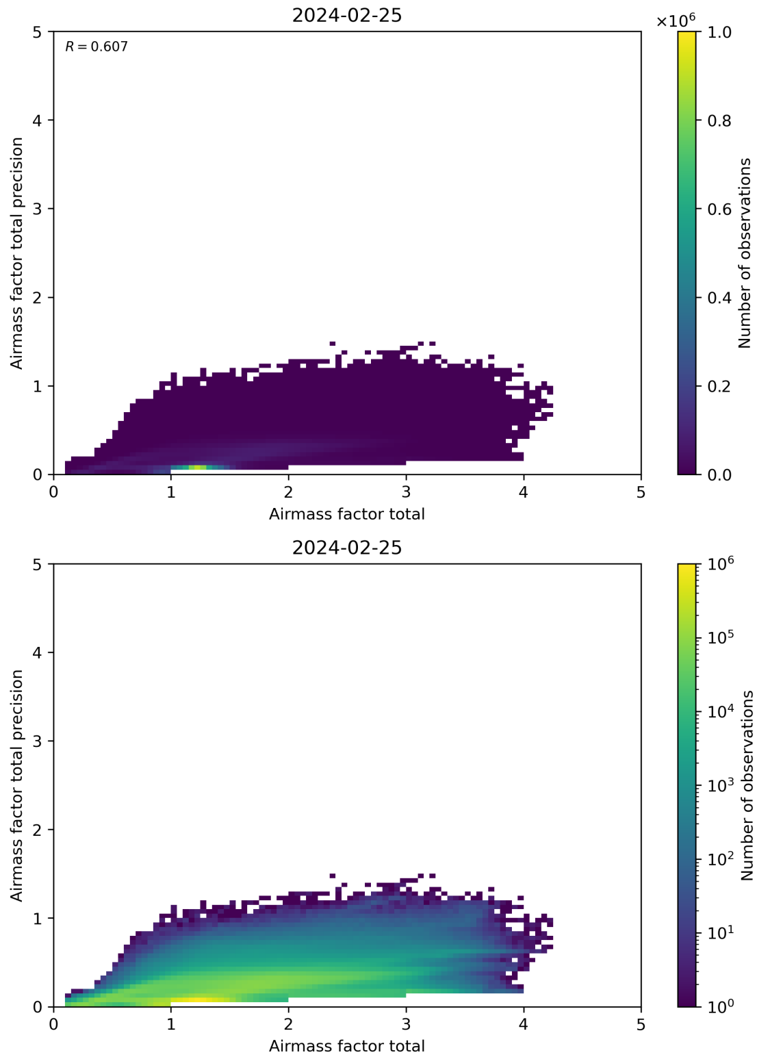
Figure 103: Scatter density plot of “Airmass factor total” against “Airmass factor total precision” for 2024-02-24 to 2024-02-26.
