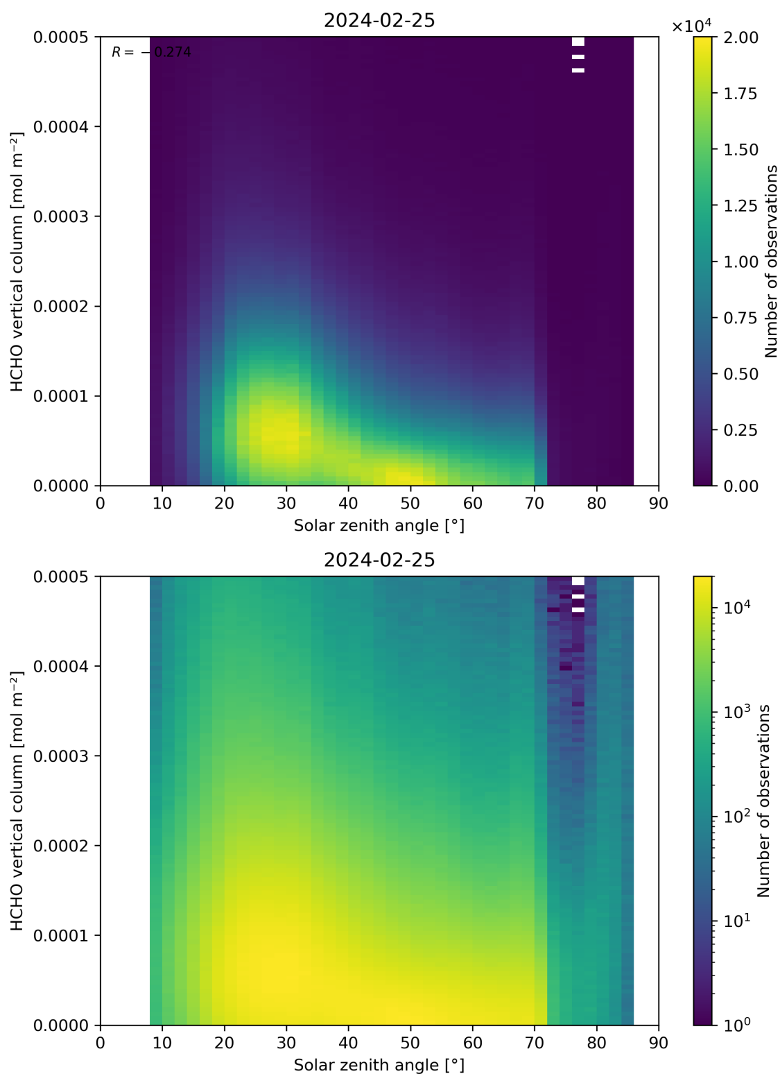
Figure 177: Scatter density plot of “Solar zenith angle” against “HCHO vertical column” for 2024-02-24 to 2024-02-26.
