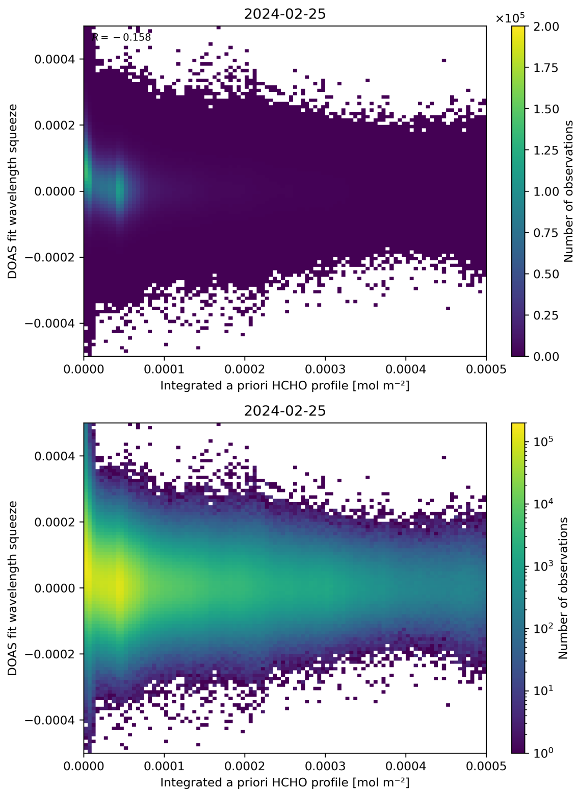
Figure 150: Scatter density plot of “Integrated a priori HCHO profile” against “DOAS fit wavelength squeeze” for 2024-02-24 to 2024-02-26.
