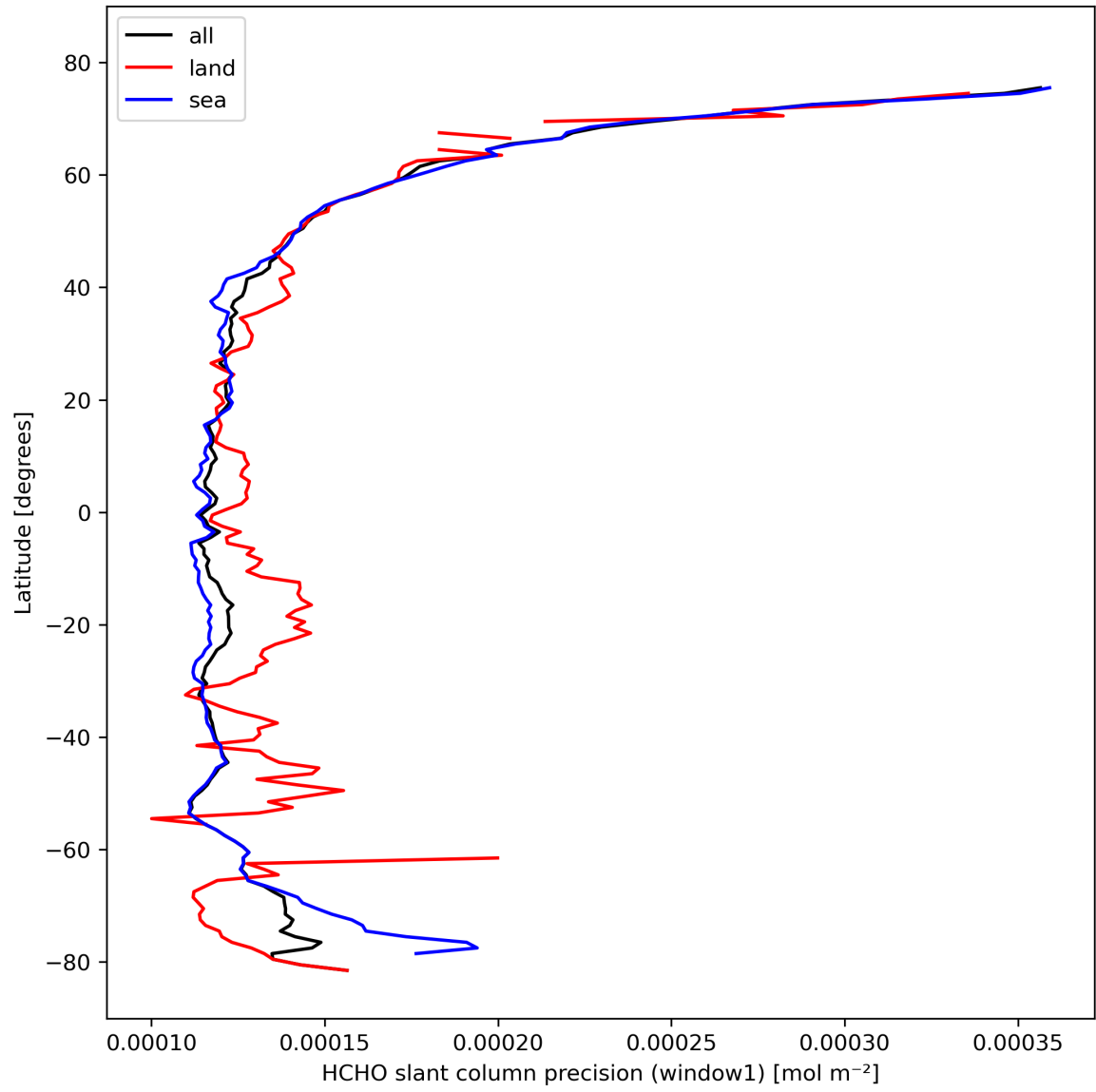
Figure 25: Zonal average of “HCHO slant column precision (window1)” for 2024-02-24 to 2024-02-26.
