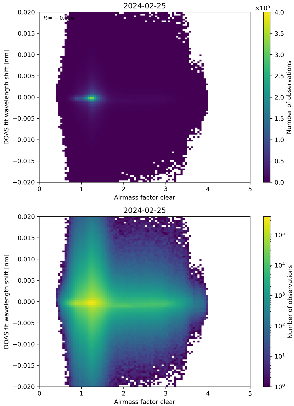
Figure 72: Scatter density plot of “Airmass factor clear” against “DOAS fit wavelength shift” for 2024-02-24 to 2024-02-26.
