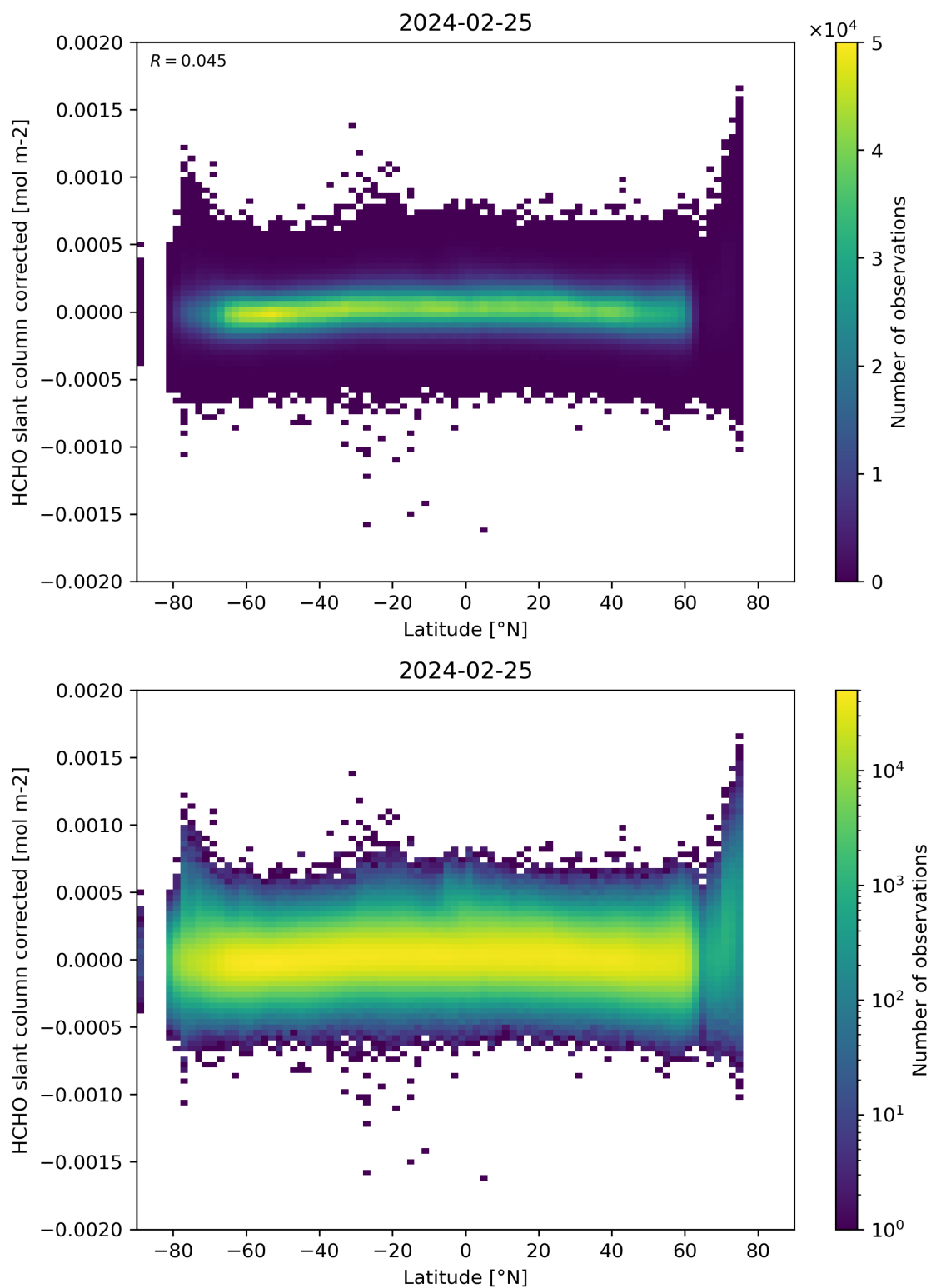
Figure 157: Scatter density plot of “Latitude” against “HCHO slant column corrected” for 2024-02-24 to 2024-02-26.
