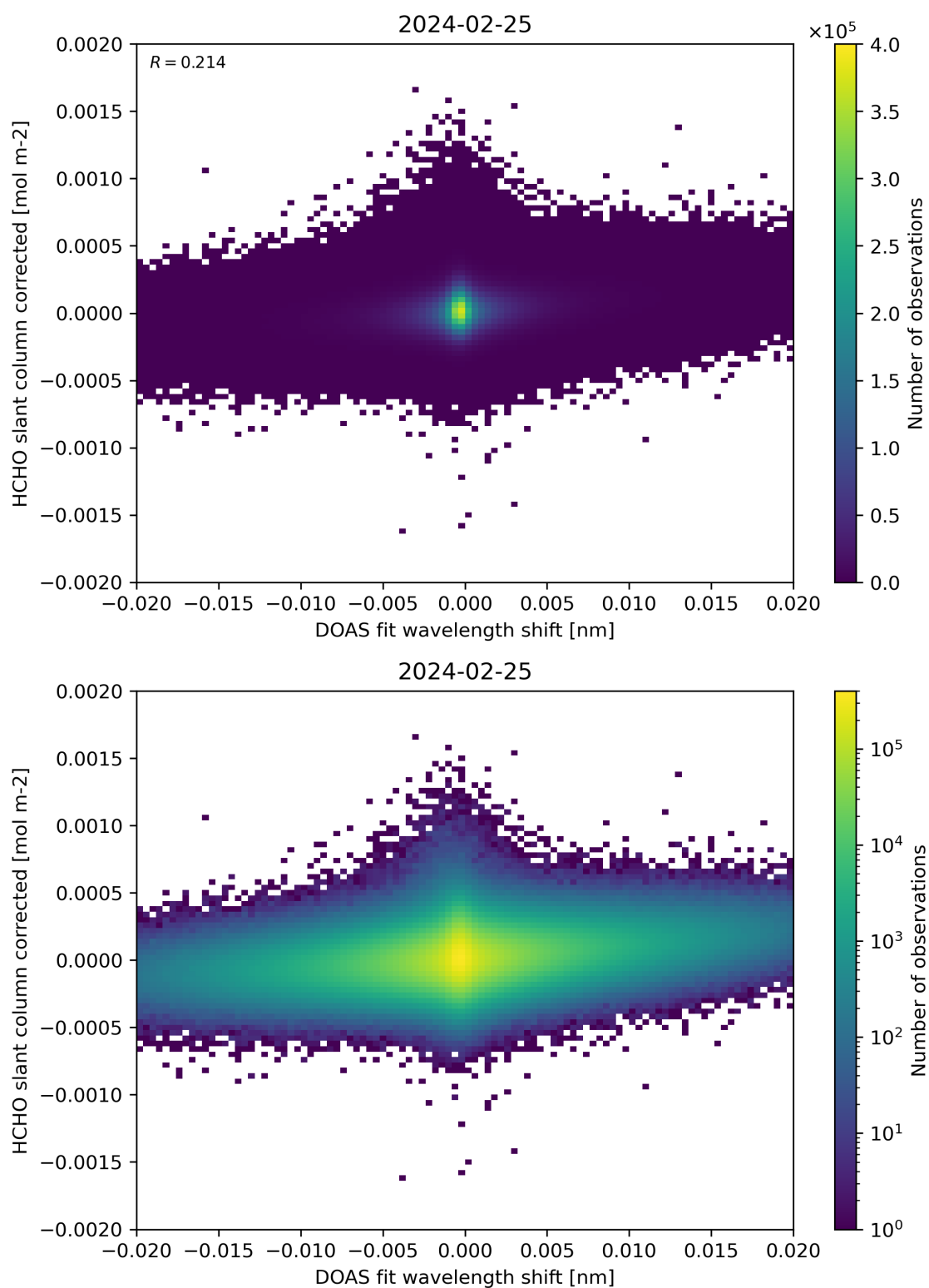
Figure 66: Scatter density plot of “DOAS fit wavelength shift” against “HCHO slant column corrected” for 2024-02-24 to 2024-02-26.
