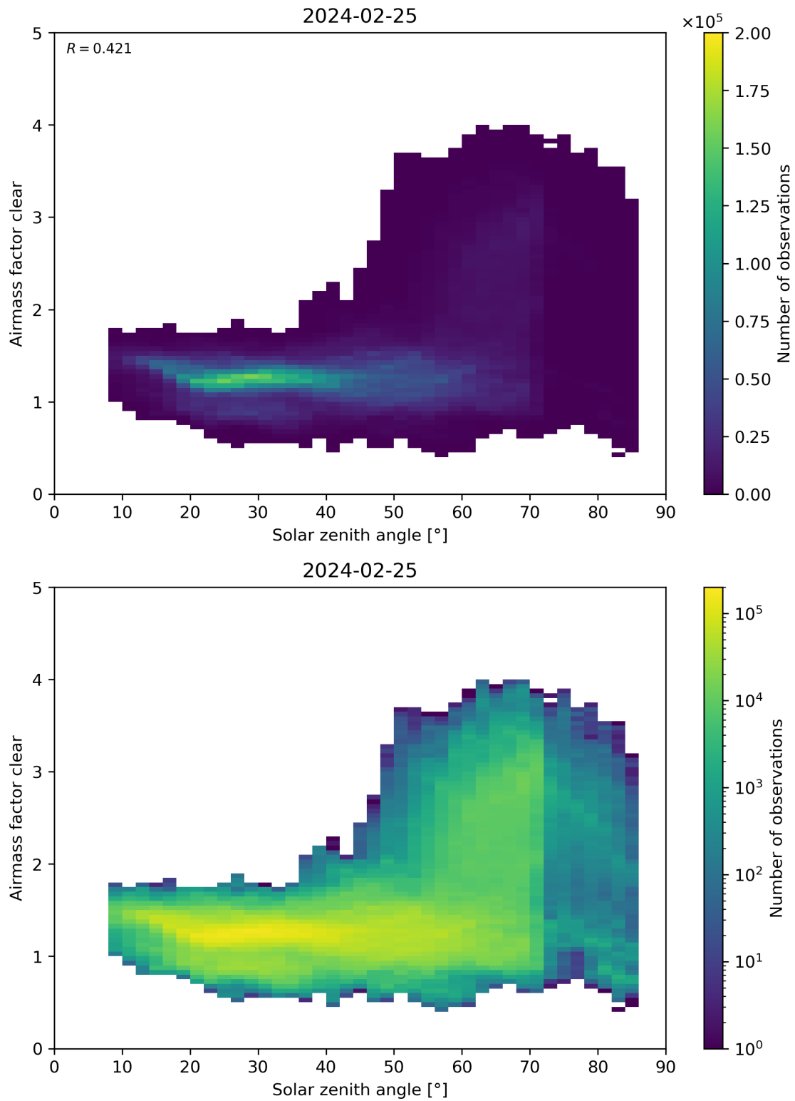
Figure 170: Scatter density plot of “Solar zenith angle” against “Airmass factor clear” for 2024-02-24 to 2024-02-26.
