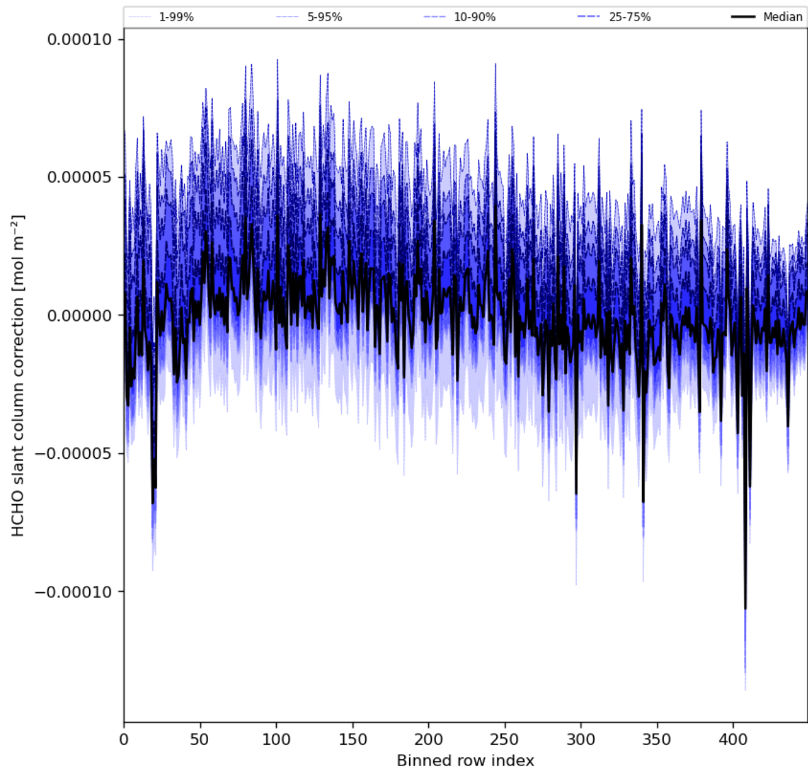
Figure 61: Along track statistics of “HCHO slant column correction” for 2024-02-24 to 2024-02-26
