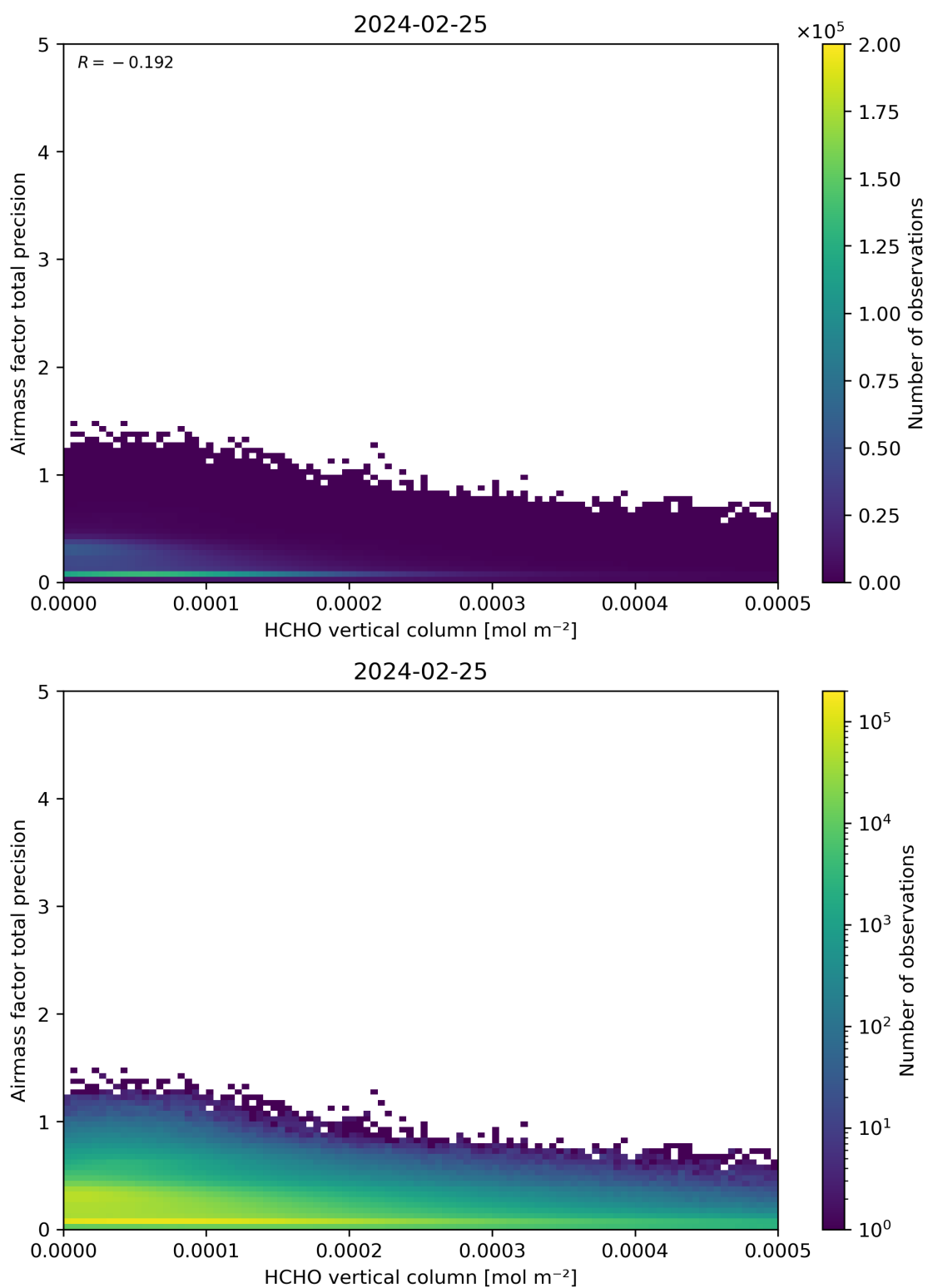
Figure 132: Scatter density plot of “HCHO vertical column” against “Airmass factor total precision” for 2024-02-24 to 2024-02-26.
