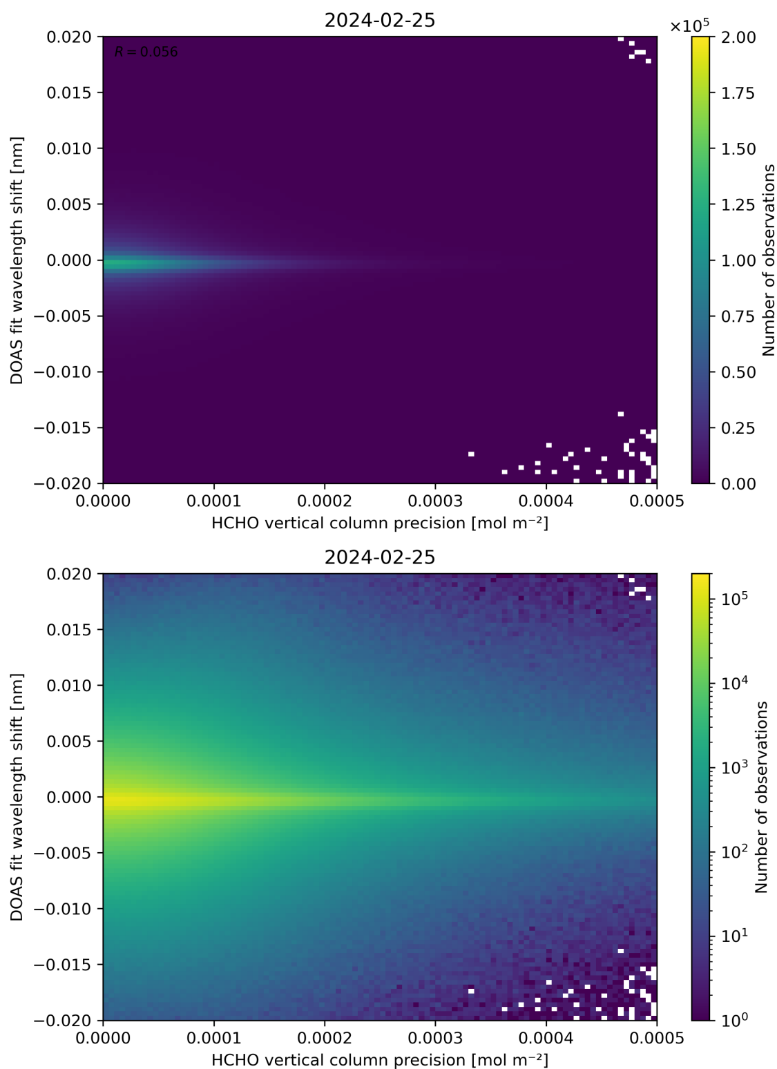
Figure 137: Scatter density plot of “HCHO vertical column precision” against “DOAS fit wavelength shift” for 2024-02-24 to 2024-02-26.
