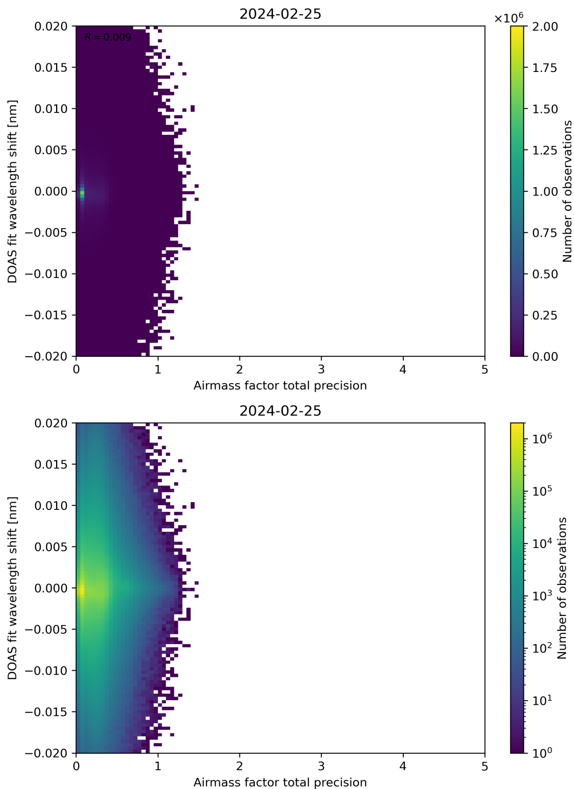
Figure 106: Scatter density plot of “Airmass factor total precision” against “DOAS fit wavelength shift” for 2024-02-24 to 2024-02-26.
