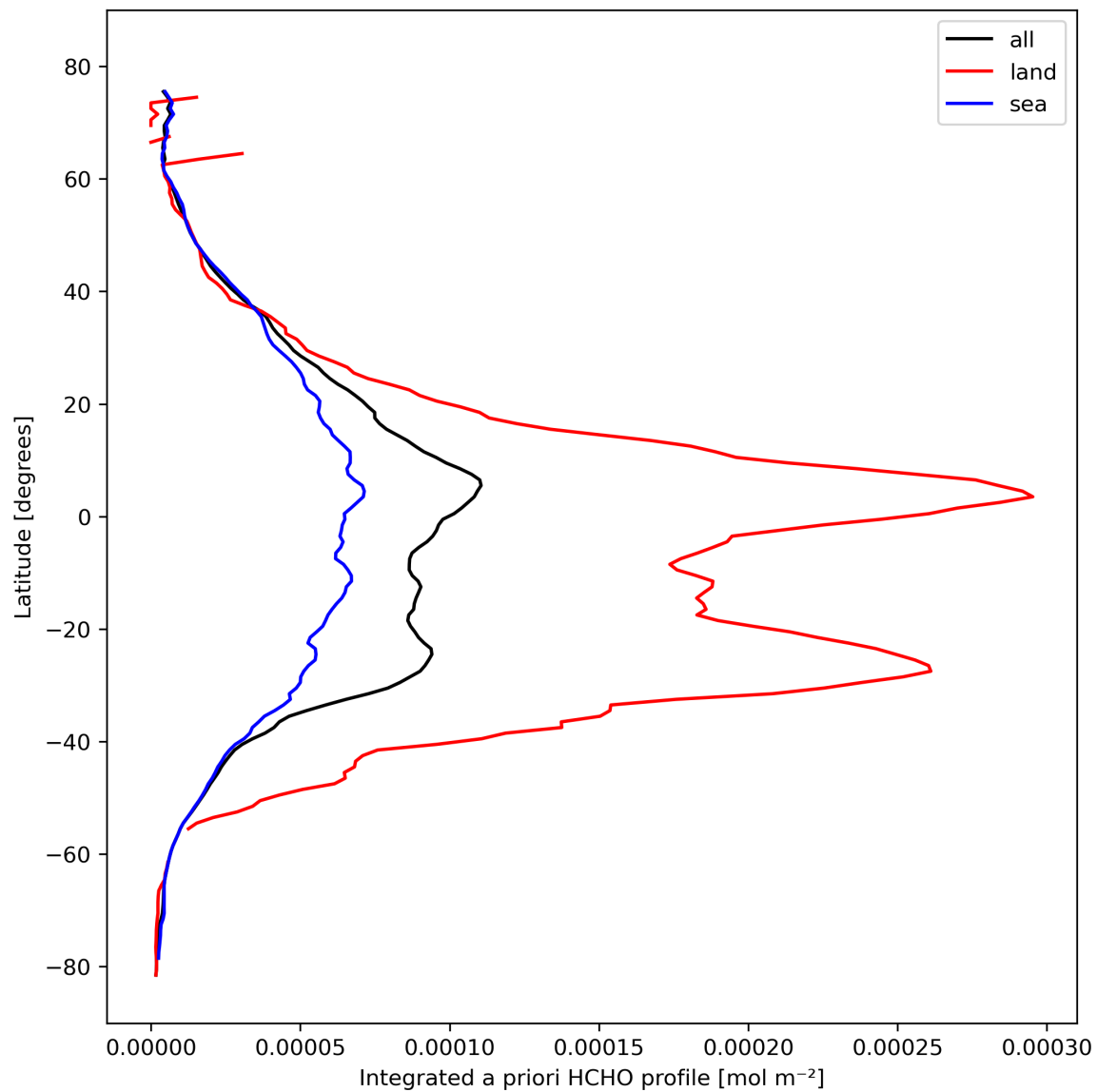
Figure 29: Zonal average of “Integrated a priori HCHO profile” for 2024-02-24 to 2024-02-26.
