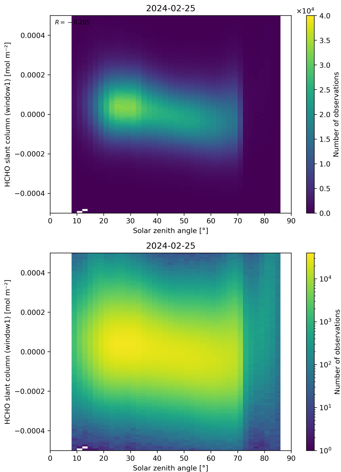
Figure 173: Scatter density plot of “Solar zenith angle” against “HCHO slant column (window1)” for 2024-02-24 to 2024-02-26.
