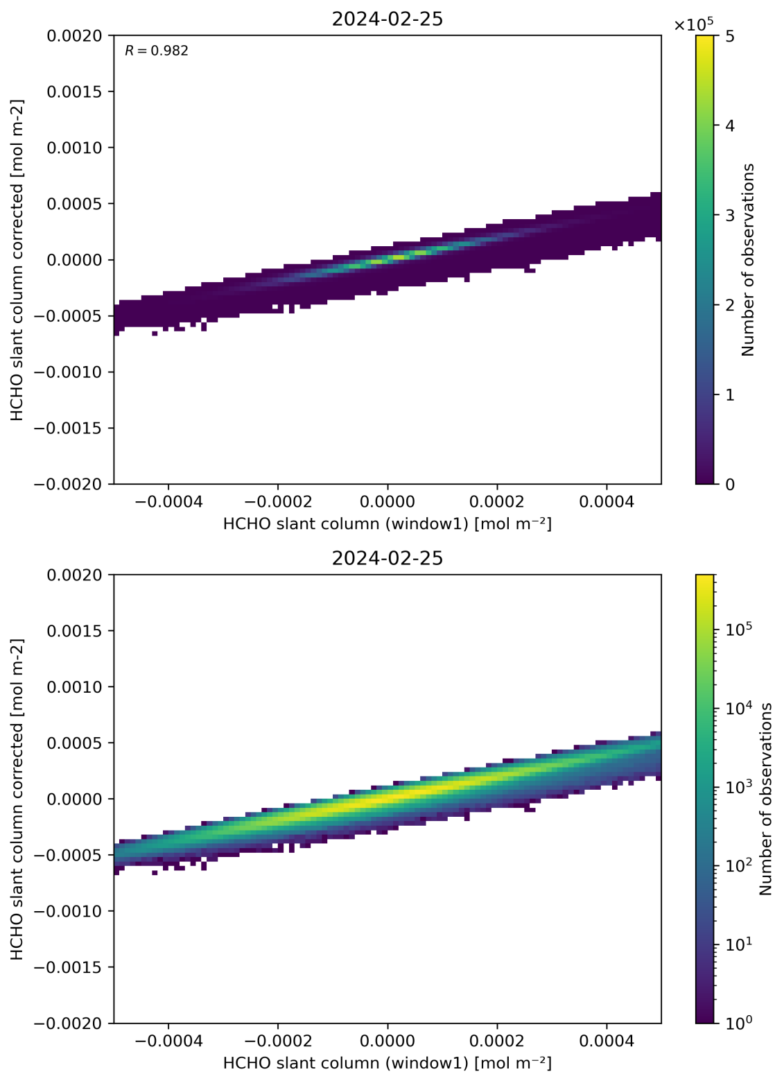
Figure 82: Scatter density plot of “HCHO slant column (window1)” against “HCHO slant column corrected” for 2024-02-24 to 2024-02-26.
