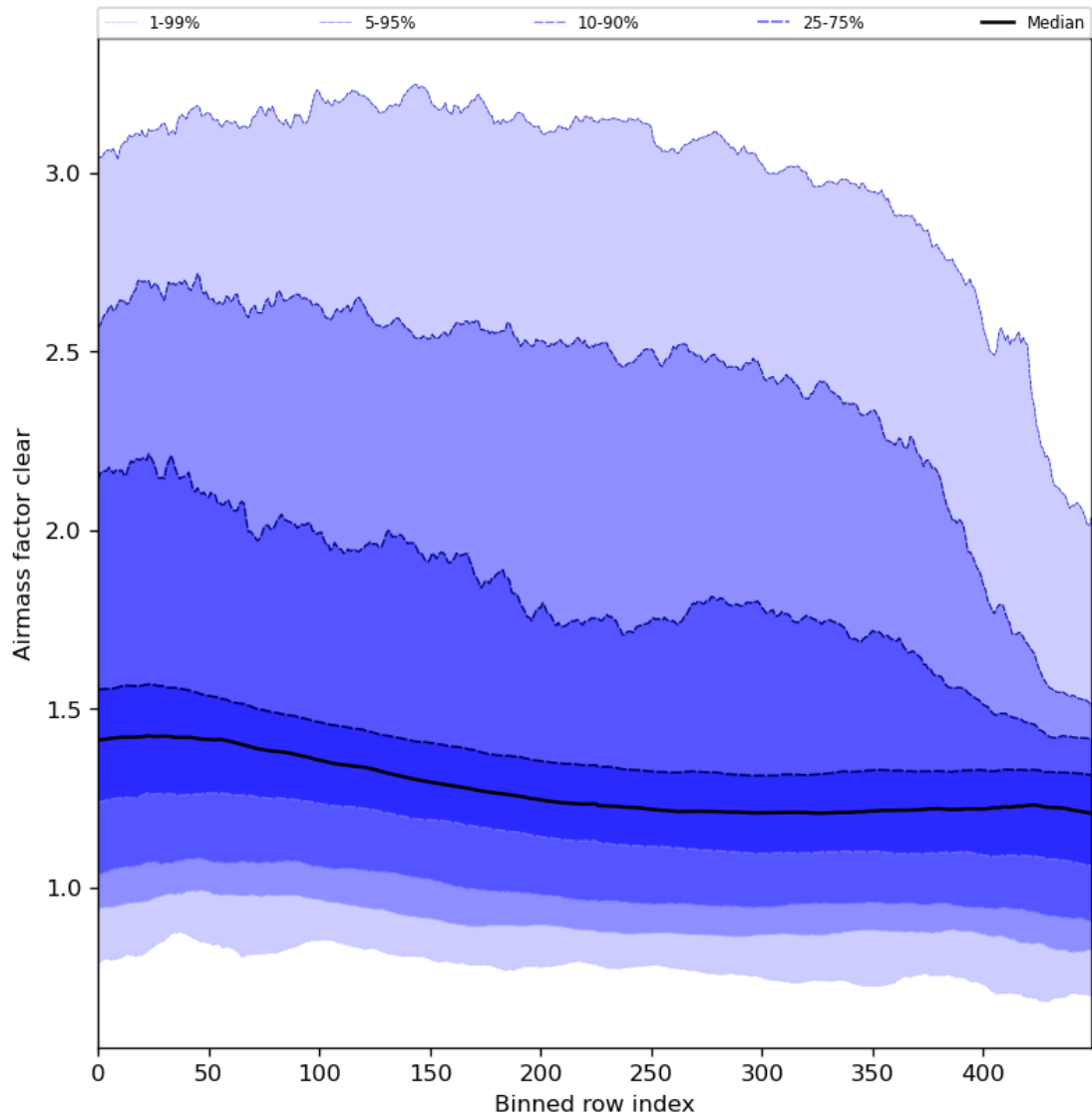
Figure 56: Along track statistics of “Airmass factor clear” for 2024-02-24 to 2024-02-26
