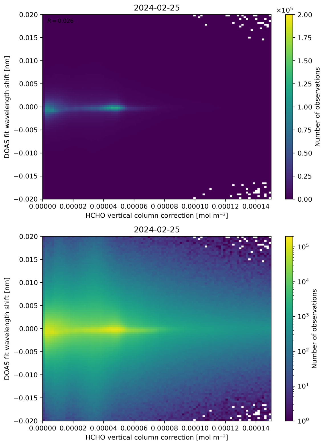
Figure 113: Scatter density plot of “HCHO vertical column correction” against “DOAS fit wavelength shift” for 2024-02-24 to 2024-02-26.
