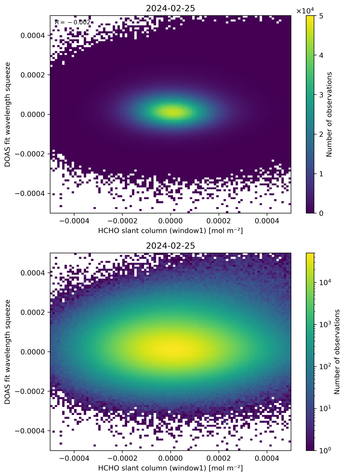
Figure 80: Scatter density plot of “HCHO slant column (window1)” against “DOAS fit wavelength squeeze” for 2024-02-24 to 2024-02-26.
