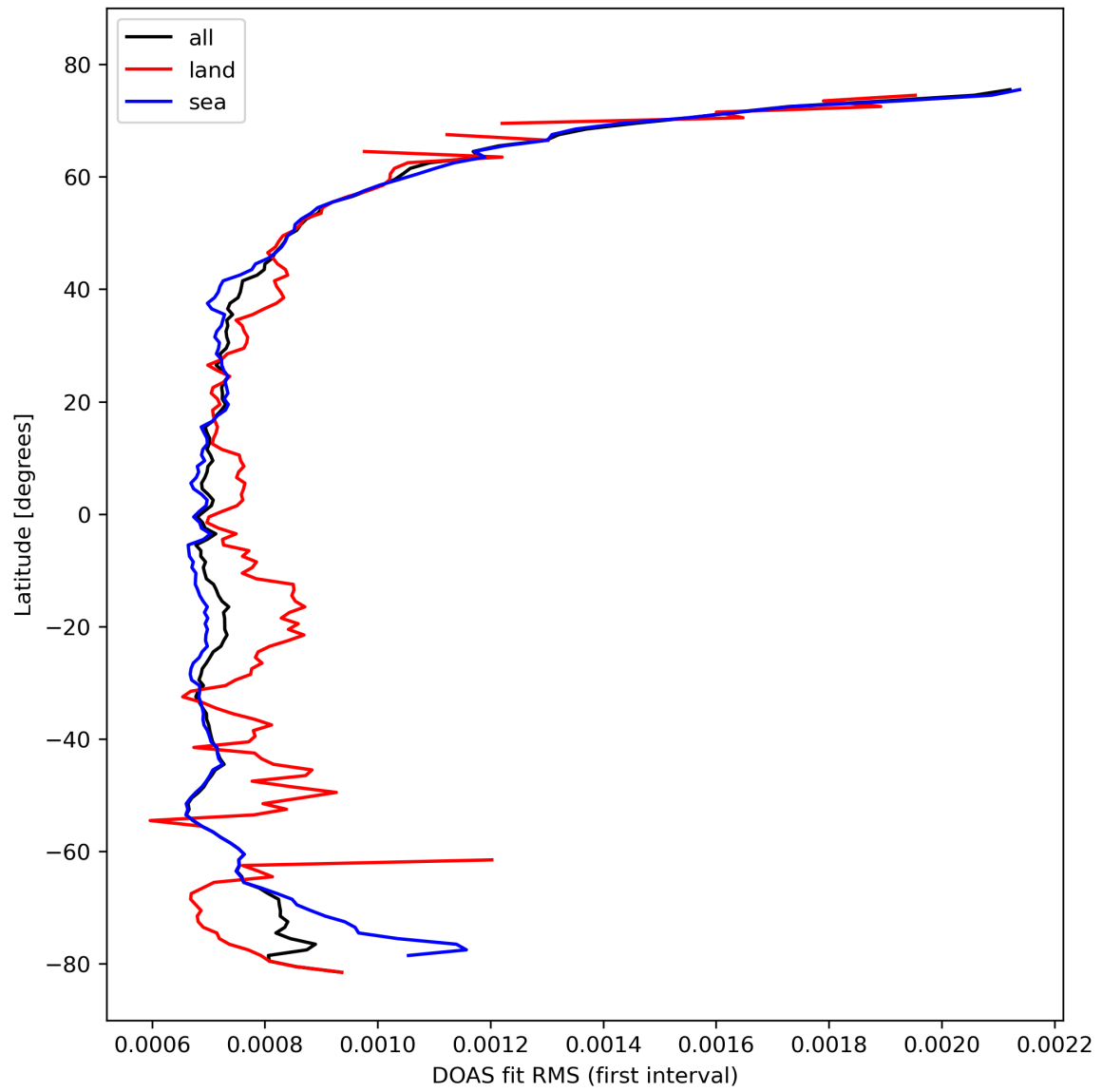
Figure 32: Zonal average of “DOAS fit RMS (first interval)” for 2024-02-24 to 2024-02-26.
