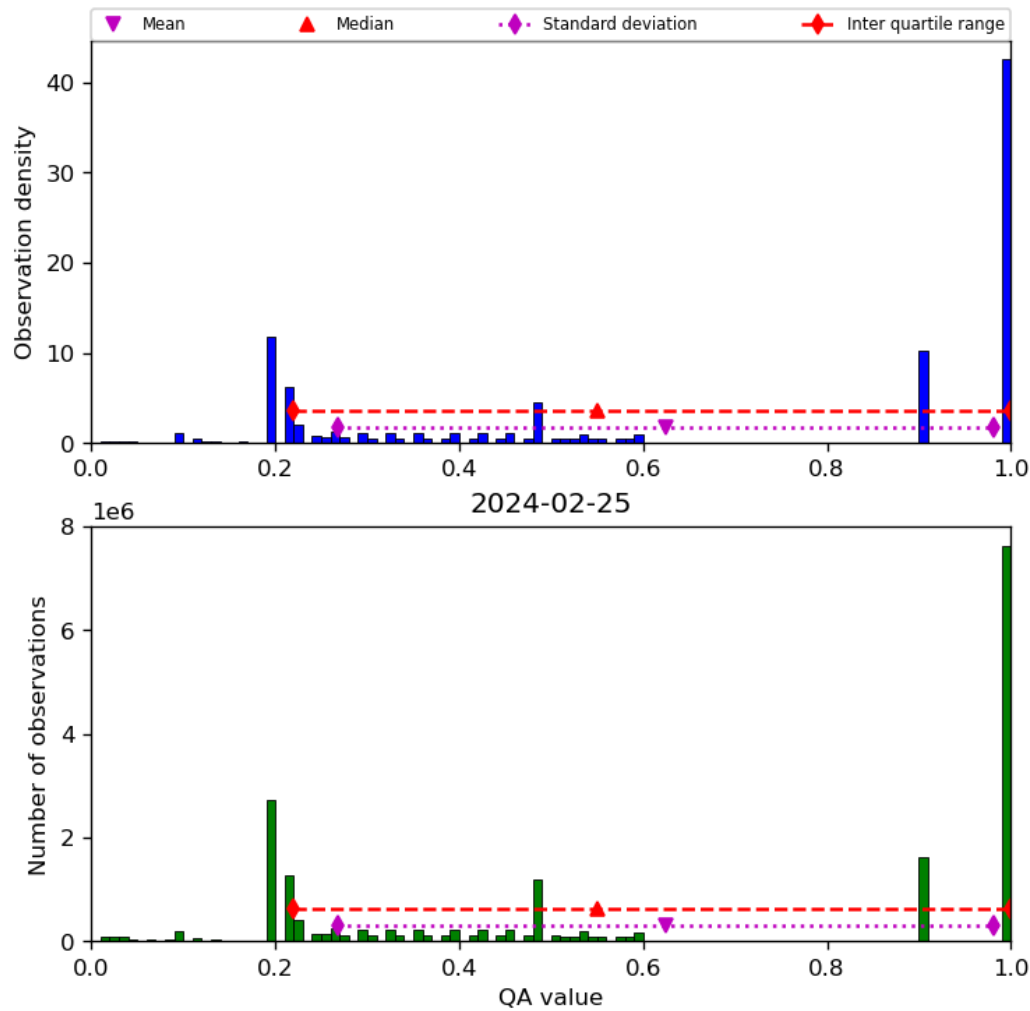
Figure 34: Histogram of “QA value” for 2024-02-24 to 2024-02-26
