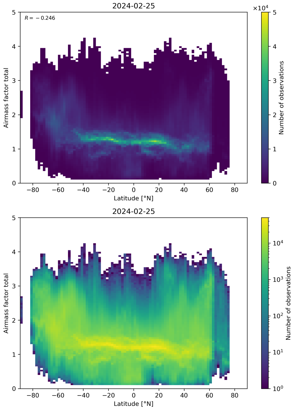
Figure 161: Scatter density plot of “Latitude” against “Airmass factor total” for 2024-02-24 to 2024-02-26.
