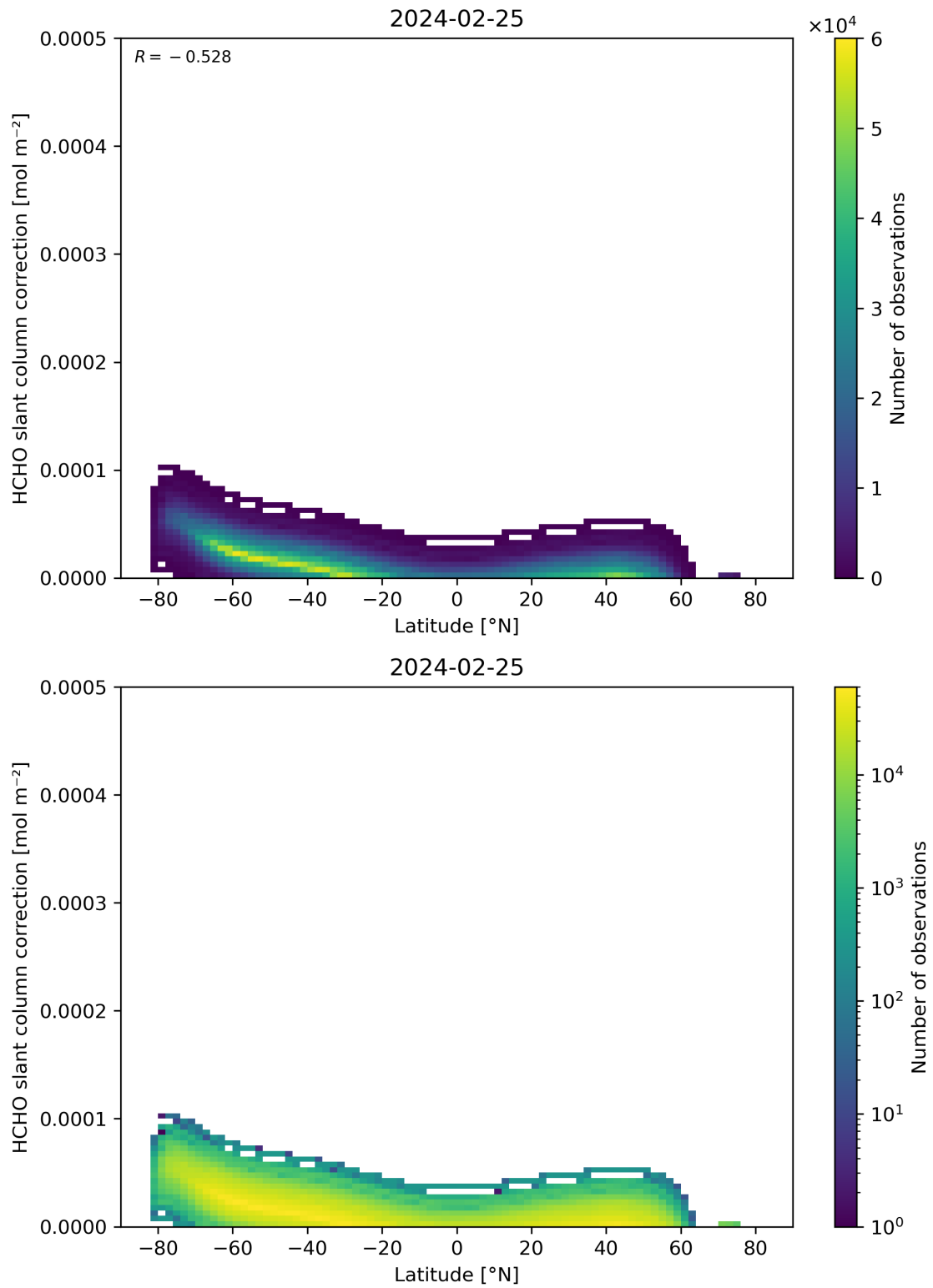
Figure 158: Scatter density plot of “Latitude” against “HCHO slant column correction” for 2024-02-24 to 2024-02-26.
