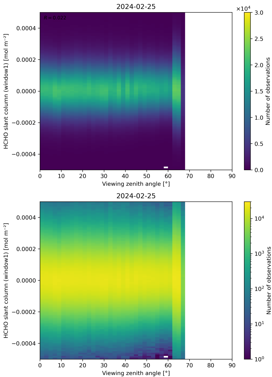
Figure 188: Scatter density plot of “Viewing zenith angle” against “HCHO slant column (window1)” for 2024-02-24 to 2024-02-26.
