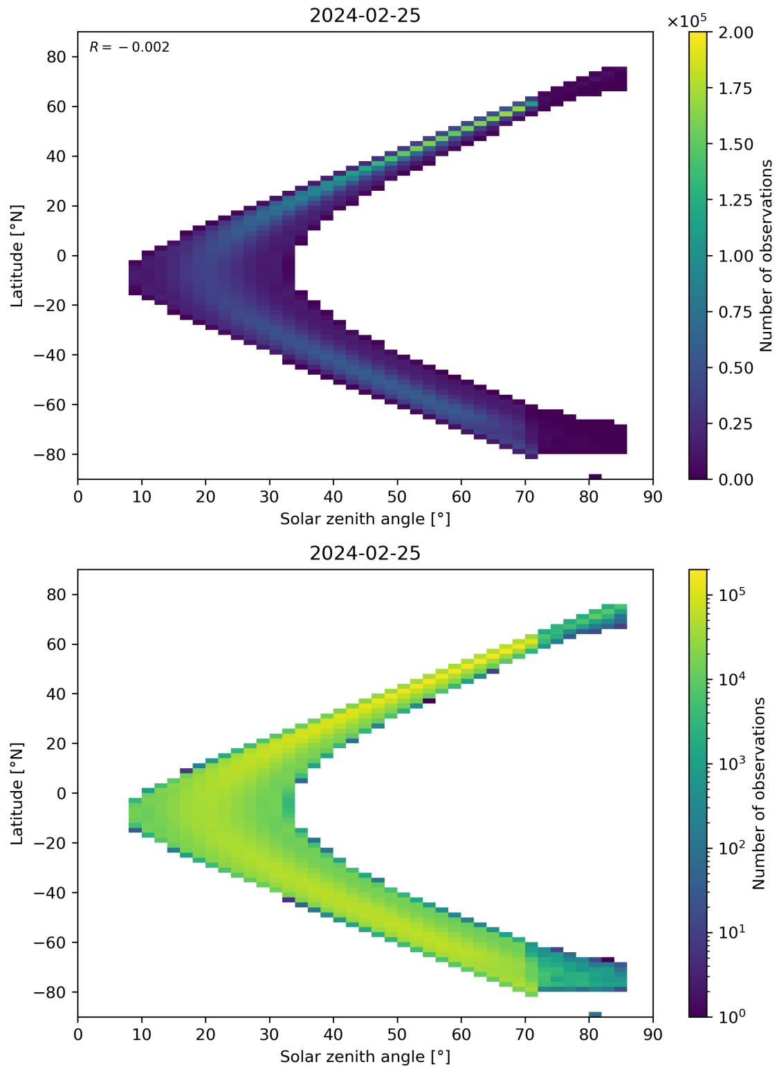
Figure 181: Scatter density plot of “Solar zenith angle” against “Latitude” for 2024-02-24 to 2024-02-26.
