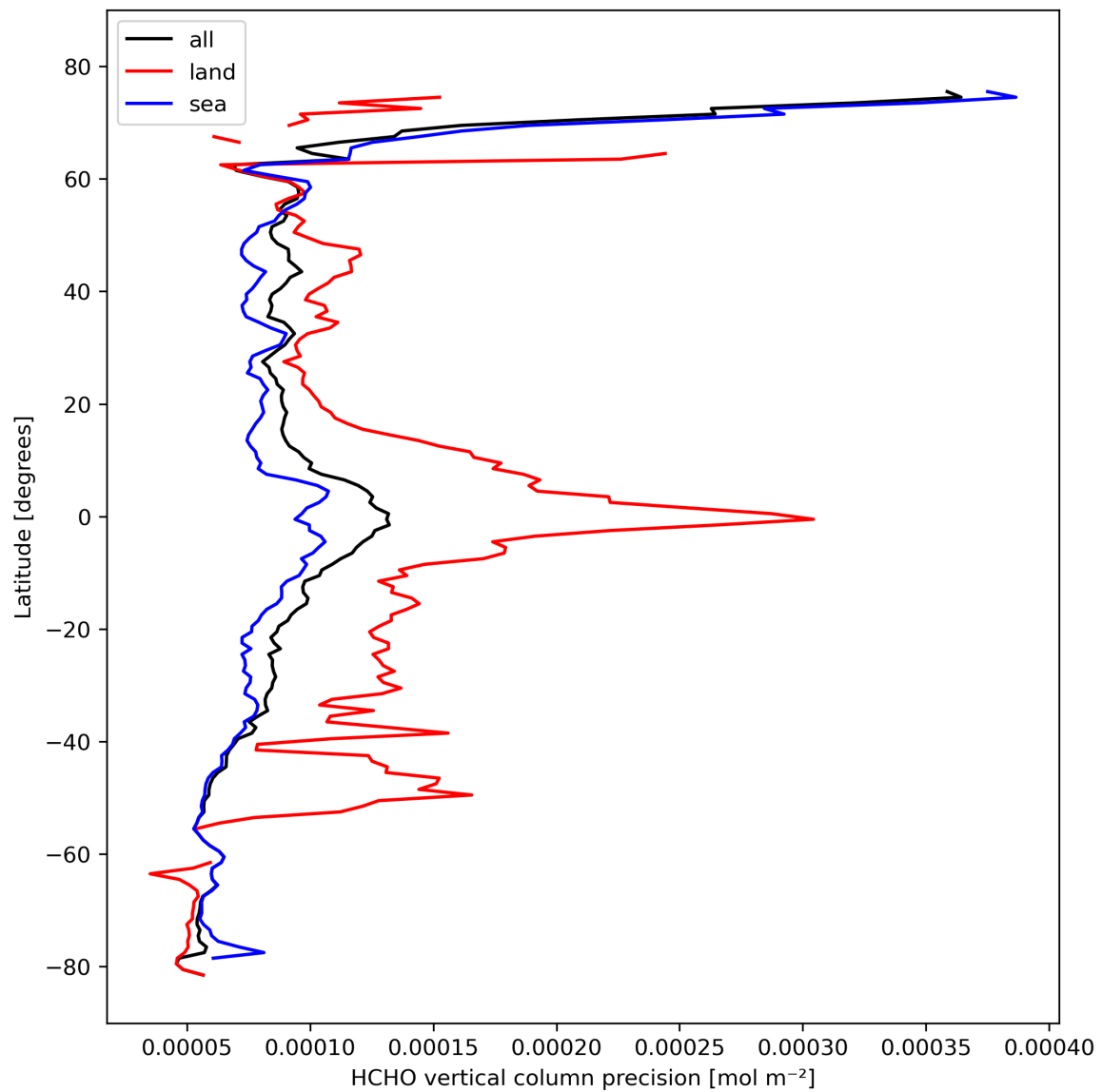
Figure 22: Zonal average of “HCHO vertical column precision” for 2024-02-24 to 2024-02-26.
