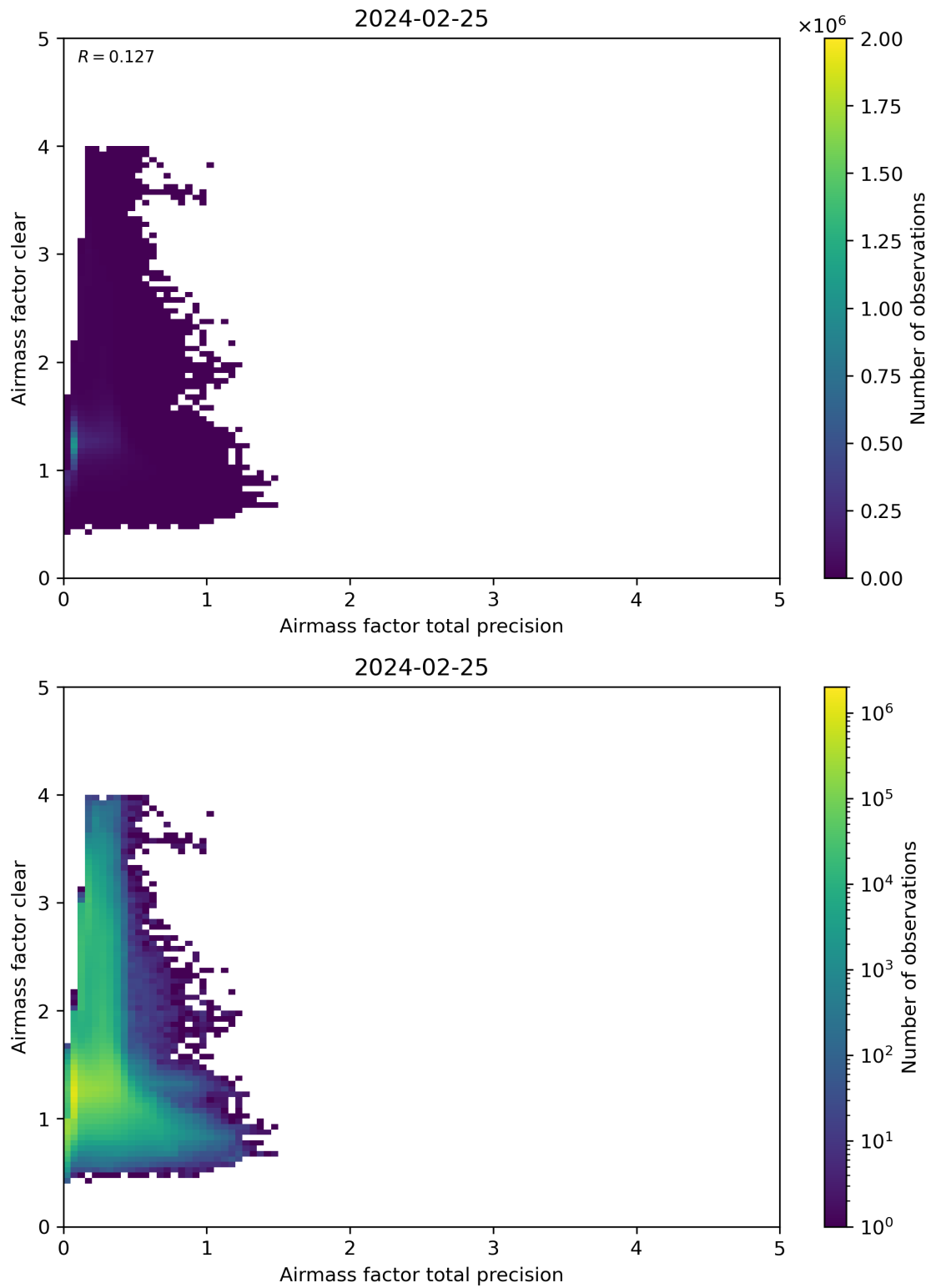
Figure 108: Scatter density plot of “Airmass factor total precision” against “Airmass factor clear” for 2024-02-24 to 2024-02-26.
