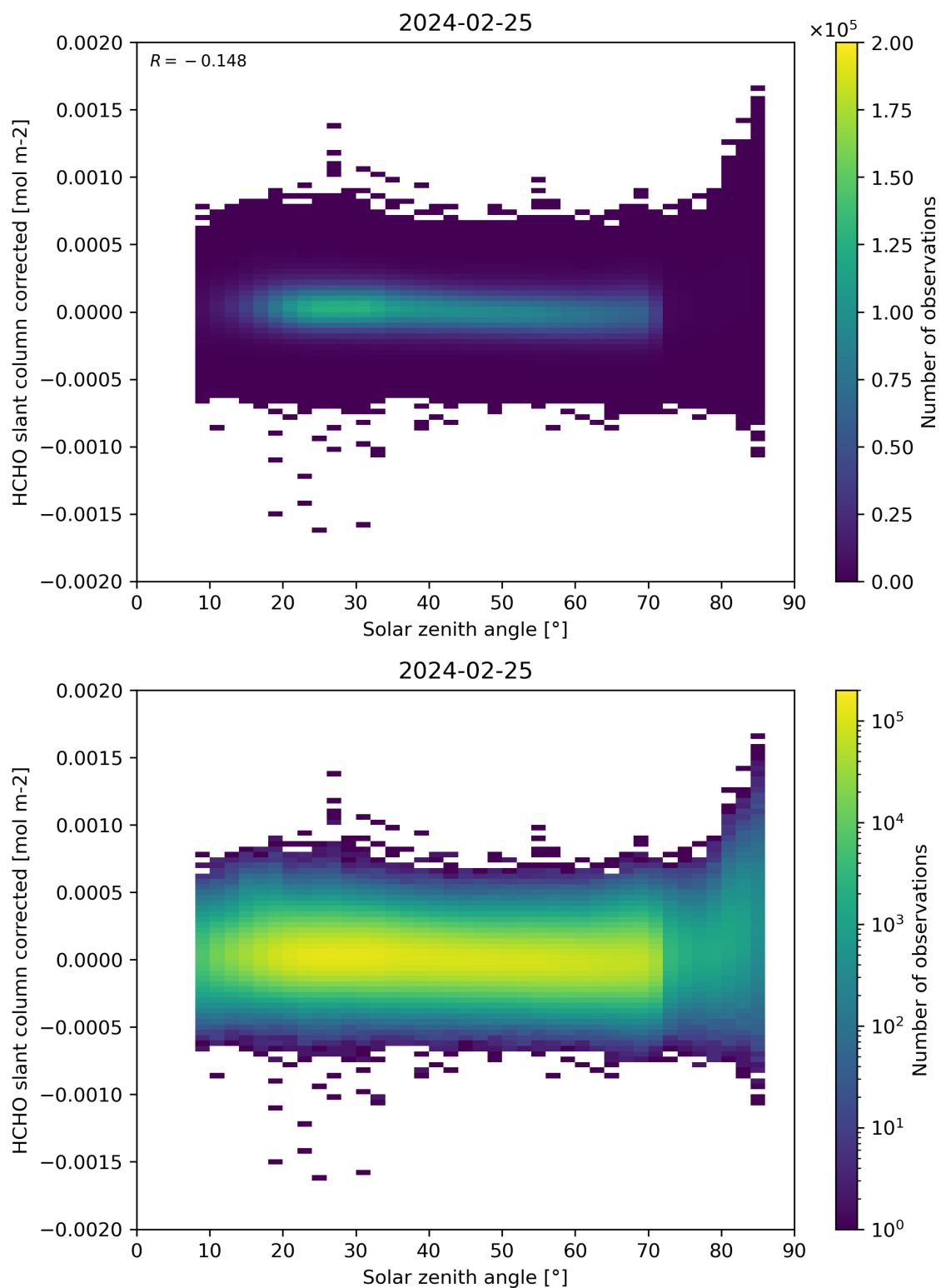
Figure 171: Scatter density plot of “Solar zenith angle” against “HCHO slant column corrected” for 2024-02-24 to 2024-02-26.
