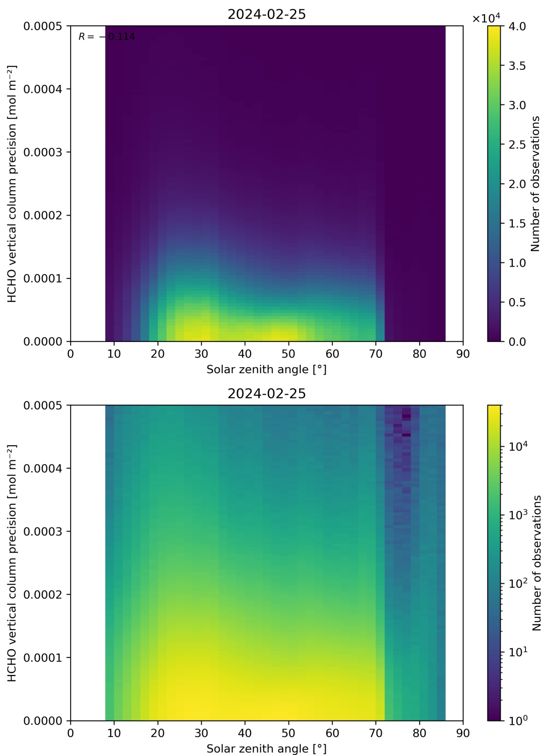
Figure 179: Scatter density plot of “Solar zenith angle” against “HCHO vertical column precision” for 2024-02-24 to 2024-02-26.
