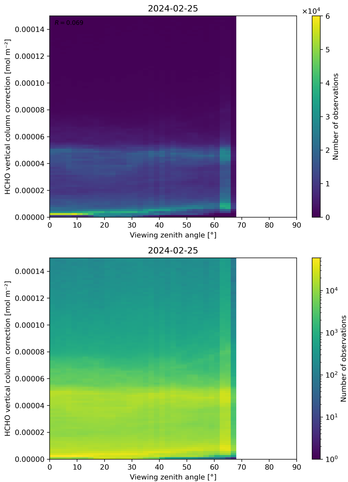
Figure 193: Scatter density plot of “Viewing zenith angle” against “HCHO vertical column correction” for 2024-02-24 to 2024-02-26.
