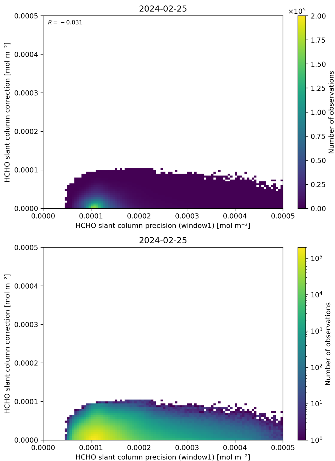
Figure 93: Scatter density plot of “HCHO slant column precision (window1)” against “HCHO slant column correction” for 2024-02-24 to 2024-02-26.
