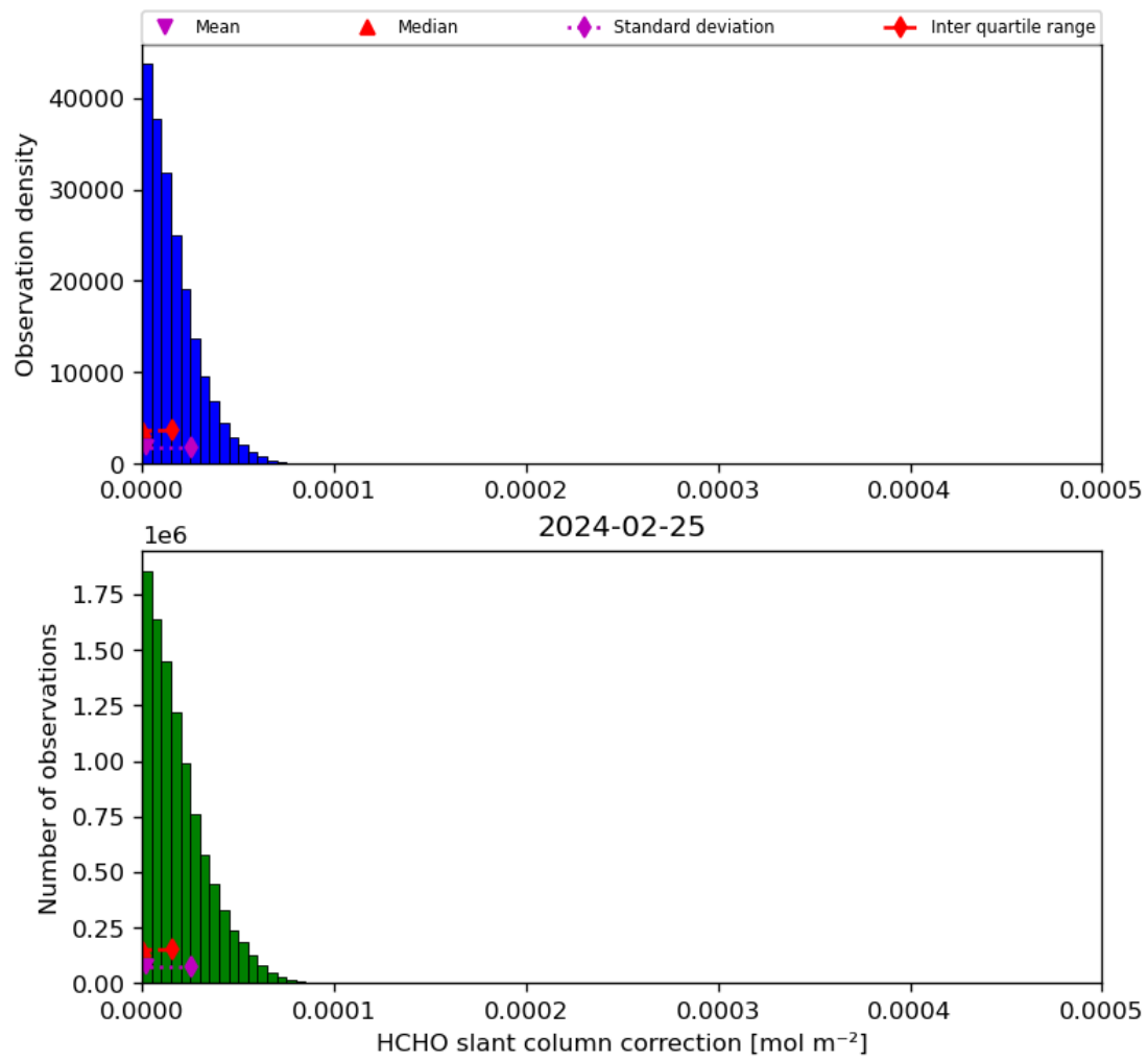
Figure 47: Histogram of “HCHO slant column correction” for 2024-02-24 to 2024-02-26
