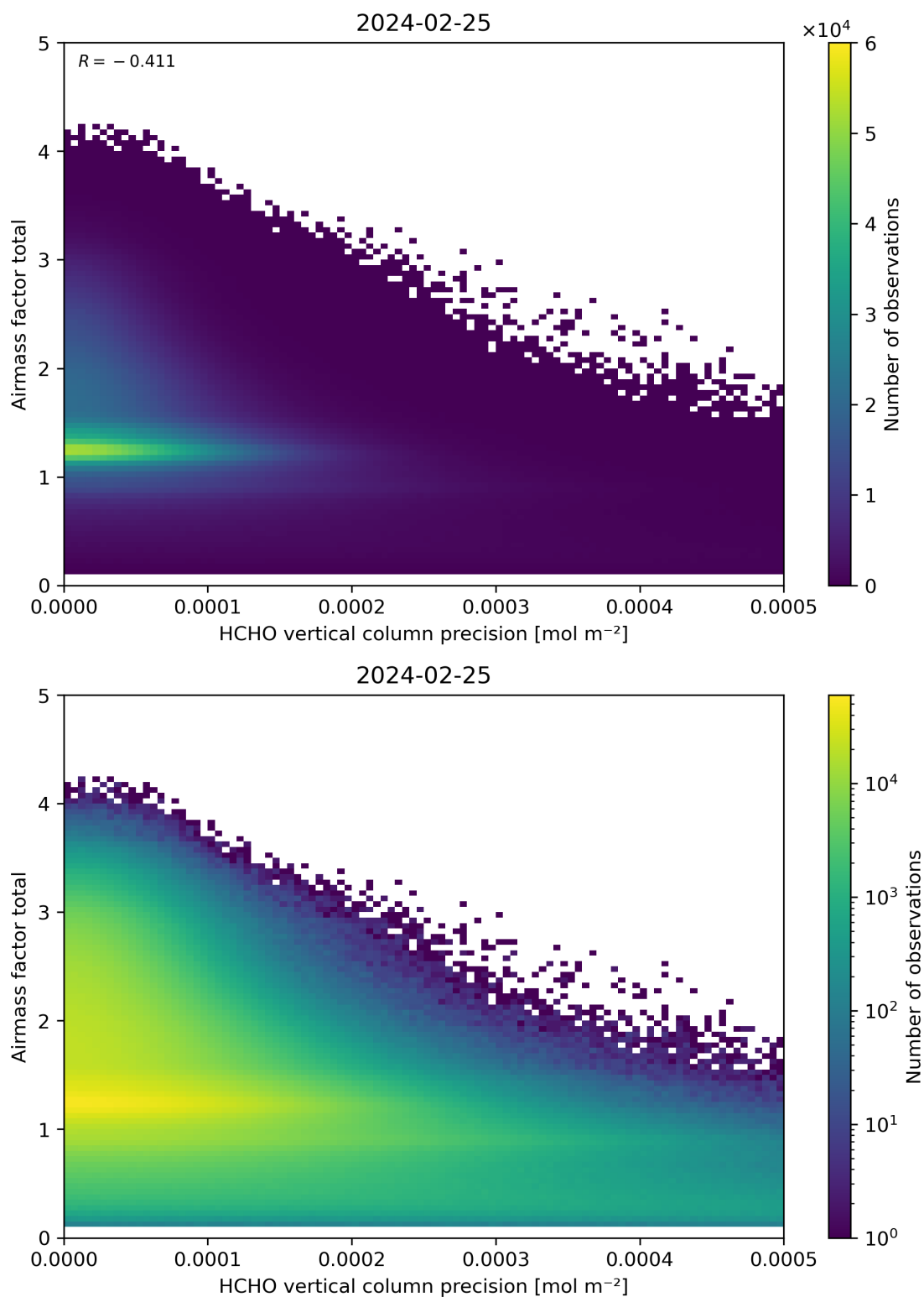
Figure 144: Scatter density plot of “HCHO vertical column precision” against “Airmass factor total” for 2024-02-24 to 2024-02-26.
