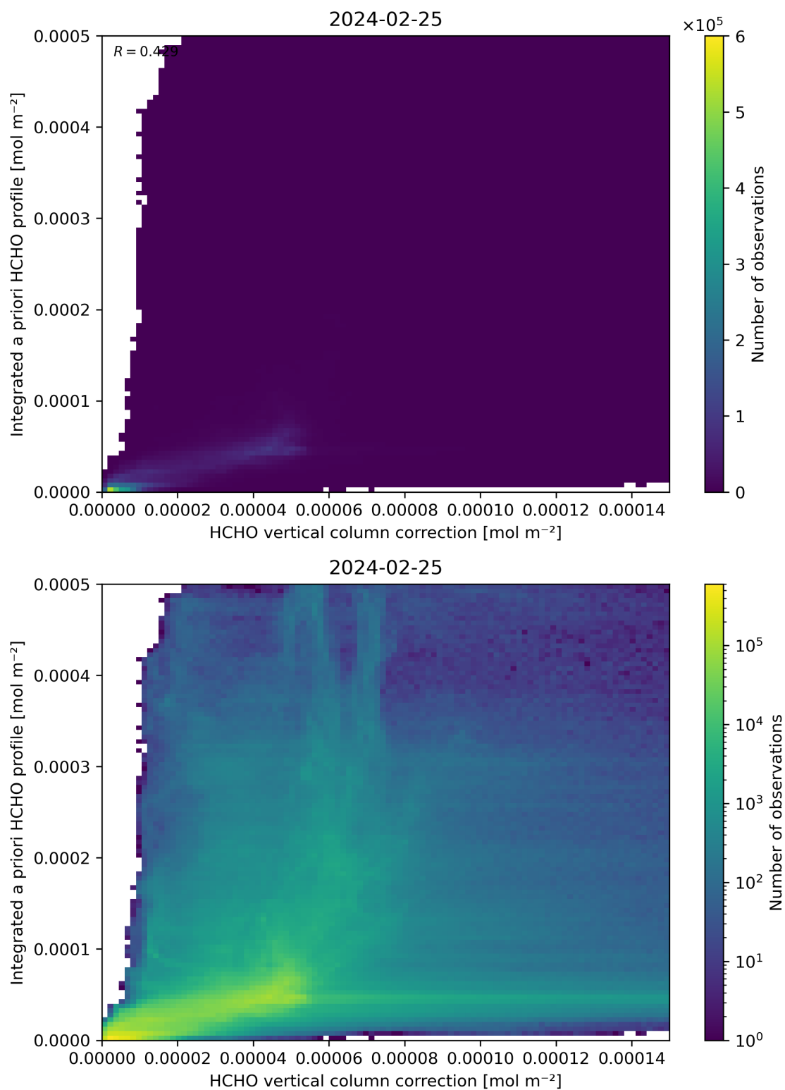
Figure 122: Scatter density plot of “HCHO vertical column correction” against “Integrated a priori HCHO profile” for 2024-02-24 to 2024-02-26.
