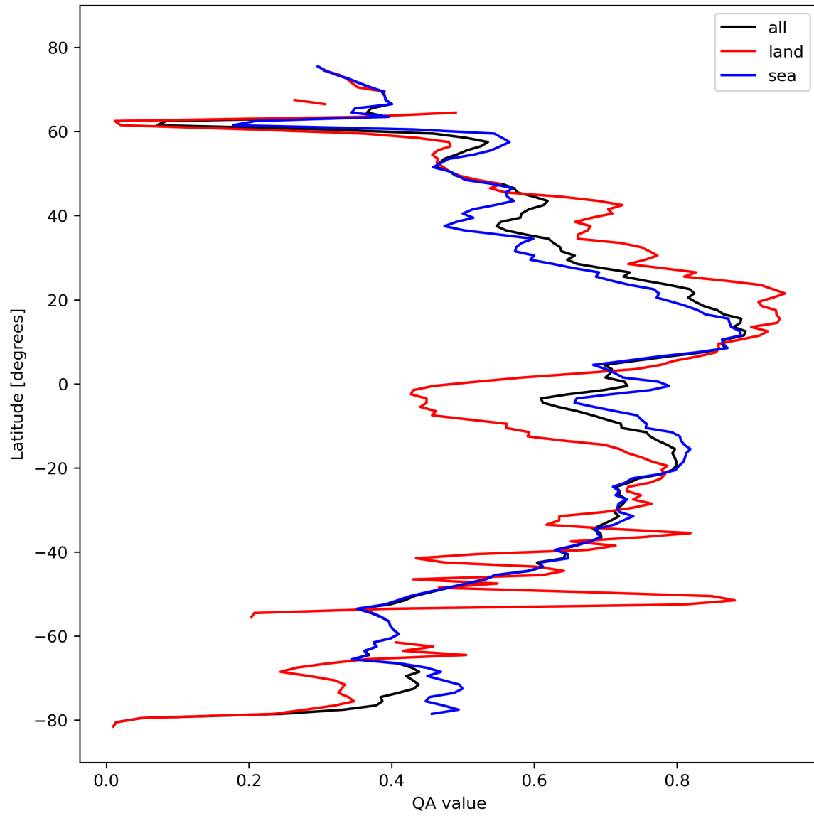
Figure 20: Zonal average of “QA value” for 2024-02-24 to 2024-02-26.
