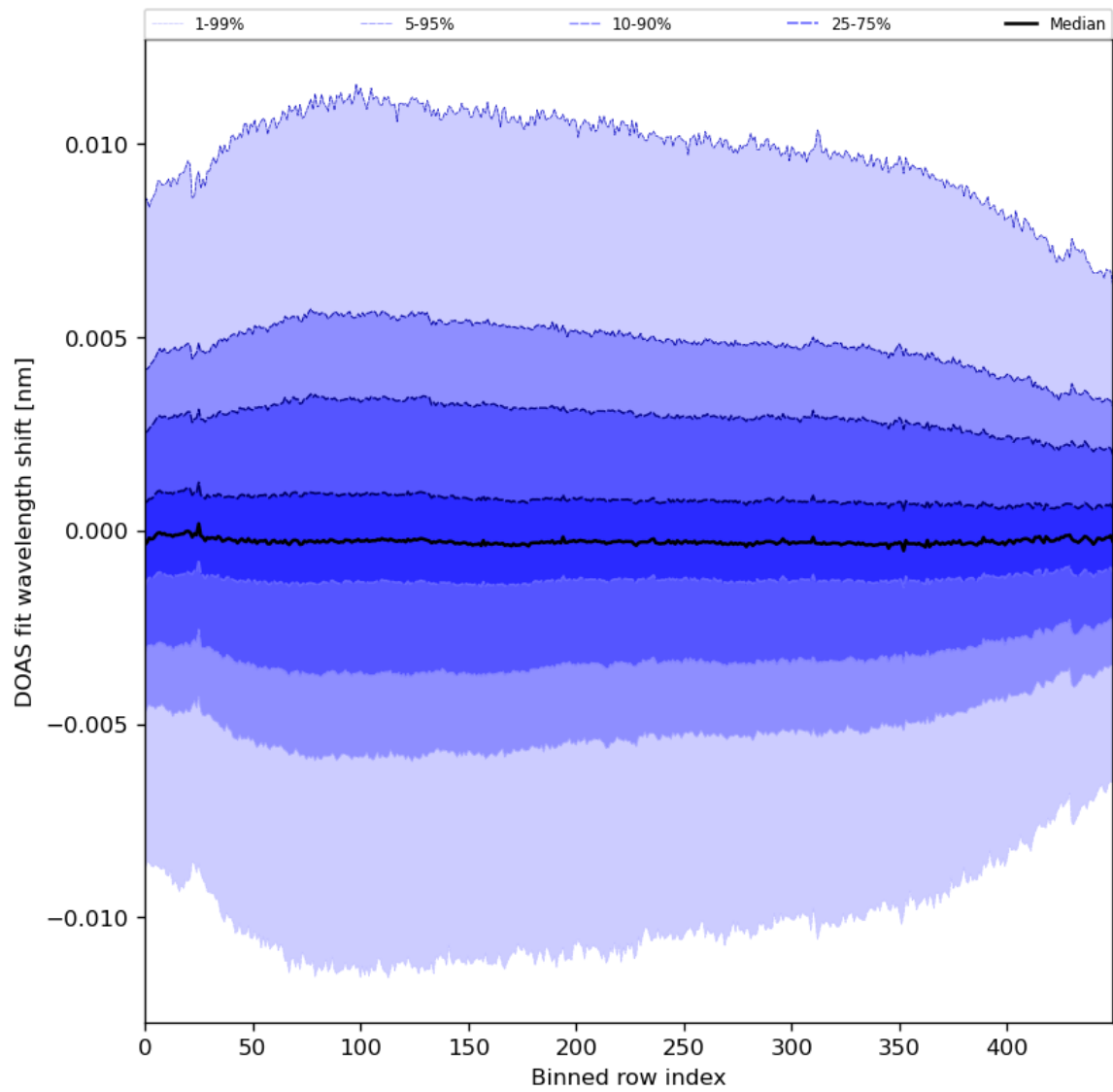
Figure 58: Along track statistics of “DOAS fit wavelength shift” for 2024-02-24 to 2024-02-26
