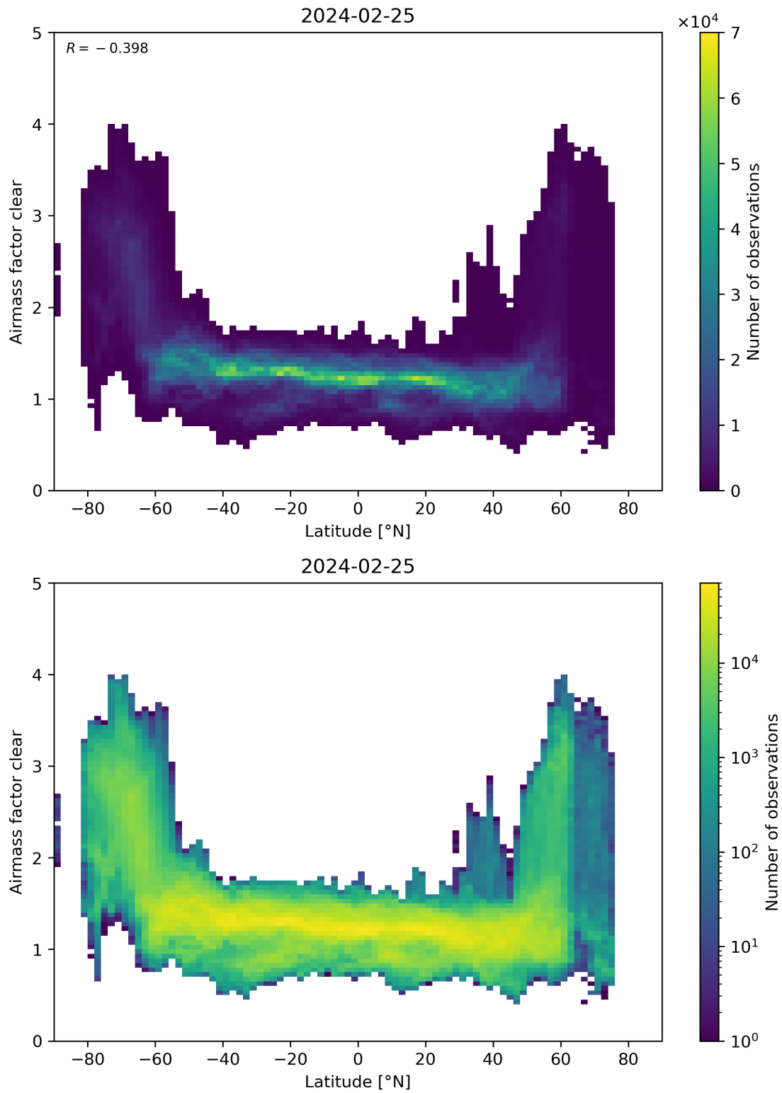
Figure 156: Scatter density plot of “Latitude” against “Airmass factor clear” for 2024-02-24 to 2024-02-26.
