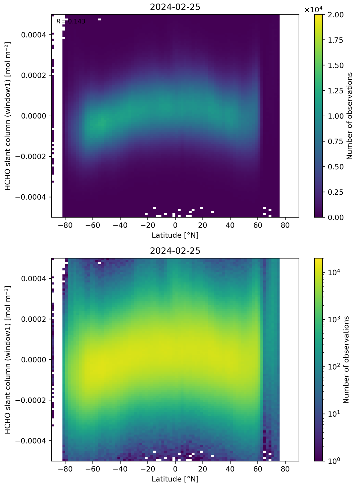
Figure 159: Scatter density plot of “Latitude” against “HCHO slant column (window1)” for 2024-02-24 to 2024-02-26.
