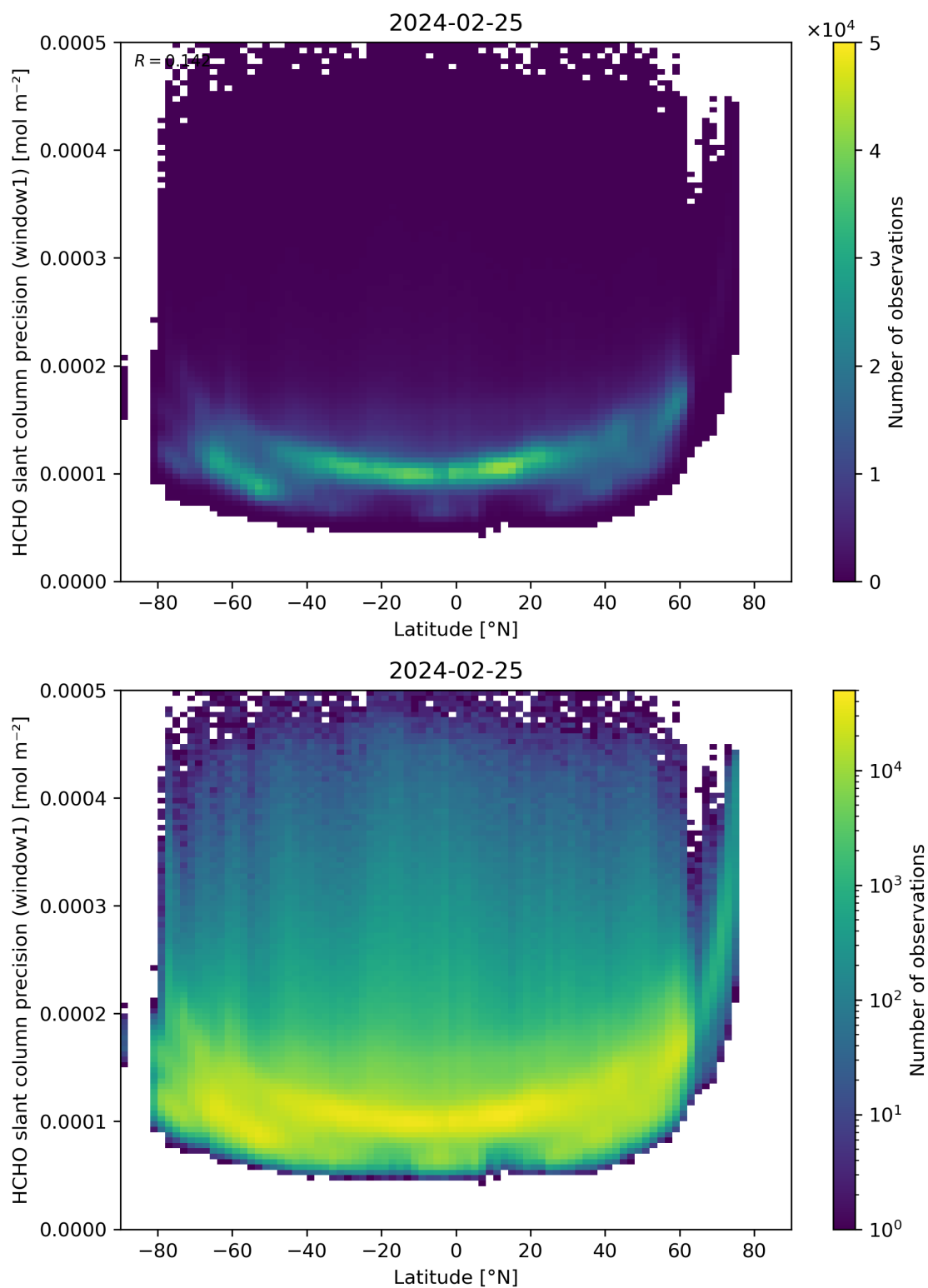
Figure 160: Scatter density plot of “Latitude” against “HCHO slant column precision (window1)” for 2024-02-24 to 2024-02-26.
