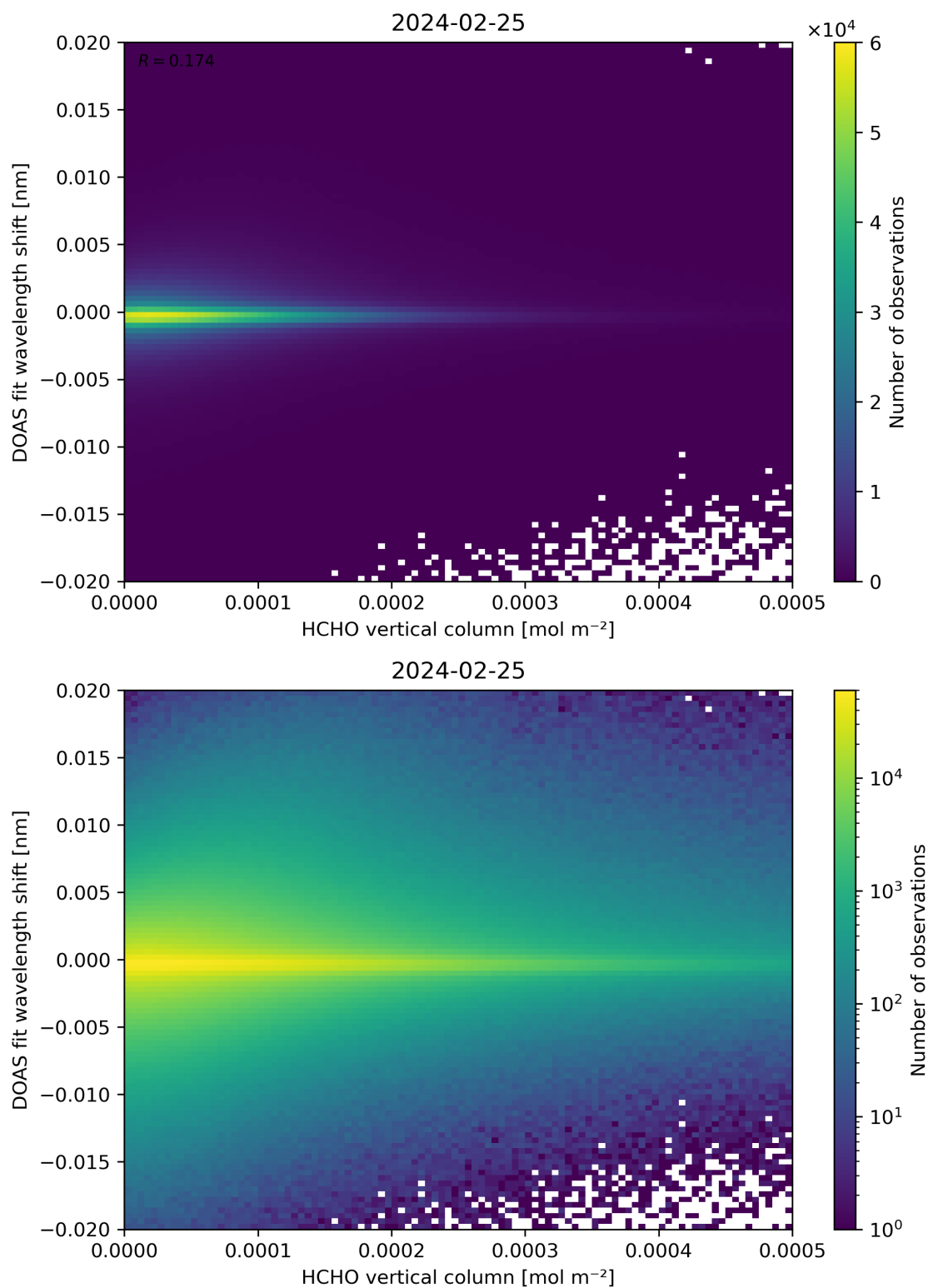
Figure 124: Scatter density plot of “HCHO vertical column” against “DOAS fit wavelength shift” for 2024-02-24 to 2024-02-26.
