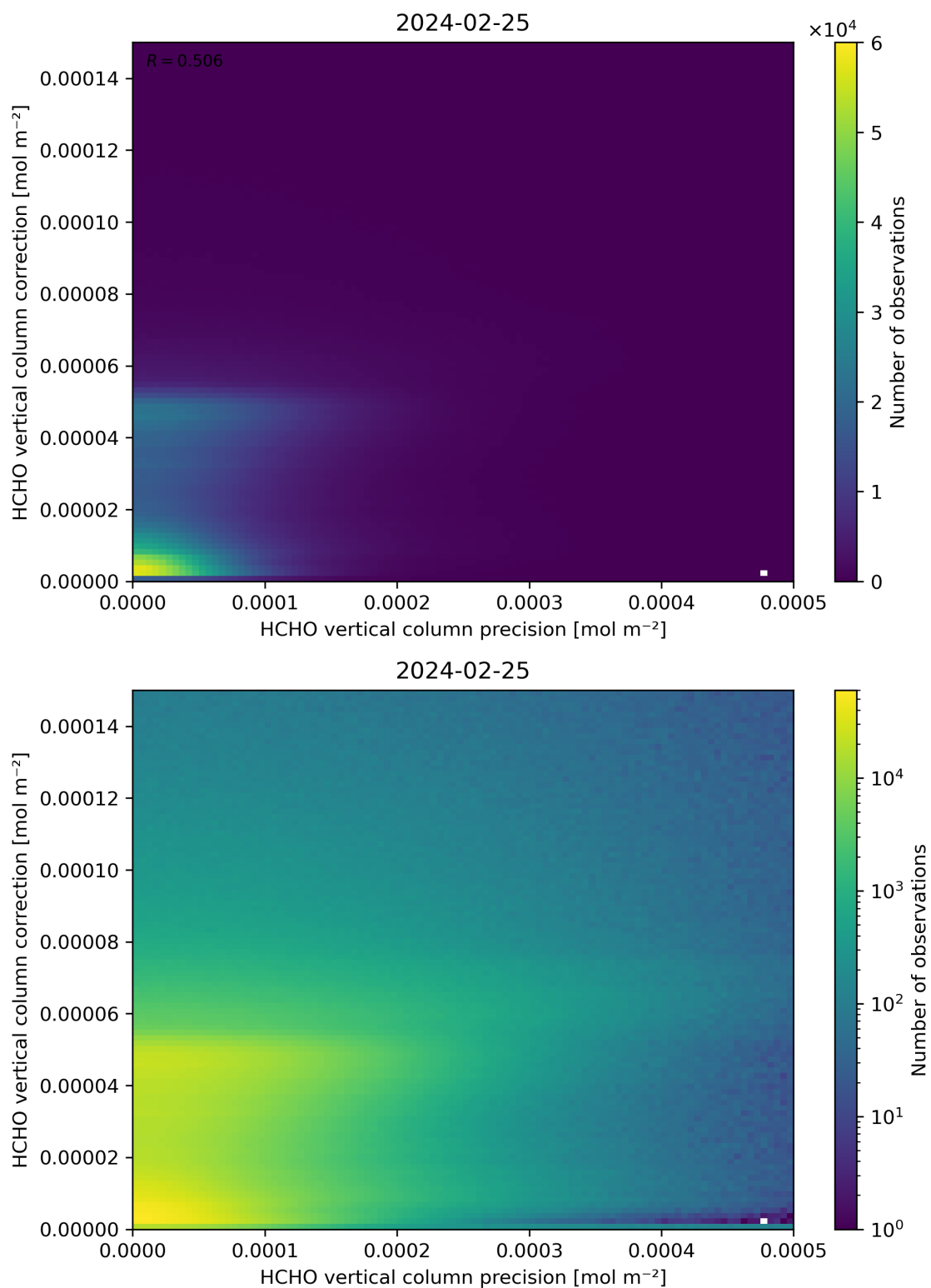
Figure 146: Scatter density plot of “HCHO vertical column precision” against “HCHO vertical column correction” for 2024-02-24 to 2024-02-26.
