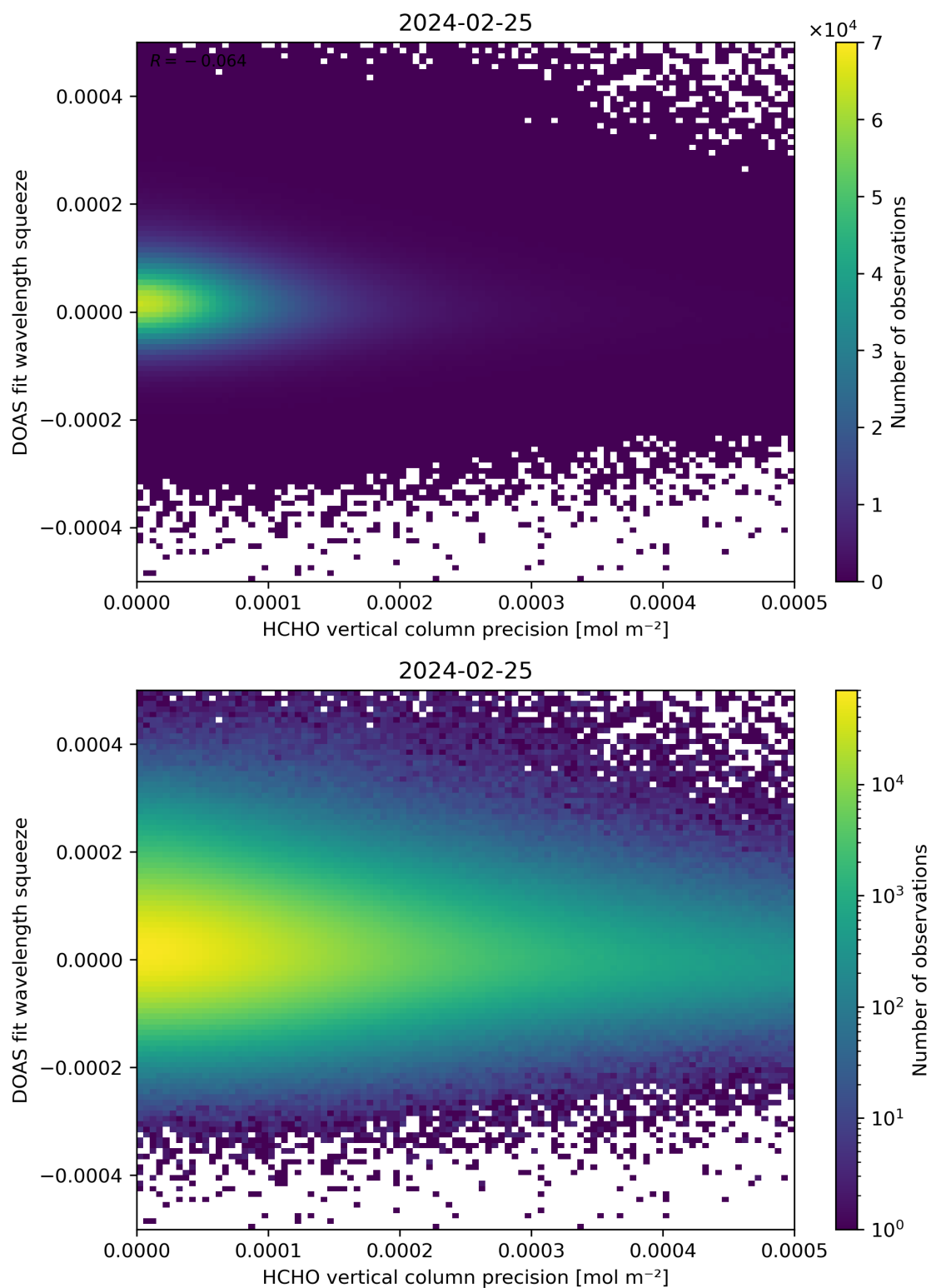
Figure 138: Scatter density plot of “HCHO vertical column precision” against “DOAS fit wavelength squeeze” for 2024-02-24 to 2024-02-26.
