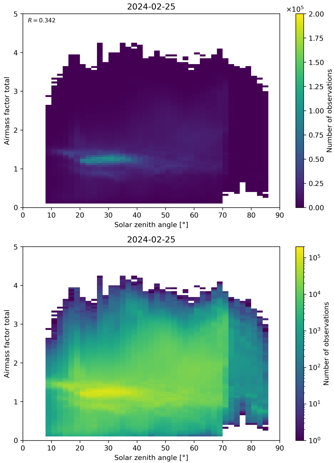
Figure 175: Scatter density plot of “Solar zenith angle” against “Airmass factor total” for 2024-02-24 to 2024-02-26.
