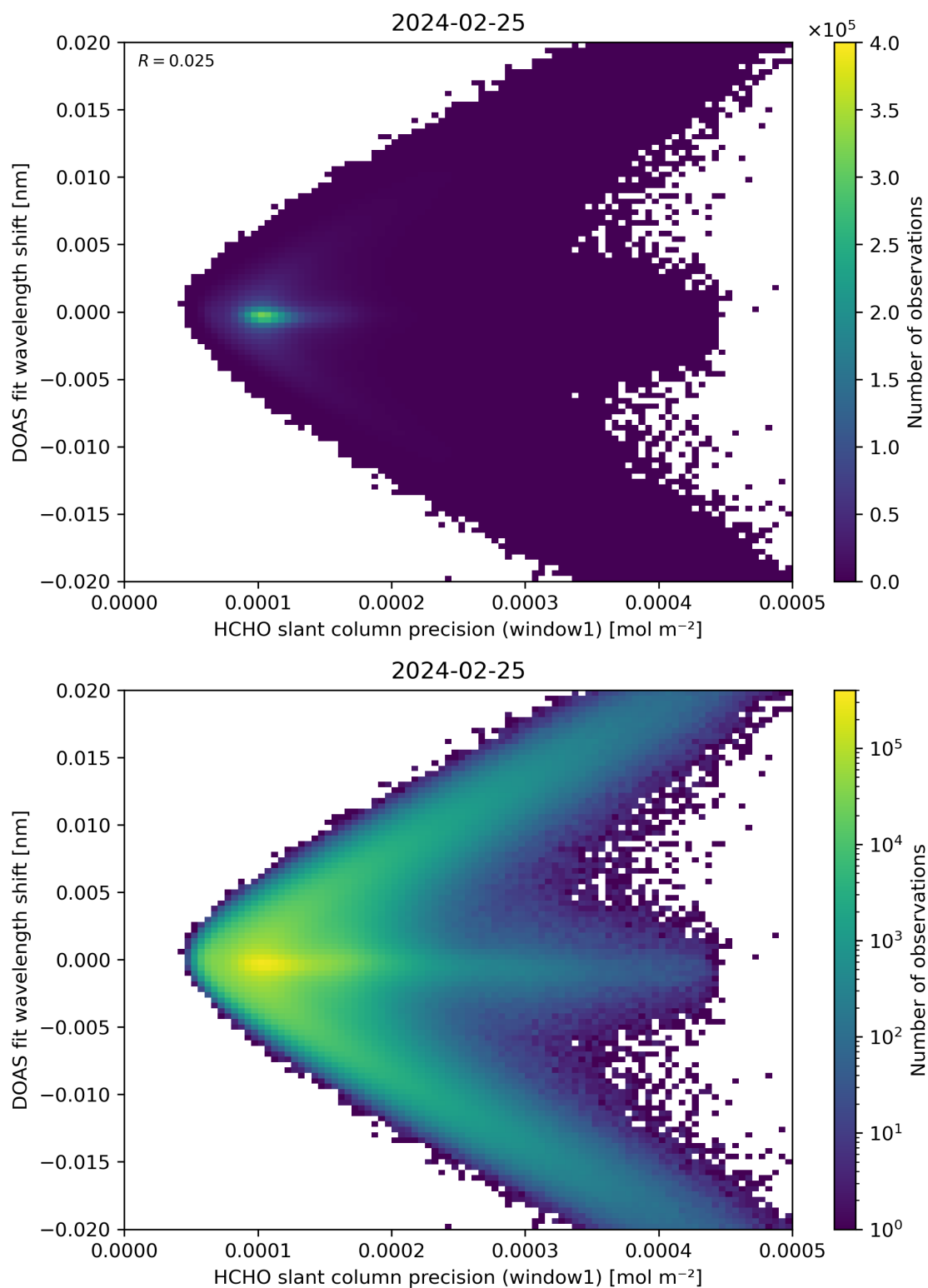
Figure 89: Scatter density plot of “HCHO slant column precision (window1)” against “DOAS fit wavelength shift” for 2024-02-24 to 2024-02-26.
