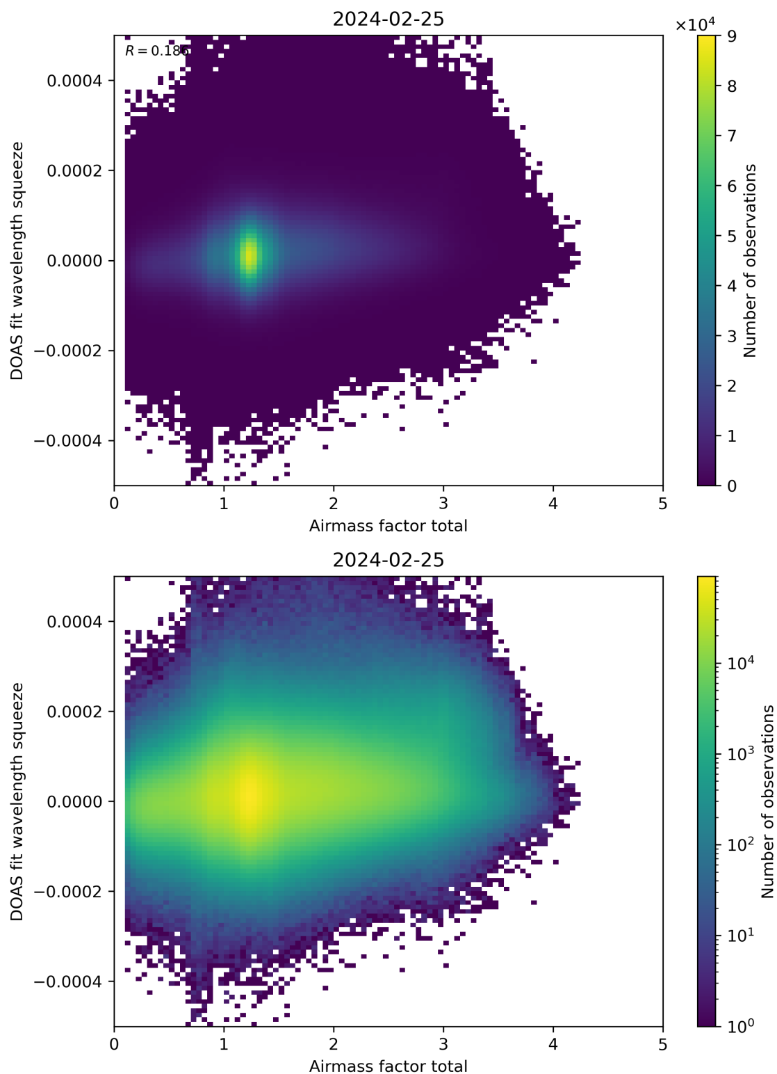
Figure 99: Scatter density plot of “Airmass factor total” against “DOAS fit wavelength squeeze” for 2024-02-24 to 2024-02-26.
