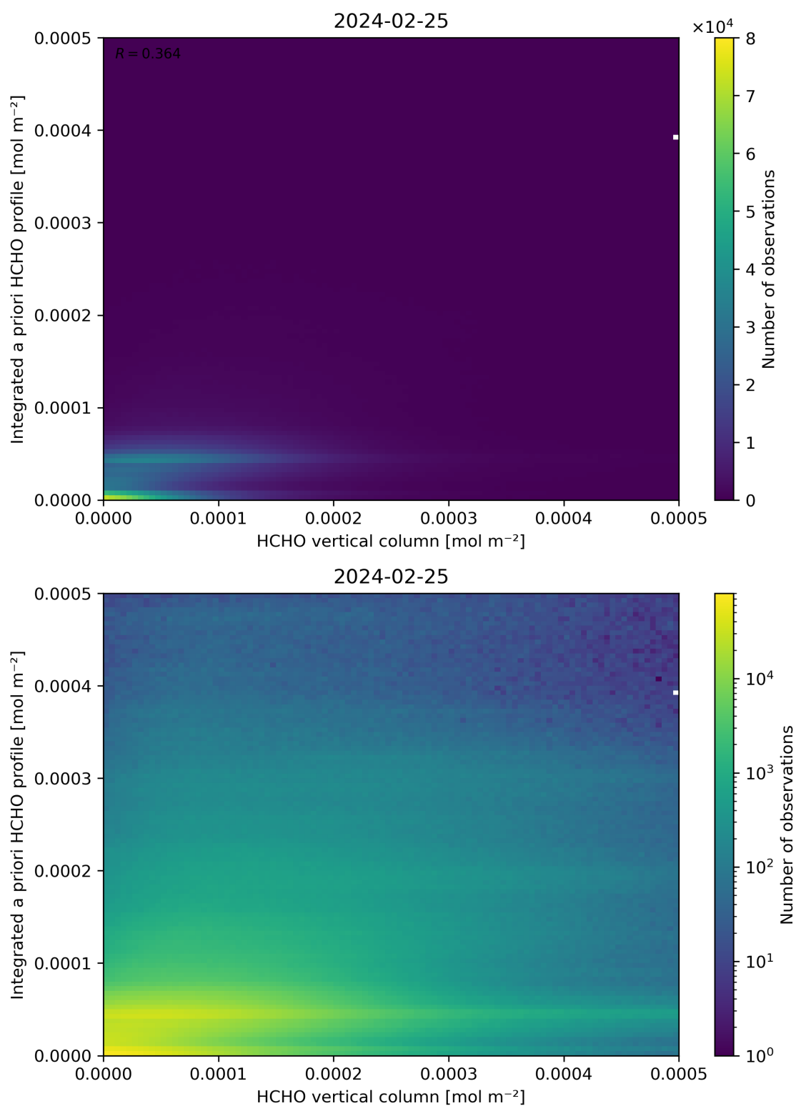
Figure 135: Scatter density plot of “HCHO vertical column” against “Integrated a priori HCHO profile” for 2024-02-24 to 2024-02-26.
