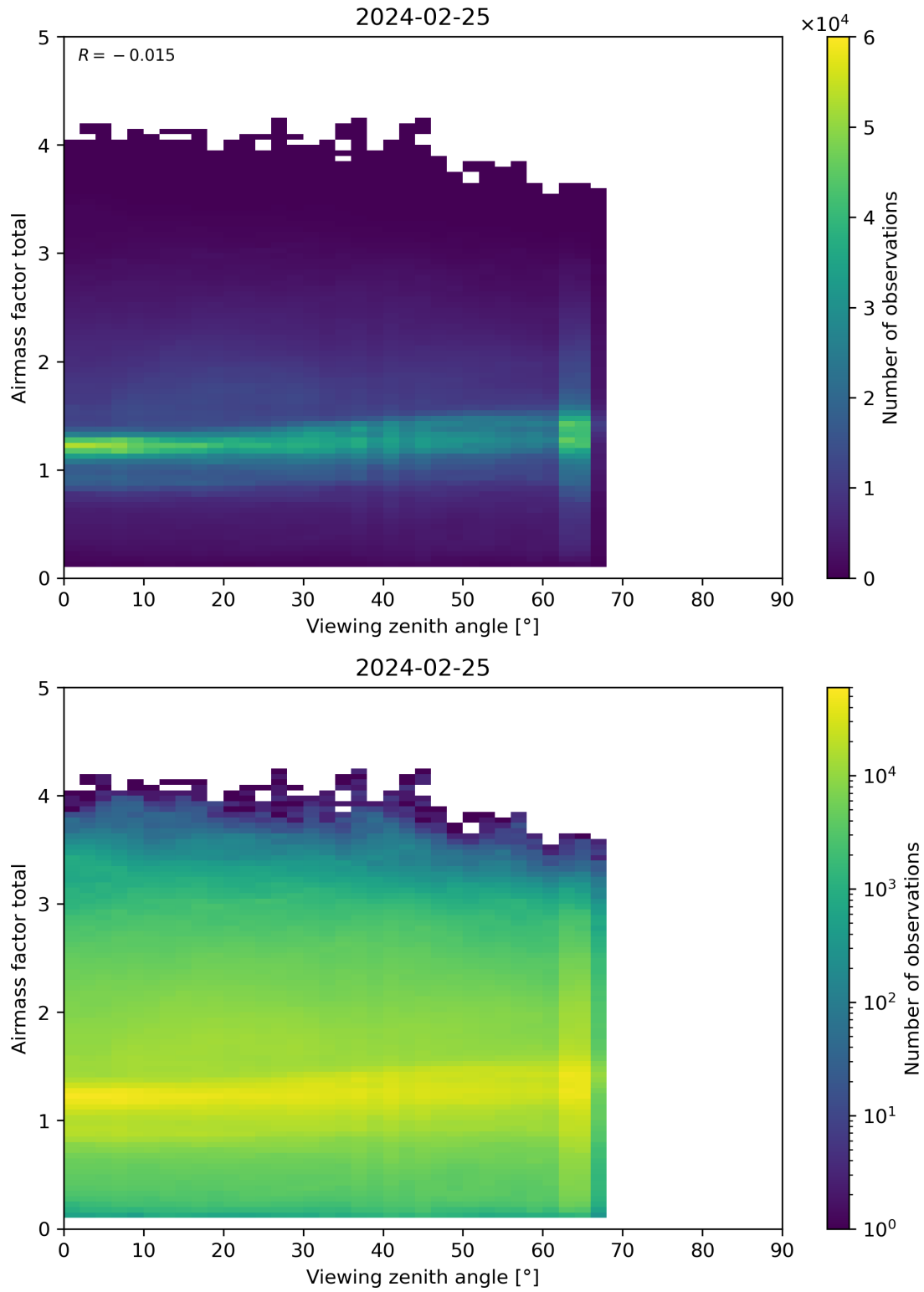
Figure 190: Scatter density plot of “Viewing zenith angle” against “Airmass factor total” for 2024-02-24 to 2024-02-26.
