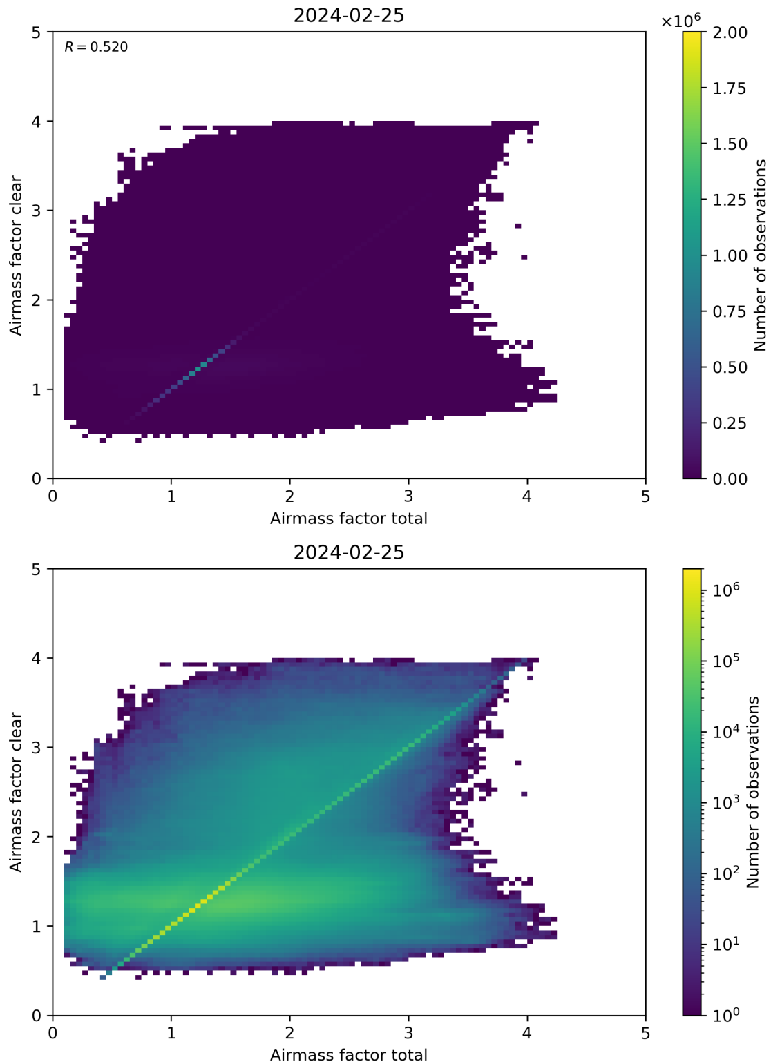
Figure 100: Scatter density plot of “Airmass factor total” against “Airmass factor clear” for 2024-02-24 to 2024-02-26.
