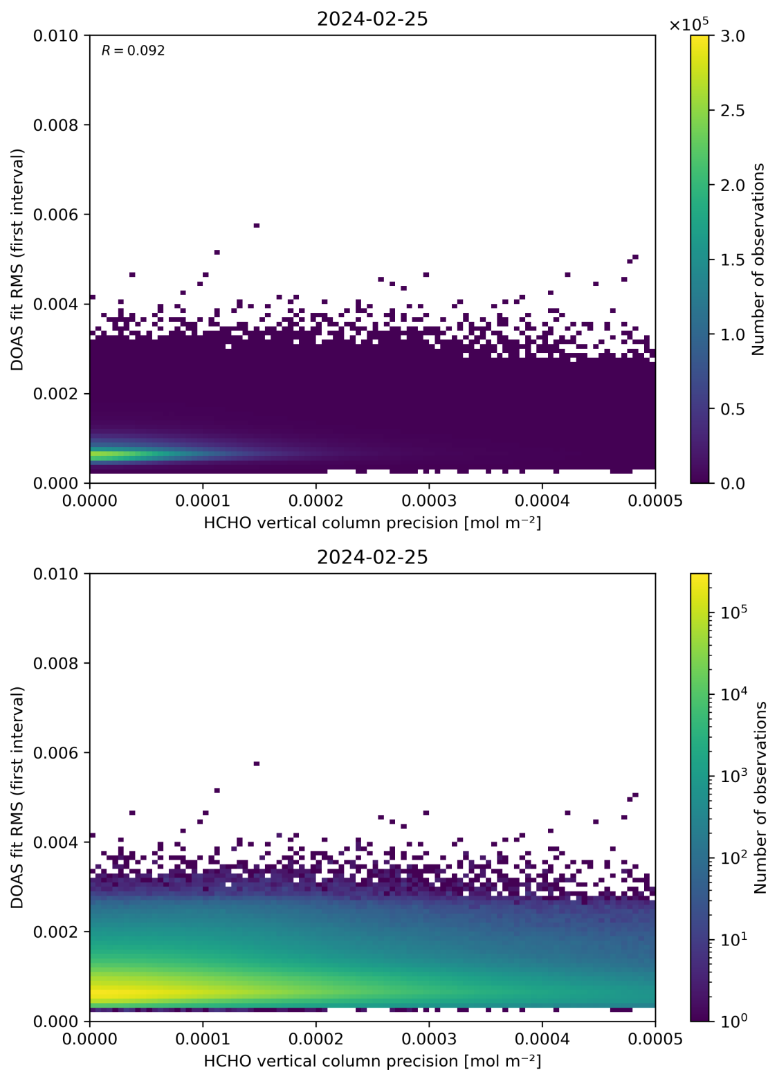
Figure 136: Scatter density plot of “HCHO vertical column precision” against “DOAS fit RMS (first interval)” for 2024-02-24 to 2024-02-26.
