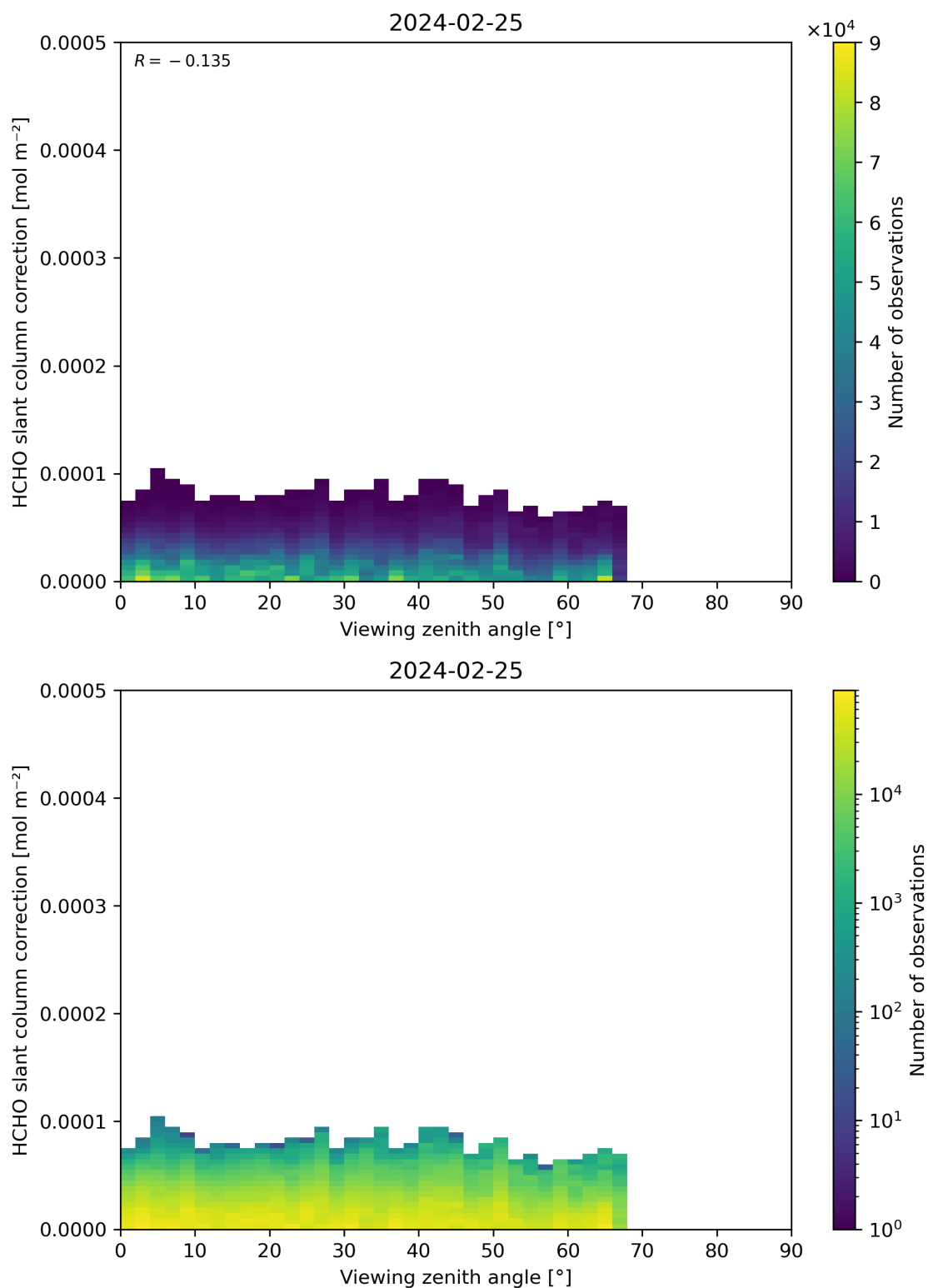
Figure 187: Scatter density plot of “Viewing zenith angle” against “HCHO slant column correction” for 2024-02-24 to 2024-02-26.
