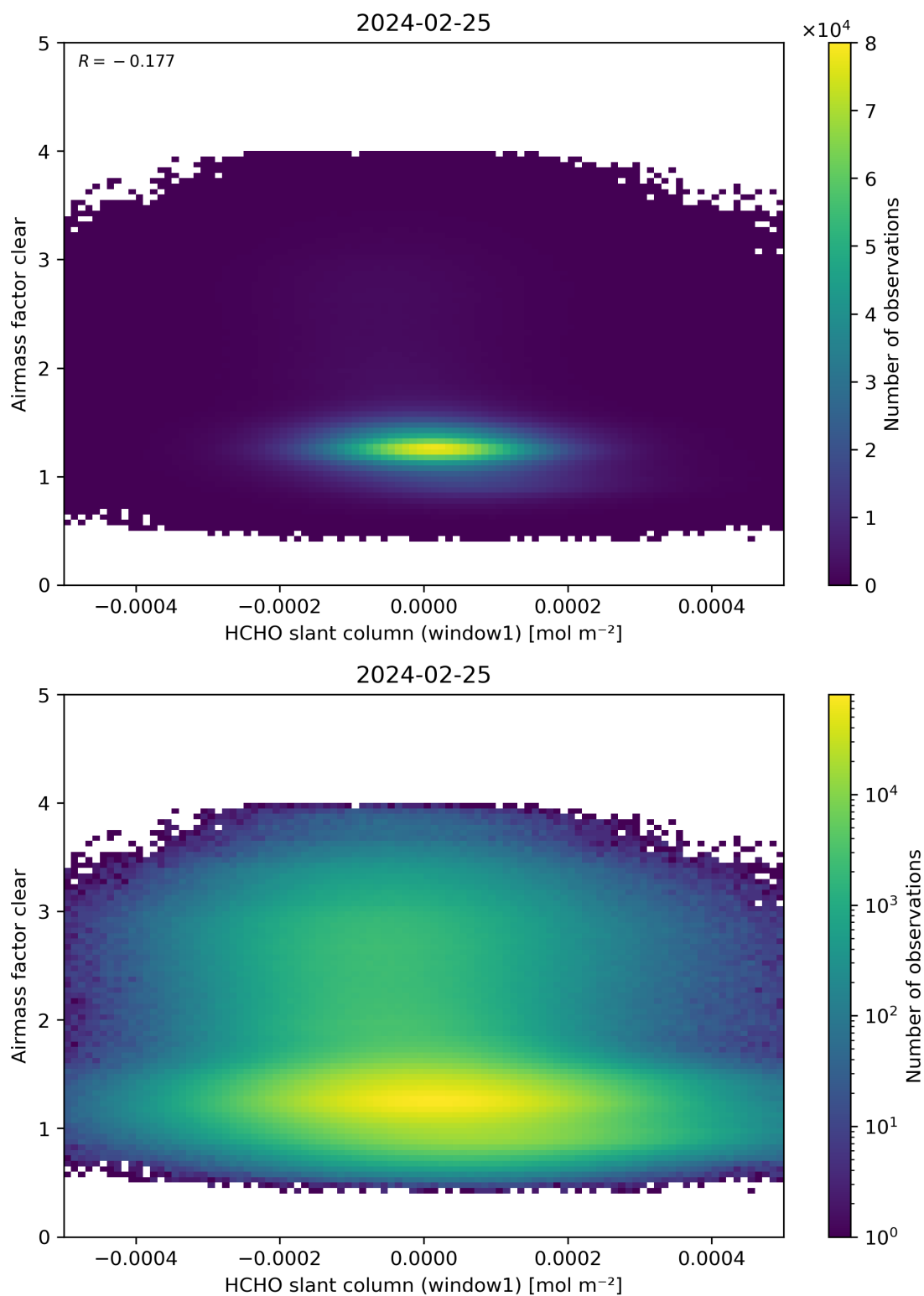
Figure 81: Scatter density plot of “HCHO slant column (window1)” against “Airmass factor clear” for 2024-02-24 to 2024-02-26.
