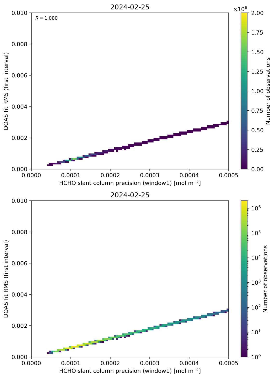
Figure 88: Scatter density plot of “HCHO slant column precision (window1)” against “DOAS fit RMS (first interval)” for 2024-02-24 to 2024-02-26.
