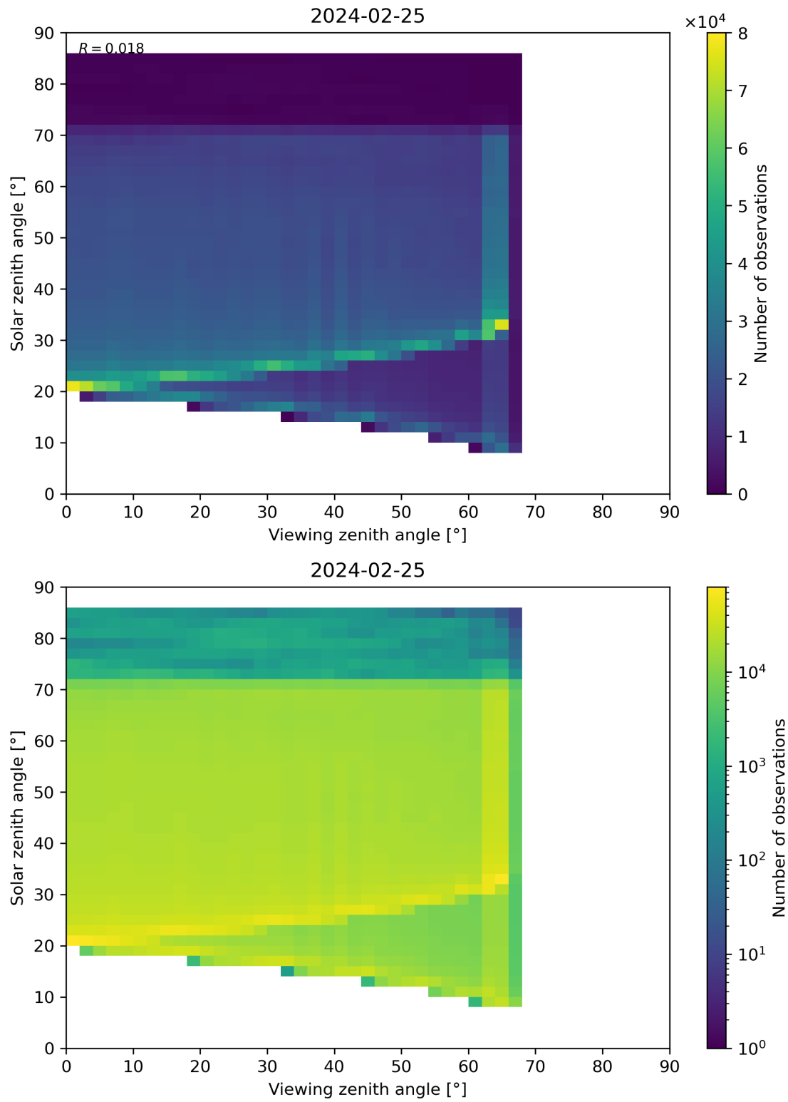
Figure 197: Scatter density plot of “Viewing zenith angle” against “Solar zenith angle” for 2024-02-24 to 2024-02-26.
