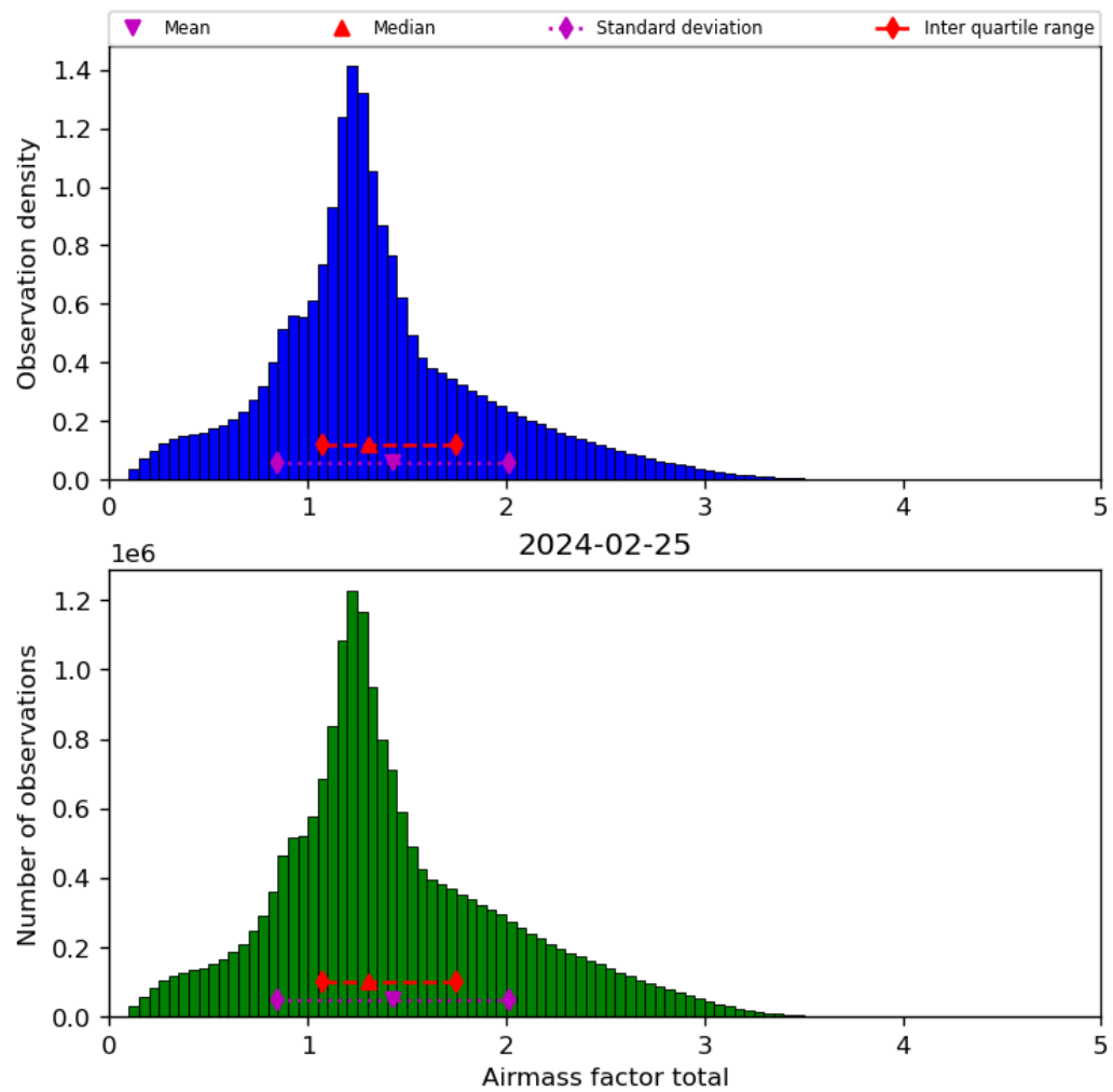
Figure 40: Histogram of “Airmass factor total” for 2024-02-24 to 2024-02-26
