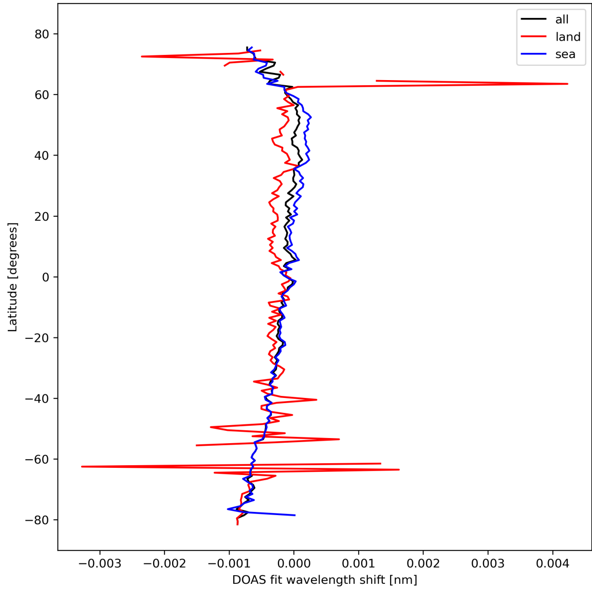
Figure 30: Zonal average of “DOAS fit wavelength shift” for 2024-02-24 to 2024-02-26.
