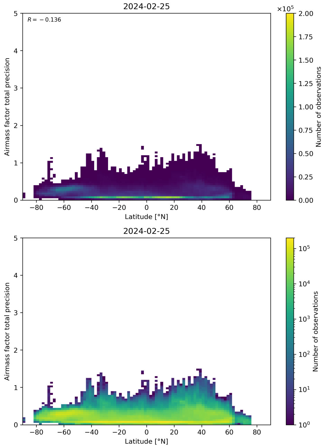
Figure 162: Scatter density plot of “Latitude” against “Airmass factor total precision” for 2024-02-24 to 2024-02-26.
