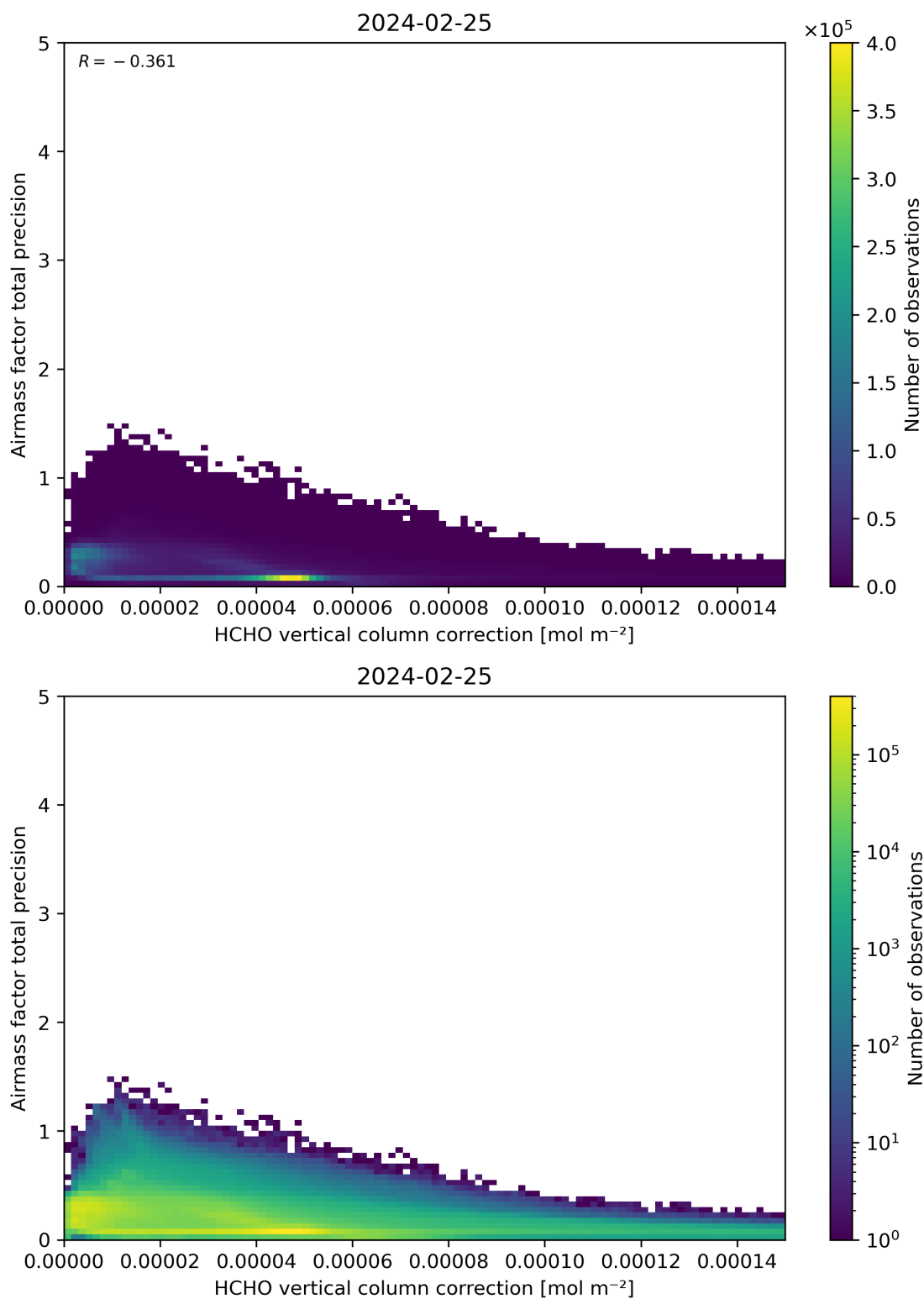
Figure 121: Scatter density plot of “HCHO vertical column correction” against “Airmass factor total precision” for 2024-02-24 to 2024-02-26.
