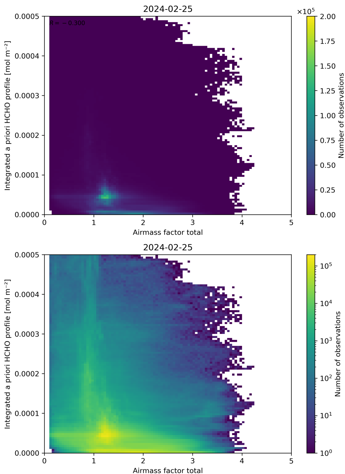
Figure 104: Scatter density plot of “Airmass factor total” against “Integrated a priori HCHO profile” for 2024-02-24 to 2024-02-26.
