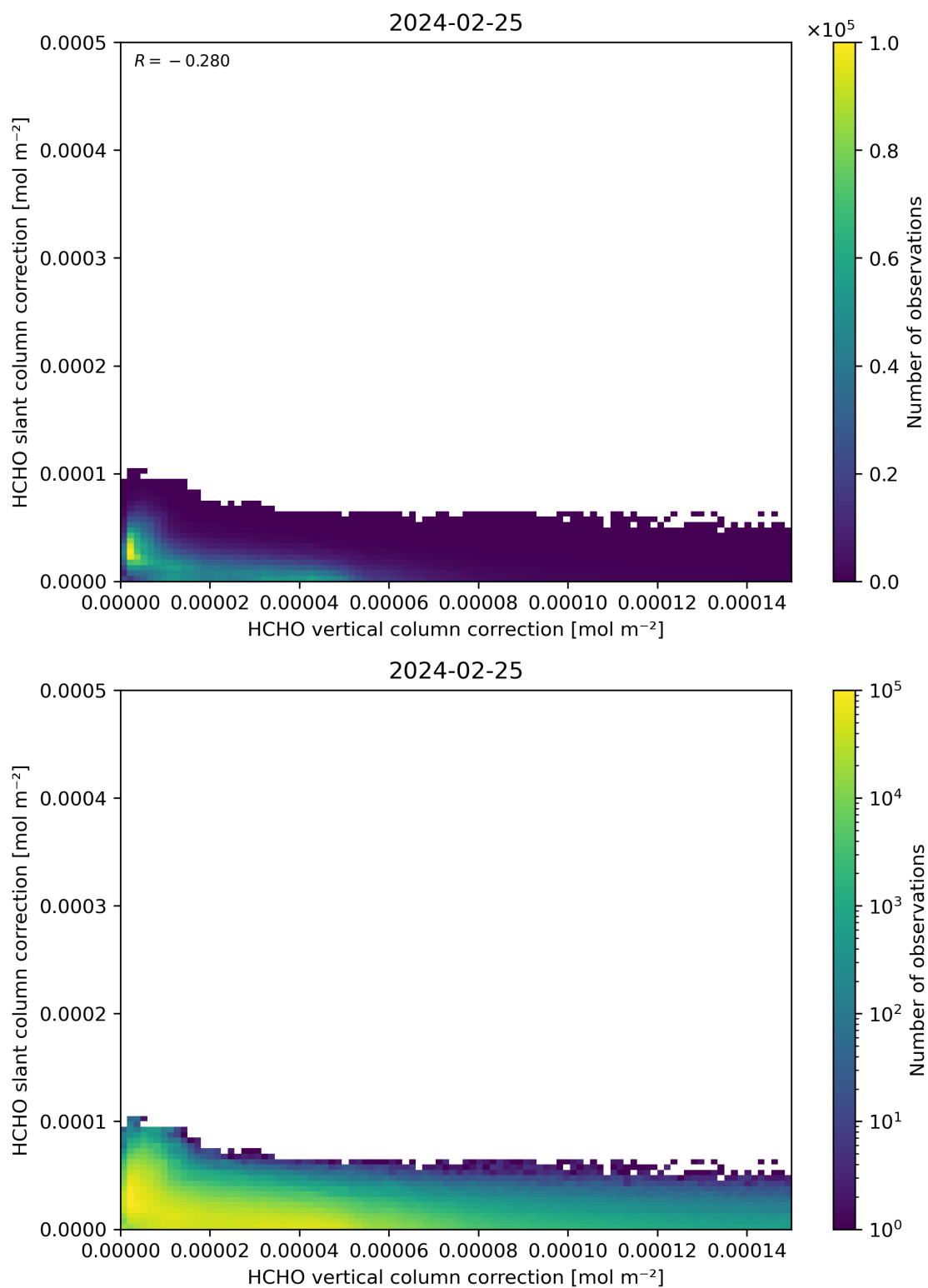
Figure 117: Scatter density plot of “HCHO vertical column correction” against “HCHO slant column correction” for 2024-02-24 to 2024-02-26.
