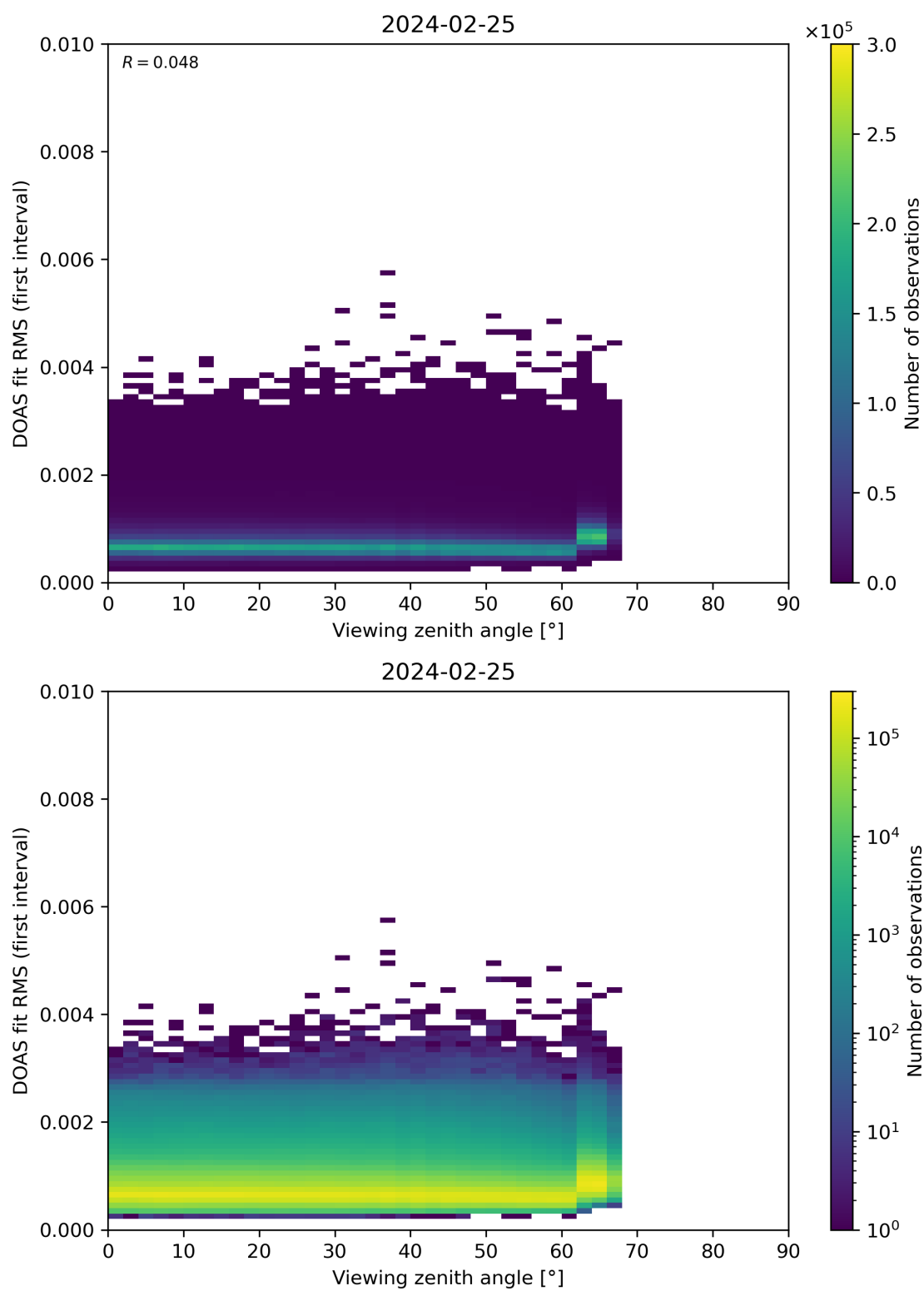
Figure 182: Scatter density plot of “Viewing zenith angle” against “DOAS fit RMS (first interval)” for 2024-02-24 to 2024-02-26.
