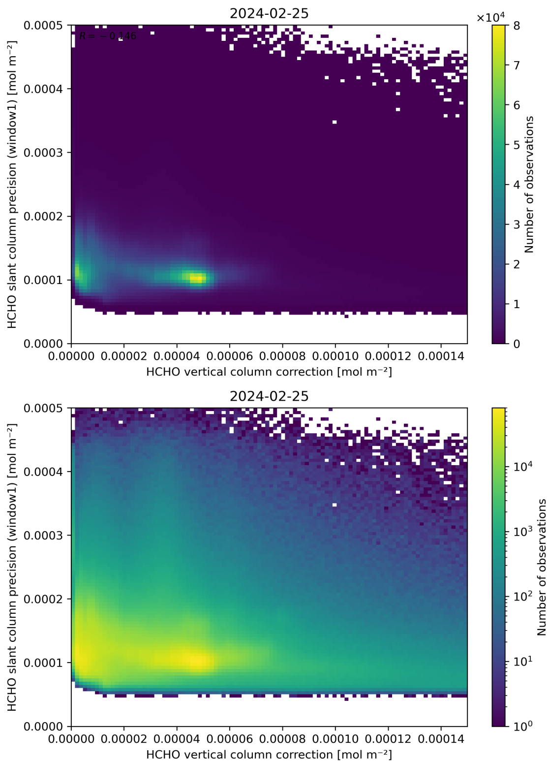
Figure 119: Scatter density plot of “HCHO vertical column correction” against “HCHO slant column precision (window1)” for 2024-02-24 to 2024-02-26.
