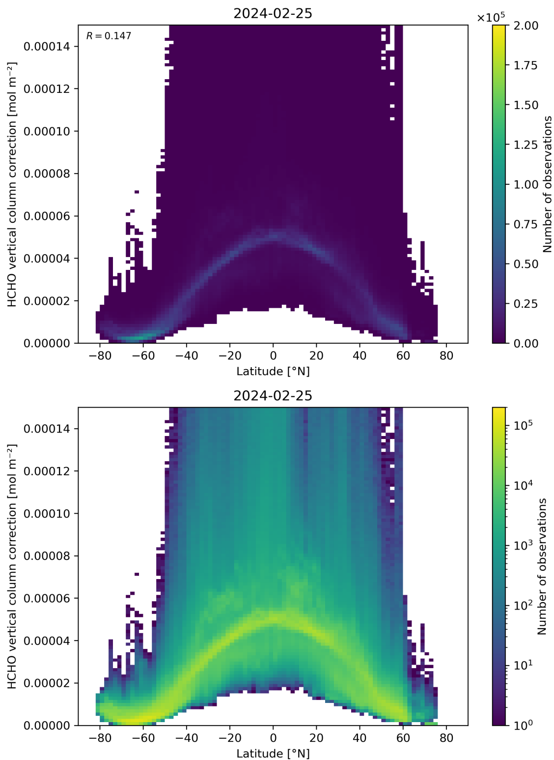
Figure 164: Scatter density plot of “Latitude” against “HCHO vertical column correction” for 2024-02-24 to 2024-02-26.
