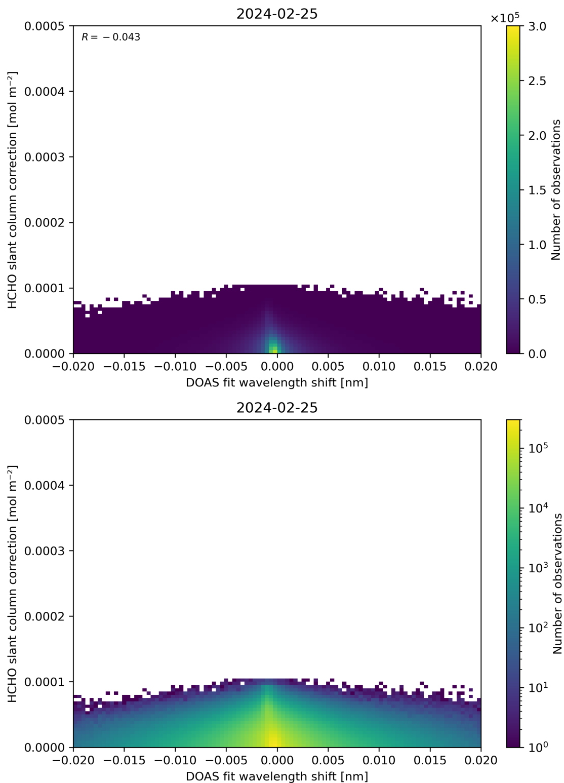
Figure 67: Scatter density plot of “DOAS fit wavelength shift” against “HCHO slant column correction” for 2024-02-24 to 2024-02-26.
