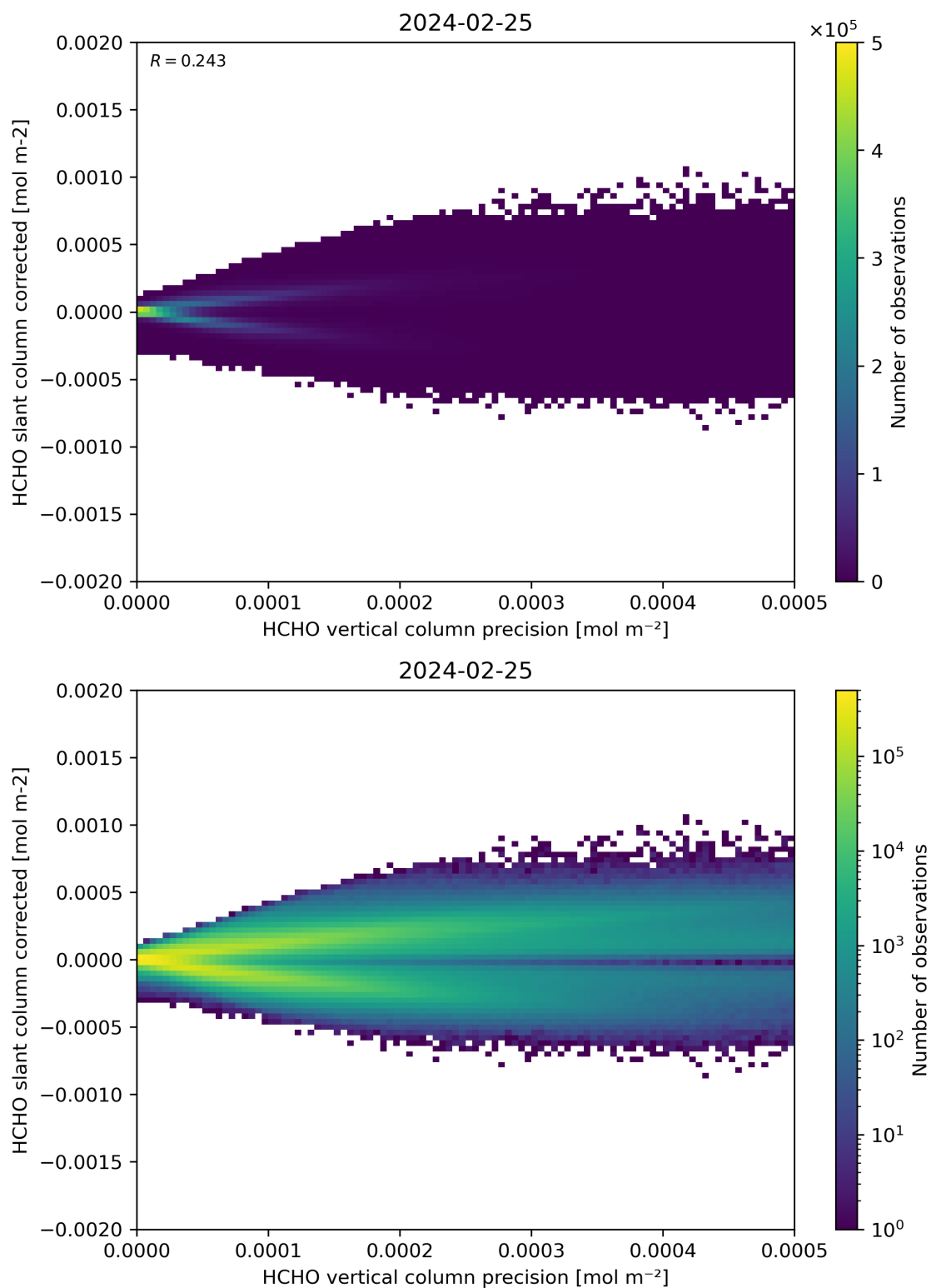
Figure 140: Scatter density plot of “HCHO vertical column precision” against “HCHO slant column corrected” for 2024-02-24 to 2024-02-26.
