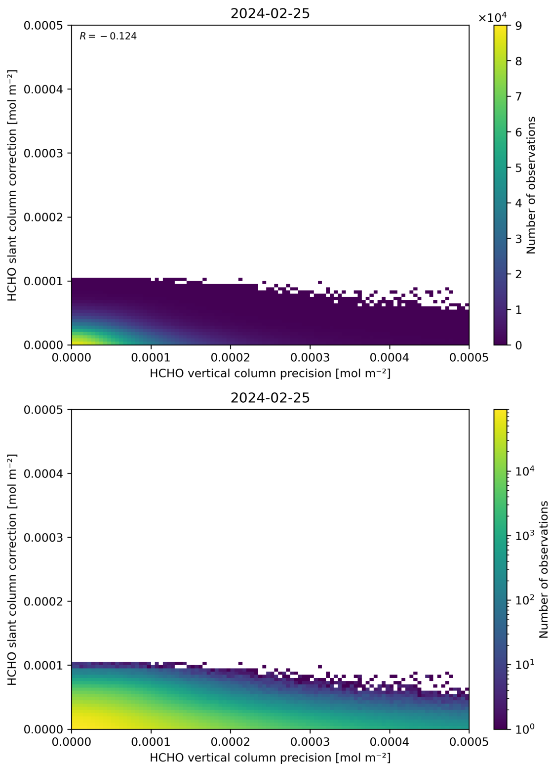
Figure 141: Scatter density plot of “HCHO vertical column precision” against “HCHO slant column correction” for 2024-02-24 to 2024-02-26.
