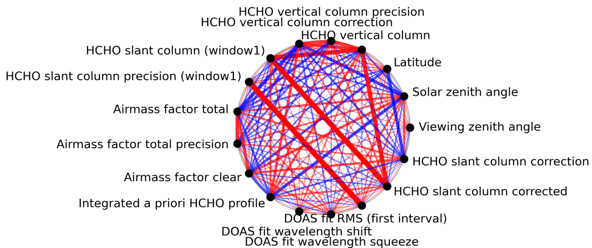
Figure 1: Map of correlation graph for 2024-02-24 to 2024-02-26.
