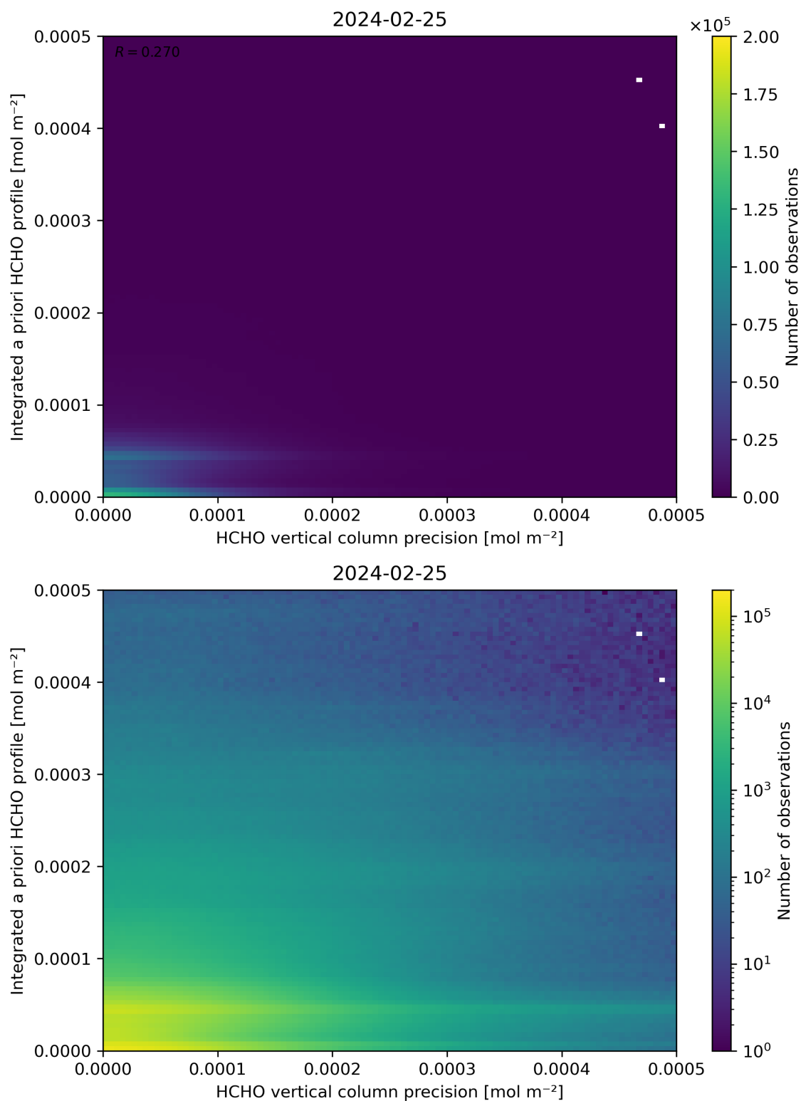
Figure 147: Scatter density plot of “HCHO vertical column precision” against “Integrated a priori HCHO profile” for 2024-02-24 to 2024-02-26.
