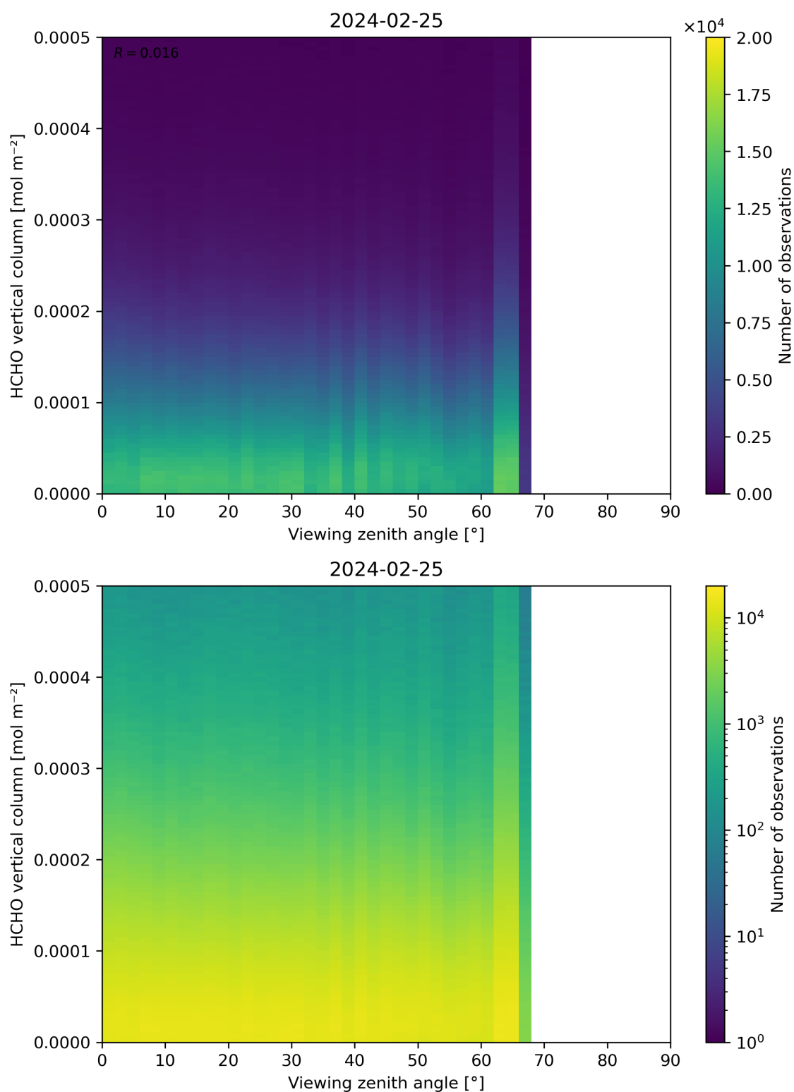
Figure 192: Scatter density plot of “Viewing zenith angle” against “HCHO vertical column” for 2024-02-24 to 2024-02-26.
