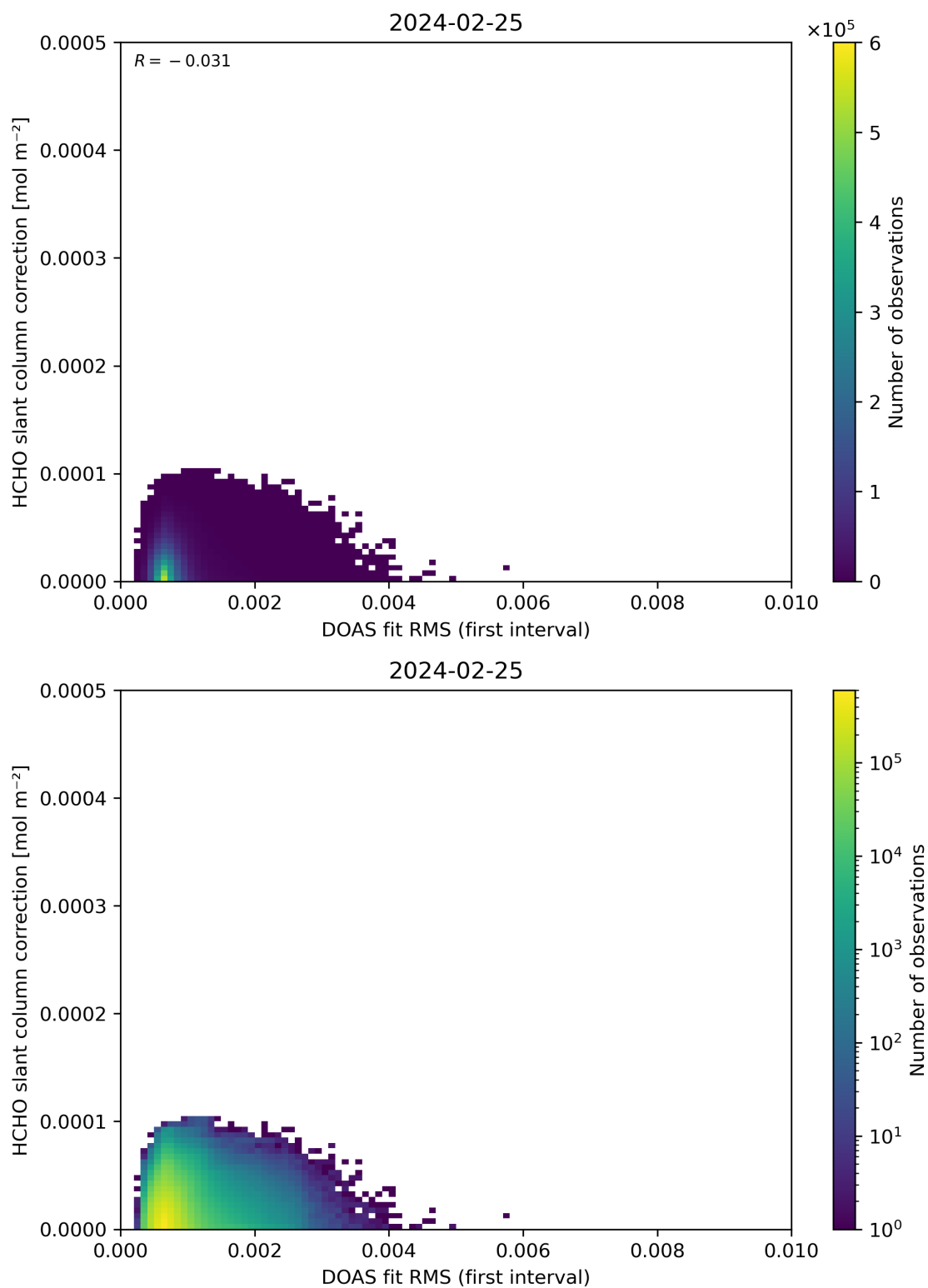
Figure 63: Scatter density plot of “DOAS fit RMS (first interval)” against “HCHO slant column correction” for 2024-02-24 to 2024-02-26.
