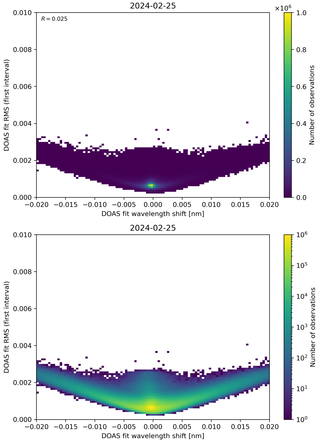
Figure 64: Scatter density plot of “DOAS fit wavelength shift” against “DOAS fit RMS (first interval)” for 2024-02-24 to 2024-02-26.
