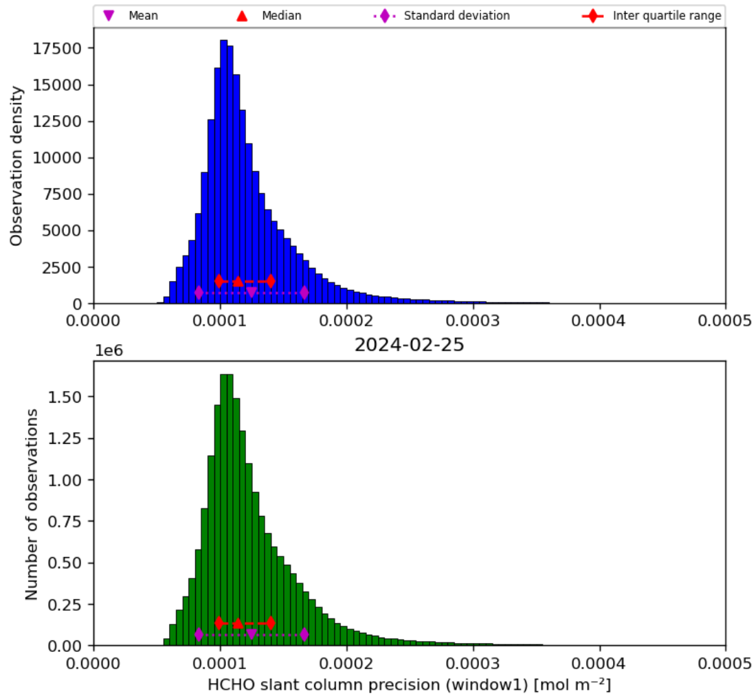
Figure 39: Histogram of “HCHO slant column precision (window1)” for 2024-02-24 to 2024-02-26
