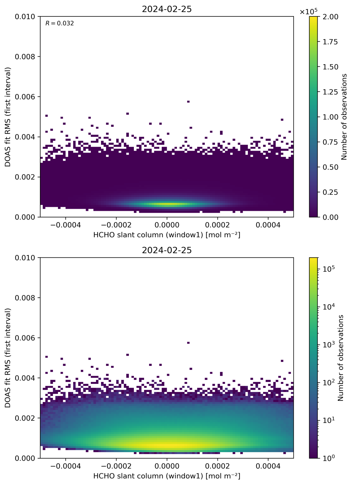
Figure 78: Scatter density plot of “HCHO slant column (window1)” against “DOAS fit RMS (first interval)” for 2024-02-24 to 2024-02-26.
