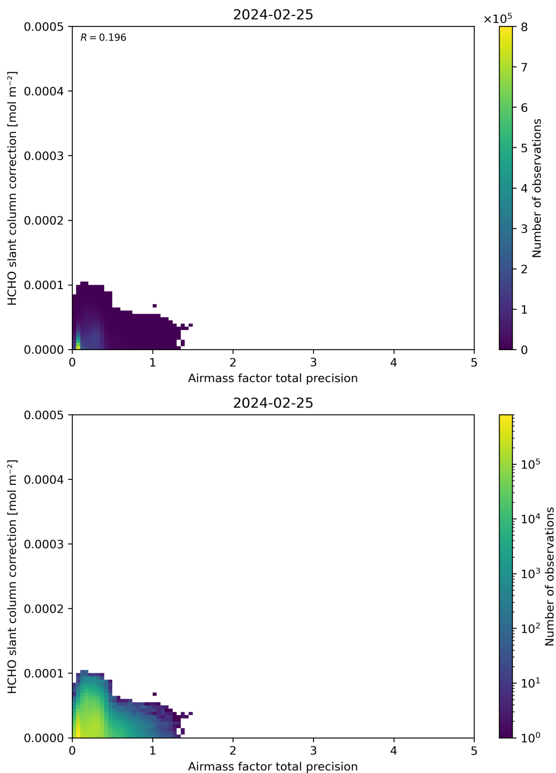
Figure 110: Scatter density plot of “Airmass factor total precision” against “HCHO slant column correction” for 2024-02-24 to 2024-02-26.
