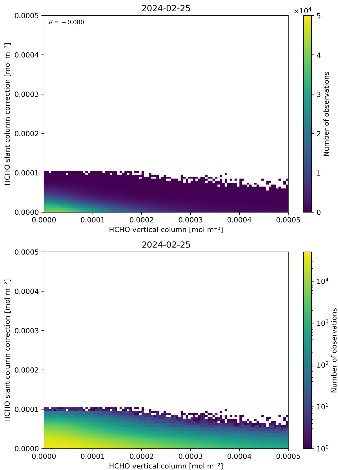
Figure 128: Scatter density plot of “HCHO vertical column” against “HCHO slant column correction” for 2024-02-24 to 2024-02-26.
