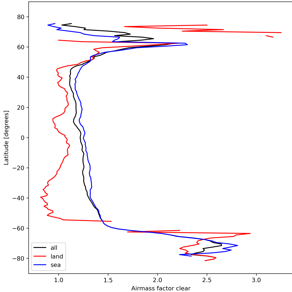
Figure 28: Zonal average of “Airmass factor clear” for 2024-02-24 to 2024-02-26.
