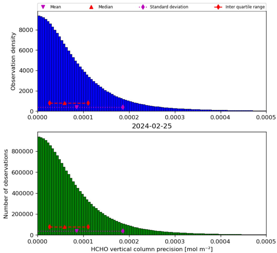
Figure 36: Histogram of “HCHO vertical column precision” for 2024-02-24 to 2024-02-26
