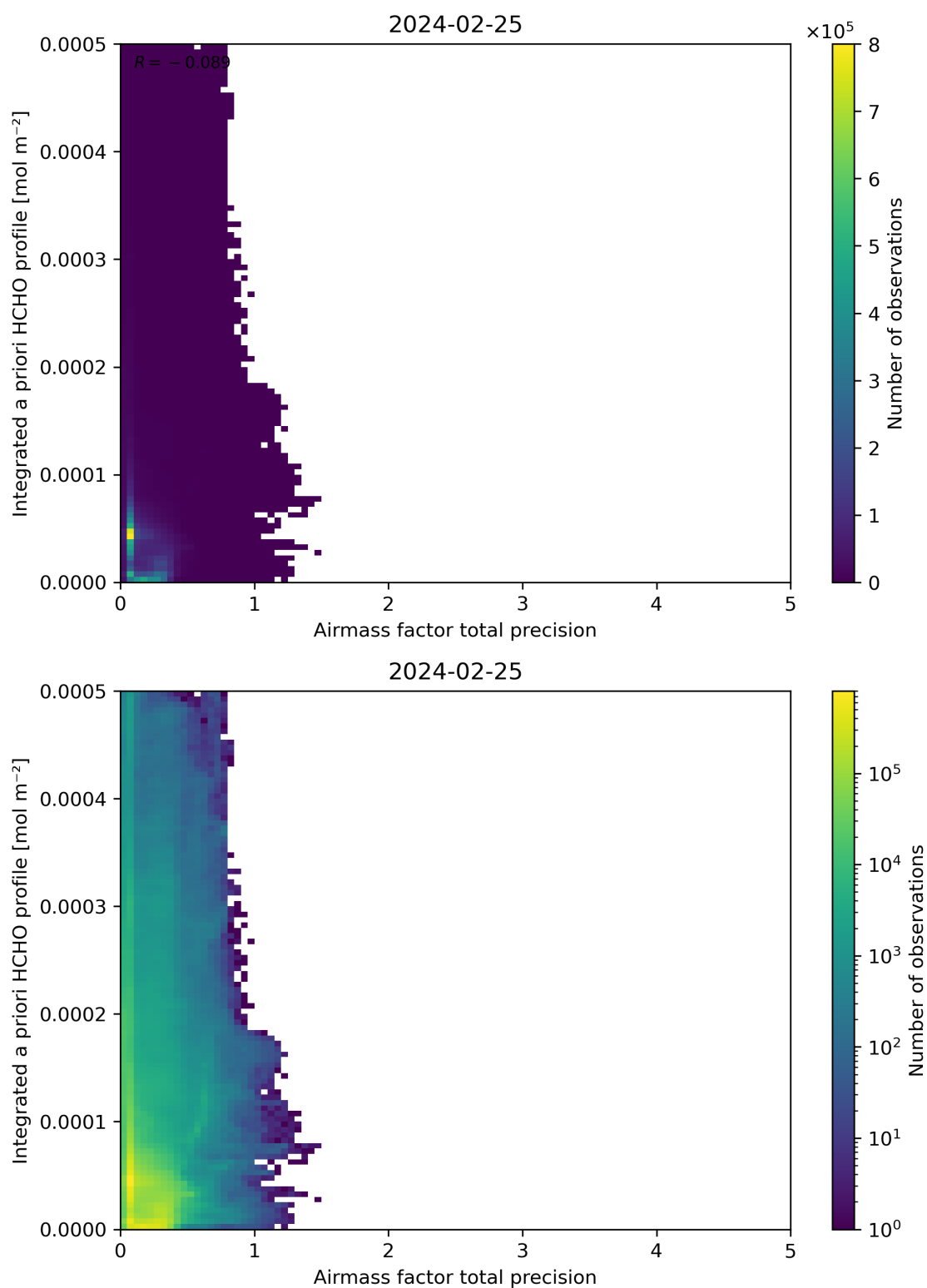
Figure 111: Scatter density plot of “Airmass factor total precision” against “Integrated a priori HCHO profile” for 2024-02-24 to 2024-02-26.
