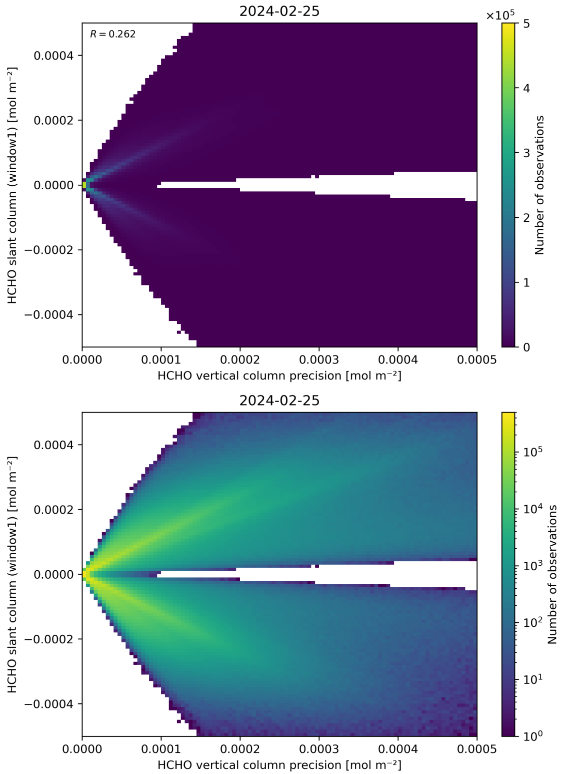
Figure 142: Scatter density plot of “HCHO vertical column precision” against “HCHO slant column (window1)” for 2024-02-24 to 2024-02-26.
