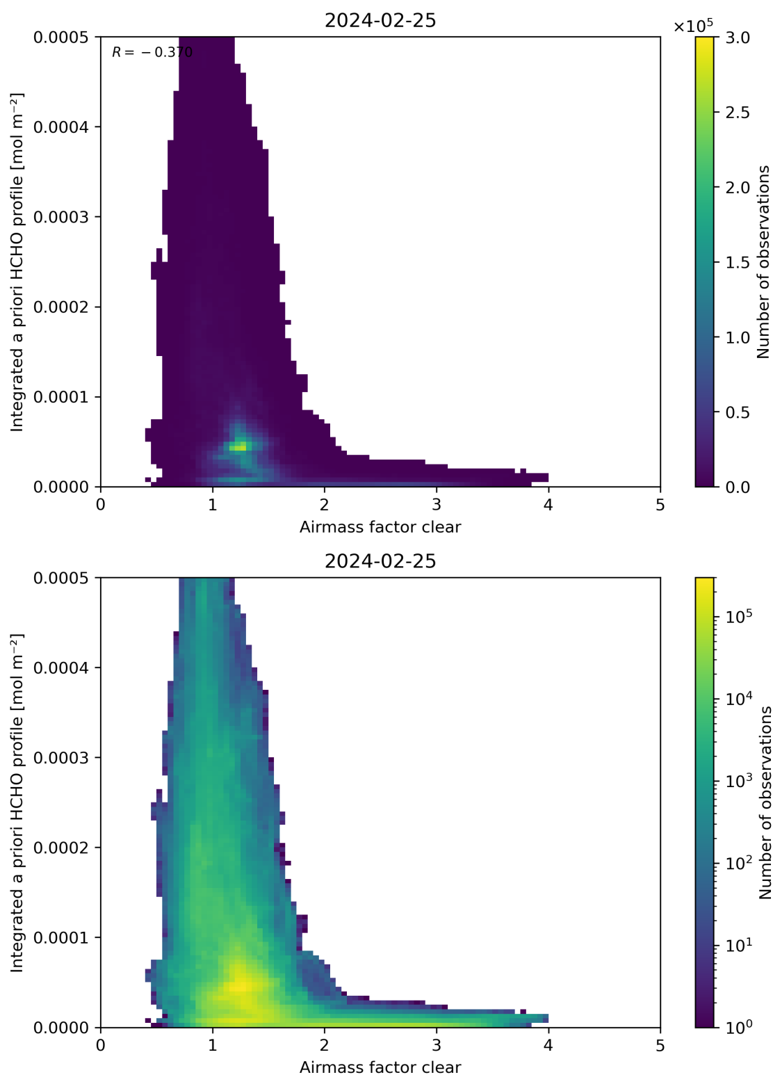
Figure 76: Scatter density plot of “Airmass factor clear” against “Integrated a priori HCHO profile” for 2024-02-24 to 2024-02-26.
