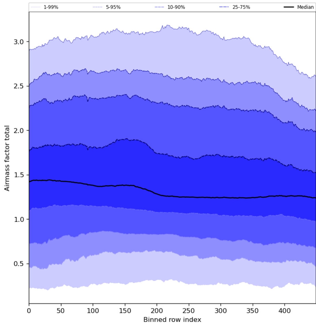
Figure 54: Along track statistics of “Airmass factor total” for 2024-02-24 to 2024-02-26
