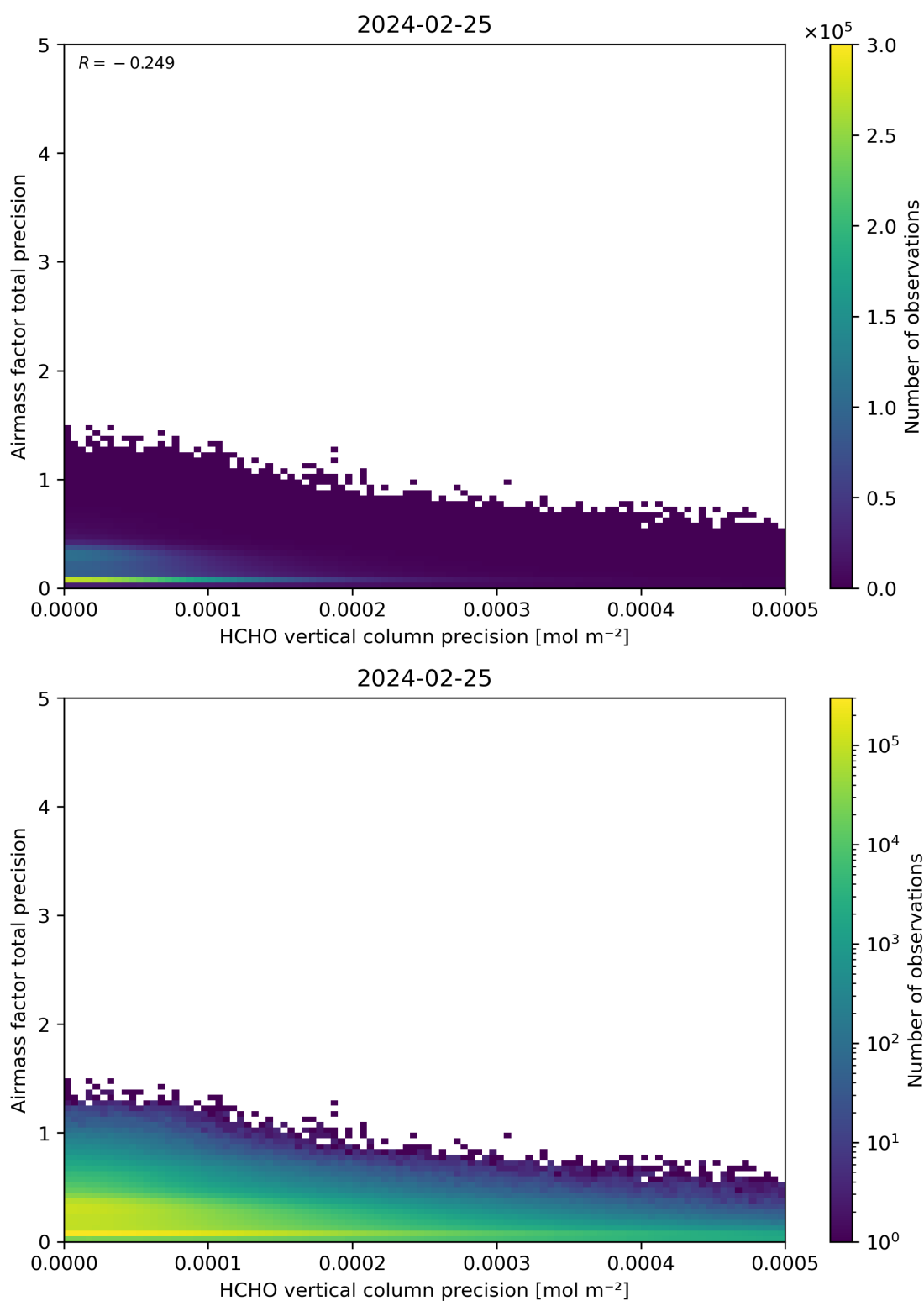
Figure 145: Scatter density plot of “HCHO vertical column precision” against “Airmass factor total precision” for 2024-02-24 to 2024-02-26.
