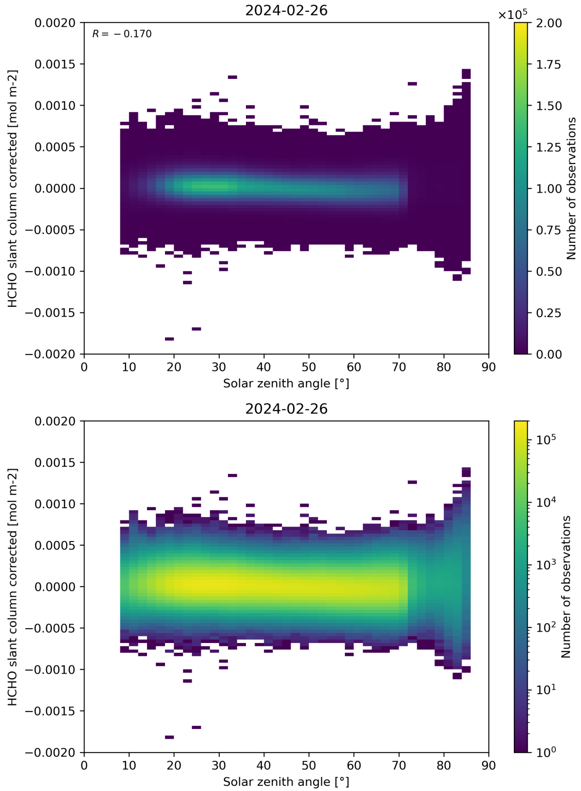
Figure 171: Scatter density plot of “Solar zenith angle” against “HCHO slant column corrected” for 2024-02-25 to 2024-02-27.
