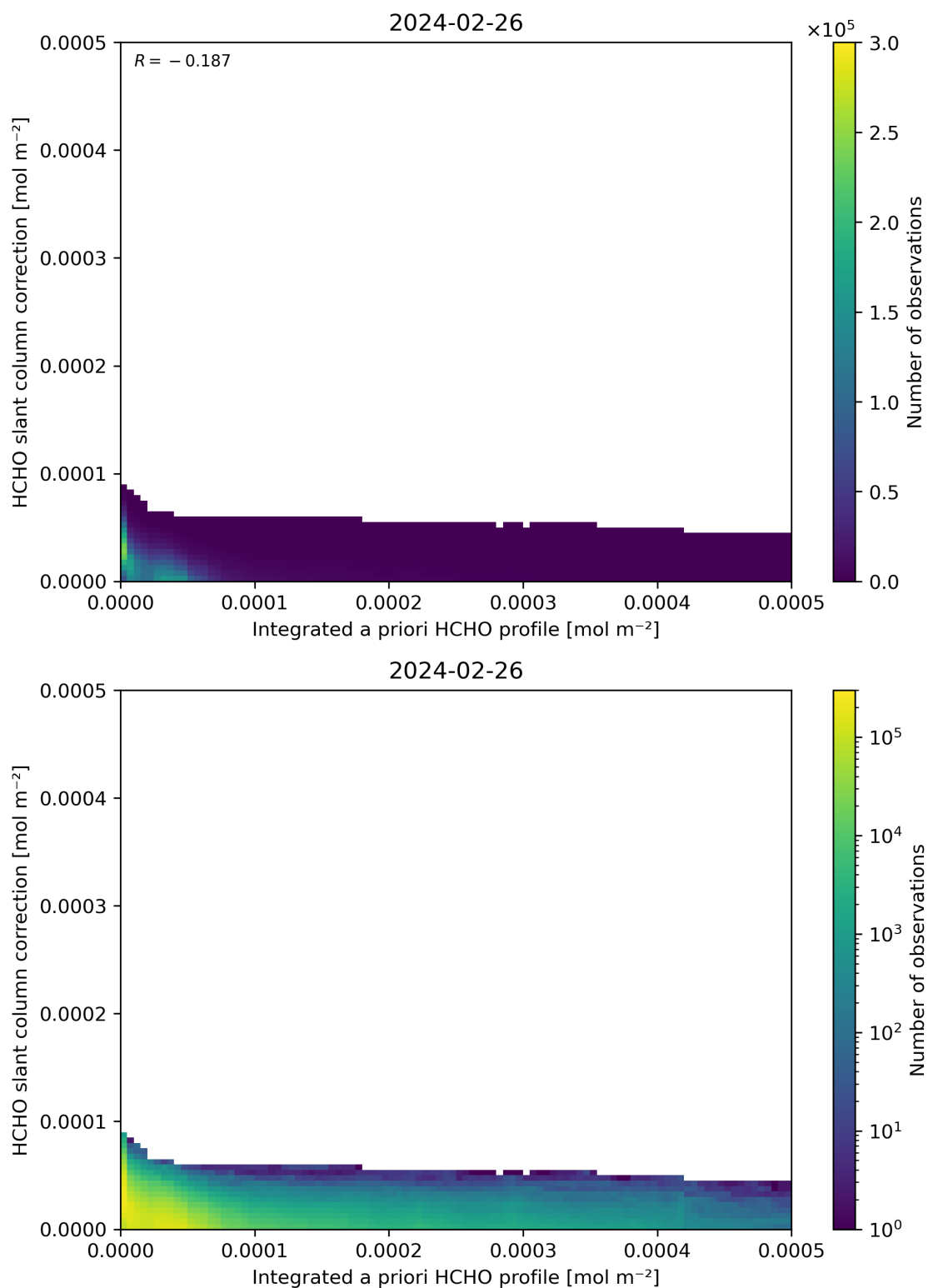
Figure 152: Scatter density plot of “Integrated a priori HCHO profile” against “HCHO slant column correction” for 2024-02-25 to 2024-02-27.
