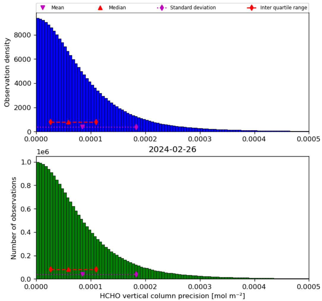
Figure 36: Histogram of “HCHO vertical column precision” for 2024-02-25 to 2024-02-27
