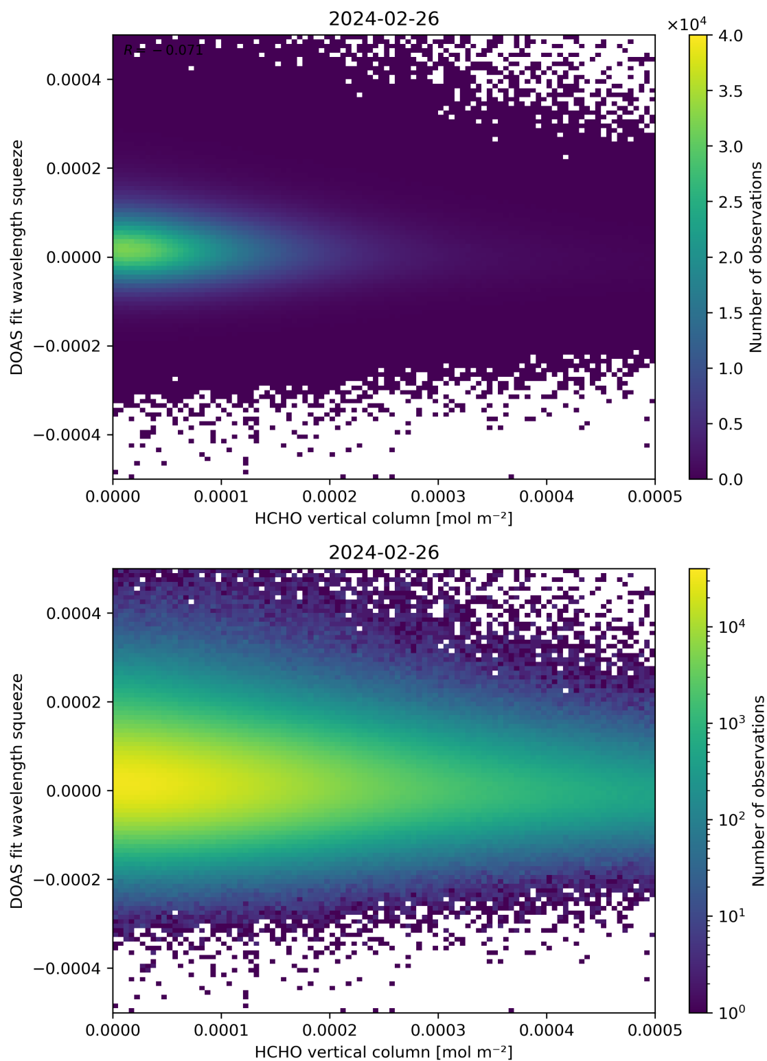
Figure 125: Scatter density plot of “HCHO vertical column” against “DOAS fit wavelength squeeze” for 2024-02-25 to 2024-02-27.
