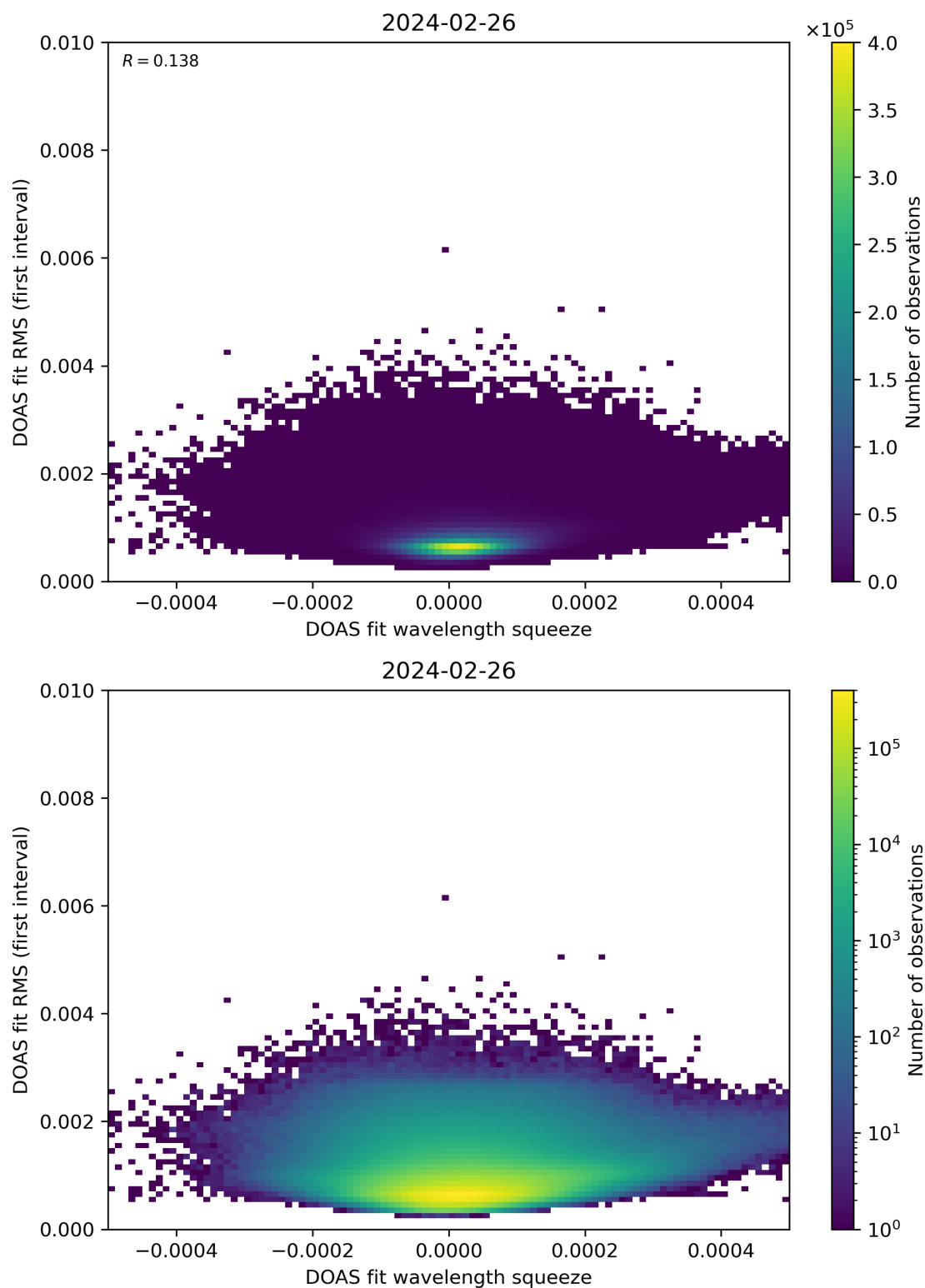
Figure 68: Scatter density plot of “DOAS fit wavelength squeeze” against “DOAS fit RMS (first interval)” for 2024-02-25 to 2024-02-27.
