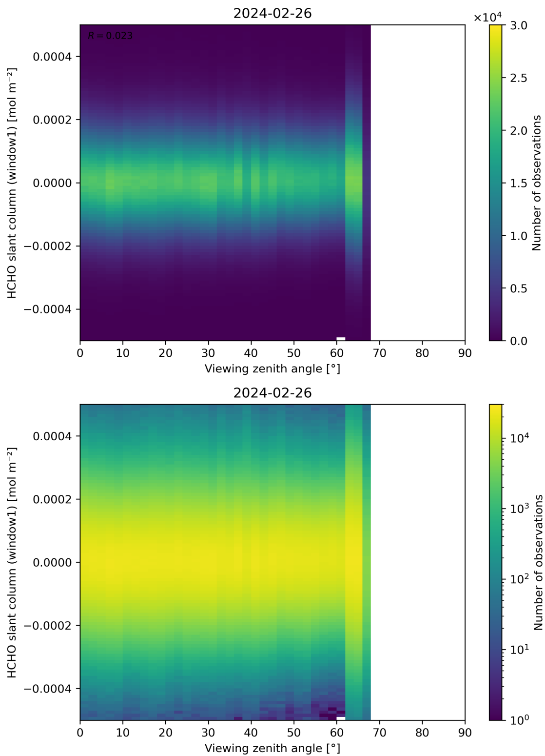
Figure 188: Scatter density plot of “Viewing zenith angle” against “HCHO slant column (window1)” for 2024-02-25 to 2024-02-27.
