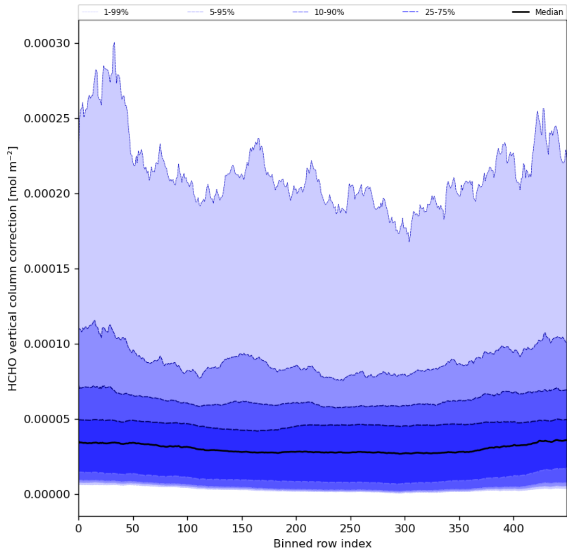
Figure 51: Along track statistics of “HCHO vertical column correction” for 2024-02-25 to 2024-02-27
