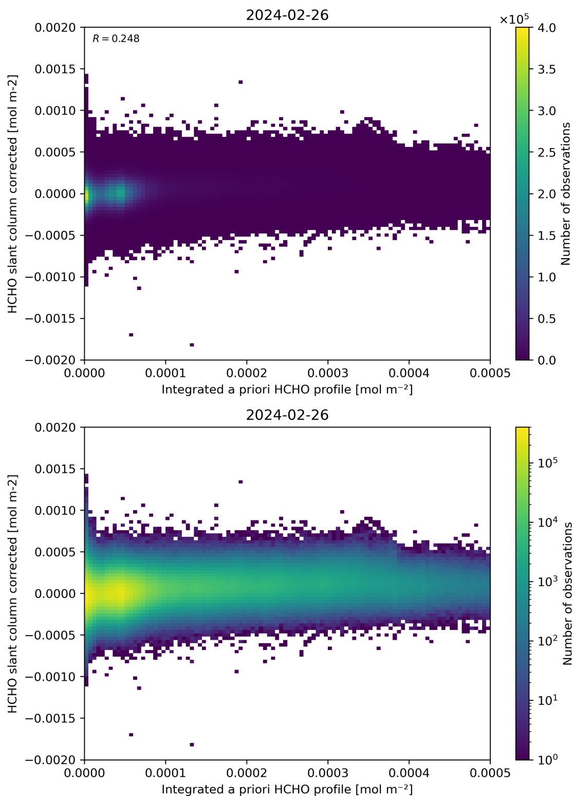
Figure 151: Scatter density plot of “Integrated a priori HCHO profile” against “HCHO slant column corrected” for 2024-02-25 to 2024-02-27.
