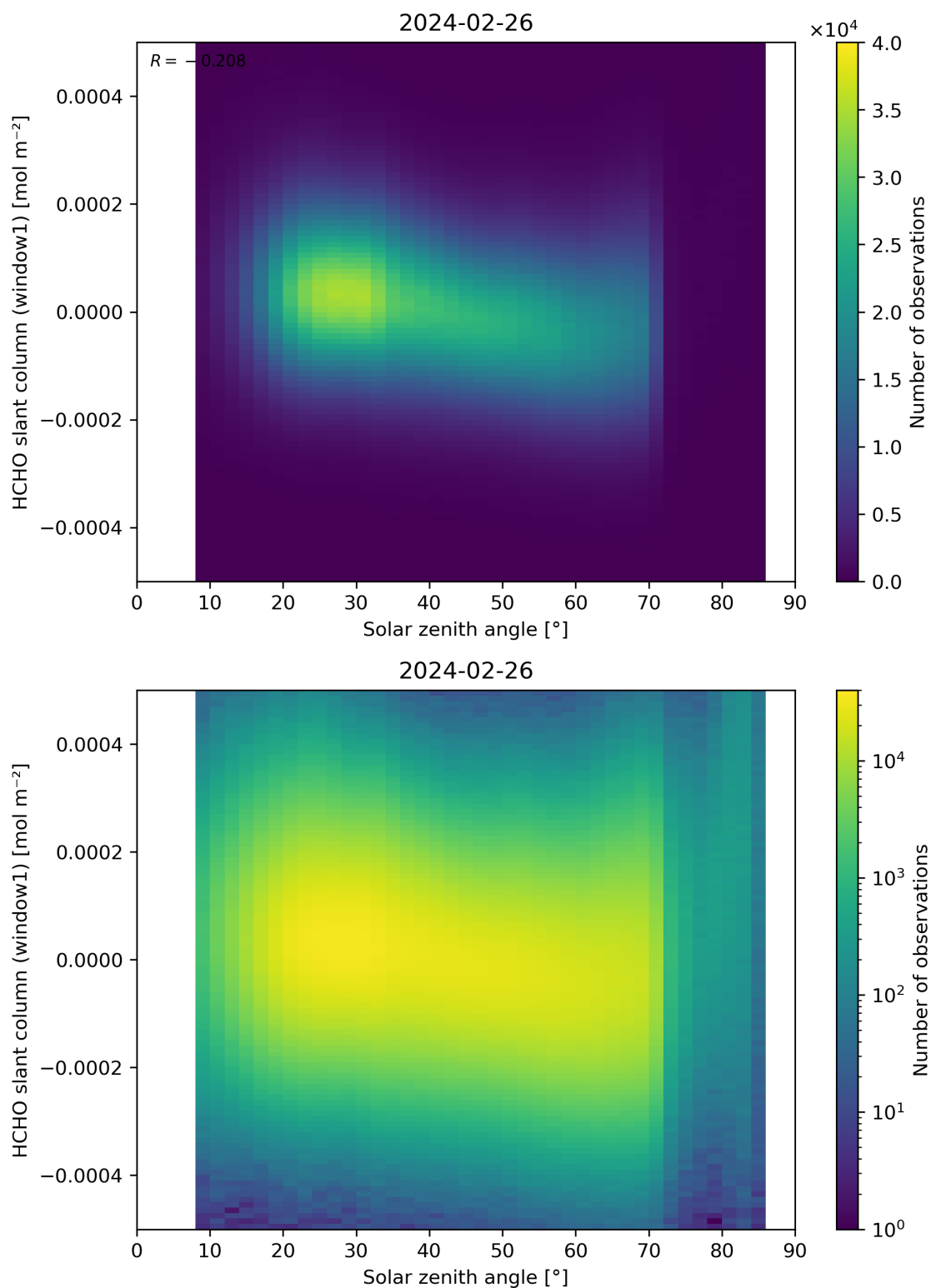
Figure 173: Scatter density plot of “Solar zenith angle” against “HCHO slant column (window1)” for 2024-02-25 to 2024-02-27.
