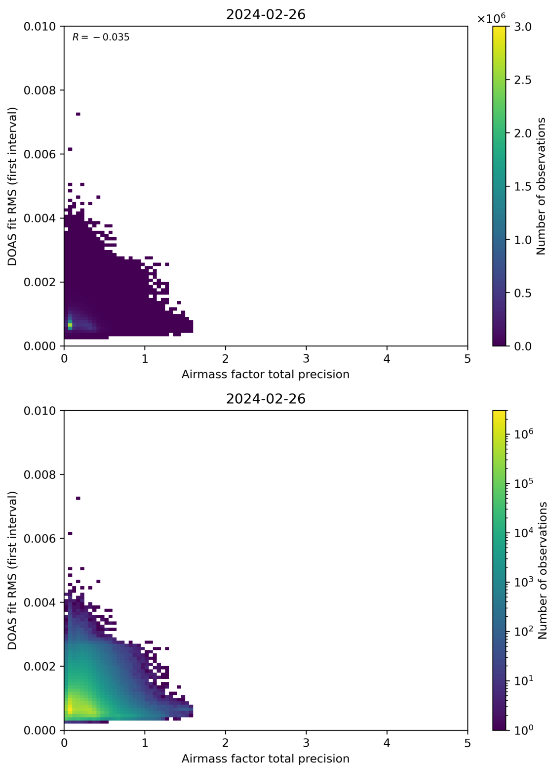
Figure 105: Scatter density plot of “Airmass factor total precision” against “DOAS fit RMS (first interval)” for 2024-02-25 to 2024-02-27.
