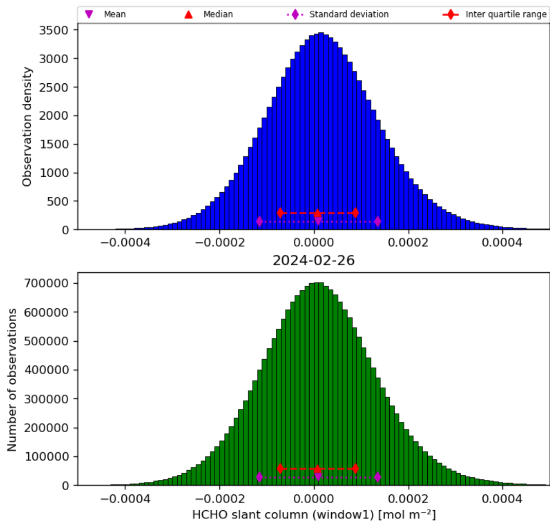
Figure 38: Histogram of “HCHO slant column (window1)” for 2024-02-25 to 2024-02-27
