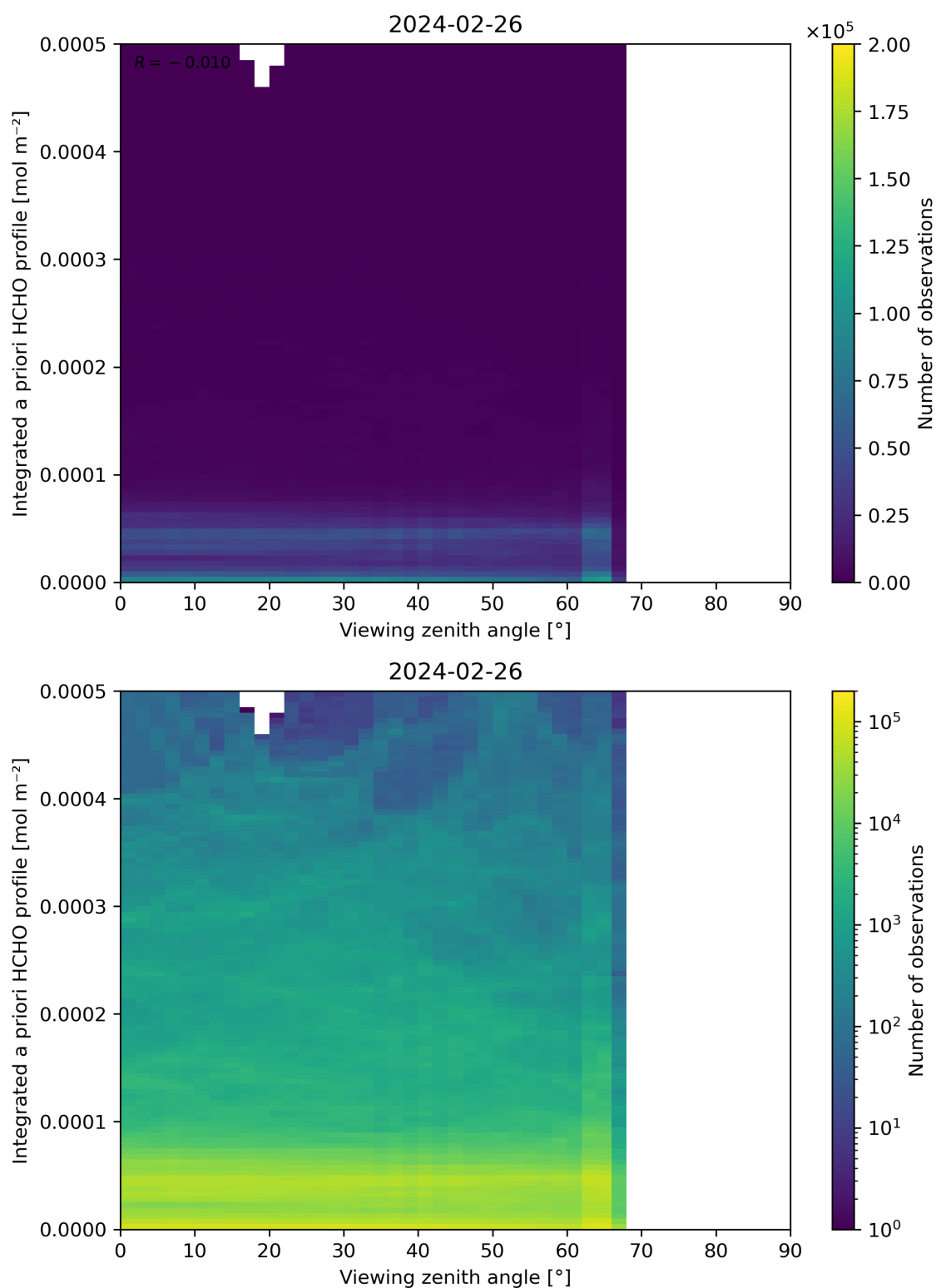
Figure 195: Scatter density plot of “Viewing zenith angle” against “Integrated a priori HCHO profile” for 2024-02-25 to 2024-02-27.
