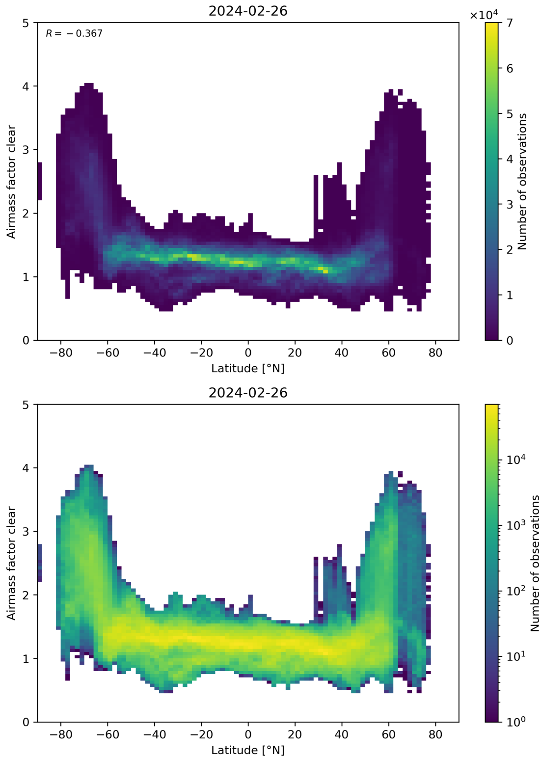
Figure 156: Scatter density plot of “Latitude” against “Airmass factor clear” for 2024-02-25 to 2024-02-27.
