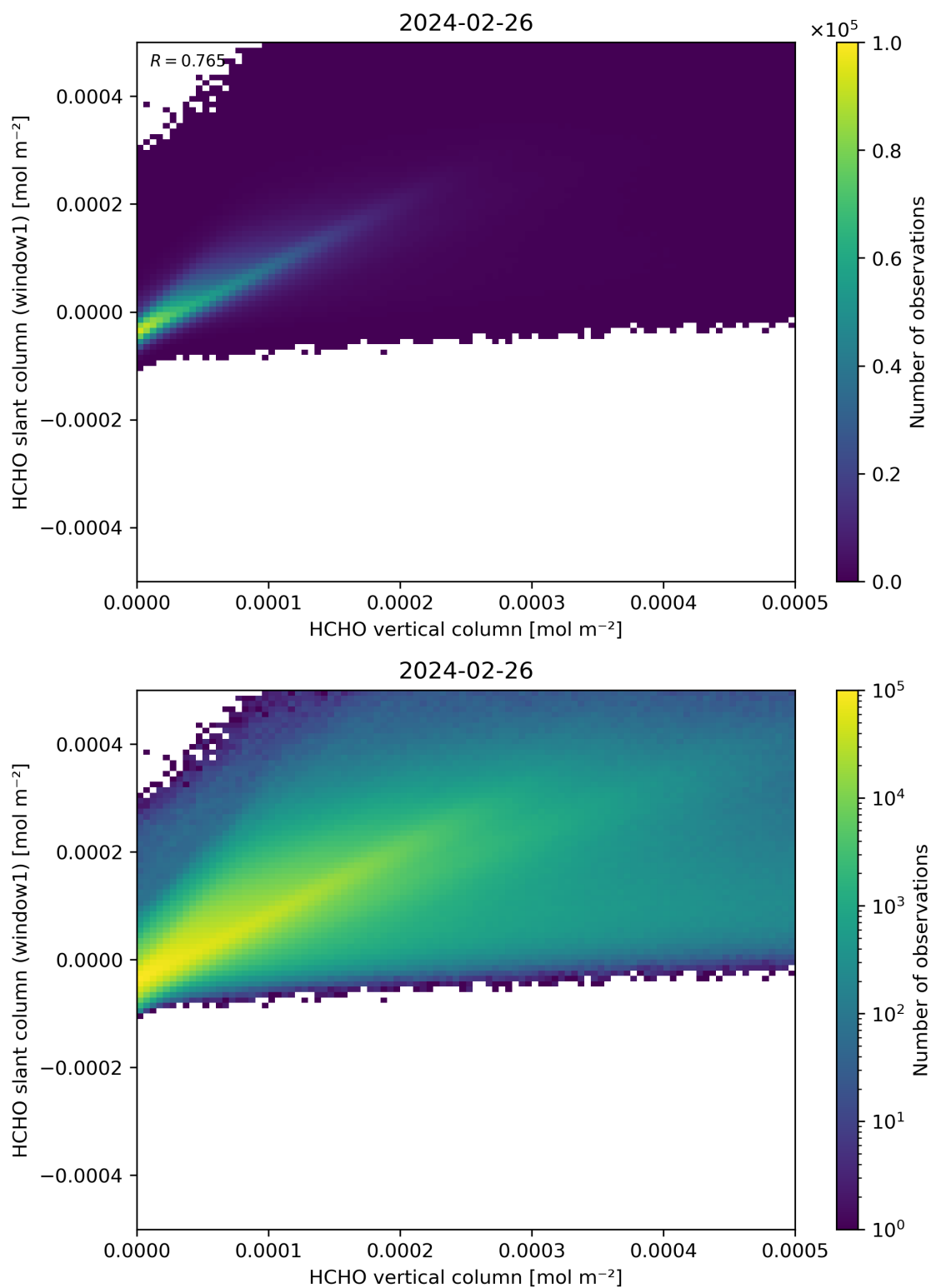
Figure 129: Scatter density plot of “HCHO vertical column” against “HCHO slant column (window1)” for 2024-02-25 to 2024-02-27.
