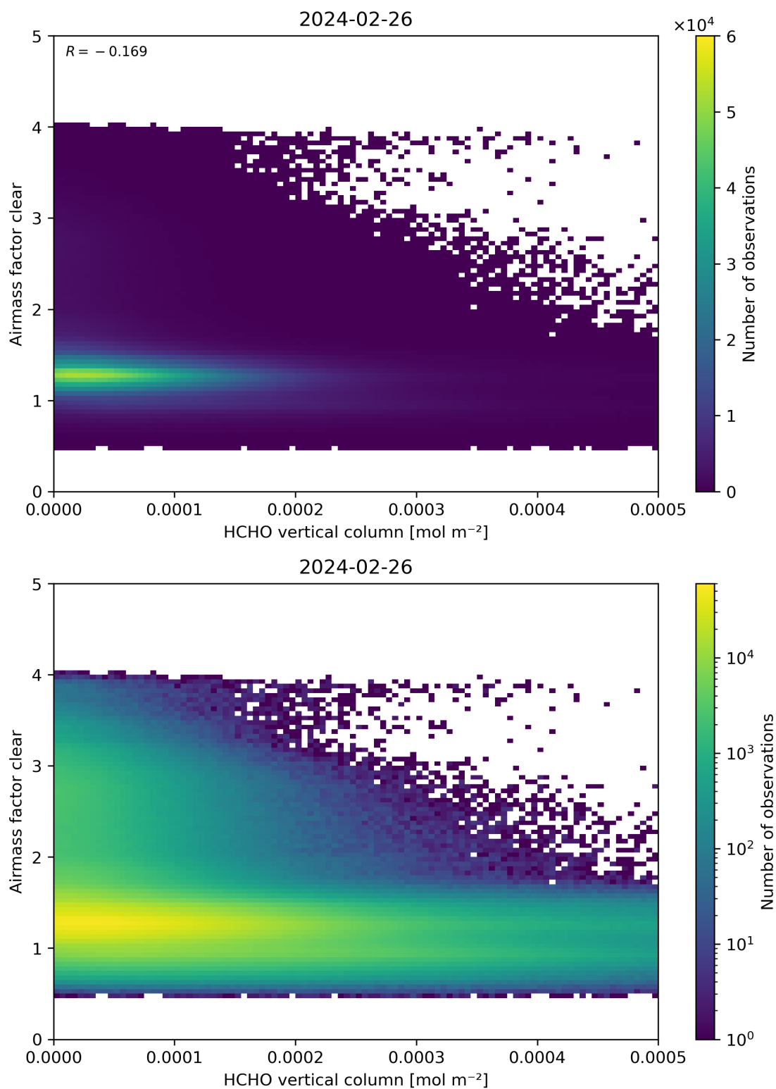
Figure 126: Scatter density plot of “HCHO vertical column” against “Airmass factor clear” for 2024-02-25 to 2024-02-27.
