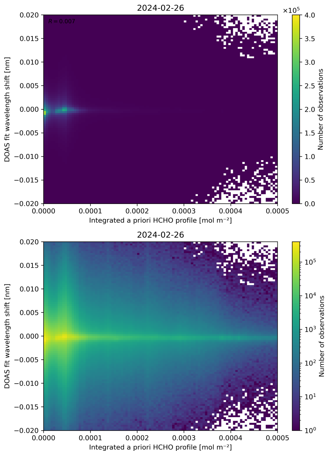
Figure 149: Scatter density plot of “Integrated a priori HCHO profile” against “DOAS fit wavelength shift” for 2024-02-25 to 2024-02-27.
