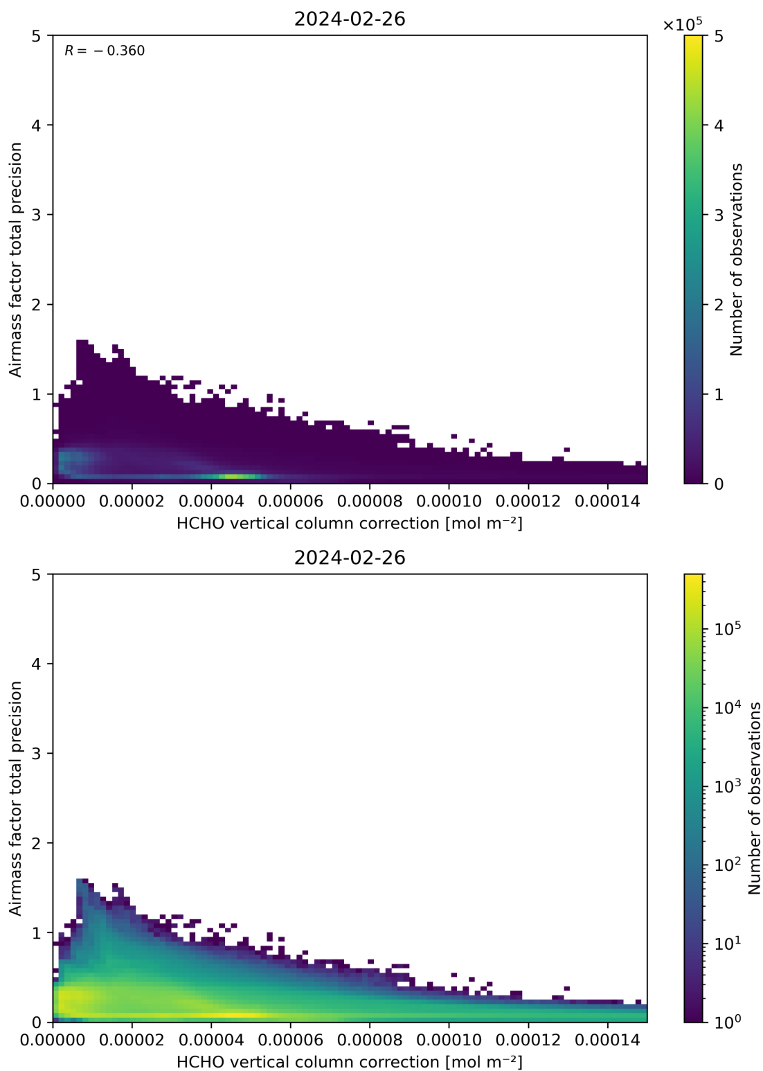
Figure 121: Scatter density plot of “HCHO vertical column correction” against “Airmass factor total precision” for 2024-02-25 to 2024-02-27.
