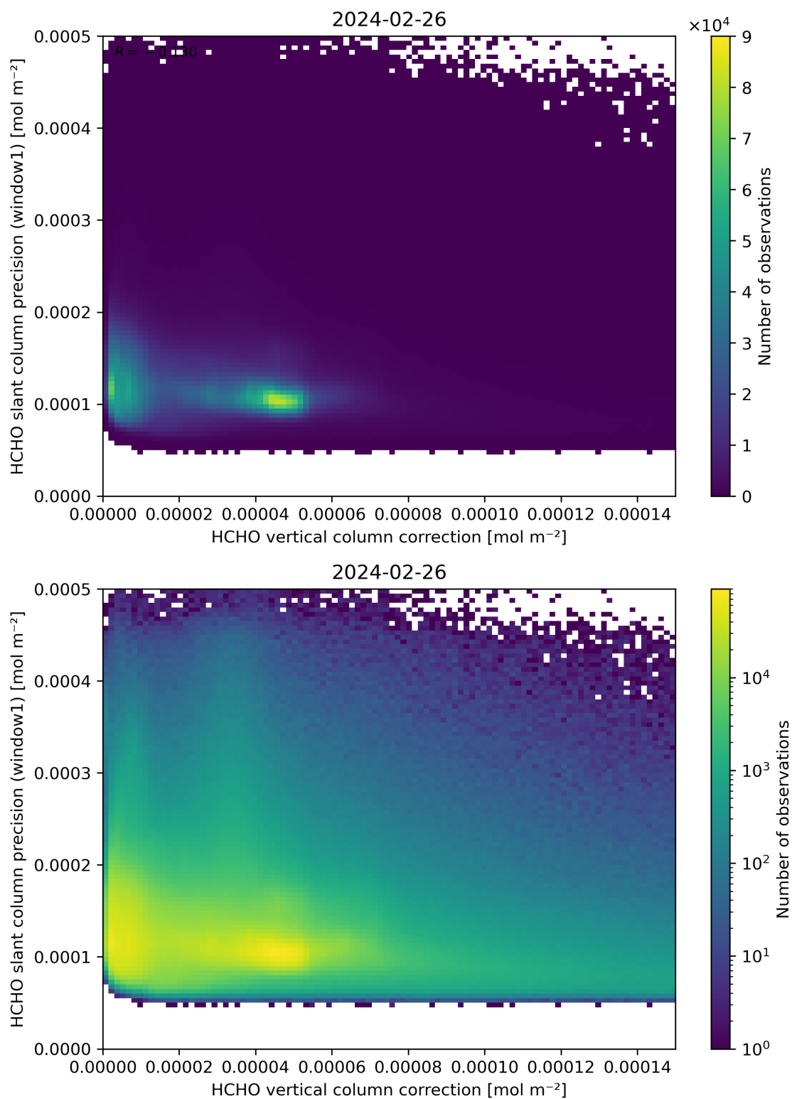
Figure 119: Scatter density plot of “HCHO vertical column correction” against “HCHO slant column precision (window1)” for 2024-02-25 to 2024-02-27.
