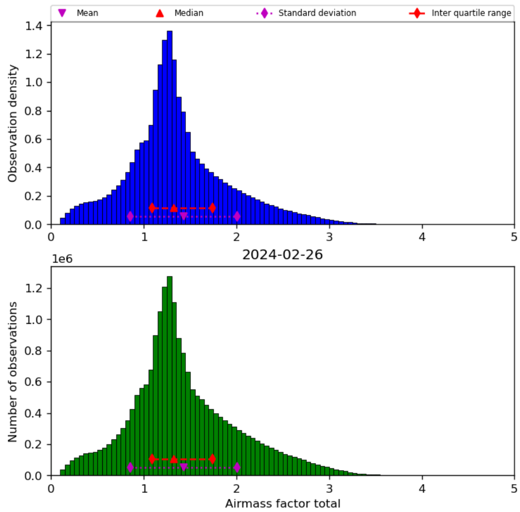
Figure 40: Histogram of “Airmass factor total” for 2024-02-25 to 2024-02-27
