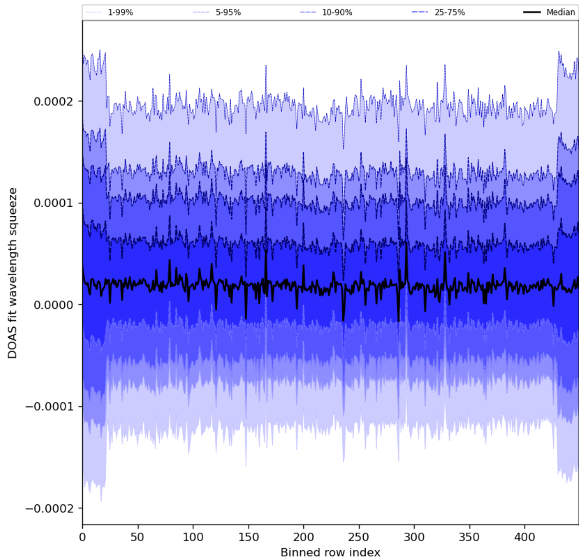
Figure 59: Along track statistics of “DOAS fit wavelength squeeze” for 2024-02-25 to 2024-02-27
