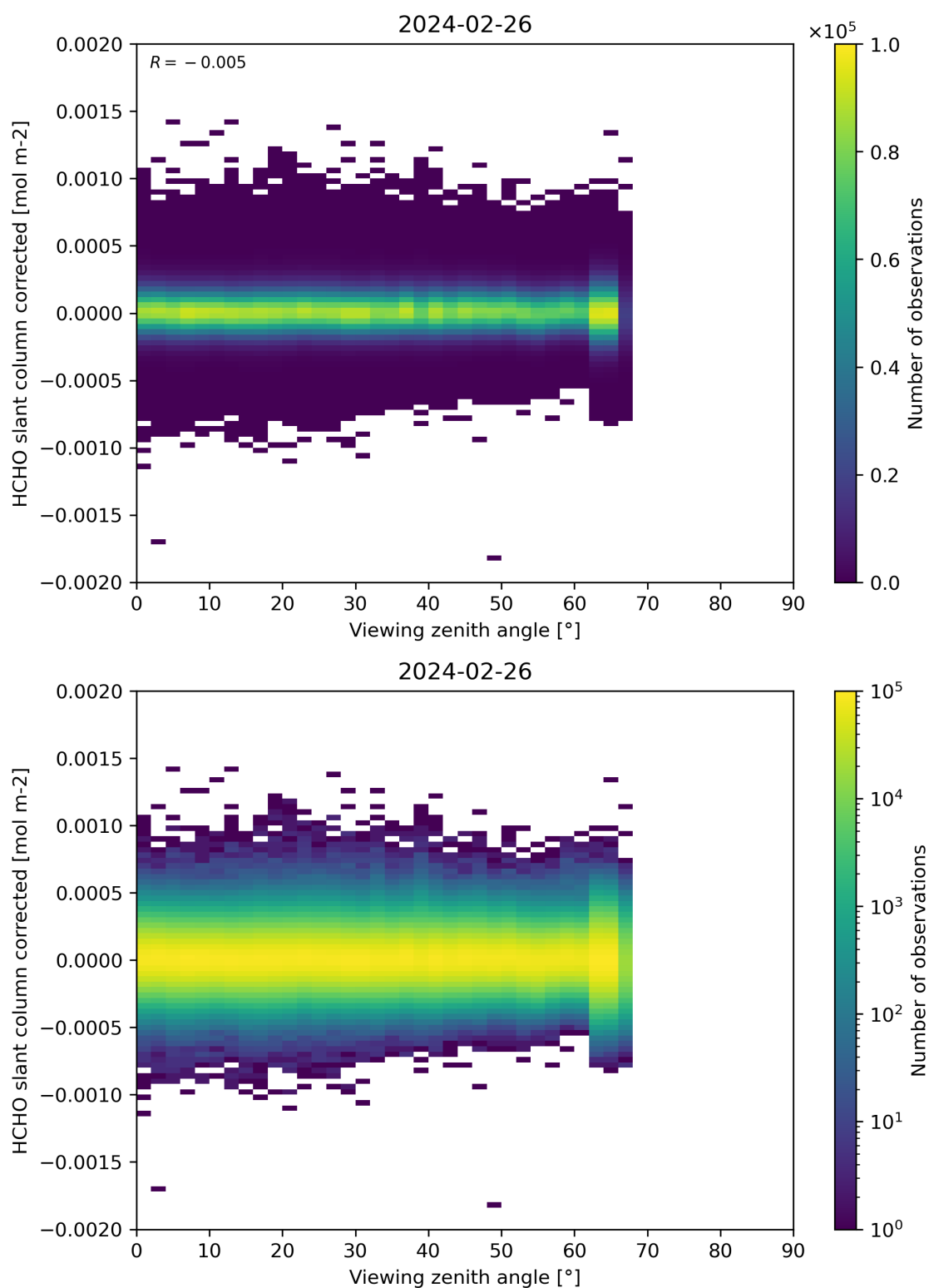
Figure 186: Scatter density plot of “Viewing zenith angle” against “HCHO slant column corrected” for 2024-02-25 to 2024-02-27.
