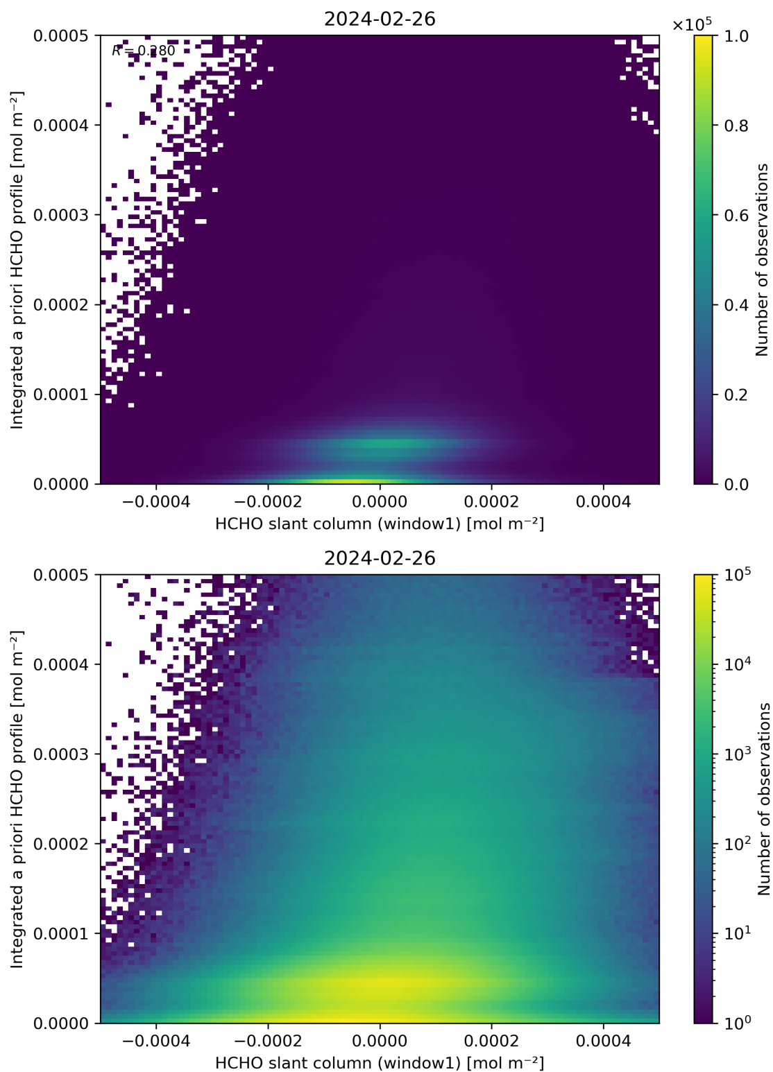
Figure 87: Scatter density plot of “HCHO slant column (window1)” against “Integrated a priori HCHO profile” for 2024-02-25 to 2024-02-27.
