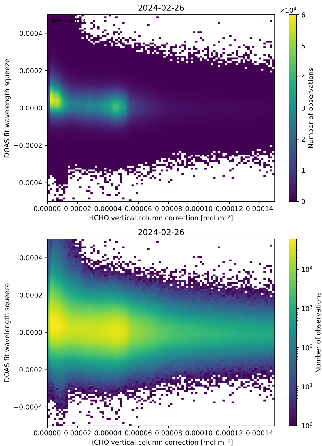
Figure 114: Scatter density plot of “HCHO vertical column correction” against “DOAS fit wavelength squeeze” for 2024-02-25 to 2024-02-27.
