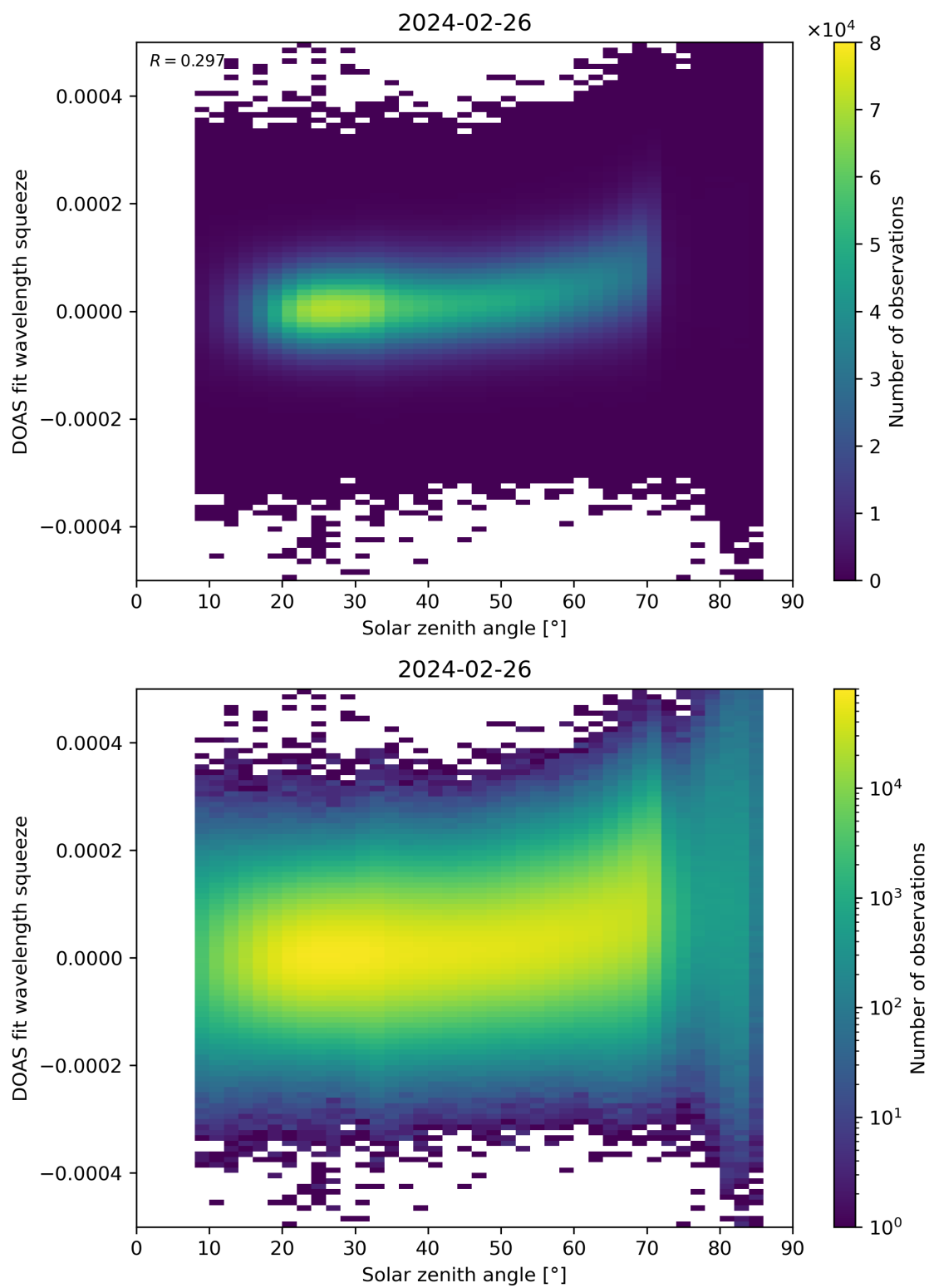
Figure 169: Scatter density plot of “Solar zenith angle” against “DOAS fit wavelength squeeze” for 2024-02-25 to 2024-02-27.
