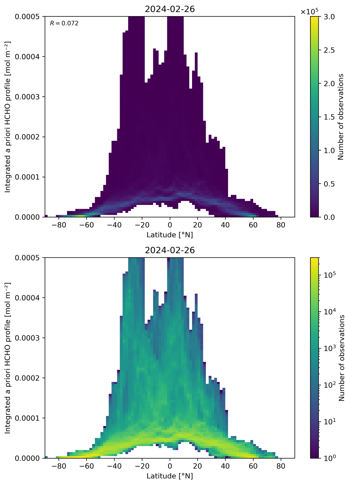
Figure 166: Scatter density plot of “Latitude” against “Integrated a priori HCHO profile” for 2024-02-25 to 2024-02-27.
