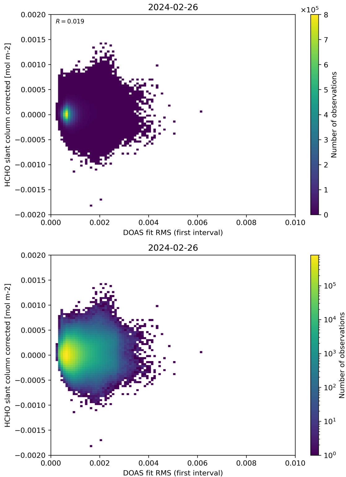
Figure 62: Scatter density plot of “DOAS fit RMS (first interval)” against “HCHO slant column corrected” for 2024-02-25 to 2024-02-27.
