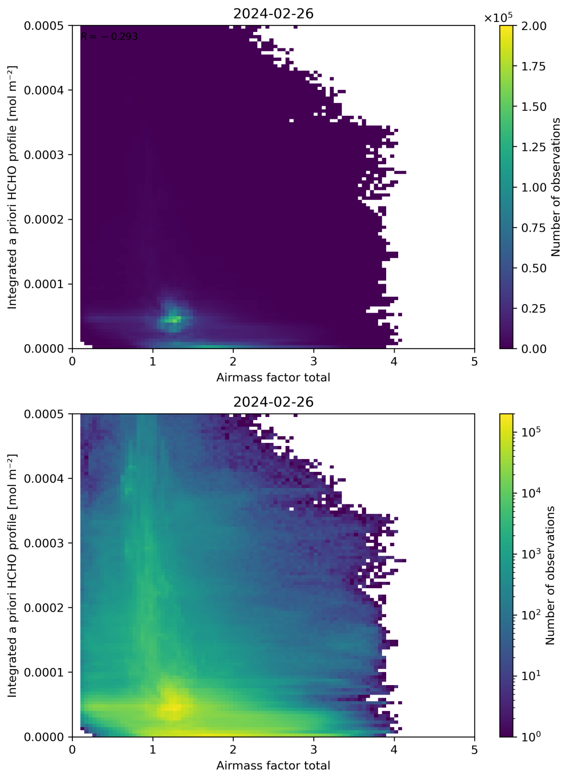
Figure 104: Scatter density plot of “Airmass factor total” against “Integrated a priori HCHO profile” for 2024-02-25 to 2024-02-27.
