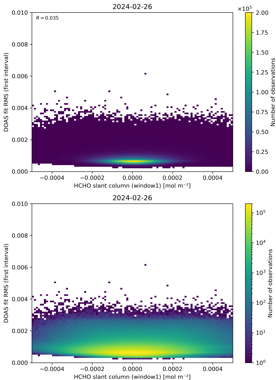
Figure 78: Scatter density plot of “HCHO slant column (window1)” against “DOAS fit RMS (first interval)” for 2024-02-25 to 2024-02-27.
