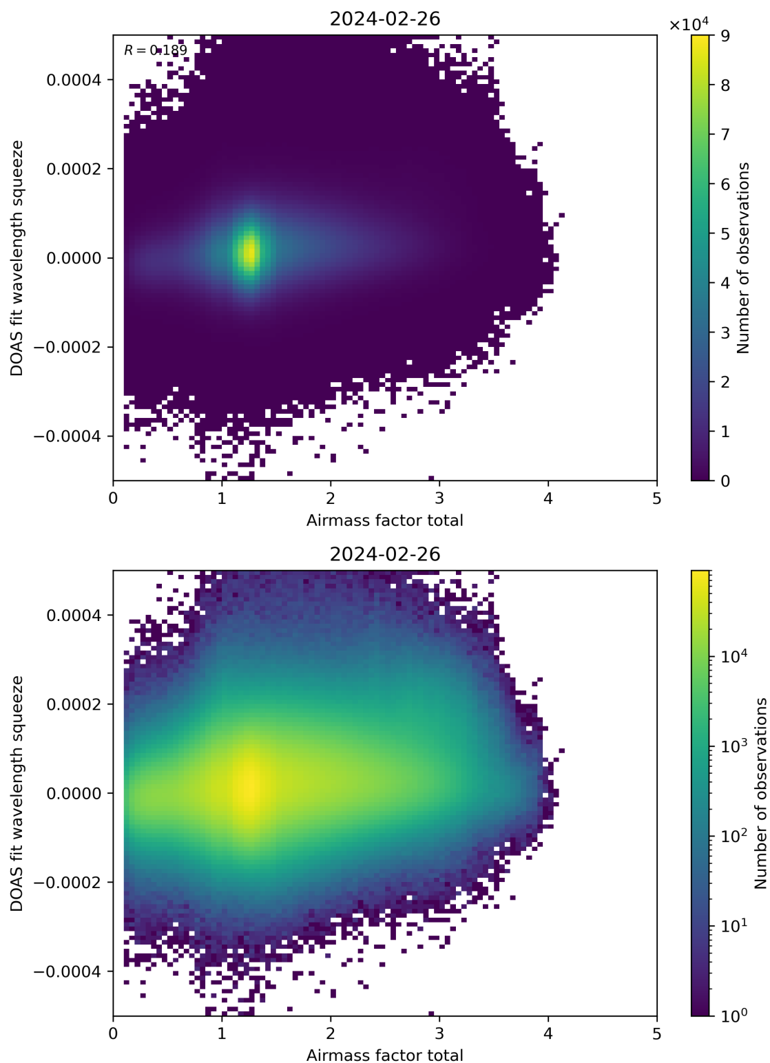
Figure 99: Scatter density plot of “Airmass factor total” against “DOAS fit wavelength squeeze” for 2024-02-25 to 2024-02-27.
