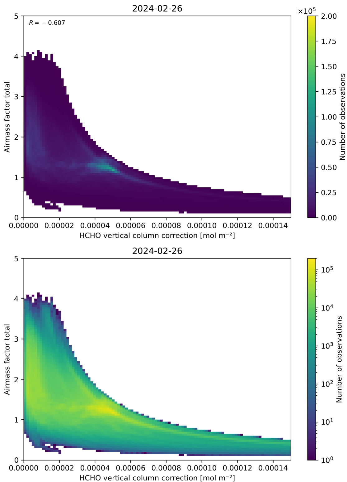
Figure 120: Scatter density plot of “HCHO vertical column correction” against “Airmass factor total” for 2024-02-25 to 2024-02-27.
