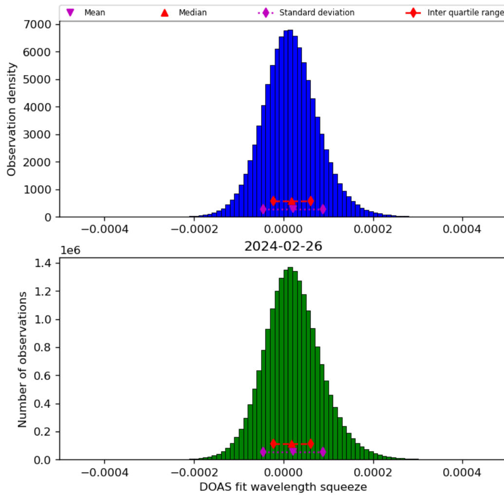
Figure 45: Histogram of “DOAS fit wavelength squeeze” for 2024-02-25 to 2024-02-27
