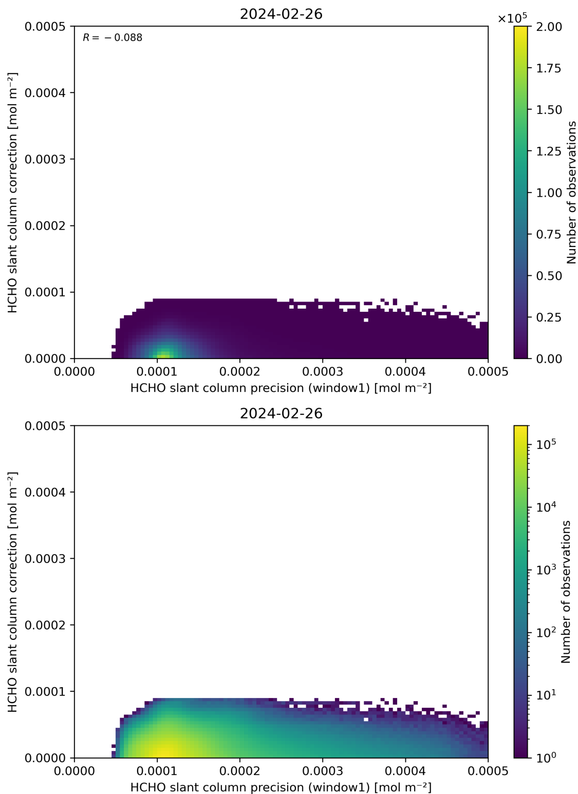
Figure 93: Scatter density plot of “HCHO slant column precision (window1)” against “HCHO slant column correction” for 2024-02-25 to 2024-02-27.
