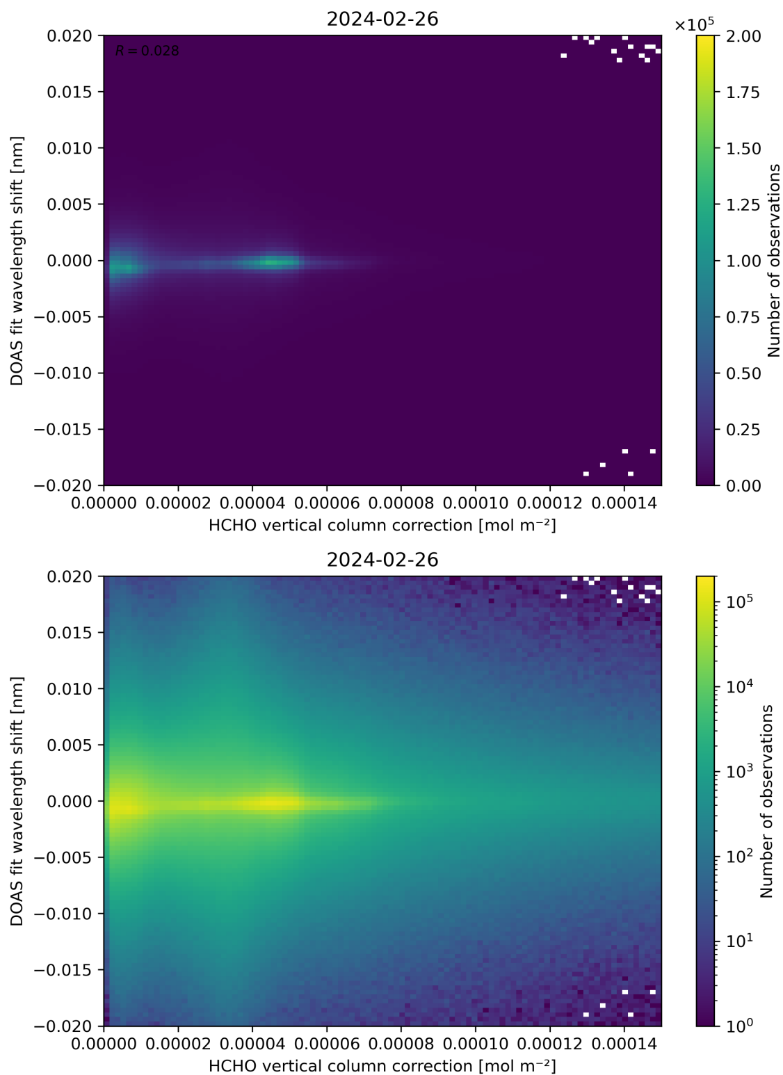
Figure 113: Scatter density plot of “HCHO vertical column correction” against “DOAS fit wavelength shift” for 2024-02-25 to 2024-02-27.
