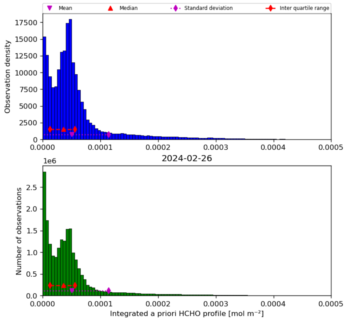
Figure 43: Histogram of “Integrated a priori HCHO profile” for 2024-02-25 to 2024-02-27
