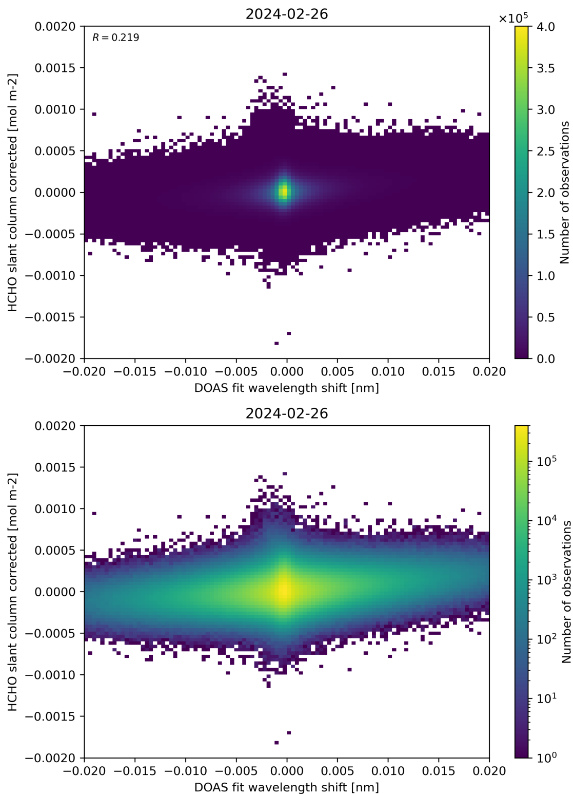
Figure 66: Scatter density plot of “DOAS fit wavelength shift” against “HCHO slant column corrected” for 2024-02-25 to 2024-02-27.
