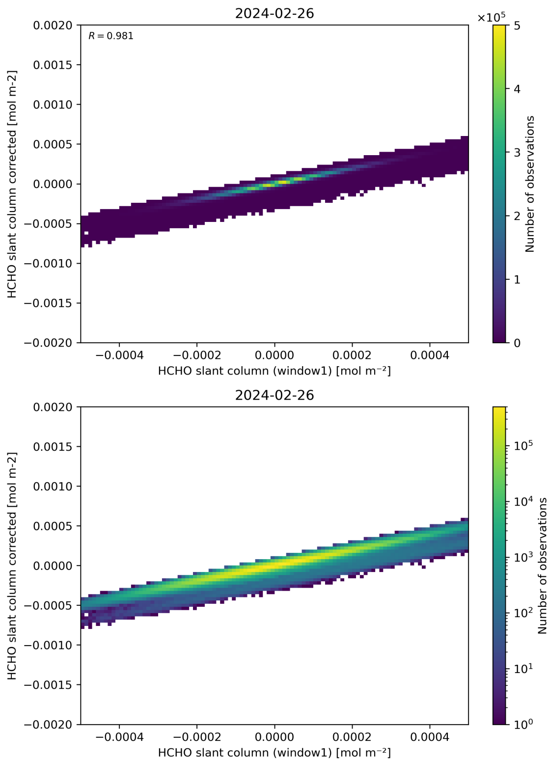
Figure 82: Scatter density plot of “HCHO slant column (window1)” against “HCHO slant column corrected” for 2024-02-25 to 2024-02-27.
