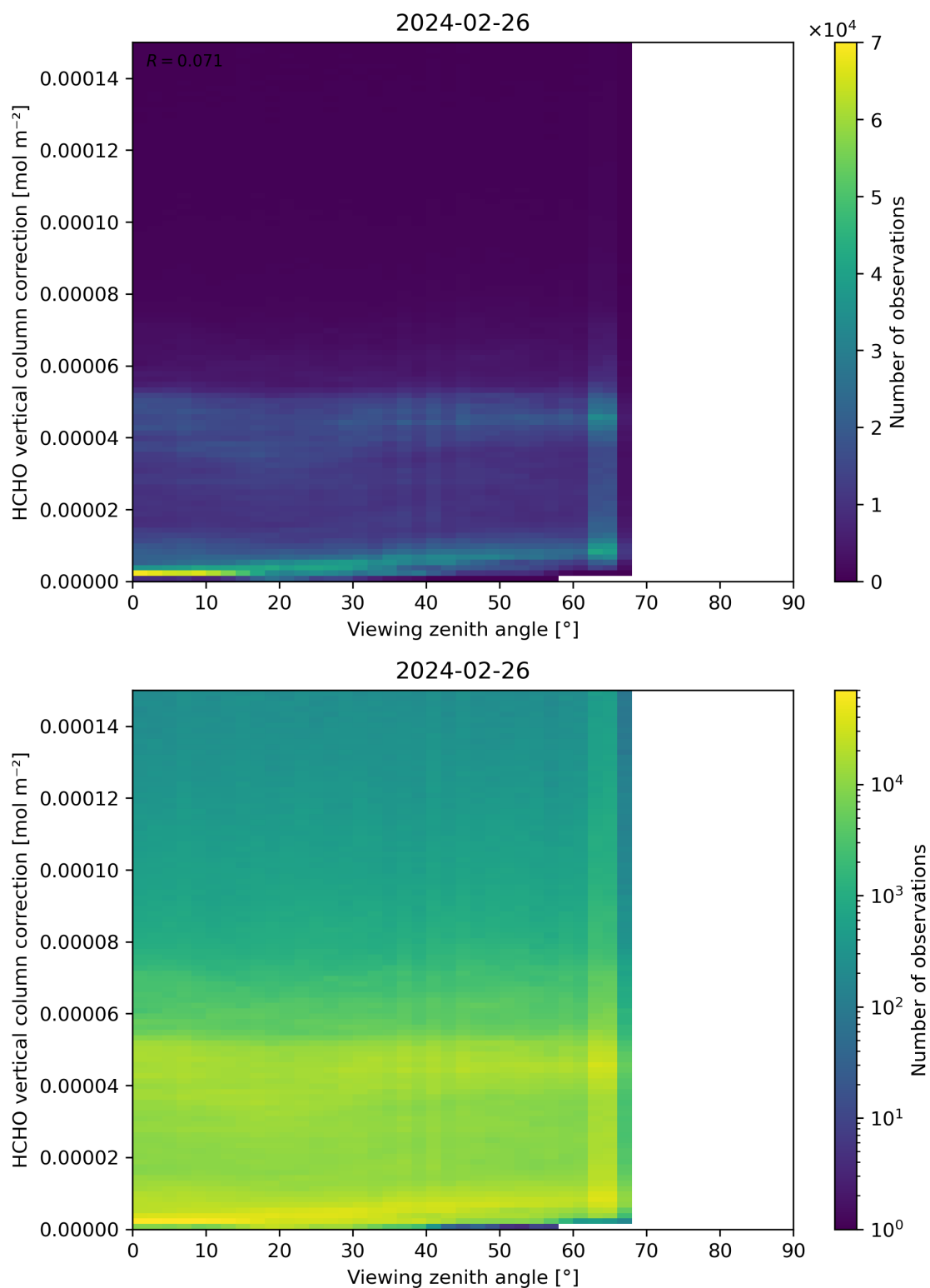
Figure 193: Scatter density plot of “Viewing zenith angle” against “HCHO vertical column correction” for 2024-02-25 to 2024-02-27.
