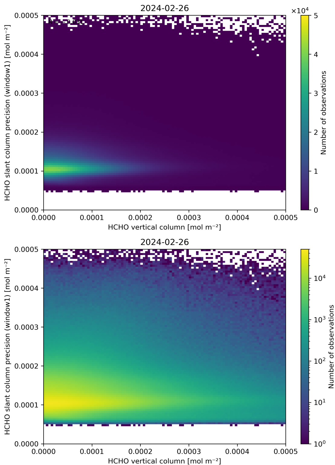
Figure 130: Scatter density plot of “HCHO vertical column” against “HCHO slant column precision (window1)” for 2024-02-25 to 2024-02-27.
