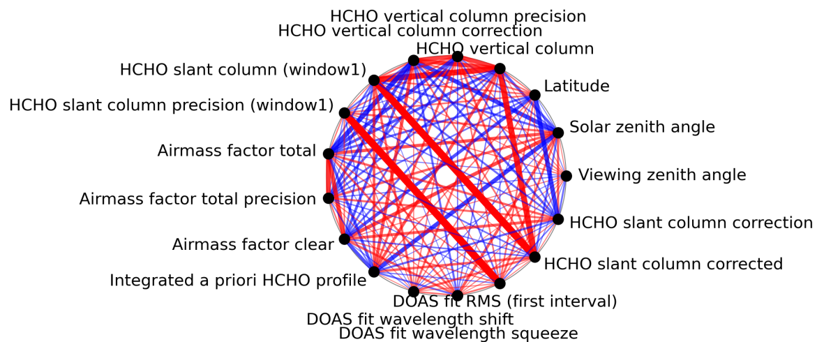
Figure 1: Map of correlation graph for 2024-02-25 to 2024-02-27.
