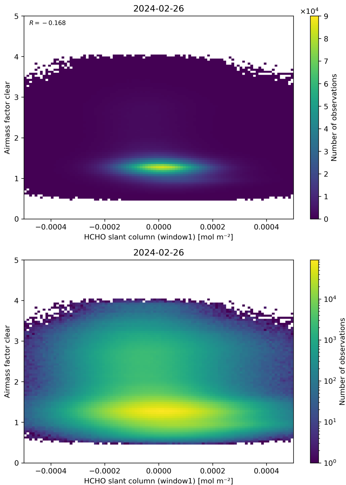
Figure 81: Scatter density plot of “HCHO slant column (window1)” against “Airmass factor clear” for 2024-02-25 to 2024-02-27.
