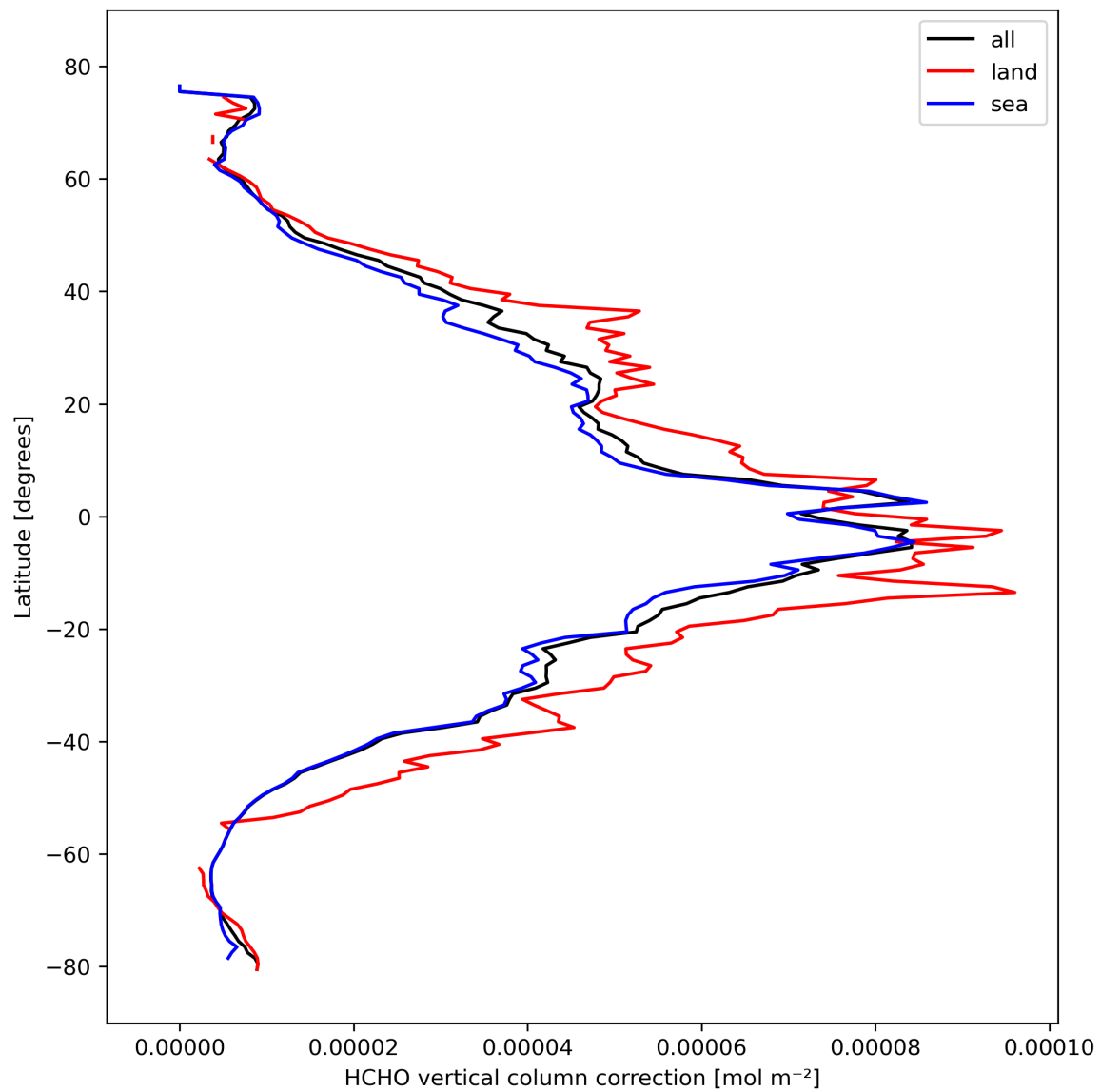
Figure 23: Zonal average of “HCHO vertical column correction” for 2024-02-25 to 2024-02-27.
