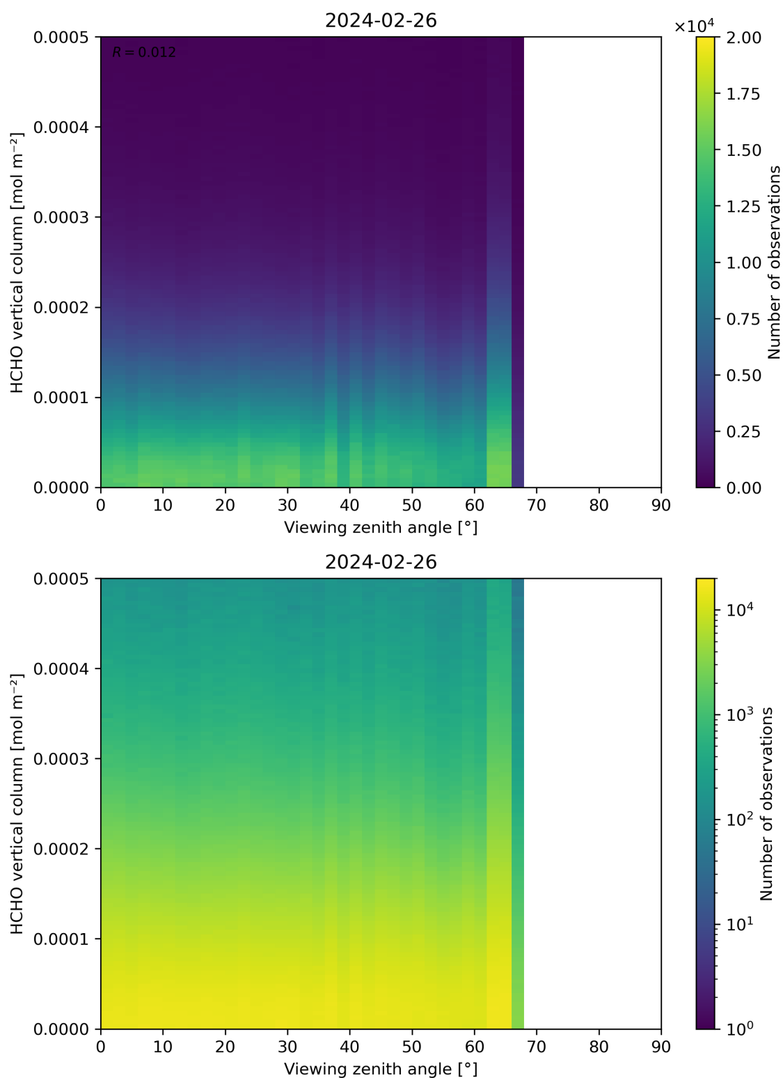
Figure 192: Scatter density plot of “Viewing zenith angle” against “HCHO vertical column” for 2024-02-25 to 2024-02-27.
