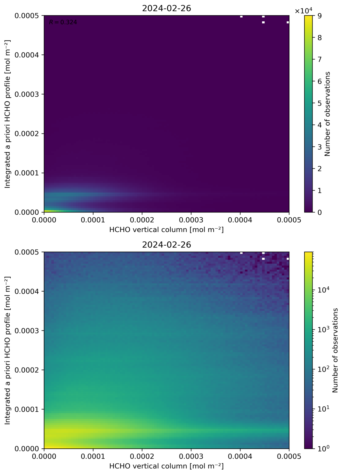
Figure 135: Scatter density plot of “HCHO vertical column” against “Integrated a priori HCHO profile” for 2024-02-25 to 2024-02-27.
