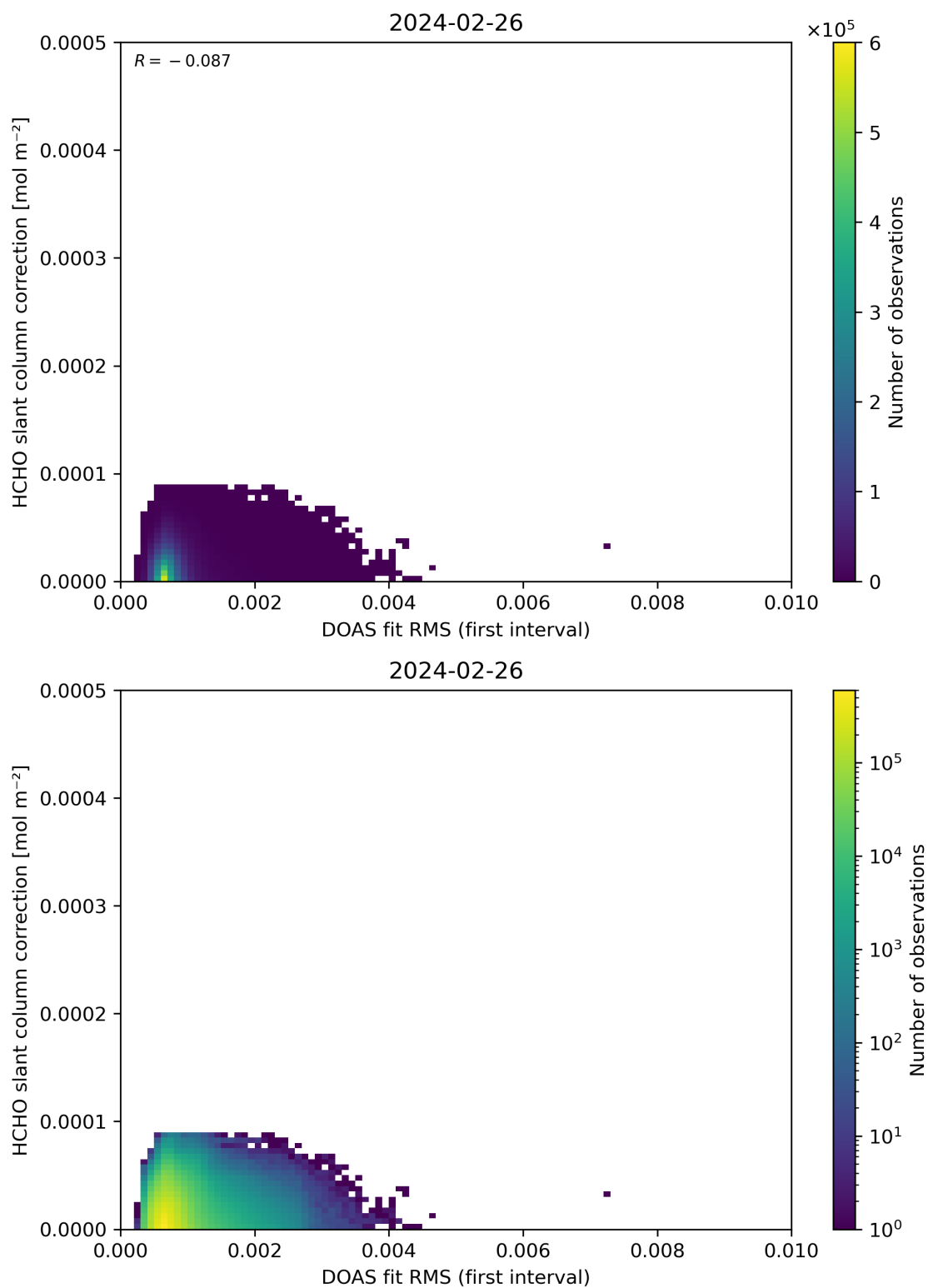
Figure 63: Scatter density plot of “DOAS fit RMS (first interval)” against “HCHO slant column correction” for 2024-02-25 to 2024-02-27.
