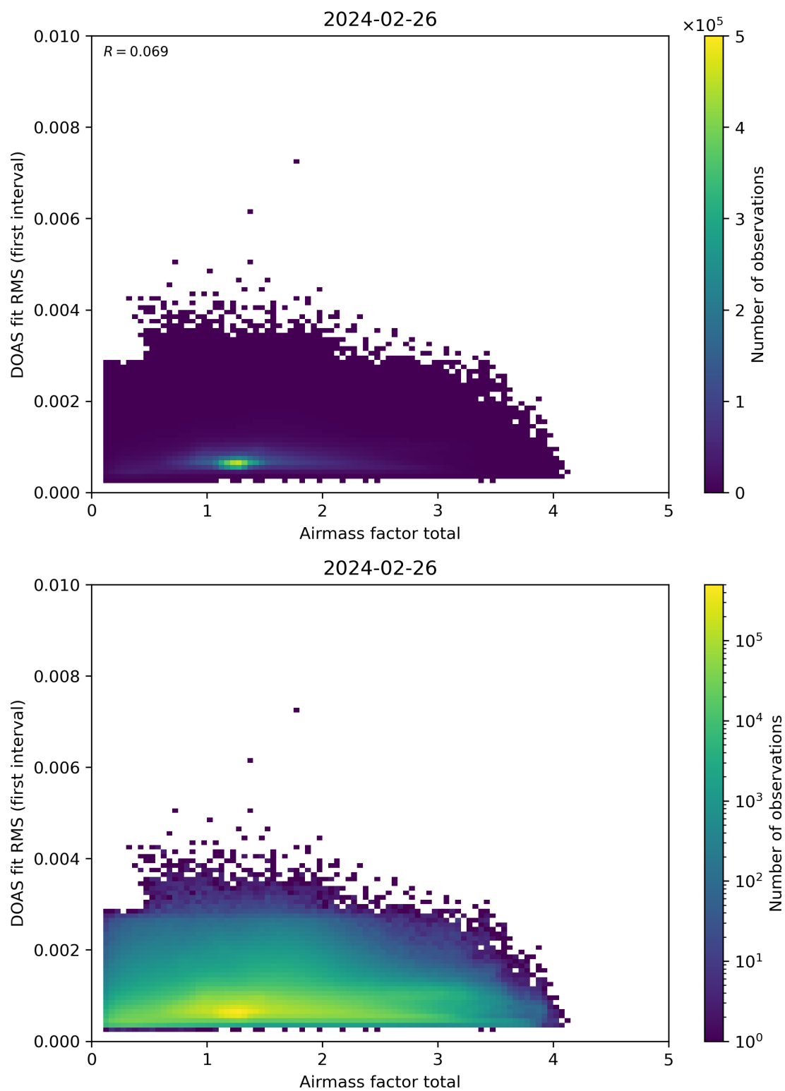
Figure 97: Scatter density plot of “Airmass factor total” against “DOAS fit RMS (first interval)” for 2024-02-25 to 2024-02-27.
