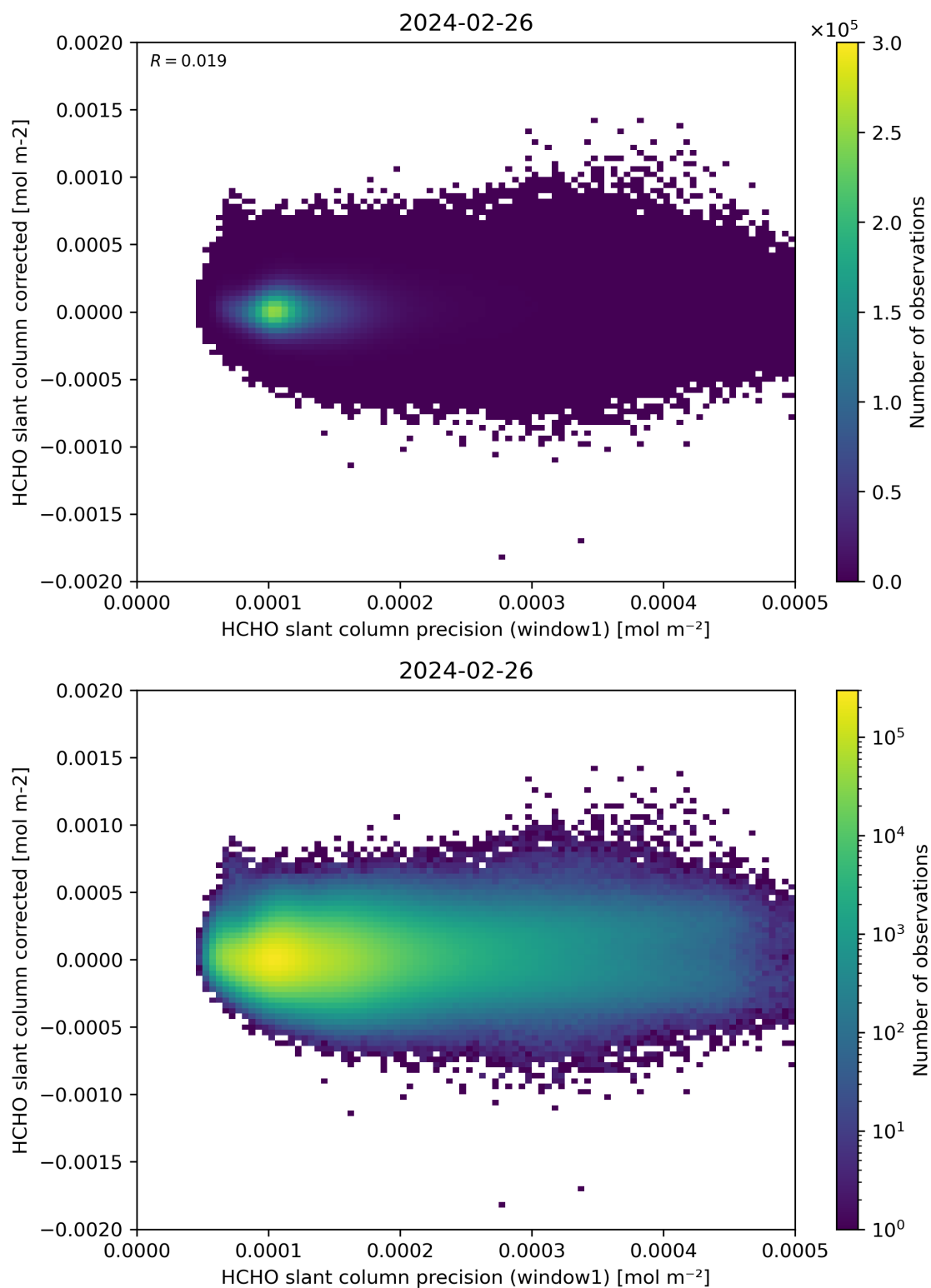
Figure 92: Scatter density plot of “HCHO slant column precision (window1)” against “HCHO slant column corrected” for 2024-02-25 to 2024-02-27.
