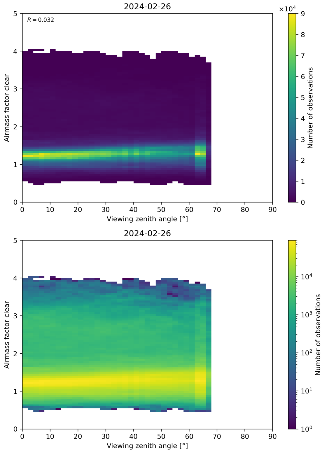
Figure 185: Scatter density plot of “Viewing zenith angle” against “Airmass factor clear” for 2024-02-25 to 2024-02-27.
