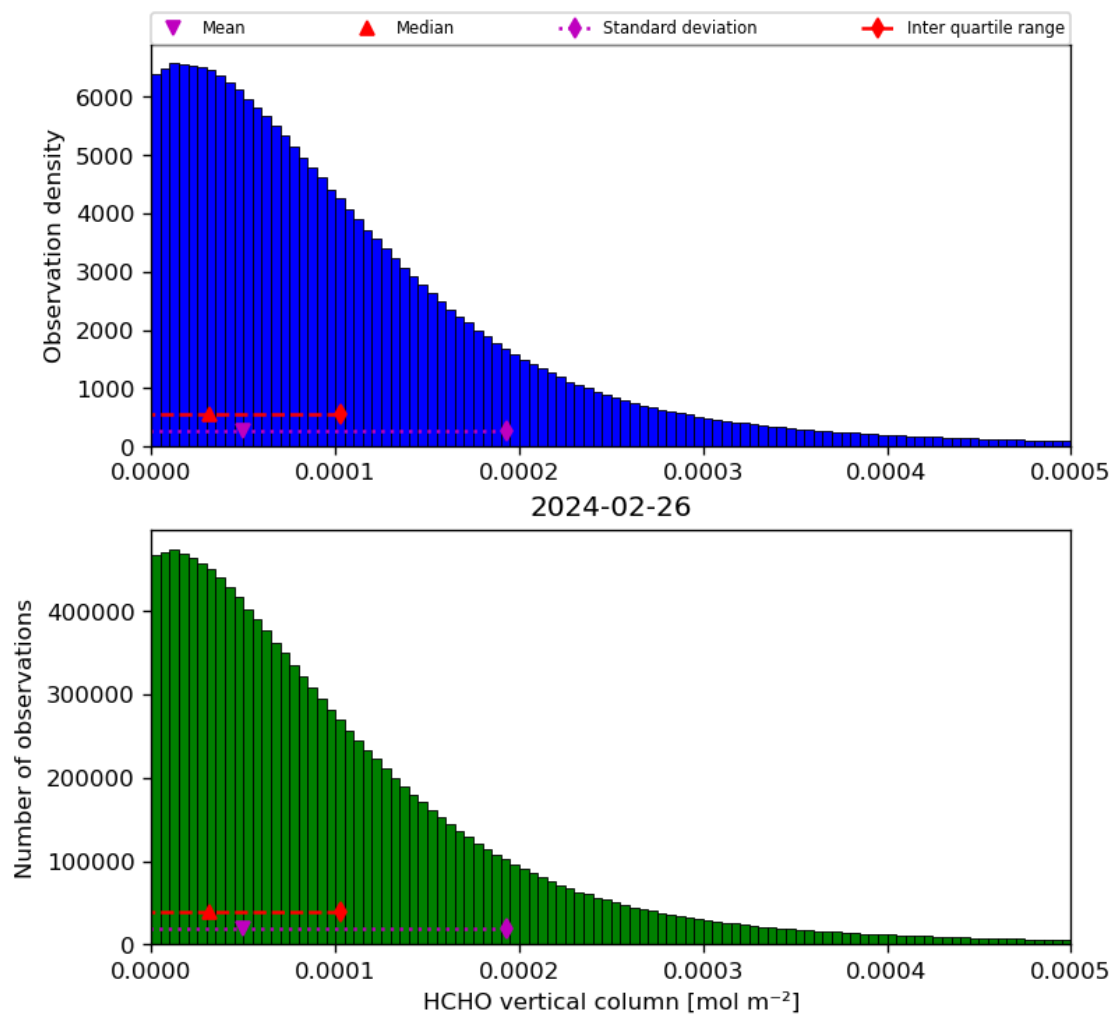
Figure 35: Histogram of “HCHO vertical column” for 2024-02-25 to 2024-02-27
