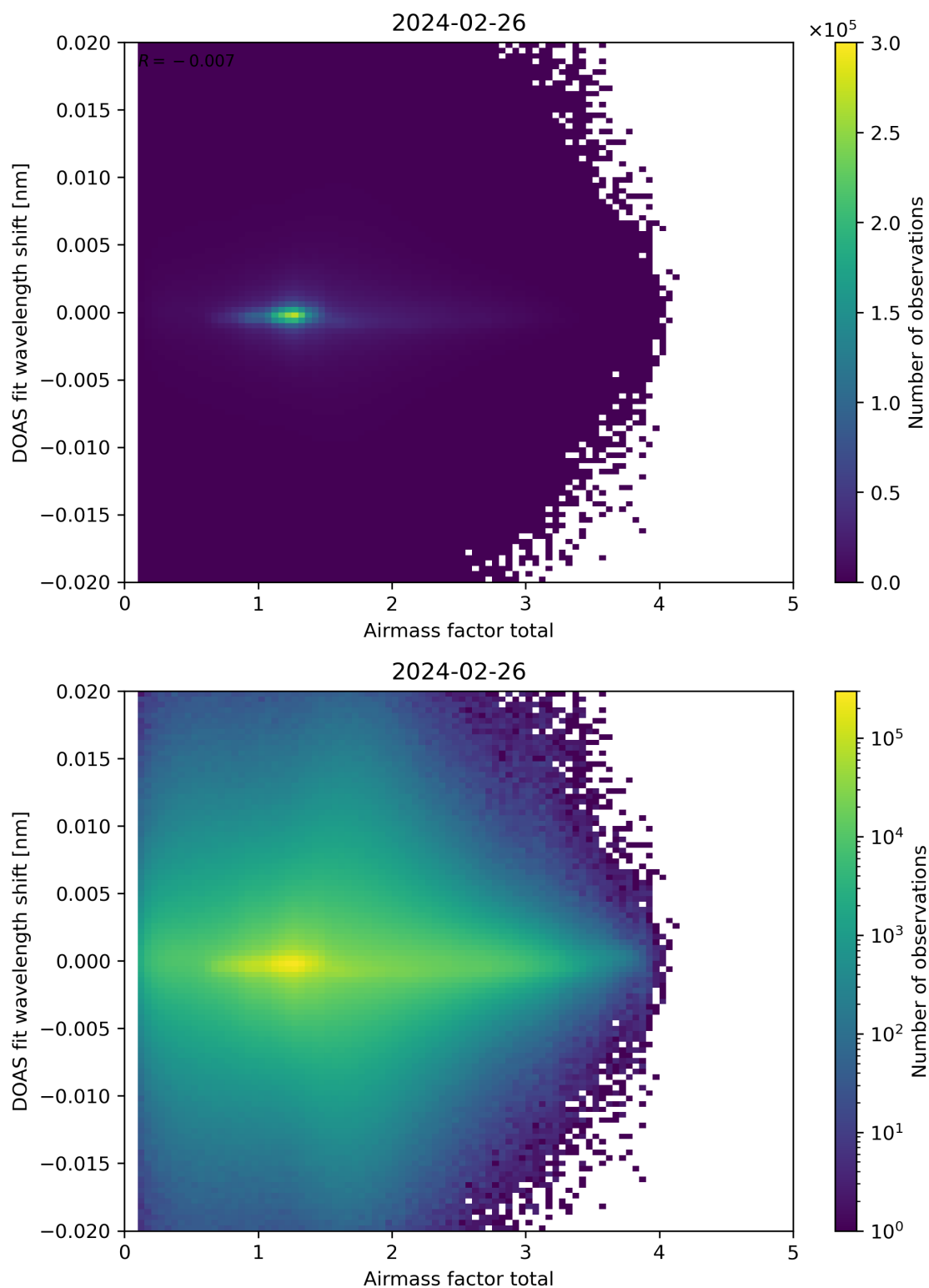
Figure 98: Scatter density plot of “Airmass factor total” against “DOAS fit wavelength shift” for 2024-02-25 to 2024-02-27.
