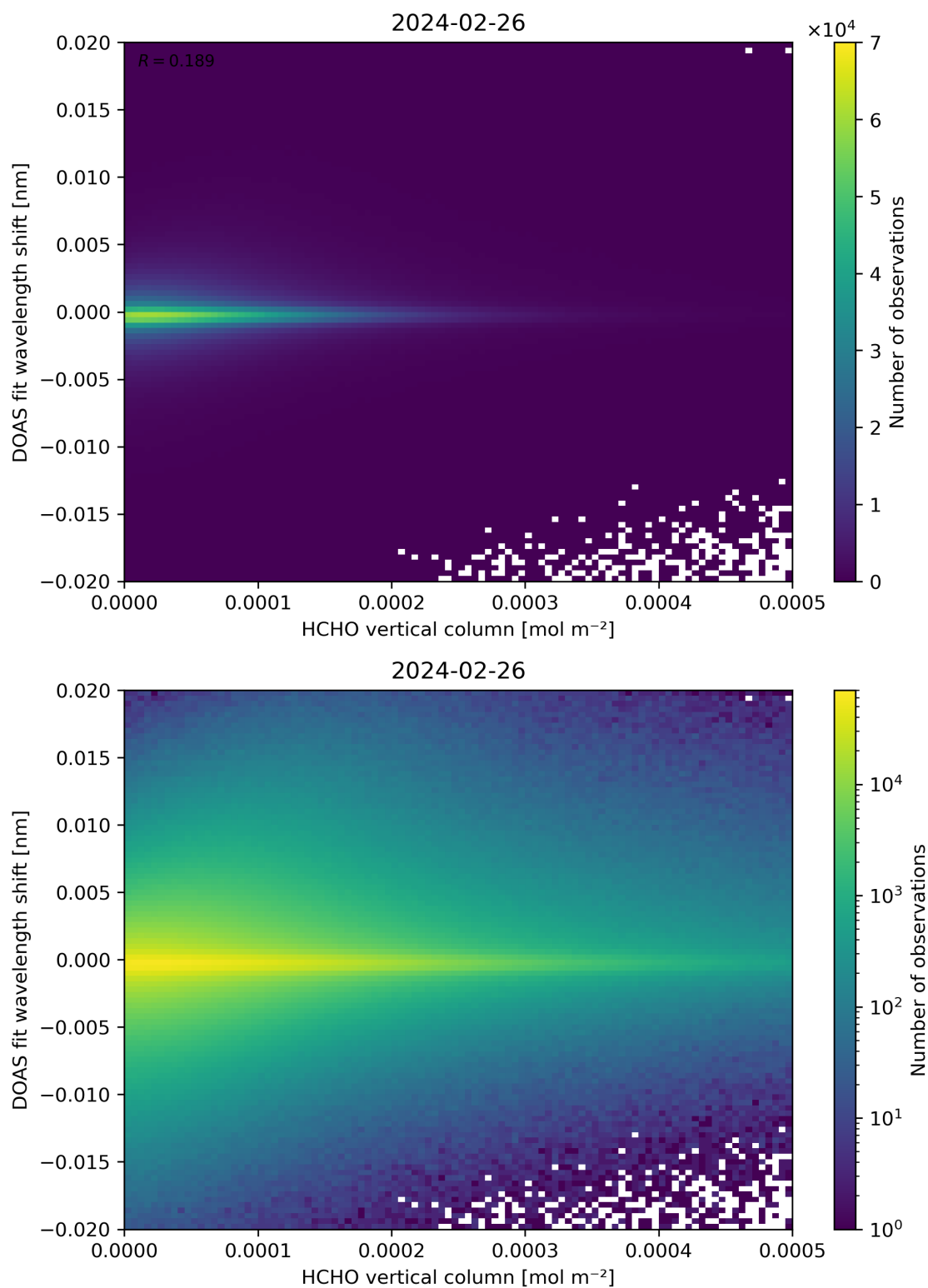
Figure 124: Scatter density plot of “HCHO vertical column” against “DOAS fit wavelength shift” for 2024-02-25 to 2024-02-27.
