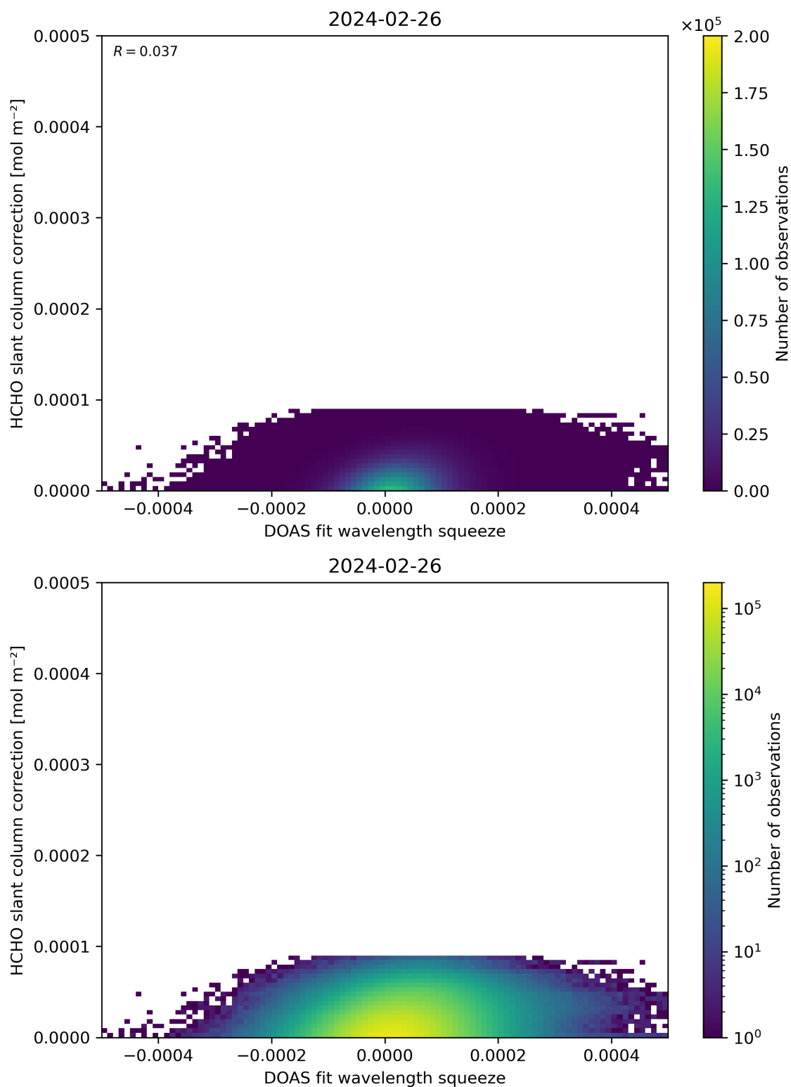
Figure 70: Scatter density plot of “DOAS fit wavelength squeeze” against “HCHO slant column correction” for 2024-02-25 to 2024-02-27.
