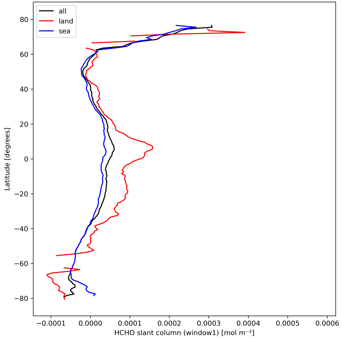
Figure 24: Zonal average of “HCHO slant column (window1)” for 2024-02-25 to 2024-02-27.
