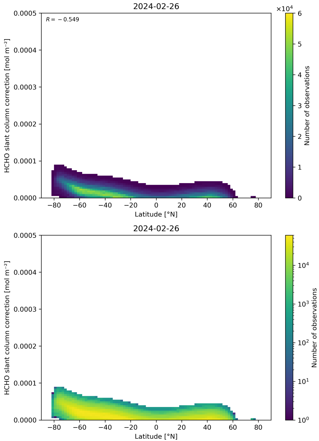
Figure 158: Scatter density plot of “Latitude” against “HCHO slant column correction” for 2024-02-25 to 2024-02-27.
