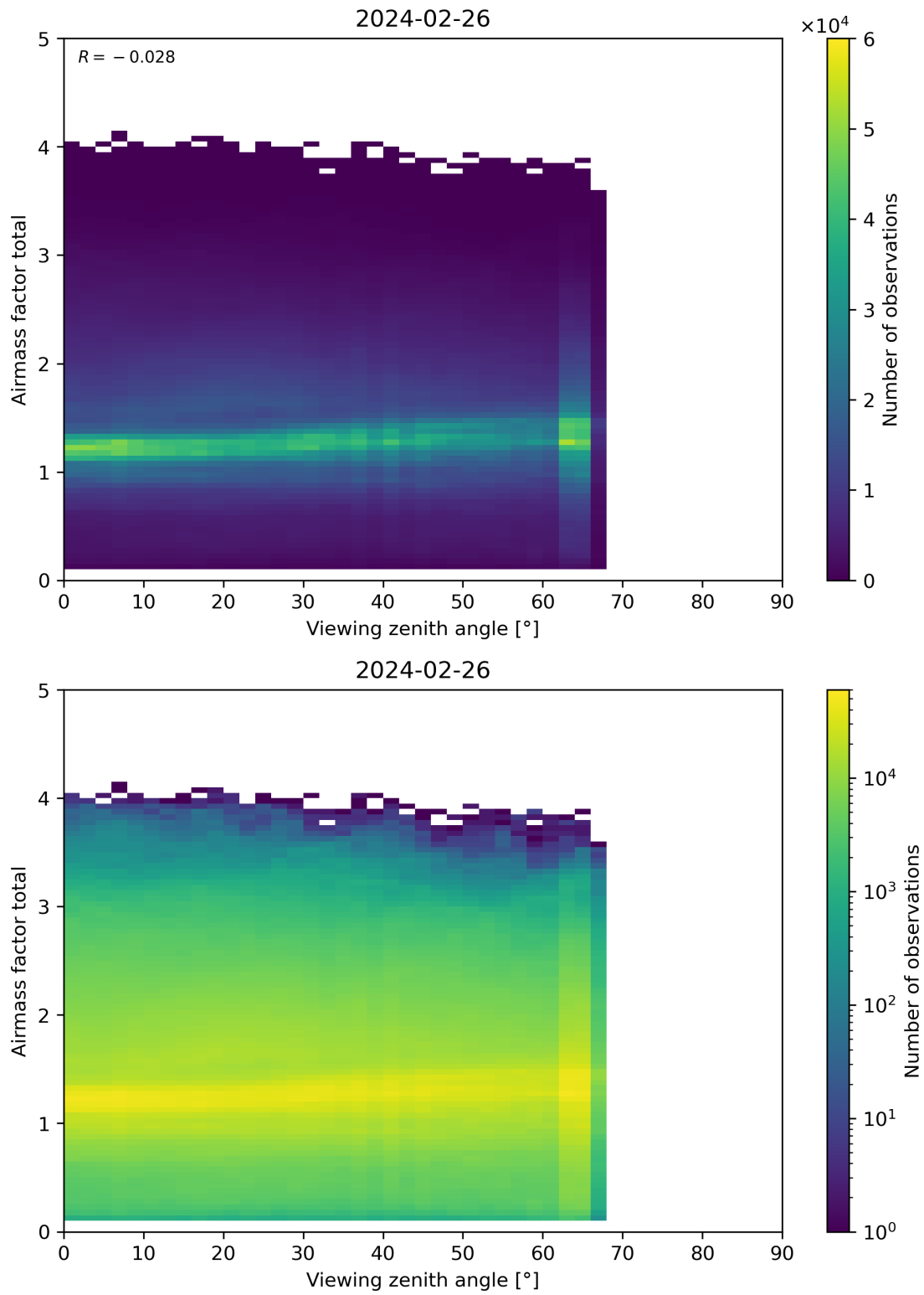
Figure 190: Scatter density plot of “Viewing zenith angle” against “Airmass factor total” for 2024-02-25 to 2024-02-27.
