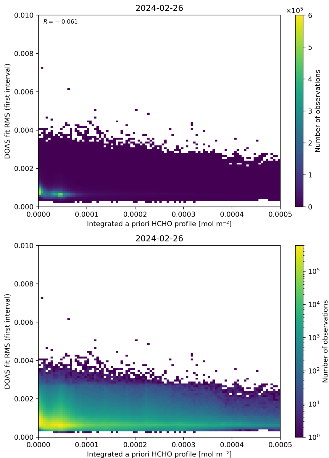
Figure 148: Scatter density plot of “Integrated a priori HCHO profile” against “DOAS fit RMS (first interval)” for 2024-02-25 to 2024-02-27.
