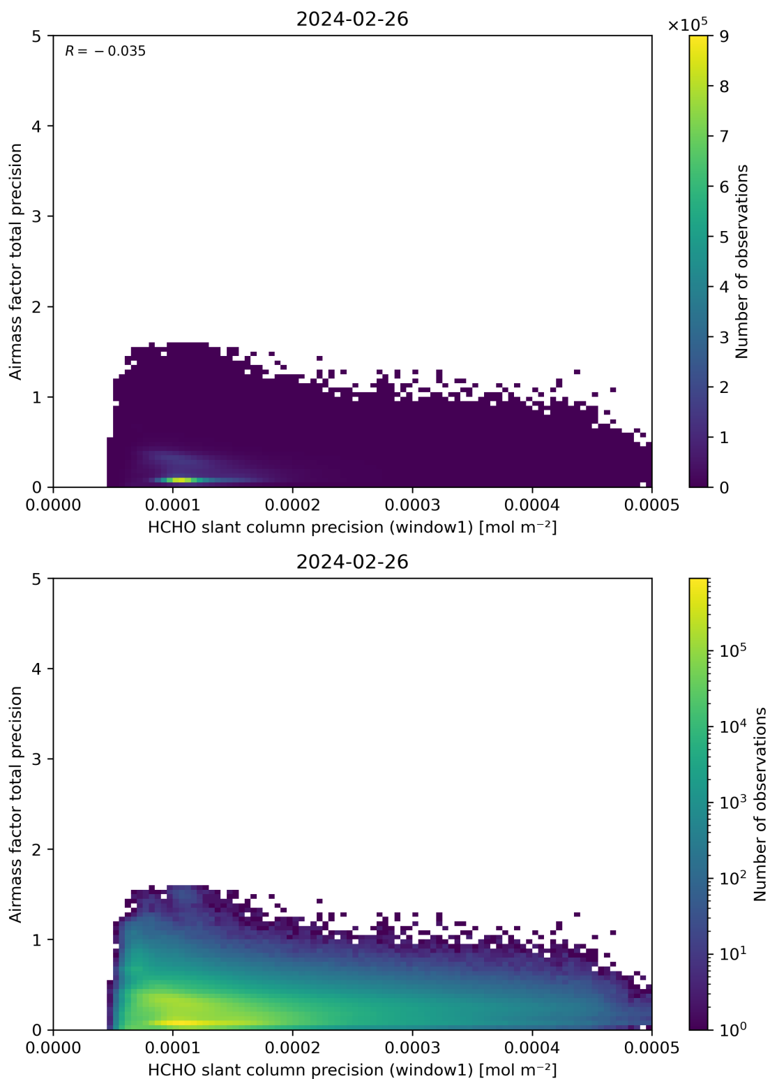
Figure 95: Scatter density plot of “HCHO slant column precision (window1)” against “Airmass factor total precision” for 2024-02-25 to 2024-02-27.
