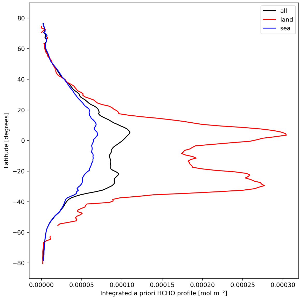
Figure 29: Zonal average of “Integrated a priori HCHO profile” for 2024-02-25 to 2024-02-27.
