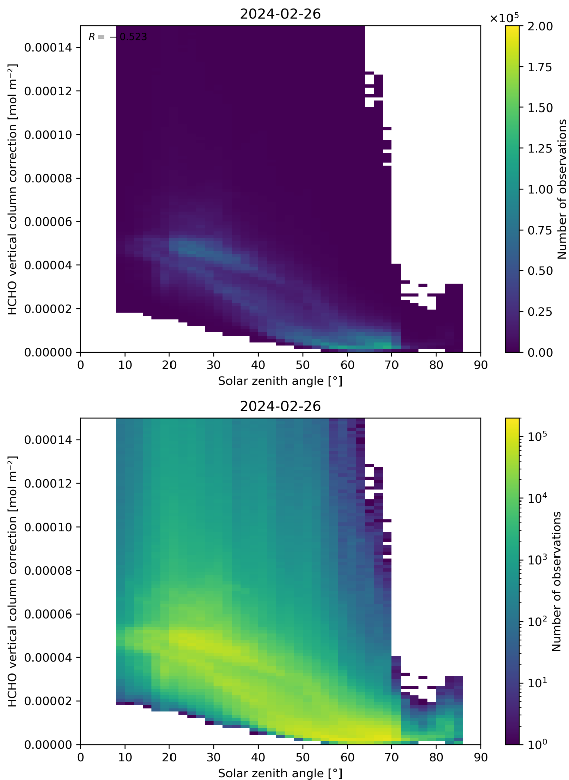
Figure 178: Scatter density plot of “Solar zenith angle” against “HCHO vertical column correction” for 2024-02-25 to 2024-02-27.
