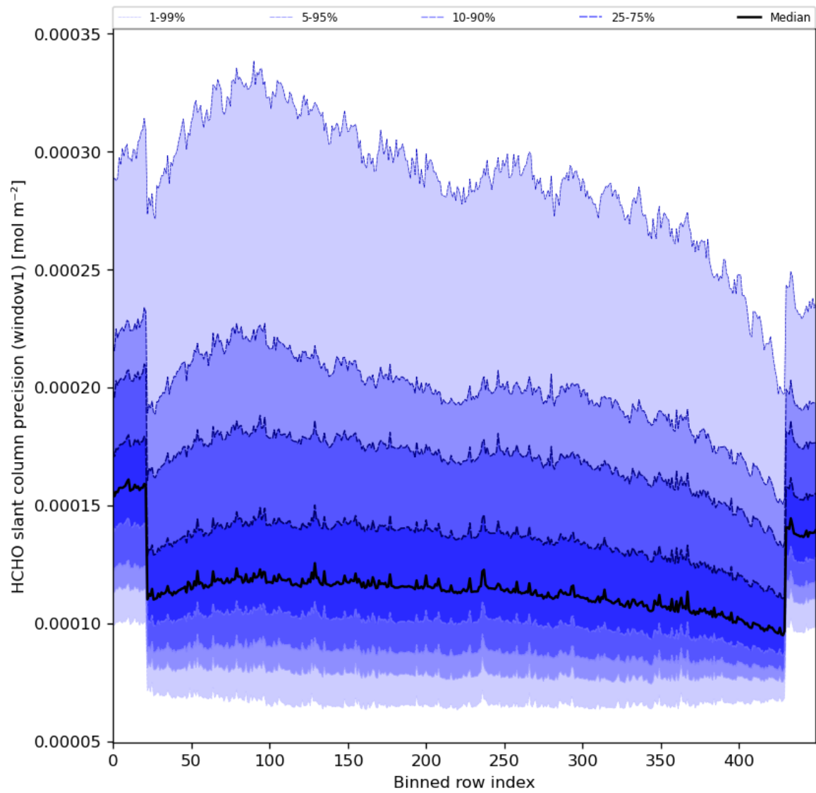
Figure 53: Along track statistics of “HCHO slant column precision (window1)” for 2024-02-25 to 2024-02-27
