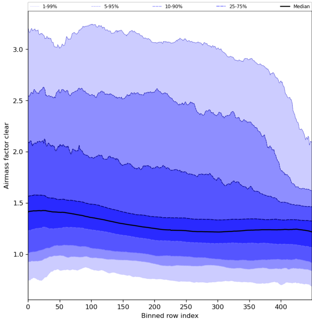
Figure 56: Along track statistics of “Airmass factor clear” for 2024-02-25 to 2024-02-27
