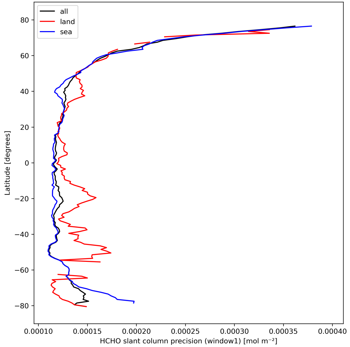
Figure 25: Zonal average of “HCHO slant column precision (window1)” for 2024-02-25 to 2024-02-27.
