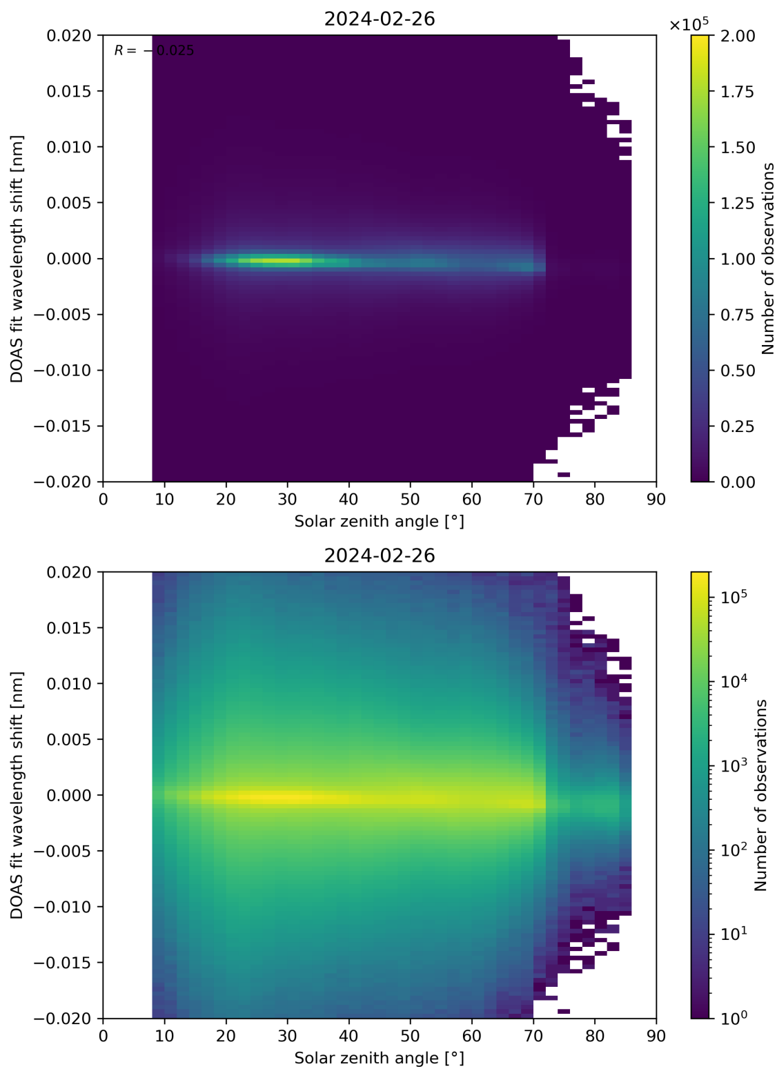
Figure 168: Scatter density plot of “Solar zenith angle” against “DOAS fit wavelength shift” for 2024-02-25 to 2024-02-27.
