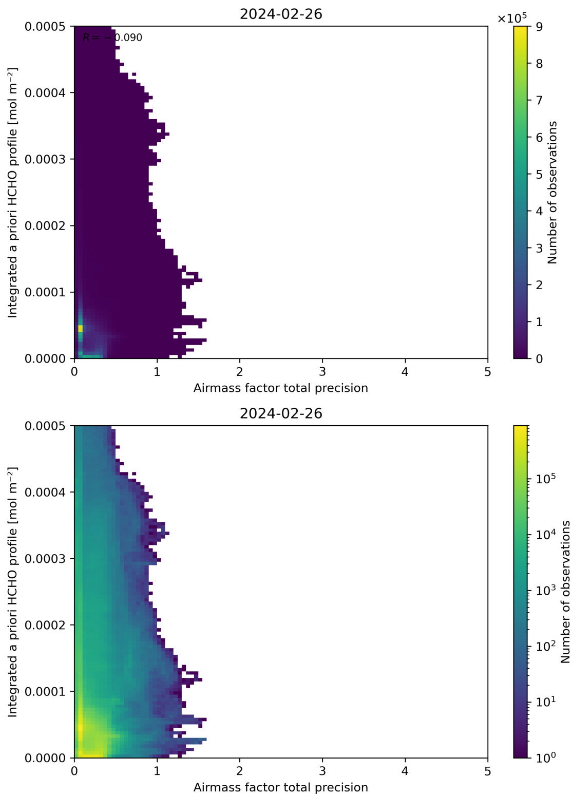
Figure 111: Scatter density plot of “Airmass factor total precision” against “Integrated a priori HCHO profile” for 2024-02-25 to 2024-02-27.
