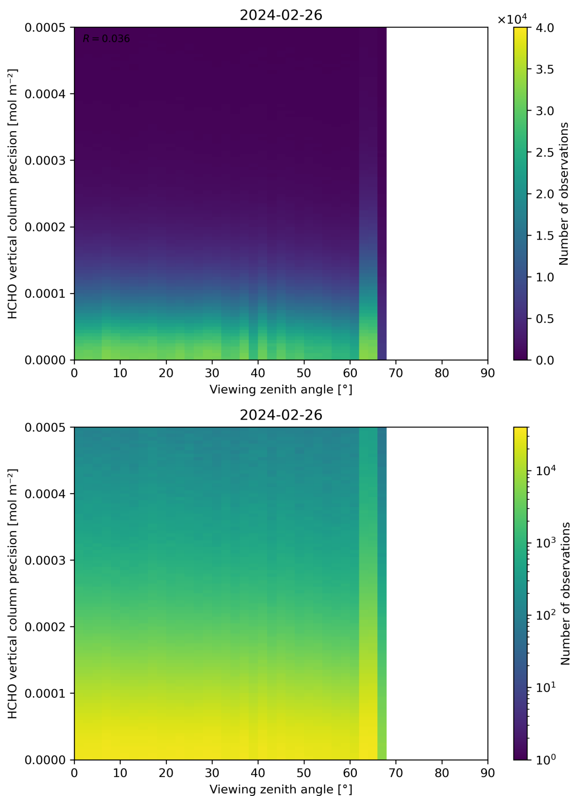
Figure 194: Scatter density plot of “Viewing zenith angle” against “HCHO vertical column precision” for 2024-02-25 to 2024-02-27.
