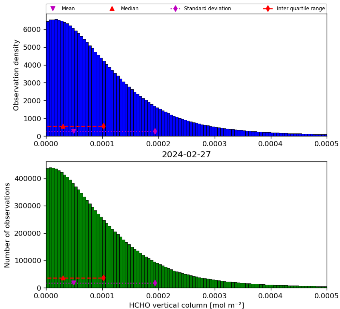
Figure 35: Histogram of “HCHO vertical column” for 2024-02-27 to 2024-02-28
