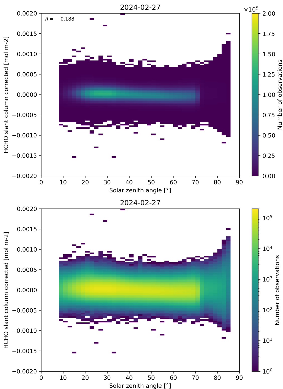
Figure 171: Scatter density plot of “Solar zenith angle” against “HCHO slant column corrected” for 2024-02-27 to 2024-02-28.
