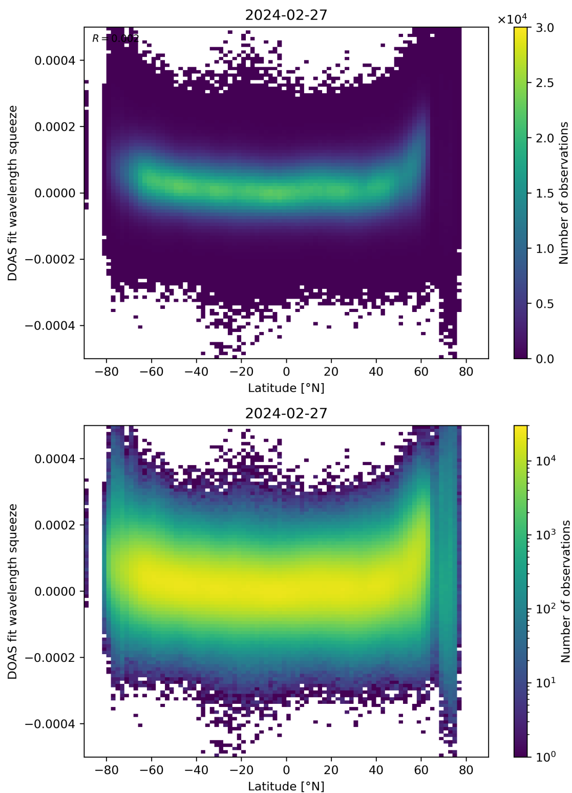
Figure 155: Scatter density plot of “Latitude” against “DOAS fit wavelength squeeze” for 2024-02-27 to 2024-02-28.
