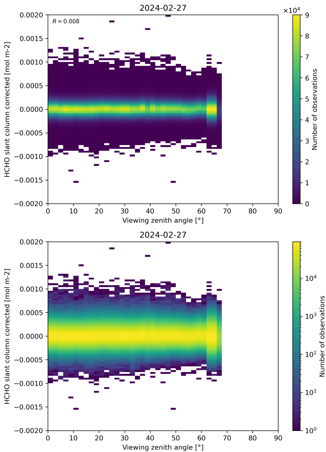
Figure 186: Scatter density plot of “Viewing zenith angle” against “HCHO slant column corrected” for 2024-02-27 to 2024-02-28.
