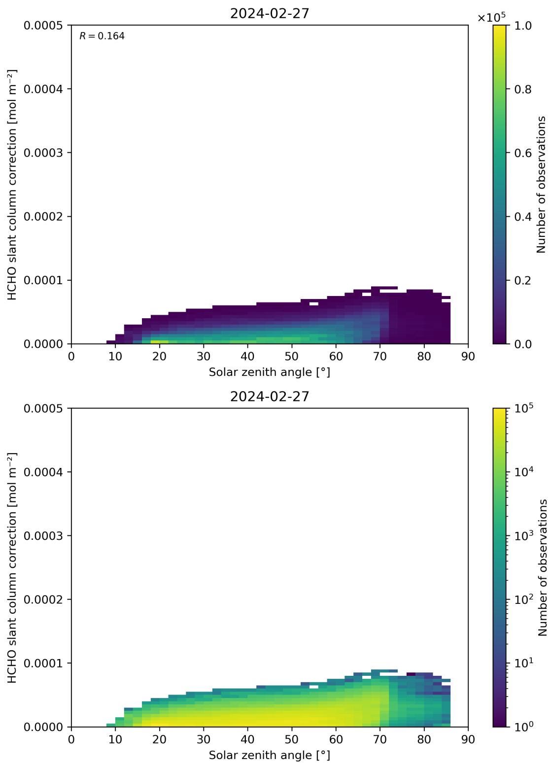
Figure 172: Scatter density plot of “Solar zenith angle” against “HCHO slant column correction” for 2024-02-27 to 2024-02-28.
