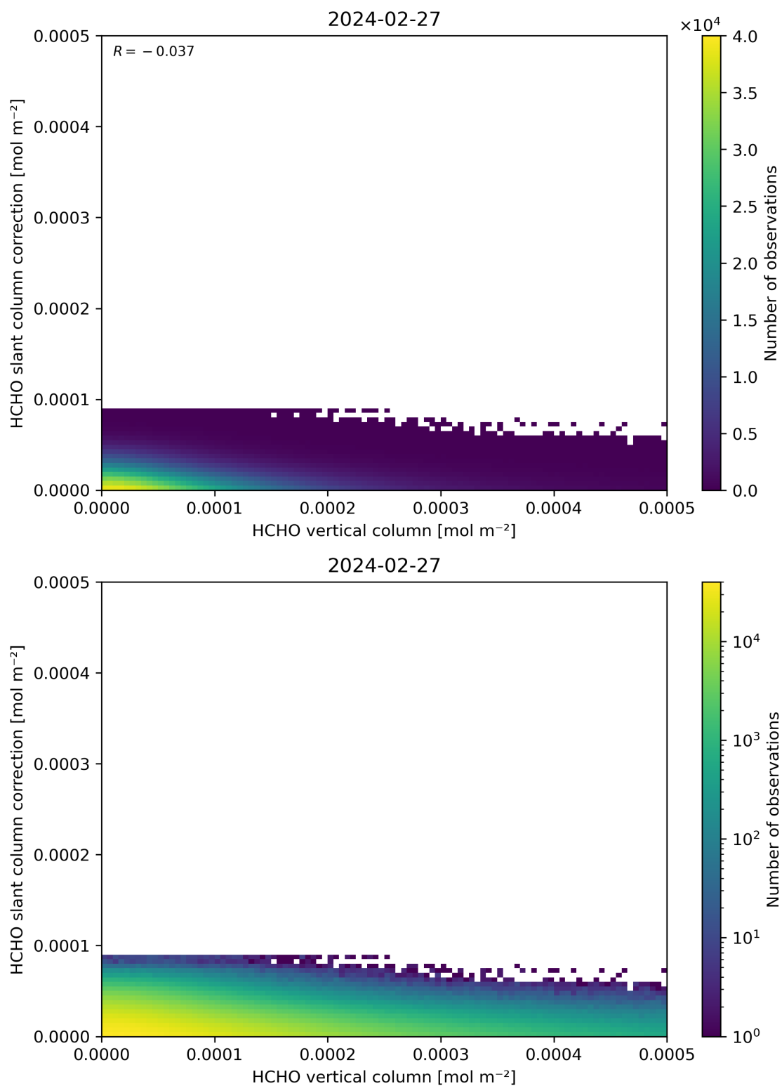
Figure 128: Scatter density plot of “HCHO vertical column” against “HCHO slant column correction” for 2024-02-27 to 2024-02-28.
