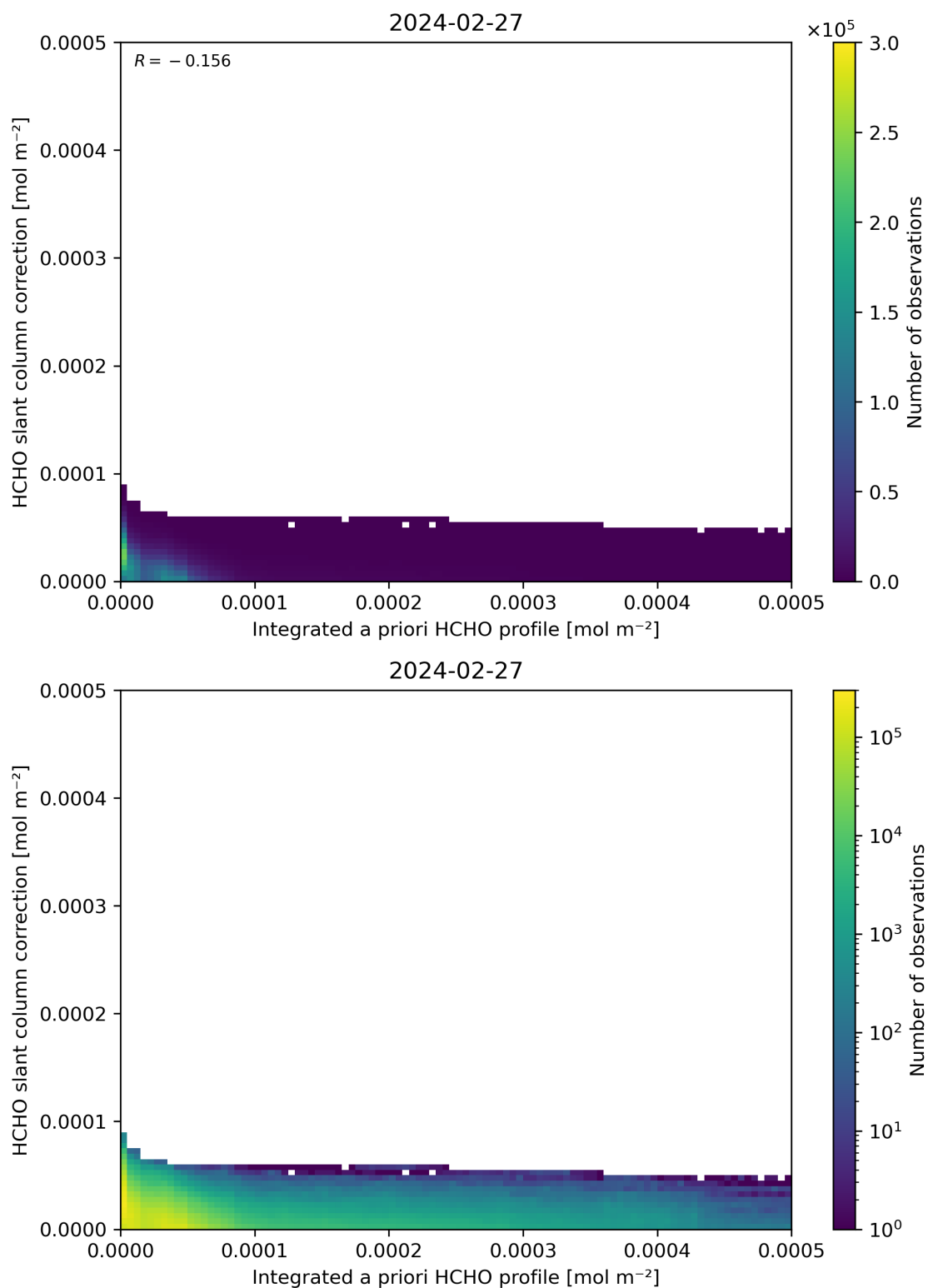
Figure 152: Scatter density plot of “Integrated a priori HCHO profile” against “HCHO slant column correction” for 2024-02-27 to 2024-02-28.
