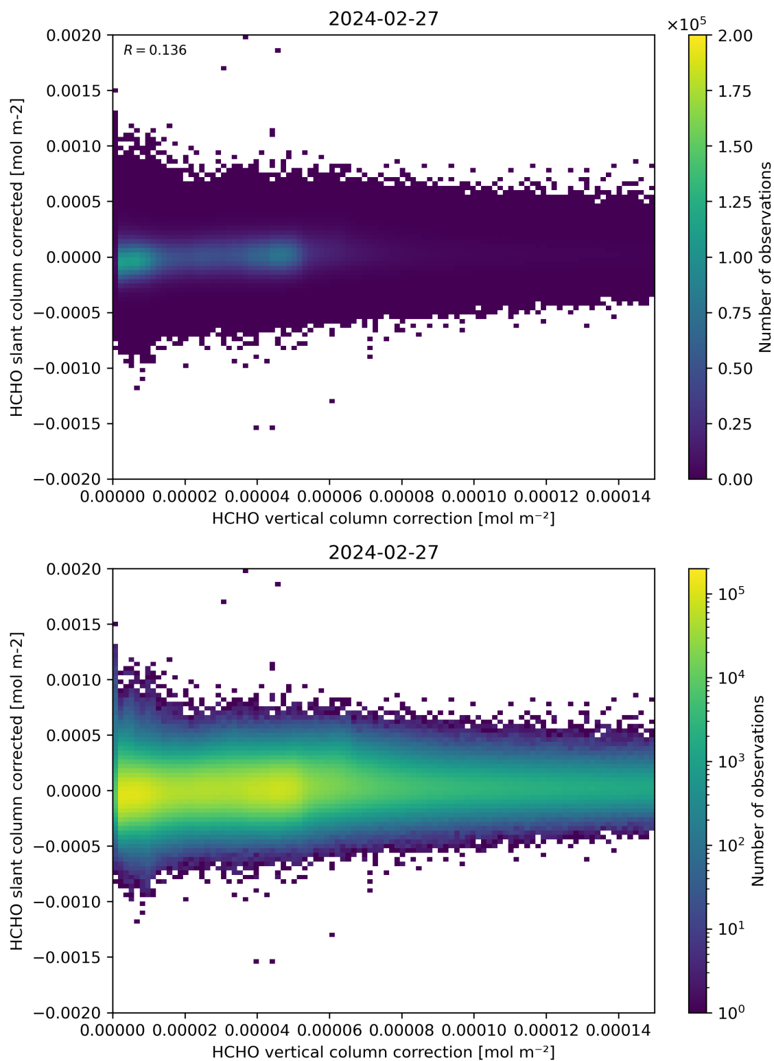
Figure 116: Scatter density plot of “HCHO vertical column correction” against “HCHO slant column corrected” for 2024-02-27 to 2024-02-28.
