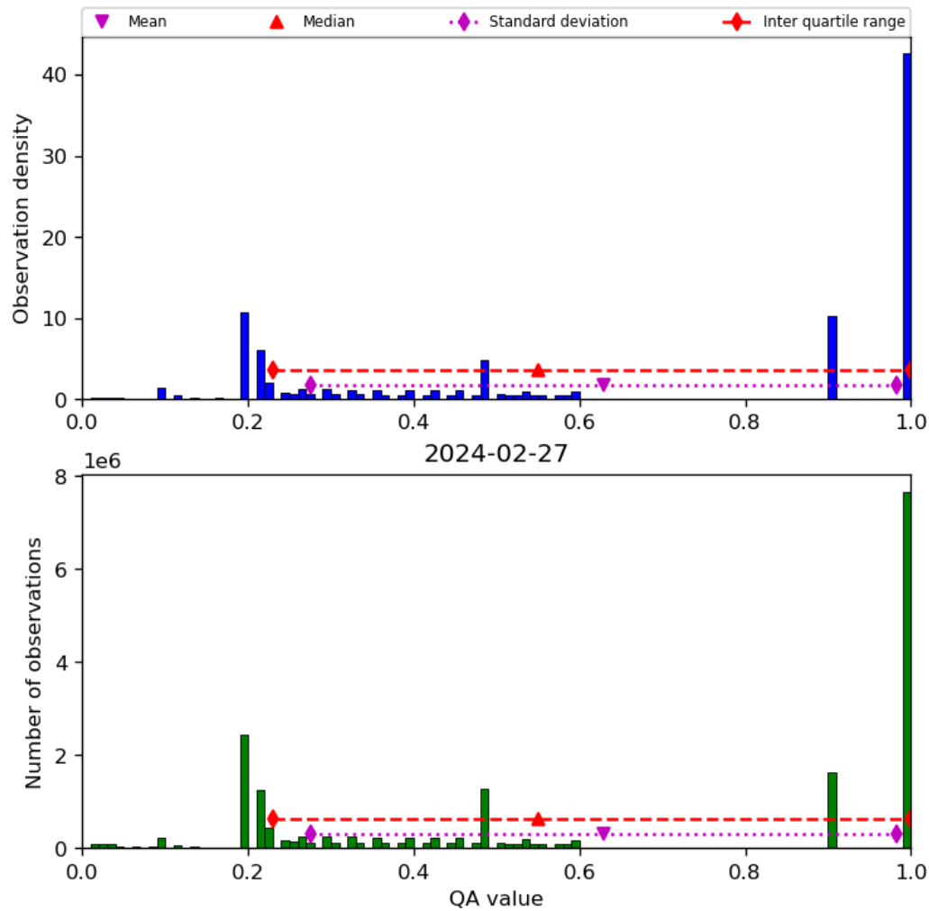
Figure 34: Histogram of “QA value” for 2024-02-27 to 2024-02-28
