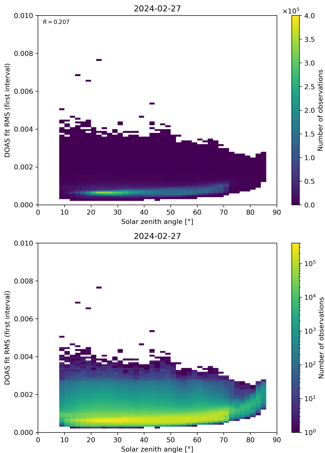
Figure 167: Scatter density plot of “Solar zenith angle” against “DOAS fit RMS (first interval)” for 2024-02-27 to 2024-02-28.
