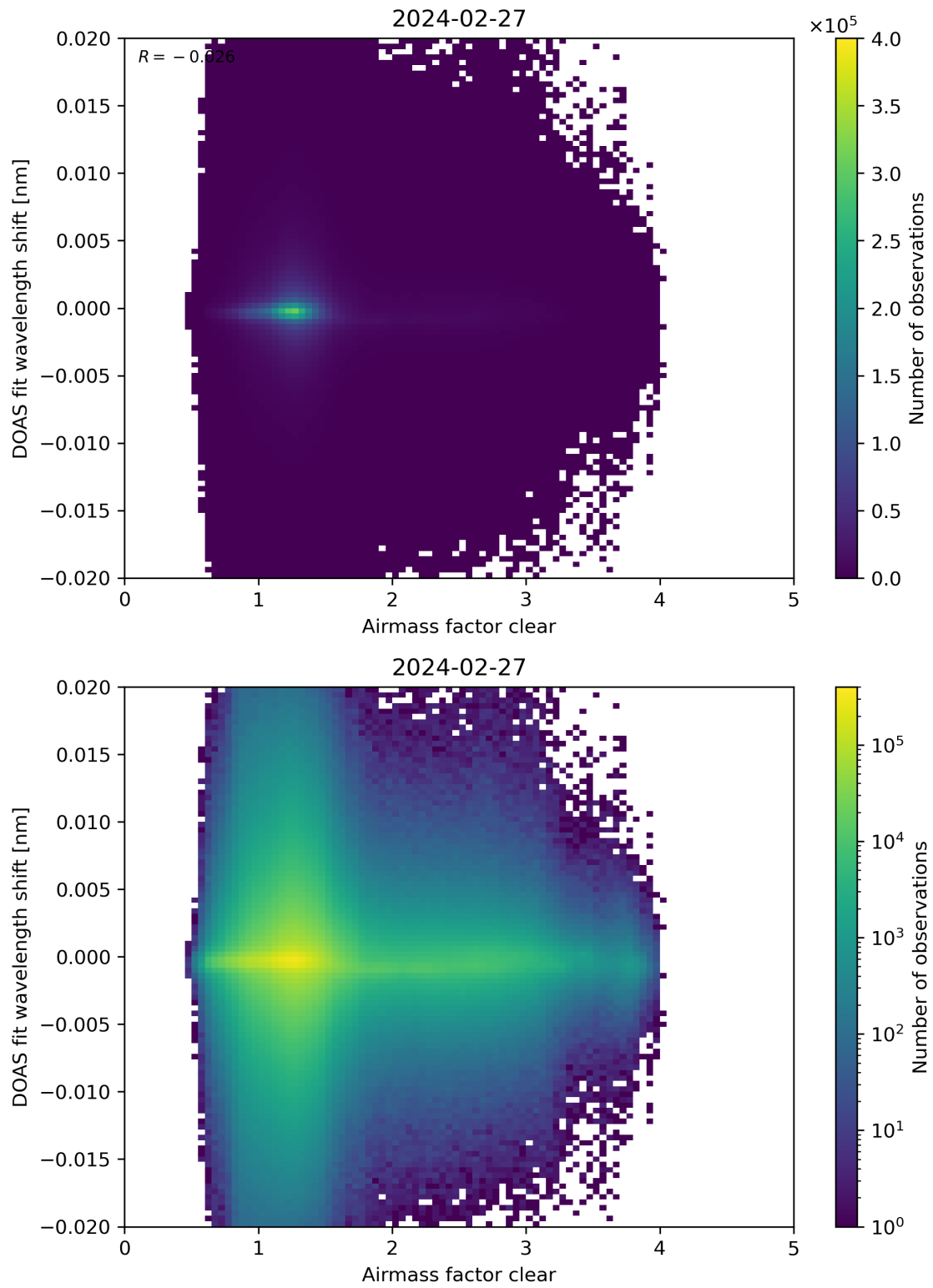
Figure 72: Scatter density plot of “Airmass factor clear” against “DOAS fit wavelength shift” for 2024-02-27 to 2024-02-28.
