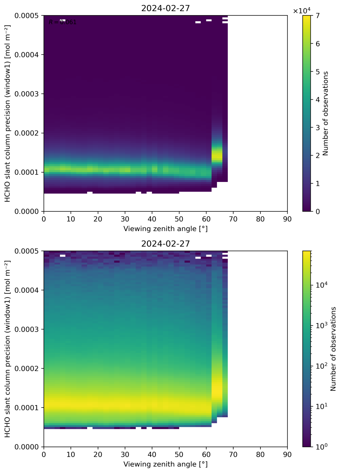
Figure 189: Scatter density plot of “Viewing zenith angle” against “HCHO slant column precision (window1)” for 2024-02-27 to 2024-02-28.
