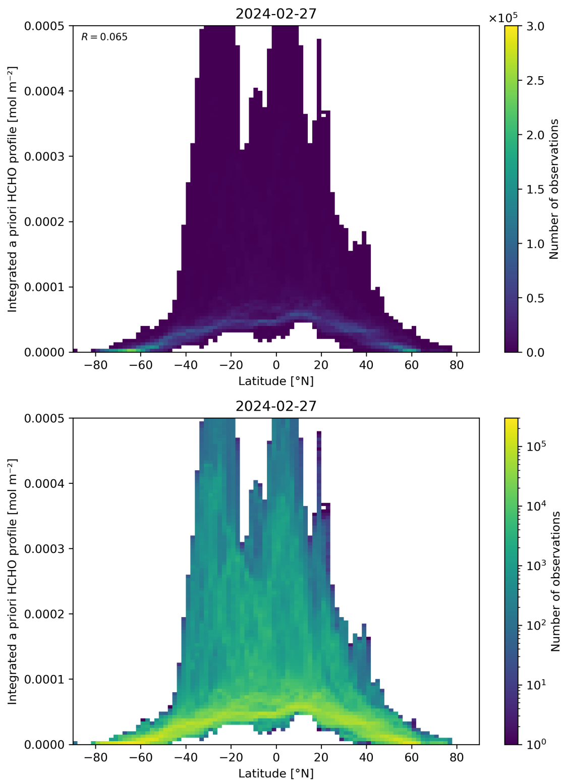
Figure 166: Scatter density plot of “Latitude” against “Integrated a priori HCHO profile” for 2024-02-27 to 2024-02-28.
