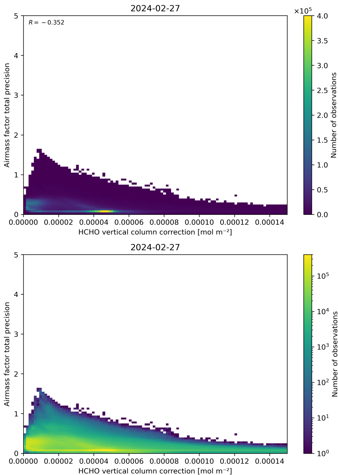
Figure 121: Scatter density plot of “HCHO vertical column correction” against “Airmass factor total precision” for 2024-02-27 to 2024-02-28.
