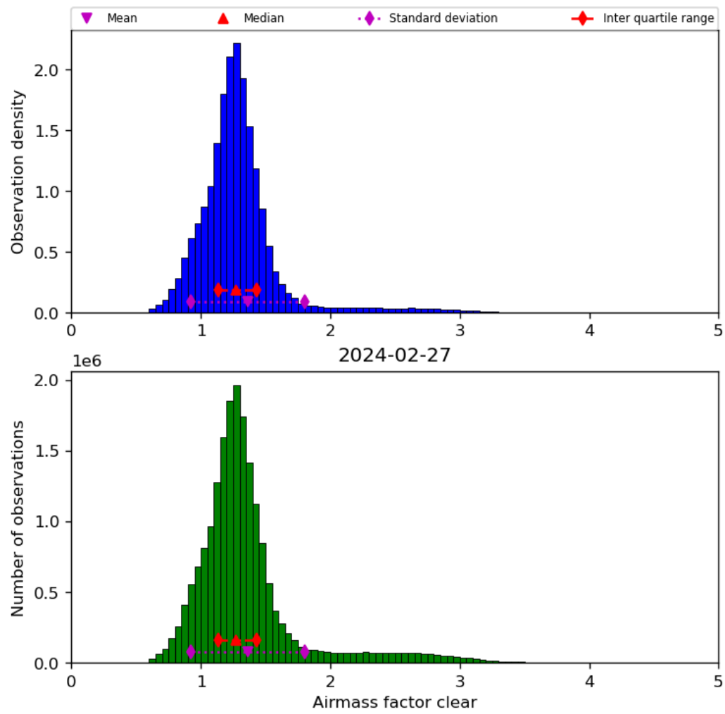
Figure 42: Histogram of “Airmass factor clear” for 2024-02-27 to 2024-02-28
