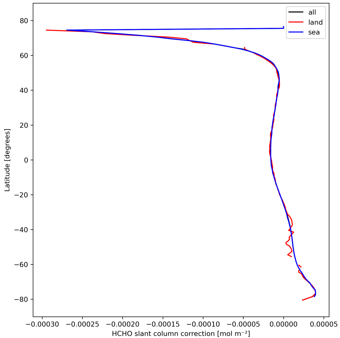
Figure 33: Zonal average of “HCHO slant column correction” for 2024-02-27 to 2024-02-28.
