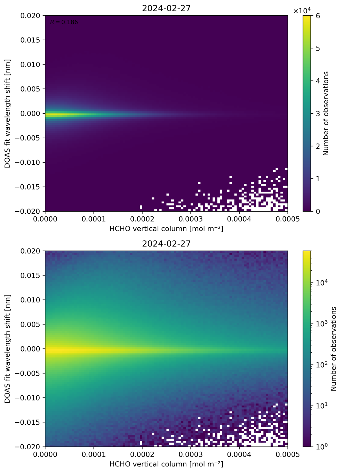
Figure 124: Scatter density plot of “HCHO vertical column” against “DOAS fit wavelength shift” for 2024-02-27 to 2024-02-28.
