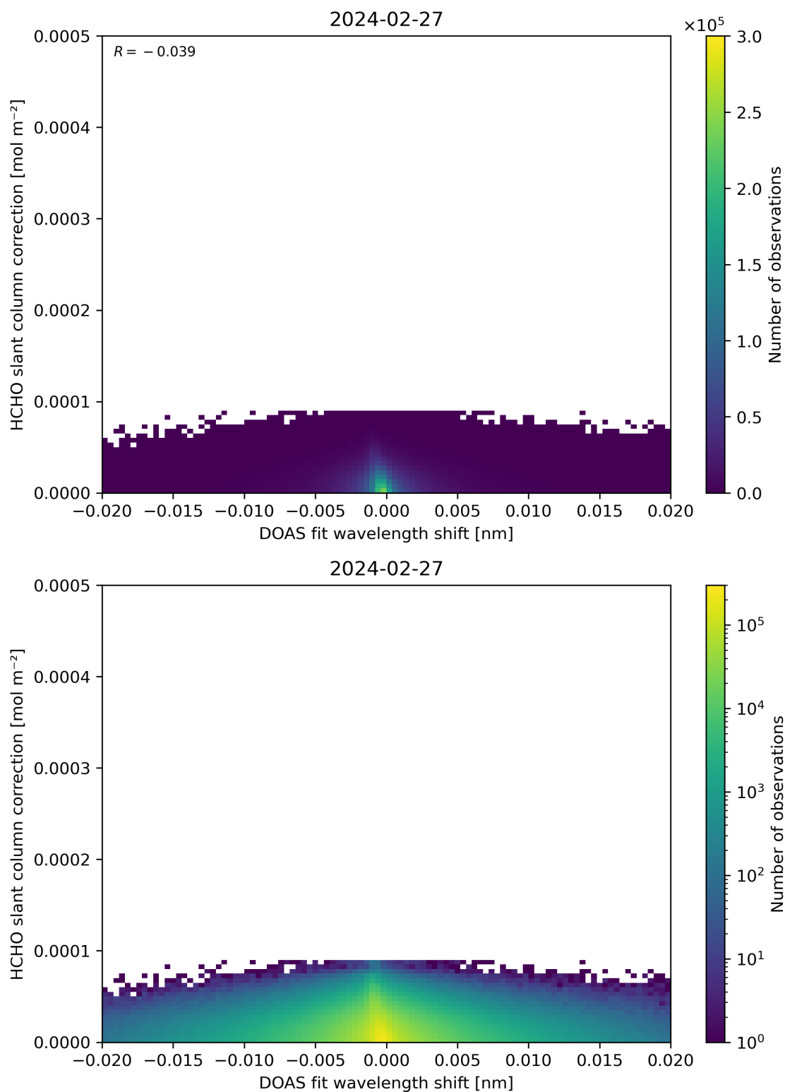
Figure 67: Scatter density plot of “DOAS fit wavelength shift” against “HCHO slant column correction” for 2024-02-27 to 2024-02-28.
