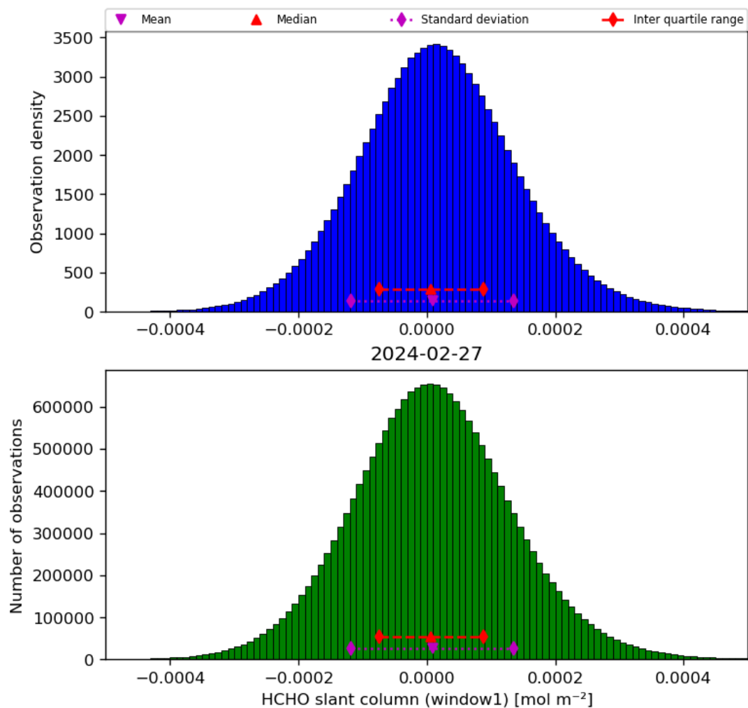
Figure 38: Histogram of “HCHO slant column (window1)” for 2024-02-27 to 2024-02-28
