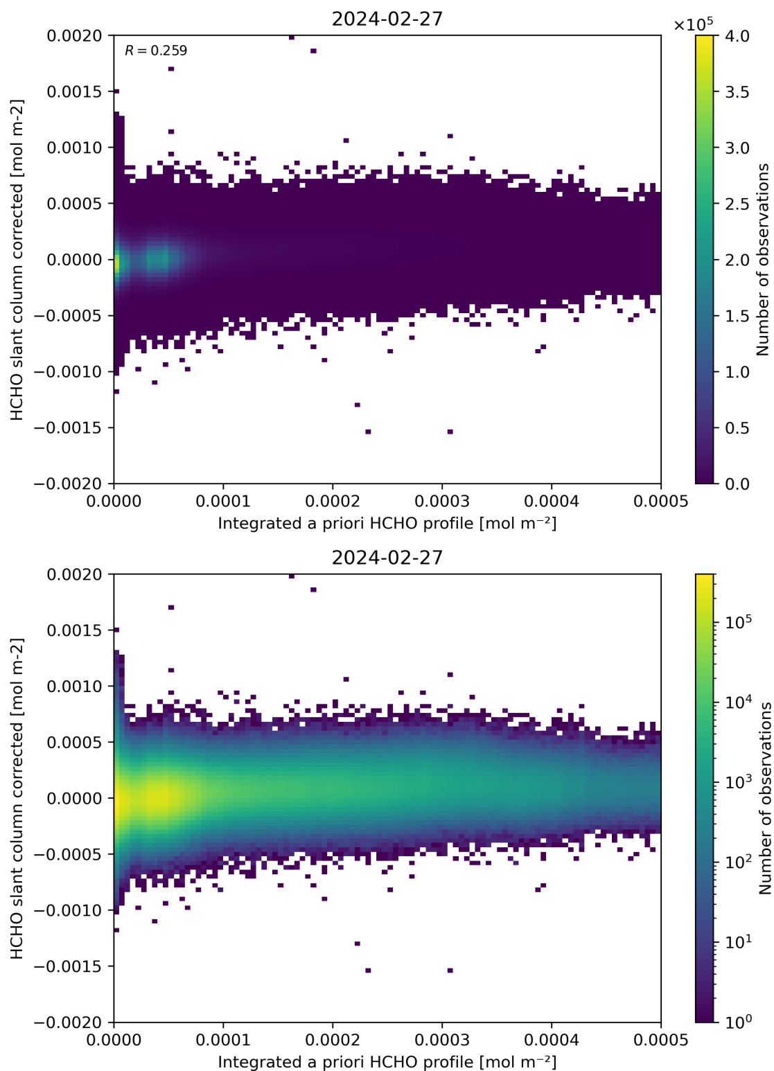
Figure 151: Scatter density plot of “Integrated a priori HCHO profile” against “HCHO slant column corrected” for 2024-02-27 to 2024-02-28.
