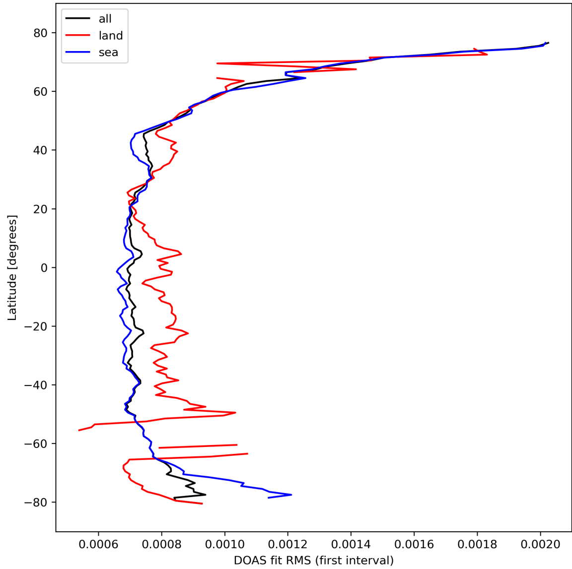
Figure 32: Zonal average of “DOAS fit RMS (first interval)” for 2024-02-27 to 2024-02-28.
