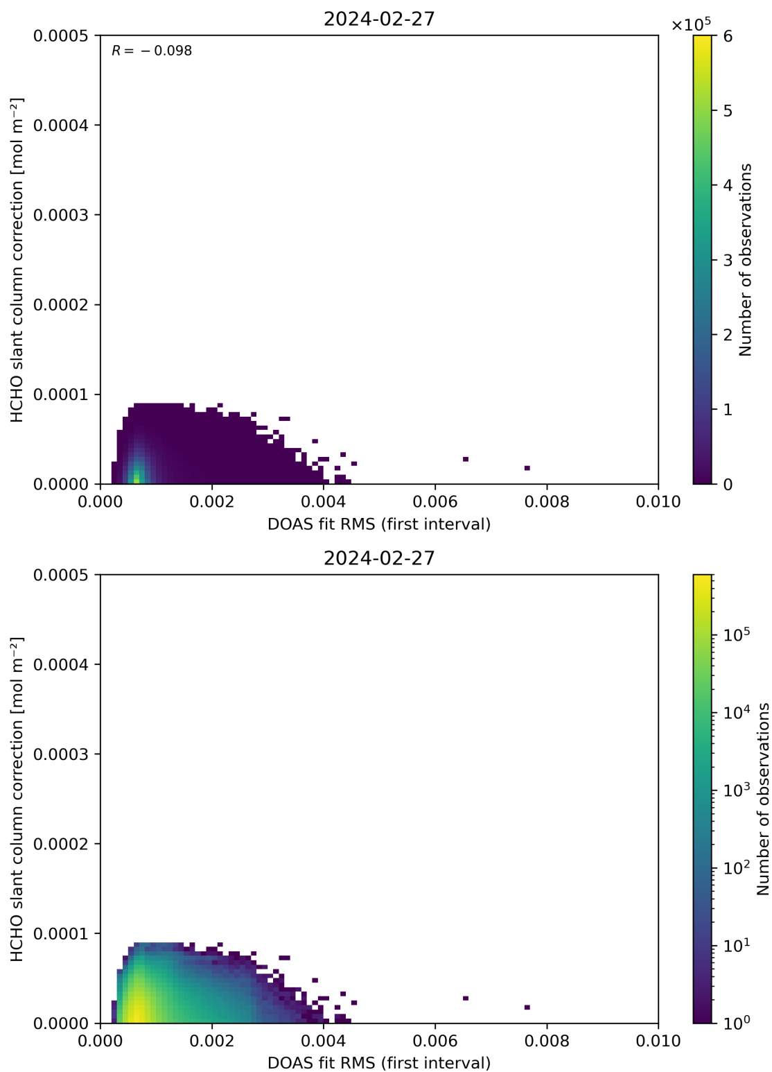
Figure 63: Scatter density plot of “DOAS fit RMS (first interval)” against “HCHO slant column correction” for 2024-02-27 to 2024-02-28.
