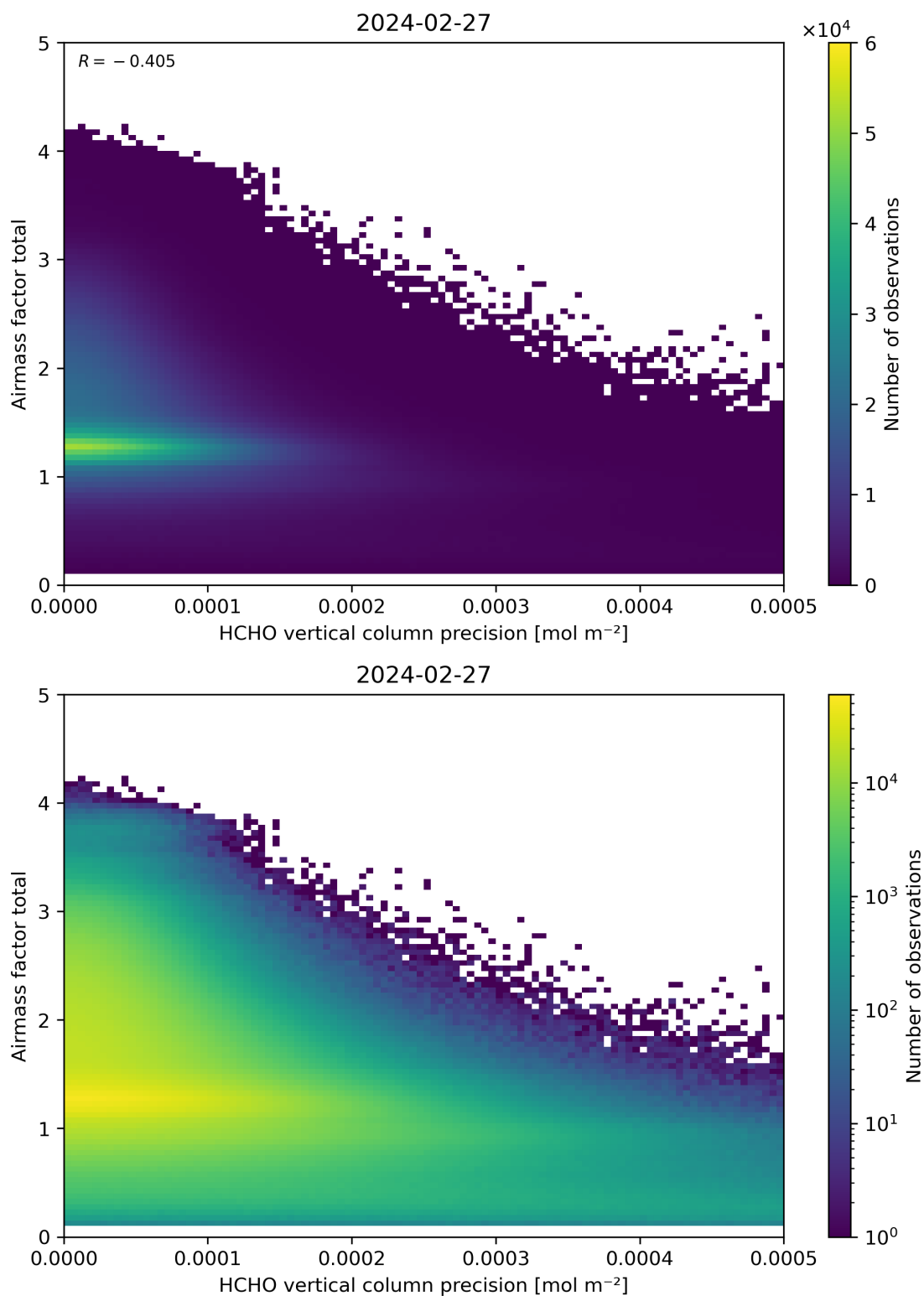
Figure 144: Scatter density plot of “HCHO vertical column precision” against “Airmass factor total” for 2024-02-27 to 2024-02-28.
