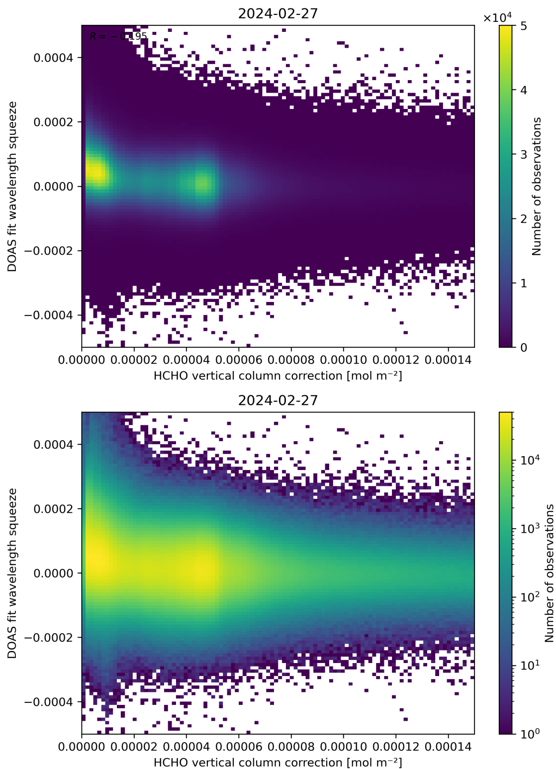
Figure 114: Scatter density plot of “HCHO vertical column correction” against “DOAS fit wavelength squeeze” for 2024-02-27 to 2024-02-28.
