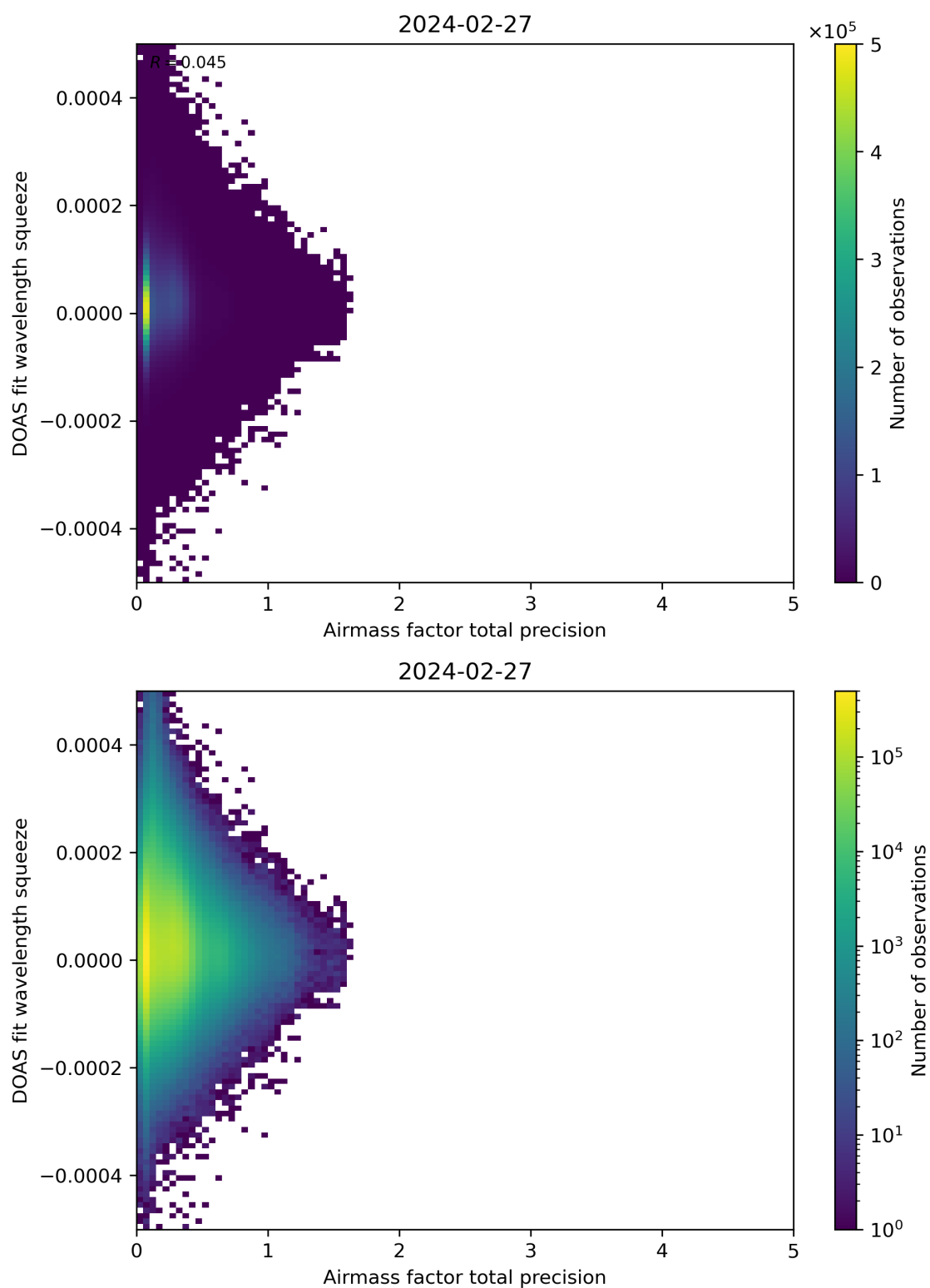
Figure 107: Scatter density plot of “Airmass factor total precision” against “DOAS fit wavelength squeeze” for 2024-02-27 to 2024-02-28.
