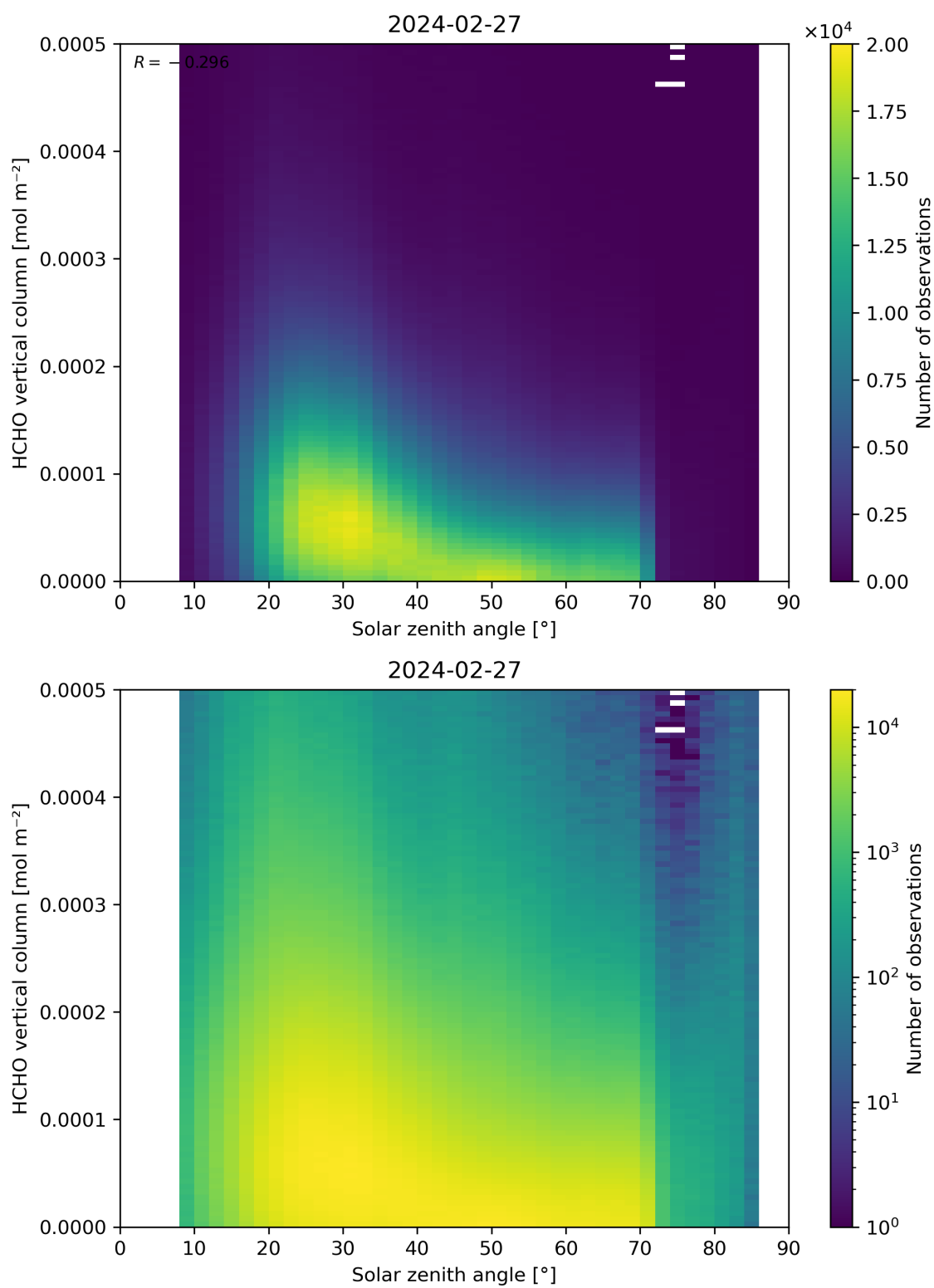
Figure 177: Scatter density plot of “Solar zenith angle” against “HCHO vertical column” for 2024-02-27 to 2024-02-28.
