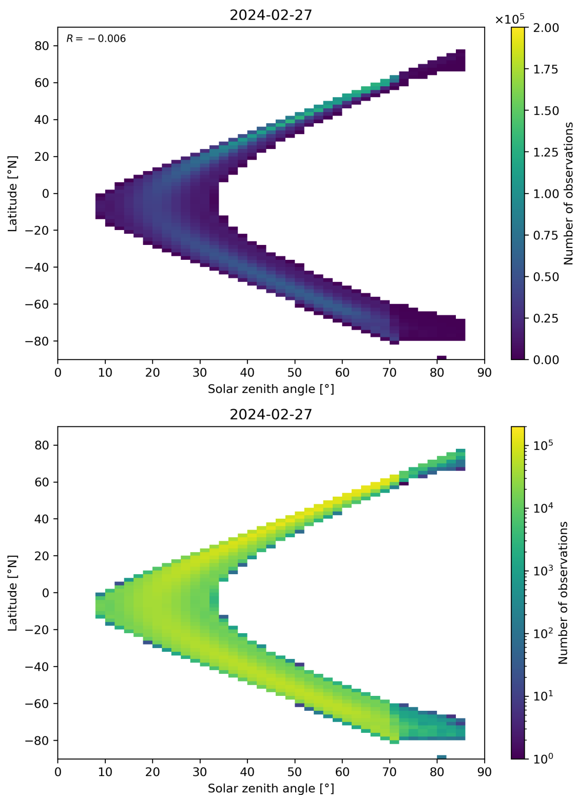
Figure 181: Scatter density plot of “Solar zenith angle” against “Latitude” for 2024-02-27 to 2024-02-28.
