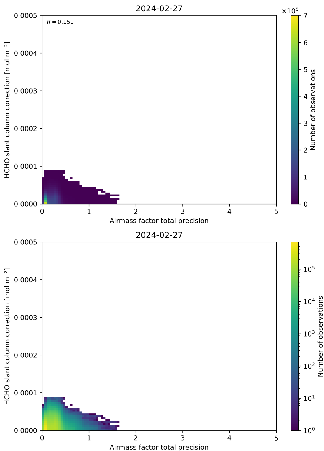
Figure 110: Scatter density plot of “Airmass factor total precision” against “HCHO slant column correction” for 2024-02-27 to 2024-02-28.
