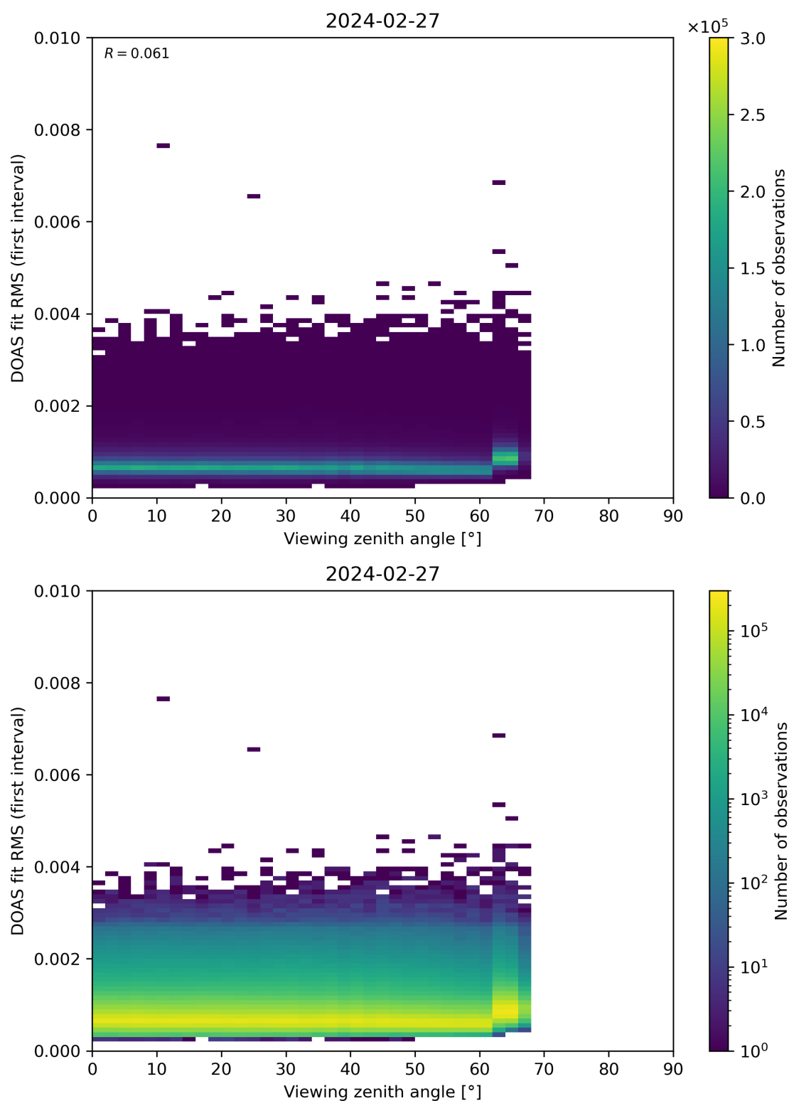
Figure 182: Scatter density plot of “Viewing zenith angle” against “DOAS fit RMS (first interval)” for 2024-02-27 to 2024-02-28.
