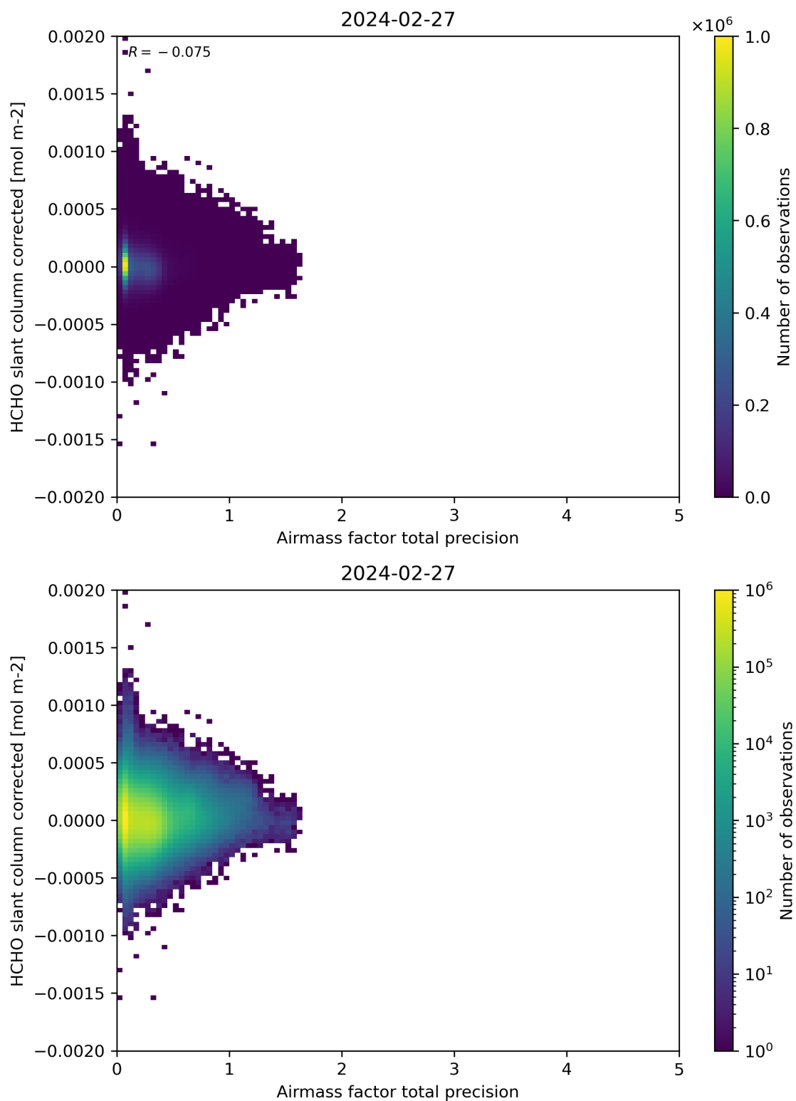
Figure 109: Scatter density plot of “Airmass factor total precision” against “HCHO slant column corrected” for 2024-02-27 to 2024-02-28.
