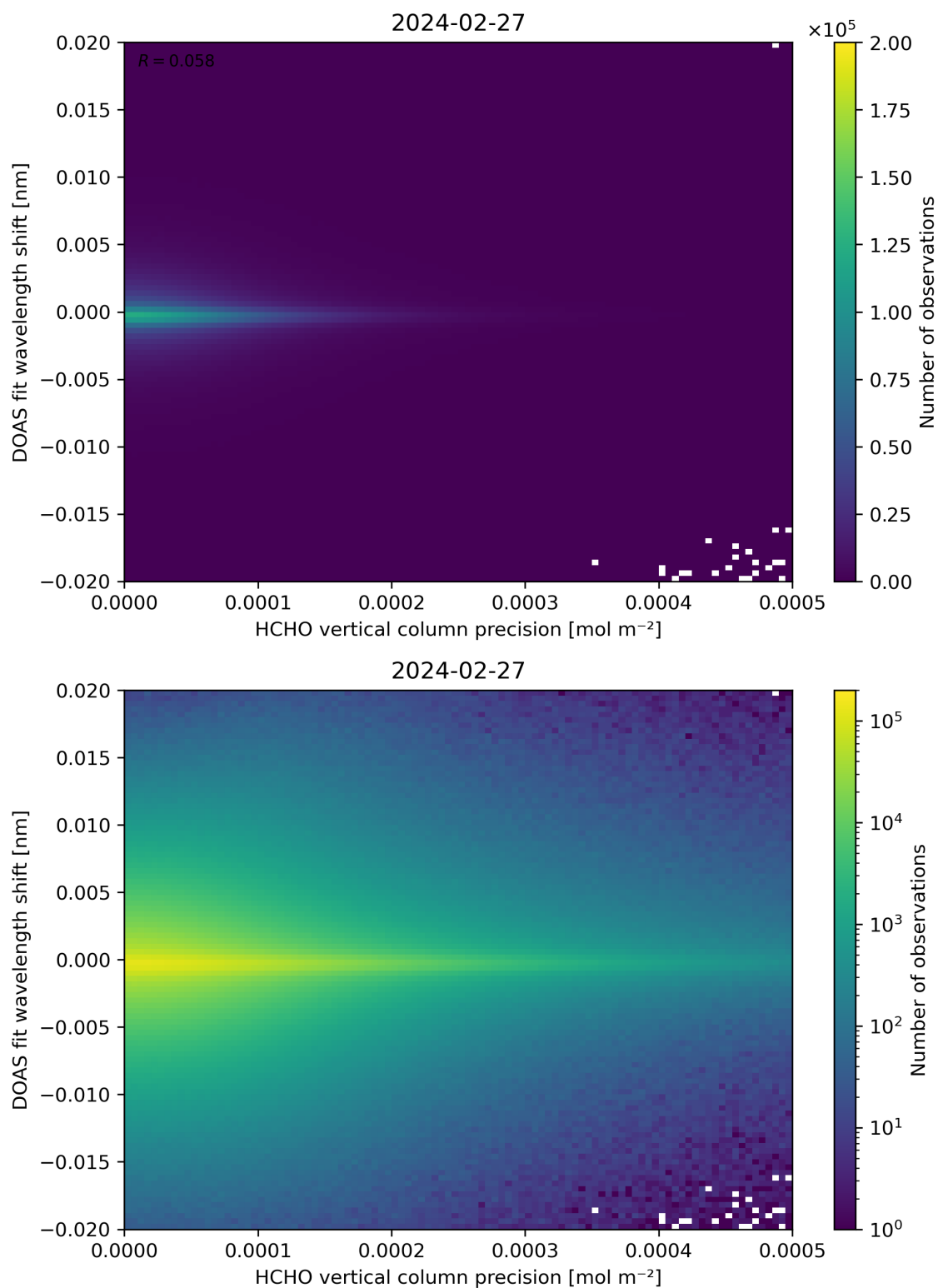
Figure 137: Scatter density plot of “HCHO vertical column precision” against “DOAS fit wavelength shift” for 2024-02-27 to 2024-02-28.
