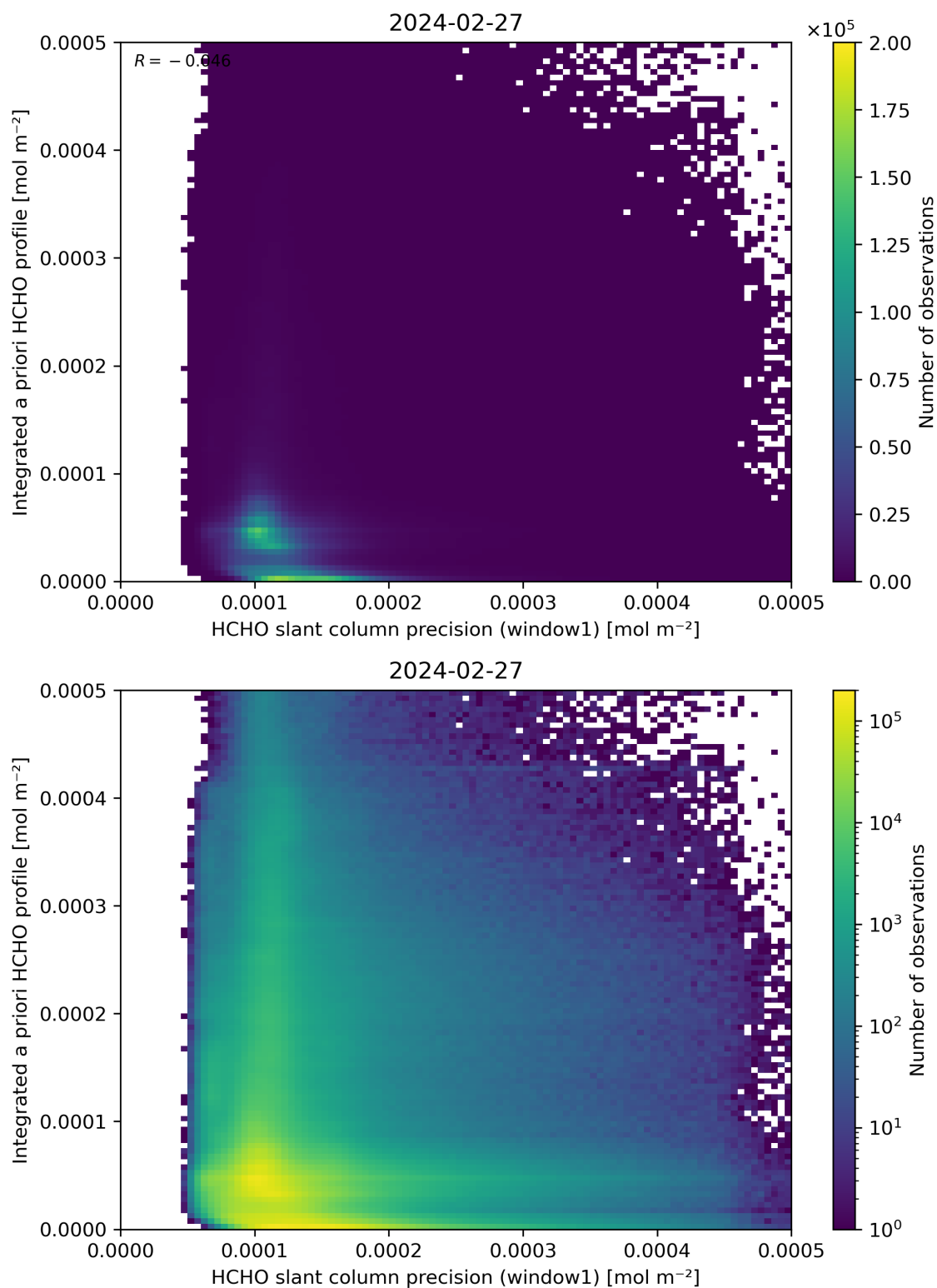
Figure 96: Scatter density plot of “HCHO slant column precision (window1)” against “Integrated a priori HCHO profile” for 2024-02-27 to 2024-02-28.
