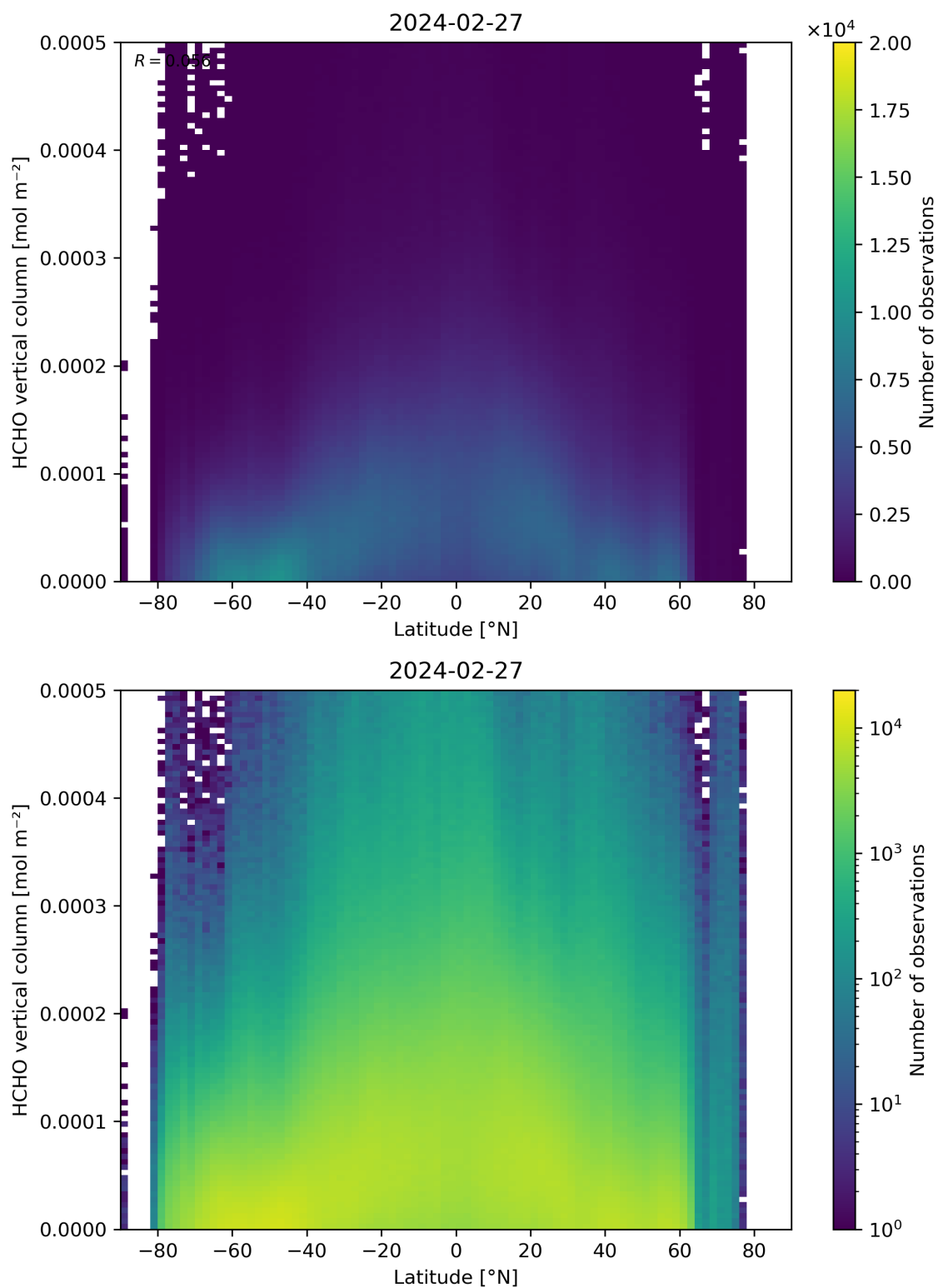
Figure 163: Scatter density plot of “Latitude” against “HCHO vertical column” for 2024-02-27 to 2024-02-28.
