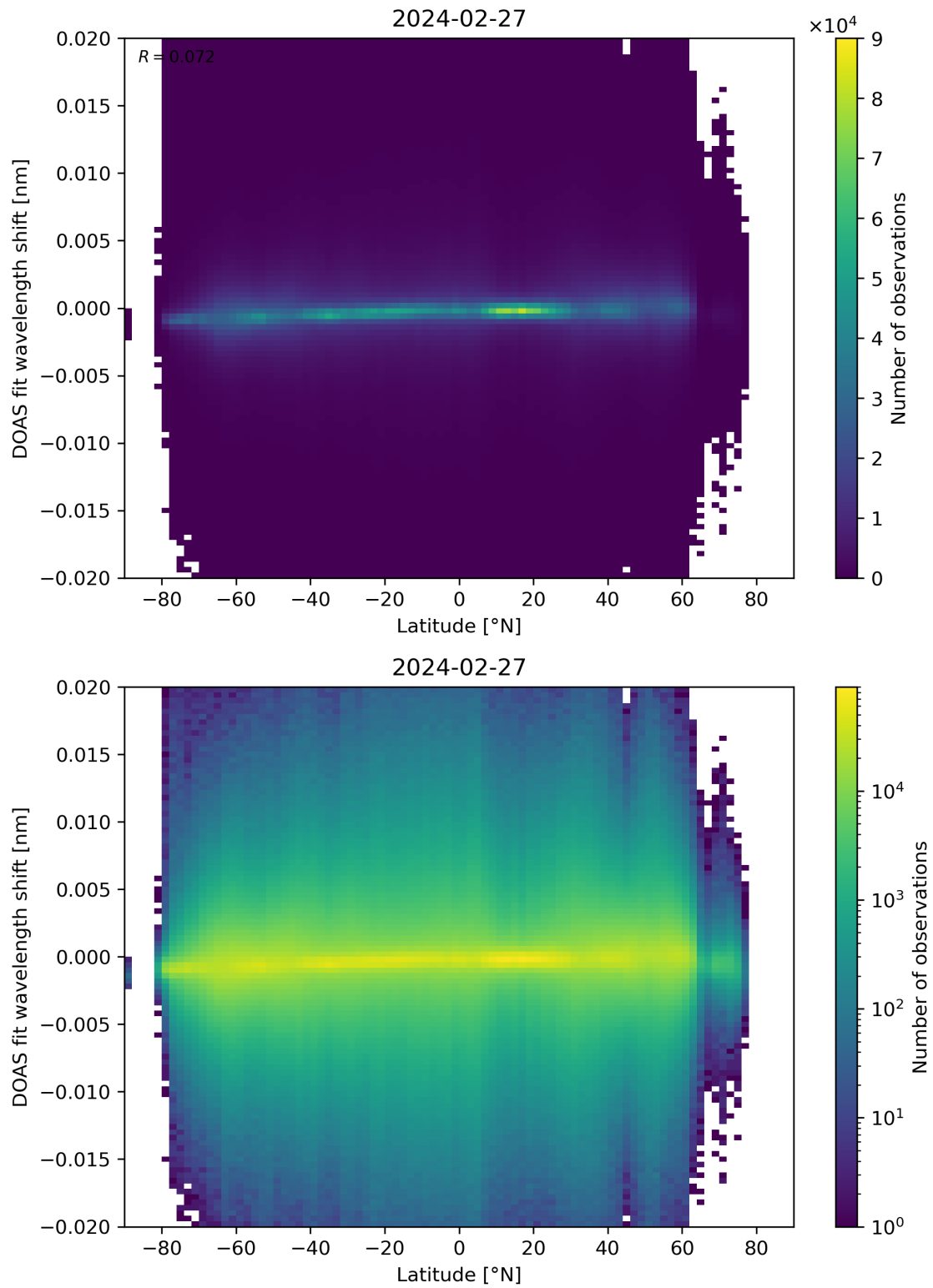
Figure 154: Scatter density plot of “Latitude” against “DOAS fit wavelength shift” for 2024-02-27 to 2024-02-28.
