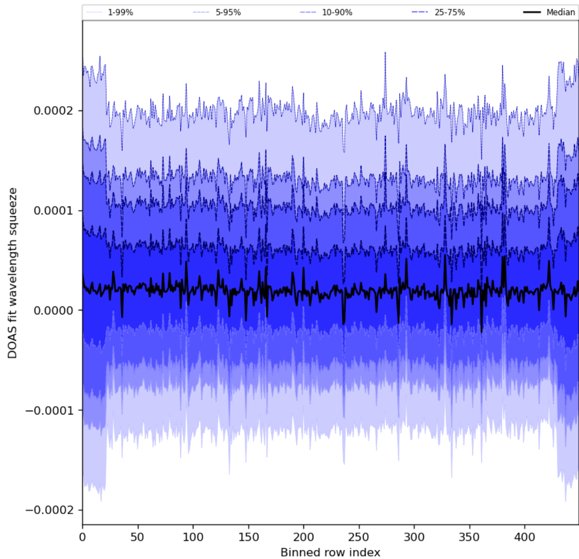
Figure 59: Along track statistics of “DOAS fit wavelength squeeze” for 2024-02-27 to 2024-02-28
