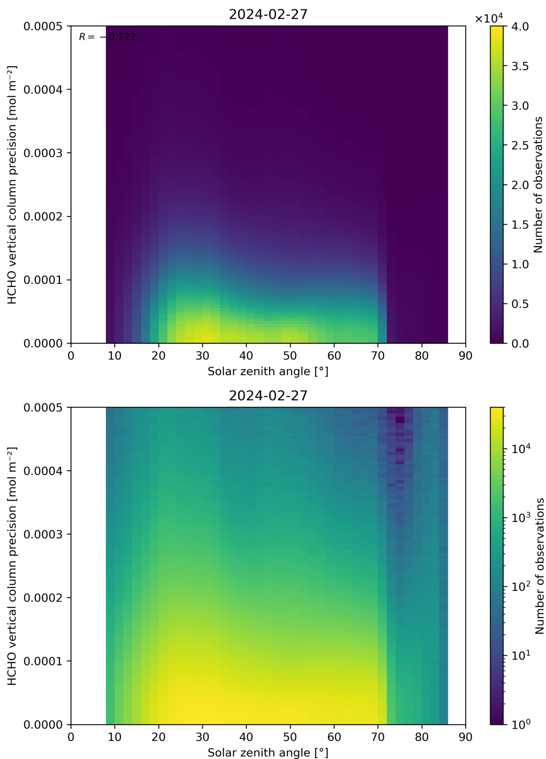
Figure 179: Scatter density plot of “Solar zenith angle” against “HCHO vertical column precision” for 2024-02-27 to 2024-02-28.
