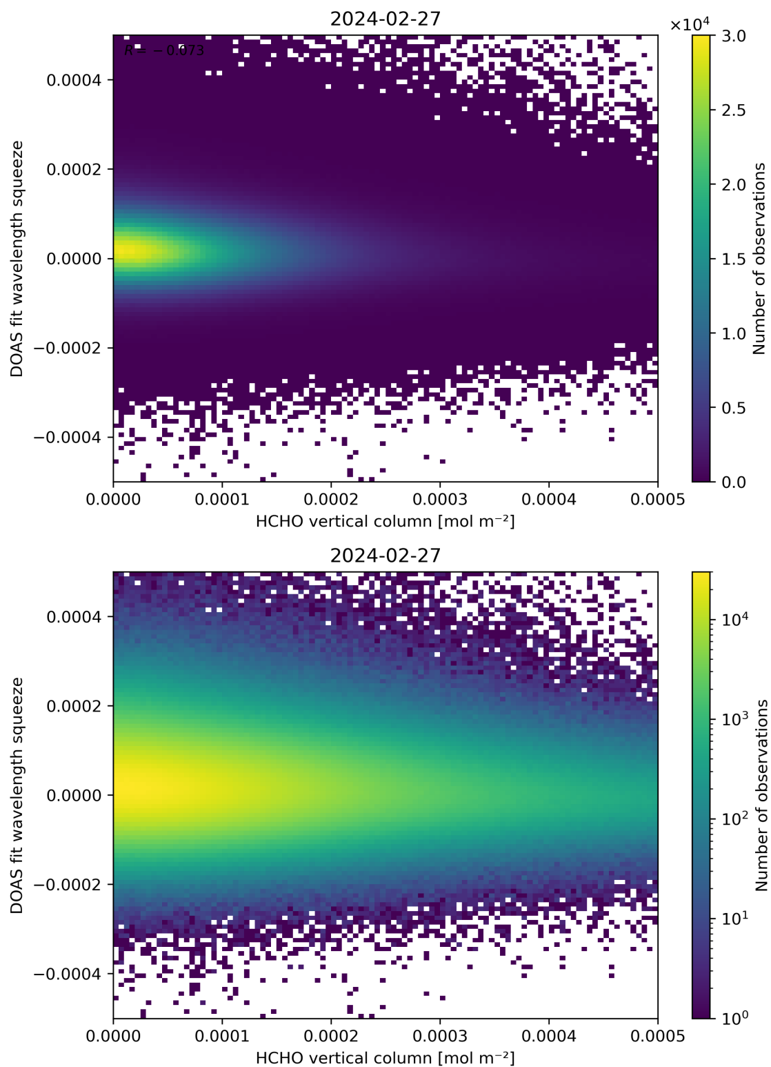
Figure 125: Scatter density plot of “HCHO vertical column” against “DOAS fit wavelength squeeze” for 2024-02-27 to 2024-02-28.
