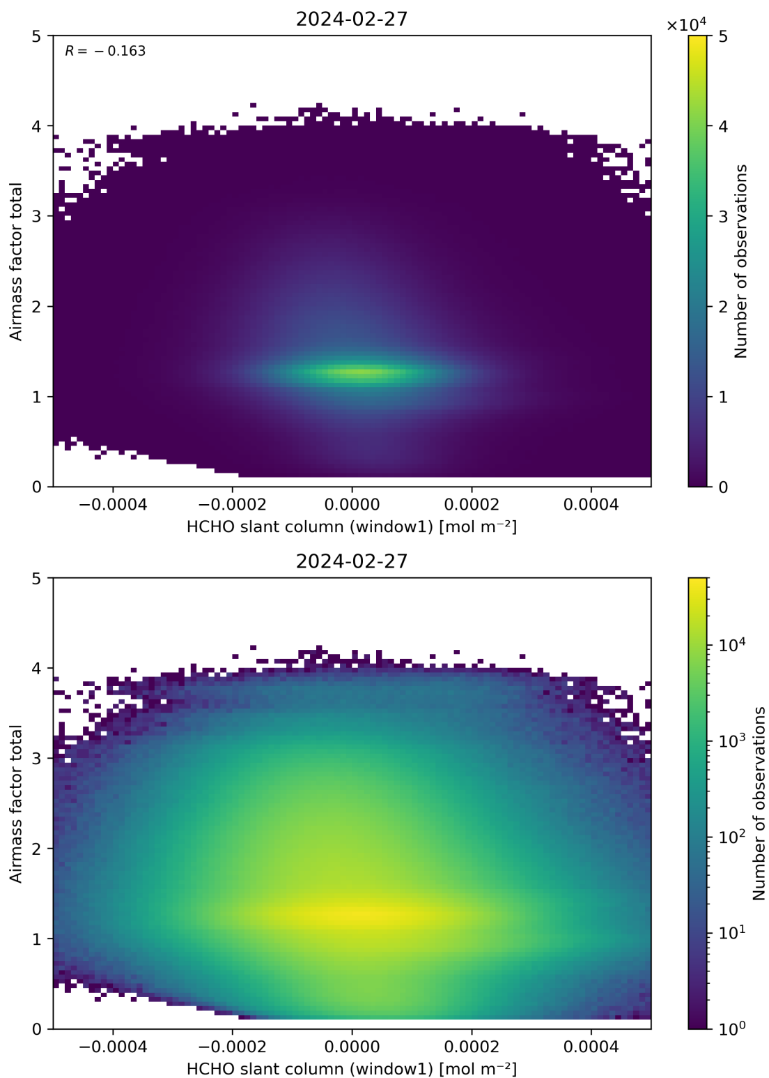
Figure 85: Scatter density plot of “HCHO slant column (window1)” against “Airmass factor total” for 2024-02-27 to 2024-02-28.
