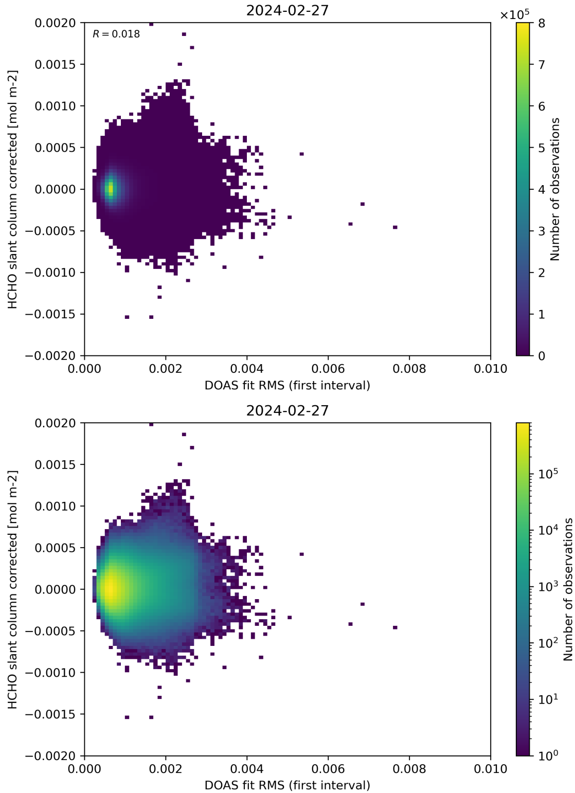
Figure 62: Scatter density plot of “DOAS fit RMS (first interval)” against “HCHO slant column corrected” for 2024-02-27 to 2024-02-28.
