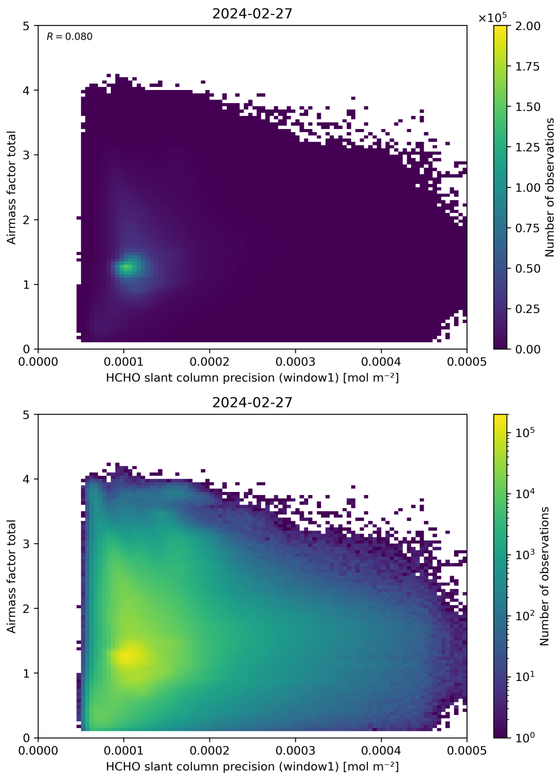
Figure 94: Scatter density plot of “HCHO slant column precision (window1)” against “Airmass factor total” for 2024-02-27 to 2024-02-28.
