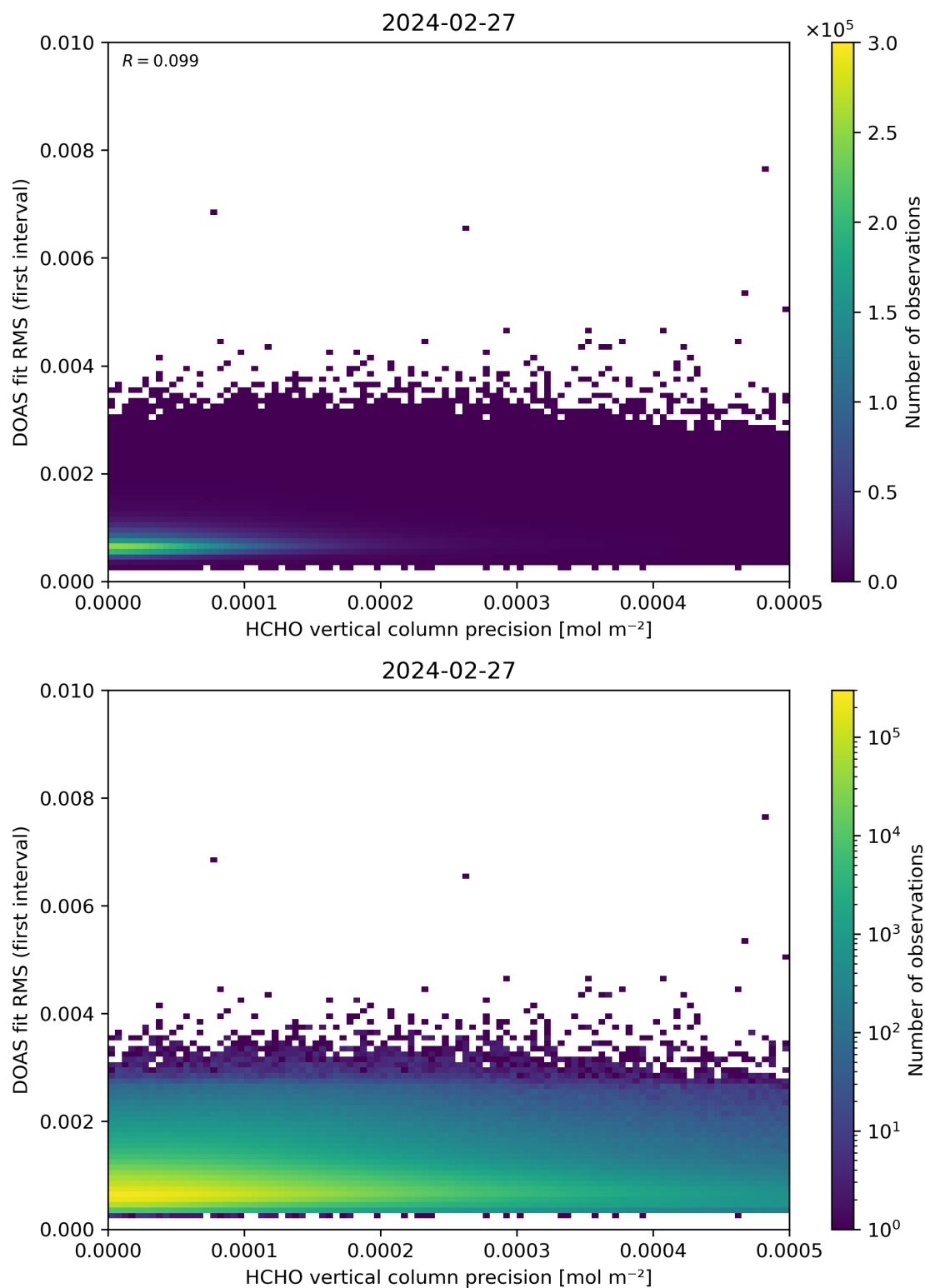
Figure 136: Scatter density plot of “HCHO vertical column precision” against “DOAS fit RMS (first interval)” for 2024-02-27 to 2024-02-28.
