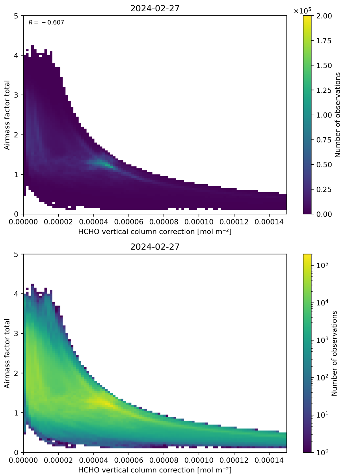
Figure 120: Scatter density plot of “HCHO vertical column correction” against “Airmass factor total” for 2024-02-27 to 2024-02-28.
