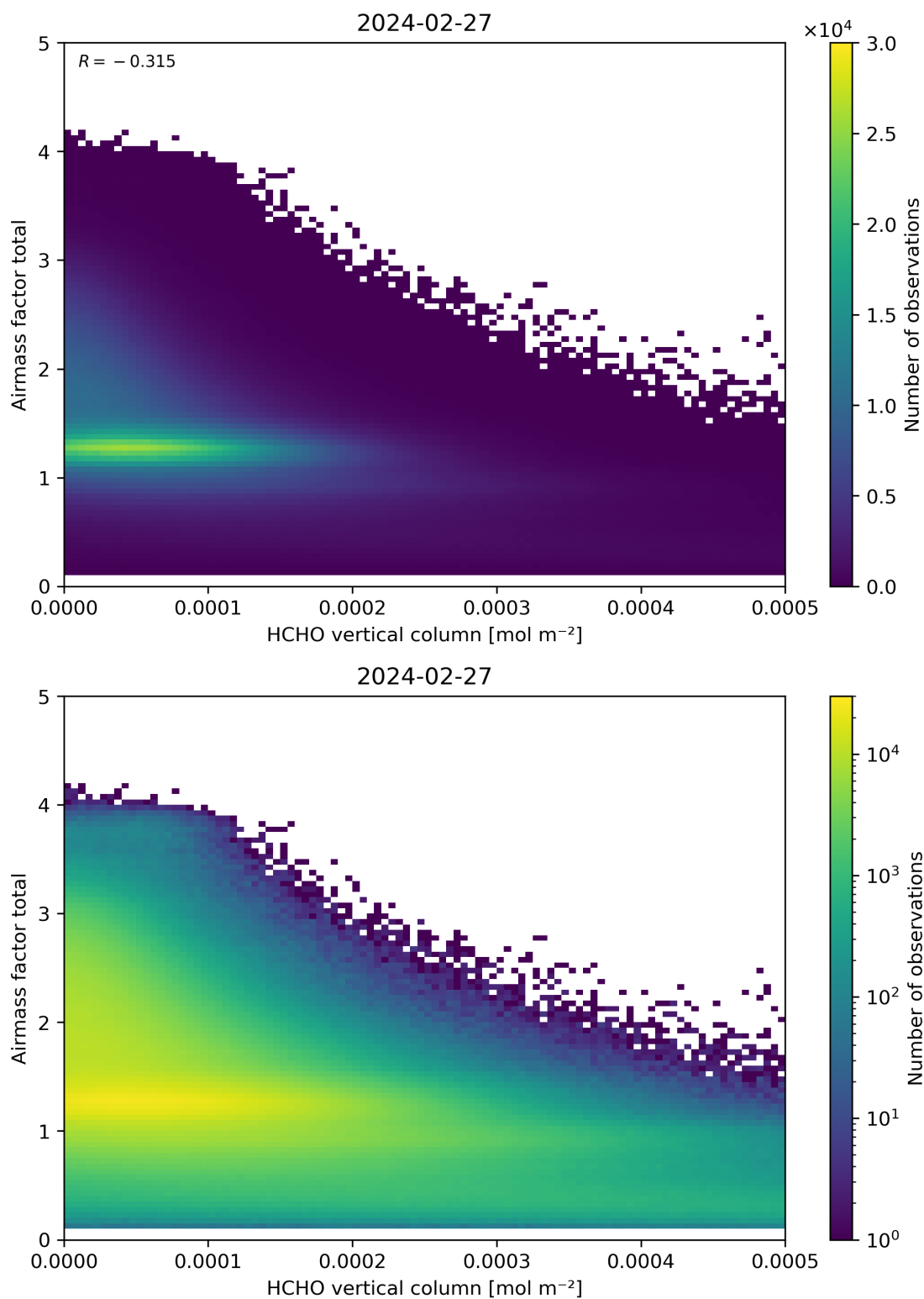
Figure 131: Scatter density plot of “HCHO vertical column” against “Airmass factor total” for 2024-02-27 to 2024-02-28.
