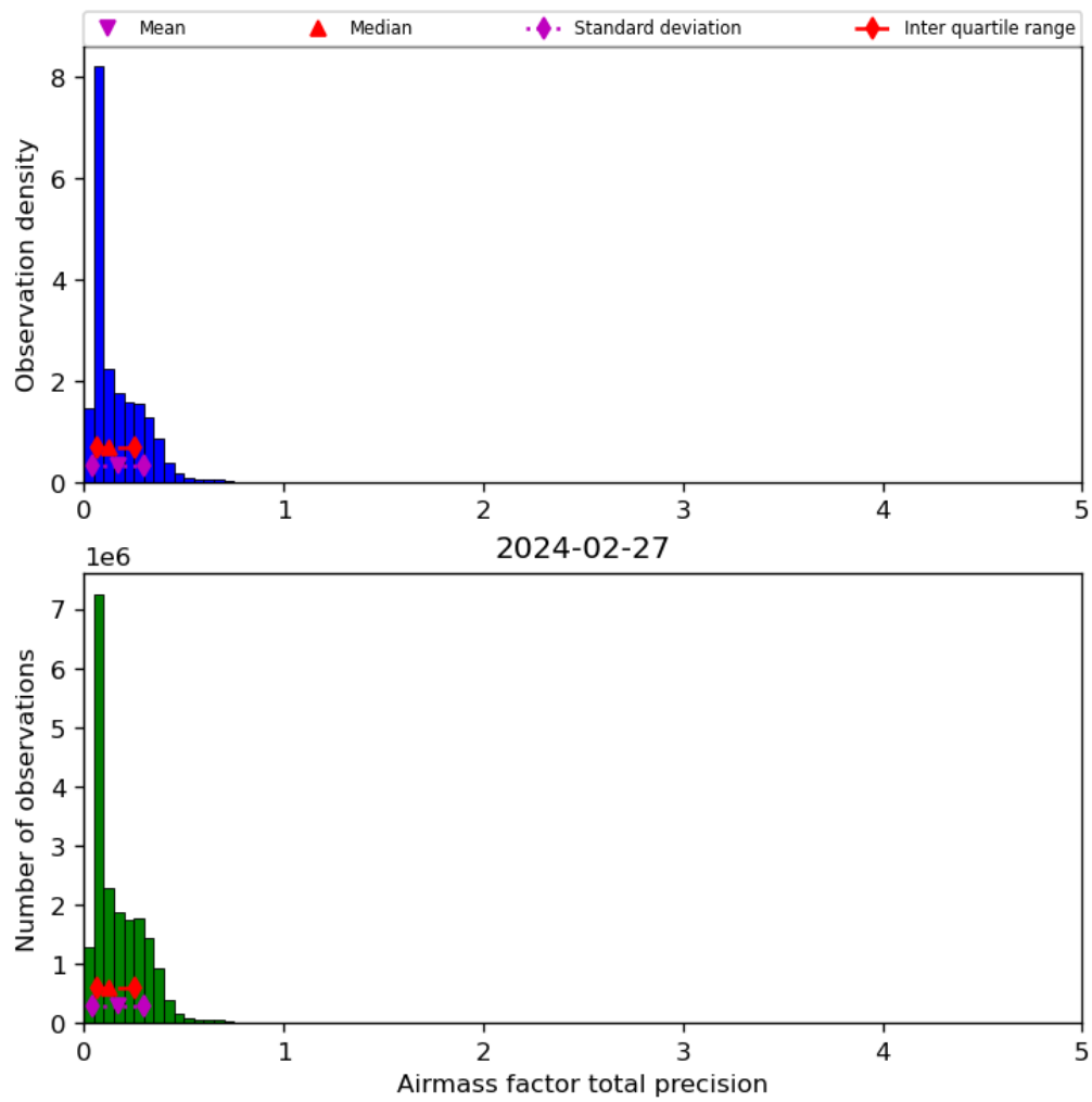
Figure 41: Histogram of “Airmass factor total precision” for 2024-02-27 to 2024-02-28
