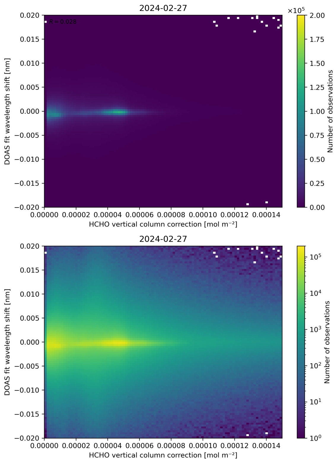
Figure 113: Scatter density plot of “HCHO vertical column correction” against “DOAS fit wavelength shift” for 2024-02-27 to 2024-02-28.
