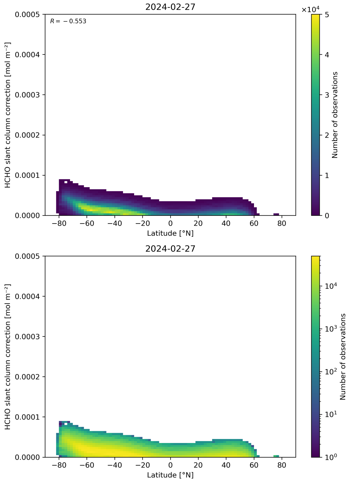
Figure 158: Scatter density plot of “Latitude” against “HCHO slant column correction” for 2024-02-27 to 2024-02-28.
