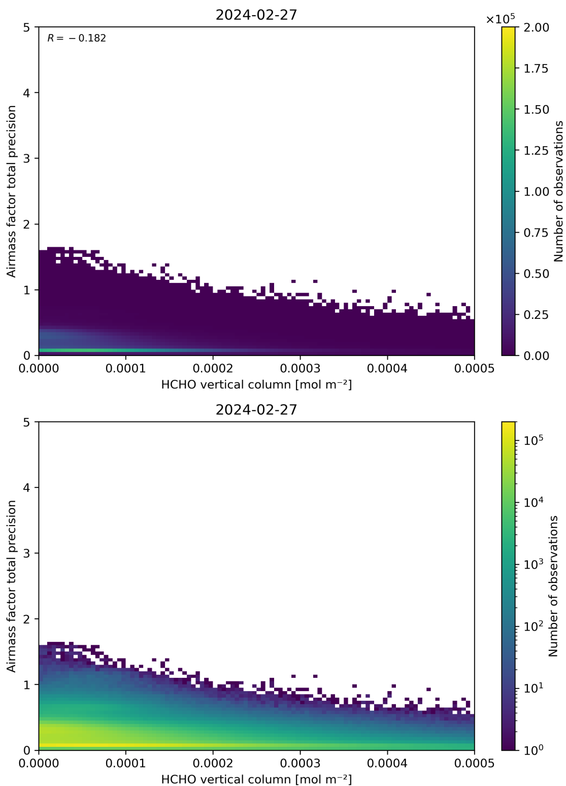
Figure 132: Scatter density plot of “HCHO vertical column” against “Airmass factor total precision” for 2024-02-27 to 2024-02-28.
