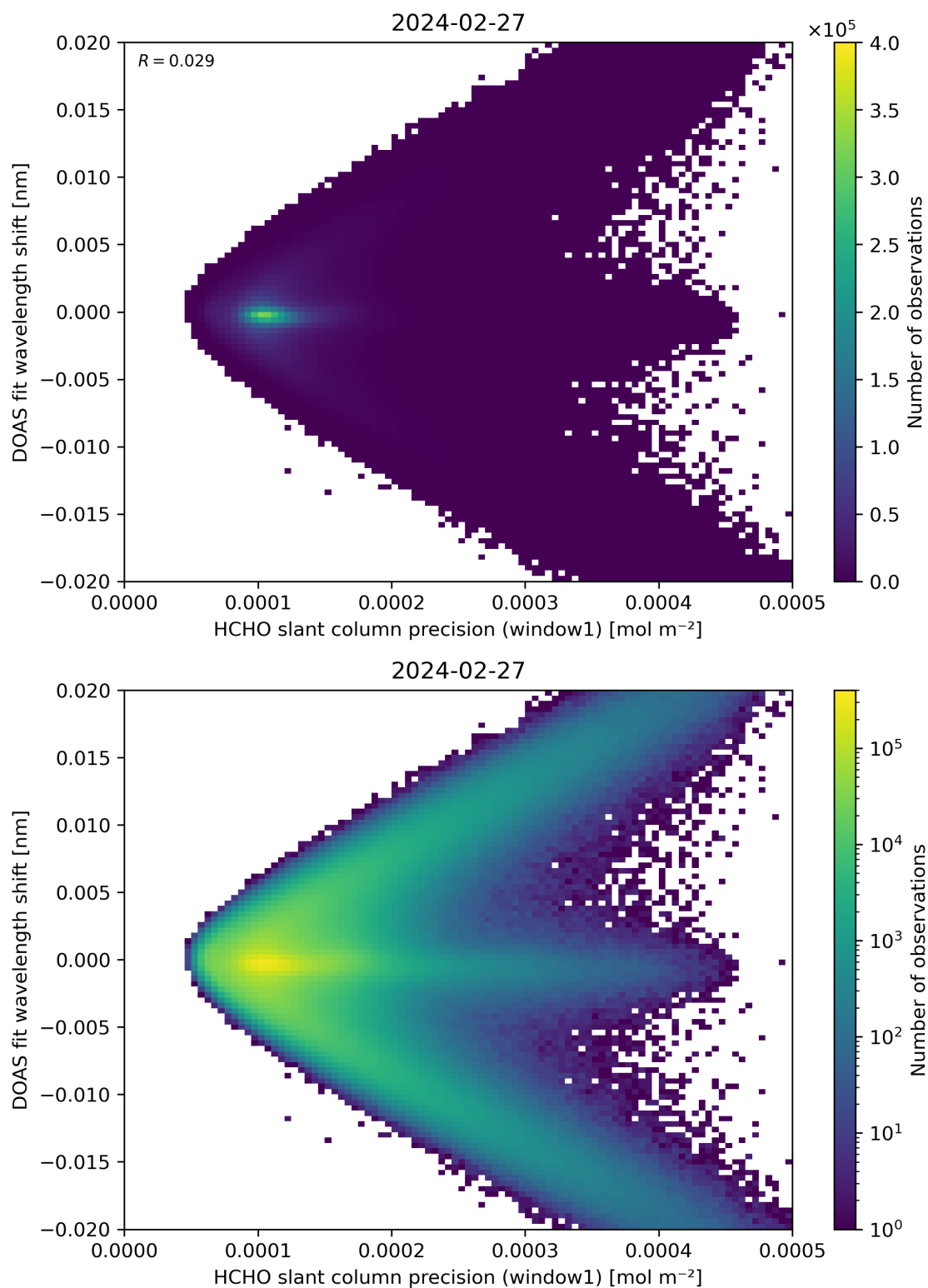
Figure 89: Scatter density plot of “HCHO slant column precision (window1)” against “DOAS fit wavelength shift” for 2024-02-27 to 2024-02-28.
