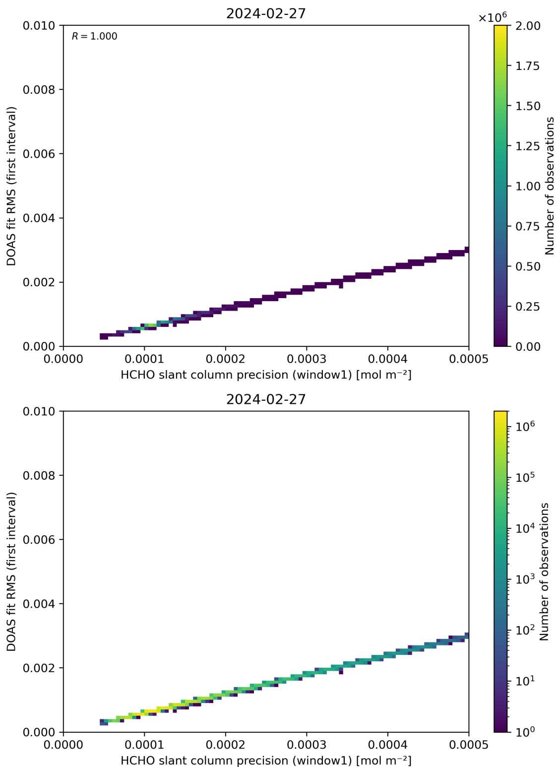
Figure 88: Scatter density plot of “HCHO slant column precision (window1)” against “DOAS fit RMS (first interval)” for 2024-02-27 to 2024-02-28.
