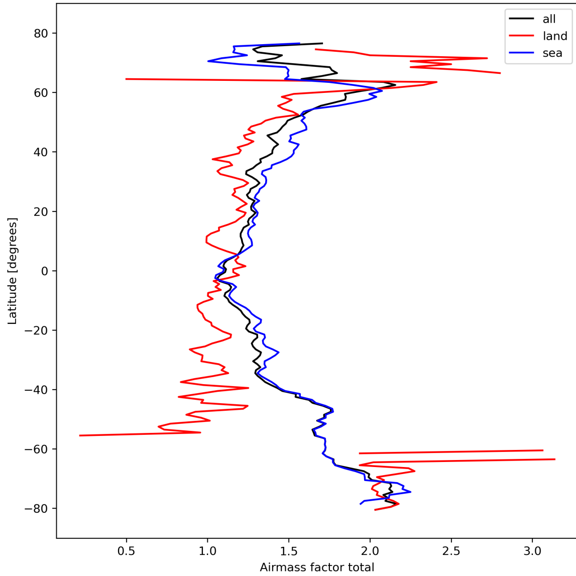
Figure 26: Zonal average of “Airmass factor total” for 2024-02-27 to 2024-02-28.
