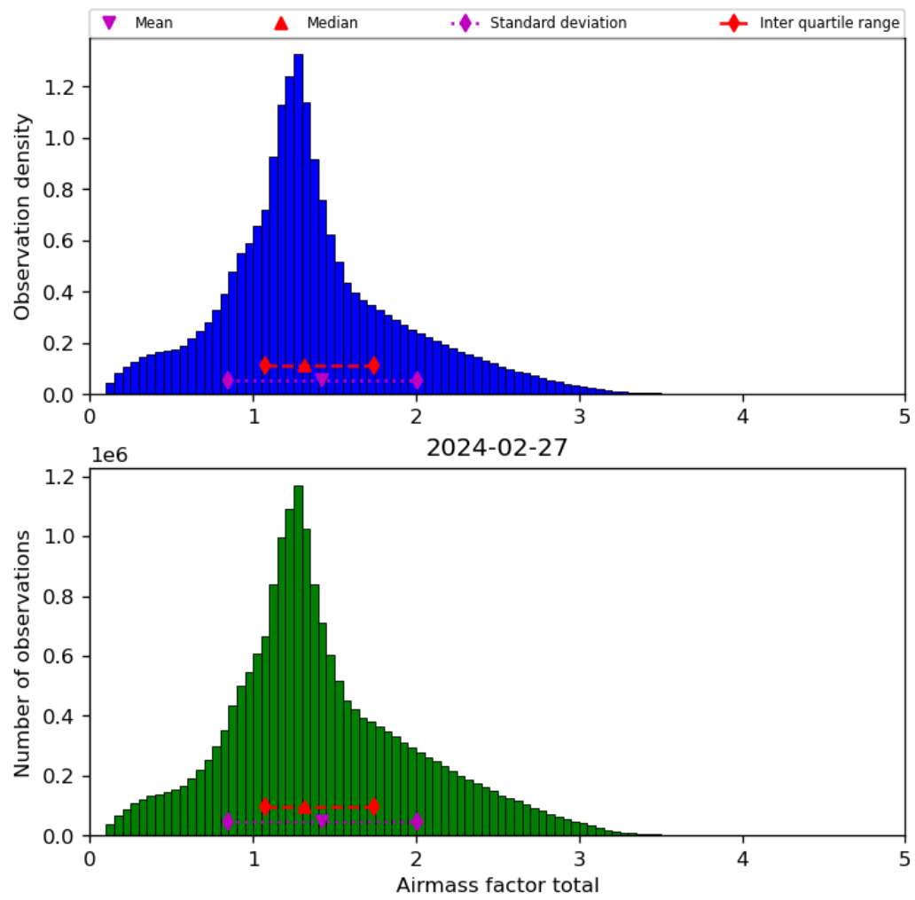
Figure 40: Histogram of “Airmass factor total” for 2024-02-27 to 2024-02-28
