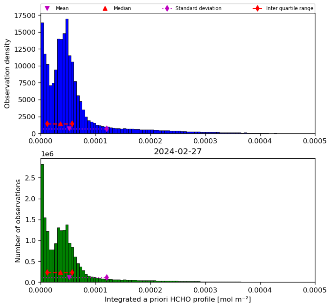
Figure 43: Histogram of “Integrated a priori HCHO profile” for 2024-02-27 to 2024-02-28
