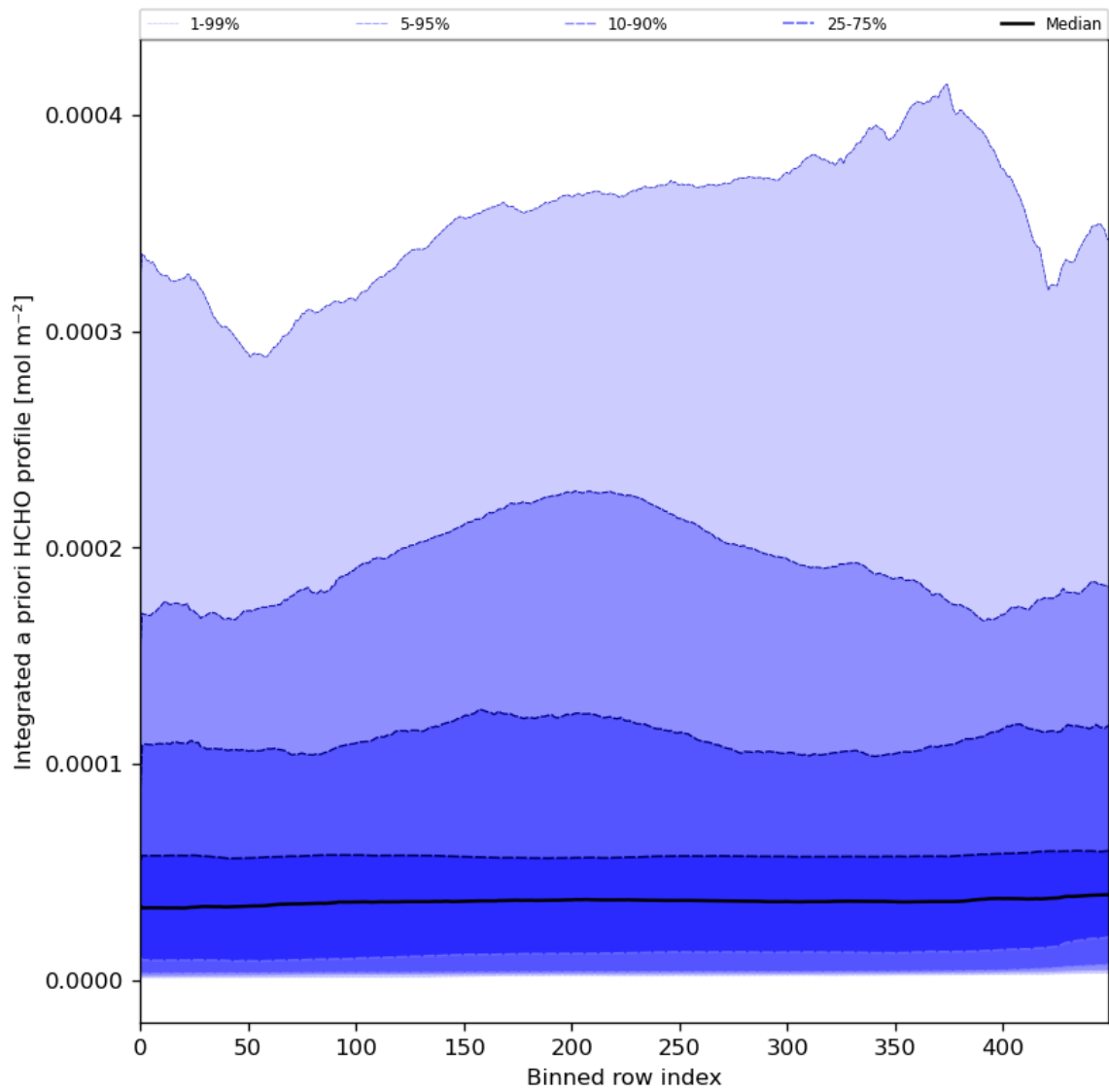
Figure 57: Along track statistics of “Integrated a priori HCHO profile” for 2024-02-27 to 2024-02-28
