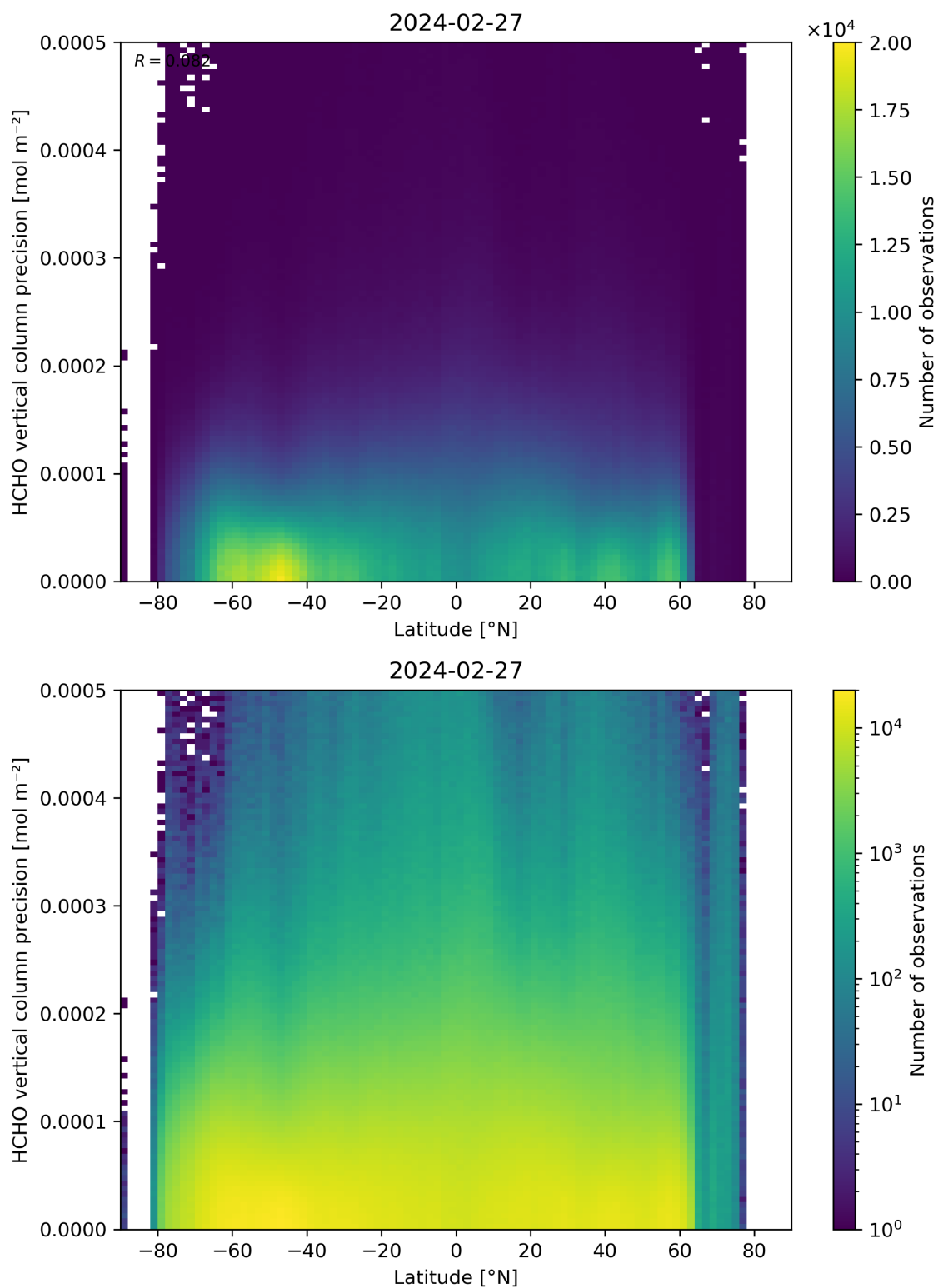
Figure 165: Scatter density plot of “Latitude” against “HCHO vertical column precision” for 2024-02-27 to 2024-02-28.
