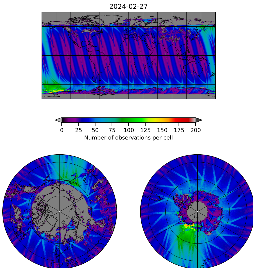
Figure 19: Map of the number of observations for 2024-02-27 to 2024-02-28
