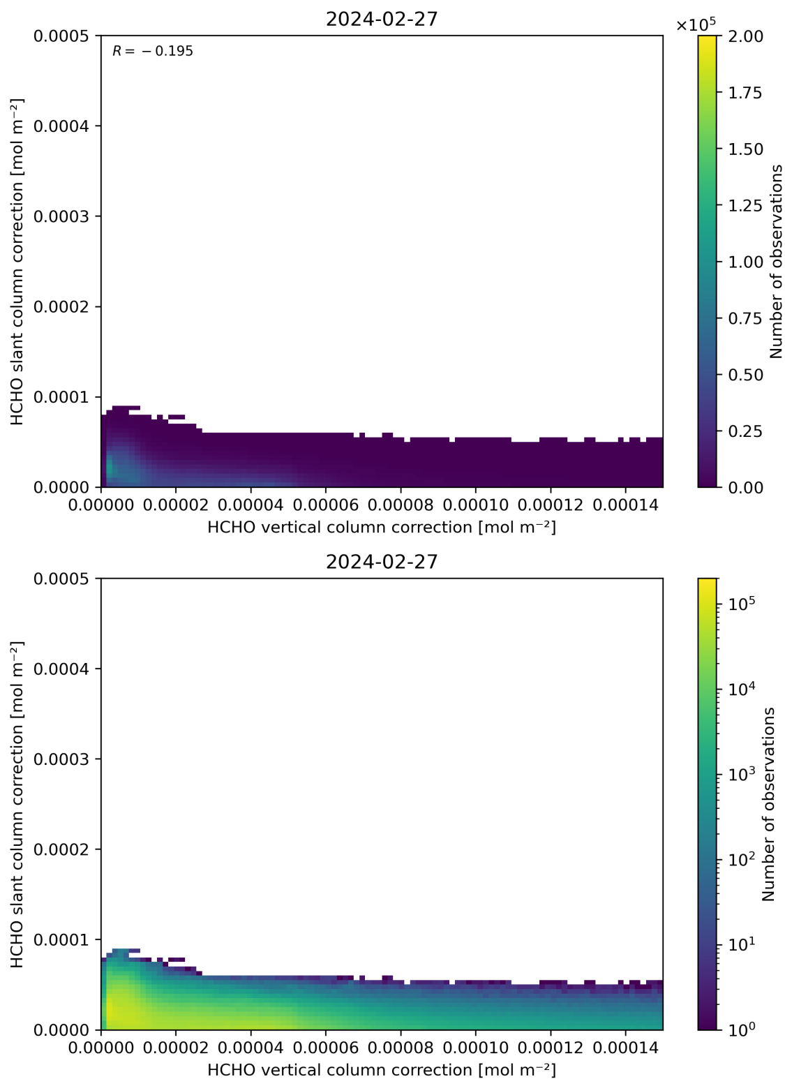
Figure 117: Scatter density plot of “HCHO vertical column correction” against “HCHO slant column correction” for 2024-02-27 to 2024-02-28.
