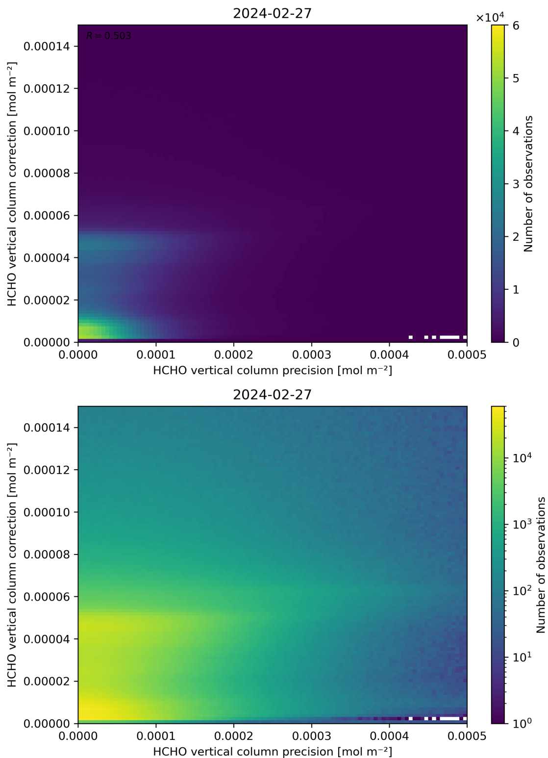
Figure 146: Scatter density plot of “HCHO vertical column precision” against “HCHO vertical column correction” for 2024-02-27 to 2024-02-28.
