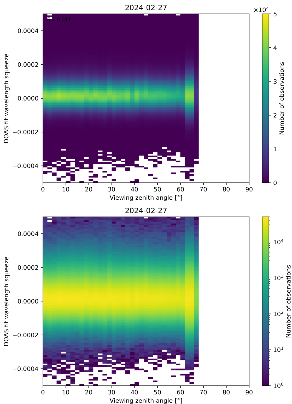
Figure 184: Scatter density plot of “Viewing zenith angle” against “DOAS fit wavelength squeeze” for 2024-02-27 to 2024-02-28.
