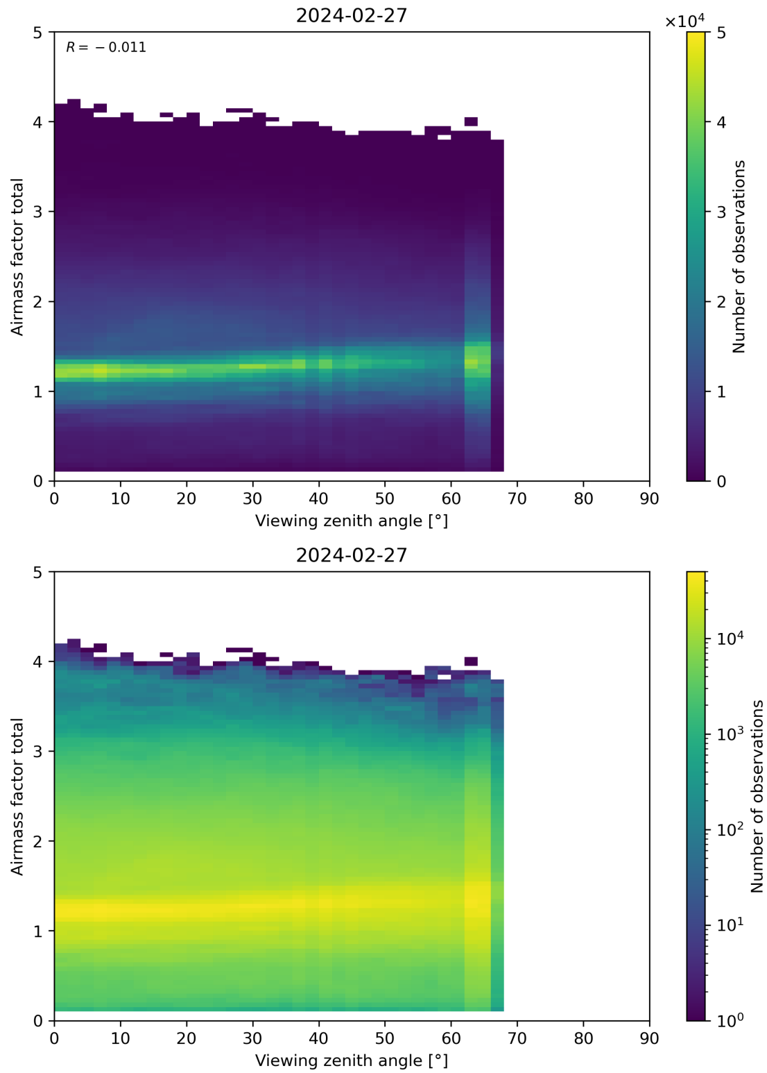
Figure 190: Scatter density plot of “Viewing zenith angle” against “Airmass factor total” for 2024-02-27 to 2024-02-28.
