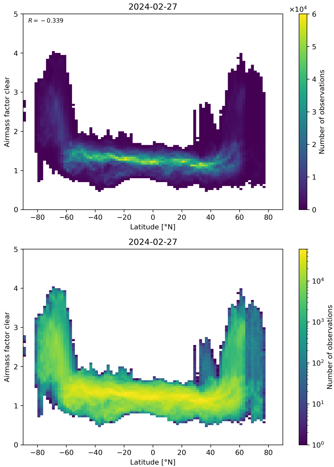
Figure 156: Scatter density plot of “Latitude” against “Airmass factor clear” for 2024-02-27 to 2024-02-28.
