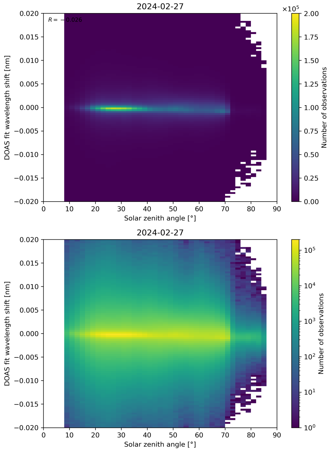
Figure 168: Scatter density plot of “Solar zenith angle” against “DOAS fit wavelength shift” for 2024-02-27 to 2024-02-28.
