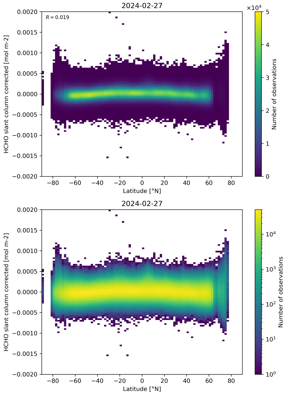
Figure 157: Scatter density plot of “Latitude” against “HCHO slant column corrected” for 2024-02-27 to 2024-02-28.
