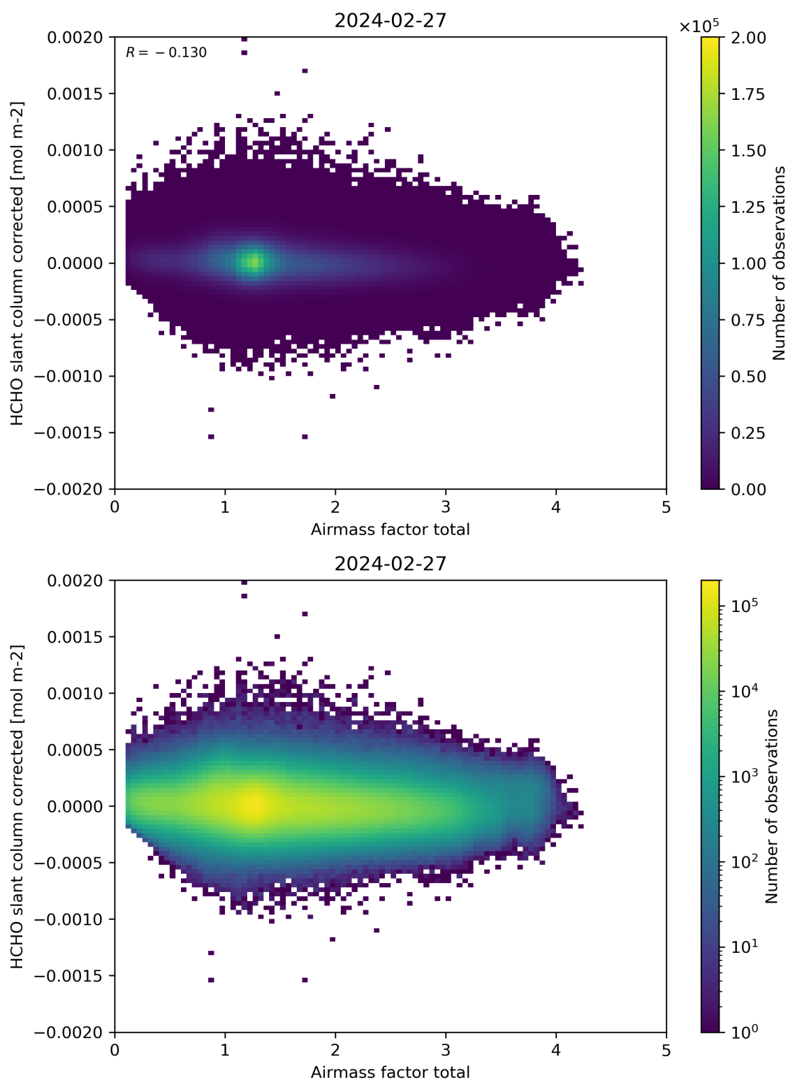
Figure 101: Scatter density plot of “Airmass factor total” against “HCHO slant column corrected” for 2024-02-27 to 2024-02-28.
