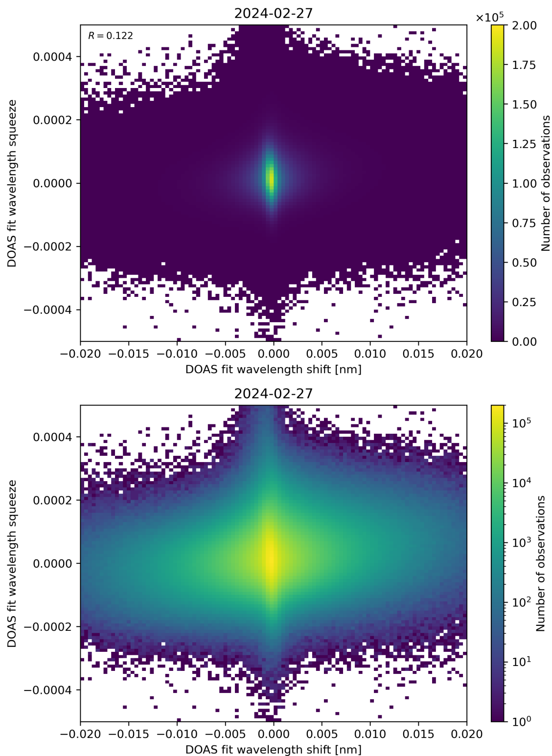
Figure 65: Scatter density plot of “DOAS fit wavelength shift” against “DOAS fit wavelength squeeze” for 2024-02-27 to 2024-02-28.
