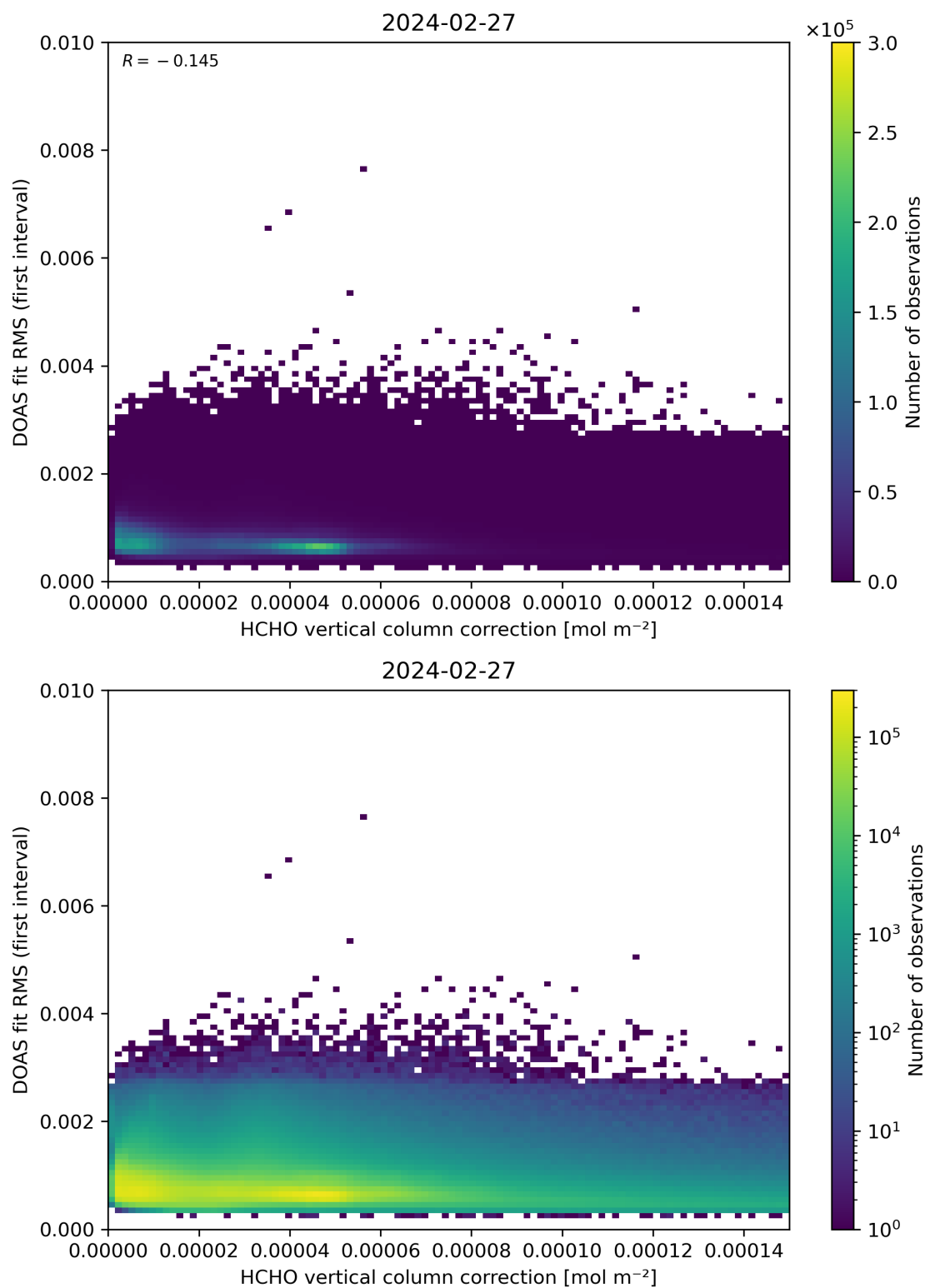
Figure 112: Scatter density plot of “HCHO vertical column correction” against “DOAS fit RMS (first interval)” for 2024-02-27 to 2024-02-28.
