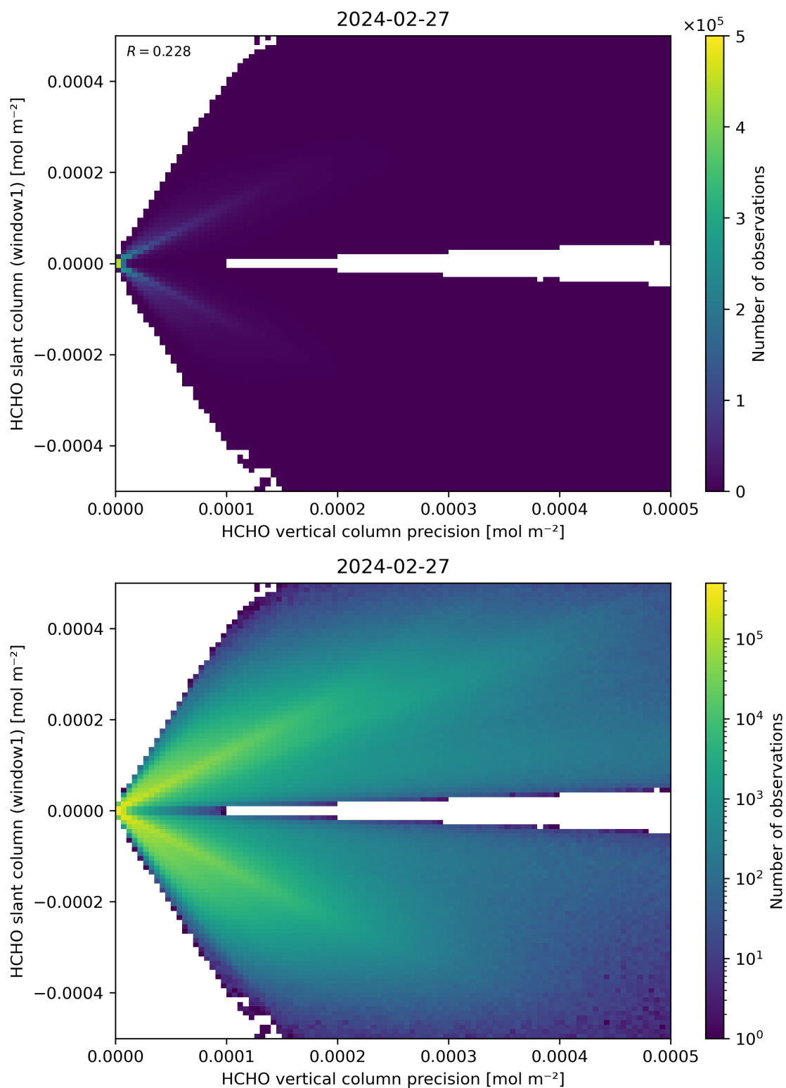
Figure 142: Scatter density plot of “HCHO vertical column precision” against “HCHO slant column (window1)” for 2024-02-27 to 2024-02-28.
