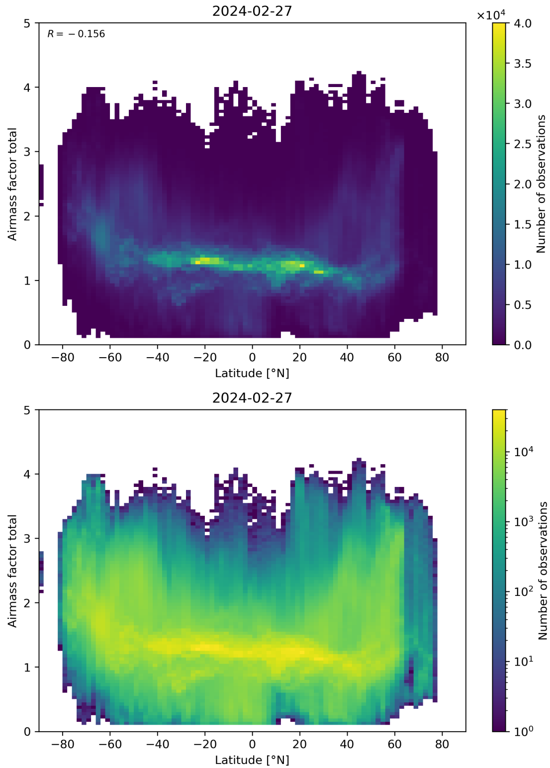
Figure 161: Scatter density plot of “Latitude” against “Airmass factor total” for 2024-02-27 to 2024-02-28.
