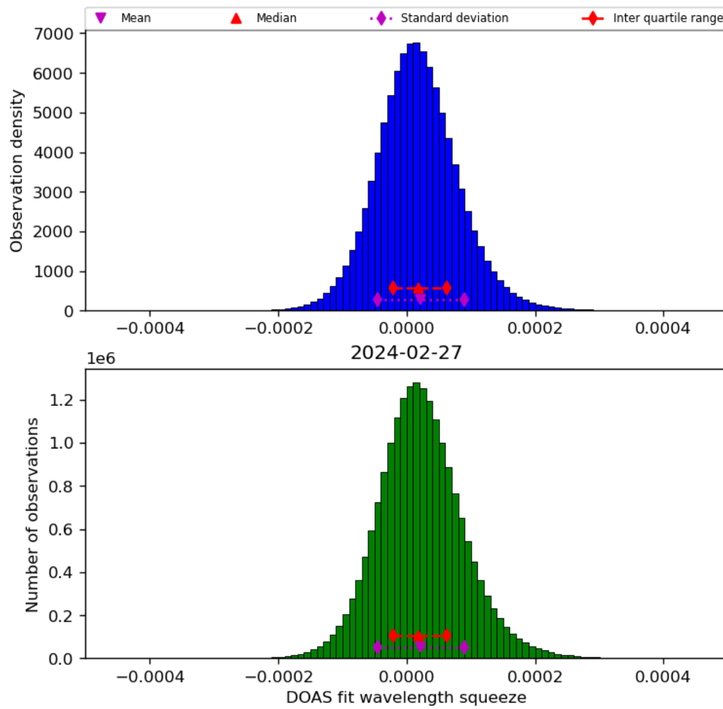
Figure 45: Histogram of “DOAS fit wavelength squeeze” for 2024-02-27 to 2024-02-28
