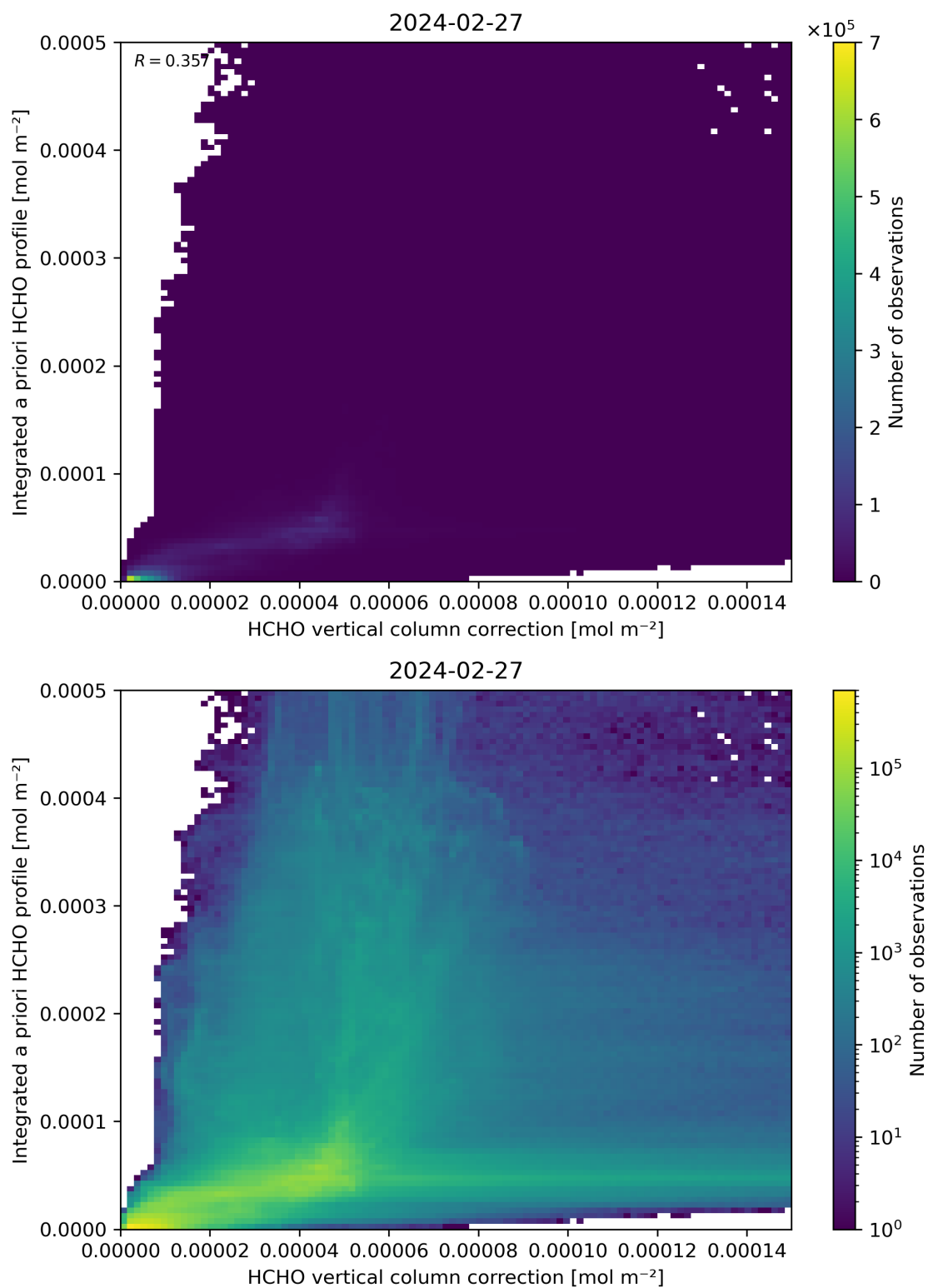
Figure 122: Scatter density plot of “HCHO vertical column correction” against “Integrated a priori HCHO profile” for 2024-02-27 to 2024-02-28.
