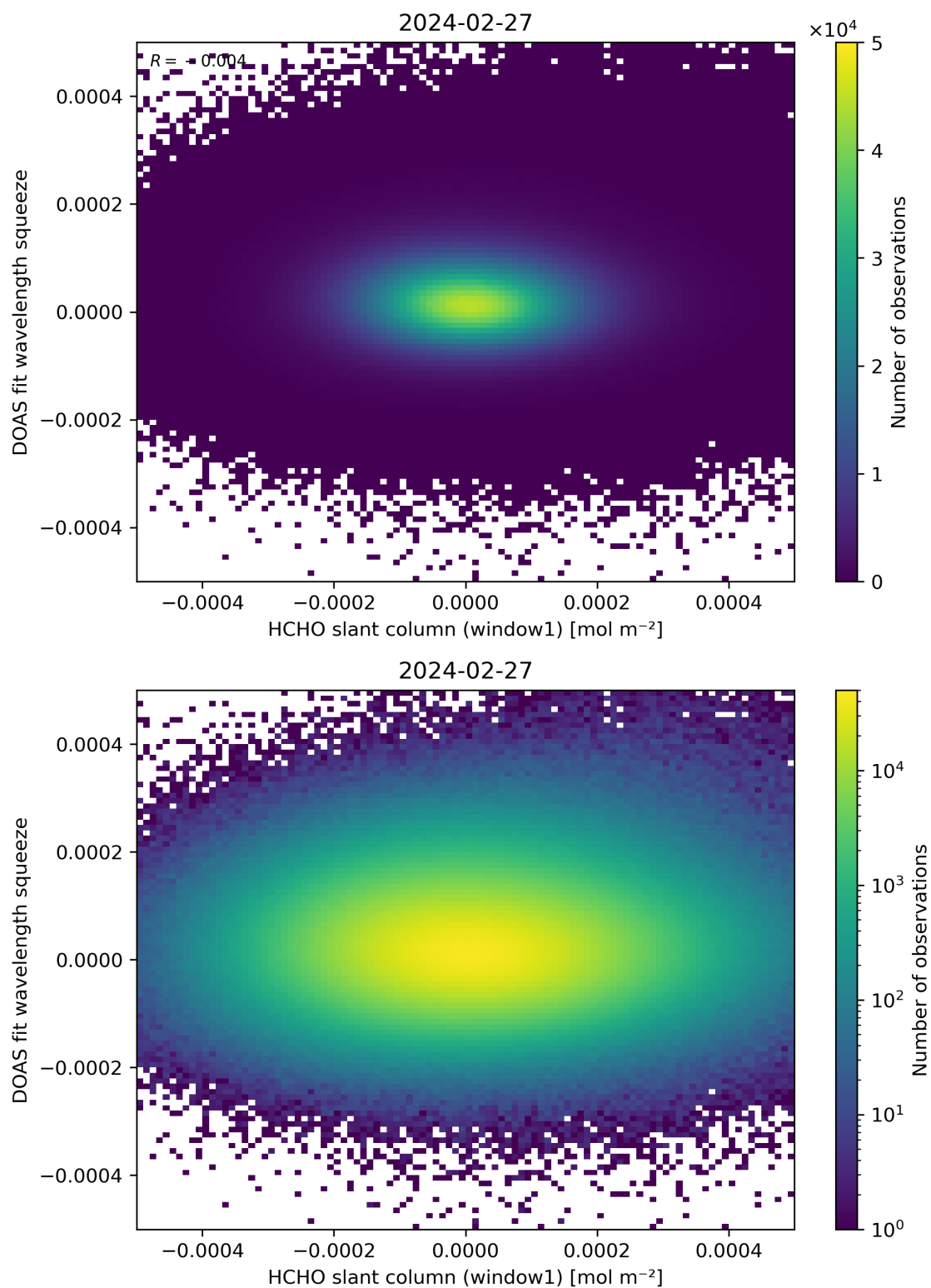
Figure 80: Scatter density plot of “HCHO slant column (window1)” against “DOAS fit wavelength squeeze” for 2024-02-27 to 2024-02-28.
