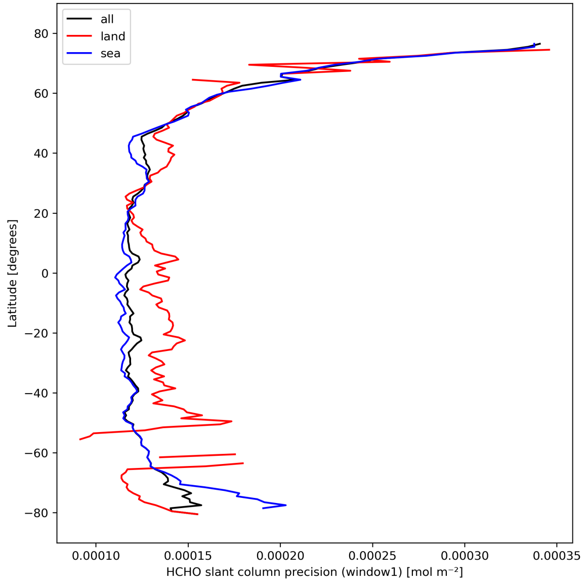
Figure 25: Zonal average of “HCHO slant column precision (window1)” for 2024-02-27 to 2024-02-28.
