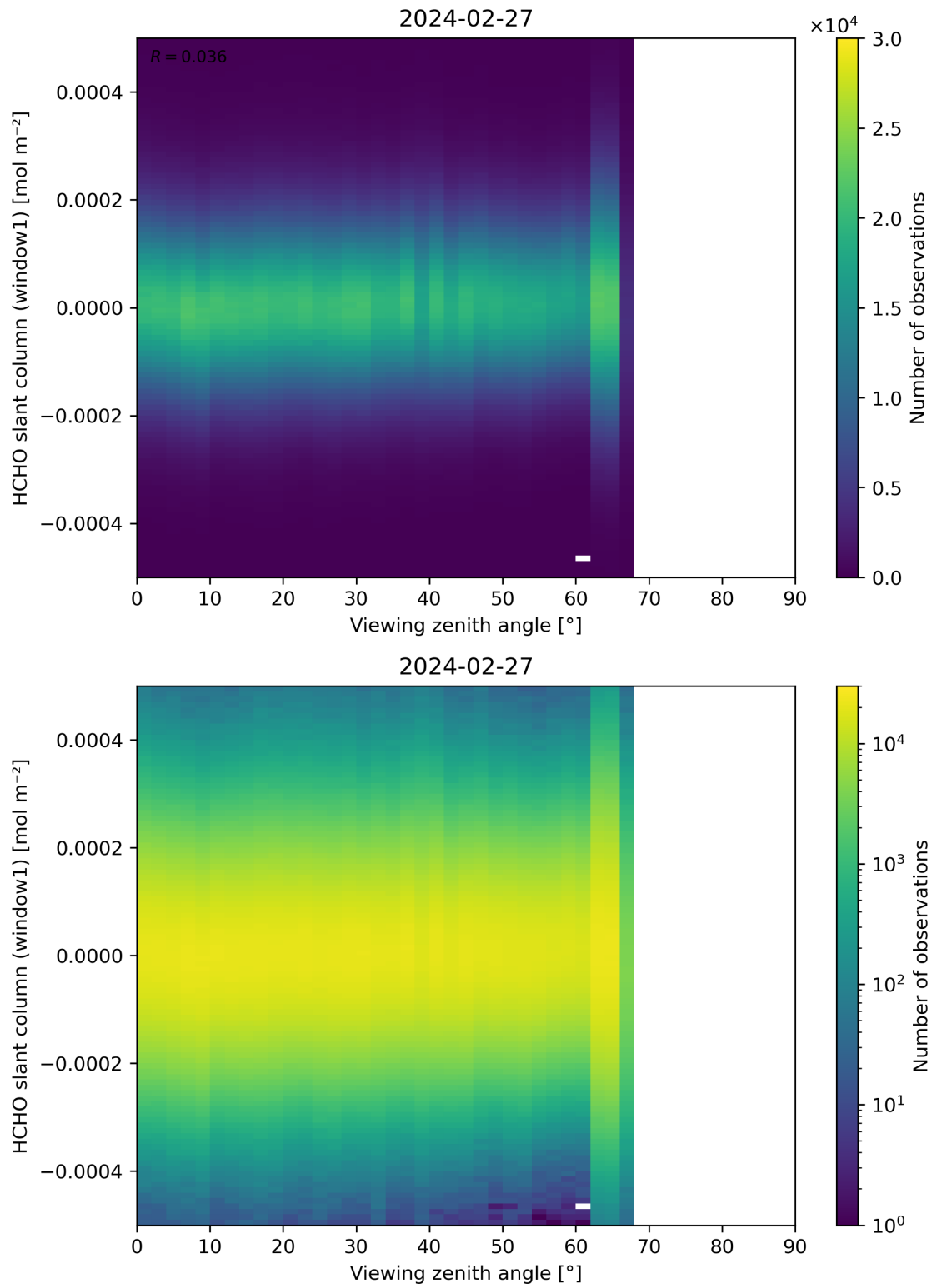
Figure 188: Scatter density plot of “Viewing zenith angle” against “HCHO slant column (window1)” for 2024-02-27 to 2024-02-28.
