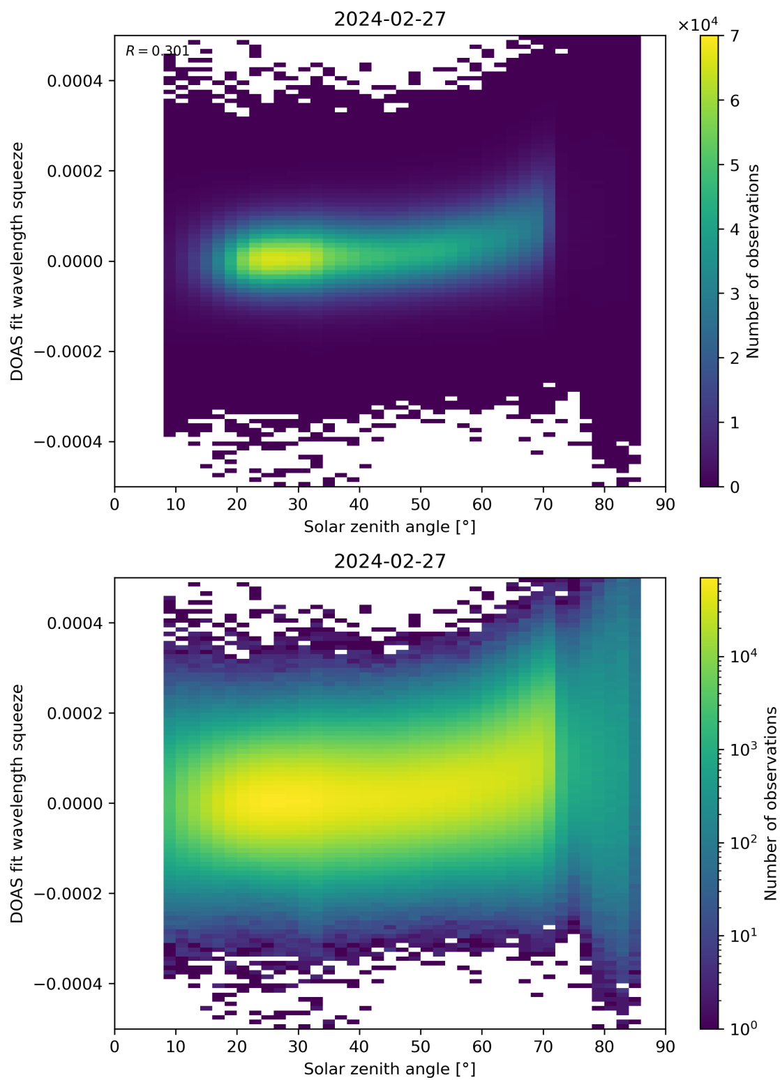
Figure 169: Scatter density plot of “Solar zenith angle” against “DOAS fit wavelength squeeze” for 2024-02-27 to 2024-02-28.
