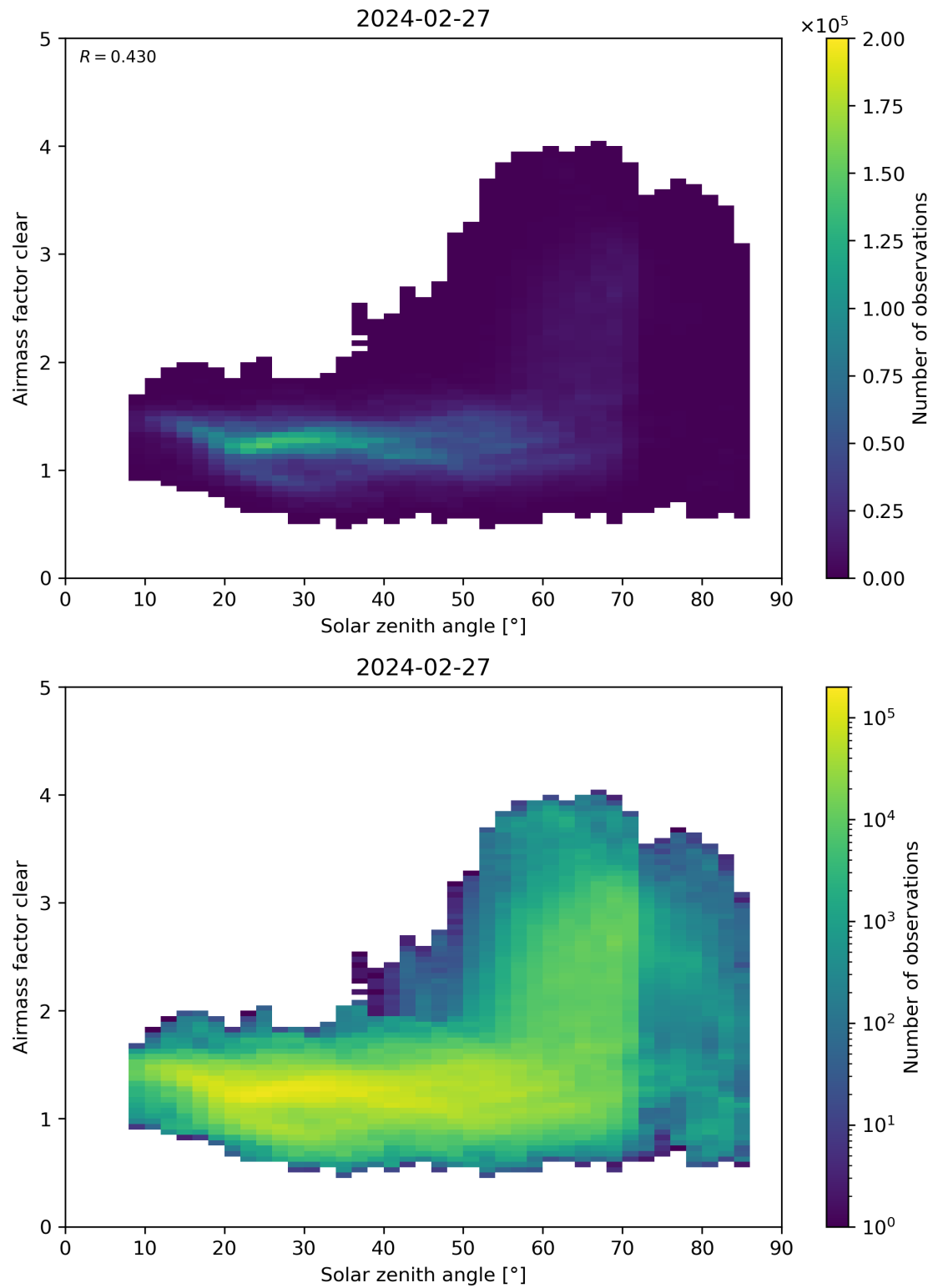
Figure 170: Scatter density plot of “Solar zenith angle” against “Airmass factor clear” for 2024-02-27 to 2024-02-28.
