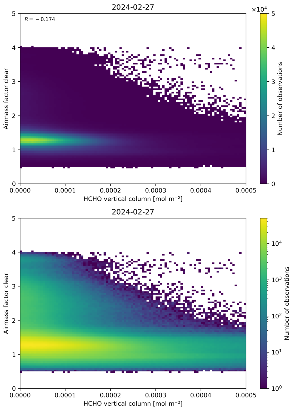
Figure 126: Scatter density plot of “HCHO vertical column” against “Airmass factor clear” for 2024-02-27 to 2024-02-28.
