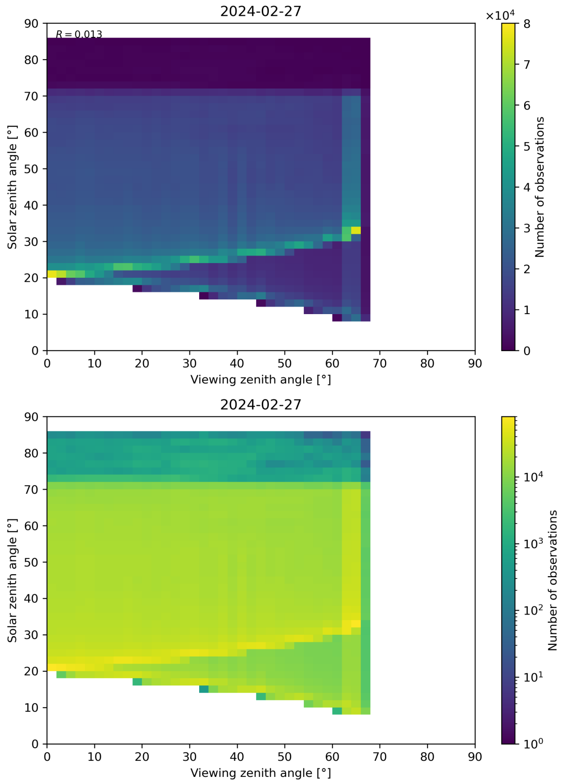
Figure 197: Scatter density plot of “Viewing zenith angle” against “Solar zenith angle” for 2024-02-27 to 2024-02-28.
