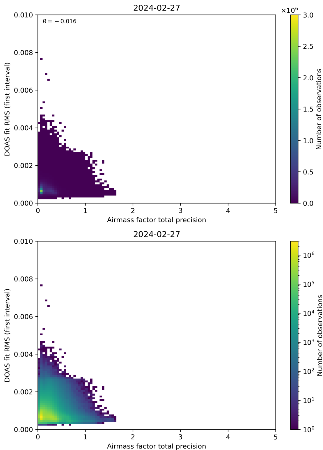
Figure 105: Scatter density plot of “Airmass factor total precision” against “DOAS fit RMS (first interval)” for 2024-02-27 to 2024-02-28.
