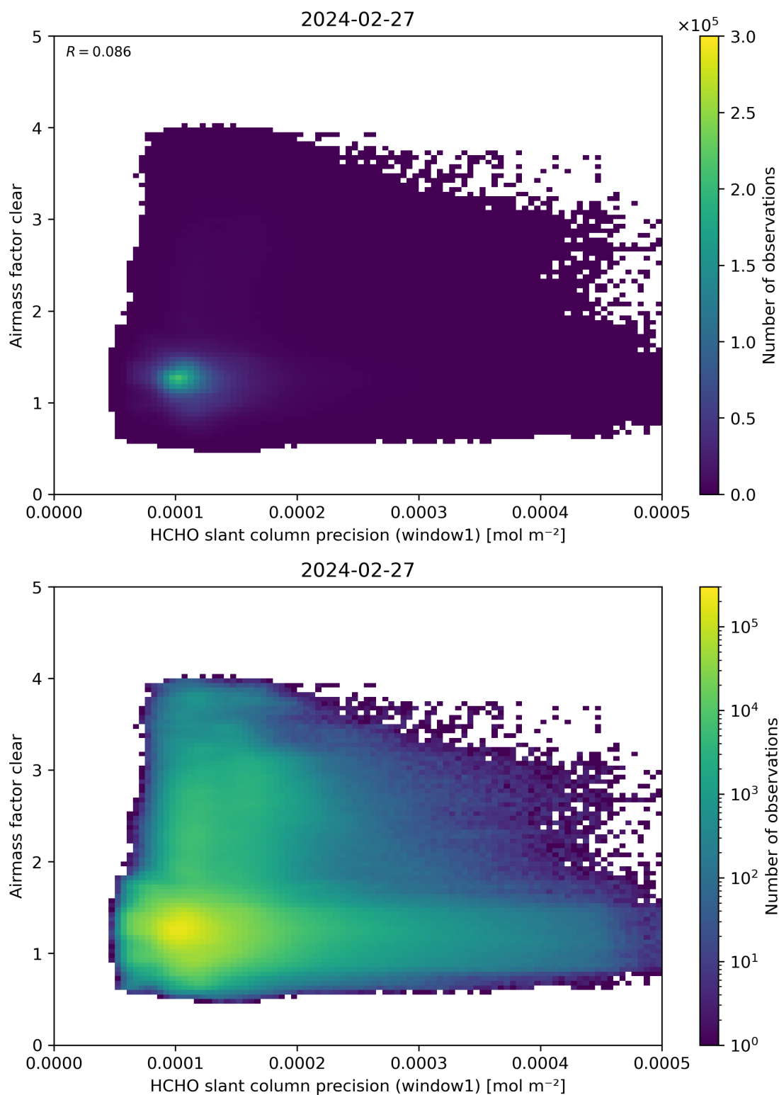
Figure 91: Scatter density plot of “HCHO slant column precision (window1)” against “Airmass factor clear” for 2024-02-27 to 2024-02-28.
