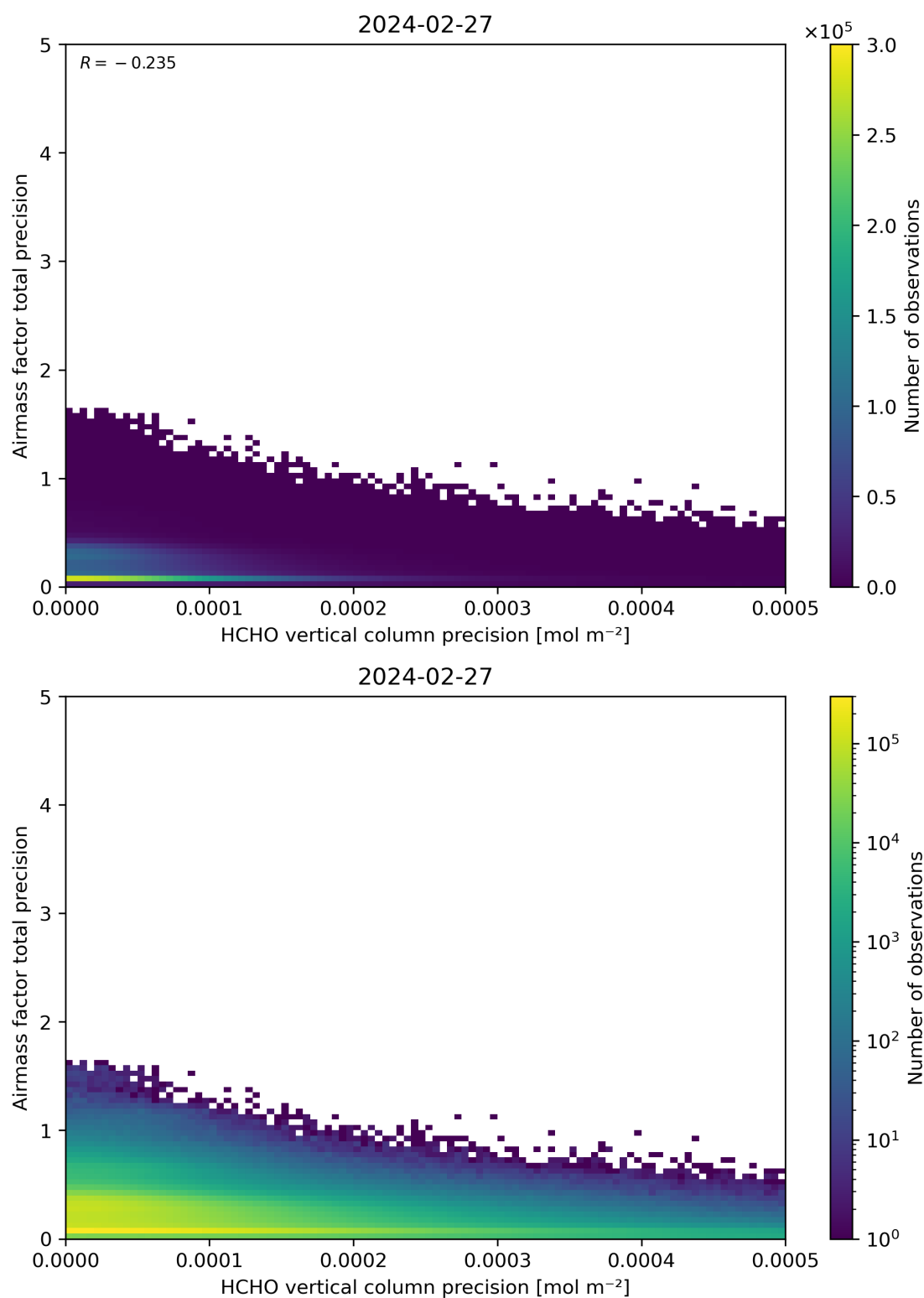
Figure 145: Scatter density plot of “HCHO vertical column precision” against “Airmass factor total precision” for 2024-02-27 to 2024-02-28.
