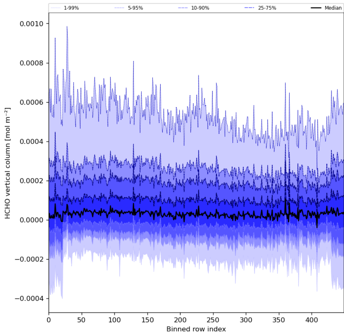
Figure 49: Along track statistics of “HCHO vertical column” for 2024-02-27 to 2024-02-28
