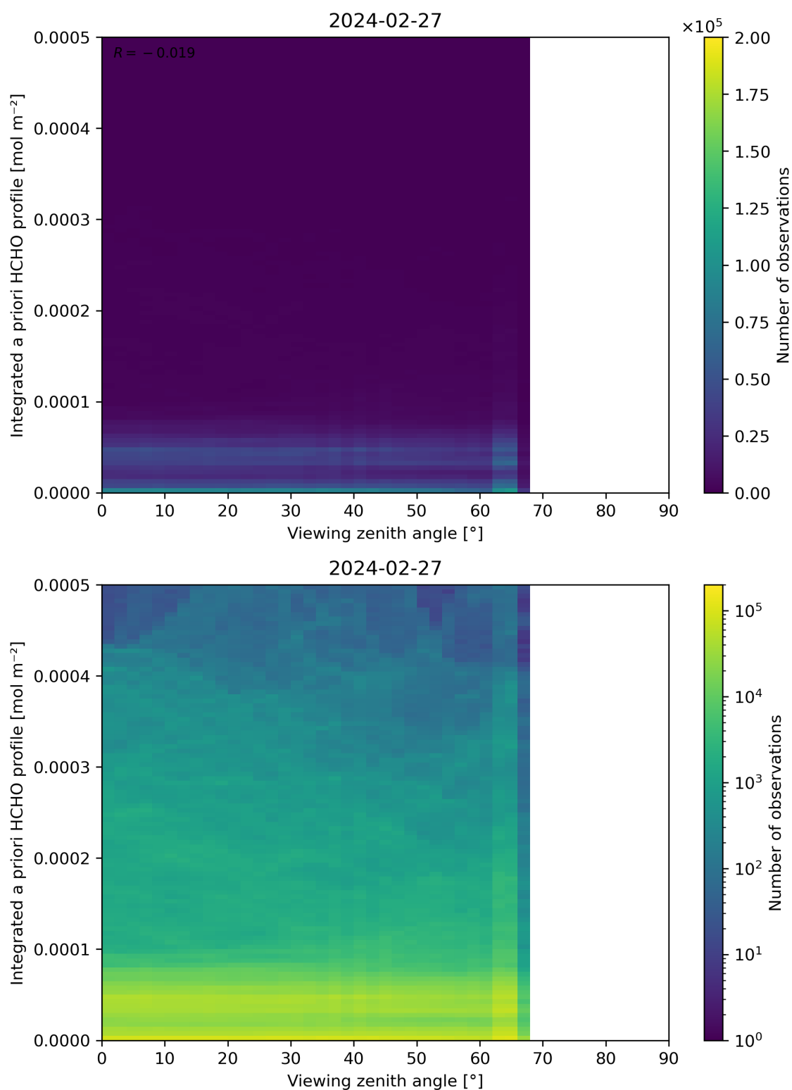
Figure 195: Scatter density plot of “Viewing zenith angle” against “Integrated a priori HCHO profile” for 2024-02-27 to 2024-02-28.
