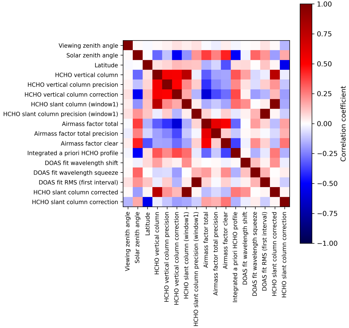
Figure 2: Map of correlation matrix for 2024-02-27 to 2024-02-28.
