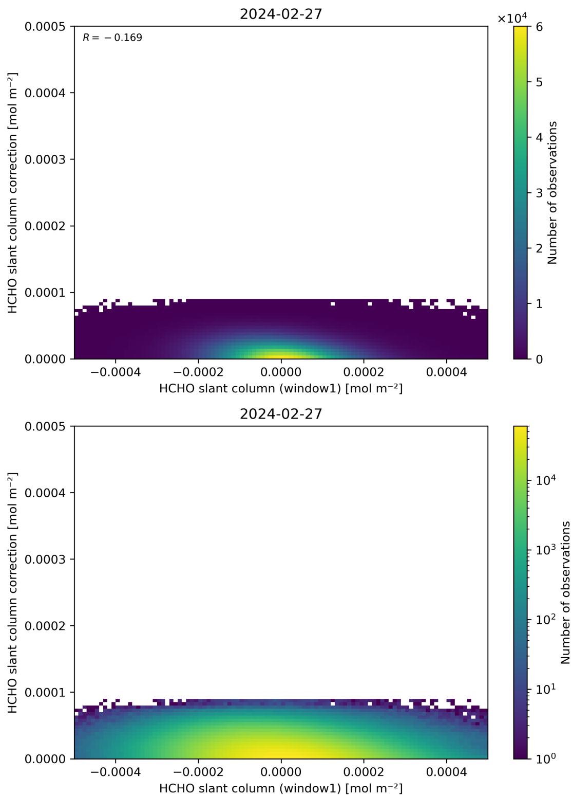
Figure 83: Scatter density plot of “HCHO slant column (window1)” against “HCHO slant column correction” for 2024-02-27 to 2024-02-28.
