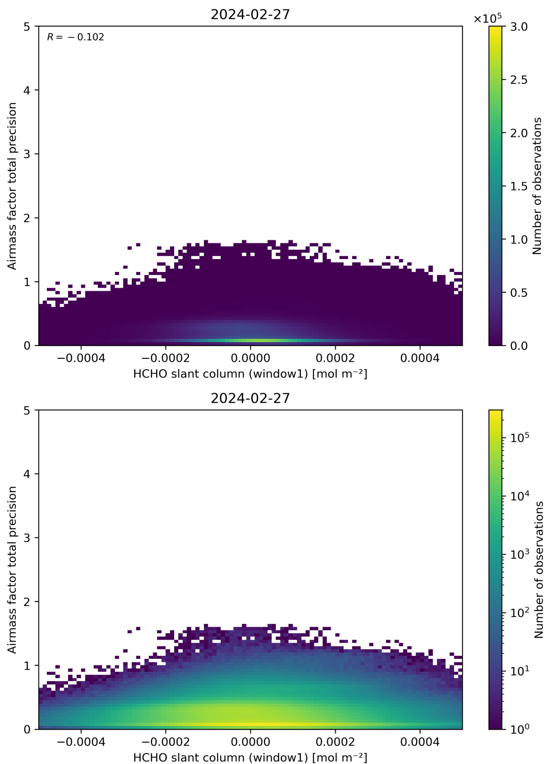
Figure 86: Scatter density plot of “HCHO slant column (window1)” against “Airmass factor total precision” for 2024-02-27 to 2024-02-28.
