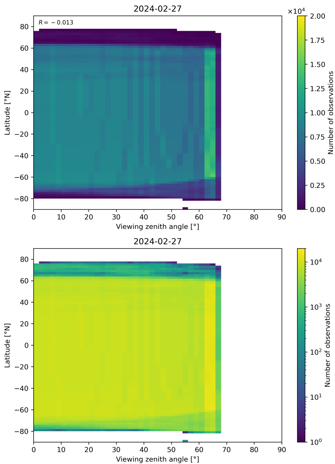
Figure 196: Scatter density plot of “Viewing zenith angle” against “Latitude” for 2024-02-27 to 2024-02-28.
