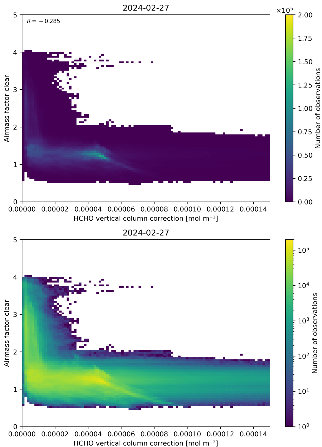
Figure 115: Scatter density plot of “HCHO vertical column correction” against “Airmass factor clear” for 2024-02-27 to 2024-02-28.
