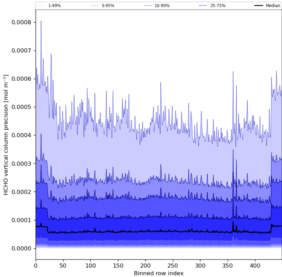
Figure 50: Along track statistics of “HCHO vertical column precision” for 2024-02-27 to 2024-02-28
