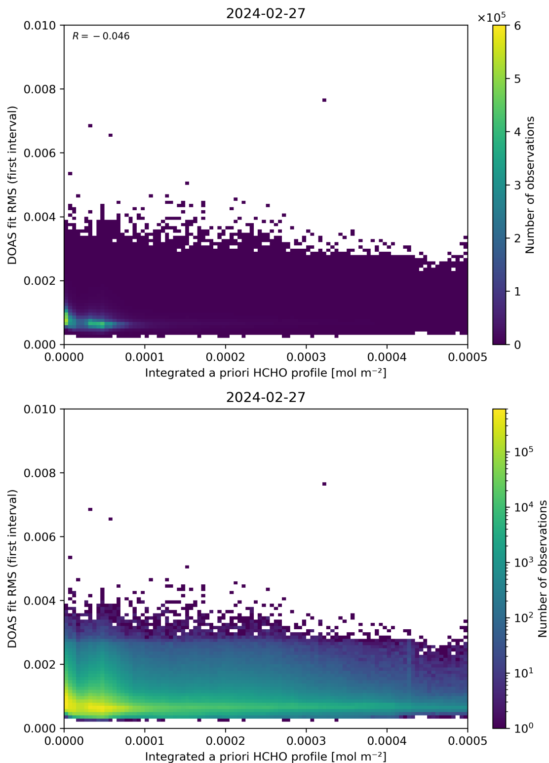
Figure 148: Scatter density plot of “Integrated a priori HCHO profile” against “DOAS fit RMS (first interval)” for 2024-02-27 to 2024-02-28.
