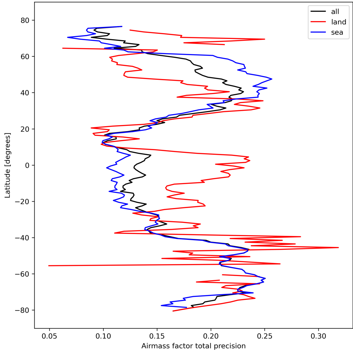
Figure 27: Zonal average of “Airmass factor total precision” for 2024-02-27 to 2024-02-28.
