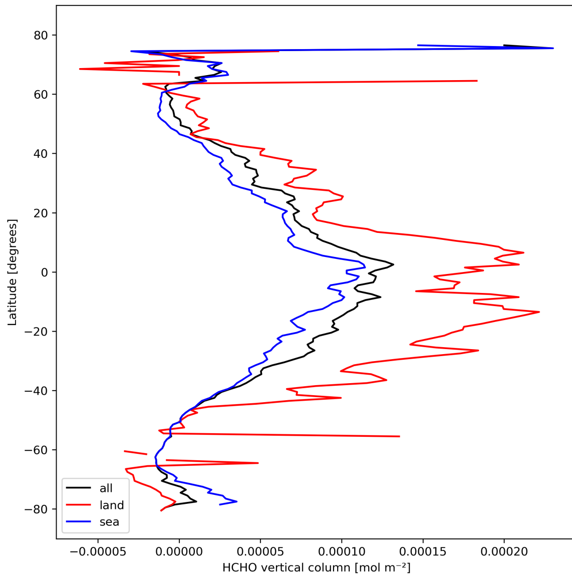
Figure 21: Zonal average of “HCHO vertical column” for 2024-02-27 to 2024-02-28.
