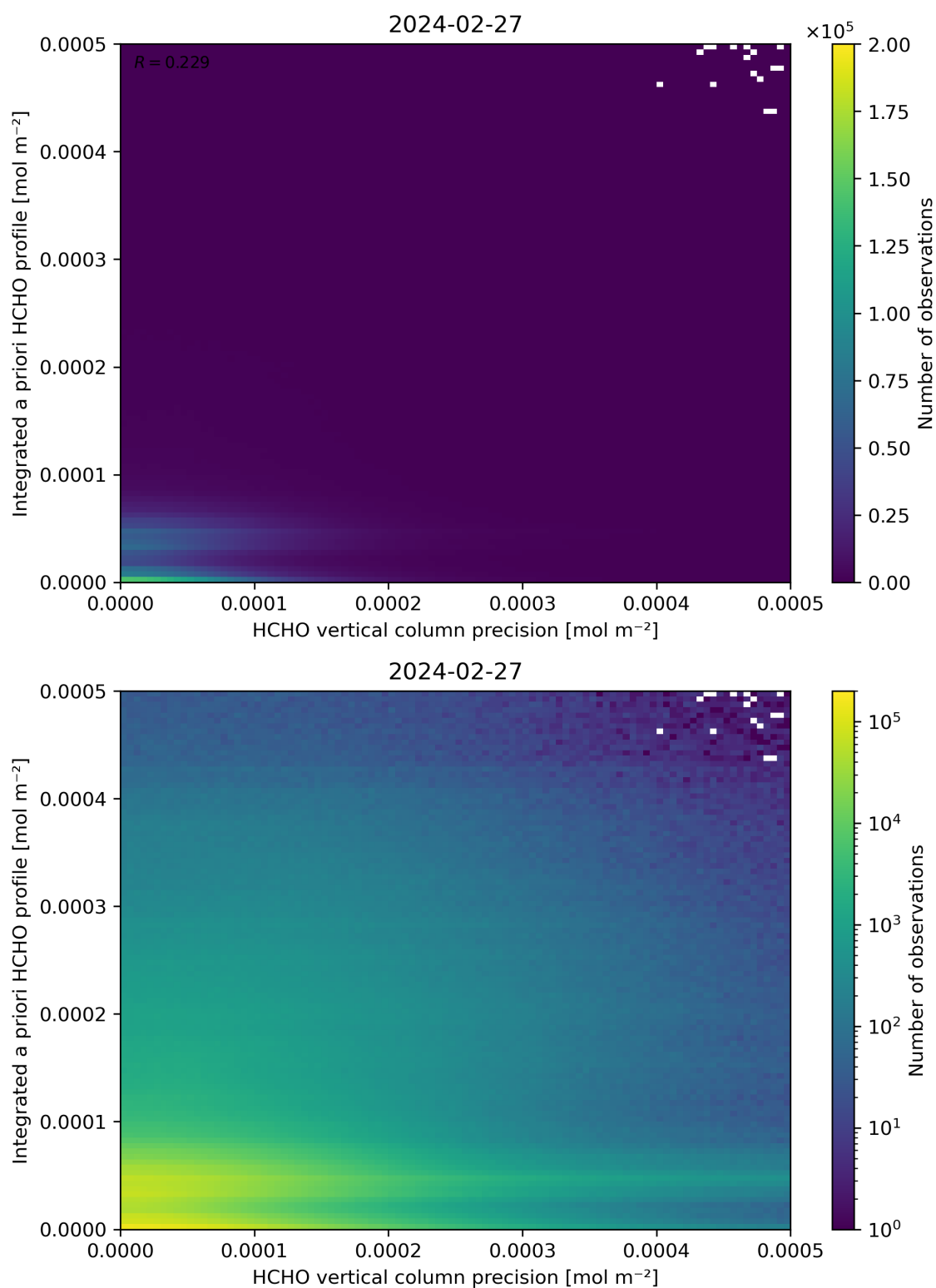
Figure 147: Scatter density plot of “HCHO vertical column precision” against “Integrated a priori HCHO profile” for 2024-02-27 to 2024-02-28.
