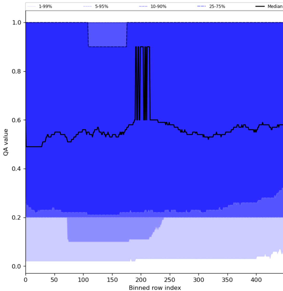
Figure 48: Along track statistics of “QA value” for 2024-02-27 to 2024-02-28
