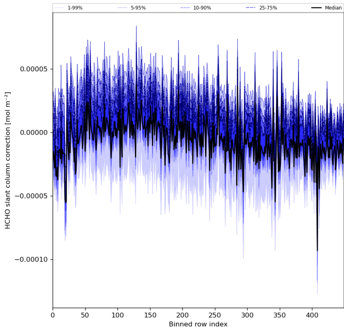
Figure 61: Along track statistics of “HCHO slant column correction” for 2024-02-27 to 2024-02-28
