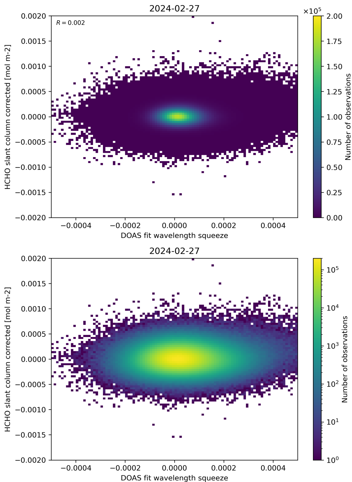
Figure 69: Scatter density plot of “DOAS fit wavelength squeeze” against “HCHO slant column corrected” for 2024-02-27 to 2024-02-28.
