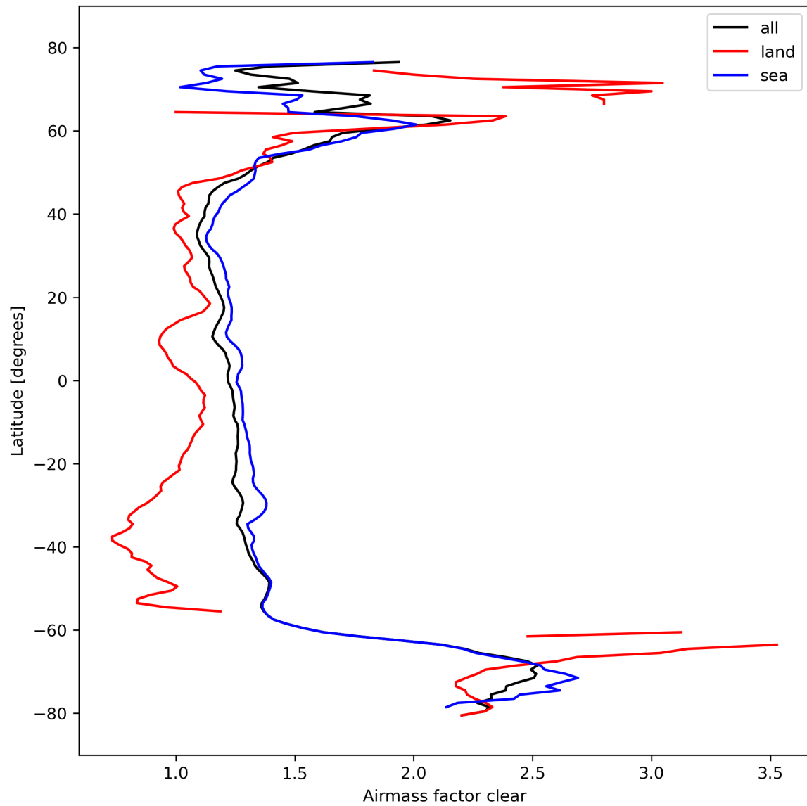
Figure 28: Zonal average of “Airmass factor clear” for 2024-02-27 to 2024-02-28.
