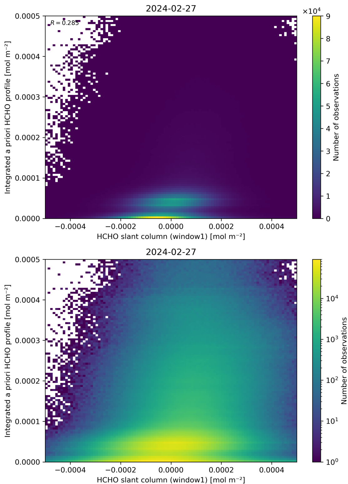
Figure 87: Scatter density plot of “HCHO slant column (window1)” against “Integrated a priori HCHO profile” for 2024-02-27 to 2024-02-28.
