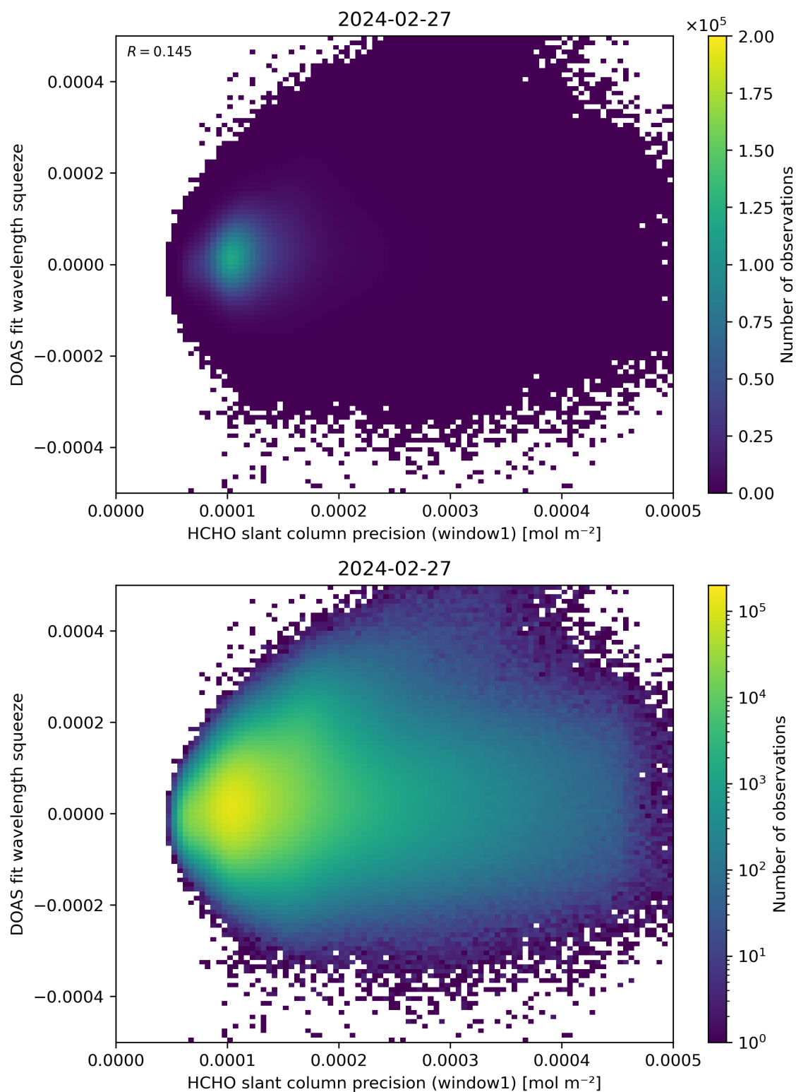
Figure 90: Scatter density plot of “HCHO slant column precision (window1)” against “DOAS fit wavelength squeeze” for 2024-02-27 to 2024-02-28.
