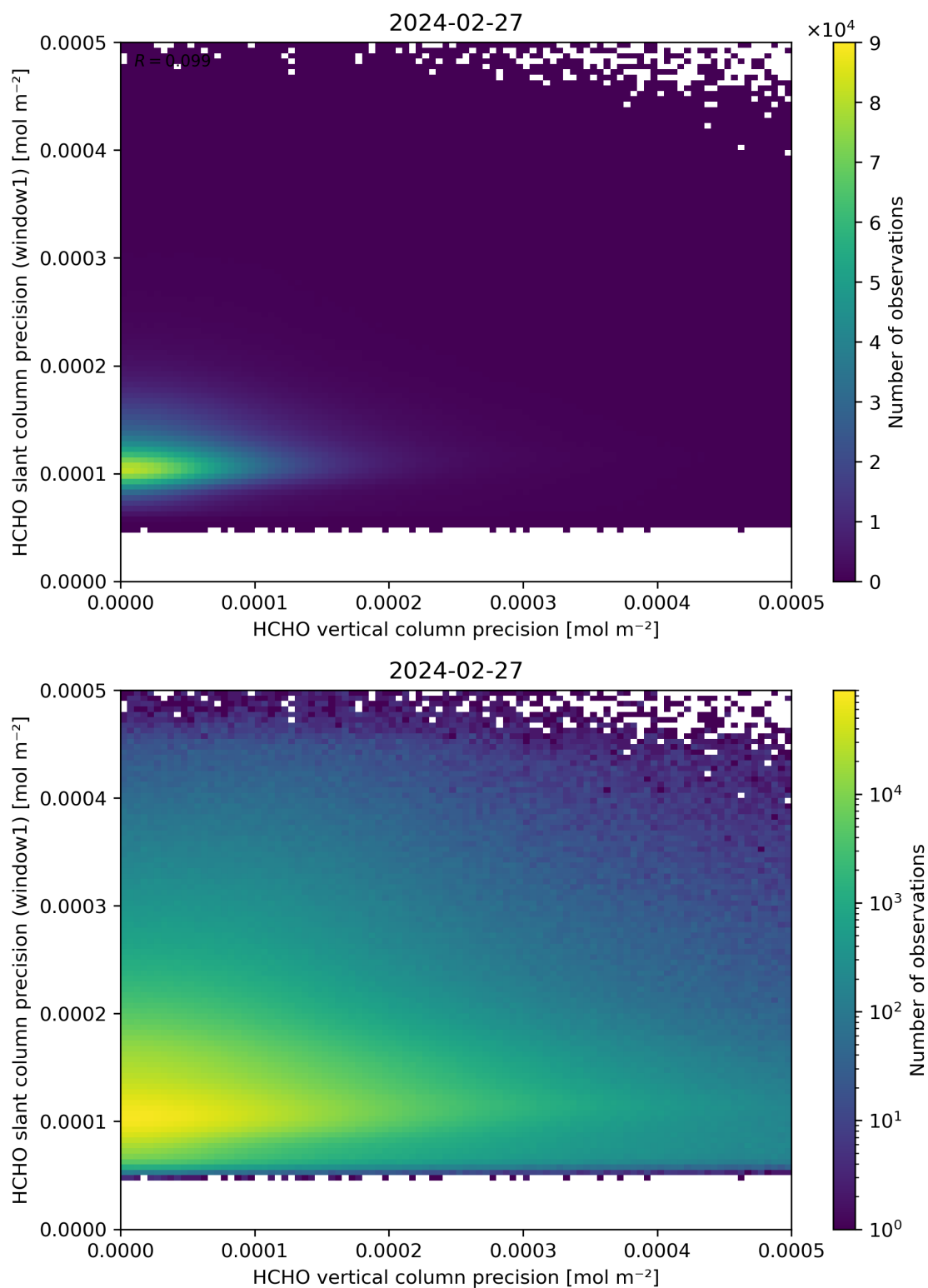
Figure 143: Scatter density plot of “HCHO vertical column precision” against “HCHO slant column precision (window1)” for 2024-02-27 to 2024-02-28.
