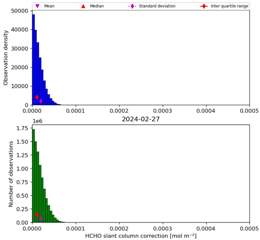
Figure 47: Histogram of “HCHO slant column correction” for 2024-02-27 to 2024-02-28
