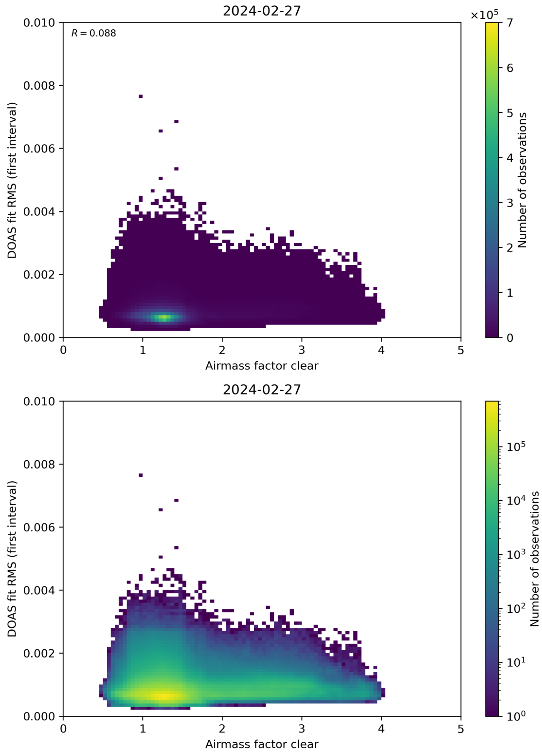
Figure 71: Scatter density plot of “Airmass factor clear” against “DOAS fit RMS (first interval)” for 2024-02-27 to 2024-02-28.
