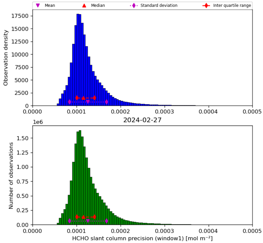
Figure 39: Histogram of “HCHO slant column precision (window1)” for 2024-02-27 to 2024-02-28
