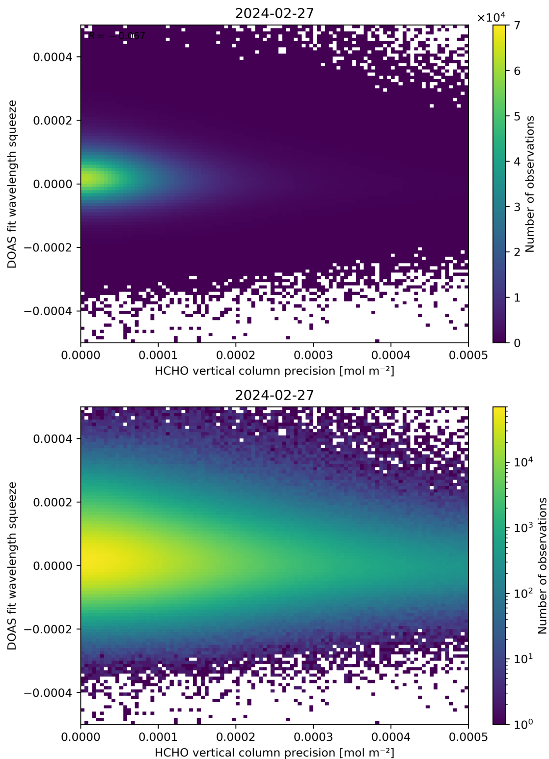
Figure 138: Scatter density plot of “HCHO vertical column precision” against “DOAS fit wavelength squeeze” for 2024-02-27 to 2024-02-28.
