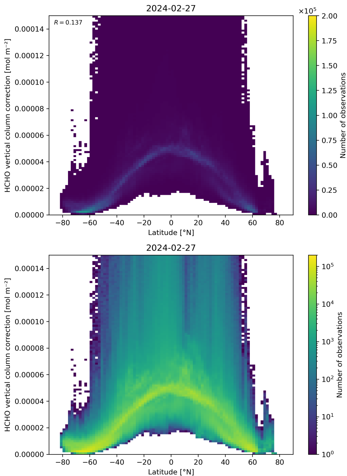
Figure 164: Scatter density plot of “Latitude” against “HCHO vertical column correction” for 2024-02-27 to 2024-02-28.
