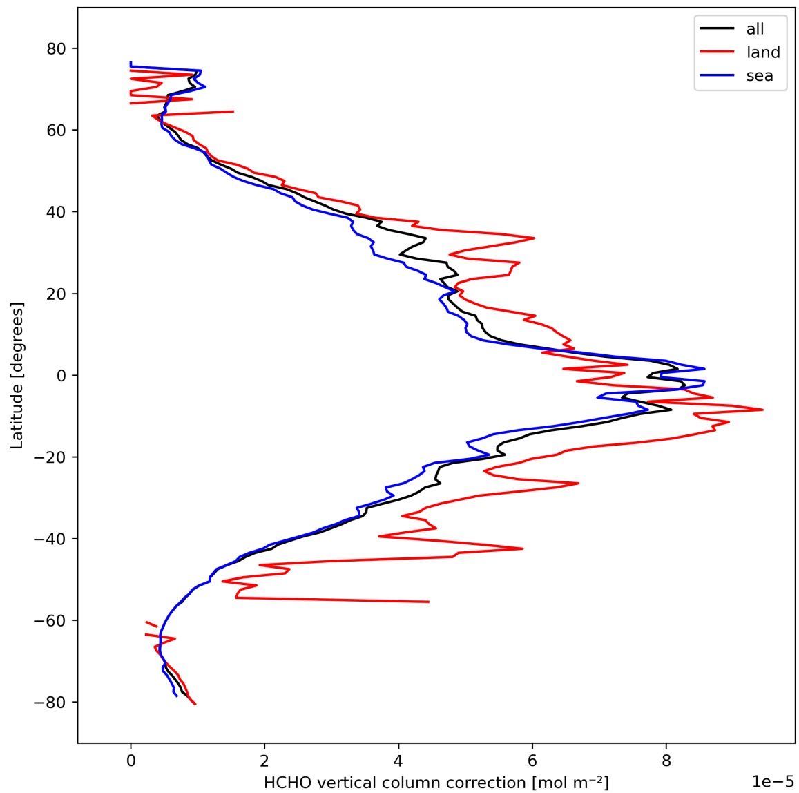
Figure 23: Zonal average of “HCHO vertical column correction” for 2024-02-27 to 2024-02-28.
