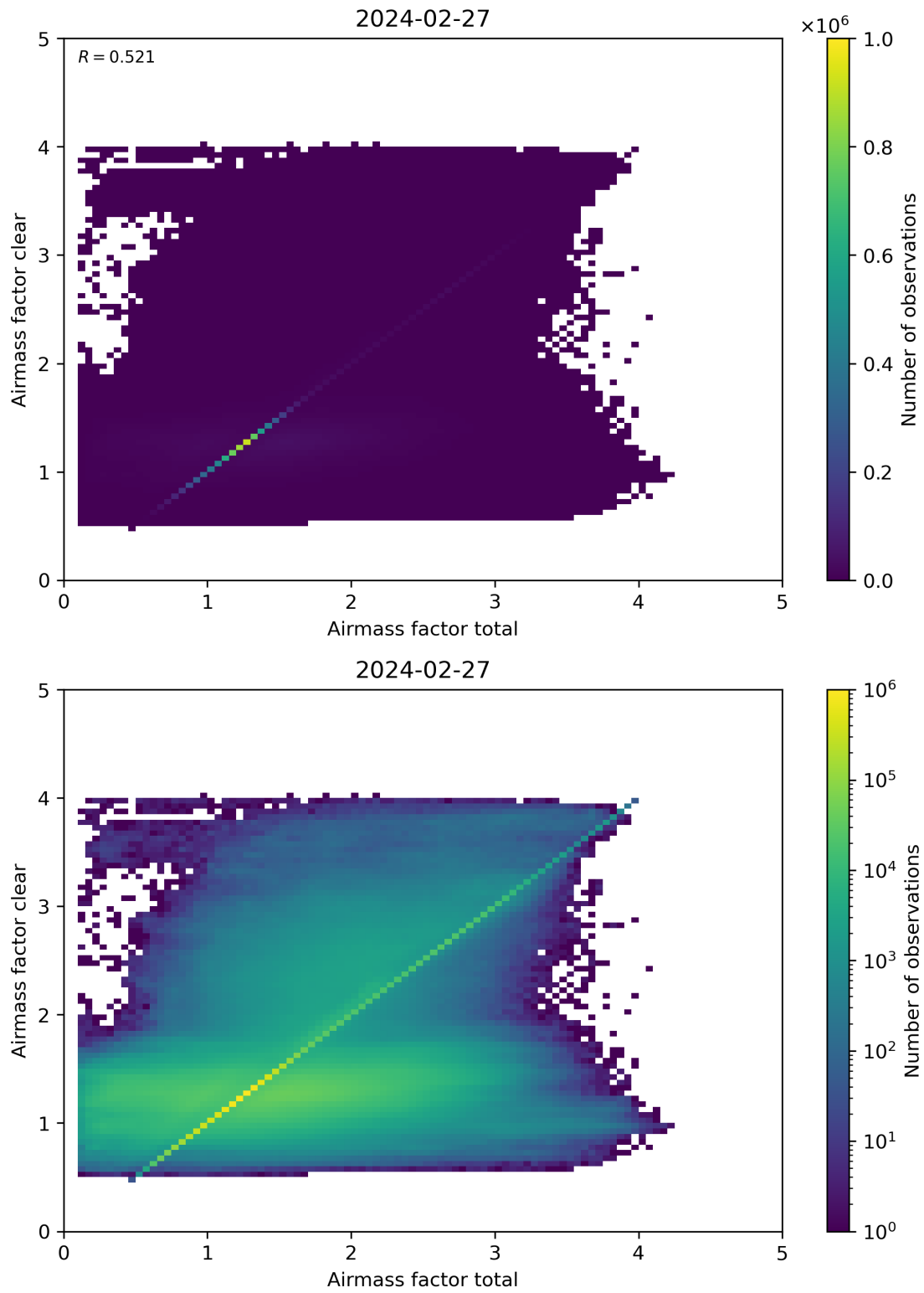
Figure 100: Scatter density plot of “Airmass factor total” against “Airmass factor clear” for 2024-02-27 to 2024-02-28.
