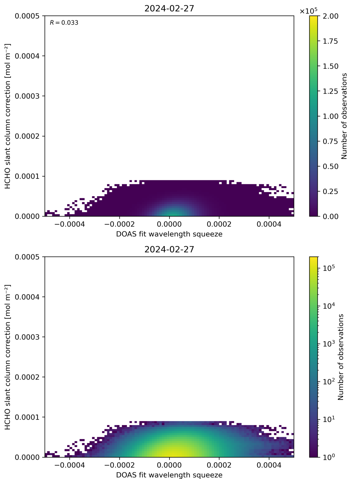
Figure 70: Scatter density plot of “DOAS fit wavelength squeeze” against “HCHO slant column correction” for 2024-02-27 to 2024-02-28.
