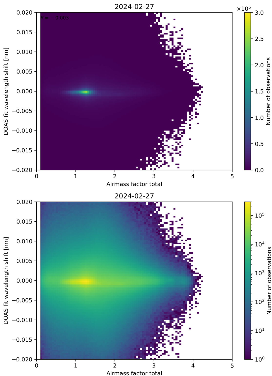
Figure 98: Scatter density plot of “Airmass factor total” against “DOAS fit wavelength shift” for 2024-02-27 to 2024-02-28.
