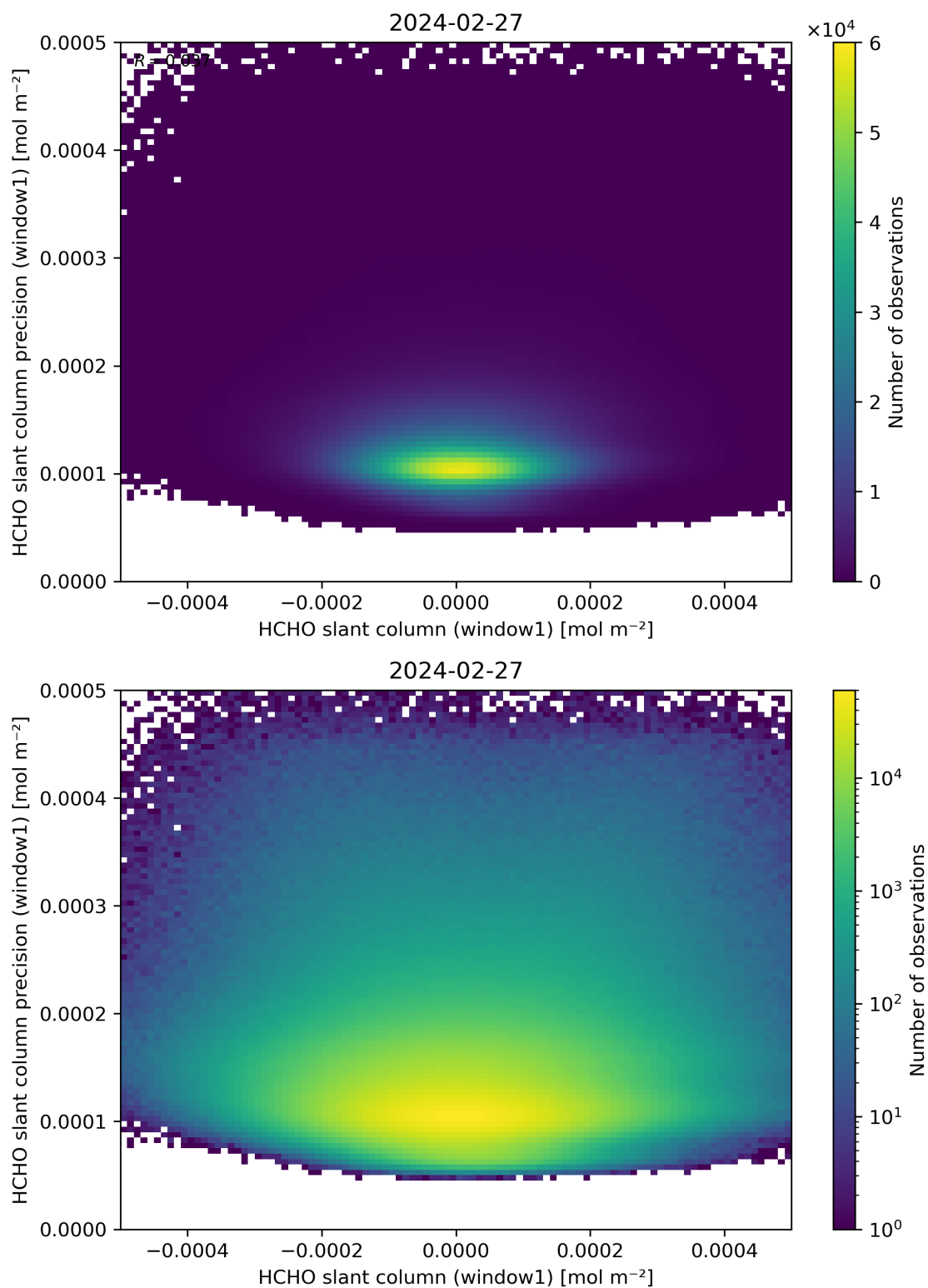
Figure 84: Scatter density plot of “HCHO slant column (window1)” against “HCHO slant column precision (window1)” for 2024-02-27 to 2024-02-28.
