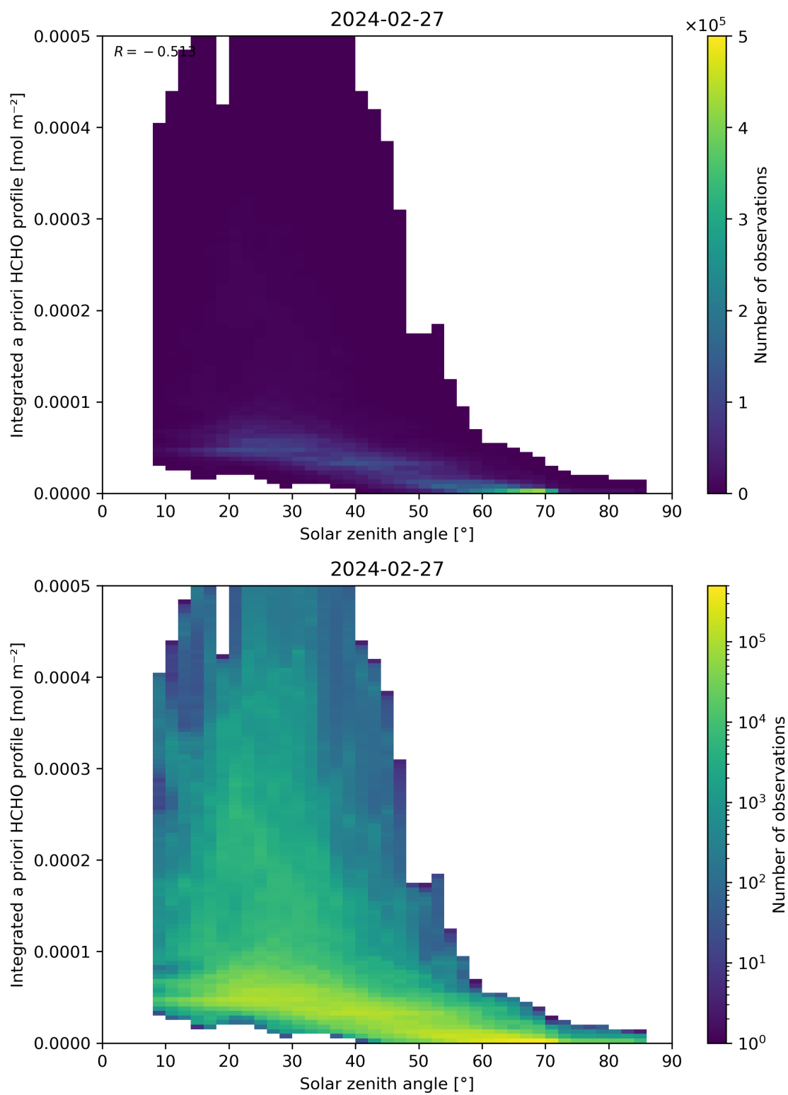
Figure 180: Scatter density plot of “Solar zenith angle” against “Integrated a priori HCHO profile” for 2024-02-27 to 2024-02-28.
