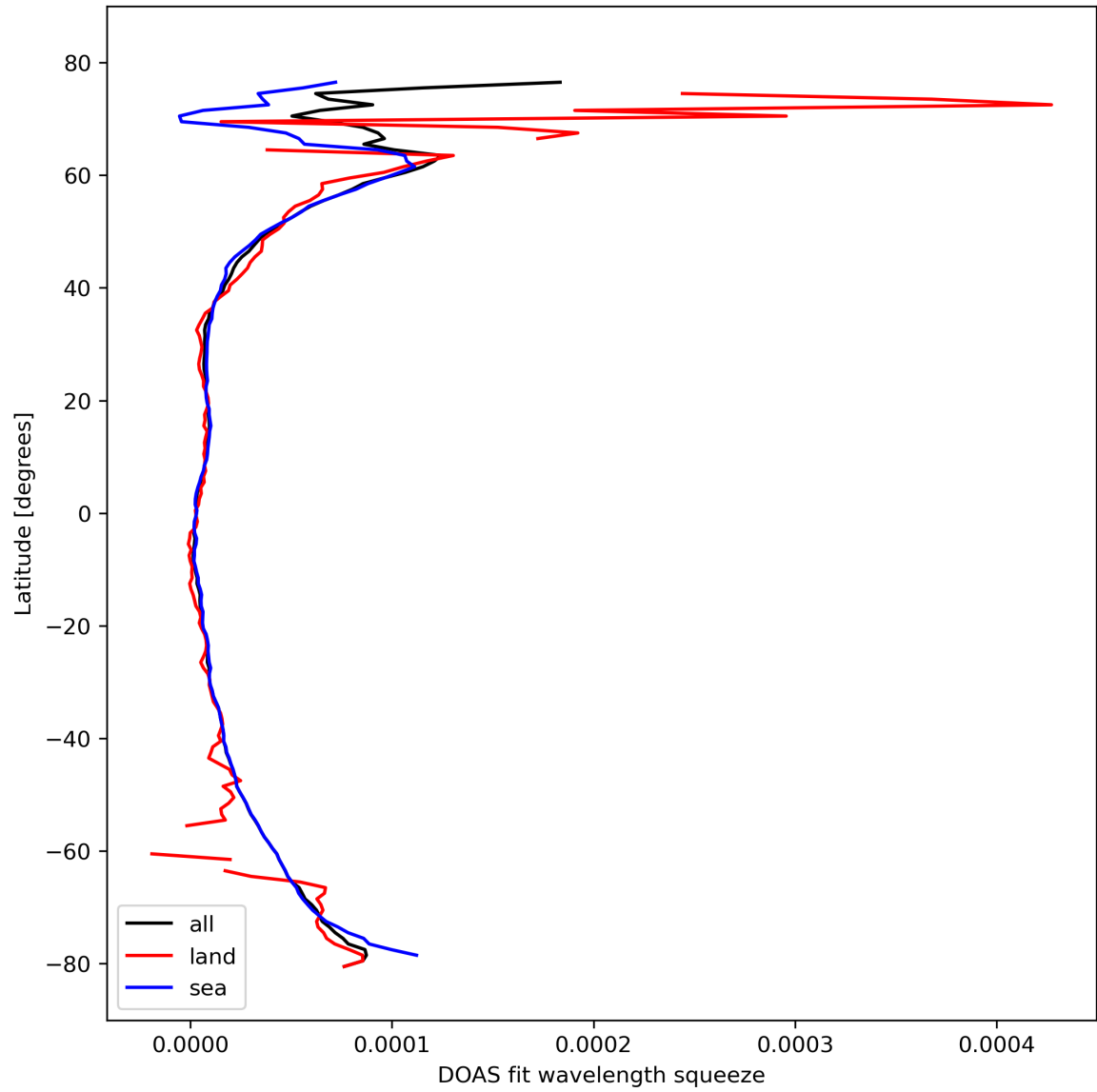
Figure 31: Zonal average of “DOAS fit wavelength squeeze” for 2024-02-27 to 2024-02-28.
