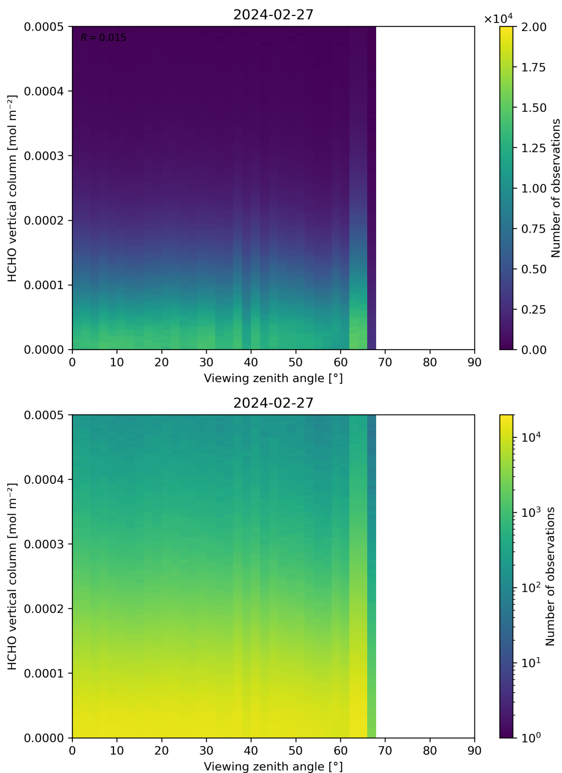
Figure 192: Scatter density plot of “Viewing zenith angle” against “HCHO vertical column” for 2024-02-27 to 2024-02-28.
