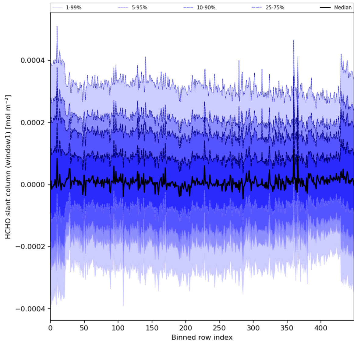
Figure 52: Along track statistics of “HCHO slant column (window1)” for 2024-02-27 to 2024-02-28
