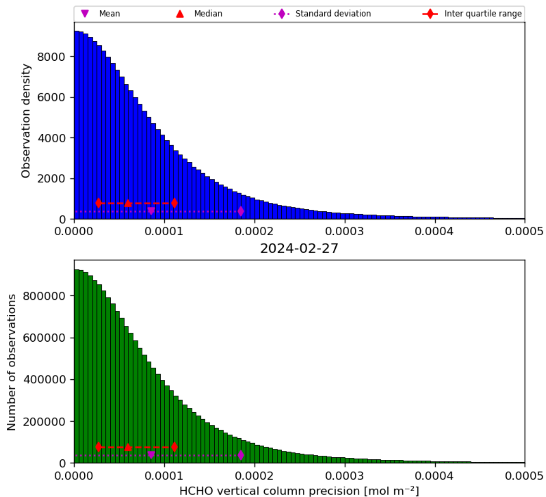
Figure 36: Histogram of “HCHO vertical column precision” for 2024-02-27 to 2024-02-28
