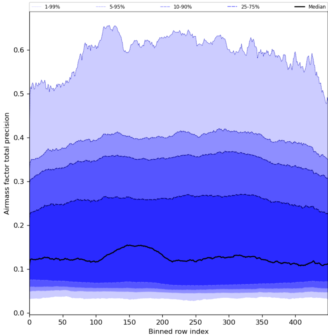
Figure 55: Along track statistics of “Airmass factor total precision” for 2024-02-27 to 2024-02-28
