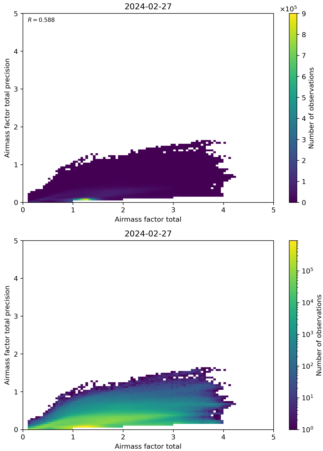
Figure 103: Scatter density plot of “Airmass factor total” against “Airmass factor total precision” for 2024-02-27 to 2024-02-28.
