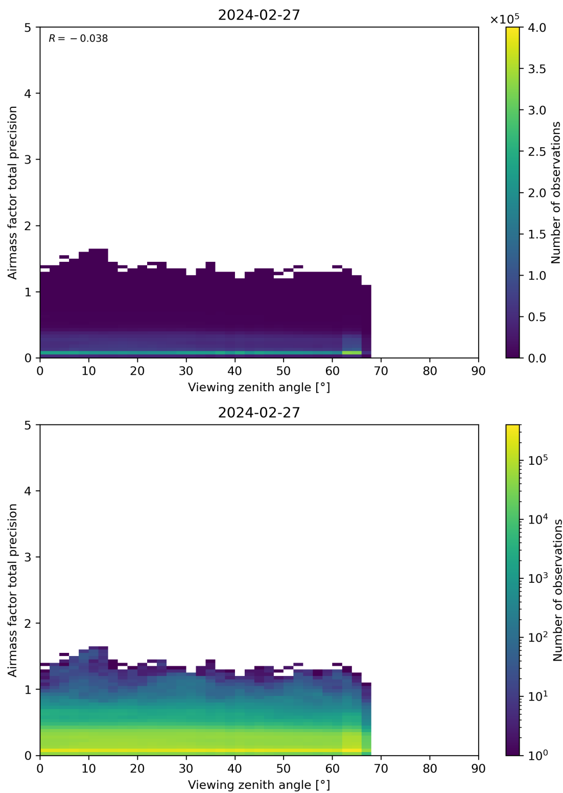
Figure 191: Scatter density plot of “Viewing zenith angle” against “Airmass factor total precision” for 2024-02-27 to 2024-02-28.
