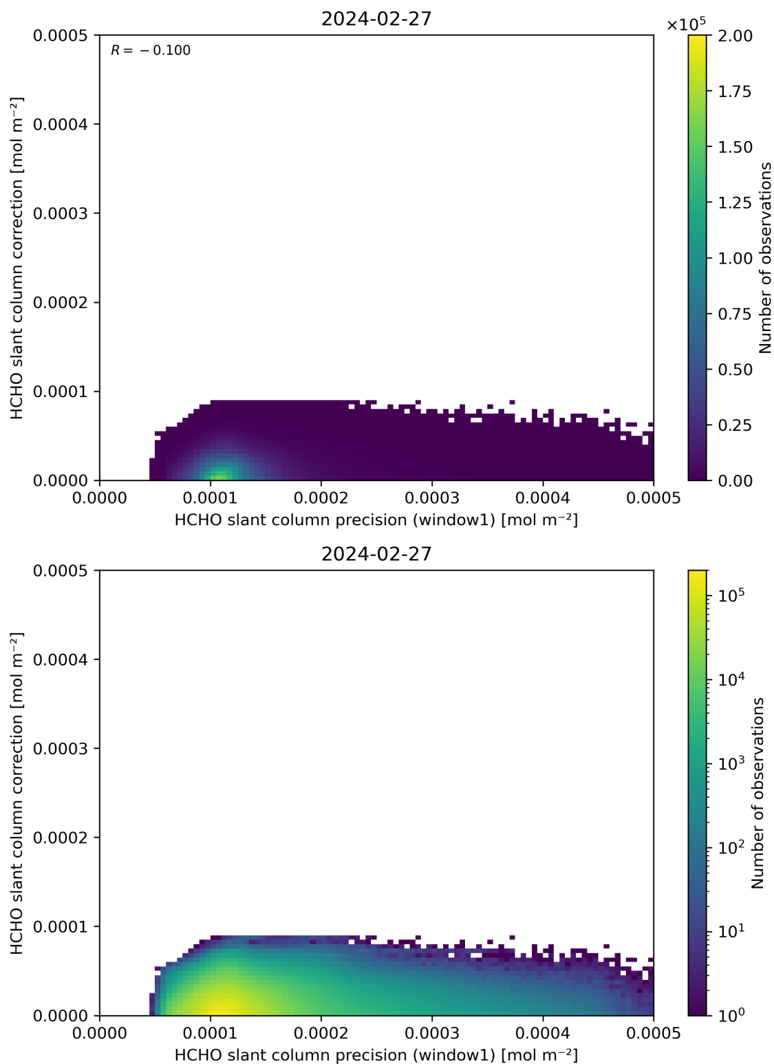
Figure 93: Scatter density plot of “HCHO slant column precision (window1)” against “HCHO slant column correction” for 2024-02-27 to 2024-02-28.
