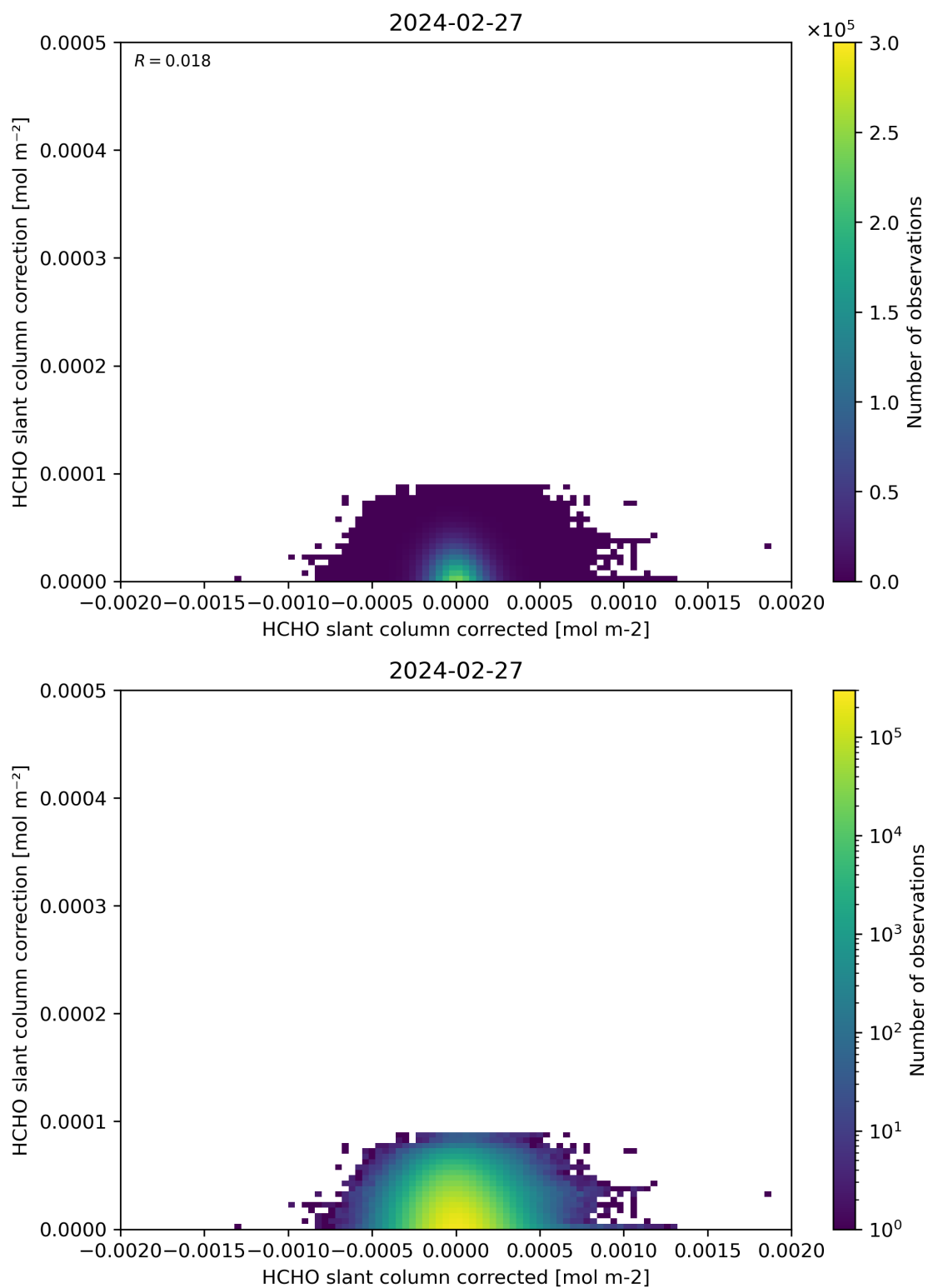
Figure 77: Scatter density plot of “HCHO slant column corrected” against “HCHO slant column correction” for 2024-02-27 to 2024-02-28.
