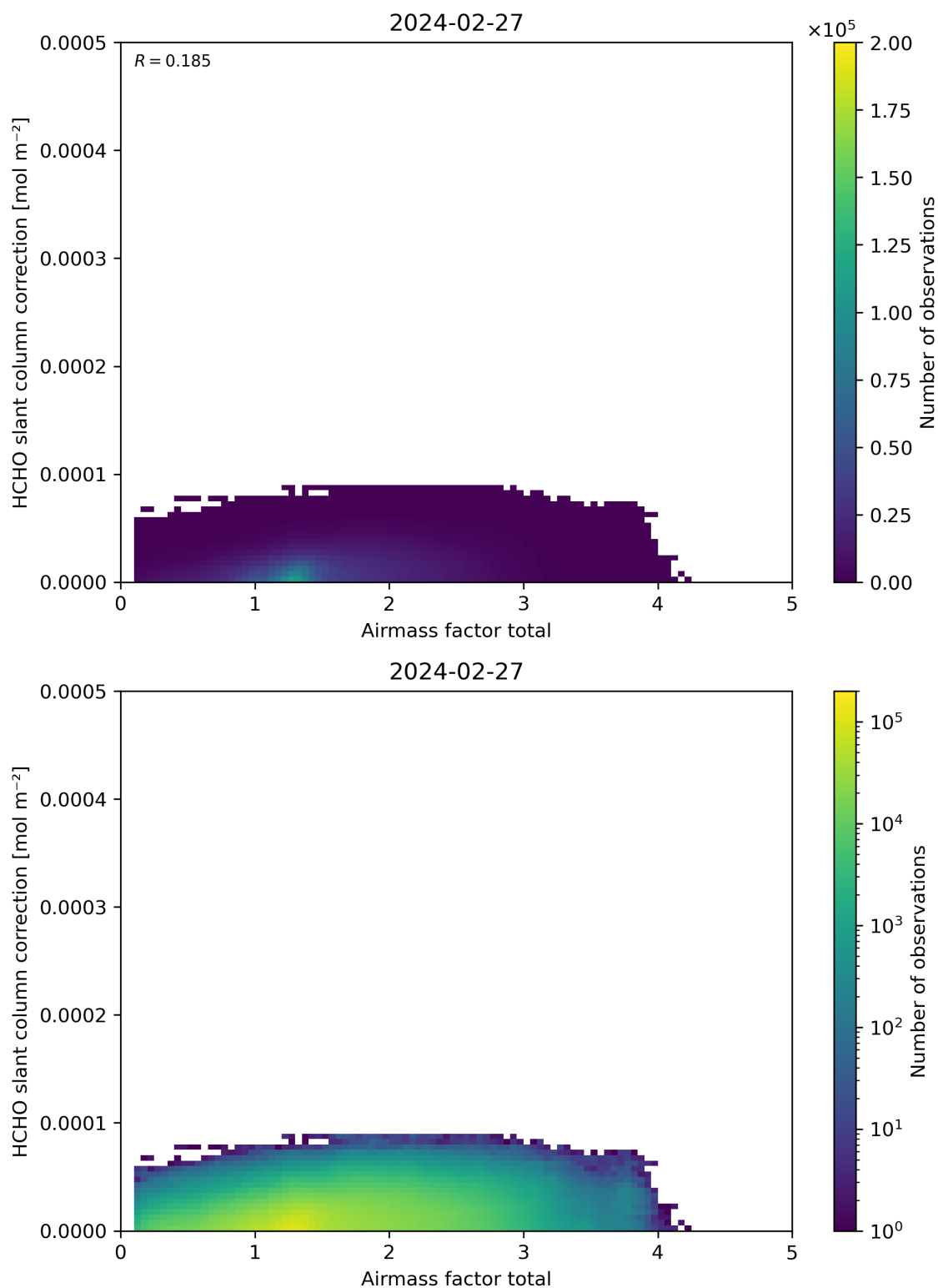
Figure 102: Scatter density plot of “Airmass factor total” against “HCHO slant column correction” for 2024-02-27 to 2024-02-28.
