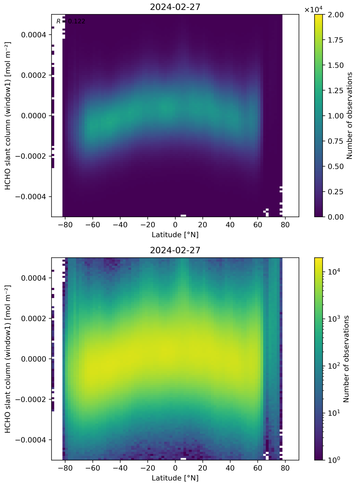
Figure 159: Scatter density plot of “Latitude” against “HCHO slant column (window1)” for 2024-02-27 to 2024-02-28.
