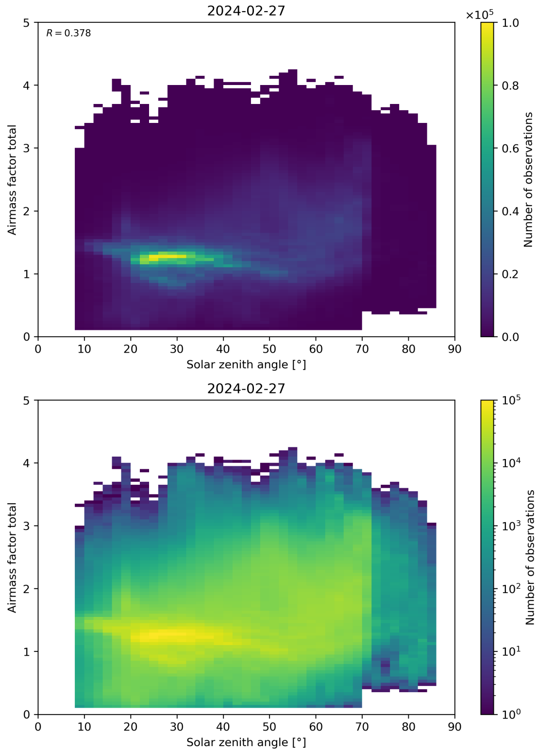
Figure 175: Scatter density plot of “Solar zenith angle” against “Airmass factor total” for 2024-02-27 to 2024-02-28.
