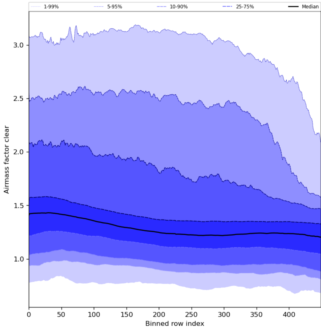
Figure 56: Along track statistics of “Airmass factor clear” for 2024-02-27 to 2024-02-28
