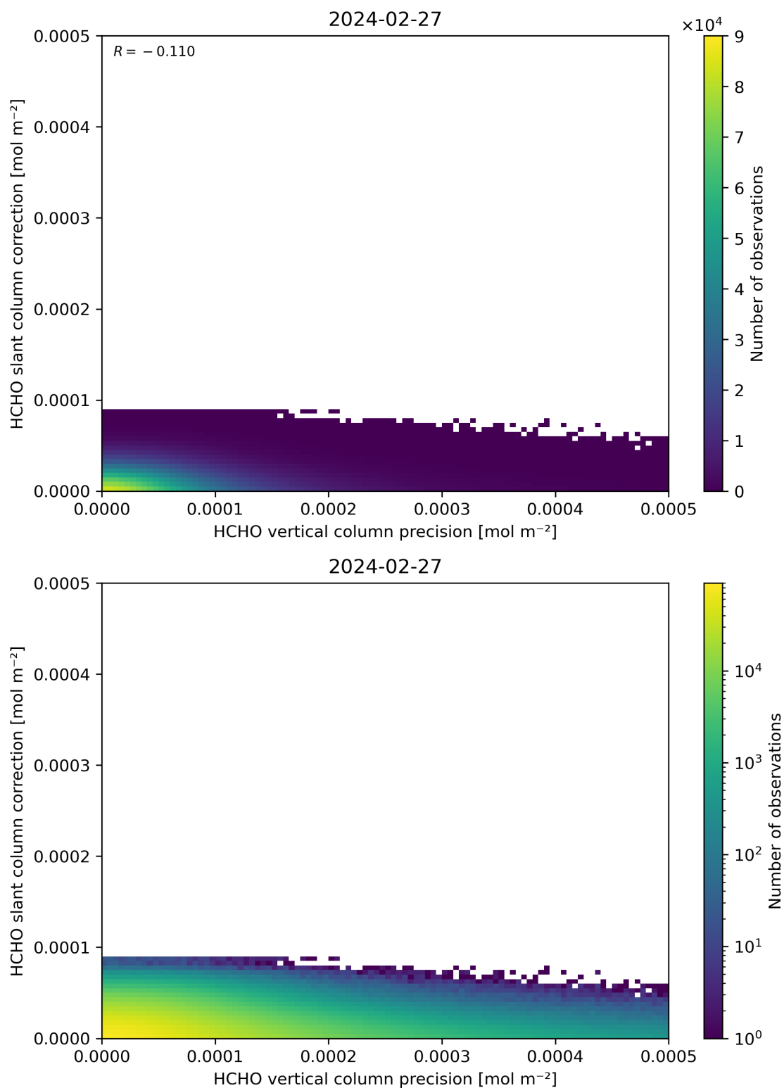
Figure 141: Scatter density plot of “HCHO vertical column precision” against “HCHO slant column correction” for 2024-02-27 to 2024-02-28.
