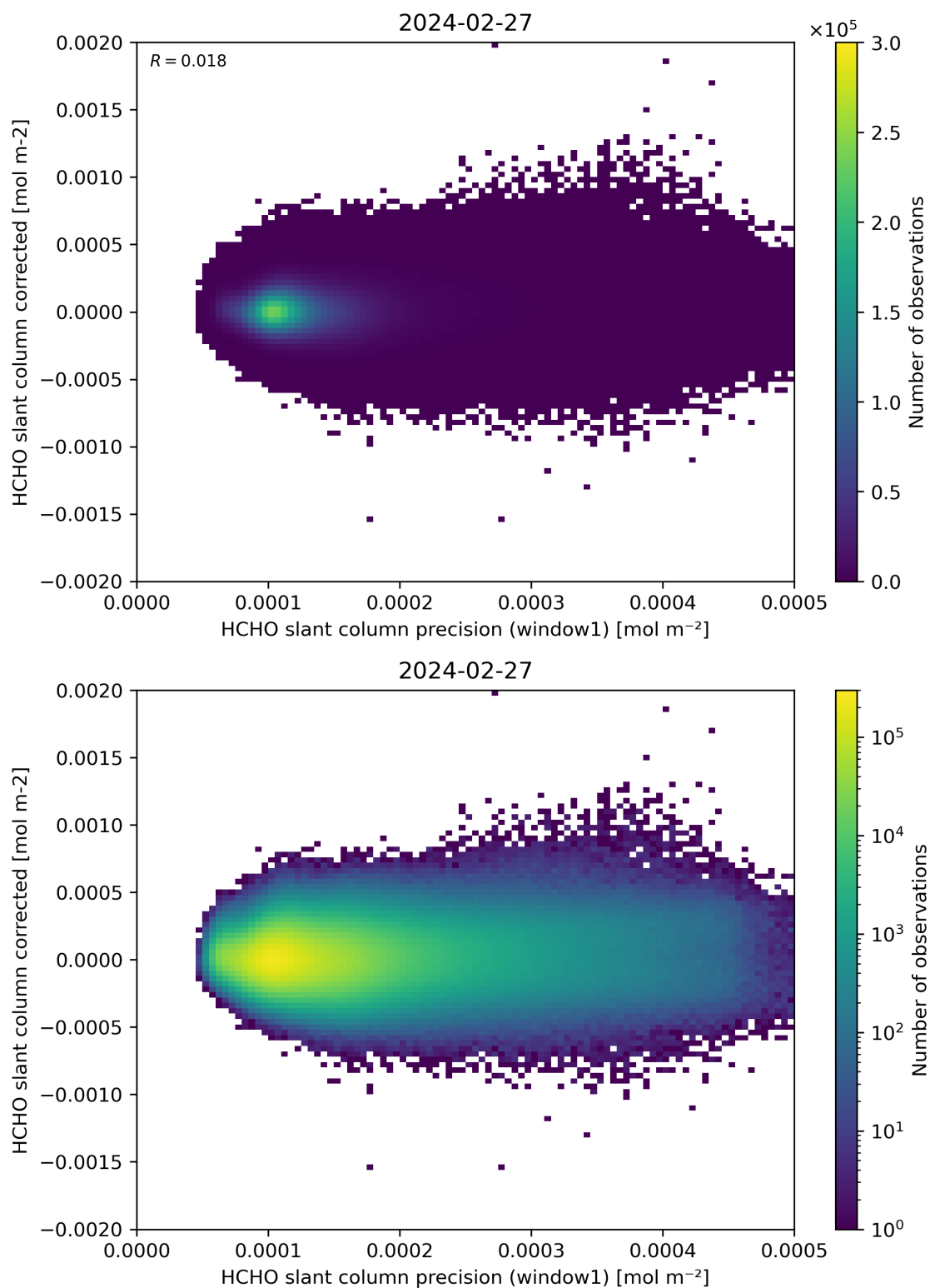
Figure 92: Scatter density plot of “HCHO slant column precision (window1)” against “HCHO slant column corrected” for 2024-02-27 to 2024-02-28.
