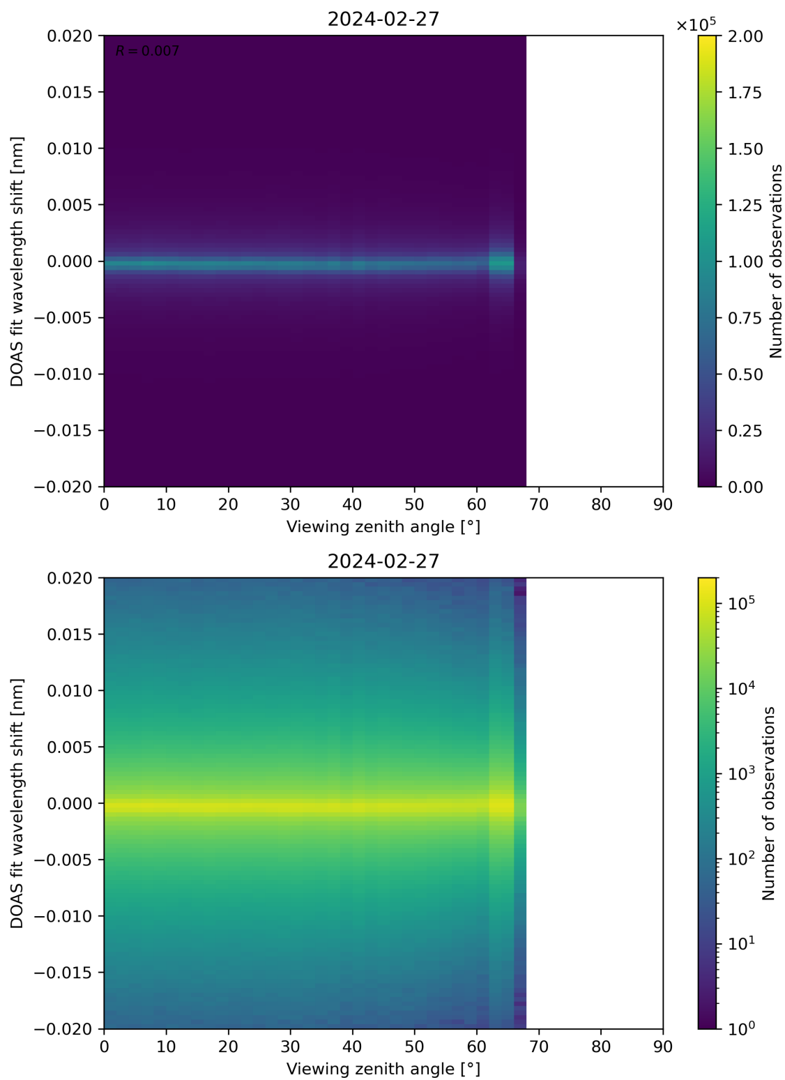
Figure 183: Scatter density plot of “Viewing zenith angle” against “DOAS fit wavelength shift” for 2024-02-27 to 2024-02-28.
