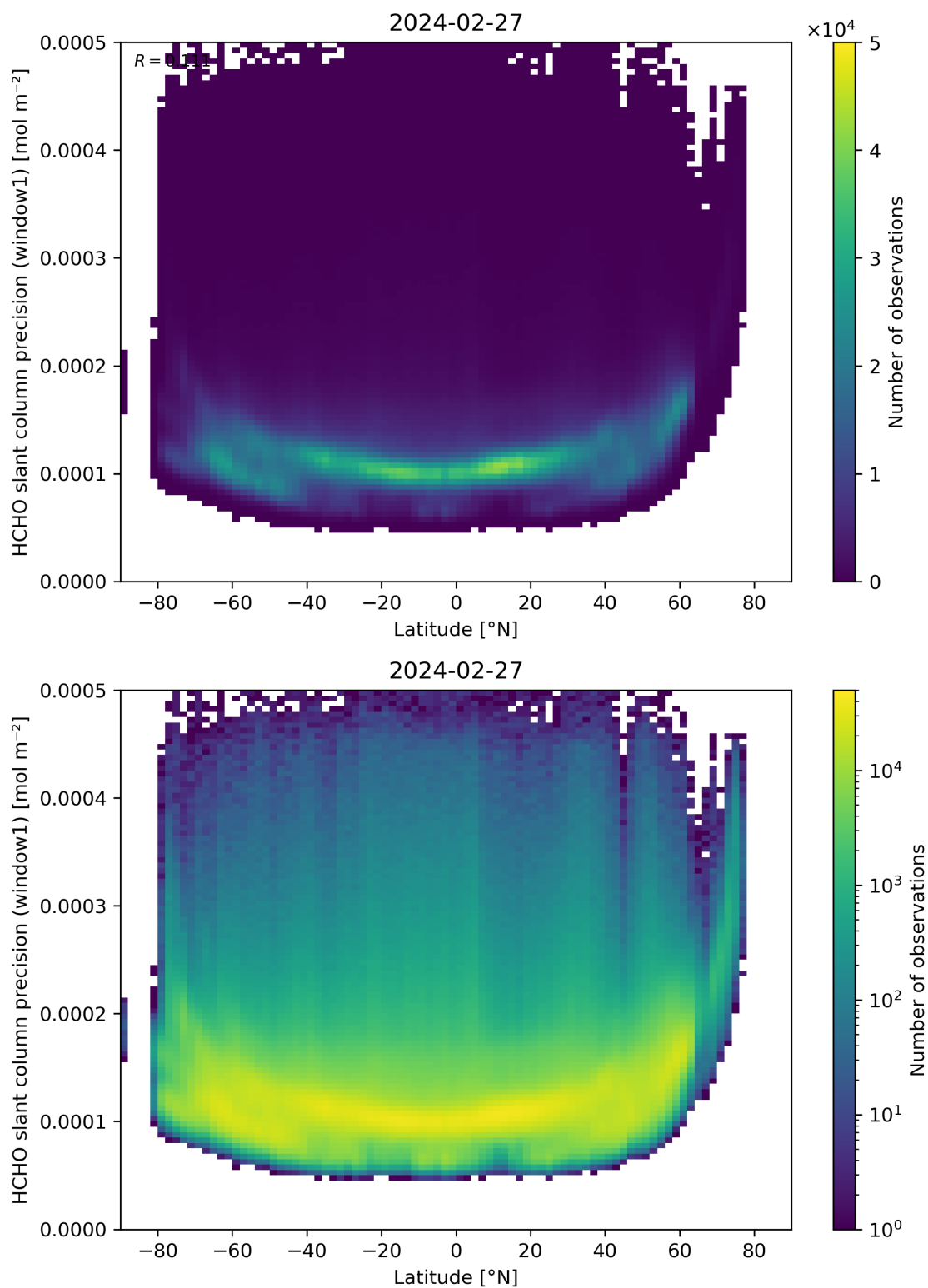
Figure 160: Scatter density plot of “Latitude” against “HCHO slant column precision (window1)” for 2024-02-27 to 2024-02-28.
