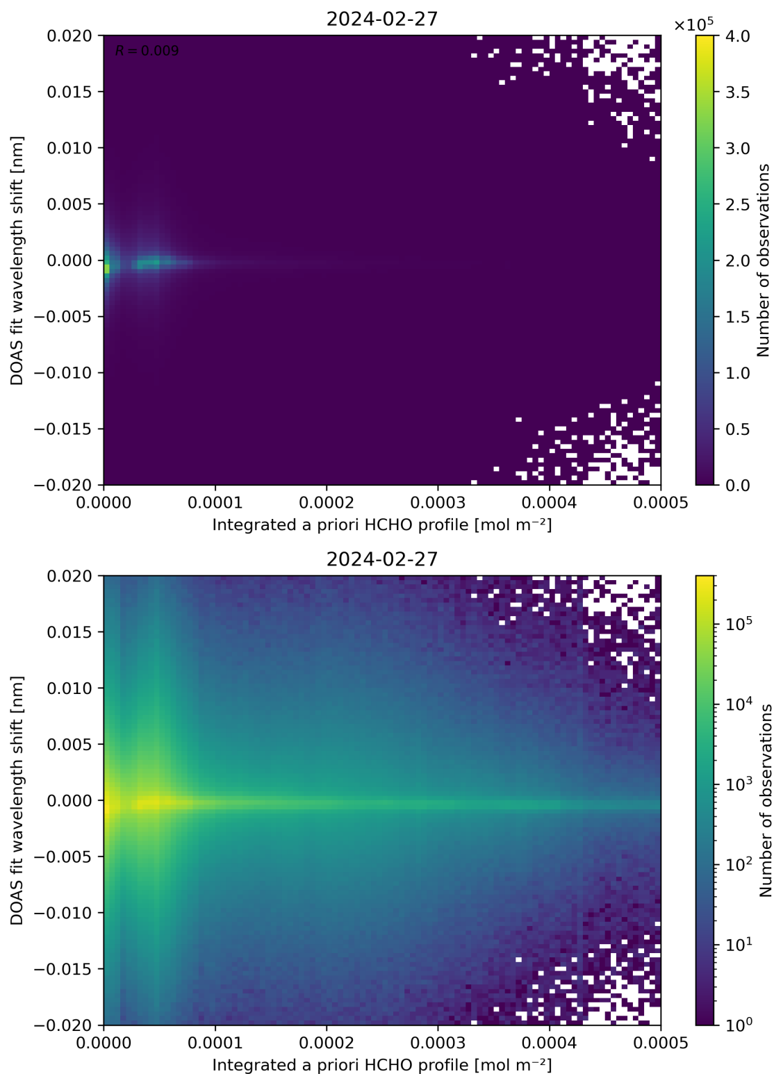
Figure 149: Scatter density plot of “Integrated a priori HCHO profile” against “DOAS fit wavelength shift” for 2024-02-27 to 2024-02-28.
