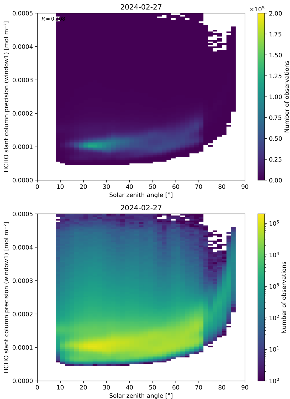
Figure 174: Scatter density plot of “Solar zenith angle” against “HCHO slant column precision (window1)” for 2024-02-27 to 2024-02-28.
