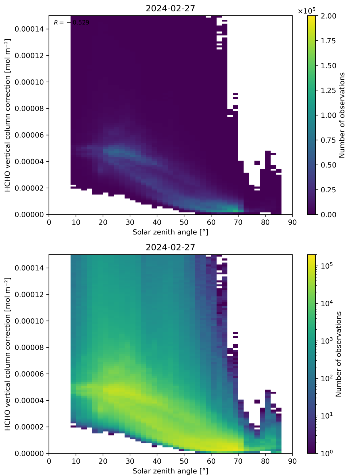
Figure 178: Scatter density plot of “Solar zenith angle” against “HCHO vertical column correction” for 2024-02-27 to 2024-02-28.
