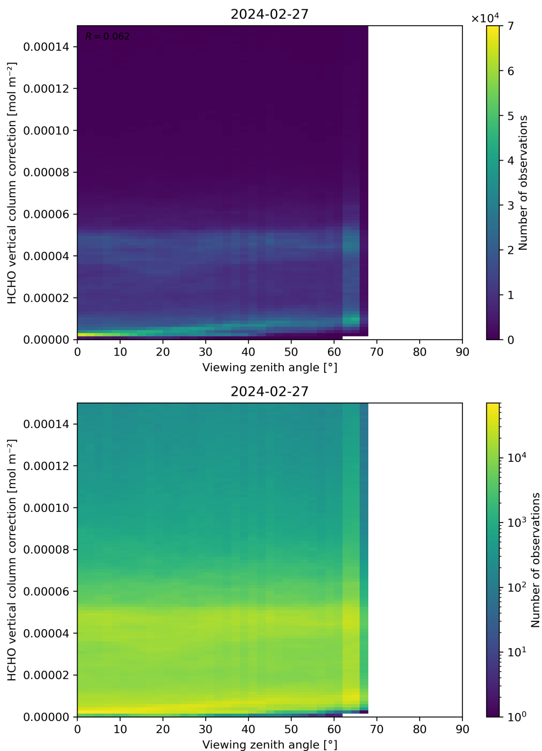
Figure 193: Scatter density plot of “Viewing zenith angle” against “HCHO vertical column correction” for 2024-02-27 to 2024-02-28.
