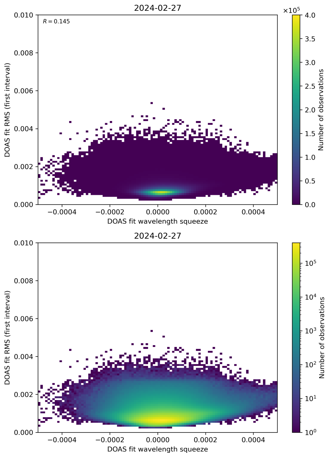
Figure 68: Scatter density plot of “DOAS fit wavelength squeeze” against “DOAS fit RMS (first interval)” for 2024-02-27 to 2024-02-28.
