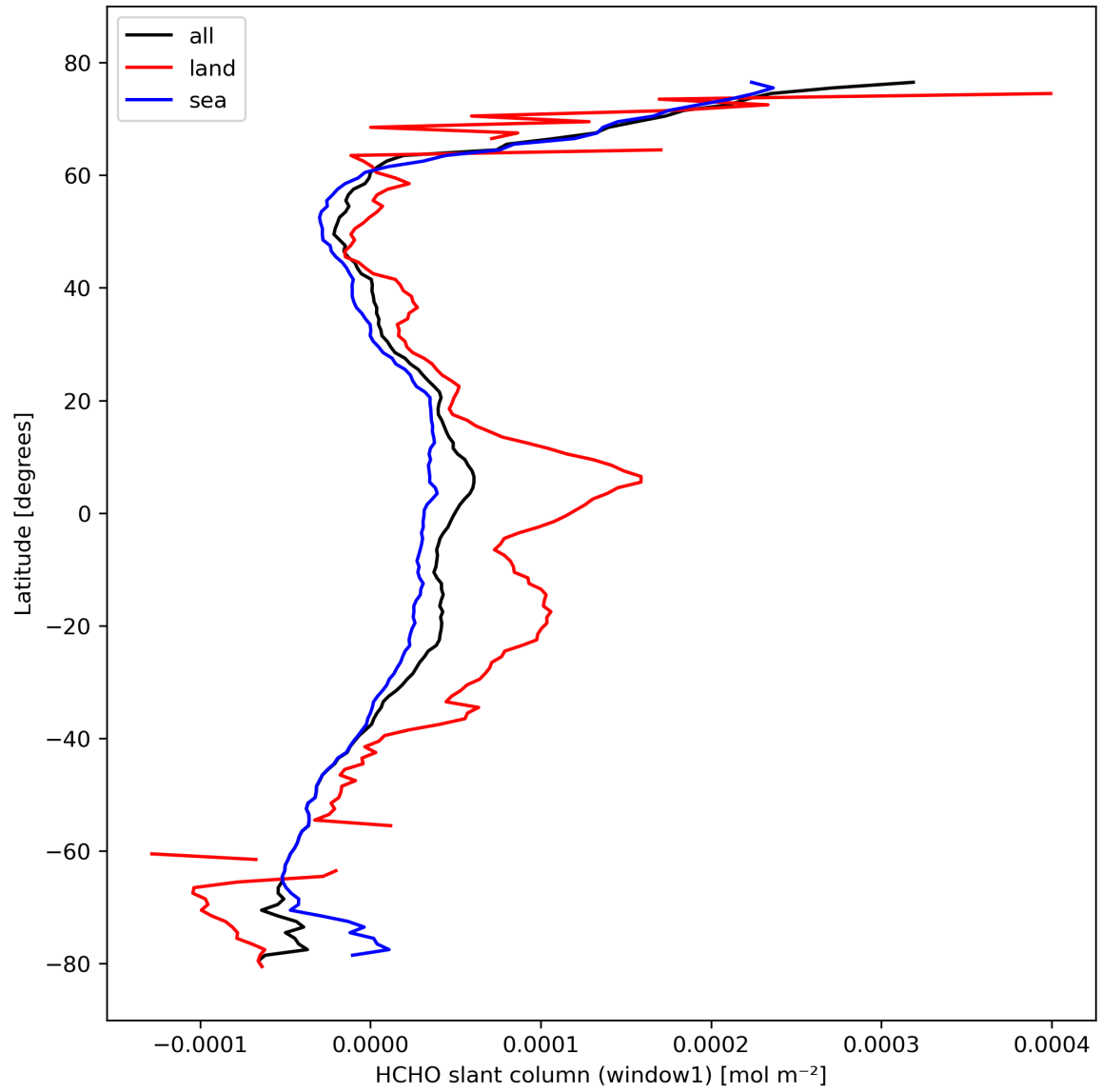
Figure 24: Zonal average of “HCHO slant column (window1)” for 2024-02-27 to 2024-02-28.
