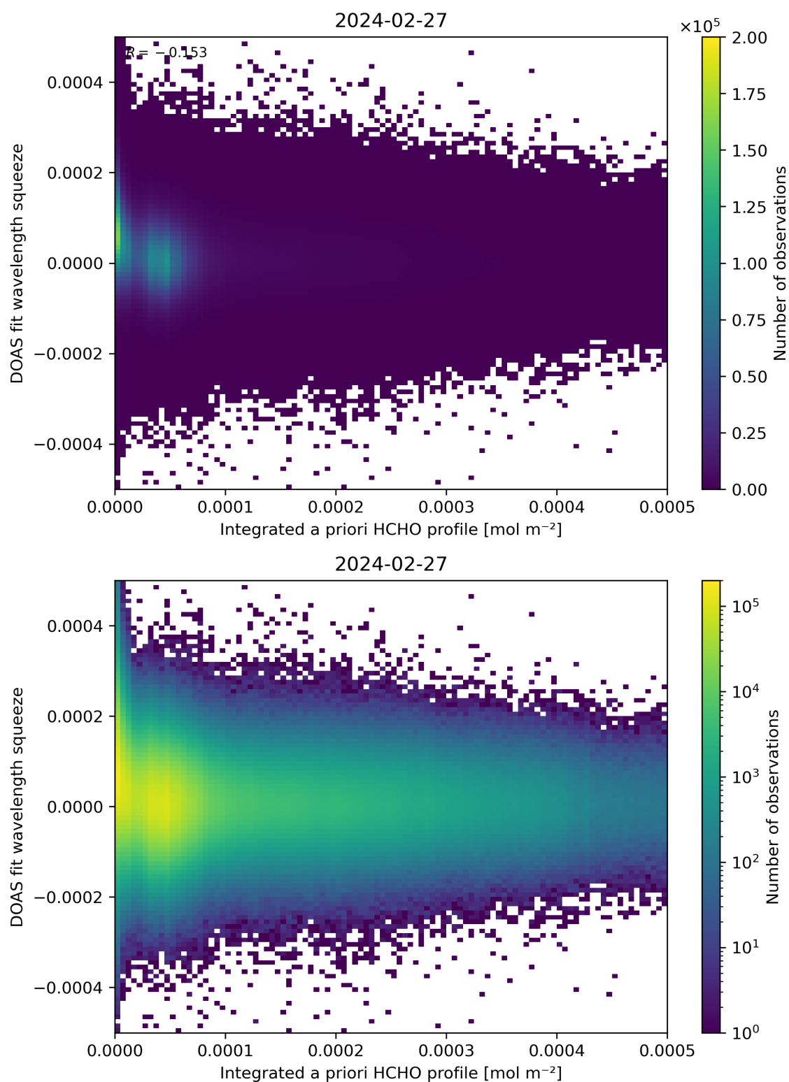
Figure 150: Scatter density plot of “Integrated a priori HCHO profile” against “DOAS fit wavelength squeeze” for 2024-02-27 to 2024-02-28.
