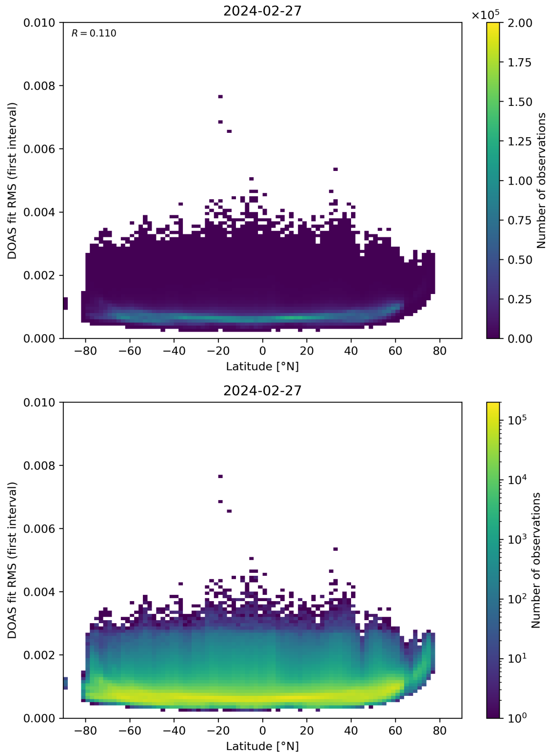
Figure 153: Scatter density plot of “Latitude” against “DOAS fit RMS (first interval)” for 2024-02-27 to 2024-02-28.
