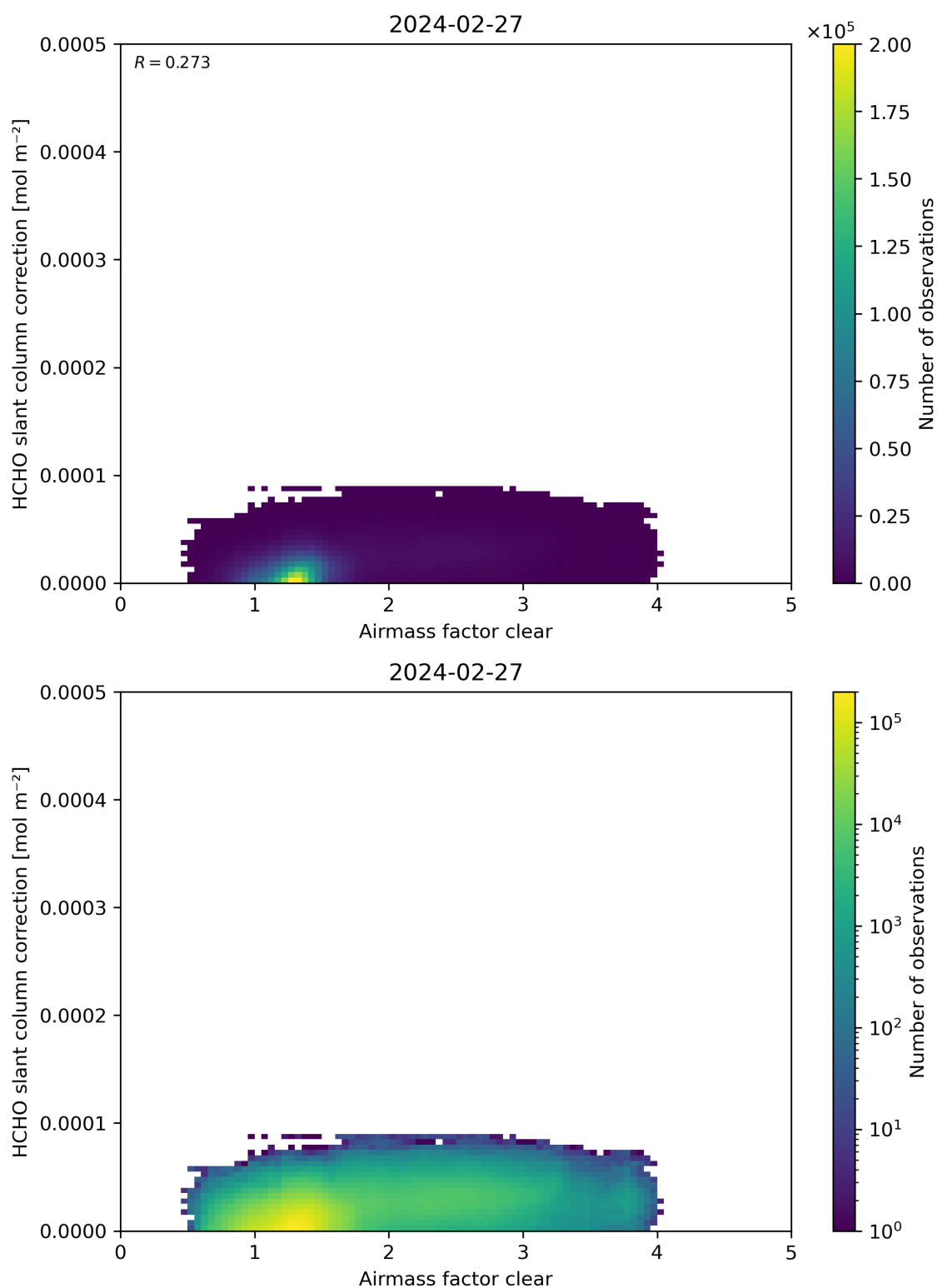
Figure 75: Scatter density plot of “Airmass factor clear” against “HCHO slant column correction” for 2024-02-27 to 2024-02-28.
