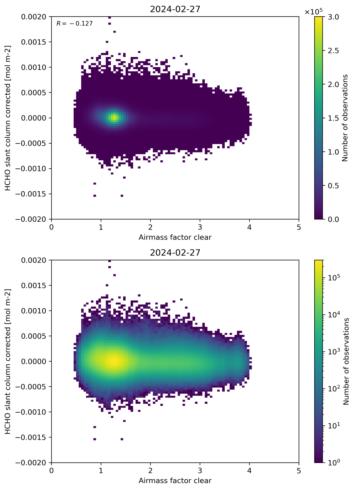
Figure 74: Scatter density plot of “Airmass factor clear” against “HCHO slant column corrected” for 2024-02-27 to 2024-02-28.
