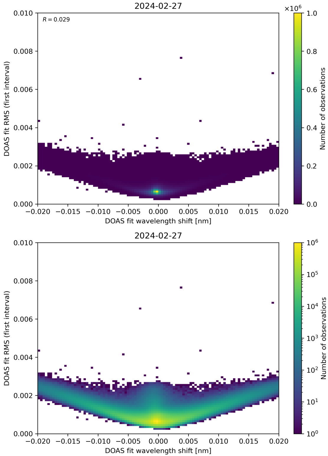
Figure 64: Scatter density plot of “DOAS fit wavelength shift” against “DOAS fit RMS (first interval)” for 2024-02-27 to 2024-02-28.
