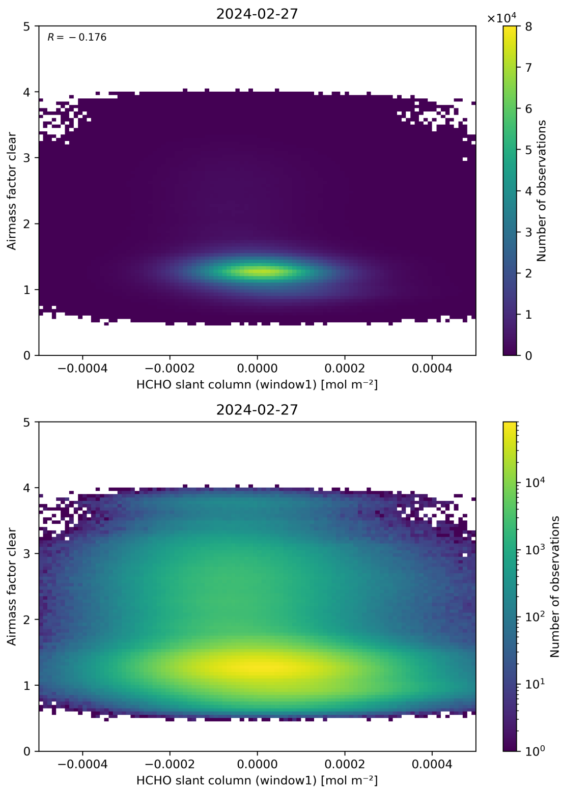
Figure 81: Scatter density plot of “HCHO slant column (window1)” against “Airmass factor clear” for 2024-02-27 to 2024-02-28.
