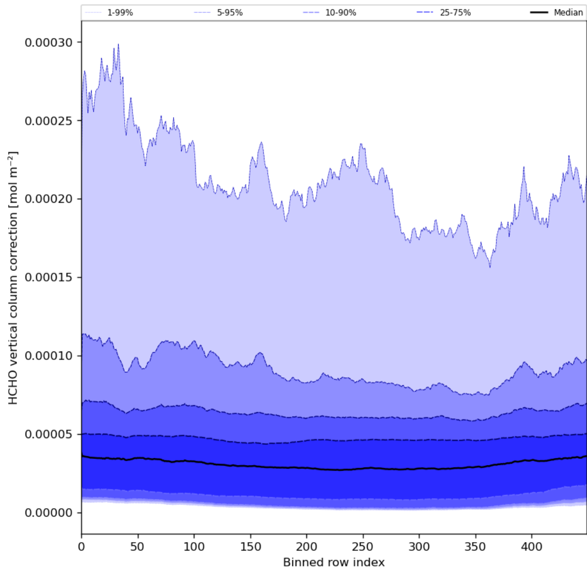
Figure 51: Along track statistics of “HCHO vertical column correction” for 2024-02-27 to 2024-02-28
