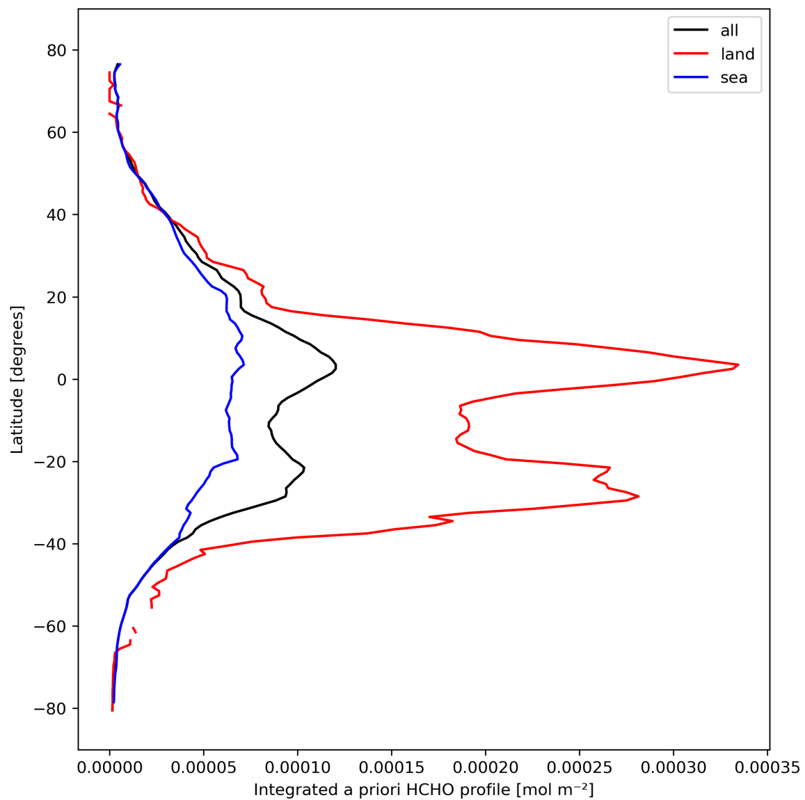
Figure 29: Zonal average of “Integrated a priori HCHO profile” for 2024-02-27 to 2024-02-28.
