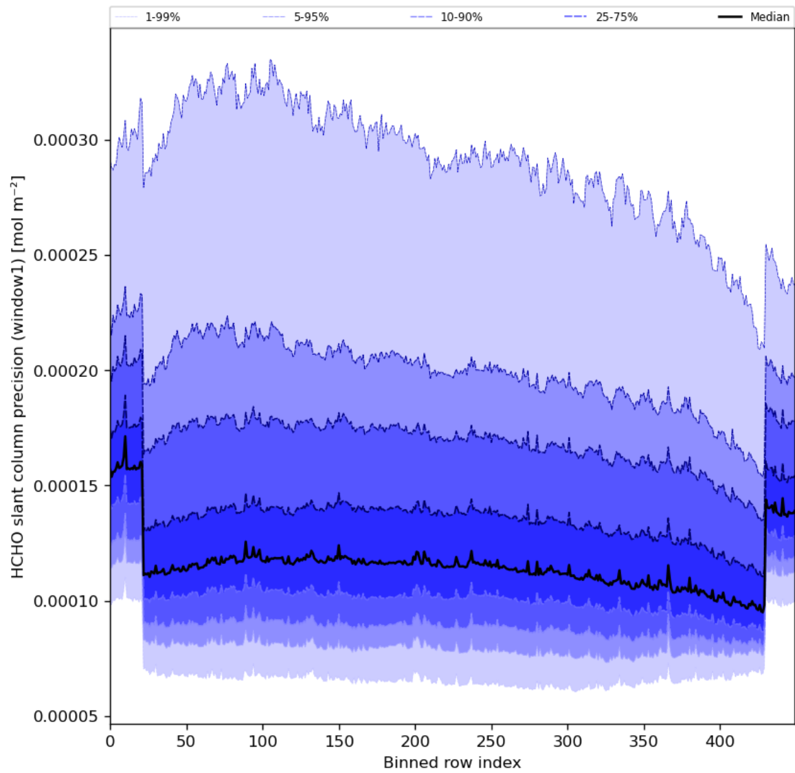
Figure 53: Along track statistics of “HCHO slant column precision (window1)” for 2024-02-27 to 2024-02-29
