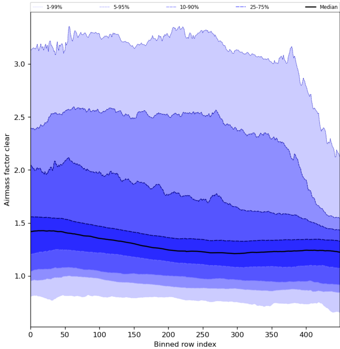
Figure 56: Along track statistics of “Airmass factor clear” for 2024-02-27 to 2024-02-29
