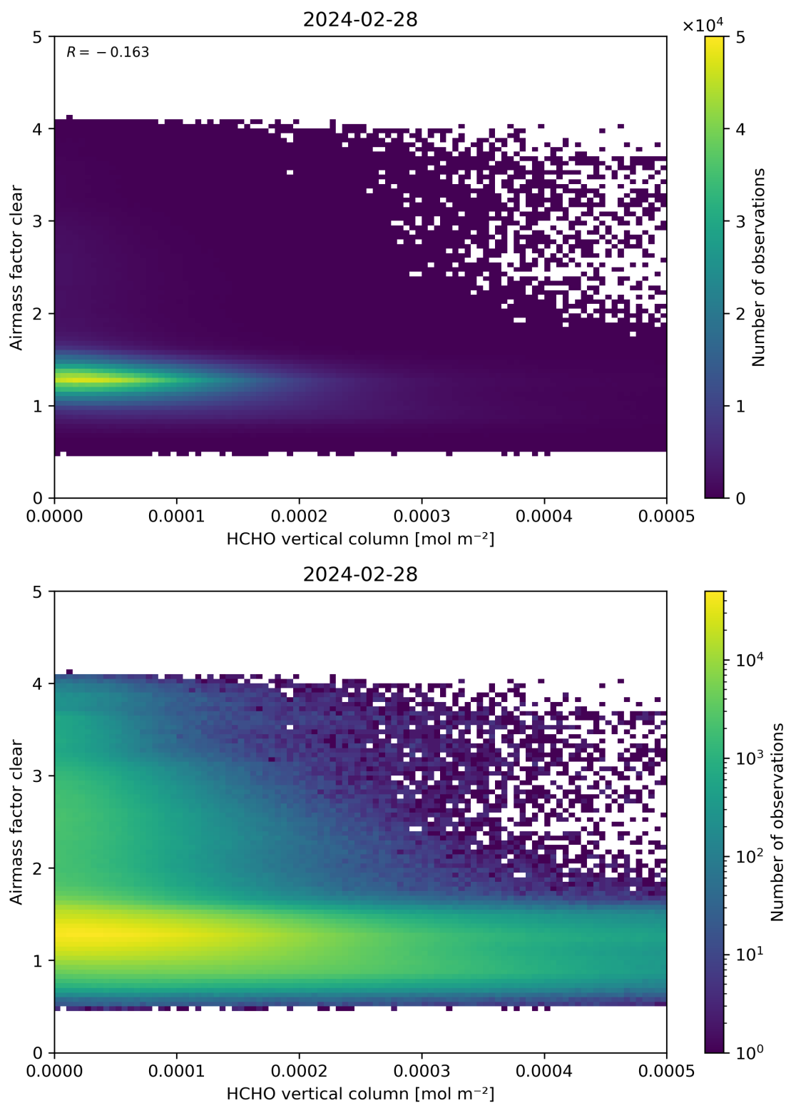
Figure 126: Scatter density plot of “HCHO vertical column” against “Airmass factor clear” for 2024-02-27 to 2024-02-29.
