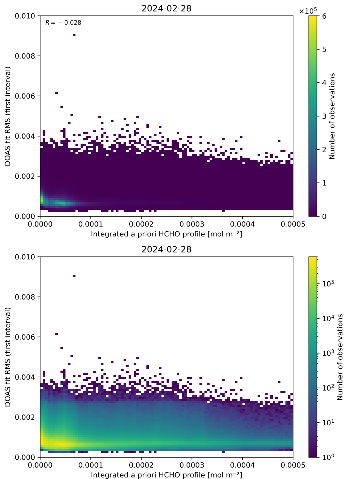
Figure 148: Scatter density plot of “Integrated a priori HCHO profile” against “DOAS fit RMS (first interval)” for 2024-02-27 to 2024-02-29.
