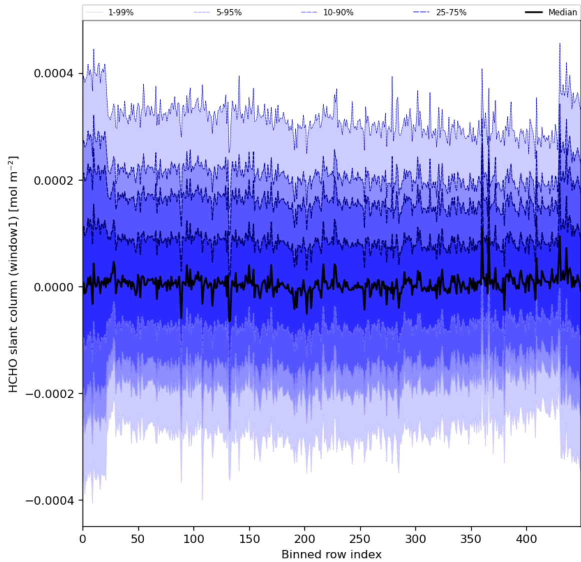
Figure 52: Along track statistics of “HCHO slant column (window1)” for 2024-02-27 to 2024-02-29
