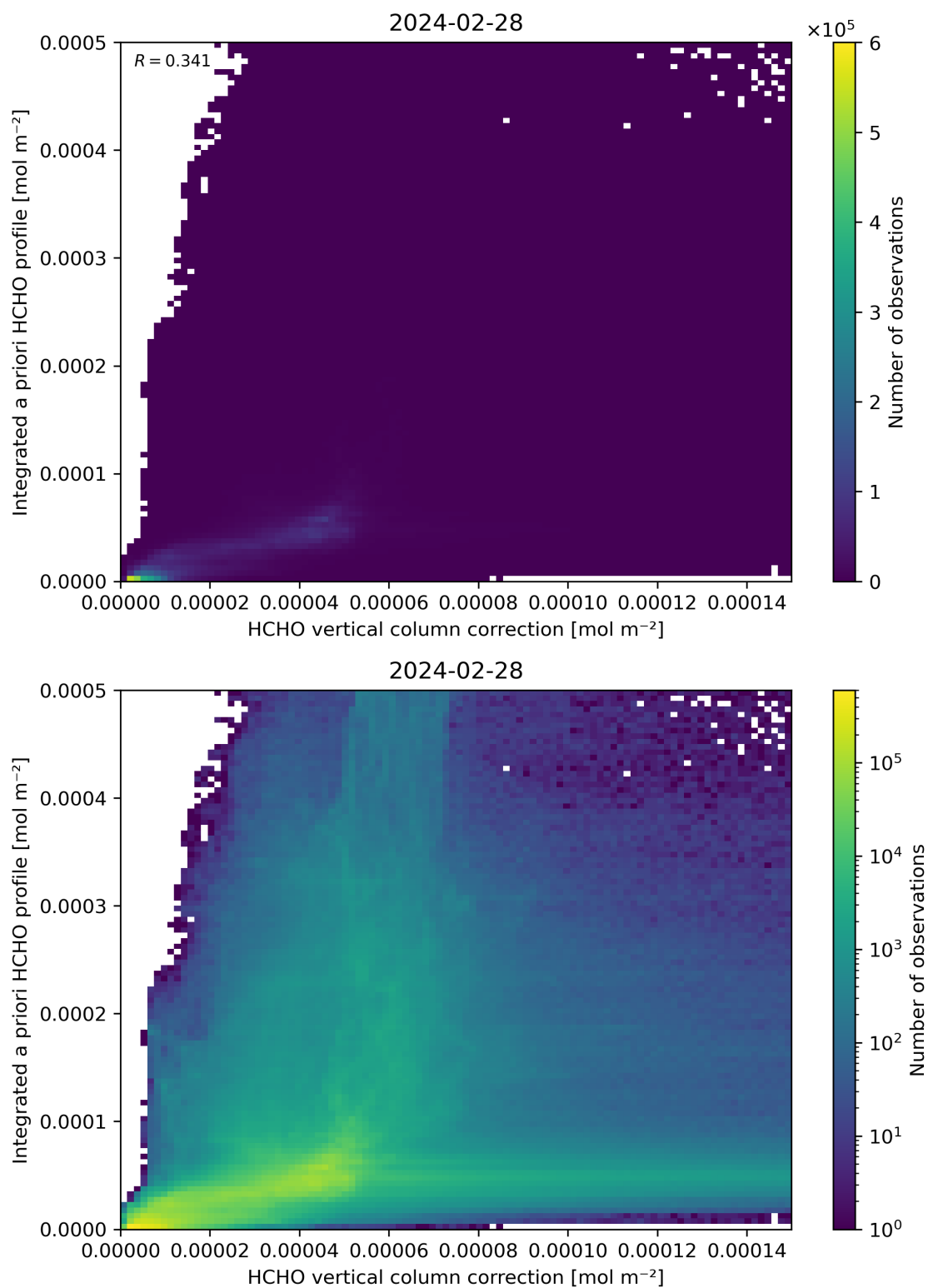
Figure 122: Scatter density plot of “HCHO vertical column correction” against “Integrated a priori HCHO profile” for 2024-02-27 to 2024-02-29.
