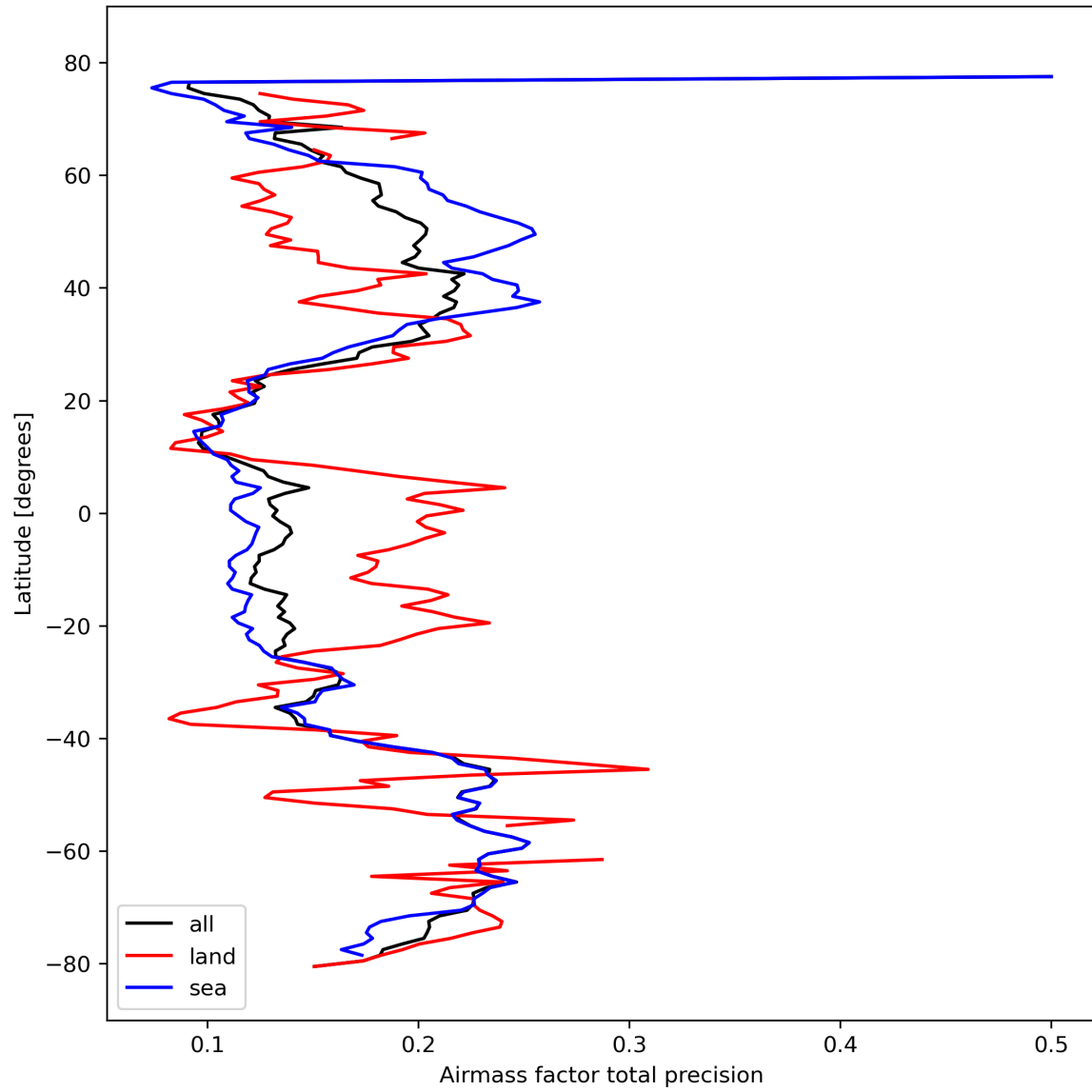
Figure 27: Zonal average of “Air mass factor total precision” for 2024-02-27 to 2024-02-29.
