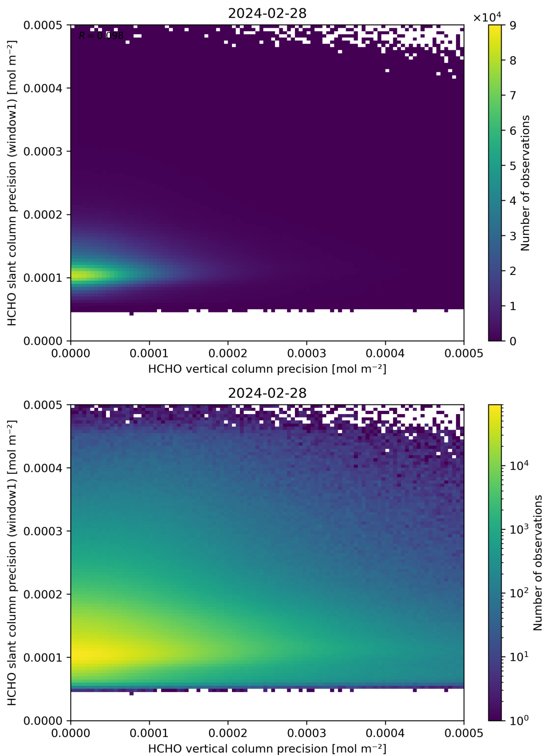
Figure 143: Scatter density plot of “HCHO vertical column precision” against “HCHO slant column precision (window1)” for 2024-02-27 to 2024-02-29.
