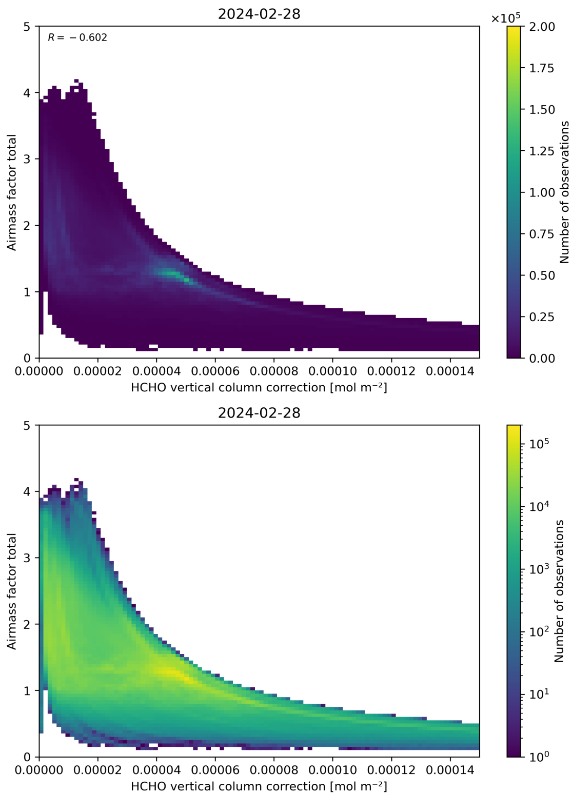
Figure 120: Scatter density plot of “HCHO vertical column correction” against “Airmass factor total” for 2024-02-27 to 2024-02-29.
