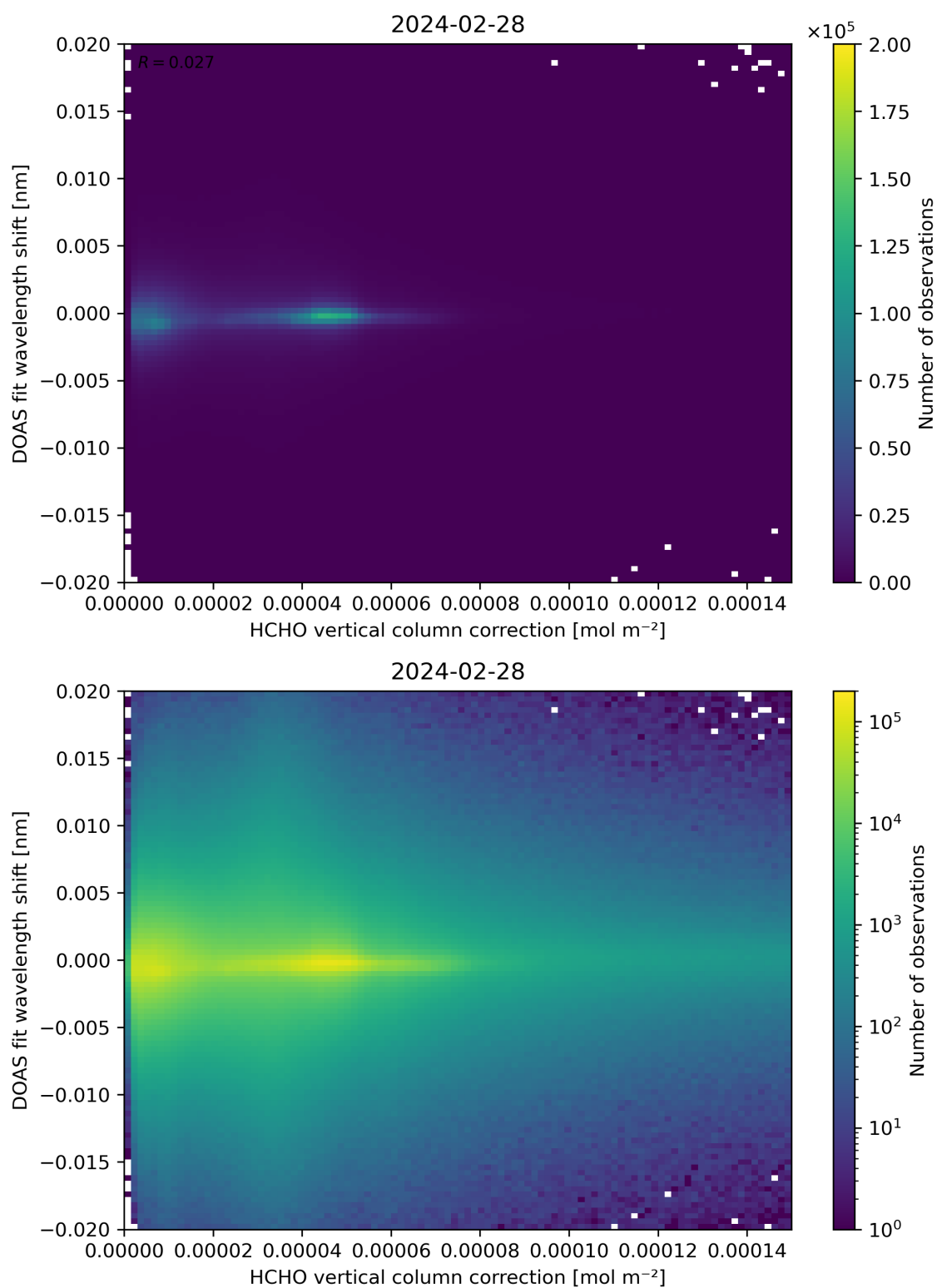
Figure 113: Scatter density plot of “HCHO vertical column correction” against “DOAS fit wavelength shift” for 2024-02-27 to 2024-02-29.
