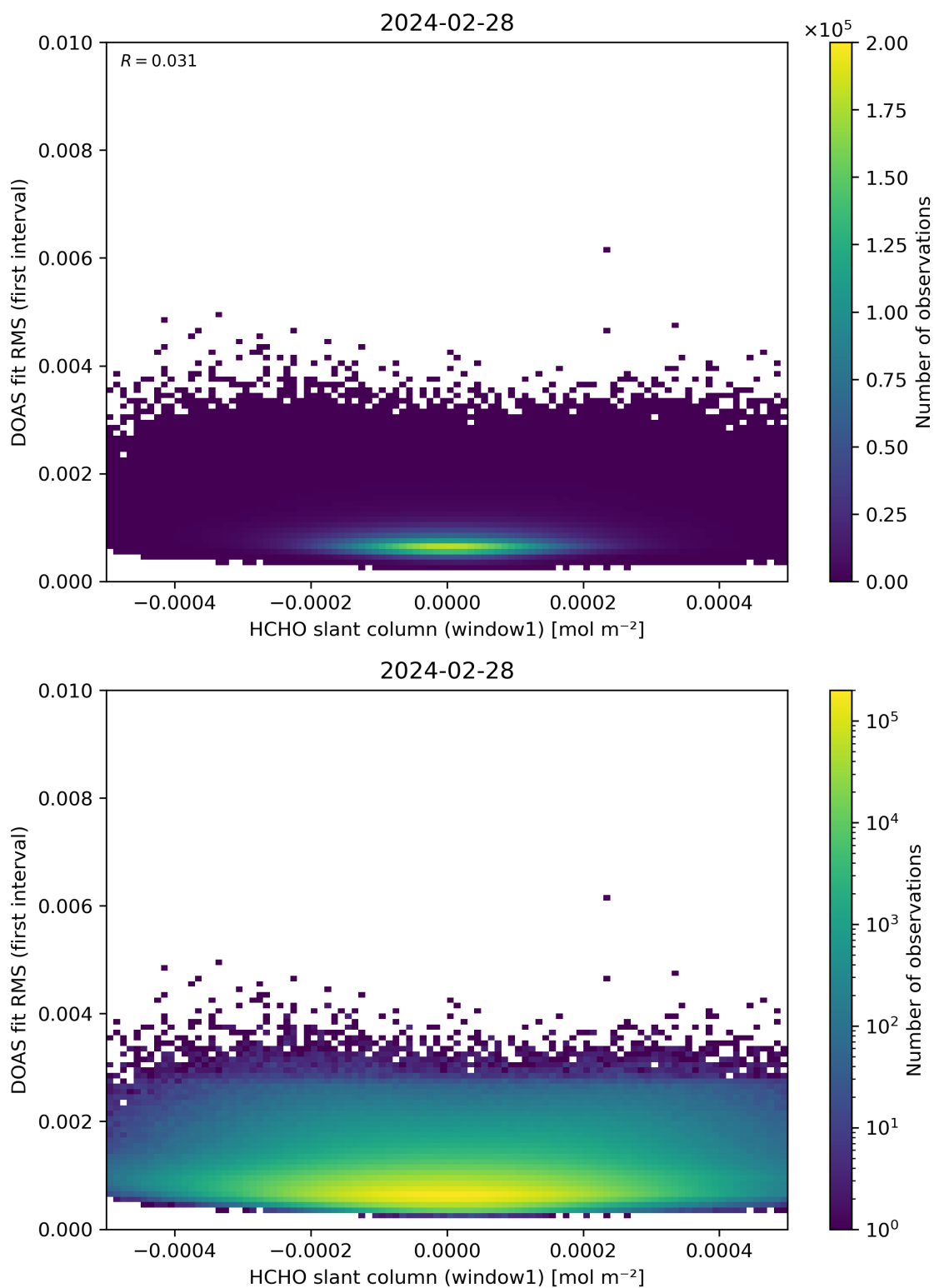
Figure 78: Scatter density plot of “HCHO slant column (window1)” against “DOAS fit RMS (first interval)” for 2024-02-27 to 2024-02-29.
