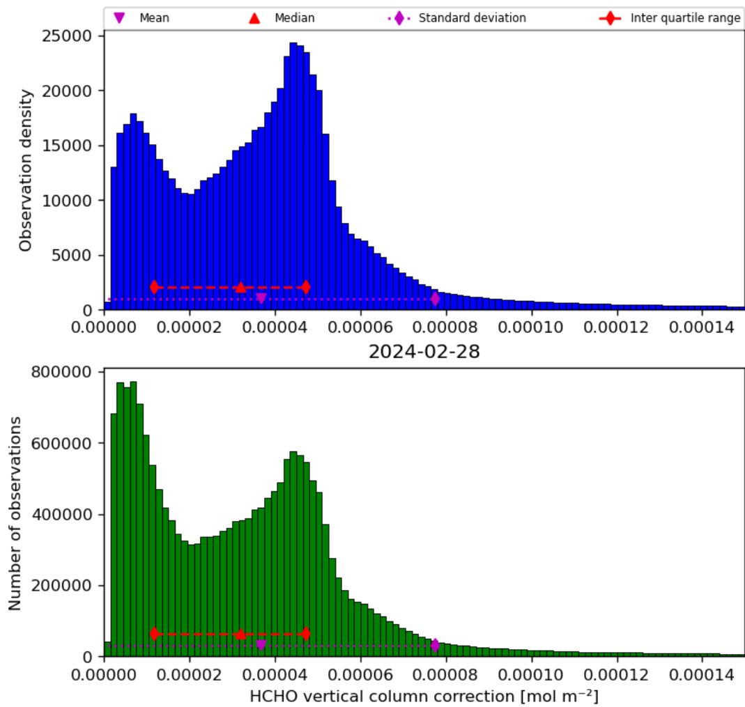
Figure 37: Histogram of “HCHO vertical column correction” for 2024-02-27 to 2024-02-29
