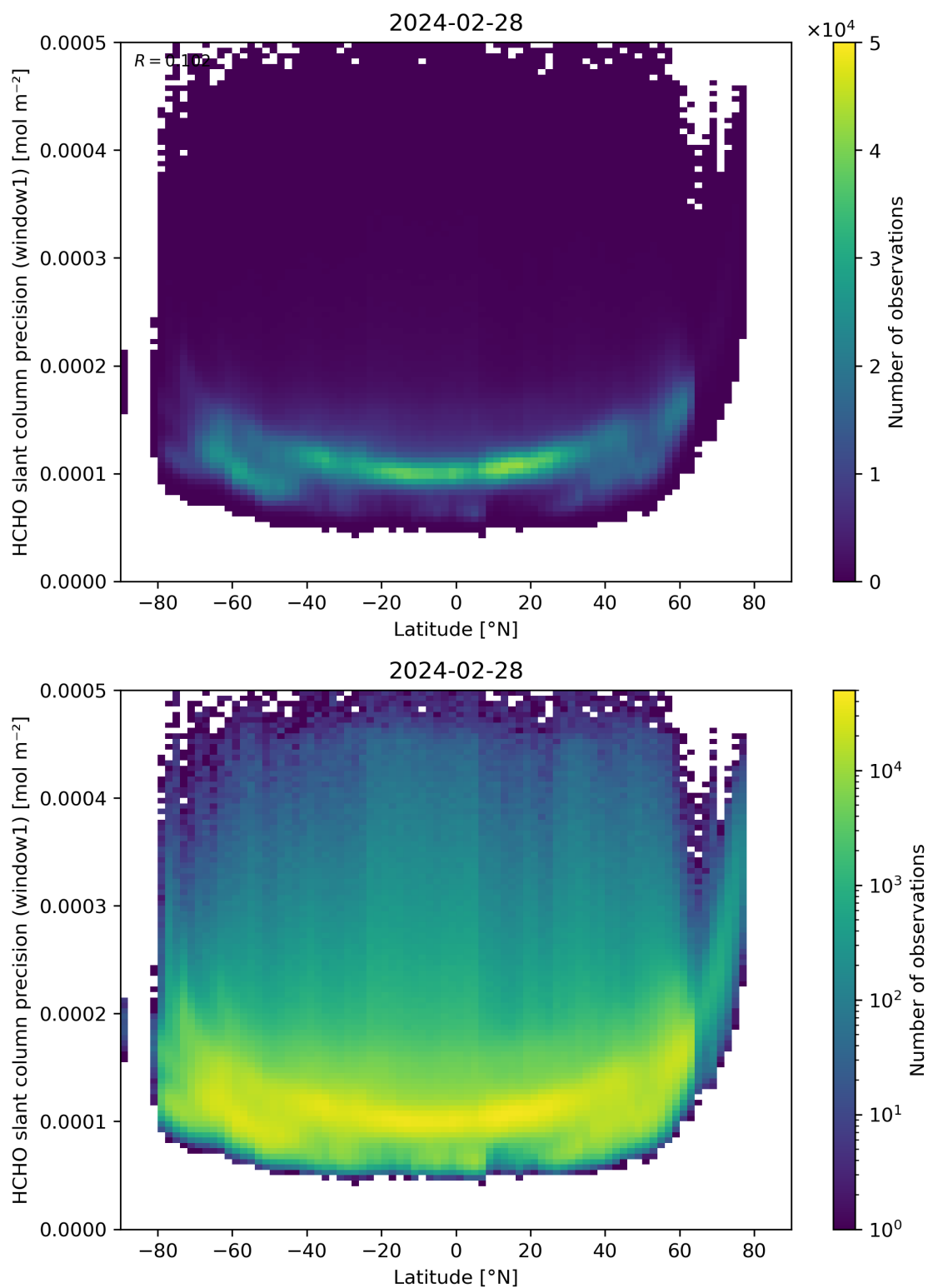
Figure 160: Scatter density plot of “Latitude” against “HCHO slant column precision (window1)” for 2024-02-27 to 2024-02-29.
