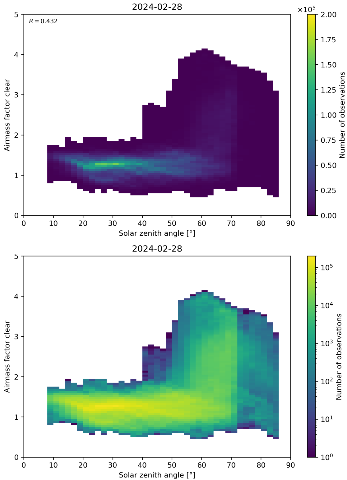
Figure 170: Scatter density plot of “Solar zenith angle” against “Airmass factor clear” for 2024-02-27 to 2024-02-29.
