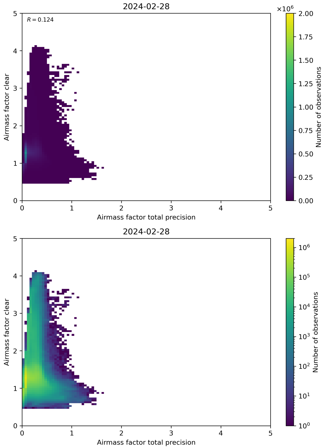
Figure 108: Scatter density plot of “Airmass factor total precision” against “Airmass factor clear” for 2024-02-27 to 2024-02-29.
