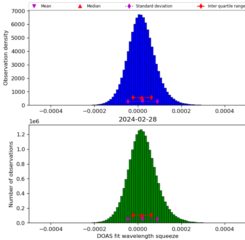
Figure 45: Histogram of “DOAS fit wavelength squeeze” for 2024-02-27 to 2024-02-29
