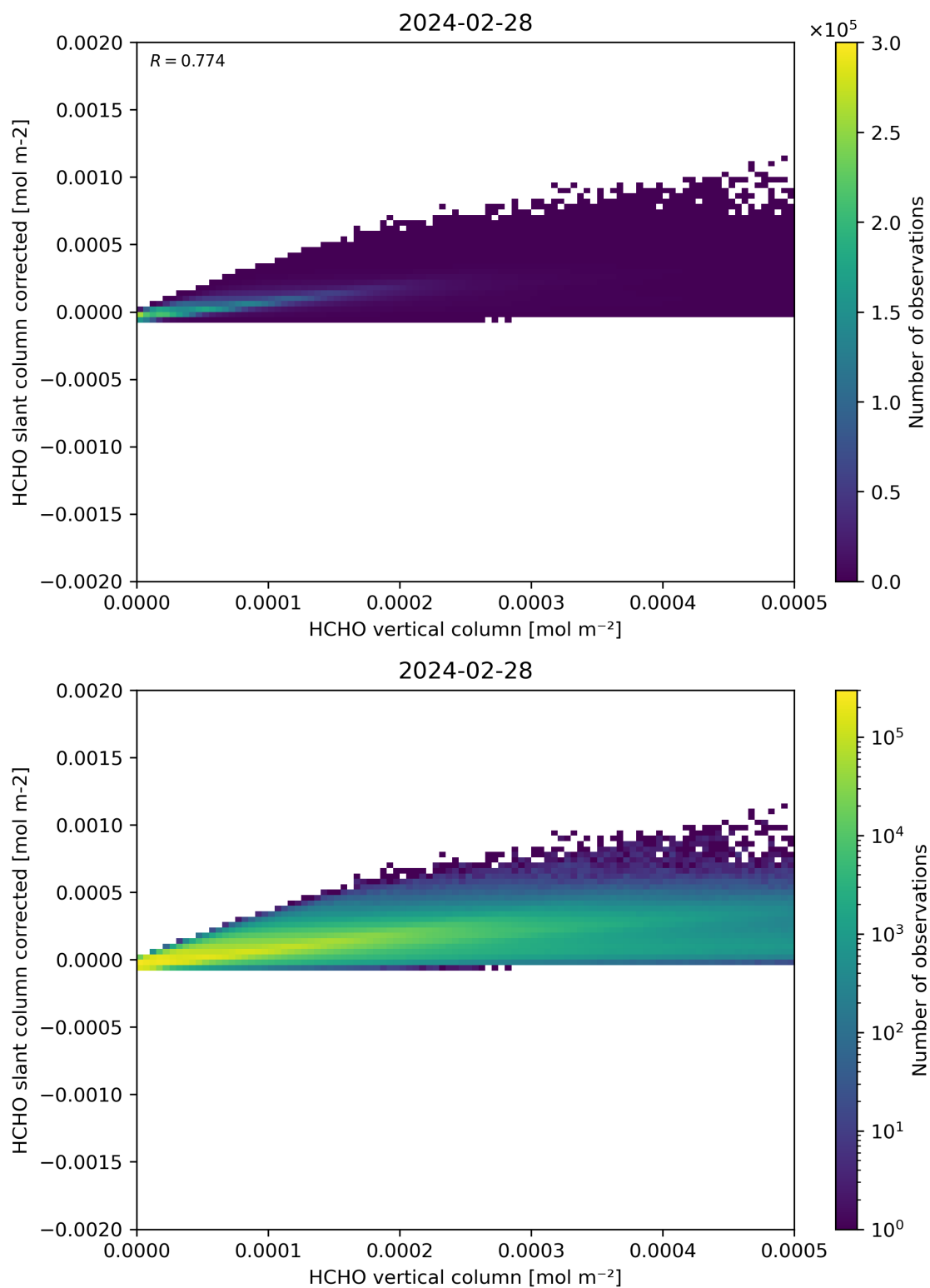
Figure 127: Scatter density plot of “HCHO vertical column” against “HCHO slant column corrected” for 2024-02-27 to 2024-02-29.
