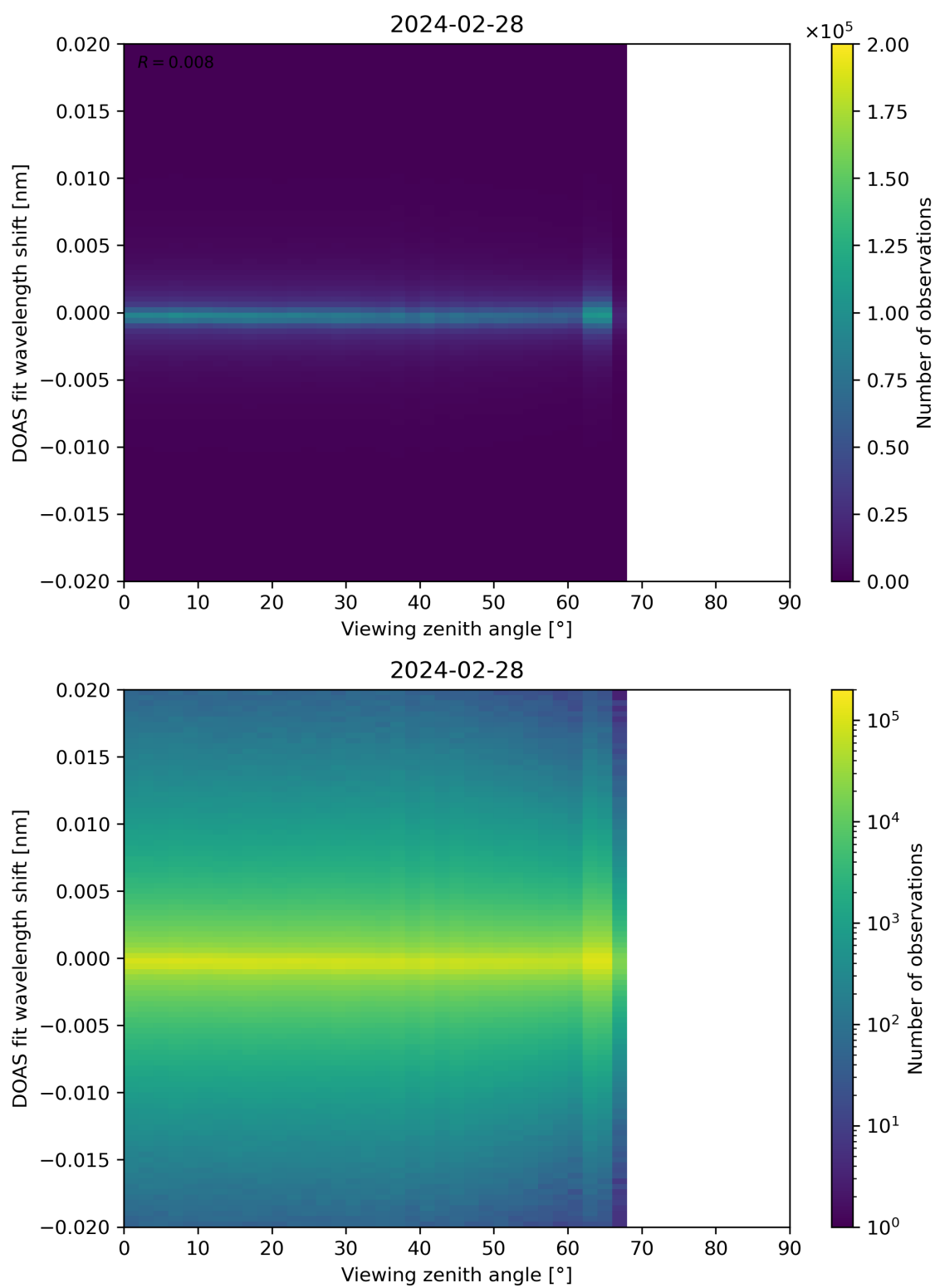
Figure 183: Scatter density plot of “Viewing zenith angle” against “DOAS fit wavelength shift” for 2024-02-27 to 2024-02-29.
