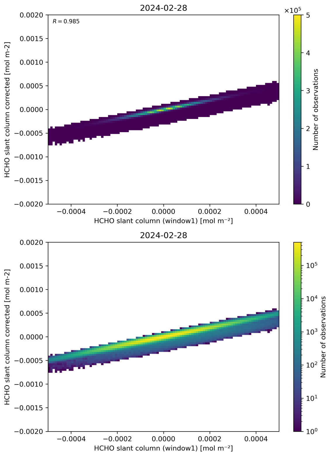
Figure 82: Scatter density plot of “HCHO slant column (window1)” against “HCHO slant column corrected” for 2024-02-27 to 2024-02-29.
