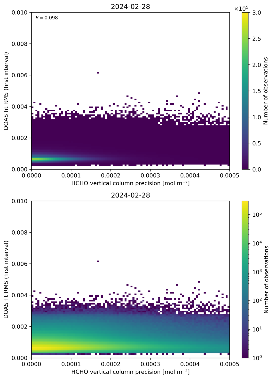
Figure 136: Scatter density plot of “HCHO vertical column precision” against “DOAS fit RMS (first interval)” for 2024-02-27 to 2024-02-29.
