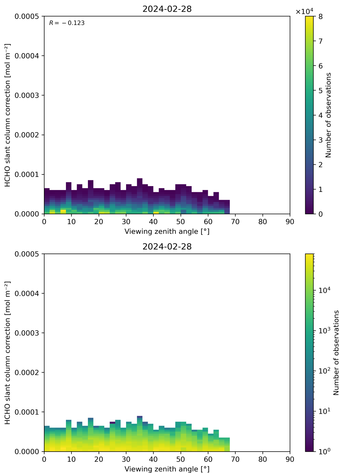
Figure 187: Scatter density plot of “Viewing zenith angle” against “HCHO slant column correction” for 2024-02-27 to 2024-02-29.
