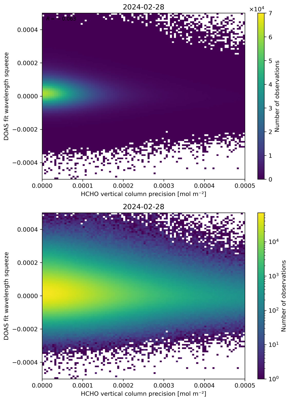
Figure 138: Scatter density plot of “HCHO vertical column precision” against “DOAS fit wavelength squeeze” for 2024-02-27 to 2024-02-29.
