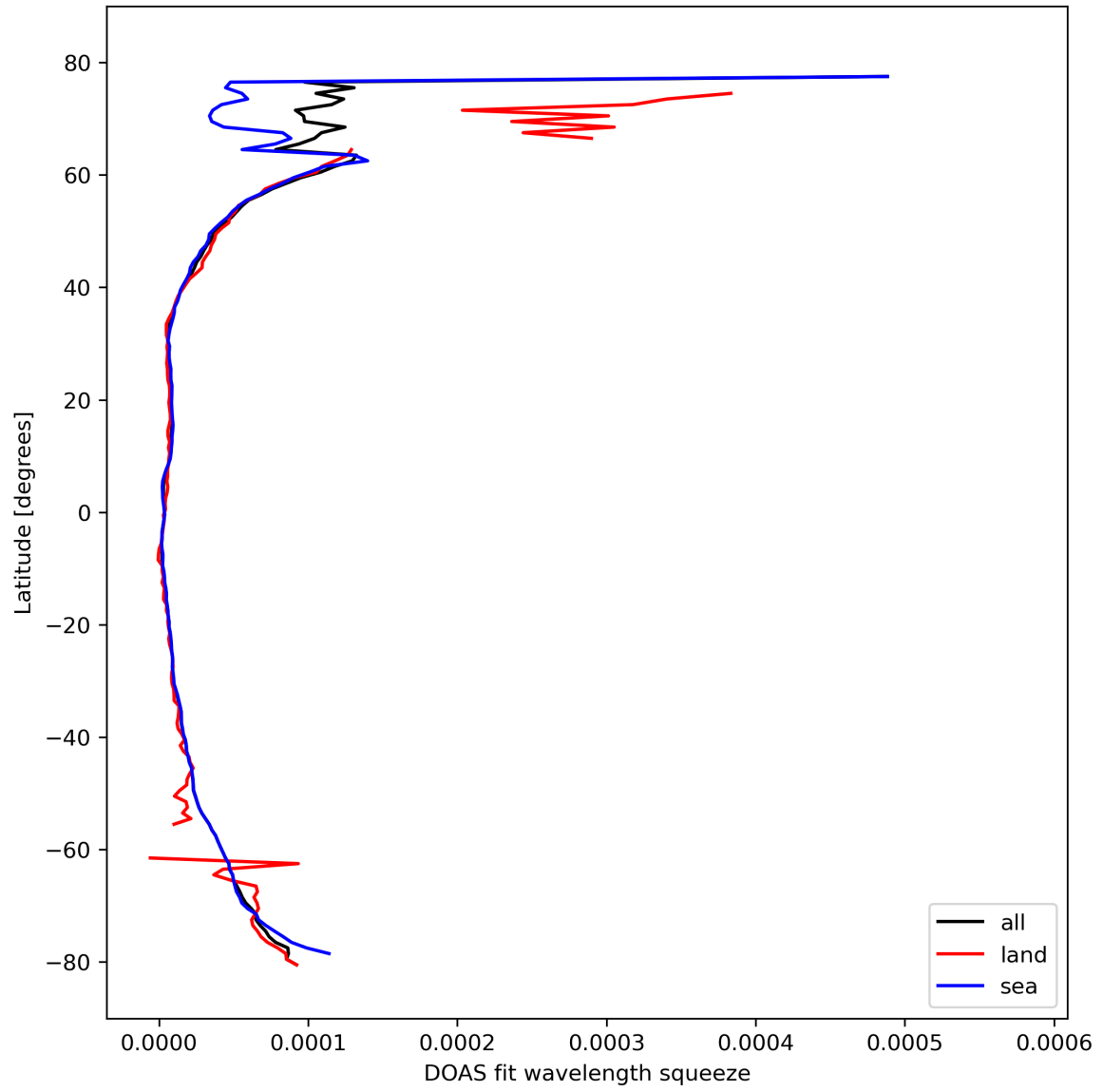
Figure 31: Zonal average of “DOAS fit wavelength squeeze” for 2024-02-27 to 2024-02-29.
