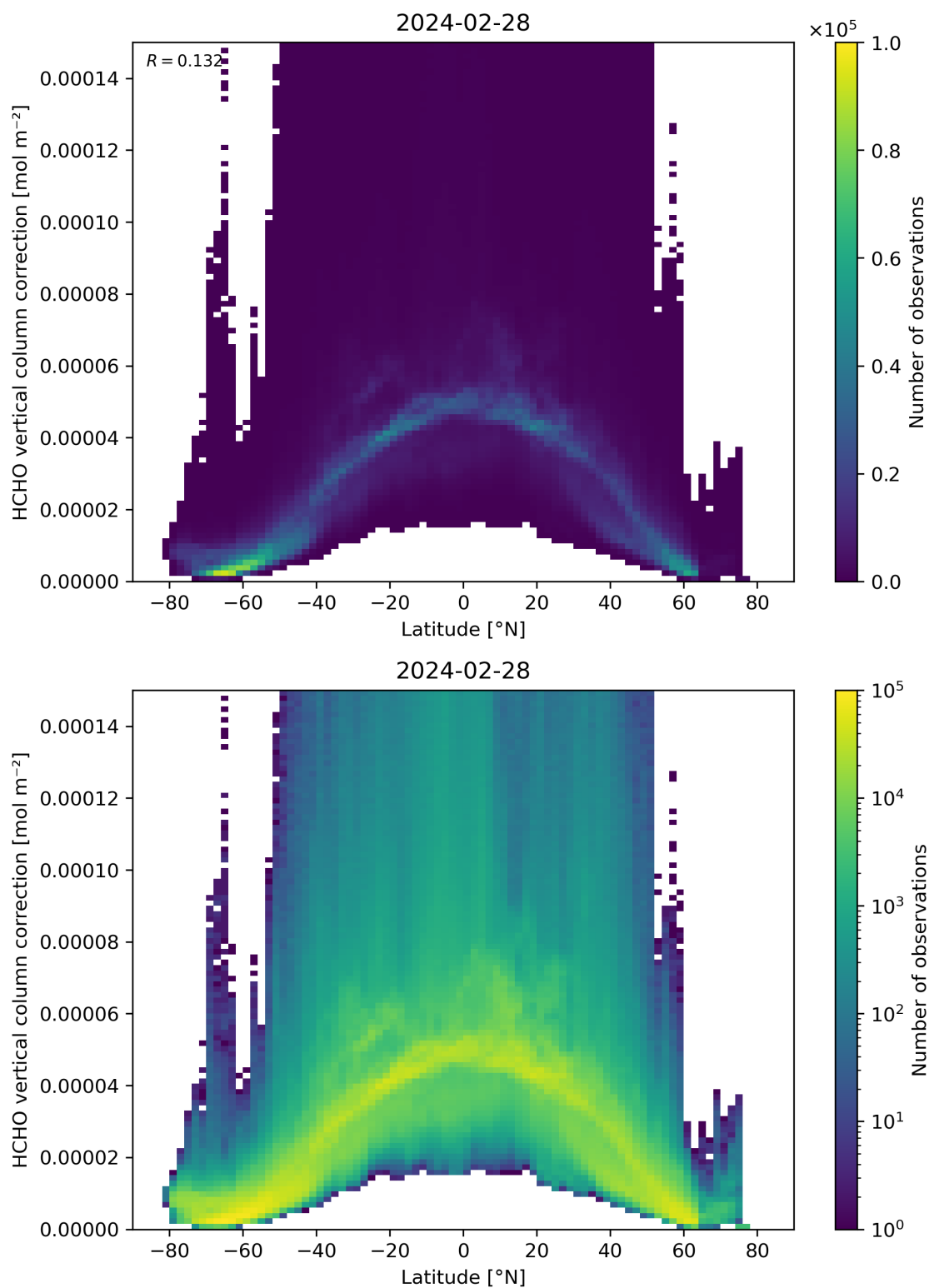
Figure 164: Scatter density plot of “Latitude” against “HCHO vertical column correction” for 2024-02-27 to 2024-02-29.
