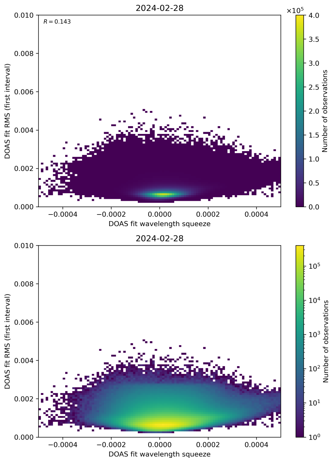
Figure 68: Scatter density plot of “DOAS fit wavelength squeeze” against “DOAS fit RMS (first interval)” for 2024-02-27 to 2024-02-29.
