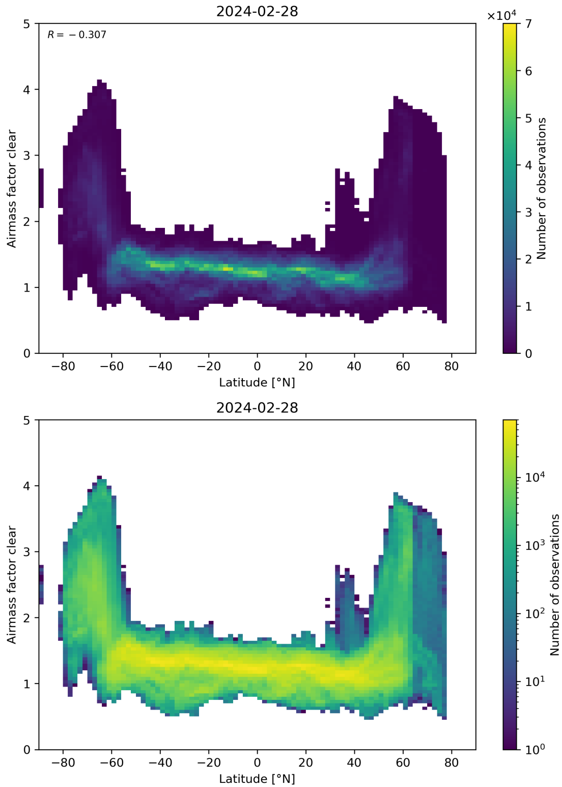
Figure 156: Scatter density plot of “Latitude” against “Airmass factor clear” for 2024-02-27 to 2024-02-29.
