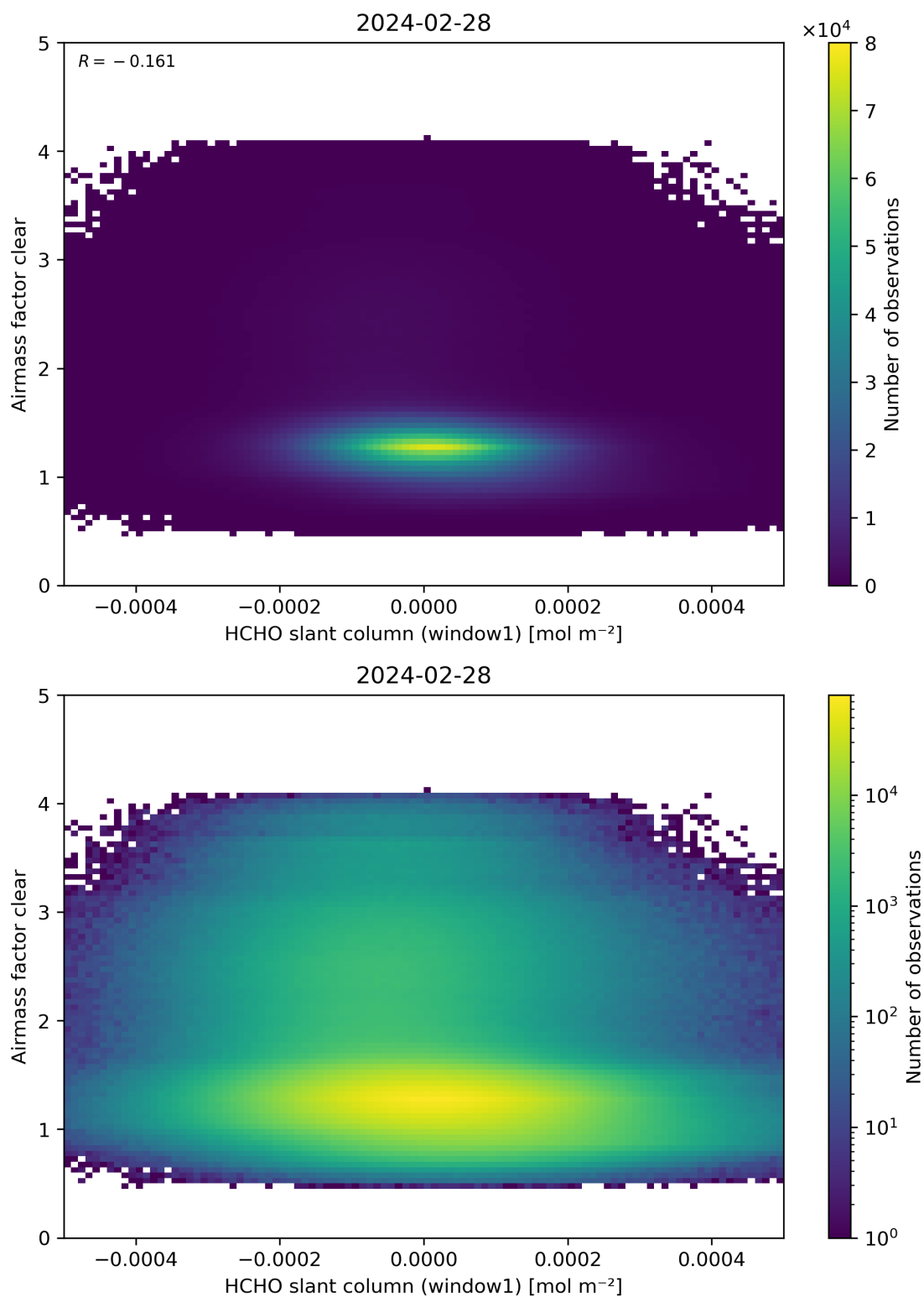
Figure 81: Scatter density plot of “HCHO slant column (window1)” against “Airmass factor clear” for 2024-02-27 to 2024-02-29.
