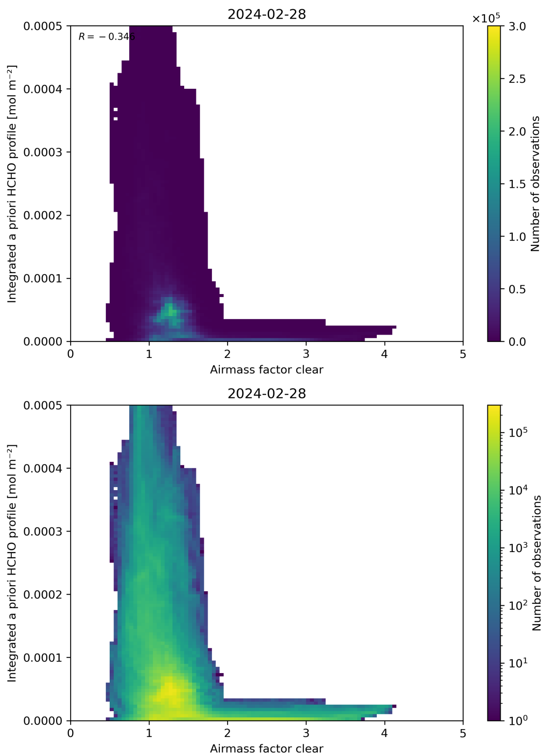
Figure 76: Scatter density plot of “Airmass factor clear” against “Integrated a priori HCHO profile” for 2024-02-27 to 2024-02-29.
