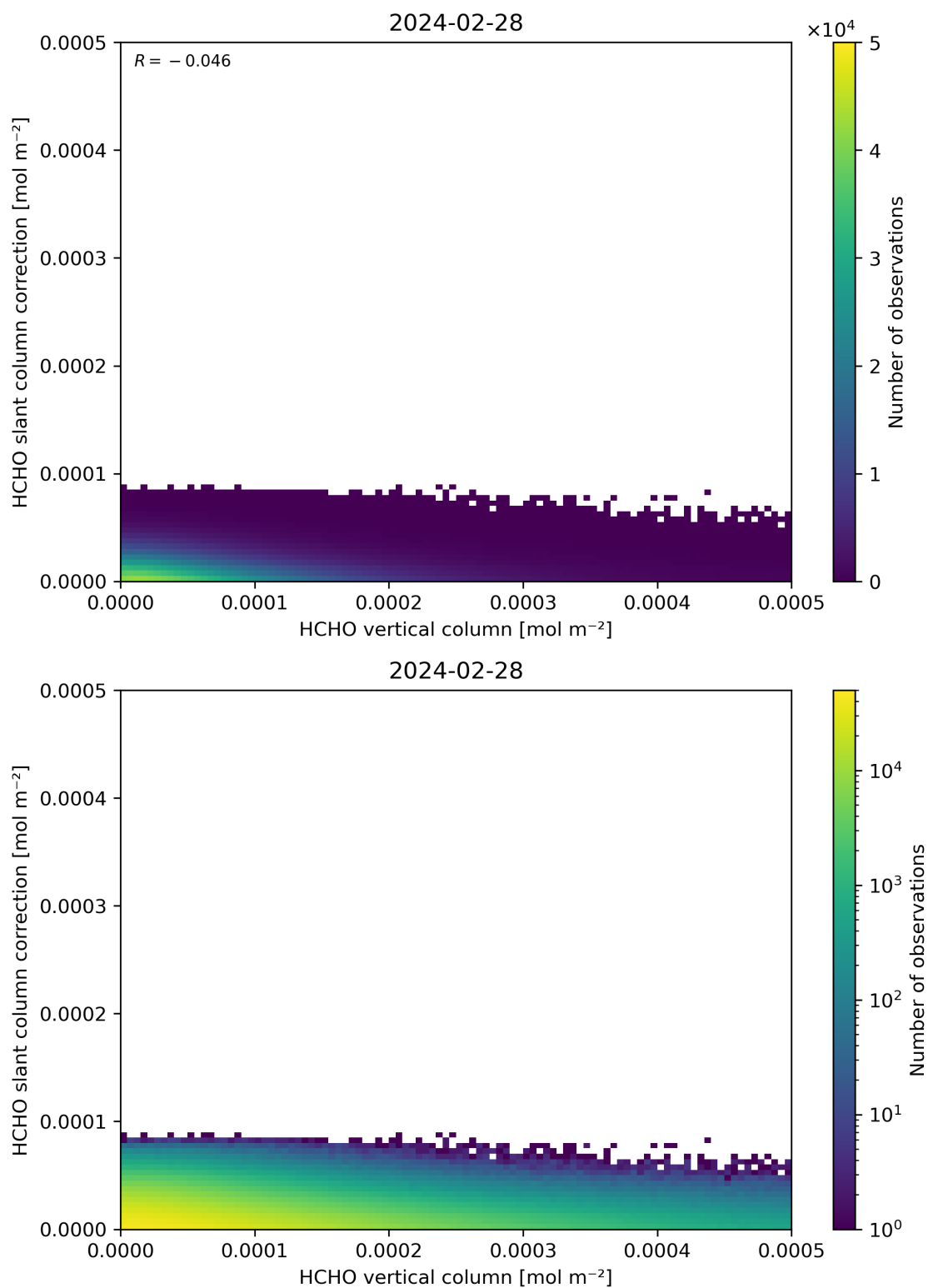
Figure 128: Scatter density plot of “HCHO vertical column” against “HCHO slant column correction” for 2024-02-27 to 2024-02-29.
