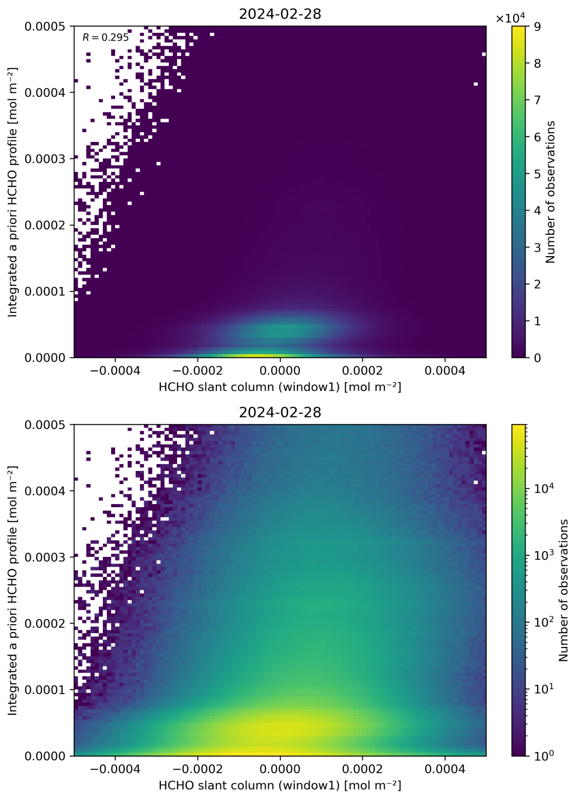
Figure 87: Scatter density plot of “HCHO slant column (window1)” against “Integrated a priori HCHO profile” for 2024-02-27 to 2024-02-29.
