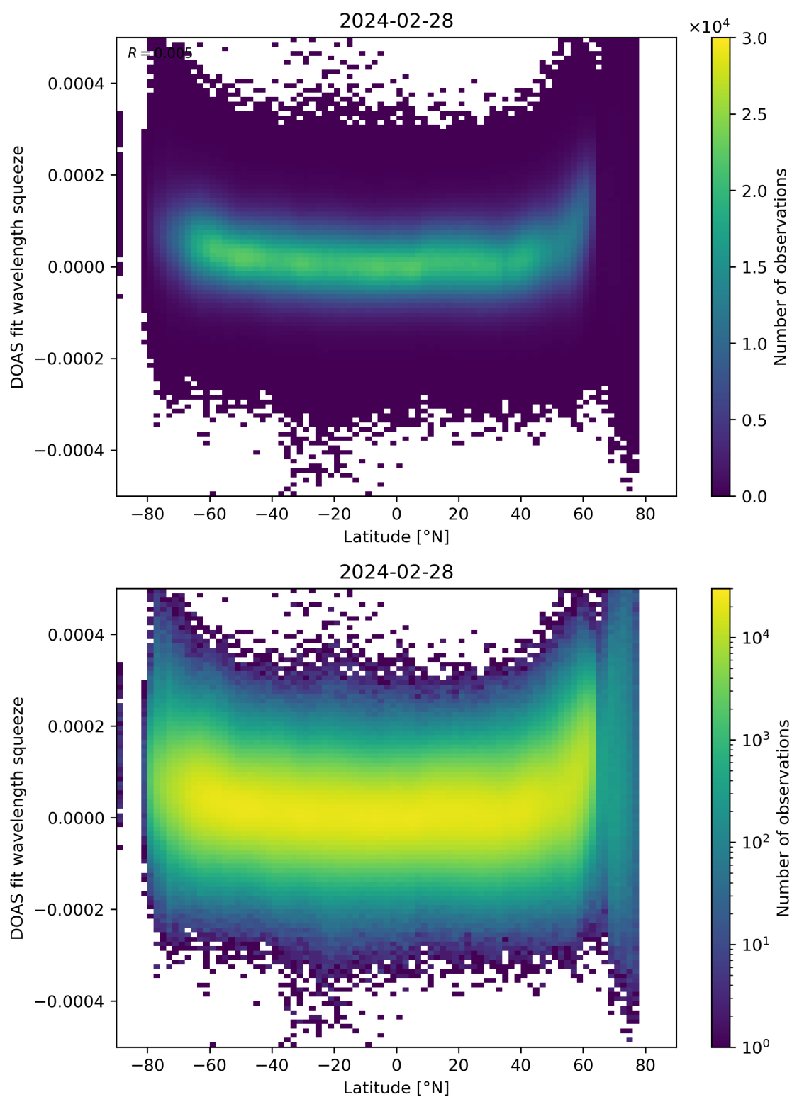
Figure 155: Scatter density plot of “Latitude” against “DOAS fit wavelength squeeze” for 2024-02-27 to 2024-02-29.
