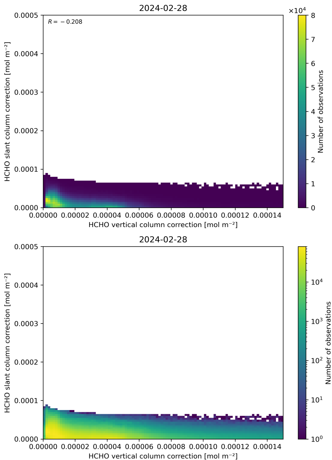
Figure 117: Scatter density plot of “HCHO vertical column correction” against “HCHO slant column correction” for 2024-02-27 to 2024-02-29.
