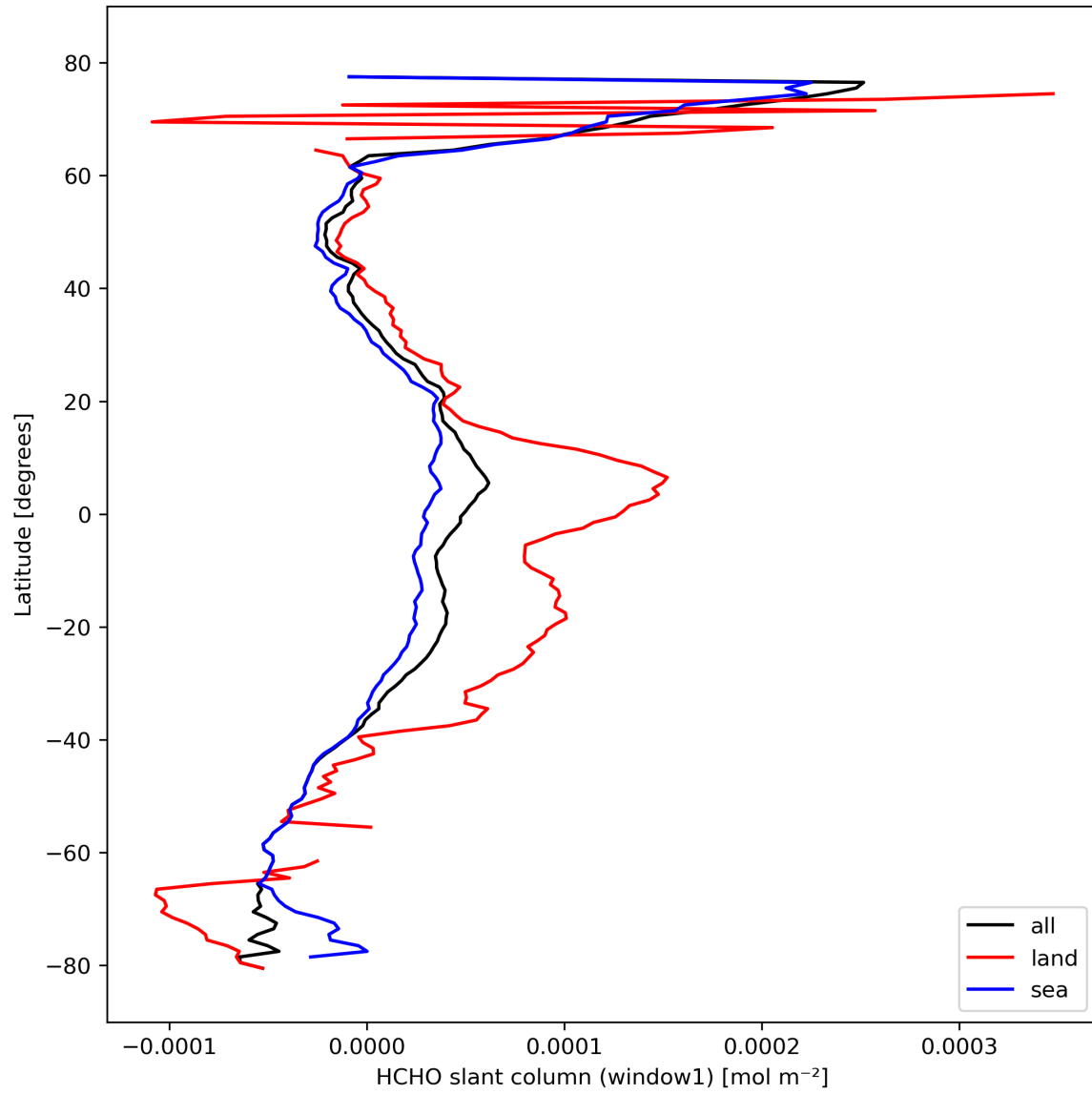
Figure 24: Zonal average of “HCHO slant column (window1)” for 2024-02-27 to 2024-02-29.
