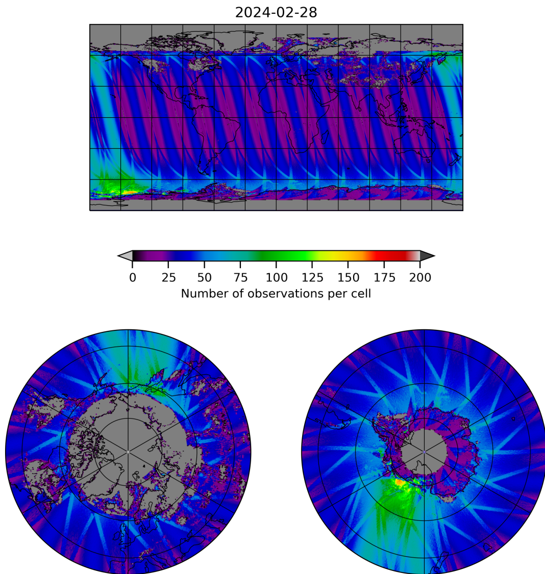
Figure 19: Map of the number of observations for 2024-02-27 to 2024-02-29
