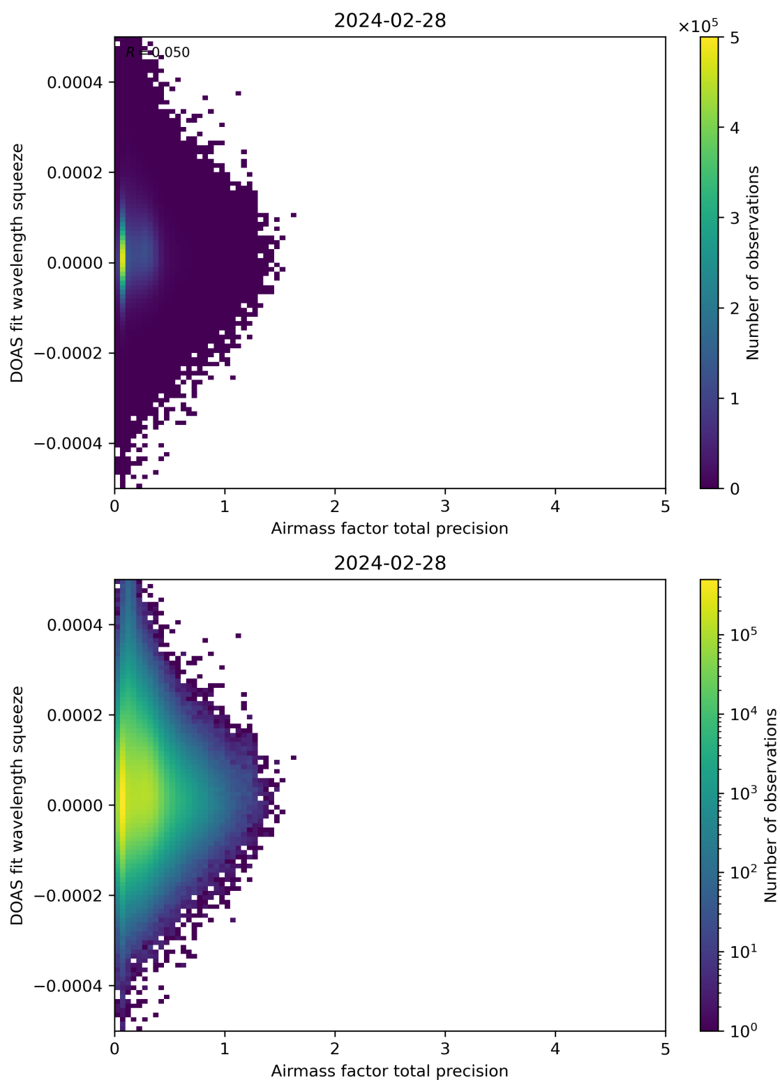
Figure 107: Scatter density plot of “Airmass factor total precision” against “DOAS fit wavelength squeeze” for 2024-02-27 to 2024-02-29.
