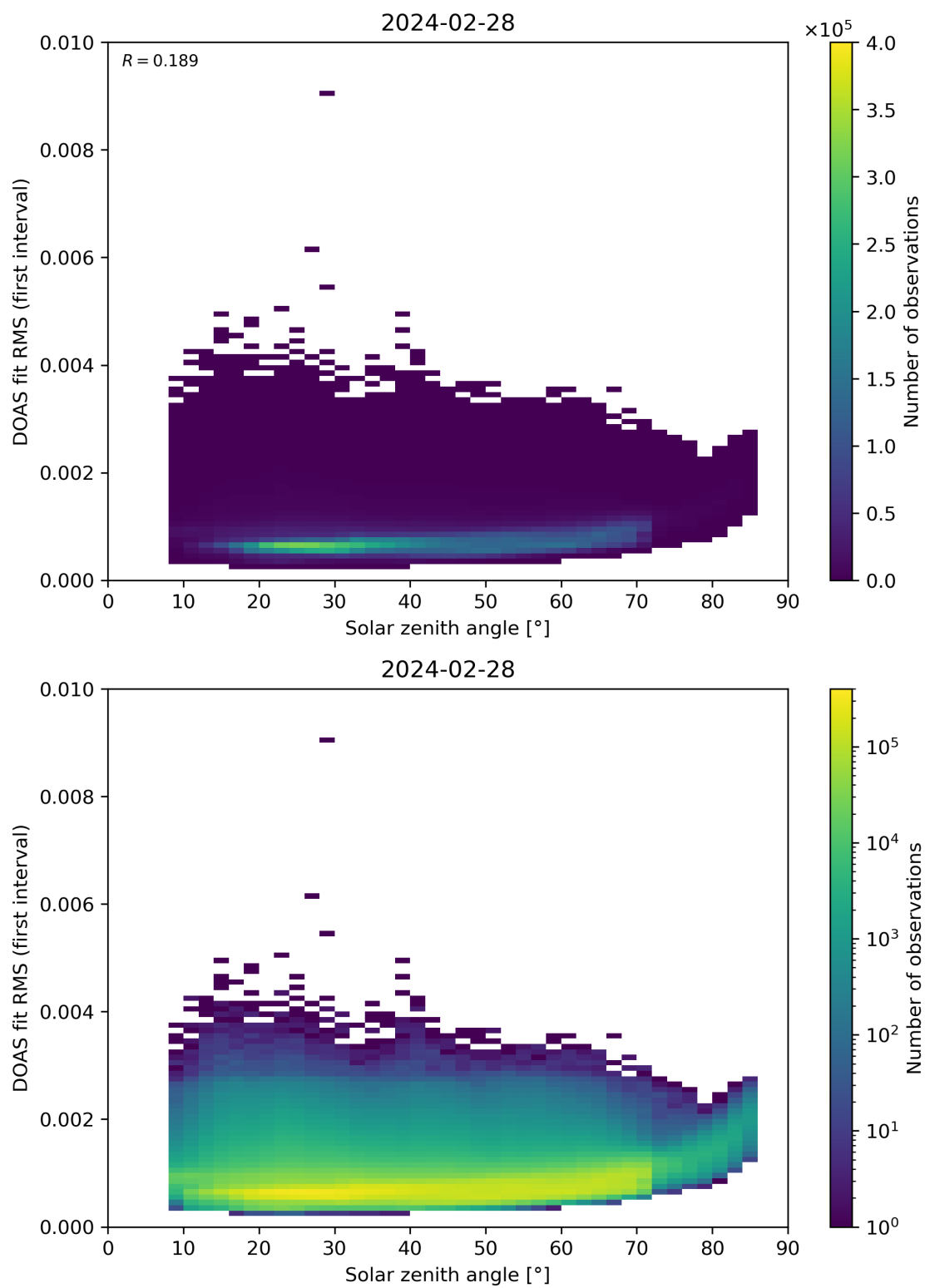
Figure 167: Scatter density plot of “Solar zenith angle” against “DOAS fit RMS (first interval)” for 2024-02-27 to 2024-02-29.
