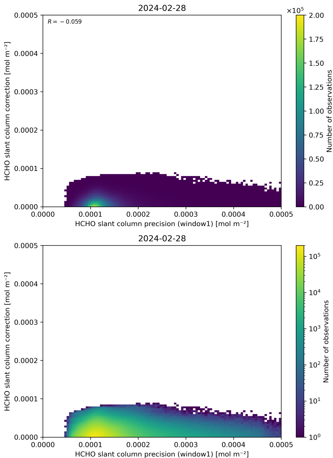
Figure 93: Scatter density plot of “HCHO slant column precision (window1)” against “HCHO slant column correction” for 2024-02-27 to 2024-02-29.
