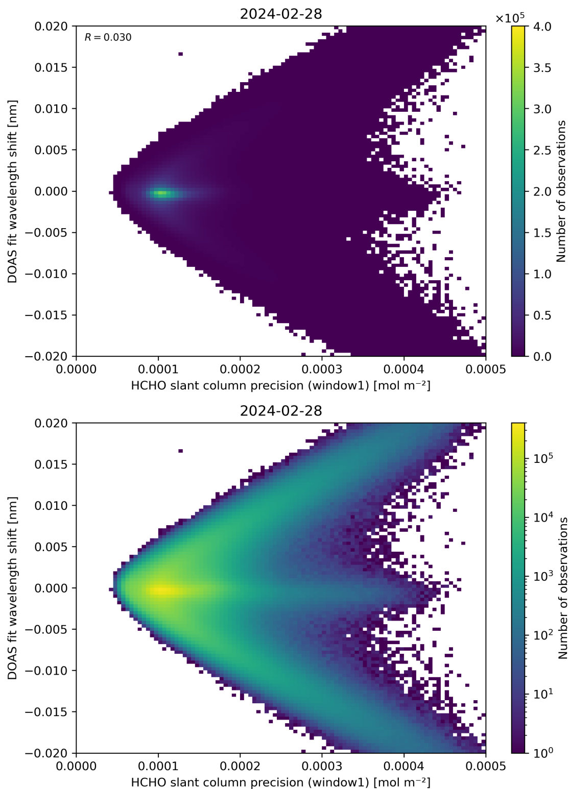
Figure 89: Scatter density plot of “HCHO slant column precision (window1)” against “DOAS fit wavelength shift” for 2024-02-27 to 2024-02-29.
