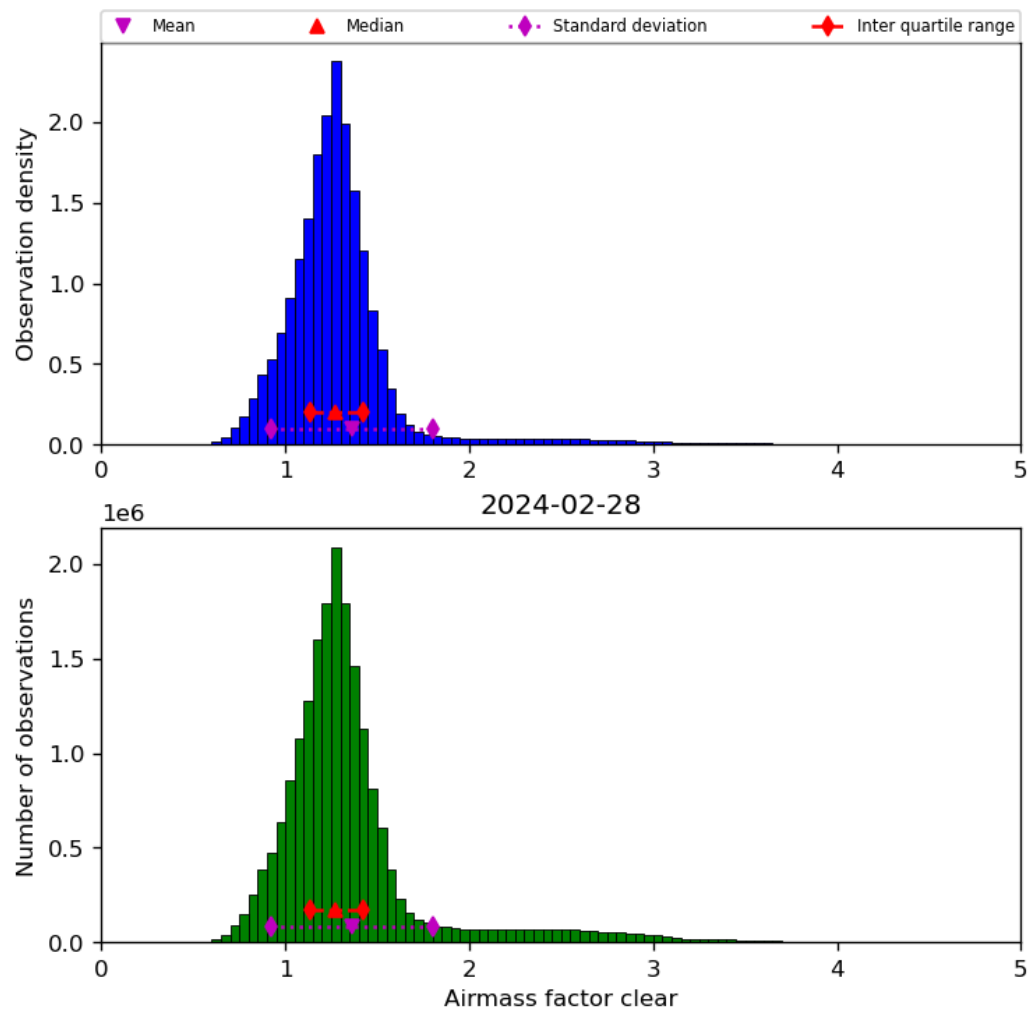
Figure 42: Histogram of “Airmass factor clear” for 2024-02-27 to 2024-02-29
