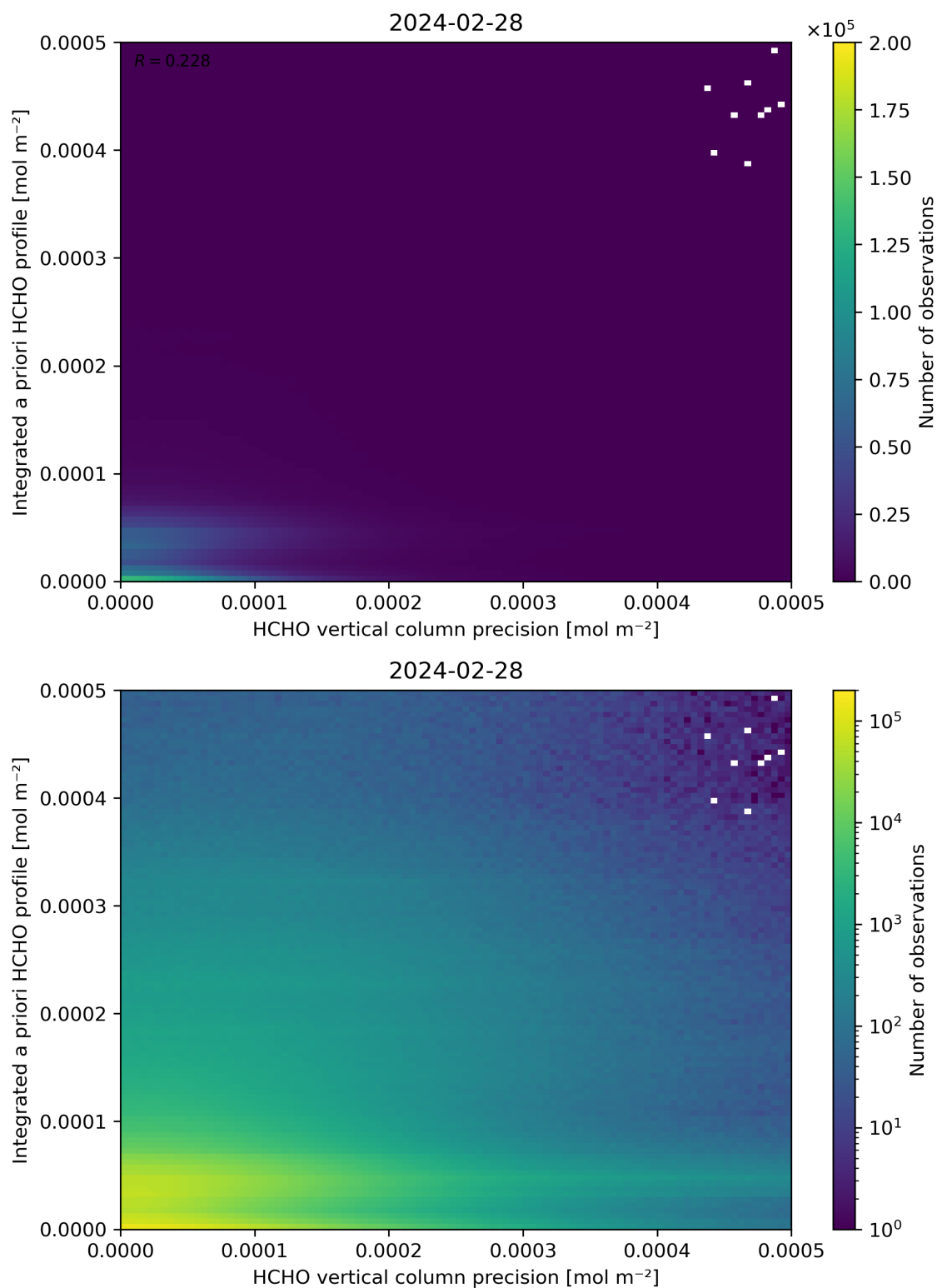
Figure 147: Scatter density plot of “HCHO vertical column precision” against “Integrated a priori HCHO profile” for 2024-02-27 to 2024-02-29.
