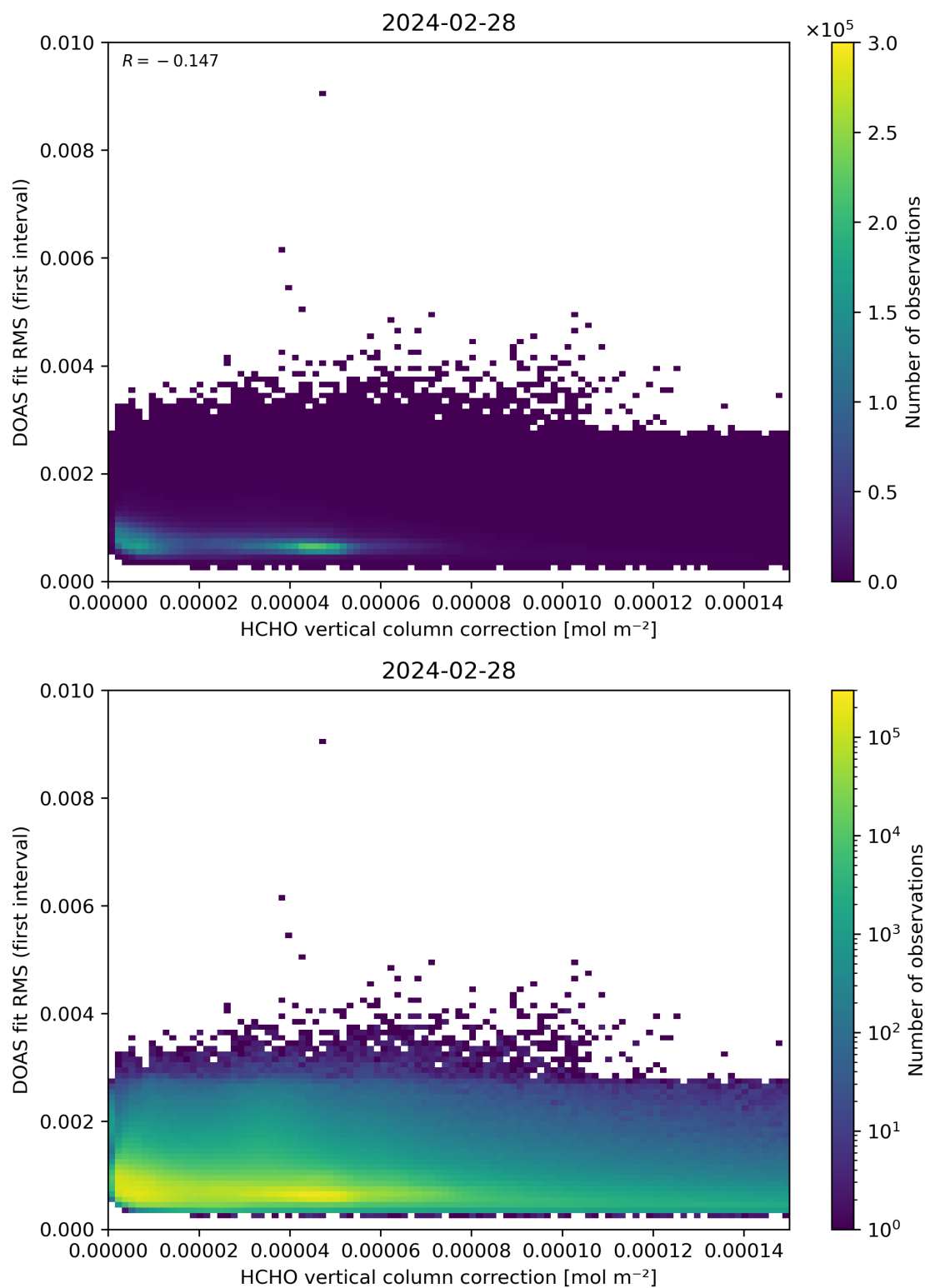
Figure 112: Scatter density plot of “HCHO vertical column correction” against “DOAS fit RMS (first interval)” for 2024-02-27 to 2024-02-29.
