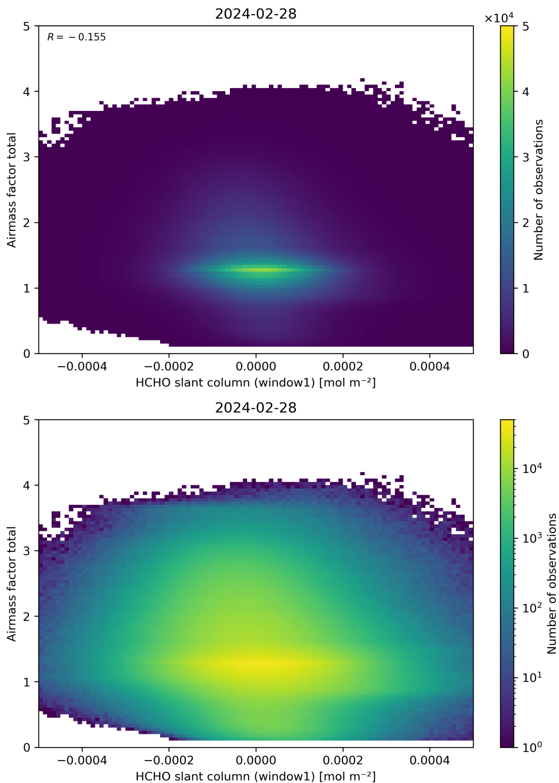
Figure 85: Scatter density plot of “HCHO slant column (window1)” against “Airmass factor total” for 2024-02-27 to 2024-02-29.
