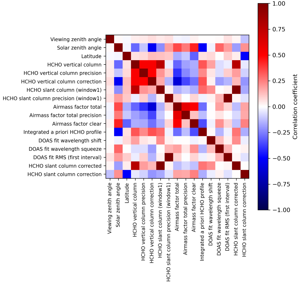
Figure 2: Map of correlation matrix for 2024-02-27 to 2024-02-29.
