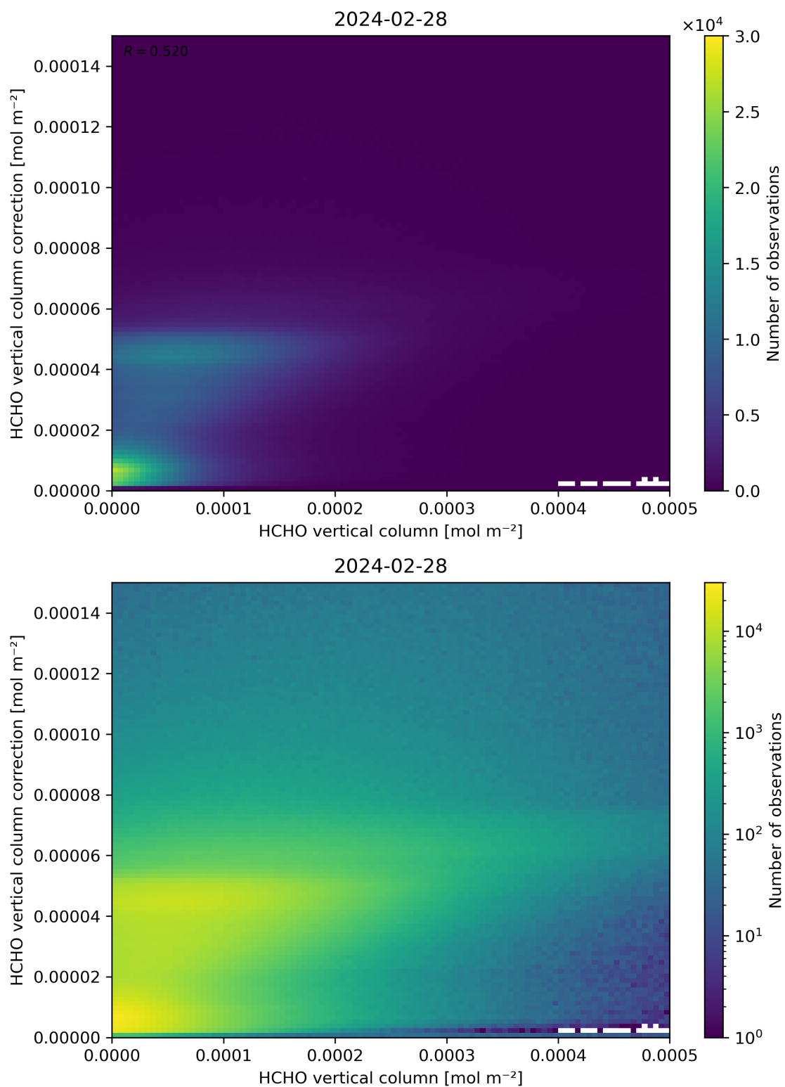
Figure 133: Scatter density plot of “HCHO vertical column” against “HCHO vertical column correction” for 2024-02-27 to 2024-02-29.
