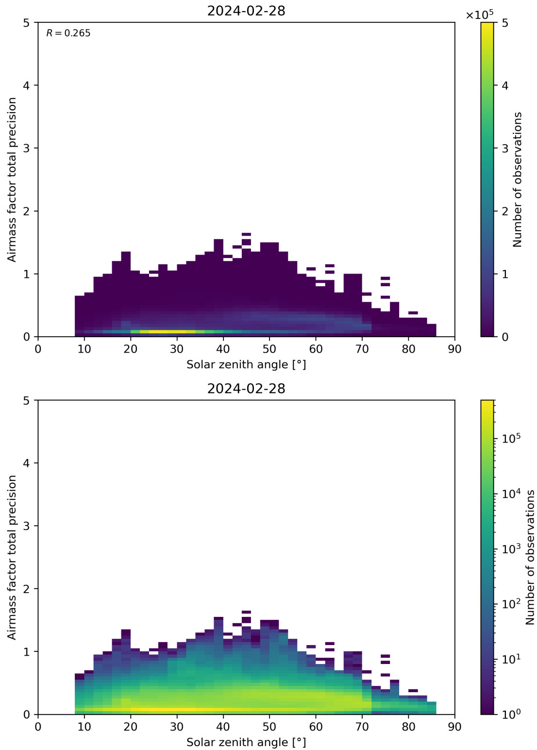
Figure 176: Scatter density plot of “Solar zenith angle” against “Airmass factor total precision” for 2024-02-27 to 2024-02-29.
