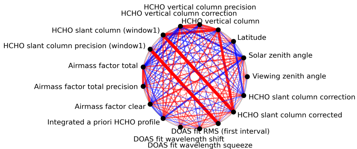
Figure 1: Map of correlation graph for 2024-02-27 to 2024-02-29.
