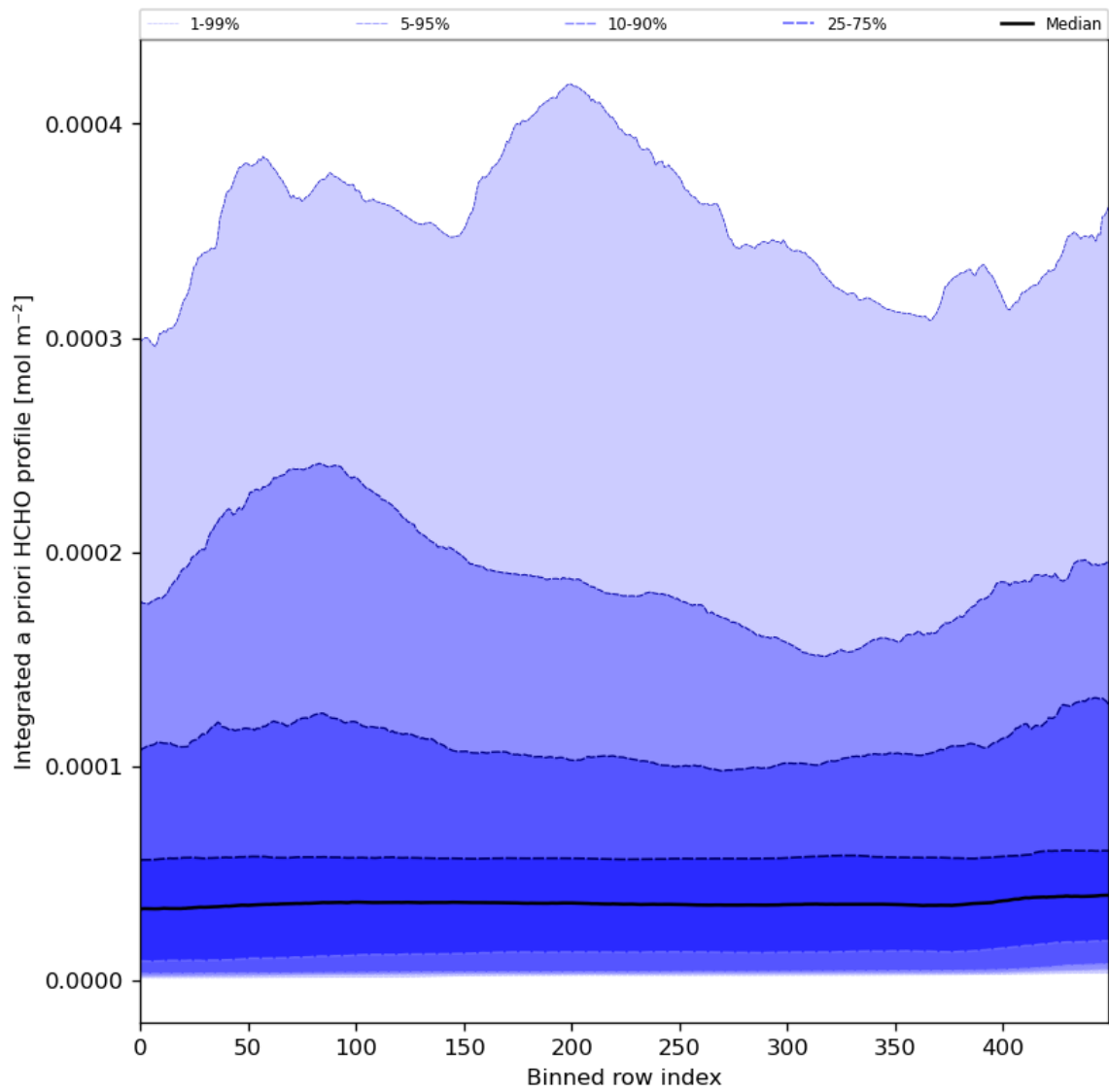
Figure 57: Along track statistics of “Integrated a priori HCHO profile” for 2024-02-27 to 2024-02-29
