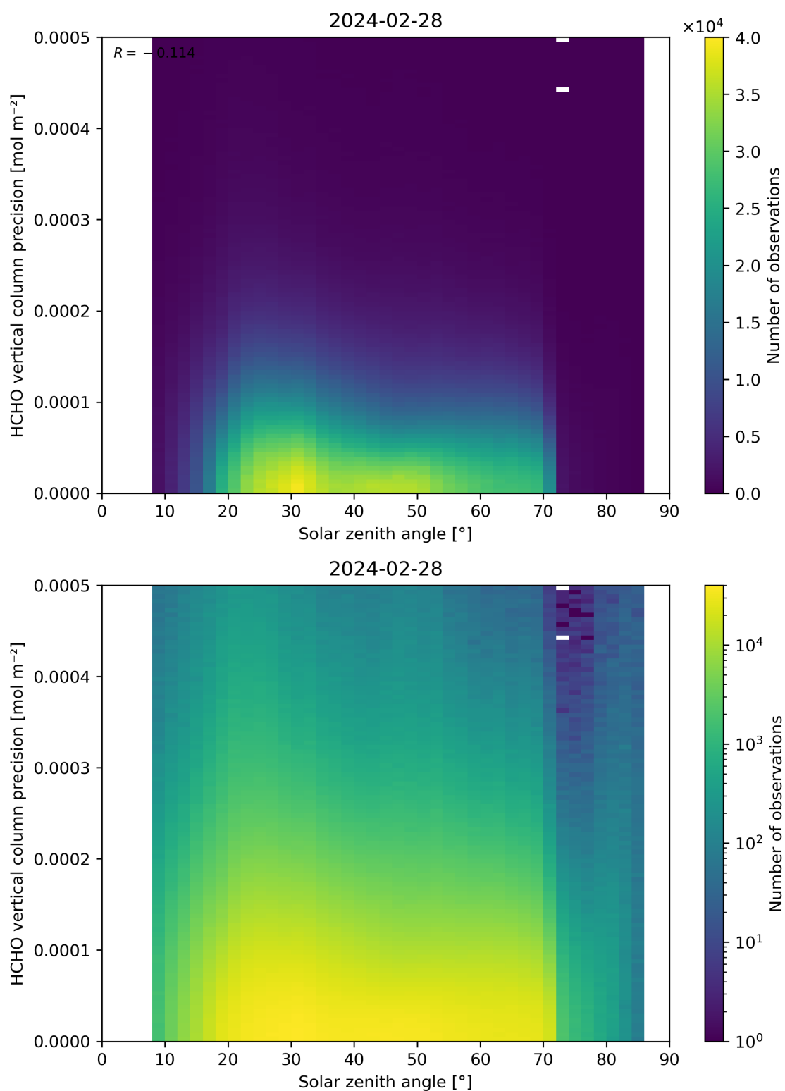
Figure 179: Scatter density plot of “Solar zenith angle” against “HCHO vertical column precision” for 2024-02-27 to 2024-02-29.
