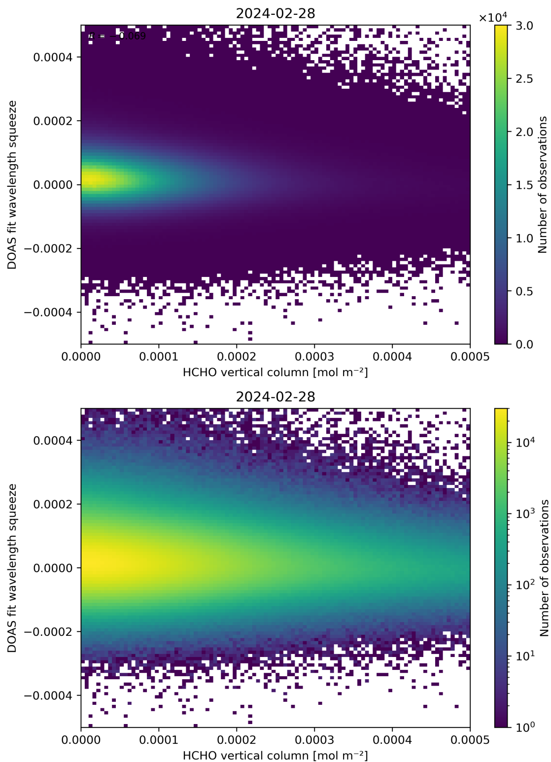
Figure 125: Scatter density plot of “HCHO vertical column” against “DOAS fit wavelength squeeze” for 2024-02-27 to 2024-02-29.
