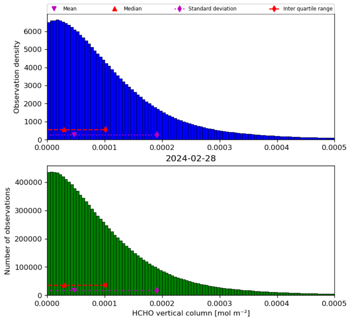
Figure 35: Histogram of “HCHO vertical column” for 2024-02-27 to 2024-02-29
