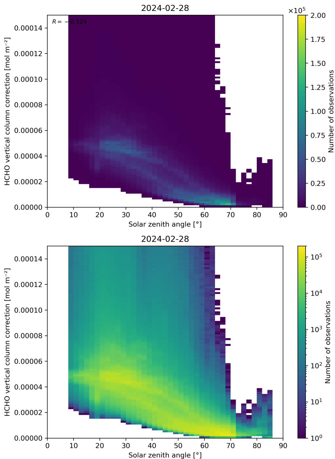
Figure 178: Scatter density plot of “Solar zenith angle” against “HCHO vertical column correction” for 2024-02-27 to 2024-02-29.
