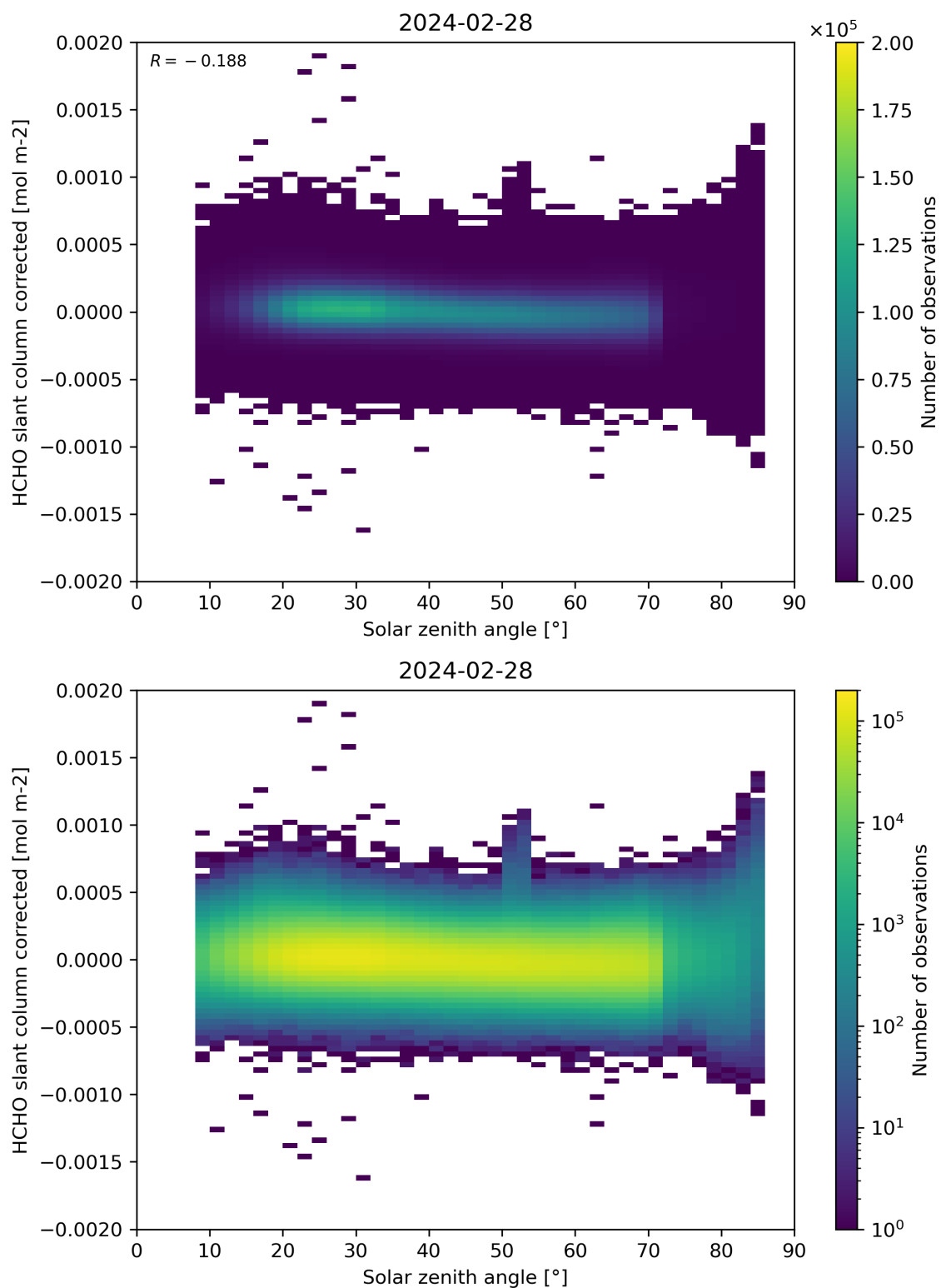
Figure 171: Scatter density plot of “Solar zenith angle” against “HCHO slant column corrected” for 2024-02-27 to 2024-02-29.
