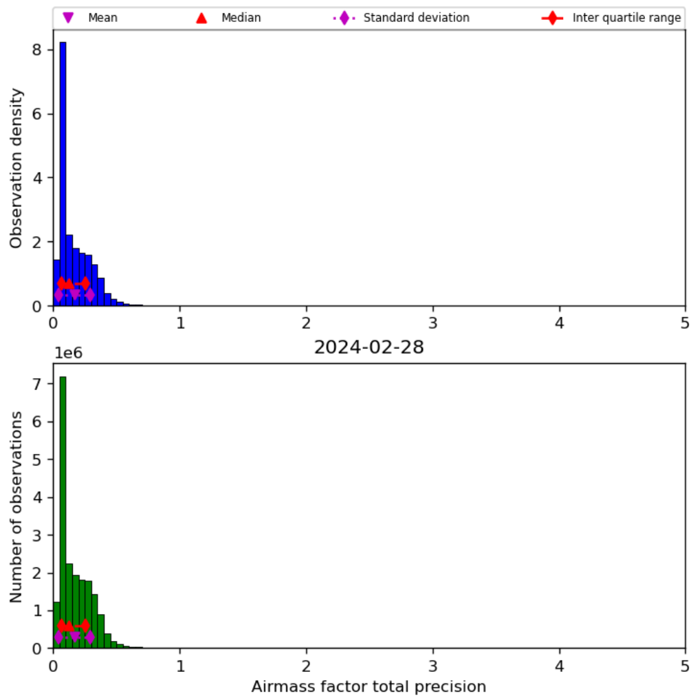
Figure 41: Histogram of “Airmass factor total precision” for 2024-02-27 to 2024-02-29
