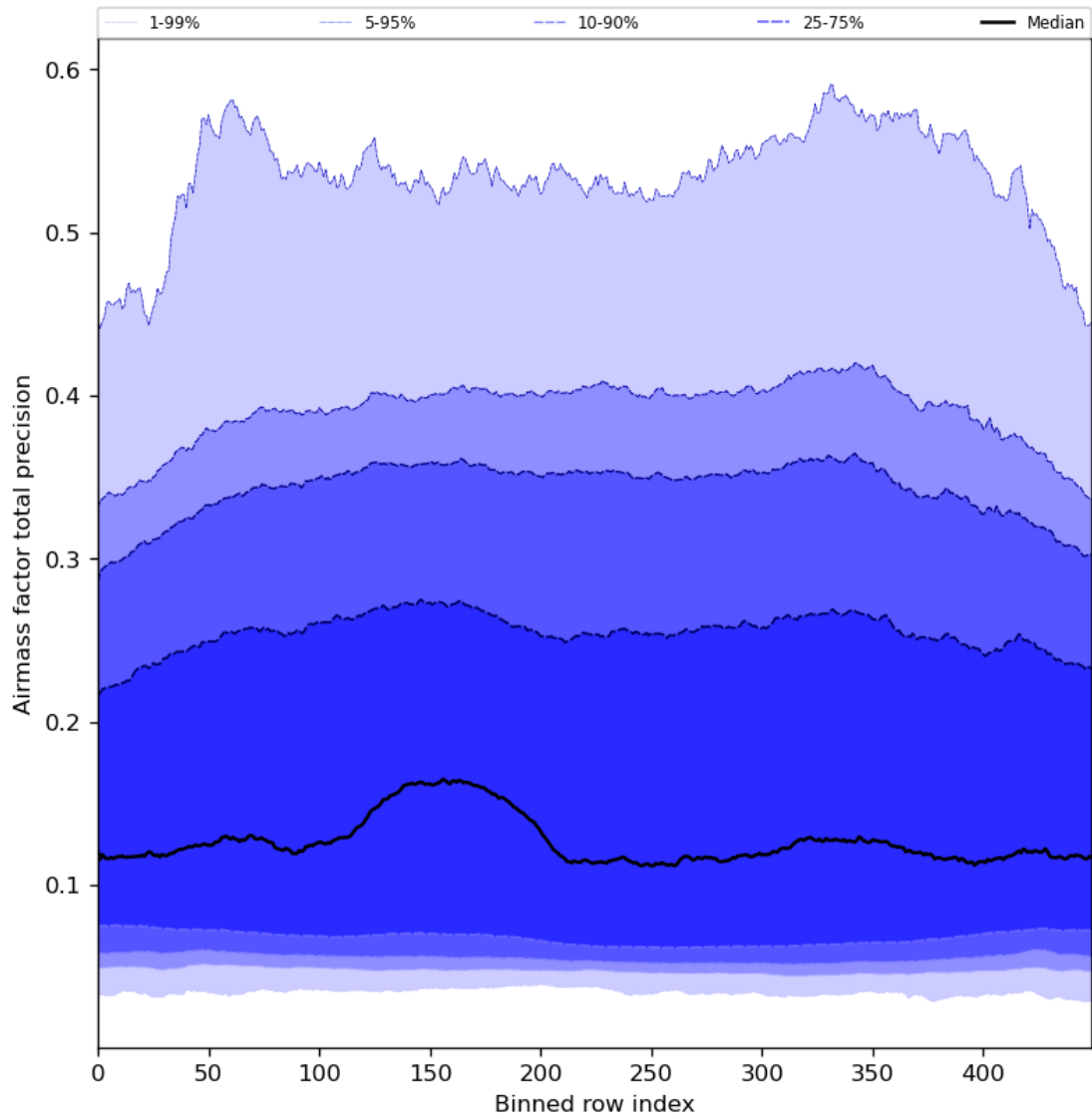
Figure 55: Along track statistics of “Airmass factor total precision” for 2024-02-27 to 2024-02-29
