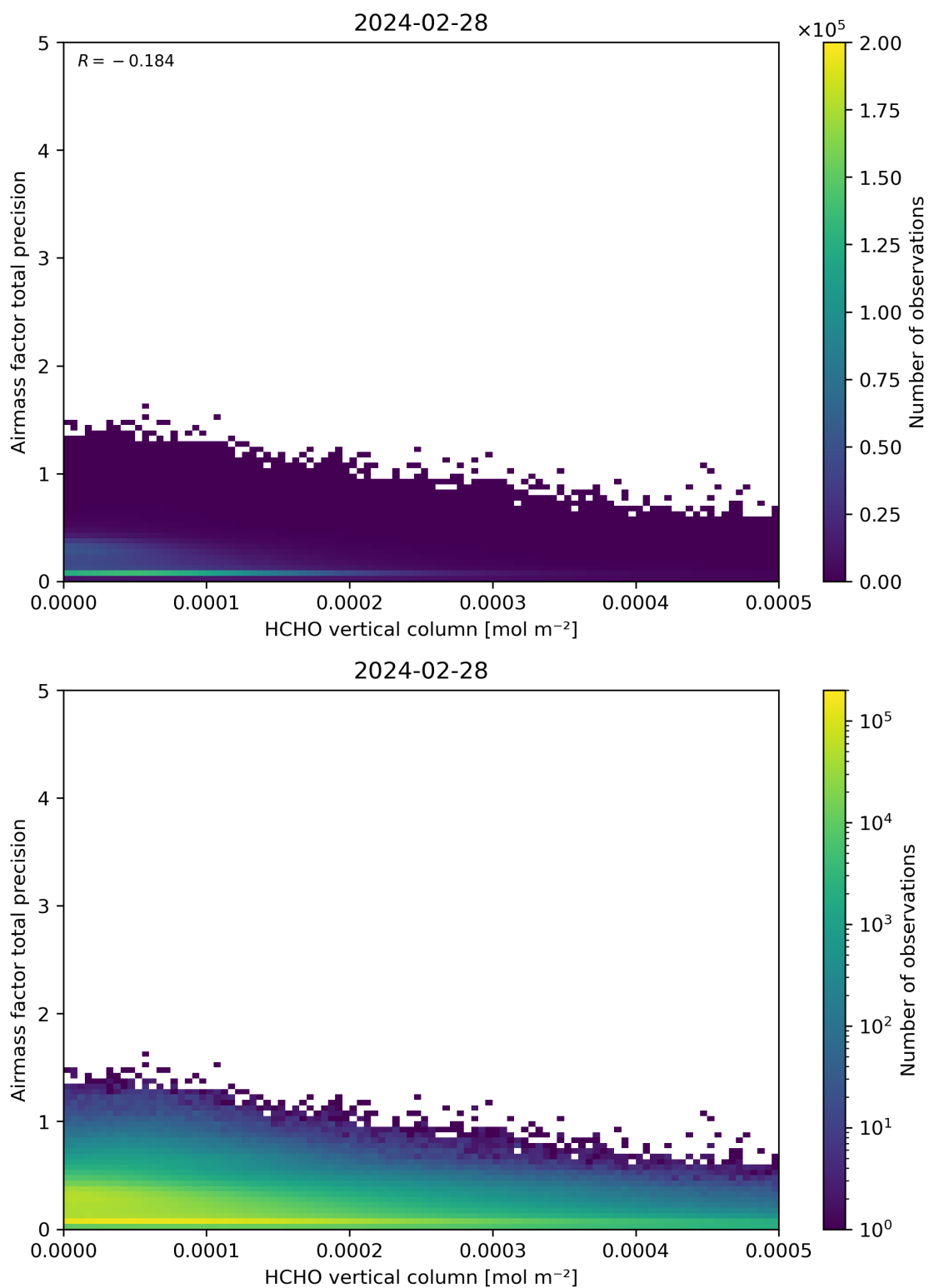
Figure 132: Scatter density plot of “HCHO vertical column” against “Airmass factor total precision” for 2024-02-27 to 2024-02-29.
