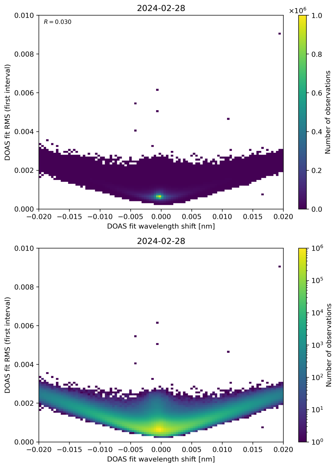
Figure 64: Scatter density plot of “DOAS fit wavelength shift” against “DOAS fit RMS (first interval)” for 2024-02-27 to 2024-02-29.
