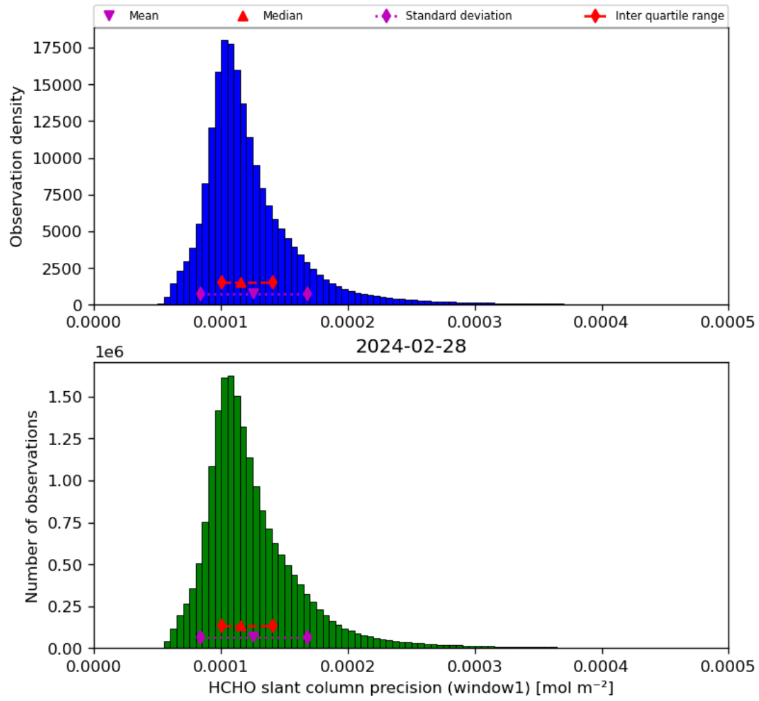
Figure 39: Histogram of “HCHO slant column precision (window1)” for 2024-02-27 to 2024-02-29
