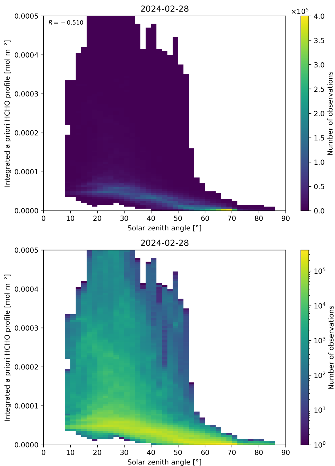
Figure 180: Scatter density plot of “Solar zenith angle” against “Integrated a priori HCHO profile” for 2024-02-27 to 2024-02-29.
