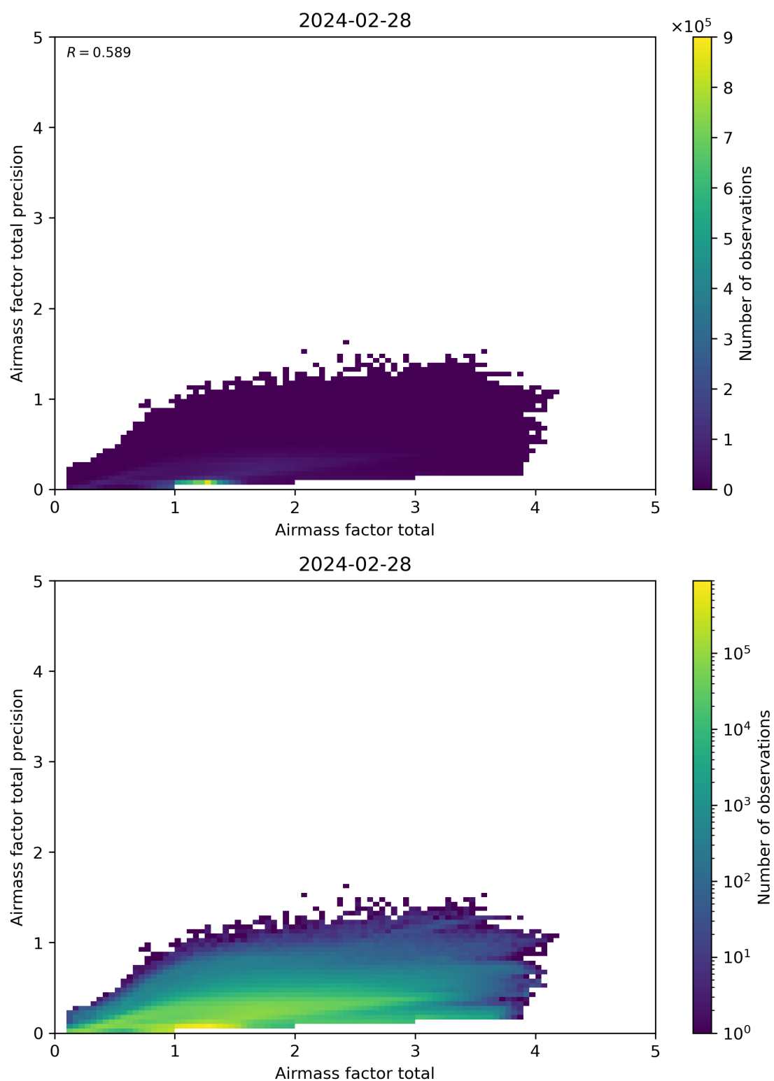
Figure 103: Scatter density plot of “Airmass factor total” against “Airmass factor total precision” for 2024-02-27 to 2024-02-29.
