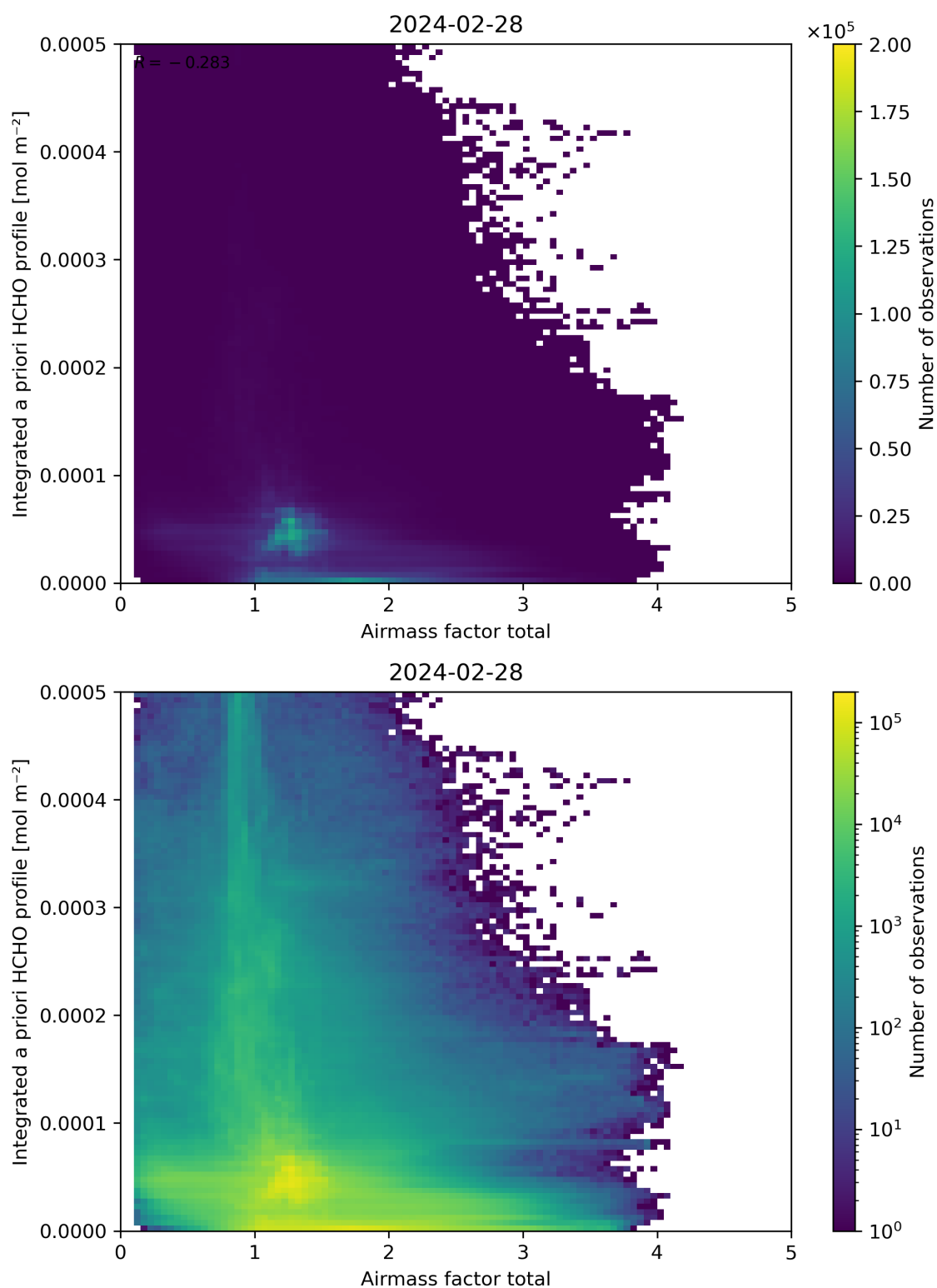
Figure 104: Scatter density plot of “Air mass factor total” against “Integrated a priori HCHO profile” for 2024-02-27 to 2024-02-29.
