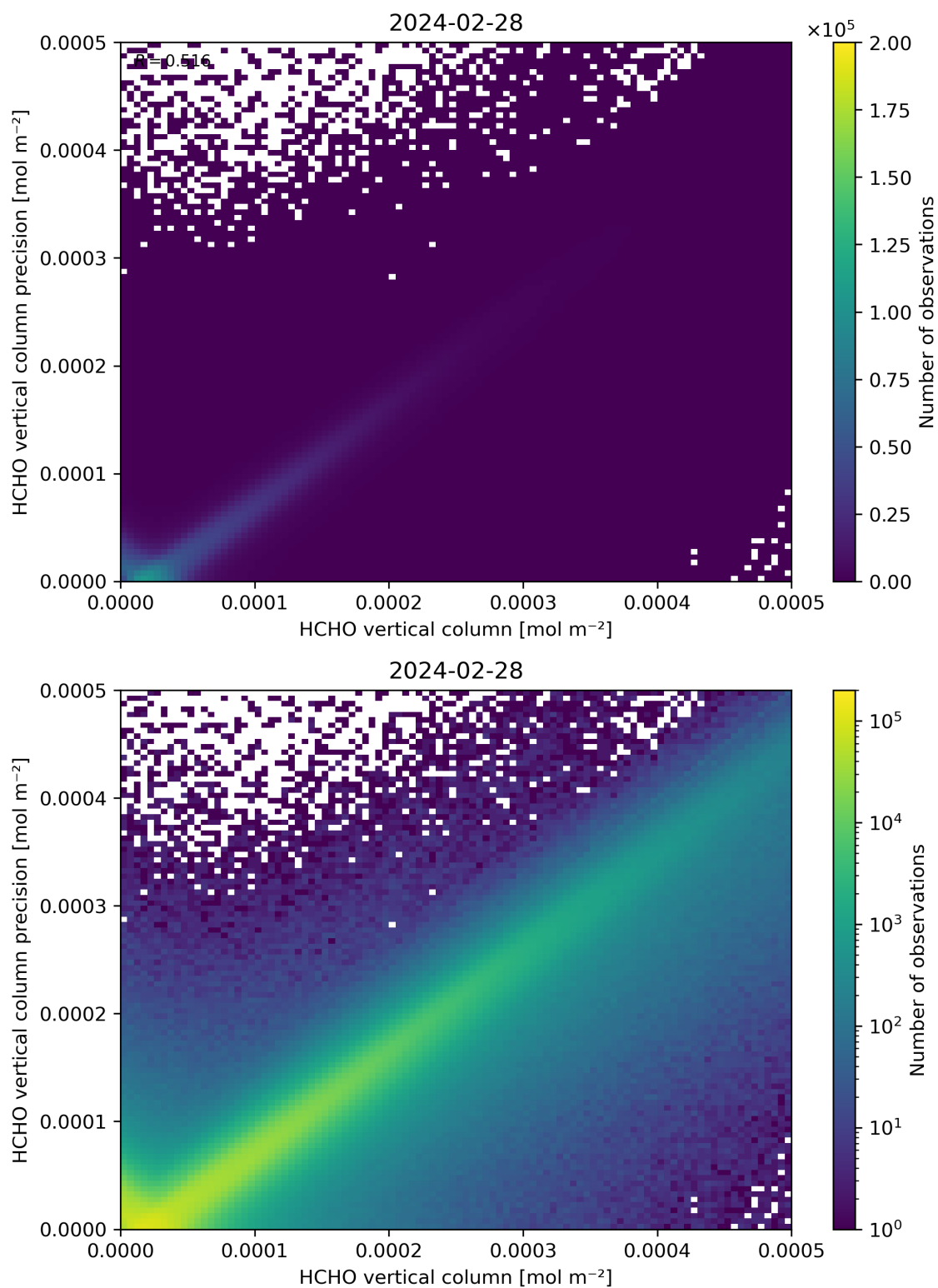
Figure 134: Scatter density plot of “HCHO vertical column” against “HCHO vertical column precision” for 2024-02-27 to 2024-02-29.
