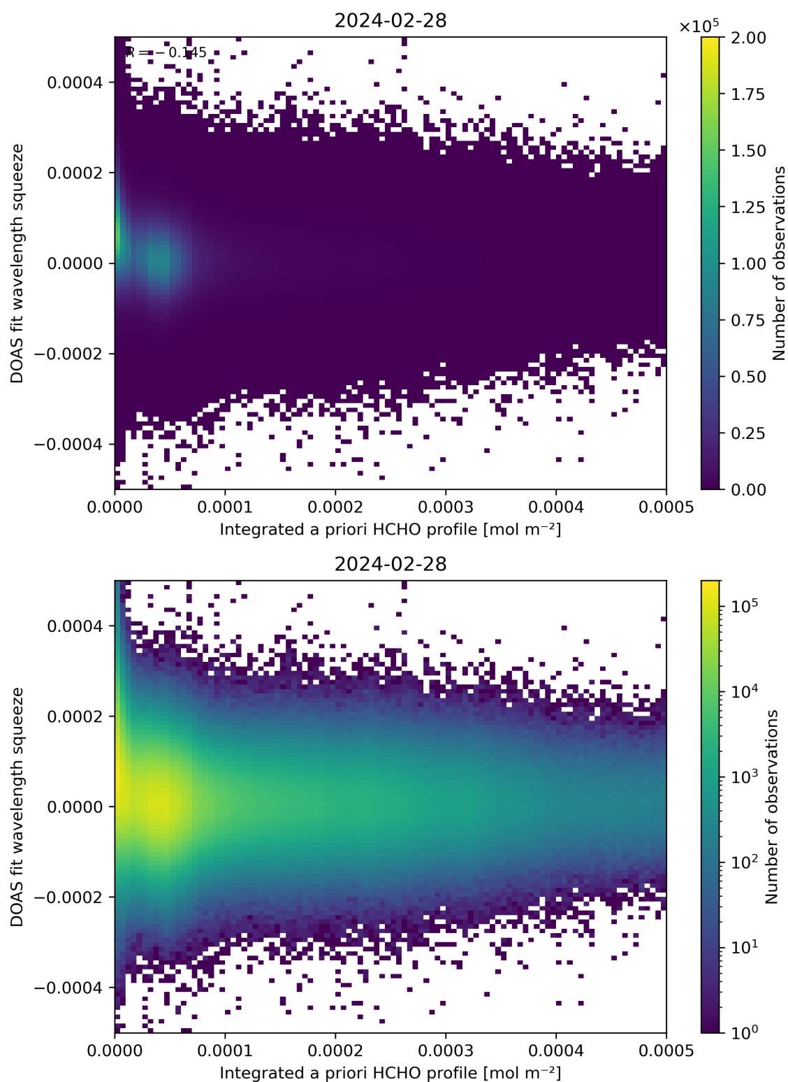
Figure 150: Scatter density plot of “Integrated a priori HCHO profile” against “DOAS fit wavelength squeeze” for 2024-02-27 to 2024-02-29.
