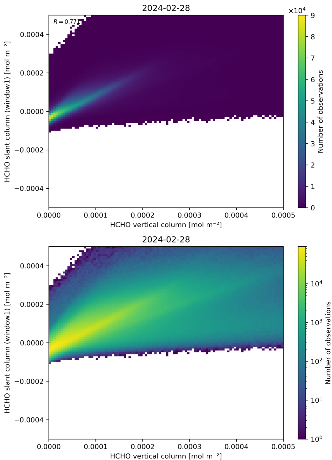
Figure 129: Scatter density plot of “HCHO vertical column” against “HCHO slant column (window1)” for 2024-02-27 to 2024-02-29.
