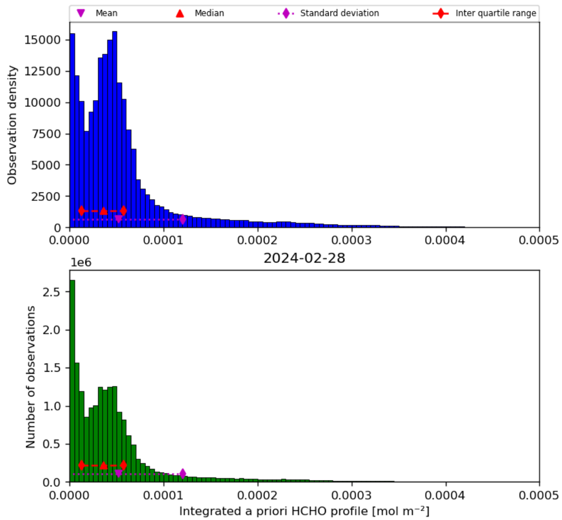
Figure 43: Histogram of “Integrated a priori HCHO profile” for 2024-02-27 to 2024-02-29
