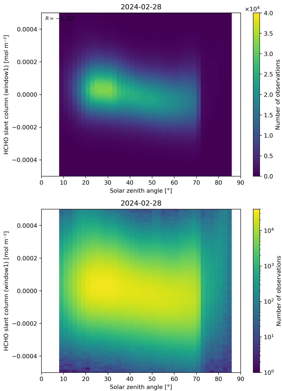
Figure 173: Scatter density plot of “Solar zenith angle” against “HCHO slant column (window1)” for 2024-02-27 to 2024-02-29.
