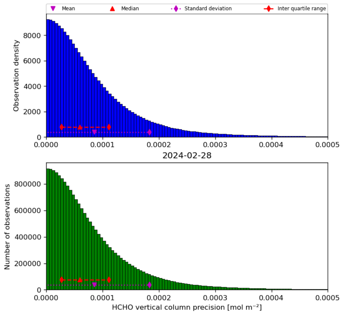
Figure 36: Histogram of “HCHO vertical column precision” for 2024-02-27 to 2024-02-29
