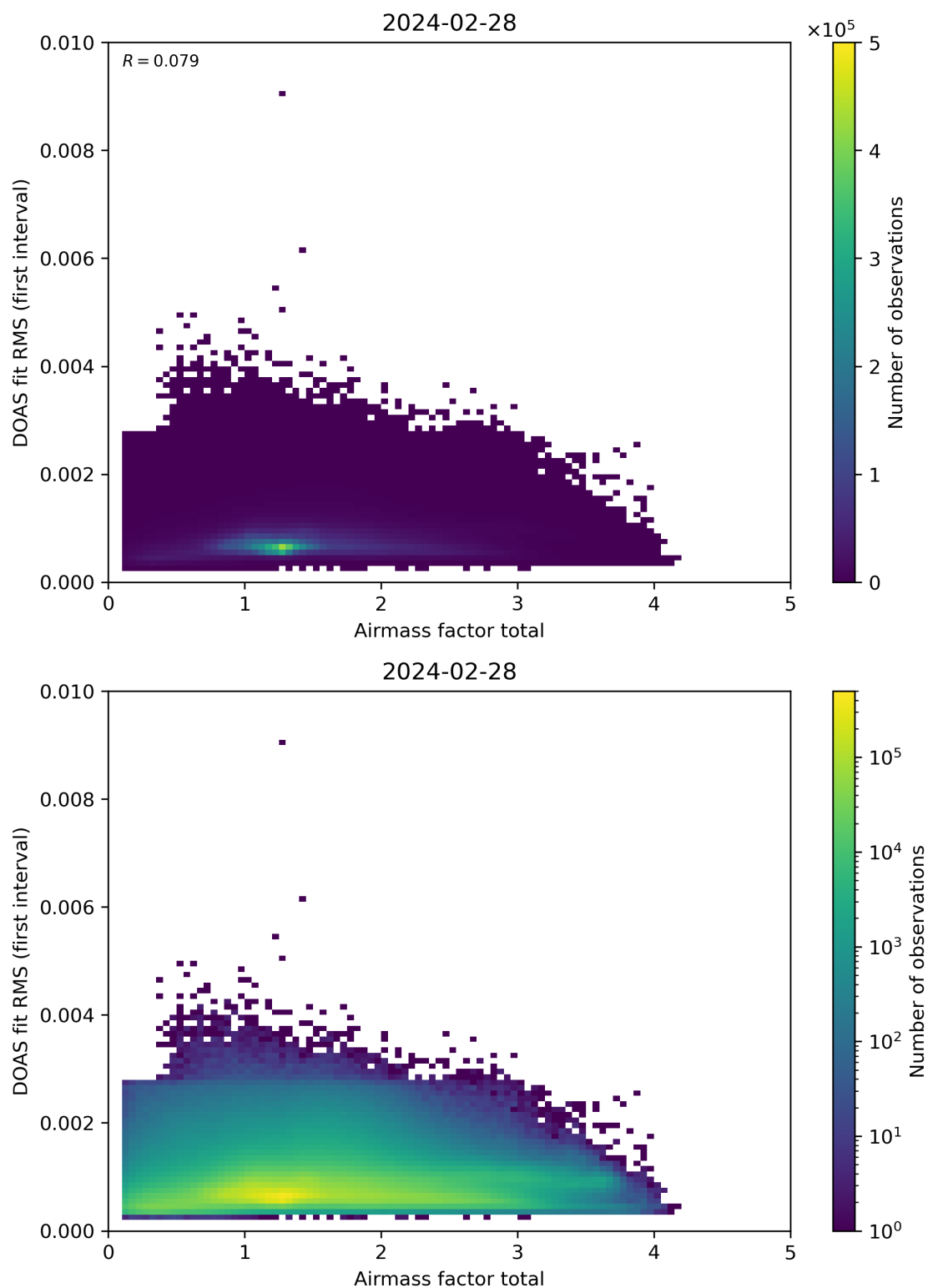
Figure 97: Scatter density plot of “Airmass factor total” against “DOAS fit RMS (first interval)” for 2024-02-27 to 2024-02-29.
