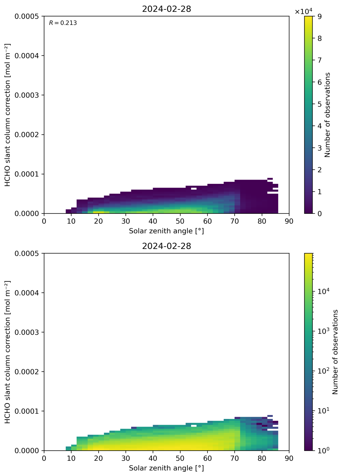
Figure 172: Scatter density plot of “Solar zenith angle” against “HCHO slant column correction” for 2024-02-27 to 2024-02-29.
