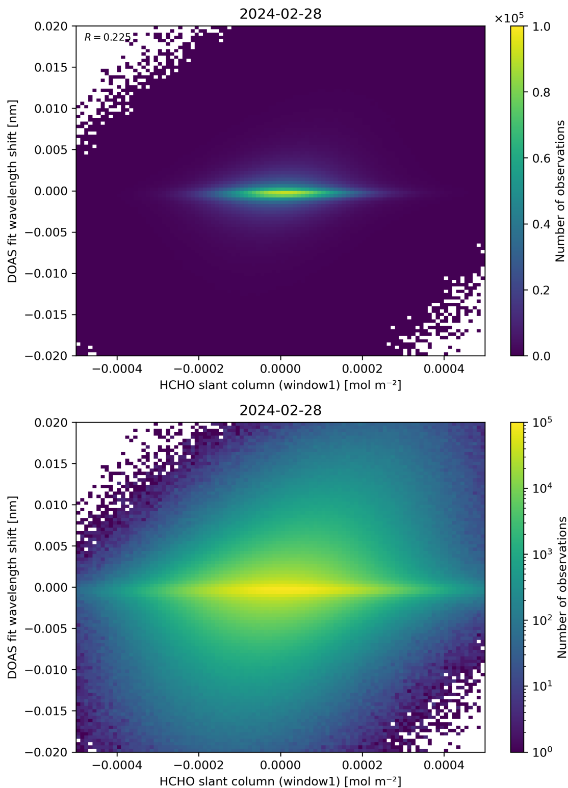
Figure 79: Scatter density plot of “HCHO slant column (window1)” against “DOAS fit wavelength shift” for 2024-02-27 to 2024-02-29.
