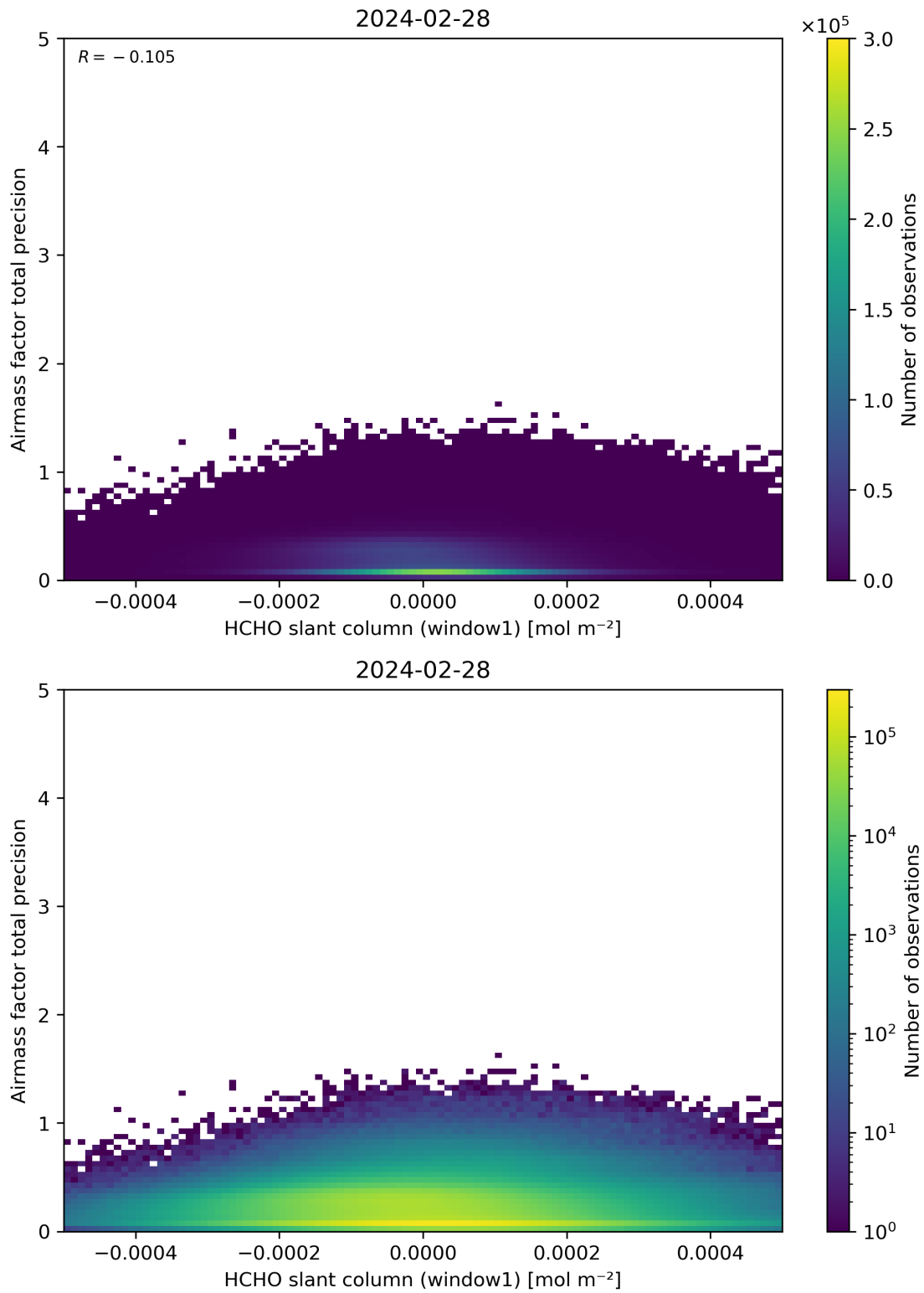
Figure 86: Scatter density plot of “HCHO slant column (window1)” against “Airmass factor total precision” for 2024-02-27 to 2024-02-29.
