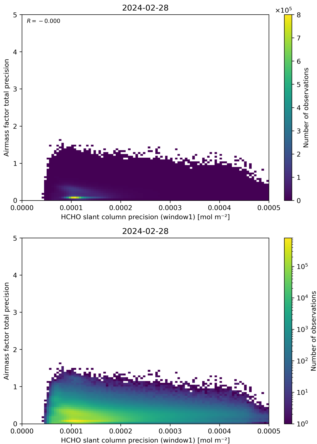
Figure 95: Scatter density plot of “HCHO slant column precision (window1)” against “Airmass factor total precision” for 2024-02-27 to 2024-02-29.
