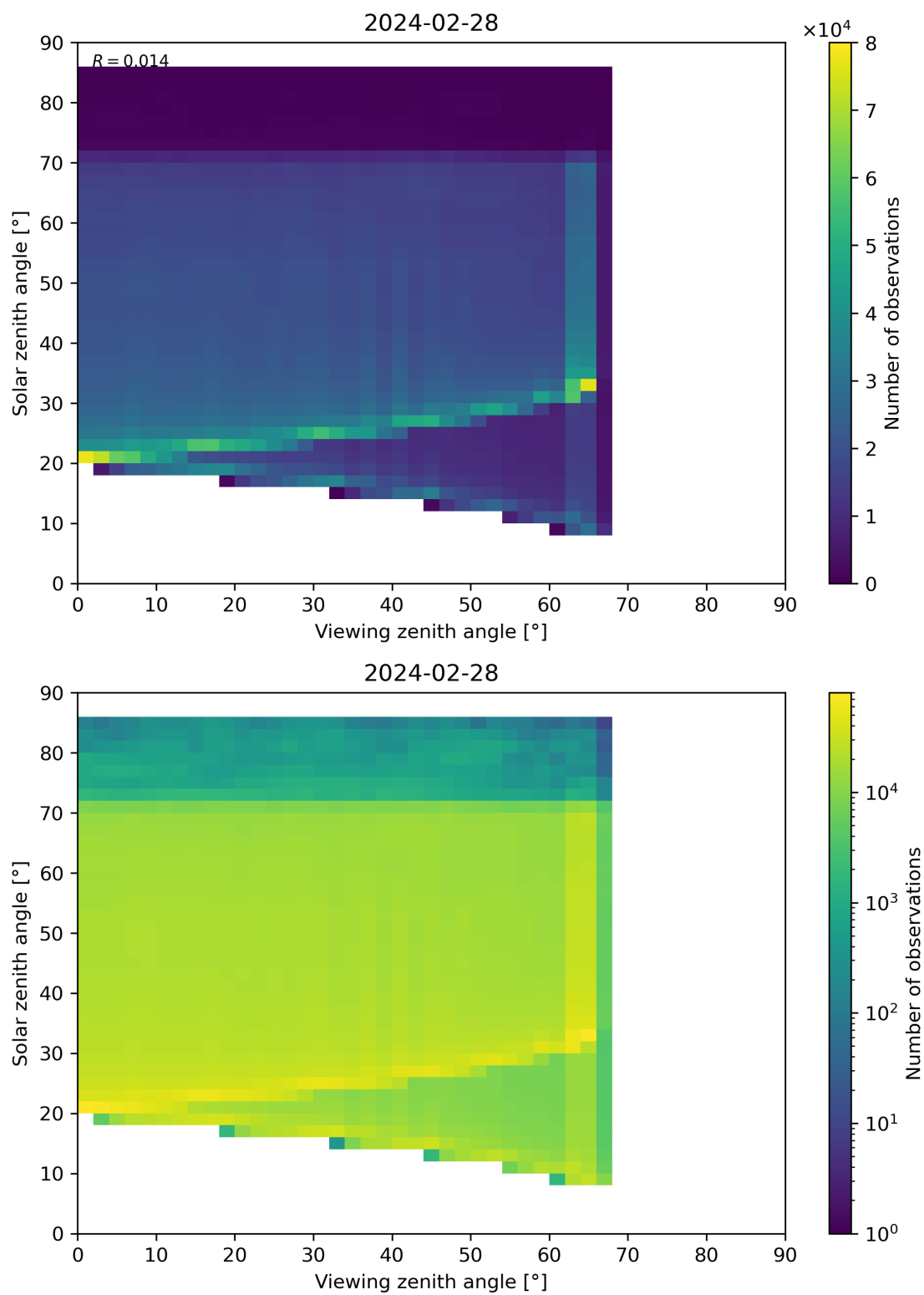
Figure 197: Scatter density plot of “Viewing zenith angle” against “Solar zenith angle” for 2024-02-27 to 2024-02-29.
