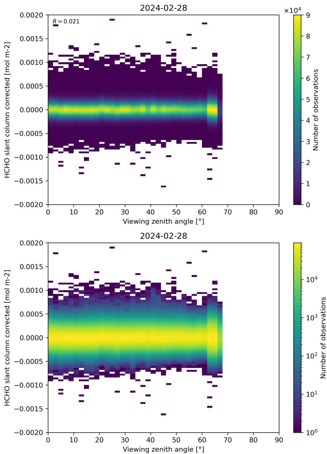
Figure 186: Scatter density plot of “Viewing zenith angle” against “HCHO slant column corrected” for 2024-02-27 to 2024-02-29.
