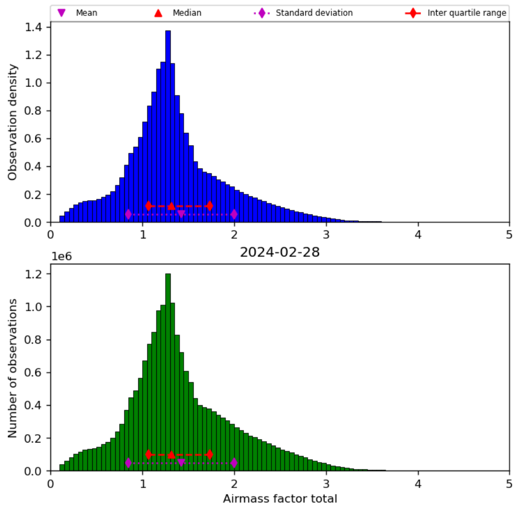
Figure 40: Histogram of “Airmass factor total” for 2024-02-27 to 2024-02-29
