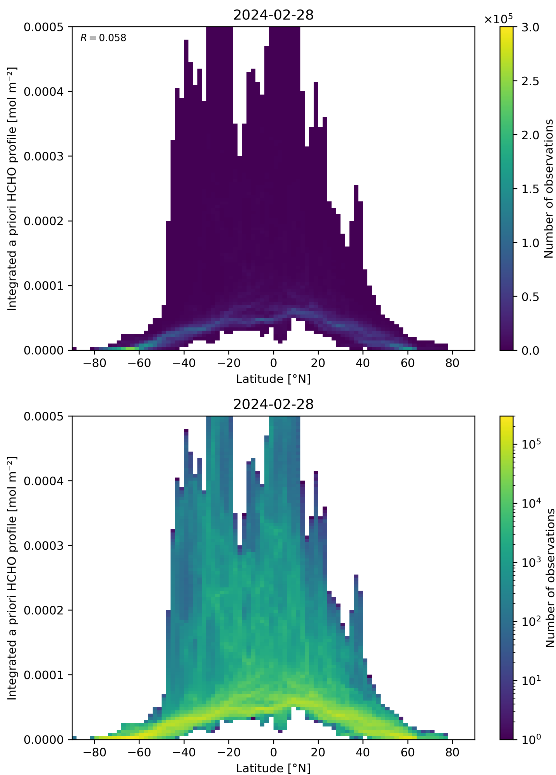
Figure 166: Scatter density plot of “Latitude” against “Integrated a priori HCHO profile” for 2024-02-27 to 2024-02-29.
