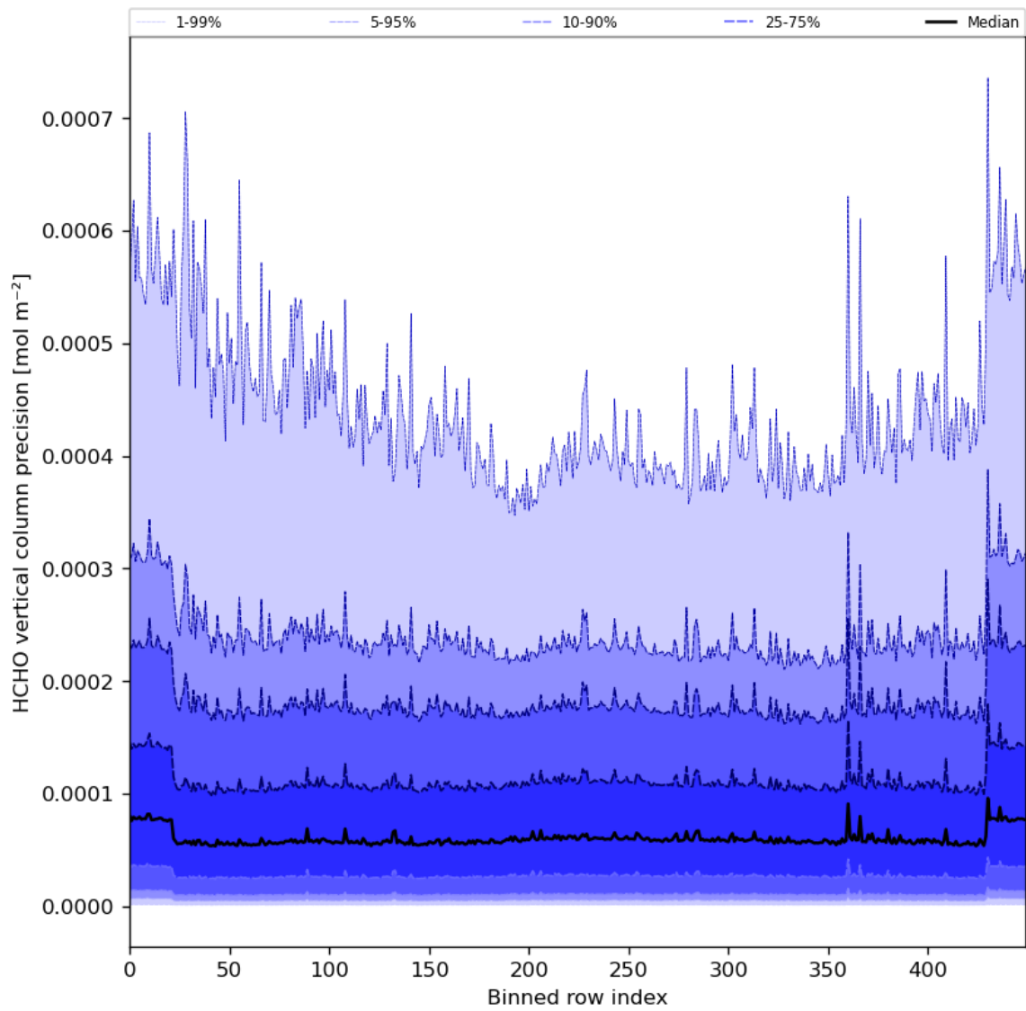
Figure 50: Along track statistics of “HCHO vertical column precision” for 2024-02-27 to 2024-02-29
