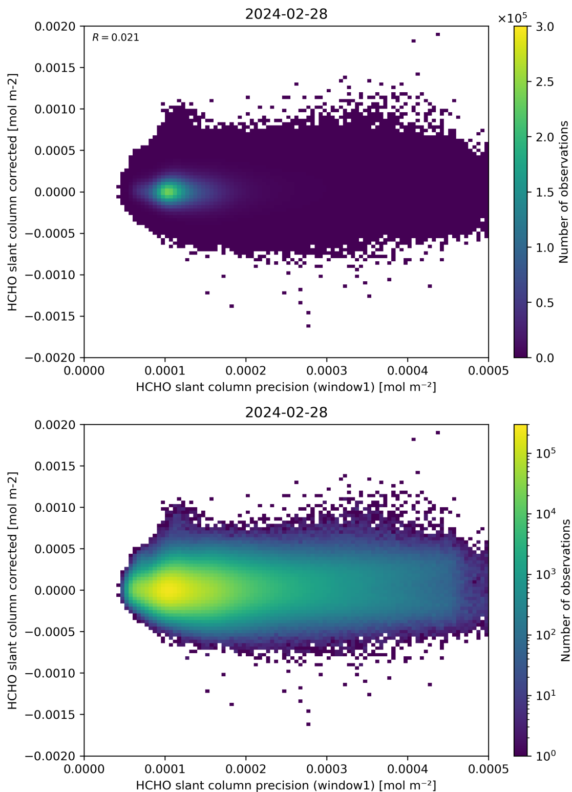
Figure 92: Scatter density plot of “HCHO slant column precision (window1)” against “HCHO slant column corrected” for 2024-02-27 to 2024-02-29.
