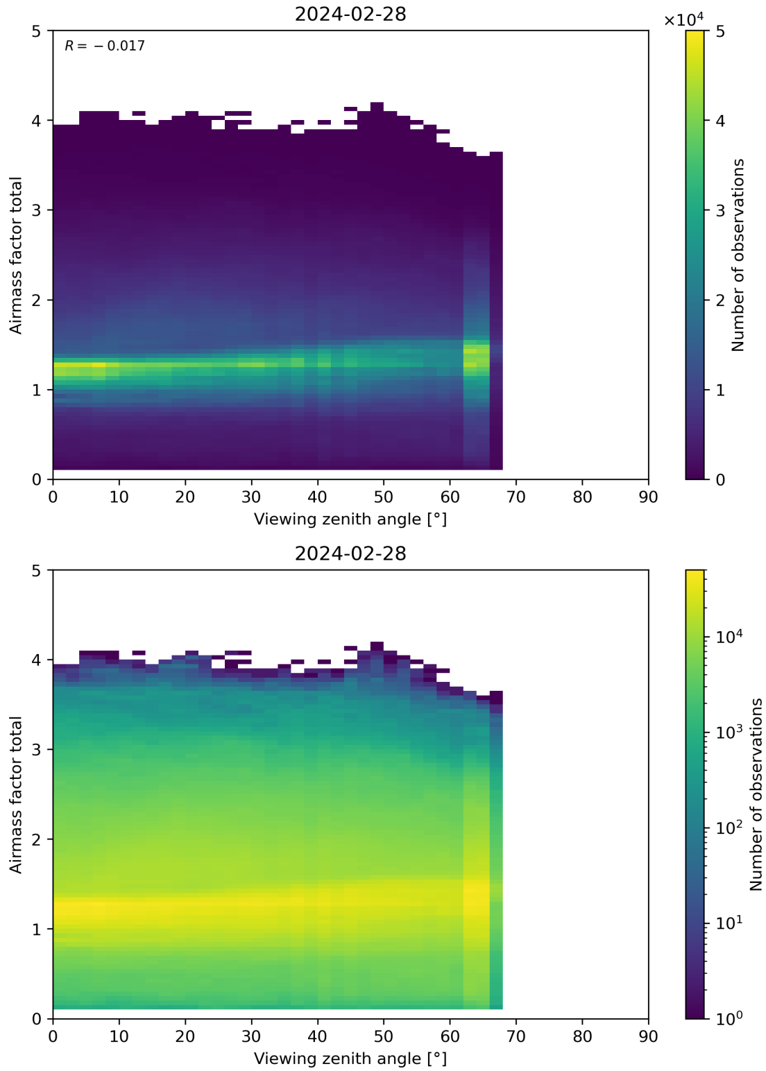
Figure 190: Scatter density plot of “Viewing zenith angle” against “Airmass factor total” for 2024-02-27 to 2024-02-29.
