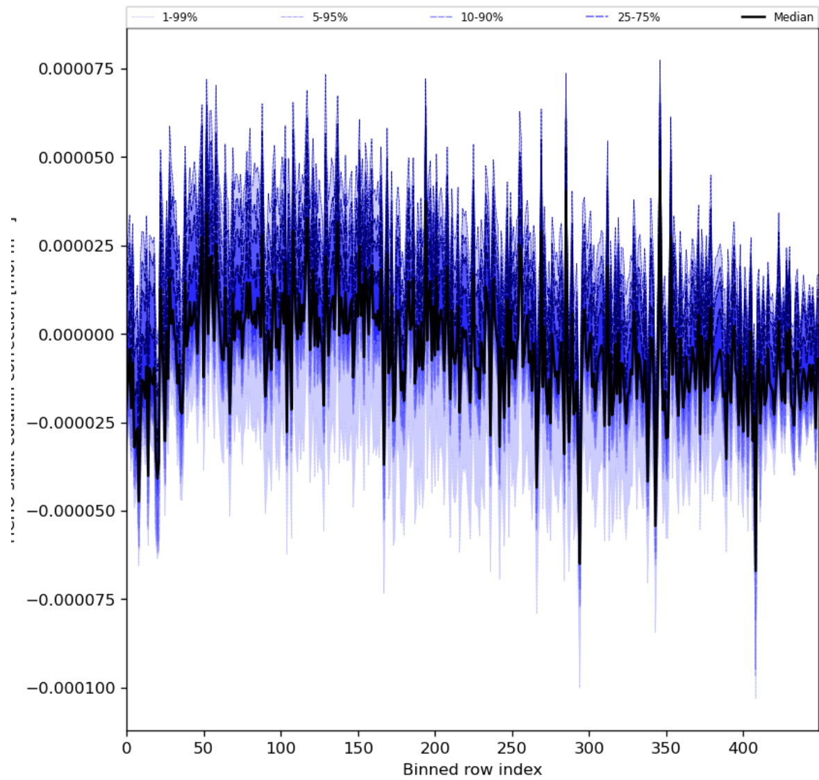
Figure 61: Along track statistics of “HCHO slant column correction” for 2024-02-27 to 2024-02-29
