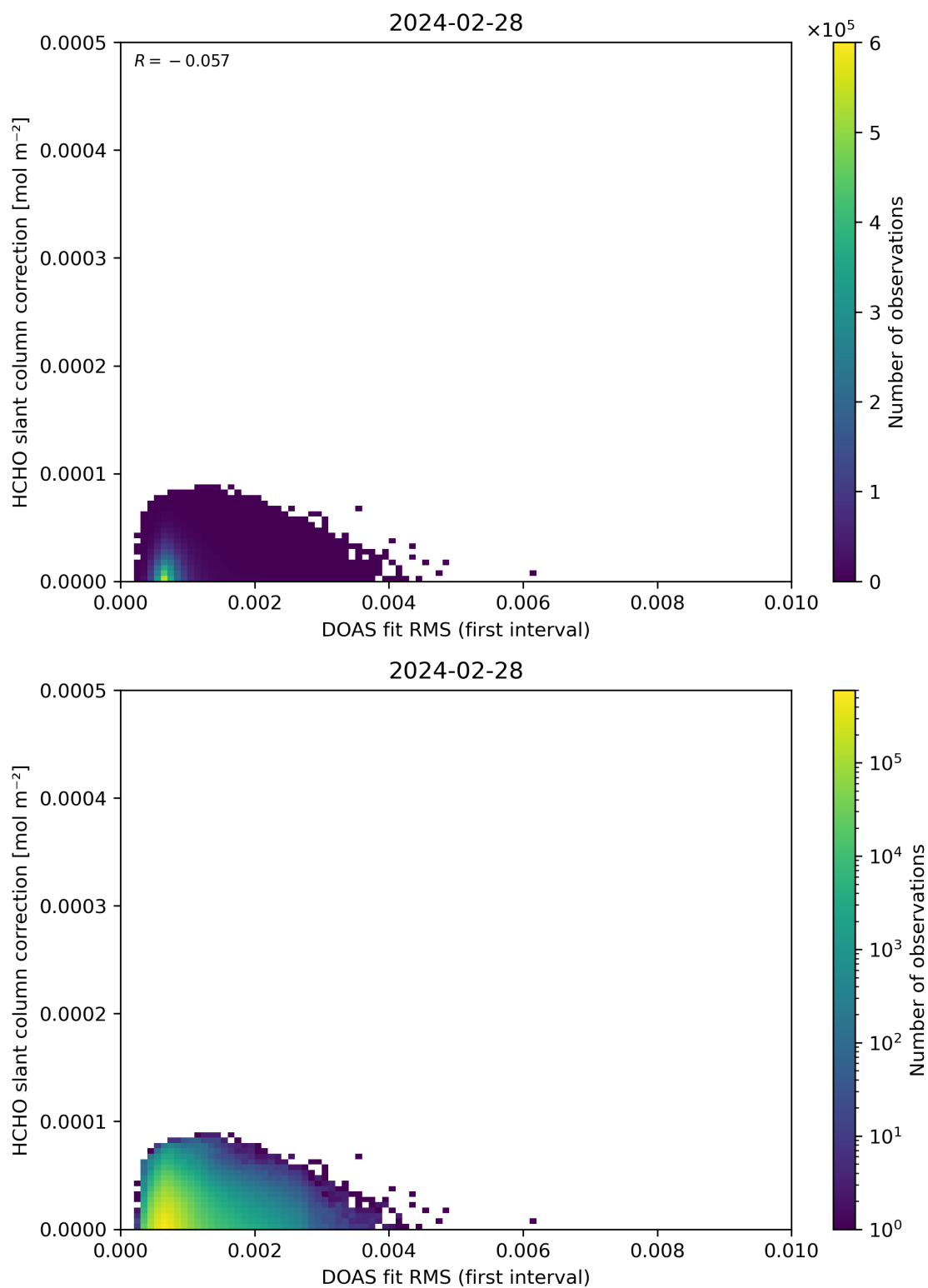
Figure 63: Scatter density plot of “DOAS fit RMS (first interval)” against “HCHO slant column correction” for 2024-02-27 to 2024-02-29.
