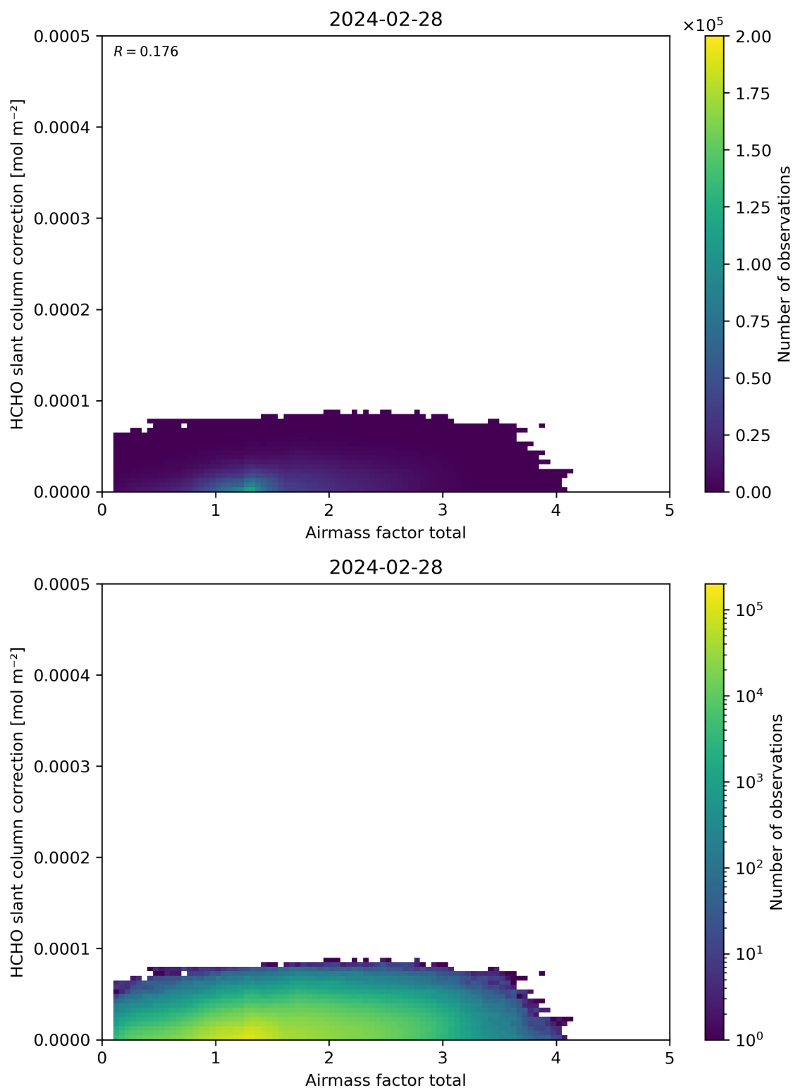
Figure 102: Scatter density plot of “Airmass factor total” against “HCHO slant column correction” for 2024-02-27 to 2024-02-29.
