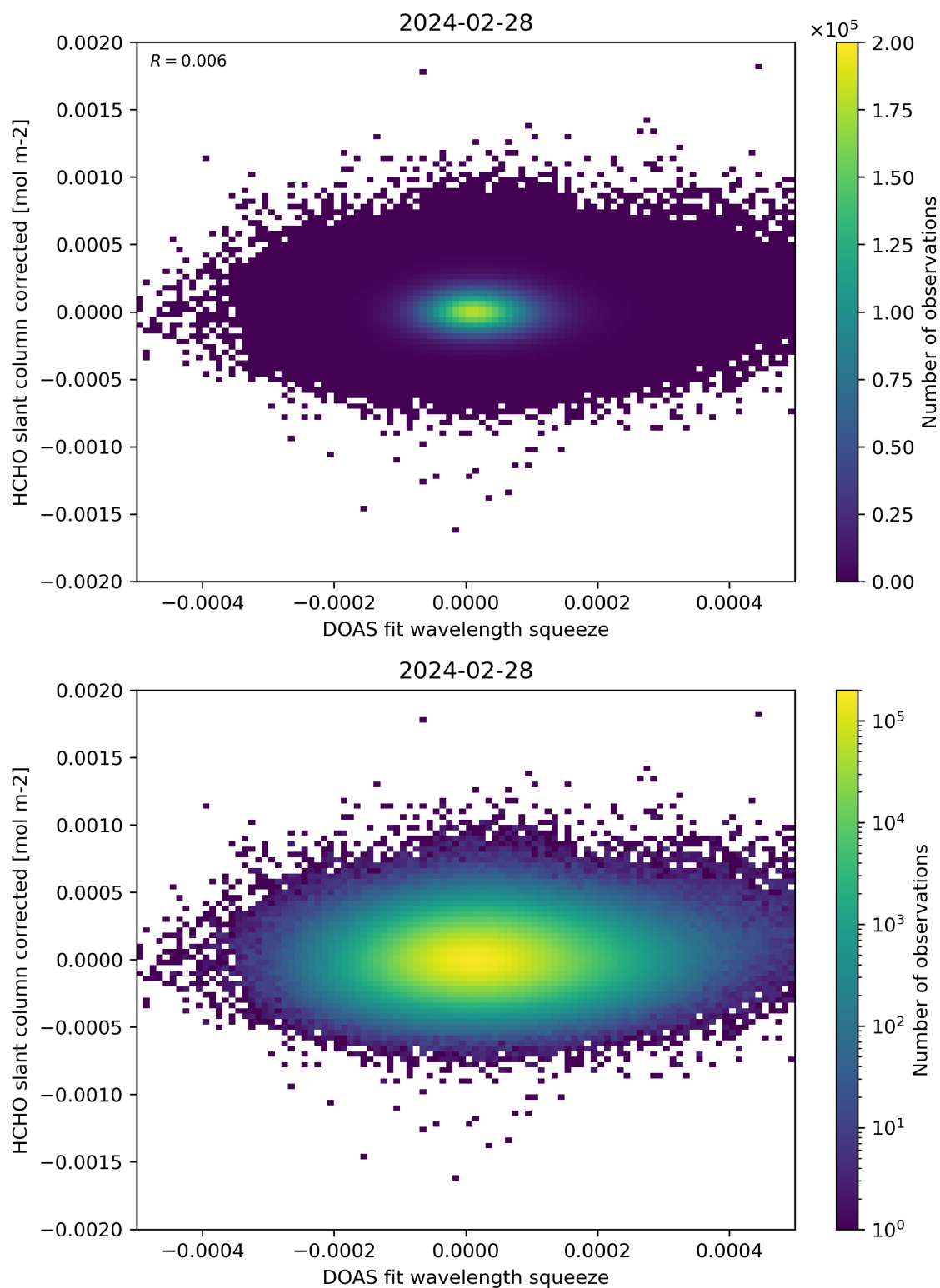
Figure 69: Scatter density plot of “DOAS fit wavelength squeeze” against “HCHO slant column corrected” for 2024-02-27 to 2024-02-29.
