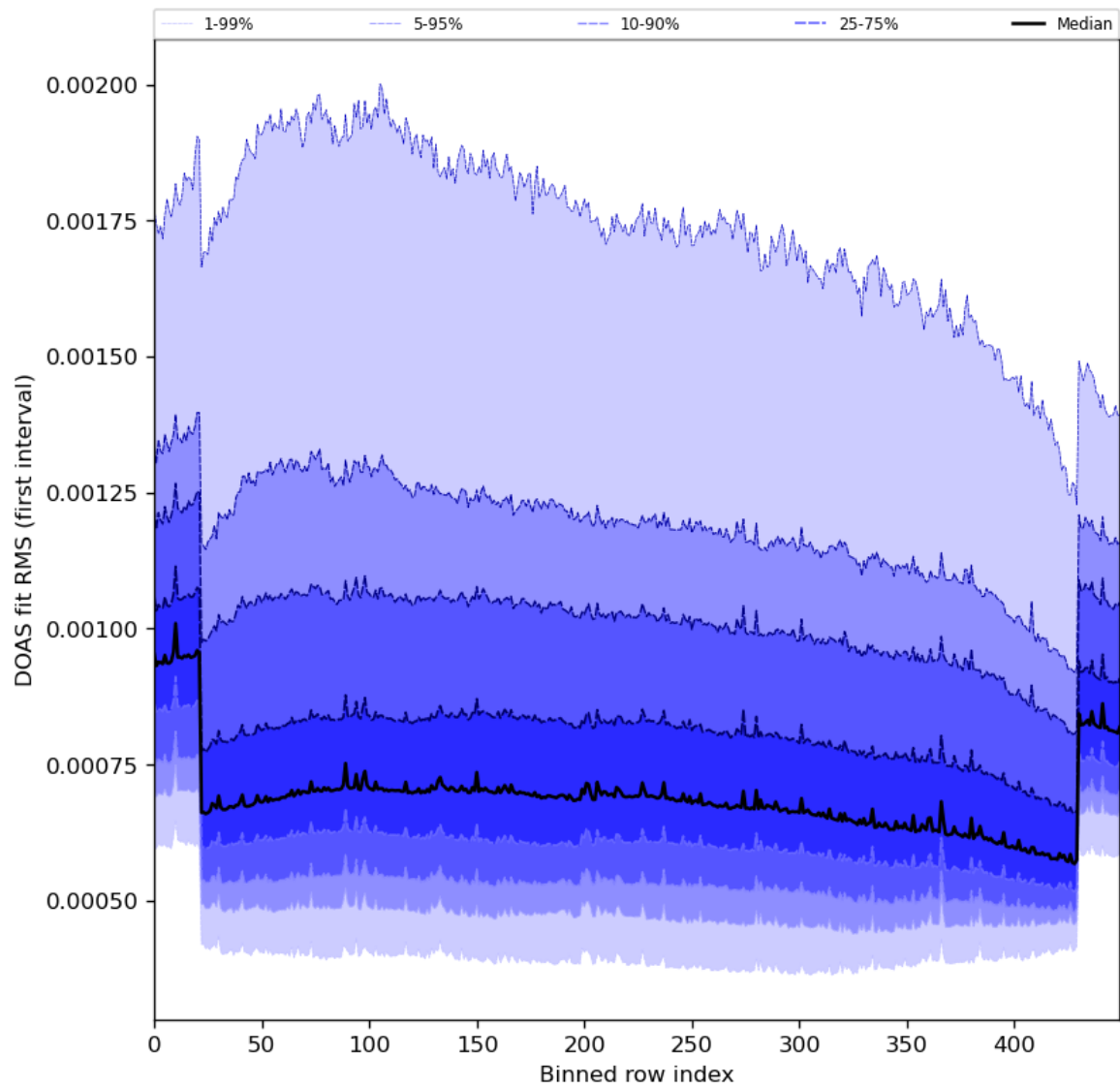
Figure 60: Along track statistics of “DOAS fit RMS (first interval)” for 2024-02-27 to 2024-02-29
