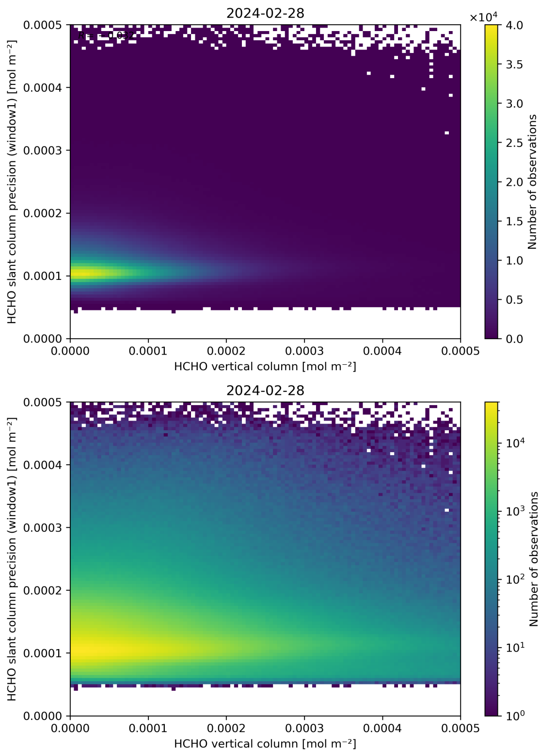
Figure 130: Scatter density plot of “HCHO vertical column” against “HCHO slant column precision (window1)” for 2024-02-27 to 2024-02-29.
