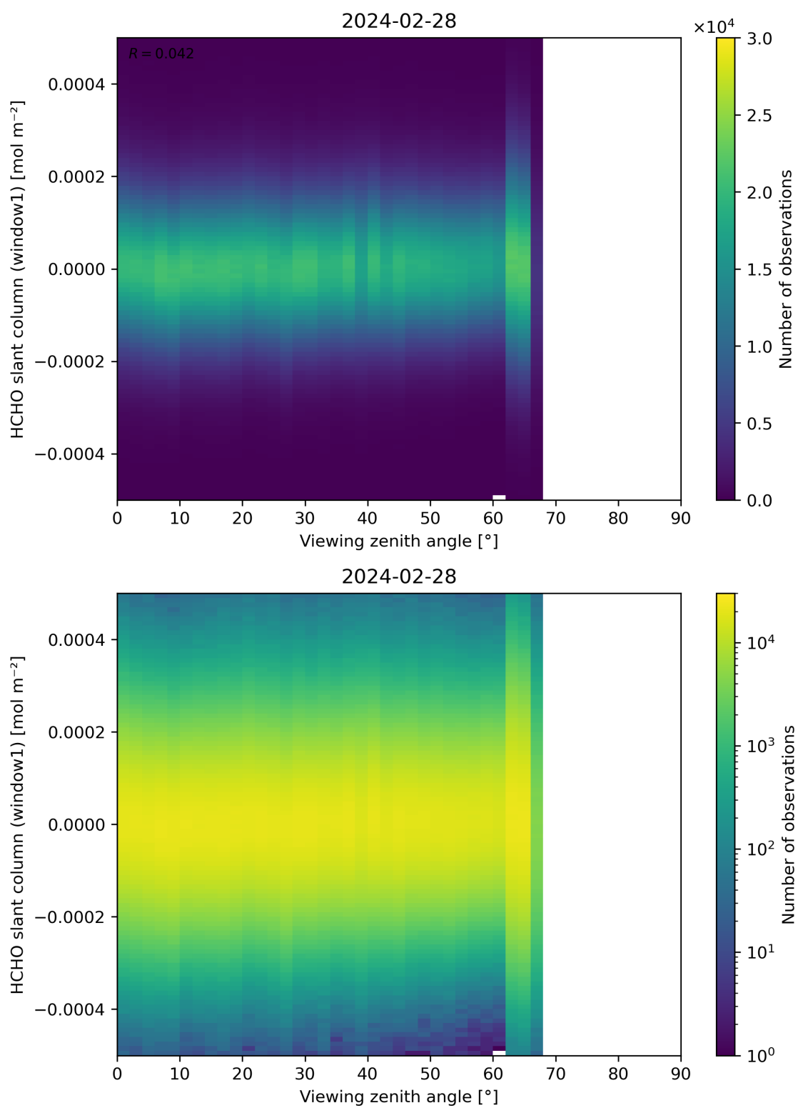
Figure 188: Scatter density plot of “Viewing zenith angle” against “HCHO slant column (window1)” for 2024-02-27 to 2024-02-29.
