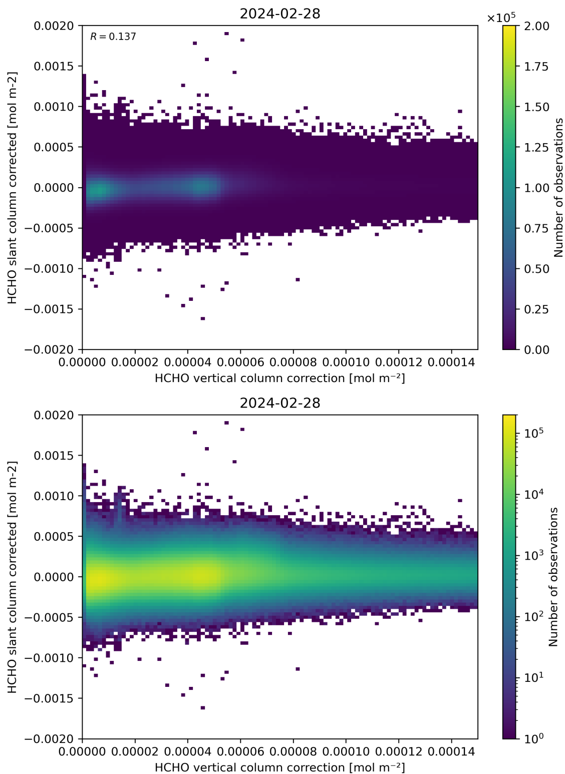
Figure 116: Scatter density plot of “HCHO vertical column correction” against “HCHO slant column corrected” for 2024-02-27 to 2024-02-29.
