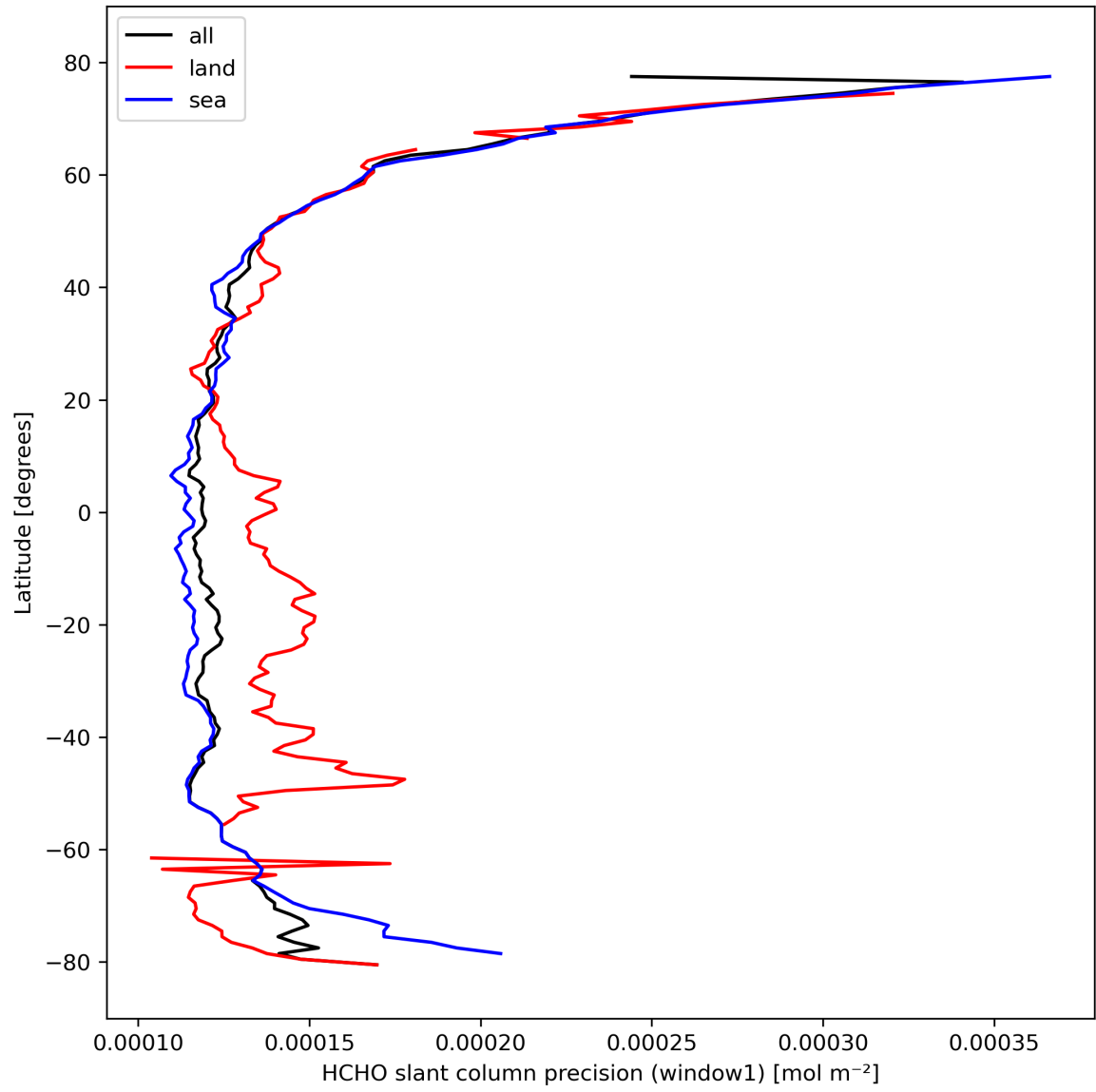
Figure 25: Zonal average of “HCHO slant column precision (window1)” for 2024-02-27 to 2024-02-29.
