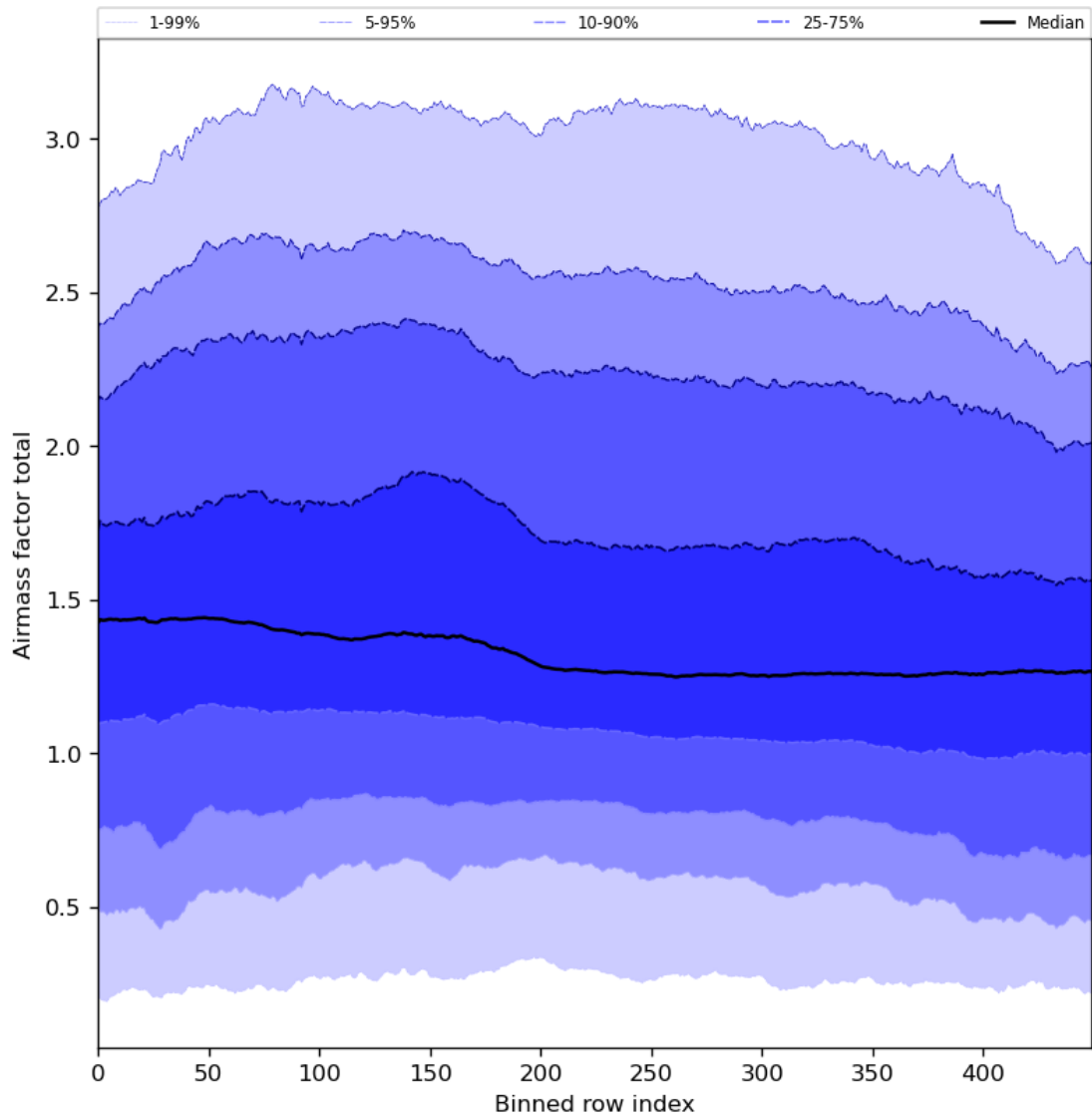
Figure 54: Along track statistics of “Airmass factor total” for 2024-02-27 to 2024-02-29
