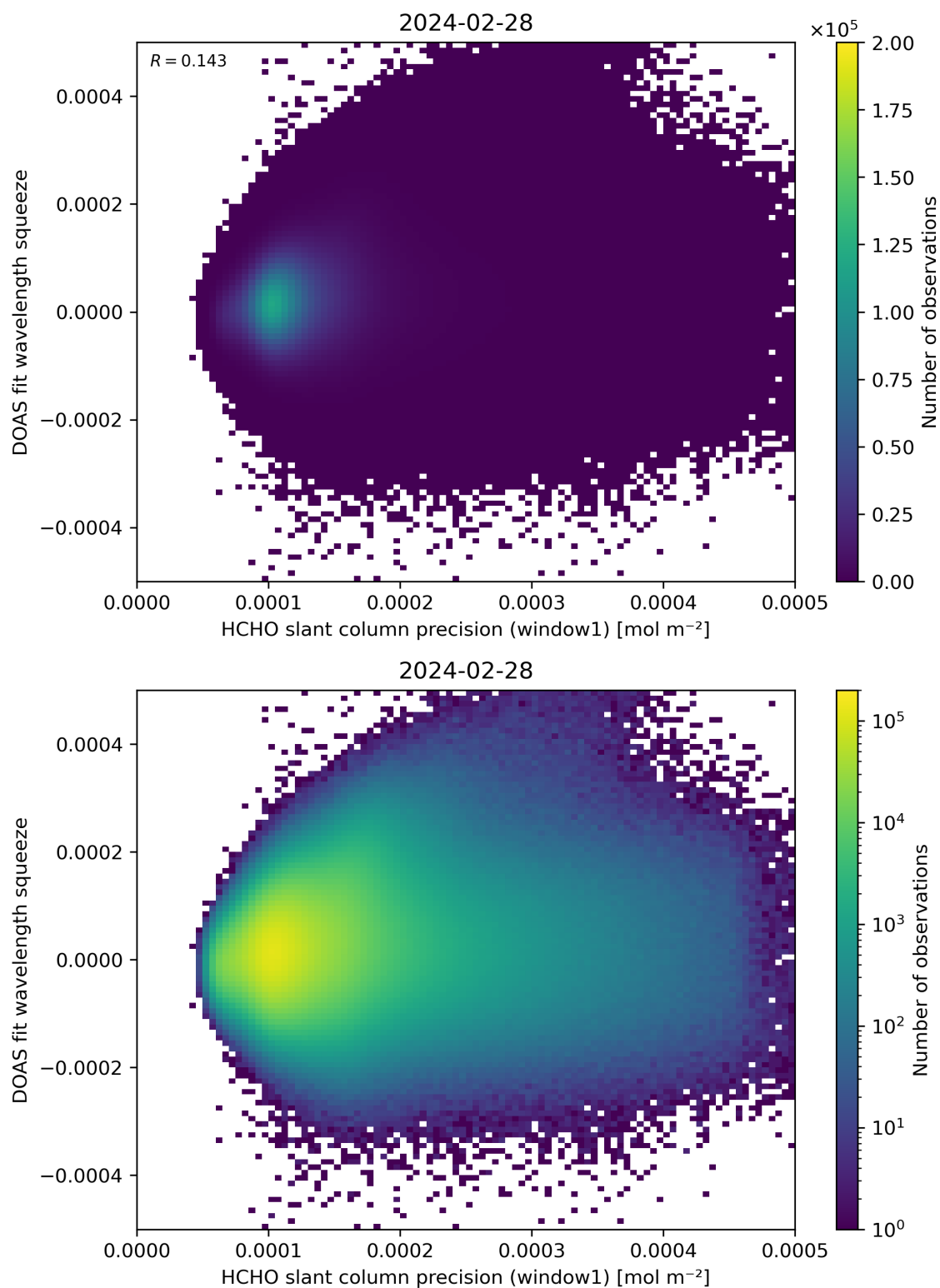
Figure 90: Scatter density plot of “HCHO slant column precision (window1)” against “DOAS fit wavelength squeeze” for 2024-02-27 to 2024-02-29.
