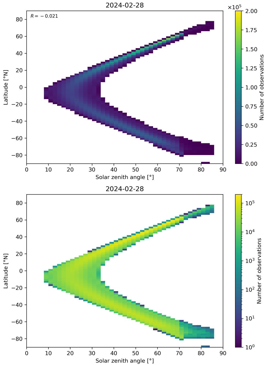
Figure 181: Scatter density plot of “Solar zenith angle” against “Latitude” for 2024-02-27 to 2024-02-29.
