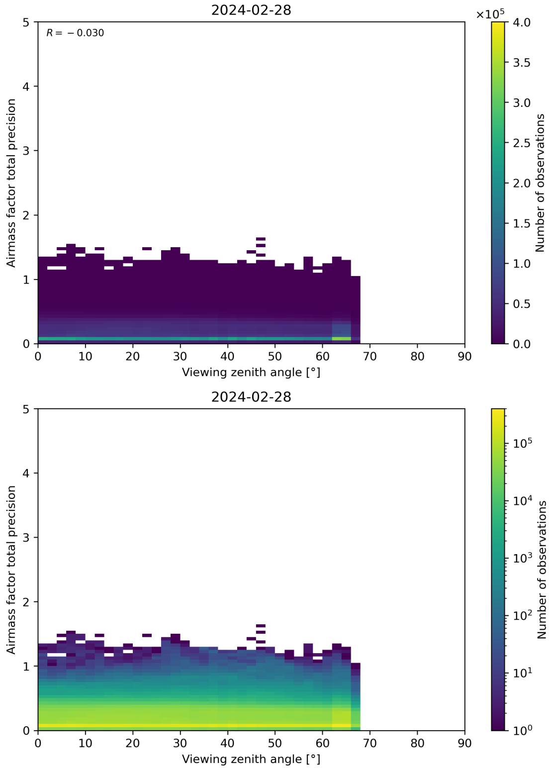
Figure 191: Scatter density plot of “Viewing zenith angle” against “Airmass factor total precision” for 2024-02-27 to 2024-02-29.
