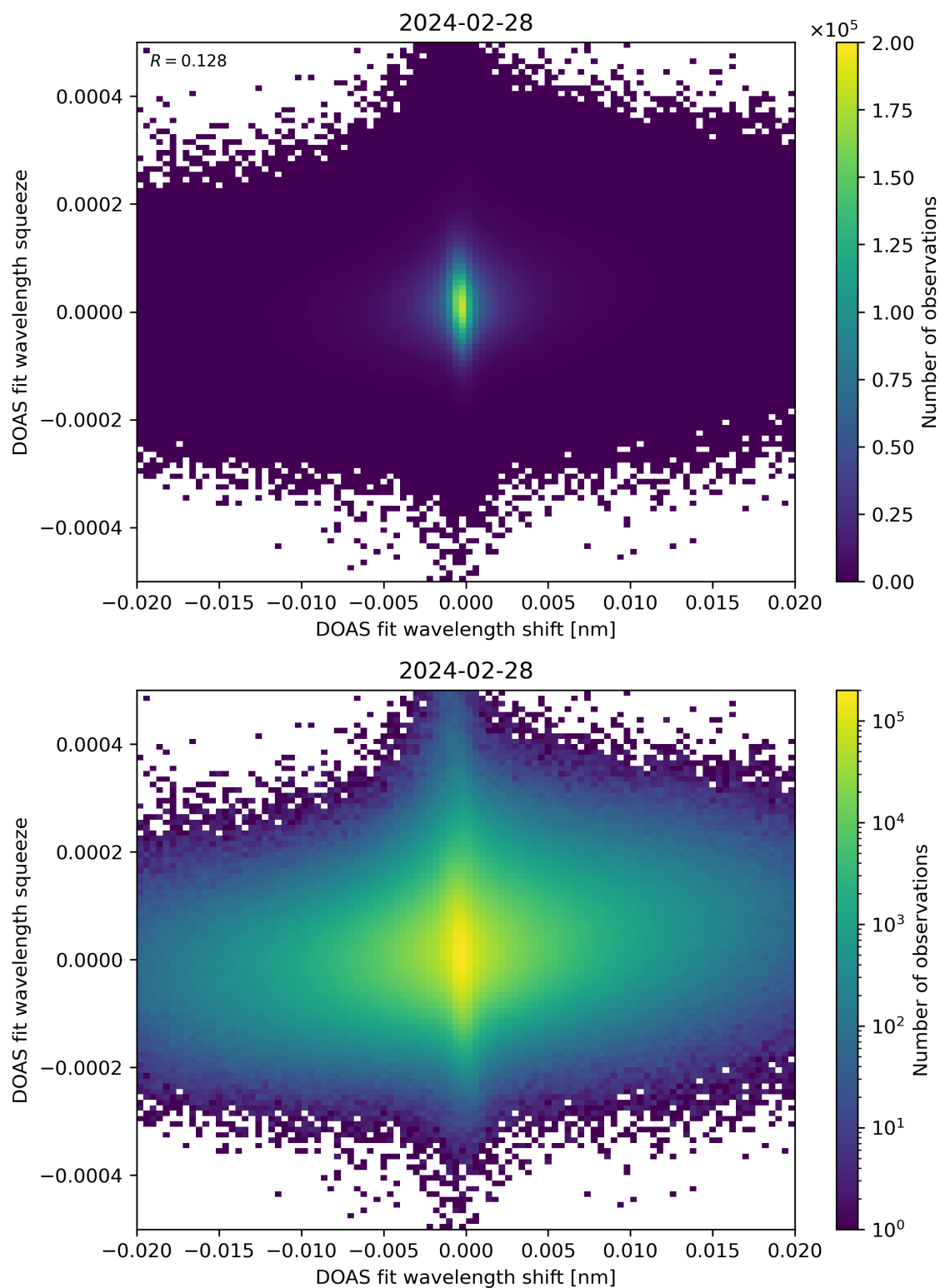
Figure 65: Scatter density plot of “DOAS fit wavelength shift” against “DOAS fit wavelength squeeze” for 2024-02-27 to 2024-02-29.
