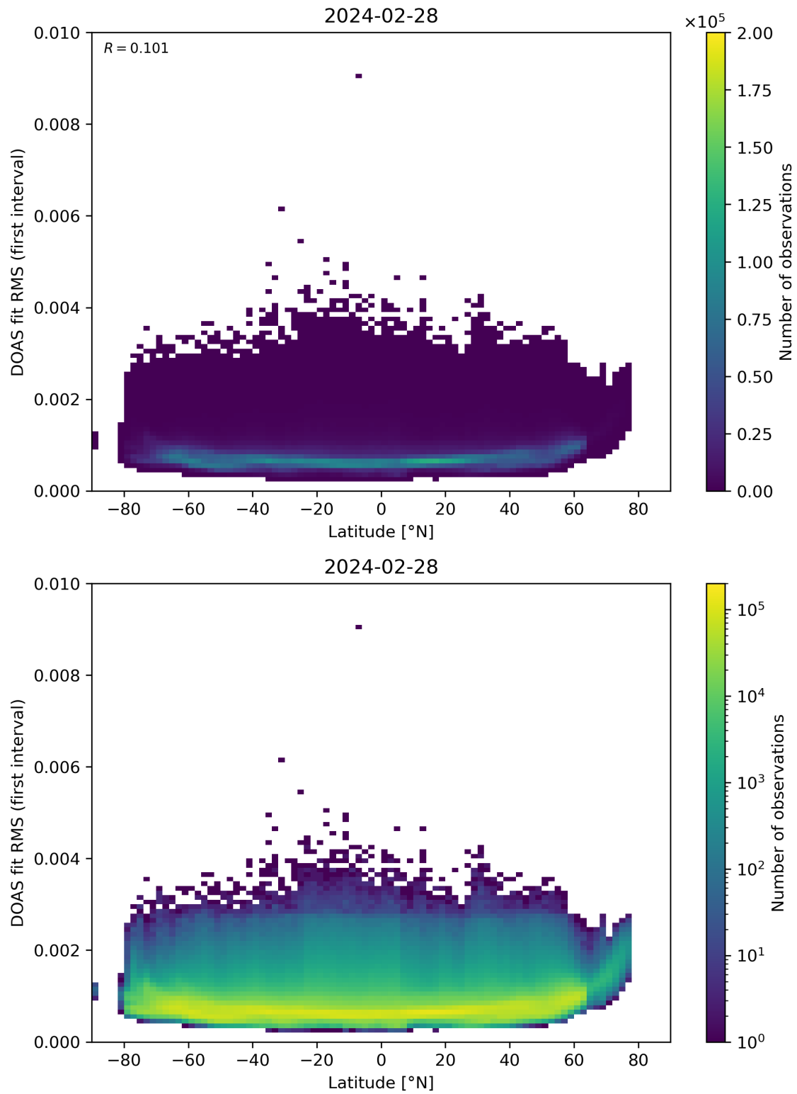
Figure 153: Scatter density plot of “Latitude” against “DOAS fit RMS (first interval)” for 2024-02-27 to 2024-02-29.
