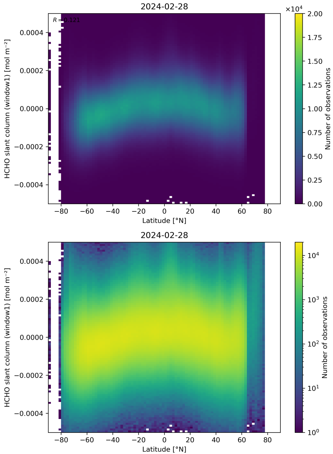
Figure 159: Scatter density plot of “Latitude” against “HCHO slant column (window1)” for 2024-02-27 to 2024-02-29.
