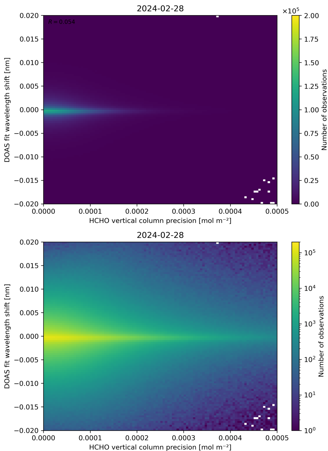
Figure 137: Scatter density plot of “HCHO vertical column precision” against “DOAS fit wavelength shift” for 2024-02-27 to 2024-02-29.
