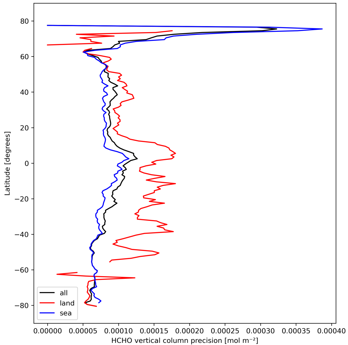
Figure 22: Zonal average of “HCHO vertical column precision” for 2024-02-27 to 2024-02-29.
