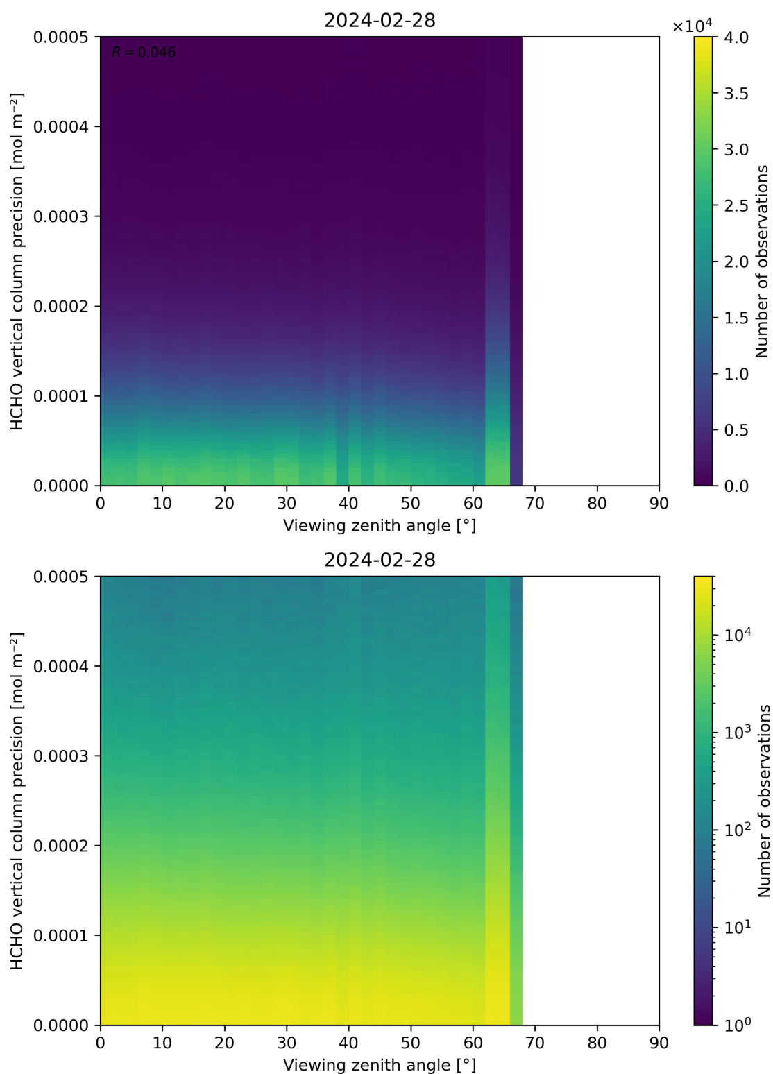
Figure 194: Scatter density plot of “Viewing zenith angle” against “HCHO vertical column precision” for 2024-02-27 to 2024-02-29.
