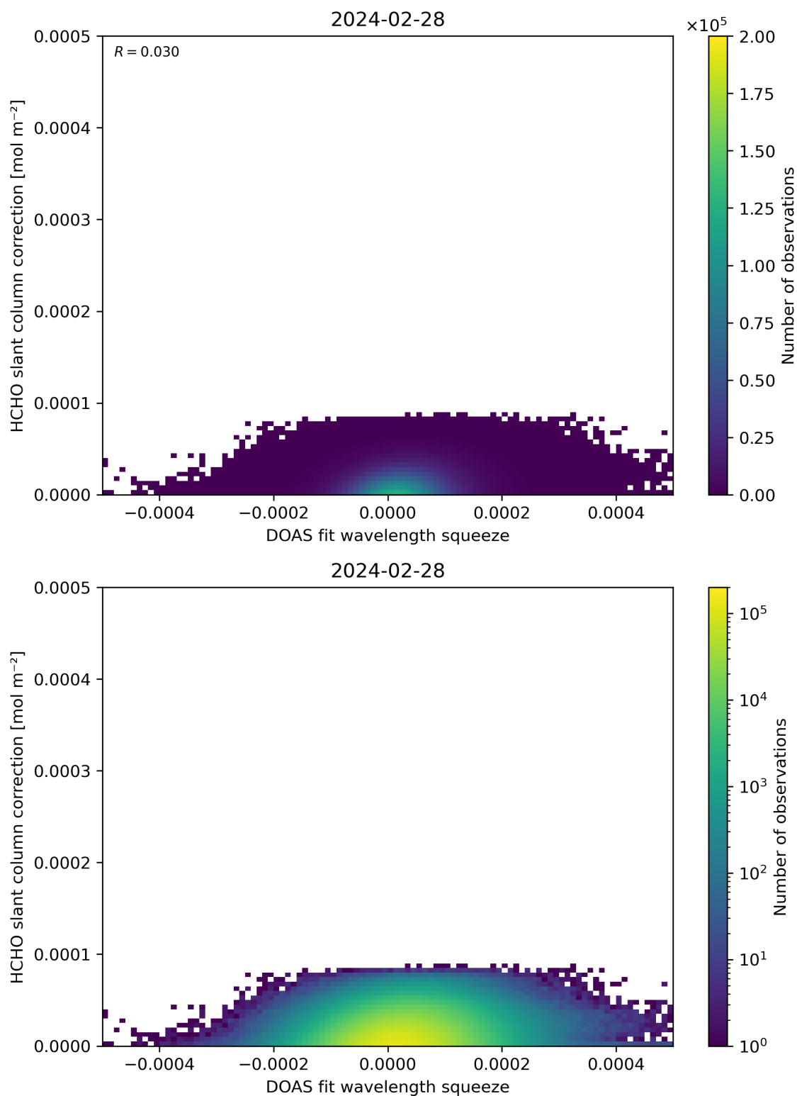
Figure 70: Scatter density plot of “DOAS fit wavelength squeeze” against “HCHO slant column correction” for 2024-02-27 to 2024-02-29.
