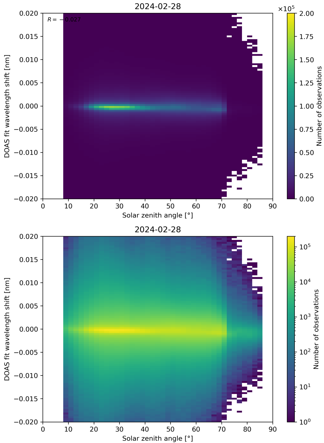
Figure 168: Scatter density plot of “Solar zenith angle” against “DOAS fit wavelength shift” for 2024-02-27 to 2024-02-29.
