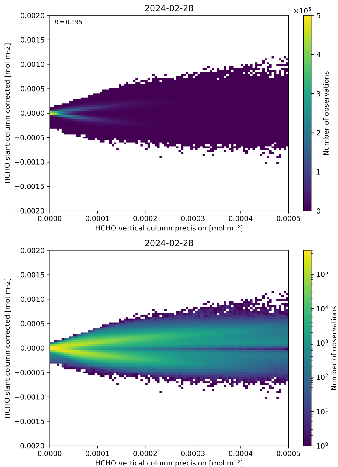
Figure 140: Scatter density plot of “HCHO vertical column precision” against “HCHO slant column corrected” for 2024-02-27 to 2024-02-29.
