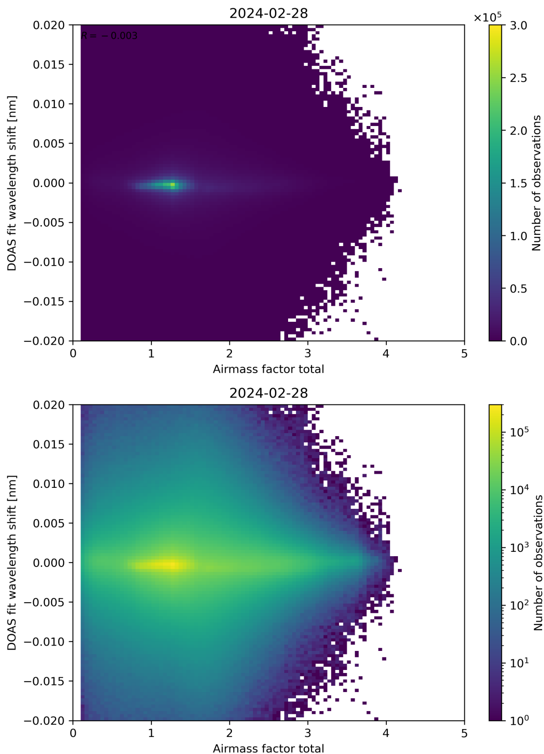
Figure 98: Scatter density plot of “Airmass factor total” against “DOAS fit wavelength shift” for 2024-02-27 to 2024-02-29.
