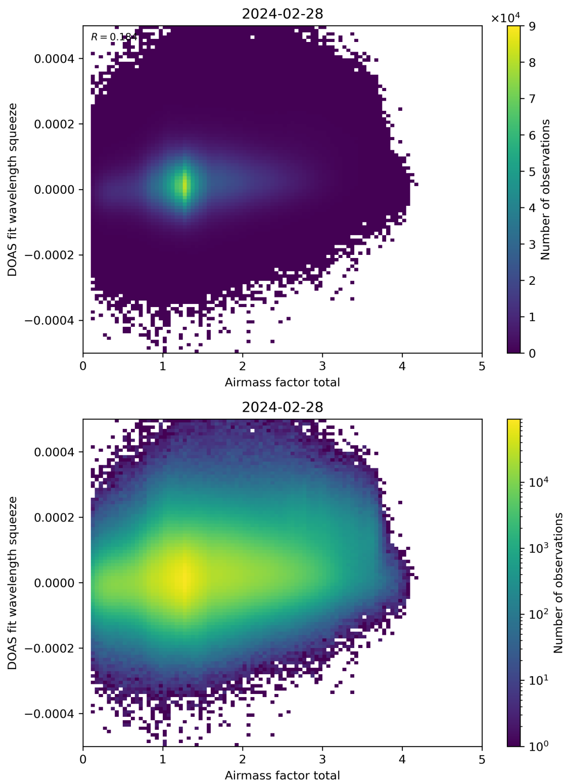
Figure 99: Scatter density plot of “Airmass factor total” against “DOAS fit wavelength squeeze” for 2024-02-27 to 2024-02-29.
