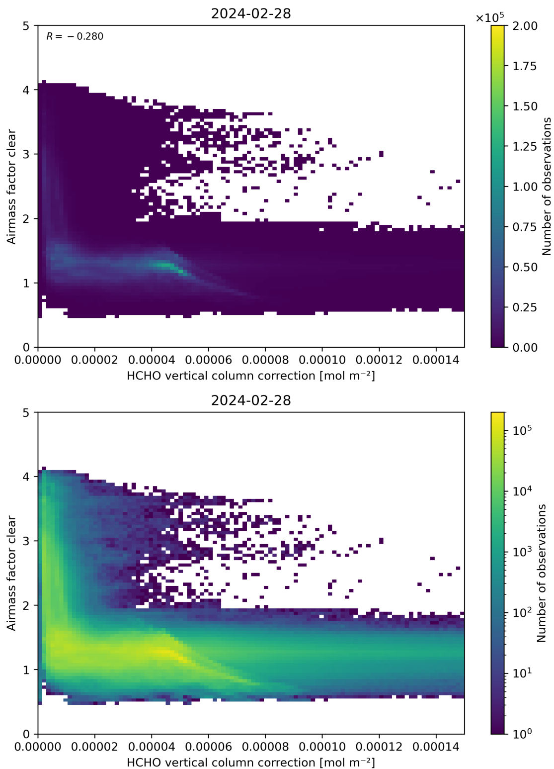
Figure 115: Scatter density plot of “HCHO vertical column correction” against “Airmass factor clear” for 2024-02-27 to 2024-02-29.
