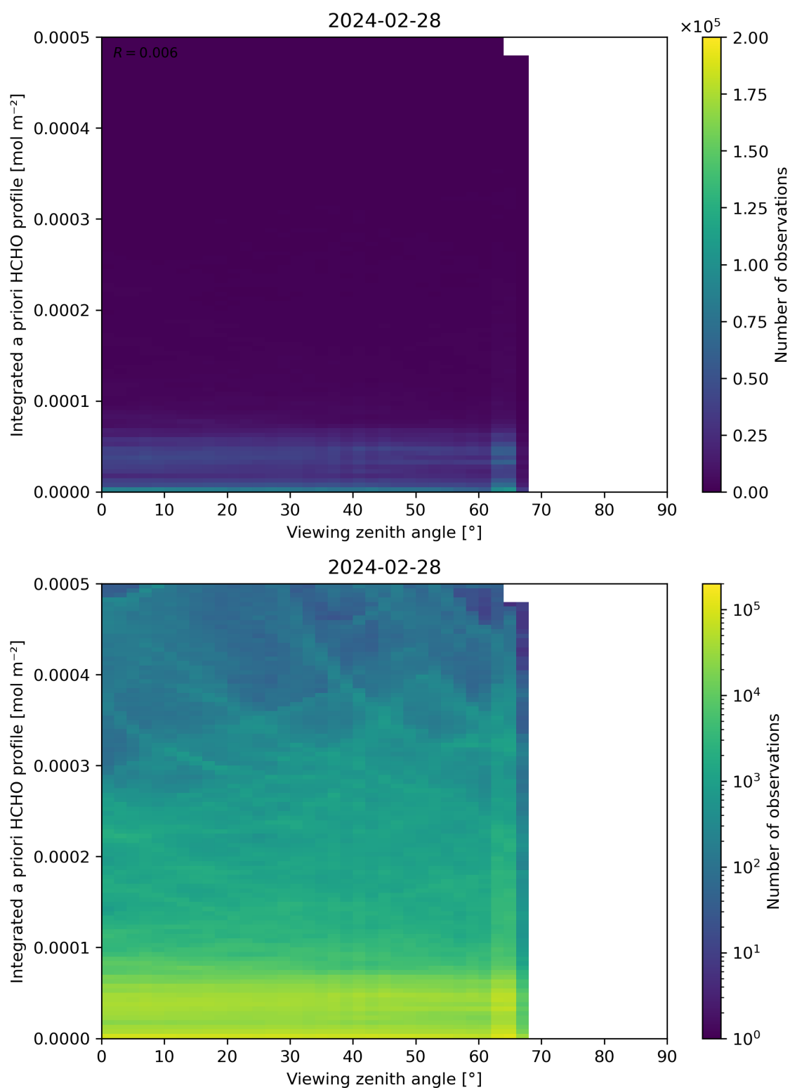
Figure 195: Scatter density plot of “Viewing zenith angle” against “Integrated a priori HCHO profile” for 2024-02-27 to 2024-02-29.
