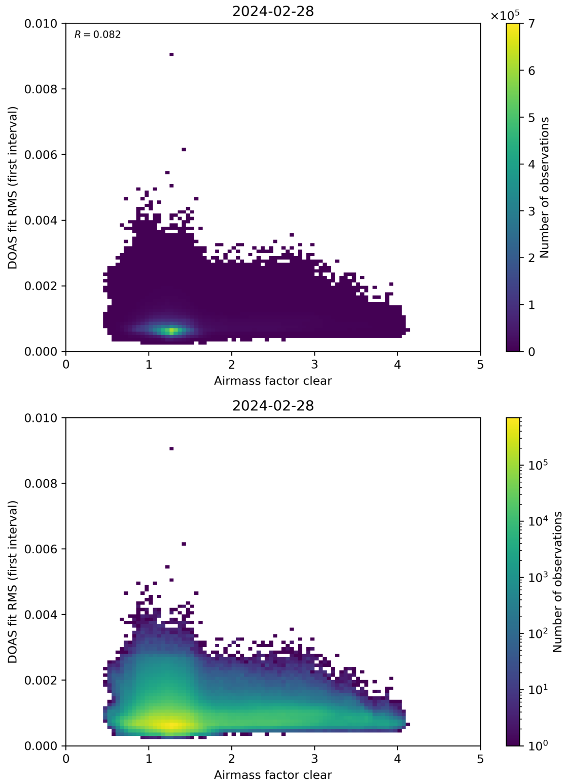
Figure 71: Scatter density plot of “Airmass factor clear” against “DOAS fit RMS (first interval)” for 2024-02-27 to 2024-02-29.
