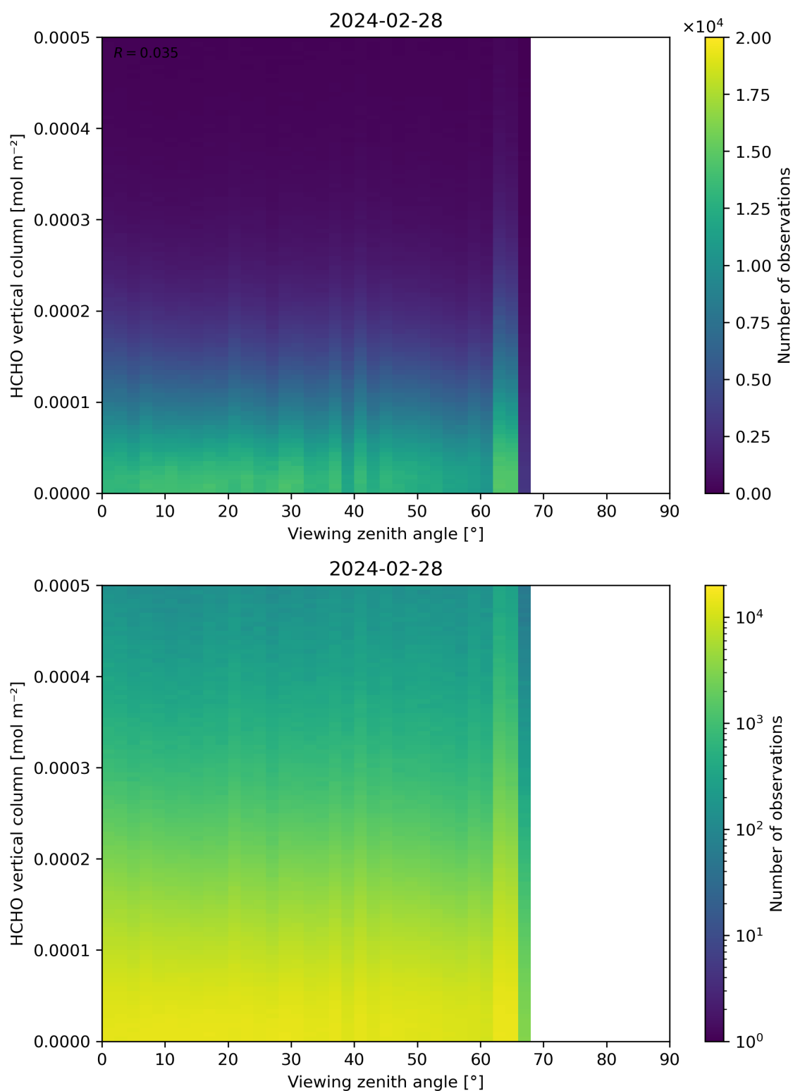
Figure 192: Scatter density plot of “Viewing zenith angle” against “HCHO vertical column” for 2024-02-27 to 2024-02-29.
