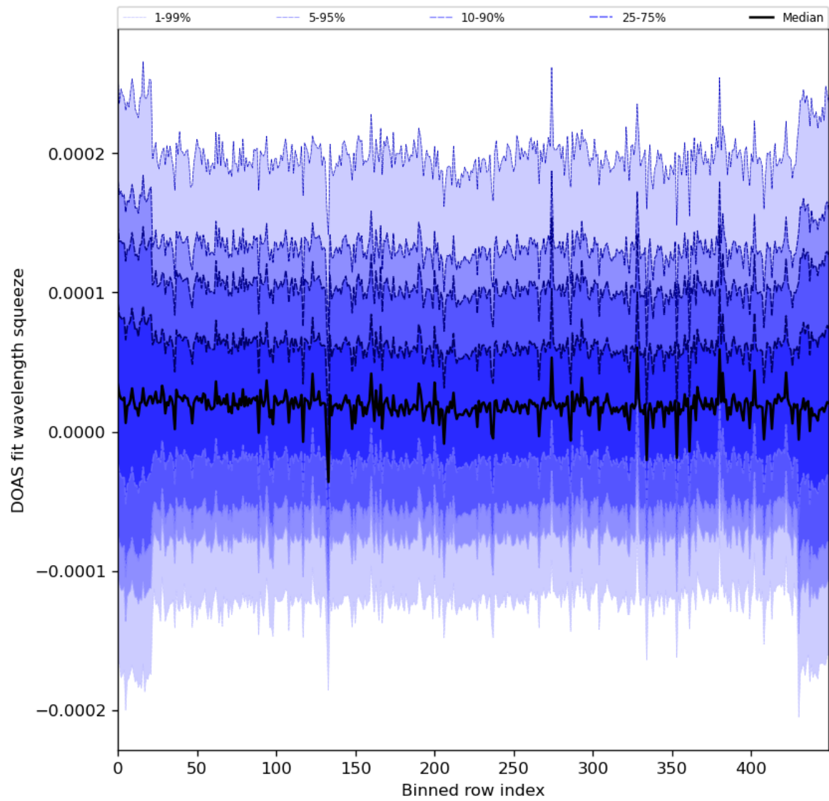
Figure 59: Along track statistics of “DOAS fit wavelength squeeze” for 2024-02-27 to 2024-02-29
