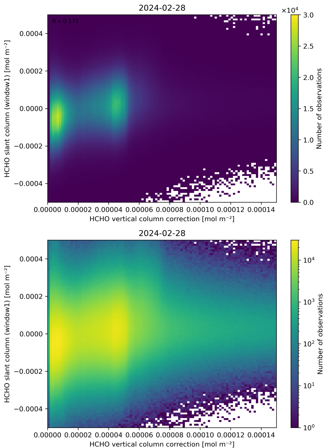
Figure 118: Scatter density plot of “HCHO vertical column correction” against “HCHO slant column (window1)” for 2024-02-27 to 2024-02-29.
