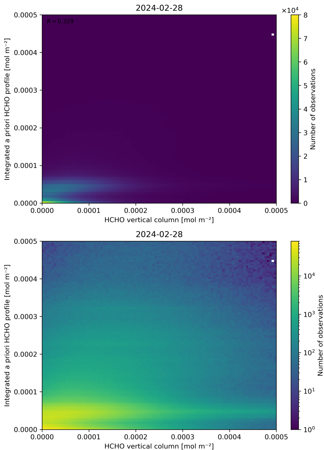
Figure 135: Scatter density plot of “HCHO vertical column” against “Integrated a priori HCHO profile” for 2024-02-27 to 2024-02-29.
