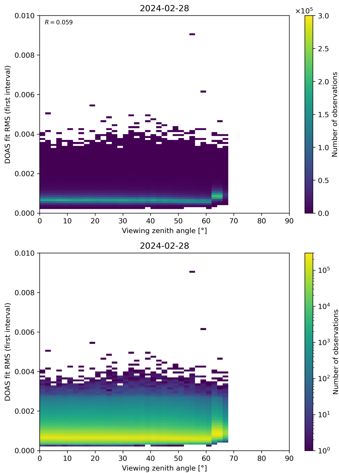
Figure 182: Scatter density plot of “Viewing zenith angle” against “DOAS fit RMS (first interval)” for 2024-02-27 to 2024-02-29.
