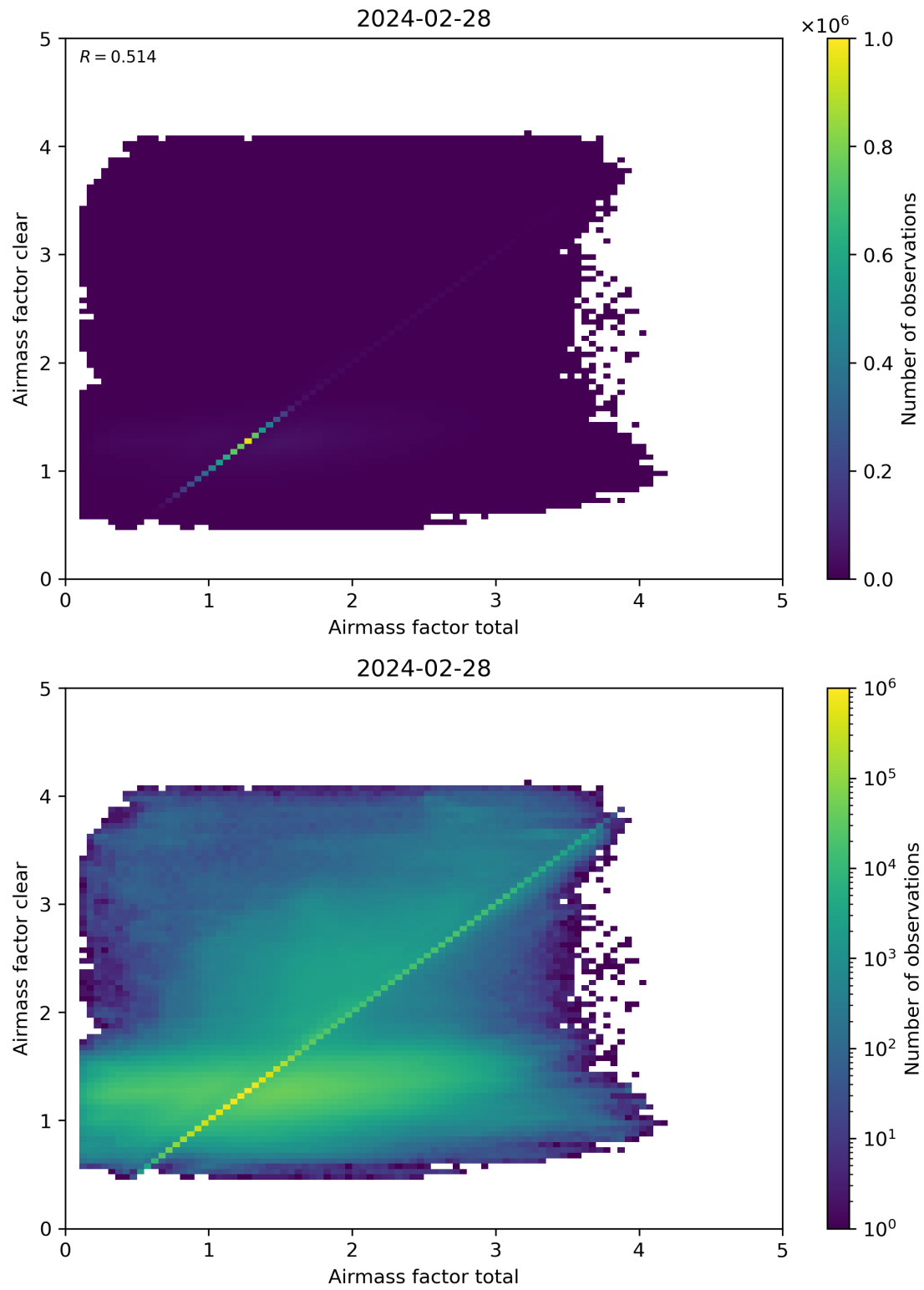
Figure 100: Scatter density plot of “Airmass factor total” against “Airmass factor clear” for 2024-02-27 to 2024-02-29.
