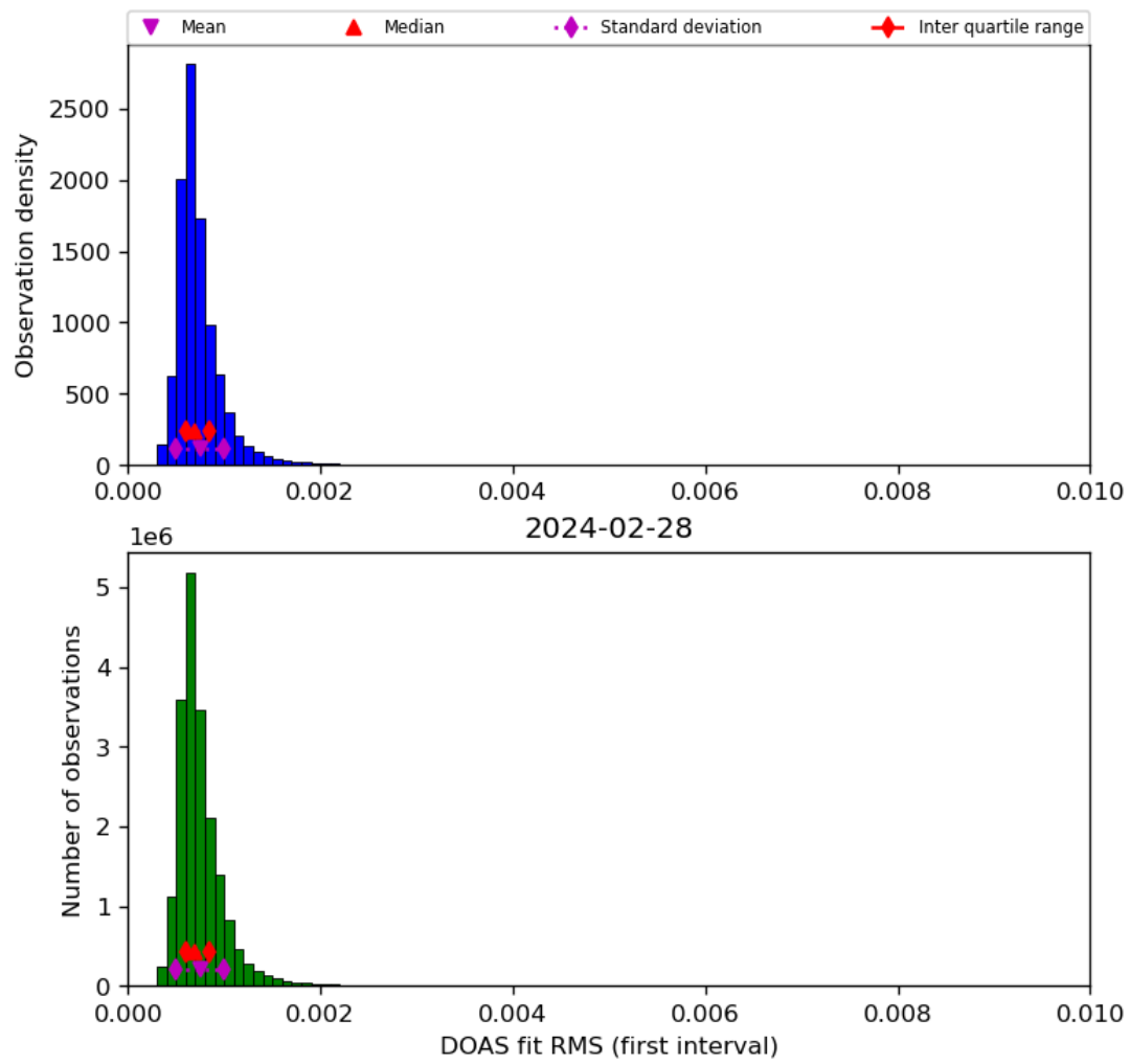
Figure 46: Histogram of “DOAS fit RMS (first interval)” for 2024-02-27 to 2024-02-29
