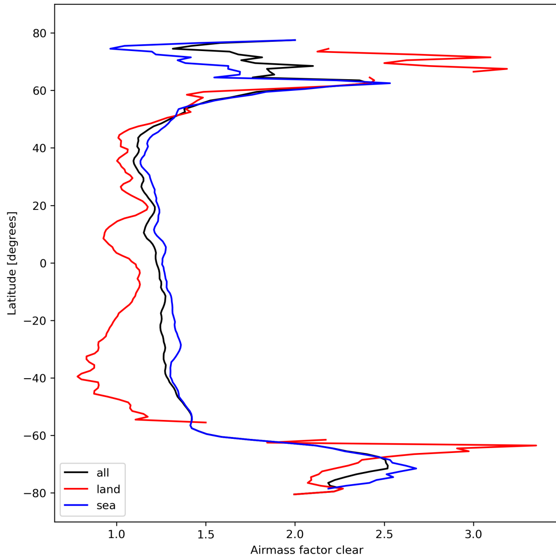
Figure 28: Zonal average of “Airmass factor clear” for 2024-02-27 to 2024-02-29.
