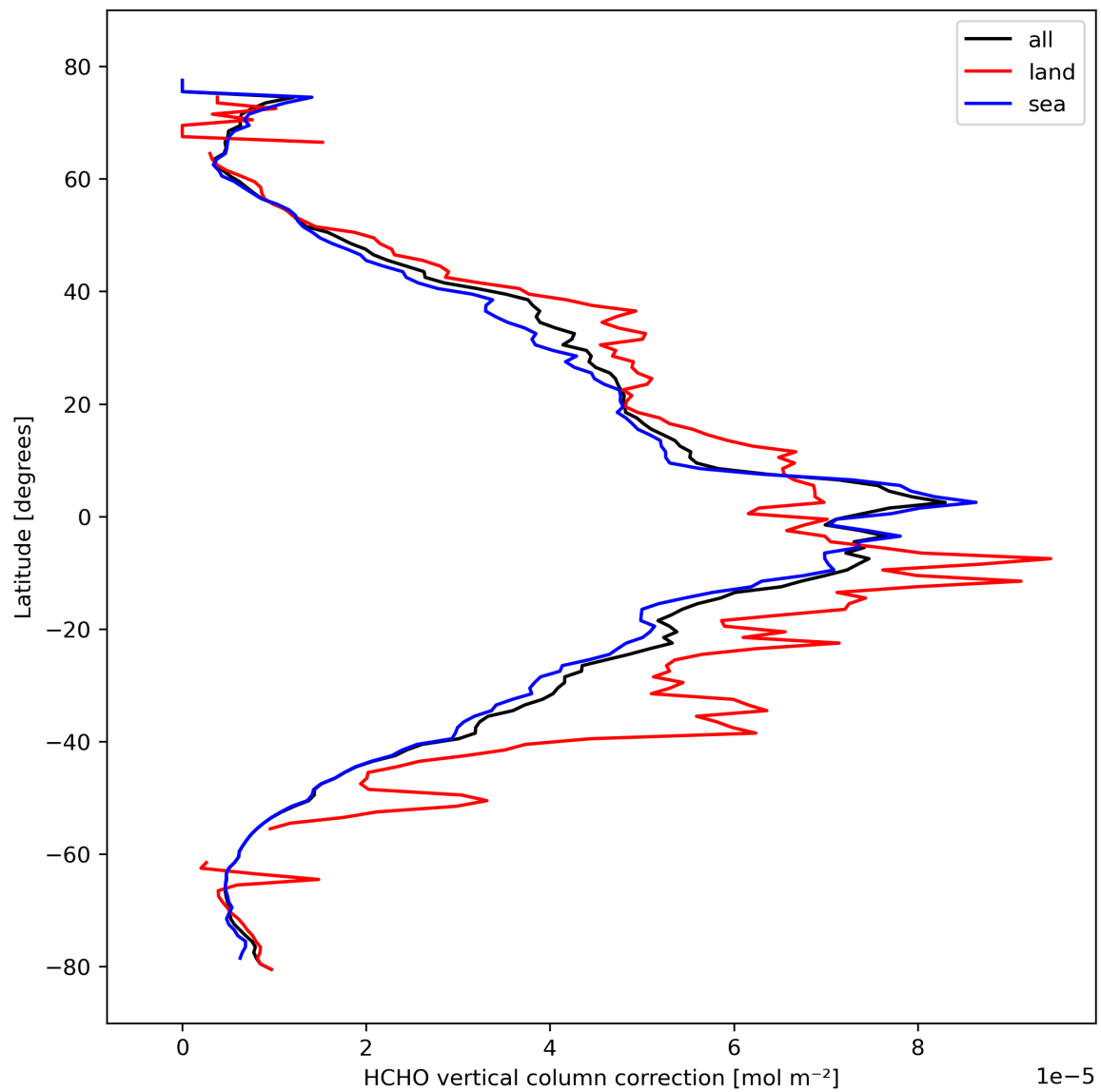
Figure 23: Zonal average of “HCHO vertical column correction” for 2024-02-27 to 2024-02-29.
