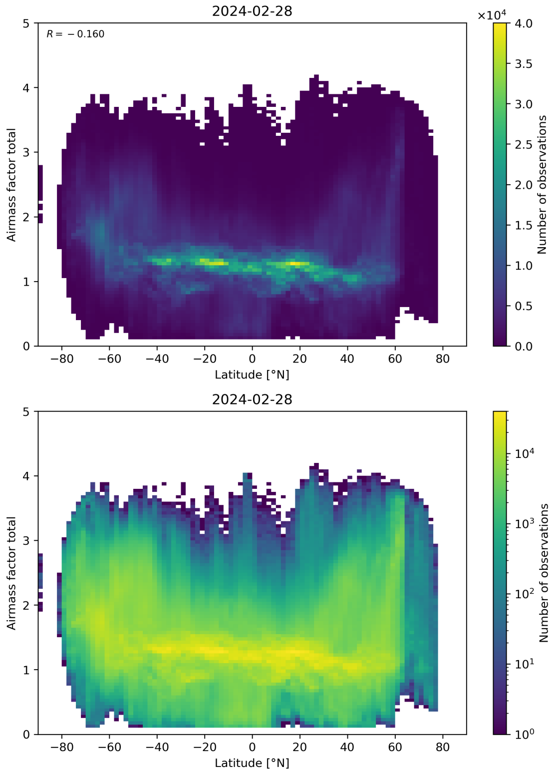
Figure 161: Scatter density plot of “Latitude” against “Airmass factor total” for 2024-02-27 to 2024-02-29.
