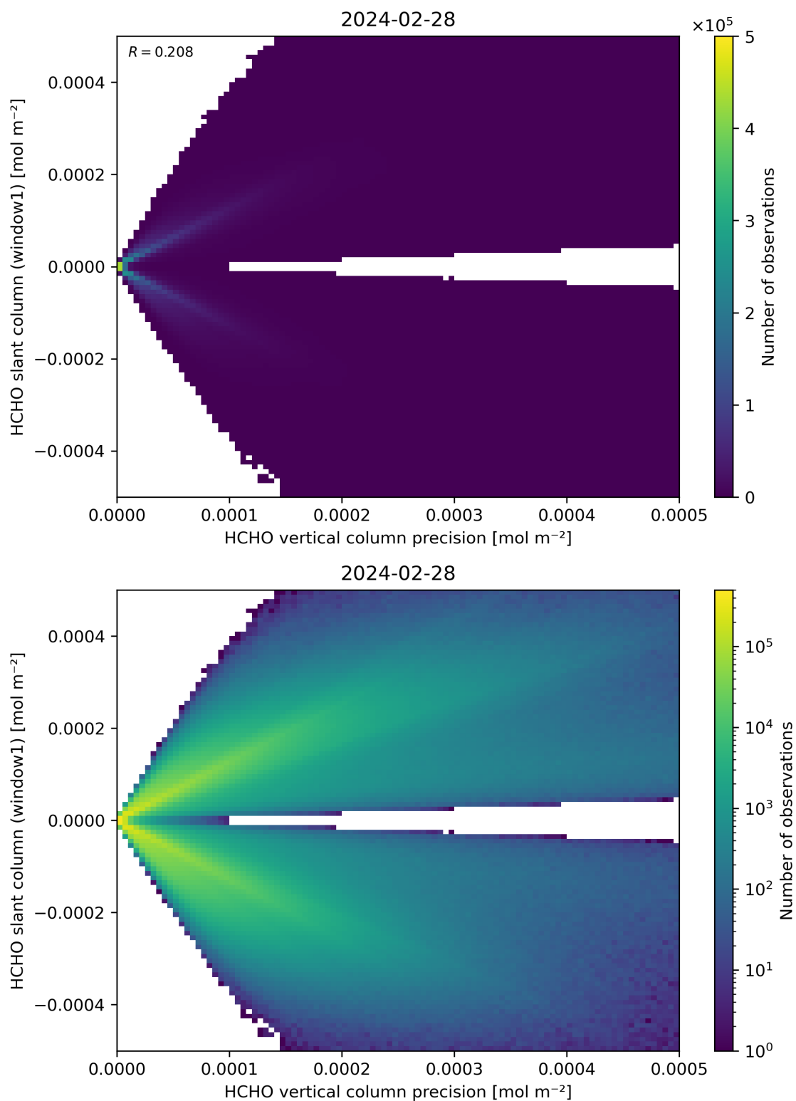
Figure 142: Scatter density plot of “HCHO vertical column precision” against “HCHO slant column (window1)” for 2024-02-27 to 2024-02-29.
