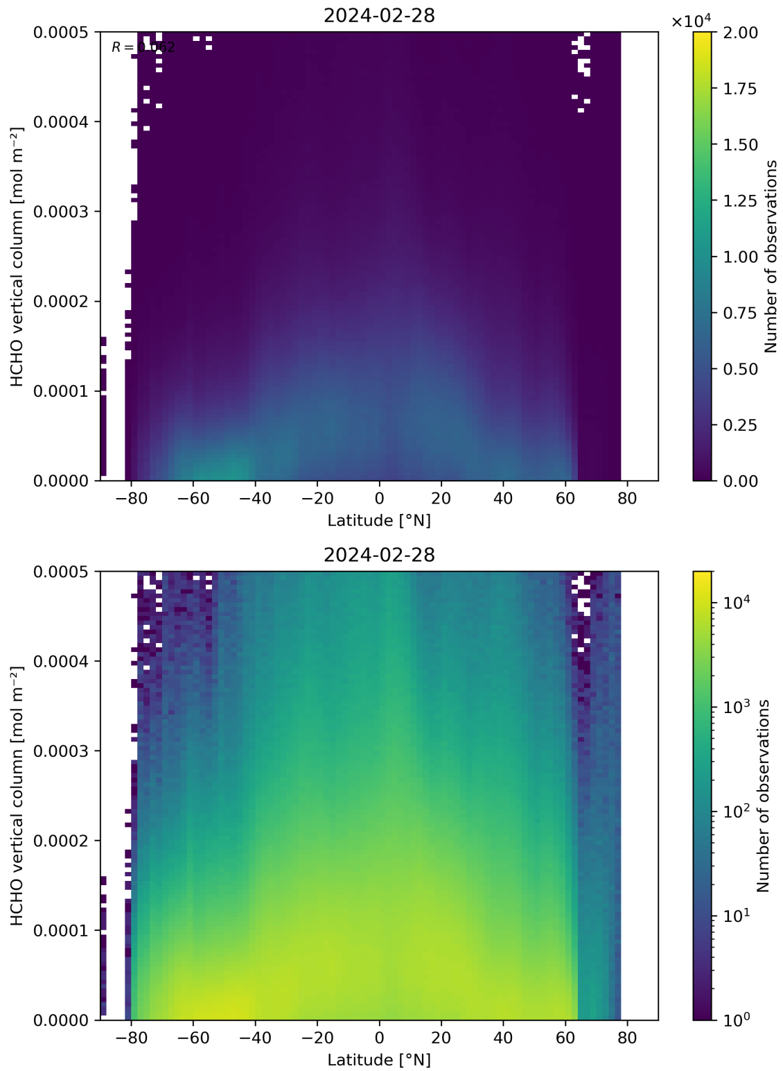
Figure 163: Scatter density plot of “Latitude” against “HCHO vertical column” for 2024-02-27 to 2024-02-29.
