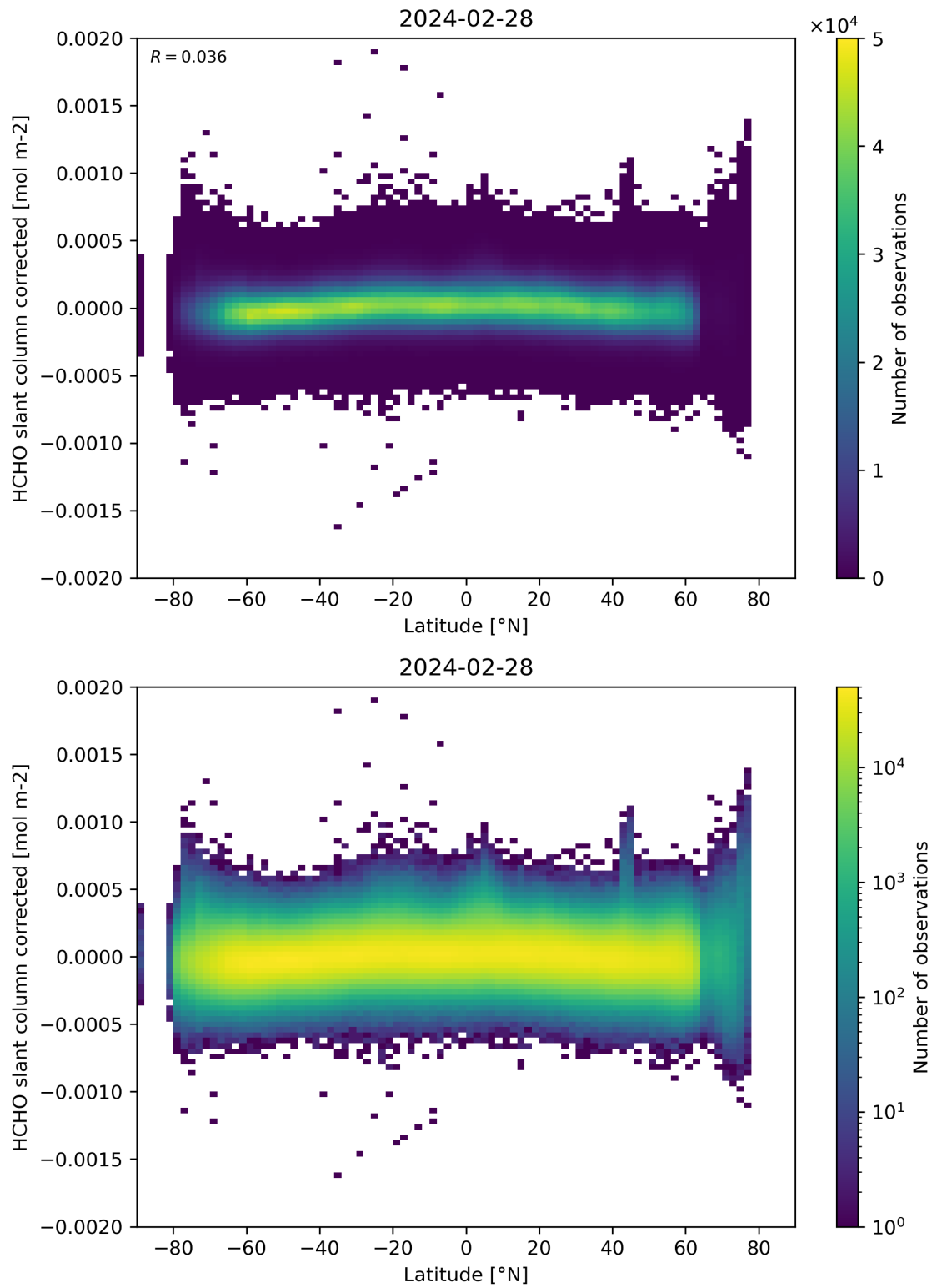
Figure 157: Scatter density plot of “Latitude” against “HCHO slant column corrected” for 2024-02-27 to 2024-02-29.
