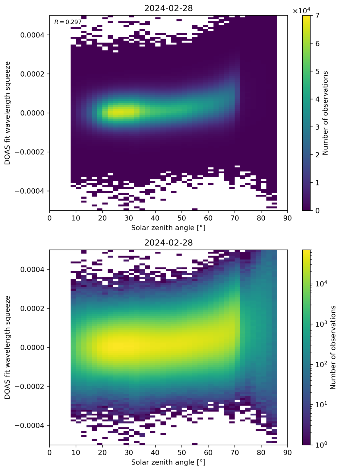
Figure 169: Scatter density plot of “Solar zenith angle” against “DOAS fit wavelength squeeze” for 2024-02-27 to 2024-02-29.
