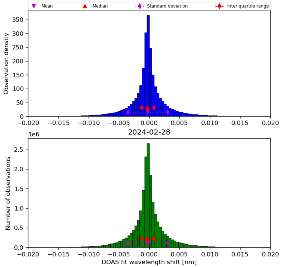
Figure 44: Histogram of “DOAS fit wavelength shift” for 2024-02-27 to 2024-02-29
