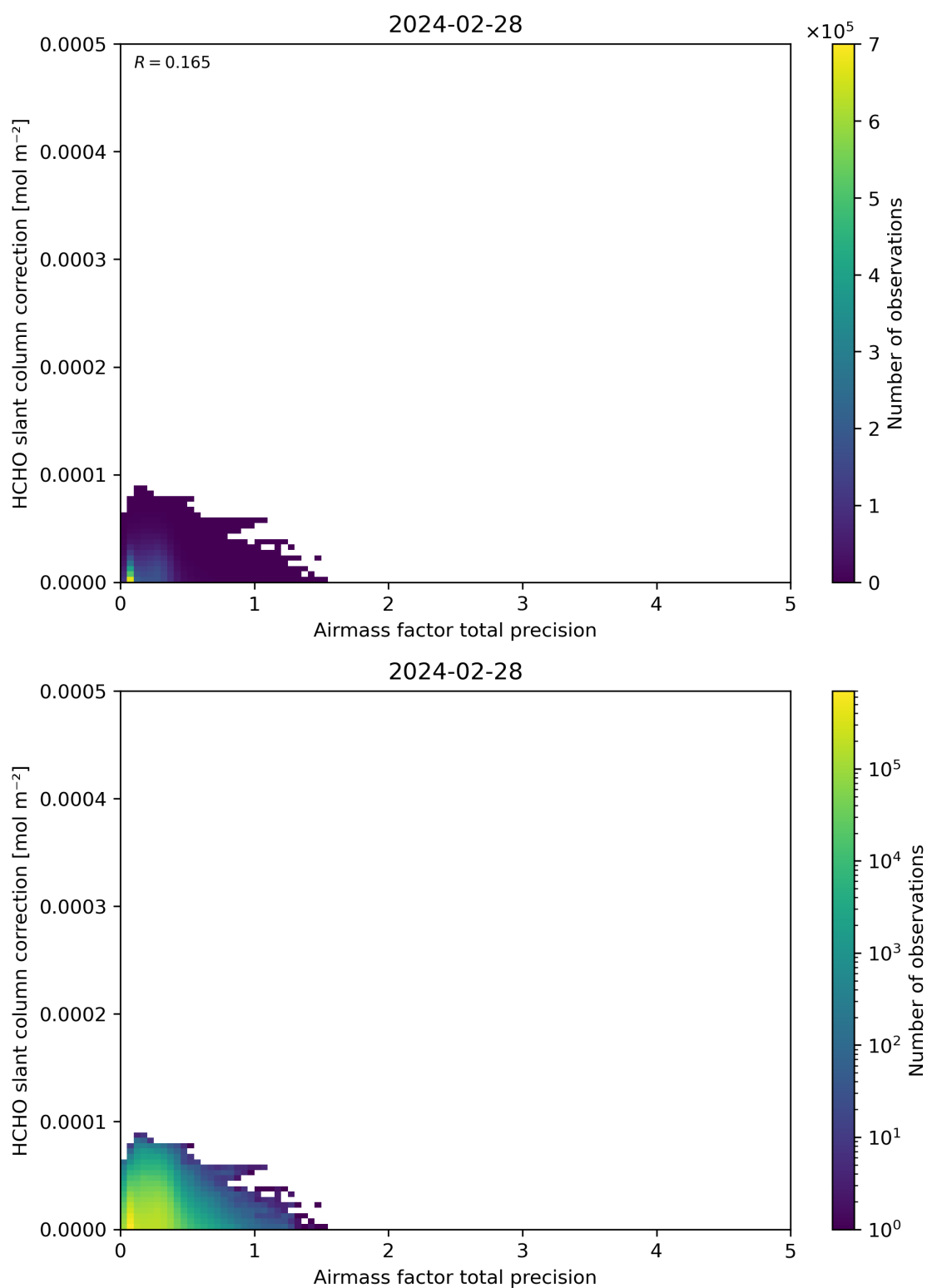
Figure 110: Scatter density plot of “Airmass factor total precision” against “HCHO slant column correction” for 2024-02-27 to 2024-02-29.
