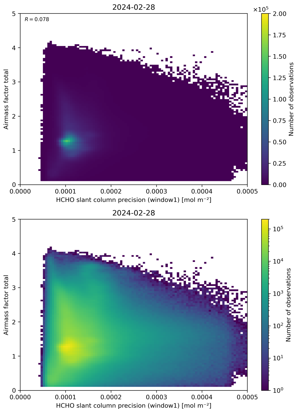
Figure 94: Scatter density plot of “HCHO slant column precision (window1)” against “Airmass factor total” for 2024-02-27 to 2024-02-29.
