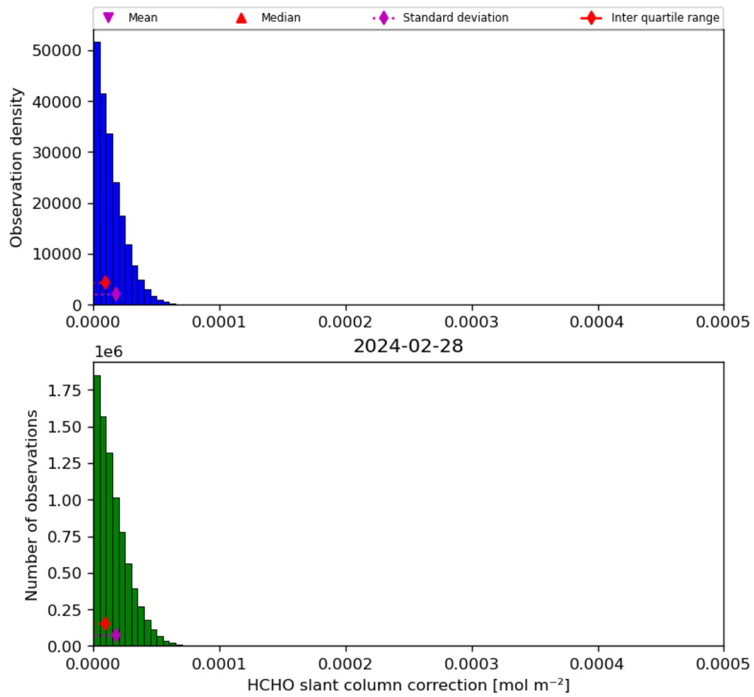
Figure 47: Histogram of “HCHO slant column correction” for 2024-02-27 to 2024-02-29
