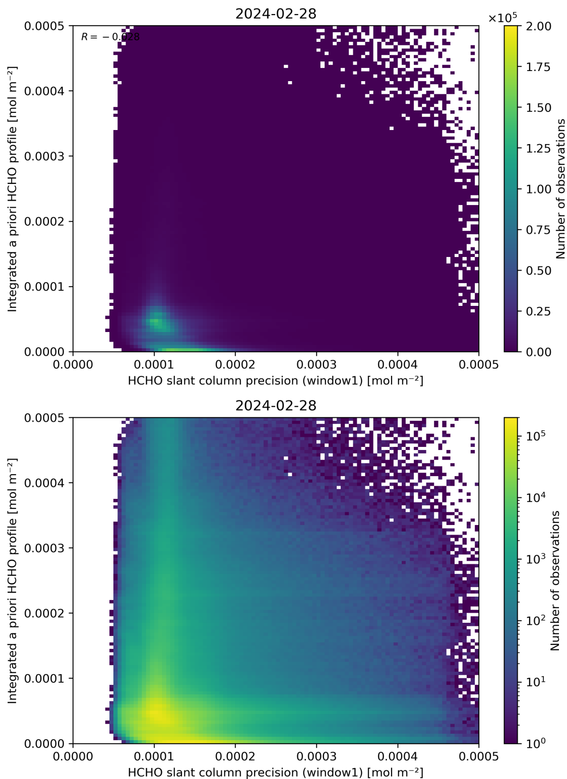
Figure 96: Scatter density plot of “HCHO slant column precision (window1)” against “Integrated a priori HCHO profile” for 2024-02-27 to 2024-02-29.
