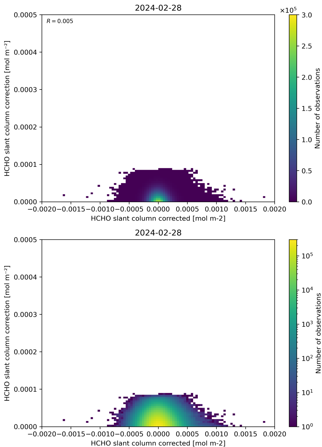
Figure 77: Scatter density plot of “HCHO slant column corrected” against “HCHO slant column correction” for 2024-02-27 to 2024-02-29.
