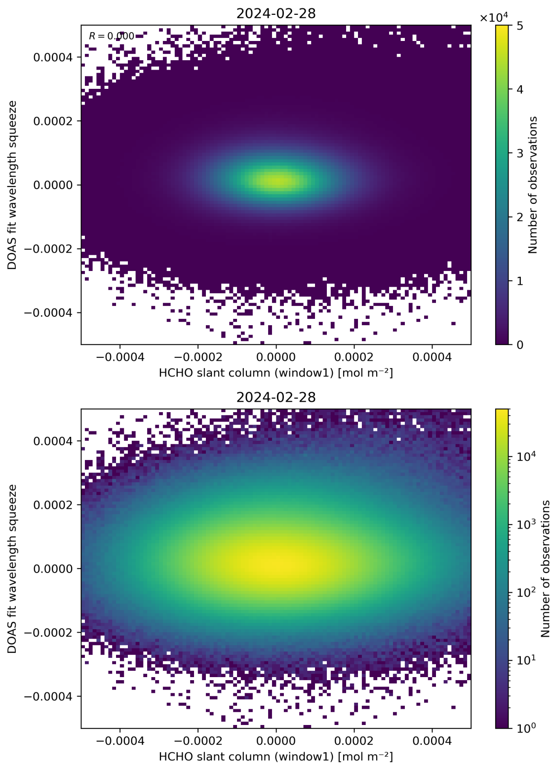
Figure 80: Scatter density plot of “HCHO slant column (window1)” against “DOAS fit wavelength squeeze” for 2024-02-27 to 2024-02-29.
