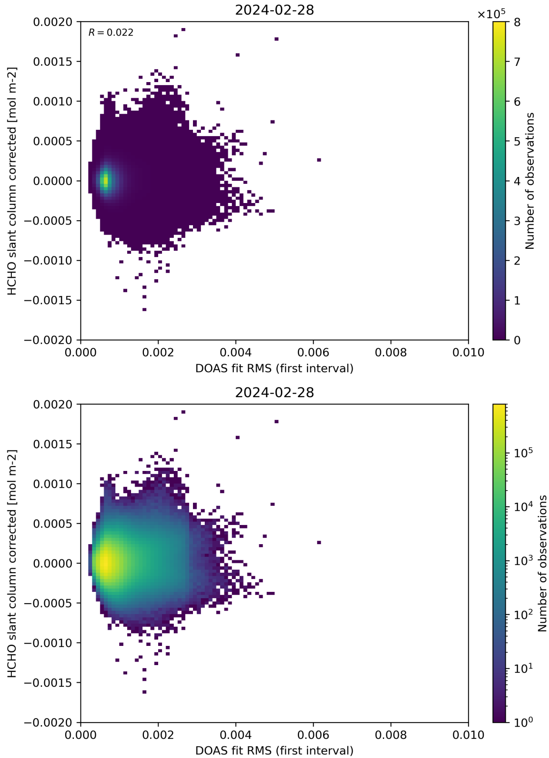
Figure 62: Scatter density plot of “DOAS fit RMS (first interval)” against “HCHO slant column corrected” for 2024-02-27 to 2024-02-29.
