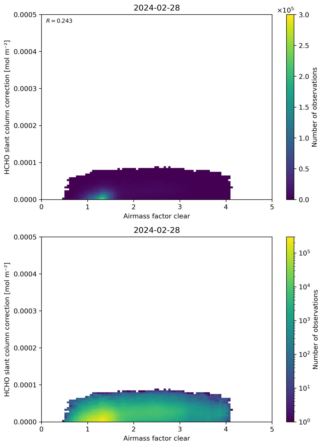
Figure 75: Scatter density plot of “Airmass factor clear” against “HCHO slant column correction” for 2024-02-27 to 2024-02-29.
