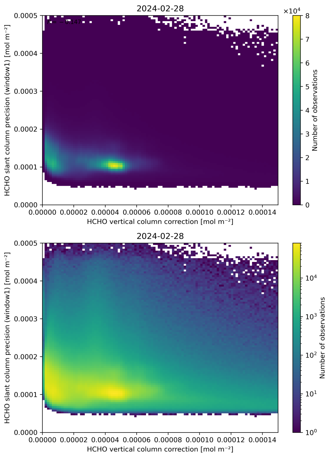
Figure 119: Scatter density plot of “HCHO vertical column correction” against “HCHO slant column precision (window1)” for 2024-02-27 to 2024-02-29.
