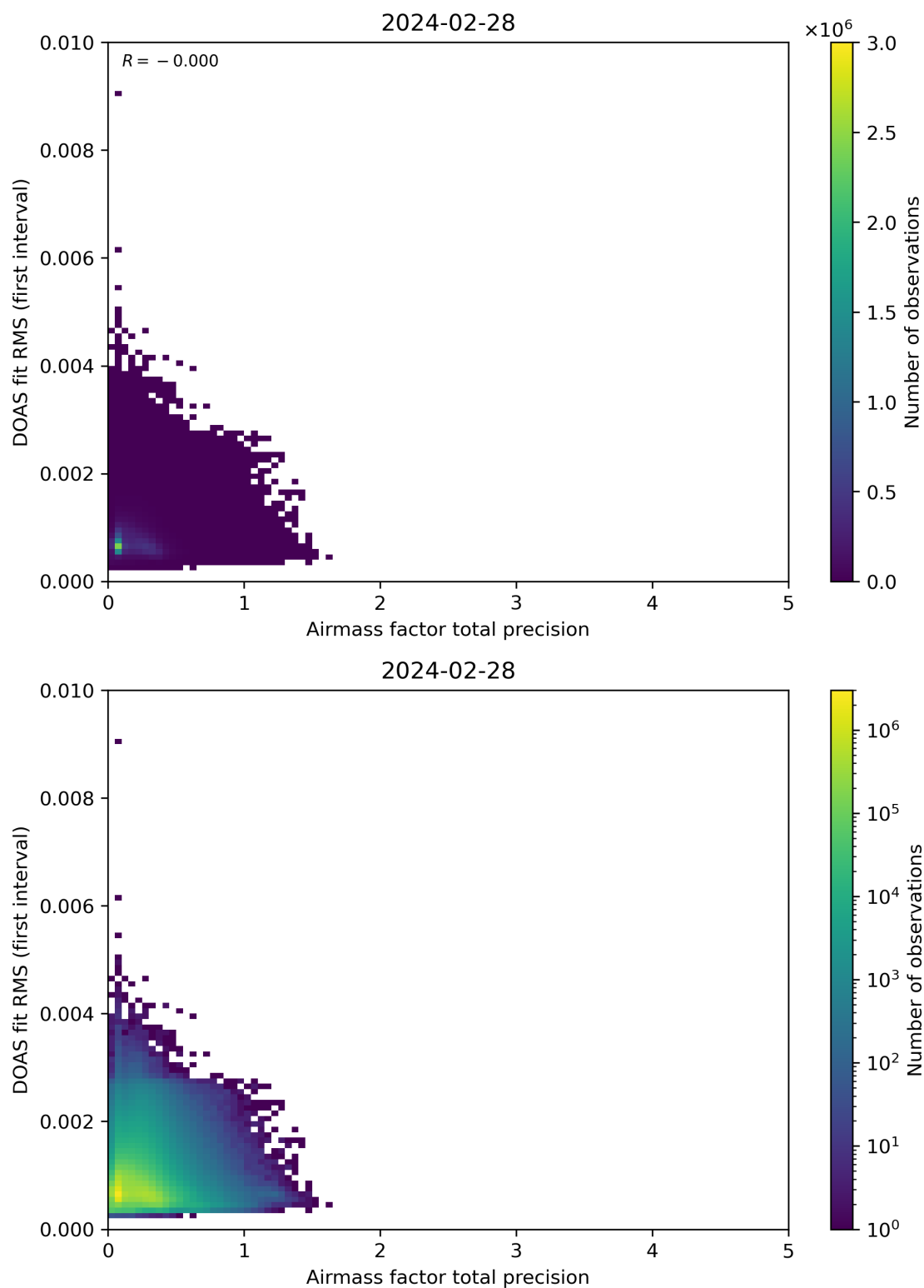
Figure 105: Scatter density plot of “Airmass factor total precision” against “DOAS fit RMS (first interval)” for 2024-02-27 to 2024-02-29.
