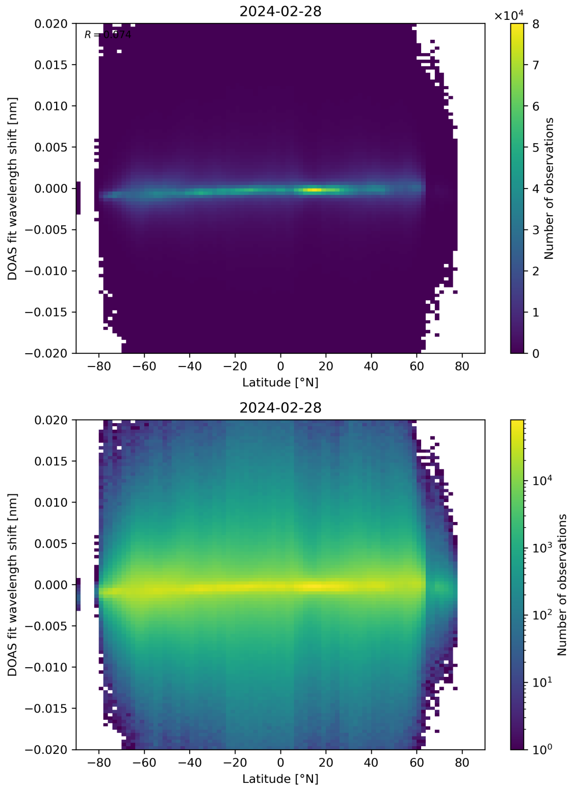
Figure 154: Scatter density plot of “Latitude” against “DOAS fit wavelength shift” for 2024-02-27 to 2024-02-29.
