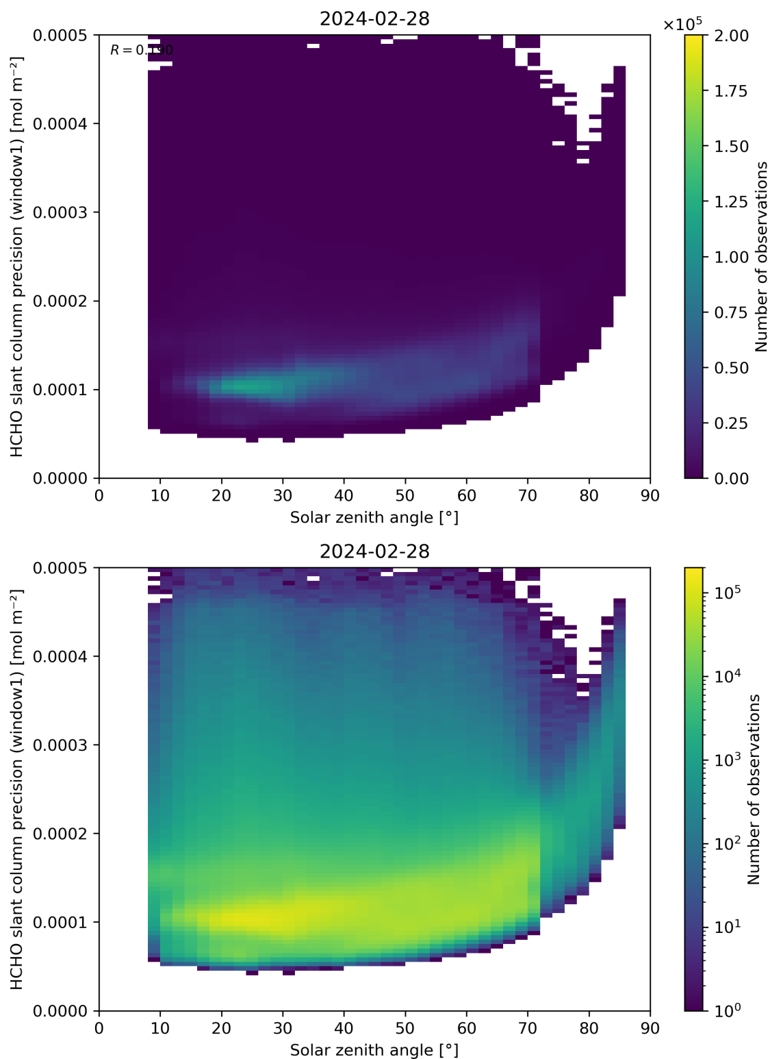
Figure 174: Scatter density plot of “Solar zenith angle” against “HCHO slant column precision (window1)” for 2024-02-27 to 2024-02-29.
