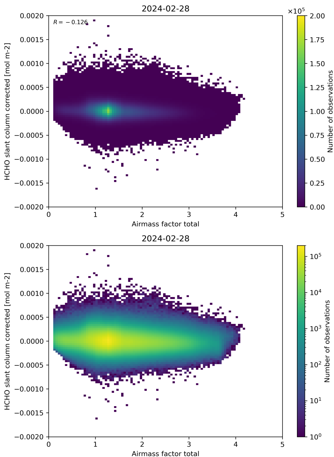
Figure 101: Scatter density plot of “Airmass factor total” against “HCHO slant column corrected” for 2024-02-27 to 2024-02-29.
