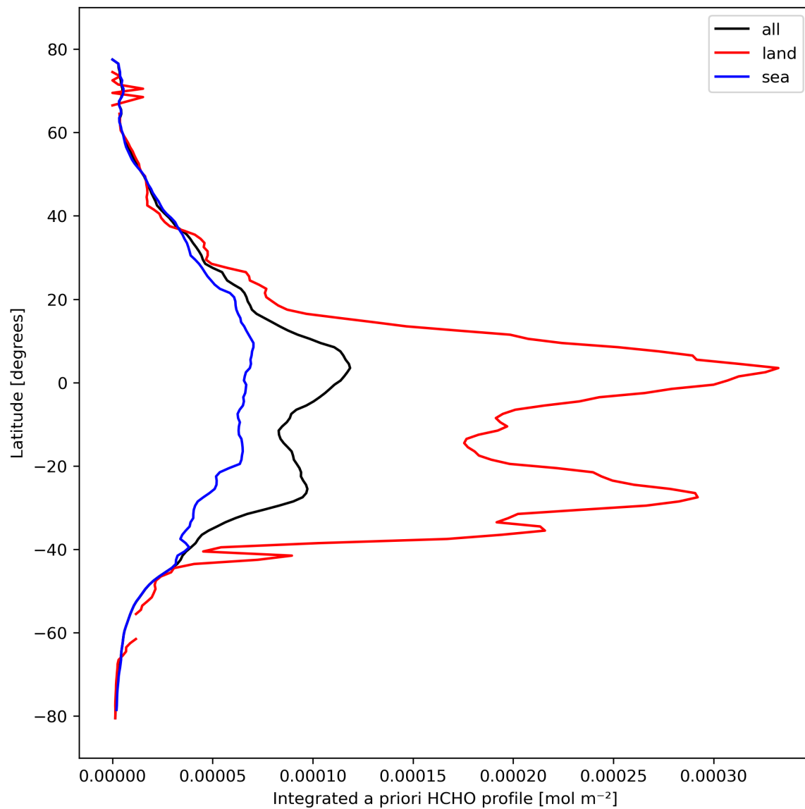
Figure 29: Zonal average of “Integrated a priori HCHO profile” for 2024-02-27 to 2024-02-29.
