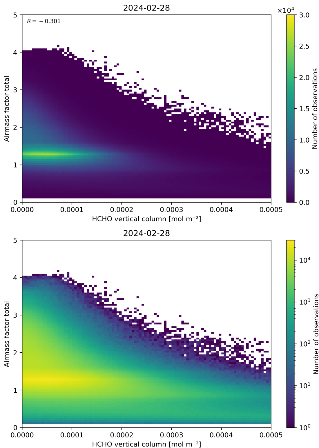
Figure 131: Scatter density plot of “HCHO vertical column” against “Airmass factor total” for 2024-02-27 to 2024-02-29.
