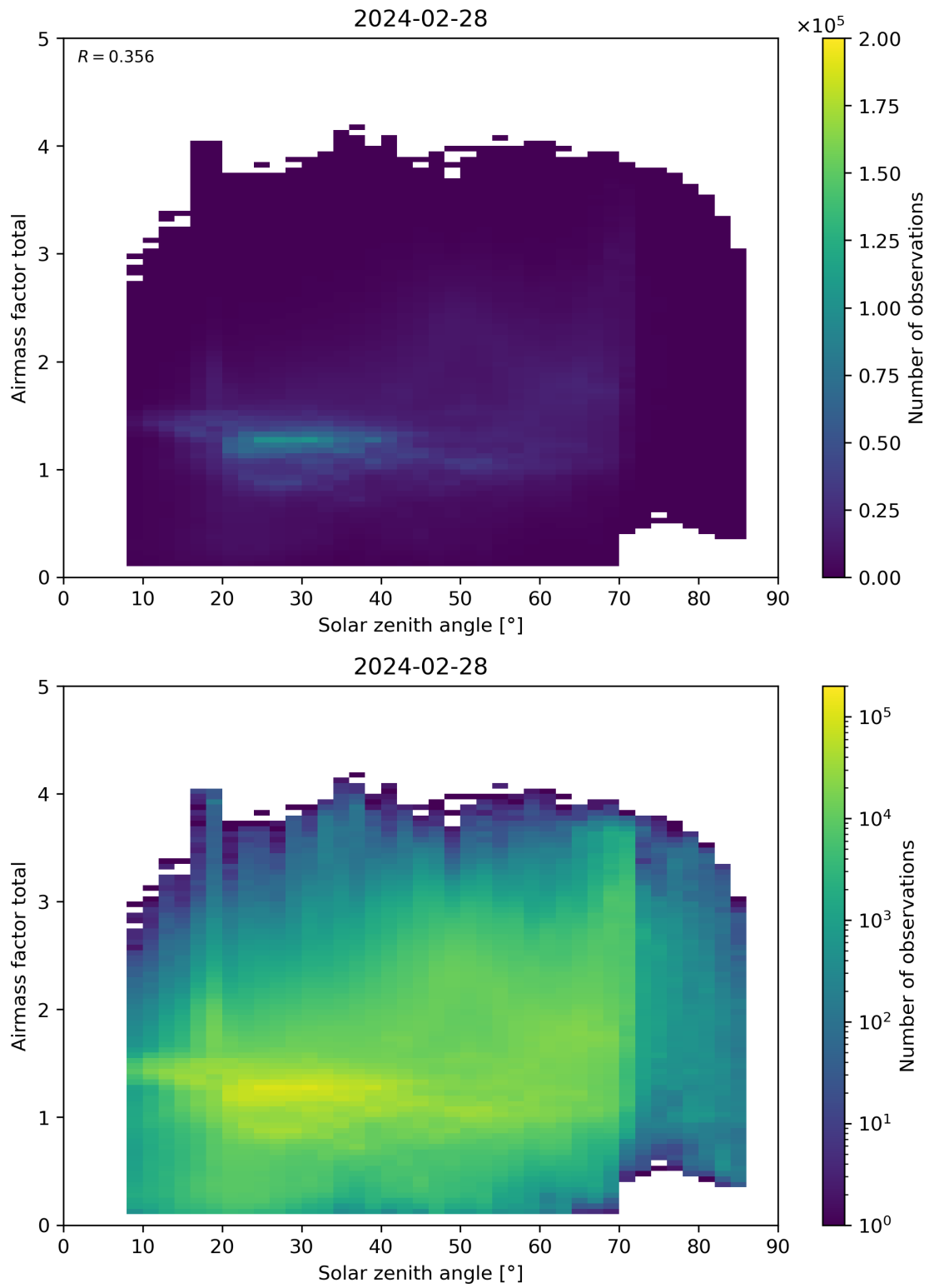
Figure 175: Scatter density plot of “Solar zenith angle” against “Airmass factor total” for 2024-02-27 to 2024-02-29.
