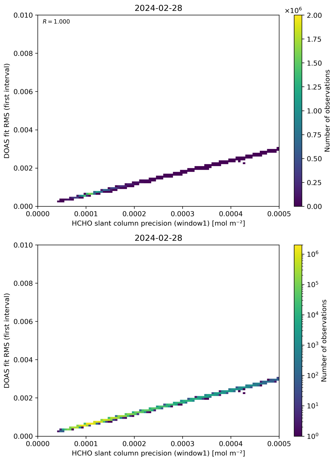
Figure 88: Scatter density plot of “HCHO slant column precision (window1)” against “DOAS fit RMS (first interval)” for 2024-02-27 to 2024-02-29.
