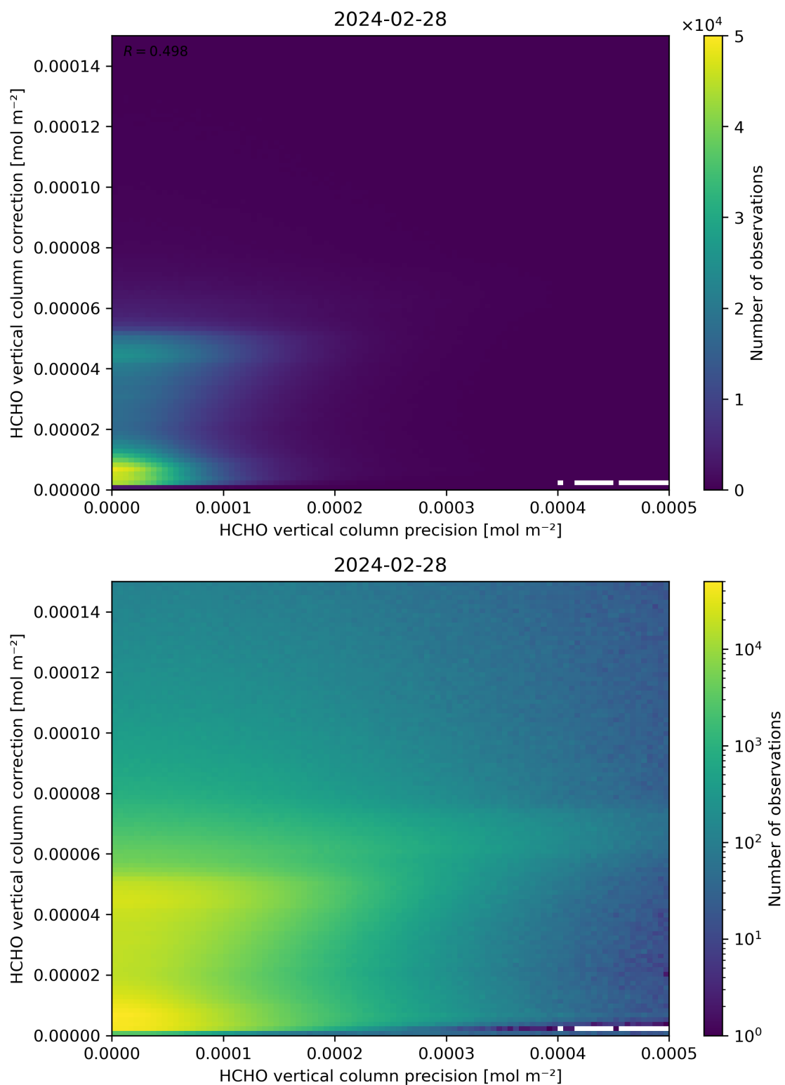
Figure 146: Scatter density plot of “HCHO vertical column precision” against “HCHO vertical column correction” for 2024-02-27 to 2024-02-29.
