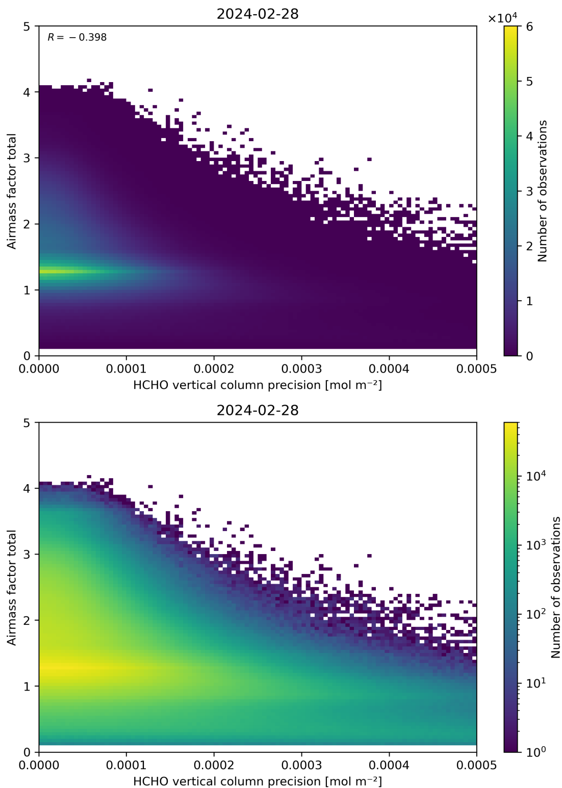
Figure 144: Scatter density plot of “HCHO vertical column precision” against “Airmass factor total” for 2024-02-27 to 2024-02-29.
