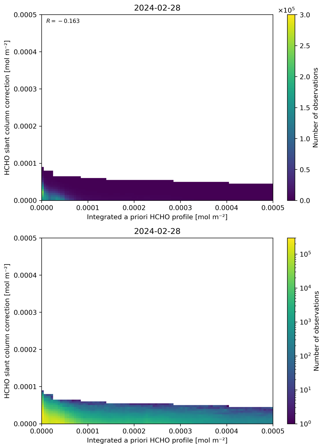
Figure 152: Scatter density plot of “Integrated a priori HCHO profile” against “HCHO slant column correction” for 2024-02-27 to 2024-02-29.
