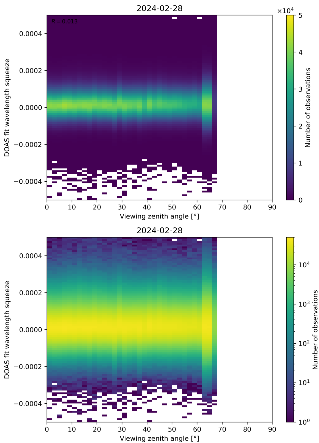
Figure 184: Scatter density plot of “Viewing zenith angle” against “DOAS fit wavelength squeeze” for 2024-02-27 to 2024-02-29.
