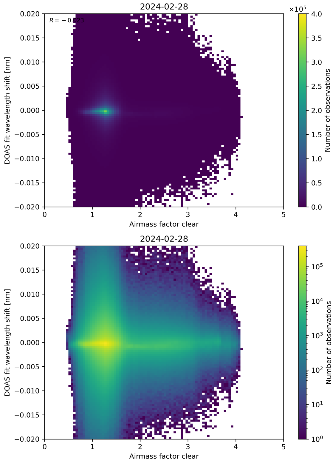
Figure 72: Scatter density plot of “Airmass factor clear” against “DOAS fit wavelength shift” for 2024-02-27 to 2024-02-29.
