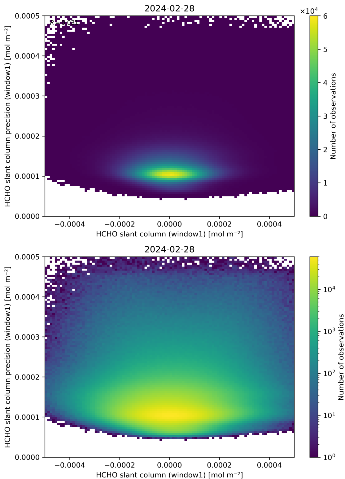
Figure 84: Scatter density plot of “HCHO slant column (window1)” against “HCHO slant column precision (window1)” for 2024-02-27 to 2024-02-29.
