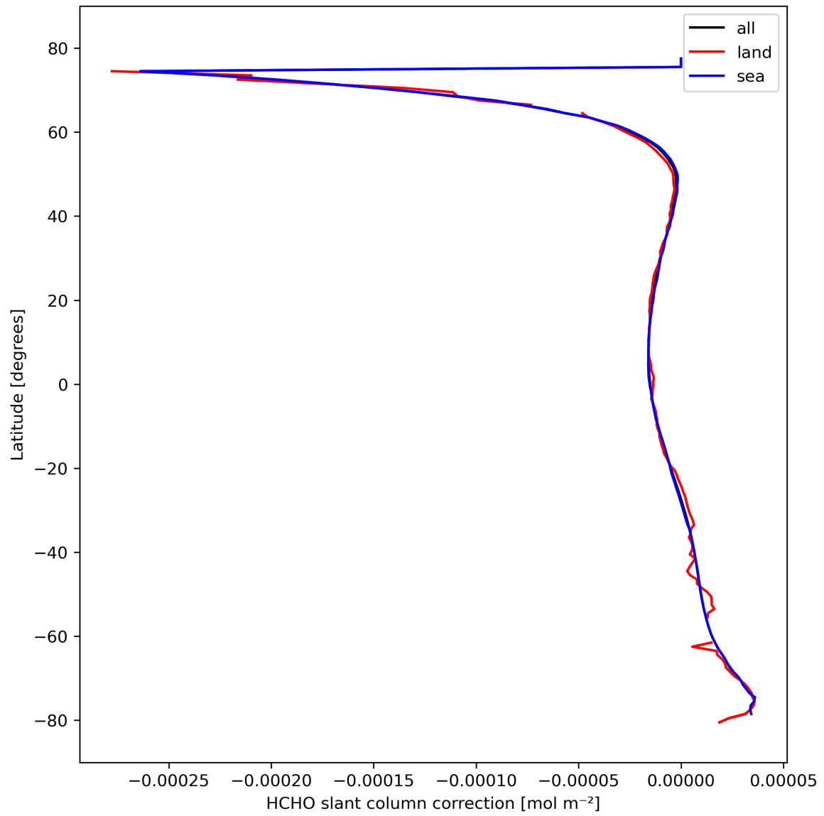
Figure 33: Zonal average of “HCHO slant column correction” for 2024-02-27 to 2024-02-29.
