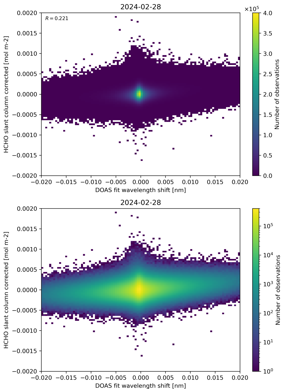
Figure 66: Scatter density plot of “DOAS fit wavelength shift” against “HCHO slant column corrected” for 2024-02-27 to 2024-02-29.
