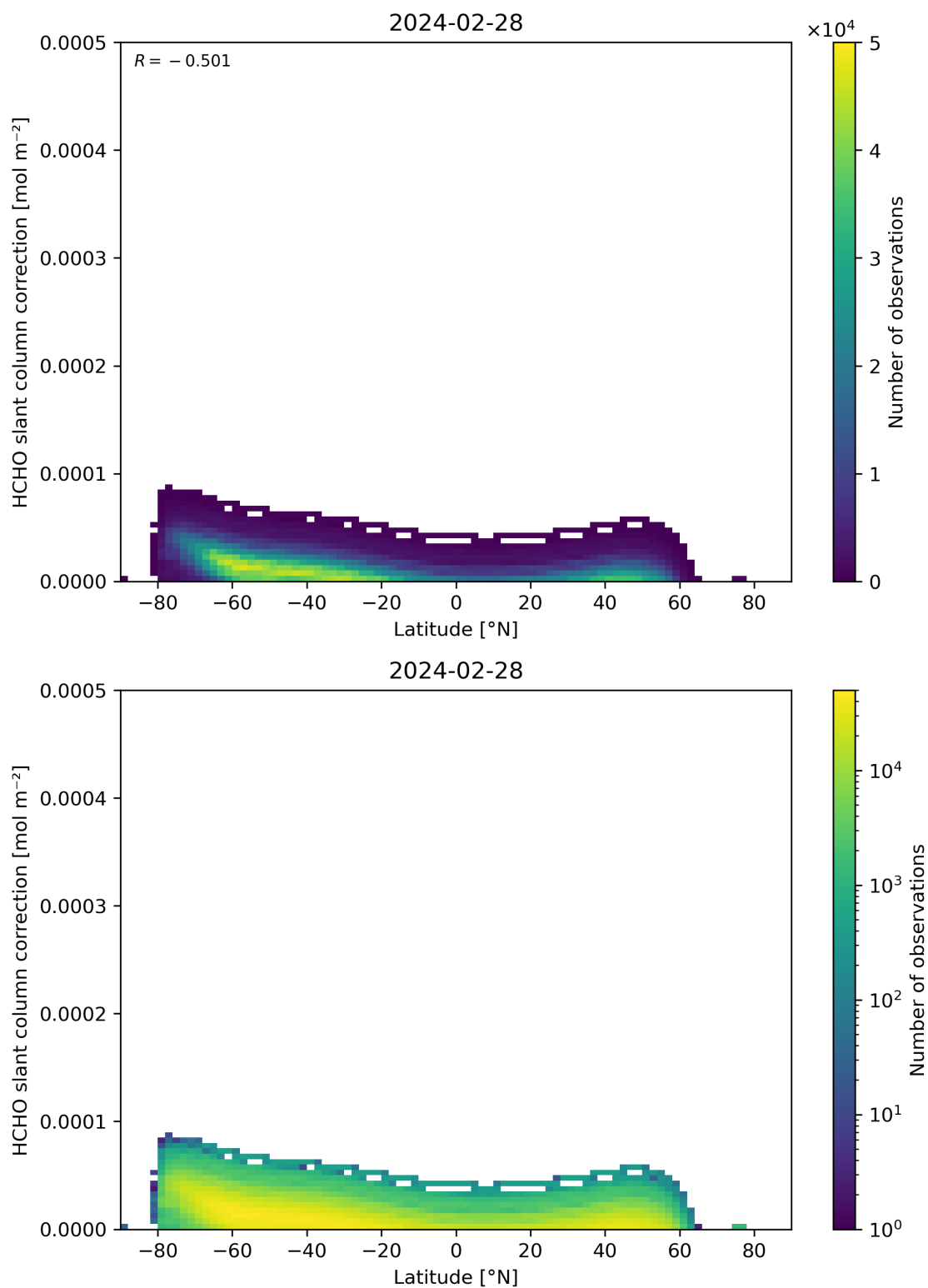
Figure 158: Scatter density plot of “Latitude” against “HCHO slant column correction” for 2024-02-27 to 2024-02-29.
