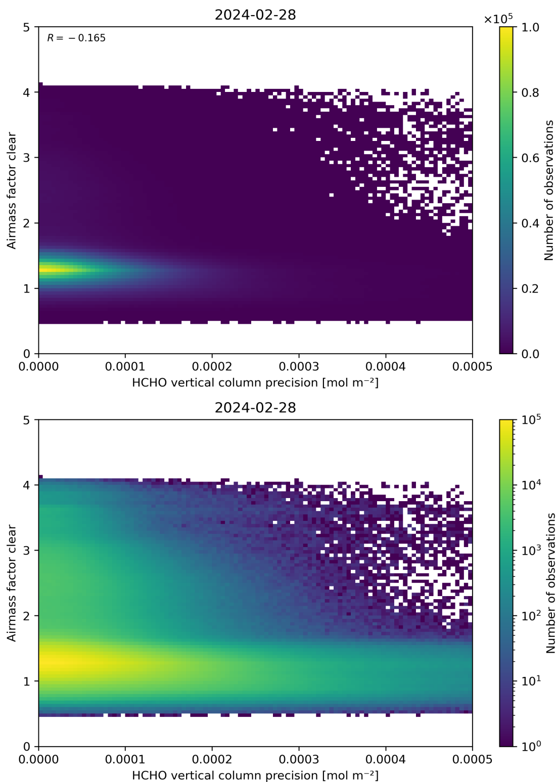
Figure 139: Scatter density plot of “HCHO vertical column precision” against “Airmass factor clear” for 2024-02-27 to 2024-02-29.
