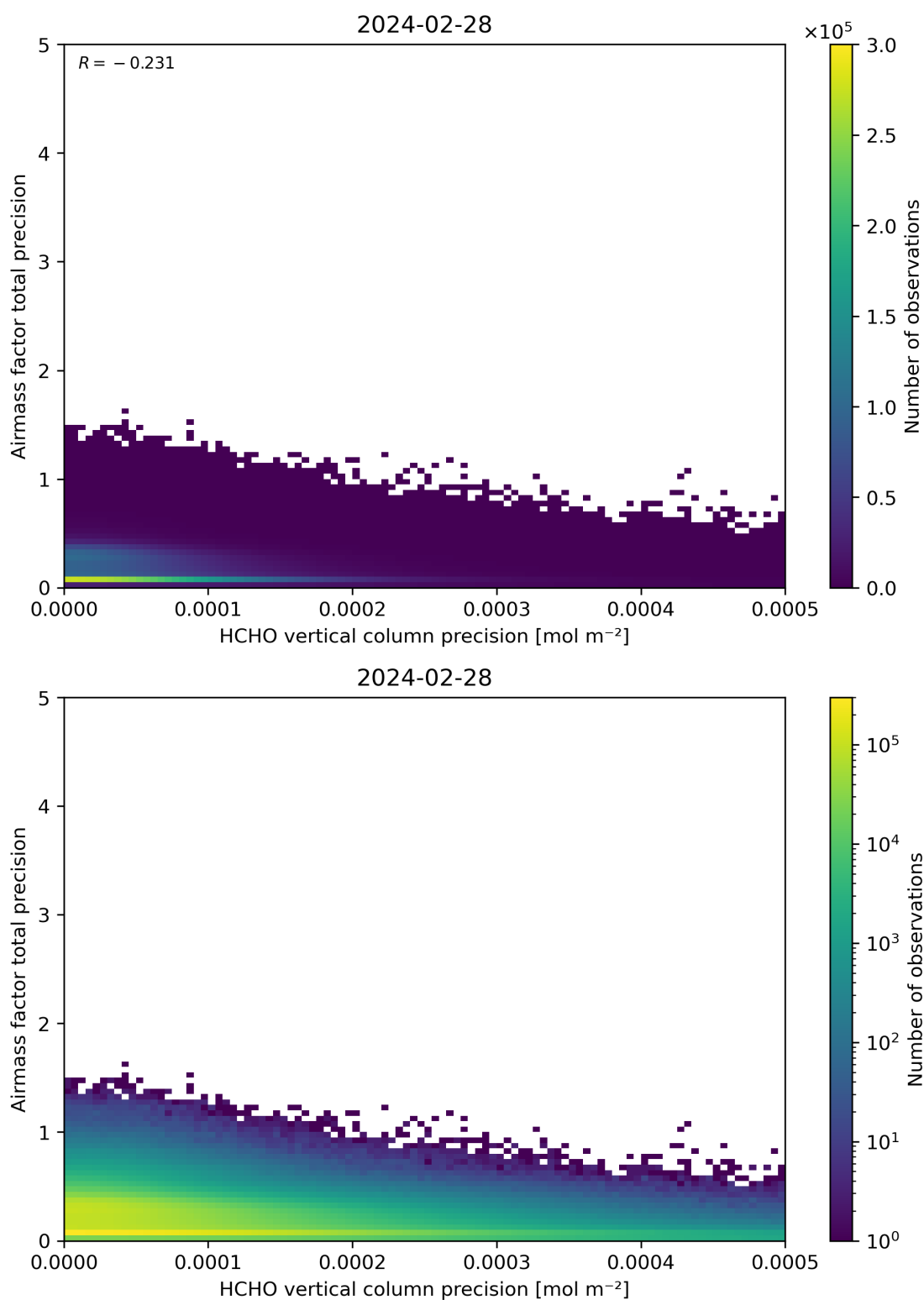
Figure 145: Scatter density plot of “HCHO vertical column precision” against “Airmass factor total precision” for 2024-02-27 to 2024-02-29.
