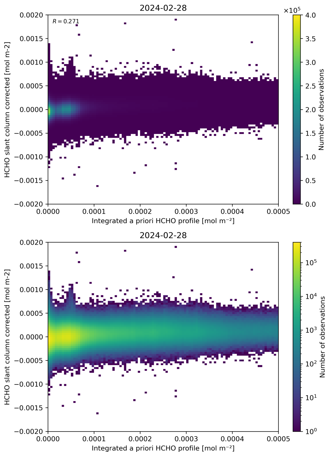
Figure 151: Scatter density plot of “Integrated a priori HCHO profile” against “HCHO slant column corrected” for 2024-02-27 to 2024-02-29.
