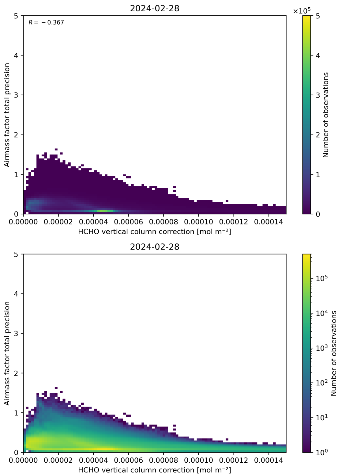
Figure 121: Scatter density plot of “HCHO vertical column correction” against “Airmass factor total precision” for 2024-02-27 to 2024-02-29.
