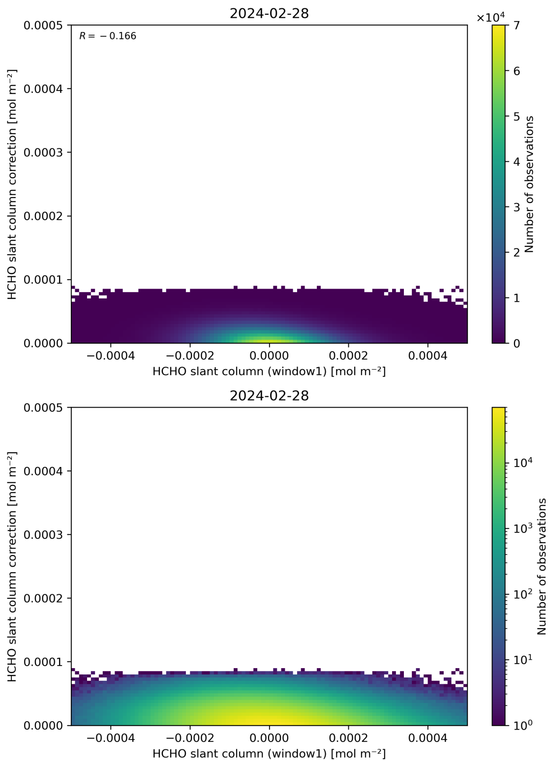
Figure 83: Scatter density plot of “HCHO slant column (window1)” against “HCHO slant column correction” for 2024-02-27 to 2024-02-29.
