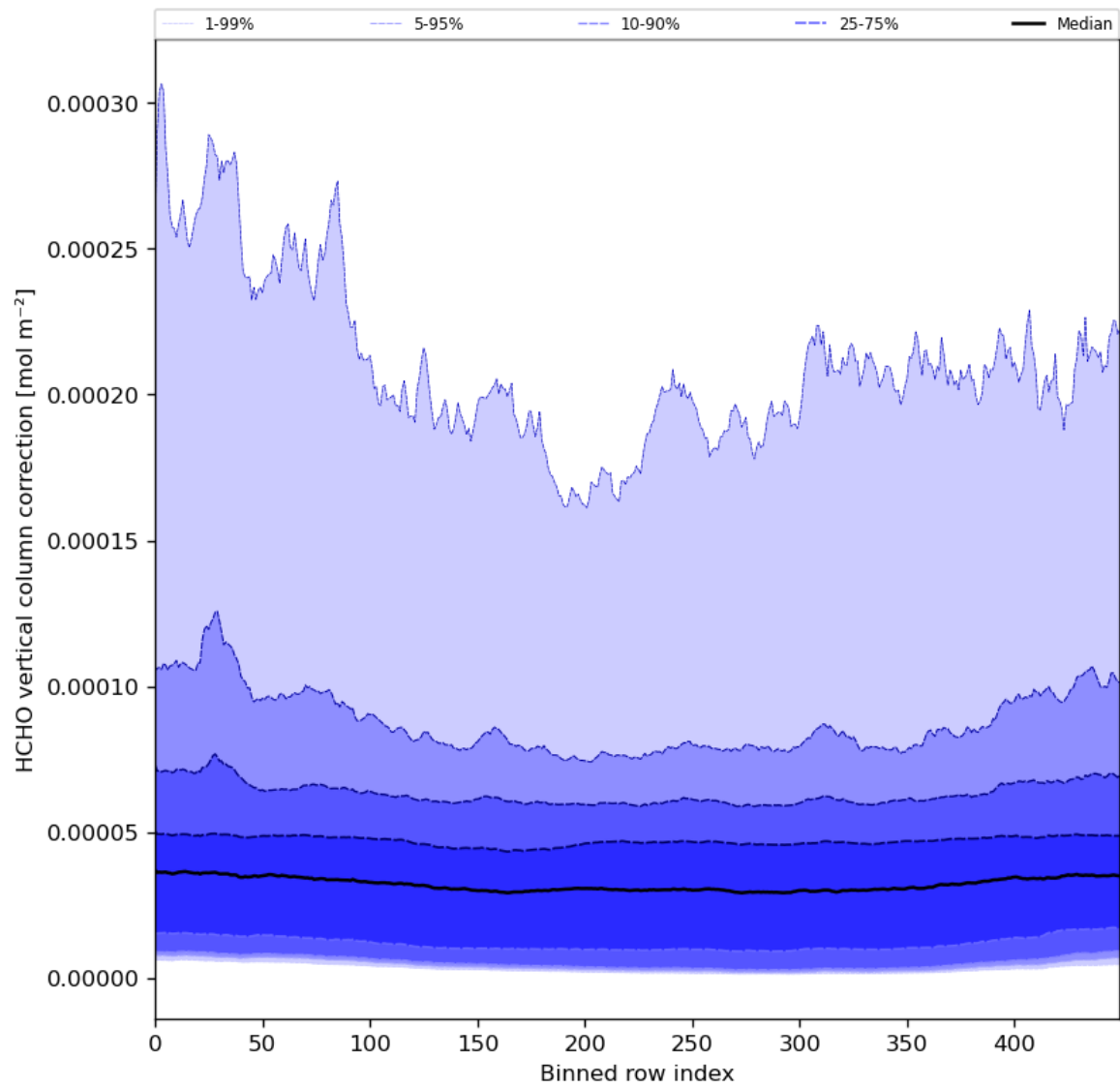
Figure 51: Along track statistics of “HCHO vertical column correction” for 2024-02-27 to 2024-02-29
