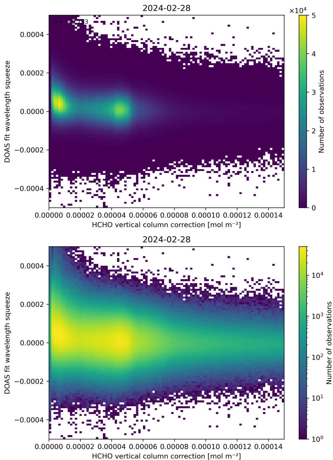
Figure 114: Scatter density plot of “HCHO vertical column correction” against “DOAS fit wavelength squeeze” for 2024-02-27 to 2024-02-29.
