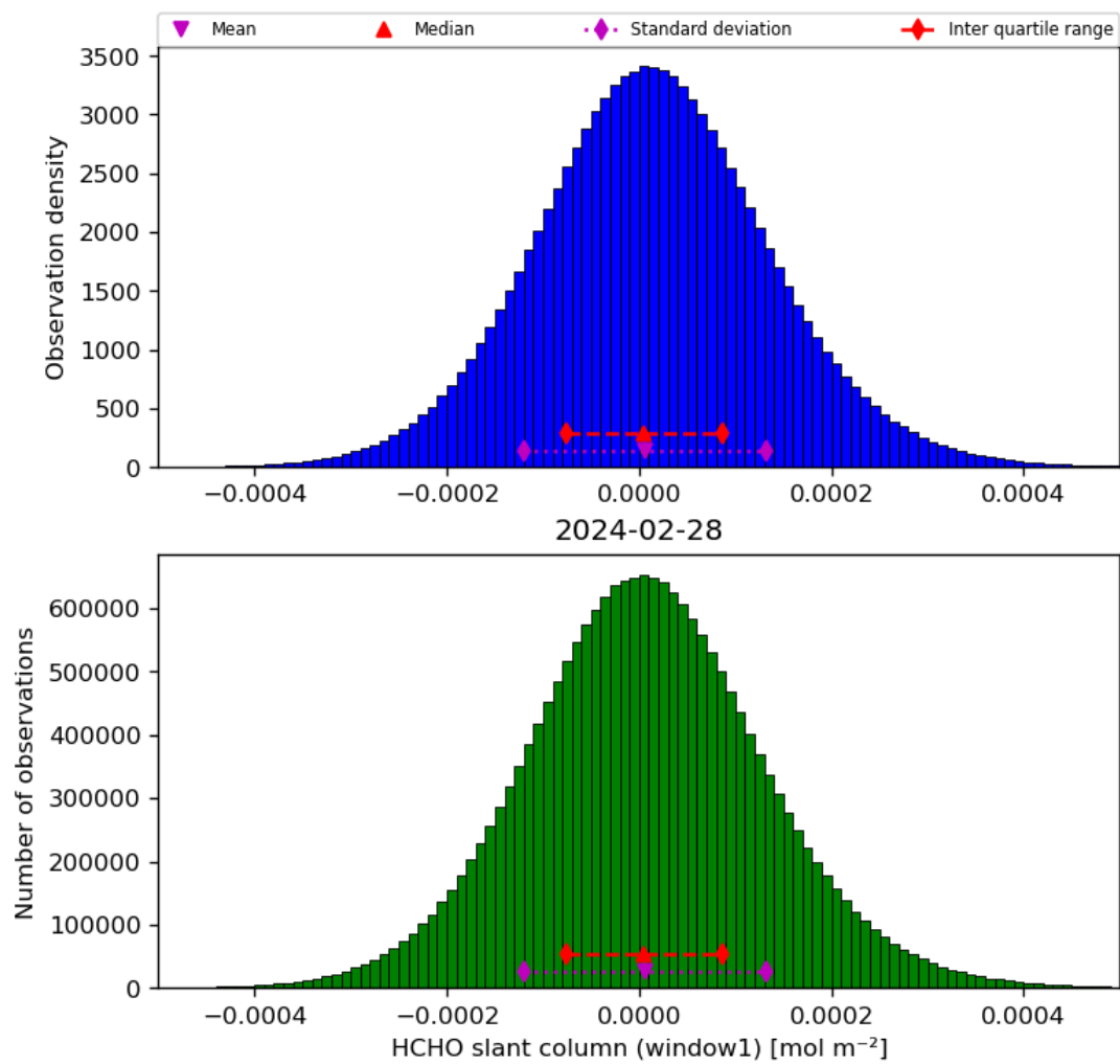
Figure 38: Histogram of “HCHO slant column (window1)” for 2024-02-27 to 2024-02-29
