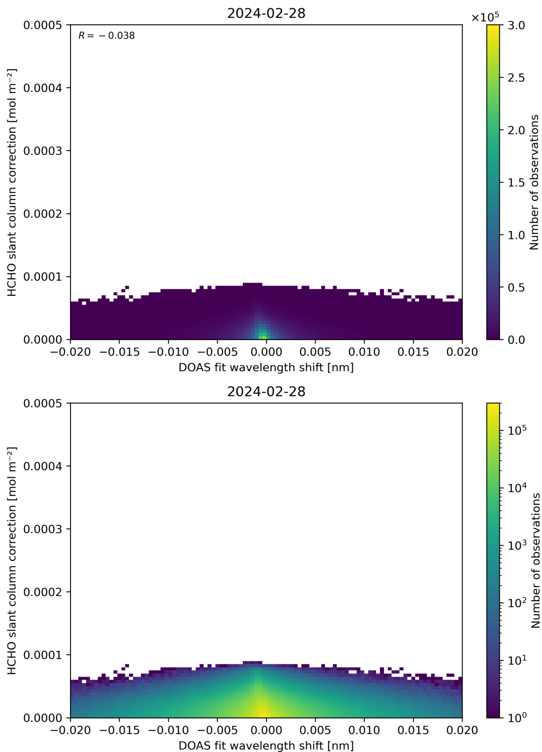
Figure 67: Scatter density plot of “DOAS fit wavelength shift” against “HCHO slant column correction” for 2024-02-27 to 2024-02-29.
