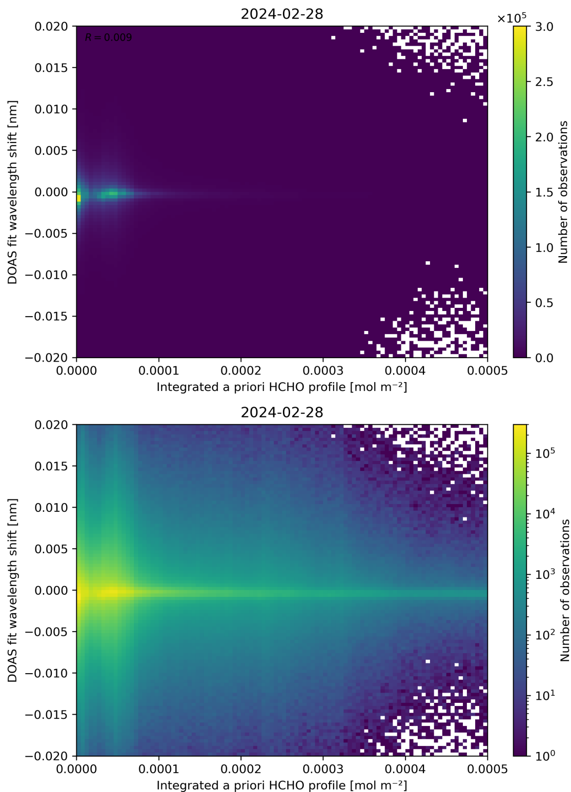
Figure 149: Scatter density plot of “Integrated a priori HCHO profile” against “DOAS fit wavelength shift” for 2024-02-27 to 2024-02-29.
