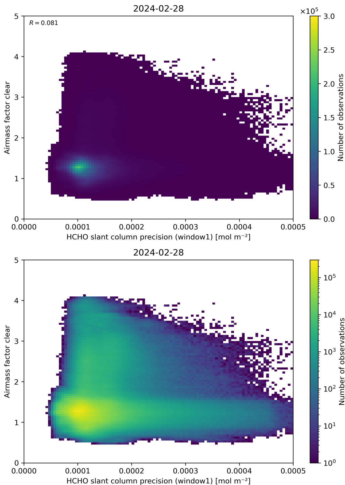
Figure 91: Scatter density plot of “HCHO slant column precision (window1)” against “Airmass factor clear” for 2024-02-27 to 2024-02-29.
