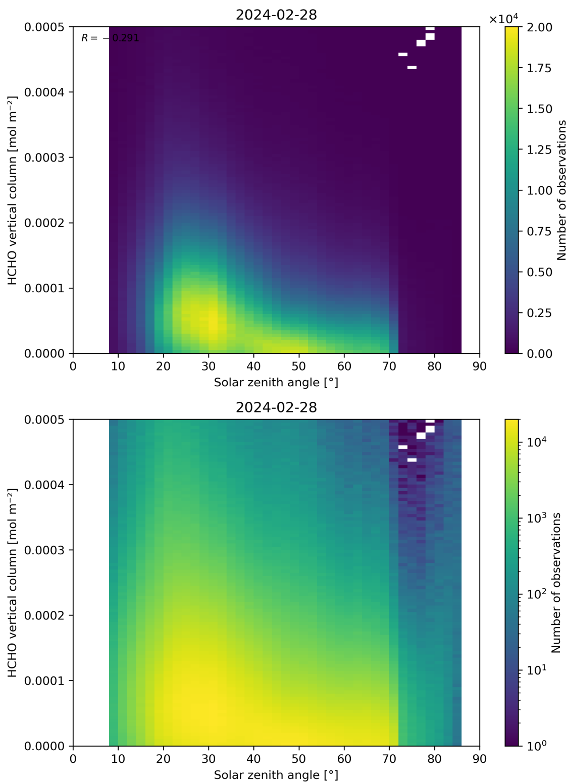
Figure 177: Scatter density plot of “Solar zenith angle” against “HCHO vertical column” for 2024-02-27 to 2024-02-29.
