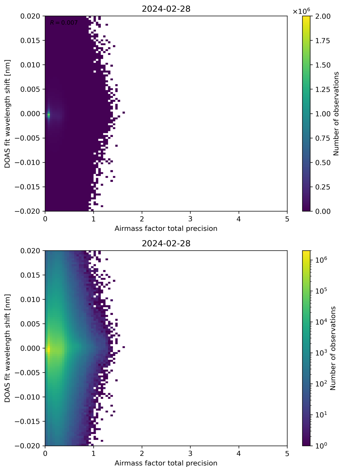
Figure 106: Scatter density plot of “Airmass factor total precision” against “DOAS fit wavelength shift” for 2024-02-27 to 2024-02-29.
