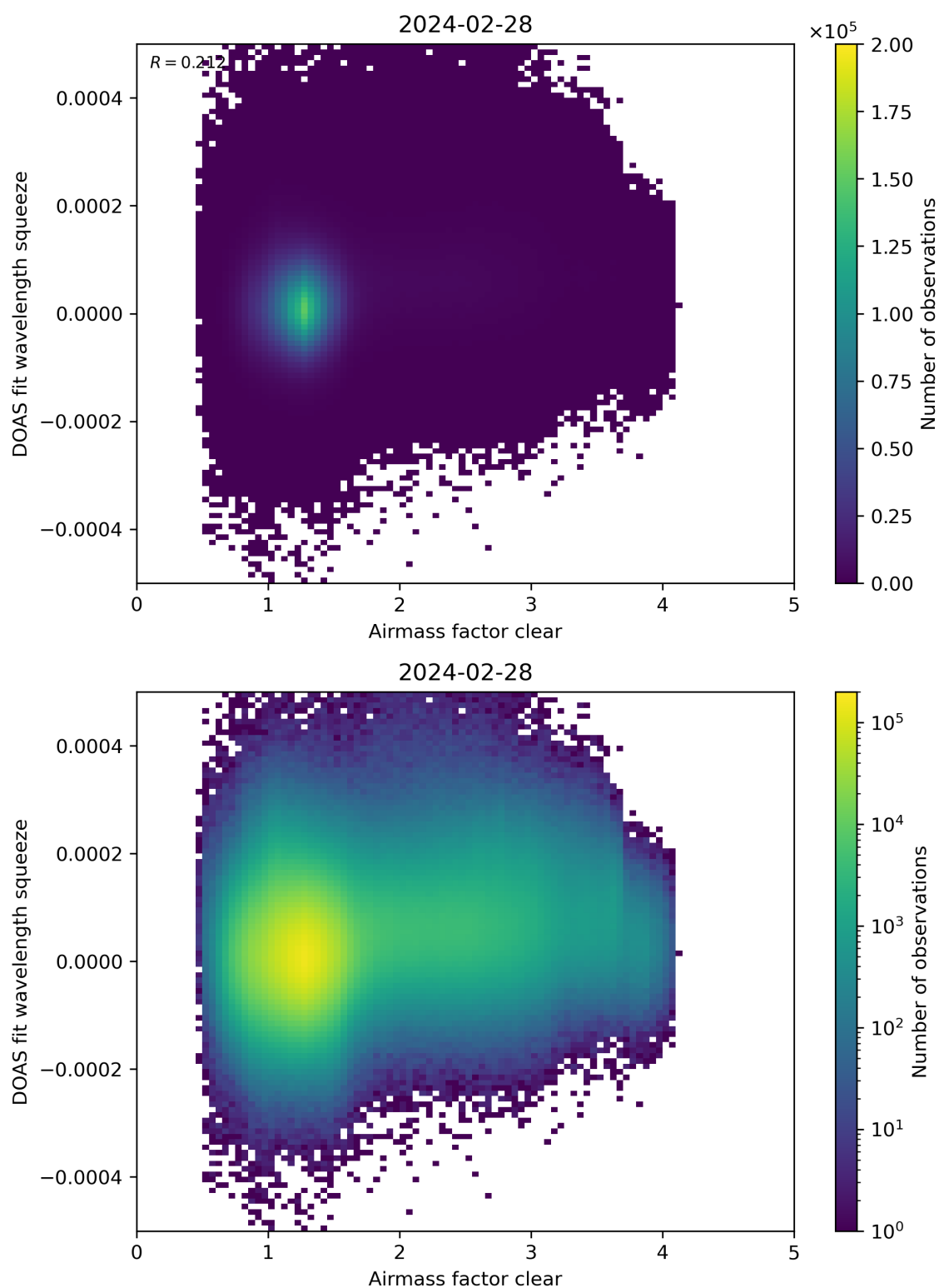
Figure 73: Scatter density plot of “Airmass factor clear” against “DOAS fit wavelength squeeze” for 2024-02-27 to 2024-02-29.
