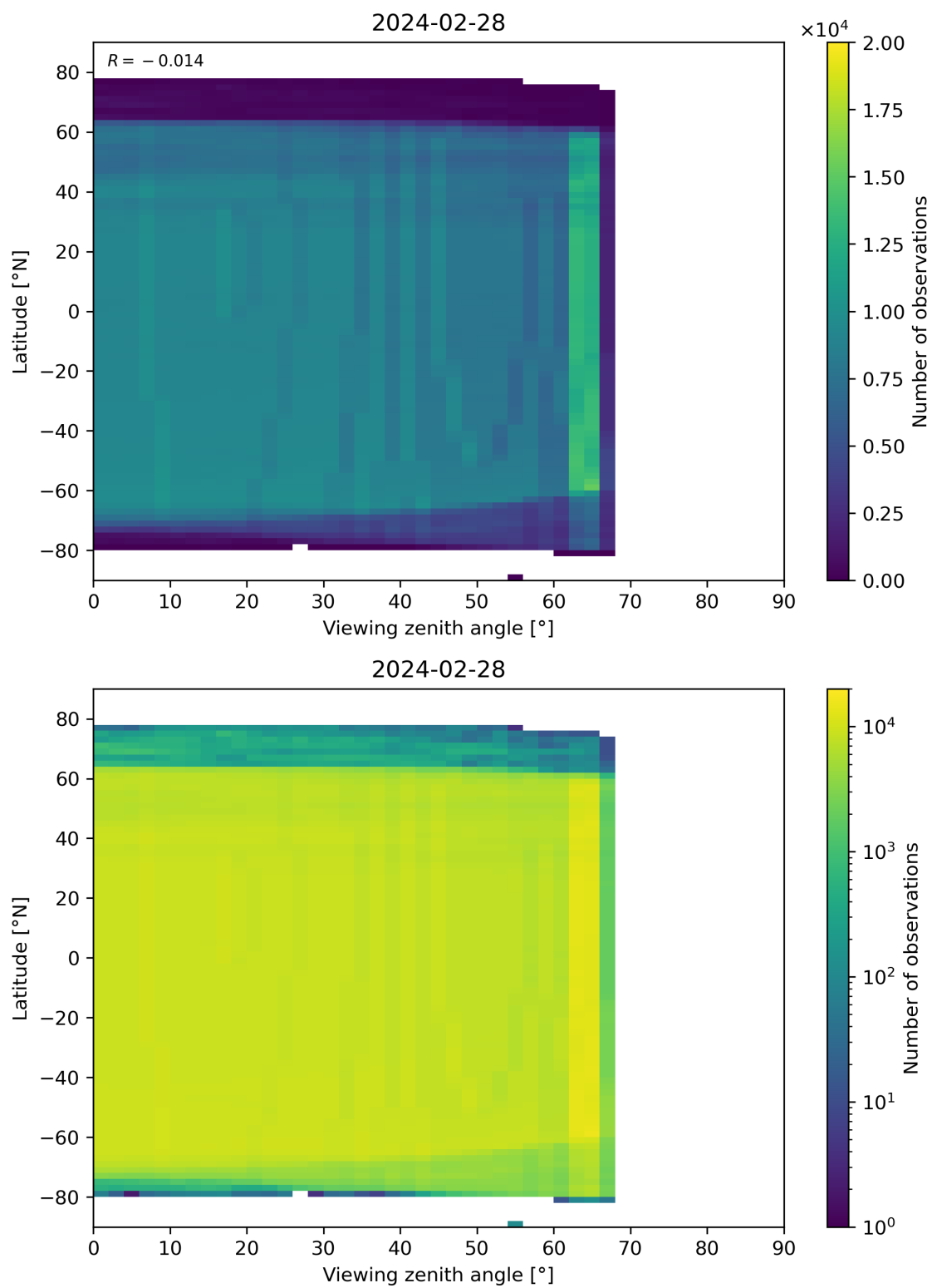
Figure 196: Scatter density plot of “Viewing zenith angle” against “Latitude” for 2024-02-27 to 2024-02-29.
