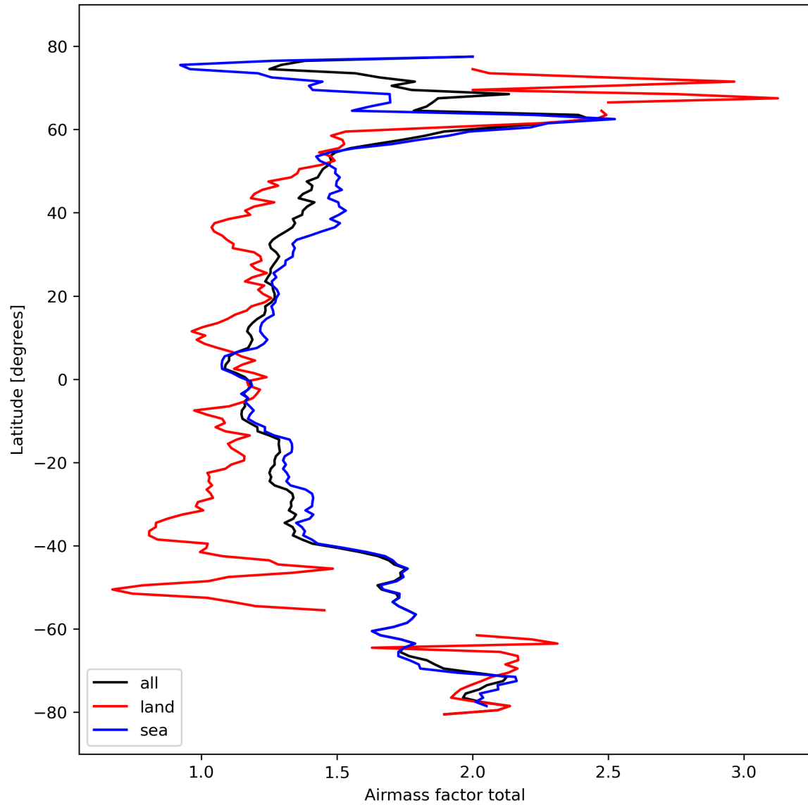
Figure 26: Zonal average of “Airmass factor total” for 2024-02-27 to 2024-02-29.
