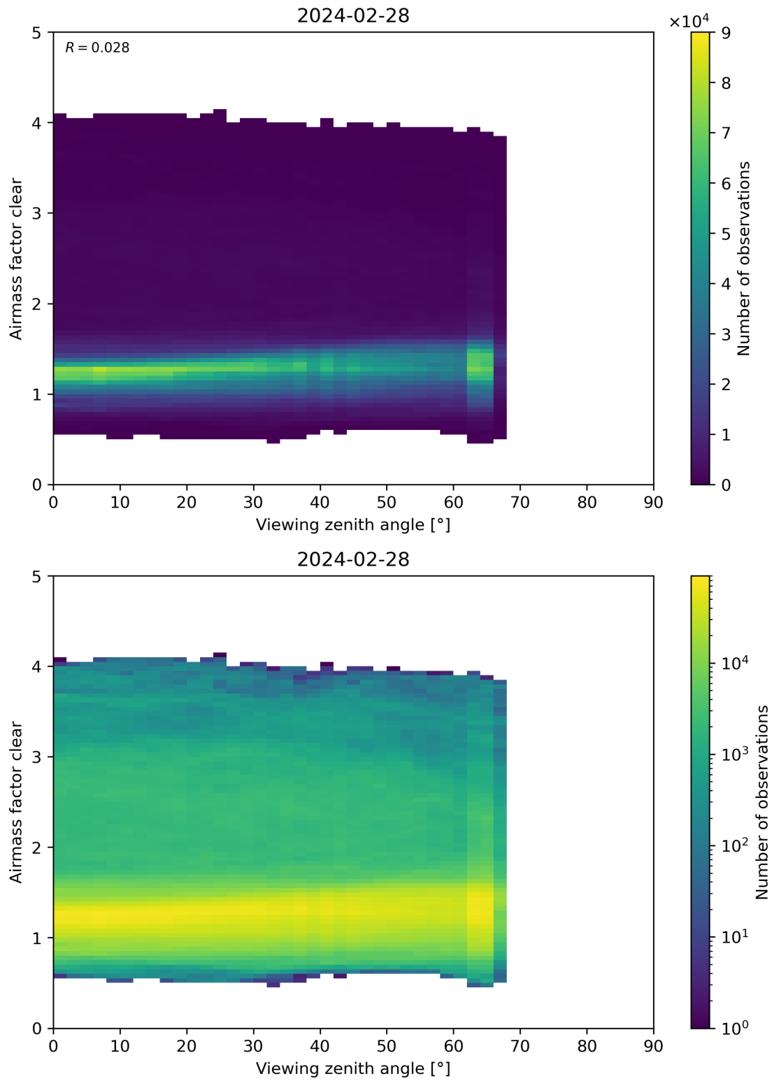
Figure 185: Scatter density plot of “Viewing zenith angle” against “Airmass factor clear” for 2024-02-27 to 2024-02-29.
