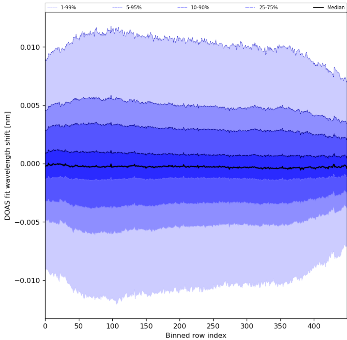
Figure 58: Along track statistics of “DOAS fit wavelength shift” for 2024-02-27 to 2024-02-29
