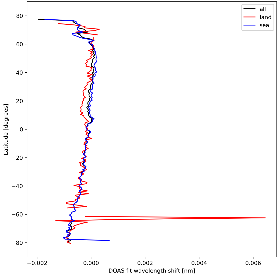
Figure 30: Zonal average of “DOAS fit wavelength shift” for 2024-02-27 to 2024-02-29.
