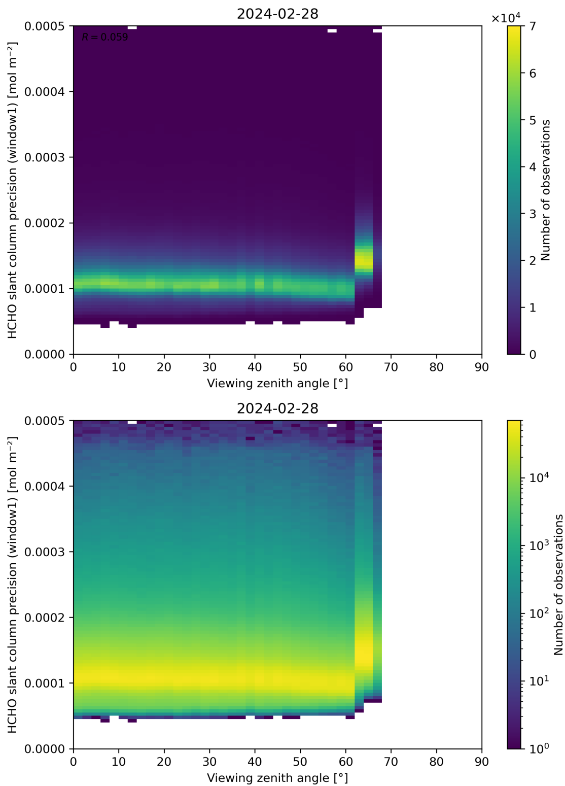
Figure 189: Scatter density plot of “Viewing zenith angle” against “HCHO slant column precision (window1)” for 2024-02-27 to 2024-02-29.
