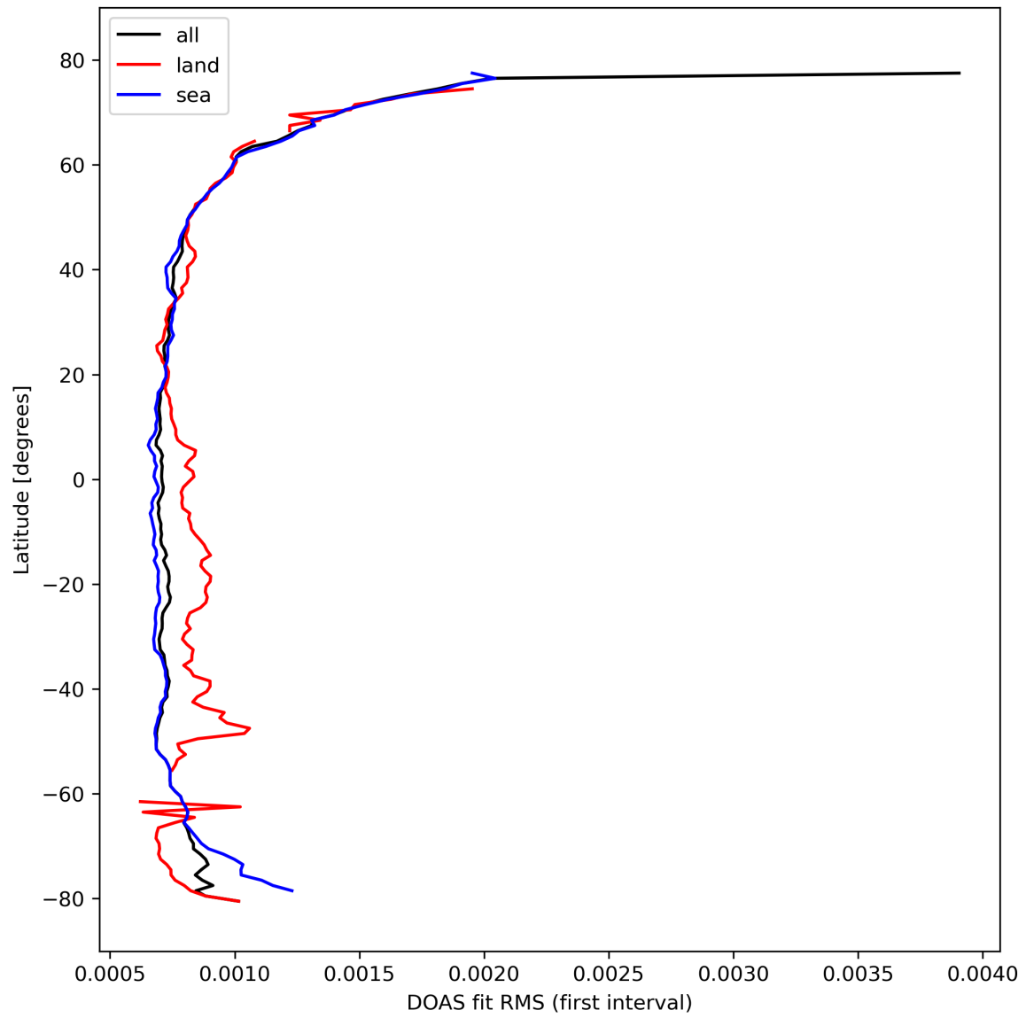
Figure 32: Zonal average of “DOAS fit RMS (first interval)” for 2024-02-27 to 2024-02-29.
