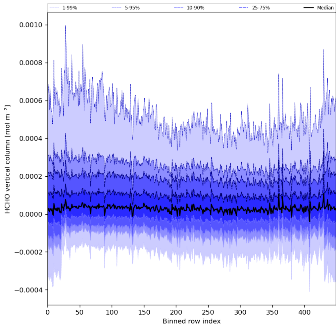
Figure 49: Along track statistics of “HCHO vertical column” for 2024-02-27 to 2024-02-29
