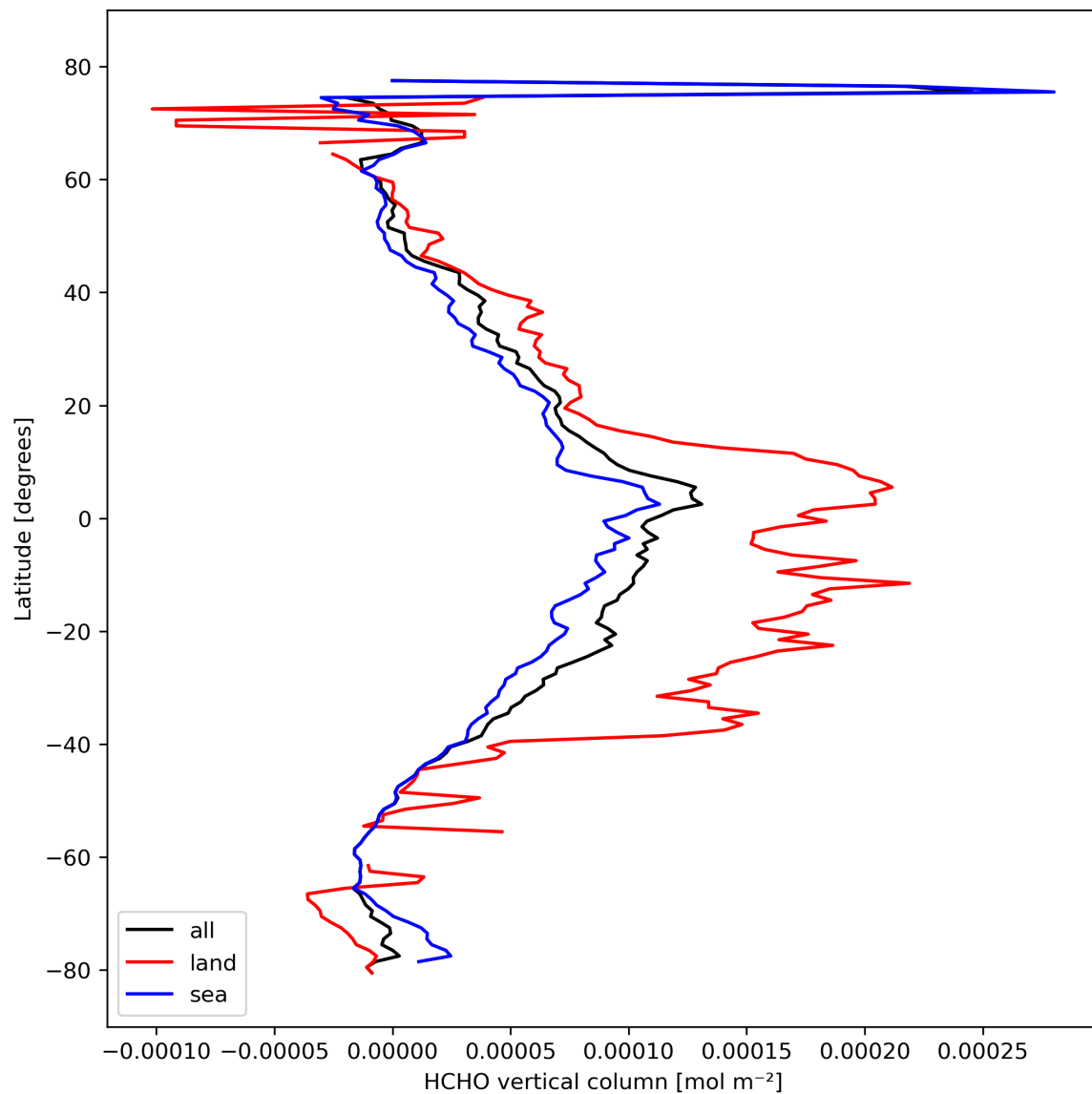
Figure 21: Zonal average of “HCHO vertical column” for 2024-02-27 to 2024-02-29.
