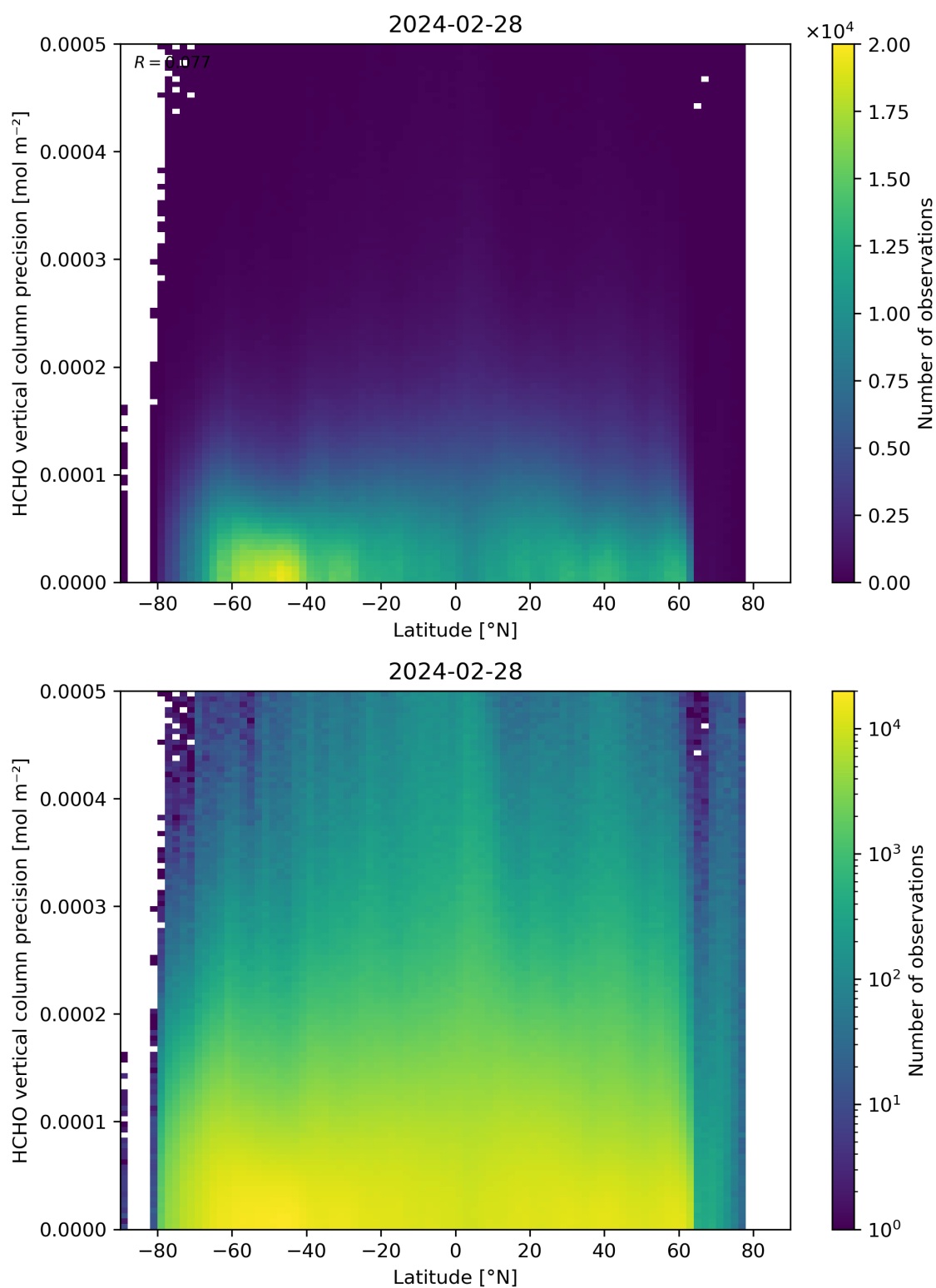
Figure 165: Scatter density plot of “Latitude” against “HCHO vertical column precision” for 2024-02-27 to 2024-02-29.
