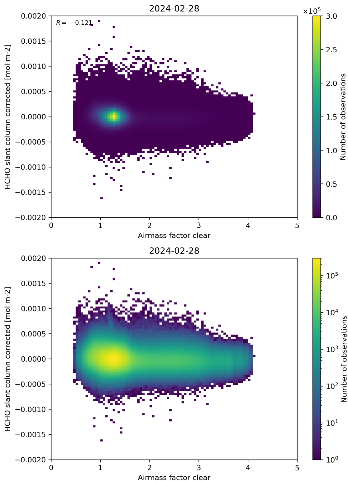
Figure 74: Scatter density plot of “Airmass factor clear” against “HCHO slant column corrected” for 2024-02-27 to 2024-02-29.
