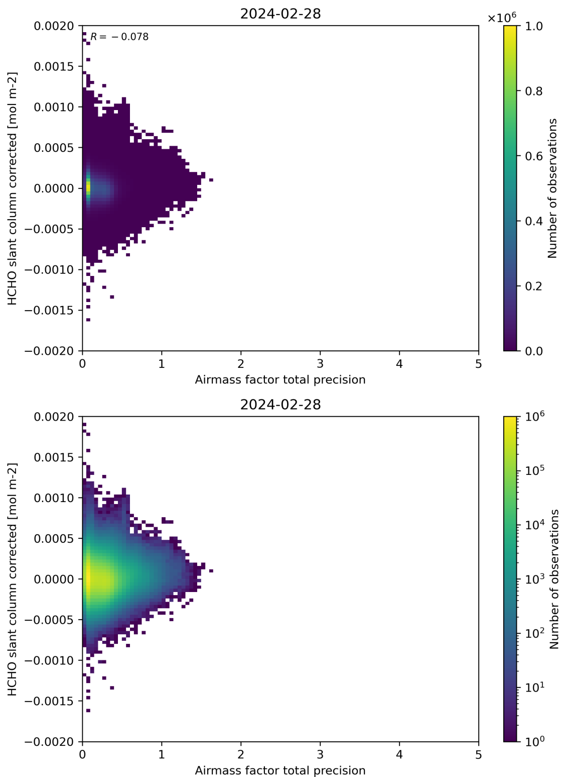
Figure 109: Scatter density plot of “Airmass factor total precision” against “HCHO slant column corrected” for 2024-02-27 to 2024-02-29.
