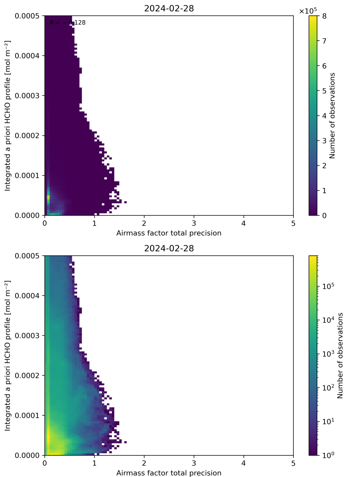
Figure 111: Scatter density plot of “Airmass factor total precision” against “Integrated a priori HCHO profile” for 2024-02-27 to 2024-02-29.
