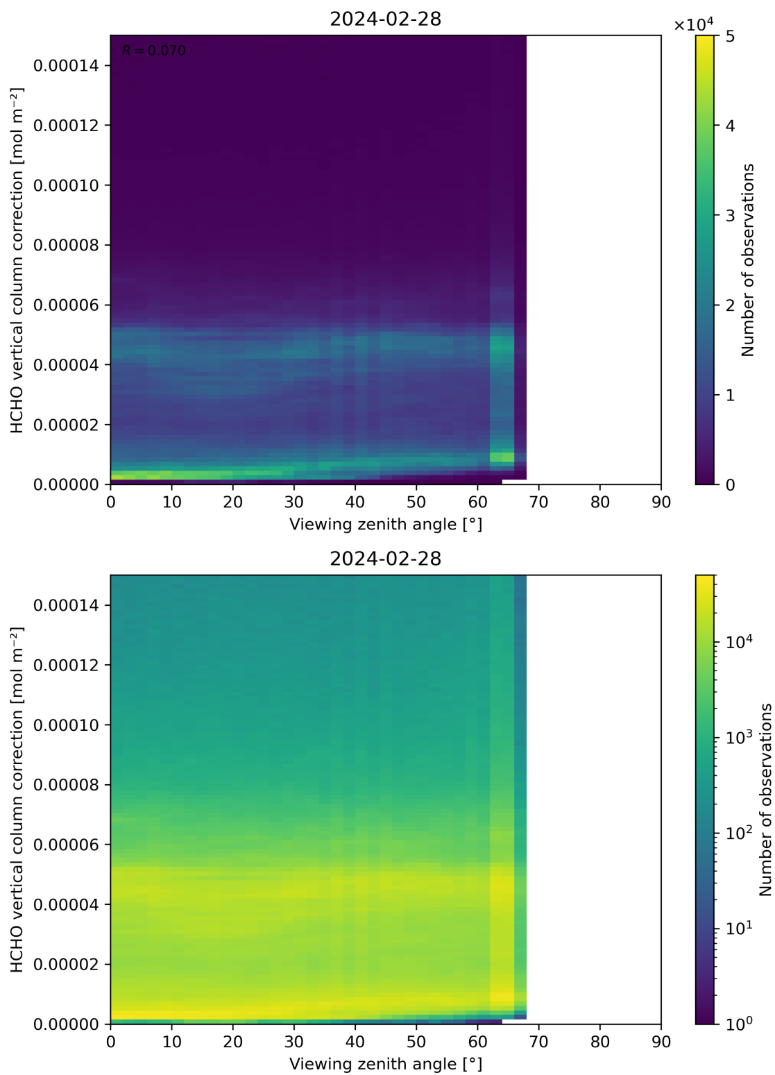
Figure 193: Scatter density plot of “Viewing zenith angle” against “HCHO vertical column correction” for 2024-02-27 to 2024-02-29.
