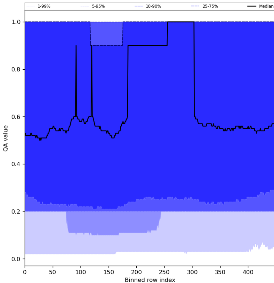
Figure 48: Along track statistics of “QA value” for 2024-02-27 to 2024-02-29
