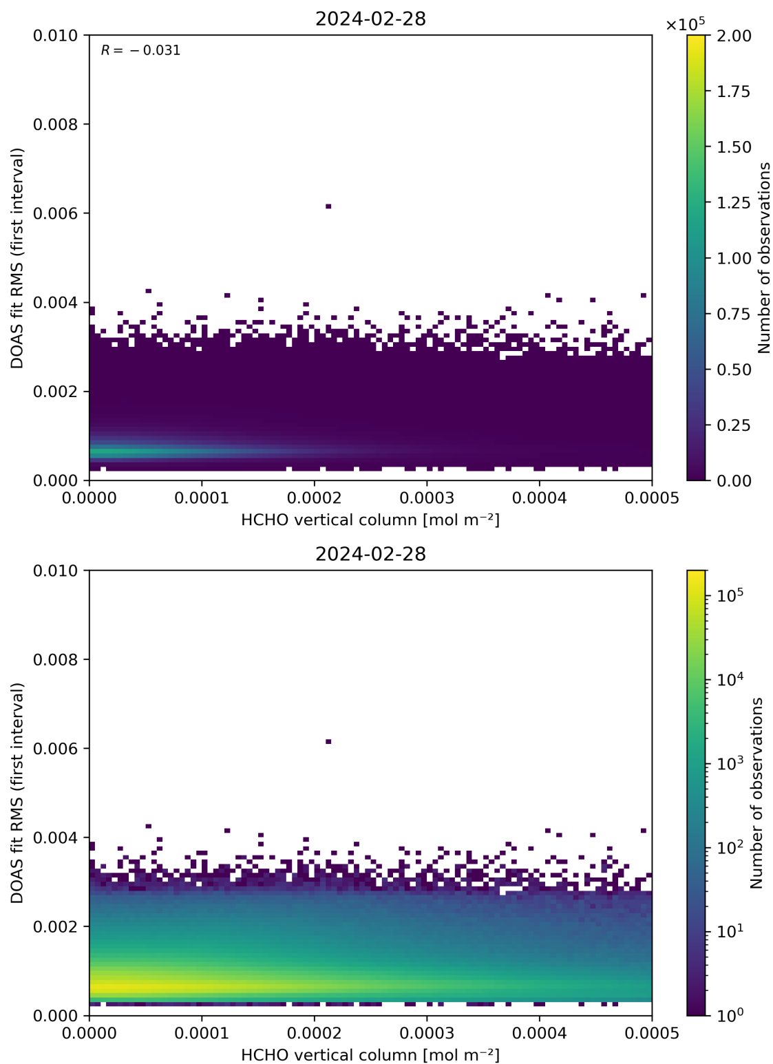
Figure 123: Scatter density plot of “HCHO vertical column” against “DOAS fit RMS (first interval)” for 2024-02-27 to 2024-02-29.
