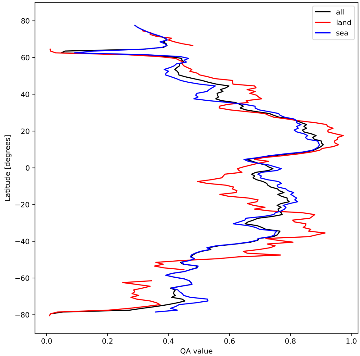
Figure 20: Zonal average of “QA value” for 2024-02-27 to 2024-02-29.
