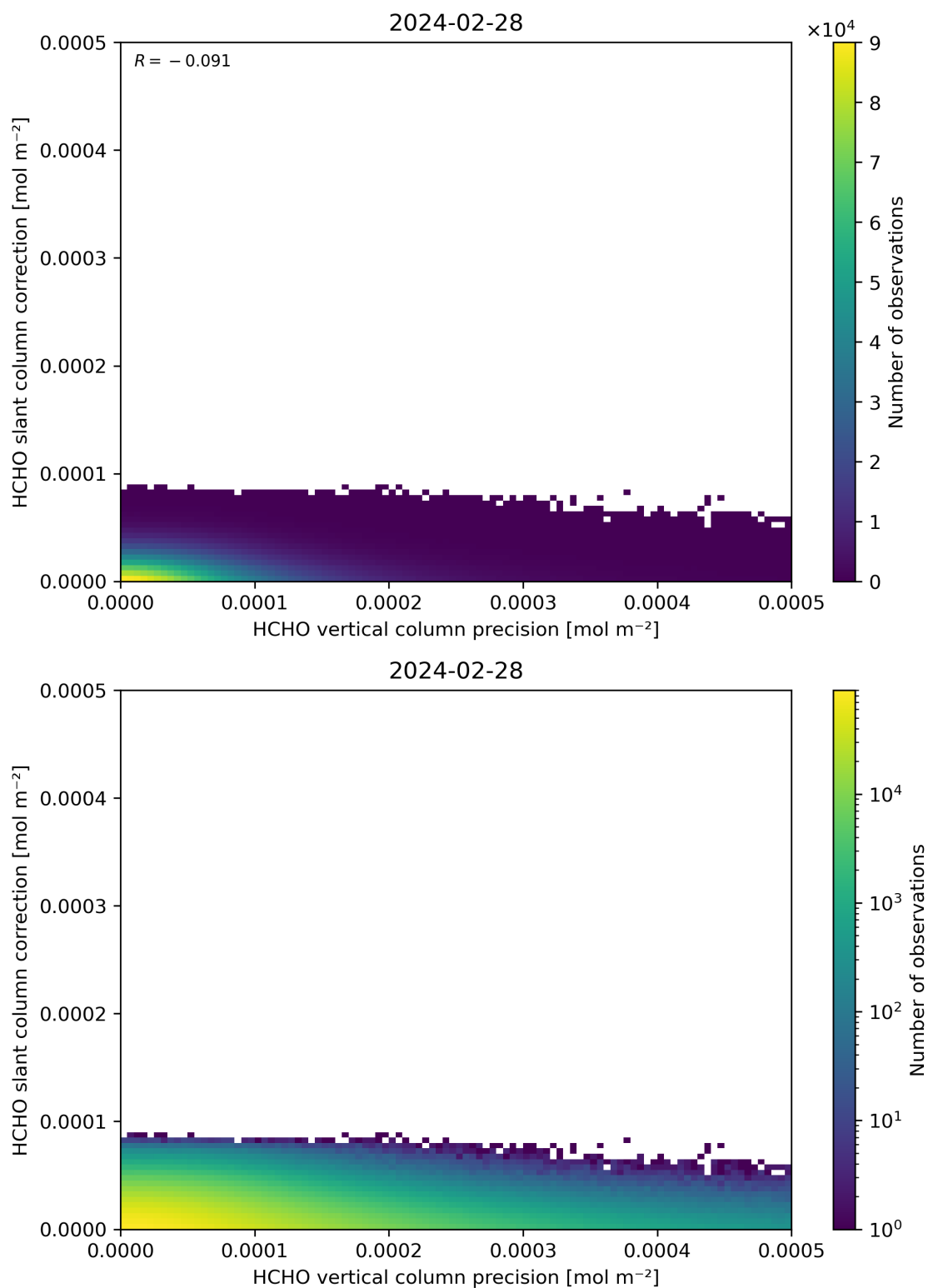
Figure 141: Scatter density plot of “HCHO vertical column precision” against “HCHO slant column correction” for 2024-02-27 to 2024-02-29.
