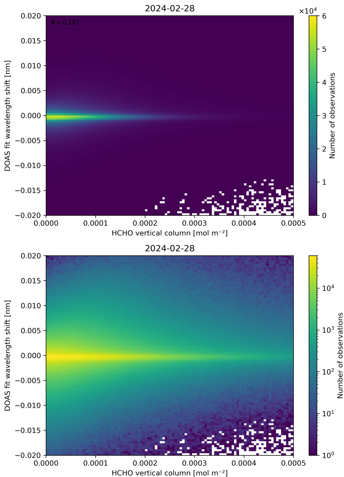
Figure 124: Scatter density plot of “HCHO vertical column” against “DOAS fit wavelength shift” for 2024-02-27 to 2024-02-29.
