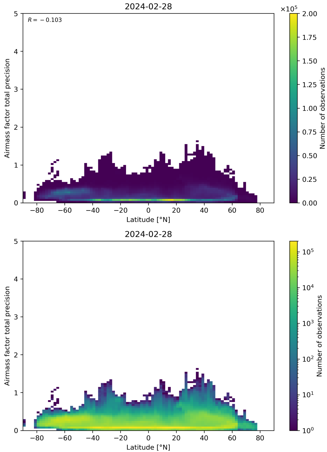
Figure 162: Scatter density plot of “Latitude” against “Airmass factor total precision” for 2024-02-27 to 2024-02-29.
