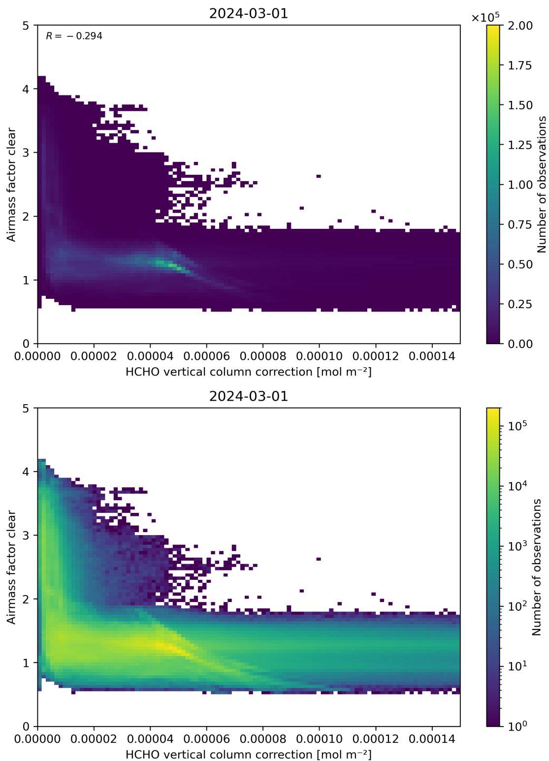
Figure 115: Scatter density plot of “HCHO vertical column correction” against “Airmass factor clear” for 2024-02-29 to 2024-03-02.
