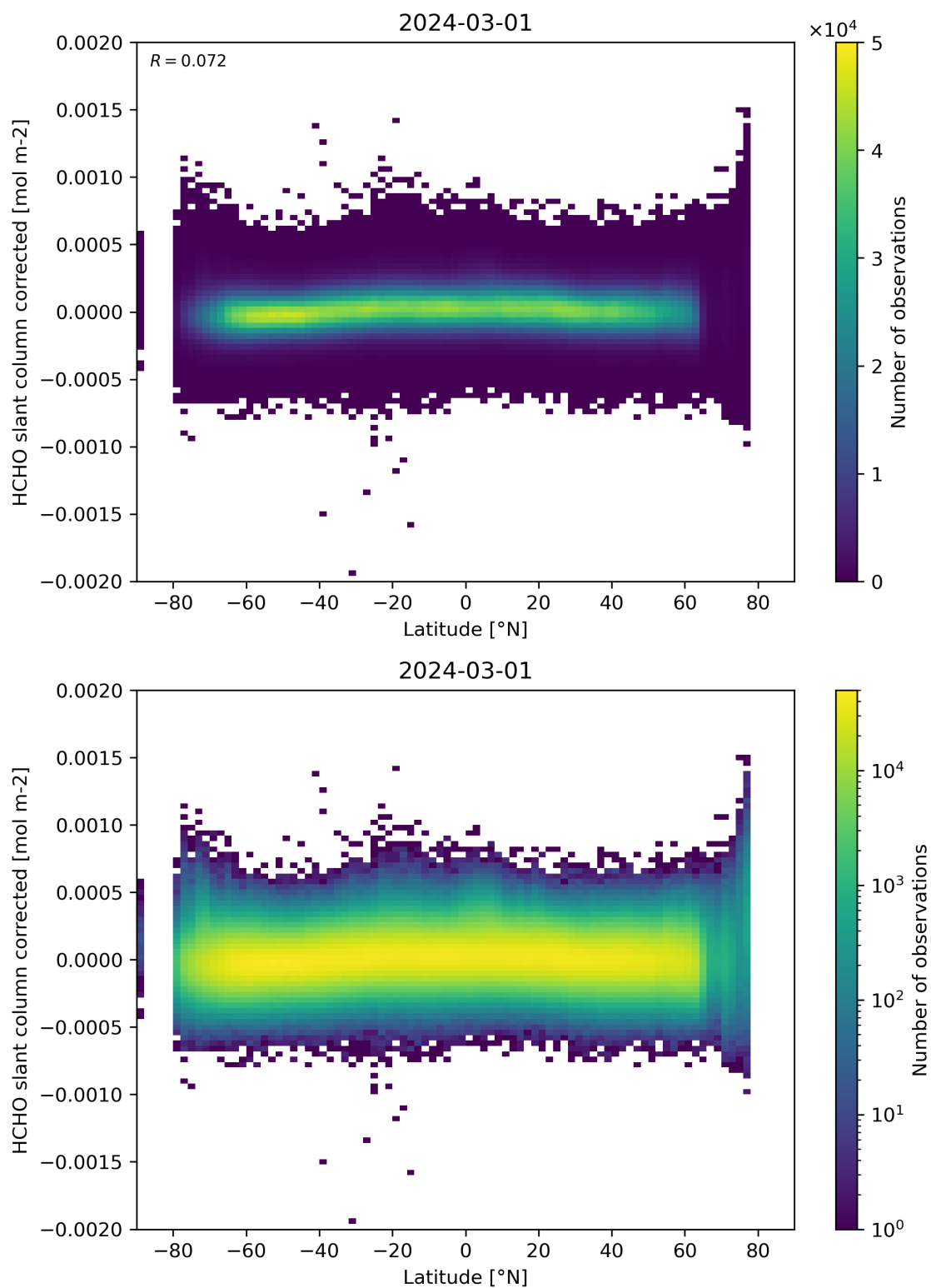
Figure 157: Scatter density plot of “Latitude” against “HCHO slant column corrected” for 2024-02-29 to 2024-03-02.
