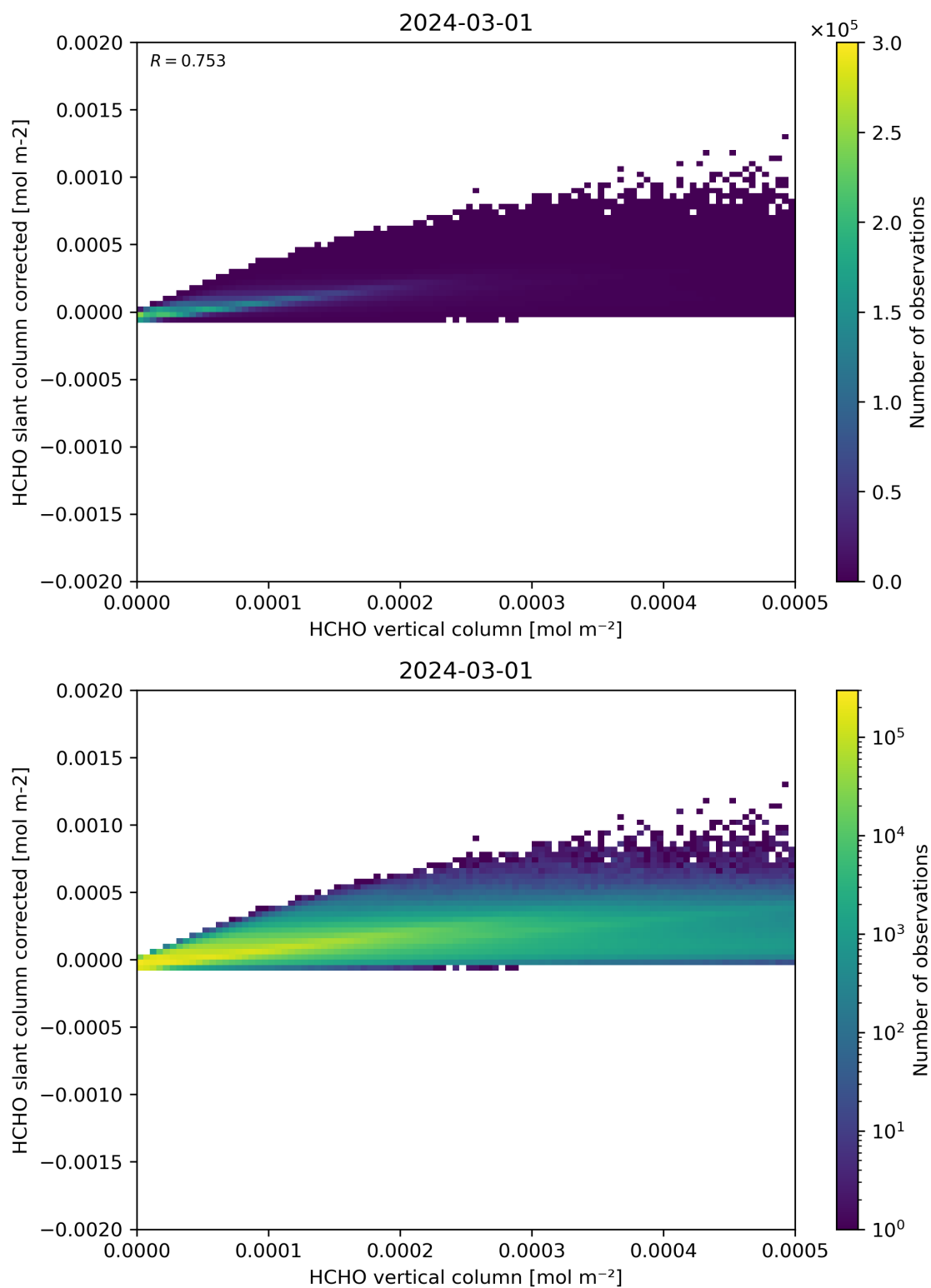
Figure 127: Scatter density plot of “HCHO vertical column” against “HCHO slant column corrected” for 2024-02-29 to 2024-03-02.
