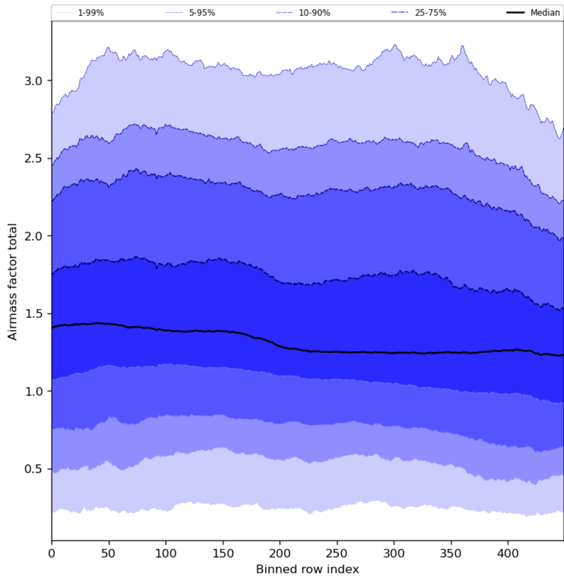
Figure 54: Along track statistics of “Airmass factor total” for 2024-02-29 to 2024-03-02
