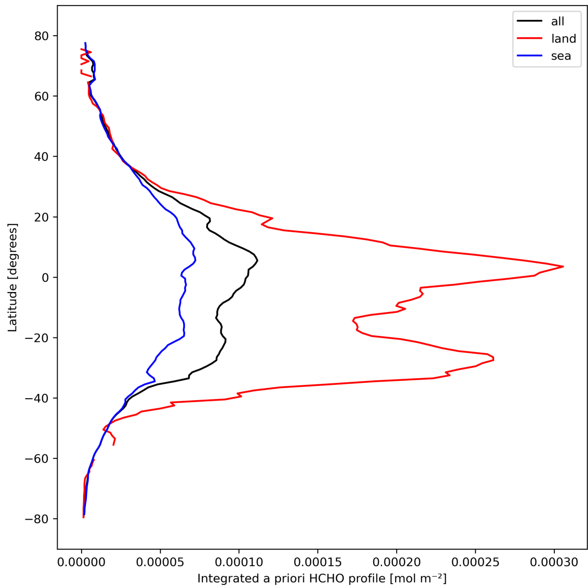
Figure 29: Zonal average of “Integrated a priori HCHO profile” for 2024-02-29 to 2024-03-02.
