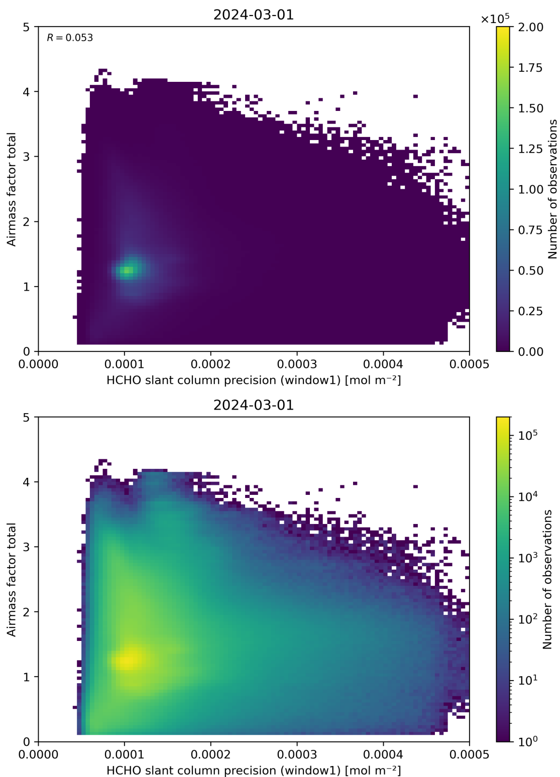
Figure 94: Scatter density plot of “HCHO slant column precision (window1)” against “Airmass factor total” for 2024-02-29 to 2024-03-02.
