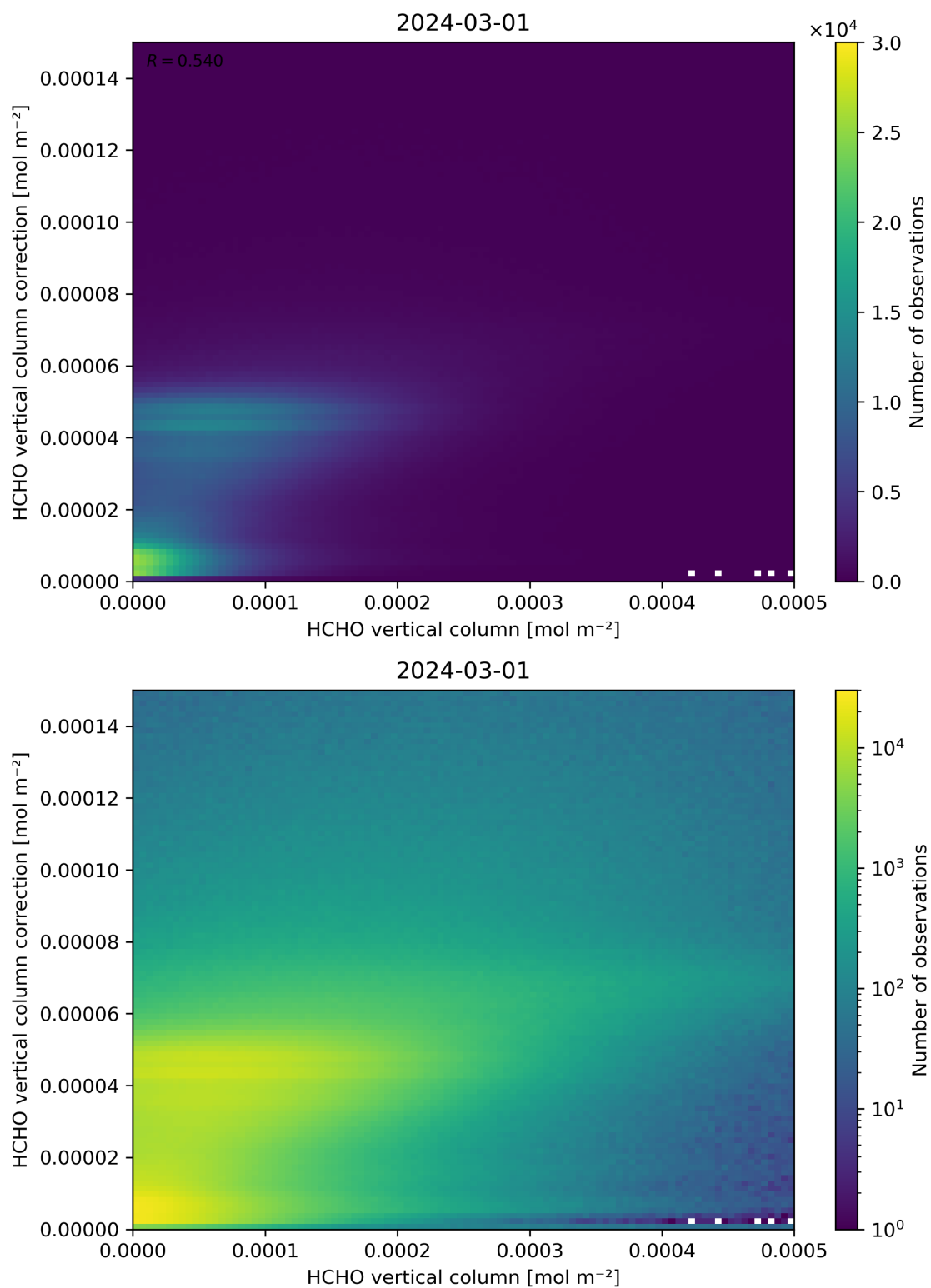
Figure 133: Scatter density plot of “HCHO vertical column” against “HCHO vertical column correction” for 2024-02-29 to 2024-03-02.
