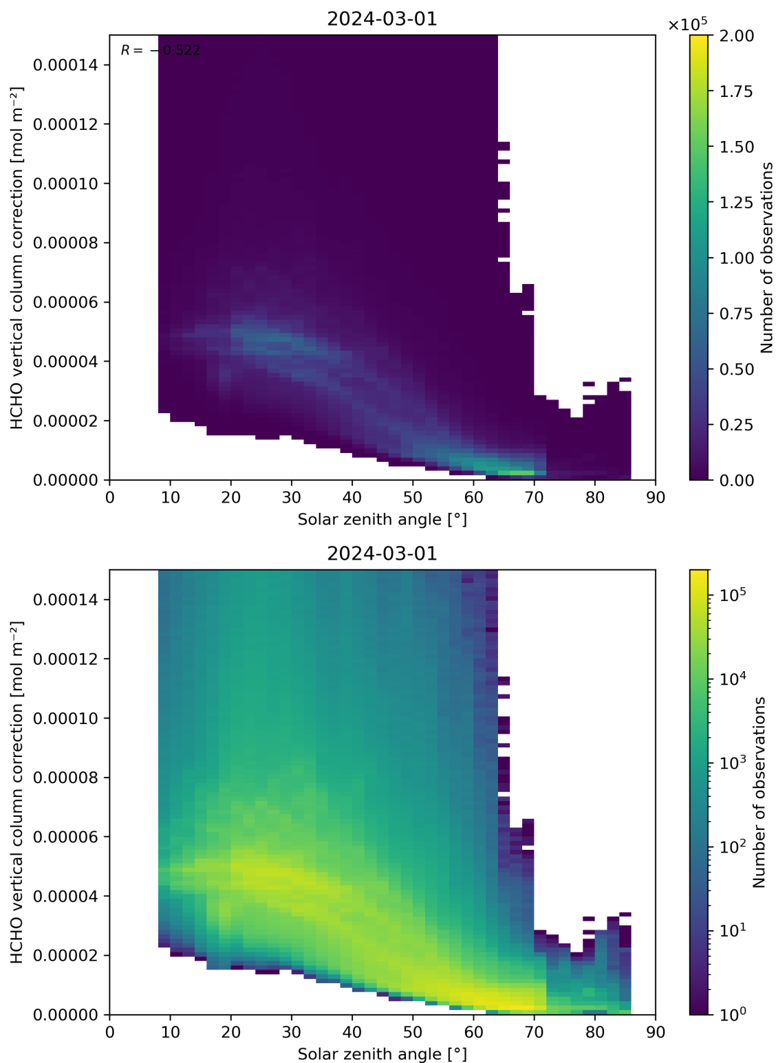
Figure 178: Scatter density plot of “Solar zenith angle” against “HCHO vertical column correction” for 2024-02-29 to 2024-03-02.
