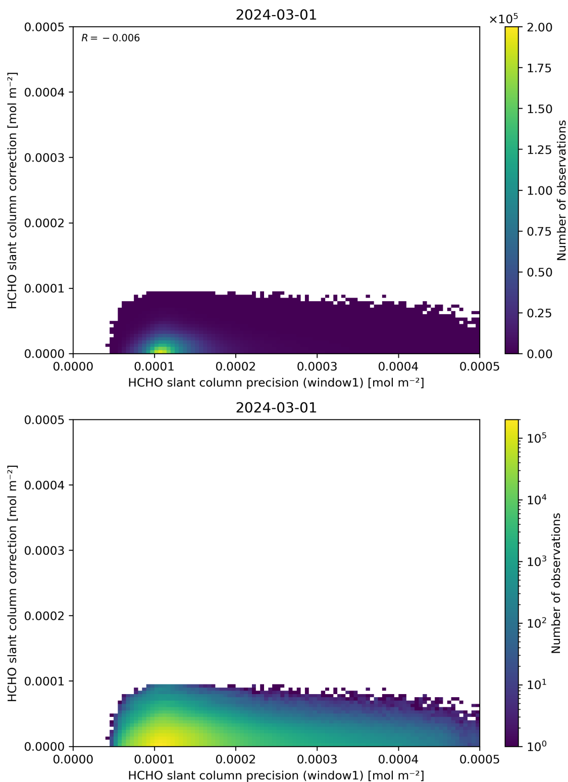
Figure 93: Scatter density plot of “HCHO slant column precision (window1)” against “HCHO slant column correction” for 2024-02-29 to 2024-03-02.
