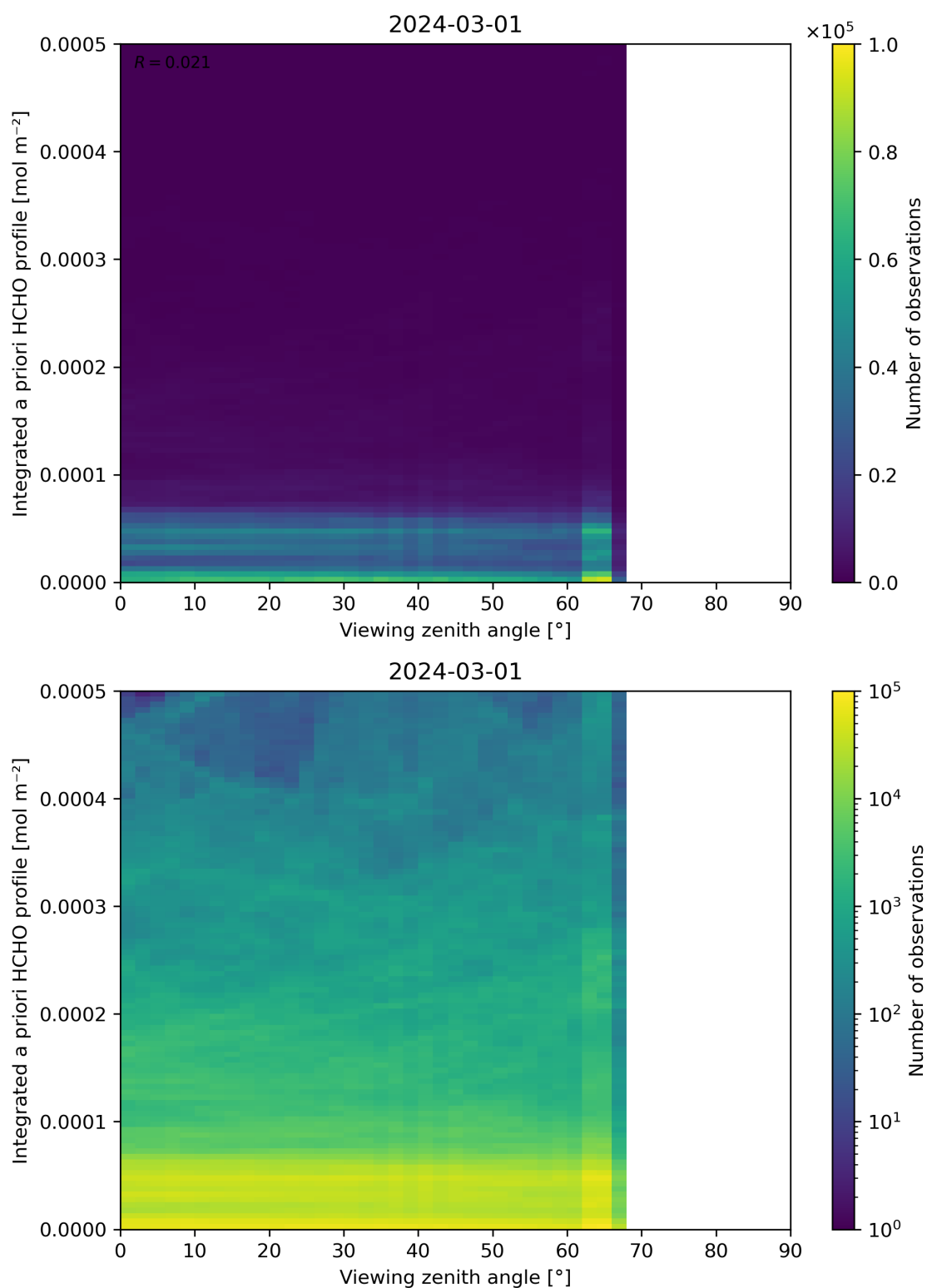
Figure 195: Scatter density plot of “Viewing zenith angle” against “Integrated a priori HCHO profile” for 2024-02-29 to 2024-03-02.
