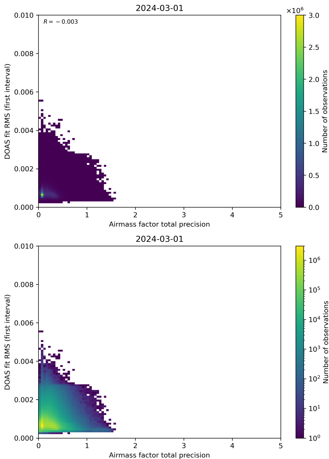
Figure 105: Scatter density plot of “Airmass factor total precision” against “DOAS fit RMS (first interval)” for 2024-02-29 to 2024-03-02.
