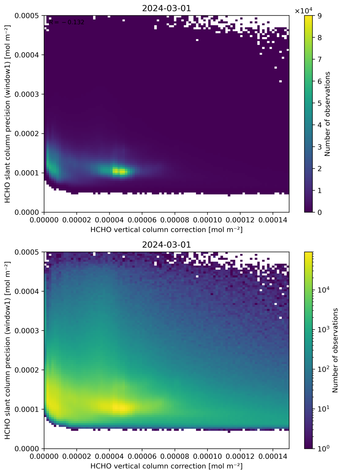
Figure 119: Scatter density plot of “HCHO vertical column correction” against “HCHO slant column precision (window1)” for 2024-02-29 to 2024-03-02.
