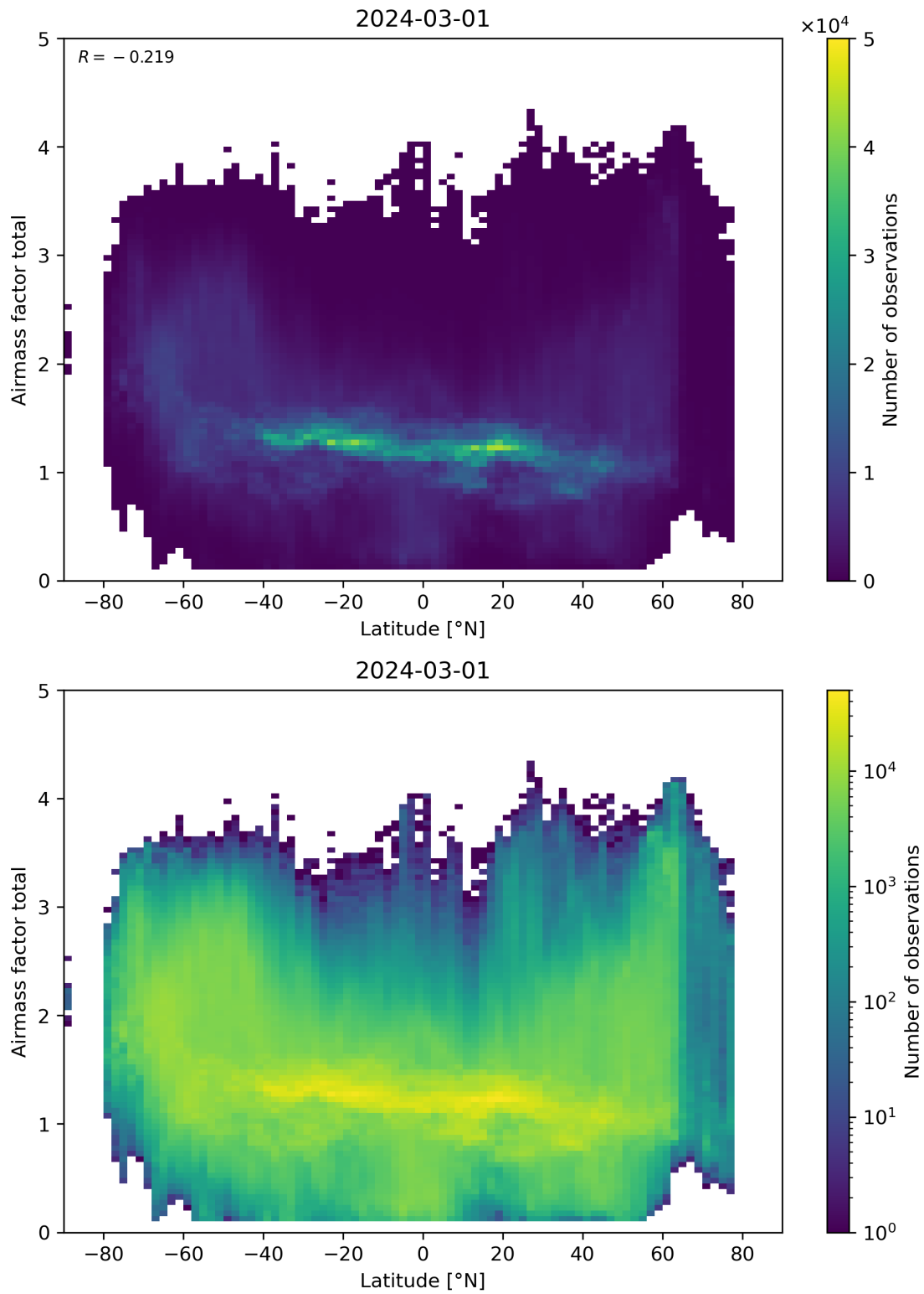
Figure 161: Scatter density plot of “Latitude” against “Airmass factor total” for 2024-02-29 to 2024-03-02.
