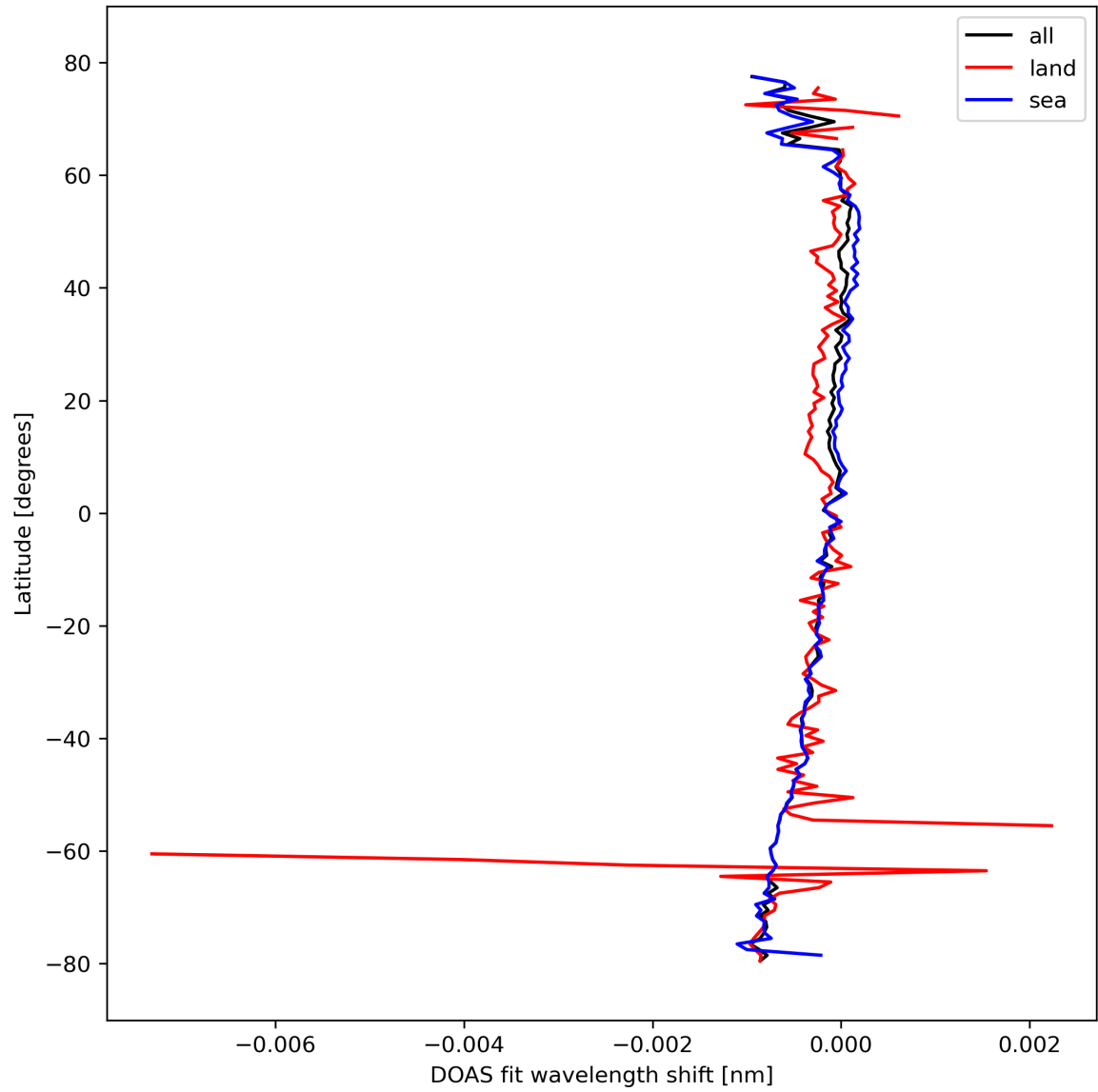
Figure 30: Zonal average of "DOAS fit wavelength shift" for 2024-02-29 to 2024-03-02.
