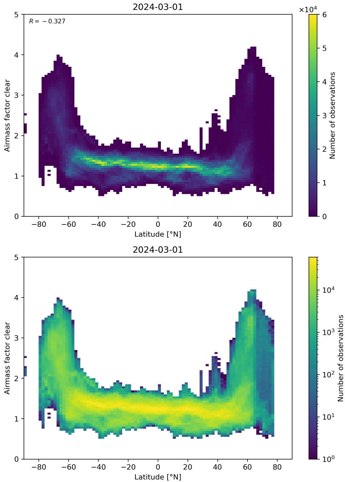
Figure 156: Scatter density plot of “Latitude” against “Airmass factor clear” for 2024-02-29 to 2024-03-02.
