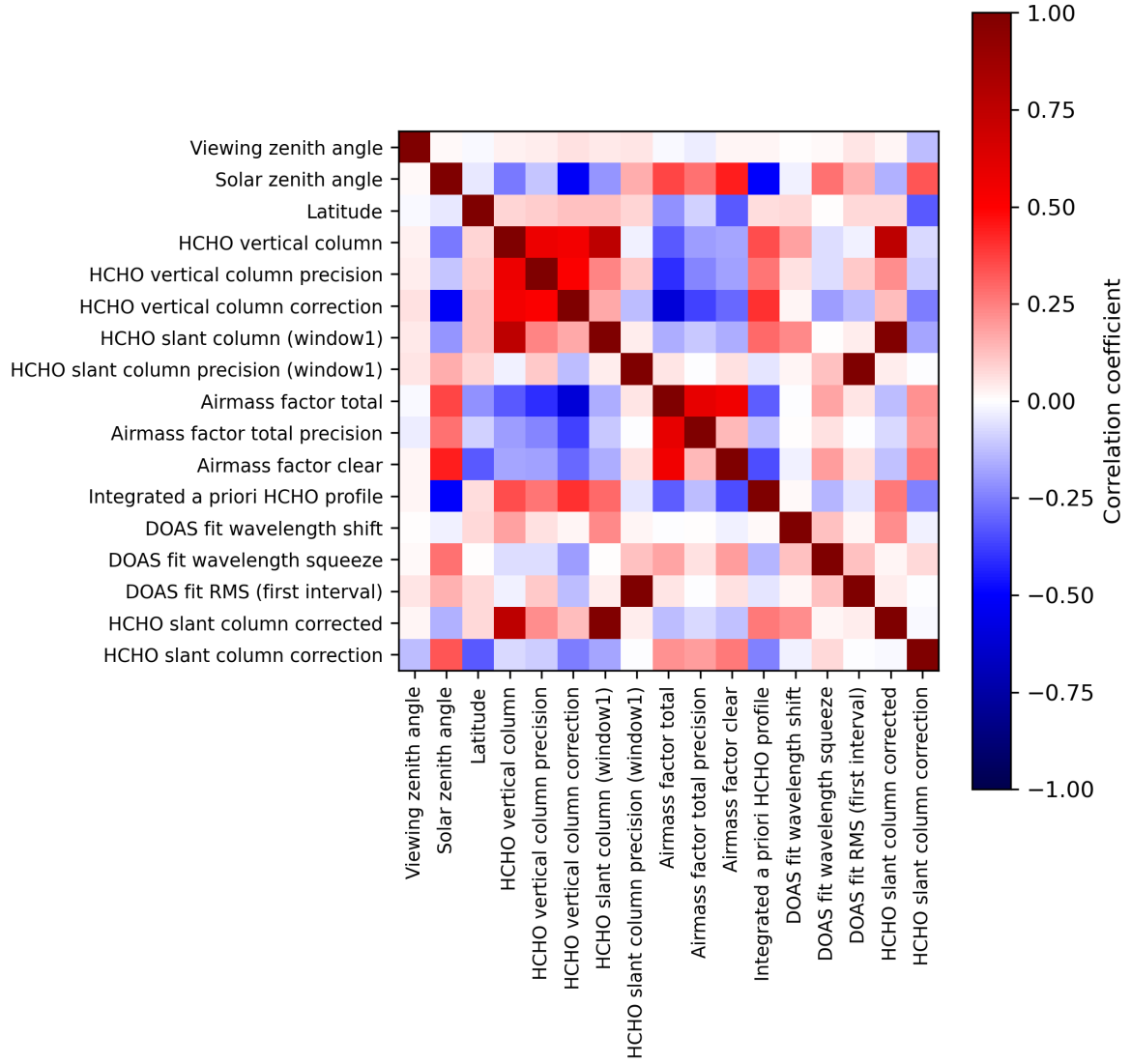
Figure 2: Map of correlation matrix for 2024-02-29 to 2024-03-02.
