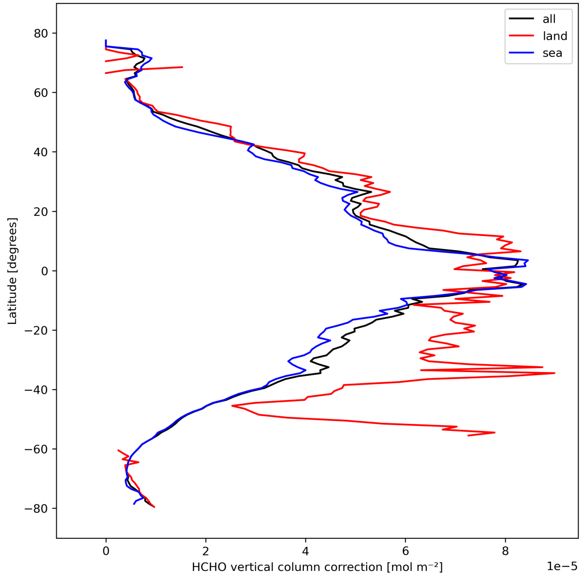
Figure 23: Zonal average of “HCHO vertical column correction” for 2024-02-29 to 2024-03-02.
