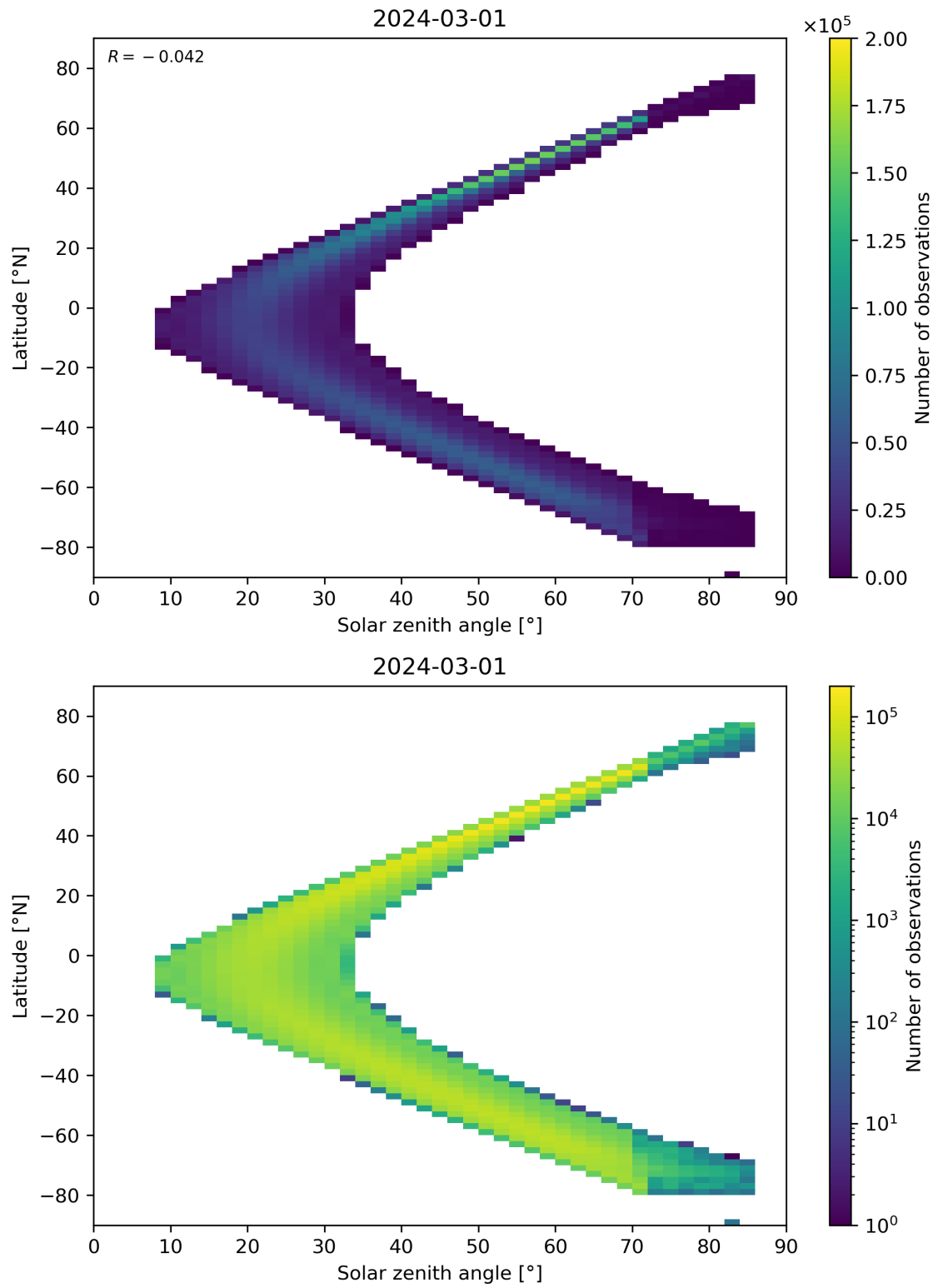
Figure 181: Scatter density plot of “Solar zenith angle” against “Latitude” for 2024-02-29 to 2024-03-02.
