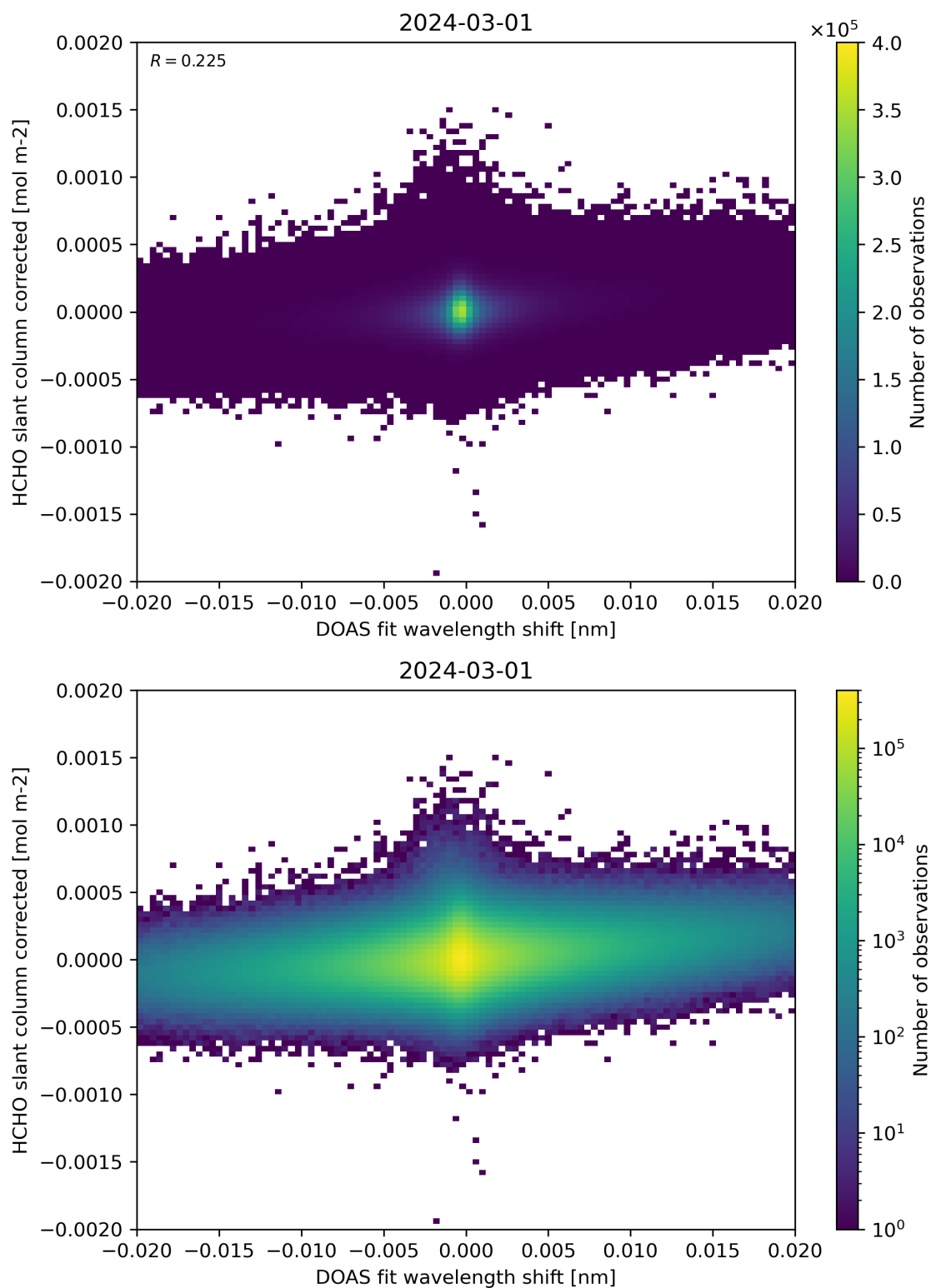
Figure 66: Scatter density plot of “DOAS fit wavelength shift” against “HCHO slant column corrected” for 2024-02-29 to 2024-03-02.
