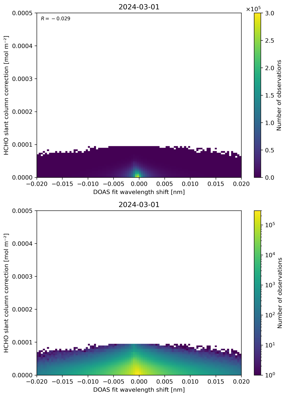
Figure 67: Scatter density plot of “DOAS fit wavelength shift” against “HCHO slant column correction” for 2024-02-29 to 2024-03-02.
