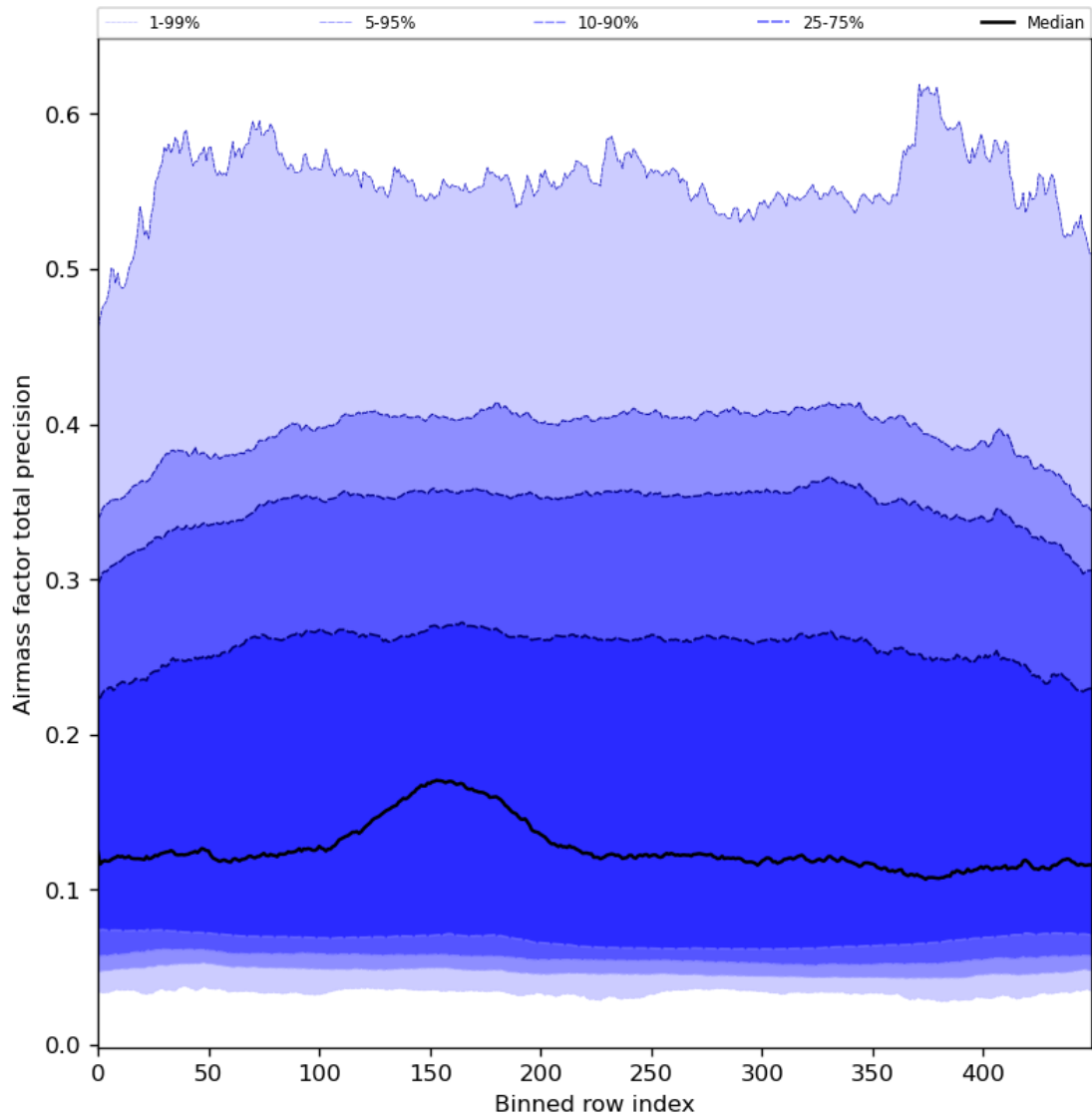
Figure 55: Along track statistics of “Airmass factor total precision” for 2024-02-29 to 2024-03-02
