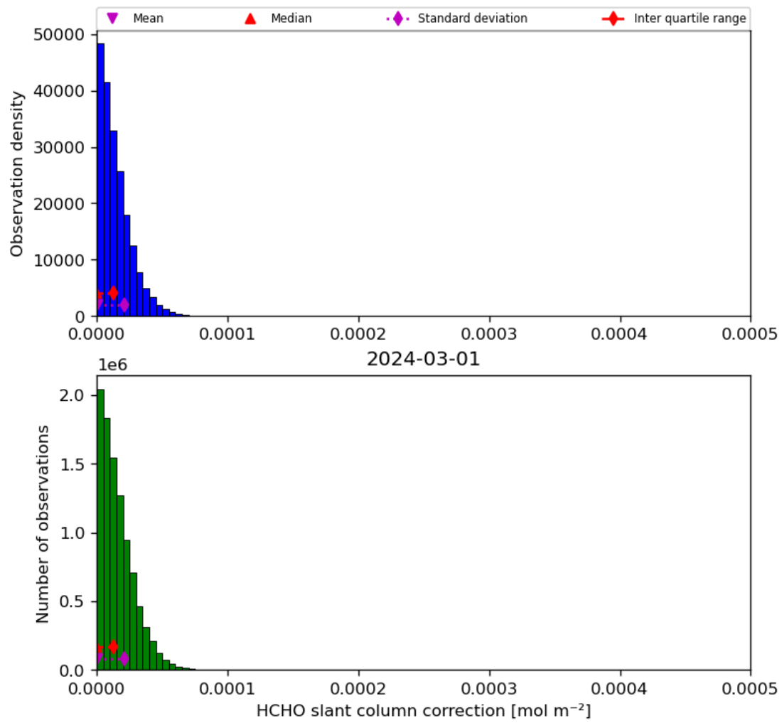
Figure 47: Histogram of “HCHO slant column correction” for 2024-02-29 to 2024-03-02
