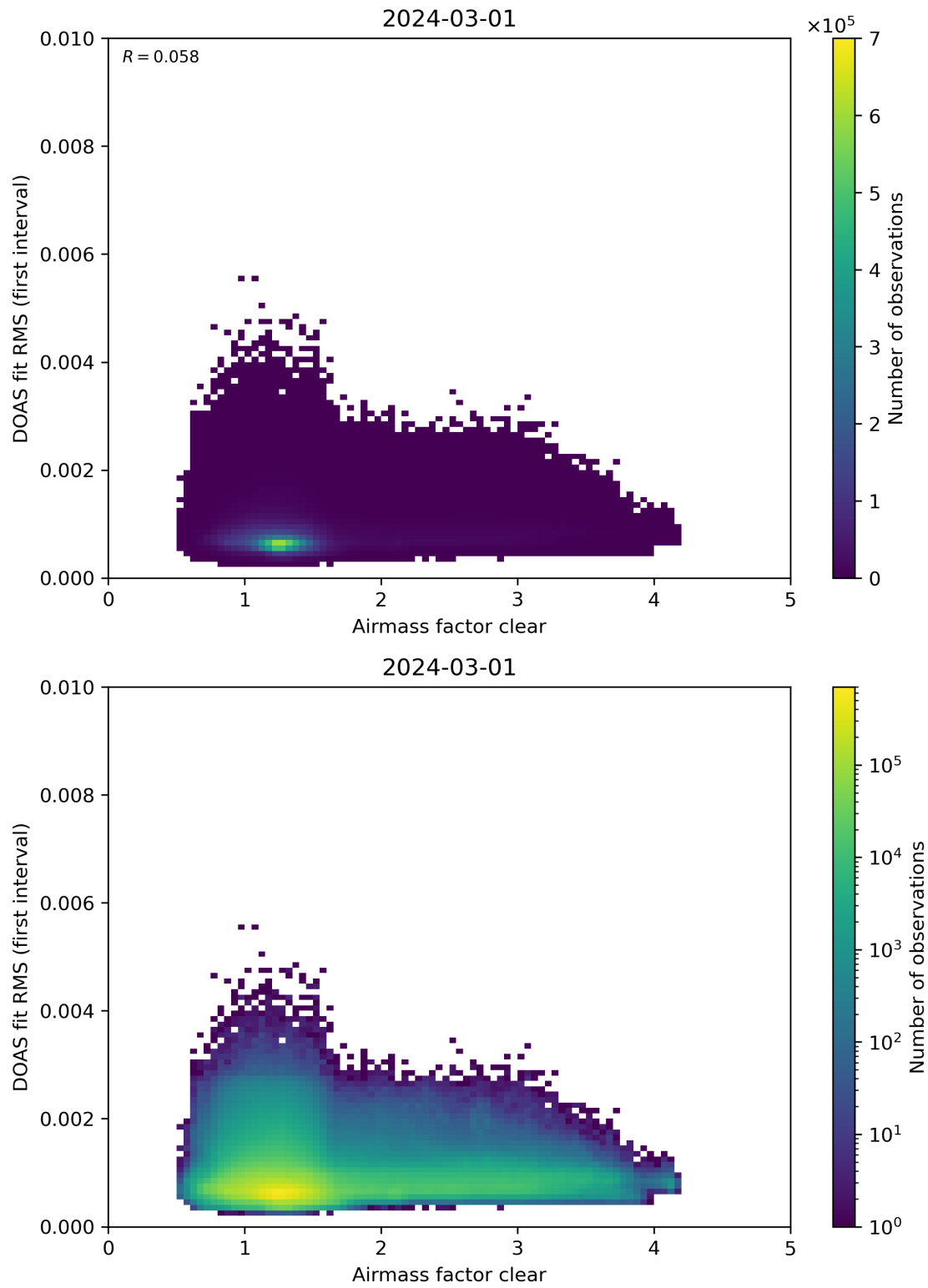
Figure 71: Scatter density plot of “Airmass factor clear” against “DOAS fit RMS (first interval)” for 2024-02-29 to 2024-03-02.
