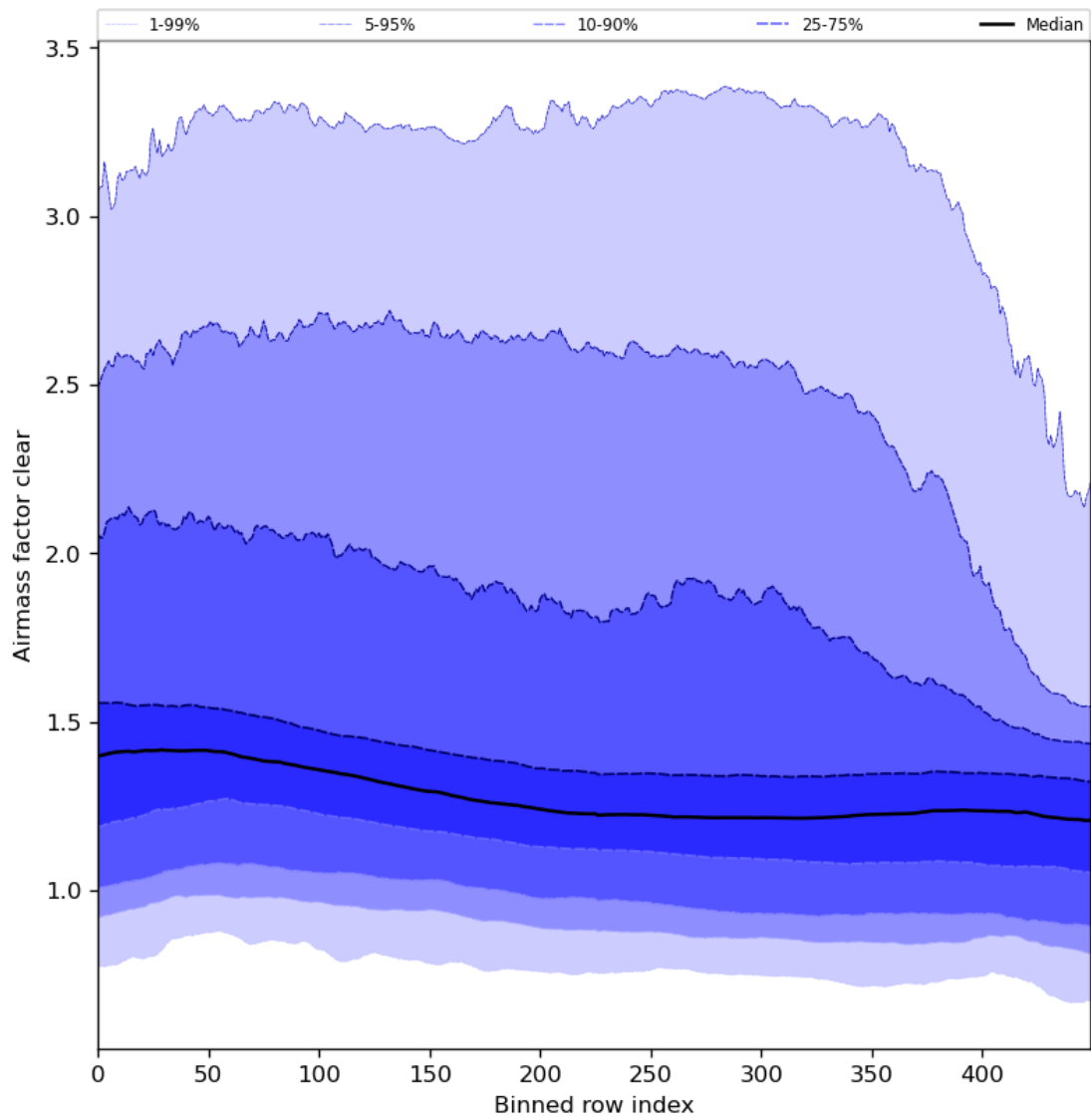
Figure 56: Along track statistics of “Airmass factor clear” for 2024-02-29 to 2024-03-02
