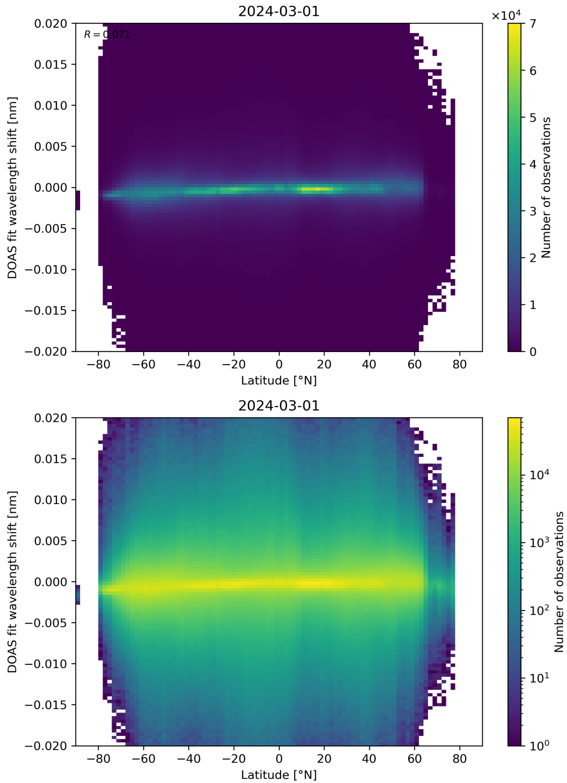
Figure 154: Scatter density plot of “Latitude” against “DOAS fit wavelength shift” for 2024-02-29 to 2024-03-02.
