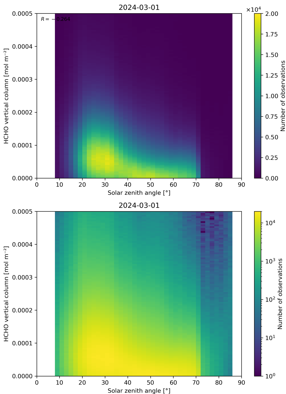
Figure 177: Scatter density plot of “Solar zenith angle” against “HCHO vertical column” for 2024-02-29 to 2024-03-02.
