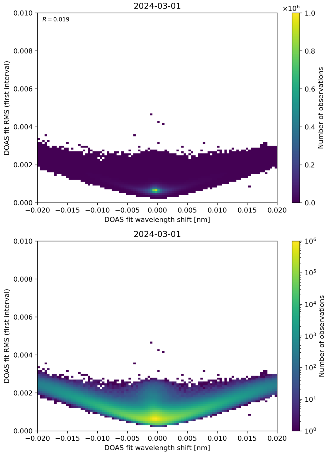
Figure 64: Scatter density plot of “DOAS fit wavelength shift” against “DOAS fit RMS (first interval)” for 2024-02-29 to 2024-03-02.
