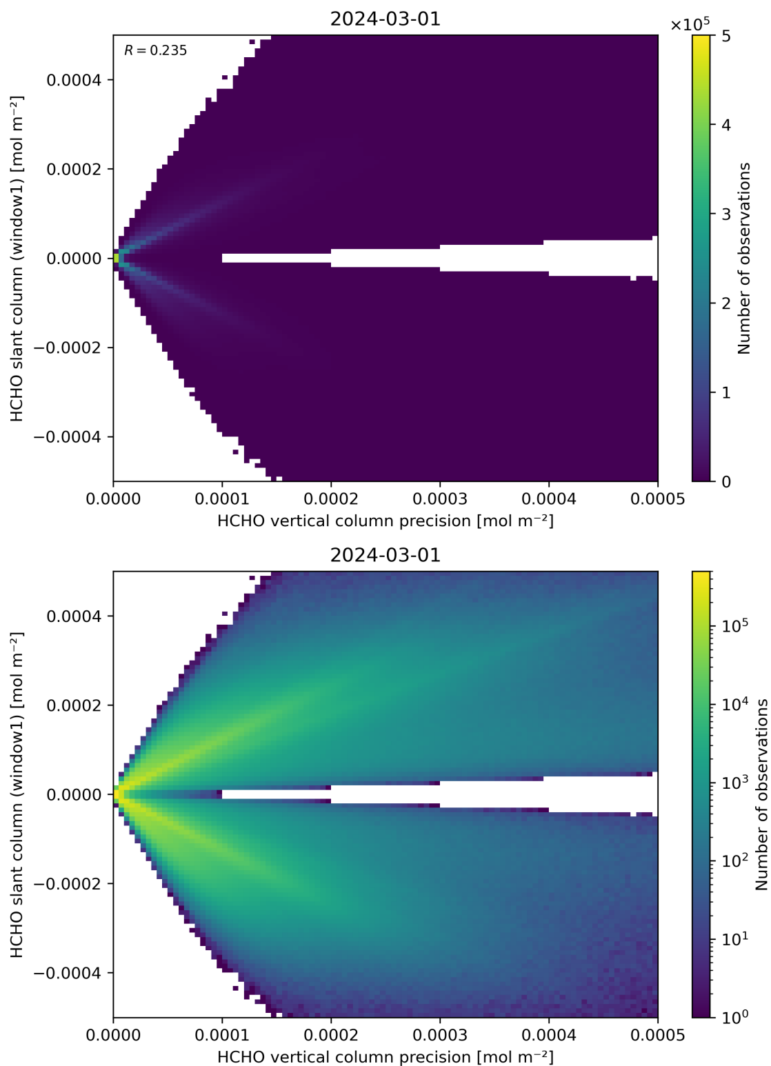
Figure 142: Scatter density plot of “HCHO vertical column precision” against “HCHO slant column (window1)” for 2024-02-29 to 2024-03-02.
