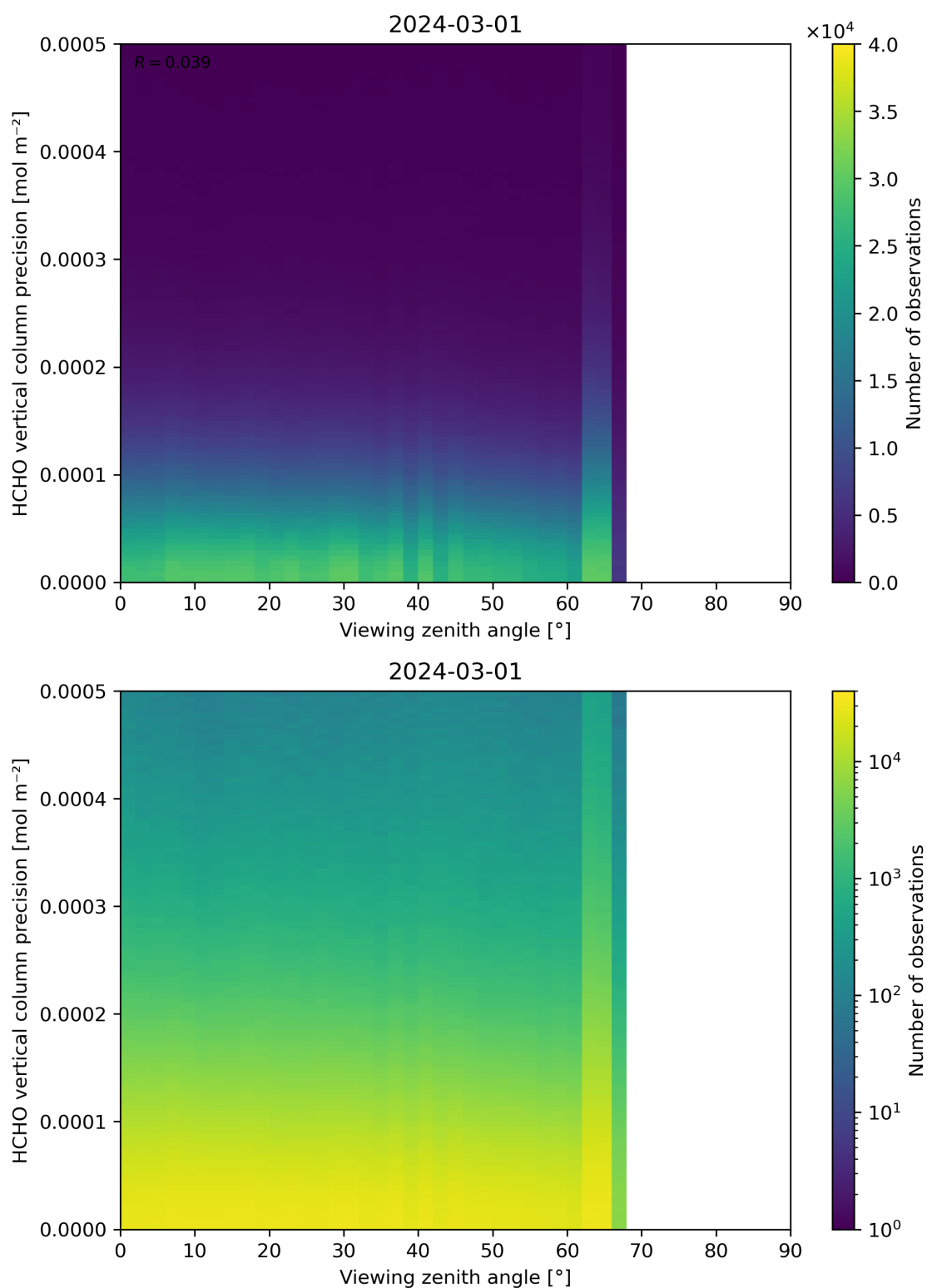
Figure 194: Scatter density plot of “Viewing zenith angle” against “HCHO vertical column precision” for 2024-02-29 to 2024-03-02.
