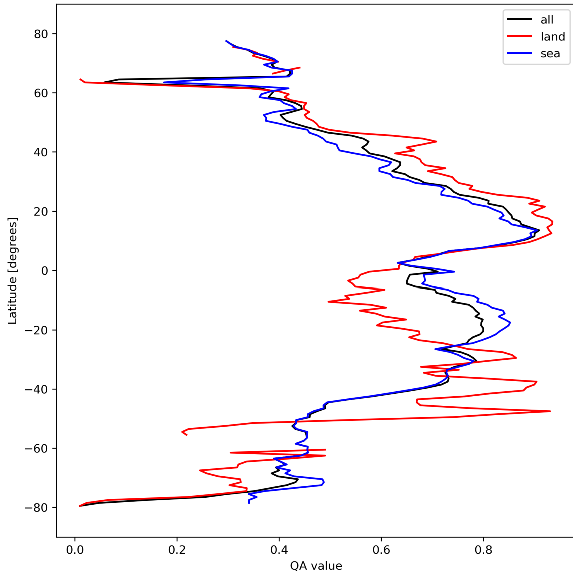
Figure 20: Zonal average of “QA value” for 2024-02-29 to 2024-03-02.
