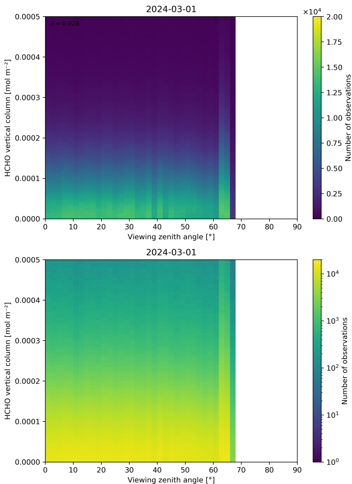
Figure 192: Scatter density plot of “Viewing zenith angle” against “HCHO vertical column” for 2024-02-29 to 2024-03-02.
