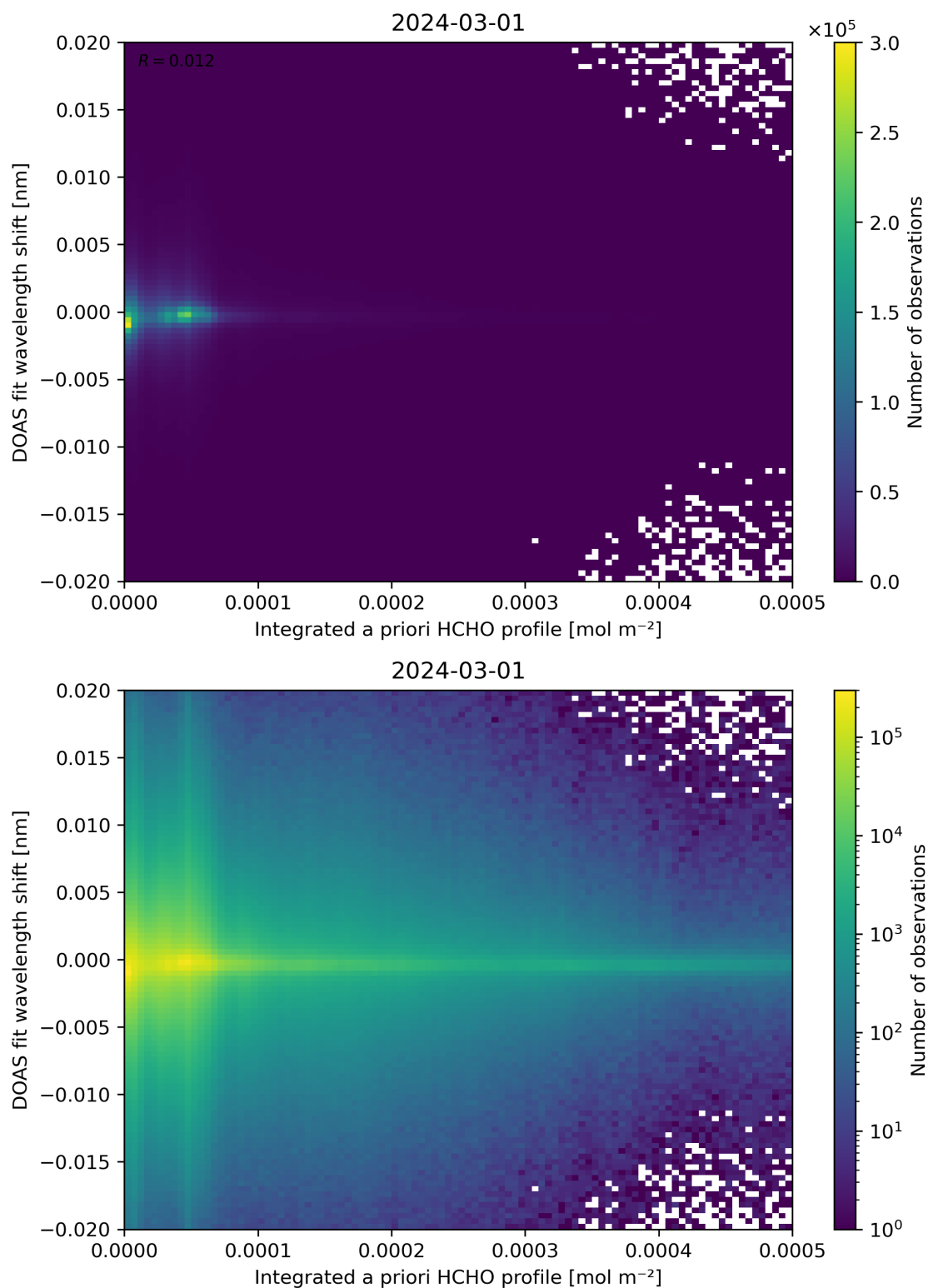
Figure 149: Scatter density plot of “Integrated a priori HCHO profile” against “DOAS fit wavelength shift” for 2024-02-29 to 2024-03-02.
