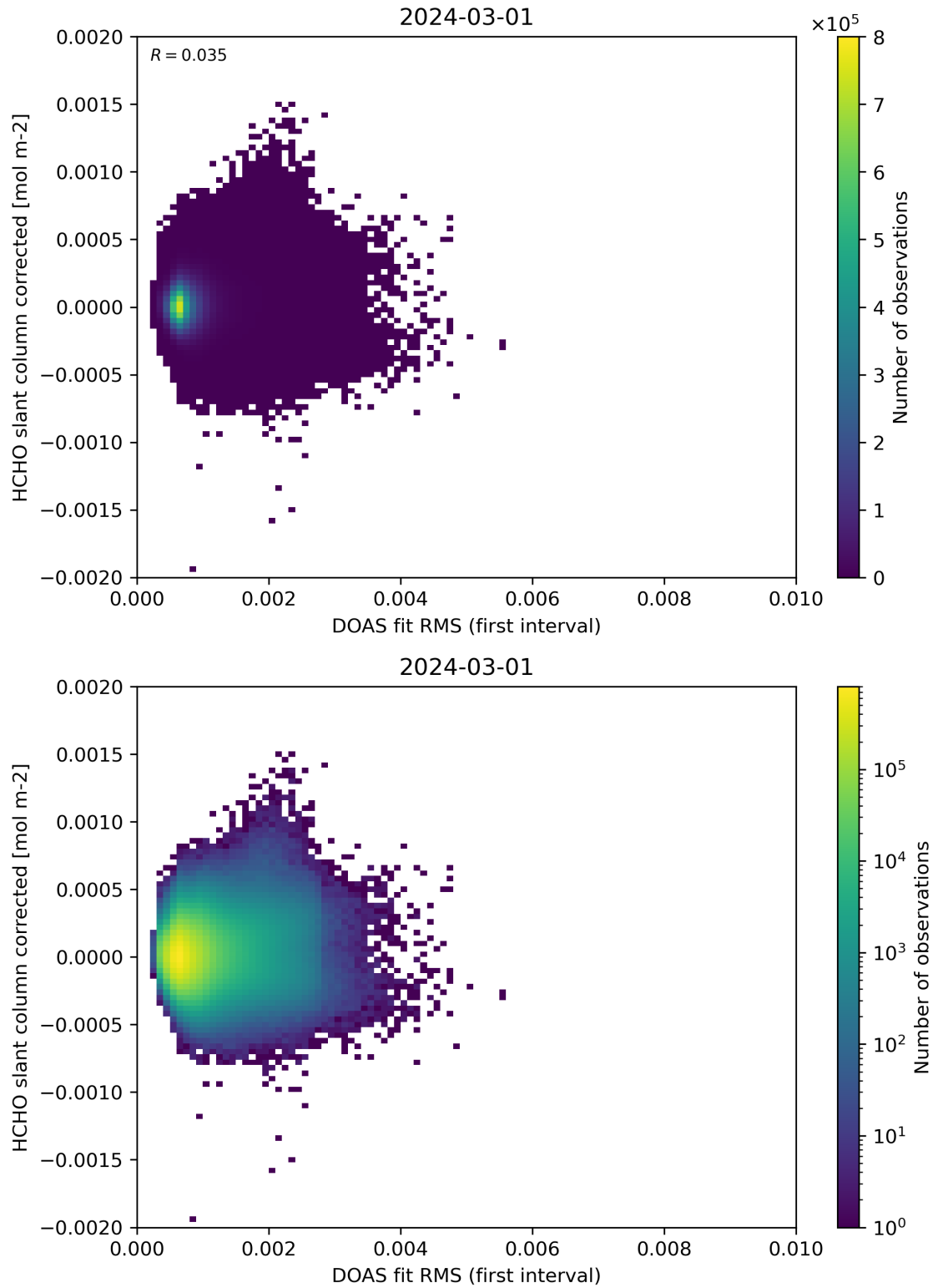
Figure 62: Scatter density plot of “DOAS fit RMS (first interval)” against “HCHO slant column corrected” for 2024-02-29 to 2024-03-02.
