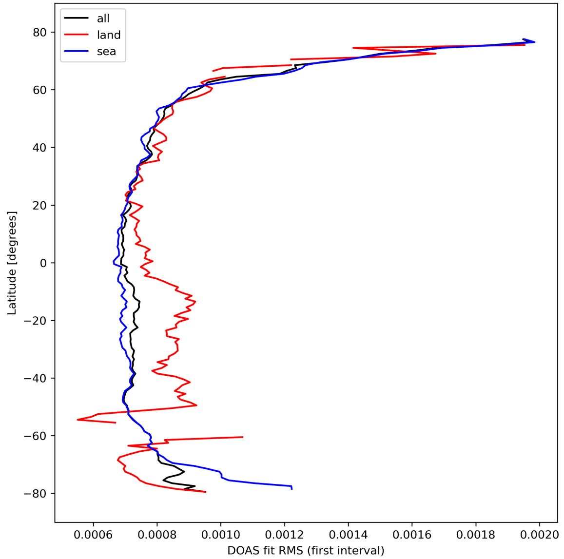
Figure 32: Zonal average of “DOAS fit RMS (first interval)” for 2024-02-29 to 2024-03-02.
