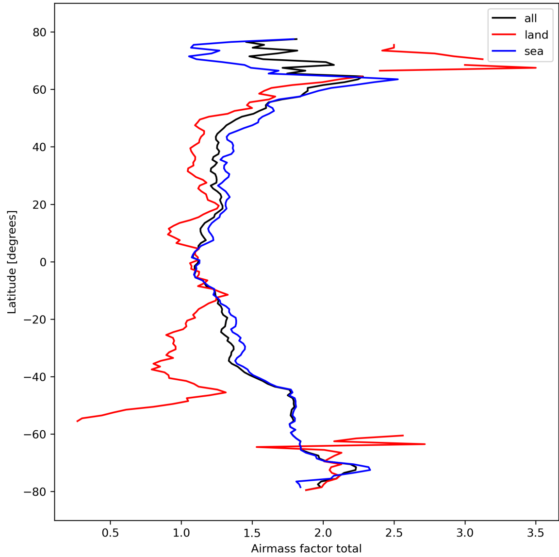
Figure 26: Zonal average of “Airmass factor total” for 2024-02-29 to 2024-03-02.
