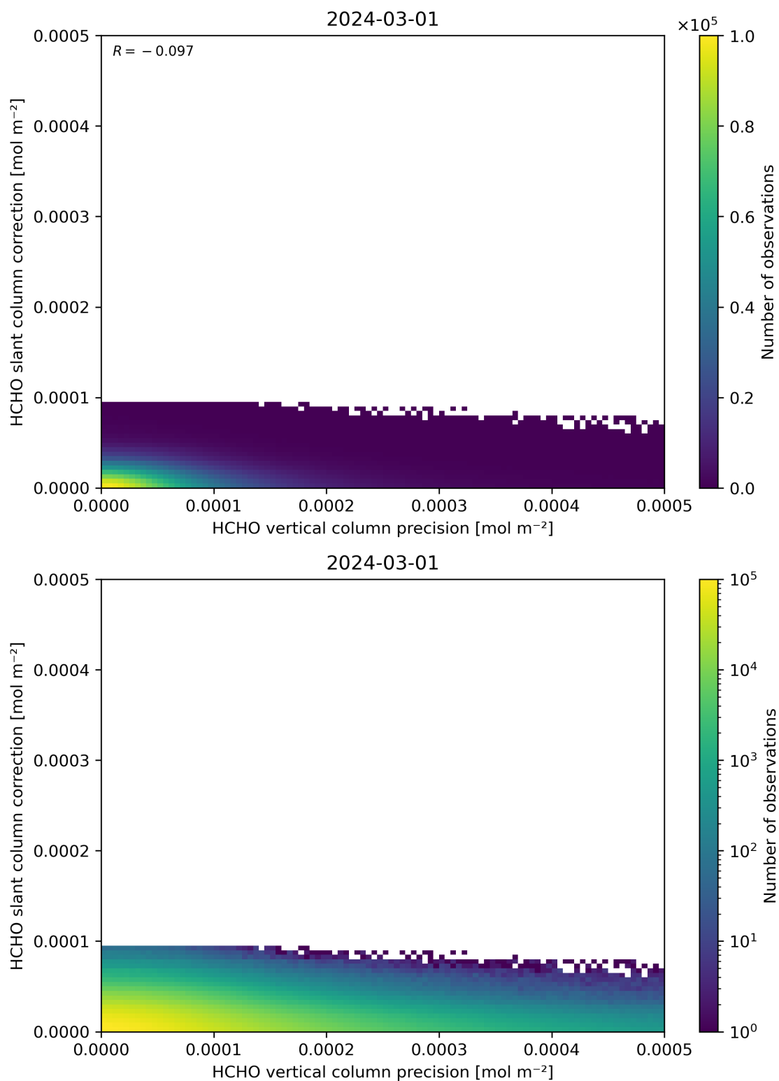
Figure 141: Scatter density plot of “HCHO vertical column precision” against “HCHO slant column correction” for 2024-02-29 to 2024-03-02.
