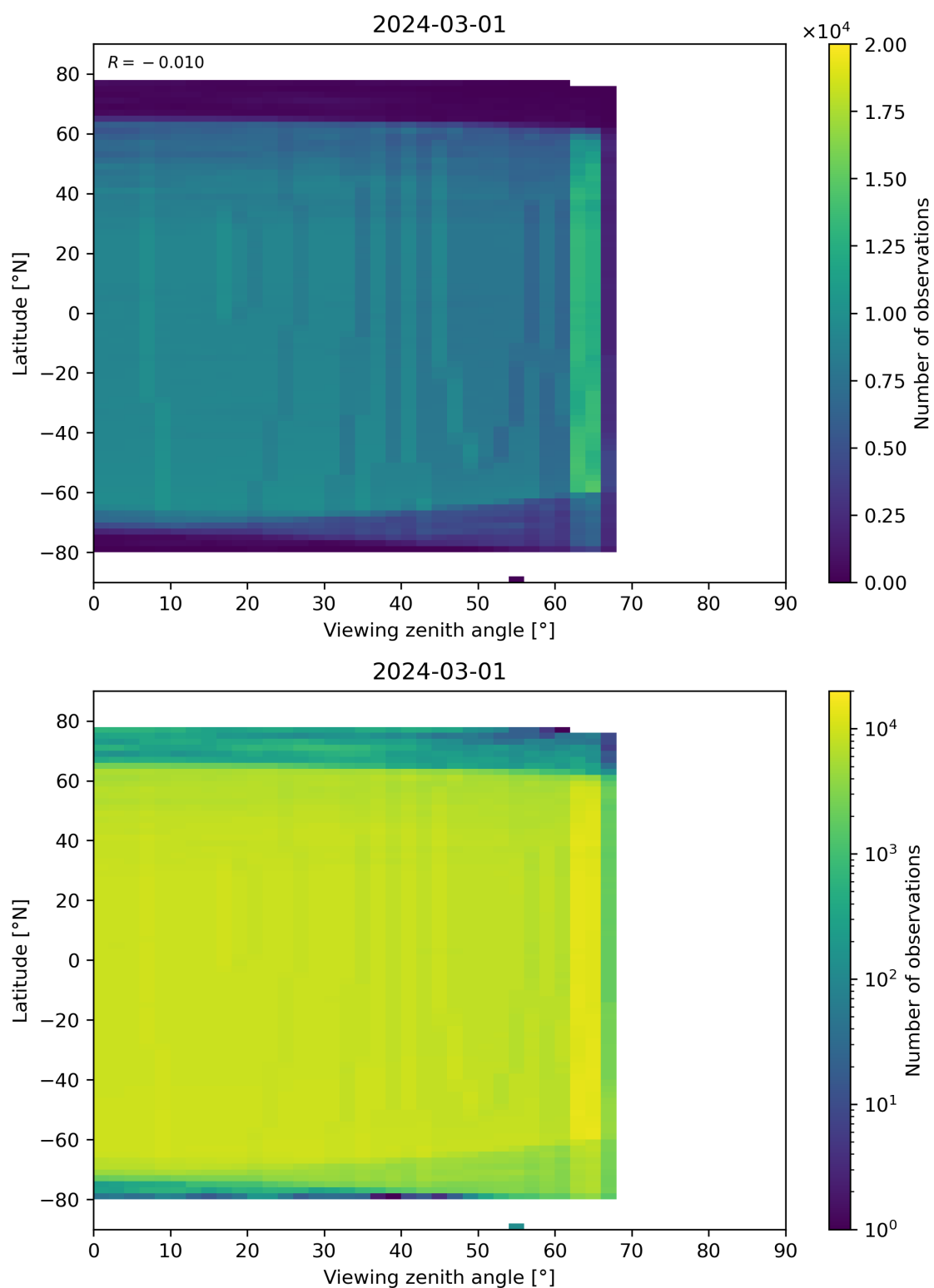
Figure 196: Scatter density plot of “Viewing zenith angle” against “Latitude” for 2024-02-29 to 2024-03-02.
