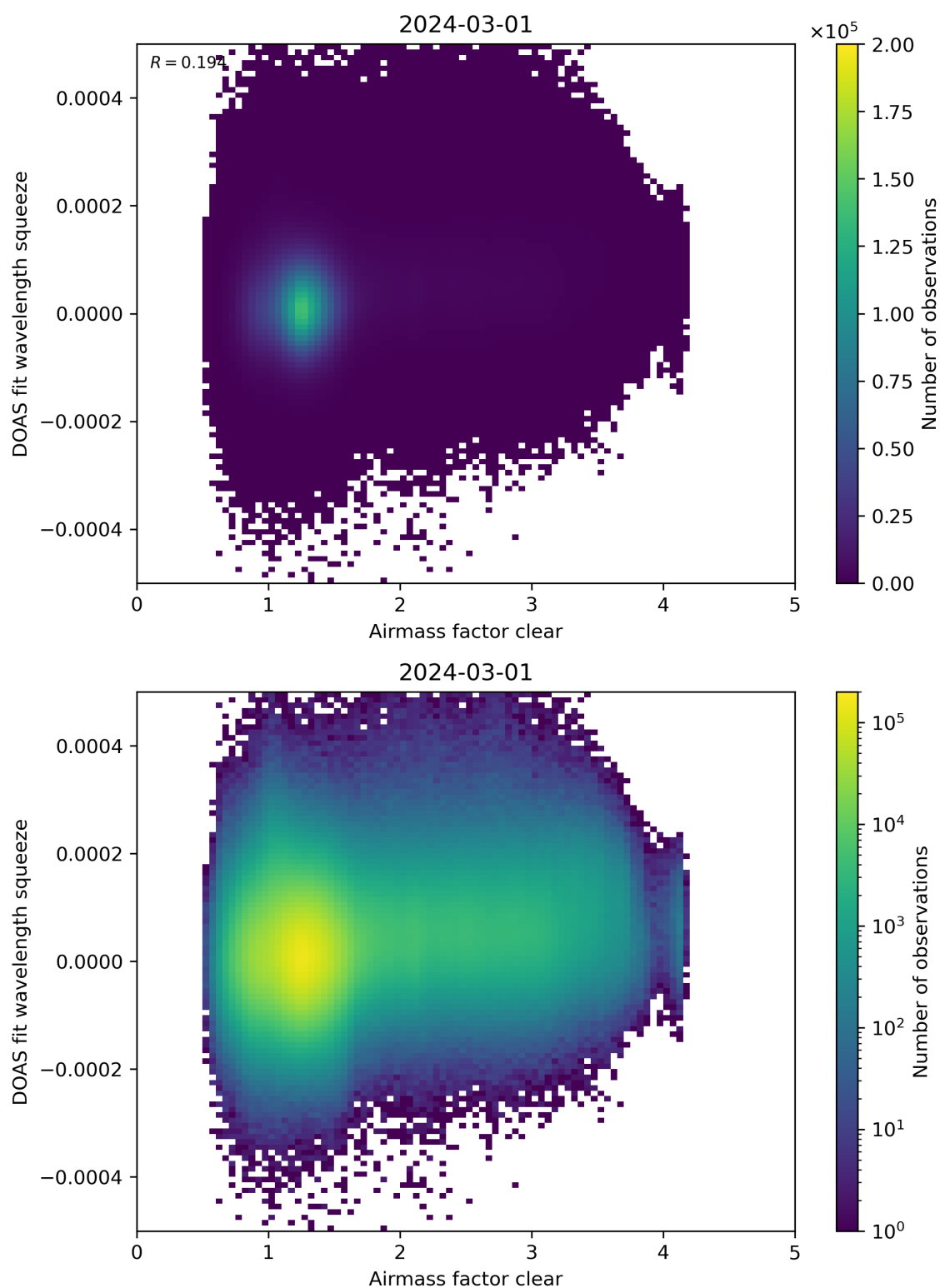
Figure 73: Scatter density plot of “Airmass factor clear” against “DOAS fit wavelength squeeze” for 2024-02-29 to 2024-03-02.
