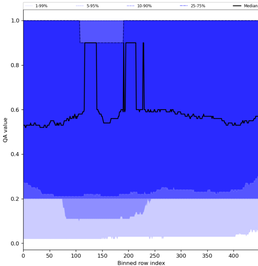
Figure 48: Along track statistics of “QA value” for 2024-02-29 to 2024-03-02
