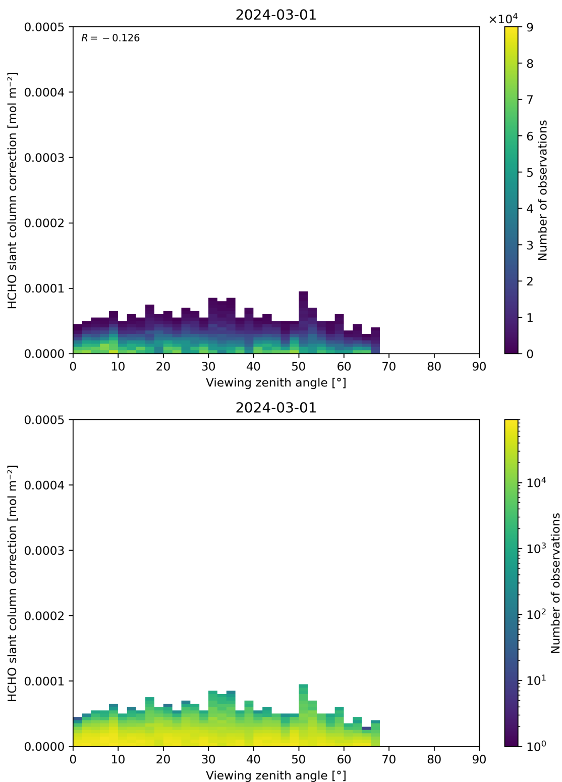
Figure 187: Scatter density plot of “Viewing zenith angle” against “HCHO slant column correction” for 2024-02-29 to 2024-03-02.
