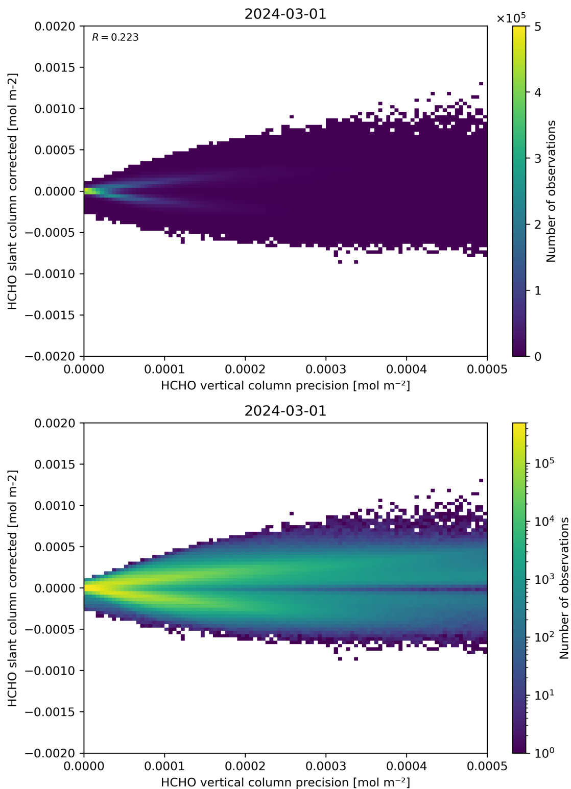
Figure 140: Scatter density plot of “HCHO vertical column precision” against “HCHO slant column corrected” for 2024-02-29 to 2024-03-02.
