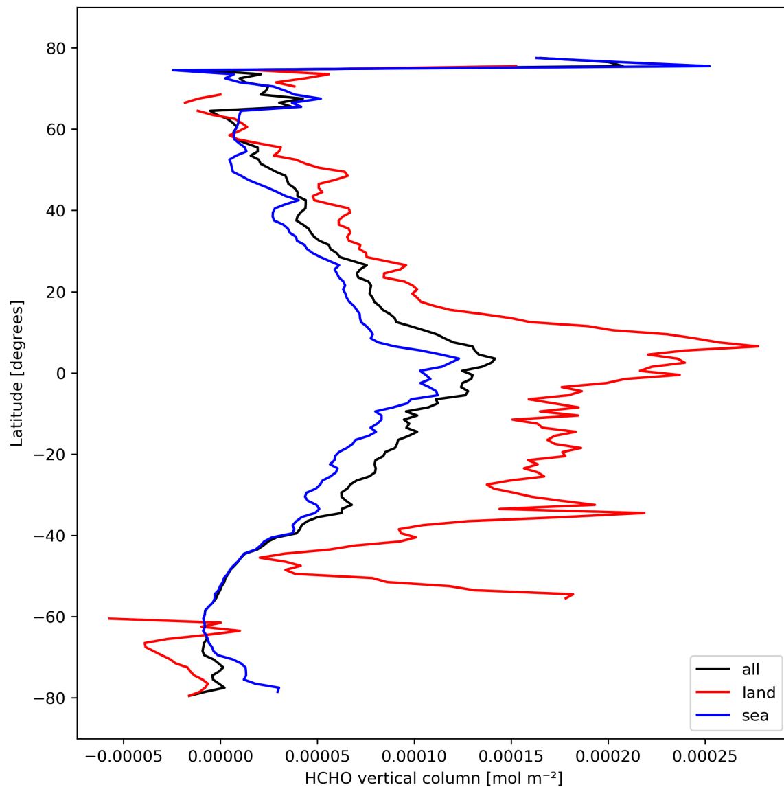
Figure 21: Zonal average of “HCHO vertical column” for 2024-02-29 to 2024-03-02.
