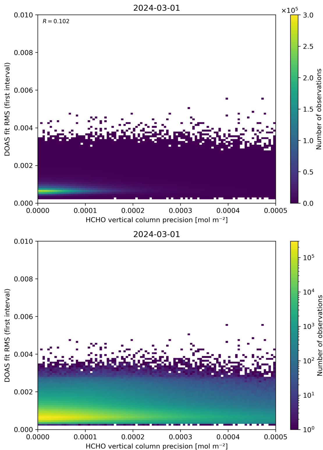
Figure 136: Scatter density plot of “HCHO vertical column precision” against “DOAS fit RMS (first interval)” for 2024-02-29 to 2024-03-02.
