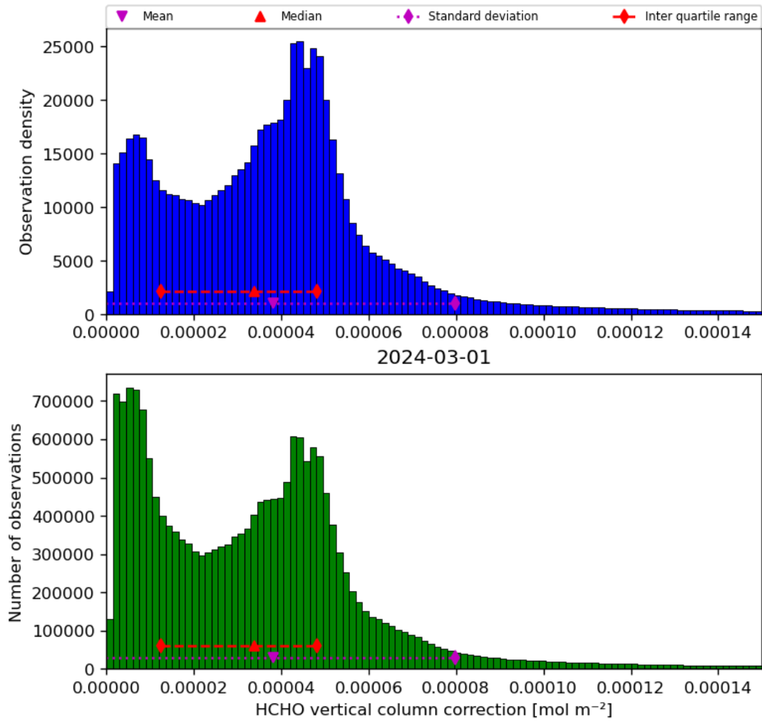
Figure 37: Histogram of “HCHO vertical column correction” for 2024-02-29 to 2024-03-02
