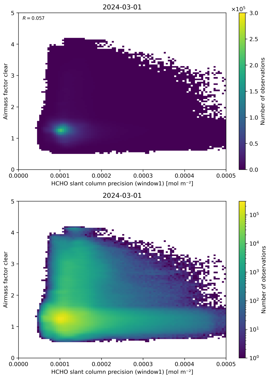
Figure 91: Scatter density plot of “HCHO slant column precision (window1)” against “Airmass factor clear” for 2024-02-29 to 2024-03-02.
