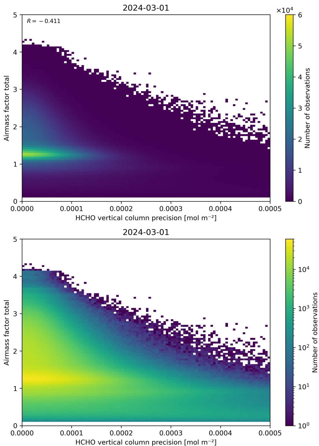
Figure 144: Scatter density plot of “HCHO vertical column precision” against “Airmass factor total” for 2024-02-29 to 2024-03-02.
