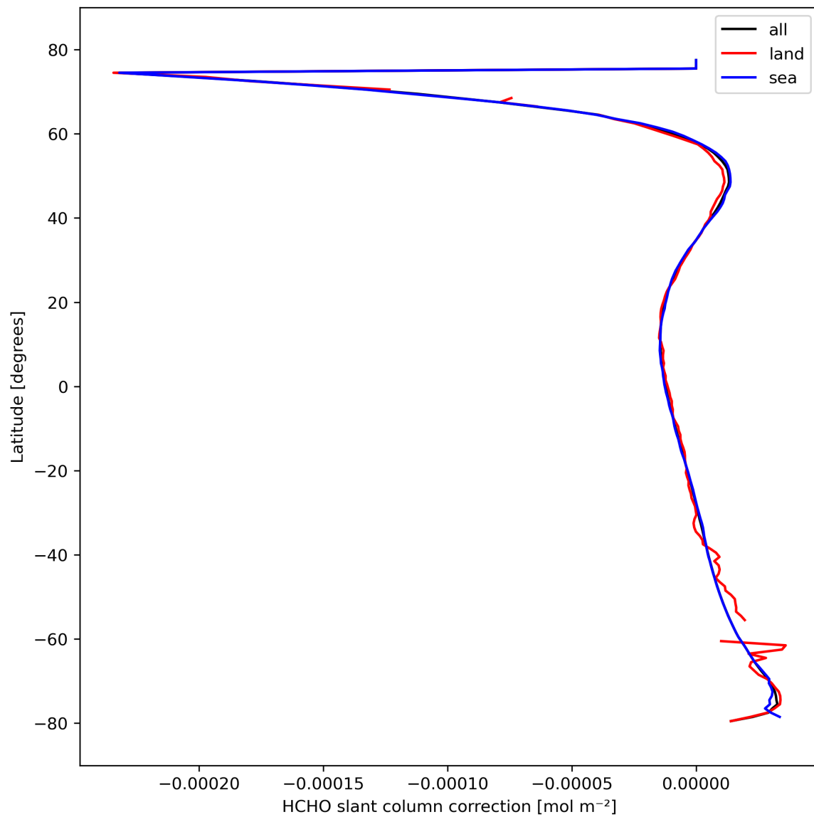
Figure 33: Zonal average of “HCHO slant column correction” for 2024-02-29 to 2024-03-02.
