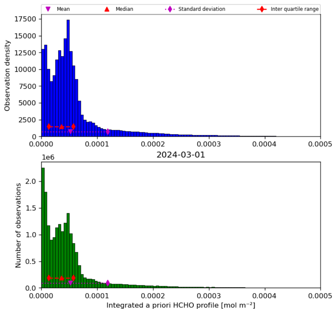
Figure 43: Histogram of “Integrated a priori HCHO profile” for 2024-02-29 to 2024-03-02
