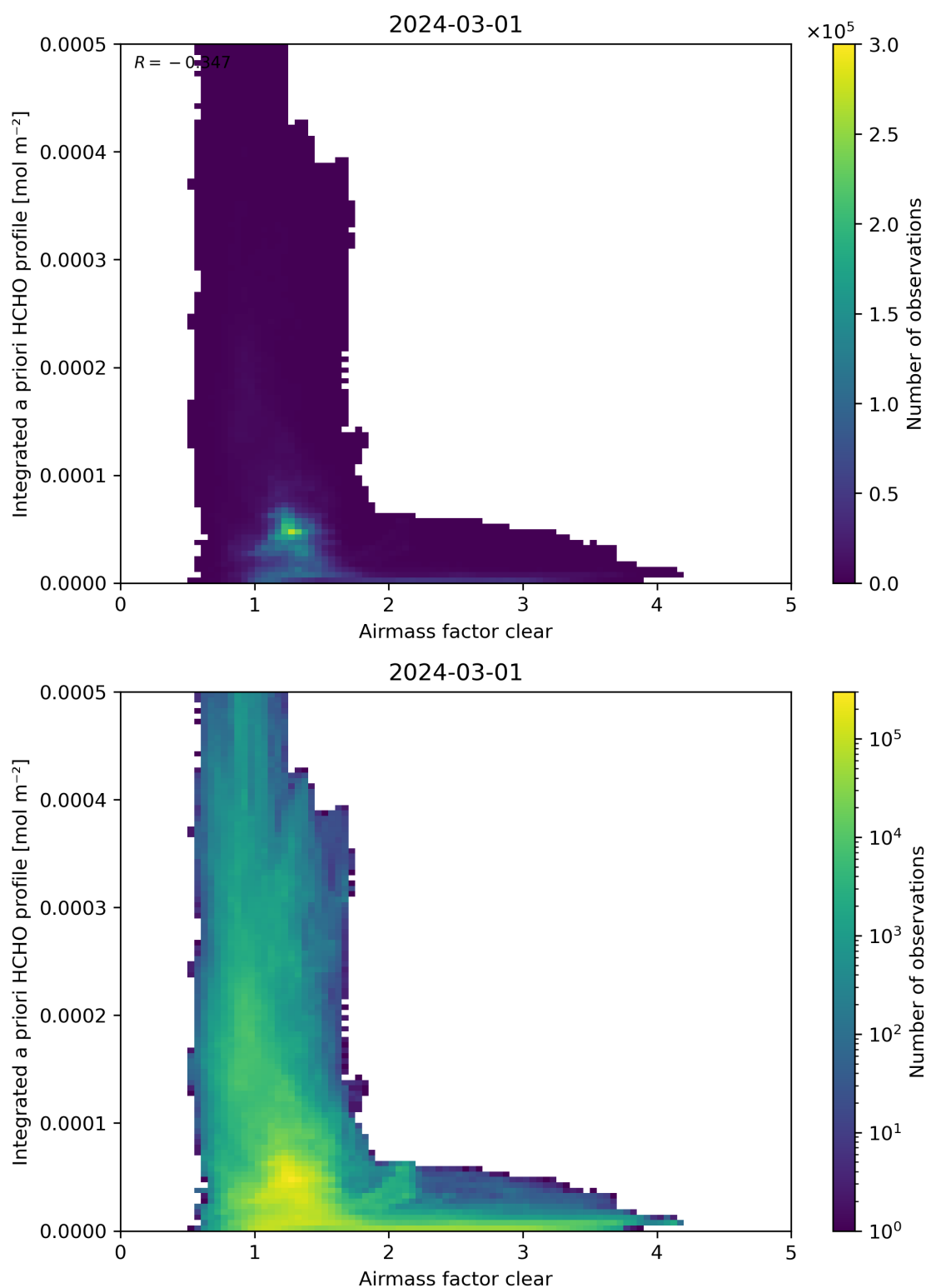
Figure 76: Scatter density plot of “Airmass factor clear” against “Integrated a priori HCHO profile” for 2024-02-29 to 2024-03-02.
