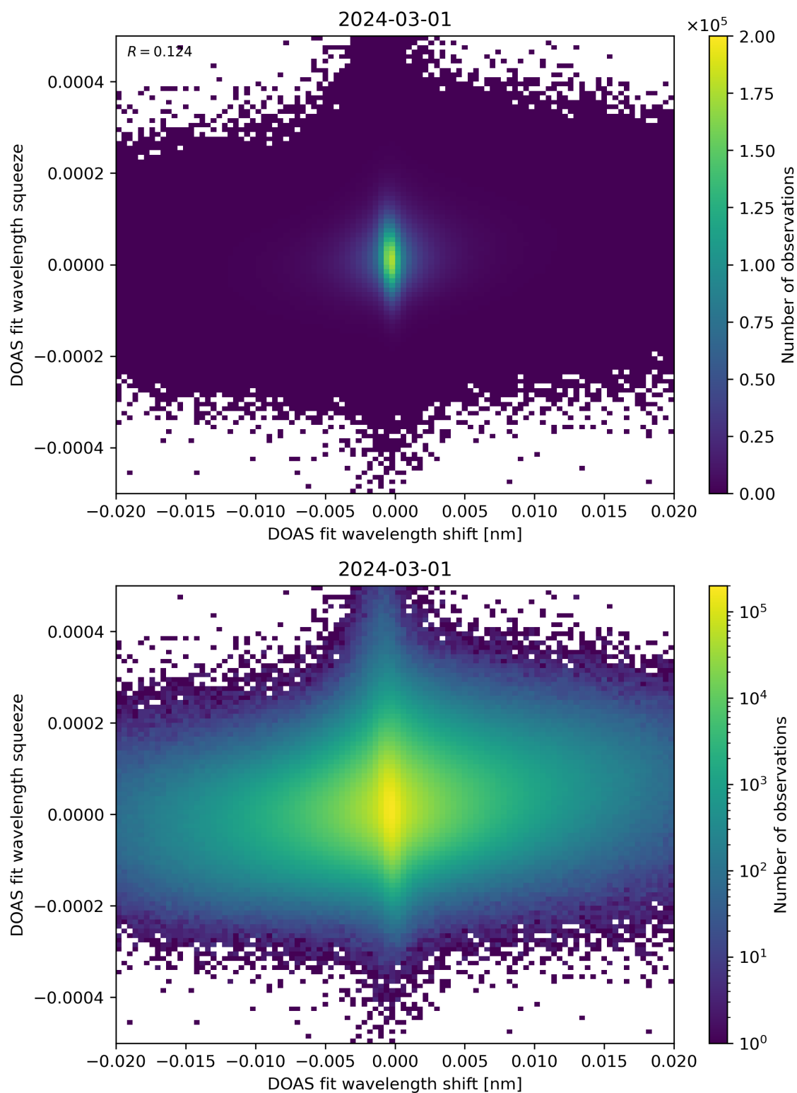
Figure 65: Scatter density plot of “DOAS fit wavelength shift” against “DOAS fit wavelength squeeze” for 2024-02-29 to 2024-03-02.
