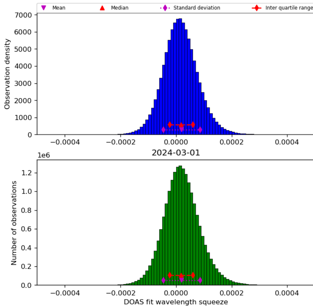
Figure 45: Histogram of “DOAS fit wavelength squeeze” for 2024-02-29 to 2024-03-02
