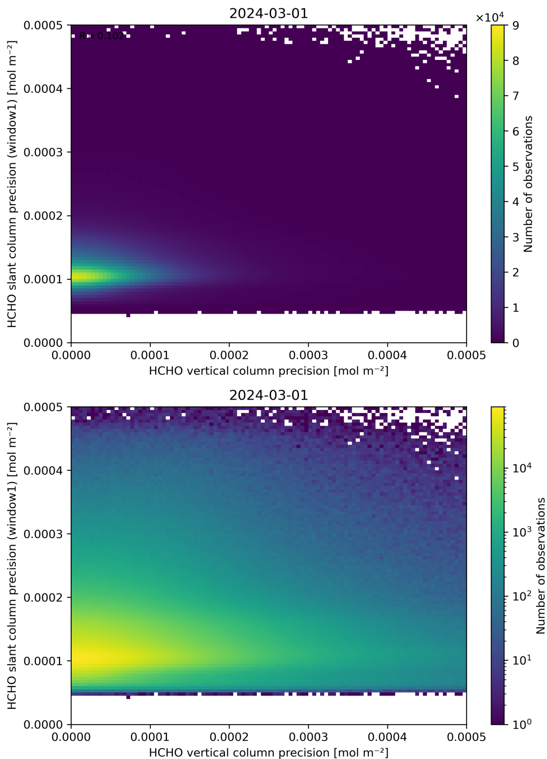
Figure 143: Scatter density plot of “HCHO vertical column precision” against “HCHO slant column precision (window1)” for 2024-02-29 to 2024-03-02.
