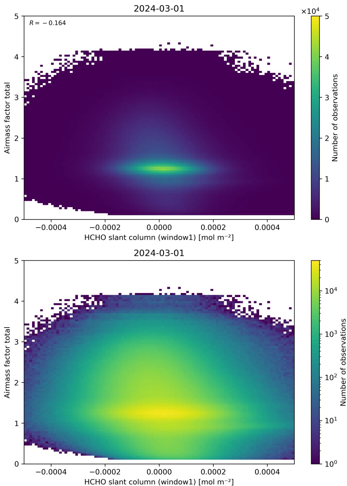
Figure 85: Scatter density plot of “HCHO slant column (window1)” against “Airmass factor total” for 2024-02-29 to 2024-03-02.
