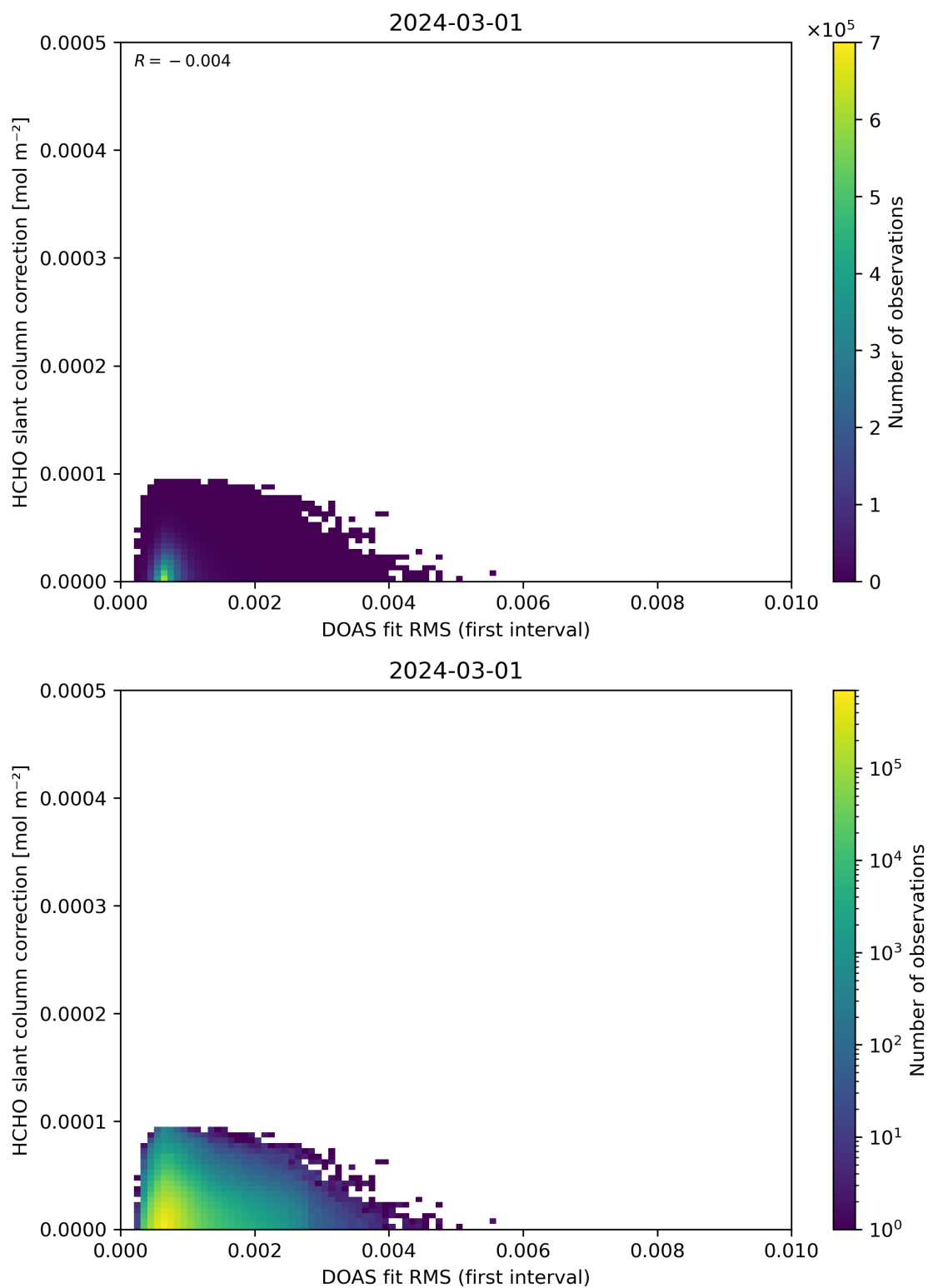
Figure 63: Scatter density plot of “DOAS fit RMS (first interval)” against “HCHO slant column correction” for 2024-02-29 to 2024-03-02.
