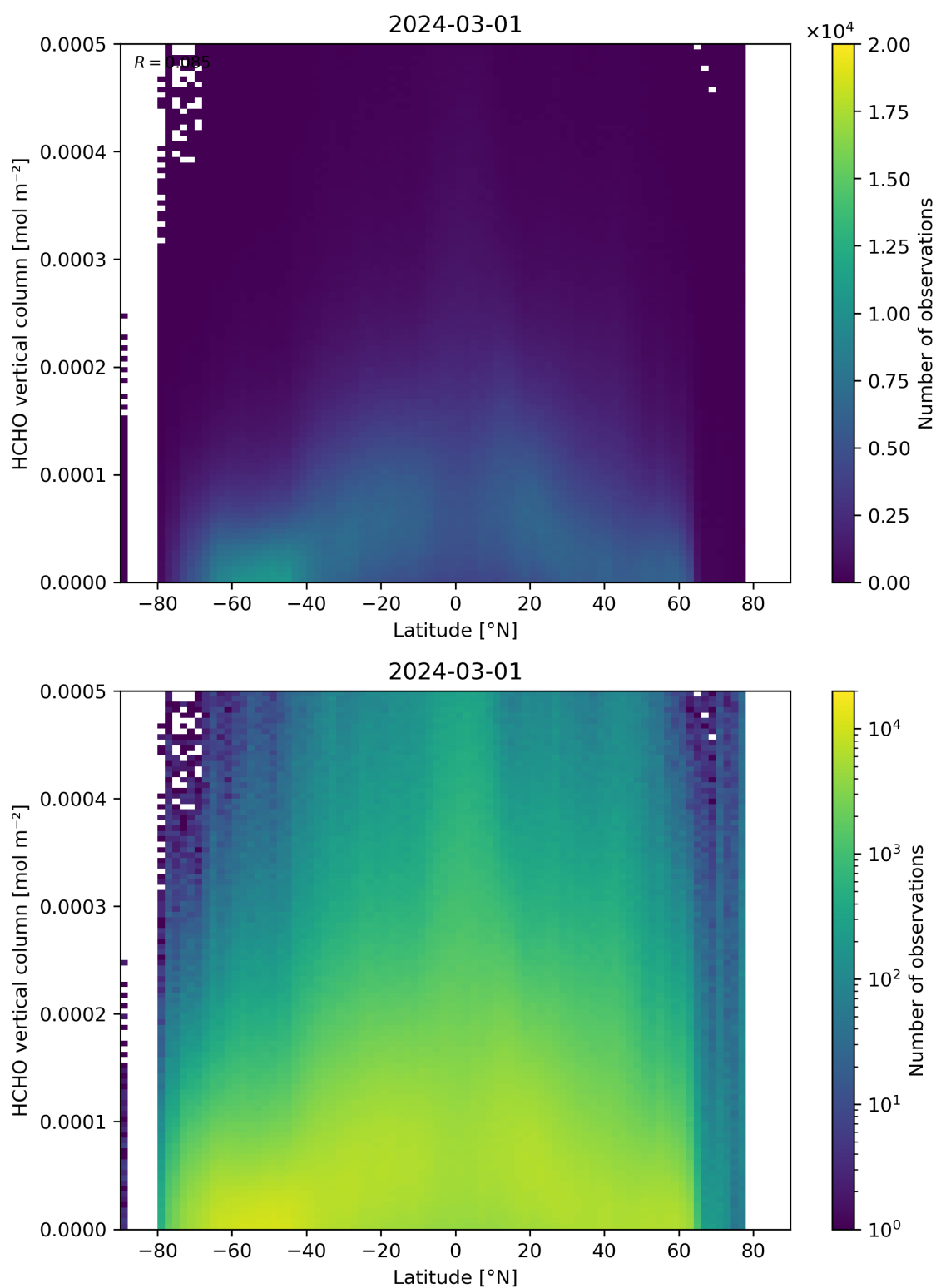
Figure 163: Scatter density plot of “Latitude” against “HCHO vertical column” for 2024-02-29 to 2024-03-02.
