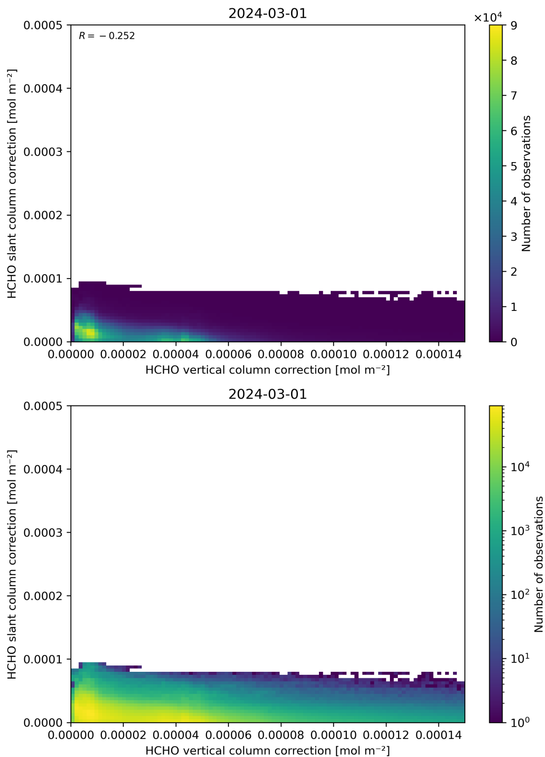
Figure 117: Scatter density plot of “HCHO vertical column correction” against “HCHO slant column correction” for 2024-02-29 to 2024-03-02.
