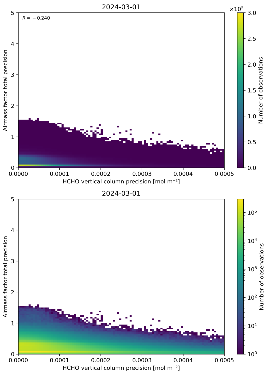
Figure 145: Scatter density plot of “HCHO vertical column precision” against “Airmass factor total precision” for 2024-02-29 to 2024-03-02.
