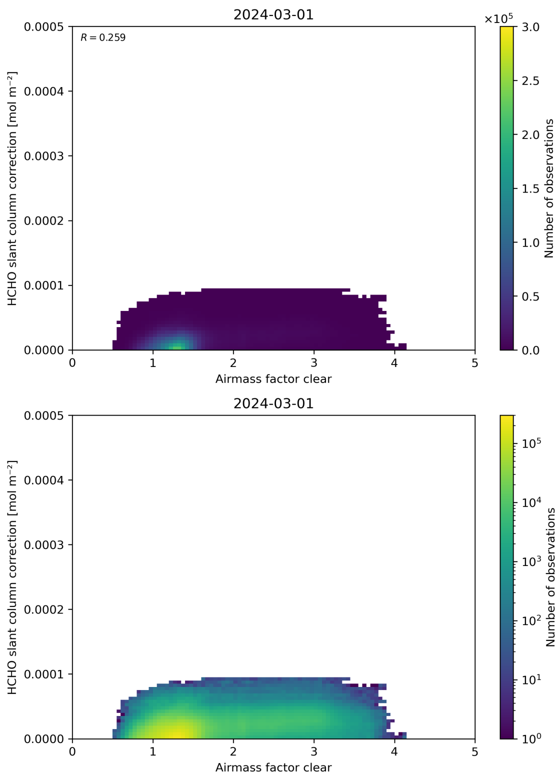
Figure 75: Scatter density plot of “Airmass factor clear” against “HCHO slant column correction” for 2024-02-29 to 2024-03-02.
