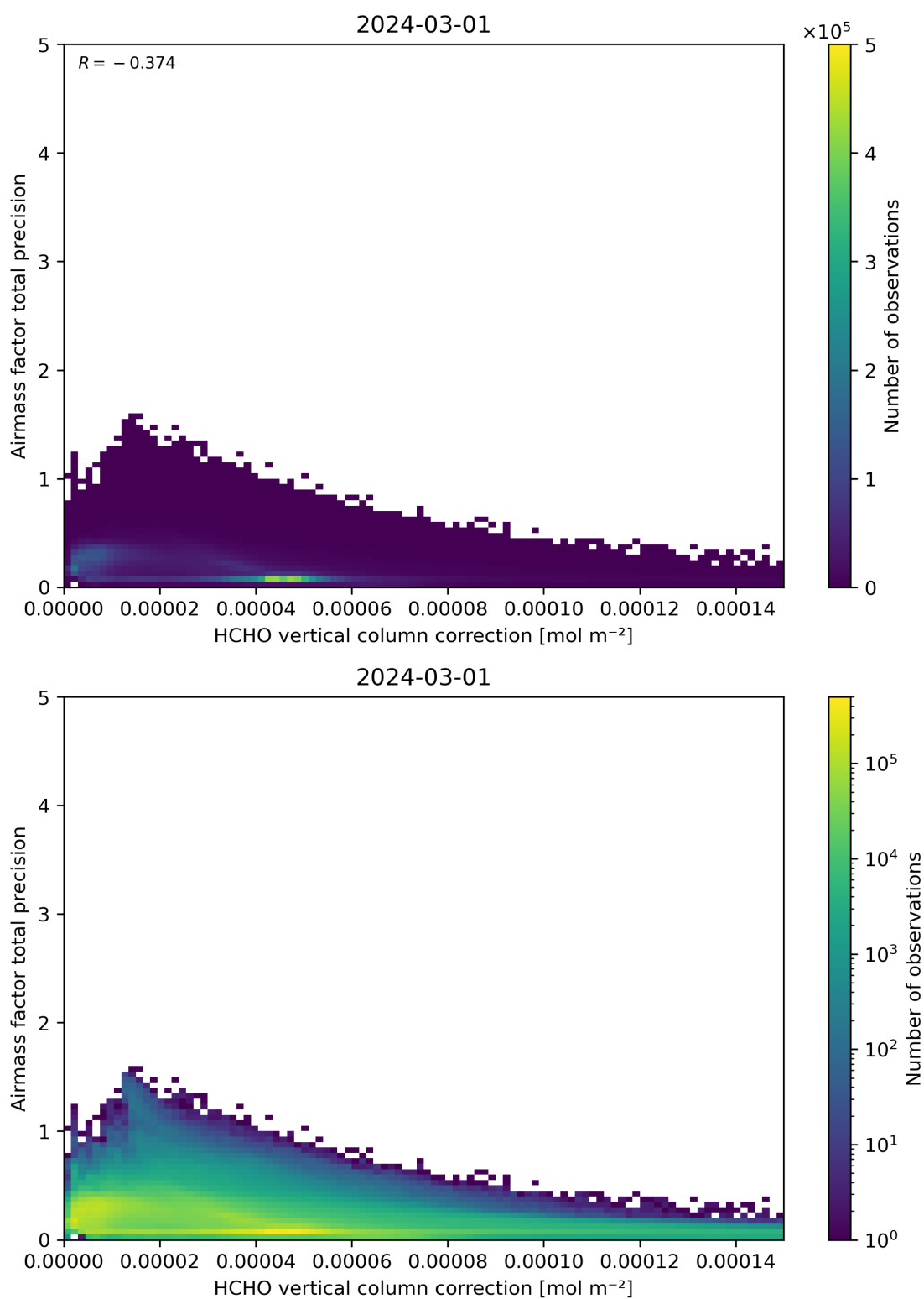
Figure 121: Scatter density plot of “HCHO vertical column correction” against “Airmass factor total precision” for 2024-02-29 to 2024-03-02.
