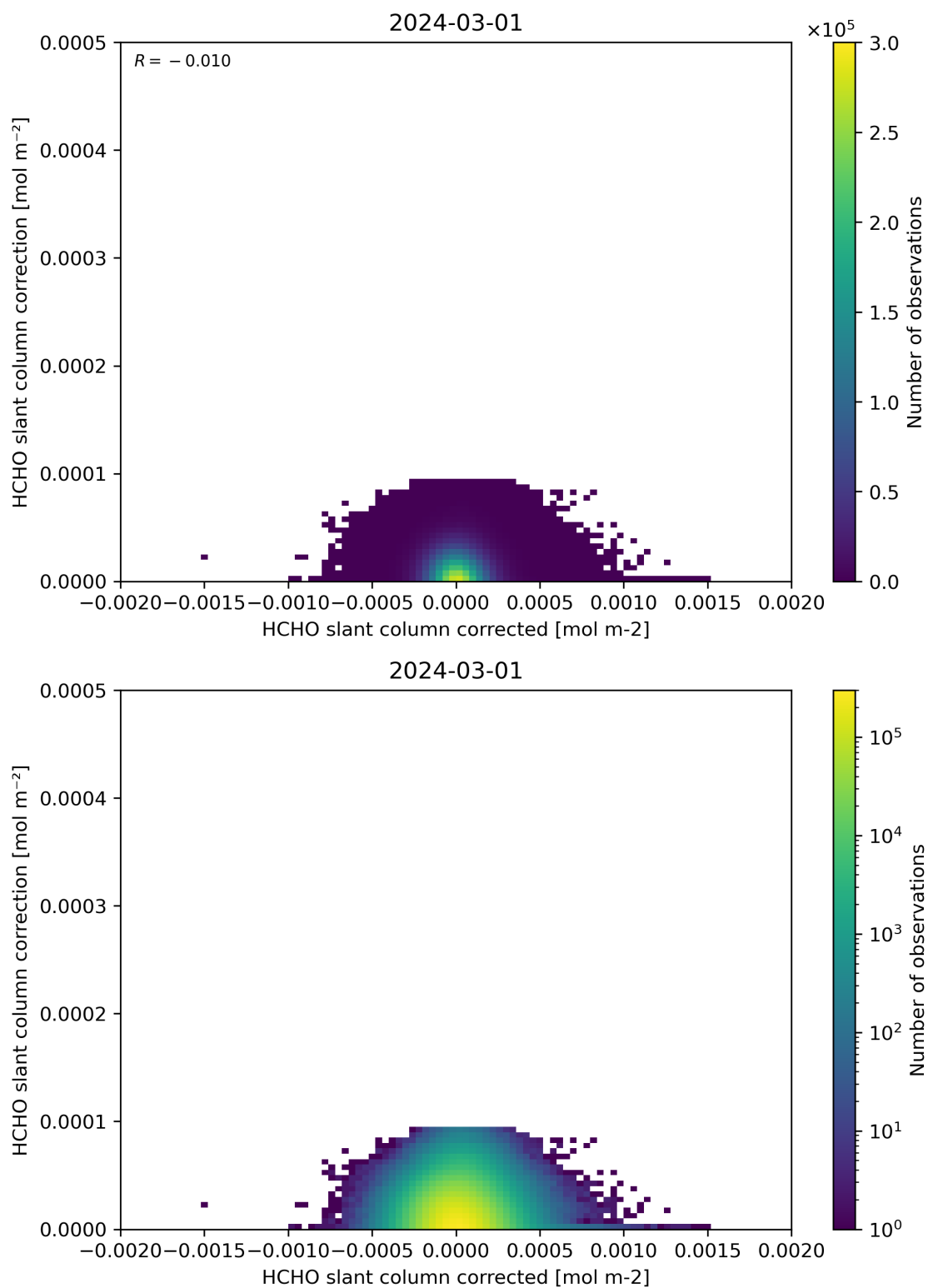
Figure 77: Scatter density plot of “HCHO slant column corrected” against “HCHO slant column correction” for 2024-02-29 to 2024-03-02.
