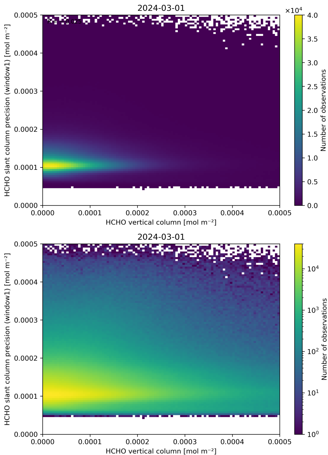
Figure 130: Scatter density plot of “HCHO vertical column” against “HCHO slant column precision (window1)” for 2024-02-29 to 2024-03-02.
