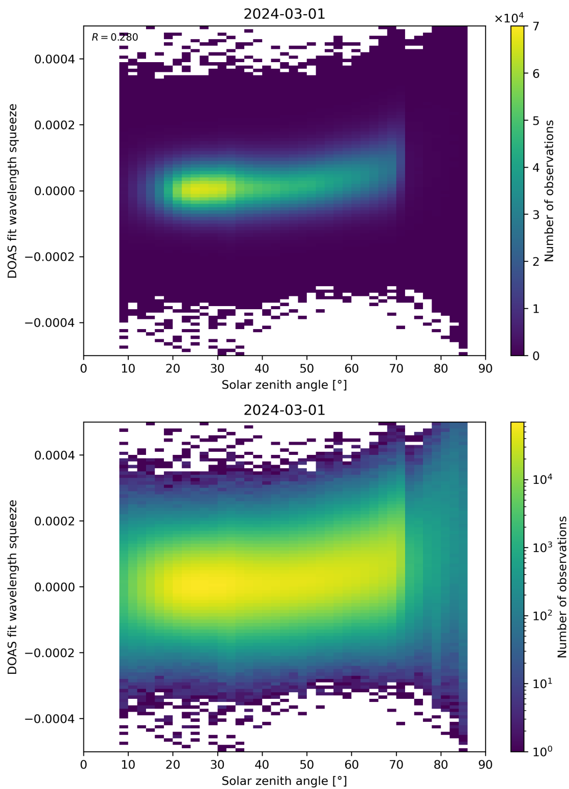
Figure 169: Scatter density plot of “Solar zenith angle” against “DOAS fit wavelength squeeze” for 2024-02-29 to 2024-03-02.
