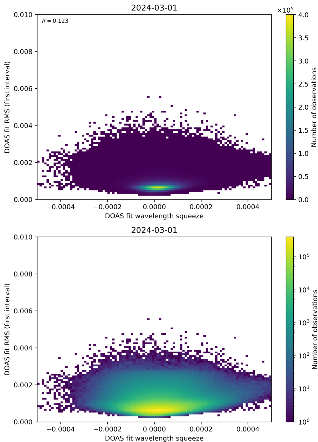
Figure 68: Scatter density plot of “DOAS fit wavelength squeeze” against “DOAS fit RMS (first interval)” for 2024-02-29 to 2024-03-02.
