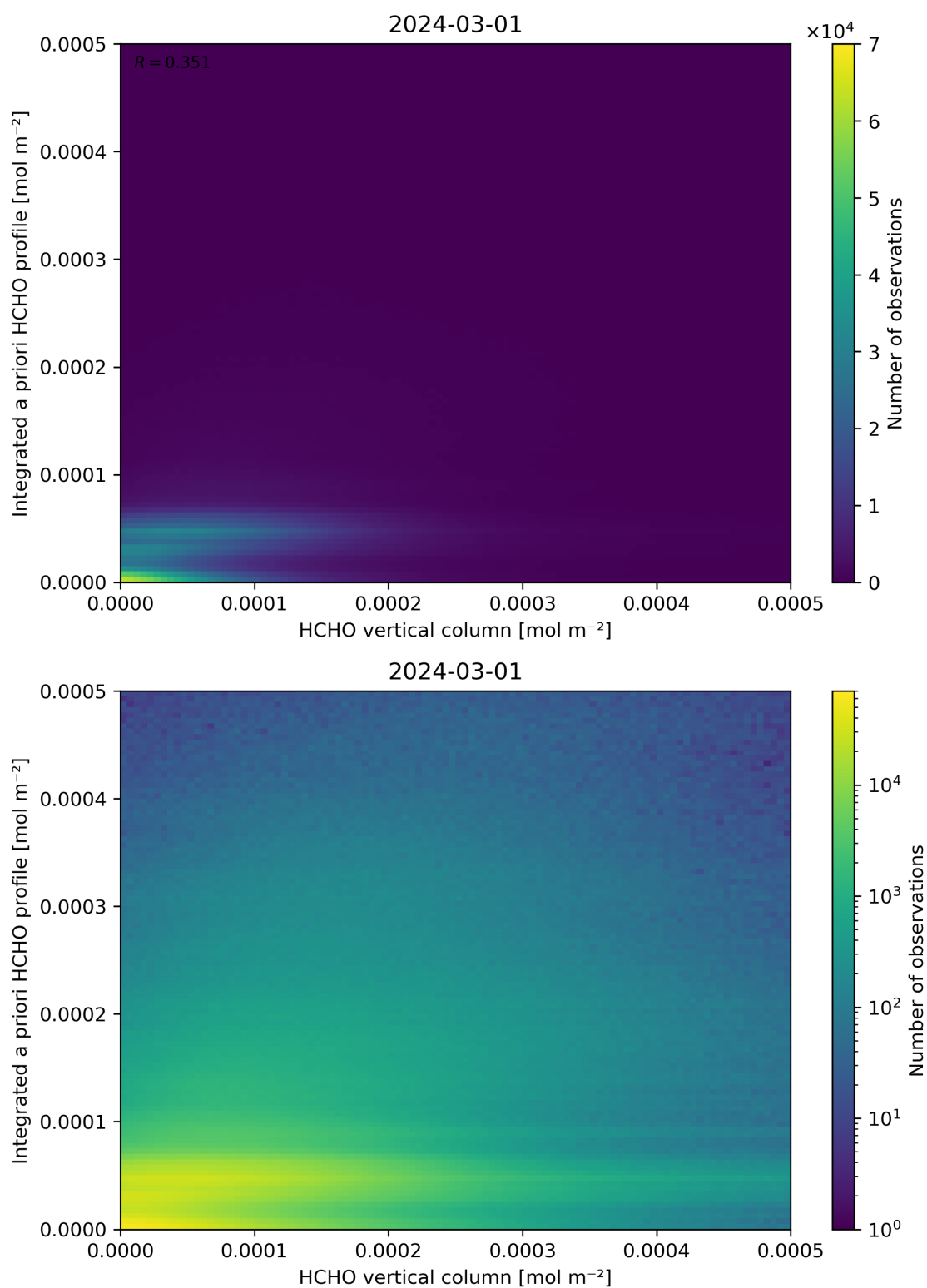
Figure 135: Scatter density plot of “HCHO vertical column” against “Integrated a priori HCHO profile” for 2024-02-29 to 2024-03-02.
