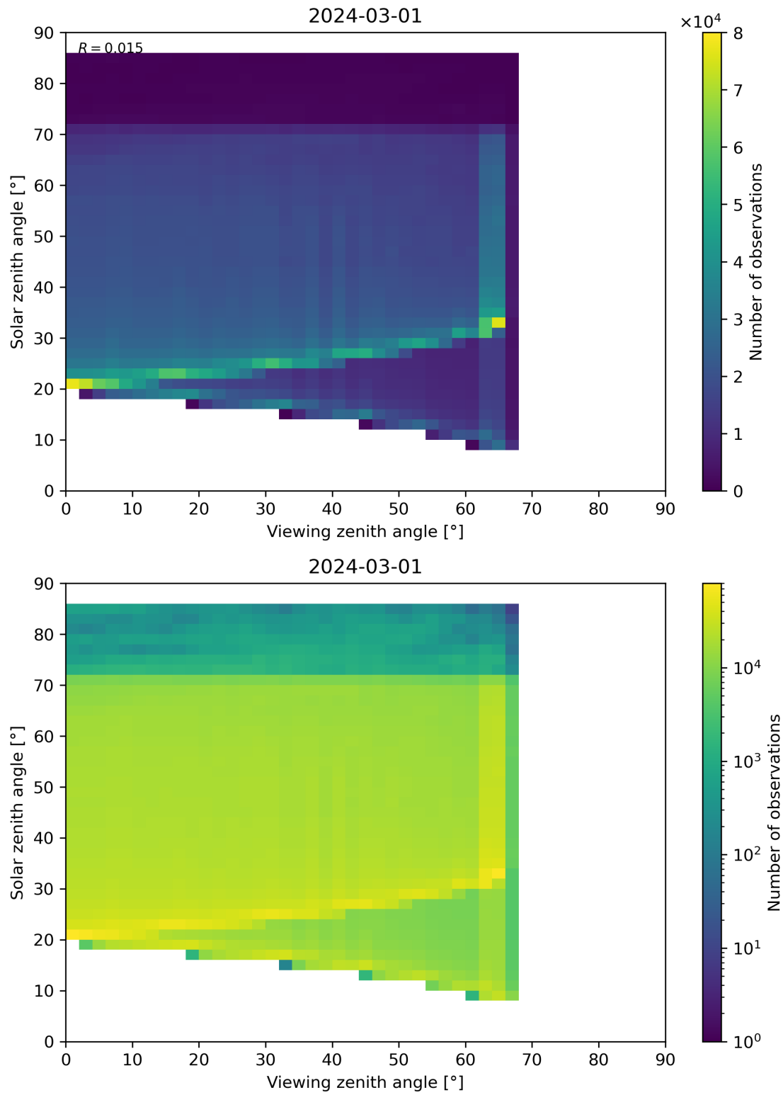
Figure 197: Scatter density plot of “Viewing zenith angle” against “Solar zenith angle” for 2024-02-29 to 2024-03-02.
