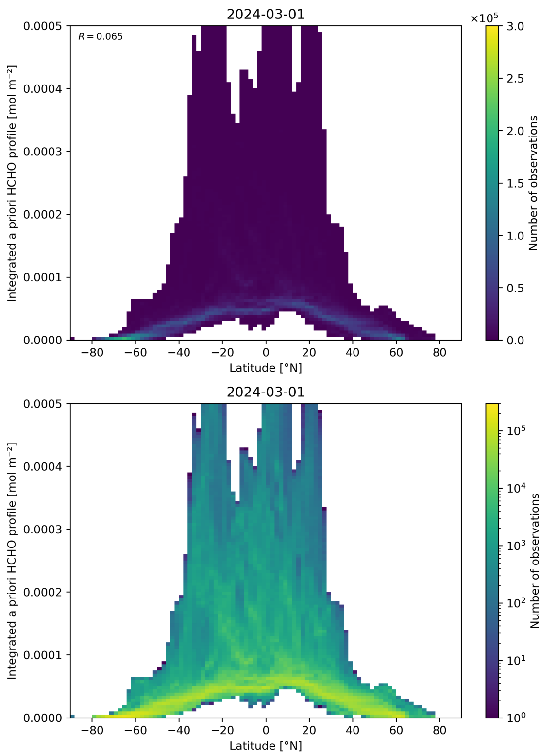
Figure 166: Scatter density plot of “Latitude” against “Integrated a priori HCHO profile” for 2024-02-29 to 2024-03-02.
