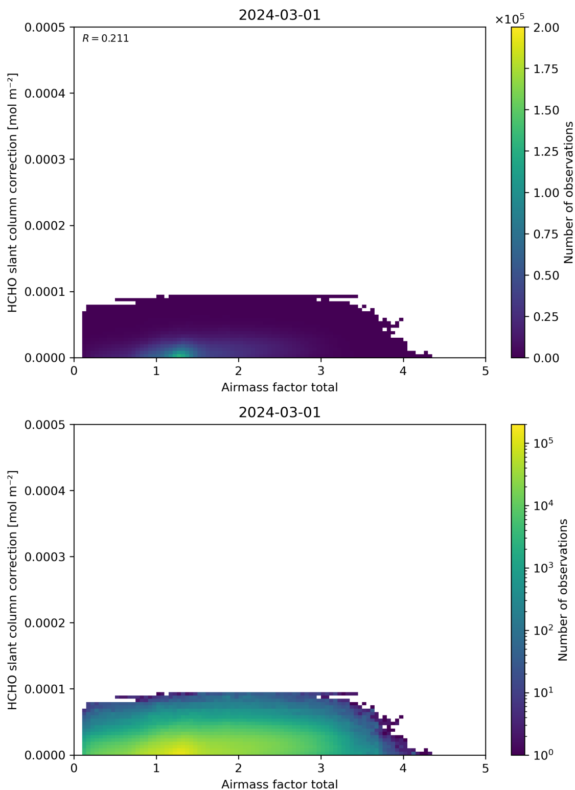
Figure 102: Scatter density plot of “Airmass factor total” against “HCHO slant column correction” for 2024-02-29 to 2024-03-02.
