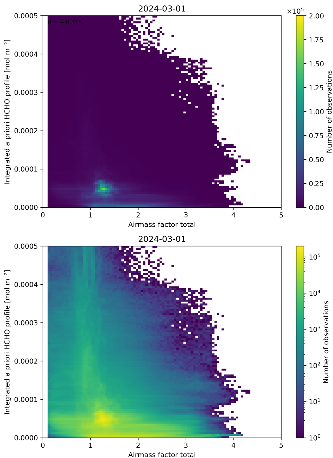
Figure 104: Scatter density plot of “Airmass factor total” against “Integrated a priori HCHO profile” for 2024-02-29 to 2024-03-02.
