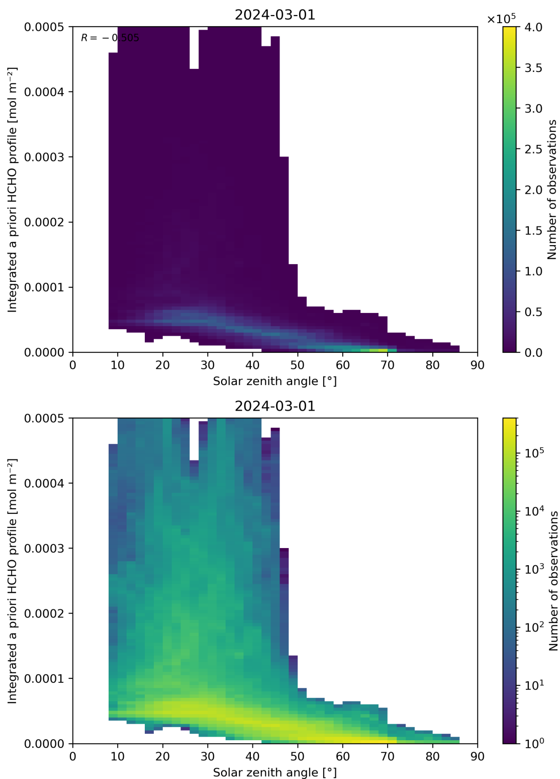
Figure 180: Scatter density plot of “Solar zenith angle” against “Integrated a priori HCHO profile” for 2024-02-29 to 2024-03-02.
