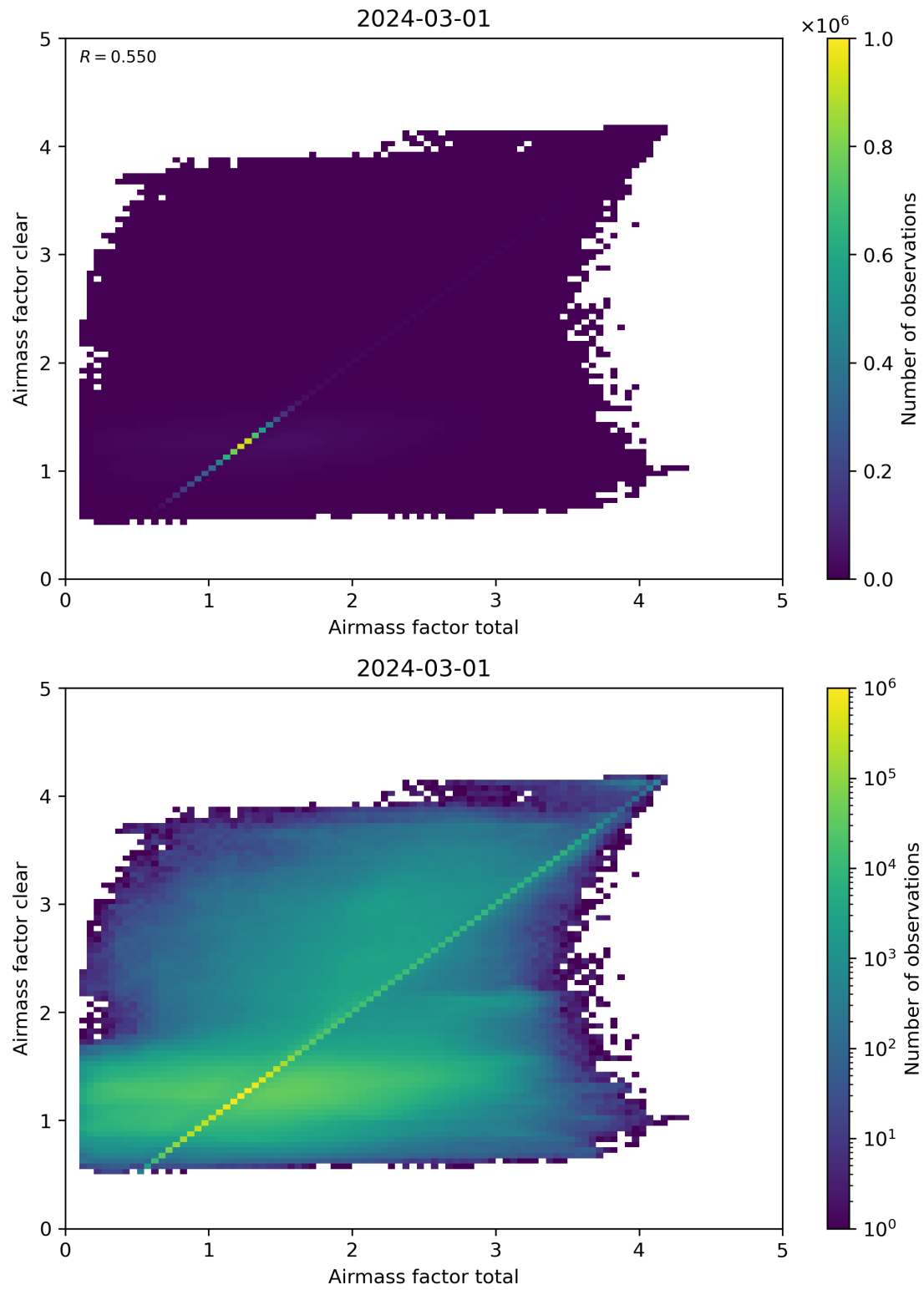
Figure 100: Scatter density plot of “Airmass factor total” against “Airmass factor clear” for 2024-02-29 to 2024-03-02.
