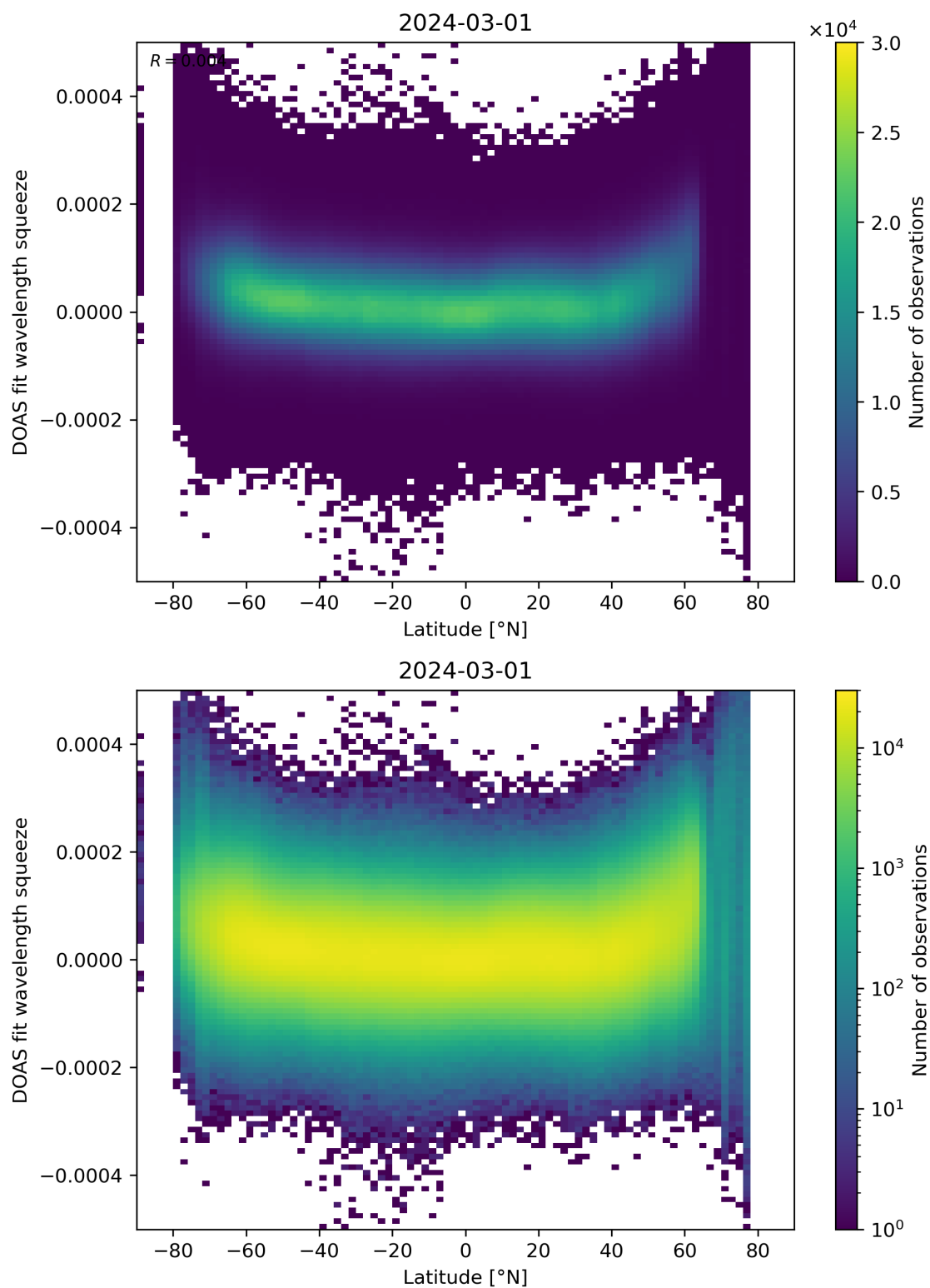
Figure 155: Scatter density plot of “Latitude” against “DOAS fit wavelength squeeze” for 2024-02-29 to 2024-03-02.
