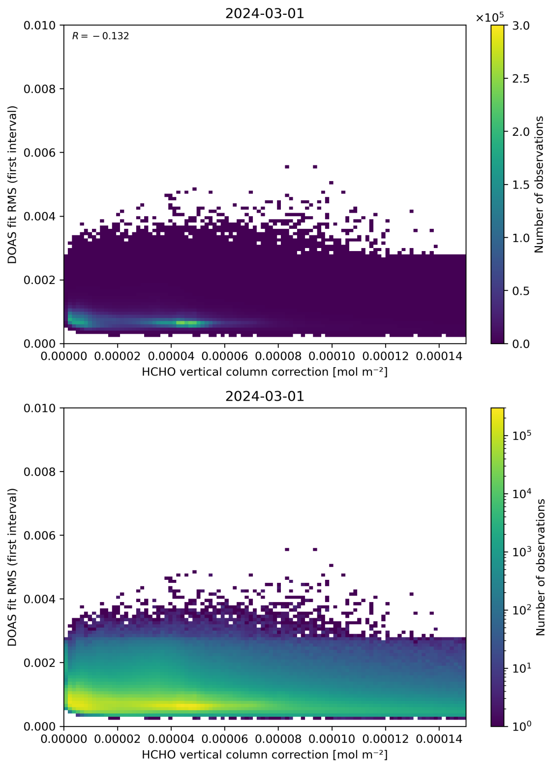
Figure 112: Scatter density plot of “HCHO vertical column correction” against “DOAS fit RMS (first interval)” for 2024-02-29 to 2024-03-02.
