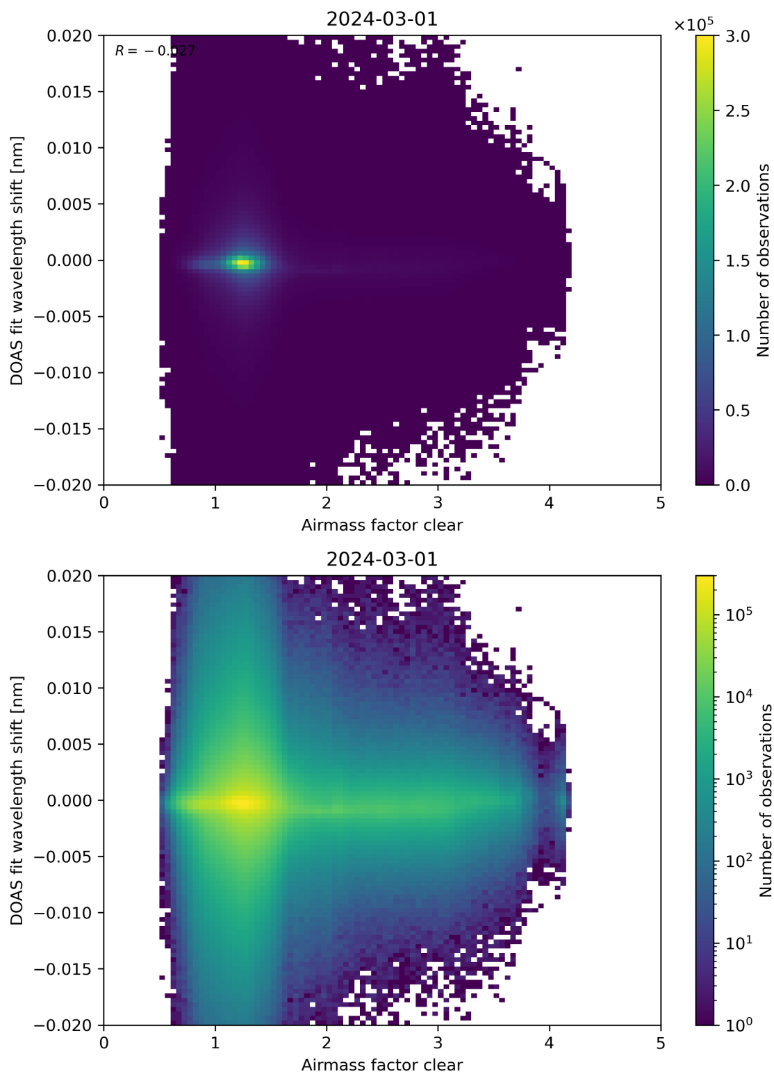
Figure 72: Scatter density plot of “Airmass factor clear” against “DOAS fit wavelength shift” for 2024-02-29 to 2024-03-02.
