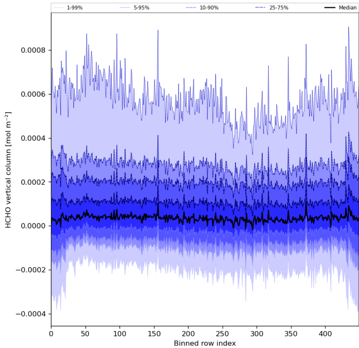
Figure 49: Along track statistics of “HCHO vertical column” for 2024-02-29 to 2024-03-02
