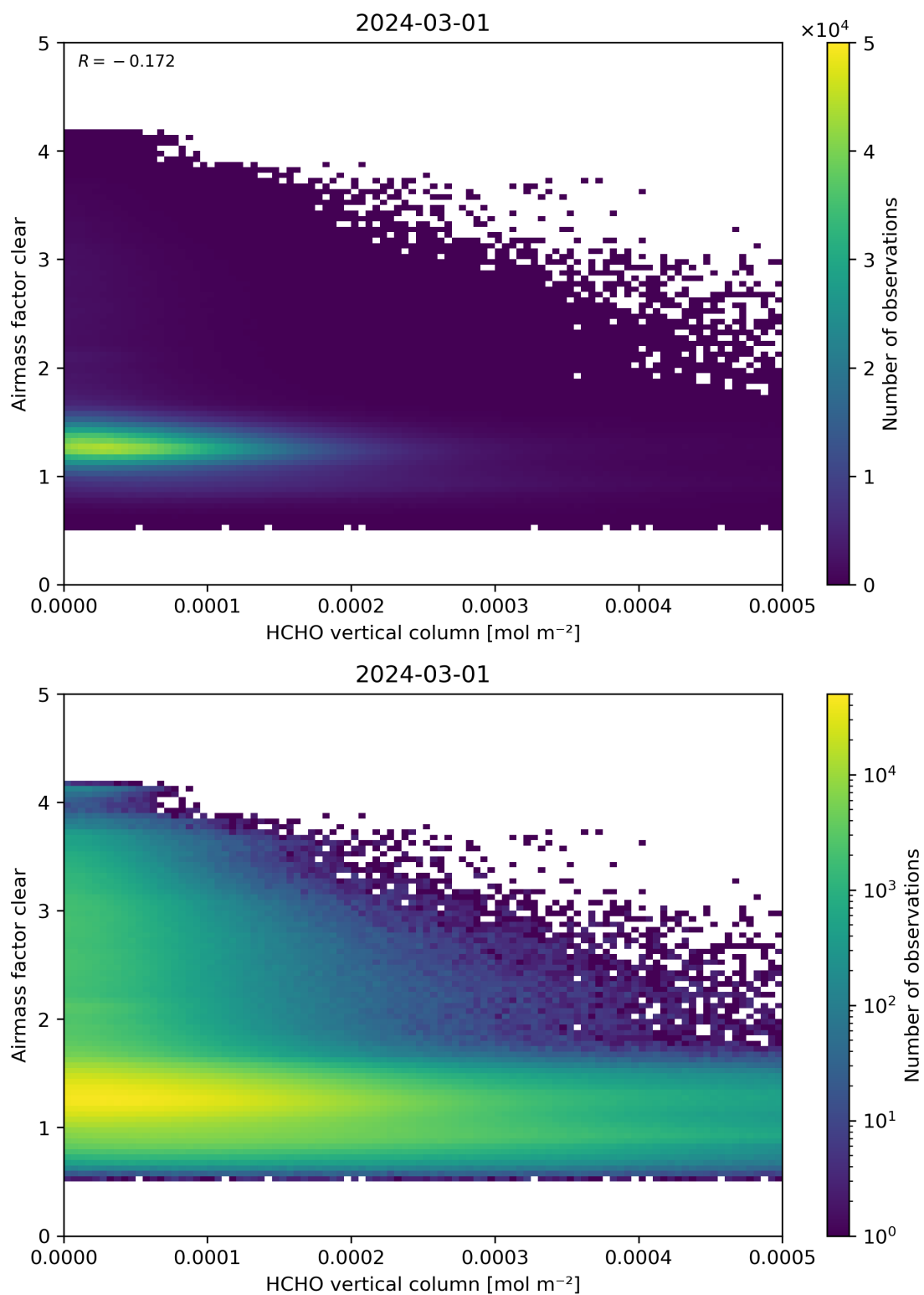
Figure 126: Scatter density plot of “HCHO vertical column” against “Airmass factor clear” for 2024-02-29 to 2024-03-02.
