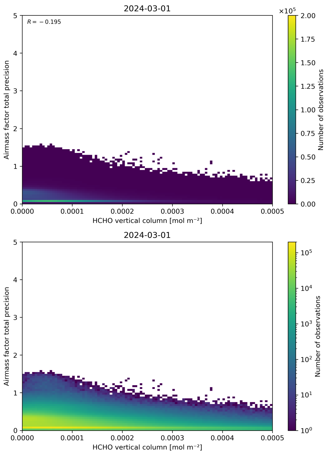
Figure 132: Scatter density plot of “HCHO vertical column” against “Airmass factor total precision” for 2024-02-29 to 2024-03-02.
