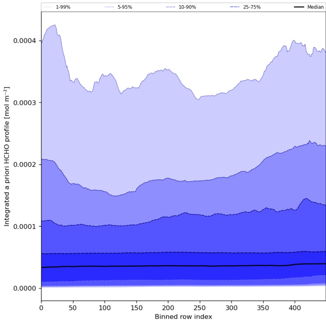
Figure 57: Along track statistics of “Integrated a priori HCHO profile” for 2024-02-29 to 2024-03-02
