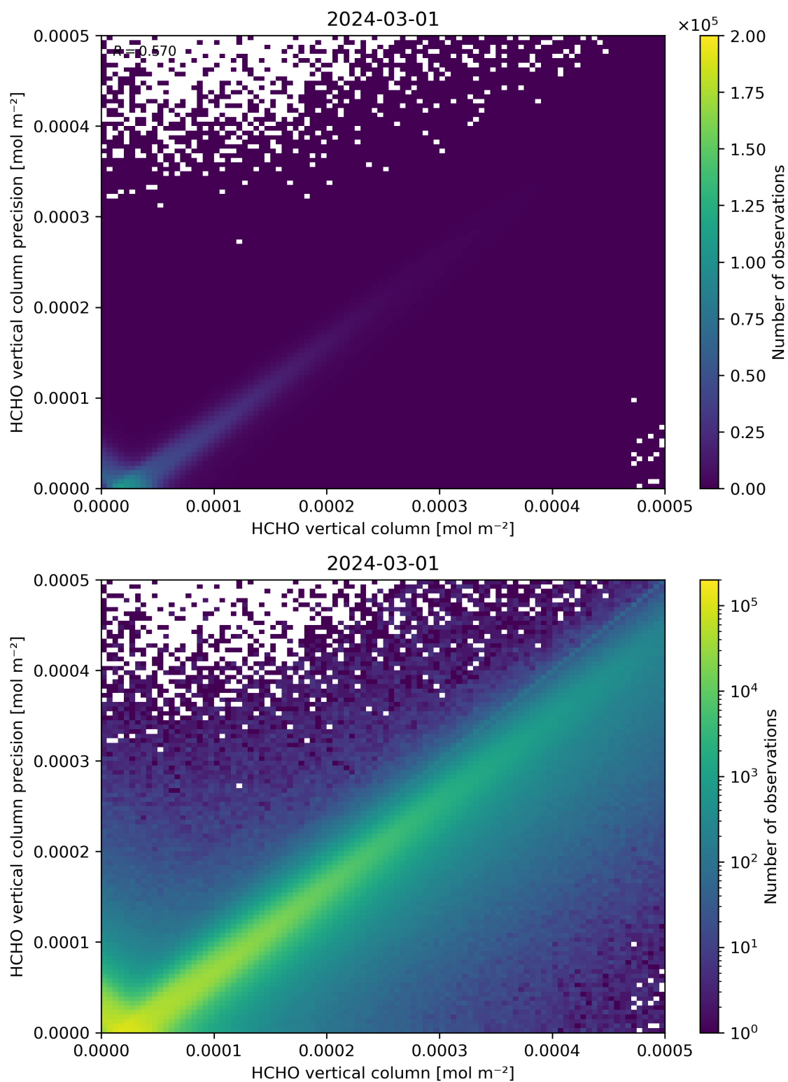
Figure 134: Scatter density plot of “HCHO vertical column” against “HCHO vertical column precision” for 2024-02-29 to 2024-03-02.
