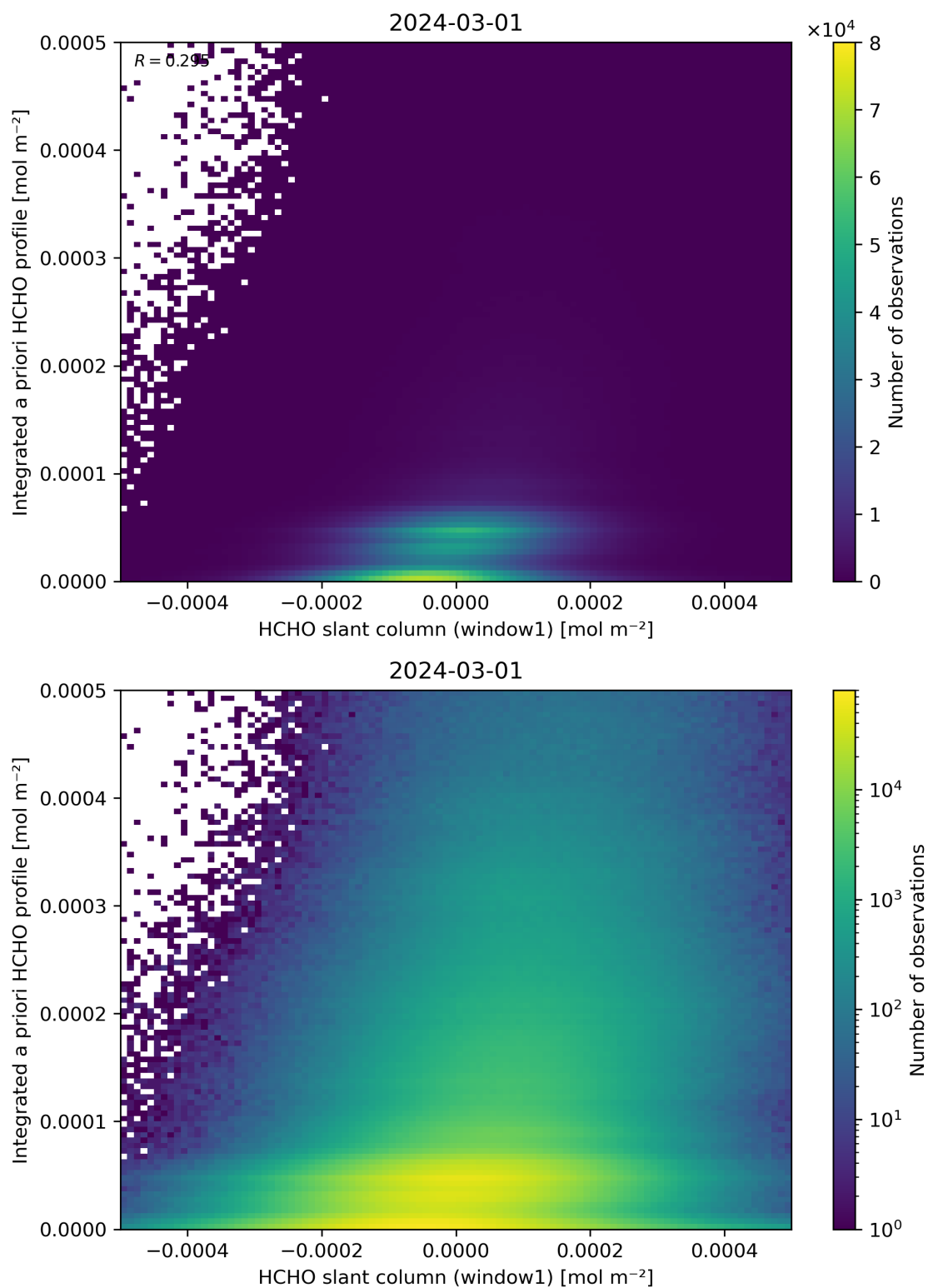
Figure 87: Scatter density plot of “HCHO slant column (window1)” against “Integrated a priori HCHO profile” for 2024-02-29 to 2024-03-02.
