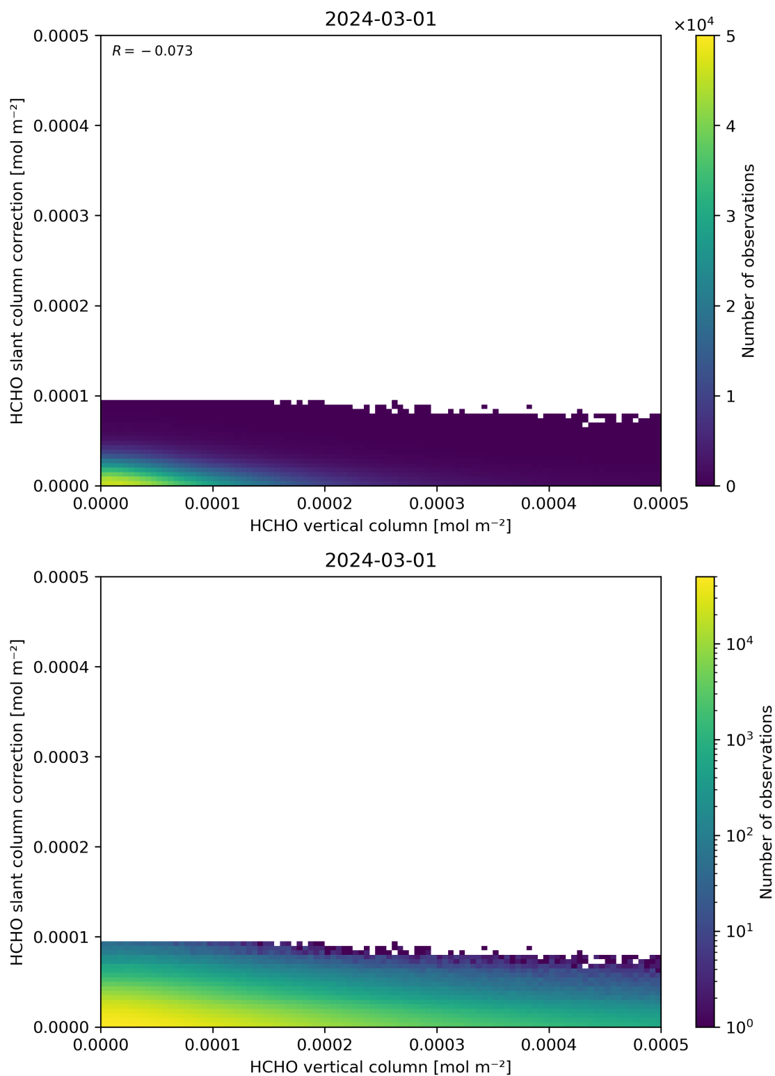
Figure 128: Scatter density plot of “HCHO vertical column” against “HCHO slant column correction” for 2024-02-29 to 2024-03-02.
