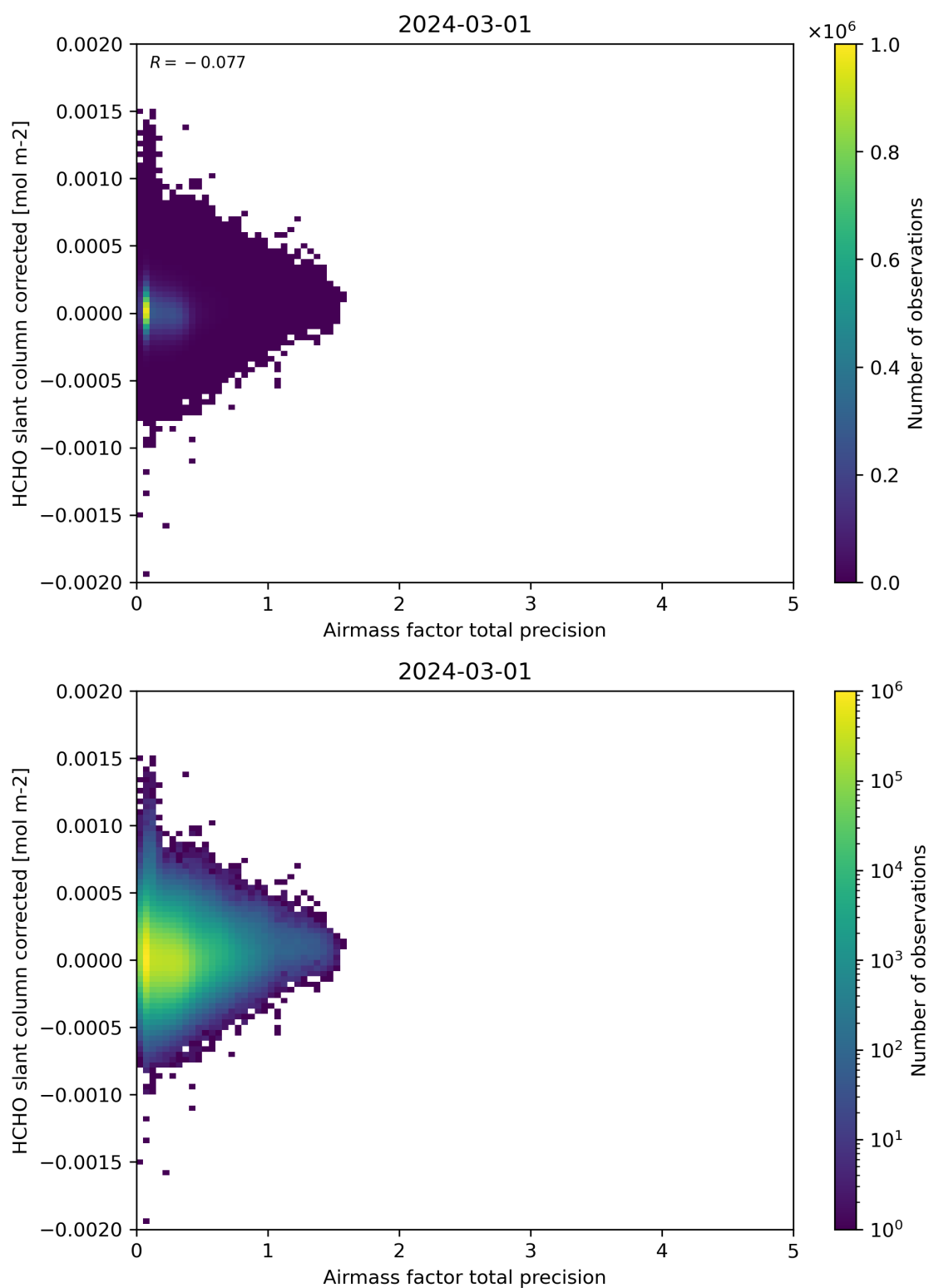
Figure 109: Scatter density plot of “Airmass factor total precision” against “HCHO slant column corrected” for 2024-02-29 to 2024-03-02.
