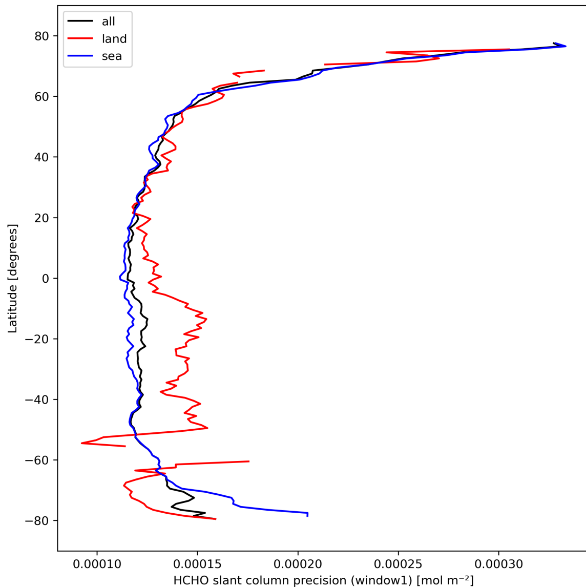
Figure 25: Zonal average of “HCHO slant column precision (window1)” for 2024-02-29 to 2024-03-02.
