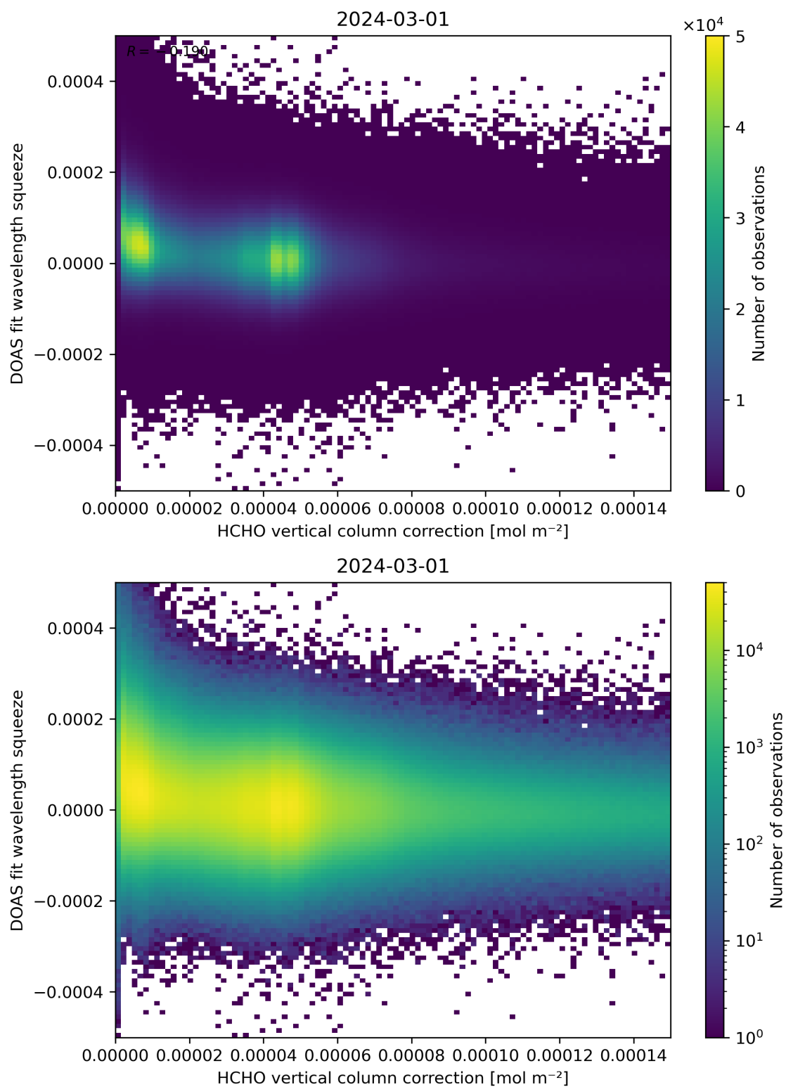
Figure 114: Scatter density plot of “HCHO vertical column correction” against “DOAS fit wavelength squeeze” for 2024-02-29 to 2024-03-02.
