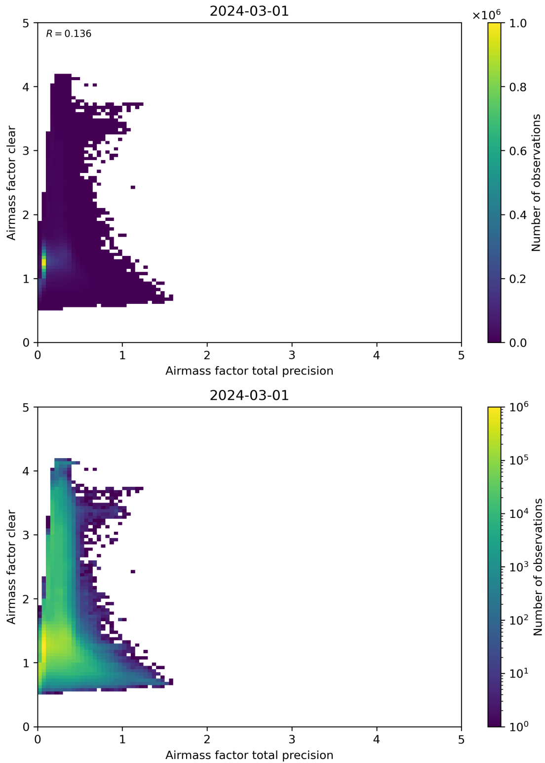
Figure 108: Scatter density plot of “Airmass factor total precision” against “Airmass factor clear” for 2024-02-29 to 2024-03-02.
