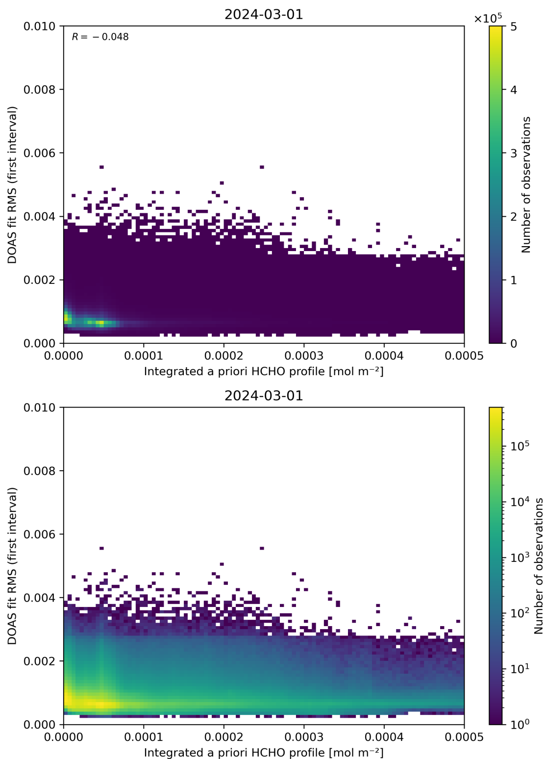
Figure 148: Scatter density plot of “Integrated a priori HCHO profile” against “DOAS fit RMS (first interval)” for 2024-02-29 to 2024-03-02.
