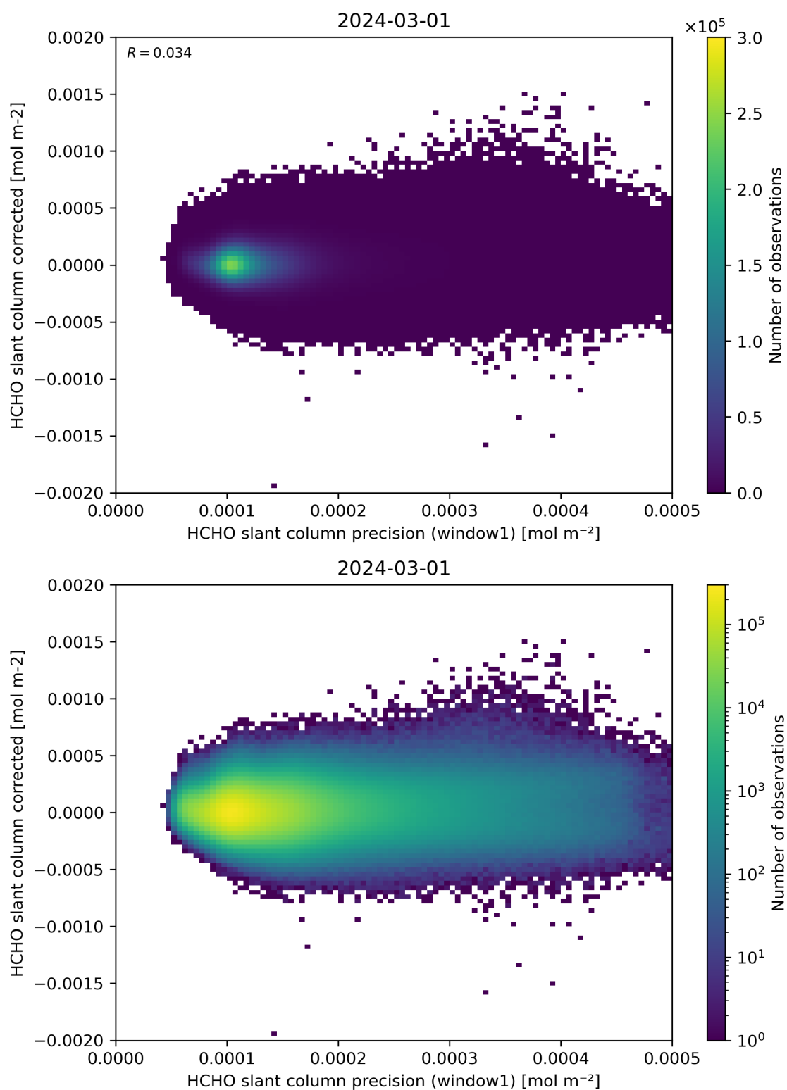
Figure 92: Scatter density plot of “HCHO slant column precision (window1)” against “HCHO slant column corrected” for 2024-02-29 to 2024-03-02.
