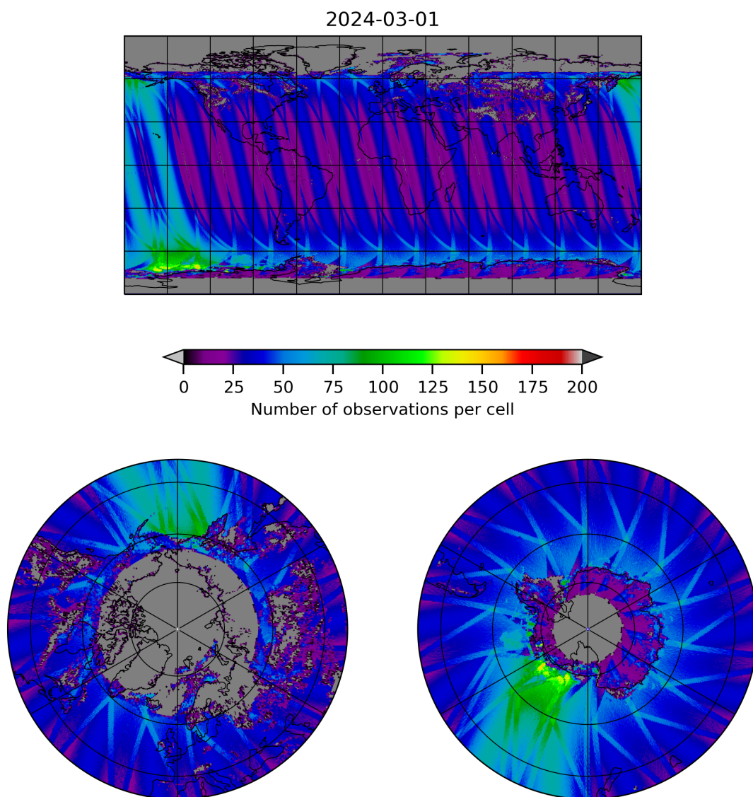
Figure 19: Map of the number of observations for 2024-02-29 to 2024-03-02
