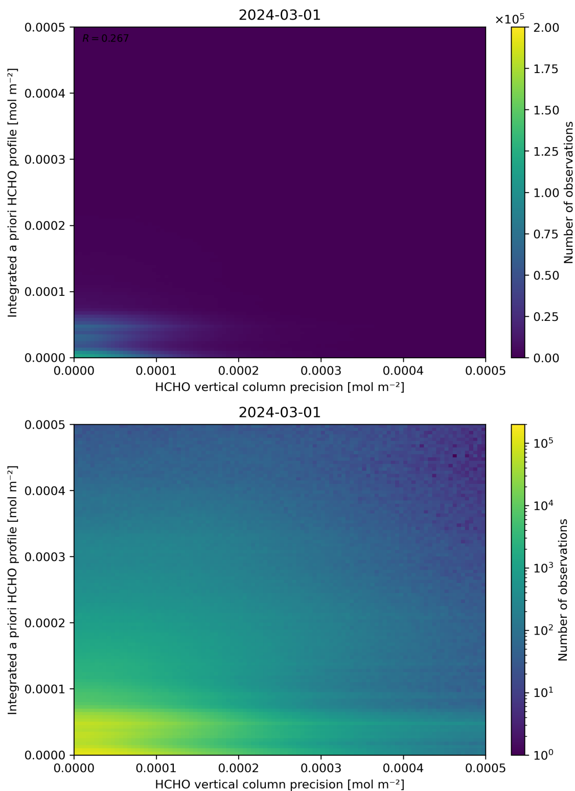
Figure 147: Scatter density plot of “HCHO vertical column precision” against “Integrated a priori HCHO profile” for 2024-02-29 to 2024-03-02.
