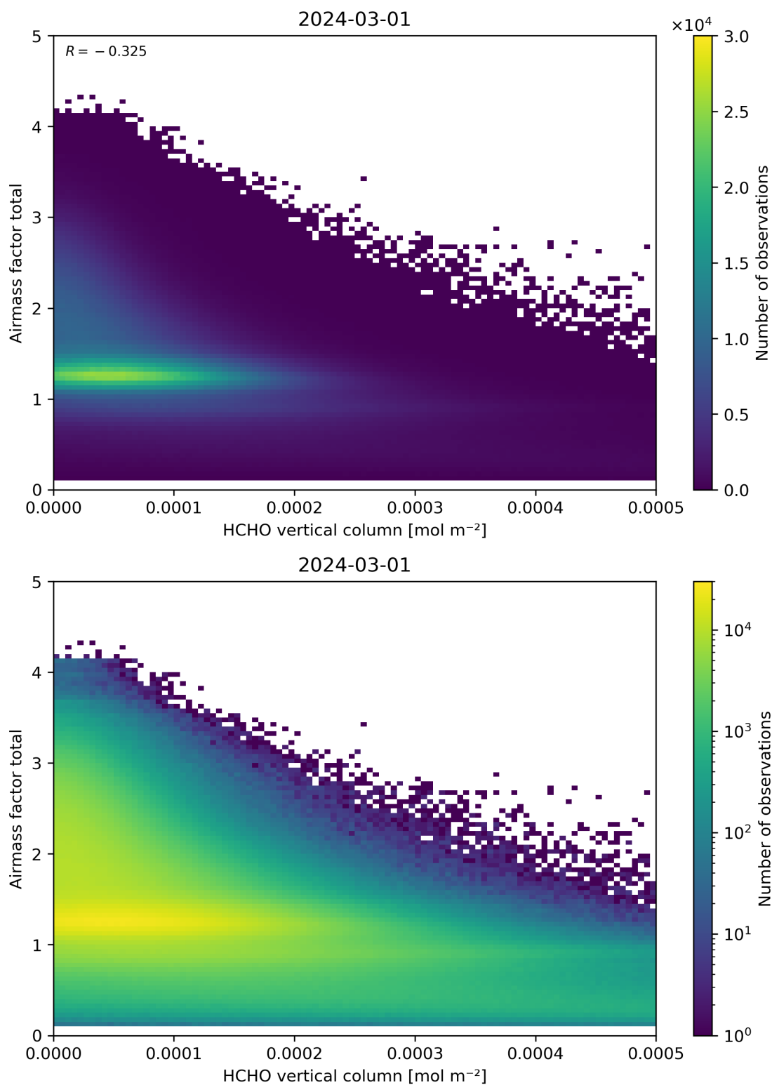
Figure 131: Scatter density plot of “HCHO vertical column” against “Airmass factor total” for 2024-02-29 to 2024-03-02.
