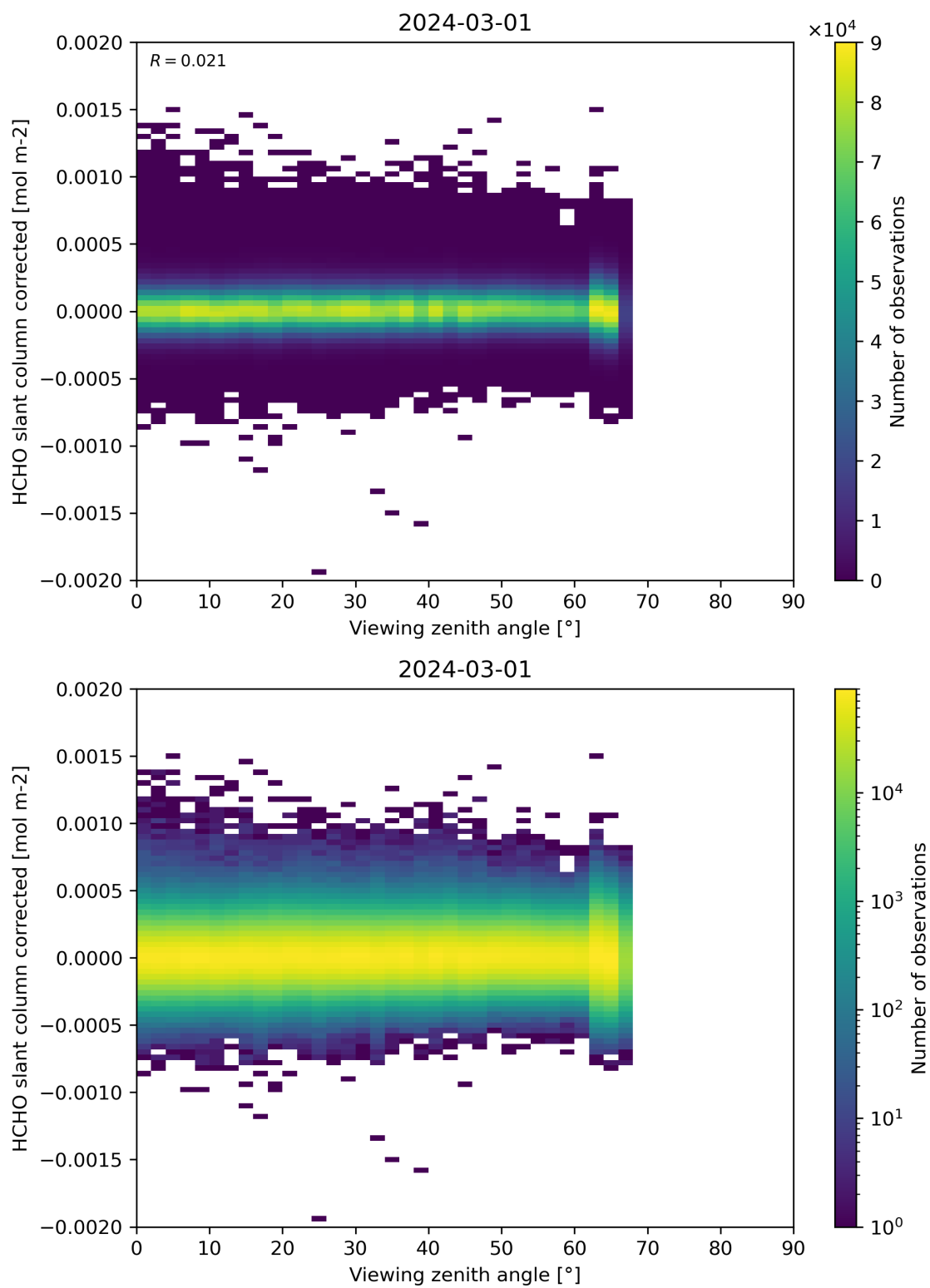
Figure 186: Scatter density plot of “Viewing zenith angle” against “HCHO slant column corrected” for 2024-02-29 to 2024-03-02.
