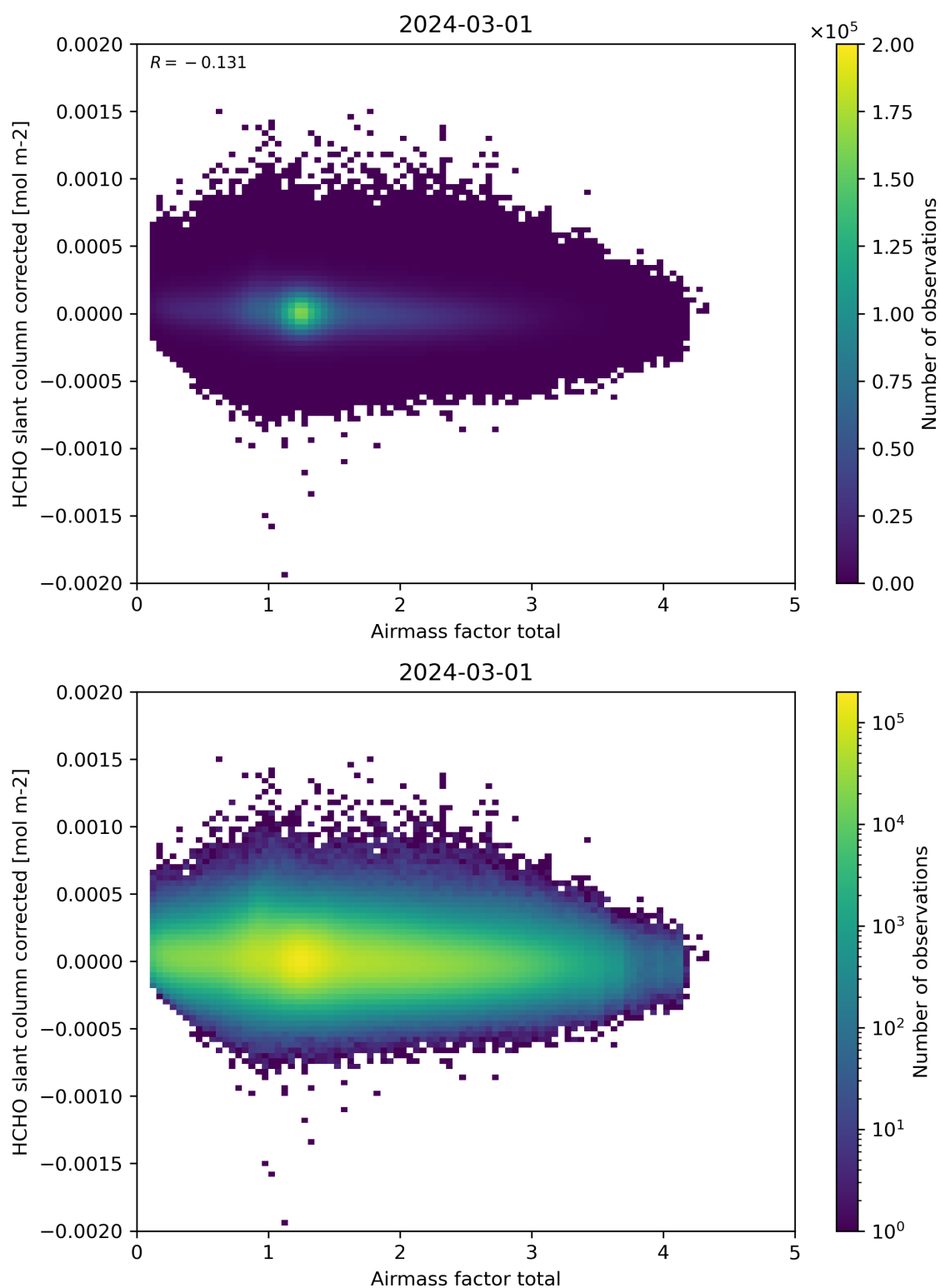
Figure 101: Scatter density plot of “Airmass factor total” against “HCHO slant column corrected” for 2024-02-29 to 2024-03-02.
