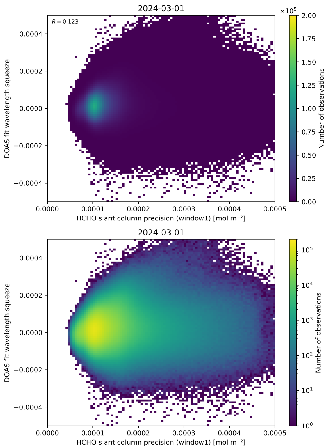
Figure 90: Scatter density plot of “HCHO slant column precision (window1)” against “DOAS fit wavelength squeeze” for 2024-02-29 to 2024-03-02.
