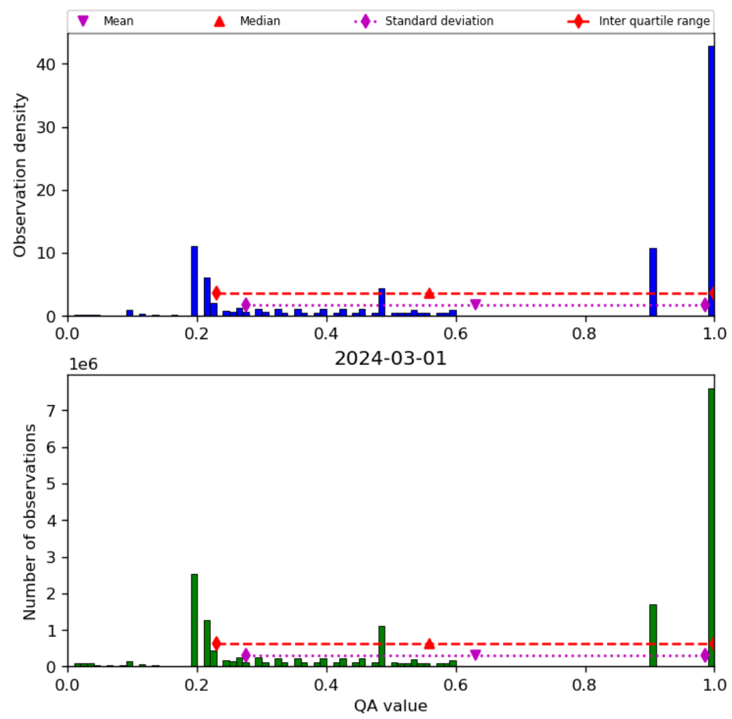
Figure 34: Histogram of “QA value” for 2024-02-29 to 2024-03-02
