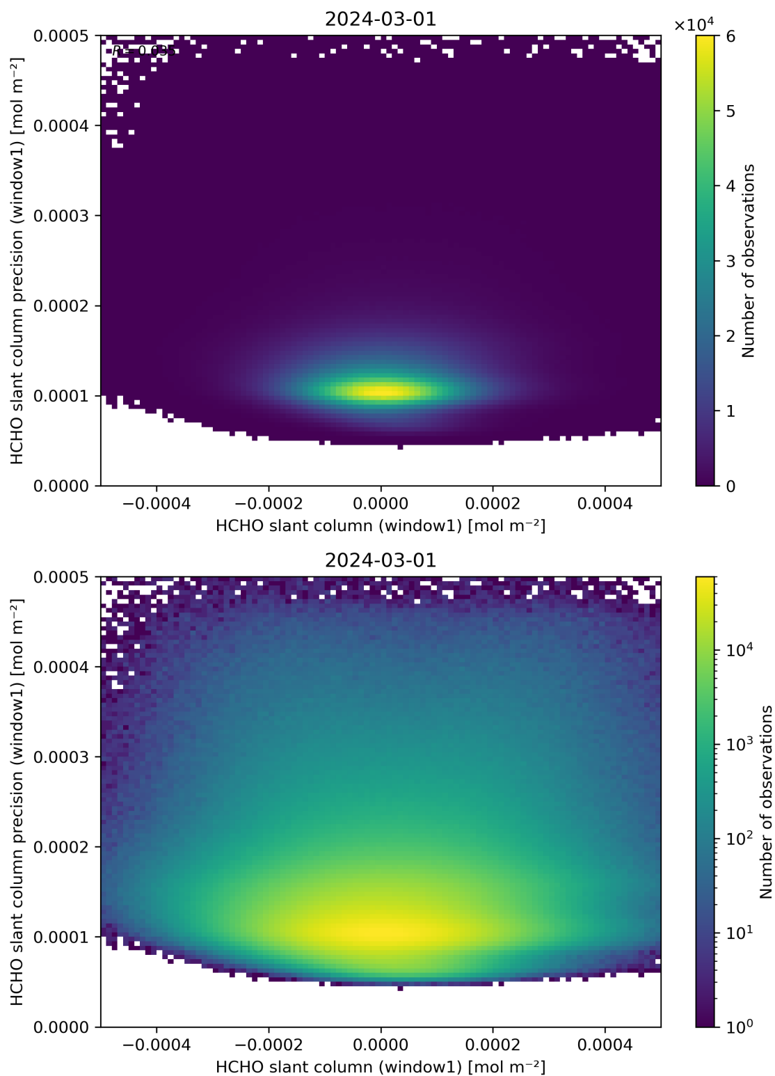
Figure 84: Scatter density plot of “HCHO slant column (window1)” against “HCHO slant column precision (window1)” for 2024-02-29 to 2024-03-02.
