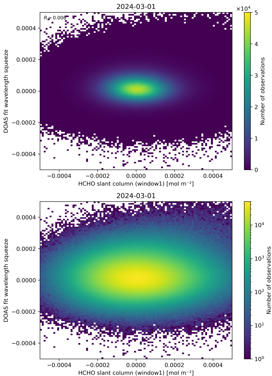
Figure 80: Scatter density plot of “HCHO slant column (window1)” against “DOAS fit wavelength squeeze” for 2024-02-29 to 2024-03-02.
