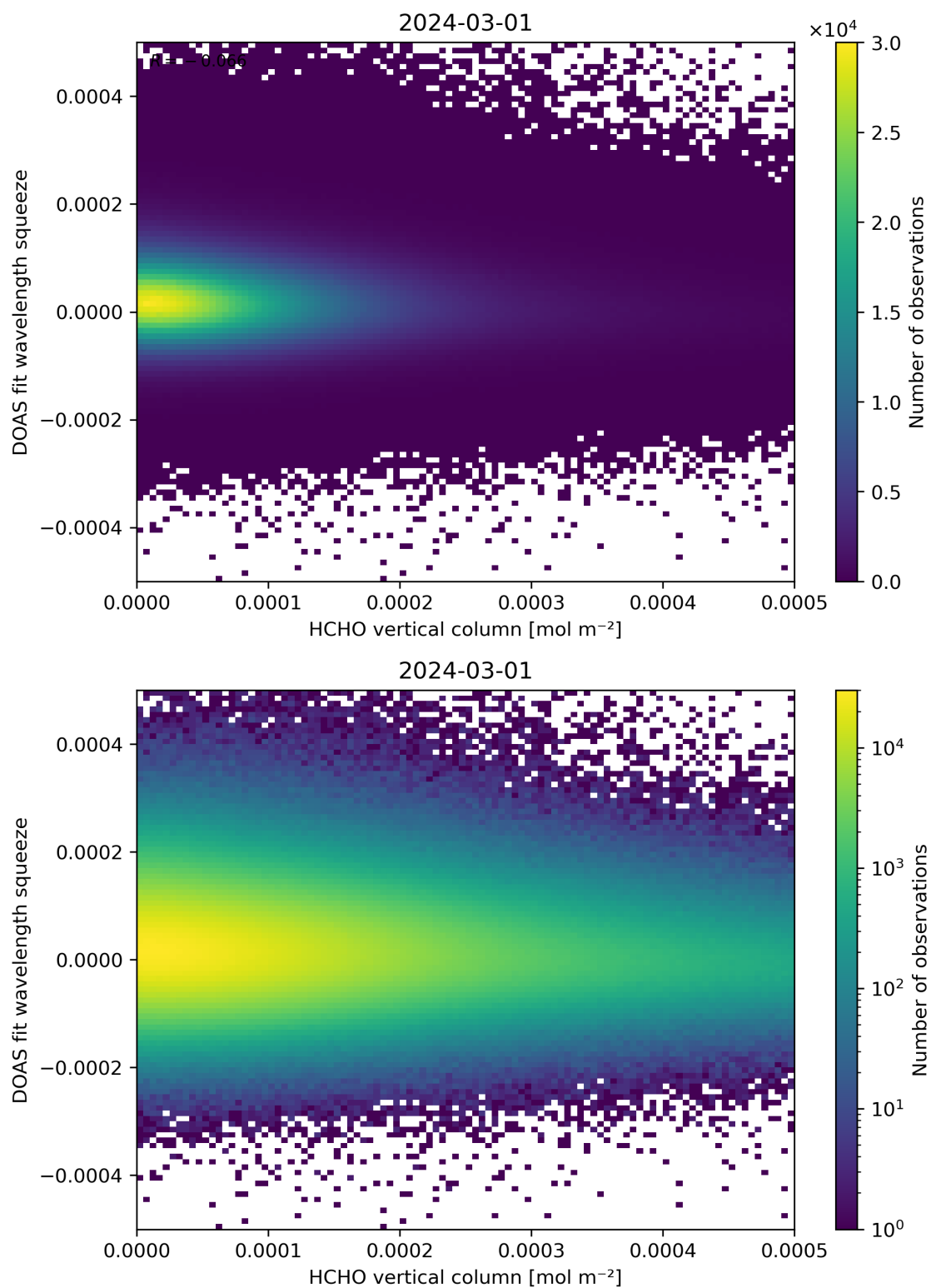
Figure 125: Scatter density plot of “HCHO vertical column” against “DOAS fit wavelength squeeze” for 2024-02-29 to 2024-03-02.
