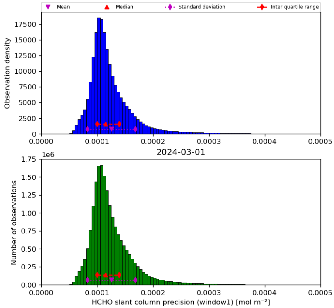
Figure 39: Histogram of “HCHO slant column precision (window1)” for 2024-02-29 to 2024-03-02
