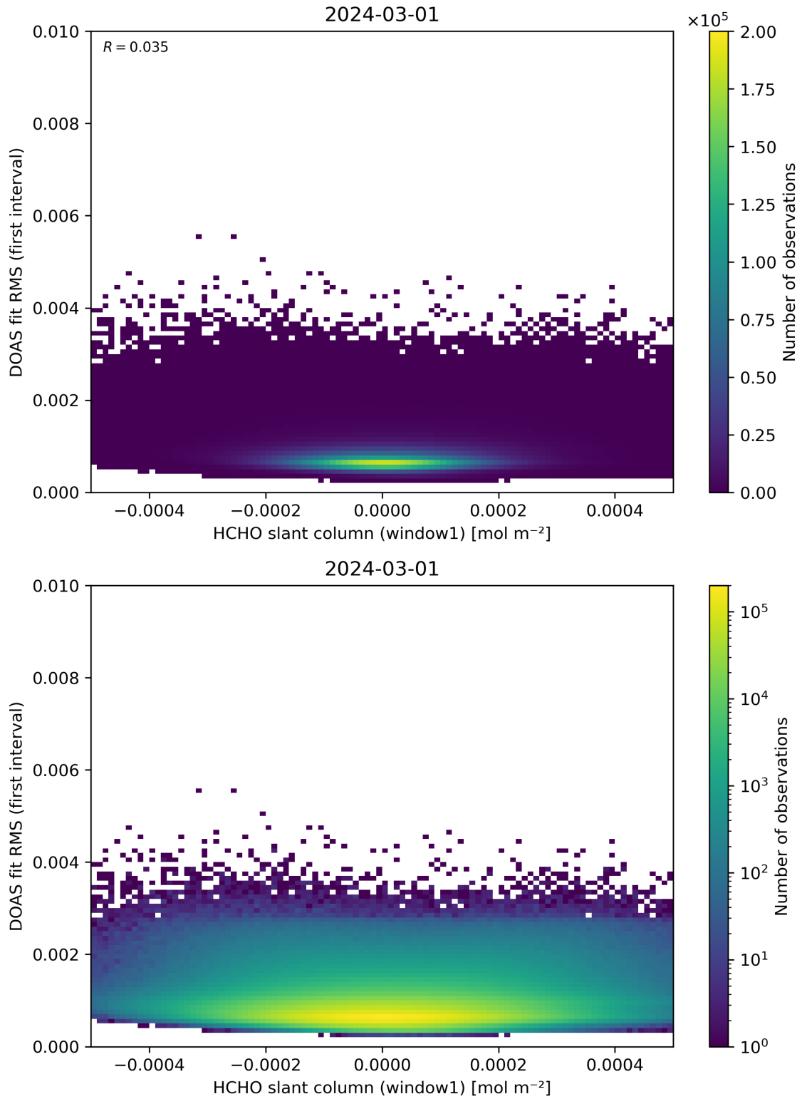
Figure 78: Scatter density plot of “HCHO slant column (window1)” against “DOAS fit RMS (first interval)” for 2024-02-29 to 2024-03-02.
