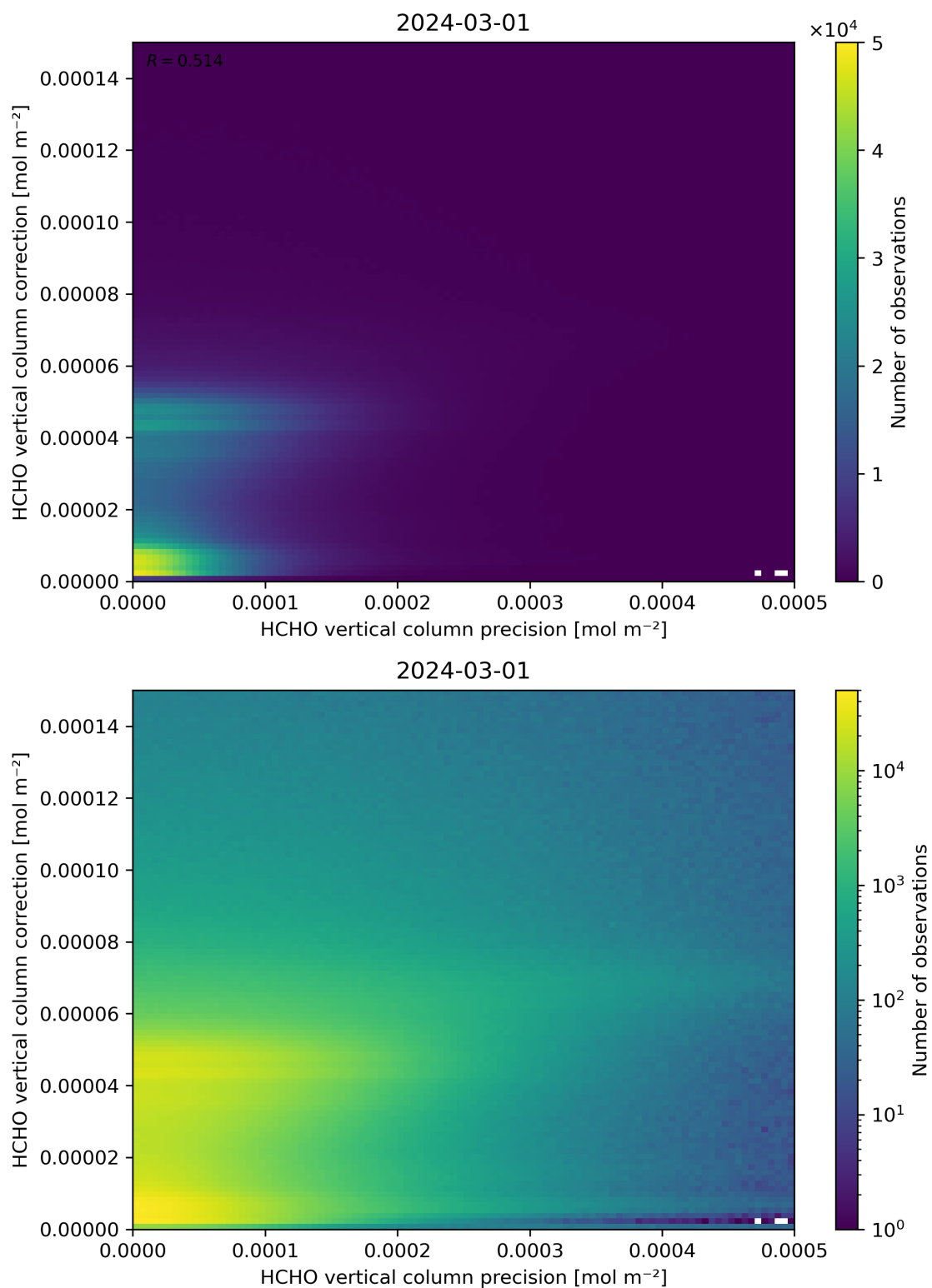
Figure 146: Scatter density plot of “HCHO vertical column precision” against “HCHO vertical column correction” for 2024-02-29 to 2024-03-02.
