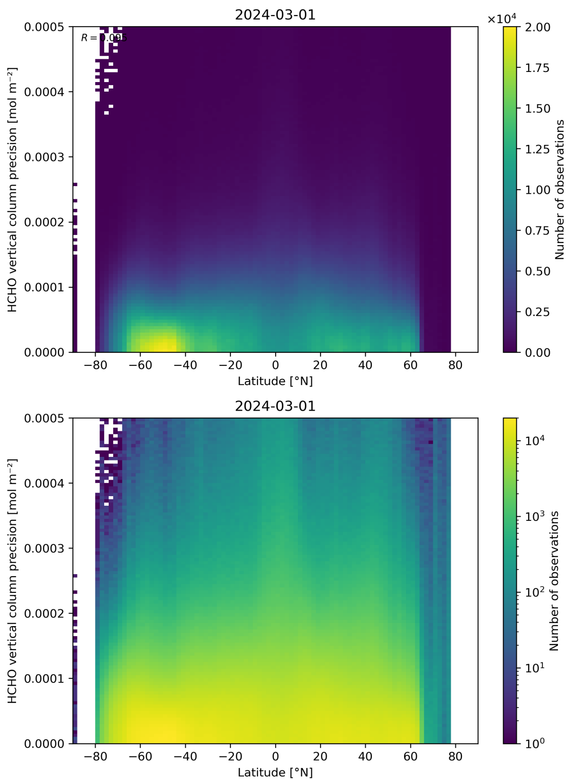
Figure 165: Scatter density plot of “Latitude” against “HCHO vertical column precision” for 2024-02-29 to 2024-03-02.
