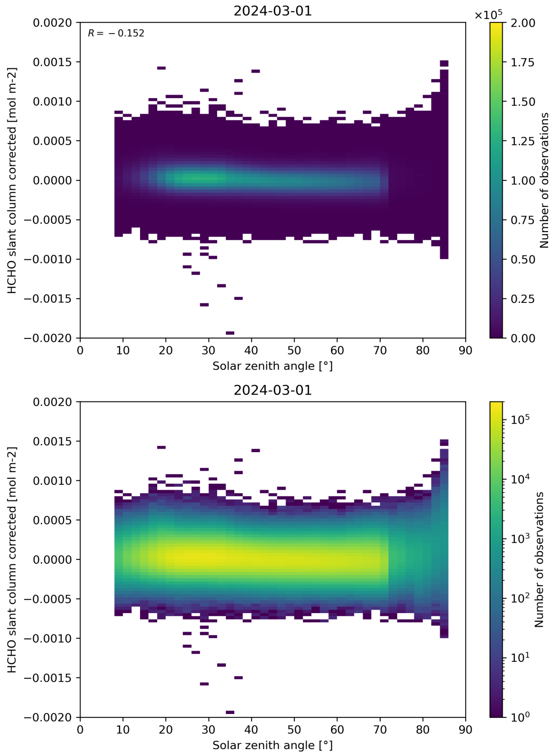
Figure 171: Scatter density plot of “Solar zenith angle” against “HCHO slant column corrected” for 2024-02-29 to 2024-03-02.
