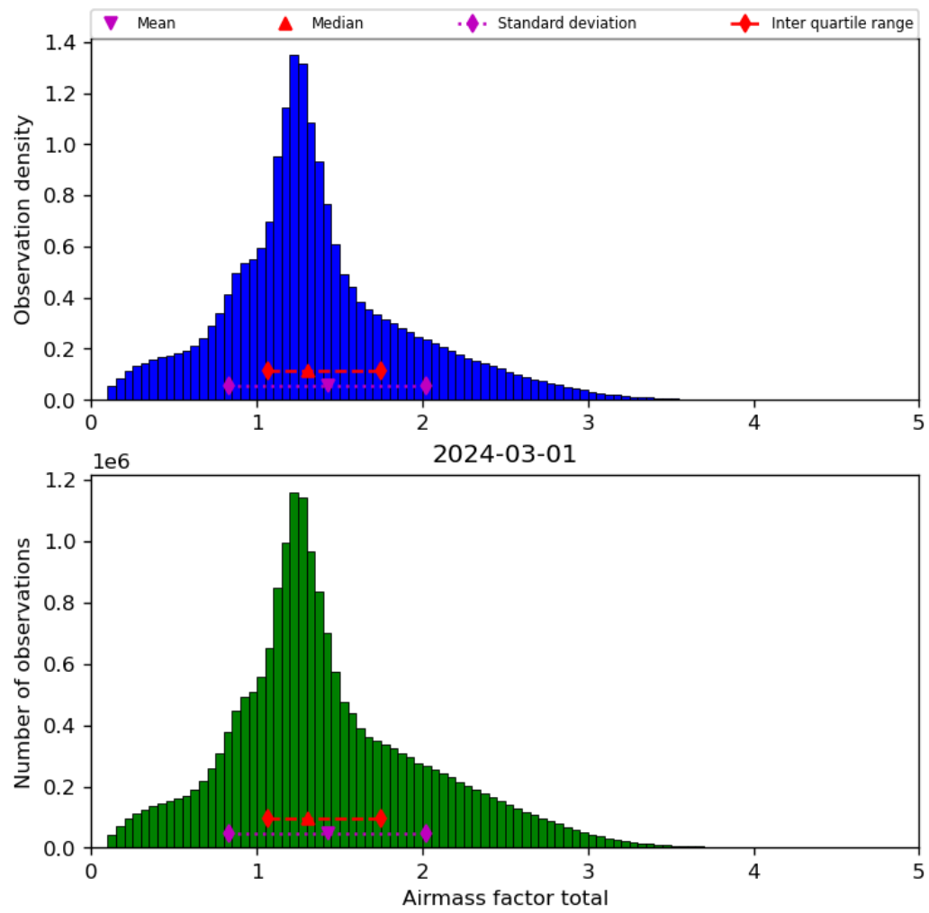
Figure 40: Histogram of “Airmass factor total” for 2024-02-29 to 2024-03-02
