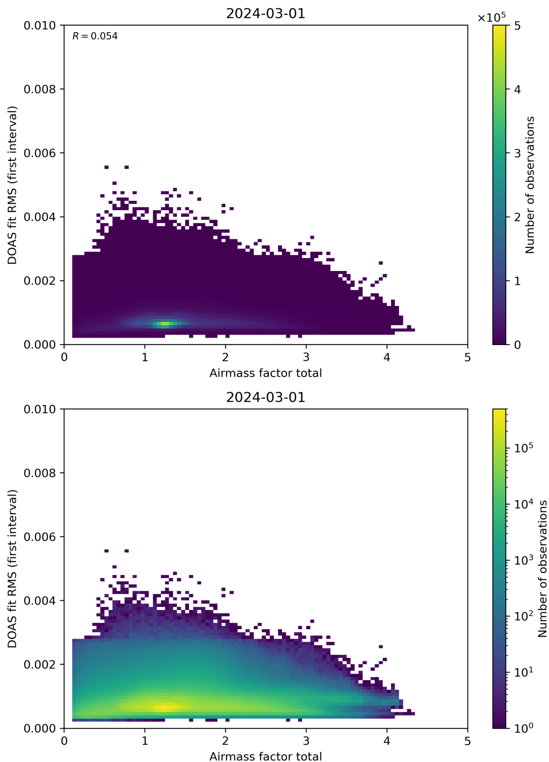
Figure 97: Scatter density plot of “Airmass factor total” against “DOAS fit RMS (first interval)” for 2024-02-29 to 2024-03-02.
