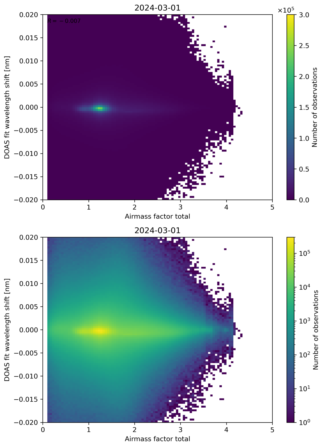
Figure 98: Scatter density plot of “Airmass factor total” against “DOAS fit wavelength shift” for 2024-02-29 to 2024-03-02.
