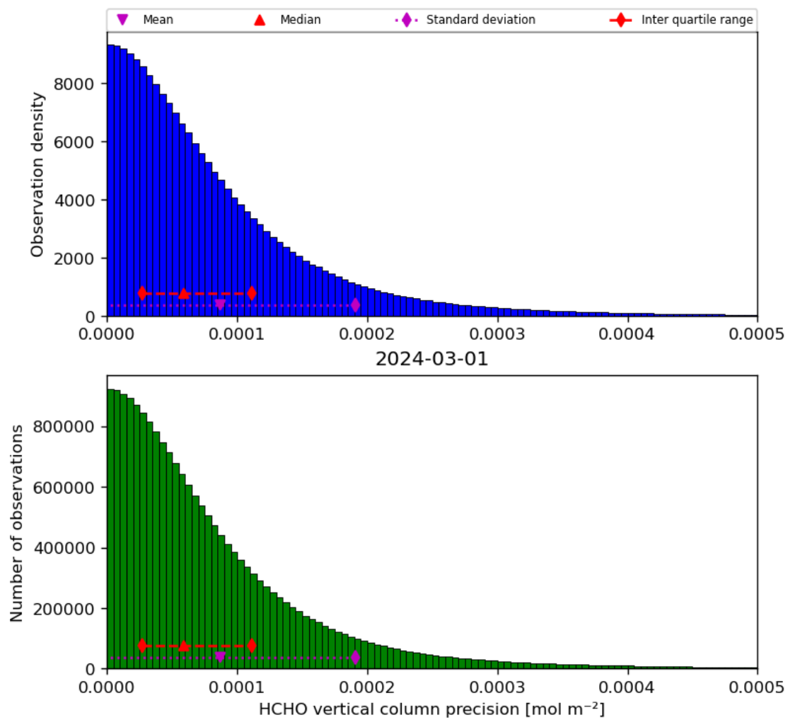
Figure 36: Histogram of “HCHO vertical column precision” for 2024-02-29 to 2024-03-02
