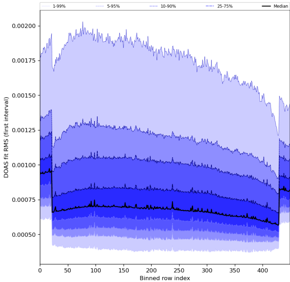
Figure 60: Along track statistics of “DOAS fit RMS (first interval)” for 2024-02-29 to 2024-03-02
