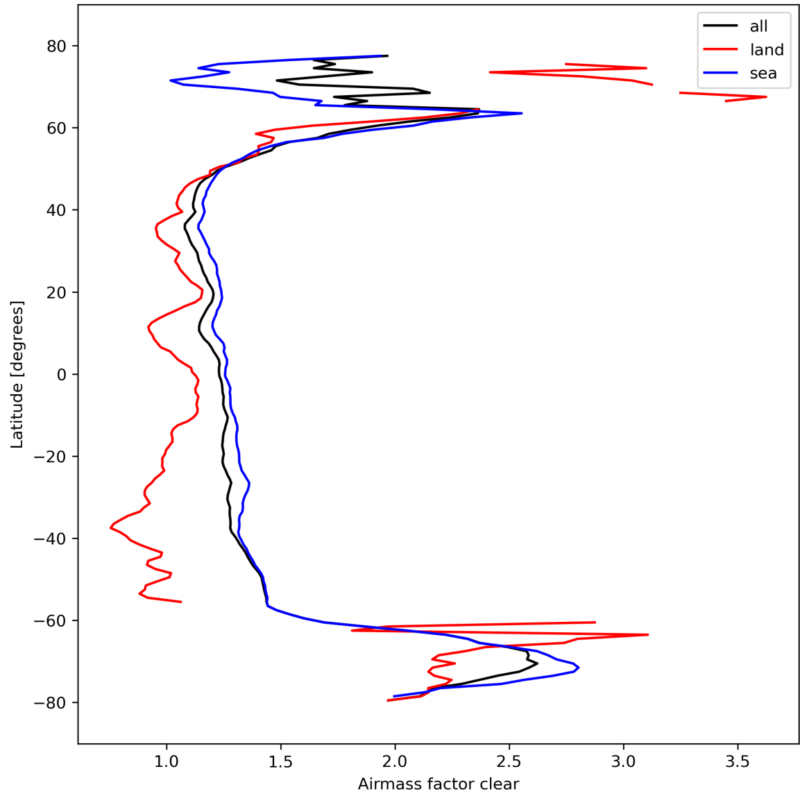
Figure 28: Zonal average of “Airmass factor clear” for 2024-02-29 to 2024-03-02.
