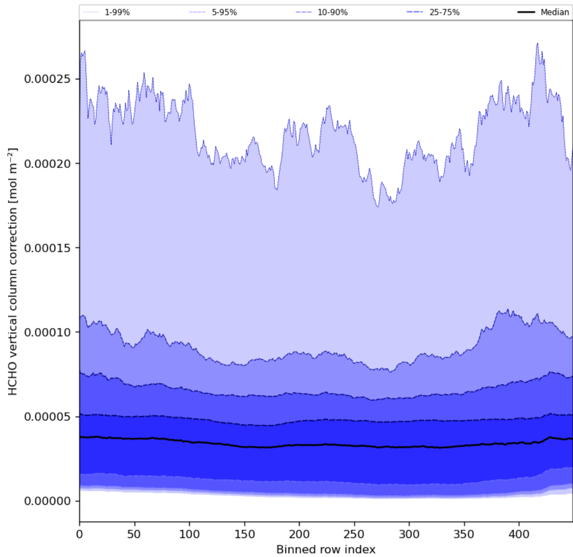
Figure 51: Along track statistics of "HCHO vertical column correction" for 2024-02-29 to 2024-03-02
