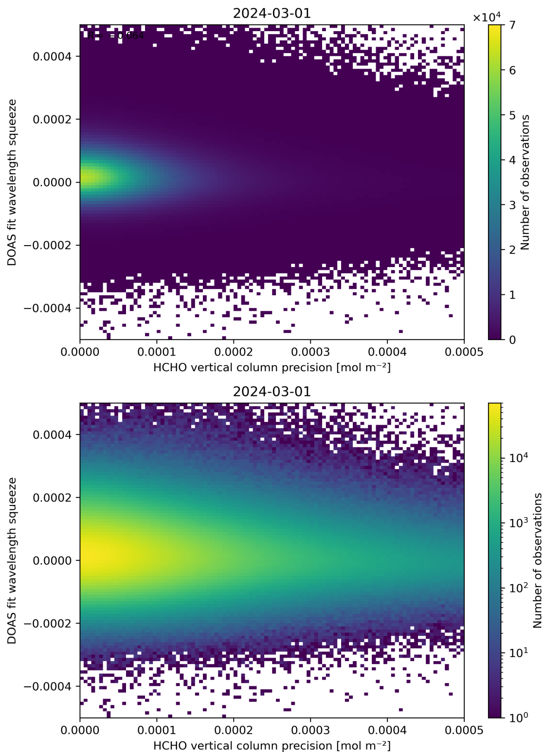
Figure 138: Scatter density plot of “HCHO vertical column precision” against “DOAS fit wavelength squeeze” for 2024-02-29 to 2024-03-02.
