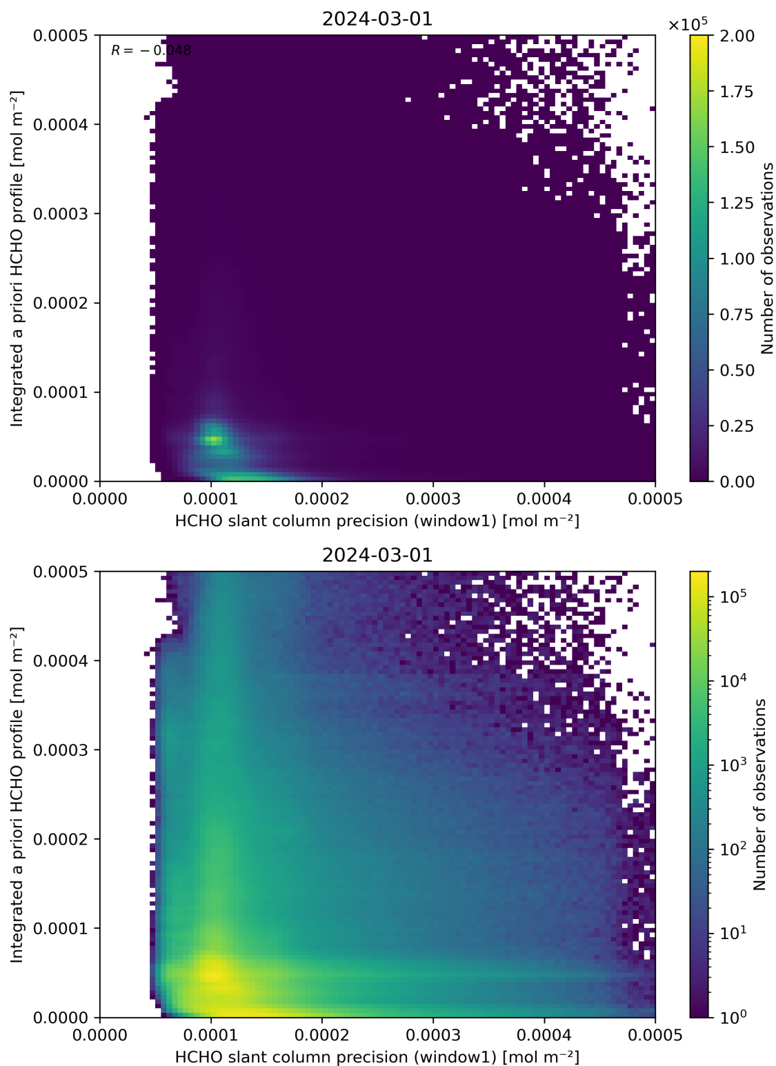
Figure 96: Scatter density plot of “HCHO slant column precision (window1)” against “Integrated a priori HCHO profile” for 2024-02-29 to 2024-03-02.
