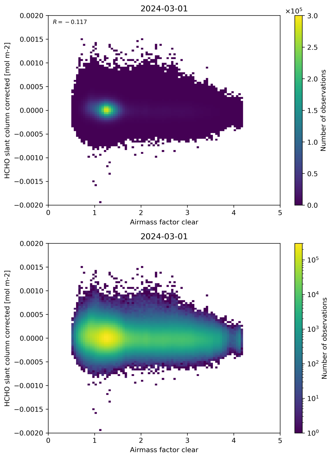
Figure 74: Scatter density plot of “Airmass factor clear” against “HCHO slant column corrected” for 2024-02-29 to 2024-03-02.
