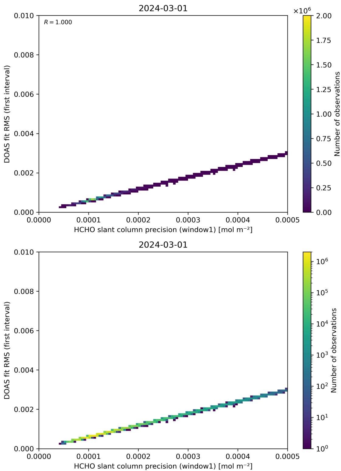
Figure 88: Scatter density plot of “HCHO slant column precision (window1)” against “DOAS fit RMS (first interval)” for 2024-02-29 to 2024-03-02.
