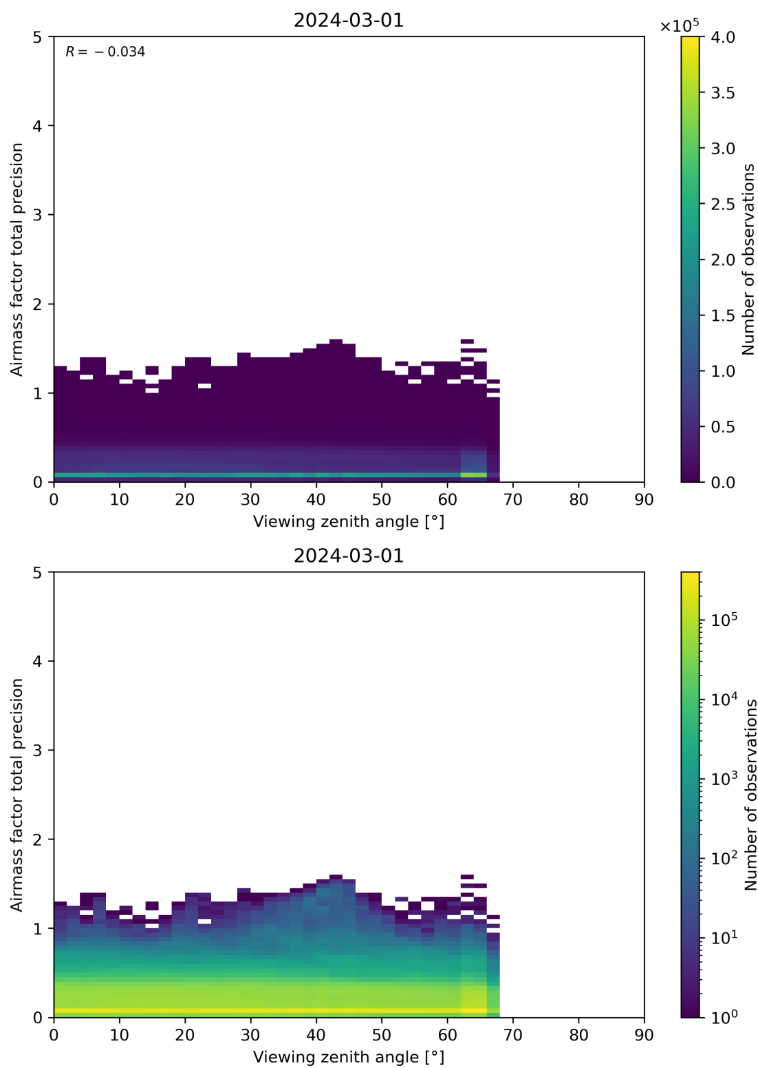
Figure 191: Scatter density plot of “Viewing zenith angle” against “Airmass factor total precision” for 2024-02-29 to 2024-03-02.
