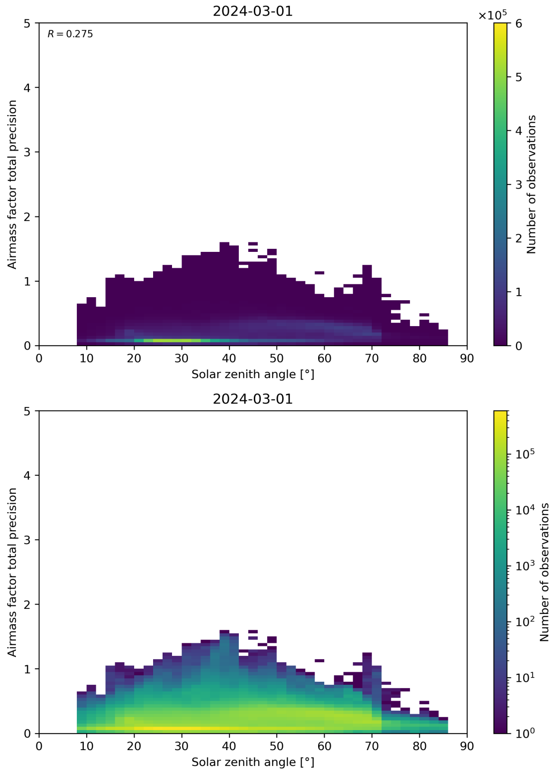
Figure 176: Scatter density plot of “Solar zenith angle” against “Airmass factor total precision” for 2024-02-29 to 2024-03-02.
