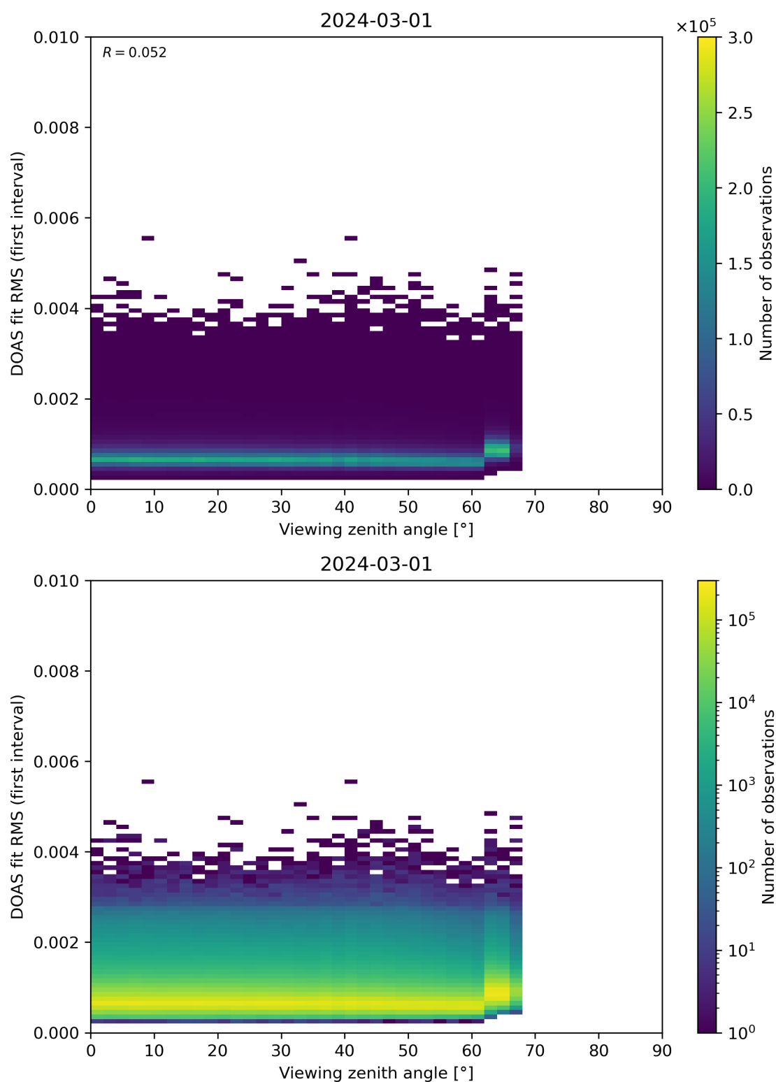
Figure 182: Scatter density plot of “Viewing zenith angle” against “DOAS fit RMS (first interval)” for 2024-02-29 to 2024-03-02.
