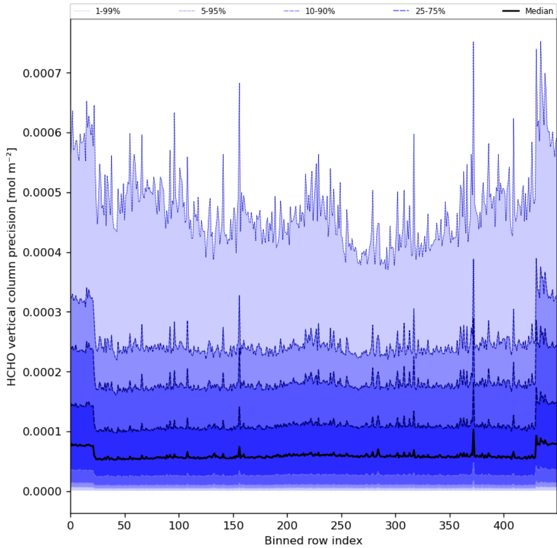
Figure 50: Along track statistics of "HCHO vertical column precision" for 2024-02-29 to 2024-03-02
