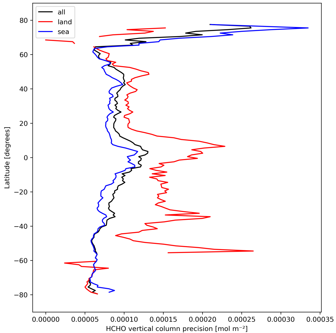
Figure 22: Zonal average of “HCHO vertical column precision” for 2024-02-29 to 2024-03-02.
