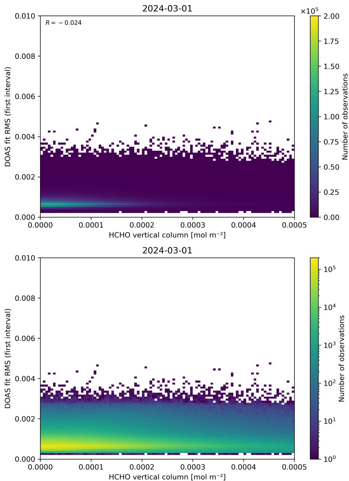
Figure 123: Scatter density plot of “HCHO vertical column” against “DOAS fit RMS (first interval)” for 2024-02-29 to 2024-03-02.
