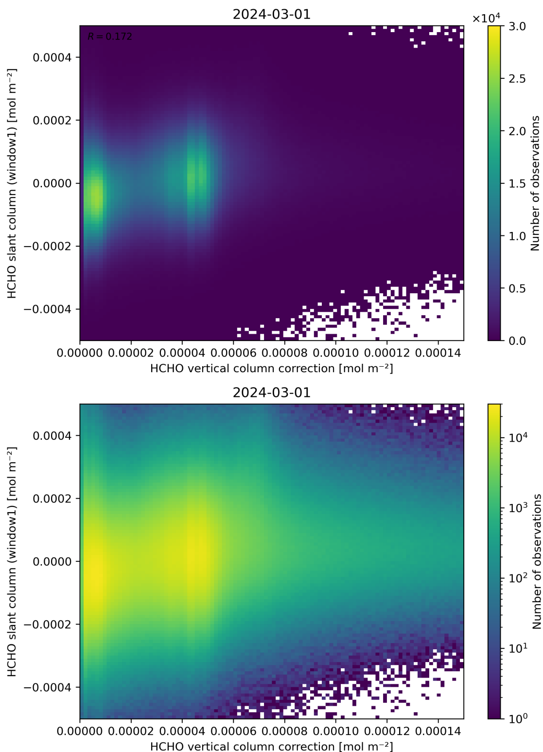
Figure 118: Scatter density plot of “HCHO vertical column correction” against “HCHO slant column (window1)” for 2024-02-29 to 2024-03-02.
