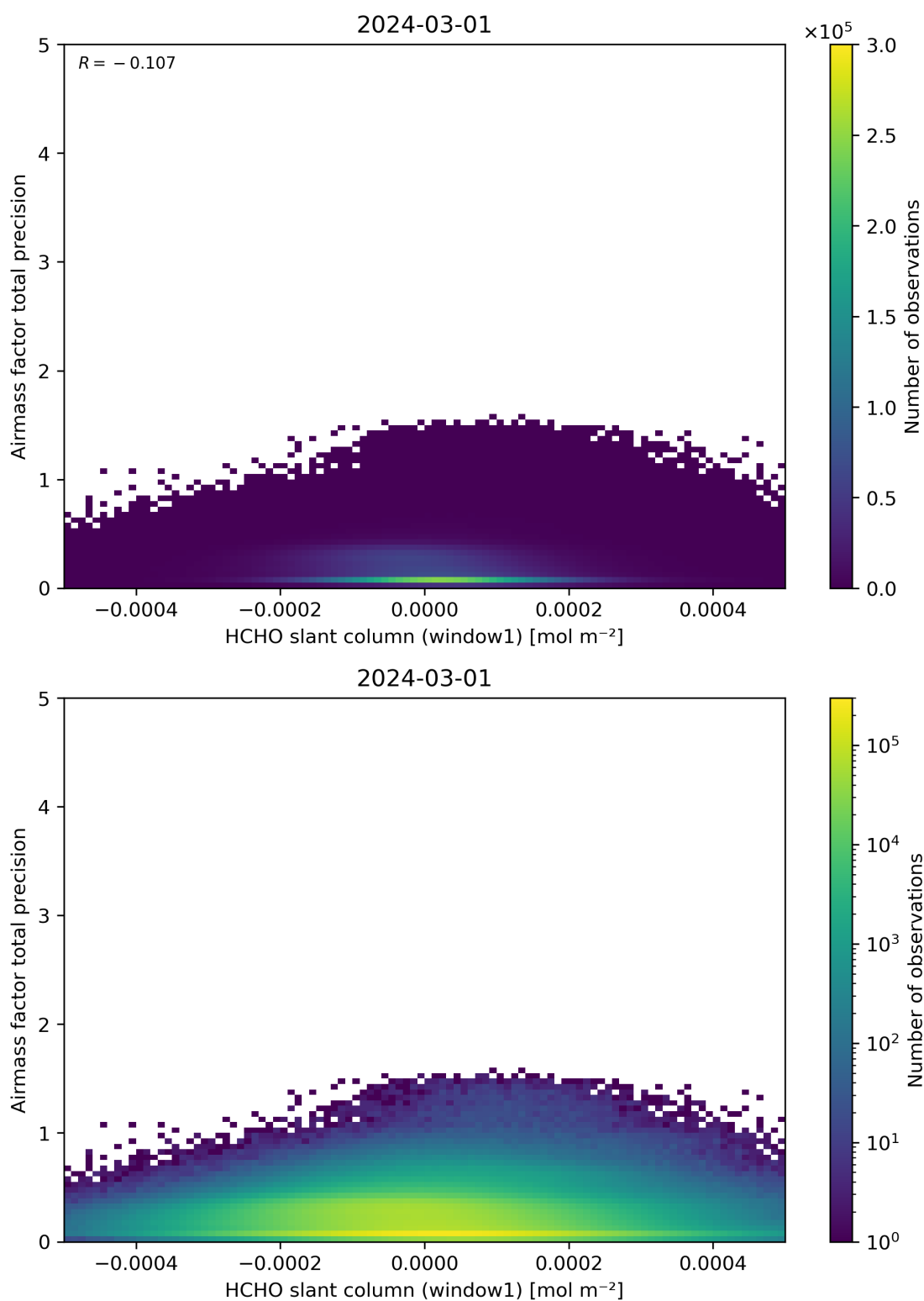
Figure 86: Scatter density plot of “HCHO slant column (window1)” against “Airmass factor total precision” for 2024-02-29 to 2024-03-02.
