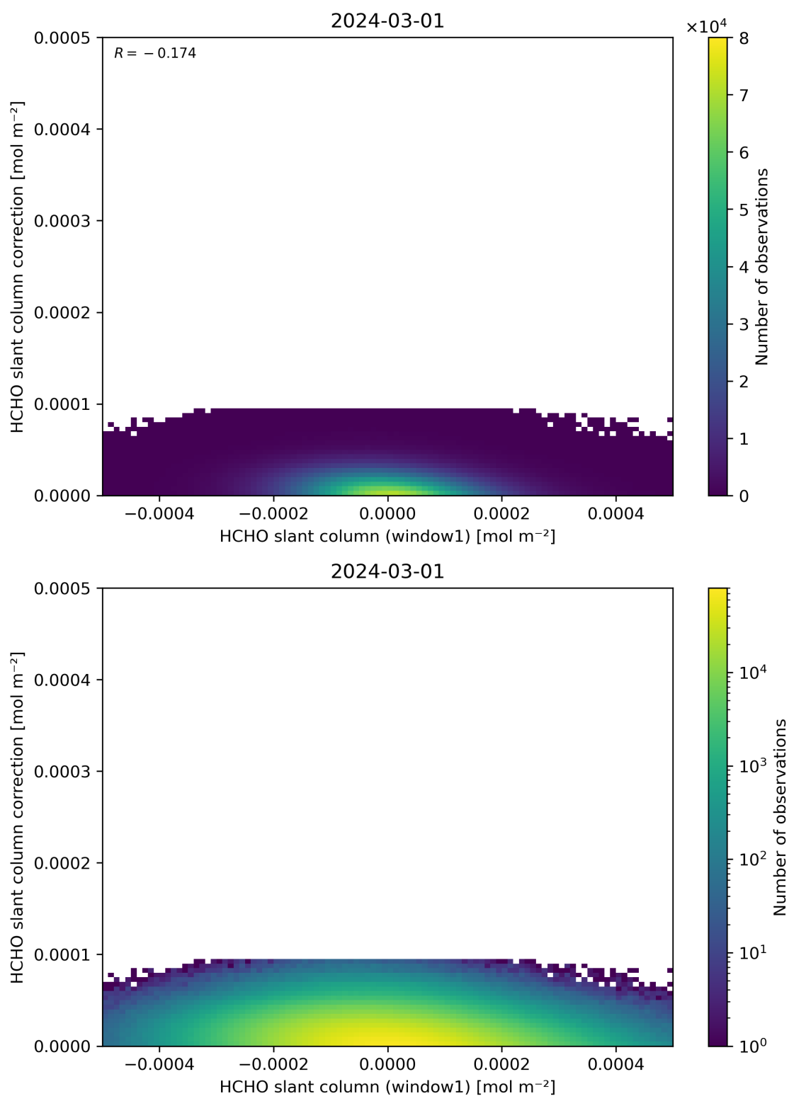
Figure 83: Scatter density plot of “HCHO slant column (window1)” against “HCHO slant column correction” for 2024-02-29 to 2024-03-02.
