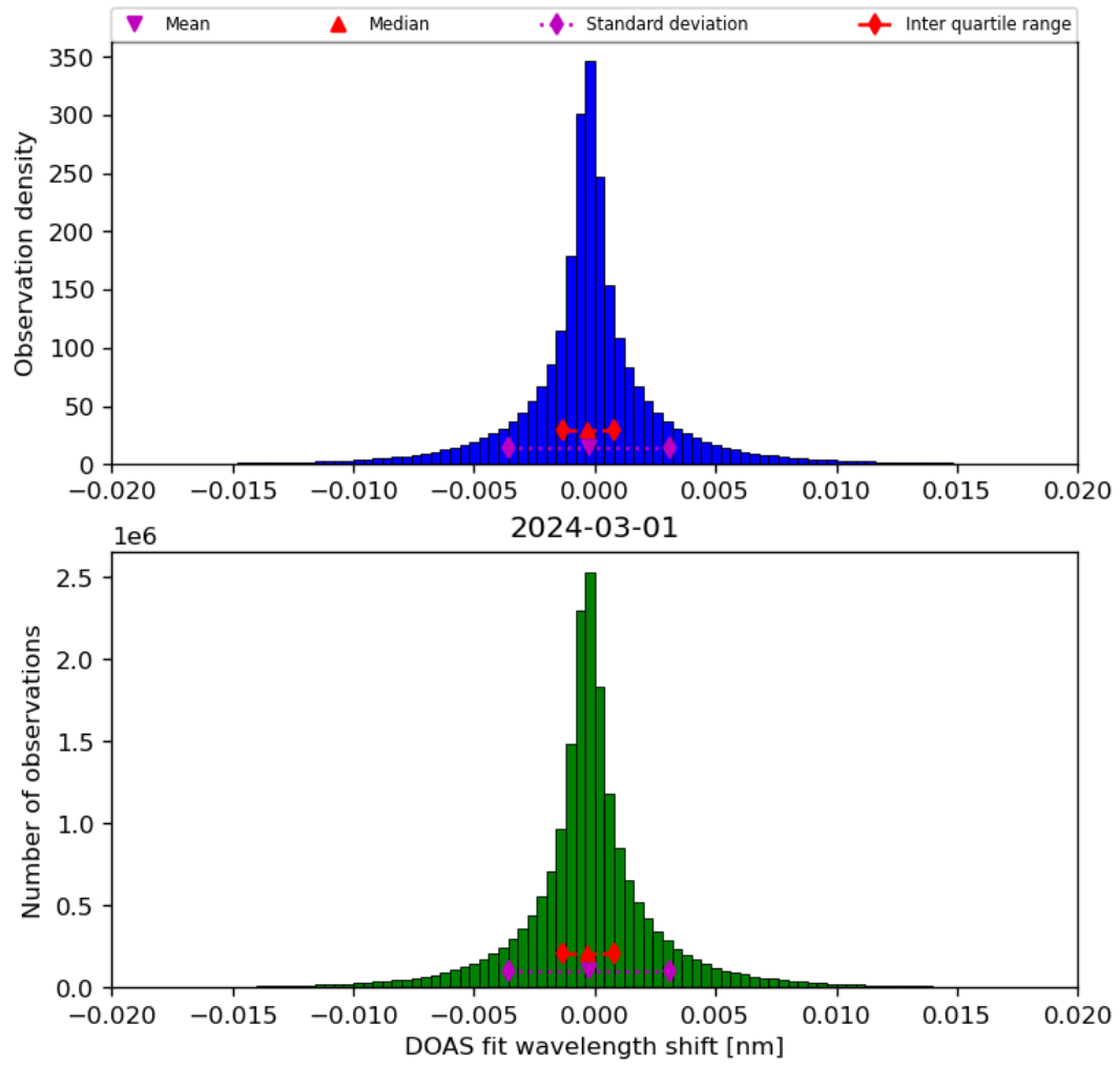
Figure 44: Histogram of “DOAS fit wavelength shift” for 2024-02-29 to 2024-03-02
