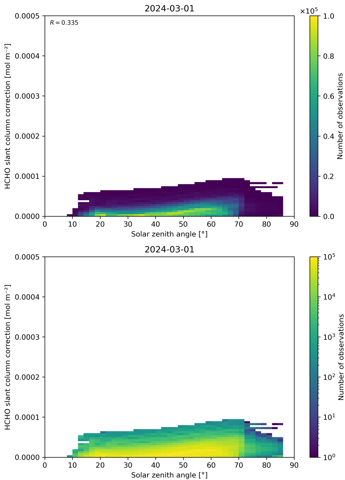
Figure 172: Scatter density plot of “Solar zenith angle” against “HCHO slant column correction” for 2024-02-29 to 2024-03-02.
