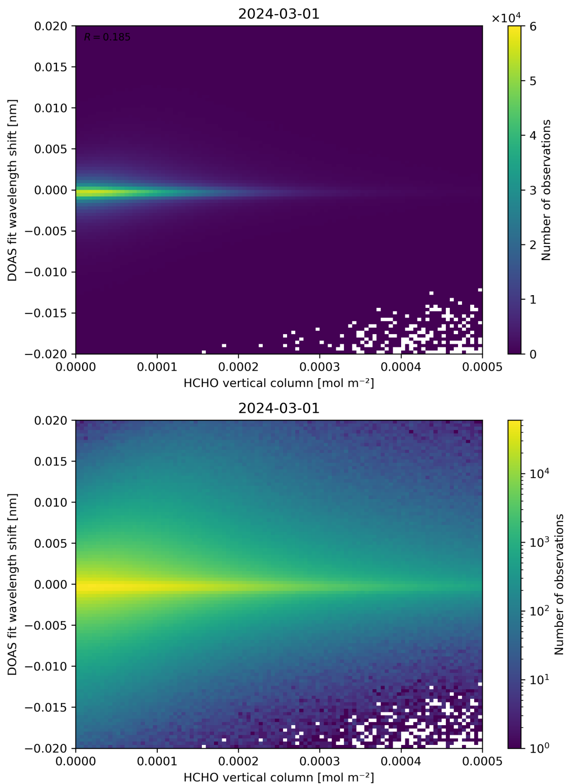
Figure 124: Scatter density plot of “HCHO vertical column” against “DOAS fit wavelength shift” for 2024-02-29 to 2024-03-02.
