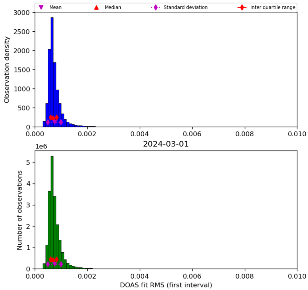
Figure 46: Histogram of “DOAS fit RMS (first interval)” for 2024-02-29 to 2024-03-02
