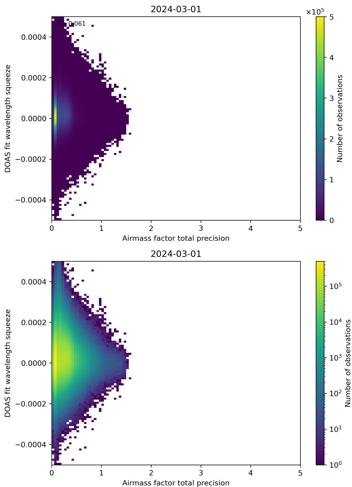
Figure 107: Scatter density plot of “Airmass factor total precision” against “DOAS fit wavelength squeeze” for 2024-02-29 to 2024-03-02.
