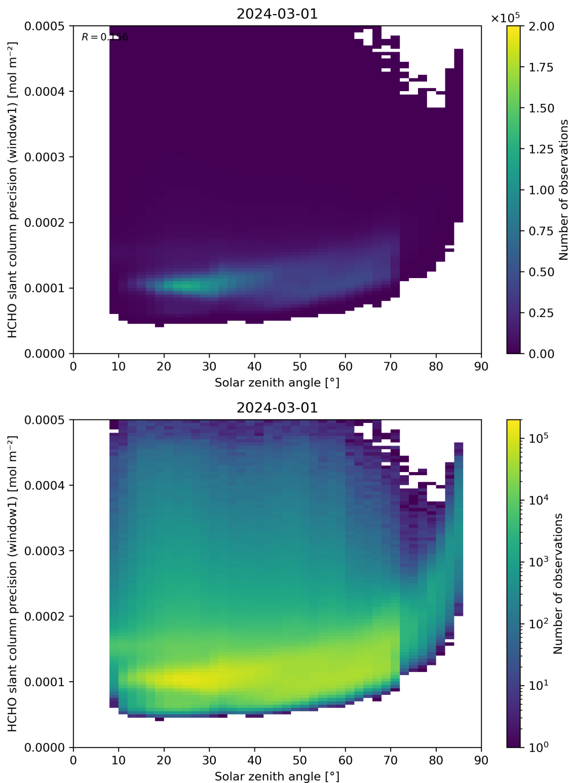
Figure 174: Scatter density plot of “Solar zenith angle” against “HCHO slant column precision (window1)” for 2024-02-29 to 2024-03-02.
