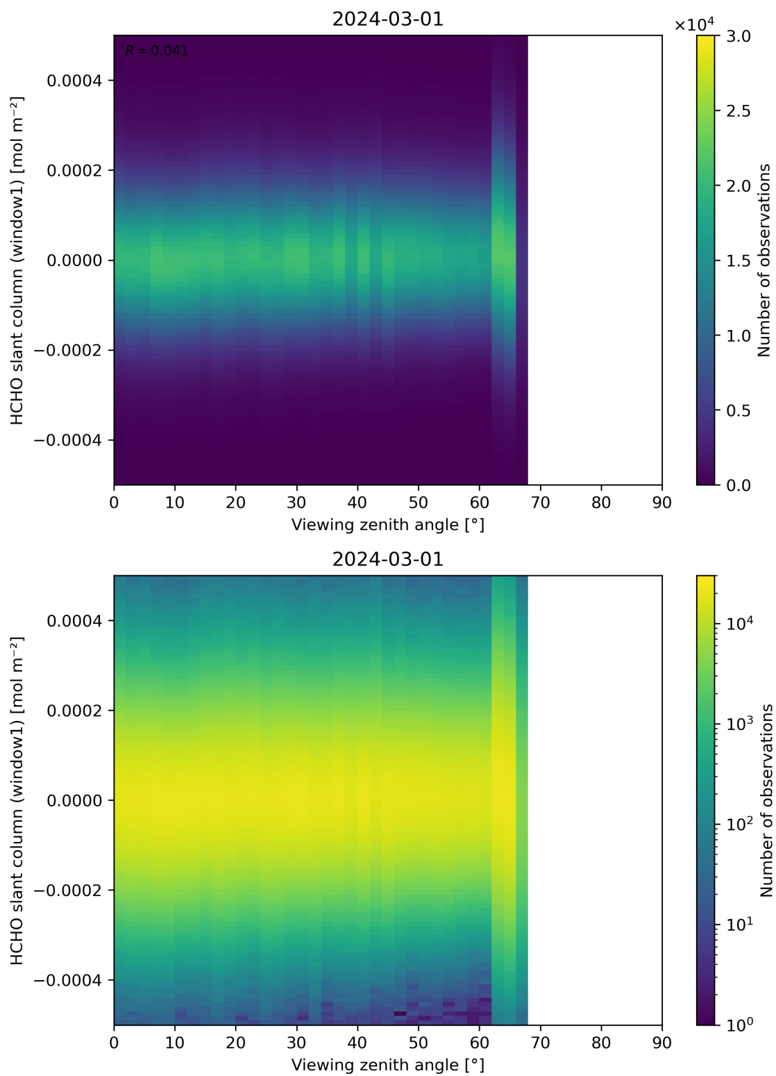
Figure 188: Scatter density plot of “Viewing zenith angle” against “HCHO slant column (window1)” for 2024-02-29 to 2024-03-02.
