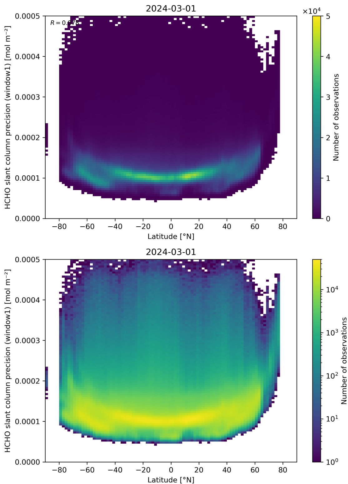
Figure 160: Scatter density plot of “Latitude” against “HCHO slant column precision (window1)” for 2024-02-29 to 2024-03-02.
