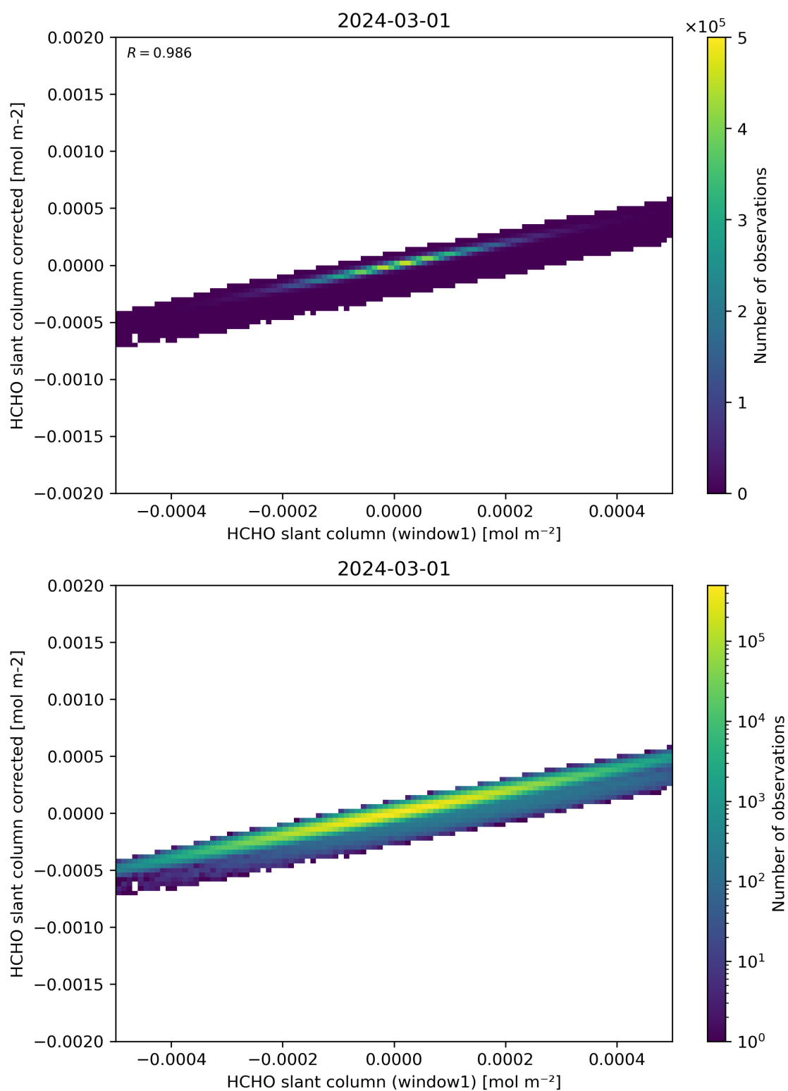
Figure 82: Scatter density plot of “HCHO slant column (window1)” against “HCHO slant column corrected” for 2024-02-29 to 2024-03-02.
