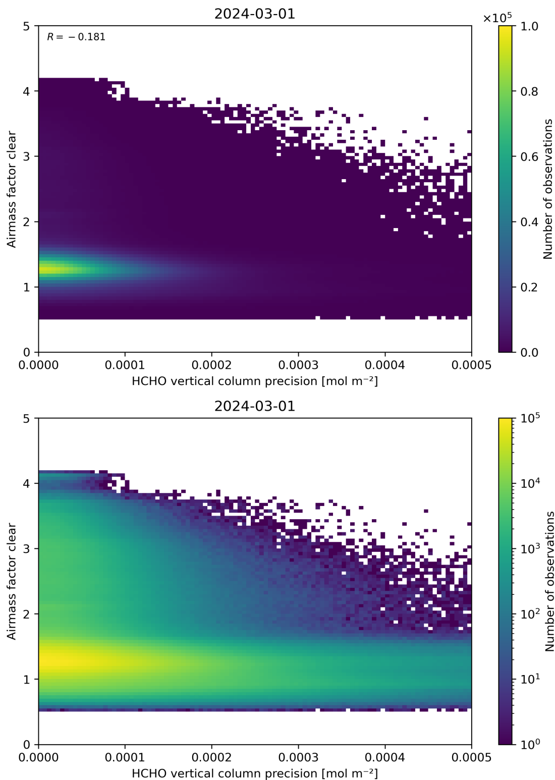
Figure 139: Scatter density plot of “HCHO vertical column precision” against “Airmass factor clear” for 2024-02-29 to 2024-03-02.
