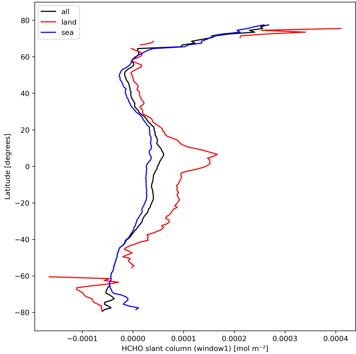
Figure 24: Zonal average of “HCHO slant column (window1)” for 2024-02-29 to 2024-03-02.
