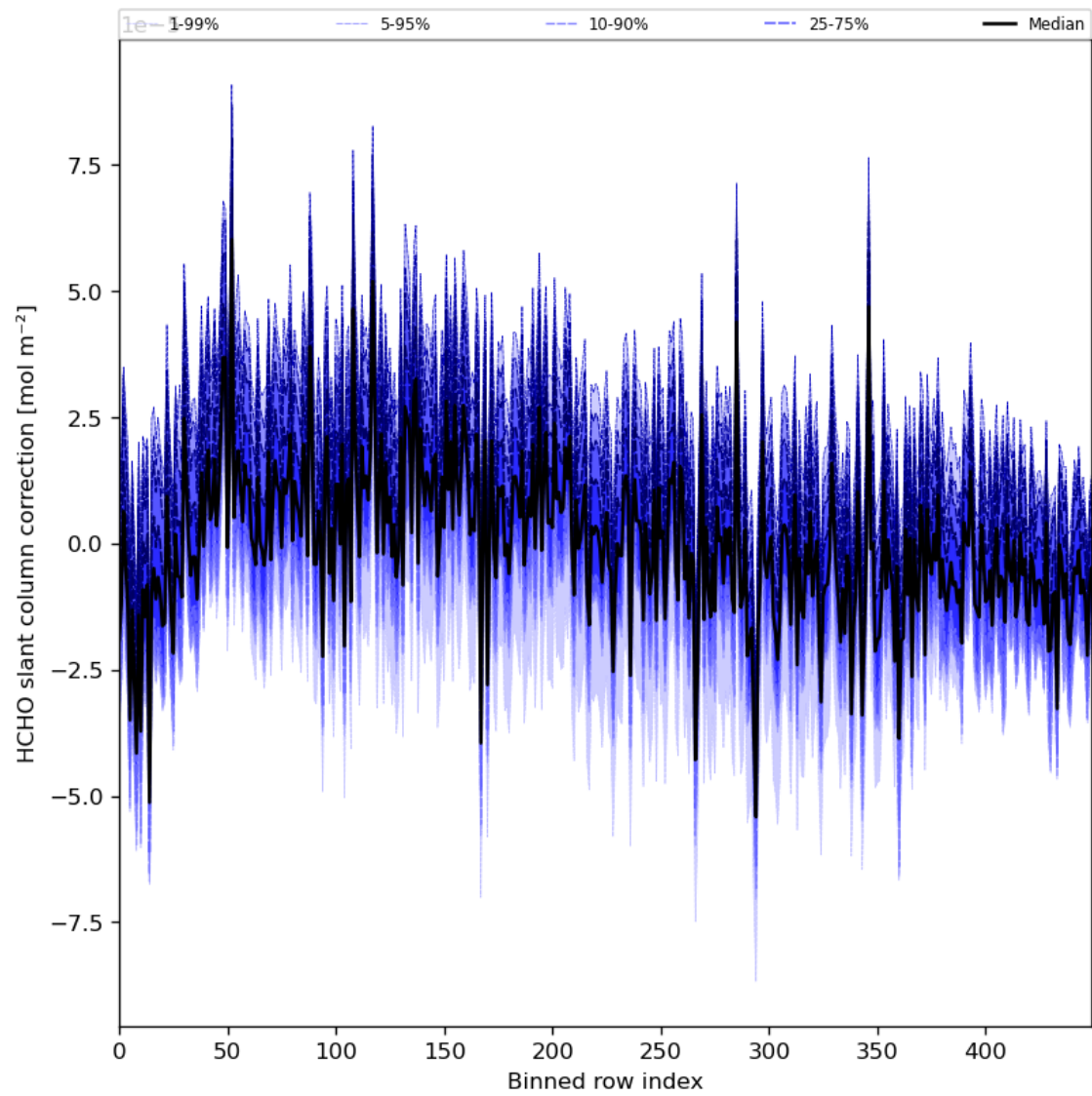
Figure 61: Along track statistics of “HCHO slant column correction” for 2024-02-29 to 2024-03-02
