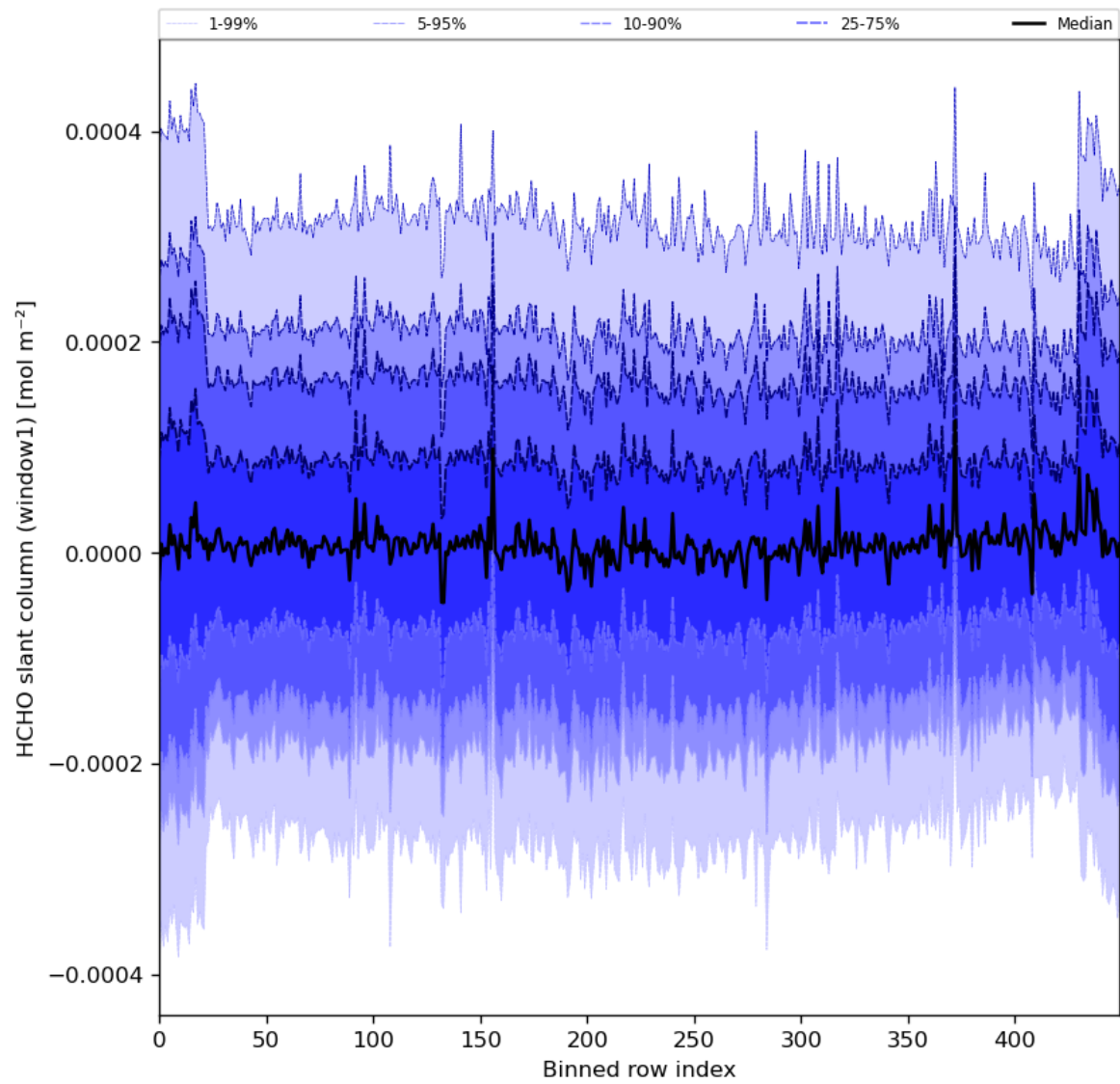
Figure 52: Along track statistics of “HCHO slant column (window1)” for 2024-02-29 to 2024-03-02
