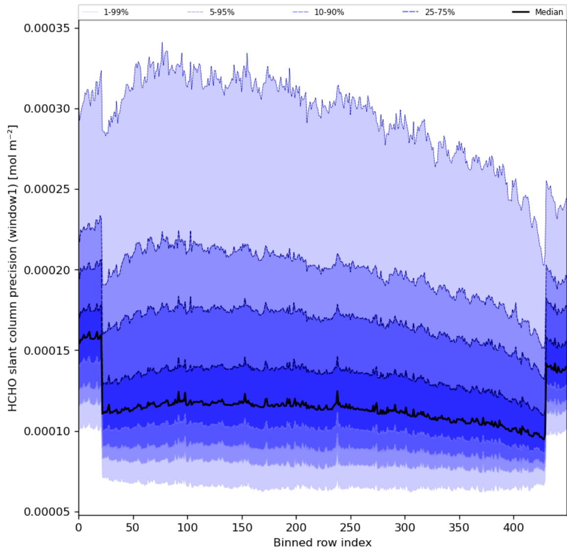
Figure 53: Along track statistics of “HCHO slant column precision (window1)” for 2024-02-29 to 2024-03-02
