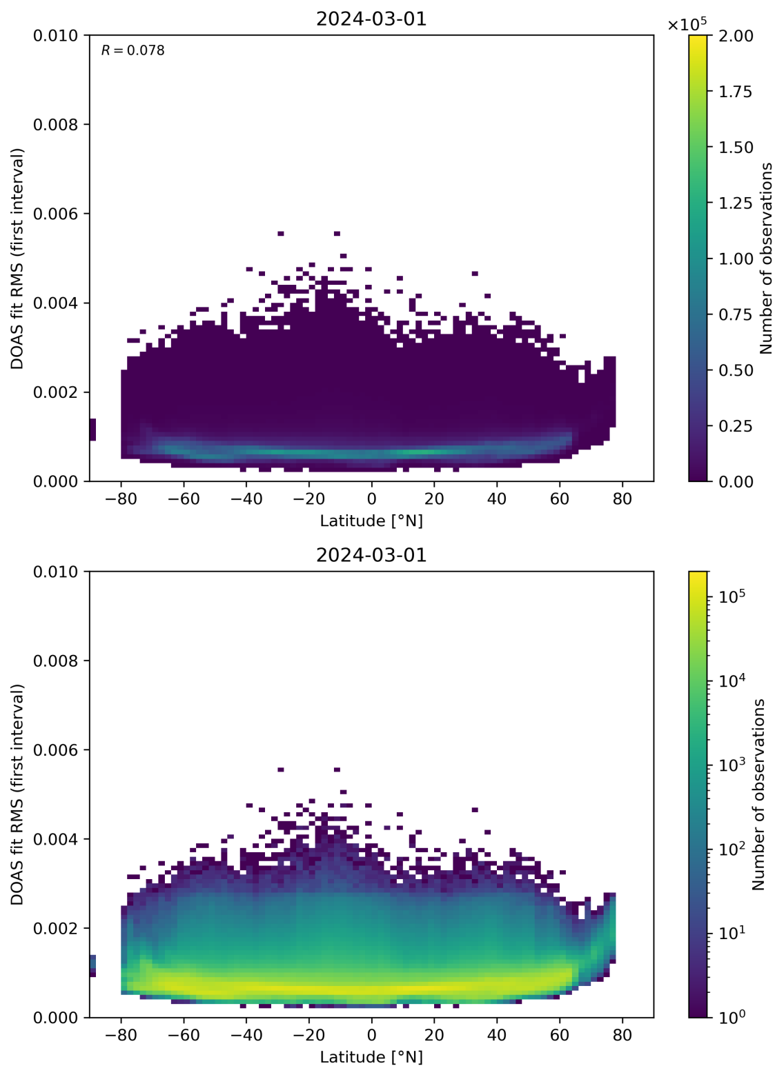
Figure 153: Scatter density plot of “Latitude” against “DOAS fit RMS (first interval)” for 2024-02-29 to 2024-03-02.
