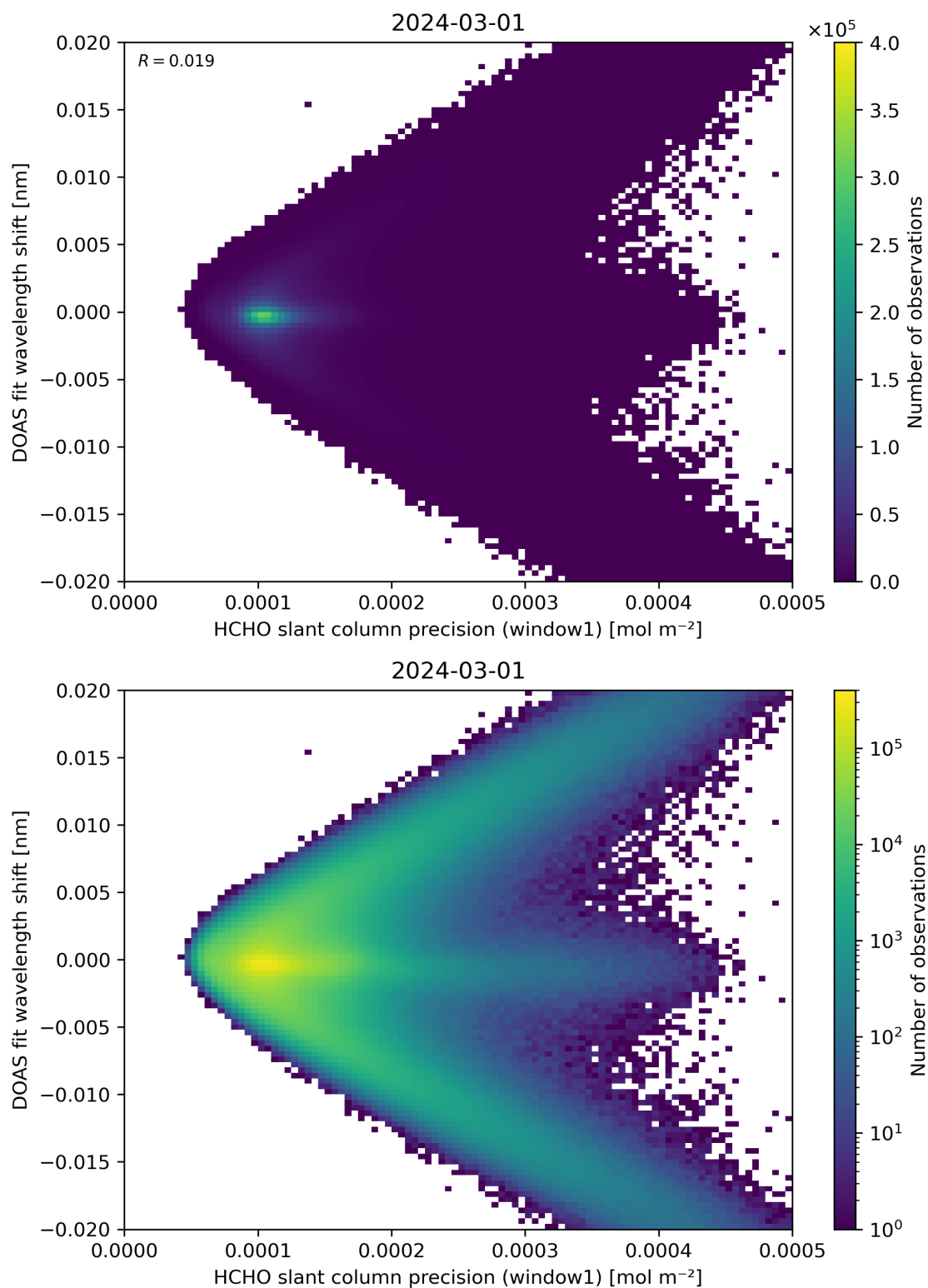
Figure 89: Scatter density plot of “HCHO slant column precision (window1)” against “DOAS fit wavelength shift” for 2024-02-29 to 2024-03-02.
