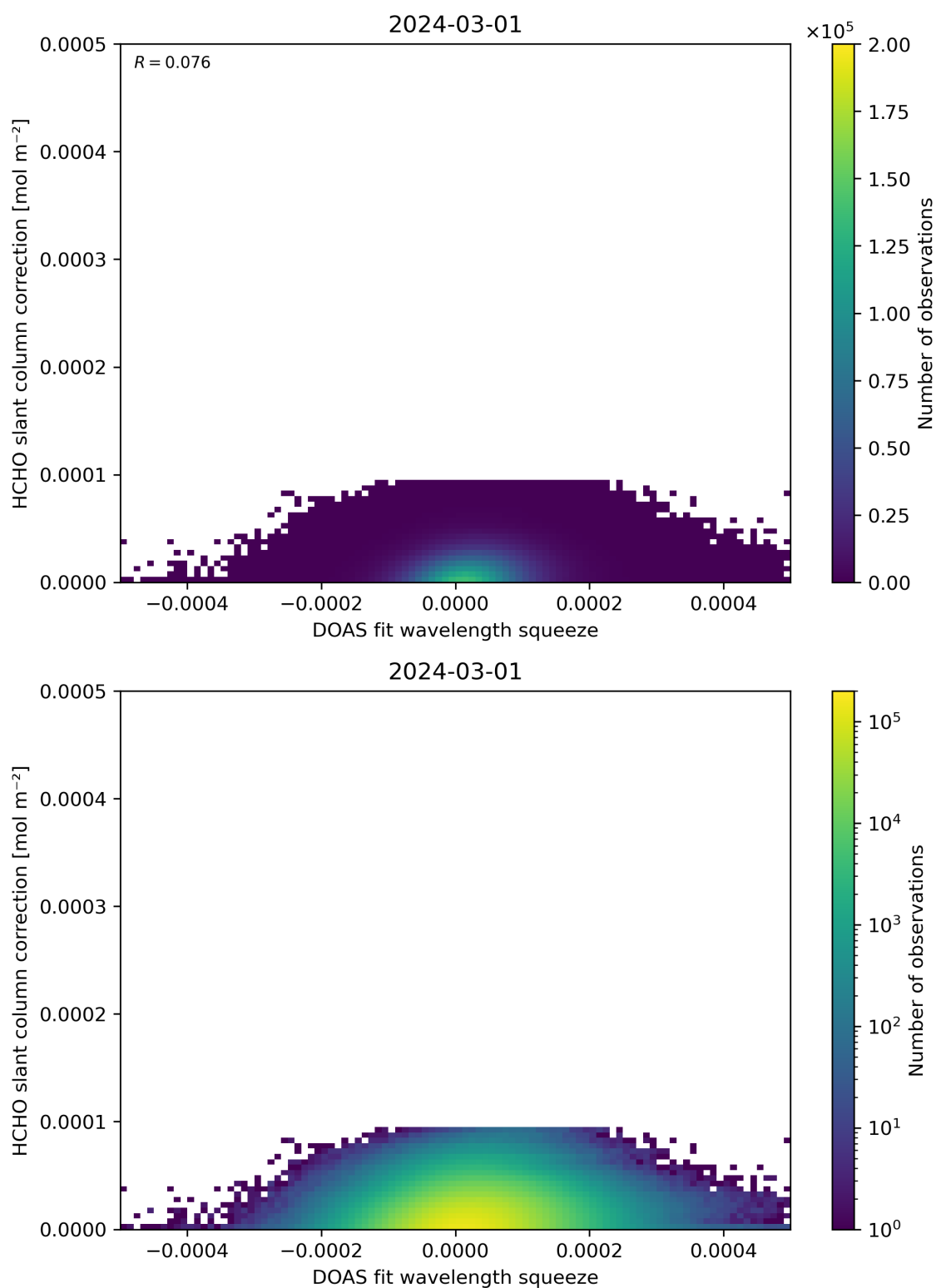
Figure 70: Scatter density plot of “DOAS fit wavelength squeeze” against “HCHO slant column correction” for 2024-02-29 to 2024-03-02.
