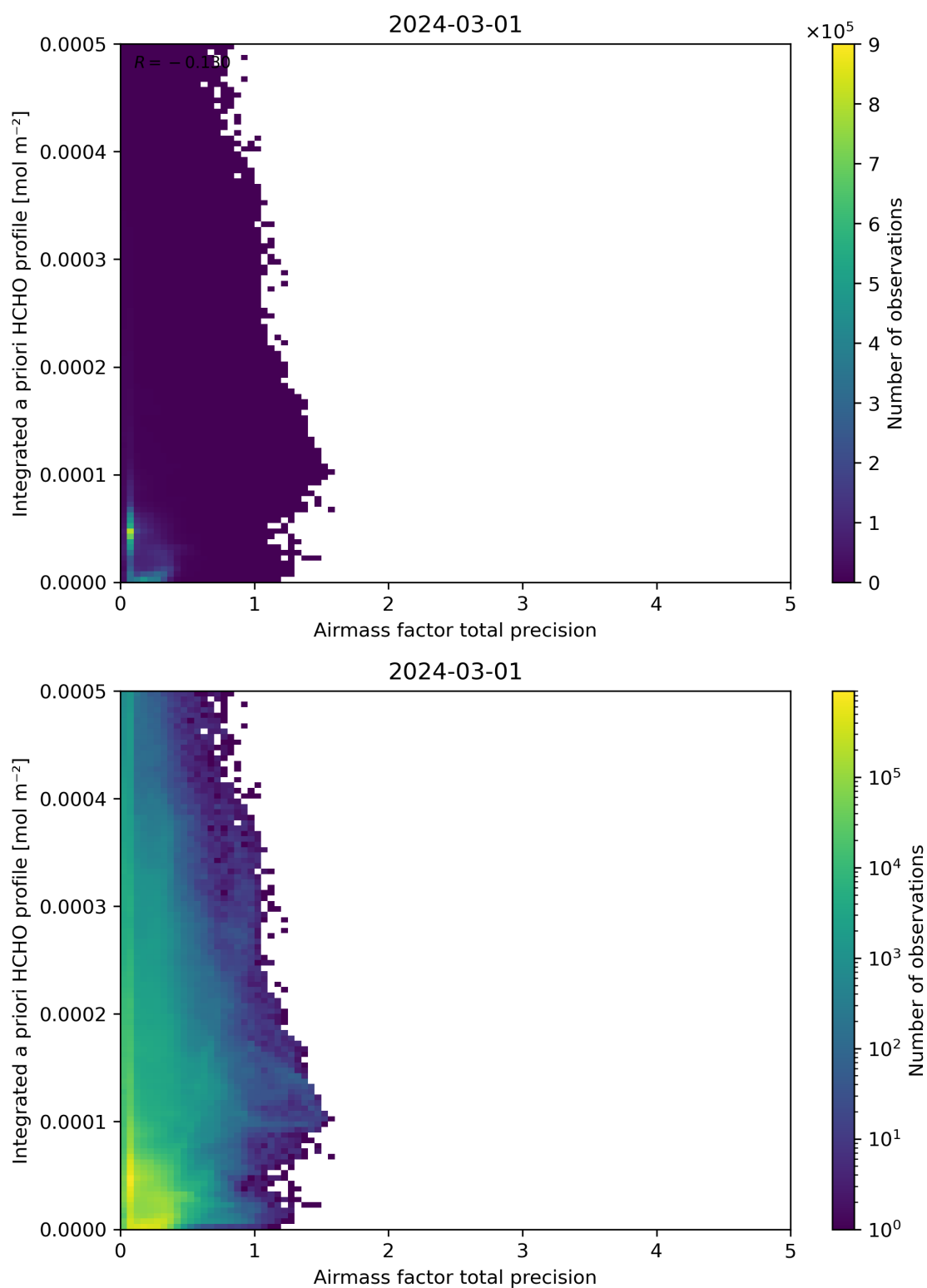
Figure 111: Scatter density plot of “Airmass factor total precision” against “Integrated a priori HCHO profile” for 2024-02-29 to 2024-03-02.
