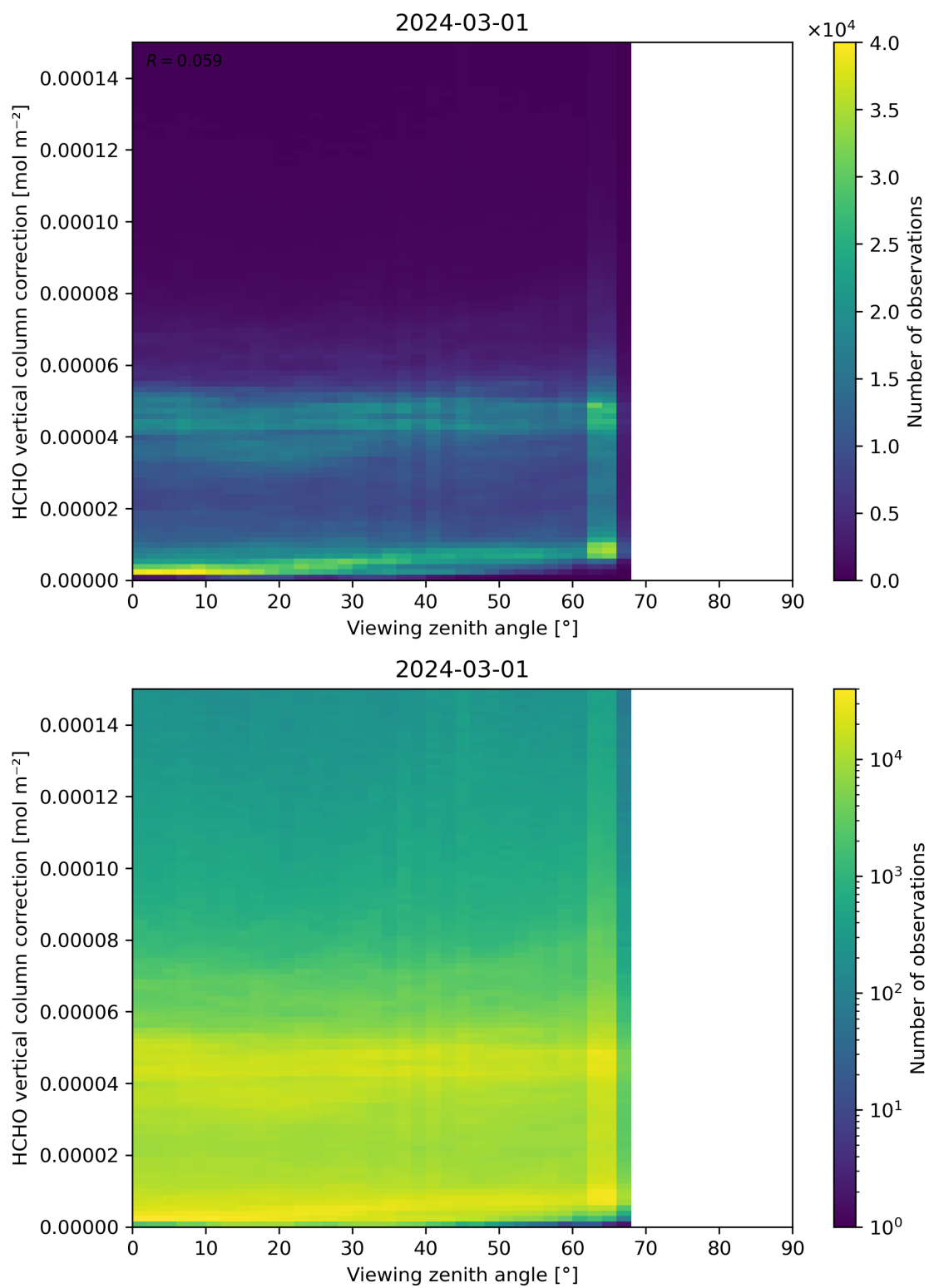
Figure 193: Scatter density plot of “Viewing zenith angle” against “HCHO vertical column correction” for 2024-02-29 to 2024-03-02.
