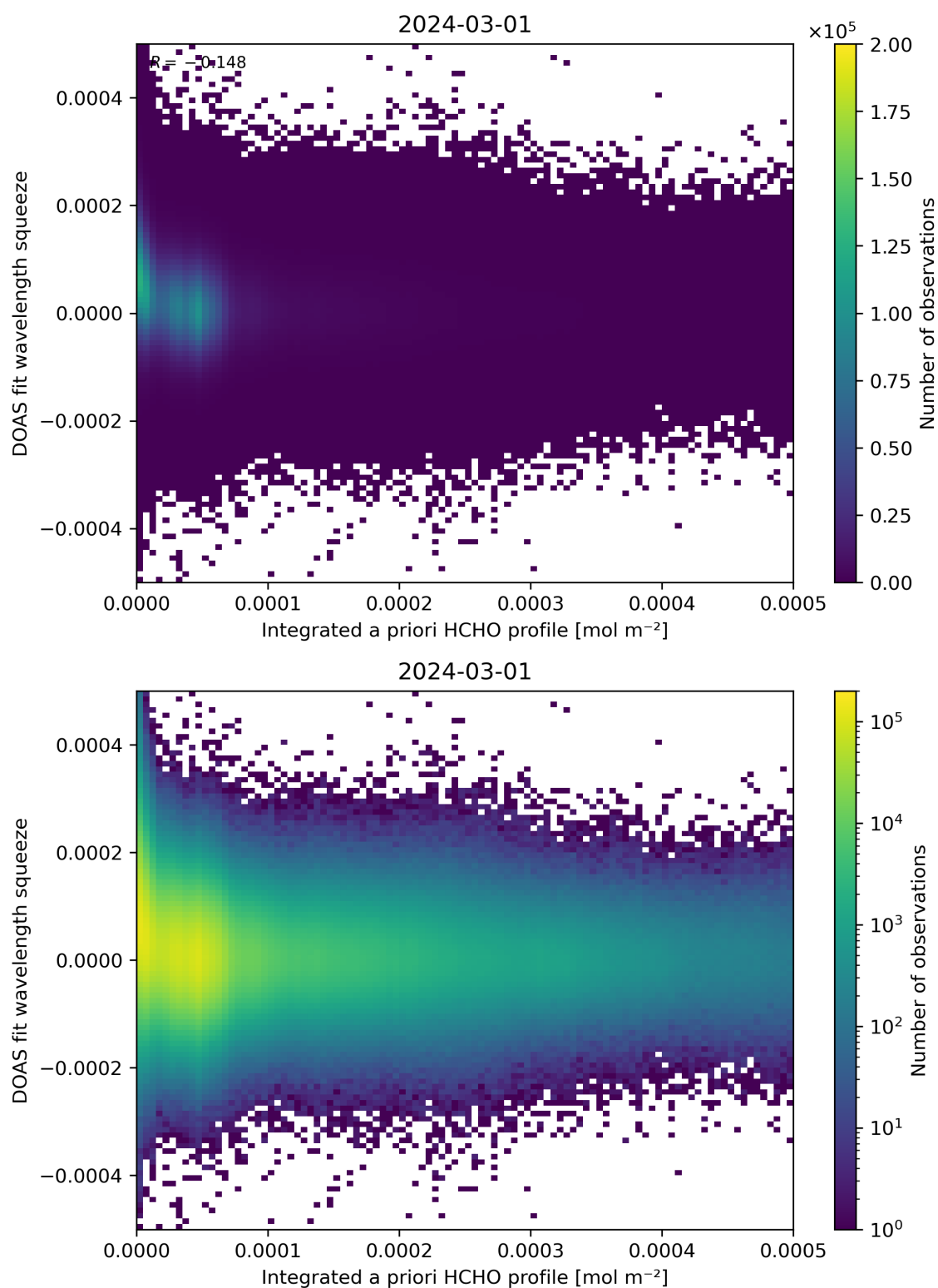
Figure 150: Scatter density plot of “Integrated a priori HCHO profile” against “DOAS fit wavelength squeeze” for 2024-02-29 to 2024-03-02.
