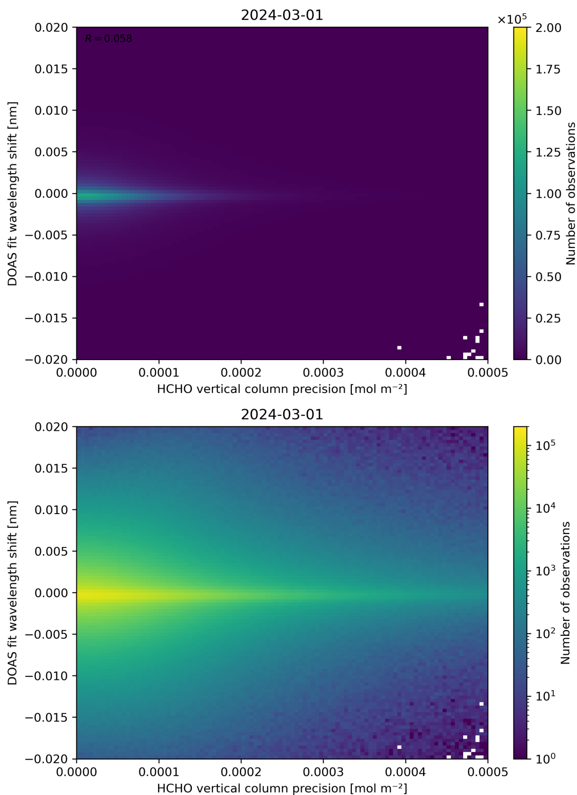
Figure 137: Scatter density plot of “HCHO vertical column precision” against “DOAS fit wavelength shift” for 2024-02-29 to 2024-03-02.
