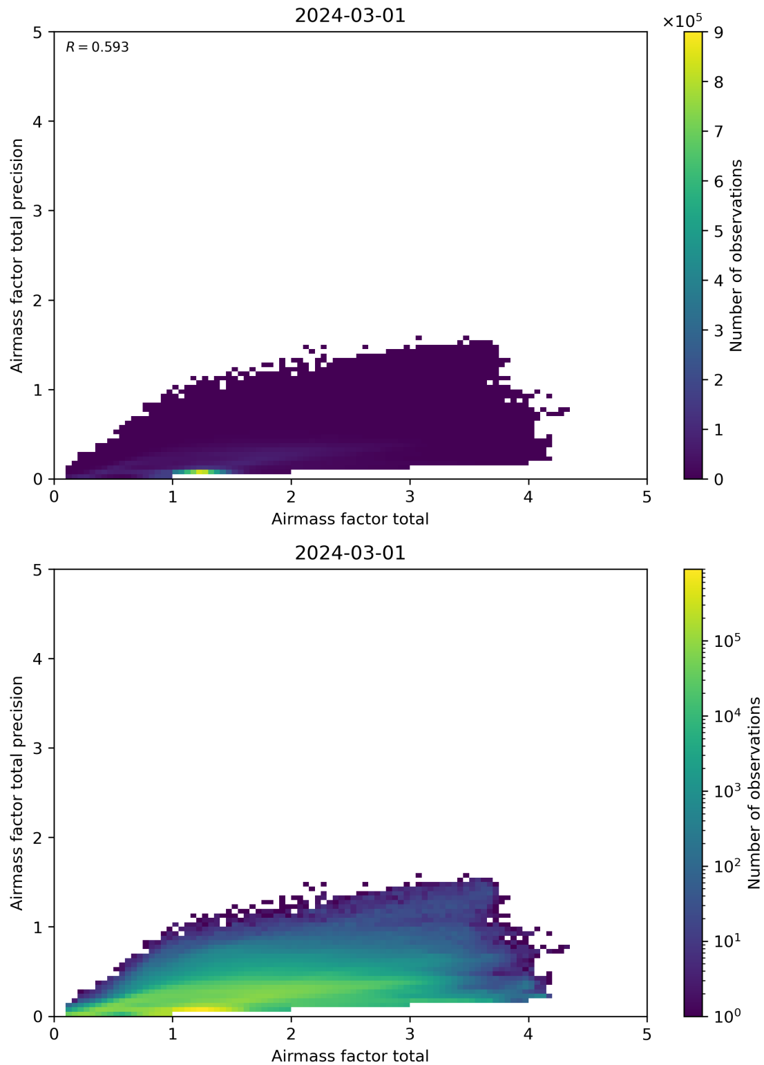
Figure 103: Scatter density plot of “Airmass factor total” against “Airmass factor total precision” for 2024-02-29 to 2024-03-02.
