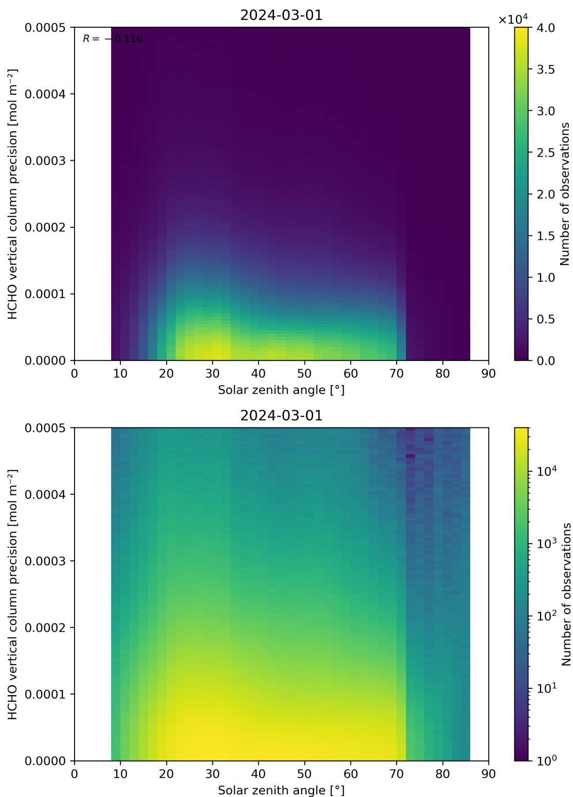
Figure 179: Scatter density plot of “Solar zenith angle” against “HCHO vertical column precision” for 2024-02-29 to 2024-03-02.
