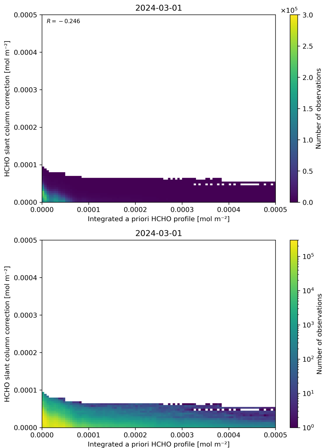
Figure 152: Scatter density plot of “Integrated a priori HCHO profile” against “HCHO slant column correction” for 2024-02-29 to 2024-03-02.
