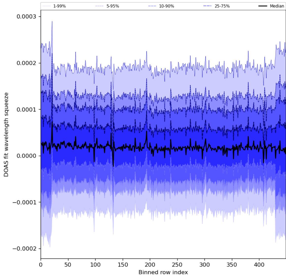
Figure 59: Along track statistics of “DOAS fit wavelength squeeze” for 2024-02-29 to 2024-03-02
