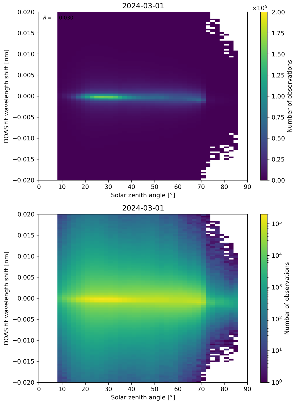
Figure 168: Scatter density plot of “Solar zenith angle” against “DOAS fit wavelength shift” for 2024-02-29 to 2024-03-02.
