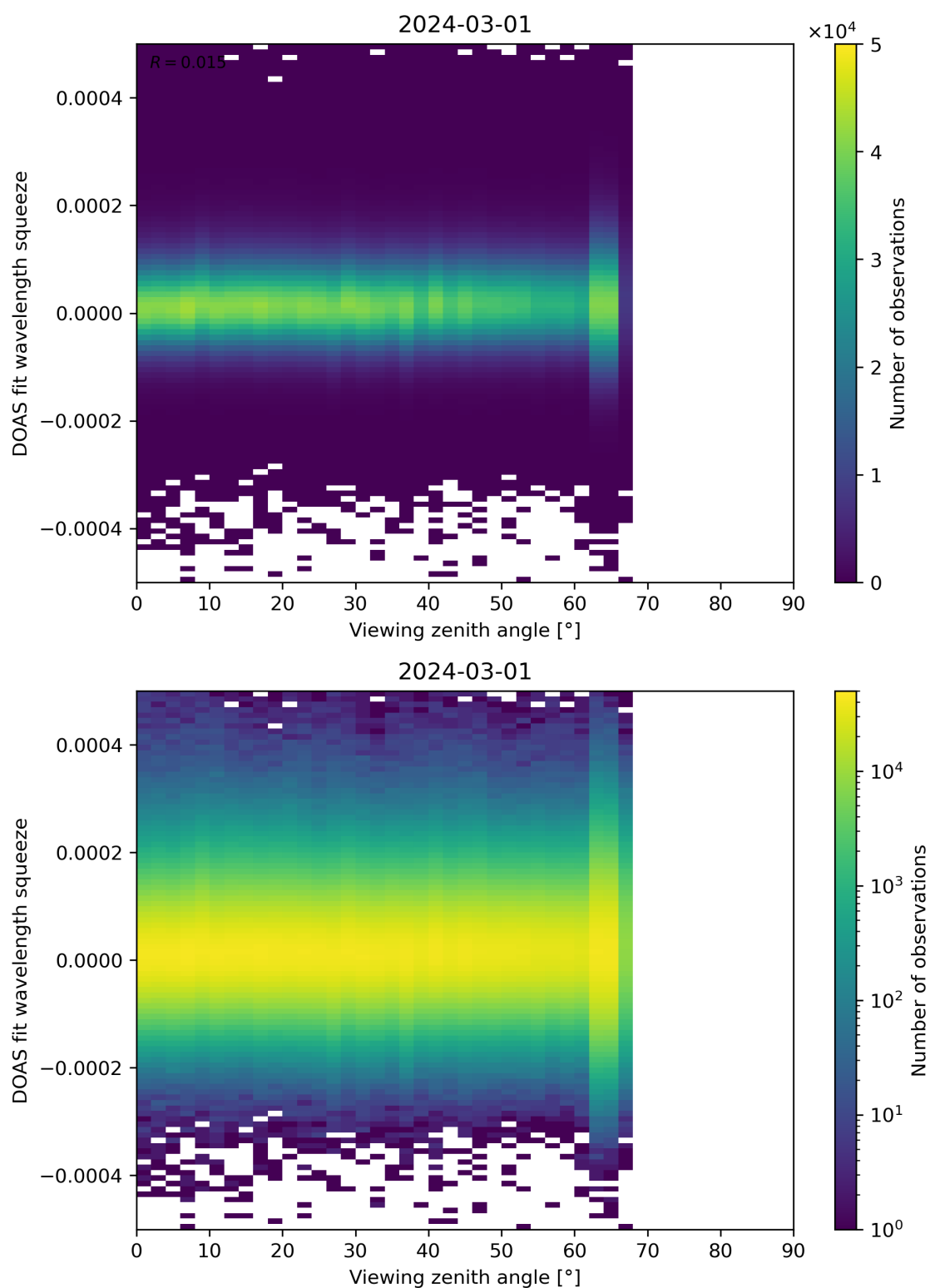
Figure 184: Scatter density plot of “Viewing zenith angle” against “DOAS fit wavelength squeeze” for 2024-02-29 to 2024-03-02.
