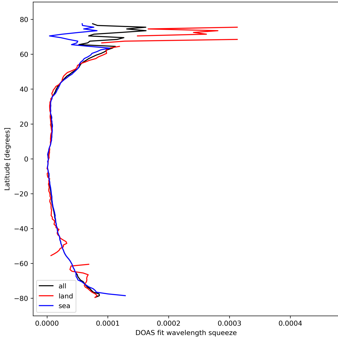
Figure 31: Zonal average of “DOAS fit wavelength squeeze” for 2024-02-29 to 2024-03-02.
