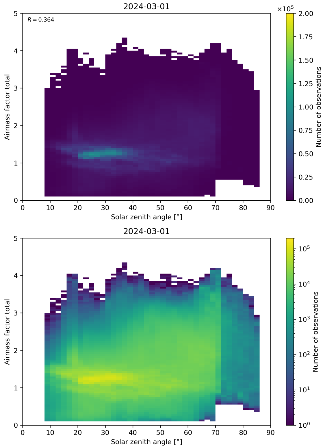
Figure 175: Scatter density plot of “Solar zenith angle” against “Airmass factor total” for 2024-02-29 to 2024-03-02.
