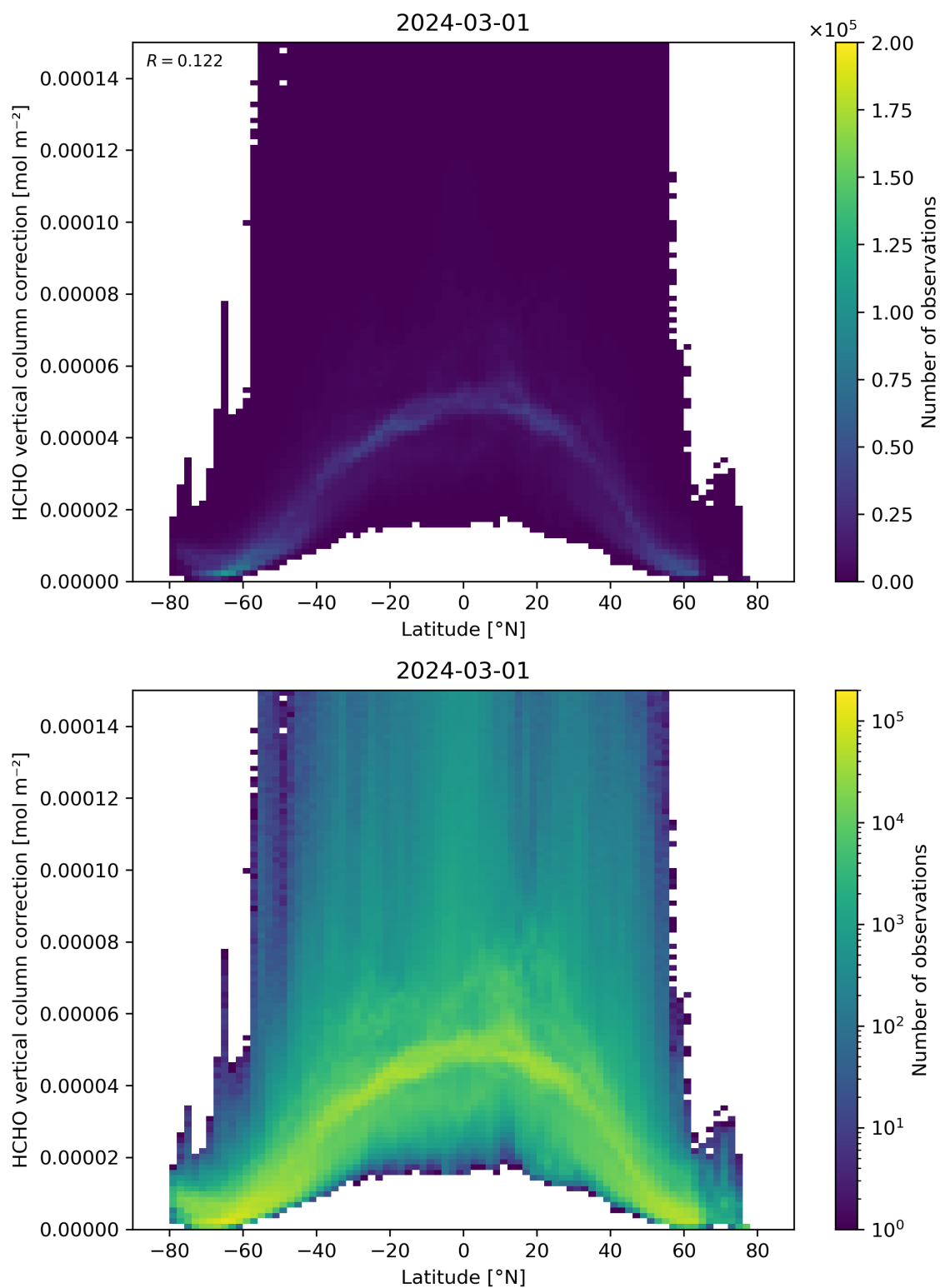
Figure 164: Scatter density plot of “Latitude” against “HCHO vertical column correction” for 2024-02-29 to 2024-03-02.
