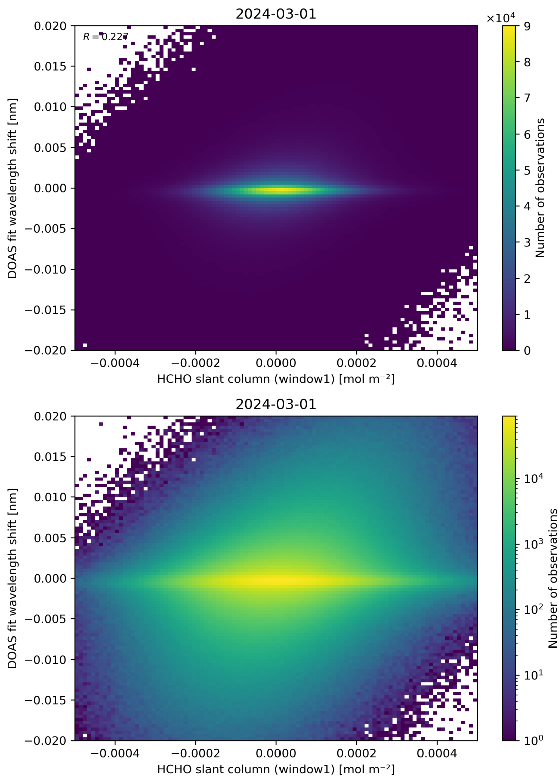
Figure 79: Scatter density plot of “HCHO slant column (window1)” against “DOAS fit wavelength shift” for 2024-02-29 to 2024-03-02.
