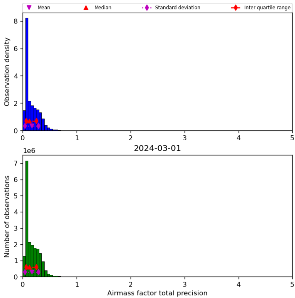
Figure 41: Histogram of “Airmass factor total precision” for 2024-02-29 to 2024-03-02
