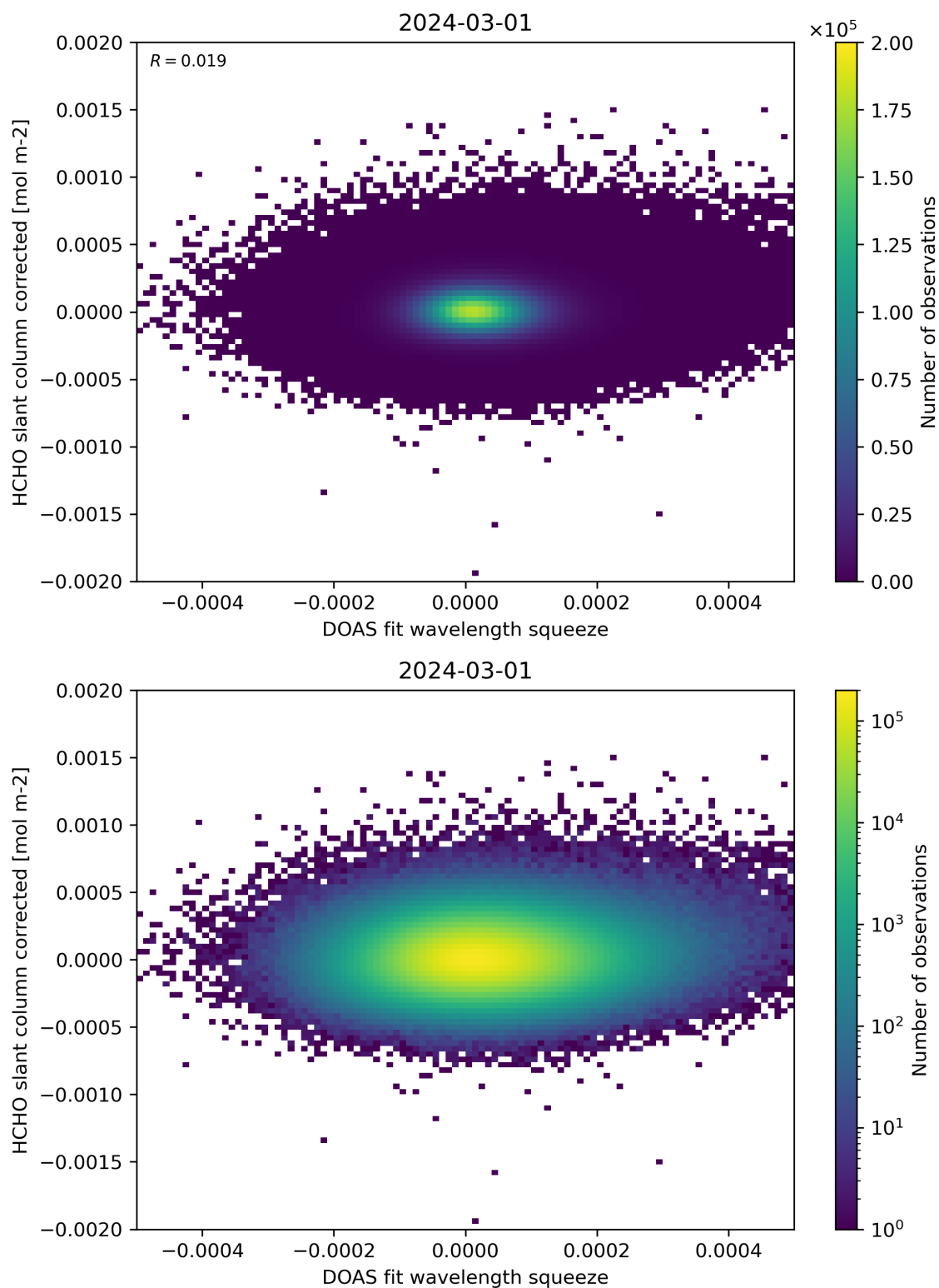
Figure 69: Scatter density plot of “DOAS fit wavelength squeeze” against “HCHO slant column corrected” for 2024-02-29 to 2024-03-02.
