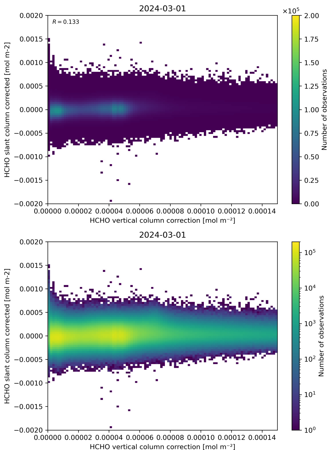
Figure 116: Scatter density plot of “HCHO vertical column correction” against “HCHO slant column corrected” for 2024-02-29 to 2024-03-02.
