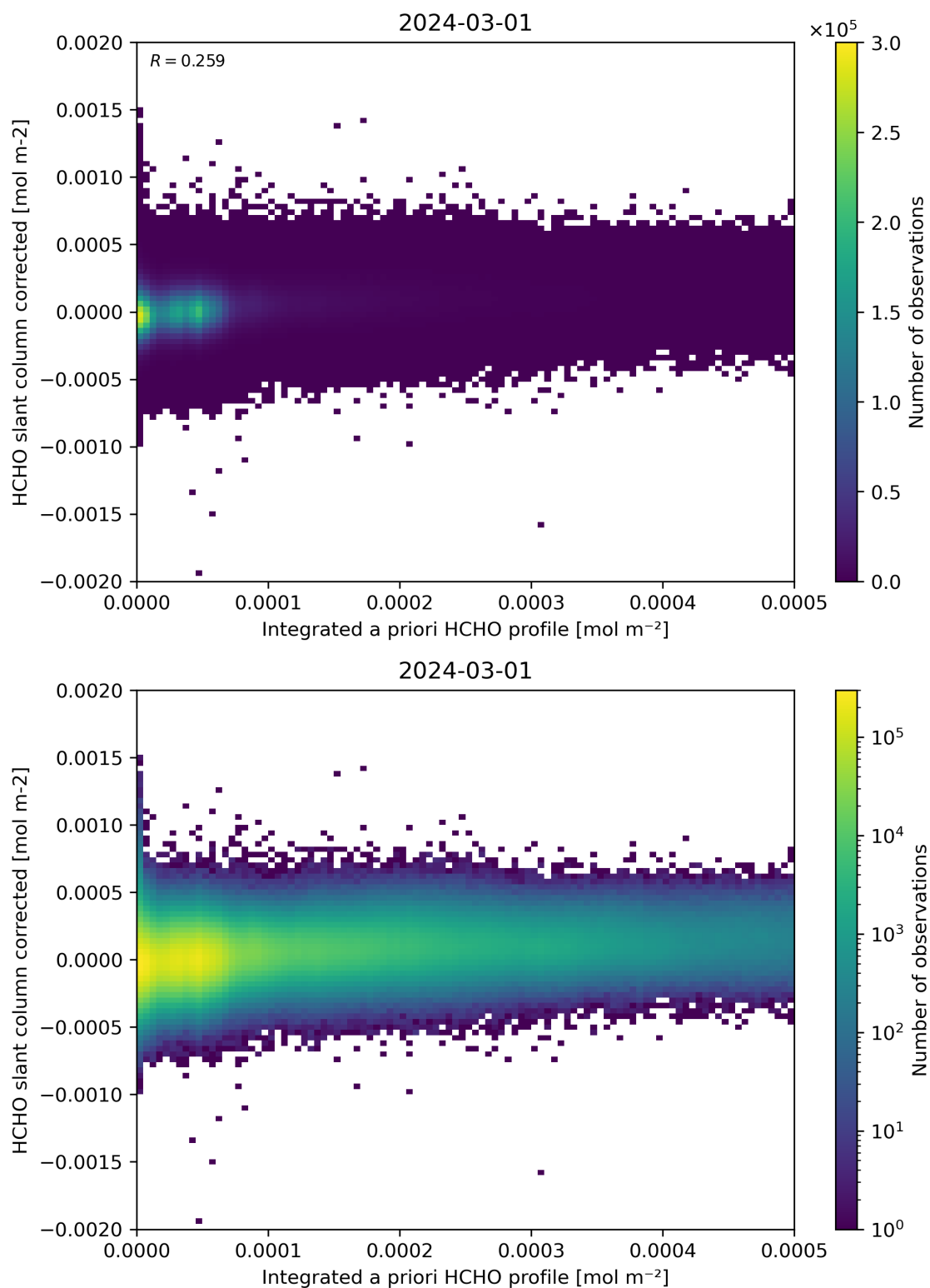
Figure 151: Scatter density plot of “Integrated a priori HCHO profile” against “HCHO slant column corrected” for 2024-02-29 to 2024-03-02.
