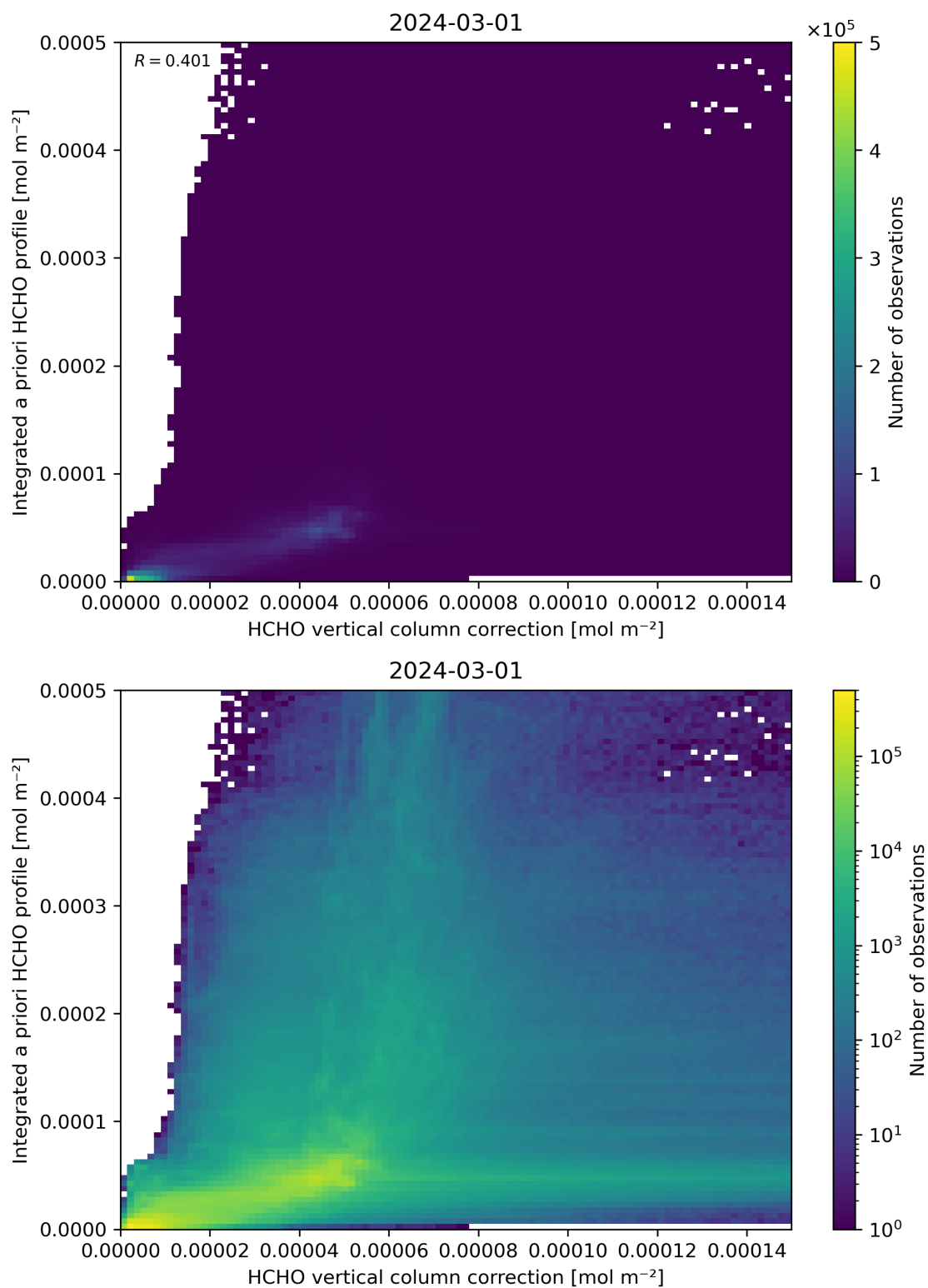
Figure 122: Scatter density plot of “HCHO vertical column correction” against “Integrated a priori HCHO profile” for 2024-02-29 to 2024-03-02.
