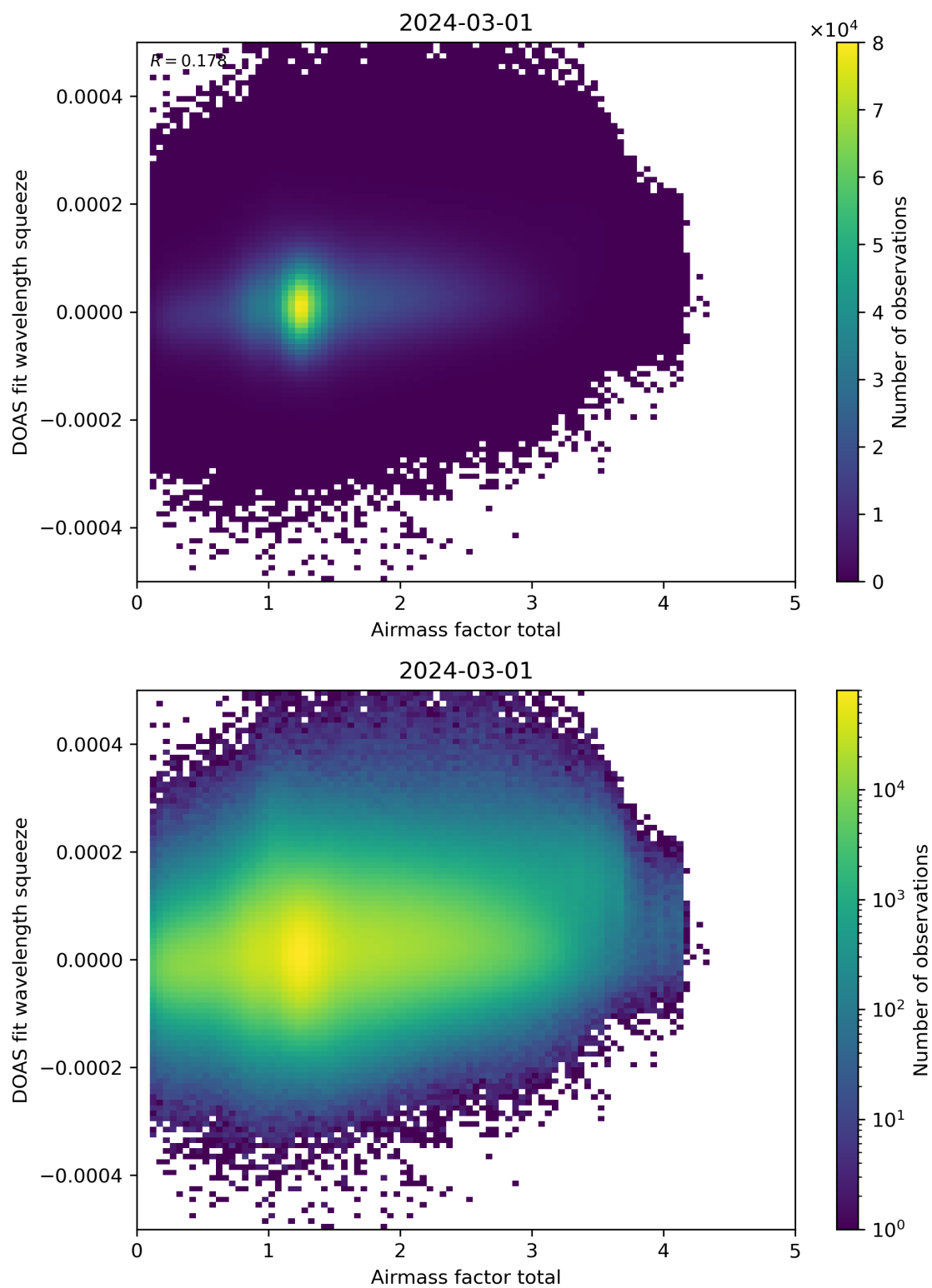
Figure 99: Scatter density plot of “Airmass factor total” against “DOAS fit wavelength squeeze” for 2024-02-29 to 2024-03-02.
