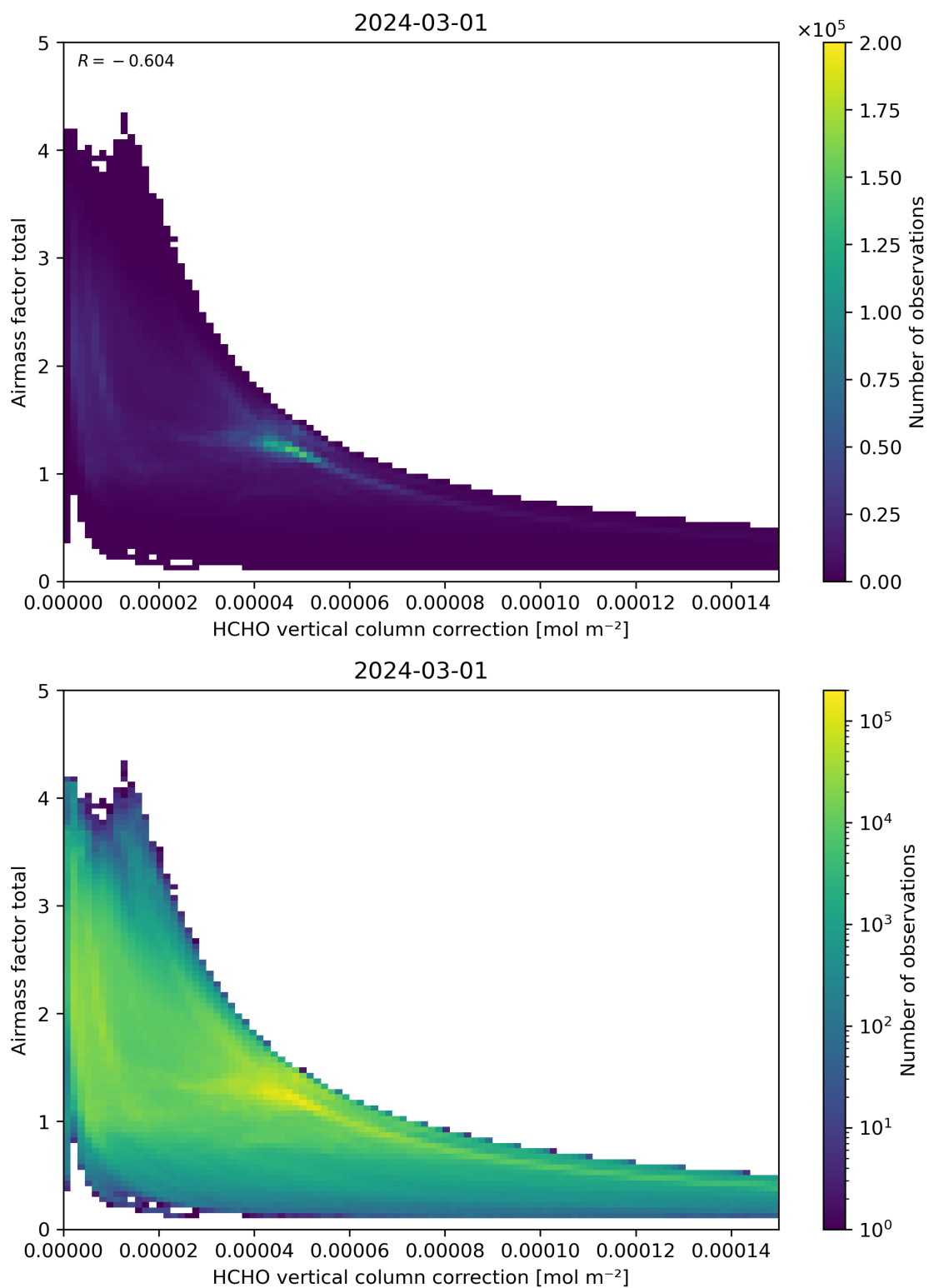
Figure 120: Scatter density plot of “HCHO vertical column correction” against “Airmass factor total” for 2024-02-29 to 2024-03-02.
