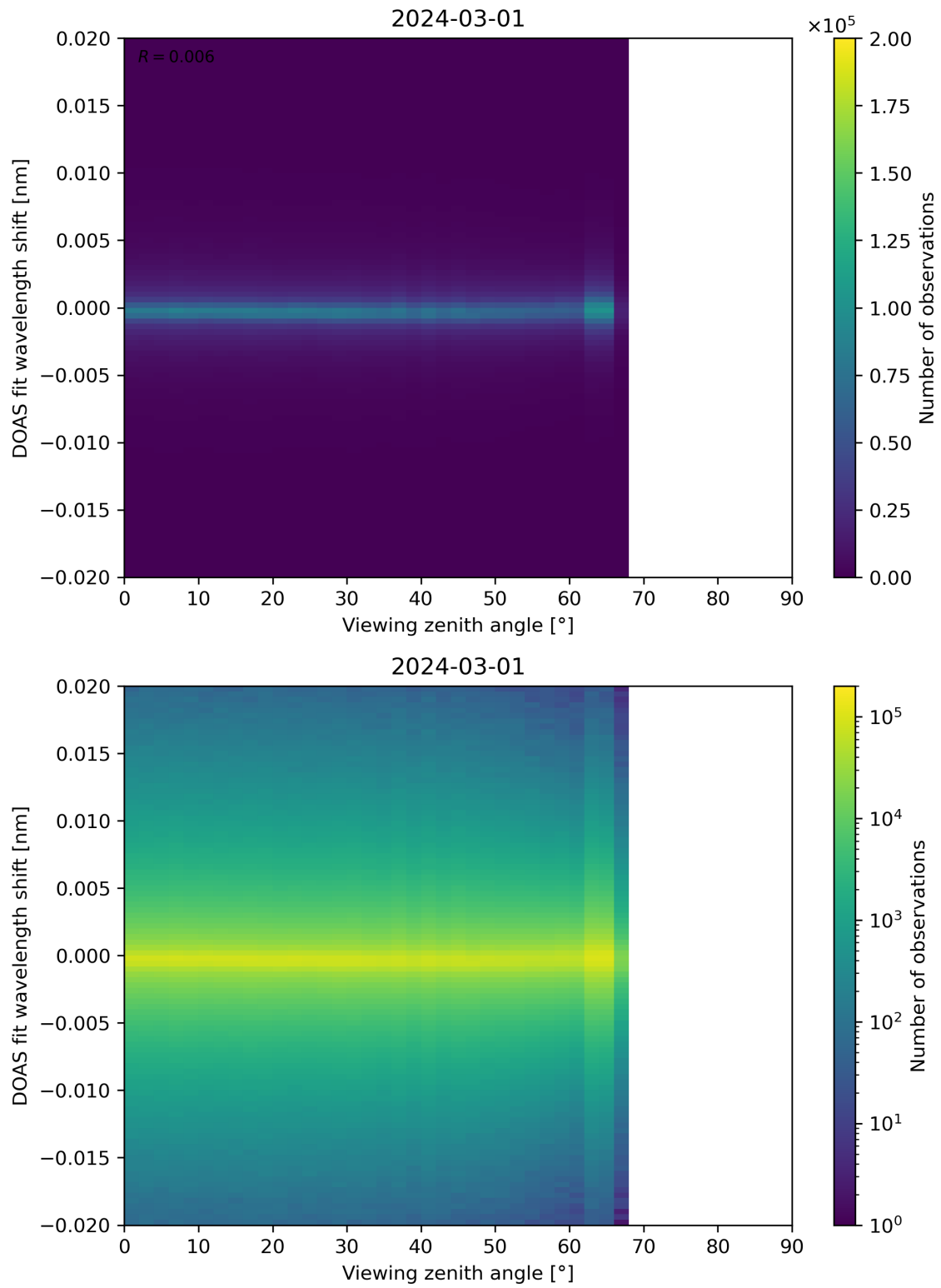
Figure 183: Scatter density plot of “Viewing zenith angle” against “DOAS fit wavelength shift” for 2024-02-29 to 2024-03-02.
