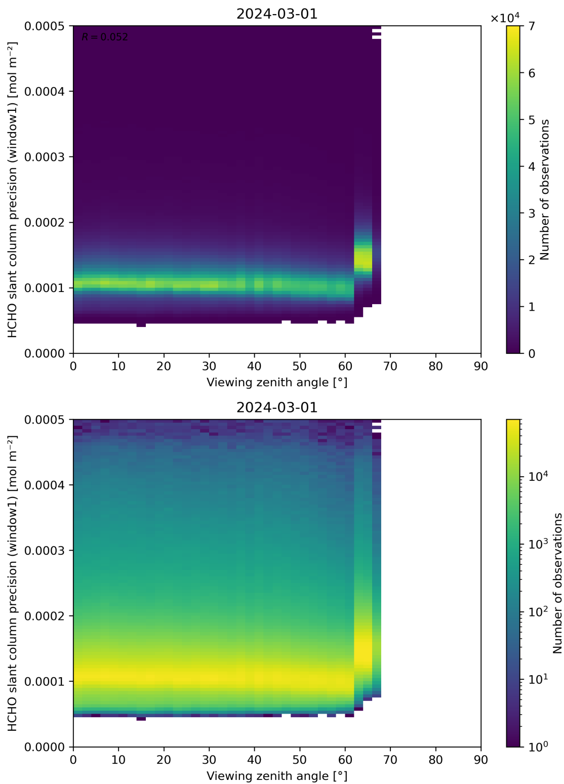
Figure 189: Scatter density plot of “Viewing zenith angle” against “HCHO slant column precision (window1)” for 2024-02-29 to 2024-03-02.
