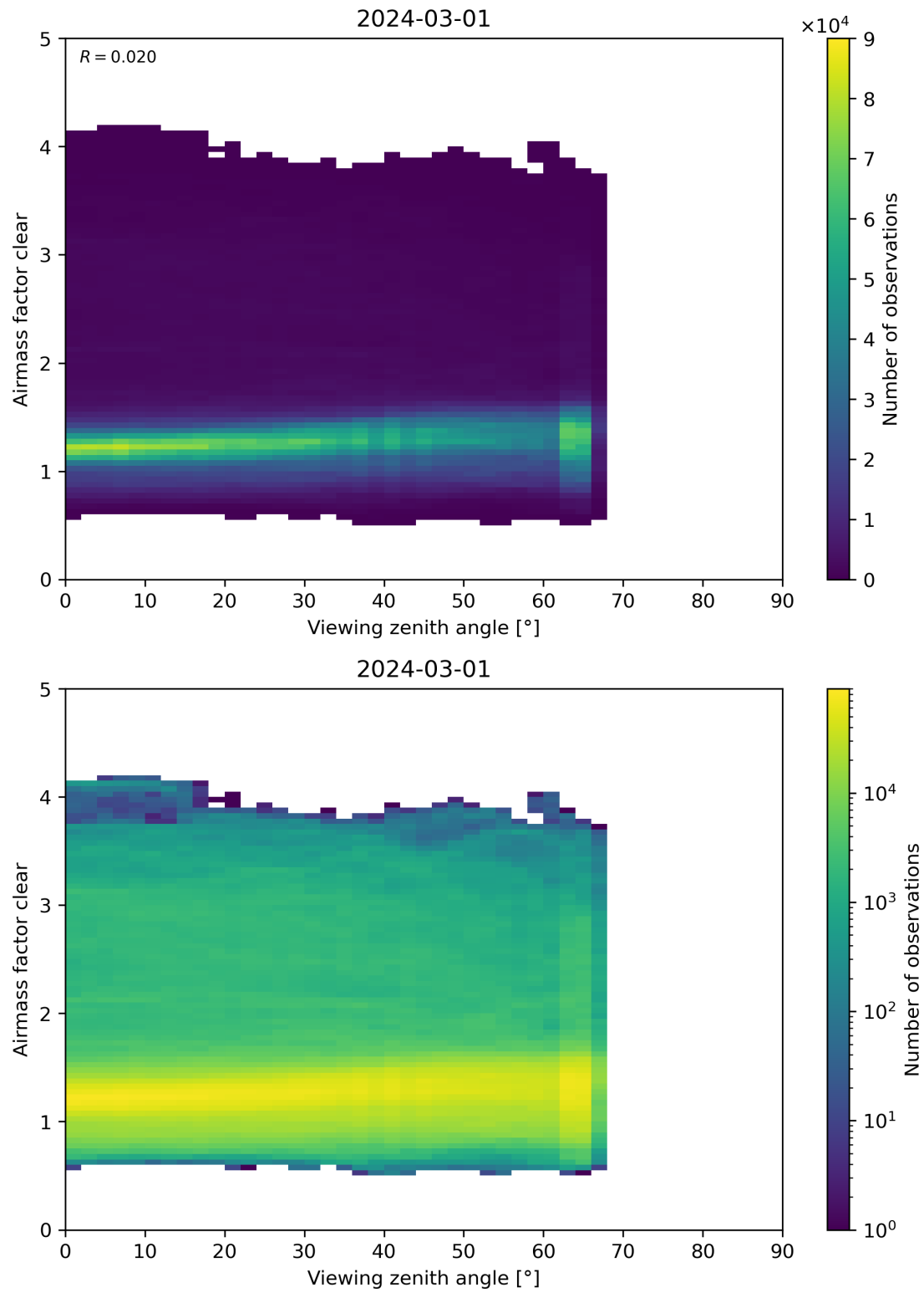
Figure 185: Scatter density plot of “Viewing zenith angle” against “Airmass factor clear” for 2024-02-29 to 2024-03-02.
