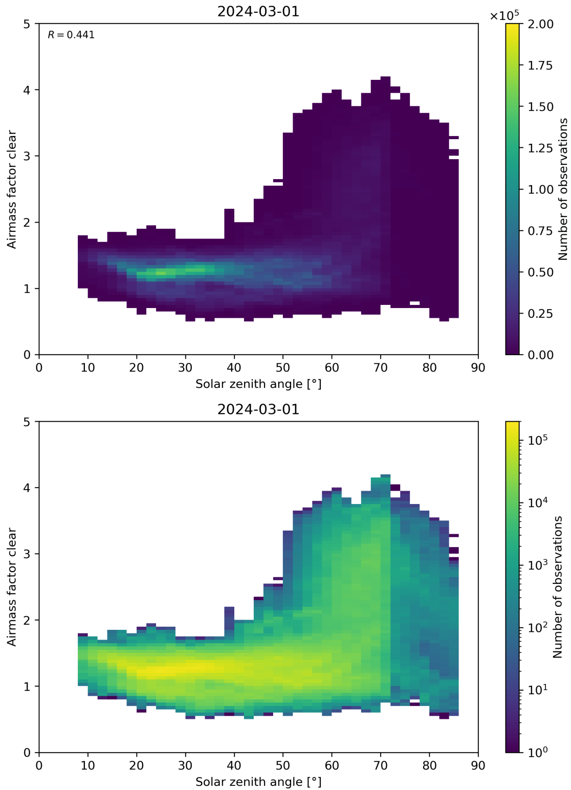
Figure 170: Scatter density plot of “Solar zenith angle” against “Airmass factor clear” for 2024-02-29 to 2024-03-02.
