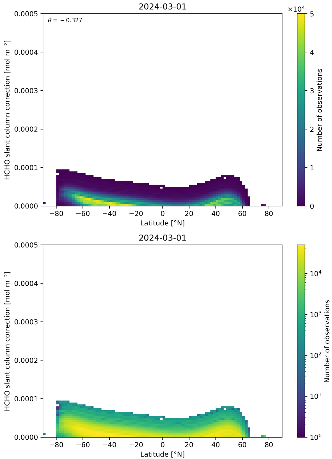
Figure 158: Scatter density plot of “Latitude” against “HCHO slant column correction” for 2024-02-29 to 2024-03-02.
