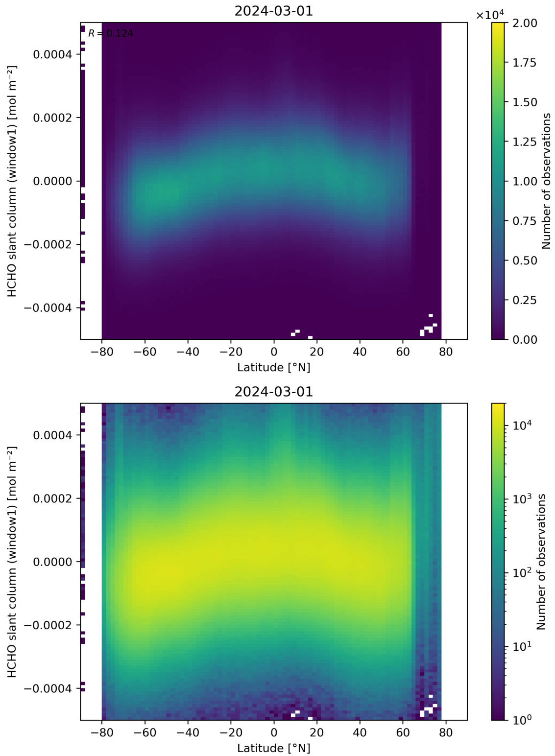
Figure 159: Scatter density plot of “Latitude” against “HCHO slant column (window1)” for 2024-02-29 to 2024-03-02.
