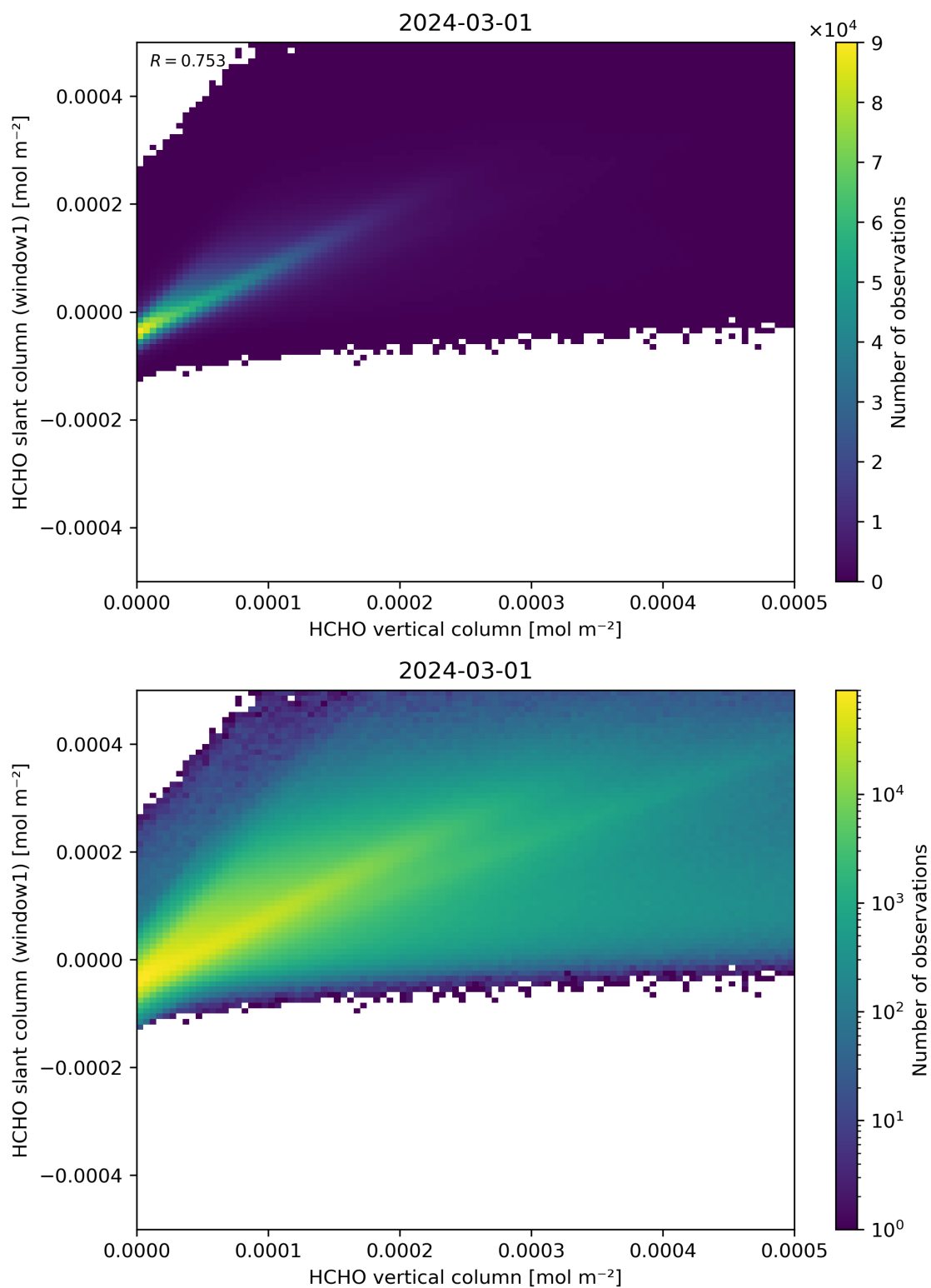
Figure 129: Scatter density plot of “HCHO vertical column” against “HCHO slant column (window1)” for 2024-02-29 to 2024-03-02.
