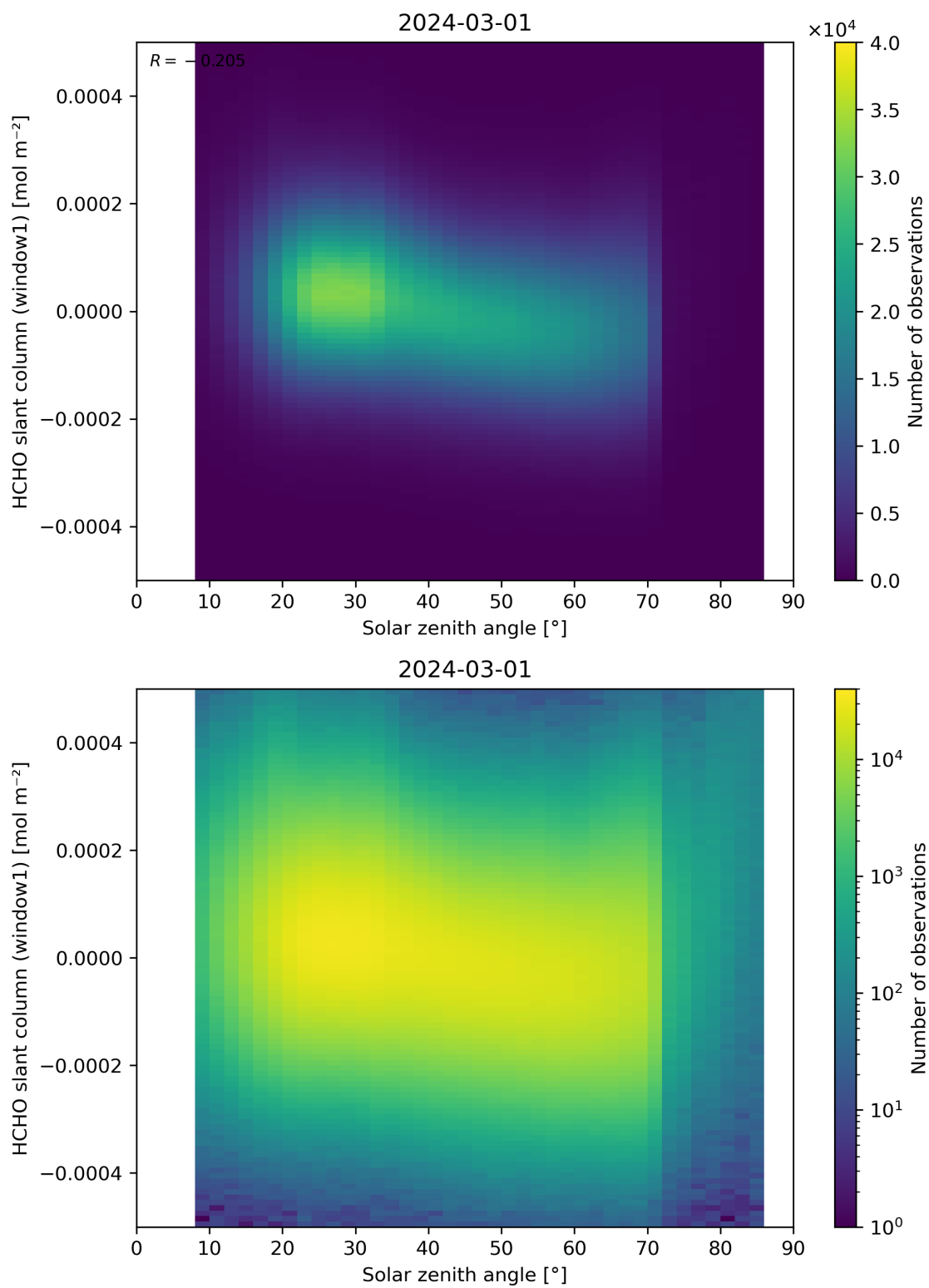
Figure 173: Scatter density plot of “Solar zenith angle” against “HCHO slant column (window1)” for 2024-02-29 to 2024-03-02.
