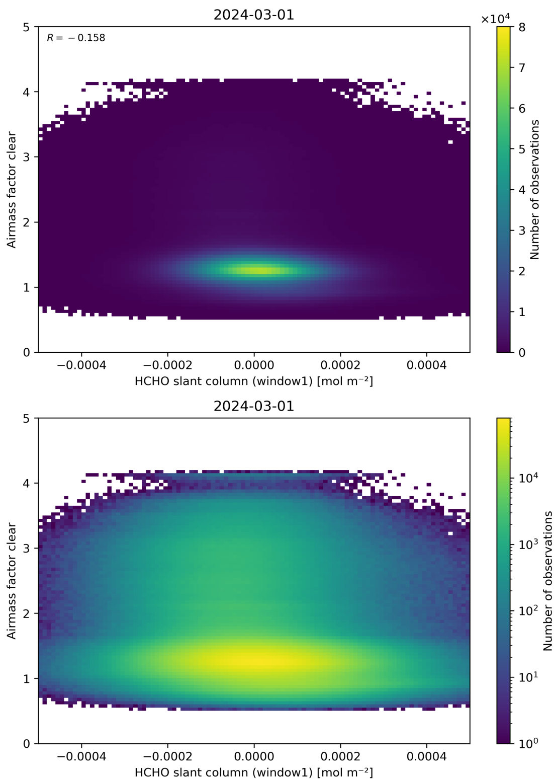
Figure 81: Scatter density plot of “HCHO slant column (window1)” against “Airmass factor clear” for 2024-02-29 to 2024-03-02.
