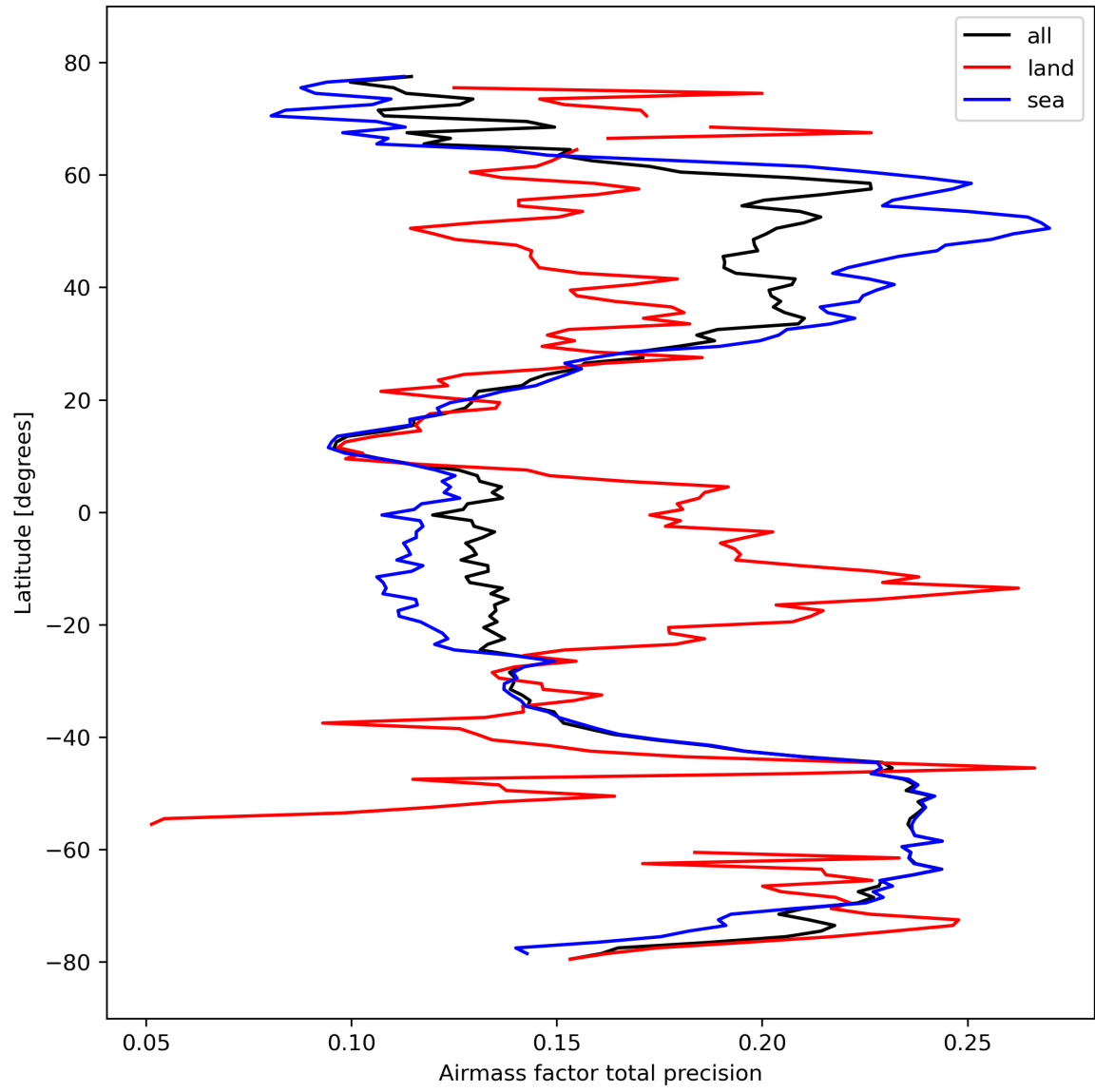
Figure 27: Zonal average of “Airmass factor total precision” for 2024-02-29 to 2024-03-02.
