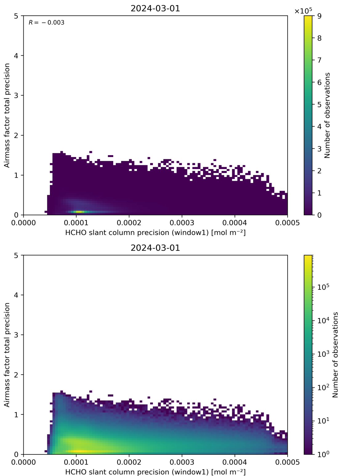
Figure 95: Scatter density plot of “HCHO slant column precision (window1)” against “Airmass factor total precision” for 2024-02-29 to 2024-03-02.
