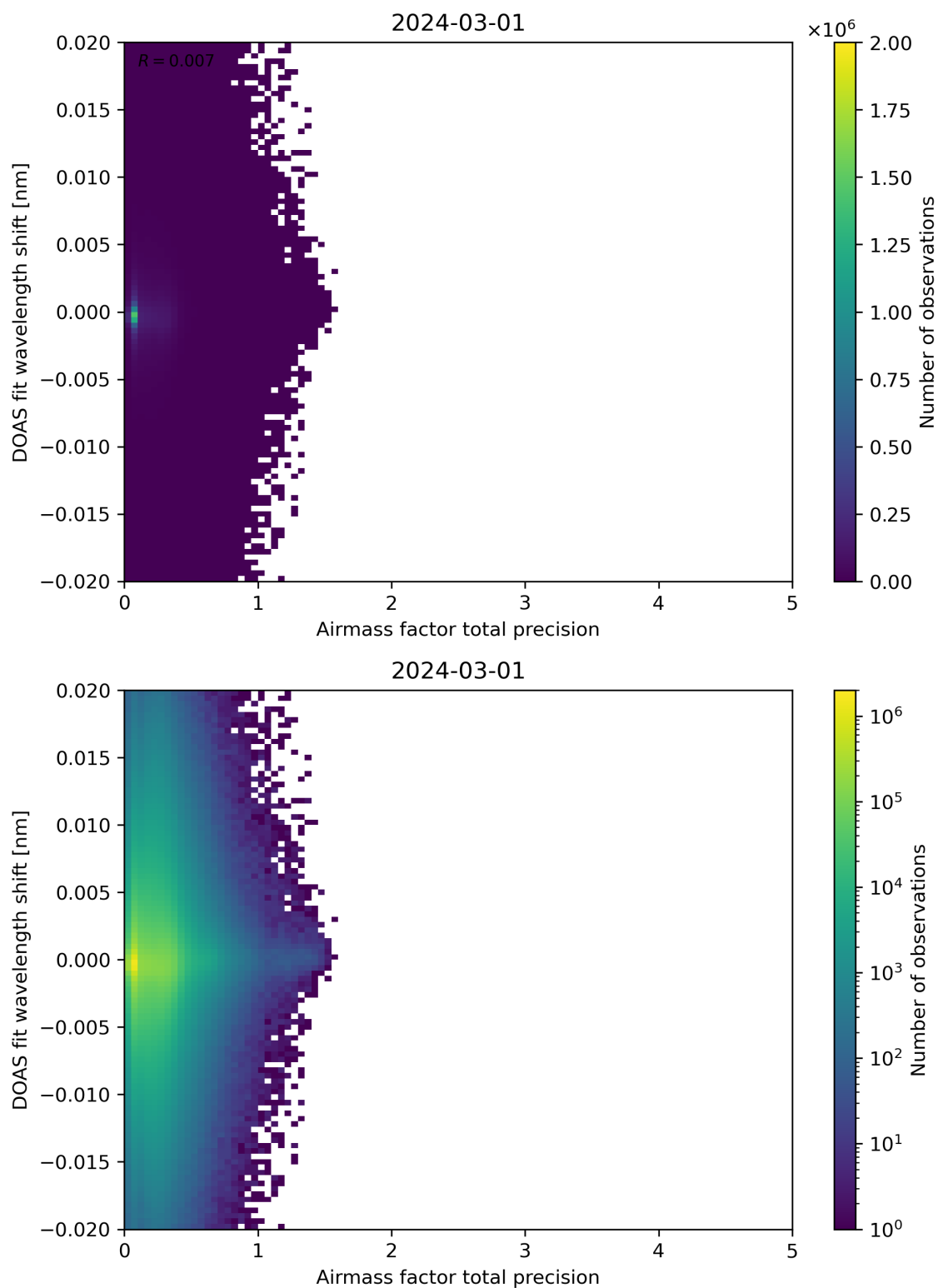
Figure 106: Scatter density plot of “Airmass factor total precision” against “DOAS fit wavelength shift” for 2024-02-29 to 2024-03-02.
