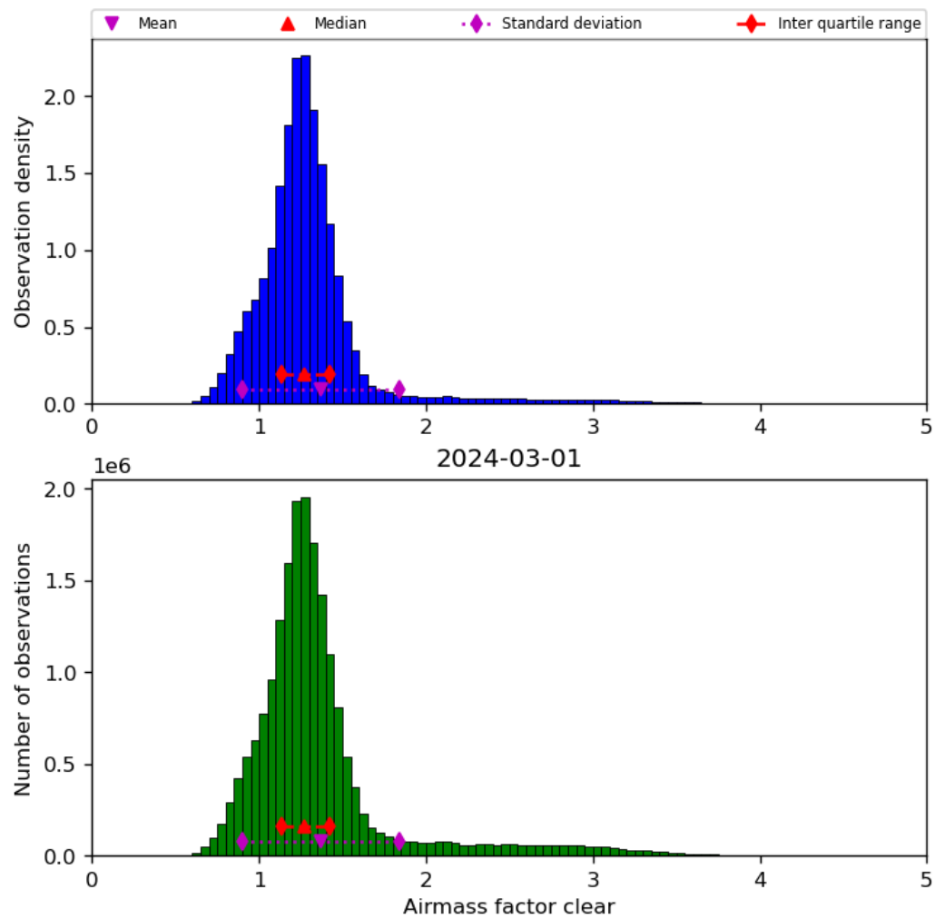
Figure 42: Histogram of “Airmass factor clear” for 2024-02-29 to 2024-03-02
