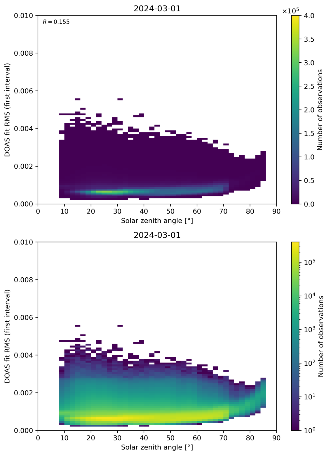
Figure 167: Scatter density plot of “Solar zenith angle” against “DOAS fit RMS (first interval)” for 2024-02-29 to 2024-03-02.
