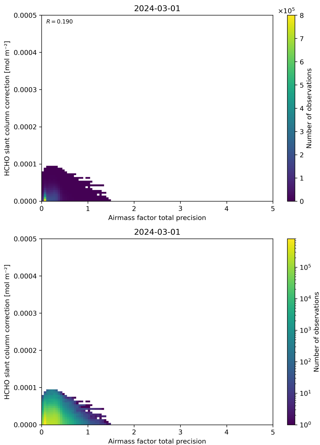
Figure 110: Scatter density plot of “Airmass factor total precision” against “HCHO slant column correction” for 2024-02-29 to 2024-03-02.
