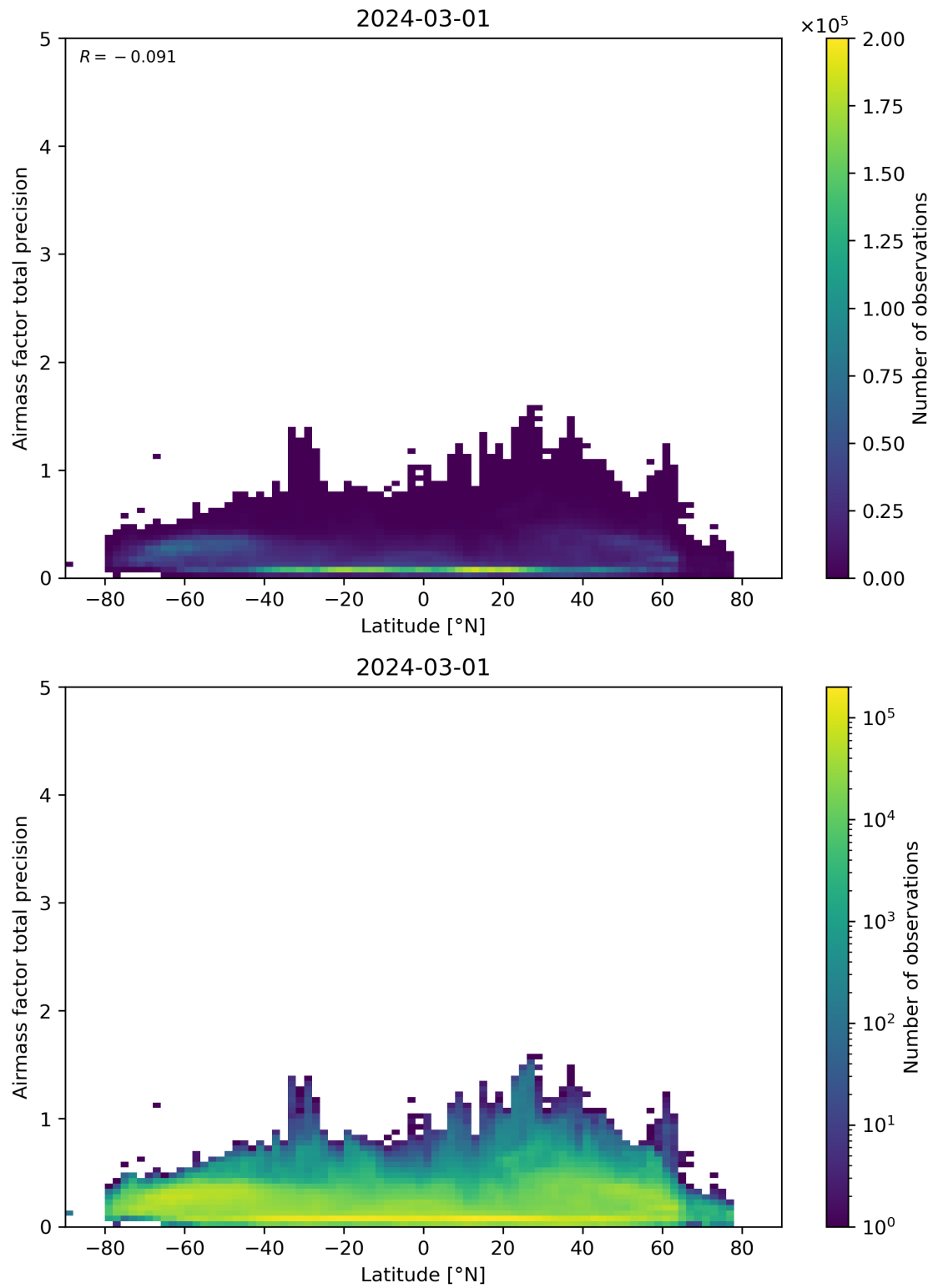
Figure 162: Scatter density plot of “Latitude” against “Airmass factor total precision” for 2024-02-29 to 2024-03-02.
