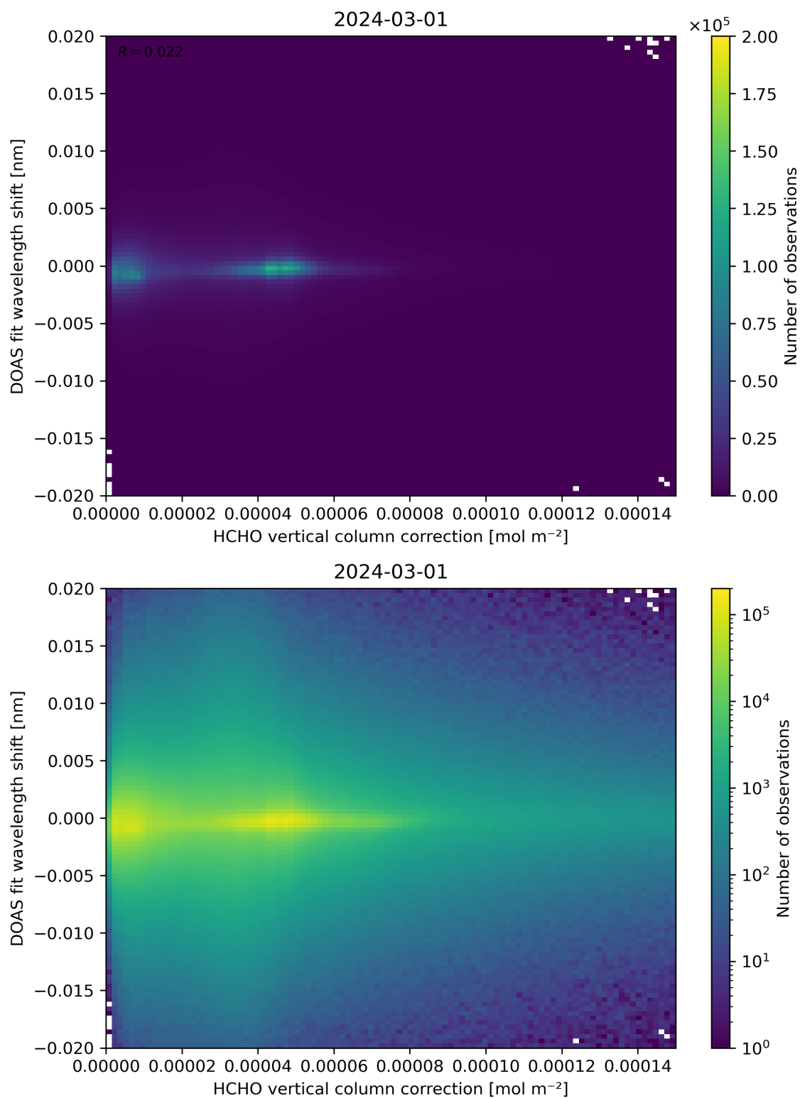
Figure 113: Scatter density plot of “HCHO vertical column correction” against “DOAS fit wavelength shift” for 2024-02-29 to 2024-03-02.
