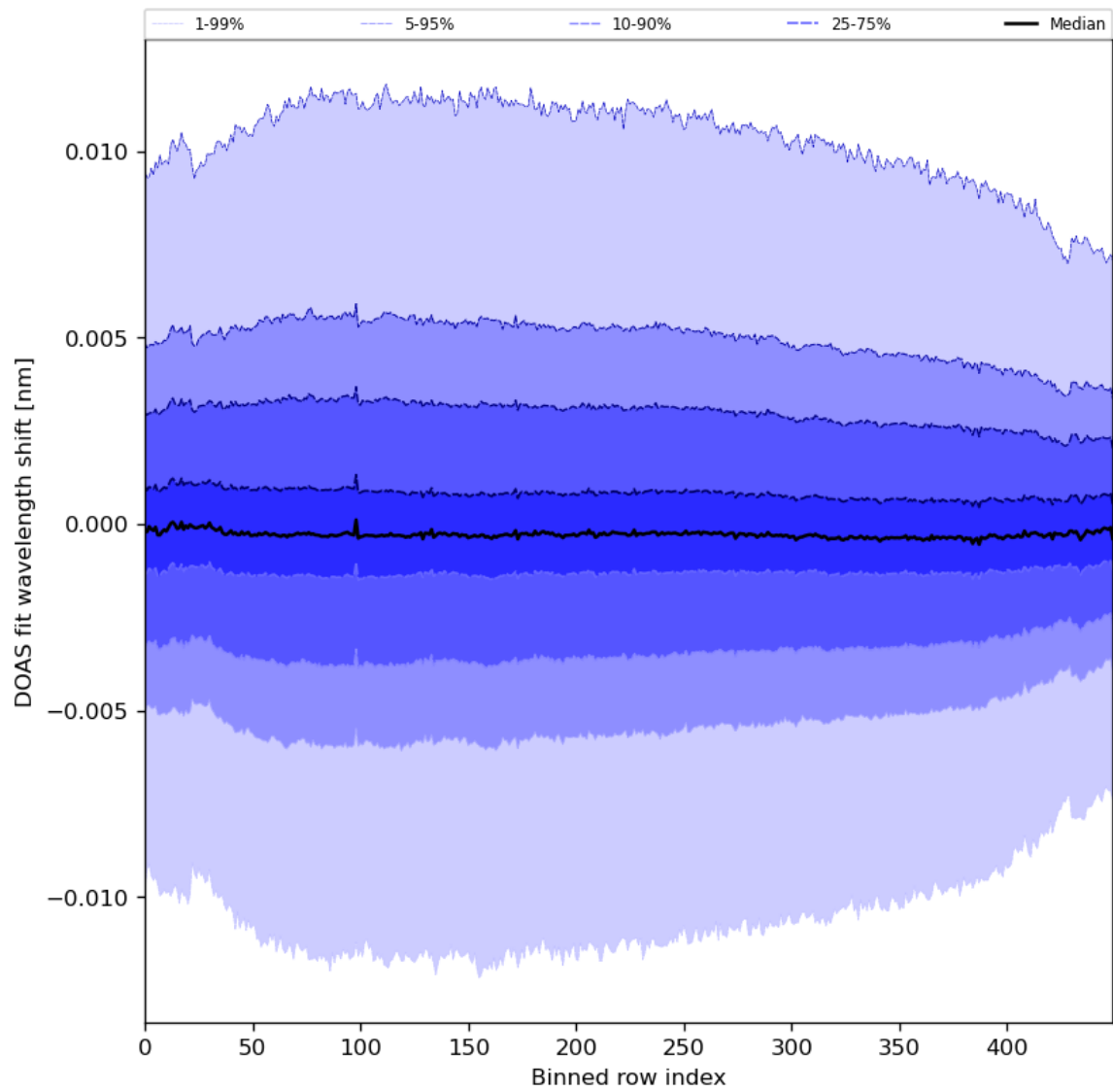
Figure 58: Along track statistics of “DOAS fit wavelength shift” for 2024-02-29 to 2024-03-02
