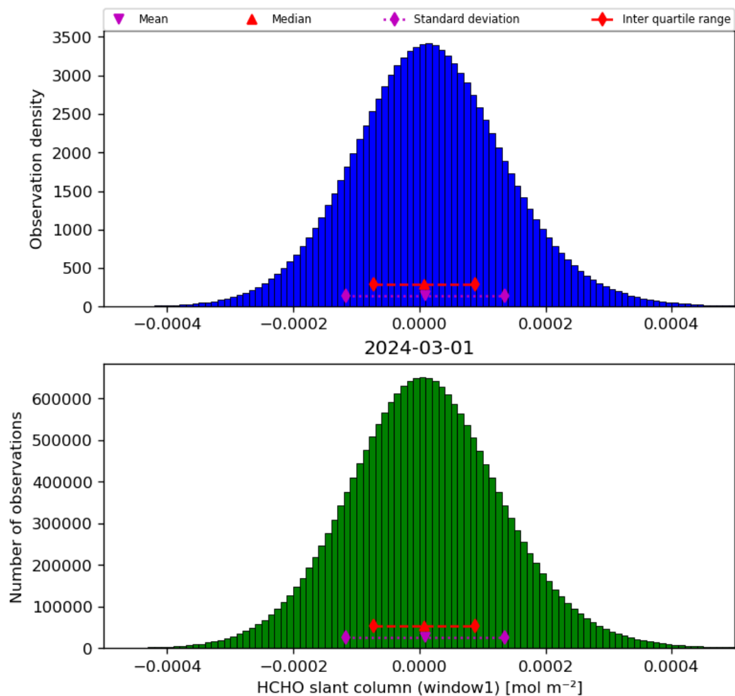
Figure 38: Histogram of “HCHO slant column (window1)” for 2024-02-29 to 2024-03-02
