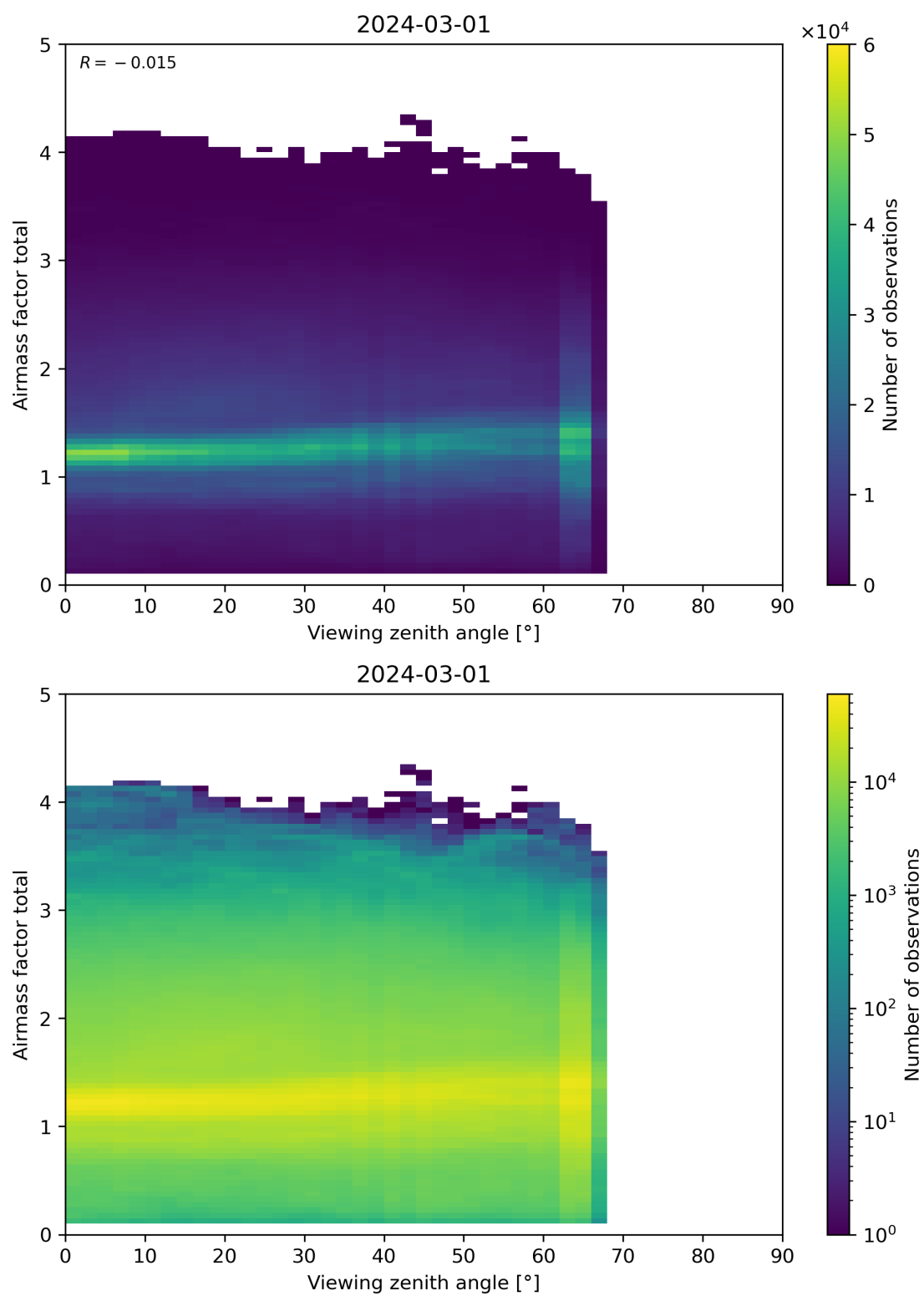
Figure 190: Scatter density plot of “Viewing zenith angle” against “Airmass factor total” for 2024-02-29 to 2024-03-02.
