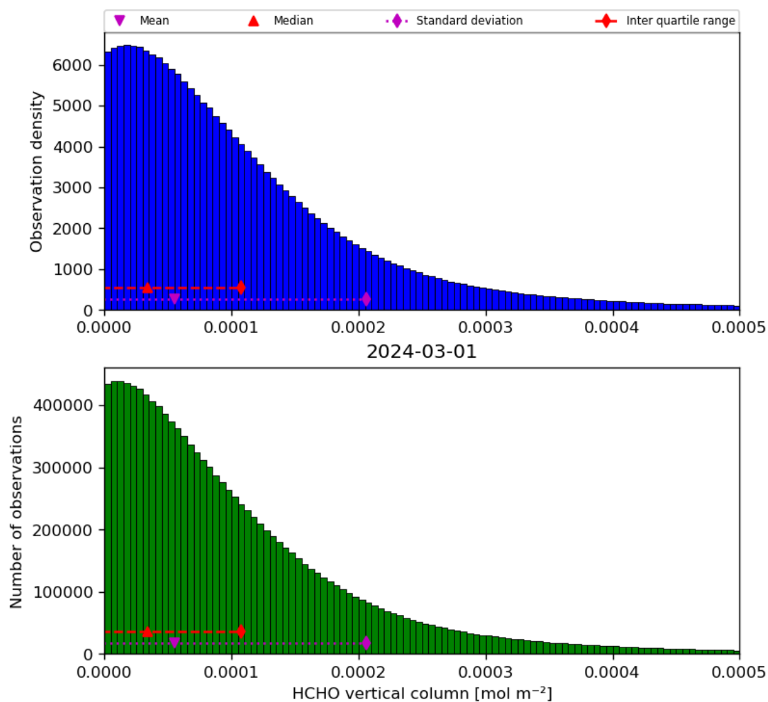
Figure 35: Histogram of “HCHO vertical column” for 2024-02-29 to 2024-03-02
