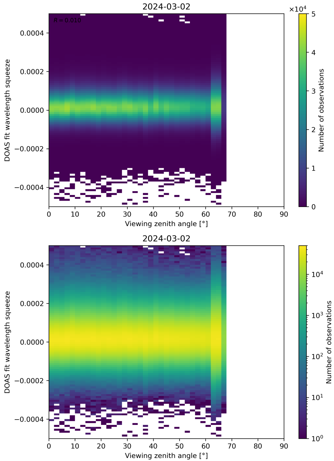
Figure 184: Scatter density plot of “Viewing zenith angle” against “DOAS fit wavelength squeeze” for 2024-03-01 to 2024-03-03.
