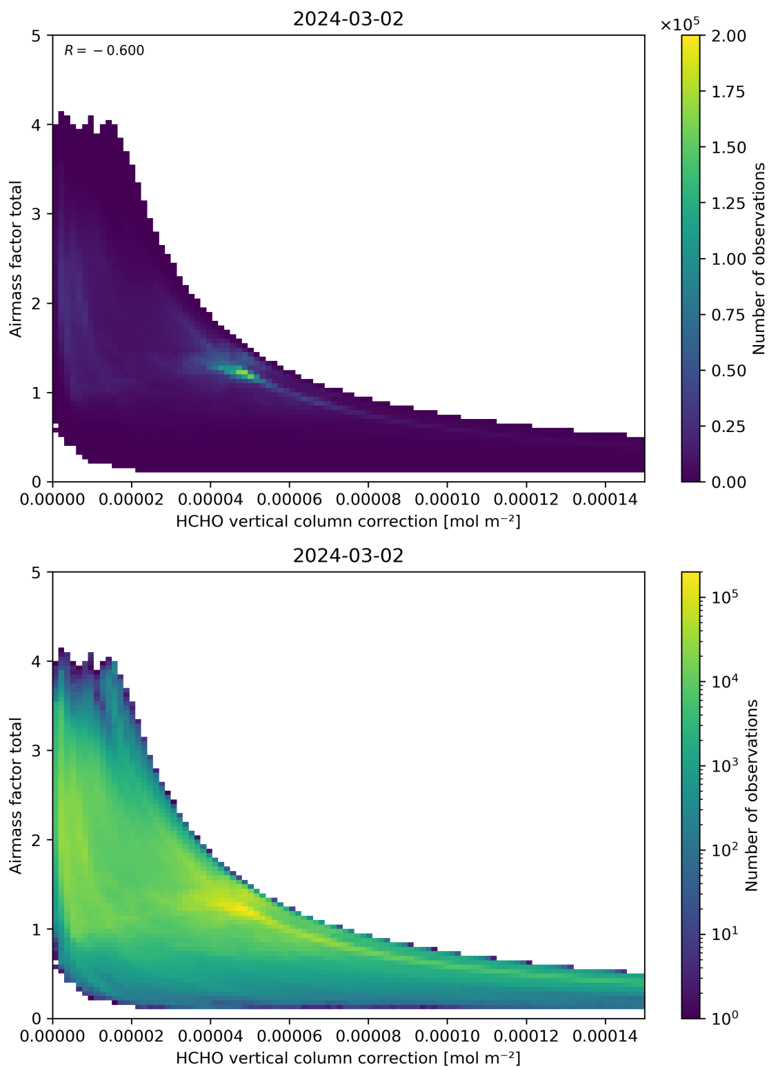
Figure 120: Scatter density plot of “HCHO vertical column correction” against “Airmass factor total” for 2024-03-01 to 2024-03-03.
