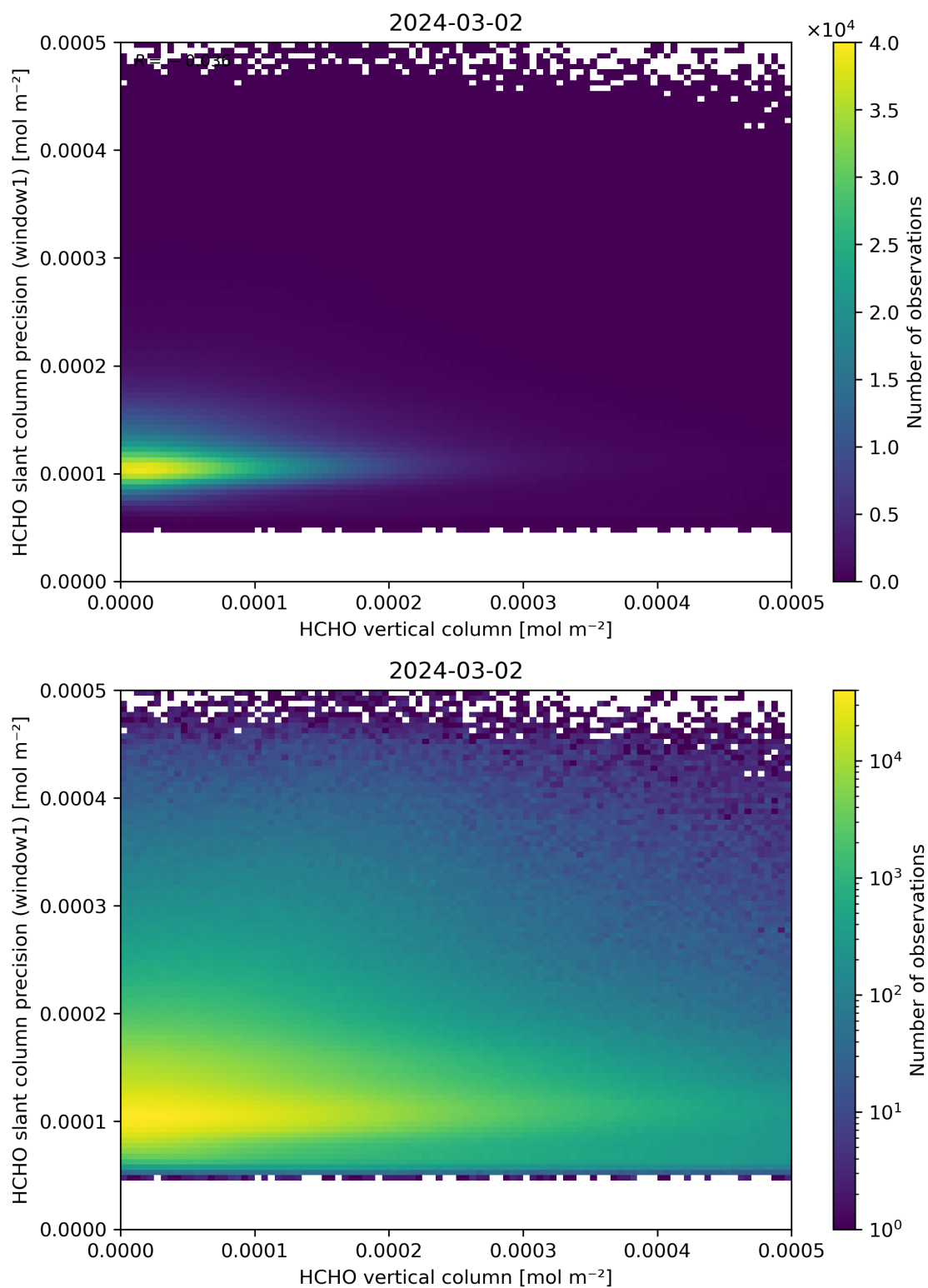
Figure 130: Scatter density plot of “HCHO vertical column” against “HCHO slant column precision (window1)” for 2024-03-01 to 2024-03-03.
