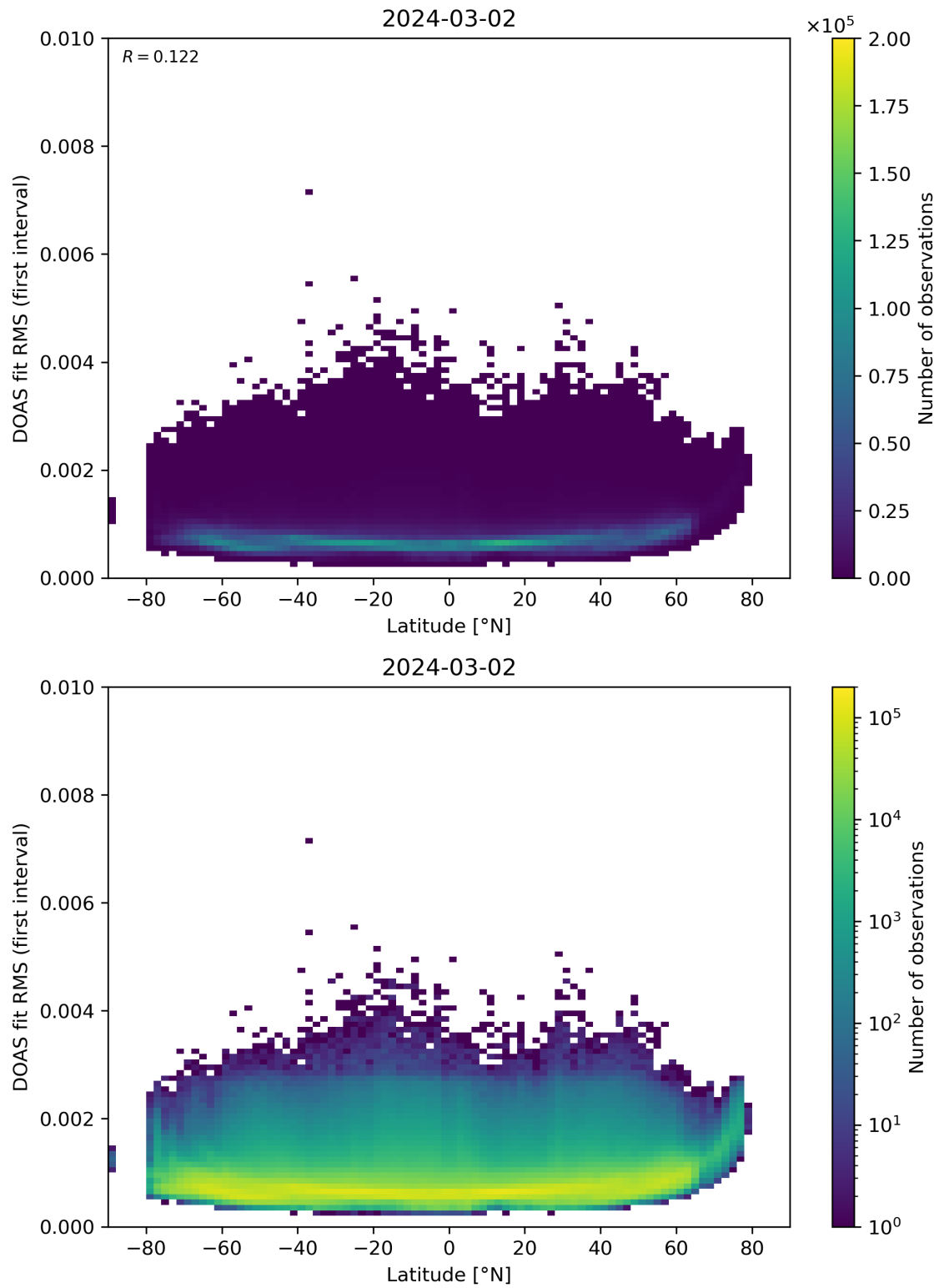
Figure 153: Scatter density plot of “Latitude” against “DOAS fit RMS (first interval)” for 2024-03-01 to 2024-03-03.
