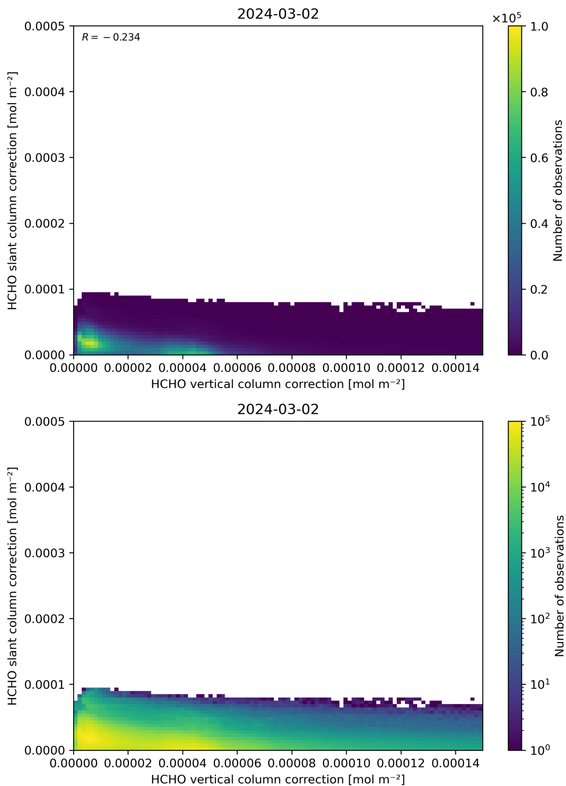
Figure 117: Scatter density plot of “HCHO vertical column correction” against “HCHO slant column correction” for 2024-03-01 to 2024-03-03.
