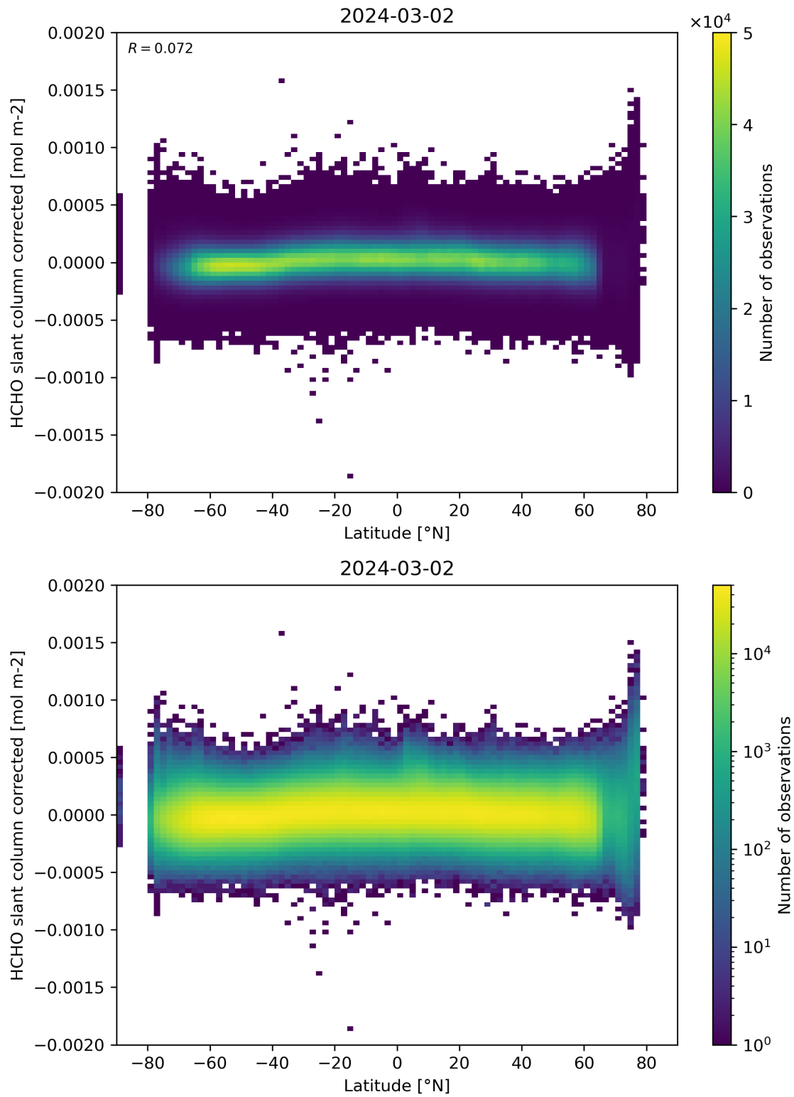
Figure 157: Scatter density plot of “Latitude” against “HCHO slant column corrected” for 2024-03-01 to 2024-03-03.
