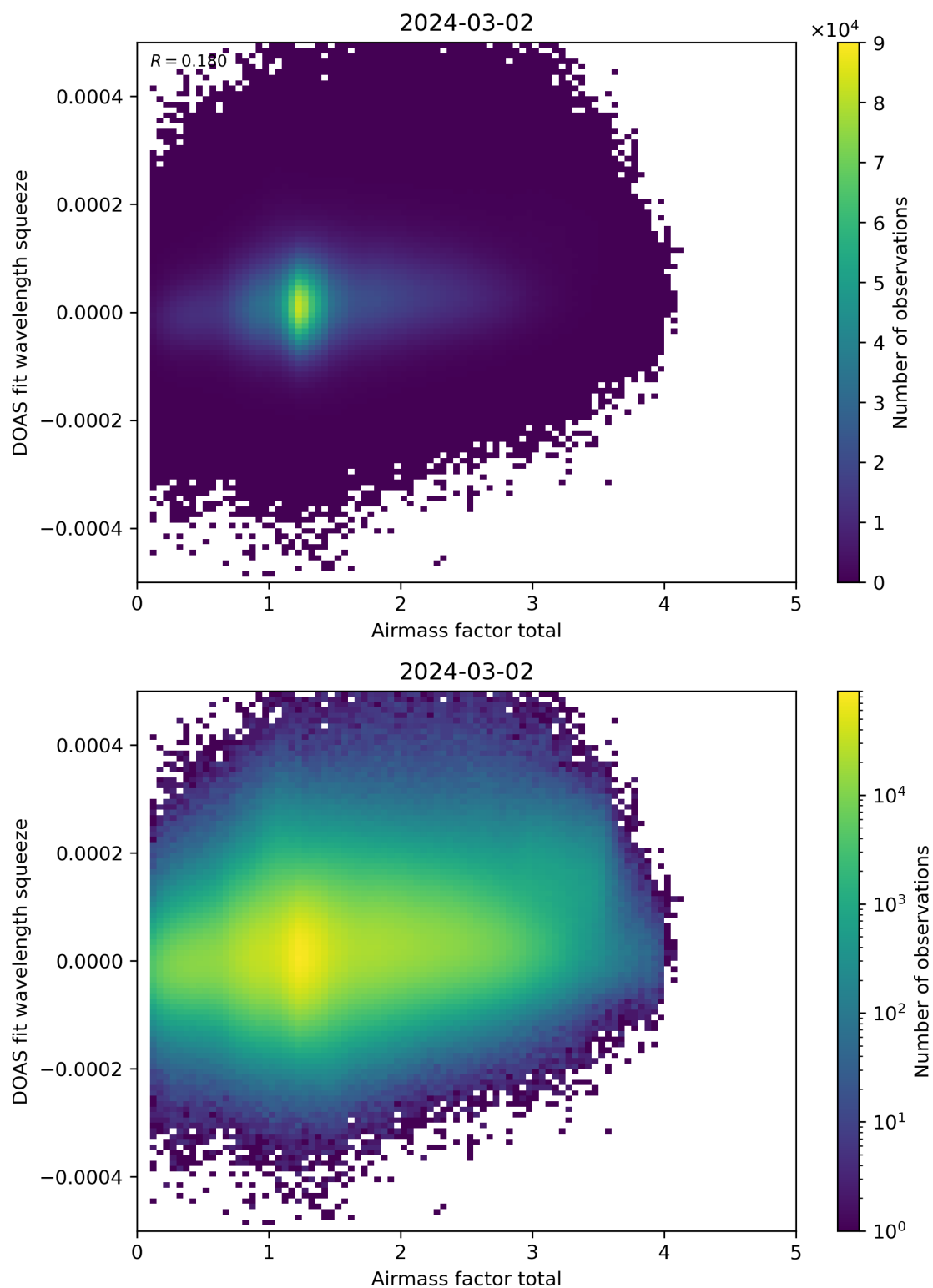
Figure 99: Scatter density plot of “Airmass factor total” against “DOAS fit wavelength squeeze” for 2024-03-01 to 2024-03-03.
