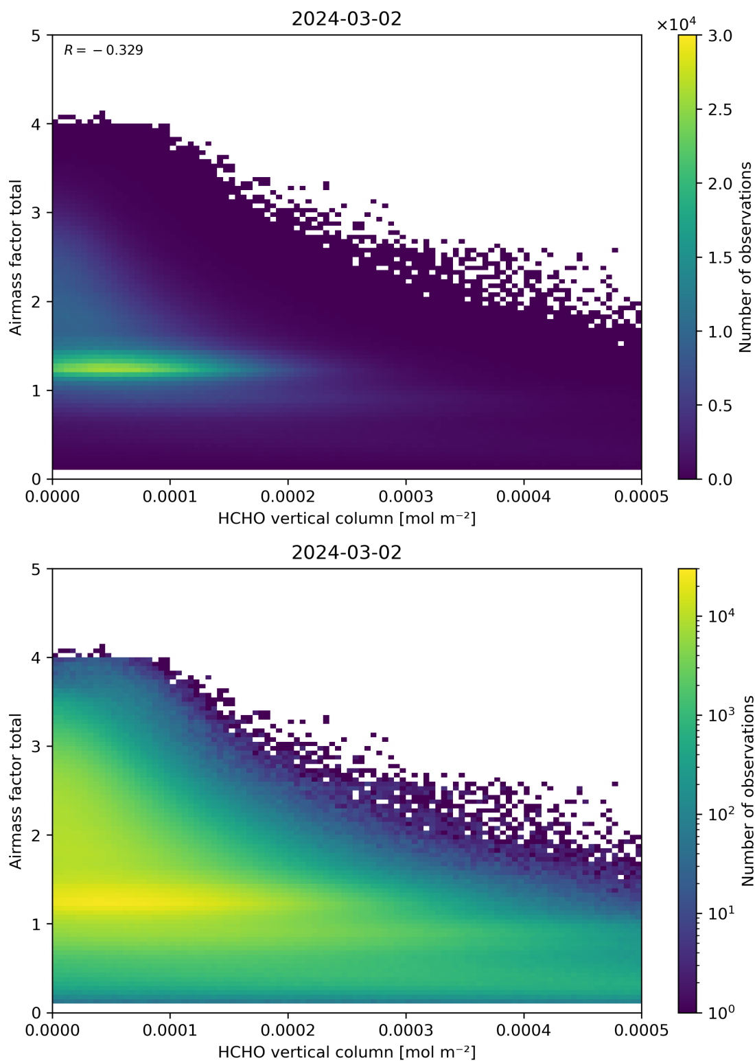
Figure 131: Scatter density plot of “HCHO vertical column” against “Airmass factor total” for 2024-03-01 to 2024-03-03.
