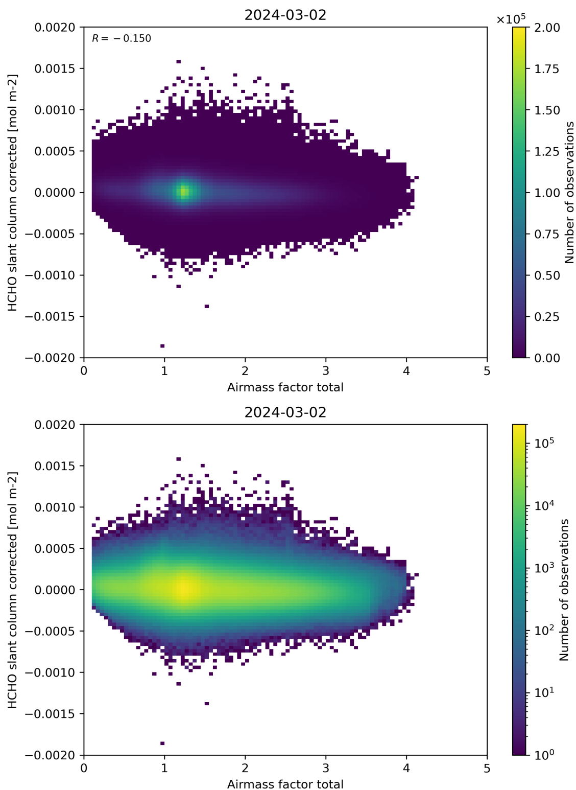
Figure 101: Scatter density plot of “Airmass factor total” against “HCHO slant column corrected” for 2024-03-01 to 2024-03-03.
