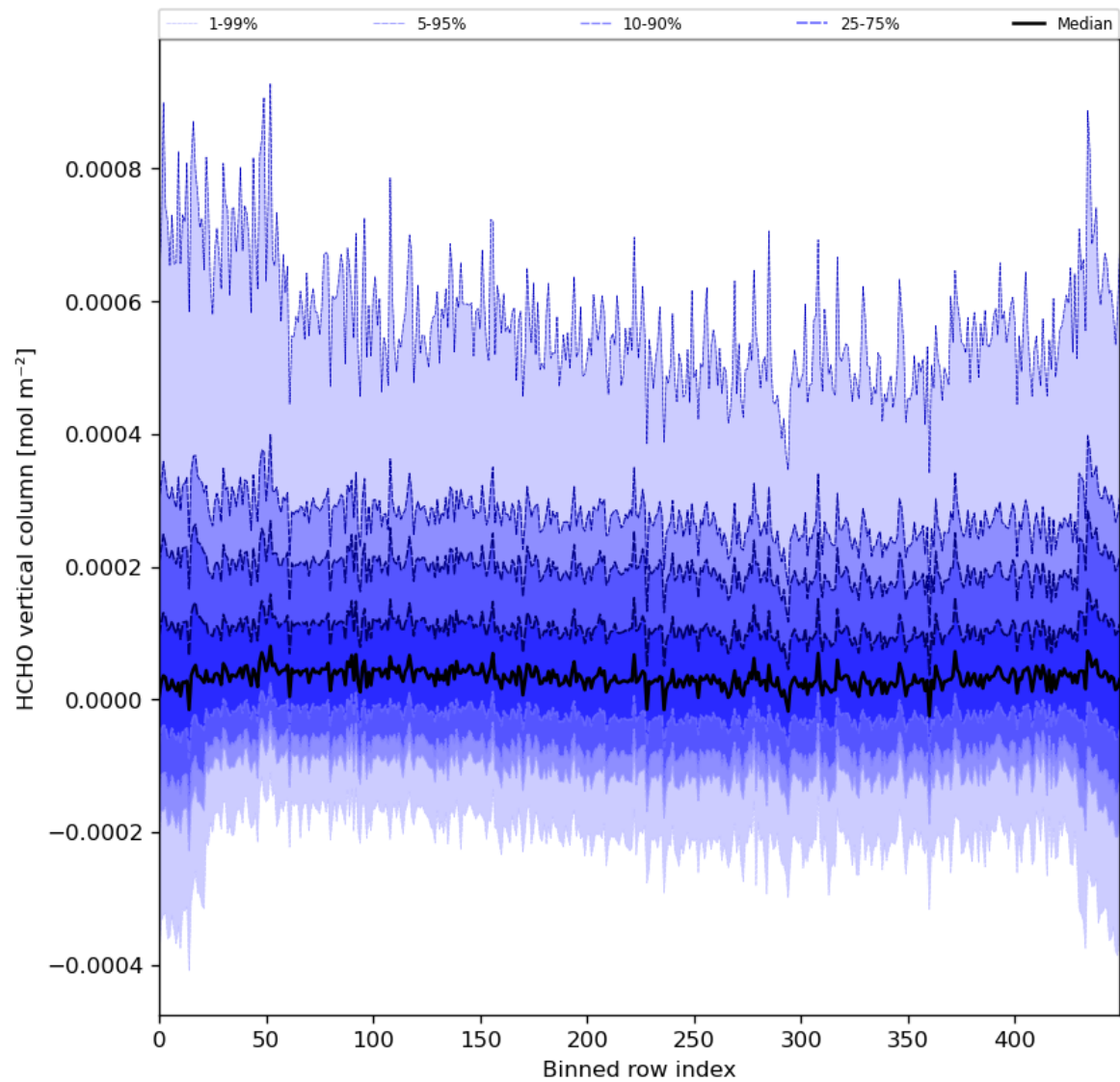
Figure 49: Along track statistics of “HCHO vertical column” for 2024-03-01 to 2024-03-03
