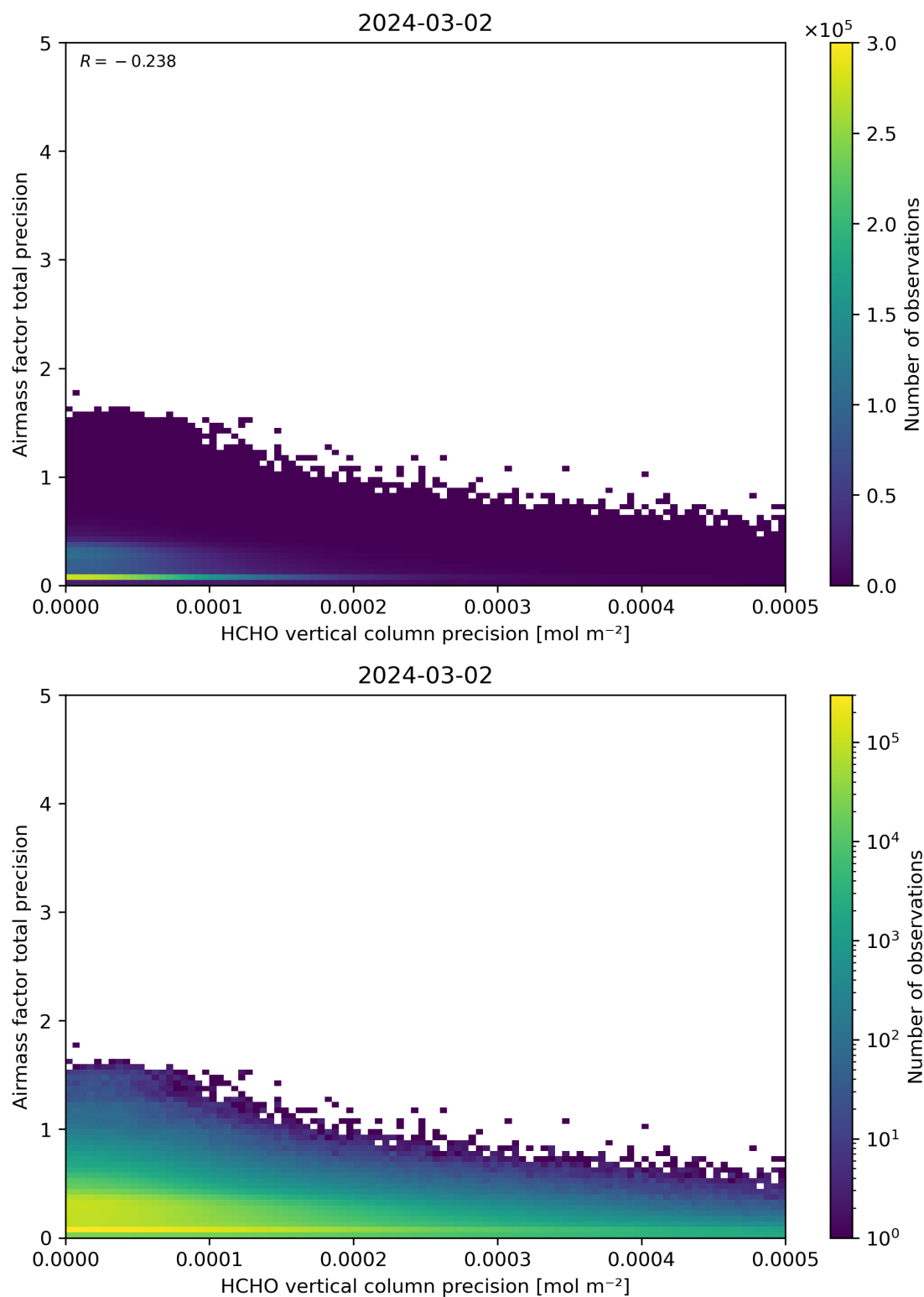
Figure 145: Scatter density plot of “HCHO vertical column precision” against “Airmass factor total precision” for 2024-03-01 to 2024-03-03.
