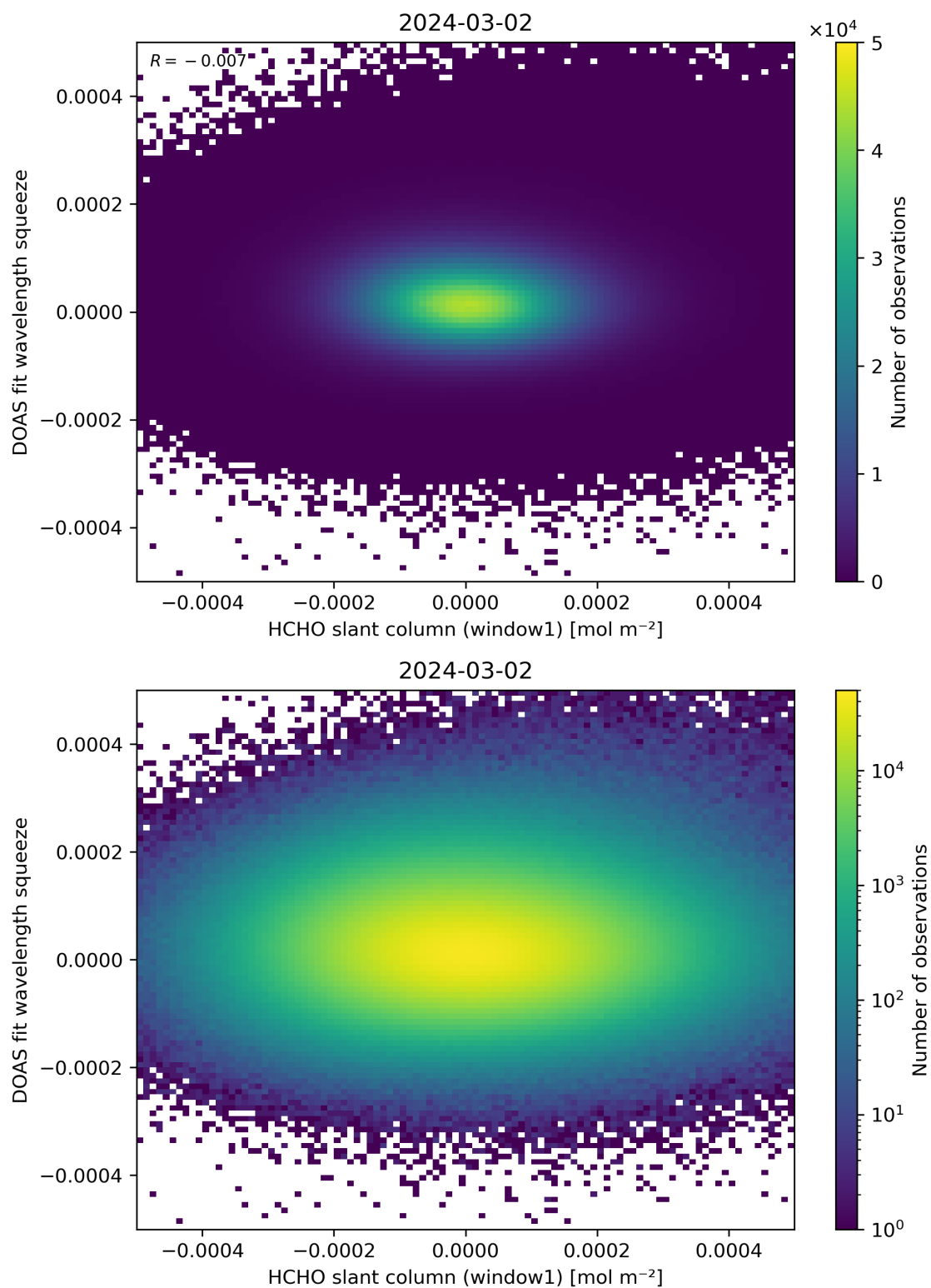
Figure 80: Scatter density plot of “HCHO slant column (window1)” against “DOAS fit wavelength squeeze” for 2024-03-01 to 2024-03-03.
