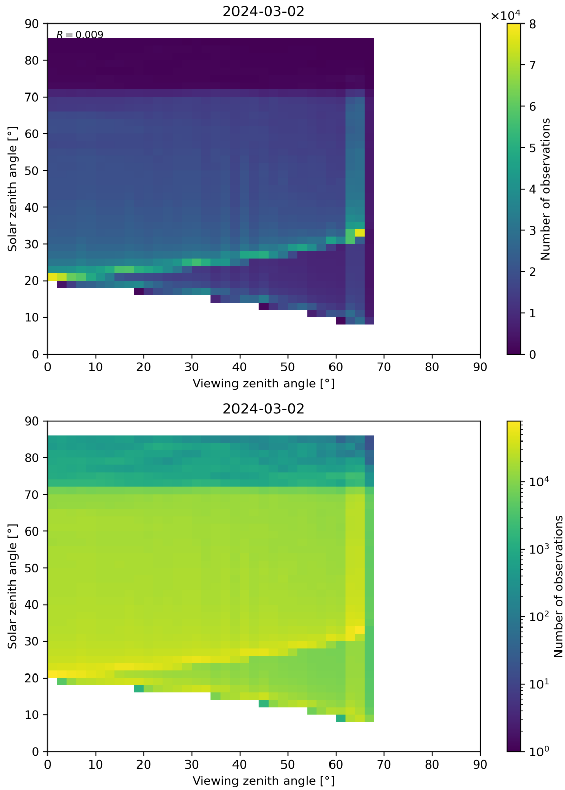
Figure 197: Scatter density plot of “Viewing zenith angle” against “Solar zenith angle” for 2024-03-01 to 2024-03-03.
