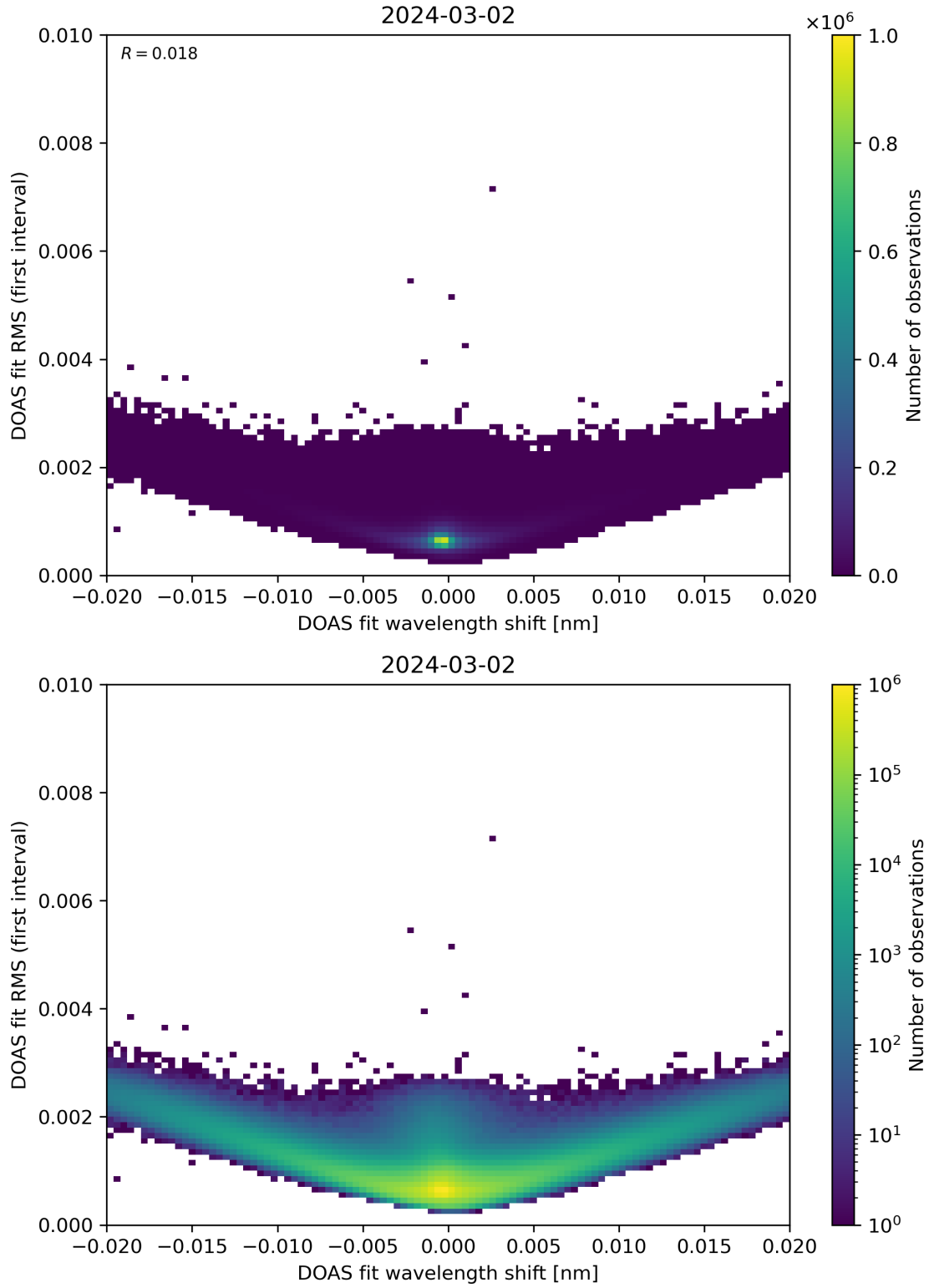
Figure 64: Scatter density plot of “DOAS fit wavelength shift” against “DOAS fit RMS (first interval)” for 2024-03-01 to 2024-03-03.
