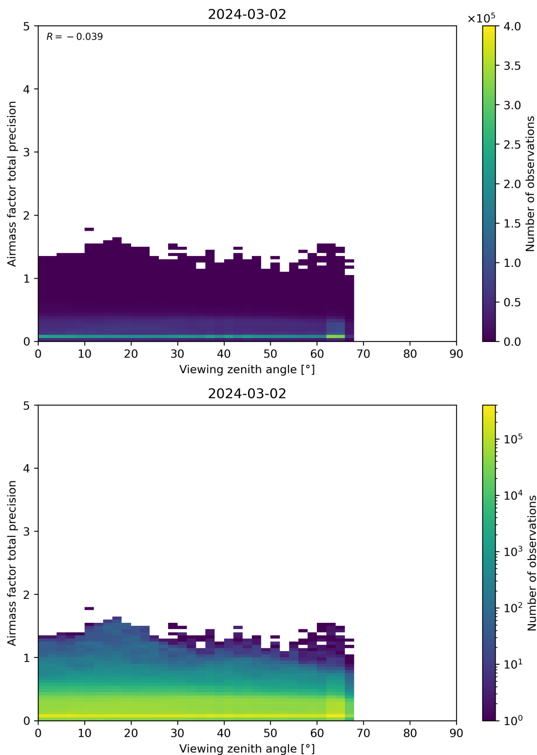
Figure 191: Scatter density plot of “Viewing zenith angle” against “Airmass factor total precision” for 2024-03-01 to 2024-03-03.
