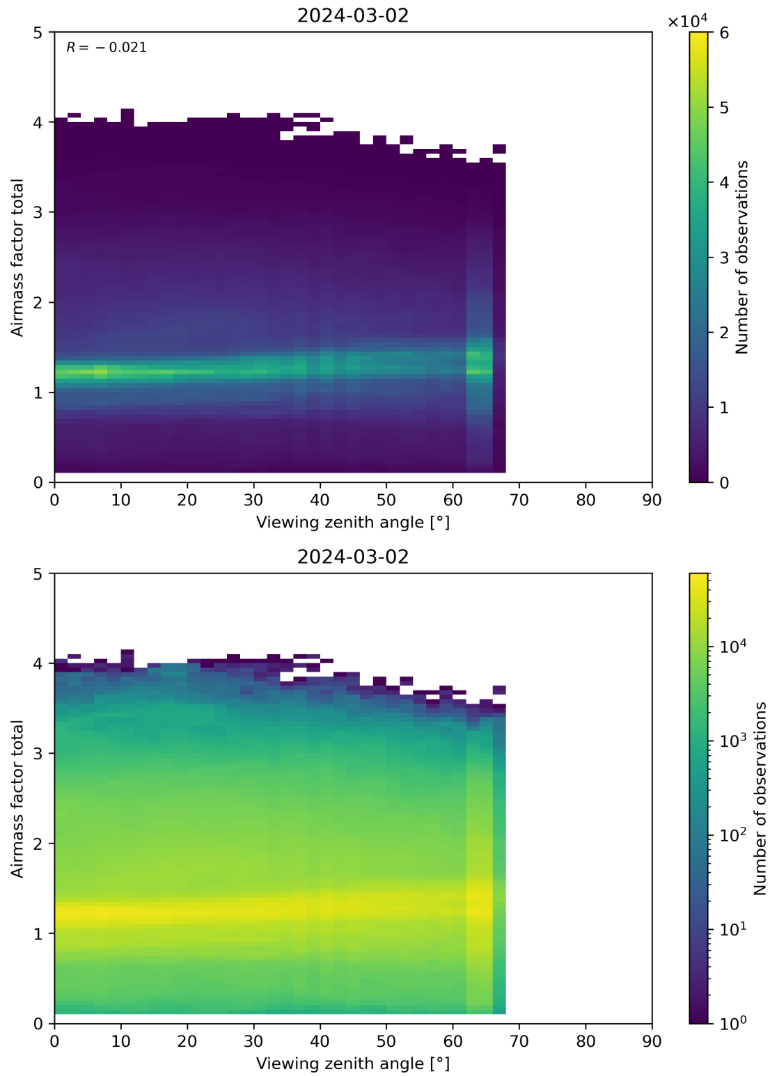
Figure 190: Scatter density plot of “Viewing zenith angle” against “Airmass factor total” for 2024-03-01 to 2024-03-03.
