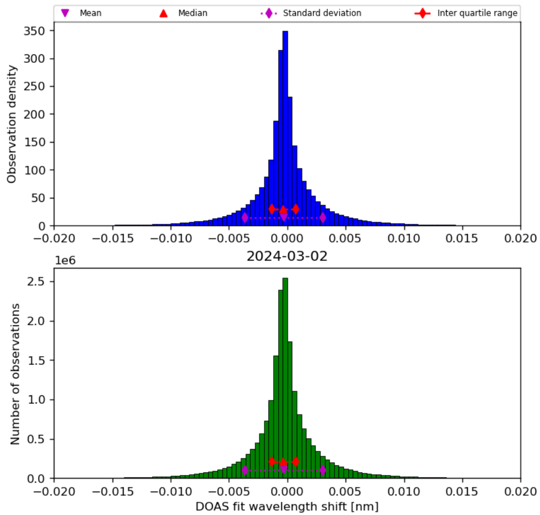
Figure 44: Histogram of “DOAS fit wavelength shift” for 2024-03-01 to 2024-03-03
