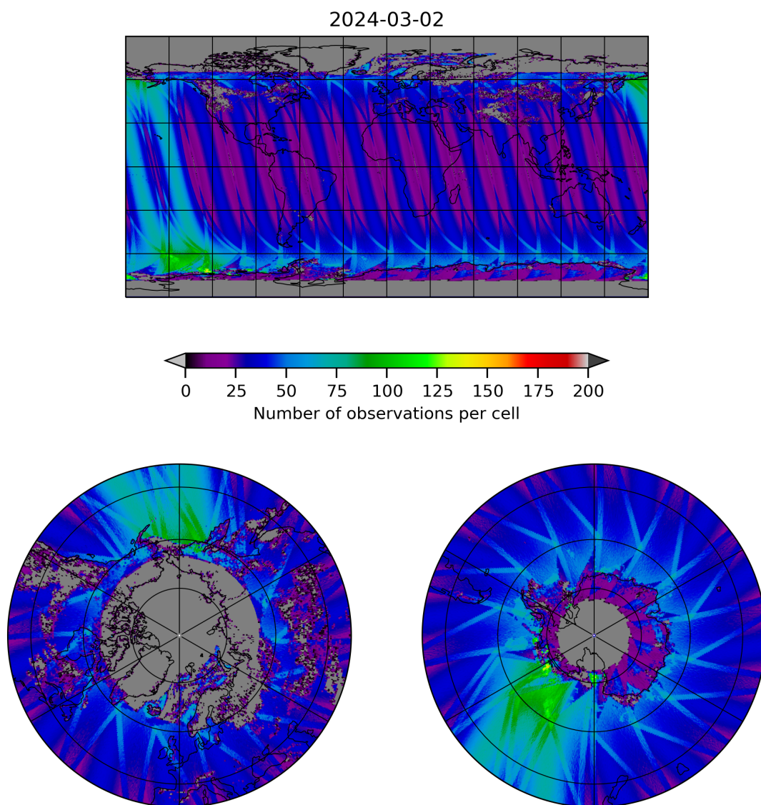
Figure 19: Map of the number of observations for 2024-03-01 to 2024-03-03
