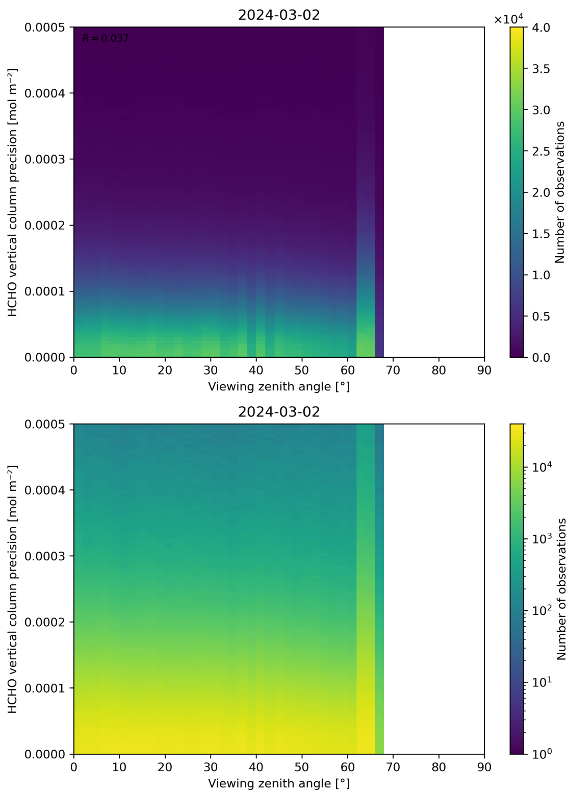
Figure 194: Scatter density plot of “Viewing zenith angle” against “HCHO vertical column precision” for 2024-03-01 to 2024-03-03.
