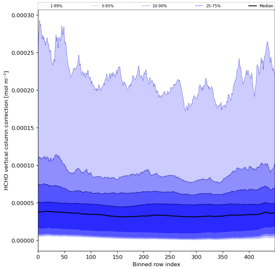
Figure 51: Along track statistics of “HCHO vertical column correction” for 2024-03-01 to 2024-03-03
