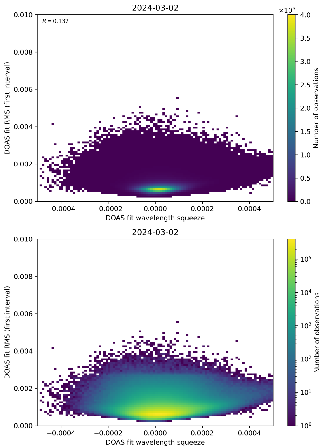
Figure 68: Scatter density plot of “DOAS fit wavelength squeeze” against “DOAS fit RMS (first interval)” for 2024-03-01 to 2024-03-03.
