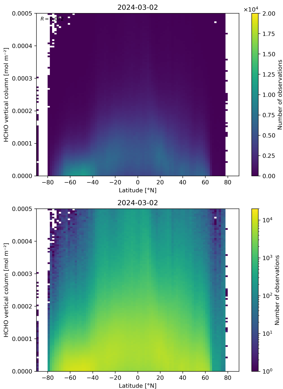
Figure 163: Scatter density plot of “Latitude” against “HCHO vertical column” for 2024-03-01 to 2024-03-03.
