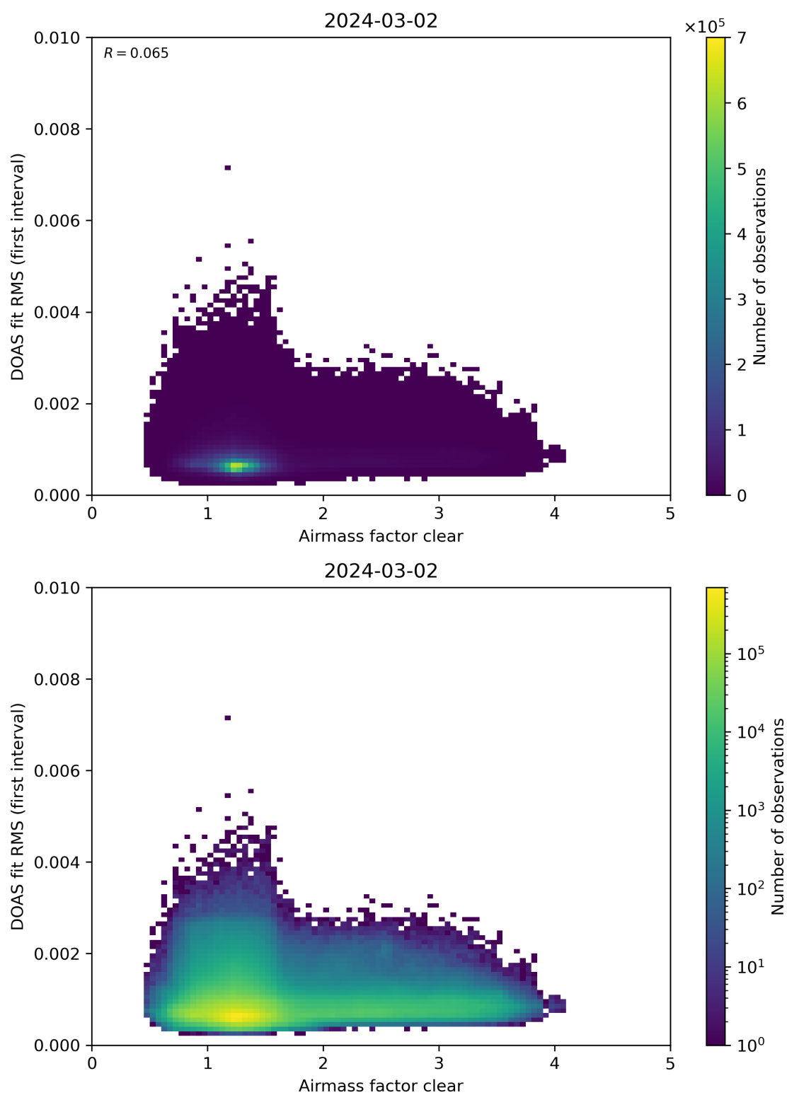
Figure 71: Scatter density plot of “Airmass factor clear” against “DOAS fit RMS (first interval)” for 2024-03-01 to 2024-03-03.
