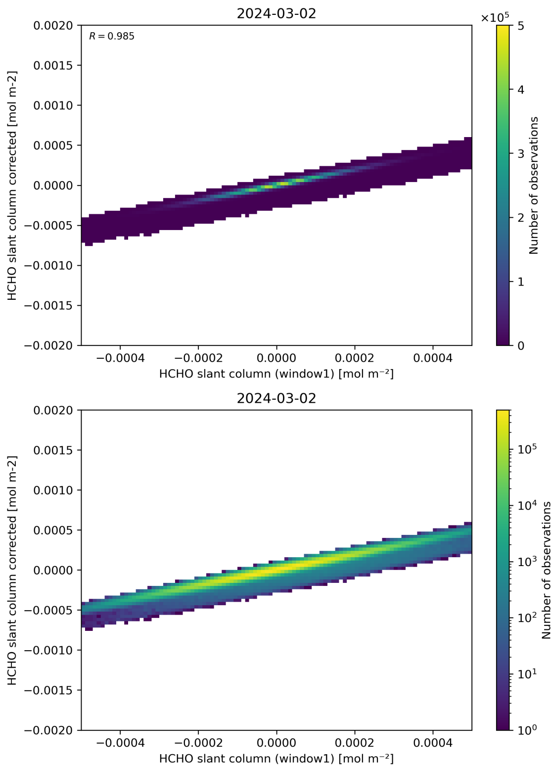
Figure 82: Scatter density plot of “HCHO slant column (window1)” against “HCHO slant column corrected” for 2024-03-01 to 2024-03-03.
