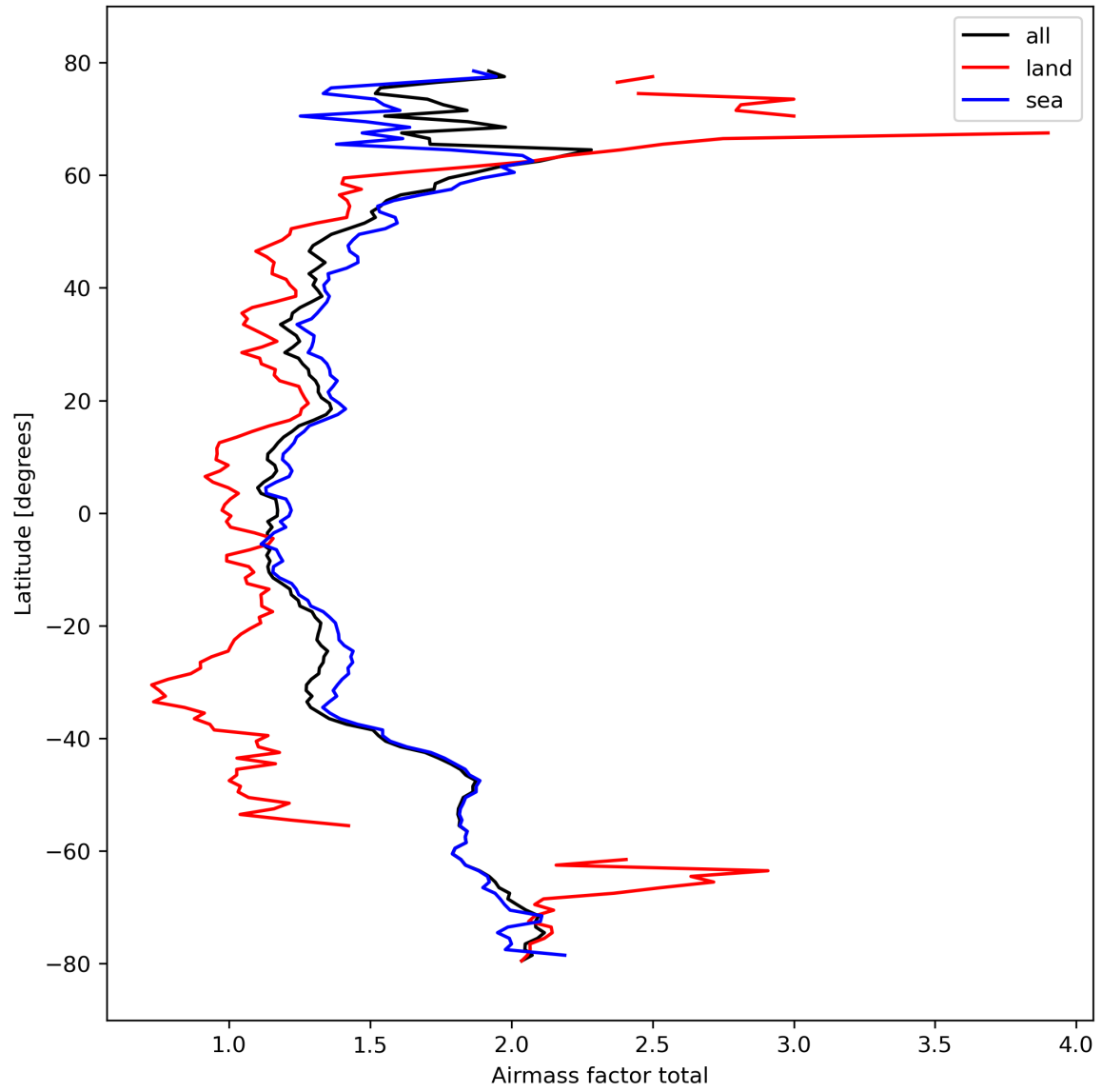
Figure 26: Zonal average of “Airmass factor total” for 2024-03-01 to 2024-03-03.
