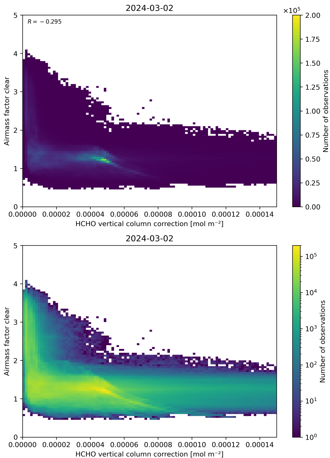
Figure 115: Scatter density plot of “HCHO vertical column correction” against “Airmass factor clear” for 2024-03-01 to 2024-03-03.
