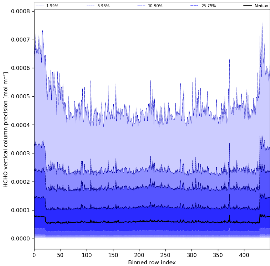
Figure 50: Along track statistics of “HCHO vertical column precision” for 2024-03-01 to 2024-03-03
