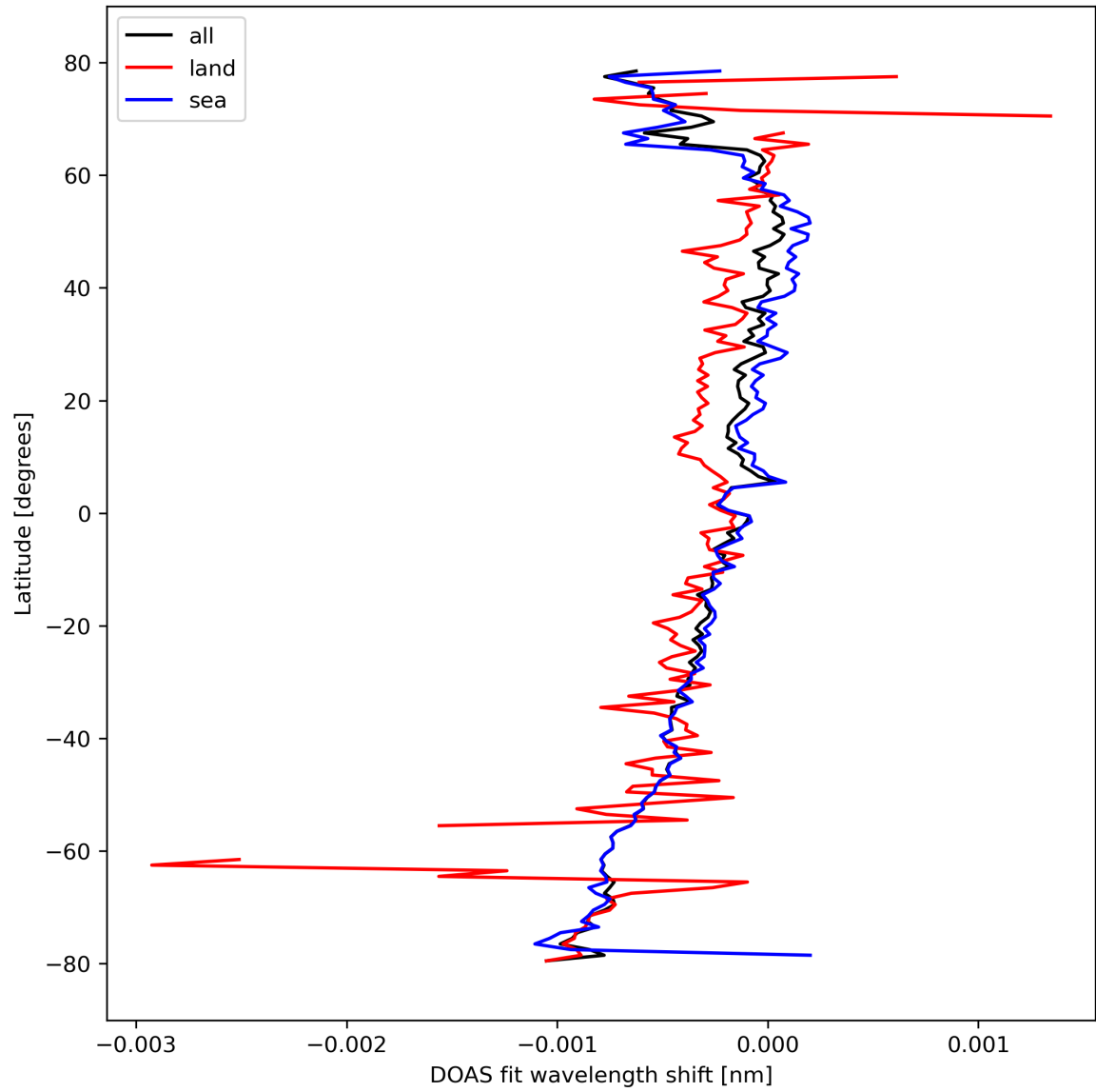
Figure 30: Zonal average of “DOAS fit wavelength shift” for 2024-03-01 to 2024-03-03.
