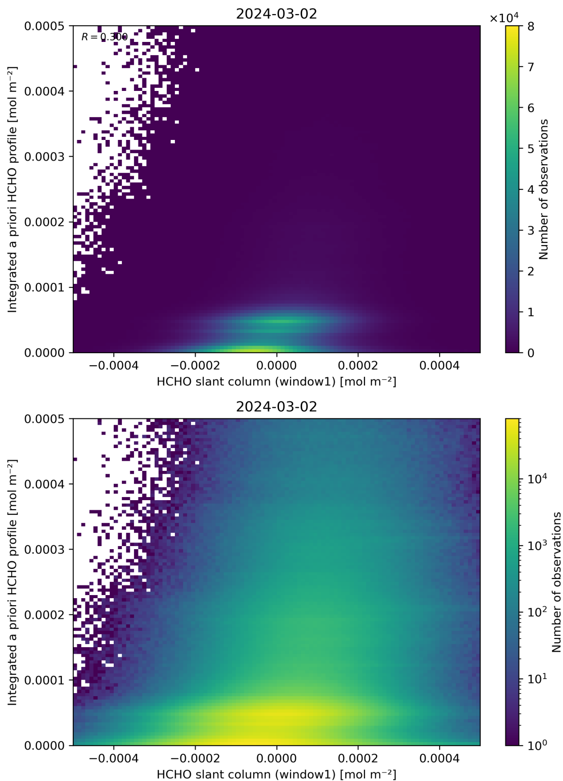
Figure 87: Scatter density plot of “HCHO slant column (window1)” against “Integrated a priori HCHO profile” for 2024-03-01 to 2024-03-03.
