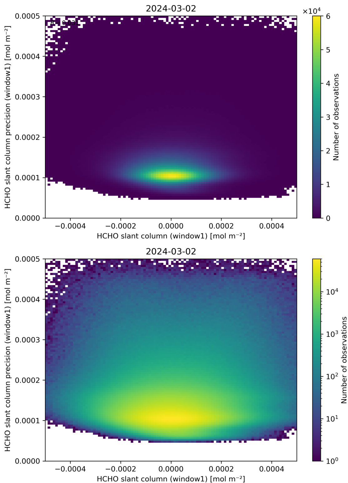
Figure 84: Scatter density plot of “HCHO slant column (window1)” against “HCHO slant column precision (window1)” for 2024-03-01 to 2024-03-03.
