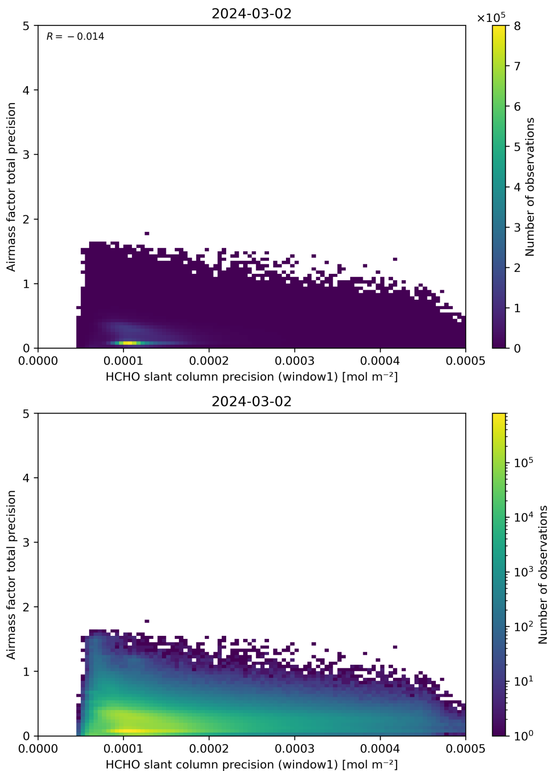
Figure 95: Scatter density plot of “HCHO slant column precision (window1)” against “Airmass factor total precision” for 2024-03-01 to 2024-03-03.
