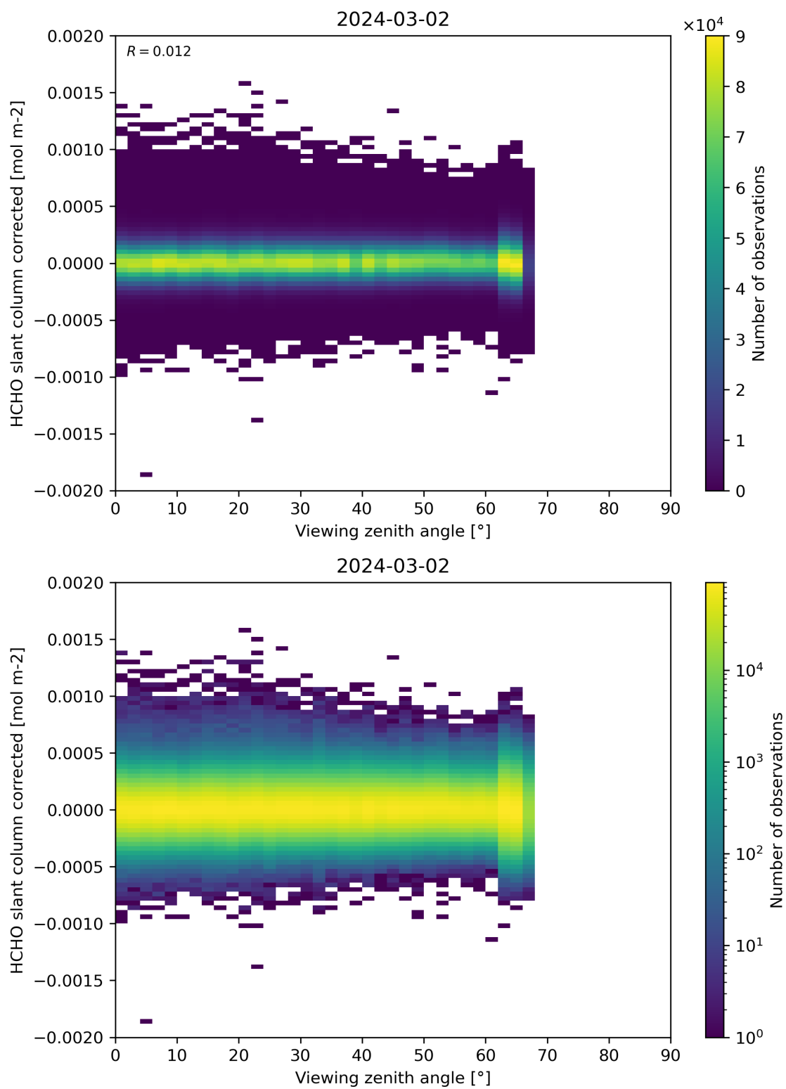
Figure 186: Scatter density plot of “Viewing zenith angle” against “HCHO slant column corrected” for 2024-03-01 to 2024-03-03.
