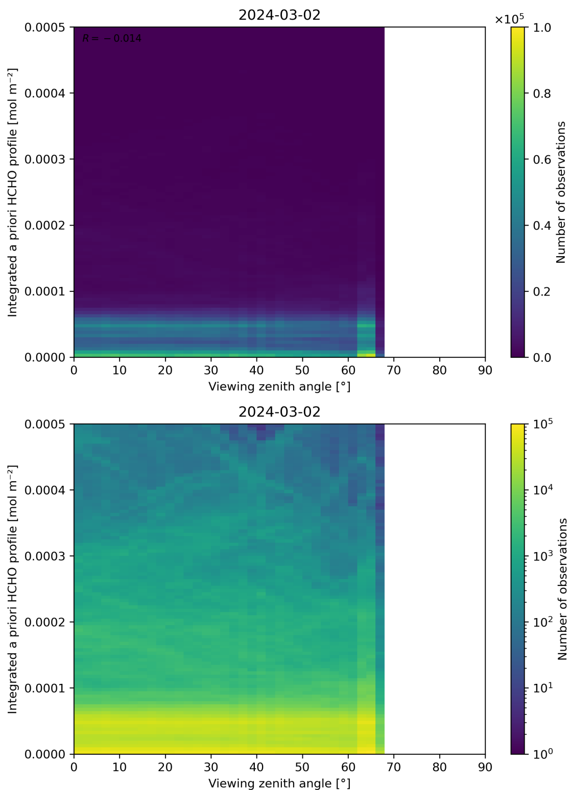
Figure 195: Scatter density plot of “Viewing zenith angle” against “Integrated a priori HCHO profile” for 2024-03-01 to 2024-03-03.
