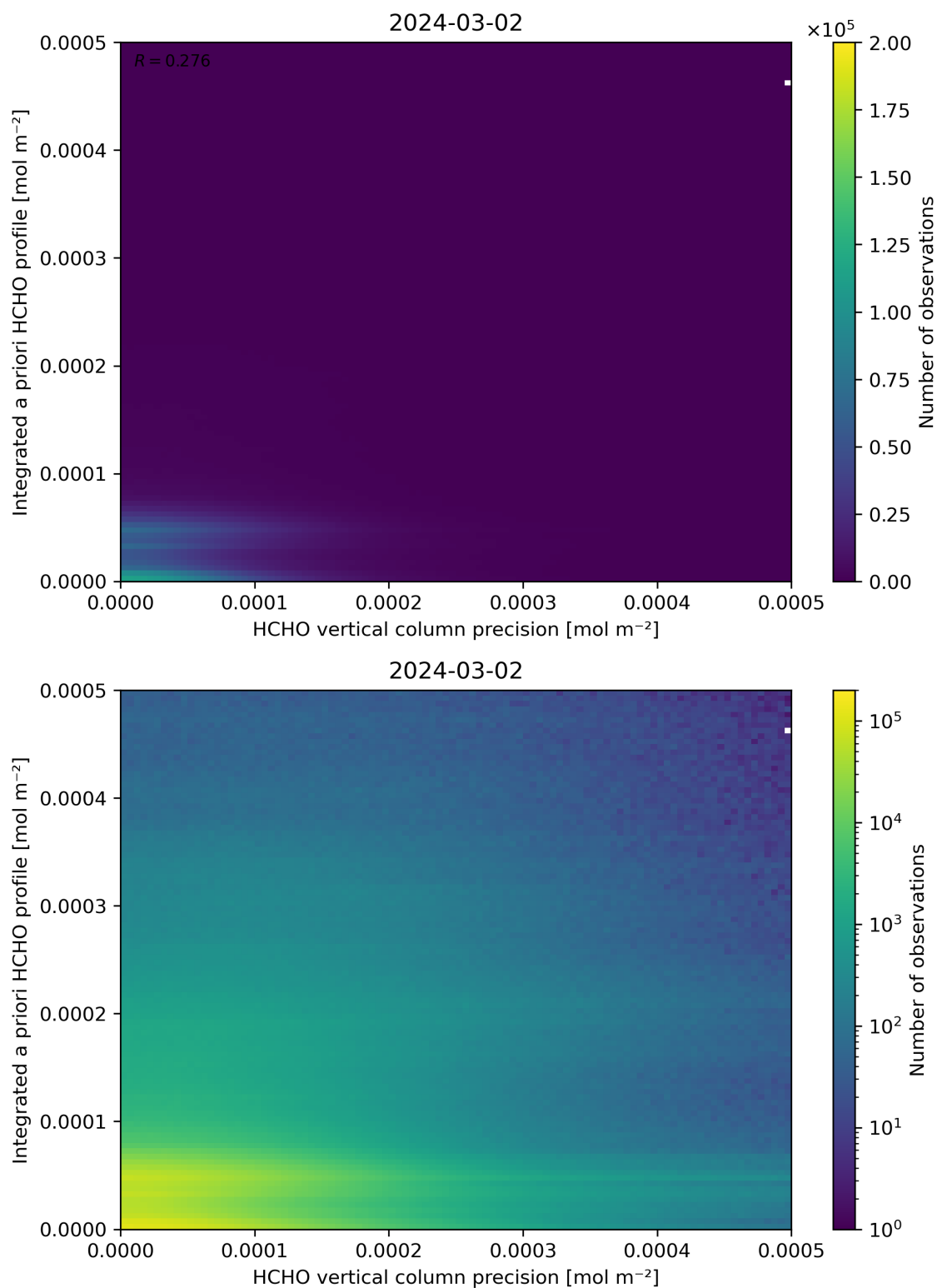
Figure 147: Scatter density plot of “HCHO vertical column precision” against “Integrated a priori HCHO profile” for 2024-03-01 to 2024-03-03.
