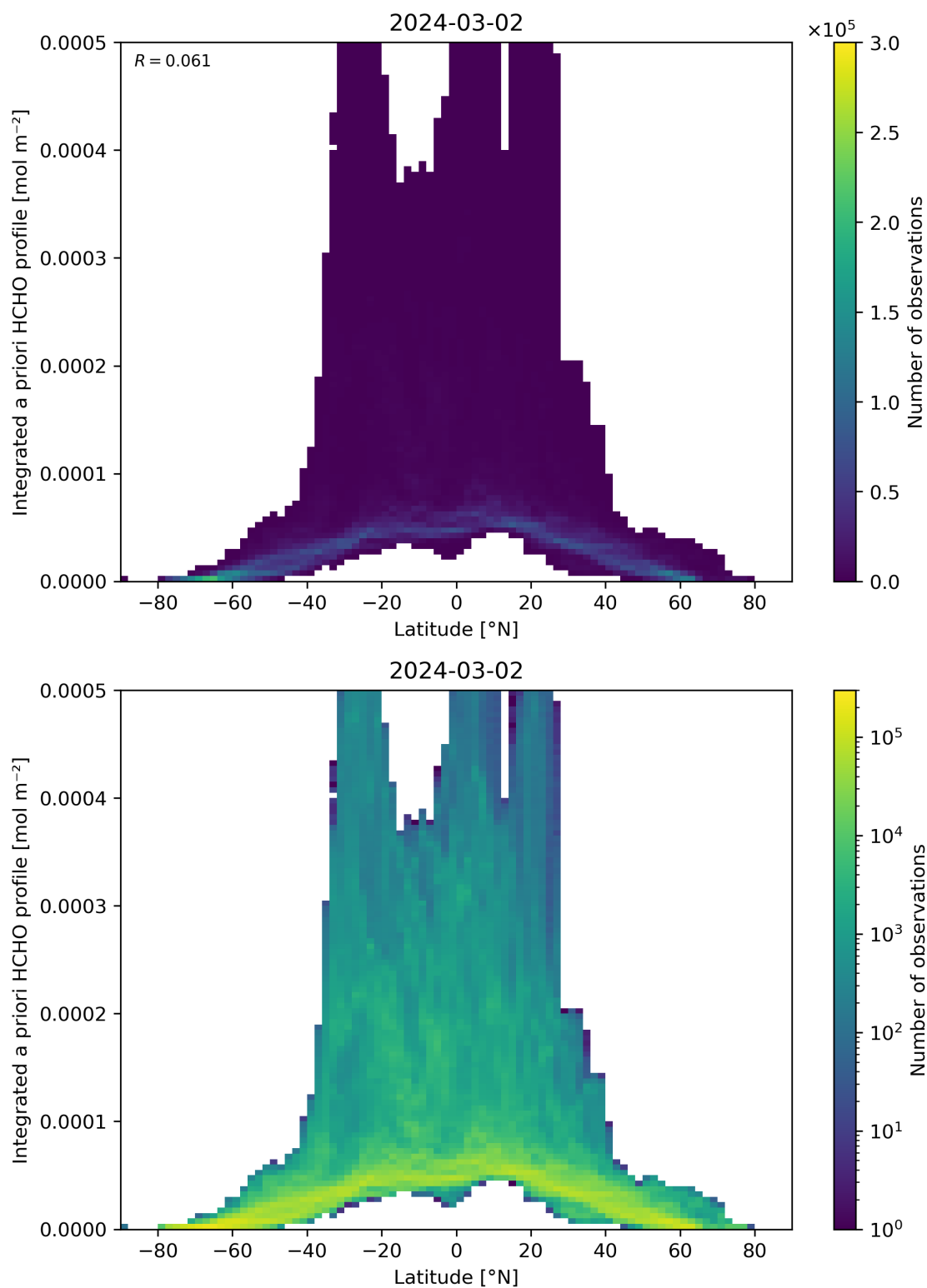
Figure 166: Scatter density plot of “Latitude” against “Integrated a priori HCHO profile” for 2024-03-01 to 2024-03-03.
