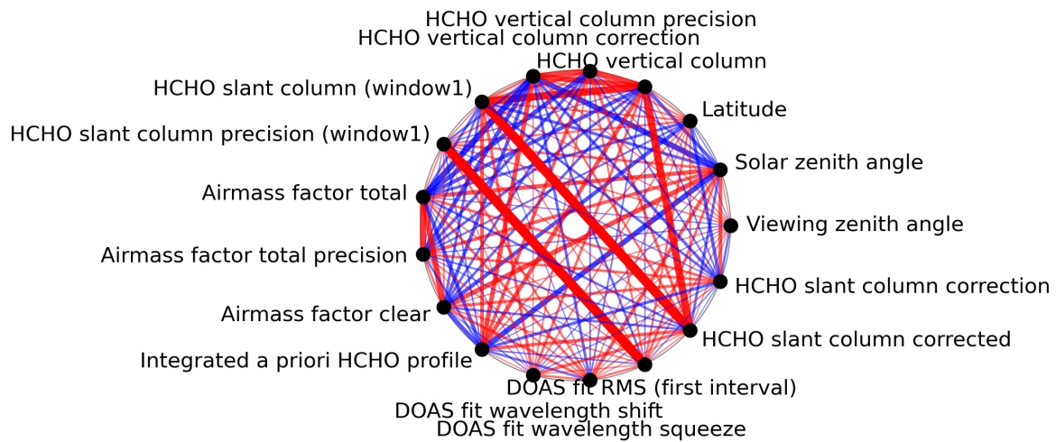
Figure 1: Map of correlation graph for 2024-03-01 to 2024-03-03.
