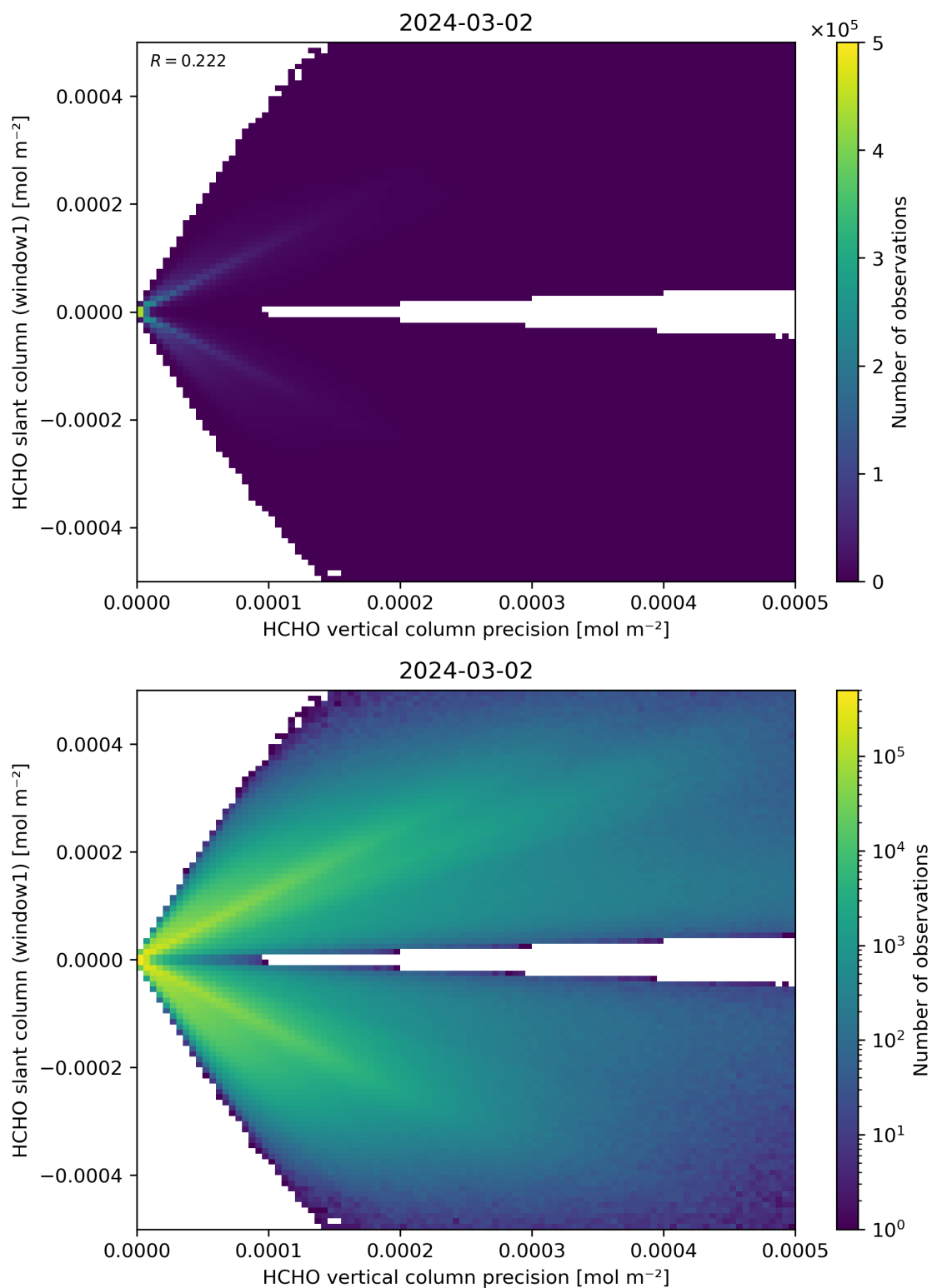
Figure 142: Scatter density plot of “HCHO vertical column precision” against “HCHO slant column (window1)” for 2024-03-01 to 2024-03-03.
