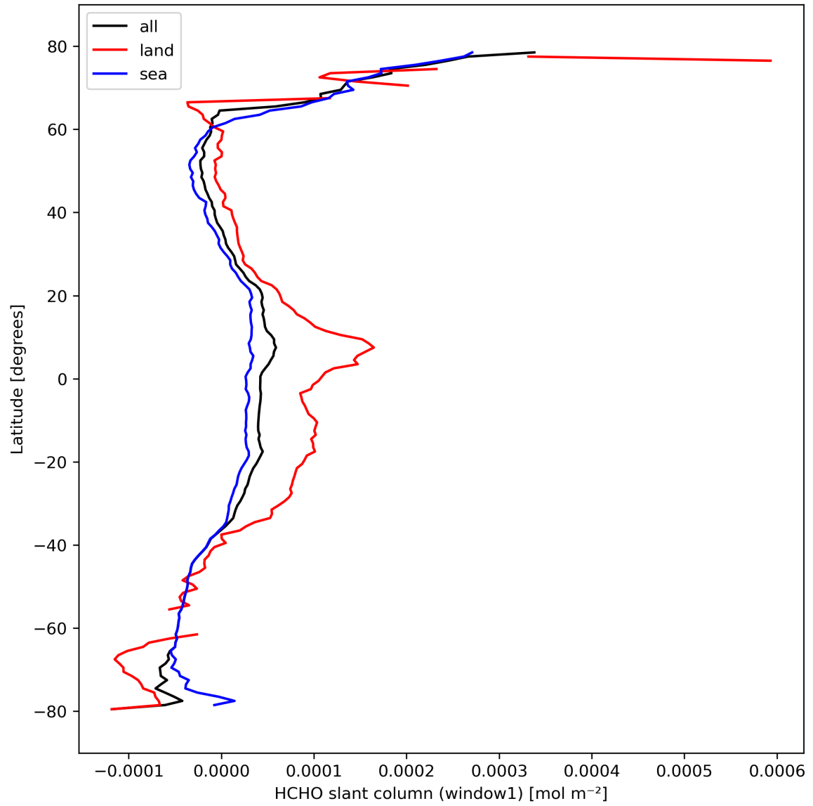
Figure 24: Zonal average of “HCHO slant column (window1)” for 2024-03-01 to 2024-03-03.
