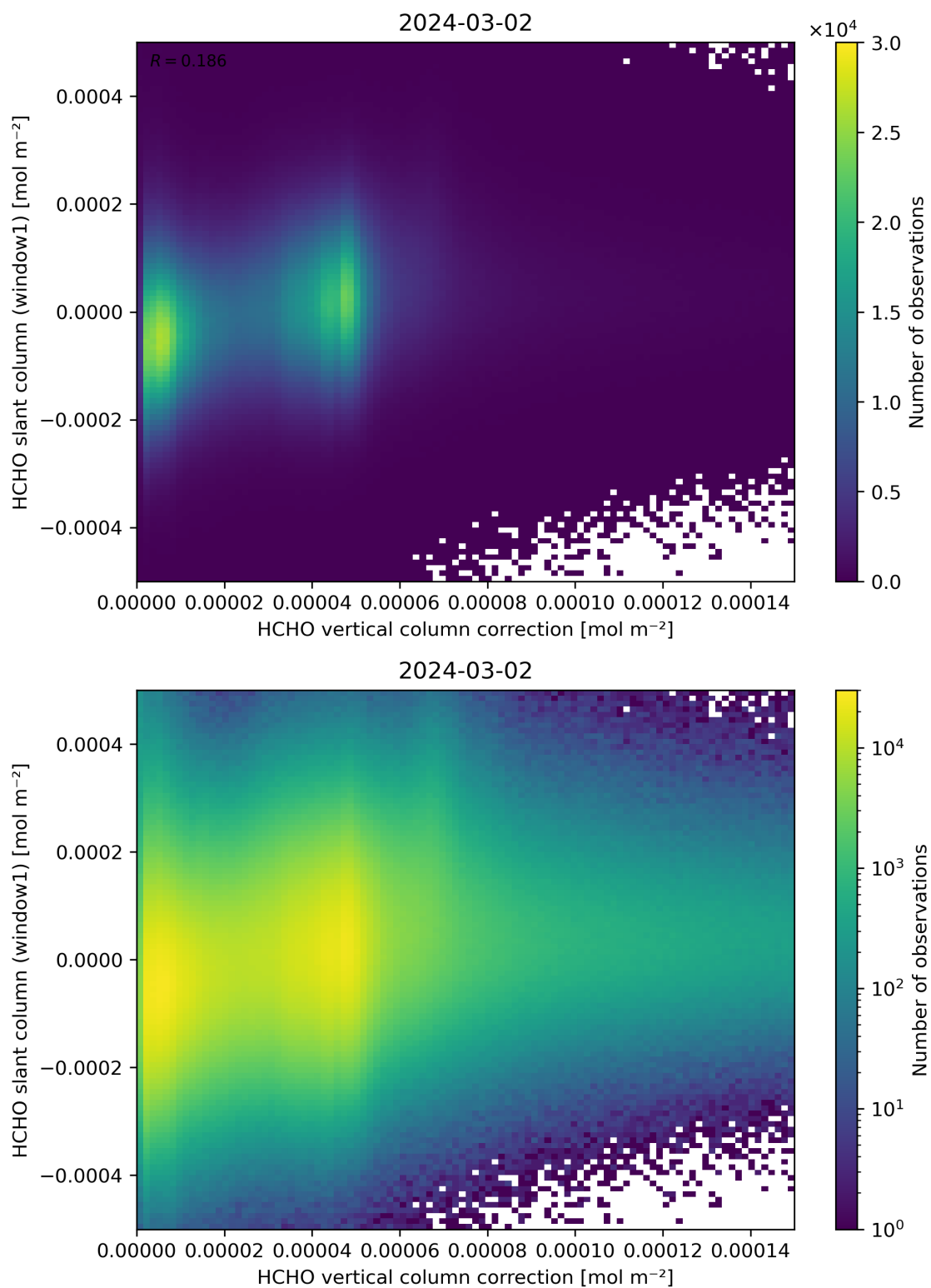
Figure 118: Scatter density plot of “HCHO vertical column correction” against “HCHO slant column (window1)” for 2024-03-01 to 2024-03-03.
