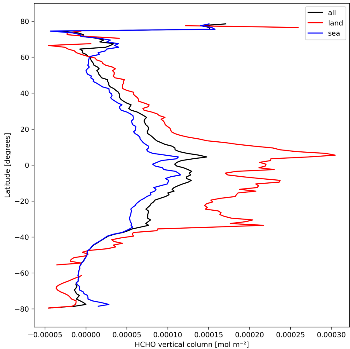
Figure 21: Zonal average of “HCHO vertical column” for 2024-03-01 to 2024-03-03.
