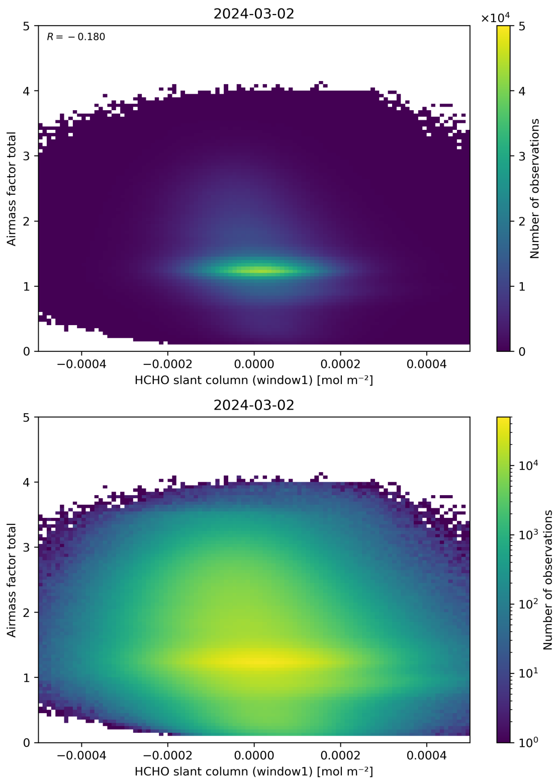
Figure 85: Scatter density plot of “HCHO slant column (window1)” against “Airmass factor total” for 2024-03-01 to 2024-03-03.
