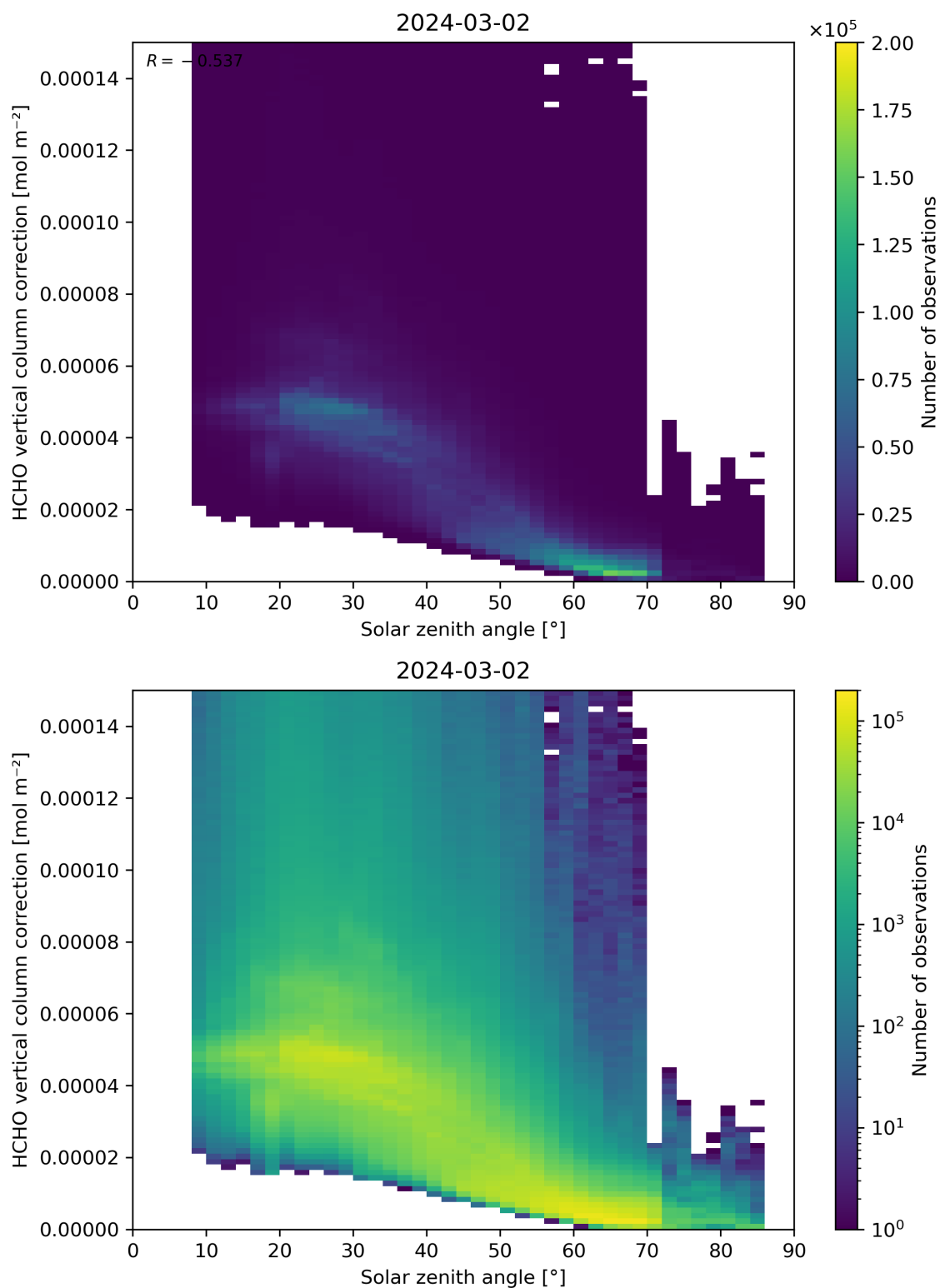
Figure 178: Scatter density plot of “Solar zenith angle” against “HCHO vertical column correction” for 2024-03-01 to 2024-03-03.
