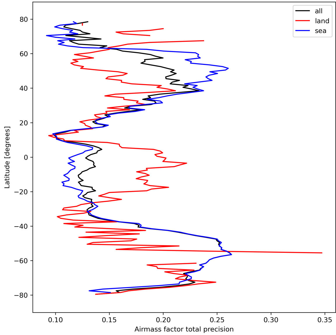
Figure 27: Zonal average of “Airmass factor total precision” for 2024-03-01 to 2024-03-03.
