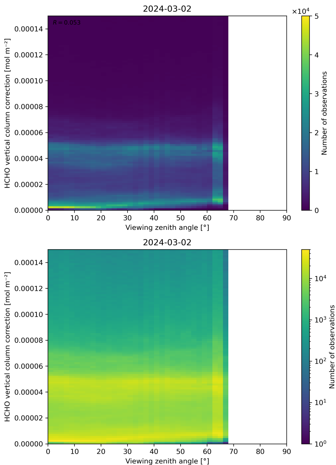
Figure 193: Scatter density plot of “Viewing zenith angle” against “HCHO vertical column correction” for 2024-03-01 to 2024-03-03.
