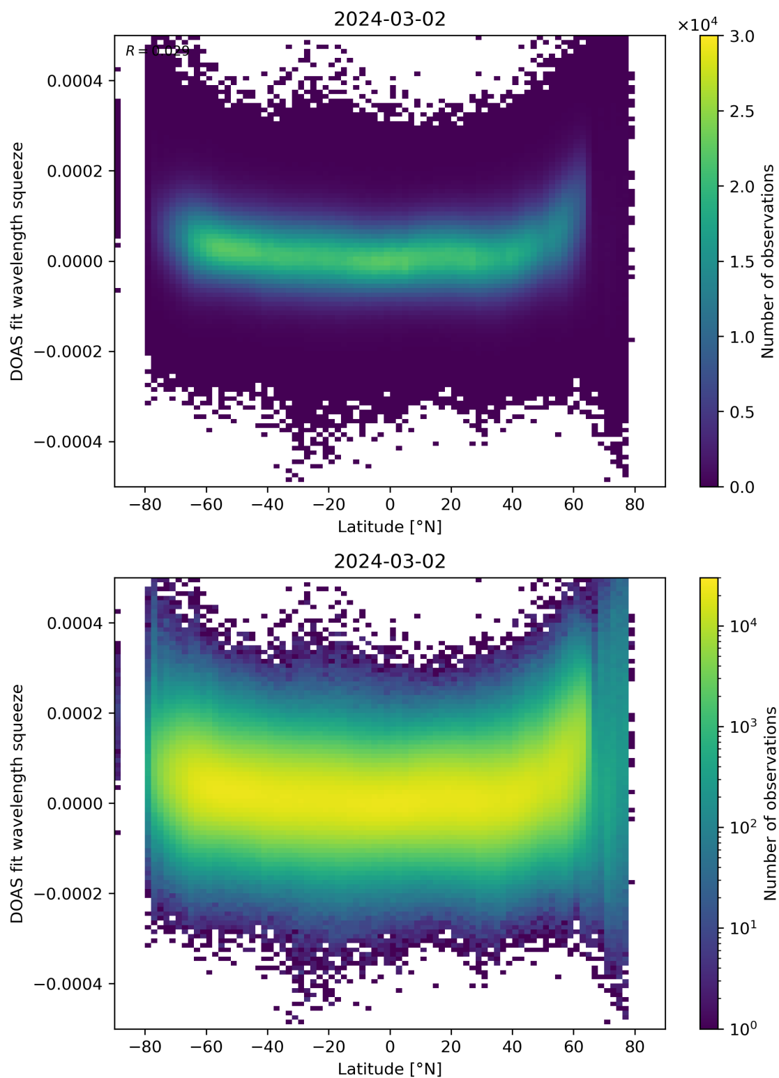
Figure 155: Scatter density plot of “Latitude” against “DOAS fit wavelength squeeze” for 2024-03-01 to 2024-03-03.
