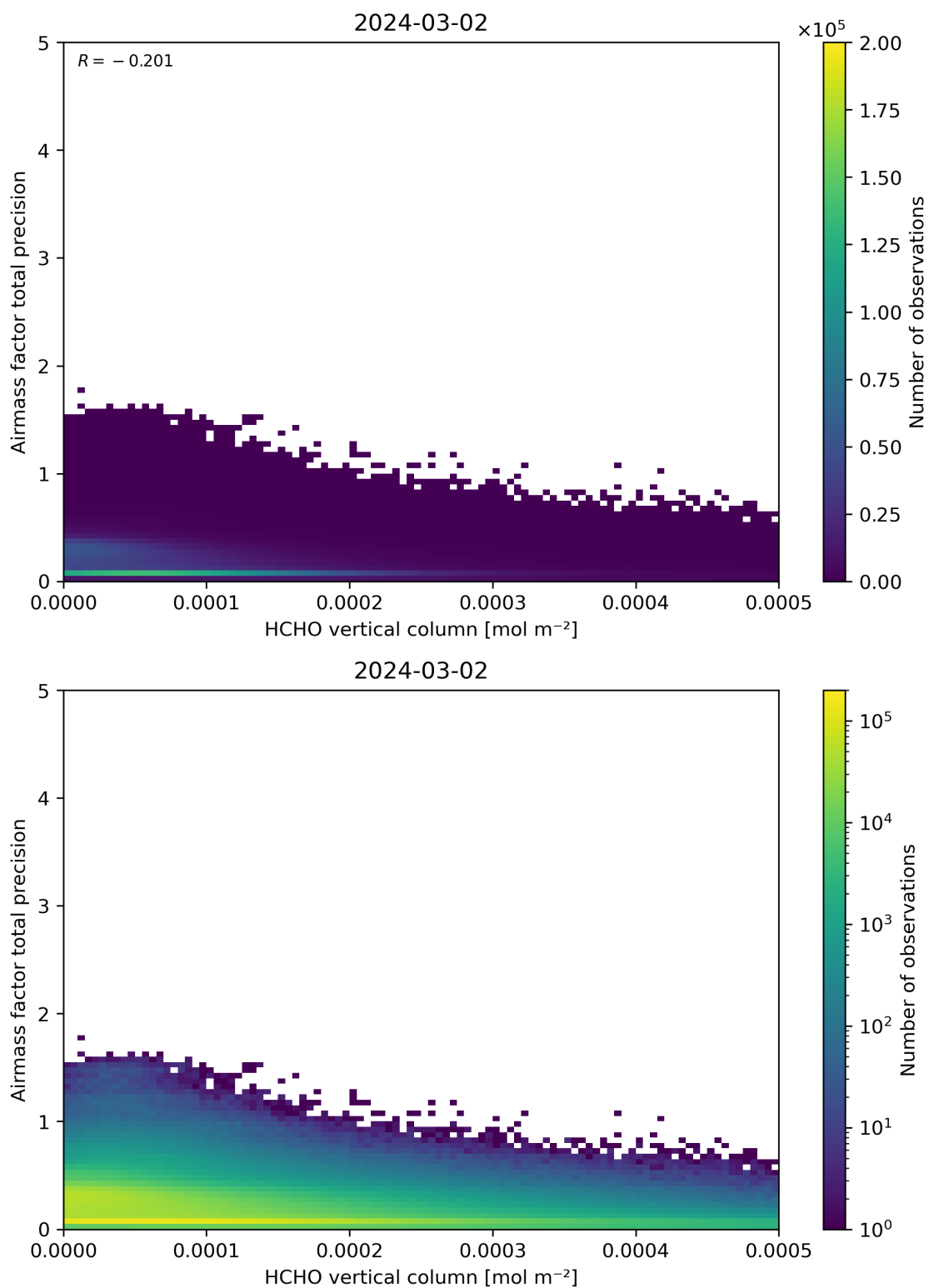
Figure 132: Scatter density plot of “HCHO vertical column” against “Airmass factor total precision” for 2024-03-01 to 2024-03-03.
