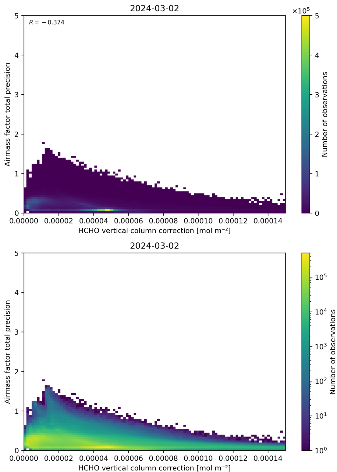
Figure 121: Scatter density plot of “HCHO vertical column correction” against “Airmass factor total precision” for 2024-03-01 to 2024-03-03.
