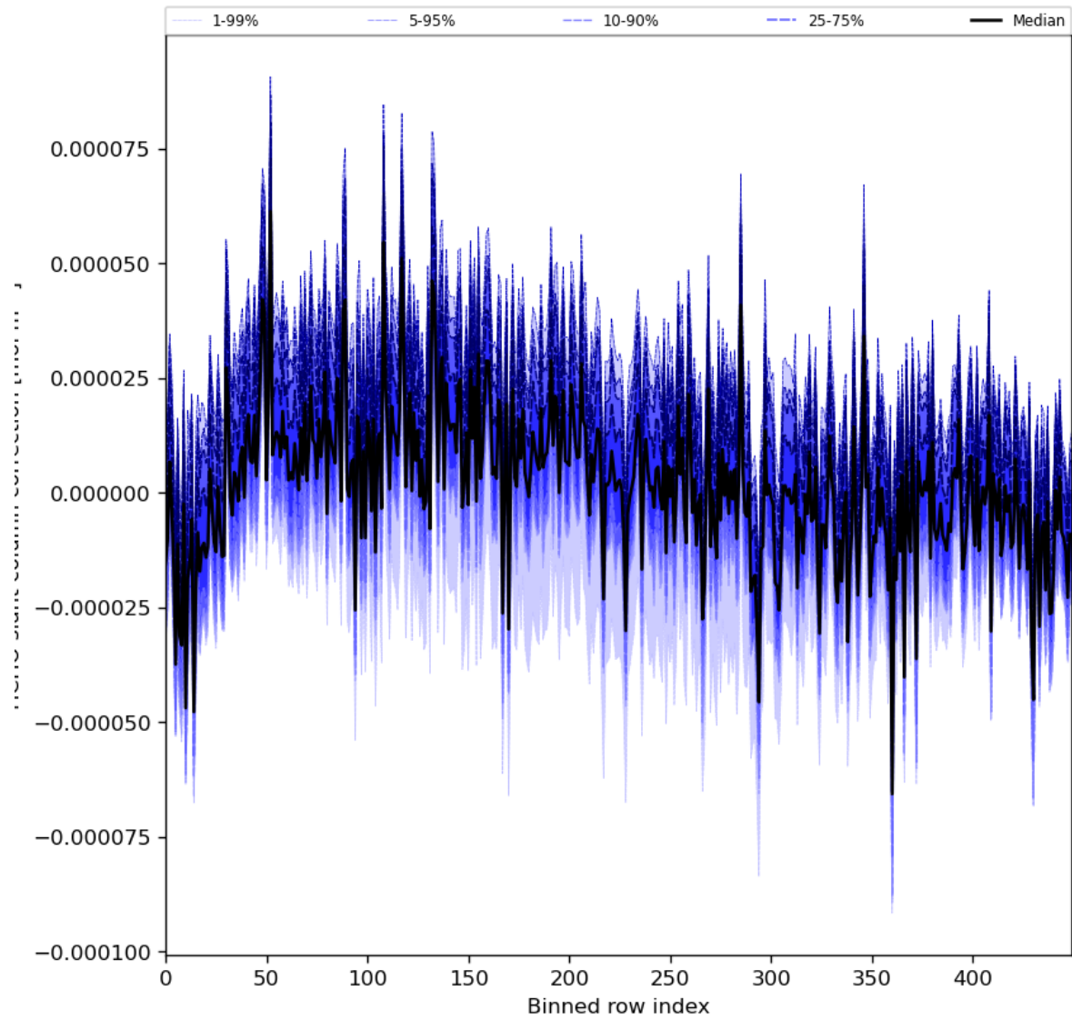
Figure 61: Along track statistics of “HCHO slant column correction” for 2024-03-01 to 2024-03-03
