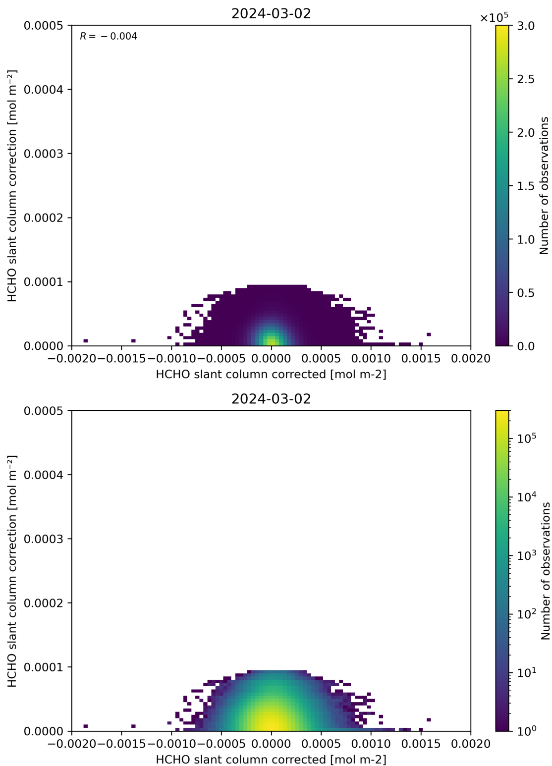
Figure 77: Scatter density plot of “HCHO slant column corrected” against “HCHO slant column correction” for 2024-03-01 to 2024-03-03.
