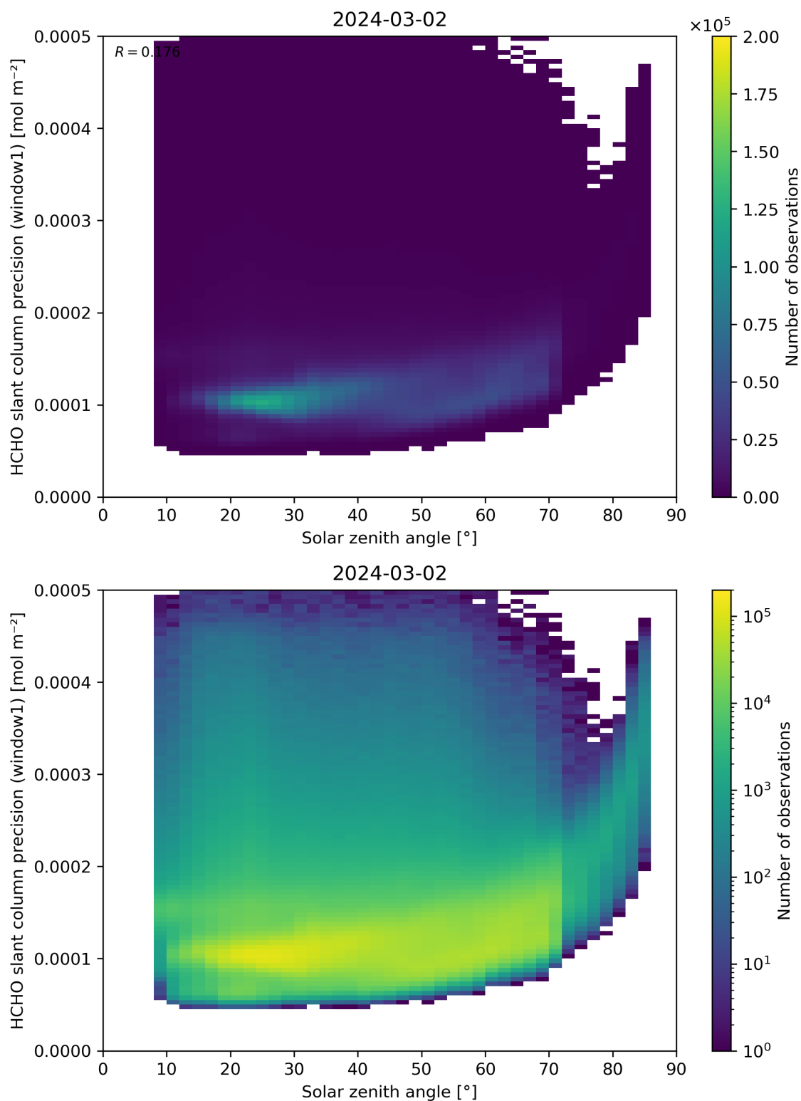
Figure 174: Scatter density plot of “Solar zenith angle” against “HCHO slant column precision (window1)” for 2024-03-01 to 2024-03-03.
