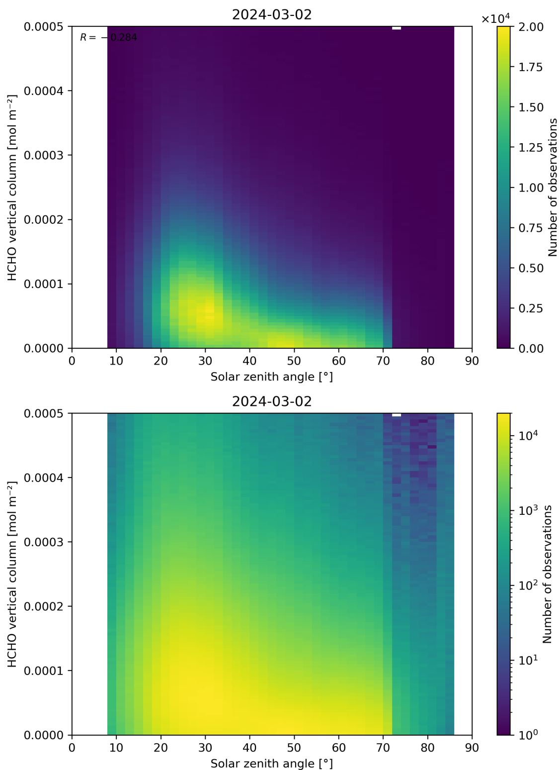
Figure 177: Scatter density plot of “Solar zenith angle” against “HCHO vertical column” for 2024-03-01 to 2024-03-03.
