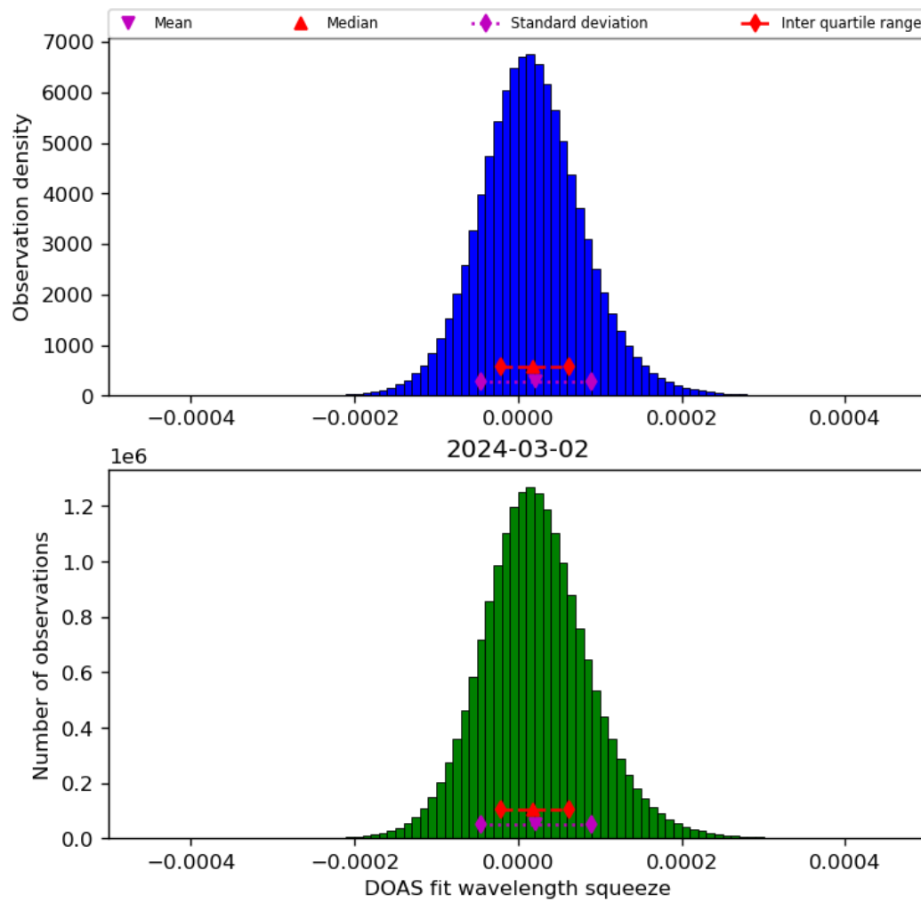
Figure 45: Histogram of “DOAS fit wavelength squeeze” for 2024-03-01 to 2024-03-03
