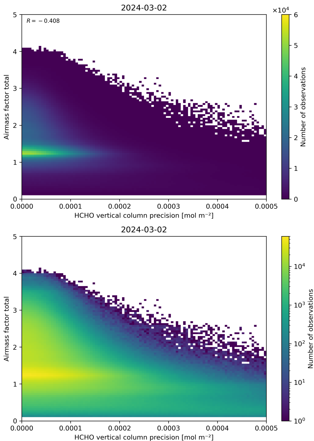
Figure 144: Scatter density plot of “HCHO vertical column precision” against “Airmass factor total” for 2024-03-01 to 2024-03-03.
