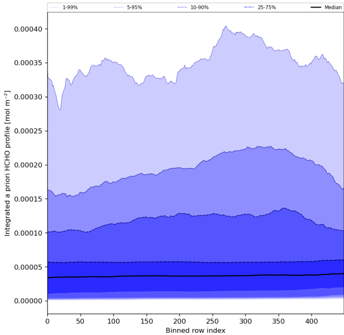
Figure 57: Along track statistics of "Integrated a priori HCHO profile" for 2024-03-01 to 2024-03-03
