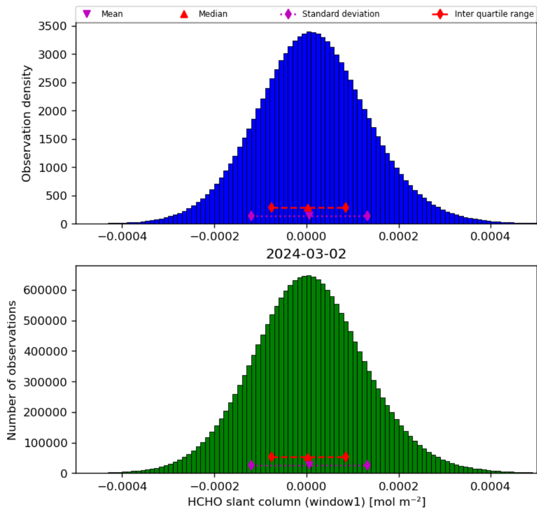
Figure 38: Histogram of “HCHO slant column (window1)” for 2024-03-01 to 2024-03-03
