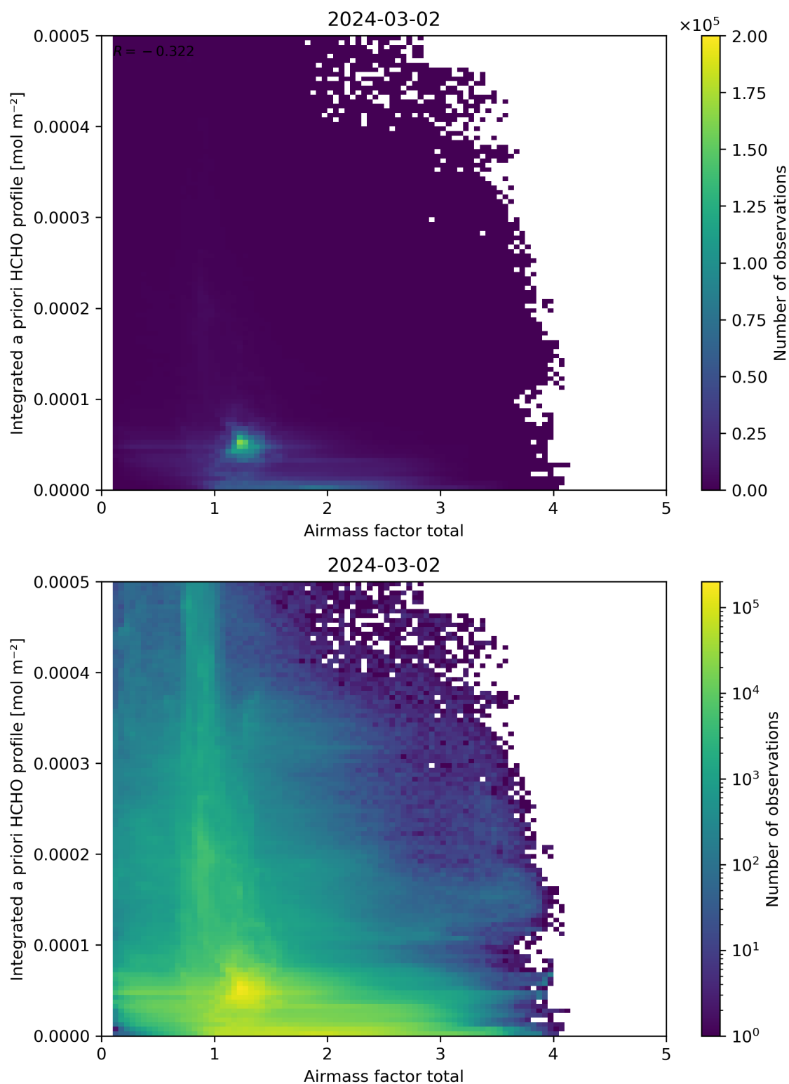
Figure 104: Scatter density plot of “Airmass factor total” against “Integrated a priori HCHO profile” for 2024-03-01 to 2024-03-03.
