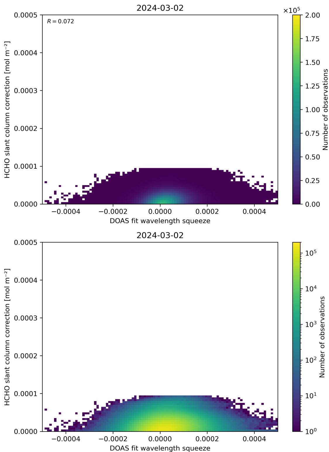
Figure 70: Scatter density plot of “DOAS fit wavelength squeeze” against “HCHO slant column correction” for 2024-03-01 to 2024-03-03.
