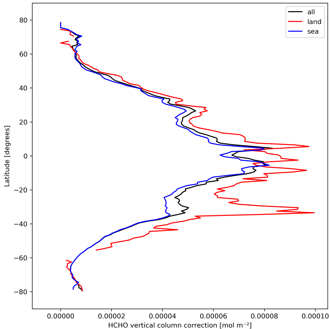
Figure 23: Zonal average of “HCHO vertical column correction” for 2024-03-01 to 2024-03-03.
