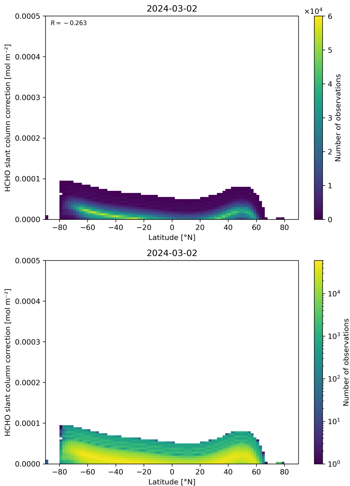
Figure 158: Scatter density plot of “Latitude” against “HCHO slant column correction” for 2024-03-01 to 2024-03-03.
