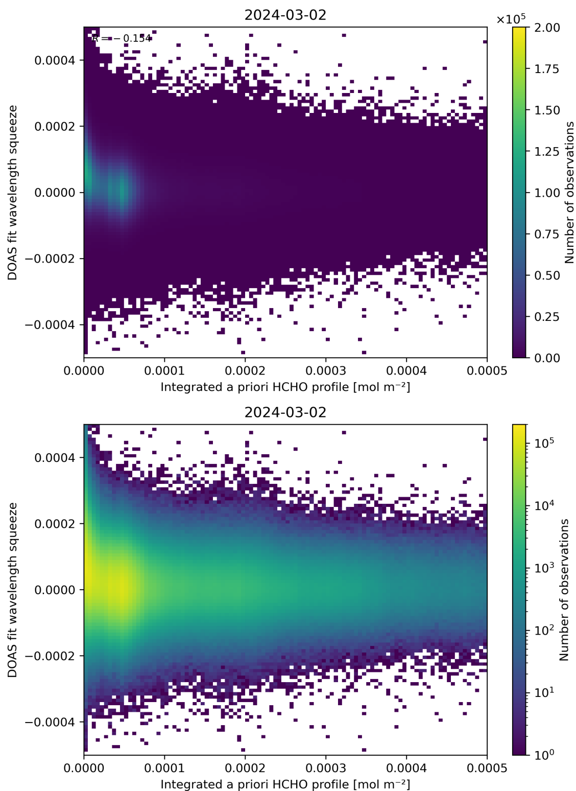
Figure 150: Scatter density plot of “Integrated a priori HCHO profile” against “DOAS fit wavelength squeeze” for 2024-03-01 to 2024-03-03.
