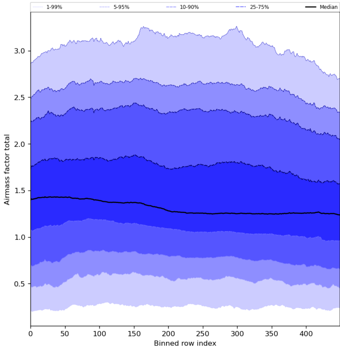
Figure 54: Along track statistics of “Airmass factor total” for 2024-03-01 to 2024-03-03
