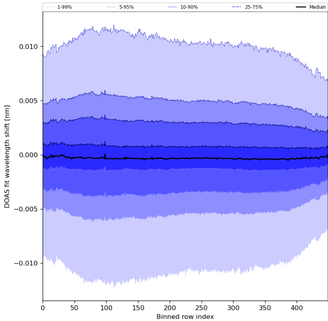
Figure 58: Along track statistics of “DOAS fit wavelength shift” for 2024-03-01 to 2024-03-03
