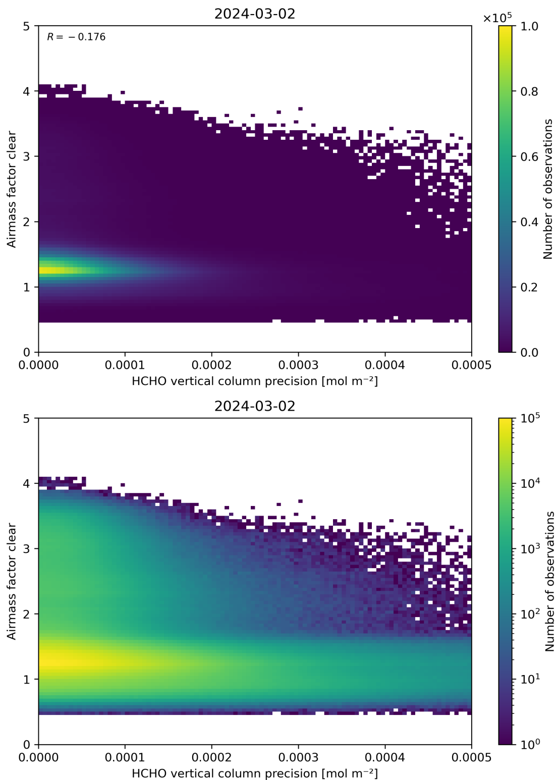
Figure 139: Scatter density plot of “HCHO vertical column precision” against “Airmass factor clear” for 2024-03-01 to 2024-03-03.
