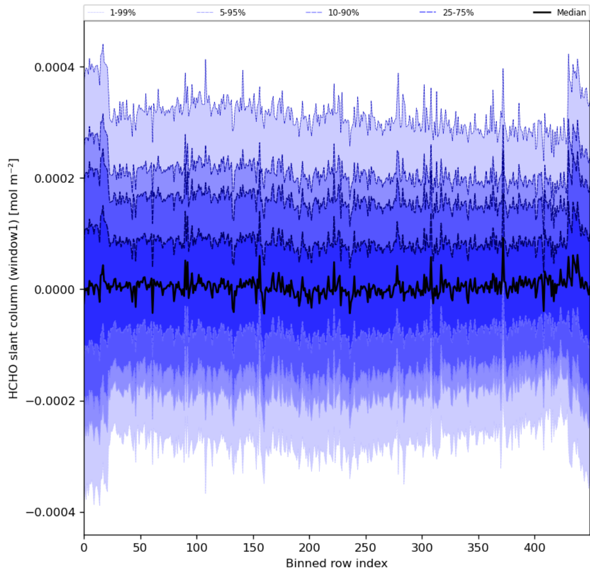
Figure 52: Along track statistics of “HCHO slant column (window1)” for 2024-03-01 to 2024-03-03
