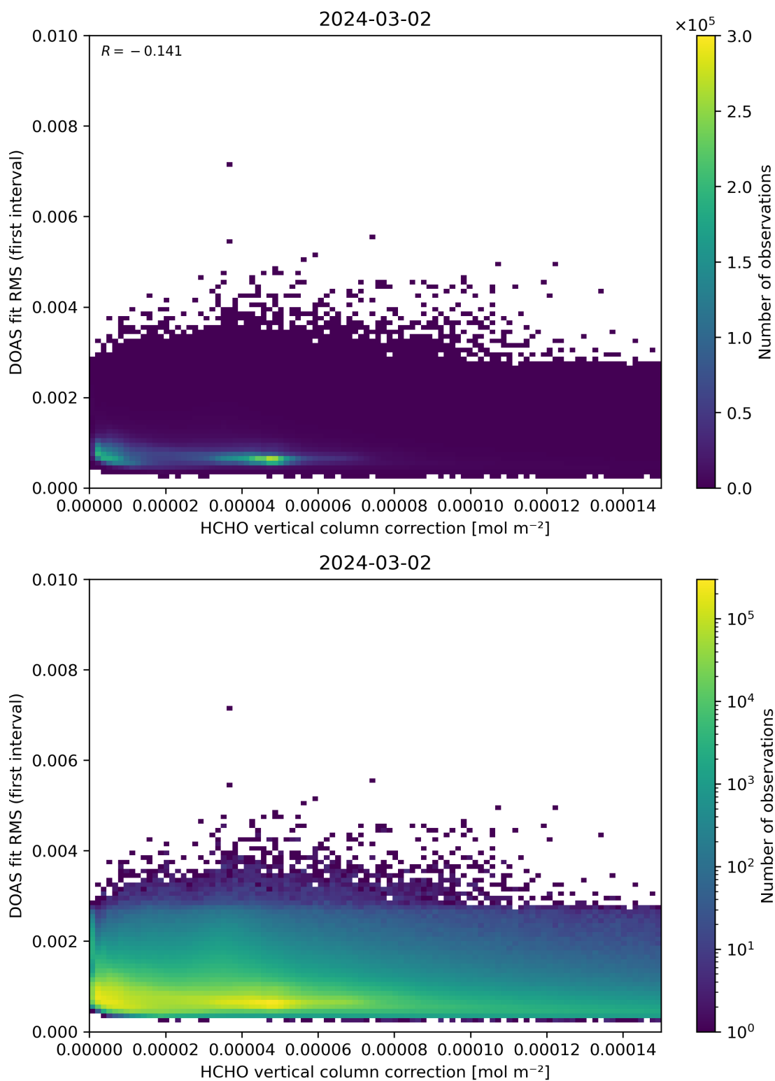
Figure 112: Scatter density plot of “HCHO vertical column correction” against “DOAS fit RMS (first interval)” for 2024-03-01 to 2024-03-03.
