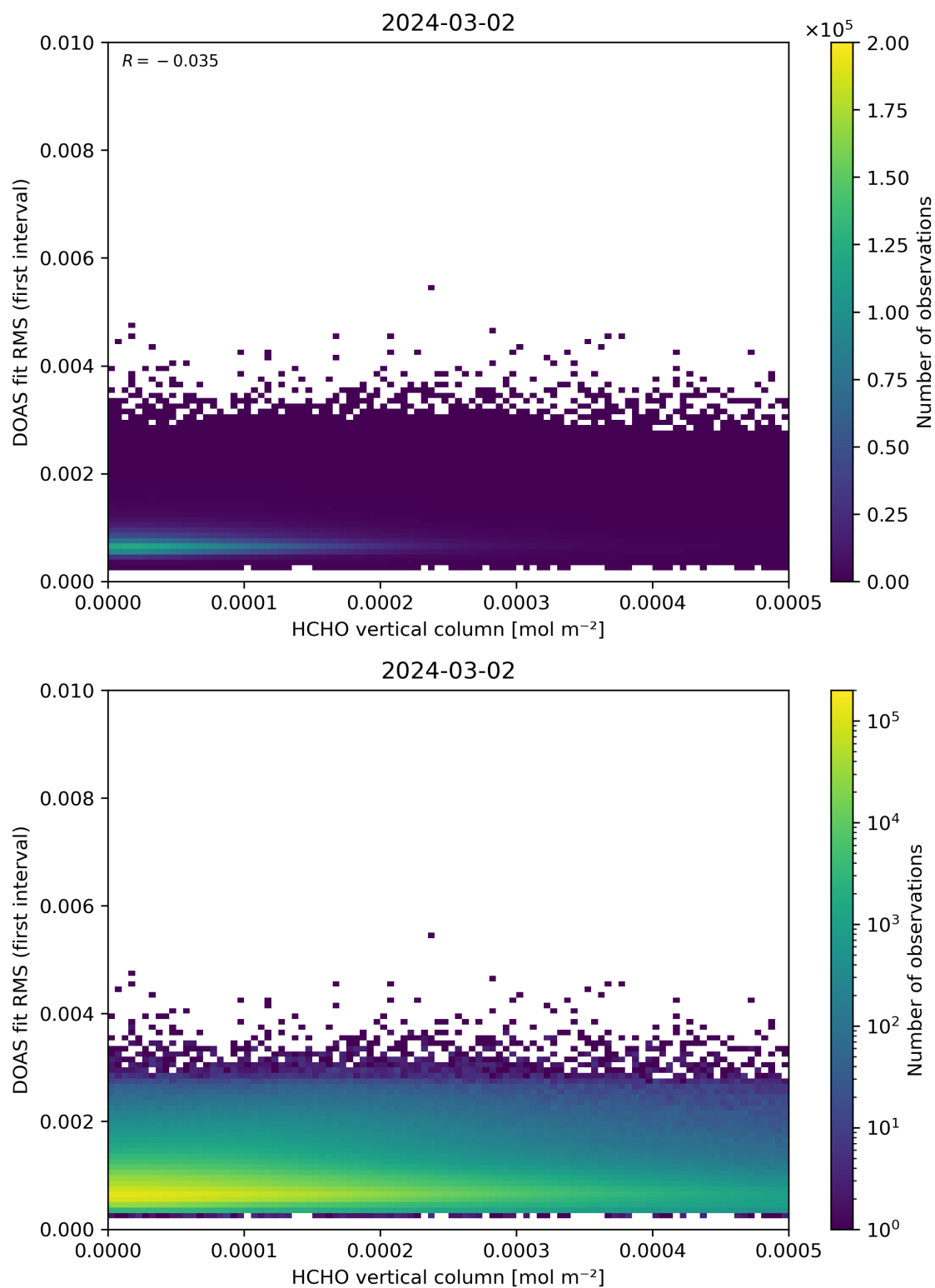
Figure 123: Scatter density plot of “HCHO vertical column” against “DOAS fit RMS (first interval)” for 2024-03-01 to 2024-03-03.
