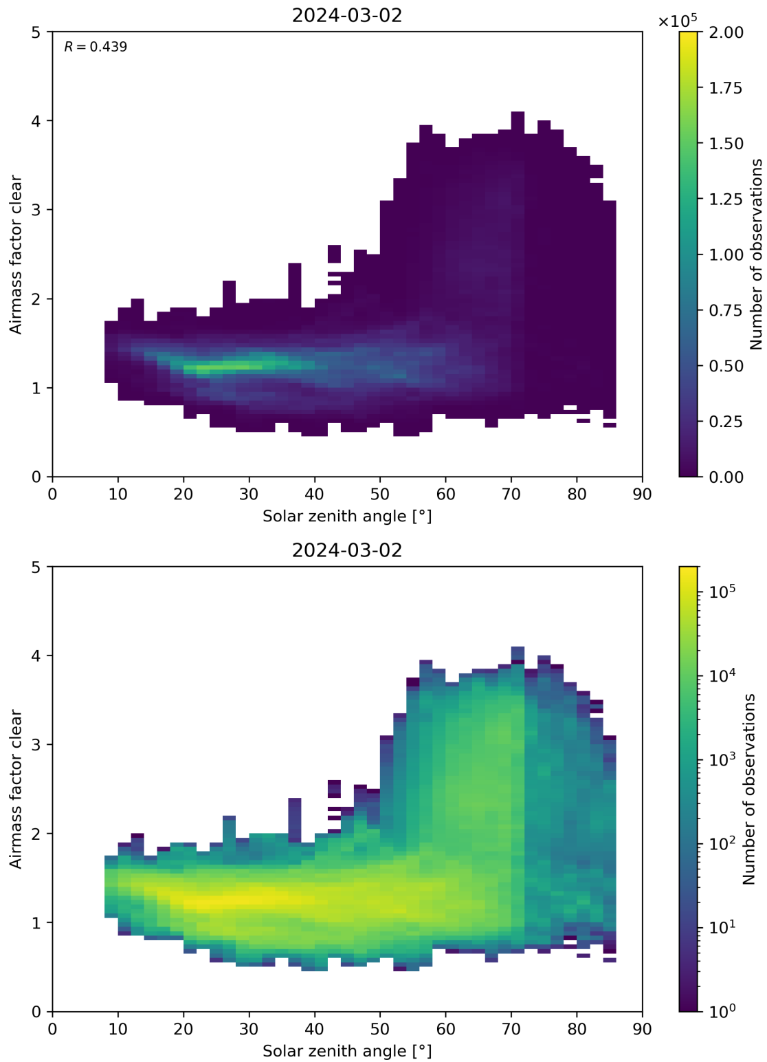
Figure 170: Scatter density plot of “Solar zenith angle” against “Airmass factor clear” for 2024-03-01 to 2024-03-03.
