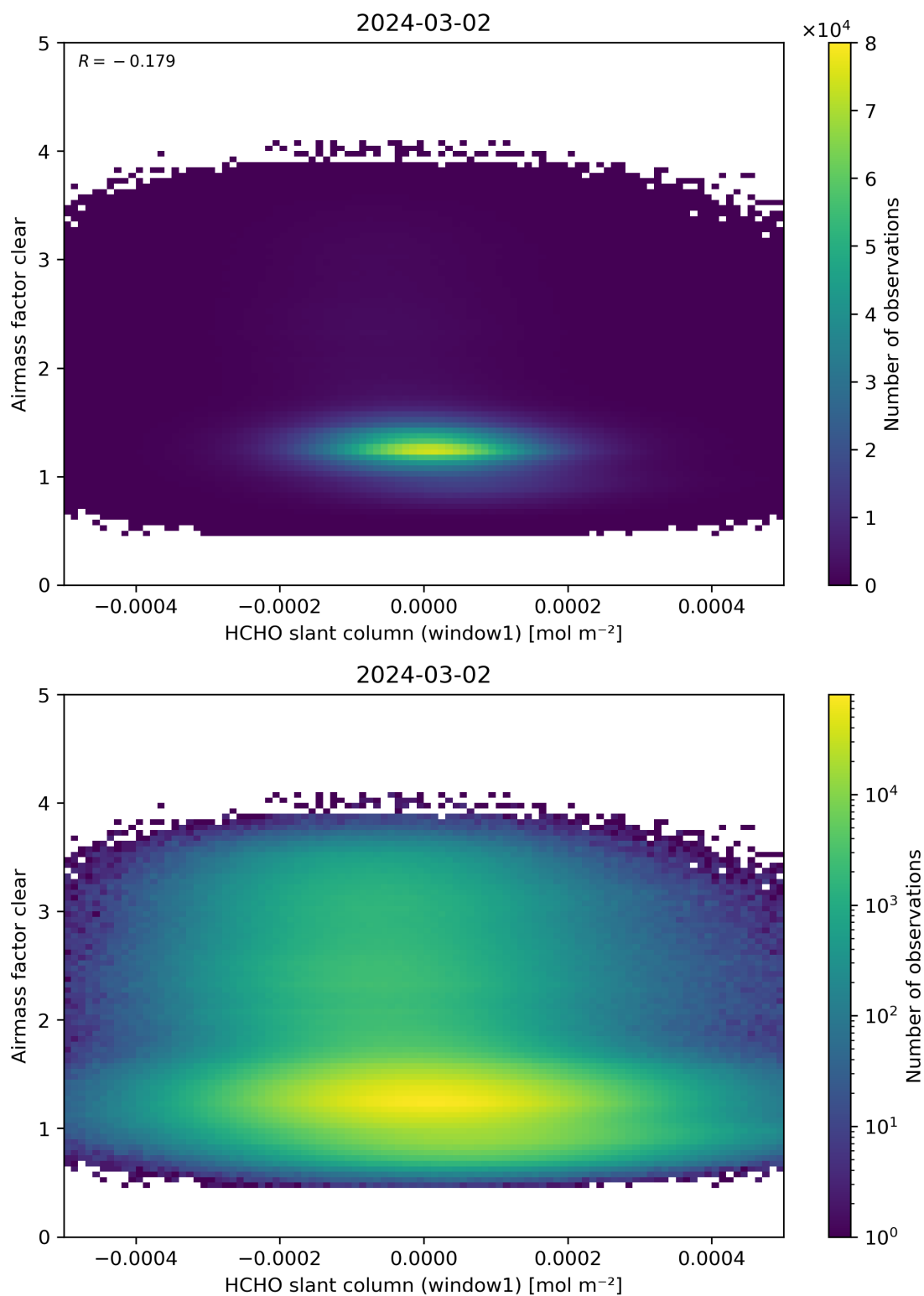
Figure 81: Scatter density plot of “HCHO slant column (window1)” against “Airmass factor clear” for 2024-03-01 to 2024-03-03.
