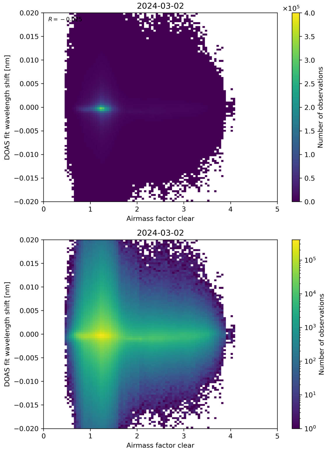
Figure 72: Scatter density plot of “Airmass factor clear” against “DOAS fit wavelength shift” for 2024-03-01 to 2024-03-03.
