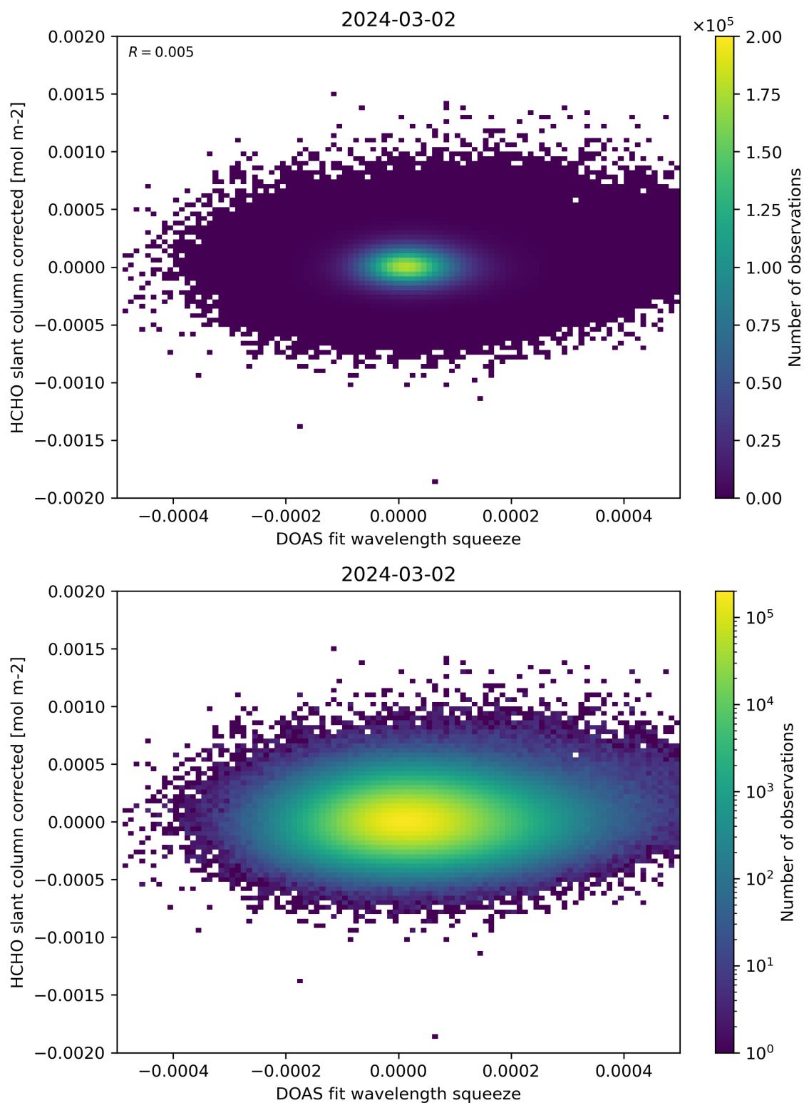
Figure 69: Scatter density plot of “DOAS fit wavelength squeeze” against “HCHO slant column corrected” for 2024-03-01 to 2024-03-03.
