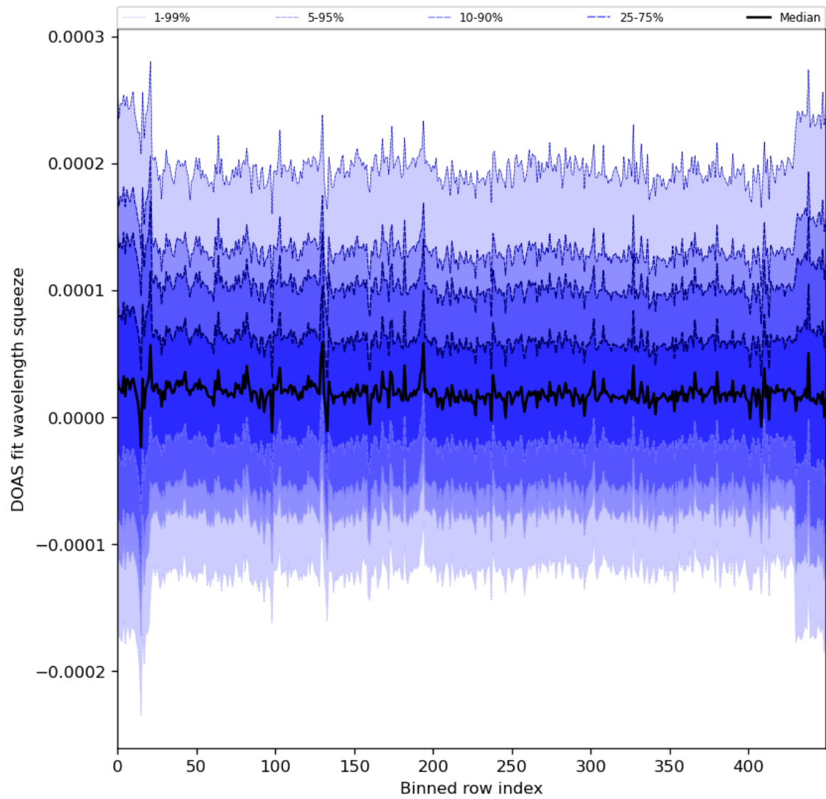
Figure 59: Along track statistics of “DOAS fit wavelength squeeze” for 2024-03-01 to 2024-03-03
