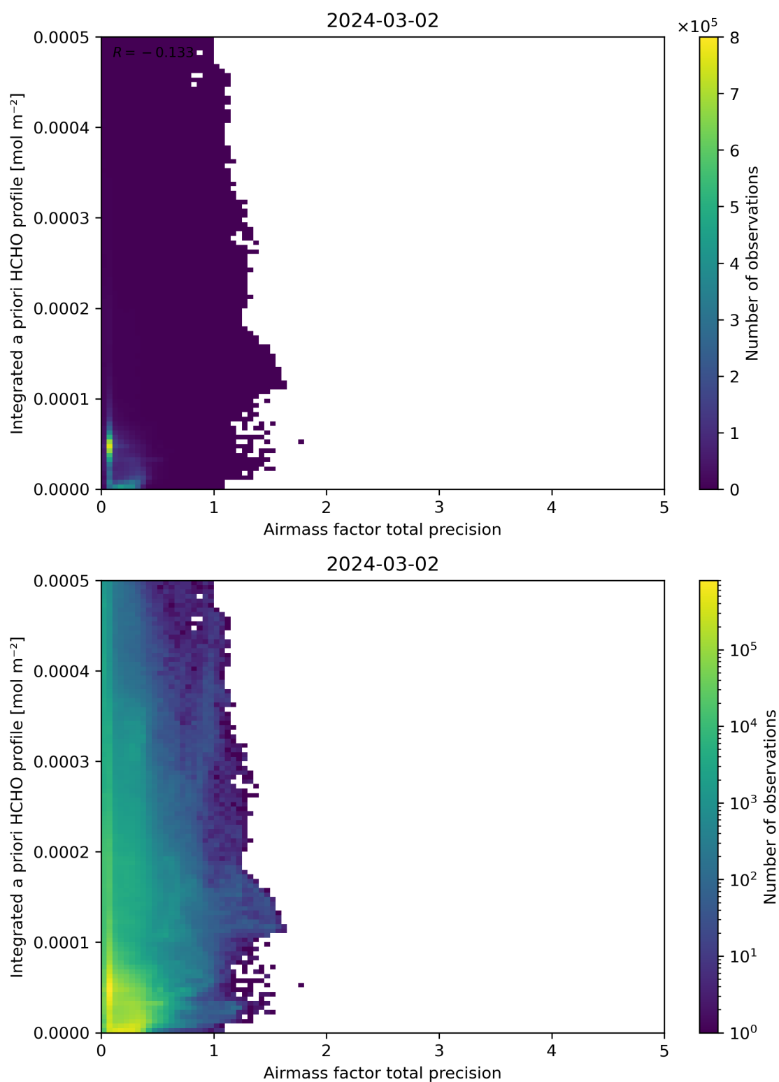
Figure 111: Scatter density plot of “Airmass factor total precision” against “Integrated a priori HCHO profile” for 2024-03-01 to 2024-03-03.
