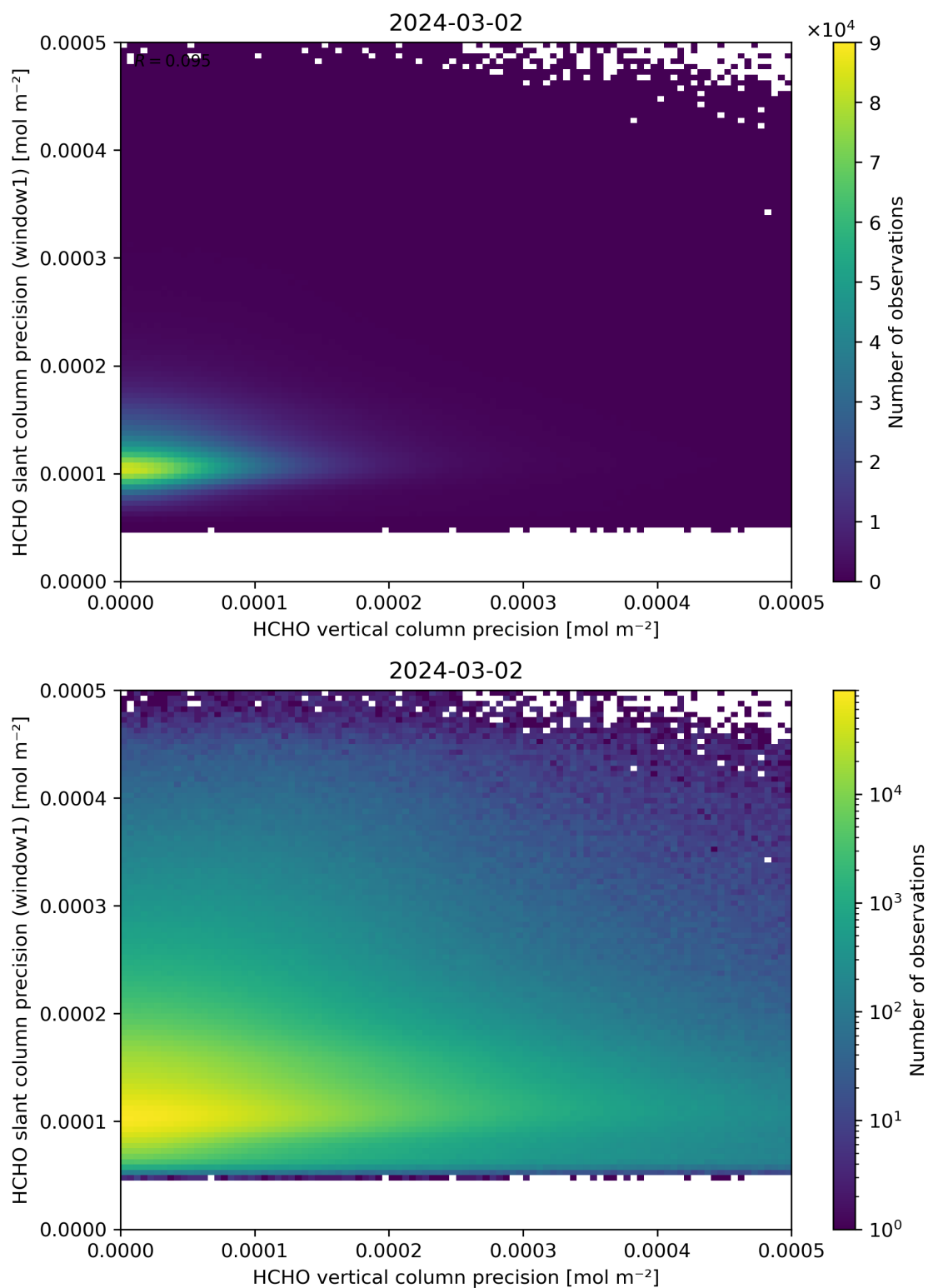
Figure 143: Scatter density plot of “HCHO vertical column precision” against “HCHO slant column precision (window1)” for 2024-03-01 to 2024-03-03.
