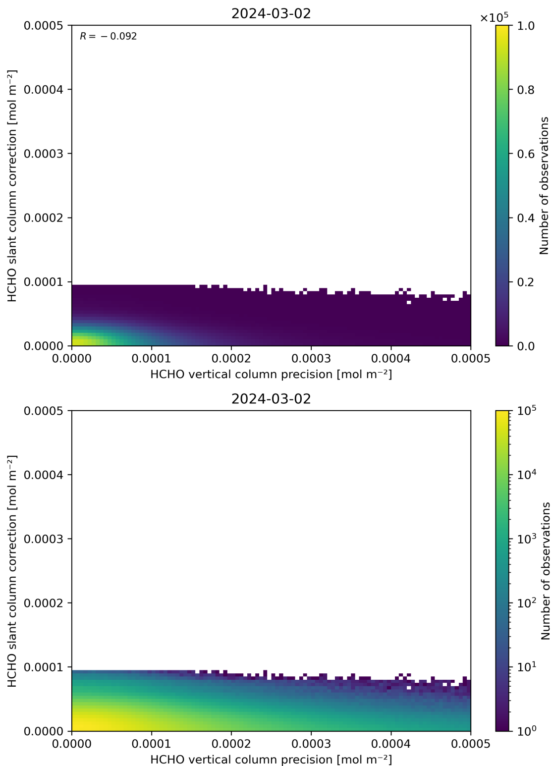
Figure 141: Scatter density plot of “HCHO vertical column precision” against “HCHO slant column correction” for 2024-03-01 to 2024-03-03.
