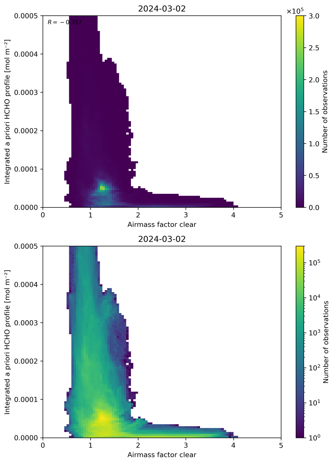
Figure 76: Scatter density plot of “Airmass factor clear” against “Integrated a priori HCHO profile” for 2024-03-01 to 2024-03-03.
