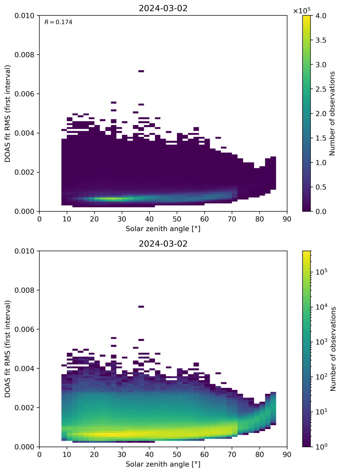
Figure 167: Scatter density plot of “Solar zenith angle” against “DOAS fit RMS (first interval)” for 2024-03-01 to 2024-03-03.
