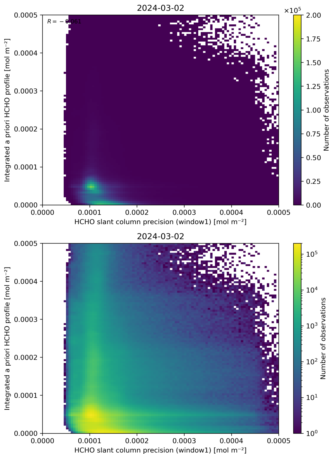
Figure 96: Scatter density plot of “HCHO slant column precision (window1)” against “Integrated a priori HCHO profile” for 2024-03-01 to 2024-03-03.
