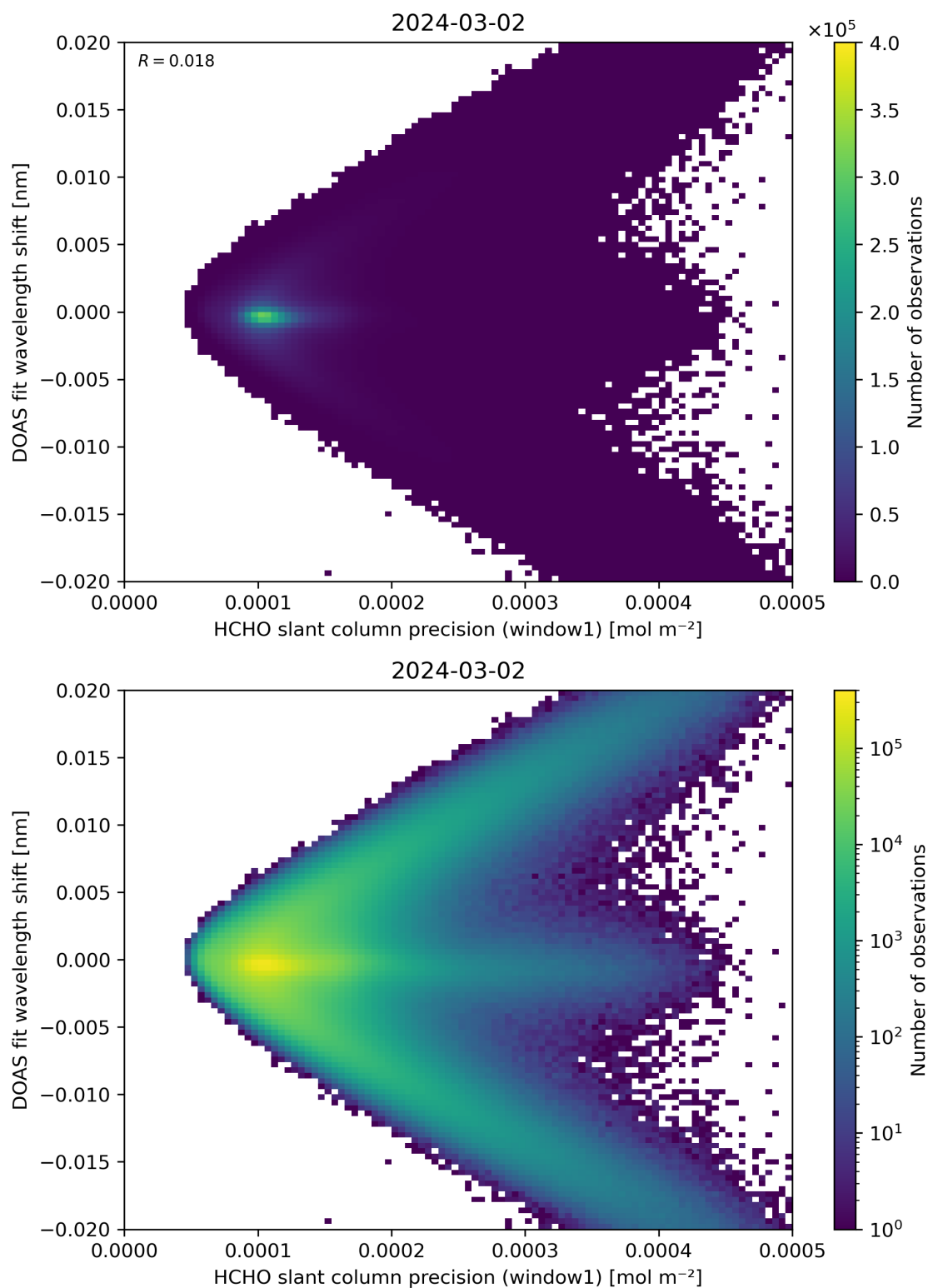
Figure 89: Scatter density plot of “HCHO slant column precision (window1)” against “DOAS fit wavelength shift” for 2024-03-01 to 2024-03-03.
