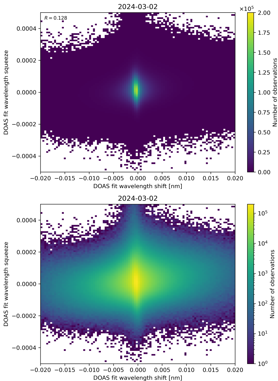
Figure 65: Scatter density plot of “DOAS fit wavelength shift” against “DOAS fit wavelength squeeze” for 2024-03-01 to 2024-03-03.
