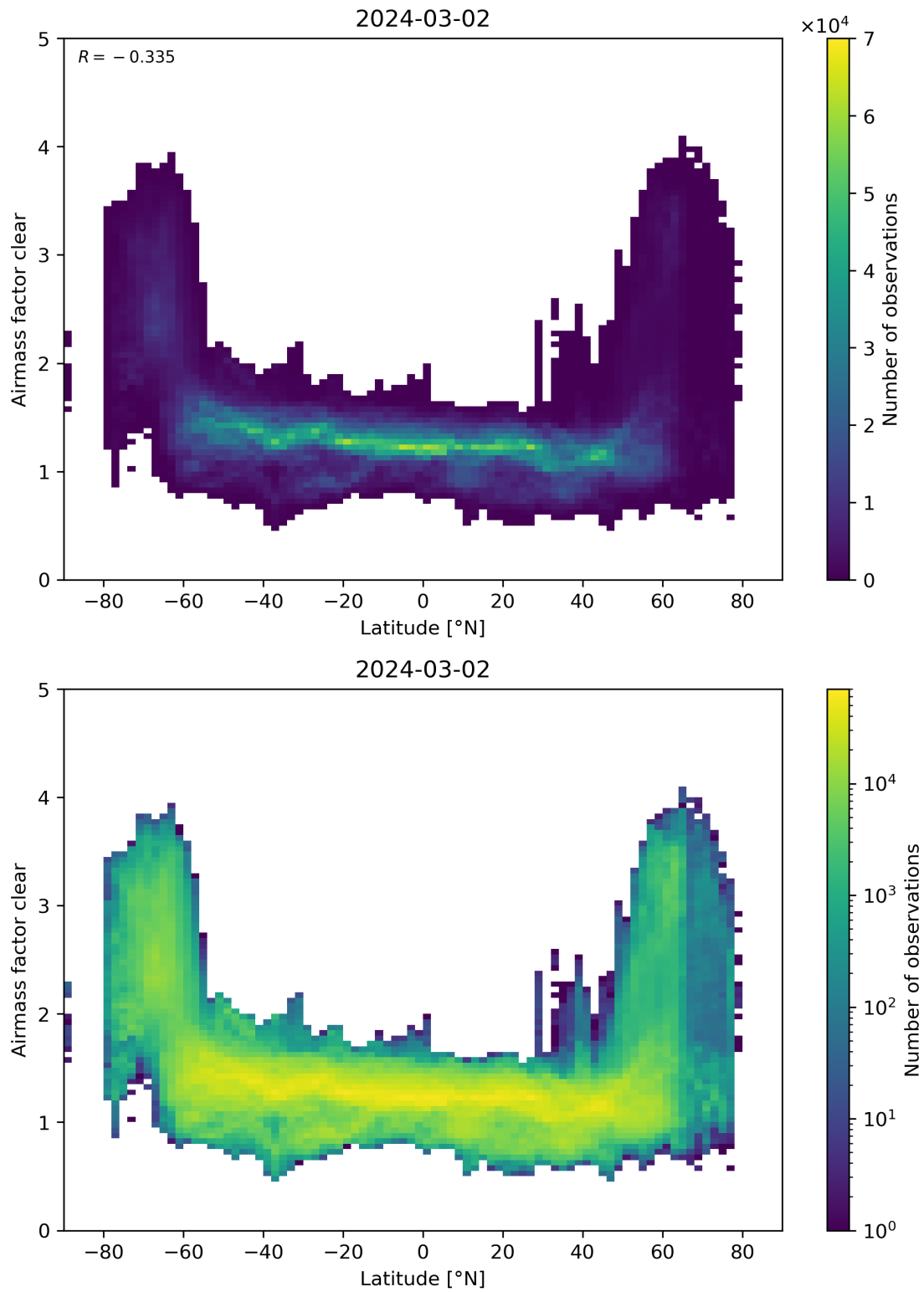
Figure 156: Scatter density plot of “Latitude” against “Airmass factor clear” for 2024-03-01 to 2024-03-03.
