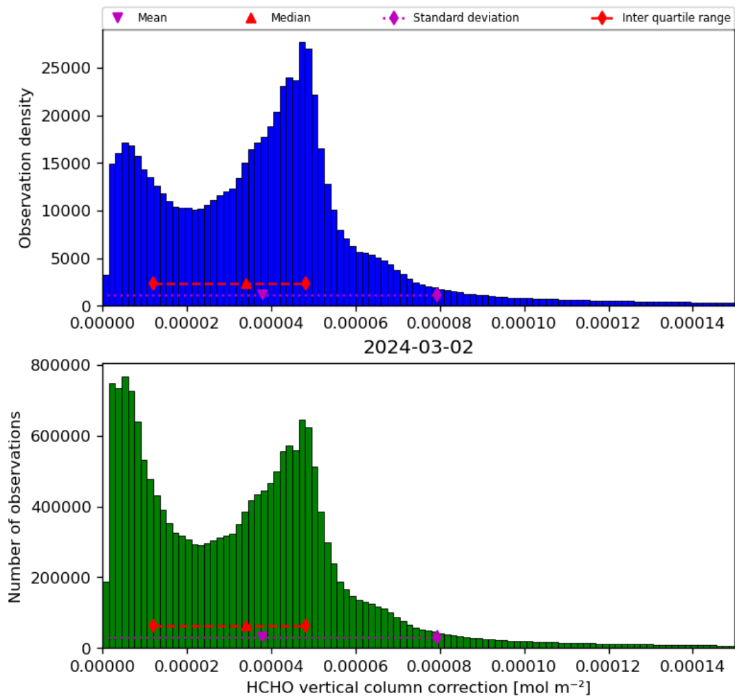
Figure 37: Histogram of “HCHO vertical column correction” for 2024-03-01 to 2024-03-03
