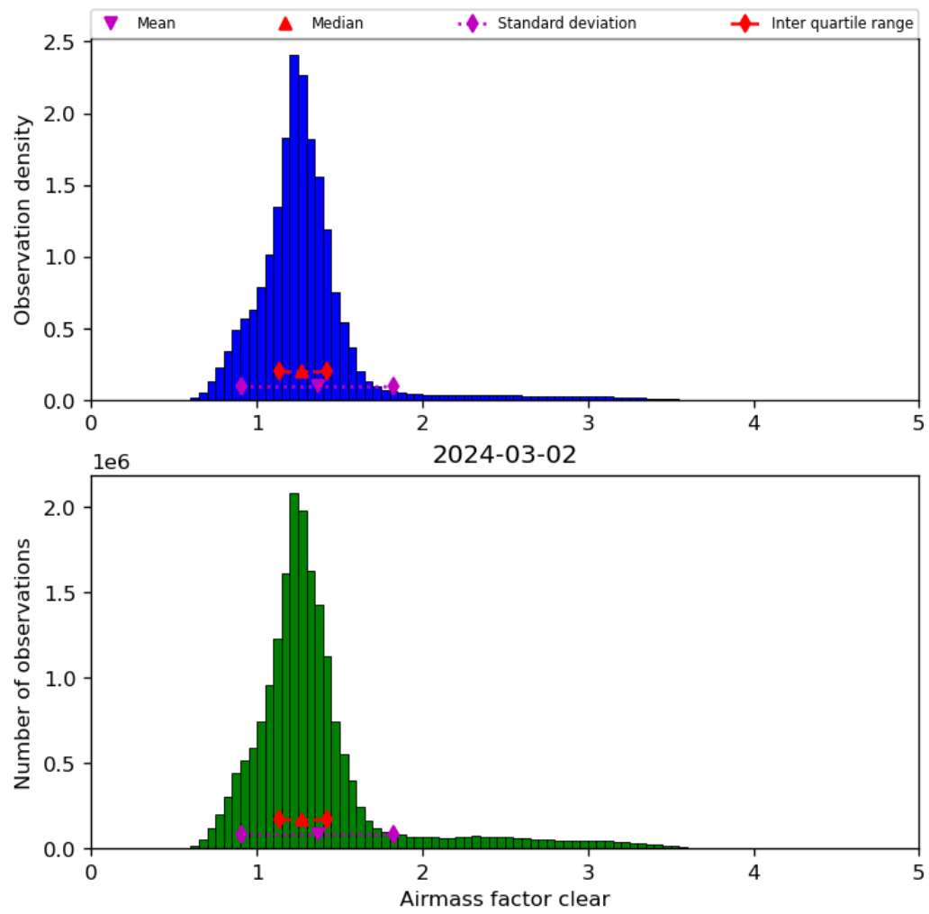
Figure 42: Histogram of “Airmass factor clear” for 2024-03-01 to 2024-03-03
