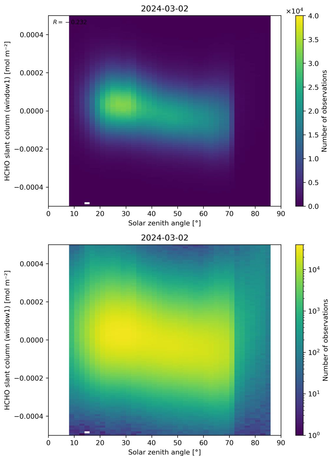
Figure 173: Scatter density plot of “Solar zenith angle” against “HCHO slant column (window1)” for 2024-03-01 to 2024-03-03.
