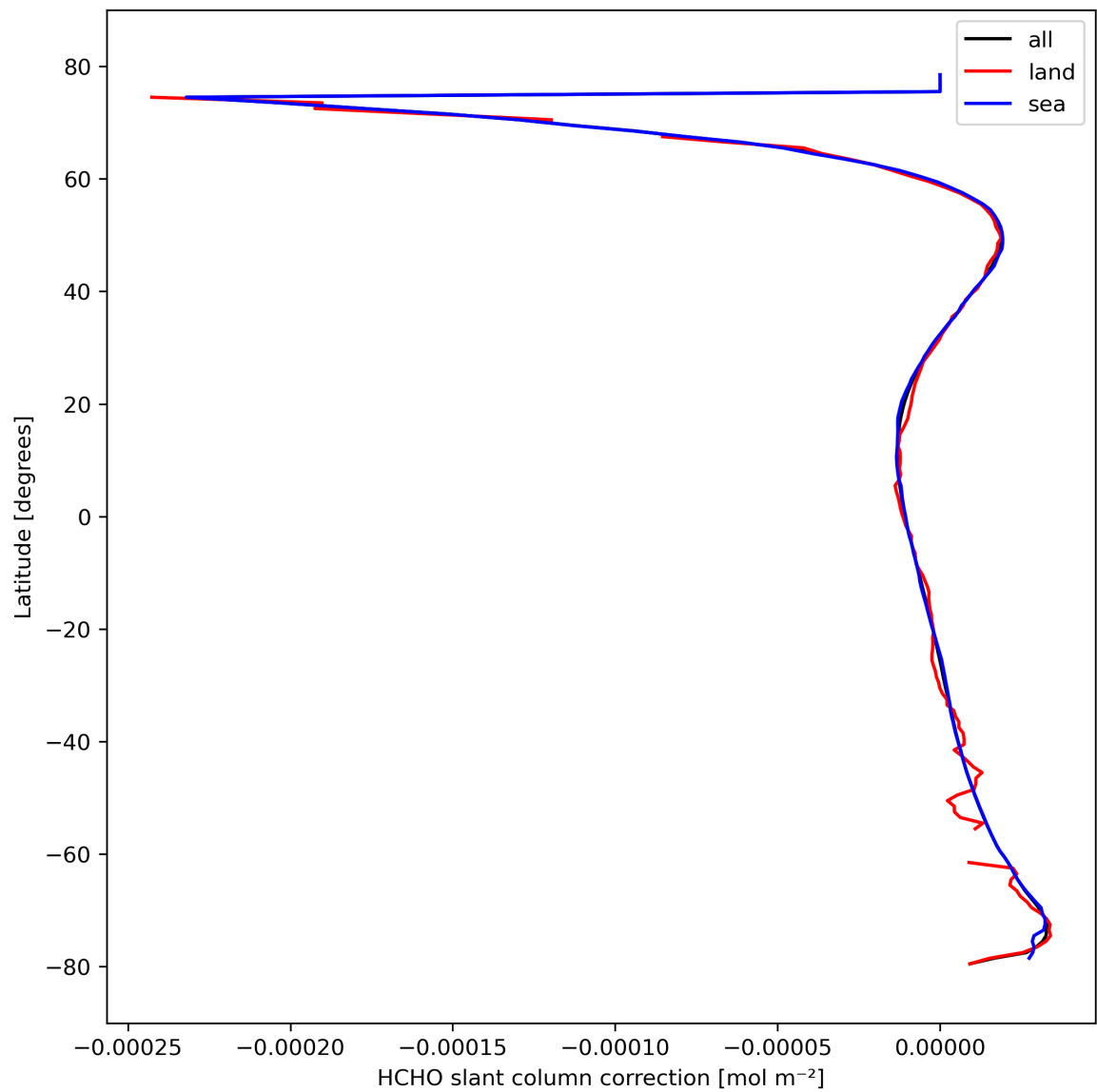
Figure 33: Zonal average of “HCHO slant column correction” for 2024-03-01 to 2024-03-03.
