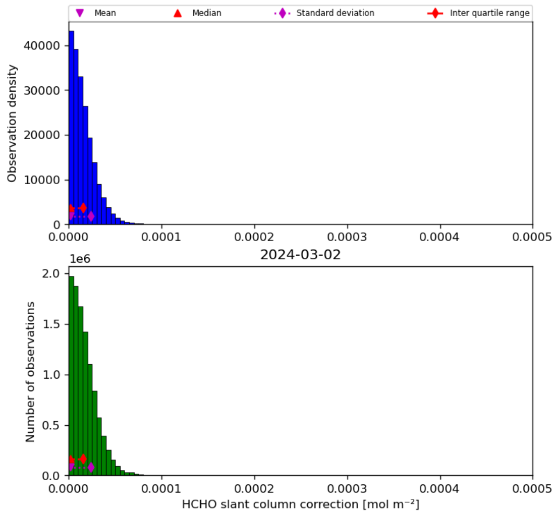
Figure 47: Histogram of “HCHO slant column correction” for 2024-03-01 to 2024-03-03
