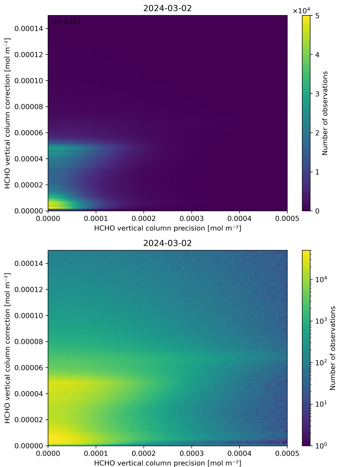
Figure 146: Scatter density plot of “HCHO vertical column precision” against “HCHO vertical column correction” for 2024-03-01 to 2024-03-03.
