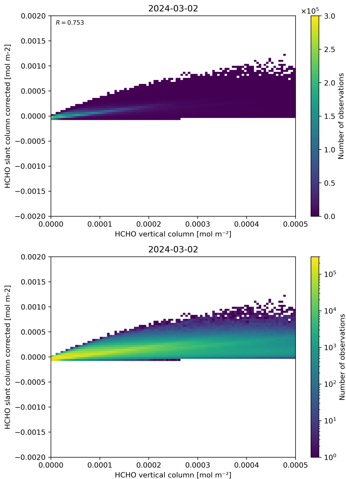
Figure 127: Scatter density plot of “HCHO vertical column” against “HCHO slant column corrected” for 2024-03-01 to 2024-03-03.
