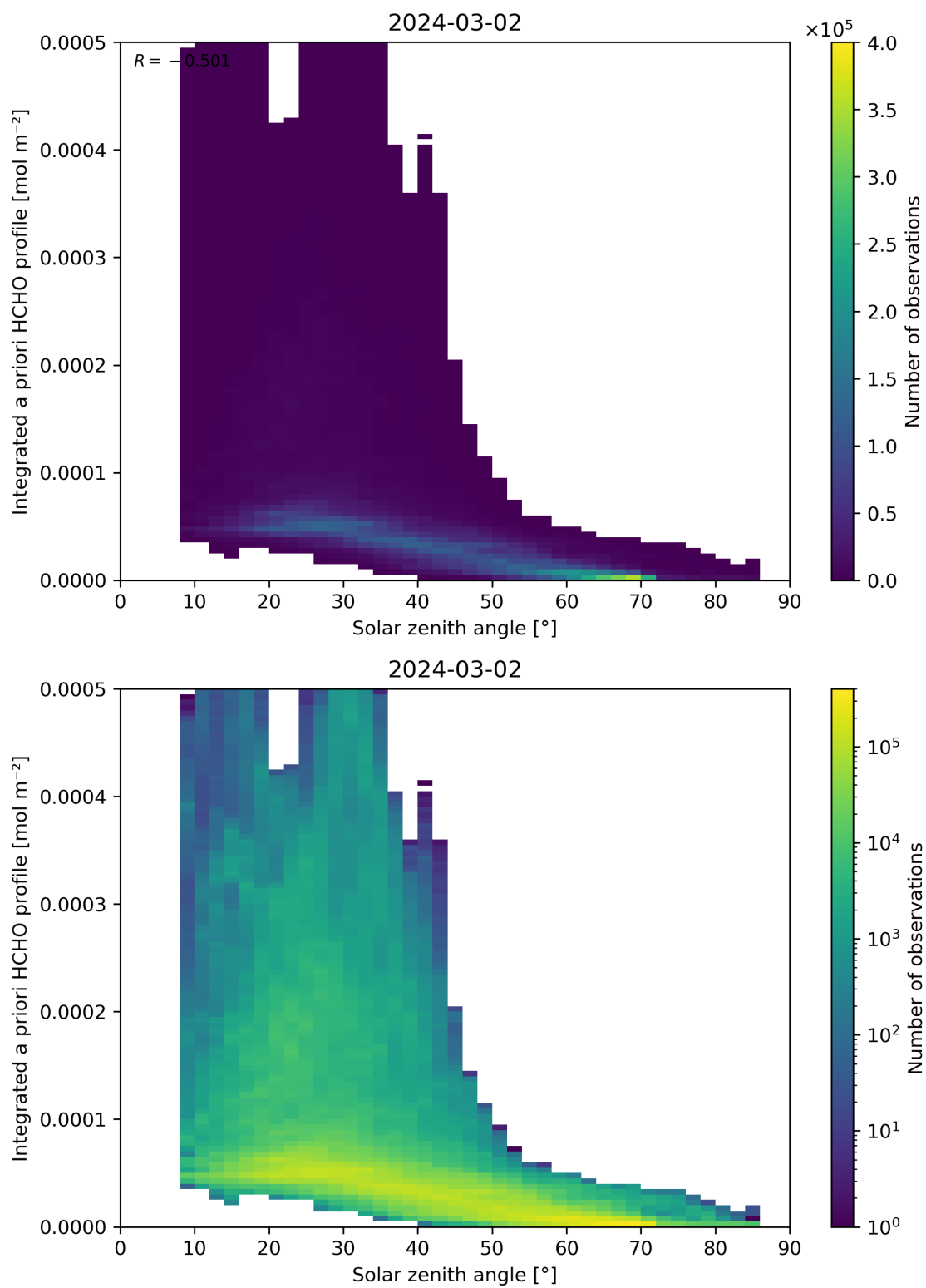
Figure 180: Scatter density plot of “Solar zenith angle” against “Integrated a priori HCHO profile” for 2024-03-01 to 2024-03-03.
