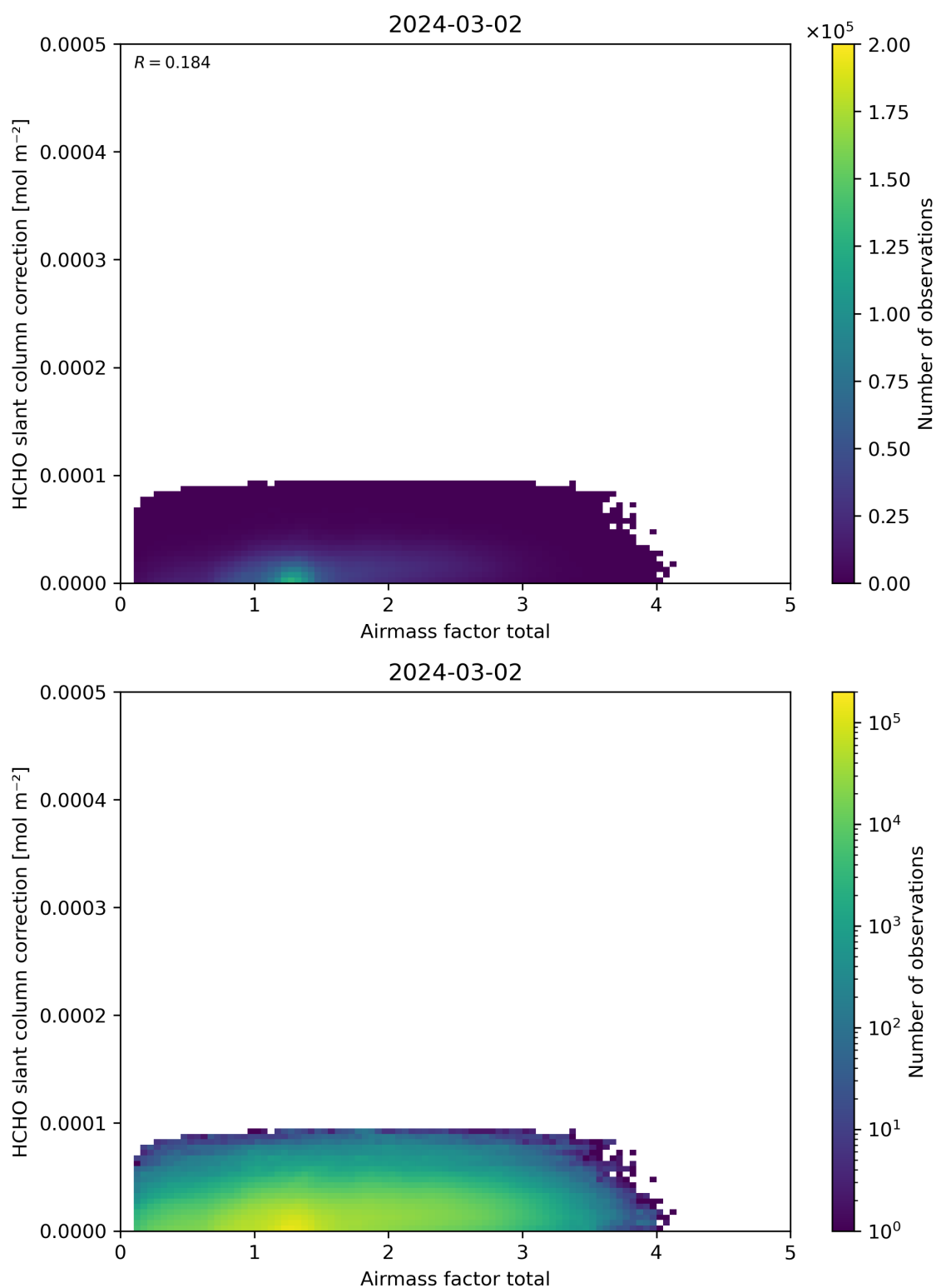
Figure 102: Scatter density plot of “Airmass factor total” against “HCHO slant column correction” for 2024-03-01 to 2024-03-03.
