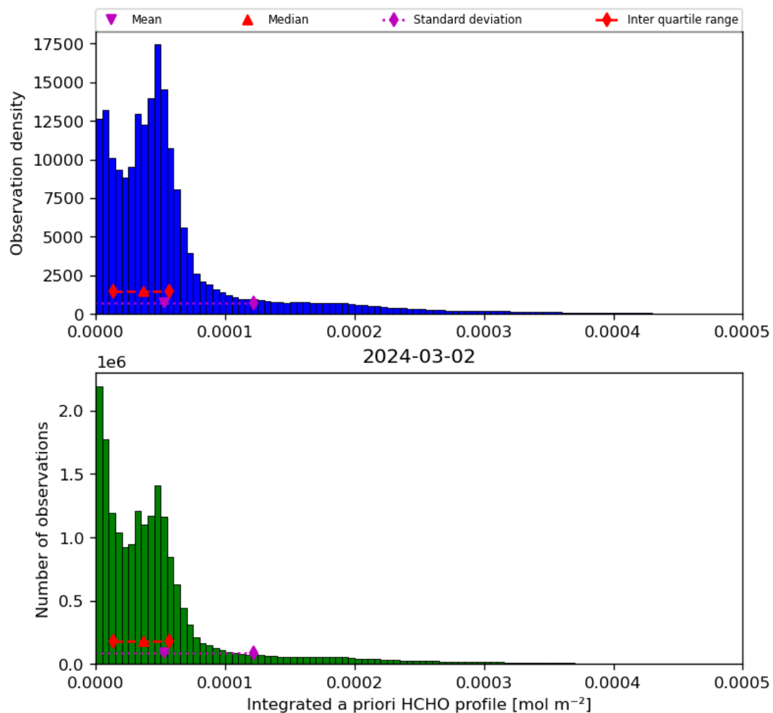
Figure 43: Histogram of “Integrated a priori HCHO profile” for 2024-03-01 to 2024-03-03
