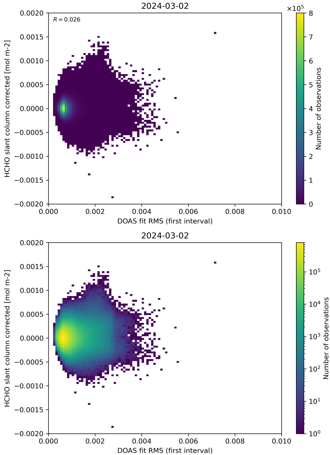
Figure 62: Scatter density plot of “DOAS fit RMS (first interval)” against “HCHO slant column corrected” for 2024-03-01 to 2024-03-03.
