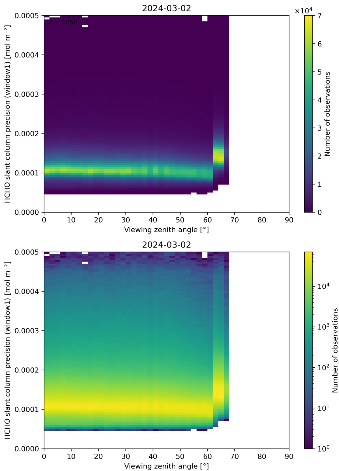
Figure 189: Scatter density plot of “Viewing zenith angle” against “HCHO slant column precision (window1)” for 2024-03-01 to 2024-03-03.
