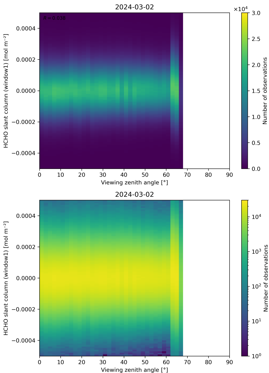
Figure 188: Scatter density plot of “Viewing zenith angle” against “HCHO slant column (window1)” for 2024-03-01 to 2024-03-03.
