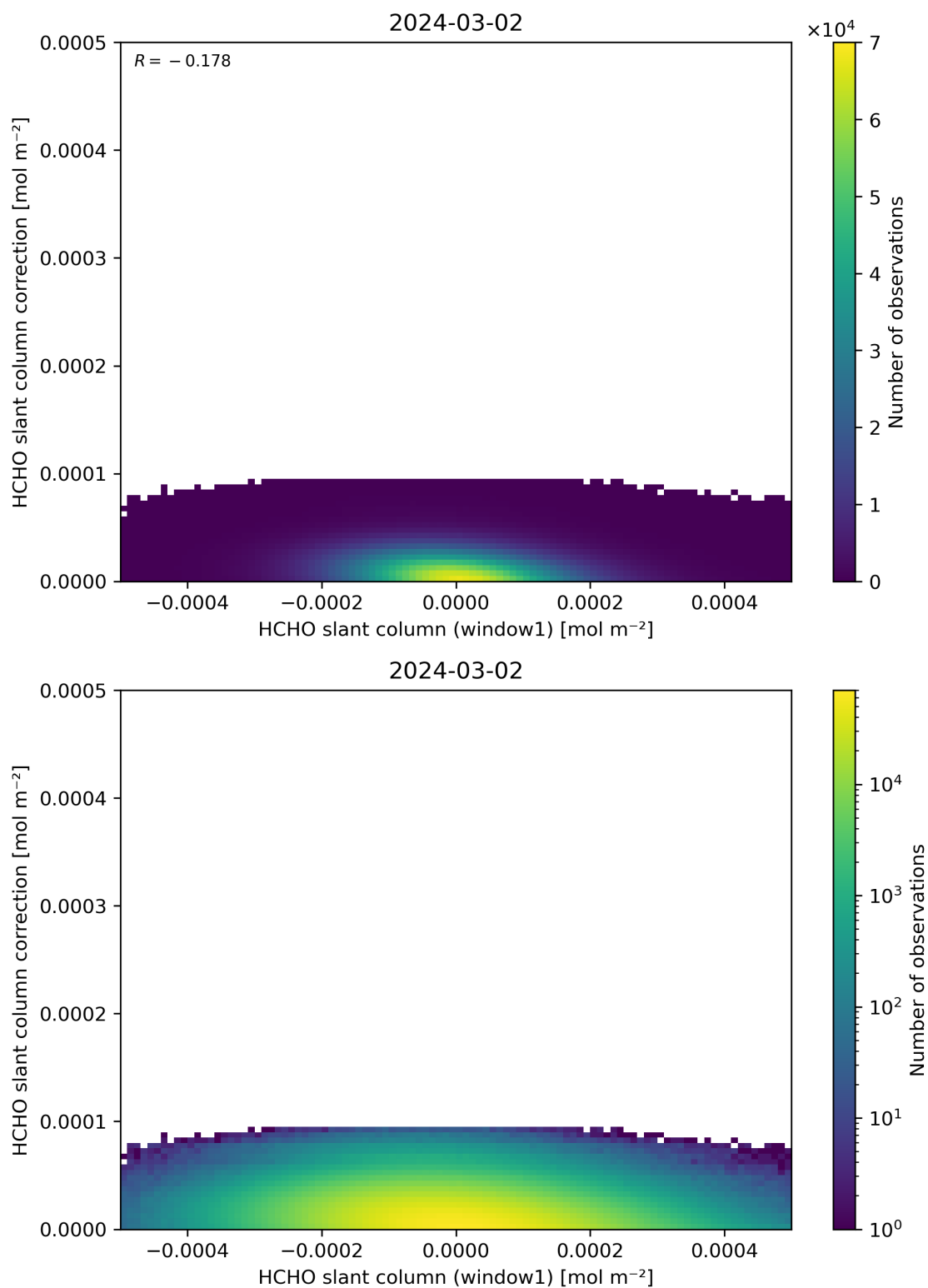
Figure 83: Scatter density plot of “HCHO slant column (window1)” against “HCHO slant column correction” for 2024-03-01 to 2024-03-03.
