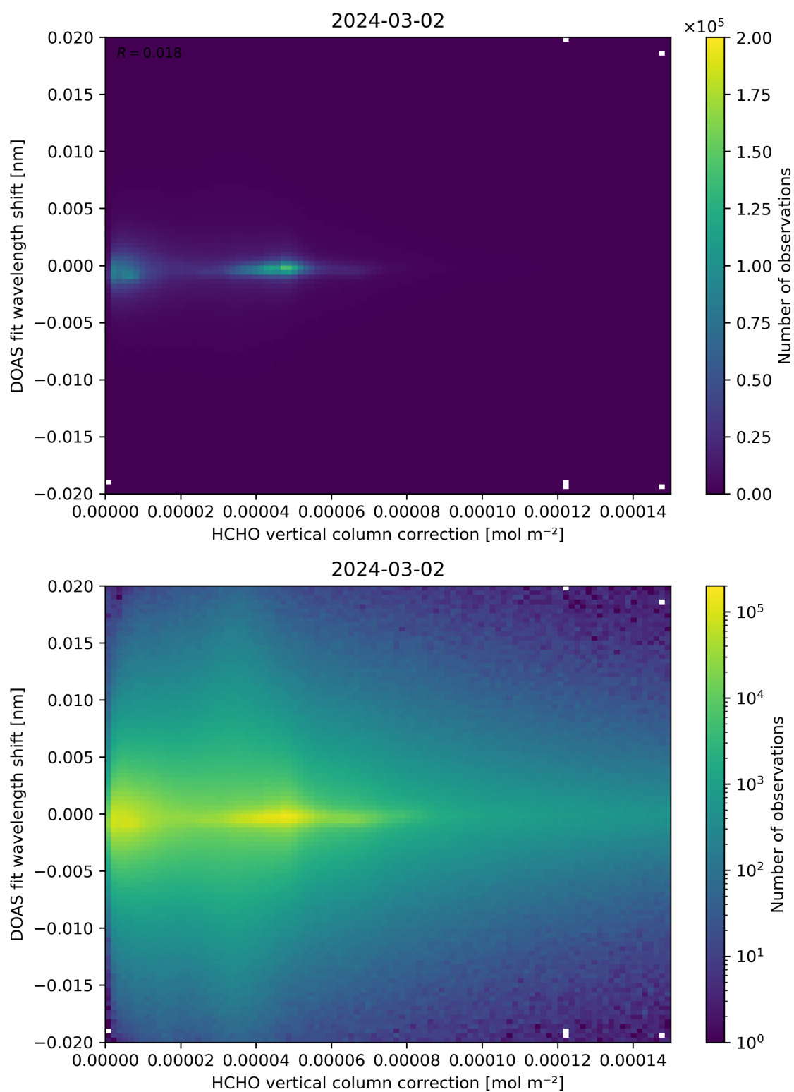
Figure 113: Scatter density plot of “HCHO vertical column correction” against “DOAS fit wavelength shift” for 2024-03-01 to 2024-03-03.
