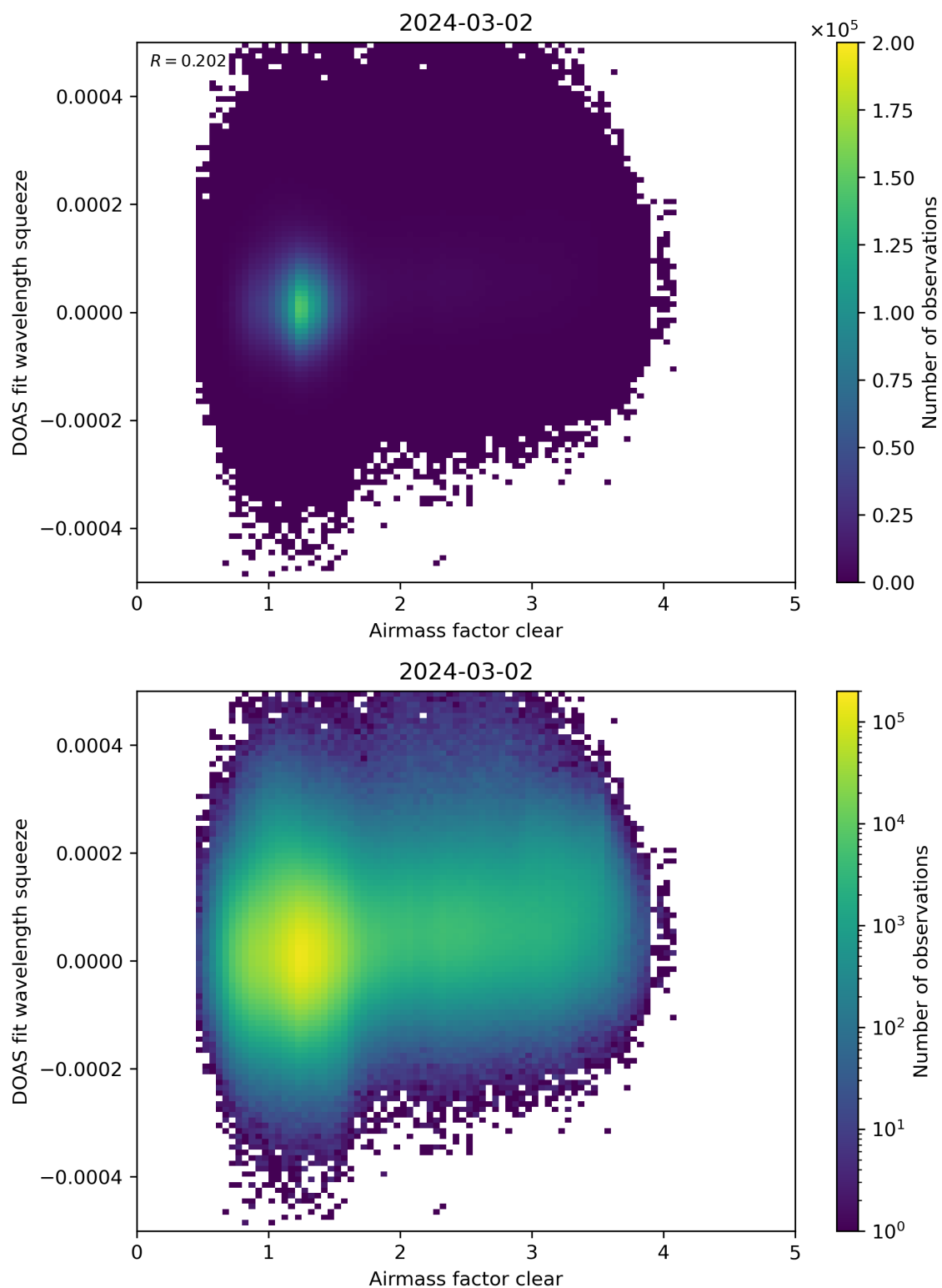
Figure 73: Scatter density plot of “Airmass factor clear” against “DOAS fit wavelength squeeze” for 2024-03-01 to 2024-03-03.
