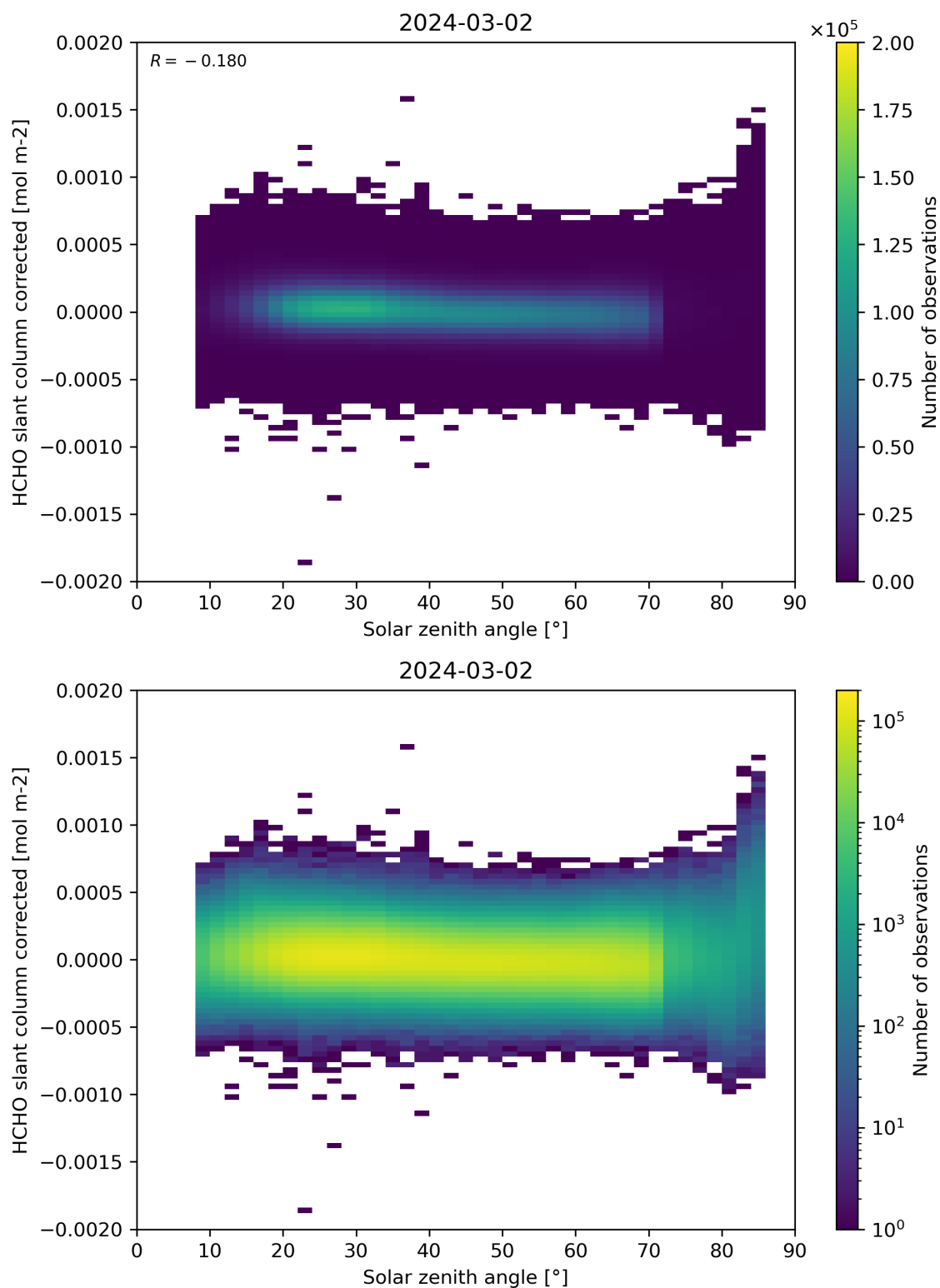
Figure 171: Scatter density plot of “Solar zenith angle” against “HCHO slant column corrected” for 2024-03-01 to 2024-03-03.
