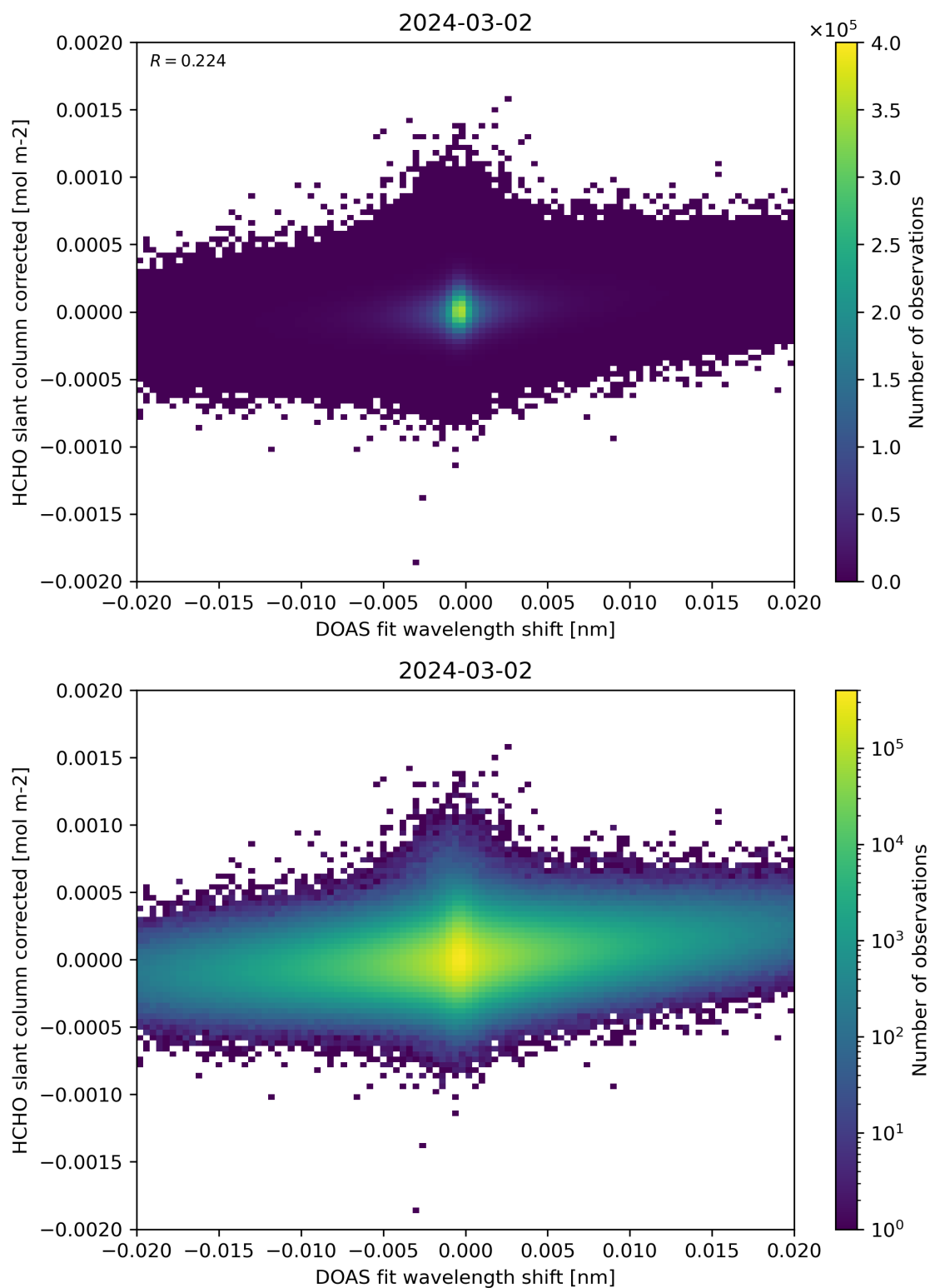
Figure 66: Scatter density plot of “DOAS fit wavelength shift” against “HCHO slant column corrected” for 2024-03-01 to 2024-03-03.
