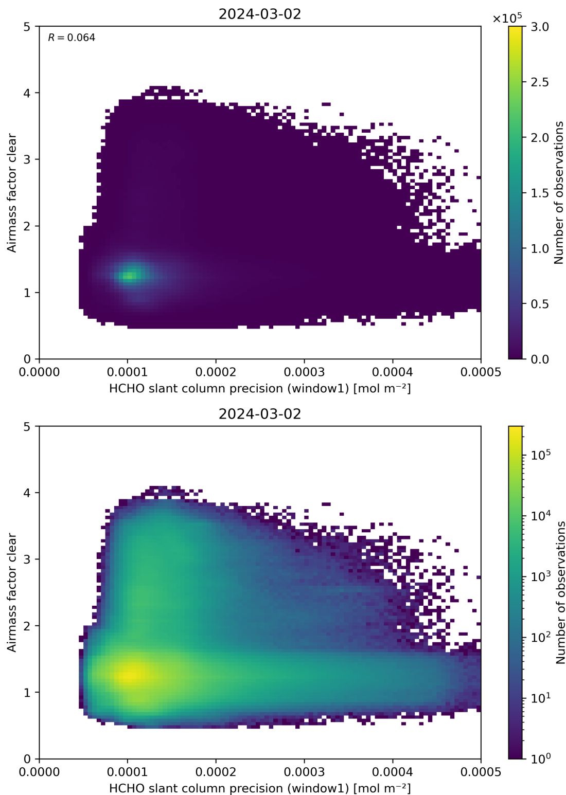
Figure 91: Scatter density plot of “HCHO slant column precision (window1)” against “Airmass factor clear” for 2024-03-01 to 2024-03-03.
