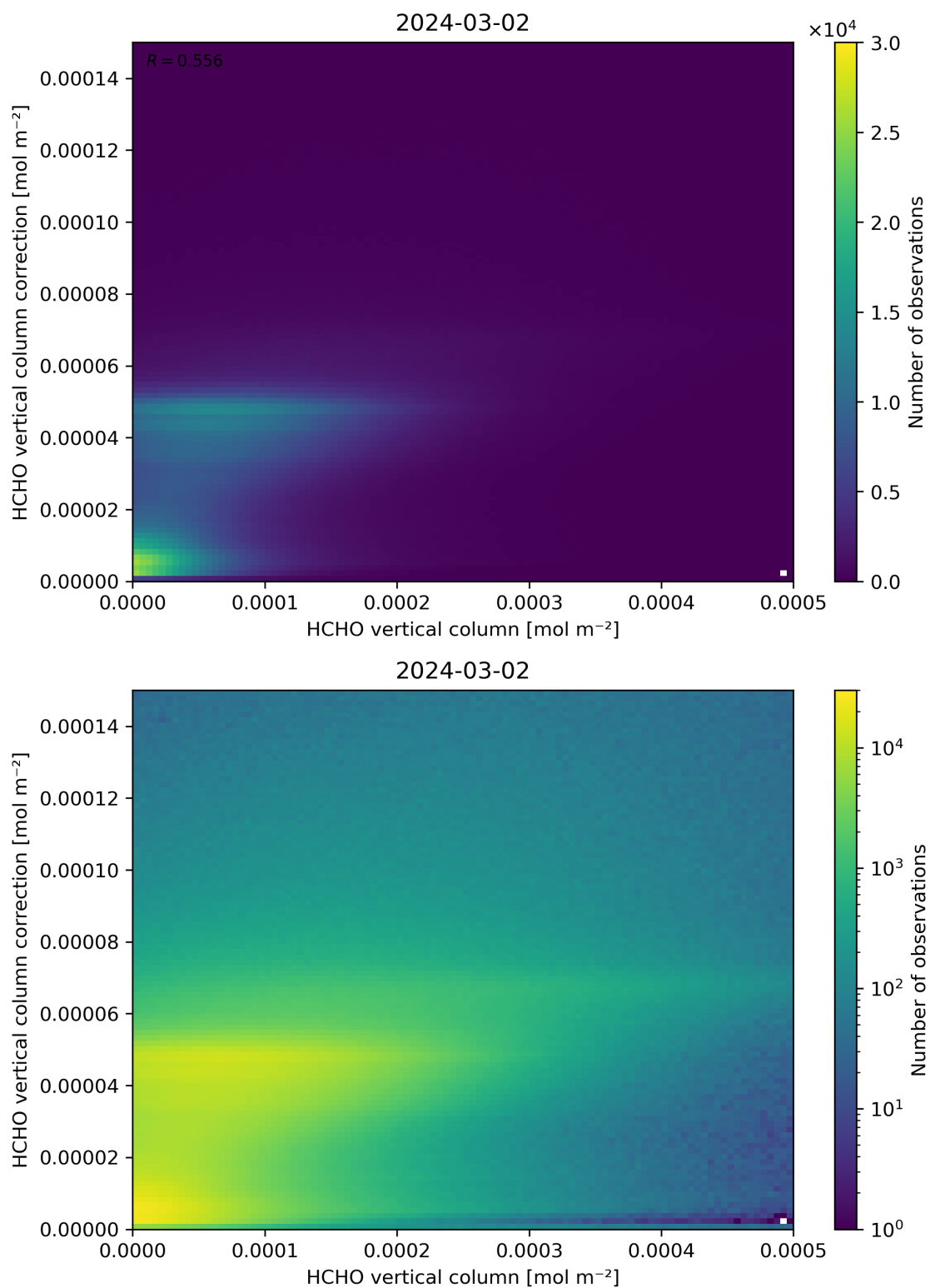
Figure 133: Scatter density plot of “HCHO vertical column” against “HCHO vertical column correction” for 2024-03-01 to 2024-03-03.
