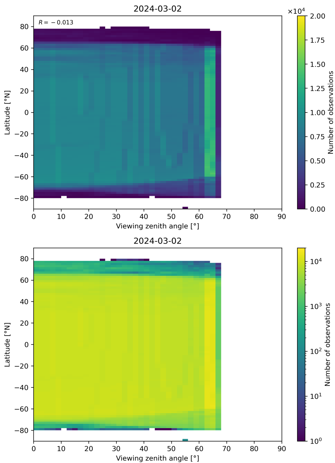
Figure 196: Scatter density plot of “Viewing zenith angle” against “Latitude” for 2024-03-01 to 2024-03-03.
