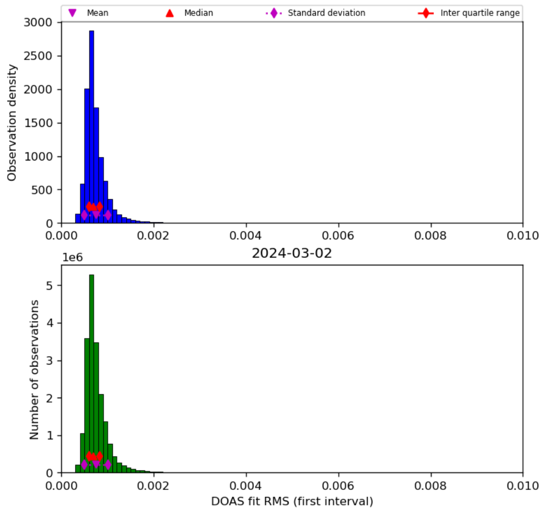
Figure 46: Histogram of “DOAS fit RMS (first interval)” for 2024-03-01 to 2024-03-03
