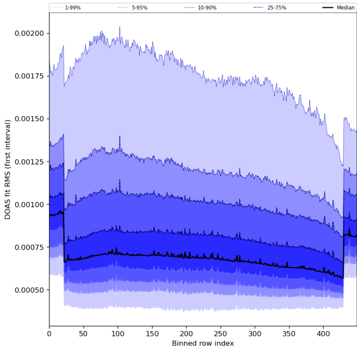
Figure 60: Along track statistics of “DOAS fit RMS (first interval)” for 2024-03-01 to 2024-03-03
