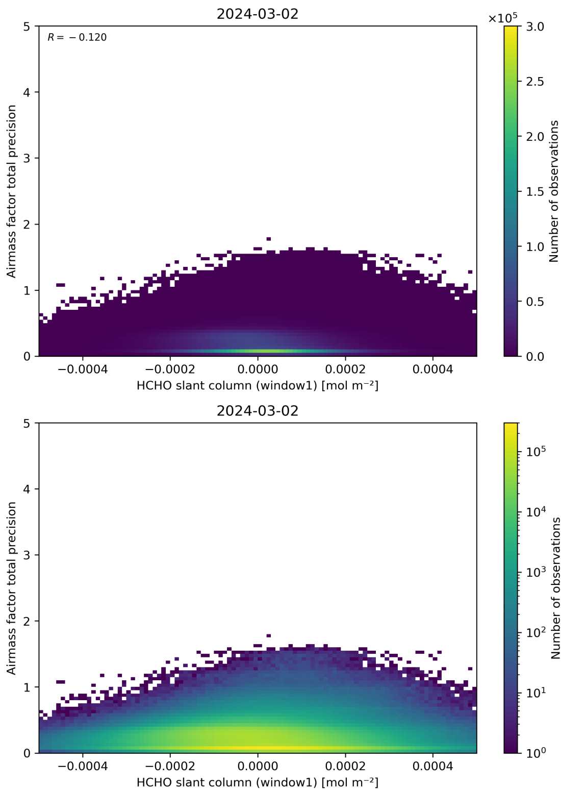
Figure 86: Scatter density plot of “HCHO slant column (window1)” against “Airmass factor total precision” for 2024-03-01 to 2024-03-03.
