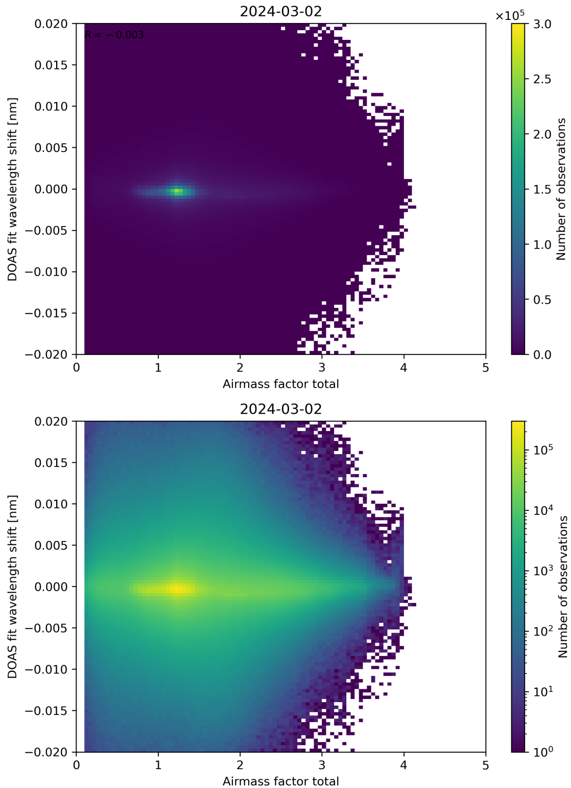
Figure 98: Scatter density plot of “Airmass factor total” against “DOAS fit wavelength shift” for 2024-03-01 to 2024-03-03.
