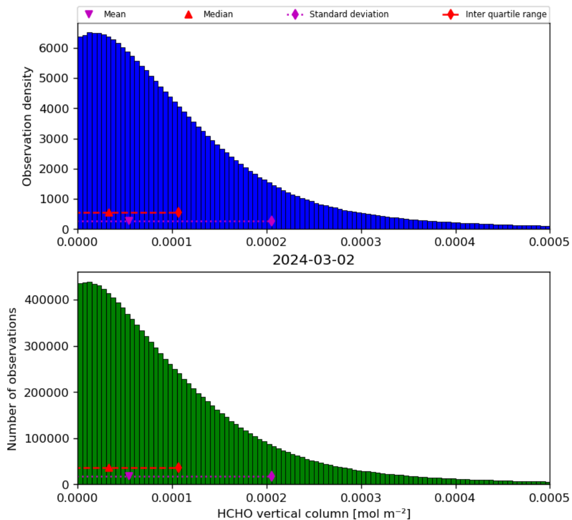
Figure 35: Histogram of “HCHO vertical column” for 2024-03-01 to 2024-03-03
