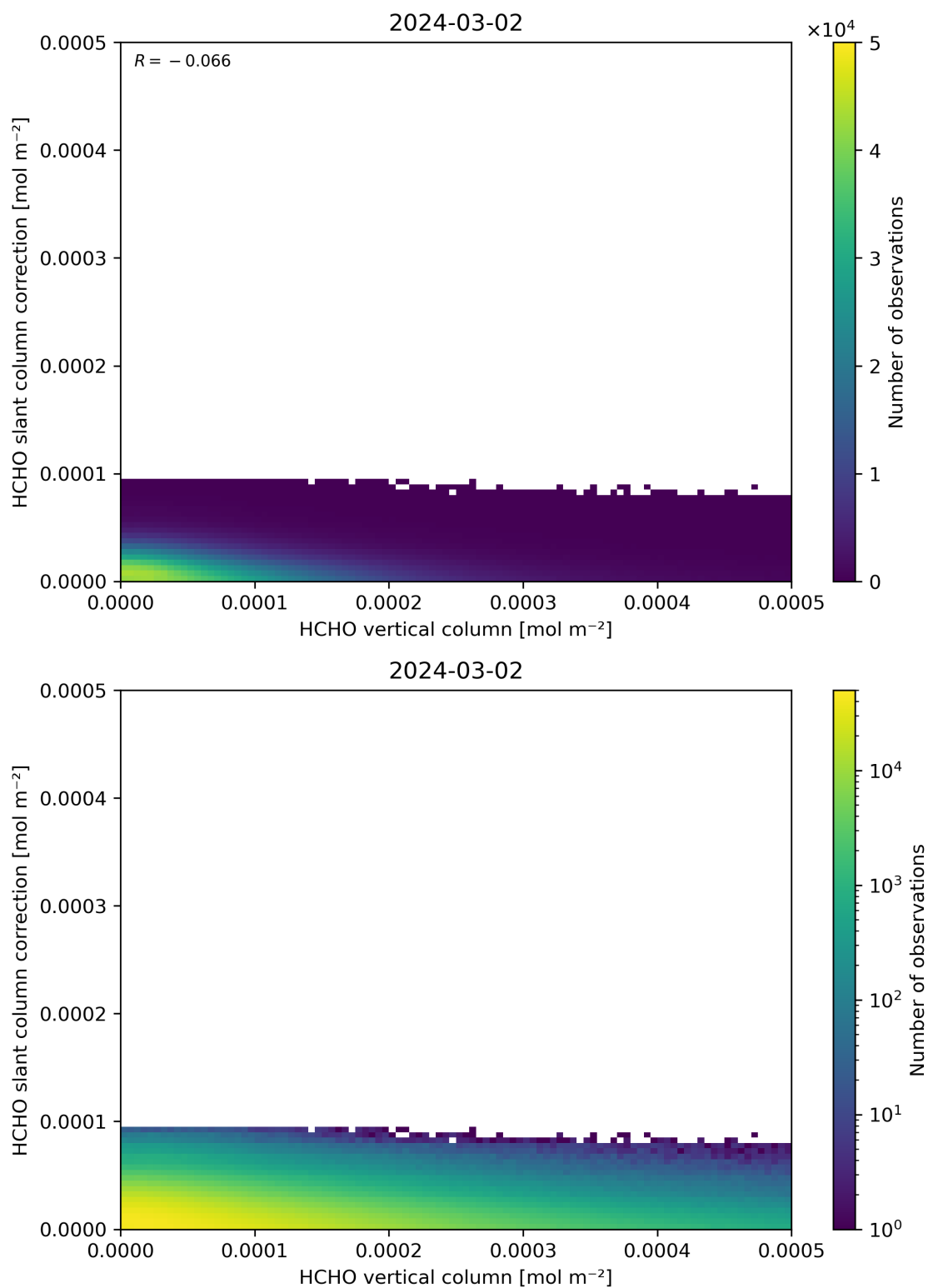
Figure 128: Scatter density plot of “HCHO vertical column” against “HCHO slant column correction” for 2024-03-01 to 2024-03-03.
