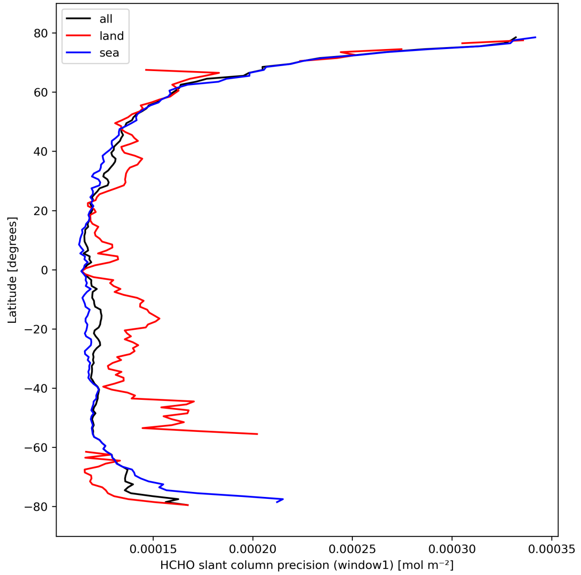
Figure 25: Zonal average of “HCHO slant column precision (window1)” for 2024-03-01 to 2024-03-03.
