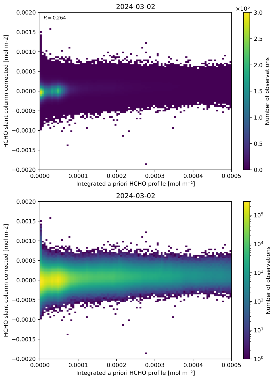
Figure 151: Scatter density plot of “Integrated a priori HCHO profile” against “HCHO slant column corrected” for 2024-03-01 to 2024-03-03.
