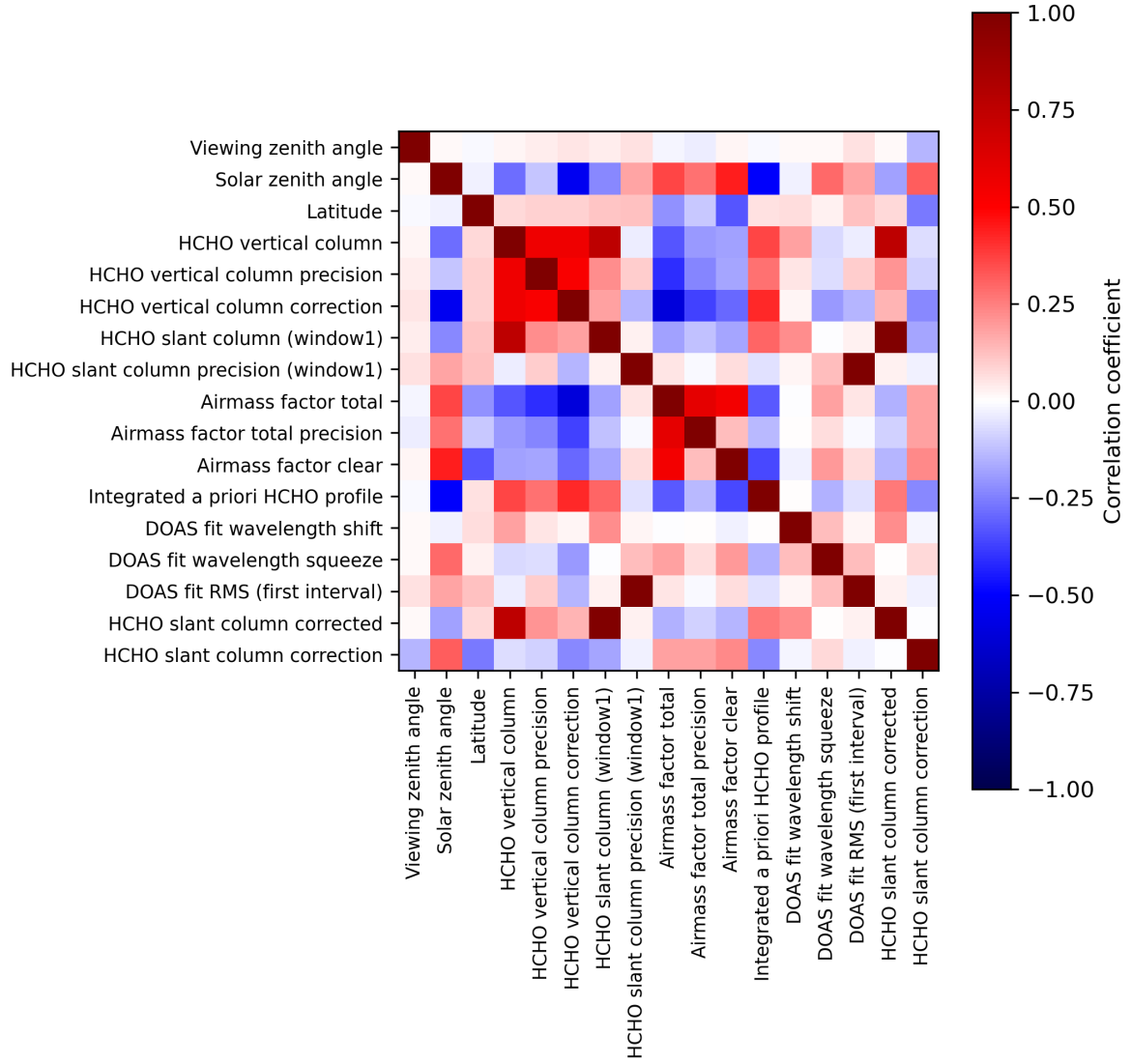
Figure 2: Map of correlation matrix for 2024-03-01 to 2024-03-03.
