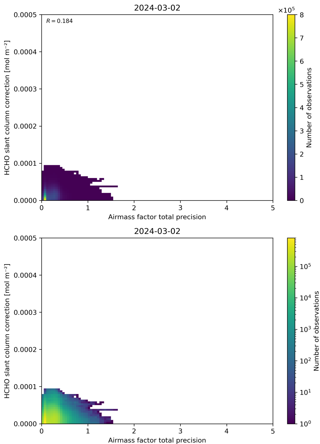
Figure 110: Scatter density plot of “Airmass factor total precision” against “HCHO slant column correction” for 2024-03-01 to 2024-03-03.
