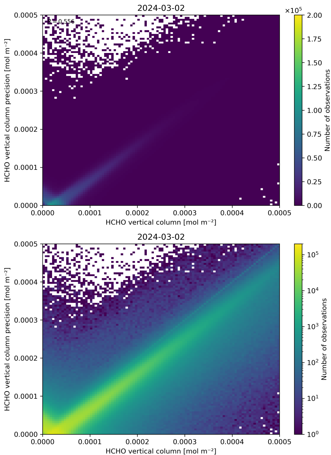
Figure 134: Scatter density plot of “HCHO vertical column” against “HCHO vertical column precision” for 2024-03-01 to 2024-03-03.
