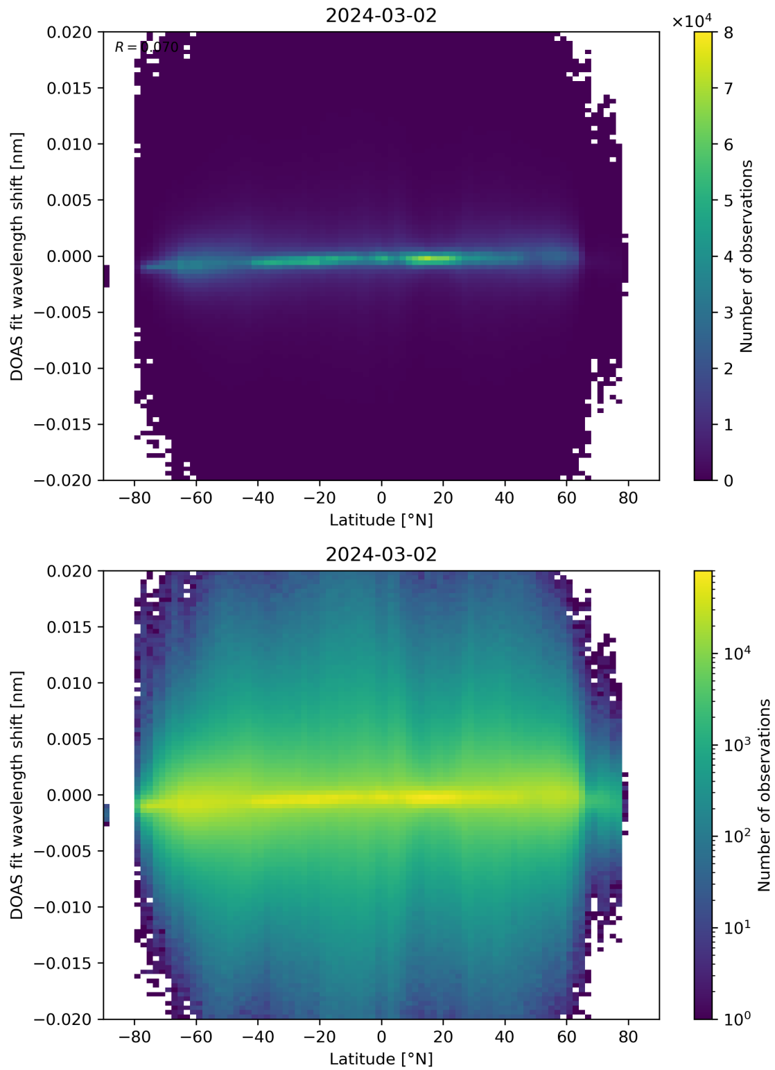
Figure 154: Scatter density plot of “Latitude” against “DOAS fit wavelength shift” for 2024-03-01 to 2024-03-03.
