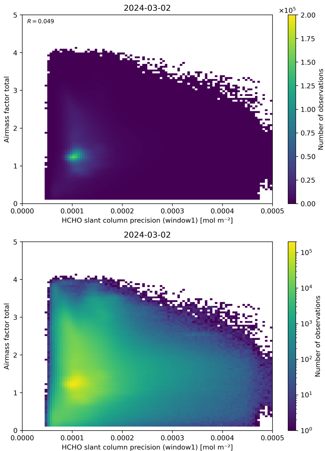
Figure 94: Scatter density plot of “HCHO slant column precision (window1)” against “Airmass factor total” for 2024-03-01 to 2024-03-03.
