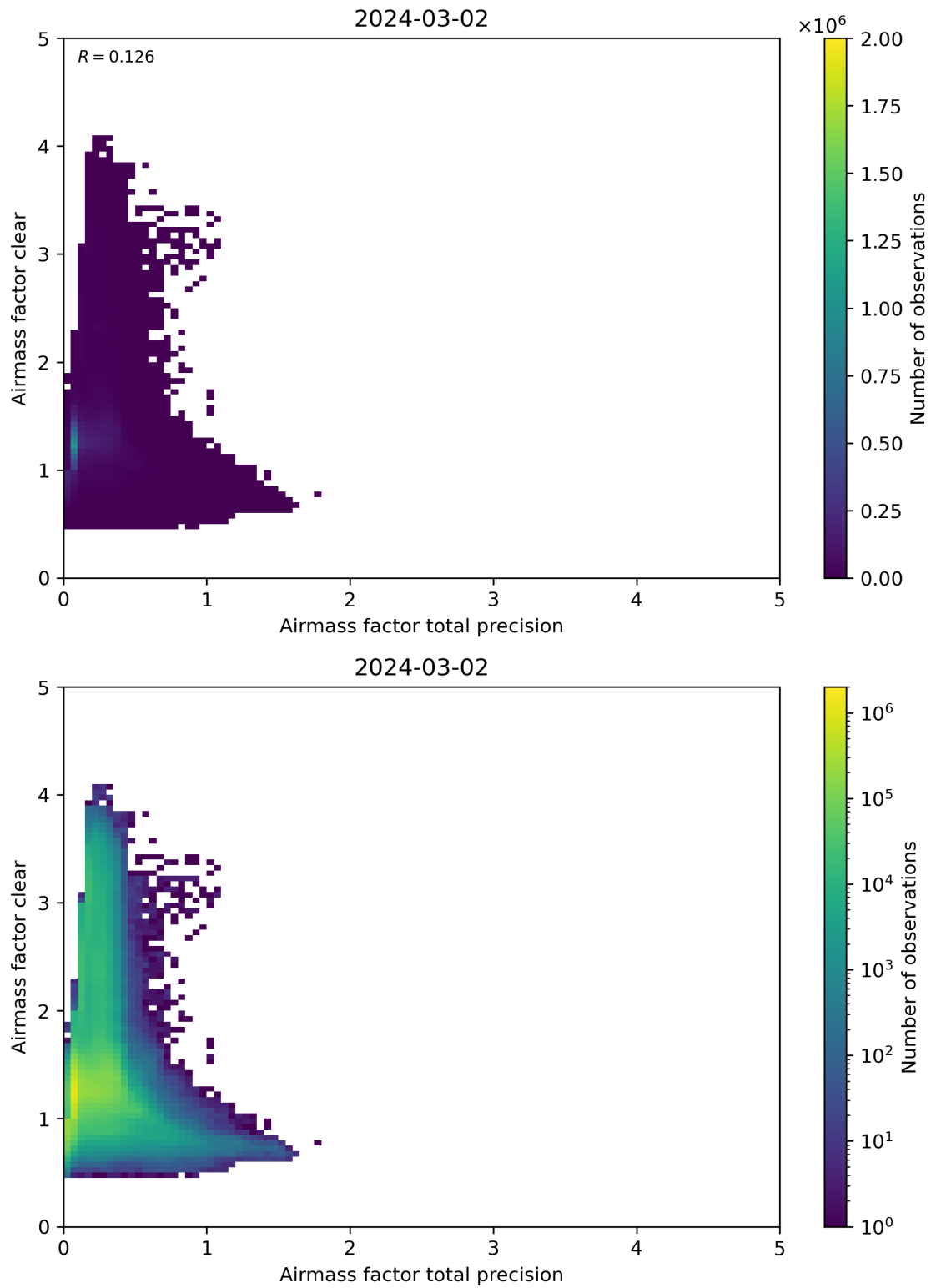
Figure 108: Scatter density plot of “Airmass factor total precision” against “Airmass factor clear” for 2024-03-01 to 2024-03-03.
