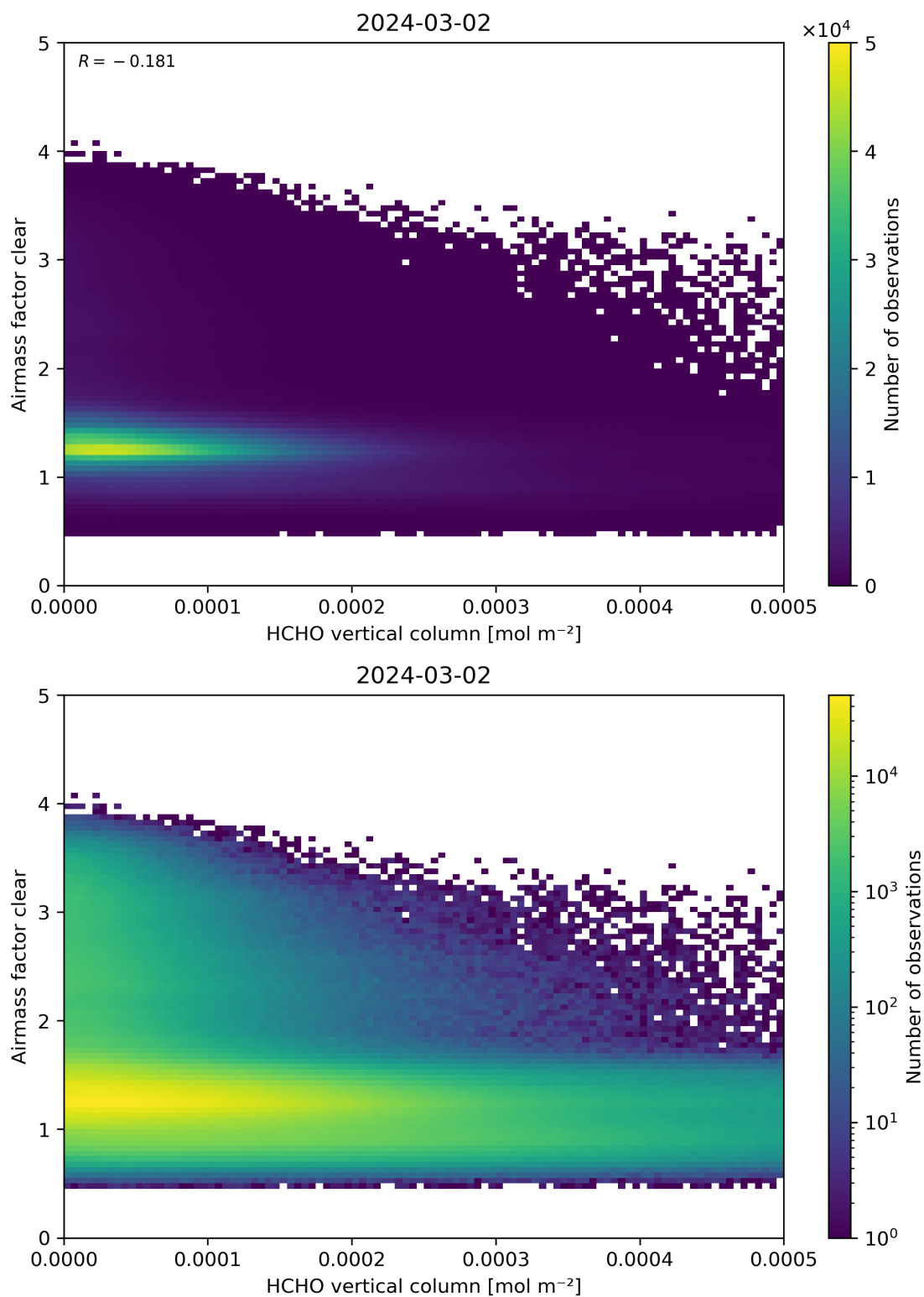
Figure 126: Scatter density plot of “HCHO vertical column” against “Airmass factor clear” for 2024-03-01 to 2024-03-03.
