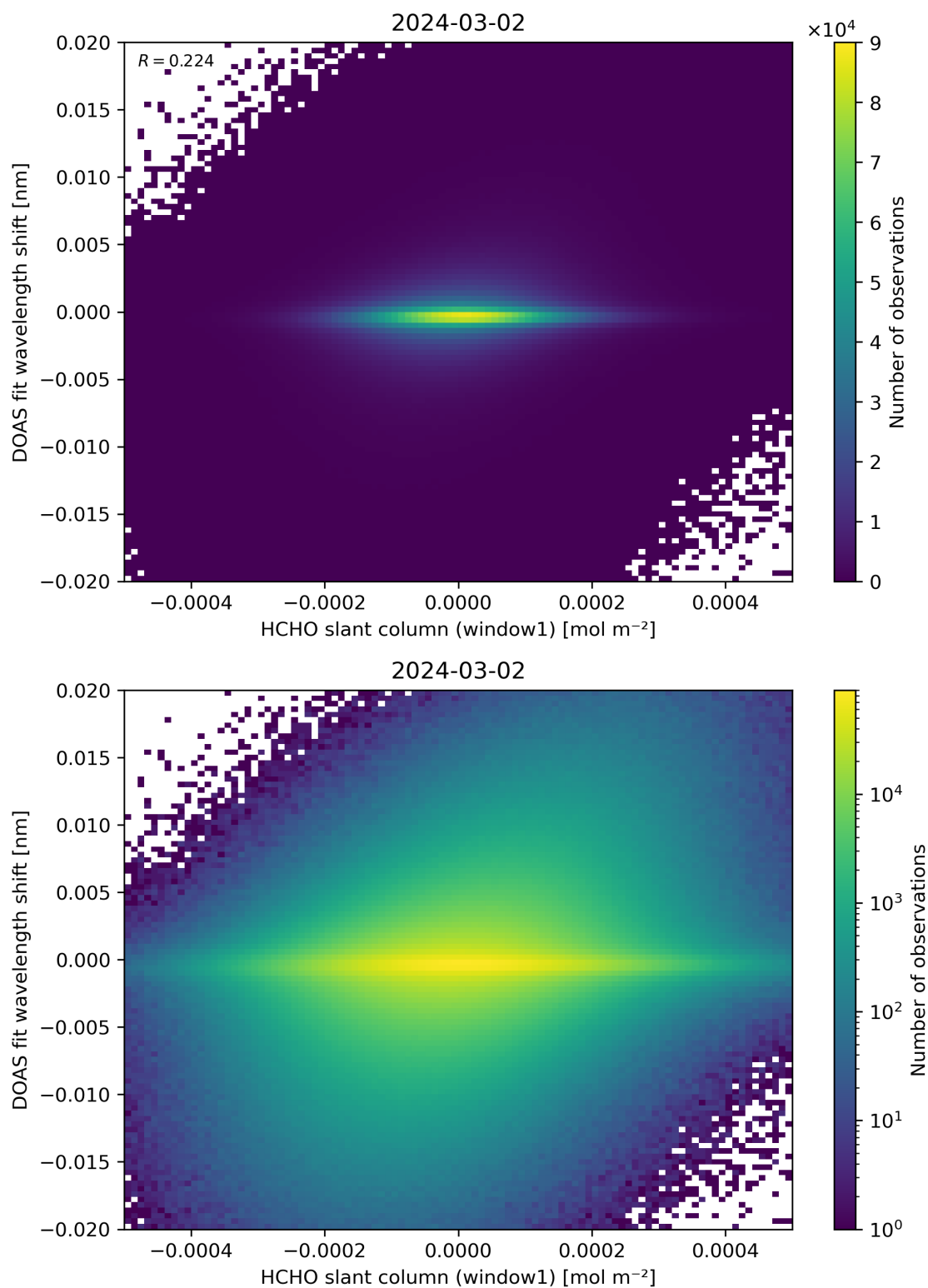
Figure 79: Scatter density plot of “HCHO slant column (window1)” against “DOAS fit wavelength shift” for 2024-03-01 to 2024-03-03.
