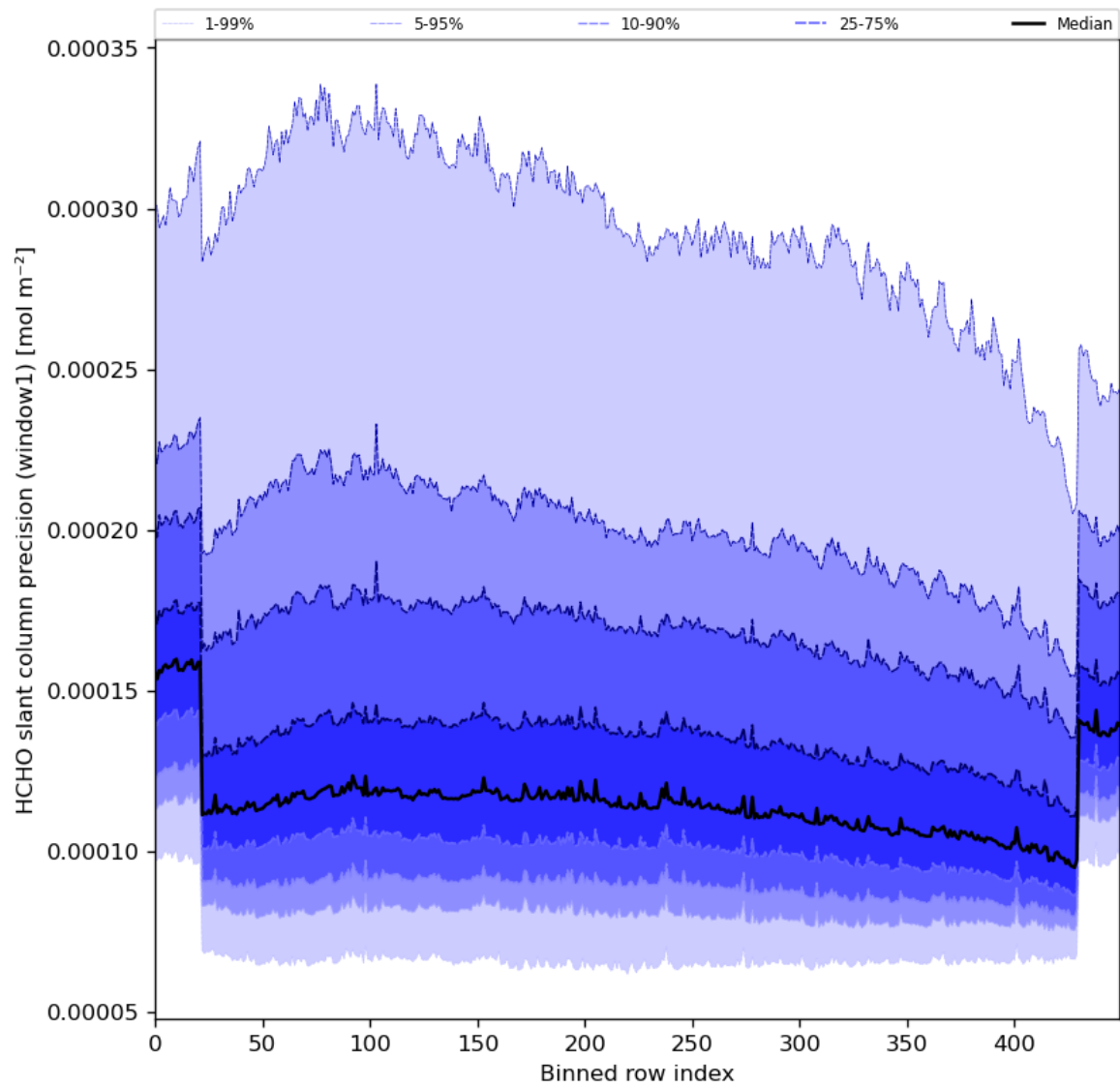
Figure 53: Along track statistics of “HCHO slant column precision (window1)” for 2024-03-01 to 2024-03-03
