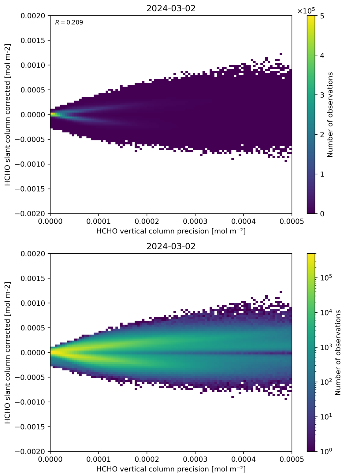
Figure 140: Scatter density plot of “HCHO vertical column precision” against “HCHO slant column corrected” for 2024-03-01 to 2024-03-03.
