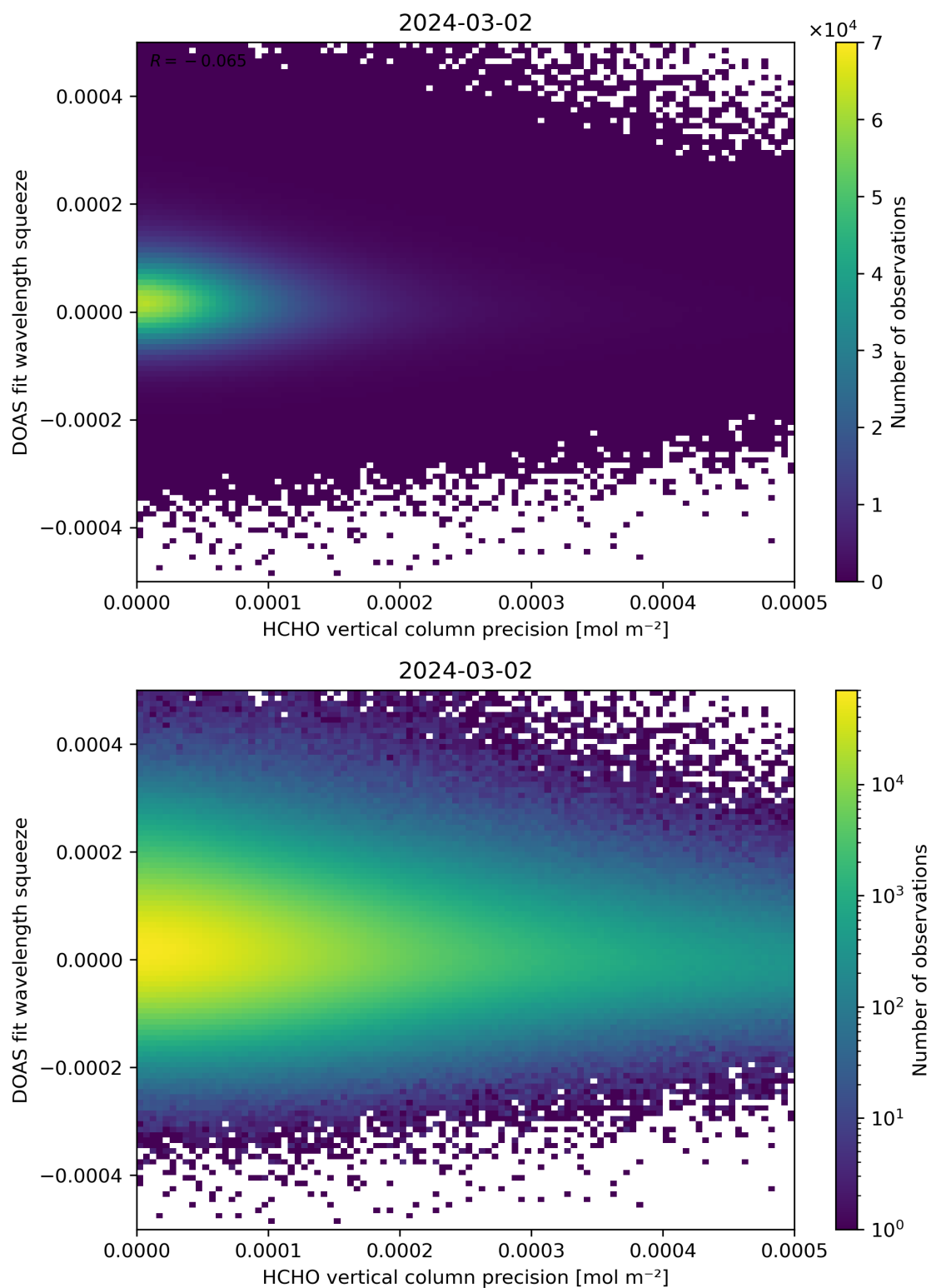
Figure 138: Scatter density plot of “HCHO vertical column precision” against “DOAS fit wavelength squeeze” for 2024-03-01 to 2024-03-03.
