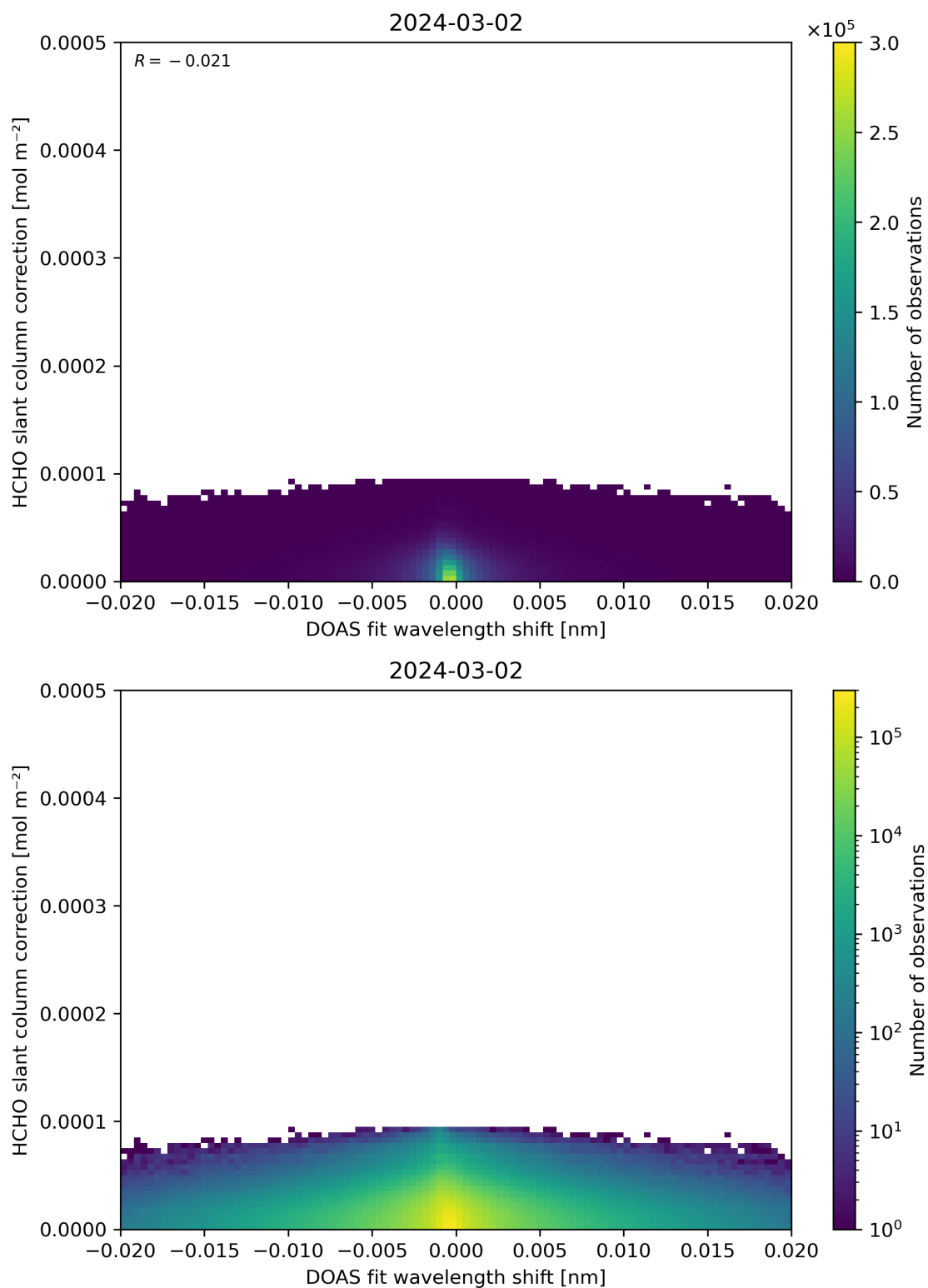
Figure 67: Scatter density plot of “DOAS fit wavelength shift” against “HCHO slant column correction” for 2024-03-01 to 2024-03-03.
