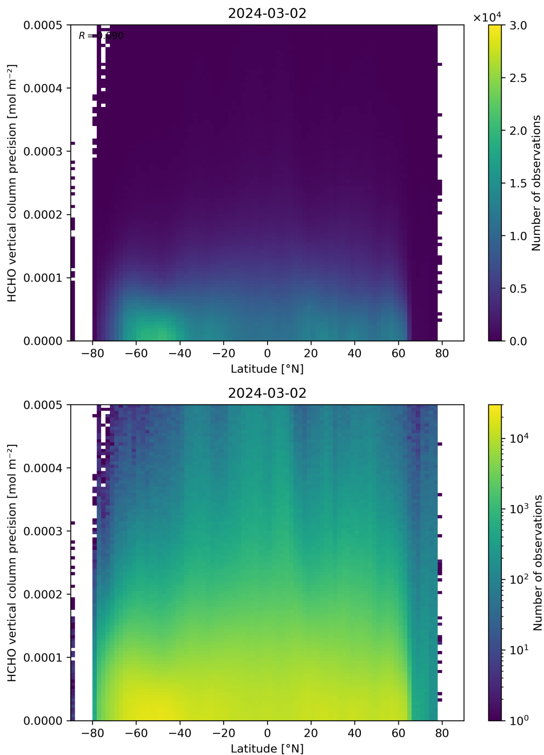
Figure 165: Scatter density plot of “Latitude” against “HCHO vertical column precision” for 2024-03-01 to 2024-03-03.
