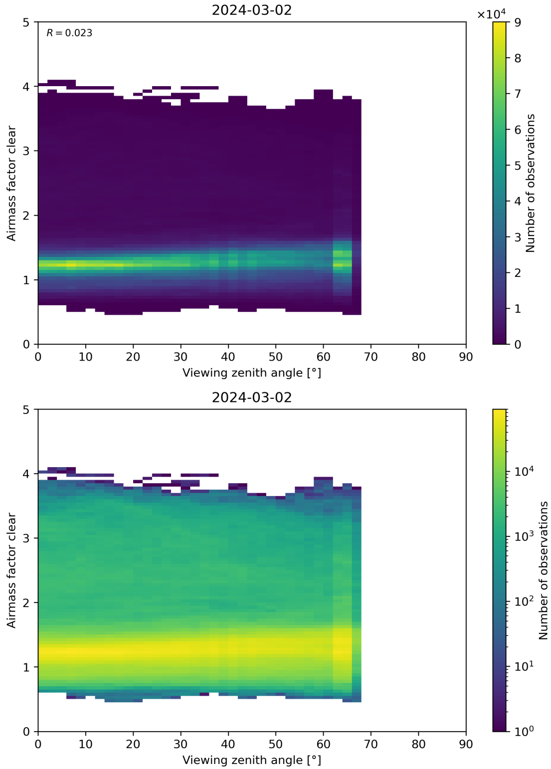
Figure 185: Scatter density plot of “Viewing zenith angle” against “Airmass factor clear” for 2024-03-01 to 2024-03-03.
