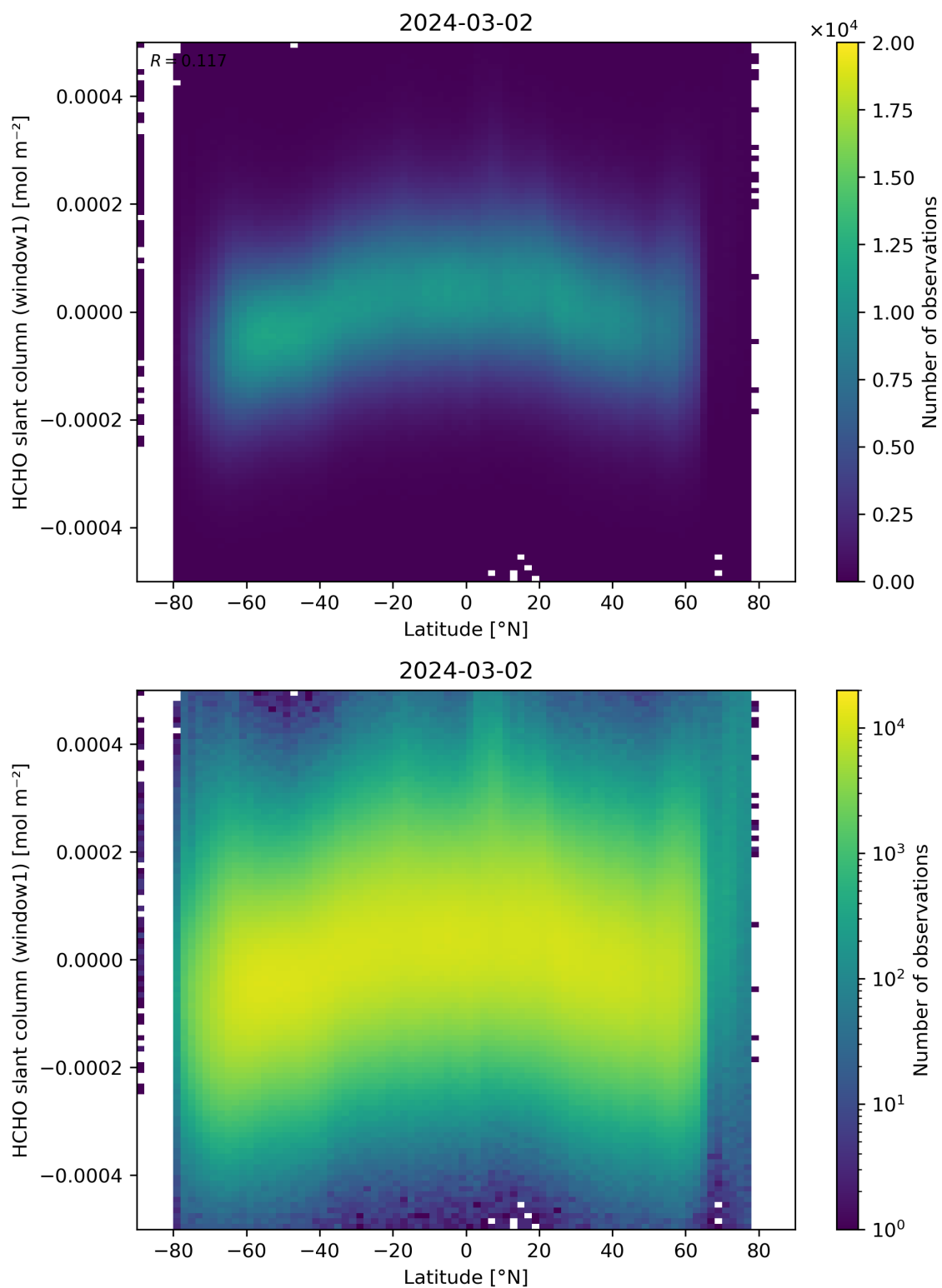
Figure 159: Scatter density plot of “Latitude” against “HCHO slant column (window1)” for 2024-03-01 to 2024-03-03.
