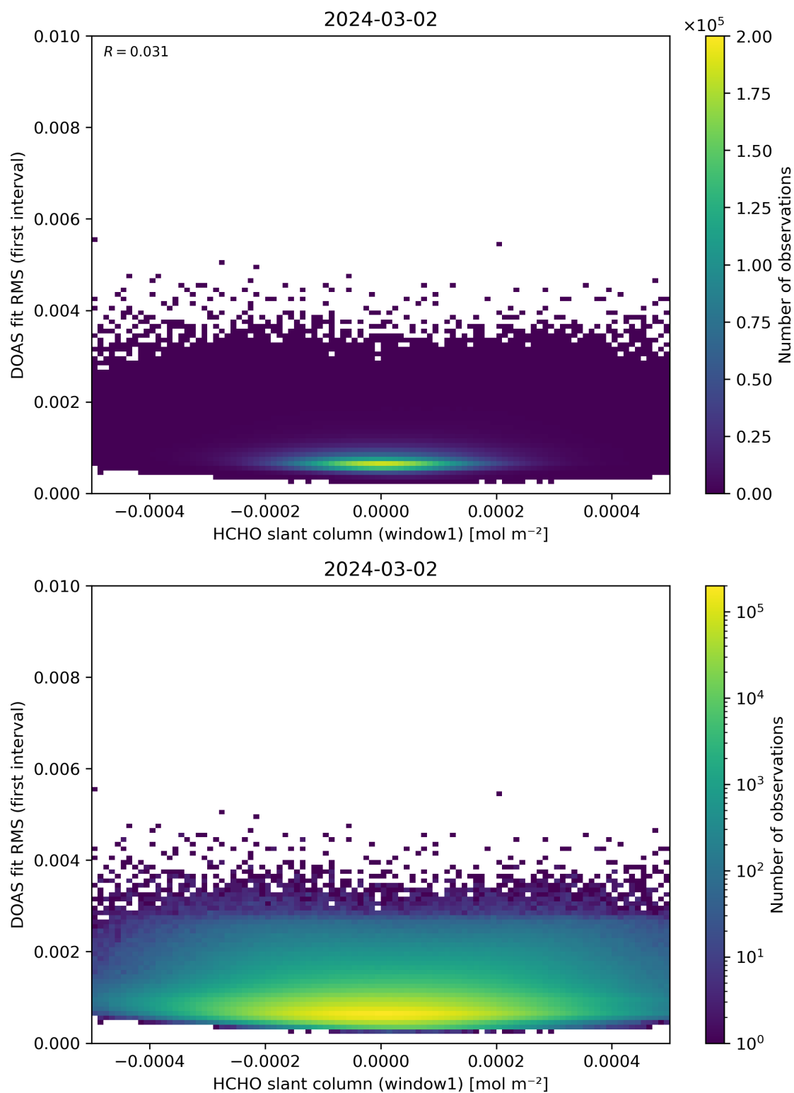
Figure 78: Scatter density plot of “HCHO slant column (window1)” against “DOAS fit RMS (first interval)” for 2024-03-01 to 2024-03-03.
