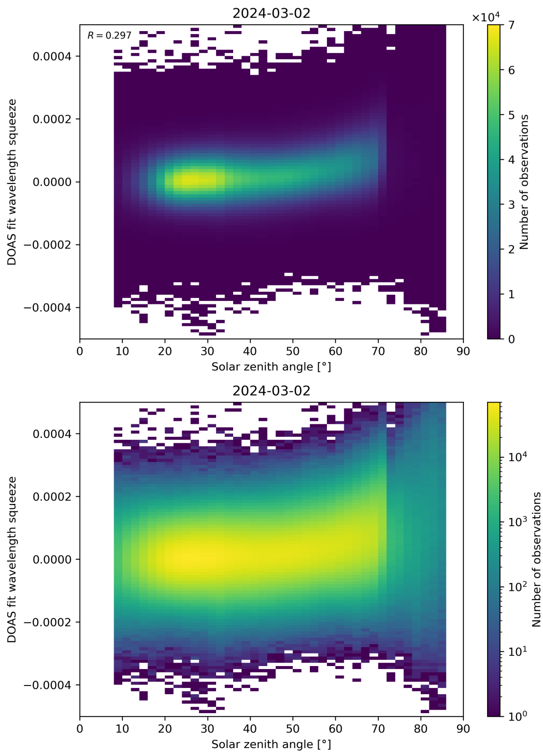
Figure 169: Scatter density plot of “Solar zenith angle” against “DOAS fit wavelength squeeze” for 2024-03-01 to 2024-03-03.
