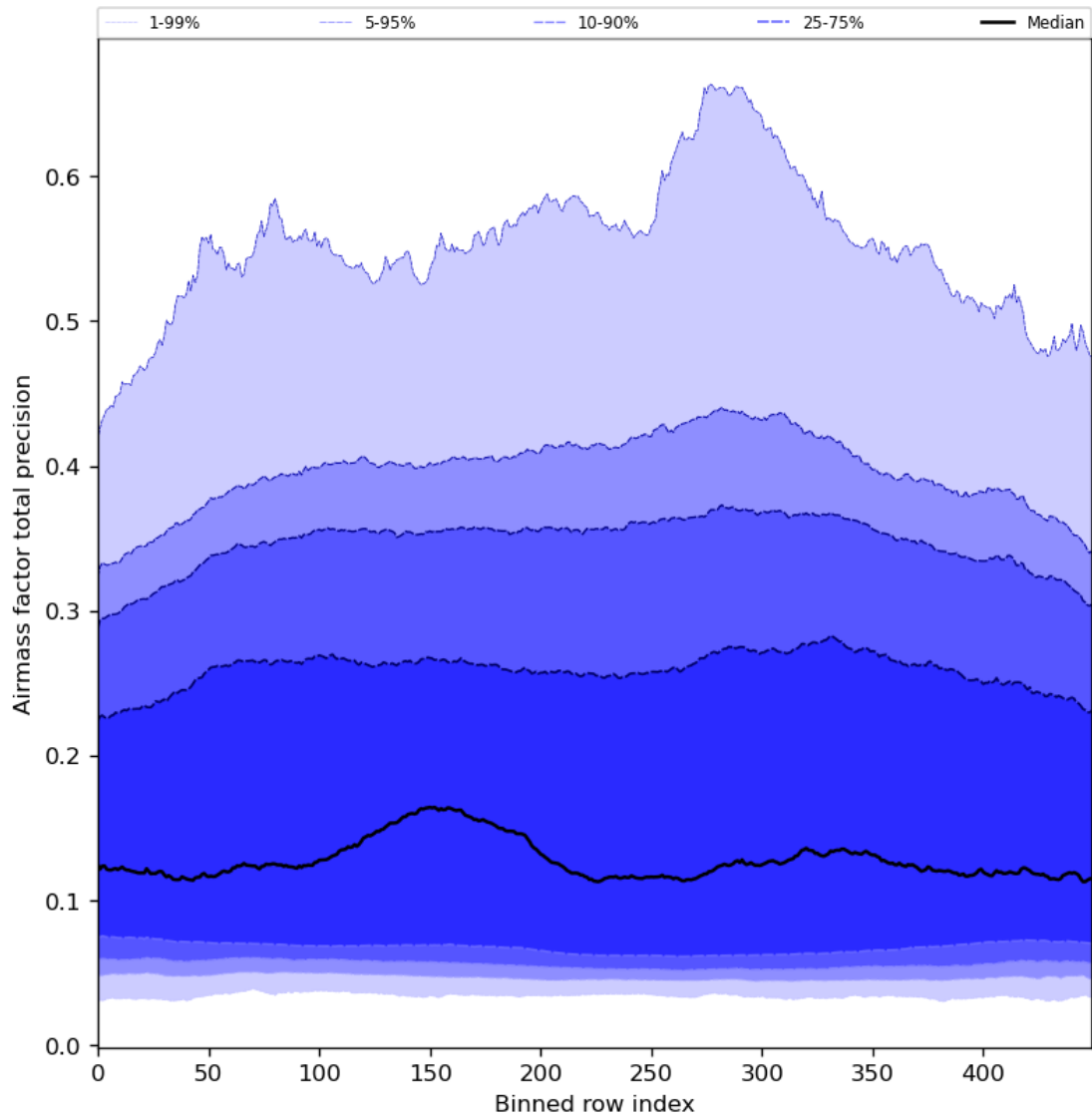
Figure 55: Along track statistics of “Airmass factor total precision” for 2024-03-01 to 2024-03-03
