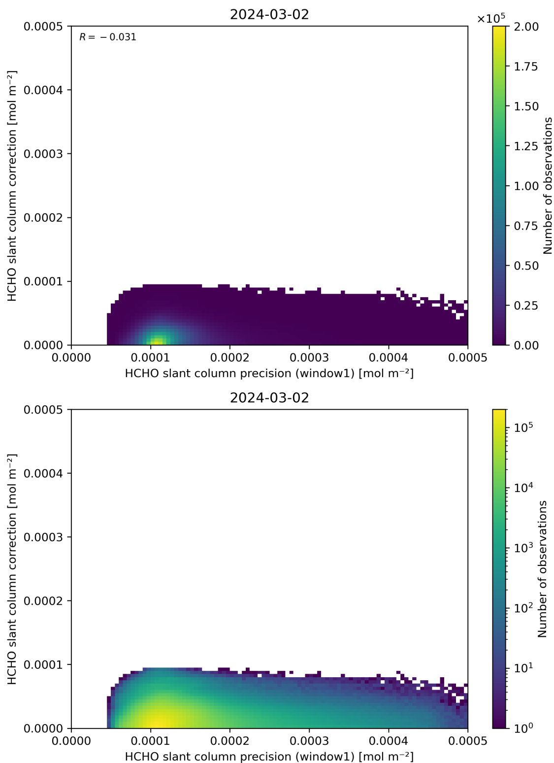
Figure 93: Scatter density plot of “HCHO slant column precision (window1)” against “HCHO slant column correction” for 2024-03-01 to 2024-03-03.
