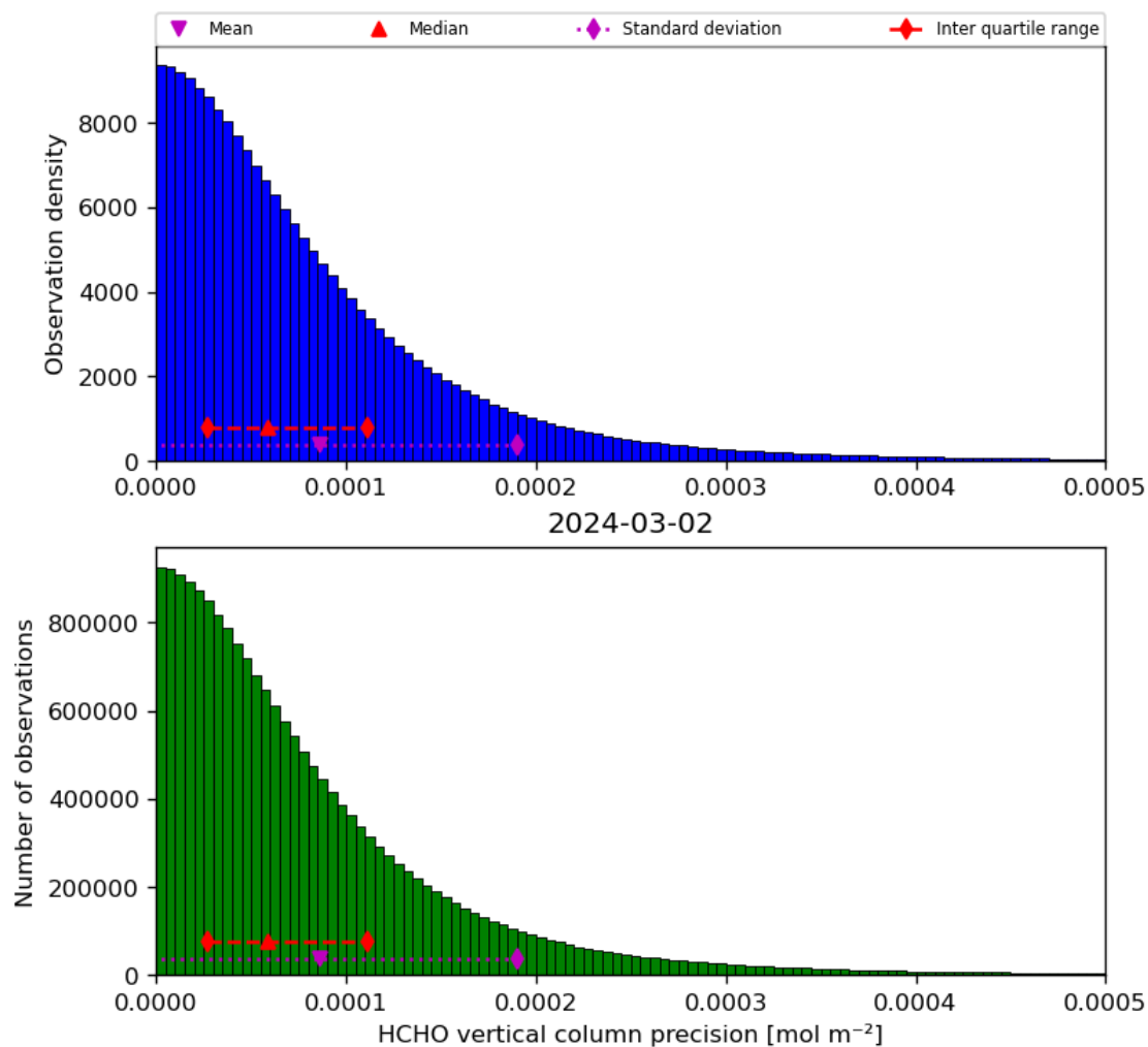
Figure 36: Histogram of “HCHO vertical column precision” for 2024-03-01 to 2024-03-03
