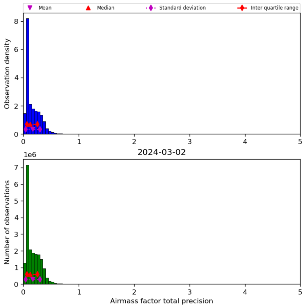
Figure 41: Histogram of “Airmass factor total precision” for 2024-03-01 to 2024-03-03
