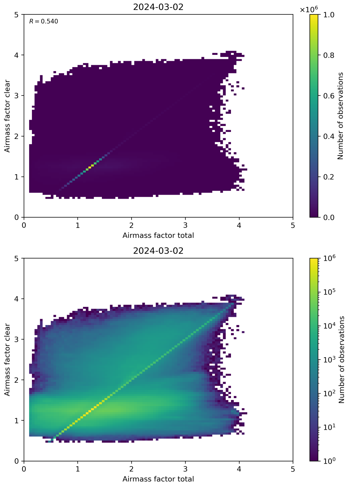
Figure 100: Scatter density plot of “Airmass factor total” against “Airmass factor clear” for 2024-03-01 to 2024-03-03.
