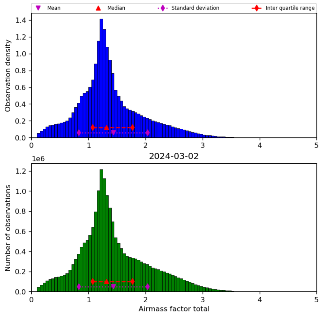
Figure 40: Histogram of “Airmass factor total” for 2024-03-01 to 2024-03-03
