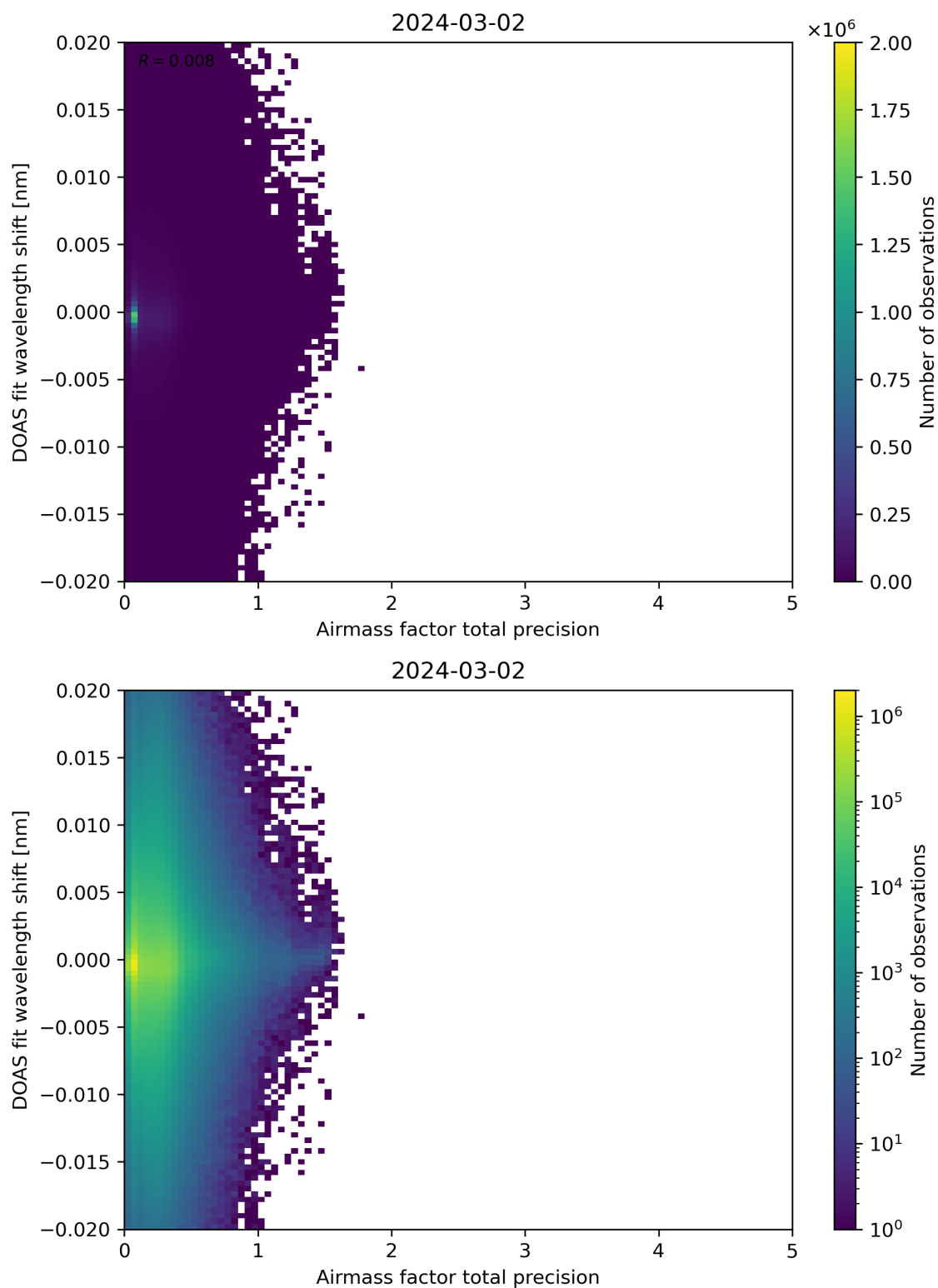
Figure 106: Scatter density plot of “Airmass factor total precision” against “DOAS fit wavelength shift” for 2024-03-01 to 2024-03-03.
