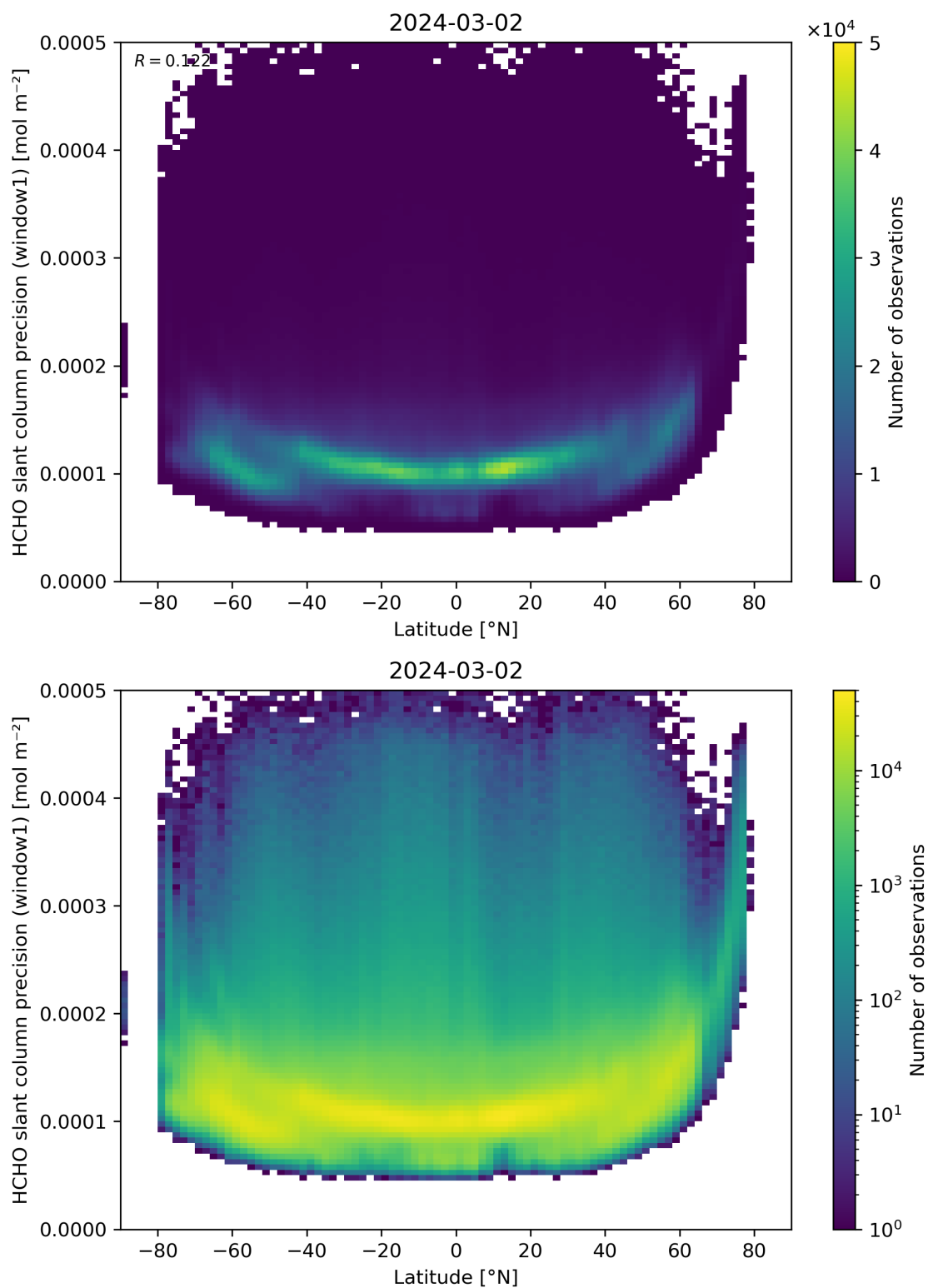
Figure 160: Scatter density plot of “Latitude” against “HCHO slant column precision (window1)” for 2024-03-01 to 2024-03-03.
