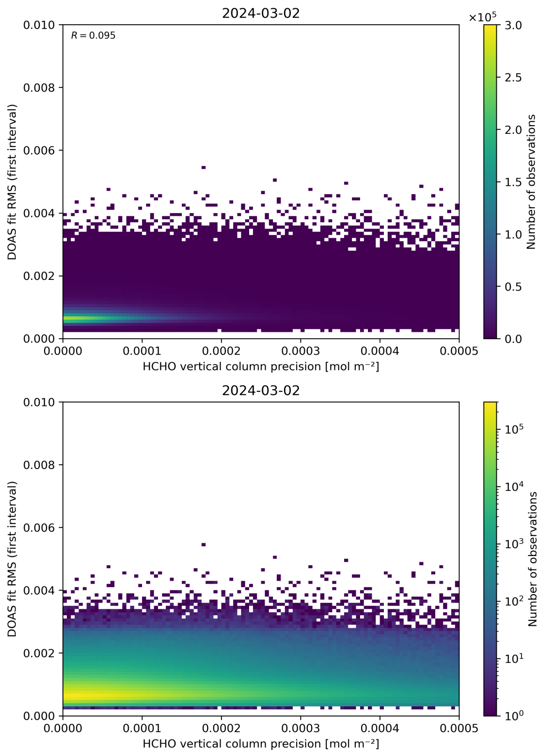
Figure 136: Scatter density plot of “HCHO vertical column precision” against “DOAS fit RMS (first interval)” for 2024-03-01 to 2024-03-03.
