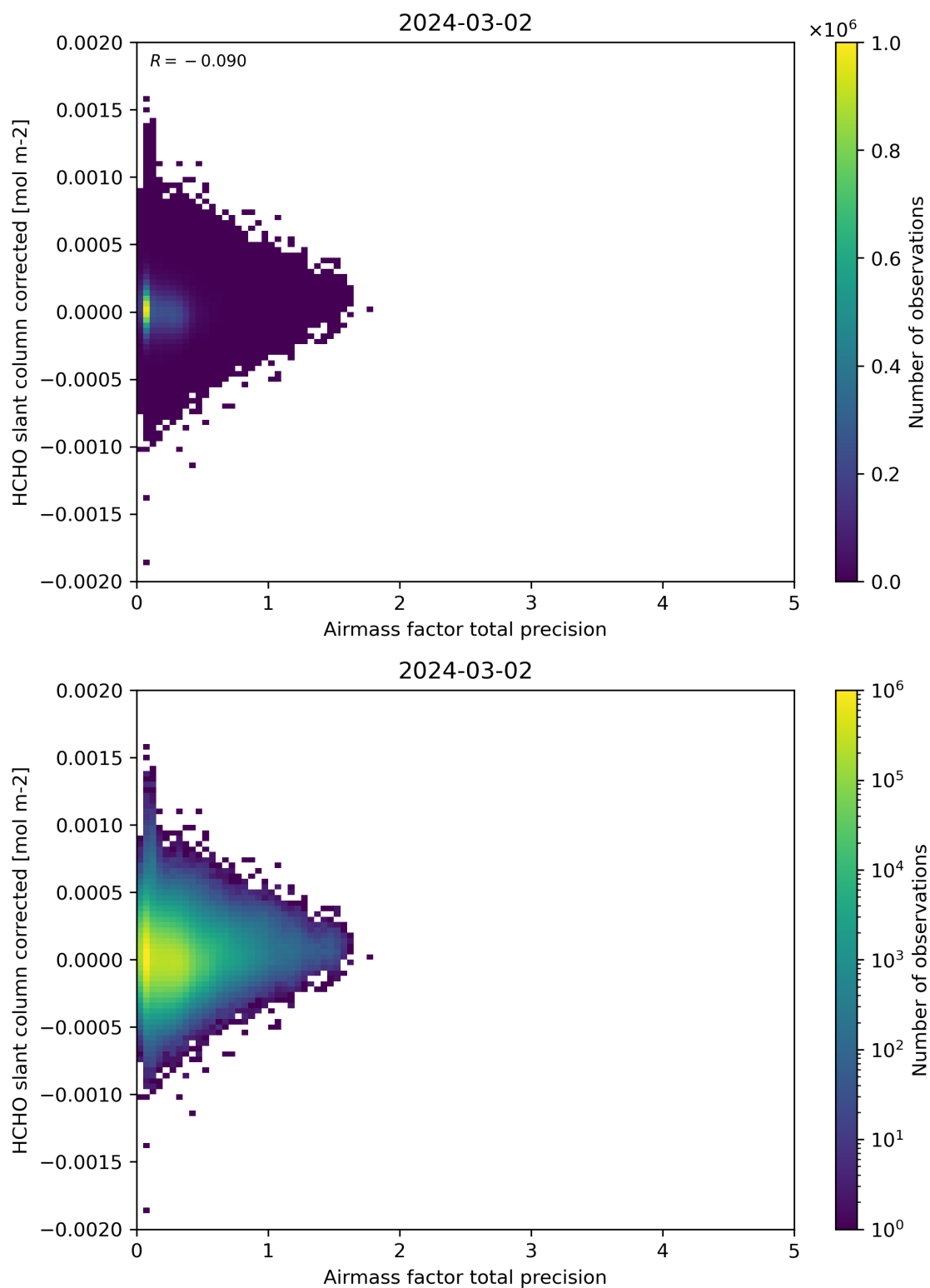
Figure 109: Scatter density plot of “Airmass factor total precision” against “HCHO slant column corrected” for 2024-03-01 to 2024-03-03.
