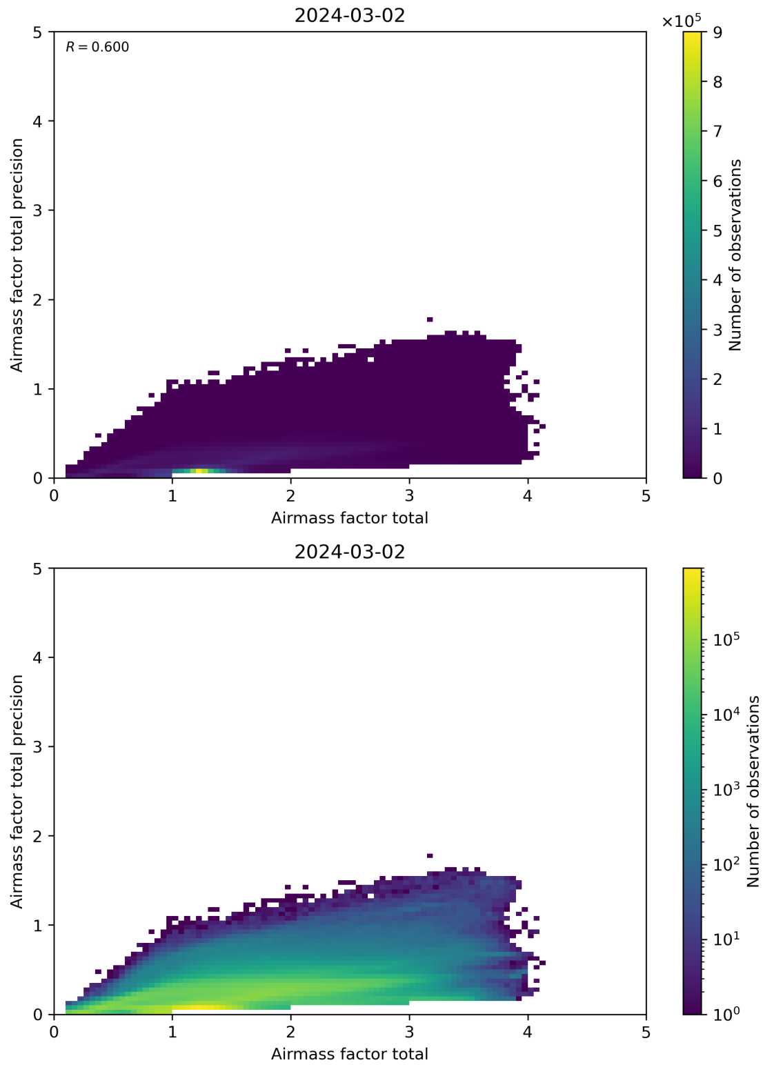
Figure 103: Scatter density plot of “Airmass factor total” against “Airmass factor total precision” for 2024-03-01 to 2024-03-03.
