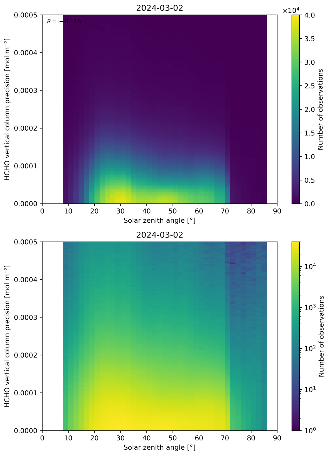
Figure 179: Scatter density plot of “Solar zenith angle” against “HCHO vertical column precision” for 2024-03-01 to 2024-03-03.
