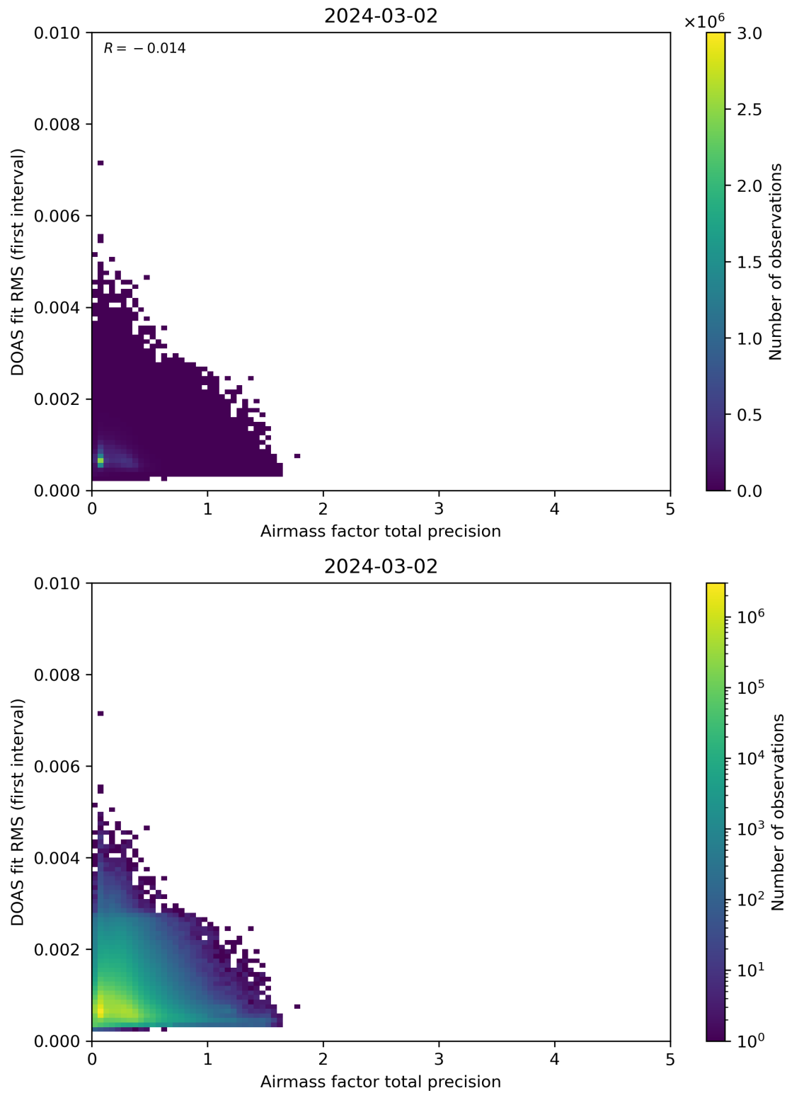
Figure 105: Scatter density plot of “Airmass factor total precision” against “DOAS fit RMS (first interval)” for 2024-03-01 to 2024-03-03.
