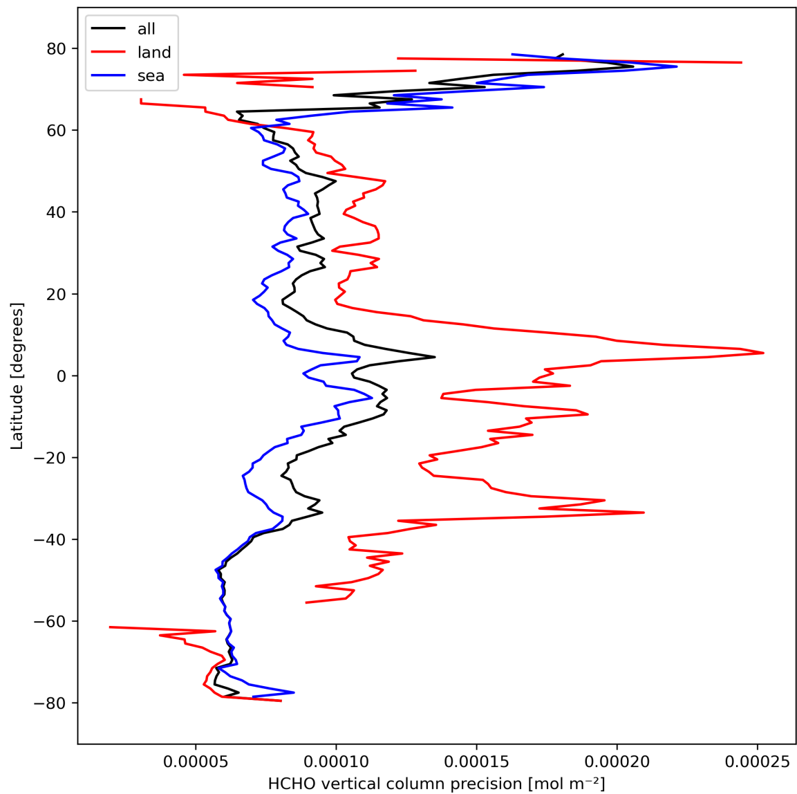
Figure 22: Zonal average of “HCHO vertical column precision” for 2024-03-01 to 2024-03-03.
