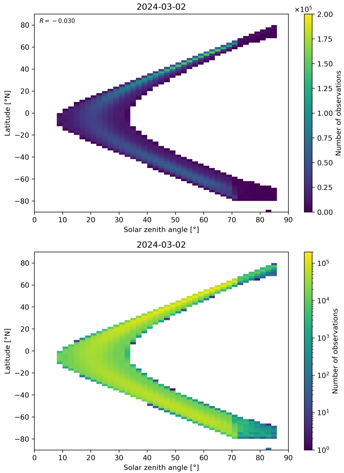
Figure 181: Scatter density plot of “Solar zenith angle” against “Latitude” for 2024-03-01 to 2024-03-03.
