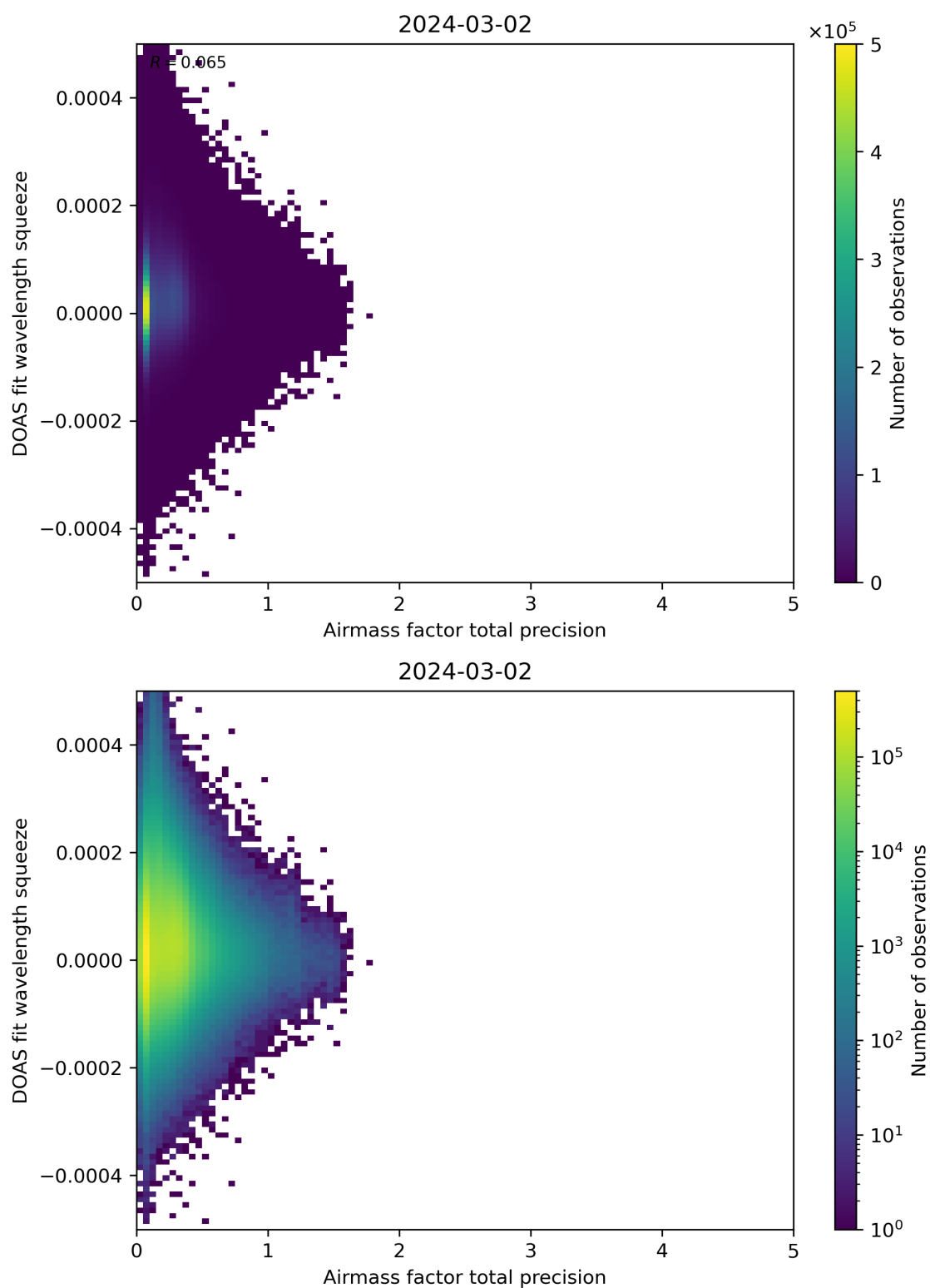
Figure 107: Scatter density plot of “Airmass factor total precision” against “DOAS fit wavelength squeeze” for 2024-03-01 to 2024-03-03.
