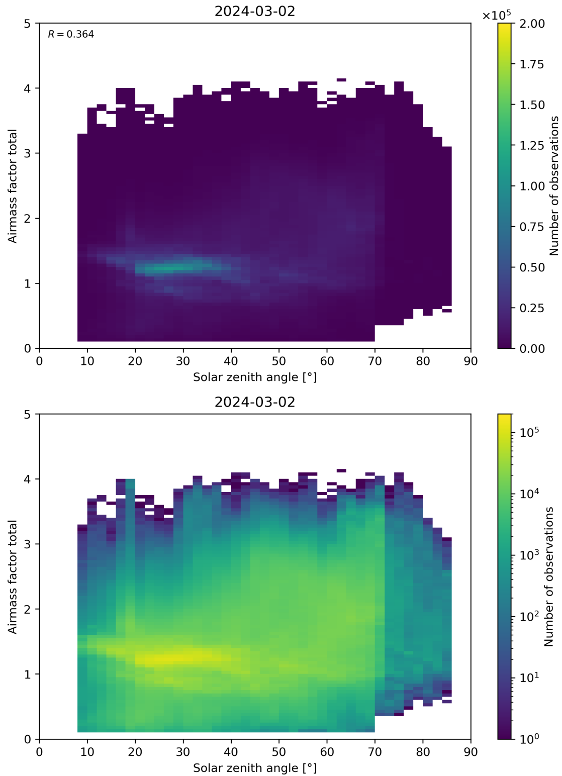
Figure 175: Scatter density plot of “Solar zenith angle” against “Airmass factor total” for 2024-03-01 to 2024-03-03.
