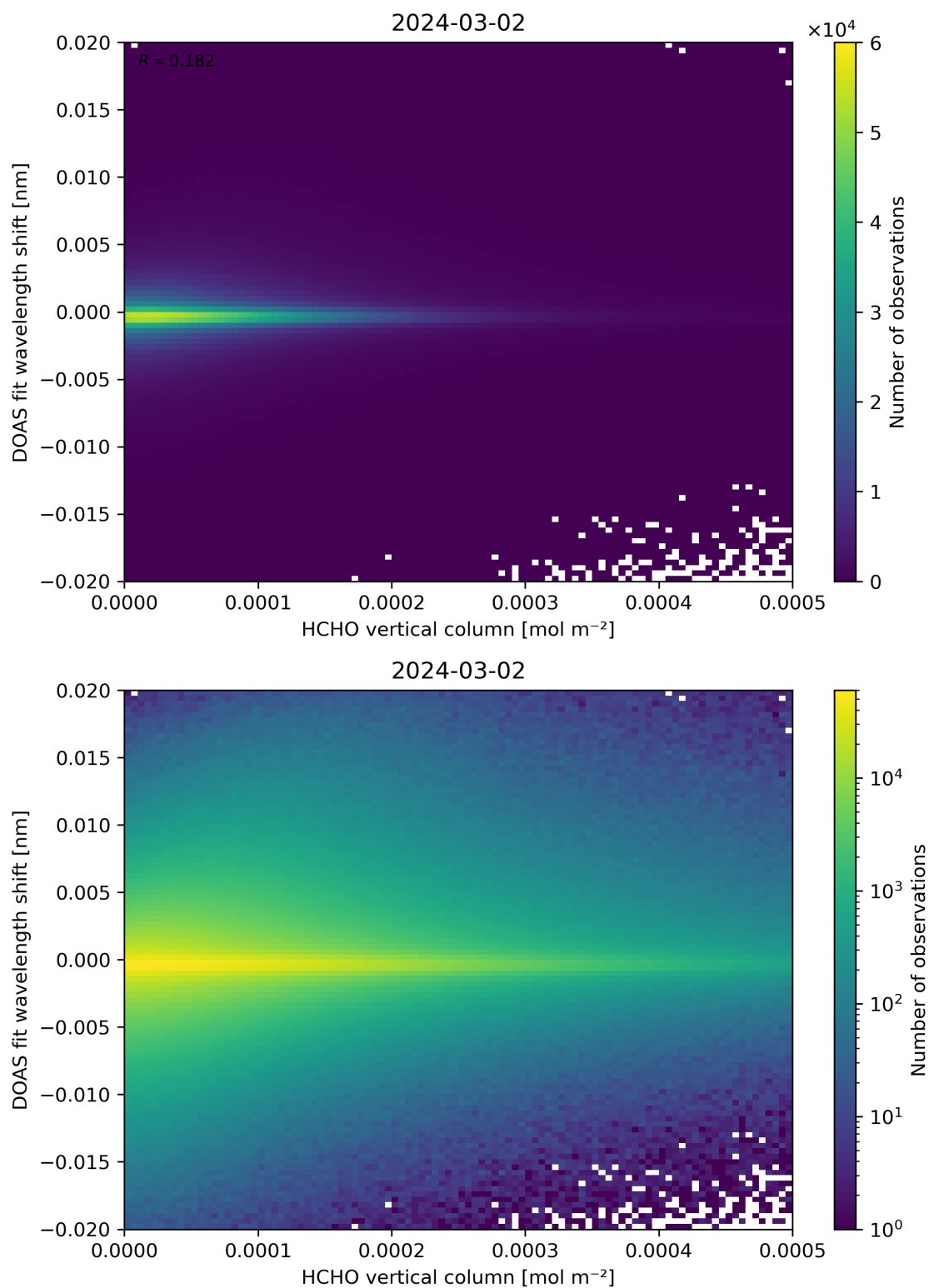
Figure 124: Scatter density plot of “HCHO vertical column” against “DOAS fit wavelength shift” for 2024-03-01 to 2024-03-03.
