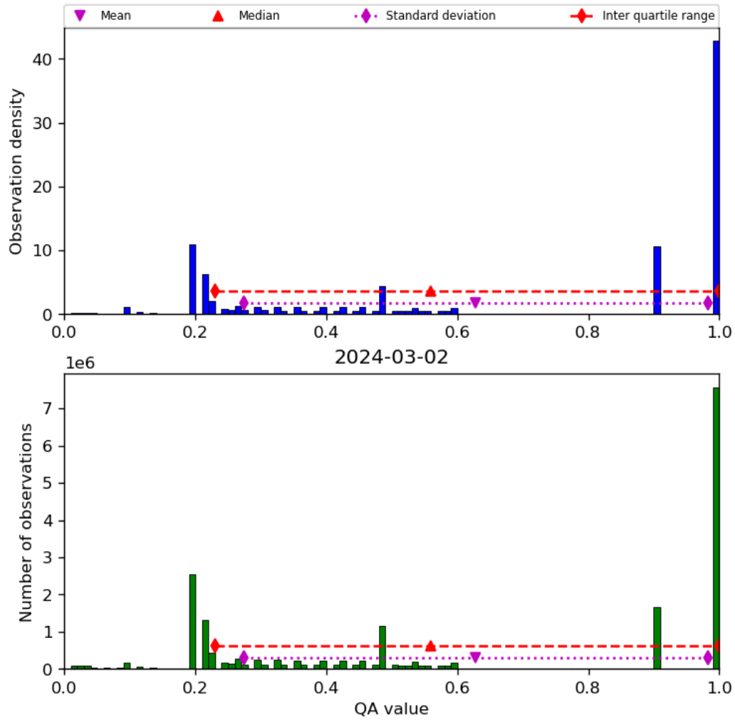
Figure 34: Histogram of “QA value” for 2024-03-01 to 2024-03-03
