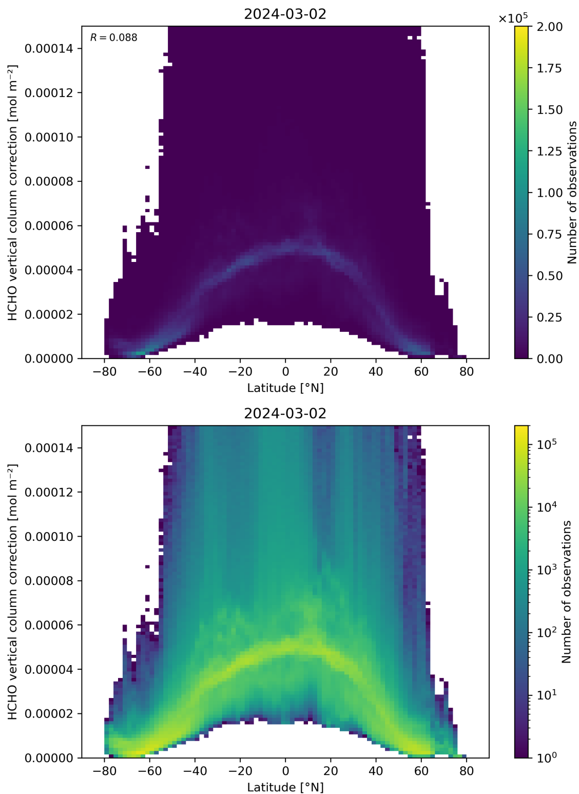
Figure 164: Scatter density plot of “Latitude” against “HCHO vertical column correction” for 2024-03-01 to 2024-03-03.
