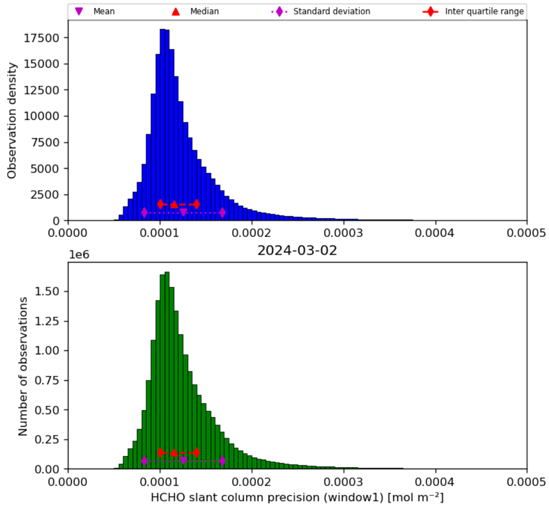
Figure 39: Histogram of “HCHO slant column precision (window1)” for 2024-03-01 to 2024-03-03
