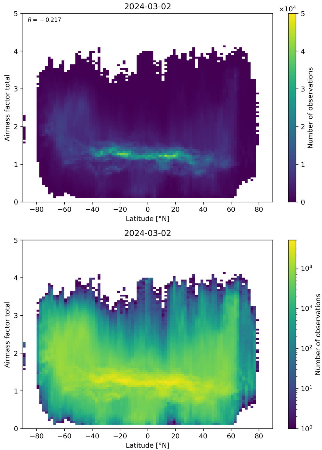
Figure 161: Scatter density plot of “Latitude” against “Airmass factor total” for 2024-03-01 to 2024-03-03.
