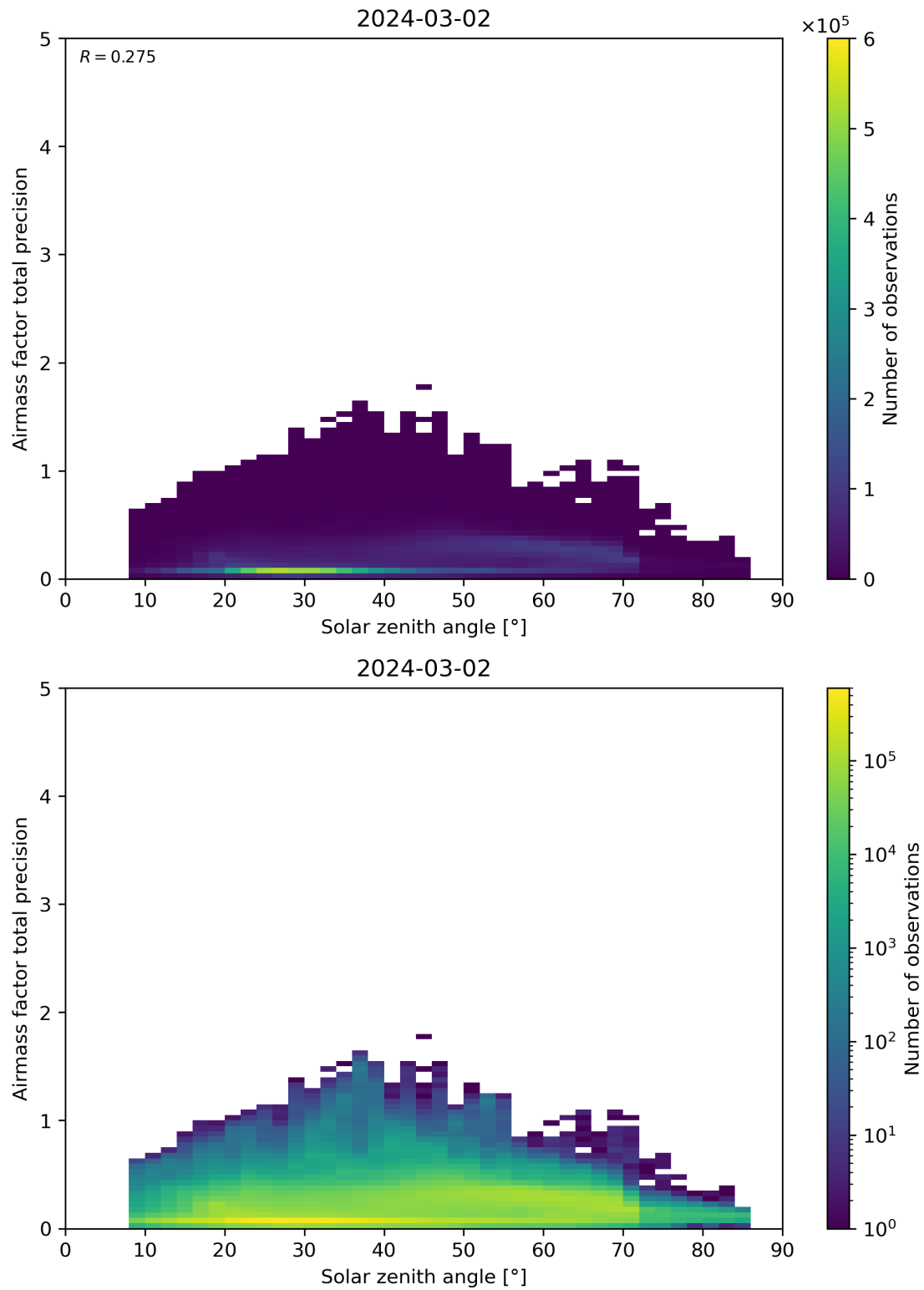
Figure 176: Scatter density plot of “Solar zenith angle” against “Airmass factor total precision” for 2024-03-01 to 2024-03-03.
