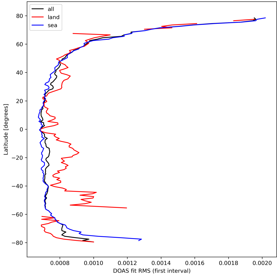
Figure 32: Zonal average of "DOAS fit RMS (first interval)" for 2024-03-01 to 2024-03-03.
