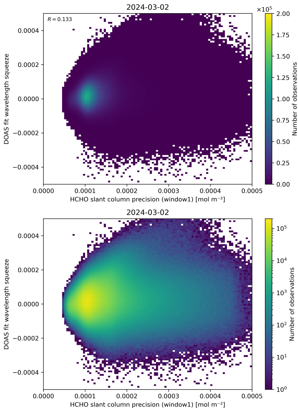
Figure 90: Scatter density plot of “HCHO slant column precision (window1)” against “DOAS fit wavelength squeeze” for 2024-03-01 to 2024-03-03.
