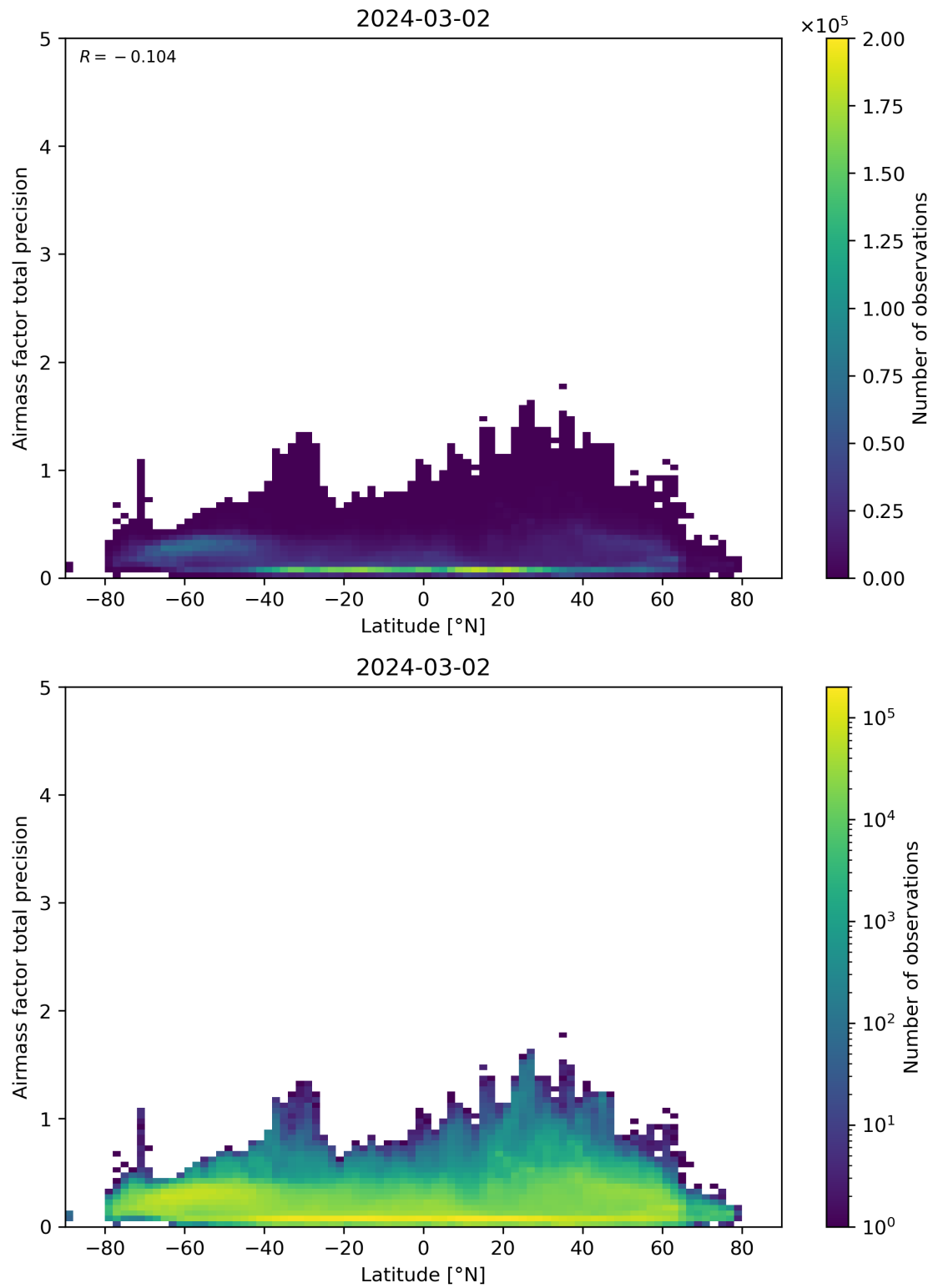
Figure 162: Scatter density plot of “Latitude” against “Airmass factor total precision” for 2024-03-01 to 2024-03-03.
