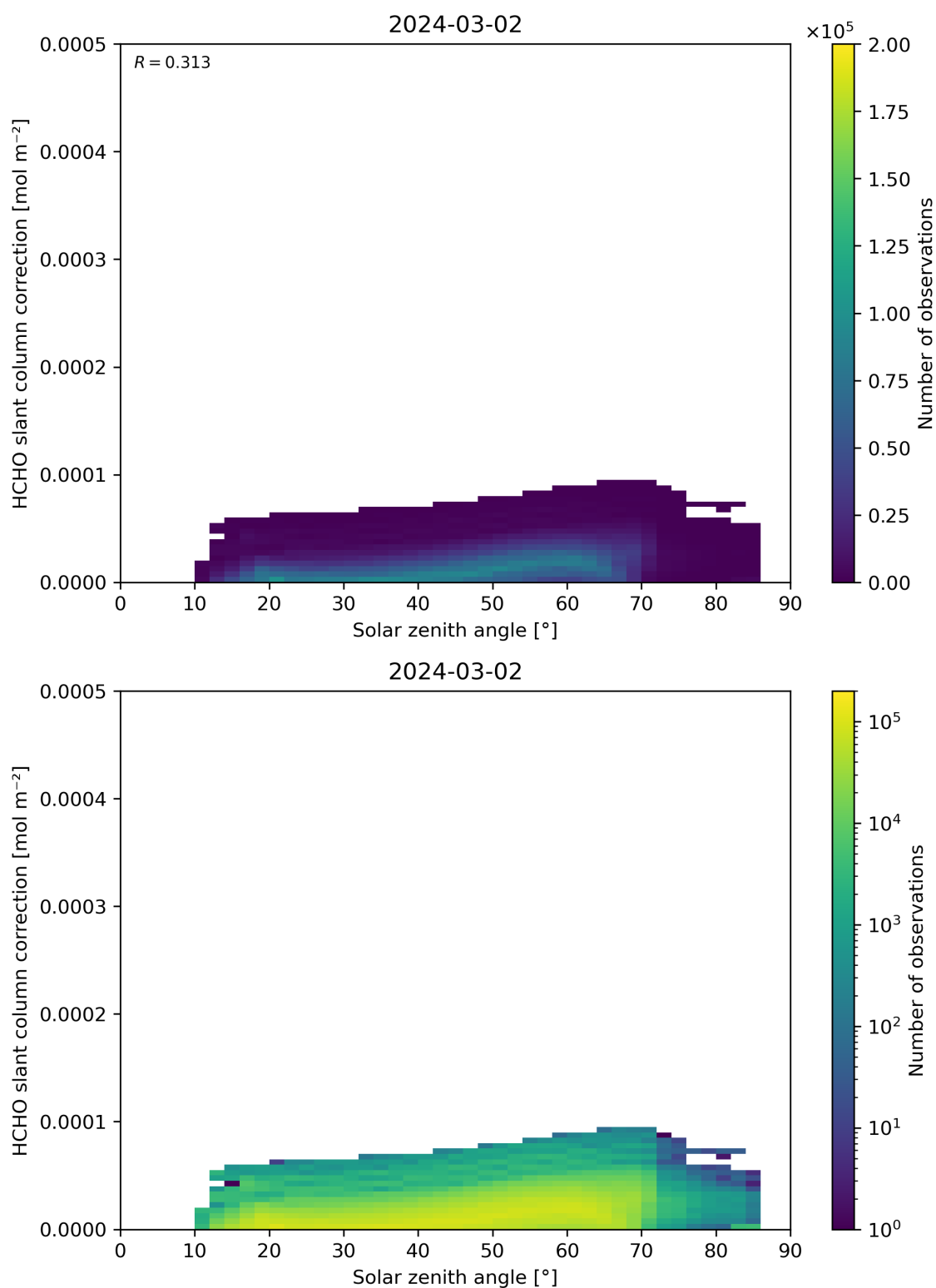
Figure 172: Scatter density plot of “Solar zenith angle” against “HCHO slant column correction” for 2024-03-01 to 2024-03-03.
