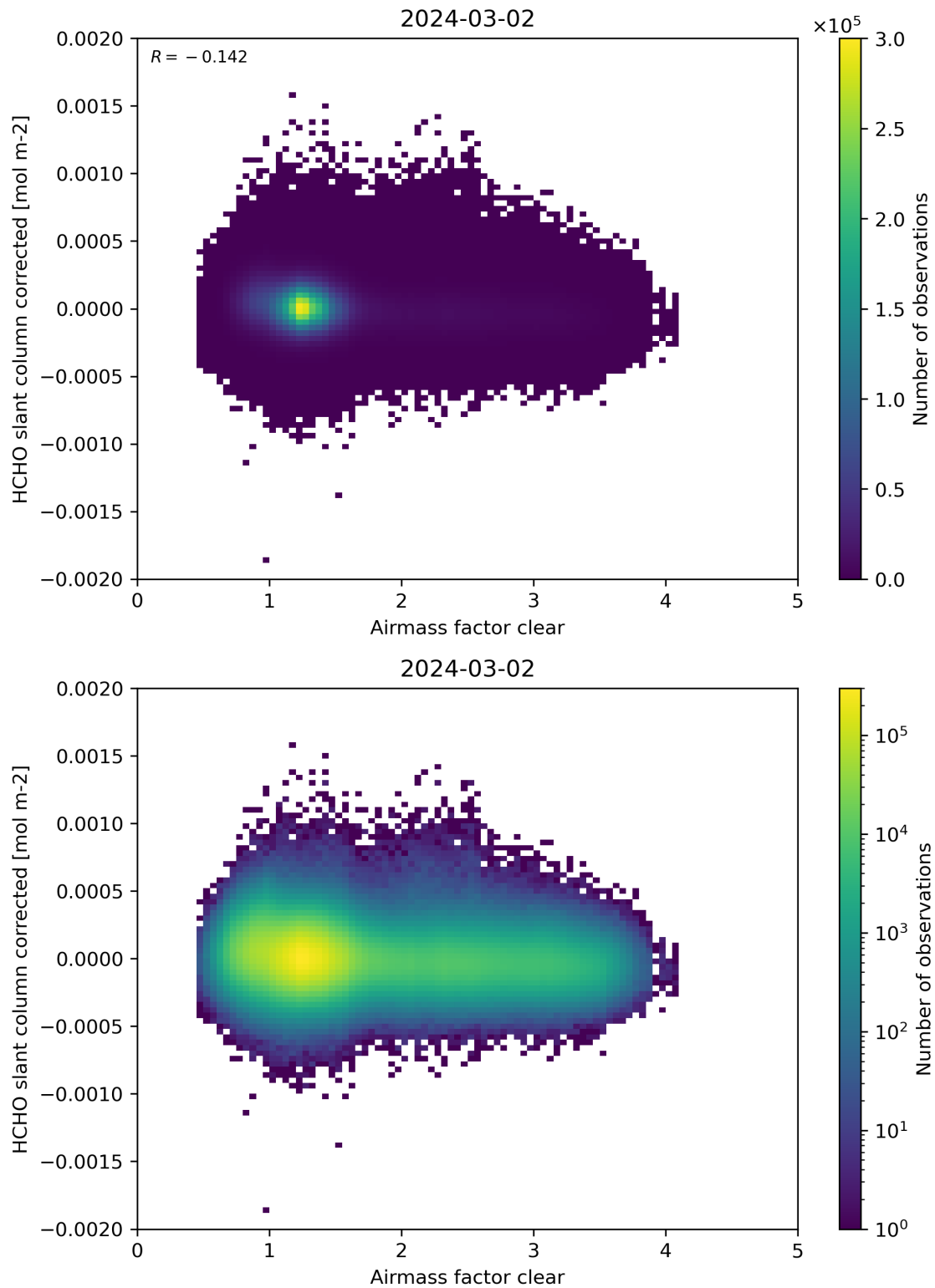
Figure 74: Scatter density plot of “Airmass factor clear” against “HCHO slant column corrected” for 2024-03-01 to 2024-03-03.
