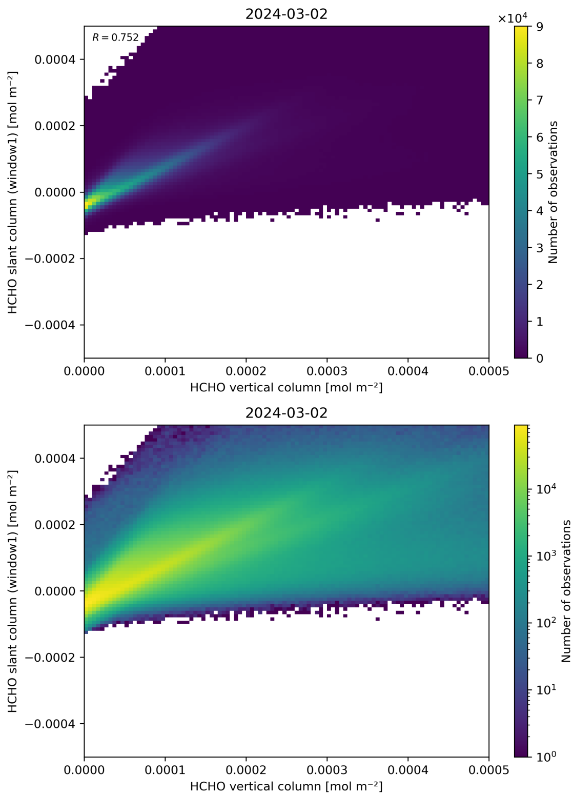
Figure 129: Scatter density plot of “HCHO vertical column” against “HCHO slant column (window1)” for 2024-03-01 to 2024-03-03.
