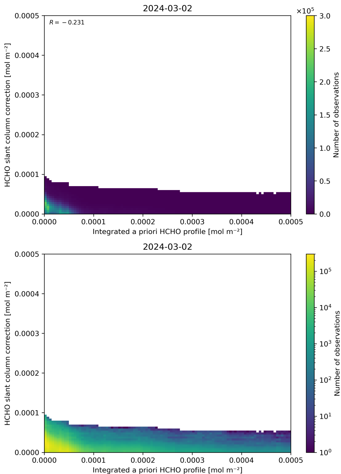
Figure 152: Scatter density plot of “Integrated a priori HCHO profile” against “HCHO slant column correction” for 2024-03-01 to 2024-03-03.
