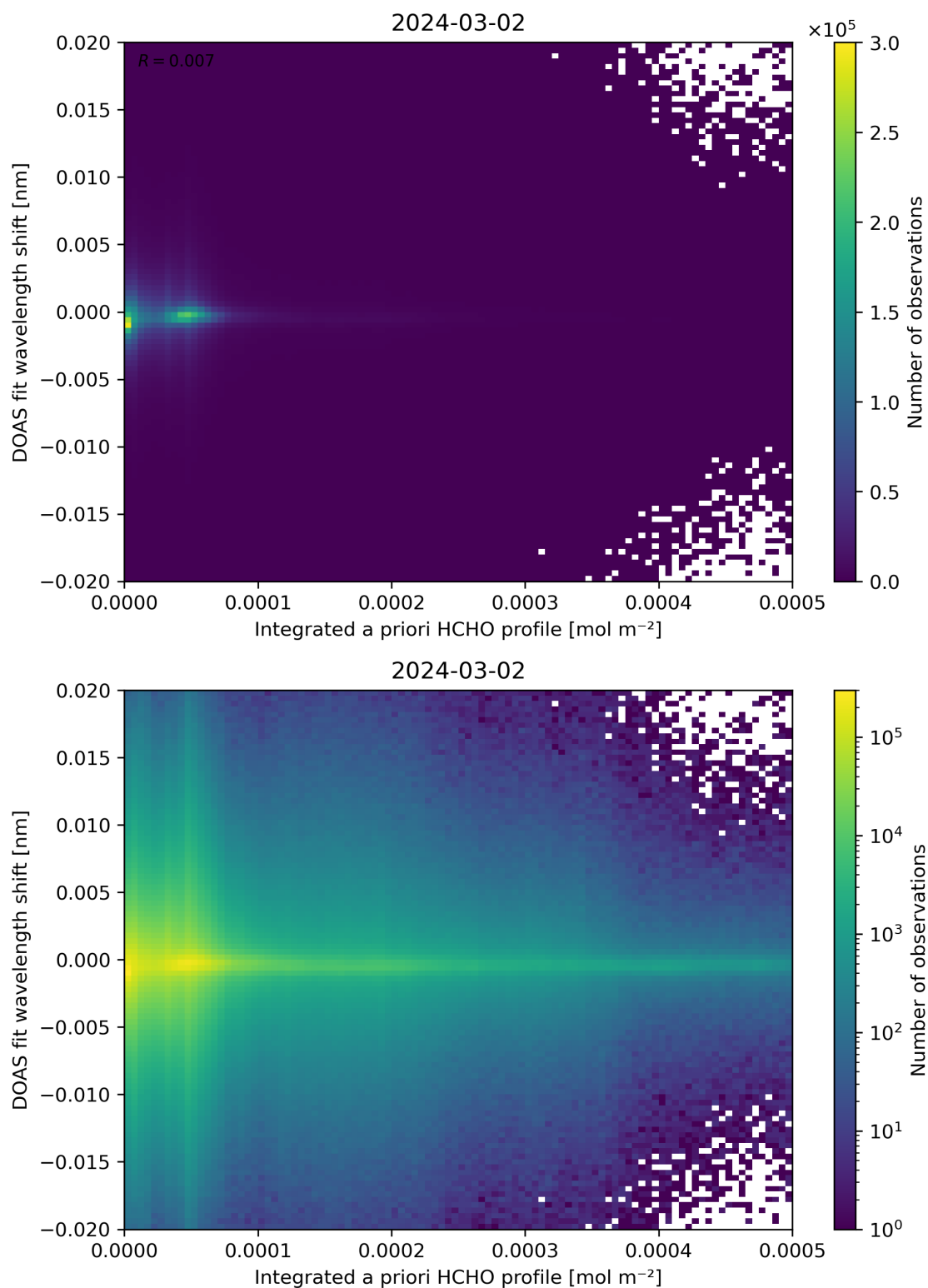
Figure 149: Scatter density plot of “Integrated a priori HCHO profile” against “DOAS fit wavelength shift” for 2024-03-01 to 2024-03-03.
