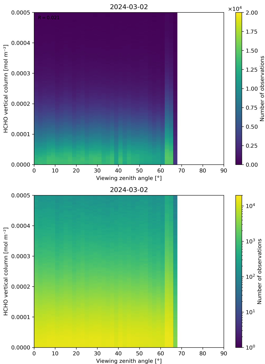
Figure 192: Scatter density plot of “Viewing zenith angle” against “HCHO vertical column” for 2024-03-01 to 2024-03-03.
