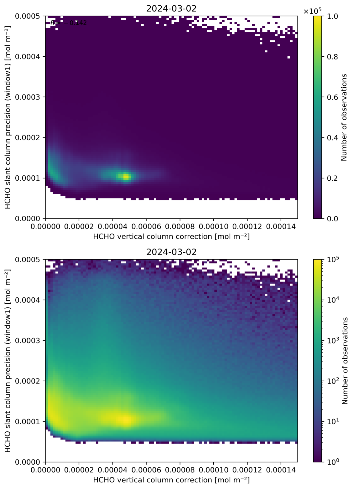
Figure 119: Scatter density plot of “HCHO vertical column correction” against “HCHO slant column precision (window1)” for 2024-03-01 to 2024-03-03.
