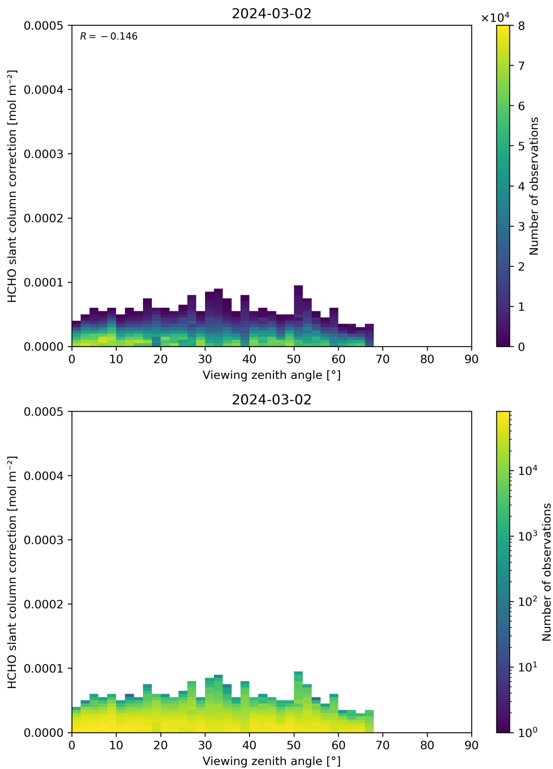
Figure 187: Scatter density plot of “Viewing zenith angle” against “HCHO slant column correction” for 2024-03-01 to 2024-03-03.
