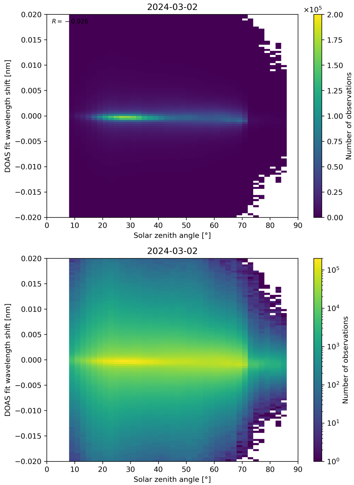
Figure 168: Scatter density plot of “Solar zenith angle” against “DOAS fit wavelength shift” for 2024-03-01 to 2024-03-03.
