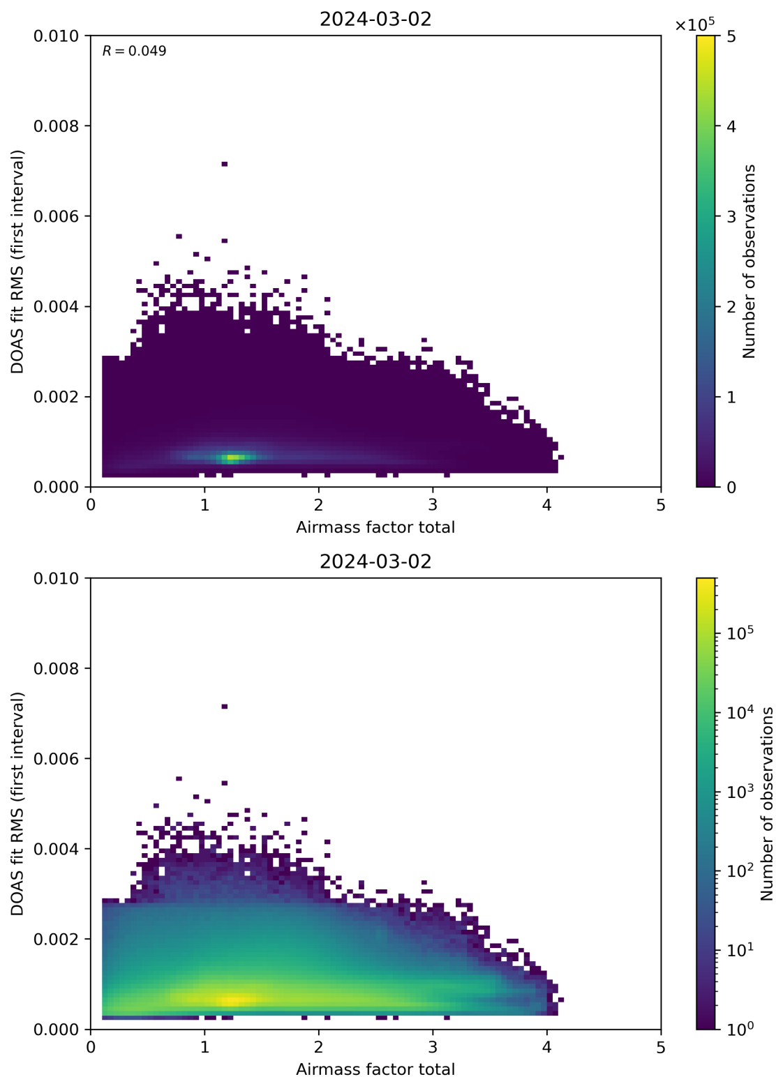
Figure 97: Scatter density plot of “Airmass factor total” against “DOAS fit RMS (first interval)” for 2024-03-01 to 2024-03-03.
