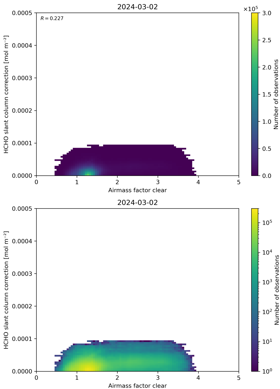
Figure 75: Scatter density plot of “Airmass factor clear” against “HCHO slant column correction” for 2024-03-01 to 2024-03-03.
