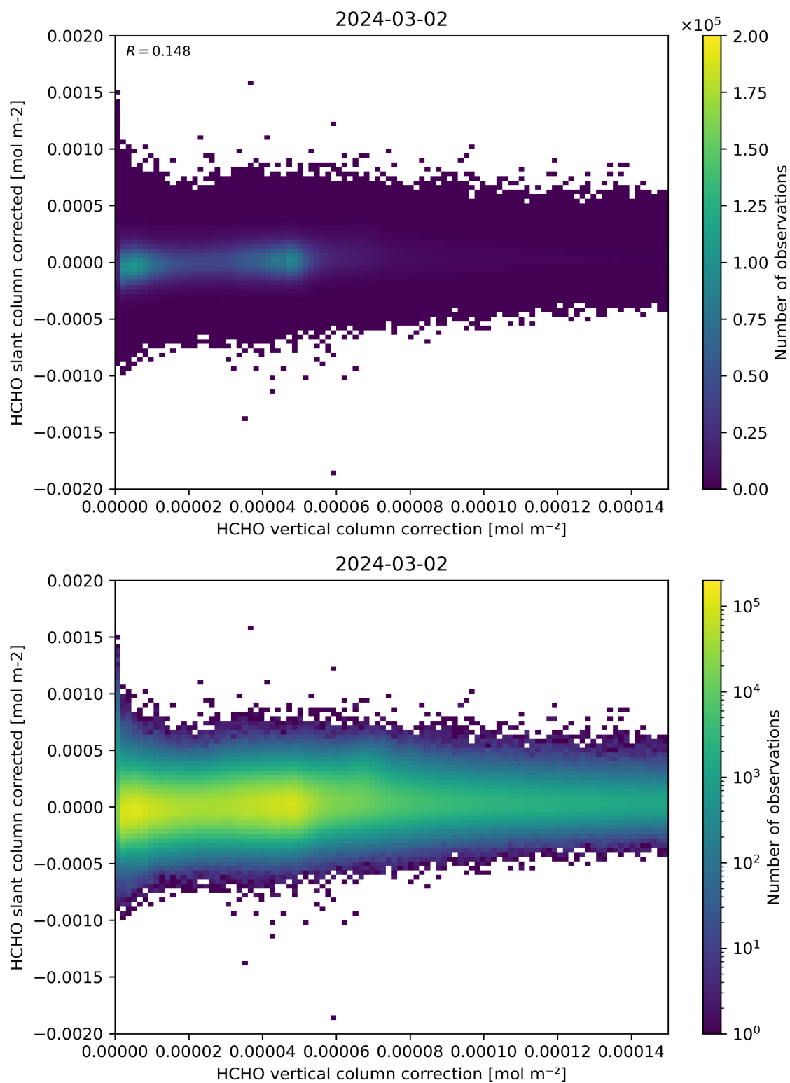
Figure 116: Scatter density plot of “HCHO vertical column correction” against “HCHO slant column corrected” for 2024-03-01 to 2024-03-03.
