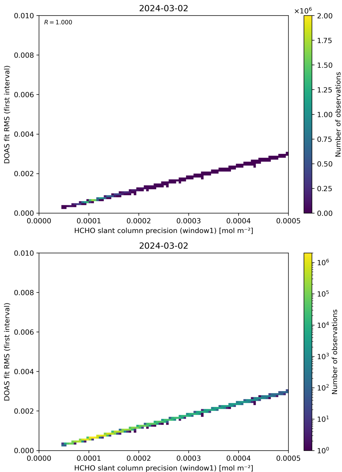
Figure 88: Scatter density plot of “HCHO slant column precision (window1)” against “DOAS fit RMS (first interval)” for 2024-03-01 to 2024-03-03.
