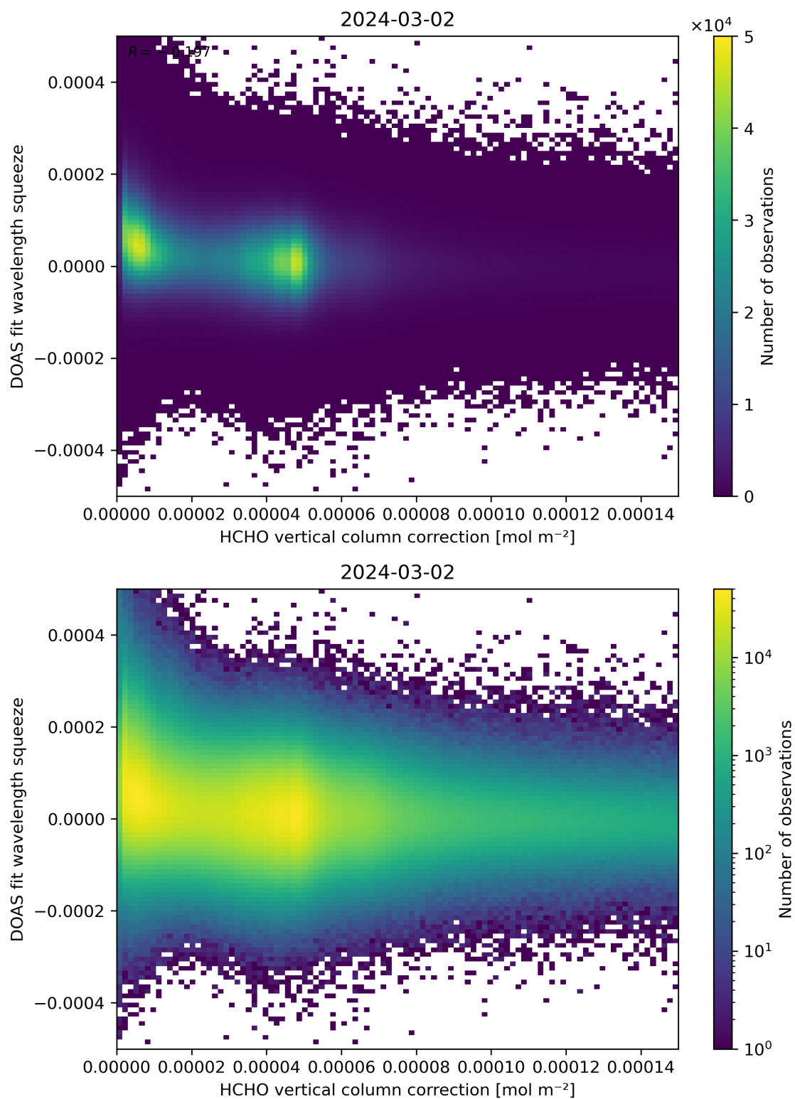
Figure 114: Scatter density plot of “HCHO vertical column correction” against “DOAS fit wavelength squeeze” for 2024-03-01 to 2024-03-03.
