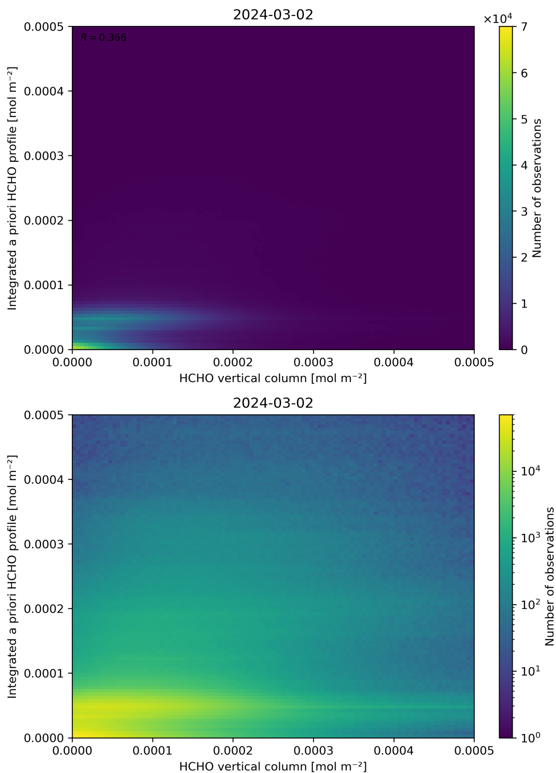
Figure 135: Scatter density plot of “HCHO vertical column” against “Integrated a priori HCHO profile” for 2024-03-01 to 2024-03-03.
