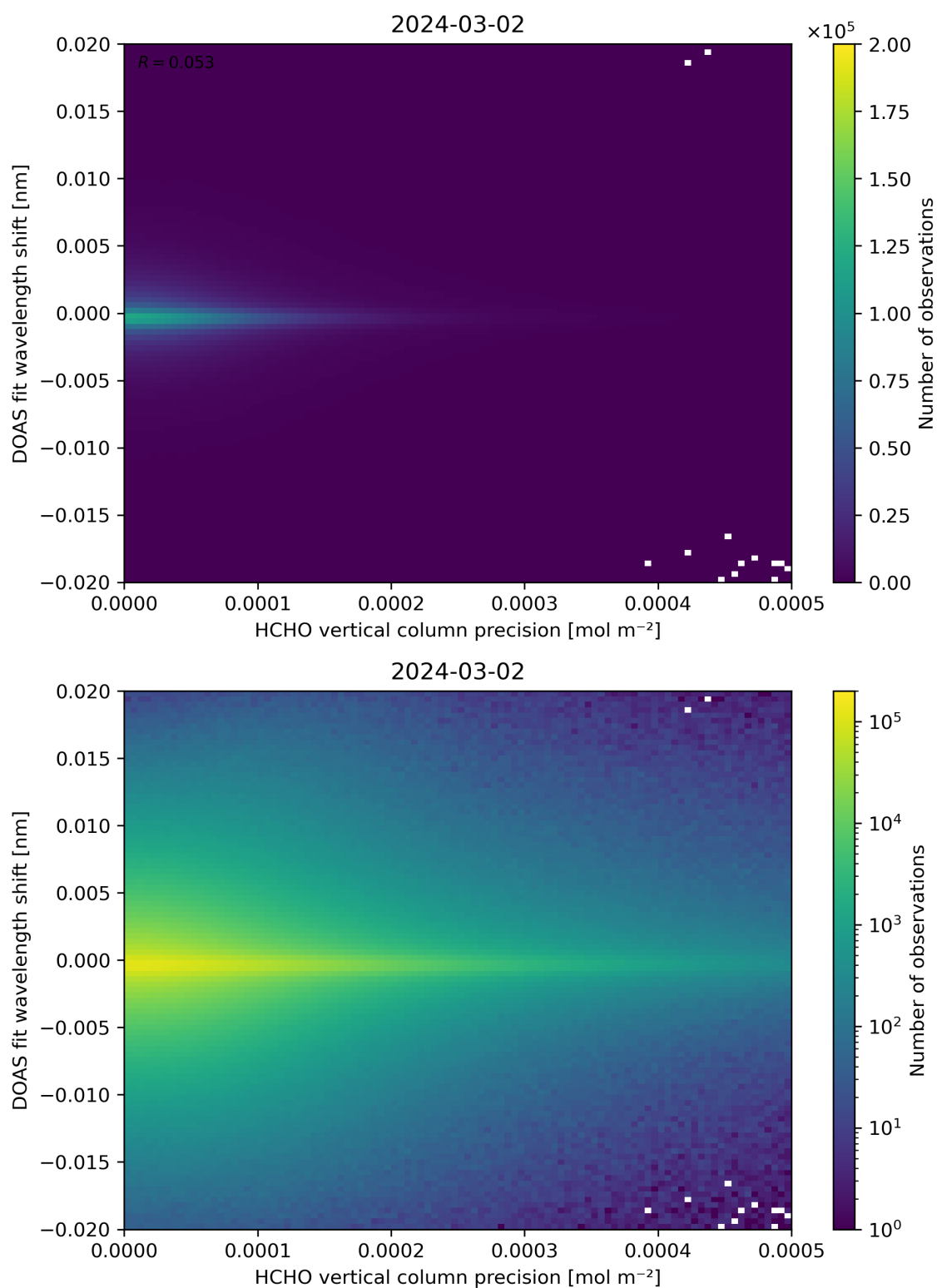
Figure 137: Scatter density plot of “HCHO vertical column precision” against “DOAS fit wavelength shift” for 2024-03-01 to 2024-03-03.
