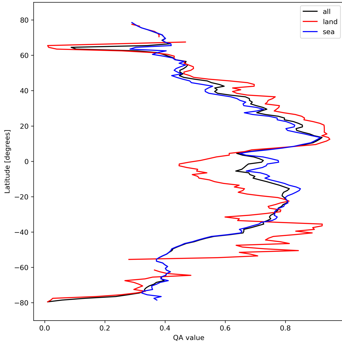
Figure 20: Zonal average of “QA value” for 2024-03-01 to 2024-03-03.
