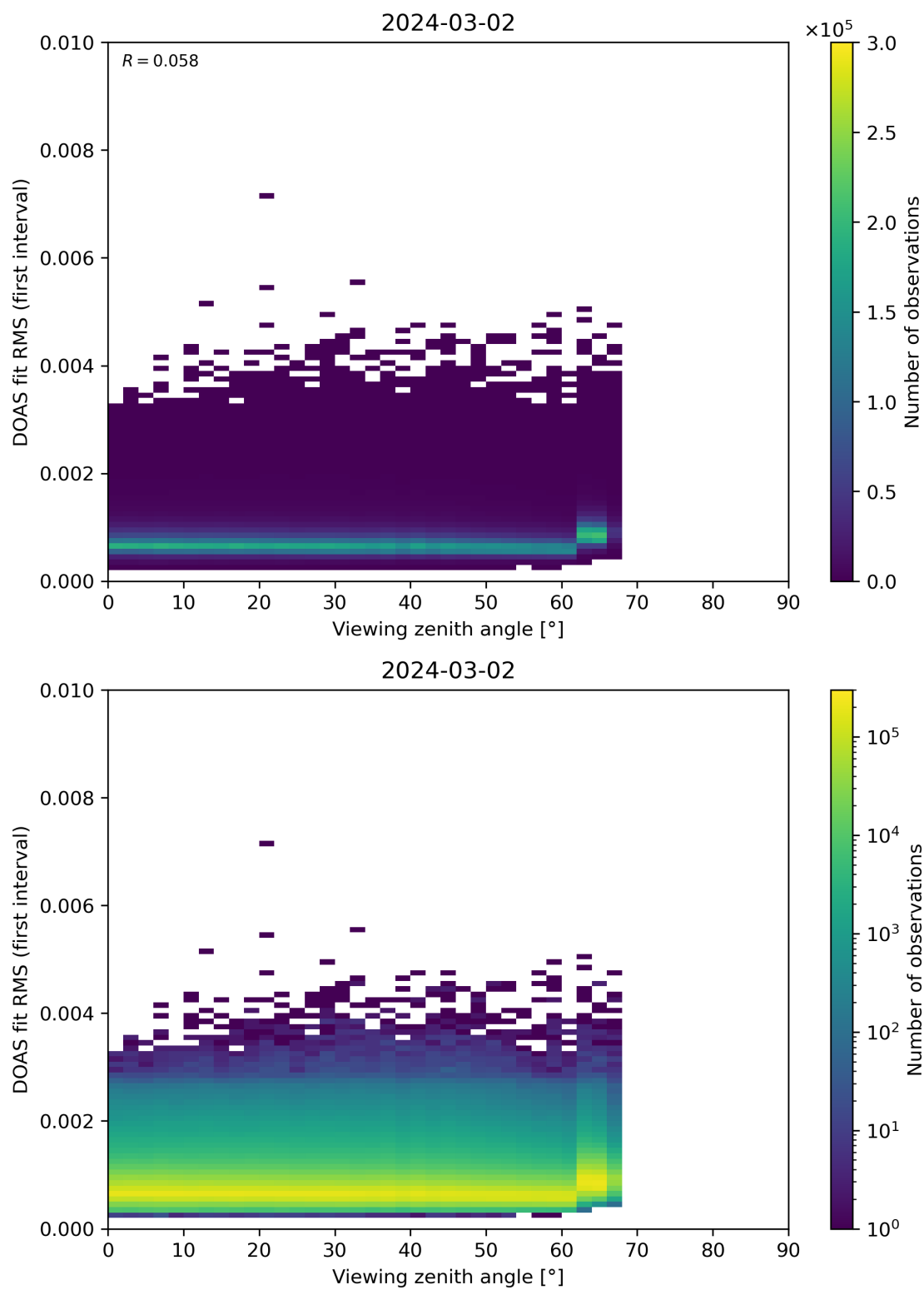
Figure 182: Scatter density plot of “Viewing zenith angle” against “DOAS fit RMS (first interval)” for 2024-03-01 to 2024-03-03.
