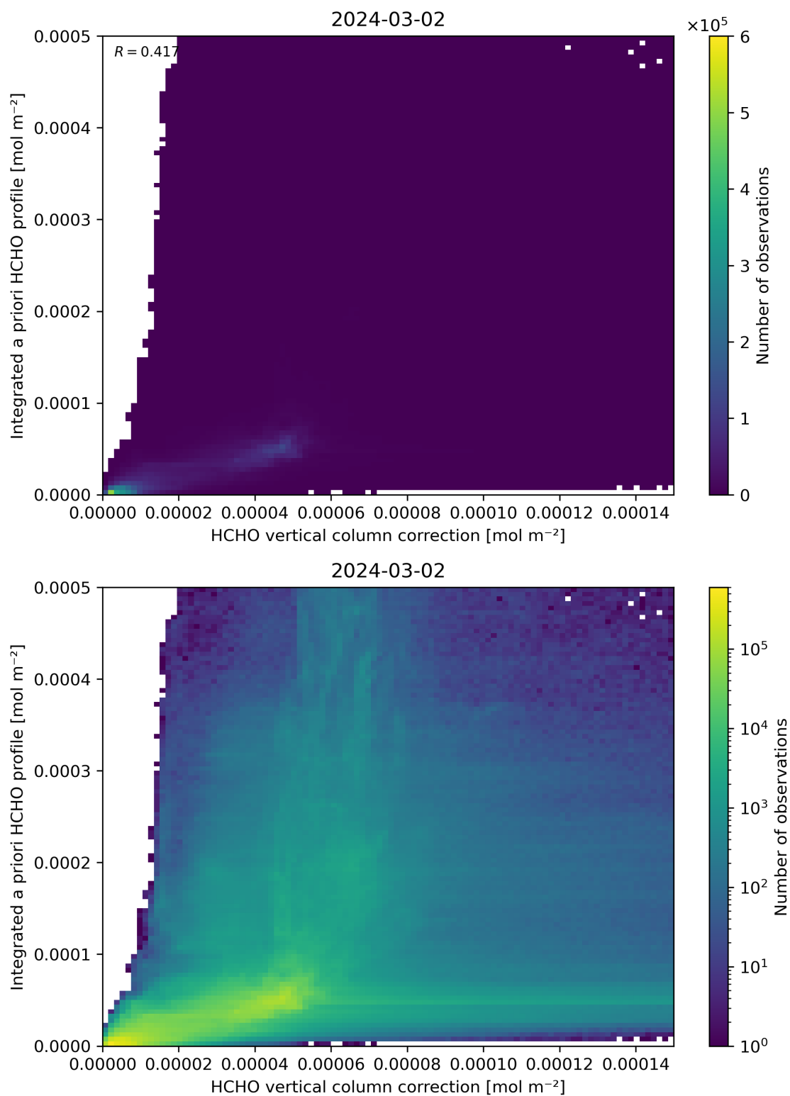
Figure 122: Scatter density plot of “HCHO vertical column correction” against “Integrated a priori HCHO profile” for 2024-03-01 to 2024-03-03.
