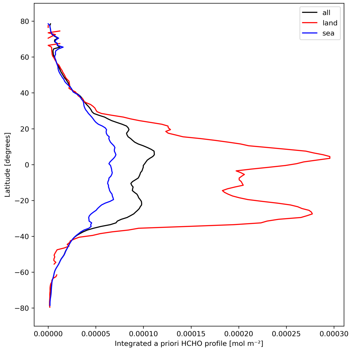
Figure 29: Zonal average of “Integrated a priori HCHO profile” for 2024-03-01 to 2024-03-03.
