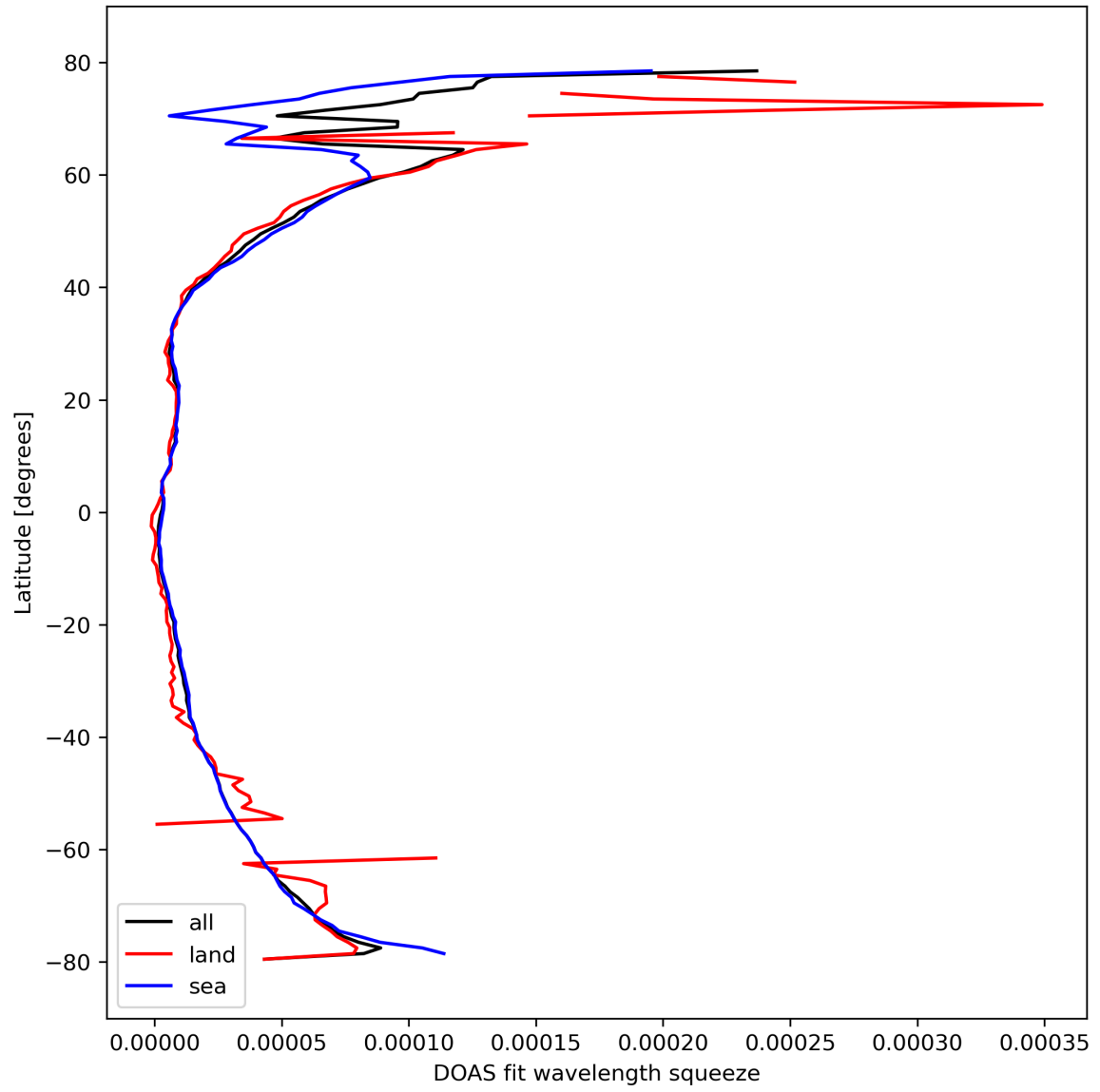
Figure 31: Zonal average of “DOAS fit wavelength squeeze” for 2024-03-01 to 2024-03-03.
