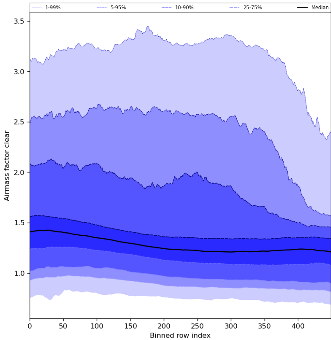
Figure 56: Along track statistics of “Airmass factor clear” for 2024-03-01 to 2024-03-03
