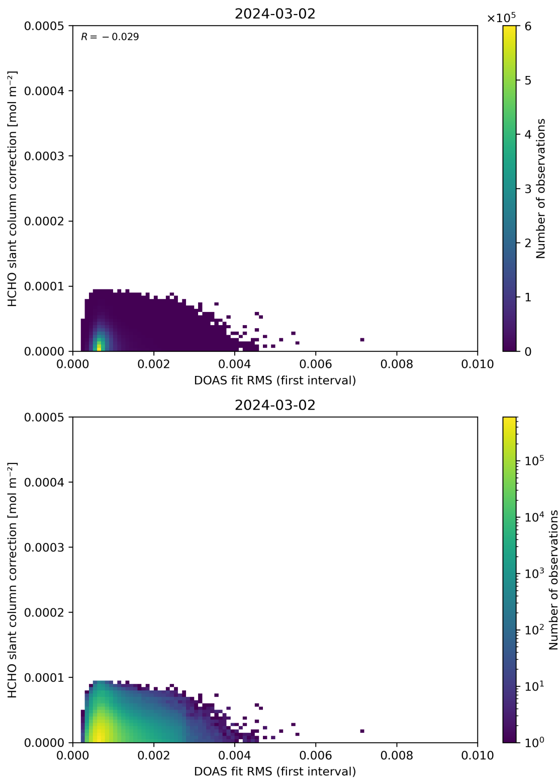
Figure 63: Scatter density plot of “DOAS fit RMS (first interval)” against “HCHO slant column correction” for 2024-03-01 to 2024-03-03.
