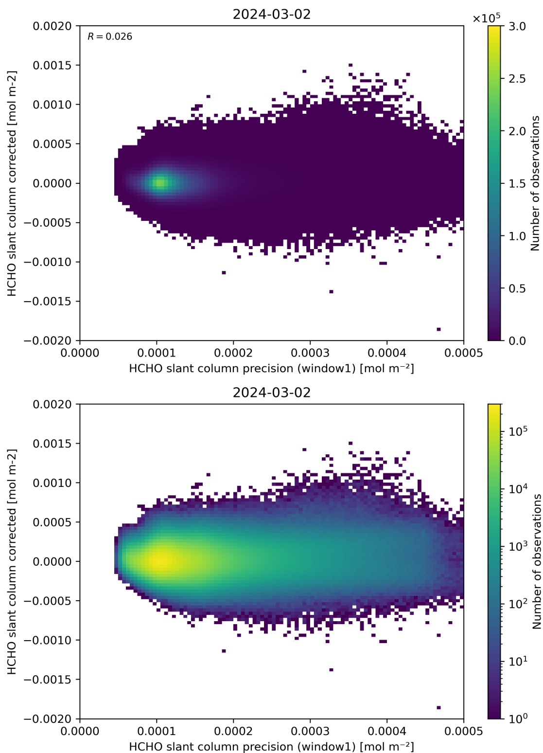
Figure 92: Scatter density plot of “HCHO slant column precision (window1)” against “HCHO slant column corrected” for 2024-03-01 to 2024-03-03.
