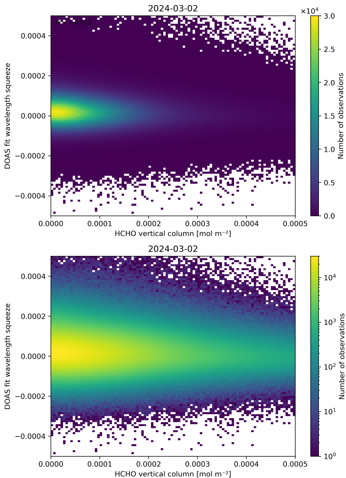
Figure 125: Scatter density plot of “HCHO vertical column” against “DOAS fit wavelength squeeze” for 2024-03-01 to 2024-03-03.
