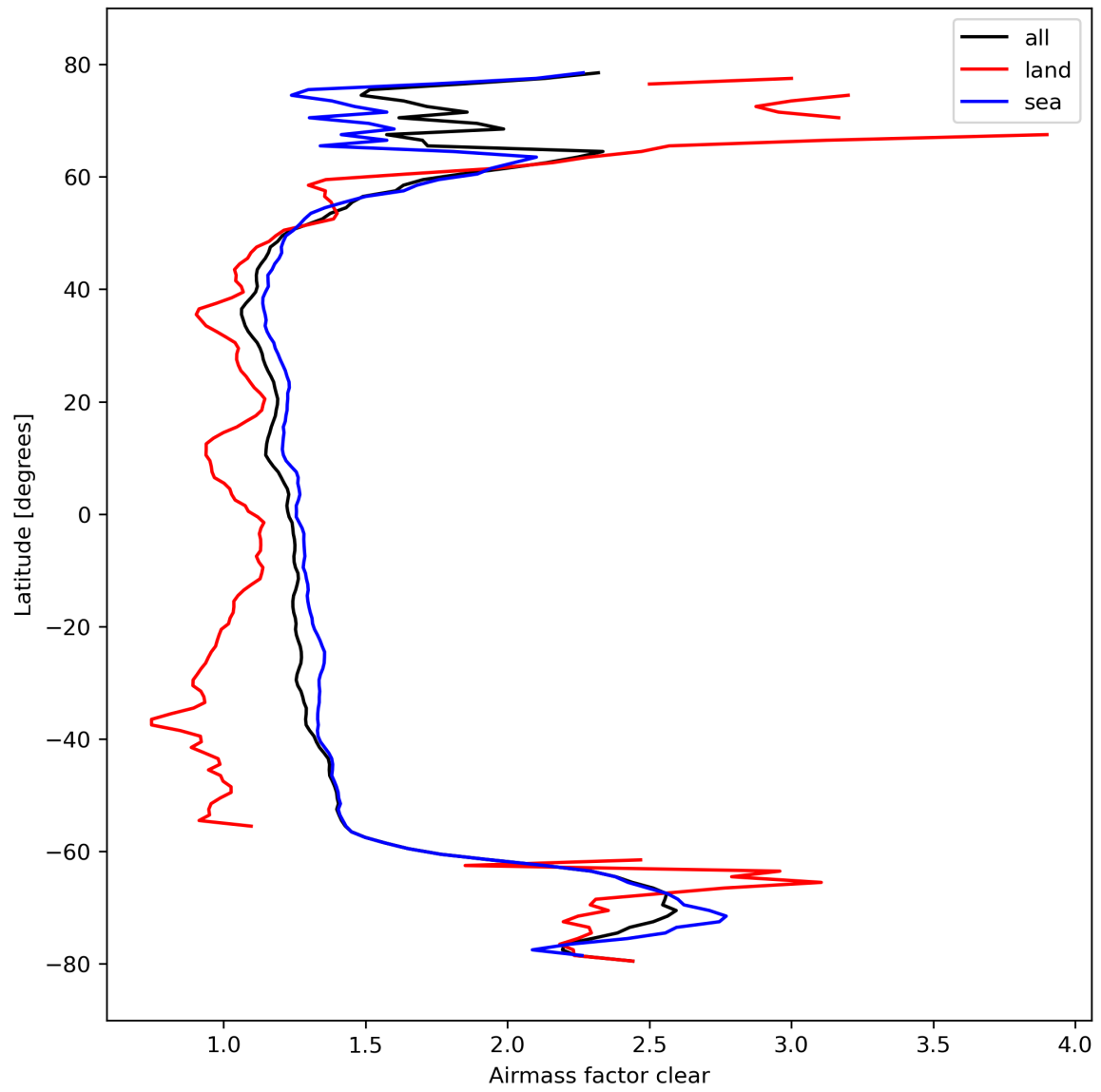
Figure 28: Zonal average of “Airmass factor clear” for 2024-03-01 to 2024-03-03.
