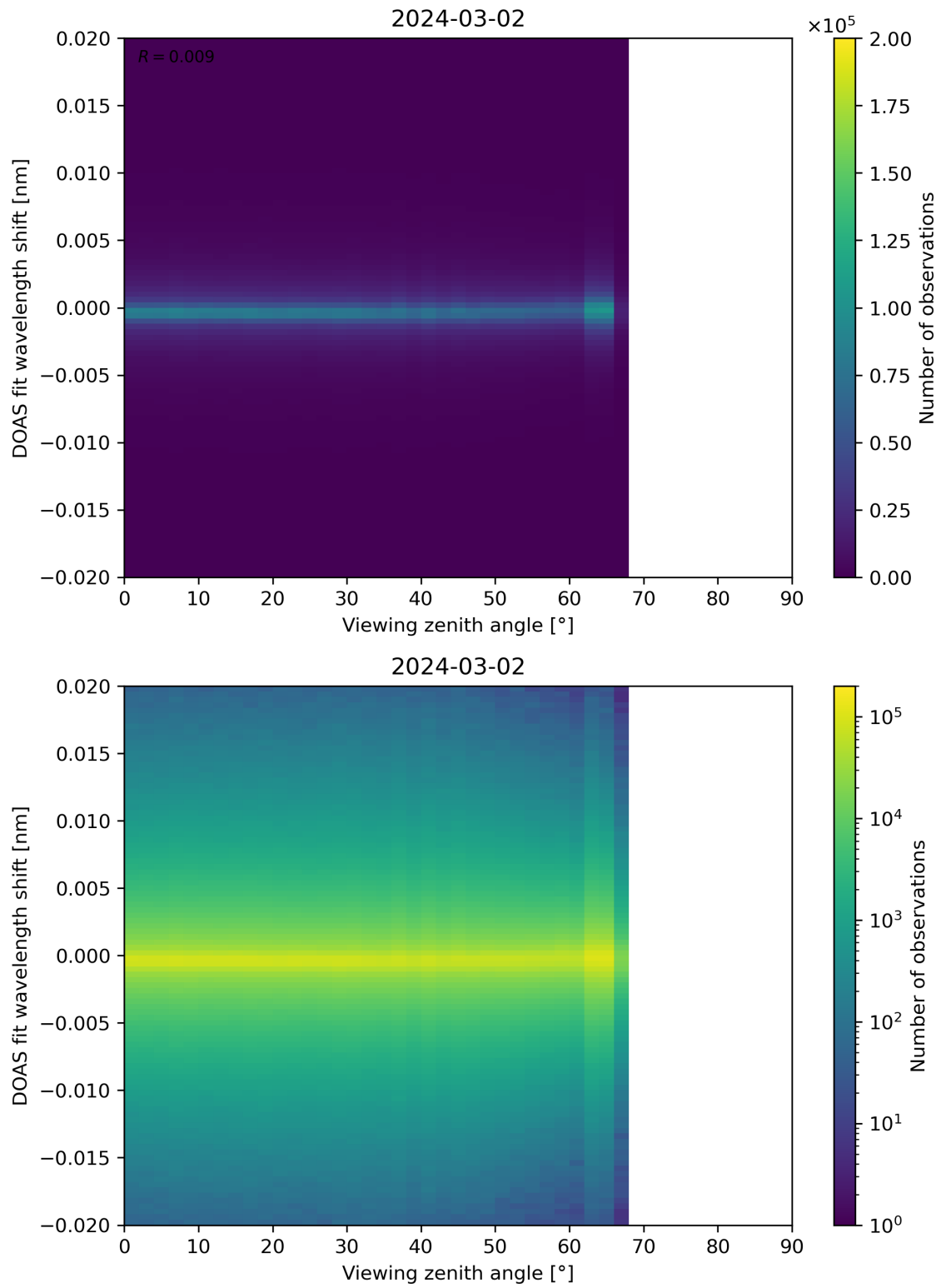
Figure 183: Scatter density plot of “Viewing zenith angle” against “DOAS fit wavelength shift” for 2024-03-01 to 2024-03-03.
