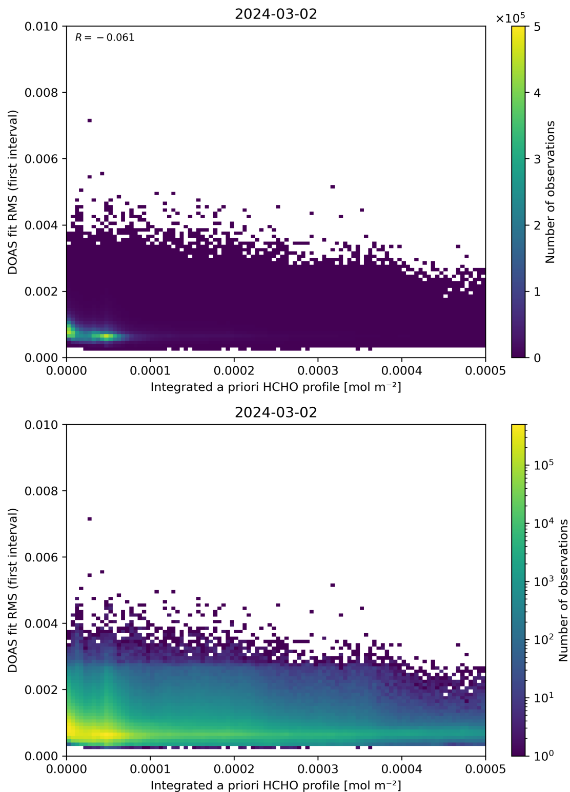
Figure 148: Scatter density plot of “Integrated a priori HCHO profile” against “DOAS fit RMS (first interval)” for 2024-03-01 to 2024-03-03.
