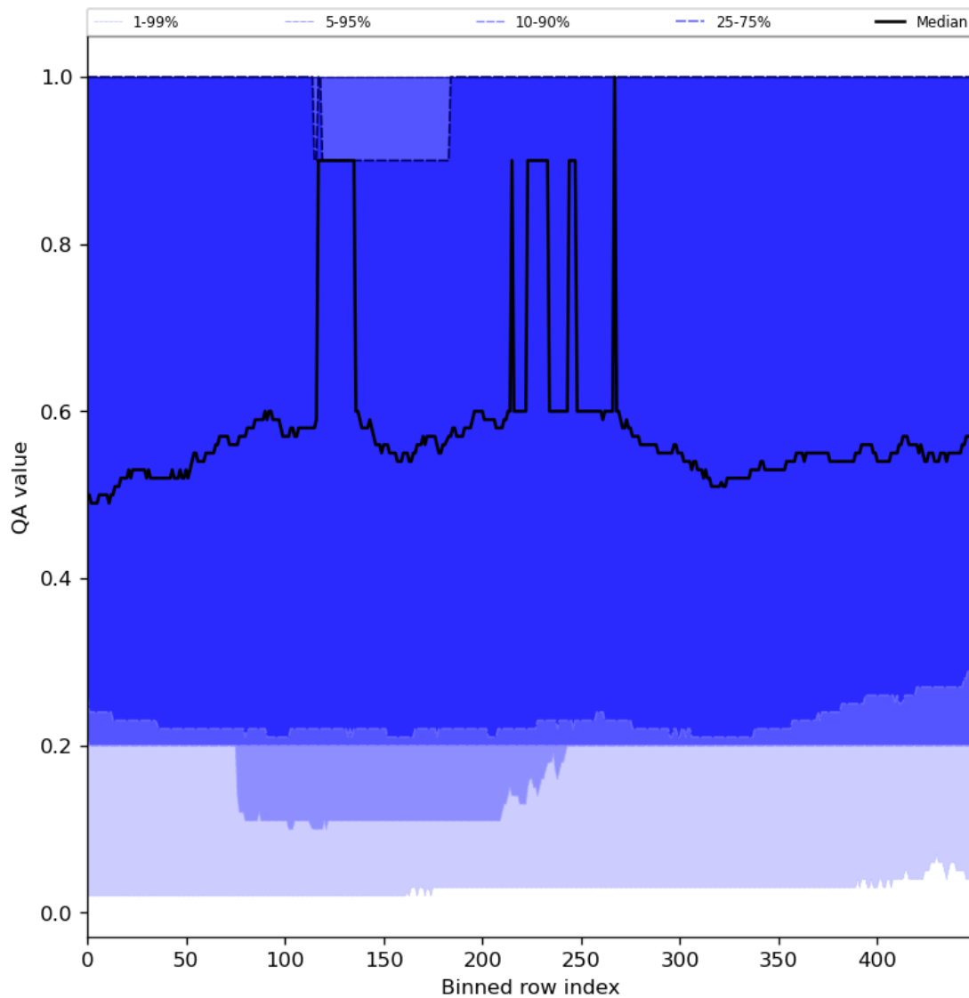
Figure 48: Along track statistics of “QA value” for 2024-03-01 to 2024-03-03
