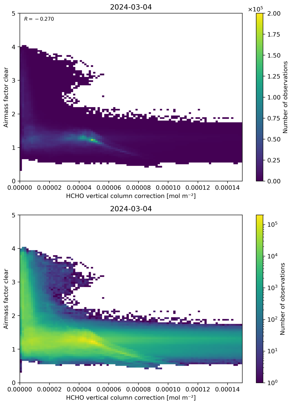
Figure 115: Scatter density plot of “HCHO vertical column correction” against “Airmass factor clear” for 2024-03-04 to 2024-03-05.
