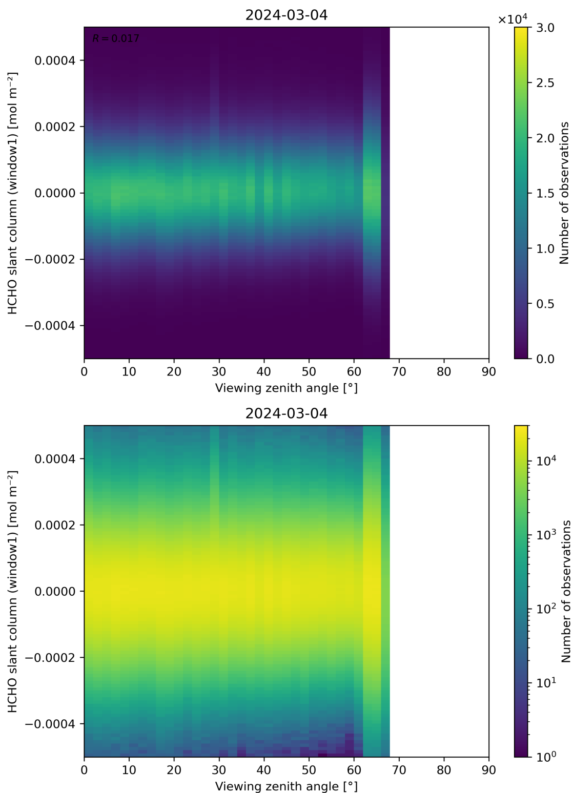
Figure 188: Scatter density plot of “Viewing zenith angle” against “HCHO slant column (window1)” for 2024-03-04 to 2024-03-05.
