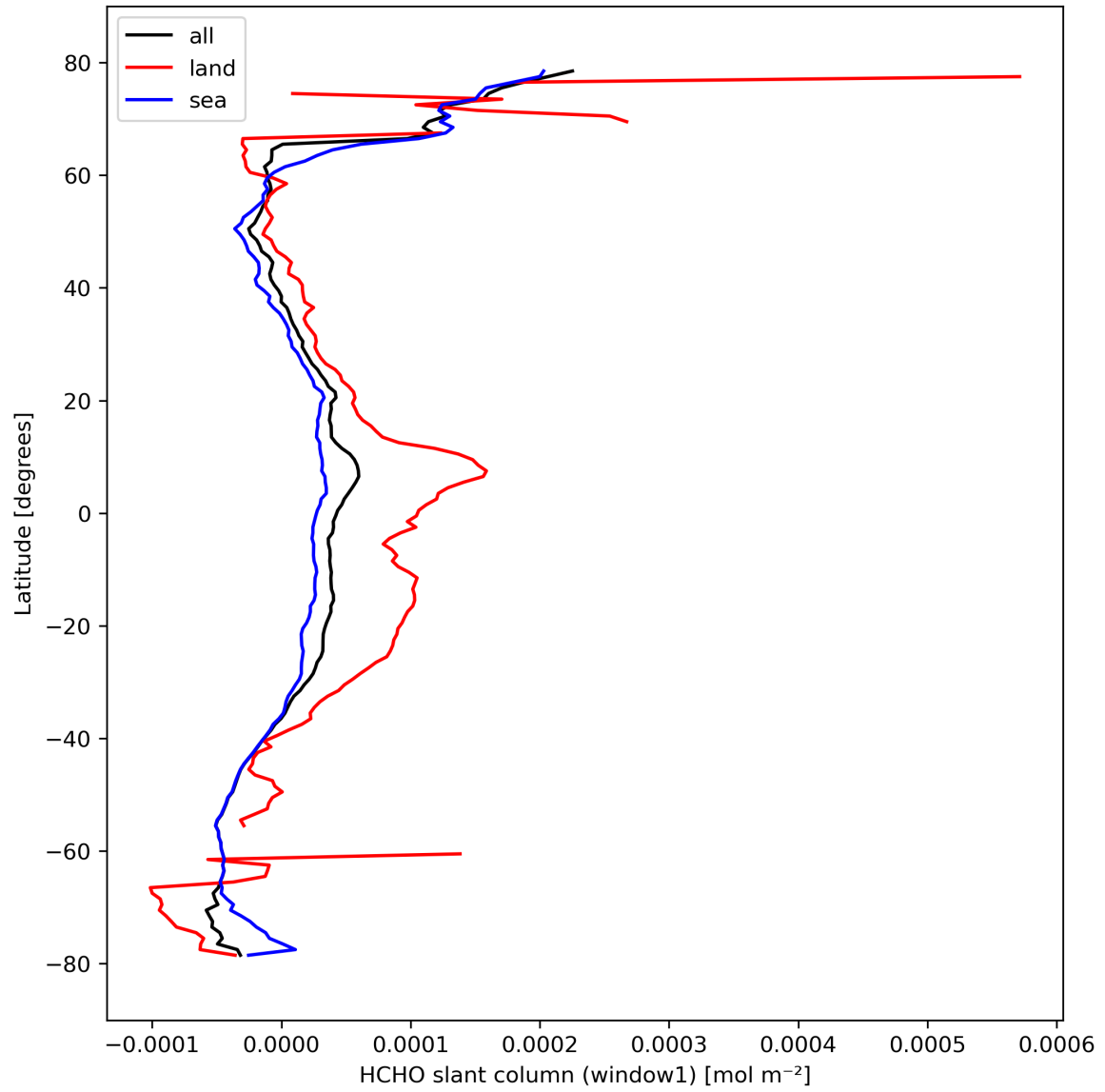
Figure 24: Zonal average of “HCHO slant column (window1)” for 2024-03-04 to 2024-03-05.
