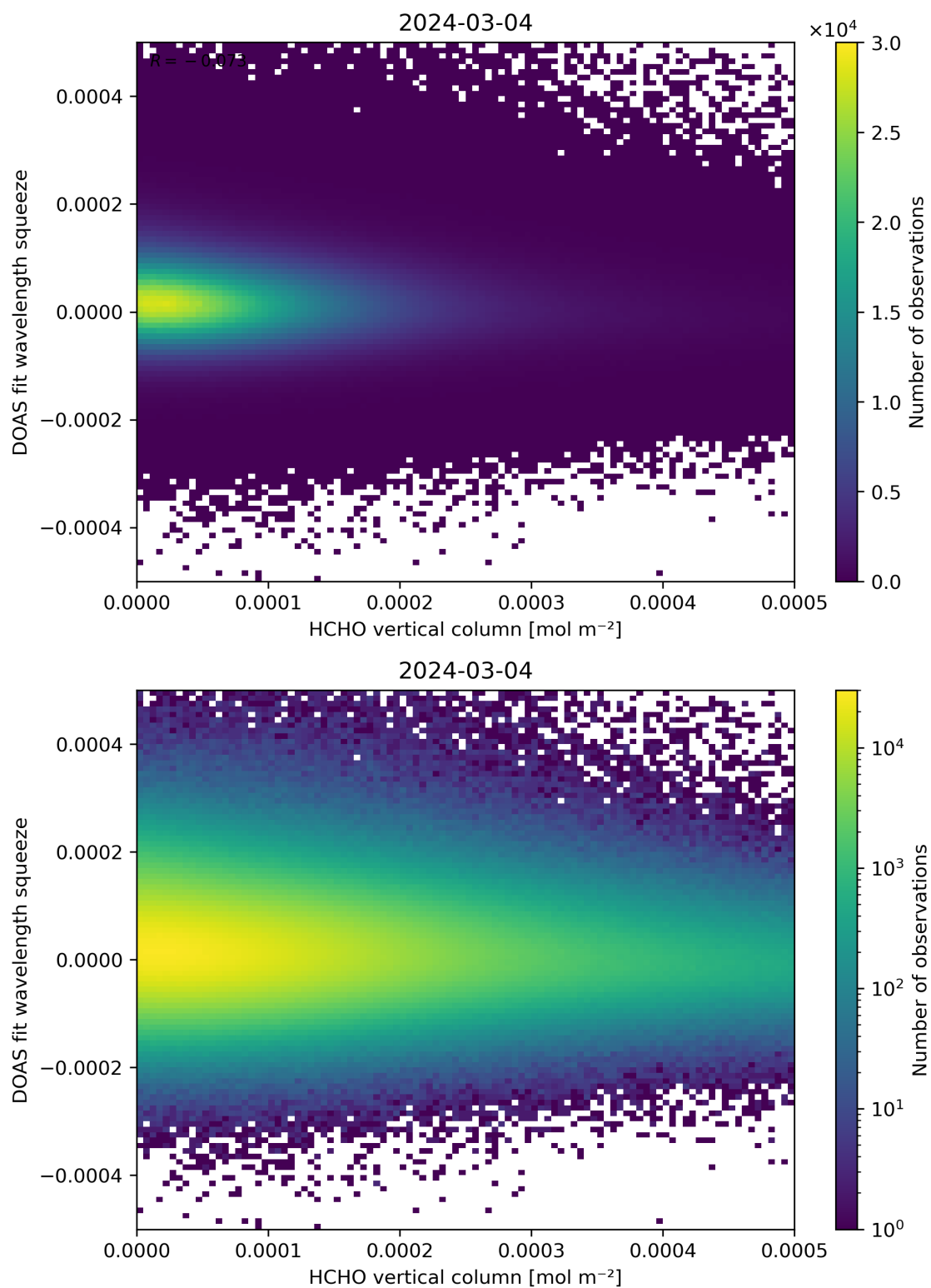
Figure 125: Scatter density plot of “HCHO vertical column” against “DOAS fit wavelength squeeze” for 2024-03-04 to 2024-03-05.
