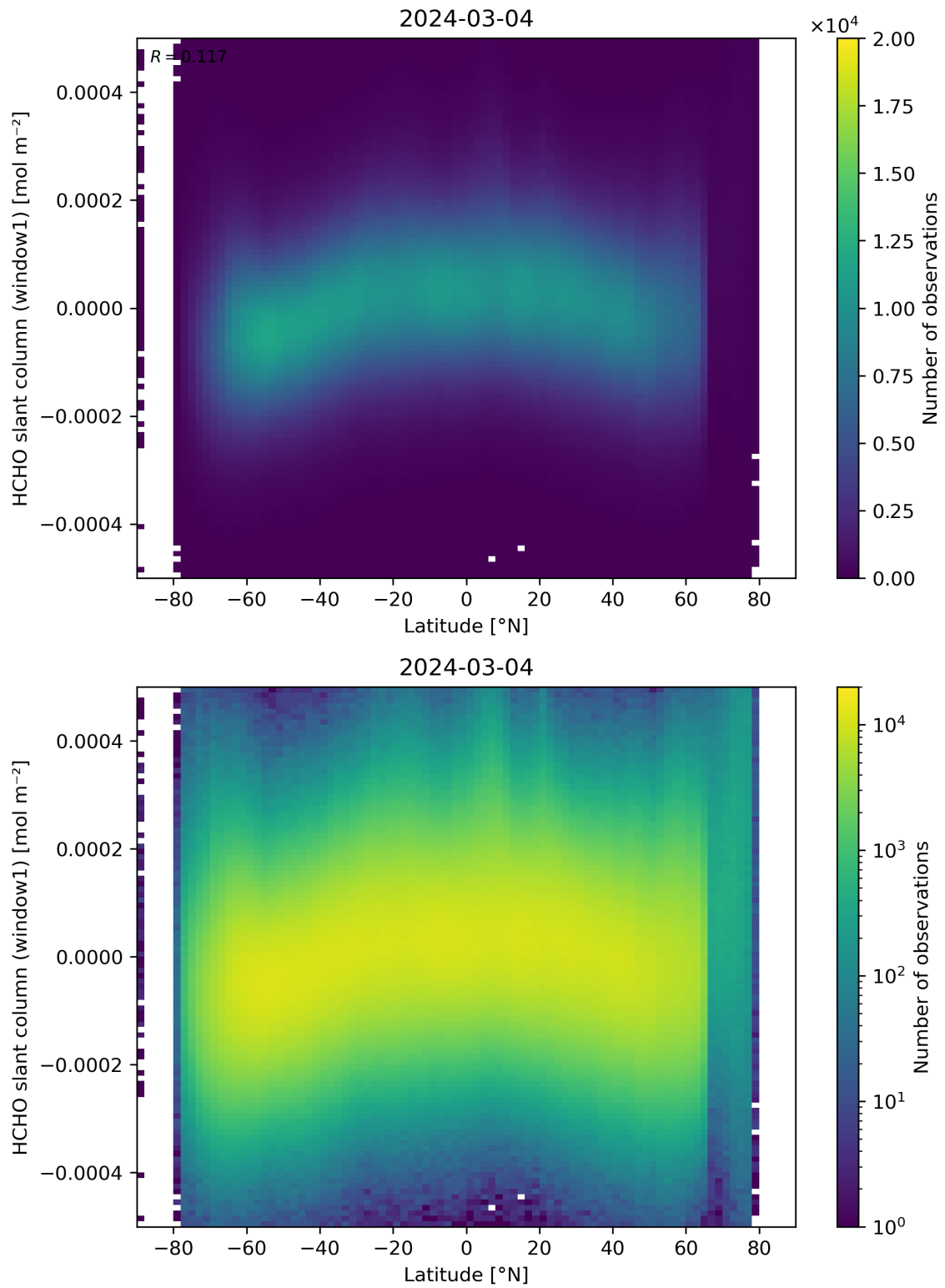
Figure 159: Scatter density plot of “Latitude” against “HCHO slant column (window1)” for 2024-03-04 to 2024-03-05.
