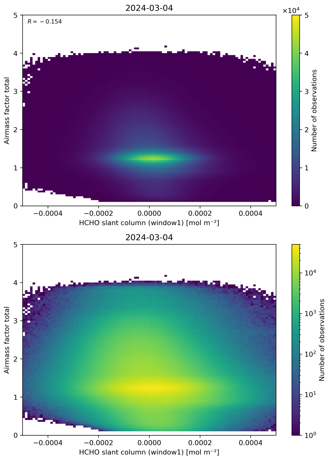
Figure 85: Scatter density plot of “HCHO slant column (window1)” against “Airmass factor total” for 2024-03-04 to 2024-03-05.
