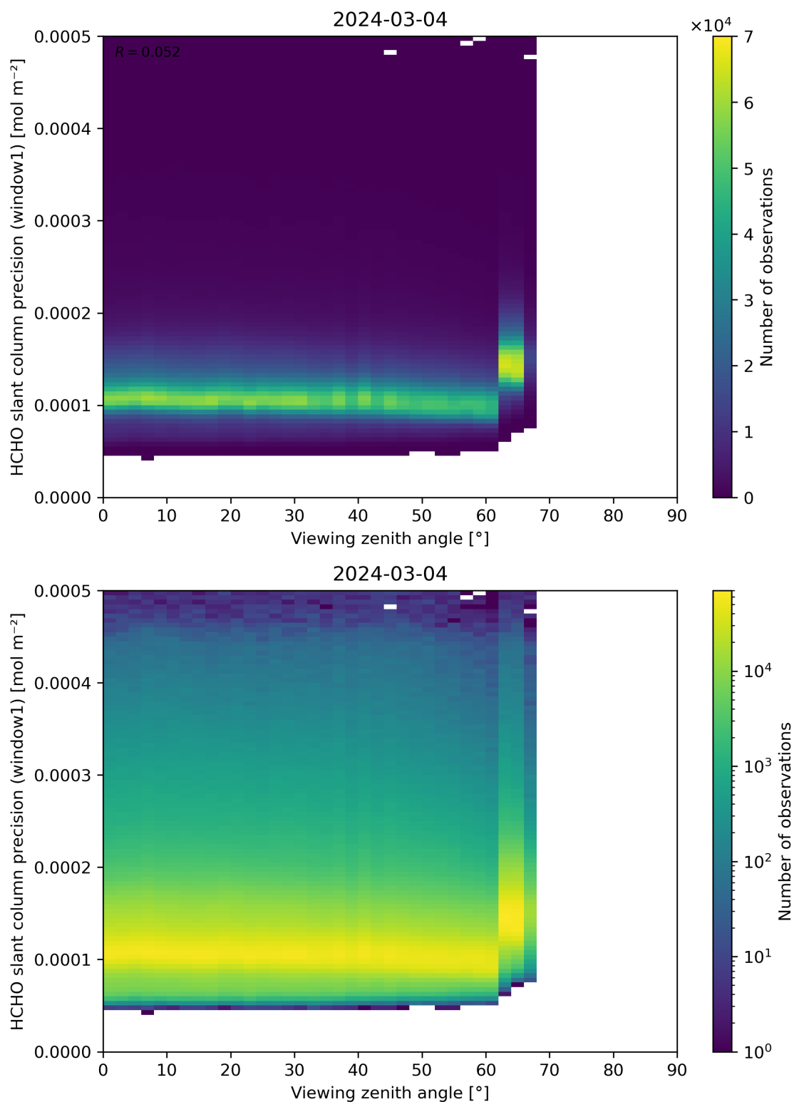
Figure 189: Scatter density plot of “Viewing zenith angle” against “HCHO slant column precision (window1)” for 2024-03-04 to 2024-03-05.
