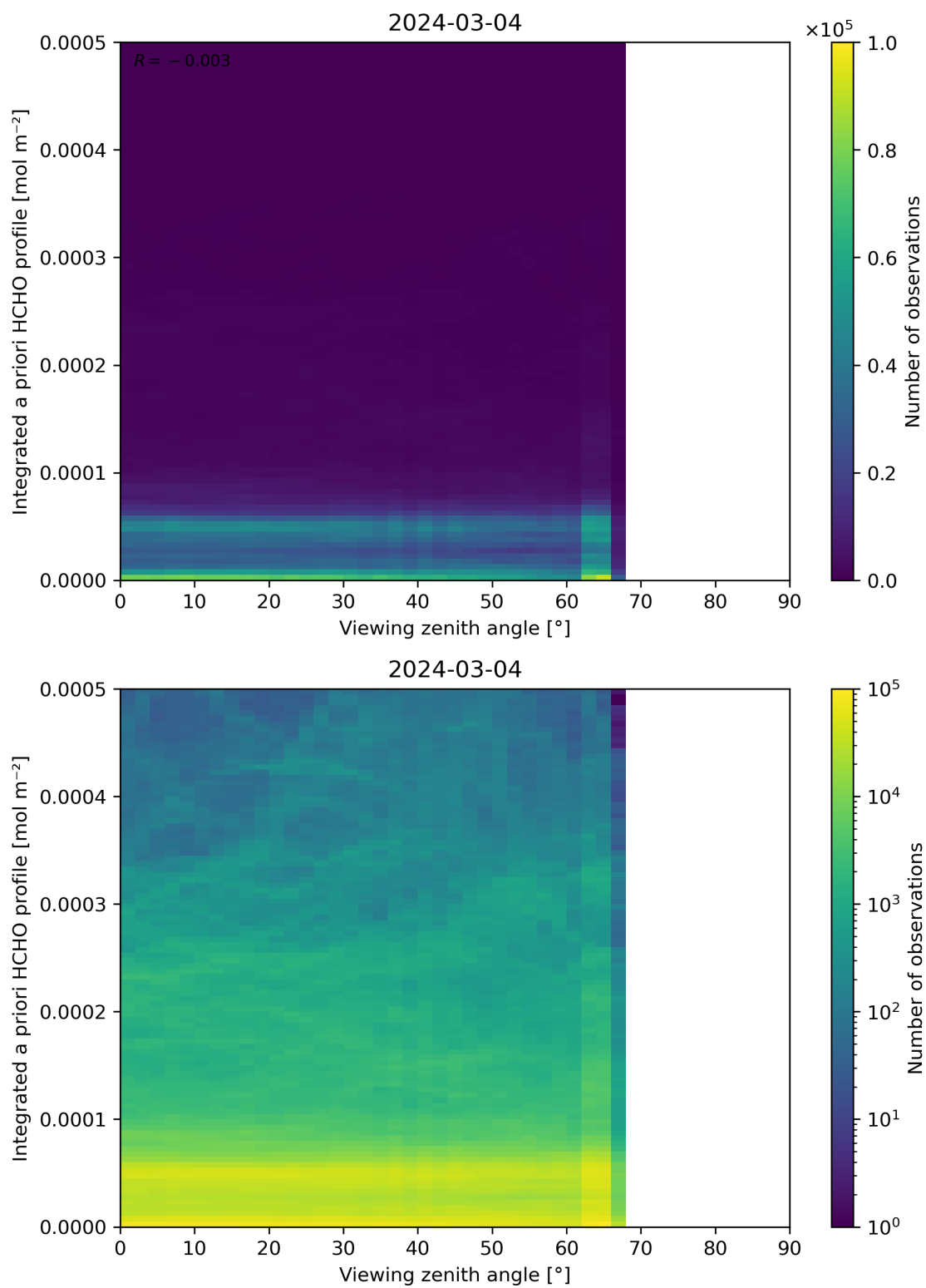
Figure 195: Scatter density plot of “Viewing zenith angle” against “Integrated a priori HCHO profile” for 2024-03-04 to 2024-03-05.
