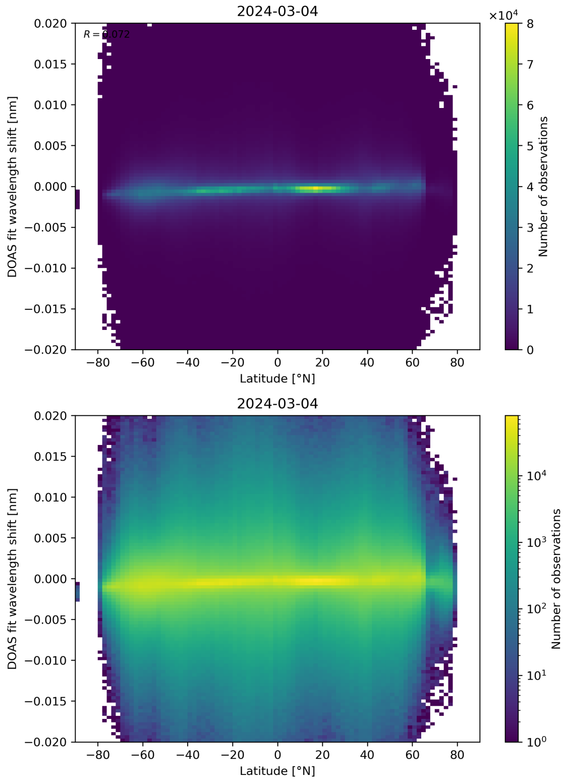
Figure 154: Scatter density plot of “Latitude” against “DOAS fit wavelength shift” for 2024-03-04 to 2024-03-05.
