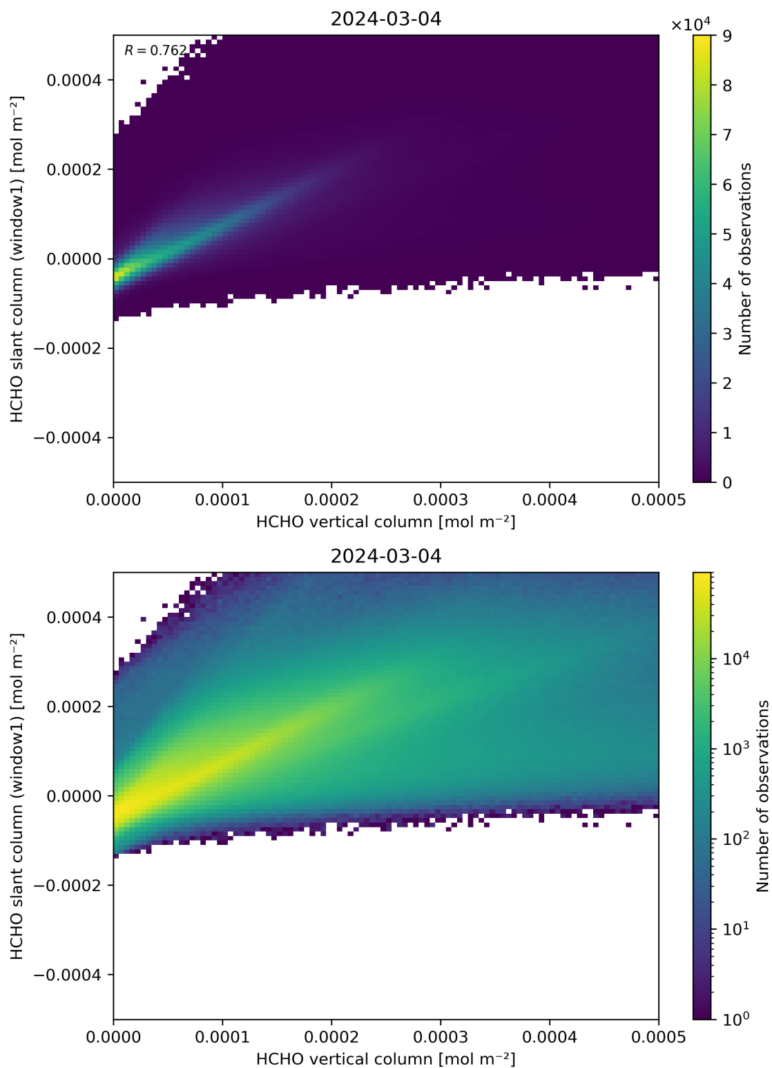
Figure 129: Scatter density plot of “HCHO vertical column” against “HCHO slant column (window1)” for 2024-03-04 to 2024-03-05.
