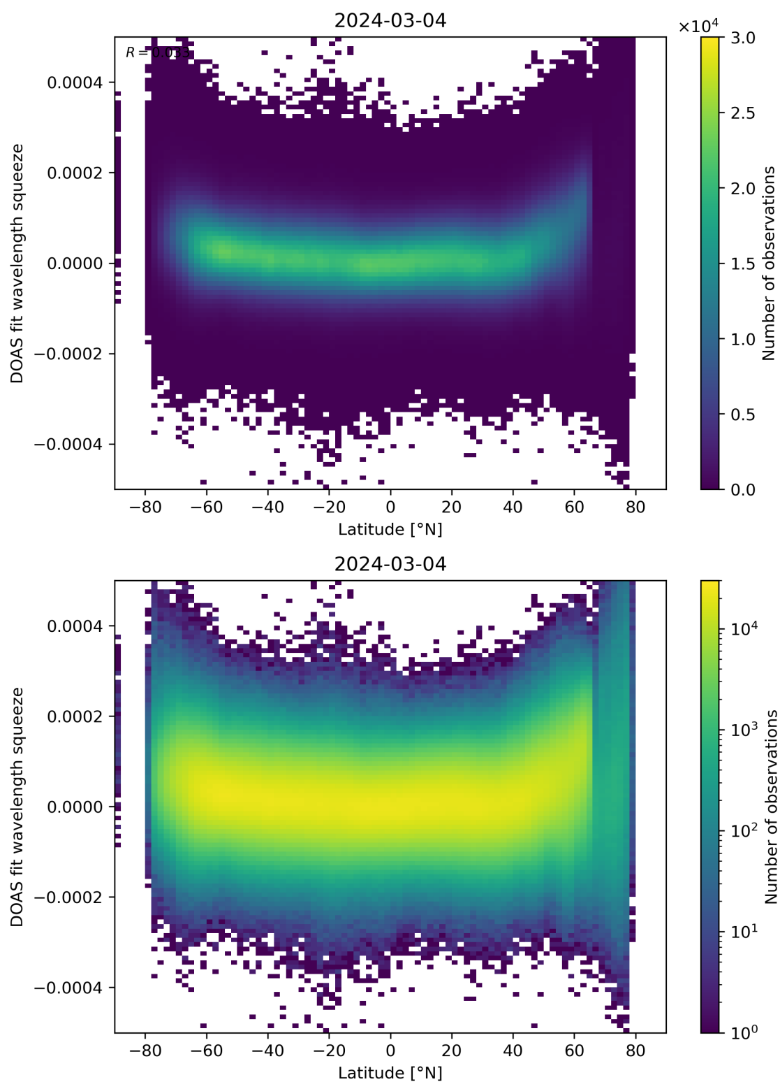
Figure 155: Scatter density plot of “Latitude” against “DOAS fit wavelength squeeze” for 2024-03-04 to 2024-03-05.
