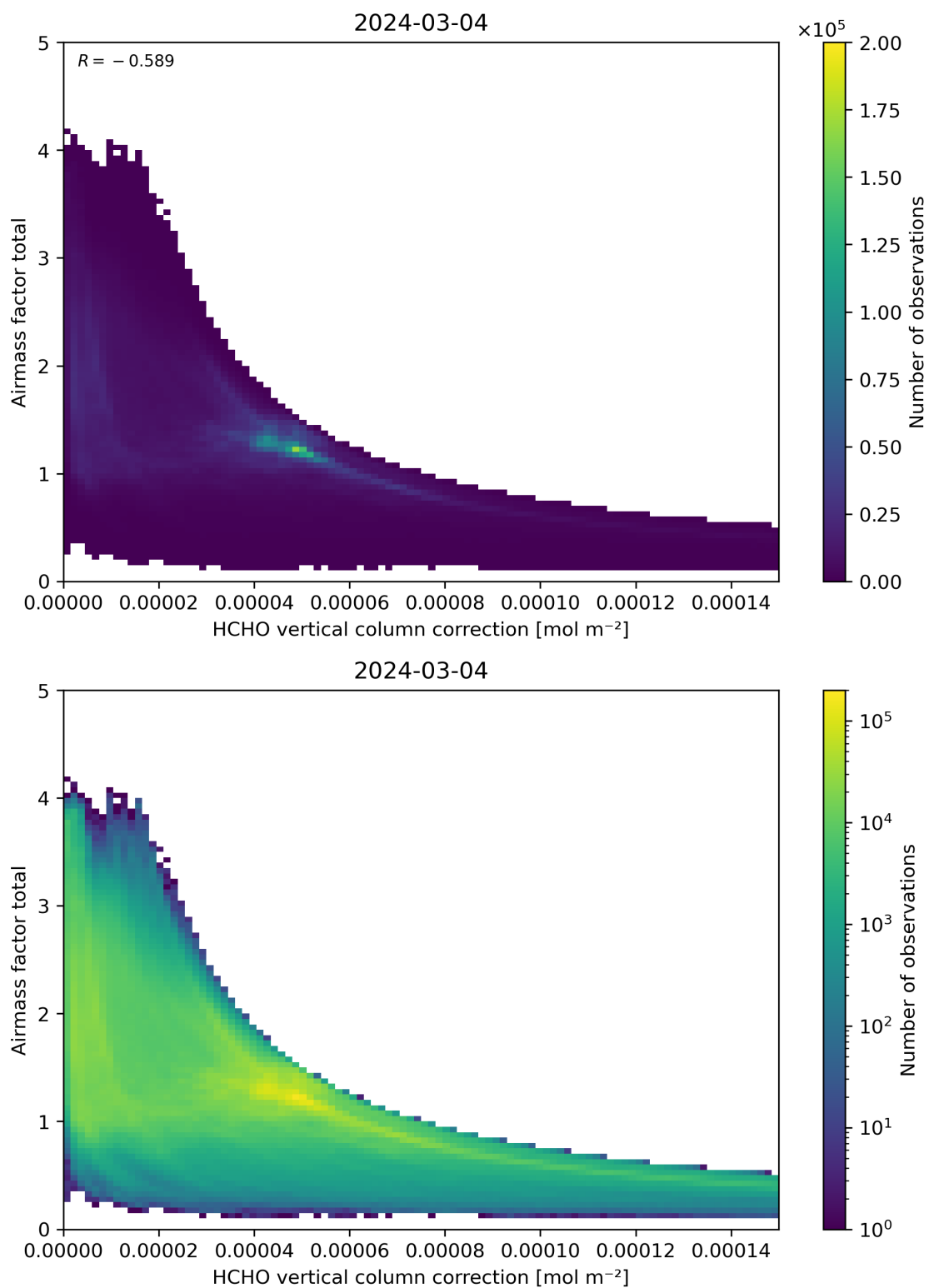
Figure 120: Scatter density plot of “HCHO vertical column correction” against “Airmass factor total” for 2024-03-04 to 2024-03-05.
