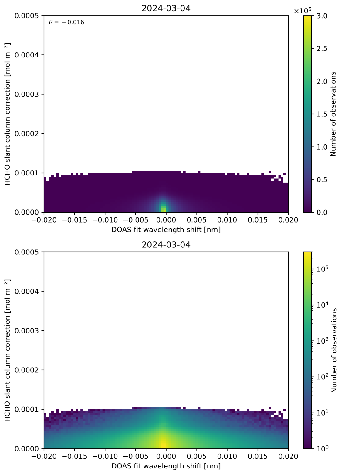
Figure 67: Scatter density plot of “DOAS fit wavelength shift” against “HCHO slant column correction” for 2024-03-04 to 2024-03-05.
