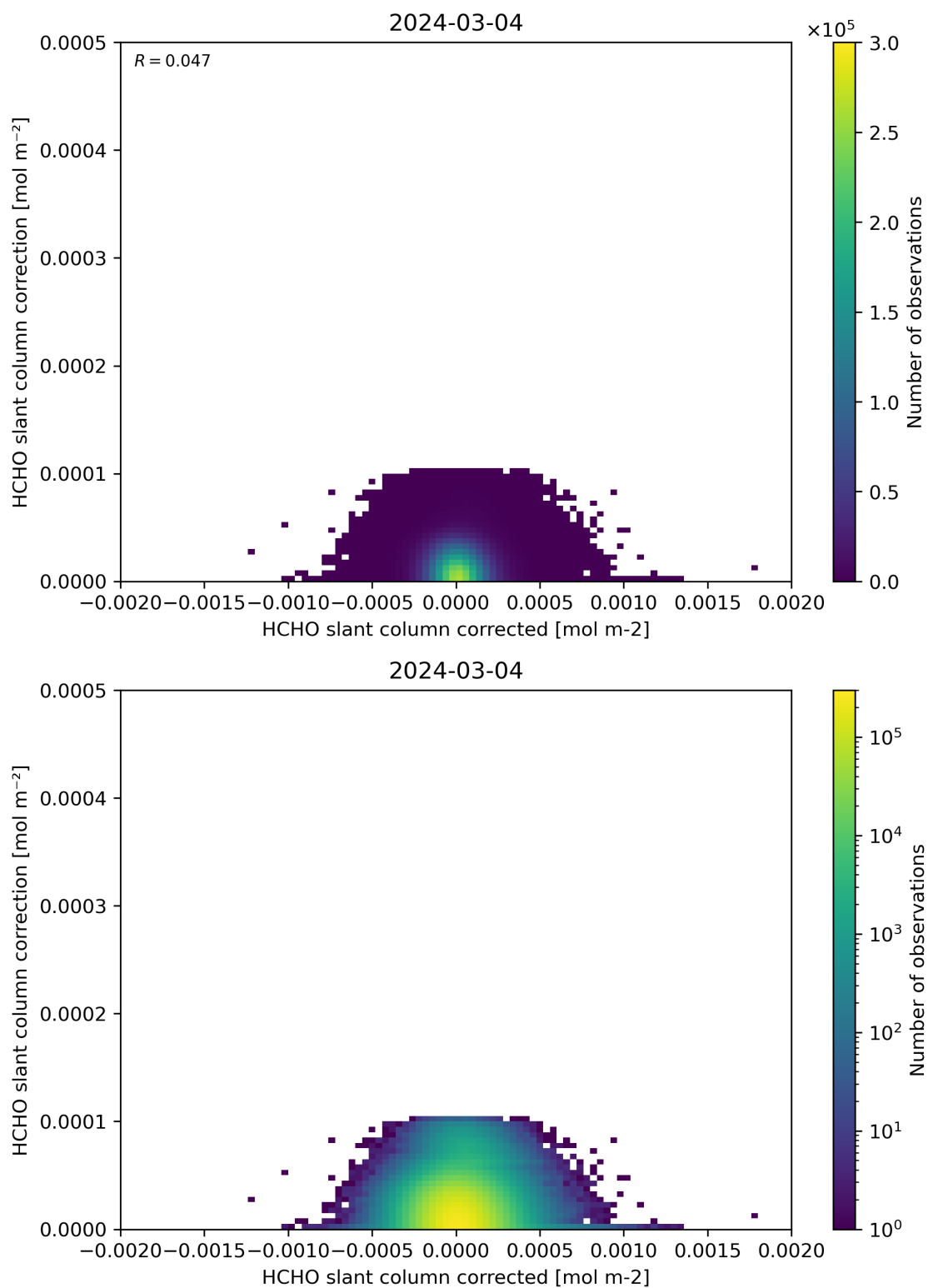
Figure 77: Scatter density plot of “HCHO slant column corrected” against “HCHO slant column correction” for 2024-03-04 to 2024-03-05.
