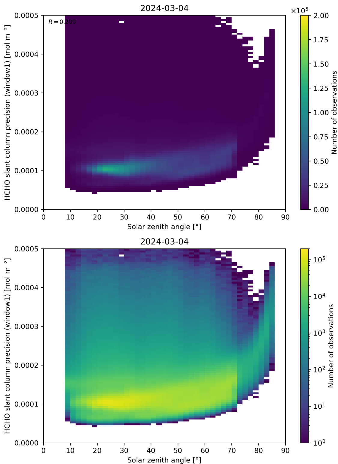
Figure 174: Scatter density plot of “Solar zenith angle” against “HCHO slant column precision (window1)” for 2024-03-04 to 2024-03-05.
