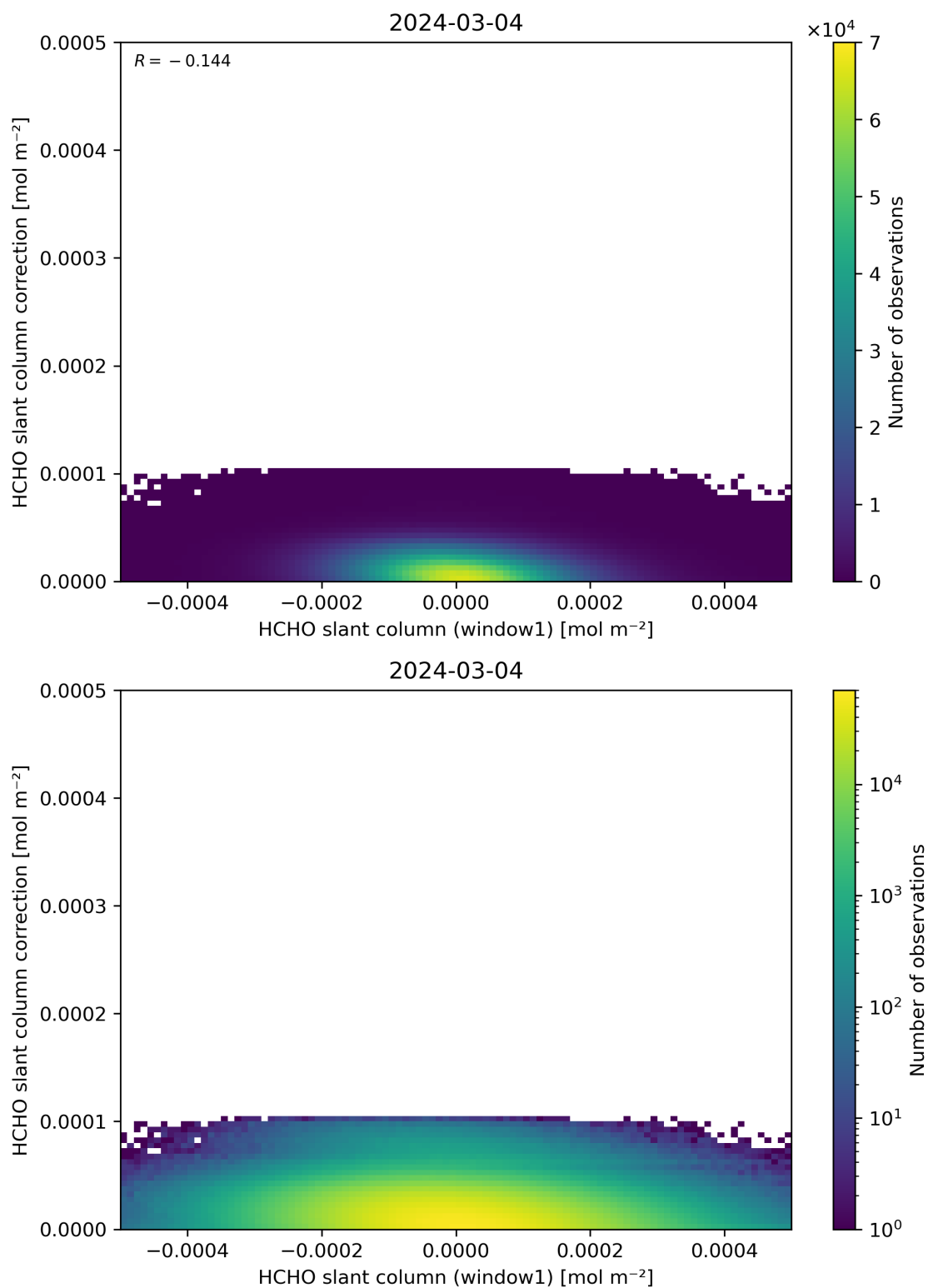
Figure 83: Scatter density plot of “HCHO slant column (window1)” against “HCHO slant column correction” for 2024-03-04 to 2024-03-05.
