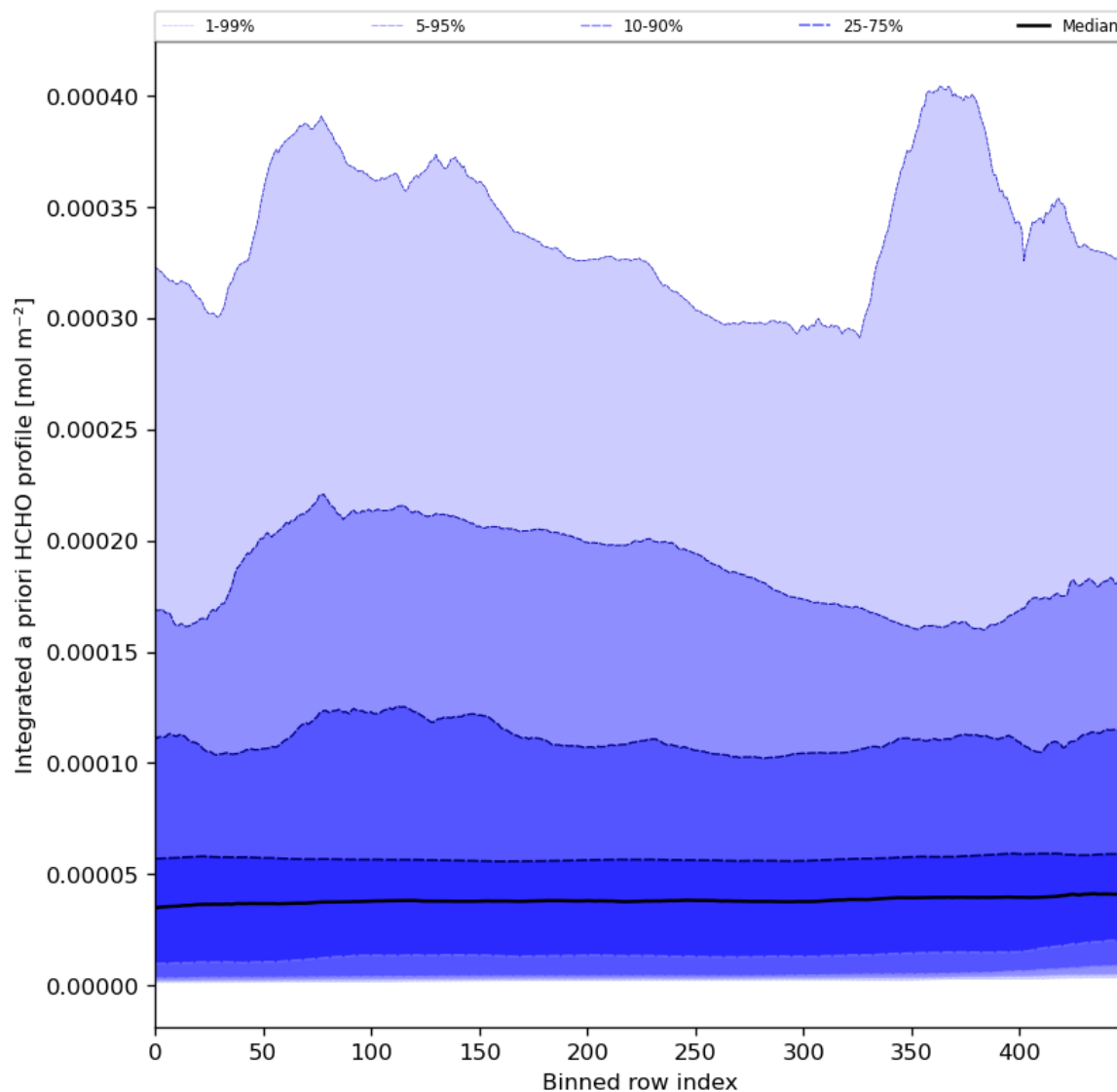
Figure 57: Along track statistics of “Integrated a priori HCHO profile” for 2024-03-04 to 2024-03-05
