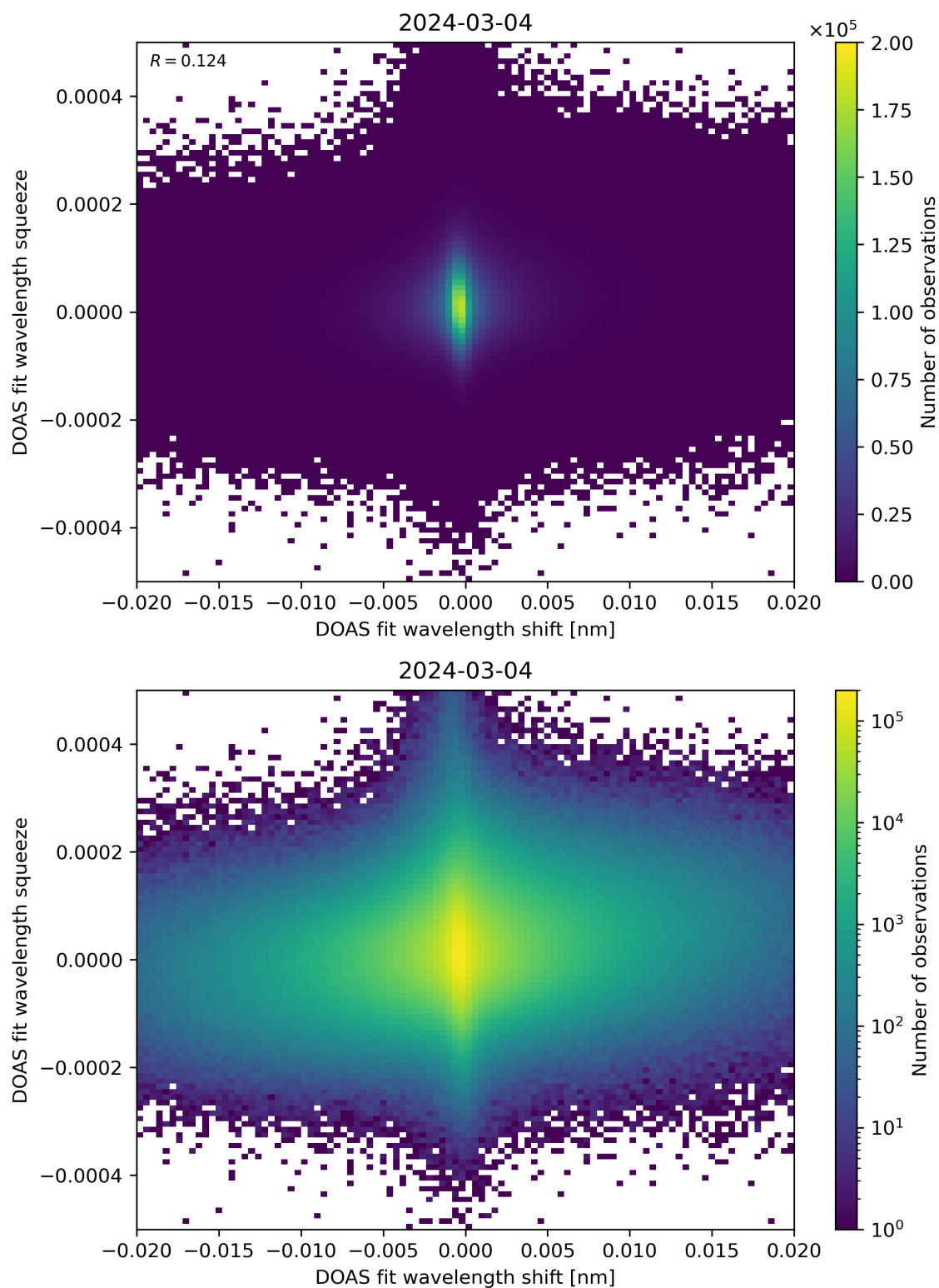
Figure 65: Scatter density plot of “DOAS fit wavelength shift” against “DOAS fit wavelength squeeze” for 2024-03-04 to 2024-03-05.
