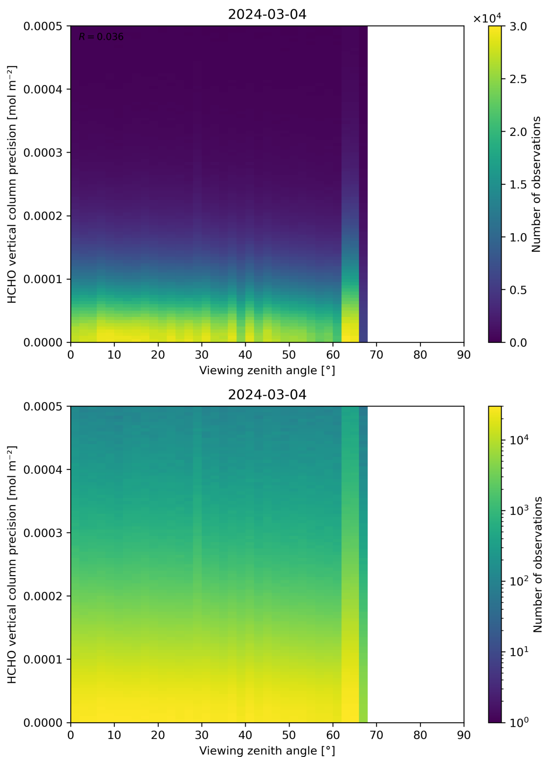
Figure 194: Scatter density plot of “Viewing zenith angle” against “HCHO vertical column precision” for 2024-03-04 to 2024-03-05.
