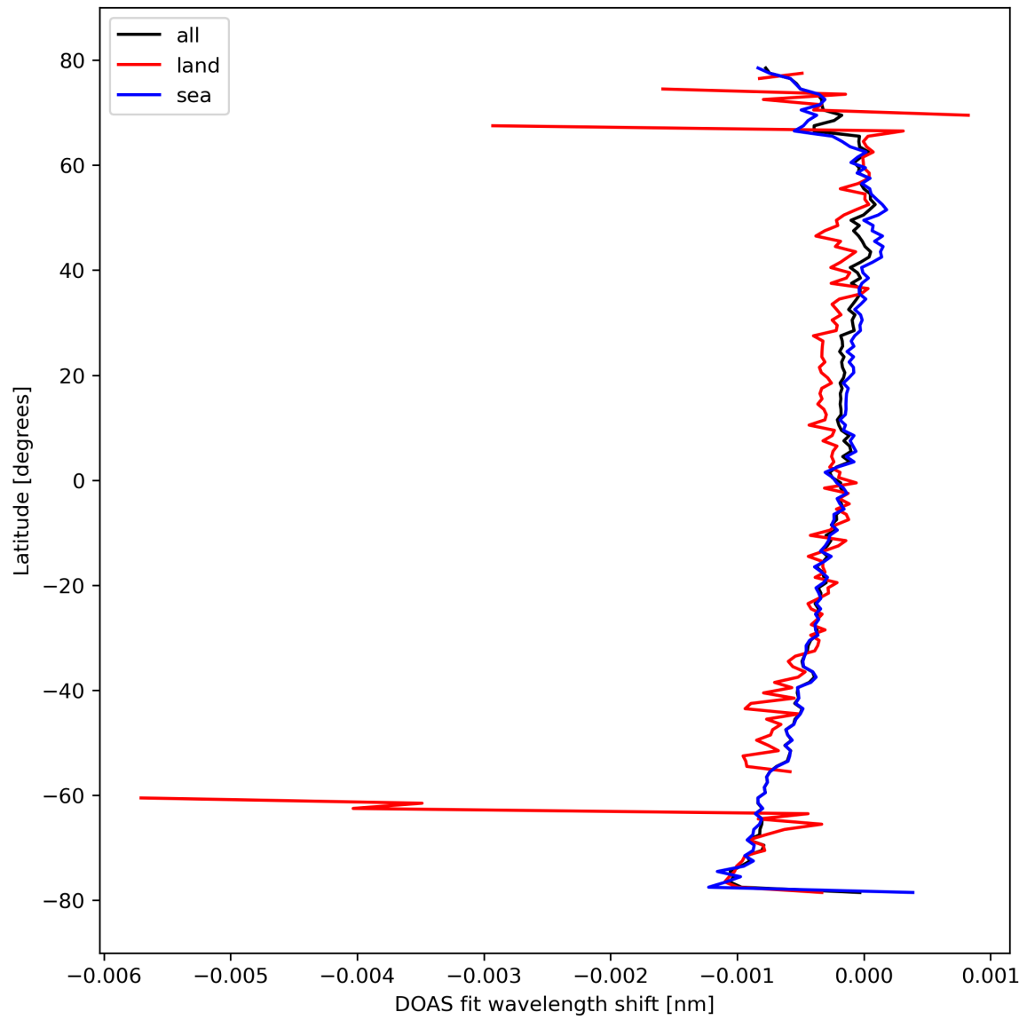
Figure 30: Zonal average of "DOAS fit wavelength shift" for 2024-03-04 to 2024-03-05.
