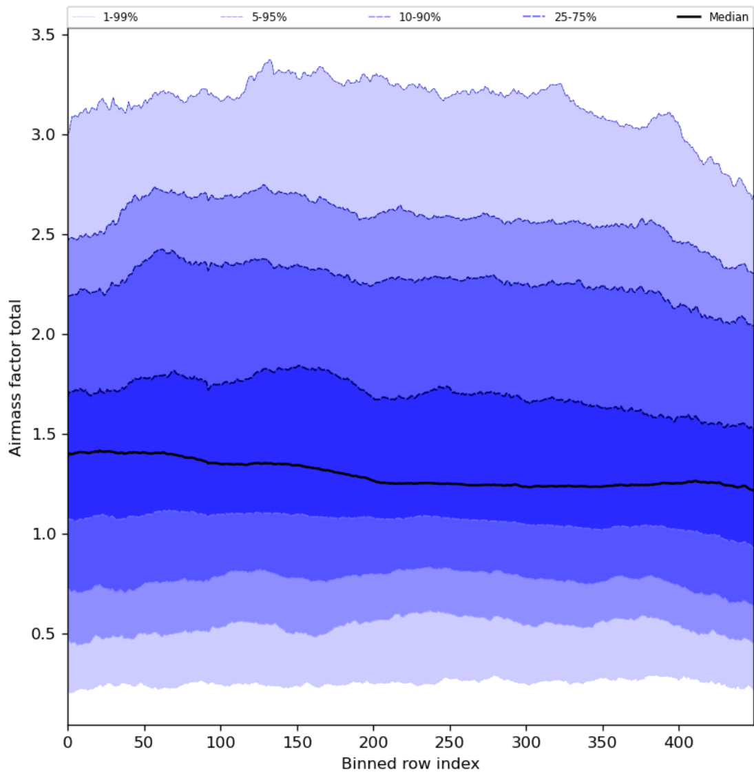
Figure 54: Along track statistics of “Airmass factor total” for 2024-03-04 to 2024-03-05
