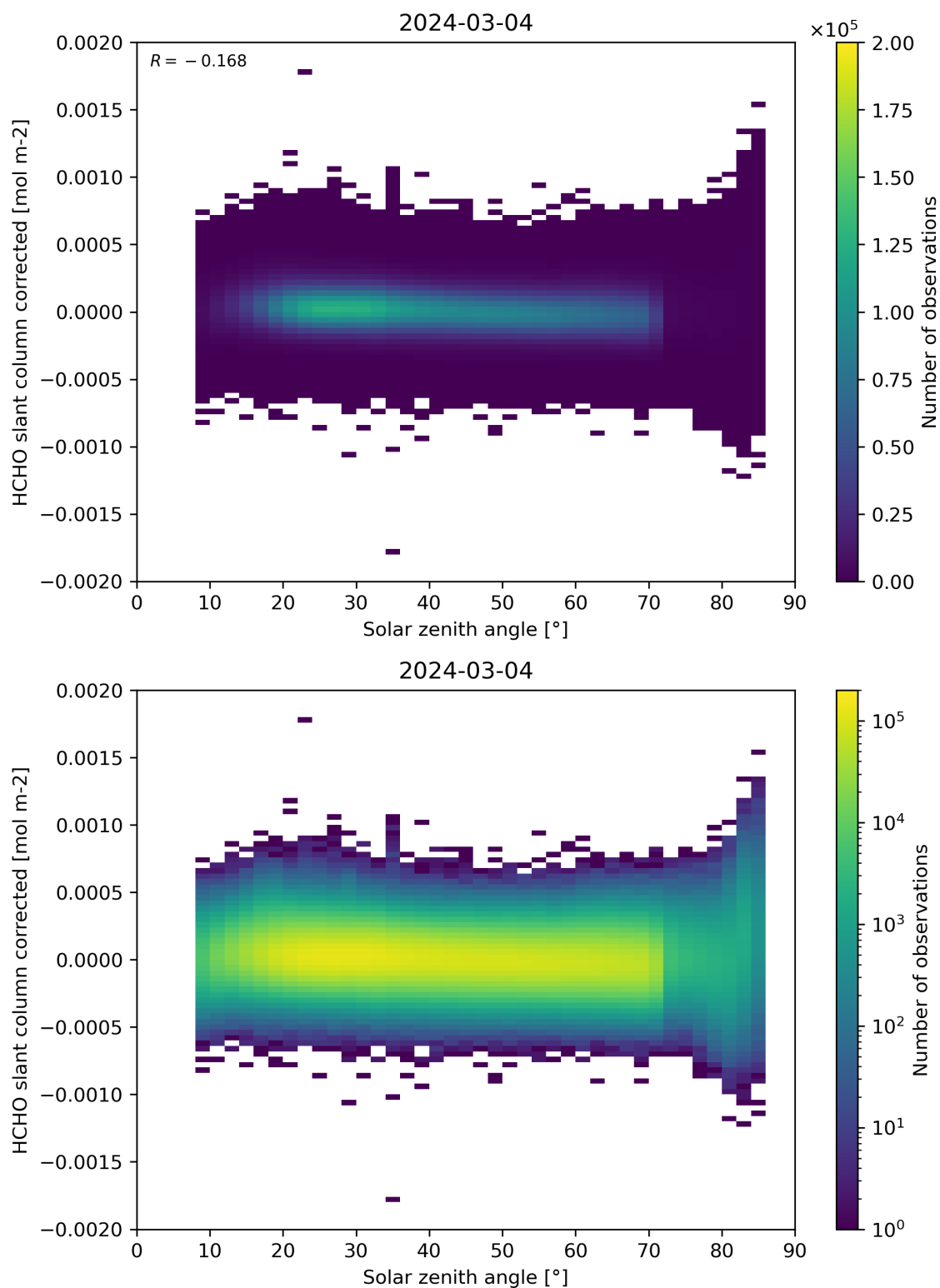
Figure 171: Scatter density plot of “Solar zenith angle” against “HCHO slant column corrected” for 2024-03-04 to 2024-03-05.
