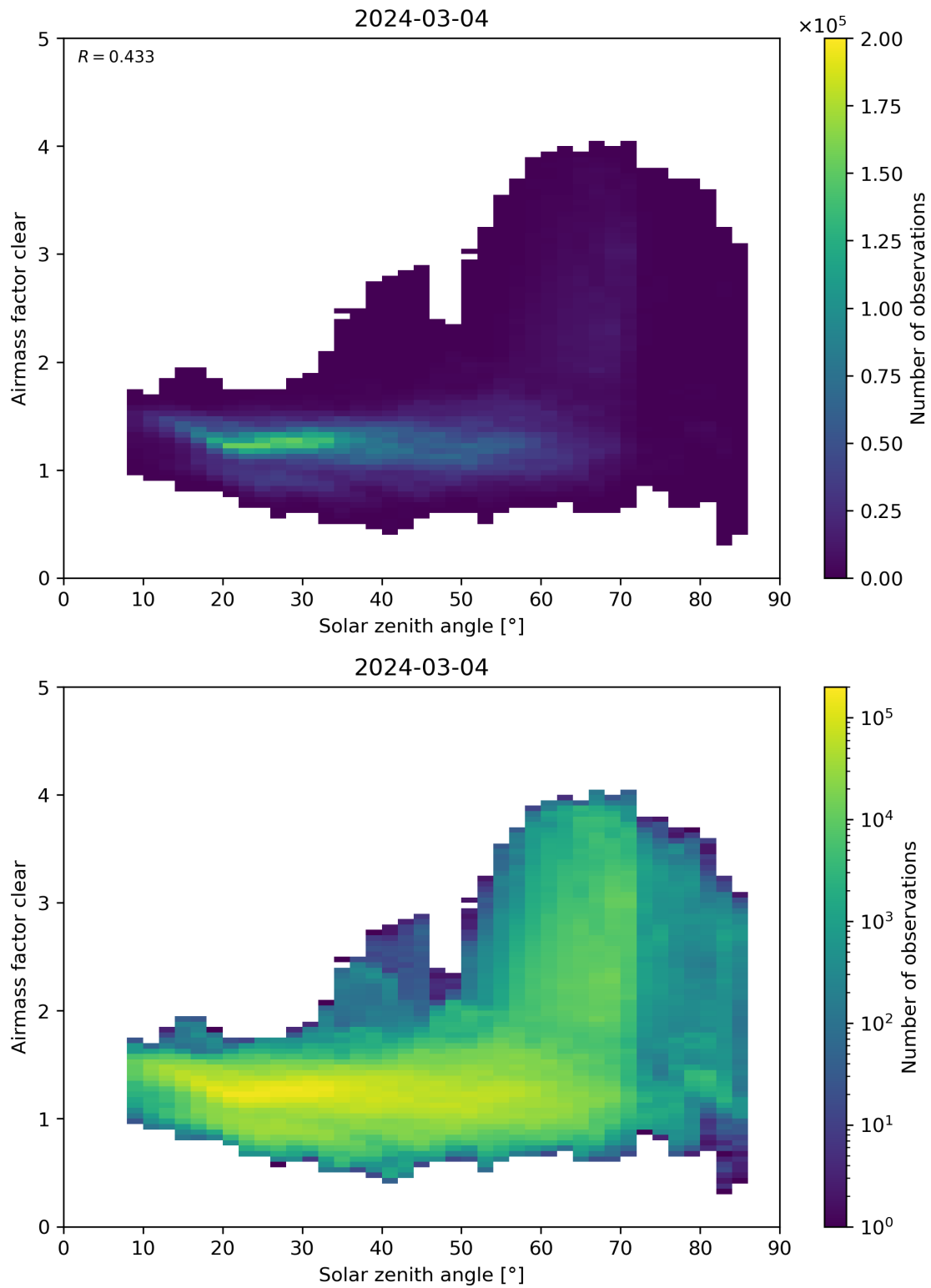
Figure 170: Scatter density plot of “Solar zenith angle” against “Airmass factor clear” for 2024-03-04 to 2024-03-05.
