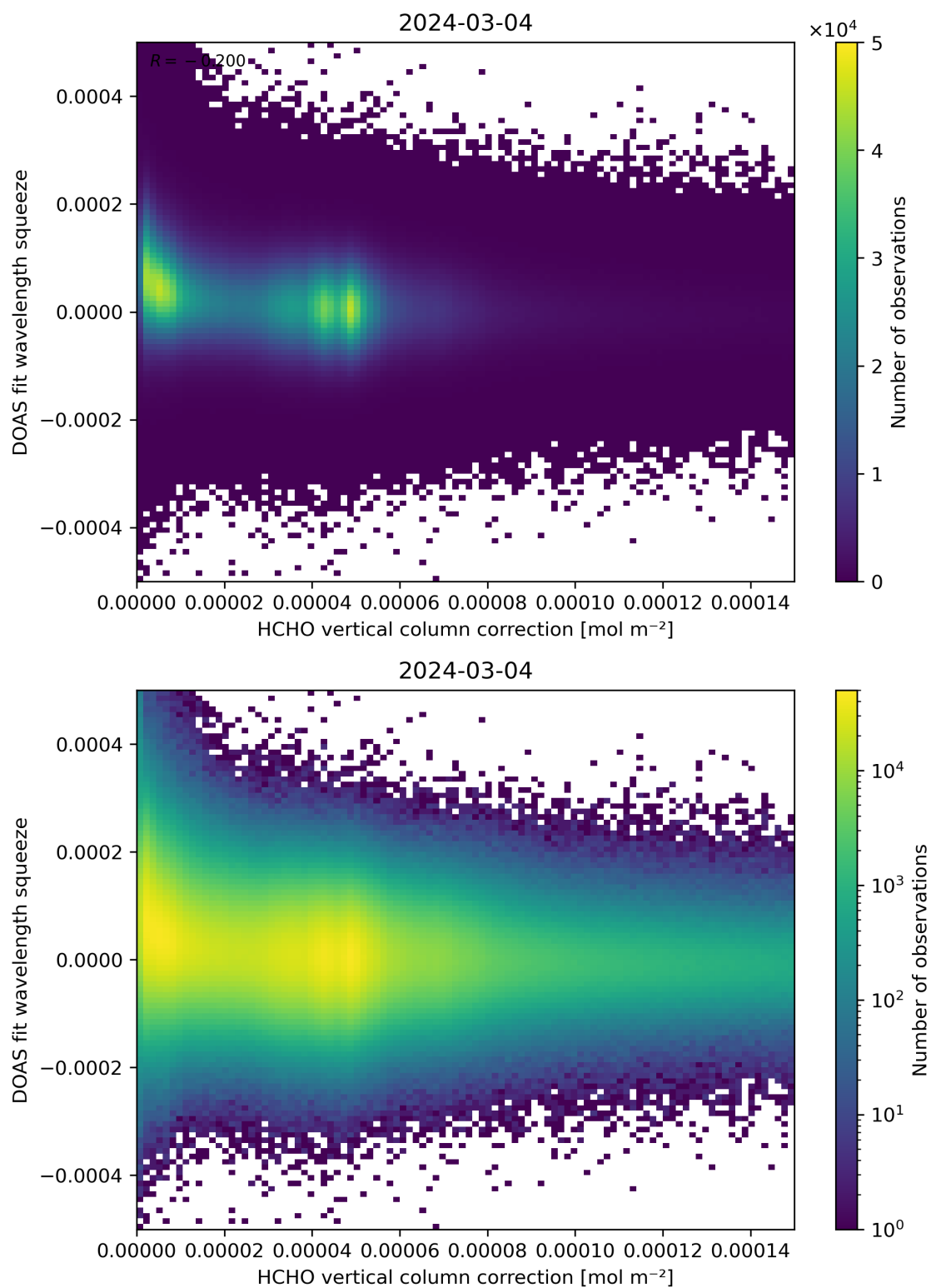
Figure 114: Scatter density plot of “HCHO vertical column correction” against “DOAS fit wavelength squeeze” for 2024-03-04 to 2024-03-05.
