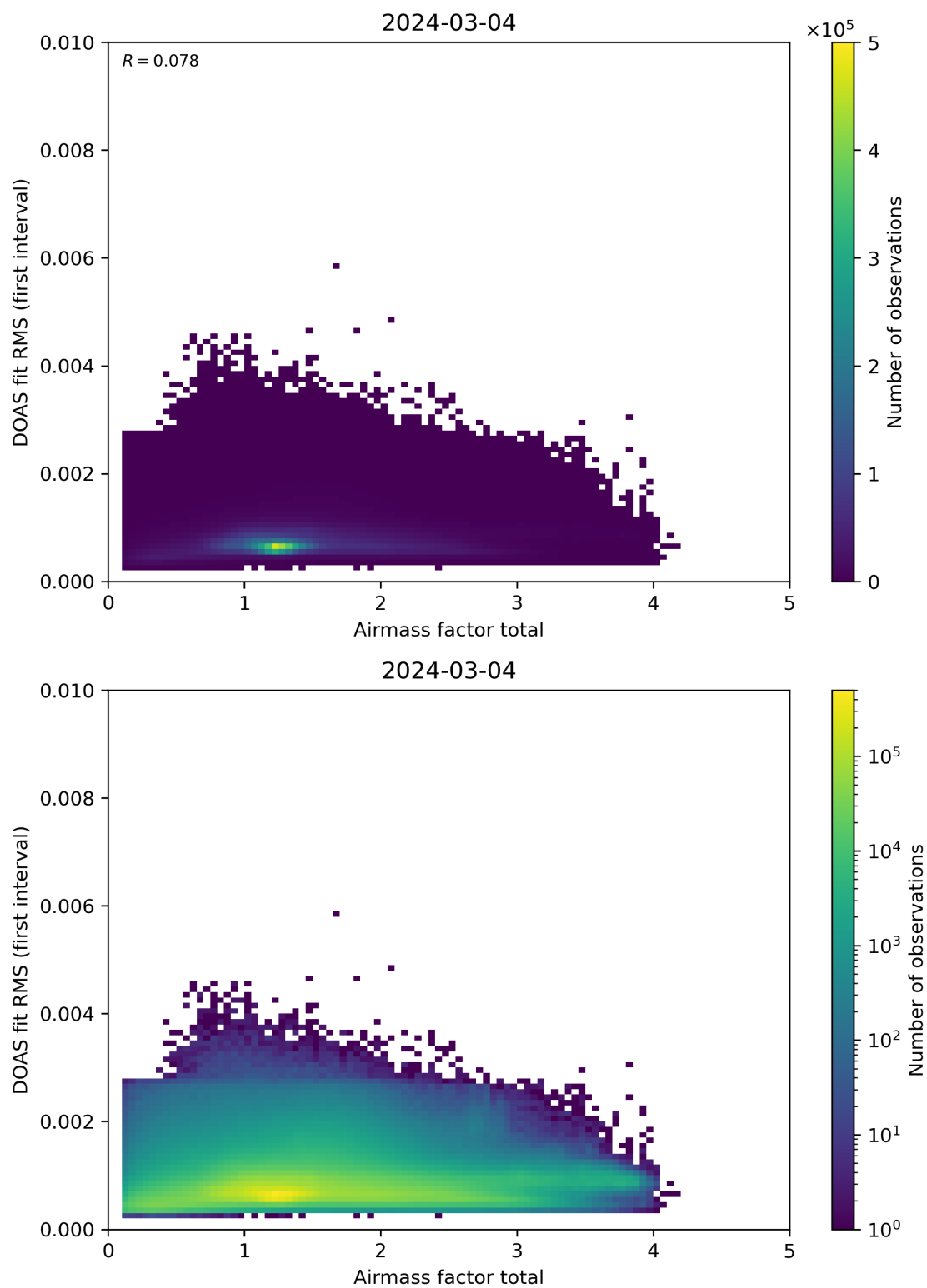
Figure 97: Scatter density plot of “Airmass factor total” against “DOAS fit RMS (first interval)” for 2024-03-04 to 2024-03-05.
