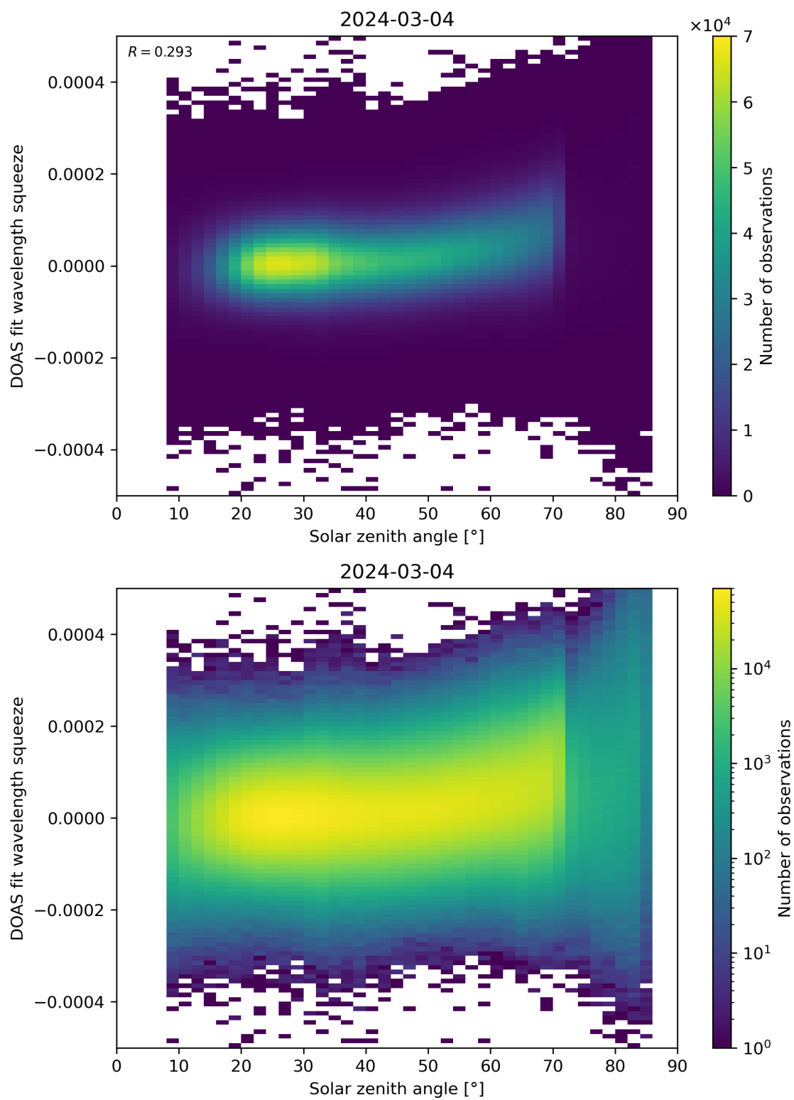
Figure 169: Scatter density plot of “Solar zenith angle” against “DOAS fit wavelength squeeze” for 2024-03-04 to 2024-03-05.
