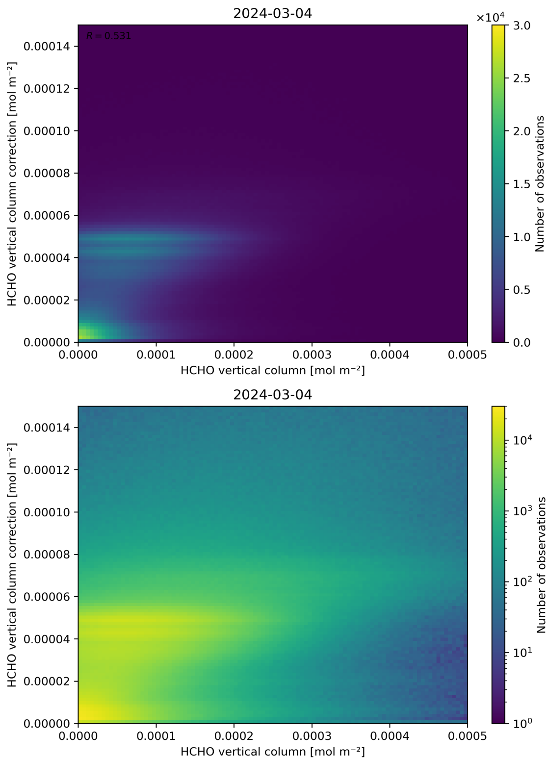
Figure 133: Scatter density plot of “HCHO vertical column” against “HCHO vertical column correction” for 2024-03-04 to 2024-03-05.
