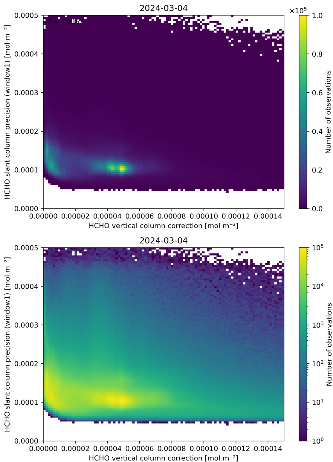
Figure 119: Scatter density plot of “HCHO vertical column correction” against “HCHO slant column precision (window1)” for 2024-03-04 to 2024-03-05.
