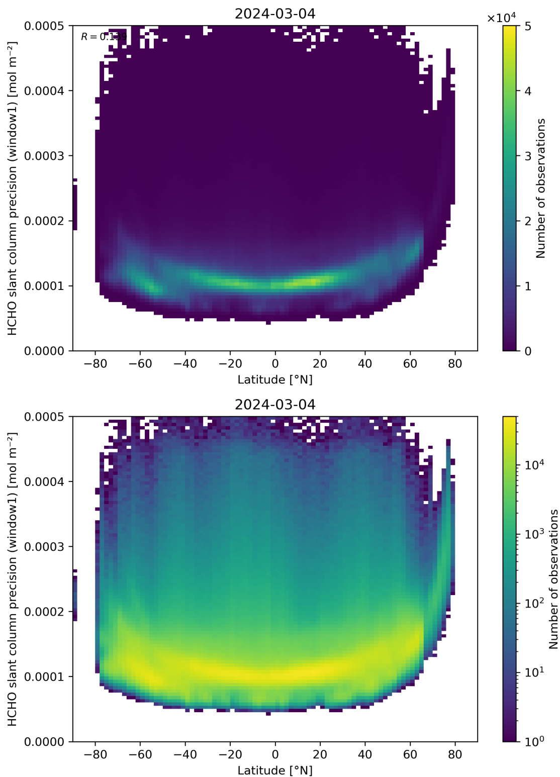
Figure 160: Scatter density plot of “Latitude” against “HCHO slant column precision (window1)” for 2024-03-04 to 2024-03-05.
