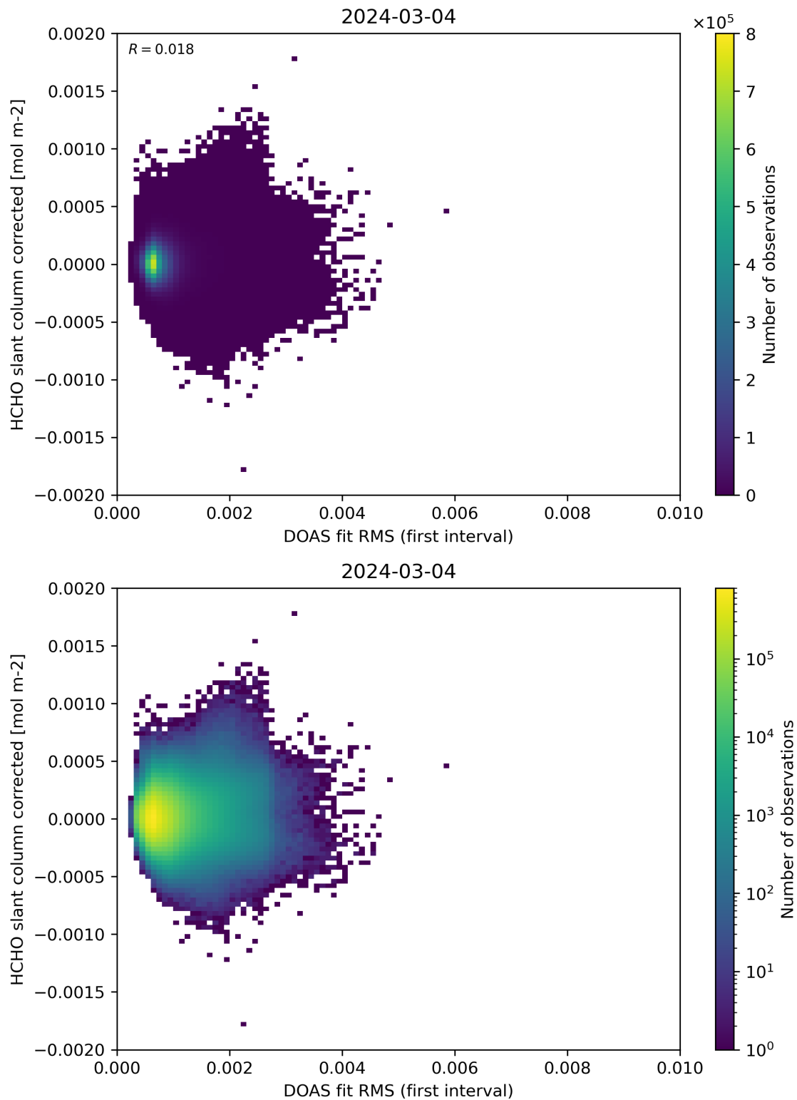
Figure 62: Scatter density plot of “DOAS fit RMS (first interval)” against “HCHO slant column corrected” for 2024-03-04 to 2024-03-05.
