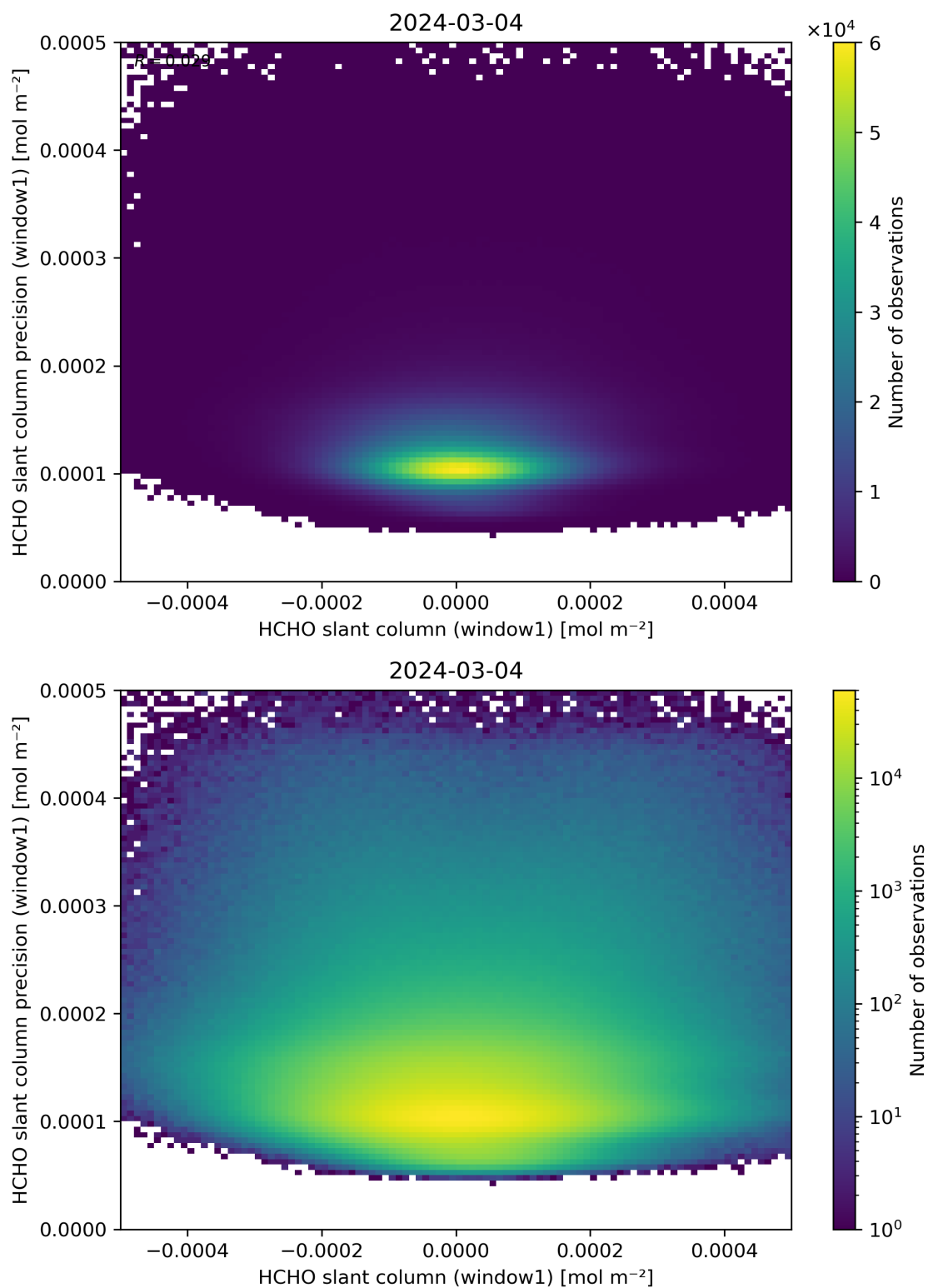
Figure 84: Scatter density plot of “HCHO slant column (window1)” against “HCHO slant column precision (window1)” for 2024-03-04 to 2024-03-05.
