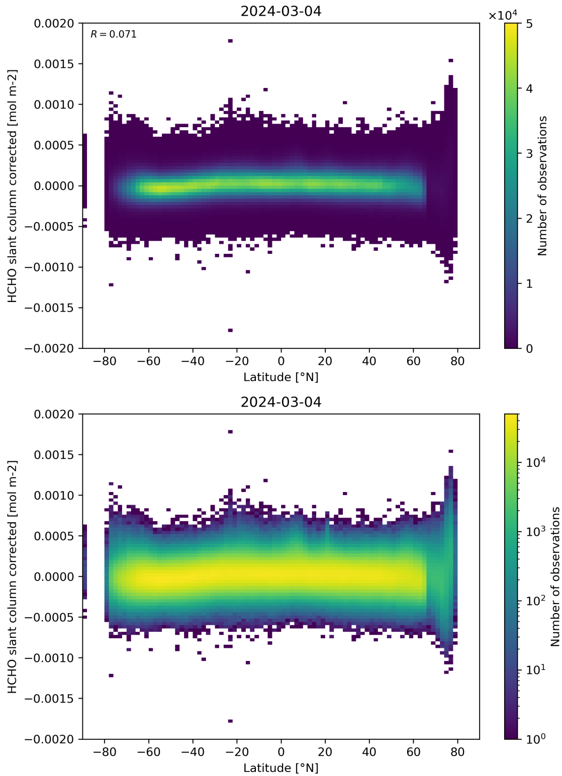
Figure 157: Scatter density plot of “Latitude” against “HCHO slant column corrected” for 2024-03-04 to 2024-03-05.
