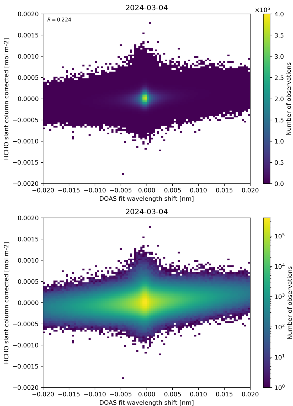
Figure 66: Scatter density plot of “DOAS fit wavelength shift” against “HCHO slant column corrected” for 2024-03-04 to 2024-03-05.
