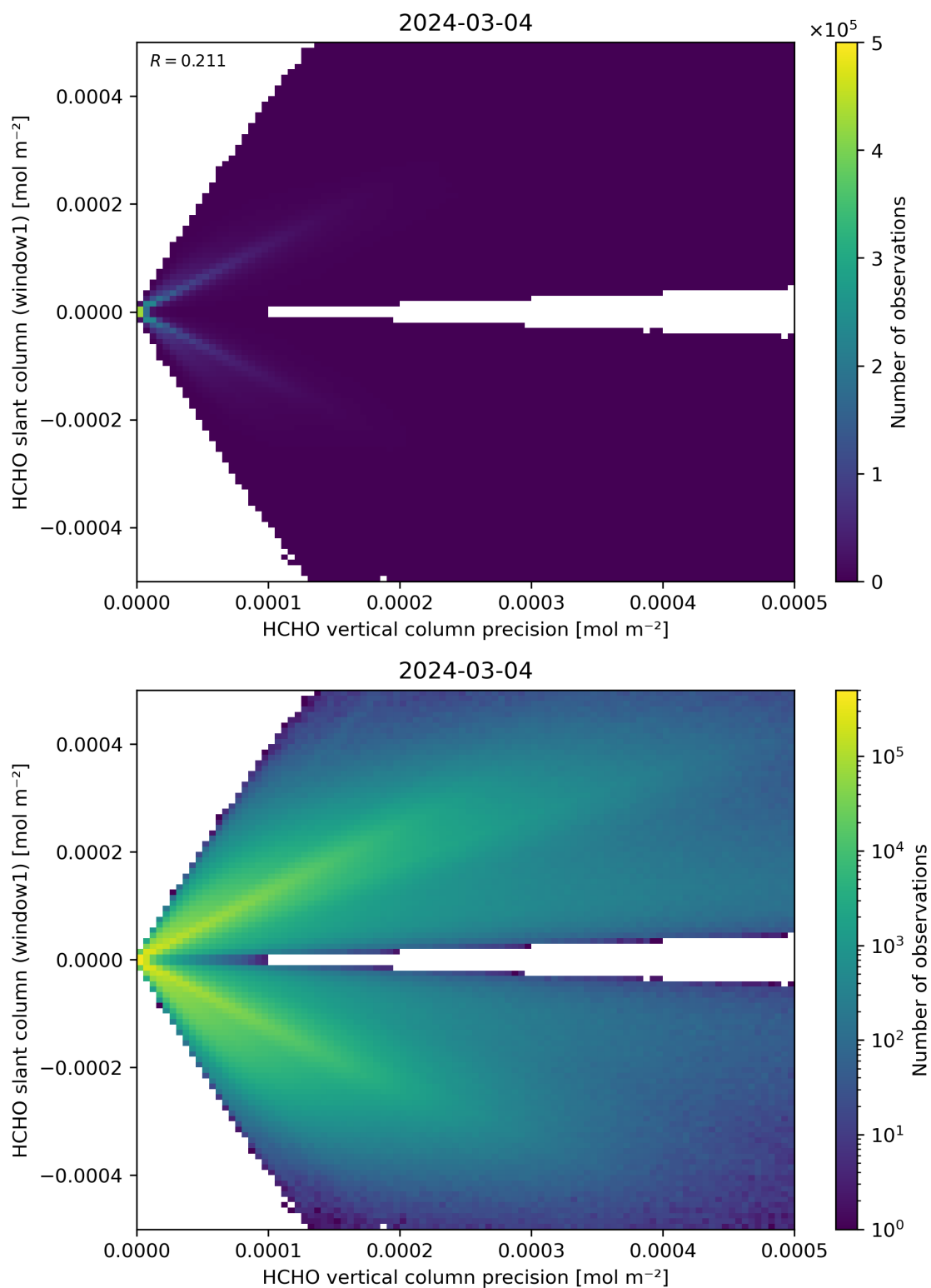
Figure 142: Scatter density plot of “HCHO vertical column precision” against “HCHO slant column (window1)” for 2024-03-04 to 2024-03-05.
