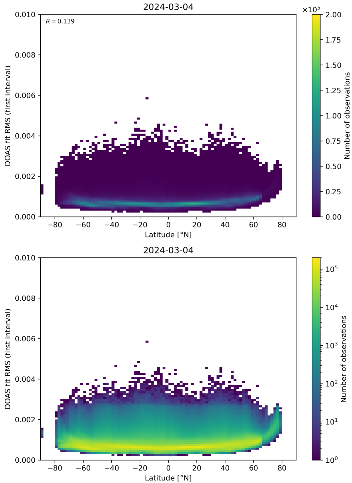
Figure 153: Scatter density plot of “Latitude” against “DOAS fit RMS (first interval)” for 2024-03-04 to 2024-03-05.
