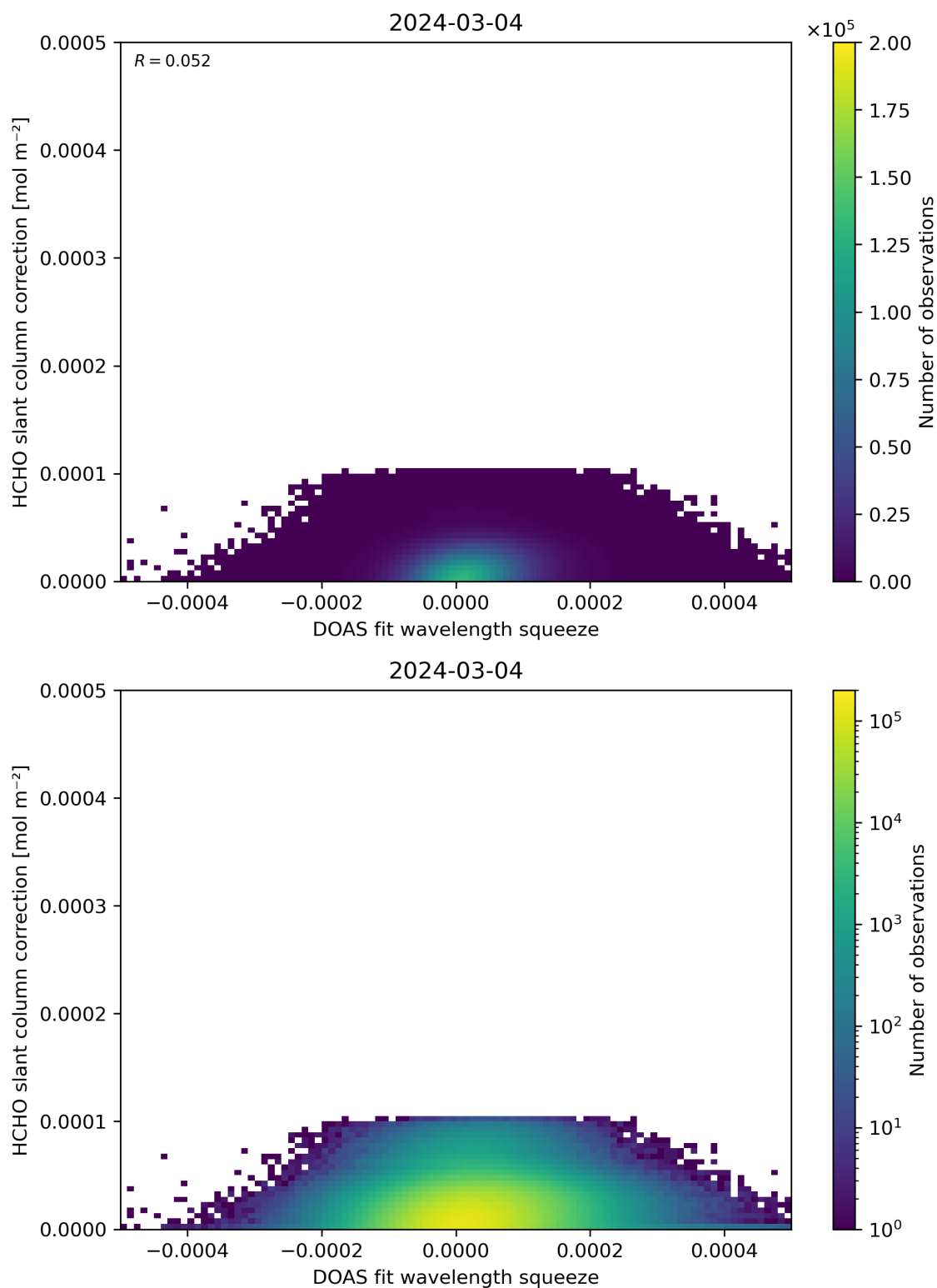
Figure 70: Scatter density plot of “DOAS fit wavelength squeeze” against “HCHO slant column correction” for 2024-03-04 to 2024-03-05.
