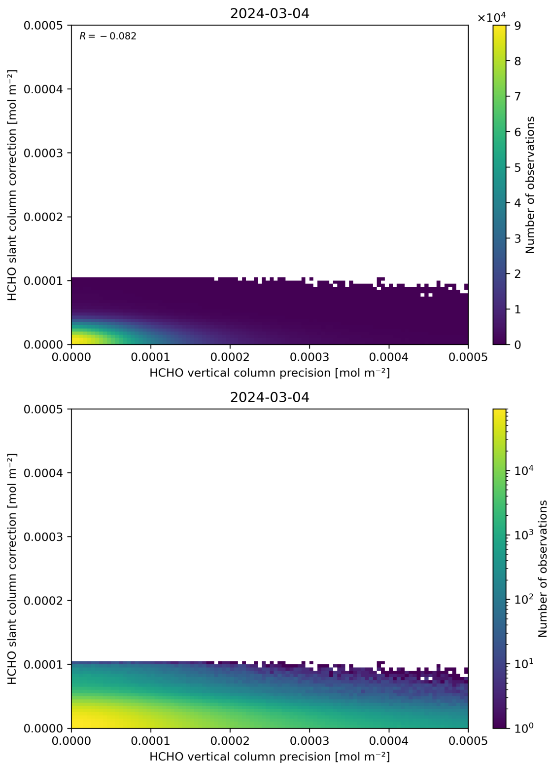
Figure 141: Scatter density plot of “HCHO vertical column precision” against “HCHO slant column correction” for 2024-03-04 to 2024-03-05.
