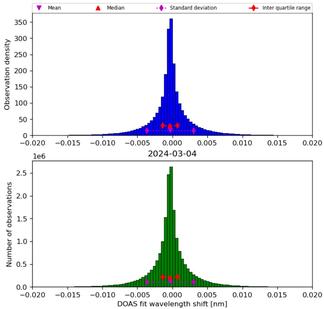
Figure 44: Histogram of “DOAS fit wavelength shift” for 2024-03-04 to 2024-03-05
