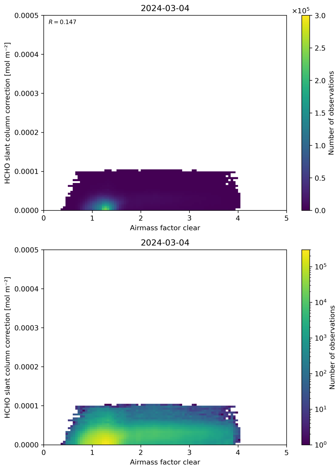
Figure 75: Scatter density plot of “Airmass factor clear” against “HCHO slant column correction” for 2024-03-04 to 2024-03-05.
