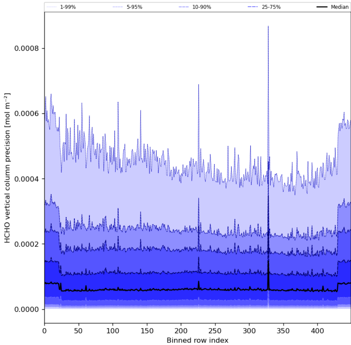
Figure 50: Along track statistics of “HCHO vertical column precision” for 2024-03-04 to 2024-03-05
