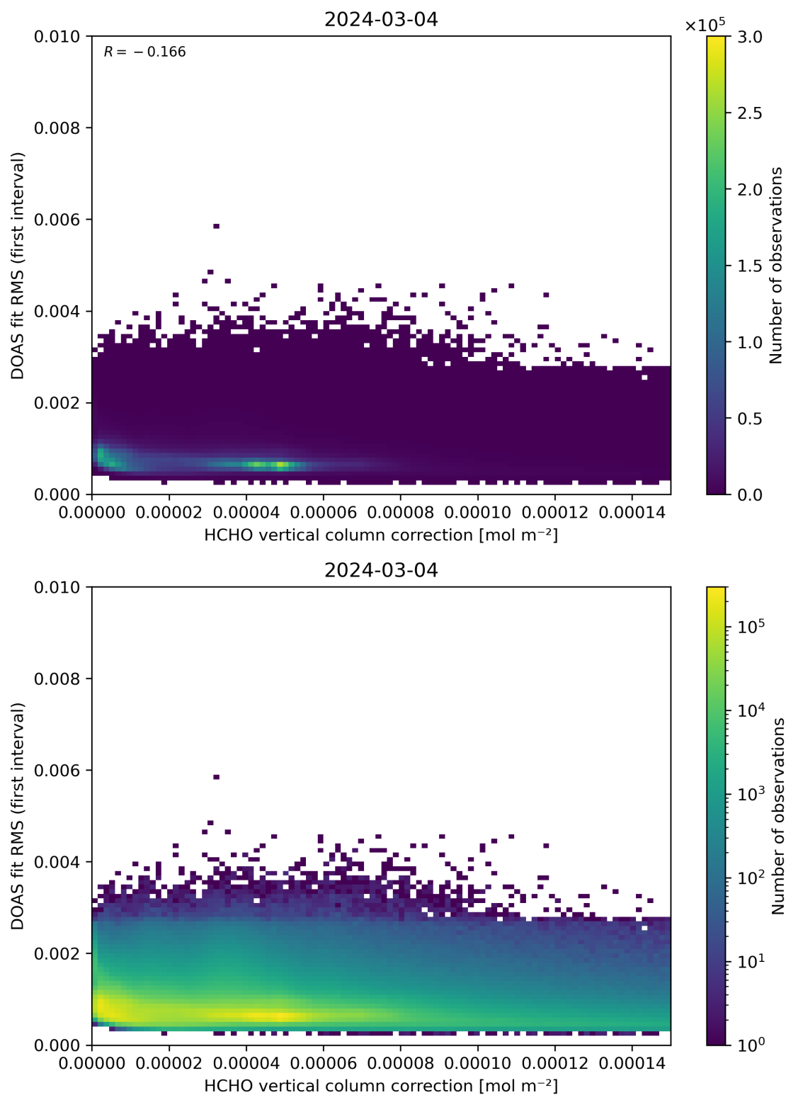
Figure 112: Scatter density plot of “HCHO vertical column correction” against “DOAS fit RMS (first interval)” for 2024-03-04 to 2024-03-05.
