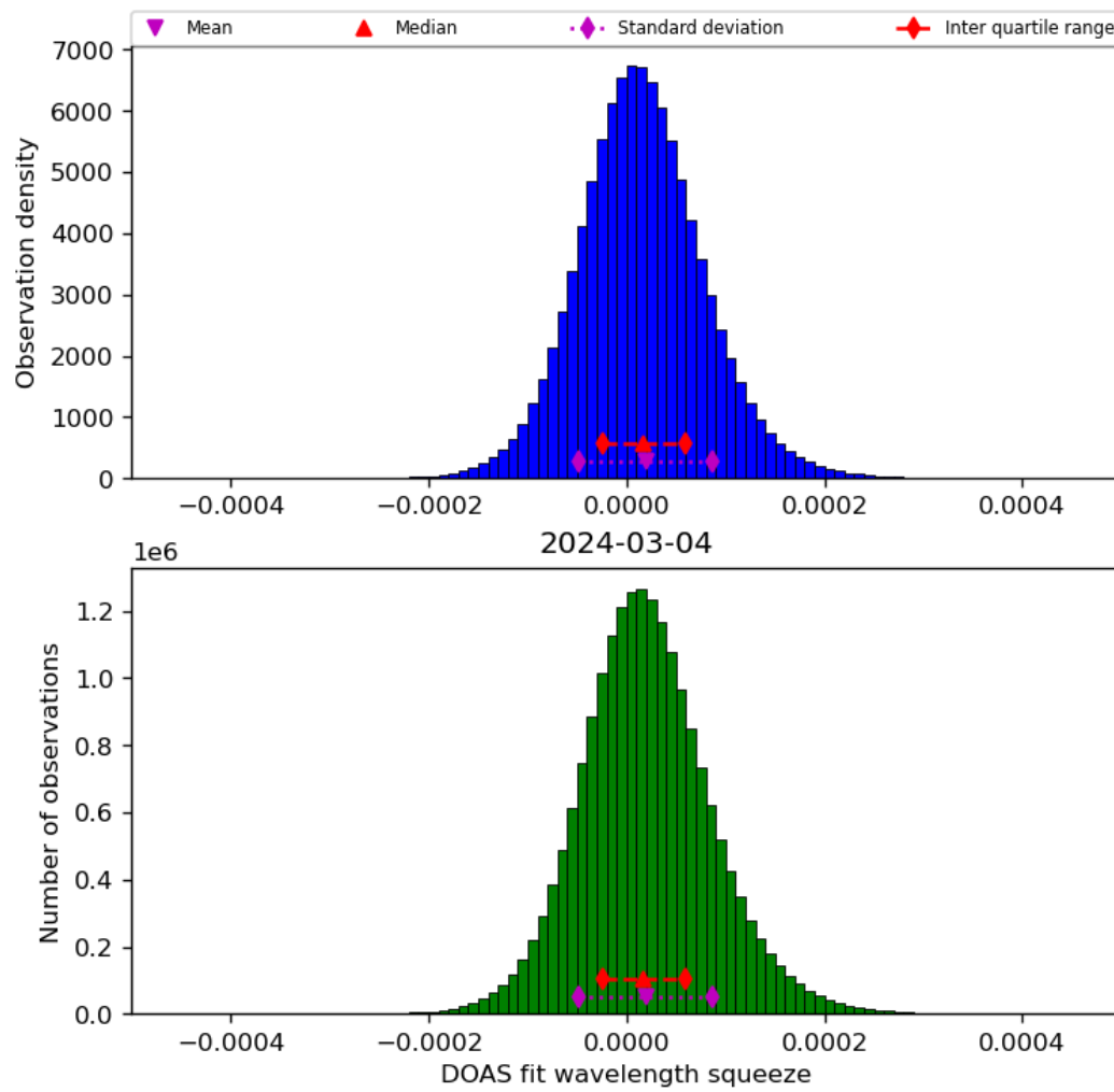
Figure 45: Histogram of “DOAS fit wavelength squeeze” for 2024-03-04 to 2024-03-05
