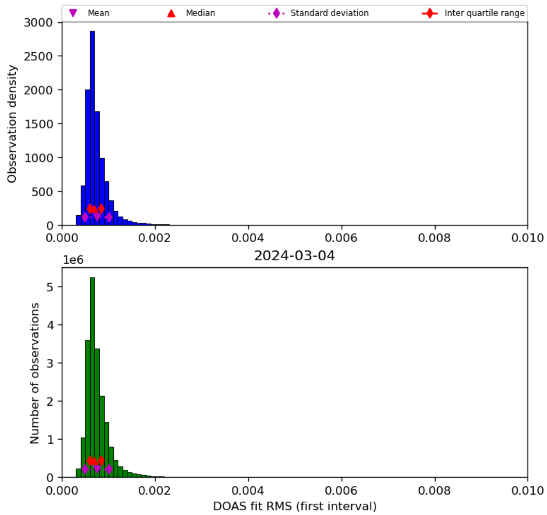
Figure 46: Histogram of “DOAS fit RMS (first interval)” for 2024-03-04 to 2024-03-05
