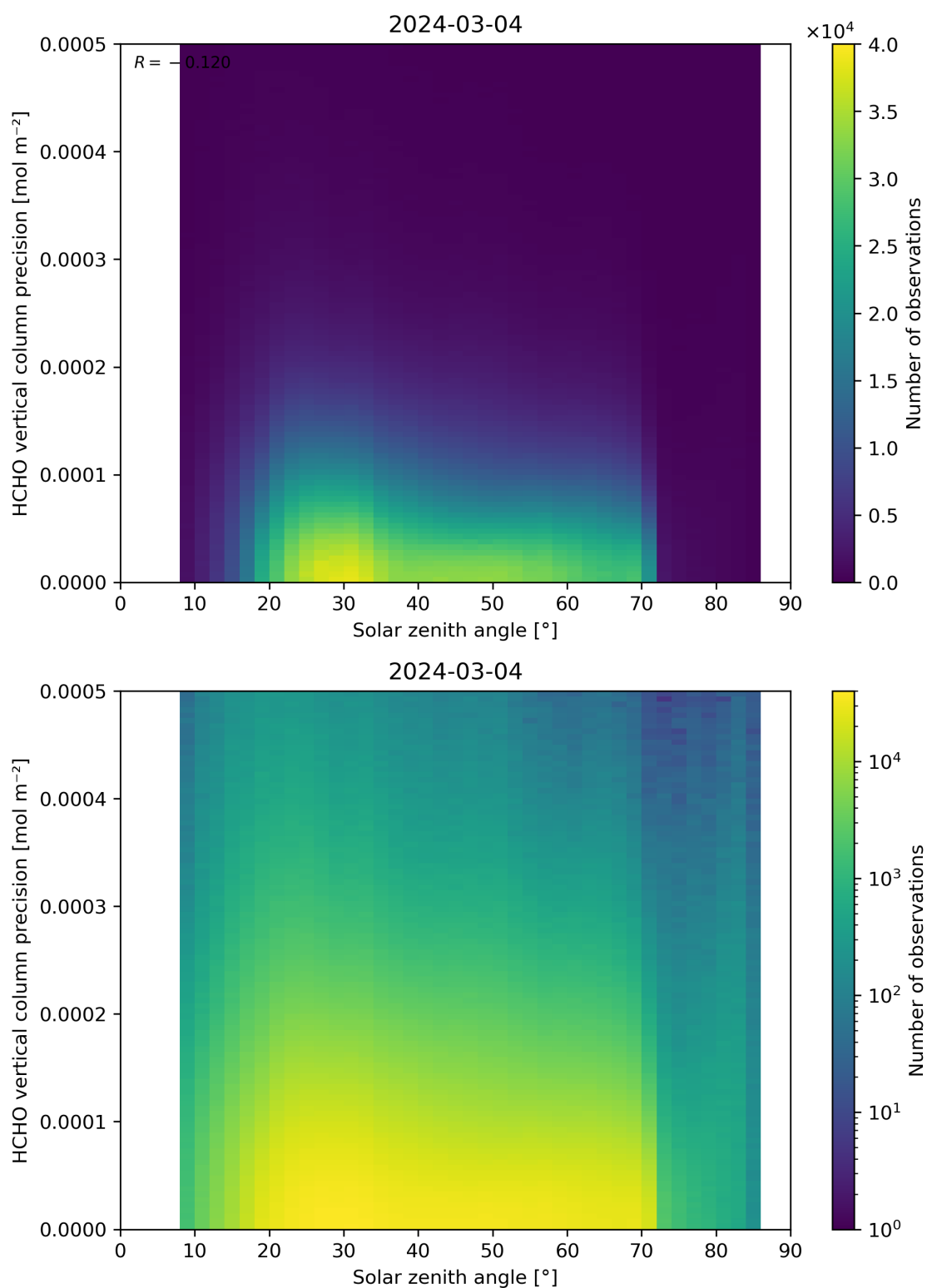
Figure 179: Scatter density plot of “Solar zenith angle” against “HCHO vertical column precision” for 2024-03-04 to 2024-03-05.
