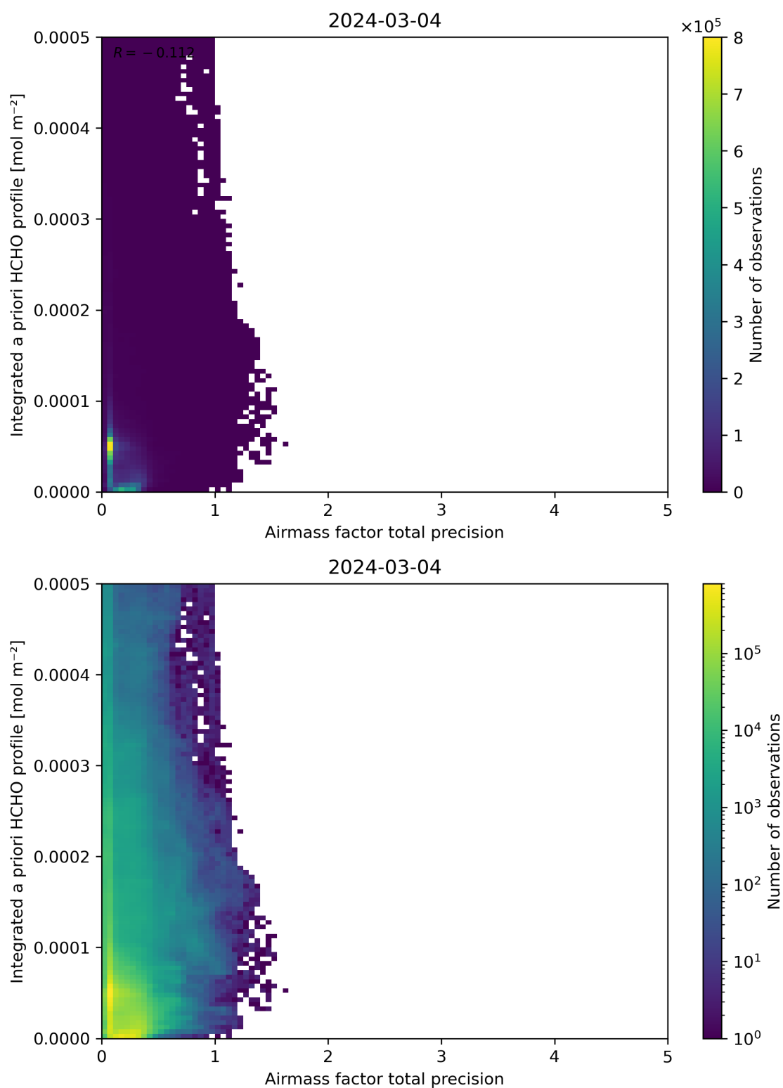
Figure 111: Scatter density plot of “Airmass factor total precision” against “Integrated a priori HCHO profile” for 2024-03-04 to 2024-03-05.
