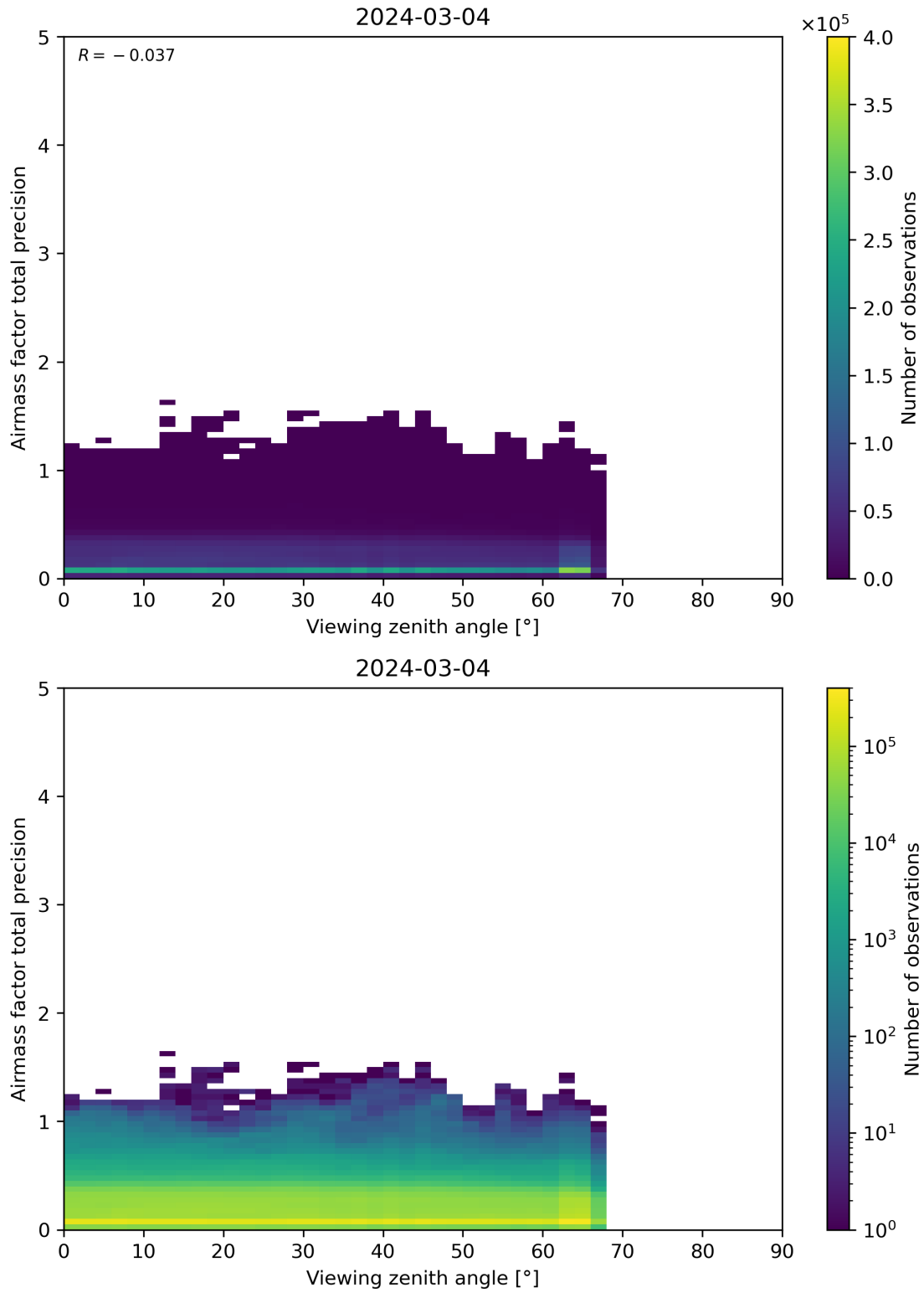
Figure 191: Scatter density plot of “Viewing zenith angle” against “Airmass factor total precision” for 2024-03-04 to 2024-03-05.
