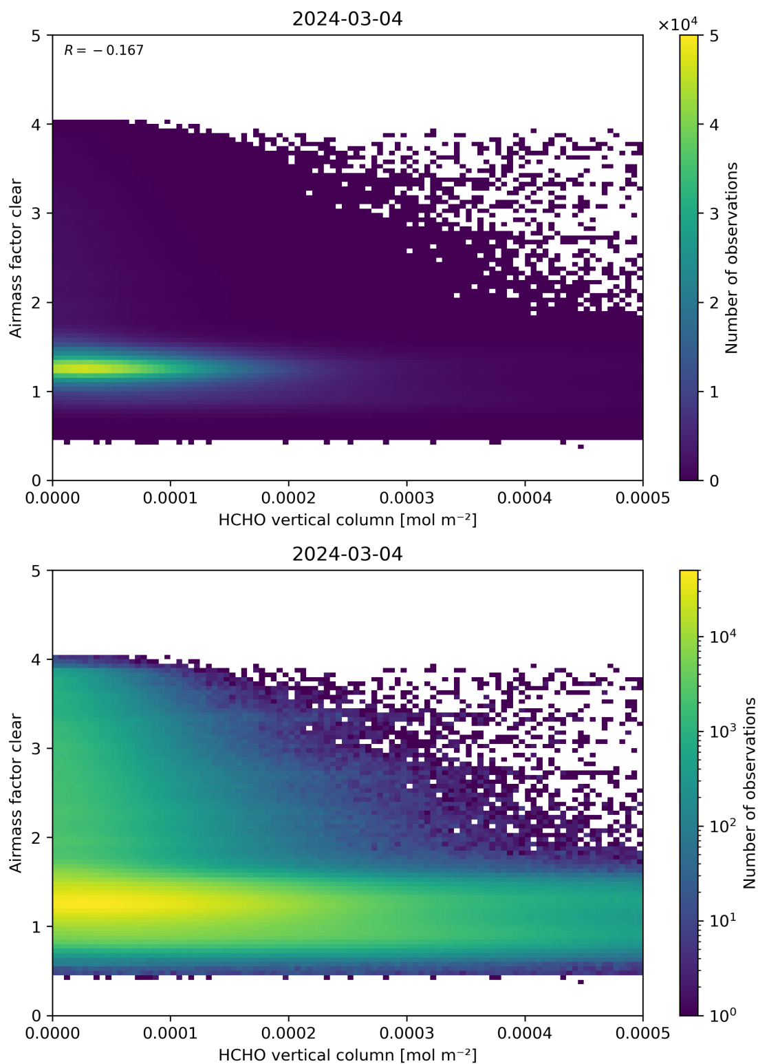
Figure 126: Scatter density plot of “HCHO vertical column” against “Airmass factor clear” for 2024-03-04 to 2024-03-05.
