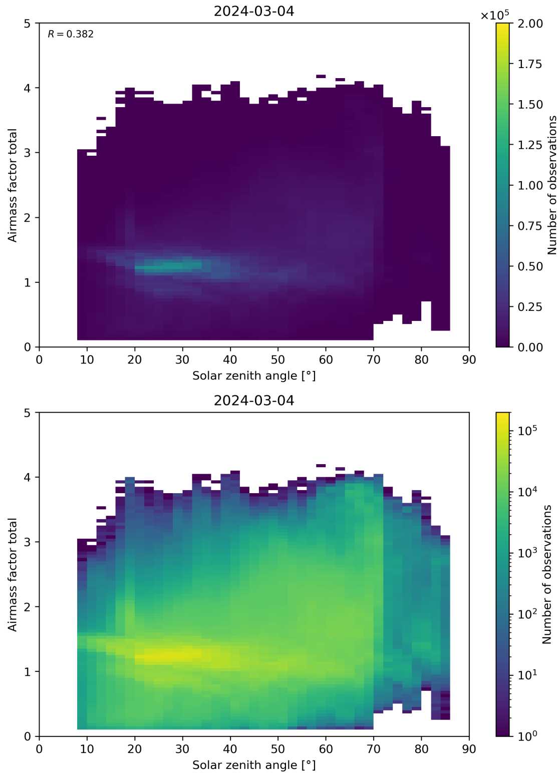
Figure 175: Scatter density plot of “Solar zenith angle” against “Airmass factor total” for 2024-03-04 to 2024-03-05.
