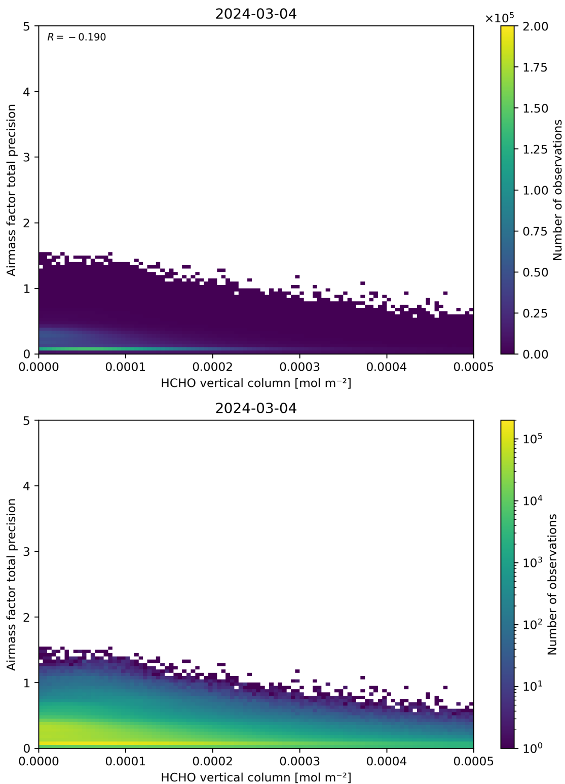
Figure 132: Scatter density plot of “HCHO vertical column” against “Airmass factor total precision” for 2024-03-04 to 2024-03-05.
