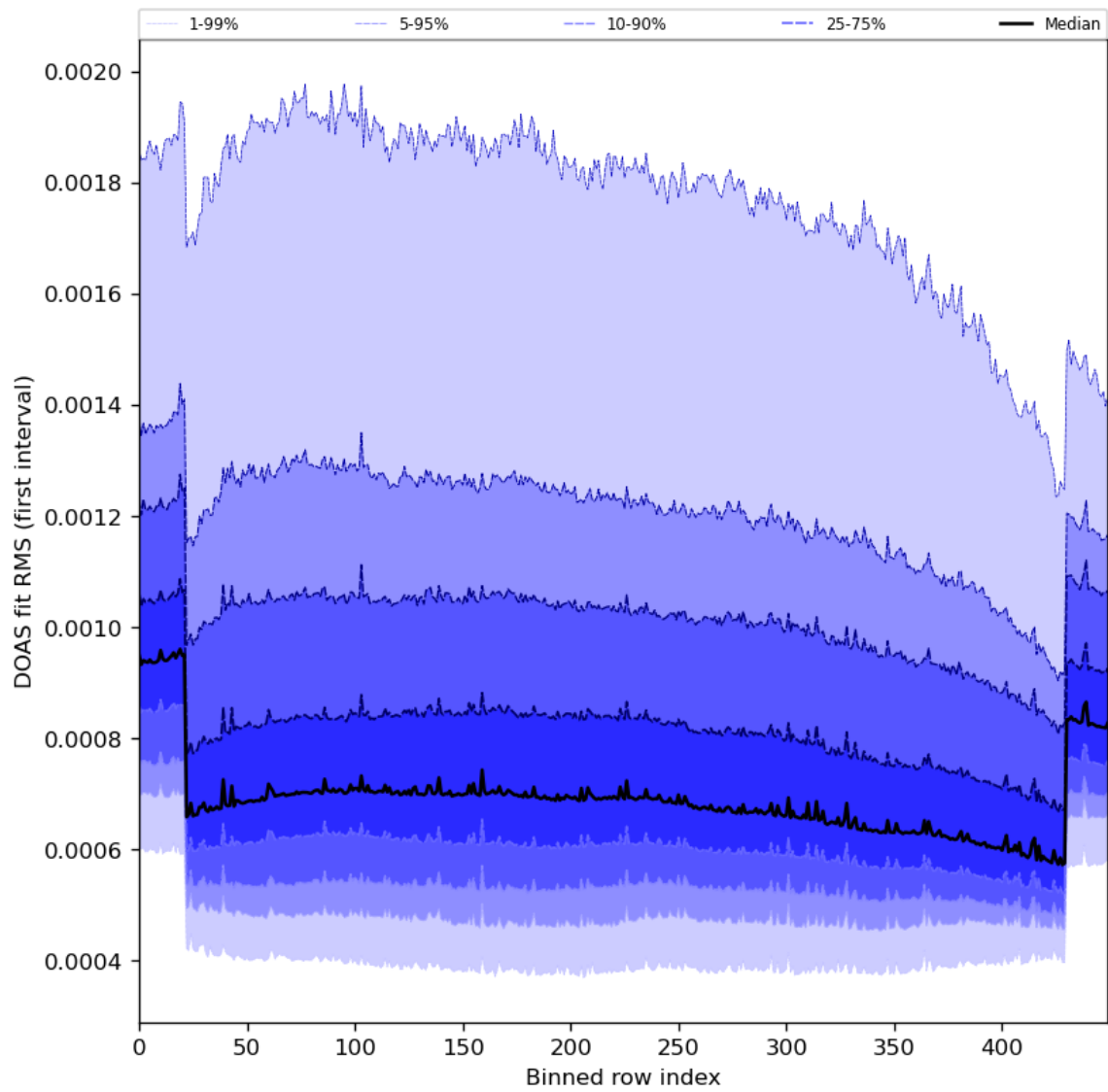
Figure 60: Along track statistics of “DOAS fit RMS (first interval)” for 2024-03-04 to 2024-03-05
