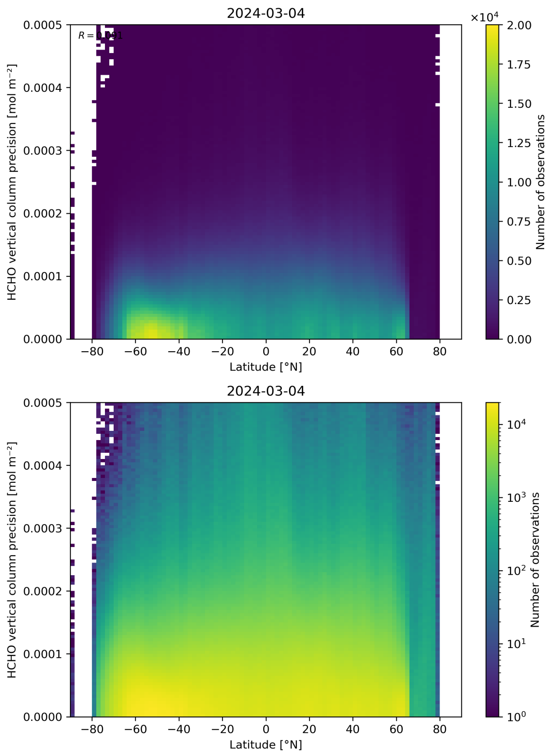
Figure 165: Scatter density plot of “Latitude” against “HCHO vertical column precision” for 2024-03-04 to 2024-03-05.
