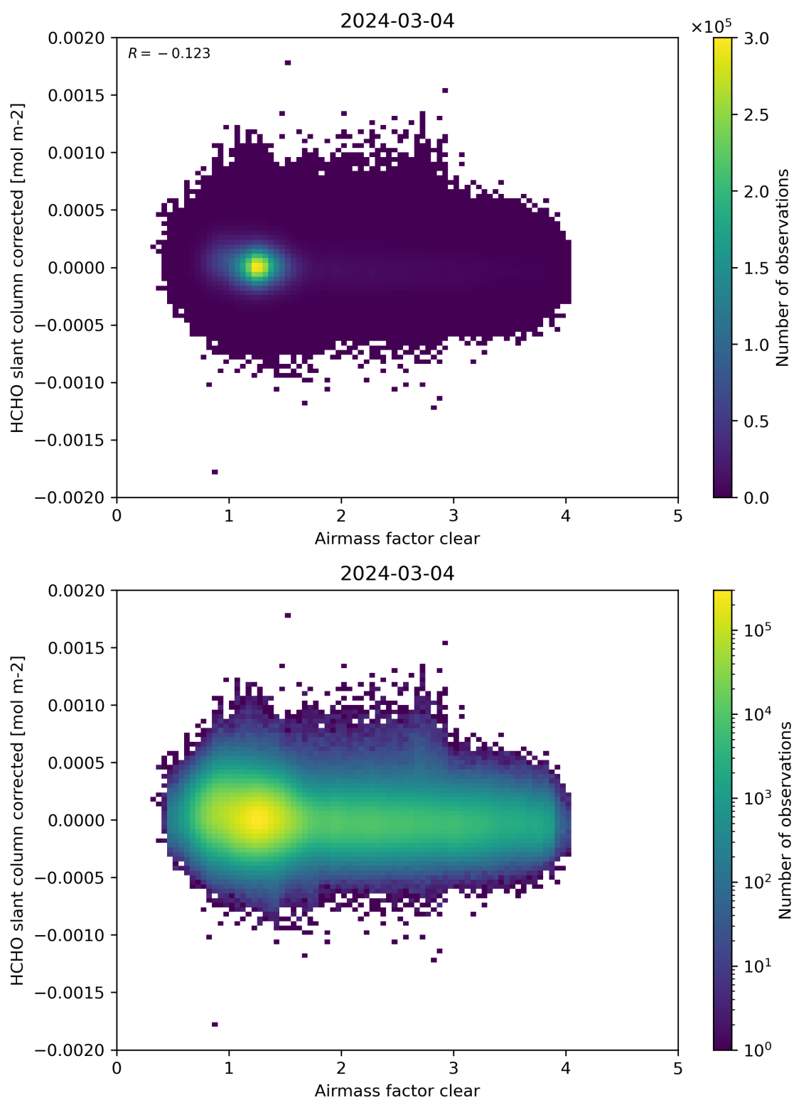
Figure 74: Scatter density plot of “Airmass factor clear” against “HCHO slant column corrected” for 2024-03-04 to 2024-03-05.
