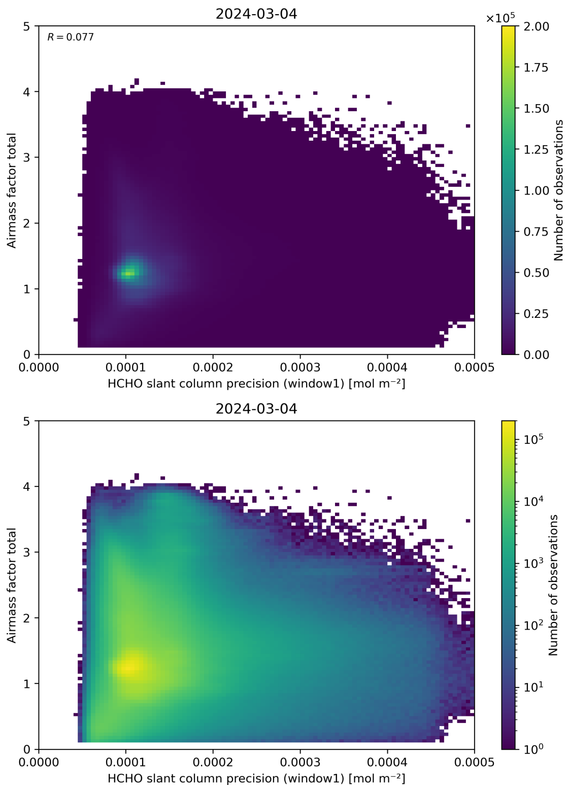
Figure 94: Scatter density plot of “HCHO slant column precision (window1)” against “Airmass factor total” for 2024-03-04 to 2024-03-05.
