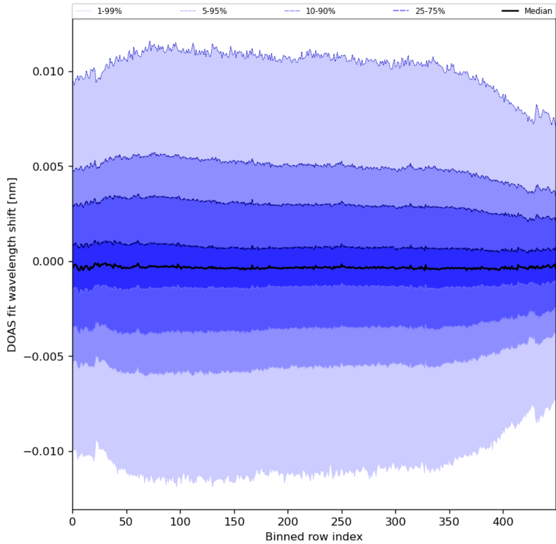
Figure 58: Along track statistics of “DOAS fit wavelength shift” for 2024-03-04 to 2024-03-05
