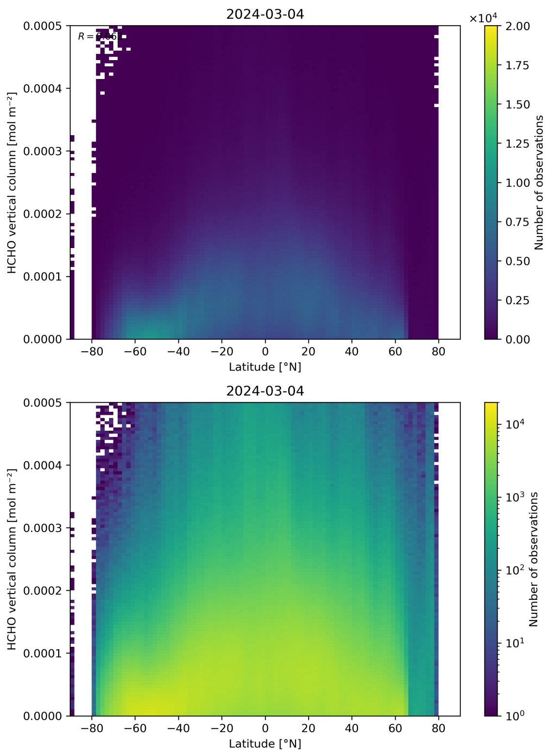
Figure 163: Scatter density plot of “Latitude” against “HCHO vertical column” for 2024-03-04 to 2024-03-05.
