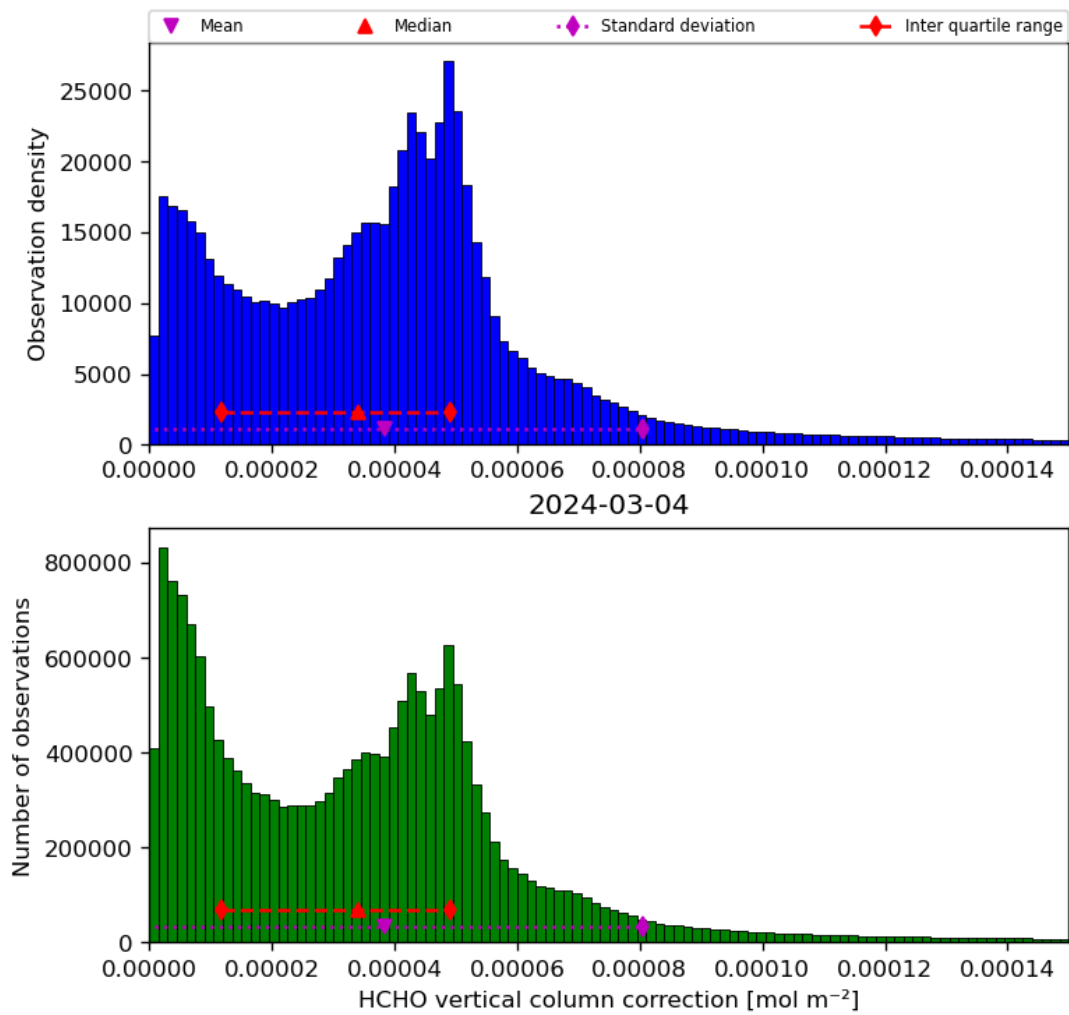
Figure 37: Histogram of “HCHO vertical column correction” for 2024-03-04 to 2024-03-05
