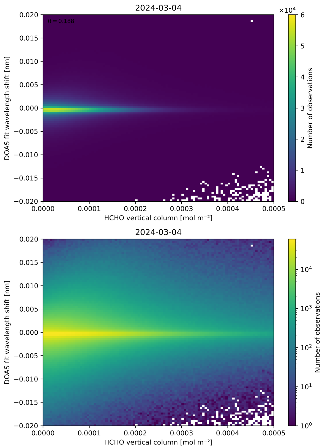
Figure 124: Scatter density plot of “HCHO vertical column” against “DOAS fit wavelength shift” for 2024-03-04 to 2024-03-05.
