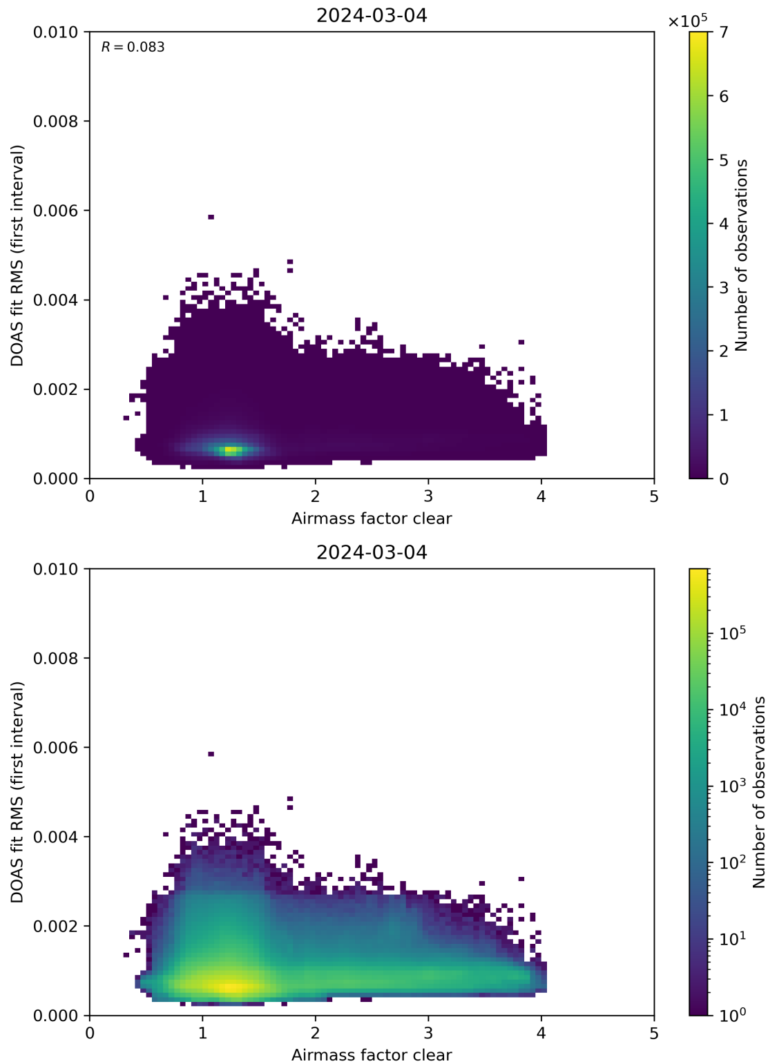
Figure 71: Scatter density plot of “Airmass factor clear” against “DOAS fit RMS (first interval)” for 2024-03-04 to 2024-03-05.
