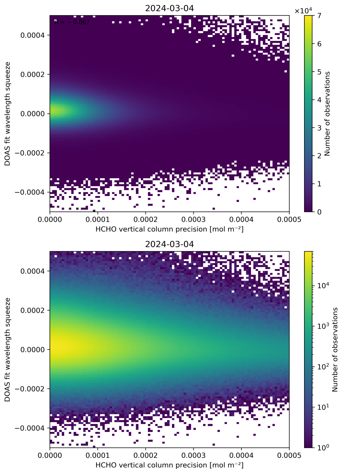
Figure 138: Scatter density plot of “HCHO vertical column precision” against “DOAS fit wavelength squeeze” for 2024-03-04 to 2024-03-05.
