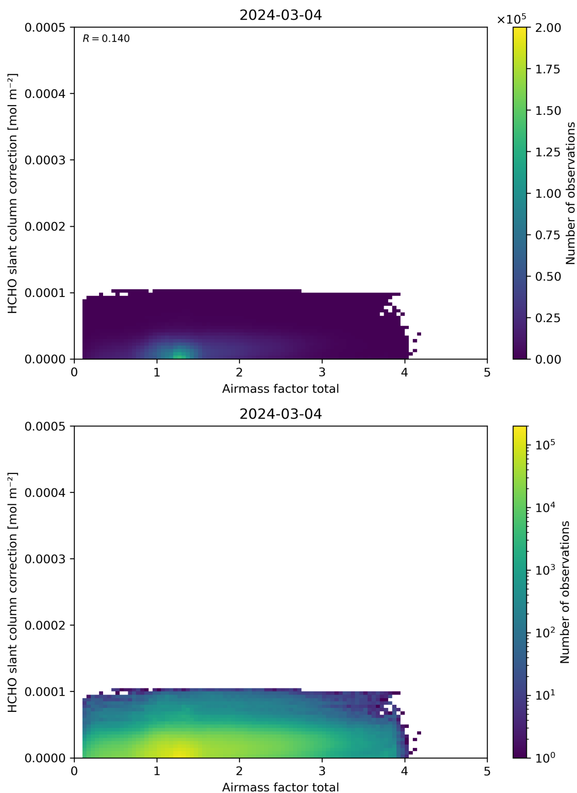
Figure 102: Scatter density plot of “Airmass factor total” against “HCHO slant column correction” for 2024-03-04 to 2024-03-05.
