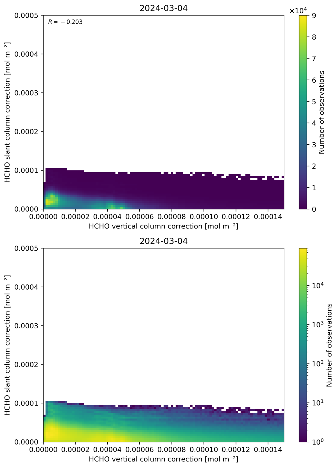
Figure 117: Scatter density plot of “HCHO vertical column correction” against “HCHO slant column correction” for 2024-03-04 to 2024-03-05.
