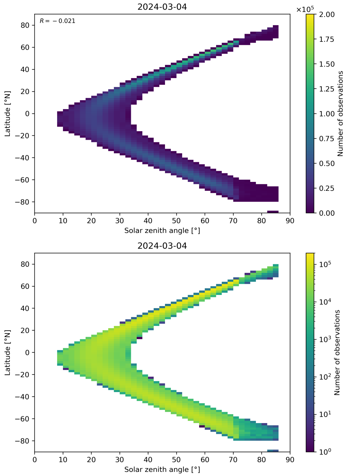
Figure 181: Scatter density plot of “Solar zenith angle” against “Latitude” for 2024-03-04 to 2024-03-05.
