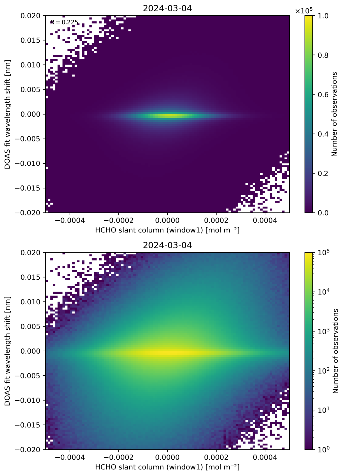
Figure 79: Scatter density plot of “HCHO slant column (window1)” against “DOAS fit wavelength shift” for 2024-03-04 to 2024-03-05.
