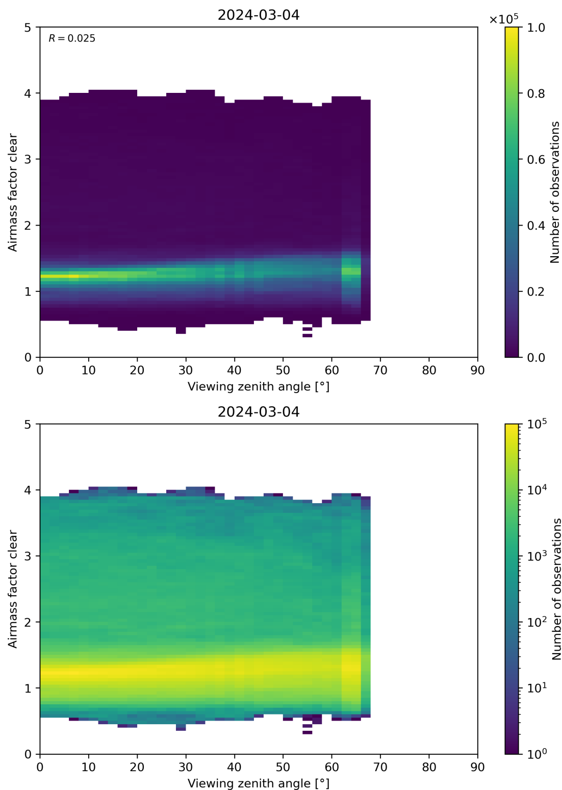
Figure 185: Scatter density plot of “Viewing zenith angle” against “Airmass factor clear” for 2024-03-04 to 2024-03-05.
