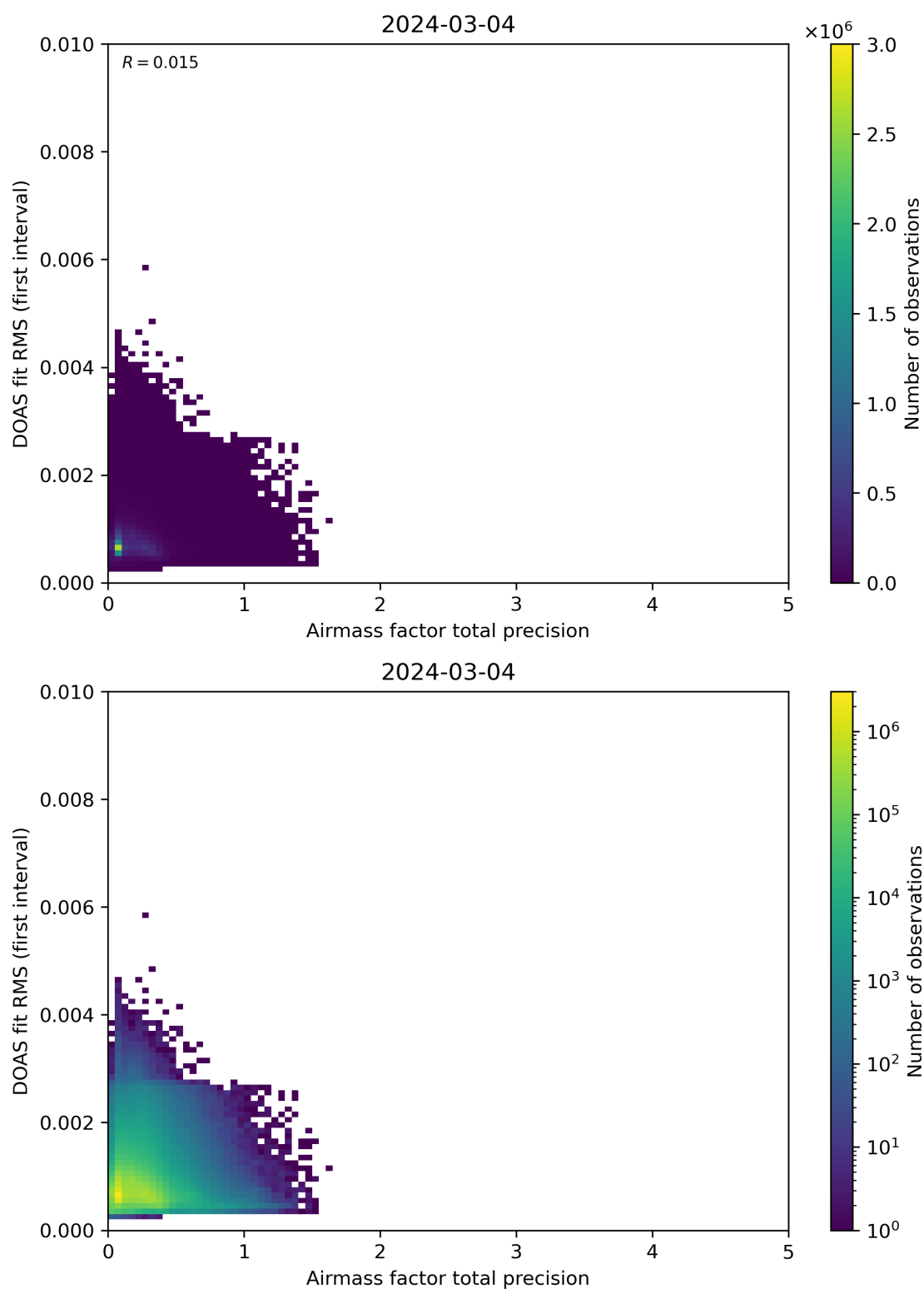
Figure 105: Scatter density plot of “Airmass factor total precision” against “DOAS fit RMS (first interval)” for 2024-03-04 to 2024-03-05.
