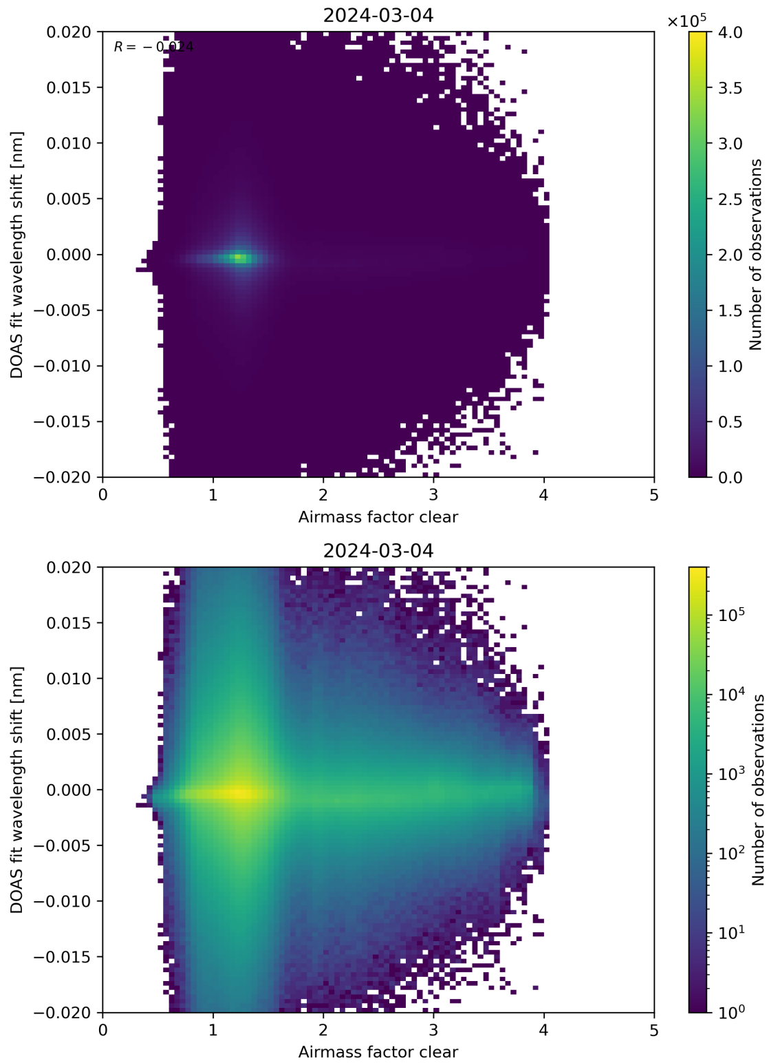
Figure 72: Scatter density plot of “Airmass factor clear” against “DOAS fit wavelength shift” for 2024-03-04 to 2024-03-05.
