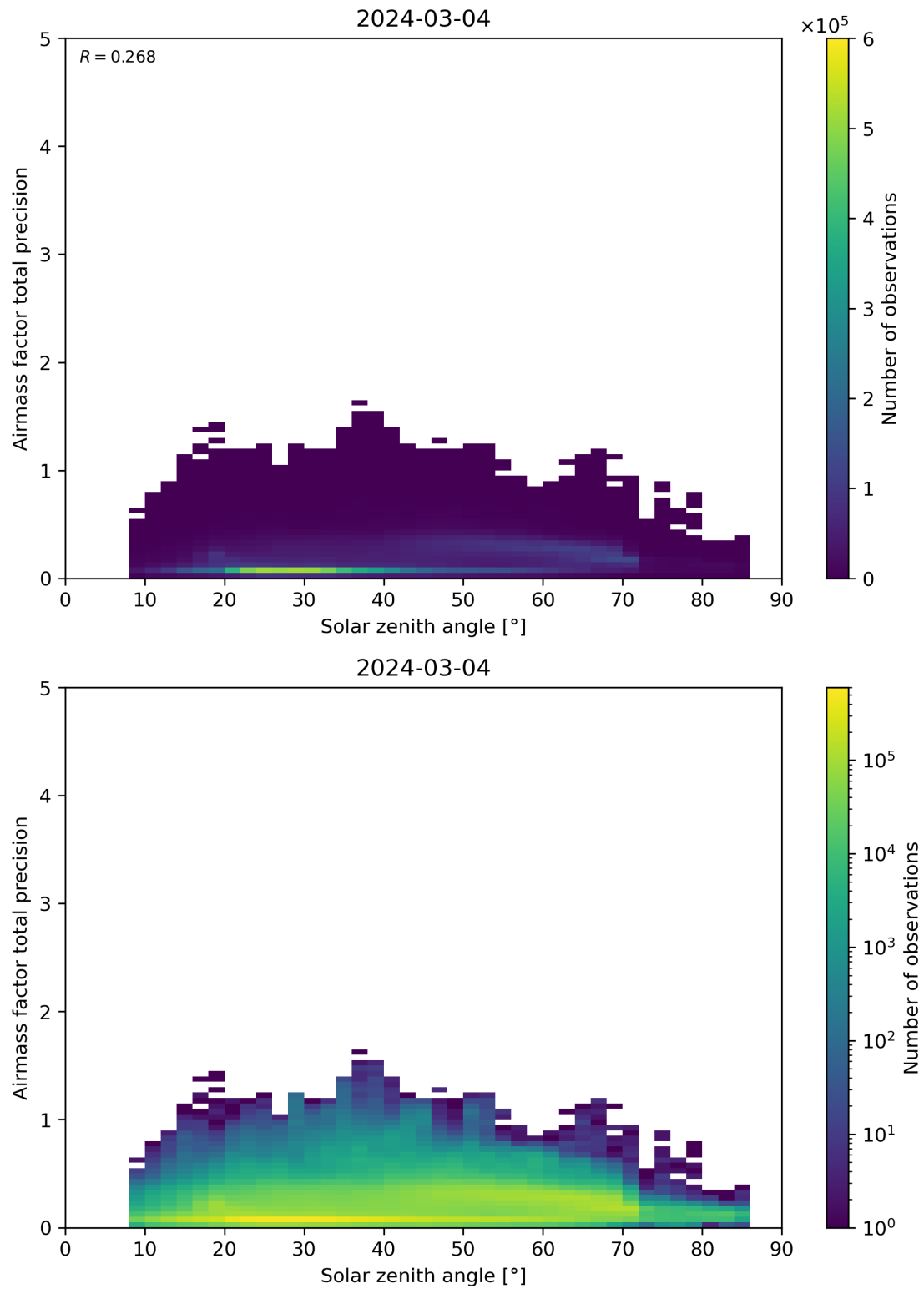
Figure 176: Scatter density plot of “Solar zenith angle” against “Airmass factor total precision” for 2024-03-04 to 2024-03-05.
