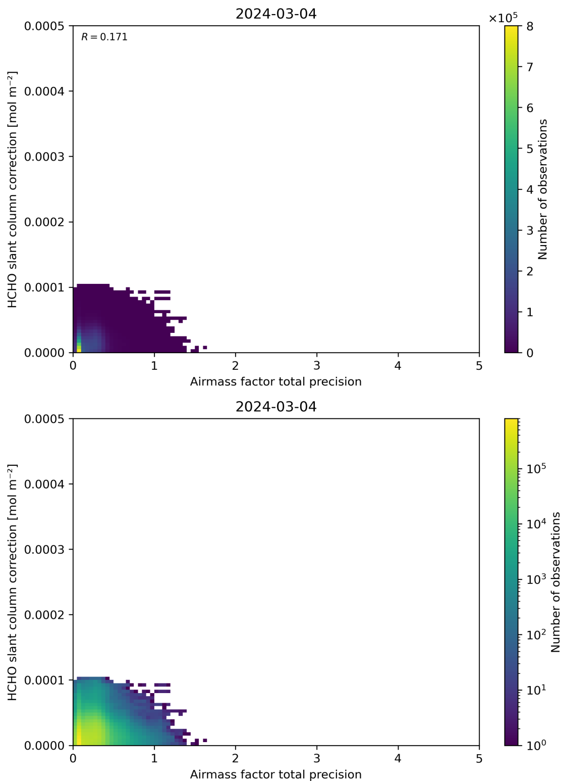
Figure 110: Scatter density plot of “Airmass factor total precision” against “HCHO slant column correction” for 2024-03-04 to 2024-03-05.
