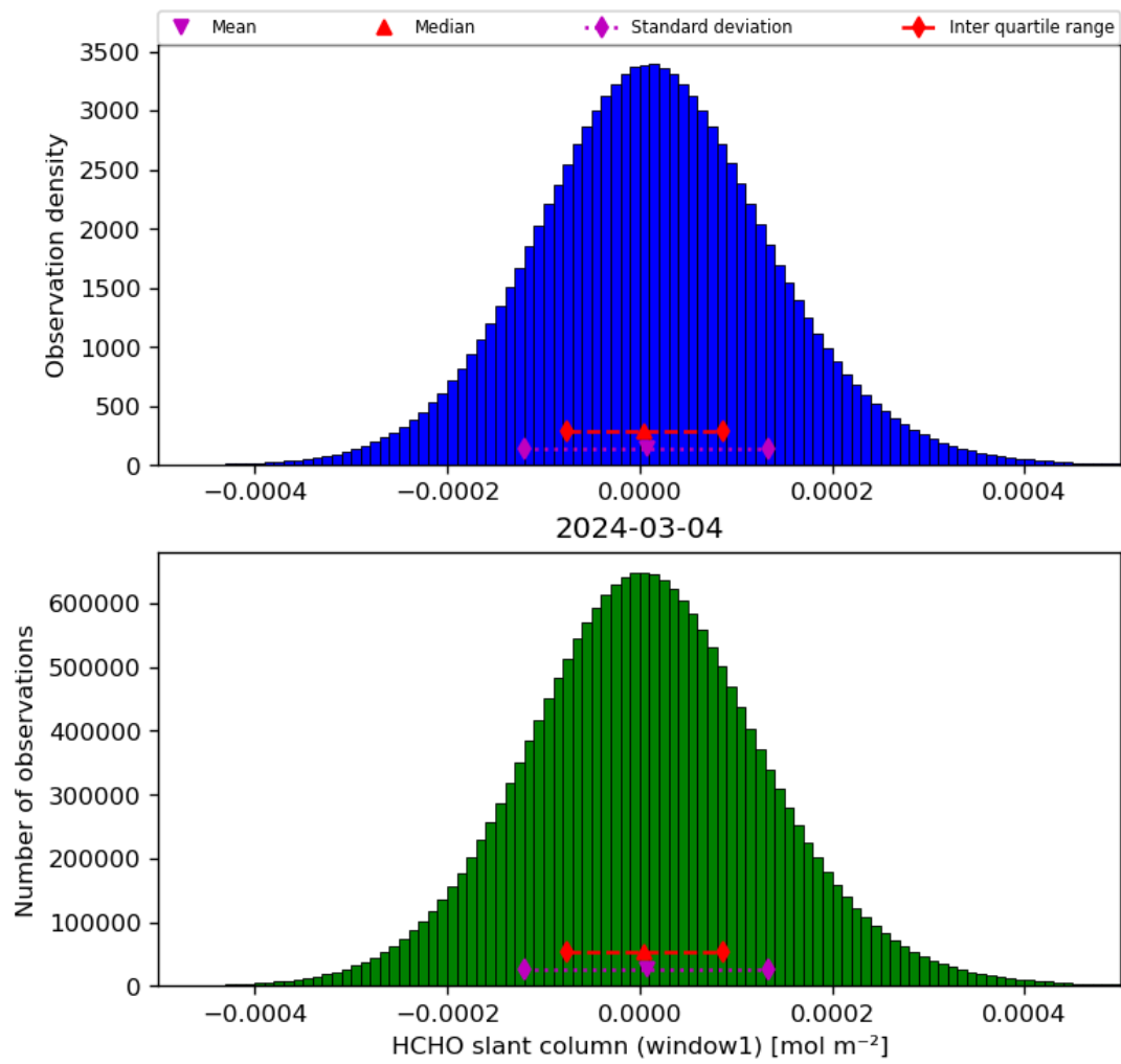
Figure 38: Histogram of “HCHO slant column (window1)” for 2024-03-04 to 2024-03-05
