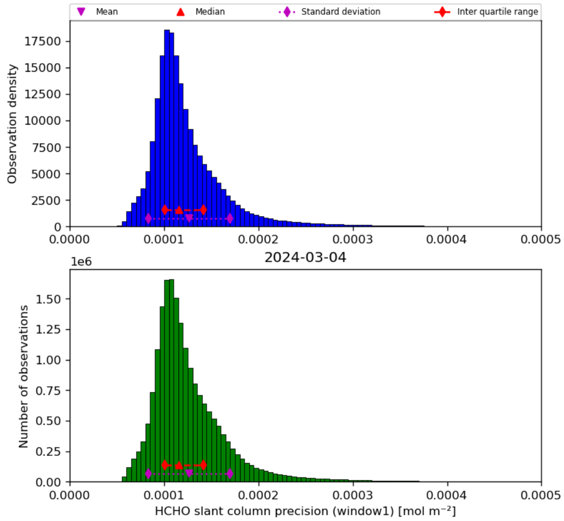
Figure 39: Histogram of “HCHO slant column precision (window1)” for 2024-03-04 to 2024-03-05
