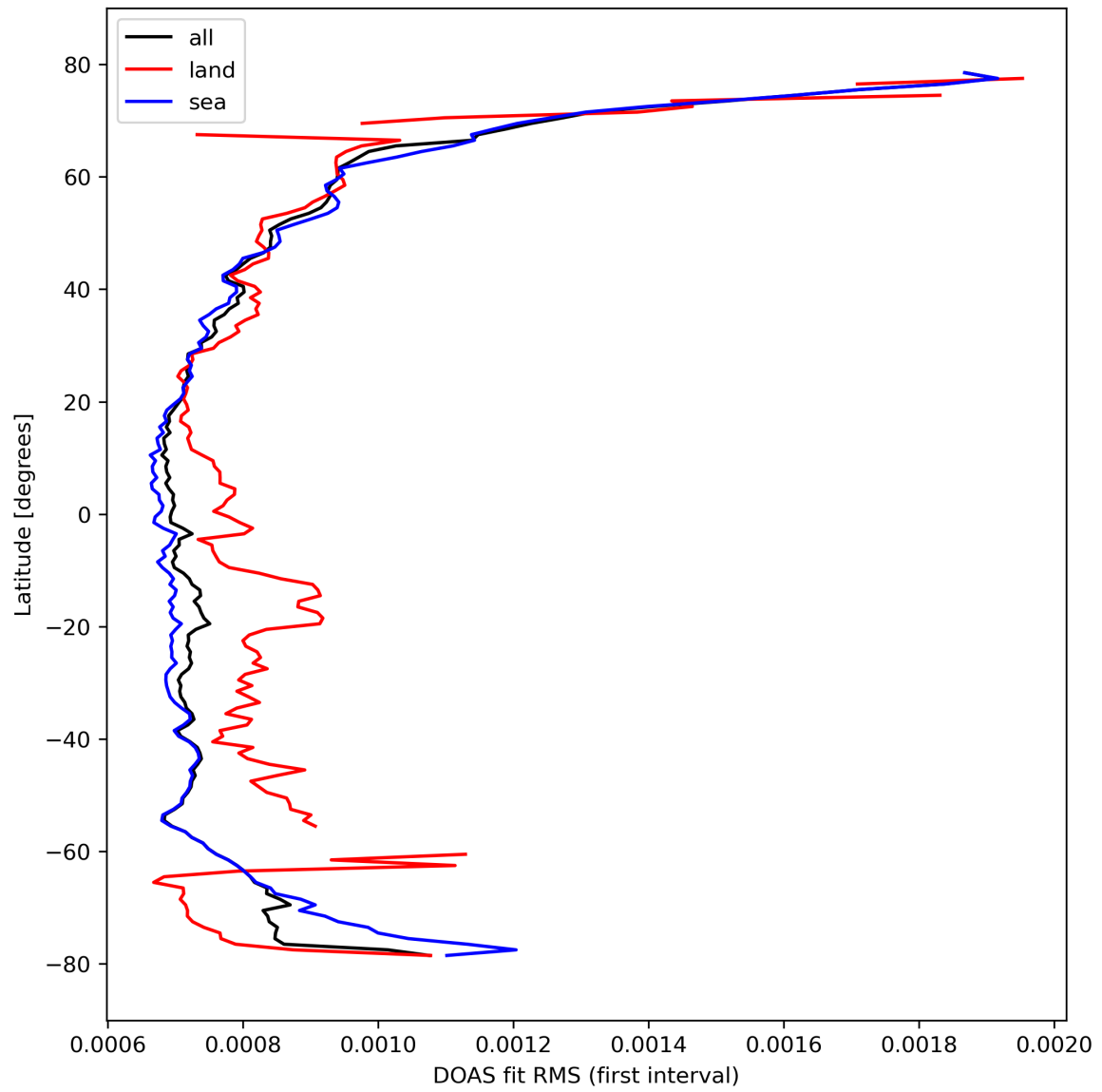
Figure 32: Zonal average of “DOAS fit RMS (first interval)” for 2024-03-04 to 2024-03-05.
