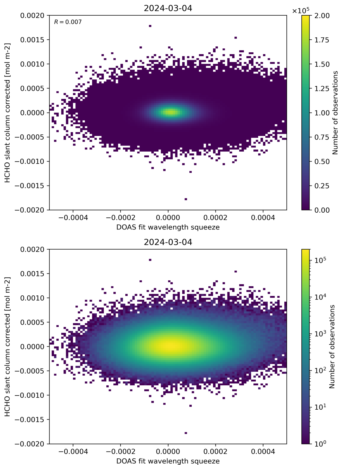
Figure 69: Scatter density plot of “DOAS fit wavelength squeeze” against “HCHO slant column corrected” for 2024-03-04 to 2024-03-05.
