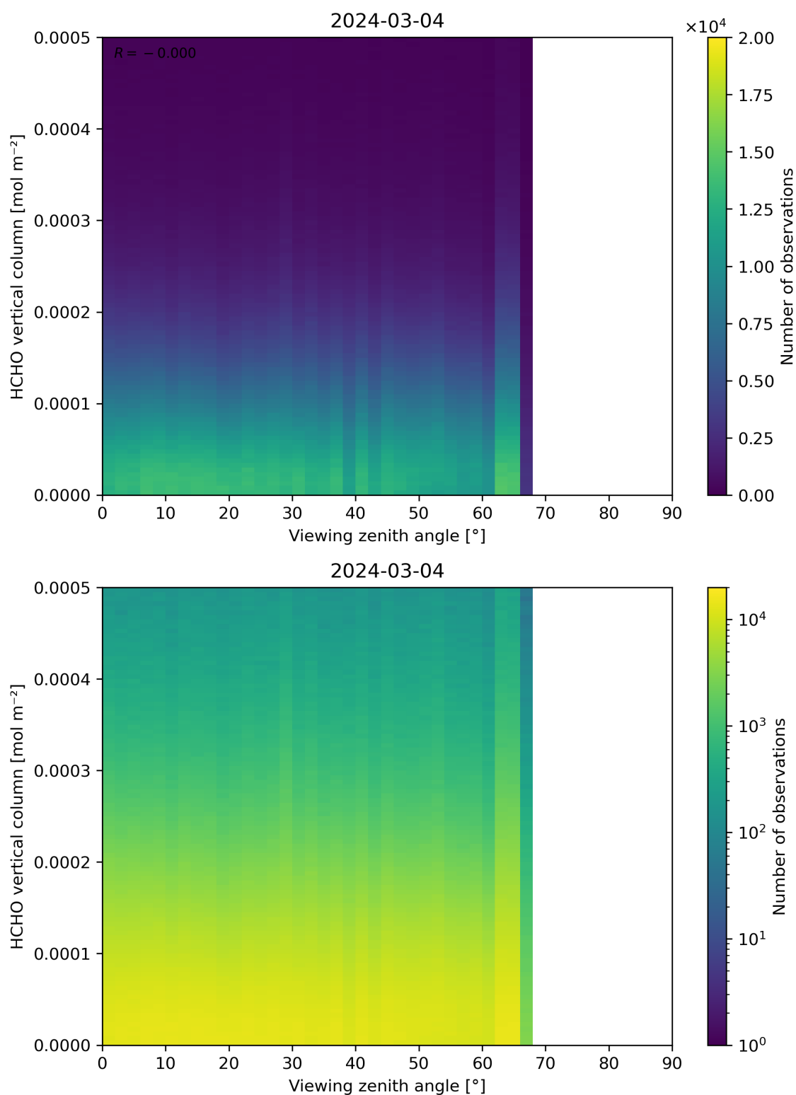
Figure 192: Scatter density plot of “Viewing zenith angle” against “HCHO vertical column” for 2024-03-04 to 2024-03-05.
