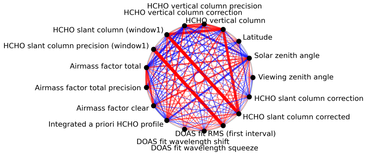
Figure 1: Map of correlation graph for 2024-03-04 to 2024-03-05.
