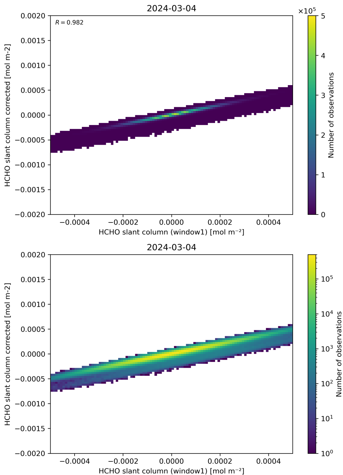
Figure 82: Scatter density plot of “HCHO slant column (window1)” against “HCHO slant column corrected” for 2024-03-04 to 2024-03-05.
