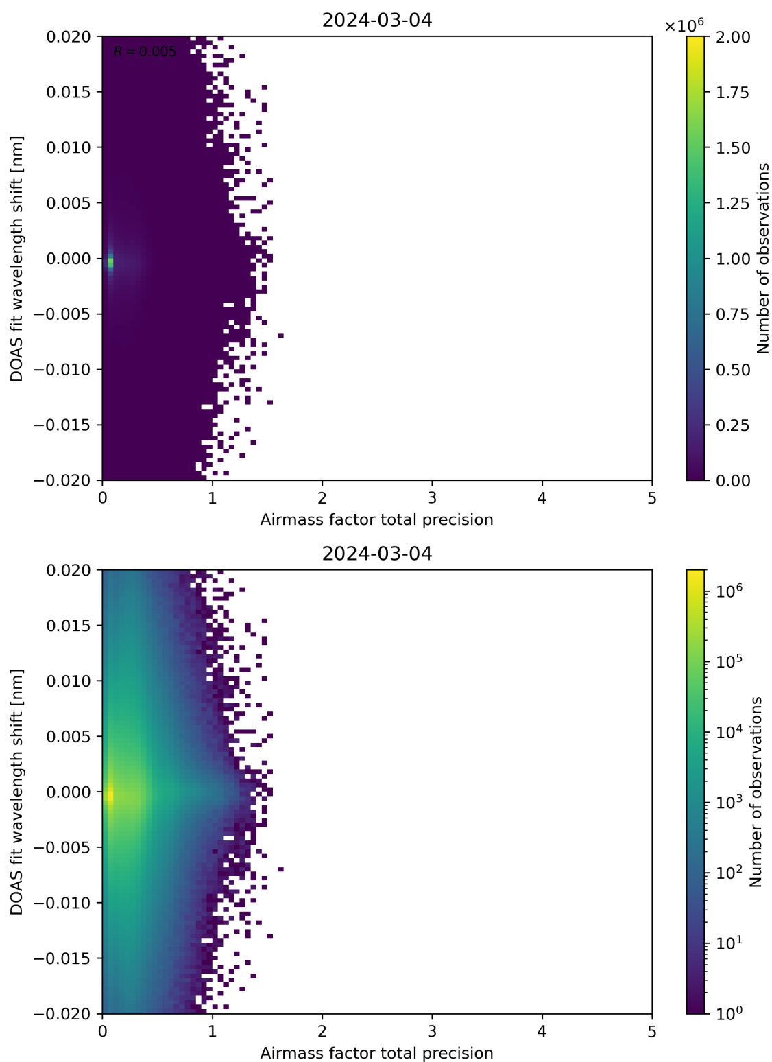
Figure 106: Scatter density plot of “Airmass factor total precision” against “DOAS fit wavelength shift” for 2024-03-04 to 2024-03-05.
