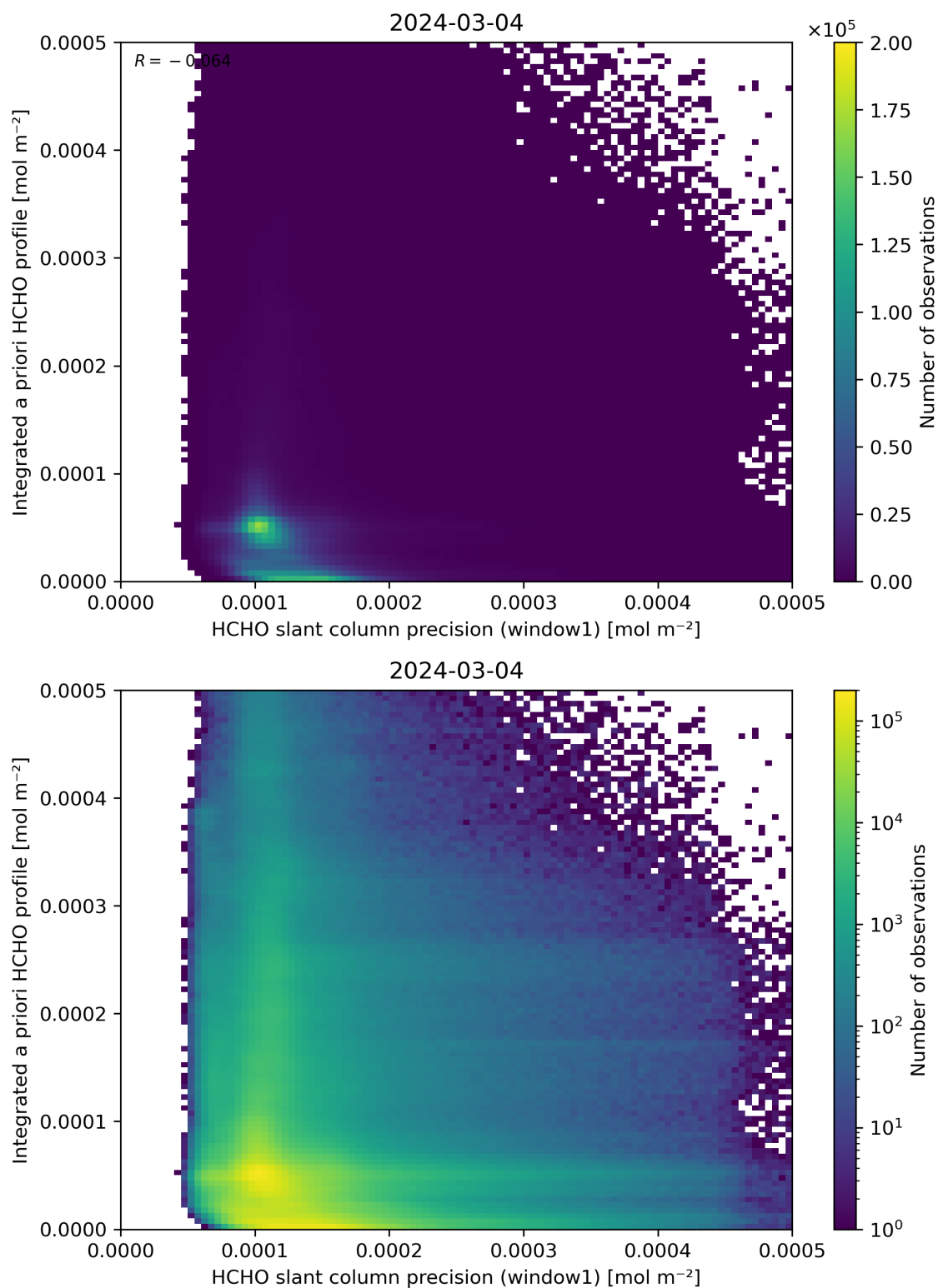
Figure 96: Scatter density plot of “HCHO slant column precision (window1)” against “Integrated a priori HCHO profile” for 2024-03-04 to 2024-03-05.
