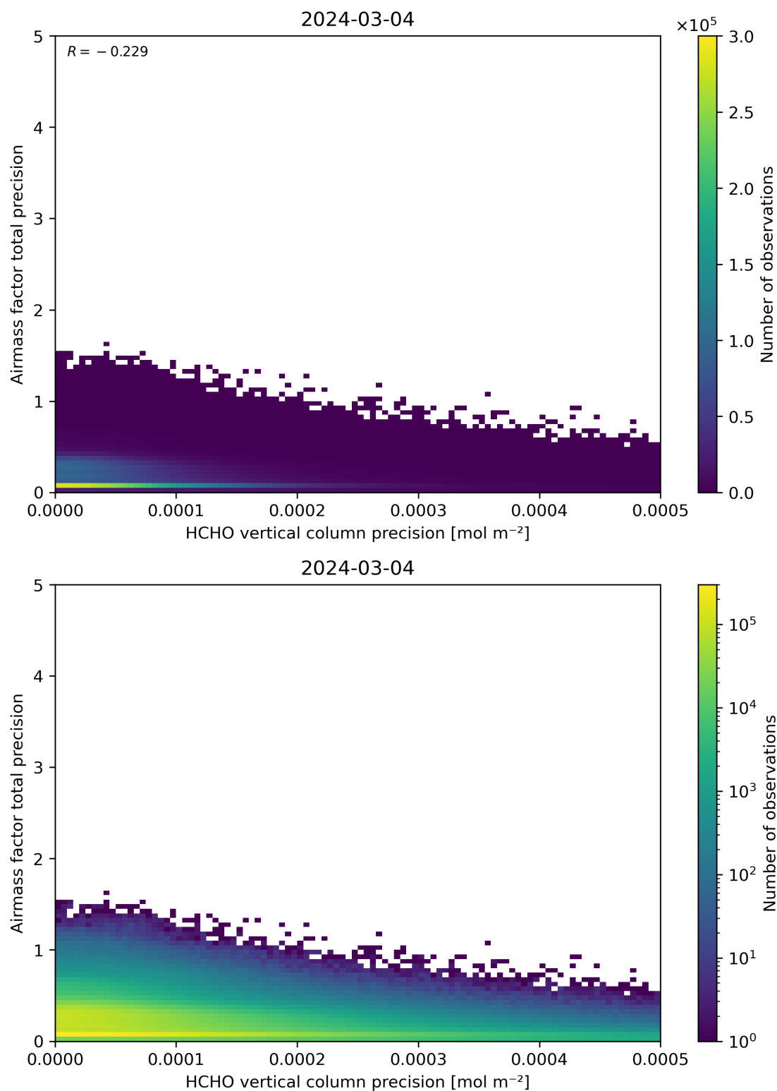
Figure 145: Scatter density plot of “HCHO vertical column precision” against “Airmass factor total precision” for 2024-03-04 to 2024-03-05.
