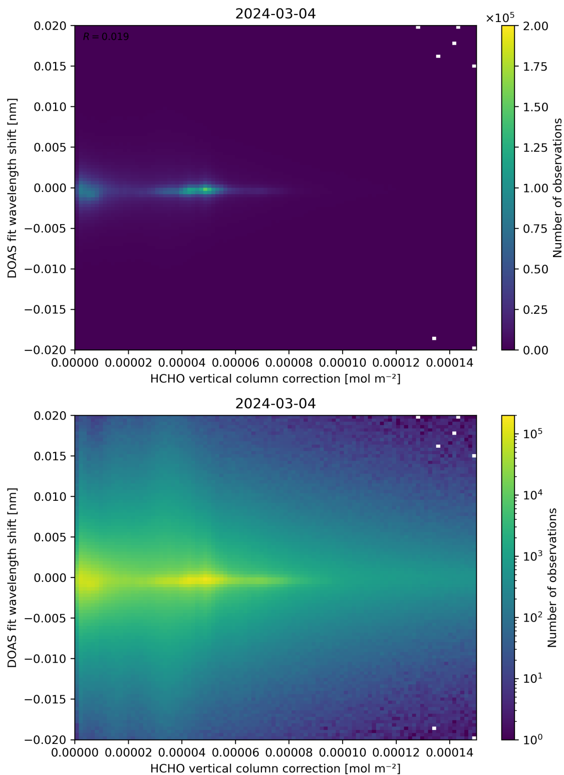
Figure 113: Scatter density plot of “HCHO vertical column correction” against “DOAS fit wavelength shift” for 2024-03-04 to 2024-03-05.
