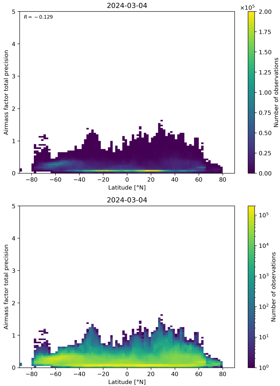
Figure 162: Scatter density plot of “Latitude” against “Airmass factor total precision” for 2024-03-04 to 2024-03-05.
