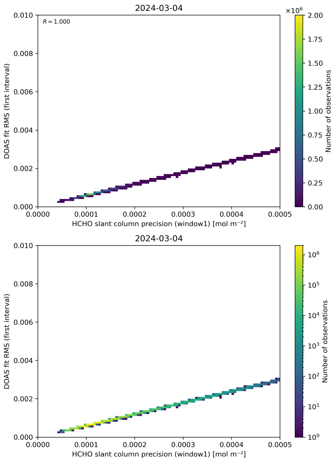
Figure 88: Scatter density plot of “HCHO slant column precision (window1)” against “DOAS fit RMS (first interval)” for 2024-03-04 to 2024-03-05.
