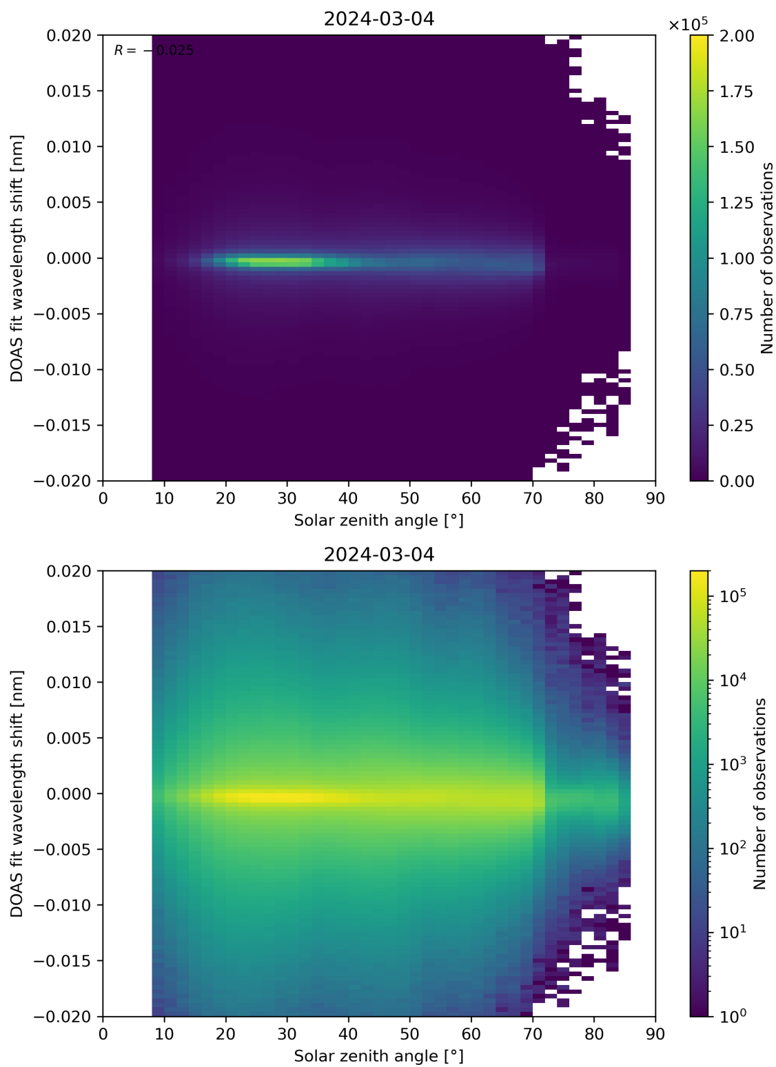
Figure 168: Scatter density plot of “Solar zenith angle” against “DOAS fit wavelength shift” for 2024-03-04 to 2024-03-05.
