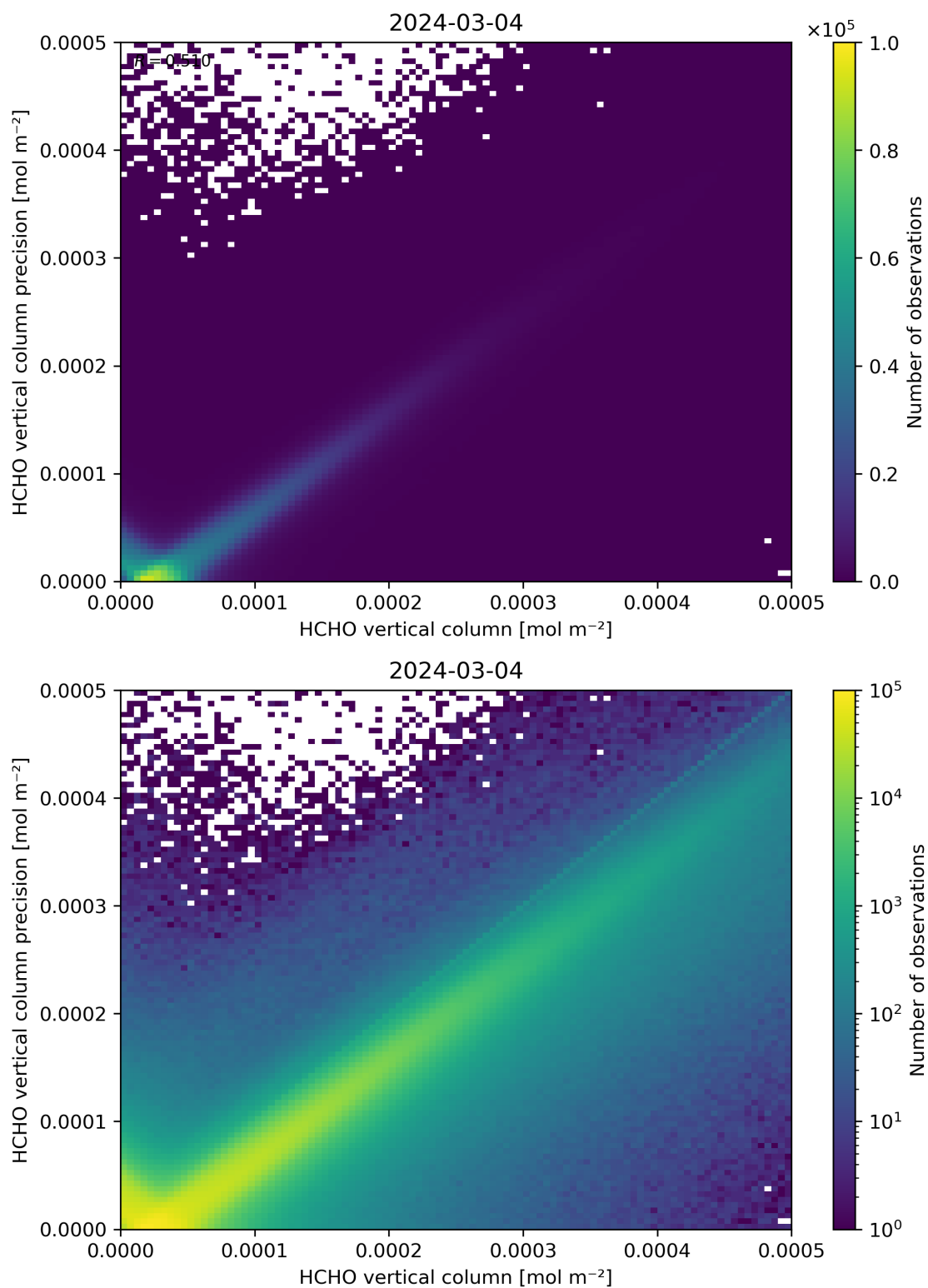
Figure 134: Scatter density plot of “HCHO vertical column” against “HCHO vertical column precision” for 2024-03-04 to 2024-03-05.
