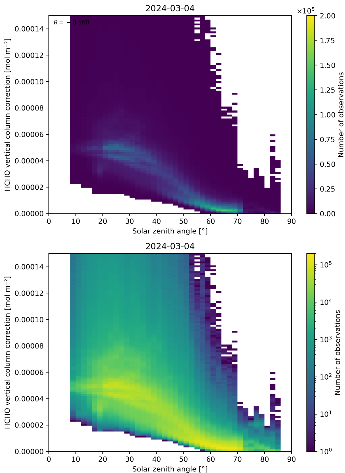
Figure 178: Scatter density plot of “Solar zenith angle” against “HCHO vertical column correction” for 2024-03-04 to 2024-03-05.
