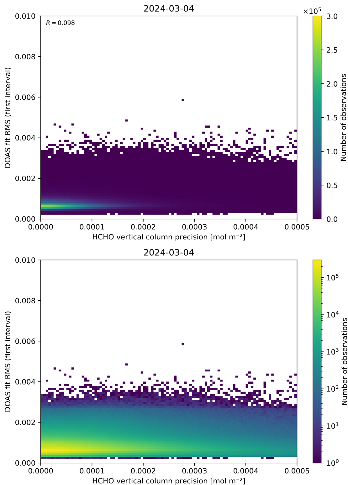
Figure 136: Scatter density plot of “HCHO vertical column precision” against “DOAS fit RMS (first interval)” for 2024-03-04 to 2024-03-05.
