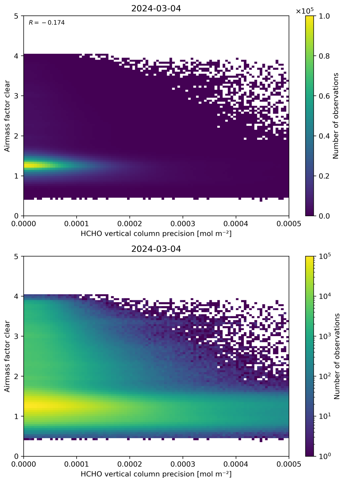
Figure 139: Scatter density plot of “HCHO vertical column precision” against “Airmass factor clear” for 2024-03-04 to 2024-03-05.
