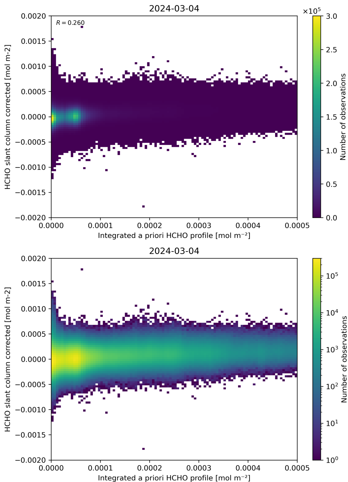
Figure 151: Scatter density plot of “Integrated a priori HCHO profile” against “HCHO slant column corrected” for 2024-03-04 to 2024-03-05.
