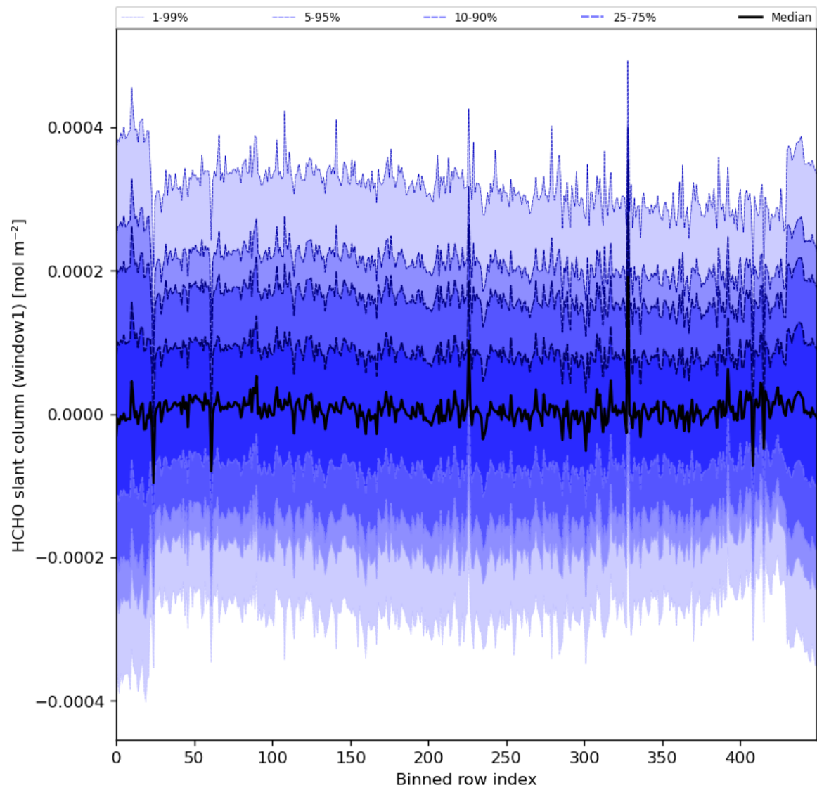
Figure 52: Along track statistics of “HCHO slant column (window1)” for 2024-03-04 to 2024-03-05
