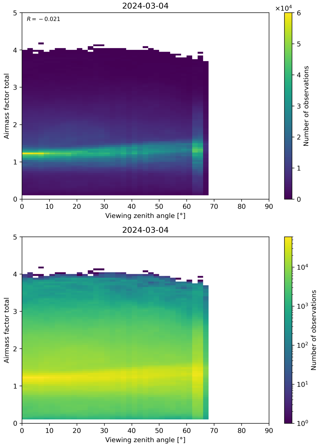
Figure 190: Scatter density plot of “Viewing zenith angle” against “Airmass factor total” for 2024-03-04 to 2024-03-05.
