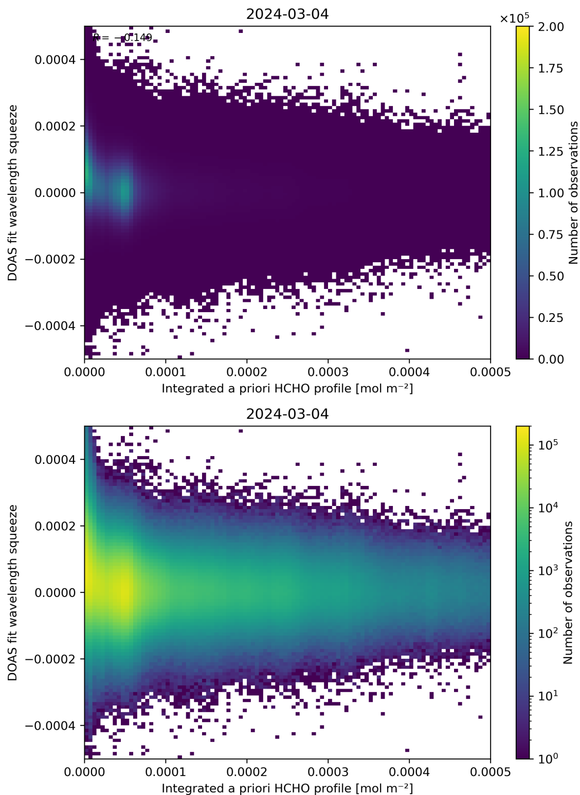
Figure 150: Scatter density plot of “Integrated a priori HCHO profile” against “DOAS fit wavelength squeeze” for 2024-03-04 to 2024-03-05.
