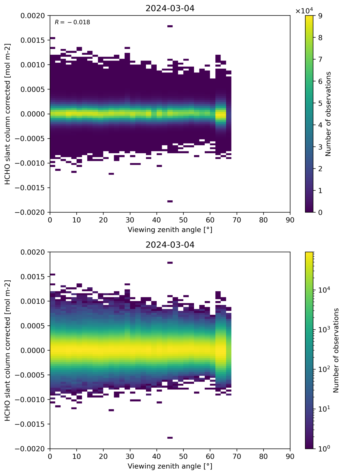
Figure 186: Scatter density plot of “Viewing zenith angle” against “HCHO slant column corrected” for 2024-03-04 to 2024-03-05.
