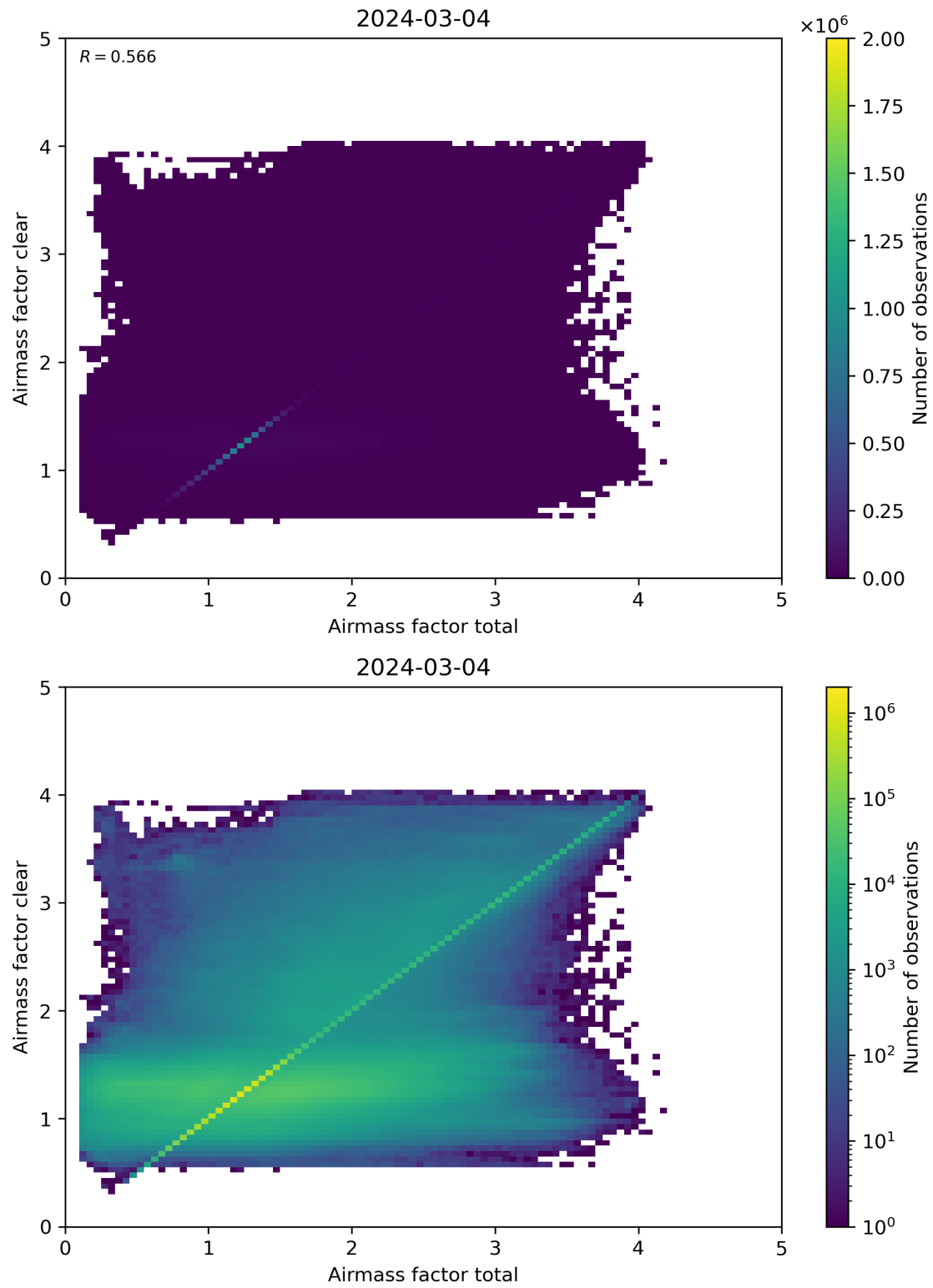
Figure 100: Scatter density plot of “Airmass factor total” against “Airmass factor clear” for 2024-03-04 to 2024-03-05.
