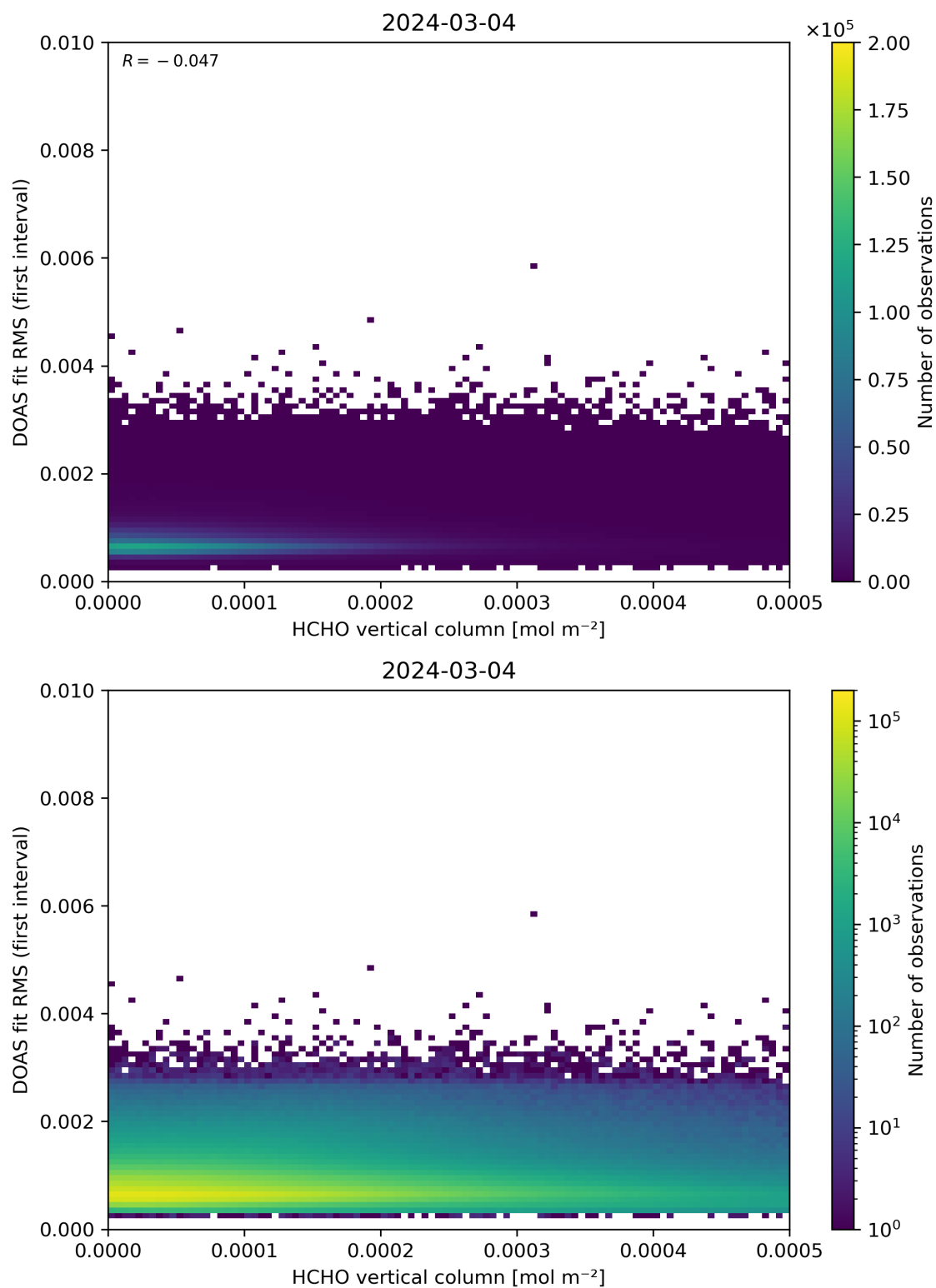
Figure 123: Scatter density plot of “HCHO vertical column” against “DOAS fit RMS (first interval)” for 2024-03-04 to 2024-03-05.
