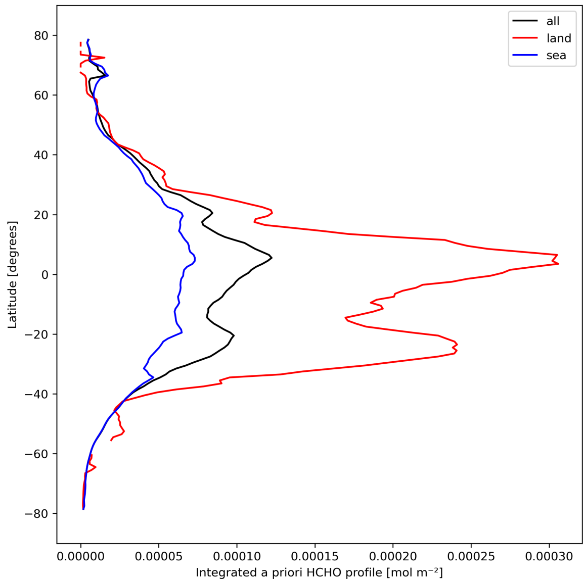
Figure 29: Zonal average of “Integrated a priori HCHO profile” for 2024-03-04 to 2024-03-05.
