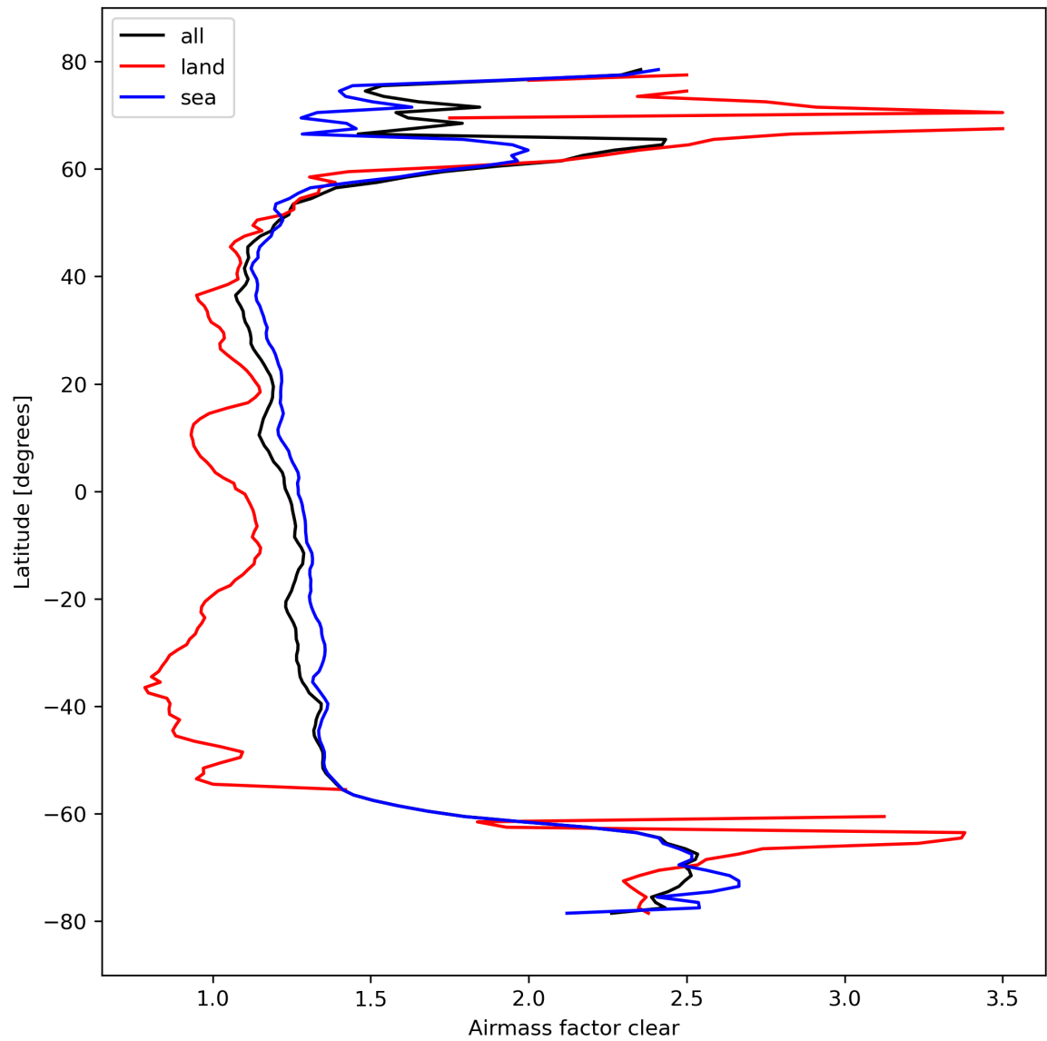
Figure 28: Zonal average of “Airmass factor clear” for 2024-03-04 to 2024-03-05.
