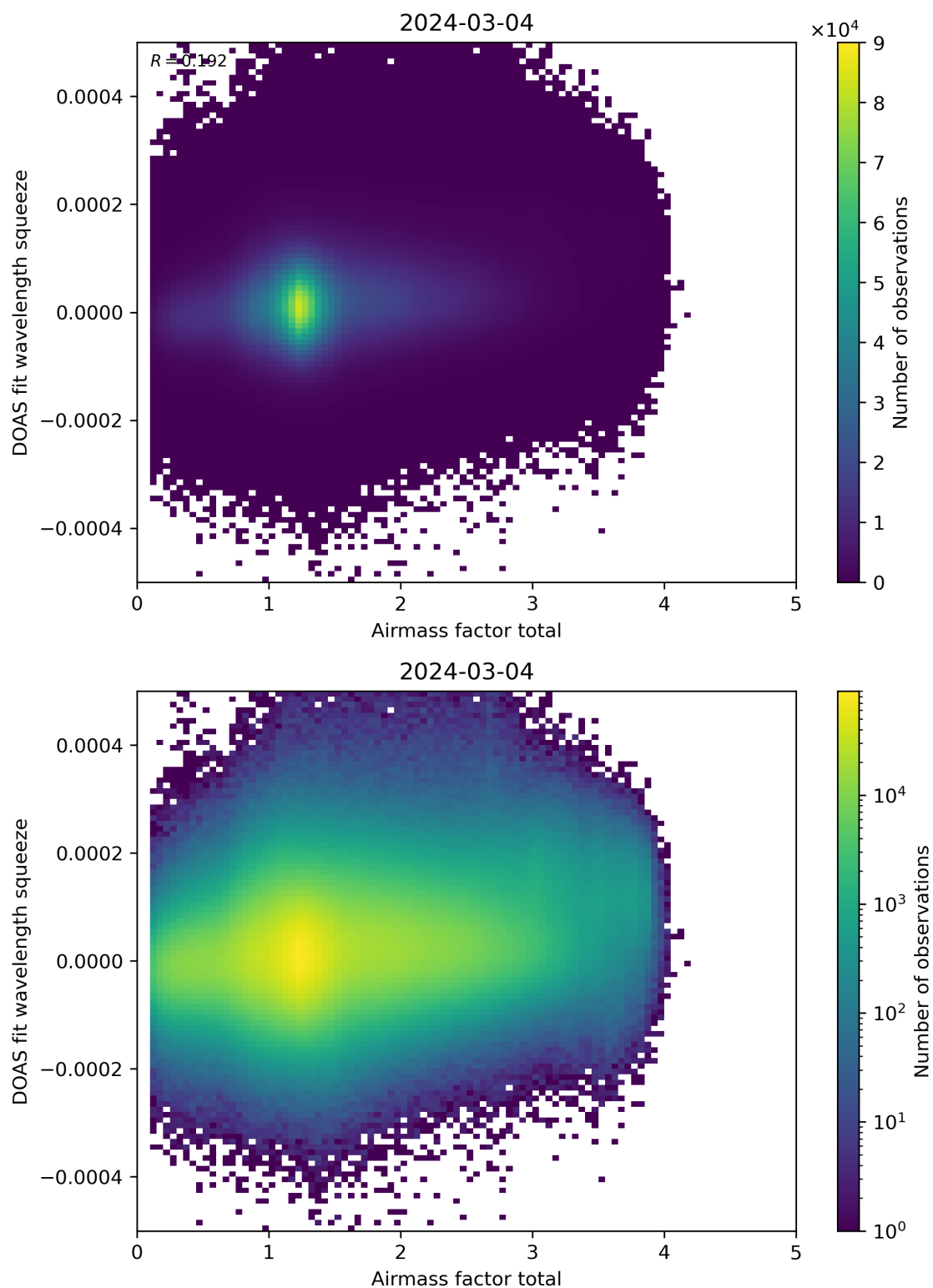
Figure 99: Scatter density plot of “Airmass factor total” against “DOAS fit wavelength squeeze” for 2024-03-04 to 2024-03-05.
