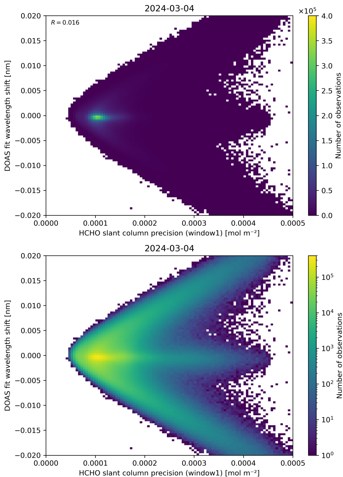
Figure 89: Scatter density plot of “HCHO slant column precision (window1)” against “DOAS fit wavelength shift” for 2024-03-04 to 2024-03-05.
