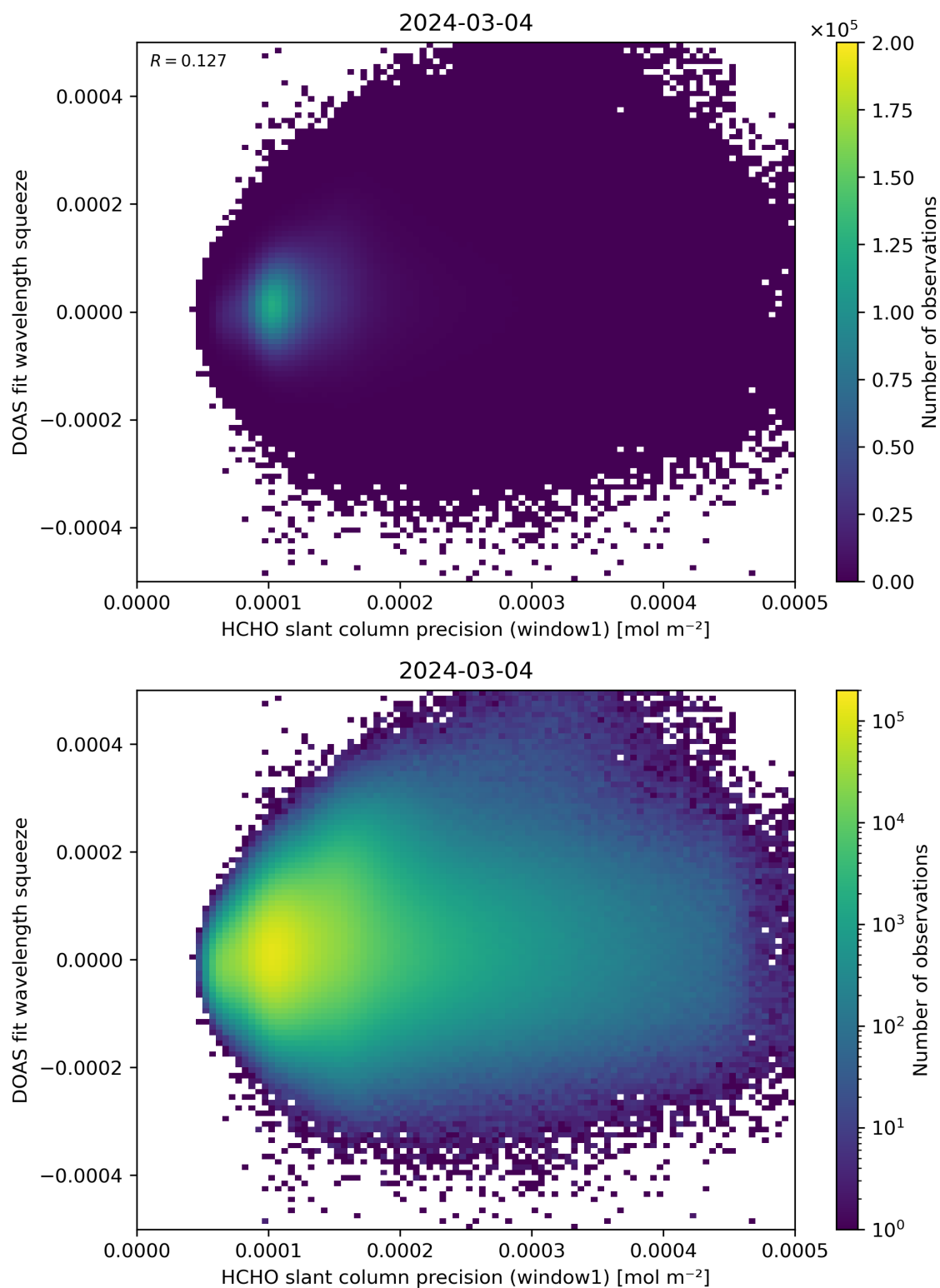
Figure 90: Scatter density plot of “HCHO slant column precision (window1)” against “DOAS fit wavelength squeeze” for 2024-03-04 to 2024-03-05.
