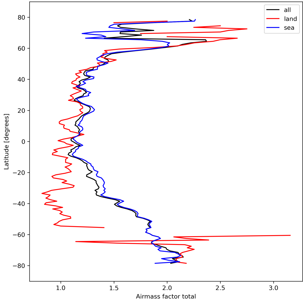
Figure 26: Zonal average of “Airmass factor total” for 2024-03-04 to 2024-03-05.
