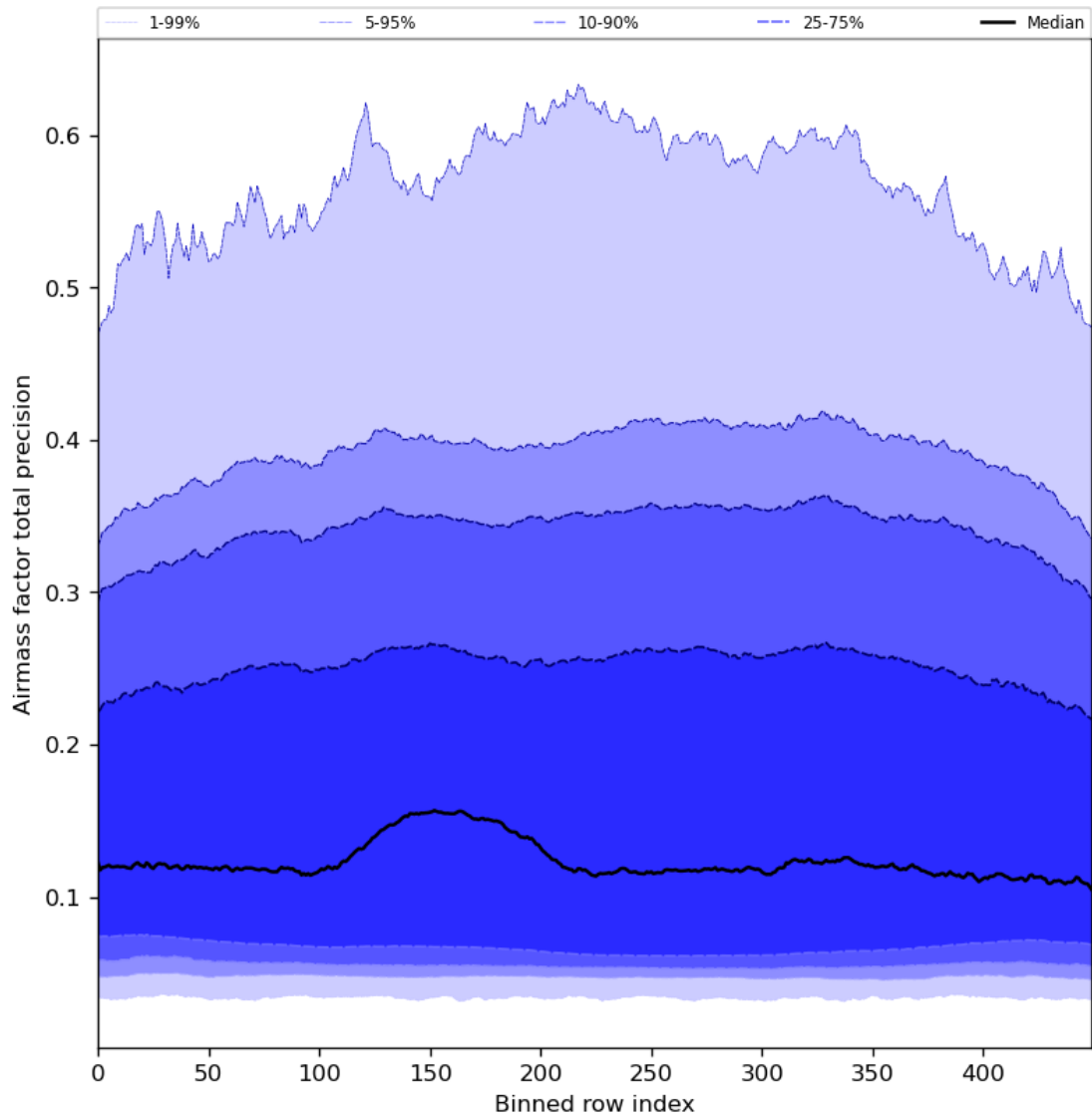
Figure 55: Along track statistics of “Airmass factor total precision” for 2024-03-04 to 2024-03-05
