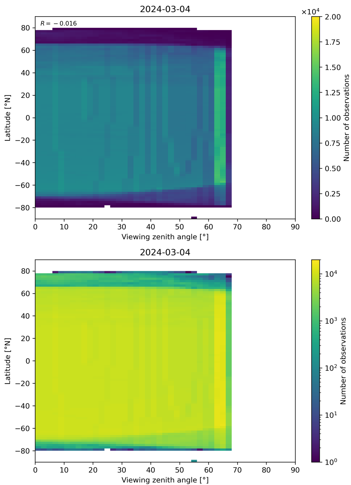
Figure 196: Scatter density plot of “Viewing zenith angle” against “Latitude” for 2024-03-04 to 2024-03-05.
