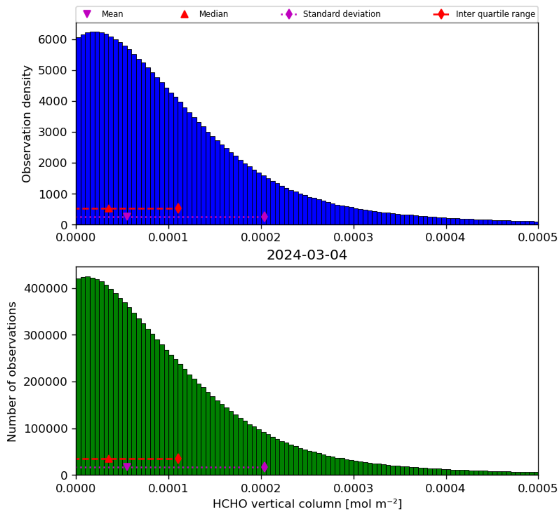
Figure 35: Histogram of “HCHO vertical column” for 2024-03-04 to 2024-03-05
