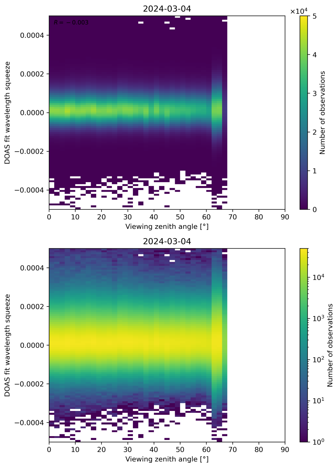
Figure 184: Scatter density plot of “Viewing zenith angle” against “DOAS fit wavelength squeeze” for 2024-03-04 to 2024-03-05.
