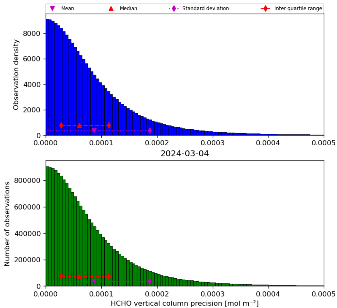
Figure 36: Histogram of “HCHO vertical column precision” for 2024-03-04 to 2024-03-05
