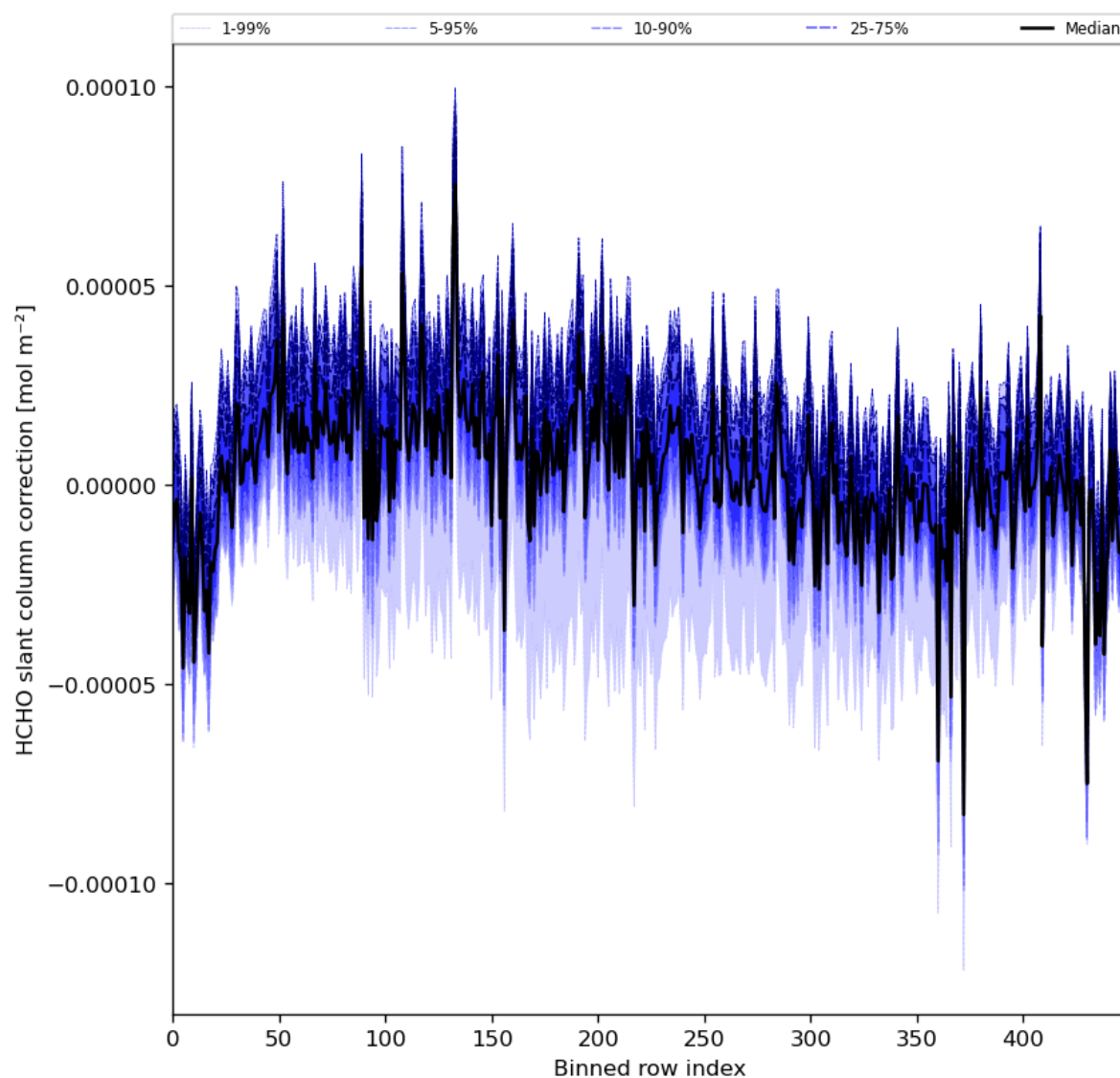
Figure 61: Along track statistics of “HCHO slant column correction” for 2024-03-04 to 2024-03-05
