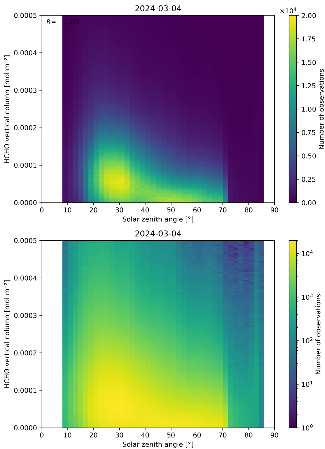
Figure 177: Scatter density plot of “Solar zenith angle” against “HCHO vertical column” for 2024-03-04 to 2024-03-05.
