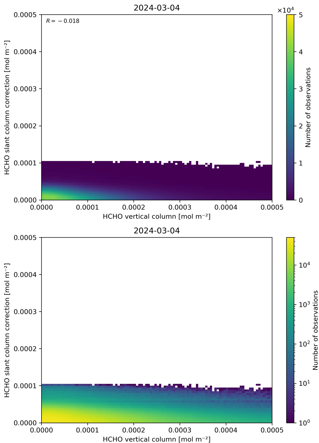
Figure 128: Scatter density plot of “HCHO vertical column” against “HCHO slant column correction” for 2024-03-04 to 2024-03-05.
