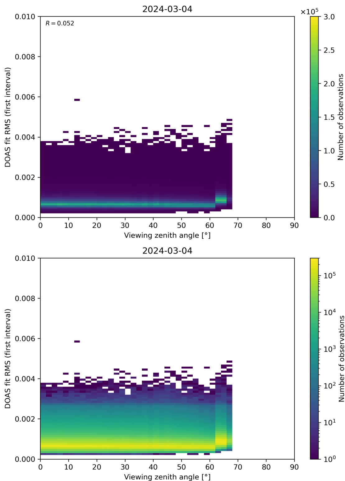
Figure 182: Scatter density plot of “Viewing zenith angle” against “DOAS fit RMS (first interval)” for 2024-03-04 to 2024-03-05.
