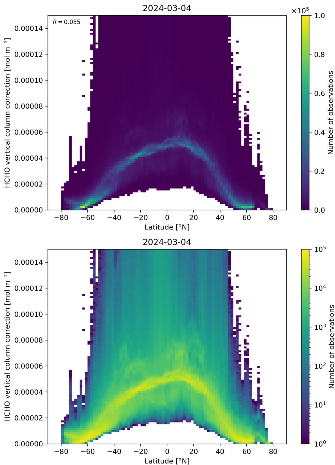
Figure 164: Scatter density plot of “Latitude” against “HCHO vertical column correction” for 2024-03-04 to 2024-03-05.
