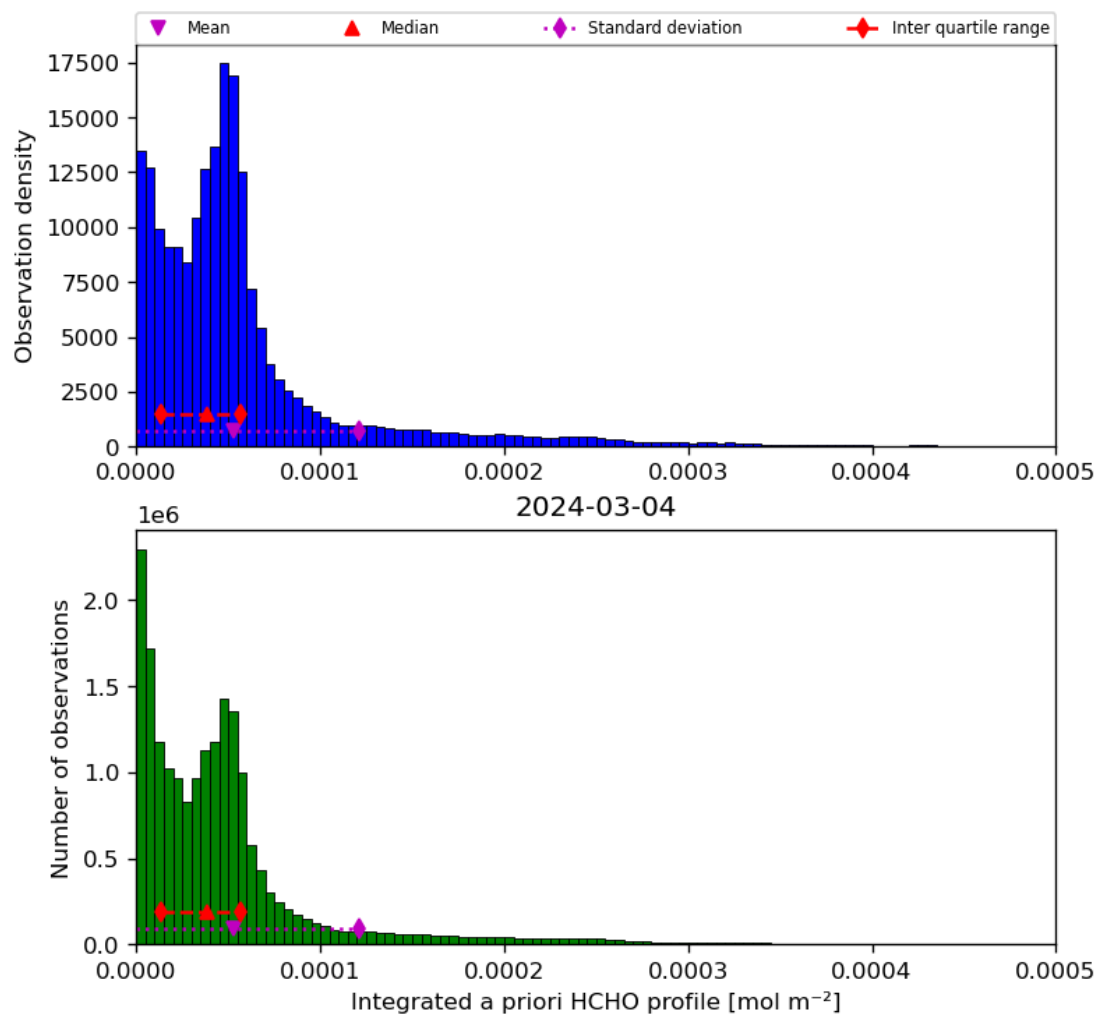
Figure 43: Histogram of “Integrated a priori HCHO profile” for 2024-03-04 to 2024-03-05
