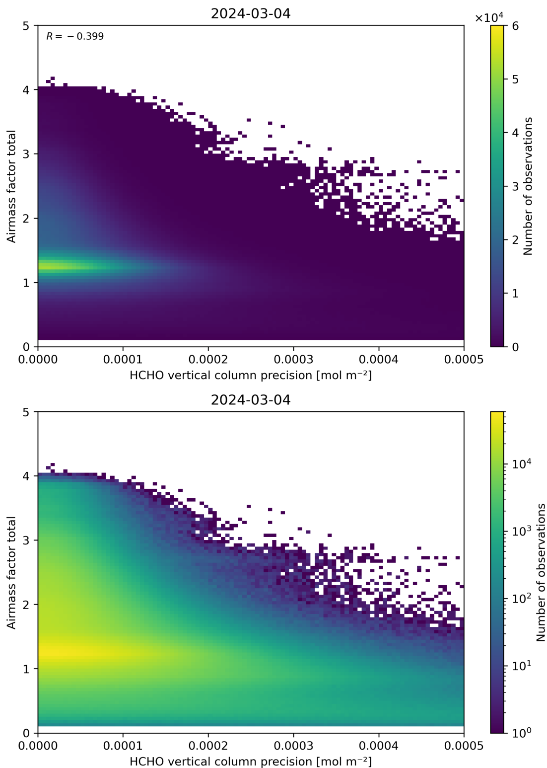
Figure 144: Scatter density plot of “HCHO vertical column precision” against “Airmass factor total” for 2024-03-04 to 2024-03-05.
