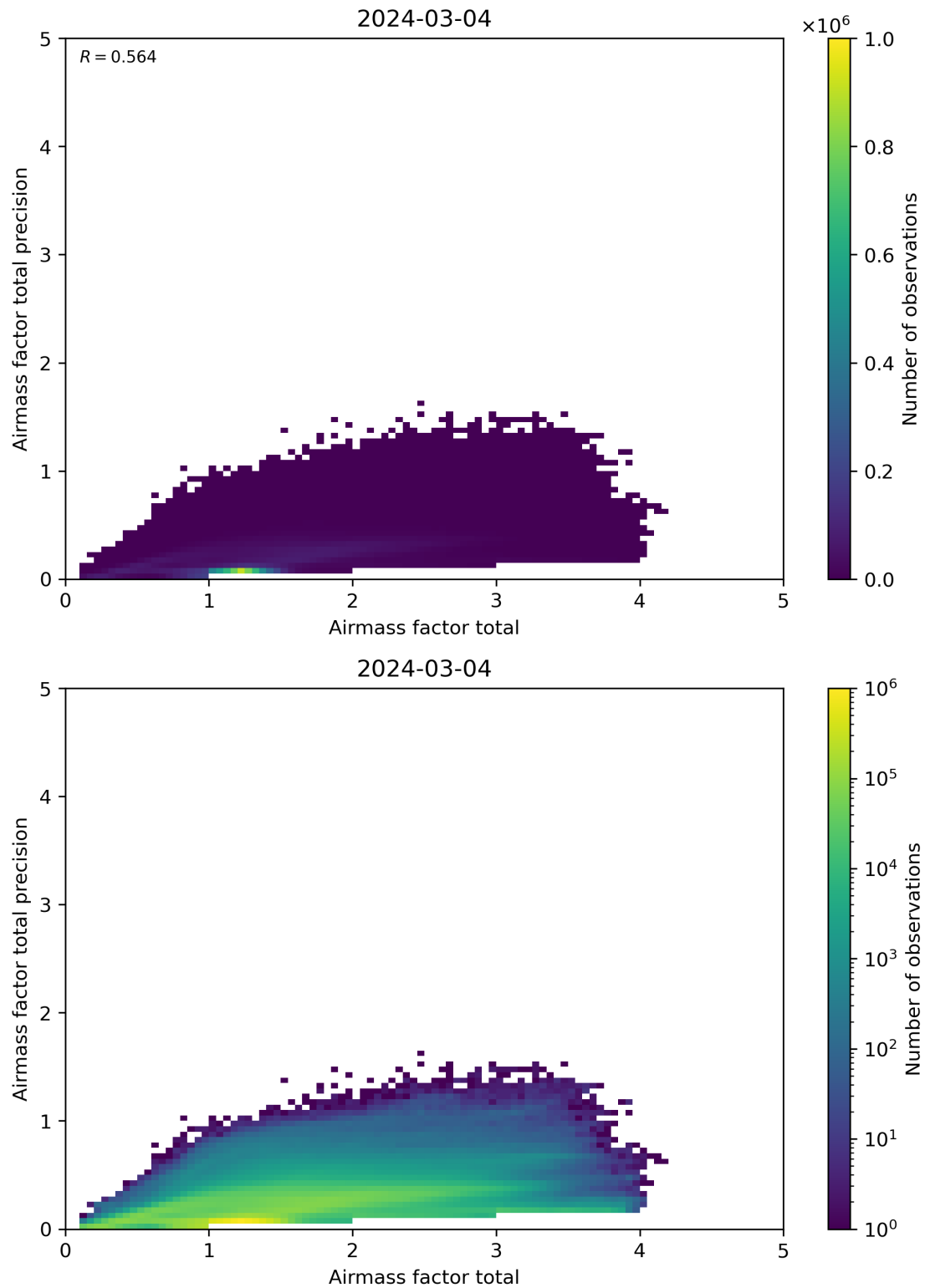
Figure 103: Scatter density plot of “Airmass factor total” against “Airmass factor total precision” for 2024-03-04 to 2024-03-05.
