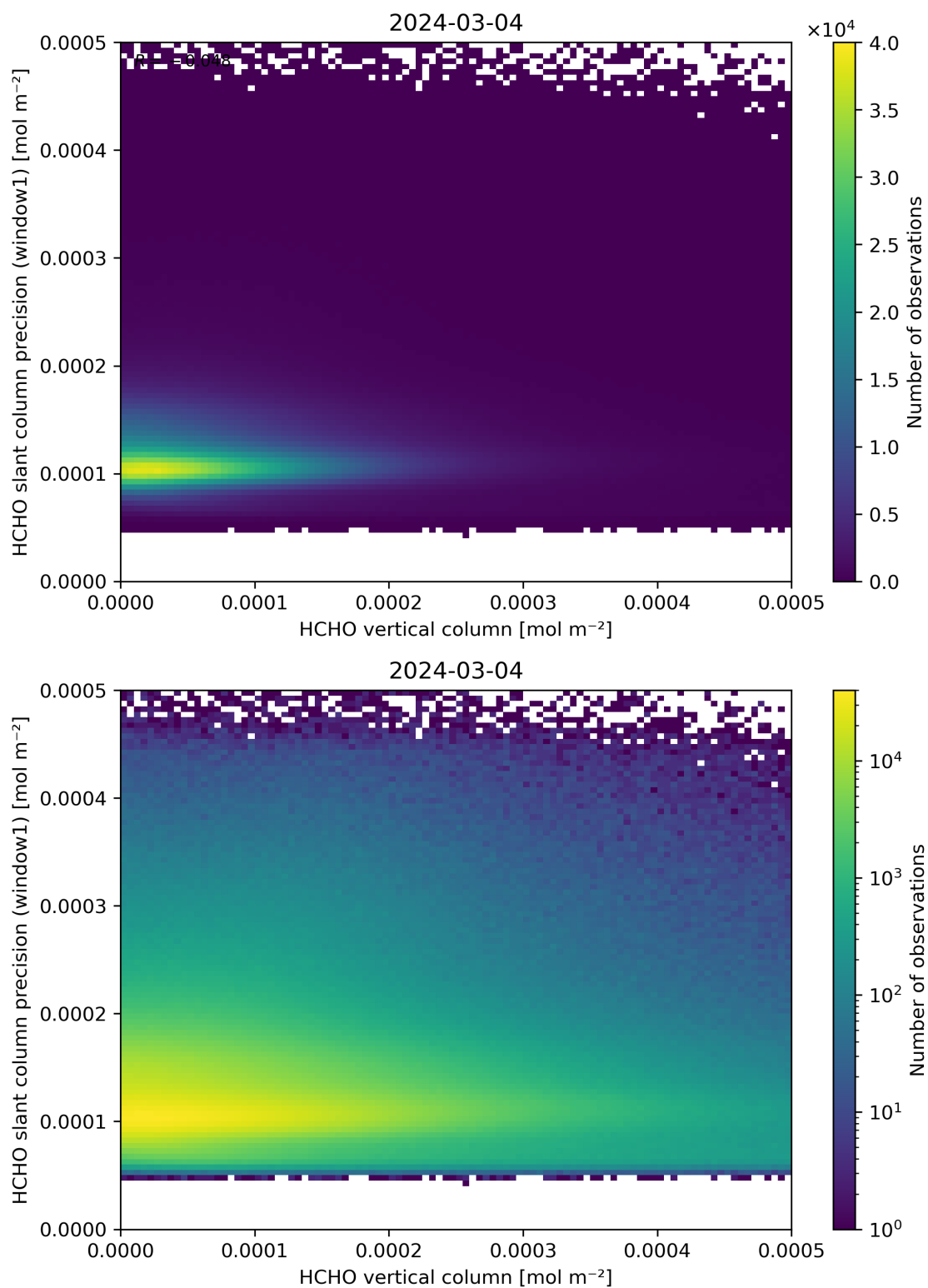
Figure 130: Scatter density plot of “HCHO vertical column” against “HCHO slant column precision (window1)” for 2024-03-04 to 2024-03-05.
