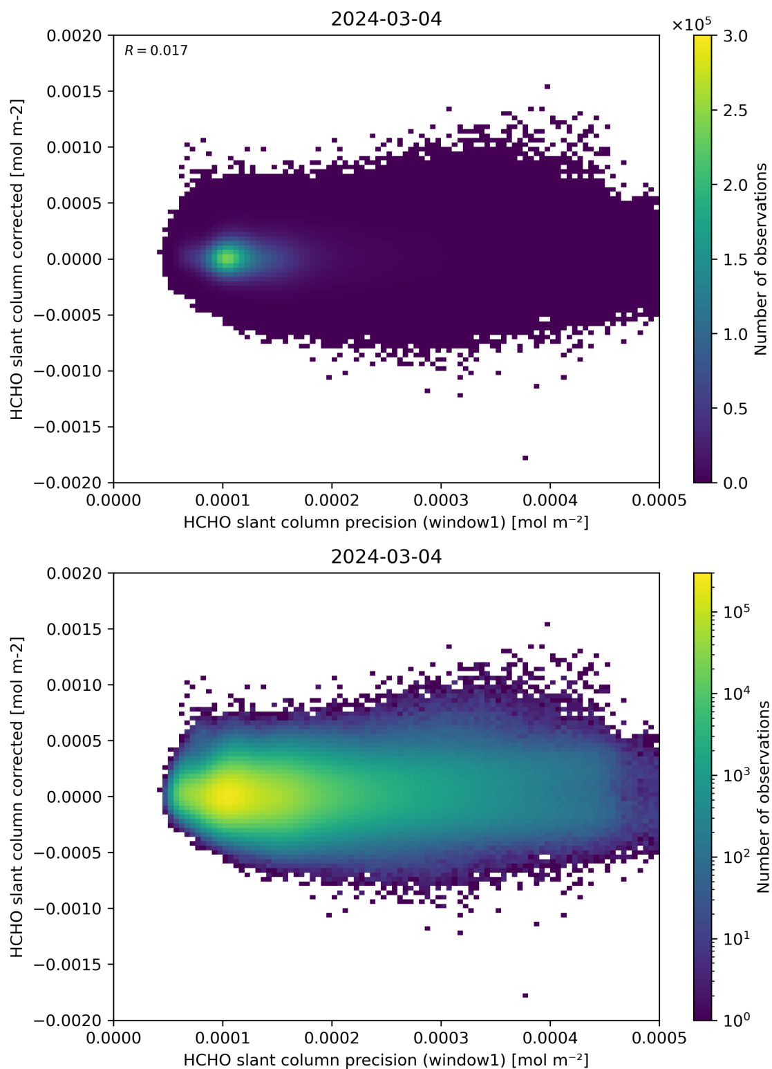
Figure 92: Scatter density plot of “HCHO slant column precision (window1)” against “HCHO slant column corrected” for 2024-03-04 to 2024-03-05.
