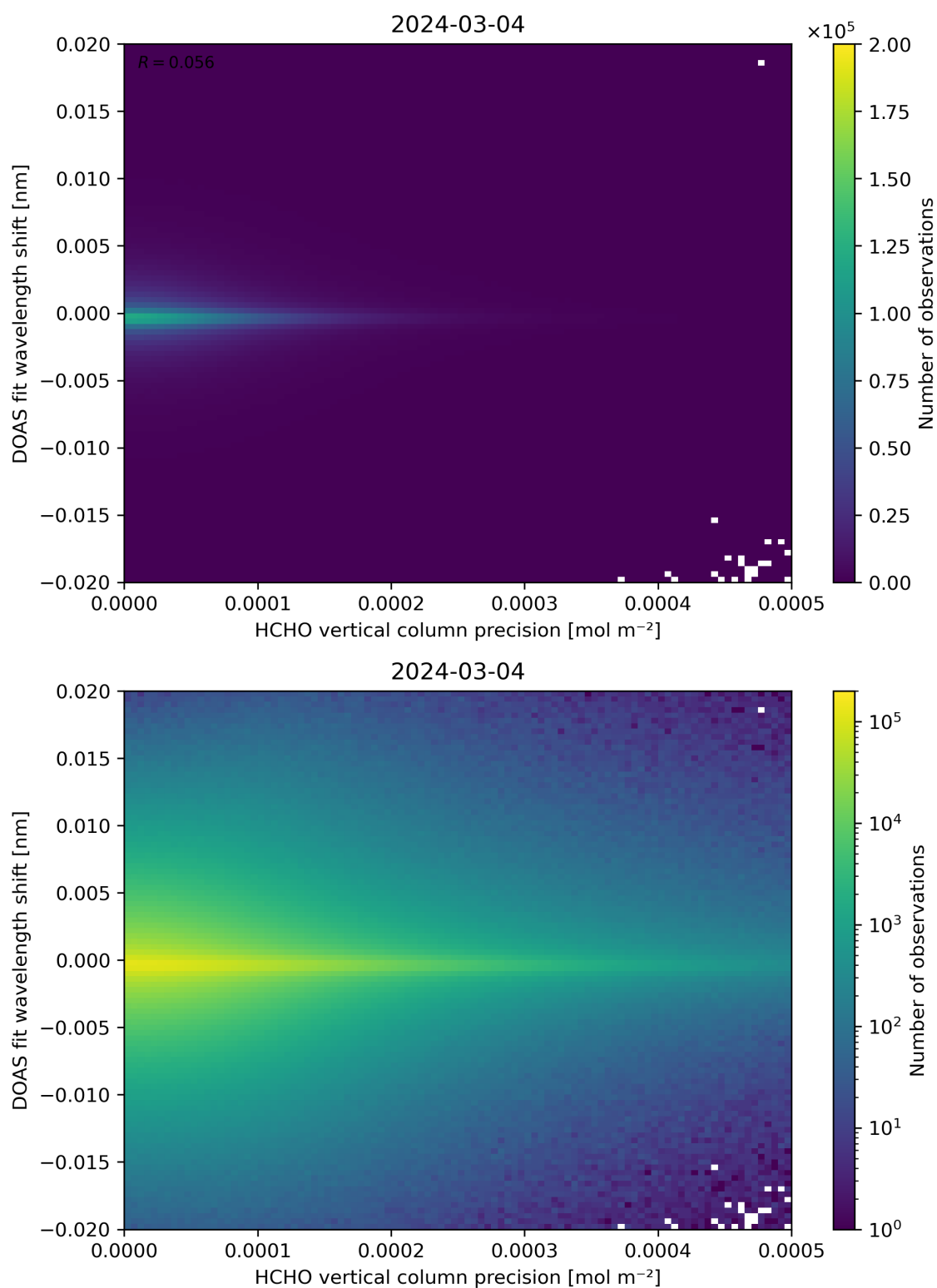
Figure 137: Scatter density plot of “HCHO vertical column precision” against “DOAS fit wavelength shift” for 2024-03-04 to 2024-03-05.
