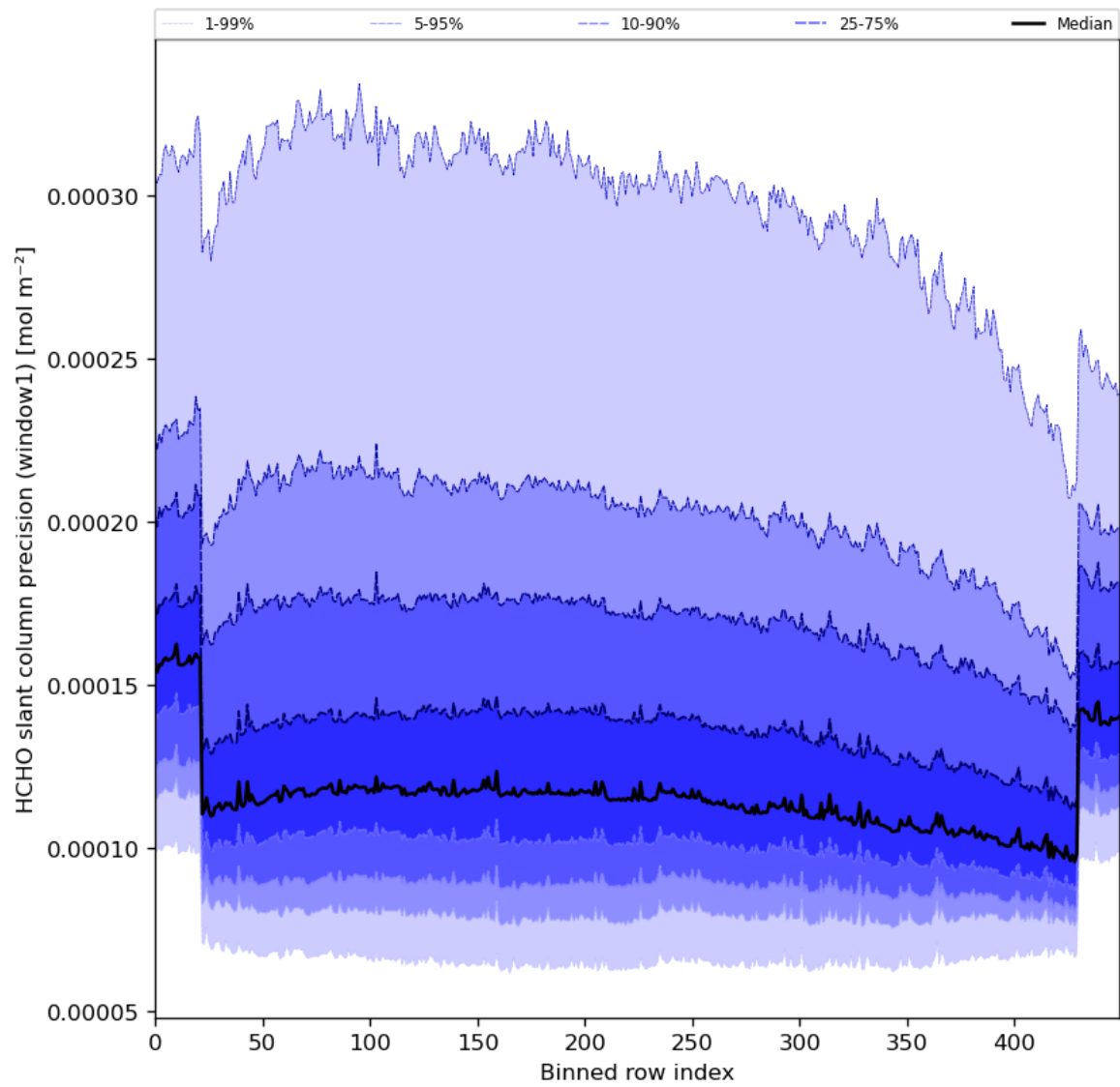
Figure 53: Along track statistics of “HCHO slant column precision (window1)” for 2024-03-04 to 2024-03-05
