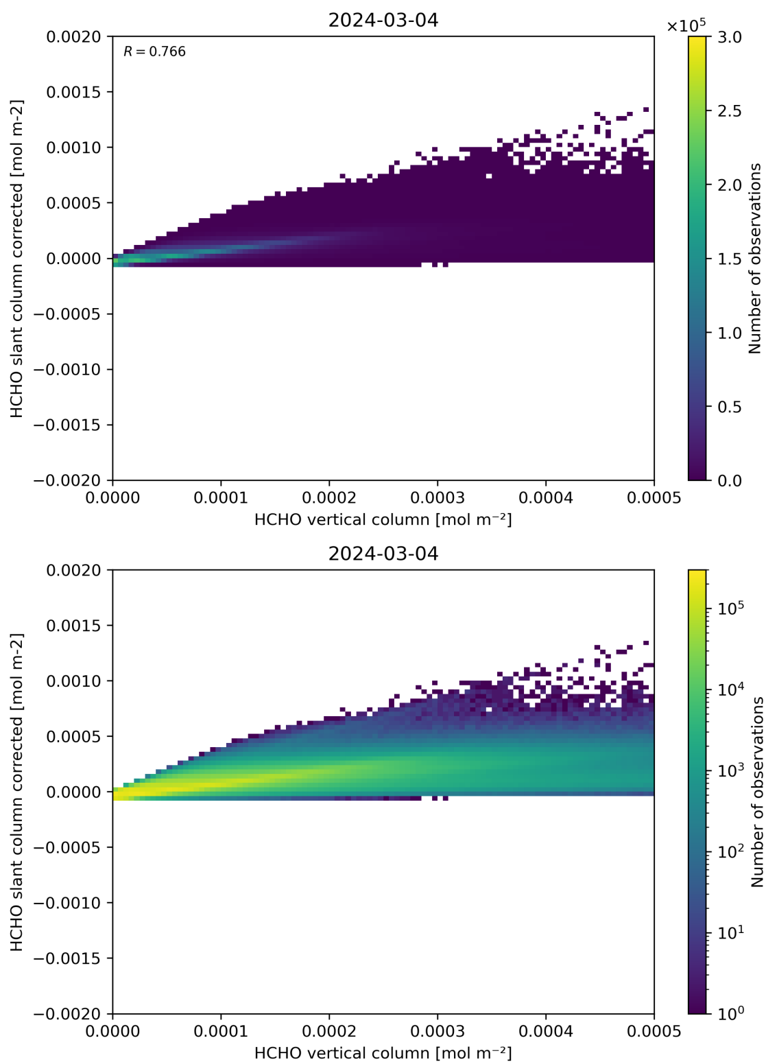
Figure 127: Scatter density plot of “HCHO vertical column” against “HCHO slant column corrected” for 2024-03-04 to 2024-03-05.
