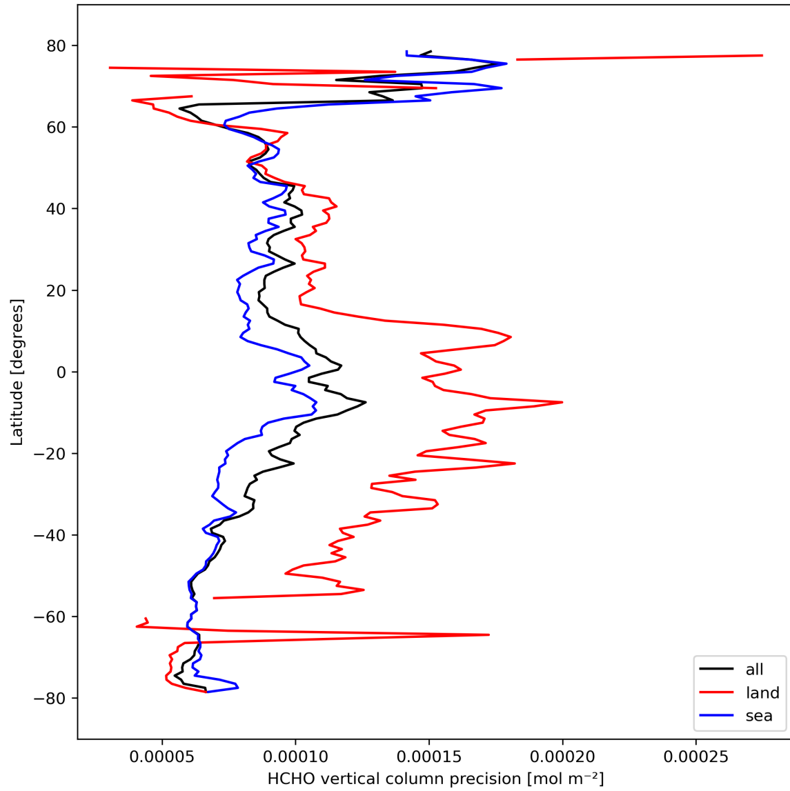
Figure 22: Zonal average of “HCHO vertical column precision” for 2024-03-04 to 2024-03-05.
