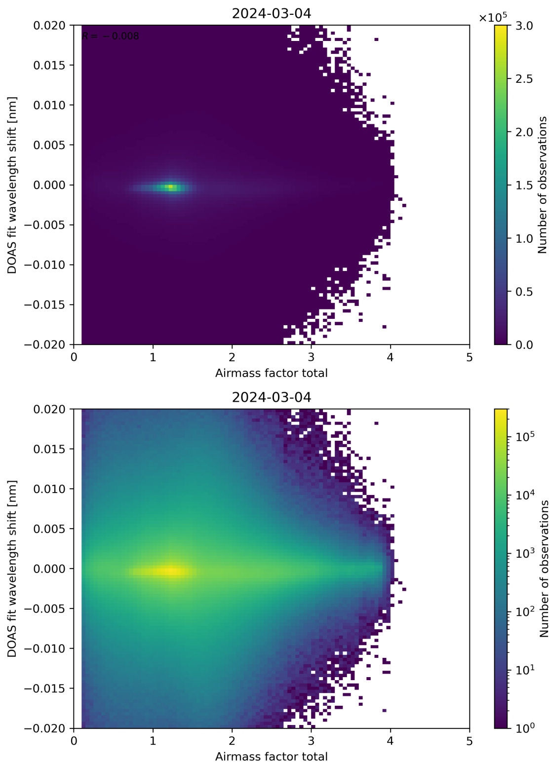
Figure 98: Scatter density plot of “Airmass factor total” against “DOAS fit wavelength shift” for 2024-03-04 to 2024-03-05.
