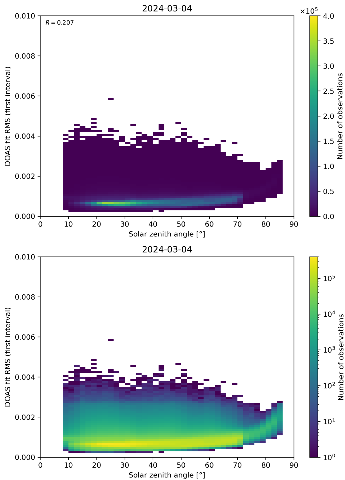
Figure 167: Scatter density plot of “Solar zenith angle” against “DOAS fit RMS (first interval)” for 2024-03-04 to 2024-03-05.
