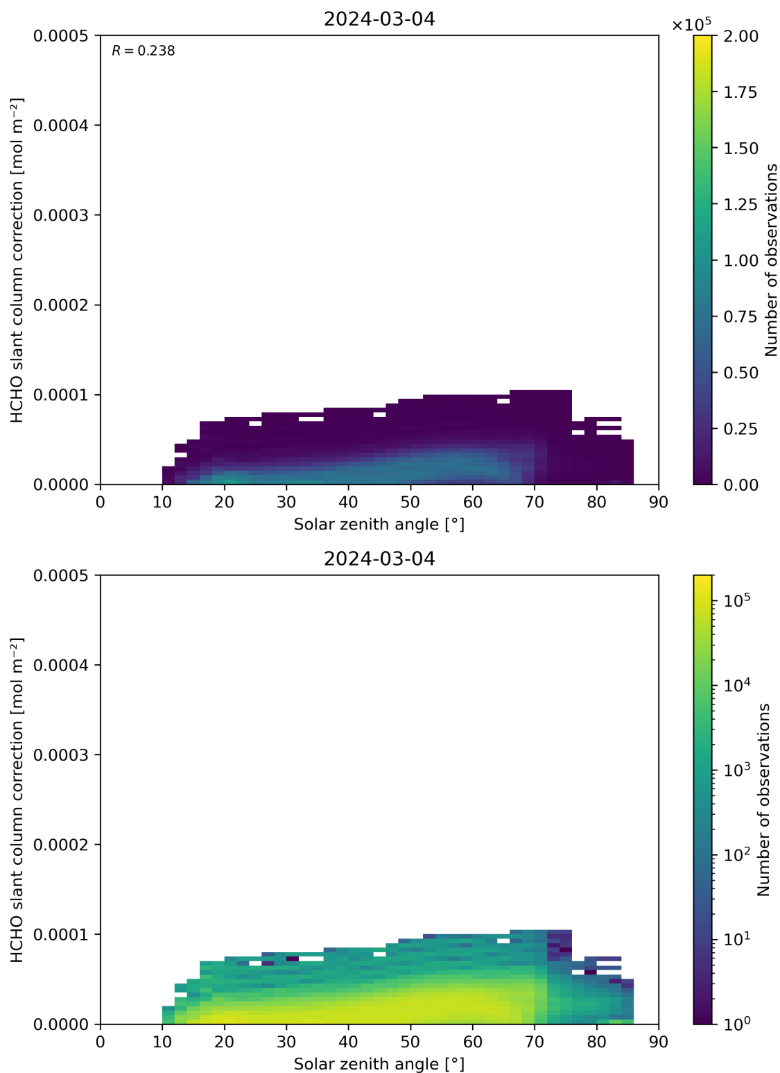
Figure 172: Scatter density plot of “Solar zenith angle” against “HCHO slant column correction” for 2024-03-04 to 2024-03-05.
