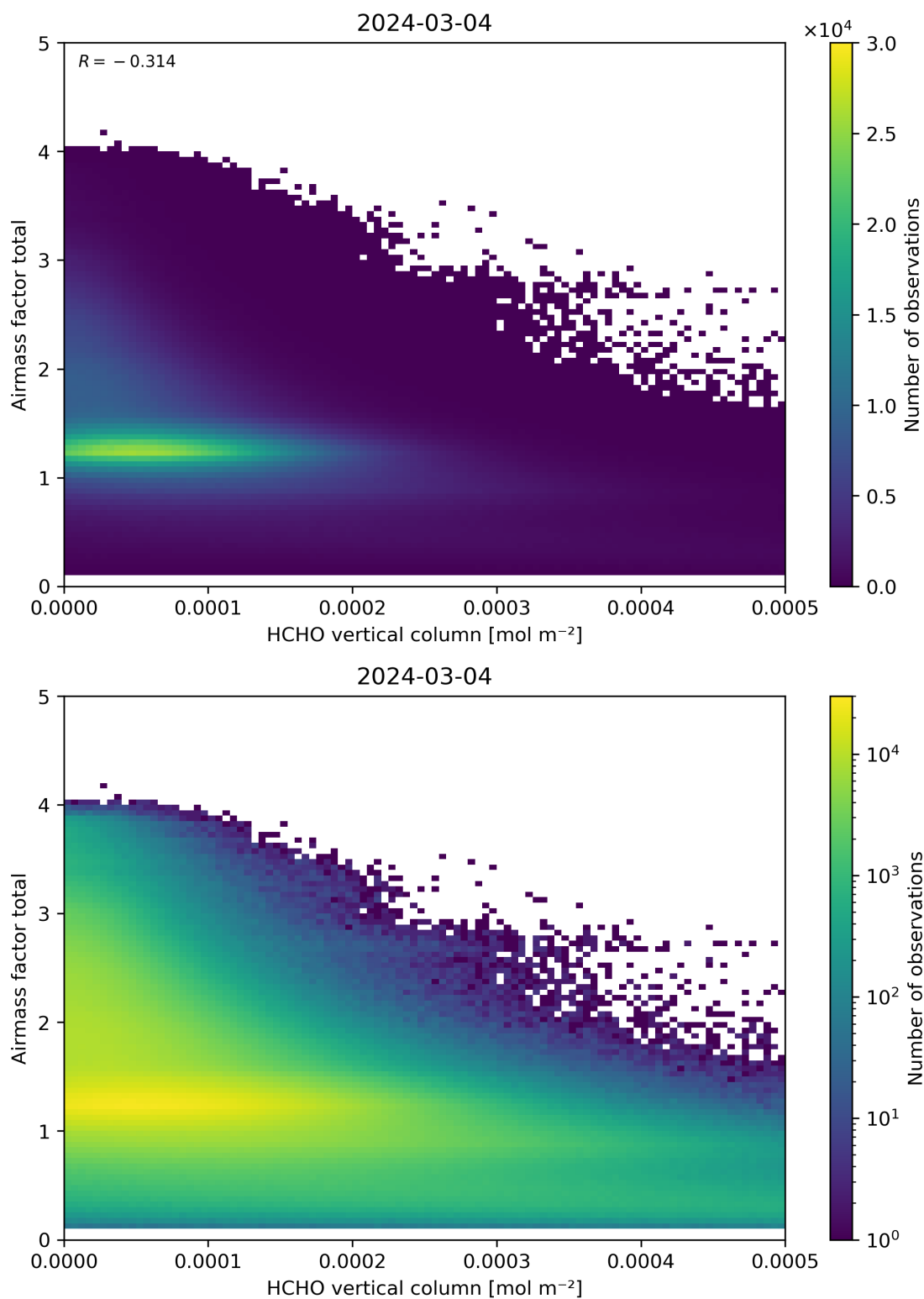
Figure 131: Scatter density plot of “HCHO vertical column” against “Airmass factor total” for 2024-03-04 to 2024-03-05.
