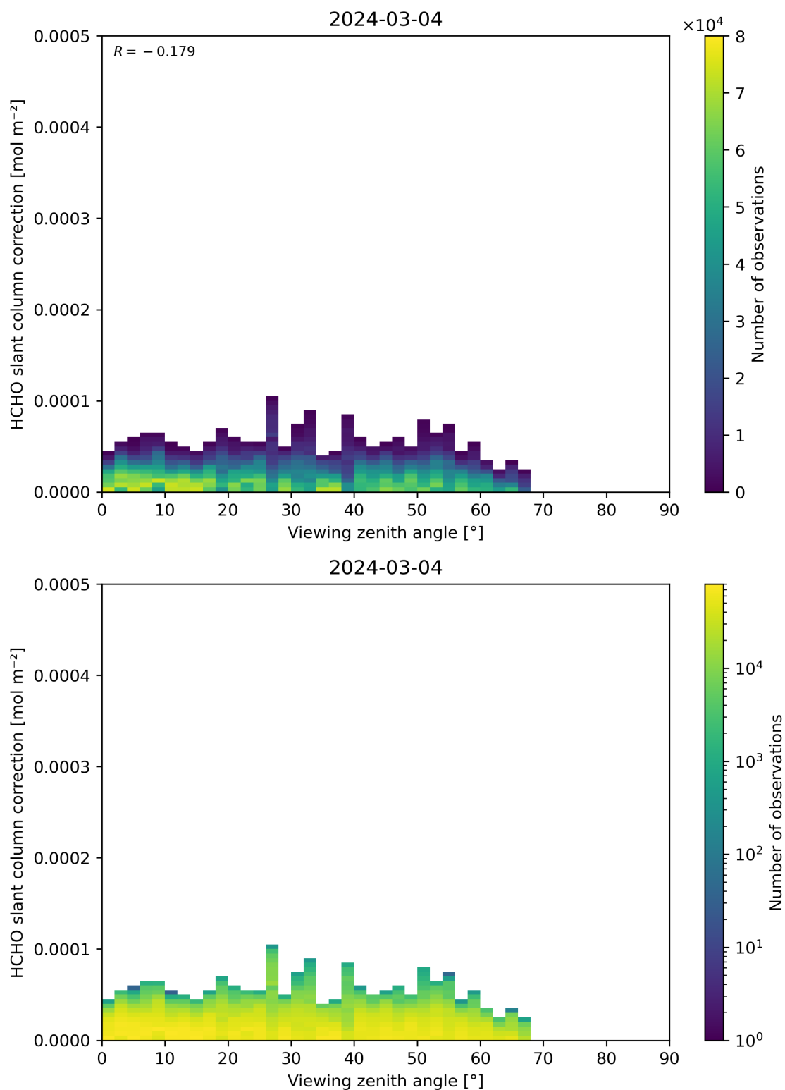
Figure 187: Scatter density plot of “Viewing zenith angle” against “HCHO slant column correction” for 2024-03-04 to 2024-03-05.
