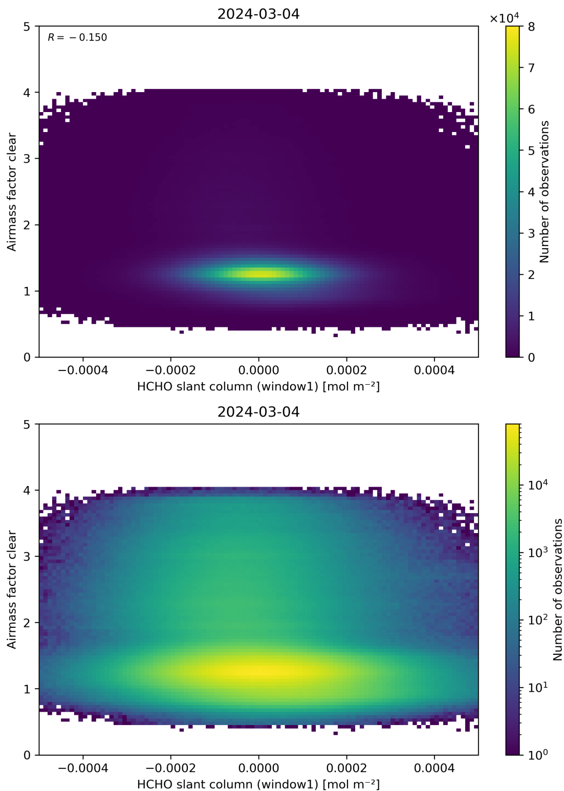
Figure 81: Scatter density plot of “HCHO slant column (window1)” against “Airmass factor clear” for 2024-03-04 to 2024-03-05.
