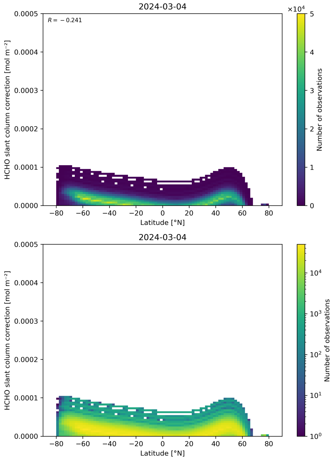
Figure 158: Scatter density plot of “Latitude” against “HCHO slant column correction” for 2024-03-04 to 2024-03-05.
