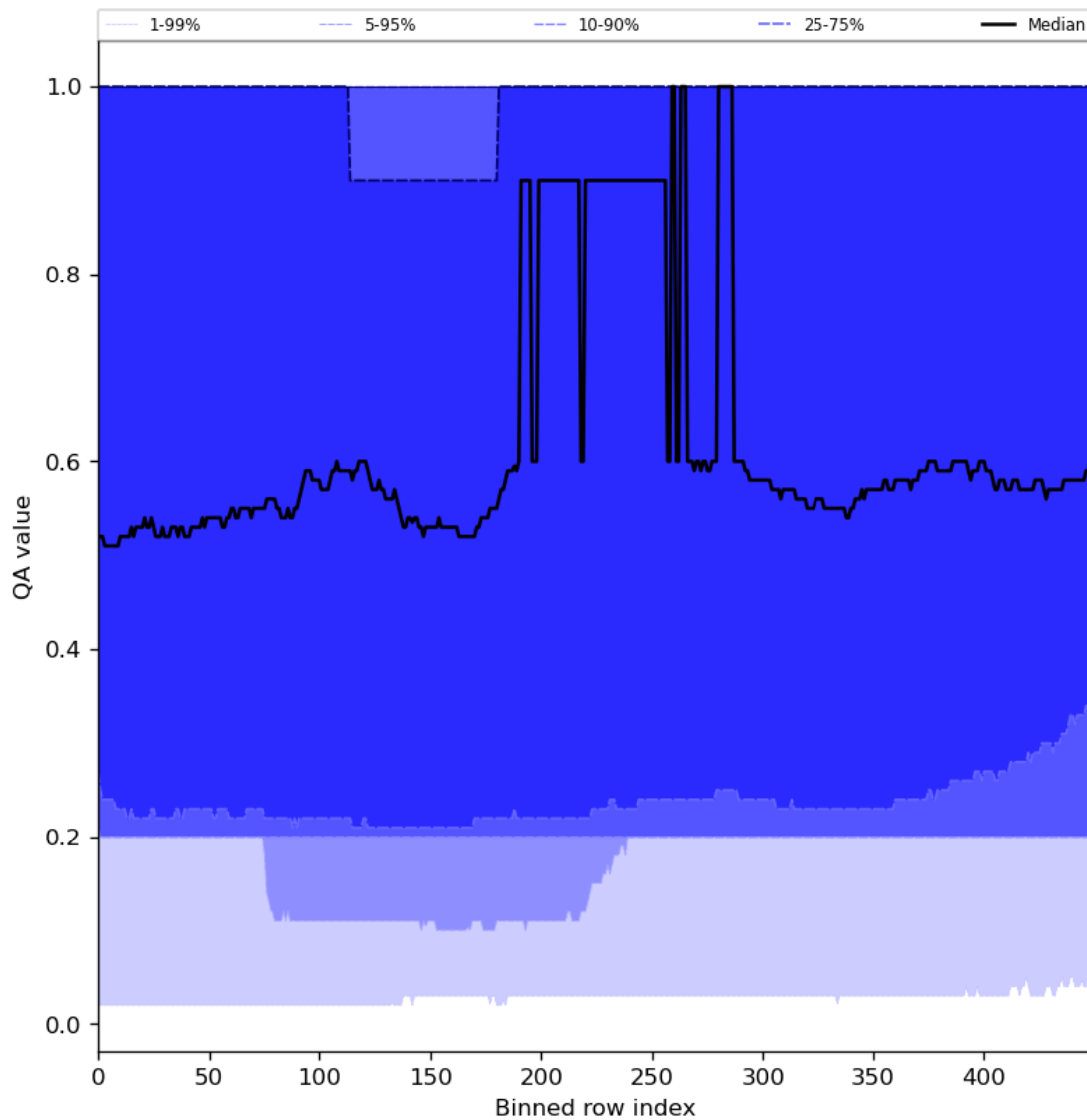
Figure 48: Along track statistics of “QA value” for 2024-03-04 to 2024-03-05
