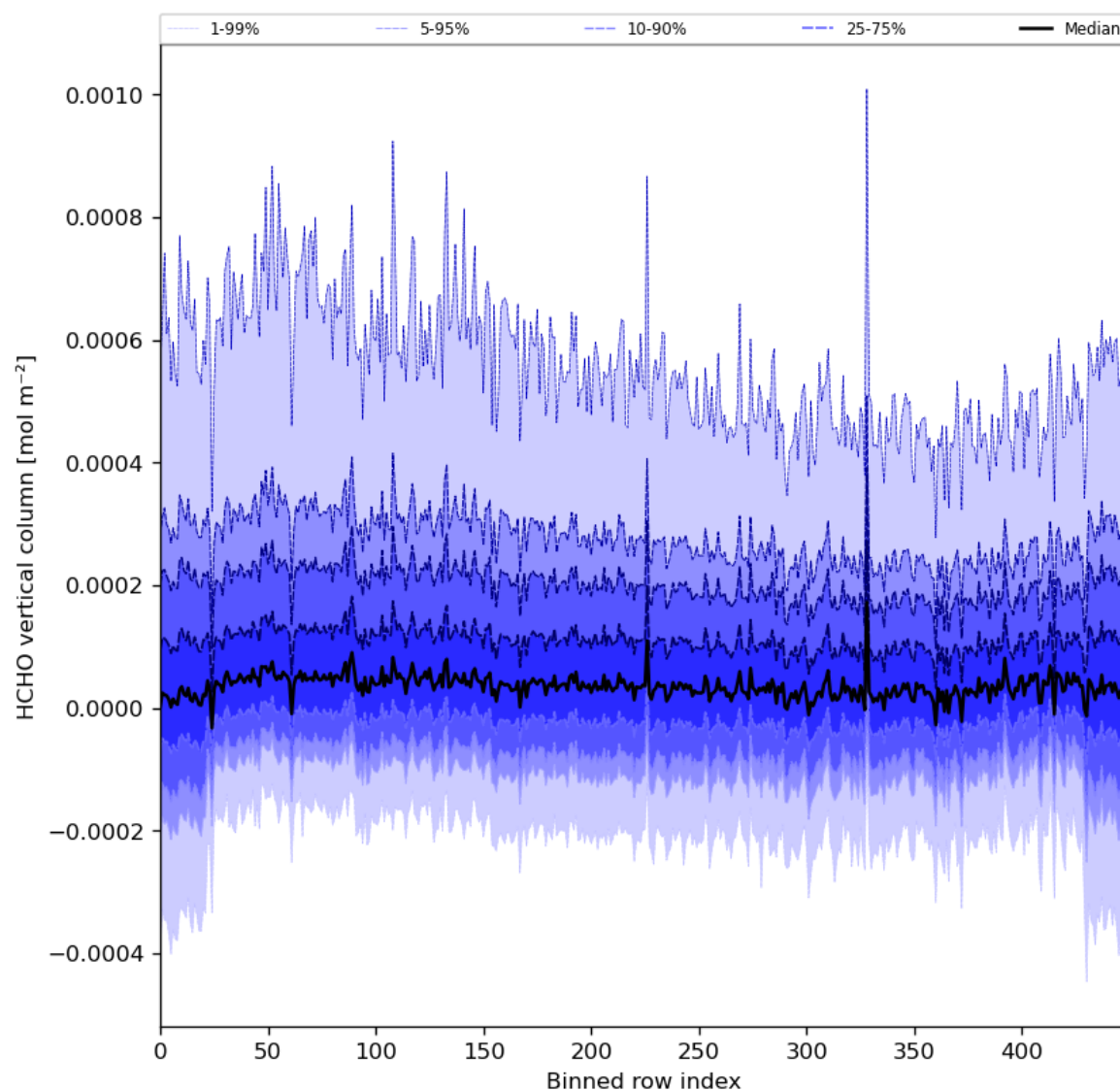
Figure 49: Along track statistics of “HCHO vertical column” for 2024-03-04 to 2024-03-05
