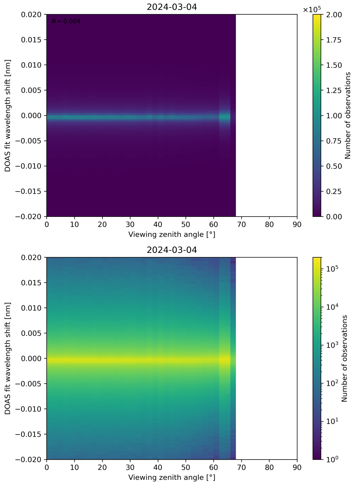
Figure 183: Scatter density plot of “Viewing zenith angle” against “DOAS fit wavelength shift” for 2024-03-04 to 2024-03-05.
