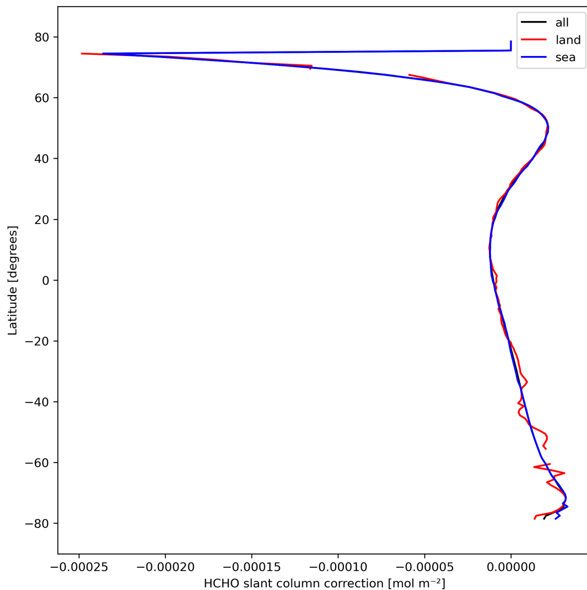
Figure 33: Zonal average of “HCHO slant column correction” for 2024-03-04 to 2024-03-05.
