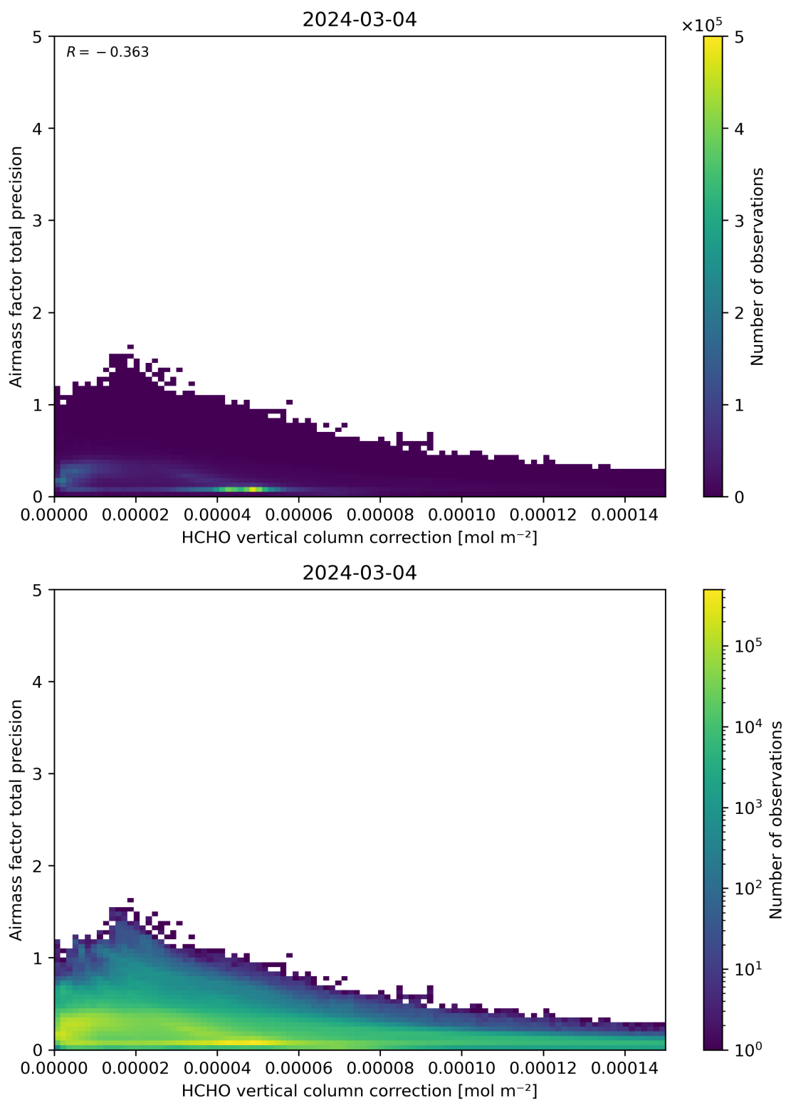
Figure 121: Scatter density plot of “HCHO vertical column correction” against “Airmass factor total precision” for 2024-03-04 to 2024-03-05.
