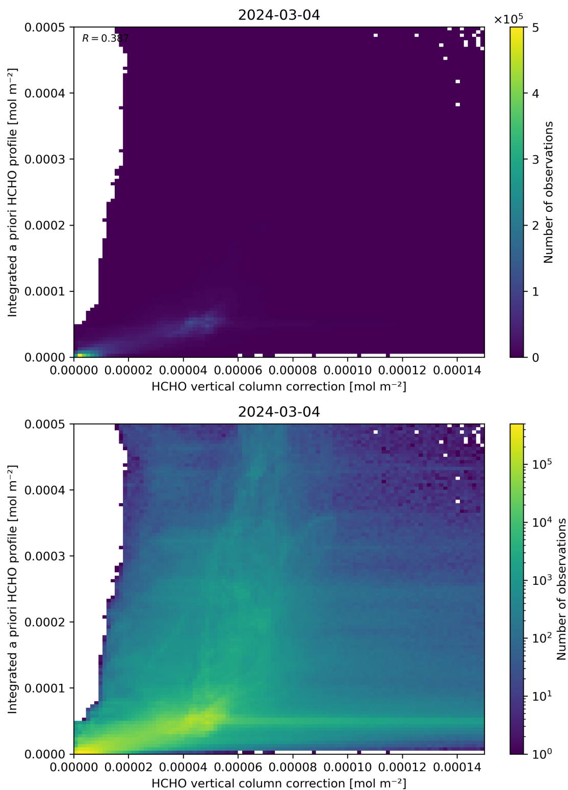
Figure 122: Scatter density plot of “HCHO vertical column correction” against “Integrated a priori HCHO profile” for 2024-03-04 to 2024-03-05.
