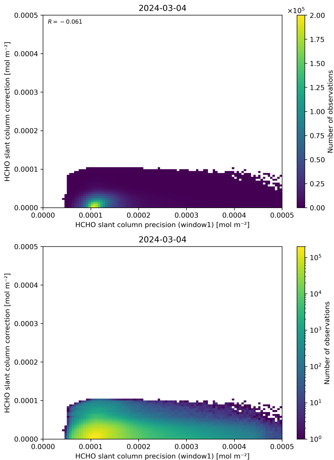
Figure 93: Scatter density plot of “HCHO slant column precision (window1)” against “HCHO slant column correction” for 2024-03-04 to 2024-03-05.
