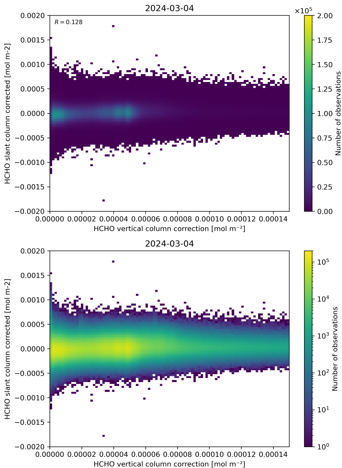
Figure 116: Scatter density plot of “HCHO vertical column correction” against “HCHO slant column corrected” for 2024-03-04 to 2024-03-05.
