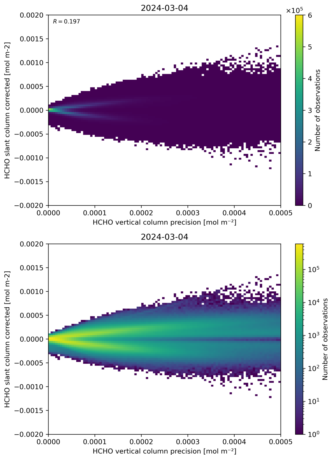
Figure 140: Scatter density plot of “HCHO vertical column precision” against “HCHO slant column corrected” for 2024-03-04 to 2024-03-05.
