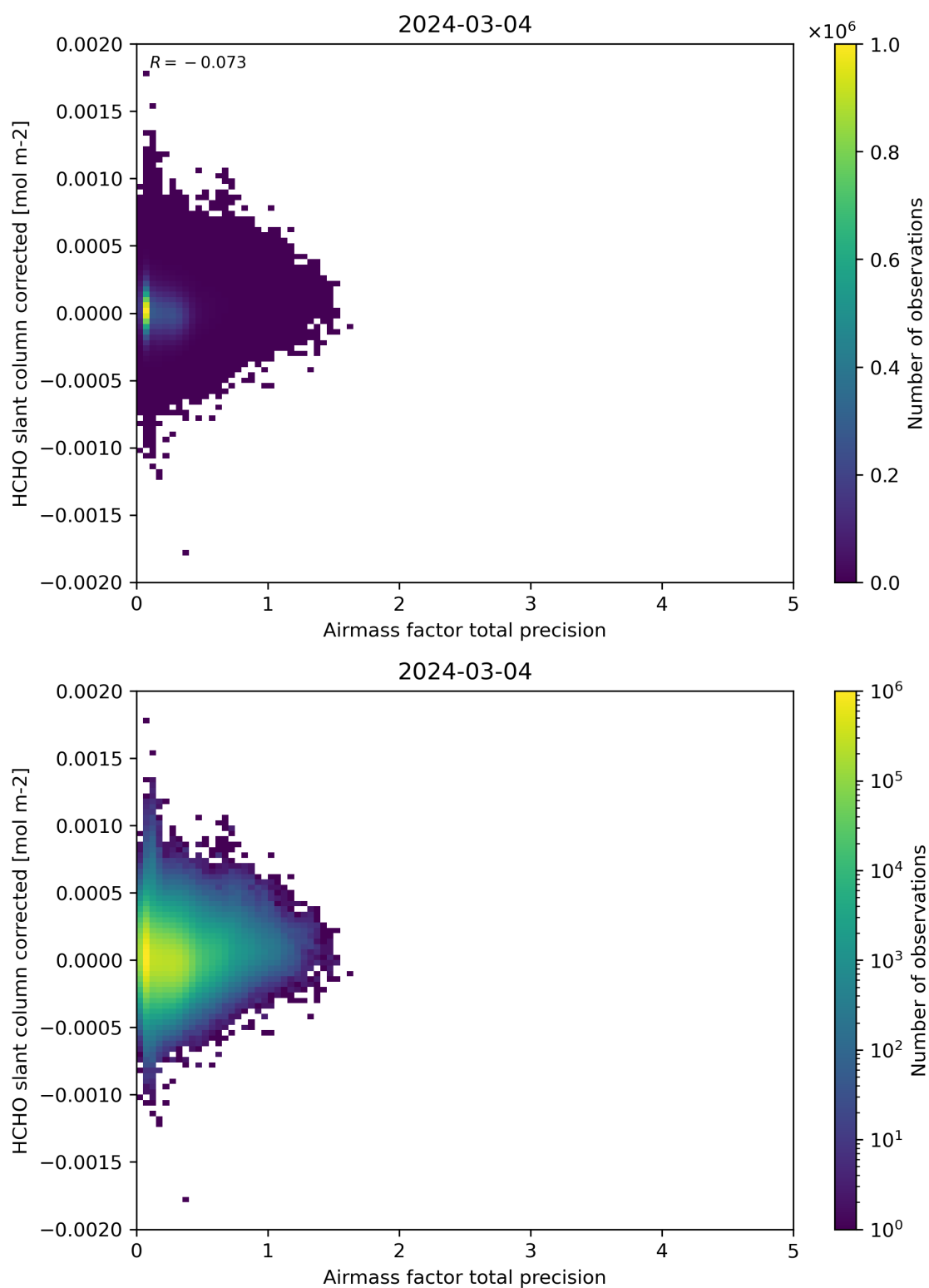
Figure 109: Scatter density plot of “Airmass factor total precision” against “HCHO slant column corrected” for 2024-03-04 to 2024-03-05.
