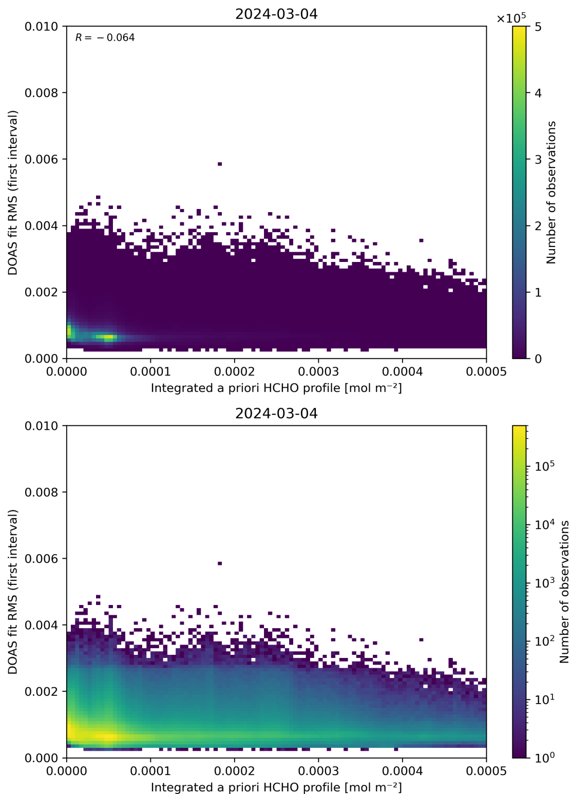
Figure 148: Scatter density plot of “Integrated a priori HCHO profile” against “DOAS fit RMS (first interval)” for 2024-03-04 to 2024-03-05.
