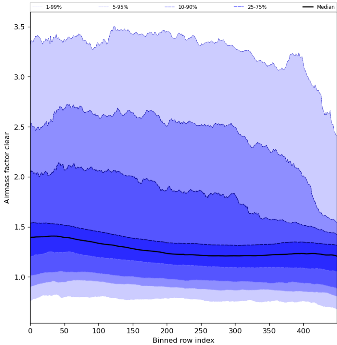
Figure 56: Along track statistics of “Airmass factor clear” for 2024-03-04 to 2024-03-05
