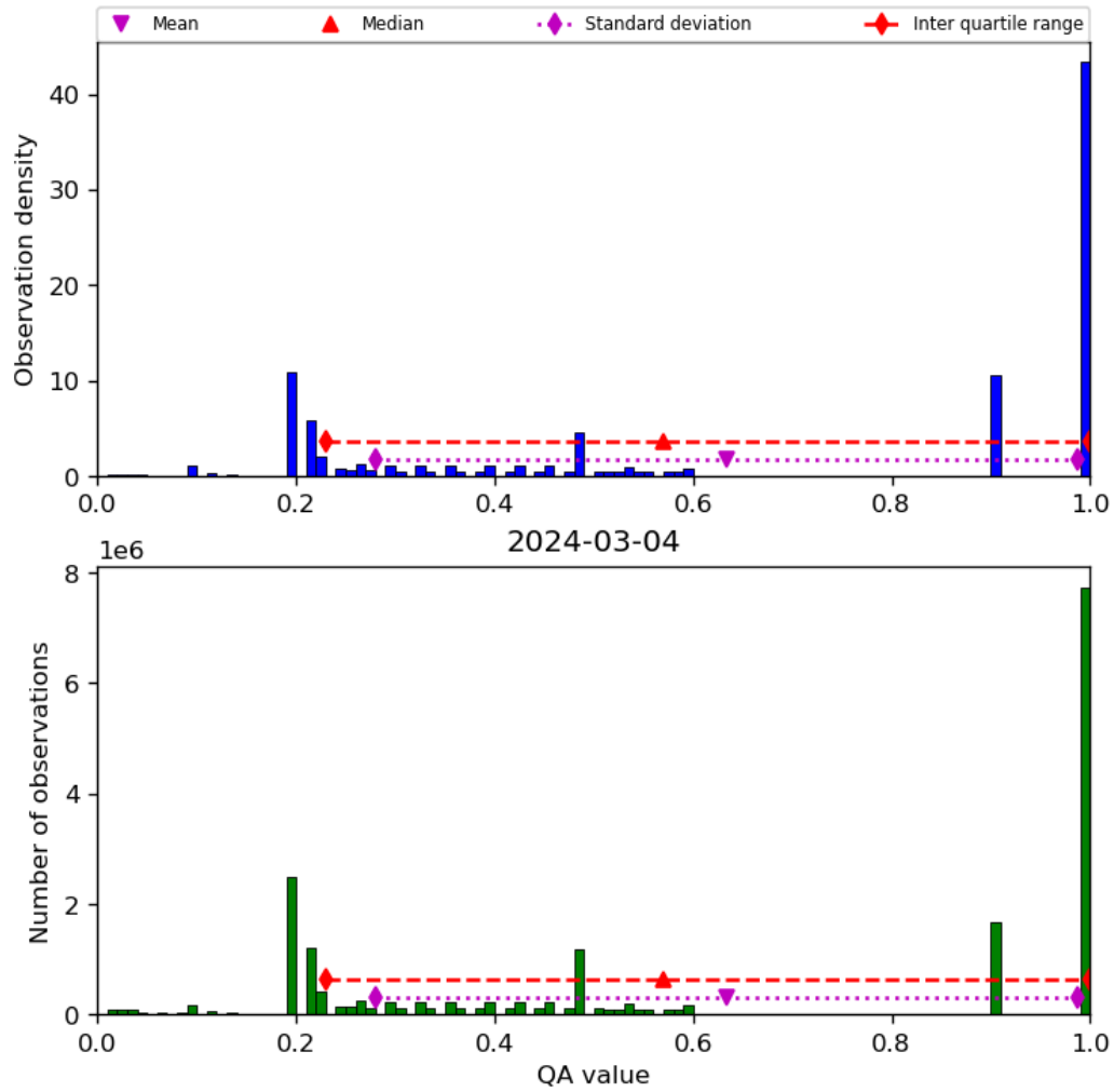
Figure 34: Histogram of “QA value” for 2024-03-04 to 2024-03-05
