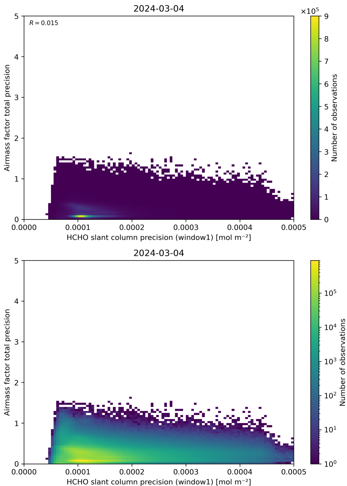
Figure 95: Scatter density plot of “HCHO slant column precision (window1)” against “Airmass factor total precision” for 2024-03-04 to 2024-03-05.
