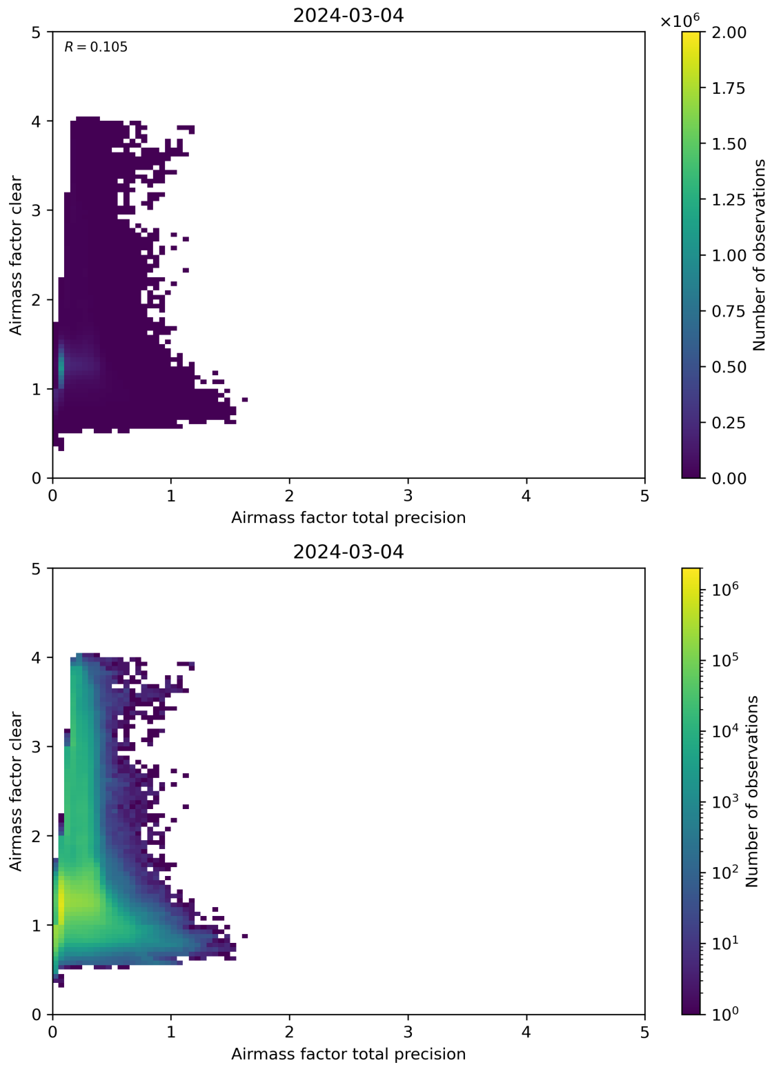
Figure 108: Scatter density plot of “Airmass factor total precision” against “Airmass factor clear” for 2024-03-04 to 2024-03-05.
