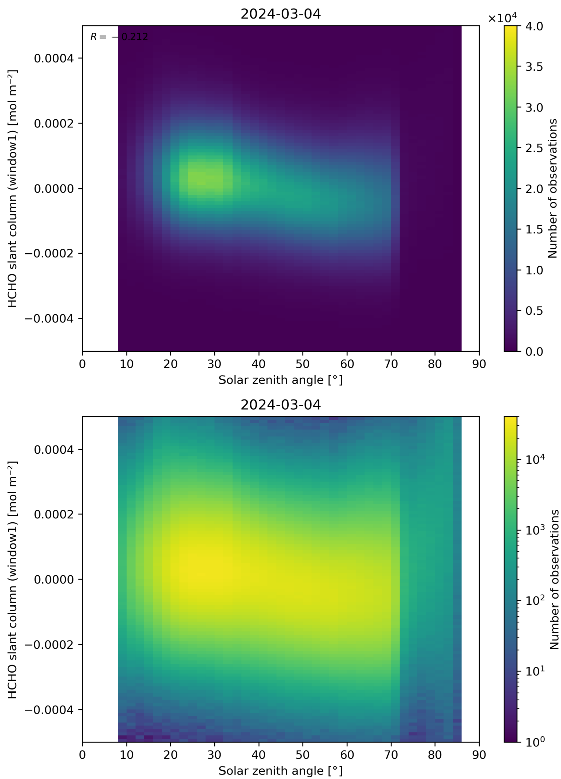
Figure 173: Scatter density plot of “Solar zenith angle” against “HCHO slant column (window1)” for 2024-03-04 to 2024-03-05.
