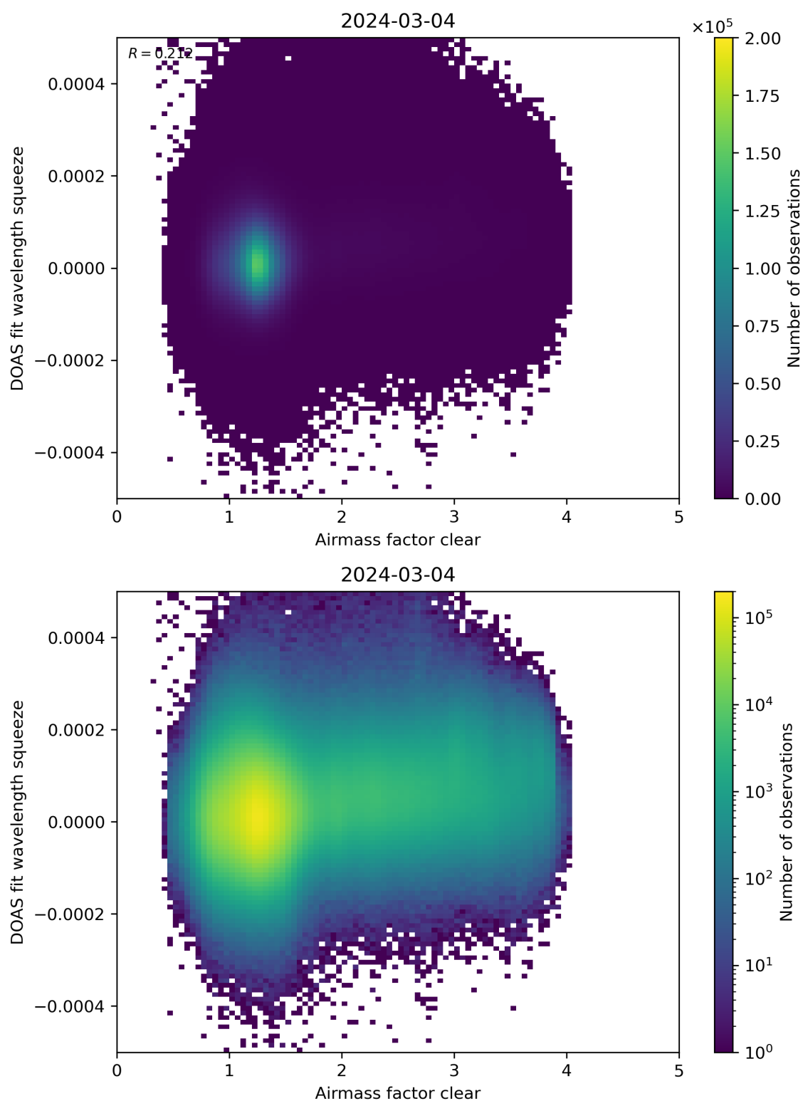
Figure 73: Scatter density plot of “Airmass factor clear” against “DOAS fit wavelength squeeze” for 2024-03-04 to 2024-03-05.
