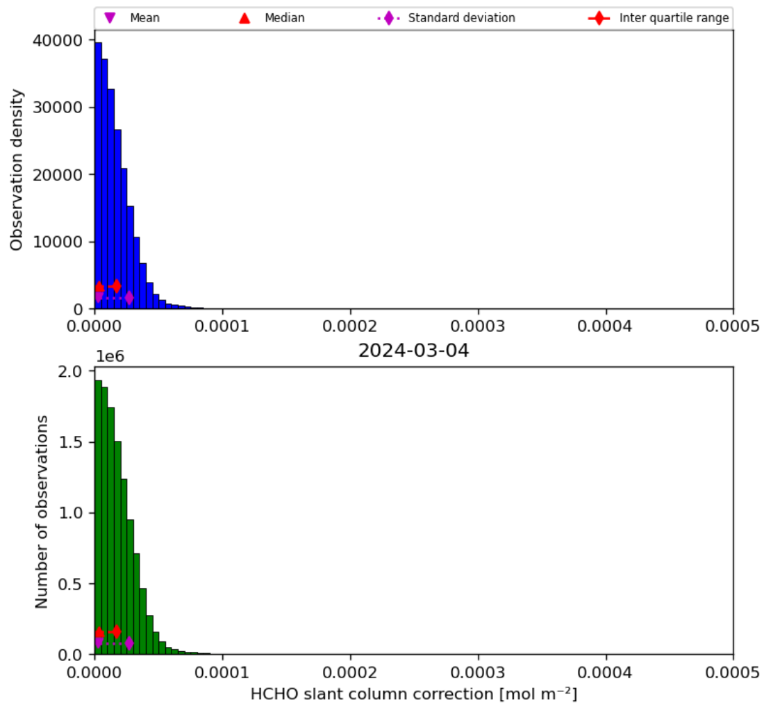
Figure 47: Histogram of “HCHO slant column correction” for 2024-03-04 to 2024-03-05
