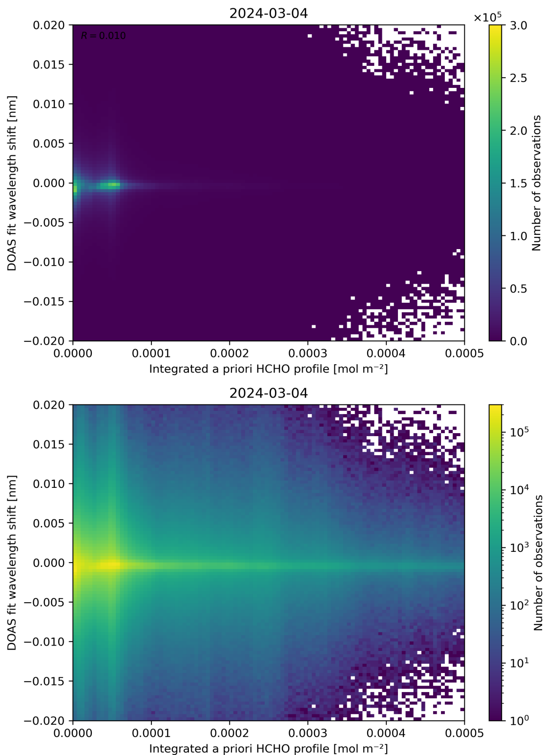
Figure 149: Scatter density plot of “Integrated a priori HCHO profile” against “DOAS fit wavelength shift” for 2024-03-04 to 2024-03-05.
