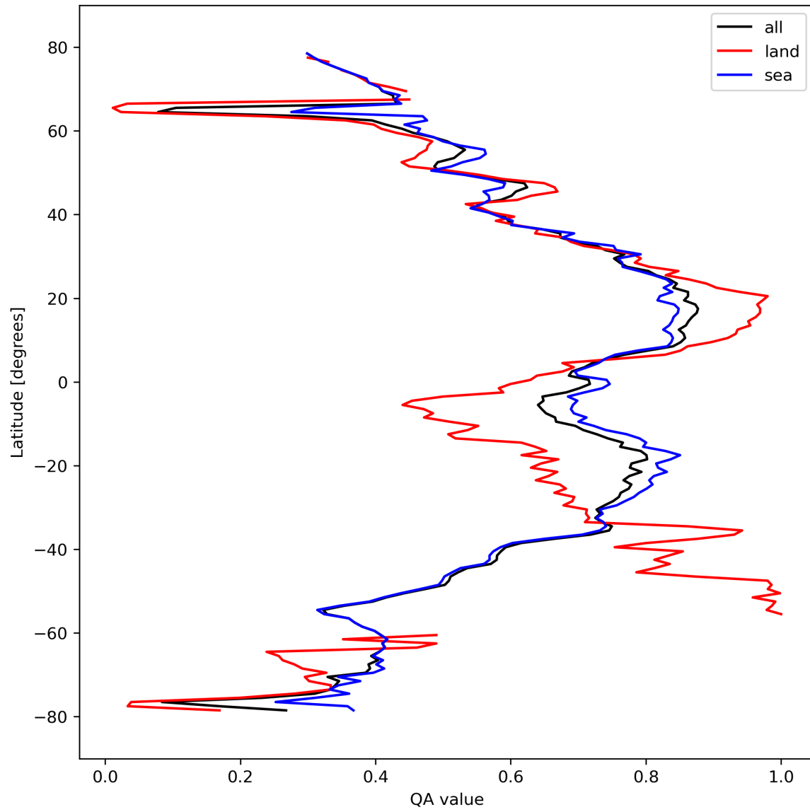
Figure 20: Zonal average of “QA value” for 2024-03-04 to 2024-03-05.
