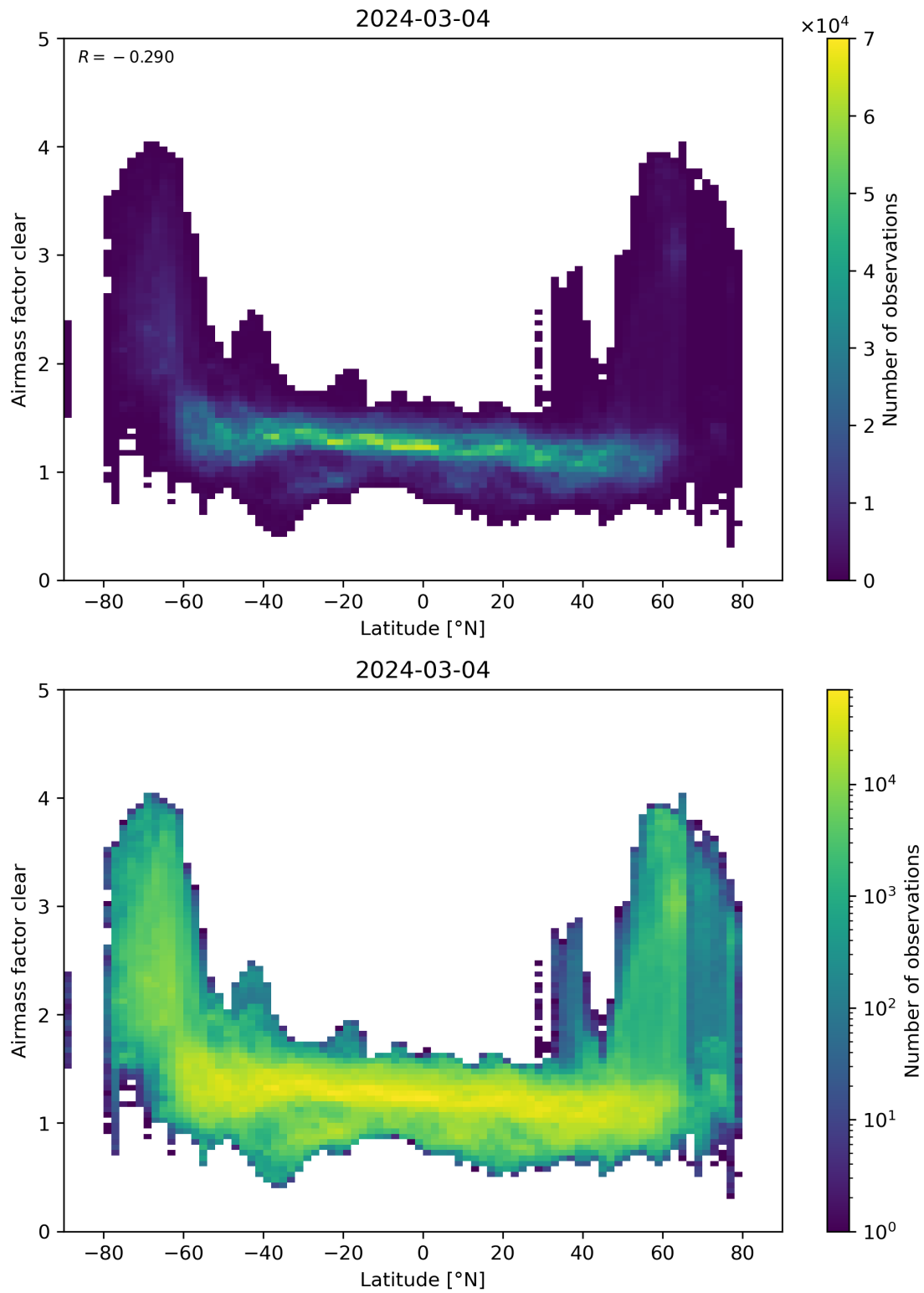
Figure 156: Scatter density plot of “Latitude” against “Airmass factor clear” for 2024-03-04 to 2024-03-05.
