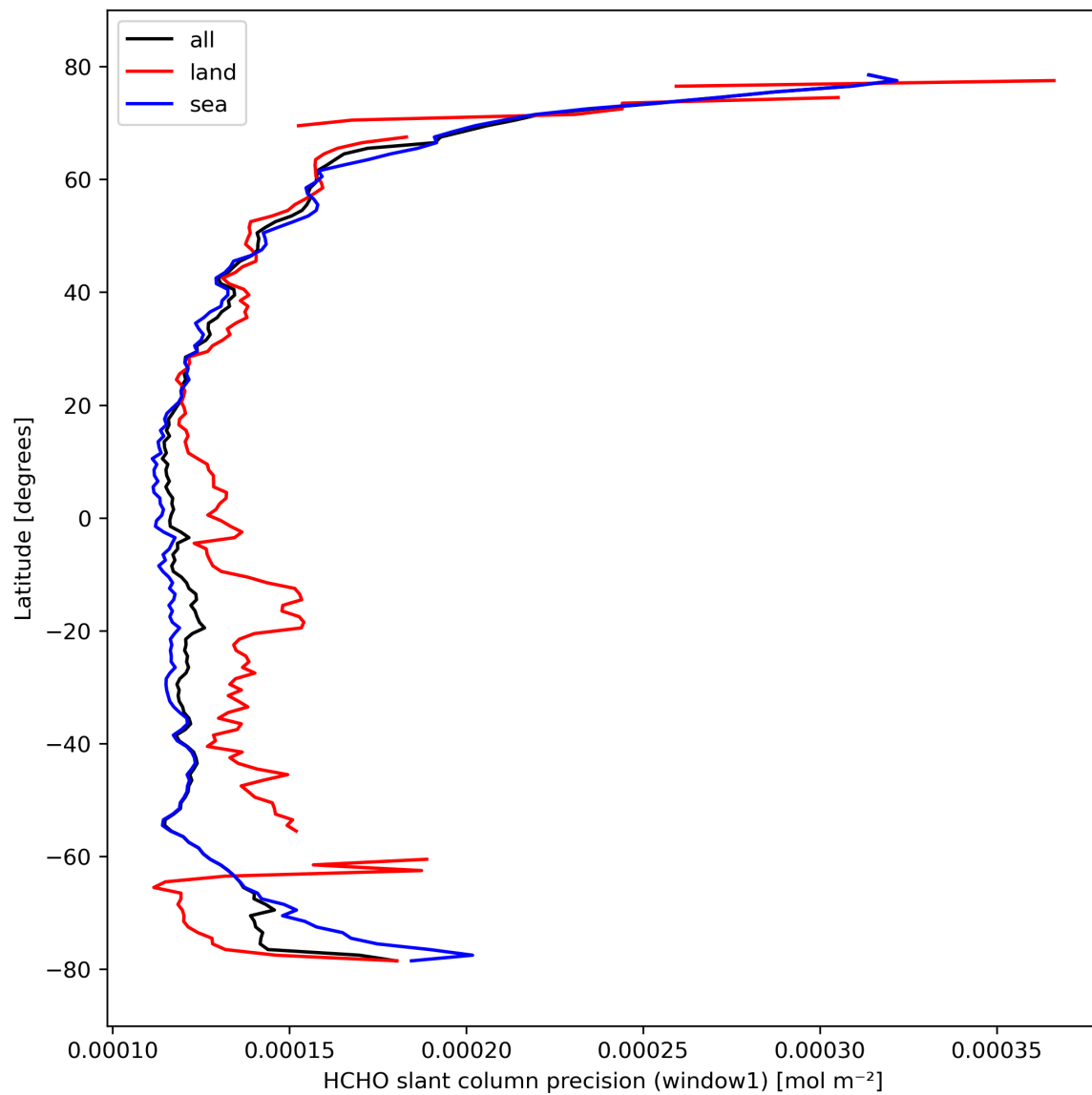
Figure 25: Zonal average of “HCHO slant column precision (window1)” for 2024-03-04 to 2024-03-05.
