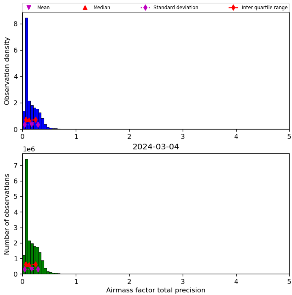
Figure 41: Histogram of “Airmass factor total precision” for 2024-03-04 to 2024-03-05
