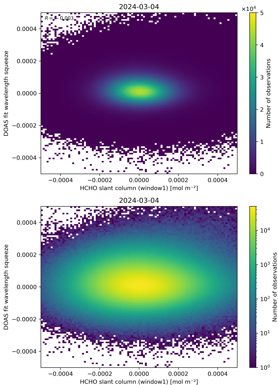
Figure 80: Scatter density plot of “HCHO slant column (window1)” against “DOAS fit wavelength squeeze” for 2024-03-04 to 2024-03-05.
