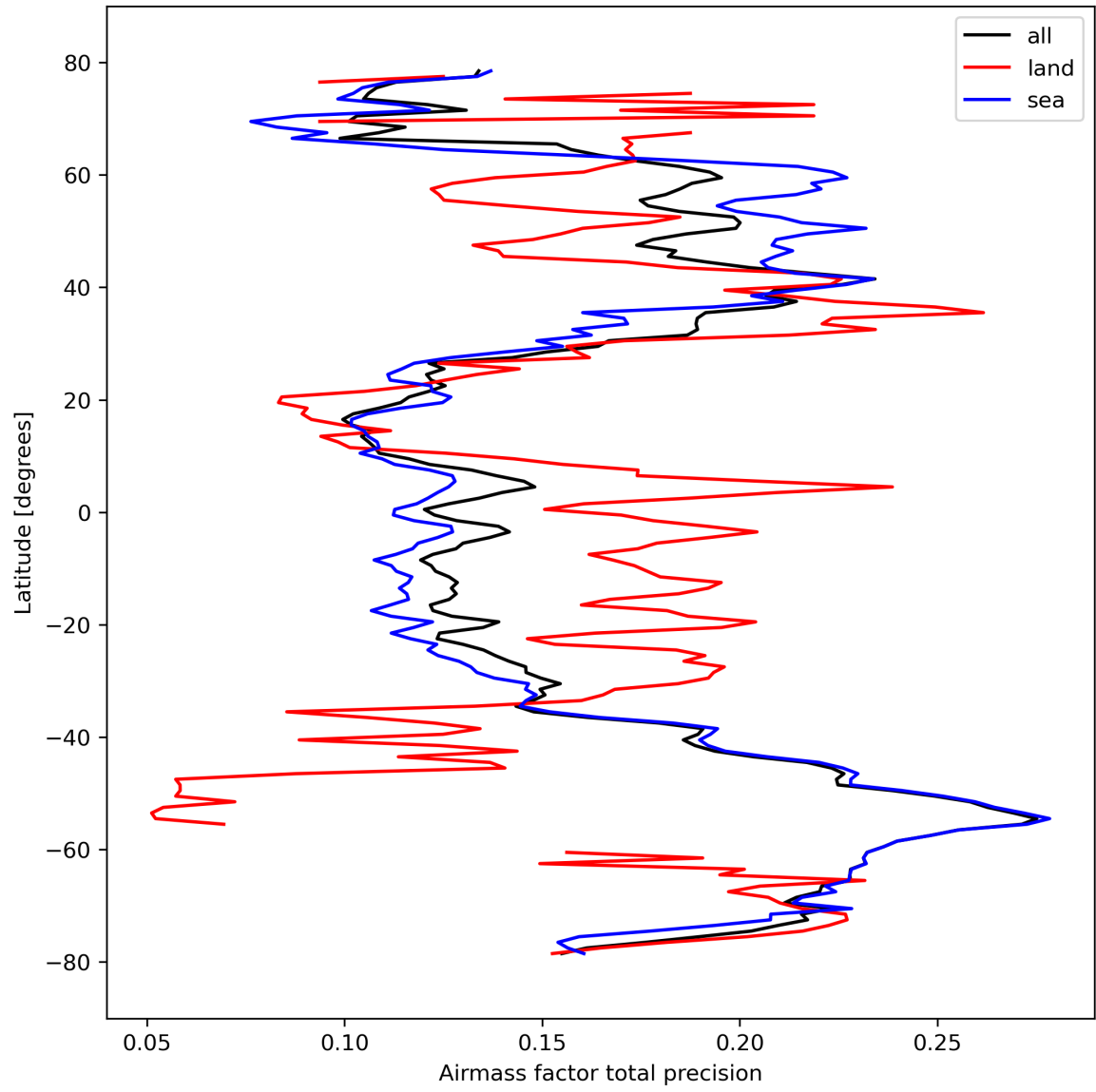
Figure 27: Zonal average of “Airmass factor total precision” for 2024-03-04 to 2024-03-05.
