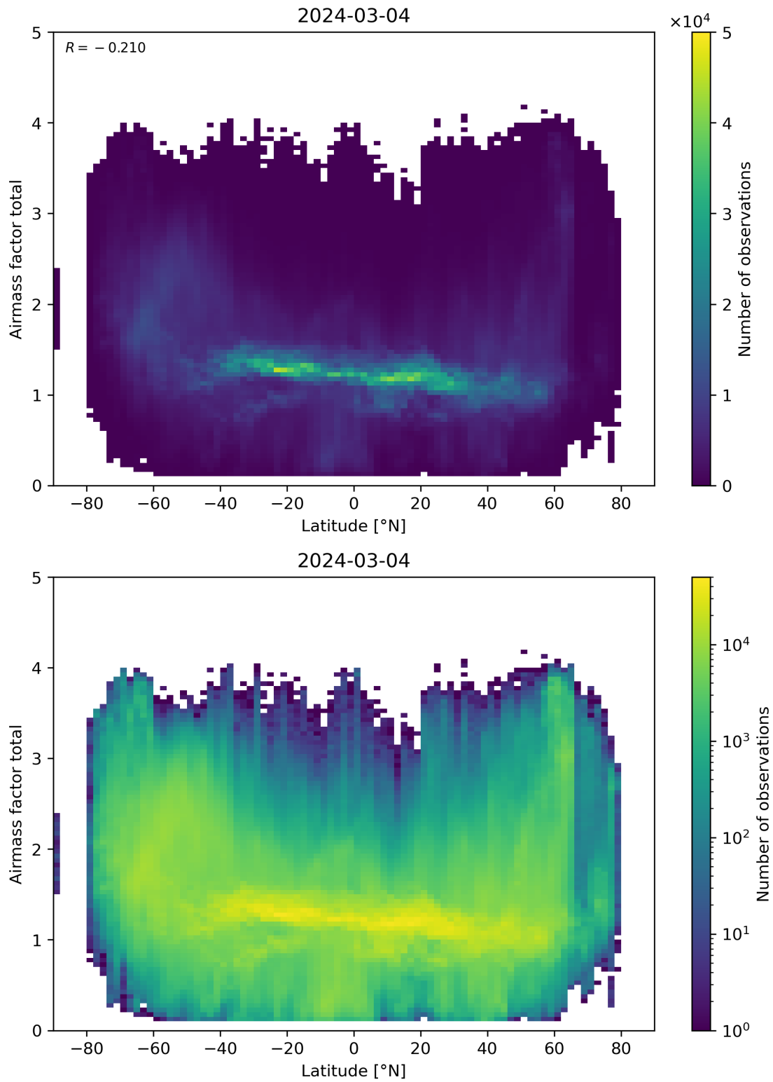
Figure 161: Scatter density plot of “Latitude” against “Airmass factor total” for 2024-03-04 to 2024-03-05.
