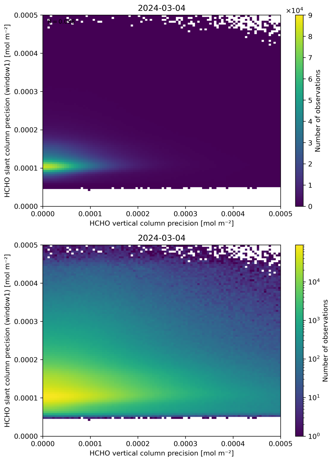
Figure 143: Scatter density plot of “HCHO vertical column precision” against “HCHO slant column precision (window1)” for 2024-03-04 to 2024-03-05.
