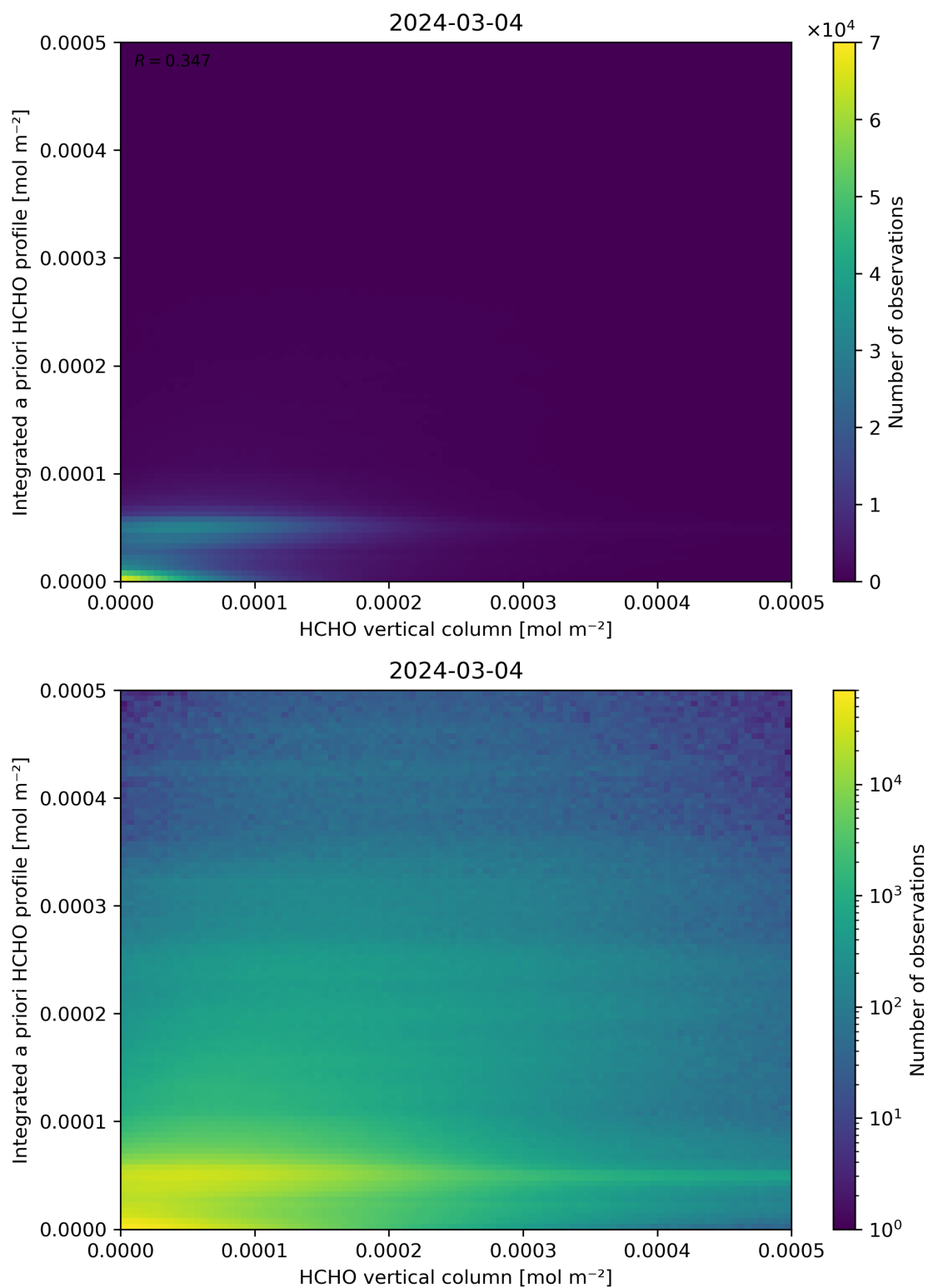
Figure 135: Scatter density plot of “HCHO vertical column” against “Integrated a priori HCHO profile” for 2024-03-04 to 2024-03-05.
