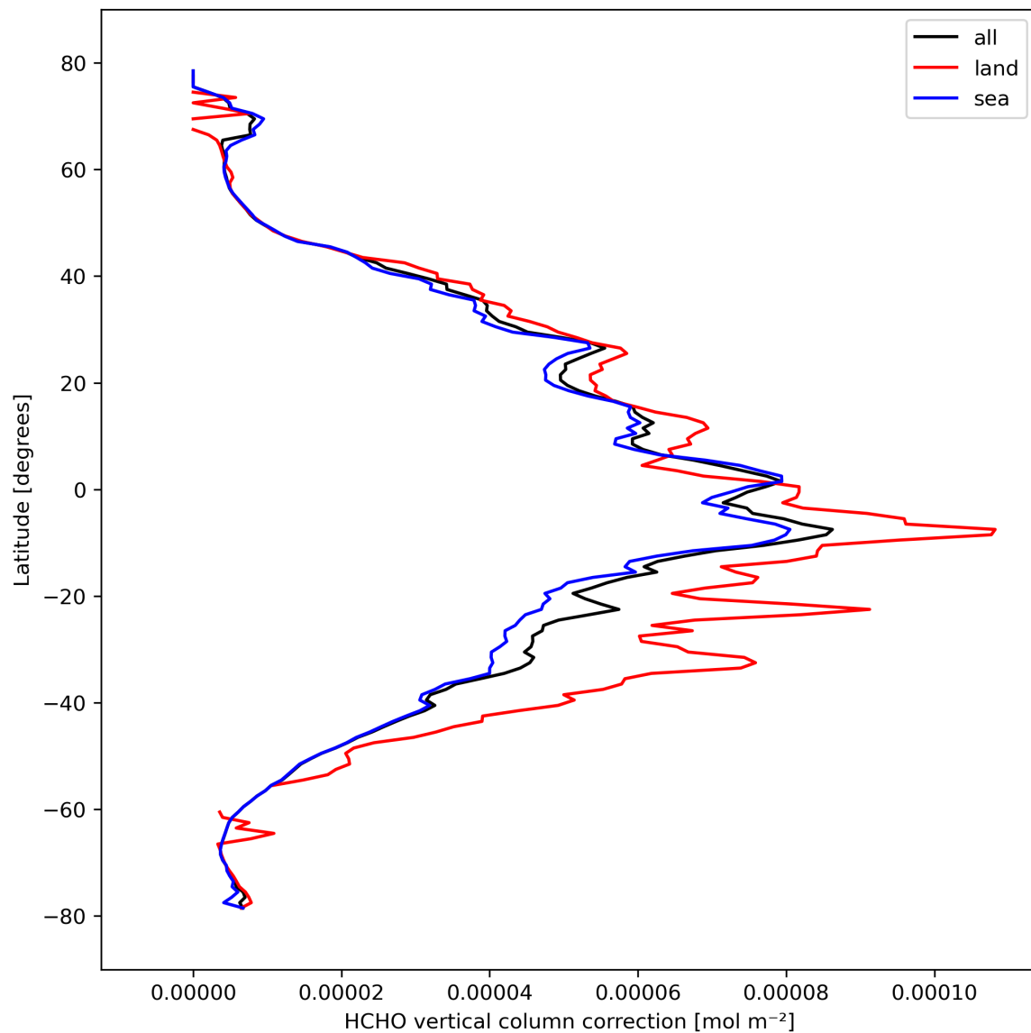
Figure 23: Zonal average of “HCHO vertical column correction” for 2024-03-04 to 2024-03-05.
