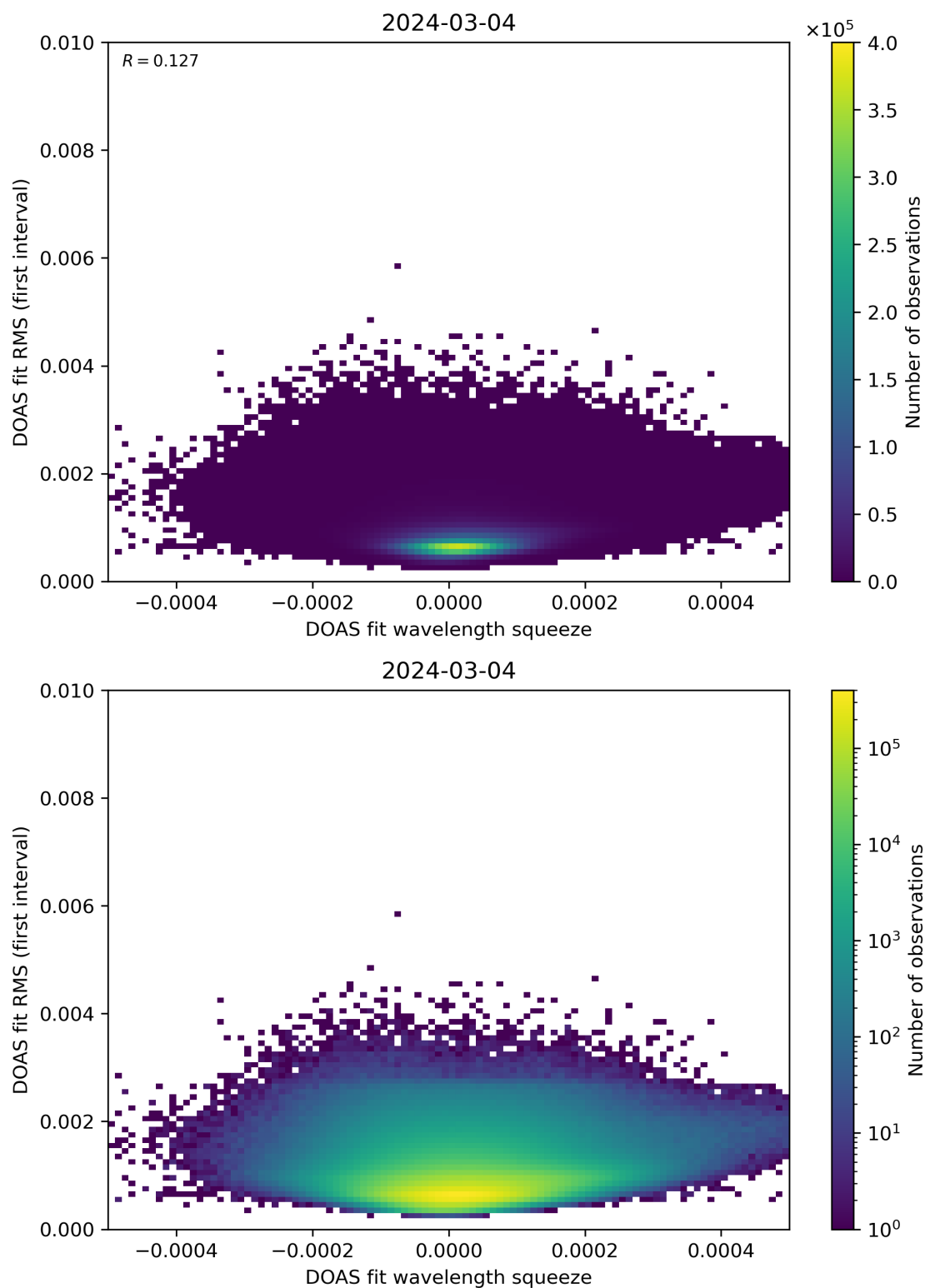
Figure 68: Scatter density plot of “DOAS fit wavelength squeeze” against “DOAS fit RMS (first interval)” for 2024-03-04 to 2024-03-05.
