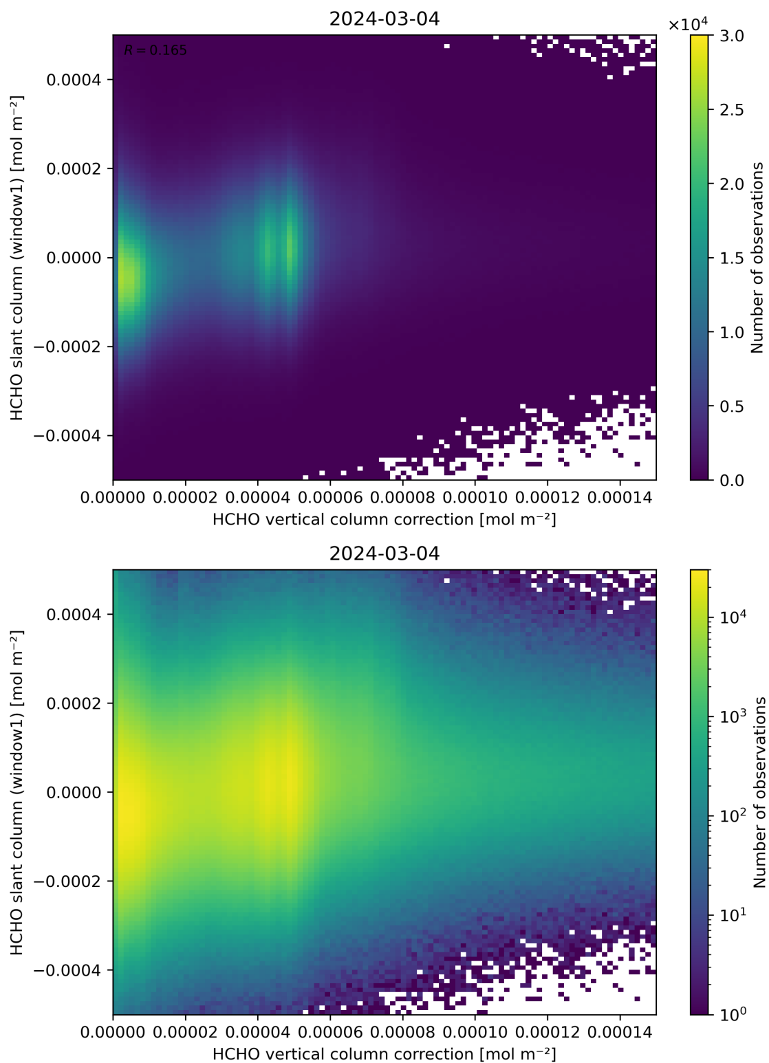
Figure 118: Scatter density plot of “HCHO vertical column correction” against “HCHO slant column (window1)” for 2024-03-04 to 2024-03-05.
