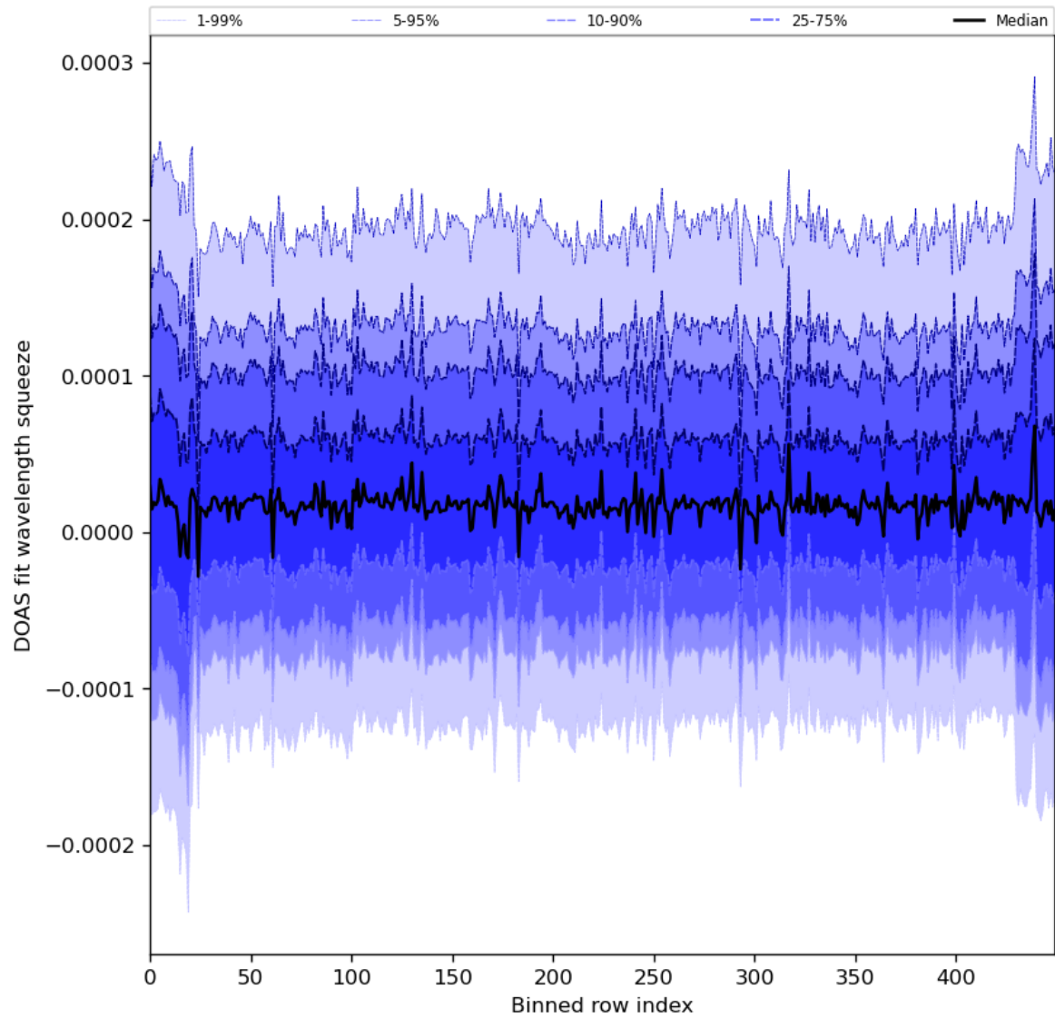
Figure 59: Along track statistics of “DOAS fit wavelength squeeze” for 2024-03-04 to 2024-03-05
