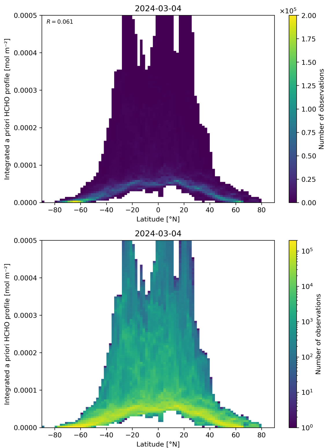
Figure 166: Scatter density plot of “Latitude” against “Integrated a priori HCHO profile” for 2024-03-04 to 2024-03-05.
