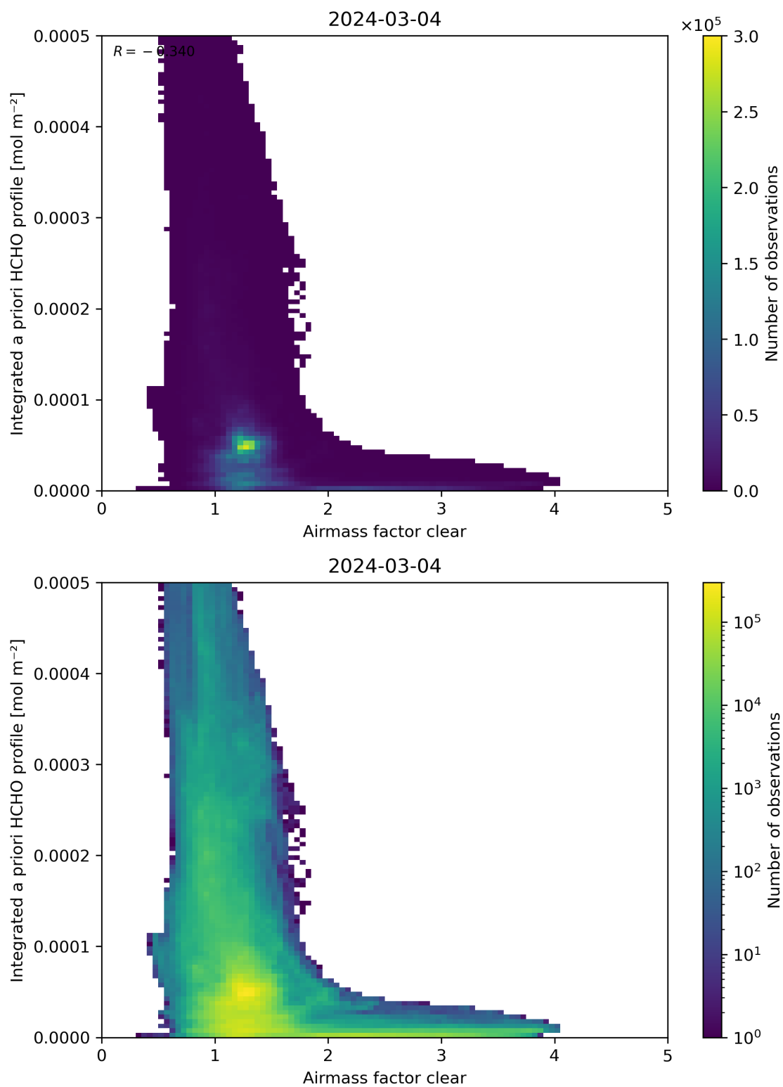
Figure 76: Scatter density plot of “Airmass factor clear” against “Integrated a priori HCHO profile” for 2024-03-04 to 2024-03-05.
