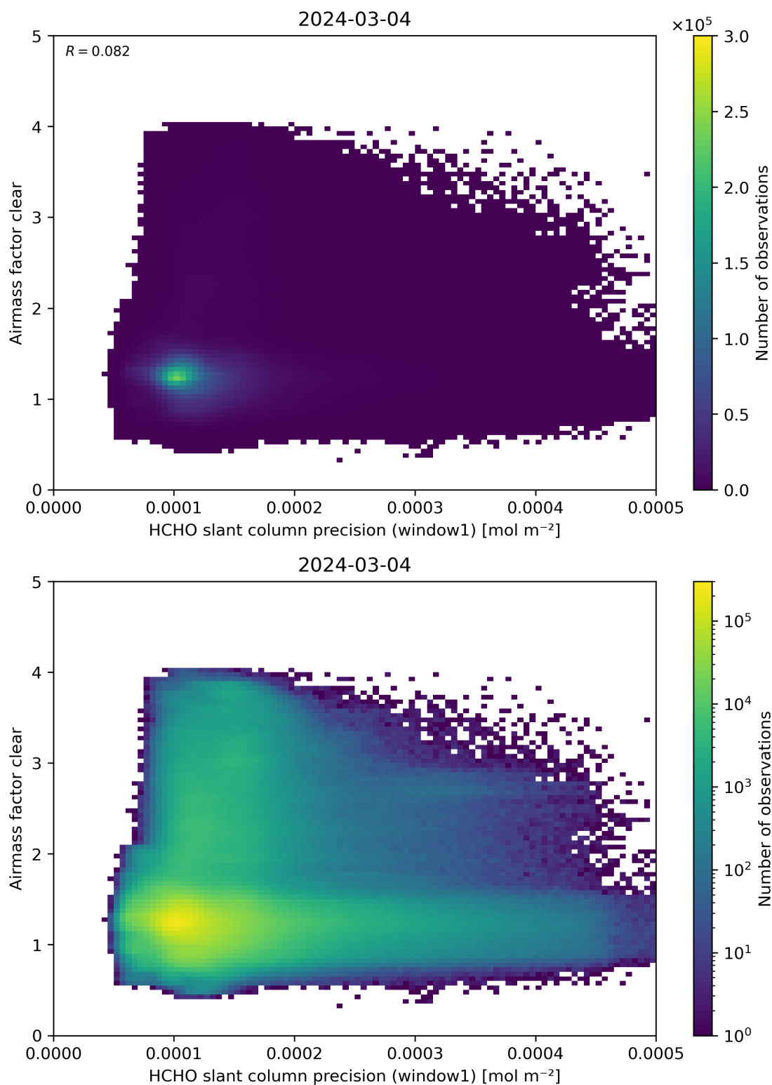
Figure 91: Scatter density plot of “HCHO slant column precision (window1)” against “Airmass factor clear” for 2024-03-04 to 2024-03-05.
