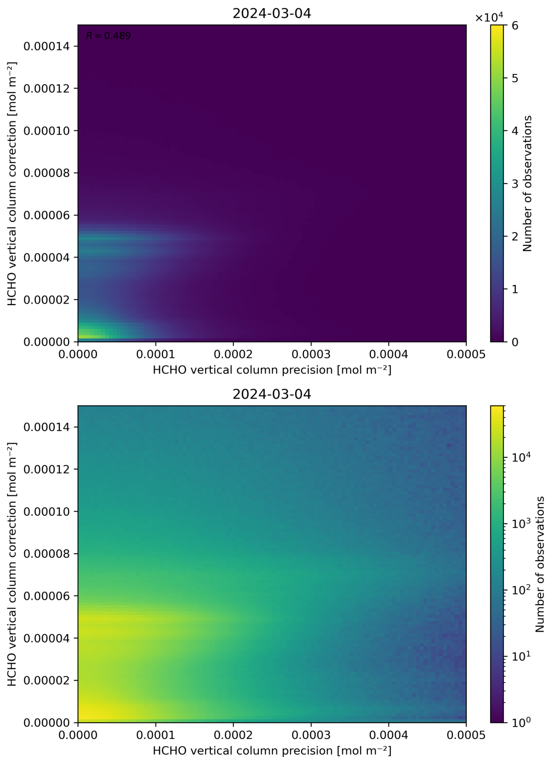
Figure 146: Scatter density plot of “HCHO vertical column precision” against “HCHO vertical column correction” for 2024-03-04 to 2024-03-05.
