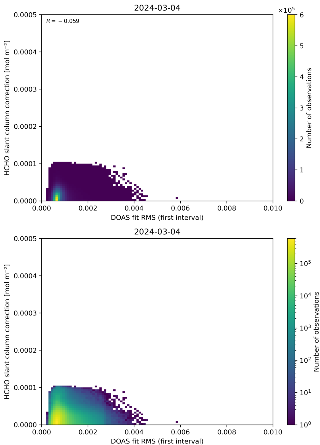
Figure 63: Scatter density plot of “DOAS fit RMS (first interval)” against “HCHO slant column correction” for 2024-03-04 to 2024-03-05.
