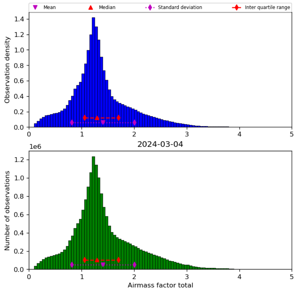
Figure 40: Histogram of “Airmass factor total” for 2024-03-04 to 2024-03-05
