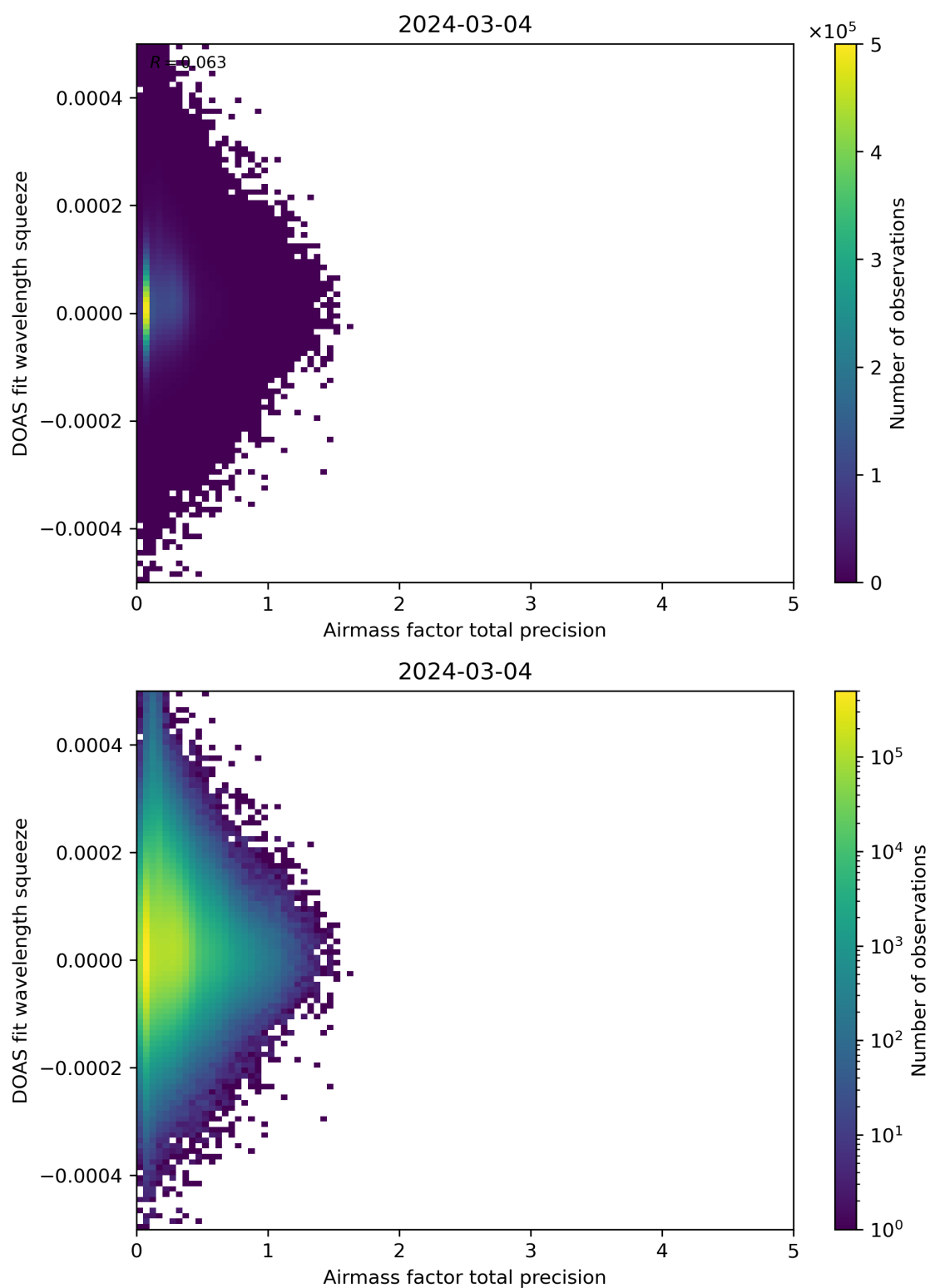
Figure 107: Scatter density plot of “Airmass factor total precision” against “DOAS fit wavelength squeeze” for 2024-03-04 to 2024-03-05.
