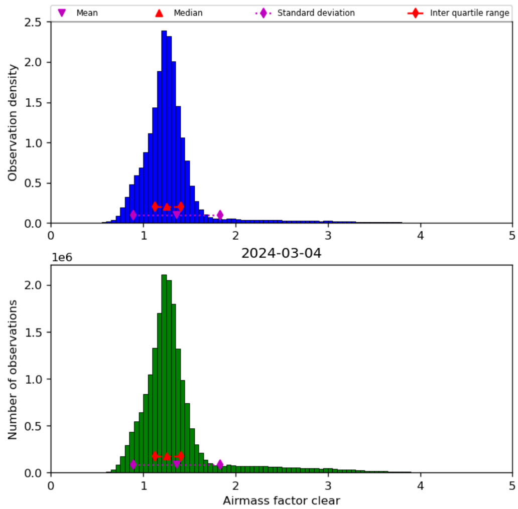
Figure 42: Histogram of “Airmass factor clear” for 2024-03-04 to 2024-03-05
