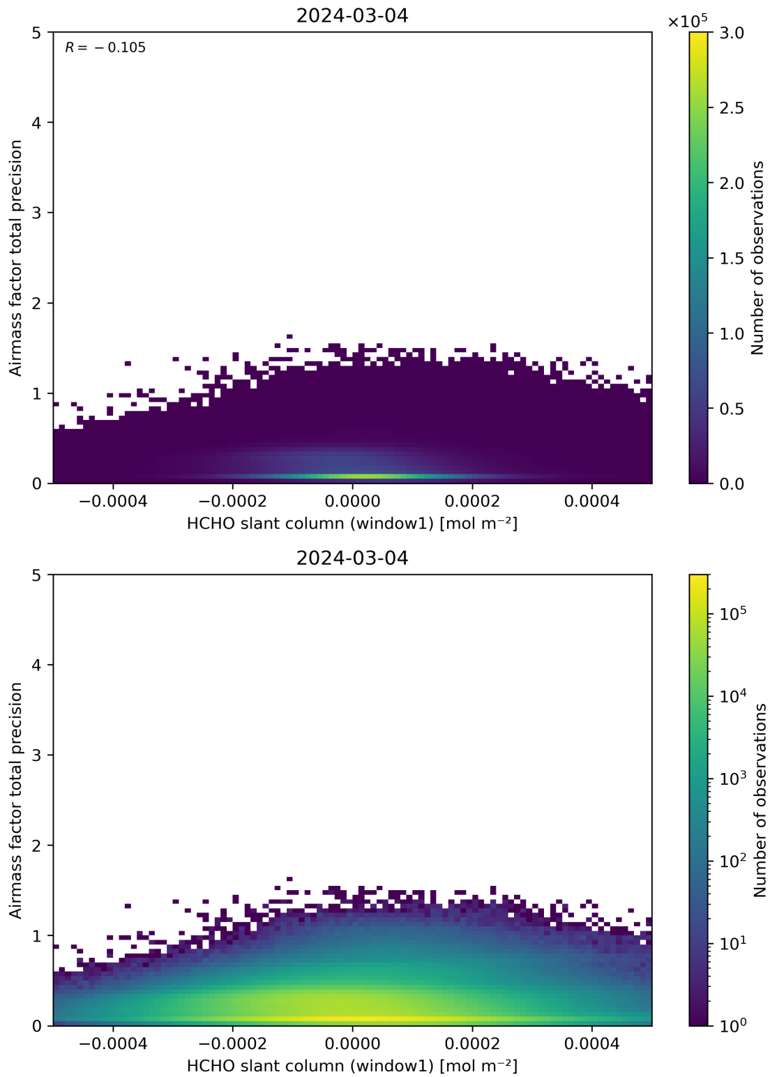
Figure 86: Scatter density plot of “HCHO slant column (window1)” against “Airmass factor total precision” for 2024-03-04 to 2024-03-05.
