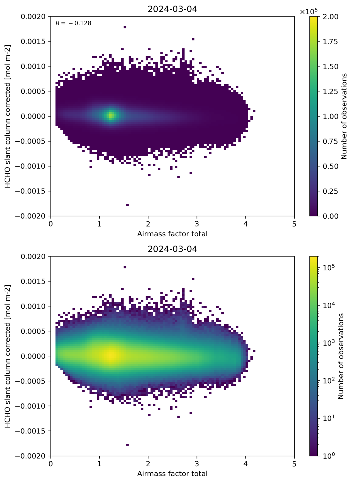
Figure 101: Scatter density plot of “Airmass factor total” against “HCHO slant column corrected” for 2024-03-04 to 2024-03-05.
