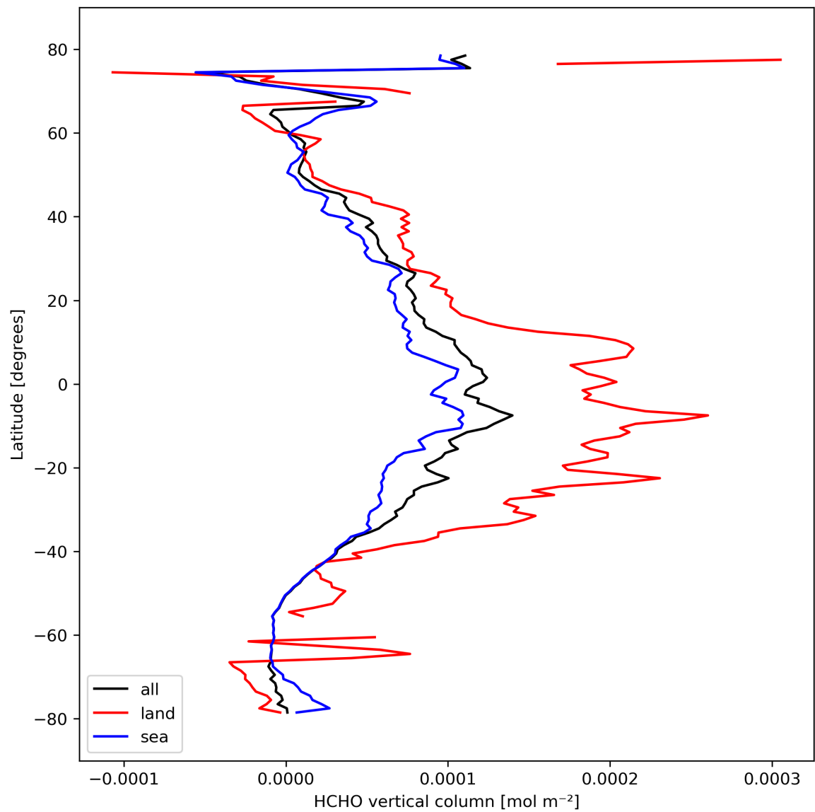
Figure 21: Zonal average of “HCHO vertical column” for 2024-03-04 to 2024-03-05.
