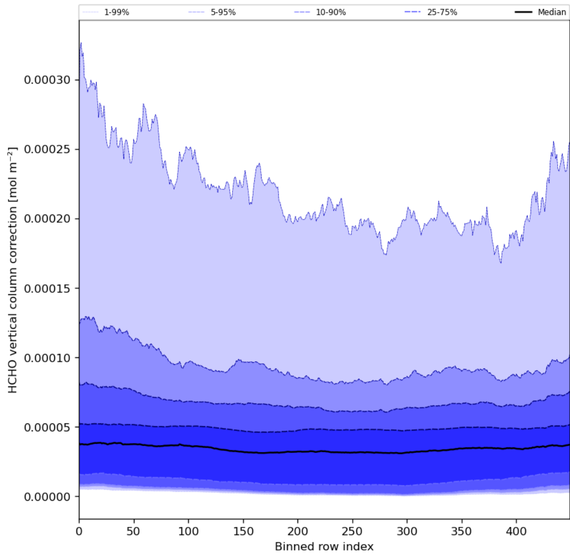
Figure 51: Along track statistics of “HCHO vertical column correction” for 2024-03-04 to 2024-03-05
