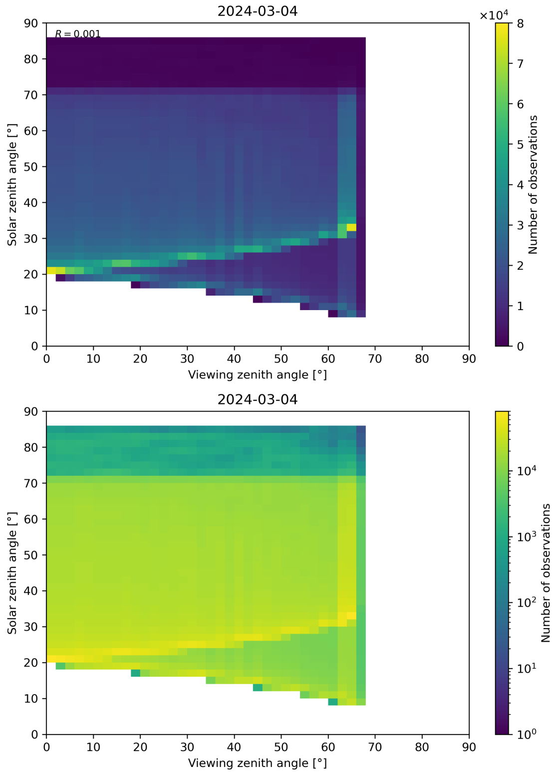
Figure 197: Scatter density plot of “Viewing zenith angle” against “Solar zenith angle” for 2024-03-04 to 2024-03-05.
