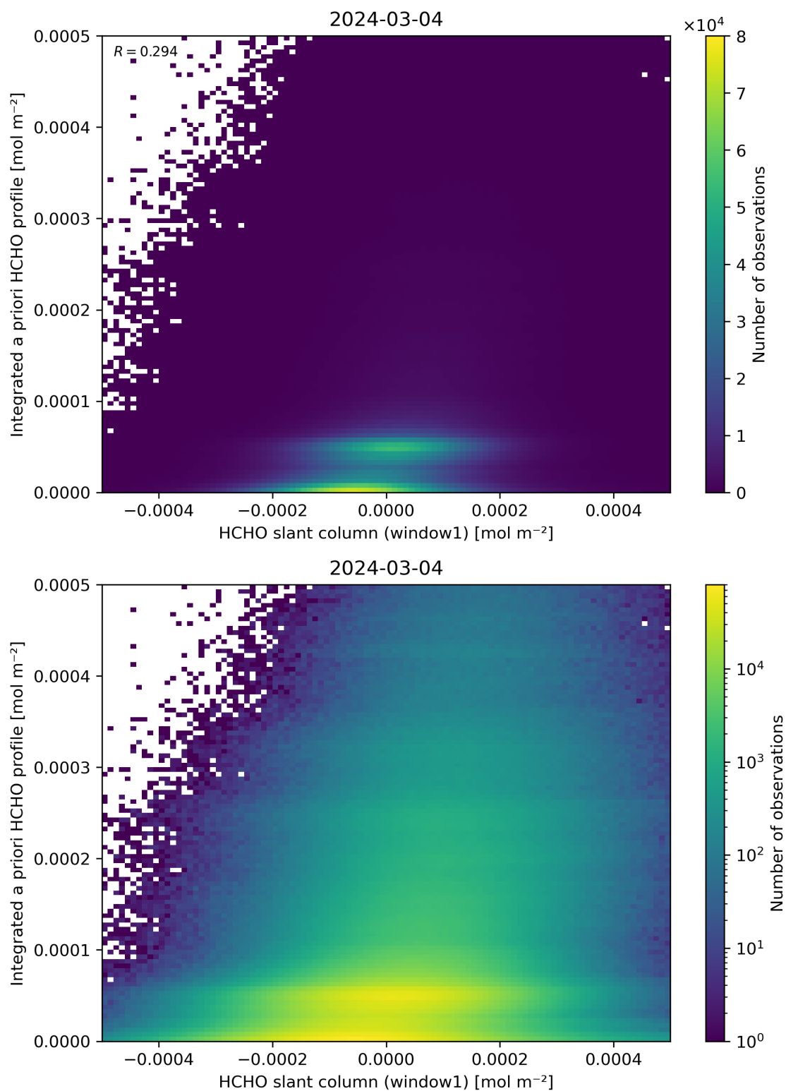
Figure 87: Scatter density plot of “HCHO slant column (window1)” against “Integrated a priori HCHO profile” for 2024-03-04 to 2024-03-05.
