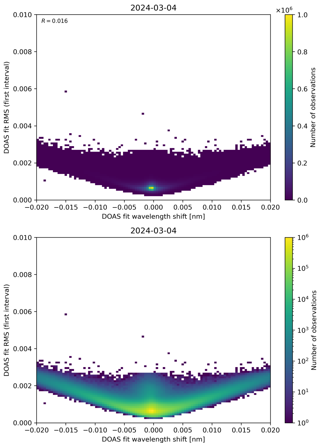
Figure 64: Scatter density plot of “DOAS fit wavelength shift” against “DOAS fit RMS (first interval)” for 2024-03-04 to 2024-03-05.
