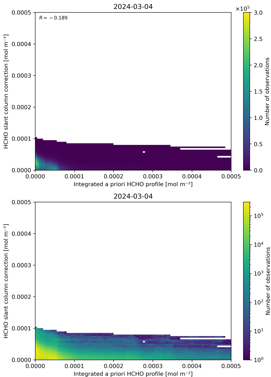
Figure 152: Scatter density plot of “Integrated a priori HCHO profile” against “HCHO slant column correction” for 2024-03-04 to 2024-03-05.
