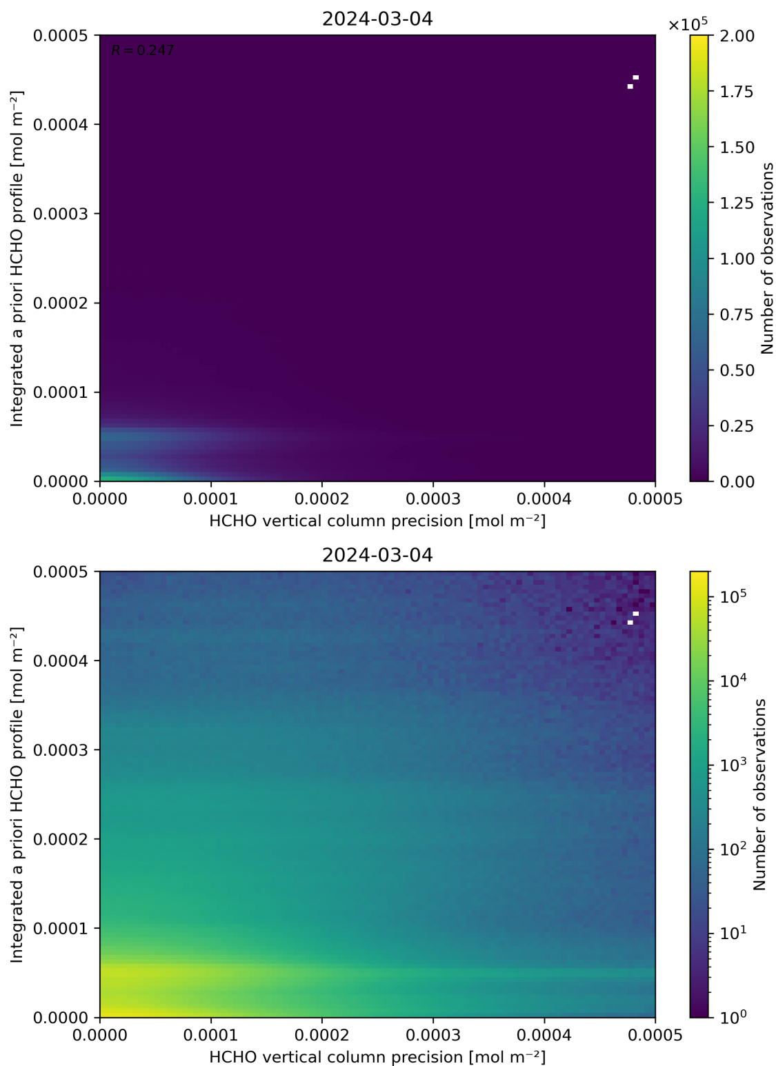
Figure 147: Scatter density plot of “HCHO vertical column precision” against “Integrated a priori HCHO profile” for 2024-03-04 to 2024-03-05.
