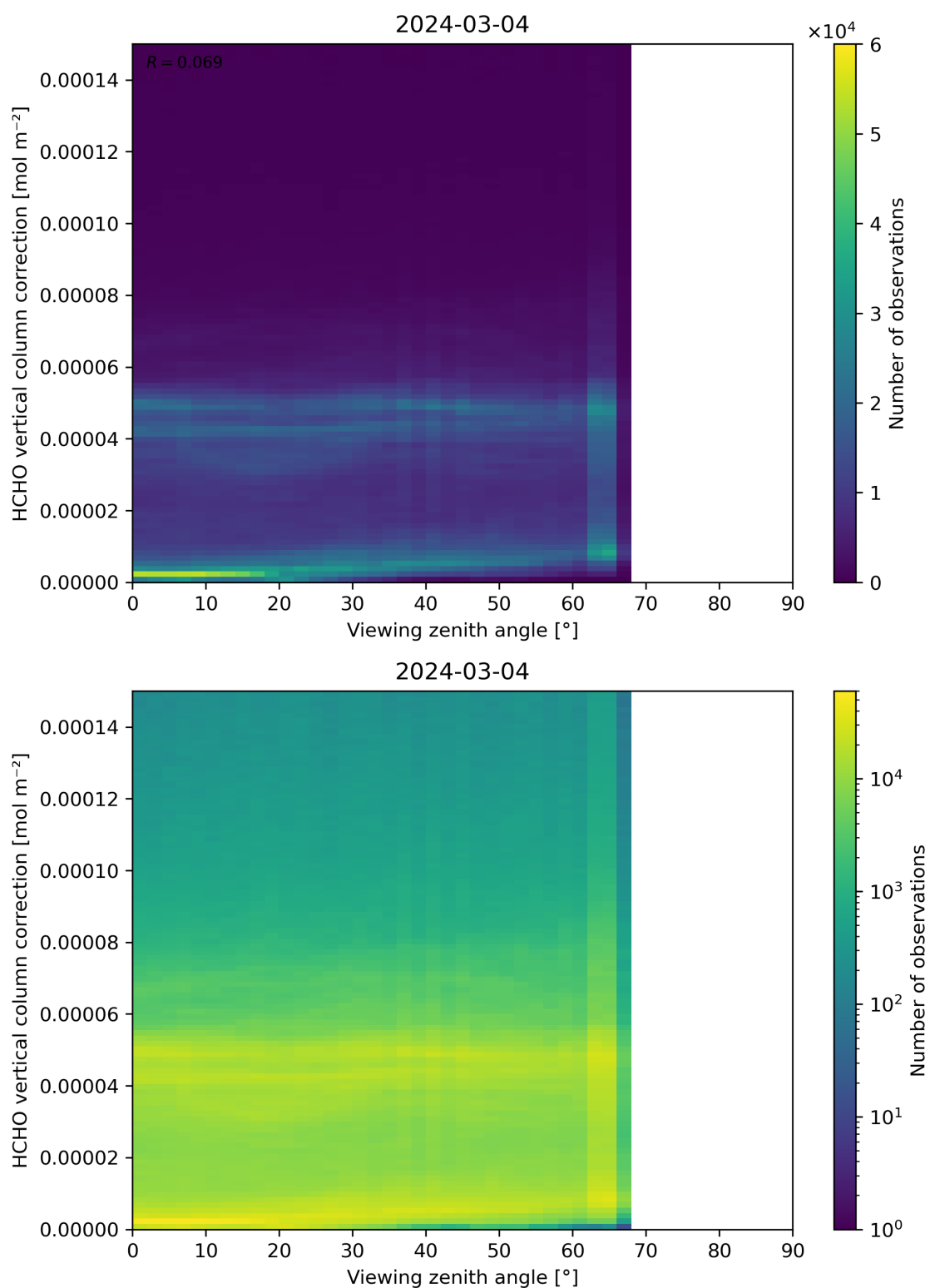
Figure 193: Scatter density plot of “Viewing zenith angle” against “HCHO vertical column correction” for 2024-03-04 to 2024-03-05.
