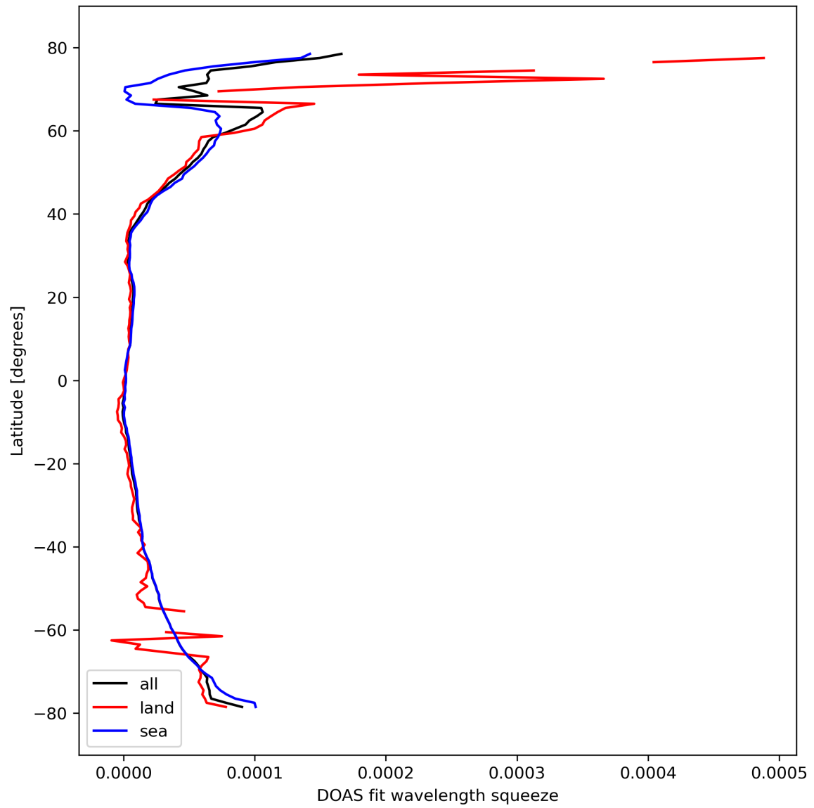
Figure 31: Zonal average of “DOAS fit wavelength squeeze” for 2024-03-04 to 2024-03-05.
