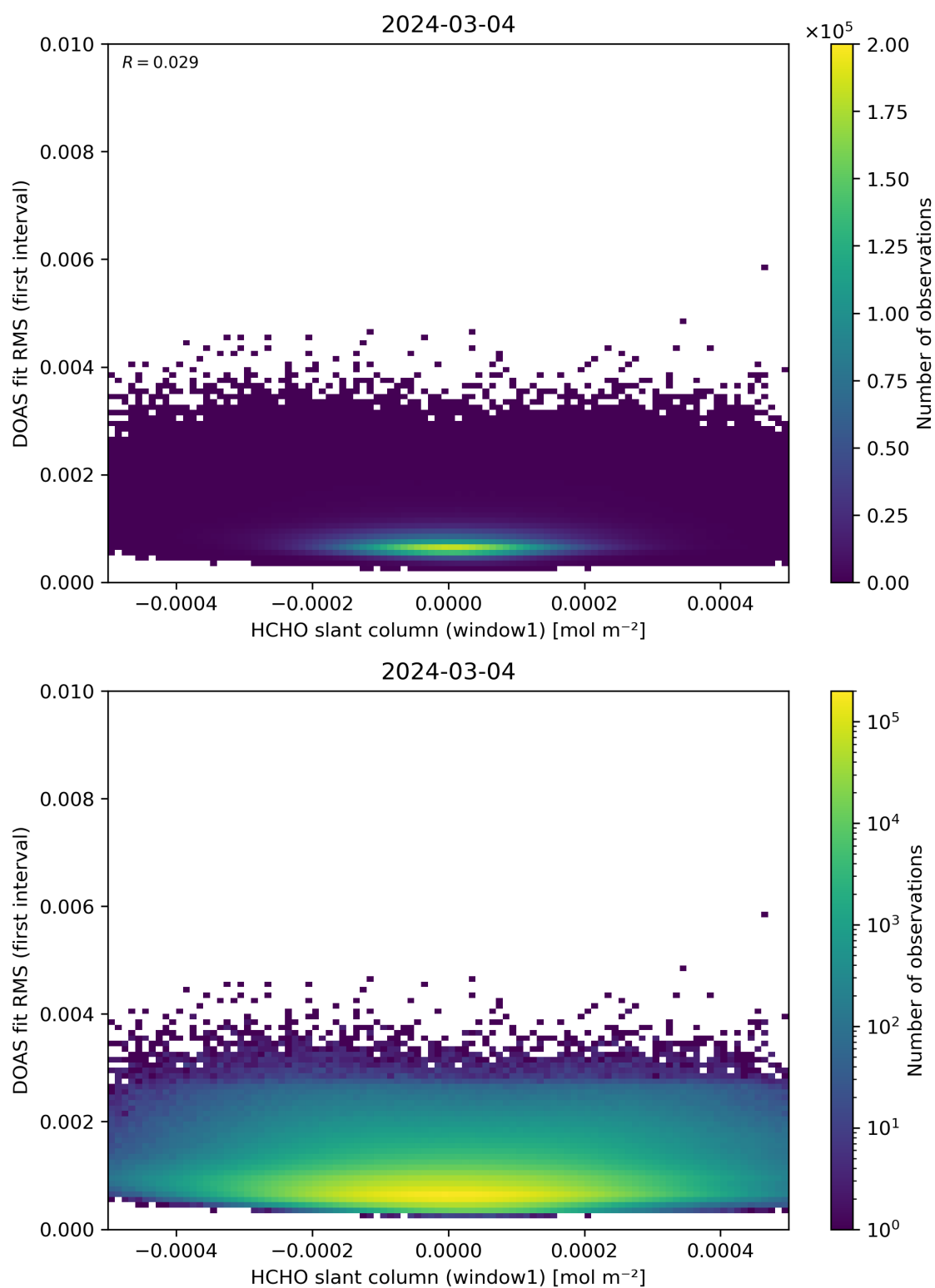
Figure 78: Scatter density plot of “HCHO slant column (window1)” against “DOAS fit RMS (first interval)” for 2024-03-04 to 2024-03-05.
