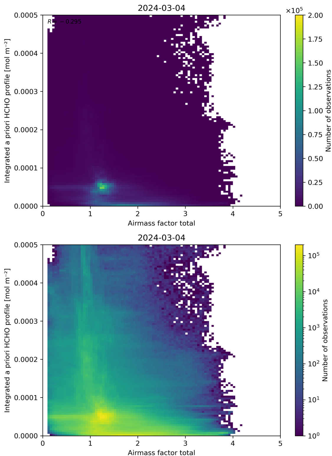
Figure 104: Scatter density plot of “Airmass factor total” against “Integrated a priori HCHO profile” for 2024-03-04 to 2024-03-05.
