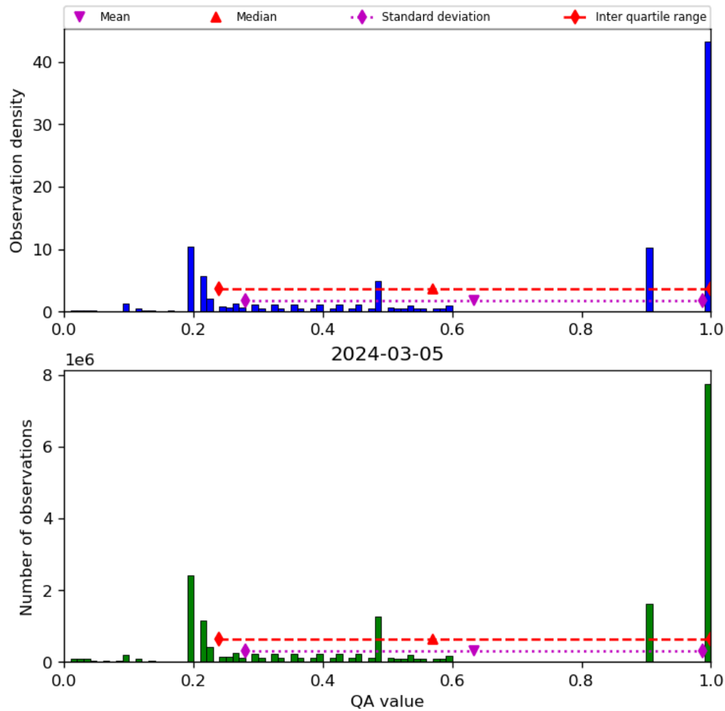
Figure 34: Histogram of “QA value” for 2024-03-04 to 2024-03-06
