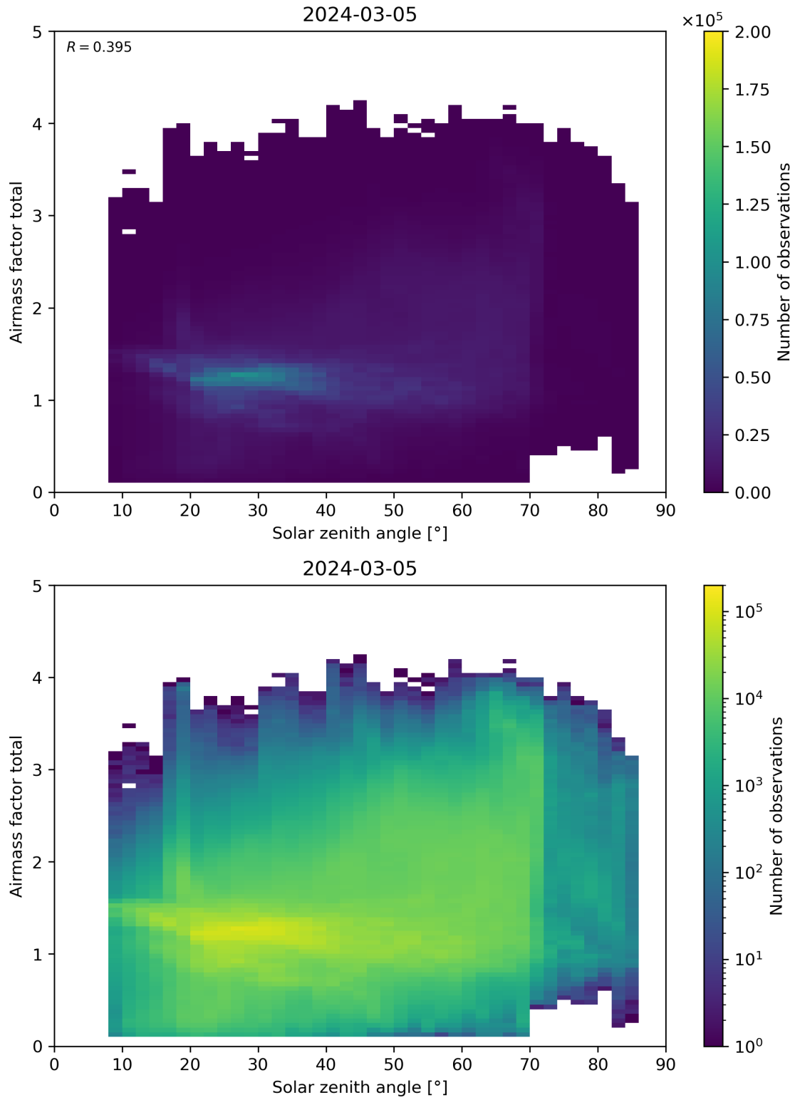
Figure 175: Scatter density plot of “Solar zenith angle” against “Airmass factor total” for 2024-03-04 to 2024-03-06.
