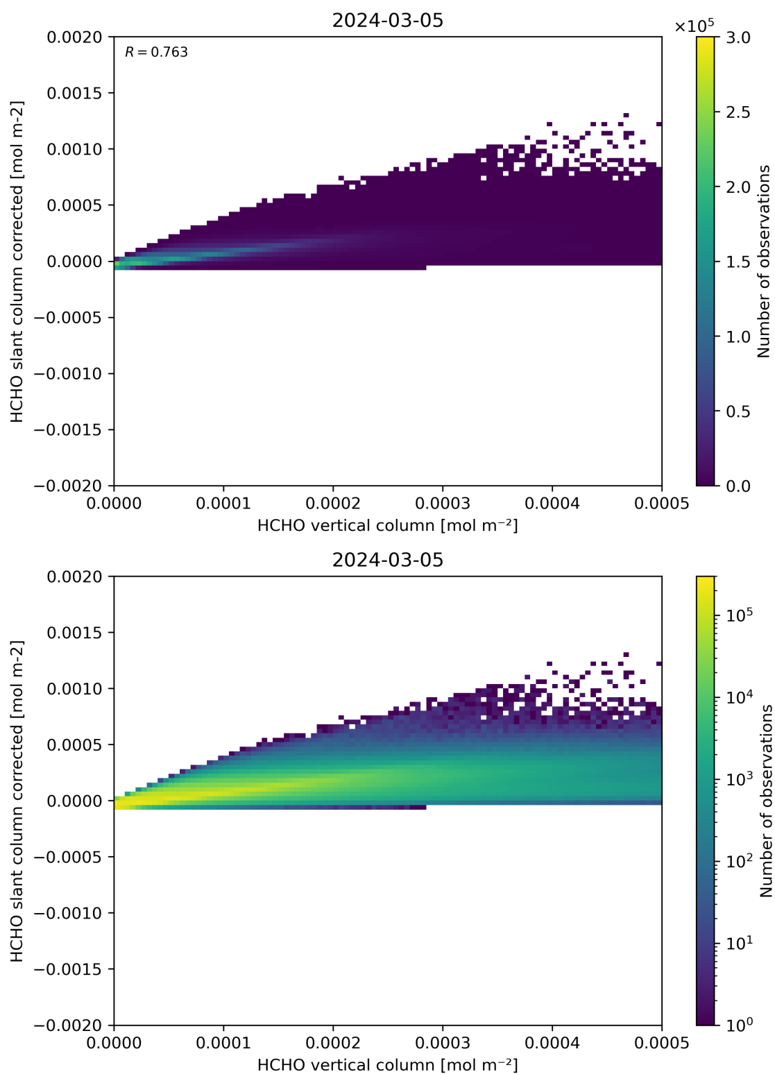
Figure 127: Scatter density plot of “HCHO vertical column” against “HCHO slant column corrected” for 2024-03-04 to 2024-03-06.
