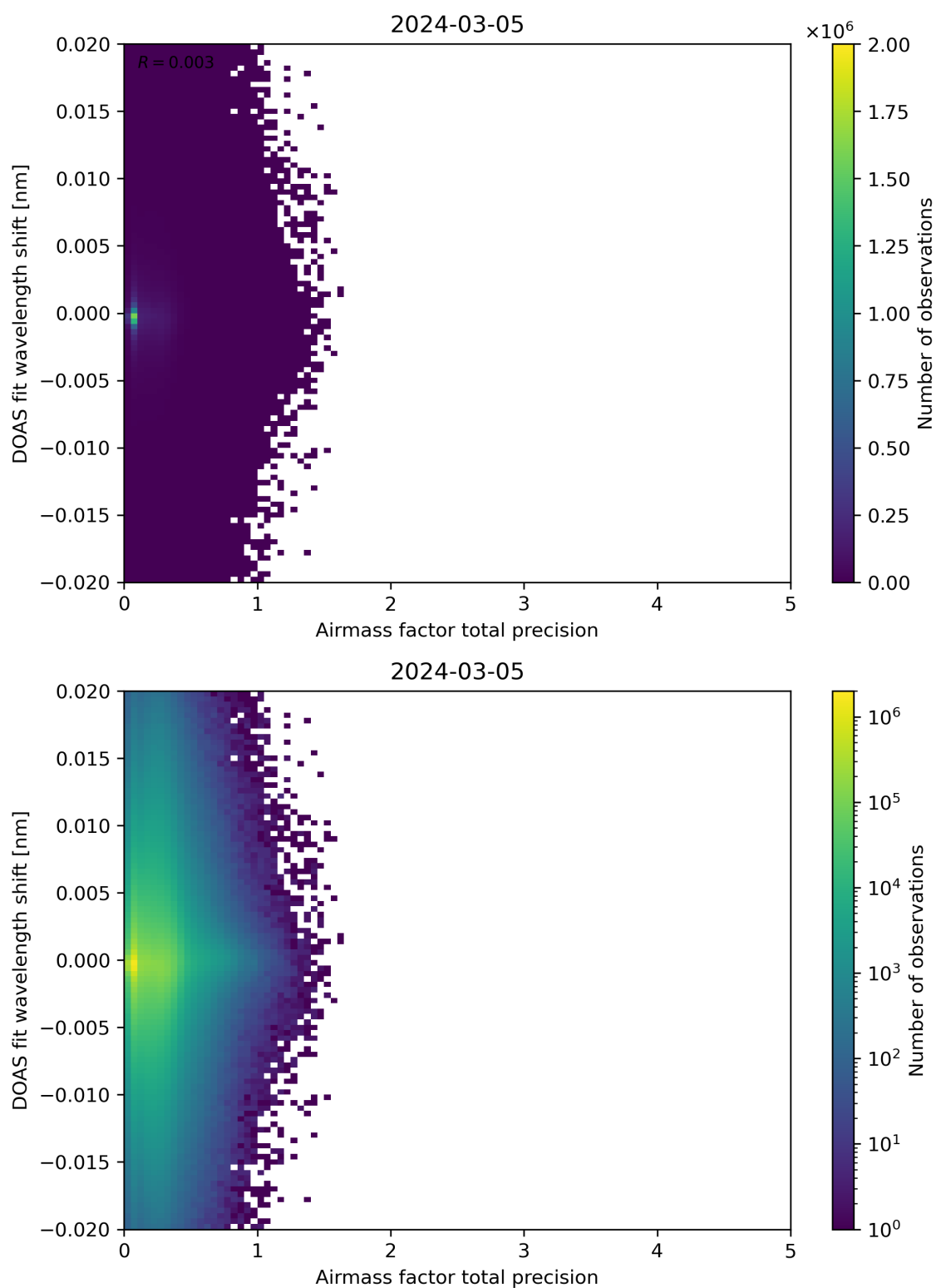
Figure 106: Scatter density plot of “Airmass factor total precision” against “DOAS fit wavelength shift” for 2024-03-04 to 2024-03-06.
