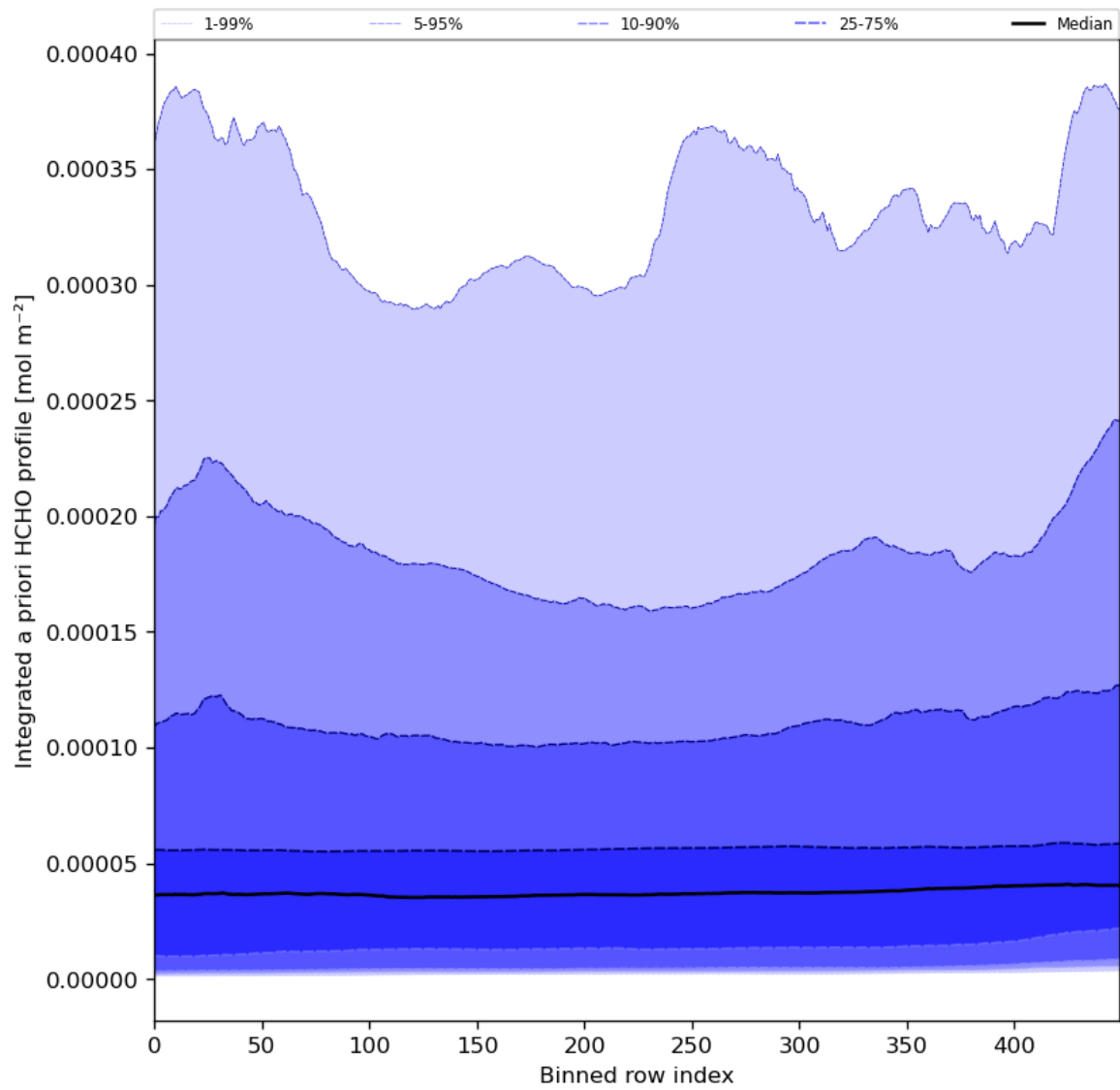
Figure 57: Along track statistics of “Integrated a priori HCHO profile” for 2024-03-04 to 2024-03-06
