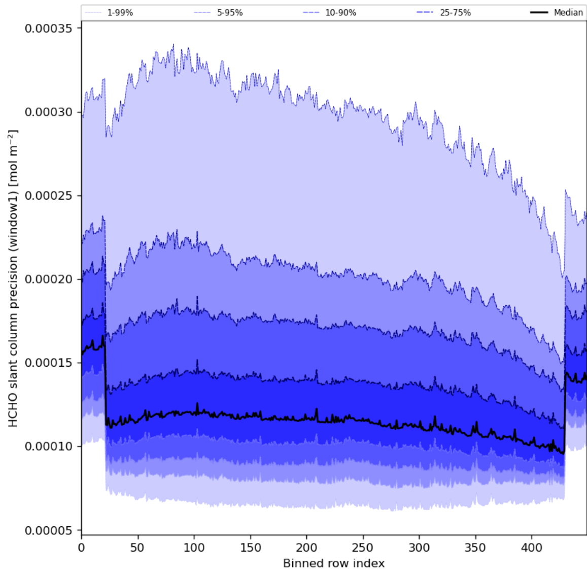
Figure 53: Along track statistics of “HCHO slant column precision (window1)” for 2024-03-04 to 2024-03-06
