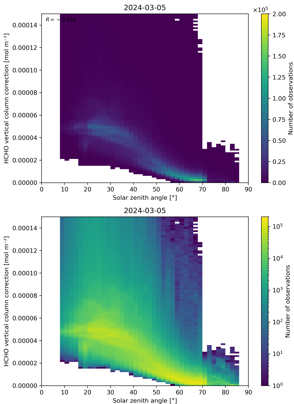
Figure 178: Scatter density plot of “Solar zenith angle” against “HCHO vertical column correction” for 2024-03-04 to 2024-03-06.
