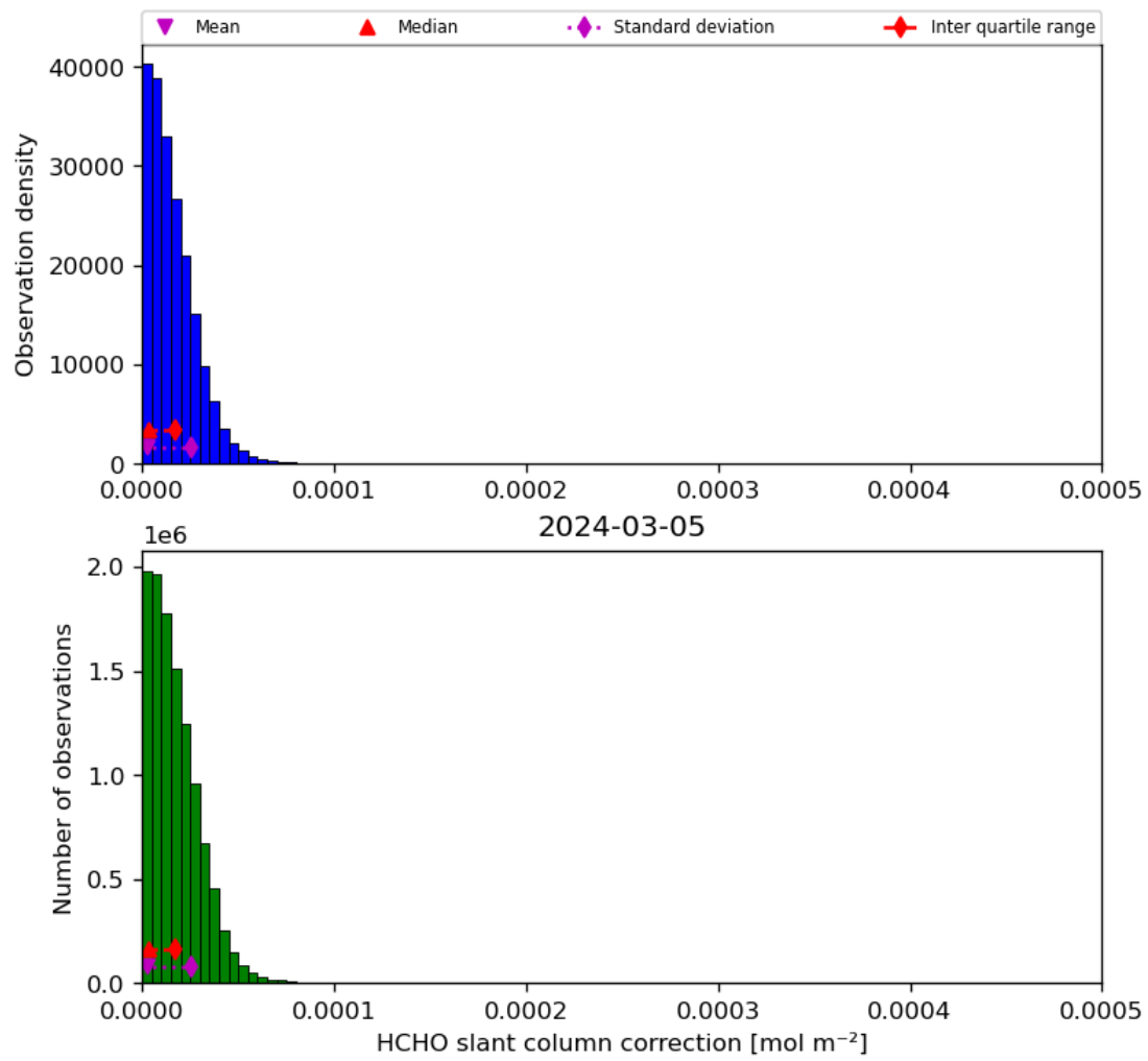
Figure 47: Histogram of “HCHO slant column correction” for 2024-03-04 to 2024-03-06
