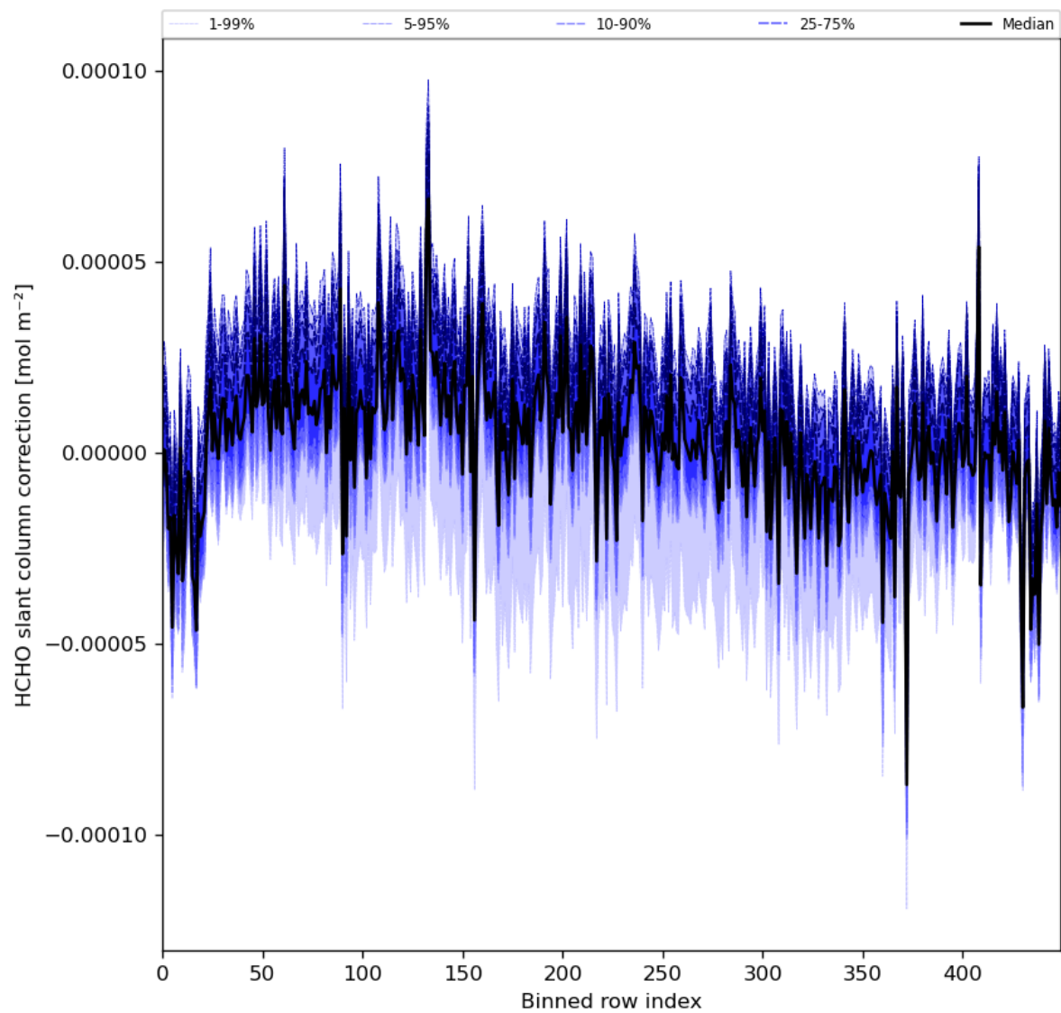
Figure 61: Along track statistics of “HCHO slant column correction” for 2024-03-04 to 2024-03-06
