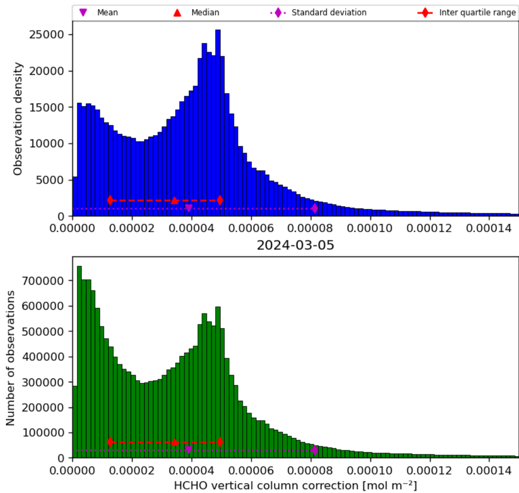
Figure 37: Histogram of “HCHO vertical column correction” for 2024-03-04 to 2024-03-06
