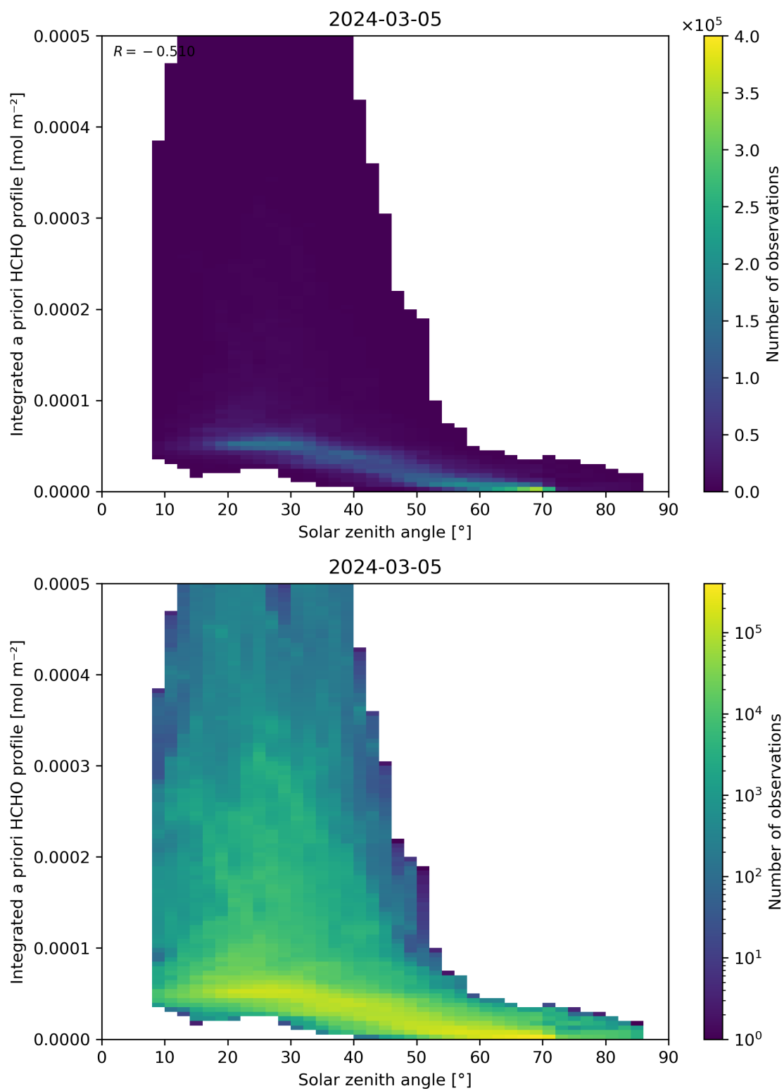
Figure 180: Scatter density plot of “Solar zenith angle” against “Integrated a priori HCHO profile” for 2024-03-04 to 2024-03-06.
