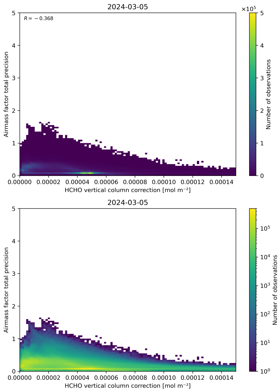
Figure 121: Scatter density plot of “HCHO vertical column correction” against “Airmass factor total precision” for 2024-03-04 to 2024-03-06.
