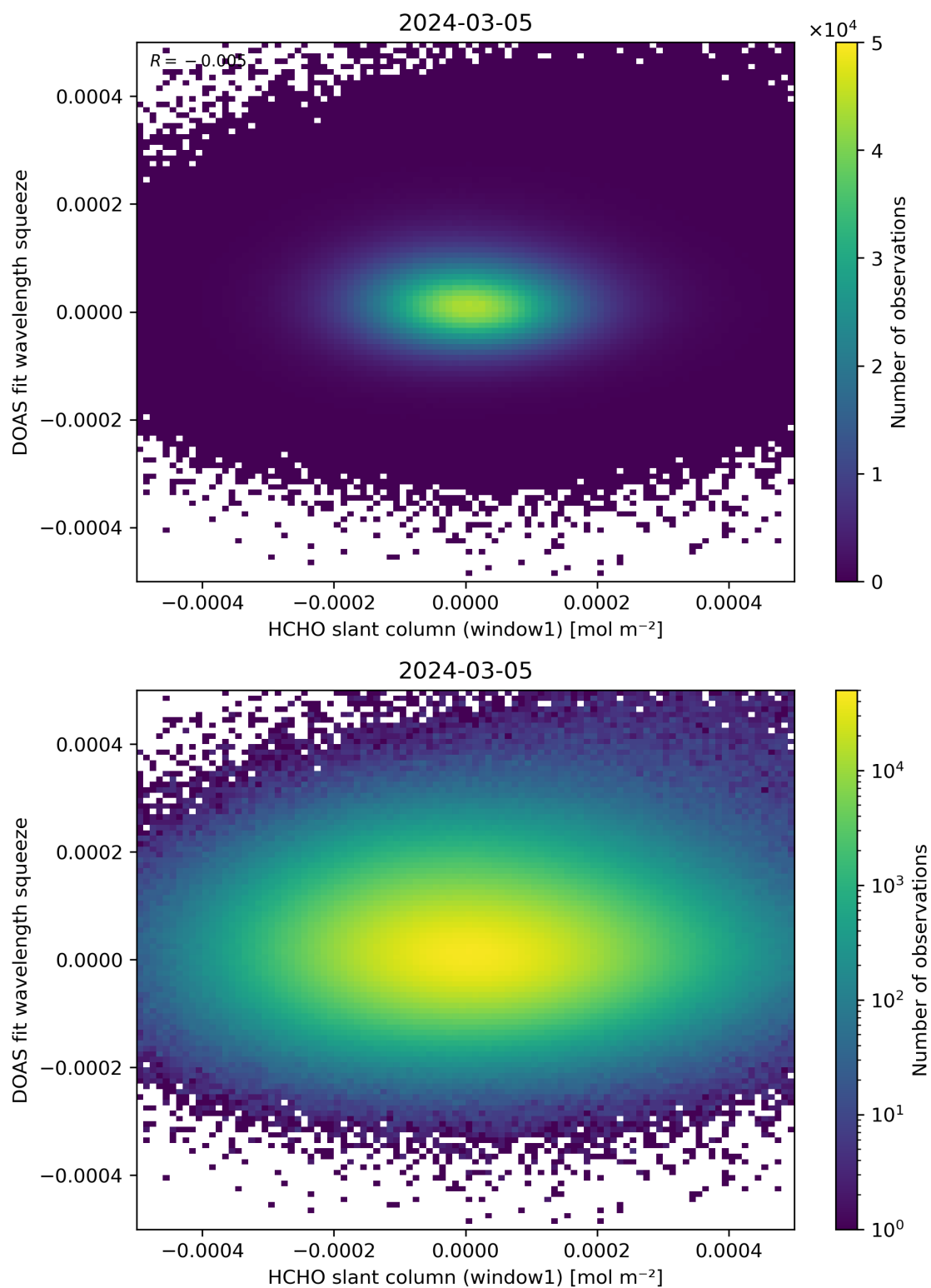
Figure 80: Scatter density plot of “HCHO slant column (window1)” against “DOAS fit wavelength squeeze” for 2024-03-04 to 2024-03-06.
