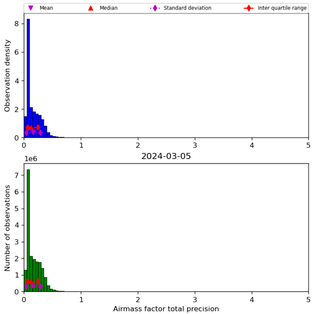
Figure 41: Histogram of “Airmass factor total precision” for 2024-03-04 to 2024-03-06
