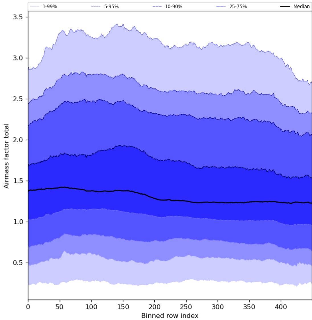
Figure 54: Along track statistics of “Airmass factor total” for 2024-03-04 to 2024-03-06
