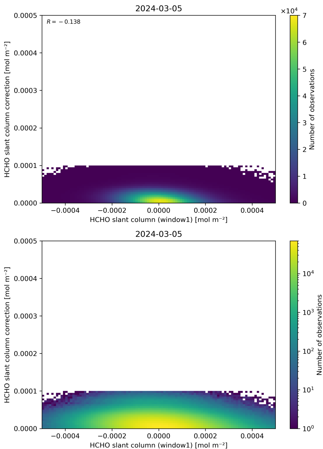
Figure 83: Scatter density plot of “HCHO slant column (window1)” against “HCHO slant column correction” for 2024-03-04 to 2024-03-06.
