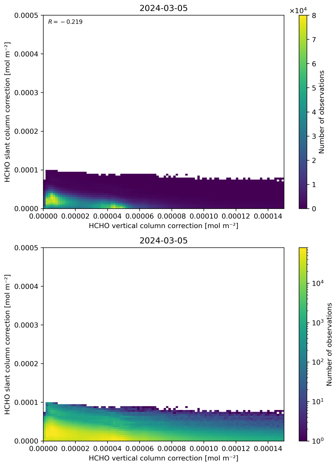
Figure 117: Scatter density plot of “HCHO vertical column correction” against “HCHO slant column correction” for 2024-03-04 to 2024-03-06.
