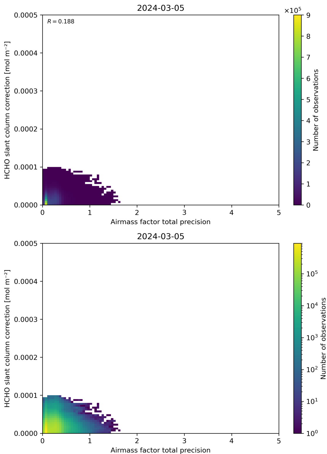
Figure 110: Scatter density plot of “Airmass factor total precision” against “HCHO slant column correction” for 2024-03-04 to 2024-03-06.
