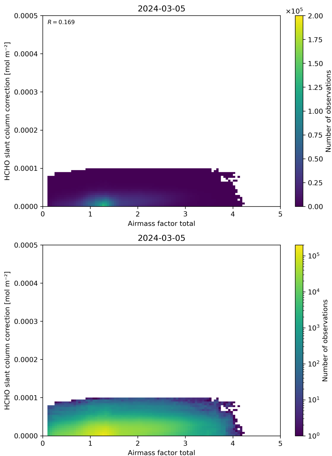
Figure 102: Scatter density plot of “Airmass factor total” against “HCHO slant column correction” for 2024-03-04 to 2024-03-06.
