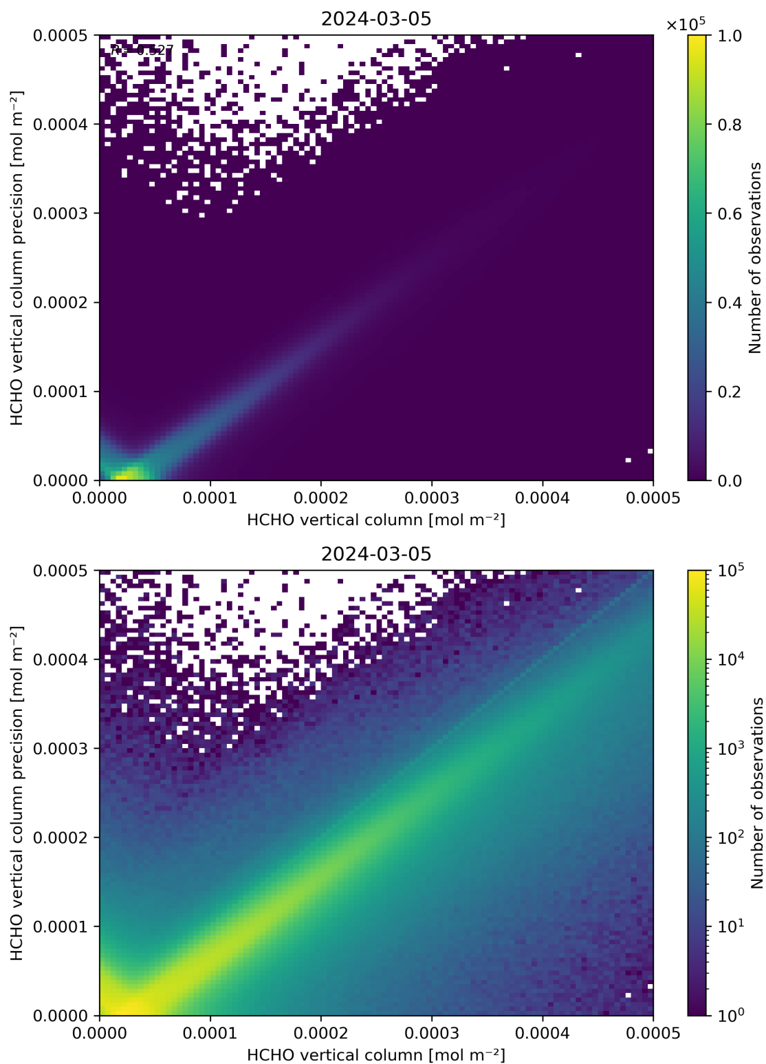
Figure 134: Scatter density plot of “HCHO vertical column” against “HCHO vertical column precision” for 2024-03-04 to 2024-03-06.
