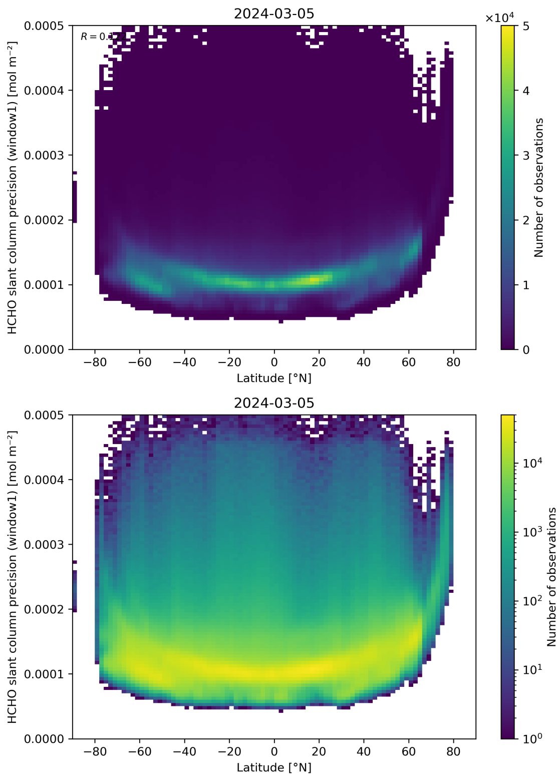
Figure 160: Scatter density plot of “Latitude” against “HCHO slant column precision (window1)” for 2024-03-04 to 2024-03-06.
