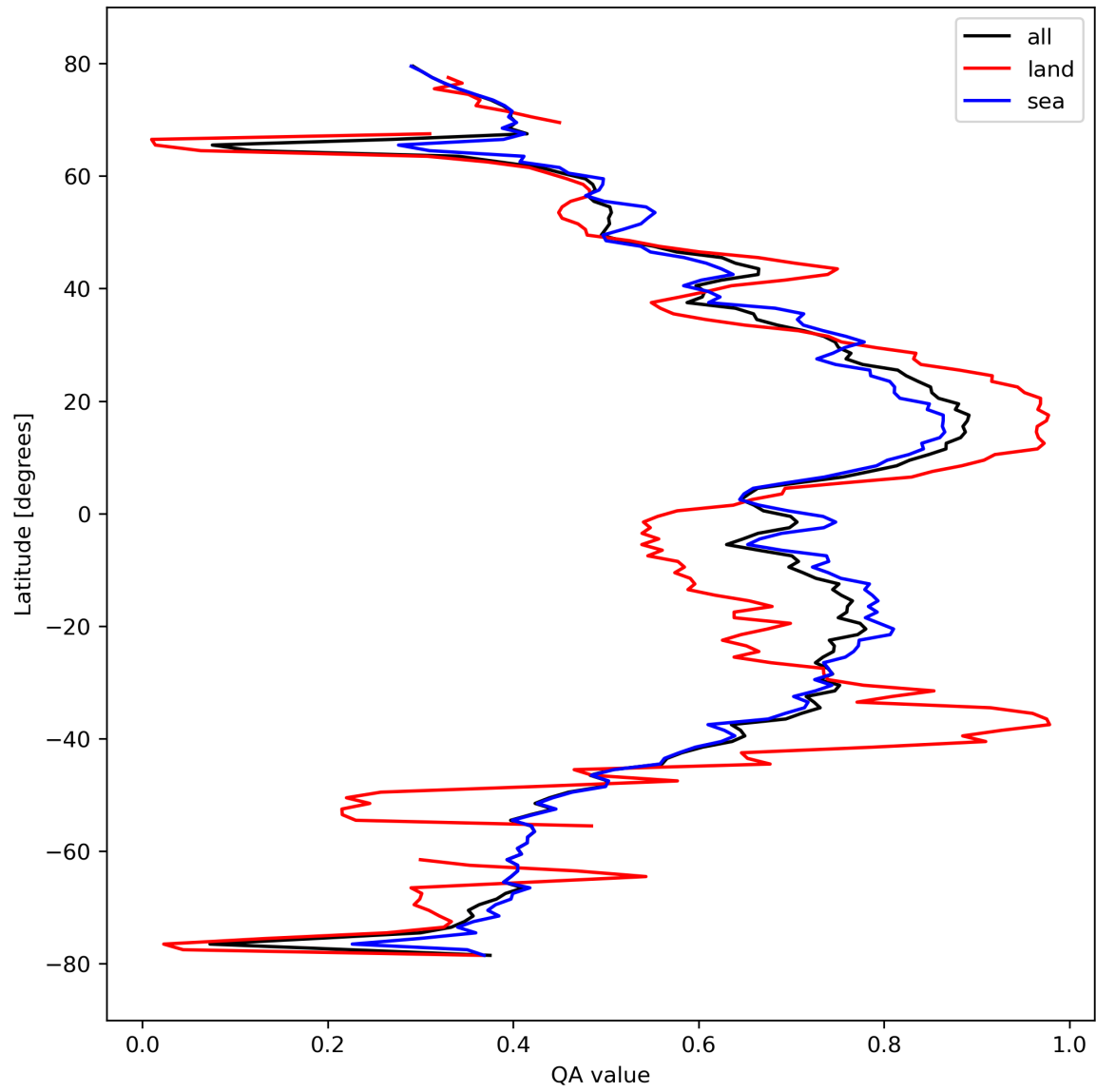
Figure 20: Zonal average of “QA value” for 2024-03-04 to 2024-03-06.
