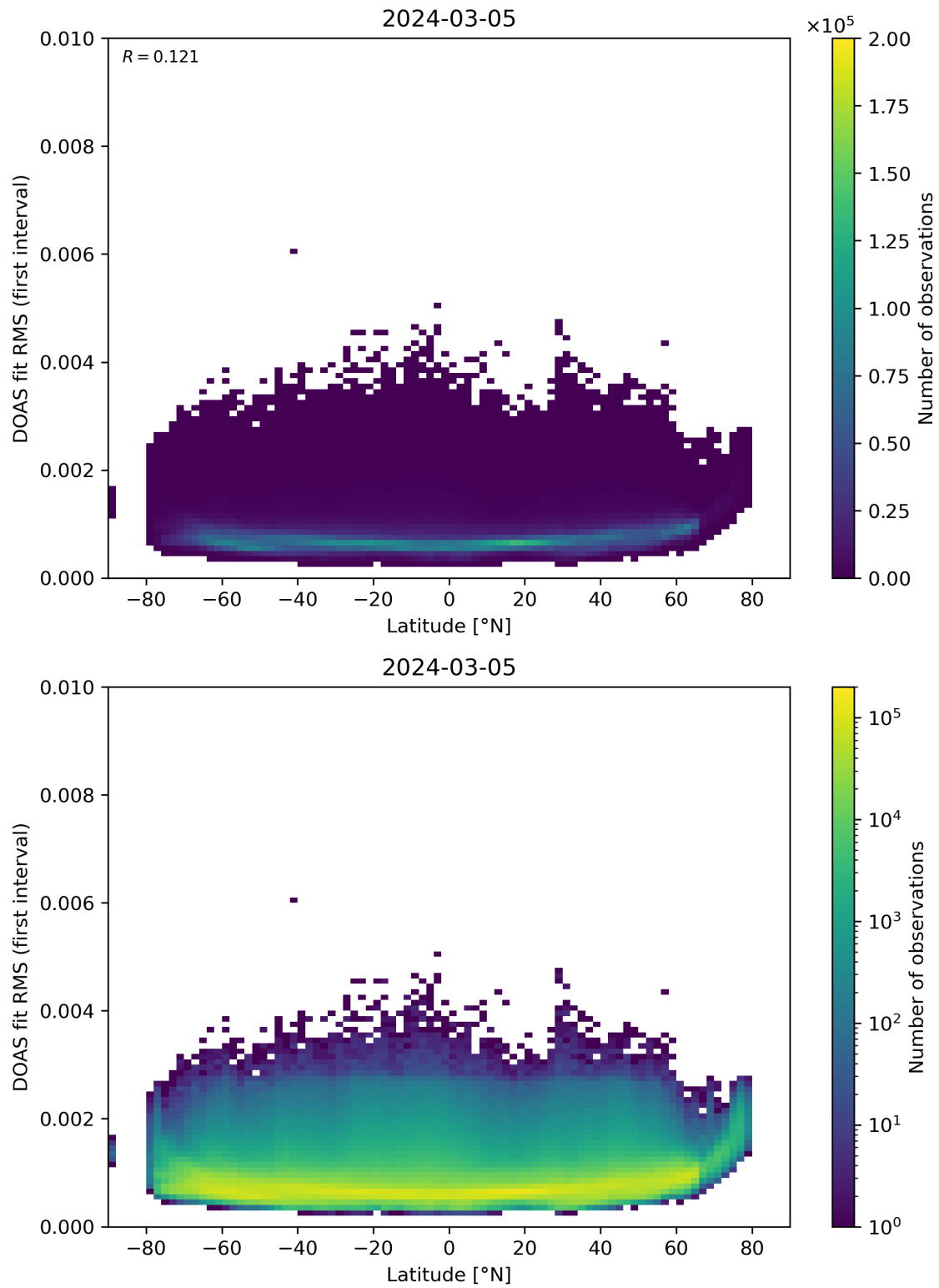
Figure 153: Scatter density plot of “Latitude” against “DOAS fit RMS (first interval)” for 2024-03-04 to 2024-03-06.
