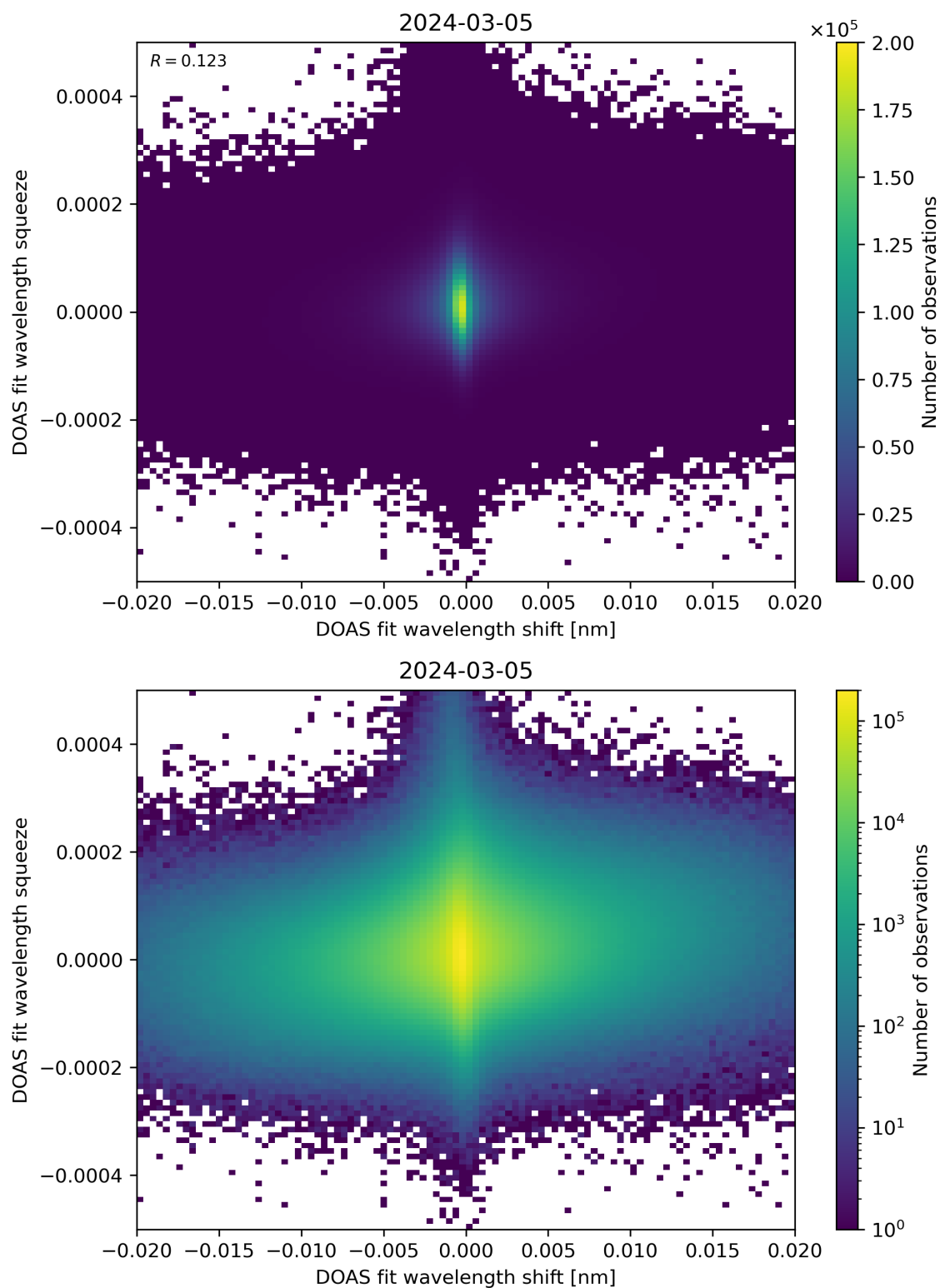
Figure 65: Scatter density plot of “DOAS fit wavelength shift” against “DOAS fit wavelength squeeze” for 2024-03-04 to 2024-03-06.
