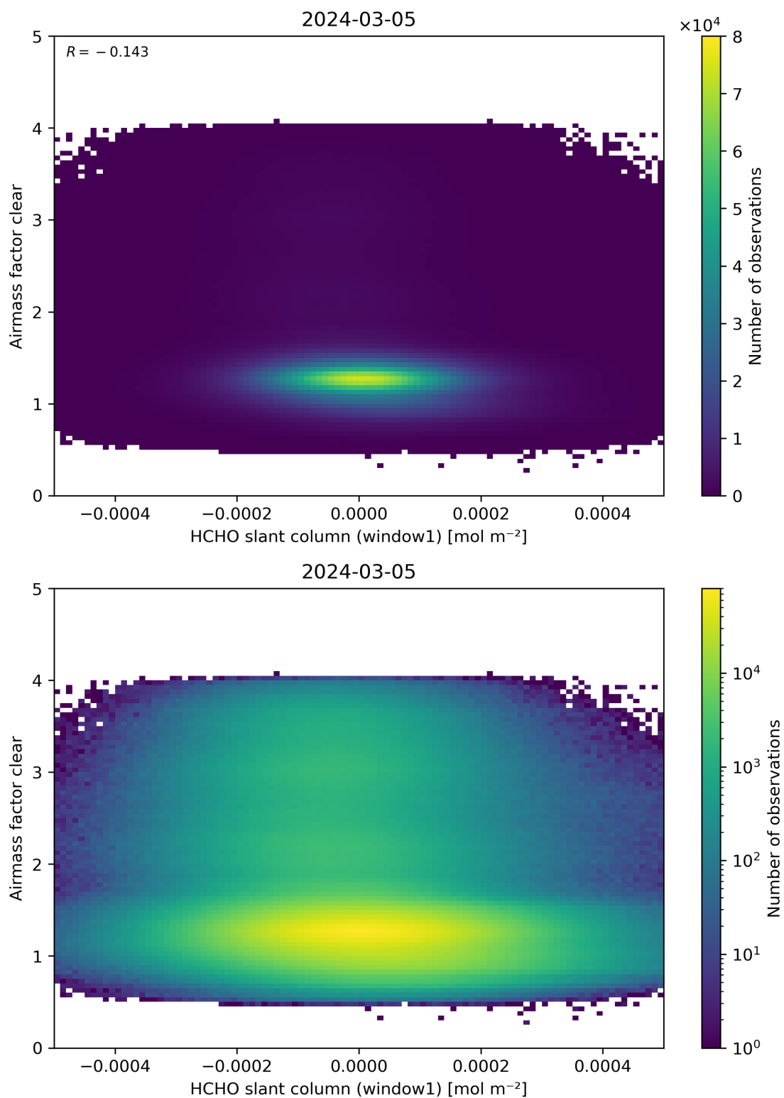
Figure 81: Scatter density plot of “HCHO slant column (window1)” against “Airmass factor clear” for 2024-03-04 to 2024-03-06.
