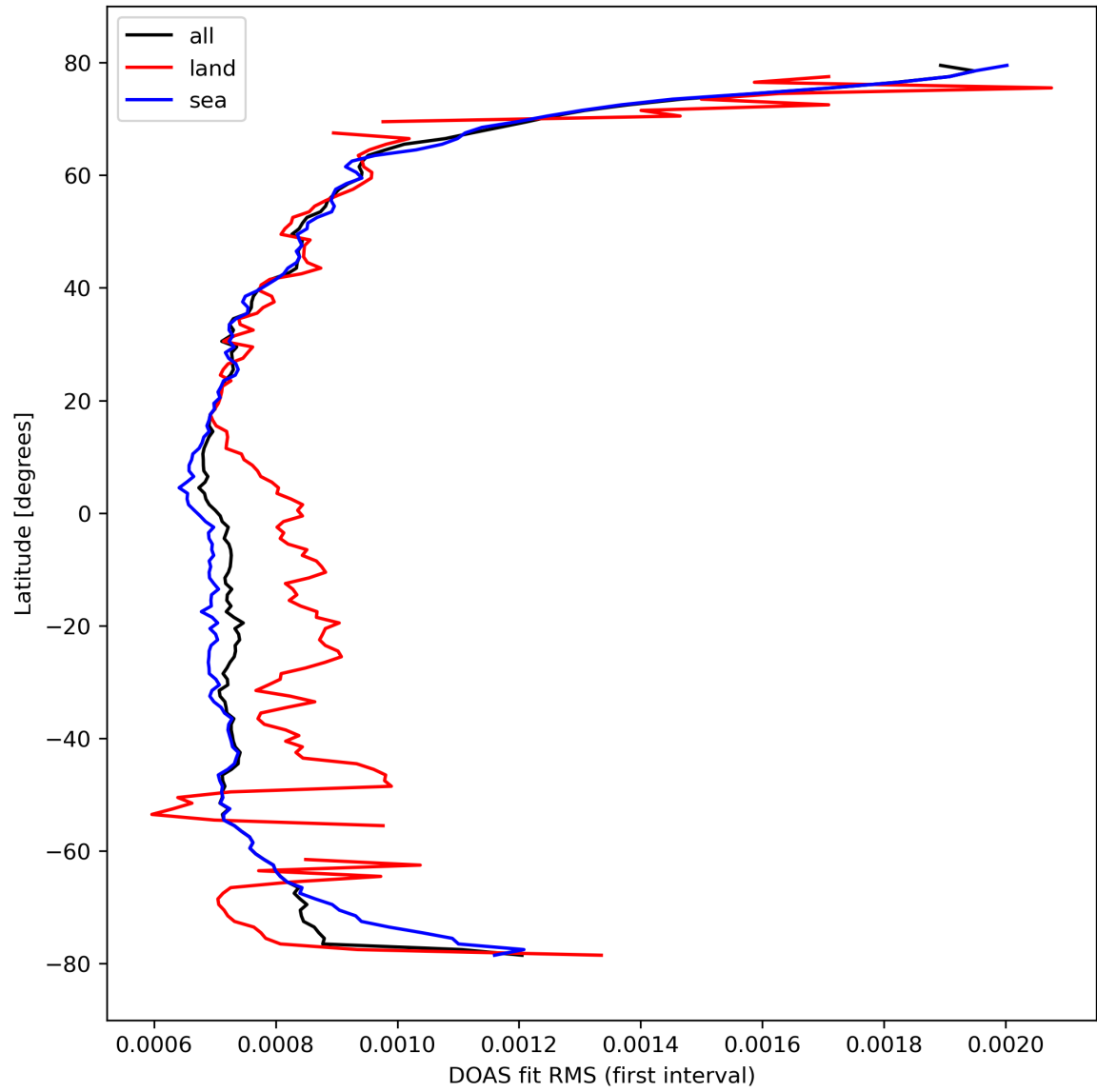
Figure 32: Zonal average of “DOAS fit RMS (first interval)” for 2024-03-04 to 2024-03-06.
