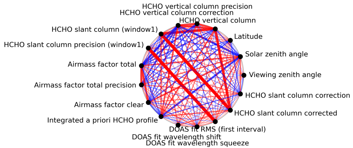
Figure 1: Map of correlation graph for 2024-03-04 to 2024-03-06.
