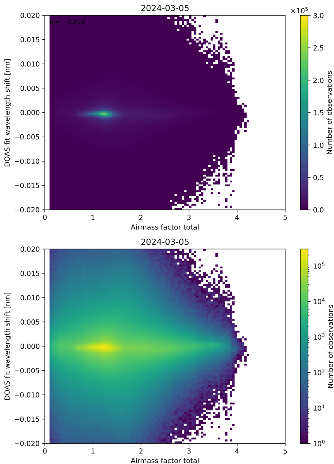
Figure 98: Scatter density plot of “Airmass factor total” against “DOAS fit wavelength shift” for 2024-03-04 to 2024-03-06.
