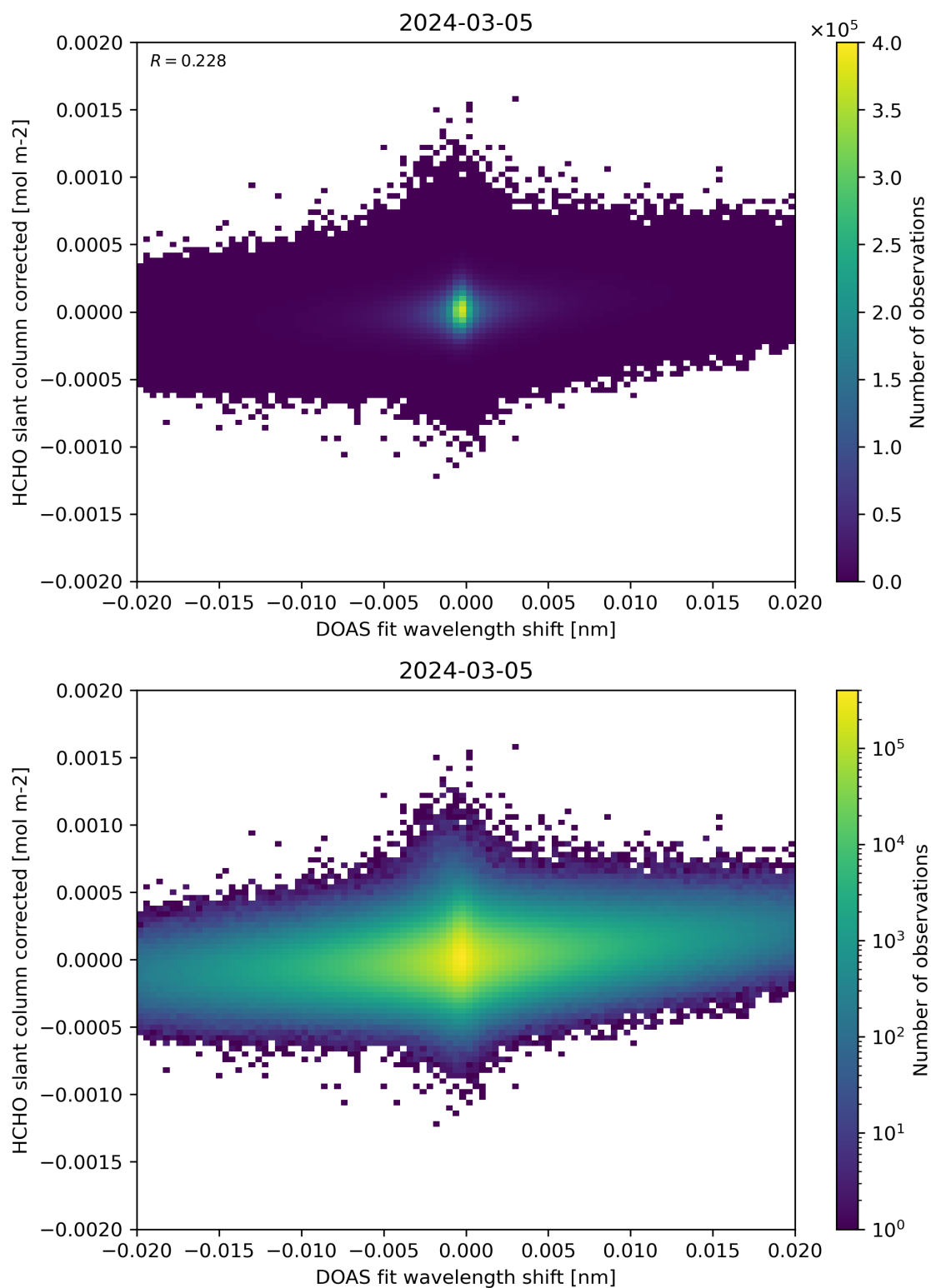
Figure 66: Scatter density plot of “DOAS fit wavelength shift” against “HCHO slant column corrected” for 2024-03-04 to 2024-03-06.
