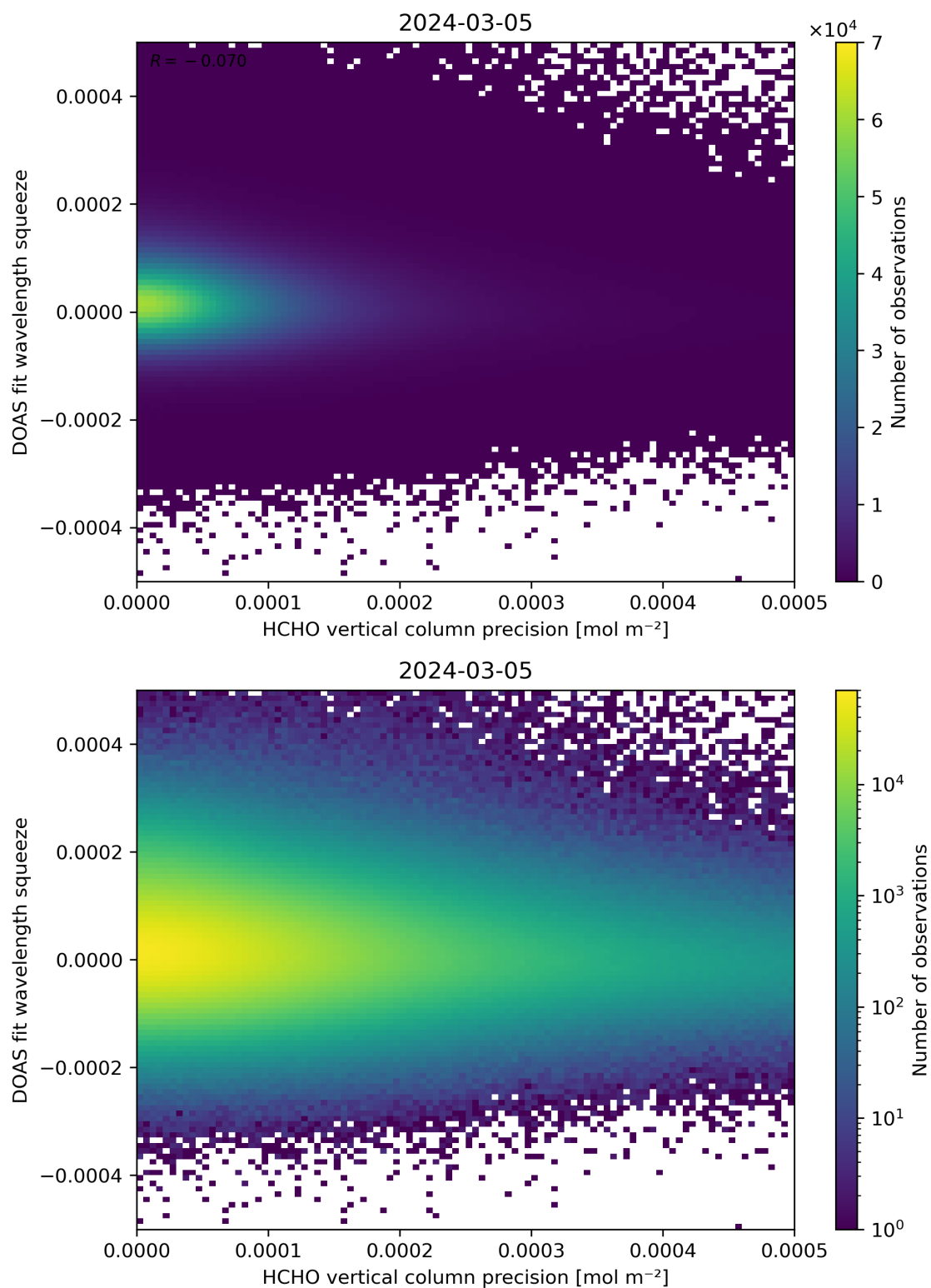
Figure 138: Scatter density plot of “HCHO vertical column precision” against “DOAS fit wavelength squeeze” for 2024-03-04 to 2024-03-06.
