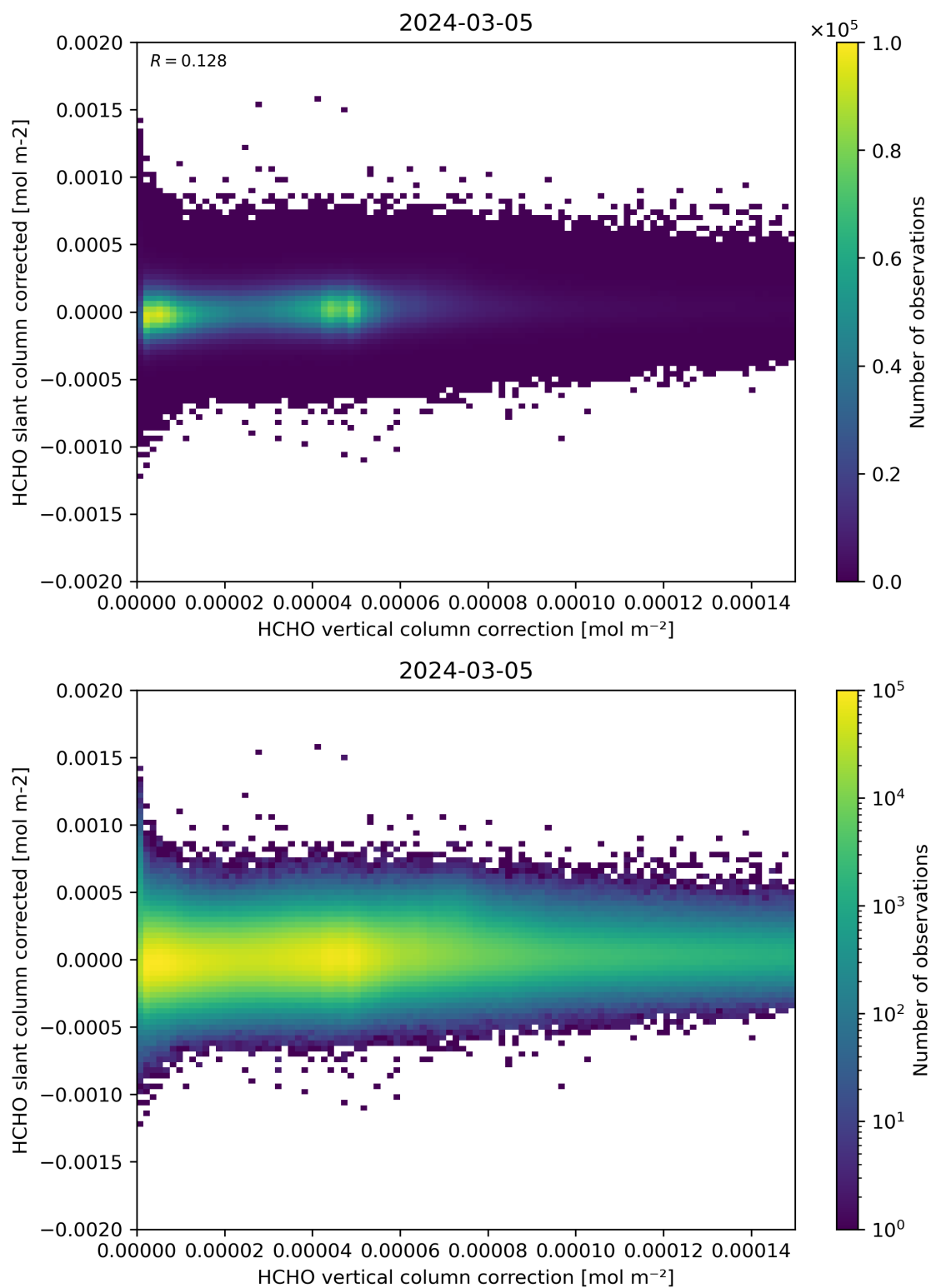
Figure 116: Scatter density plot of “HCHO vertical column correction” against “HCHO slant column corrected” for 2024-03-04 to 2024-03-06.
