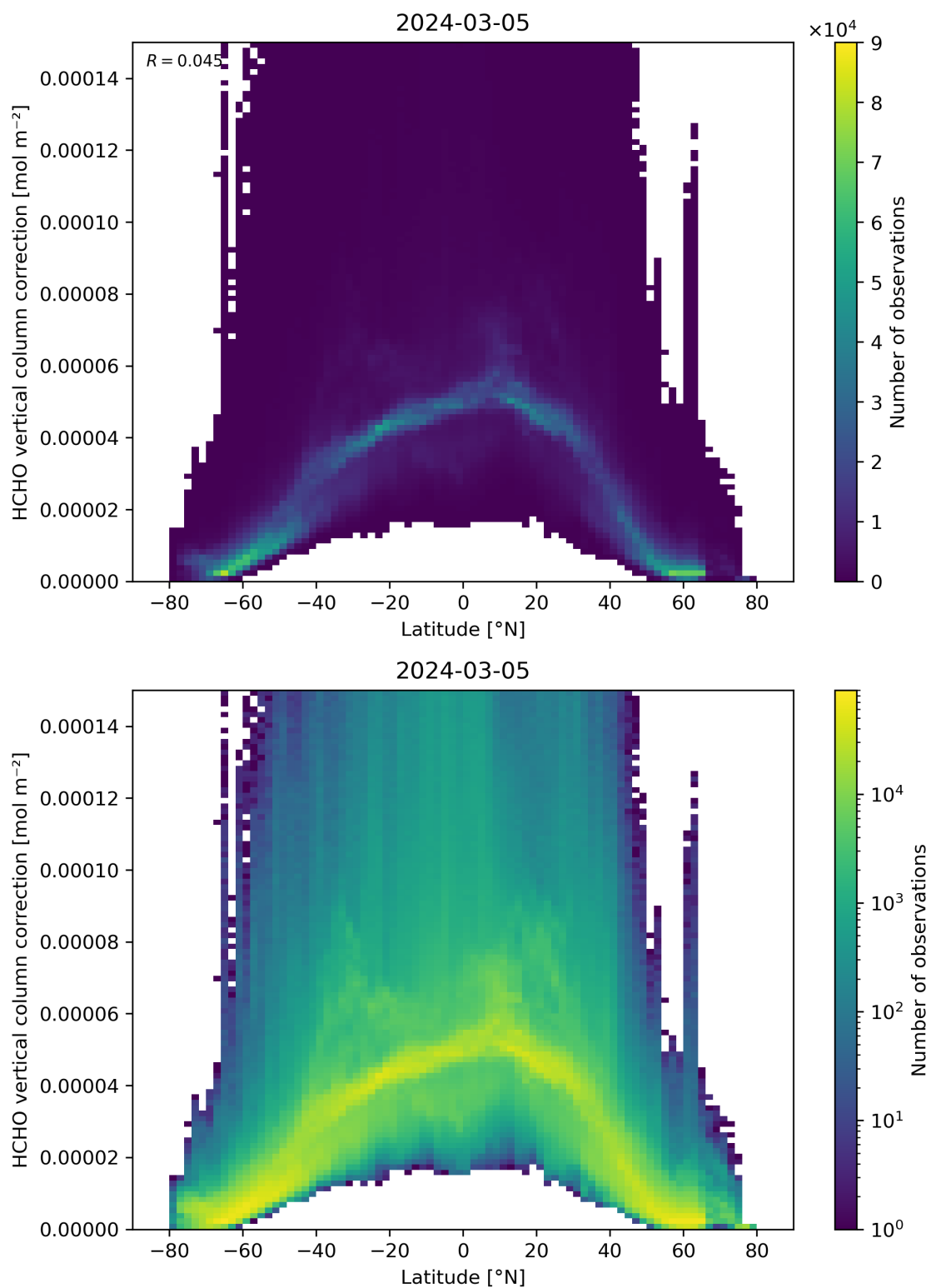
Figure 164: Scatter density plot of “Latitude” against “HCHO vertical column correction” for 2024-03-04 to 2024-03-06.
