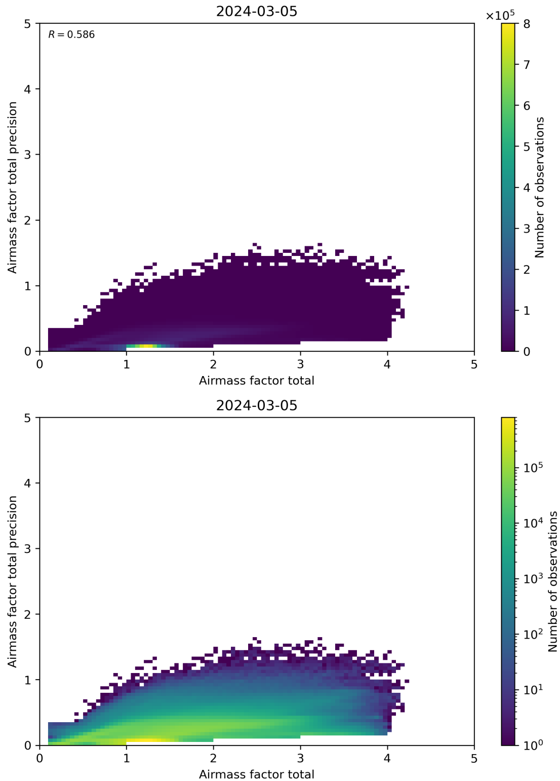
Figure 103: Scatter density plot of “Airmass factor total” against “Airmass factor total precision” for 2024-03-04 to 2024-03-06.
