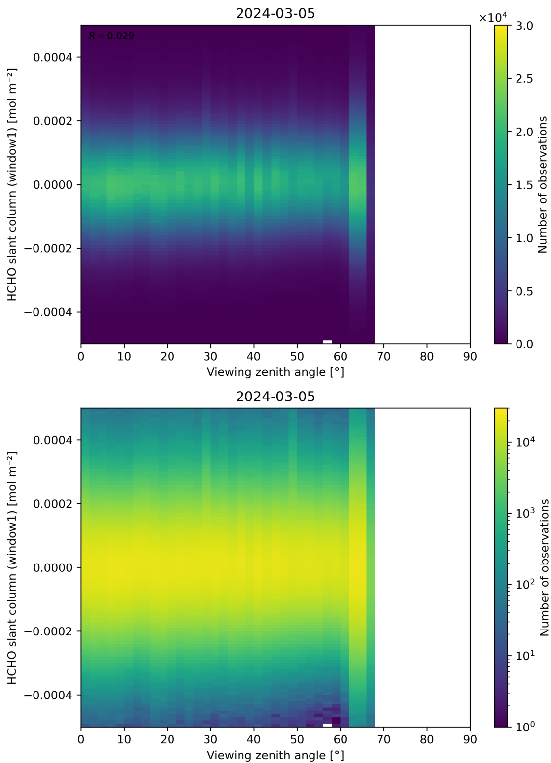
Figure 188: Scatter density plot of “Viewing zenith angle” against “HCHO slant column (window1)” for 2024-03-04 to 2024-03-06.
