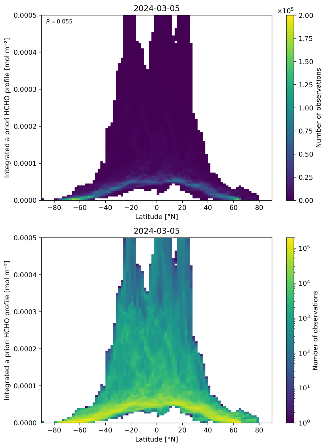
Figure 166: Scatter density plot of “Latitude” against “Integrated a priori HCHO profile” for 2024-03-04 to 2024-03-06.
