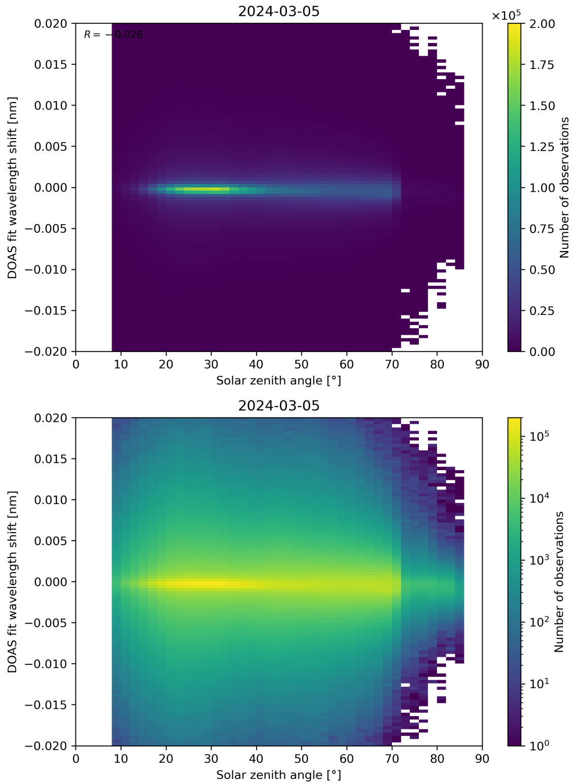
Figure 168: Scatter density plot of “Solar zenith angle” against “DOAS fit wavelength shift” for 2024-03-04 to 2024-03-06.
