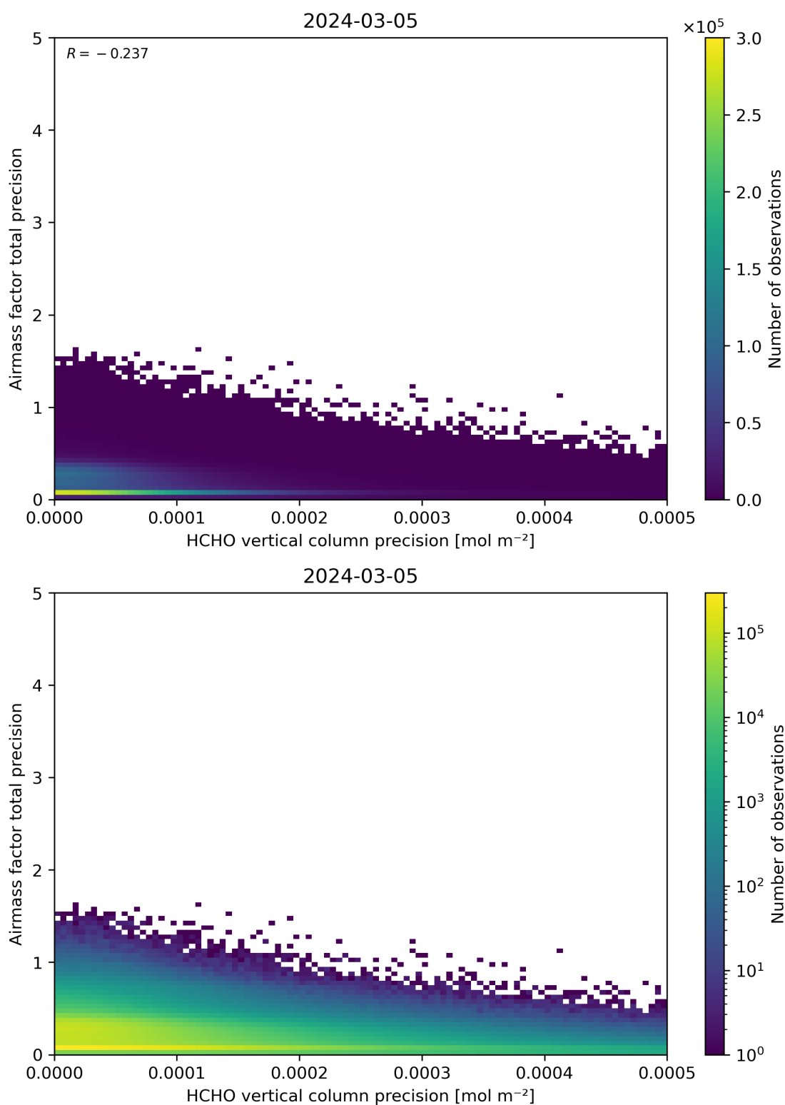
Figure 145: Scatter density plot of “HCHO vertical column precision” against “Airmass factor total precision” for 2024-03-04 to 2024-03-06.
