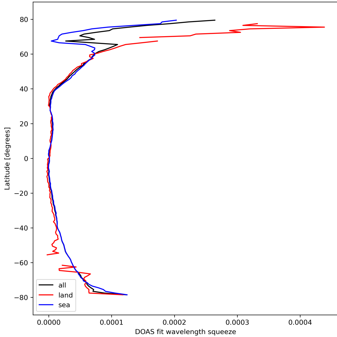
Figure 31: Zonal average of “DOAS fit wavelength squeeze” for 2024-03-04 to 2024-03-06.
