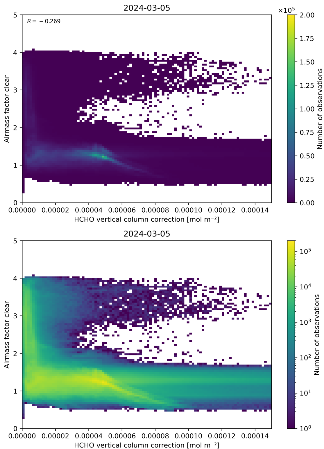
Figure 115: Scatter density plot of “HCHO vertical column correction” against “Airmass factor clear” for 2024-03-04 to 2024-03-06.
