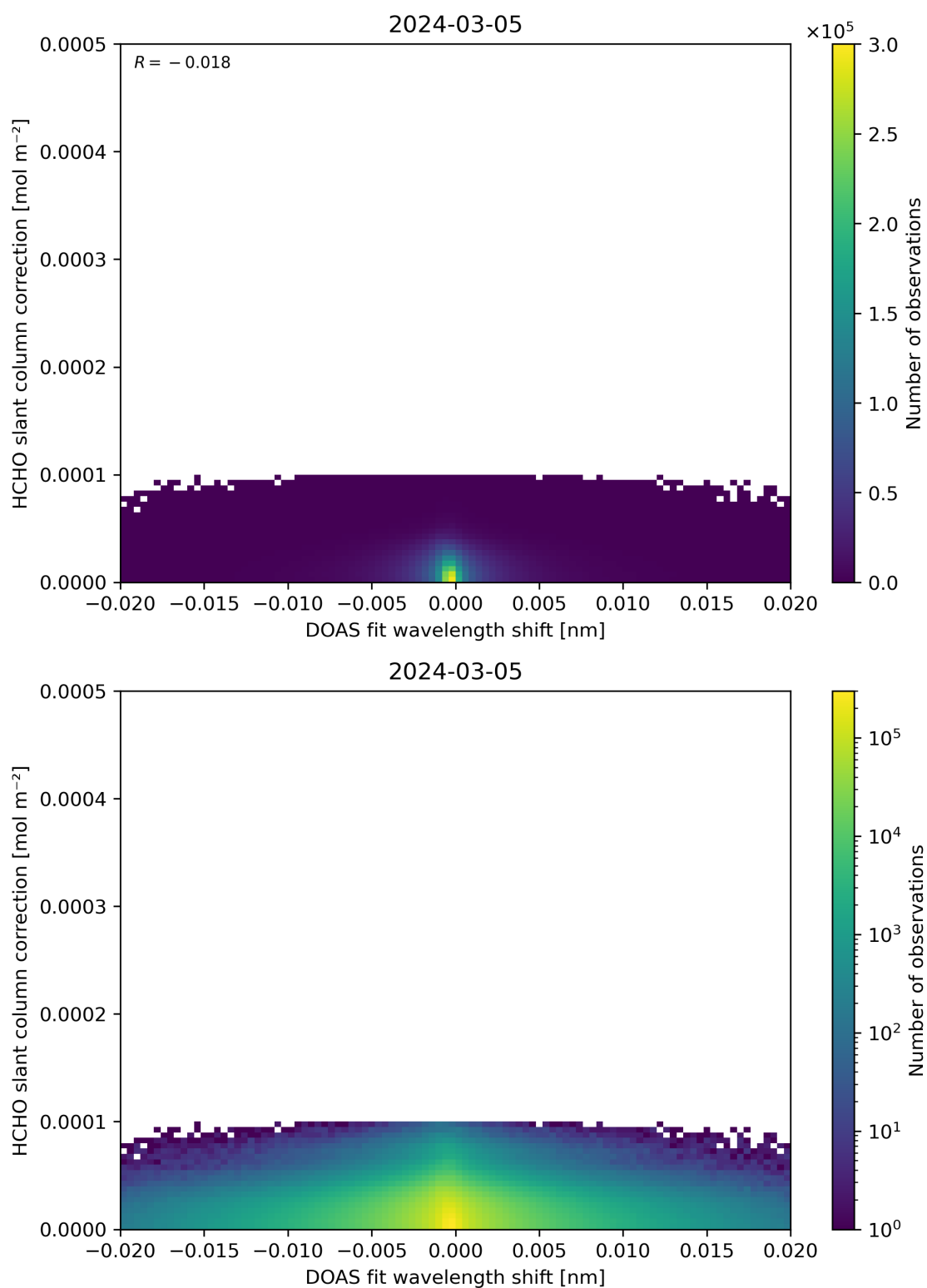
Figure 67: Scatter density plot of “DOAS fit wavelength shift” against “HCHO slant column correction” for 2024-03-04 to 2024-03-06.
