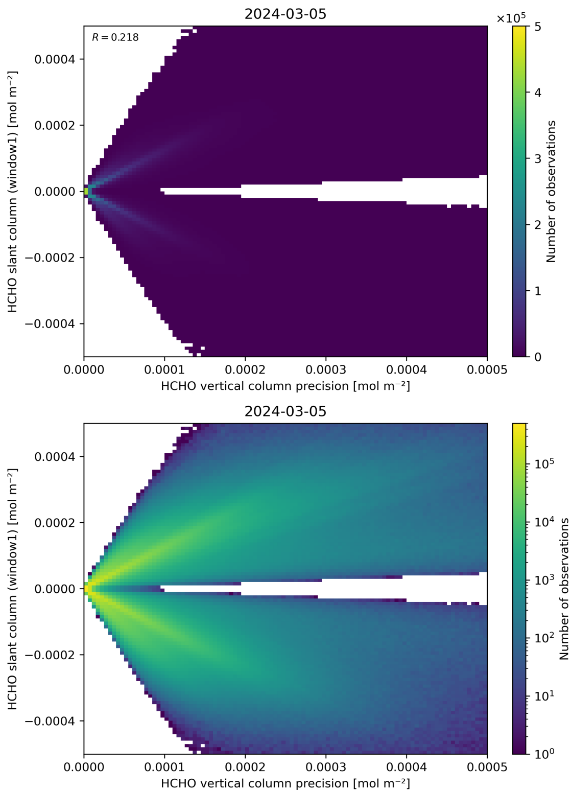
Figure 142: Scatter density plot of “HCHO vertical column precision” against “HCHO slant column (window1)” for 2024-03-04 to 2024-03-06.
