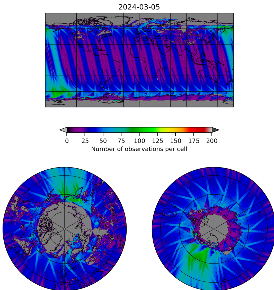
Figure 19: Map of the number of observations for 2024-03-04 to 2024-03-06
