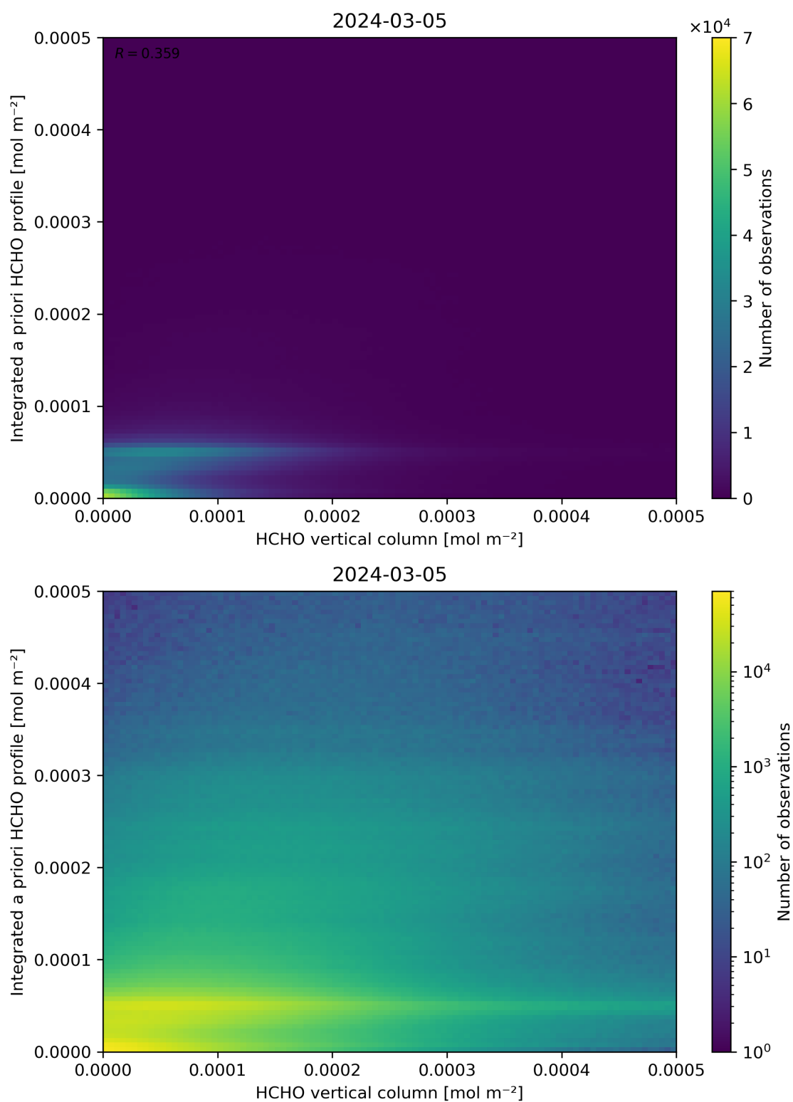
Figure 135: Scatter density plot of “HCHO vertical column” against “Integrated a priori HCHO profile” for 2024-03-04 to 2024-03-06.
