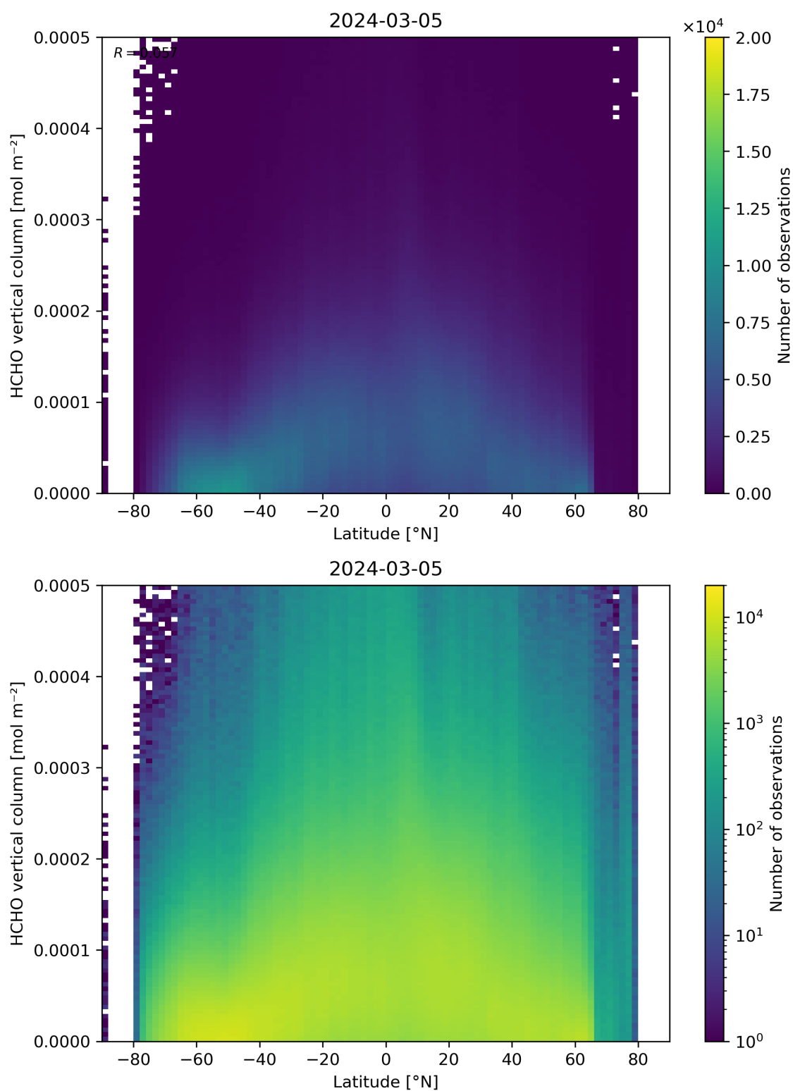
Figure 163: Scatter density plot of “Latitude” against “HCHO vertical column” for 2024-03-04 to 2024-03-06.
