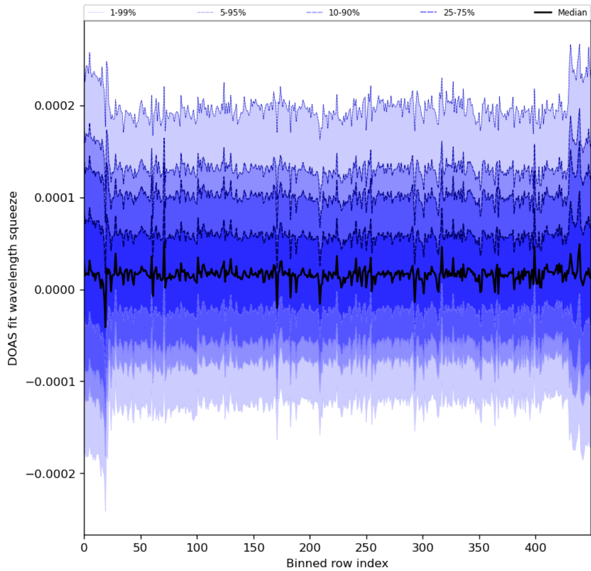
Figure 59: Along track statistics of “DOAS fit wavelength squeeze” for 2024-03-04 to 2024-03-06
