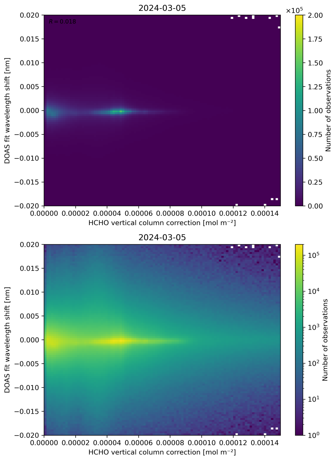
Figure 113: Scatter density plot of “HCHO vertical column correction” against “DOAS fit wavelength shift” for 2024-03-04 to 2024-03-06.
