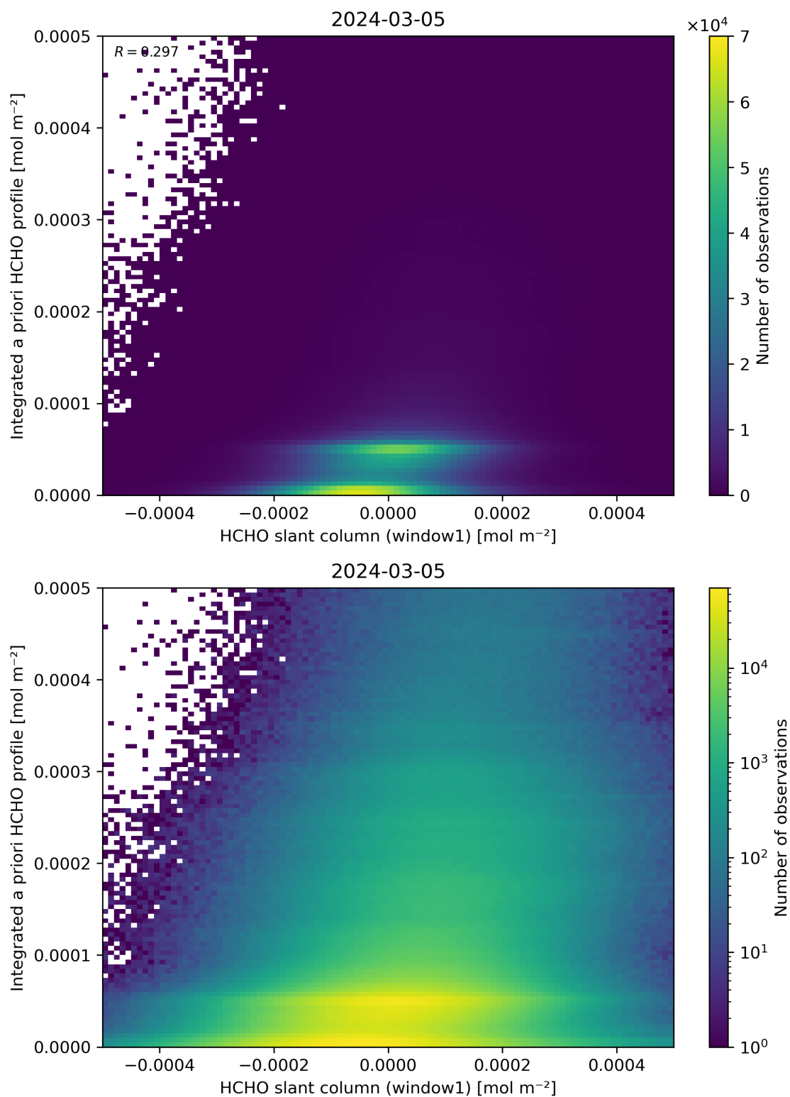
Figure 87: Scatter density plot of “HCHO slant column (window1)” against “Integrated a priori HCHO profile” for 2024-03-04 to 2024-03-06.
