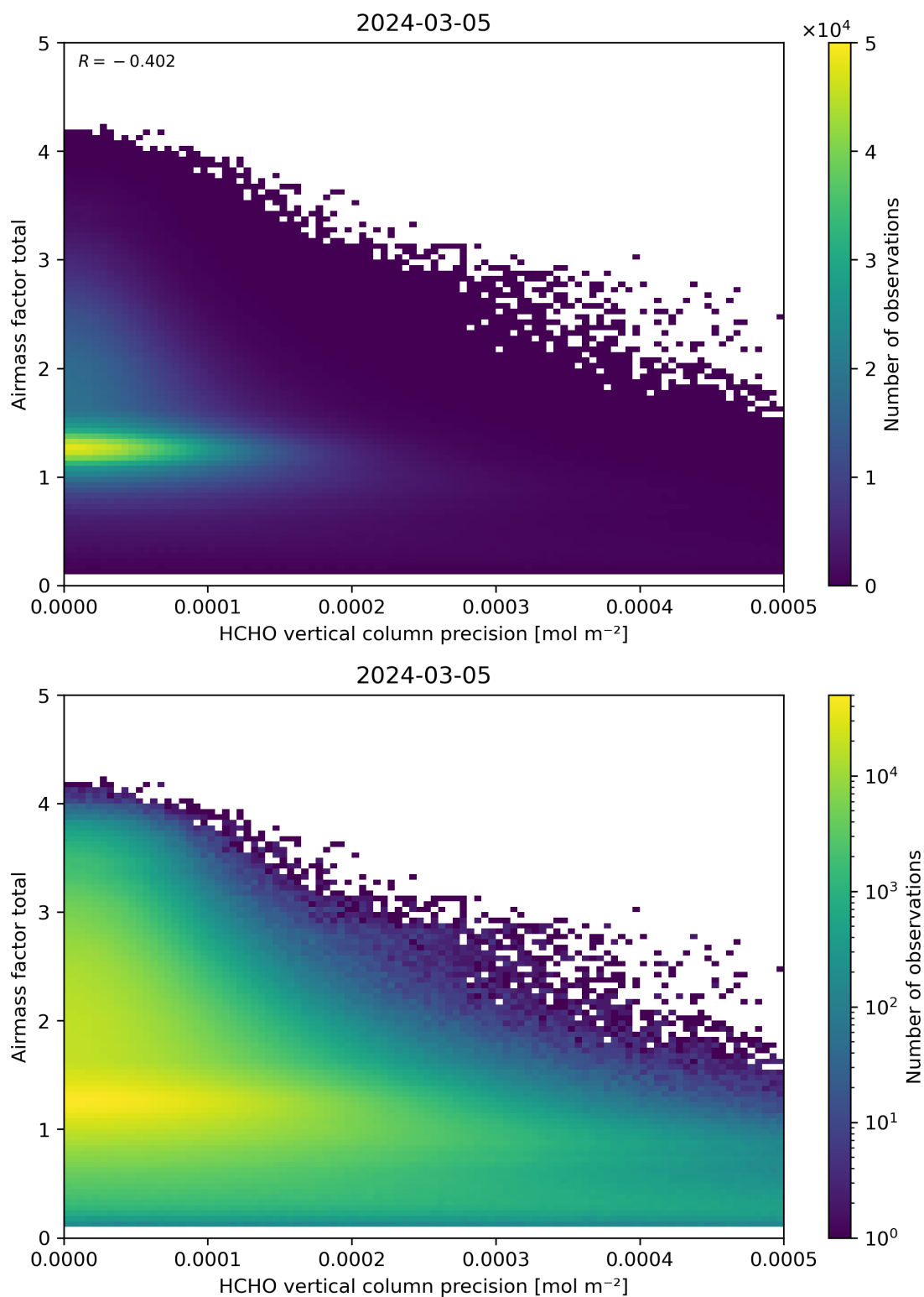
Figure 144: Scatter density plot of “HCHO vertical column precision” against “Airmass factor total” for 2024-03-04 to 2024-03-06.
