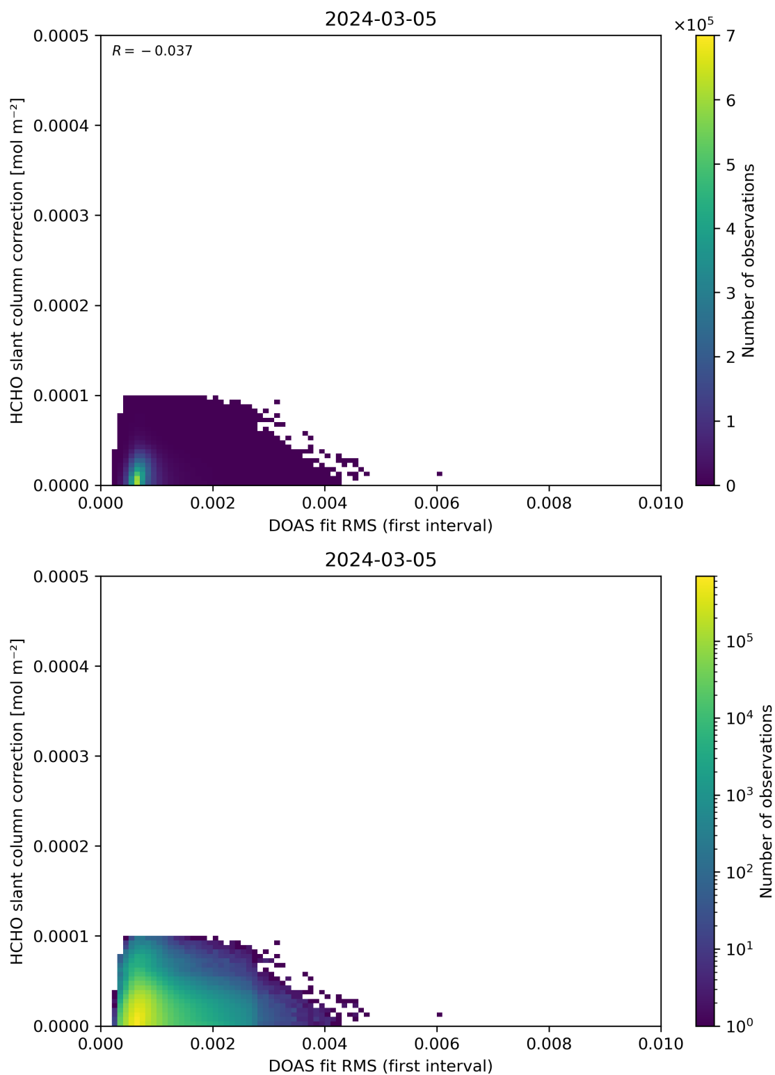
Figure 63: Scatter density plot of “DOAS fit RMS (first interval)” against “HCHO slant column correction” for 2024-03-04 to 2024-03-06.
