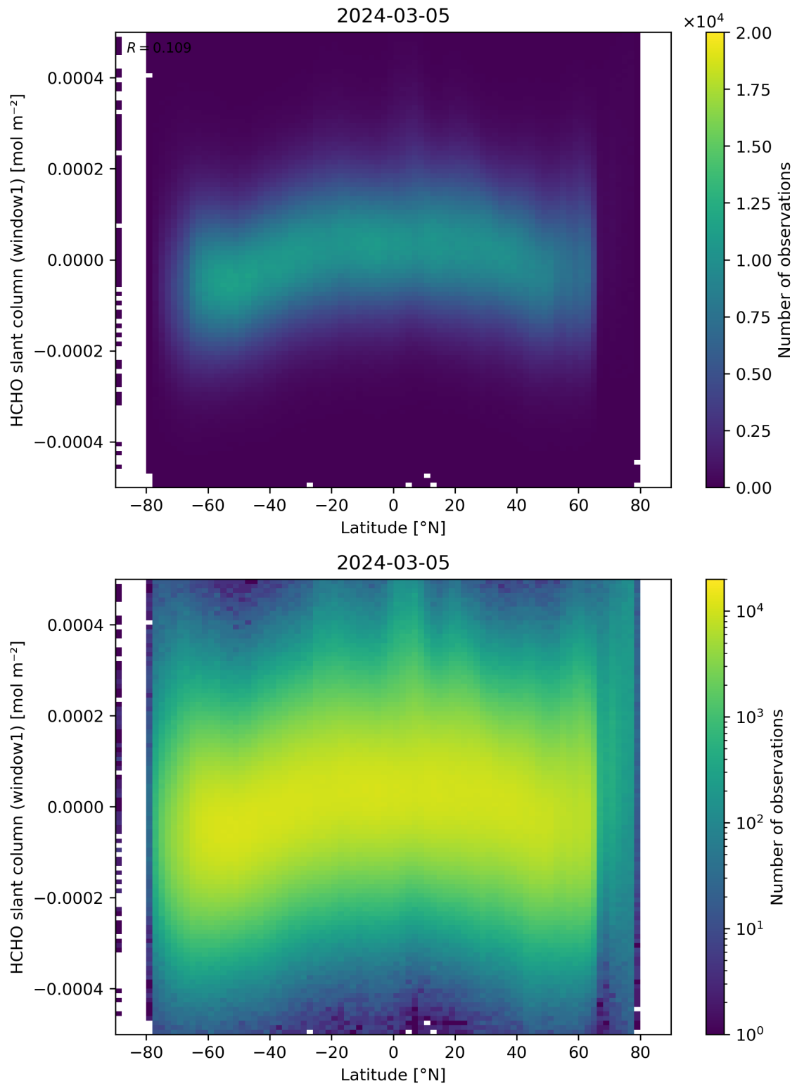
Figure 159: Scatter density plot of “Latitude” against “HCHO slant column (window1)” for 2024-03-04 to 2024-03-06.
