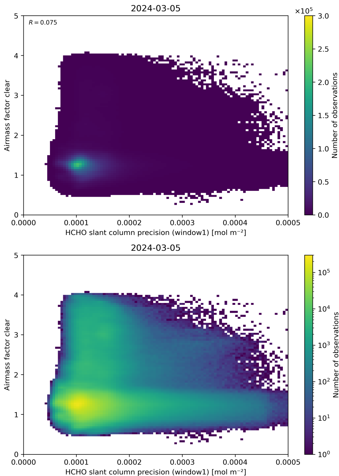
Figure 91: Scatter density plot of “HCHO slant column precision (window1)” against “Airmass factor clear” for 2024-03-04 to 2024-03-06.
