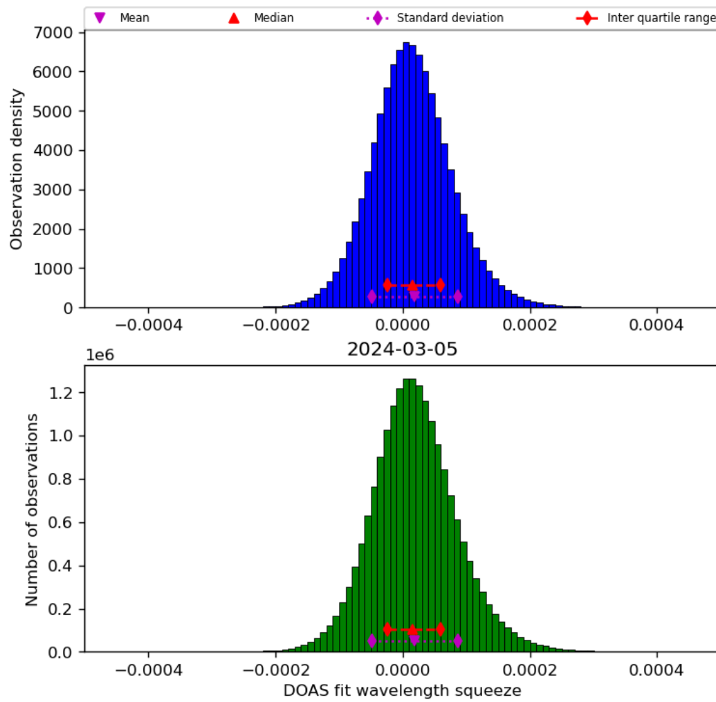
Figure 45: Histogram of “DOAS fit wavelength squeeze” for 2024-03-04 to 2024-03-06
