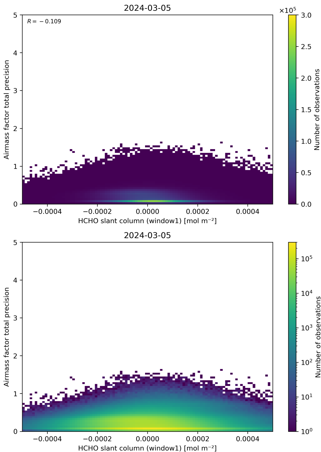
Figure 86: Scatter density plot of “HCHO slant column (window1)” against “Airmass factor total precision” for 2024-03-04 to 2024-03-06.
