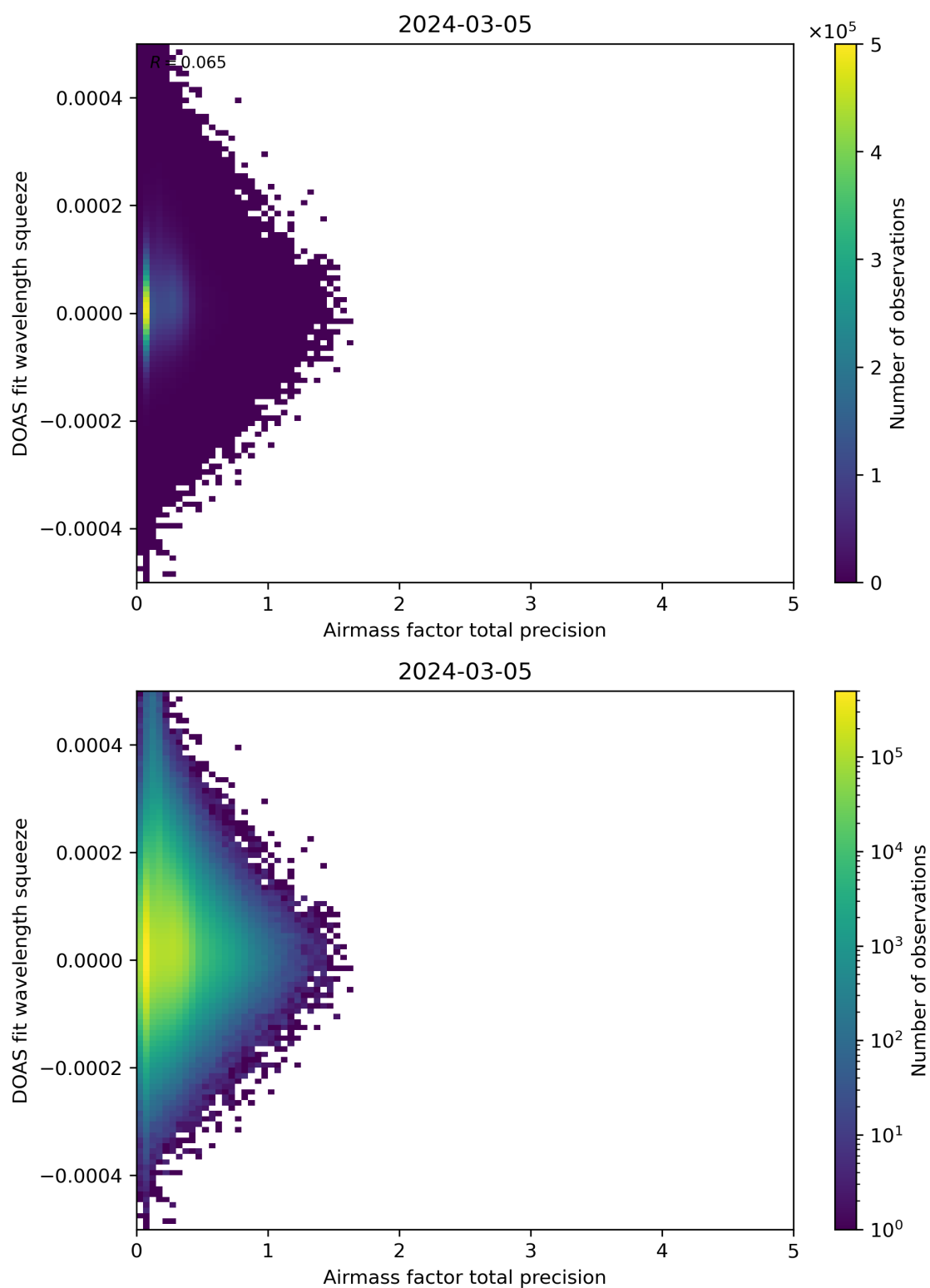
Figure 107: Scatter density plot of “Airmass factor total precision” against “DOAS fit wavelength squeeze” for 2024-03-04 to 2024-03-06.
