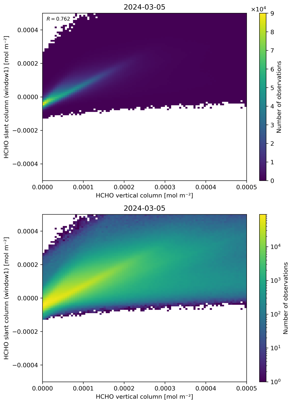
Figure 129: Scatter density plot of “HCHO vertical column” against “HCHO slant column (window1)” for 2024-03-04 to 2024-03-06.
