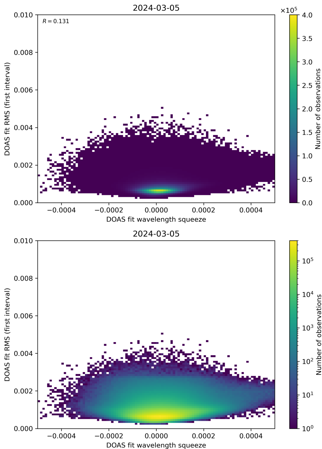
Figure 68: Scatter density plot of “DOAS fit wavelength squeeze” against “DOAS fit RMS (first interval)” for 2024-03-04 to 2024-03-06.
