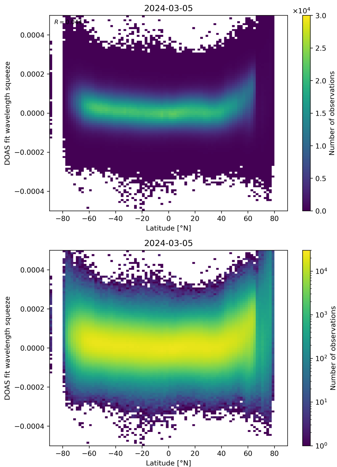
Figure 155: Scatter density plot of “Latitude” against “DOAS fit wavelength squeeze” for 2024-03-04 to 2024-03-06.
