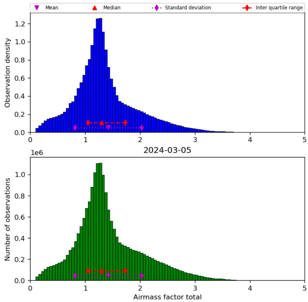
Figure 40: Histogram of “Airmass factor total” for 2024-03-04 to 2024-03-06
