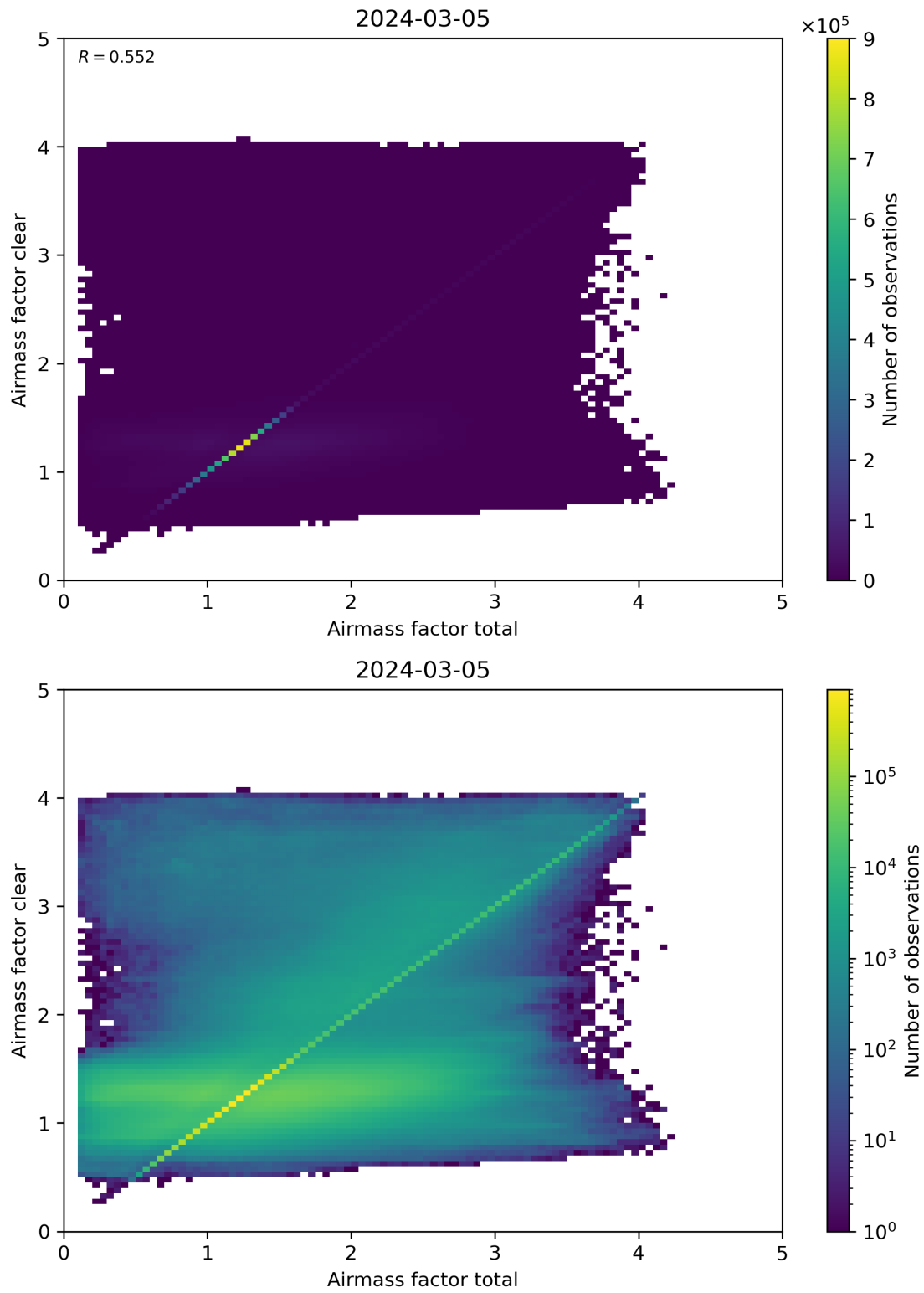
Figure 100: Scatter density plot of “Airmass factor total” against “Airmass factor clear” for 2024-03-04 to 2024-03-06.
