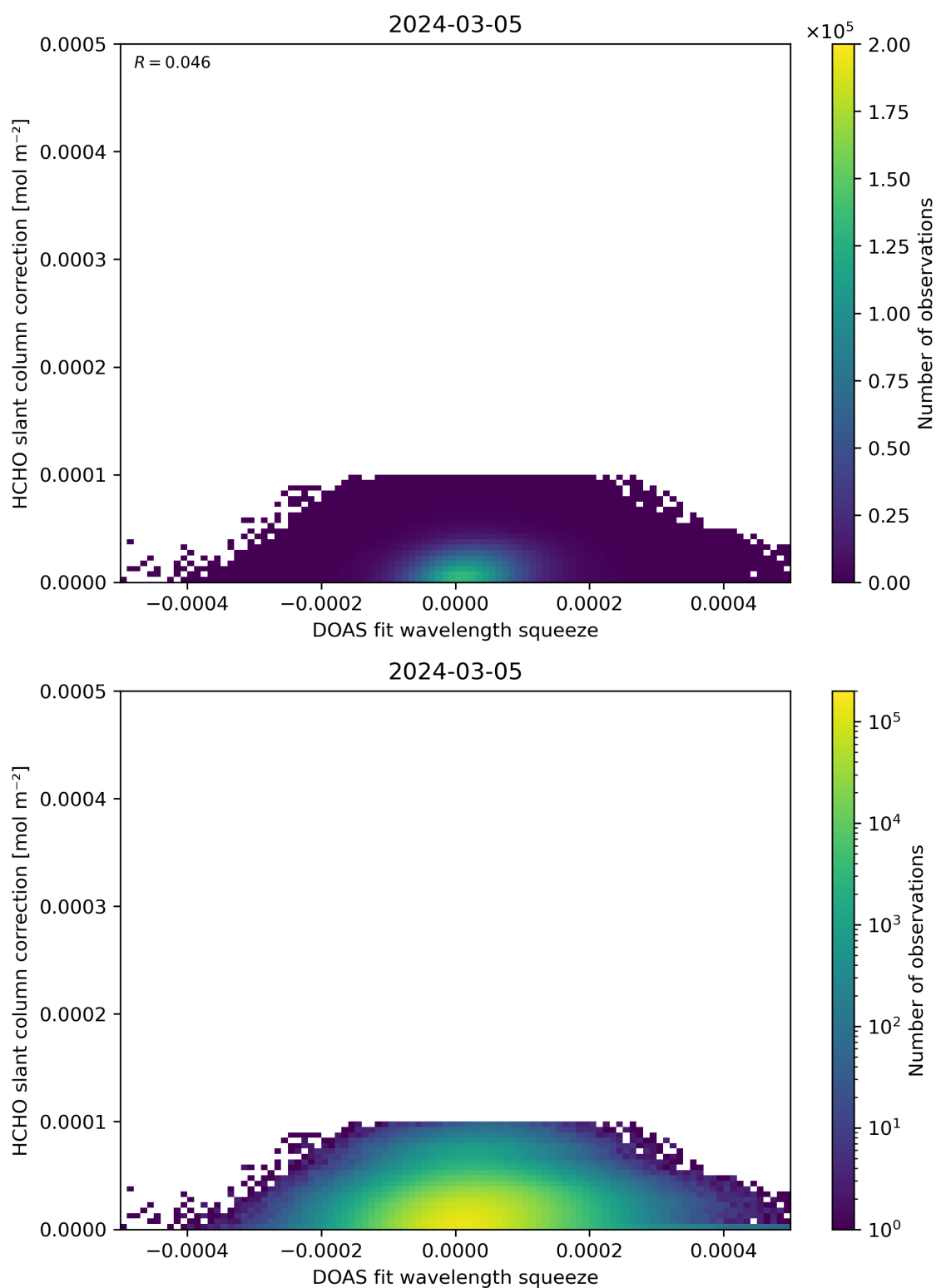
Figure 70: Scatter density plot of “DOAS fit wavelength squeeze” against “HCHO slant column correction” for 2024-03-04 to 2024-03-06.
