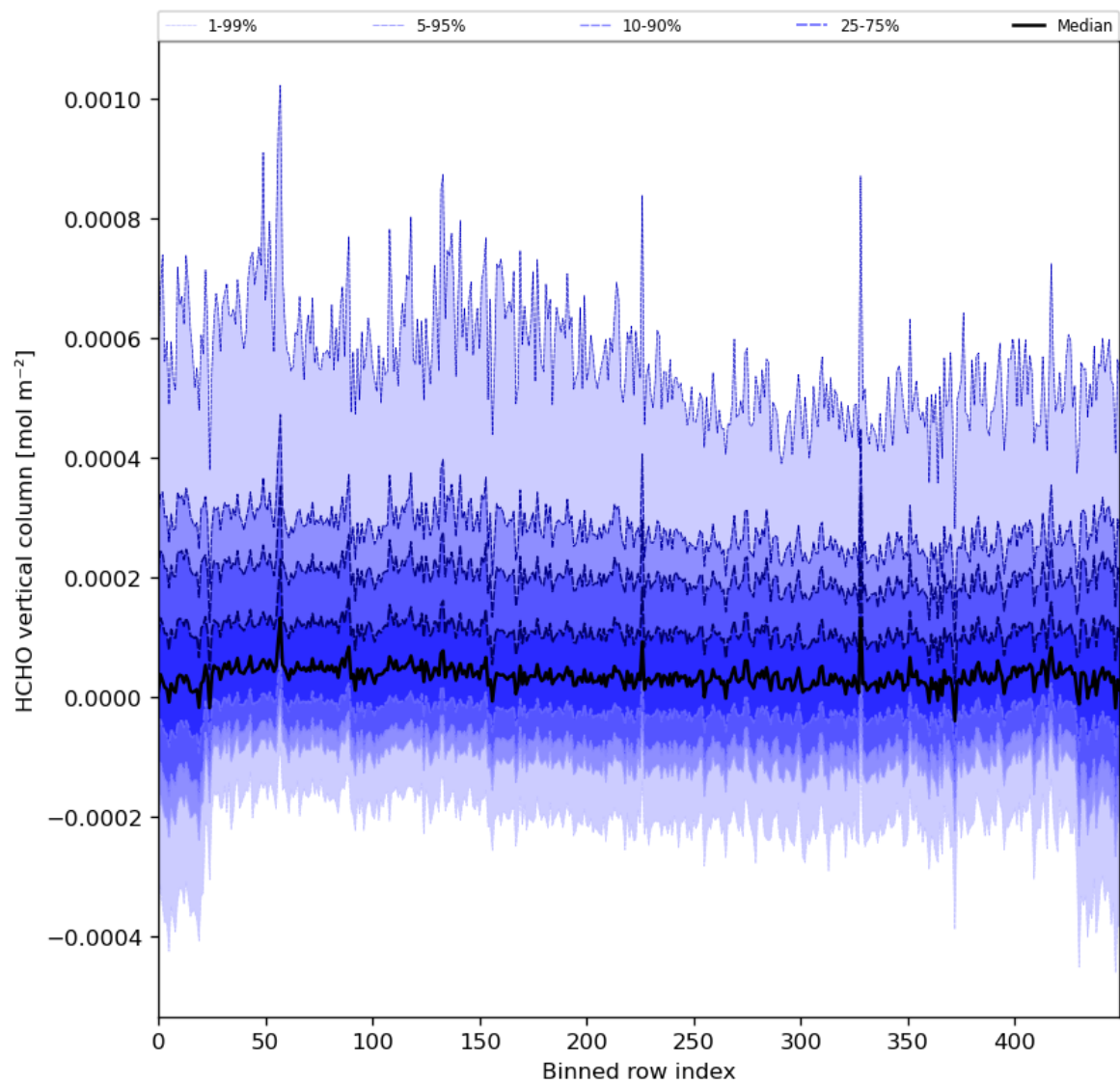
Figure 49: Along track statistics of “HCHO vertical column” for 2024-03-04 to 2024-03-06
