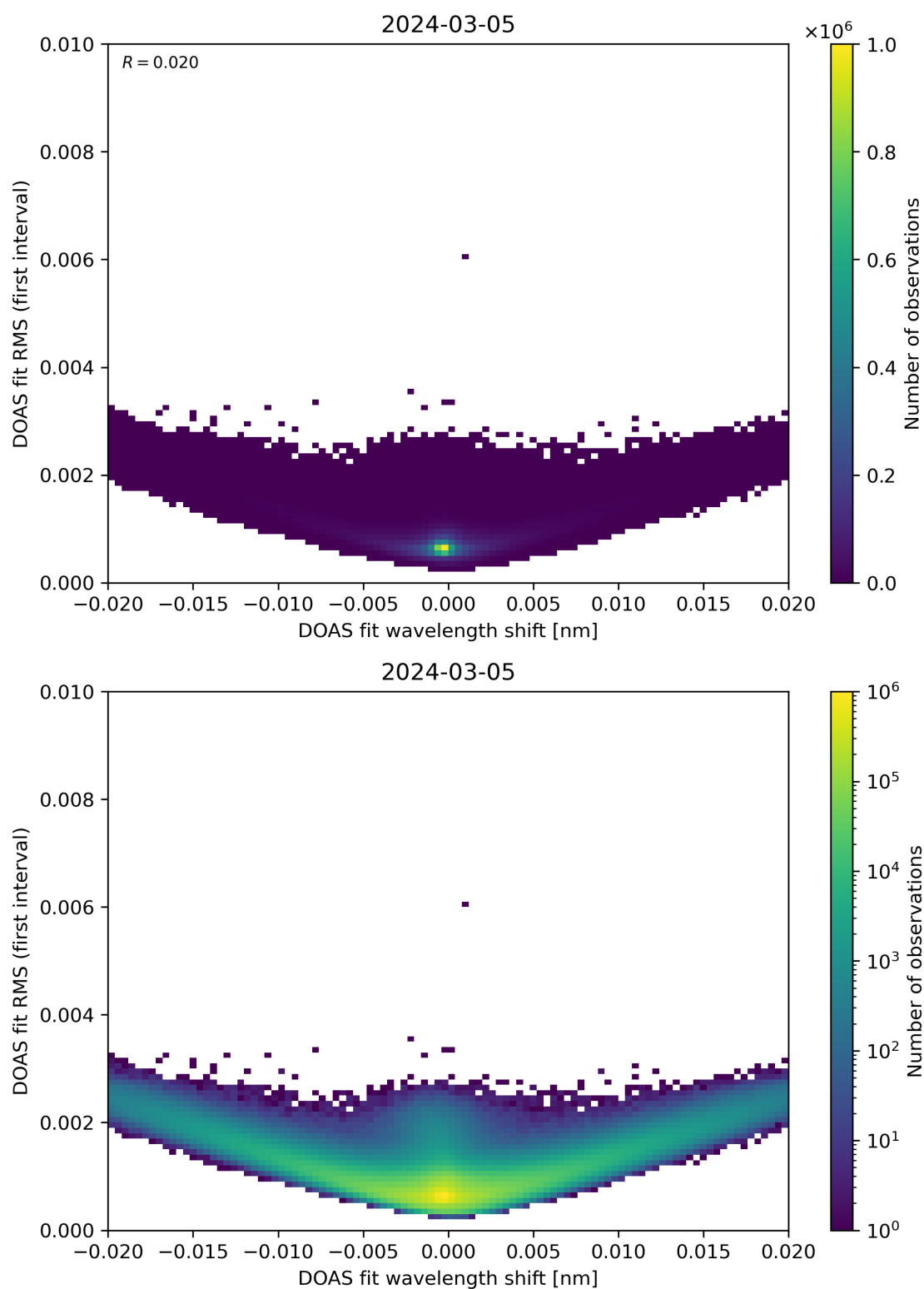
Figure 64: Scatter density plot of “DOAS fit wavelength shift” against “DOAS fit RMS (first interval)” for 2024-03-04 to 2024-03-06.
