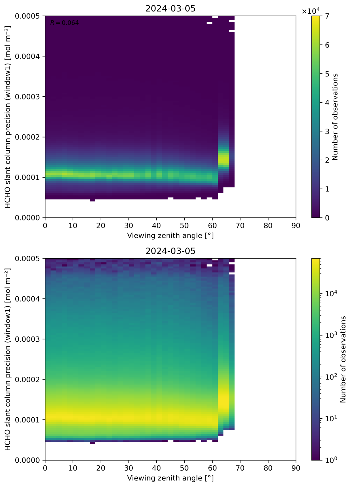
Figure 189: Scatter density plot of “Viewing zenith angle” against “HCHO slant column precision (window1)” for 2024-03-04 to 2024-03-06.
