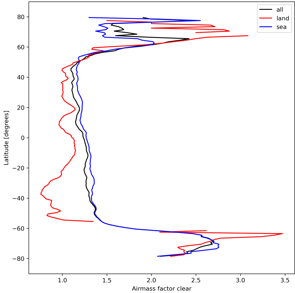
Figure 28: Zonal average of “Airmass factor clear” for 2024-03-04 to 2024-03-06.
