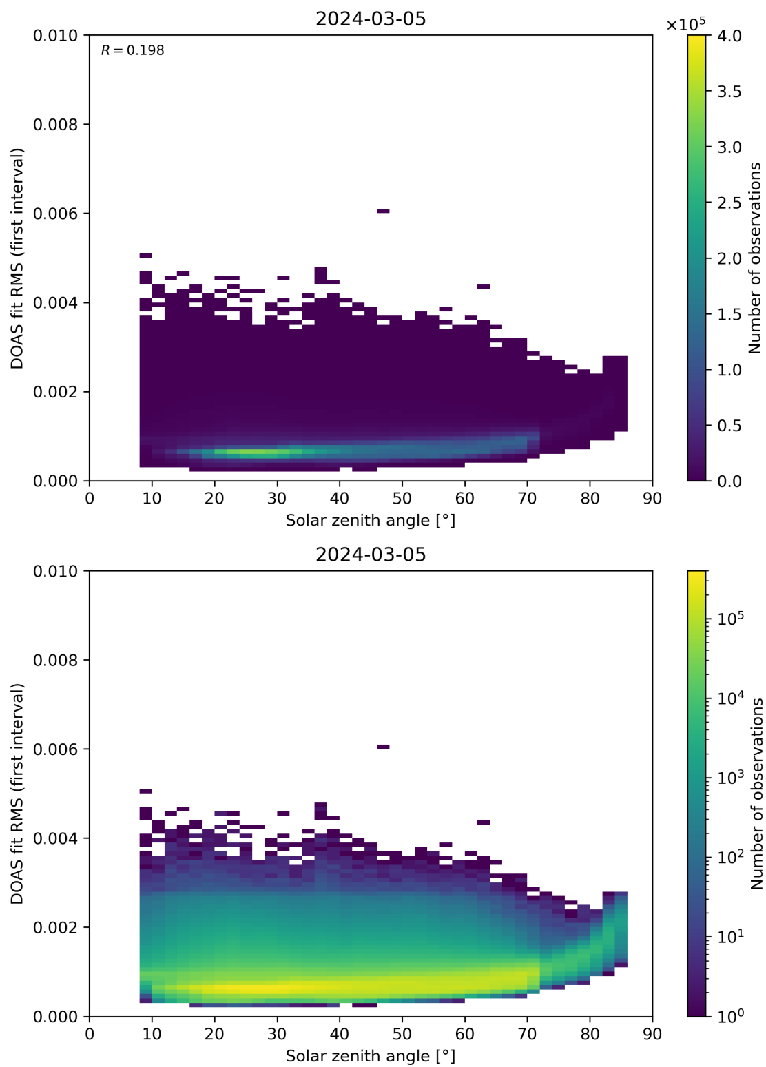
Figure 167: Scatter density plot of “Solar zenith angle” against “DOAS fit RMS (first interval)” for 2024-03-04 to 2024-03-06.
