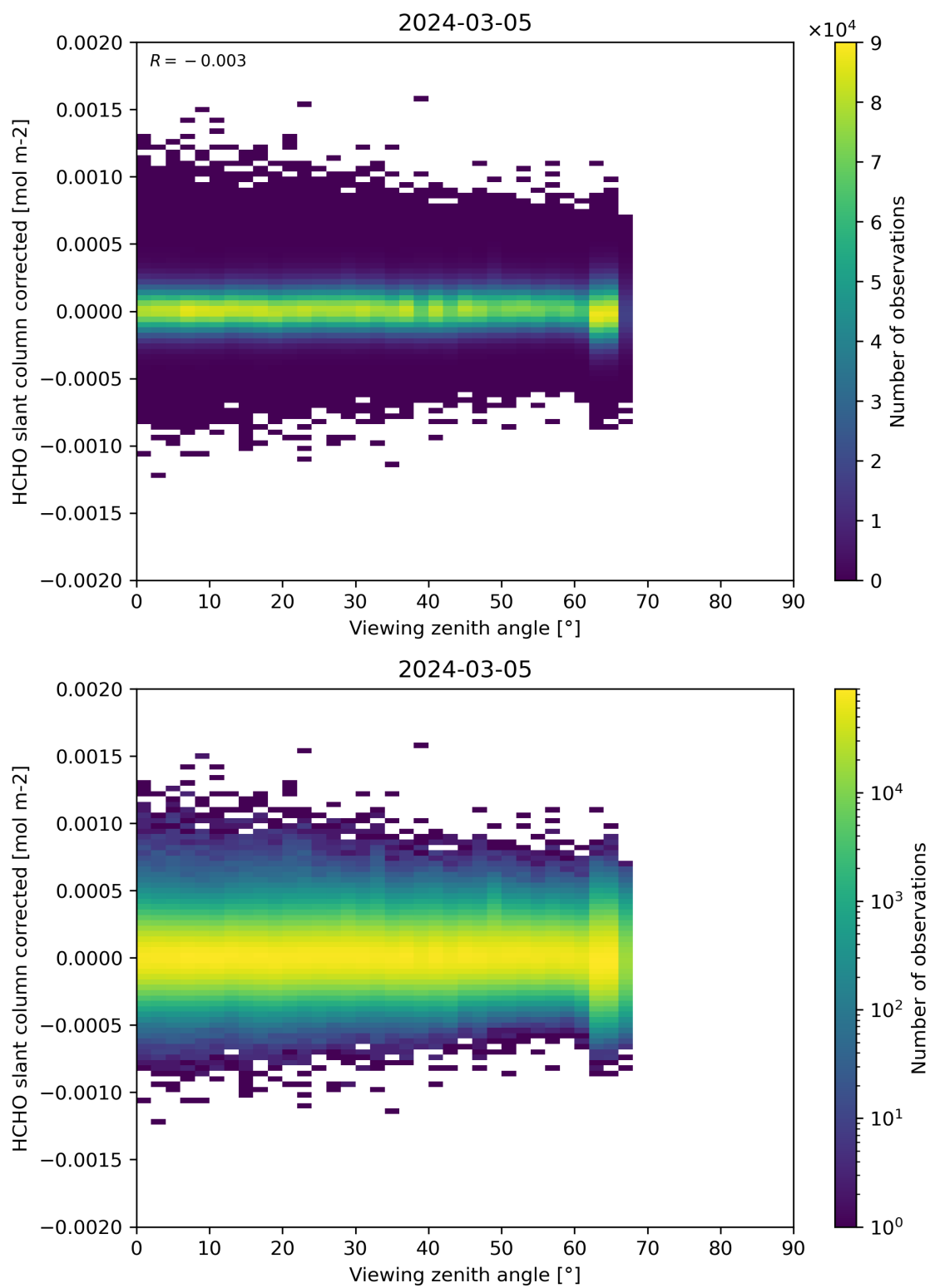
Figure 186: Scatter density plot of “Viewing zenith angle” against “HCHO slant column corrected” for 2024-03-04 to 2024-03-06.
