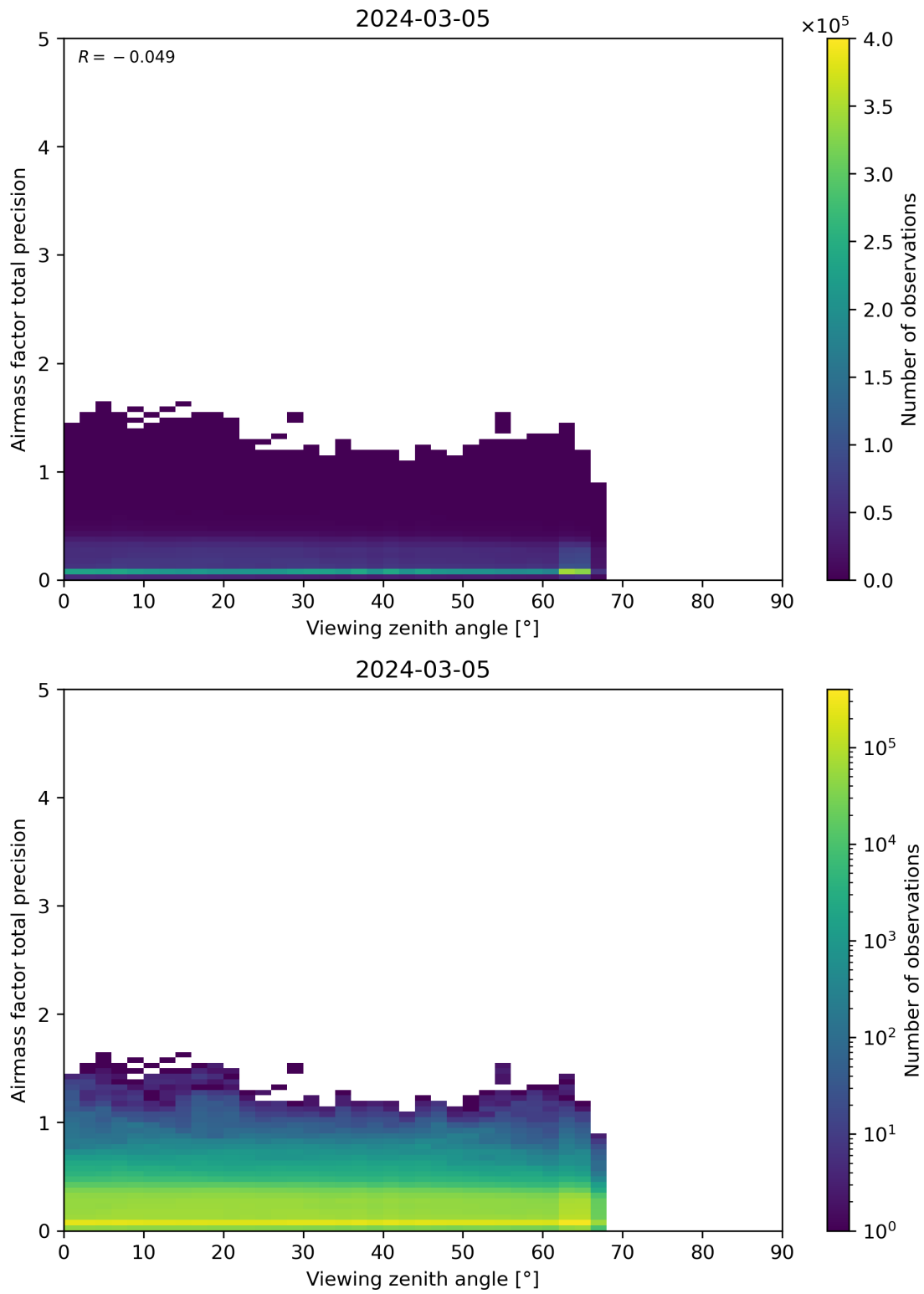
Figure 191: Scatter density plot of “Viewing zenith angle” against “Airmass factor total precision” for 2024-03-04 to 2024-03-06.
