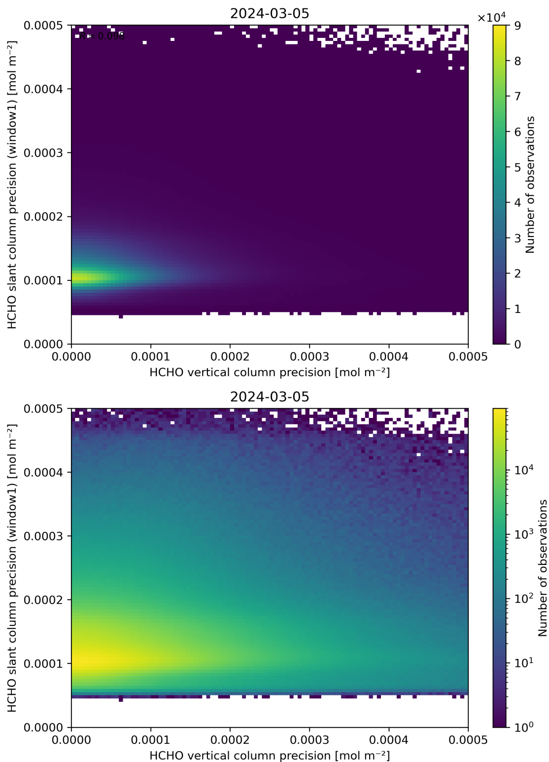
Figure 143: Scatter density plot of “HCHO vertical column precision” against “HCHO slant column precision (window1)” for 2024-03-04 to 2024-03-06.
