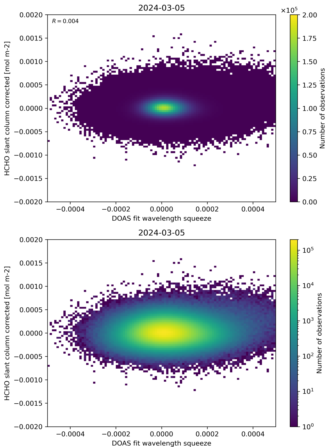
Figure 69: Scatter density plot of “DOAS fit wavelength squeeze” against “HCHO slant column corrected” for 2024-03-04 to 2024-03-06.
