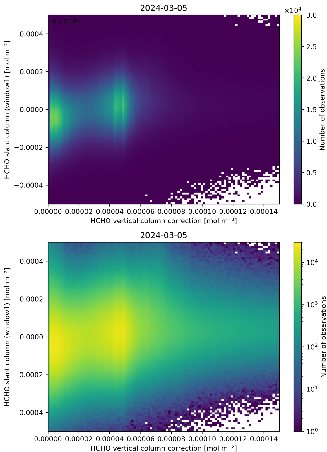
Figure 118: Scatter density plot of “HCHO vertical column correction” against “HCHO slant column (window1)” for 2024-03-04 to 2024-03-06.
