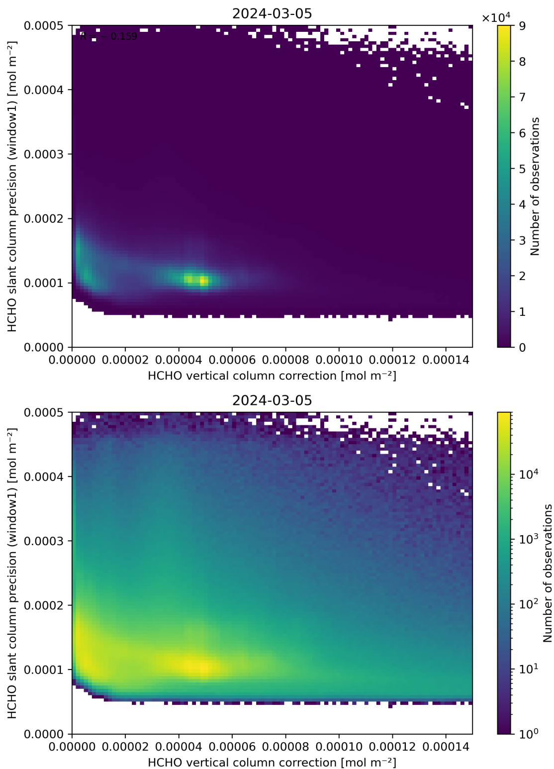
Figure 119: Scatter density plot of “HCHO vertical column correction” against “HCHO slant column precision (window1)” for 2024-03-04 to 2024-03-06.
