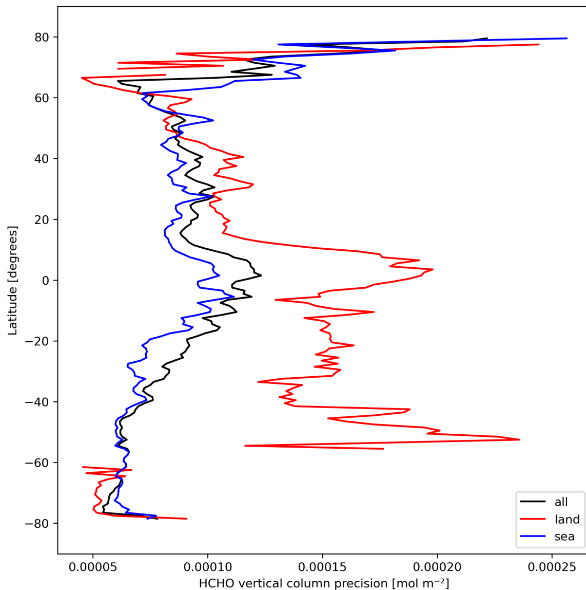
Figure 22: Zonal average of “HCHO vertical column precision” for 2024-03-04 to 2024-03-06.
