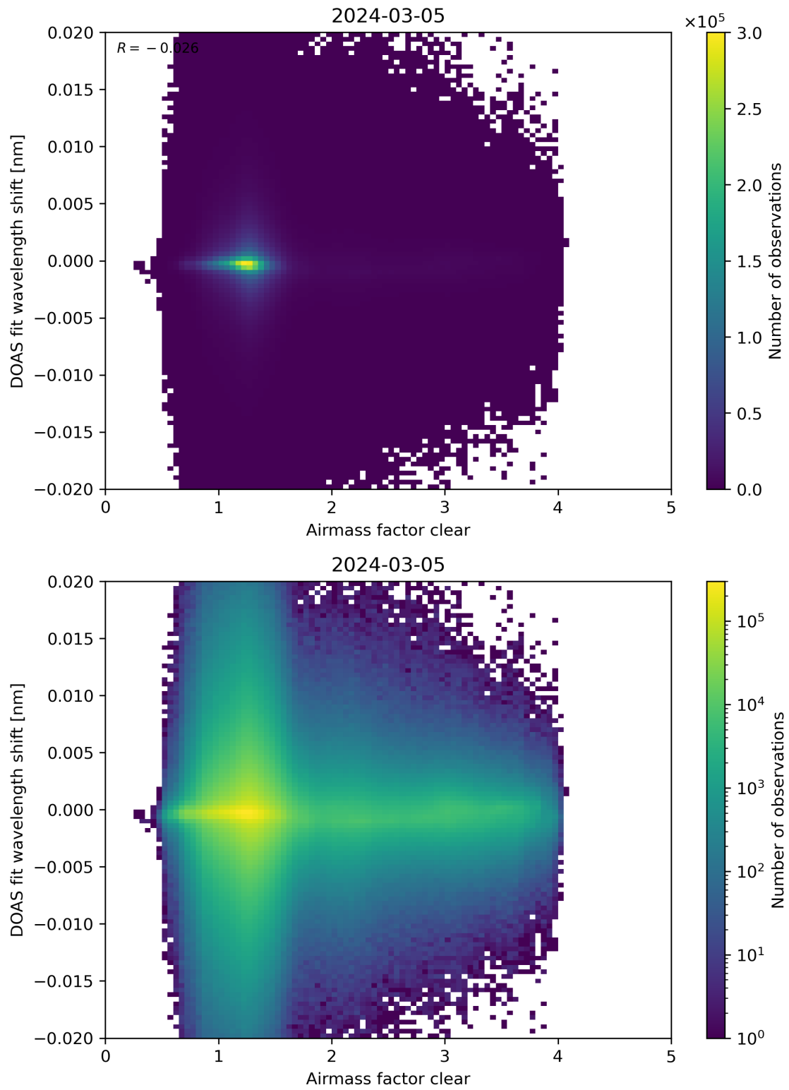
Figure 72: Scatter density plot of “Airmass factor clear” against “DOAS fit wavelength shift” for 2024-03-04 to 2024-03-06.
