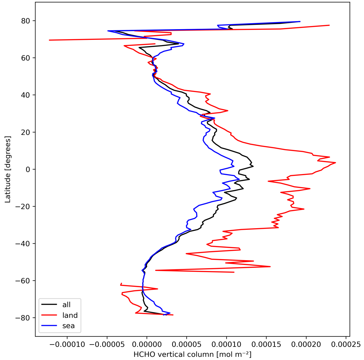
Figure 21: Zonal average of “HCHO vertical column” for 2024-03-04 to 2024-03-06.
