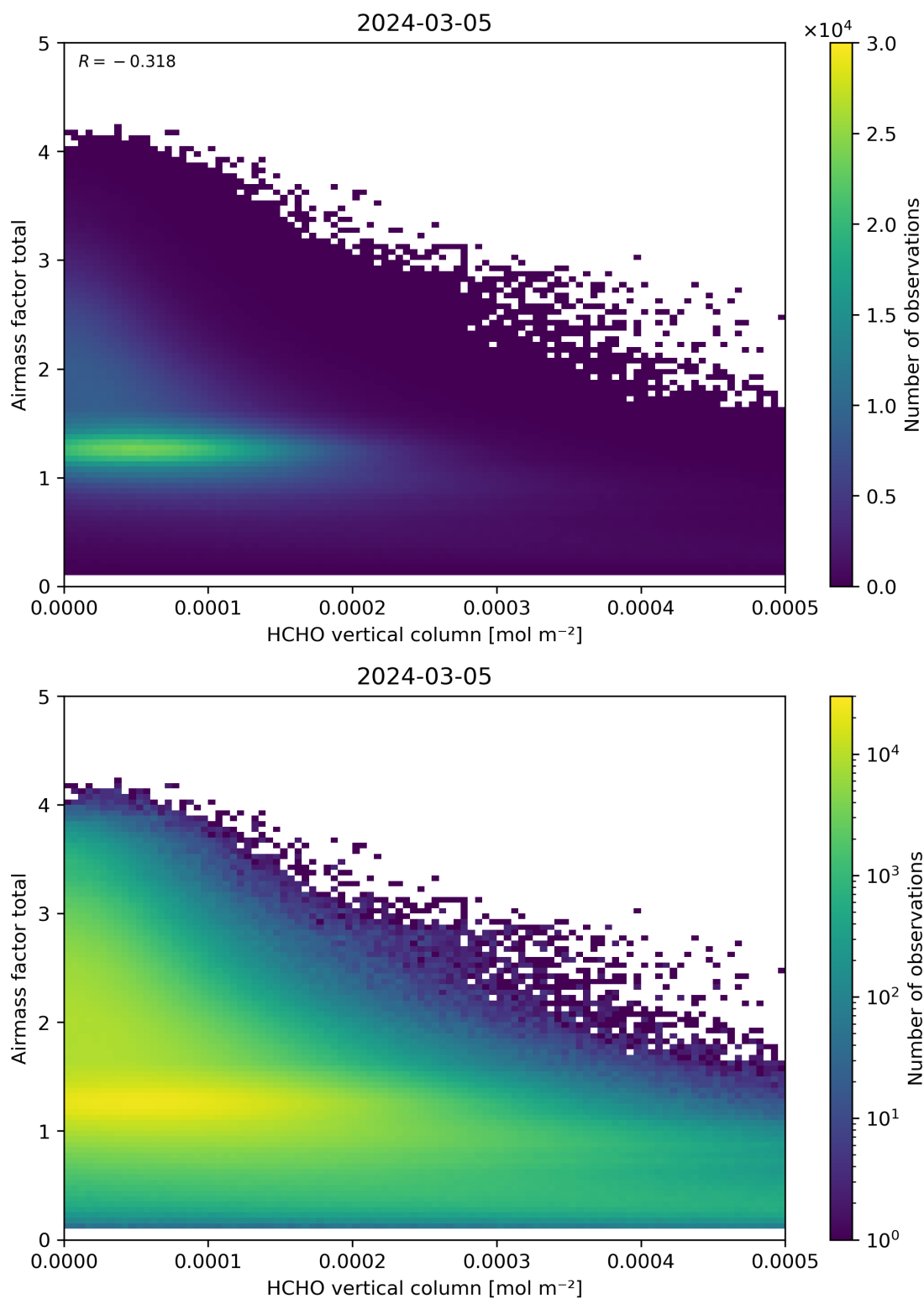
Figure 131: Scatter density plot of “HCHO vertical column” against “Airmass factor total” for 2024-03-04 to 2024-03-06.
