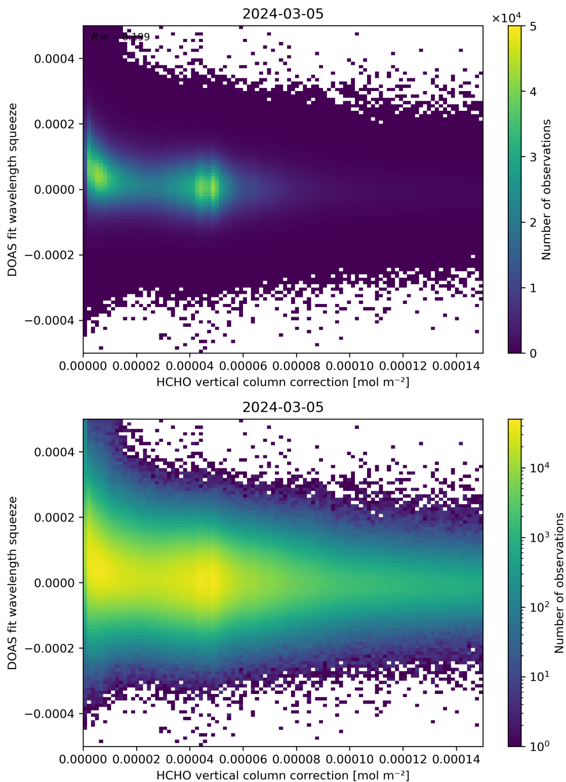
Figure 114: Scatter density plot of “HCHO vertical column correction” against “DOAS fit wavelength squeeze” for 2024-03-04 to 2024-03-06.
