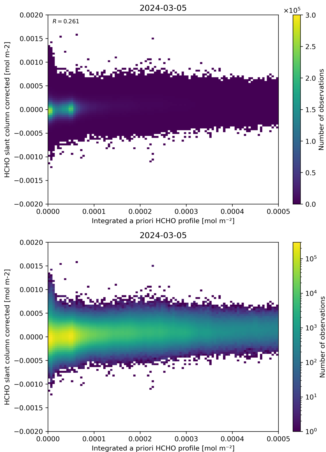
Figure 151: Scatter density plot of “Integrated a priori HCHO profile” against “HCHO slant column corrected” for 2024-03-04 to 2024-03-06.
