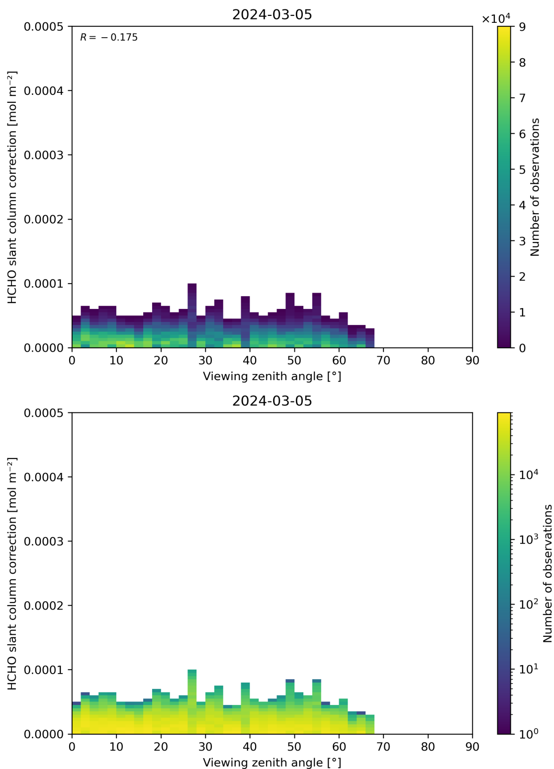
Figure 187: Scatter density plot of “Viewing zenith angle” against “HCHO slant column correction” for 2024-03-04 to 2024-03-06.
