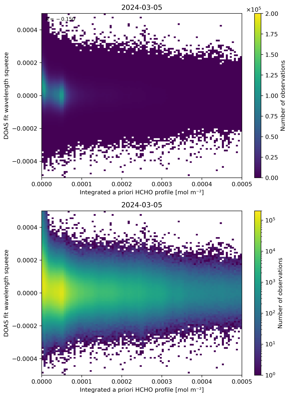
Figure 150: Scatter density plot of “Integrated a priori HCHO profile” against “DOAS fit wavelength squeeze” for 2024-03-04 to 2024-03-06.
