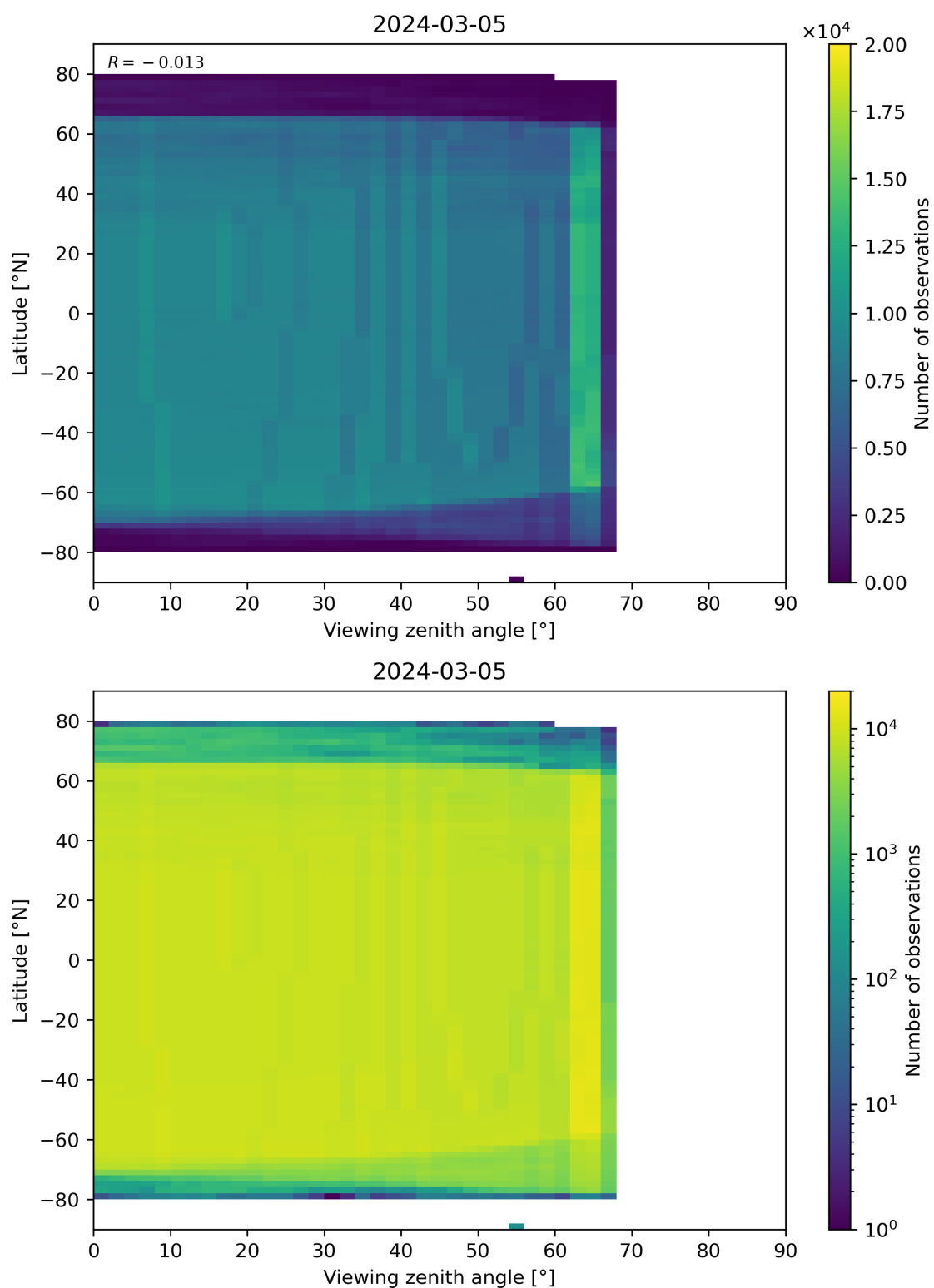
Figure 196: Scatter density plot of “Viewing zenith angle” against “Latitude” for 2024-03-04 to 2024-03-06.
