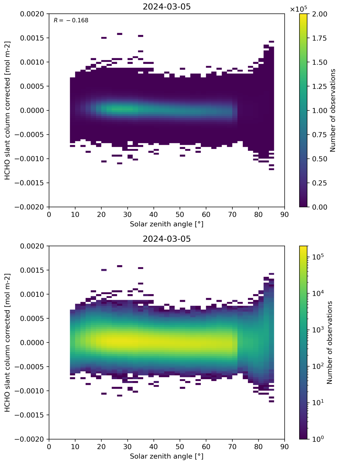
Figure 171: Scatter density plot of “Solar zenith angle” against “HCHO slant column corrected” for 2024-03-04 to 2024-03-06.
