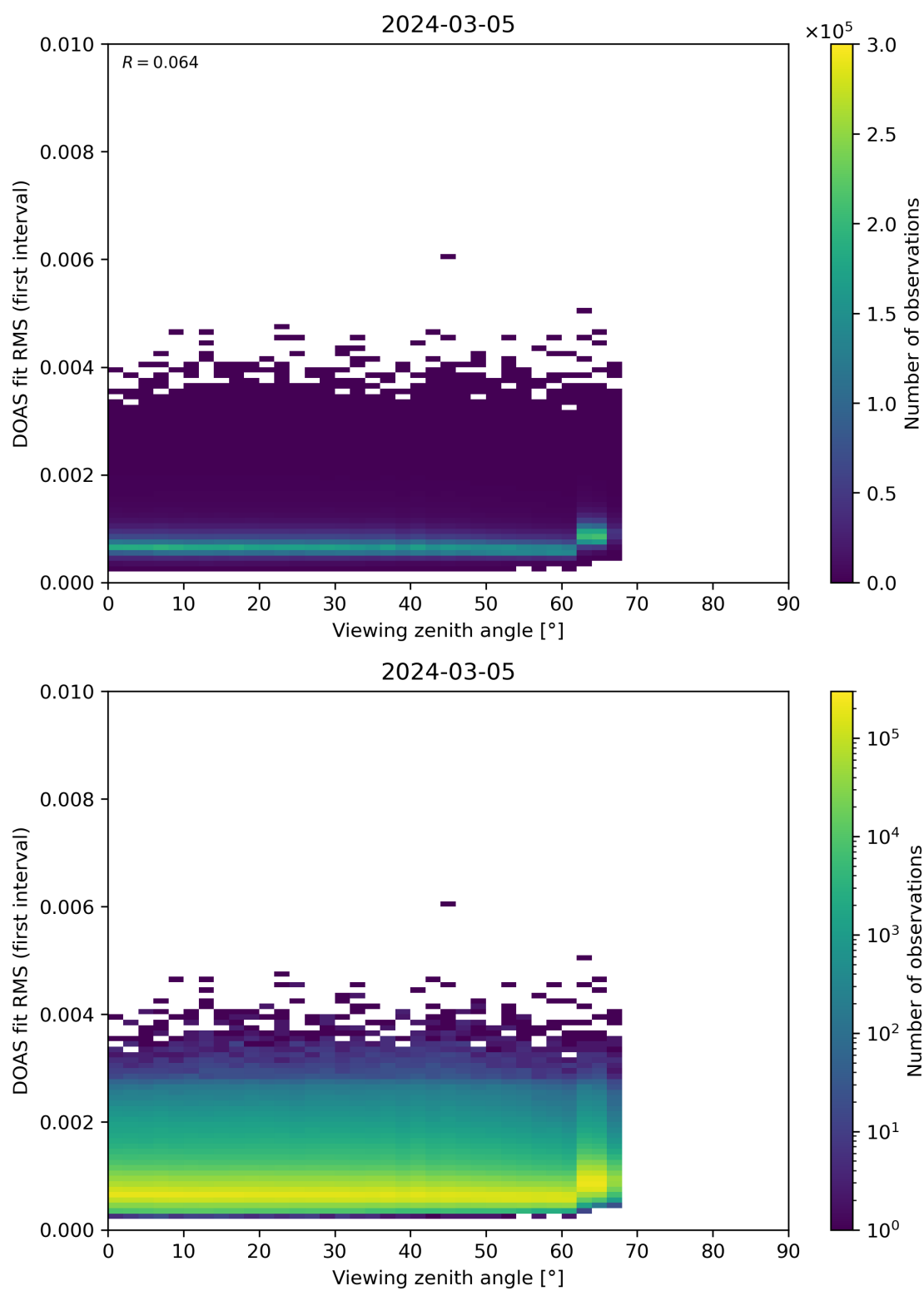
Figure 182: Scatter density plot of “Viewing zenith angle” against “DOAS fit RMS (first interval)” for 2024-03-04 to 2024-03-06.
