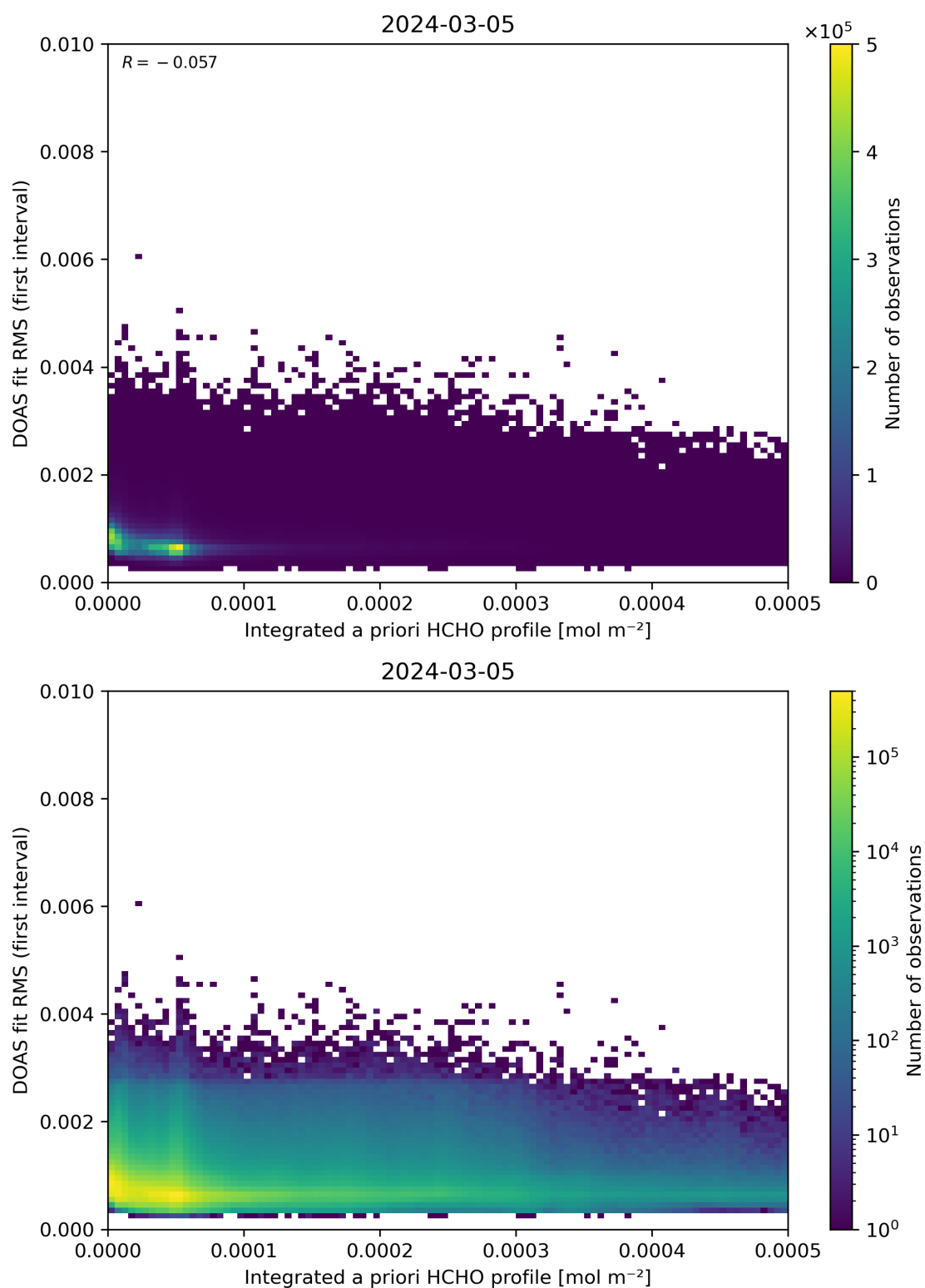
Figure 148: Scatter density plot of “Integrated a priori HCHO profile” against “DOAS fit RMS (first interval)” for 2024-03-04 to 2024-03-06.
