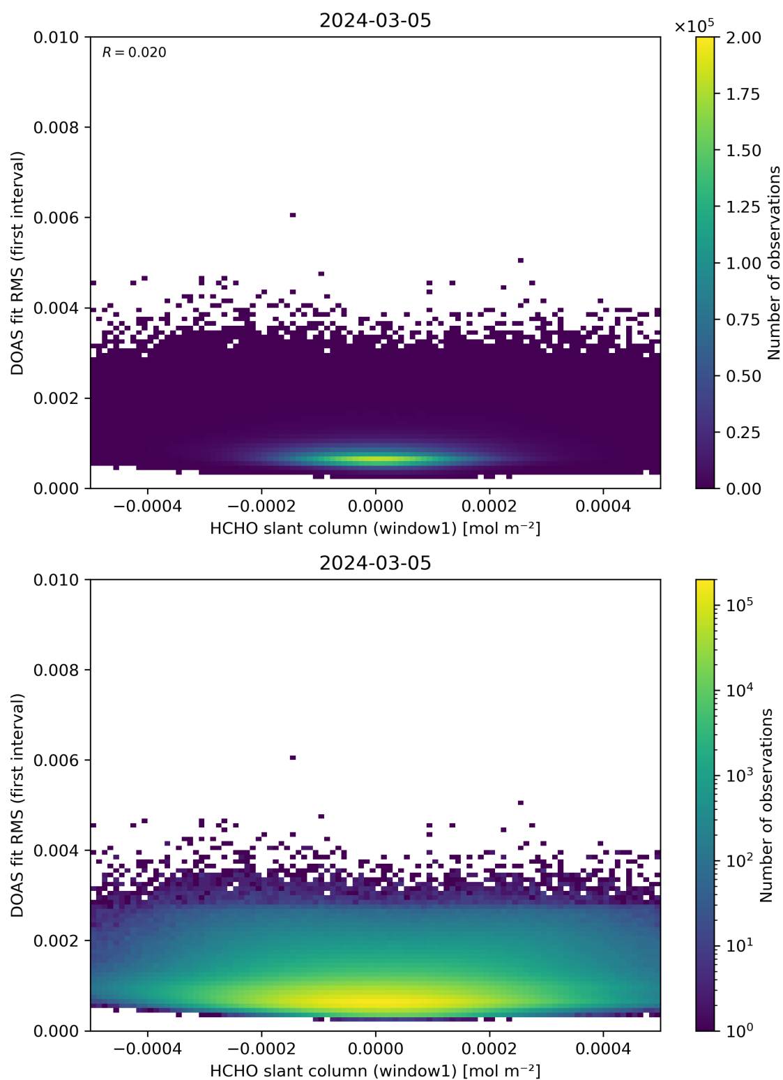
Figure 78: Scatter density plot of “HCHO slant column (window1)” against “DOAS fit RMS (first interval)” for 2024-03-04 to 2024-03-06.
