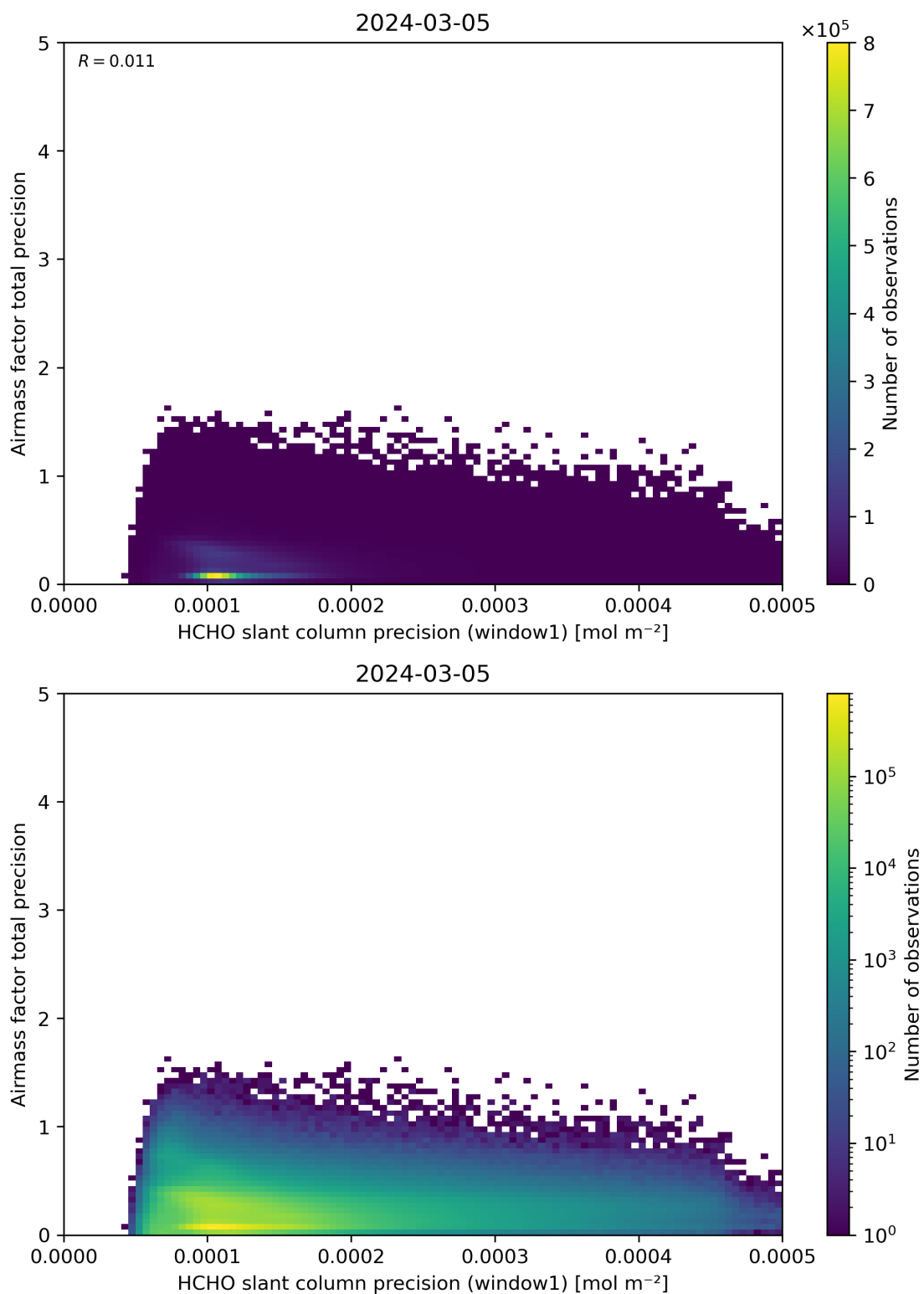
Figure 95: Scatter density plot of “HCHO slant column precision (window1)” against “Airmass factor total precision” for 2024-03-04 to 2024-03-06.
