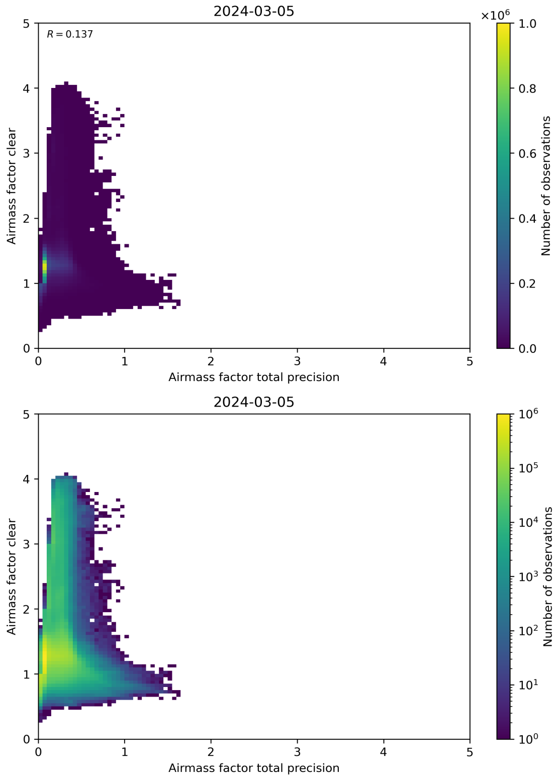
Figure 108: Scatter density plot of “Airmass factor total precision” against “Airmass factor clear” for 2024-03-04 to 2024-03-06.
