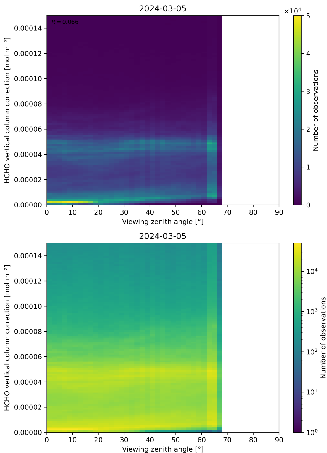
Figure 193: Scatter density plot of “Viewing zenith angle” against “HCHO vertical column correction” for 2024-03-04 to 2024-03-06.
