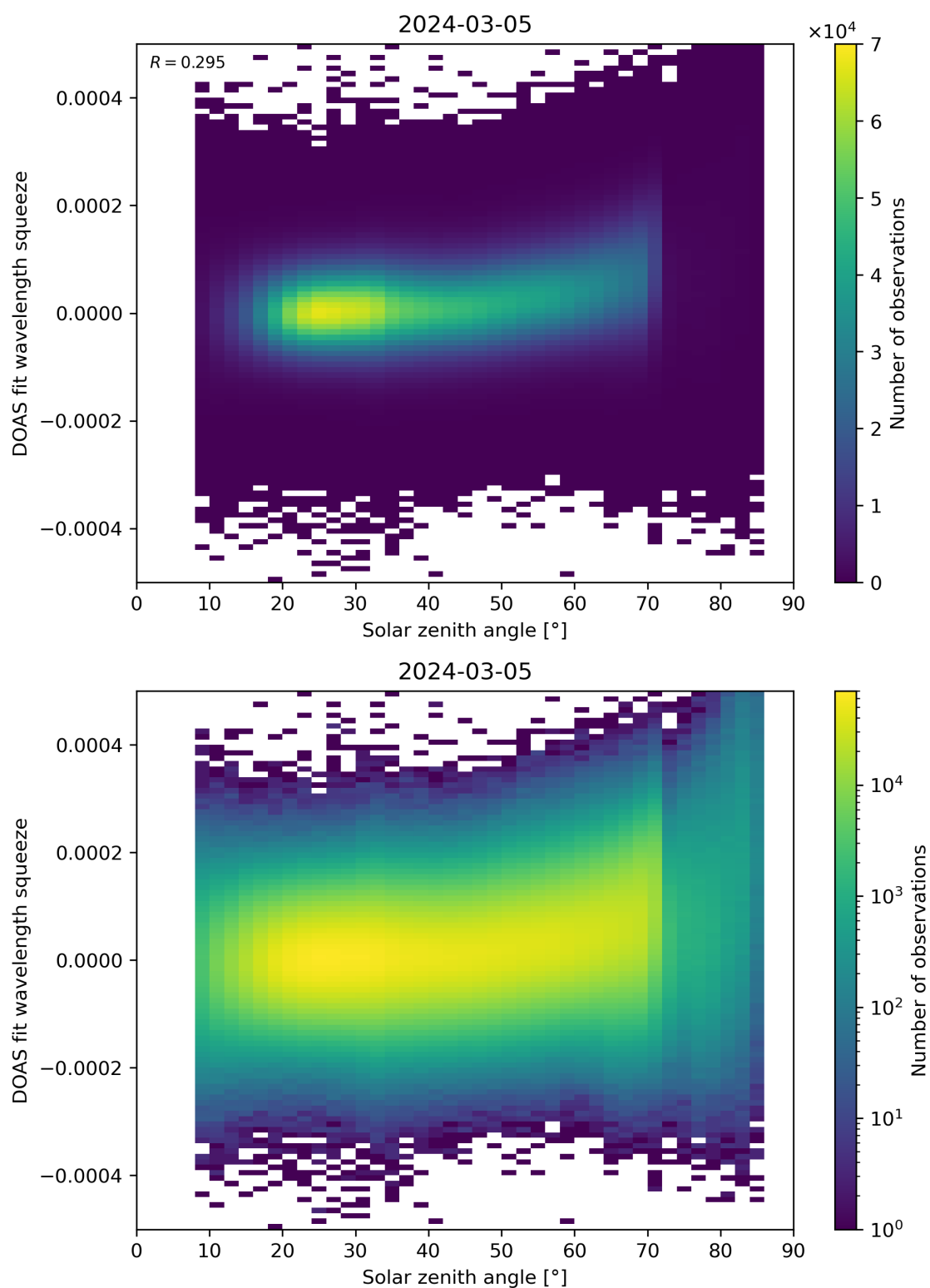
Figure 169: Scatter density plot of “Solar zenith angle” against “DOAS fit wavelength squeeze” for 2024-03-04 to 2024-03-06.
