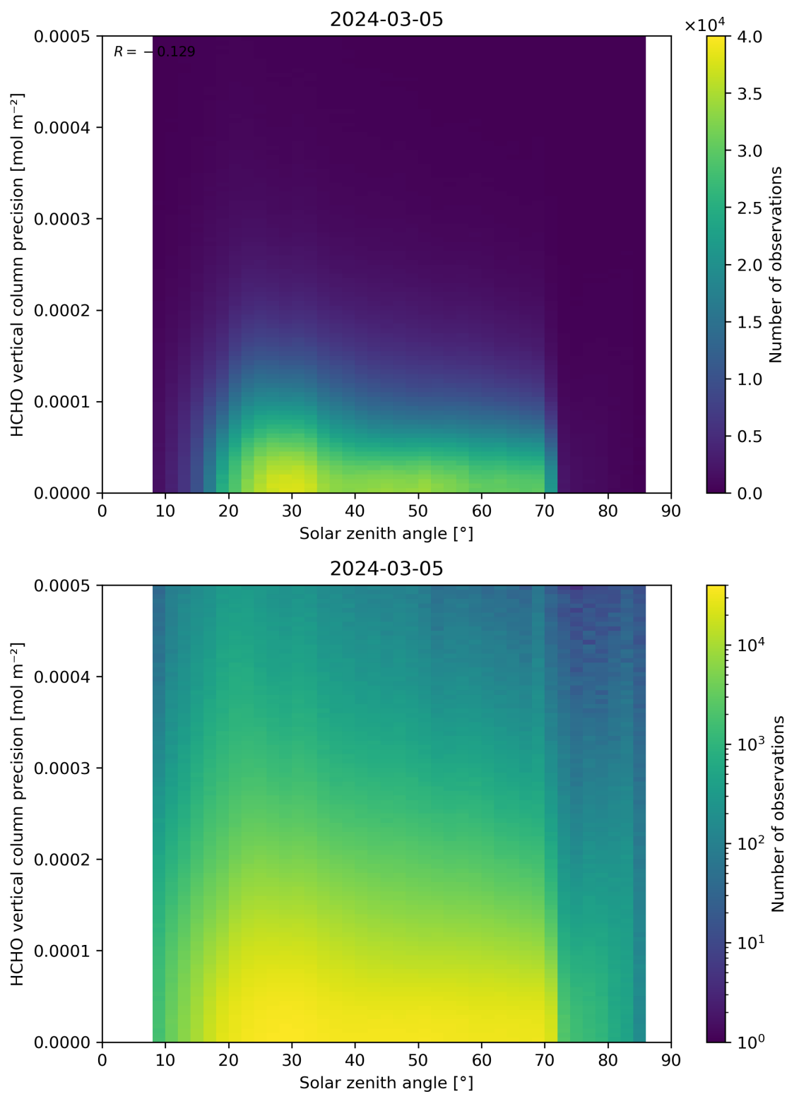
Figure 179: Scatter density plot of “Solar zenith angle” against “HCHO vertical column precision” for 2024-03-04 to 2024-03-06.
