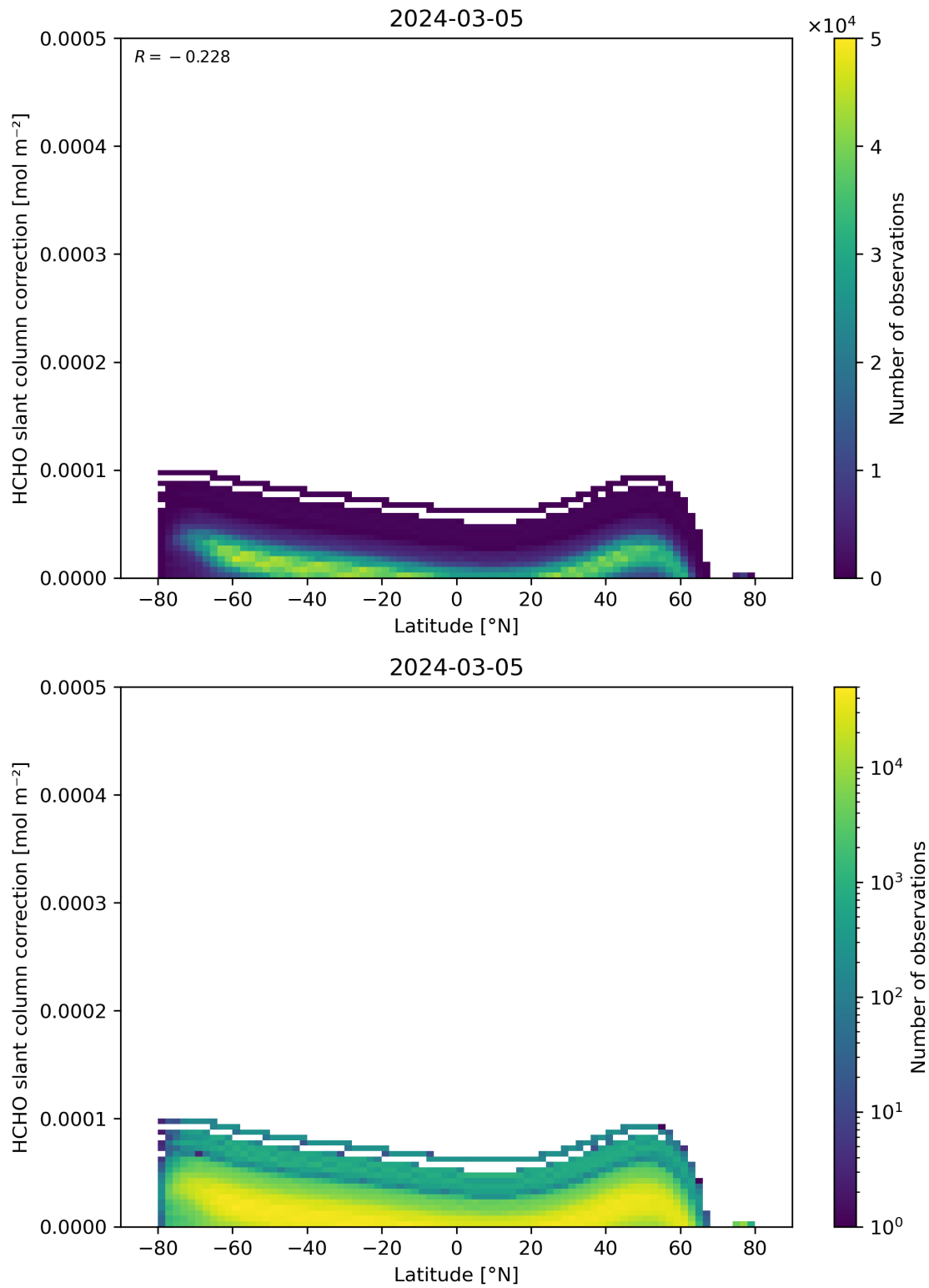
Figure 158: Scatter density plot of “Latitude” against “HCHO slant column correction” for 2024-03-04 to 2024-03-06.
