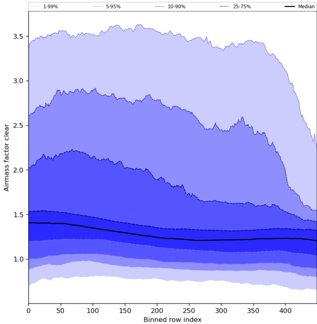
Figure 56: Along track statistics of “Airmass factor clear” for 2024-03-04 to 2024-03-06
