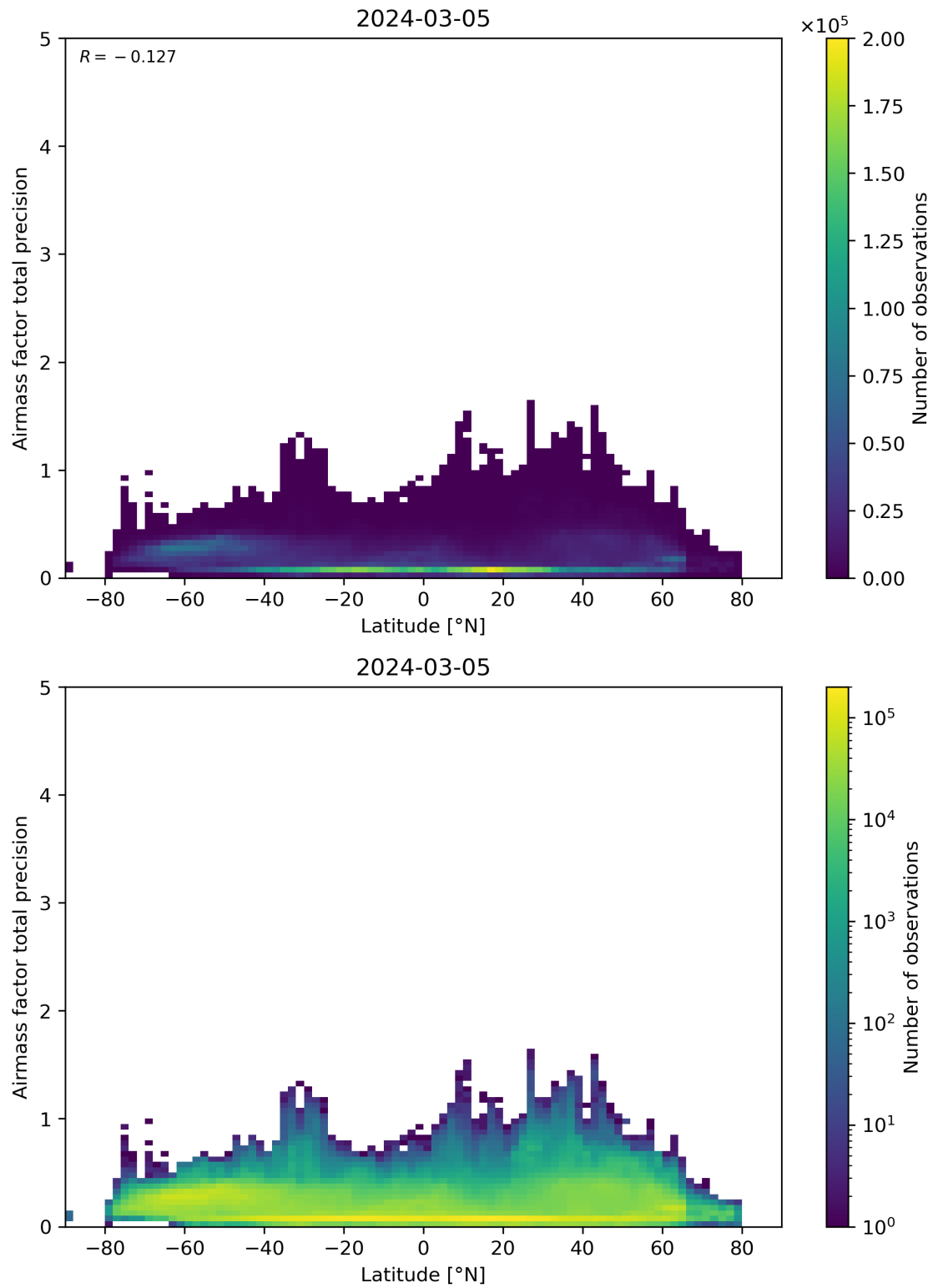
Figure 162: Scatter density plot of “Latitude” against “Airmass factor total precision” for 2024-03-04 to 2024-03-06.
