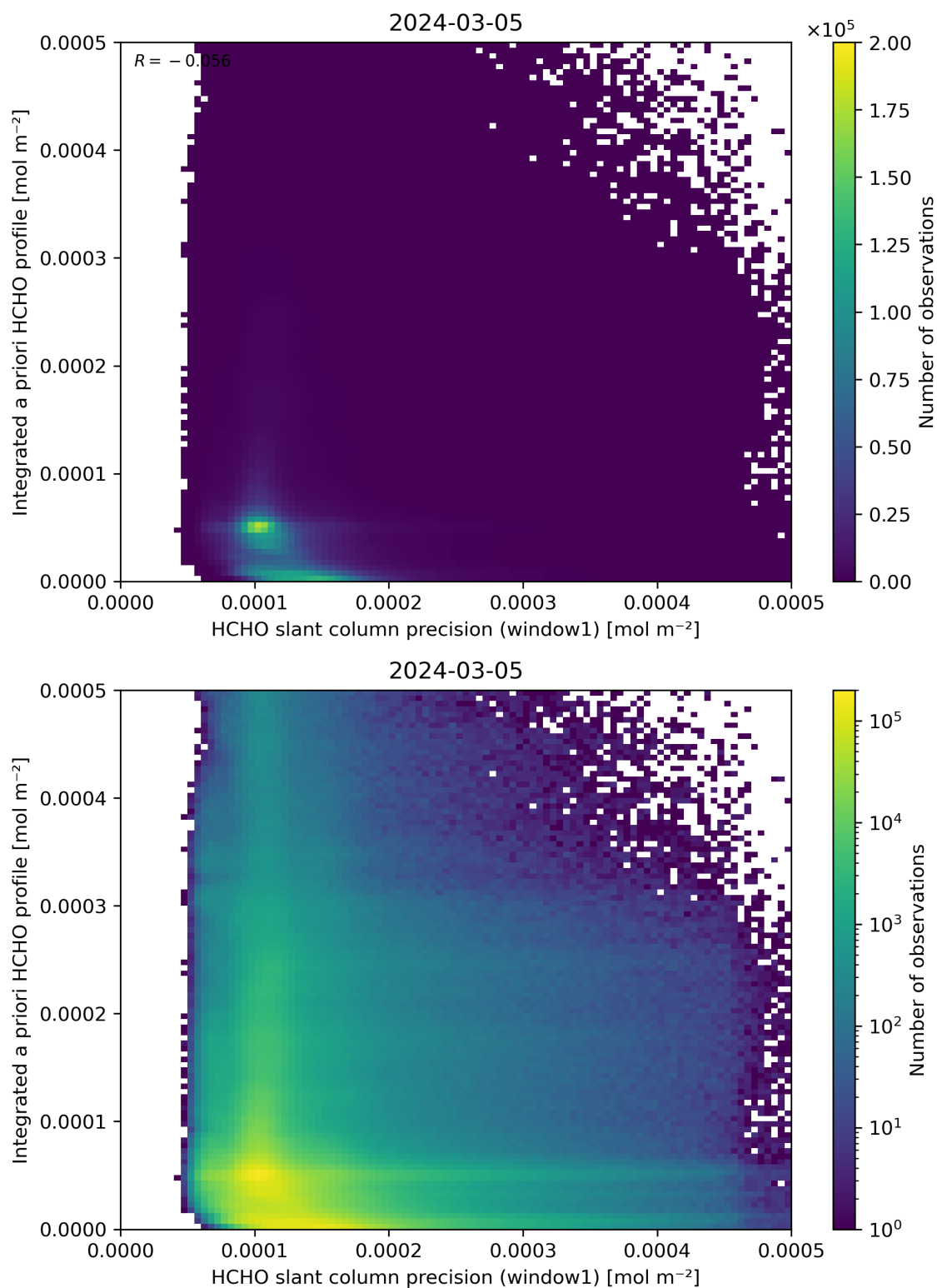
Figure 96: Scatter density plot of “HCHO slant column precision (window1)” against “Integrated a priori HCHO profile” for 2024-03-04 to 2024-03-06.
