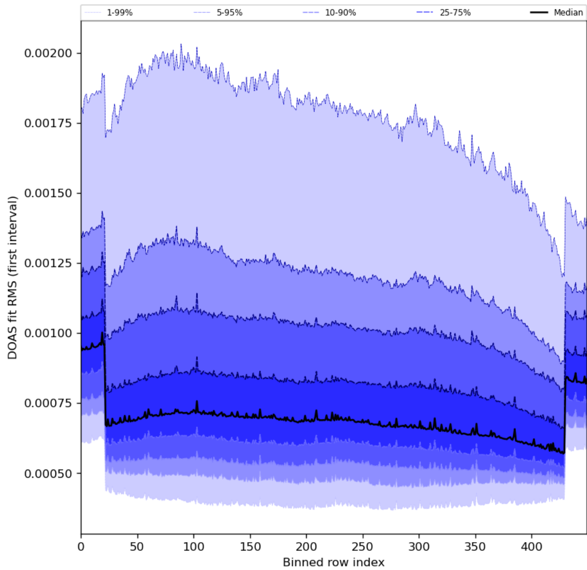
Figure 60: Along track statistics of “DOAS fit RMS (first interval)” for 2024-03-04 to 2024-03-06
