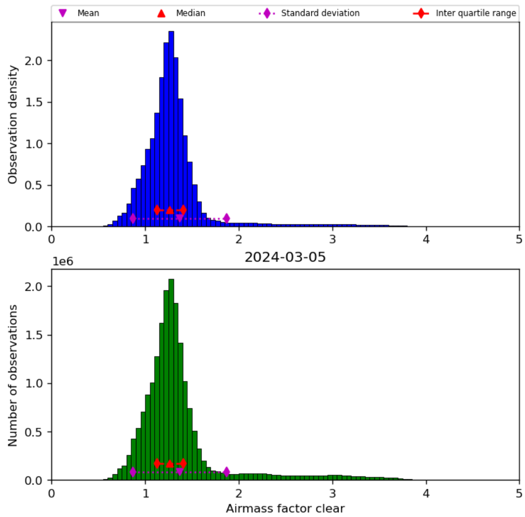
Figure 42: Histogram of “Airmass factor clear” for 2024-03-04 to 2024-03-06
