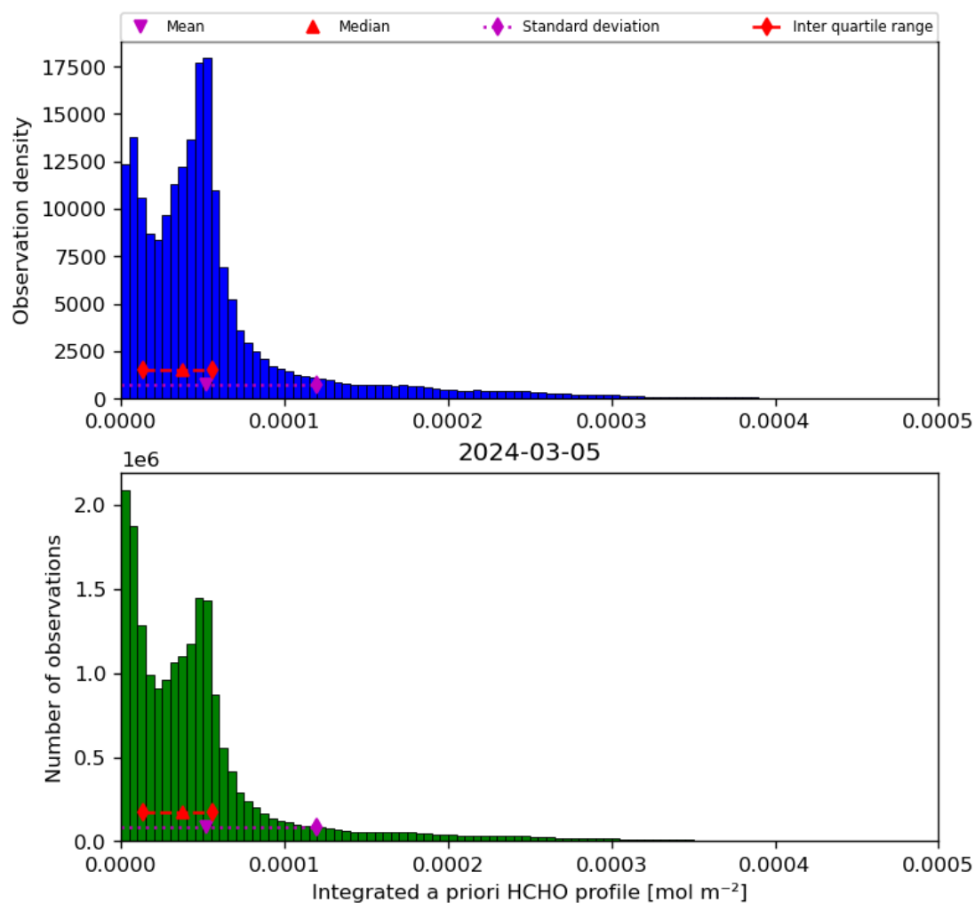
Figure 43: Histogram of “Integrated a priori HCHO profile” for 2024-03-04 to 2024-03-06
