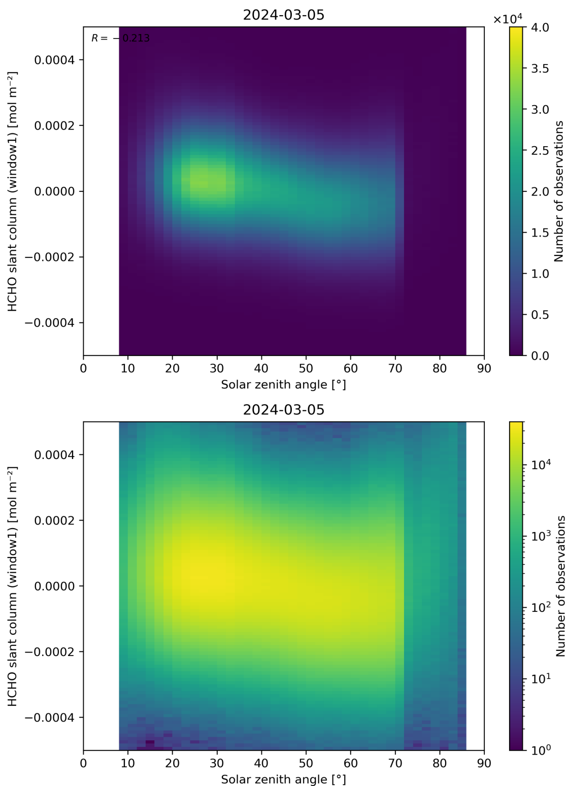
Figure 173: Scatter density plot of “Solar zenith angle” against “HCHO slant column (window1)” for 2024-03-04 to 2024-03-06.
