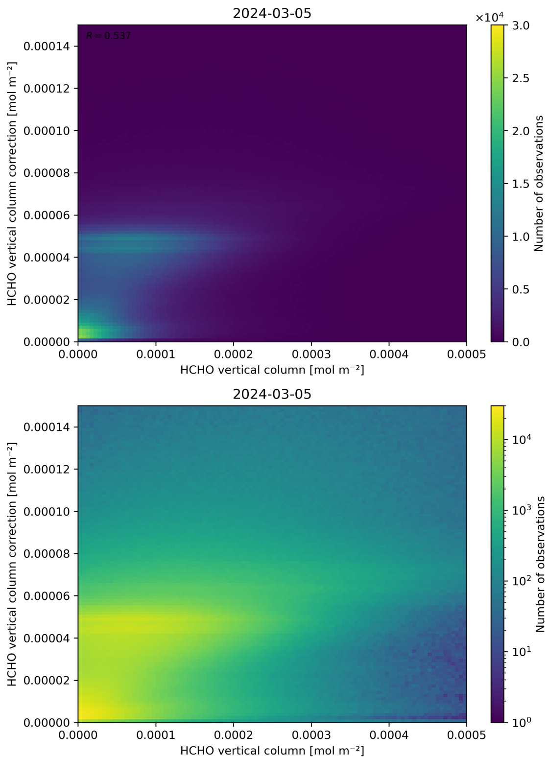
Figure 133: Scatter density plot of “HCHO vertical column” against “HCHO vertical column correction” for 2024-03-04 to 2024-03-06.
