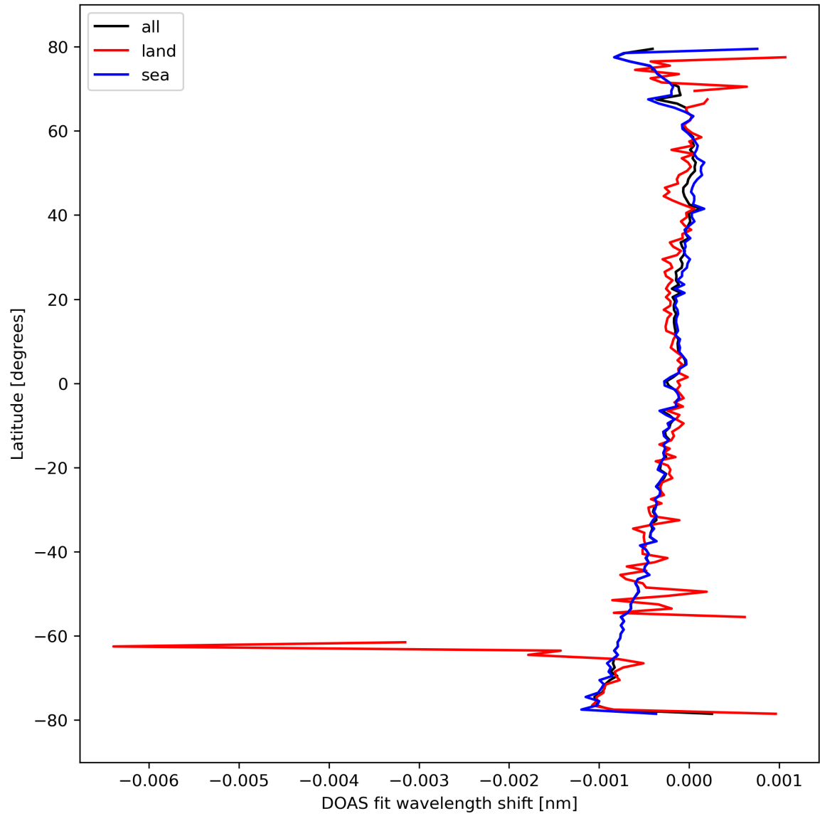
Figure 30: Zonal average of “DOAS fit wavelength shift” for 2024-03-04 to 2024-03-06.
