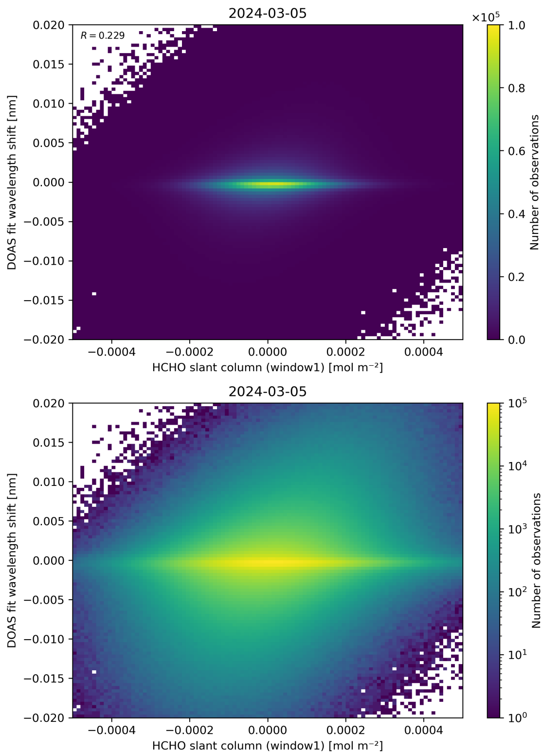
Figure 79: Scatter density plot of “HCHO slant column (window1)” against “DOAS fit wavelength shift” for 2024-03-04 to 2024-03-06.
