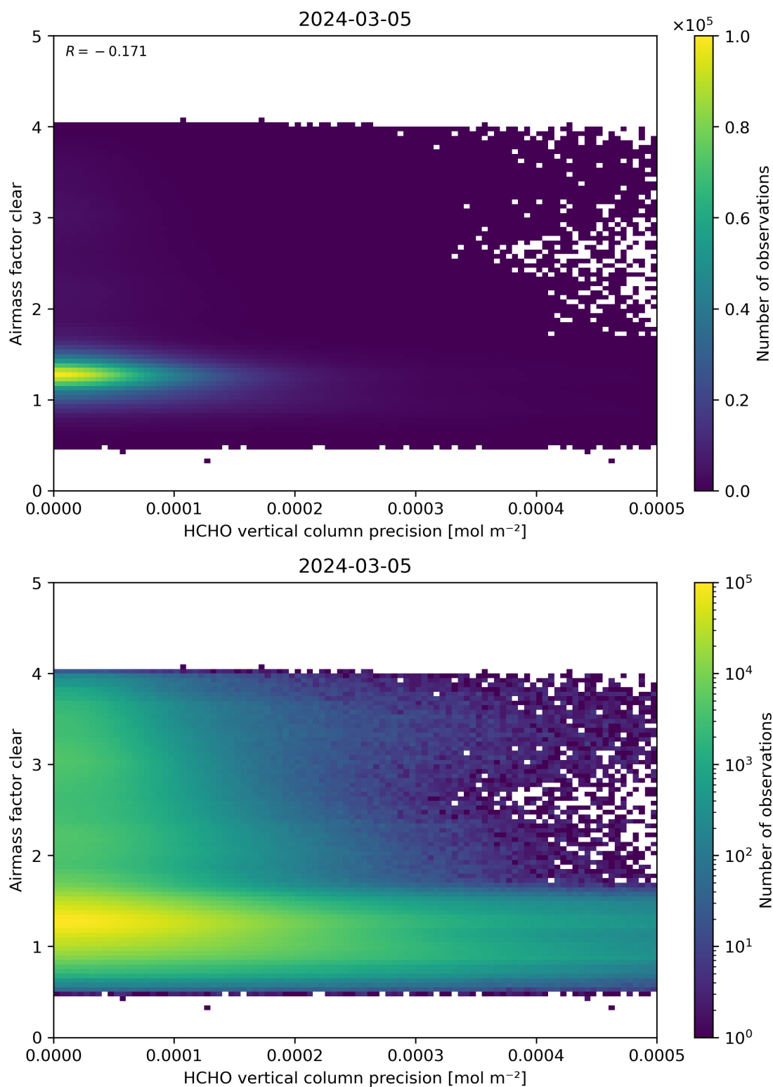
Figure 139: Scatter density plot of “HCHO vertical column precision” against “Airmass factor clear” for 2024-03-04 to 2024-03-06.
