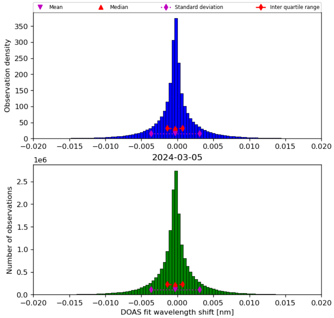
Figure 44: Histogram of “DOAS fit wavelength shift” for 2024-03-04 to 2024-03-06
