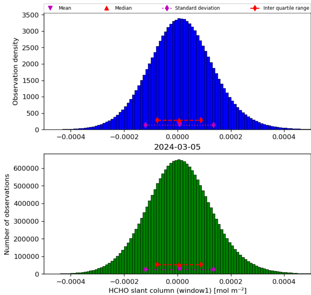
Figure 38: Histogram of “HCHO slant column (window1)” for 2024-03-04 to 2024-03-06
