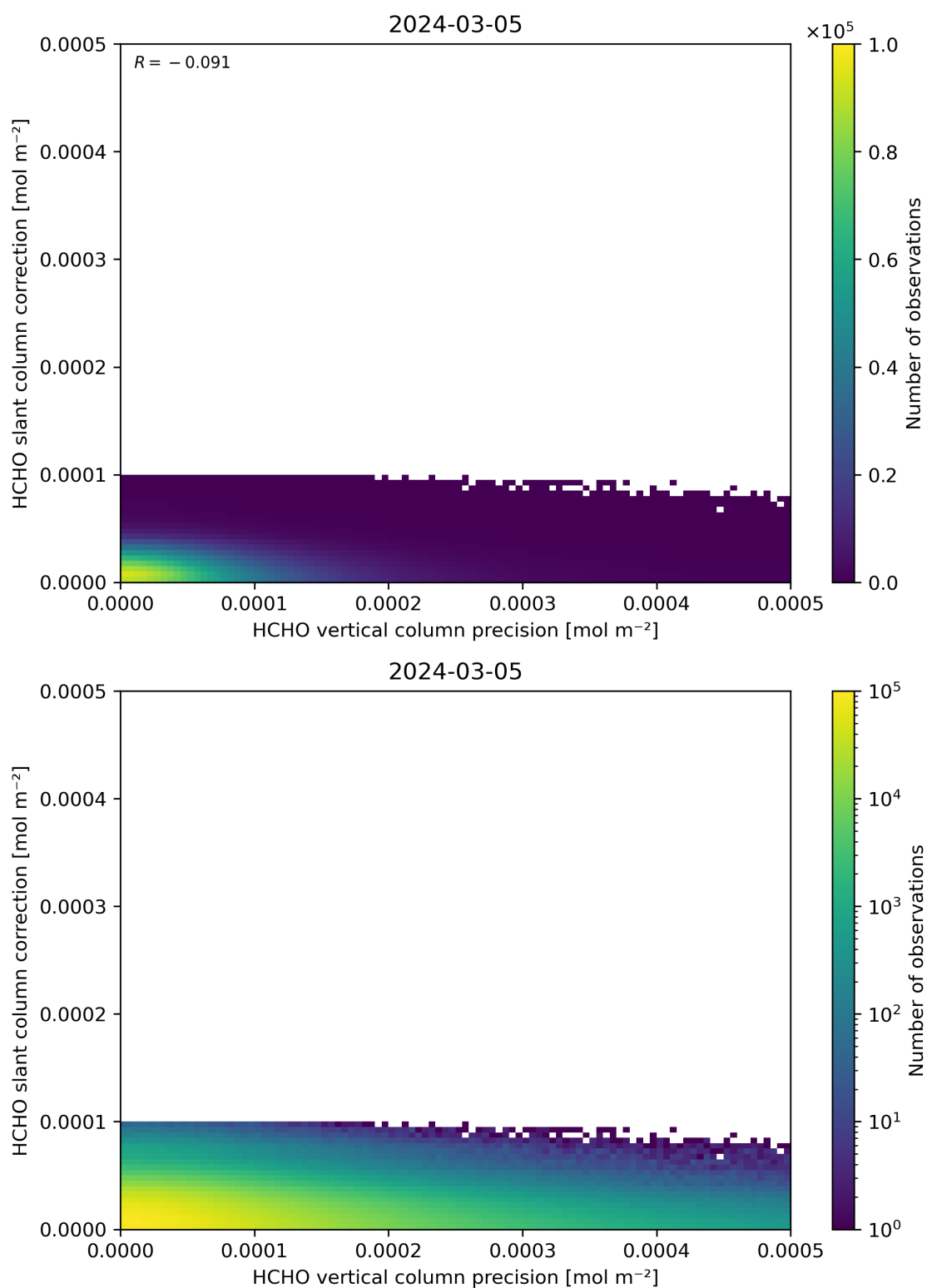
Figure 141: Scatter density plot of “HCHO vertical column precision” against “HCHO slant column correction” for 2024-03-04 to 2024-03-06.
