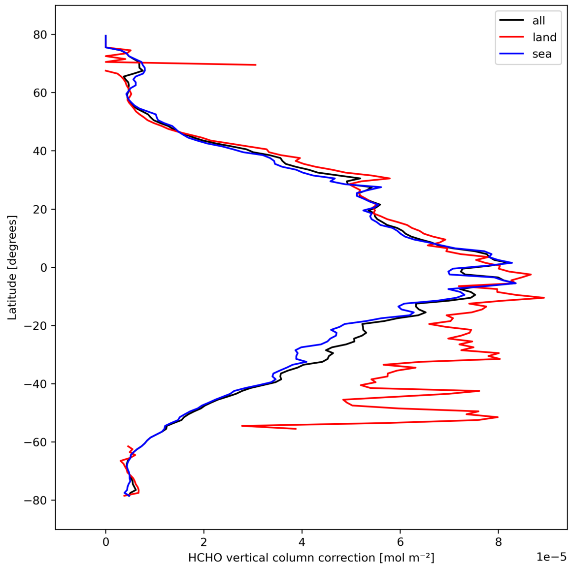
Figure 23: Zonal average of “HCHO vertical column correction” for 2024-03-04 to 2024-03-06.
