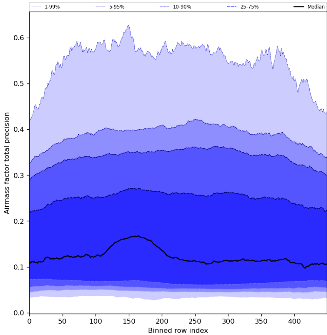
Figure 55: Along track statistics of “Airmass factor total precision” for 2024-03-04 to 2024-03-06
