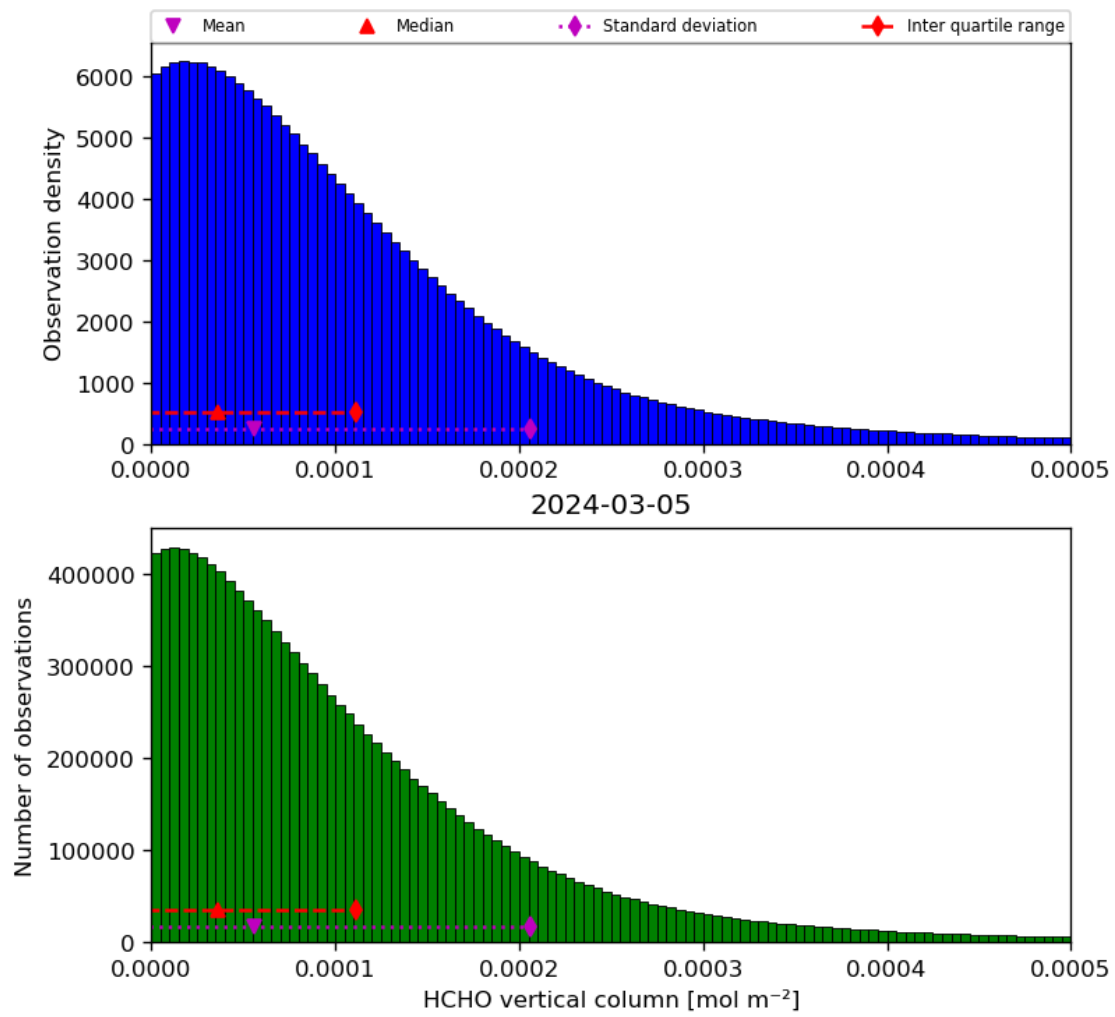
Figure 35: Histogram of “HCHO vertical column” for 2024-03-04 to 2024-03-06
