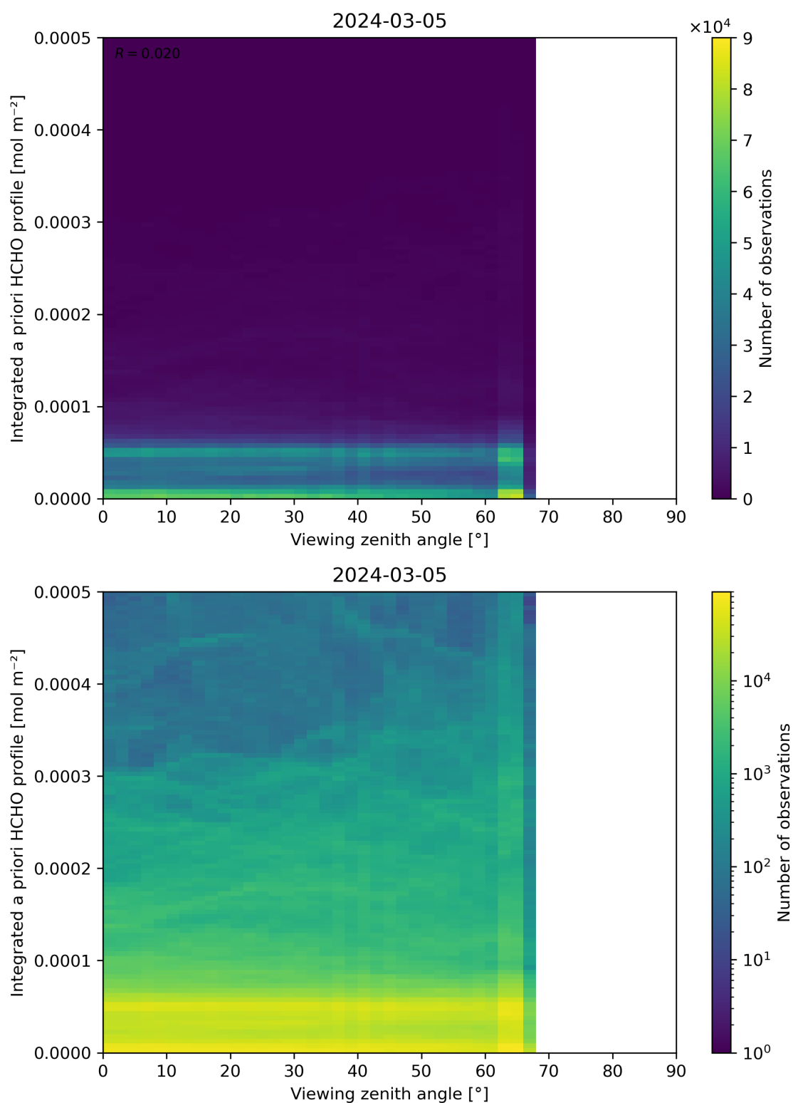
Figure 195: Scatter density plot of “Viewing zenith angle” against “Integrated a priori HCHO profile” for 2024-03-04 to 2024-03-06.
