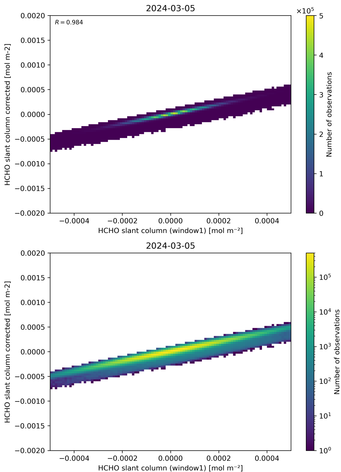
Figure 82: Scatter density plot of “HCHO slant column (window1)” against “HCHO slant column corrected” for 2024-03-04 to 2024-03-06.
