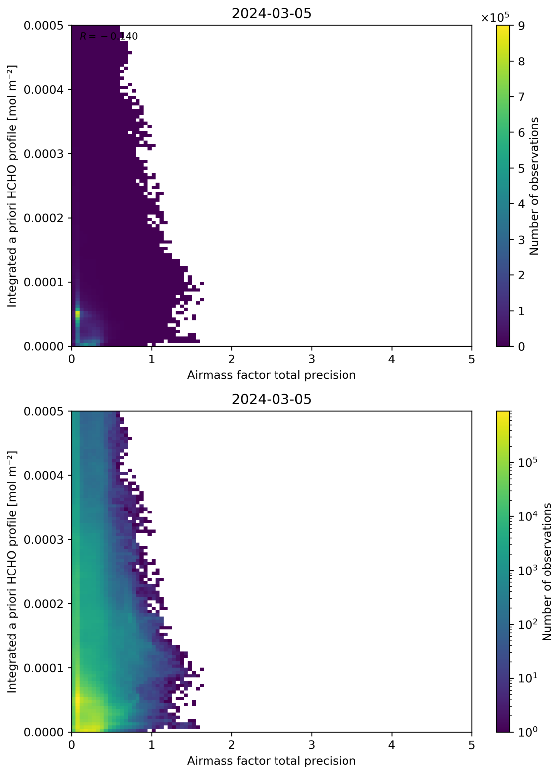
Figure 111: Scatter density plot of “Airmass factor total precision” against “Integrated a priori HCHO profile” for 2024-03-04 to 2024-03-06.
