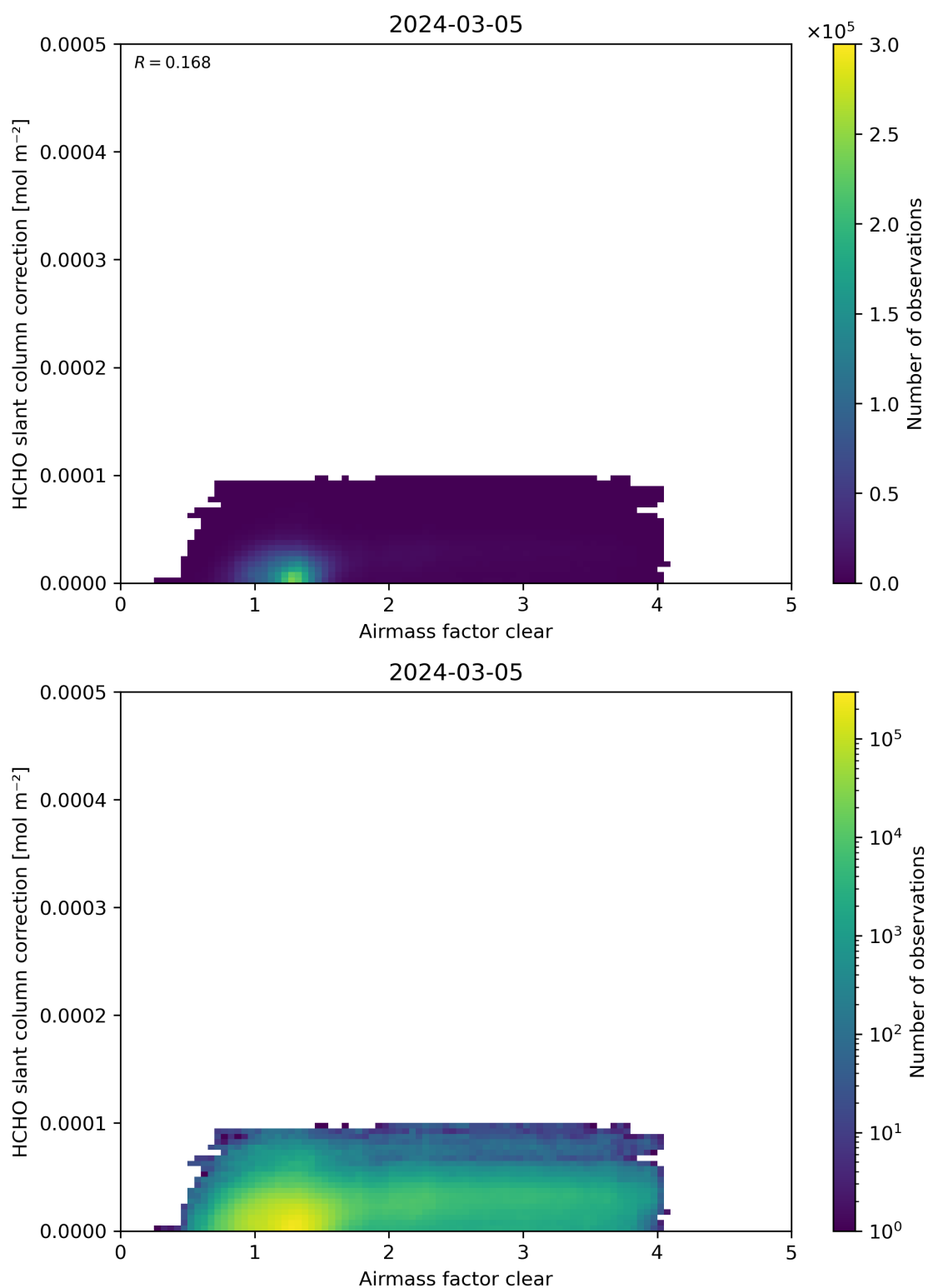
Figure 75: Scatter density plot of “Airmass factor clear” against “HCHO slant column correction” for 2024-03-04 to 2024-03-06.
