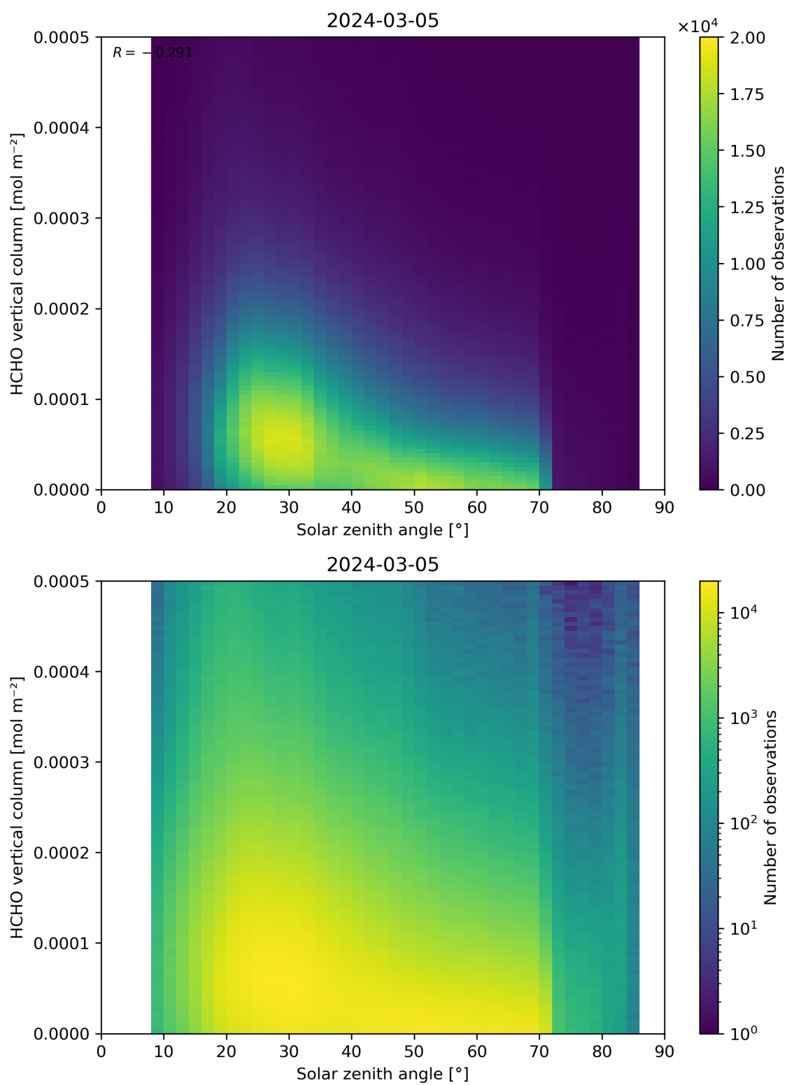
Figure 177: Scatter density plot of “Solar zenith angle” against “HCHO vertical column” for 2024-03-04 to 2024-03-06.
