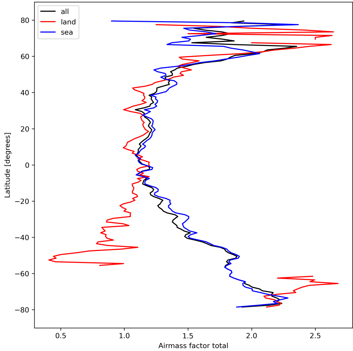
Figure 26: Zonal average of “Airmass factor total” for 2024-03-04 to 2024-03-06.
