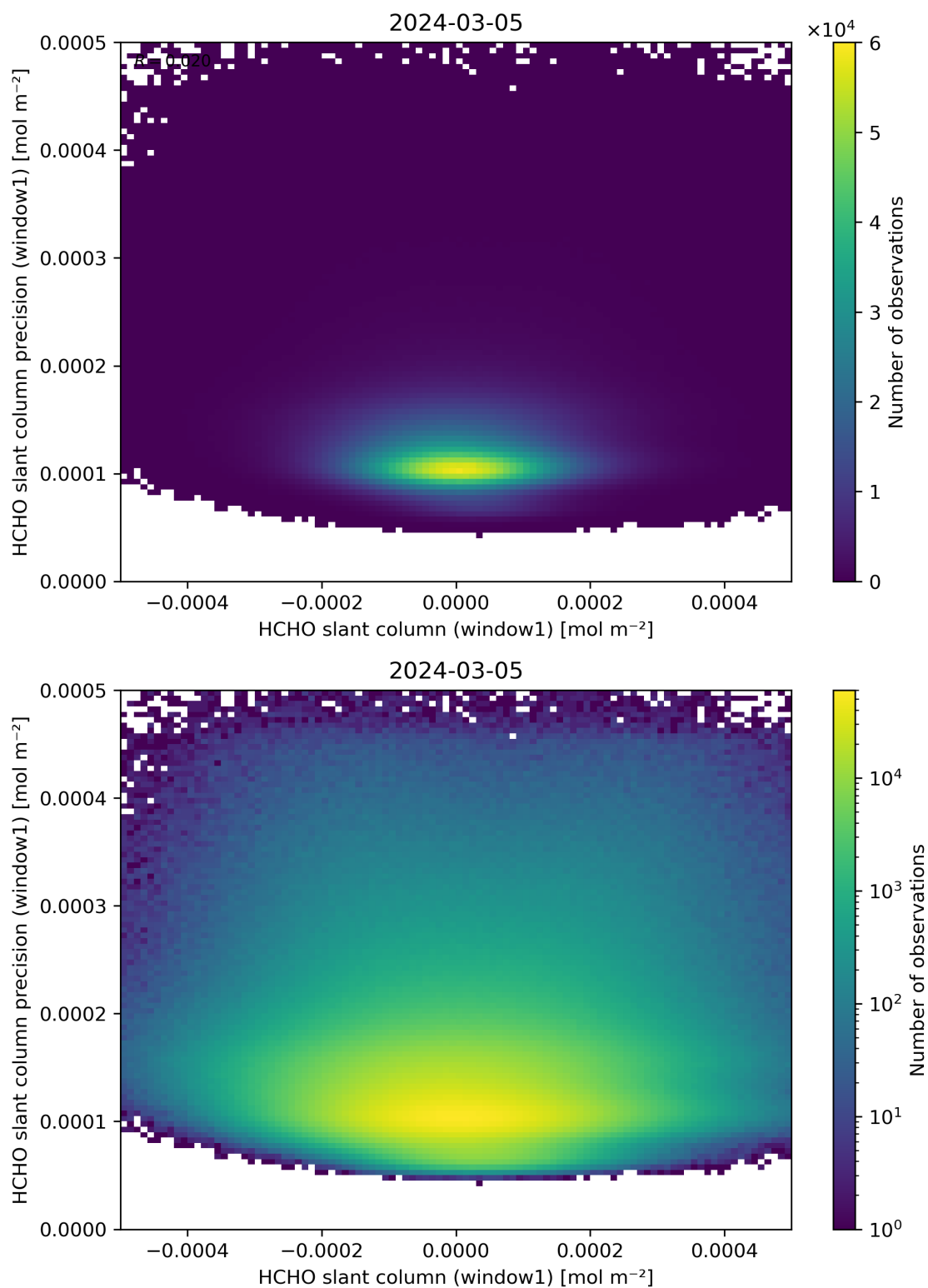
Figure 84: Scatter density plot of “HCHO slant column (window1)” against “HCHO slant column precision (window1)” for 2024-03-04 to 2024-03-06.
