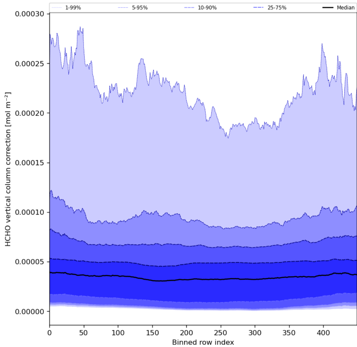
Figure 51: Along track statistics of “HCHO vertical column correction” for 2024-03-04 to 2024-03-06
