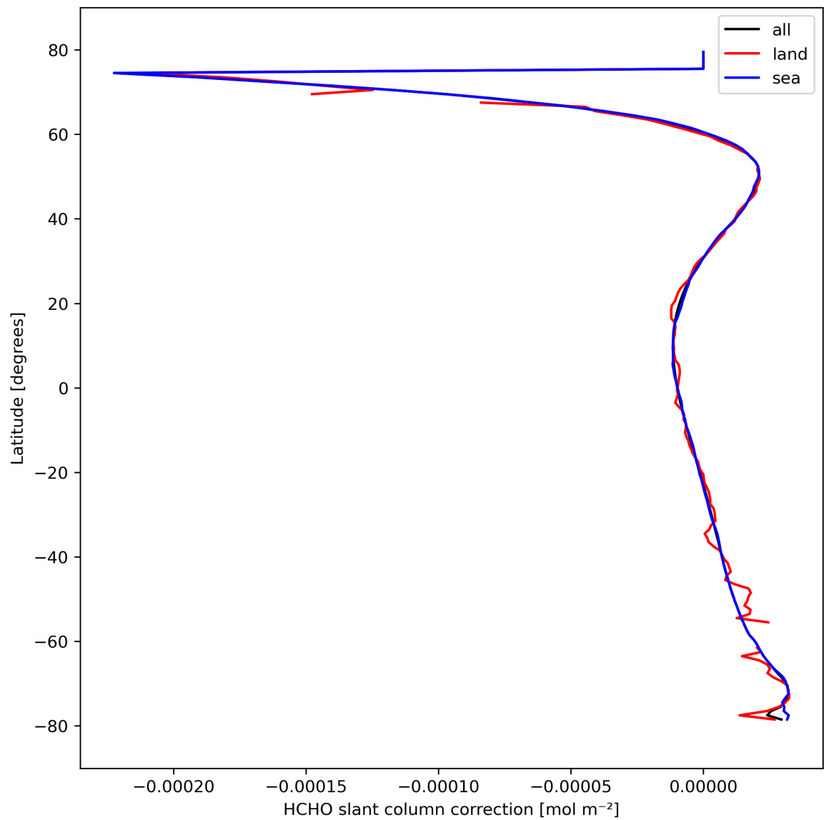
Figure 33: Zonal average of “HCHO slant column correction” for 2024-03-04 to 2024-03-06.
