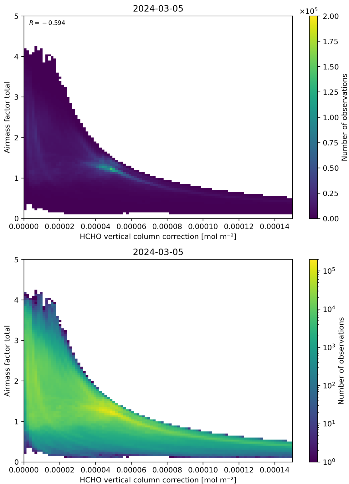
Figure 120: Scatter density plot of “HCHO vertical column correction” against “Airmass factor total” for 2024-03-04 to 2024-03-06.
