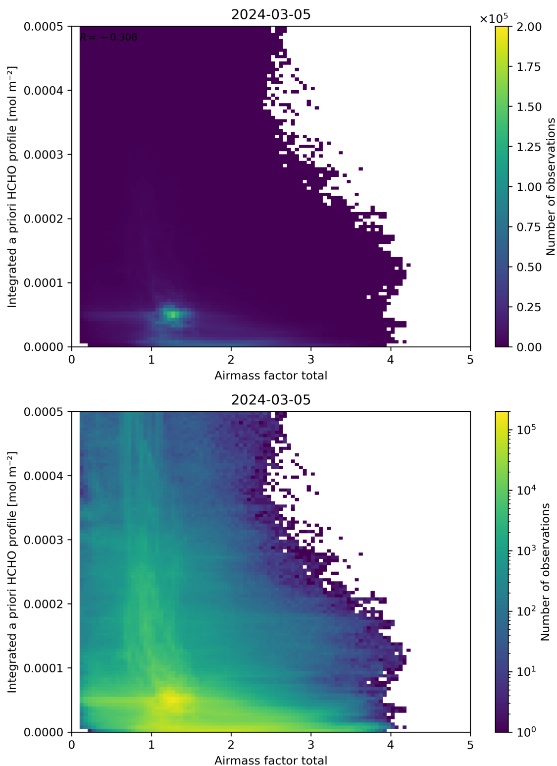
Figure 104: Scatter density plot of “Airmass factor total” against “Integrated a priori HCHO profile” for 2024-03-04 to 2024-03-06.
