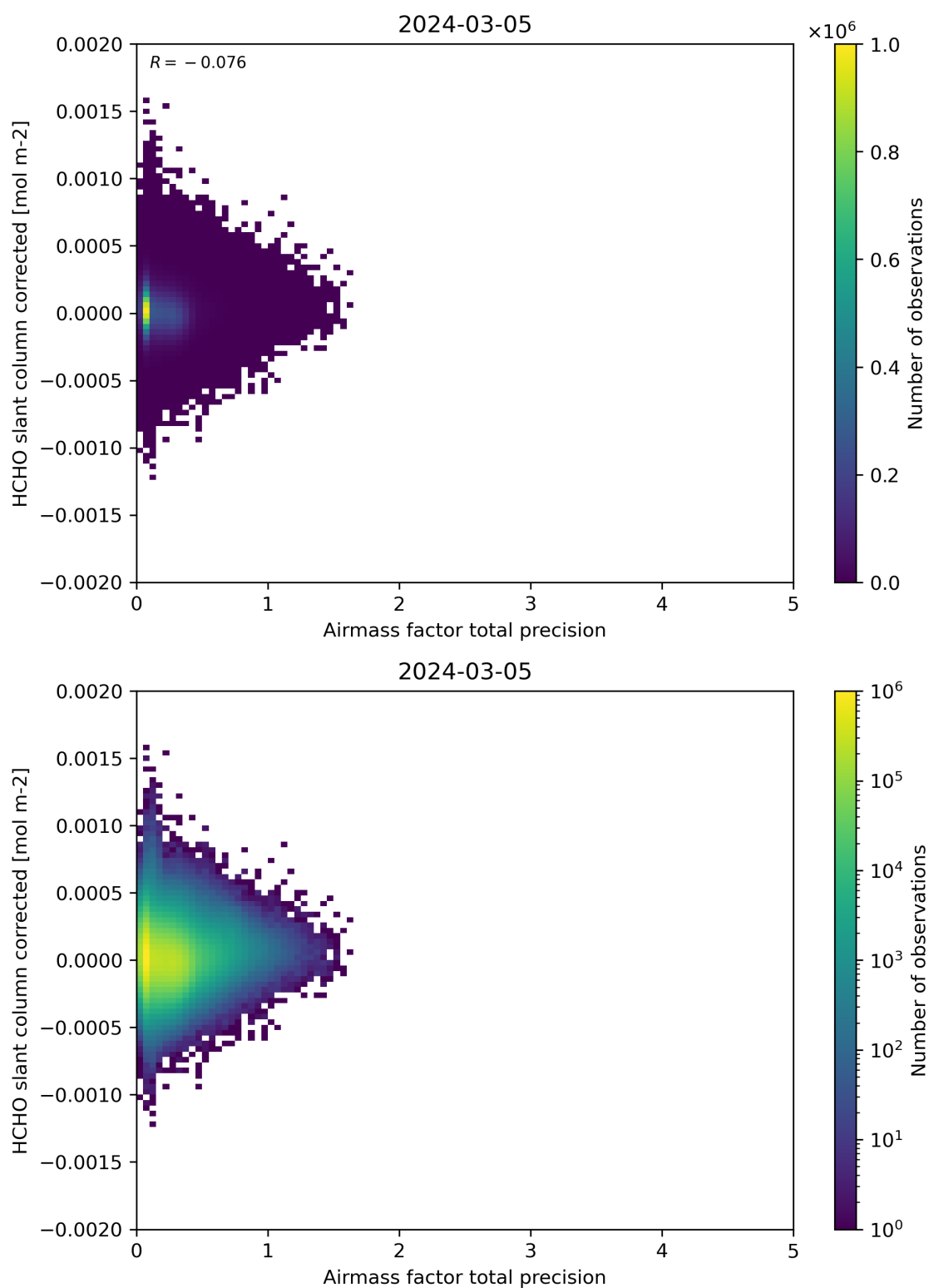
Figure 109: Scatter density plot of “Airmass factor total precision” against “HCHO slant column corrected” for 2024-03-04 to 2024-03-06.
