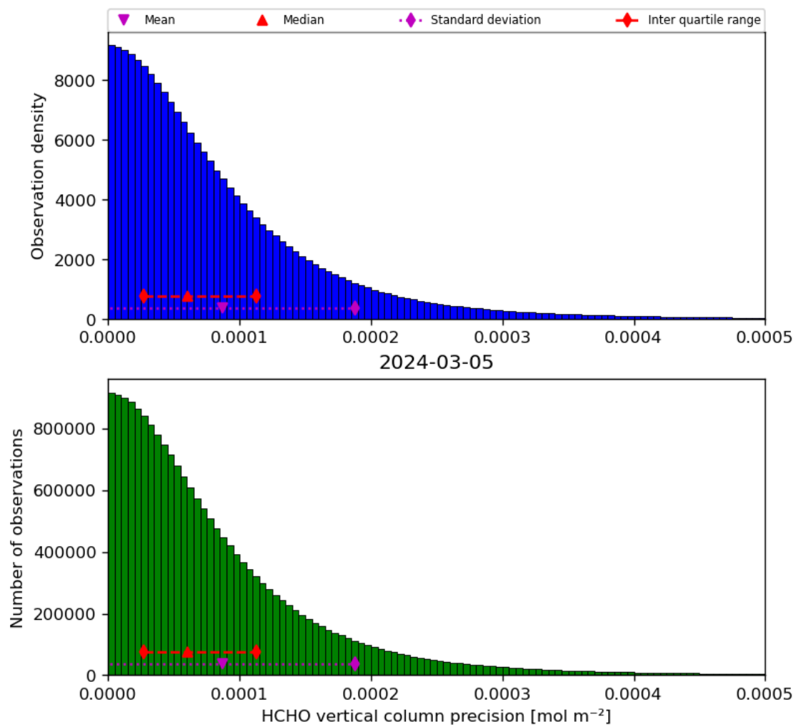
Figure 36: Histogram of “HCHO vertical column precision” for 2024-03-04 to 2024-03-06
