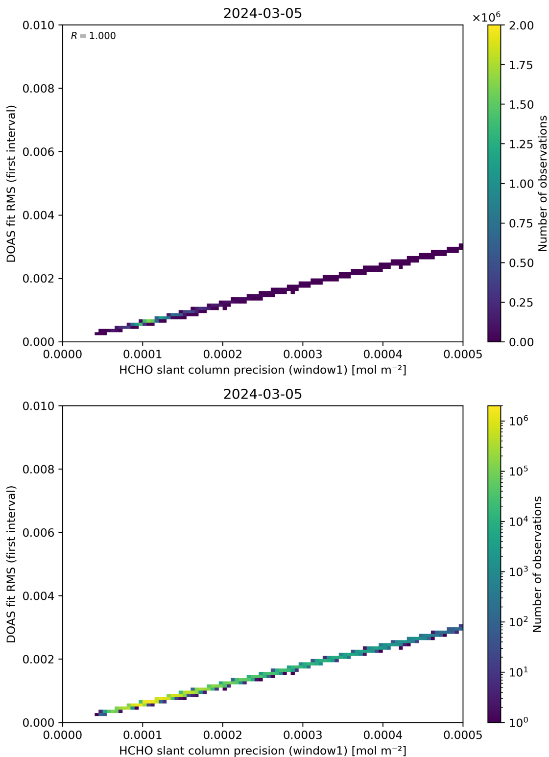
Figure 88: Scatter density plot of “HCHO slant column precision (window1)” against “DOAS fit RMS (first interval)” for 2024-03-04 to 2024-03-06.
