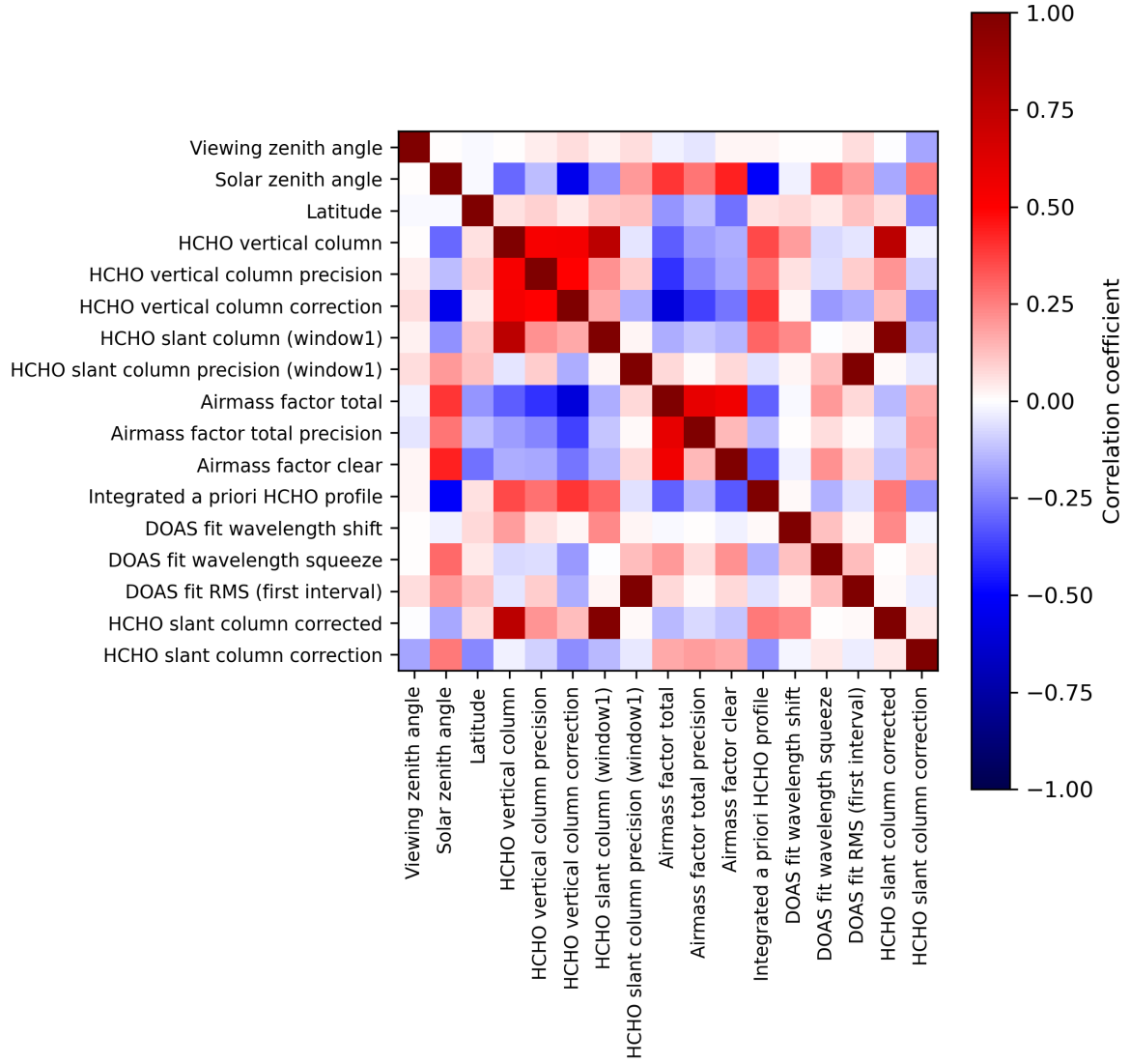
Figure 2: Map of correlation matrix for 2024-03-04 to 2024-03-06.
