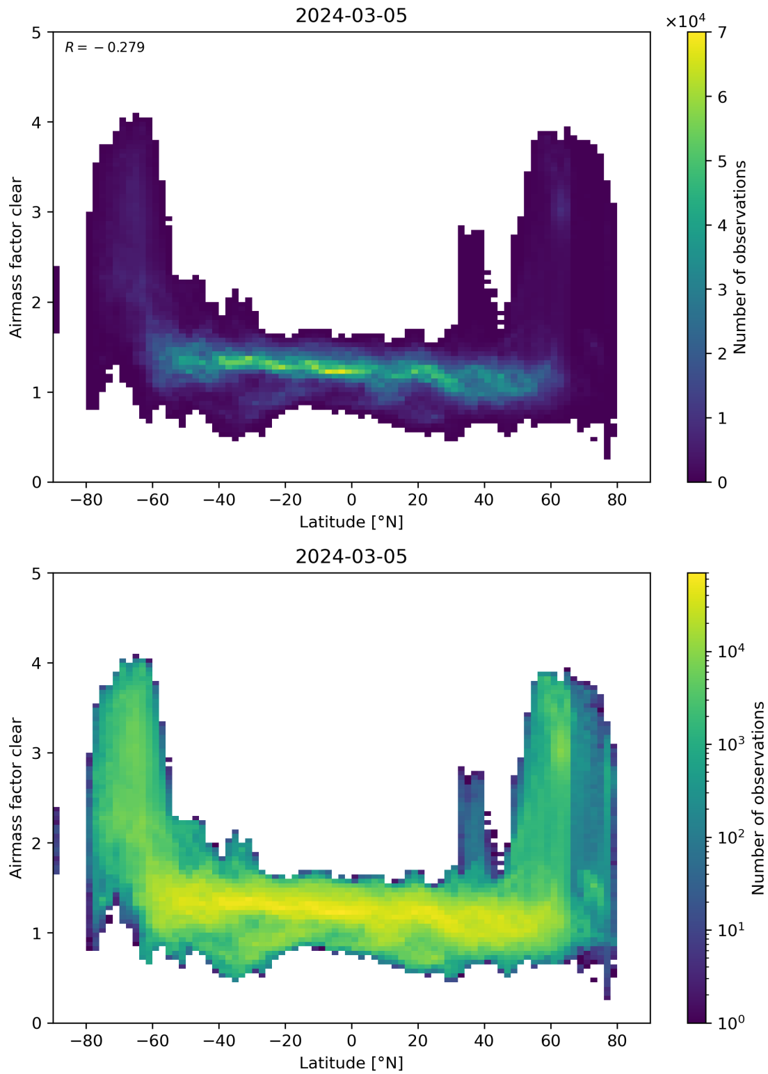
Figure 156: Scatter density plot of “Latitude” against “Airmass factor clear” for 2024-03-04 to 2024-03-06.
