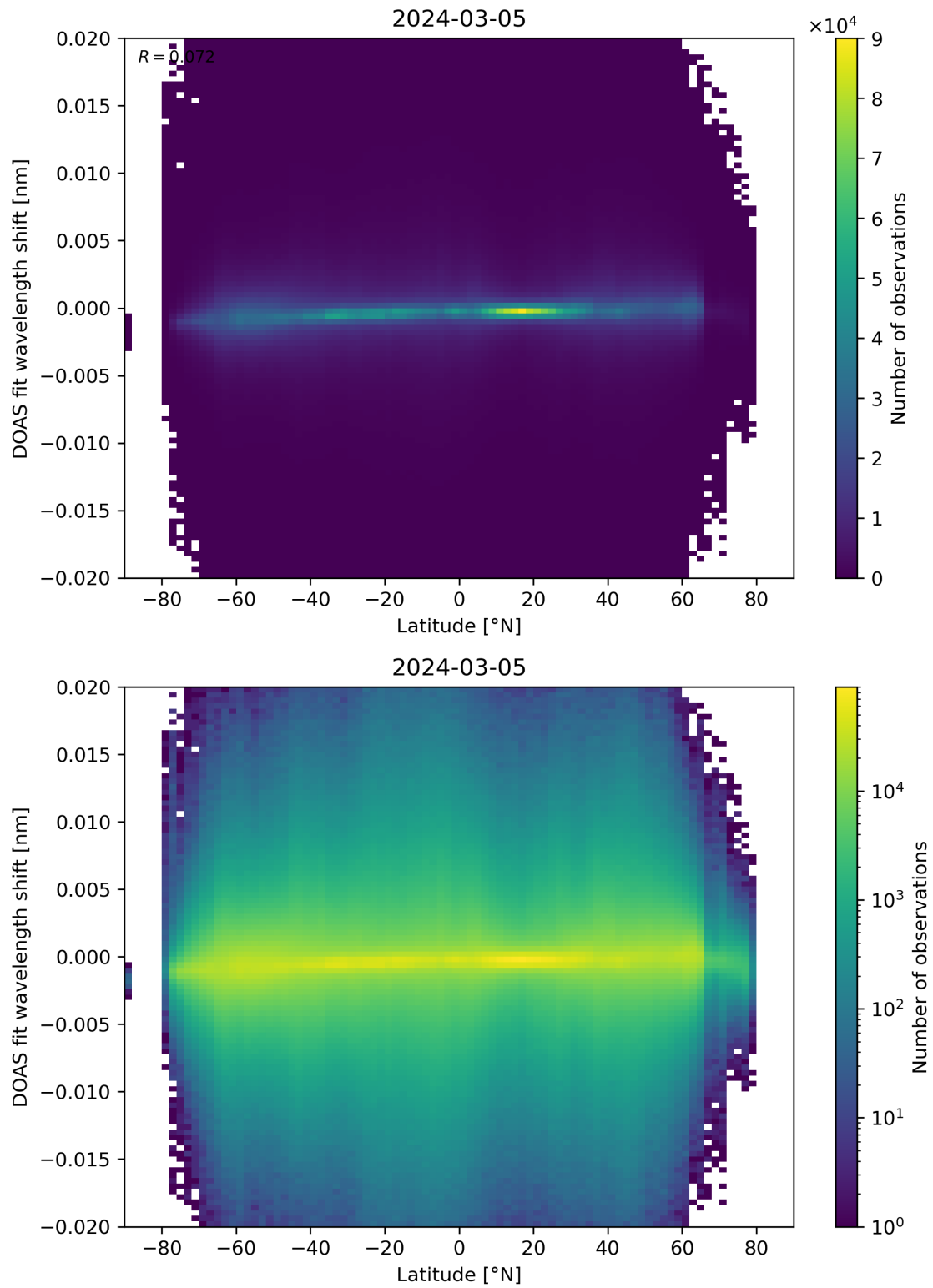
Figure 154: Scatter density plot of “Latitude” against “DOAS fit wavelength shift” for 2024-03-04 to 2024-03-06.
