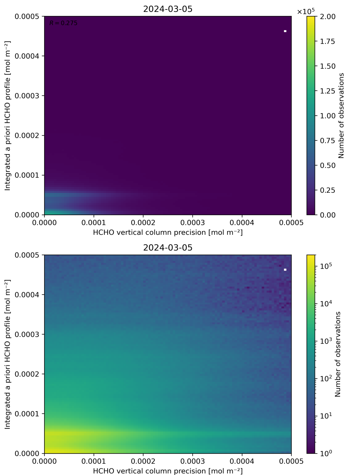
Figure 147: Scatter density plot of “HCHO vertical column precision” against “Integrated a priori HCHO profile” for 2024-03-04 to 2024-03-06.
