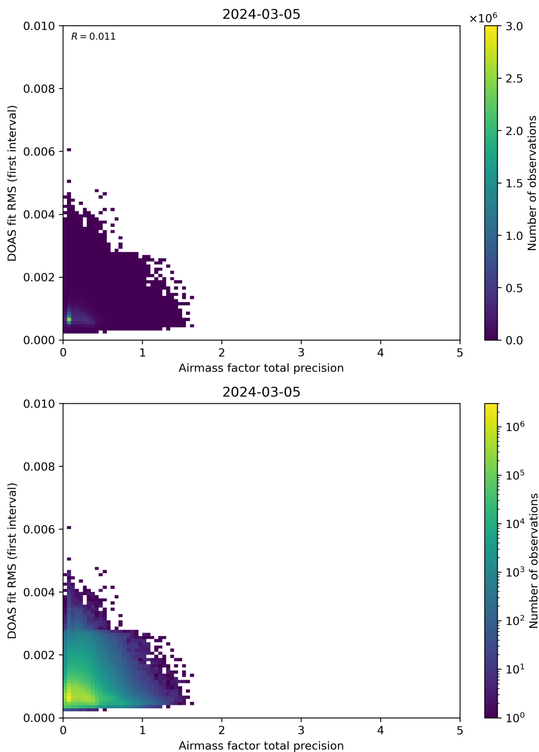
Figure 105: Scatter density plot of “Airmass factor total precision” against “DOAS fit RMS (first interval)” for 2024-03-04 to 2024-03-06.
