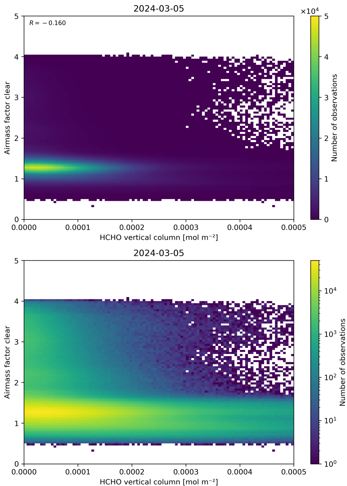
Figure 126: Scatter density plot of “HCHO vertical column” against “Airmass factor clear” for 2024-03-04 to 2024-03-06.
