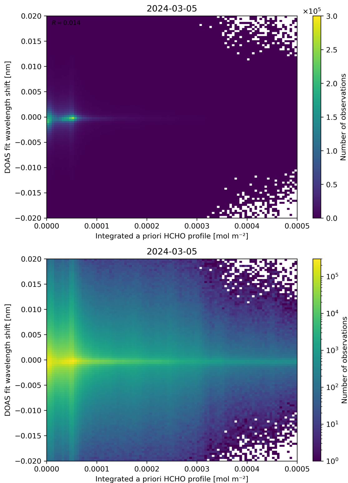
Figure 149: Scatter density plot of “Integrated a priori HCHO profile” against “DOAS fit wavelength shift” for 2024-03-04 to 2024-03-06.
