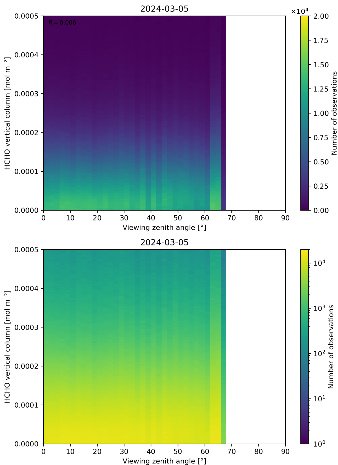
Figure 192: Scatter density plot of “Viewing zenith angle” against “HCHO vertical column” for 2024-03-04 to 2024-03-06.
