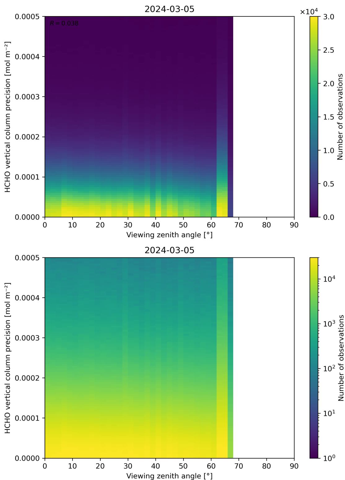
Figure 194: Scatter density plot of “Viewing zenith angle” against “HCHO vertical column precision” for 2024-03-04 to 2024-03-06.
