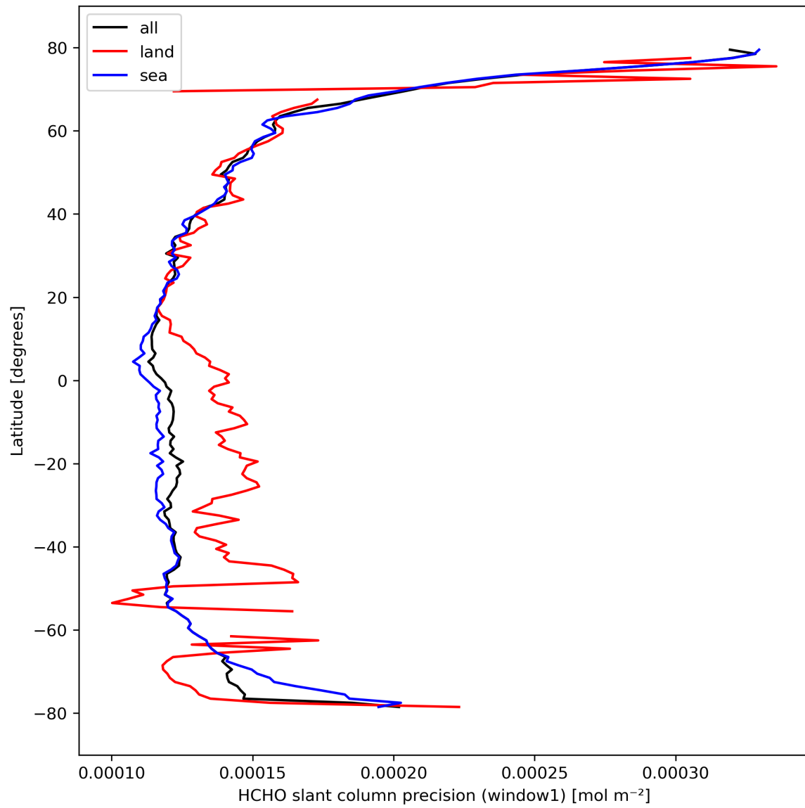
Figure 25: Zonal average of “HCHO slant column precision (window1)” for 2024-03-04 to 2024-03-06.
