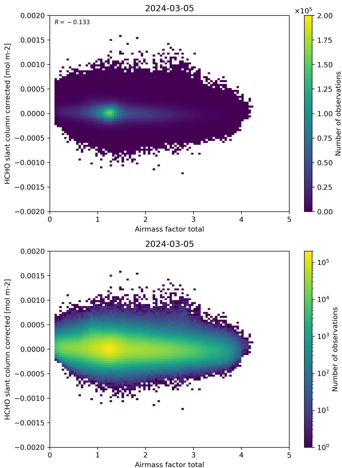
Figure 101: Scatter density plot of “Airmass factor total” against “HCHO slant column corrected” for 2024-03-04 to 2024-03-06.
