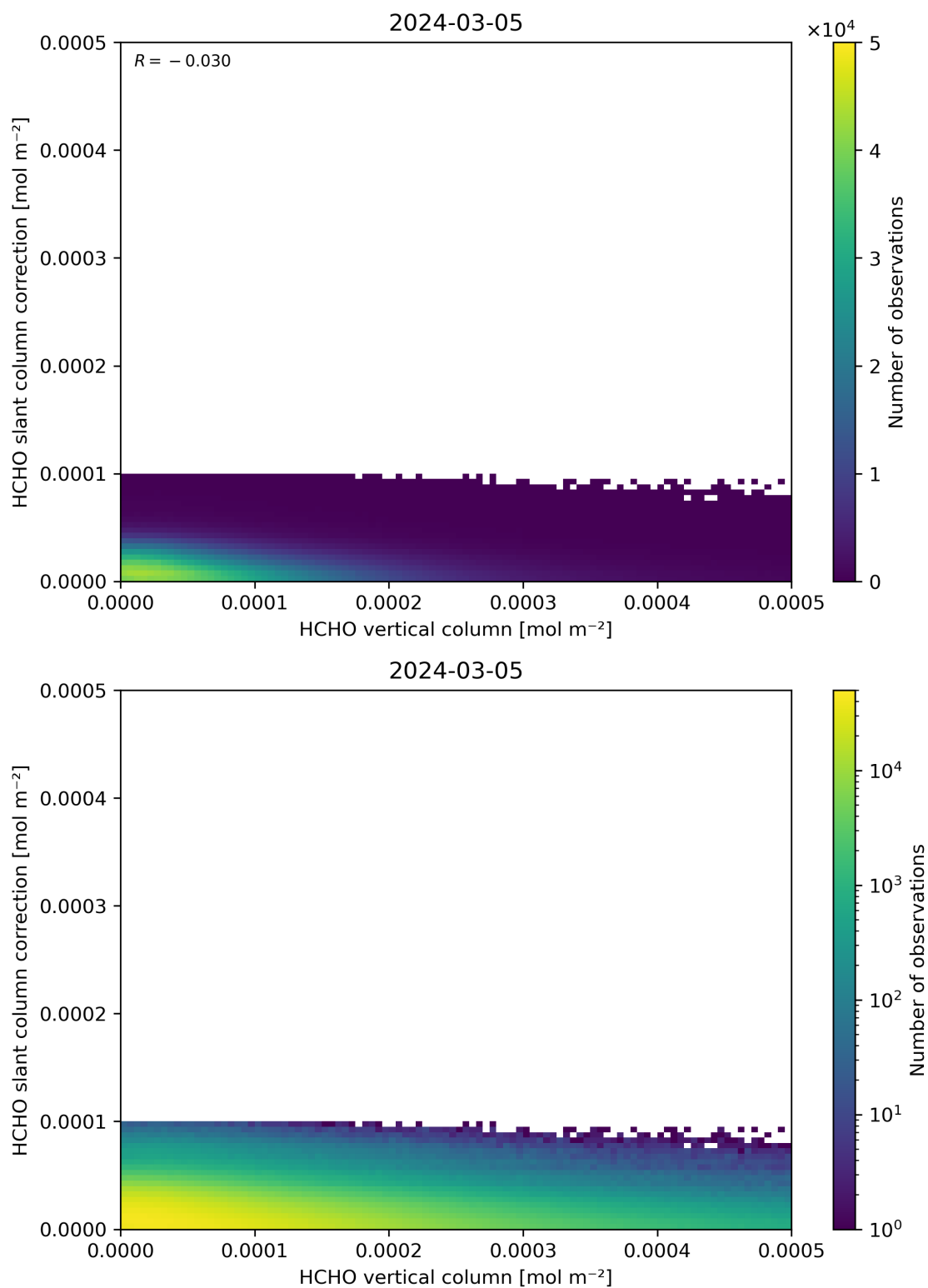
Figure 128: Scatter density plot of “HCHO vertical column” against “HCHO slant column correction” for 2024-03-04 to 2024-03-06.
