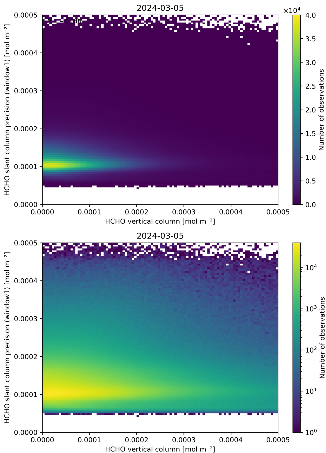
Figure 130: Scatter density plot of “HCHO vertical column” against “HCHO slant column precision (window1)” for 2024-03-04 to 2024-03-06.
