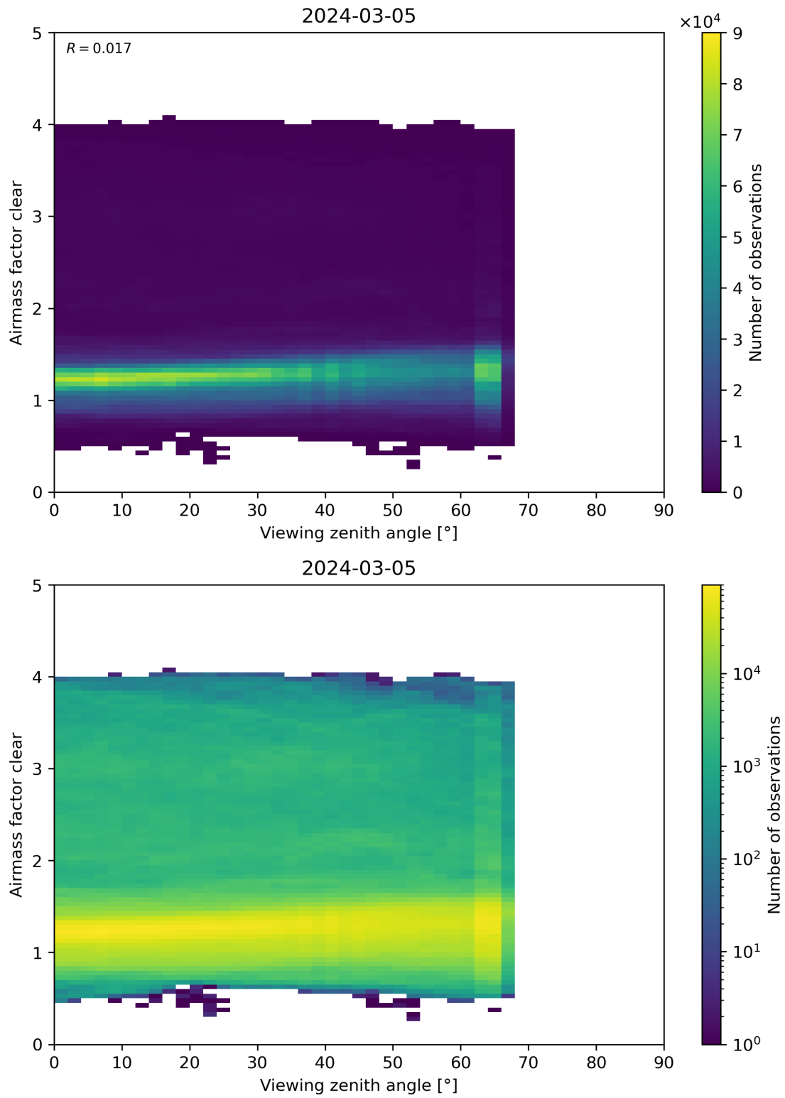
Figure 185: Scatter density plot of “Viewing zenith angle” against “Airmass factor clear” for 2024-03-04 to 2024-03-06.
