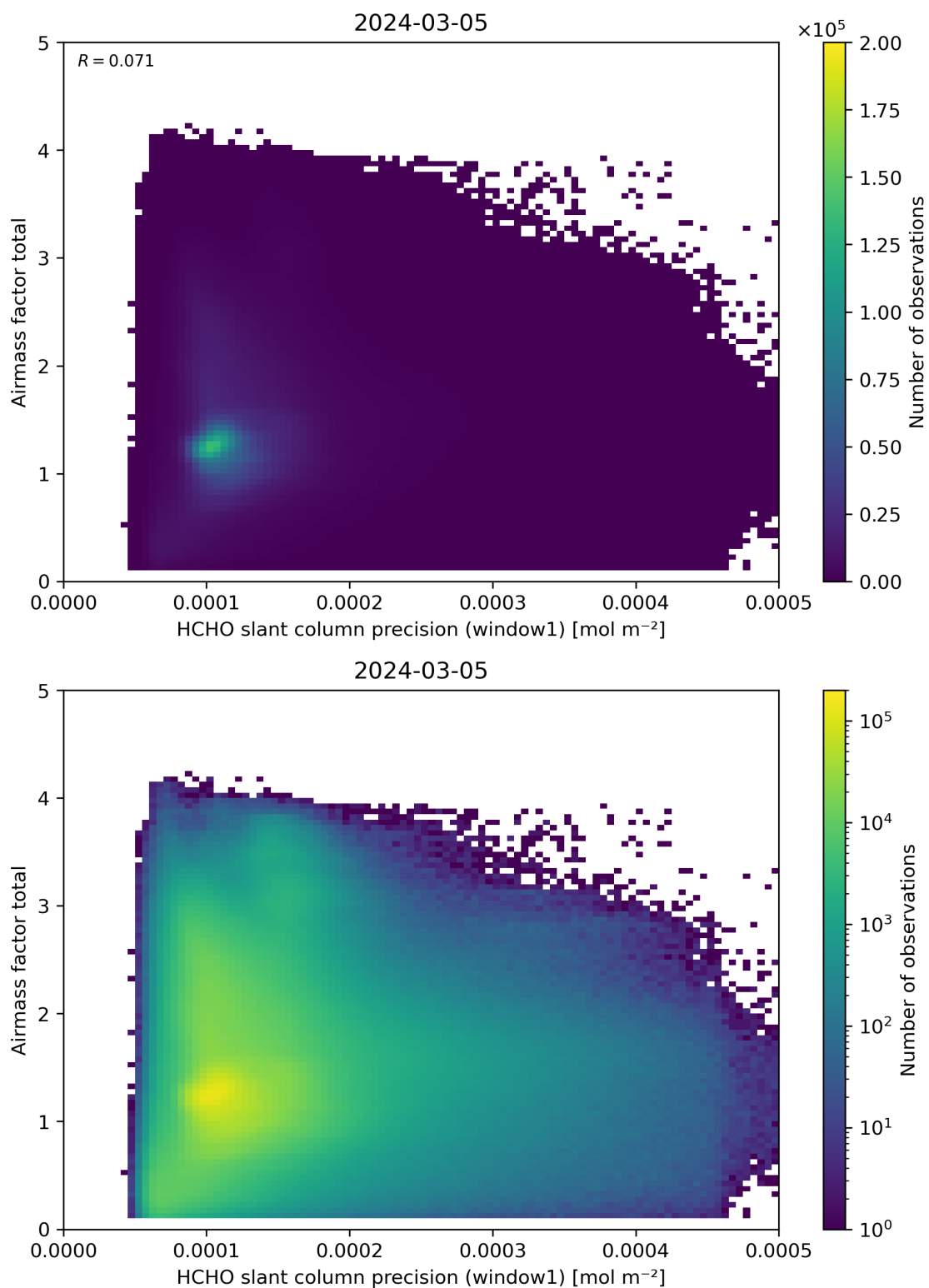
Figure 94: Scatter density plot of “HCHO slant column precision (window1)” against “Airmass factor total” for 2024-03-04 to 2024-03-06.
