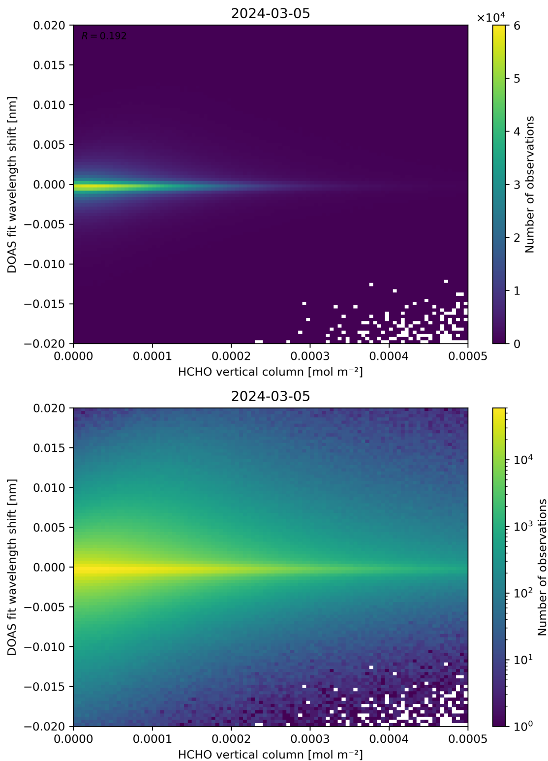
Figure 124: Scatter density plot of “HCHO vertical column” against “DOAS fit wavelength shift” for 2024-03-04 to 2024-03-06.
