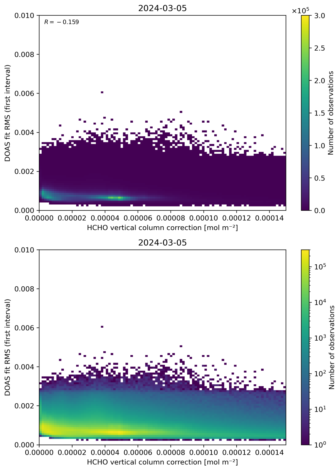
Figure 112: Scatter density plot of “HCHO vertical column correction” against “DOAS fit RMS (first interval)” for 2024-03-04 to 2024-03-06.
