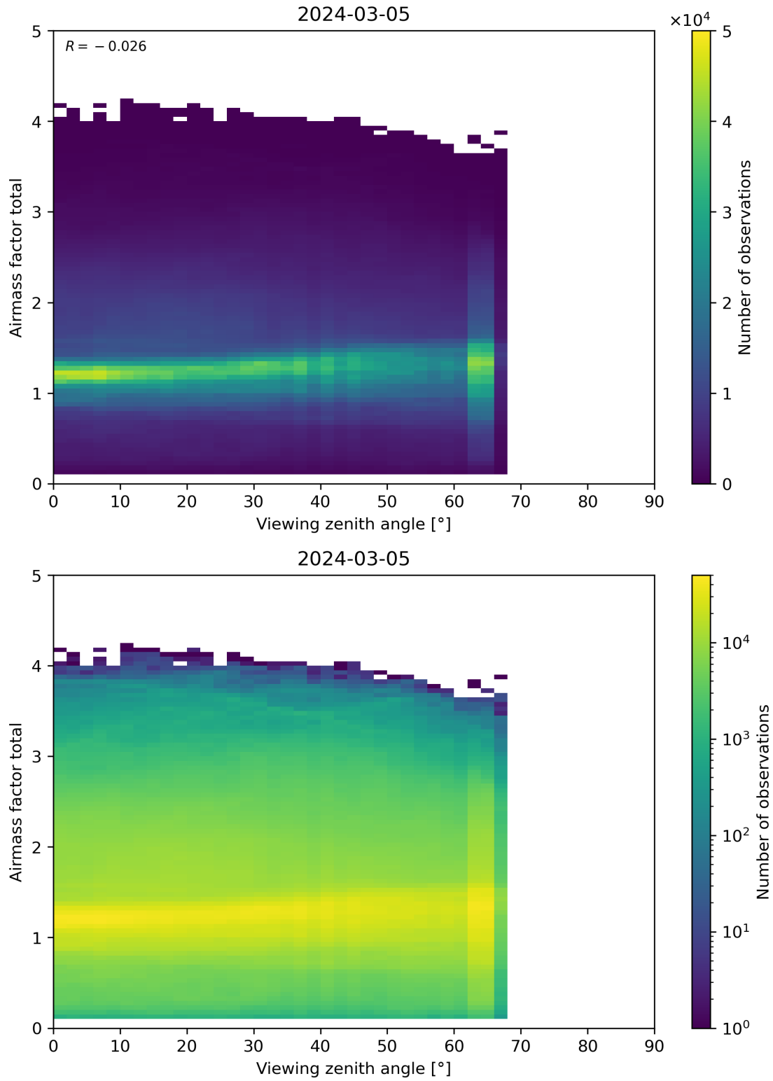
Figure 190: Scatter density plot of “Viewing zenith angle” against “Airmass factor total” for 2024-03-04 to 2024-03-06.
