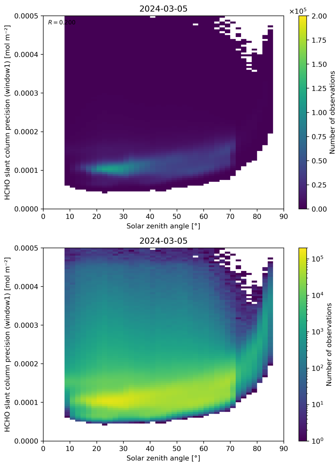
Figure 174: Scatter density plot of “Solar zenith angle” against “HCHO slant column precision (window1)” for 2024-03-04 to 2024-03-06.
