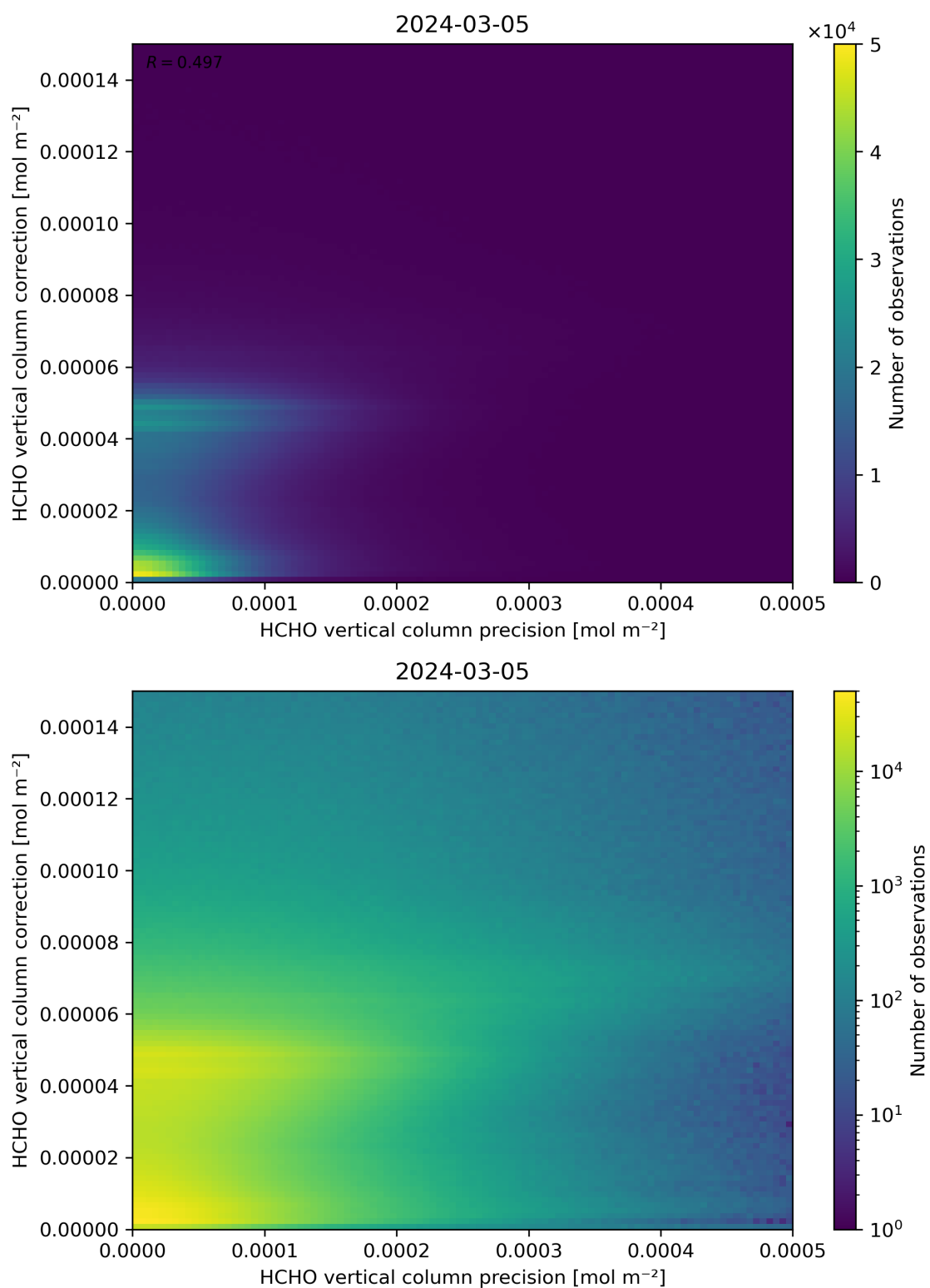
Figure 146: Scatter density plot of “HCHO vertical column precision” against “HCHO vertical column correction” for 2024-03-04 to 2024-03-06.
