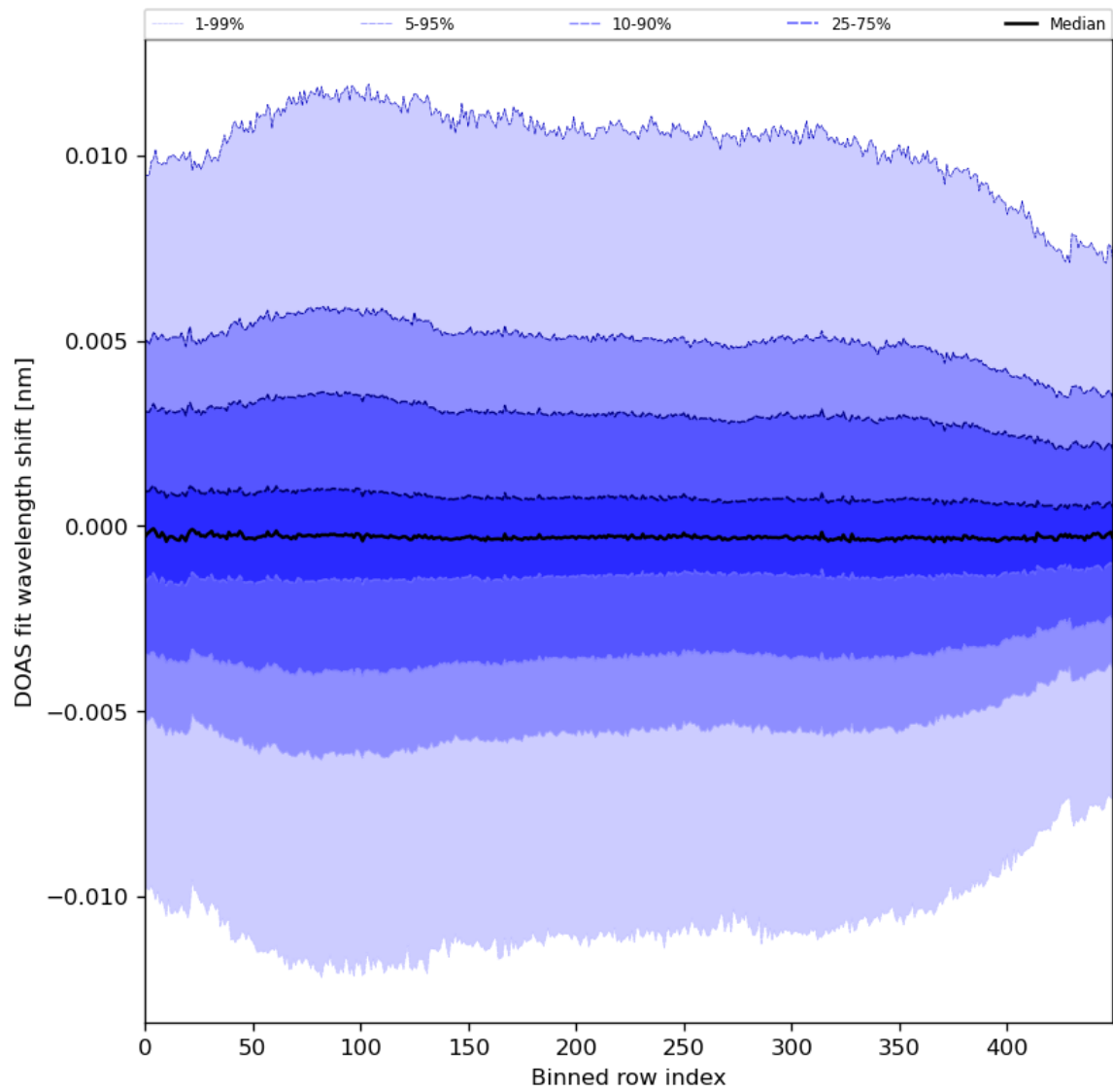
Figure 58: Along track statistics of “DOAS fit wavelength shift” for 2024-03-04 to 2024-03-06
