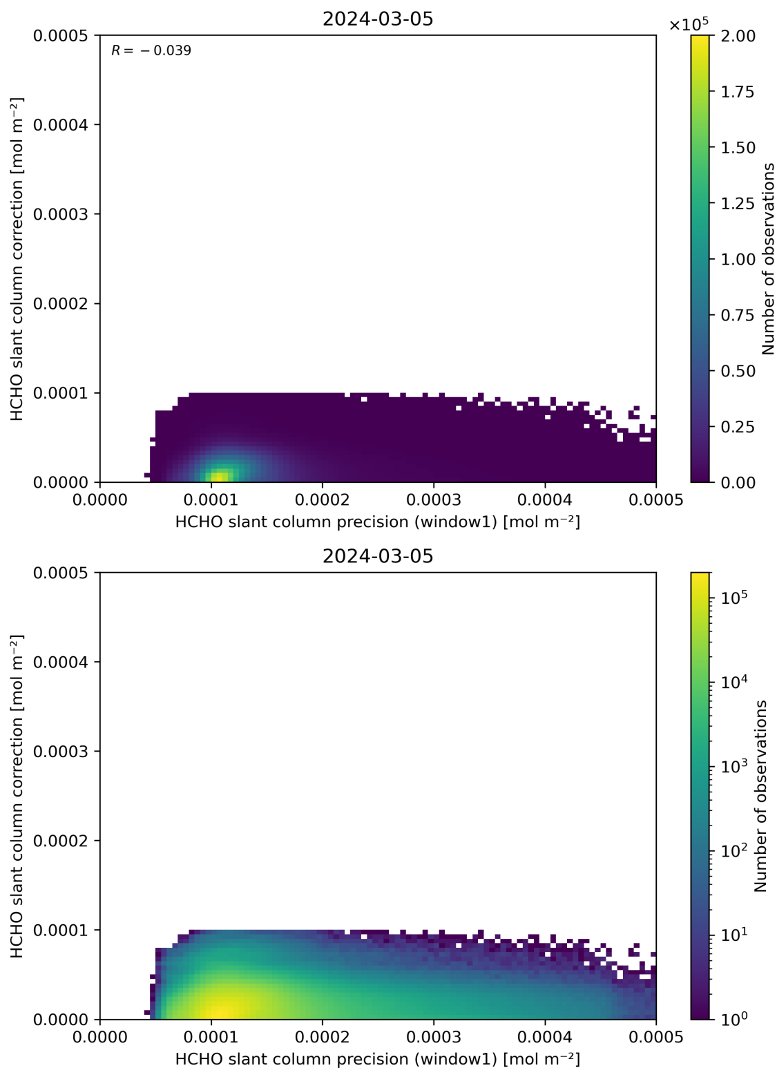
Figure 93: Scatter density plot of “HCHO slant column precision (window1)” against “HCHO slant column correction” for 2024-03-04 to 2024-03-06.
