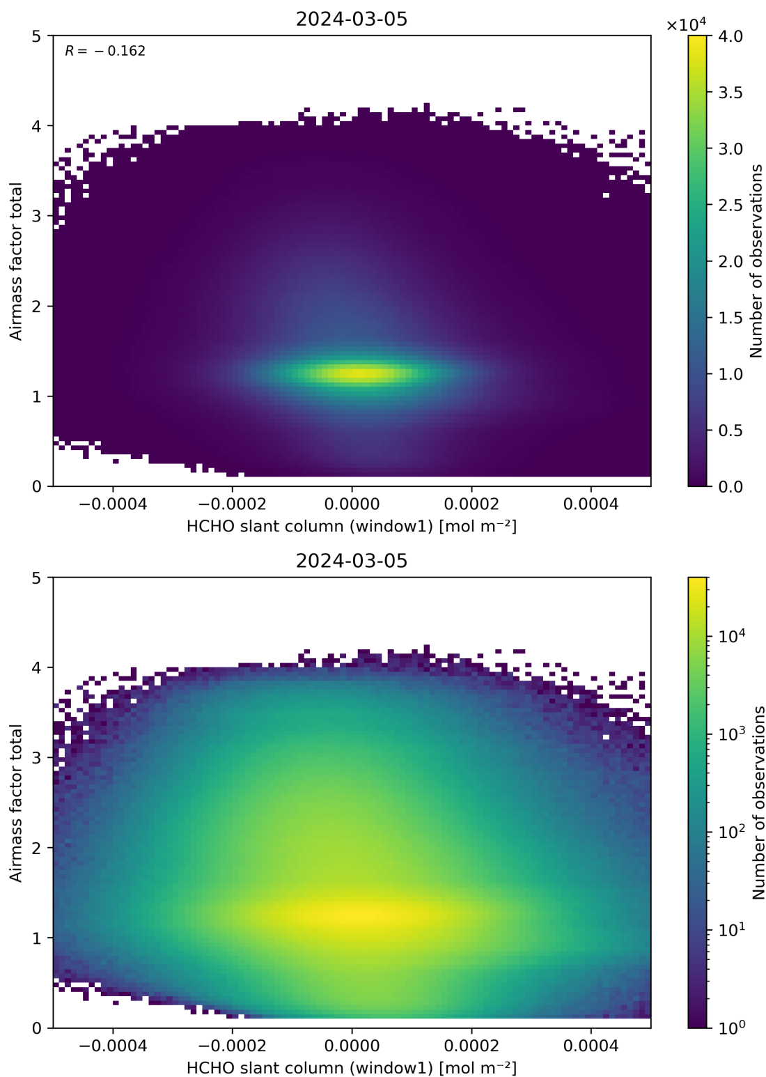
Figure 85: Scatter density plot of “HCHO slant column (window1)” against “Airmass factor total” for 2024-03-04 to 2024-03-06.
