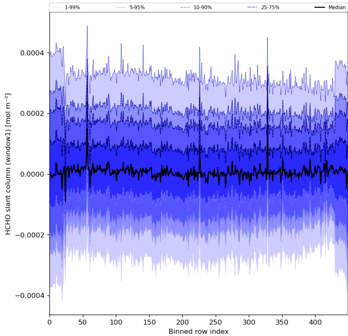
Figure 52: Along track statistics of "HCHO slant column (window1)" for 2024-03-04 to 2024-03-06
