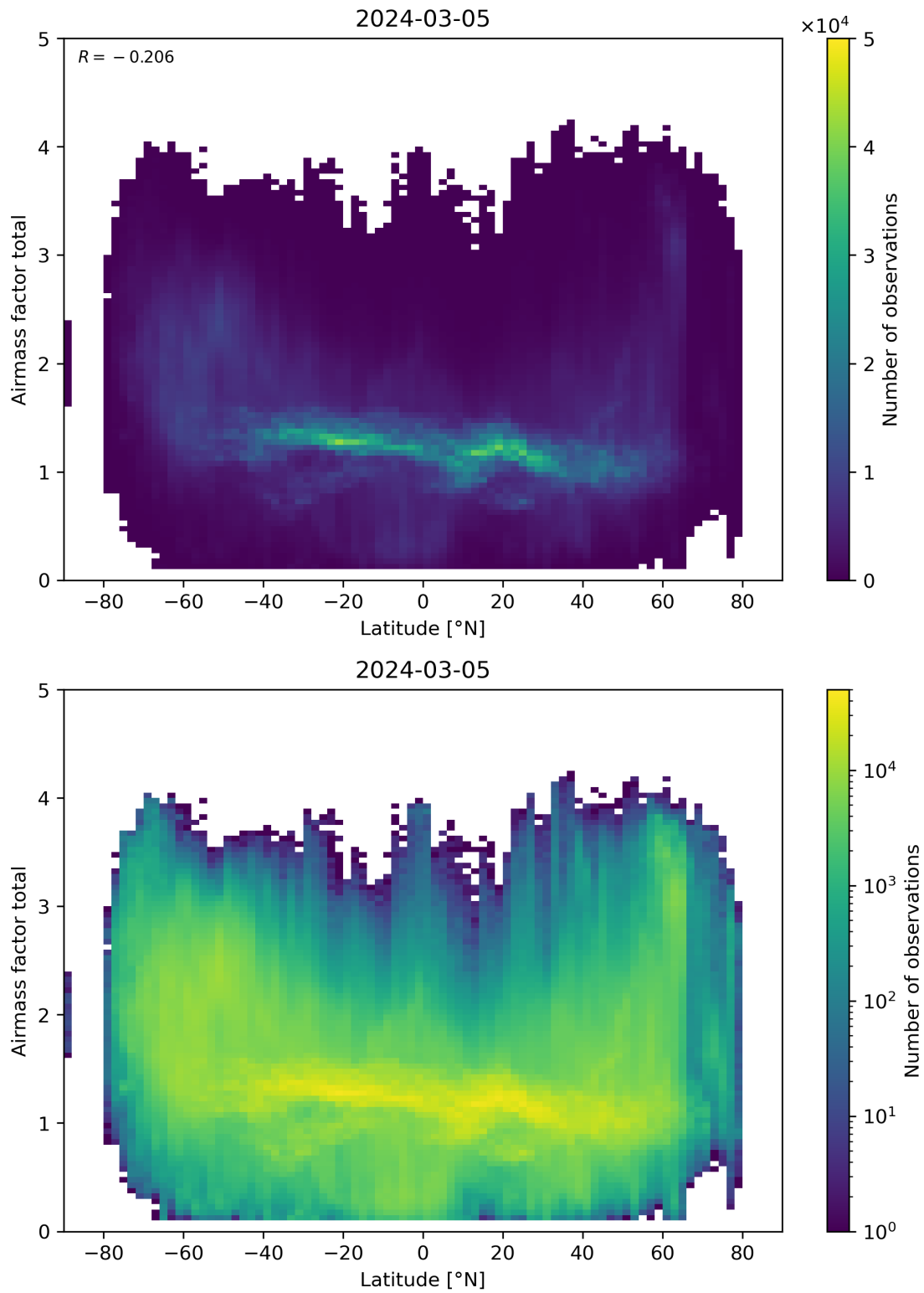
Figure 161: Scatter density plot of “Latitude” against “Airmass factor total” for 2024-03-04 to 2024-03-06.
