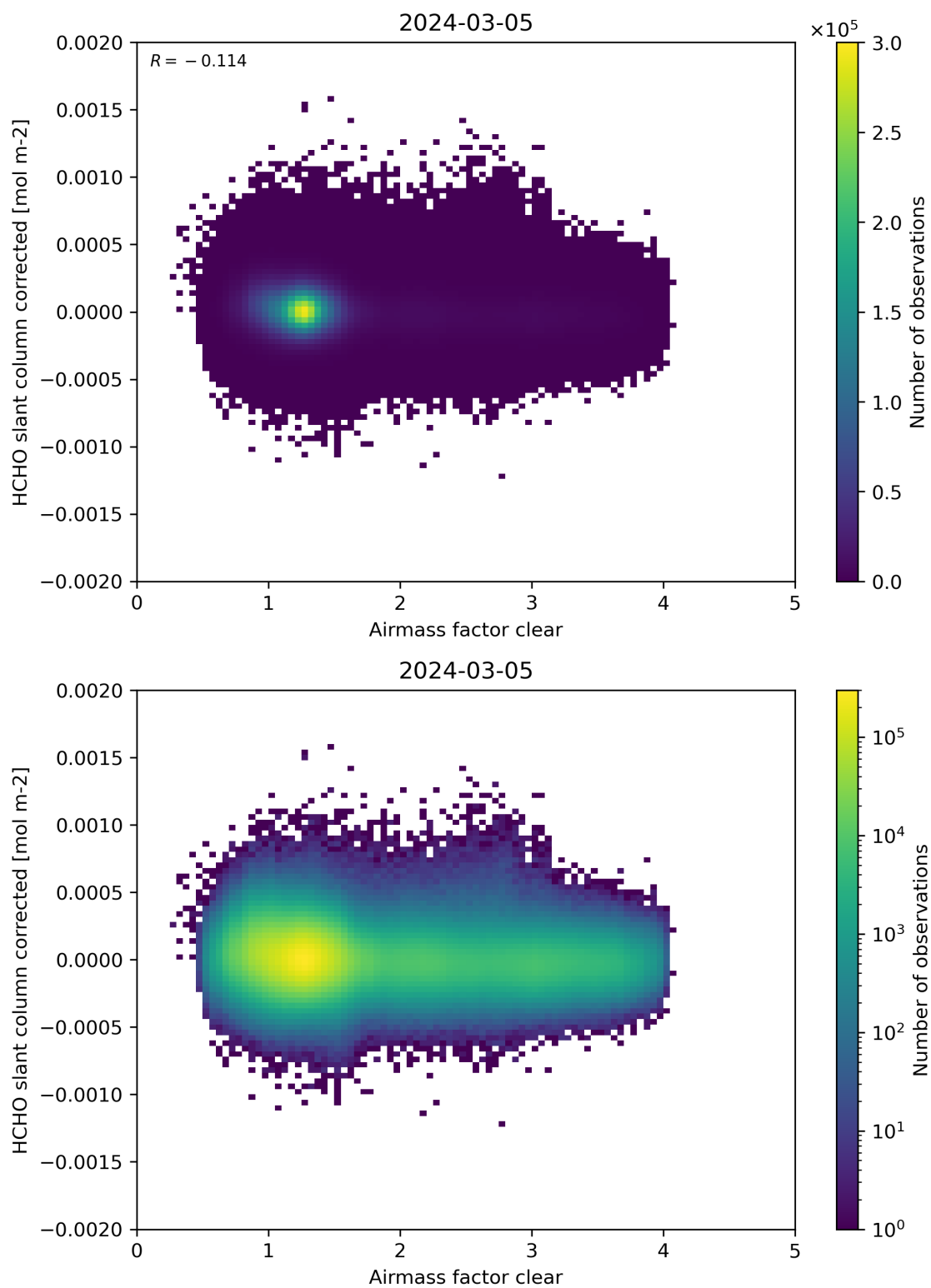
Figure 74: Scatter density plot of “Airmass factor clear” against “HCHO slant column corrected” for 2024-03-04 to 2024-03-06.
