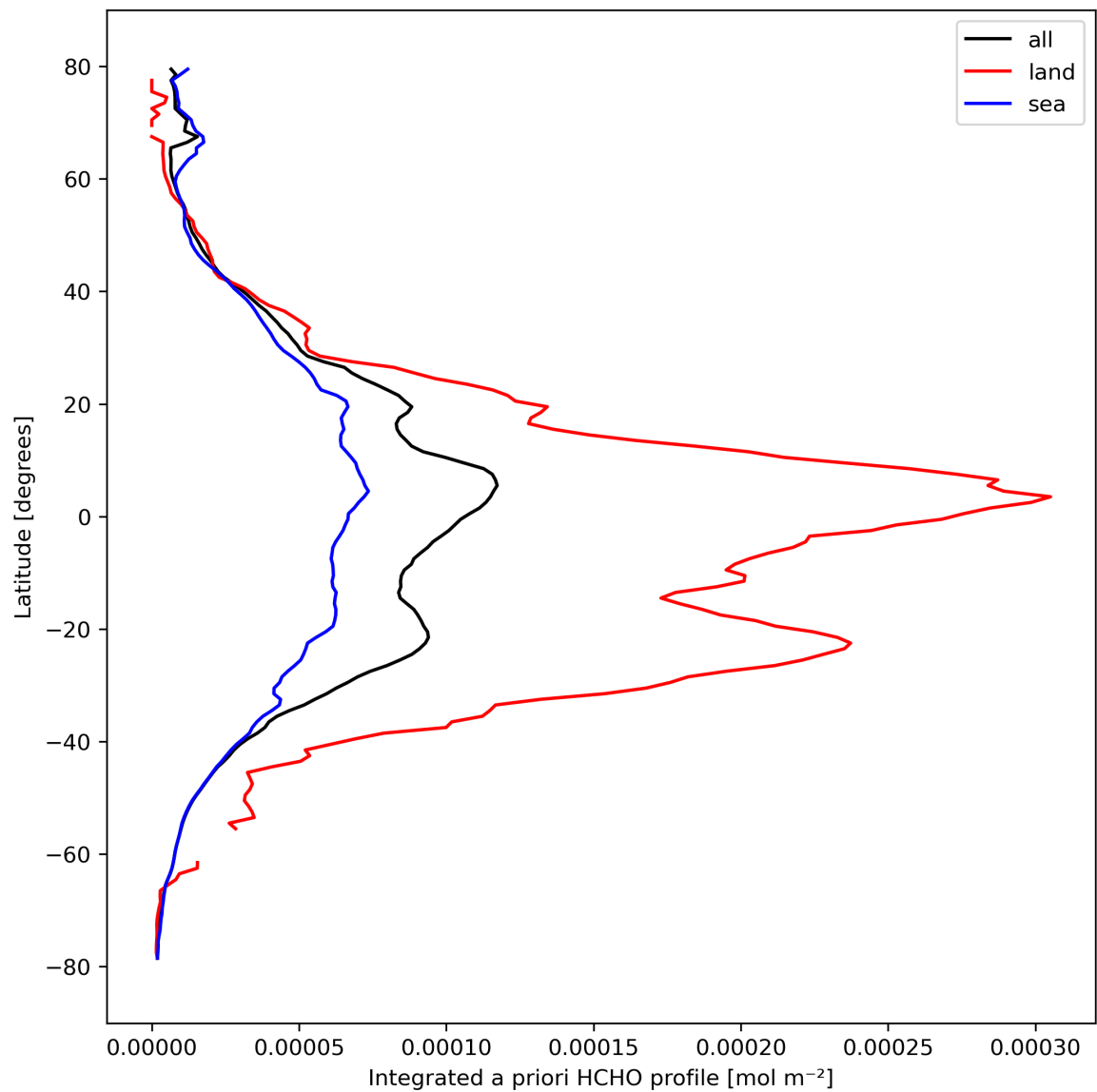
Figure 29: Zonal average of “Integrated a priori HCHO profile” for 2024-03-04 to 2024-03-06.
