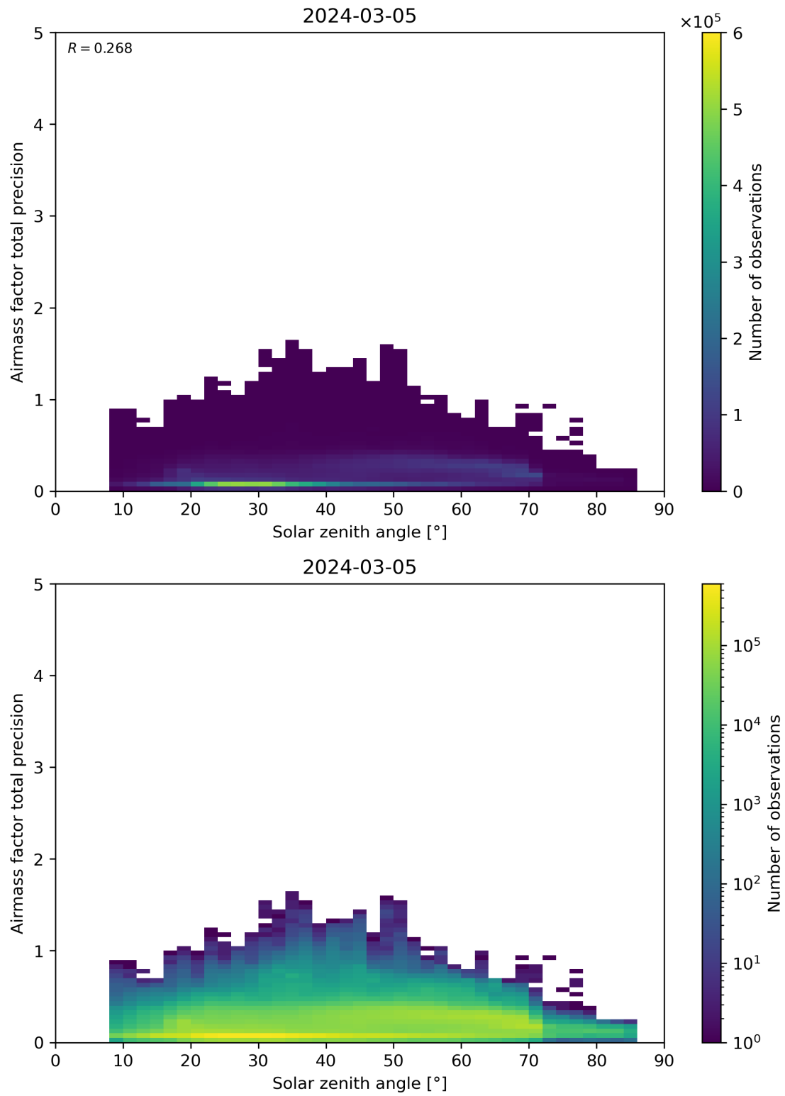
Figure 176: Scatter density plot of “Solar zenith angle” against “Airmass factor total precision” for 2024-03-04 to 2024-03-06.
