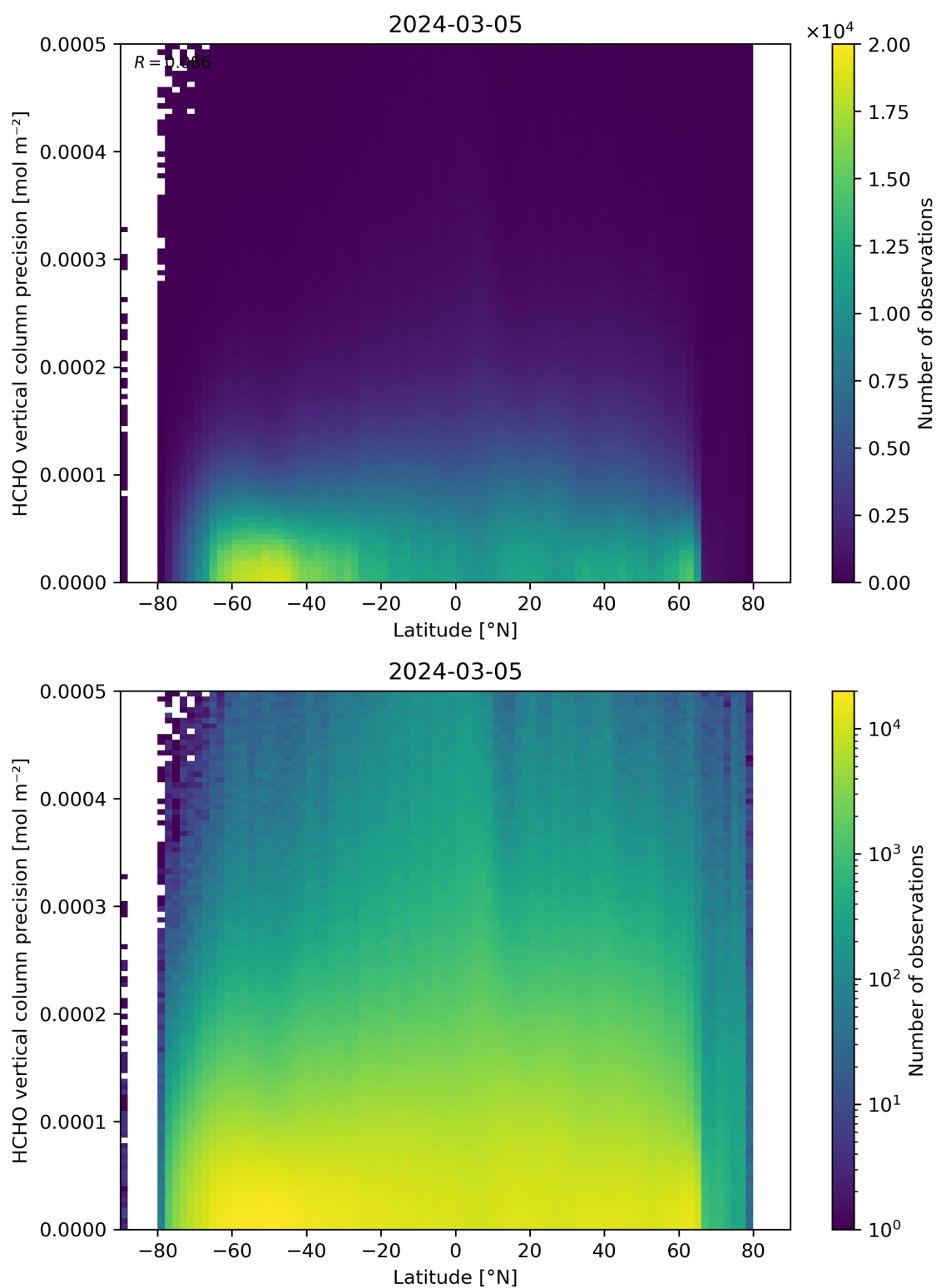
Figure 165: Scatter density plot of “Latitude” against “HCHO vertical column precision” for 2024-03-04 to 2024-03-06.
