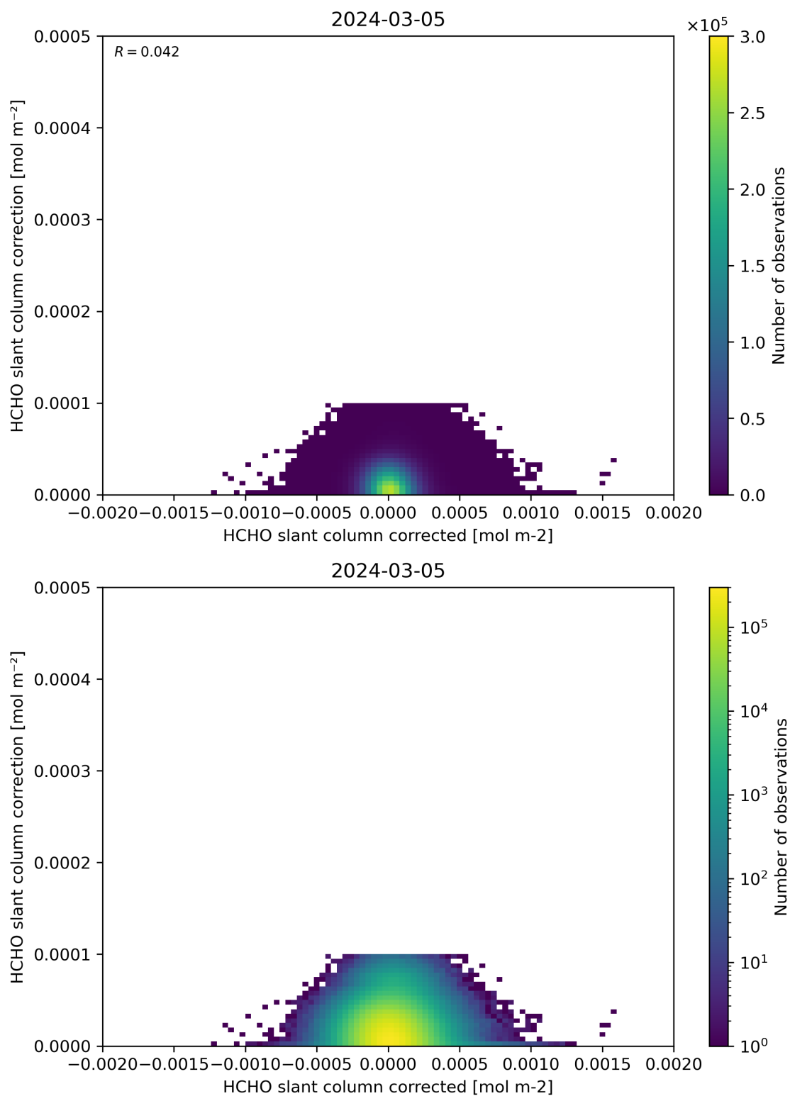
Figure 77: Scatter density plot of “HCHO slant column corrected” against “HCHO slant column correction” for 2024-03-04 to 2024-03-06.
