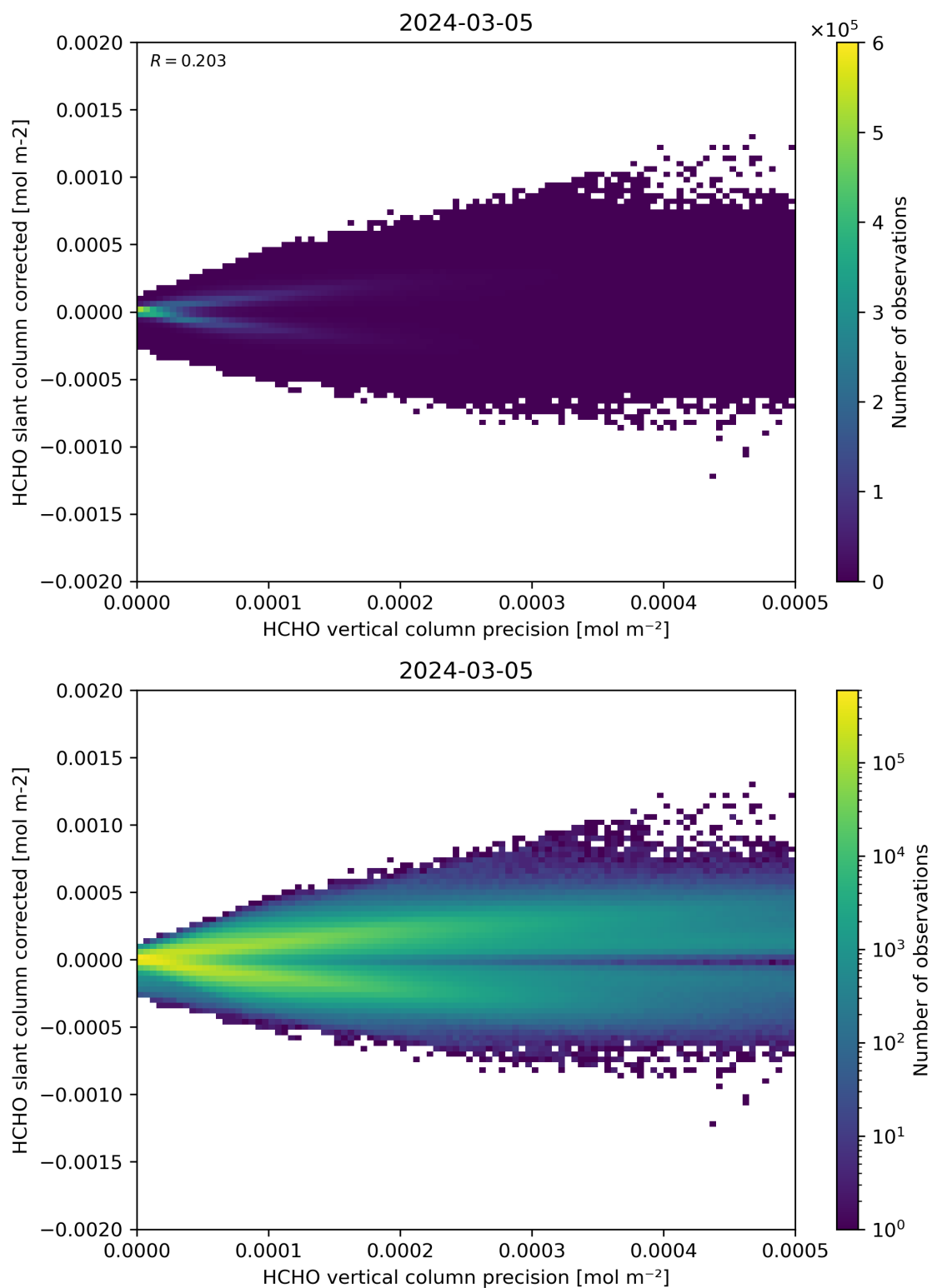
Figure 140: Scatter density plot of “HCHO vertical column precision” against “HCHO slant column corrected” for 2024-03-04 to 2024-03-06.
