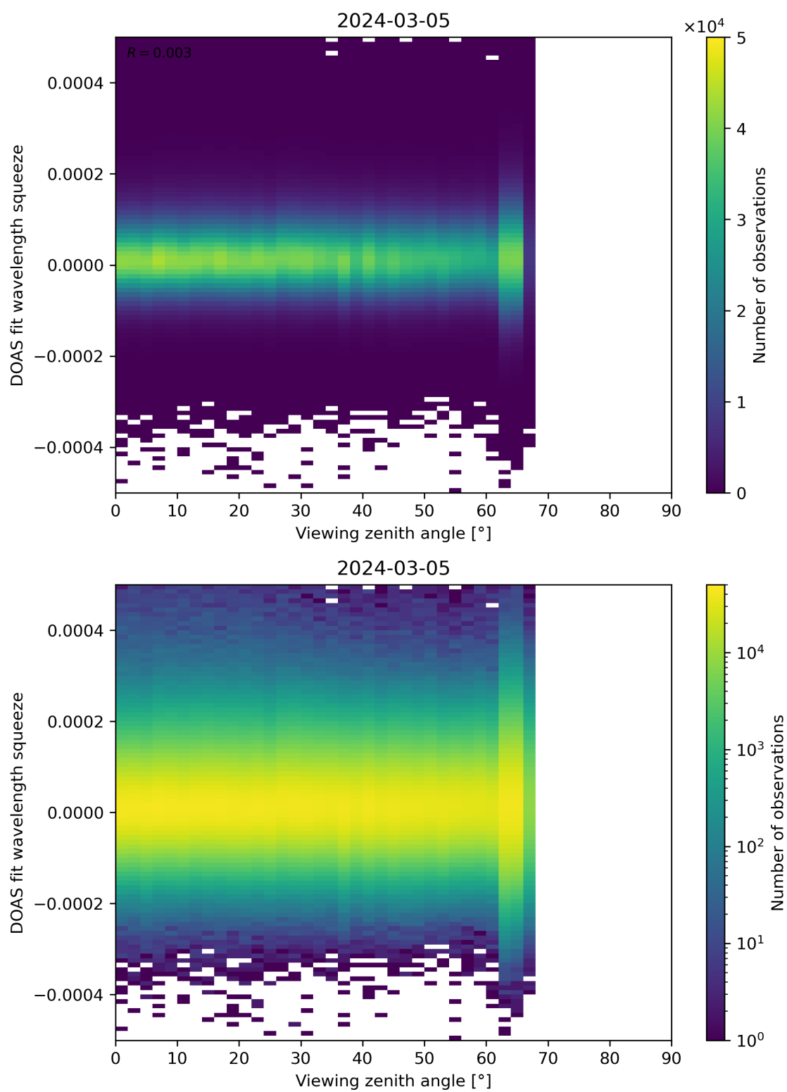
Figure 184: Scatter density plot of “Viewing zenith angle” against “DOAS fit wavelength squeeze” for 2024-03-04 to 2024-03-06.
