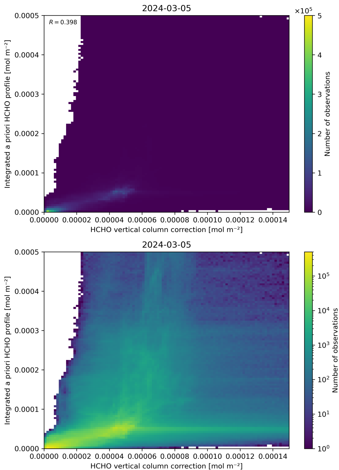
Figure 122: Scatter density plot of “HCHO vertical column correction” against “Integrated a priori HCHO profile” for 2024-03-04 to 2024-03-06.
