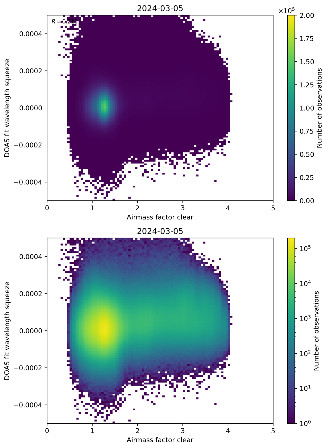
Figure 73: Scatter density plot of “Airmass factor clear” against “DOAS fit wavelength squeeze” for 2024-03-04 to 2024-03-06.
