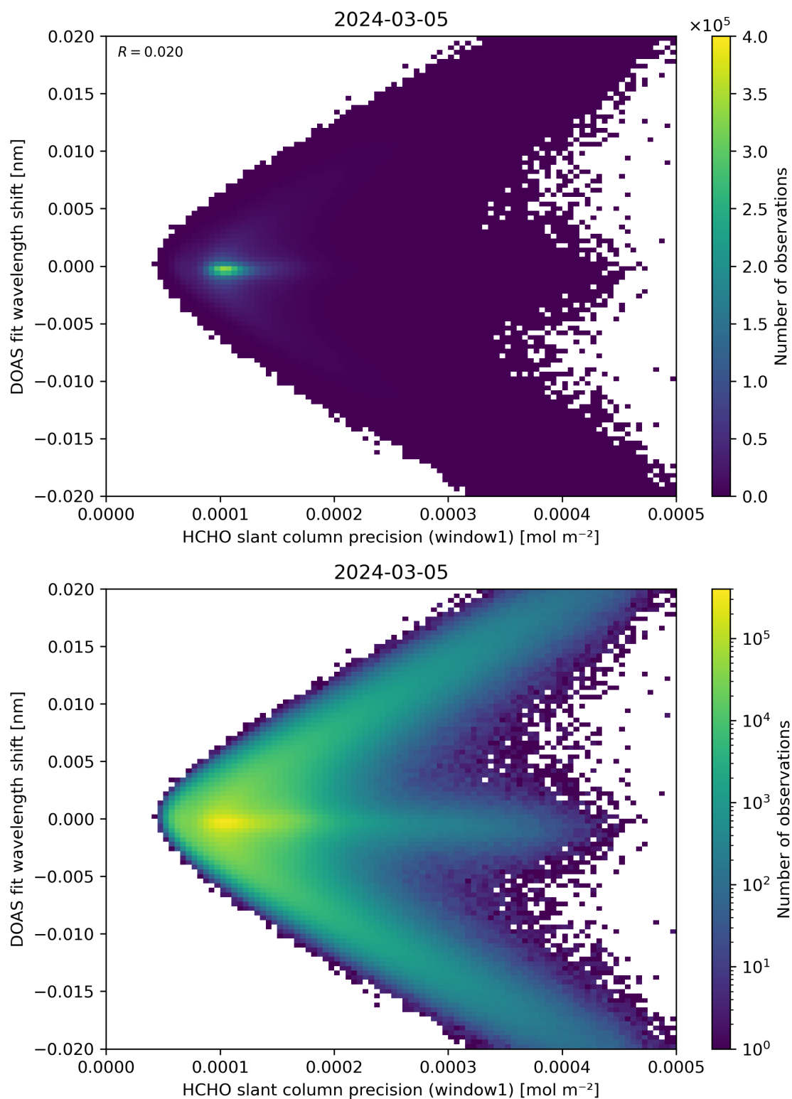
Figure 89: Scatter density plot of “HCHO slant column precision (window1)” against “DOAS fit wavelength shift” for 2024-03-04 to 2024-03-06.
