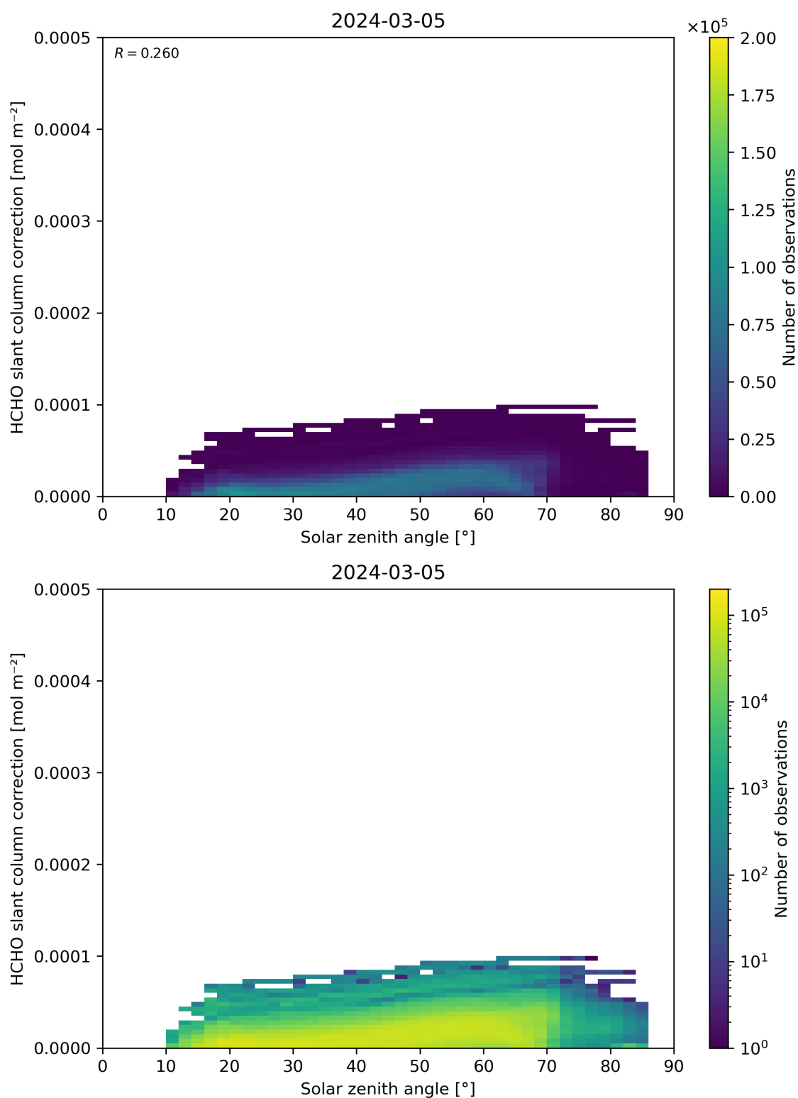
Figure 172: Scatter density plot of “Solar zenith angle” against “HCHO slant column correction” for 2024-03-04 to 2024-03-06.
