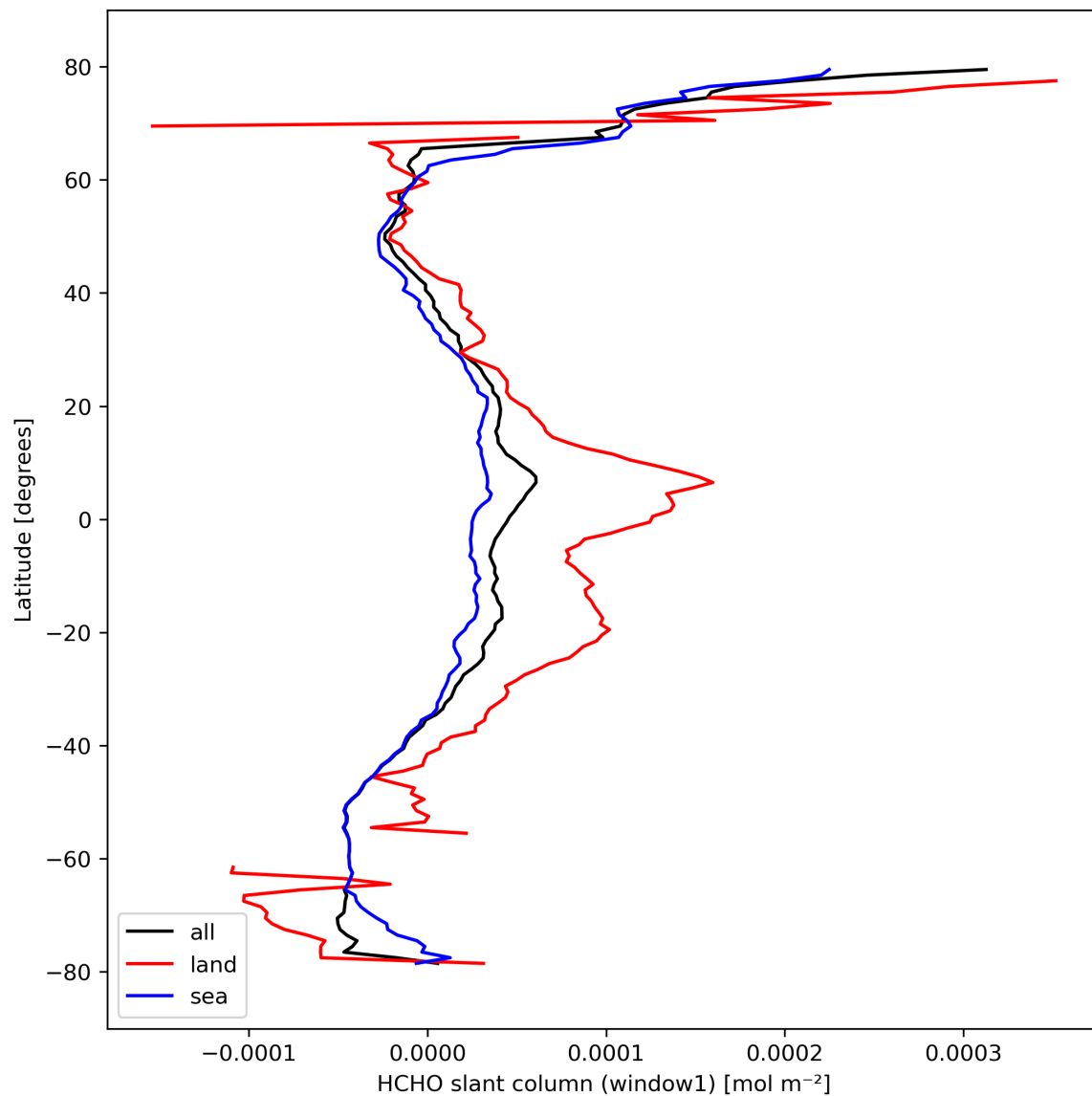
Figure 24: Zonal average of “HCHO slant column (window1)” for 2024-03-04 to 2024-03-06.
