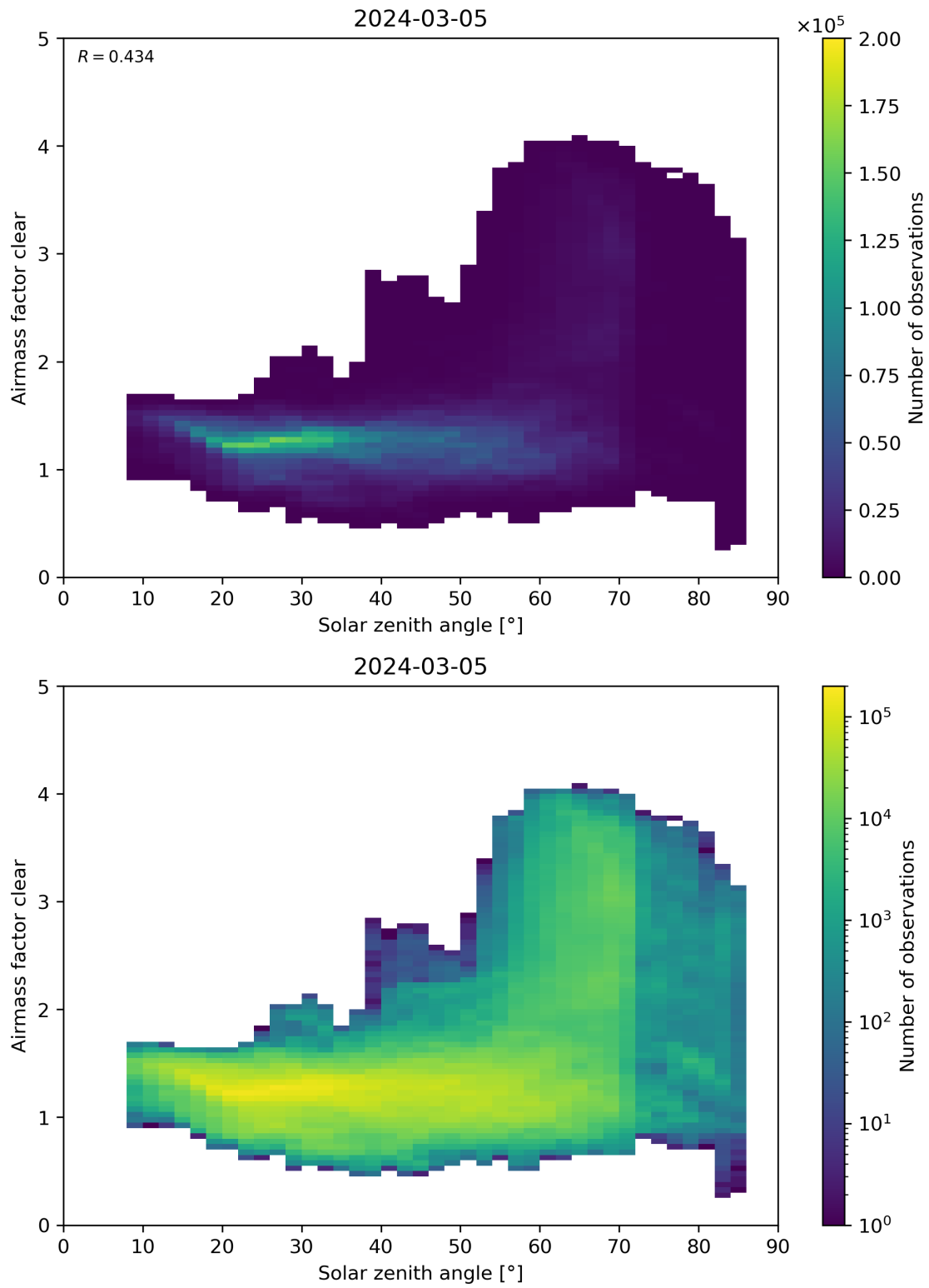
Figure 170: Scatter density plot of “Solar zenith angle” against “Airmass factor clear” for 2024-03-04 to 2024-03-06.
