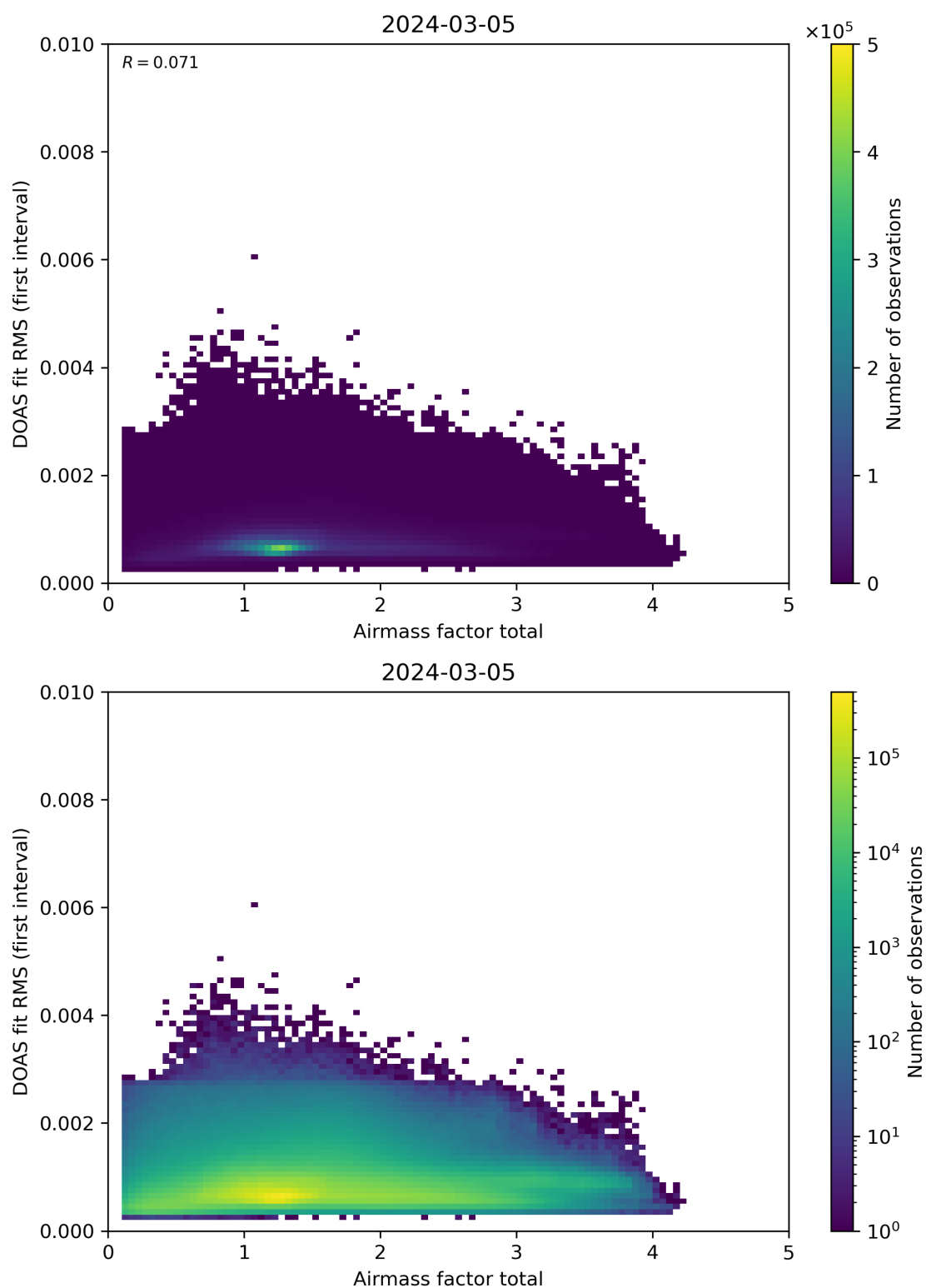
Figure 97: Scatter density plot of “Airmass factor total” against “DOAS fit RMS (first interval)” for 2024-03-04 to 2024-03-06.
