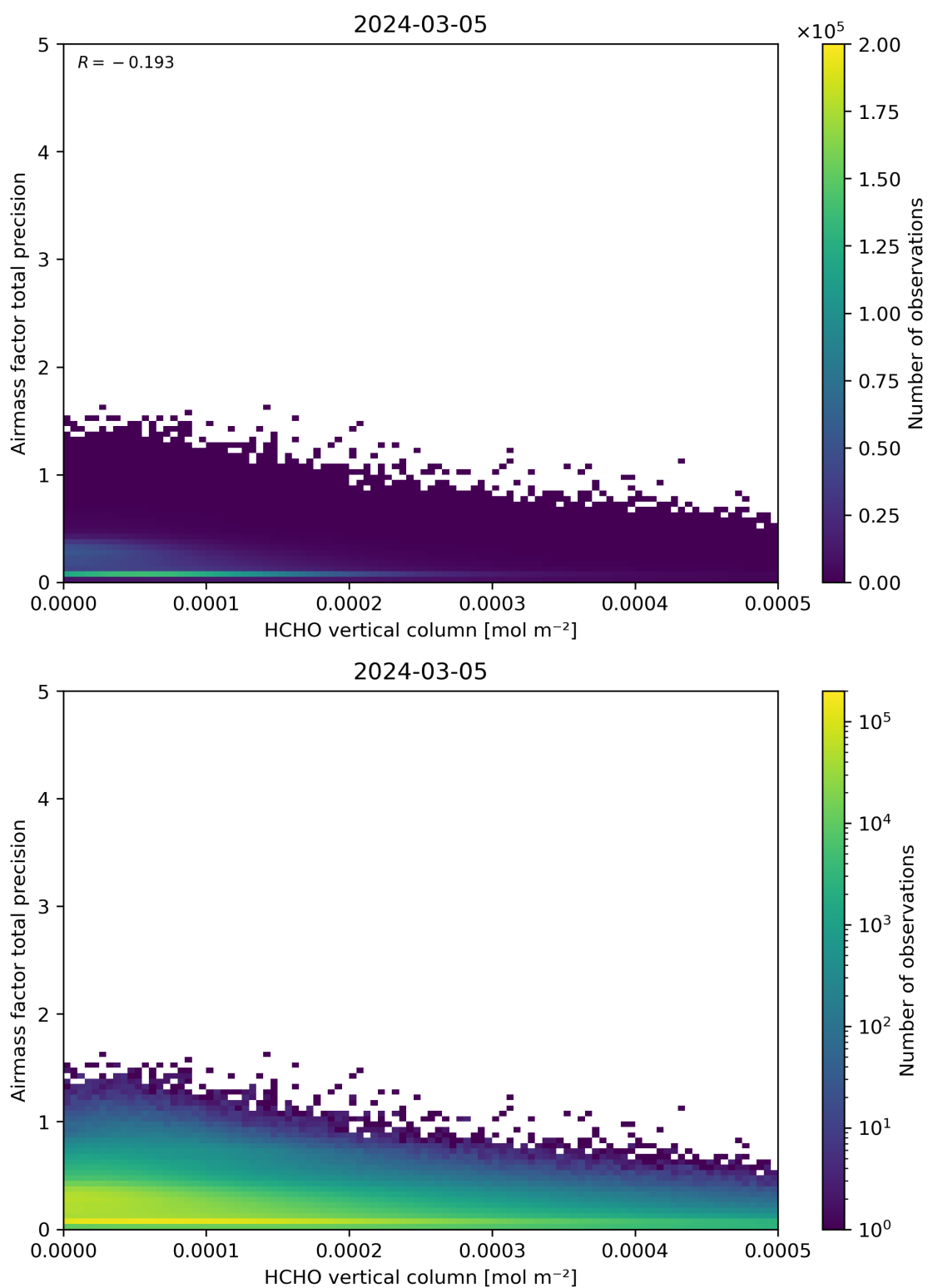
Figure 132: Scatter density plot of “HCHO vertical column” against “Airmass factor total precision” for 2024-03-04 to 2024-03-06.
