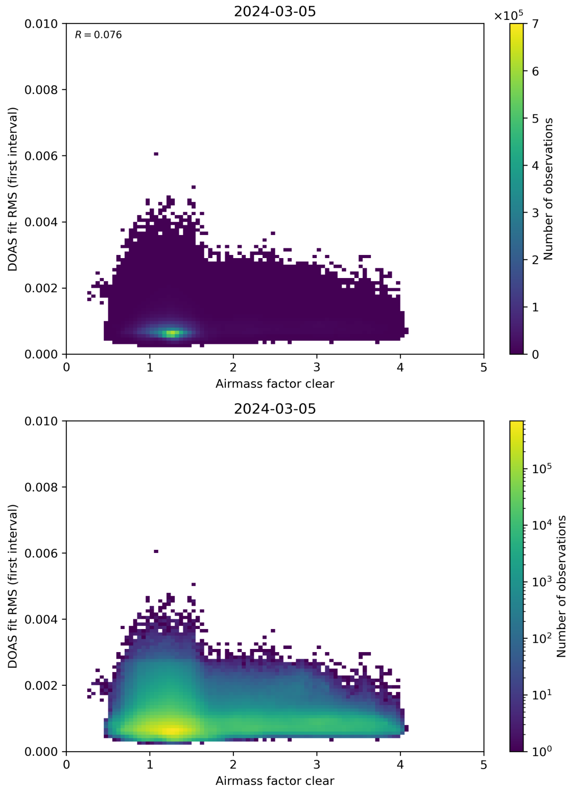
Figure 71: Scatter density plot of “Airmass factor clear” against “DOAS fit RMS (first interval)” for 2024-03-04 to 2024-03-06.
