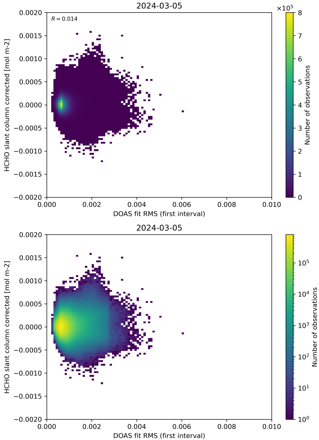
Figure 62: Scatter density plot of “DOAS fit RMS (first interval)” against “HCHO slant column corrected” for 2024-03-04 to 2024-03-06.
