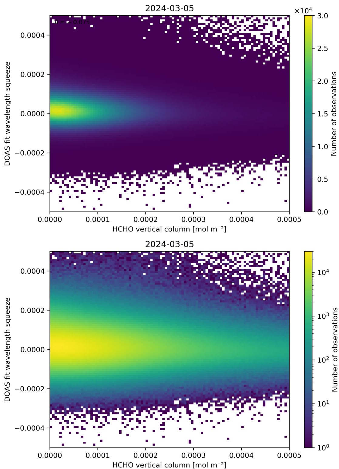
Figure 125: Scatter density plot of “HCHO vertical column” against “DOAS fit wavelength squeeze” for 2024-03-04 to 2024-03-06.
