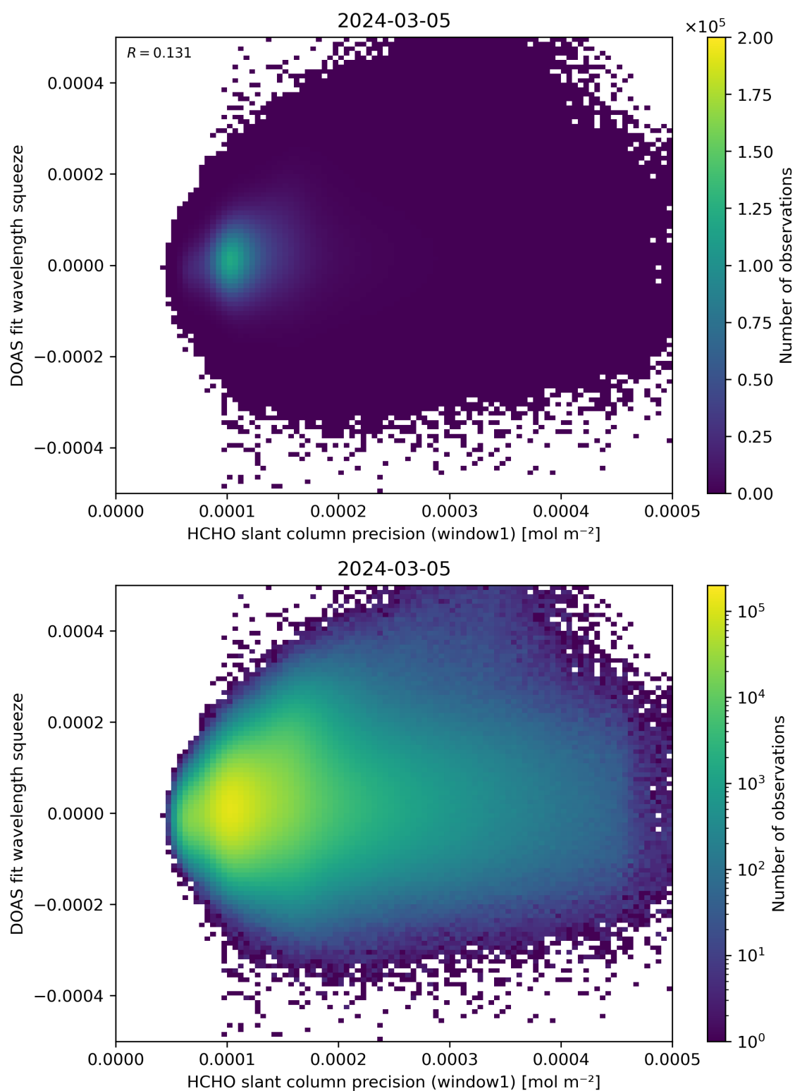
Figure 90: Scatter density plot of “HCHO slant column precision (window1)” against “DOAS fit wavelength squeeze” for 2024-03-04 to 2024-03-06.
