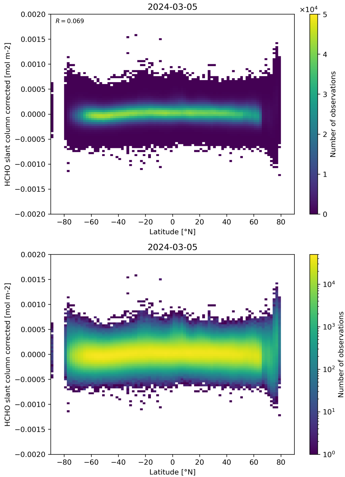
Figure 157: Scatter density plot of “Latitude” against “HCHO slant column corrected” for 2024-03-04 to 2024-03-06.
