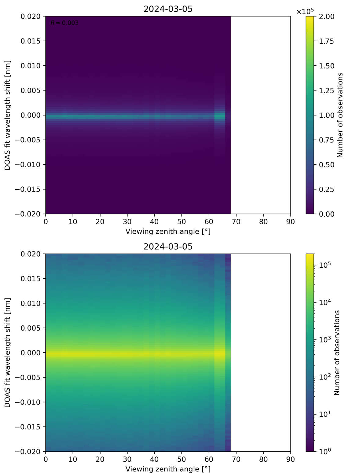
Figure 183: Scatter density plot of “Viewing zenith angle” against “DOAS fit wavelength shift” for 2024-03-04 to 2024-03-06.
