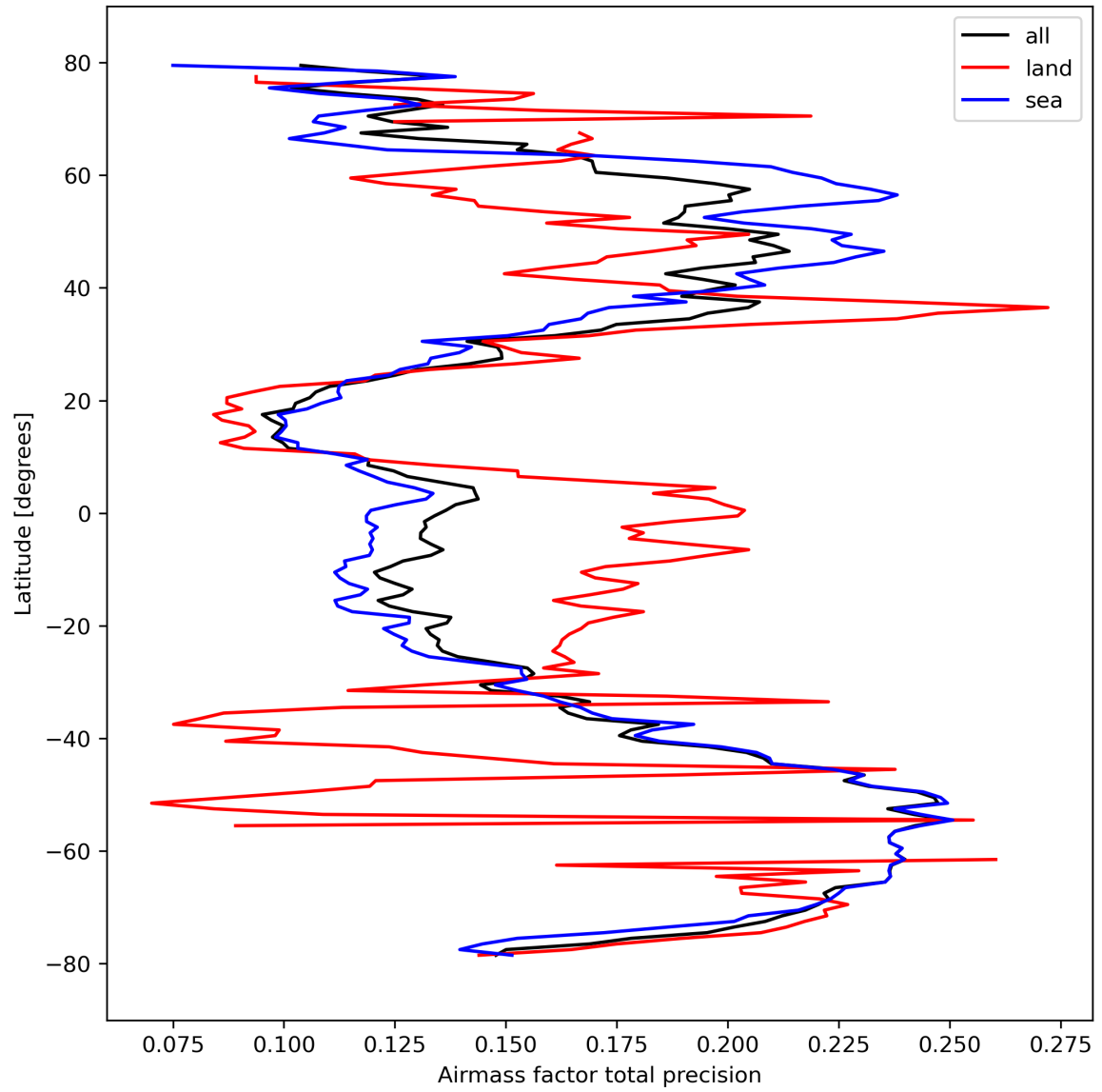
Figure 27: Zonal average of “Airmass factor total precision” for 2024-03-04 to 2024-03-06.
