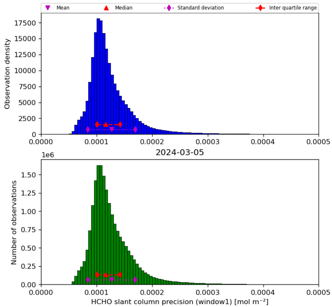
Figure 39: Histogram of “HCHO slant column precision (window1)” for 2024-03-04 to 2024-03-06
