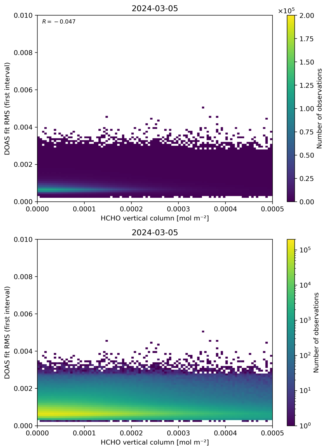
Figure 123: Scatter density plot of “HCHO vertical column” against “DOAS fit RMS (first interval)” for 2024-03-04 to 2024-03-06.
