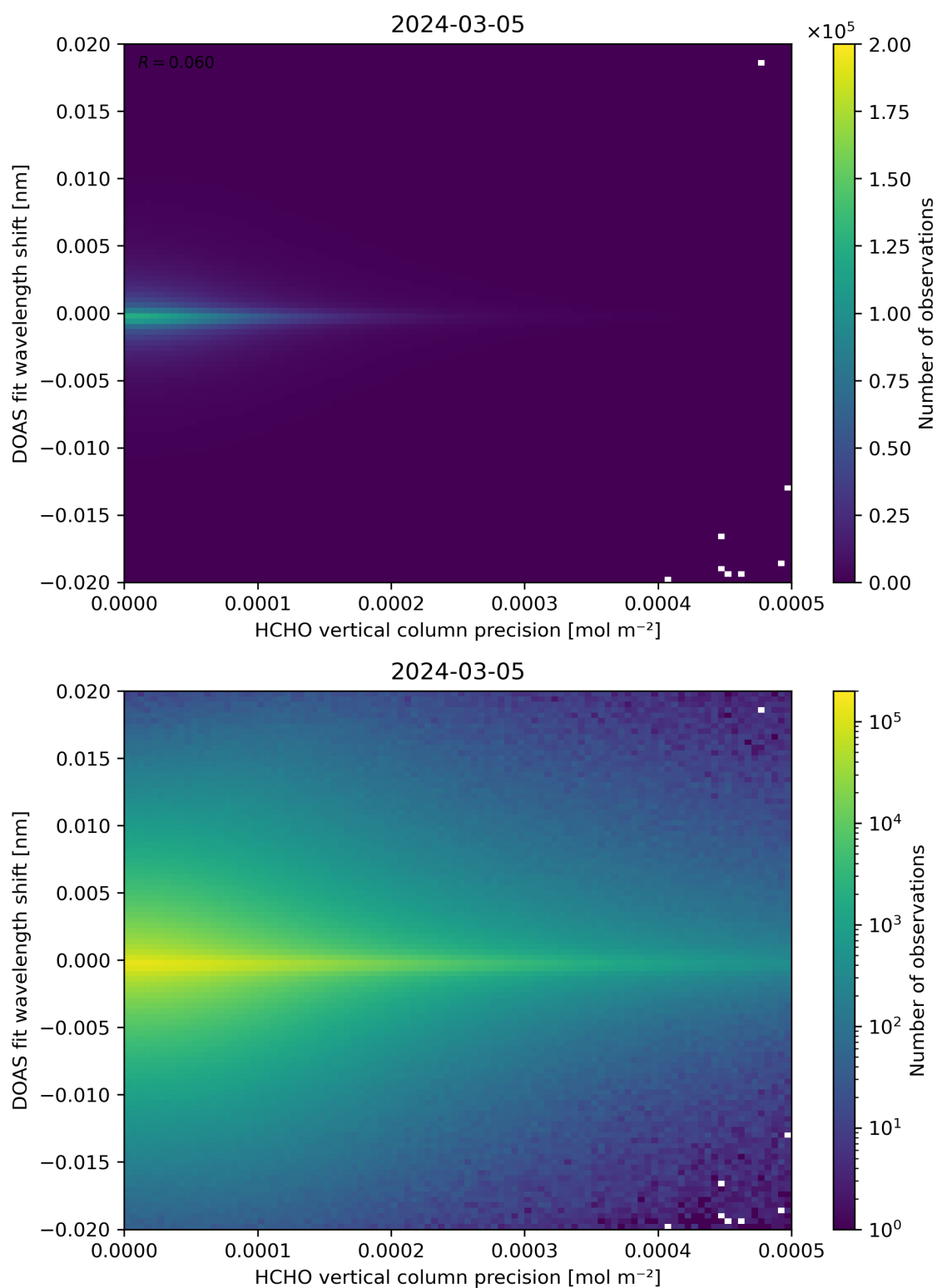
Figure 137: Scatter density plot of “HCHO vertical column precision” against “DOAS fit wavelength shift” for 2024-03-04 to 2024-03-06.
