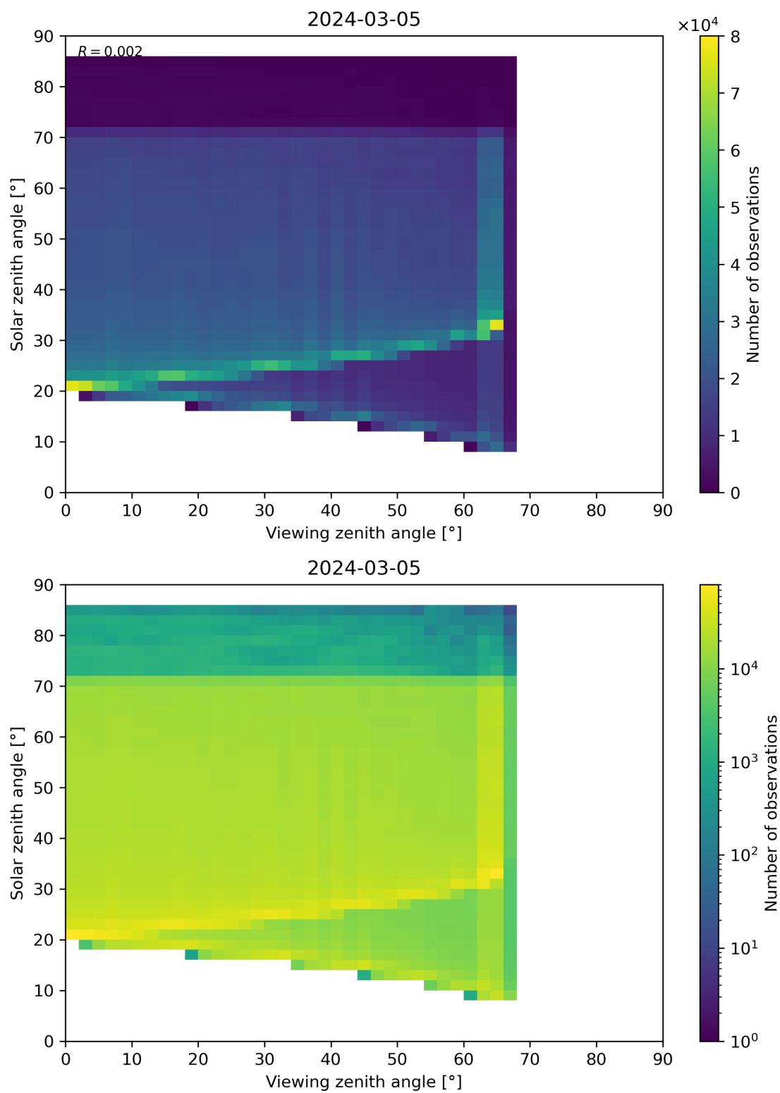
Figure 197: Scatter density plot of “Viewing zenith angle” against “Solar zenith angle” for 2024-03-04 to 2024-03-06.
