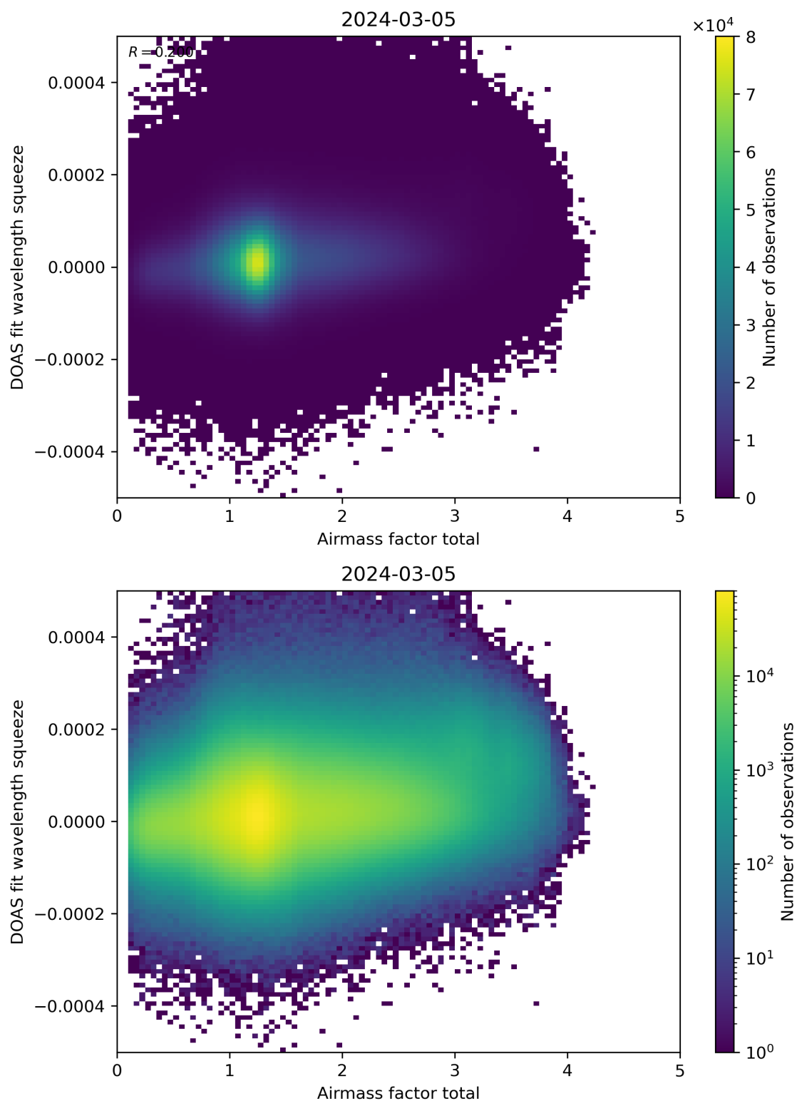
Figure 99: Scatter density plot of “Airmass factor total” against “DOAS fit wavelength squeeze” for 2024-03-04 to 2024-03-06.
