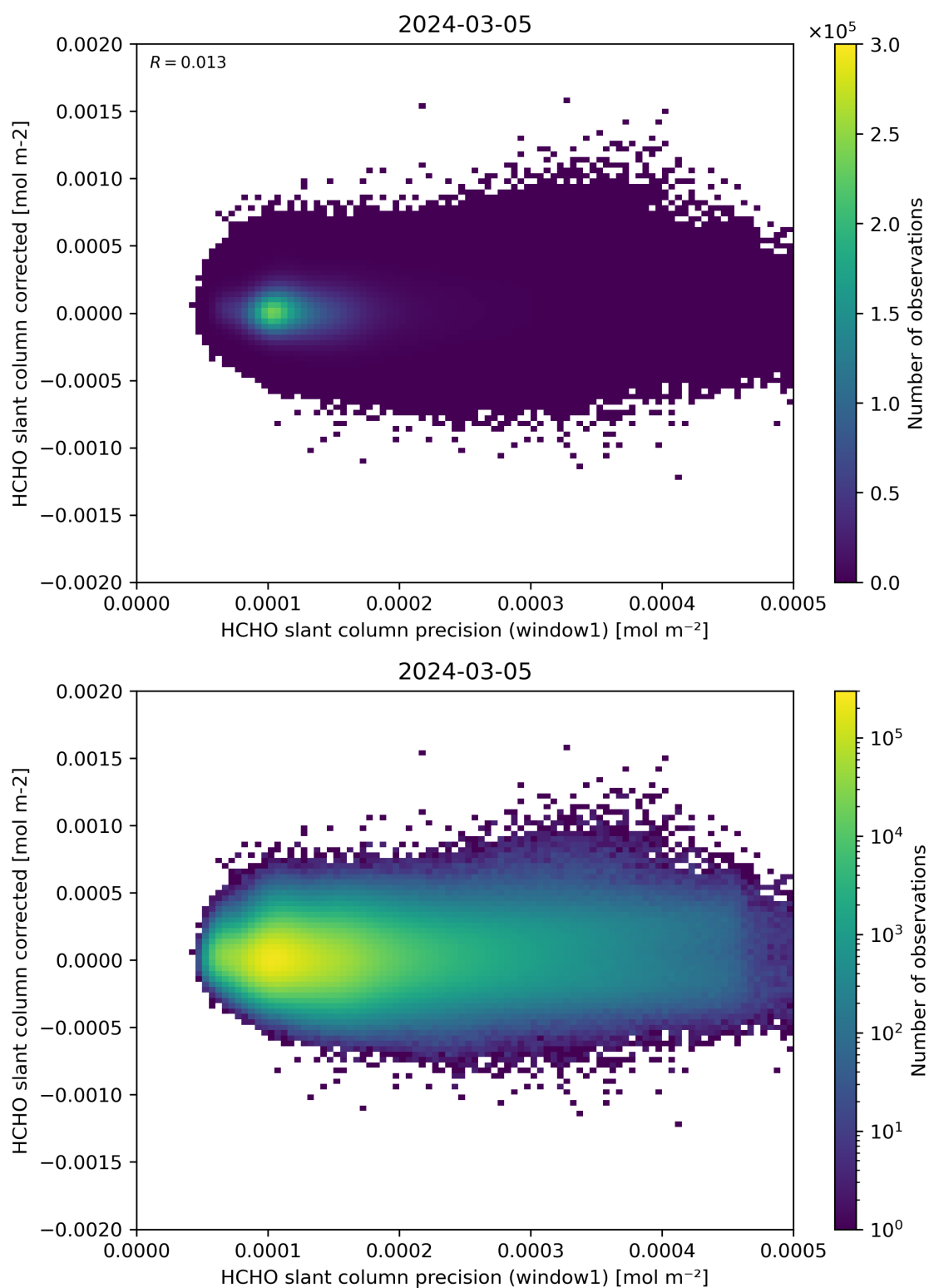
Figure 92: Scatter density plot of “HCHO slant column precision (window1)” against “HCHO slant column corrected” for 2024-03-04 to 2024-03-06.
