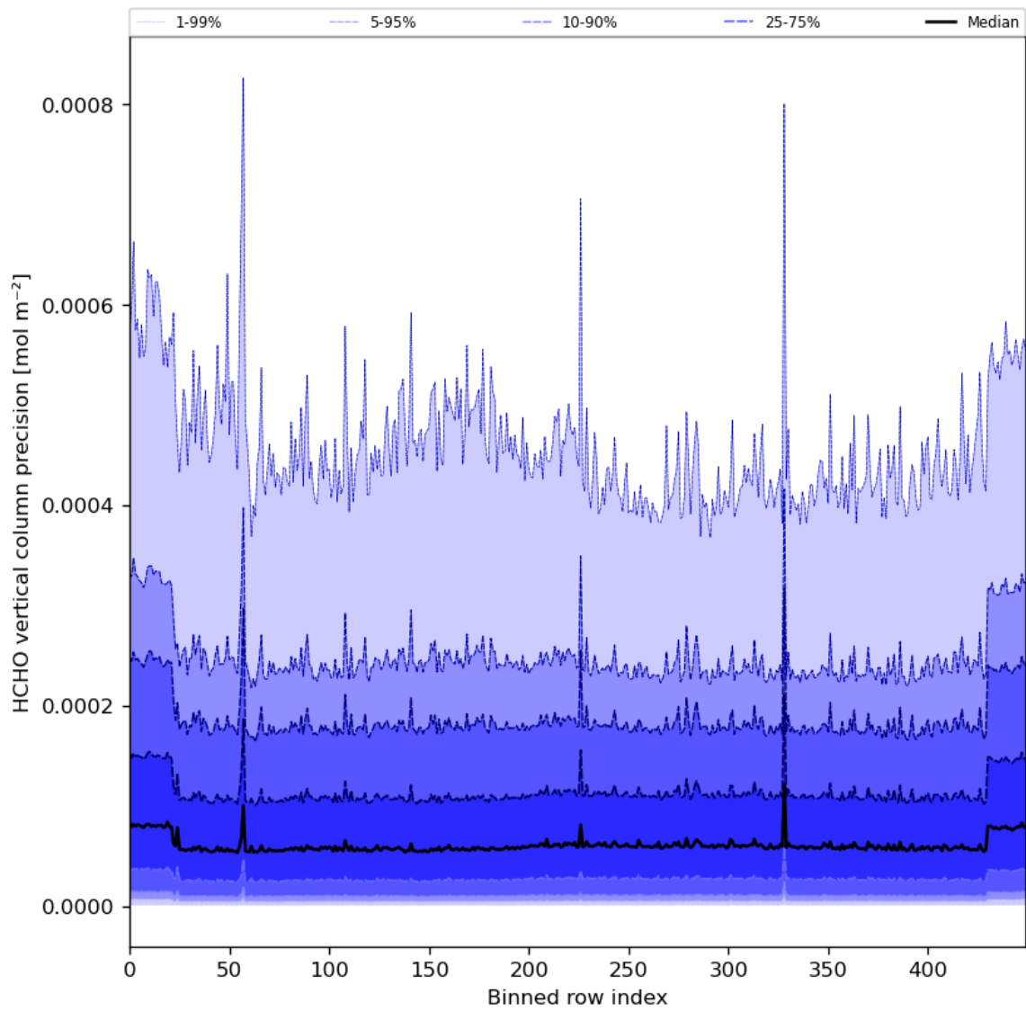
Figure 50: Along track statistics of “HCHO vertical column precision” for 2024-03-04 to 2024-03-06
