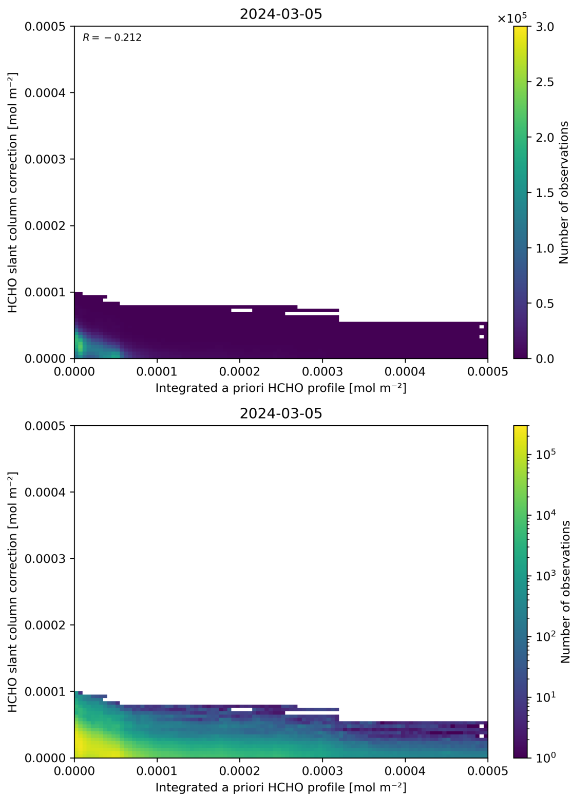
Figure 152: Scatter density plot of “Integrated a priori HCHO profile” against “HCHO slant column correction” for 2024-03-04 to 2024-03-06.
