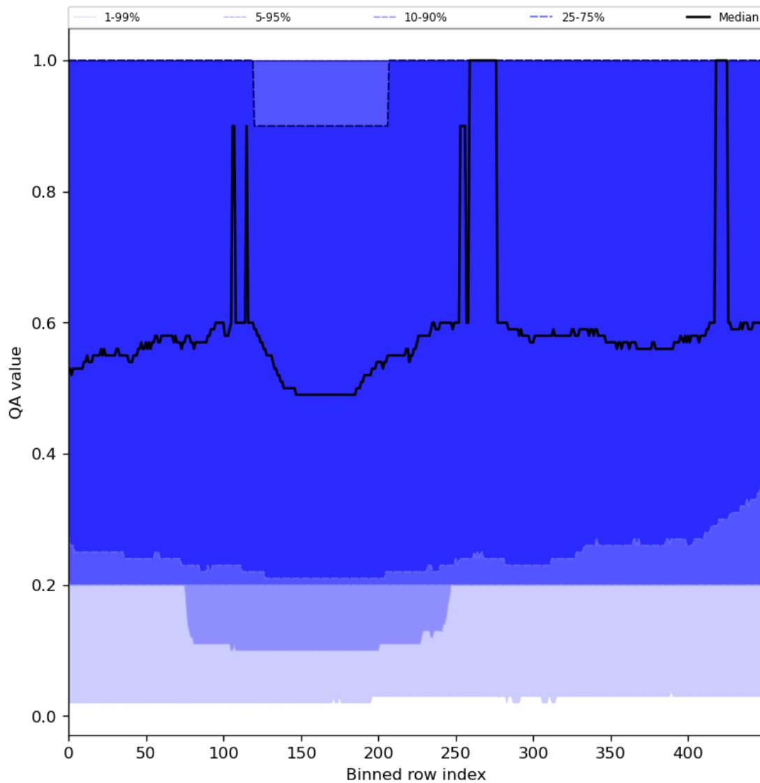
Figure 48: Along track statistics of “QA value” for 2024-03-04 to 2024-03-06
