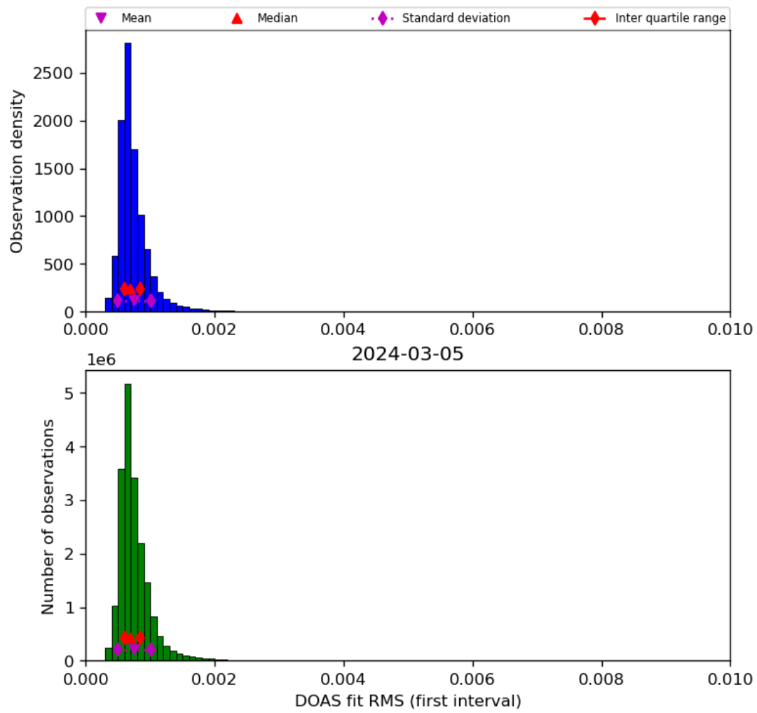
Figure 46: Histogram of “DOAS fit RMS (first interval)” for 2024-03-04 to 2024-03-06
