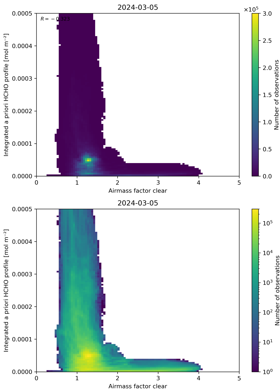
Figure 76: Scatter density plot of “Airmass factor clear” against “Integrated a priori HCHO profile” for 2024-03-04 to 2024-03-06.
