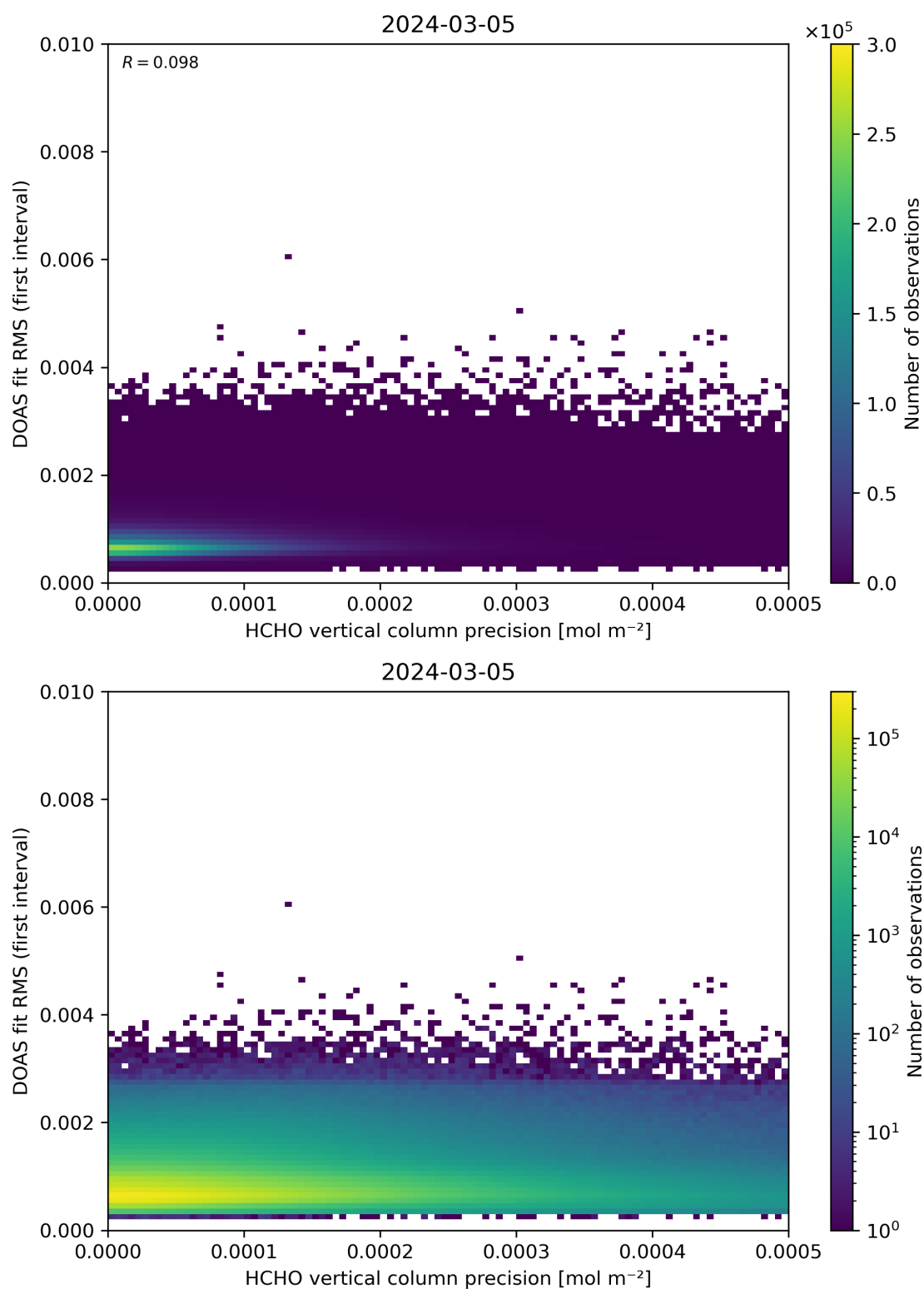
Figure 136: Scatter density plot of “HCHO vertical column precision” against “DOAS fit RMS (first interval)” for 2024-03-04 to 2024-03-06.
