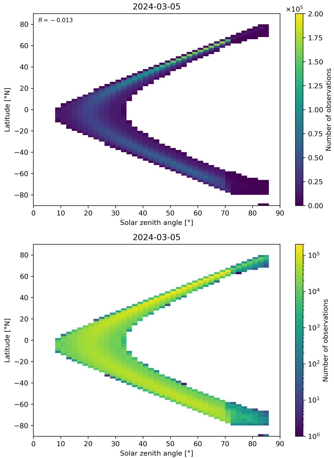
Figure 181: Scatter density plot of “Solar zenith angle” against “Latitude” for 2024-03-04 to 2024-03-06.
