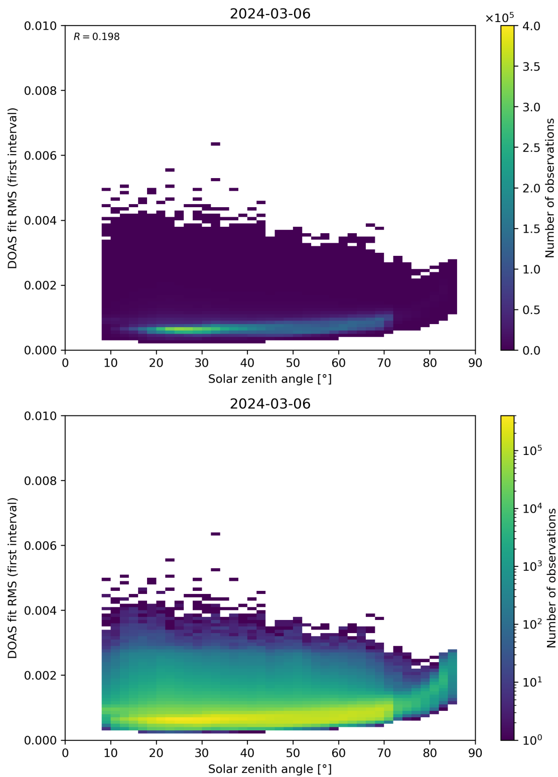
Figure 167: Scatter density plot of “Solar zenith angle” against “DOAS fit RMS (first interval)” for 2024-03-05 to 2024-03-07.
