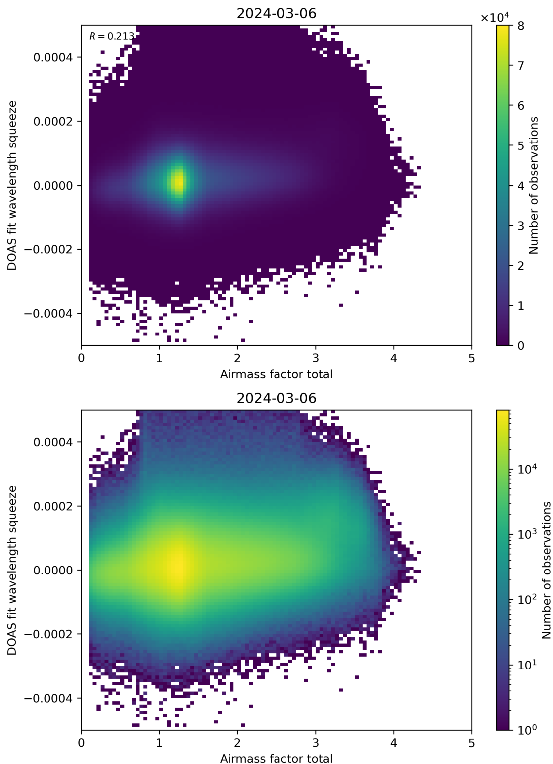
Figure 99: Scatter density plot of “Airmass factor total” against “DOAS fit wavelength squeeze” for 2024-03-05 to 2024-03-07.
