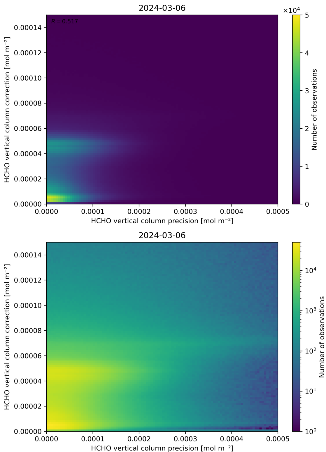
Figure 146: Scatter density plot of “HCHO vertical column precision” against “HCHO vertical column correction” for 2024-03-05 to 2024-03-07.
