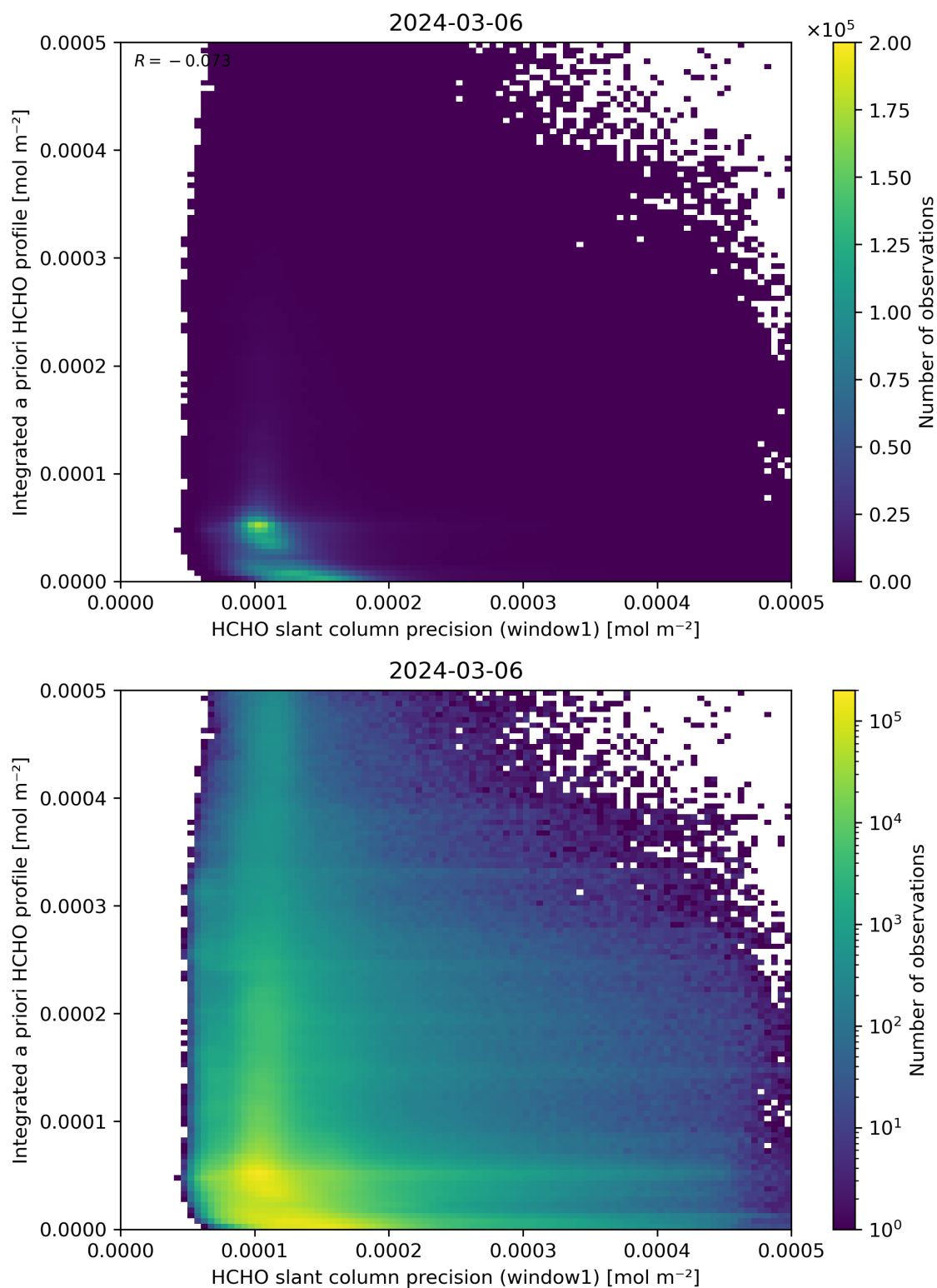
Figure 96: Scatter density plot of “HCHO slant column precision (window1)” against “Integrated a priori HCHO profile” for 2024-03-05 to 2024-03-07.
