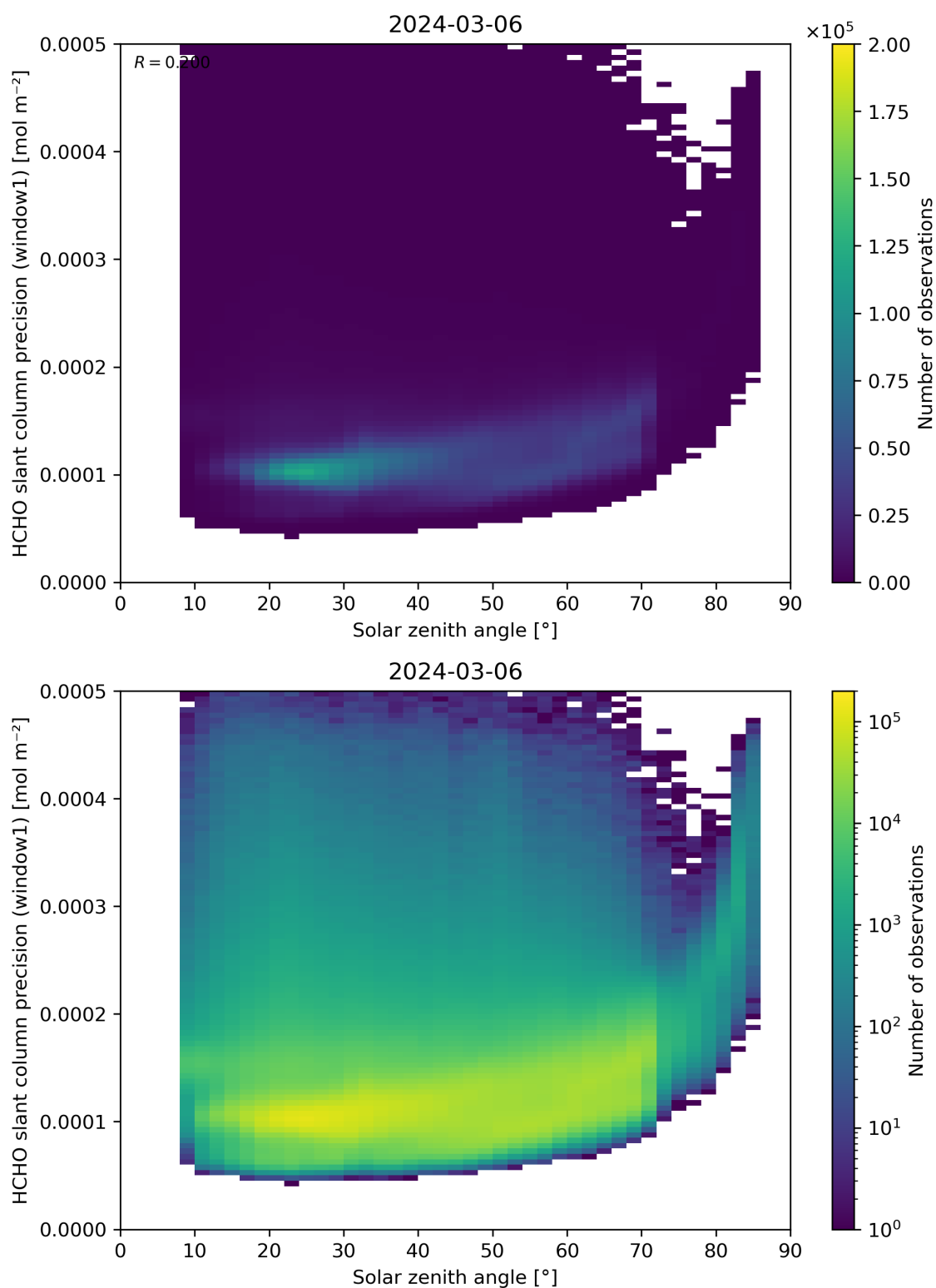
Figure 174: Scatter density plot of “Solar zenith angle” against “HCHO slant column precision (window1)” for 2024-03-05 to 2024-03-07.
