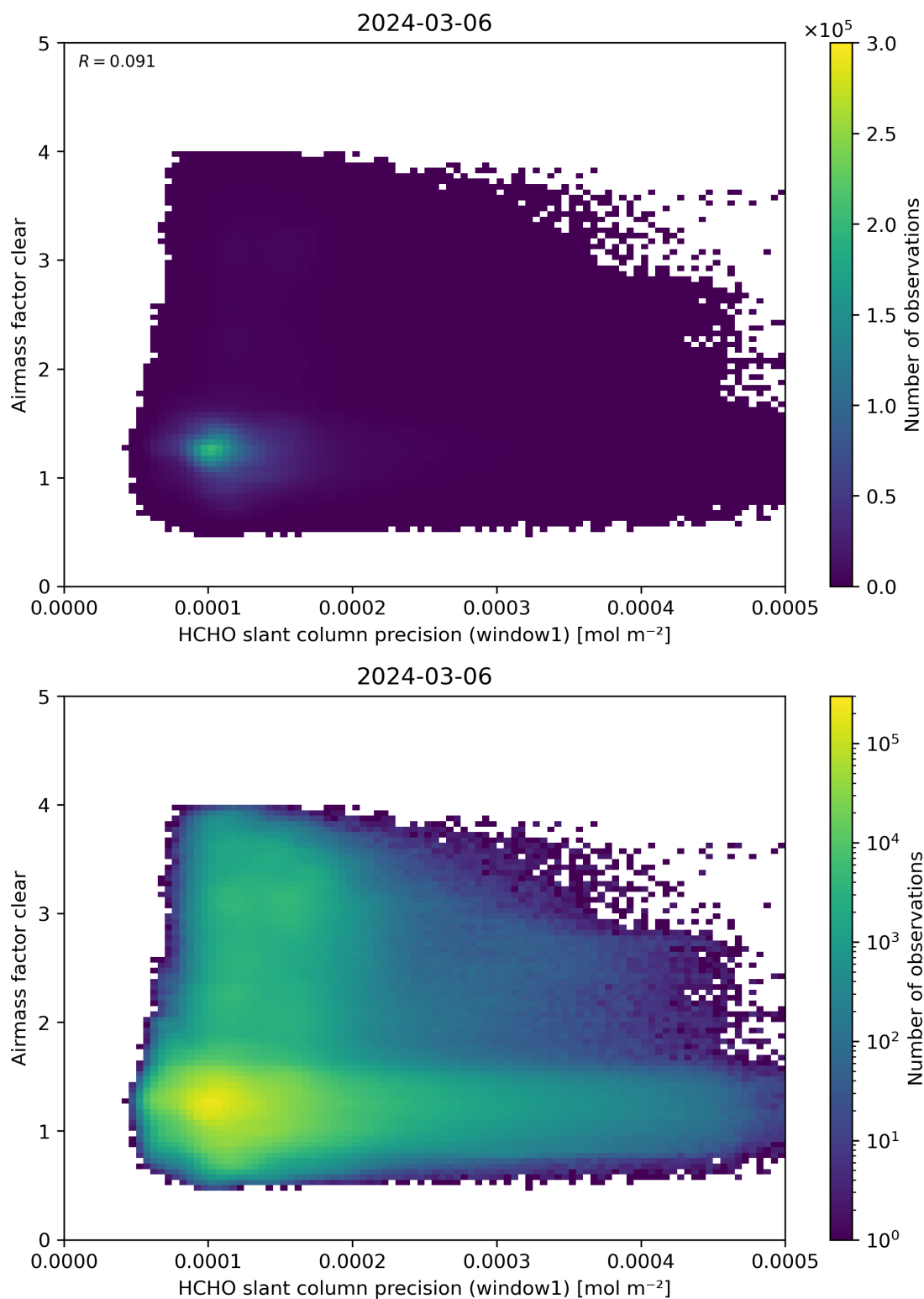
Figure 91: Scatter density plot of “HCHO slant column precision (window1)” against “Airmass factor clear” for 2024-03-05 to 2024-03-07.
