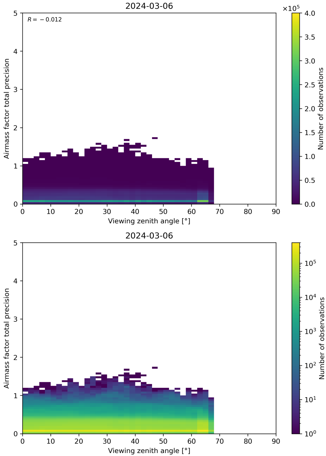
Figure 191: Scatter density plot of “Viewing zenith angle” against “Airmass factor total precision” for 2024-03-05 to 2024-03-07.
