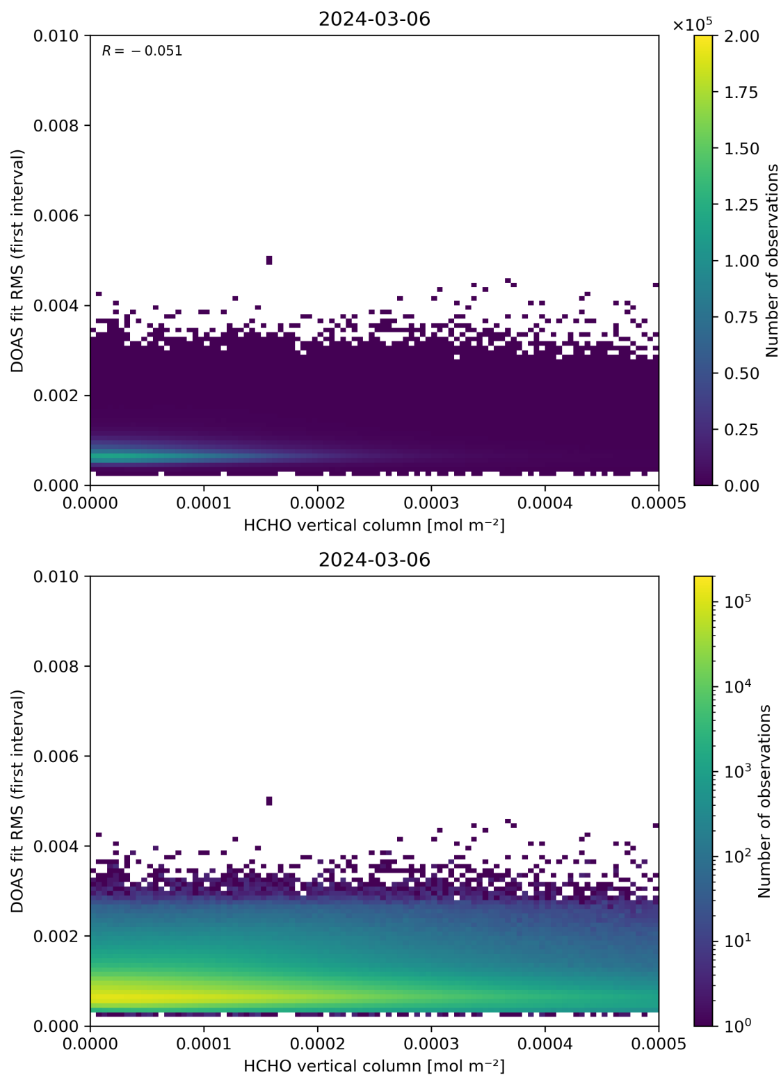
Figure 123: Scatter density plot of “HCHO vertical column” against “DOAS fit RMS (first interval)” for 2024-03-05 to 2024-03-07.
