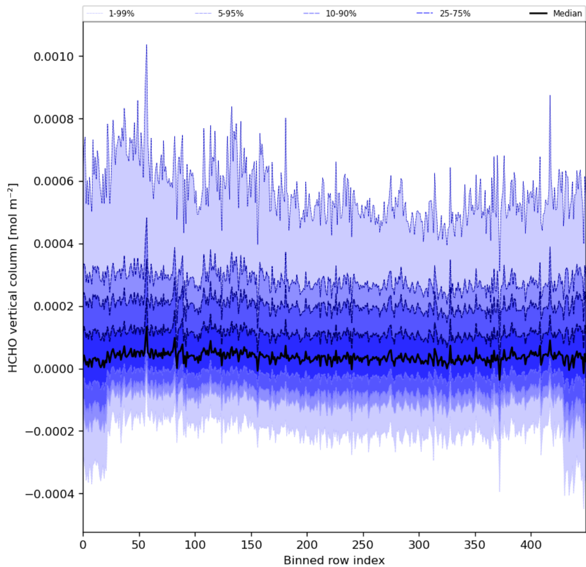
Figure 49: Along track statistics of “HCHO vertical column” for 2024-03-05 to 2024-03-07
