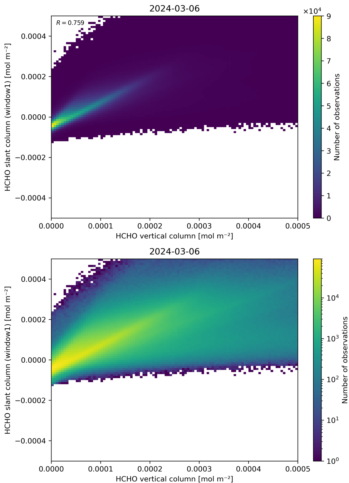
Figure 129: Scatter density plot of “HCHO vertical column” against “HCHO slant column (window1)” for 2024-03-05 to 2024-03-07.
