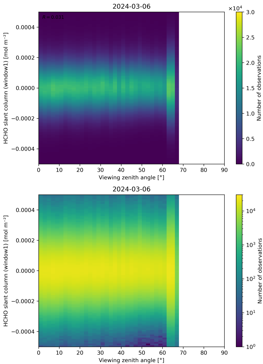
Figure 188: Scatter density plot of “Viewing zenith angle” against “HCHO slant column (window1)” for 2024-03-05 to 2024-03-07.
