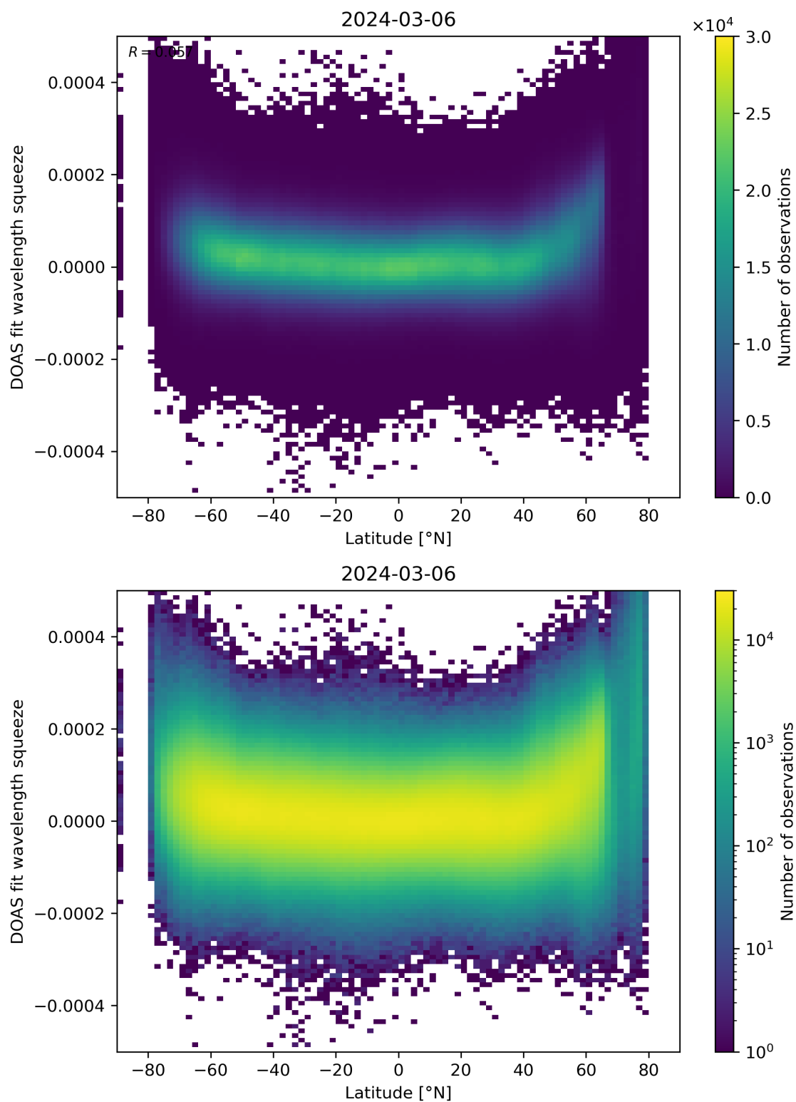
Figure 155: Scatter density plot of “Latitude” against “DOAS fit wavelength squeeze” for 2024-03-05 to 2024-03-07.
