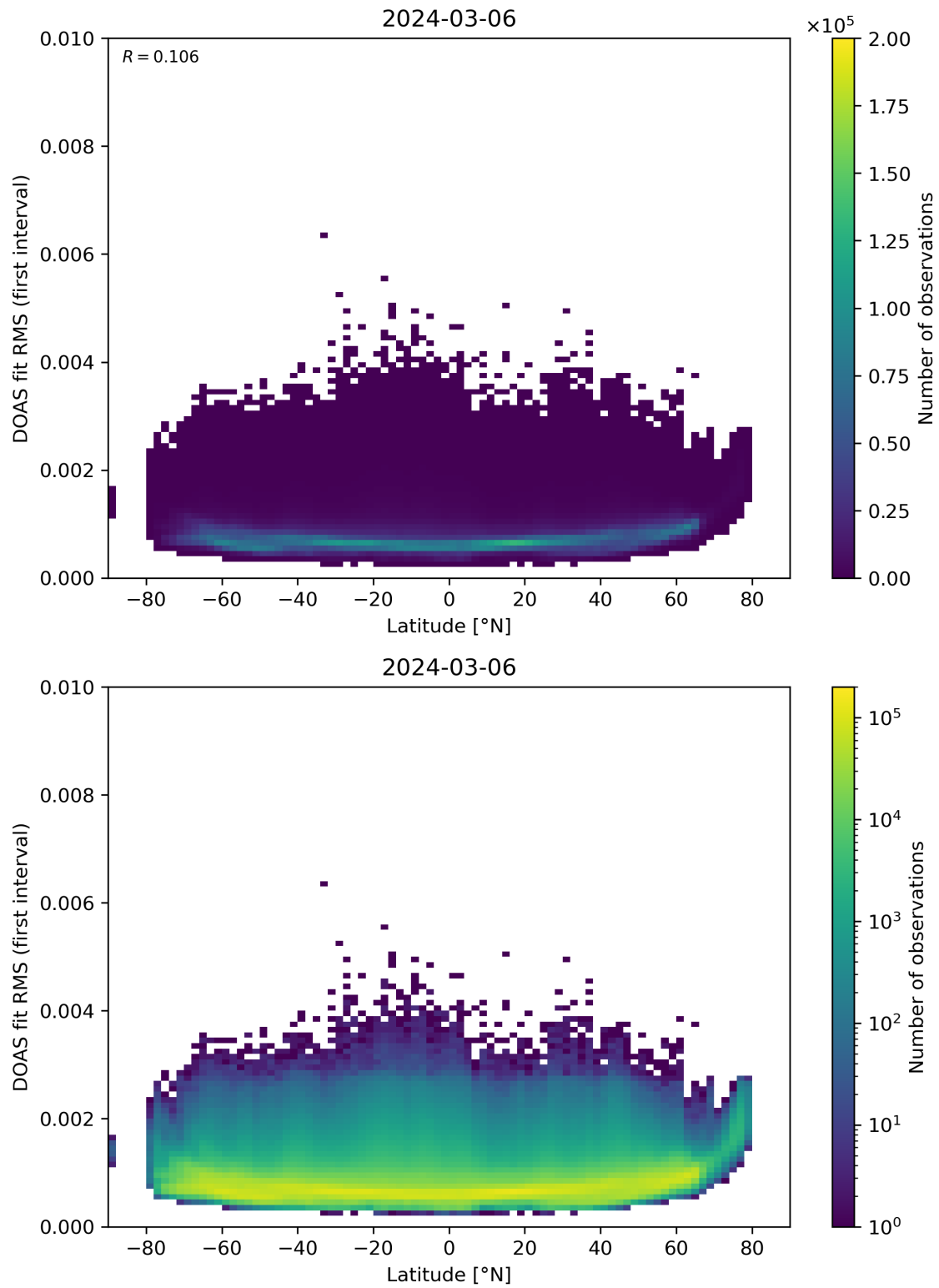
Figure 153: Scatter density plot of “Latitude” against “DOAS fit RMS (first interval)” for 2024-03-05 to 2024-03-07.
