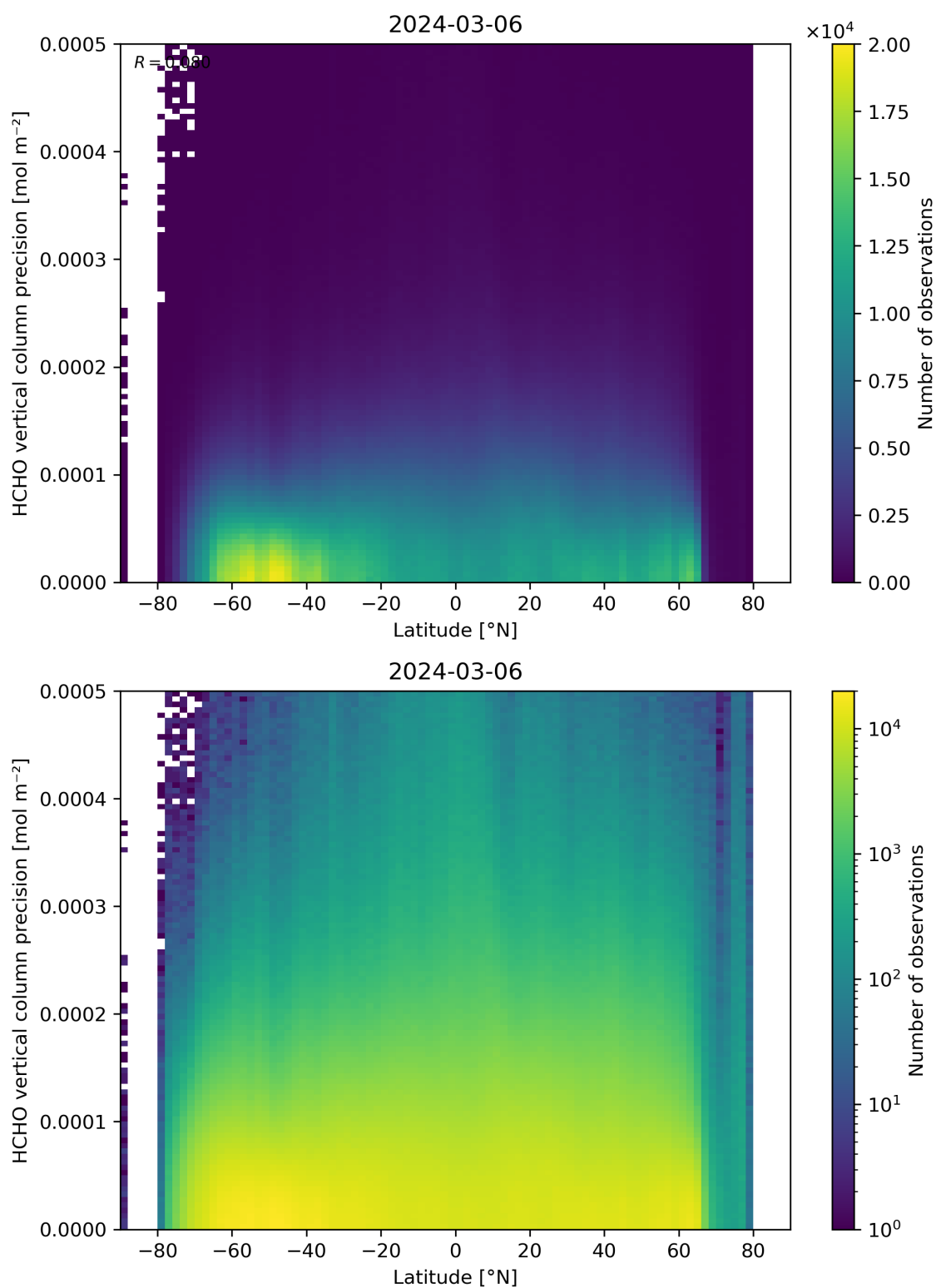
Figure 165: Scatter density plot of “Latitude” against “HCHO vertical column precision” for 2024-03-05 to 2024-03-07.
