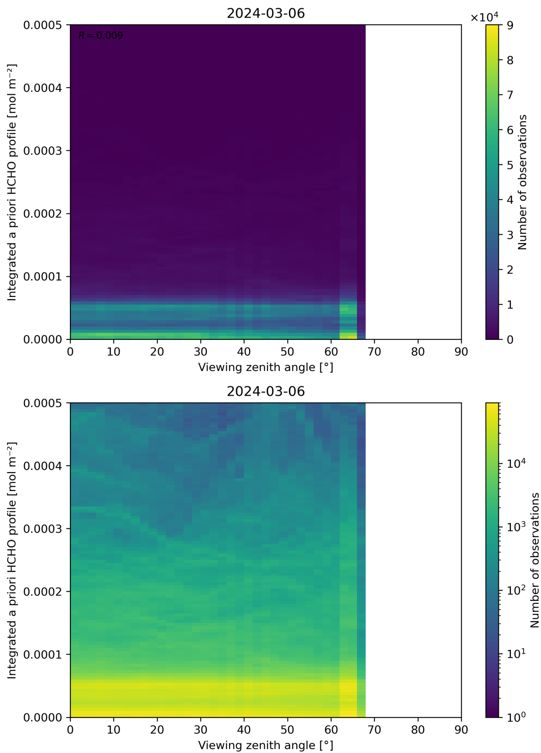
Figure 195: Scatter density plot of “Viewing zenith angle” against “Integrated a priori HCHO profile” for 2024-03-05 to 2024-03-07.
