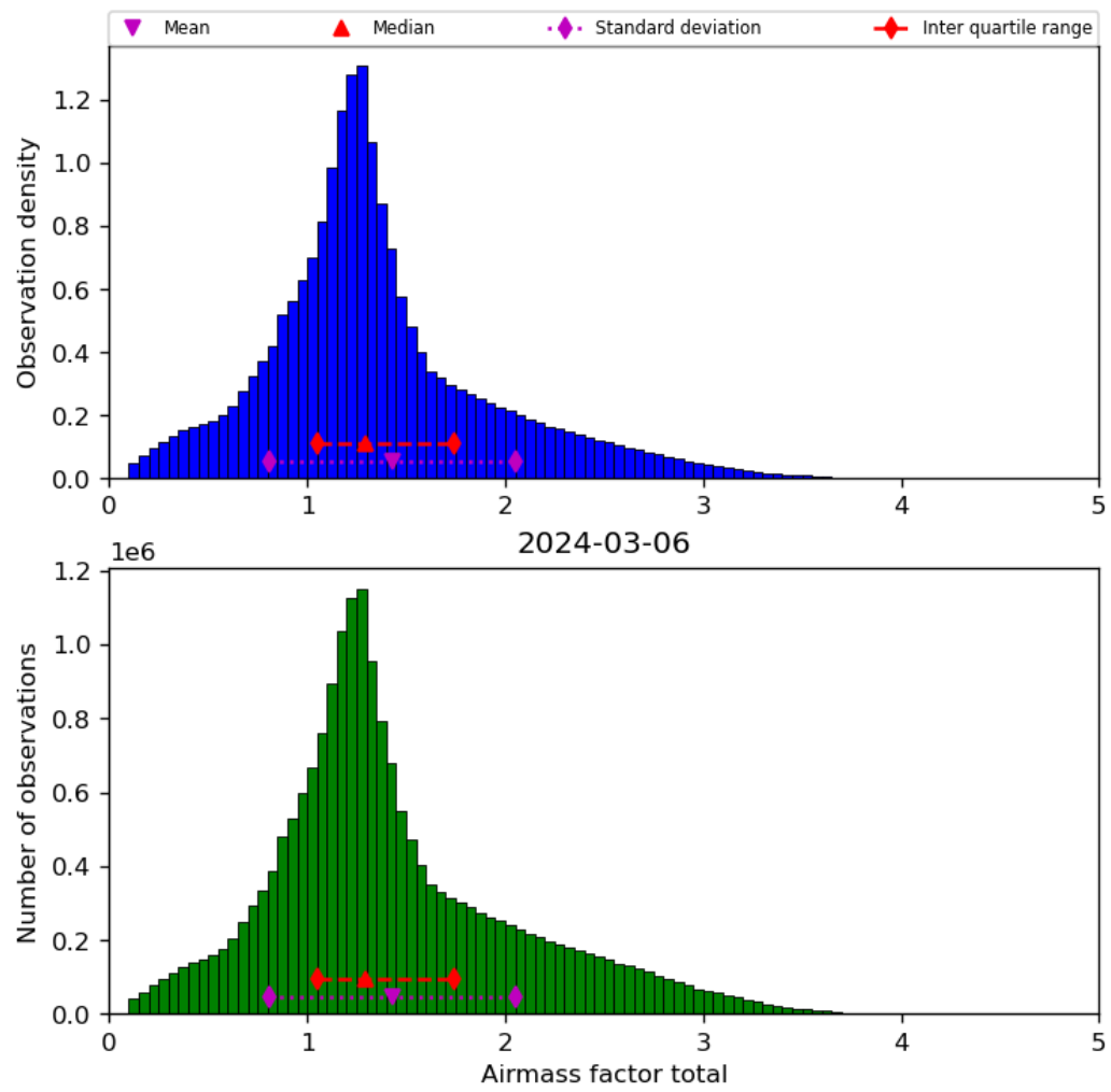
Figure 40: Histogram of “Airmass factor total” for 2024-03-05 to 2024-03-07
