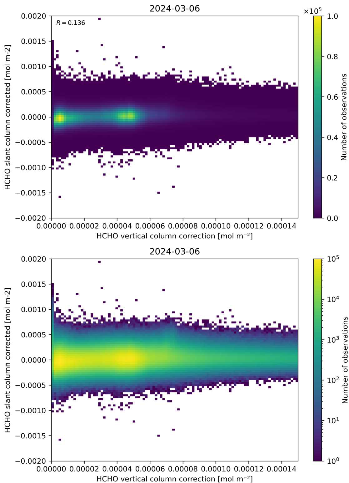
Figure 116: Scatter density plot of “HCHO vertical column correction” against “HCHO slant column corrected” for 2024-03-05 to 2024-03-07.
