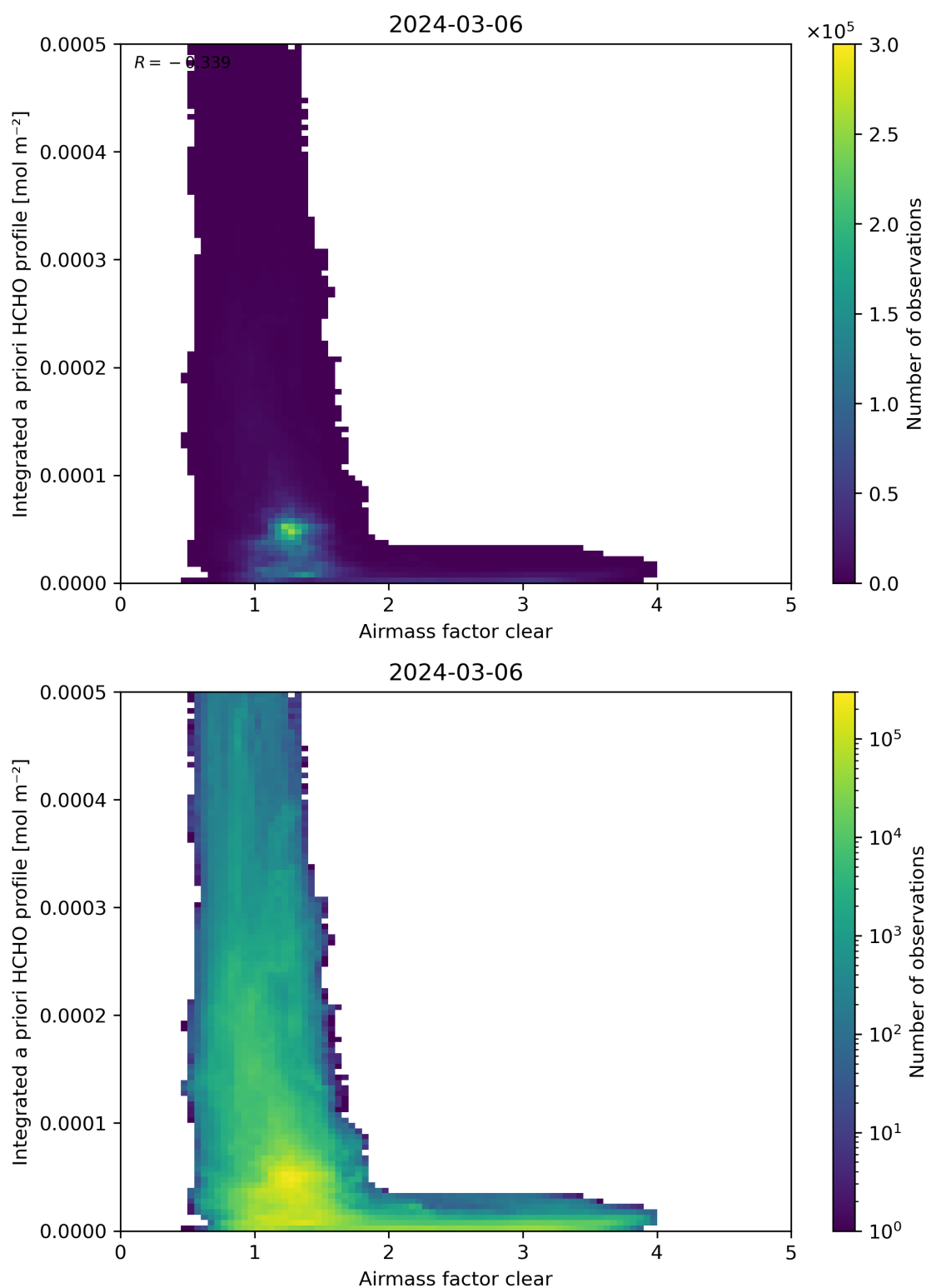
Figure 76: Scatter density plot of “Airmass factor clear” against “Integrated a priori HCHO profile” for 2024-03-05 to 2024-03-07.
