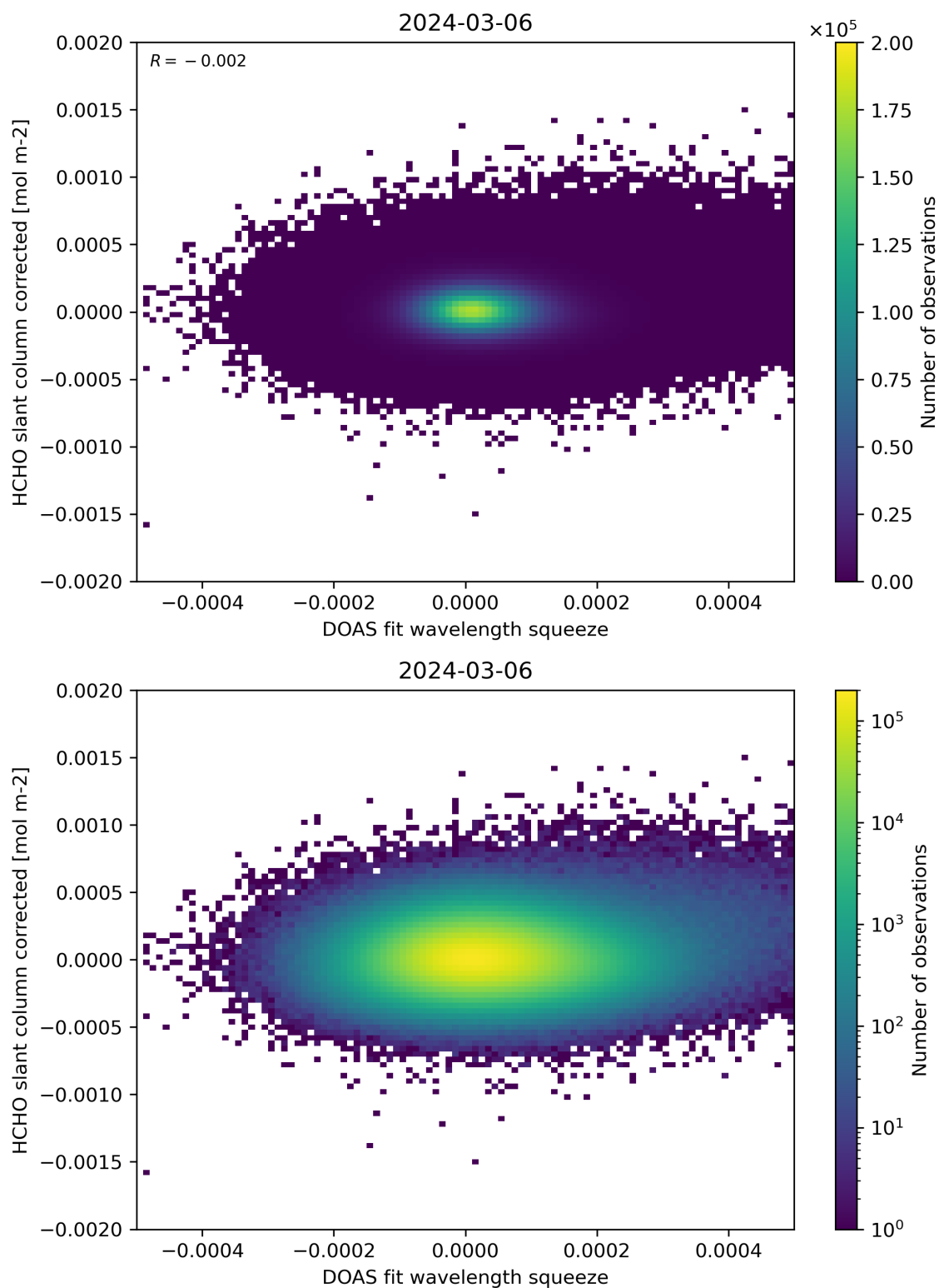
Figure 69: Scatter density plot of “DOAS fit wavelength squeeze” against “HCHO slant column corrected” for 2024-03-05 to 2024-03-07.
