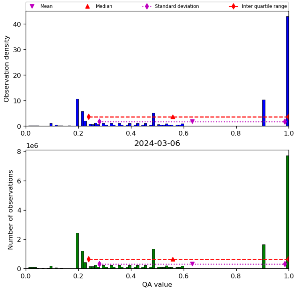
Figure 34: Histogram of “QA value” for 2024-03-05 to 2024-03-07
