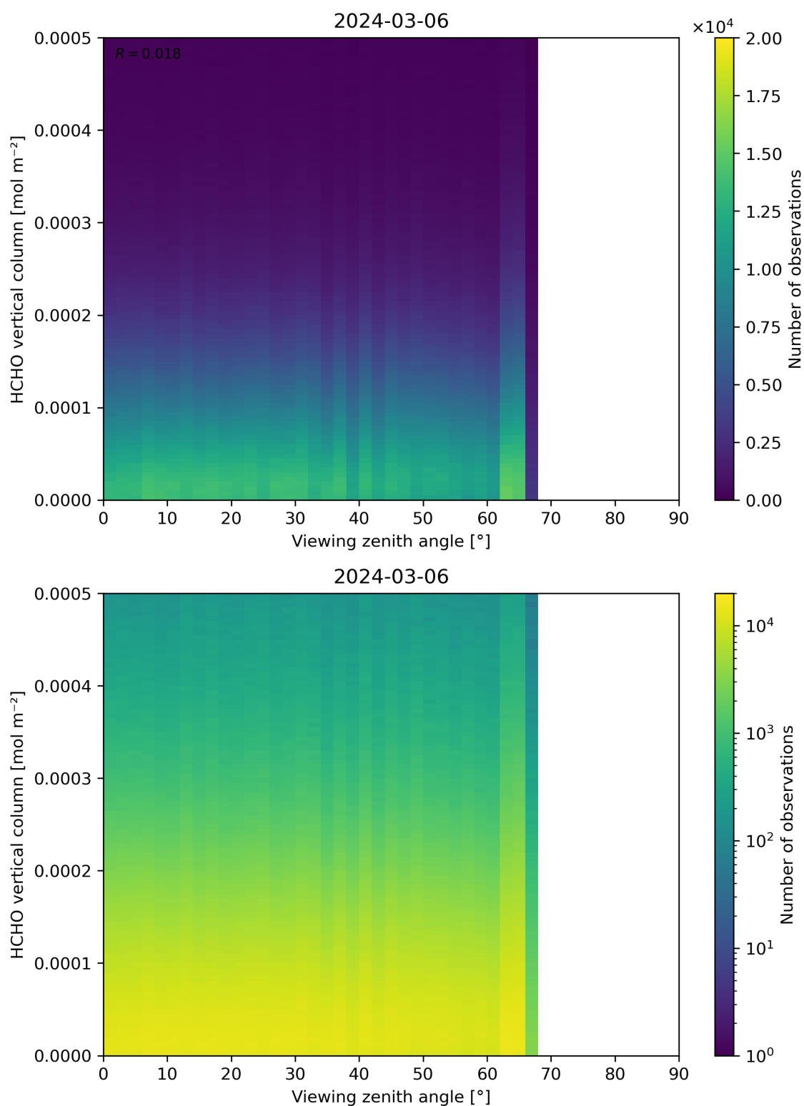
Figure 192: Scatter density plot of “Viewing zenith angle” against “HCHO vertical column” for 2024-03-05 to 2024-03-07.
