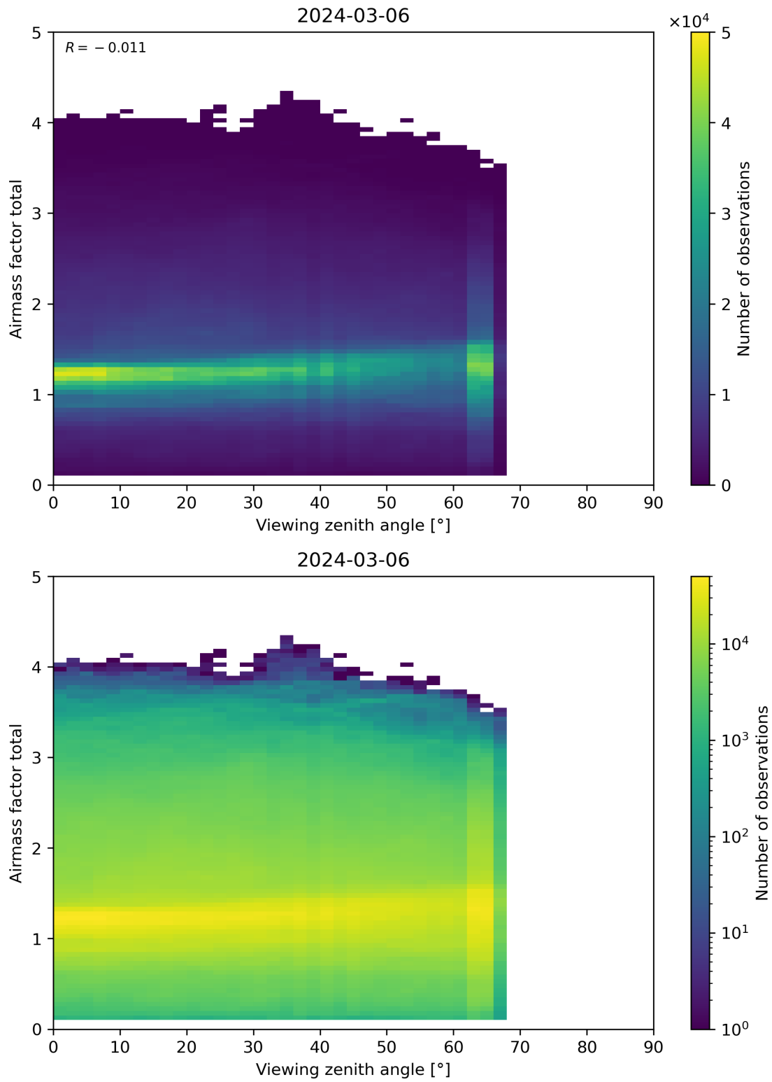
Figure 190: Scatter density plot of “Viewing zenith angle” against “Airmass factor total” for 2024-03-05 to 2024-03-07.
