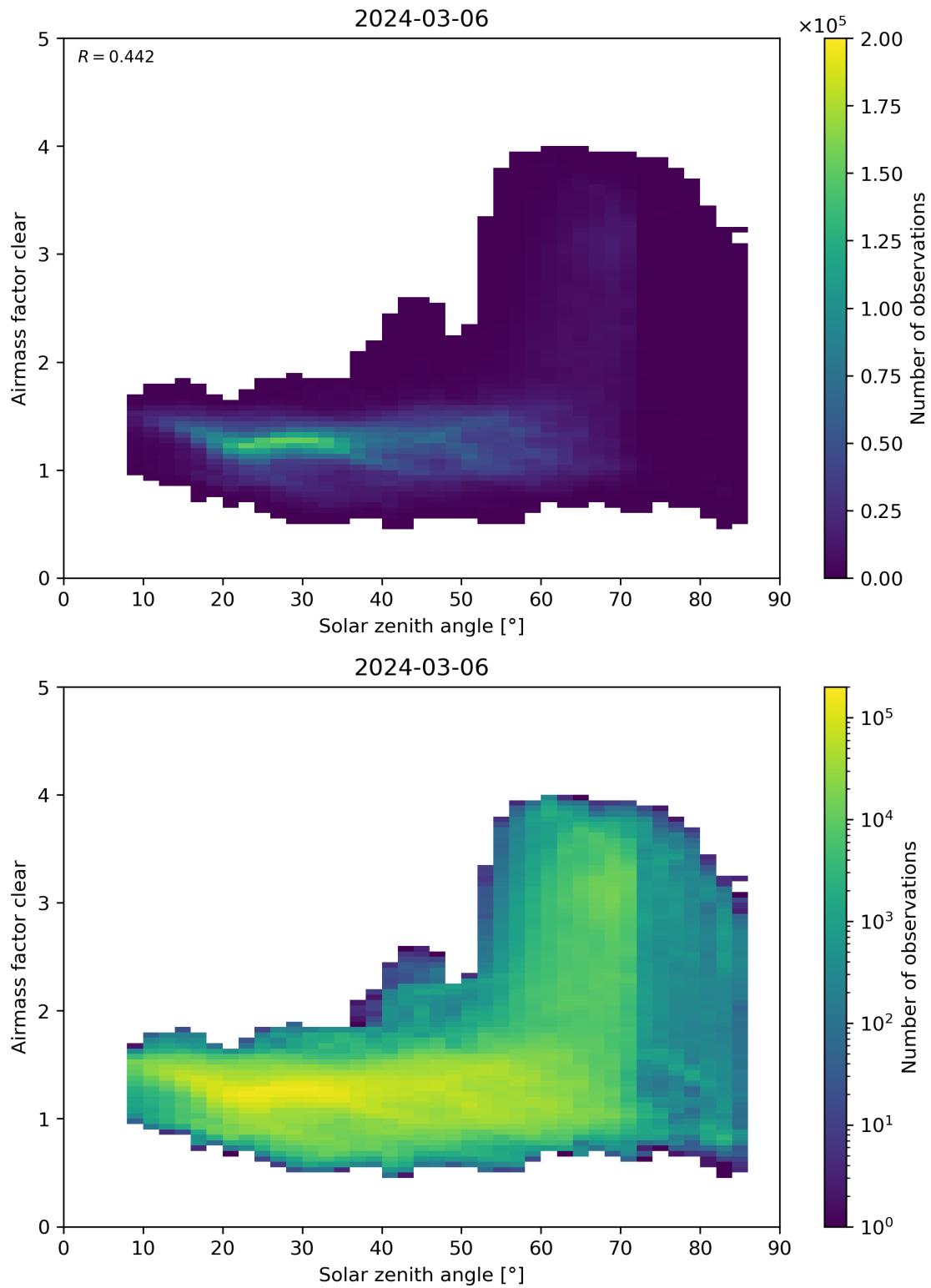
Figure 170: Scatter density plot of “Solar zenith angle” against “Airmass factor clear” for 2024-03-05 to 2024-03-07.
