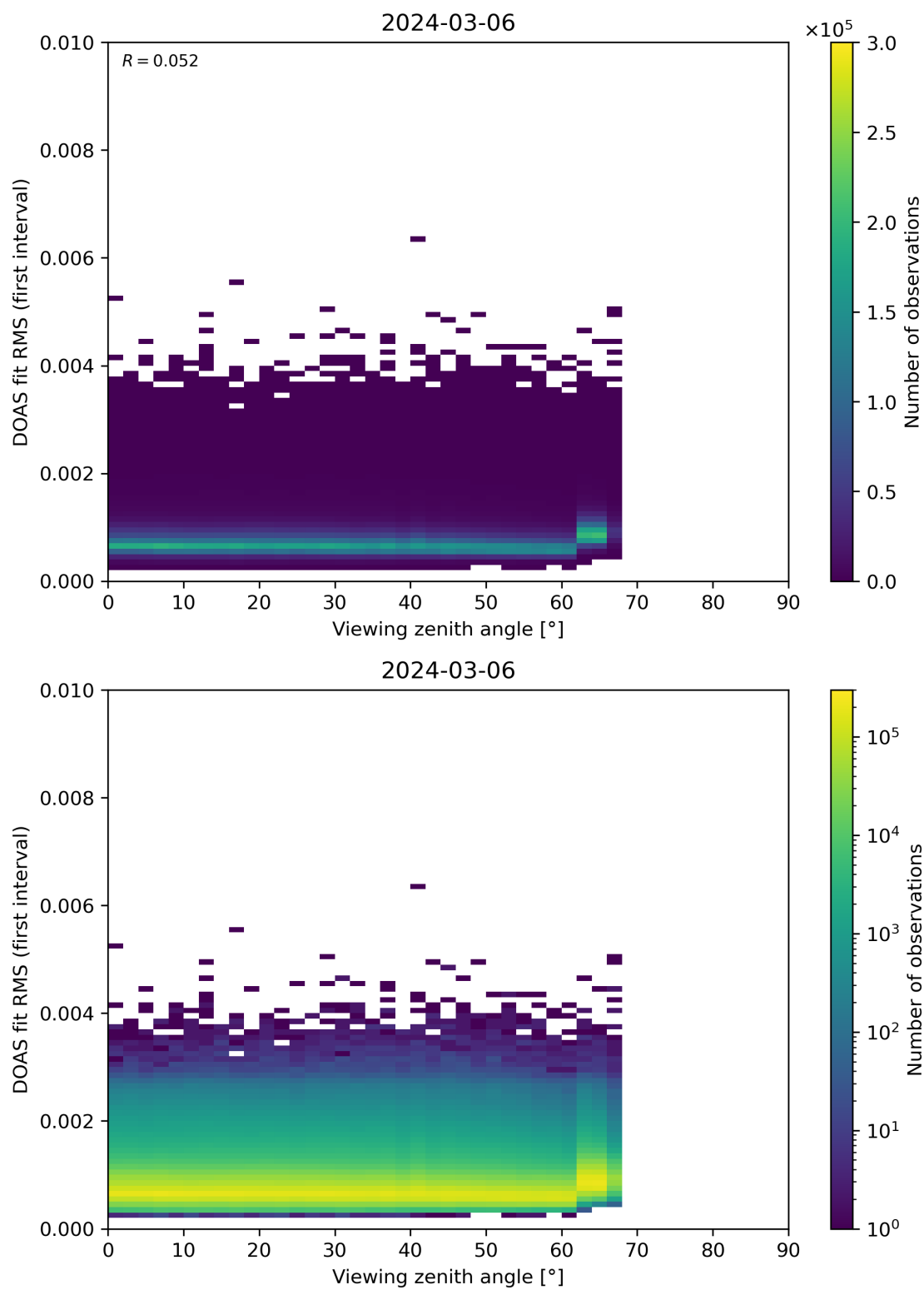
Figure 182: Scatter density plot of “Viewing zenith angle” against “DOAS fit RMS (first interval)” for 2024-03-05 to 2024-03-07.
