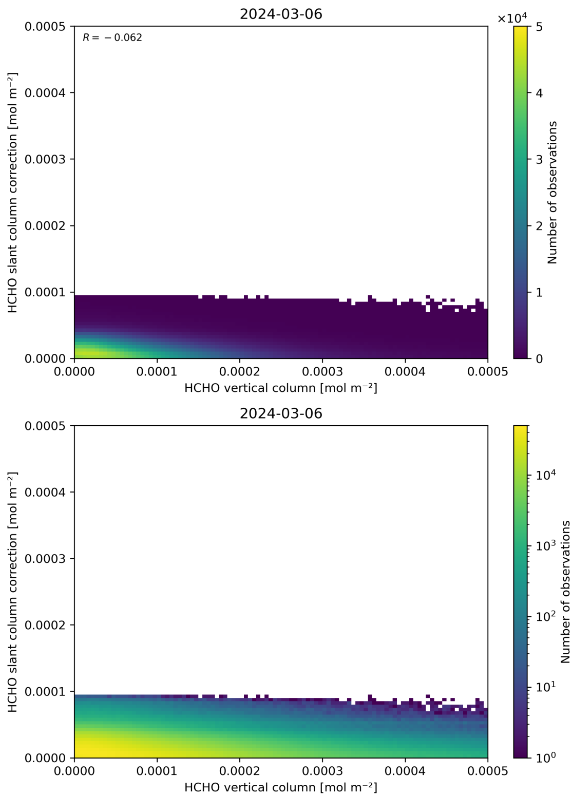
Figure 128: Scatter density plot of “HCHO vertical column” against “HCHO slant column correction” for 2024-03-05 to 2024-03-07.
