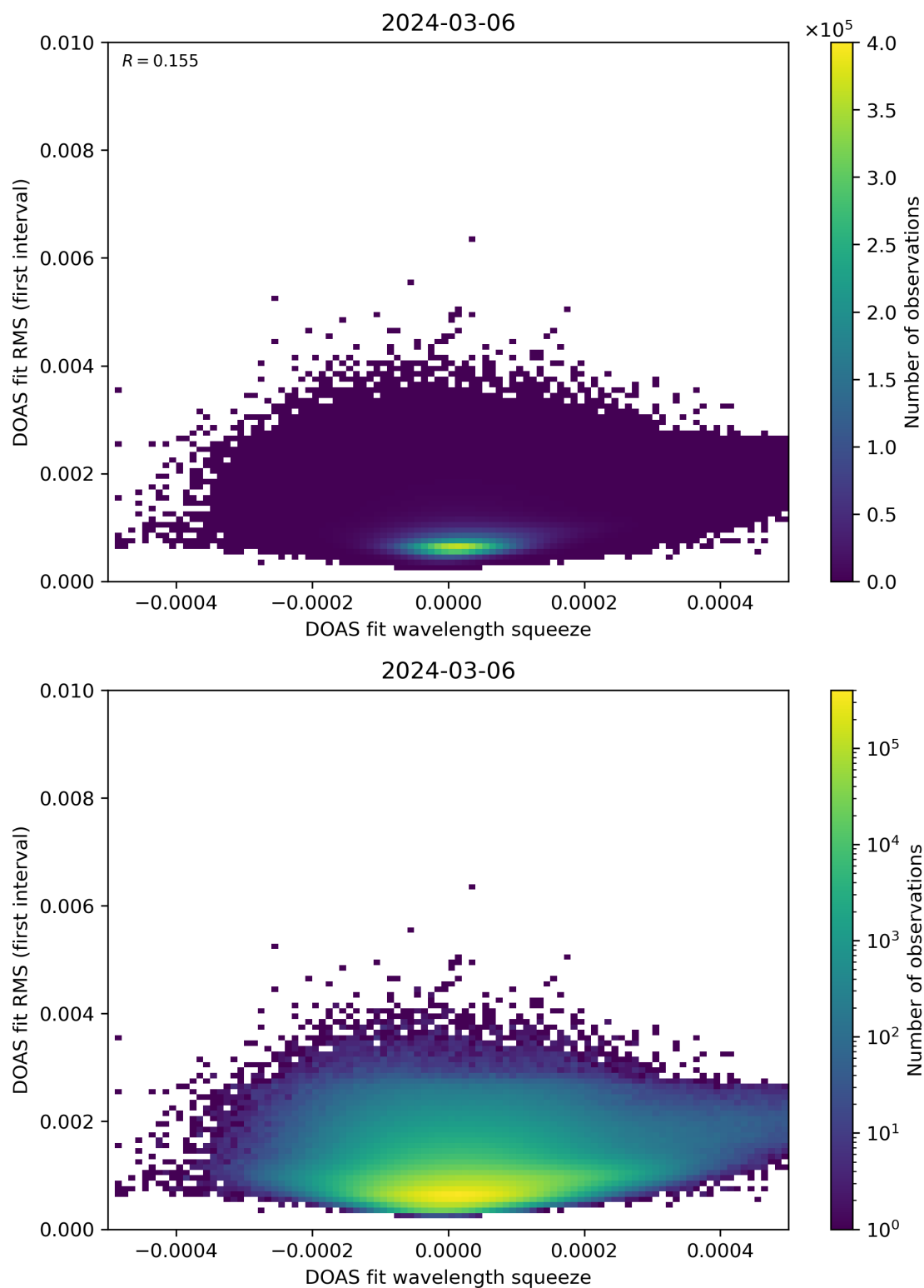
Figure 68: Scatter density plot of “DOAS fit wavelength squeeze” against “DOAS fit RMS (first interval)” for 2024-03-05 to 2024-03-07.
