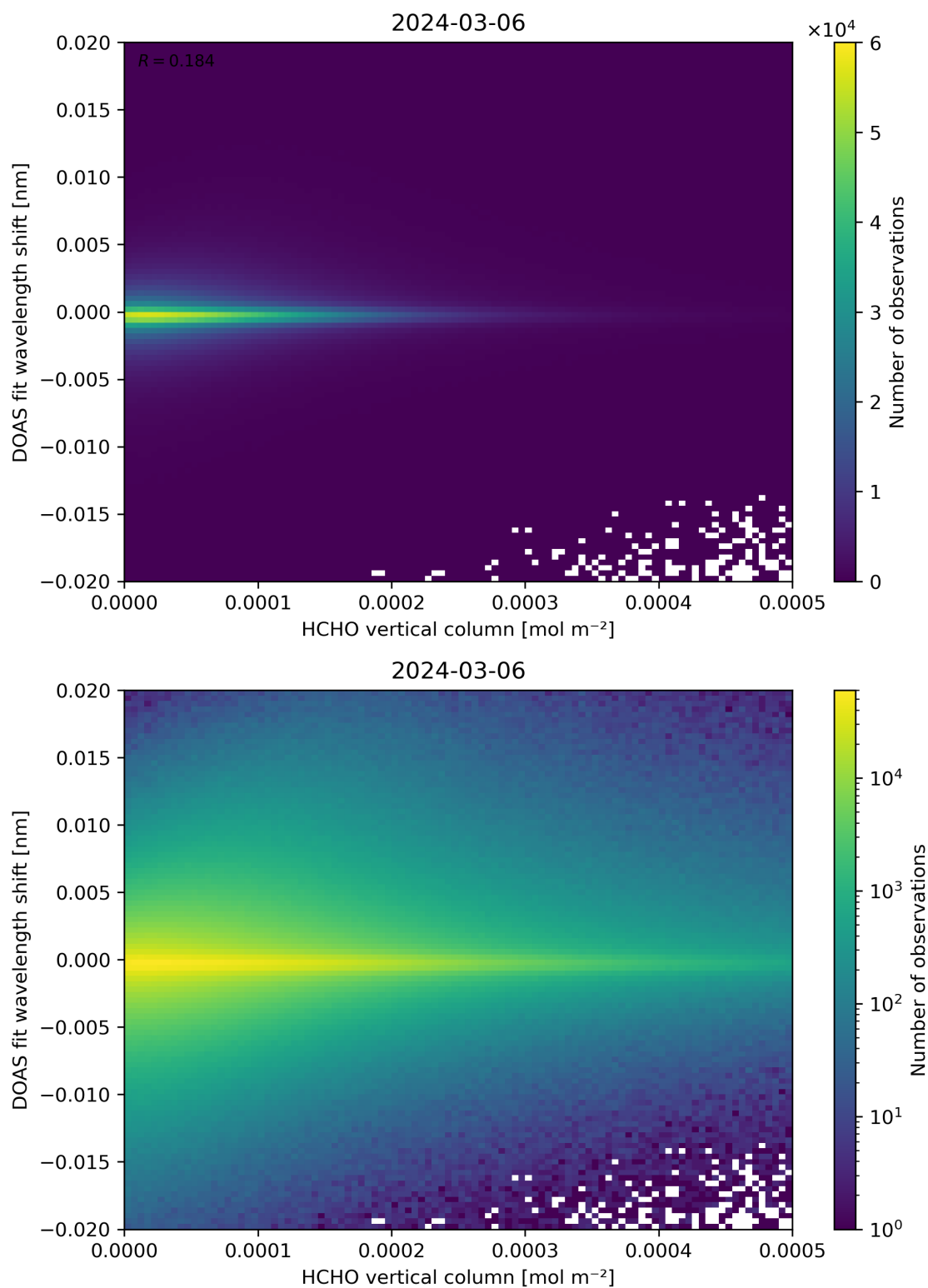
Figure 124: Scatter density plot of “HCHO vertical column” against “DOAS fit wavelength shift” for 2024-03-05 to 2024-03-07.
