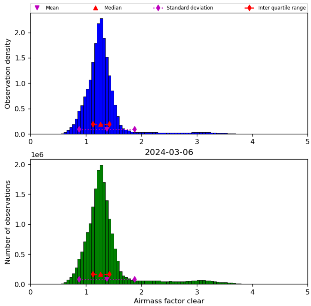
Figure 42: Histogram of “Airmass factor clear” for 2024-03-05 to 2024-03-07
