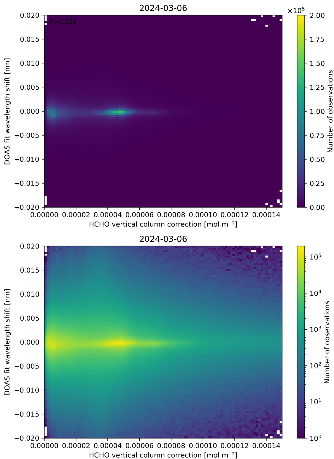
Figure 113: Scatter density plot of “HCHO vertical column correction” against “DOAS fit wavelength shift” for 2024-03-05 to 2024-03-07.
