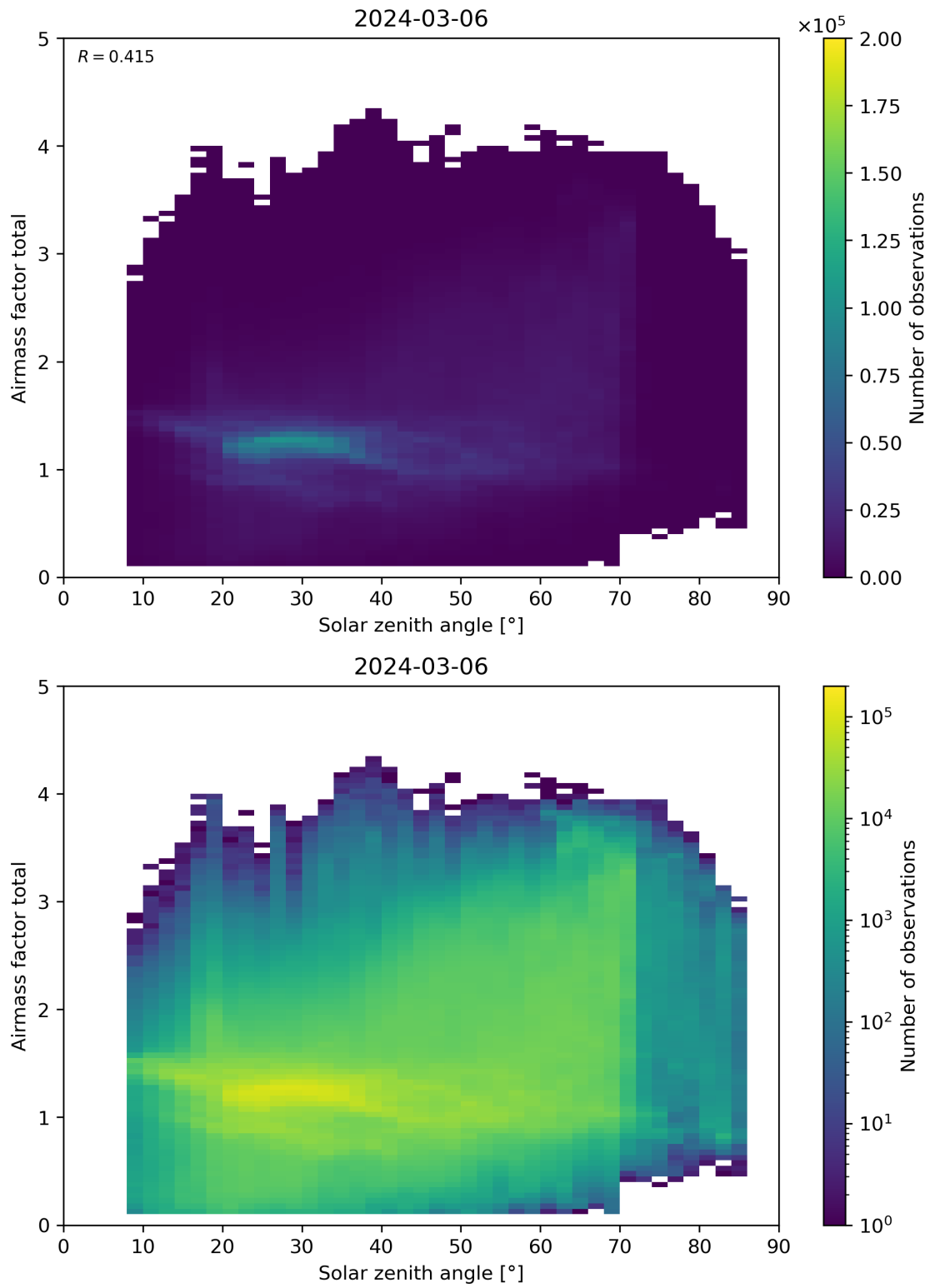
Figure 175: Scatter density plot of “Solar zenith angle” against “Airmass factor total” for 2024-03-05 to 2024-03-07.
