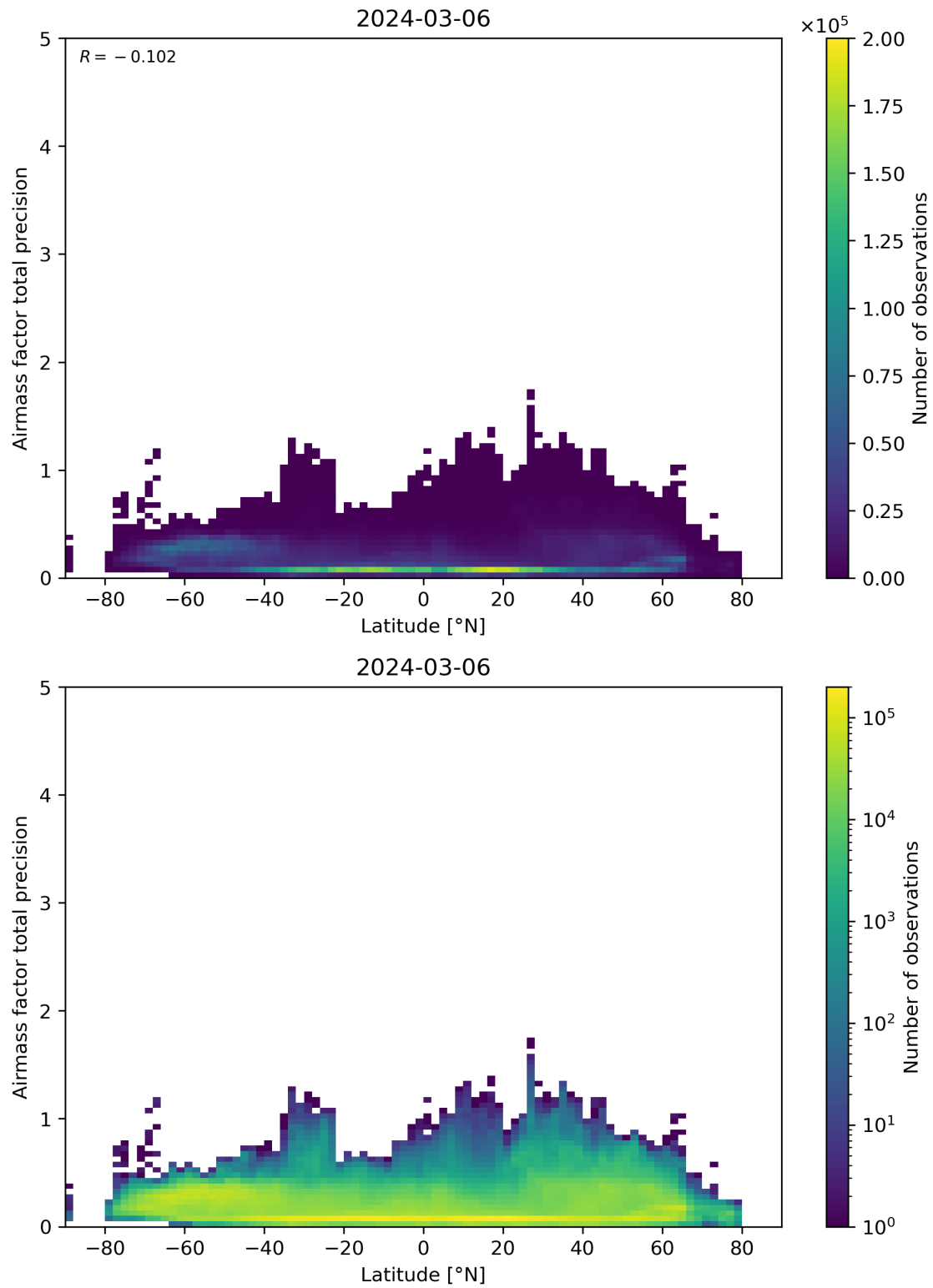
Figure 162: Scatter density plot of “Latitude” against “Airmass factor total precision” for 2024-03-05 to 2024-03-07.
