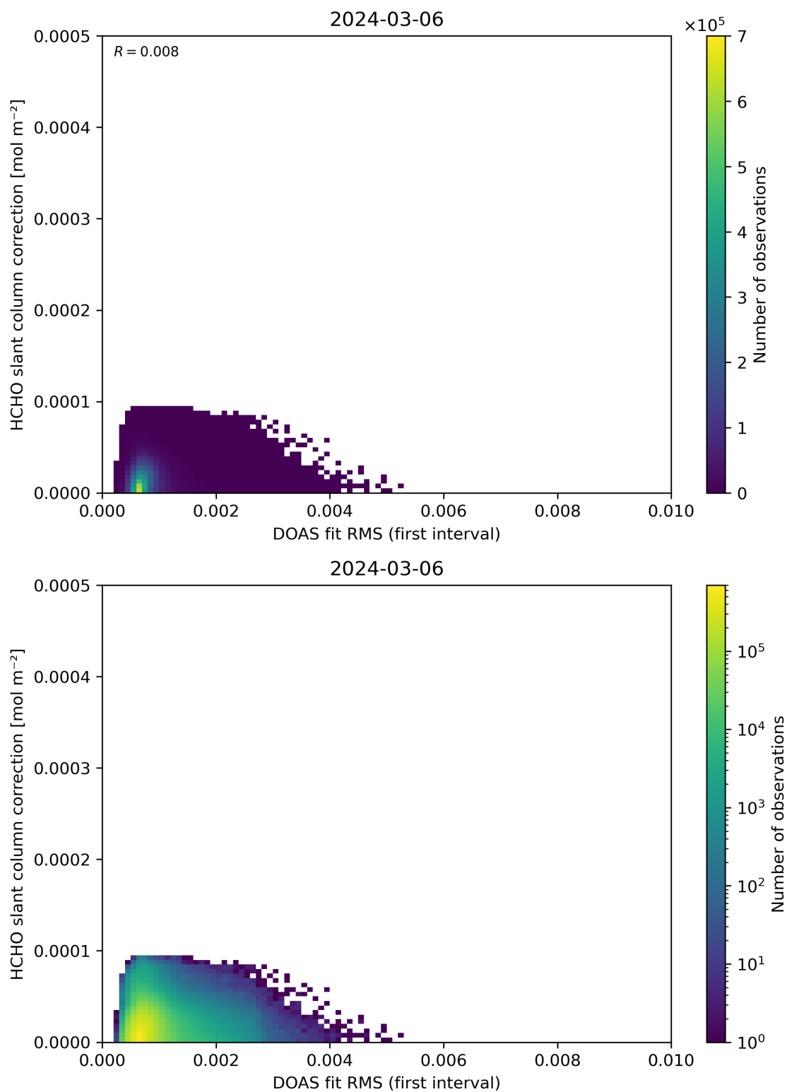
Figure 63: Scatter density plot of “DOAS fit RMS (first interval)” against “HCHO slant column correction” for 2024-03-05 to 2024-03-07.
