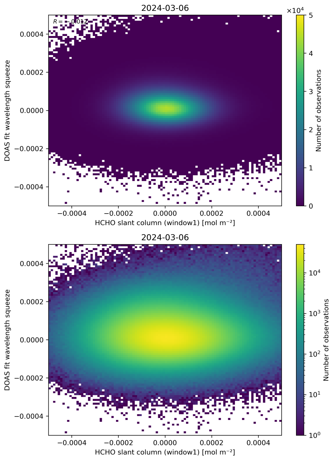
Figure 80: Scatter density plot of “HCHO slant column (window1)” against “DOAS fit wavelength squeeze” for 2024-03-05 to 2024-03-07.
