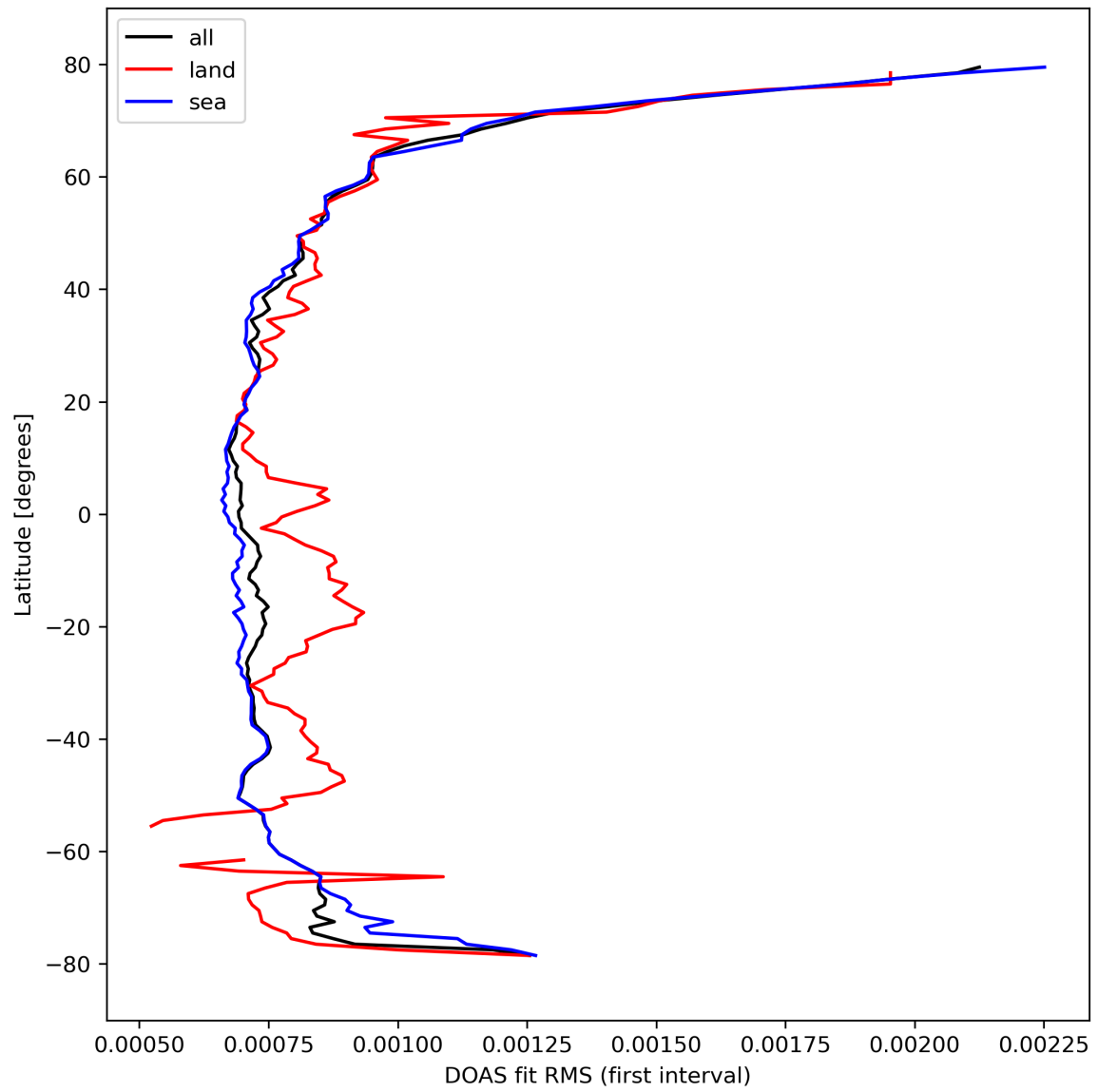
Figure 32: Zonal average of “DOAS fit RMS (first interval)” for 2024-03-05 to 2024-03-07.
