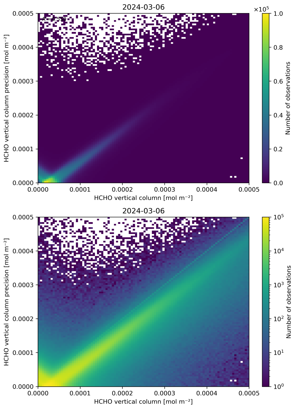
Figure 134: Scatter density plot of “HCHO vertical column” against “HCHO vertical column precision” for 2024-03-05 to 2024-03-07.
