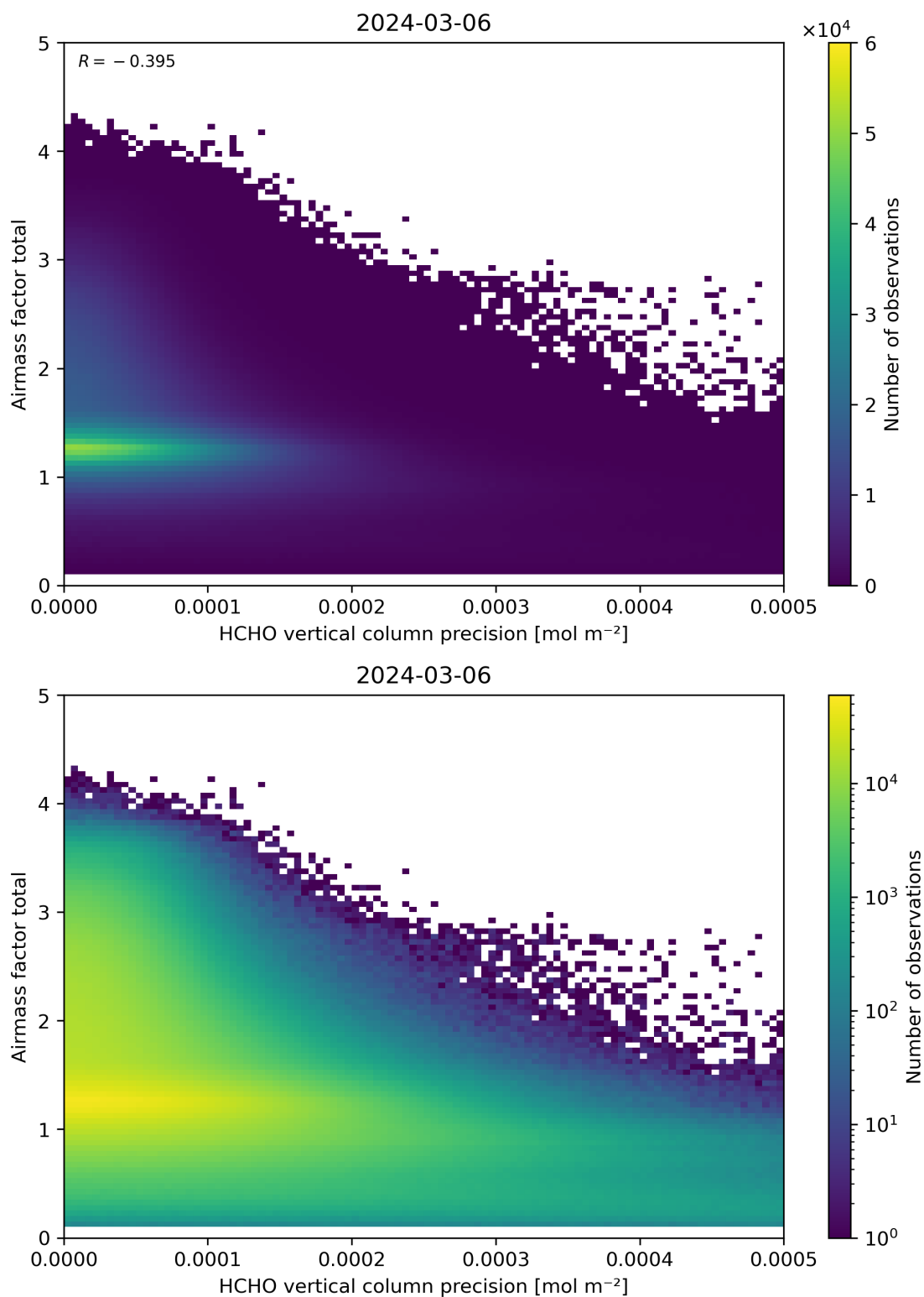
Figure 144: Scatter density plot of “HCHO vertical column precision” against “Airmass factor total” for 2024-03-05 to 2024-03-07.
