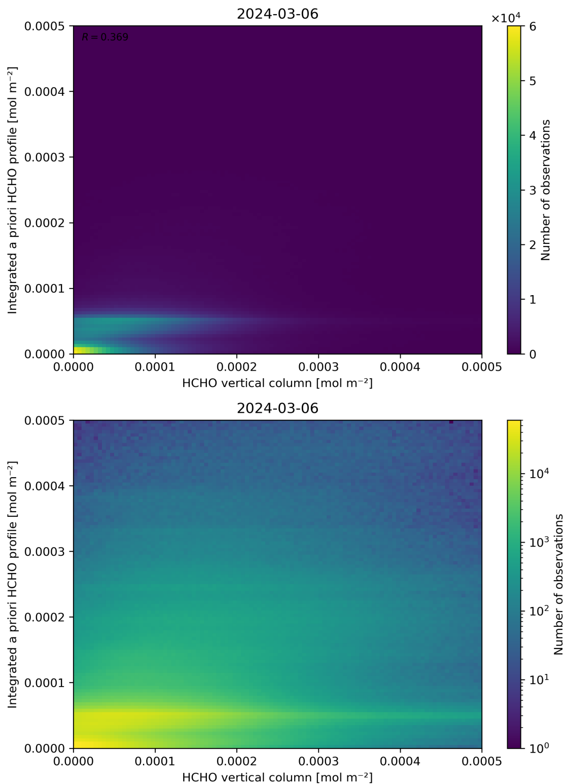
Figure 135: Scatter density plot of “HCHO vertical column” against “Integrated a priori HCHO profile” for 2024-03-05 to 2024-03-07.
