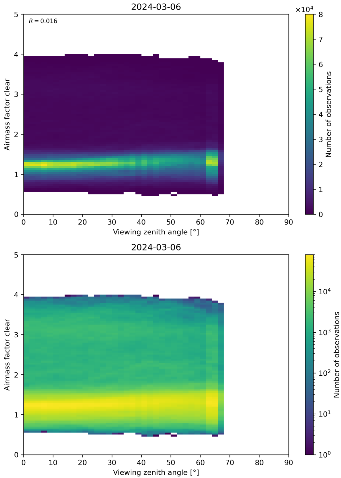
Figure 185: Scatter density plot of “Viewing zenith angle” against “Airmass factor clear” for 2024-03-05 to 2024-03-07.
