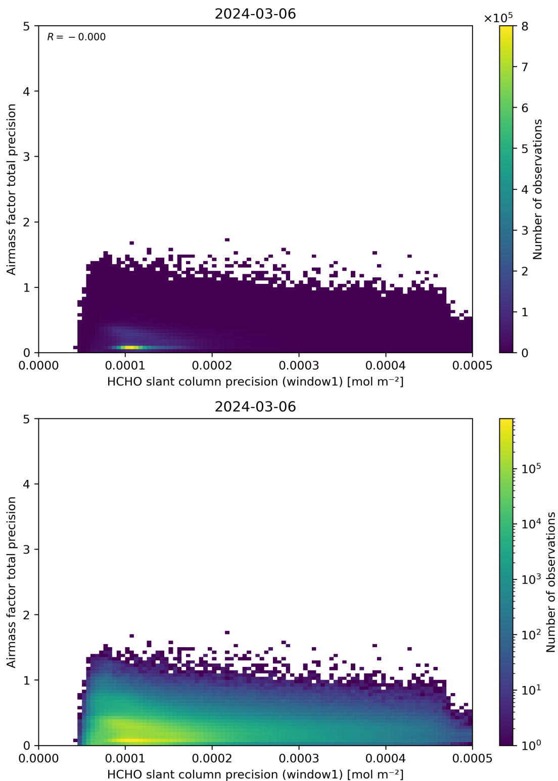
Figure 95: Scatter density plot of “HCHO slant column precision (window1)” against “Airmass factor total precision” for 2024-03-05 to 2024-03-07.
