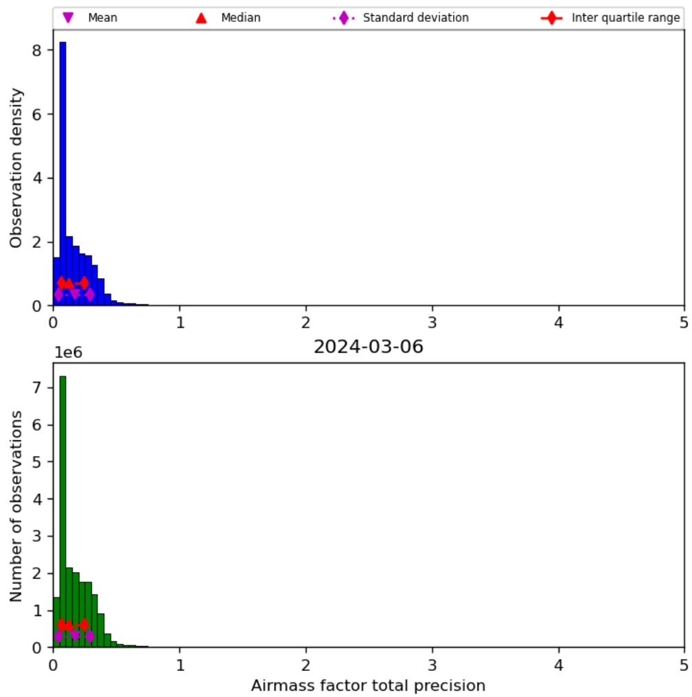
Figure 41: Histogram of “Airmass factor total precision” for 2024-03-05 to 2024-03-07
