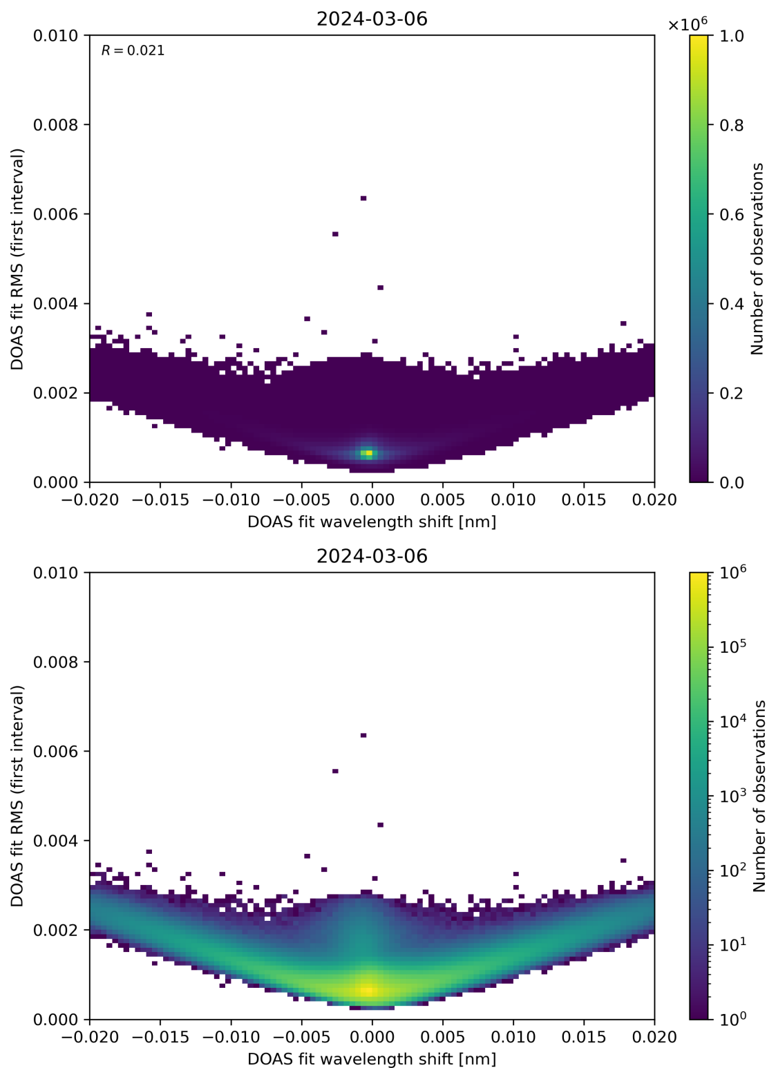
Figure 64: Scatter density plot of “DOAS fit wavelength shift” against “DOAS fit RMS (first interval)” for 2024-03-05 to 2024-03-07.
