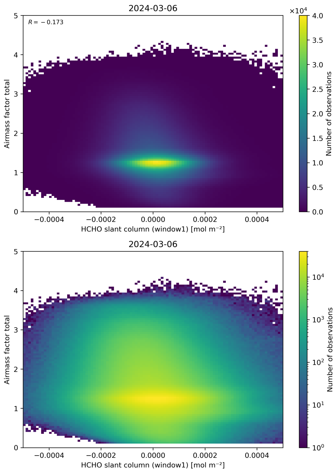
Figure 85: Scatter density plot of “HCHO slant column (window1)” against “Airmass factor total” for 2024-03-05 to 2024-03-07.
