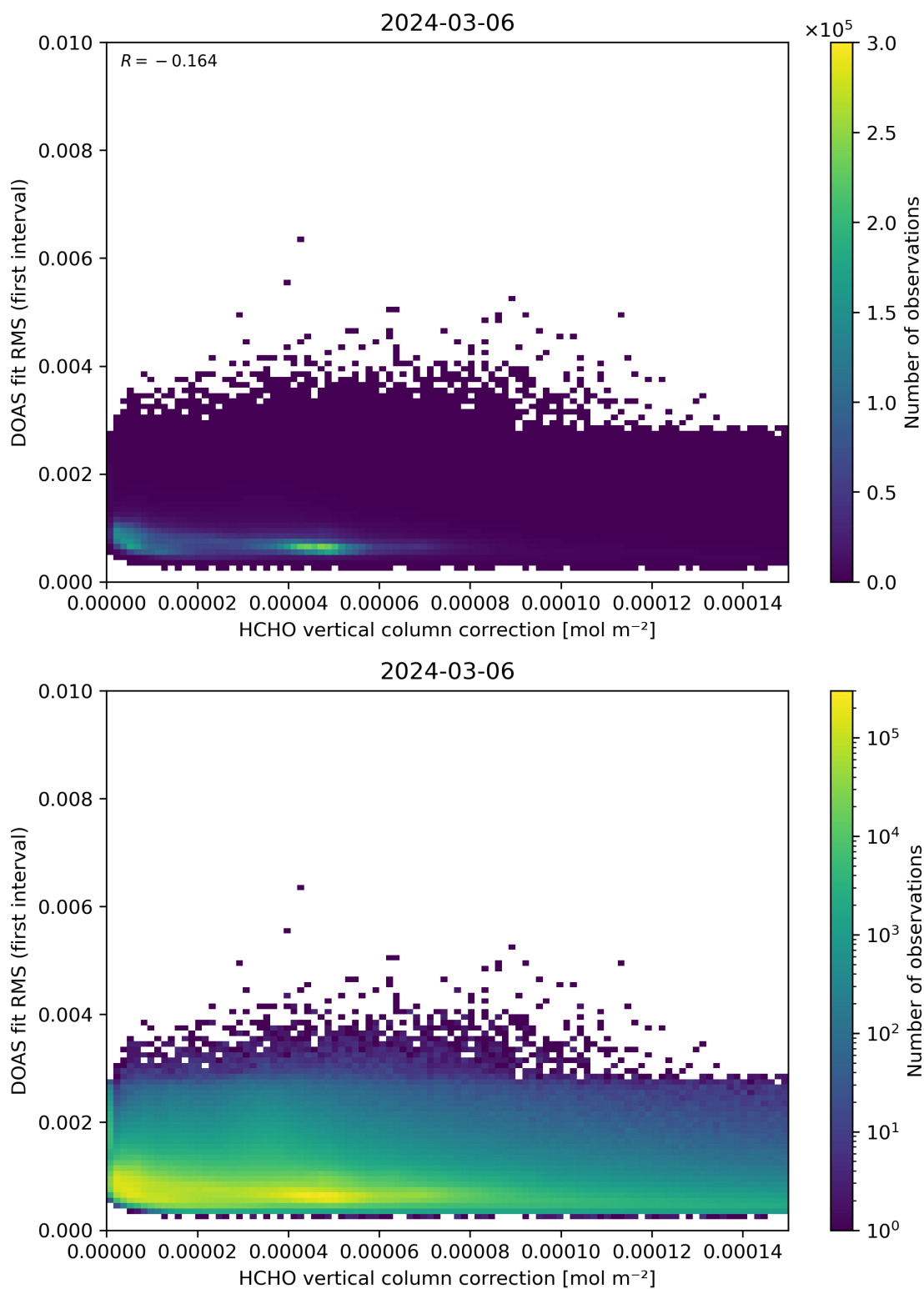
Figure 112: Scatter density plot of “HCHO vertical column correction” against “DOAS fit RMS (first interval)” for 2024-03-05 to 2024-03-07.
