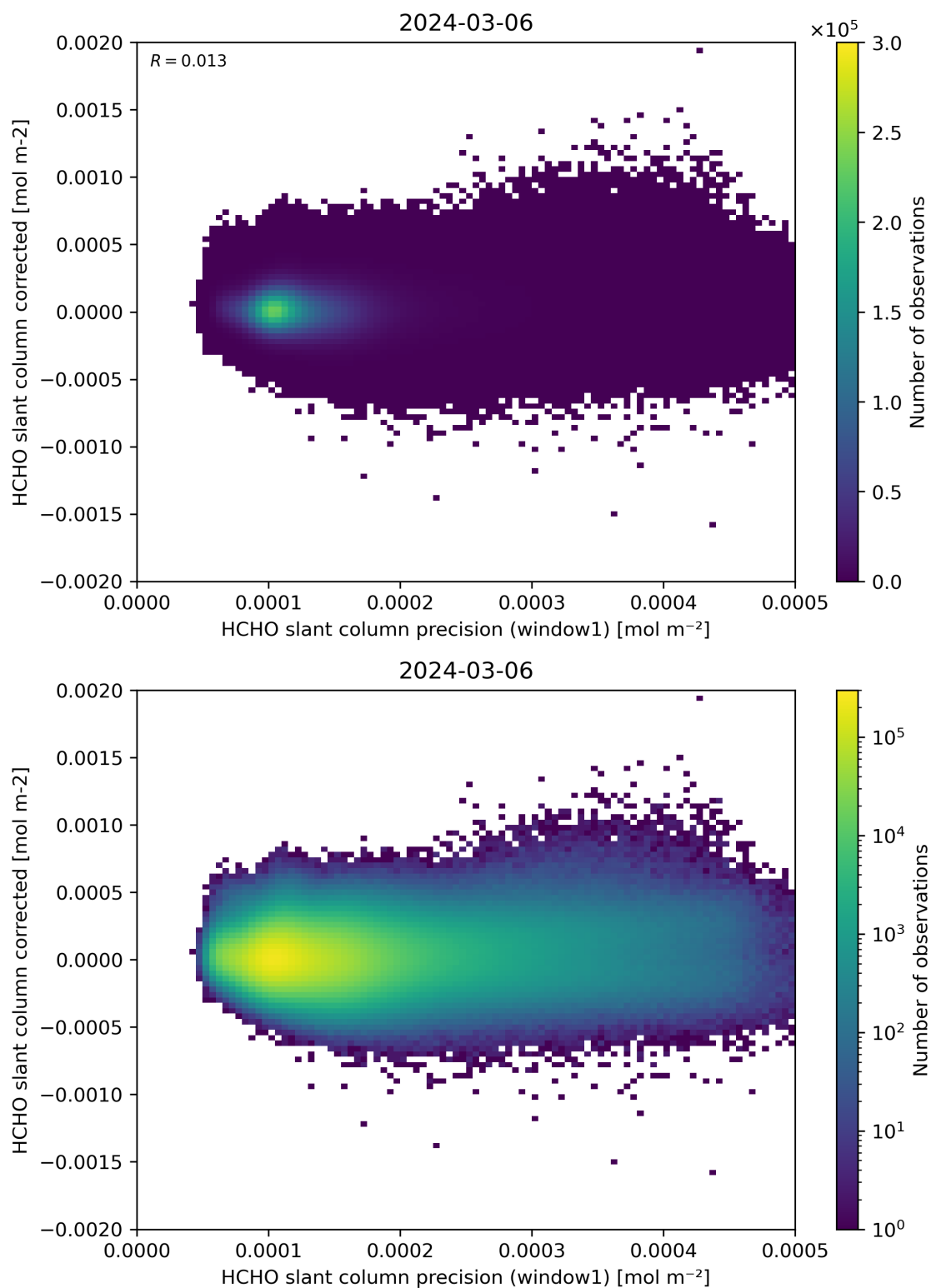
Figure 92: Scatter density plot of “HCHO slant column precision (window1)” against “HCHO slant column corrected” for 2024-03-05 to 2024-03-07.
