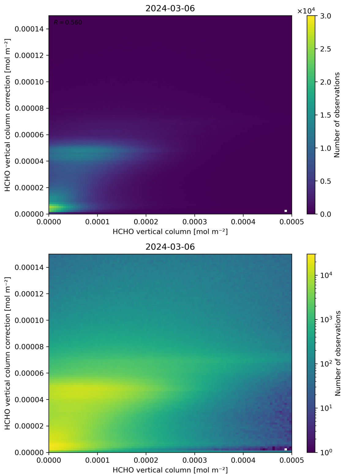
Figure 133: Scatter density plot of “HCHO vertical column” against “HCHO vertical column correction” for 2024-03-05 to 2024-03-07.
