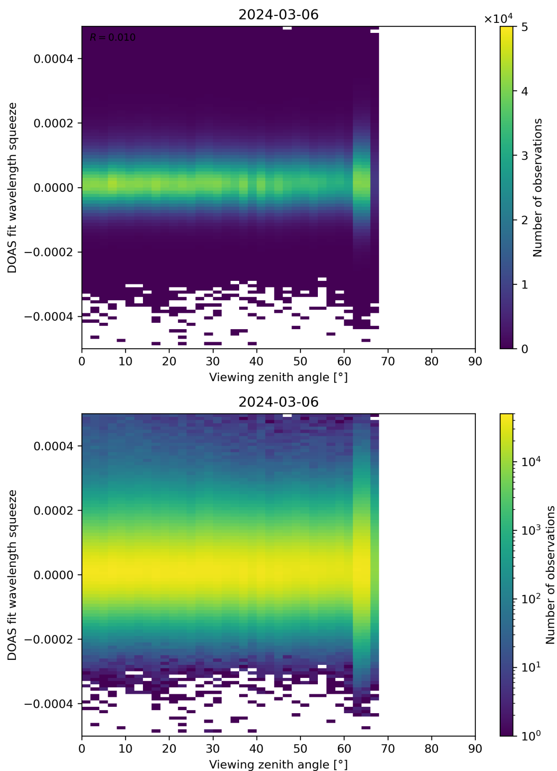
Figure 184: Scatter density plot of “Viewing zenith angle” against “DOAS fit wavelength squeeze” for 2024-03-05 to 2024-03-07.
