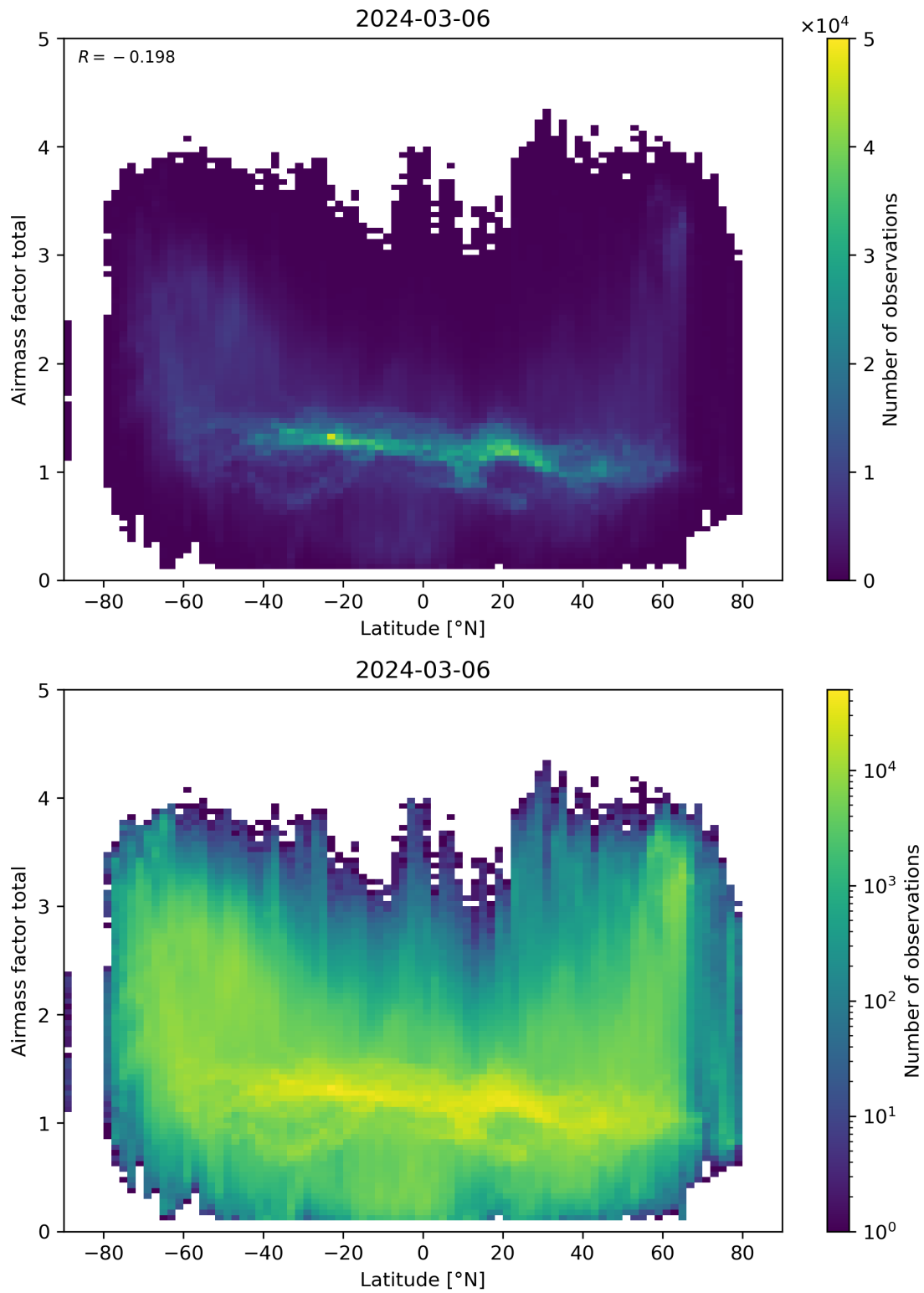
Figure 161: Scatter density plot of “Latitude” against “Airmass factor total” for 2024-03-05 to 2024-03-07.
