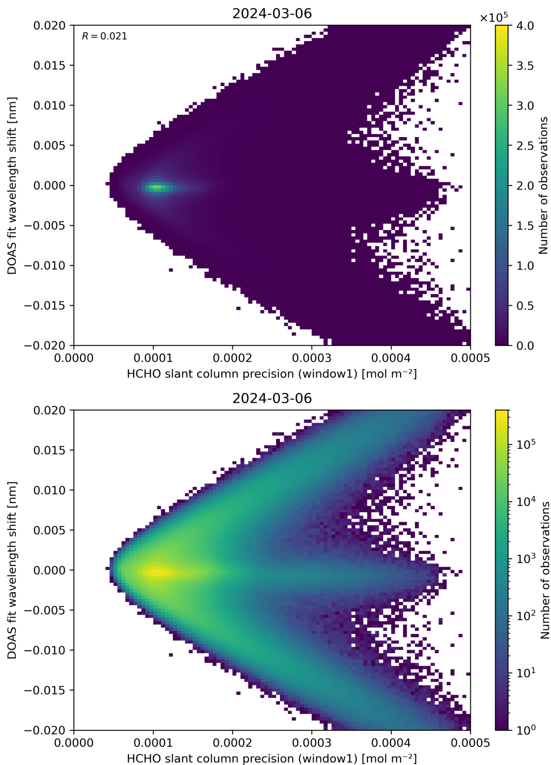
Figure 89: Scatter density plot of “HCHO slant column precision (window1)” against “DOAS fit wavelength shift” for 2024-03-05 to 2024-03-07.
