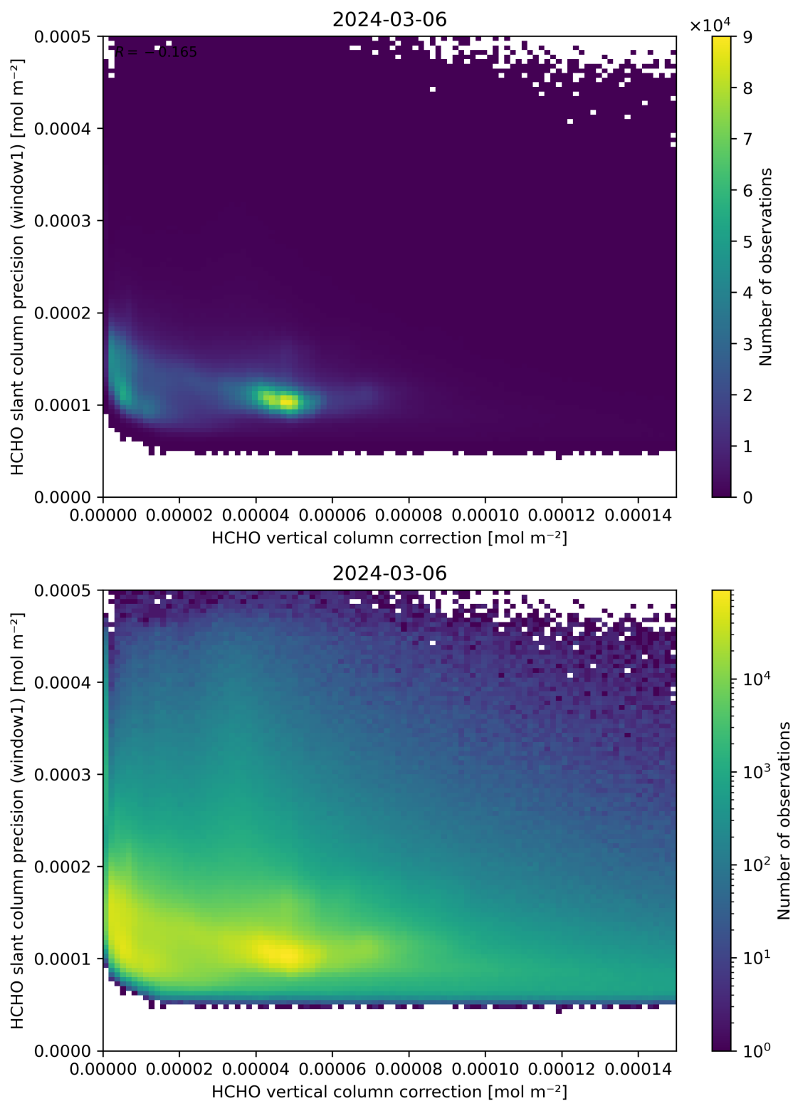
Figure 119: Scatter density plot of “HCHO vertical column correction” against “HCHO slant column precision (window1)” for 2024-03-05 to 2024-03-07.
