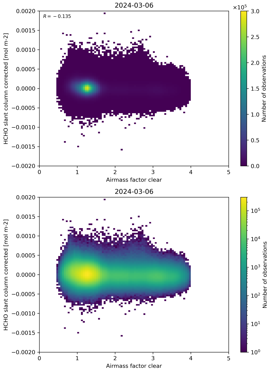
Figure 74: Scatter density plot of “Airmass factor clear” against “HCHO slant column corrected” for 2024-03-05 to 2024-03-07.
