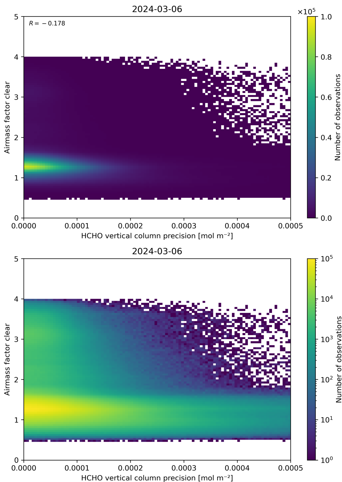
Figure 139: Scatter density plot of “HCHO vertical column precision” against “Airmass factor clear” for 2024-03-05 to 2024-03-07.
