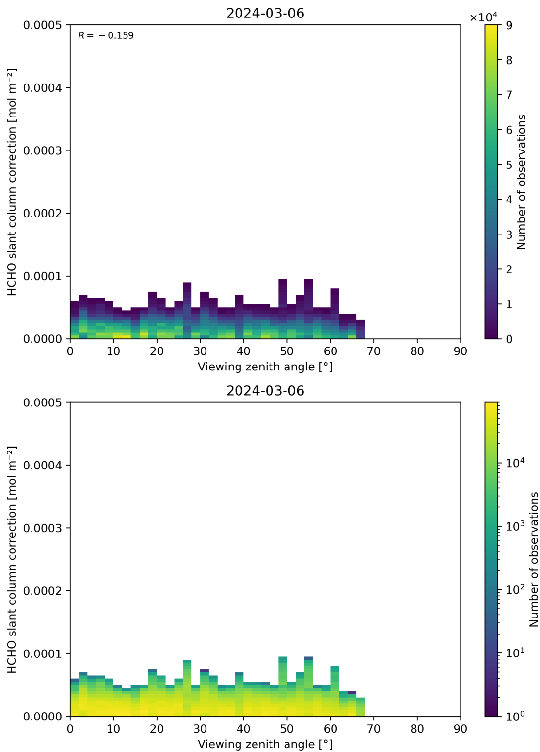
Figure 187: Scatter density plot of “Viewing zenith angle” against “HCHO slant column correction” for 2024-03-05 to 2024-03-07.
