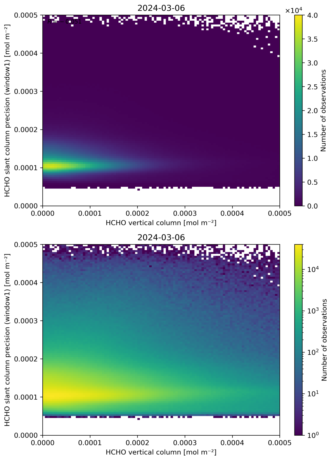
Figure 130: Scatter density plot of “HCHO vertical column” against “HCHO slant column precision (window1)” for 2024-03-05 to 2024-03-07.
