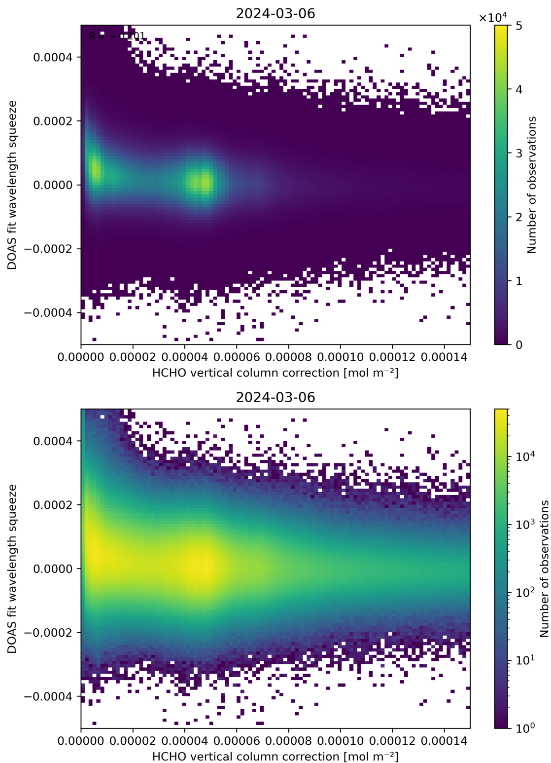
Figure 114: Scatter density plot of “HCHO vertical column correction” against “DOAS fit wavelength squeeze” for 2024-03-05 to 2024-03-07.
