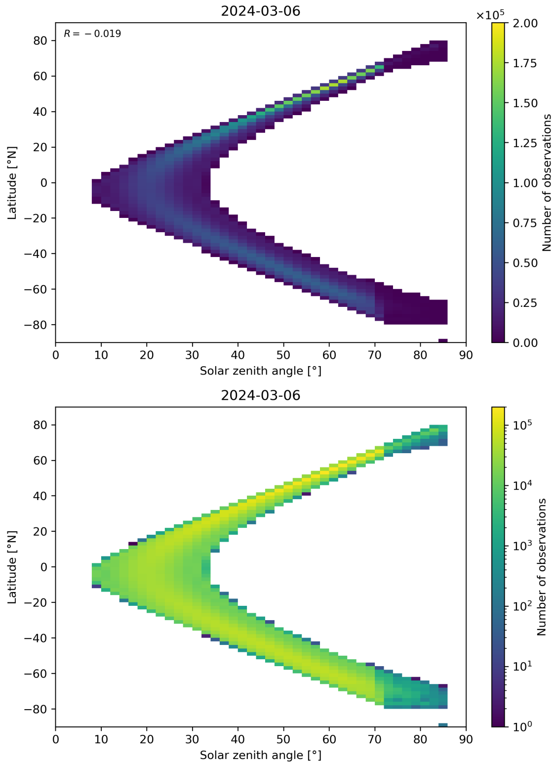
Figure 181: Scatter density plot of “Solar zenith angle” against “Latitude” for 2024-03-05 to 2024-03-07.
