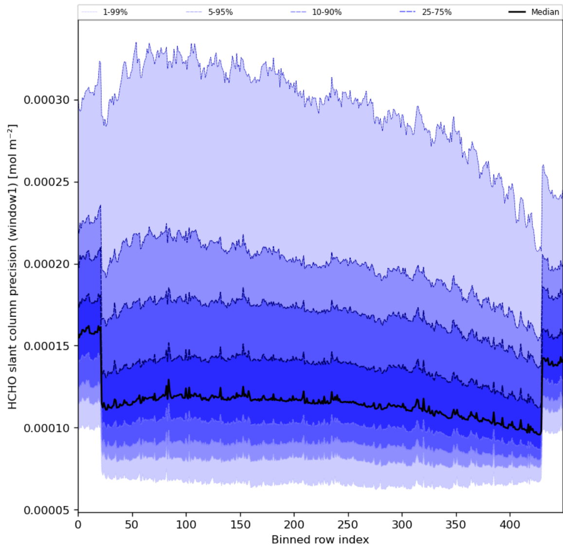
Figure 53: Along track statistics of “HCHO slant column precision (window1)” for 2024-03-05 to 2024-03-07
