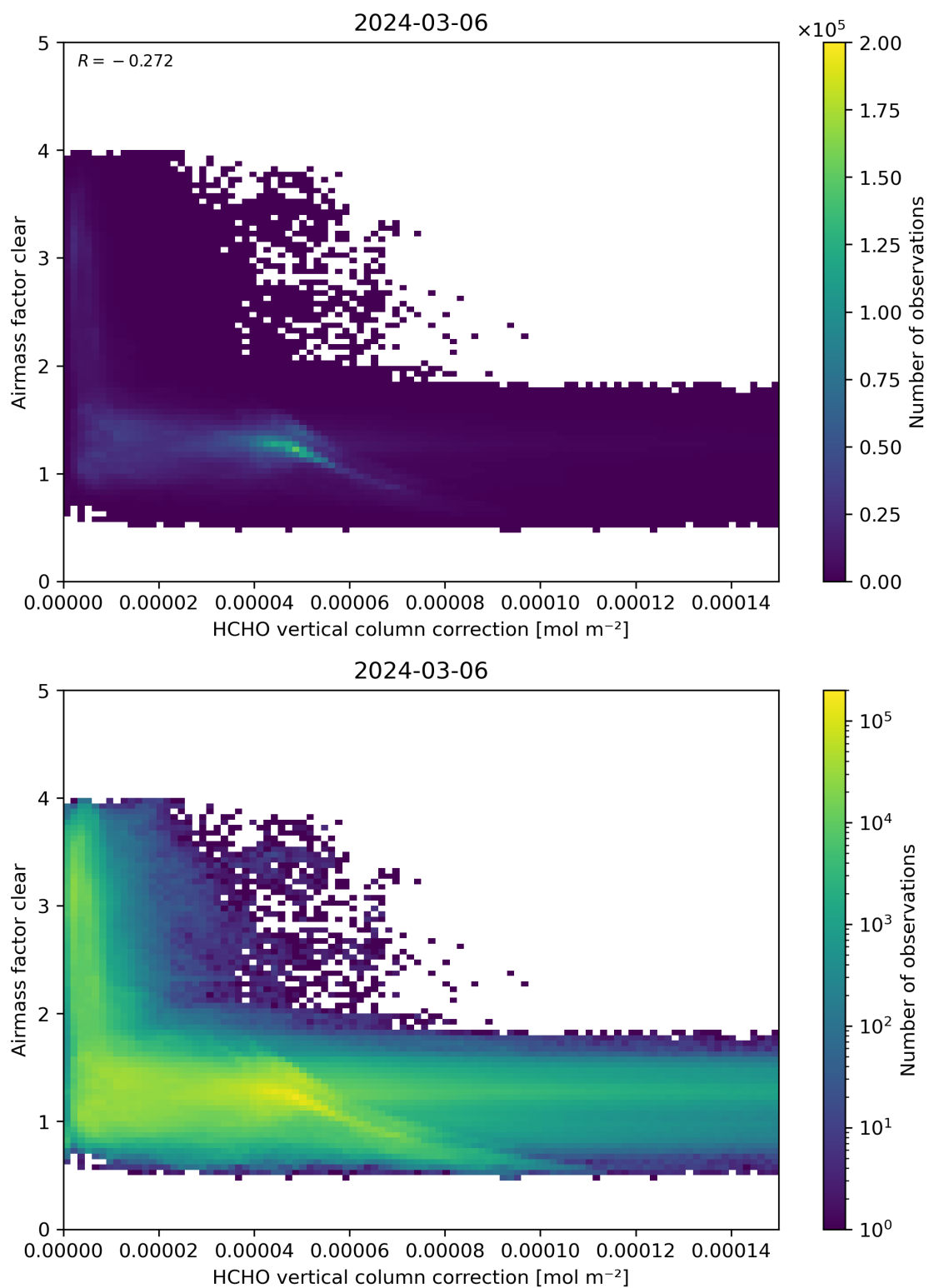
Figure 115: Scatter density plot of “HCHO vertical column correction” against “Airmass factor clear” for 2024-03-05 to 2024-03-07.
