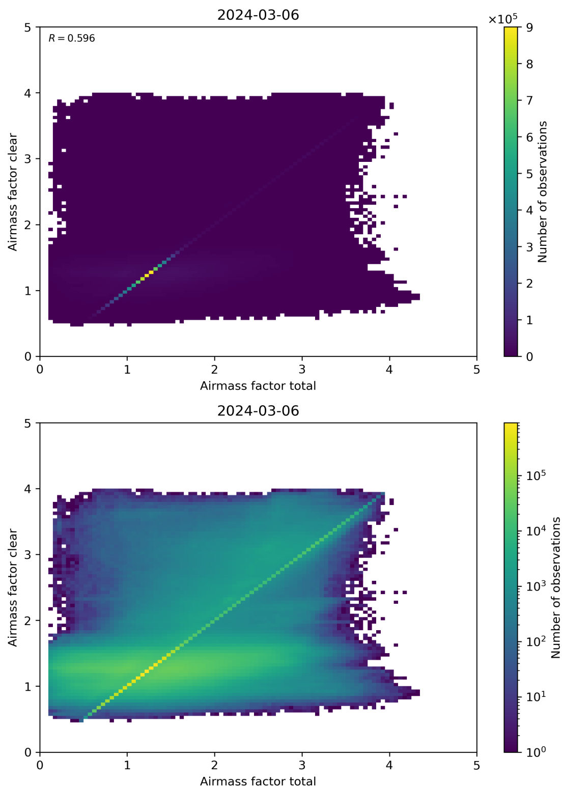
Figure 100: Scatter density plot of “Airmass factor total” against “Airmass factor clear” for 2024-03-05 to 2024-03-07.
