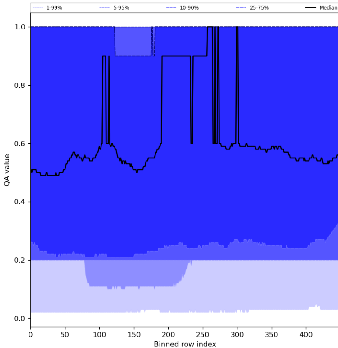
Figure 48: Along track statistics of “QA value” for 2024-03-05 to 2024-03-07
