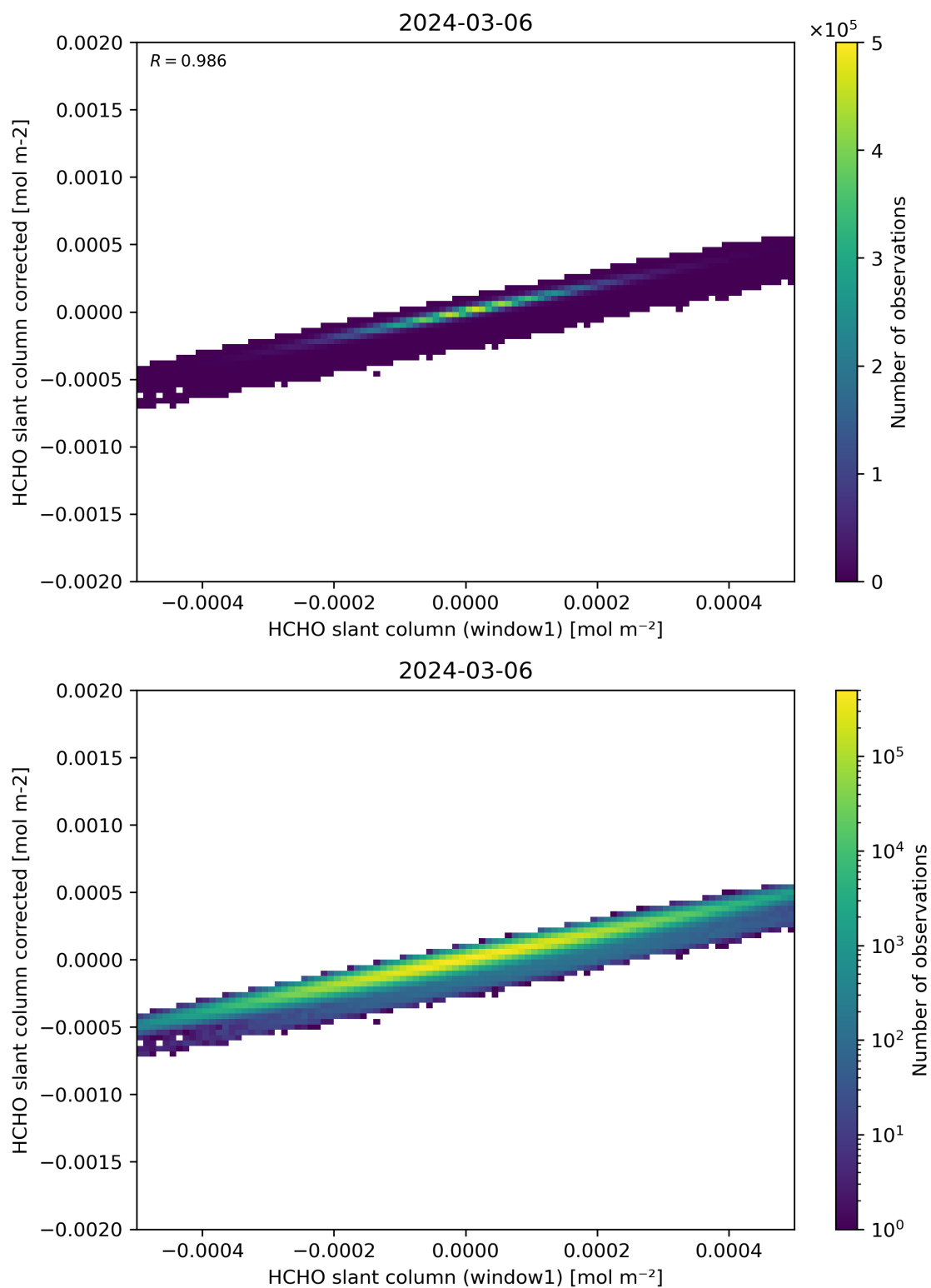
Figure 82: Scatter density plot of “HCHO slant column (window1)” against “HCHO slant column corrected” for 2024-03-05 to 2024-03-07.
