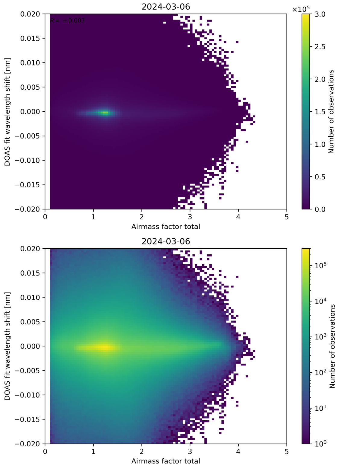
Figure 98: Scatter density plot of “Airmass factor total” against “DOAS fit wavelength shift” for 2024-03-05 to 2024-03-07.
