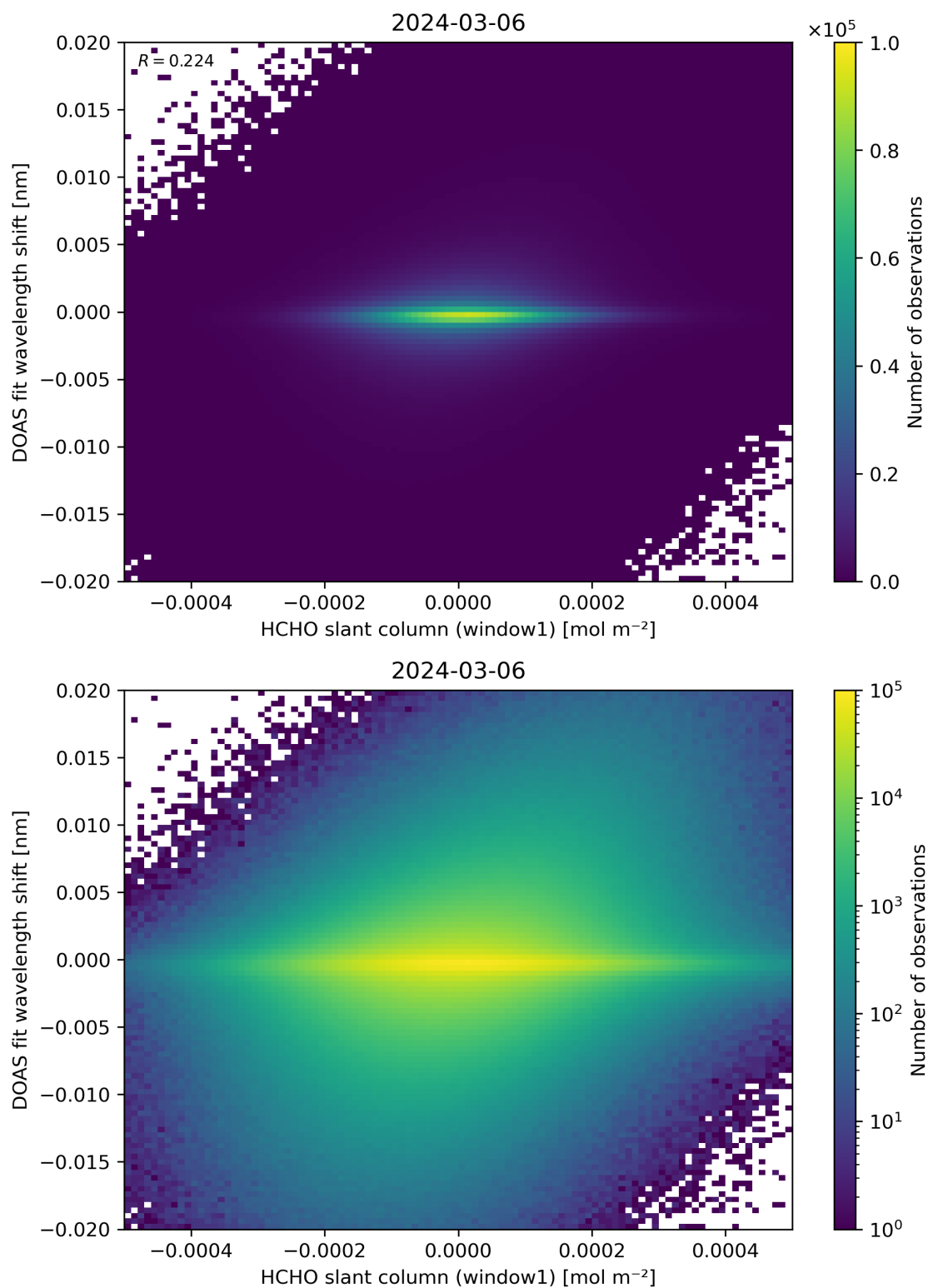
Figure 79: Scatter density plot of “HCHO slant column (window1)” against “DOAS fit wavelength shift” for 2024-03-05 to 2024-03-07.
