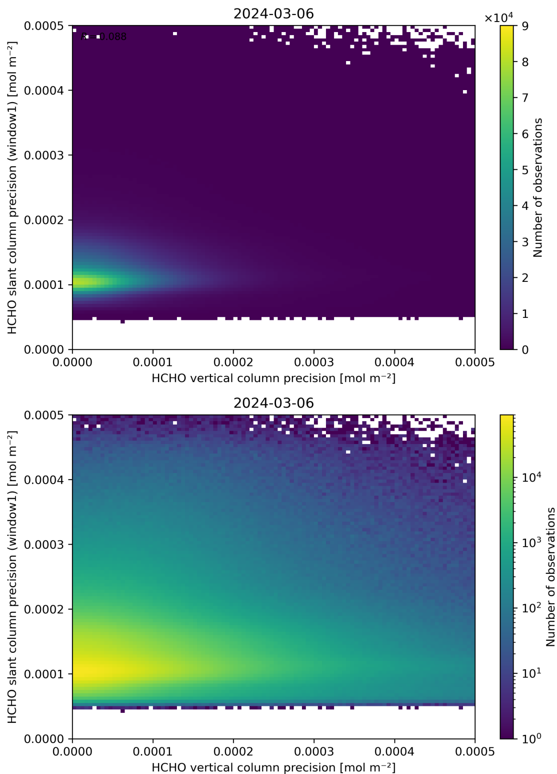
Figure 143: Scatter density plot of “HCHO vertical column precision” against “HCHO slant column precision (window1)” for 2024-03-05 to 2024-03-07.
