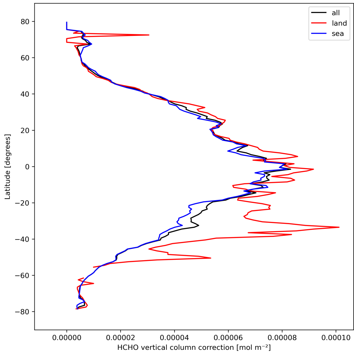
Figure 23: Zonal average of “HCHO vertical column correction” for 2024-03-05 to 2024-03-07.
