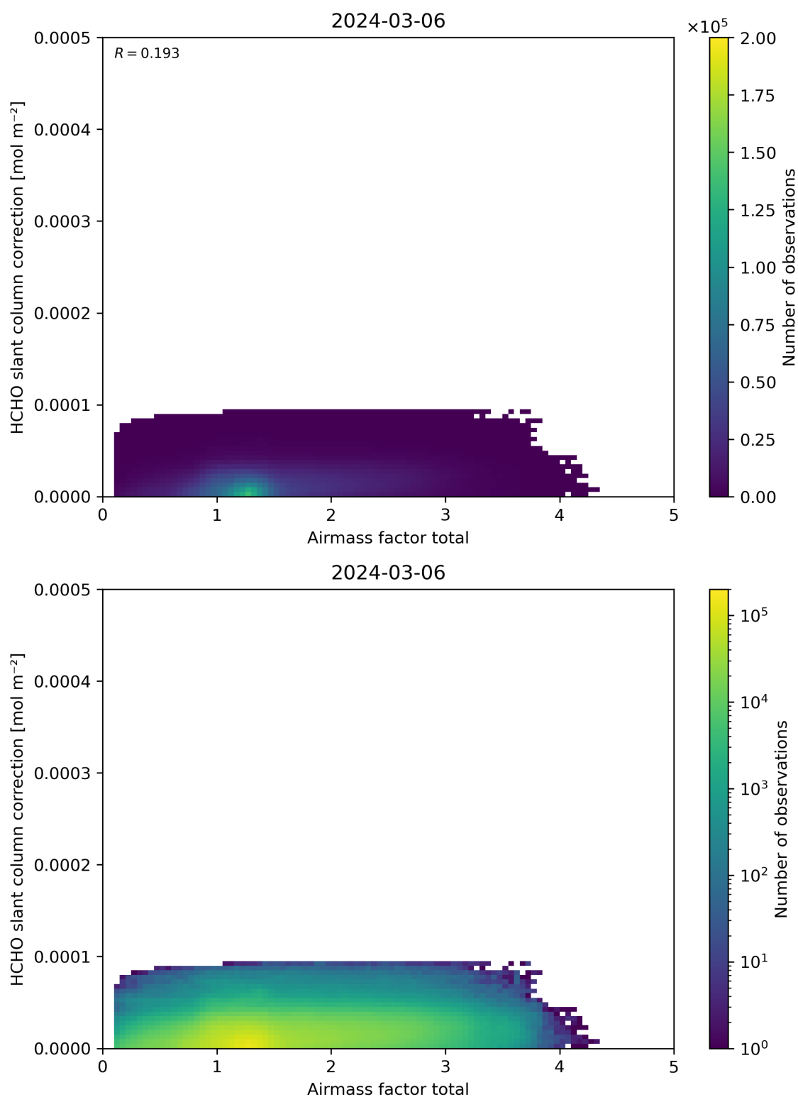
Figure 102: Scatter density plot of “Airmass factor total” against “HCHO slant column correction” for 2024-03-05 to 2024-03-07.
