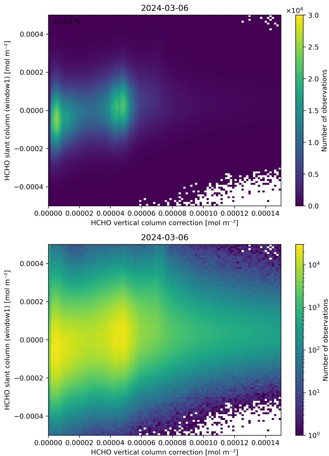
Figure 118: Scatter density plot of “HCHO vertical column correction” against “HCHO slant column (window1)” for 2024-03-05 to 2024-03-07.
