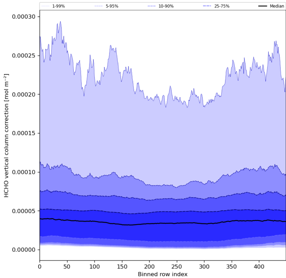
Figure 51: Along track statistics of “HCHO vertical column correction” for 2024-03-05 to 2024-03-07
