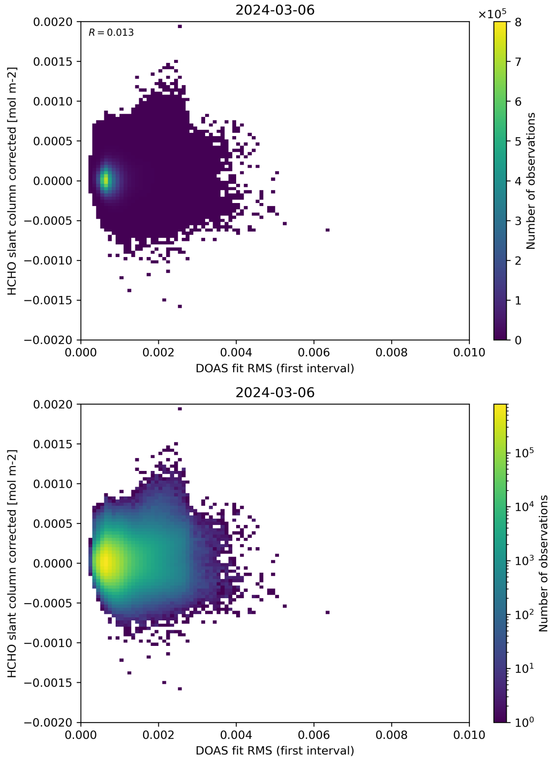
Figure 62: Scatter density plot of “DOAS fit RMS (first interval)” against “HCHO slant column corrected” for 2024-03-05 to 2024-03-07.
