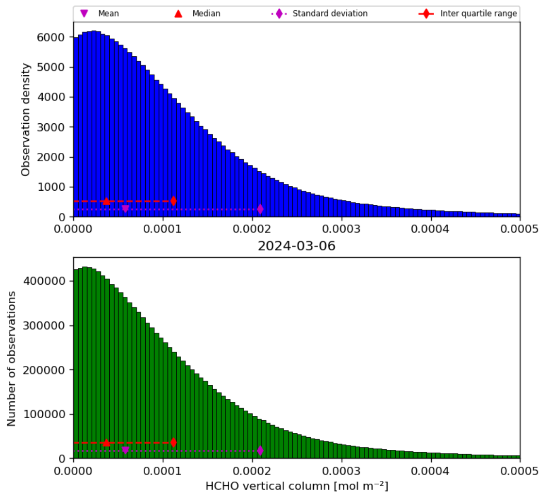
Figure 35: Histogram of “HCHO vertical column” for 2024-03-05 to 2024-03-07
