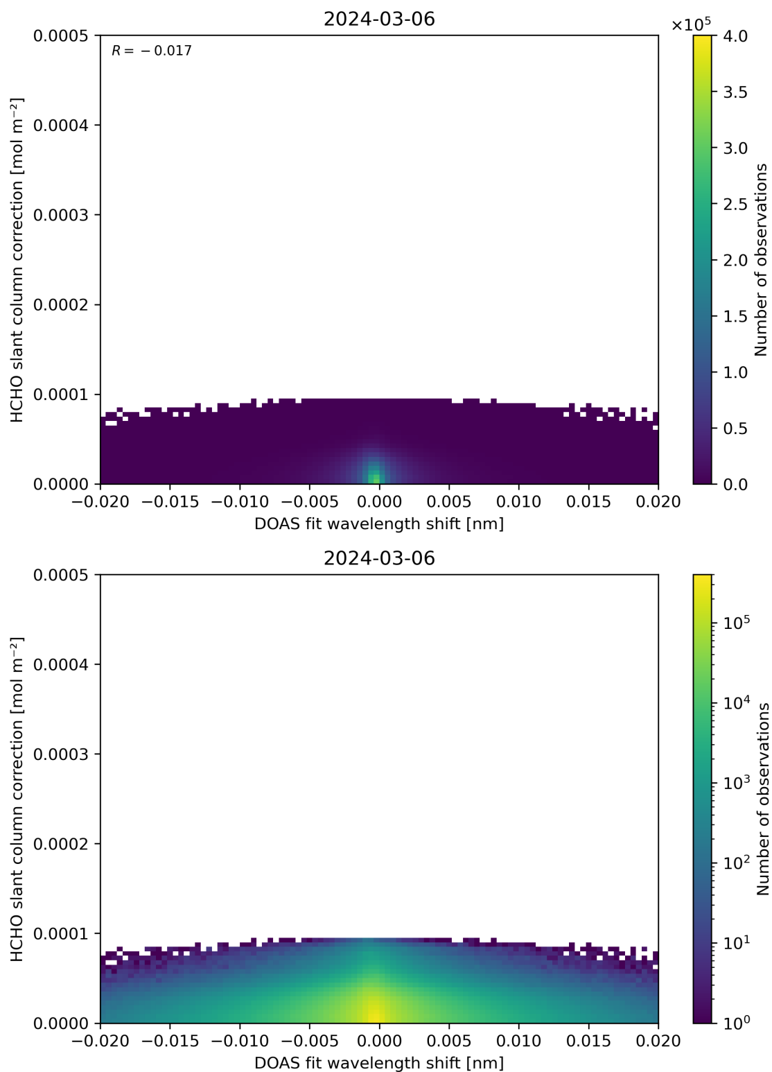
Figure 67: Scatter density plot of “DOAS fit wavelength shift” against “HCHO slant column correction” for 2024-03-05 to 2024-03-07.
