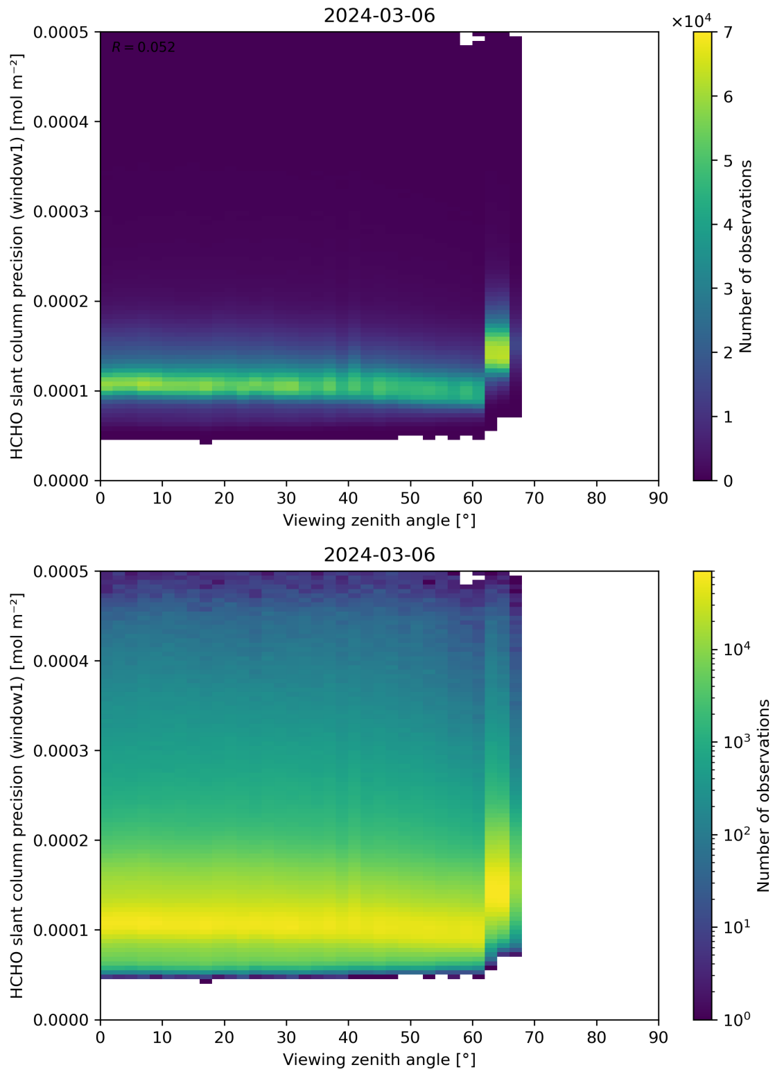
Figure 189: Scatter density plot of “Viewing zenith angle” against “HCHO slant column precision (window1)” for 2024-03-05 to 2024-03-07.
