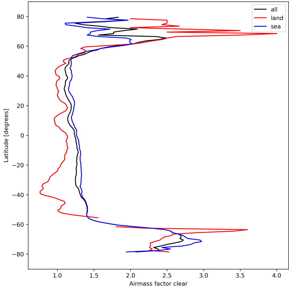
Figure 28: Zonal average of “Airmass factor clear” for 2024-03-05 to 2024-03-07.
