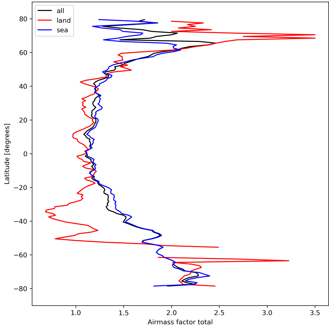
Figure 26: Zonal average of “Airmass factor total” for 2024-03-05 to 2024-03-07.
