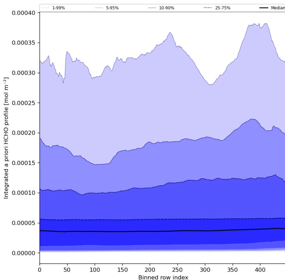
Figure 57: Along track statistics of “Integrated a priori HCHO profile” for 2024-03-05 to 2024-03-07
