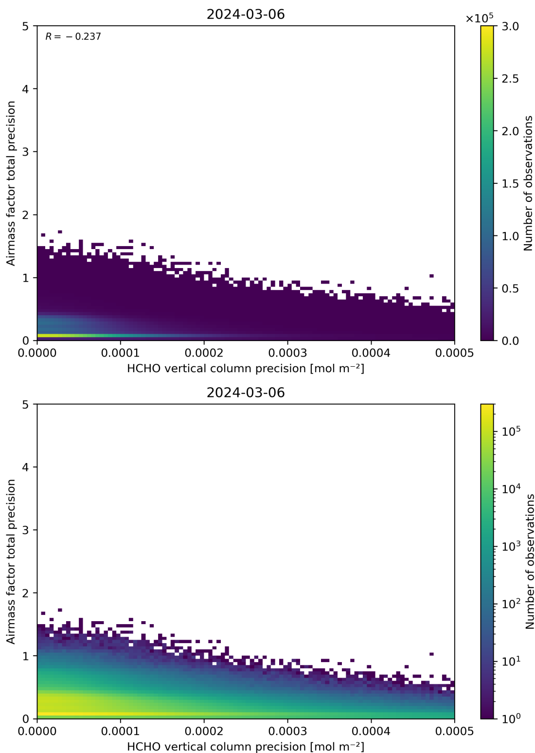
Figure 145: Scatter density plot of “HCHO vertical column precision” against “Airmass factor total precision” for 2024-03-05 to 2024-03-07.
