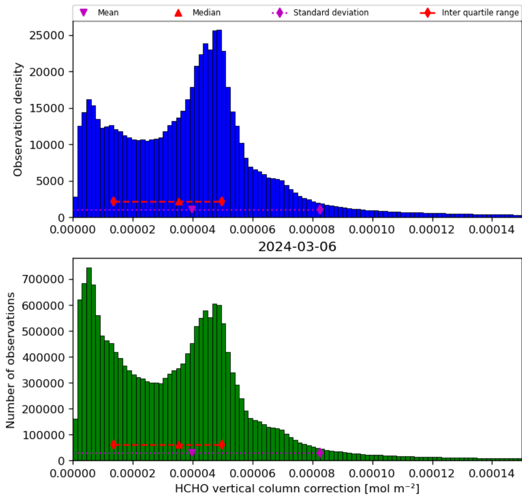
Figure 37: Histogram of “HCHO vertical column correction” for 2024-03-05 to 2024-03-07
