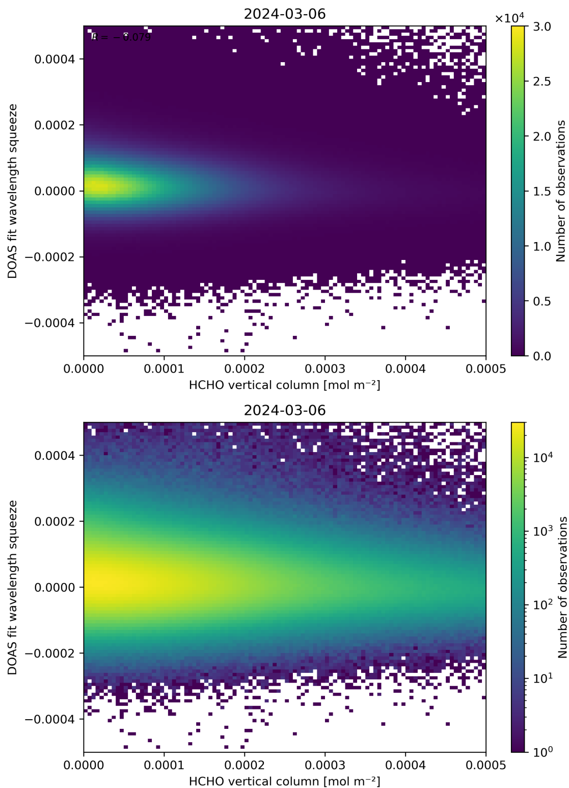
Figure 125: Scatter density plot of “HCHO vertical column” against “DOAS fit wavelength squeeze” for 2024-03-05 to 2024-03-07.
