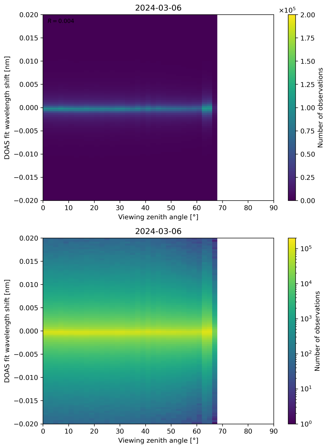
Figure 183: Scatter density plot of “Viewing zenith angle” against “DOAS fit wavelength shift” for 2024-03-05 to 2024-03-07.
