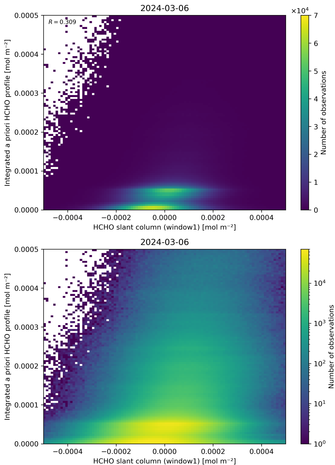
Figure 87: Scatter density plot of “HCHO slant column (window1)” against “Integrated a priori HCHO profile” for 2024-03-05 to 2024-03-07.
