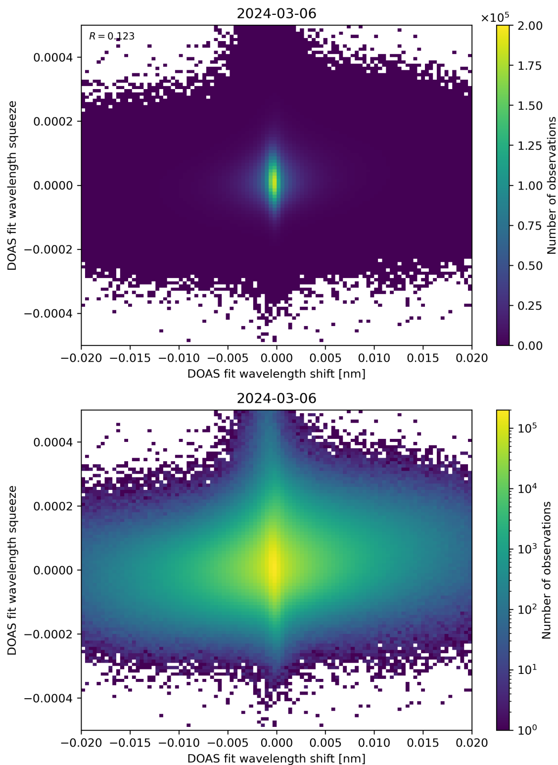
Figure 65: Scatter density plot of “DOAS fit wavelength shift” against “DOAS fit wavelength squeeze” for 2024-03-05 to 2024-03-07.
