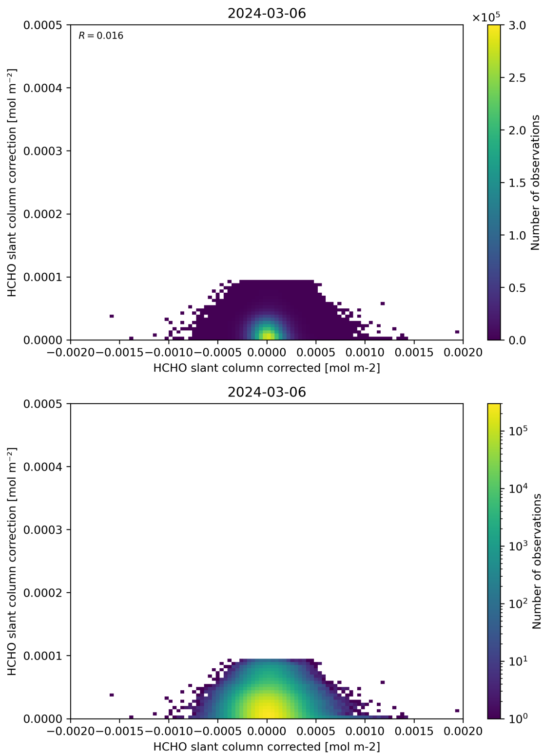
Figure 77: Scatter density plot of “HCHO slant column corrected” against “HCHO slant column correction” for 2024-03-05 to 2024-03-07.
