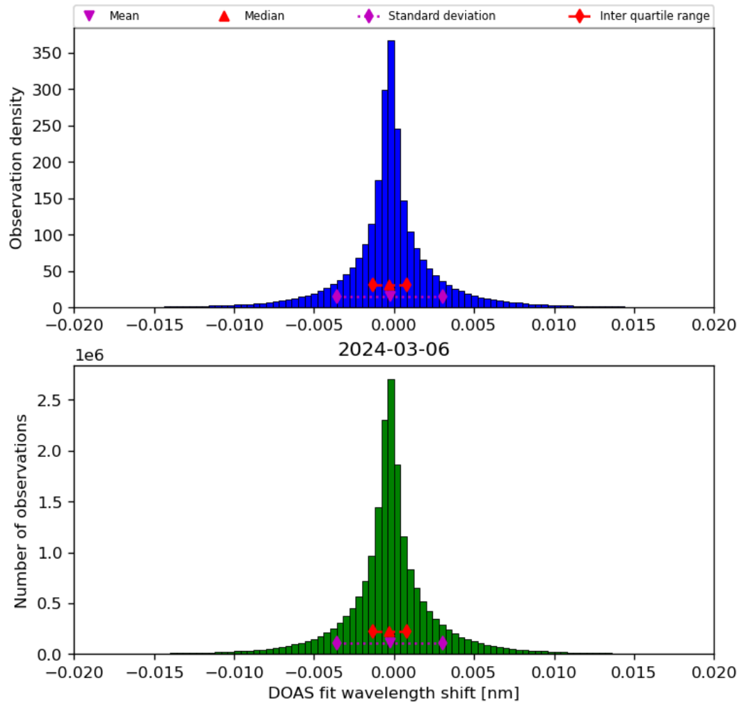
Figure 44: Histogram of “DOAS fit wavelength shift” for 2024-03-05 to 2024-03-07
