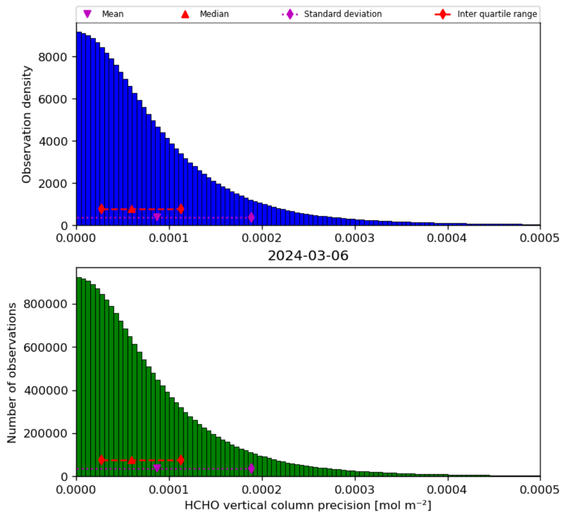
Figure 36: Histogram of “HCHO vertical column precision” for 2024-03-05 to 2024-03-07
