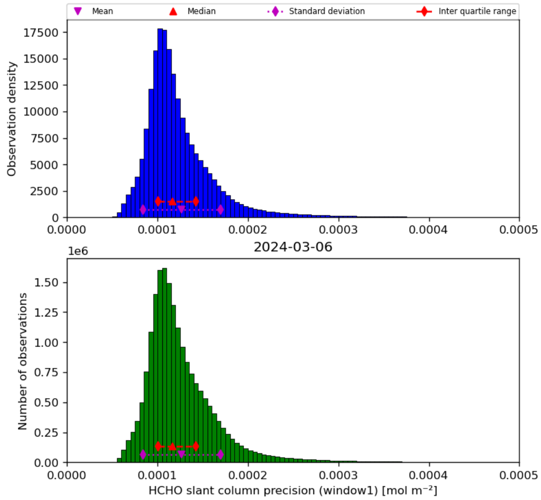
Figure 39: Histogram of “HCHO slant column precision (window1)” for 2024-03-05 to 2024-03-07
