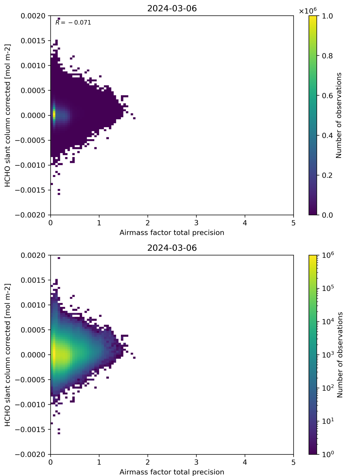
Figure 109: Scatter density plot of “Airmass factor total precision” against “HCHO slant column corrected” for 2024-03-05 to 2024-03-07.
