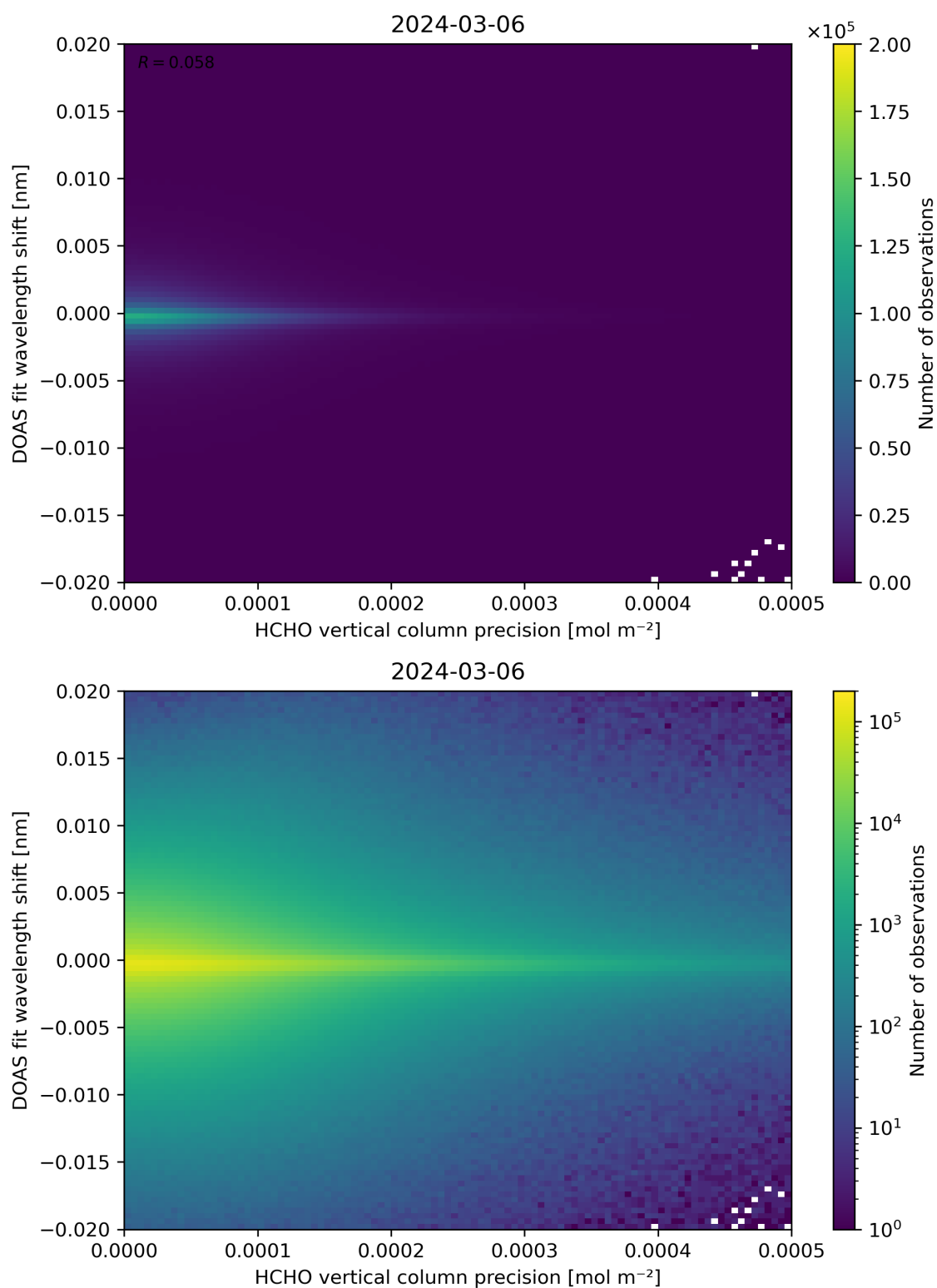
Figure 137: Scatter density plot of “HCHO vertical column precision” against “DOAS fit wavelength shift” for 2024-03-05 to 2024-03-07.
