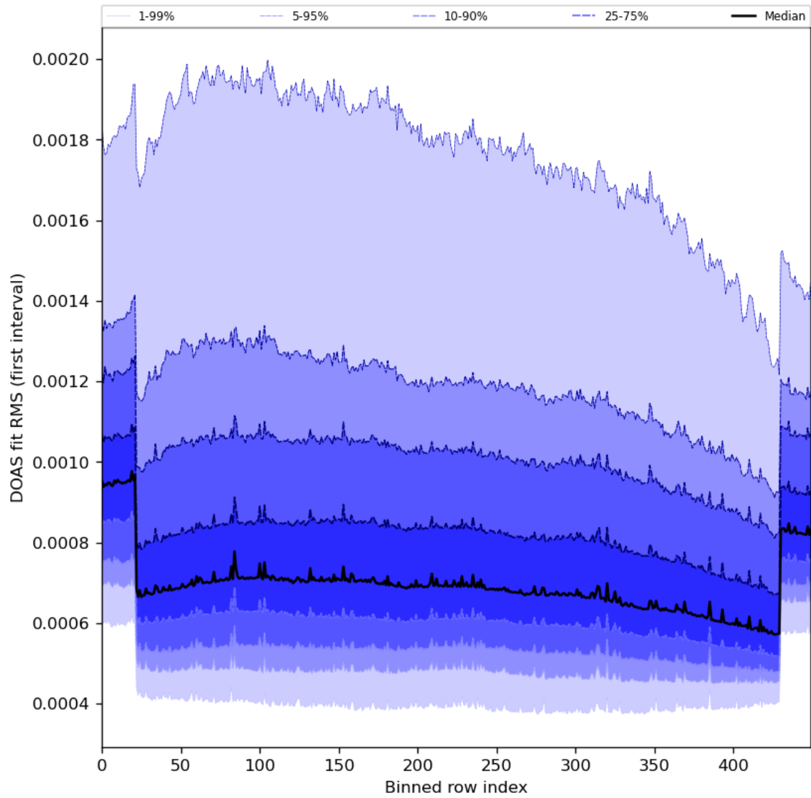
Figure 60: Along track statistics of “DOAS fit RMS (first interval)” for 2024-03-05 to 2024-03-07
