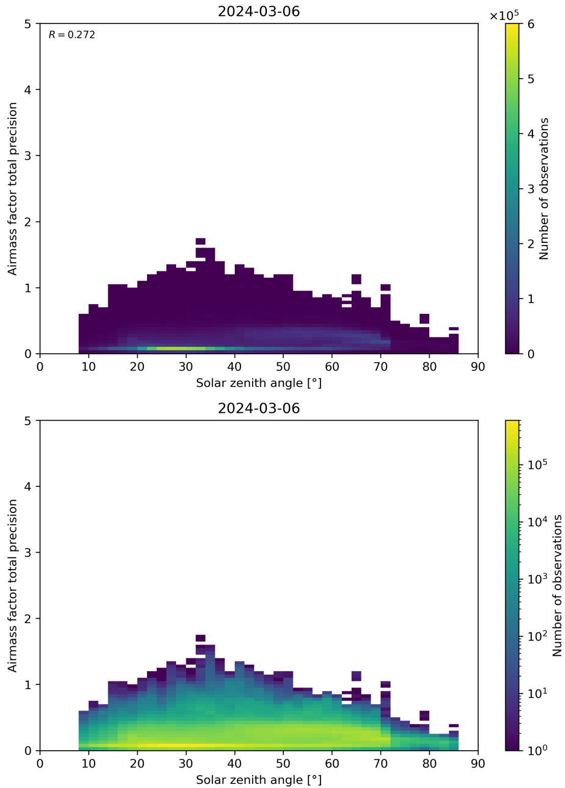
Figure 176: Scatter density plot of “Solar zenith angle” against “Airmass factor total precision” for 2024-03-05 to 2024-03-07.
