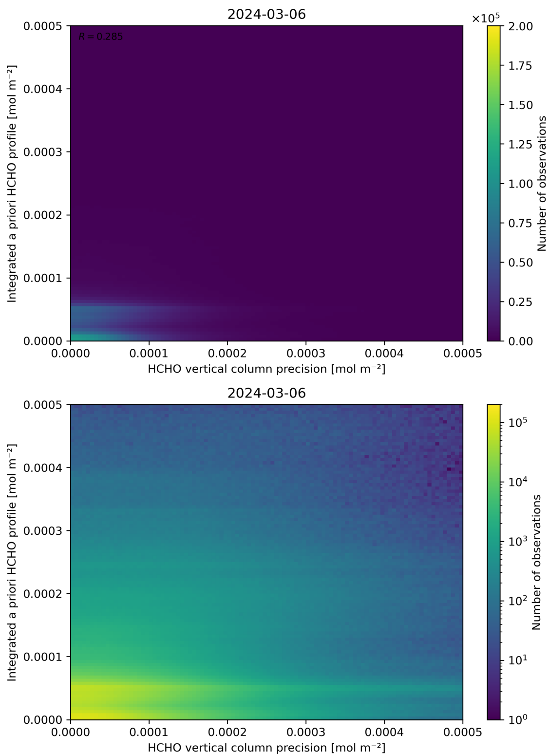
Figure 147: Scatter density plot of “HCHO vertical column precision” against “Integrated a priori HCHO profile” for 2024-03-05 to 2024-03-07.
