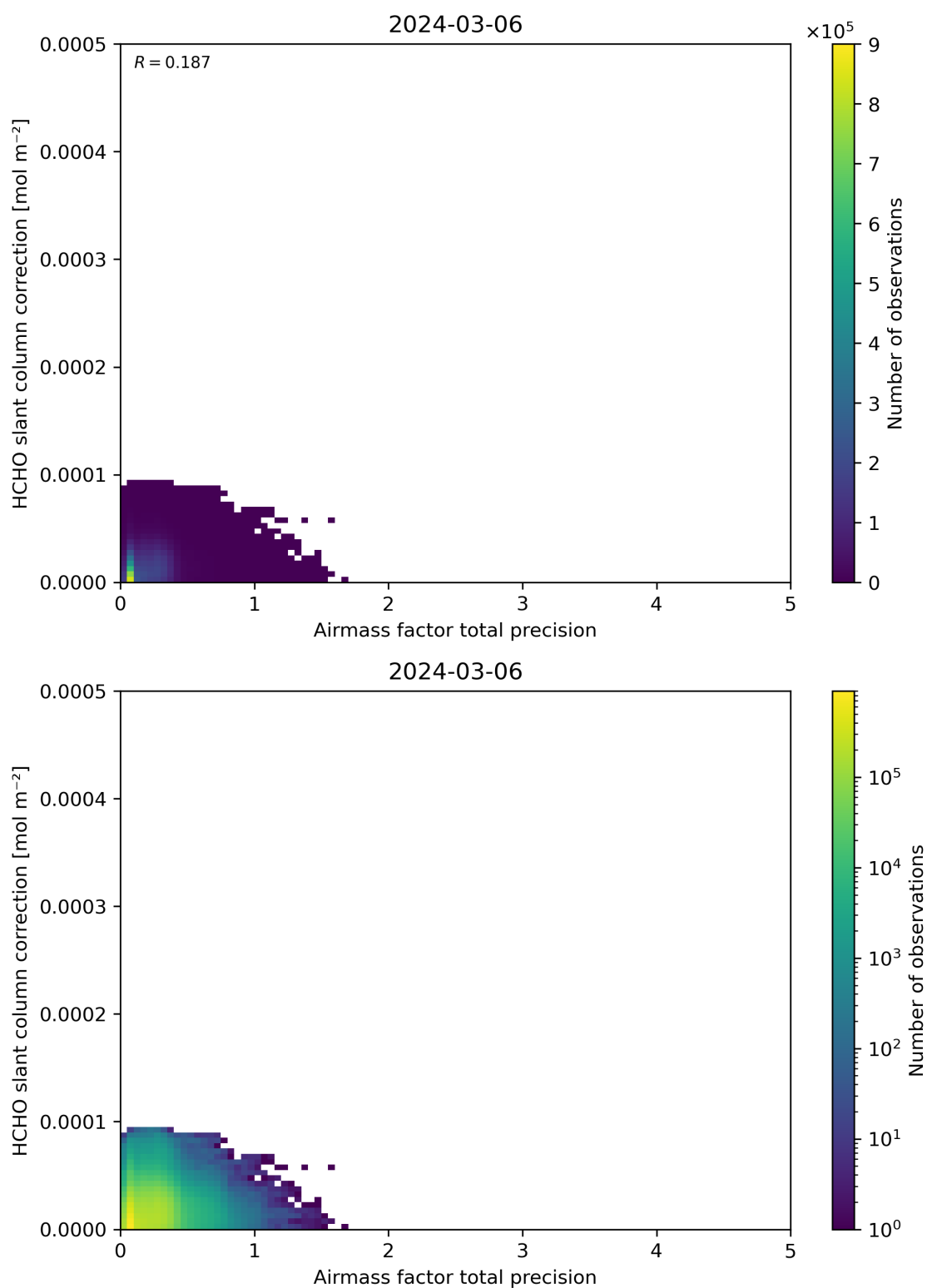
Figure 110: Scatter density plot of “Airmass factor total precision” against “HCHO slant column correction” for 2024-03-05 to 2024-03-07.
