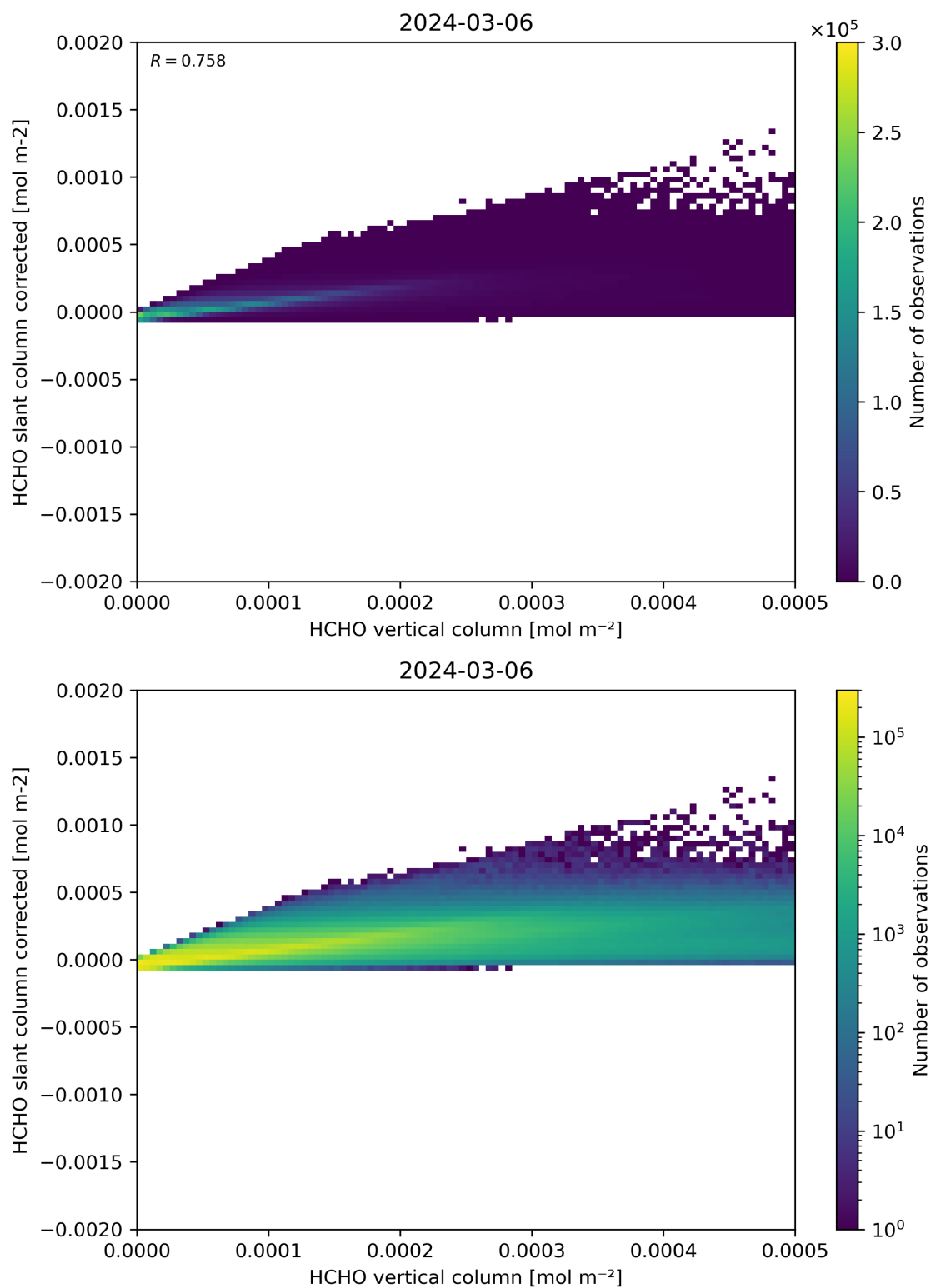
Figure 127: Scatter density plot of “HCHO vertical column” against “HCHO slant column corrected” for 2024-03-05 to 2024-03-07.
