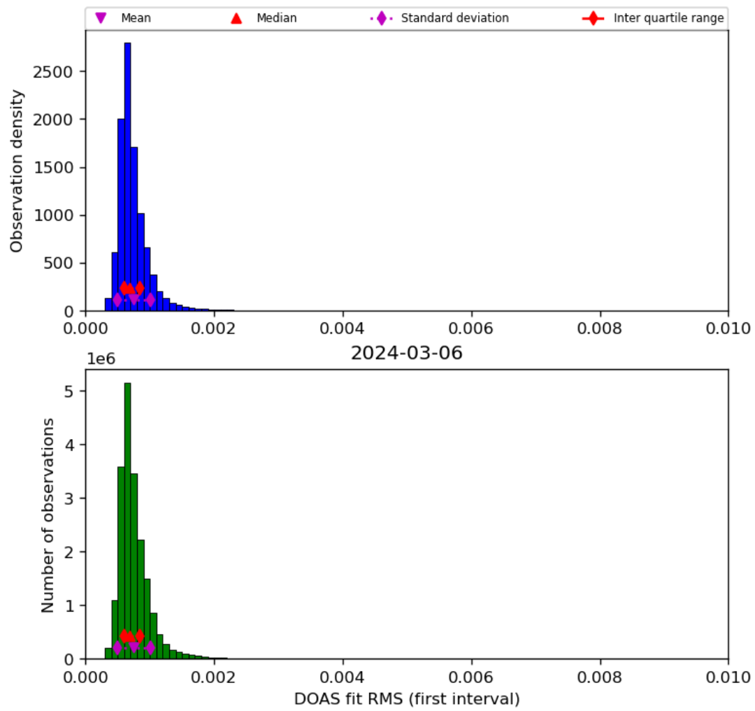
Figure 46: Histogram of “DOAS fit RMS (first interval)” for 2024-03-05 to 2024-03-07
