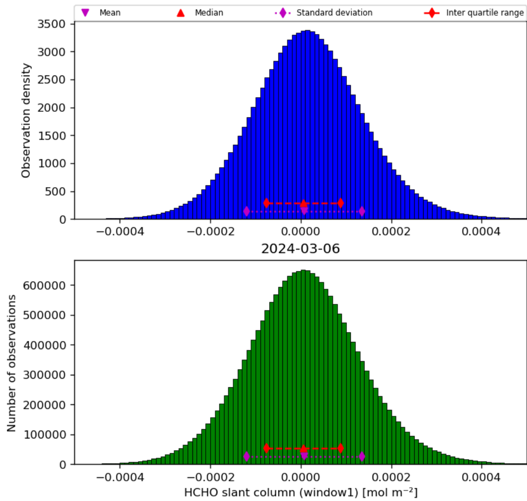
Figure 38: Histogram of “HCHO slant column (window1)” for 2024-03-05 to 2024-03-07
