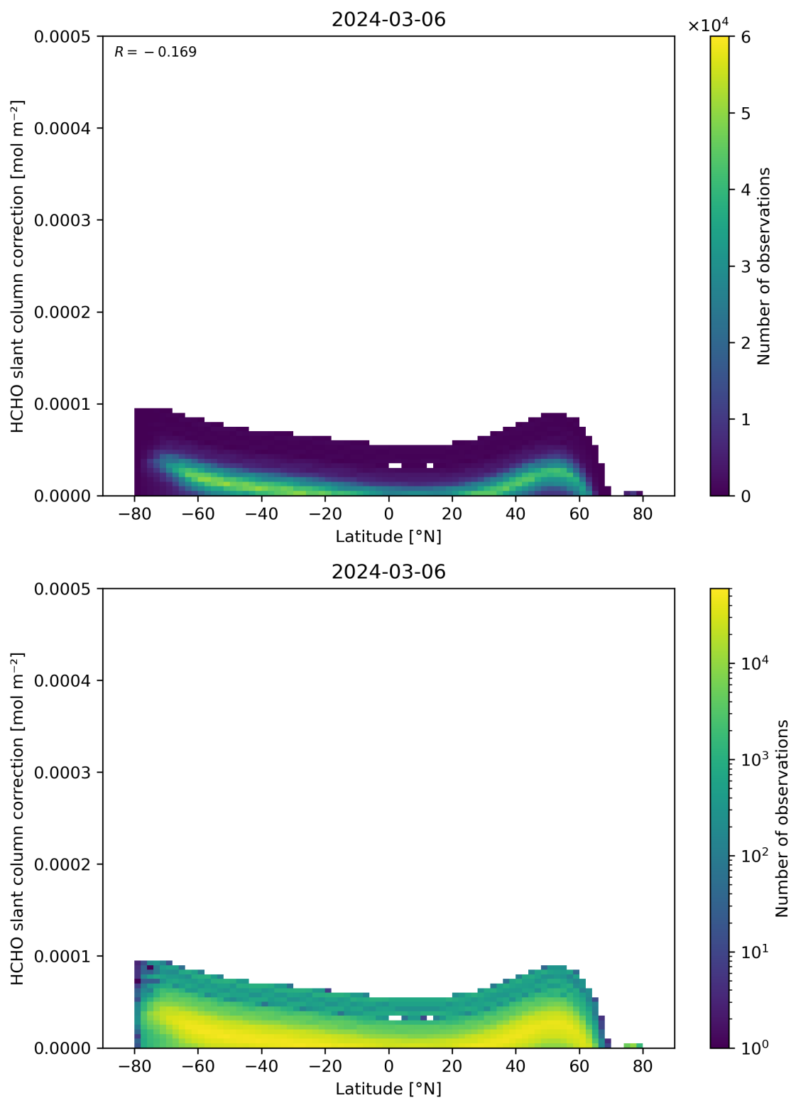
Figure 158: Scatter density plot of “Latitude” against “HCHO slant column correction” for 2024-03-05 to 2024-03-07.
