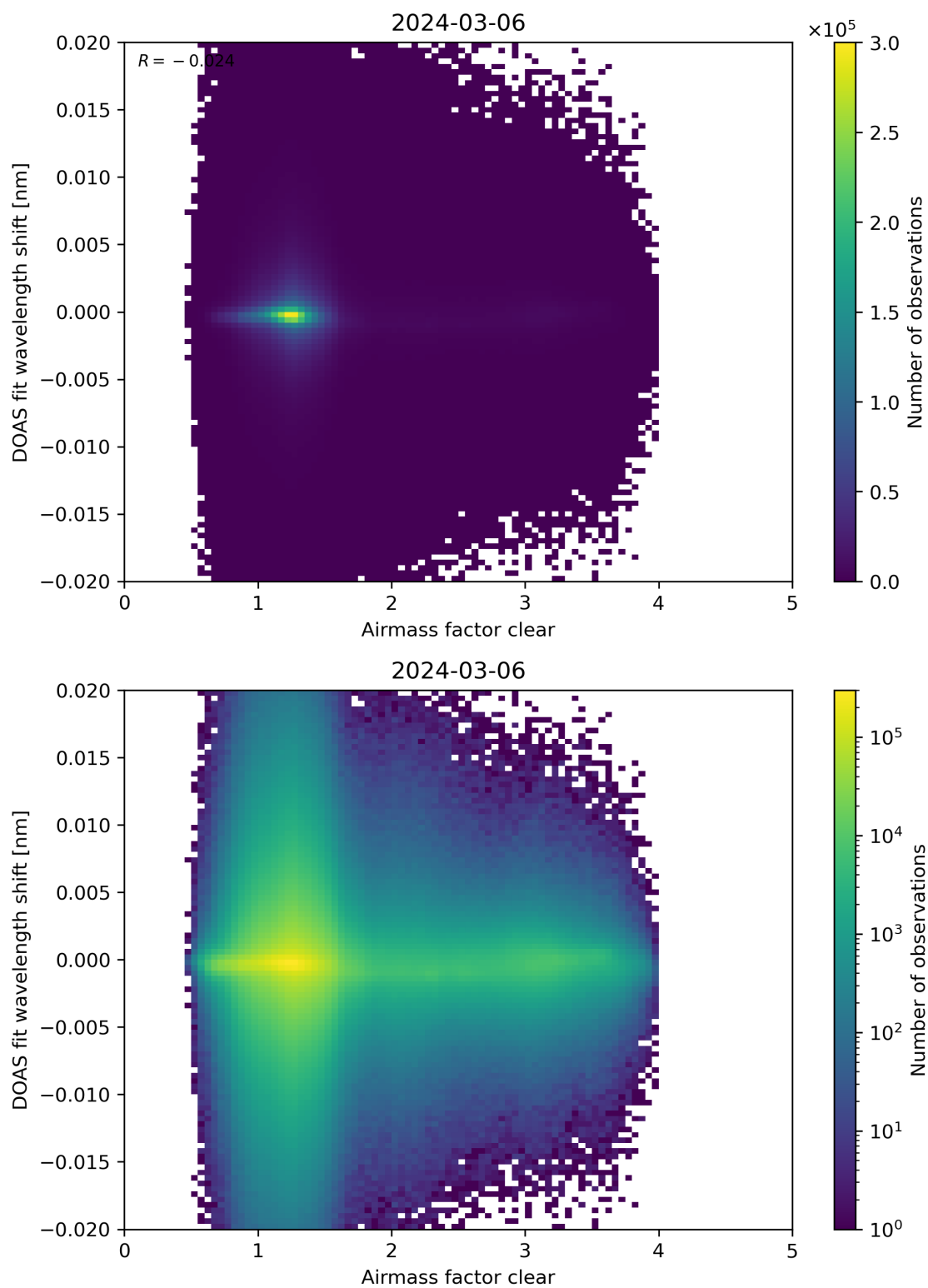
Figure 72: Scatter density plot of “Airmass factor clear” against “DOAS fit wavelength shift” for 2024-03-05 to 2024-03-07.
