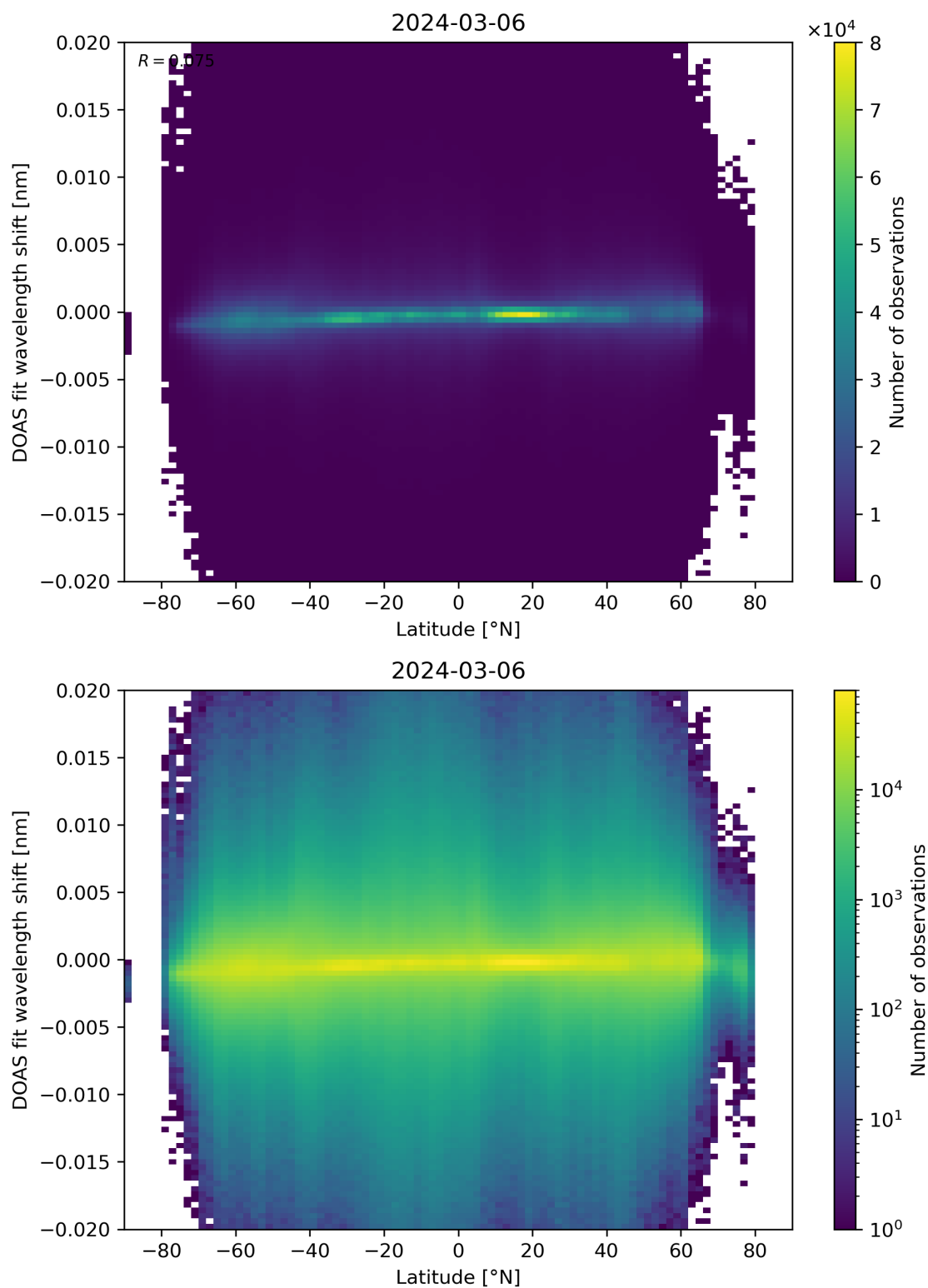
Figure 154: Scatter density plot of “Latitude” against “DOAS fit wavelength shift” for 2024-03-05 to 2024-03-07.
