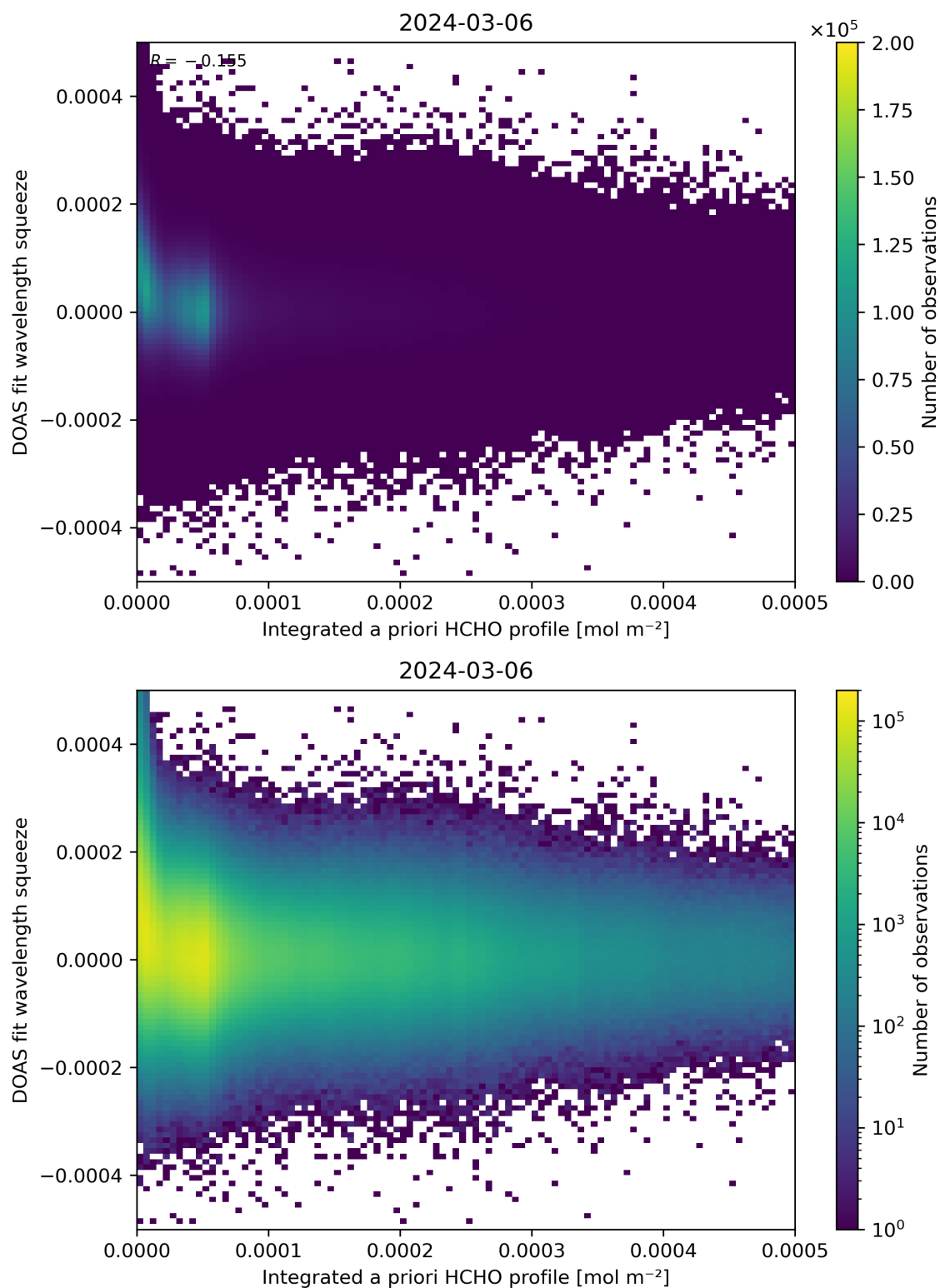
Figure 150: Scatter density plot of “Integrated a priori HCHO profile” against “DOAS fit wavelength squeeze” for 2024-03-05 to 2024-03-07.
