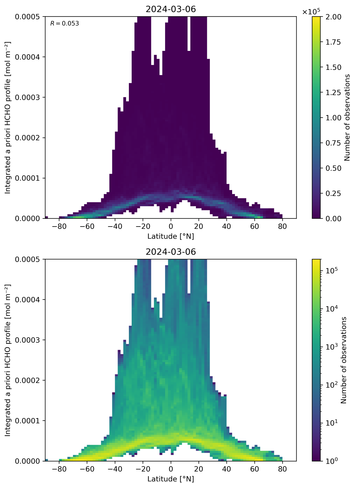
Figure 166: Scatter density plot of “Latitude” against “Integrated a priori HCHO profile” for 2024-03-05 to 2024-03-07.
