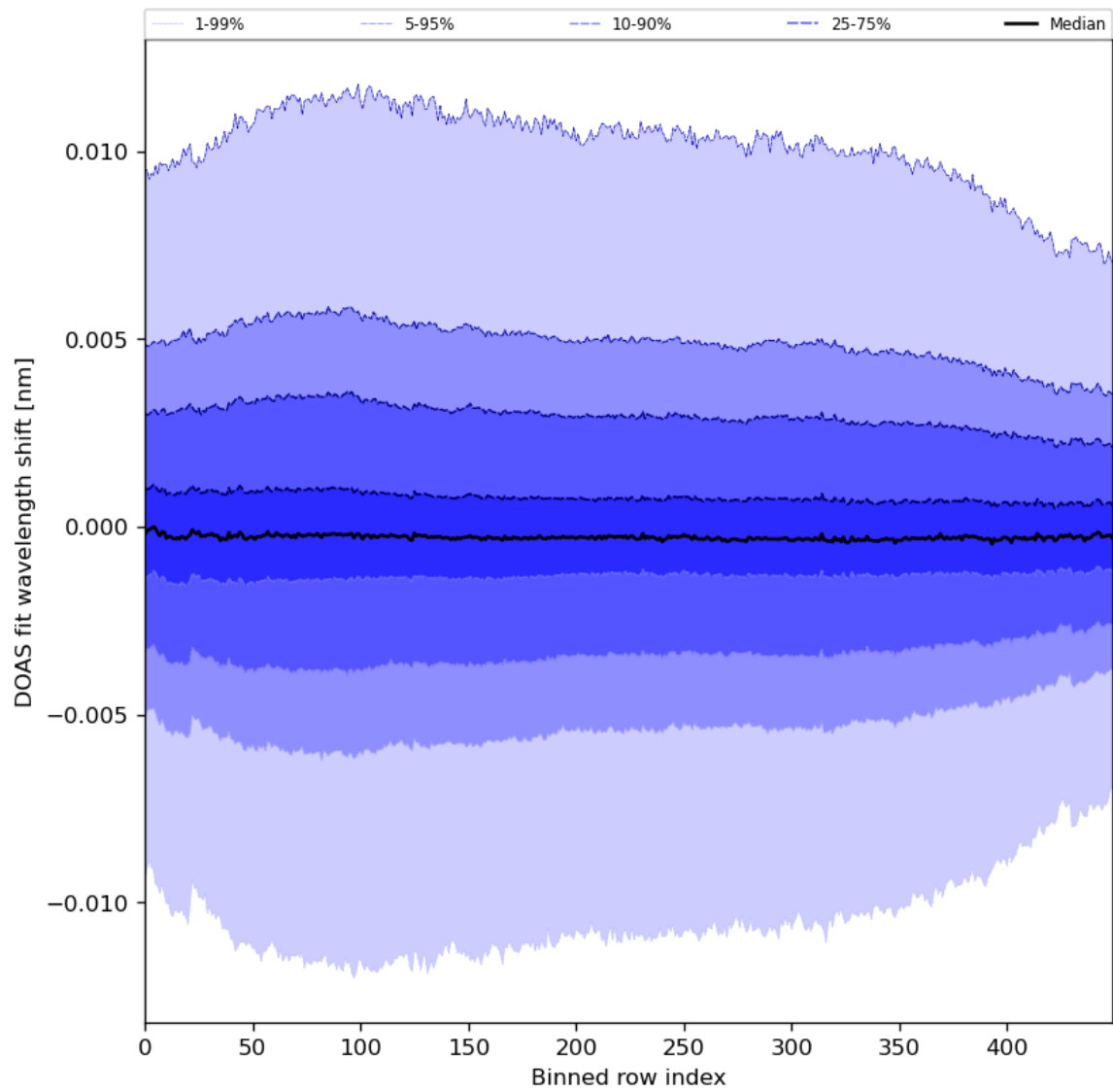
Figure 58: Along track statistics of “DOAS fit wavelength shift” for 2024-03-05 to 2024-03-07
