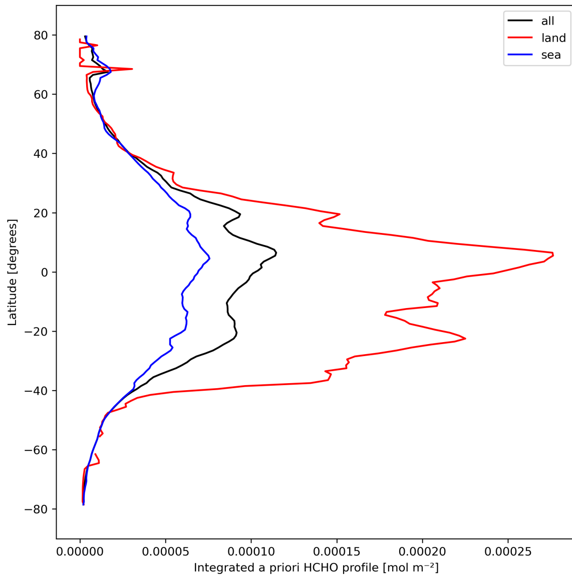
Figure 29: Zonal average of “Integrated a priori HCHO profile” for 2024-03-05 to 2024-03-07.
