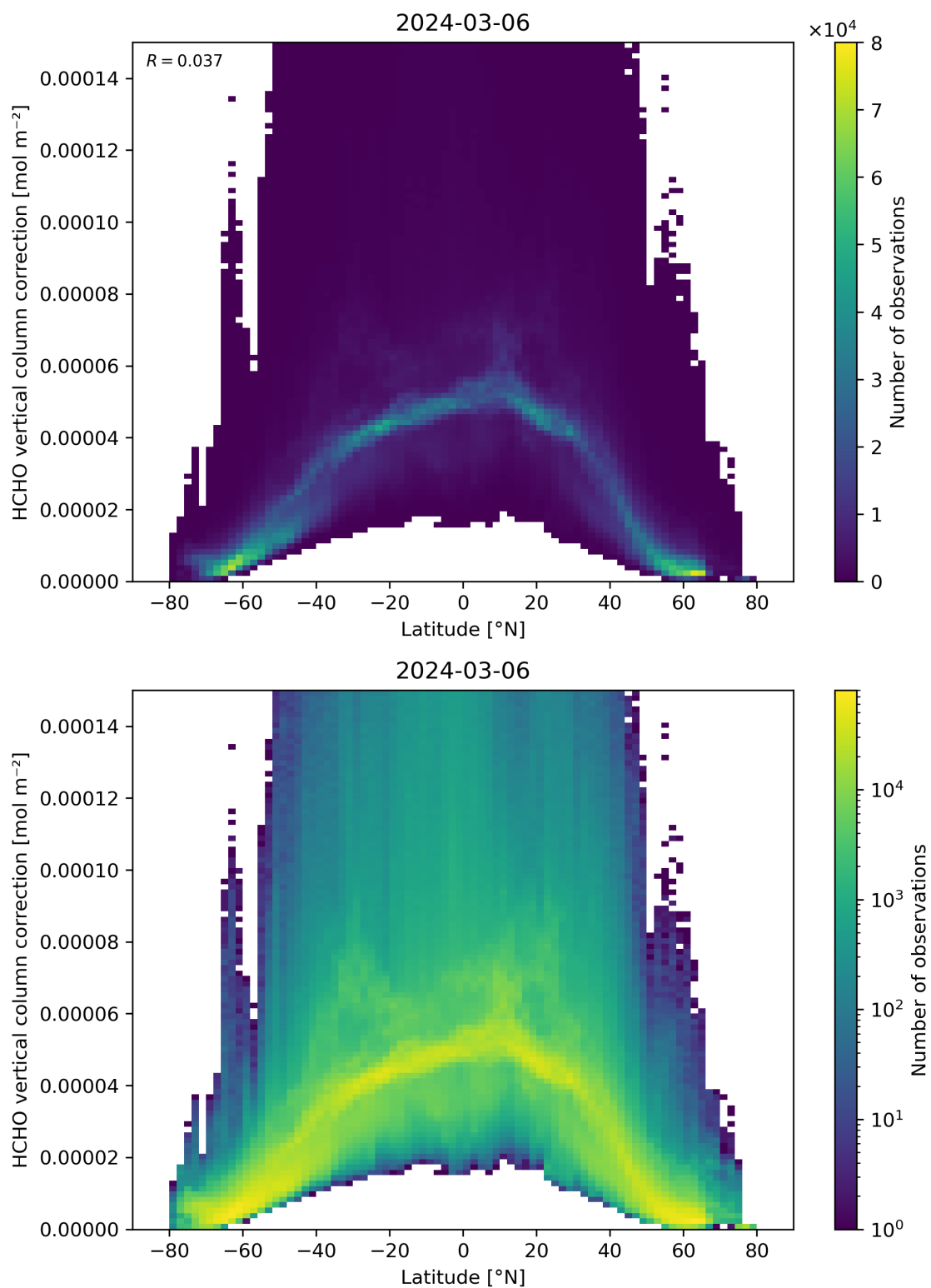
Figure 164: Scatter density plot of “Latitude” against “HCHO vertical column correction” for 2024-03-05 to 2024-03-07.
