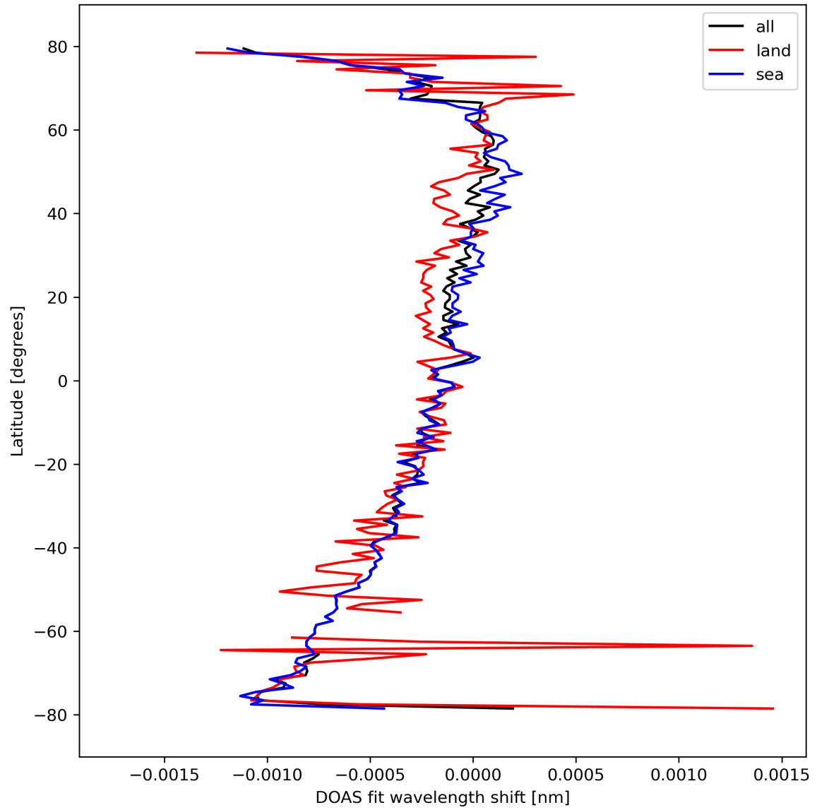
Figure 30: Zonal average of "DOAS fit wavelength shift" for 2024-03-05 to 2024-03-07.
