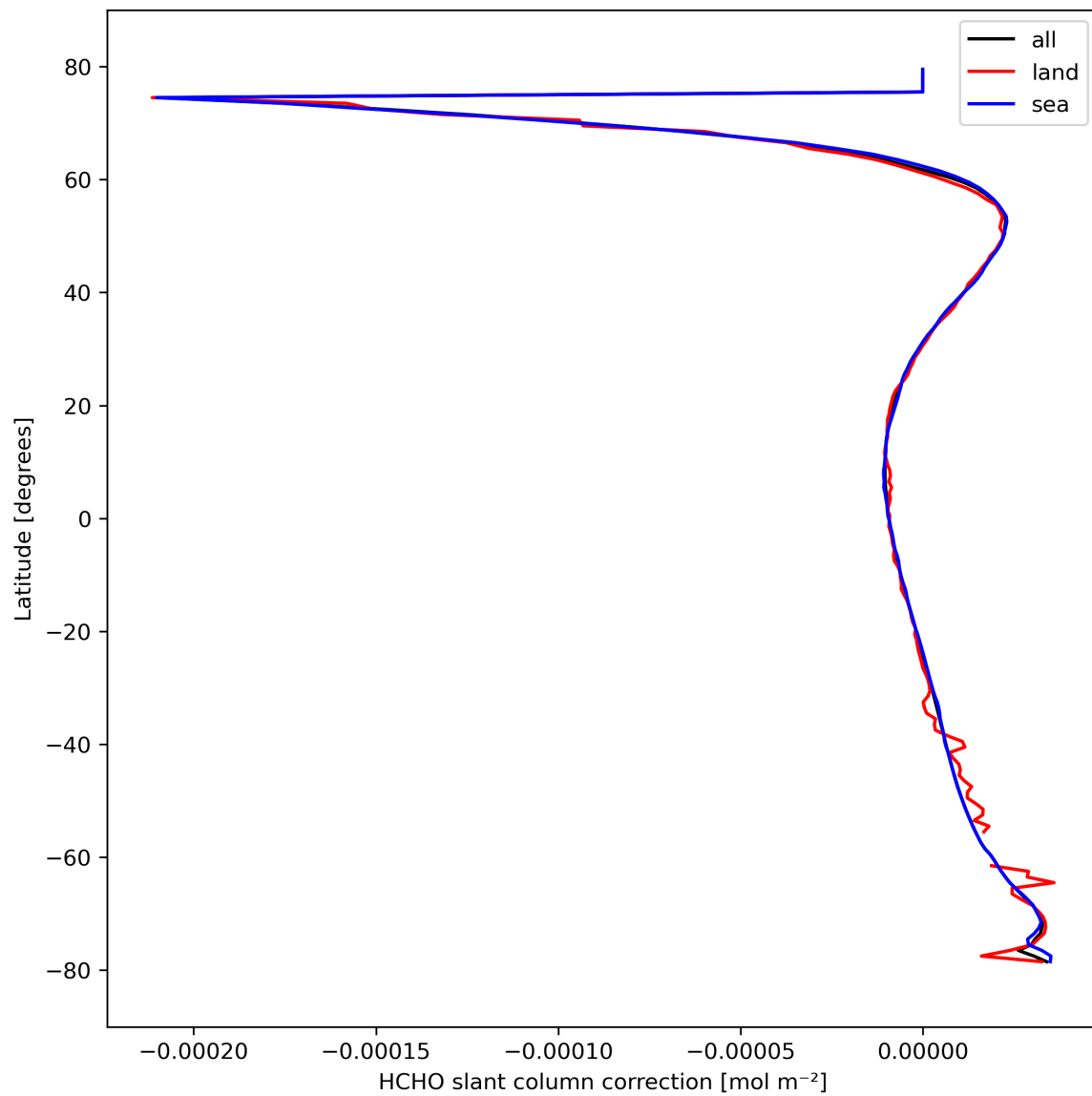
Figure 33: Zonal average of “HCHO slant column correction” for 2024-03-05 to 2024-03-07.
