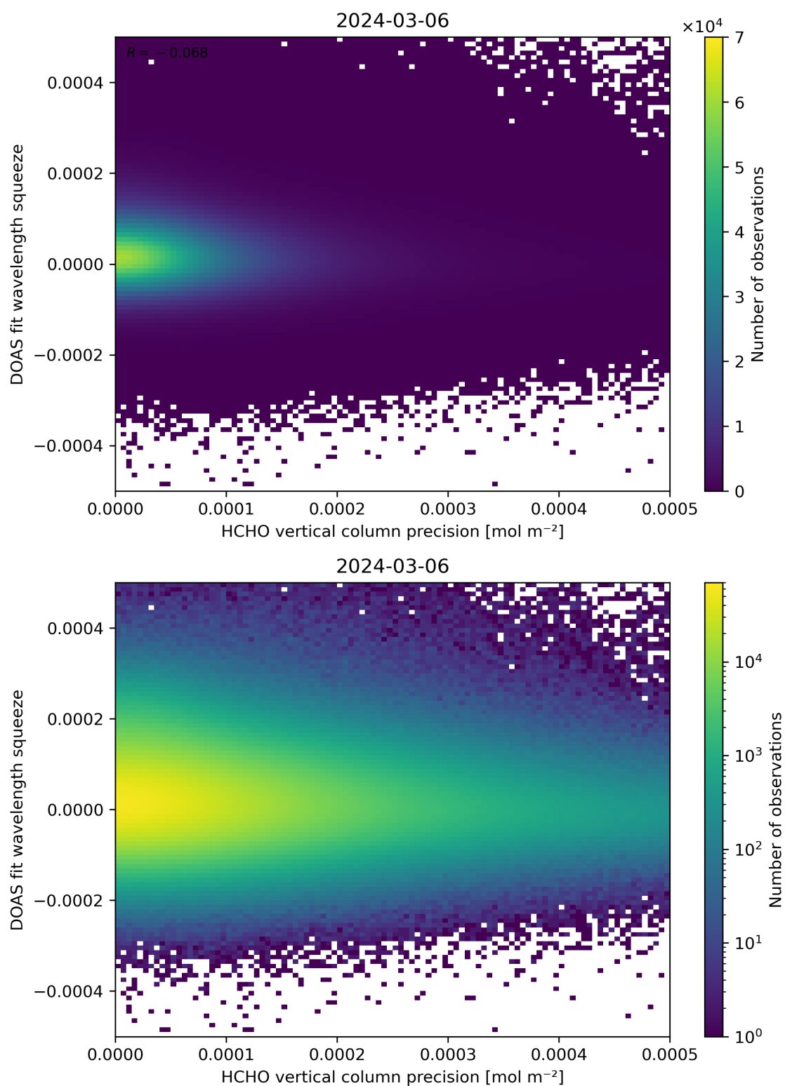
Figure 138: Scatter density plot of “HCHO vertical column precision” against “DOAS fit wavelength squeeze” for 2024-03-05 to 2024-03-07.
