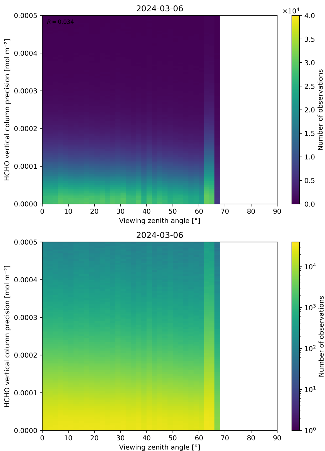
Figure 194: Scatter density plot of “Viewing zenith angle” against “HCHO vertical column precision” for 2024-03-05 to 2024-03-07.
