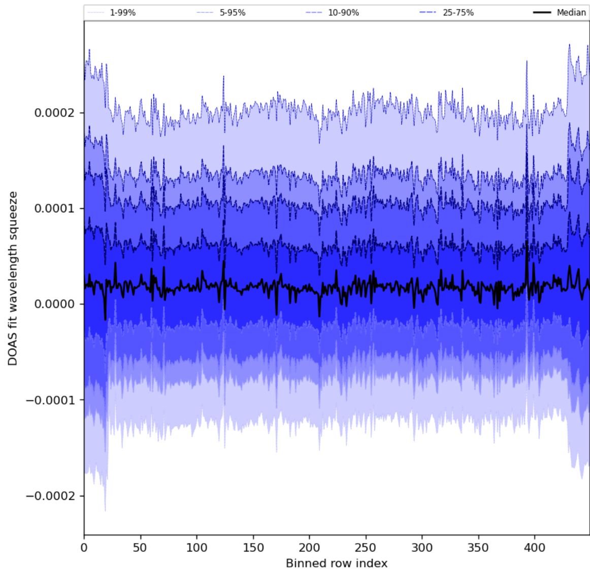
Figure 59: Along track statistics of “DOAS fit wavelength squeeze” for 2024-03-05 to 2024-03-07
