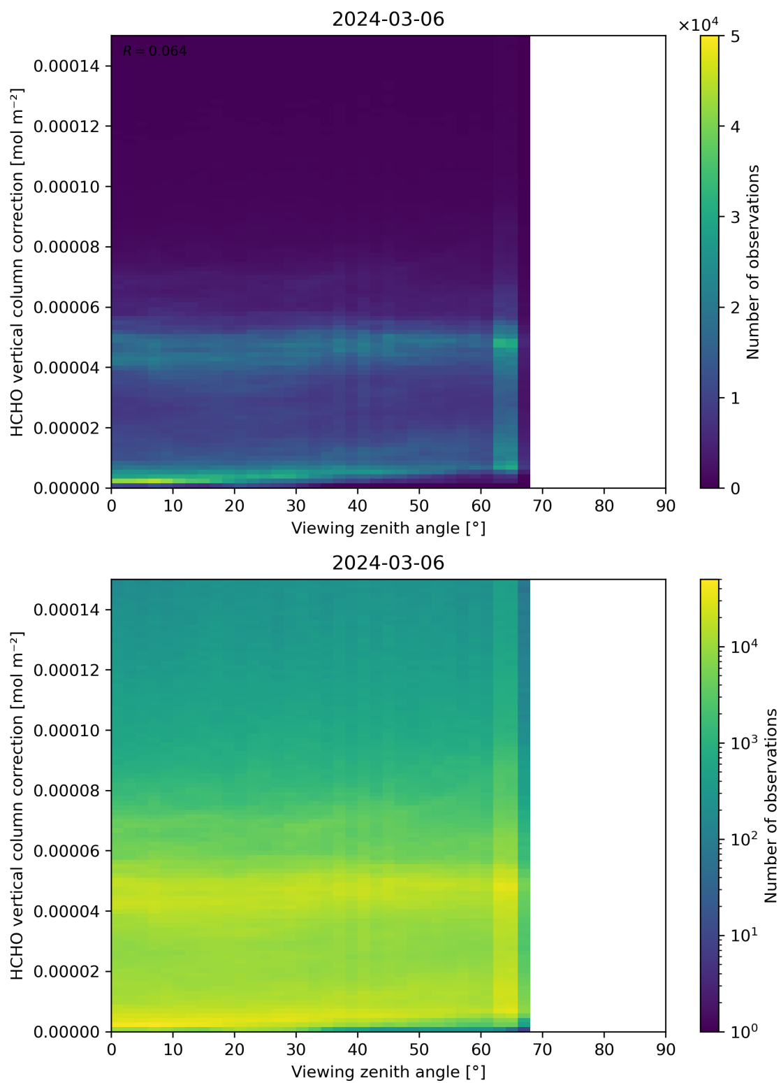
Figure 193: Scatter density plot of “Viewing zenith angle” against “HCHO vertical column correction” for 2024-03-05 to 2024-03-07.
