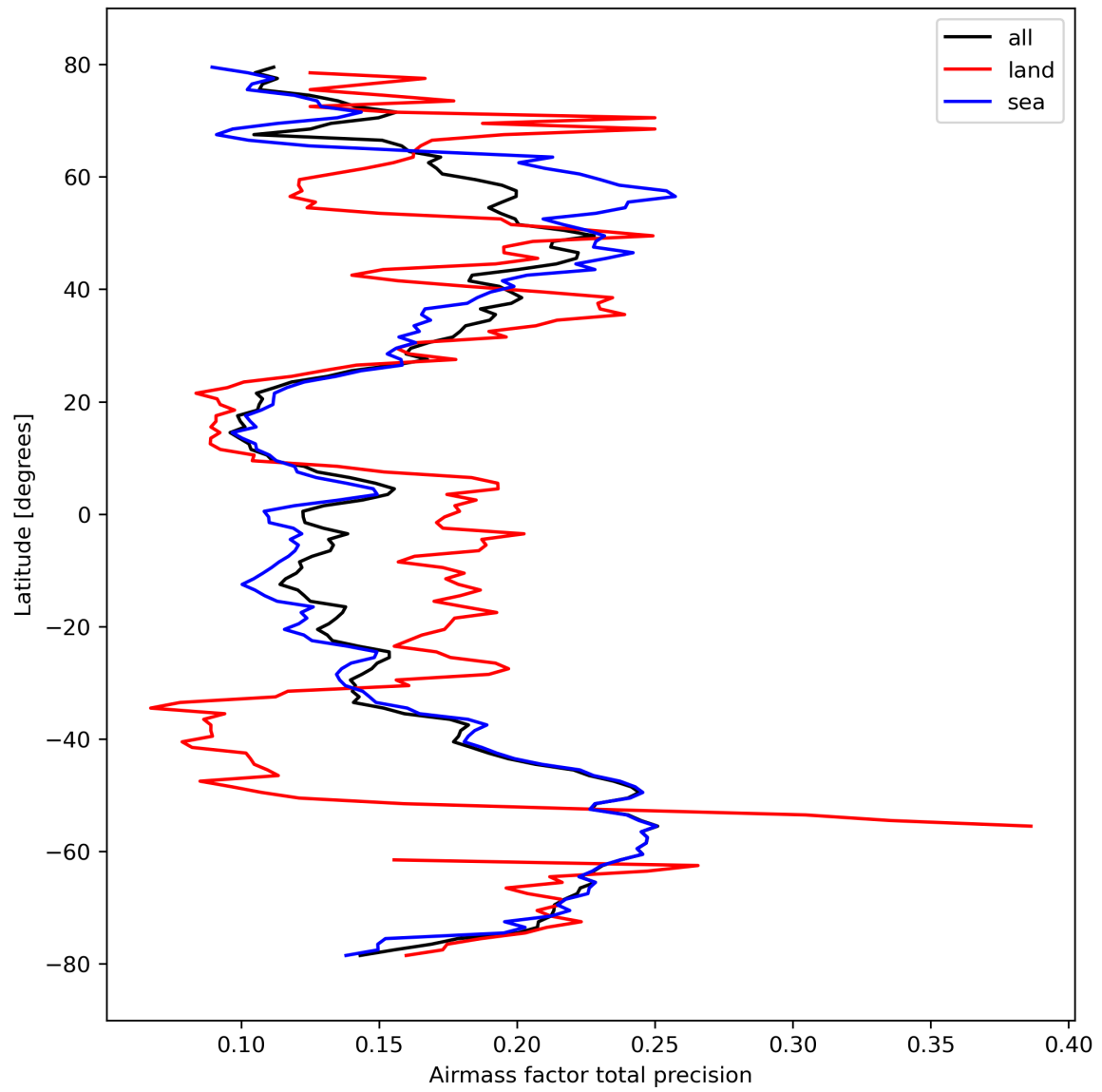
Figure 27: Zonal average of “Airmass factor total precision” for 2024-03-05 to 2024-03-07.
