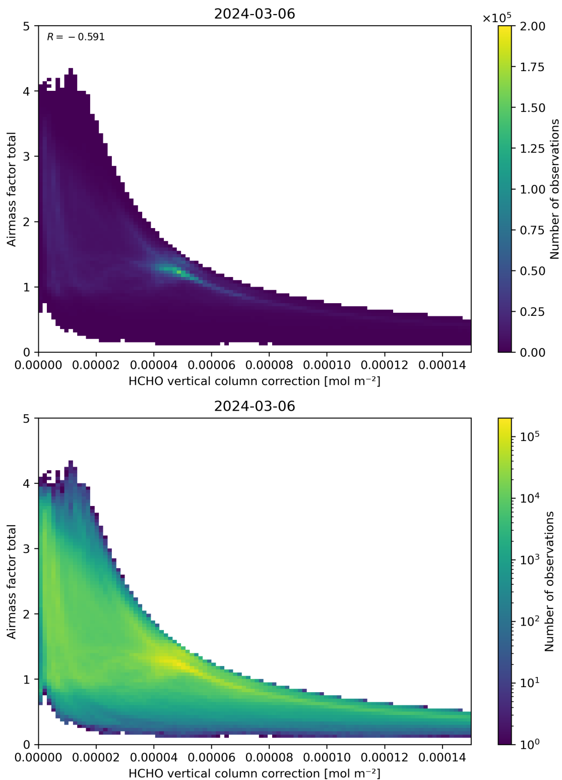
Figure 120: Scatter density plot of “HCHO vertical column correction” against “Airmass factor total” for 2024-03-05 to 2024-03-07.
