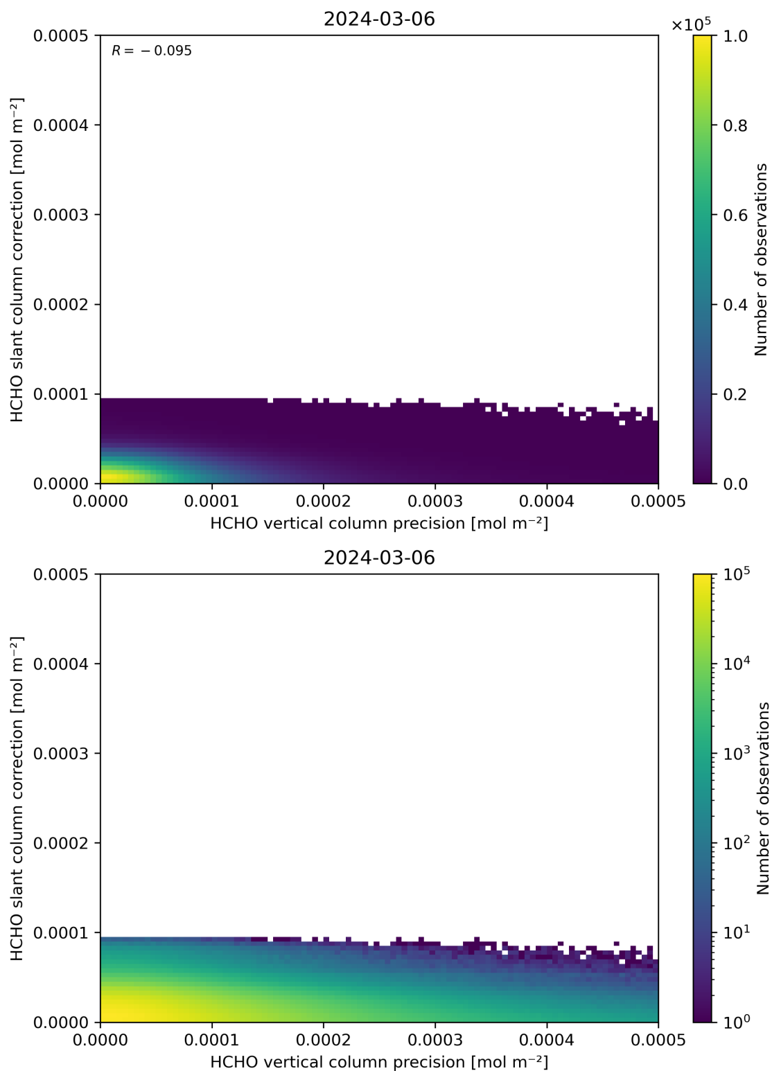
Figure 141: Scatter density plot of “HCHO vertical column precision” against “HCHO slant column correction” for 2024-03-05 to 2024-03-07.
