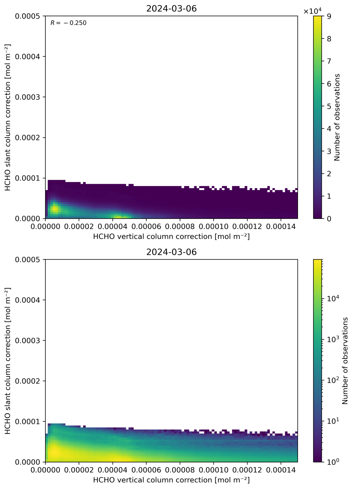
Figure 117: Scatter density plot of “HCHO vertical column correction” against “HCHO slant column correction” for 2024-03-05 to 2024-03-07.
