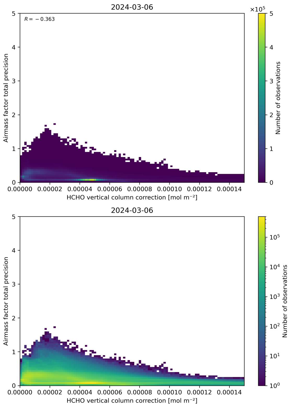
Figure 121: Scatter density plot of “HCHO vertical column correction” against “Airmass factor total precision” for 2024-03-05 to 2024-03-07.
