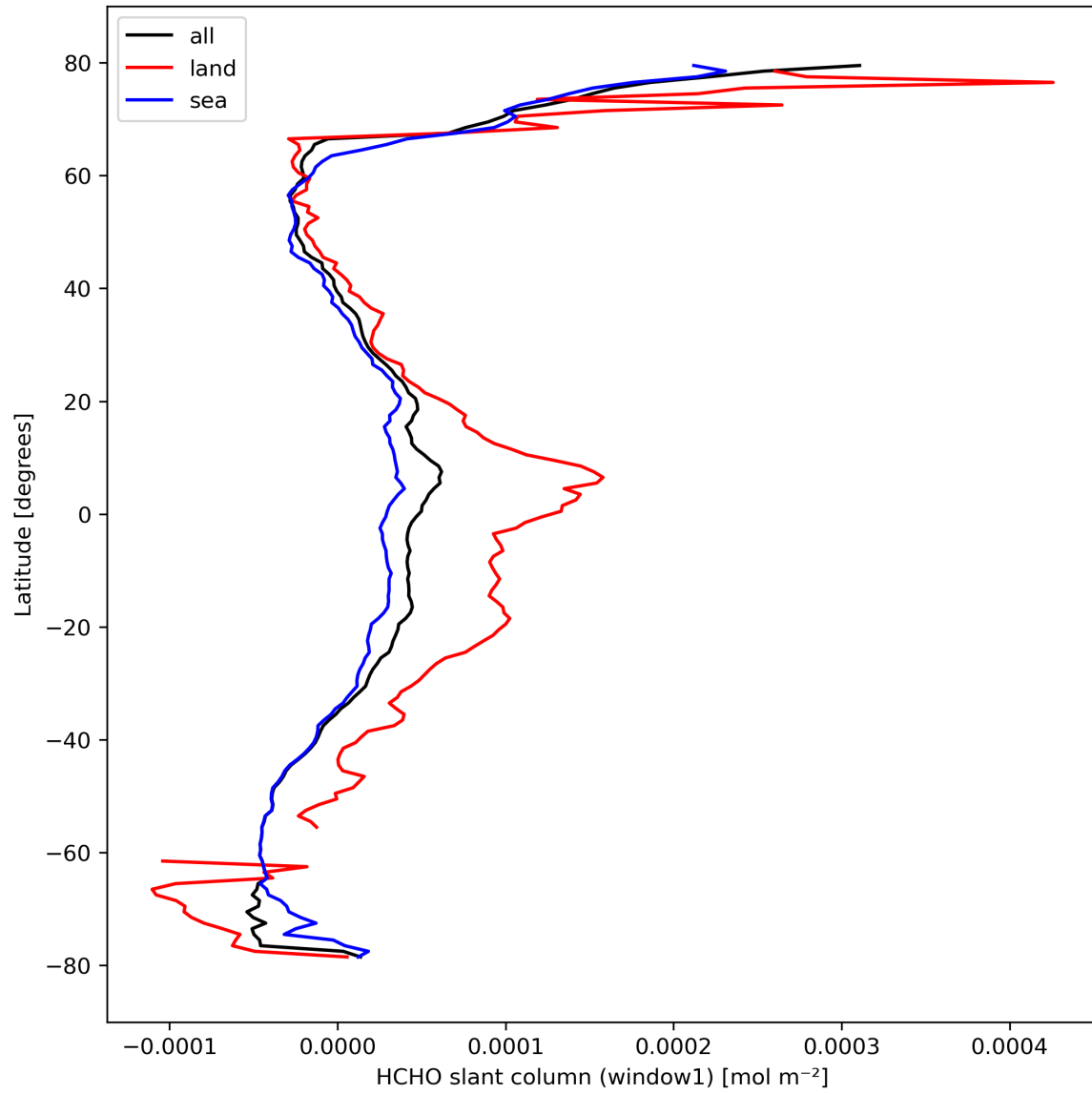
Figure 24: Zonal average of “HCHO slant column (window1)” for 2024-03-05 to 2024-03-07.
