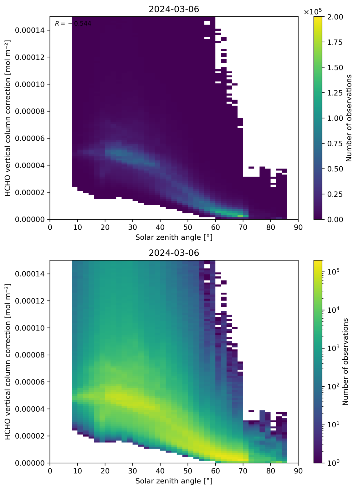
Figure 178: Scatter density plot of “Solar zenith angle” against “HCHO vertical column correction” for 2024-03-05 to 2024-03-07.
