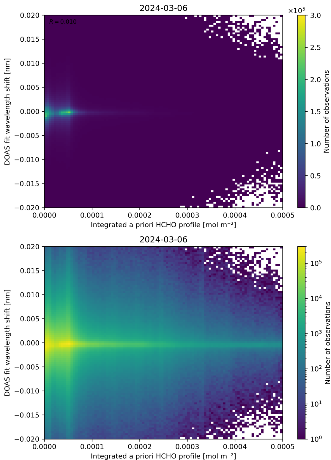
Figure 149: Scatter density plot of “Integrated a priori HCHO profile” against “DOAS fit wavelength shift” for 2024-03-05 to 2024-03-07.
