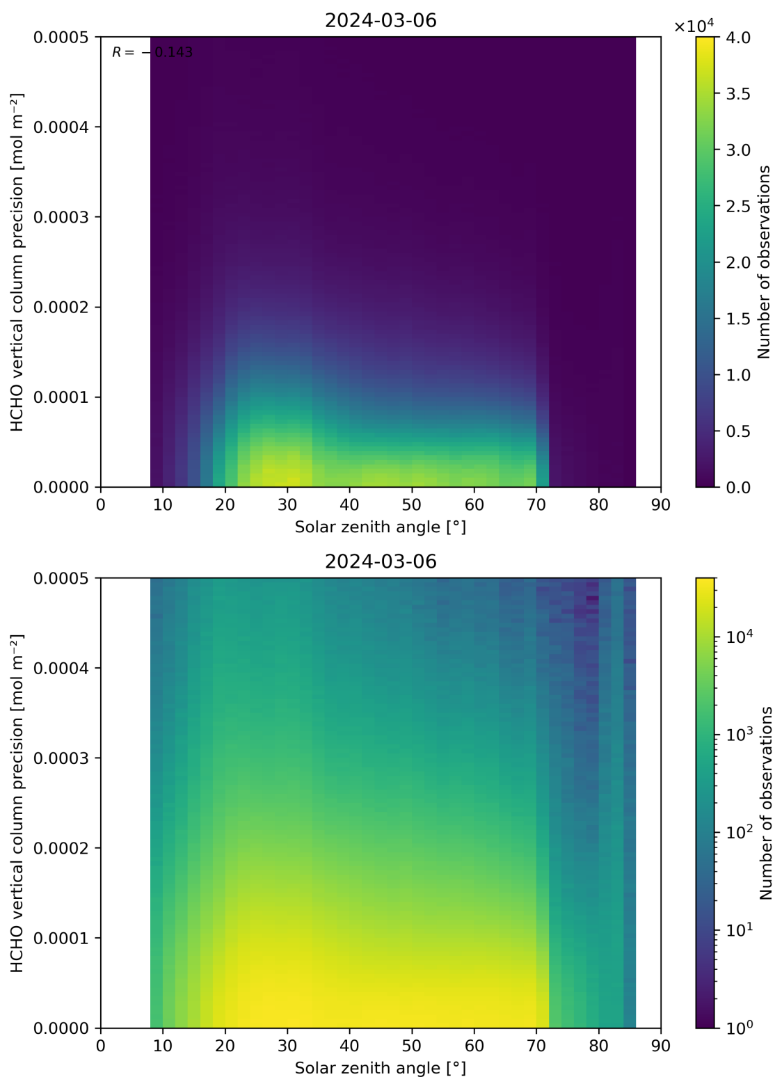
Figure 179: Scatter density plot of “Solar zenith angle” against “HCHO vertical column precision” for 2024-03-05 to 2024-03-07.
