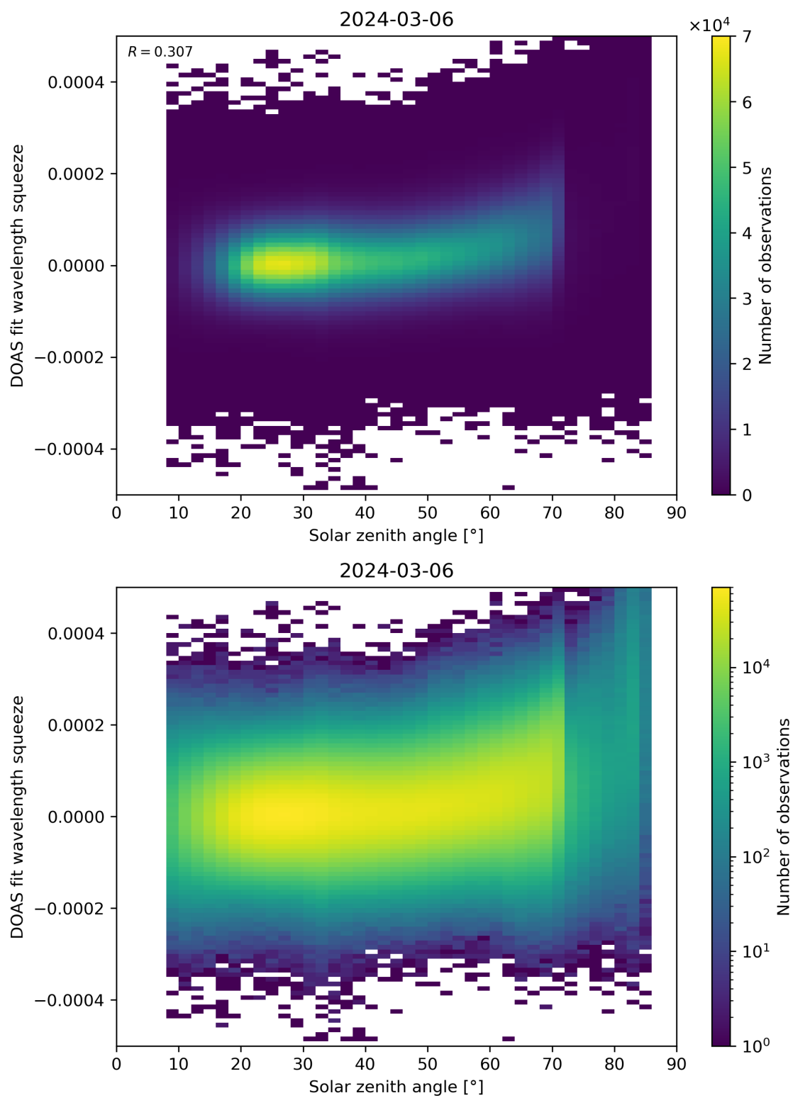
Figure 169: Scatter density plot of “Solar zenith angle” against “DOAS fit wavelength squeeze” for 2024-03-05 to 2024-03-07.
