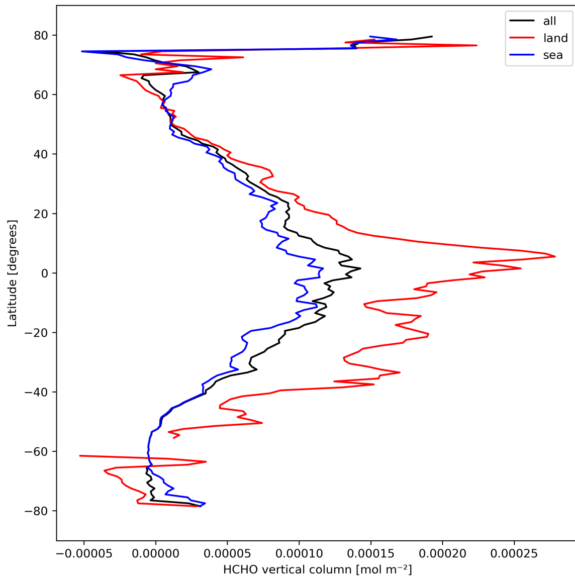
Figure 21: Zonal average of “HCHO vertical column” for 2024-03-05 to 2024-03-07.
