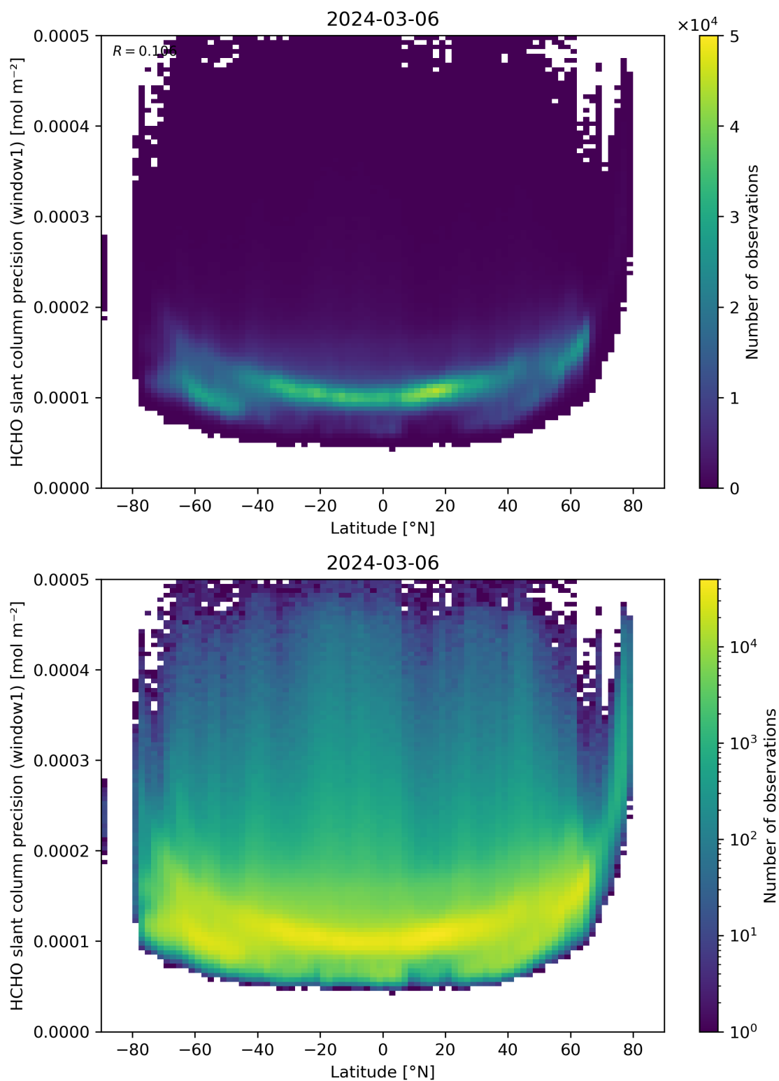
Figure 160: Scatter density plot of “Latitude” against “HCHO slant column precision (window1)” for 2024-03-05 to 2024-03-07.
