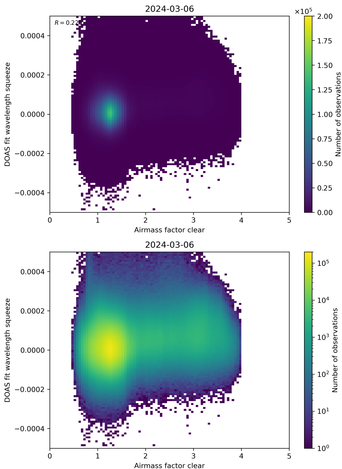
Figure 73: Scatter density plot of “Airmass factor clear” against “DOAS fit wavelength squeeze” for 2024-03-05 to 2024-03-07.
