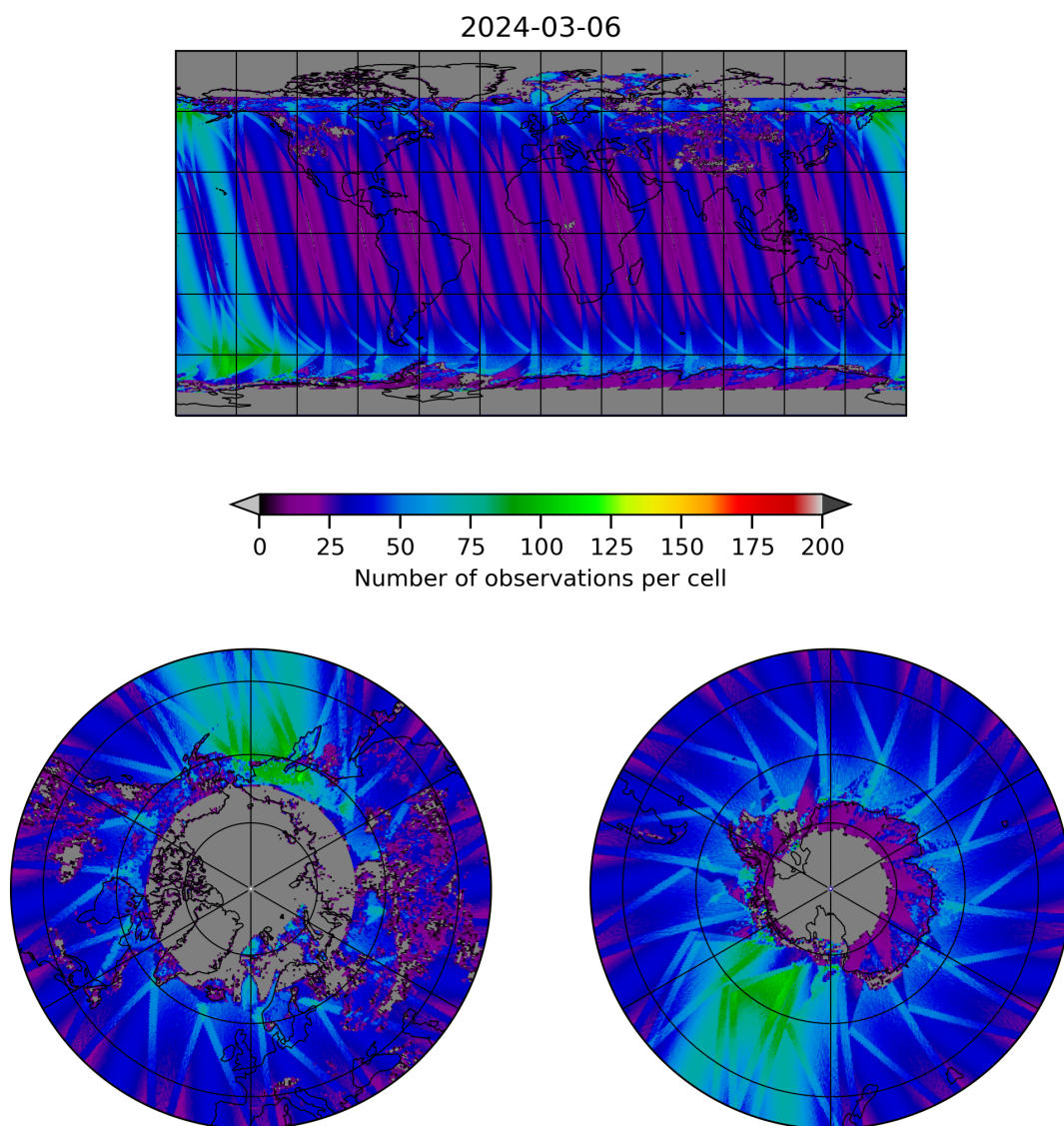
Figure 19: Map of the number of observations for 2024-03-05 to 2024-03-07
