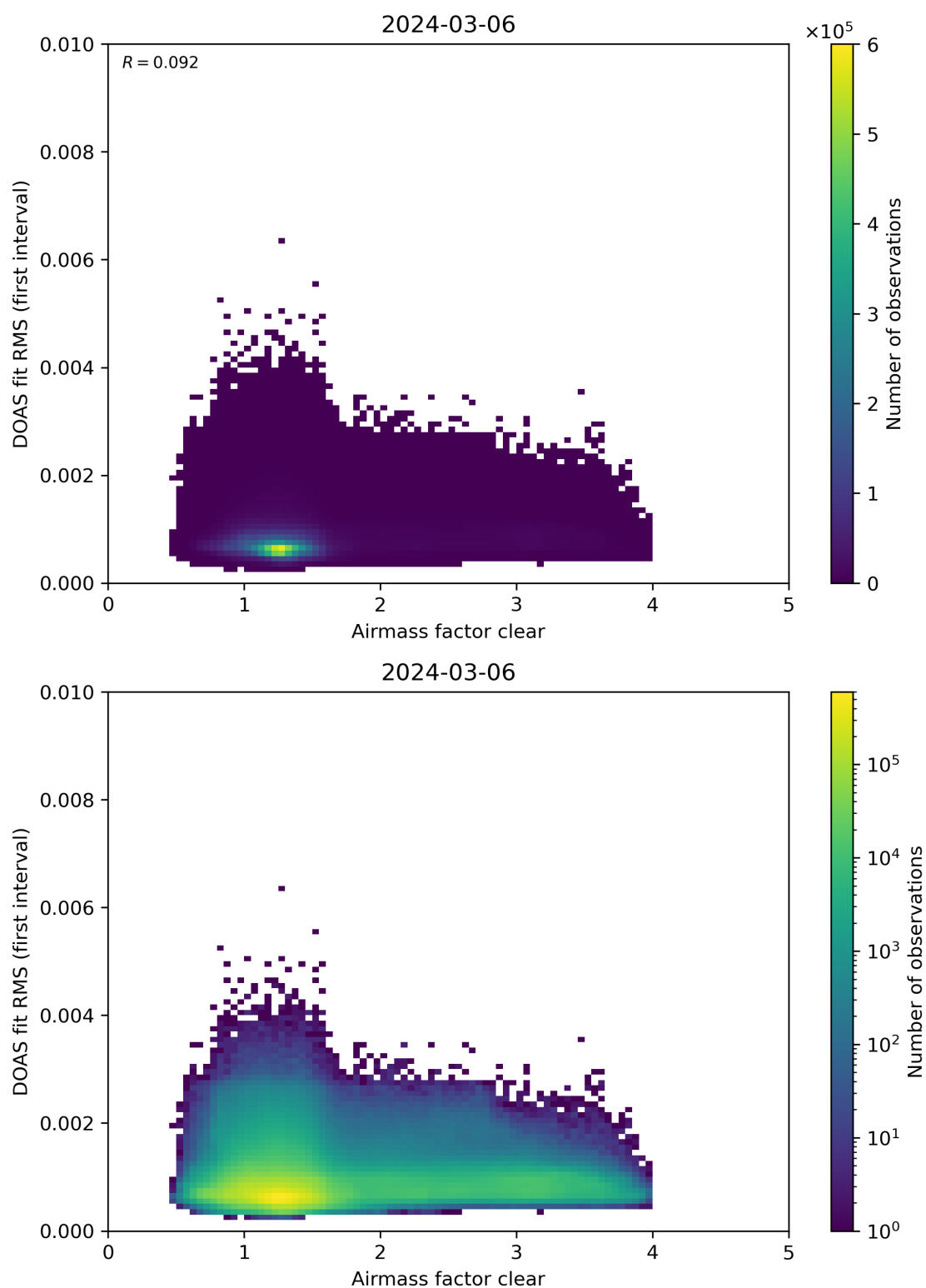
Figure 71: Scatter density plot of “Airmass factor clear” against “DOAS fit RMS (first interval)” for 2024-03-05 to 2024-03-07.
