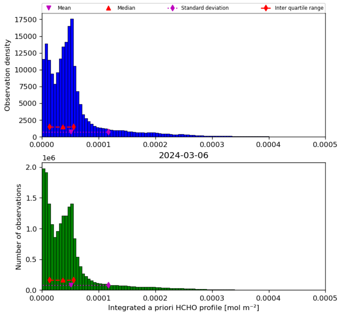
Figure 43: Histogram of “Integrated a priori HCHO profile” for 2024-03-05 to 2024-03-07
