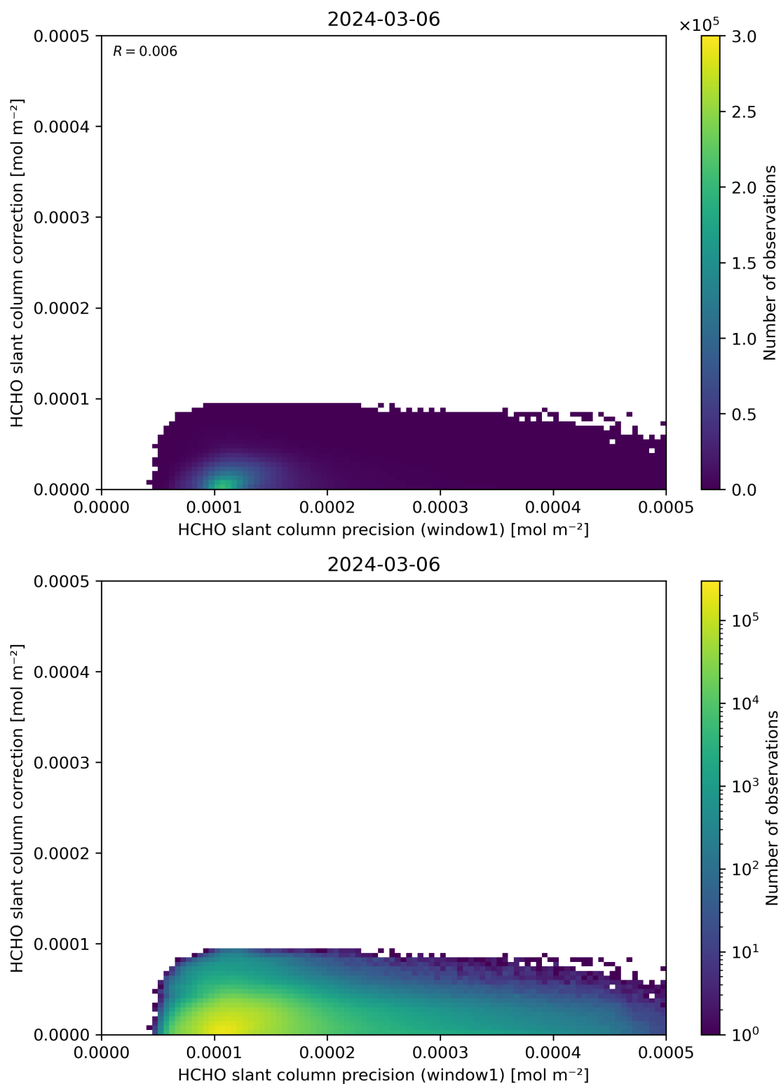
Figure 93: Scatter density plot of “HCHO slant column precision (window1)” against “HCHO slant column correction” for 2024-03-05 to 2024-03-07.
