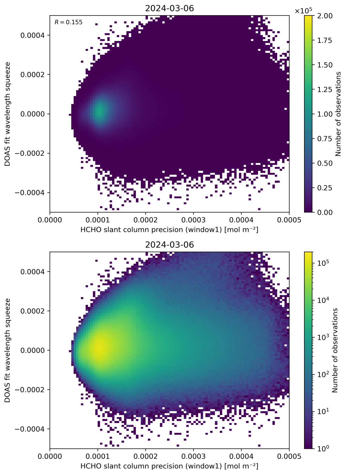
Figure 90: Scatter density plot of “HCHO slant column precision (window1)” against “DOAS fit wavelength squeeze” for 2024-03-05 to 2024-03-07.
