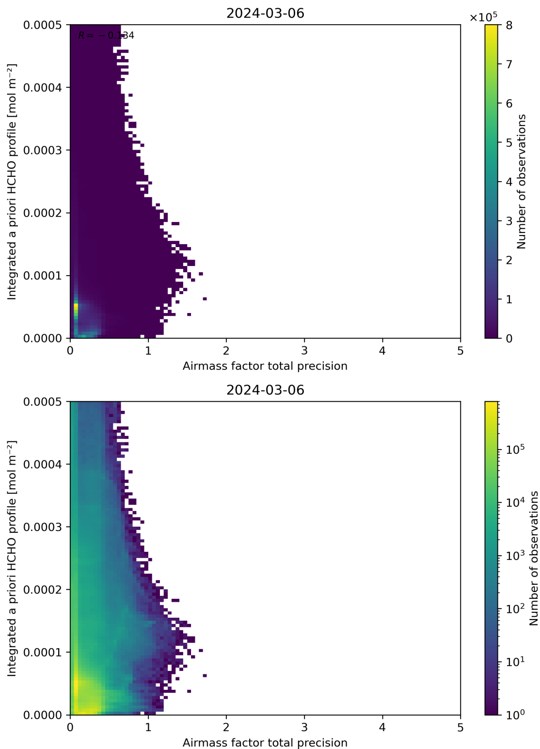
Figure 111: Scatter density plot of “Airmass factor total precision” against “Integrated a priori HCHO profile” for 2024-03-05 to 2024-03-07.
