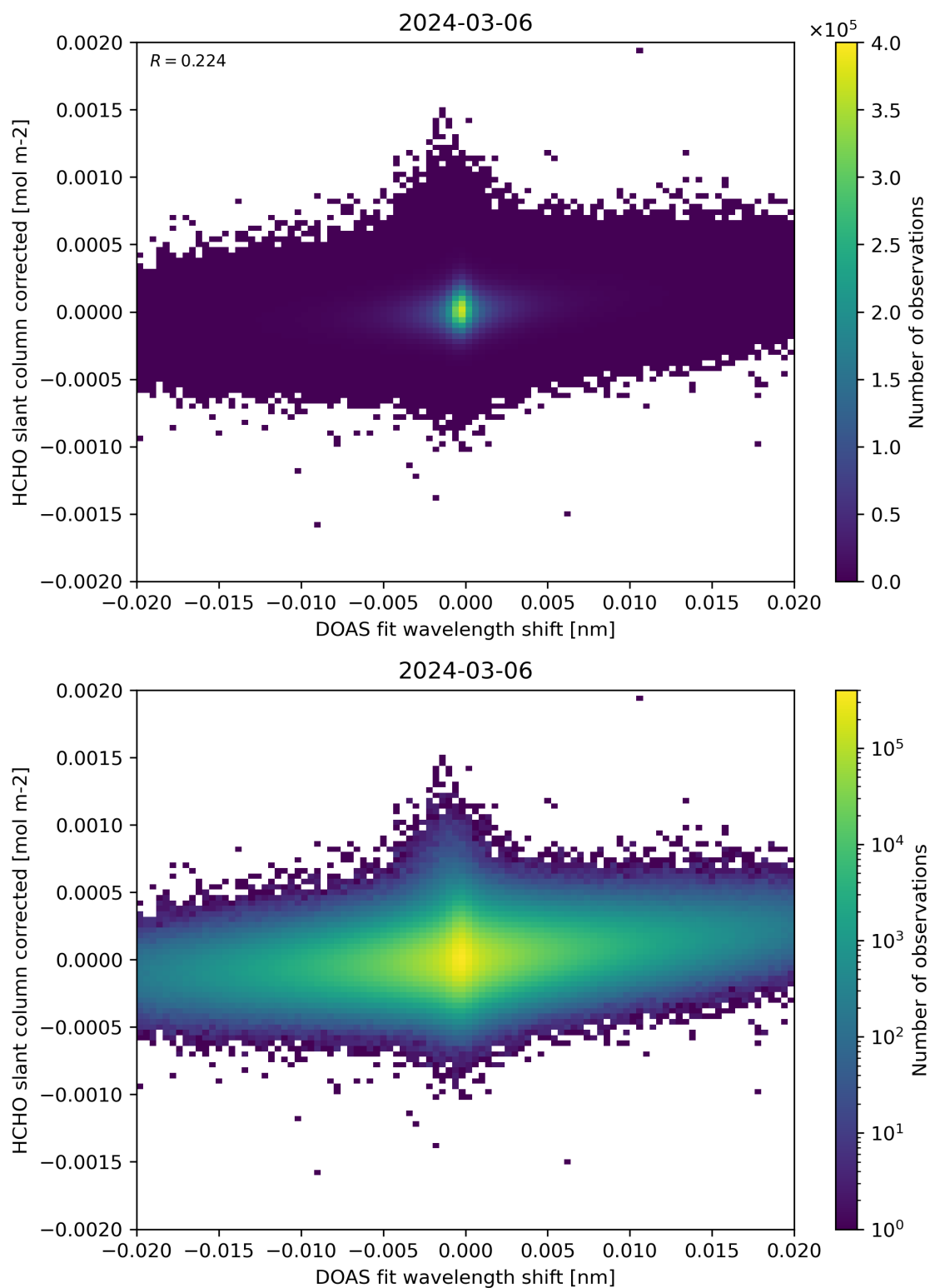
Figure 66: Scatter density plot of “DOAS fit wavelength shift” against “HCHO slant column corrected” for 2024-03-05 to 2024-03-07.
