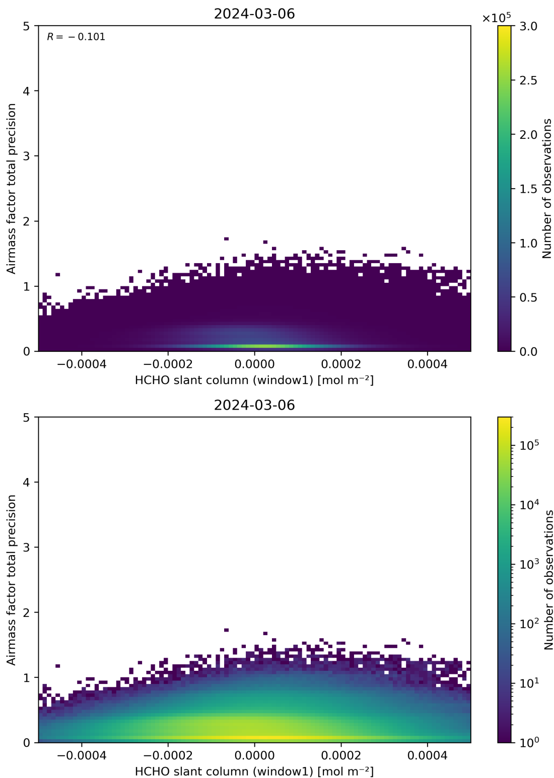
Figure 86: Scatter density plot of “HCHO slant column (window1)” against “Airmass factor total precision” for 2024-03-05 to 2024-03-07.
