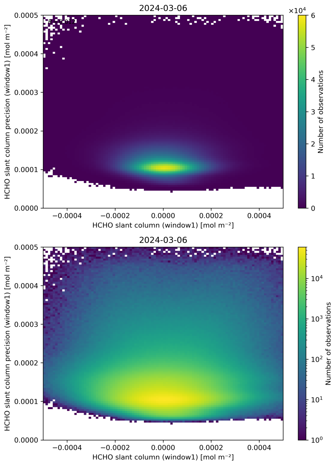
Figure 84: Scatter density plot of “HCHO slant column (window1)” against “HCHO slant column precision (window1)” for 2024-03-05 to 2024-03-07.
