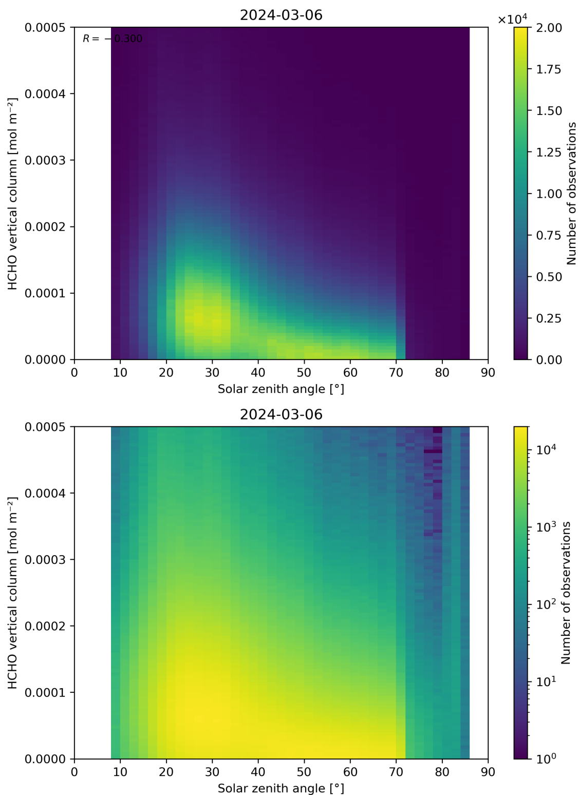
Figure 177: Scatter density plot of “Solar zenith angle” against “HCHO vertical column” for 2024-03-05 to 2024-03-07.
