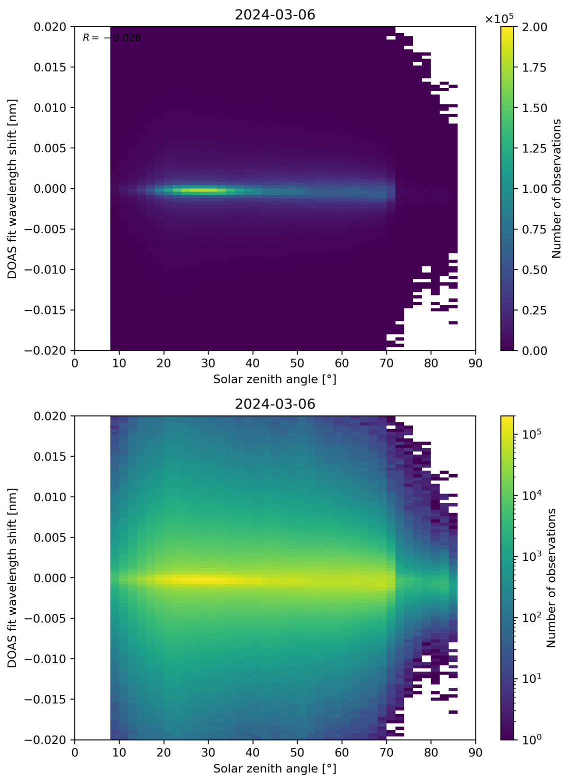
Figure 168: Scatter density plot of “Solar zenith angle” against “DOAS fit wavelength shift” for 2024-03-05 to 2024-03-07.
