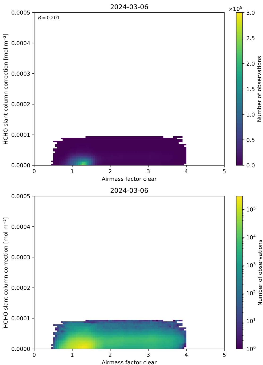
Figure 75: Scatter density plot of “Airmass factor clear” against “HCHO slant column correction” for 2024-03-05 to 2024-03-07.
