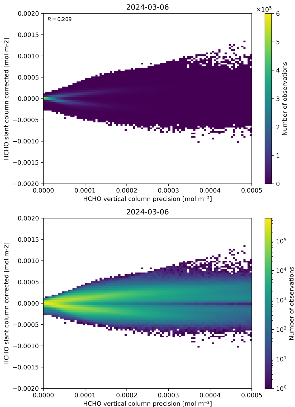
Figure 140: Scatter density plot of “HCHO vertical column precision” against “HCHO slant column corrected” for 2024-03-05 to 2024-03-07.
