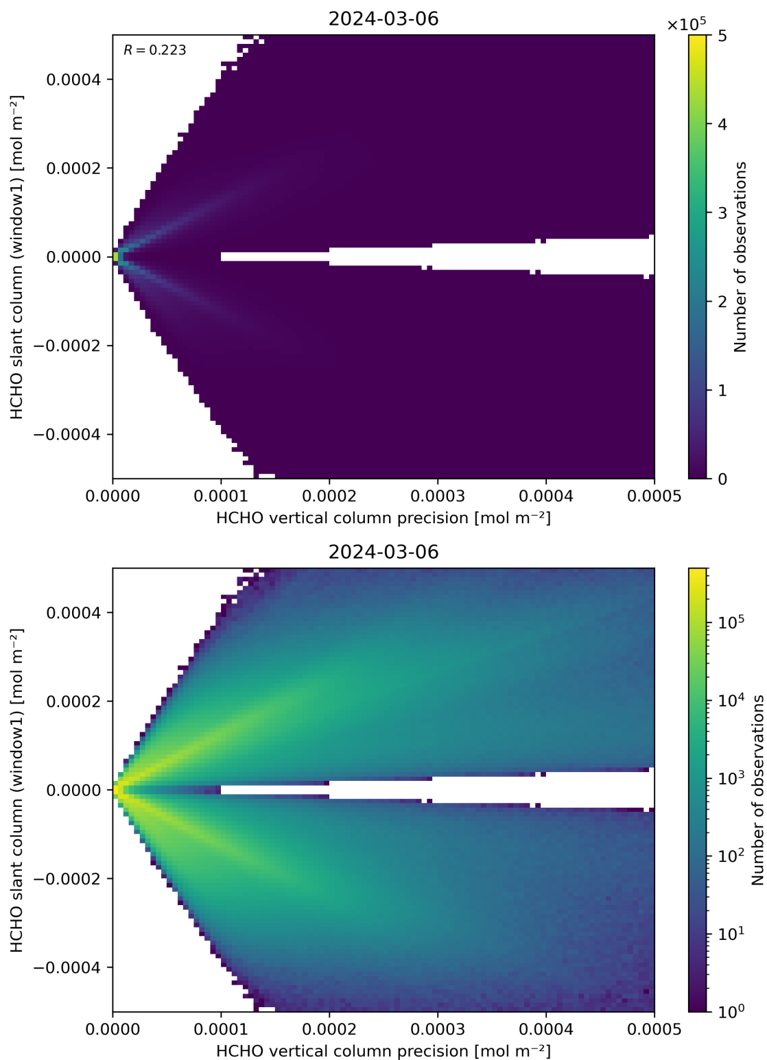
Figure 142: Scatter density plot of “HCHO vertical column precision” against “HCHO slant column (window1)” for 2024-03-05 to 2024-03-07.
