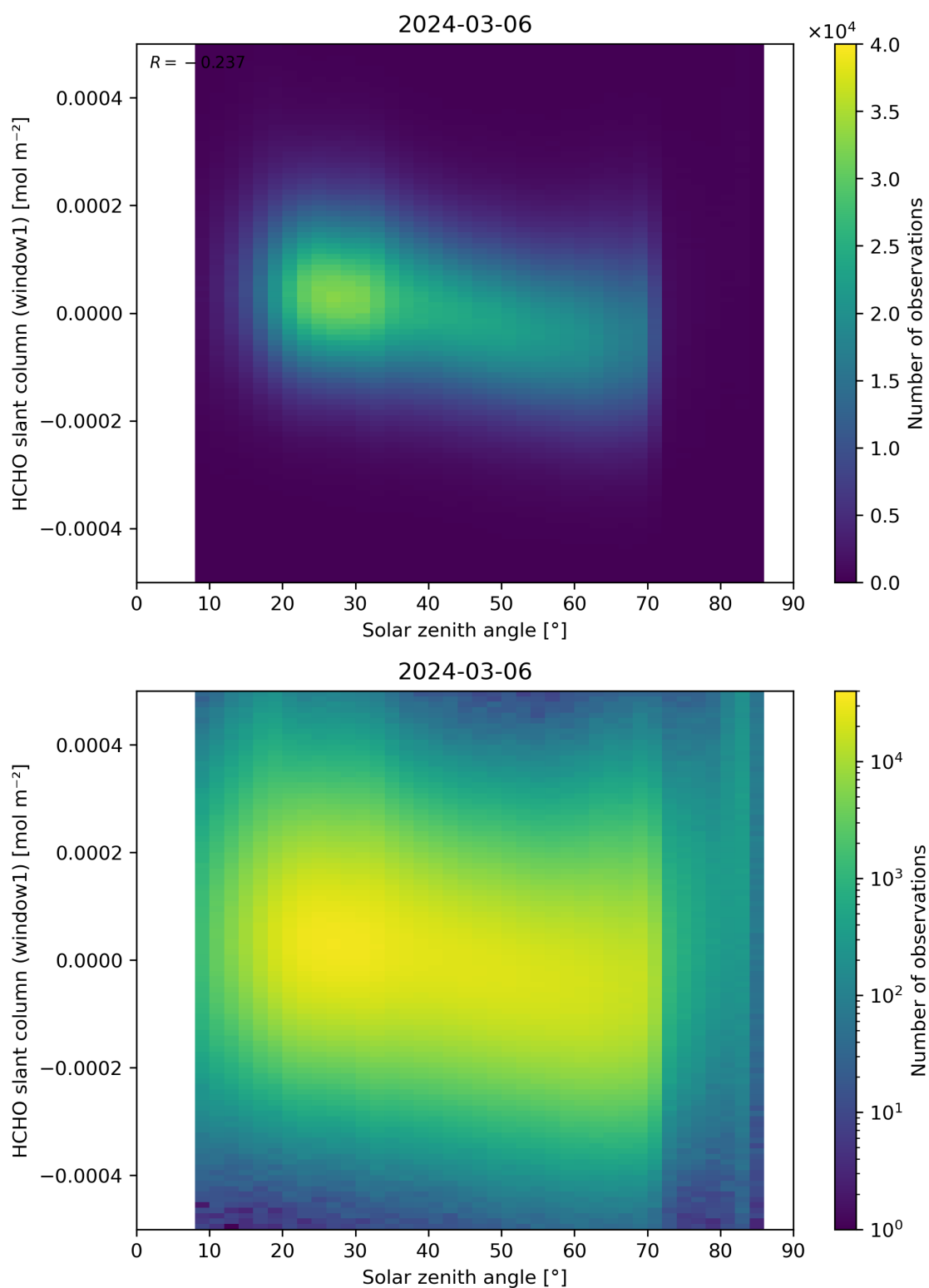
Figure 173: Scatter density plot of “Solar zenith angle” against “HCHO slant column (window1)” for 2024-03-05 to 2024-03-07.
