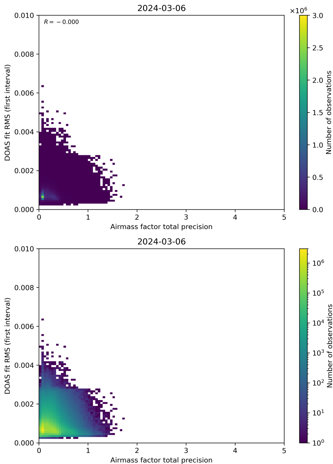
Figure 105: Scatter density plot of “Airmass factor total precision” against “DOAS fit RMS (first interval)” for 2024-03-05 to 2024-03-07.
