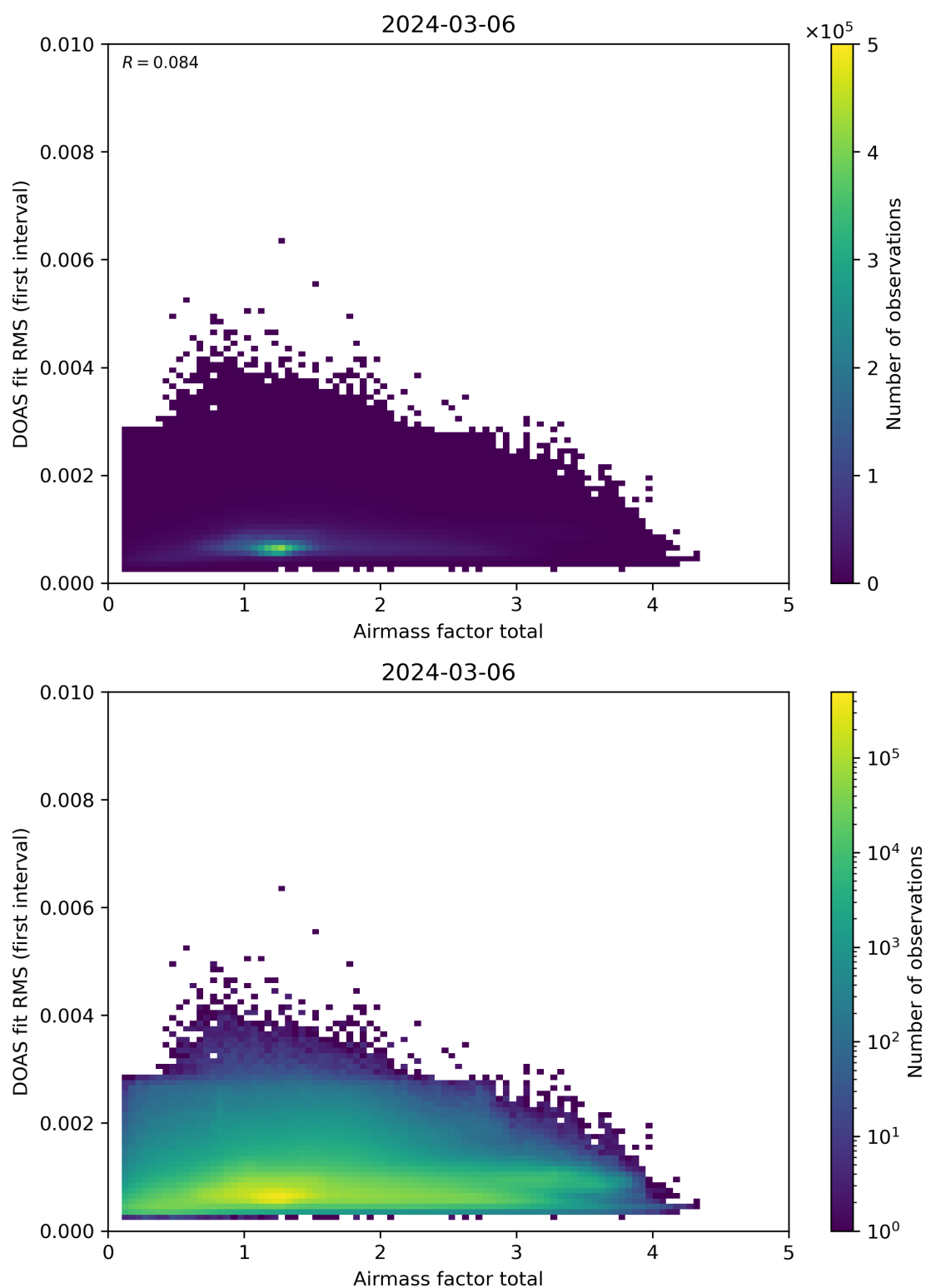
Figure 97: Scatter density plot of “Airmass factor total” against “DOAS fit RMS (first interval)” for 2024-03-05 to 2024-03-07.
