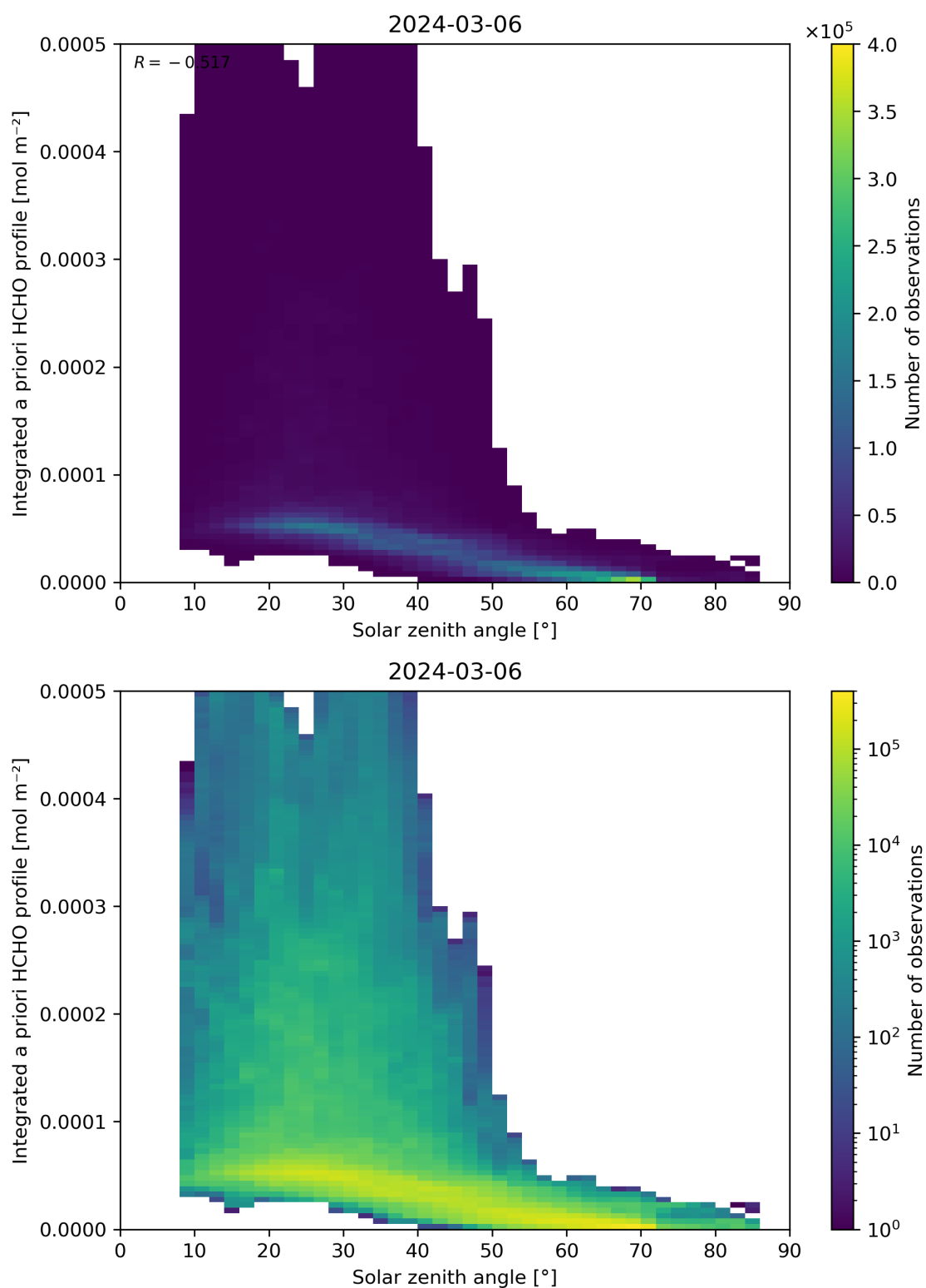
Figure 180: Scatter density plot of “Solar zenith angle” against “Integrated a priori HCHO profile” for 2024-03-05 to 2024-03-07.
