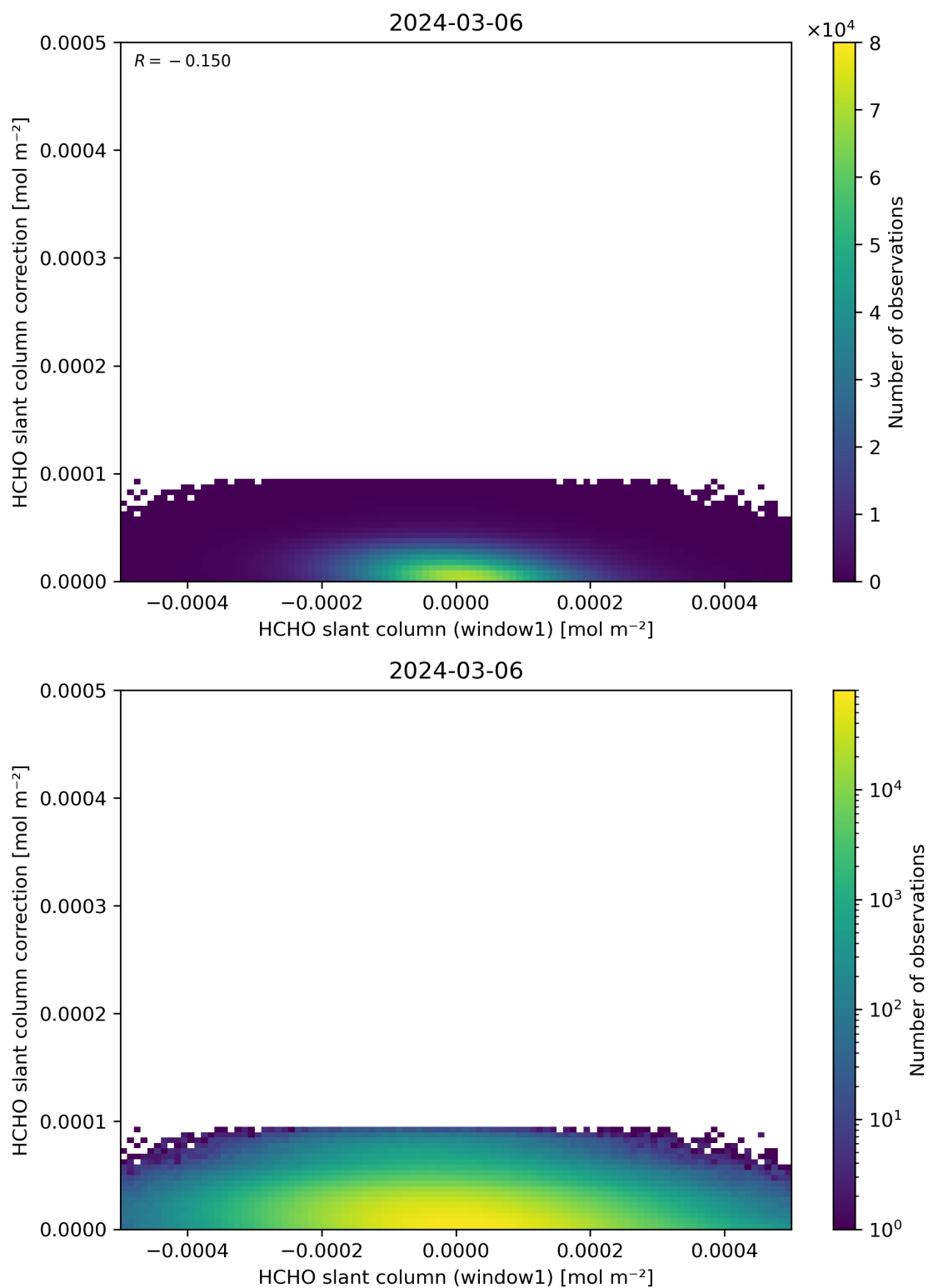
Figure 83: Scatter density plot of “HCHO slant column (window1)” against “HCHO slant column correction” for 2024-03-05 to 2024-03-07.
