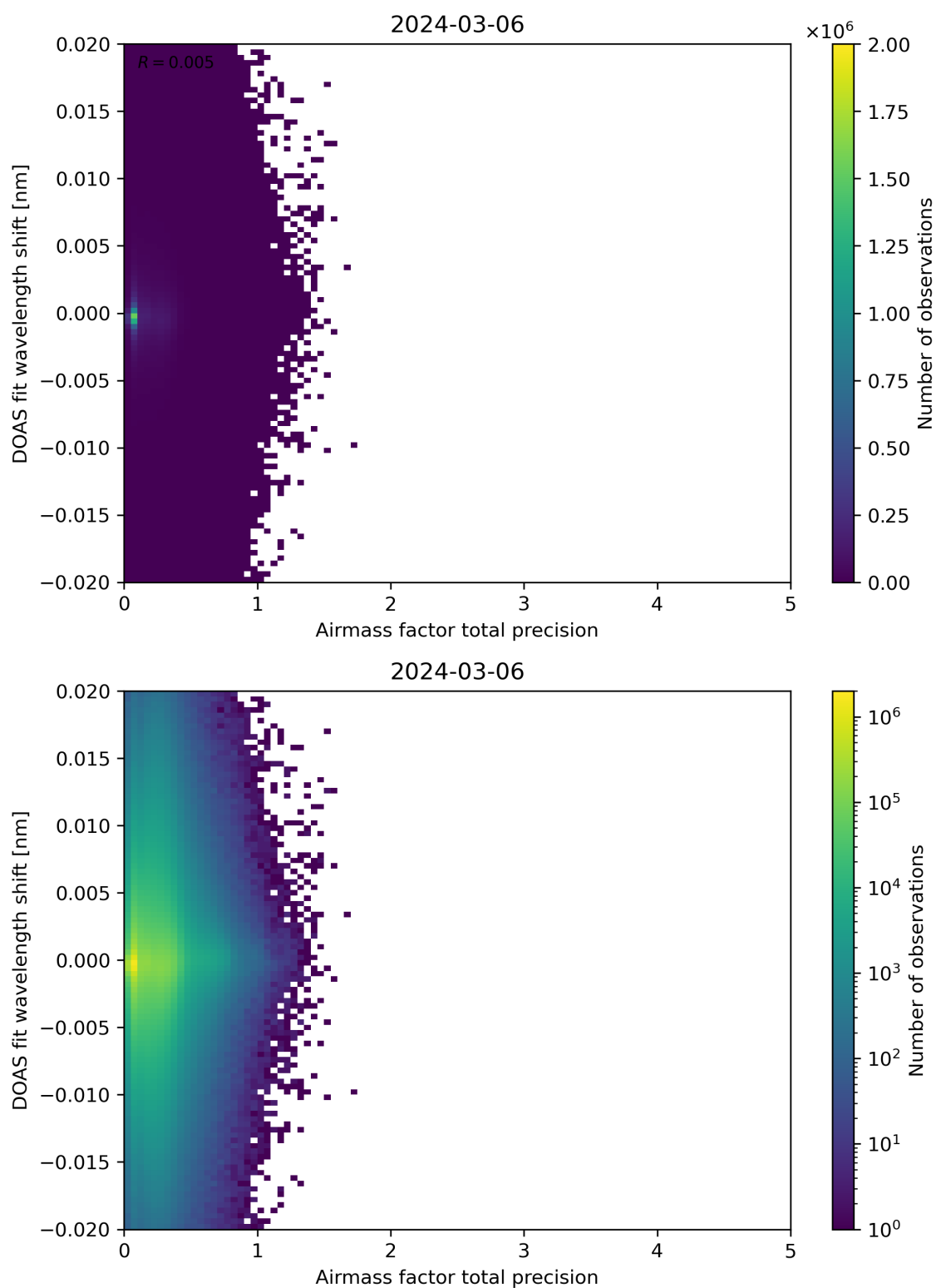
Figure 106: Scatter density plot of “Airmass factor total precision” against “DOAS fit wavelength shift” for 2024-03-05 to 2024-03-07.
