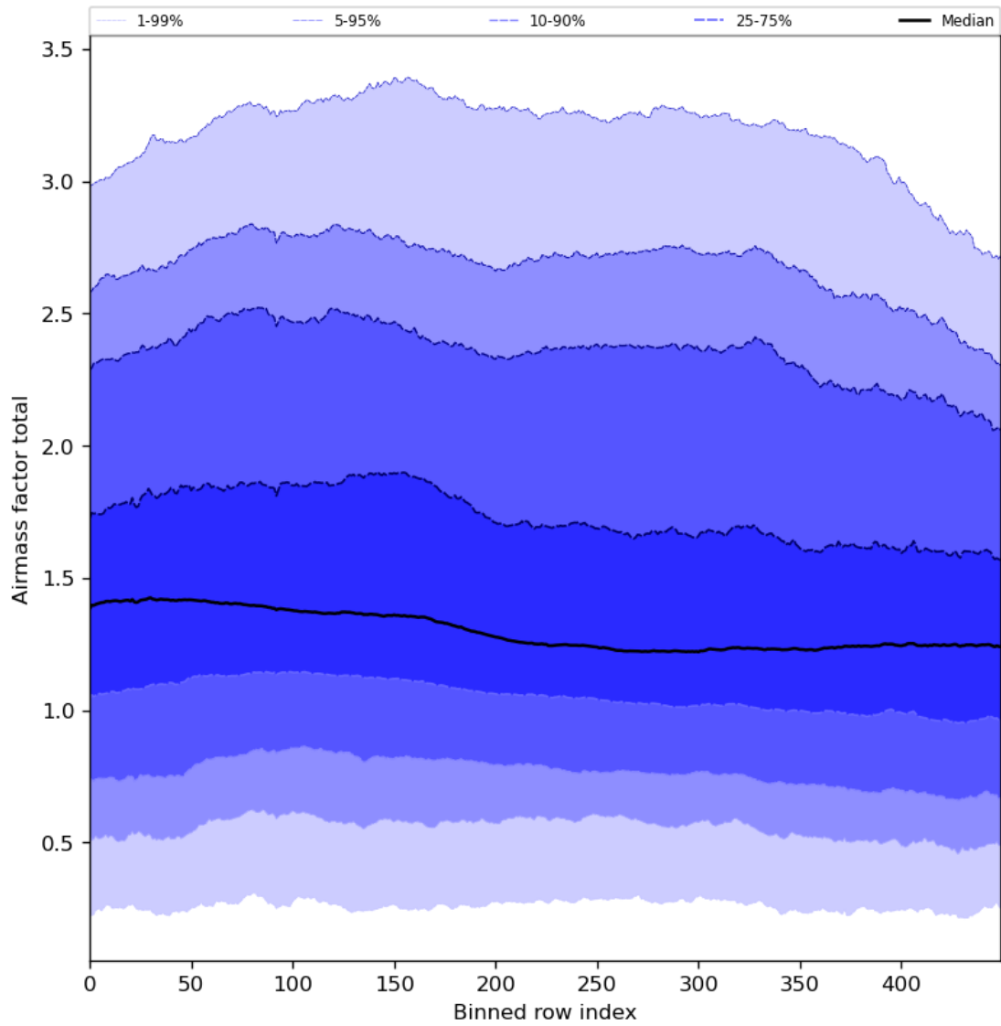
Figure 54: Along track statistics of “Airmass factor total” for 2024-03-05 to 2024-03-07
