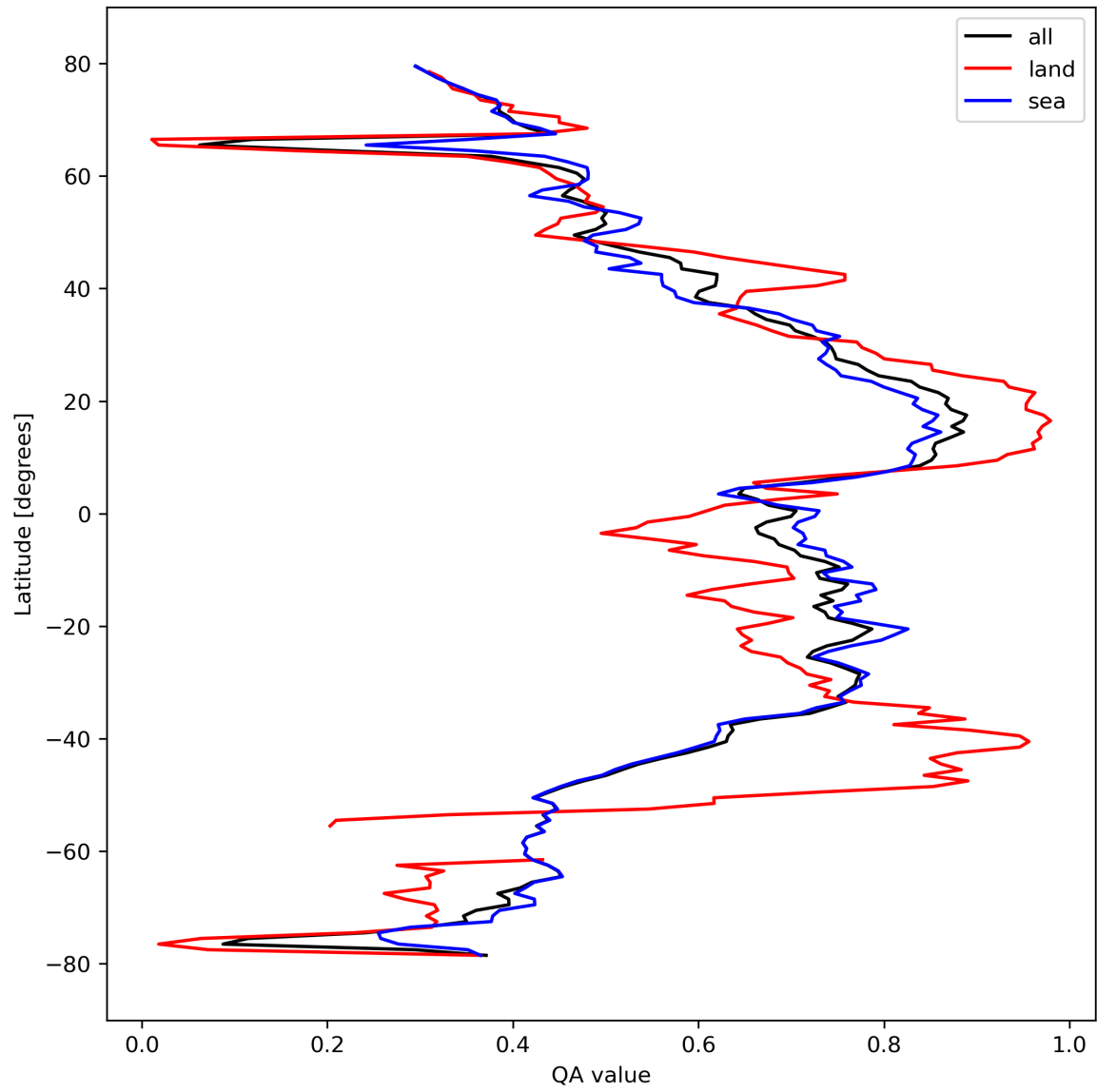
Figure 20: Zonal average of “QA value” for 2024-03-05 to 2024-03-07.
