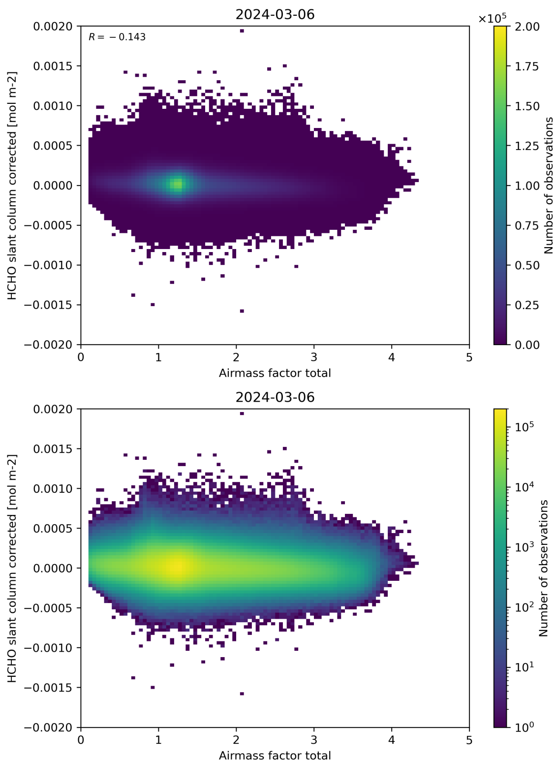
Figure 101: Scatter density plot of “Airmass factor total” against “HCHO slant column corrected” for 2024-03-05 to 2024-03-07.
