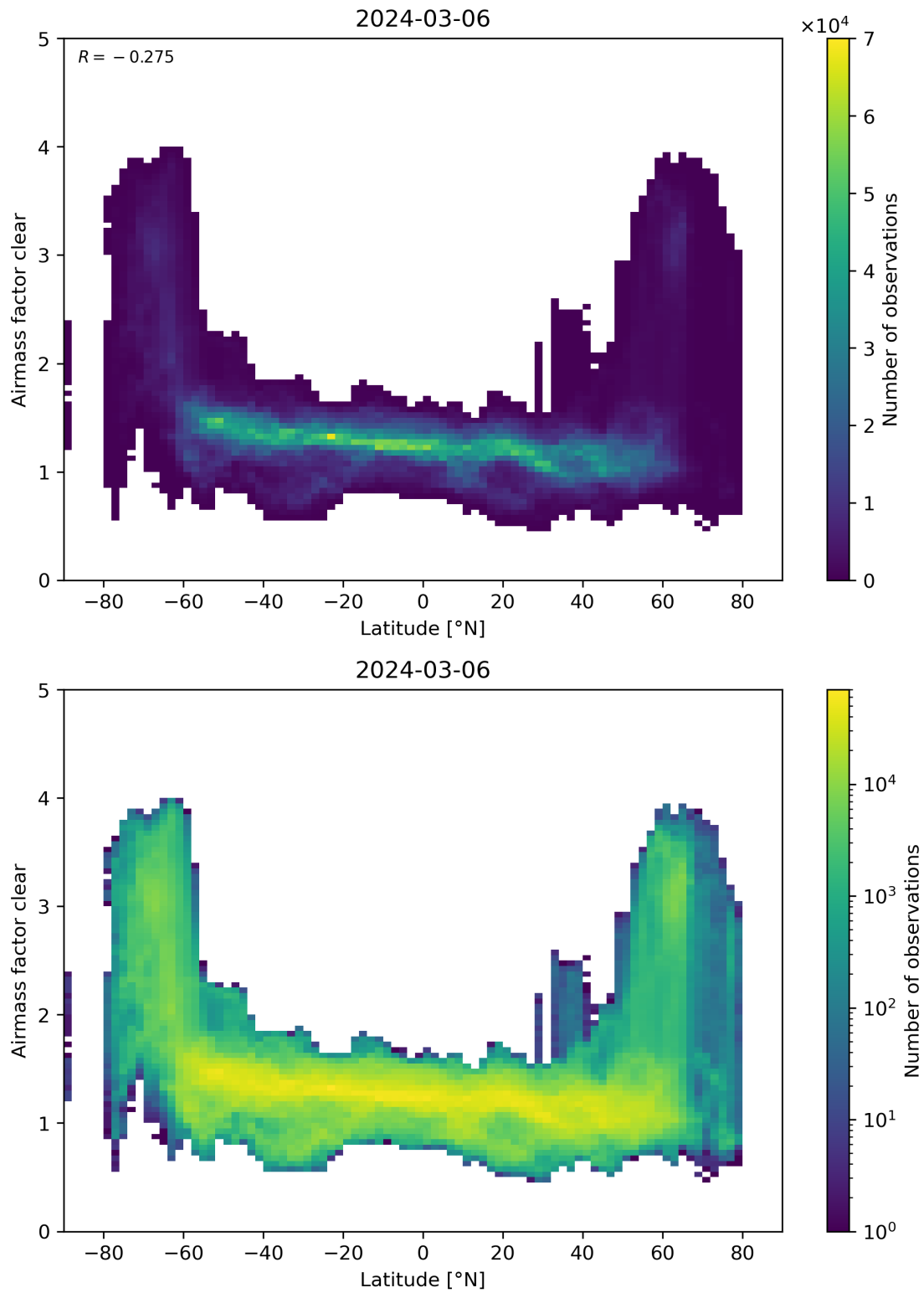
Figure 156: Scatter density plot of “Latitude” against “Airmass factor clear” for 2024-03-05 to 2024-03-07.
