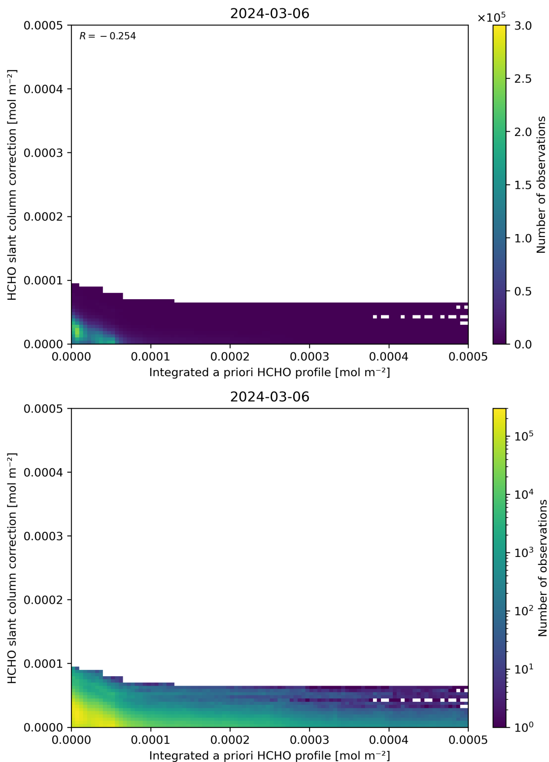
Figure 152: Scatter density plot of “Integrated a priori HCHO profile” against “HCHO slant column correction” for 2024-03-05 to 2024-03-07.
