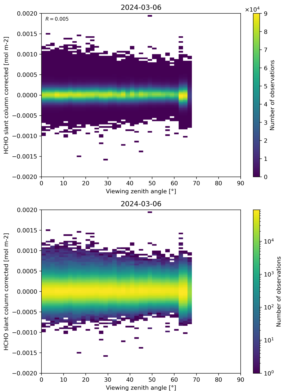
Figure 186: Scatter density plot of “Viewing zenith angle” against “HCHO slant column corrected” for 2024-03-05 to 2024-03-07.
