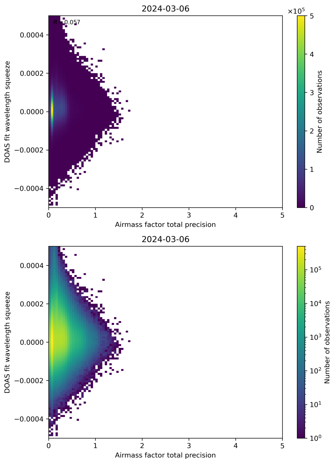
Figure 107: Scatter density plot of “Airmass factor total precision” against “DOAS fit wavelength squeeze” for 2024-03-05 to 2024-03-07.
