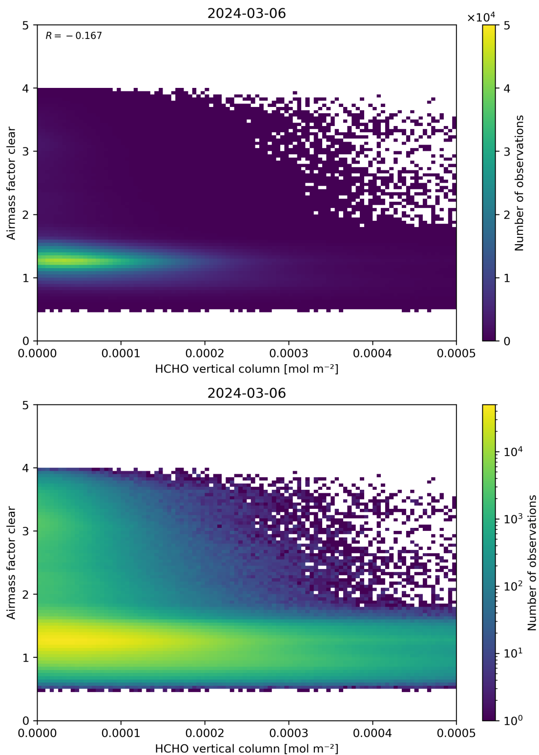
Figure 126: Scatter density plot of “HCHO vertical column” against “Airmass factor clear” for 2024-03-05 to 2024-03-07.
