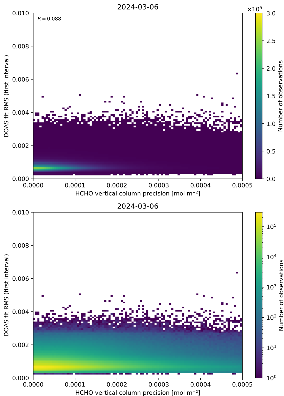
Figure 136: Scatter density plot of “HCHO vertical column precision” against “DOAS fit RMS (first interval)” for 2024-03-05 to 2024-03-07.
