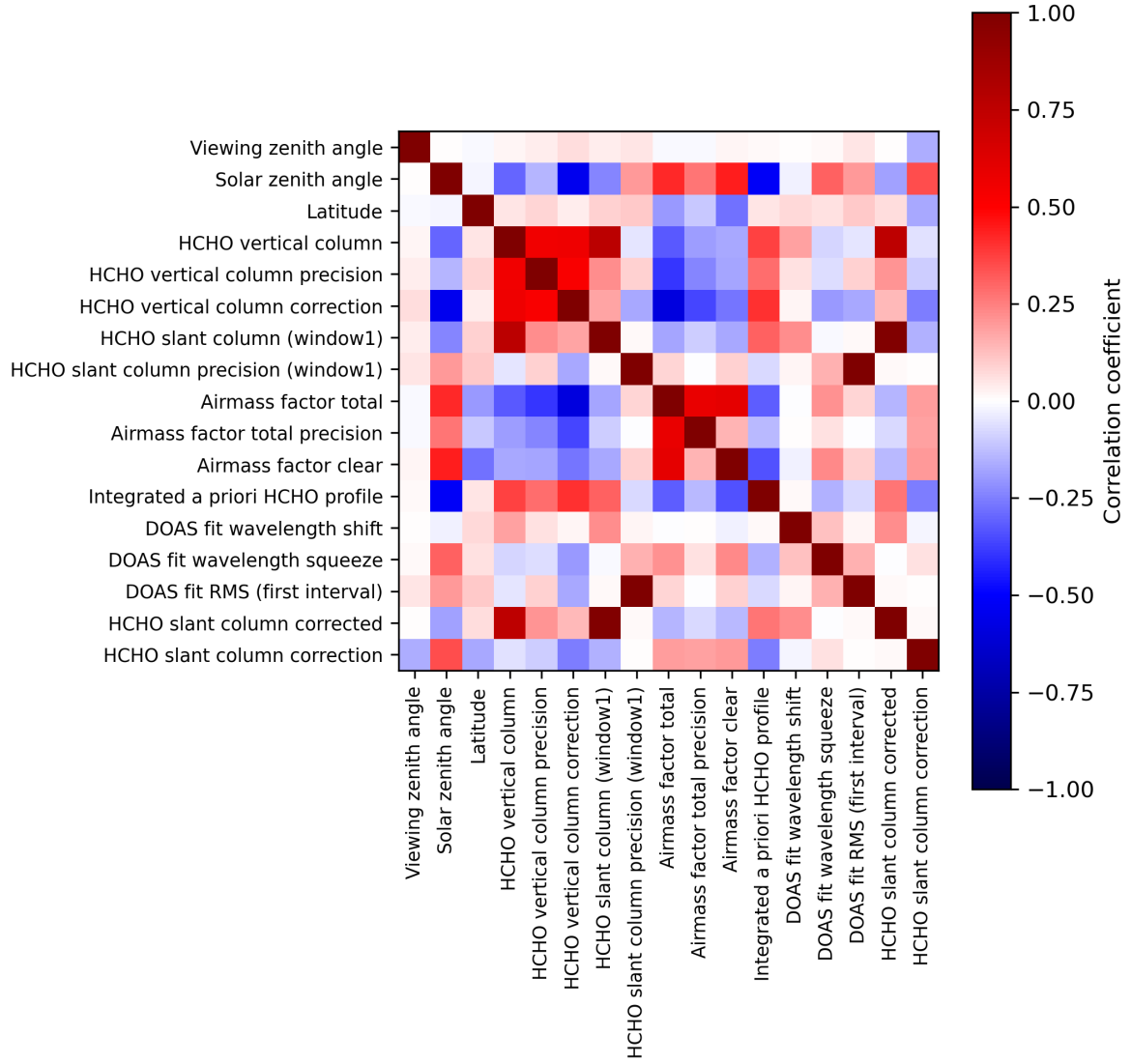
Figure 2: Map of correlation matrix for 2024-03-05 to 2024-03-07.
