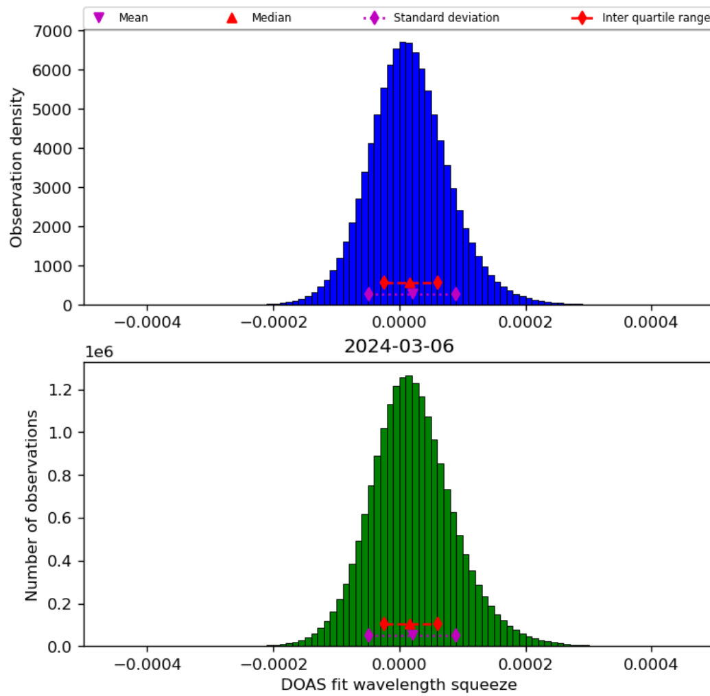
Figure 45: Histogram of “DOAS fit wavelength squeeze” for 2024-03-05 to 2024-03-07
