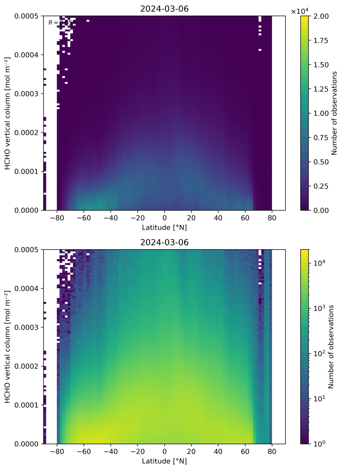
Figure 163: Scatter density plot of “Latitude” against “HCHO vertical column” for 2024-03-05 to 2024-03-07.
