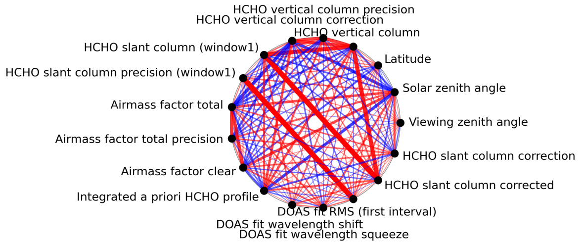
Figure 1: Map of correlation graph for 2024-03-05 to 2024-03-07.
