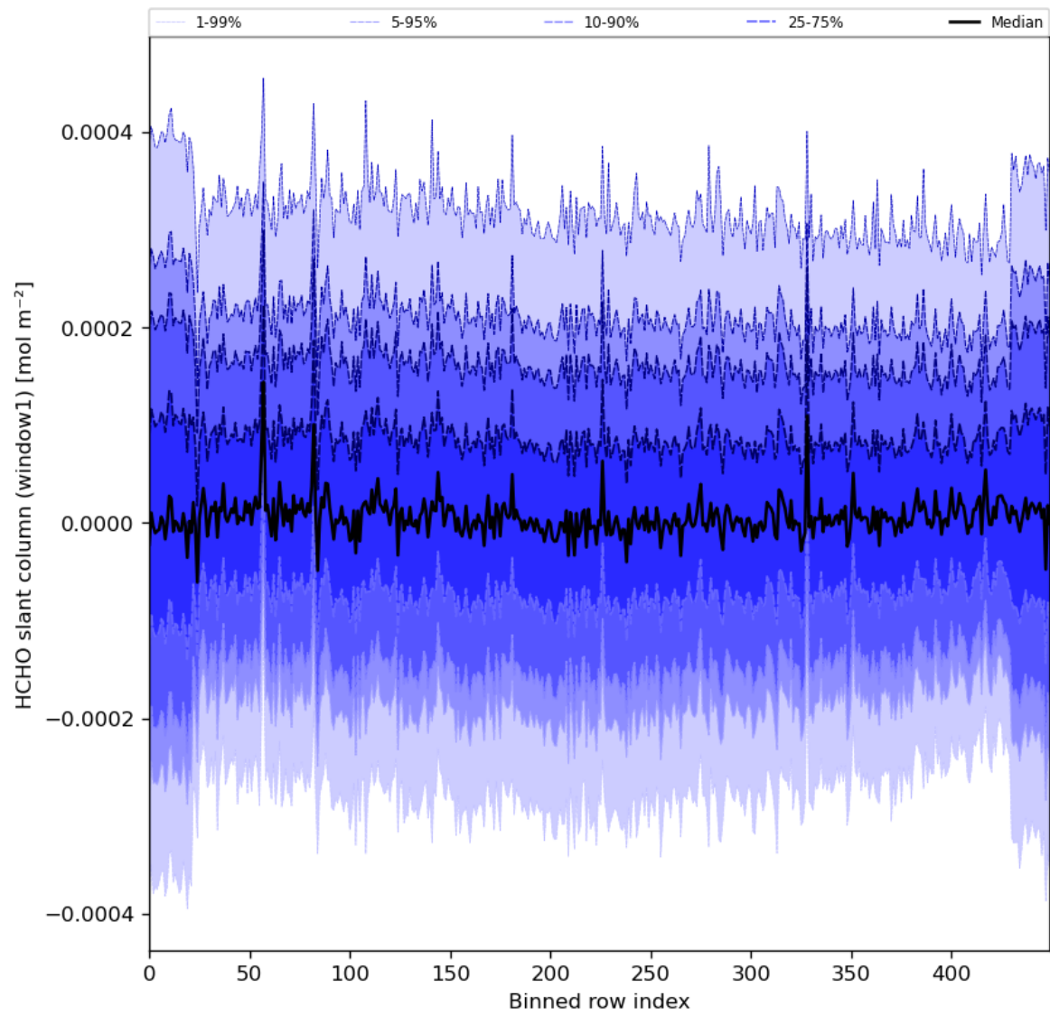
Figure 52: Along track statistics of “HCHO slant column (window1)” for 2024-03-05 to 2024-03-07
