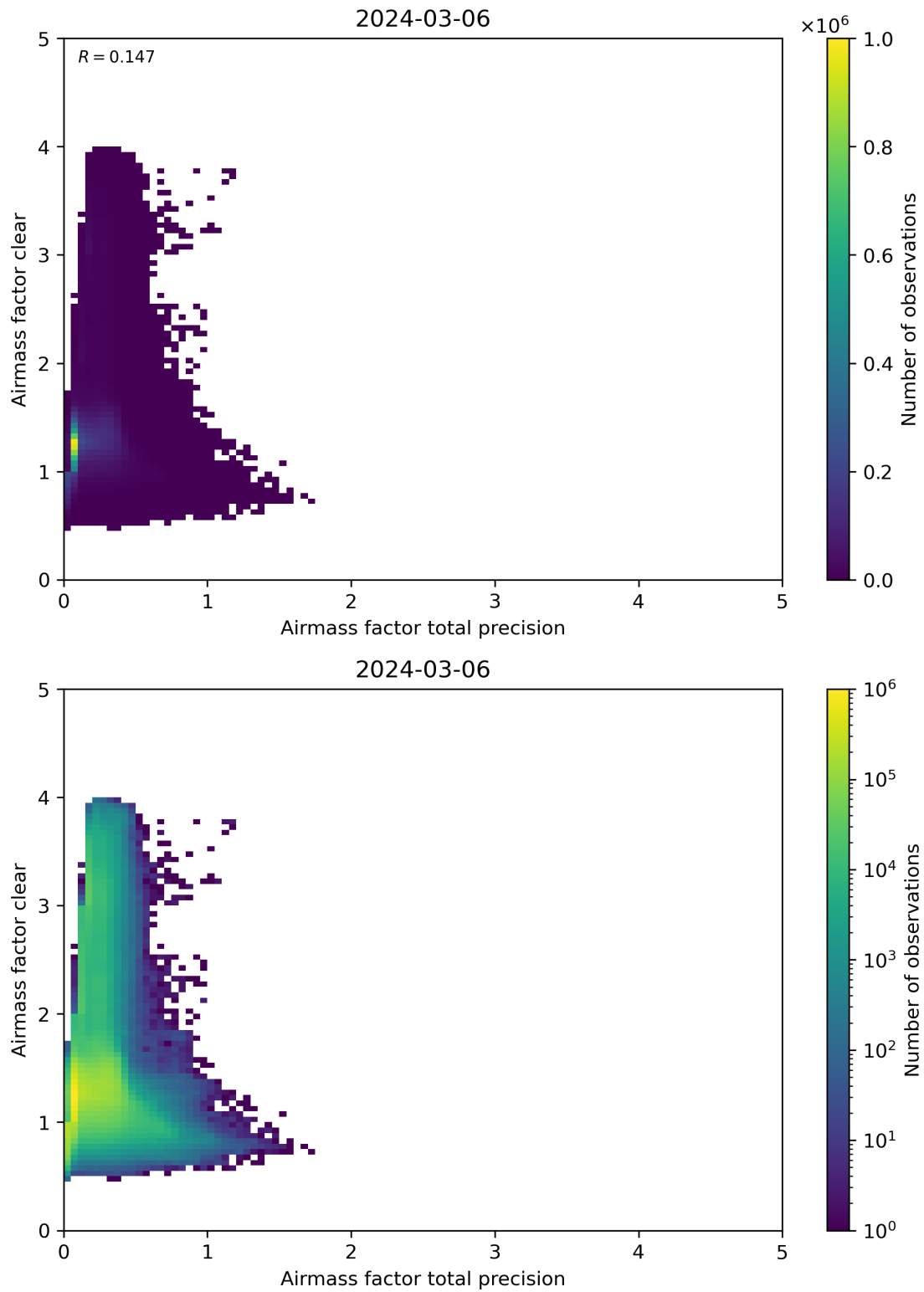
Figure 108: Scatter density plot of “Airmass factor total precision” against “Airmass factor clear” for 2024-03-05 to 2024-03-07.
