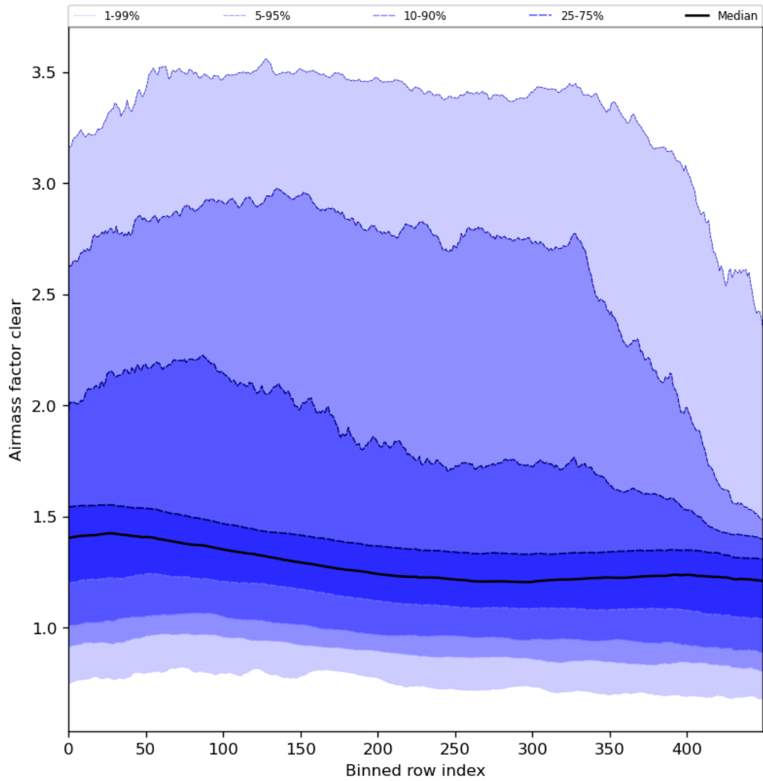
Figure 56: Along track statistics of “Airmass factor clear” for 2024-03-05 to 2024-03-07
