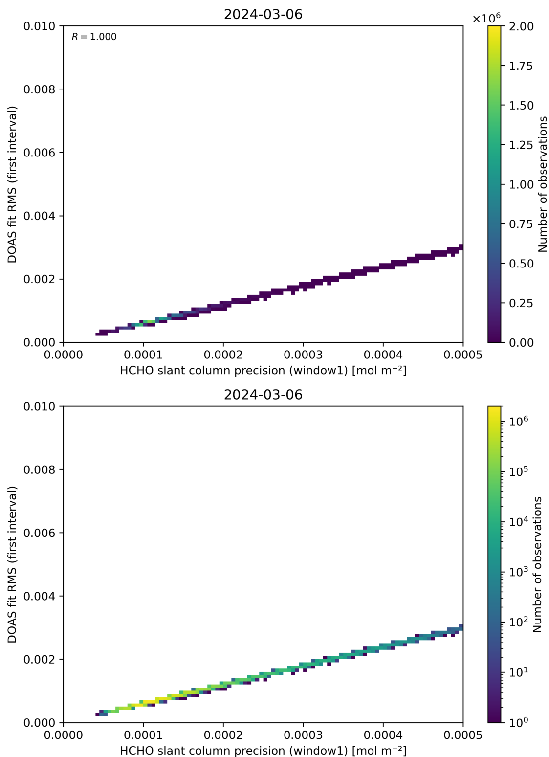
Figure 88: Scatter density plot of “HCHO slant column precision (window1)” against “DOAS fit RMS (first interval)” for 2024-03-05 to 2024-03-07.
