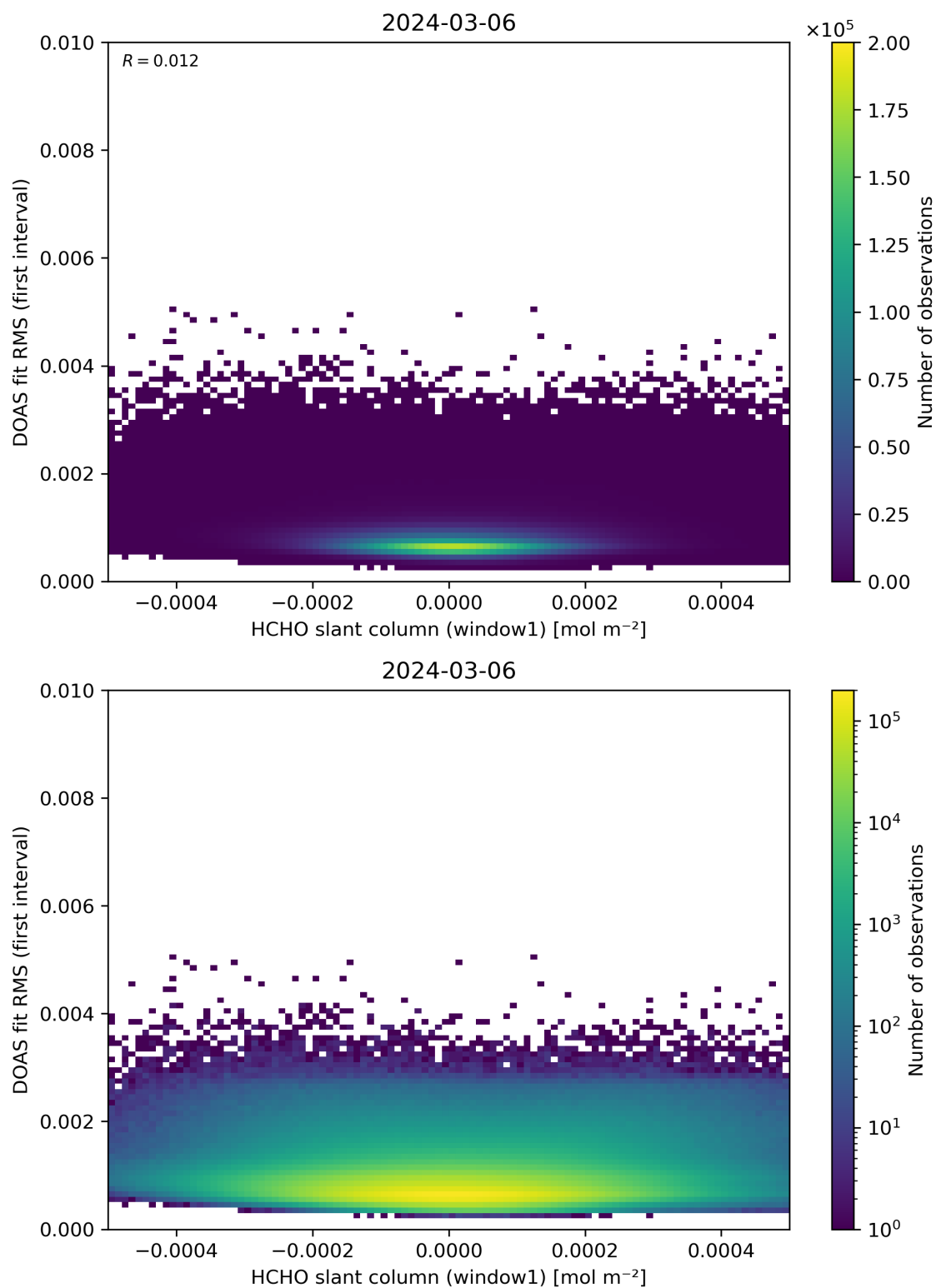
Figure 78: Scatter density plot of “HCHO slant column (window1)” against “DOAS fit RMS (first interval)” for 2024-03-05 to 2024-03-07.
