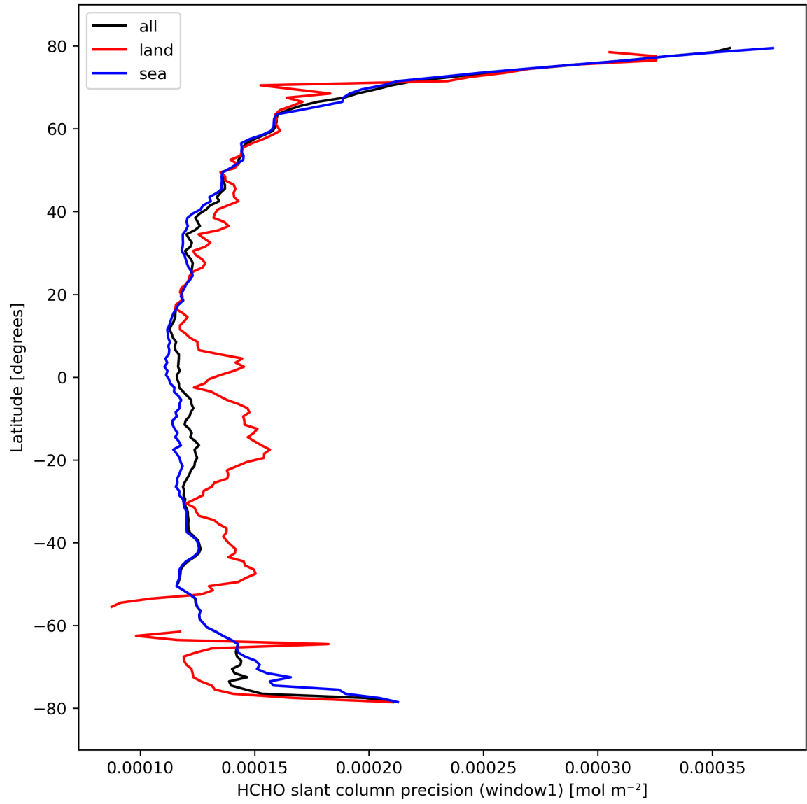
Figure 25: Zonal average of “HCHO slant column precision (window1)” for 2024-03-05 to 2024-03-07.
