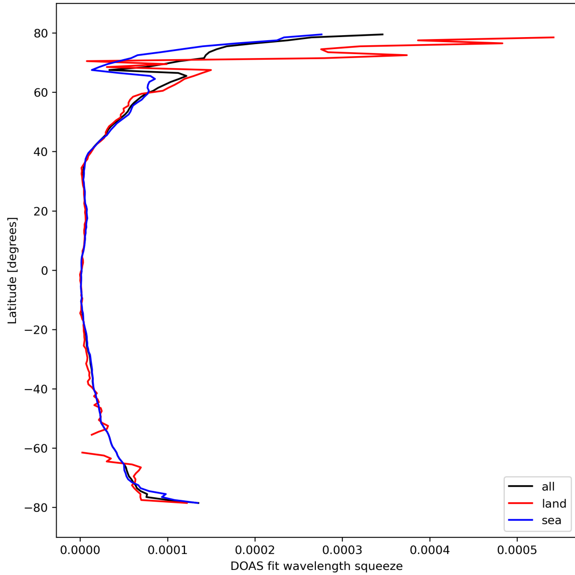
Figure 31: Zonal average of “DOAS fit wavelength squeeze” for 2024-03-05 to 2024-03-07.
