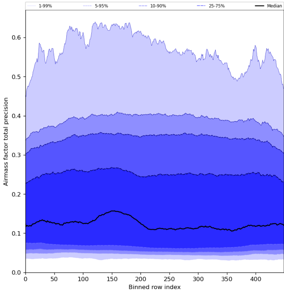
Figure 55: Along track statistics of “Airmass factor total precision” for 2024-03-05 to 2024-03-07
