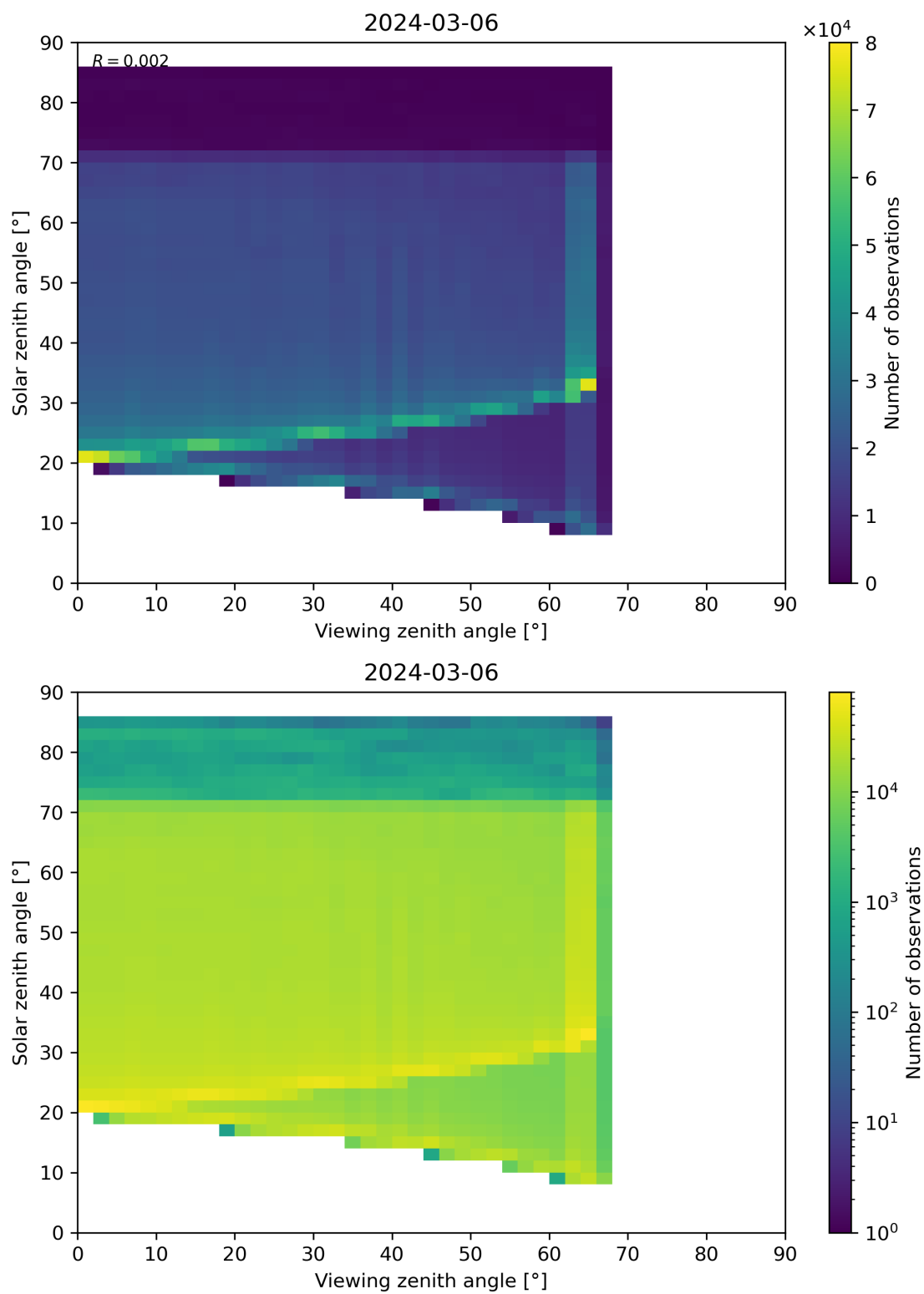
Figure 197: Scatter density plot of “Viewing zenith angle” against “Solar zenith angle” for 2024-03-05 to 2024-03-07.
