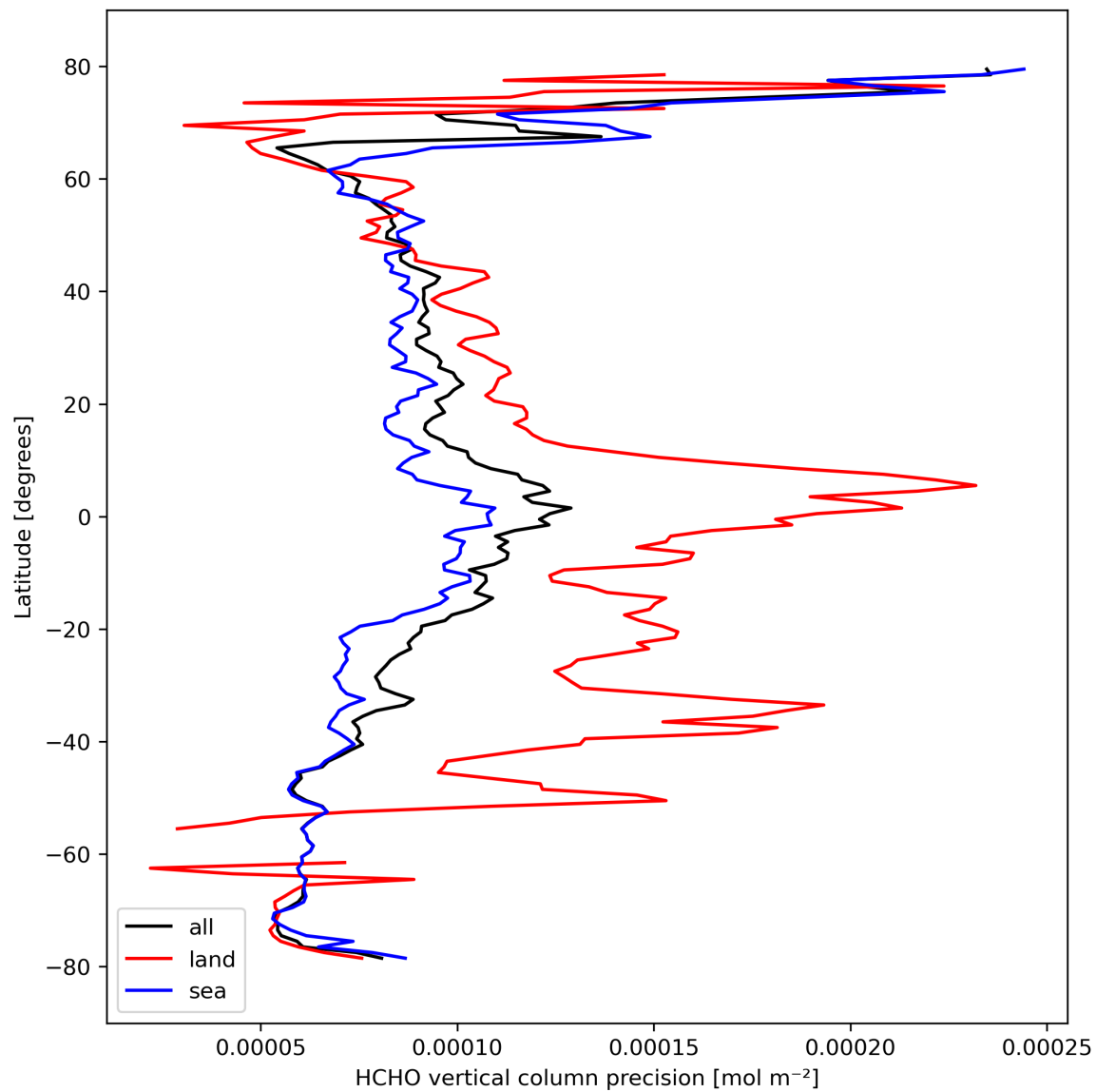
Figure 22: Zonal average of “HCHO vertical column precision” for 2024-03-05 to 2024-03-07.
