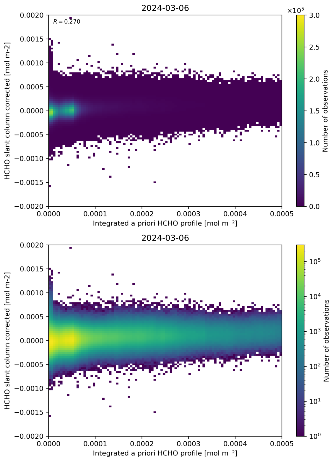
Figure 151: Scatter density plot of “Integrated a priori HCHO profile” against “HCHO slant column corrected” for 2024-03-05 to 2024-03-07.
