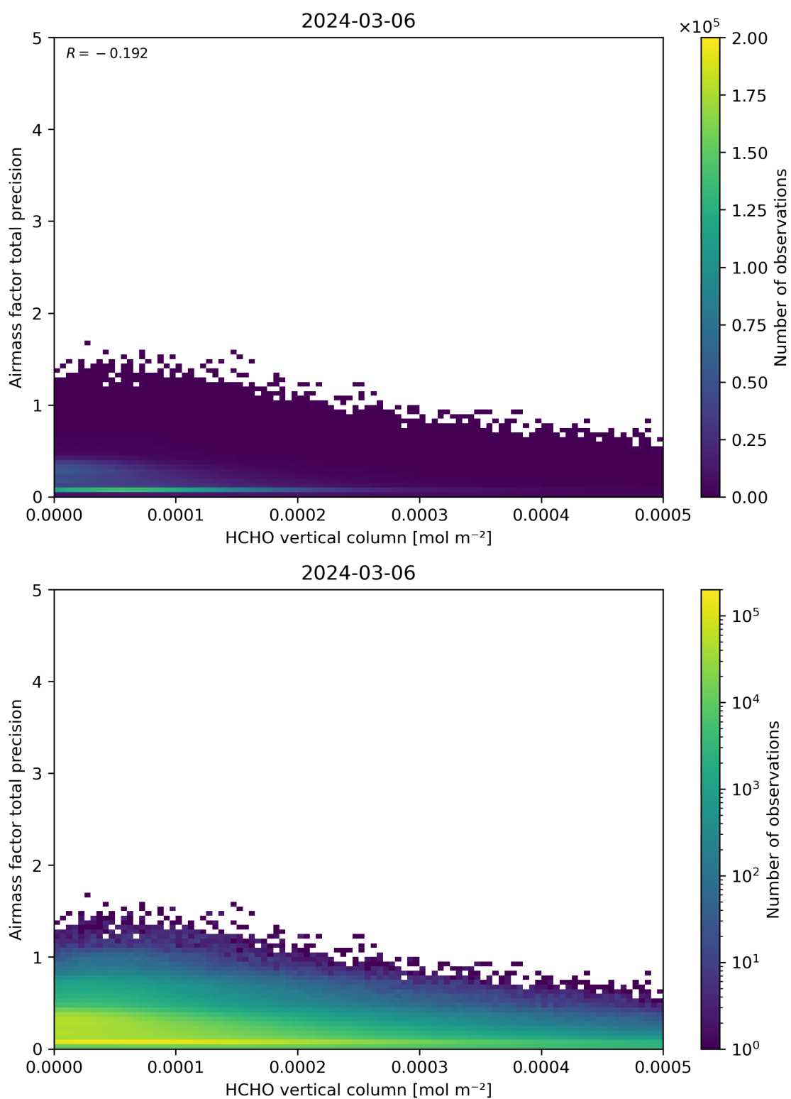
Figure 132: Scatter density plot of “HCHO vertical column” against “Airmass factor total precision” for 2024-03-05 to 2024-03-07.
