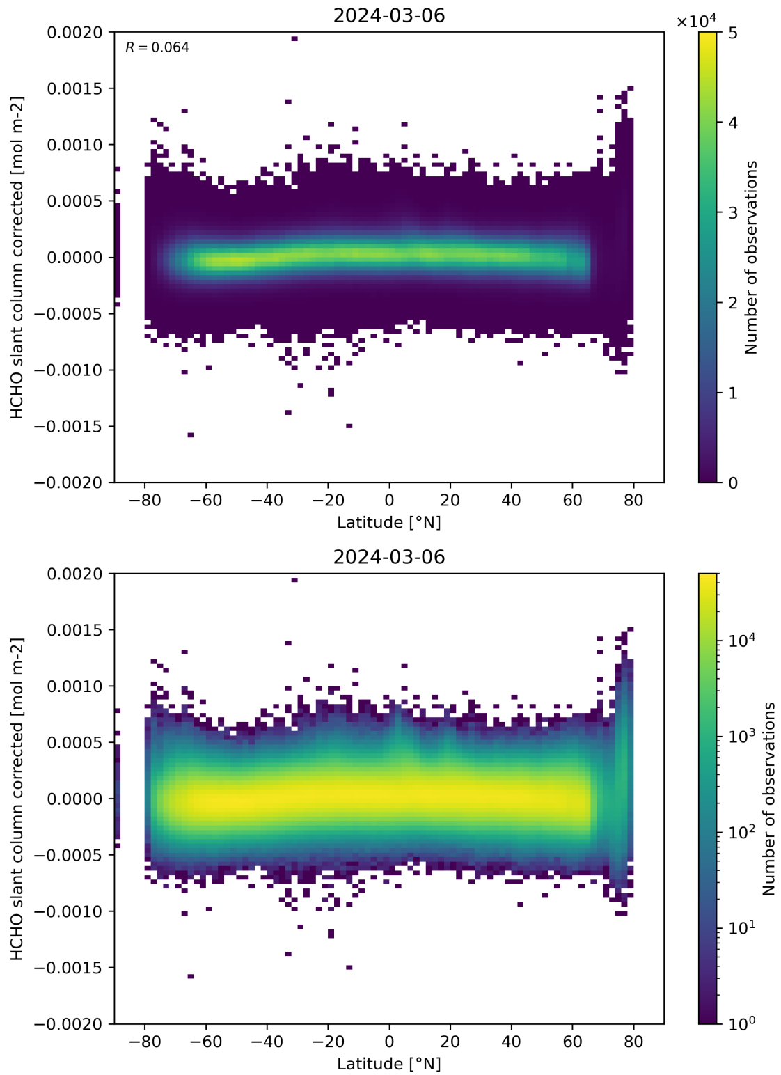
Figure 157: Scatter density plot of “Latitude” against “HCHO slant column corrected” for 2024-03-05 to 2024-03-07.
