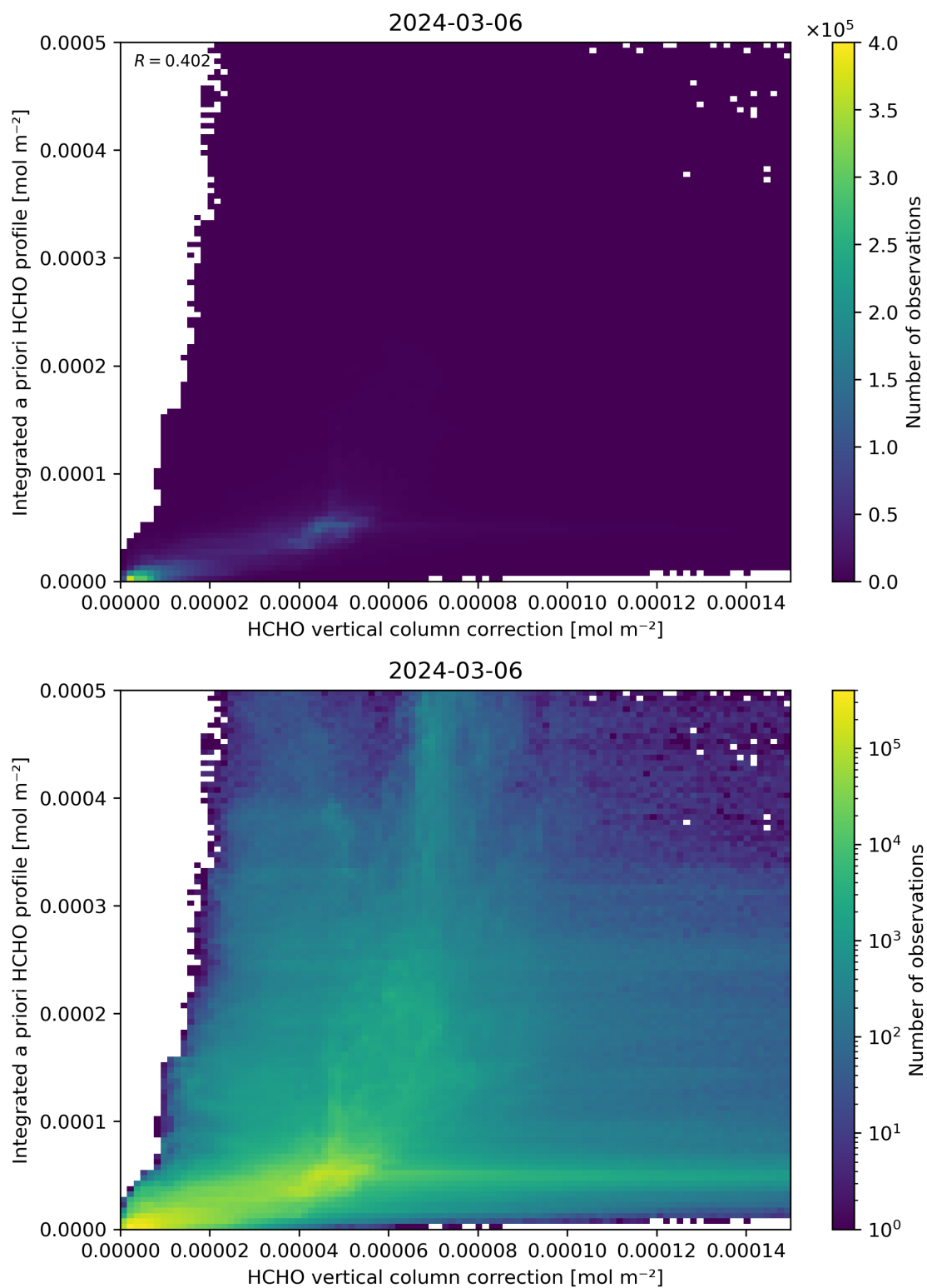
Figure 122: Scatter density plot of “HCHO vertical column correction” against “Integrated a priori HCHO profile” for 2024-03-05 to 2024-03-07.
