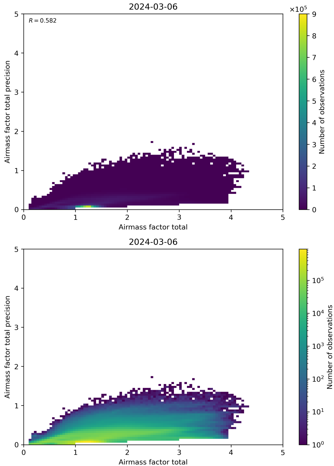
Figure 103: Scatter density plot of “Airmass factor total” against “Airmass factor total precision” for 2024-03-05 to 2024-03-07.
