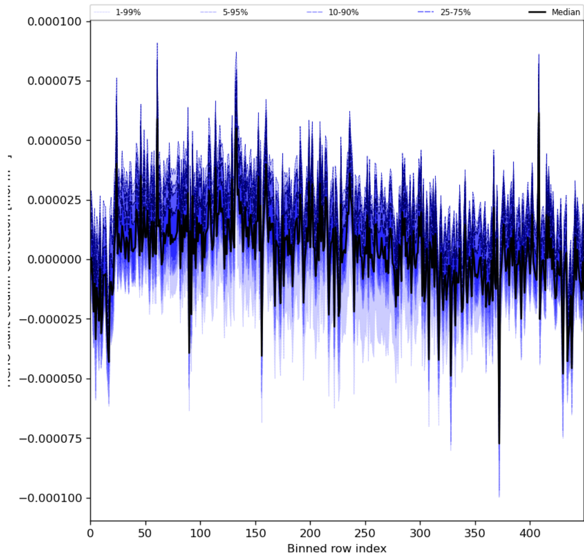
Figure 61: Along track statistics of “HCHO slant column correction” for 2024-03-05 to 2024-03-07
