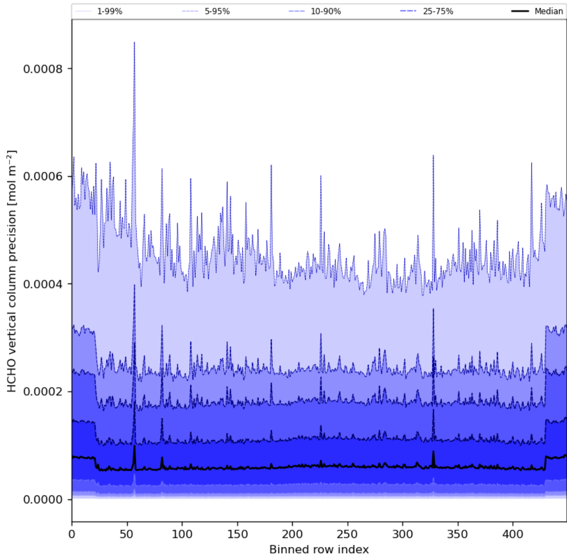
Figure 50: Along track statistics of “HCHO vertical column precision” for 2024-03-05 to 2024-03-07
