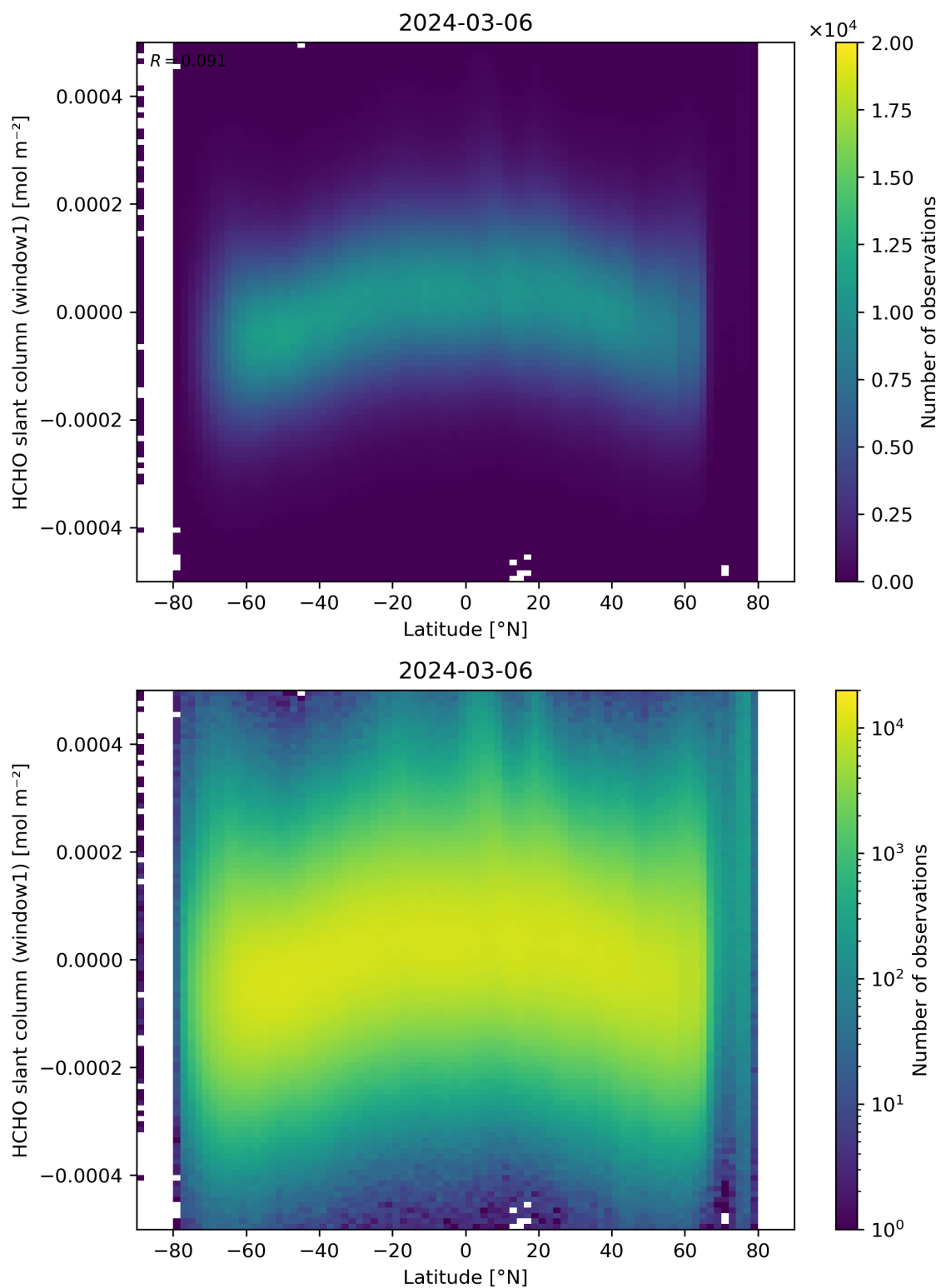
Figure 159: Scatter density plot of “Latitude” against “HCHO slant column (window1)” for 2024-03-05 to 2024-03-07.
