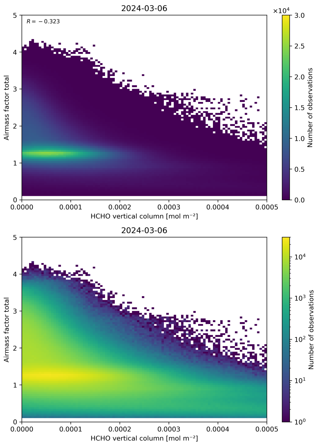
Figure 131: Scatter density plot of “HCHO vertical column” against “Airmass factor total” for 2024-03-05 to 2024-03-07.
