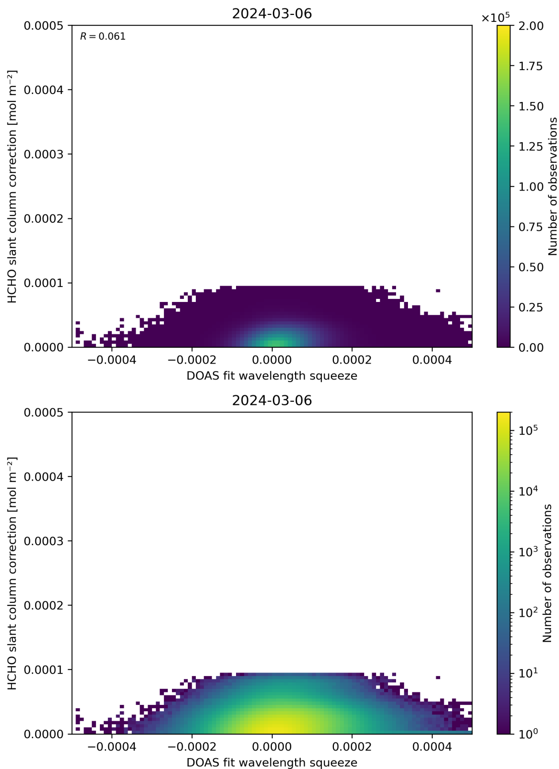
Figure 70: Scatter density plot of “DOAS fit wavelength squeeze” against “HCHO slant column correction” for 2024-03-05 to 2024-03-07.
