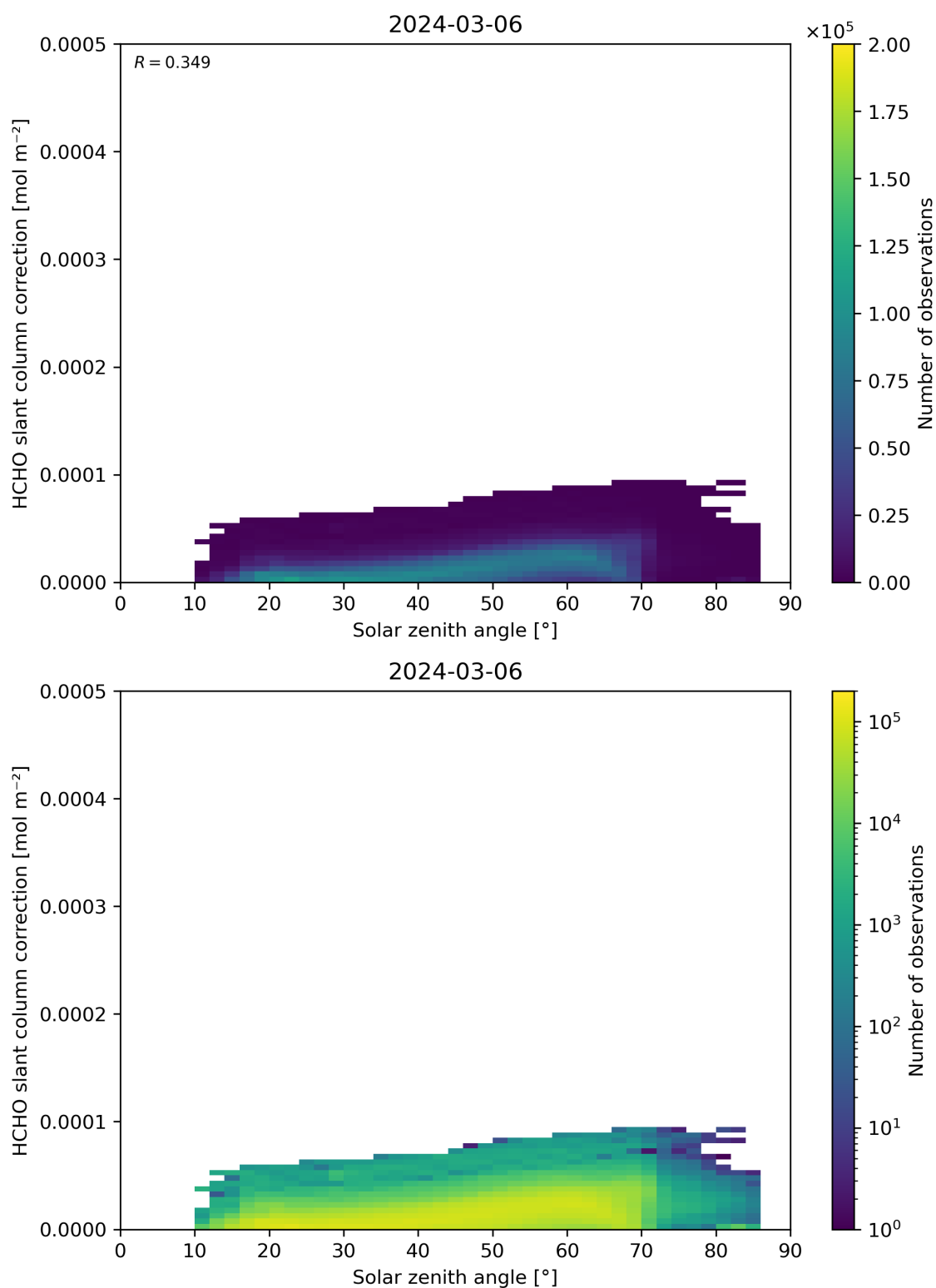
Figure 172: Scatter density plot of “Solar zenith angle” against “HCHO slant column correction” for 2024-03-05 to 2024-03-07.
