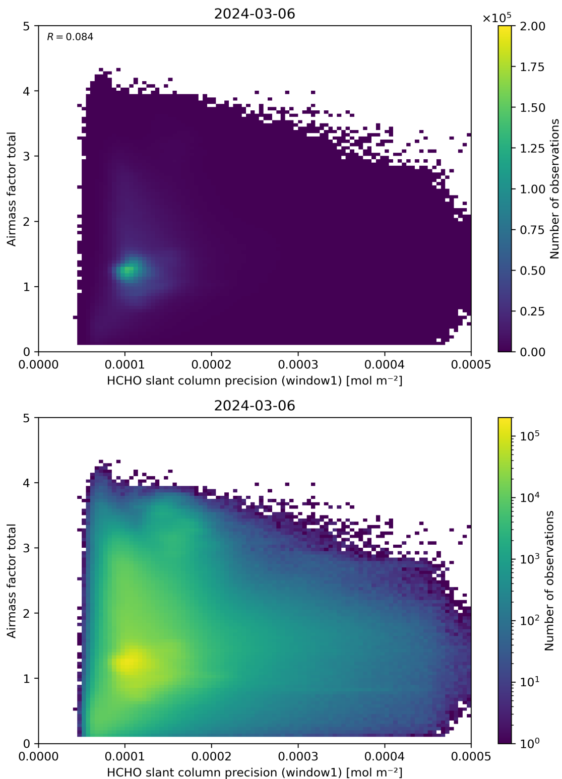
Figure 94: Scatter density plot of “HCHO slant column precision (window1)” against “Airmass factor total” for 2024-03-05 to 2024-03-07.
