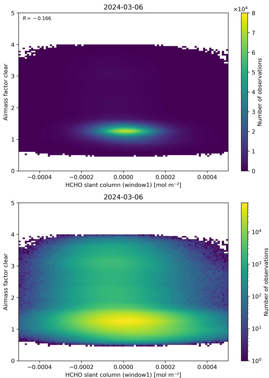
Figure 81: Scatter density plot of “HCHO slant column (window1)” against “Airmass factor clear” for 2024-03-05 to 2024-03-07.
