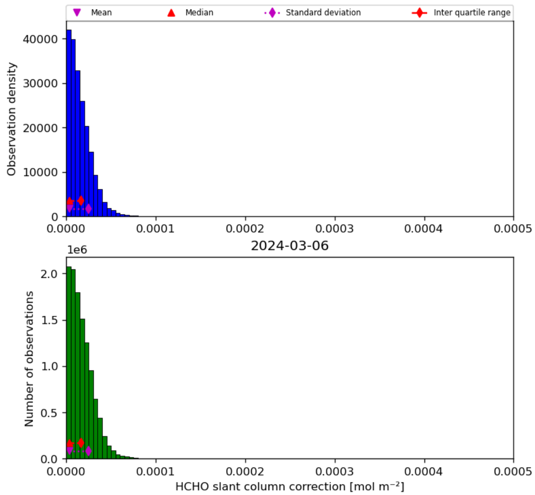
Figure 47: Histogram of “HCHO slant column correction” for 2024-03-05 to 2024-03-07
