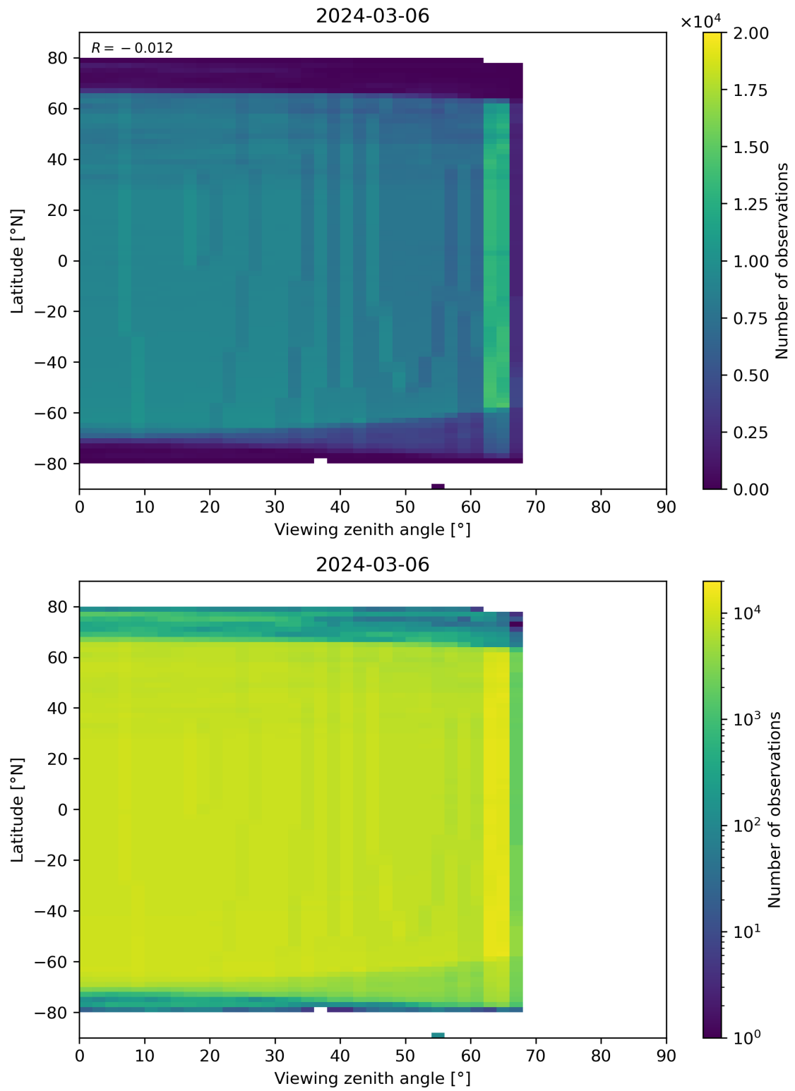
Figure 196: Scatter density plot of “Viewing zenith angle” against “Latitude” for 2024-03-05 to 2024-03-07.
