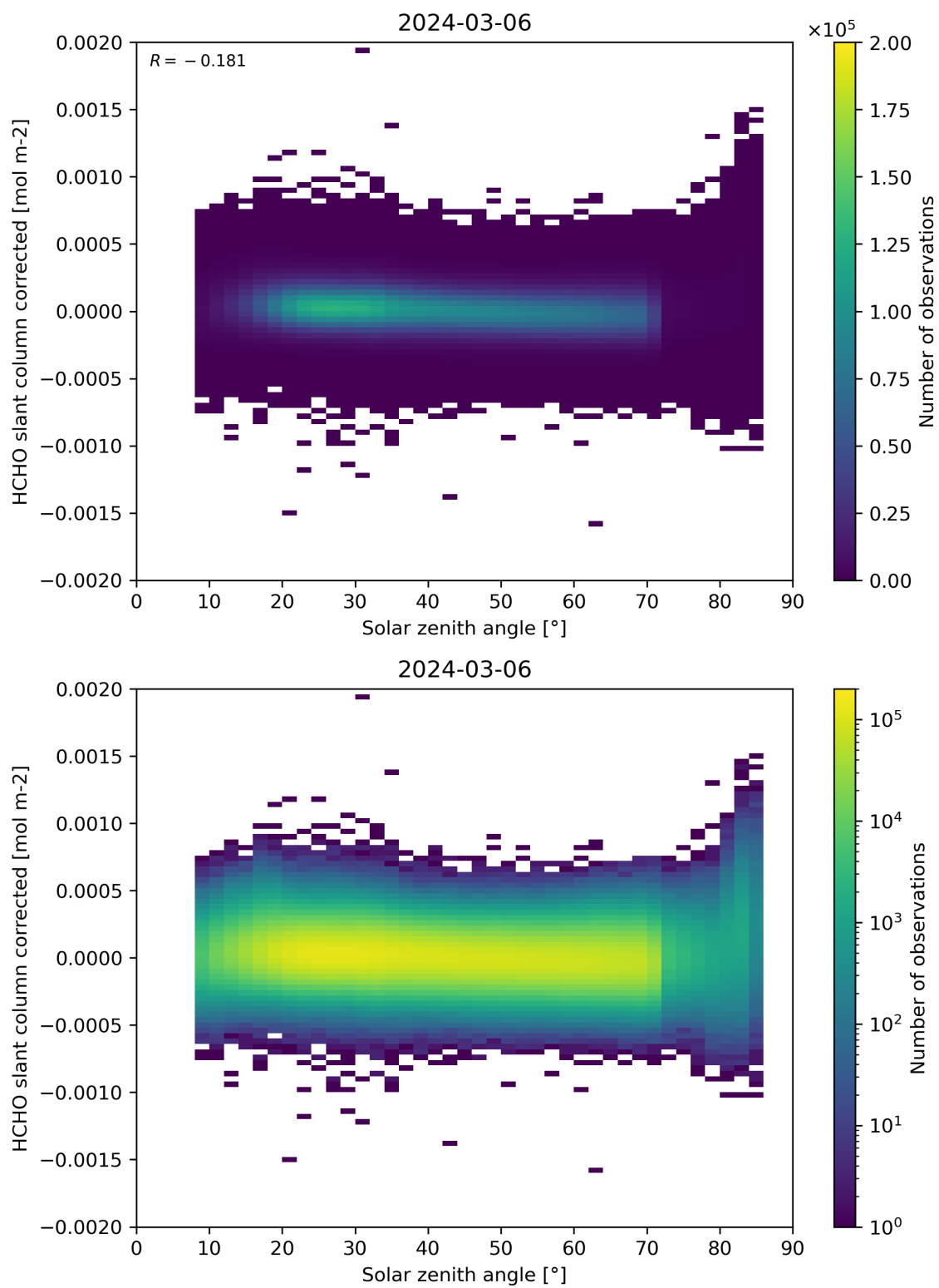
Figure 171: Scatter density plot of “Solar zenith angle” against “HCHO slant column corrected” for 2024-03-05 to 2024-03-07.
