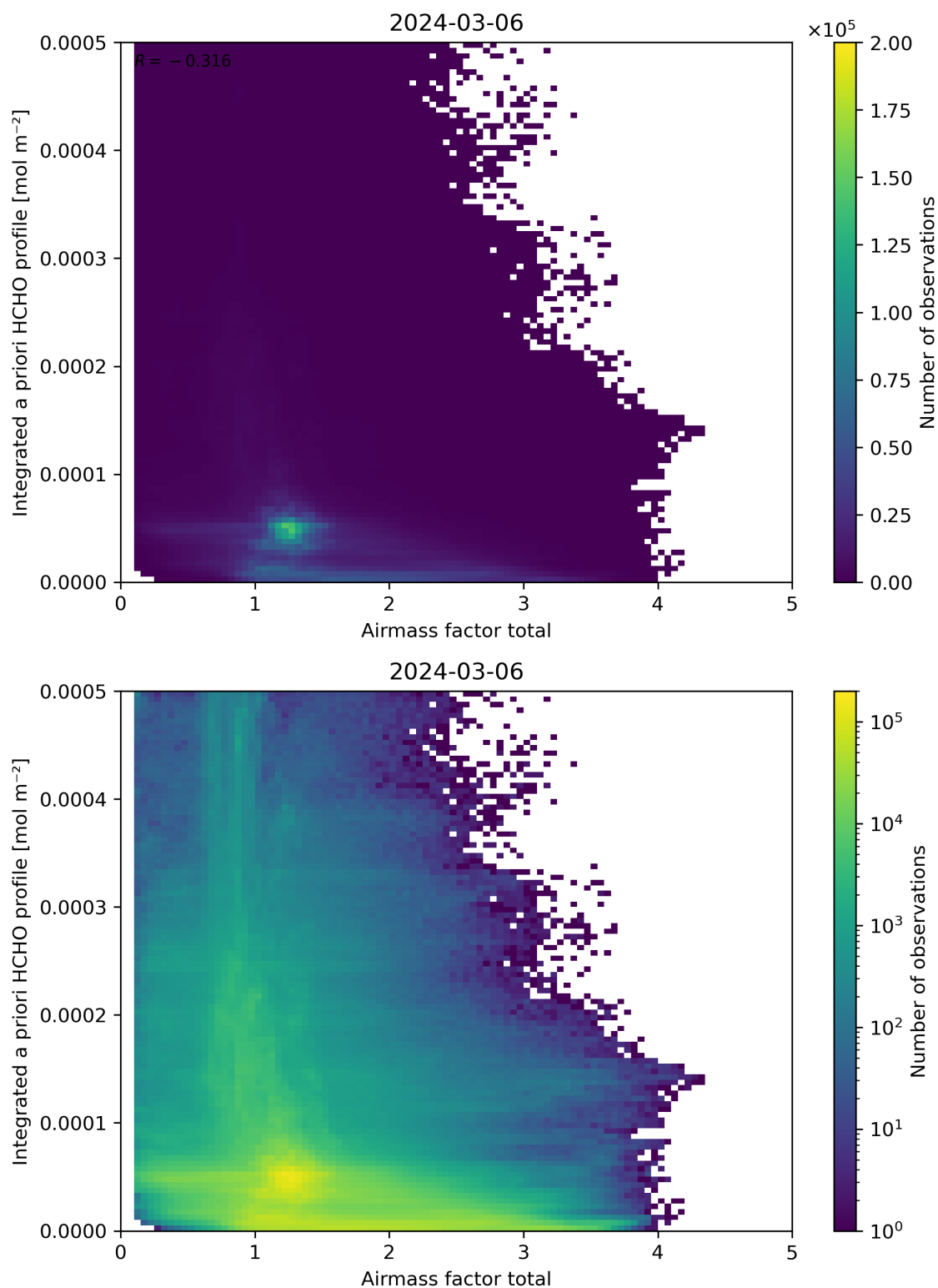
Figure 104: Scatter density plot of “Airmass factor total” against “Integrated a priori HCHO profile” for 2024-03-05 to 2024-03-07.
