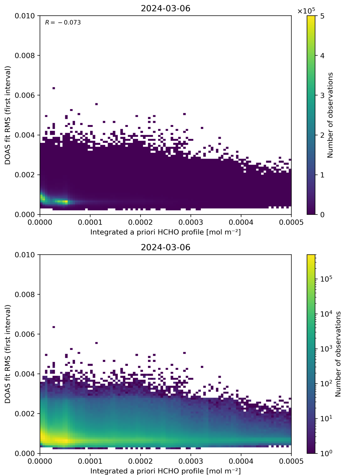
Figure 148: Scatter density plot of “Integrated a priori HCHO profile” against “DOAS fit RMS (first interval)” for 2024-03-05 to 2024-03-07.
