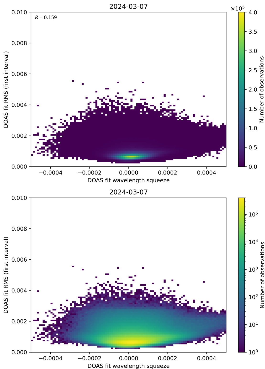
Figure 68: Scatter density plot of “DOAS fit wavelength squeeze” against “DOAS fit RMS (first interval)” for 2024-03-06 to 2024-03-08.
