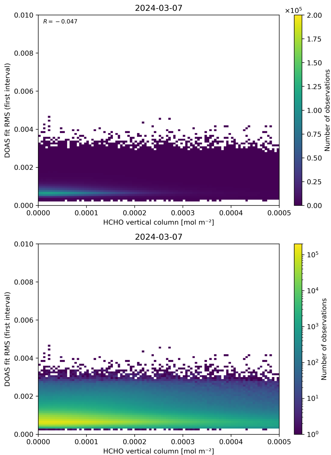
Figure 123: Scatter density plot of “HCHO vertical column” against “DOAS fit RMS (first interval)” for 2024-03-06 to 2024-03-08.
