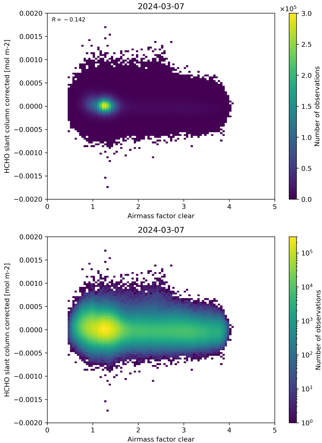
Figure 74: Scatter density plot of “Airmass factor clear” against “HCHO slant column corrected” for 2024-03-06 to 2024-03-08.
