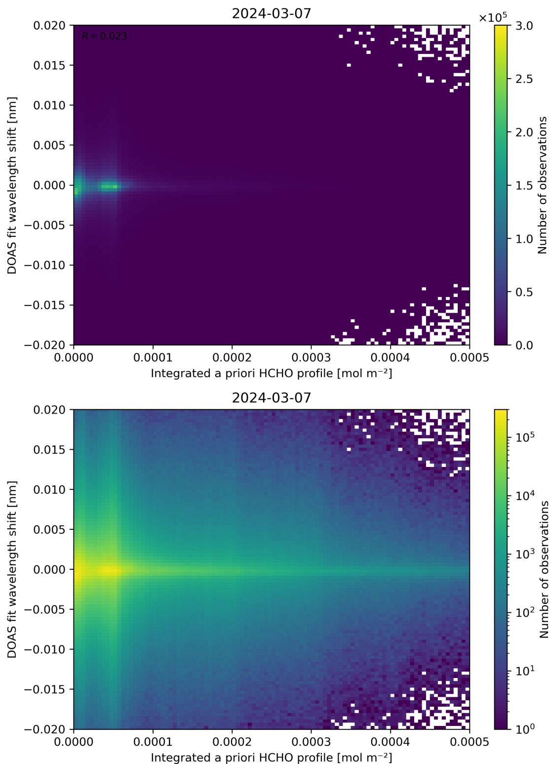
Figure 149: Scatter density plot of “Integrated a priori HCHO profile” against “DOAS fit wavelength shift” for 2024-03-06 to 2024-03-08.
