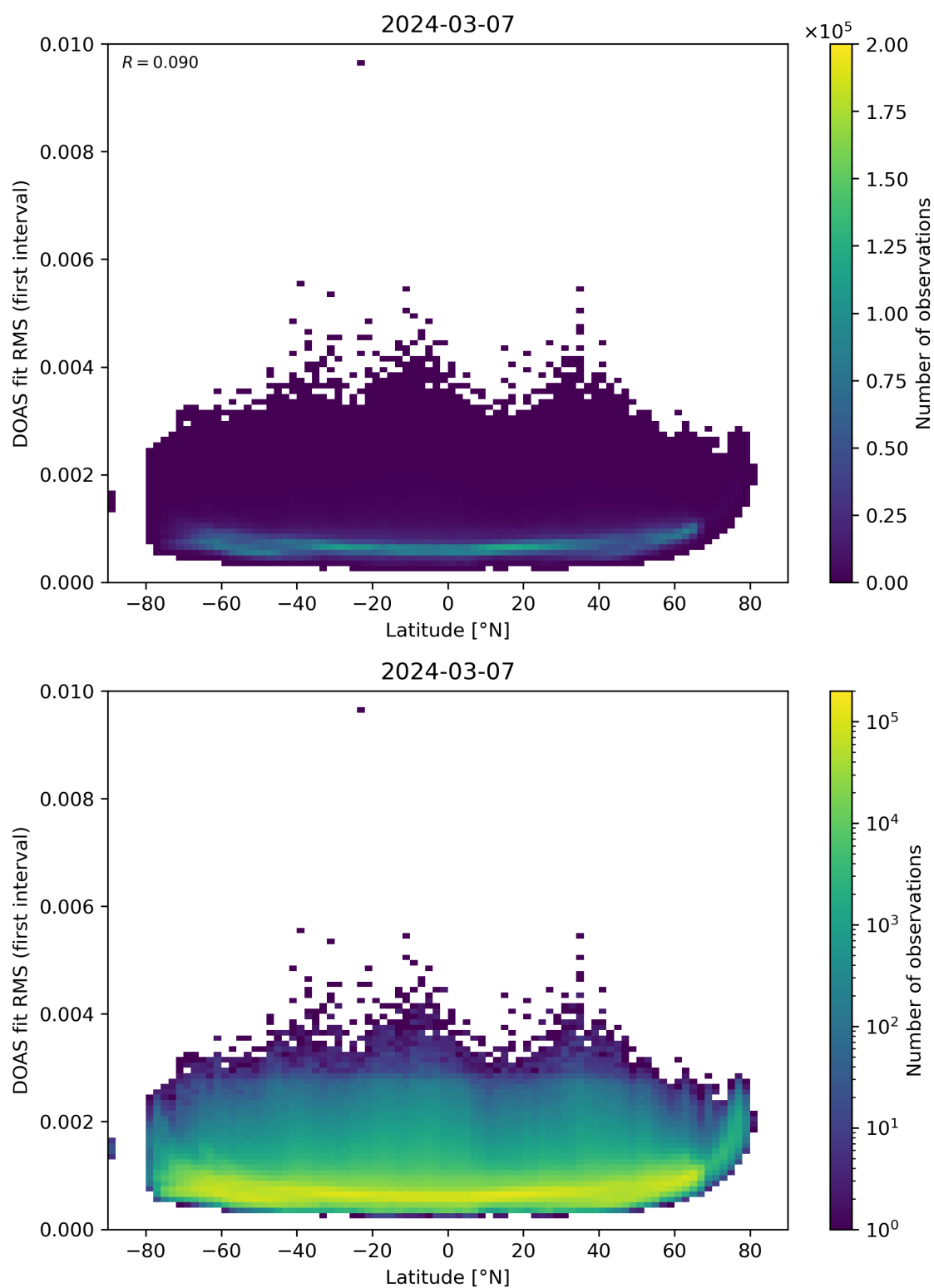
Figure 153: Scatter density plot of “Latitude” against “DOAS fit RMS (first interval)” for 2024-03-06 to 2024-03-08.
