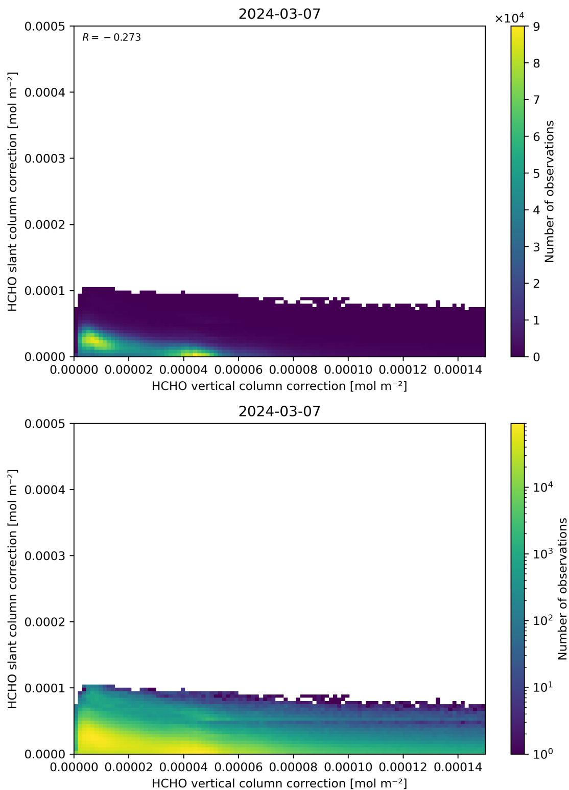
Figure 117: Scatter density plot of “HCHO vertical column correction” against “HCHO slant column correction” for 2024-03-06 to 2024-03-08.
