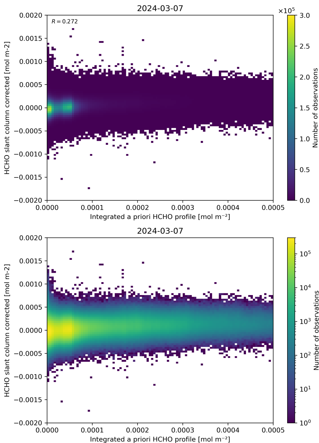
Figure 151: Scatter density plot of “Integrated a priori HCHO profile” against “HCHO slant column corrected” for 2024-03-06 to 2024-03-08.
