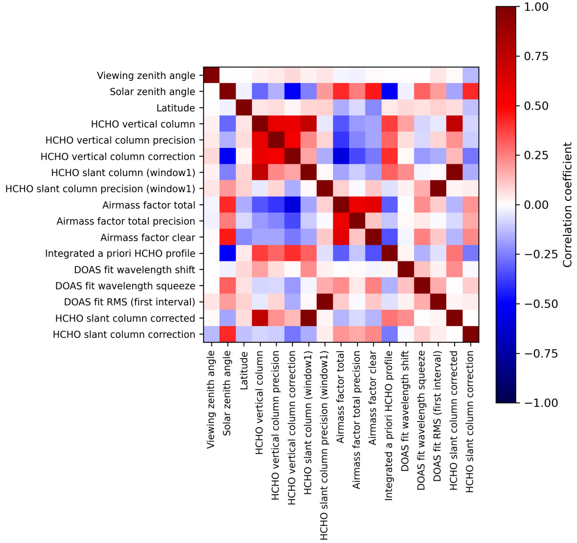
Figure 2: Map of correlation matrix for 2024-03-06 to 2024-03-08.
