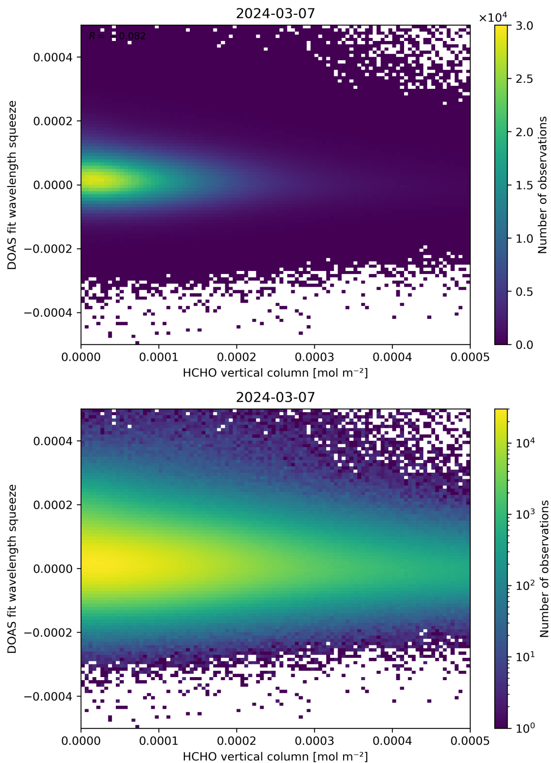
Figure 125: Scatter density plot of “HCHO vertical column” against “DOAS fit wavelength squeeze” for 2024-03-06 to 2024-03-08.
