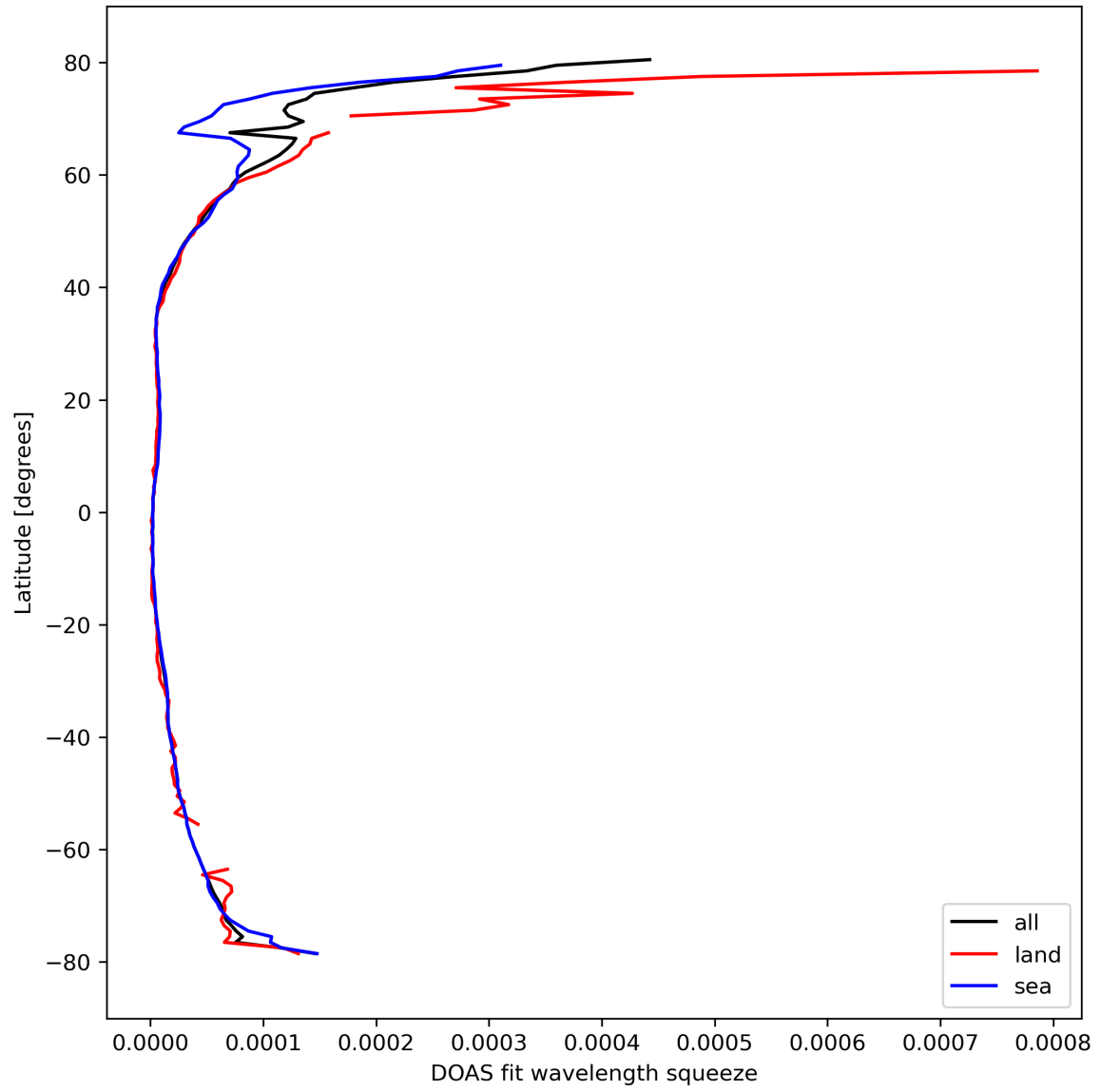
Figure 31: Zonal average of “DOAS fit wavelength squeeze” for 2024-03-06 to 2024-03-08.
