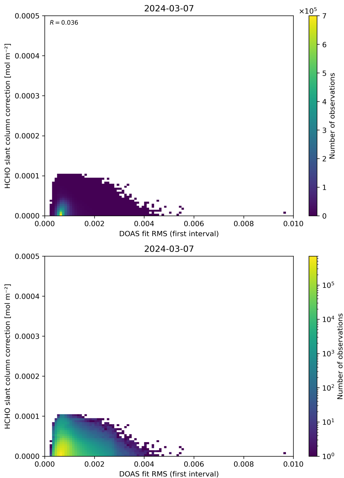
Figure 63: Scatter density plot of “DOAS fit RMS (first interval)” against “HCHO slant column correction” for 2024-03-06 to 2024-03-08.
