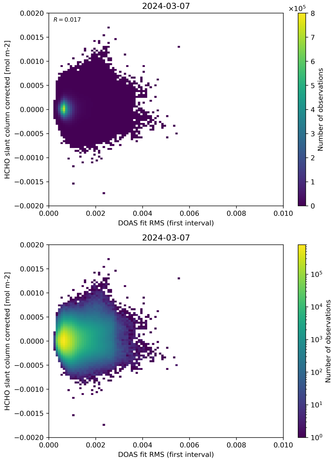
Figure 62: Scatter density plot of “DOAS fit RMS (first interval)” against “HCHO slant column corrected” for 2024-03-06 to 2024-03-08.
