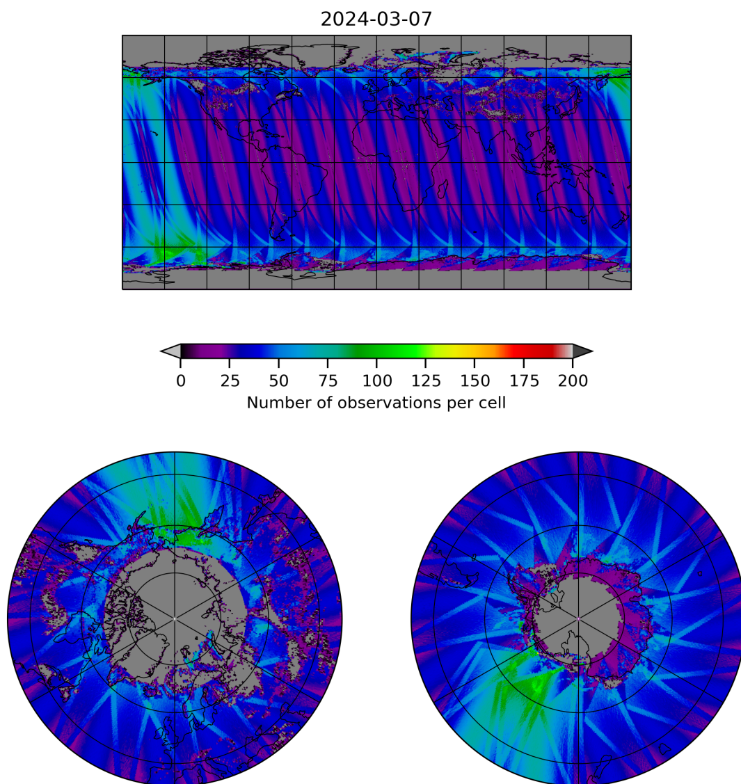
Figure 19: Map of the number of observations for 2024-03-06 to 2024-03-08
