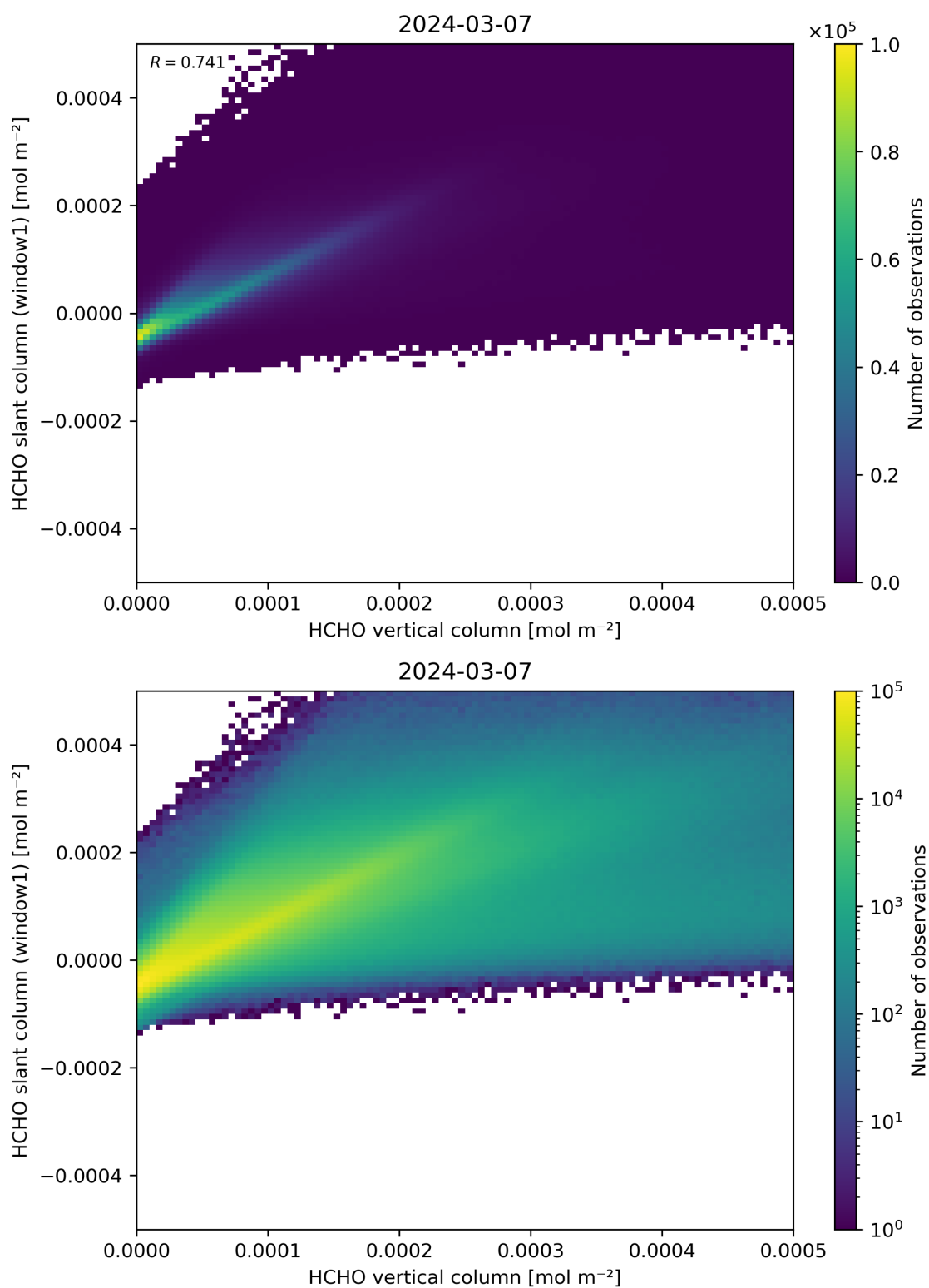
Figure 129: Scatter density plot of “HCHO vertical column” against “HCHO slant column (window1)” for 2024-03-06 to 2024-03-08.
