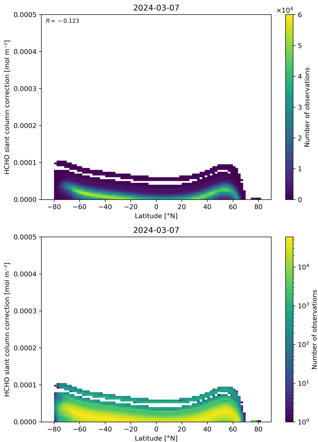
Figure 158: Scatter density plot of “Latitude” against “HCHO slant column correction” for 2024-03-06 to 2024-03-08.
