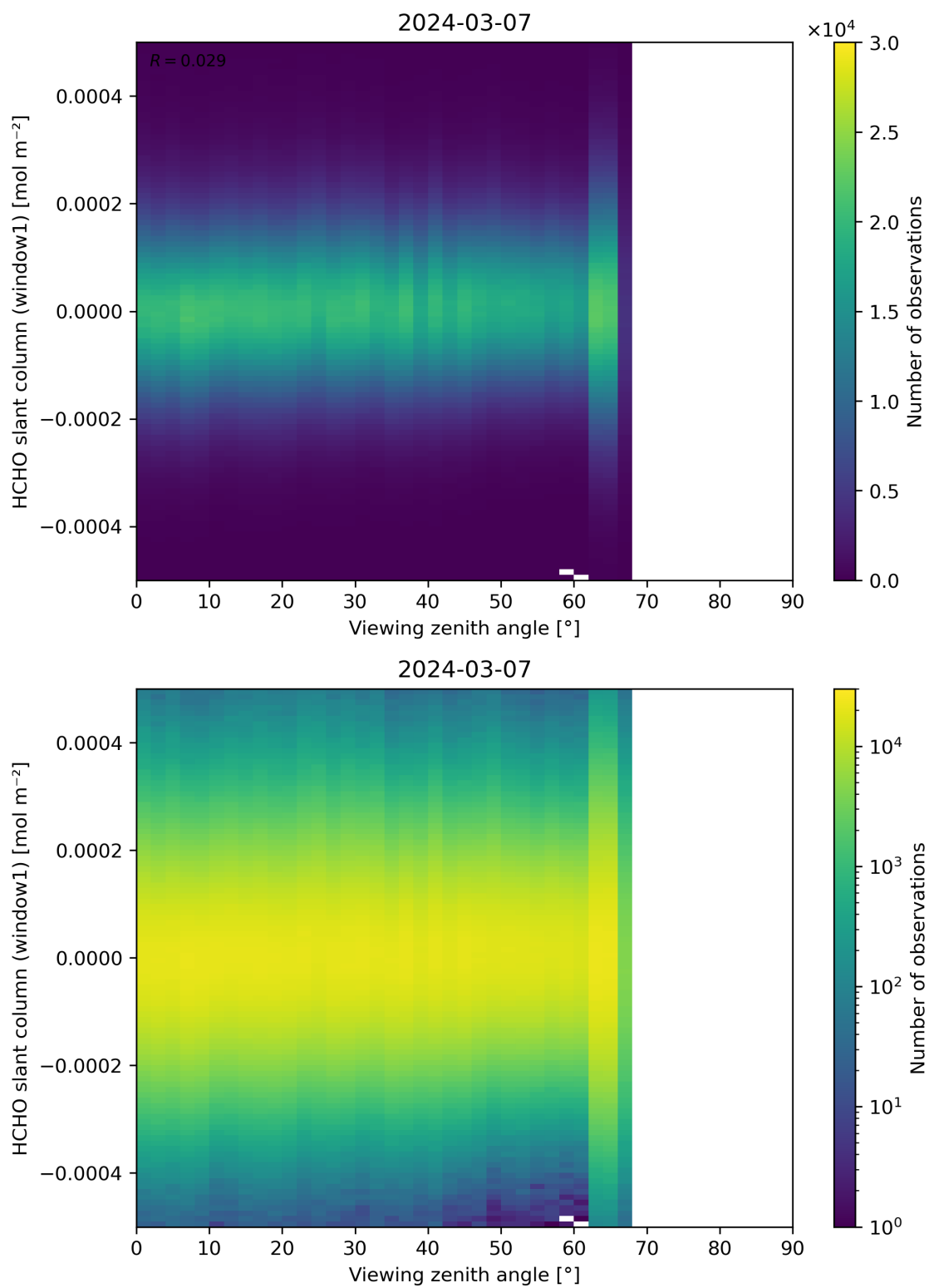
Figure 188: Scatter density plot of “Viewing zenith angle” against “HCHO slant column (window1)” for 2024-03-06 to 2024-03-08.
