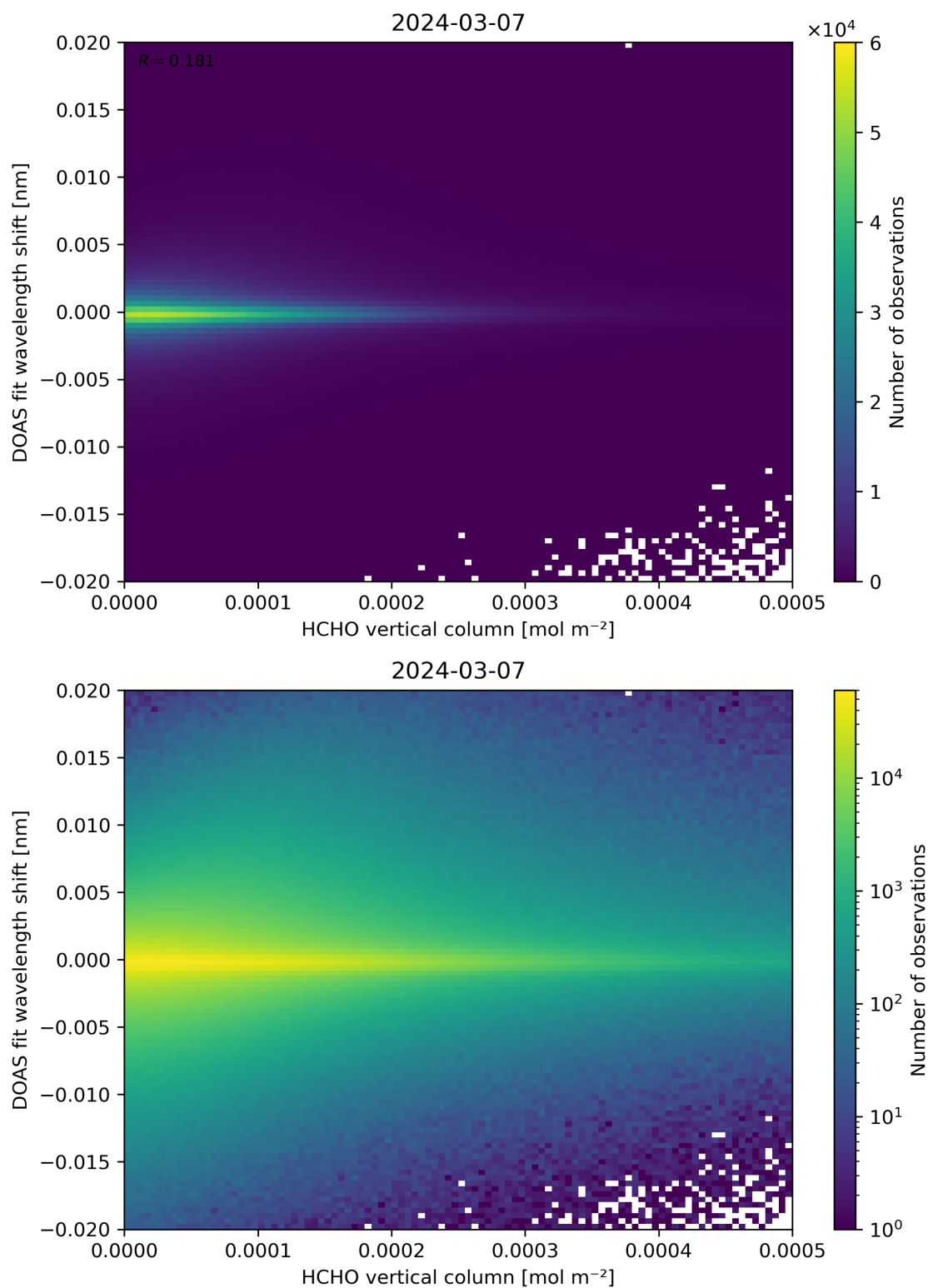
Figure 124: Scatter density plot of “HCHO vertical column” against “DOAS fit wavelength shift” for 2024-03-06 to 2024-03-08.
