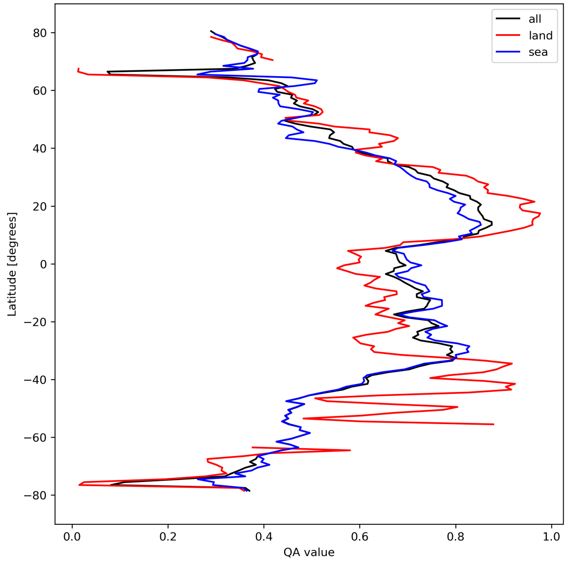
Figure 20: Zonal average of “QA value” for 2024-03-06 to 2024-03-08.
