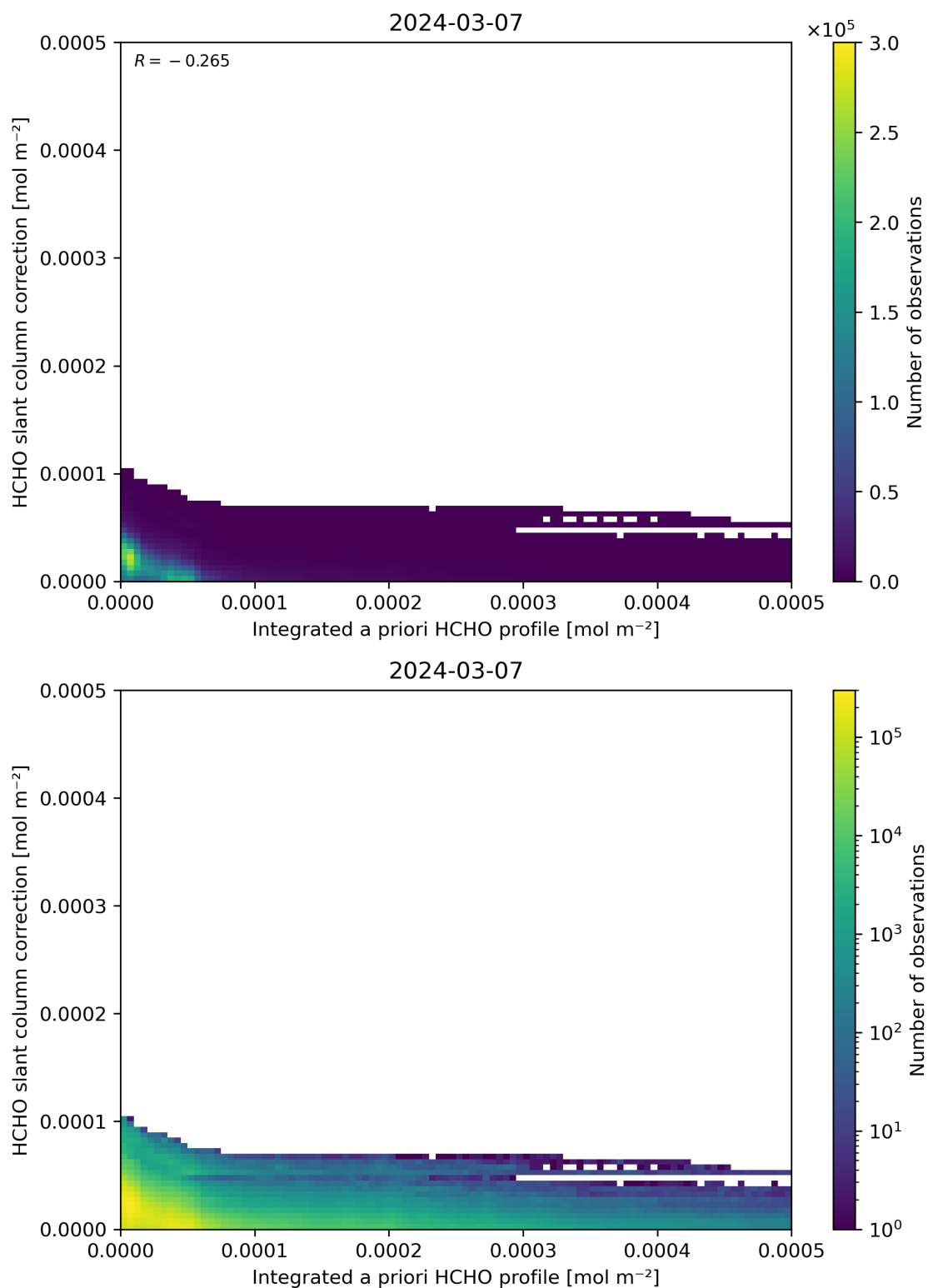
Figure 152: Scatter density plot of “Integrated a priori HCHO profile” against “HCHO slant column correction” for 2024-03-06 to 2024-03-08.
