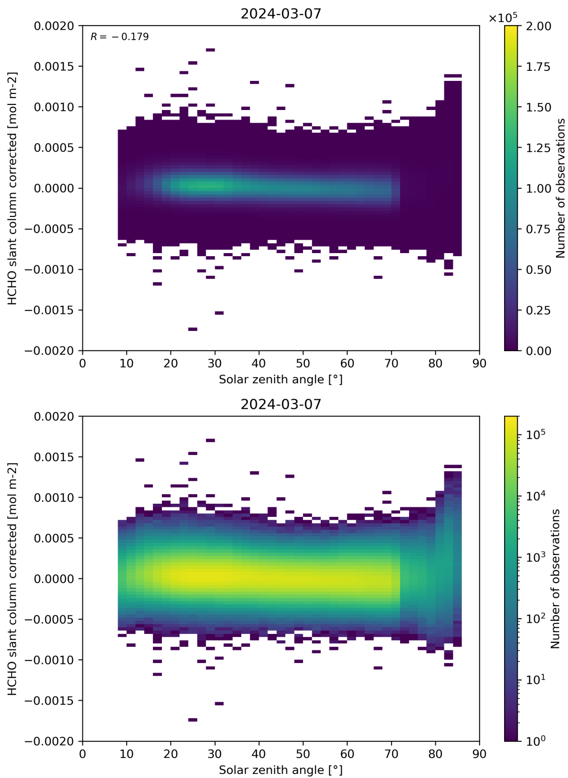
Figure 171: Scatter density plot of “Solar zenith angle” against “HCHO slant column corrected” for 2024-03-06 to 2024-03-08.
