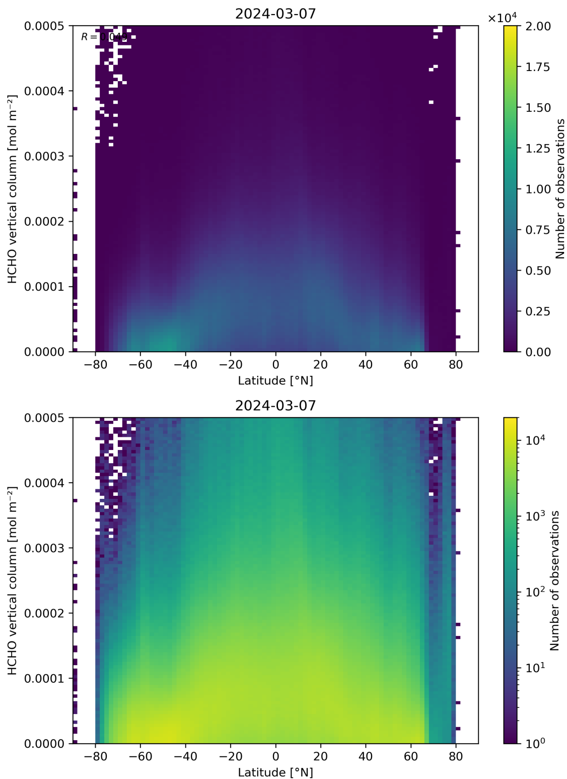
Figure 163: Scatter density plot of “Latitude” against “HCHO vertical column” for 2024-03-06 to 2024-03-08.
