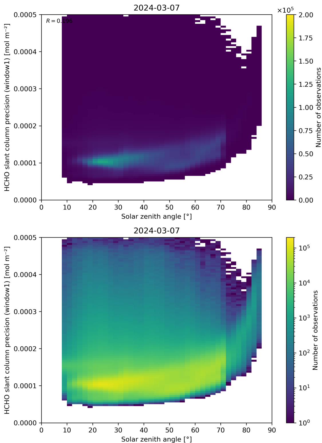
Figure 174: Scatter density plot of “Solar zenith angle” against “HCHO slant column precision (window1)” for 2024-03-06 to 2024-03-08.
