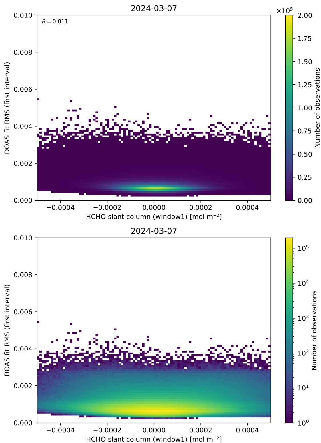
Figure 78: Scatter density plot of “HCHO slant column (window1)” against “DOAS fit RMS (first interval)” for 2024-03-06 to 2024-03-08.
