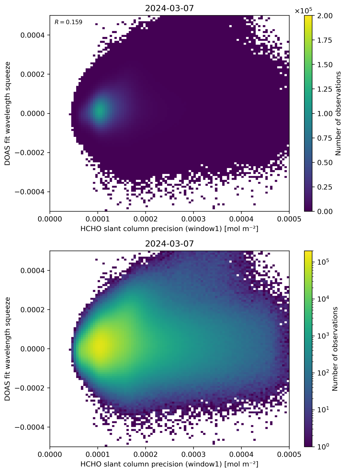
Figure 90: Scatter density plot of “HCHO slant column precision (window1)” against “DOAS fit wavelength squeeze” for 2024-03-06 to 2024-03-08.
