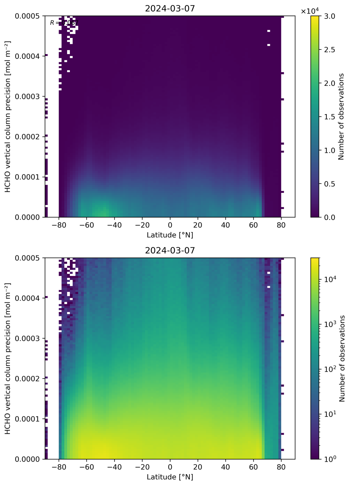
Figure 165: Scatter density plot of “Latitude” against “HCHO vertical column precision” for 2024-03-06 to 2024-03-08.
