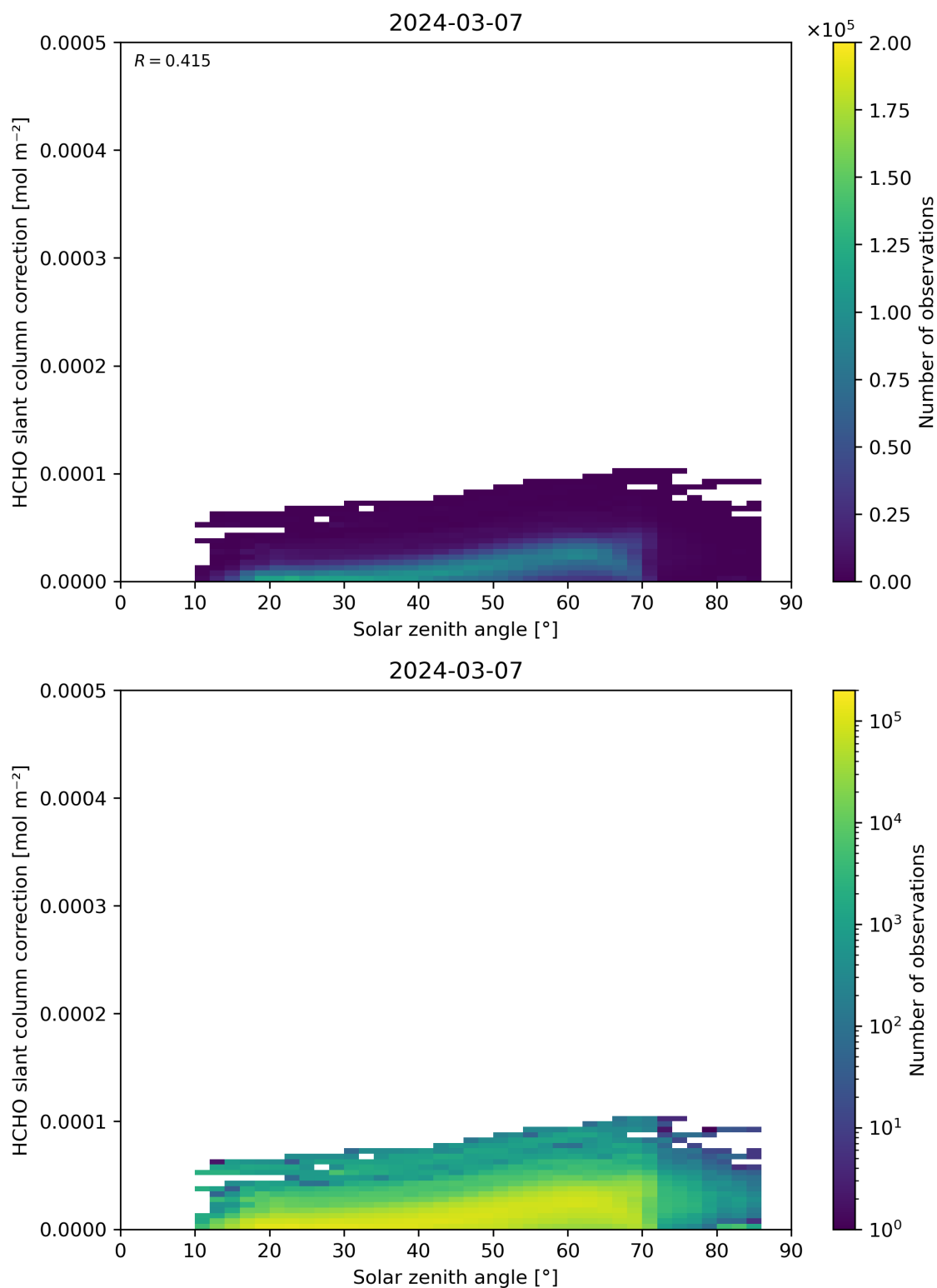
Figure 172: Scatter density plot of “Solar zenith angle” against “HCHO slant column correction” for 2024-03-06 to 2024-03-08.
