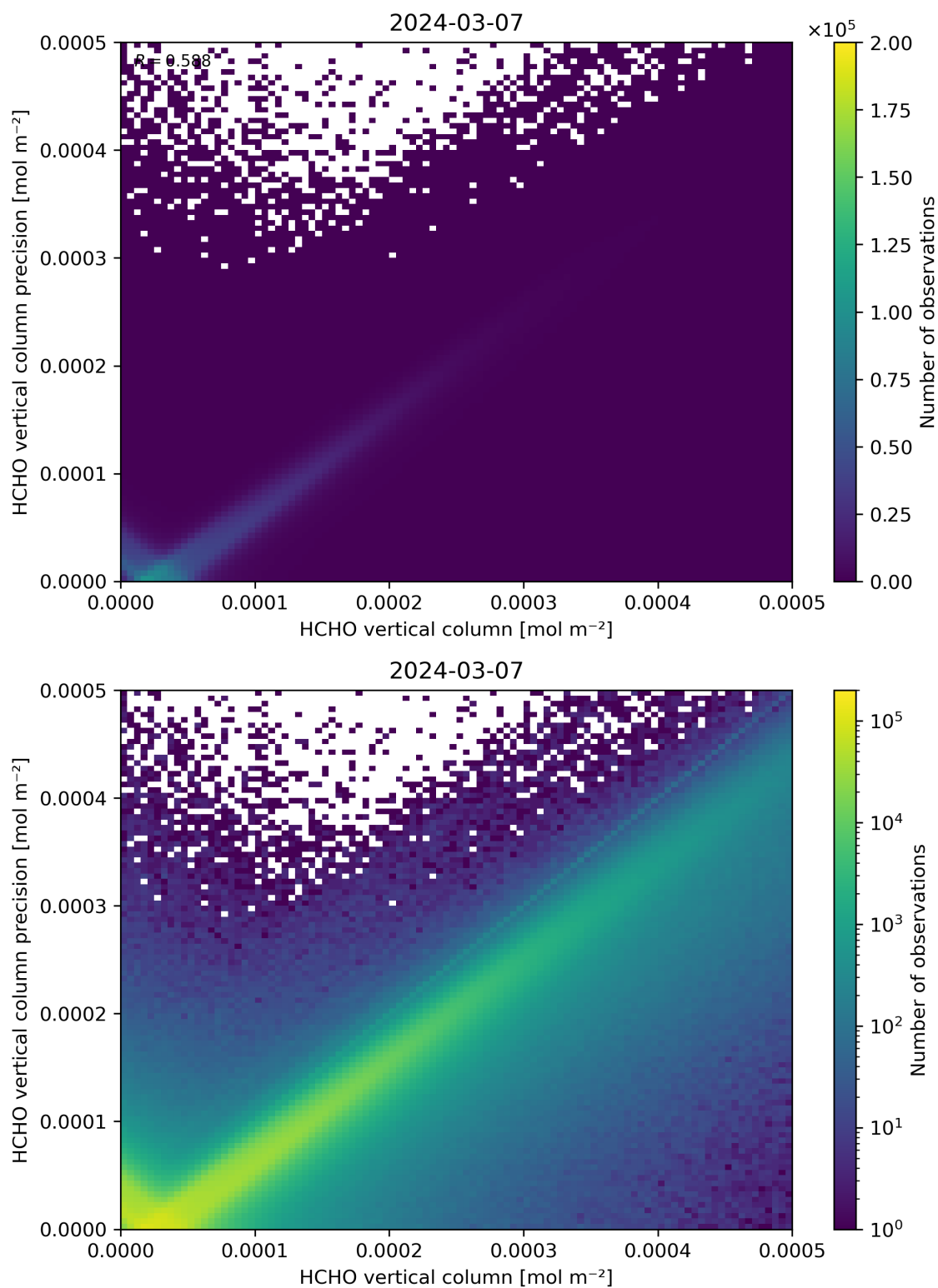
Figure 134: Scatter density plot of “HCHO vertical column” against “HCHO vertical column precision” for 2024-03-06 to 2024-03-08.
