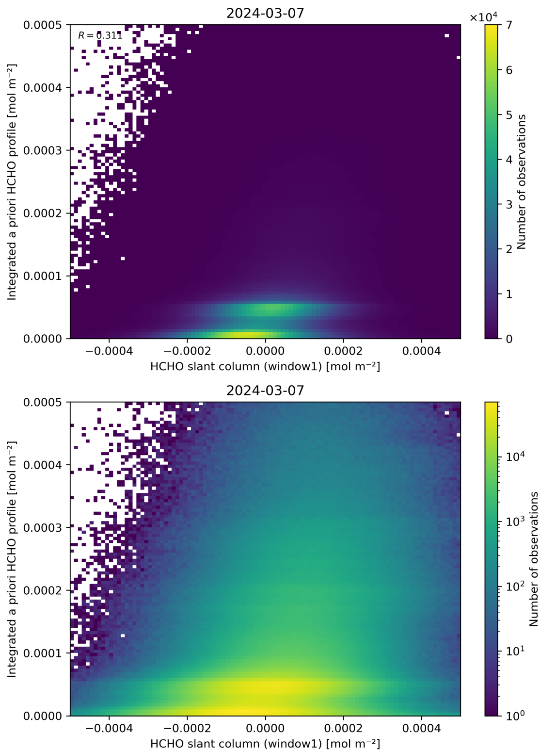
Figure 87: Scatter density plot of “HCHO slant column (window1)” against “Integrated a priori HCHO profile” for 2024-03-06 to 2024-03-08.
