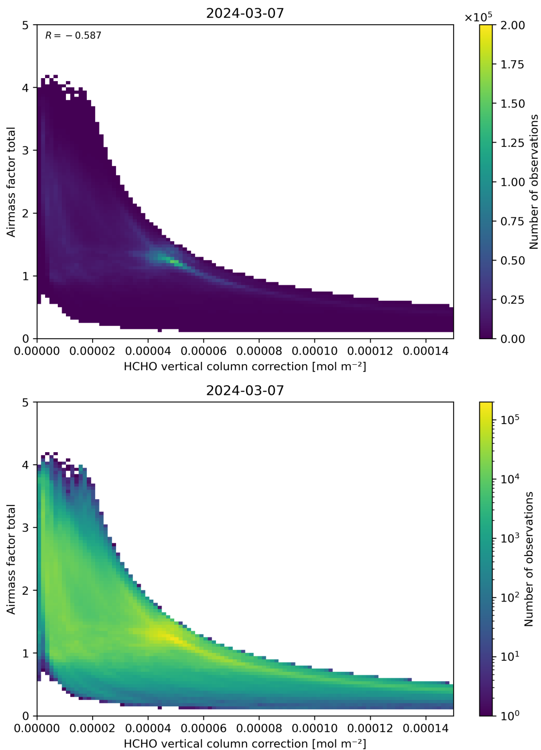
Figure 120: Scatter density plot of “HCHO vertical column correction” against “Airmass factor total” for 2024-03-06 to 2024-03-08.
