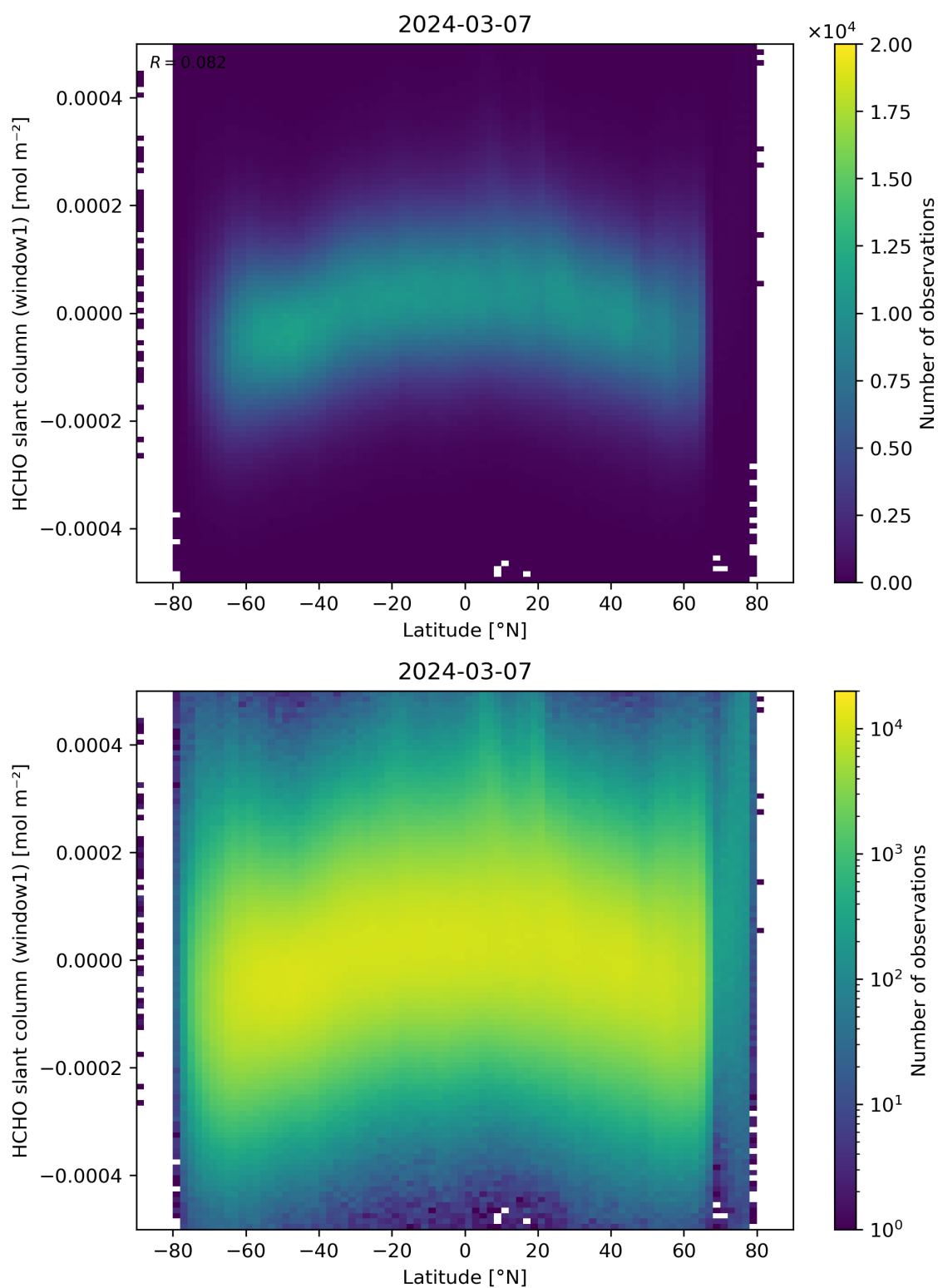
Figure 159: Scatter density plot of “Latitude” against “HCHO slant column (window1)” for 2024-03-06 to 2024-03-08.
