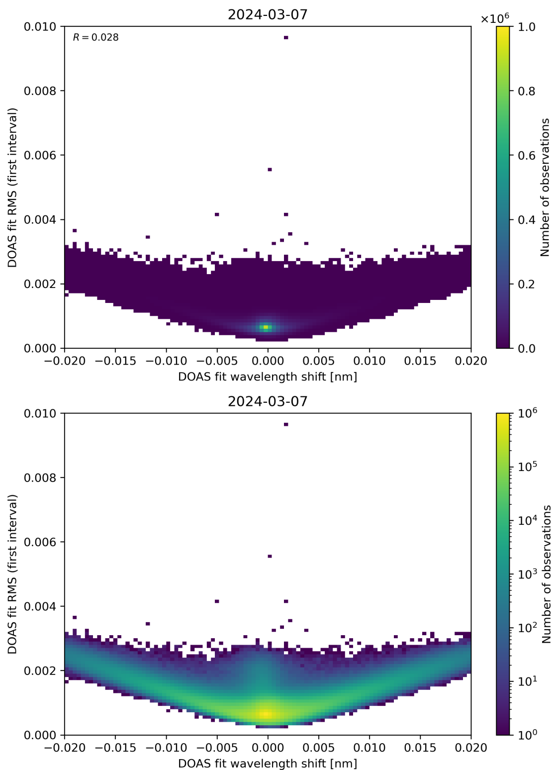
Figure 64: Scatter density plot of “DOAS fit wavelength shift” against “DOAS fit RMS (first interval)” for 2024-03-06 to 2024-03-08.
