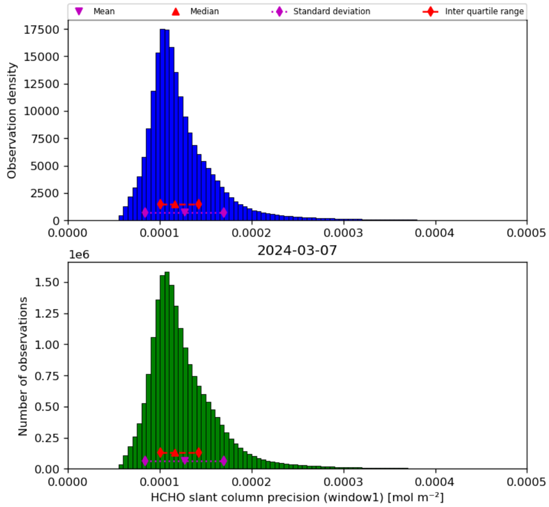
Figure 39: Histogram of “HCHO slant column precision (window1)” for 2024-03-06 to 2024-03-08
