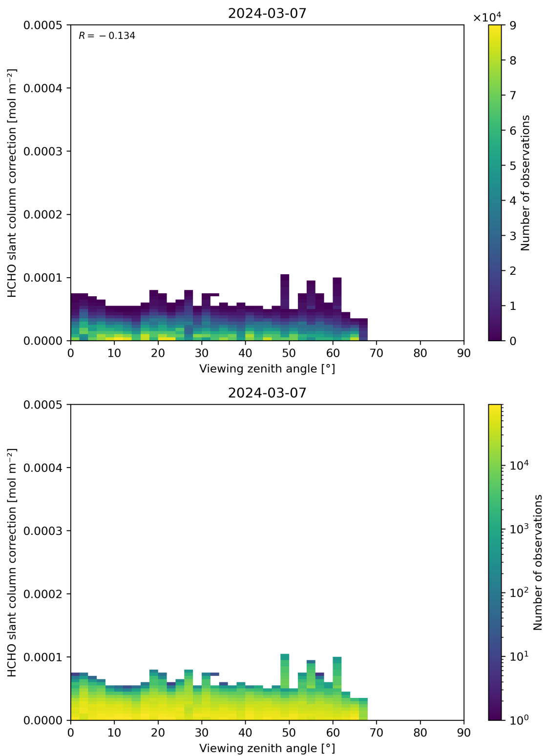
Figure 187: Scatter density plot of “Viewing zenith angle” against “HCHO slant column correction” for 2024-03-06 to 2024-03-08.
