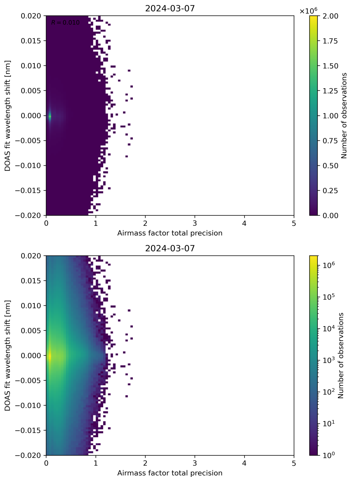
Figure 106: Scatter density plot of “Airmass factor total precision” against “DOAS fit wavelength shift” for 2024-03-06 to 2024-03-08.
