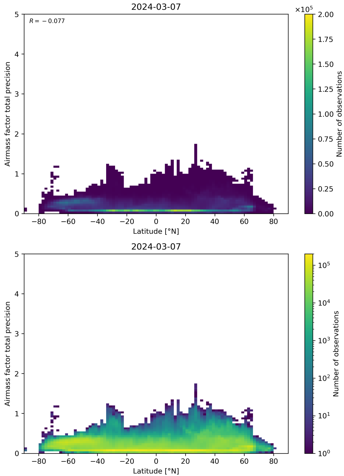
Figure 162: Scatter density plot of “Latitude” against “Airmass factor total precision” for 2024-03-06 to 2024-03-08.
