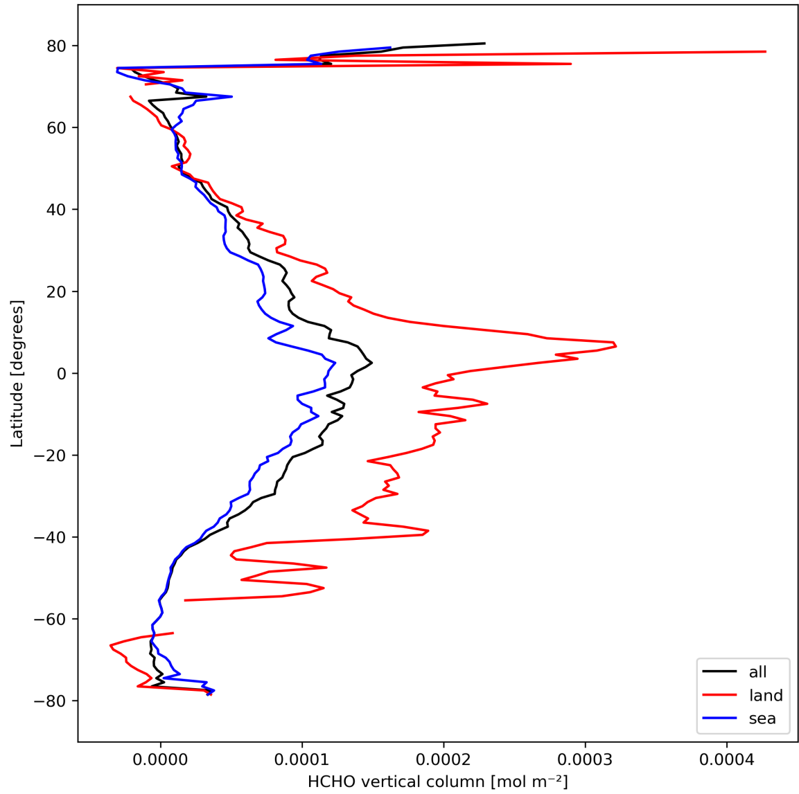
Figure 21: Zonal average of “HCHO vertical column” for 2024-03-06 to 2024-03-08.
