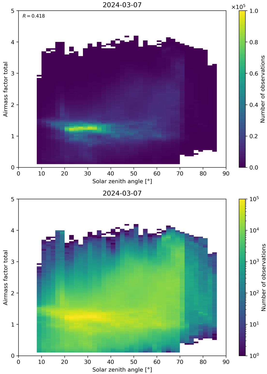
Figure 175: Scatter density plot of “Solar zenith angle” against “Airmass factor total” for 2024-03-06 to 2024-03-08.
