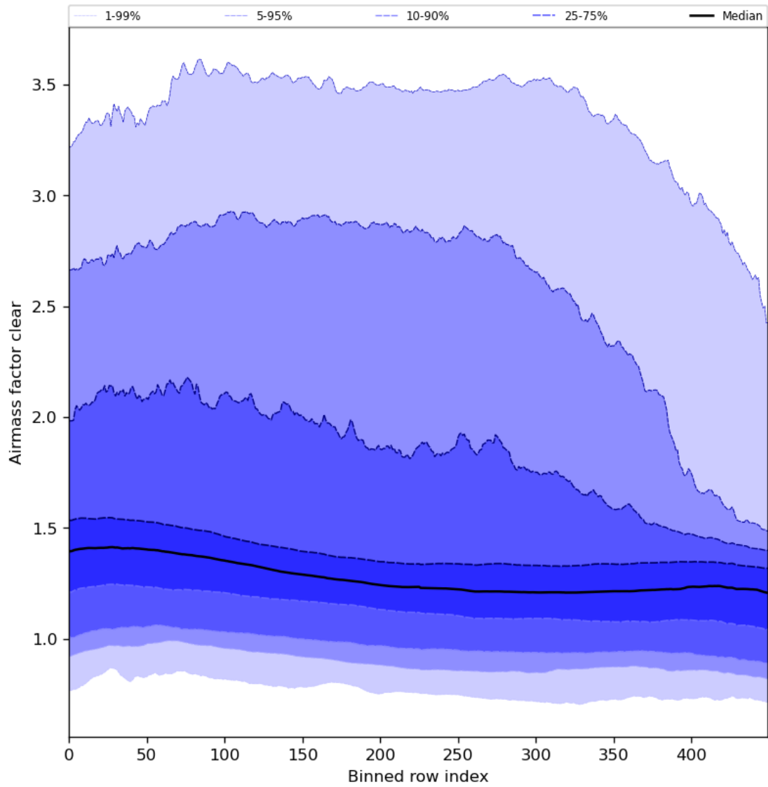
Figure 56: Along track statistics of “Airmass factor clear” for 2024-03-06 to 2024-03-08
