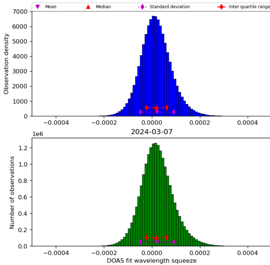
Figure 45: Histogram of “DOAS fit wavelength squeeze” for 2024-03-06 to 2024-03-08
