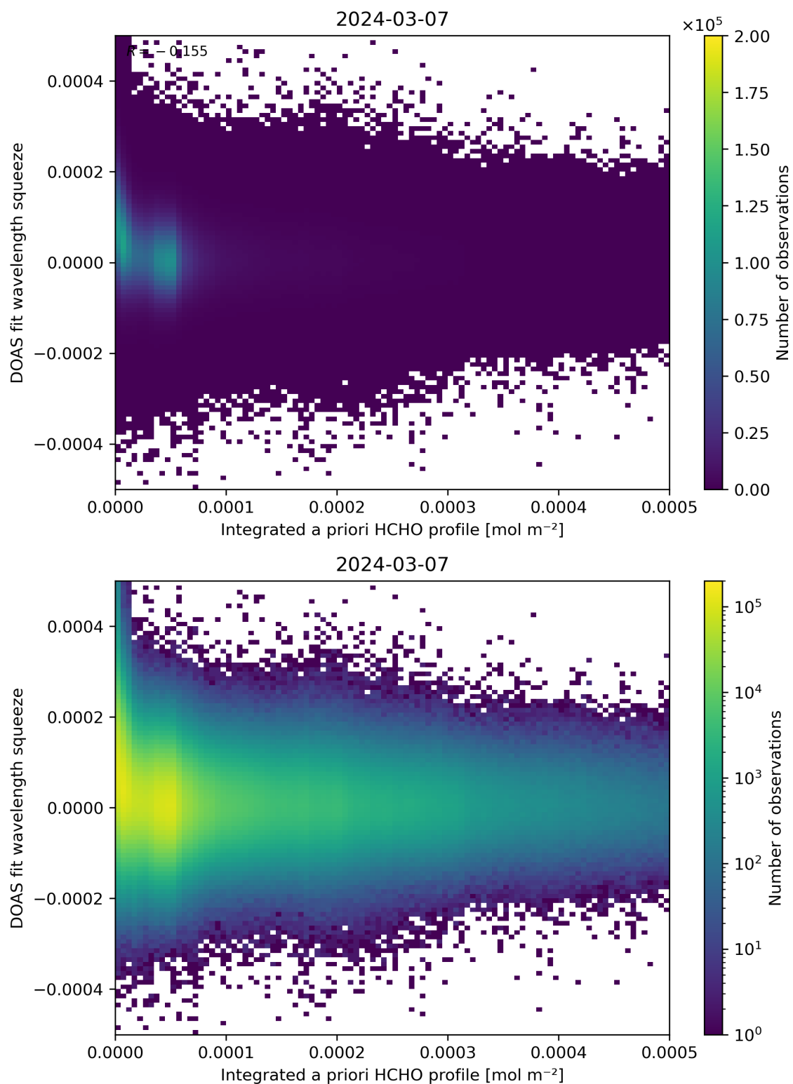
Figure 150: Scatter density plot of “Integrated a priori HCHO profile” against “DOAS fit wavelength squeeze” for 2024-03-06 to 2024-03-08.
