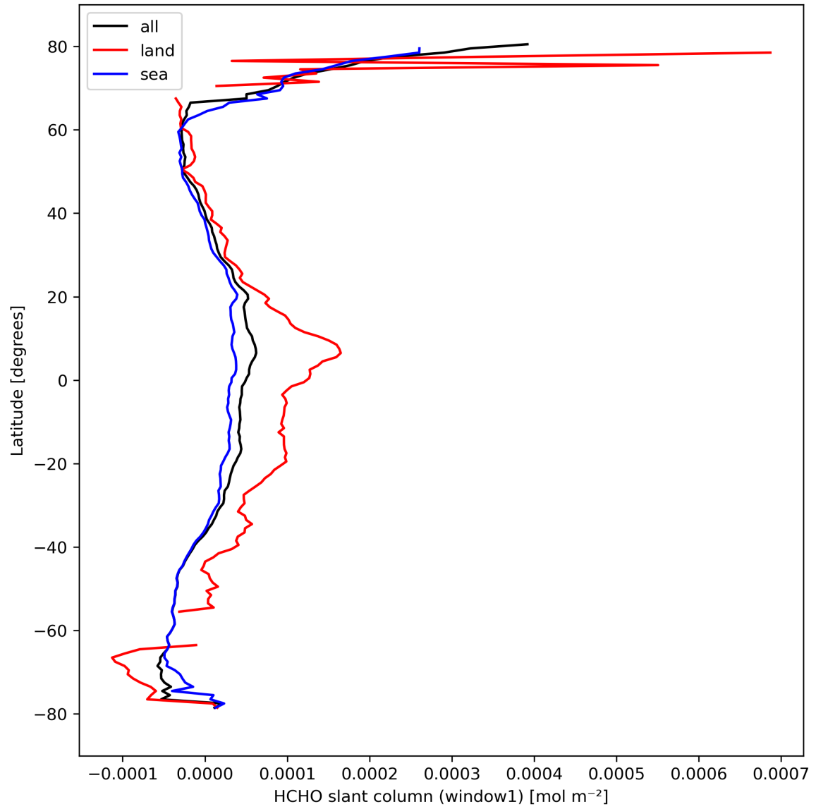
Figure 24: Zonal average of “HCHO slant column (window1)” for 2024-03-06 to 2024-03-08.
