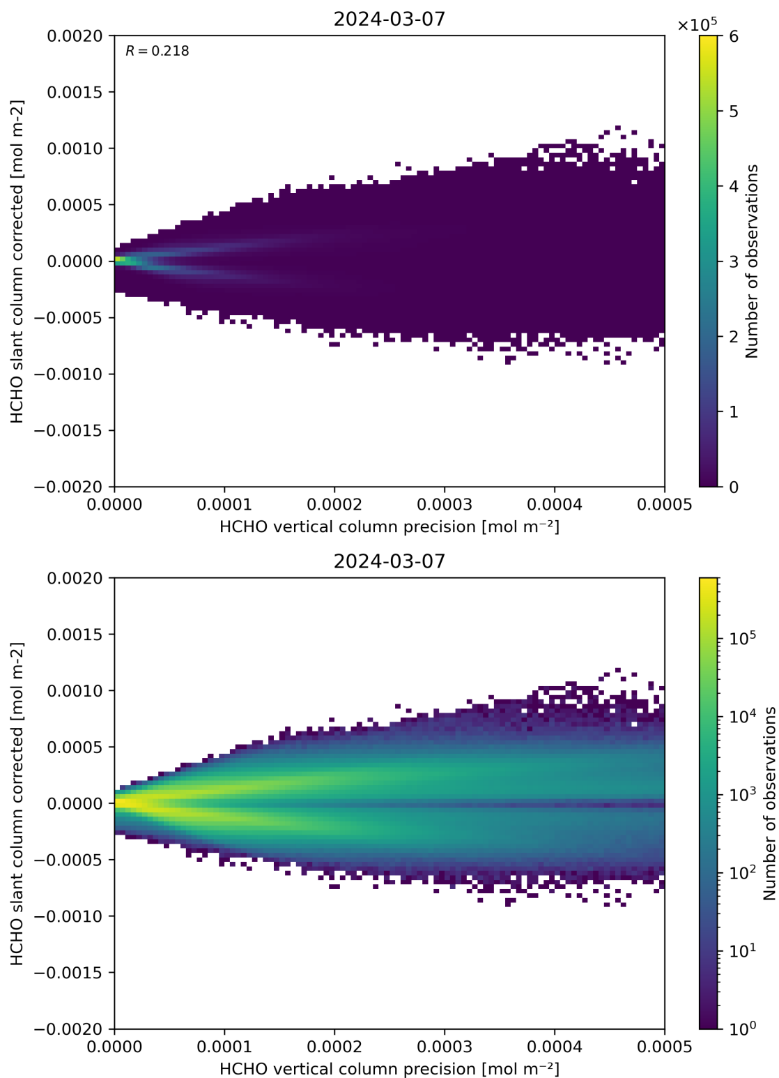
Figure 140: Scatter density plot of “HCHO vertical column precision” against “HCHO slant column corrected” for 2024-03-06 to 2024-03-08.
