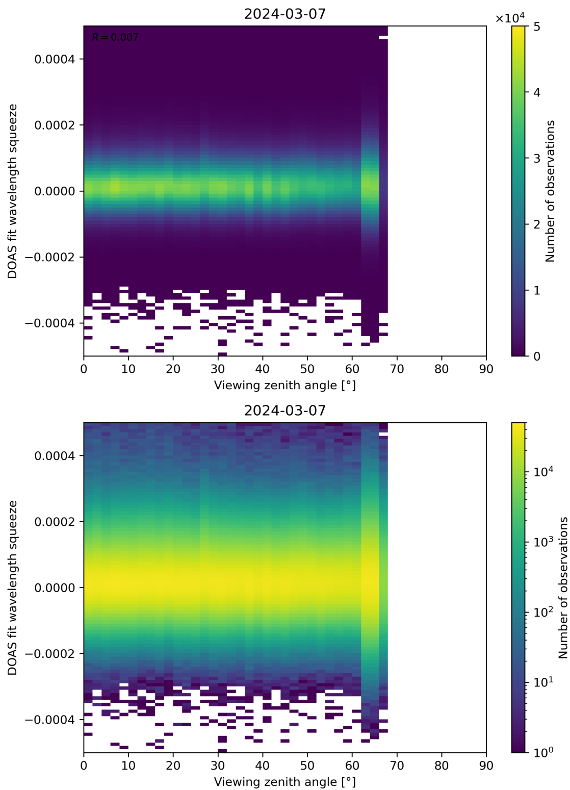
Figure 184: Scatter density plot of “Viewing zenith angle” against “DOAS fit wavelength squeeze” for 2024-03-06 to 2024-03-08.
