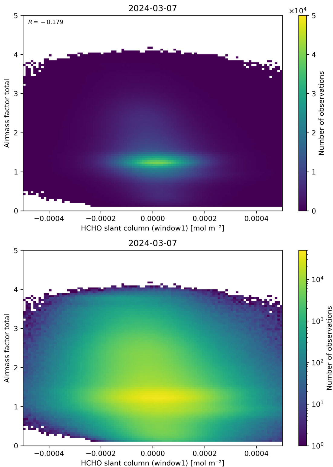
Figure 85: Scatter density plot of “HCHO slant column (window1)” against “Airmass factor total” for 2024-03-06 to 2024-03-08.
