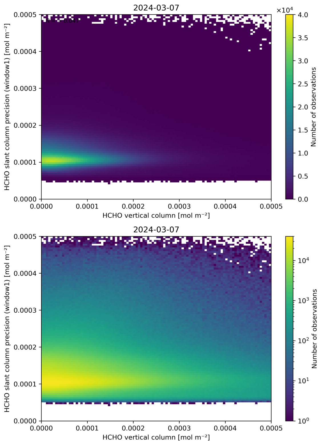
Figure 130: Scatter density plot of “HCHO vertical column” against “HCHO slant column precision (window1)” for 2024-03-06 to 2024-03-08.
