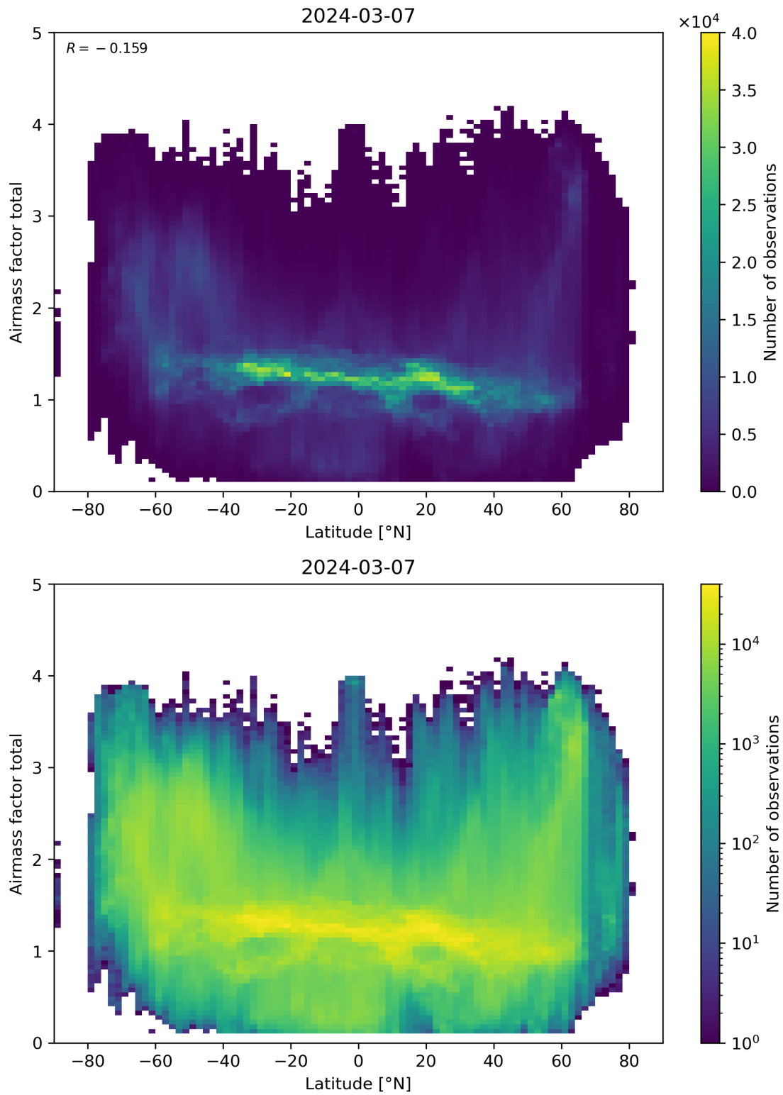
Figure 161: Scatter density plot of “Latitude” against “Airmass factor total” for 2024-03-06 to 2024-03-08.
