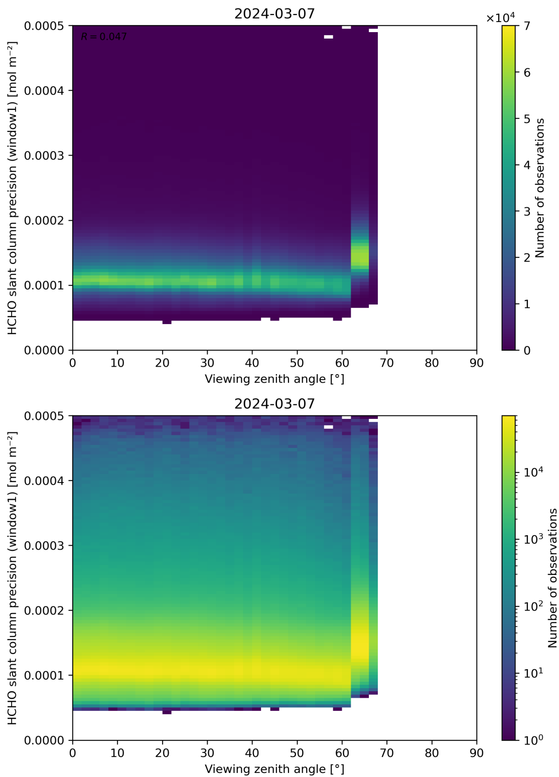
Figure 189: Scatter density plot of “Viewing zenith angle” against “HCHO slant column precision (window1)” for 2024-03-06 to 2024-03-08.
