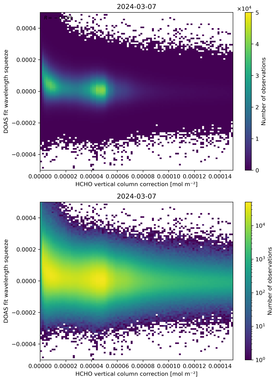
Figure 114: Scatter density plot of “HCHO vertical column correction” against “DOAS fit wavelength squeeze” for 2024-03-06 to 2024-03-08.
