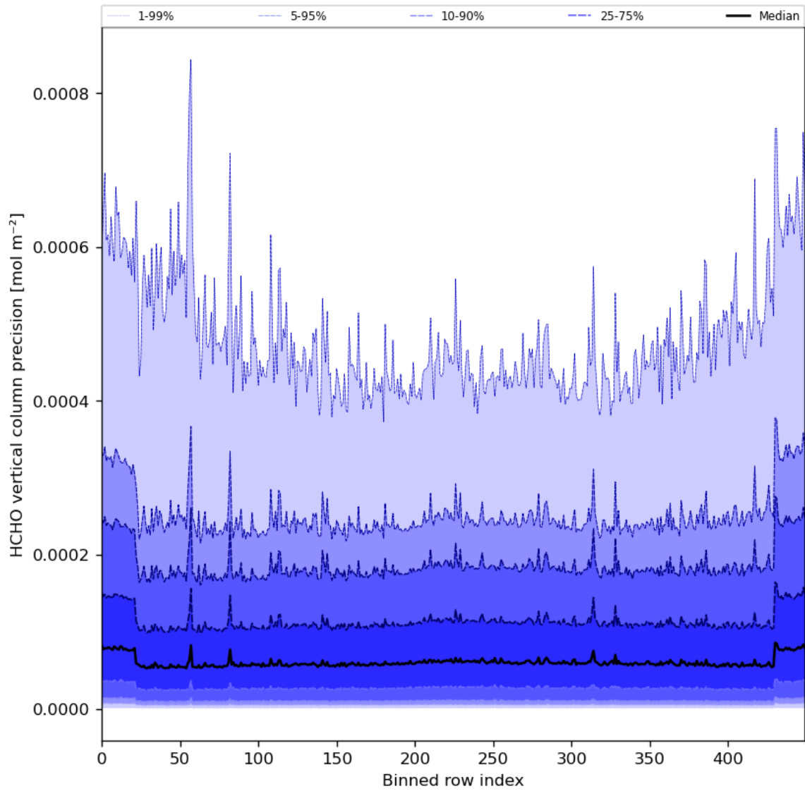
Figure 50: Along track statistics of “HCHO vertical column precision” for 2024-03-06 to 2024-03-08
