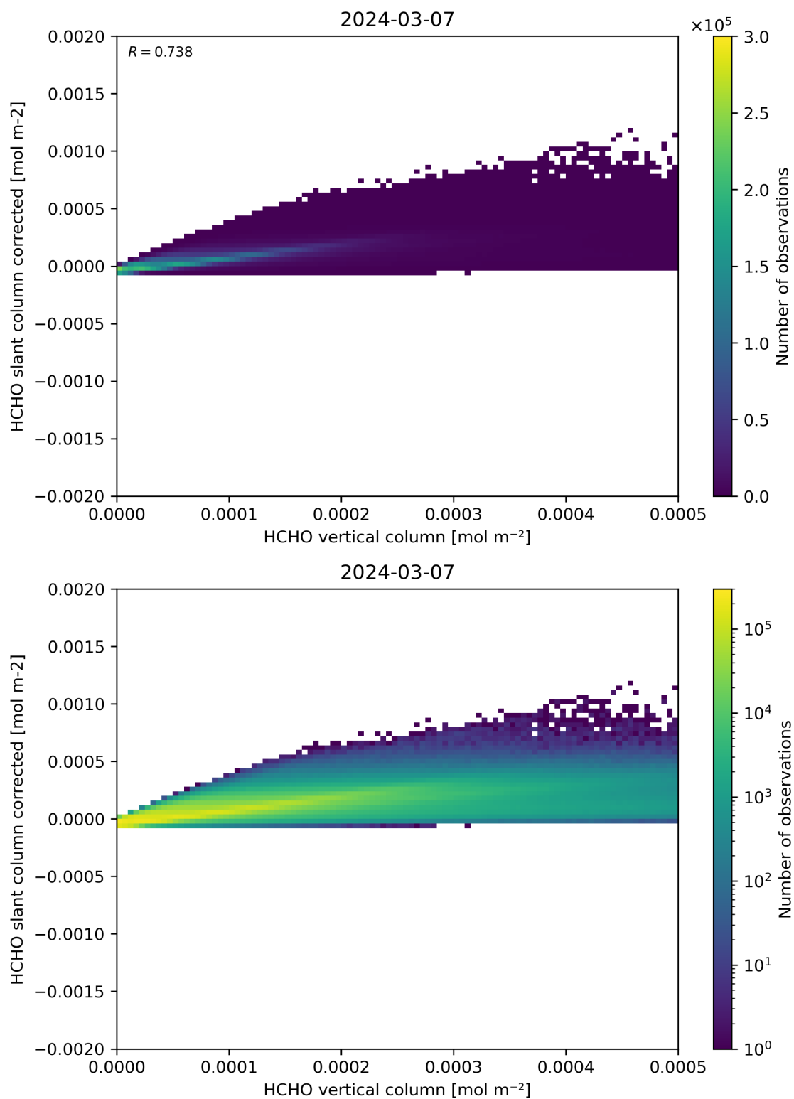
Figure 127: Scatter density plot of “HCHO vertical column” against “HCHO slant column corrected” for 2024-03-06 to 2024-03-08.
