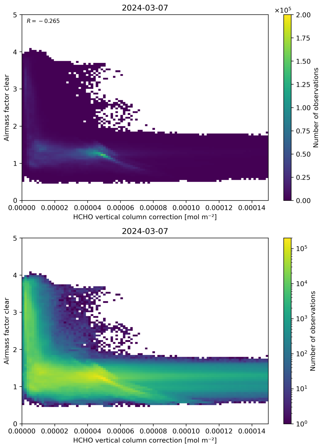
Figure 115: Scatter density plot of “HCHO vertical column correction” against “Airmass factor clear” for 2024-03-06 to 2024-03-08.
