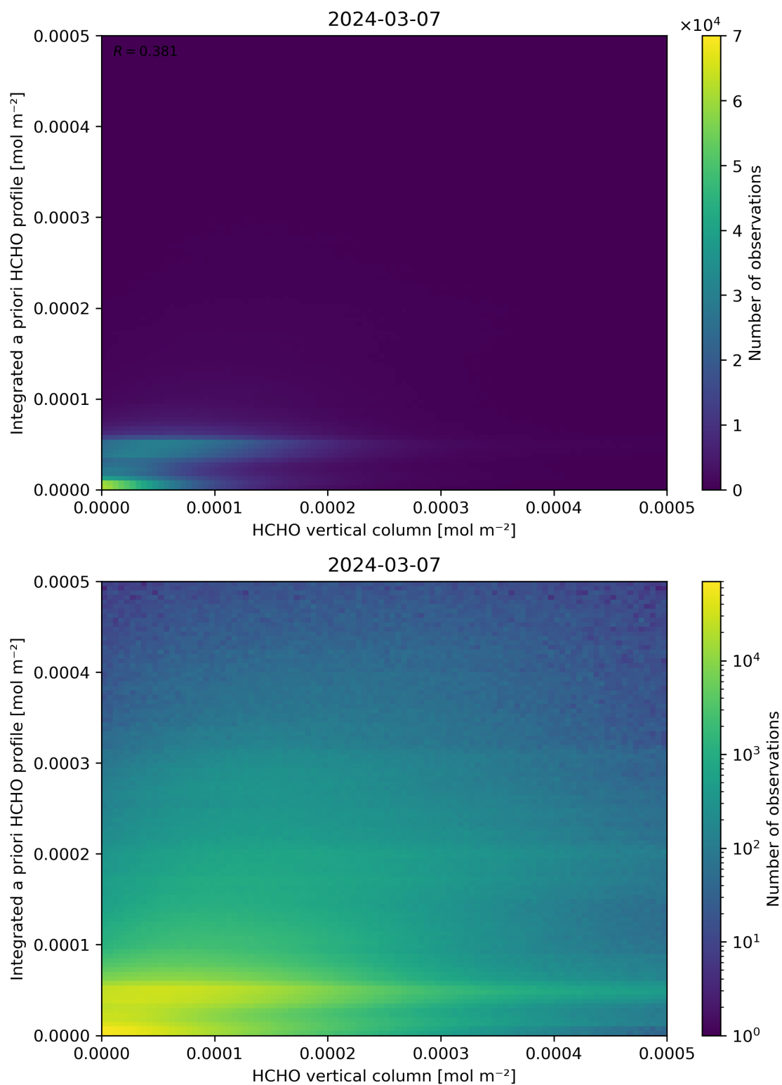
Figure 135: Scatter density plot of “HCHO vertical column” against “Integrated a priori HCHO profile” for 2024-03-06 to 2024-03-08.
