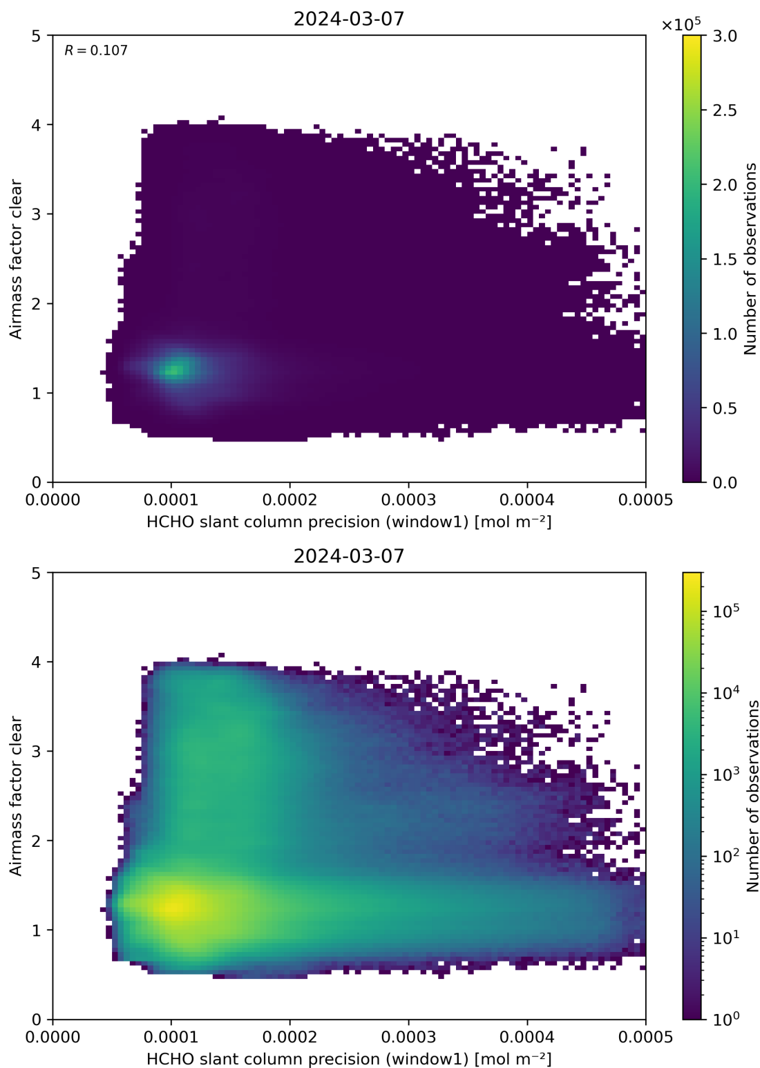
Figure 91: Scatter density plot of “HCHO slant column precision (window1)” against “Airmass factor clear” for 2024-03-06 to 2024-03-08.
