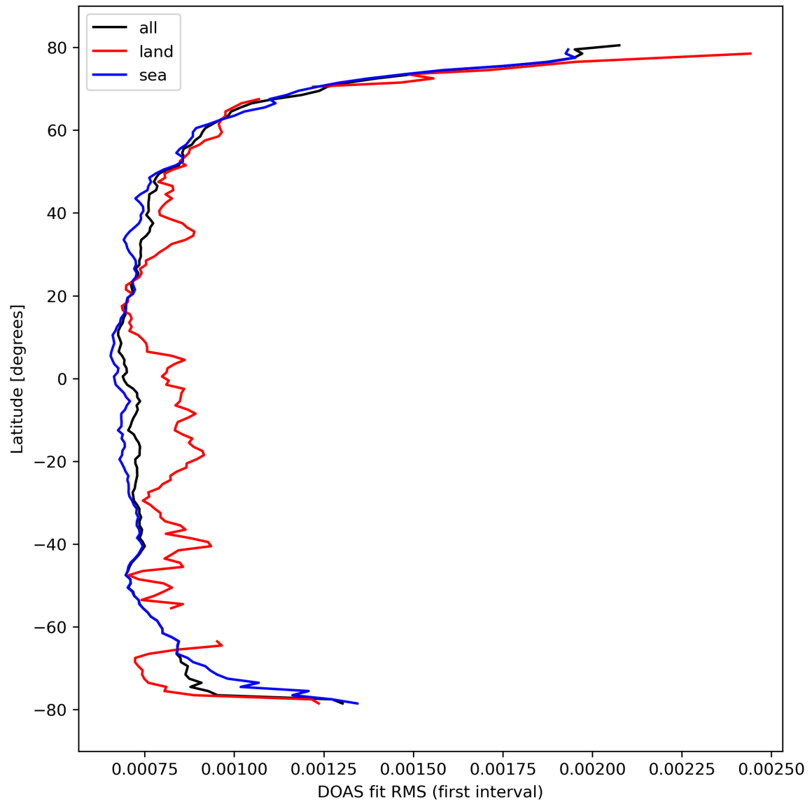
Figure 32: Zonal average of “DOAS fit RMS (first interval)” for 2024-03-06 to 2024-03-08.
