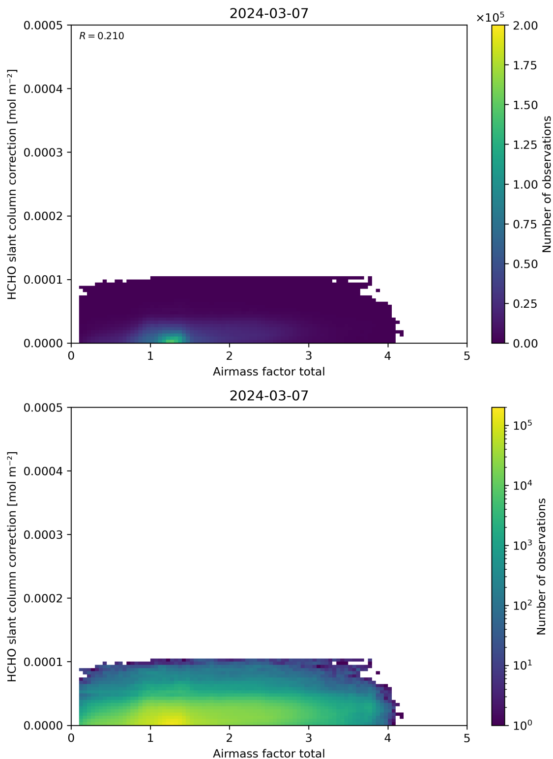
Figure 102: Scatter density plot of “Airmass factor total” against “HCHO slant column correction” for 2024-03-06 to 2024-03-08.
