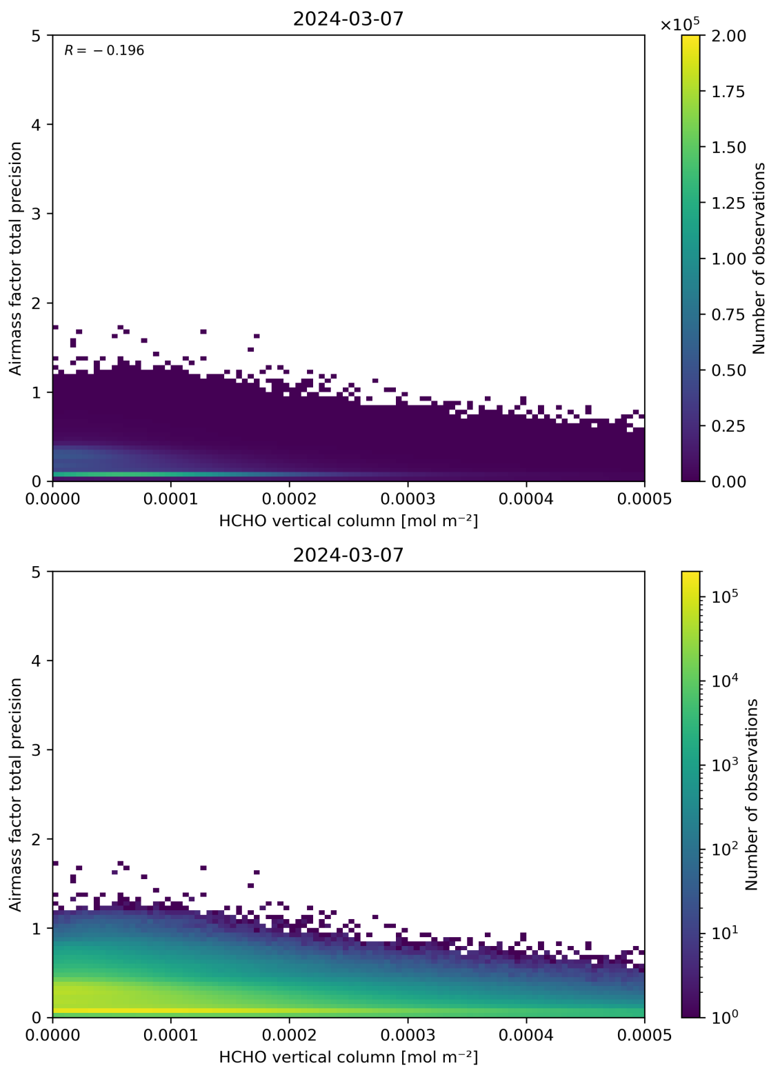
Figure 132: Scatter density plot of “HCHO vertical column” against “Airmass factor total precision” for 2024-03-06 to 2024-03-08.
