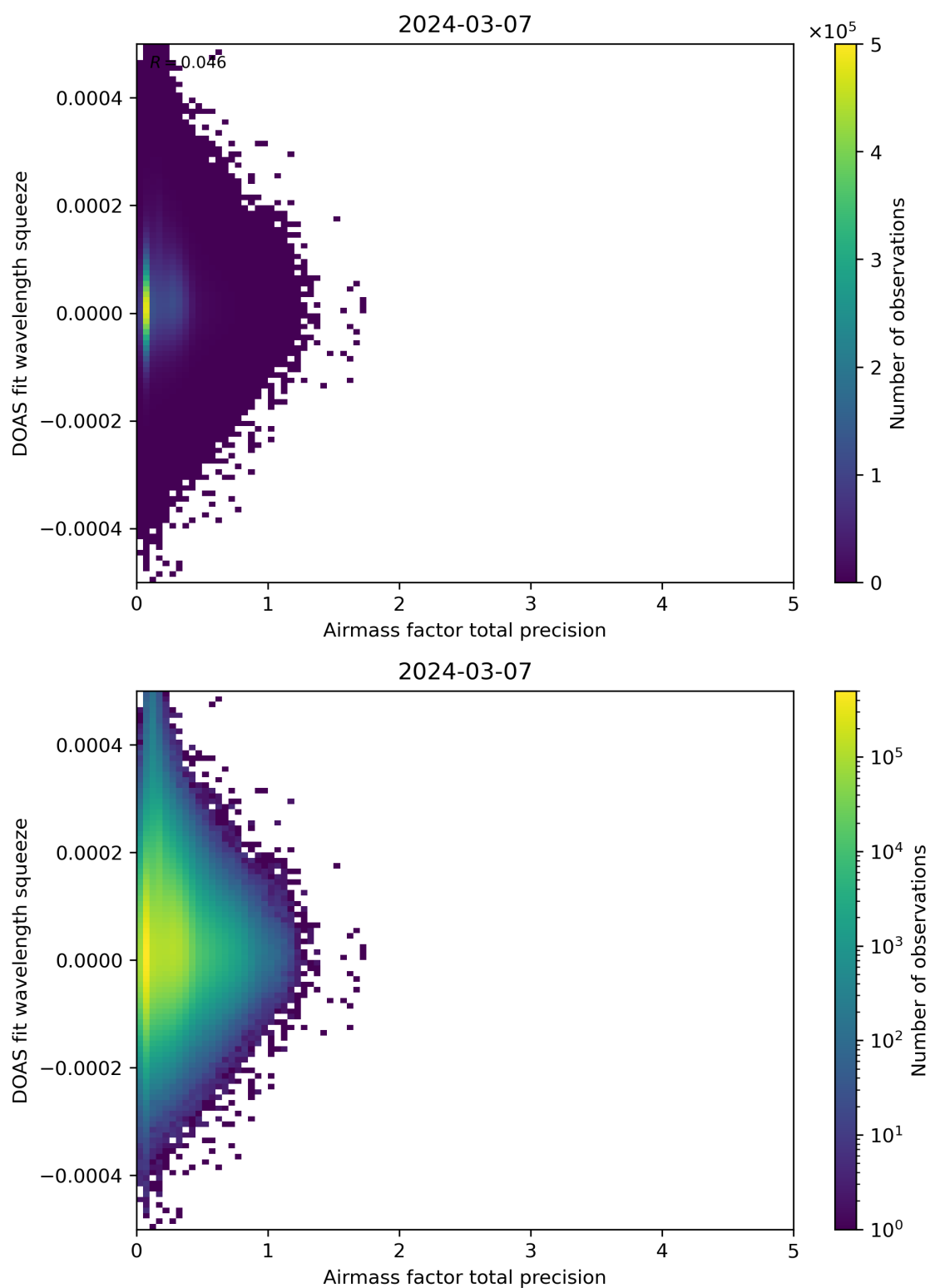
Figure 107: Scatter density plot of “Airmass factor total precision” against “DOAS fit wavelength squeeze” for 2024-03-06 to 2024-03-08.
