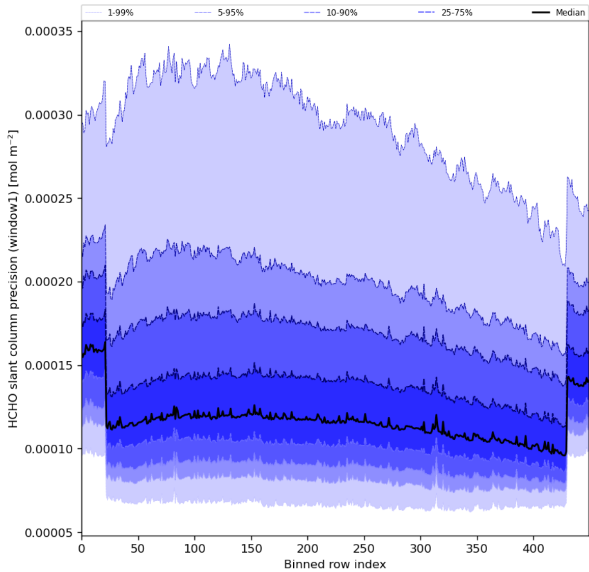
Figure 53: Along track statistics of “HCHO slant column precision (window1)” for 2024-03-06 to 2024-03-08
