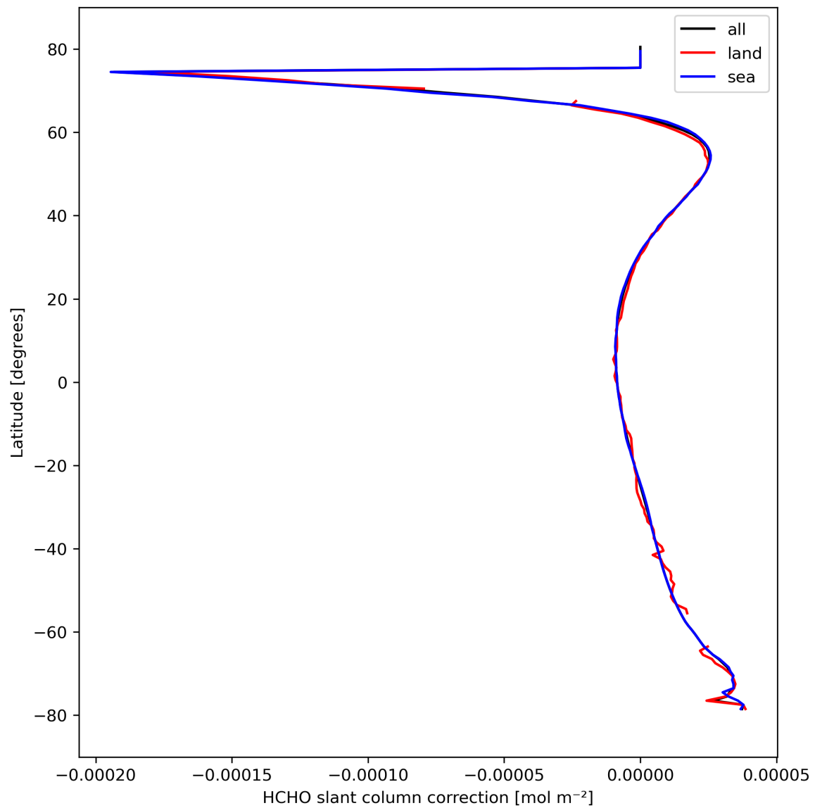
Figure 33: Zonal average of “HCHO slant column correction” for 2024-03-06 to 2024-03-08.
