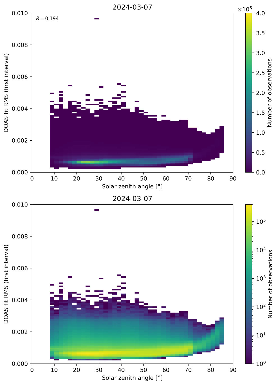
Figure 167: Scatter density plot of “Solar zenith angle” against “DOAS fit RMS (first interval)” for 2024-03-06 to 2024-03-08.
