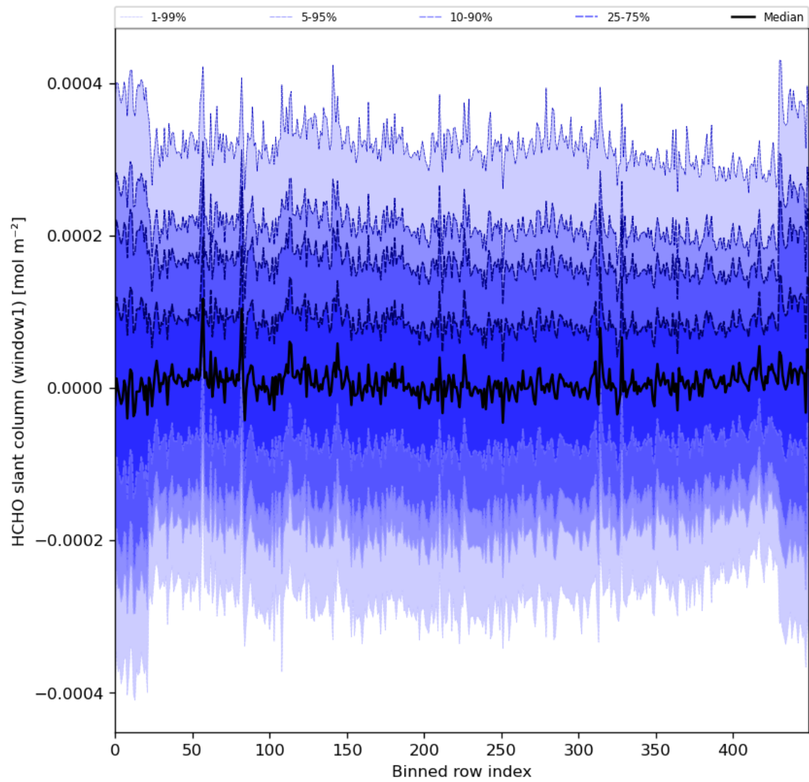
Figure 52: Along track statistics of “HCHO slant column (window1)” for 2024-03-06 to 2024-03-08
