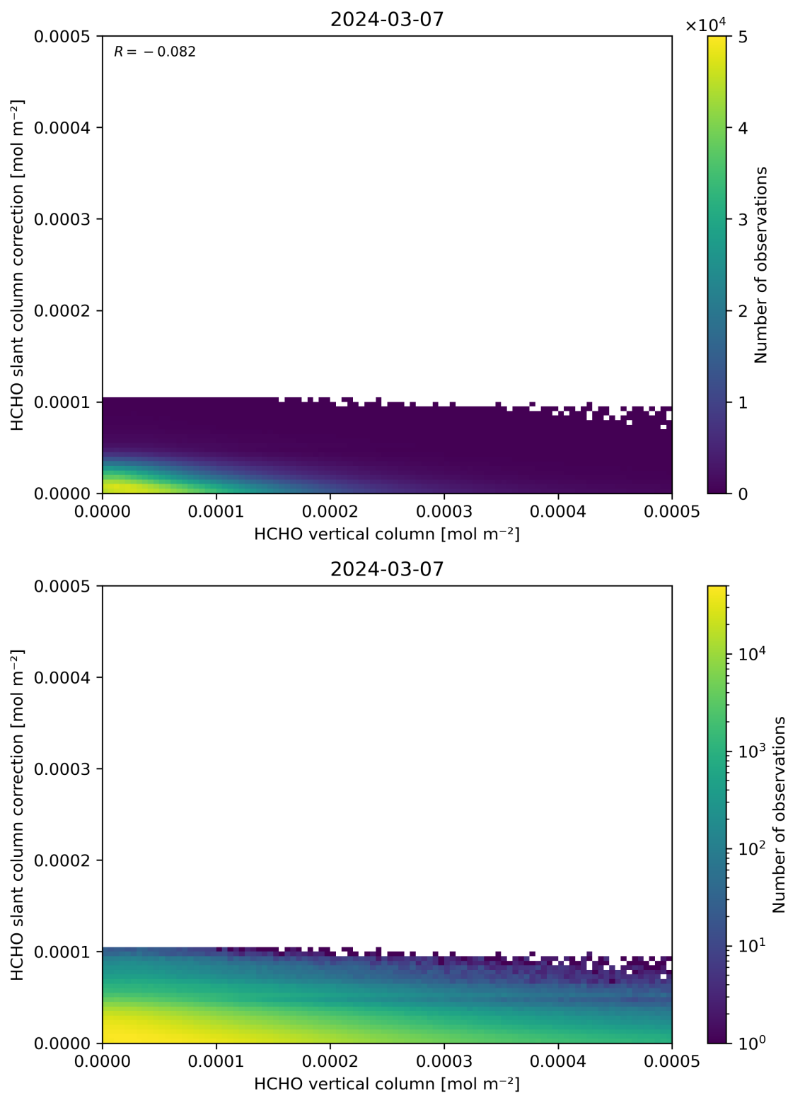
Figure 128: Scatter density plot of “HCHO vertical column” against “HCHO slant column correction” for 2024-03-06 to 2024-03-08.
