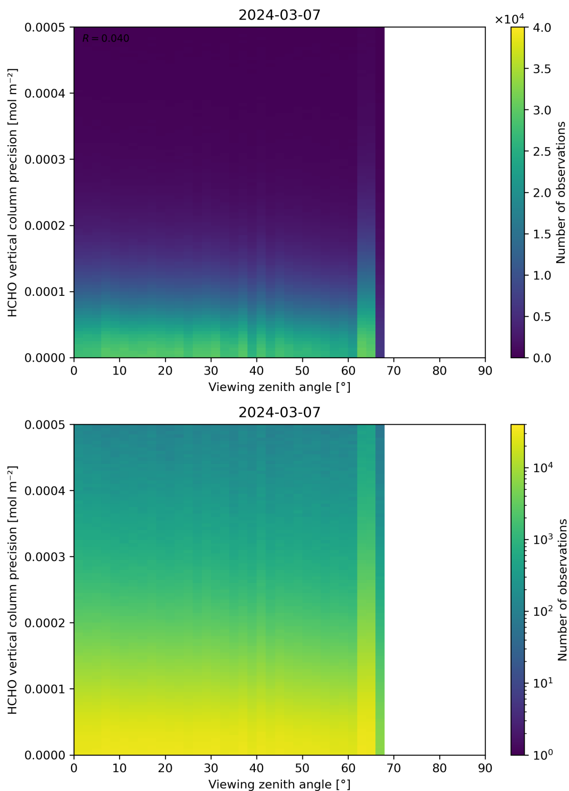
Figure 194: Scatter density plot of “Viewing zenith angle” against “HCHO vertical column precision” for 2024-03-06 to 2024-03-08.
