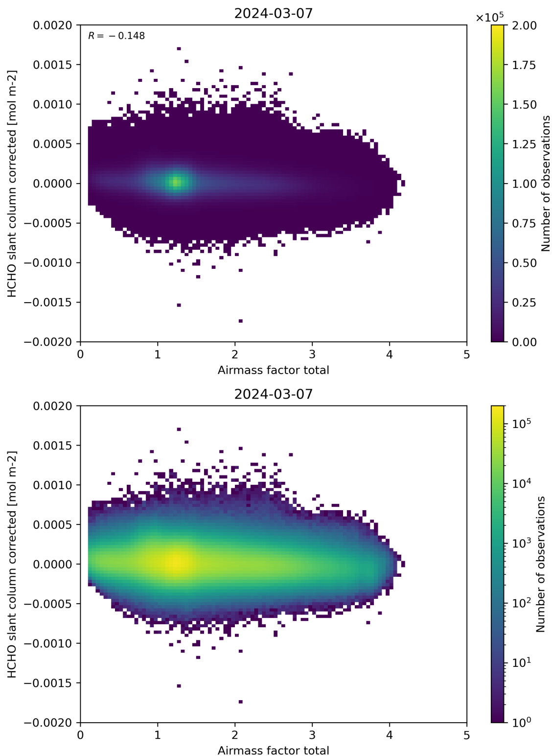
Figure 101: Scatter density plot of “Airmass factor total” against “HCHO slant column corrected” for 2024-03-06 to 2024-03-08.
