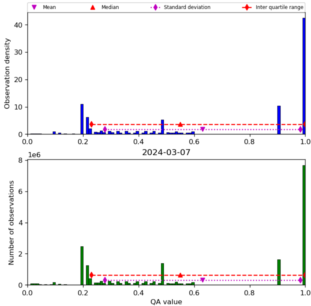
Figure 34: Histogram of “QA value” for 2024-03-06 to 2024-03-08
