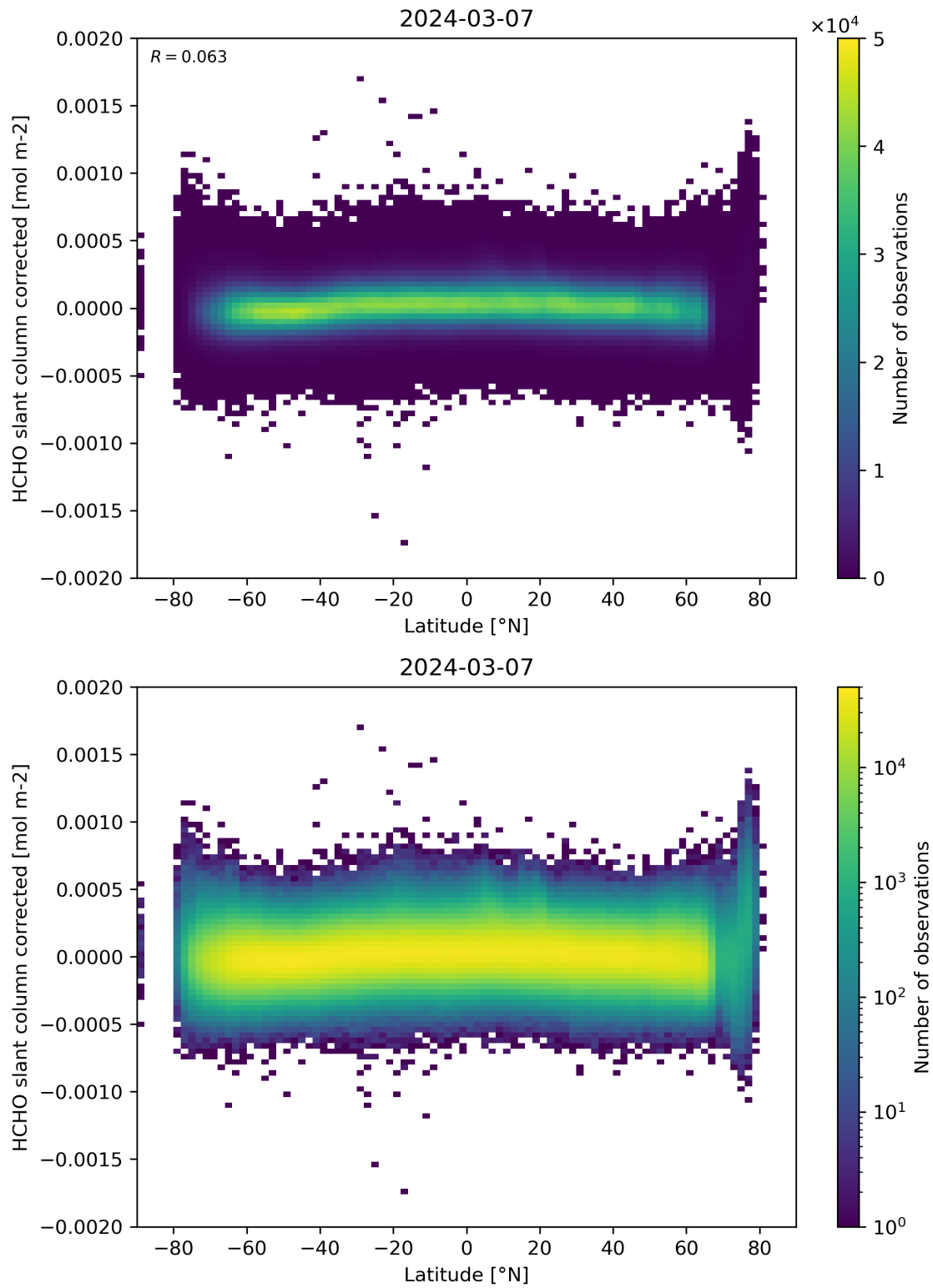
Figure 157: Scatter density plot of “Latitude” against “HCHO slant column corrected” for 2024-03-06 to 2024-03-08.
