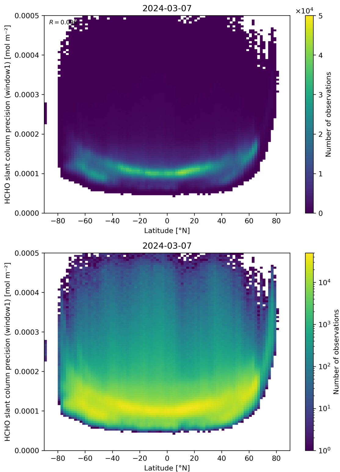
Figure 160: Scatter density plot of “Latitude” against “HCHO slant column precision (window1)” for 2024-03-06 to 2024-03-08.
