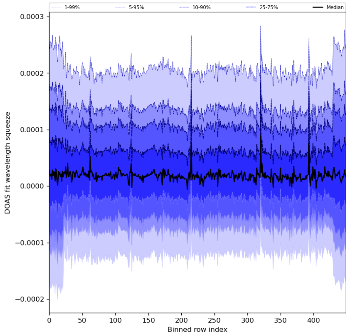
Figure 59: Along track statistics of “DOAS fit wavelength squeeze” for 2024-03-06 to 2024-03-08
