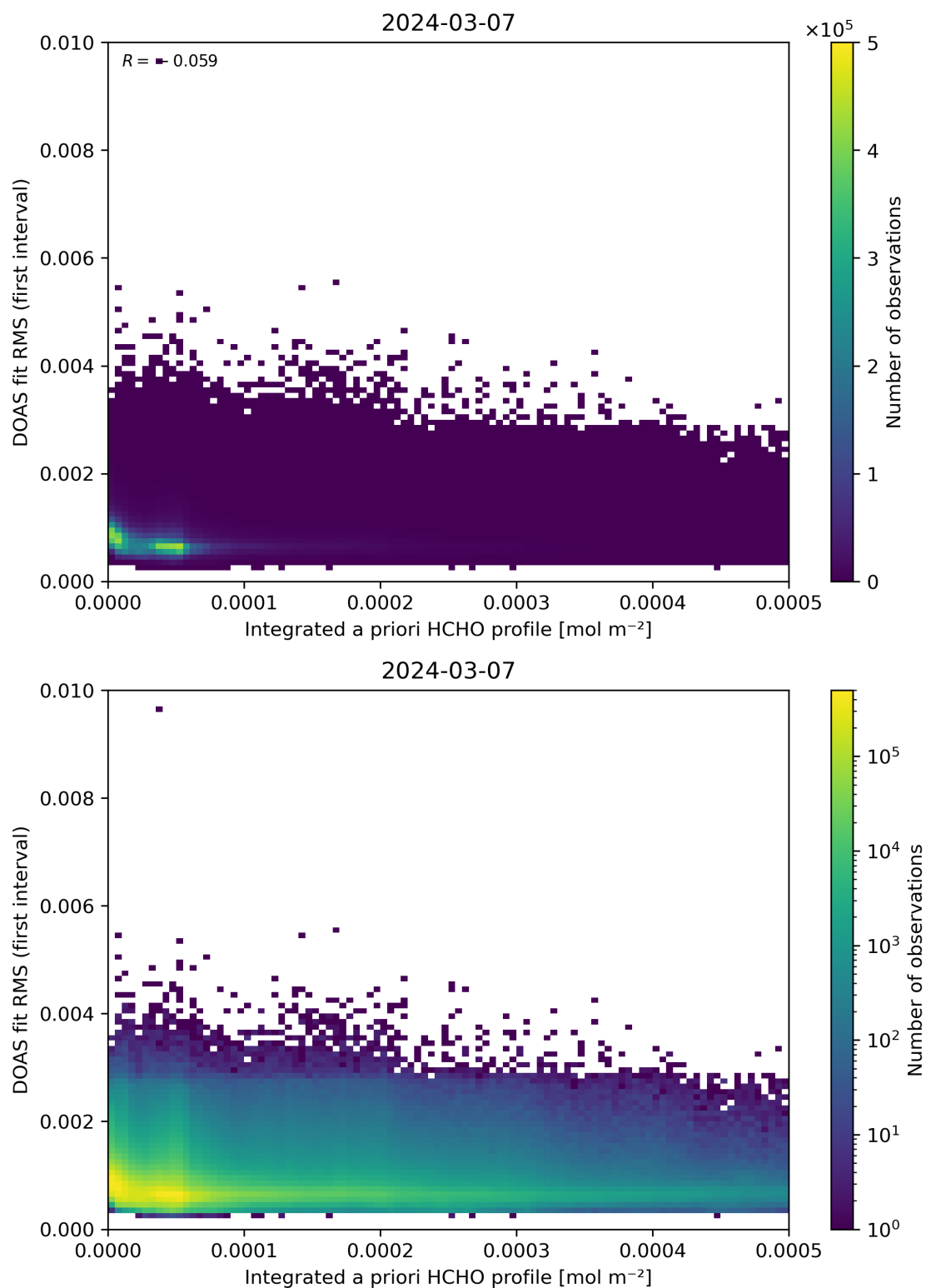
Figure 148: Scatter density plot of “Integrated a priori HCHO profile” against “DOAS fit RMS (first interval)” for 2024-03-06 to 2024-03-08.
