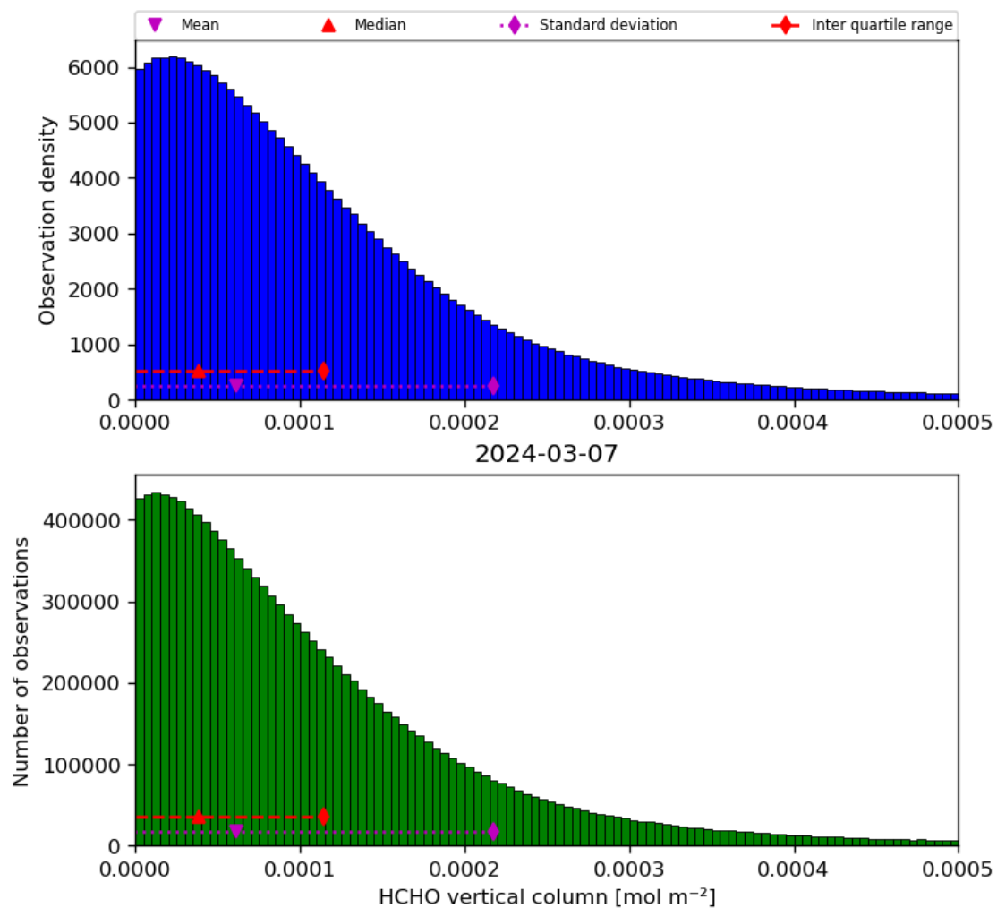
Figure 35: Histogram of “HCHO vertical column” for 2024-03-06 to 2024-03-08
