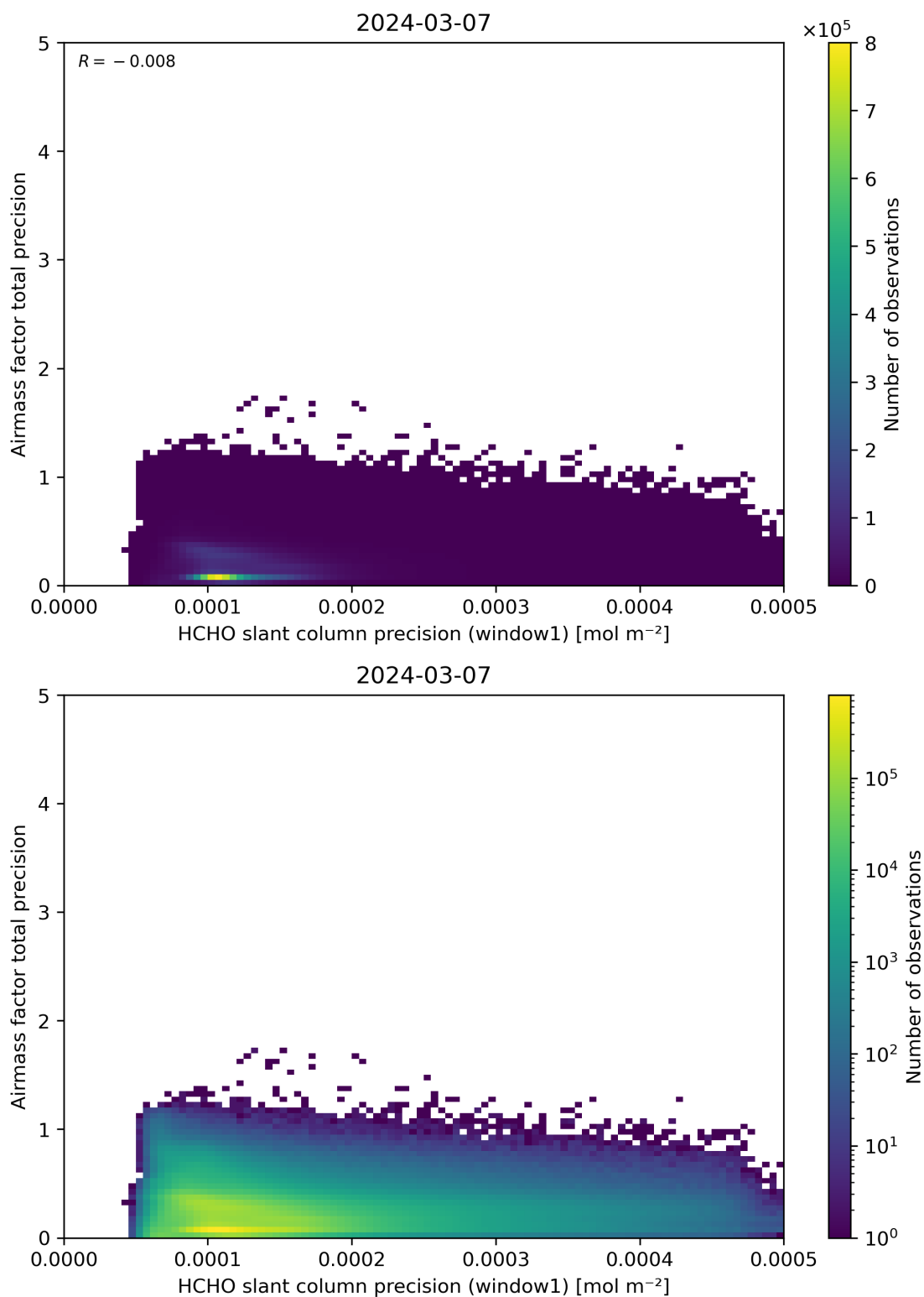
Figure 95: Scatter density plot of “HCHO slant column precision (window1)” against “Airmass factor total precision” for 2024-03-06 to 2024-03-08.
