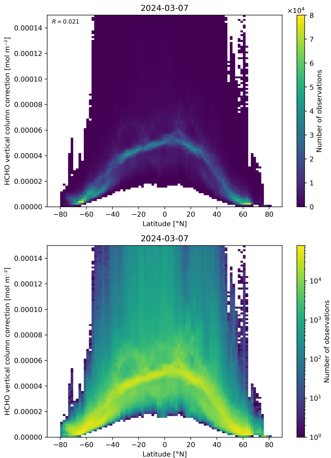
Figure 164: Scatter density plot of “Latitude” against “HCHO vertical column correction” for 2024-03-06 to 2024-03-08.
