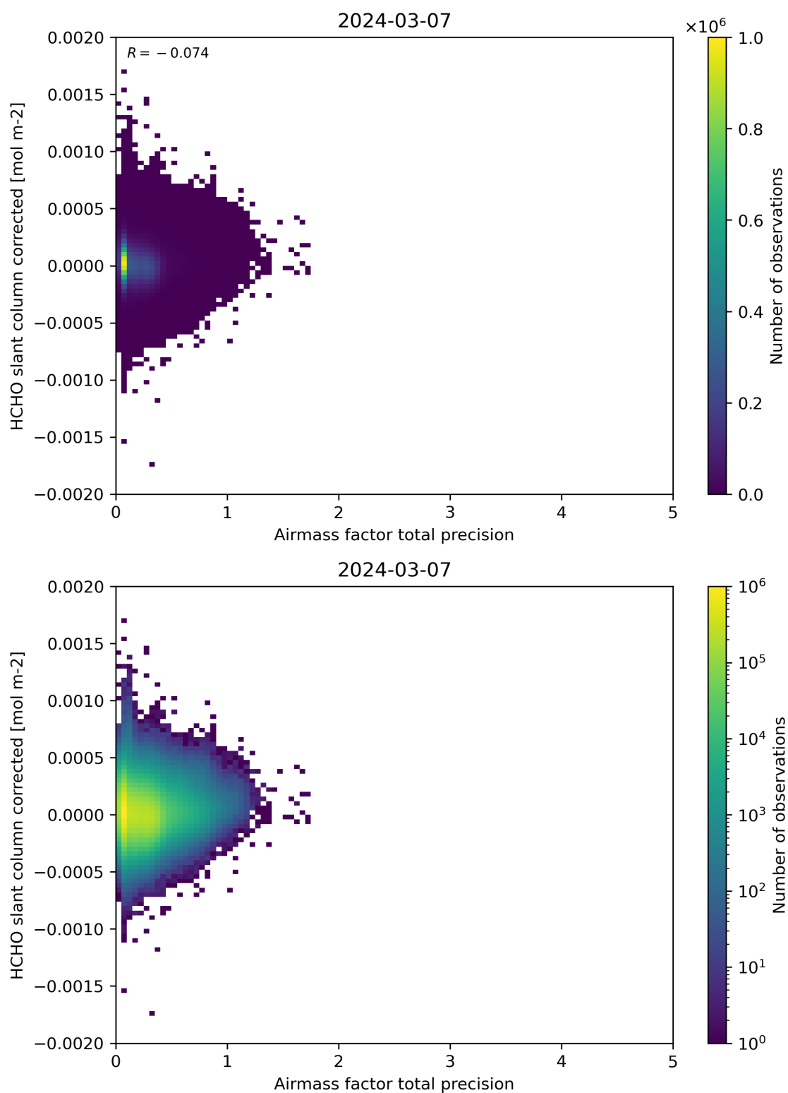
Figure 109: Scatter density plot of “Airmass factor total precision” against “HCHO slant column corrected” for 2024-03-06 to 2024-03-08.
