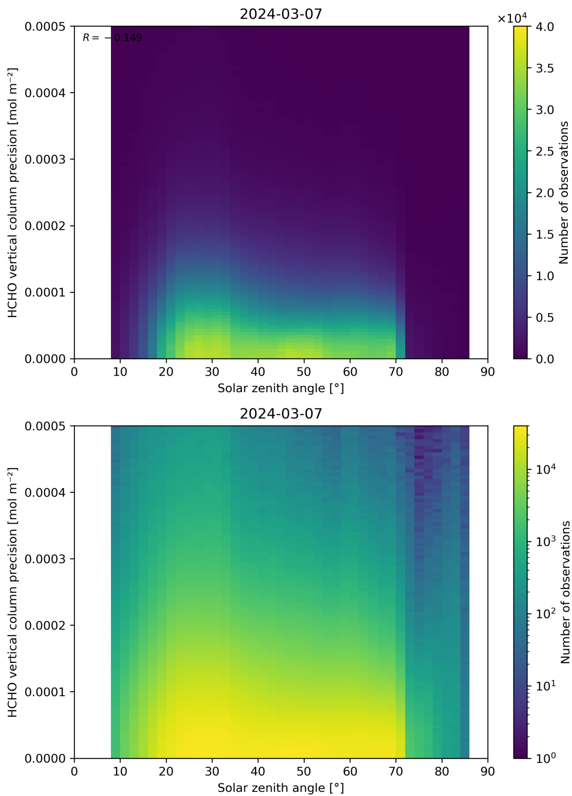
Figure 179: Scatter density plot of “Solar zenith angle” against “HCHO vertical column precision” for 2024-03-06 to 2024-03-08.
