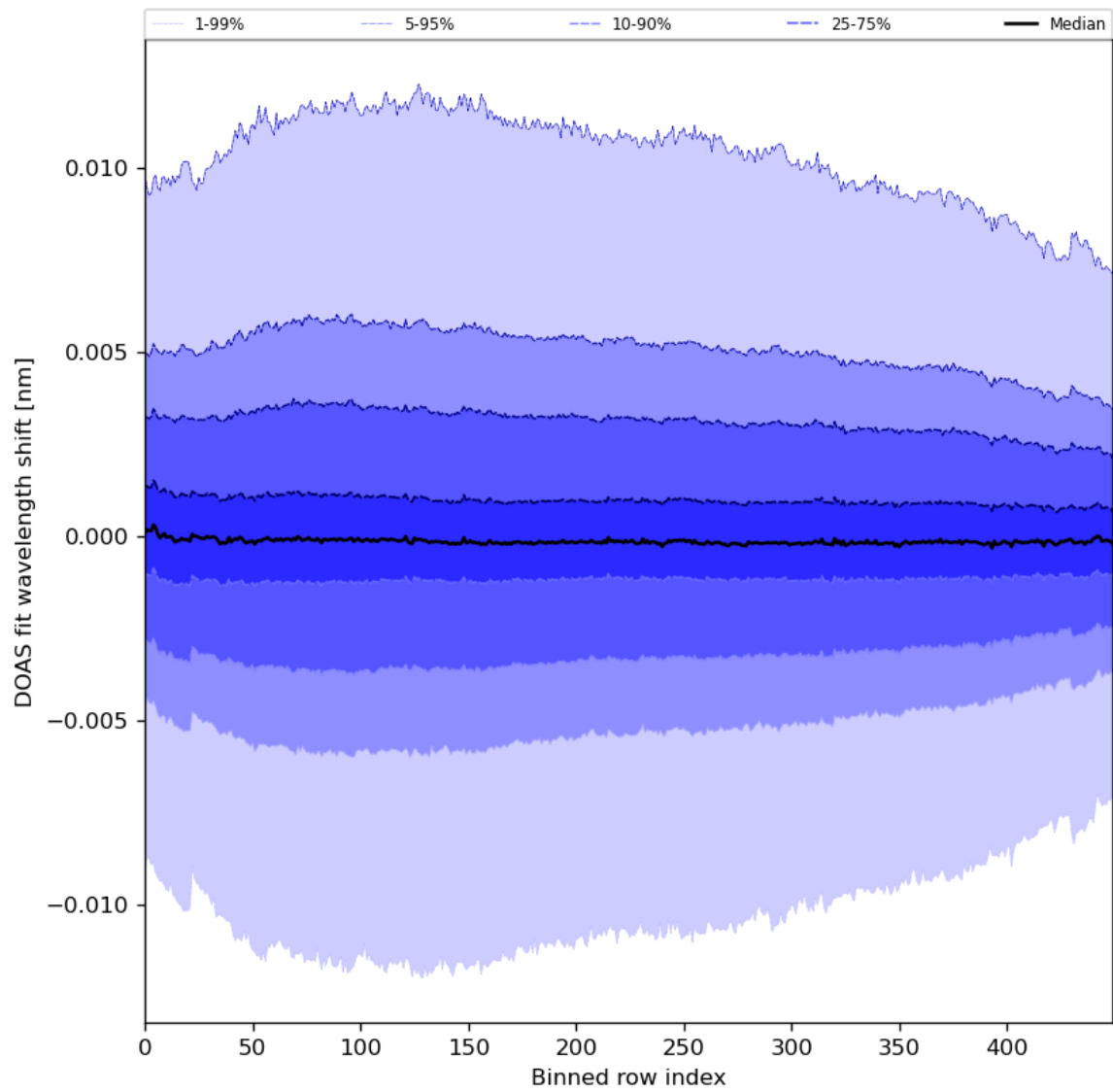
Figure 58: Along track statistics of “DOAS fit wavelength shift” for 2024-03-06 to 2024-03-08
