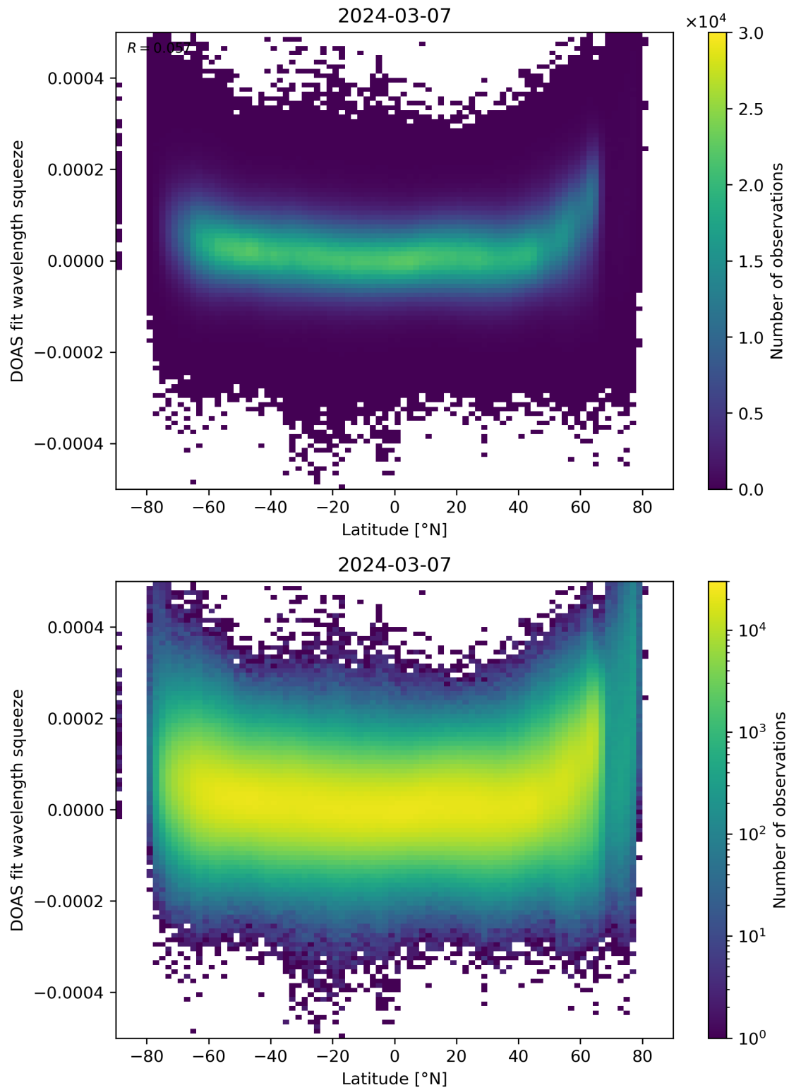
Figure 155: Scatter density plot of “Latitude” against “DOAS fit wavelength squeeze” for 2024-03-06 to 2024-03-08.
