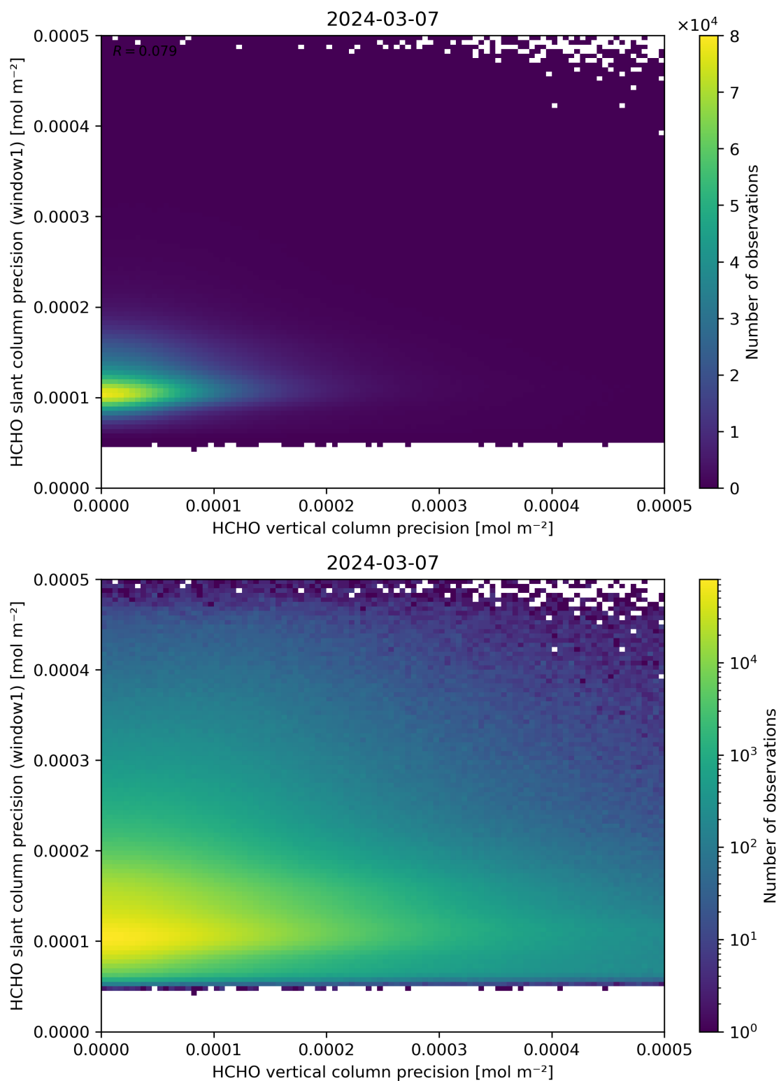
Figure 143: Scatter density plot of “HCHO vertical column precision” against “HCHO slant column precision (window1)” for 2024-03-06 to 2024-03-08.
