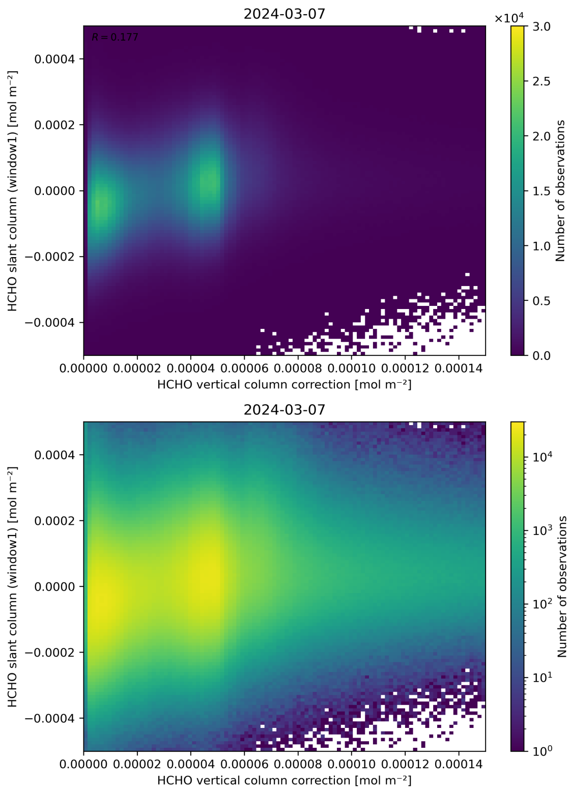
Figure 118: Scatter density plot of “HCHO vertical column correction” against “HCHO slant column (window1)” for 2024-03-06 to 2024-03-08.
