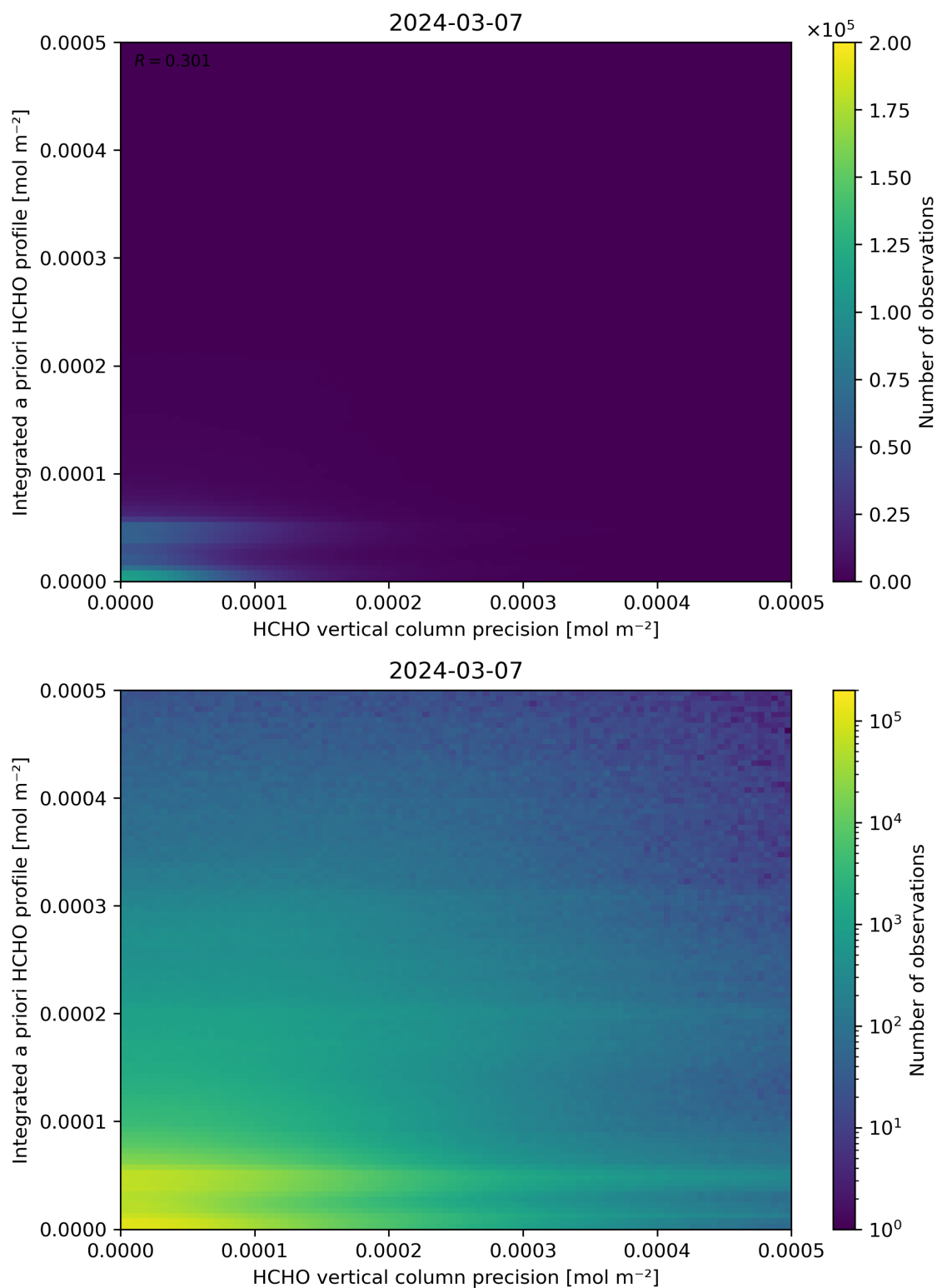
Figure 147: Scatter density plot of “HCHO vertical column precision” against “Integrated a priori HCHO profile” for 2024-03-06 to 2024-03-08.
