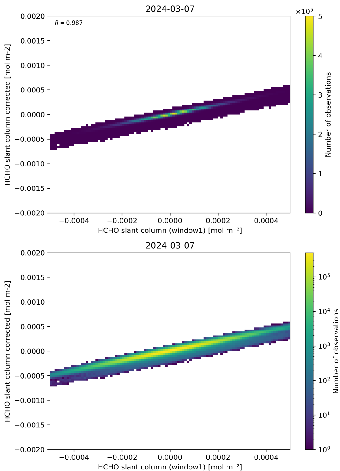
Figure 82: Scatter density plot of “HCHO slant column (window1)” against “HCHO slant column corrected” for 2024-03-06 to 2024-03-08.
