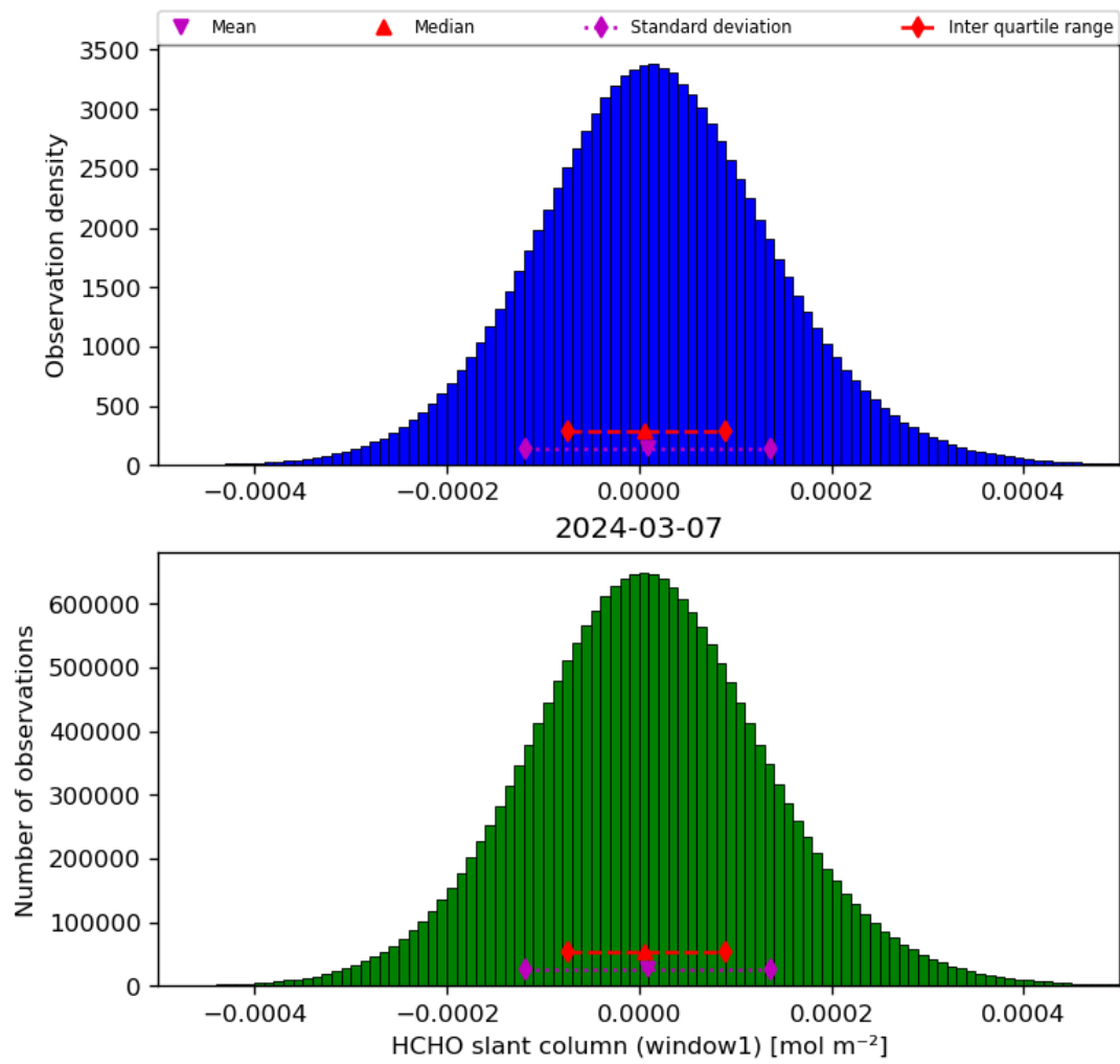
Figure 38: Histogram of “HCHO slant column (window1)” for 2024-03-06 to 2024-03-08
