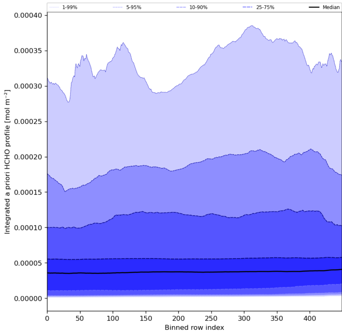
Figure 57: Along track statistics of "Integrated a priori HCHO profile" for 2024-03-06 to 2024-03-08
