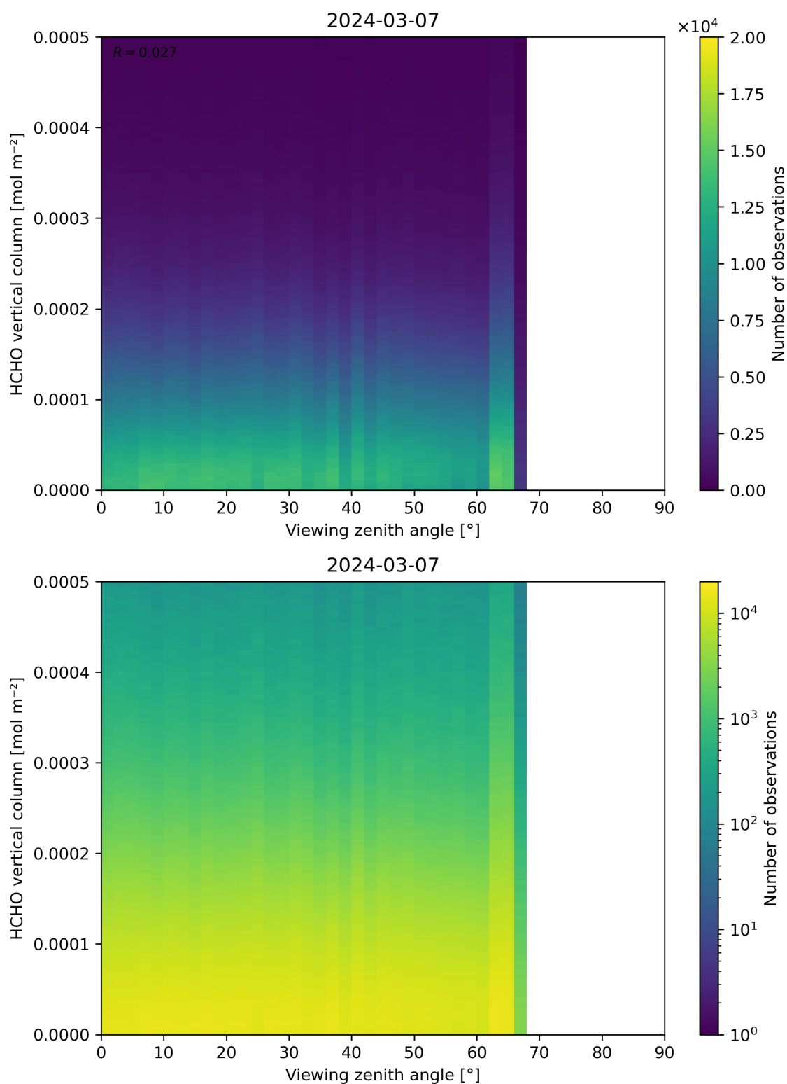
Figure 192: Scatter density plot of “Viewing zenith angle” against “HCHO vertical column” for 2024-03-06 to 2024-03-08.
