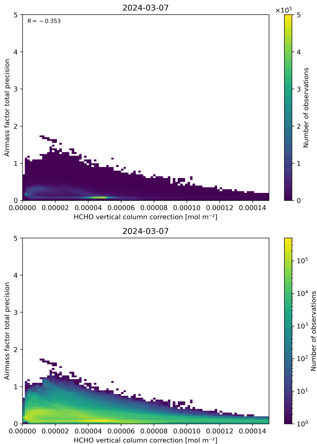
Figure 121: Scatter density plot of “HCHO vertical column correction” against “Airmass factor total precision” for 2024-03-06 to 2024-03-08.
