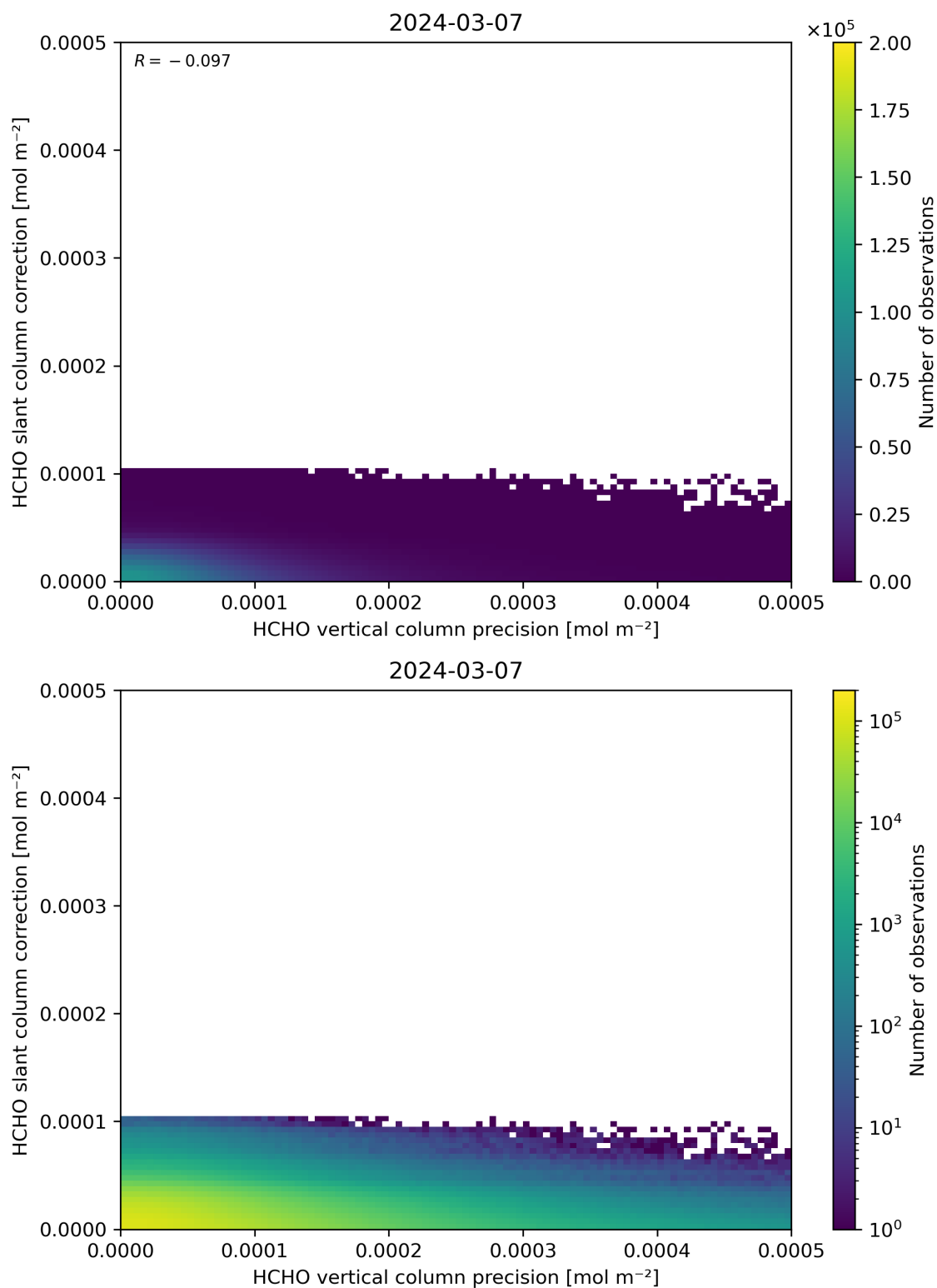
Figure 141: Scatter density plot of “HCHO vertical column precision” against “HCHO slant column correction” for 2024-03-06 to 2024-03-08.
