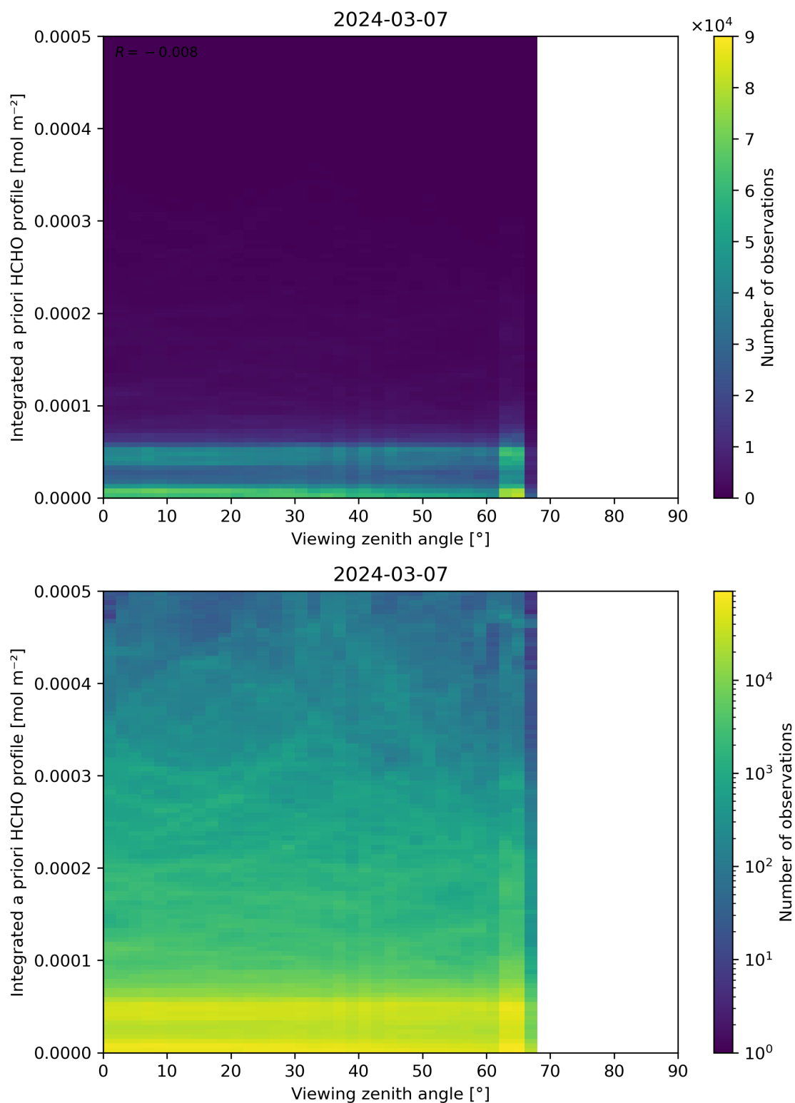
Figure 195: Scatter density plot of “Viewing zenith angle” against “Integrated a priori HCHO profile” for 2024-03-06 to 2024-03-08.
