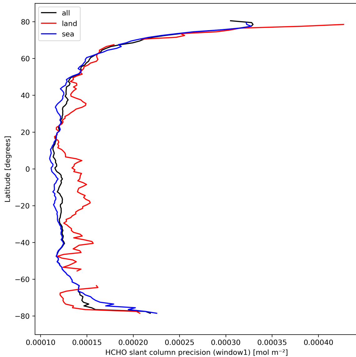
Figure 25: Zonal average of "HCHO slant column precision (window1)" for 2024-03-06 to 2024-03-08.
