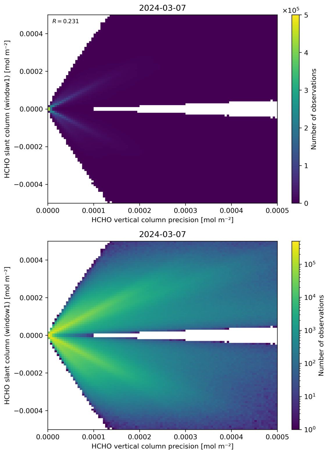
Figure 142: Scatter density plot of “HCHO vertical column precision” against “HCHO slant column (window1)” for 2024-03-06 to 2024-03-08.
