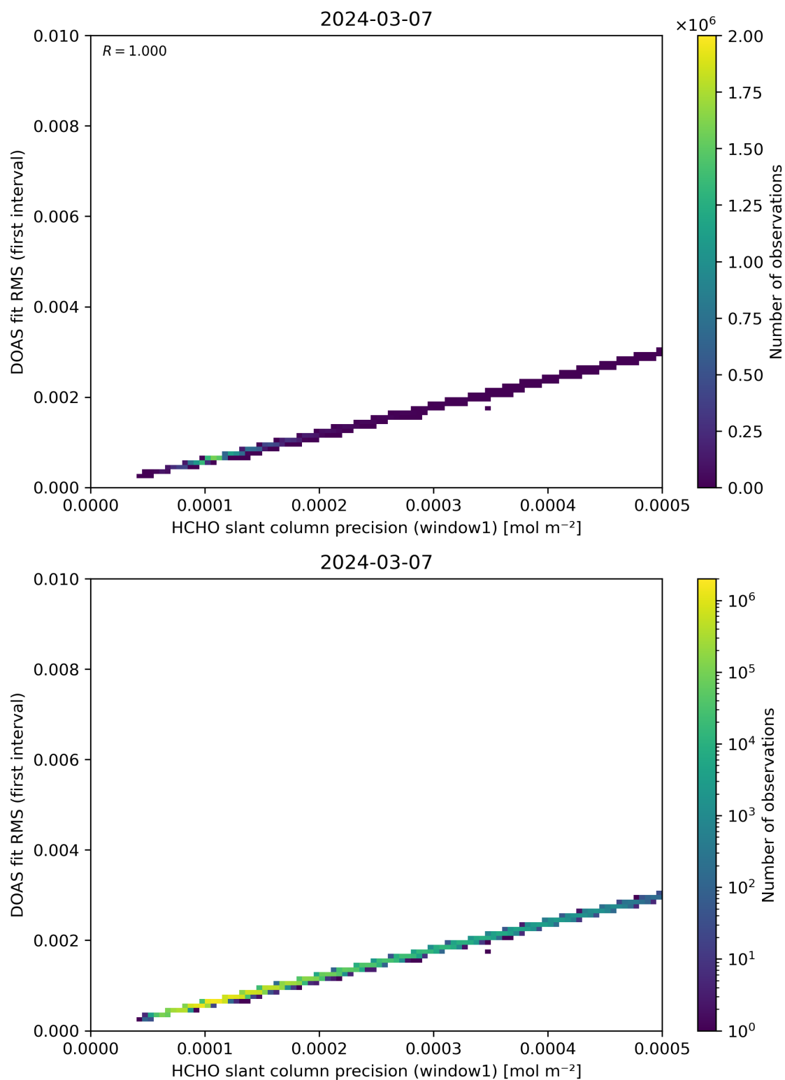
Figure 88: Scatter density plot of “HCHO slant column precision (window1)” against “DOAS fit RMS (first interval)” for 2024-03-06 to 2024-03-08.
