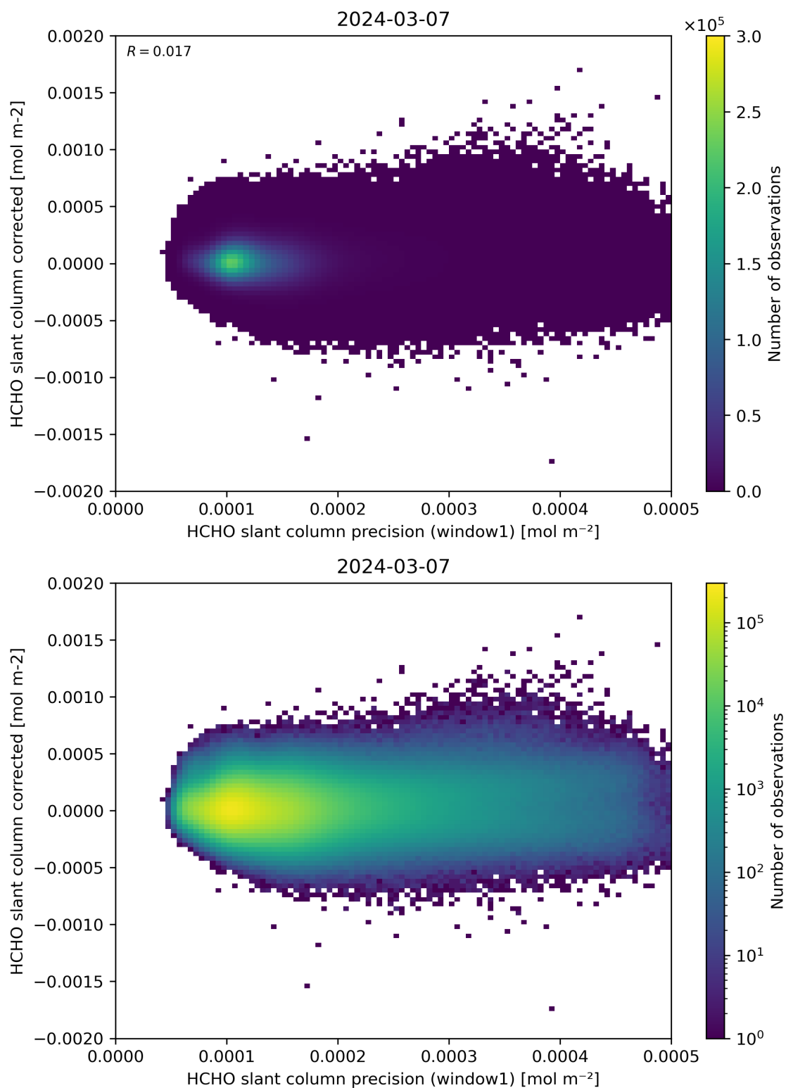
Figure 92: Scatter density plot of “HCHO slant column precision (window1)” against “HCHO slant column corrected” for 2024-03-06 to 2024-03-08.
