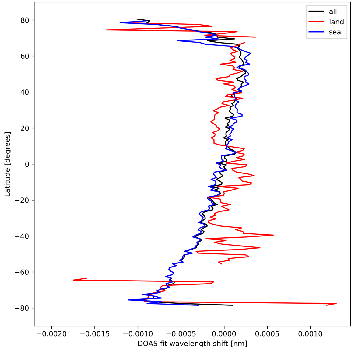
Figure 30: Zonal average of “DOAS fit wavelength shift” for 2024-03-06 to 2024-03-08.
