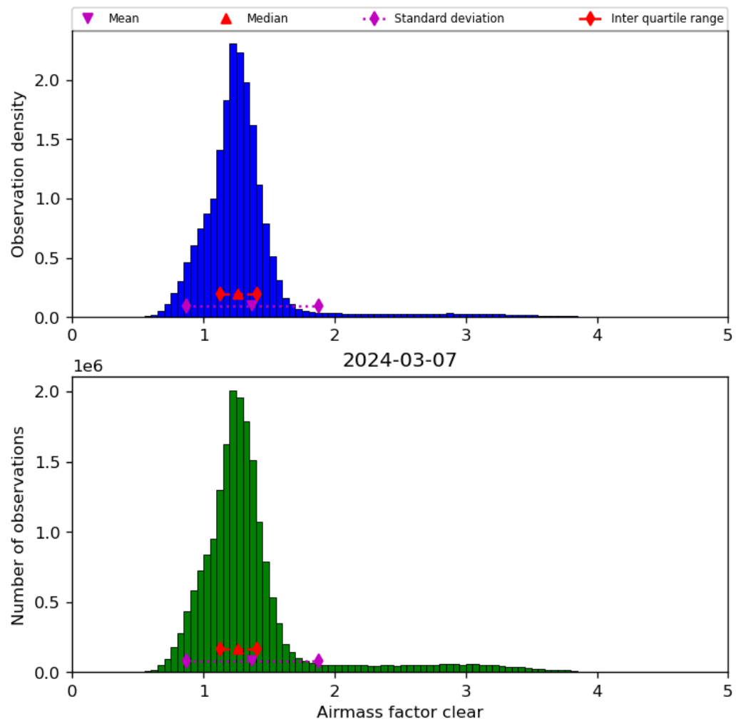
Figure 42: Histogram of “Airmass factor clear” for 2024-03-06 to 2024-03-08
