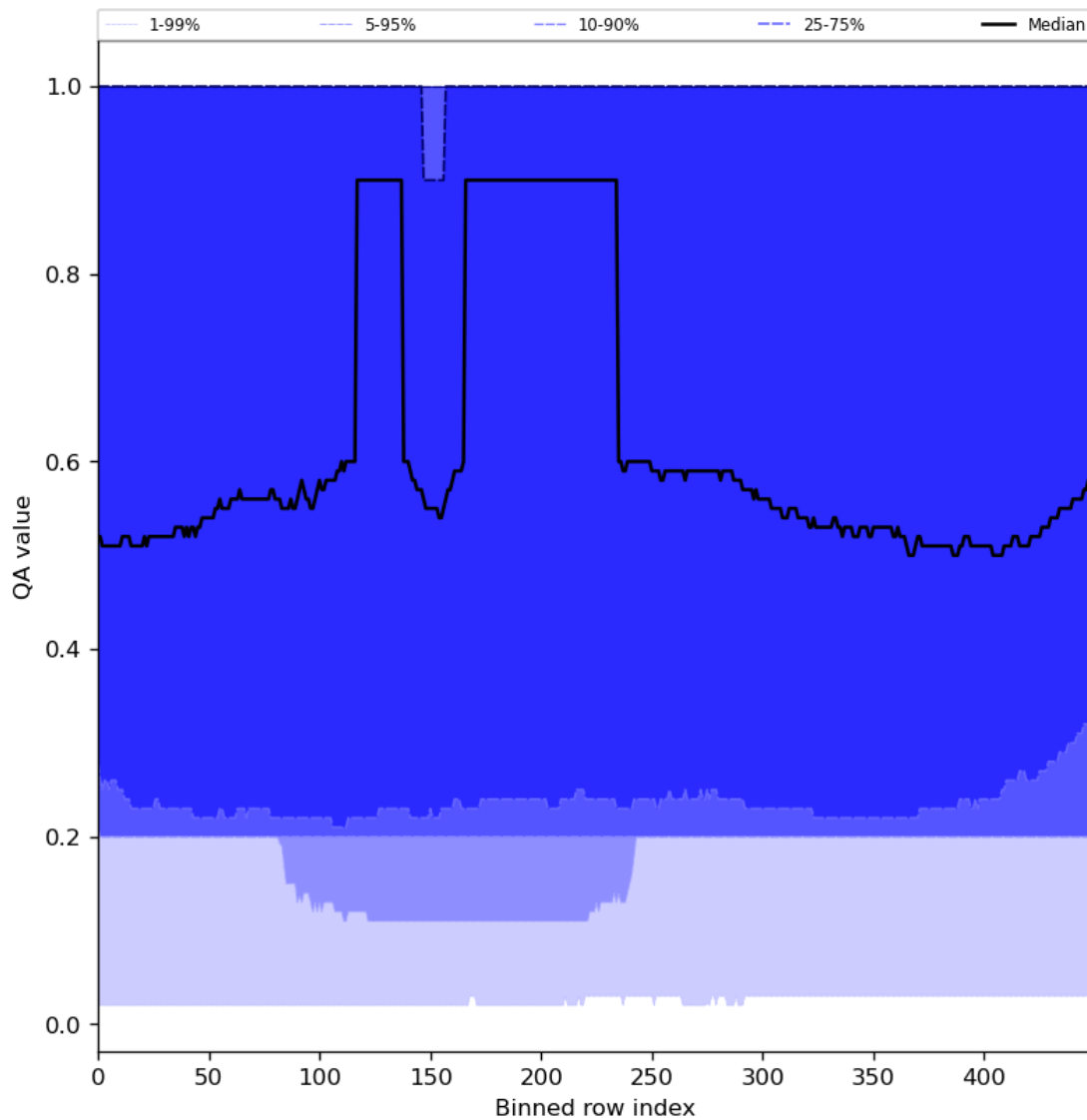
Figure 48: Along track statistics of “QA value” for 2024-03-06 to 2024-03-08
