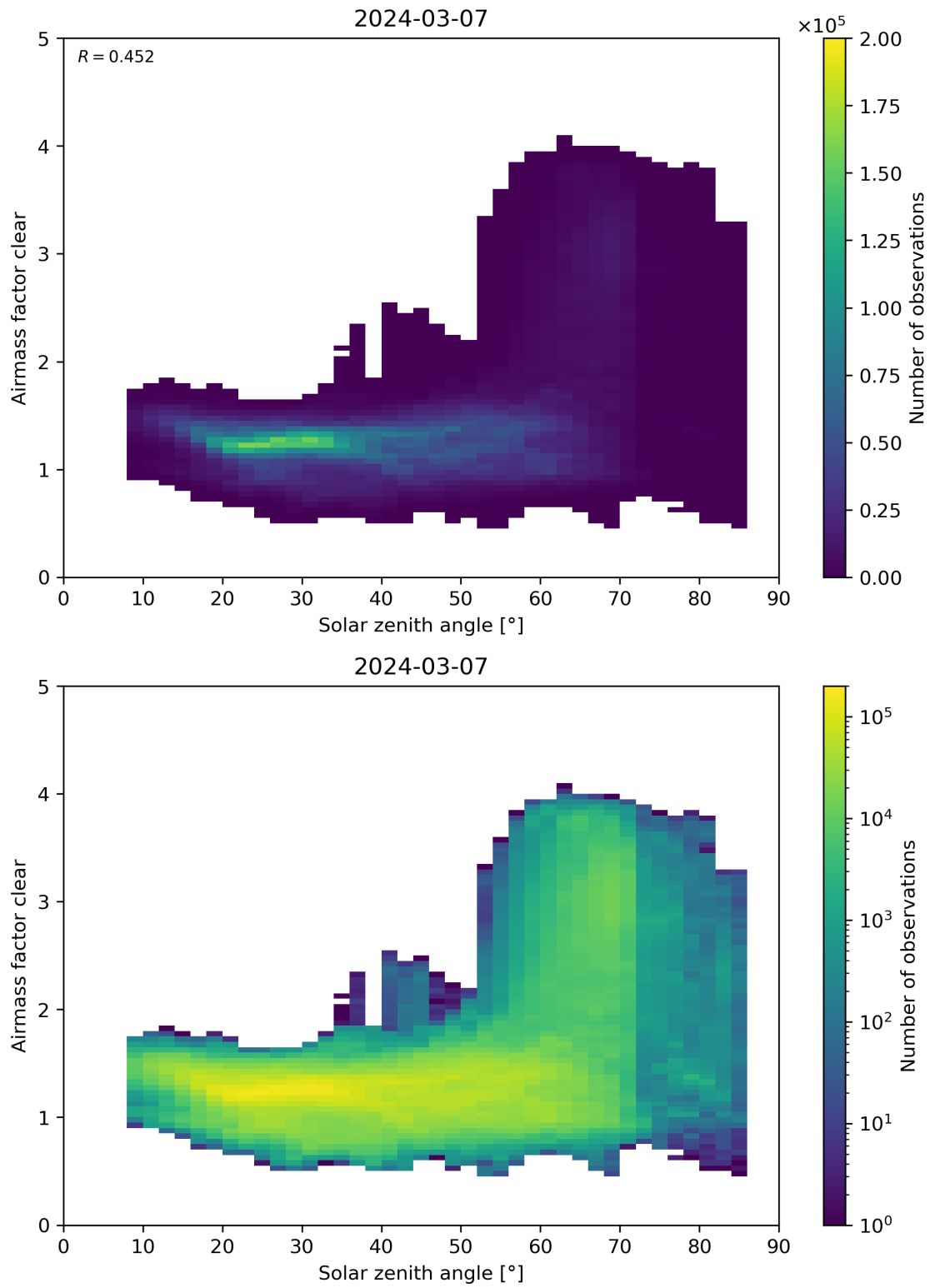
Figure 170: Scatter density plot of “Solar zenith angle” against “Airmass factor clear” for 2024-03-06 to 2024-03-08.
