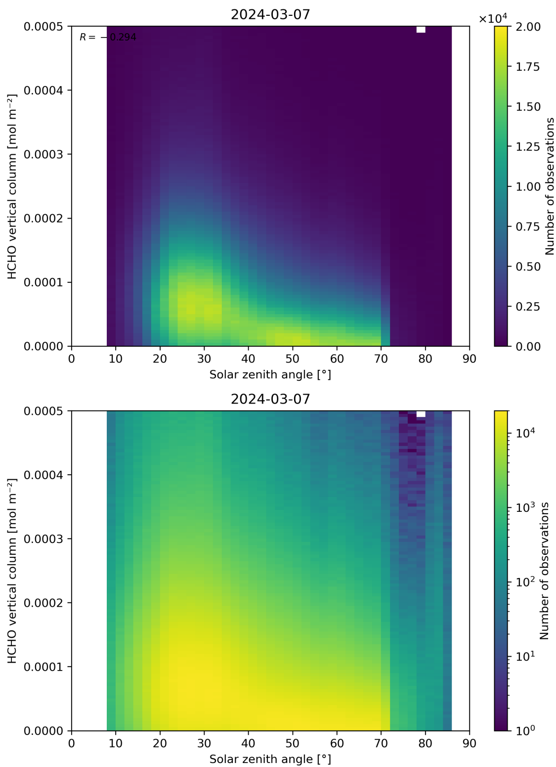
Figure 177: Scatter density plot of “Solar zenith angle” against “HCHO vertical column” for 2024-03-06 to 2024-03-08.
