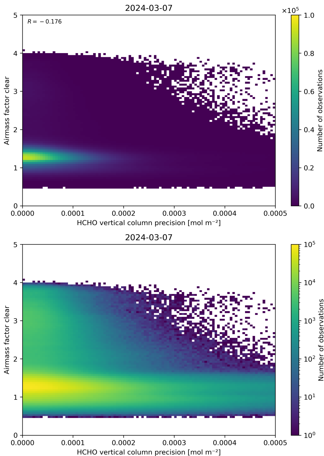
Figure 139: Scatter density plot of “HCHO vertical column precision” against “Airmass factor clear” for 2024-03-06 to 2024-03-08.
