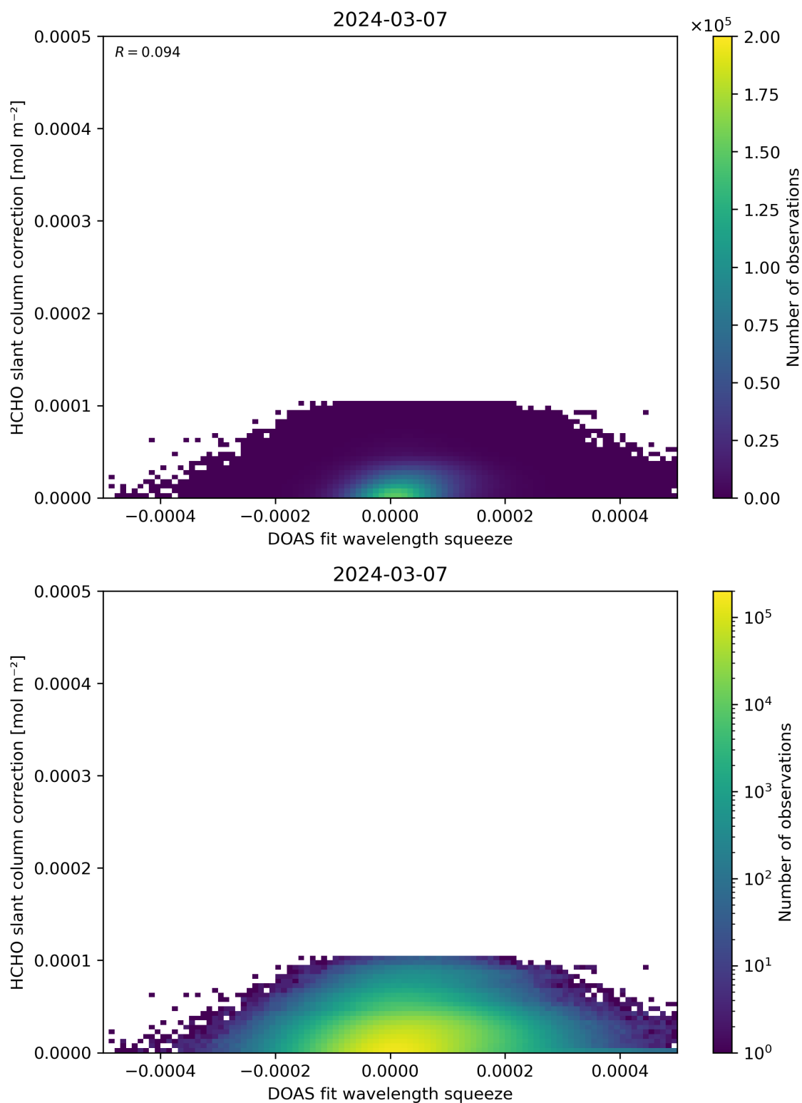
Figure 70: Scatter density plot of “DOAS fit wavelength squeeze” against “HCHO slant column correction” for 2024-03-06 to 2024-03-08.
