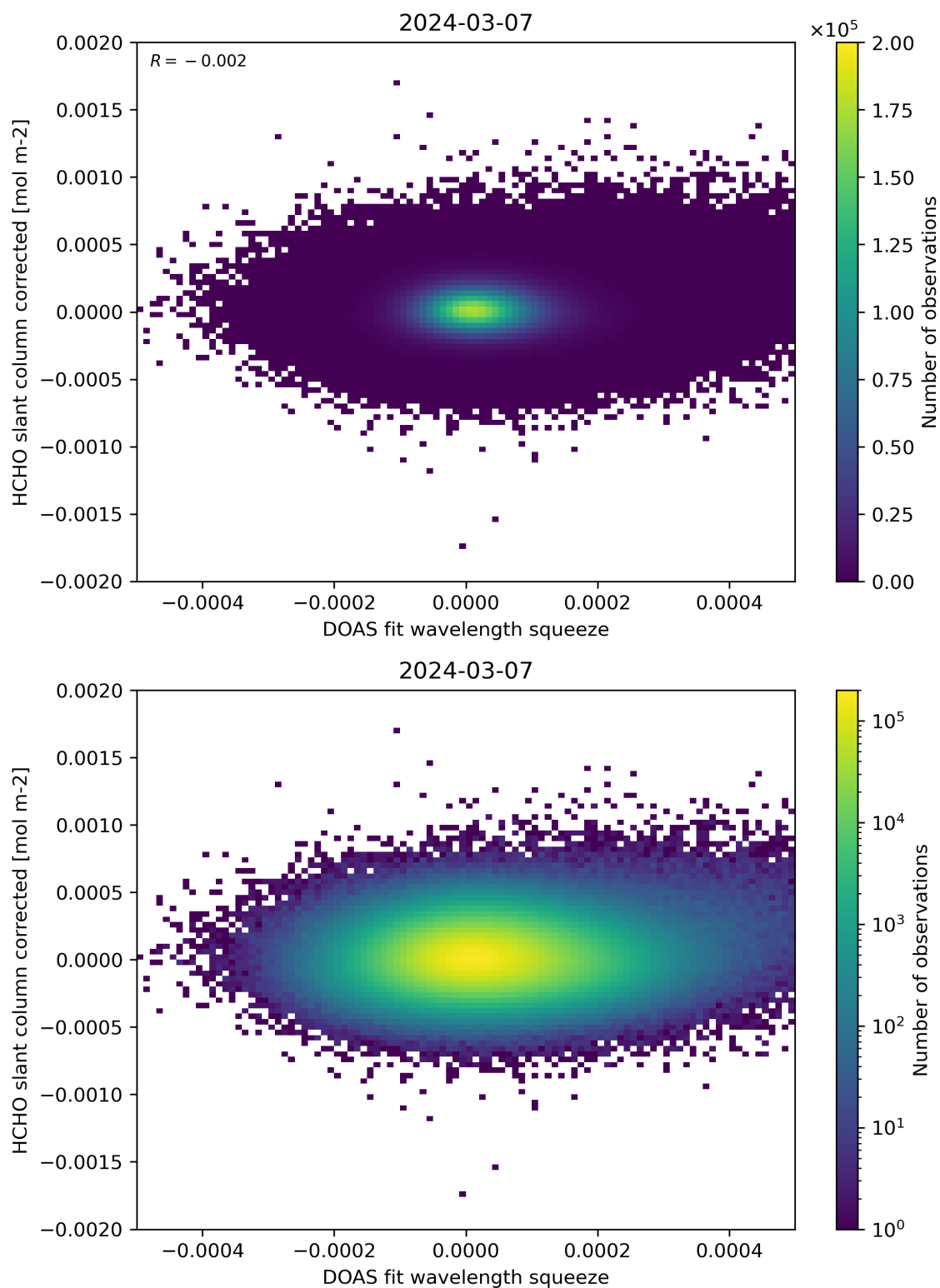
Figure 69: Scatter density plot of “DOAS fit wavelength squeeze” against “HCHO slant column corrected” for 2024-03-06 to 2024-03-08.
