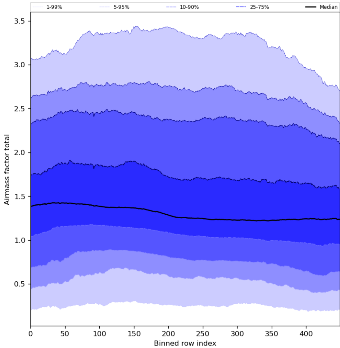
Figure 54: Along track statistics of “Airmass factor total” for 2024-03-06 to 2024-03-08
