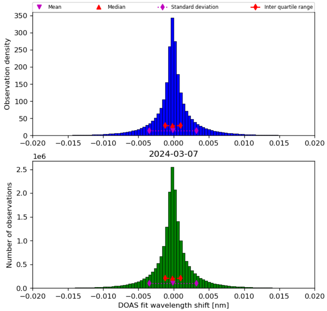
Figure 44: Histogram of “DOAS fit wavelength shift” for 2024-03-06 to 2024-03-08
