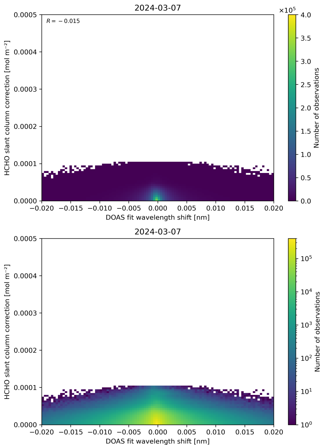
Figure 67: Scatter density plot of “DOAS fit wavelength shift” against “HCHO slant column correction” for 2024-03-06 to 2024-03-08.
