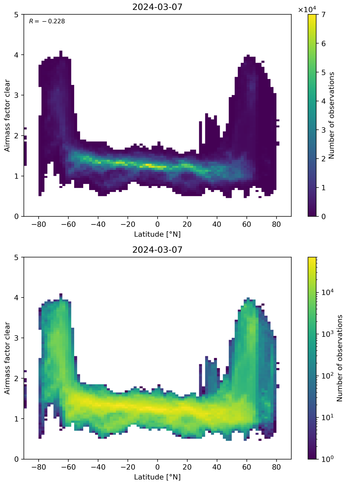
Figure 156: Scatter density plot of “Latitude” against “Airmass factor clear” for 2024-03-06 to 2024-03-08.
