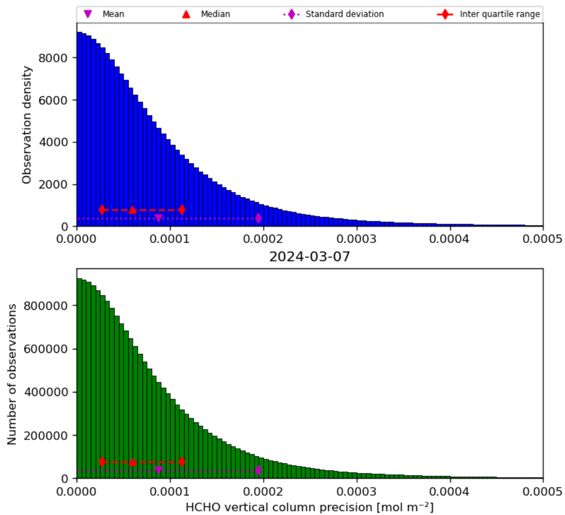
Figure 36: Histogram of “HCHO vertical column precision” for 2024-03-06 to 2024-03-08
