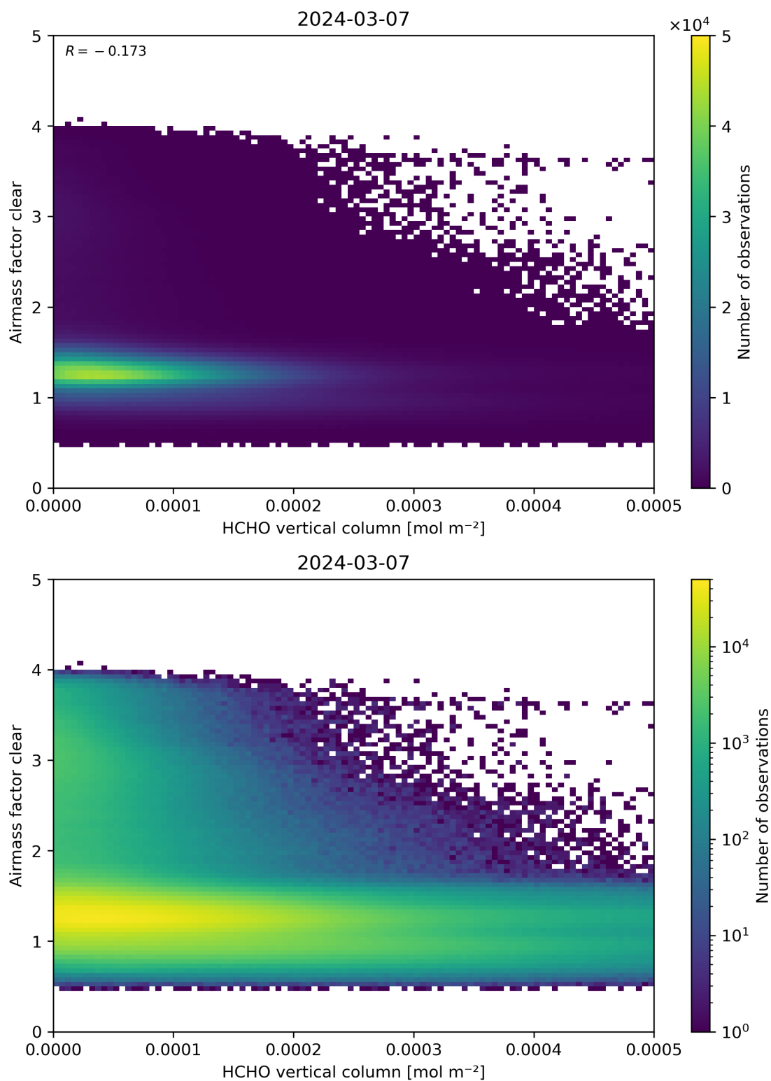
Figure 126: Scatter density plot of “HCHO vertical column” against “Airmass factor clear” for 2024-03-06 to 2024-03-08.
