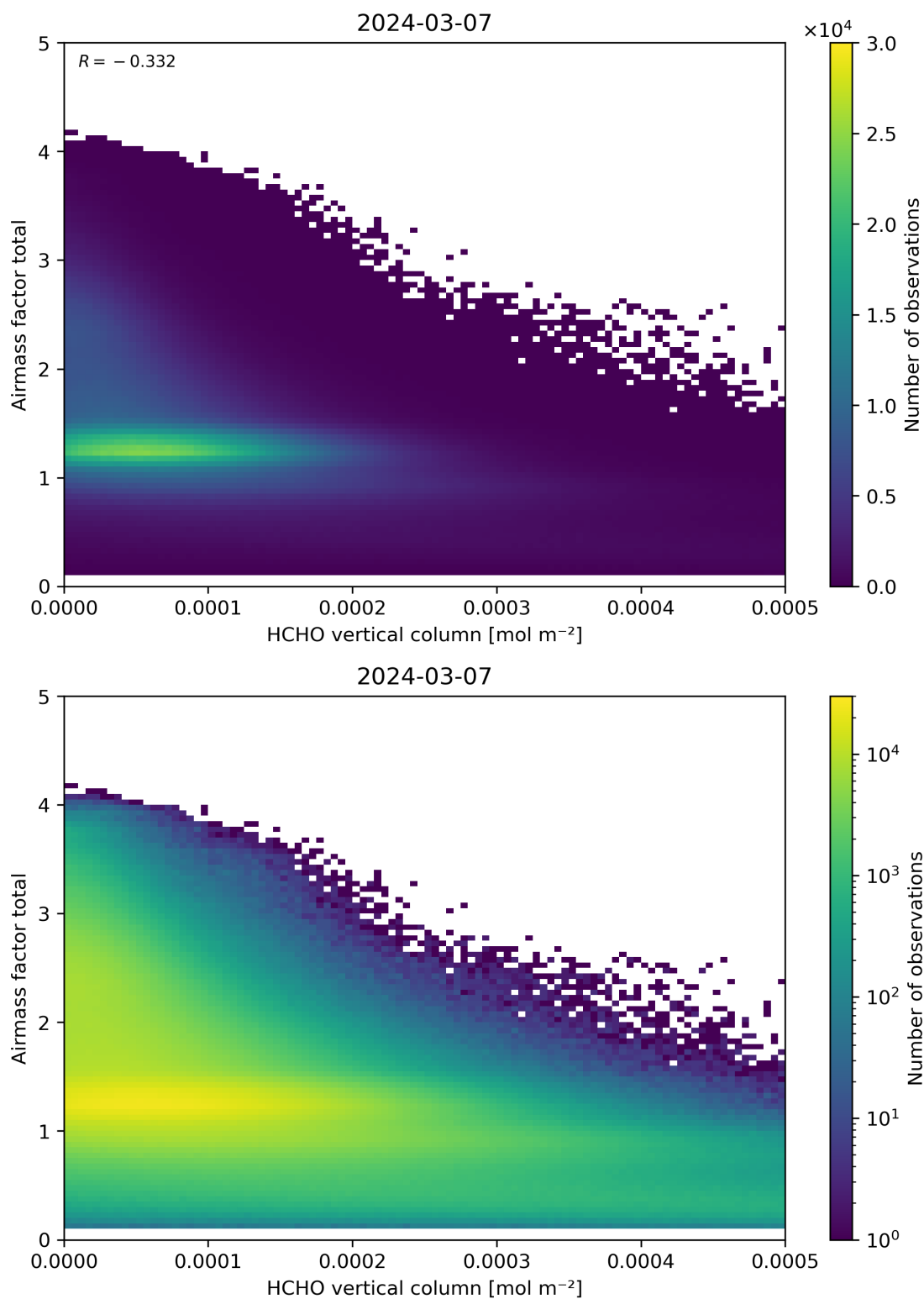
Figure 131: Scatter density plot of “HCHO vertical column” against “Airmass factor total” for 2024-03-06 to 2024-03-08.
