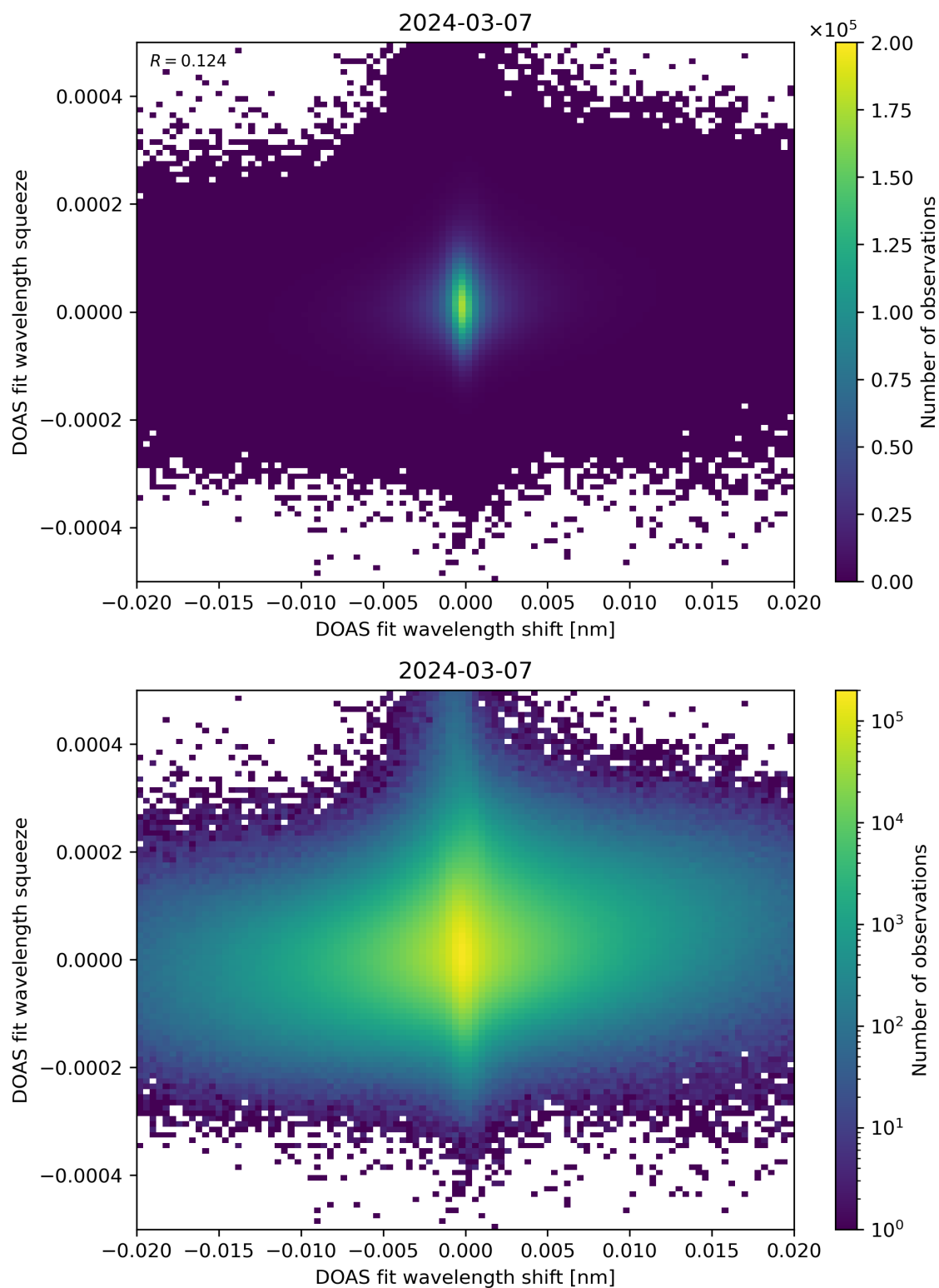
Figure 65: Scatter density plot of “DOAS fit wavelength shift” against “DOAS fit wavelength squeeze” for 2024-03-06 to 2024-03-08.
