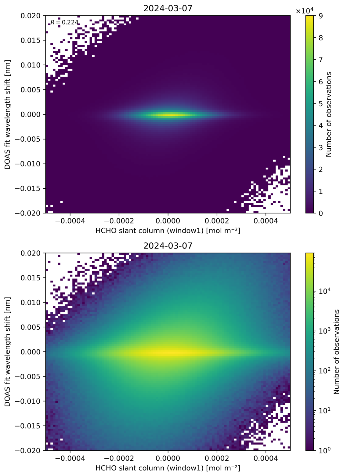
Figure 79: Scatter density plot of “HCHO slant column (window1)” against “DOAS fit wavelength shift” for 2024-03-06 to 2024-03-08.
