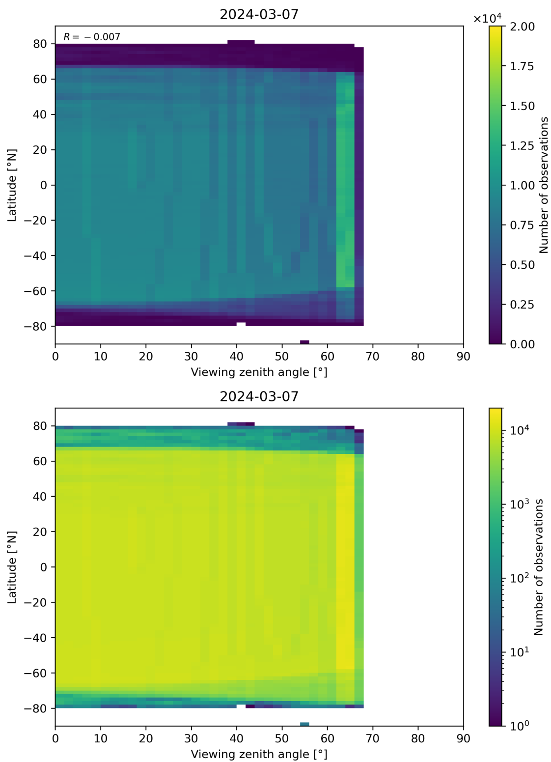
Figure 196: Scatter density plot of “Viewing zenith angle” against “Latitude” for 2024-03-06 to 2024-03-08.
