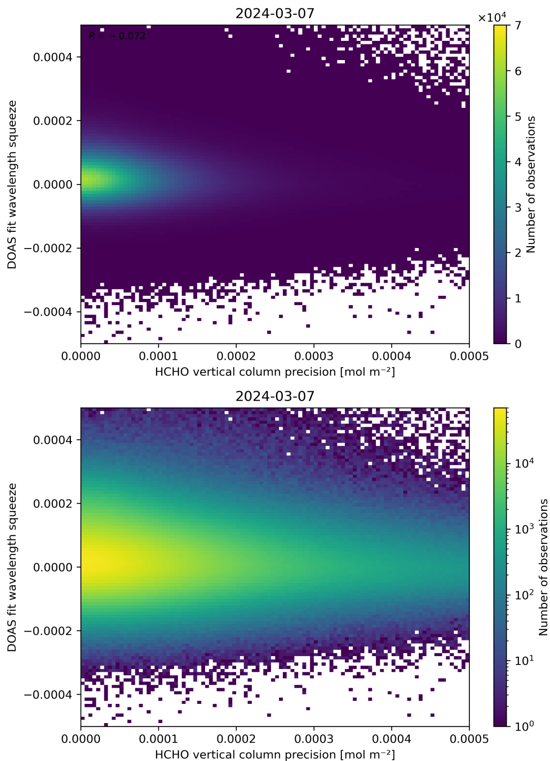
Figure 138: Scatter density plot of “HCHO vertical column precision” against “DOAS fit wavelength squeeze” for 2024-03-06 to 2024-03-08.
