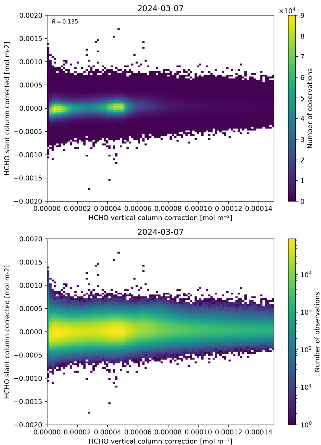
Figure 116: Scatter density plot of “HCHO vertical column correction” against “HCHO slant column corrected” for 2024-03-06 to 2024-03-08.
