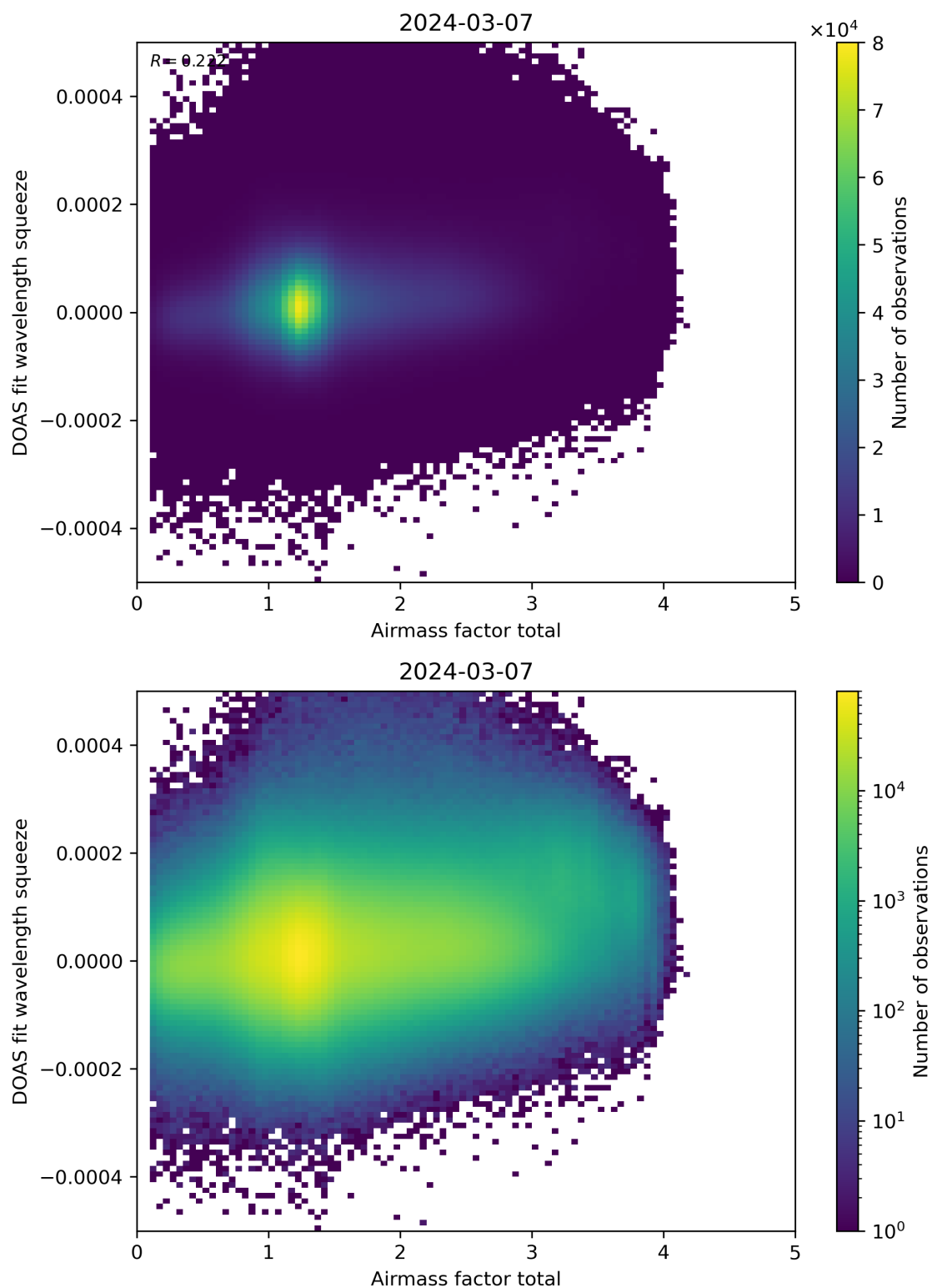
Figure 99: Scatter density plot of “Airmass factor total” against “DOAS fit wavelength squeeze” for 2024-03-06 to 2024-03-08.
