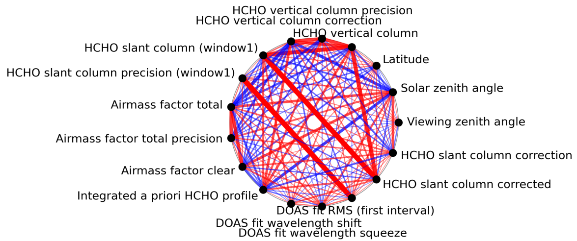
Figure 1: Map of correlation graph for 2024-03-06 to 2024-03-08.
