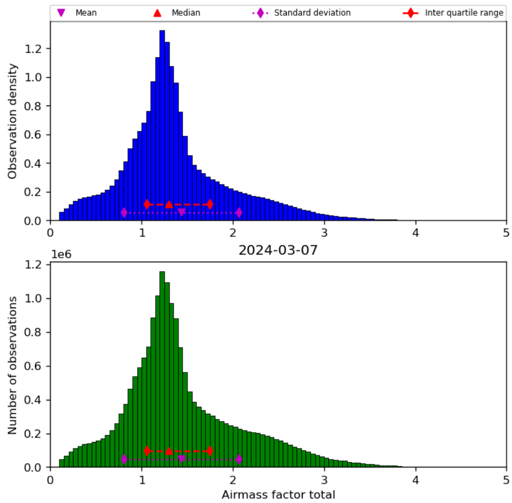
Figure 40: Histogram of “Airmass factor total” for 2024-03-06 to 2024-03-08
