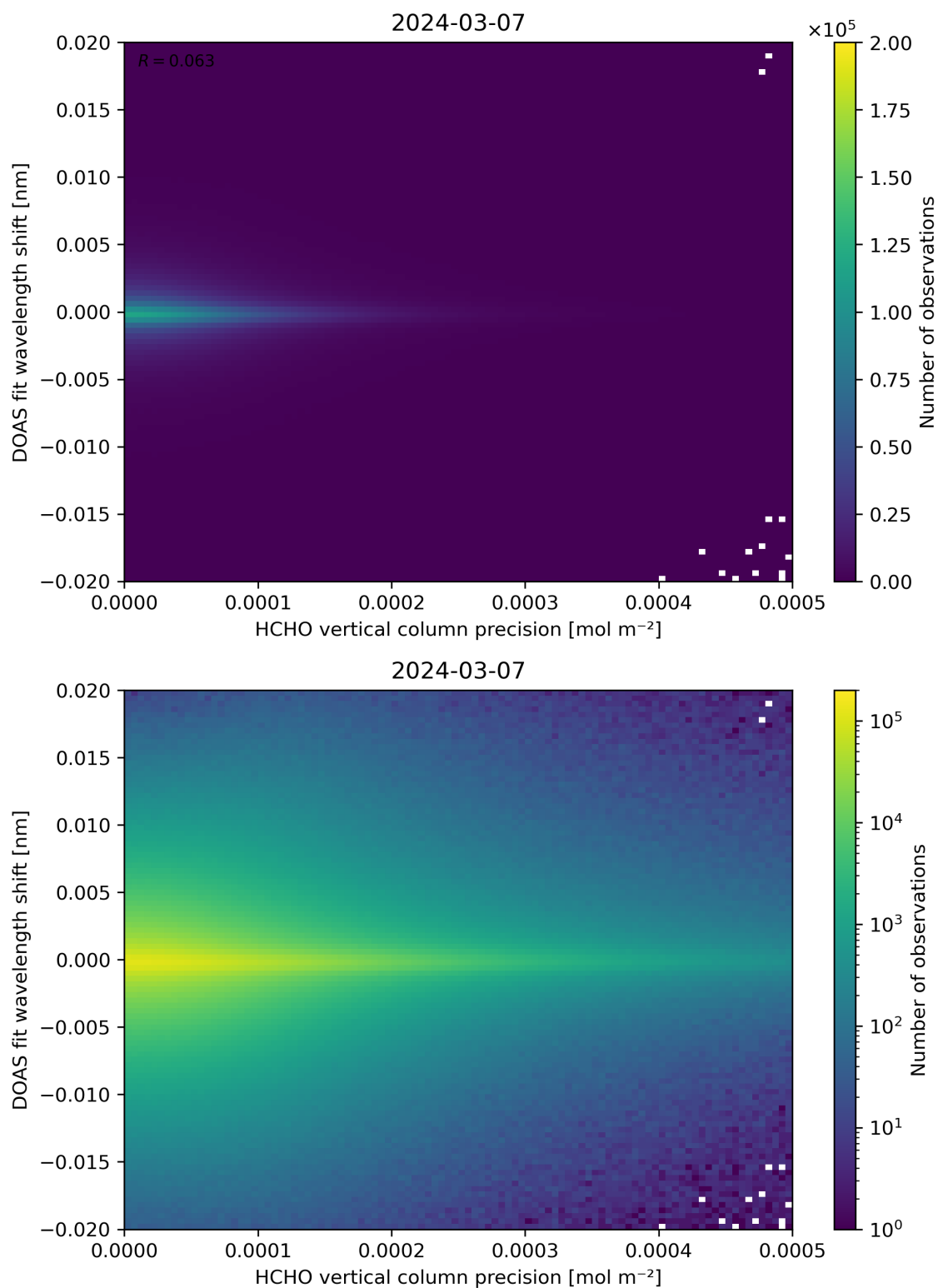
Figure 137: Scatter density plot of “HCHO vertical column precision” against “DOAS fit wavelength shift” for 2024-03-06 to 2024-03-08.
