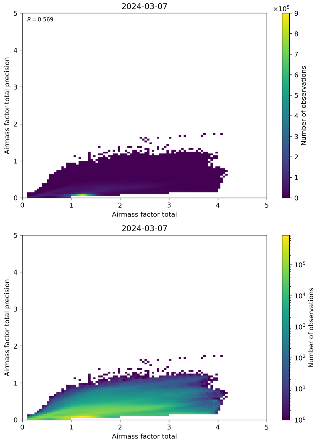
Figure 103: Scatter density plot of “Airmass factor total” against “Airmass factor total precision” for 2024-03-06 to 2024-03-08.
