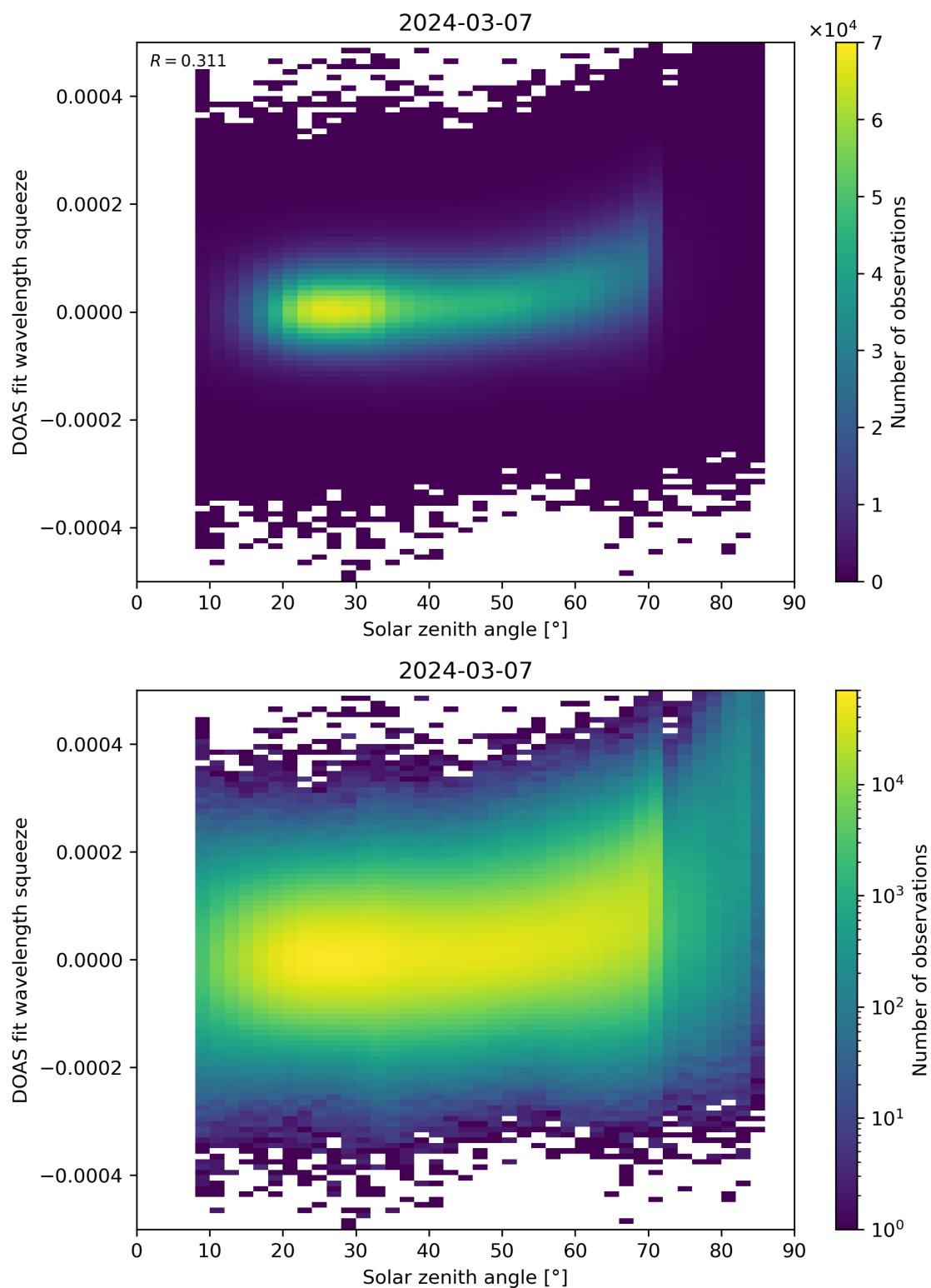
Figure 169: Scatter density plot of “Solar zenith angle” against “DOAS fit wavelength squeeze” for 2024-03-06 to 2024-03-08.
