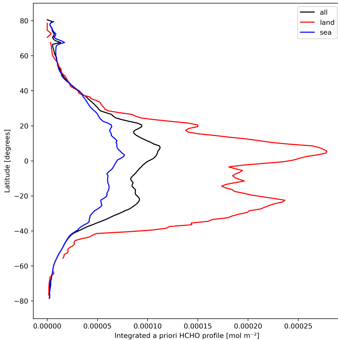
Figure 29: Zonal average of “Integrated a priori HCHO profile” for 2024-03-06 to 2024-03-08.
