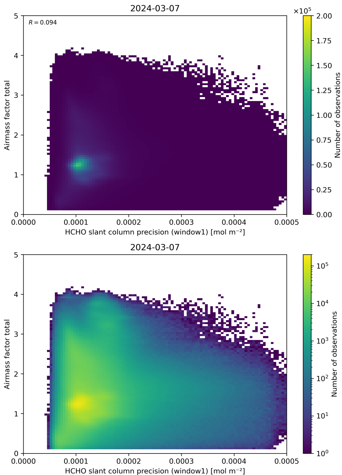
Figure 94: Scatter density plot of “HCHO slant column precision (window1)” against “Airmass factor total” for 2024-03-06 to 2024-03-08.
