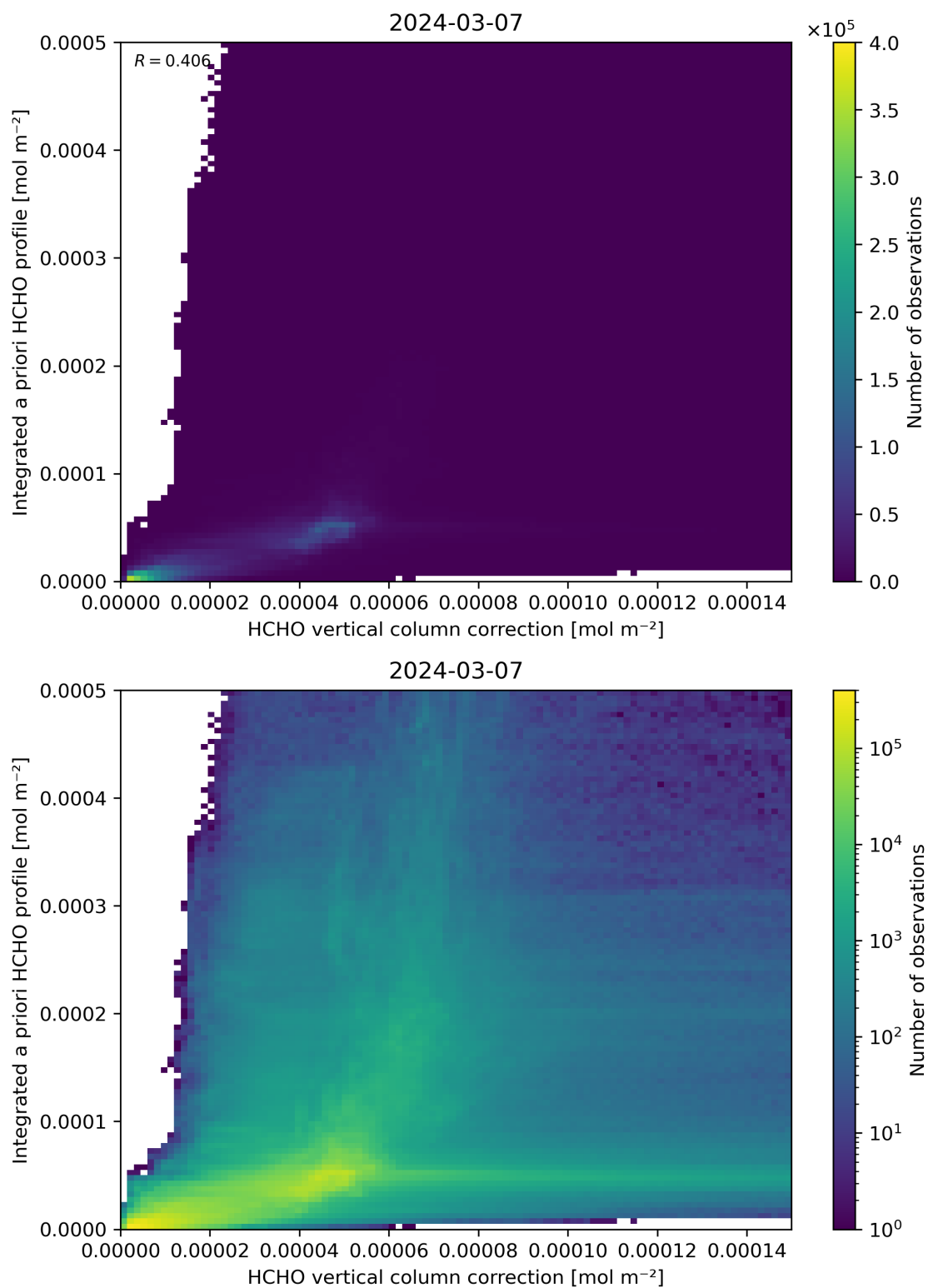
Figure 122: Scatter density plot of “HCHO vertical column correction” against “Integrated a priori HCHO profile” for 2024-03-06 to 2024-03-08.
