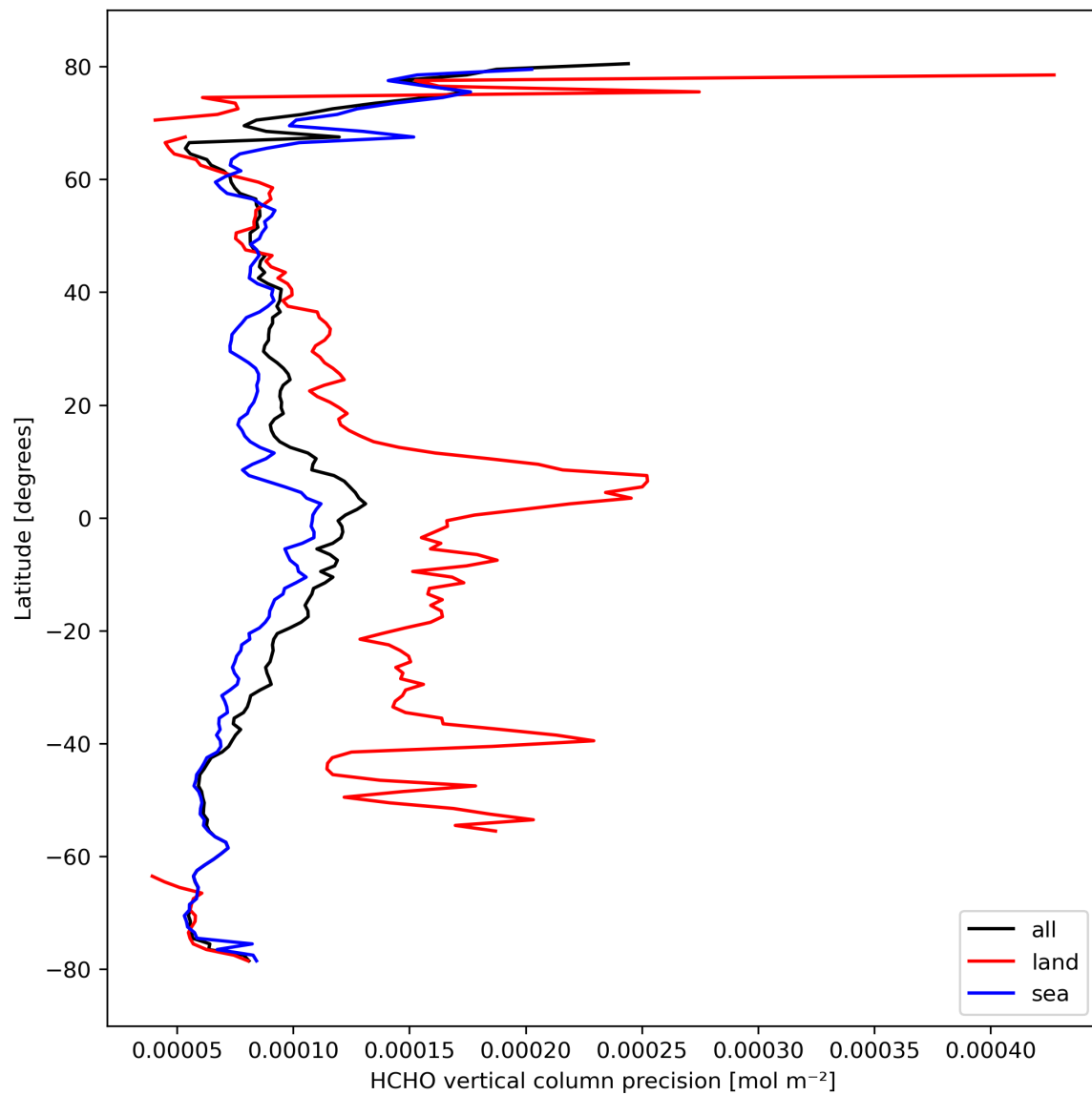
Figure 22: Zonal average of “HCHO vertical column precision” for 2024-03-06 to 2024-03-08.
