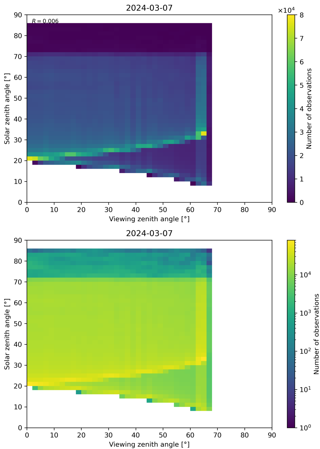
Figure 197: Scatter density plot of “Viewing zenith angle” against “Solar zenith angle” for 2024-03-06 to 2024-03-08.
