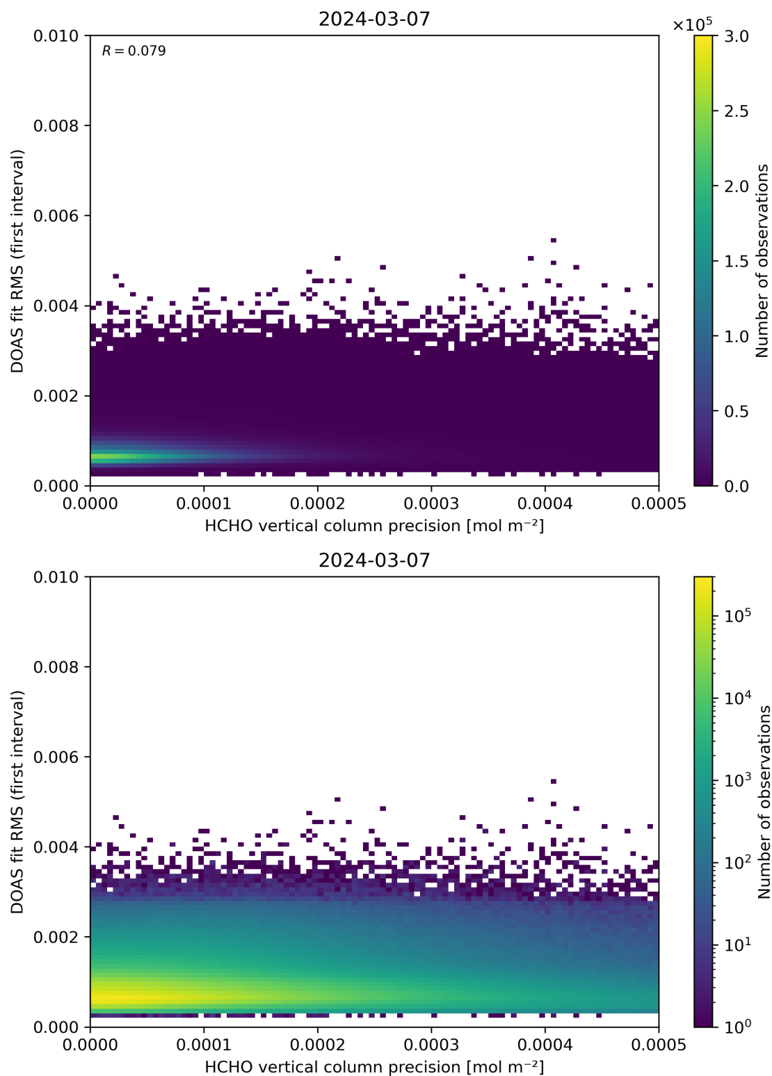
Figure 136: Scatter density plot of “HCHO vertical column precision” against “DOAS fit RMS (first interval)” for 2024-03-06 to 2024-03-08.
