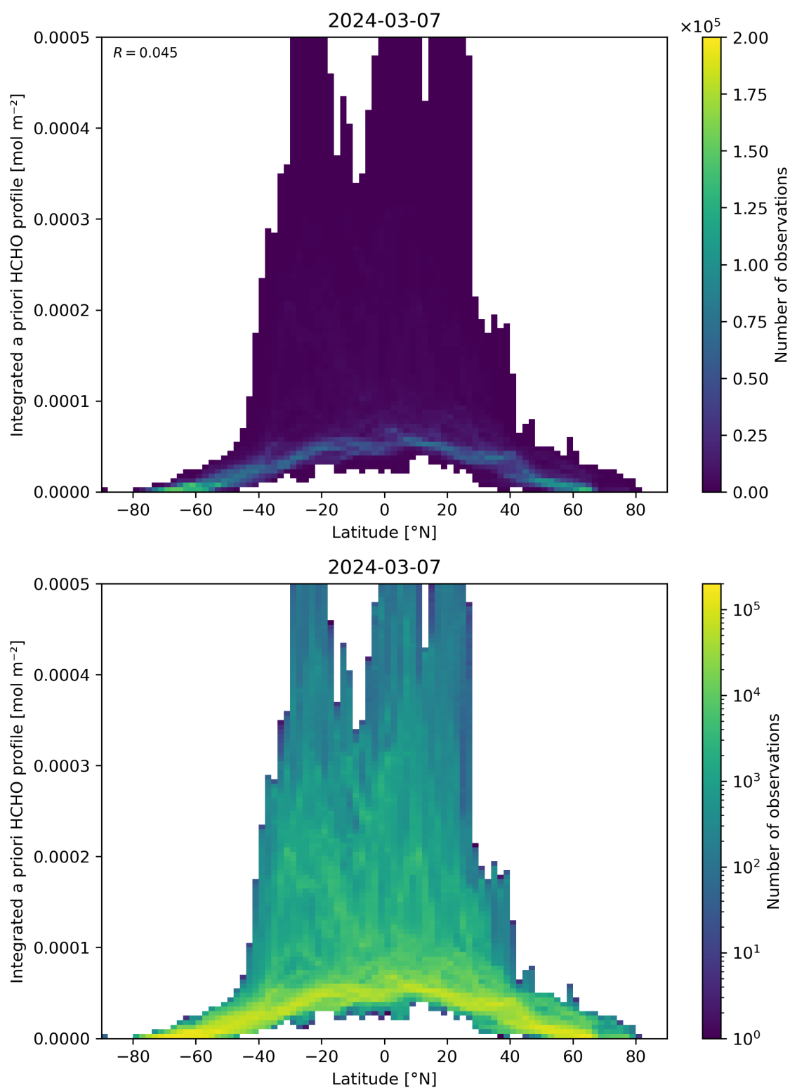
Figure 166: Scatter density plot of “Latitude” against “Integrated a priori HCHO profile” for 2024-03-06 to 2024-03-08.
