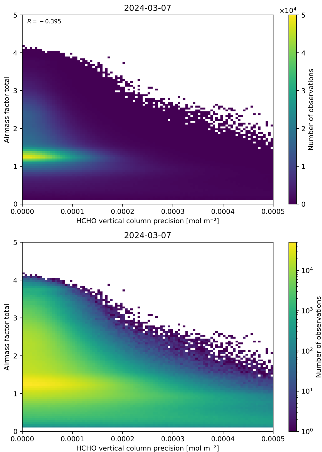
Figure 144: Scatter density plot of “HCHO vertical column precision” against “Airmass factor total” for 2024-03-06 to 2024-03-08.
