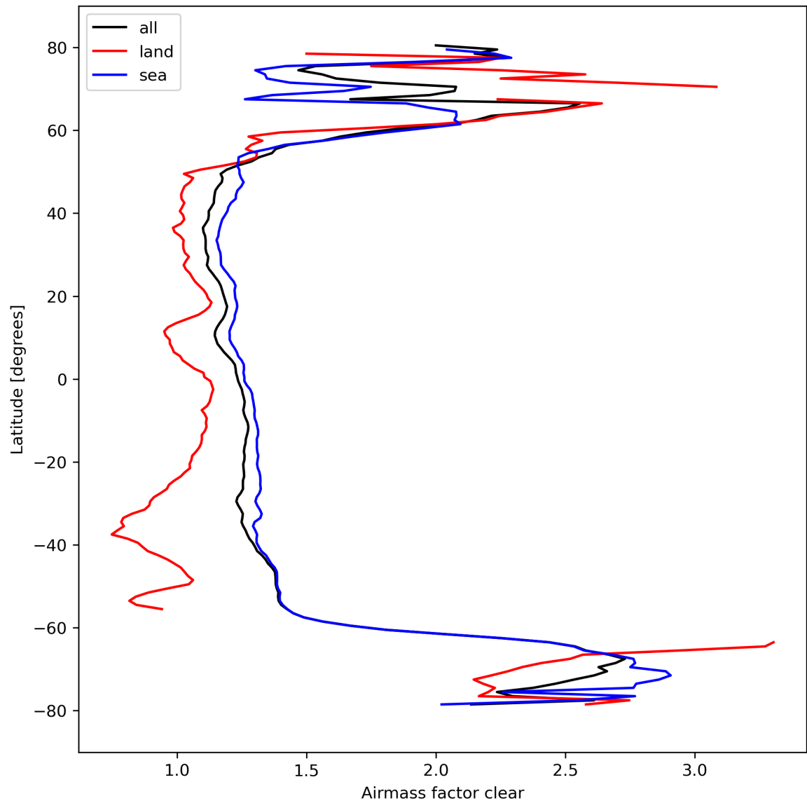
Figure 28: Zonal average of “Airmass factor clear” for 2024-03-06 to 2024-03-08.
