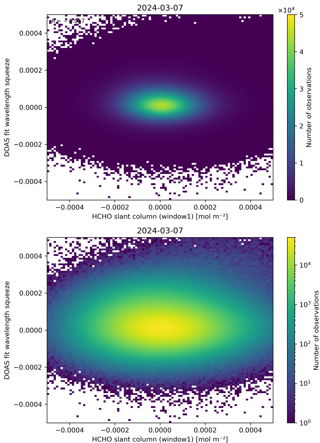
Figure 80: Scatter density plot of “HCHO slant column (window1)” against “DOAS fit wavelength squeeze” for 2024-03-06 to 2024-03-08.
