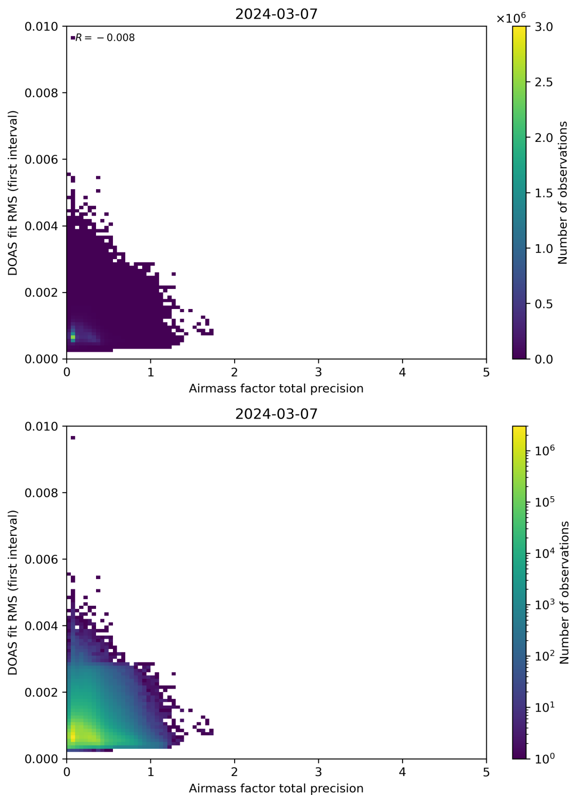
Figure 105: Scatter density plot of “Airmass factor total precision” against “DOAS fit RMS (first interval)” for 2024-03-06 to 2024-03-08.
