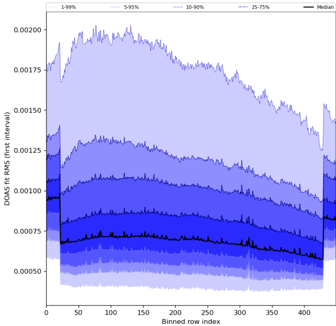
Figure 60: Along track statistics of “DOAS fit RMS (first interval)” for 2024-03-06 to 2024-03-08
