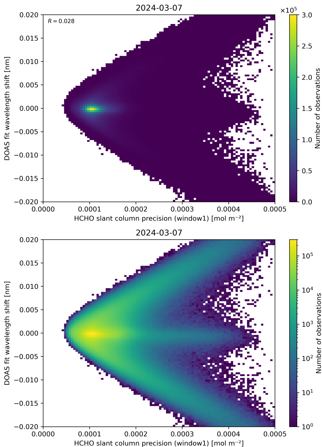
Figure 89: Scatter density plot of “HCHO slant column precision (window1)” against “DOAS fit wavelength shift” for 2024-03-06 to 2024-03-08.
