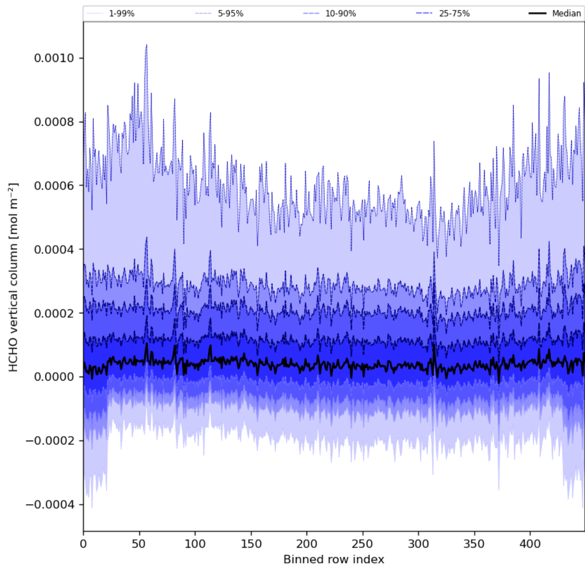
Figure 49: Along track statistics of “HCHO vertical column” for 2024-03-06 to 2024-03-08
