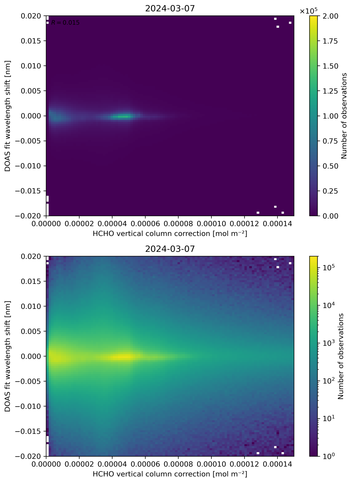
Figure 113: Scatter density plot of “HCHO vertical column correction” against “DOAS fit wavelength shift” for 2024-03-06 to 2024-03-08.
