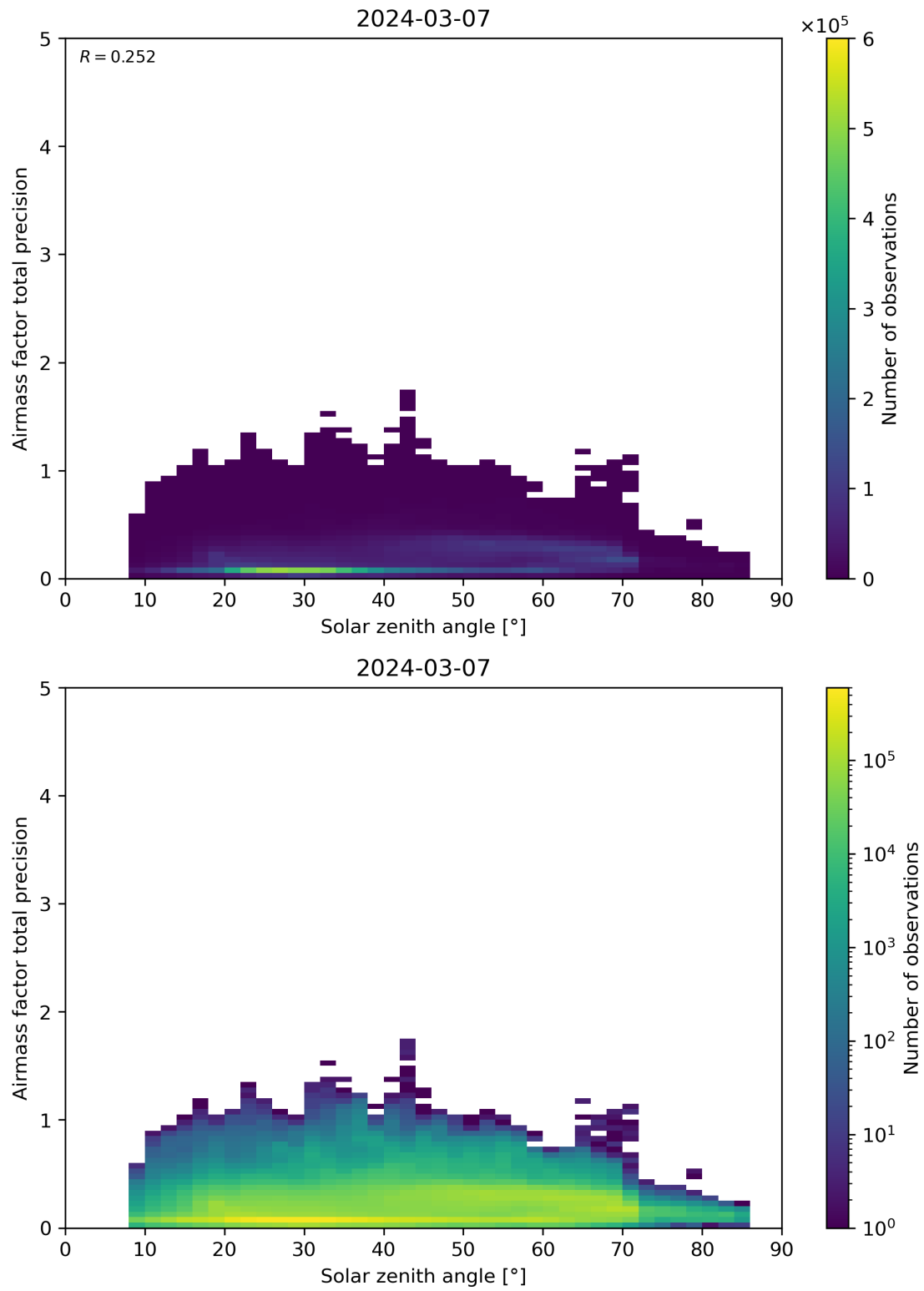
Figure 176: Scatter density plot of “Solar zenith angle” against “Airmass factor total precision” for 2024-03-06 to 2024-03-08.
