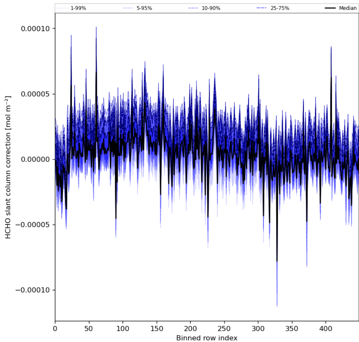
Figure 61: Along track statistics of “HCHO slant column correction” for 2024-03-06 to 2024-03-08
