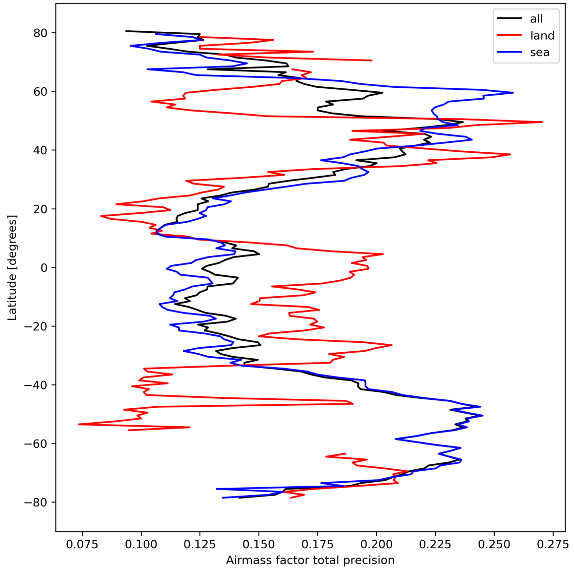
Figure 27: Zonal average of “Airmass factor total precision” for 2024-03-06 to 2024-03-08.
