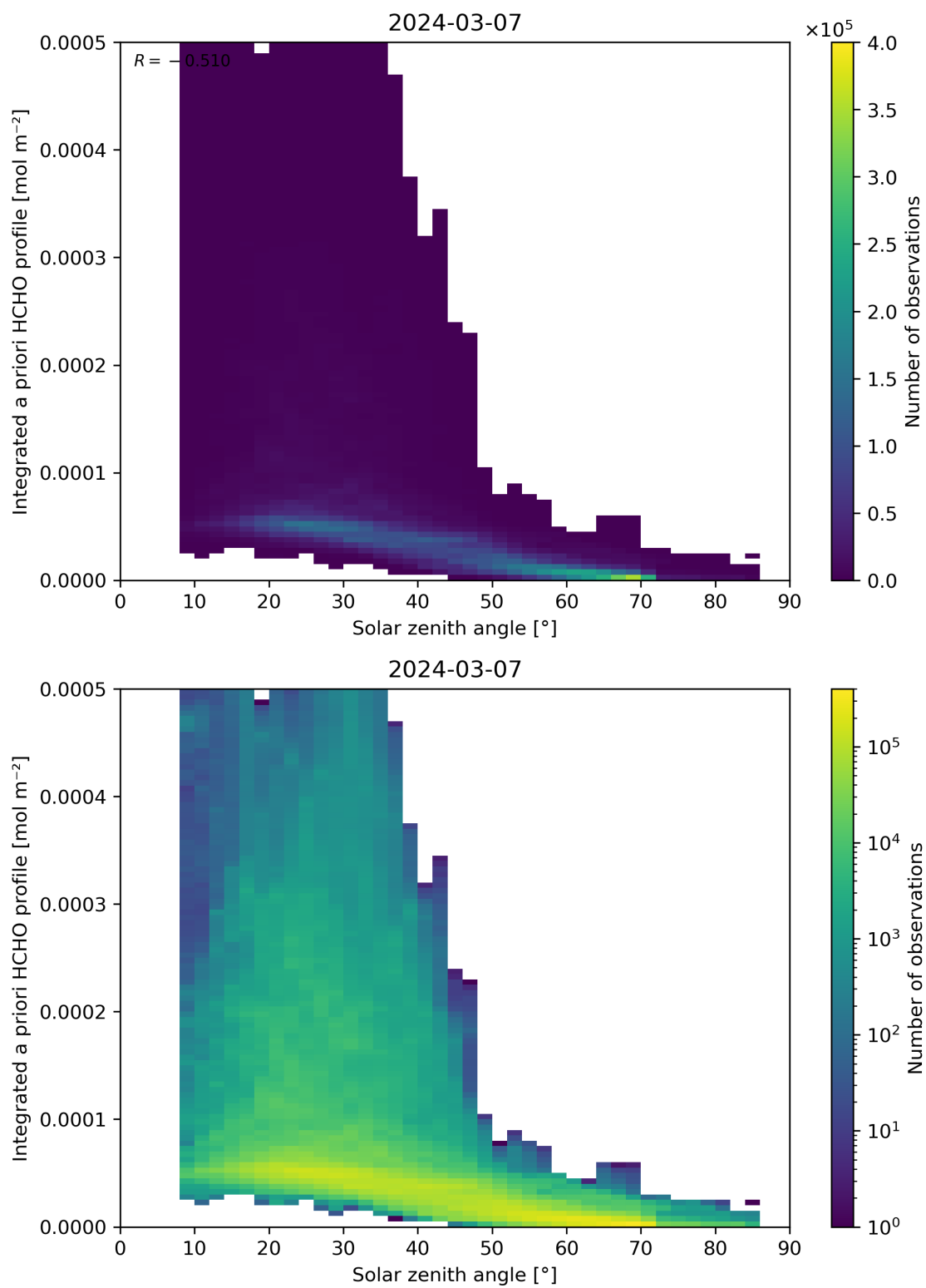
Figure 180: Scatter density plot of “Solar zenith angle” against “Integrated a priori HCHO profile” for 2024-03-06 to 2024-03-08.
