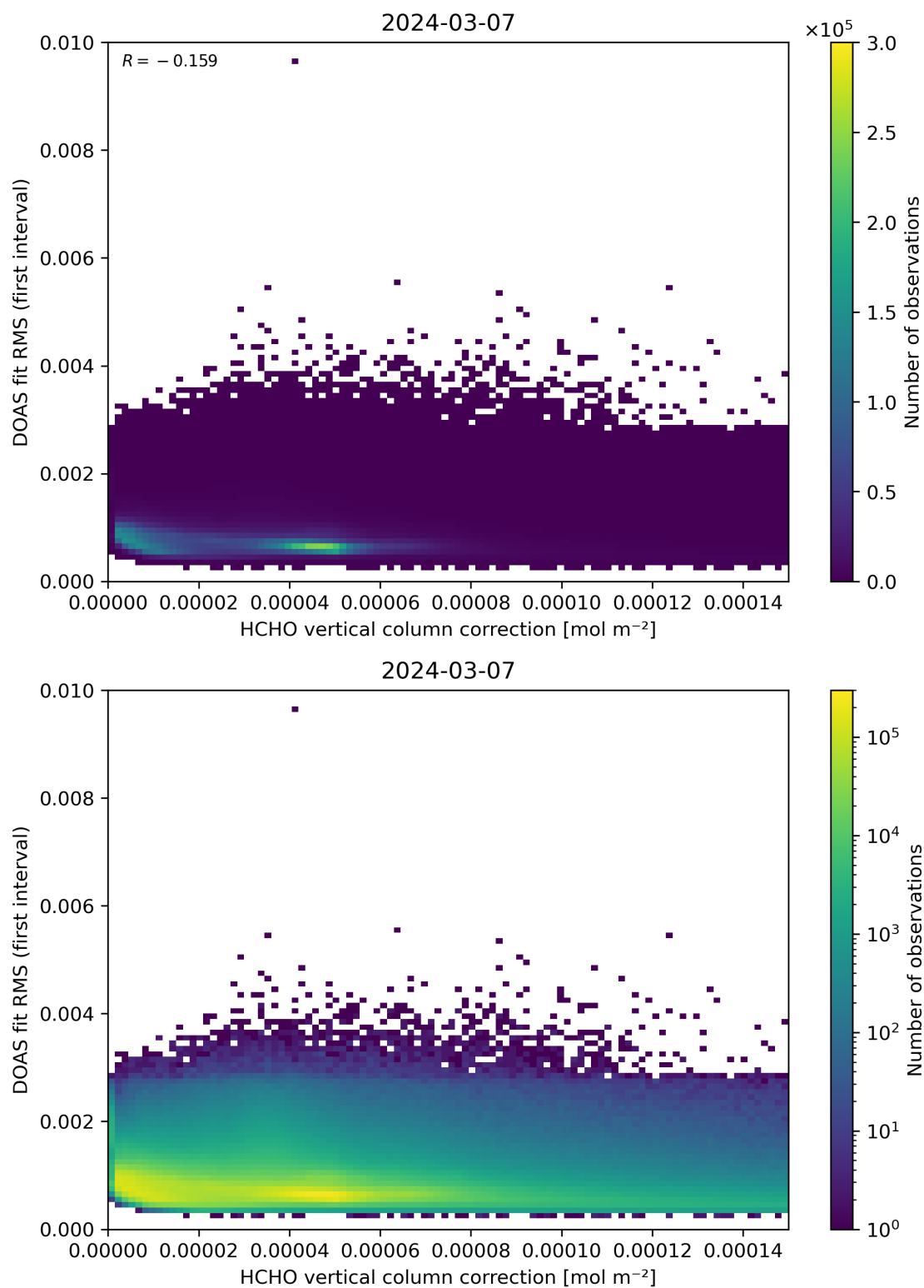
Figure 112: Scatter density plot of “HCHO vertical column correction” against “DOAS fit RMS (first interval)” for 2024-03-06 to 2024-03-08.
