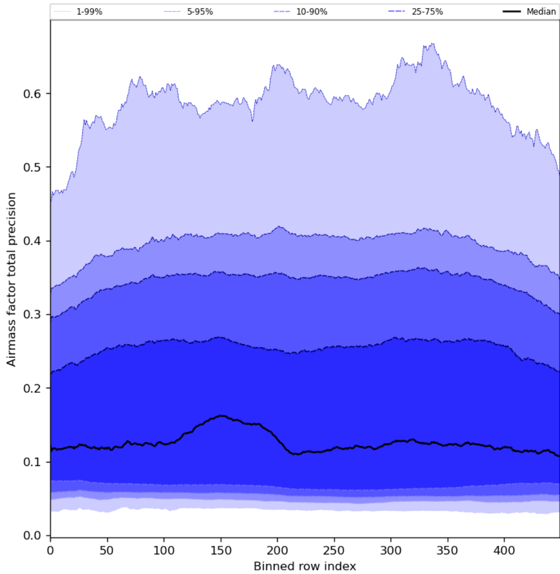
Figure 55: Along track statistics of “Airmass factor total precision” for 2024-03-06 to 2024-03-08
