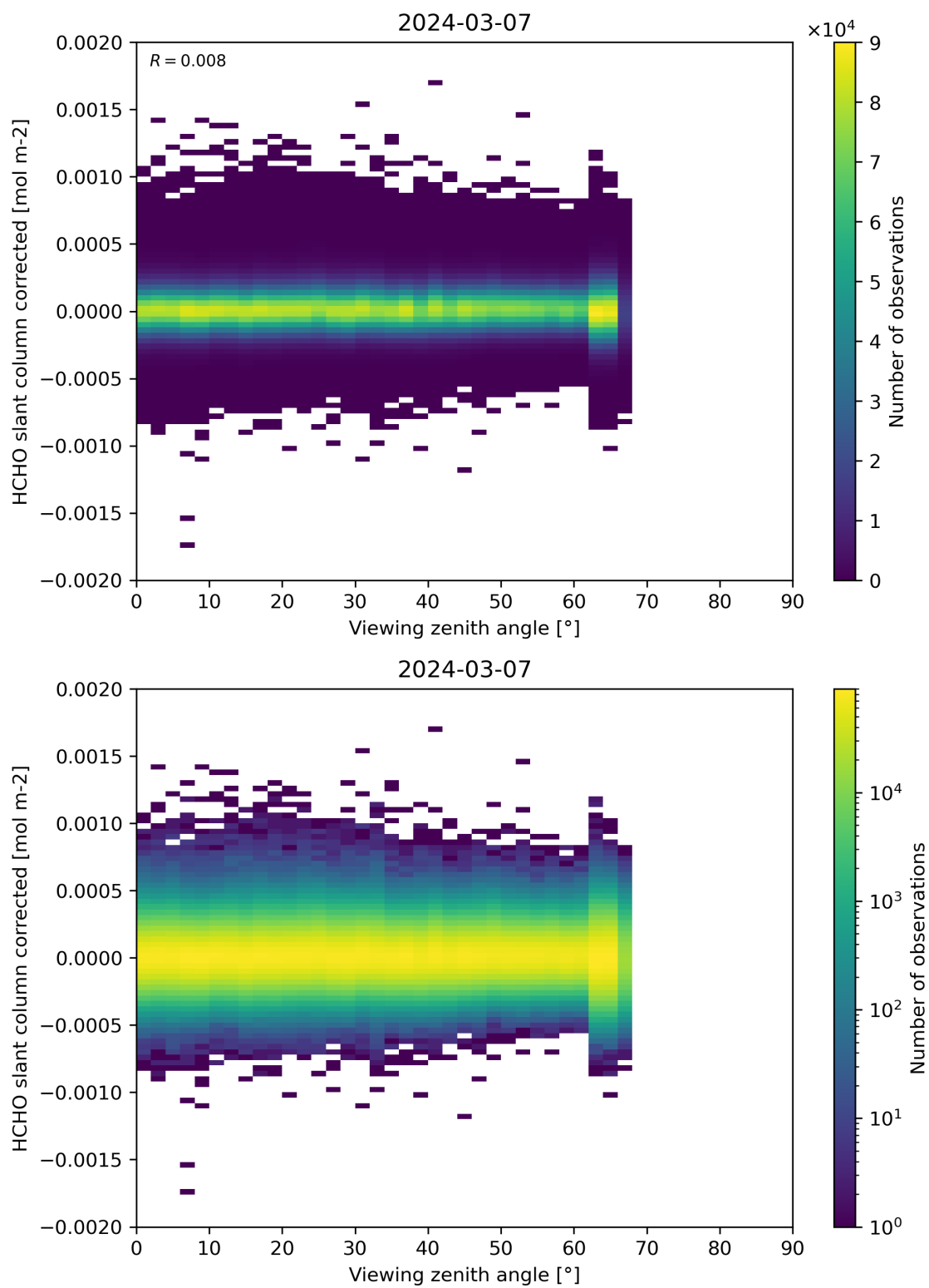
Figure 186: Scatter density plot of “Viewing zenith angle” against “HCHO slant column corrected” for 2024-03-06 to 2024-03-08.
