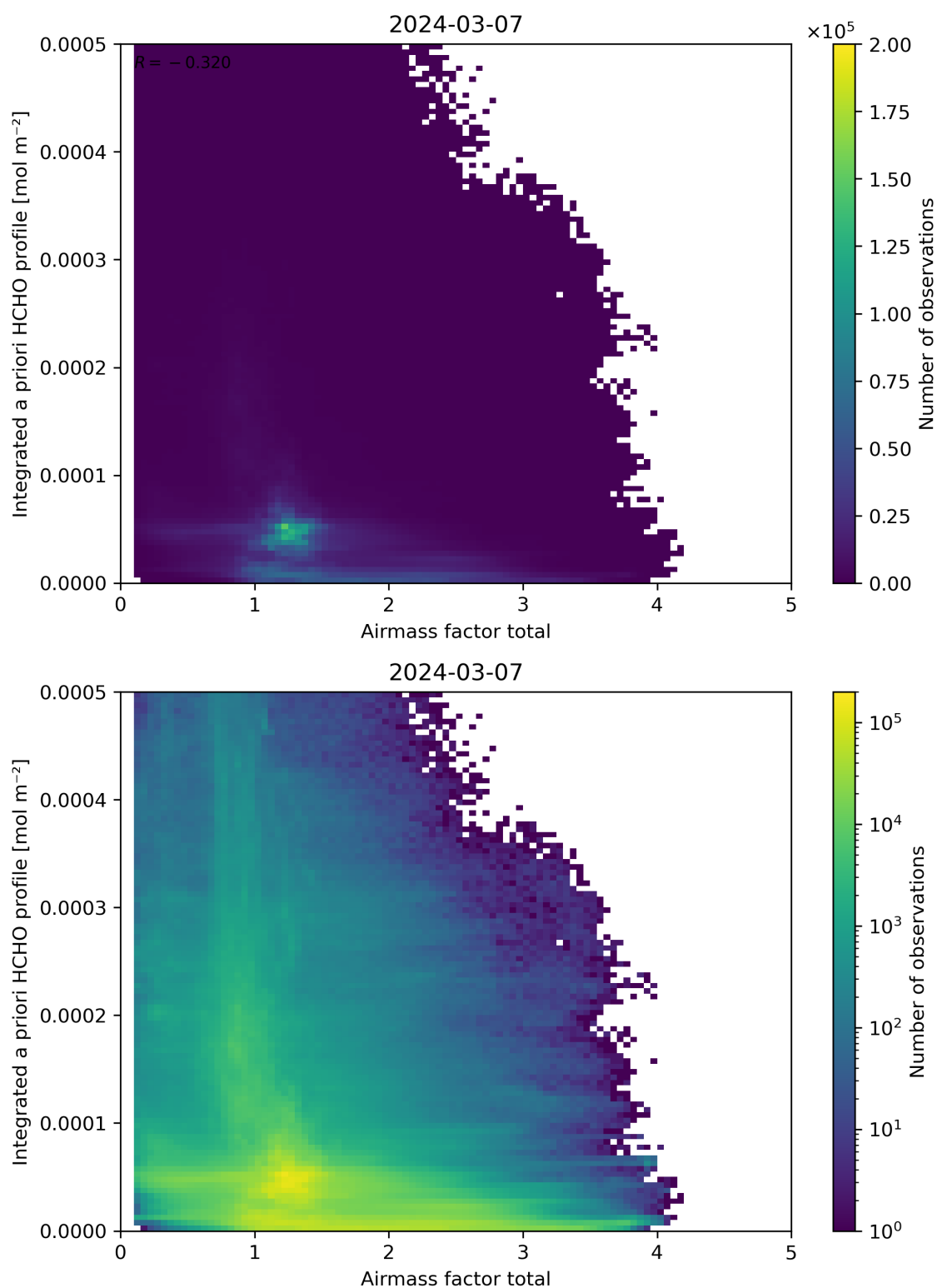
Figure 104: Scatter density plot of “Air mass factor total” against “Integrated a priori HCHO profile” for 2024-03-06 to 2024-03-08.
