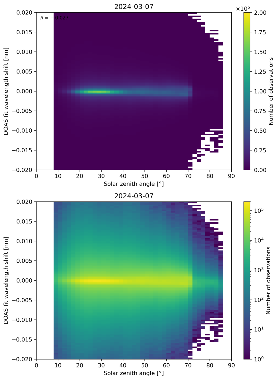
Figure 168: Scatter density plot of “Solar zenith angle” against “DOAS fit wavelength shift” for 2024-03-06 to 2024-03-08.
