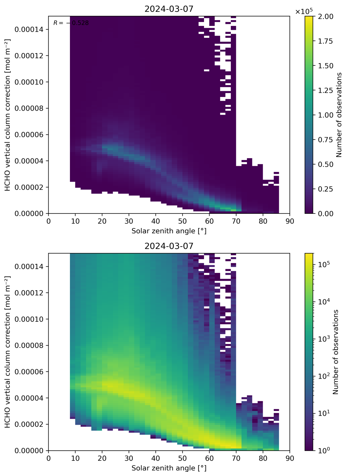
Figure 178: Scatter density plot of “Solar zenith angle” against “HCHO vertical column correction” for 2024-03-06 to 2024-03-08.
