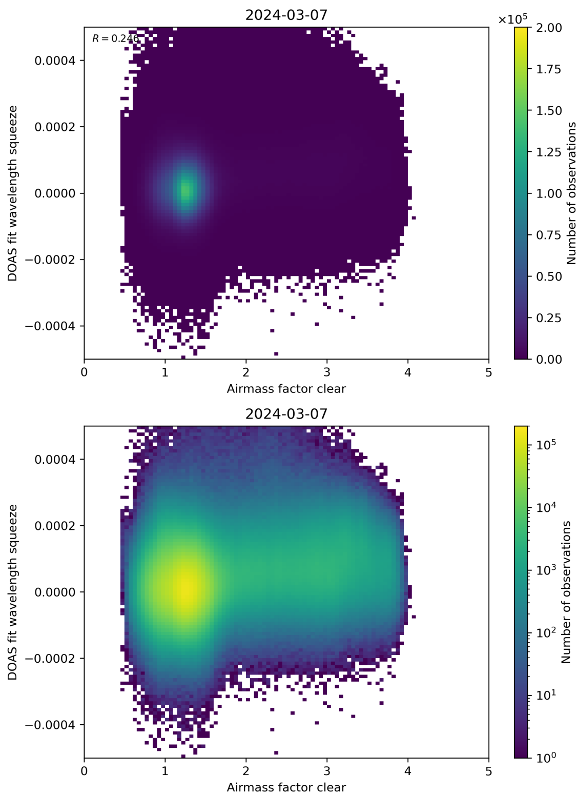
Figure 73: Scatter density plot of “Airmass factor clear” against “DOAS fit wavelength squeeze” for 2024-03-06 to 2024-03-08.
