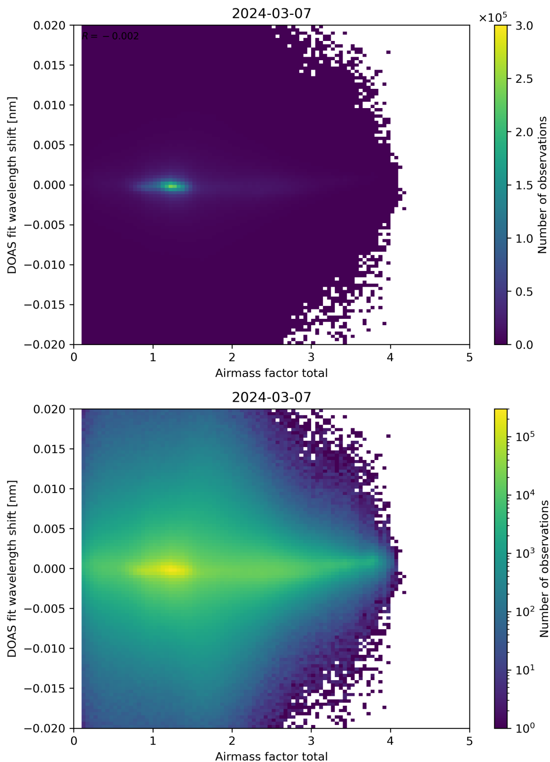
Figure 98: Scatter density plot of “Airmass factor total” against “DOAS fit wavelength shift” for 2024-03-06 to 2024-03-08.
