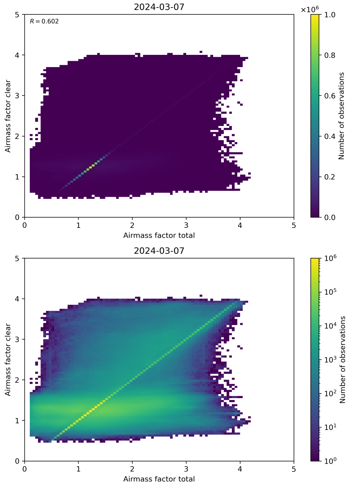
Figure 100: Scatter density plot of “Airmass factor total” against “Airmass factor clear” for 2024-03-06 to 2024-03-08.
