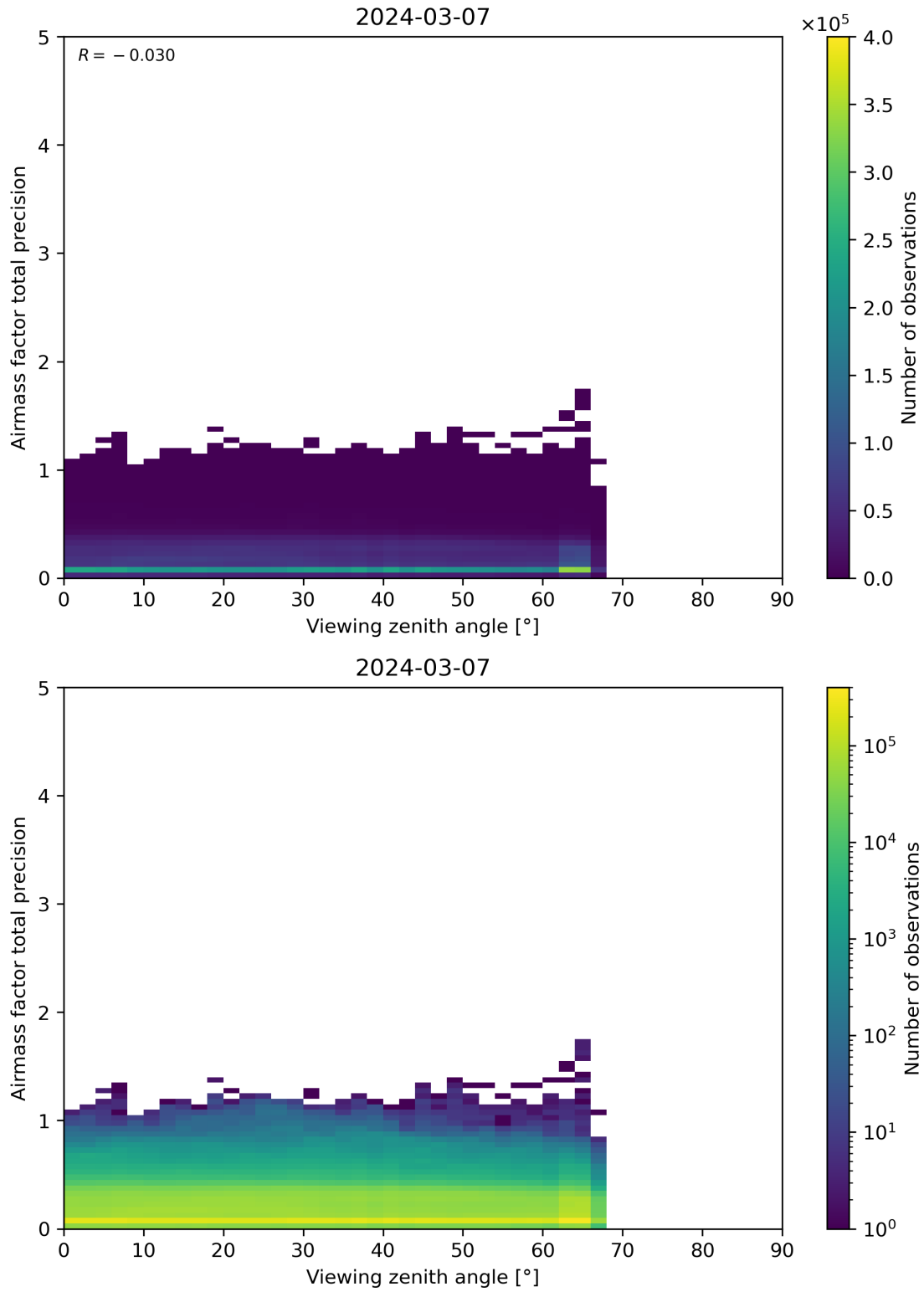
Figure 191: Scatter density plot of “Viewing zenith angle” against “Airmass factor total precision” for 2024-03-06 to 2024-03-08.
