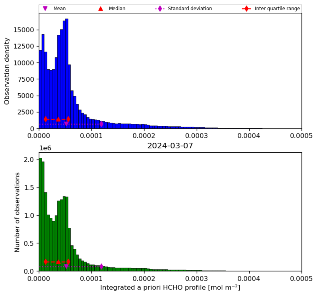
Figure 43: Histogram of “Integrated a priori HCHO profile” for 2024-03-06 to 2024-03-08
