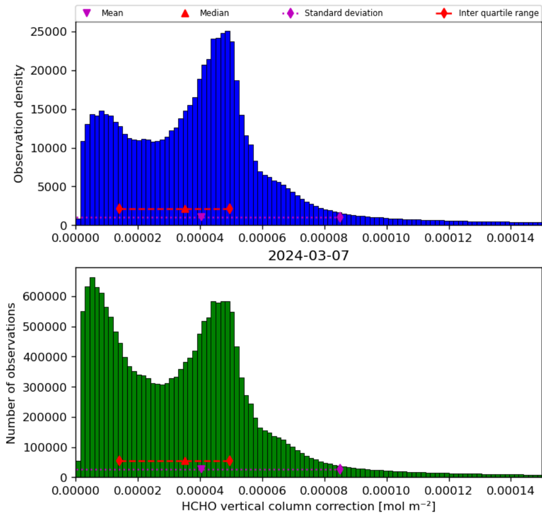
Figure 37: Histogram of “HCHO vertical column correction” for 2024-03-06 to 2024-03-08
