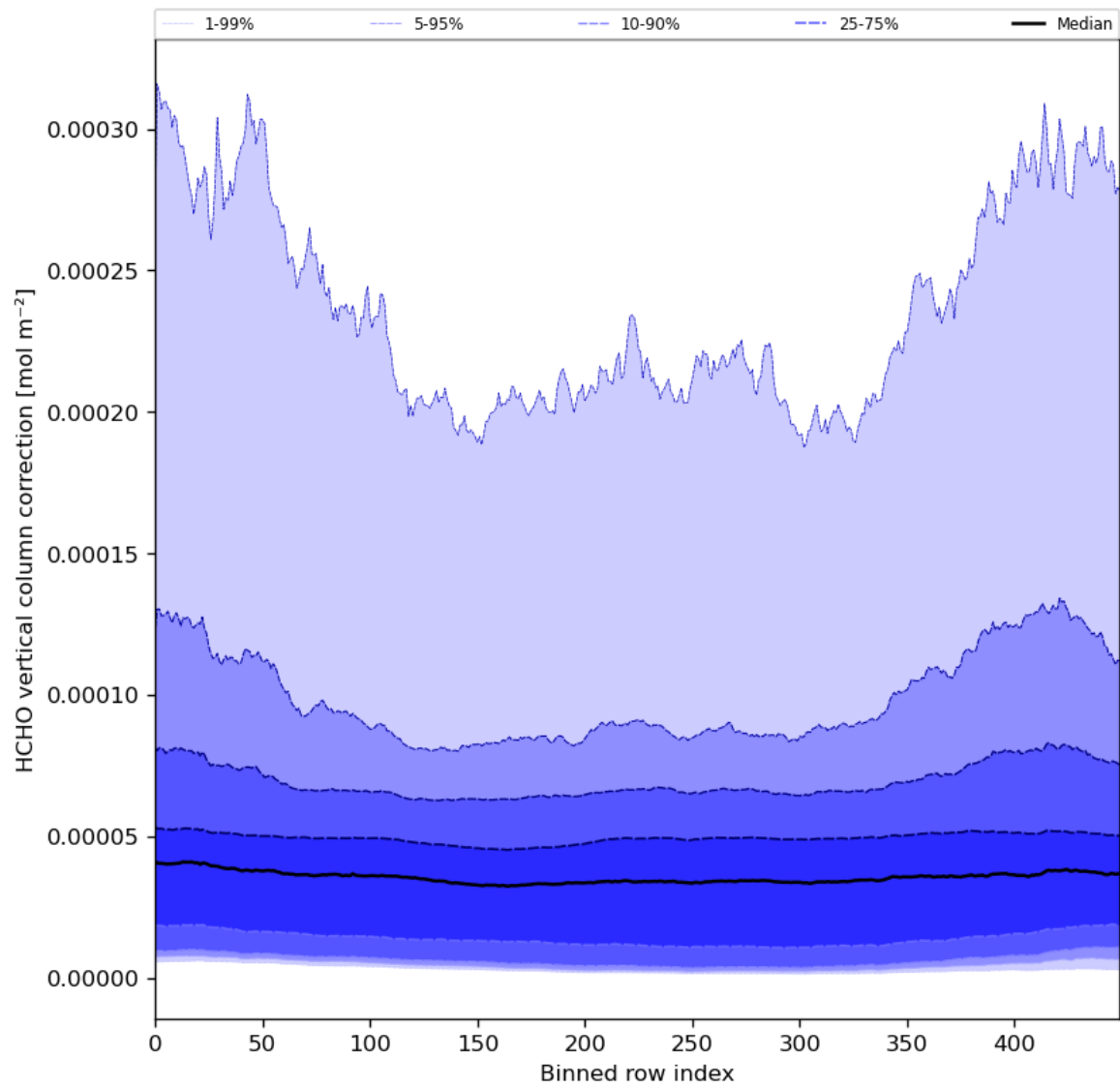
Figure 51: Along track statistics of “HCHO vertical column correction” for 2024-03-06 to 2024-03-08
