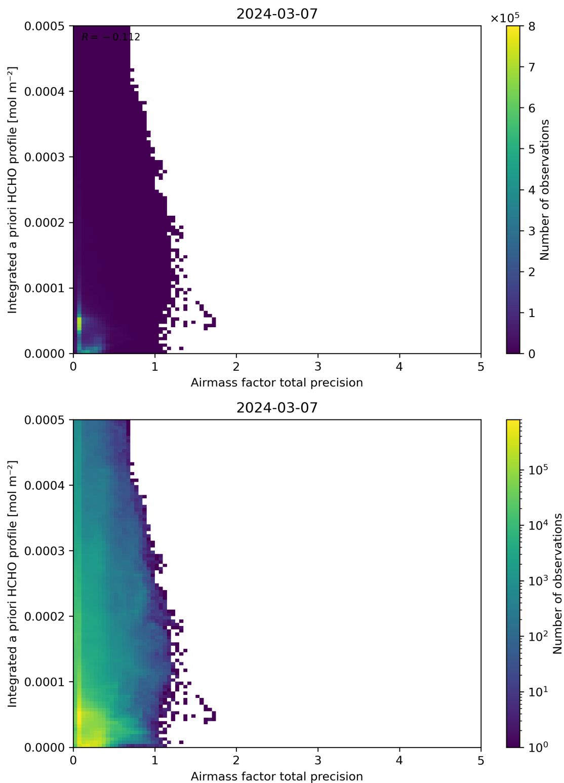
Figure 111: Scatter density plot of “Airmass factor total precision” against “Integrated a priori HCHO profile” for 2024-03-06 to 2024-03-08.
