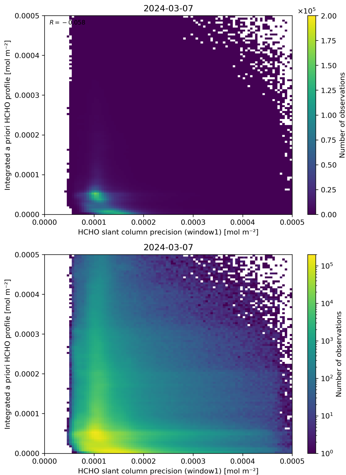
Figure 96: Scatter density plot of “HCHO slant column precision (window1)” against “Integrated a priori HCHO profile” for 2024-03-06 to 2024-03-08.
