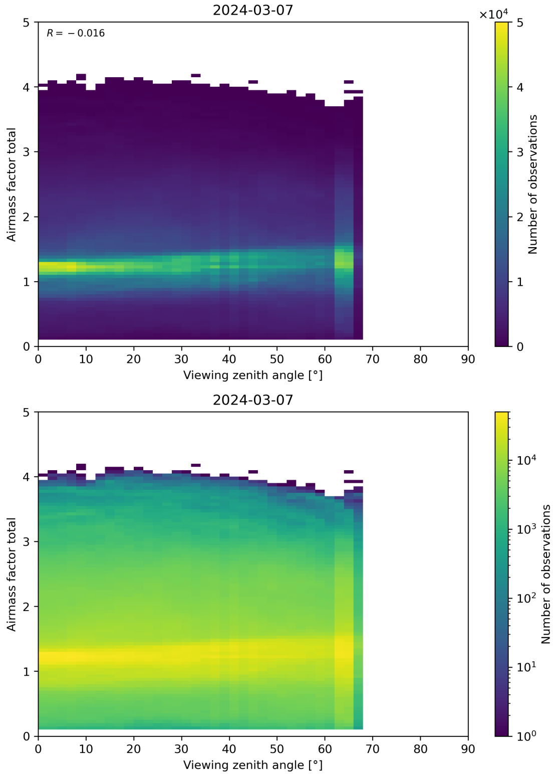
Figure 190: Scatter density plot of “Viewing zenith angle” against “Airmass factor total” for 2024-03-06 to 2024-03-08.
