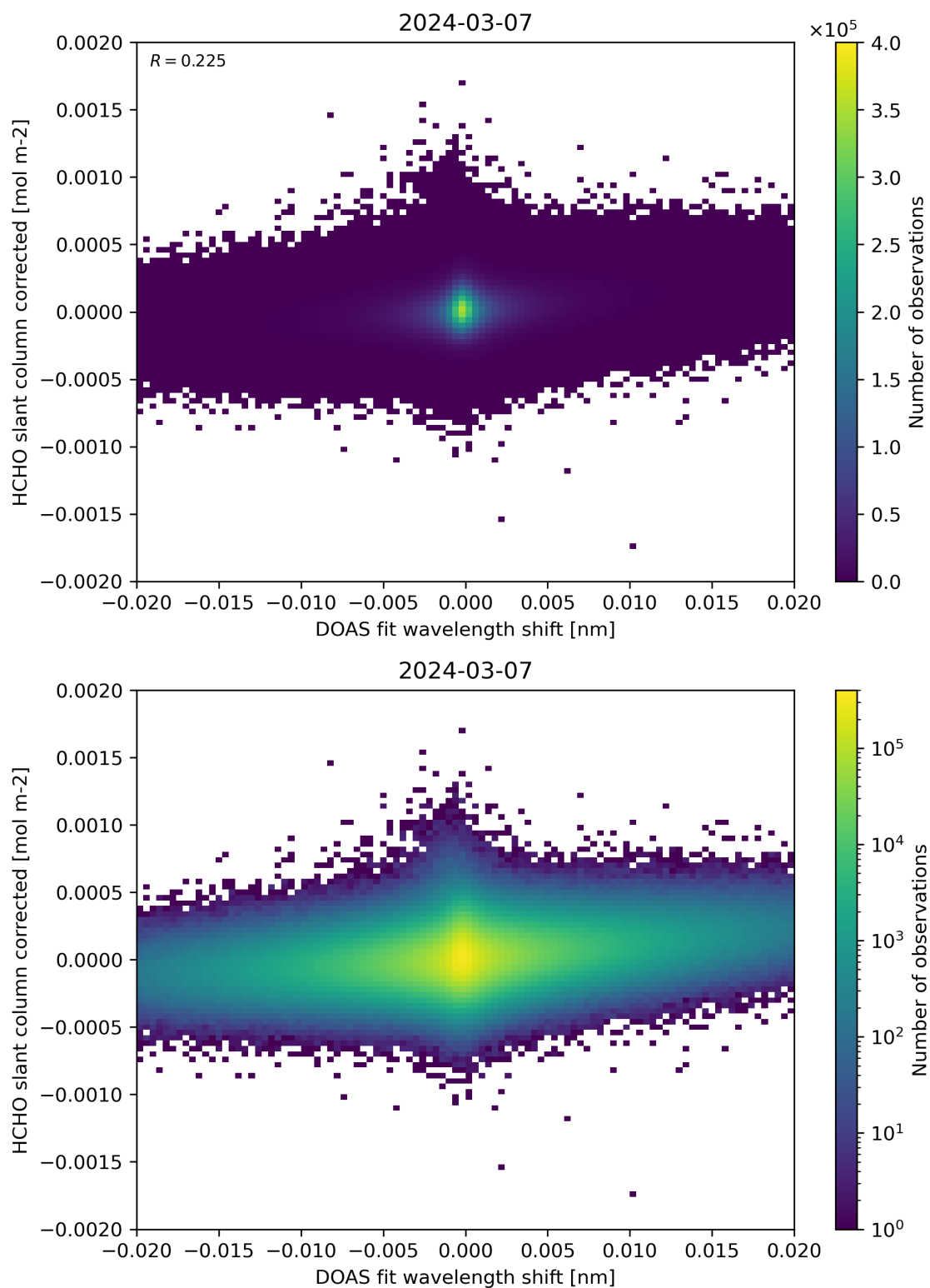
Figure 66: Scatter density plot of “DOAS fit wavelength shift” against “HCHO slant column corrected” for 2024-03-06 to 2024-03-08.
