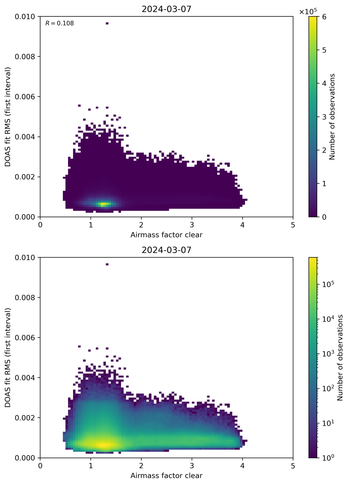
Figure 71: Scatter density plot of “Airmass factor clear” against “DOAS fit RMS (first interval)” for 2024-03-06 to 2024-03-08.
