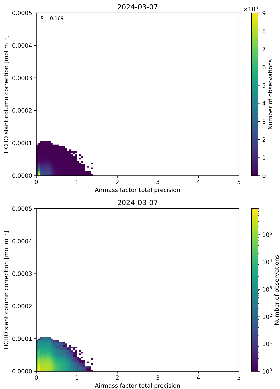
Figure 110: Scatter density plot of “Airmass factor total precision” against “HCHO slant column correction” for 2024-03-06 to 2024-03-08.
