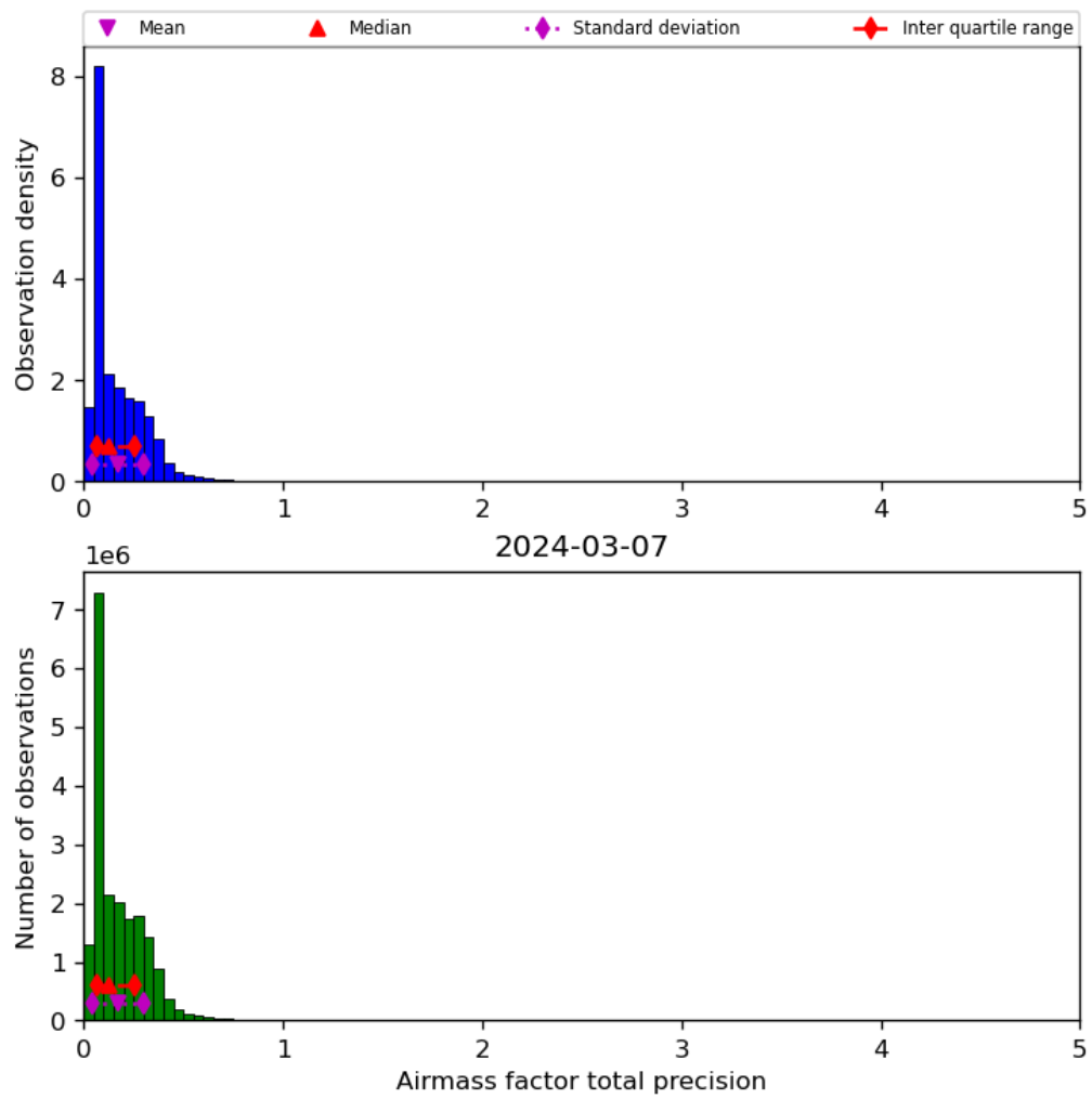
Figure 41: Histogram of “Airmass factor total precision” for 2024-03-06 to 2024-03-08
