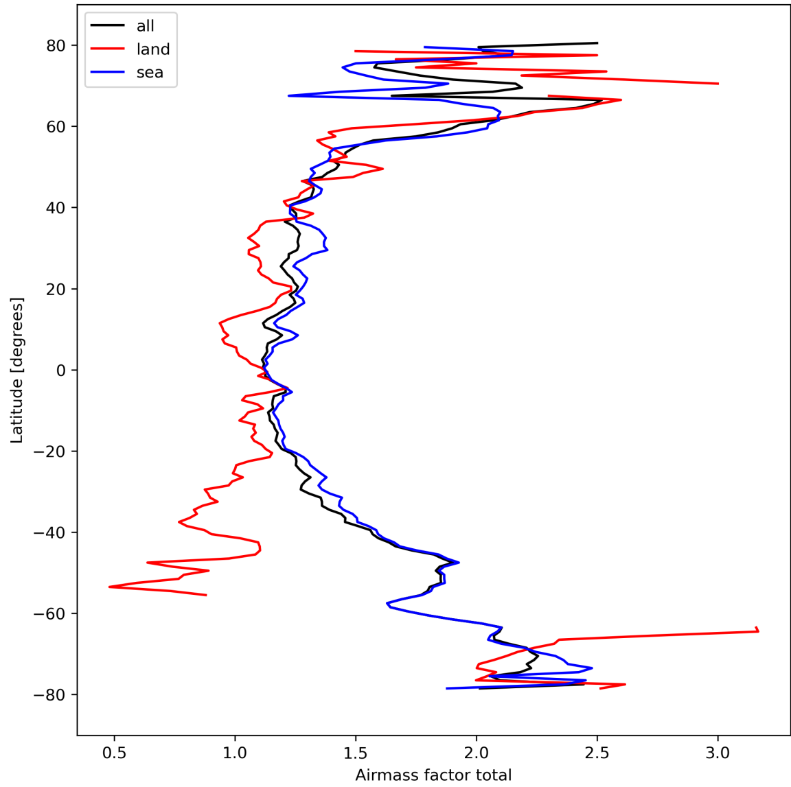
Figure 26: Zonal average of “Airmass factor total” for 2024-03-06 to 2024-03-08.
