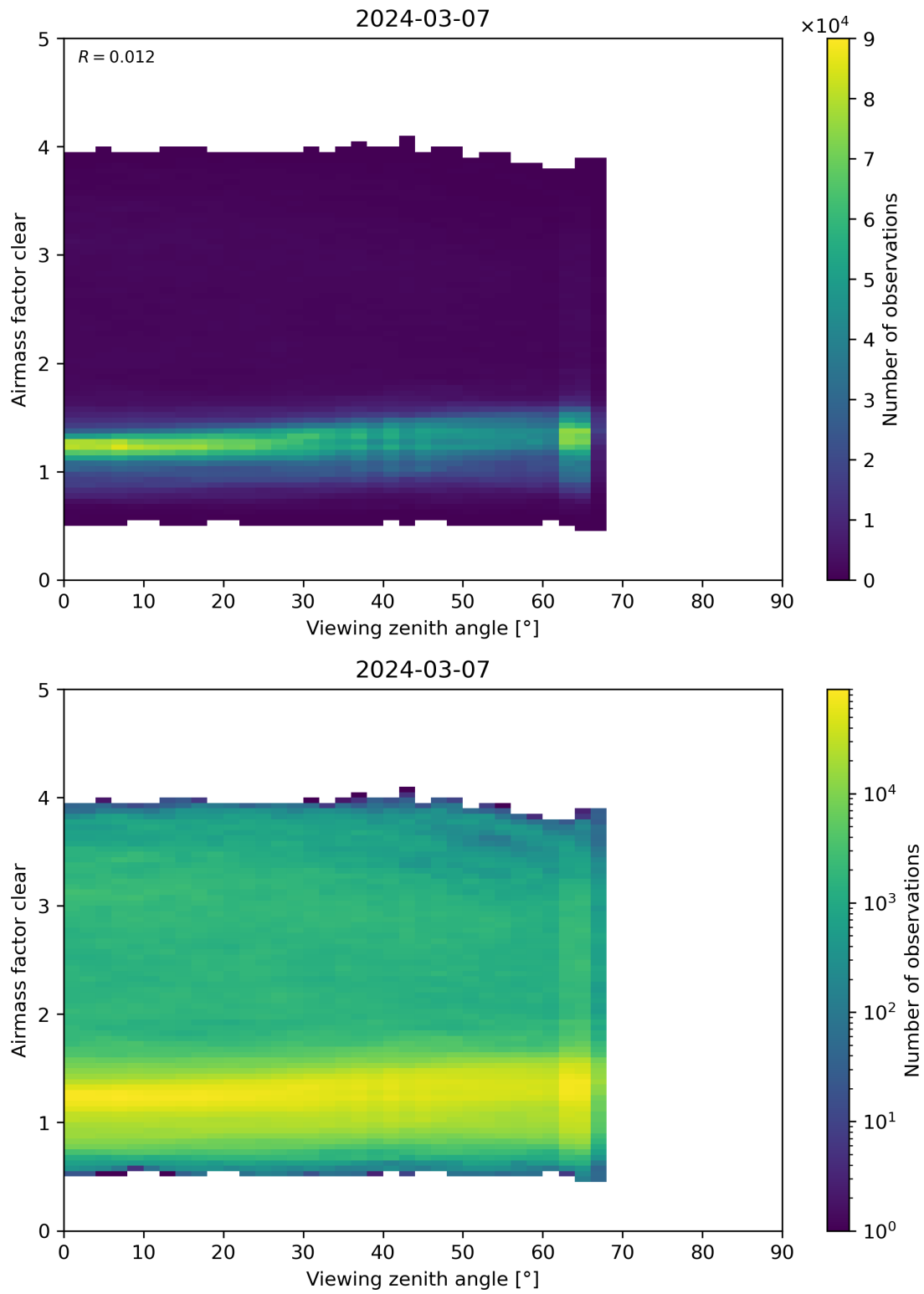
Figure 185: Scatter density plot of “Viewing zenith angle” against “Airmass factor clear” for 2024-03-06 to 2024-03-08.
