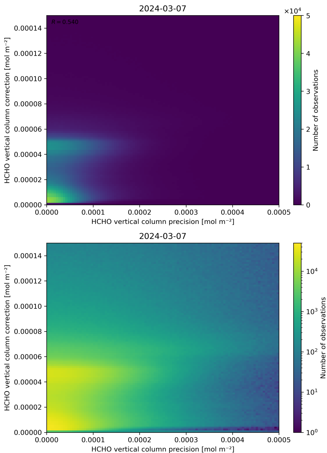
Figure 146: Scatter density plot of “HCHO vertical column precision” against “HCHO vertical column correction” for 2024-03-06 to 2024-03-08.
