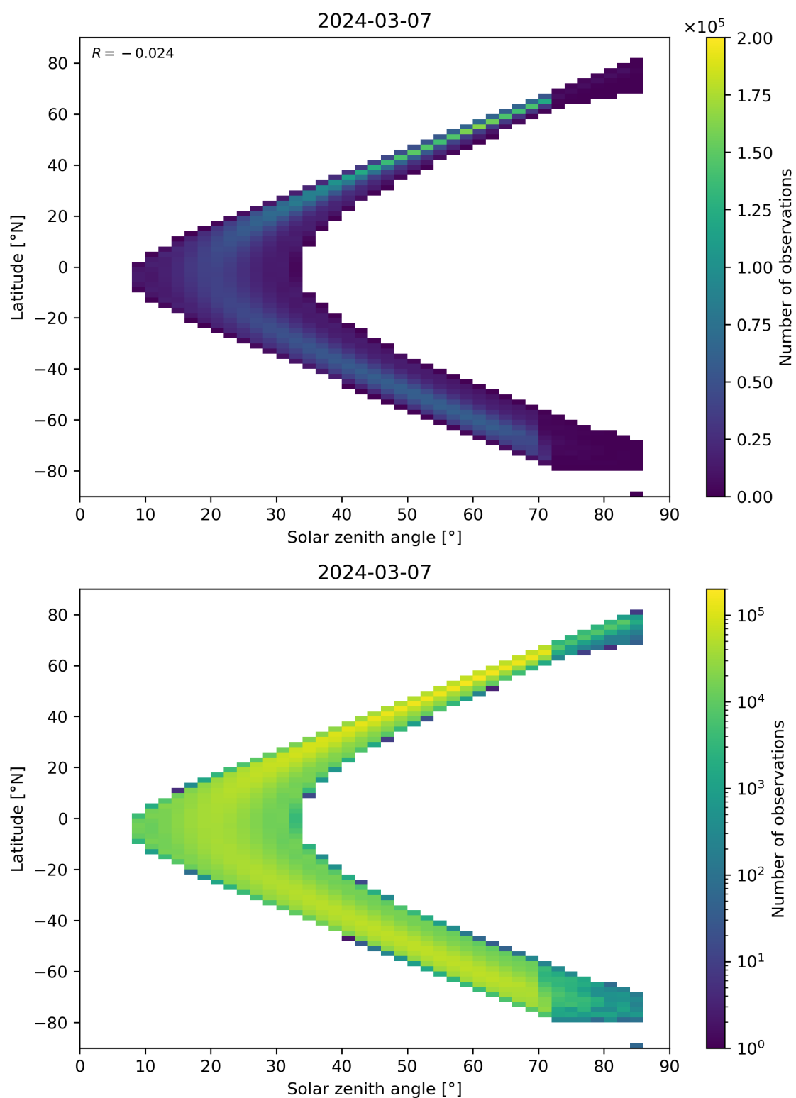
Figure 181: Scatter density plot of “Solar zenith angle” against “Latitude” for 2024-03-06 to 2024-03-08.
