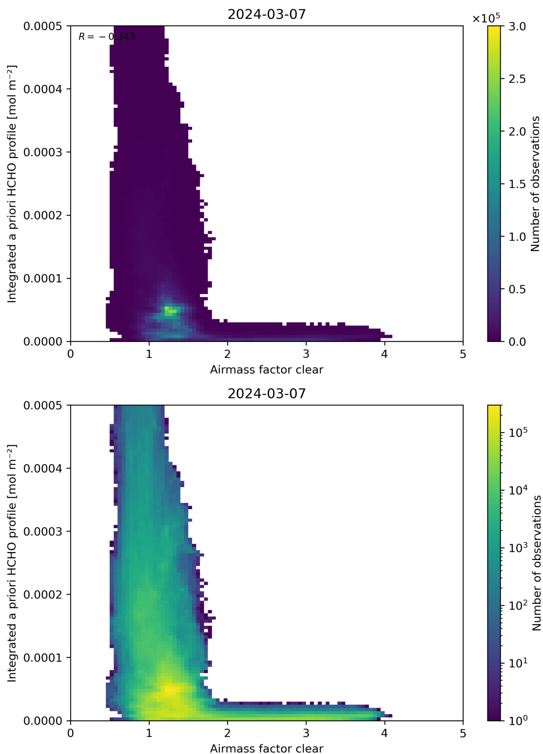
Figure 76: Scatter density plot of “Airmass factor clear” against “Integrated a priori HCHO profile” for 2024-03-06 to 2024-03-08.
