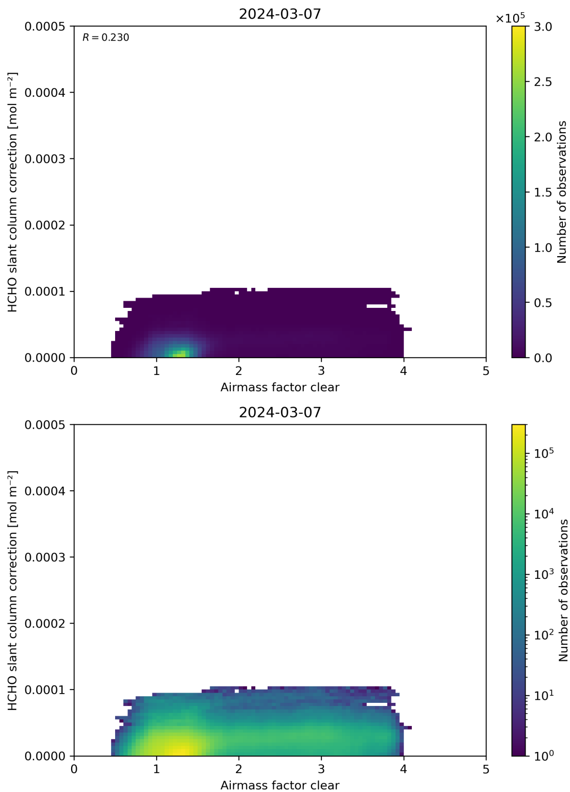
Figure 75: Scatter density plot of “Airmass factor clear” against “HCHO slant column correction” for 2024-03-06 to 2024-03-08.
