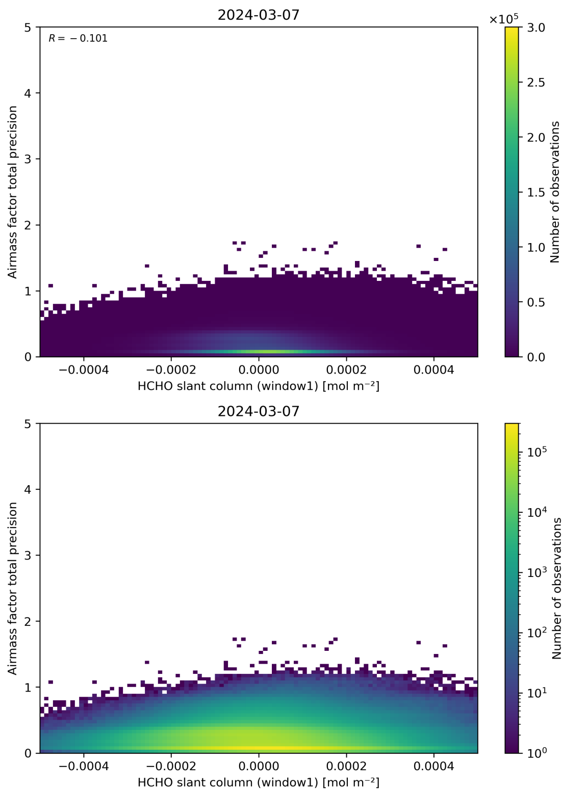
Figure 86: Scatter density plot of “HCHO slant column (window1)” against “Airmass factor total precision” for 2024-03-06 to 2024-03-08.
