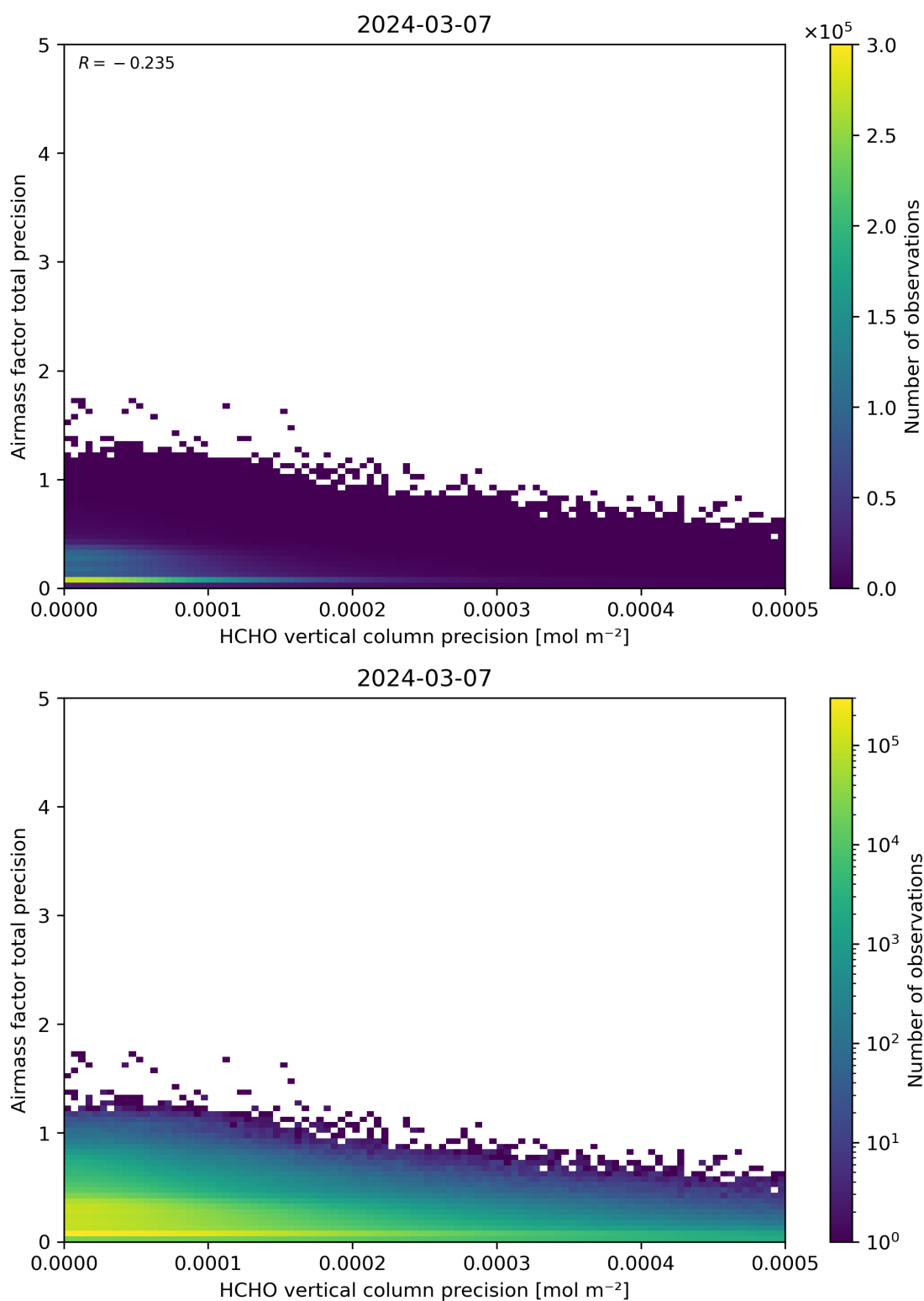
Figure 145: Scatter density plot of “HCHO vertical column precision” against “Airmass factor total precision” for 2024-03-06 to 2024-03-08.
