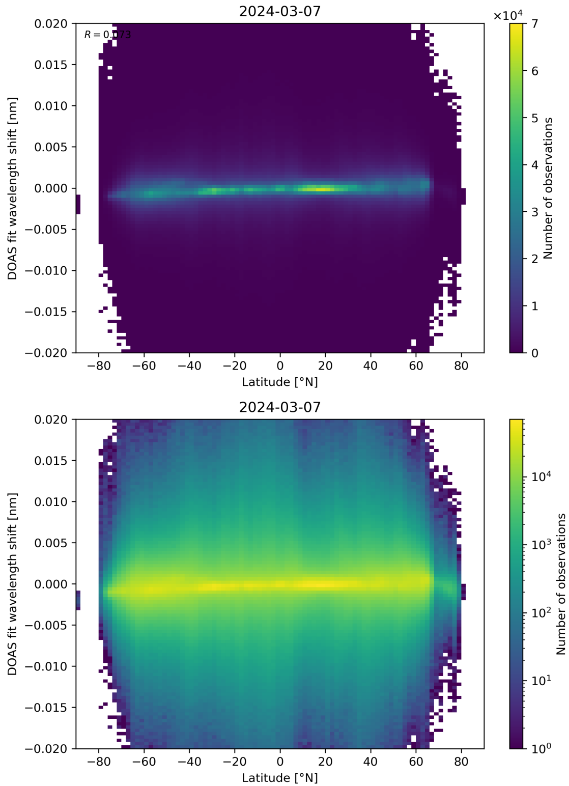
Figure 154: Scatter density plot of “Latitude” against “DOAS fit wavelength shift” for 2024-03-06 to 2024-03-08.
