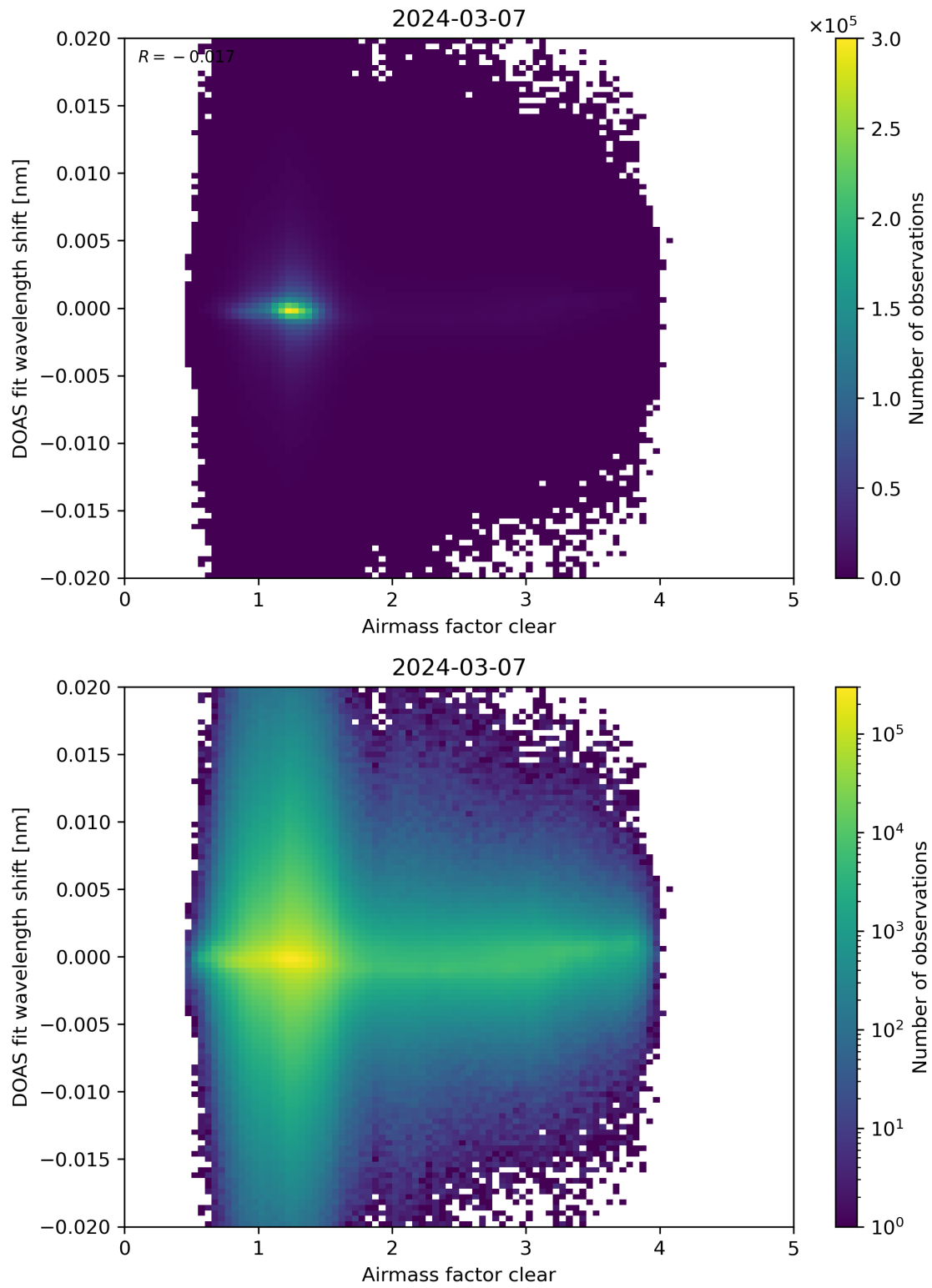
Figure 72: Scatter density plot of “Airmass factor clear” against “DOAS fit wavelength shift” for 2024-03-06 to 2024-03-08.
