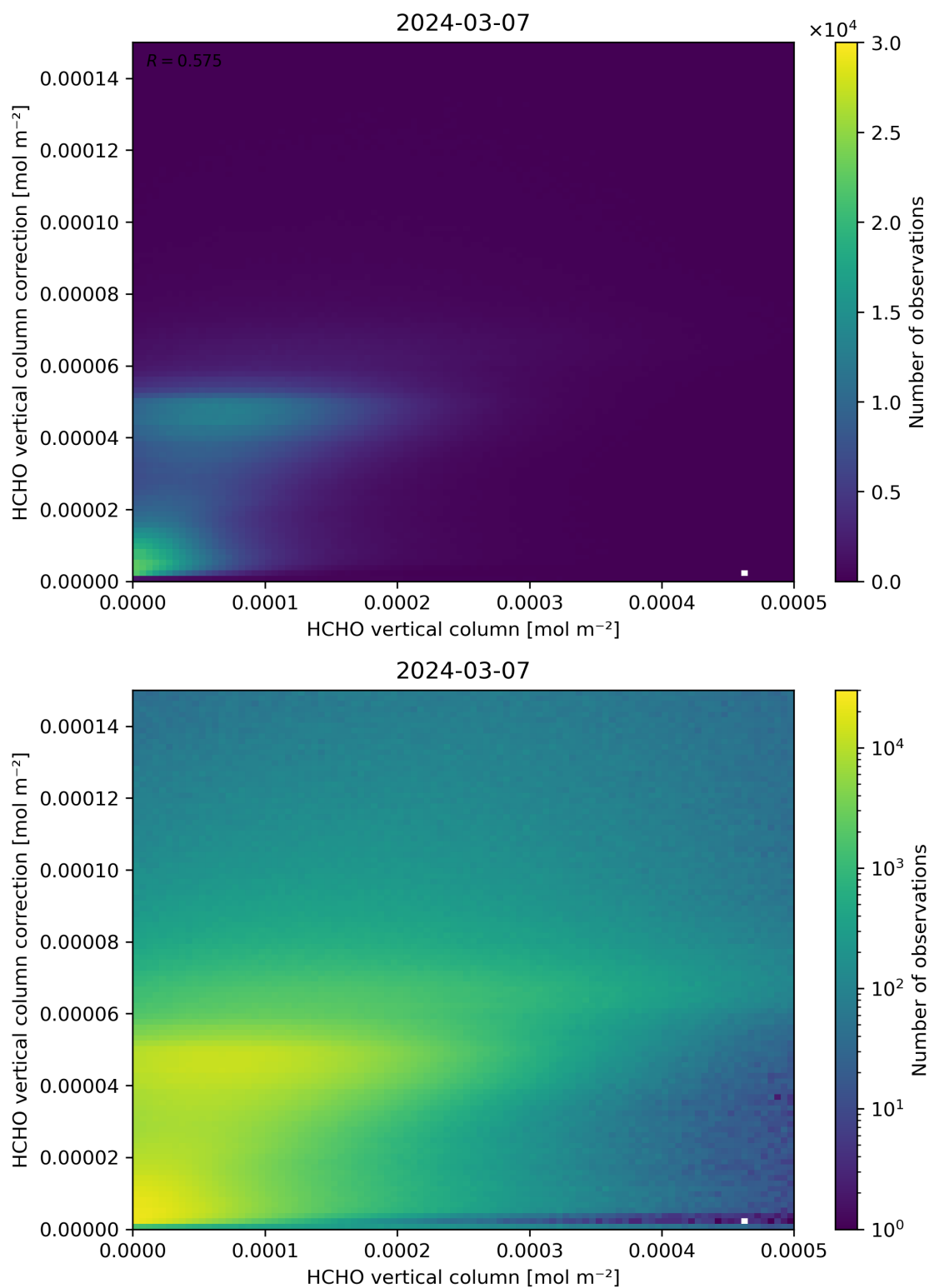
Figure 133: Scatter density plot of “HCHO vertical column” against “HCHO vertical column correction” for 2024-03-06 to 2024-03-08.
