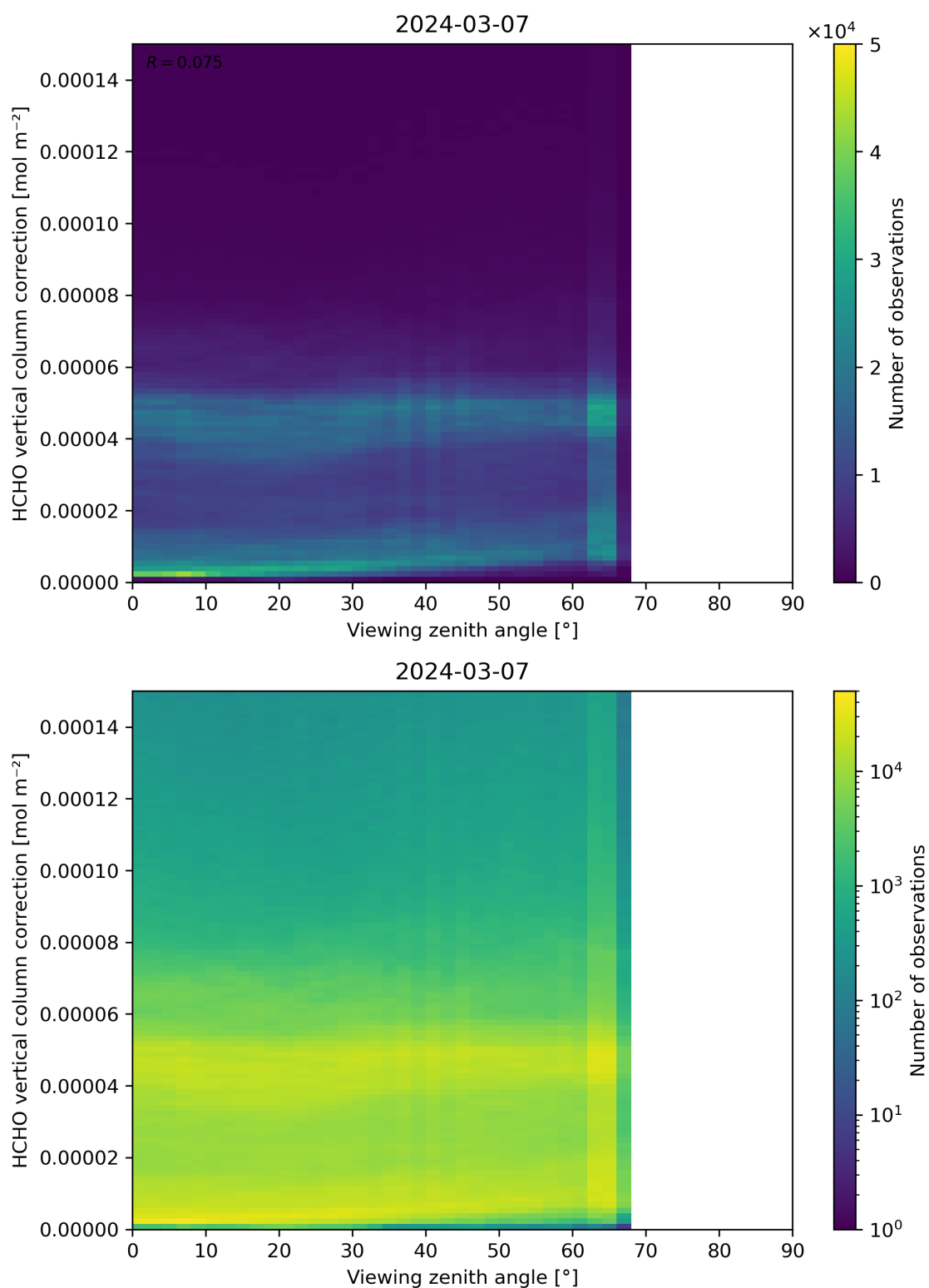
Figure 193: Scatter density plot of “Viewing zenith angle” against “HCHO vertical column correction” for 2024-03-06 to 2024-03-08.
