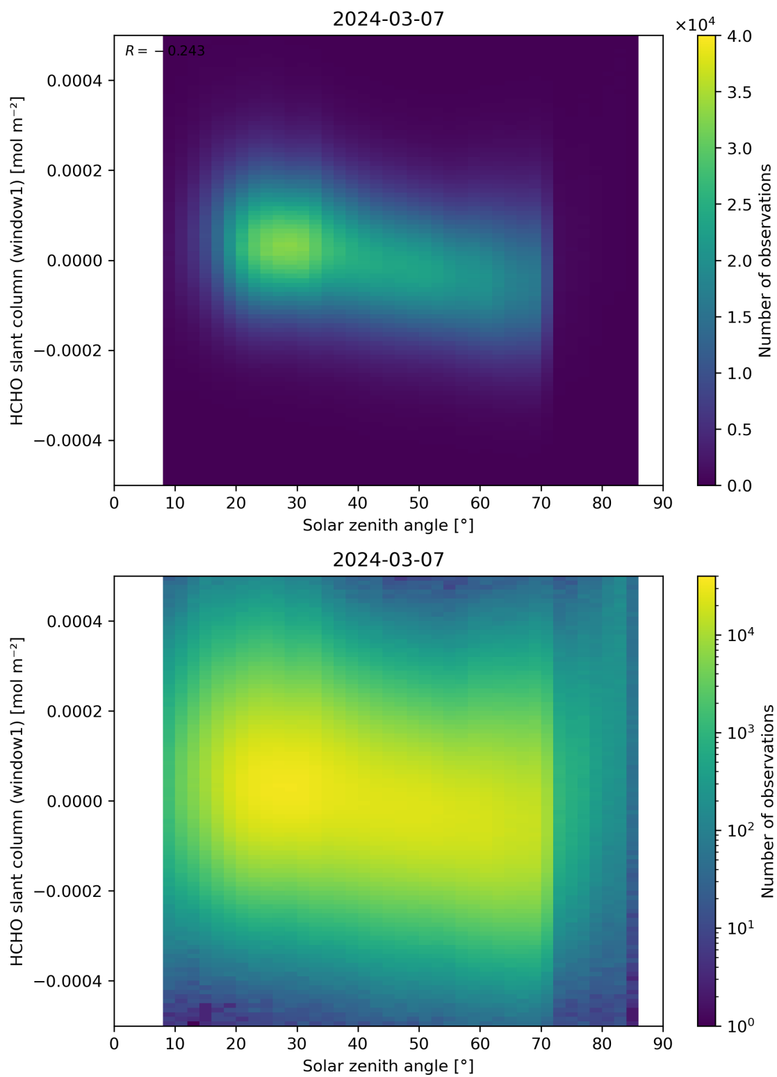
Figure 173: Scatter density plot of “Solar zenith angle” against “HCHO slant column (window1)” for 2024-03-06 to 2024-03-08.
