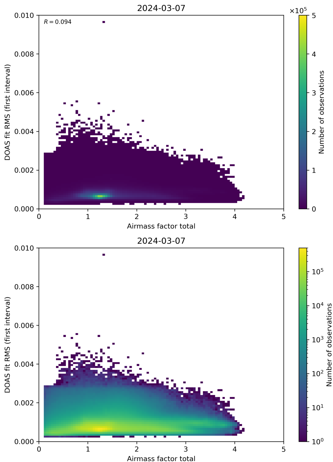
Figure 97: Scatter density plot of “Airmass factor total” against “DOAS fit RMS (first interval)” for 2024-03-06 to 2024-03-08.
