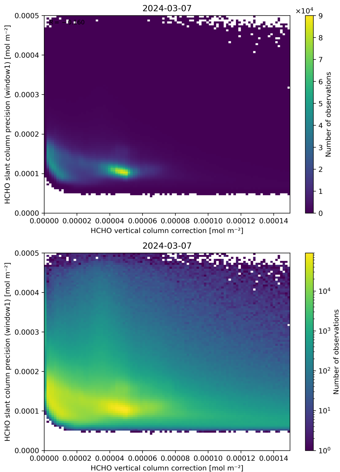
Figure 119: Scatter density plot of “HCHO vertical column correction” against “HCHO slant column precision (window1)” for 2024-03-06 to 2024-03-08.
