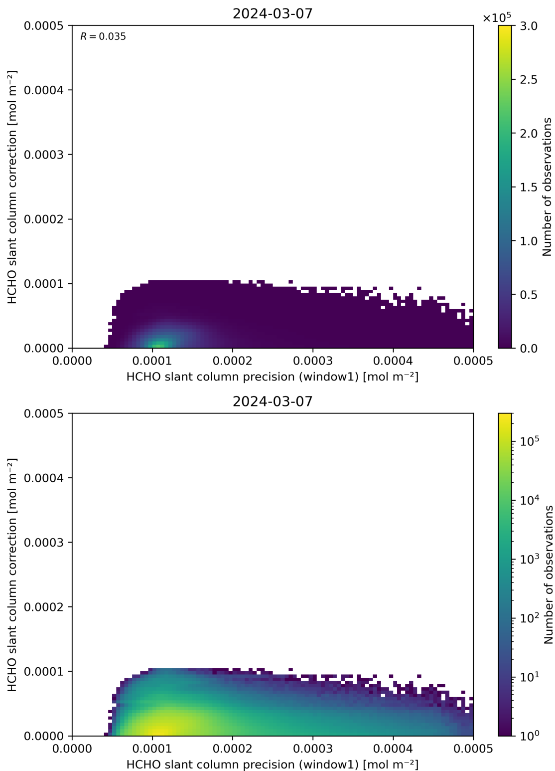
Figure 93: Scatter density plot of “HCHO slant column precision (window1)” against “HCHO slant column correction” for 2024-03-06 to 2024-03-08.
