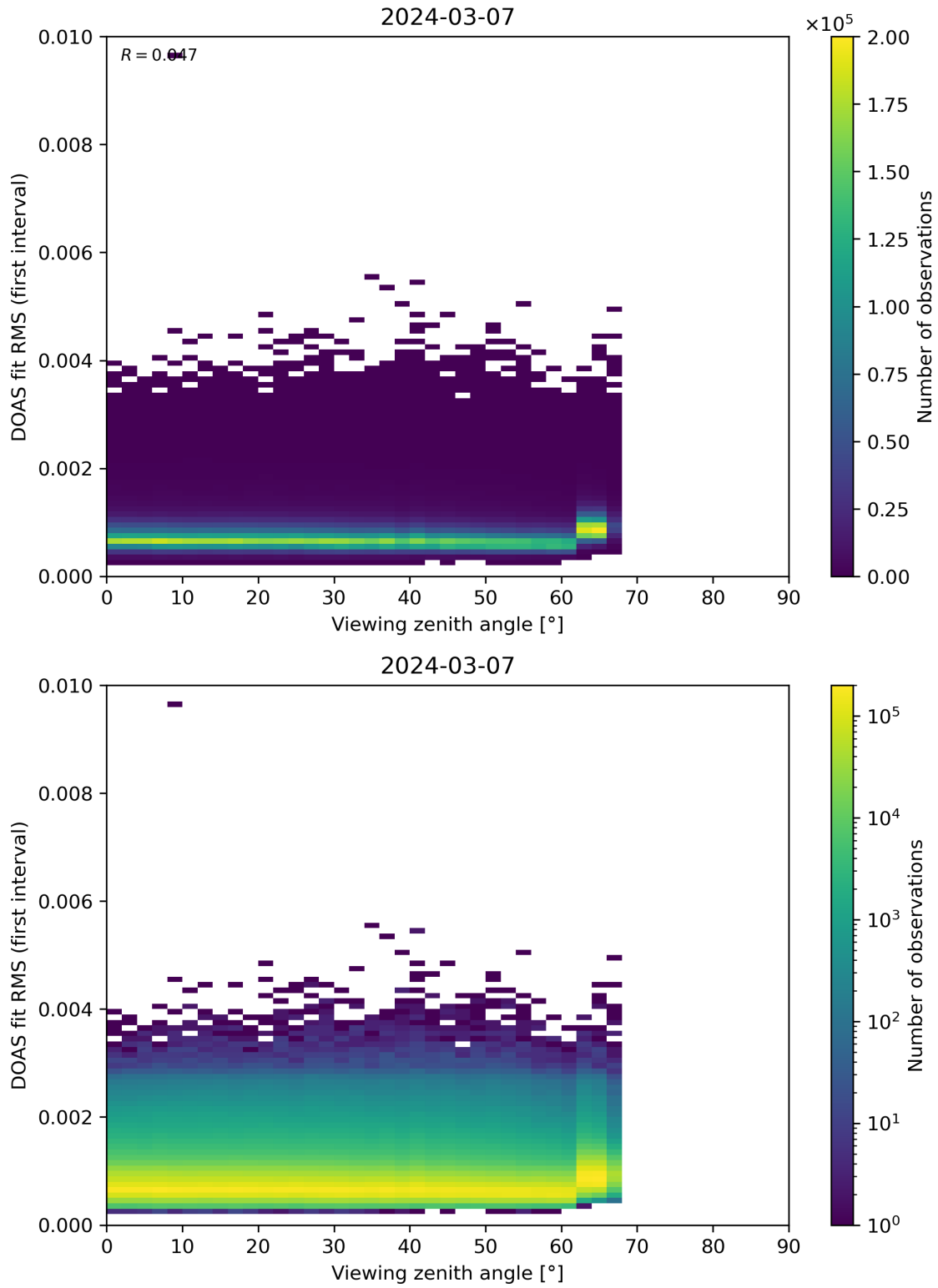
Figure 182: Scatter density plot of “Viewing zenith angle” against “DOAS fit RMS (first interval)” for 2024-03-06 to 2024-03-08.
