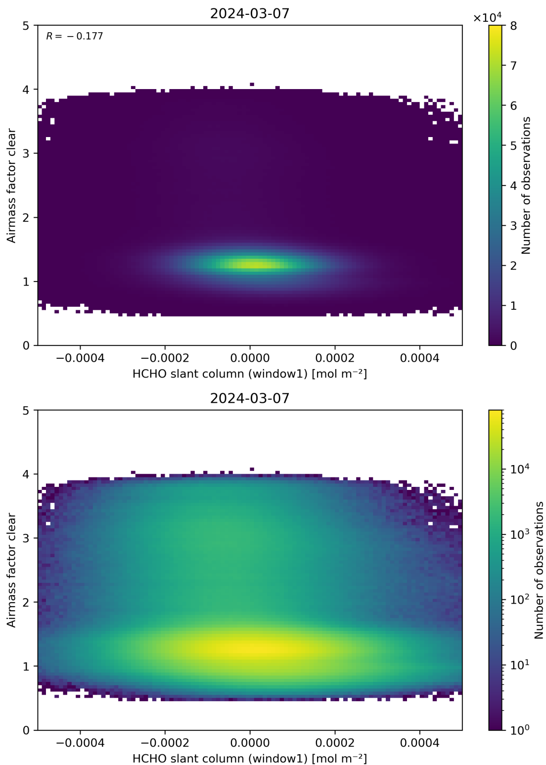
Figure 81: Scatter density plot of “HCHO slant column (window1)” against “Airmass factor clear” for 2024-03-06 to 2024-03-08.
