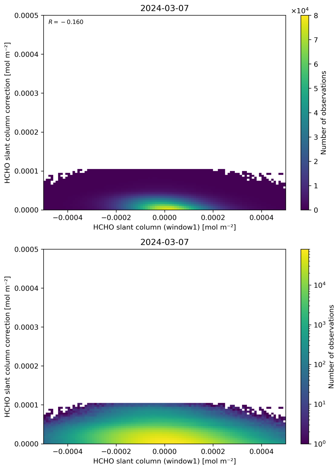
Figure 83: Scatter density plot of “HCHO slant column (window1)” against “HCHO slant column correction” for 2024-03-06 to 2024-03-08.
