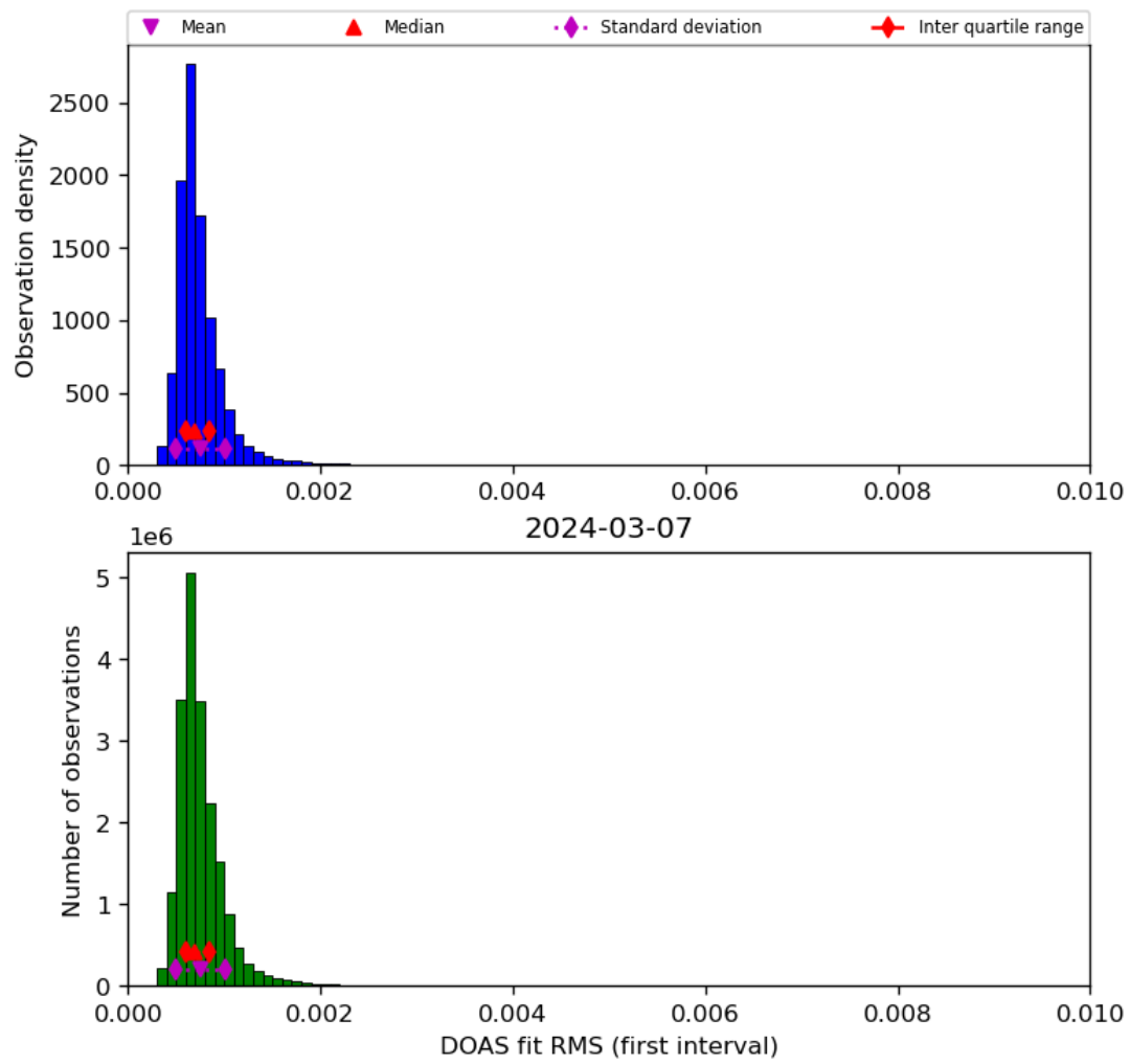
Figure 46: Histogram of “DOAS fit RMS (first interval)” for 2024-03-06 to 2024-03-08
