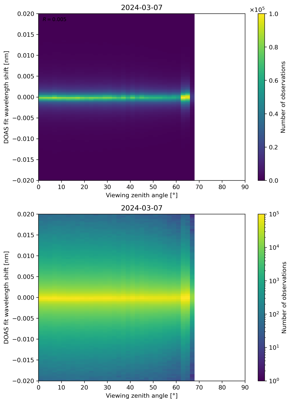
Figure 183: Scatter density plot of “Viewing zenith angle” against “DOAS fit wavelength shift” for 2024-03-06 to 2024-03-08.
