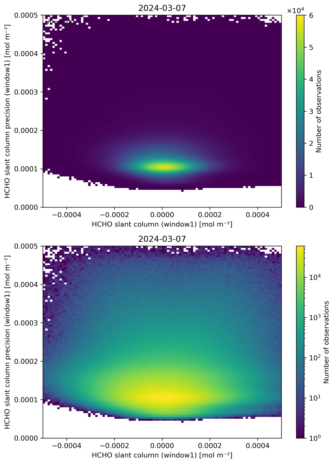
Figure 84: Scatter density plot of “HCHO slant column (window1)” against “HCHO slant column precision (window1)” for 2024-03-06 to 2024-03-08.
