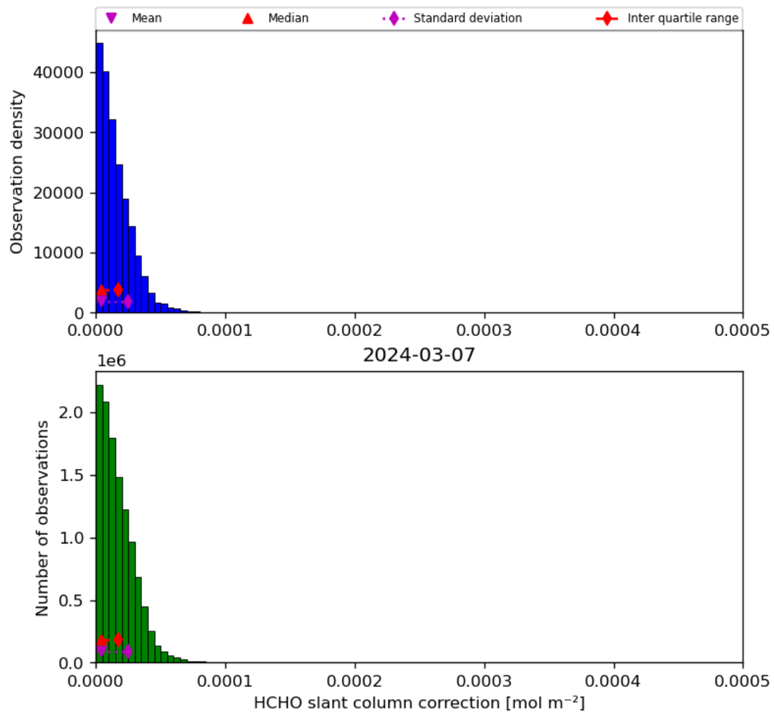
Figure 47: Histogram of “HCHO slant column correction” for 2024-03-06 to 2024-03-08
