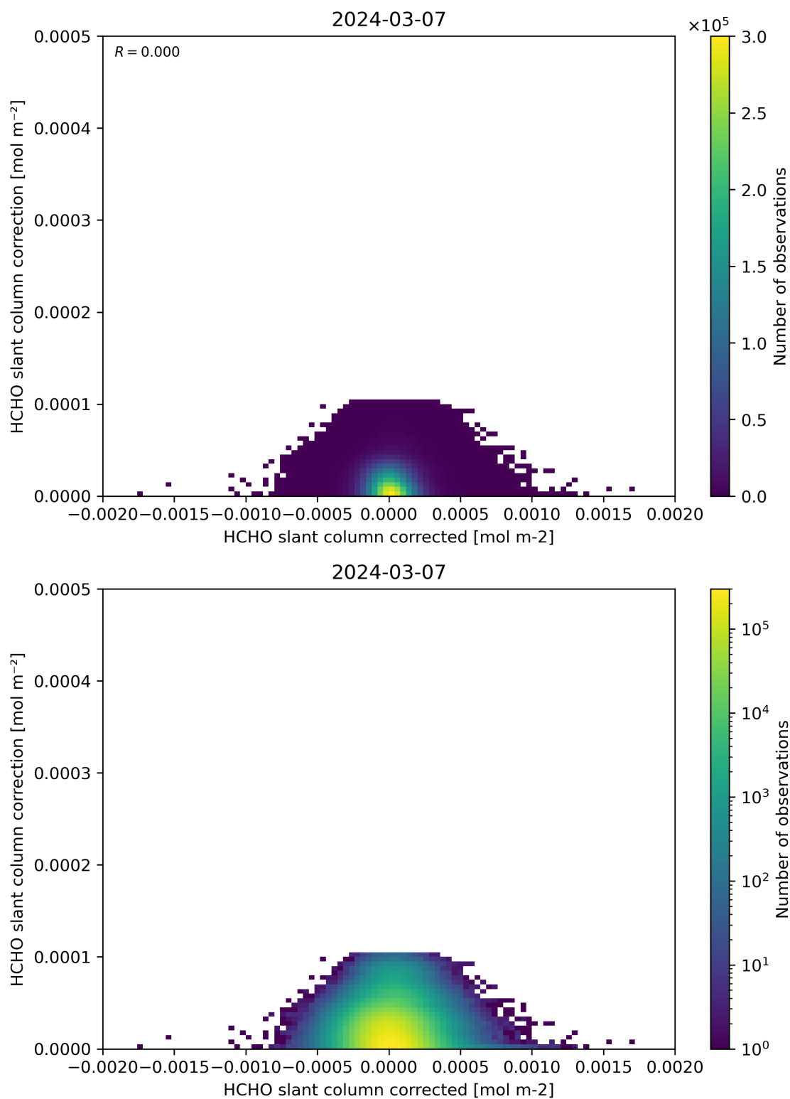
Figure 77: Scatter density plot of “HCHO slant column corrected” against “HCHO slant column correction” for 2024-03-06 to 2024-03-08.
