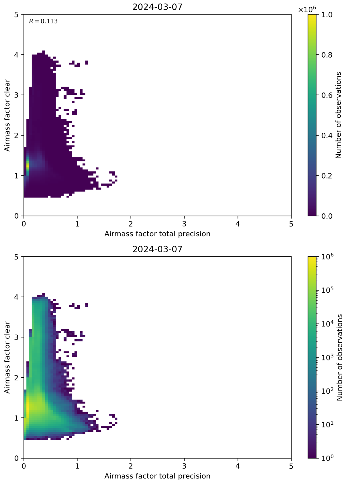
Figure 108: Scatter density plot of “Airmass factor total precision” against “Airmass factor clear” for 2024-03-06 to 2024-03-08.
