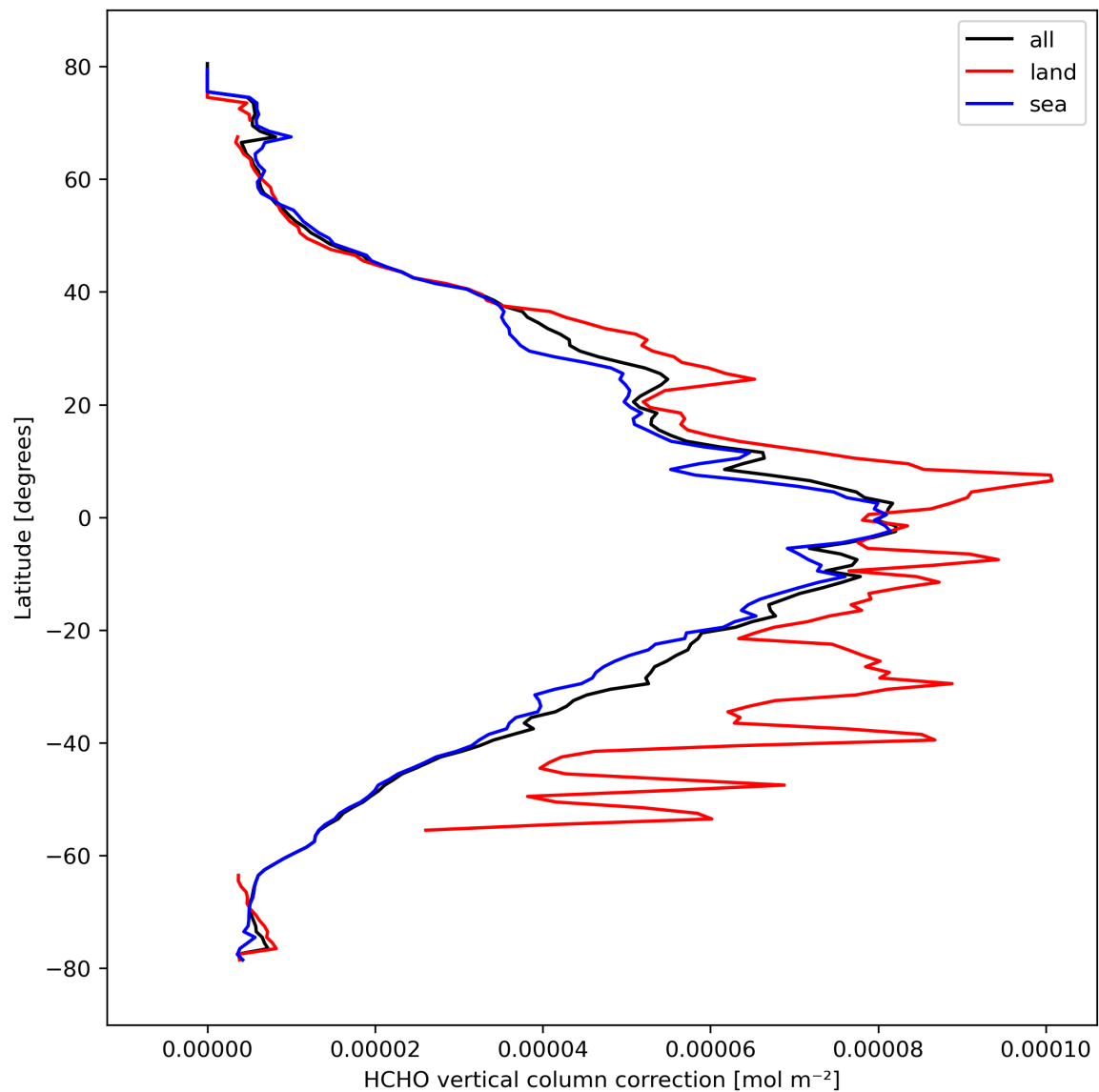
Figure 23: Zonal average of “HCHO vertical column correction” for 2024-03-06 to 2024-03-08.
