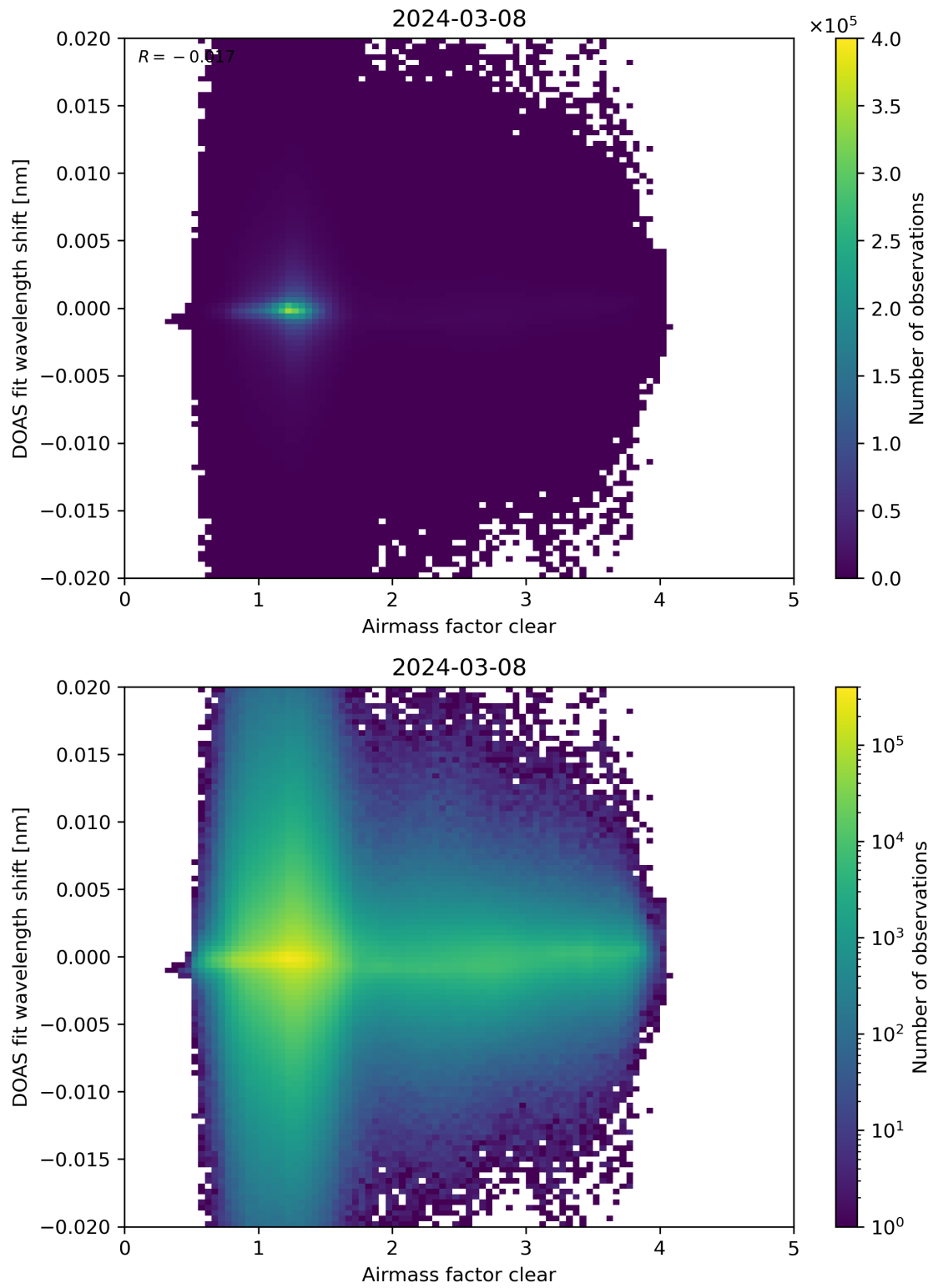
Figure 72: Scatter density plot of “Airmass factor clear” against “DOAS fit wavelength shift” for 2024-03-07 to 2024-03-09.
