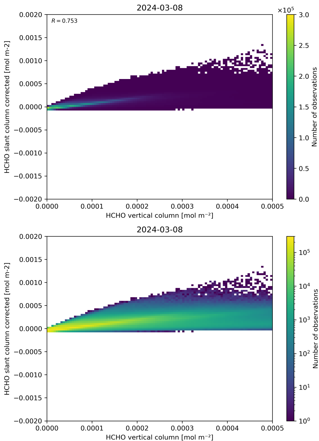
Figure 127: Scatter density plot of “HCHO vertical column” against “HCHO slant column corrected” for 2024-03-07 to 2024-03-09.
