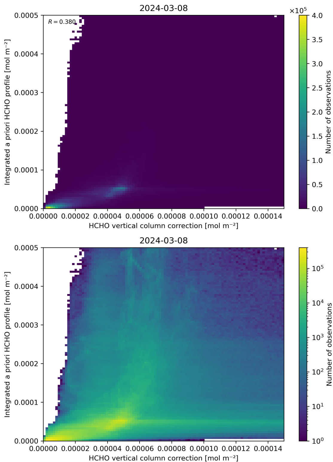
Figure 122: Scatter density plot of “HCHO vertical column correction” against “Integrated a priori HCHO profile” for 2024-03-07 to 2024-03-09.
