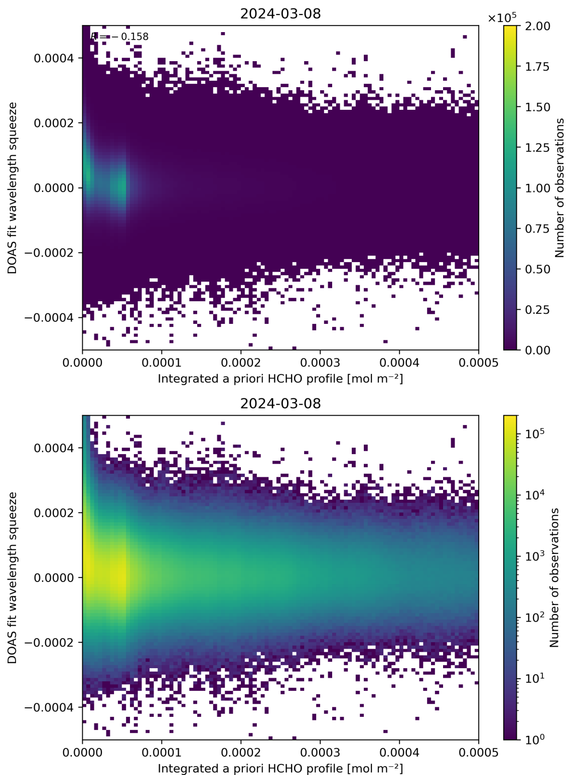
Figure 150: Scatter density plot of “Integrated a priori HCHO profile” against “DOAS fit wavelength squeeze” for 2024-03-07 to 2024-03-09.
