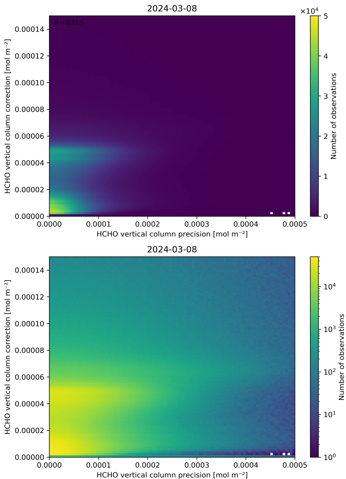
Figure 146: Scatter density plot of “HCHO vertical column precision” against “HCHO vertical column correction” for 2024-03-07 to 2024-03-09.
