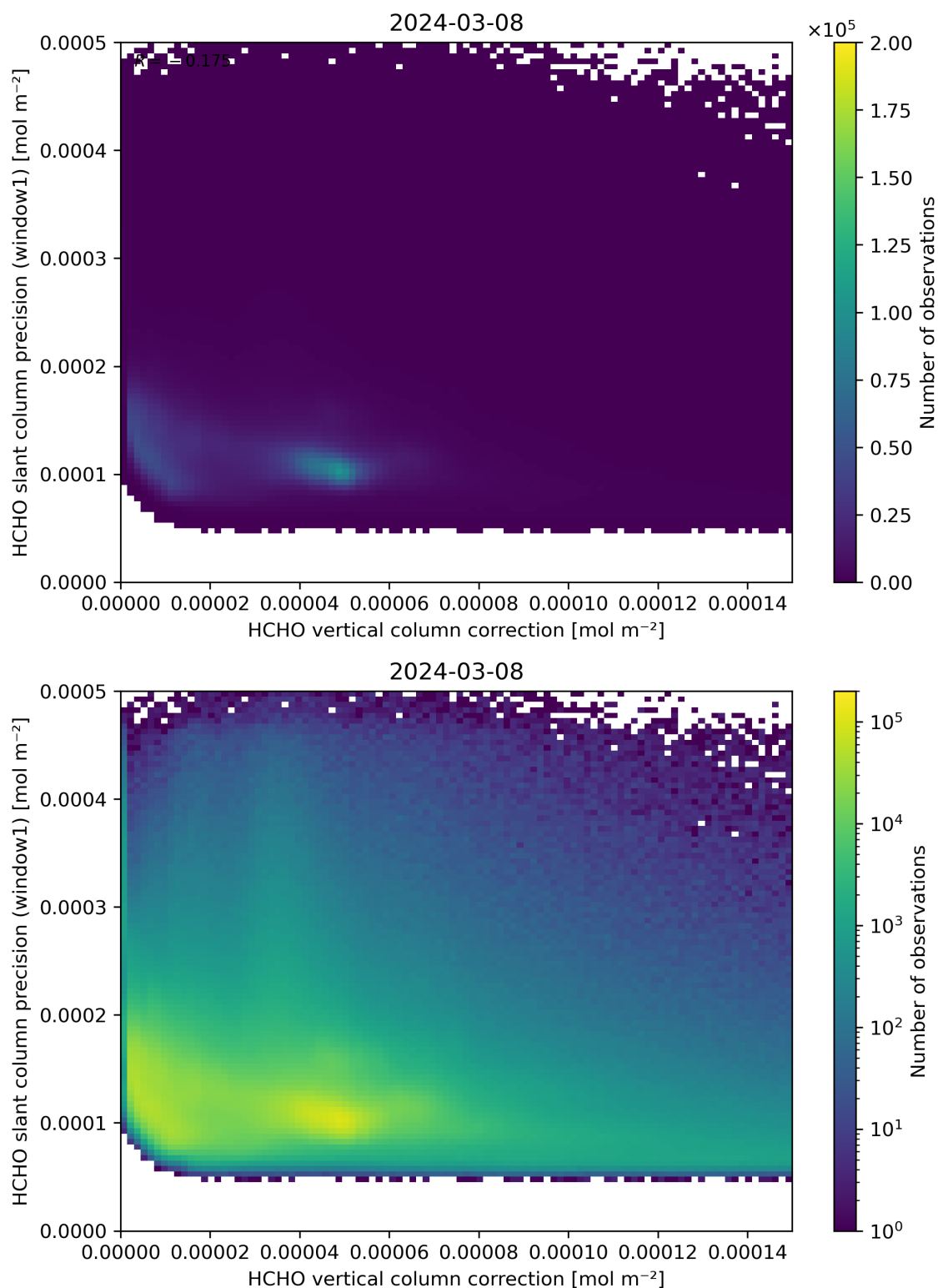
Figure 119: Scatter density plot of “HCHO vertical column correction” against “HCHO slant column precision (window1)” for 2024-03-07 to 2024-03-09.
