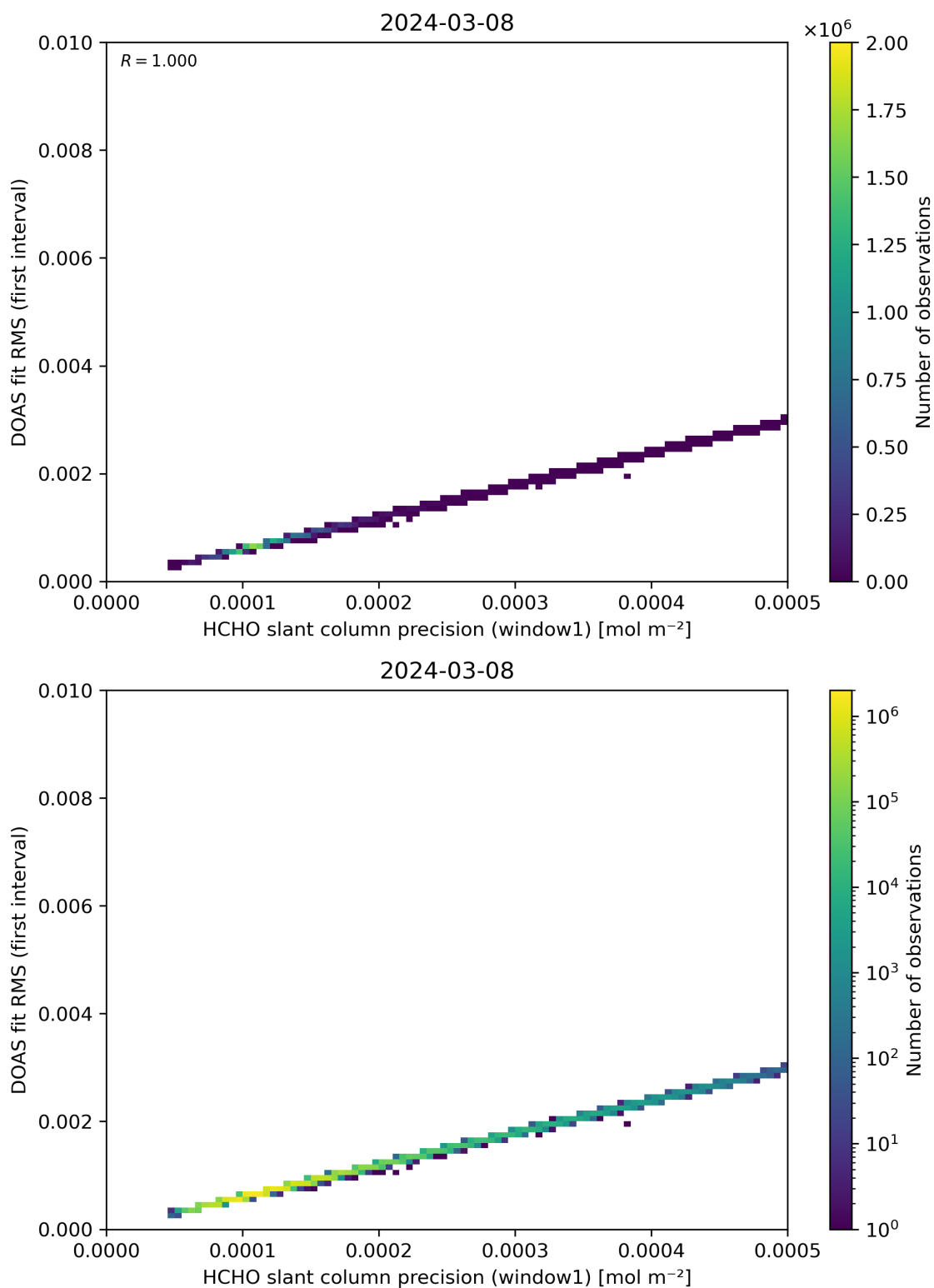
Figure 88: Scatter density plot of “HCHO slant column precision (window1)” against “DOAS fit RMS (first interval)” for 2024-03-07 to 2024-03-09.
