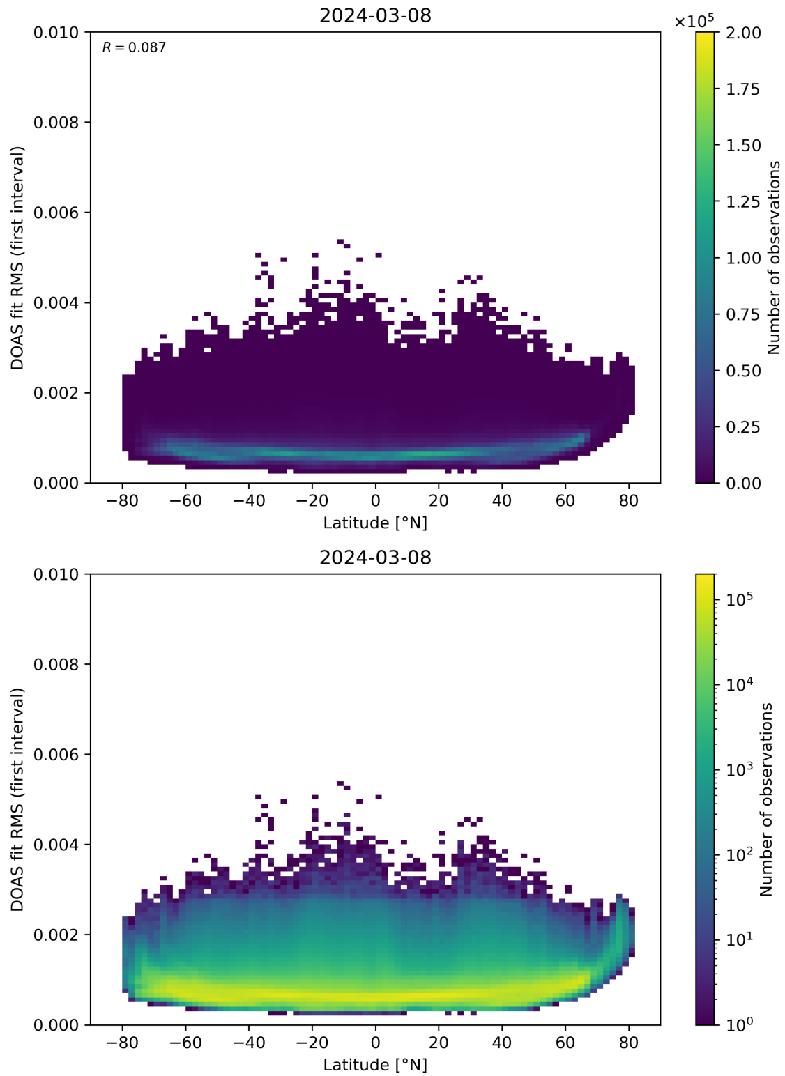
Figure 153: Scatter density plot of “Latitude” against “DOAS fit RMS (first interval)” for 2024-03-07 to 2024-03-09.
