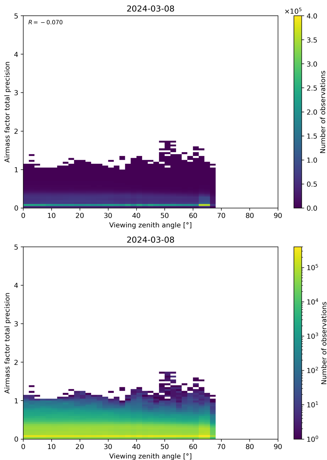
Figure 191: Scatter density plot of “Viewing zenith angle” against “Airmass factor total precision” for 2024-03-07 to 2024-03-09.
