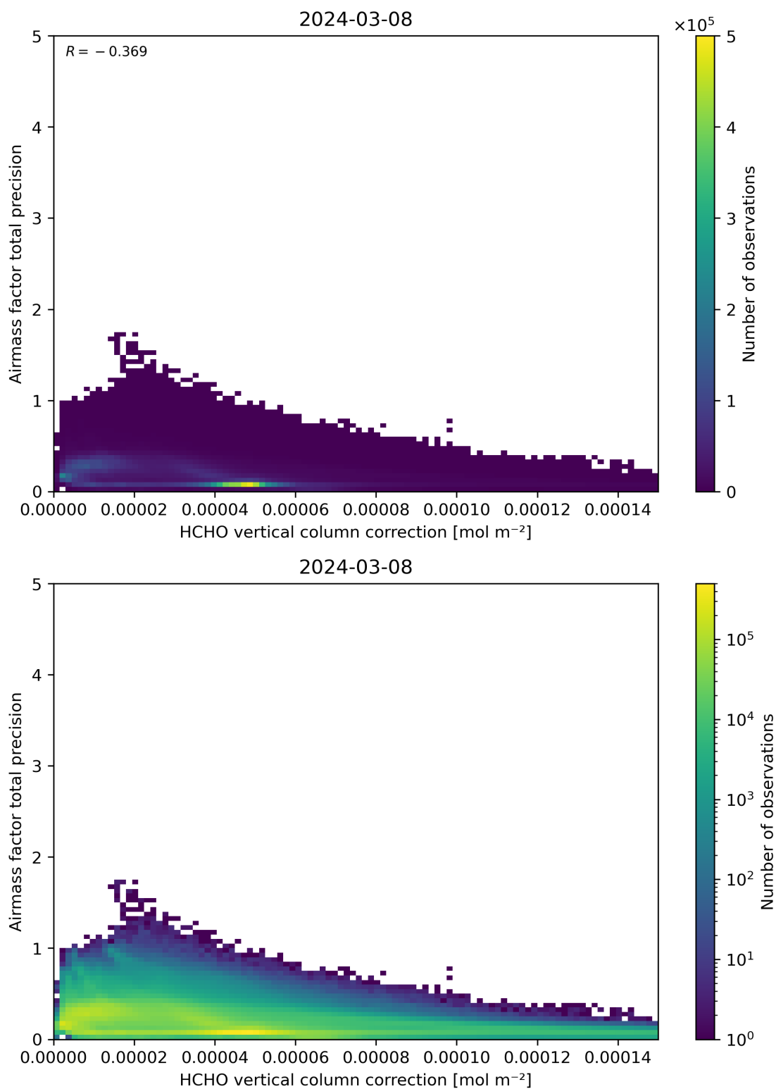
Figure 121: Scatter density plot of “HCHO vertical column correction” against “Airmass factor total precision” for 2024-03-07 to 2024-03-09.
