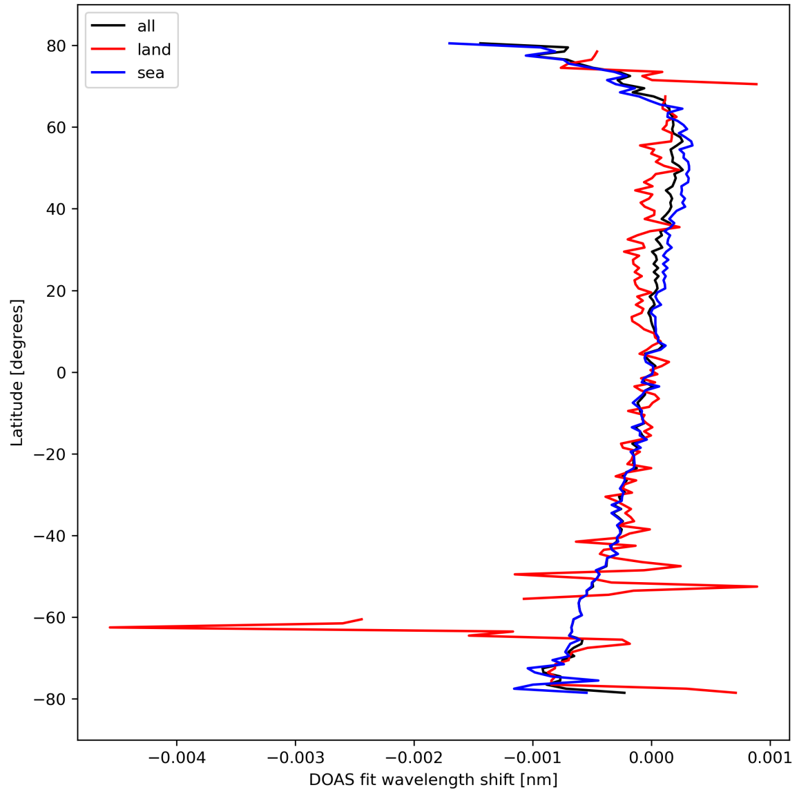
Figure 30: Zonal average of “DOAS fit wavelength shift” for 2024-03-07 to 2024-03-09.
