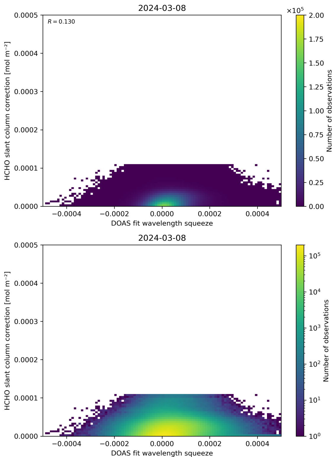
Figure 70: Scatter density plot of “DOAS fit wavelength squeeze” against “HCHO slant column correction” for 2024-03-07 to 2024-03-09.
