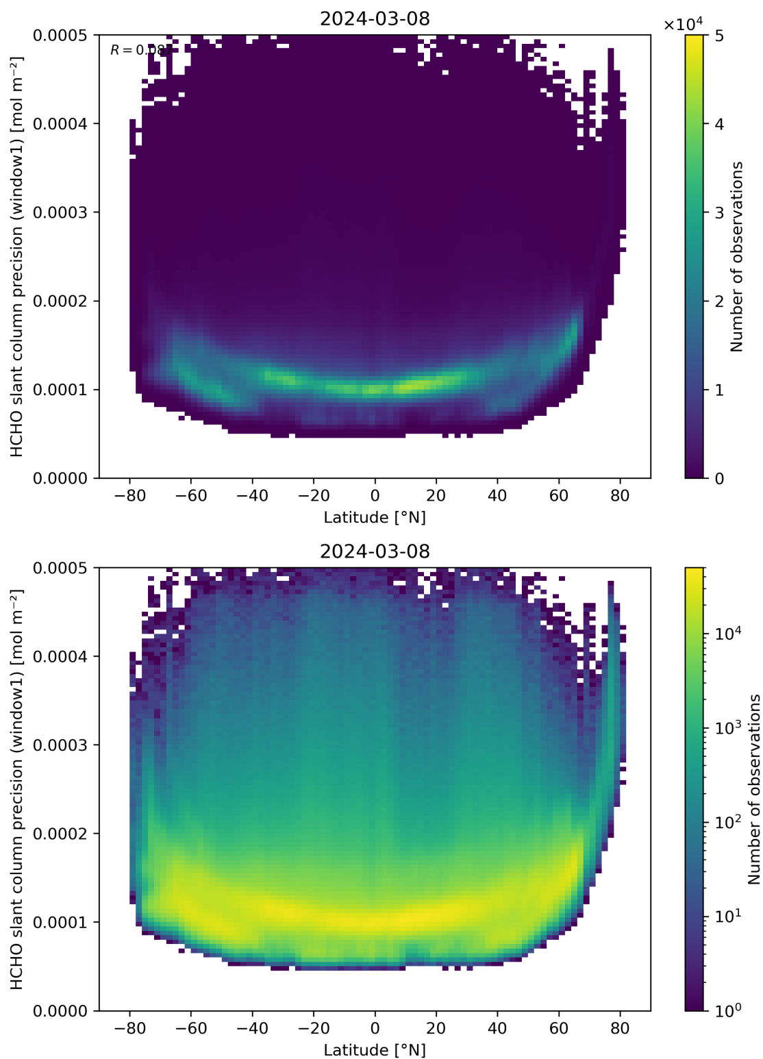
Figure 160: Scatter density plot of “Latitude” against “HCHO slant column precision (window1)” for 2024-03-07 to 2024-03-09.
