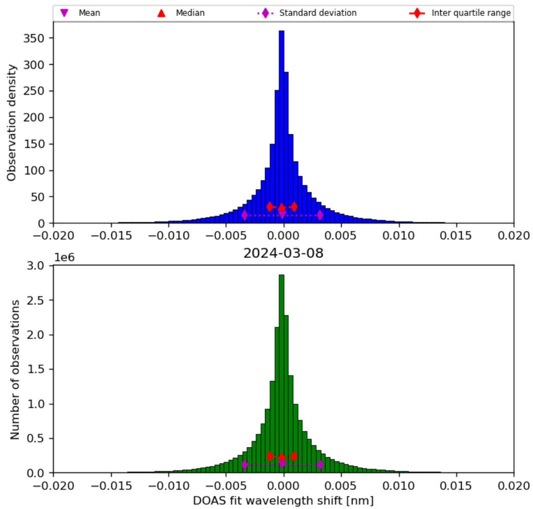
Figure 44: Histogram of “DOAS fit wavelength shift” for 2024-03-07 to 2024-03-09
