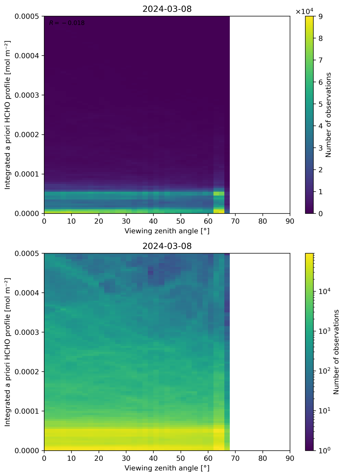
Figure 195: Scatter density plot of “Viewing zenith angle” against “Integrated a priori HCHO profile” for 2024-03-07 to 2024-03-09.
