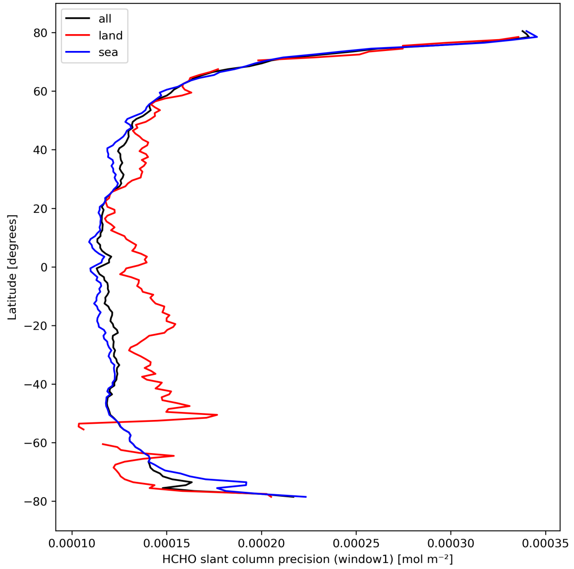
Figure 25: Zonal average of “HCHO slant column precision (window1)” for 2024-03-07 to 2024-03-09.
