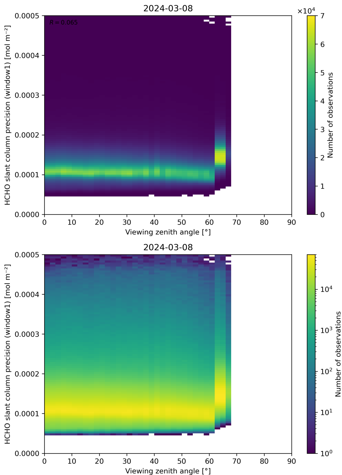
Figure 189: Scatter density plot of “Viewing zenith angle” against “HCHO slant column precision (window1)” for 2024-03-07 to 2024-03-09.
