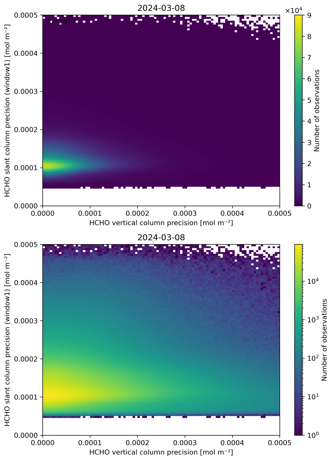
Figure 143: Scatter density plot of “HCHO vertical column precision” against “HCHO slant column precision (window1)” for 2024-03-07 to 2024-03-09.
