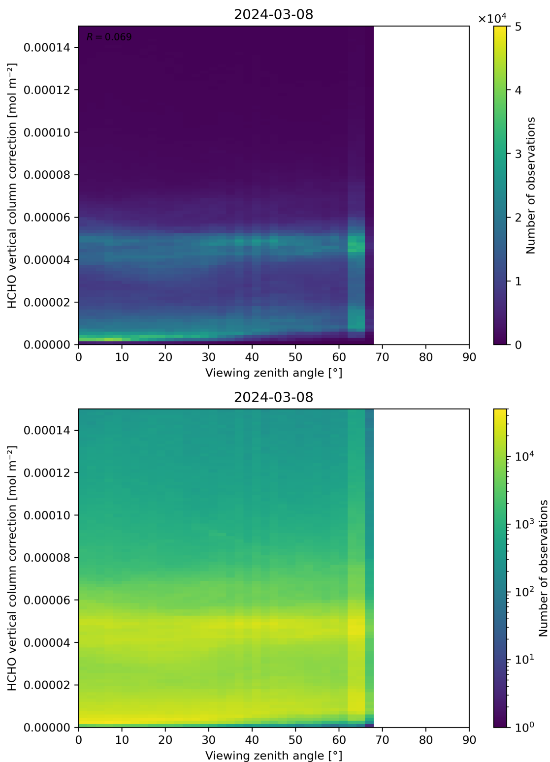
Figure 193: Scatter density plot of “Viewing zenith angle” against “HCHO vertical column correction” for 2024-03-07 to 2024-03-09.
