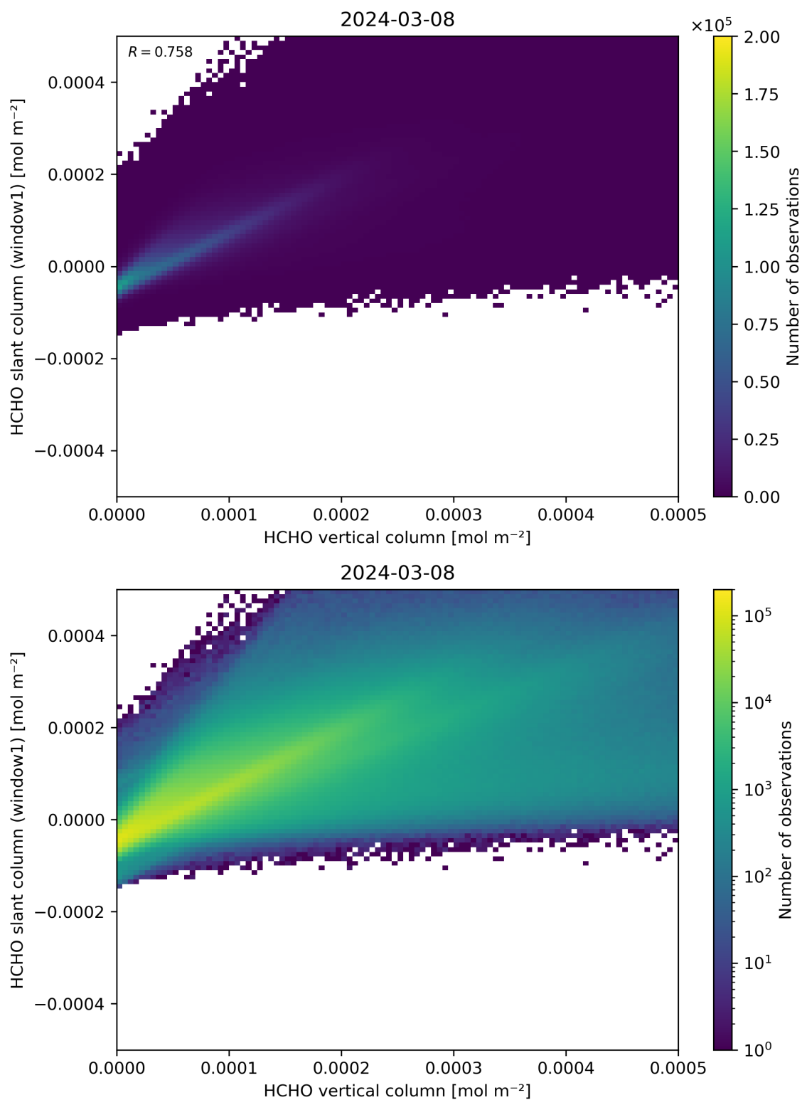
Figure 129: Scatter density plot of “HCHO vertical column” against “HCHO slant column (window1)” for 2024-03-07 to 2024-03-09.
