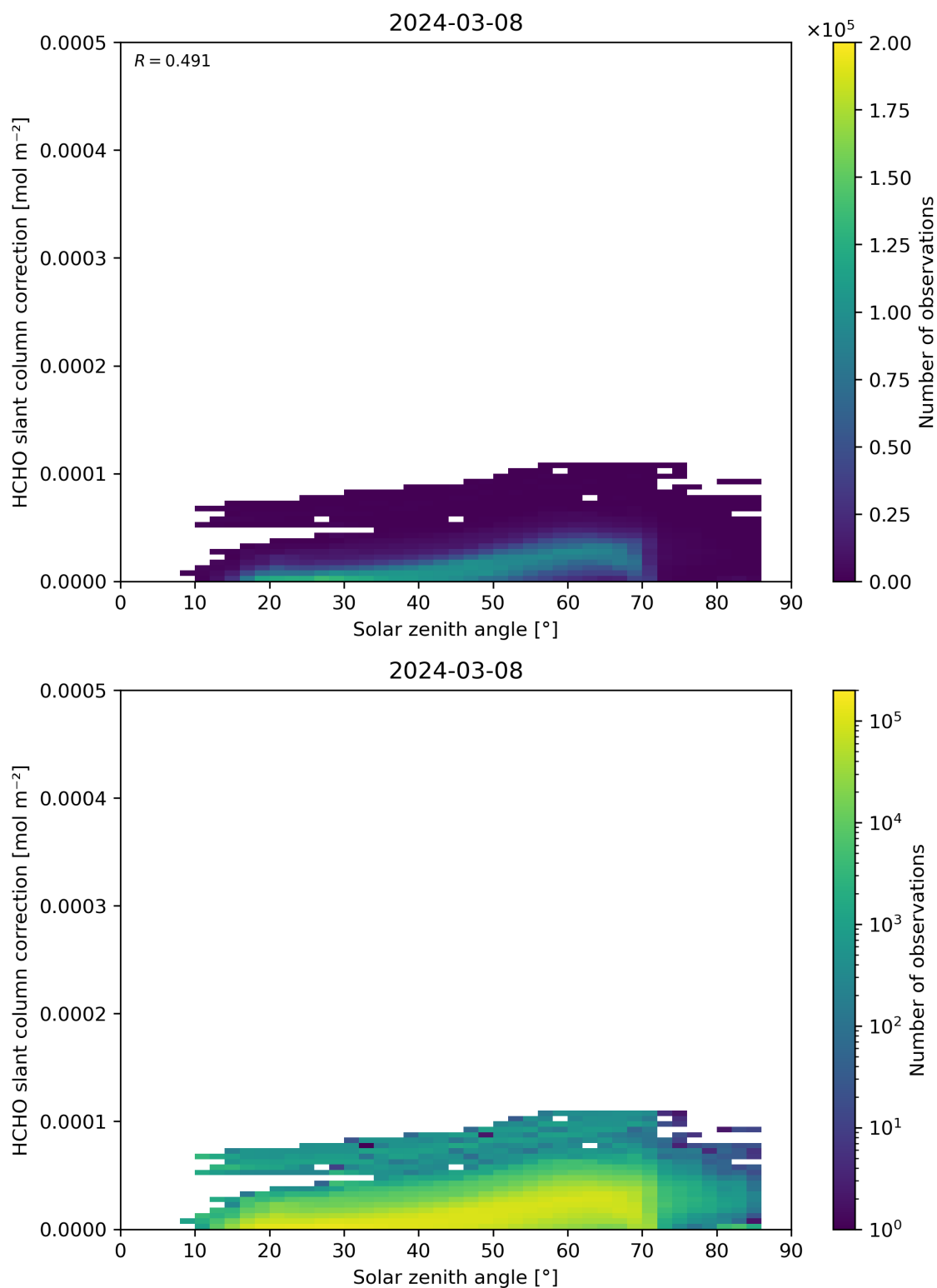
Figure 172: Scatter density plot of “Solar zenith angle” against “HCHO slant column correction” for 2024-03-07 to 2024-03-09.
