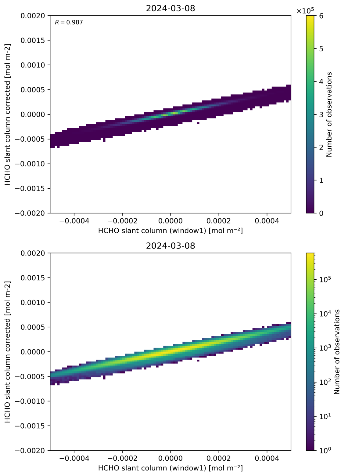
Figure 82: Scatter density plot of “HCHO slant column (window1)” against “HCHO slant column corrected” for 2024-03-07 to 2024-03-09.
