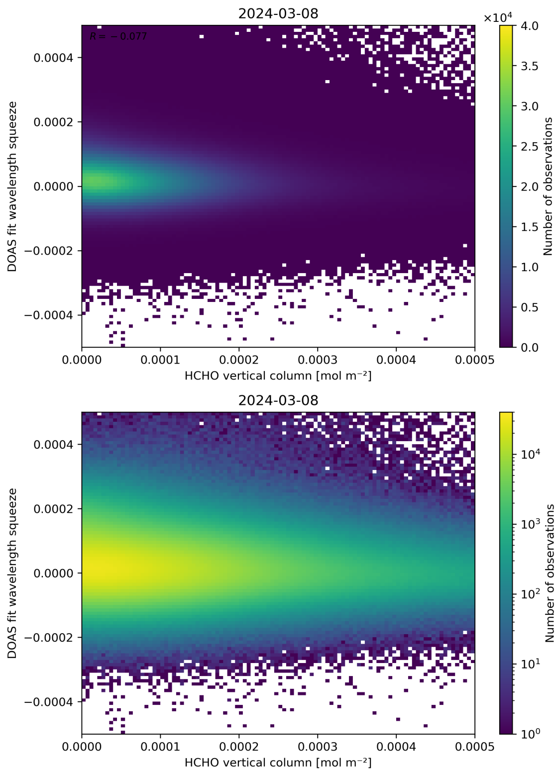
Figure 125: Scatter density plot of “HCHO vertical column” against “DOAS fit wavelength squeeze” for 2024-03-07 to 2024-03-09.
