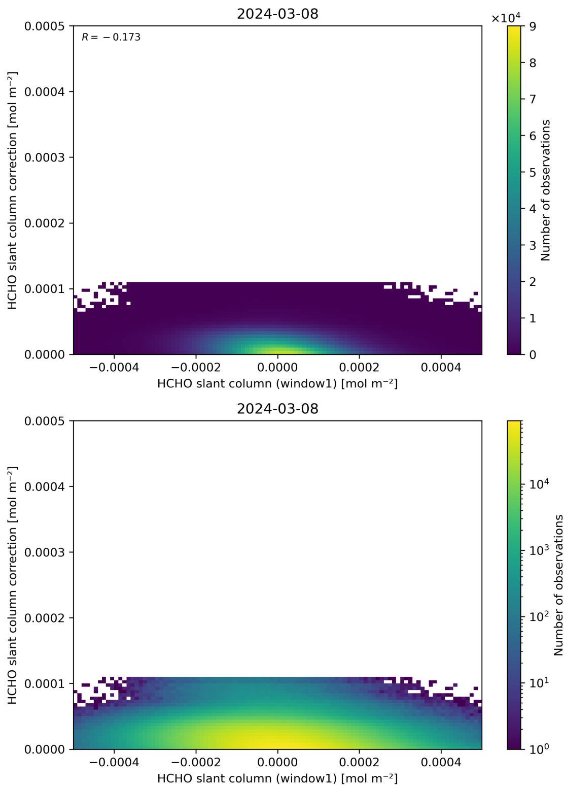
Figure 83: Scatter density plot of “HCHO slant column (window1)” against “HCHO slant column correction” for 2024-03-07 to 2024-03-09.
