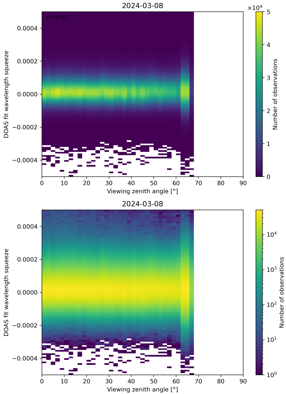
Figure 184: Scatter density plot of “Viewing zenith angle” against “DOAS fit wavelength squeeze” for 2024-03-07 to 2024-03-09.
