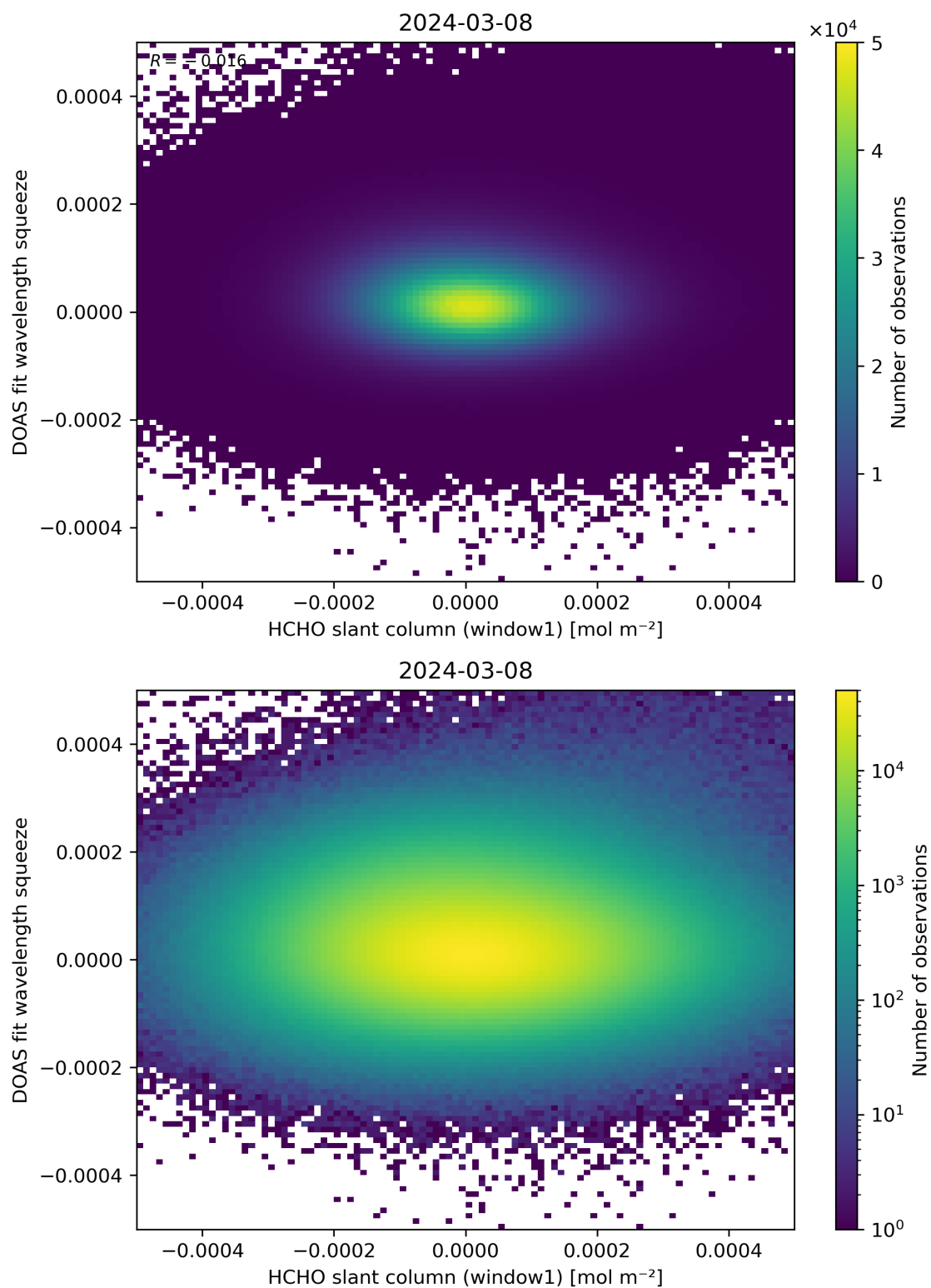
Figure 80: Scatter density plot of “HCHO slant column (window1)” against “DOAS fit wavelength squeeze” for 2024-03-07 to 2024-03-09.
