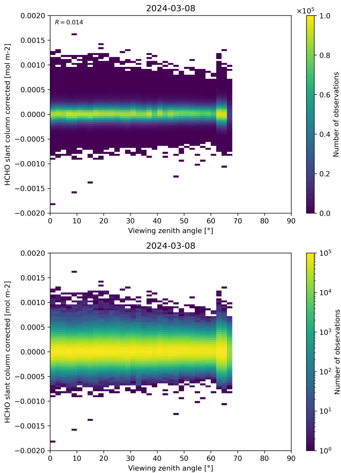
Figure 186: Scatter density plot of “Viewing zenith angle” against “HCHO slant column corrected” for 2024-03-07 to 2024-03-09.
