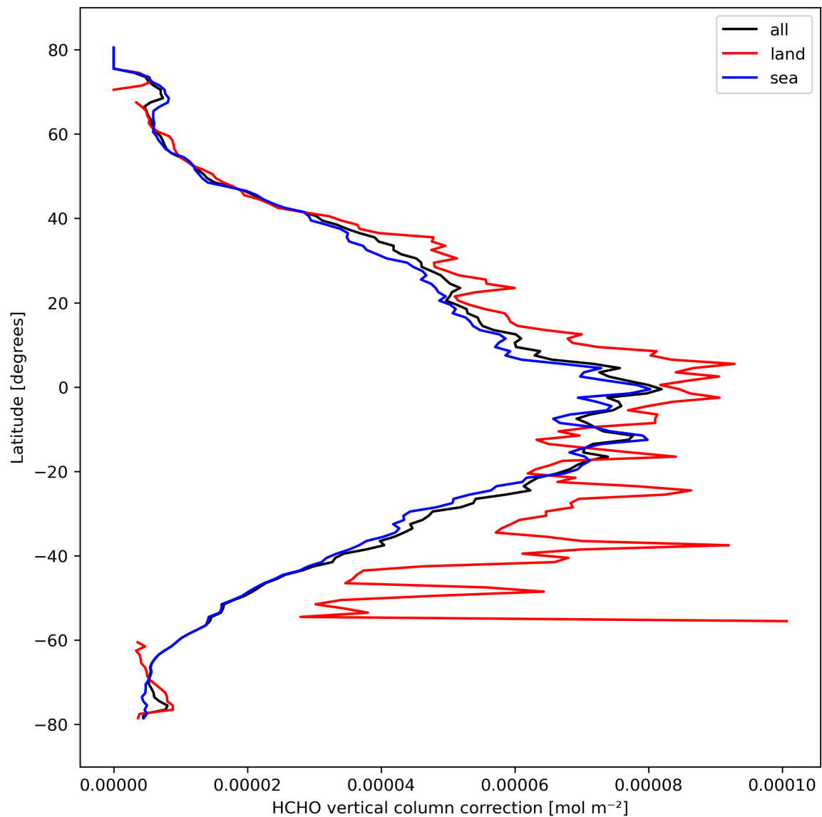
Figure 23: Zonal average of “HCHO vertical column correction” for 2024-03-07 to 2024-03-09.
