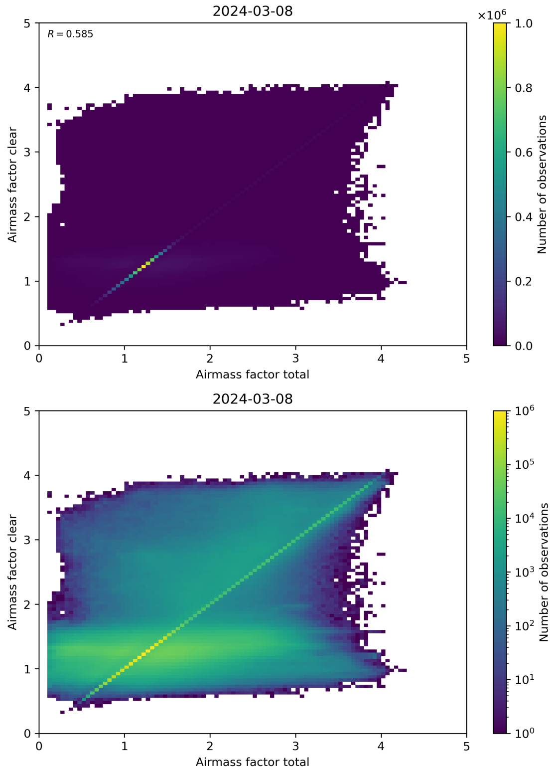
Figure 100: Scatter density plot of “Airmass factor total” against “Airmass factor clear” for 2024-03-07 to 2024-03-09.
