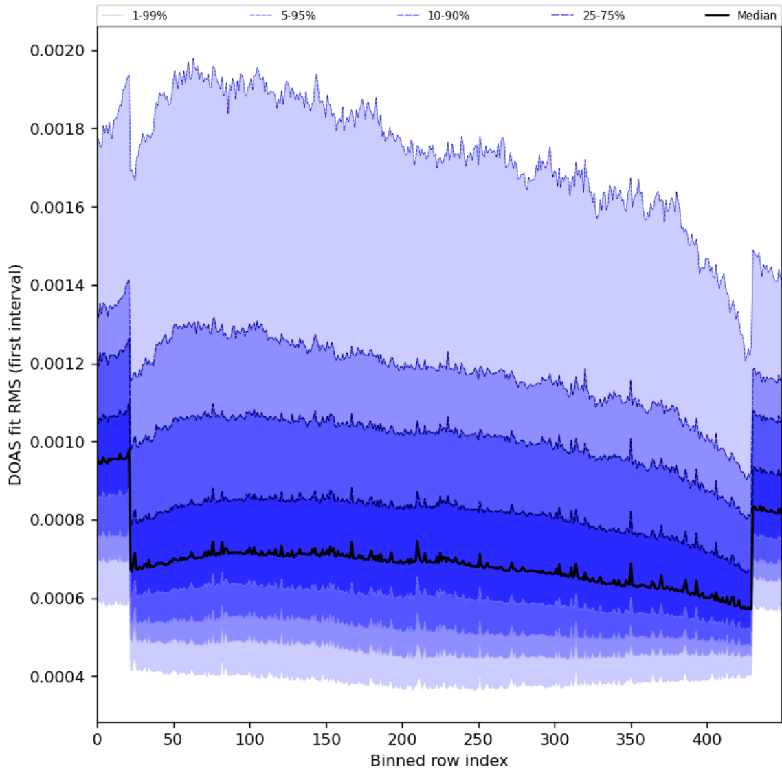
Figure 60: Along track statistics of “DOAS fit RMS (first interval)” for 2024-03-07 to 2024-03-09
