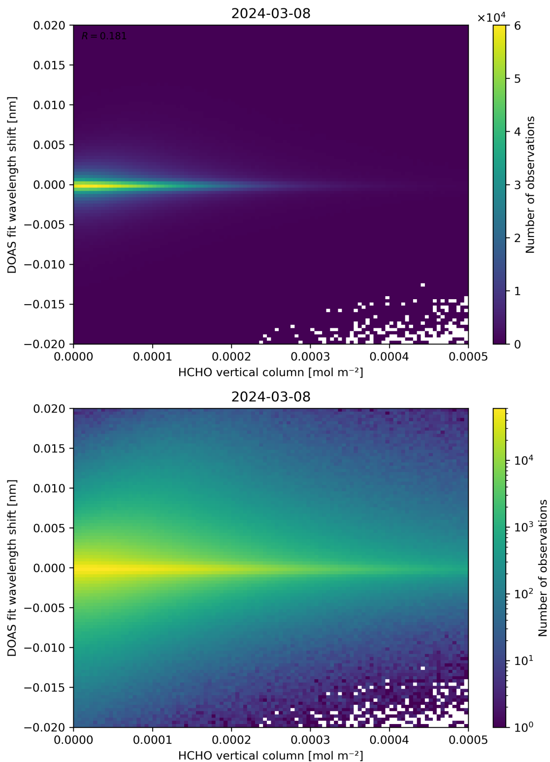
Figure 124: Scatter density plot of “HCHO vertical column” against “DOAS fit wavelength shift” for 2024-03-07 to 2024-03-09.
