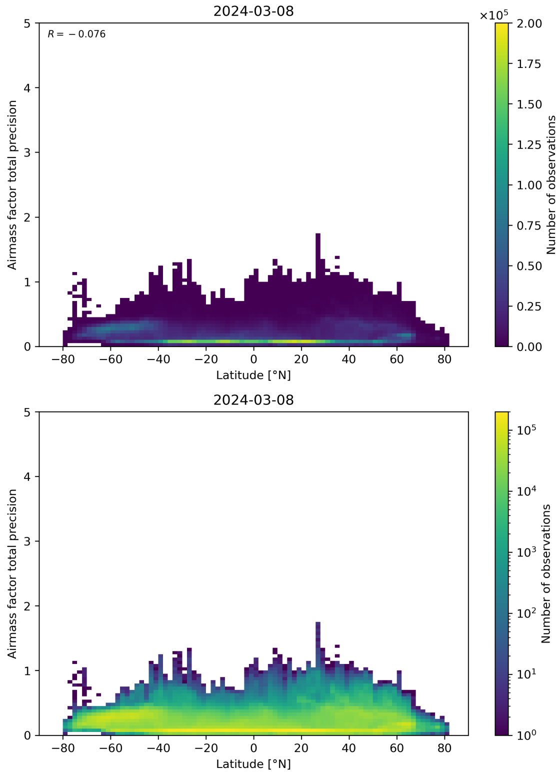
Figure 162: Scatter density plot of “Latitude” against “Airmass factor total precision” for 2024-03-07 to 2024-03-09.
