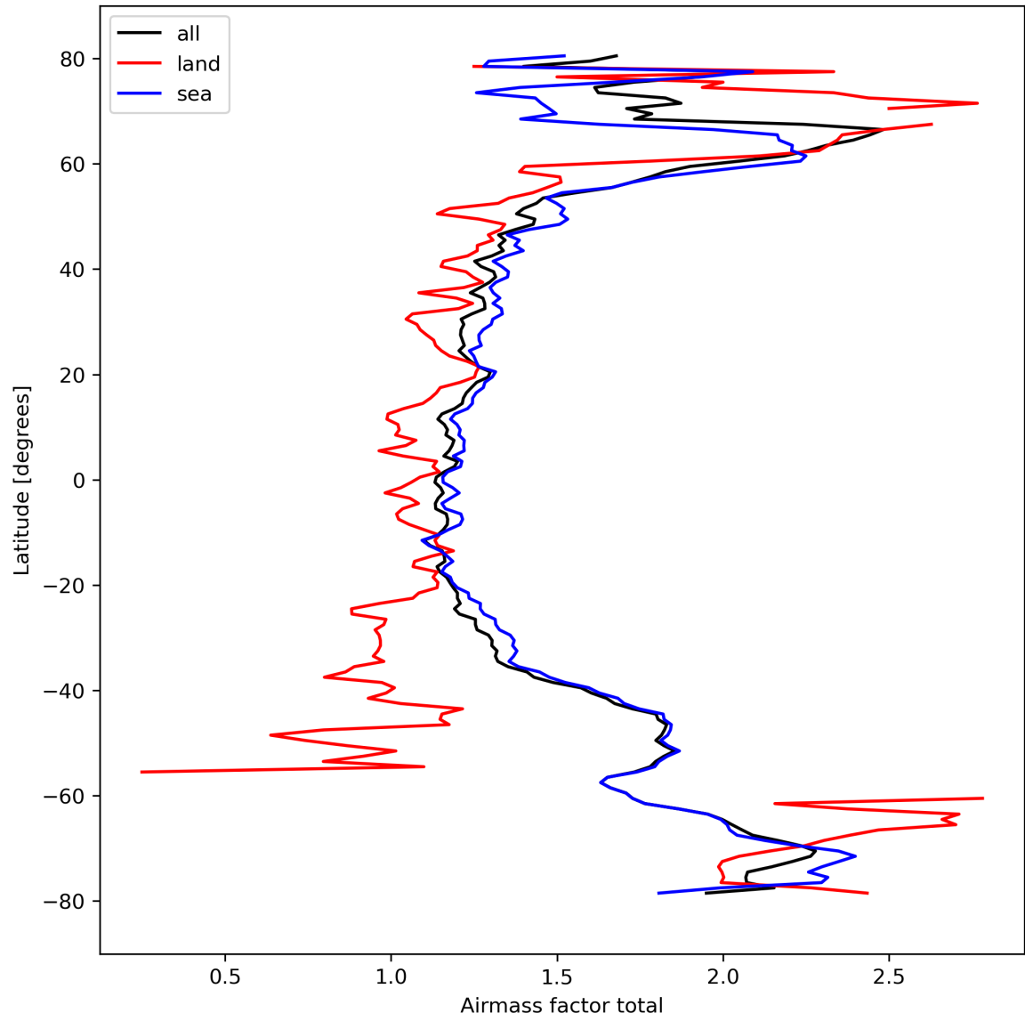
Figure 26: Zonal average of “Airmass factor total” for 2024-03-07 to 2024-03-09.
