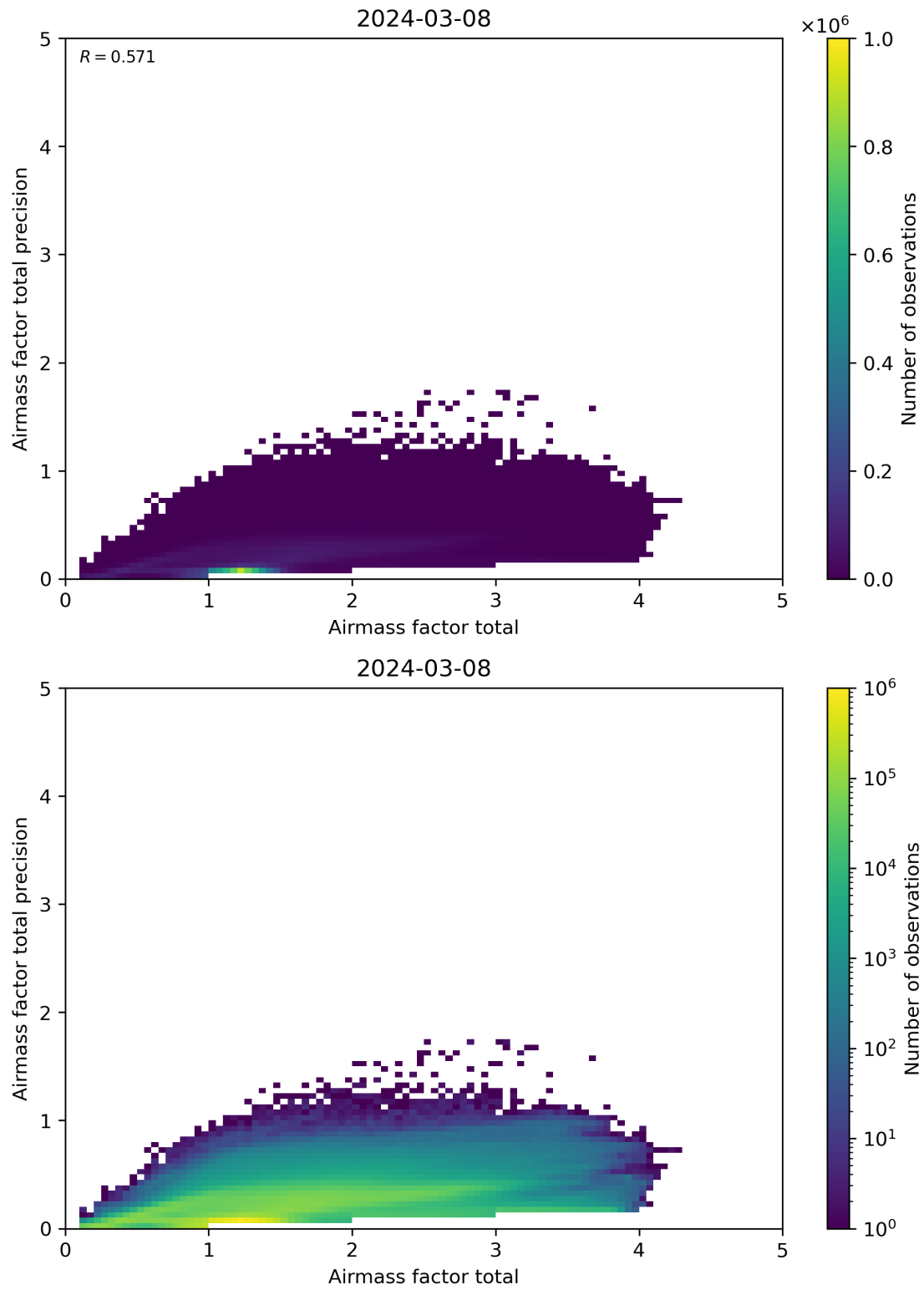
Figure 103: Scatter density plot of “Airmass factor total” against “Airmass factor total precision” for 2024-03-07 to 2024-03-09.
