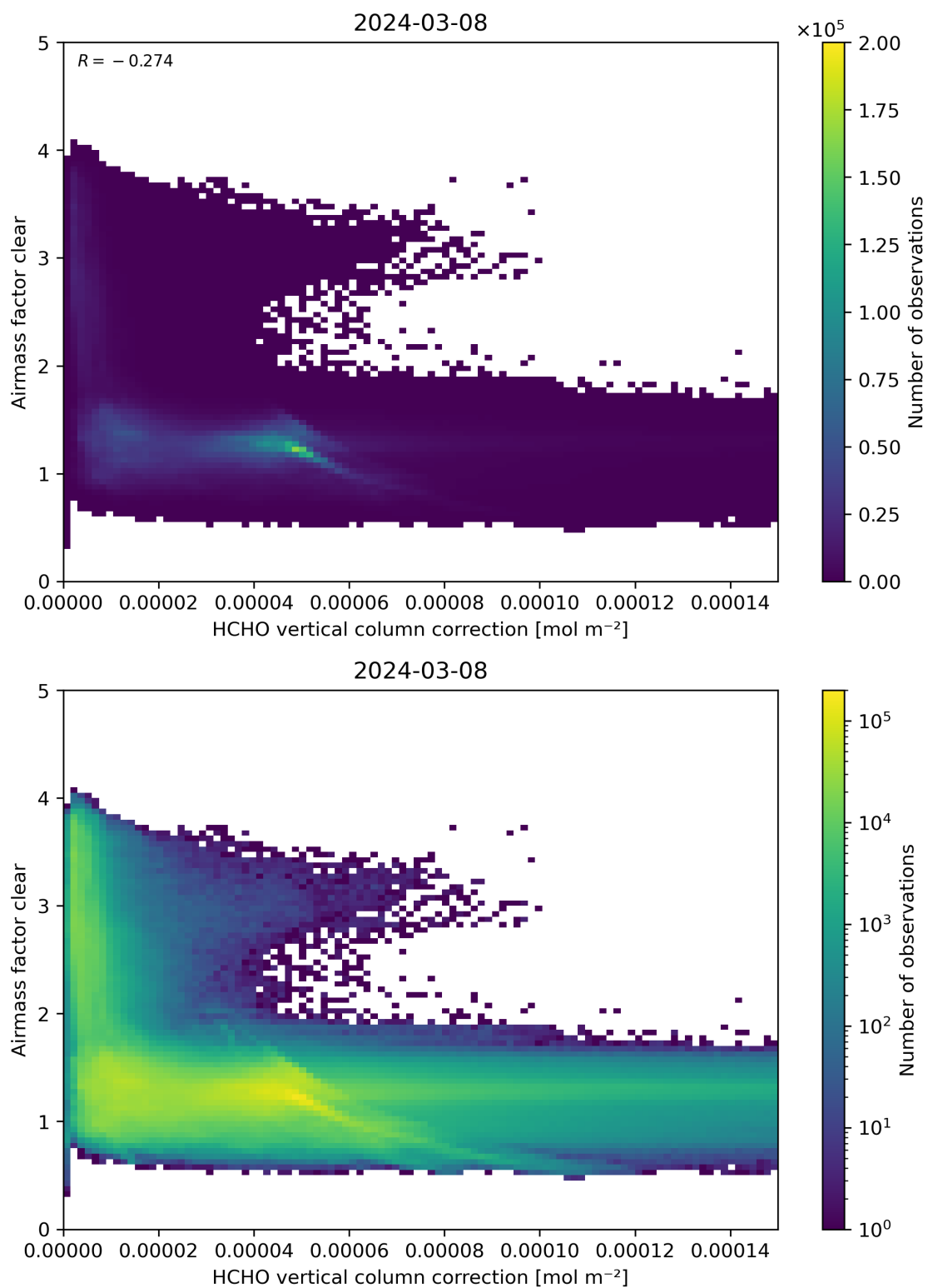
Figure 115: Scatter density plot of “HCHO vertical column correction” against “Airmass factor clear” for 2024-03-07 to 2024-03-09.
