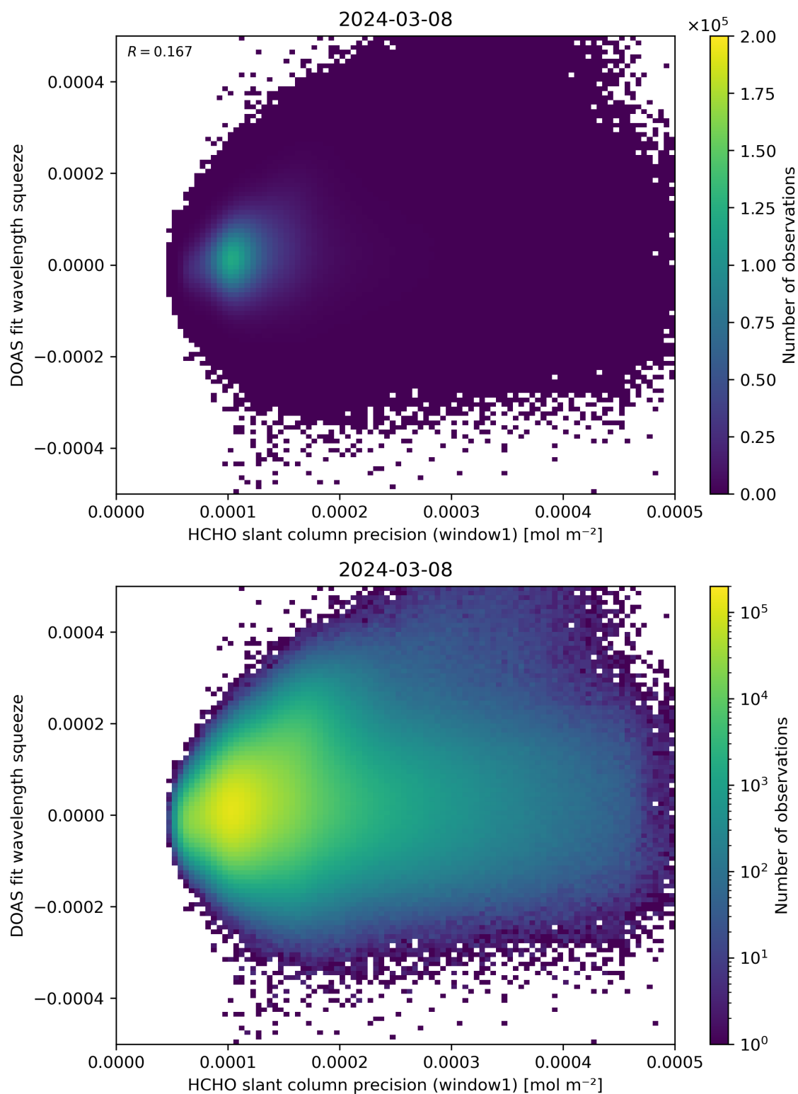
Figure 90: Scatter density plot of “HCHO slant column precision (window1)” against “DOAS fit wavelength squeeze” for 2024-03-07 to 2024-03-09.
