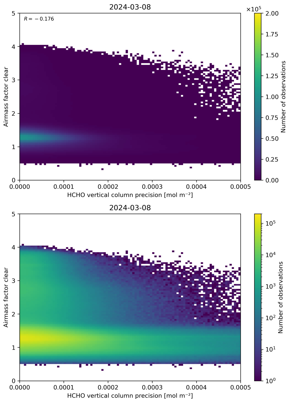
Figure 139: Scatter density plot of “HCHO vertical column precision” against “Airmass factor clear” for 2024-03-07 to 2024-03-09.
