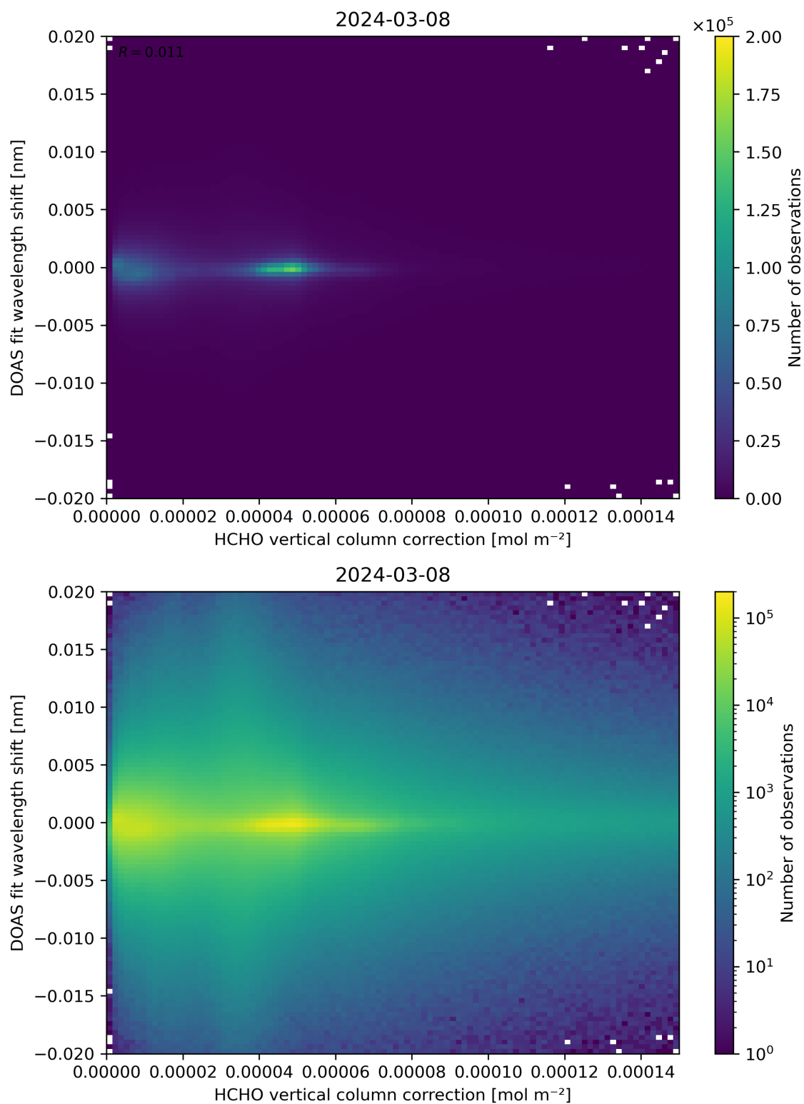
Figure 113: Scatter density plot of “HCHO vertical column correction” against “DOAS fit wavelength shift” for 2024-03-07 to 2024-03-09.
