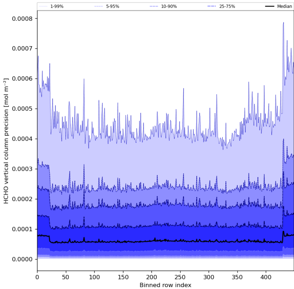
Figure 50: Along track statistics of “HCHO vertical column precision” for 2024-03-07 to 2024-03-09
