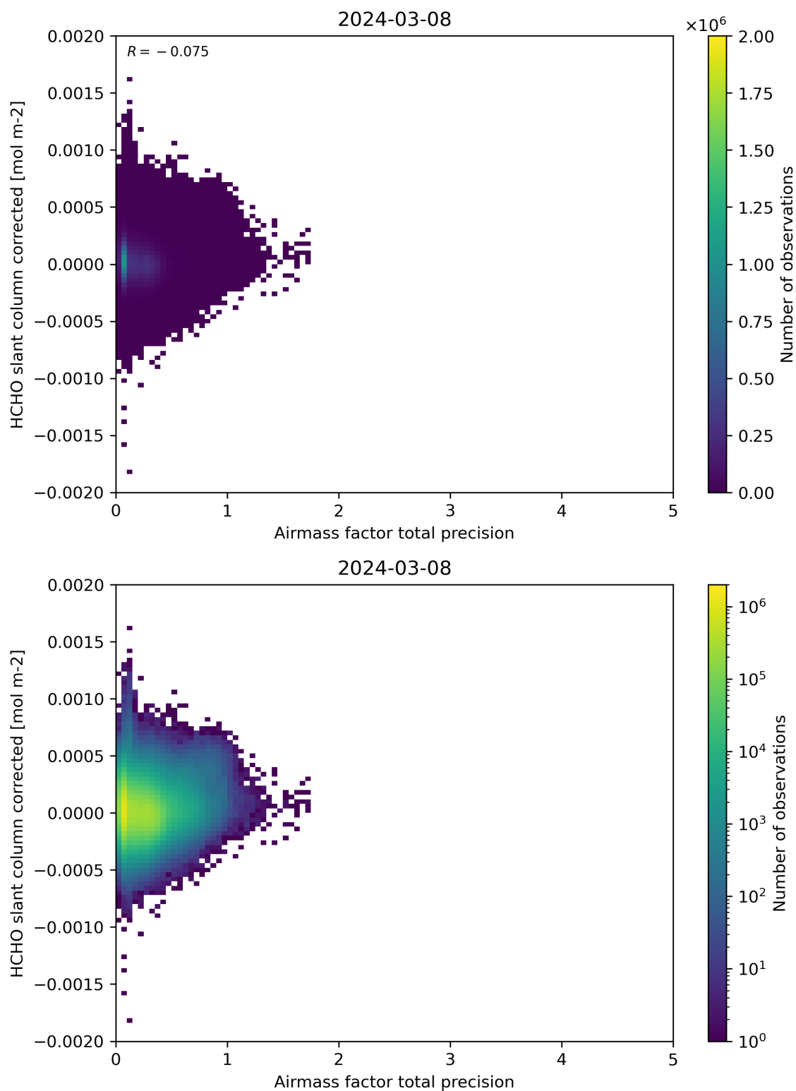
Figure 109: Scatter density plot of “Airmass factor total precision” against “HCHO slant column corrected” for 2024-03-07 to 2024-03-09.
