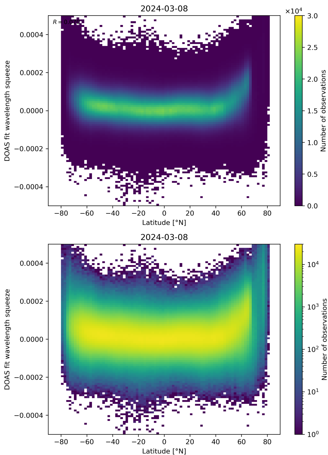
Figure 155: Scatter density plot of “Latitude” against “DOAS fit wavelength squeeze” for 2024-03-07 to 2024-03-09.
