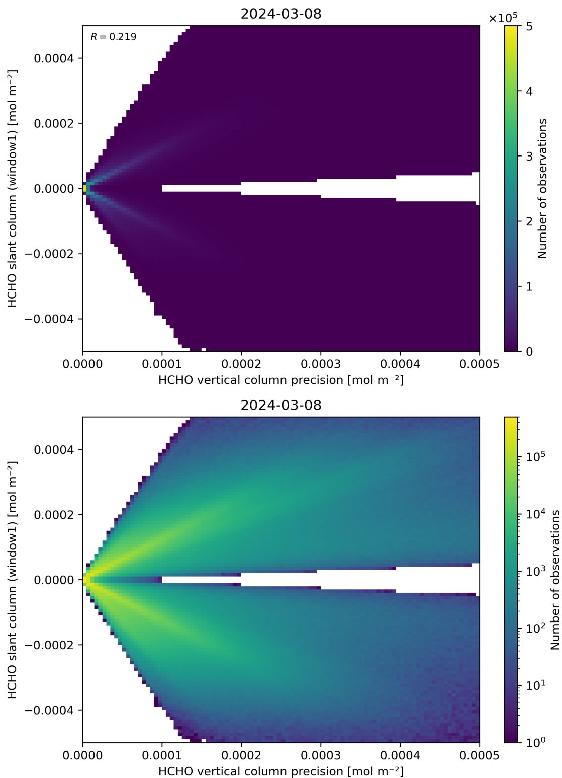
Figure 142: Scatter density plot of “HCHO vertical column precision” against “HCHO slant column (window1)” for 2024-03-07 to 2024-03-09.
