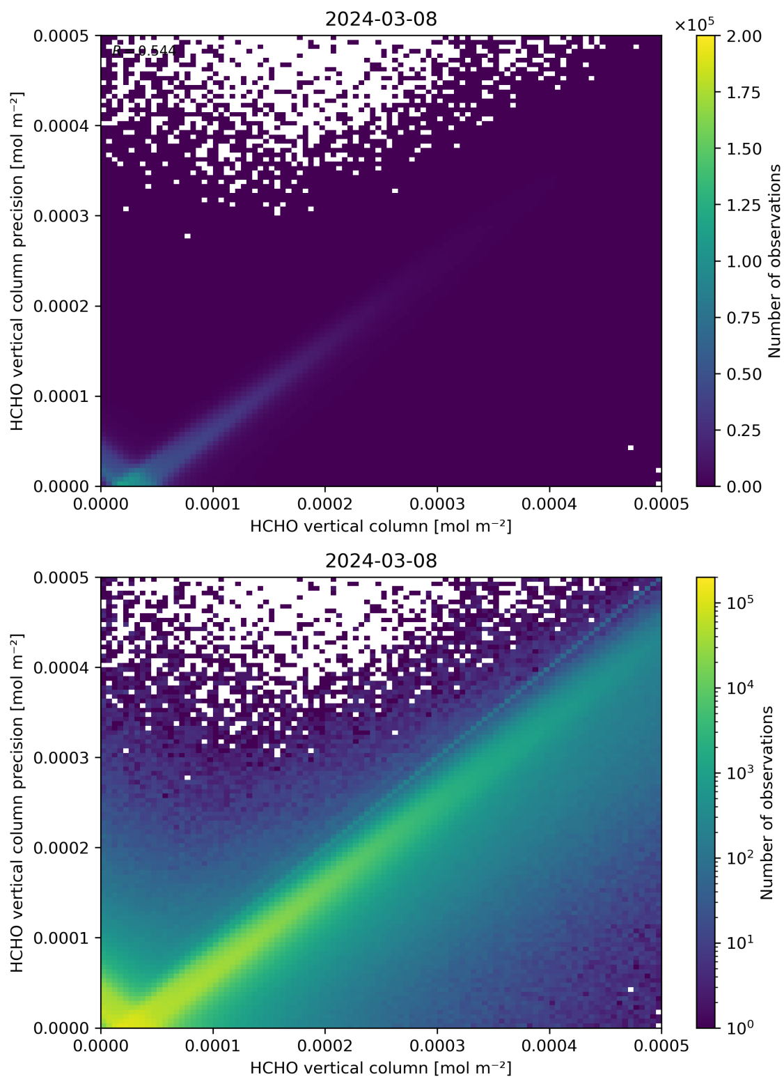
Figure 134: Scatter density plot of “HCHO vertical column” against “HCHO vertical column precision” for 2024-03-07 to 2024-03-09.
