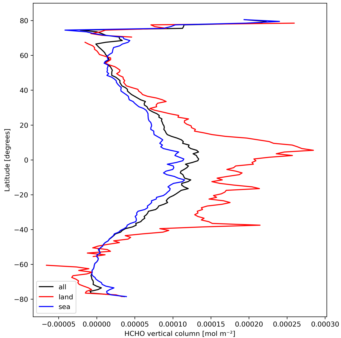
Figure 21: Zonal average of “HCHO vertical column” for 2024-03-07 to 2024-03-09.
