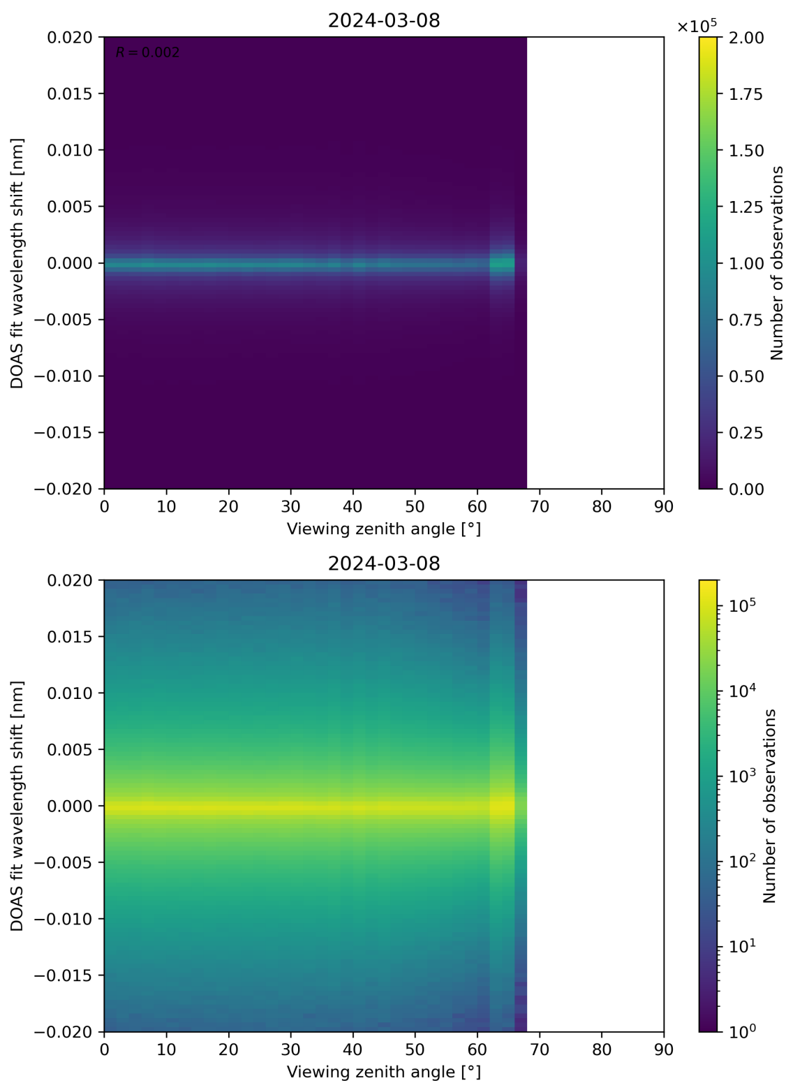
Figure 183: Scatter density plot of “Viewing zenith angle” against “DOAS fit wavelength shift” for 2024-03-07 to 2024-03-09.
