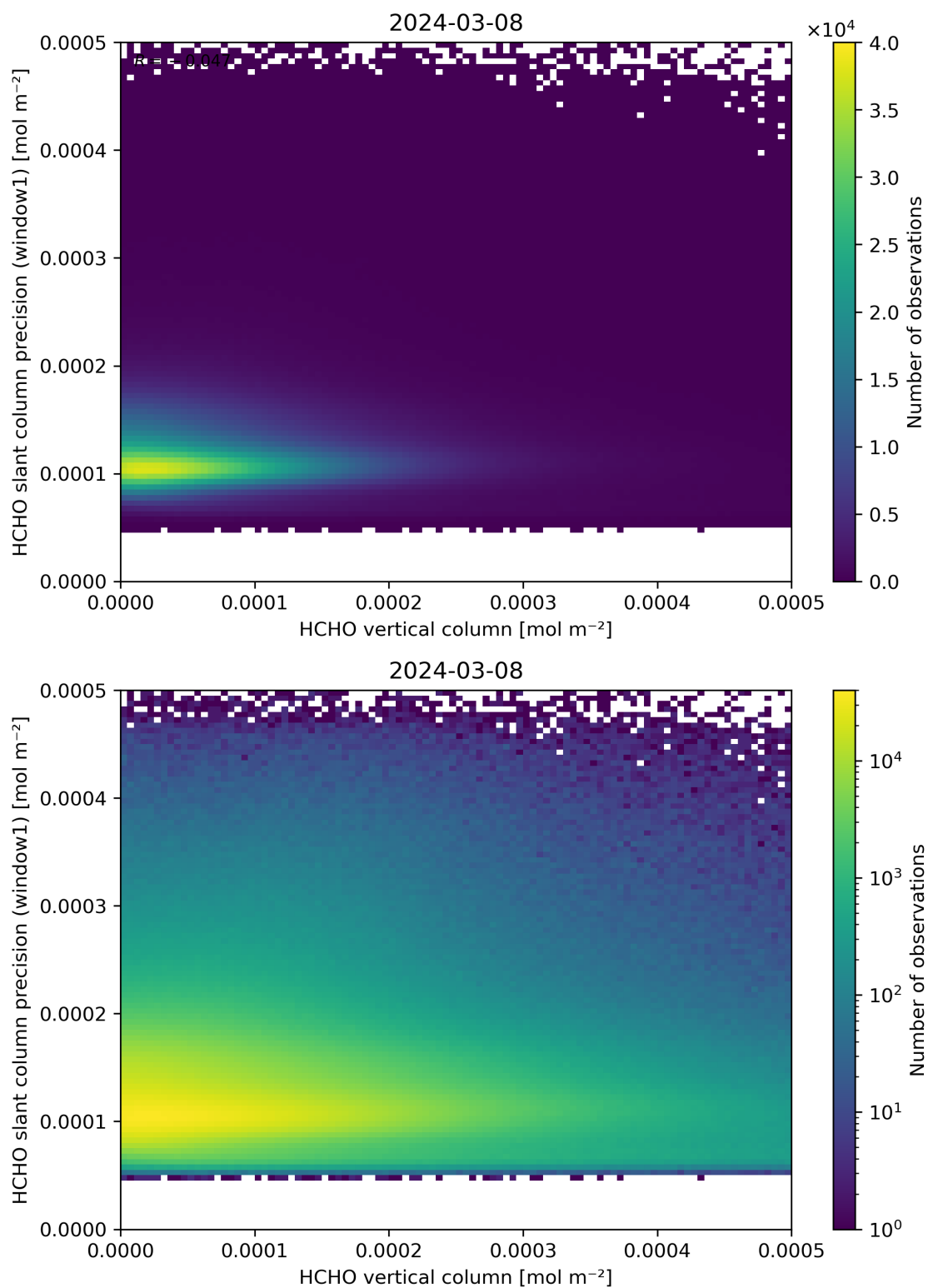
Figure 130: Scatter density plot of “HCHO vertical column” against “HCHO slant column precision (window1)” for 2024-03-07 to 2024-03-09.
