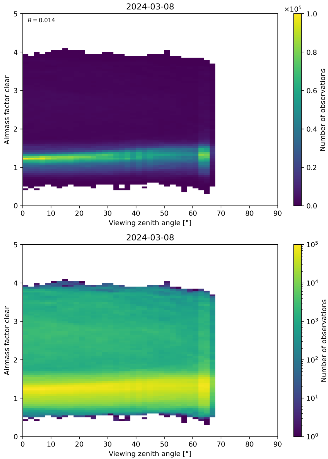
Figure 185: Scatter density plot of “Viewing zenith angle” against “Airmass factor clear” for 2024-03-07 to 2024-03-09.
