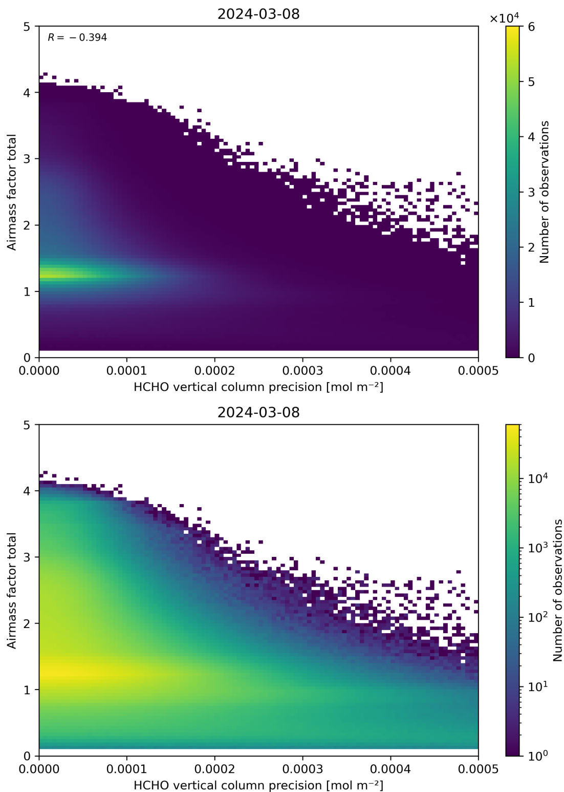
Figure 144: Scatter density plot of “HCHO vertical column precision” against “Airmass factor total” for 2024-03-07 to 2024-03-09.
