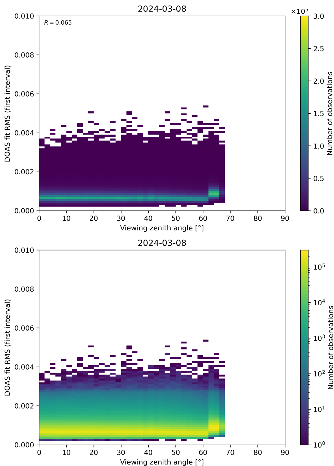
Figure 182: Scatter density plot of “Viewing zenith angle” against “DOAS fit RMS (first interval)” for 2024-03-07 to 2024-03-09.
