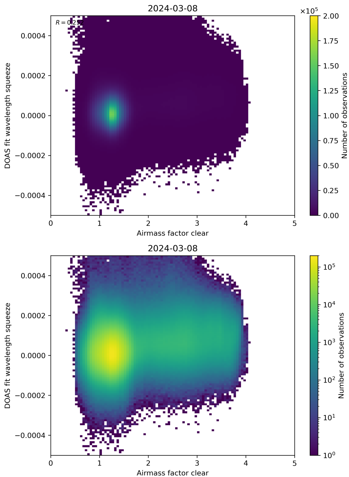
Figure 73: Scatter density plot of “Airmass factor clear” against “DOAS fit wavelength squeeze” for 2024-03-07 to 2024-03-09.
