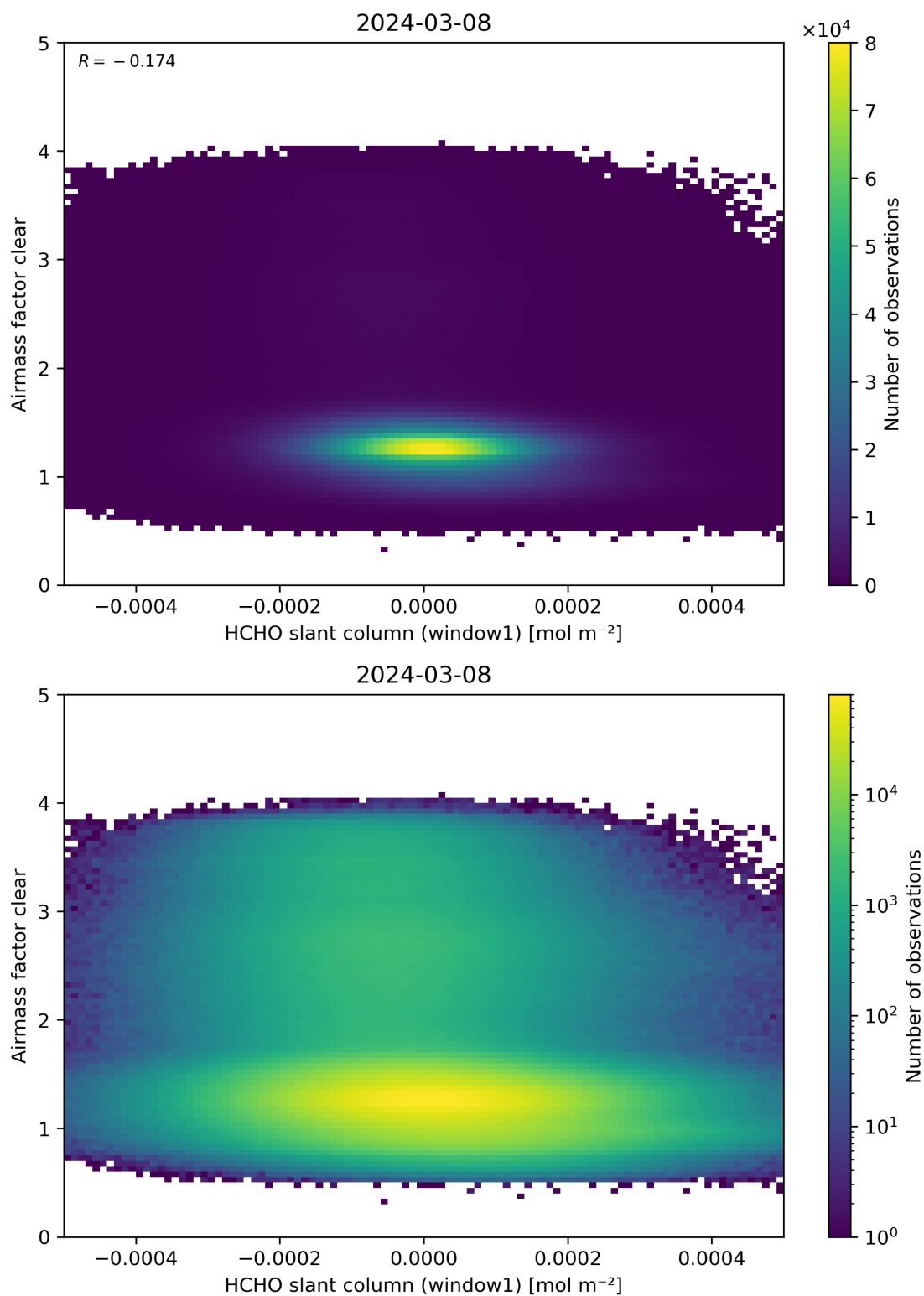
Figure 81: Scatter density plot of “HCHO slant column (window1)” against “Airmass factor clear” for 2024-03-07 to 2024-03-09.
