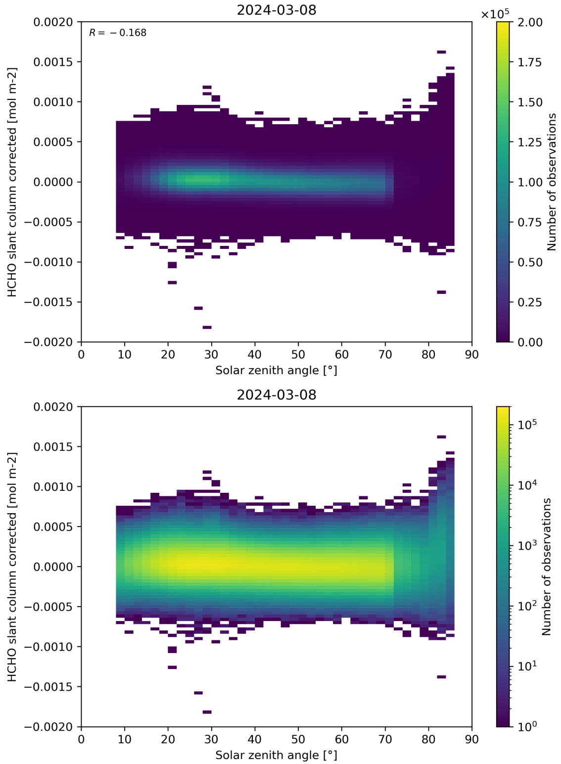
Figure 171: Scatter density plot of “Solar zenith angle” against “HCHO slant column corrected” for 2024-03-07 to 2024-03-09.
