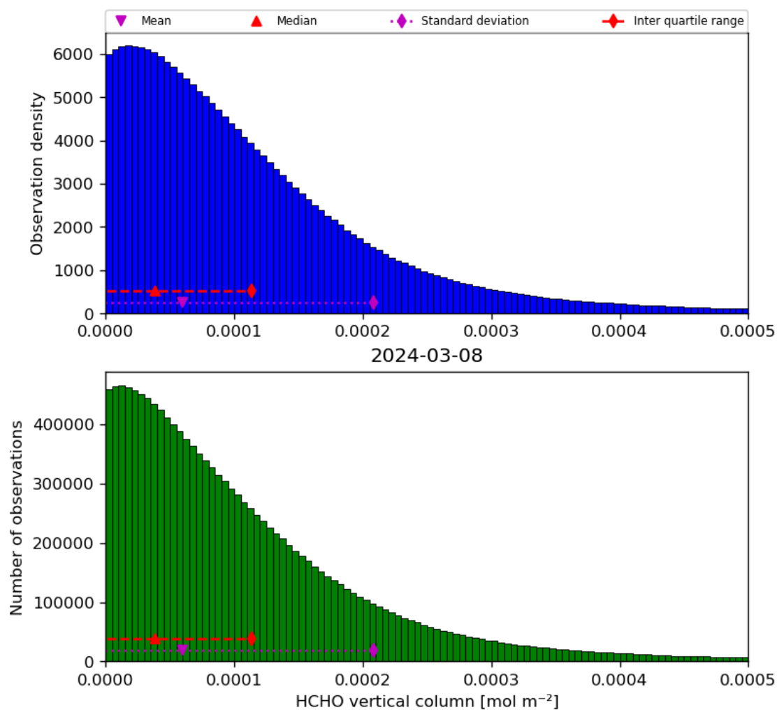
Figure 35: Histogram of “HCHO vertical column” for 2024-03-07 to 2024-03-09
