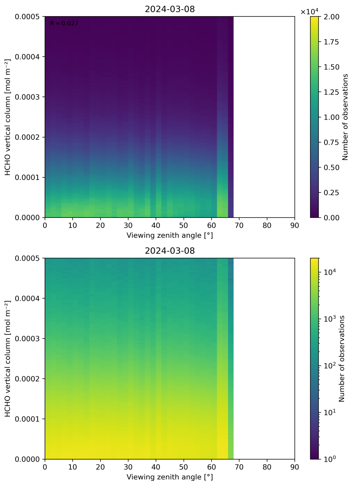
Figure 192: Scatter density plot of “Viewing zenith angle” against “HCHO vertical column” for 2024-03-07 to 2024-03-09.
