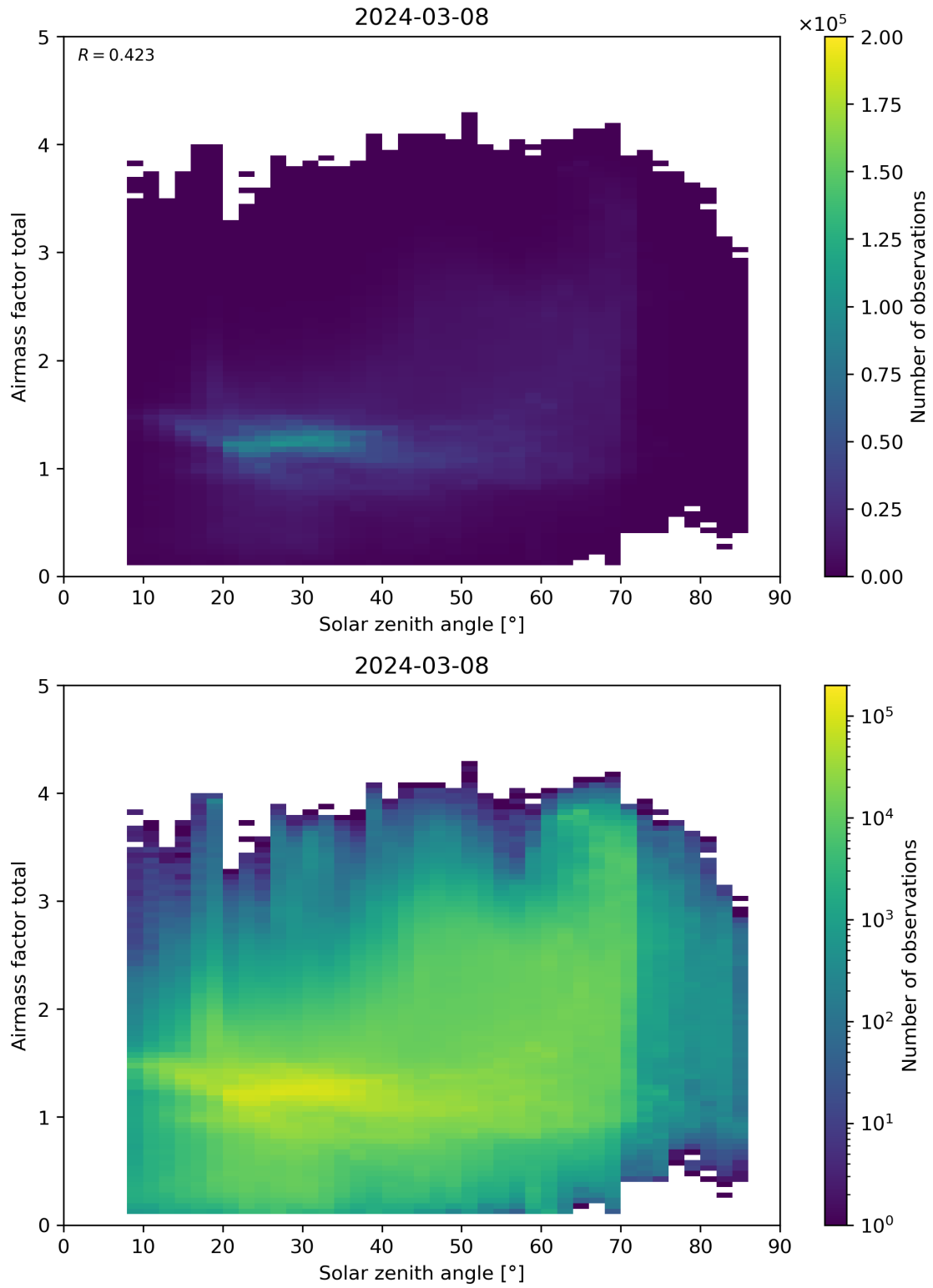
Figure 175: Scatter density plot of “Solar zenith angle” against “Airmass factor total” for 2024-03-07 to 2024-03-09.
