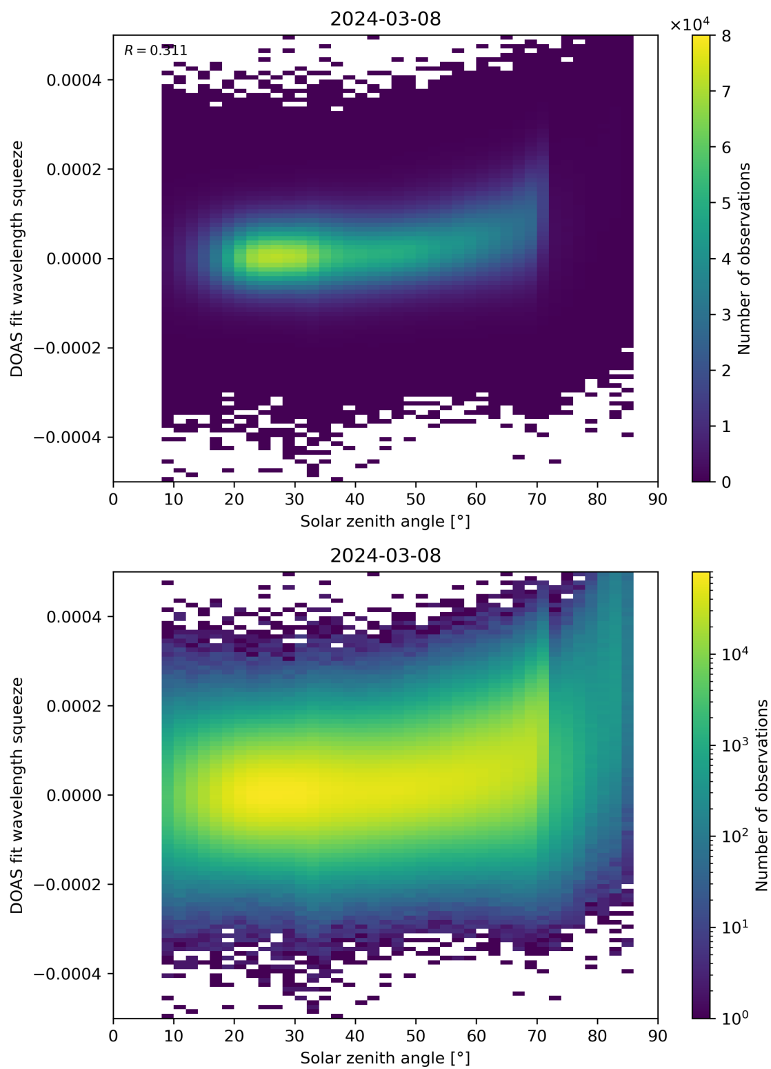
Figure 169: Scatter density plot of “Solar zenith angle” against “DOAS fit wavelength squeeze” for 2024-03-07 to 2024-03-09.
