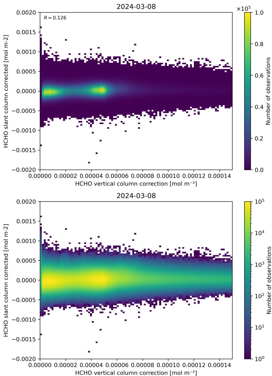
Figure 116: Scatter density plot of “HCHO vertical column correction” against “HCHO slant column corrected” for 2024-03-07 to 2024-03-09.
