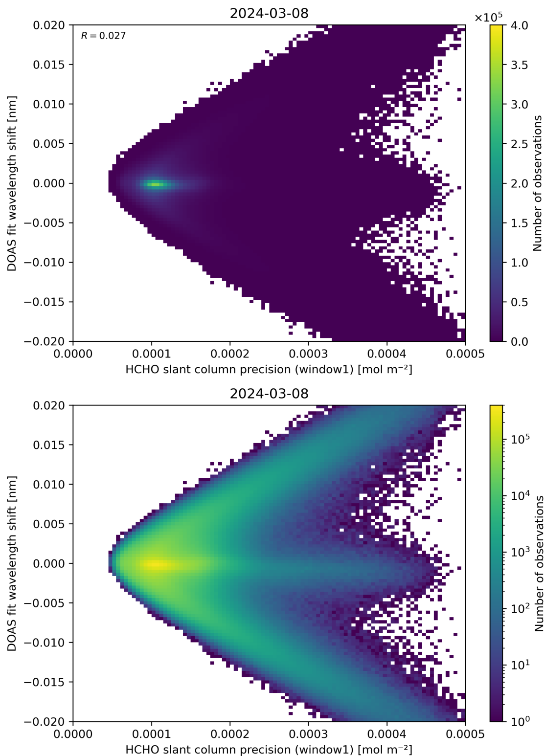
Figure 89: Scatter density plot of “HCHO slant column precision (window1)” against “DOAS fit wavelength shift” for 2024-03-07 to 2024-03-09.
