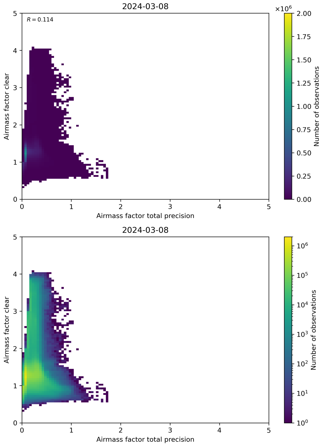
Figure 108: Scatter density plot of “Airmass factor total precision” against “Airmass factor clear” for 2024-03-07 to 2024-03-09.
