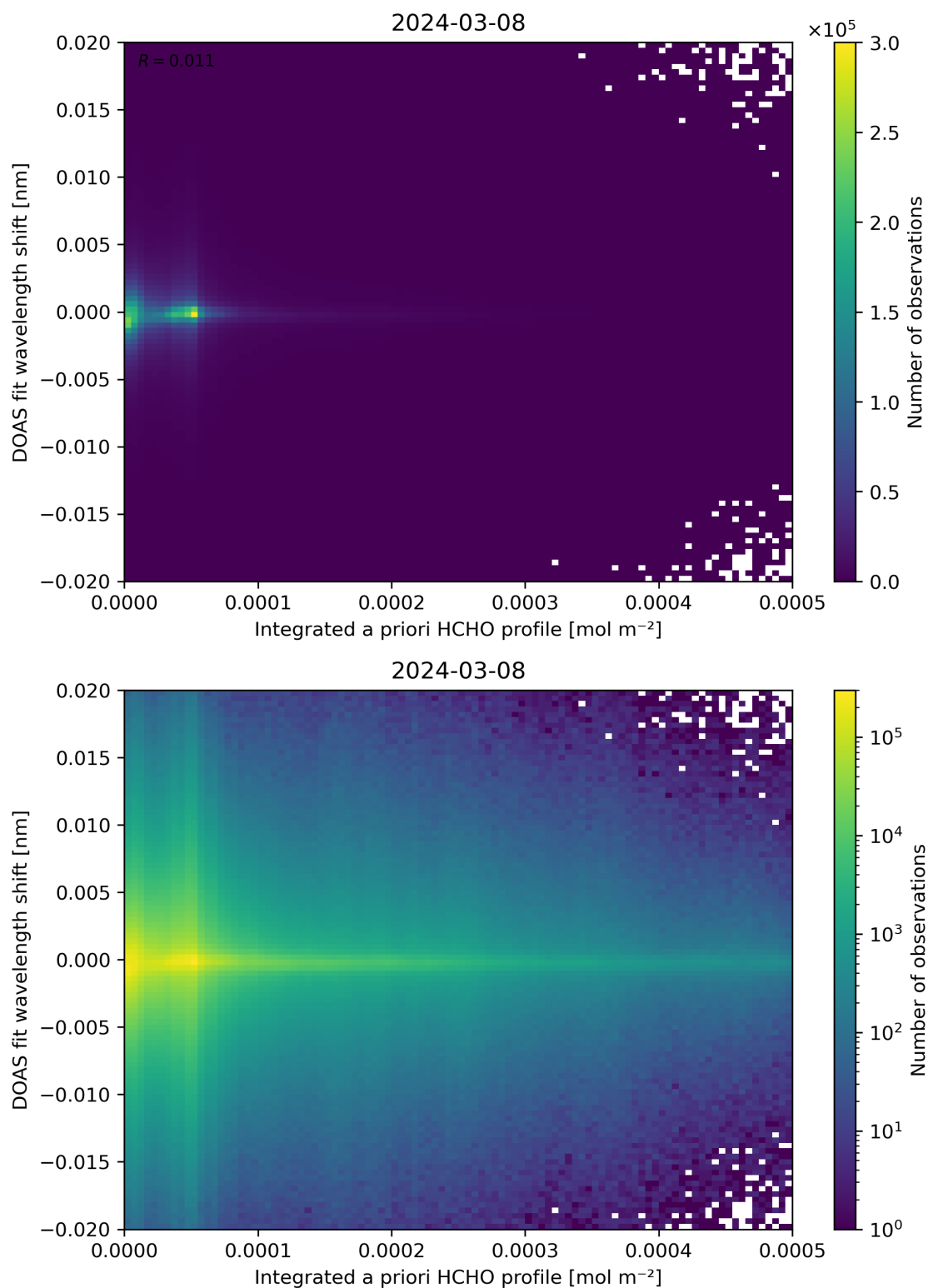
Figure 149: Scatter density plot of “Integrated a priori HCHO profile” against “DOAS fit wavelength shift” for 2024-03-07 to 2024-03-09.
