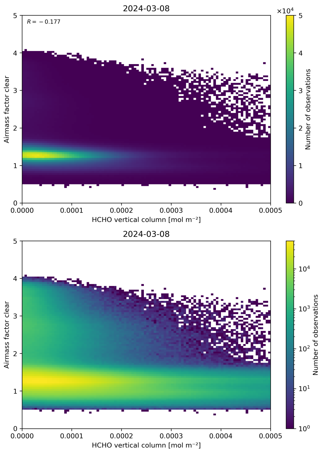
Figure 126: Scatter density plot of “HCHO vertical column” against “Airmass factor clear” for 2024-03-07 to 2024-03-09.
