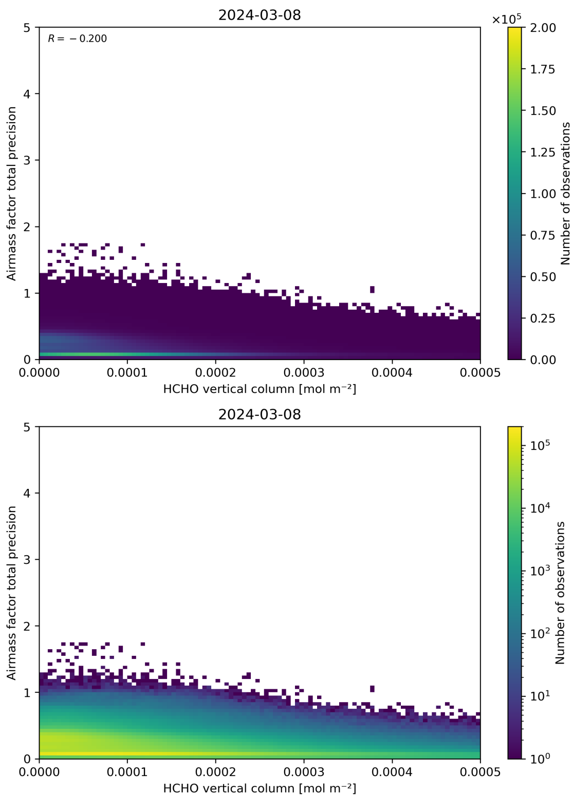
Figure 132: Scatter density plot of “HCHO vertical column” against “Airmass factor total precision” for 2024-03-07 to 2024-03-09.
