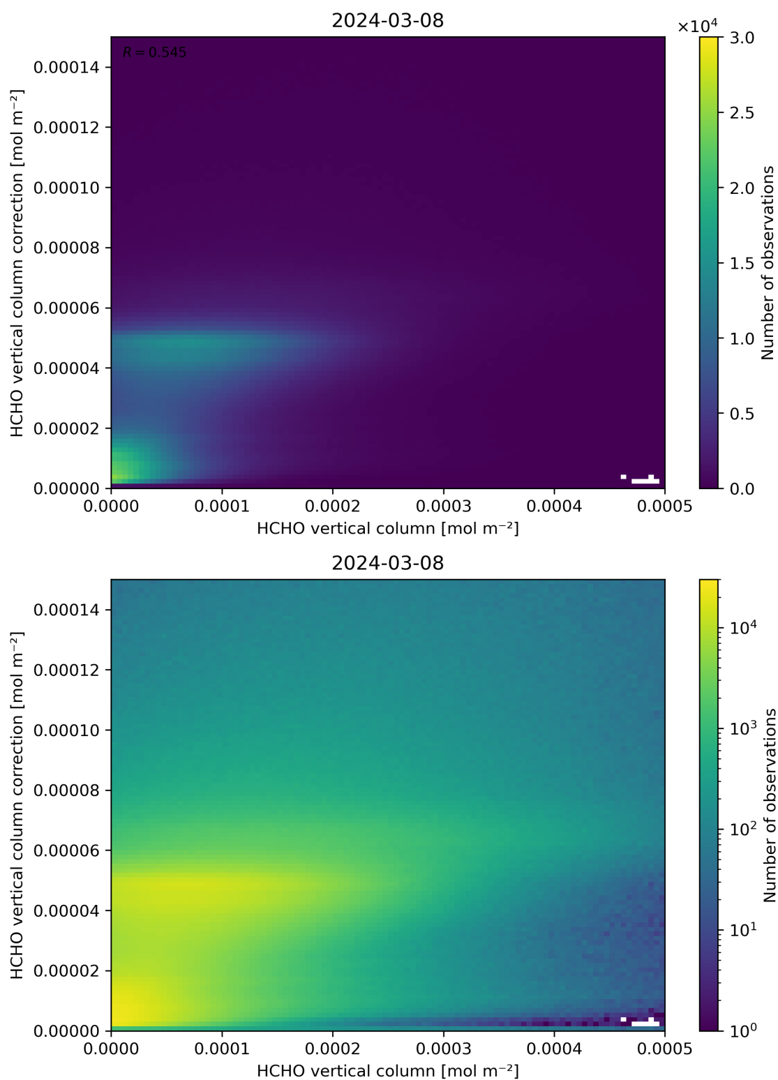
Figure 133: Scatter density plot of “HCHO vertical column” against “HCHO vertical column correction” for 2024-03-07 to 2024-03-09.
