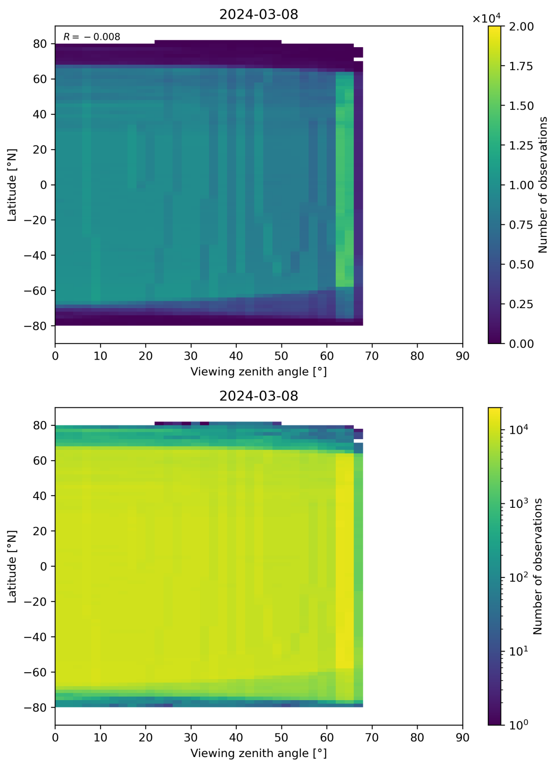
Figure 196: Scatter density plot of “Viewing zenith angle” against “Latitude” for 2024-03-07 to 2024-03-09.
