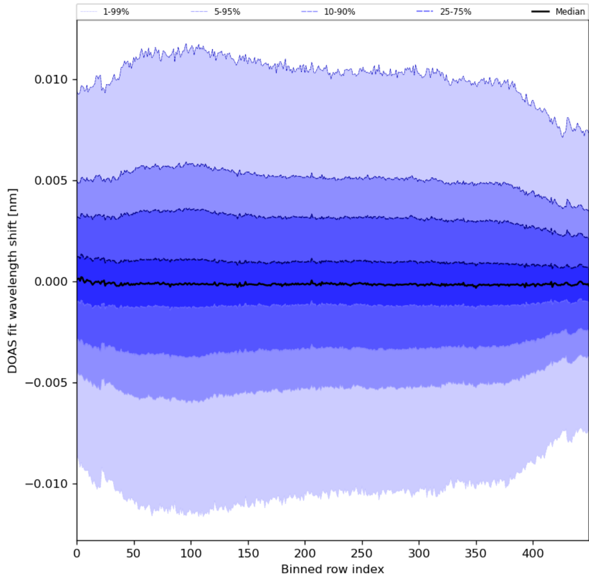
Figure 58: Along track statistics of “DOAS fit wavelength shift” for 2024-03-07 to 2024-03-09
