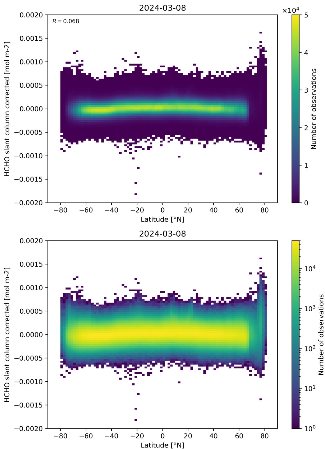
Figure 157: Scatter density plot of “Latitude” against “HCHO slant column corrected” for 2024-03-07 to 2024-03-09.
