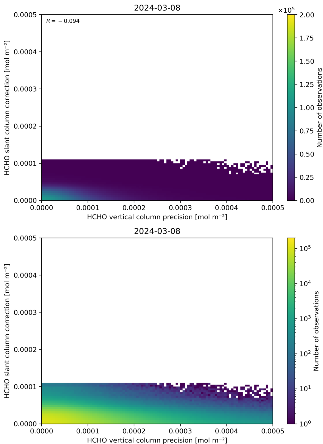
Figure 141: Scatter density plot of “HCHO vertical column precision” against “HCHO slant column correction” for 2024-03-07 to 2024-03-09.
