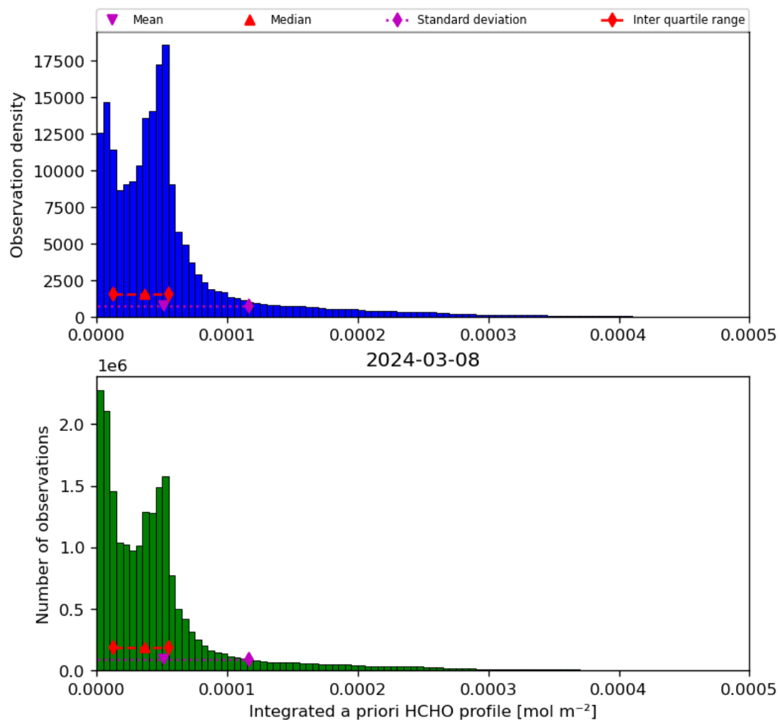
Figure 43: Histogram of “Integrated a priori HCHO profile” for 2024-03-07 to 2024-03-09
