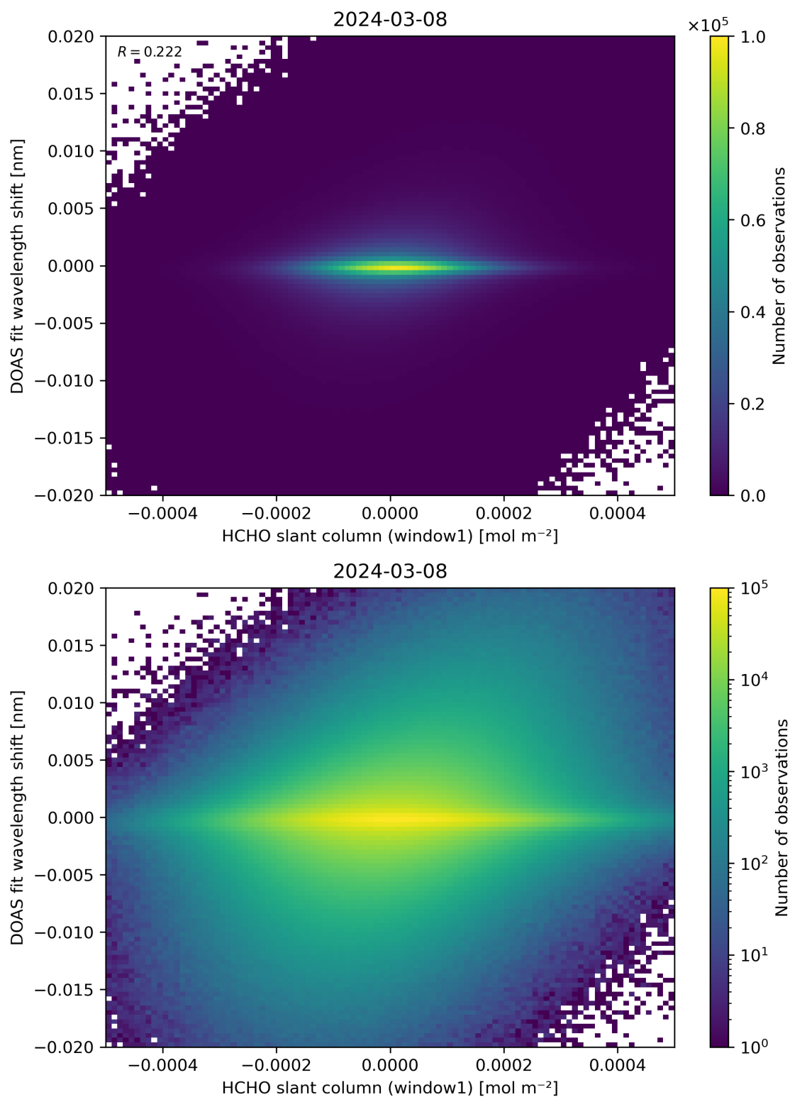
Figure 79: Scatter density plot of “HCHO slant column (window1)” against “DOAS fit wavelength shift” for 2024-03-07 to 2024-03-09.
