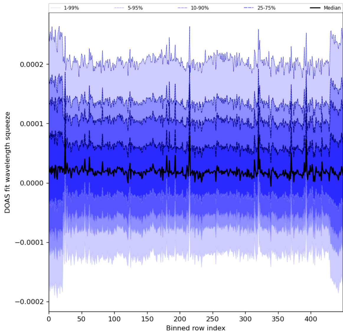
Figure 59: Along track statistics of “DOAS fit wavelength squeeze” for 2024-03-07 to 2024-03-09
