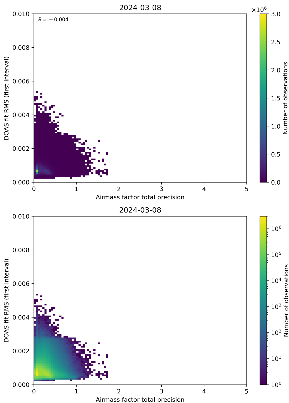
Figure 105: Scatter density plot of “Airmass factor total precision” against “DOAS fit RMS (first interval)” for 2024-03-07 to 2024-03-09.
