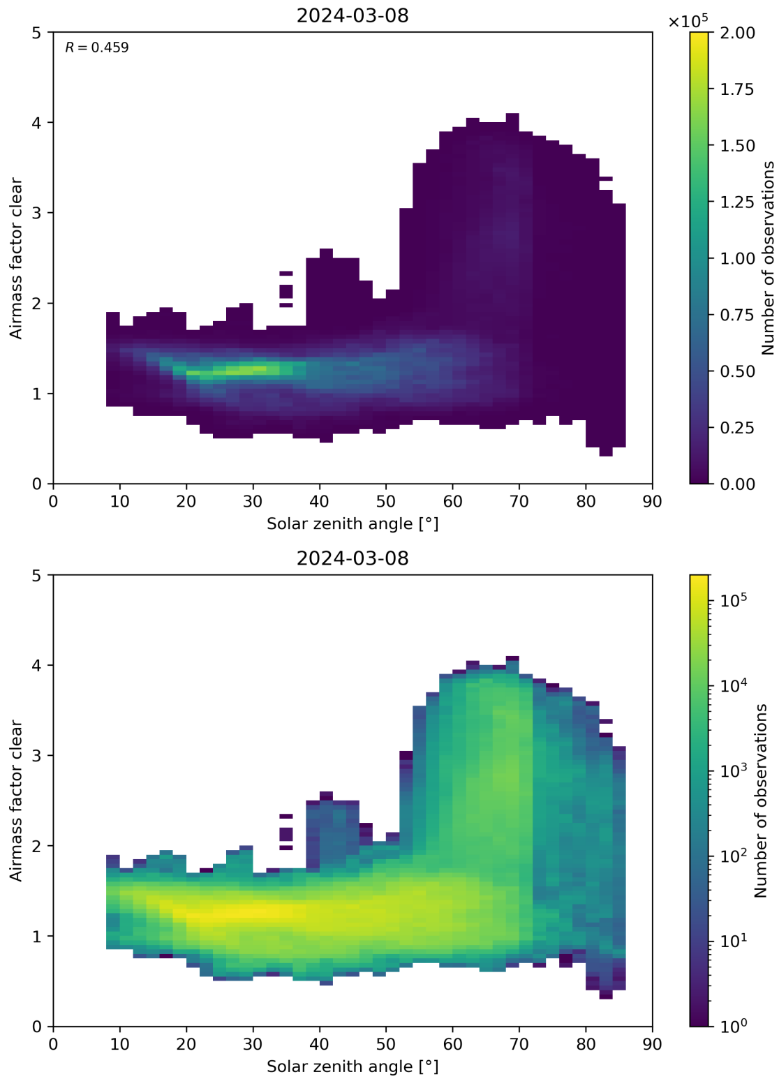
Figure 170: Scatter density plot of “Solar zenith angle” against “Airmass factor clear” for 2024-03-07 to 2024-03-09.
