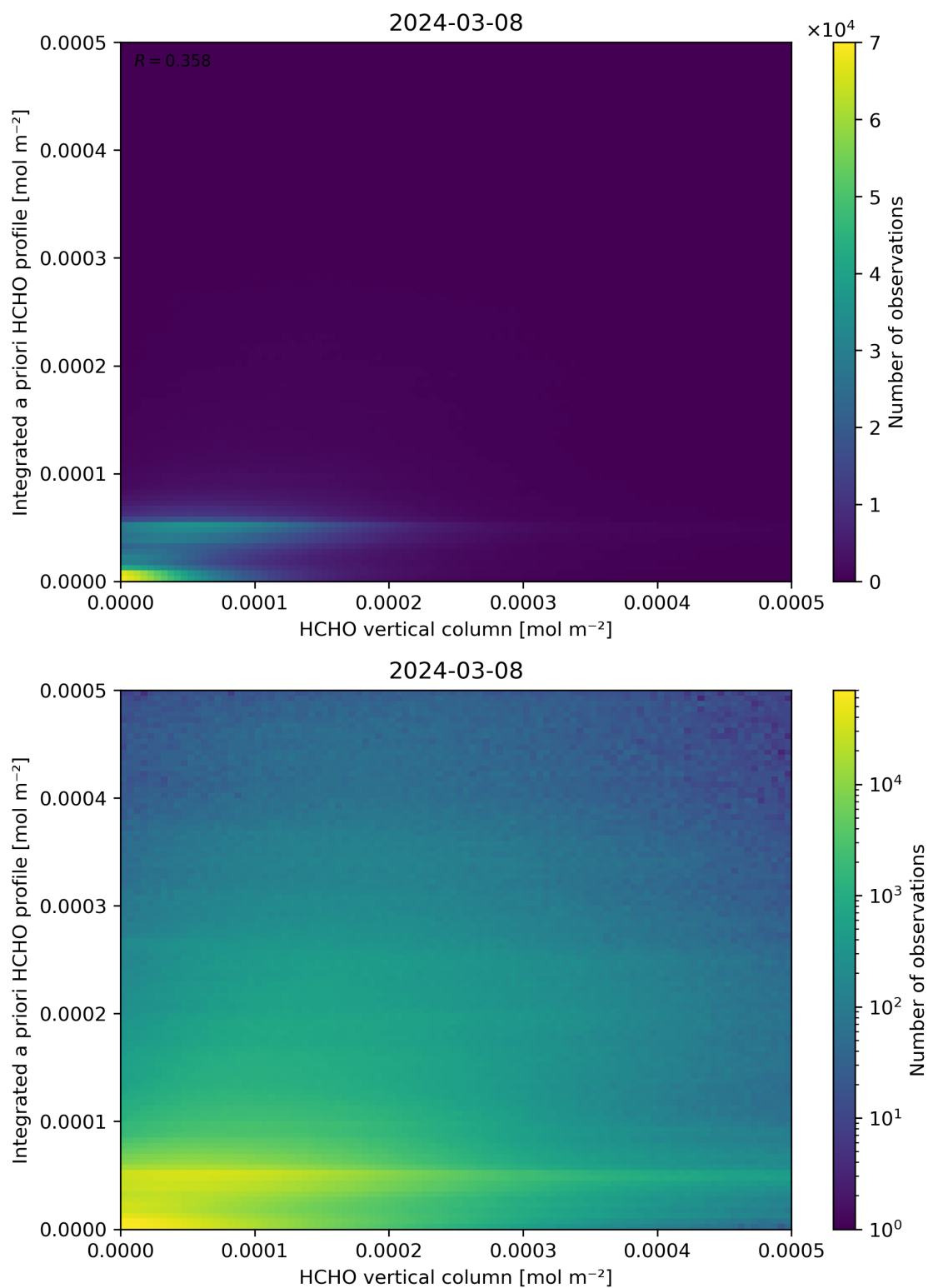
Figure 135: Scatter density plot of “HCHO vertical column” against “Integrated a priori HCHO profile” for 2024-03-07 to 2024-03-09.
