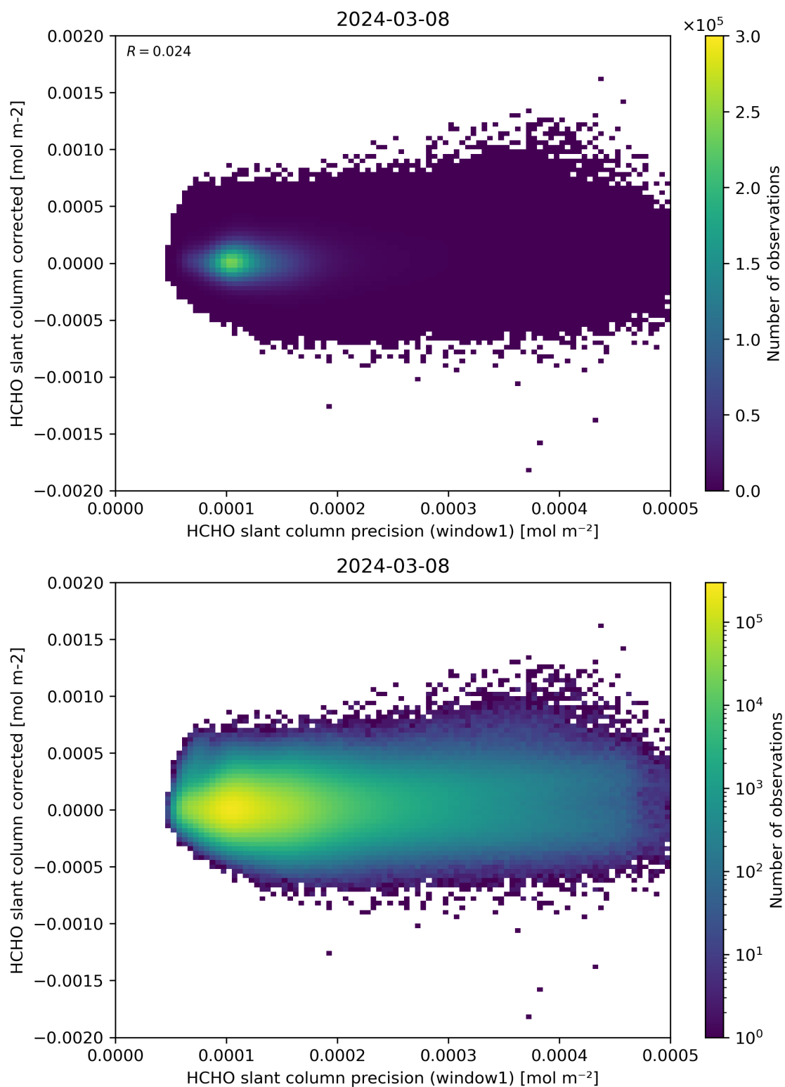
Figure 92: Scatter density plot of “HCHO slant column precision (window1)” against “HCHO slant column corrected” for 2024-03-07 to 2024-03-09.
