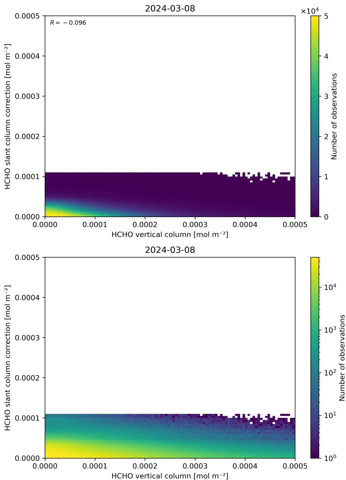
Figure 128: Scatter density plot of “HCHO vertical column” against “HCHO slant column correction” for 2024-03-07 to 2024-03-09.
