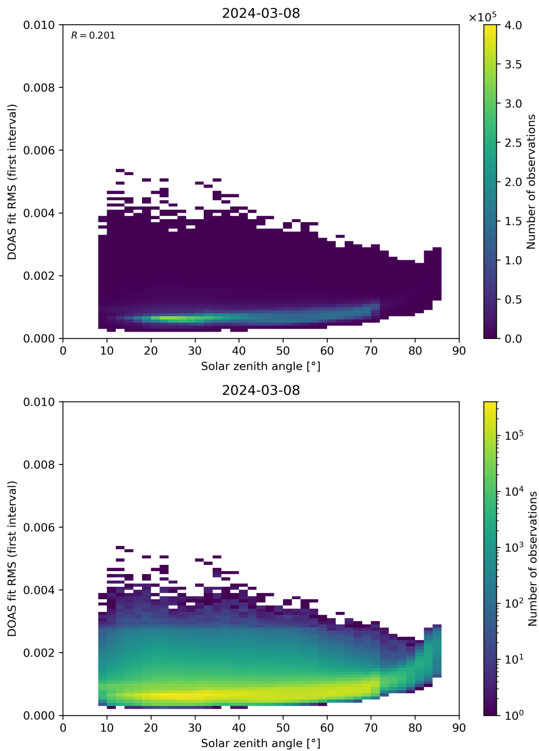
Figure 167: Scatter density plot of “Solar zenith angle” against “DOAS fit RMS (first interval)” for 2024-03-07 to 2024-03-09.
