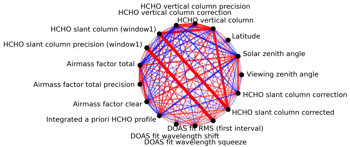
Figure 1: Map of correlation graph for 2024-03-07 to 2024-03-09.
