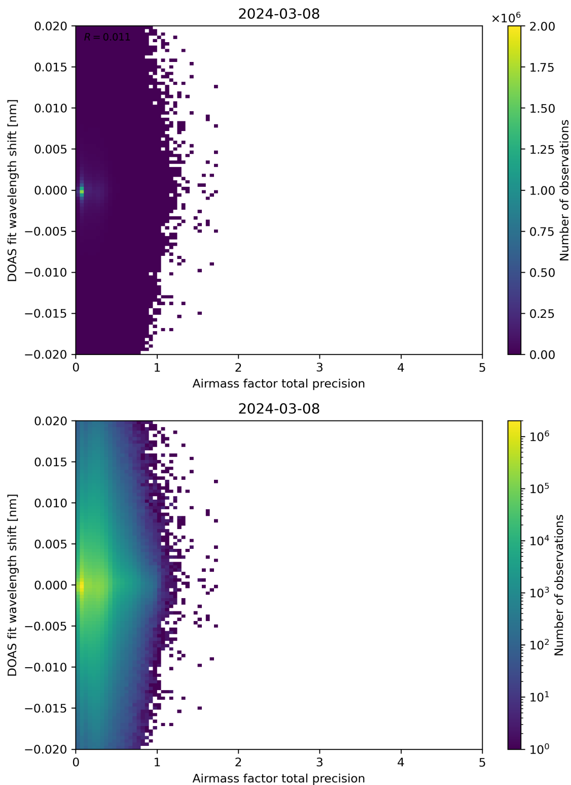
Figure 106: Scatter density plot of “Airmass factor total precision” against “DOAS fit wavelength shift” for 2024-03-07 to 2024-03-09.
