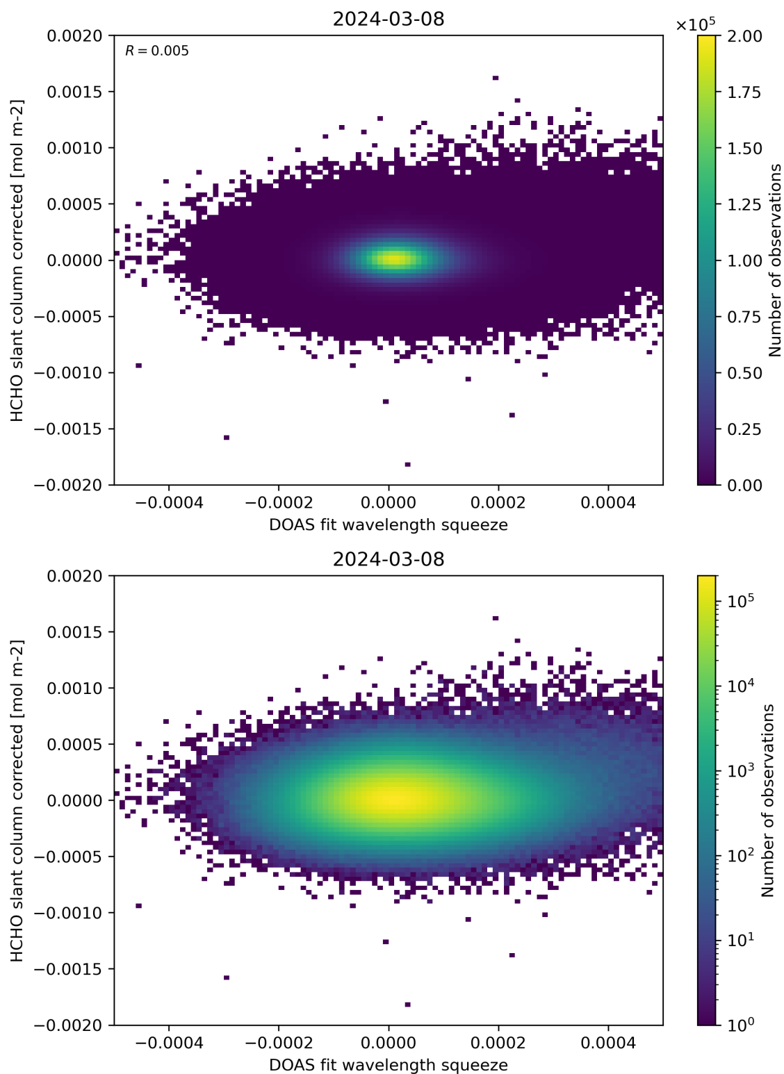
Figure 69: Scatter density plot of “DOAS fit wavelength squeeze” against “HCHO slant column corrected” for 2024-03-07 to 2024-03-09.
