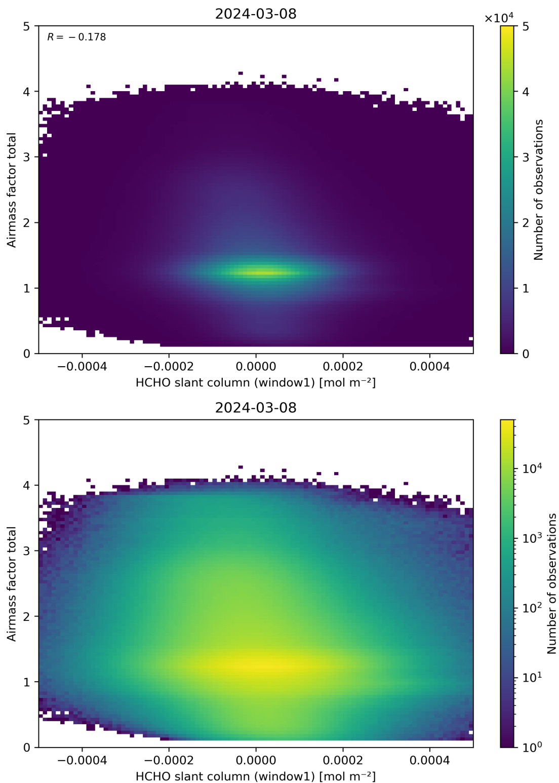
Figure 85: Scatter density plot of “HCHO slant column (window1)” against “Airmass factor total” for 2024-03-07 to 2024-03-09.
