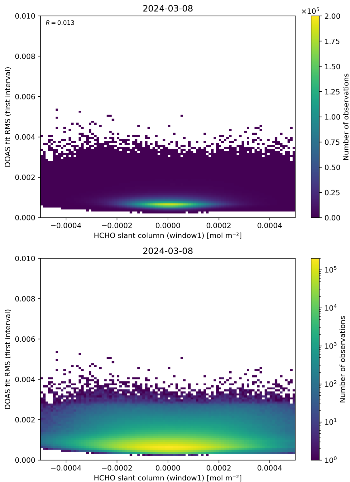
Figure 78: Scatter density plot of “HCHO slant column (window1)” against “DOAS fit RMS (first interval)” for 2024-03-07 to 2024-03-09.
