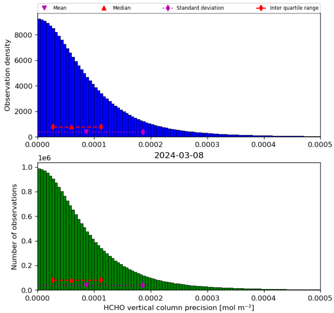
Figure 36: Histogram of “HCHO vertical column precision” for 2024-03-07 to 2024-03-09
