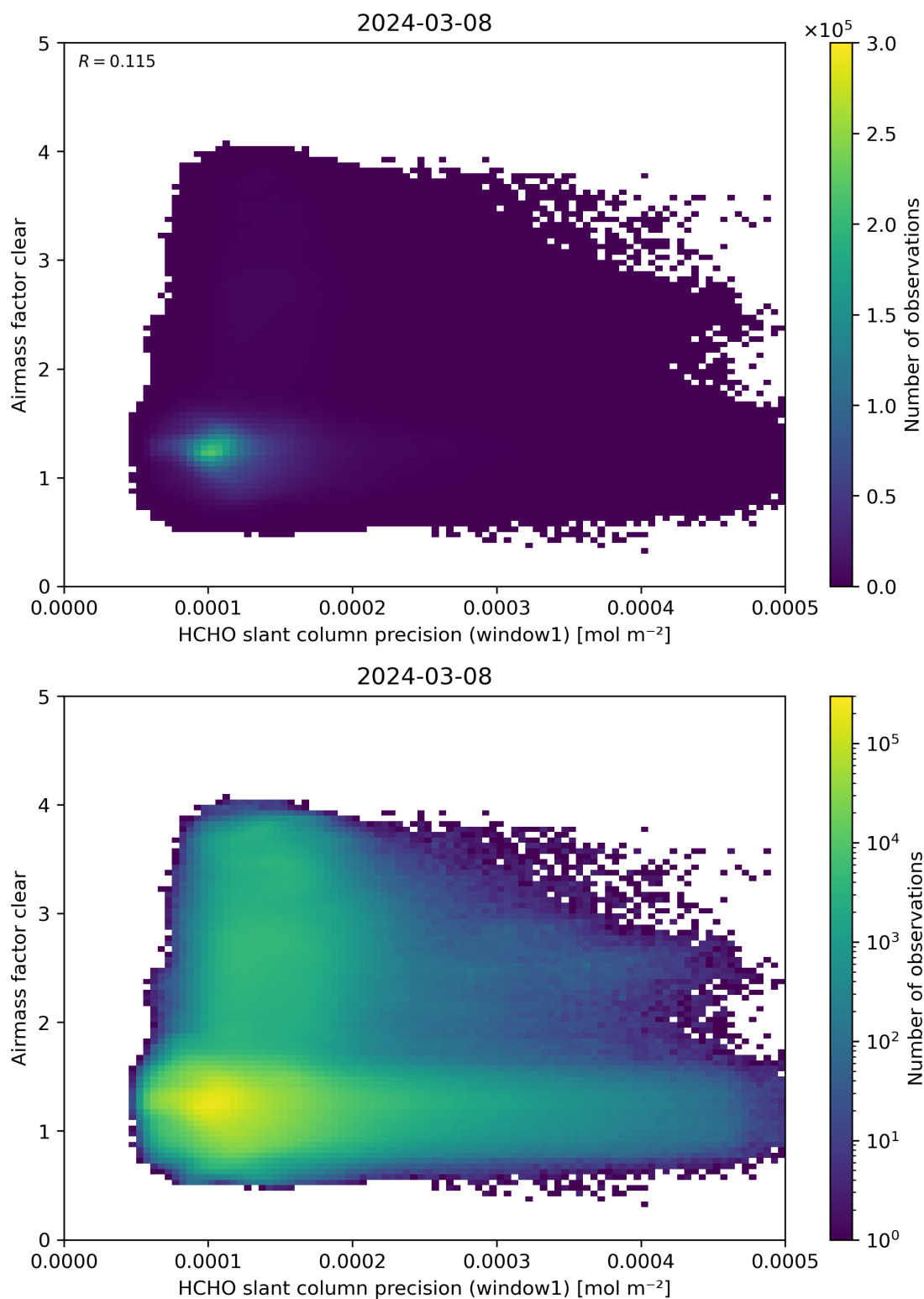
Figure 91: Scatter density plot of “HCHO slant column precision (window1)” against “Airmass factor clear” for 2024-03-07 to 2024-03-09.
