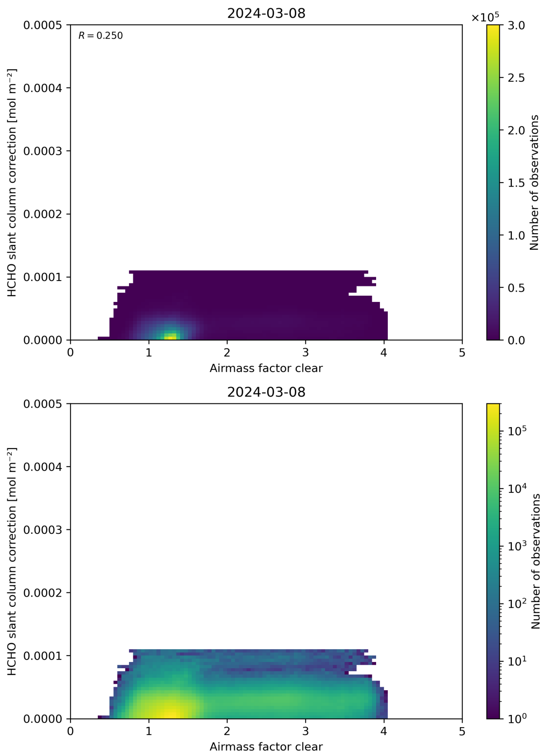
Figure 75: Scatter density plot of “Airmass factor clear” against “HCHO slant column correction” for 2024-03-07 to 2024-03-09.
