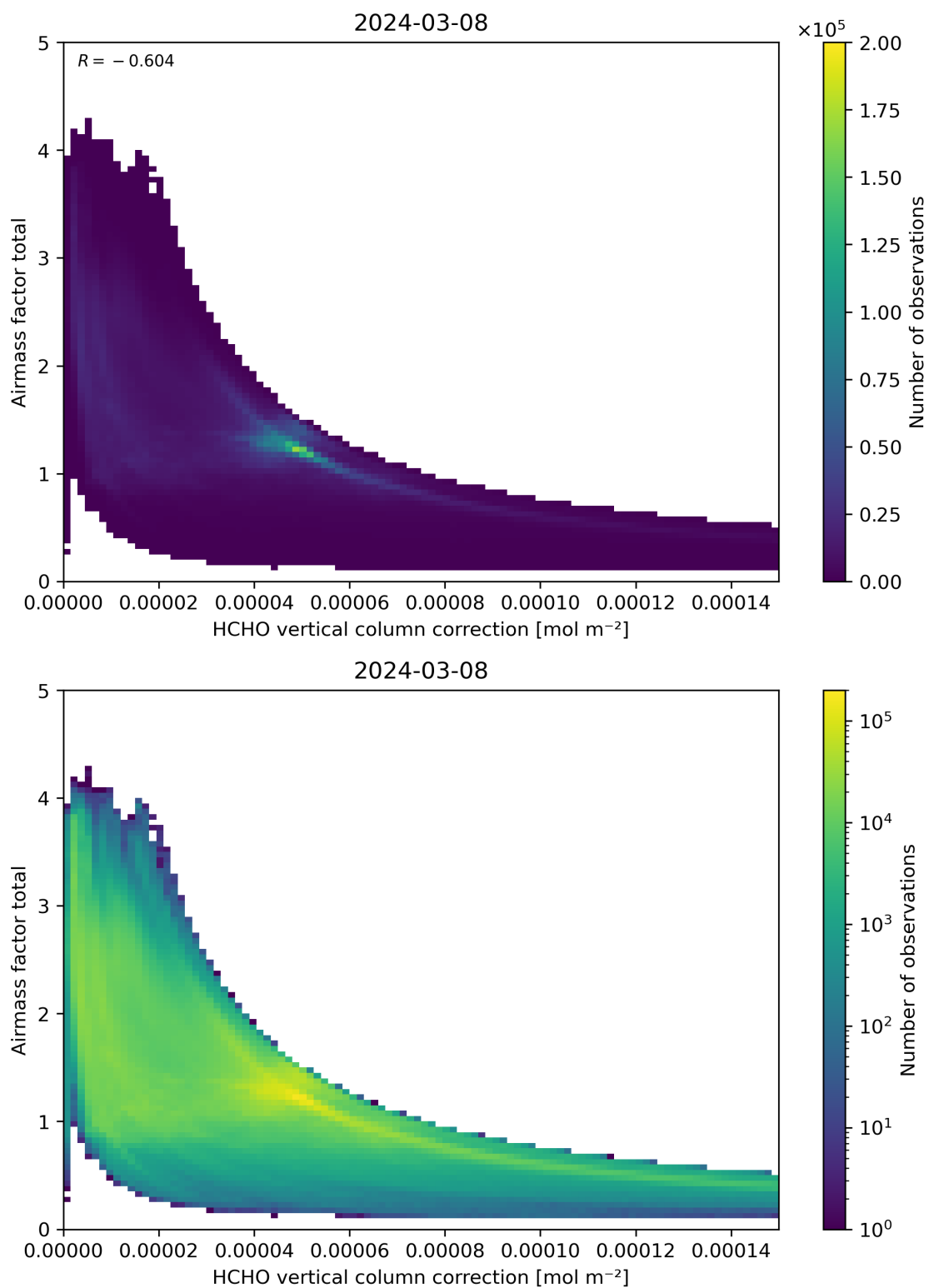
Figure 120: Scatter density plot of “HCHO vertical column correction” against “Airmass factor total” for 2024-03-07 to 2024-03-09.
