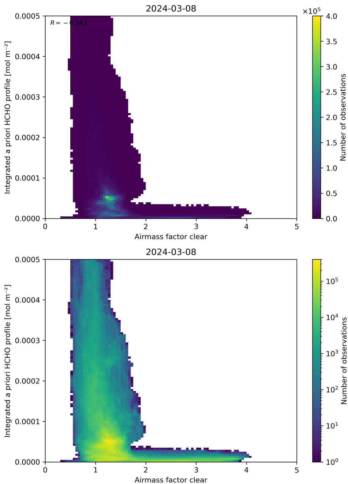
Figure 76: Scatter density plot of “Airmass factor clear” against “Integrated a priori HCHO profile” for 2024-03-07 to 2024-03-09.
