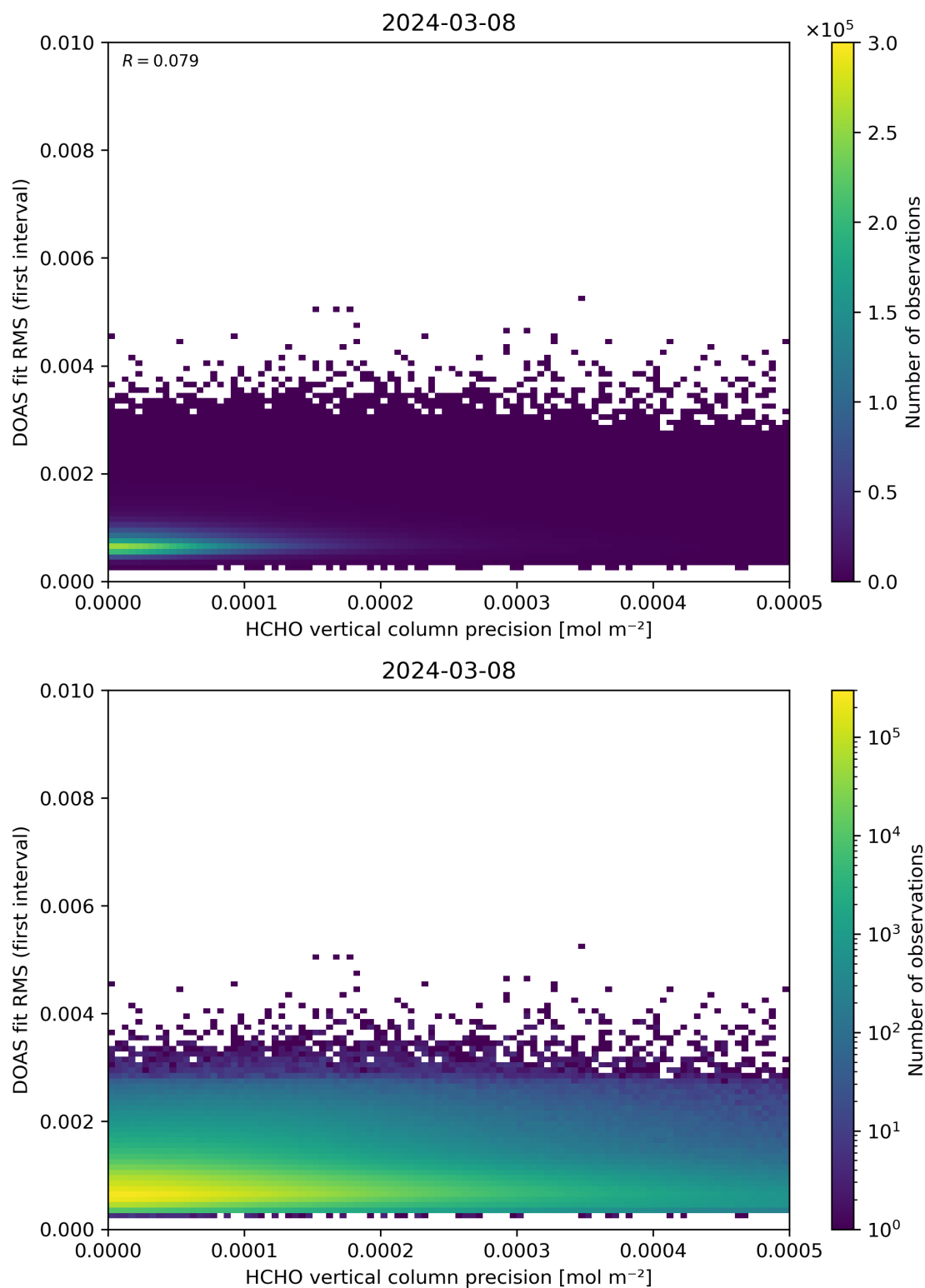
Figure 136: Scatter density plot of “HCHO vertical column precision” against “DOAS fit RMS (first interval)” for 2024-03-07 to 2024-03-09.
