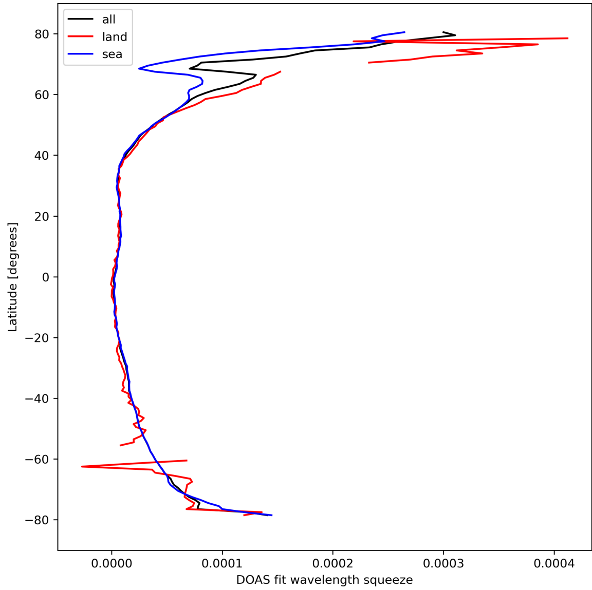
Figure 31: Zonal average of “DOAS fit wavelength squeeze” for 2024-03-07 to 2024-03-09.
