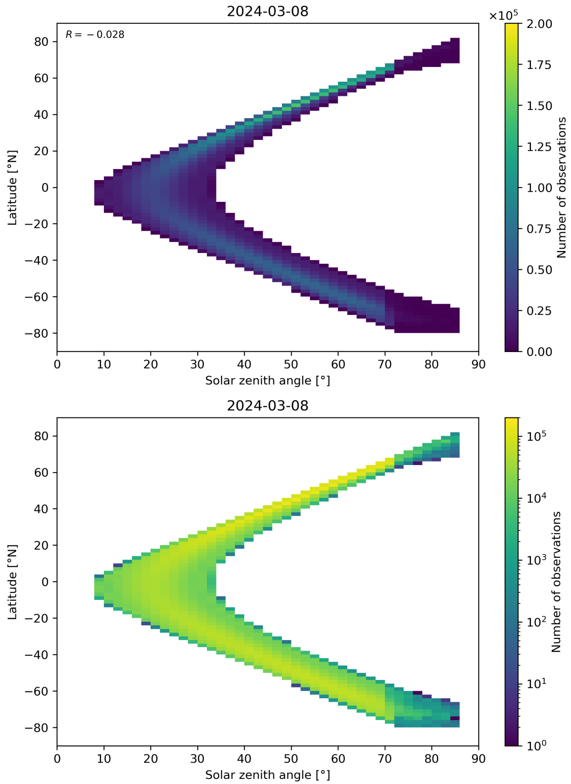
Figure 181: Scatter density plot of “Solar zenith angle” against “Latitude” for 2024-03-07 to 2024-03-09.
