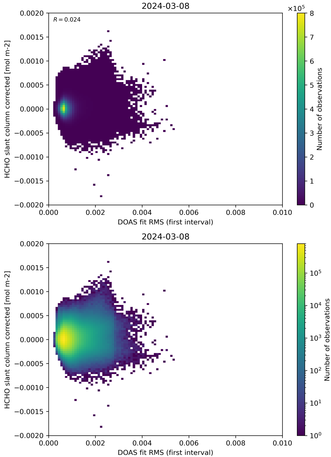
Figure 62: Scatter density plot of “DOAS fit RMS (first interval)” against “HCHO slant column corrected” for 2024-03-07 to 2024-03-09.
