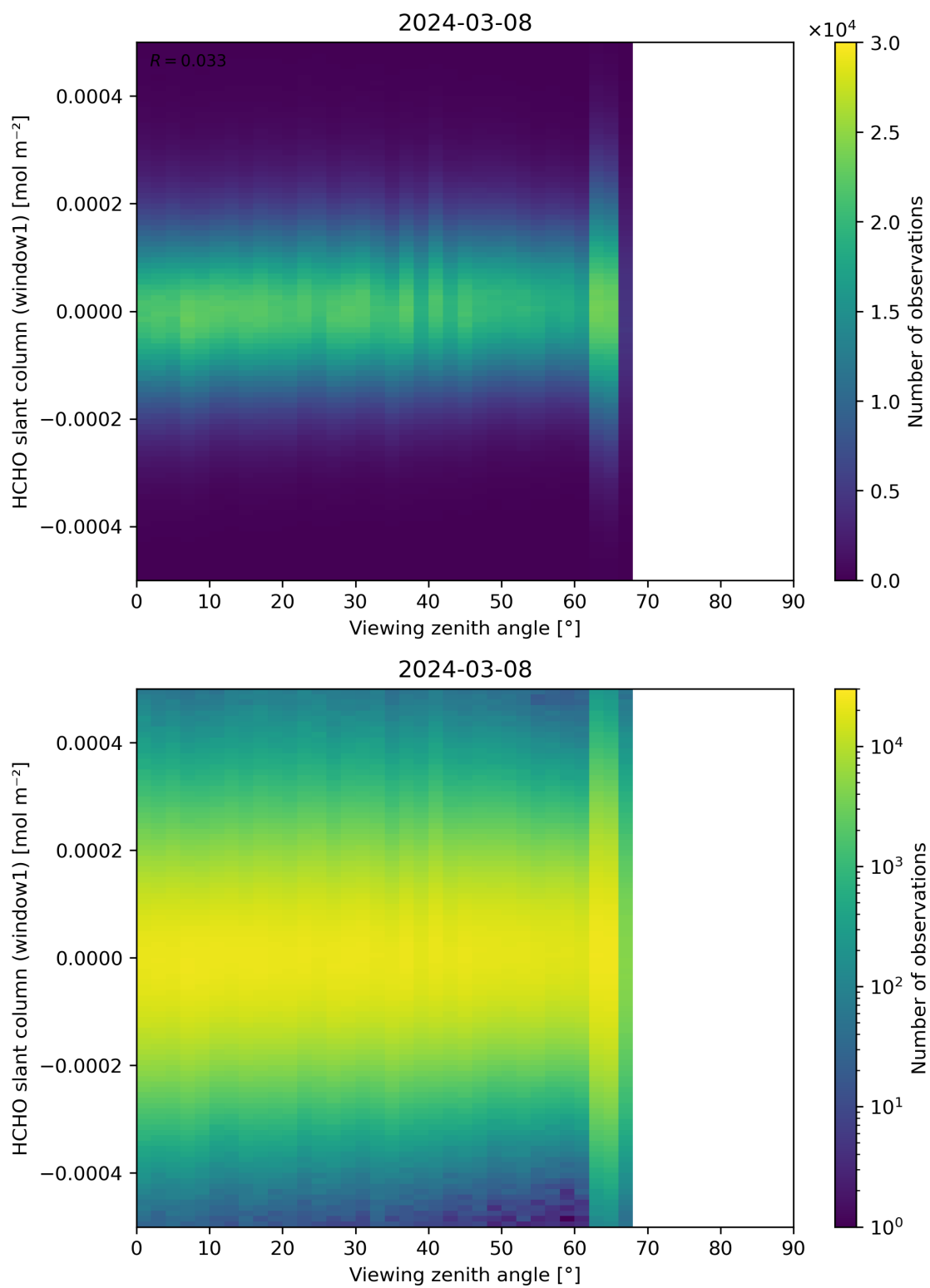
Figure 188: Scatter density plot of “Viewing zenith angle” against “HCHO slant column (window1)” for 2024-03-07 to 2024-03-09.
