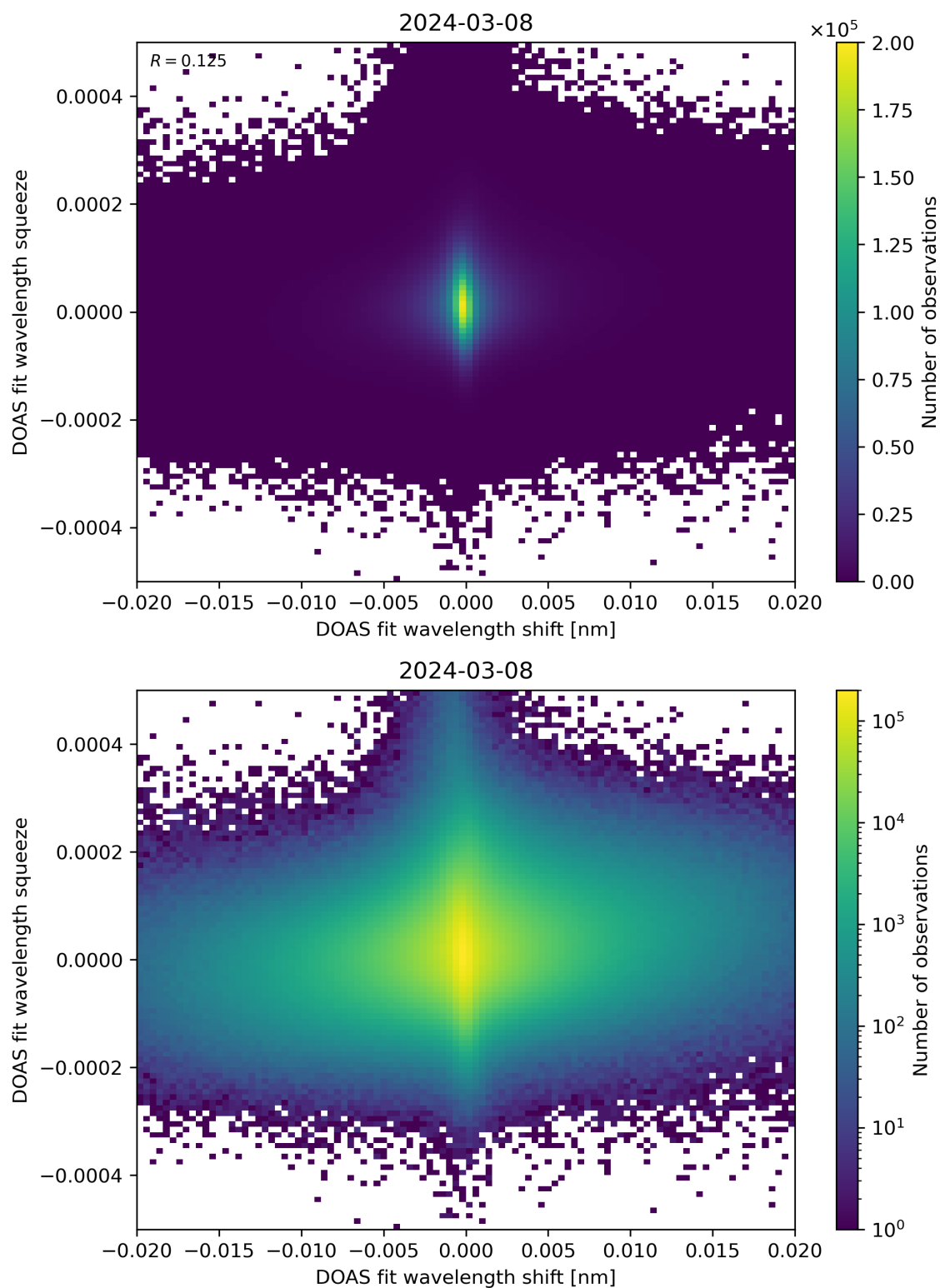
Figure 65: Scatter density plot of “DOAS fit wavelength shift” against “DOAS fit wavelength squeeze” for 2024-03-07 to 2024-03-09.
