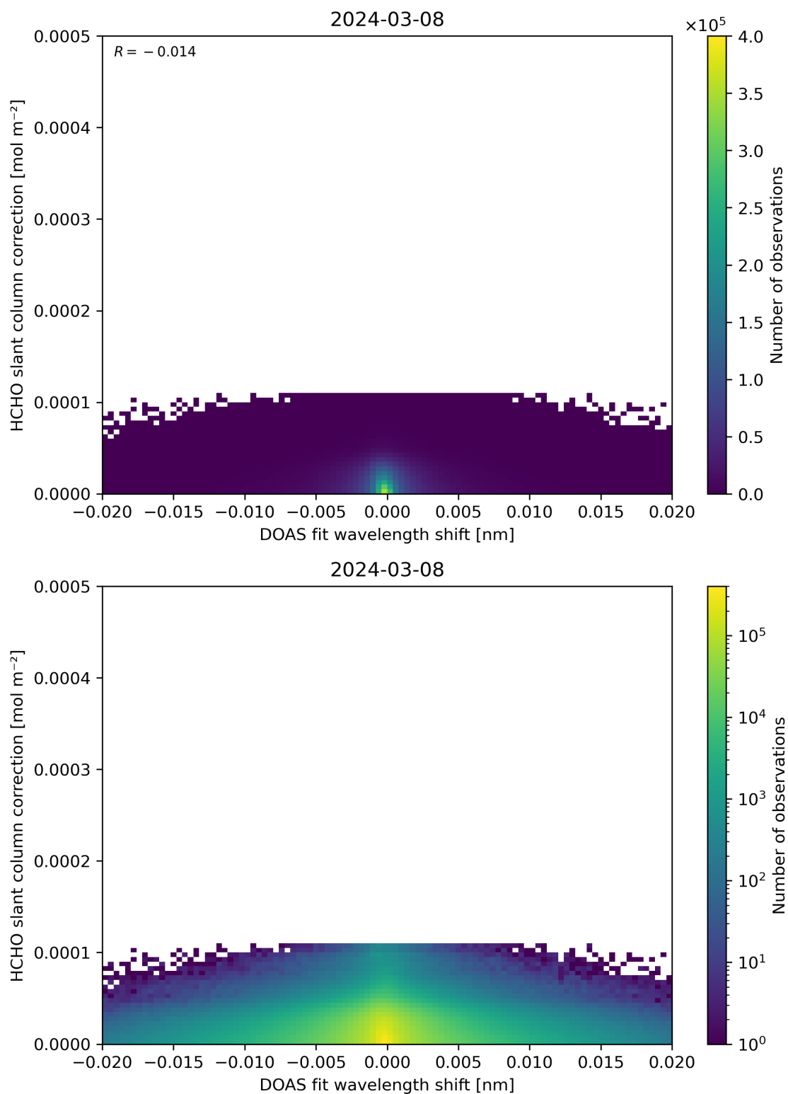
Figure 67: Scatter density plot of “DOAS fit wavelength shift” against “HCHO slant column correction” for 2024-03-07 to 2024-03-09.
