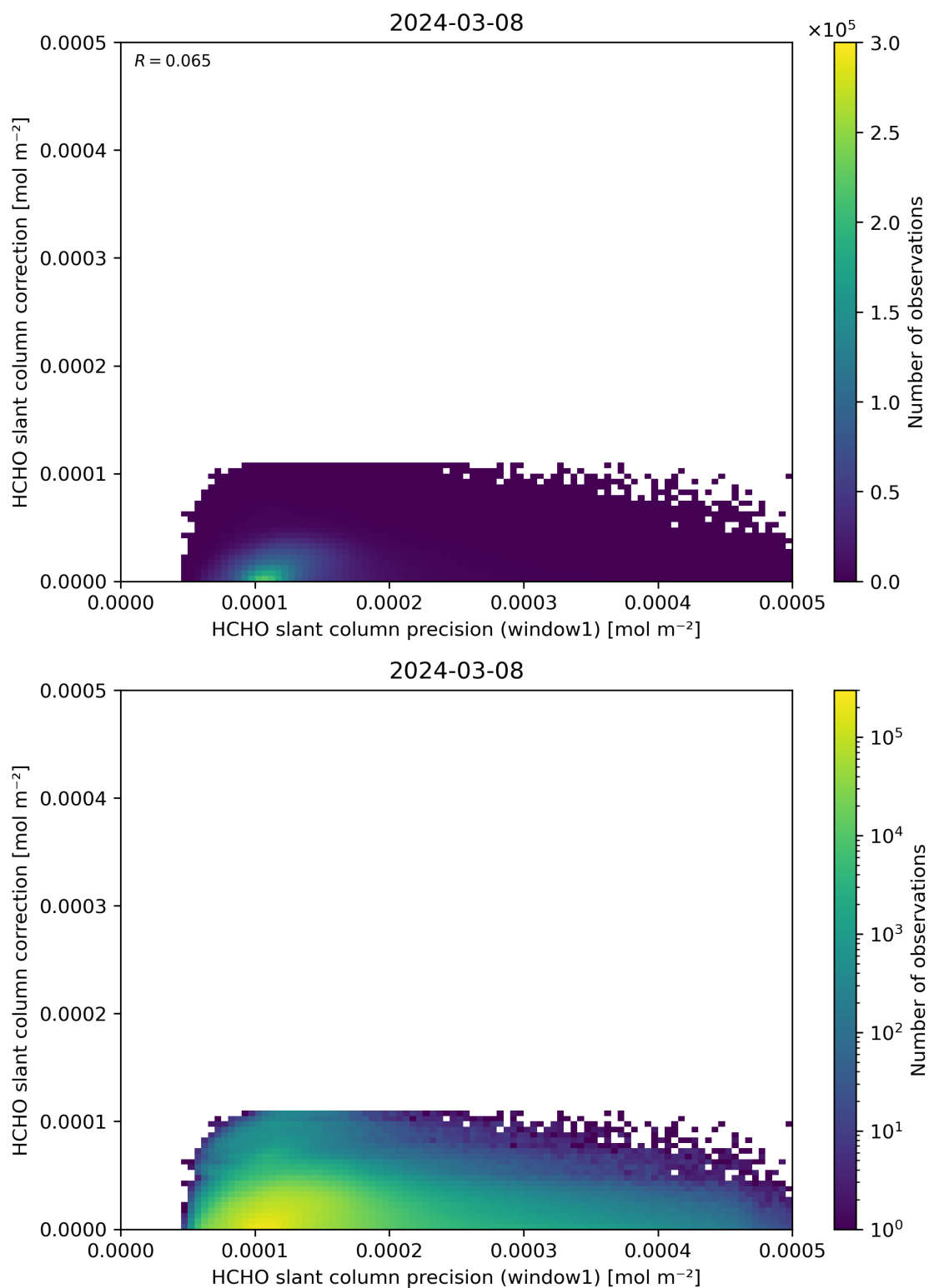
Figure 93: Scatter density plot of “HCHO slant column precision (window1)” against “HCHO slant column correction” for 2024-03-07 to 2024-03-09.
