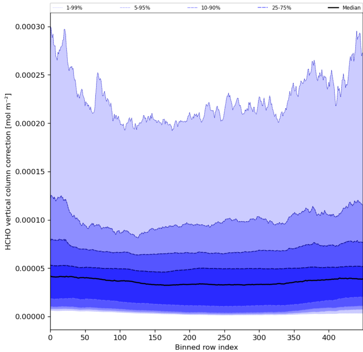
Figure 51: Along track statistics of “HCHO vertical column correction” for 2024-03-07 to 2024-03-09
