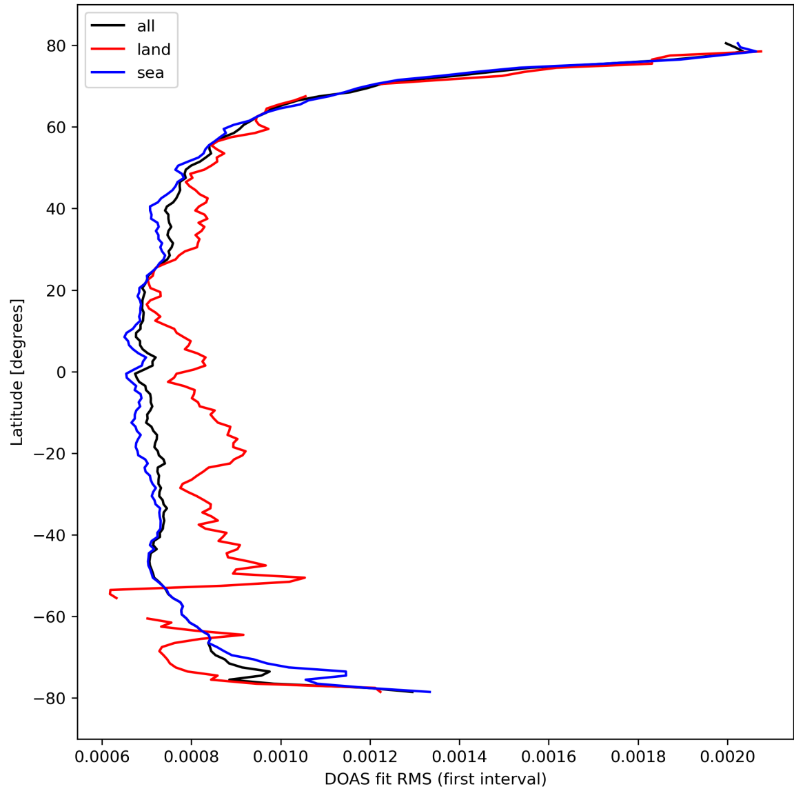
Figure 32: Zonal average of “DOAS fit RMS (first interval)” for 2024-03-07 to 2024-03-09.
