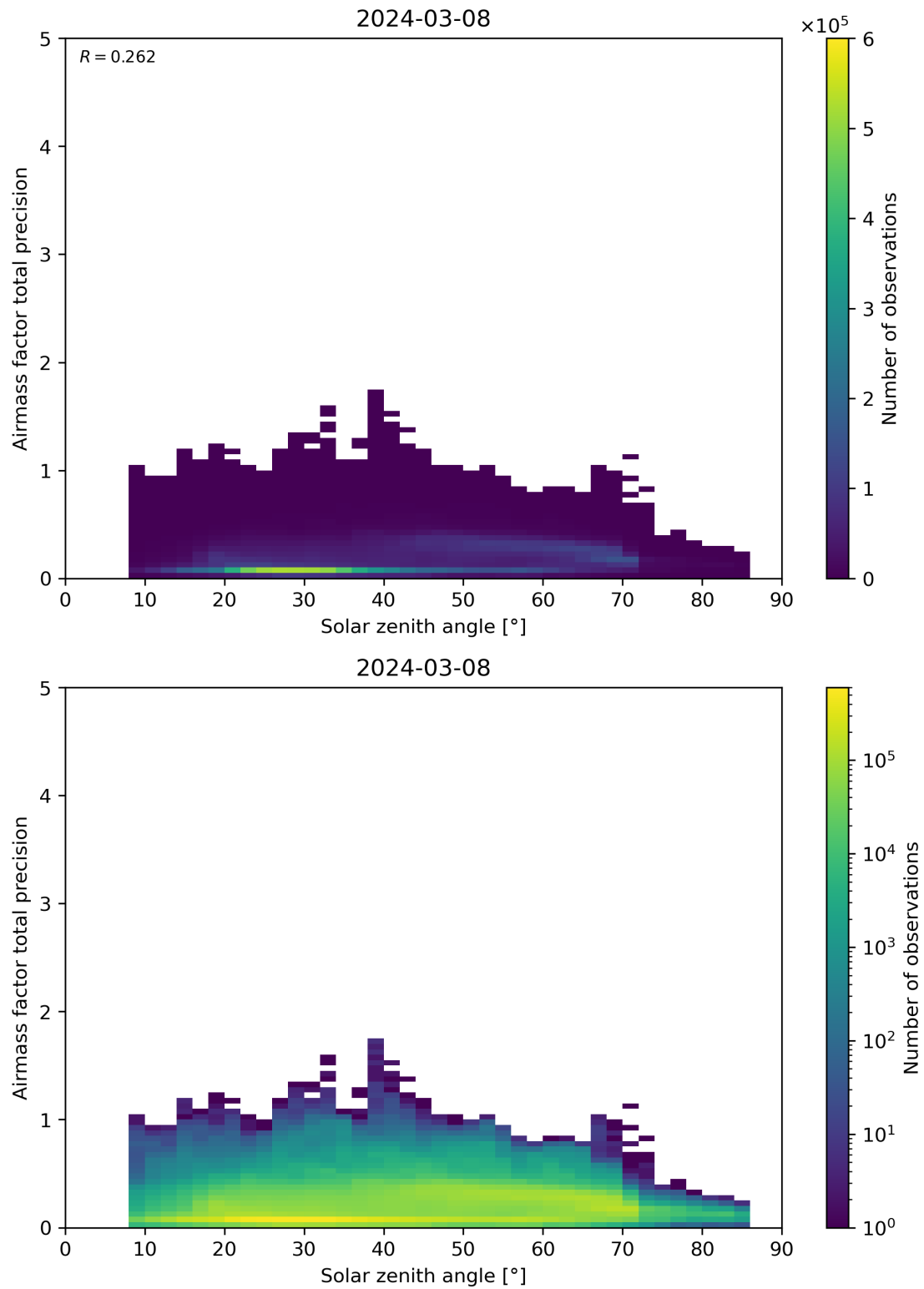
Figure 176: Scatter density plot of “Solar zenith angle” against “Airmass factor total precision” for 2024-03-07 to 2024-03-09.
