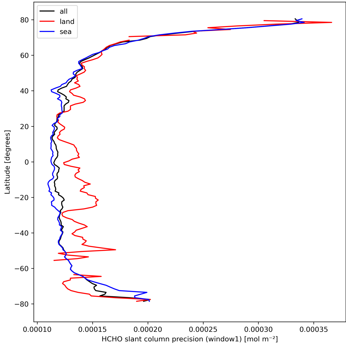
Figure 25: Zonal average of “HCHO slant column precision (window1)” for 2024-03-09 to 2024-03-10.
