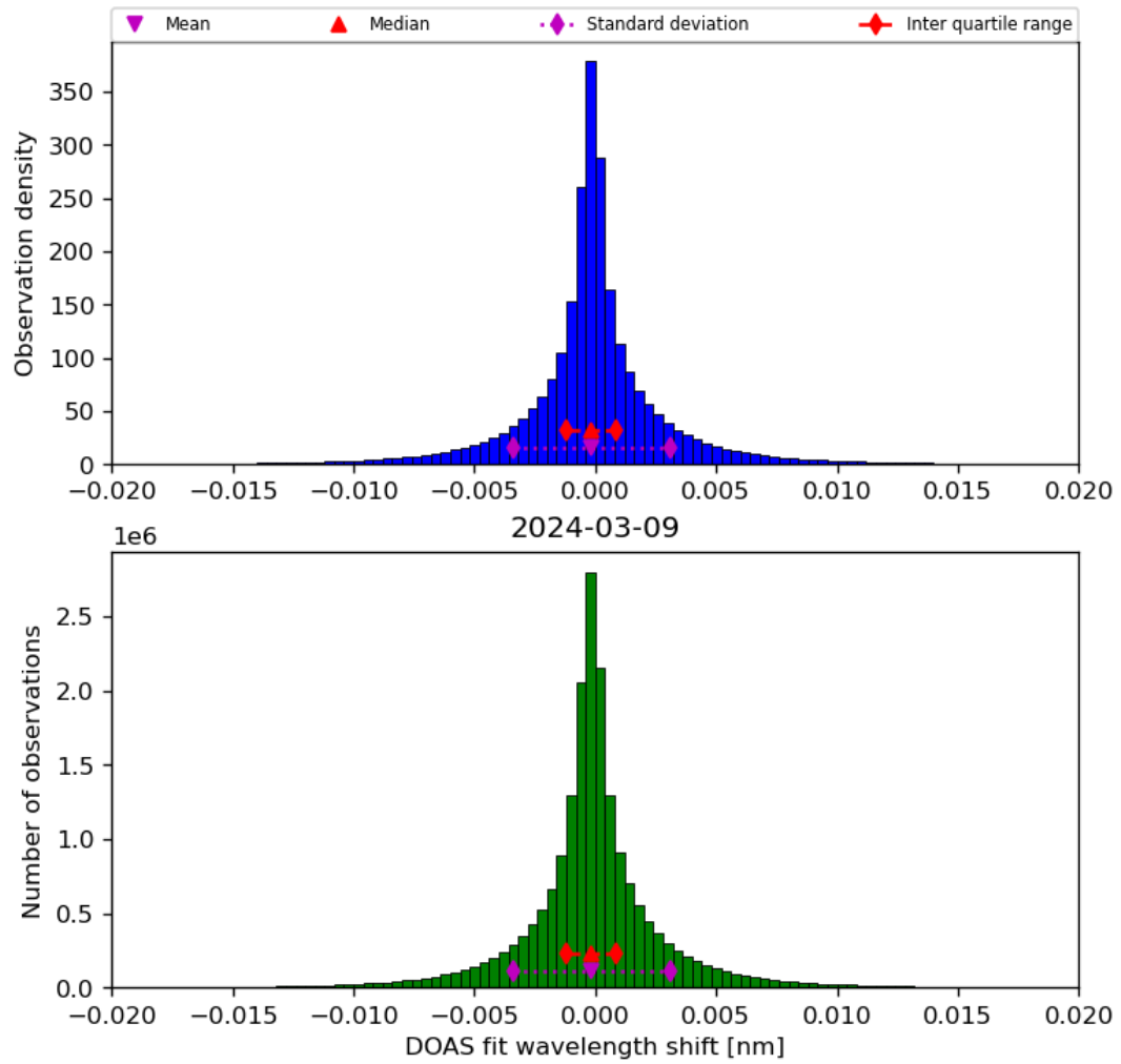
Figure 44: Histogram of “DOAS fit wavelength shift” for 2024-03-09 to 2024-03-10
