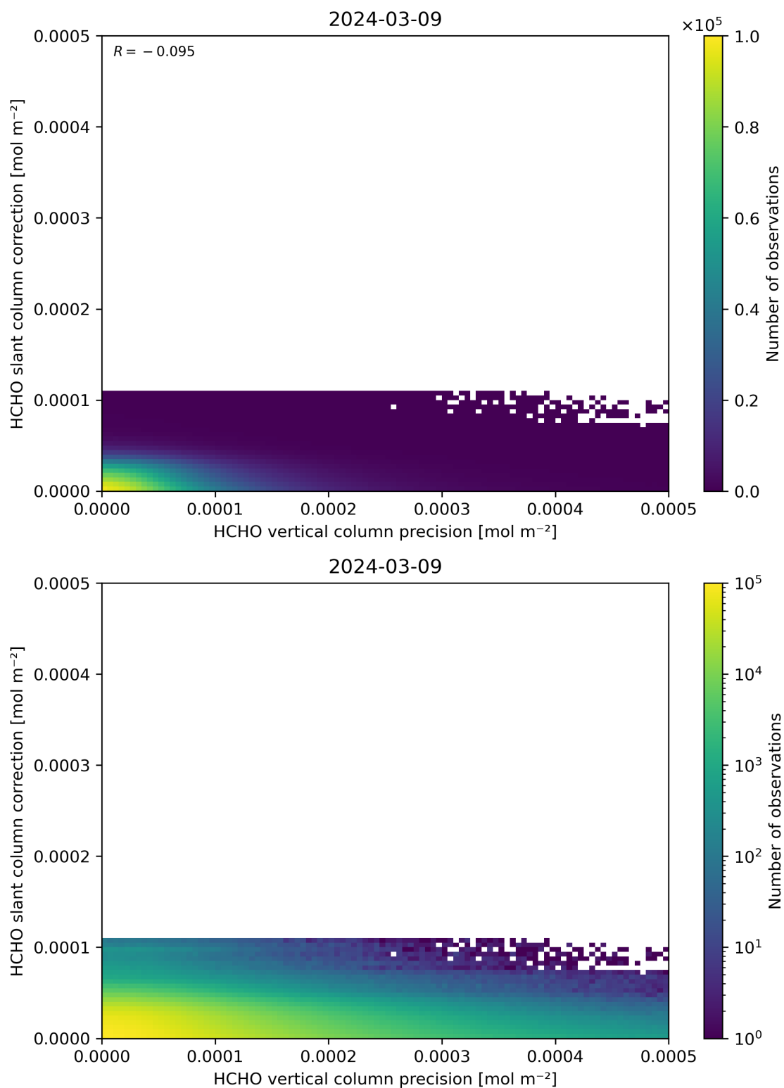
Figure 141: Scatter density plot of “HCHO vertical column precision” against “HCHO slant column correction” for 2024-03-09 to 2024-03-10.
