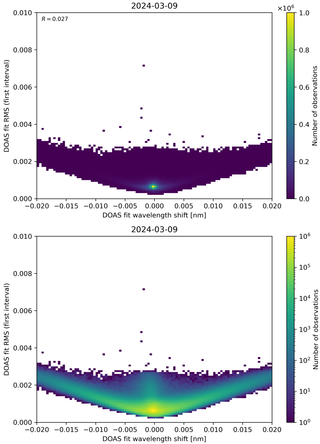
Figure 64: Scatter density plot of “DOAS fit wavelength shift” against “DOAS fit RMS (first interval)” for 2024-03-09 to 2024-03-10.
