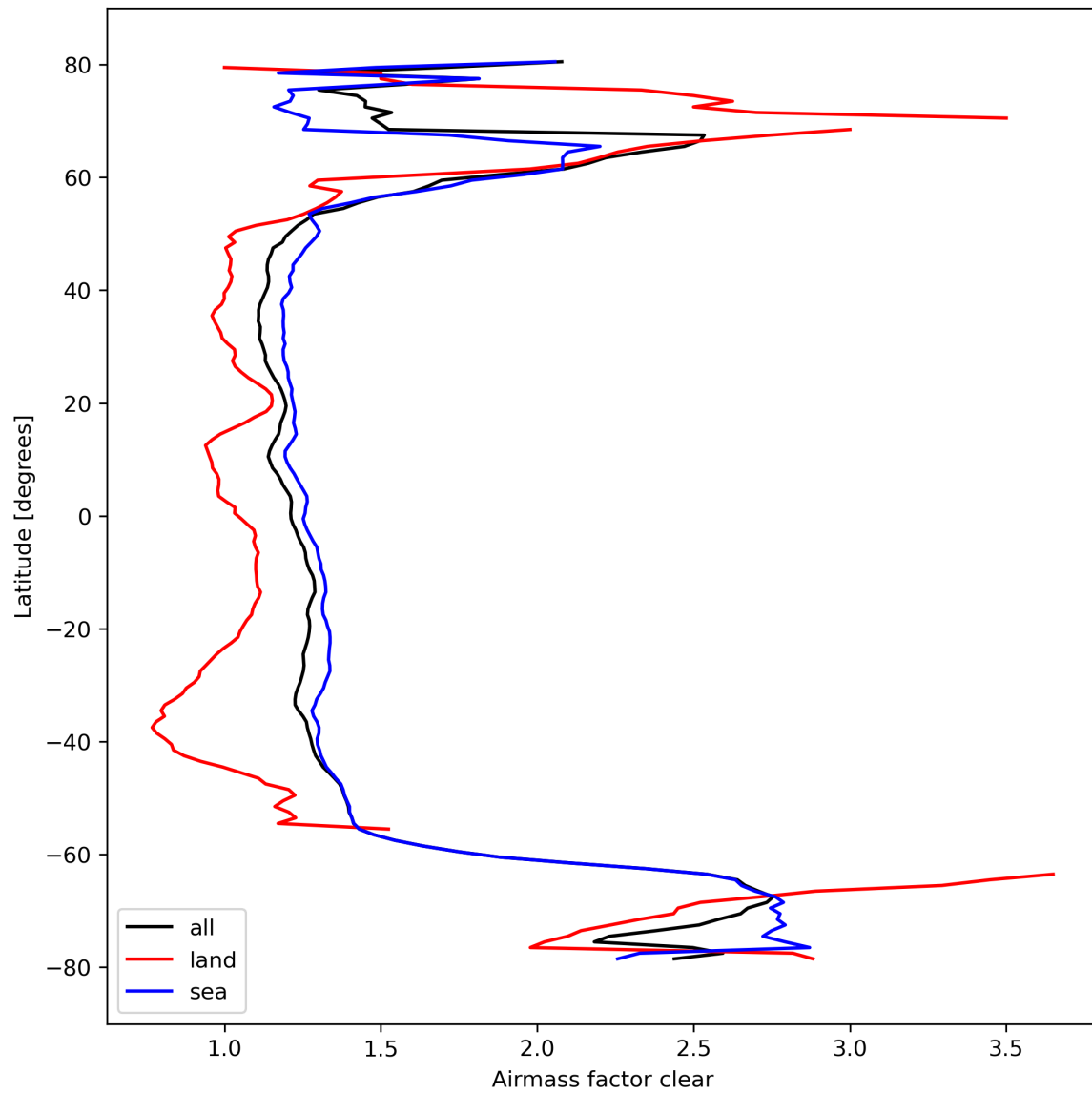
Figure 28: Zonal average of “Airmass factor clear” for 2024-03-09 to 2024-03-10.
