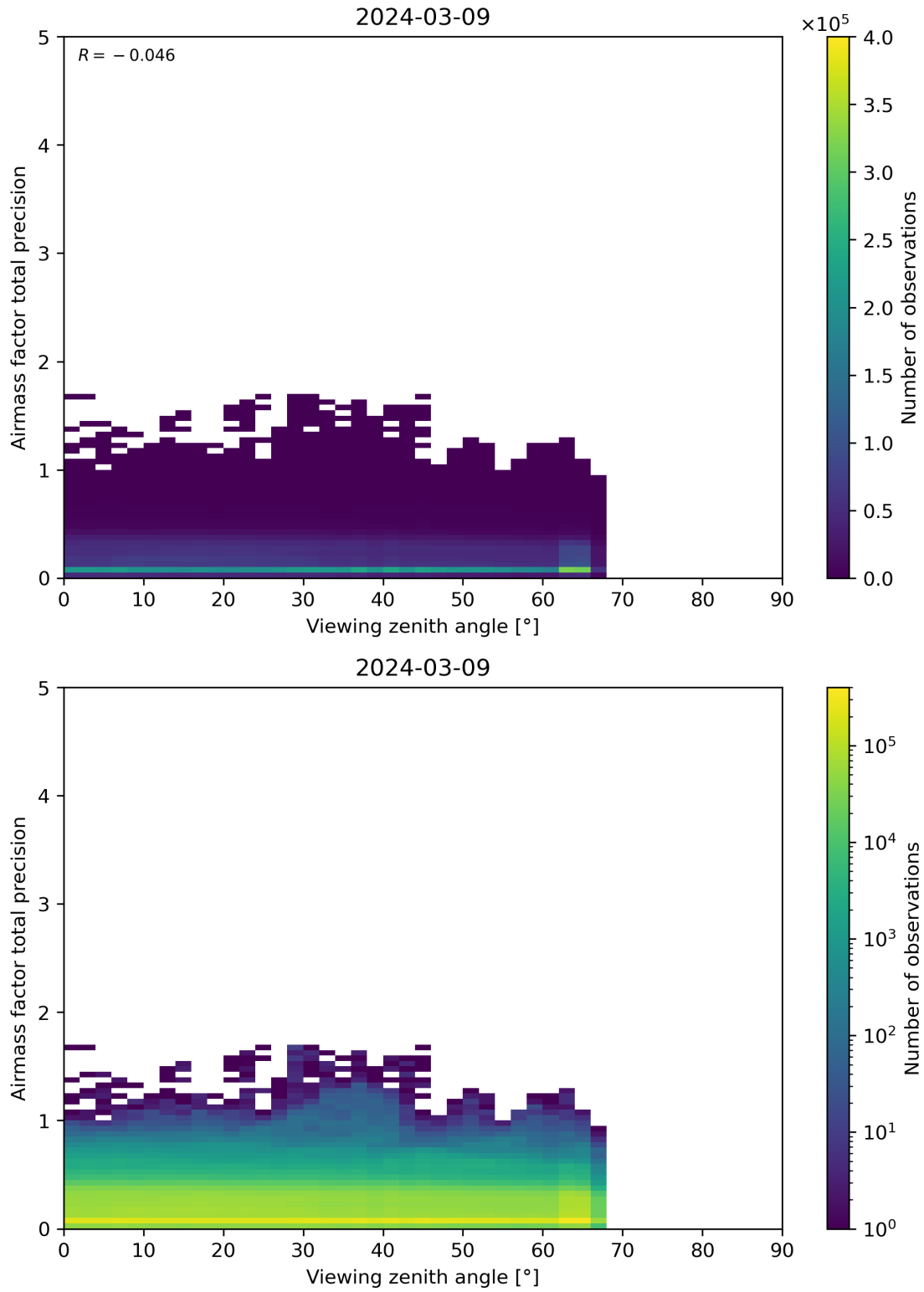
Figure 191: Scatter density plot of “Viewing zenith angle” against “Airmass factor total precision” for 2024-03-09 to 2024-03-10.
