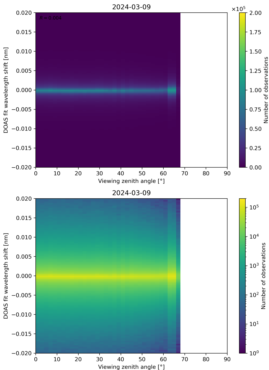
Figure 183: Scatter density plot of “Viewing zenith angle” against “DOAS fit wavelength shift” for 2024-03-09 to 2024-03-10.
