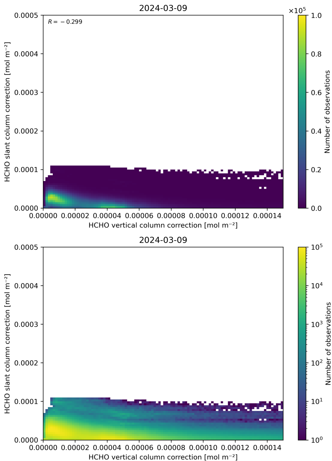
Figure 117: Scatter density plot of “HCHO vertical column correction” against “HCHO slant column correction” for 2024-03-09 to 2024-03-10.
