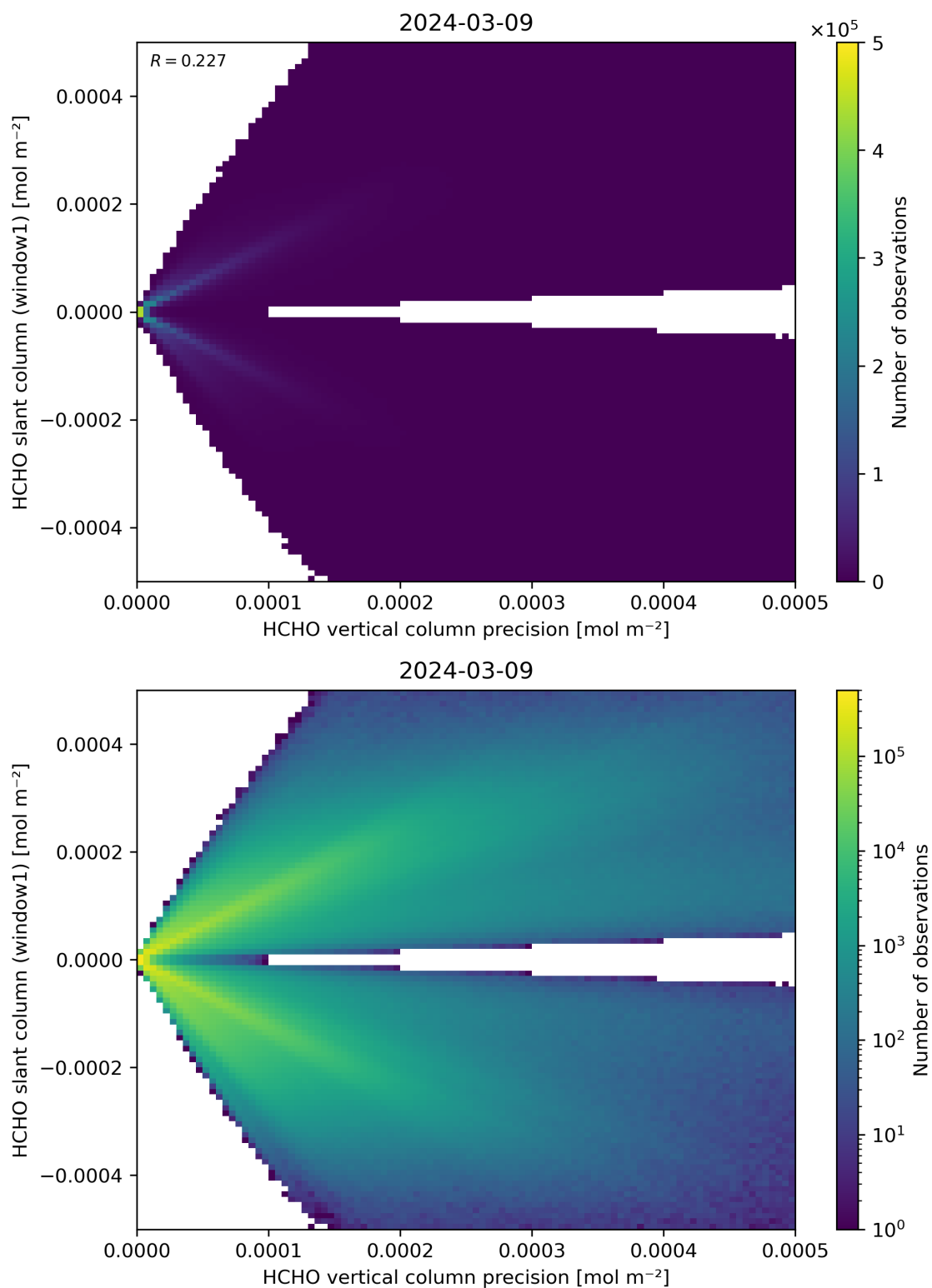
Figure 142: Scatter density plot of “HCHO vertical column precision” against “HCHO slant column (window1)” for 2024-03-09 to 2024-03-10.
