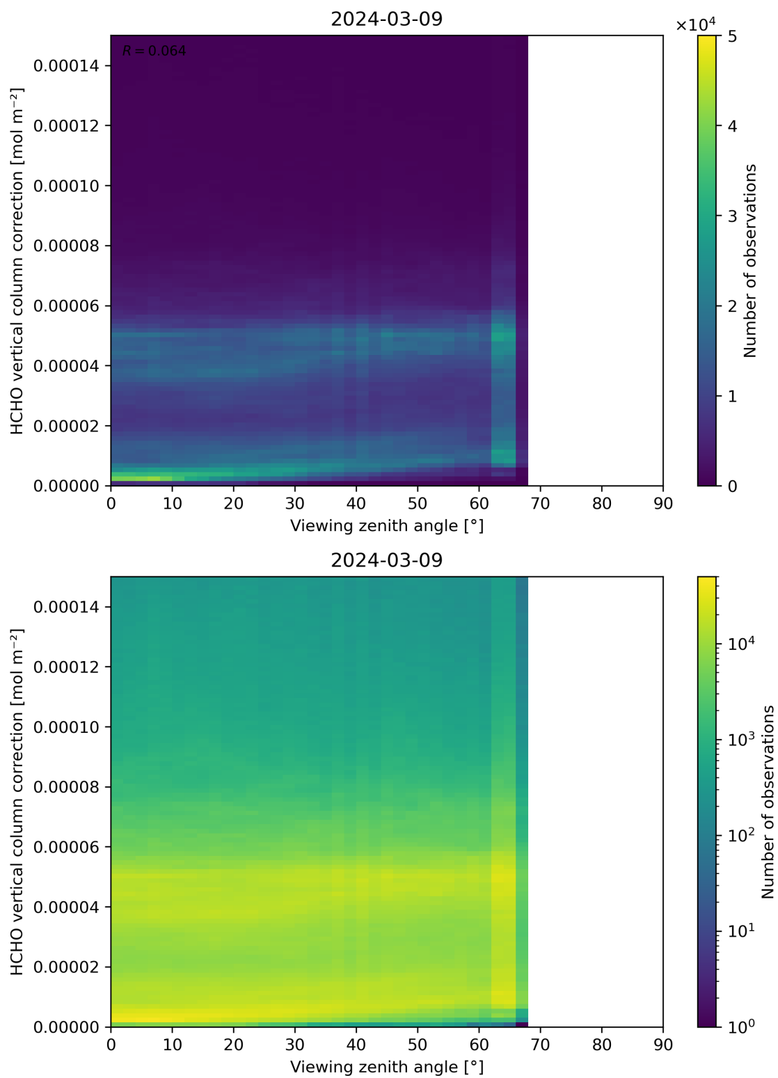
Figure 193: Scatter density plot of “Viewing zenith angle” against “HCHO vertical column correction” for 2024-03-09 to 2024-03-10.
