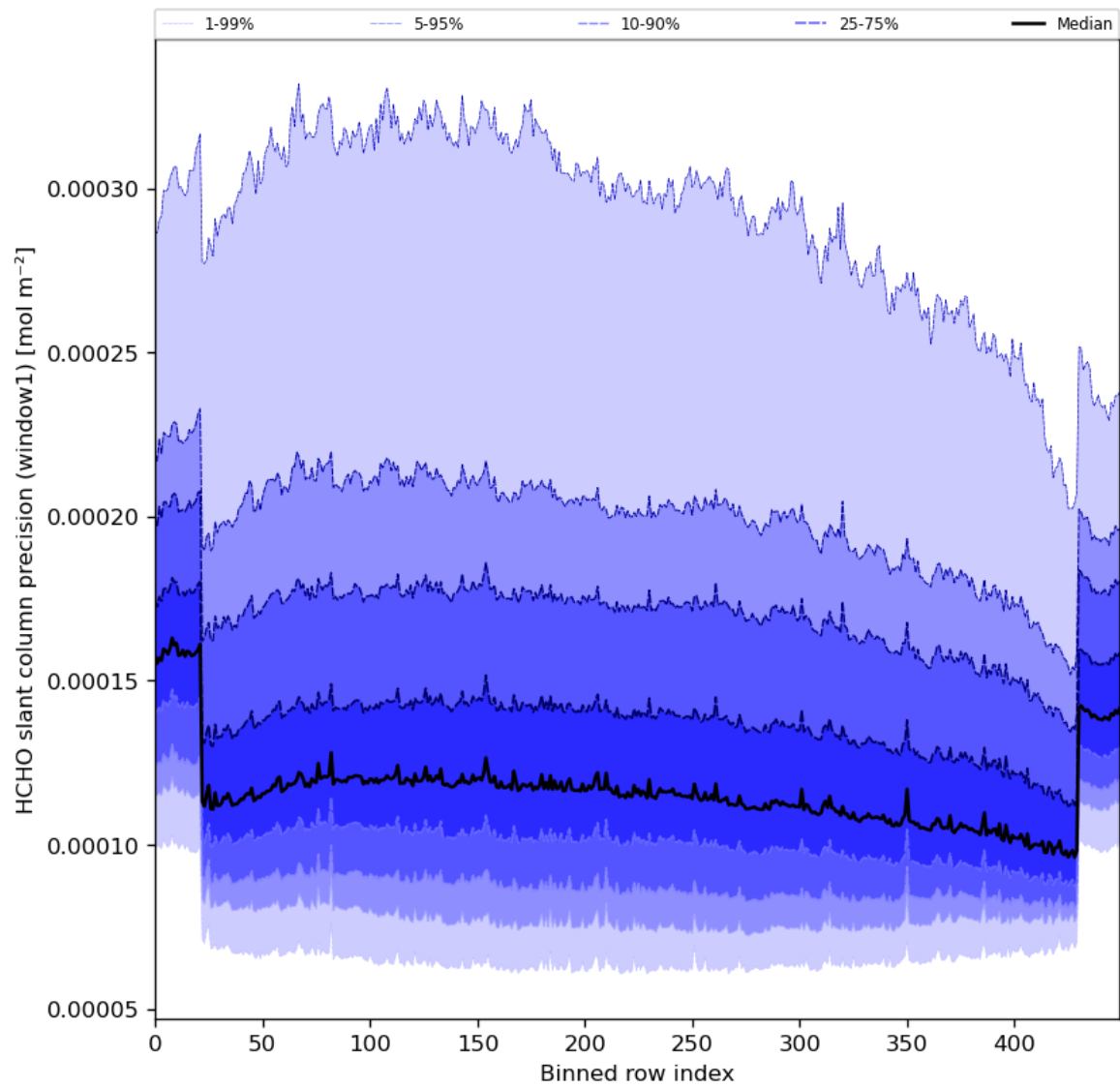
Figure 53: Along track statistics of “HCHO slant column precision (window1)” for 2024-03-09 to 2024-03-10
