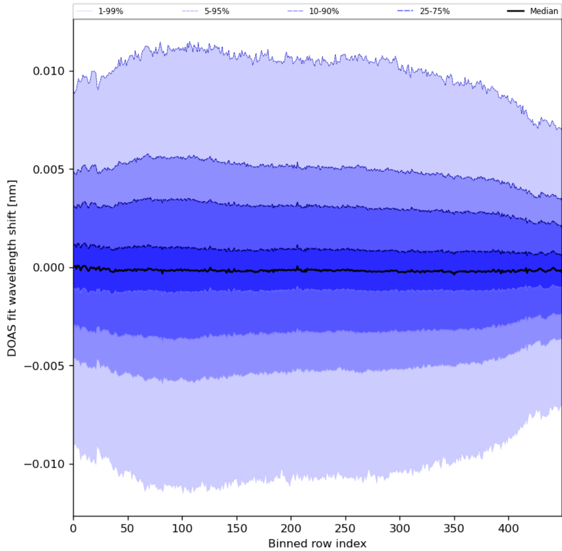
Figure 58: Along track statistics of “DOAS fit wavelength shift” for 2024-03-09 to 2024-03-10
