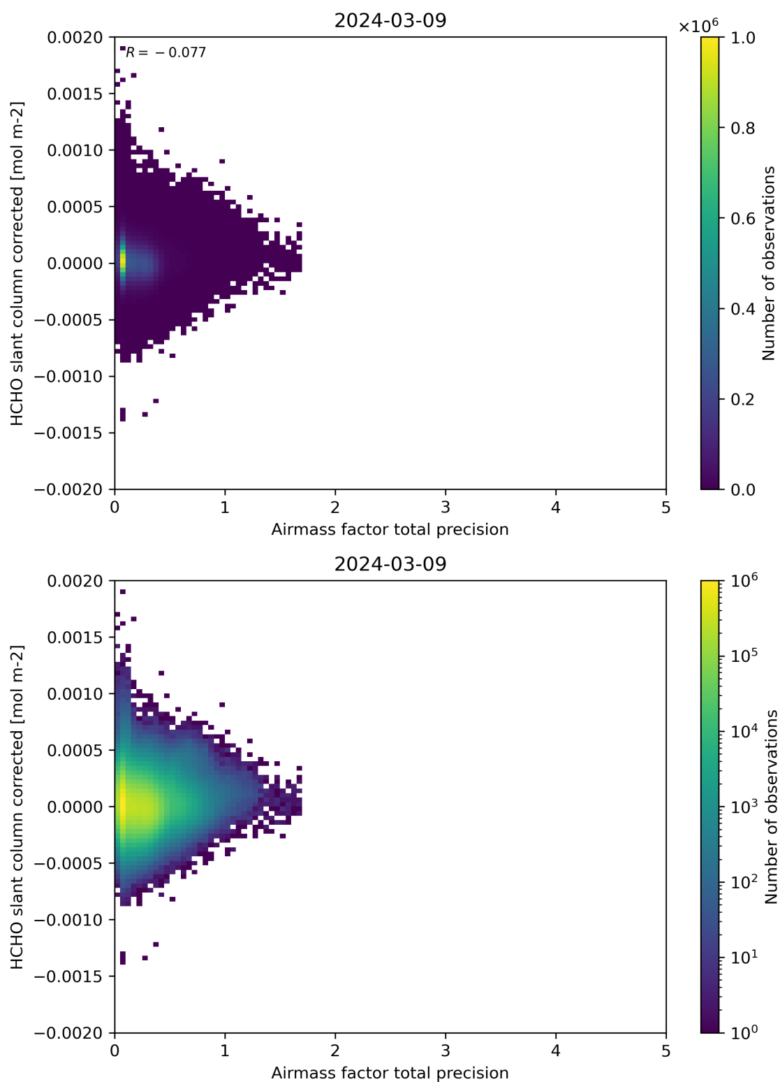
Figure 109: Scatter density plot of “Airmass factor total precision” against “HCHO slant column corrected” for 2024-03-09 to 2024-03-10.
