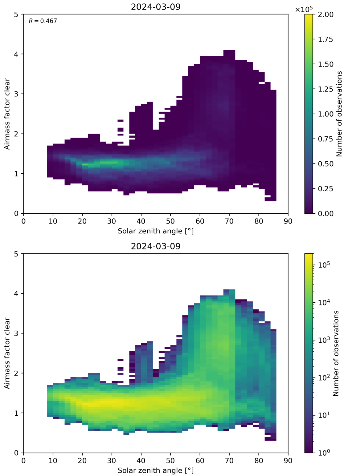
Figure 170: Scatter density plot of “Solar zenith angle” against “Airmass factor clear” for 2024-03-09 to 2024-03-10.
