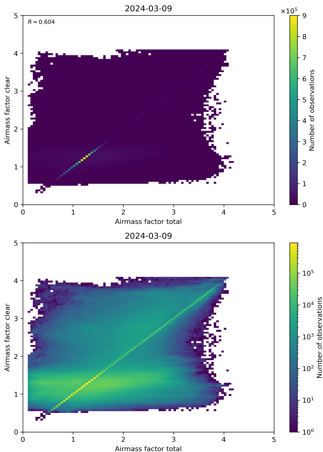
Figure 100: Scatter density plot of “Airmass factor total” against “Airmass factor clear” for 2024-03-09 to 2024-03-10.
