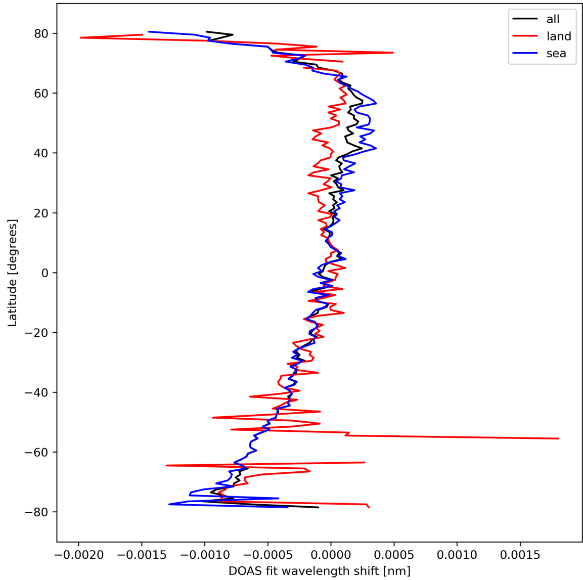
Figure 30: Zonal average of “DOAS fit wavelength shift” for 2024-03-09 to 2024-03-10.
