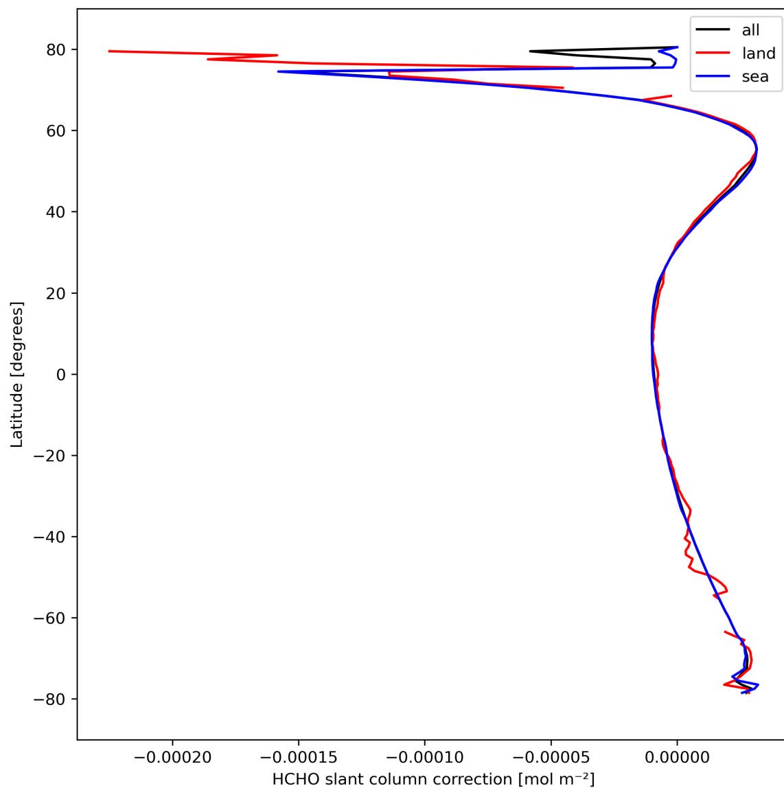
Figure 33: Zonal average of “HCHO slant column correction” for 2024-03-09 to 2024-03-10.
