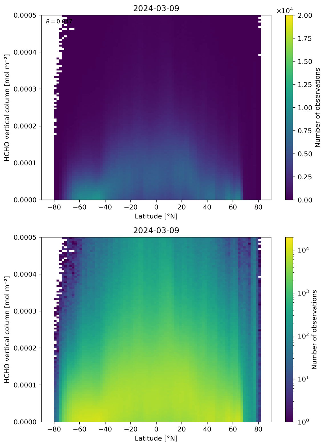
Figure 163: Scatter density plot of “Latitude” against “HCHO vertical column” for 2024-03-09 to 2024-03-10.
