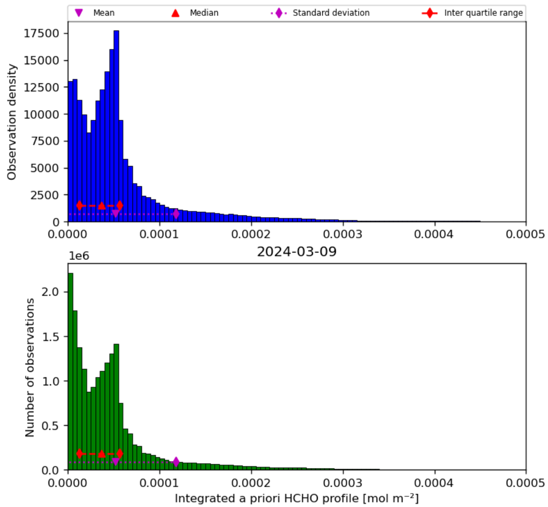
Figure 43: Histogram of “Integrated a priori HCHO profile” for 2024-03-09 to 2024-03-10
