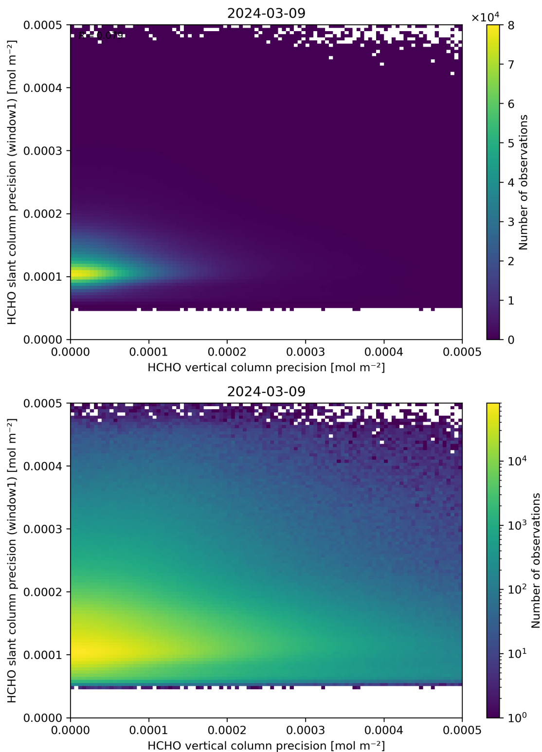
Figure 143: Scatter density plot of “HCHO vertical column precision” against “HCHO slant column precision (window1)” for 2024-03-09 to 2024-03-10.
