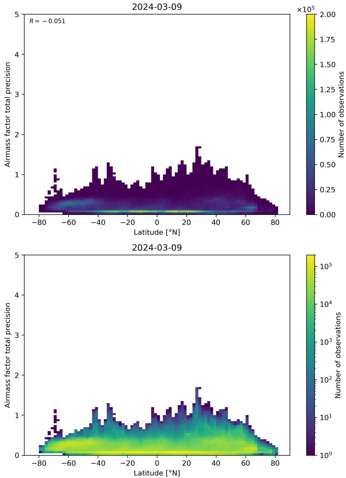
Figure 162: Scatter density plot of “Latitude” against “Airmass factor total precision” for 2024-03-09 to 2024-03-10.
