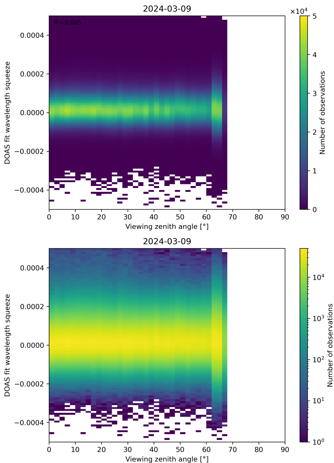
Figure 184: Scatter density plot of “Viewing zenith angle” against “DOAS fit wavelength squeeze” for 2024-03-09 to 2024-03-10.
