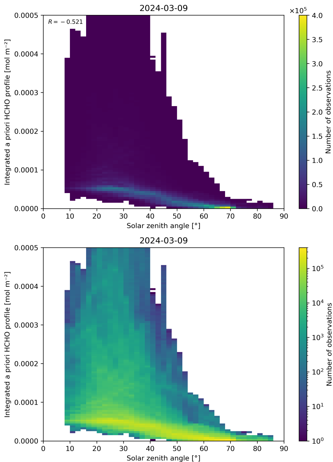
Figure 180: Scatter density plot of “Solar zenith angle” against “Integrated a priori HCHO profile” for 2024-03-09 to 2024-03-10.
