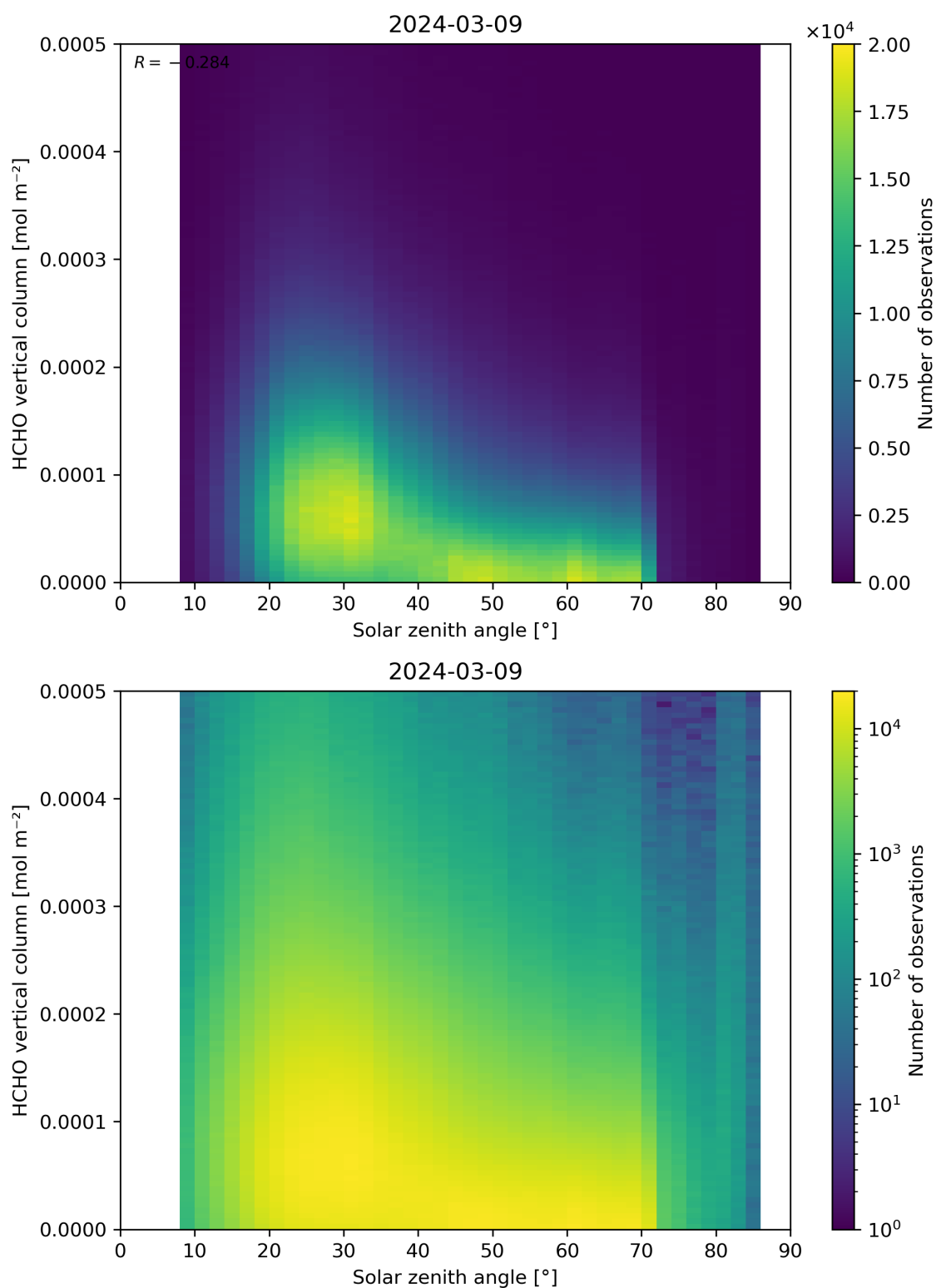
Figure 177: Scatter density plot of “Solar zenith angle” against “HCHO vertical column” for 2024-03-09 to 2024-03-10.
