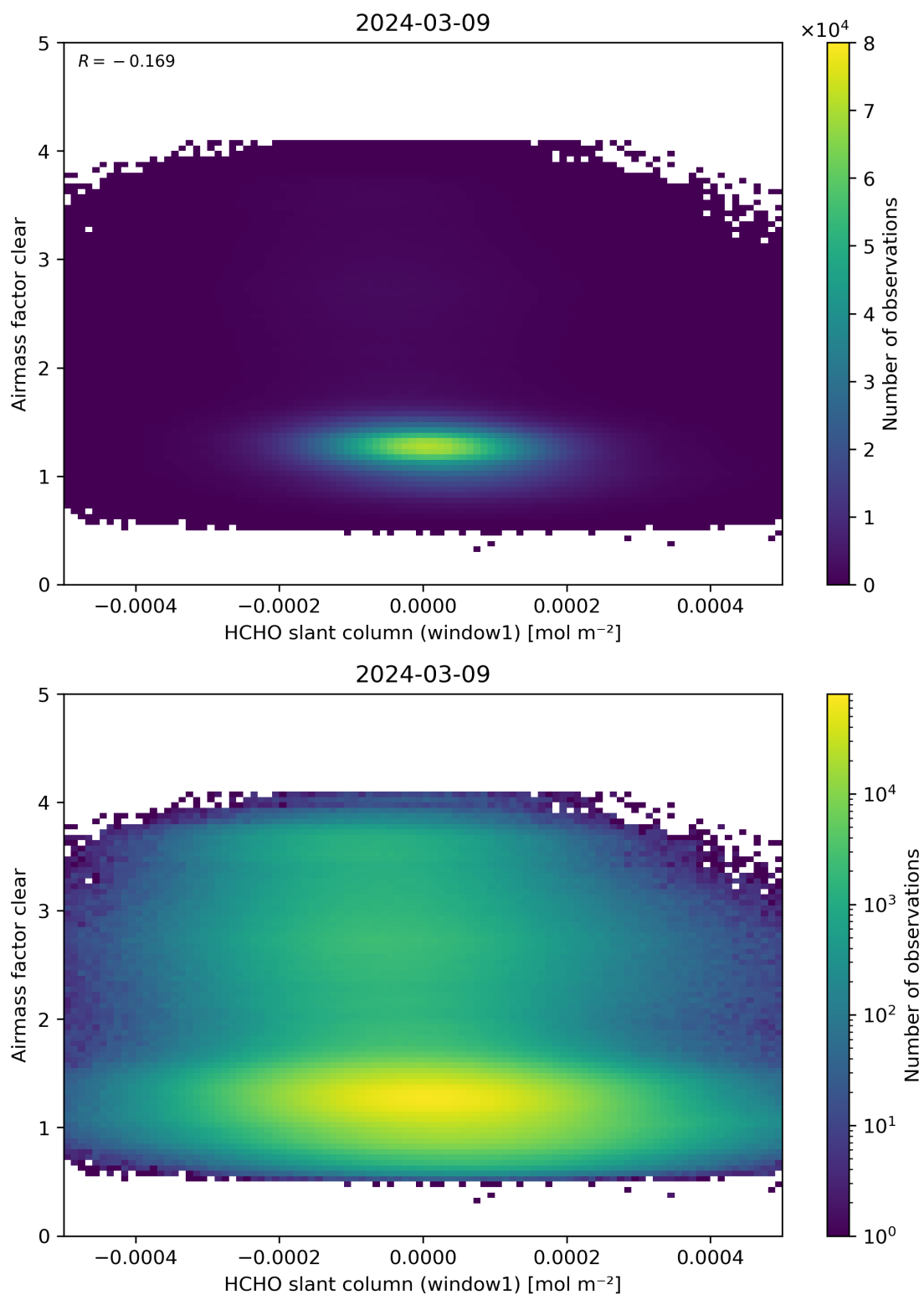
Figure 81: Scatter density plot of “HCHO slant column (window1)” against “Airmass factor clear” for 2024-03-09 to 2024-03-10.
