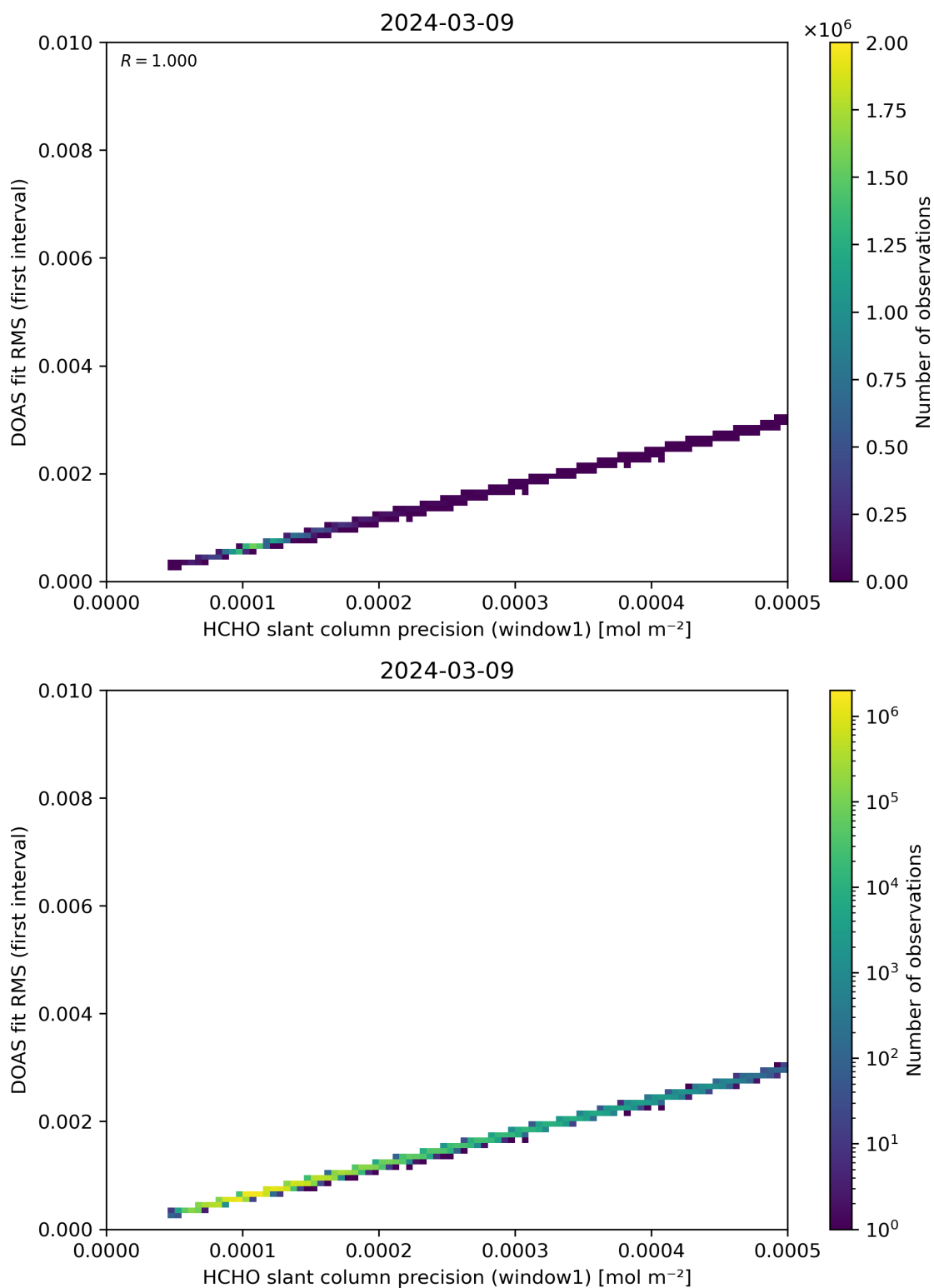
Figure 88: Scatter density plot of “HCHO slant column precision (window1)” against “DOAS fit RMS (first interval)” for 2024-03-09 to 2024-03-10.
