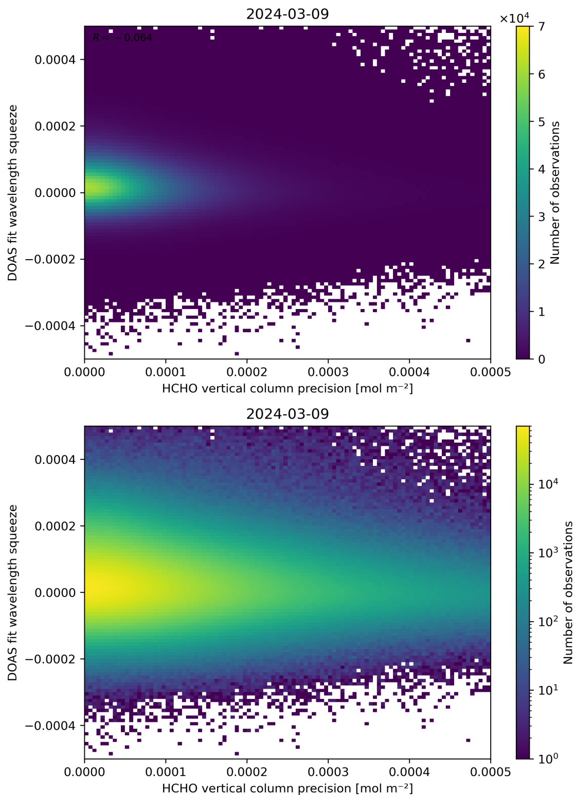
Figure 138: Scatter density plot of “HCHO vertical column precision” against “DOAS fit wavelength squeeze” for 2024-03-09 to 2024-03-10.
