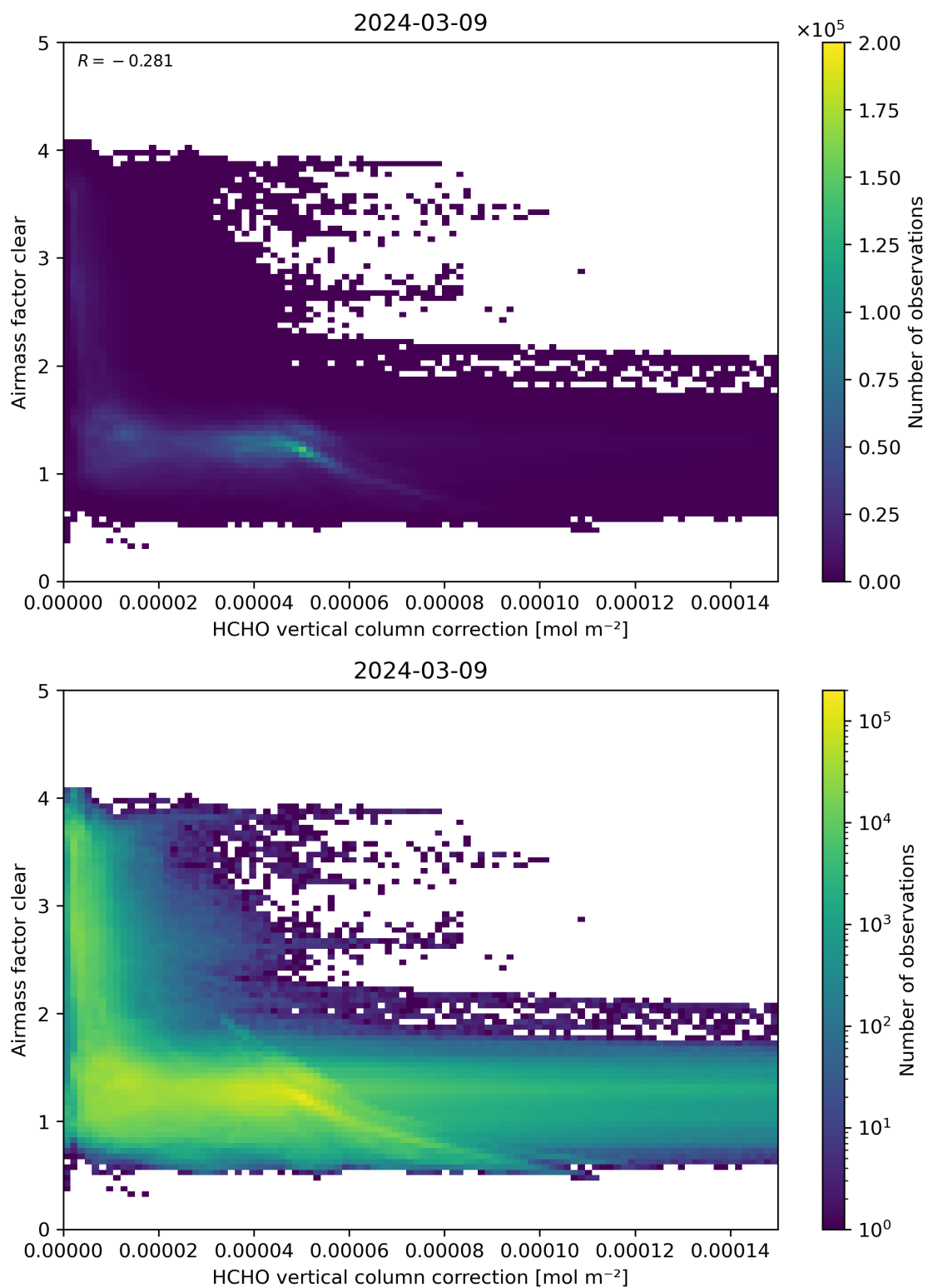
Figure 115: Scatter density plot of “HCHO vertical column correction” against “Airmass factor clear” for 2024-03-09 to 2024-03-10.
