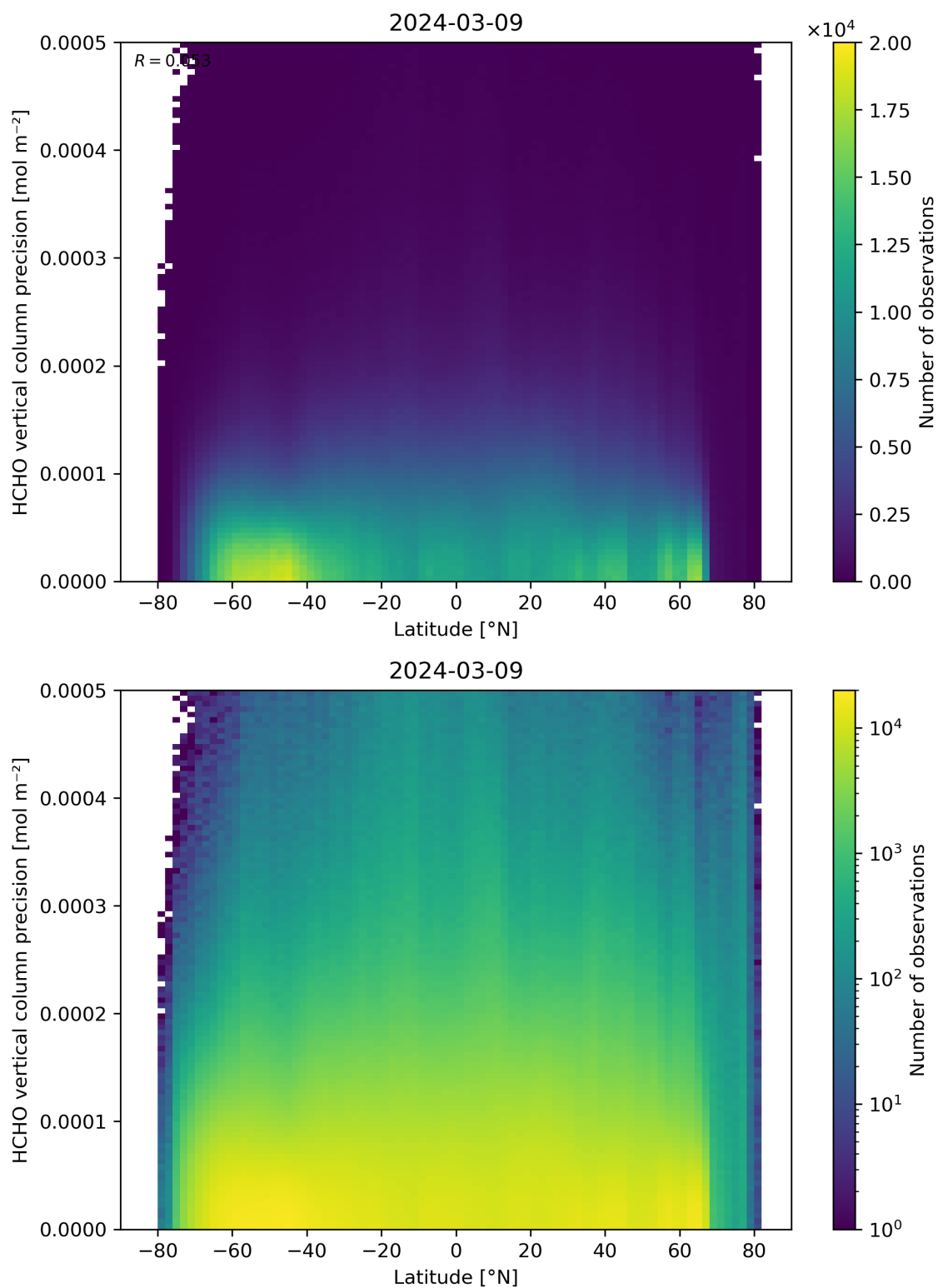
Figure 165: Scatter density plot of “Latitude” against “HCHO vertical column precision” for 2024-03-09 to 2024-03-10.
