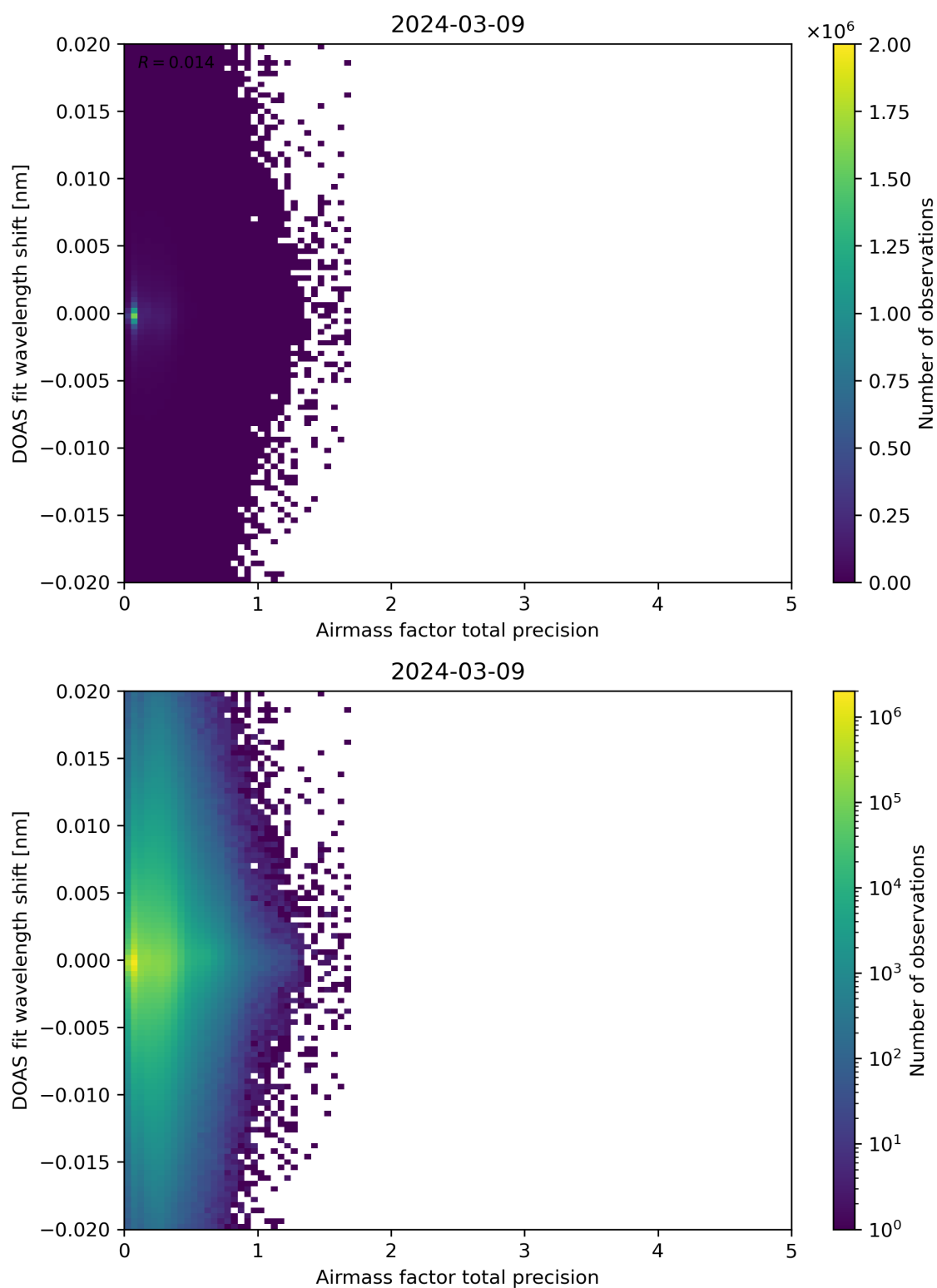
Figure 106: Scatter density plot of “Airmass factor total precision” against “DOAS fit wavelength shift” for 2024-03-09 to 2024-03-10.
