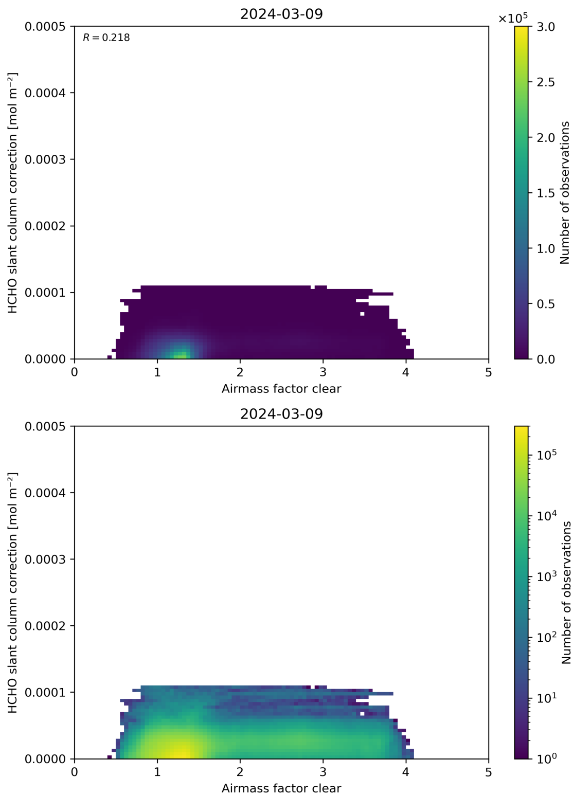
Figure 75: Scatter density plot of “Air mass factor clear” against “HCHO slant column correction” for 2024-03-09 to 2024-03-10.
