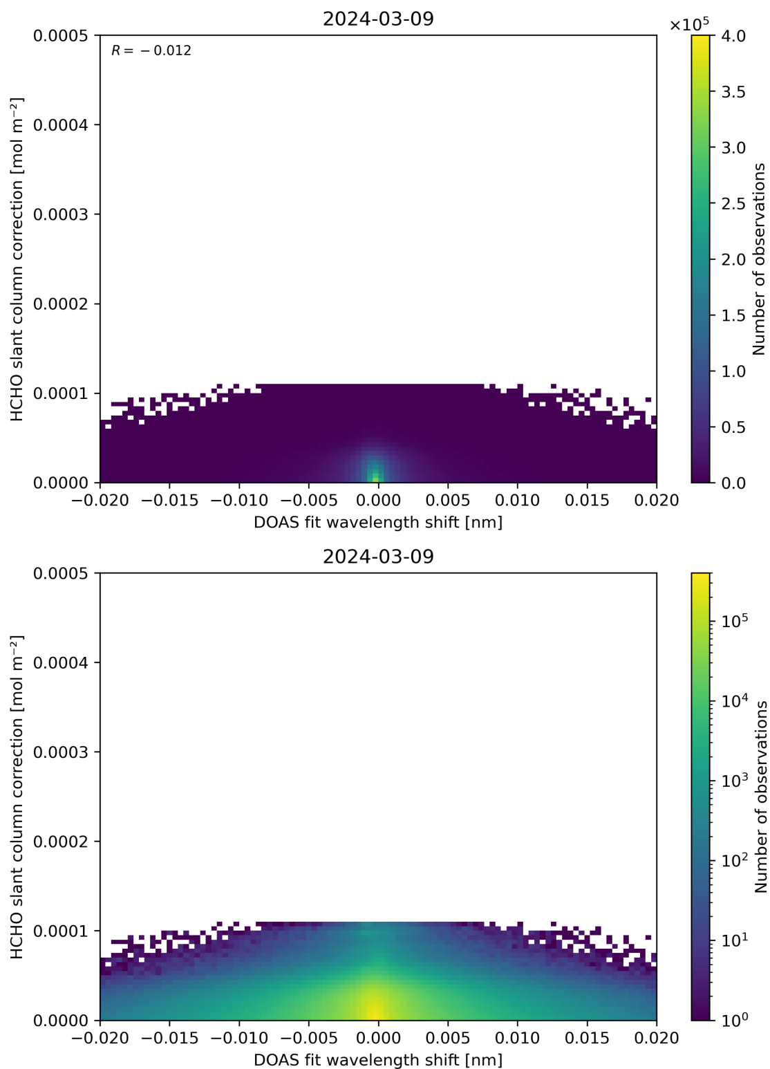
Figure 67: Scatter density plot of “DOAS fit wavelength shift” against “HCHO slant column correction” for 2024-03-09 to 2024-03-10.
