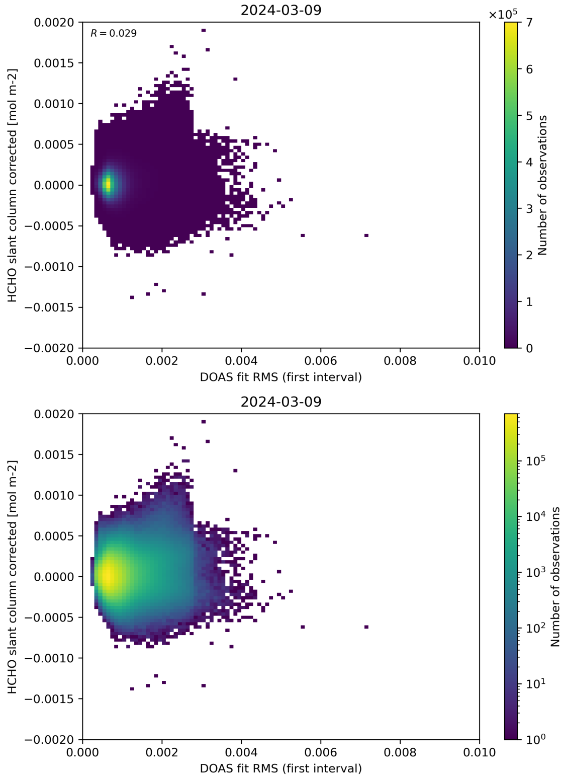
Figure 62: Scatter density plot of “DOAS fit RMS (first interval)” against “HCHO slant column corrected” for 2024-03-09 to 2024-03-10.
