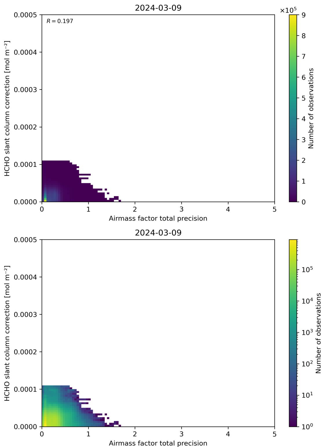
Figure 110: Scatter density plot of “Airmass factor total precision” against “HCHO slant column correction” for 2024-03-09 to 2024-03-10.
