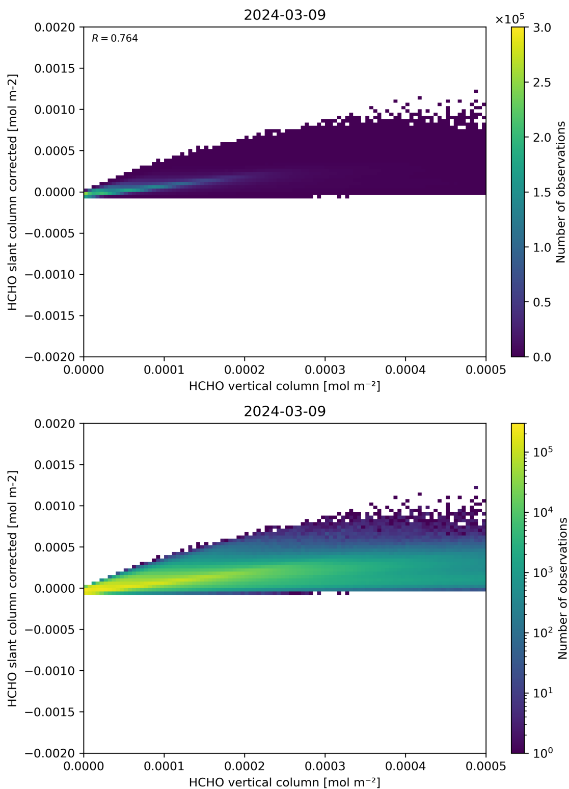
Figure 127: Scatter density plot of “HCHO vertical column” against “HCHO slant column corrected” for 2024-03-09 to 2024-03-10.
