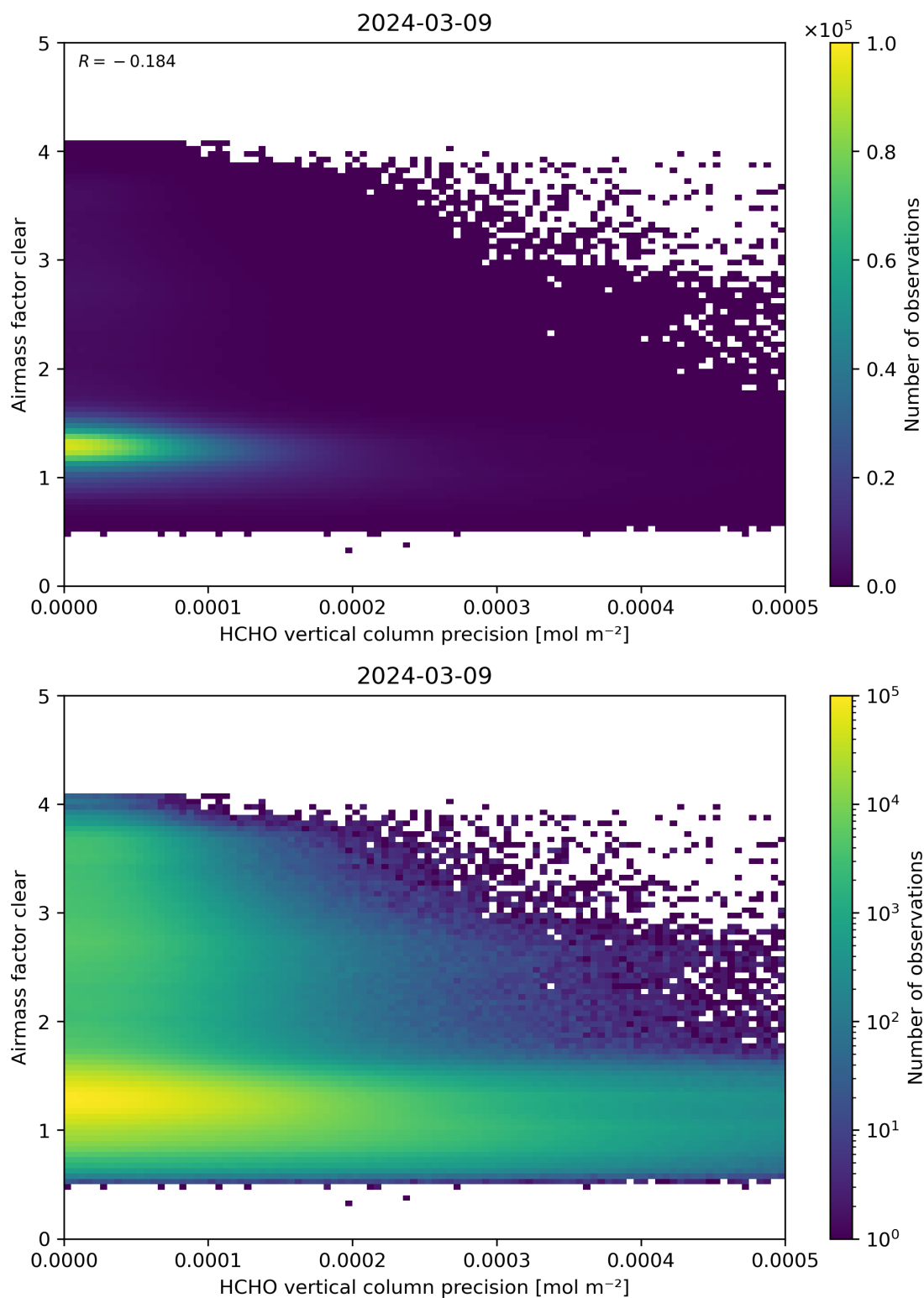
Figure 139: Scatter density plot of “HCHO vertical column precision” against “Airmass factor clear” for 2024-03-09 to 2024-03-10.
