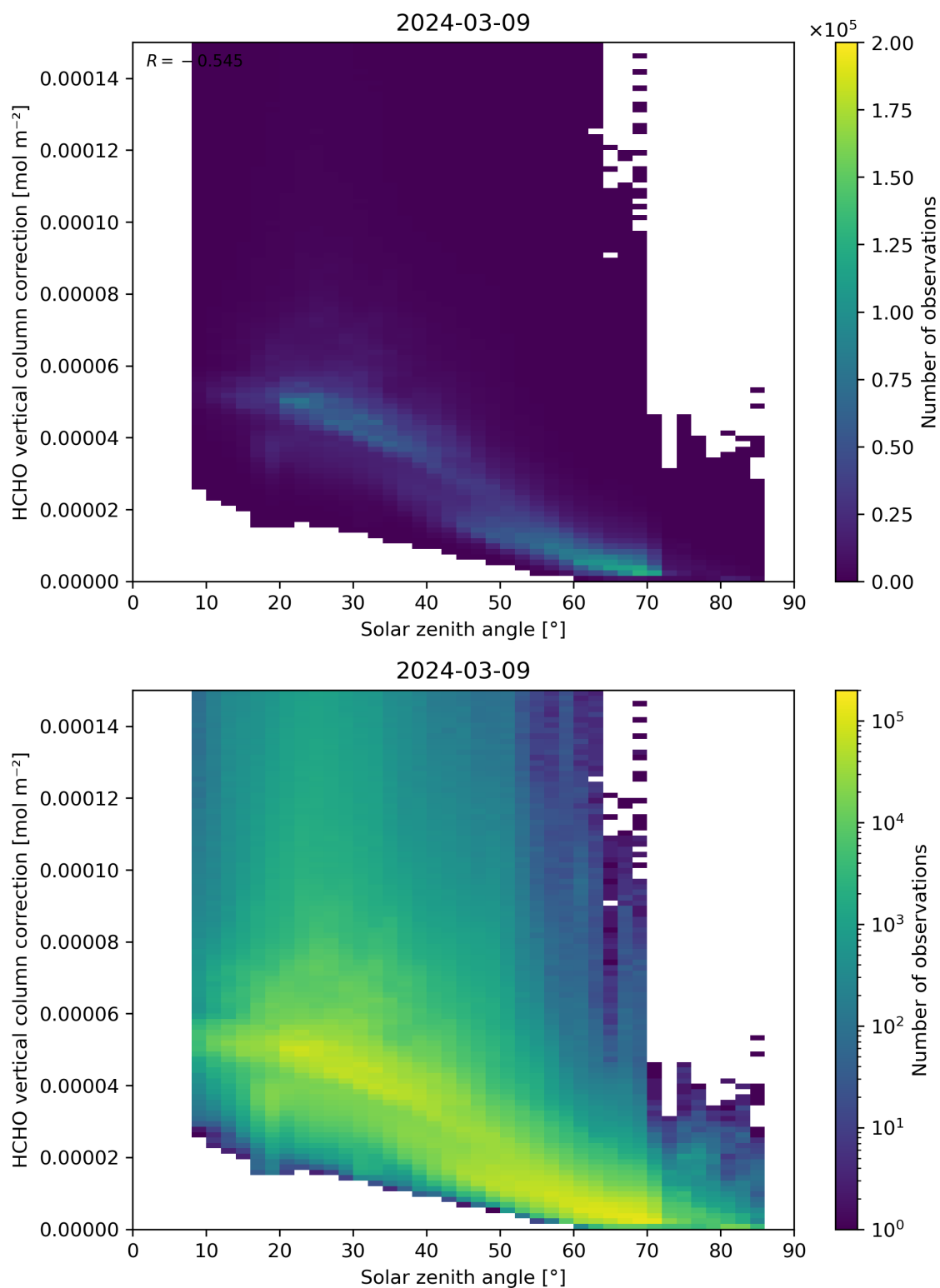
Figure 178: Scatter density plot of “Solar zenith angle” against “HCHO vertical column correction” for 2024-03-09 to 2024-03-10.
