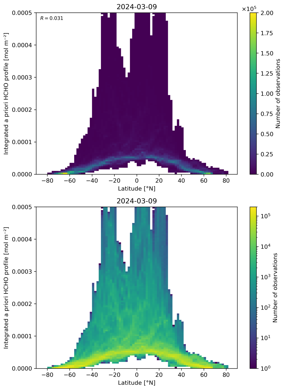
Figure 166: Scatter density plot of “Latitude” against “Integrated a priori HCHO profile” for 2024-03-09 to 2024-03-10.
