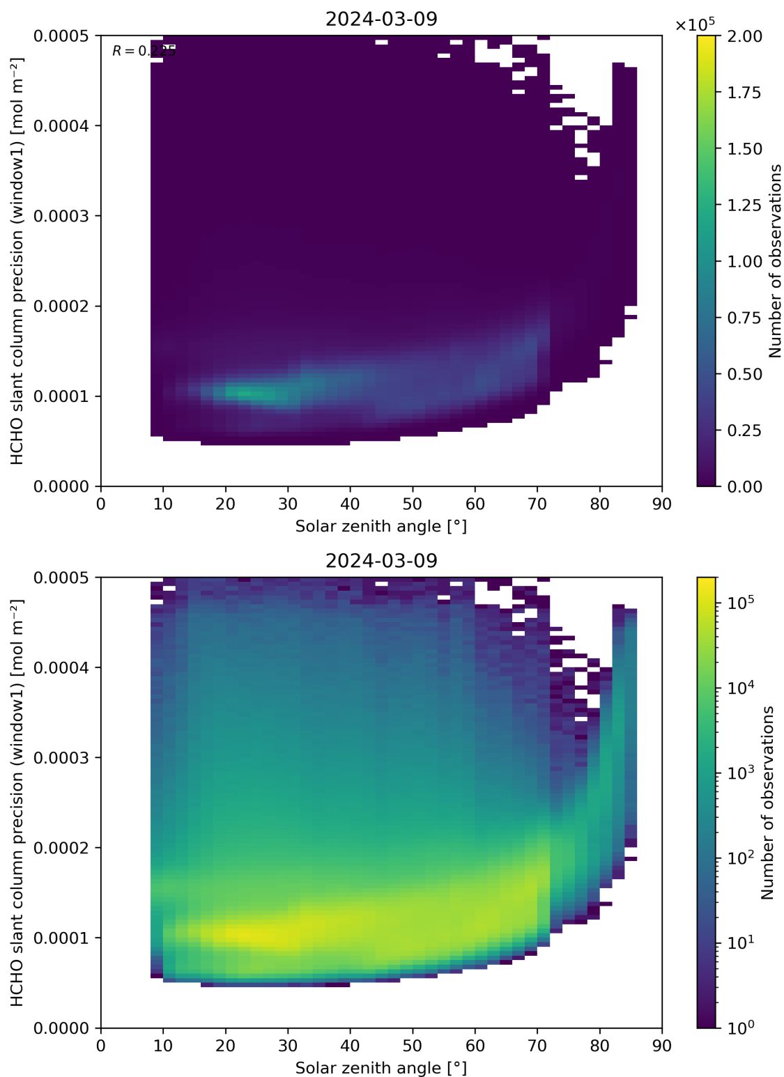
Figure 174: Scatter density plot of “Solar zenith angle” against “HCHO slant column precision (window1)” for 2024-03-09 to 2024-03-10.
