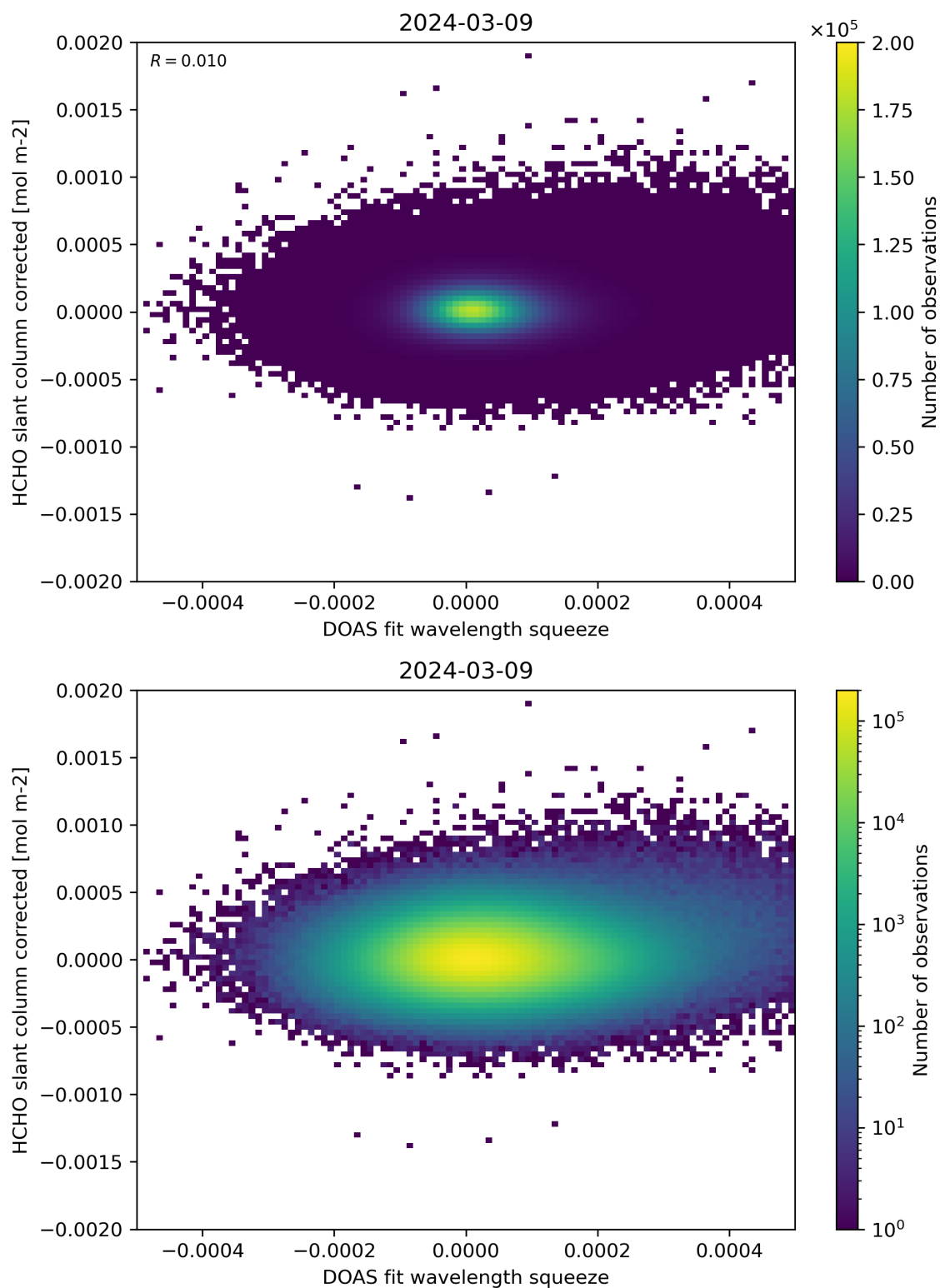
Figure 69: Scatter density plot of “DOAS fit wavelength squeeze” against “HCHO slant column corrected” for 2024-03-09 to 2024-03-10.
