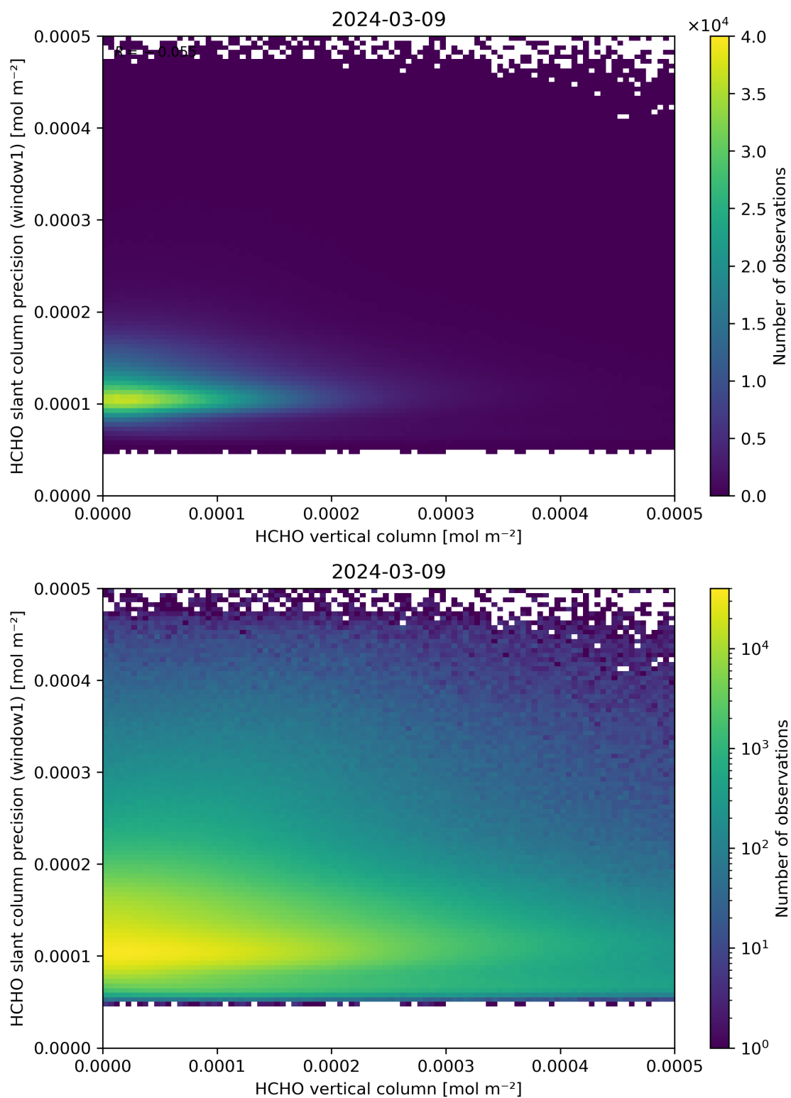
Figure 130: Scatter density plot of “HCHO vertical column” against “HCHO slant column precision (window1)” for 2024-03-09 to 2024-03-10.
