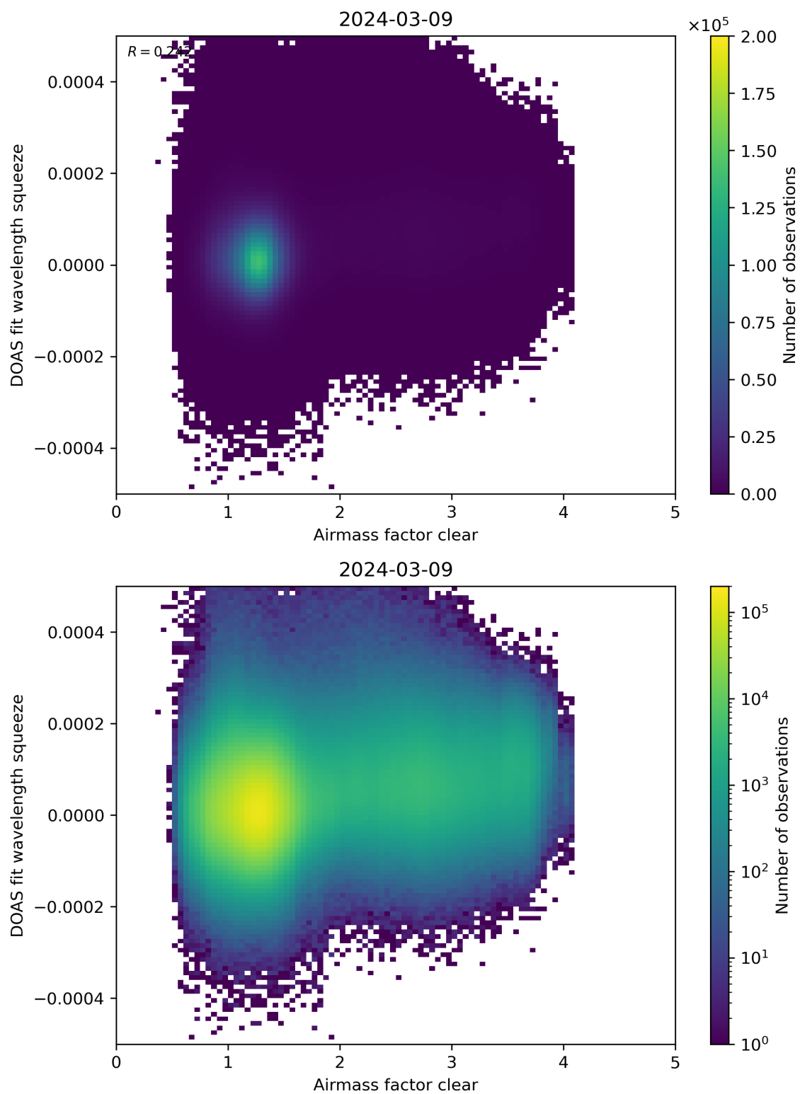
Figure 73: Scatter density plot of “Airmass factor clear” against “DOAS fit wavelength squeeze” for 2024-03-09 to 2024-03-10.
