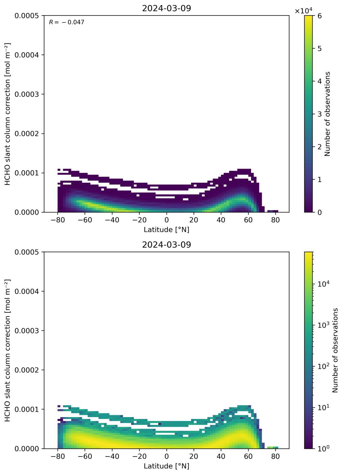
Figure 158: Scatter density plot of “Latitude” against “HCHO slant column correction” for 2024-03-09 to 2024-03-10.
