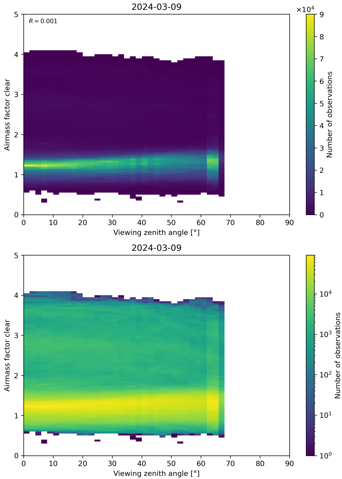
Figure 185: Scatter density plot of “Viewing zenith angle” against “Airmass factor clear” for 2024-03-09 to 2024-03-10.
