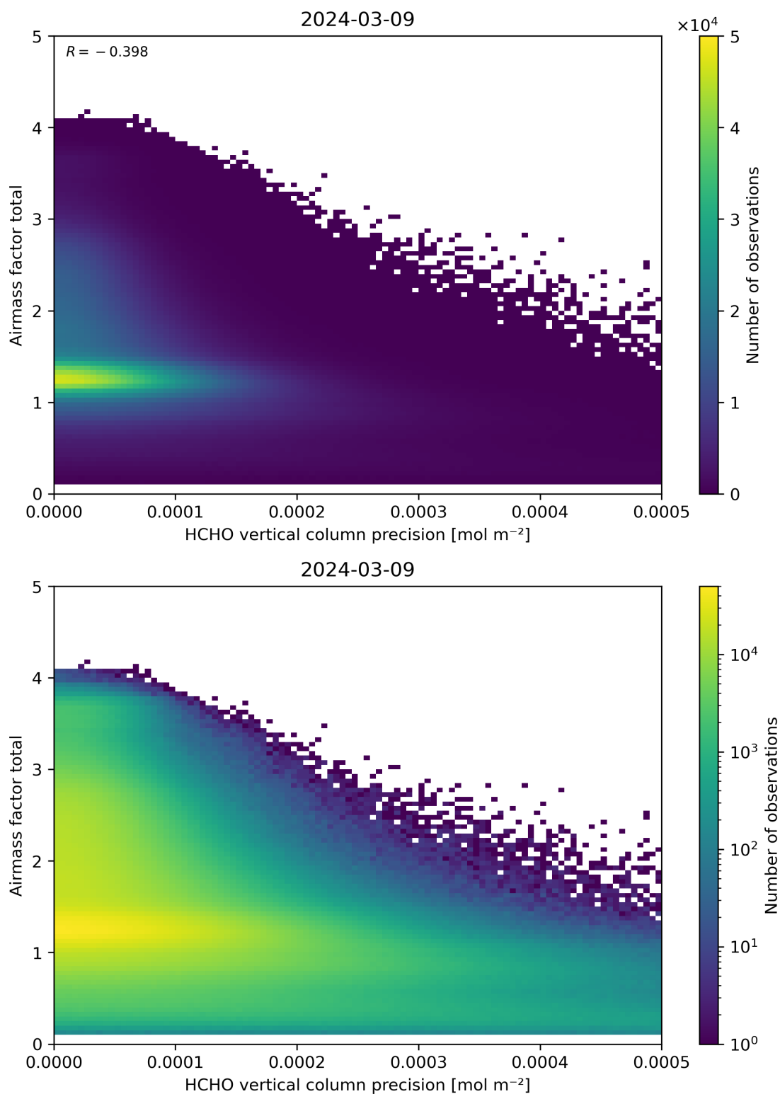
Figure 144: Scatter density plot of “HCHO vertical column precision” against “Airmass factor total” for 2024-03-09 to 2024-03-10.
