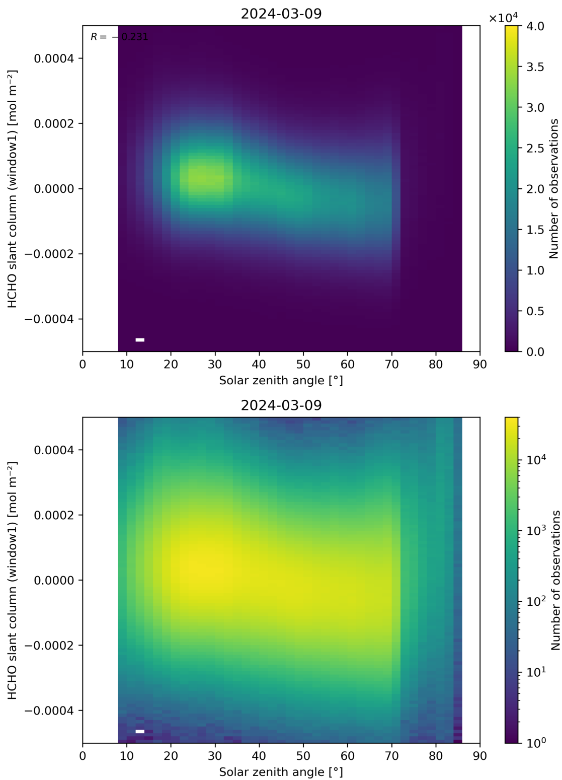
Figure 173: Scatter density plot of “Solar zenith angle” against “HCHO slant column (window1)” for 2024-03-09 to 2024-03-10.
