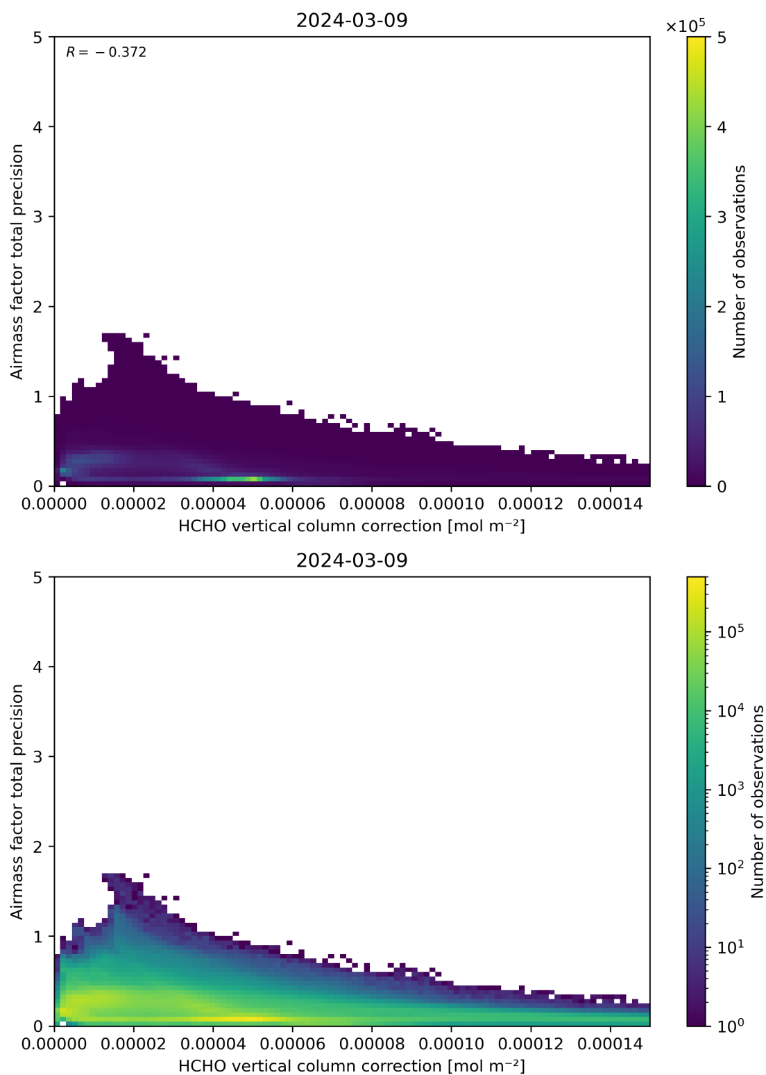
Figure 121: Scatter density plot of “HCHO vertical column correction” against “Airmass factor total precision” for 2024-03-09 to 2024-03-10.
