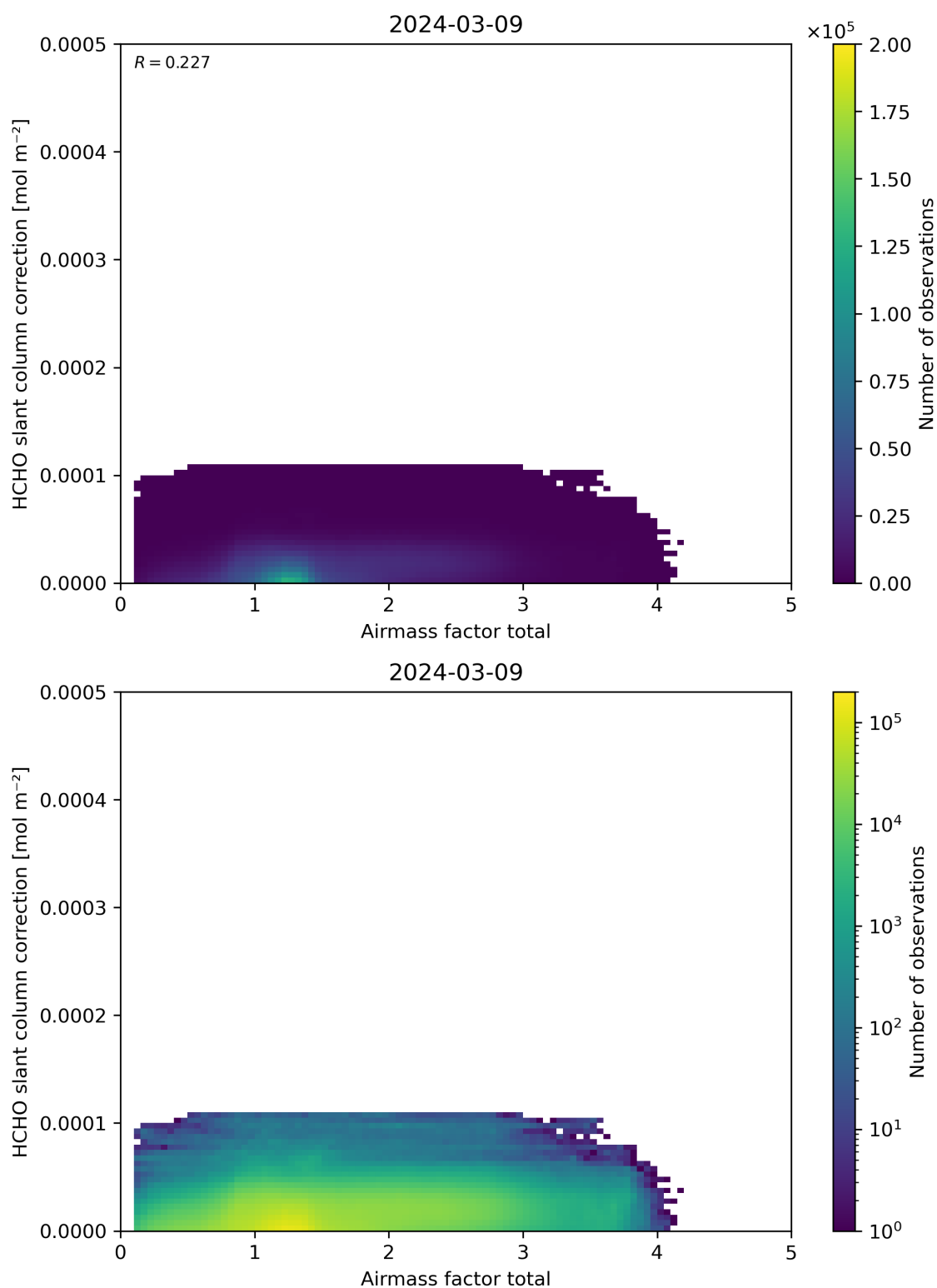
Figure 102: Scatter density plot of “Airmass factor total” against “HCHO slant column correction” for 2024-03-09 to 2024-03-10.
