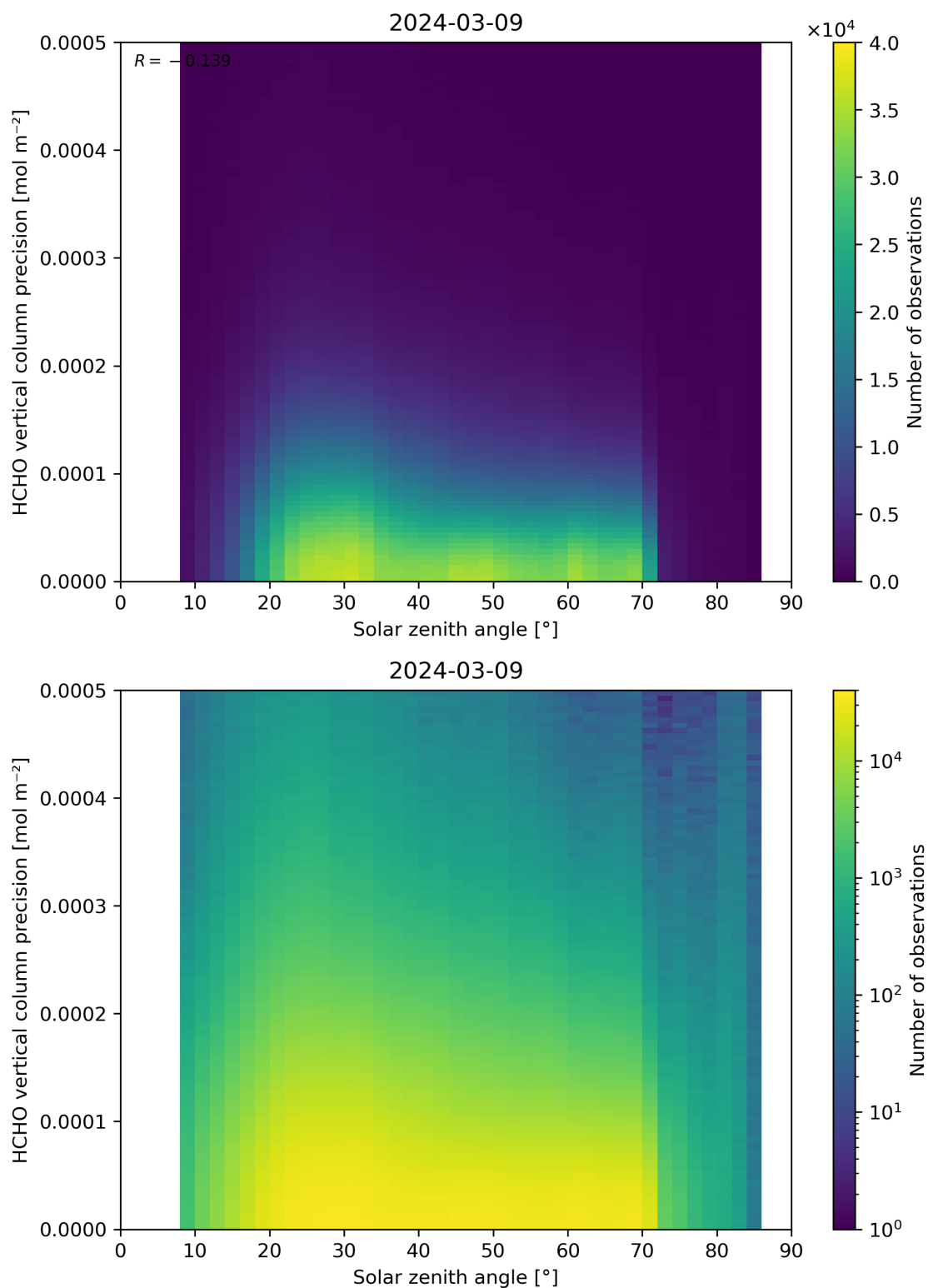
Figure 179: Scatter density plot of “Solar zenith angle” against “HCHO vertical column precision” for 2024-03-09 to 2024-03-10.
