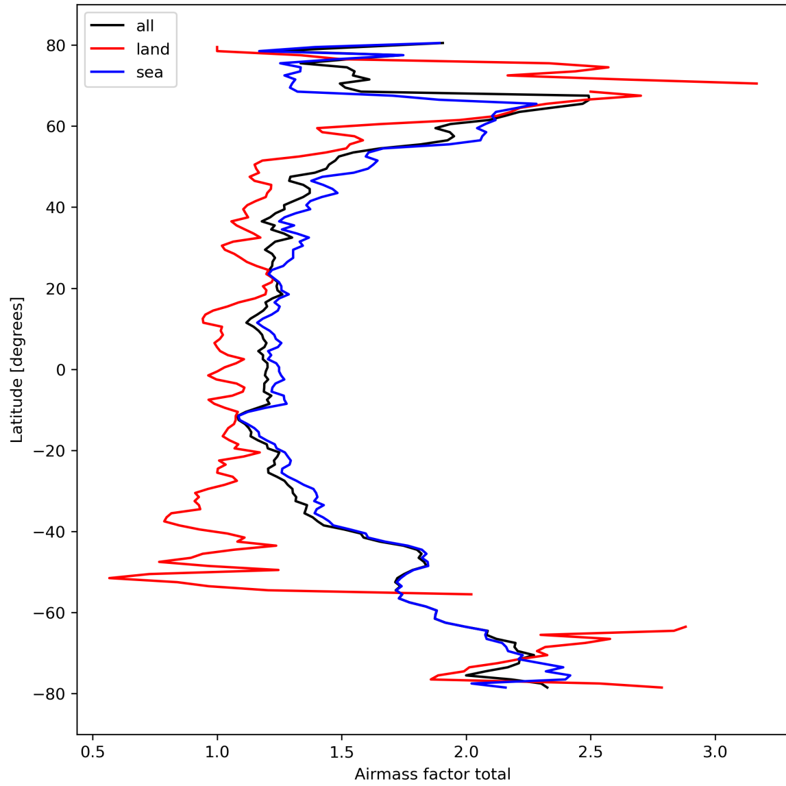
Figure 26: Zonal average of “Airmass factor total” for 2024-03-09 to 2024-03-10.
