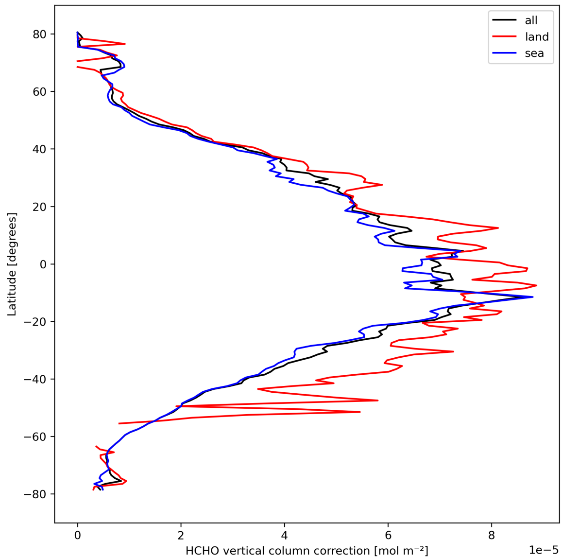
Figure 23: Zonal average of “HCHO vertical column correction” for 2024-03-09 to 2024-03-10.
