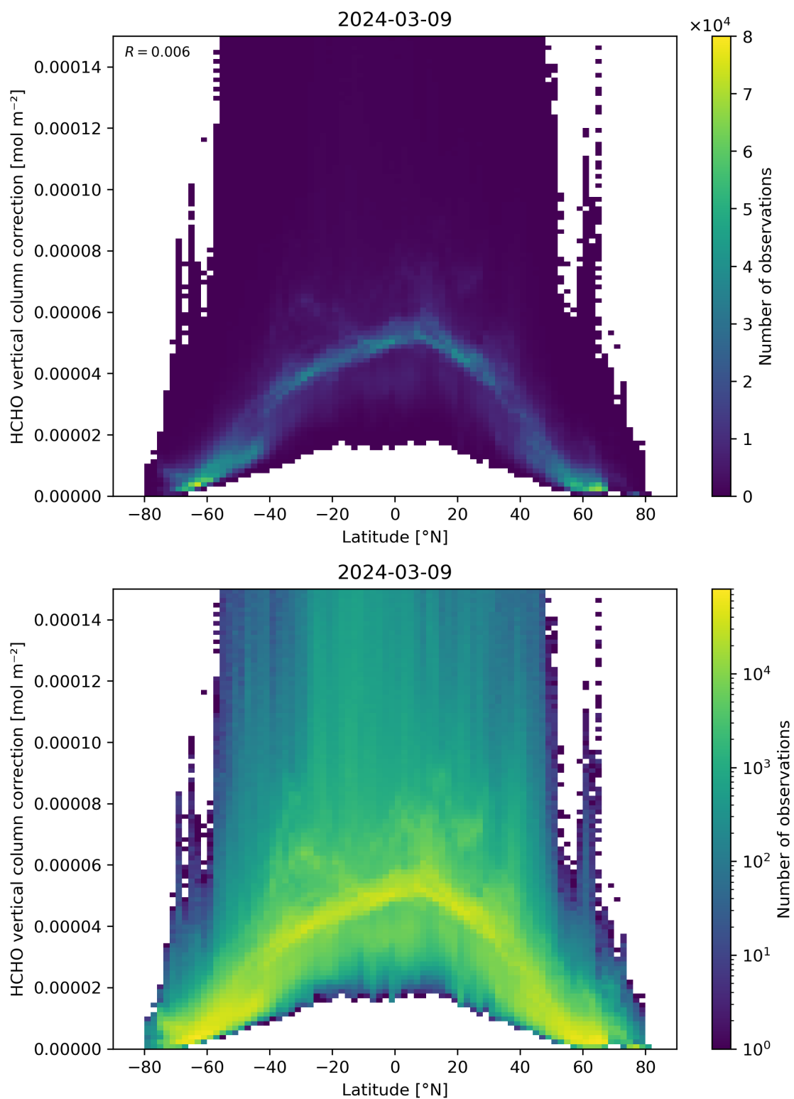
Figure 164: Scatter density plot of “Latitude” against “HCHO vertical column correction” for 2024-03-09 to 2024-03-10.
