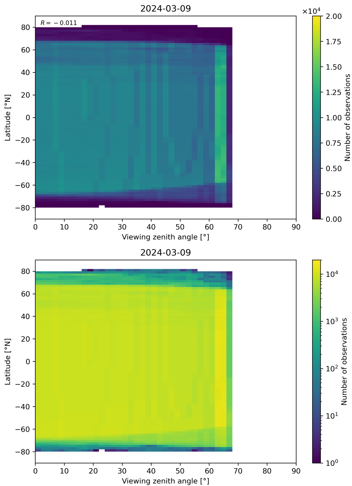
Figure 196: Scatter density plot of “Viewing zenith angle” against “Latitude” for 2024-03-09 to 2024-03-10.
