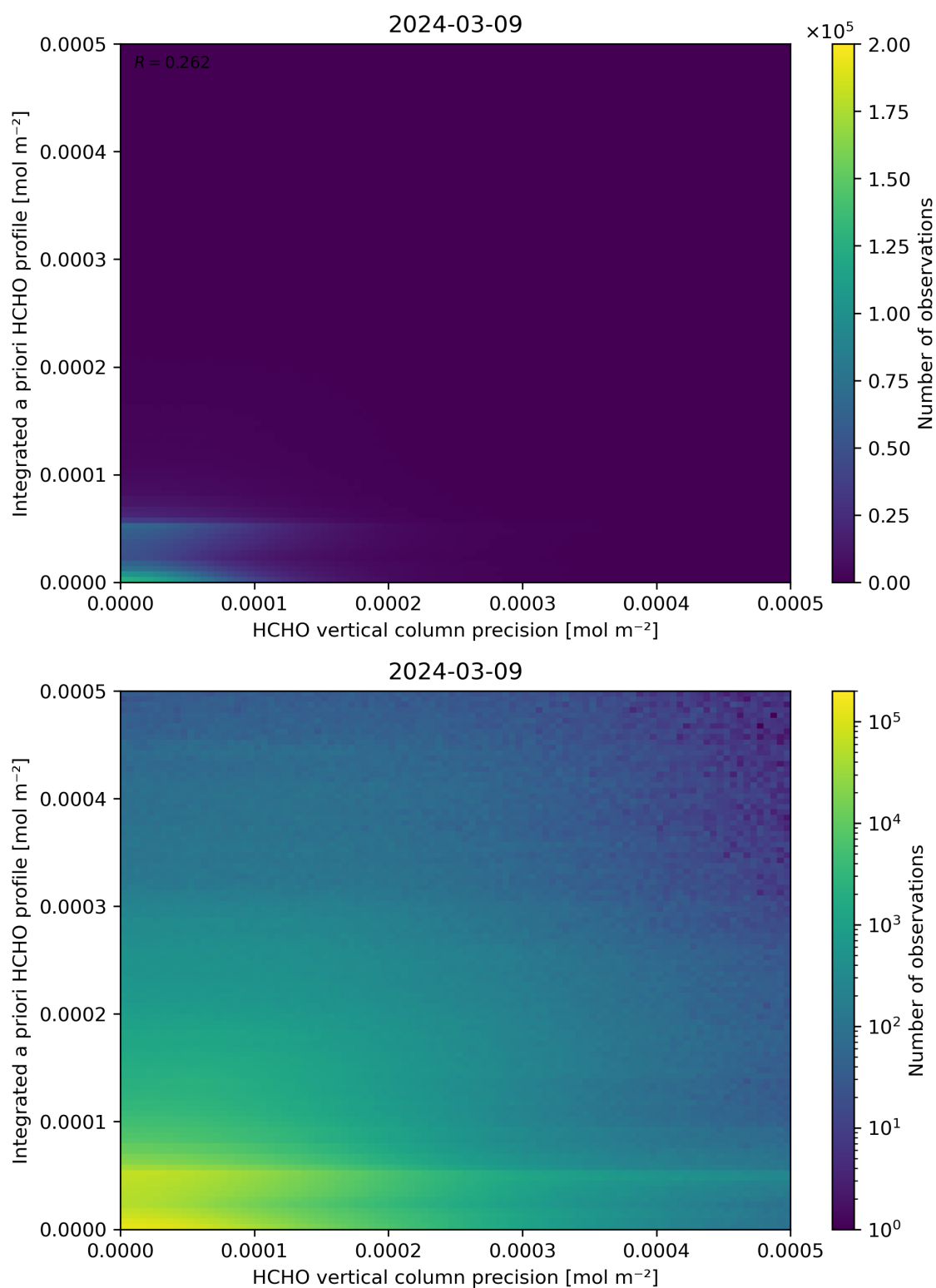
Figure 147: Scatter density plot of “HCHO vertical column precision” against “Integrated a priori HCHO profile” for 2024-03-09 to 2024-03-10.
