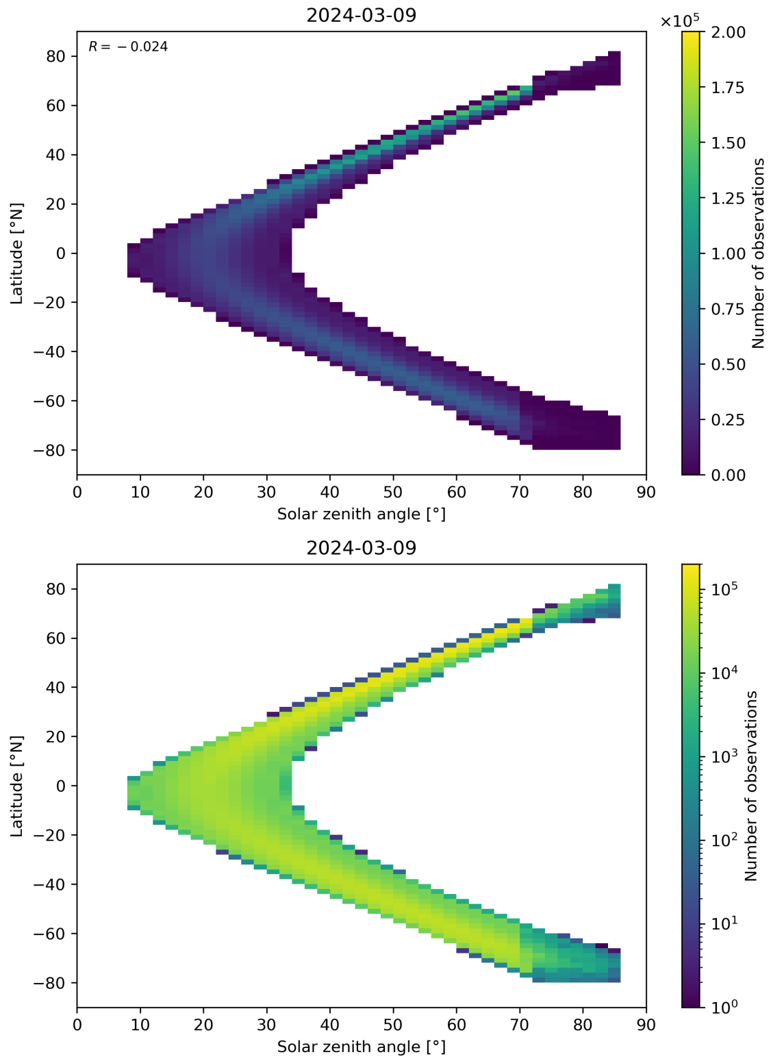
Figure 181: Scatter density plot of “Solar zenith angle” against “Latitude” for 2024-03-09 to 2024-03-10.
