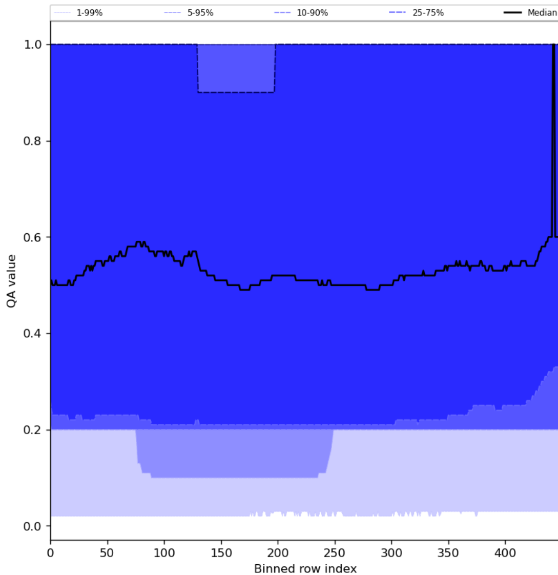
Figure 48: Along track statistics of “QA value” for 2024-03-09 to 2024-03-10
