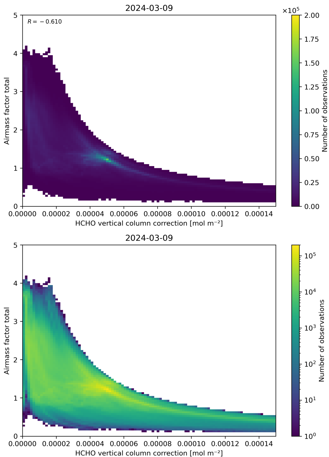
Figure 120: Scatter density plot of “HCHO vertical column correction” against “Airmass factor total” for 2024-03-09 to 2024-03-10.
