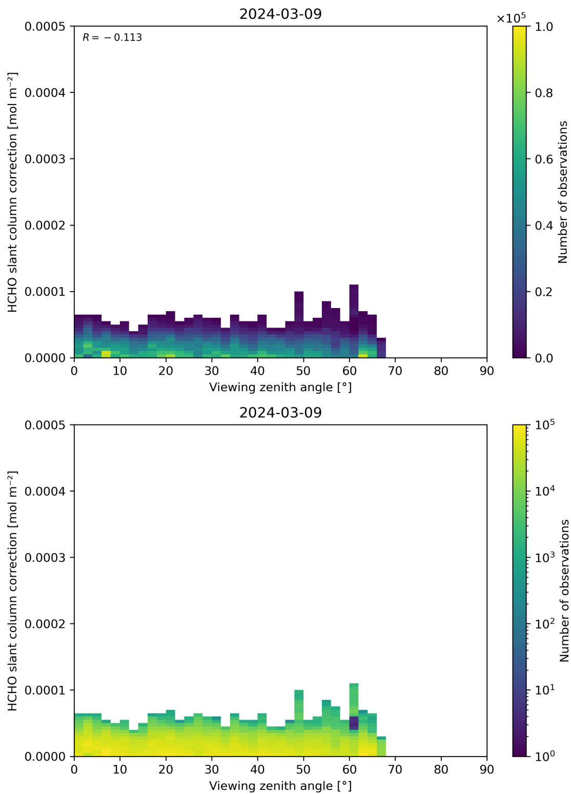
Figure 187: Scatter density plot of “Viewing zenith angle” against “HCHO slant column correction” for 2024-03-09 to 2024-03-10.
