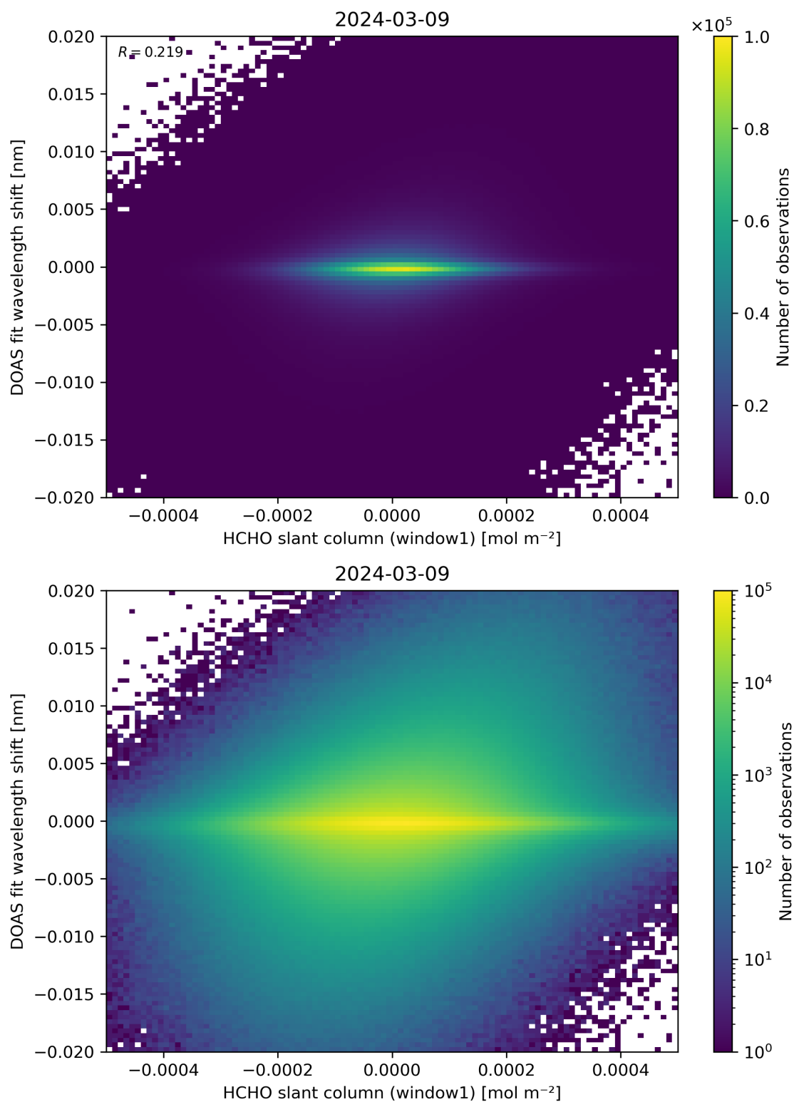
Figure 79: Scatter density plot of “HCHO slant column (window1)” against “DOAS fit wavelength shift” for 2024-03-09 to 2024-03-10.
