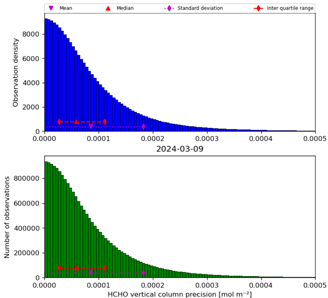
Figure 36: Histogram of “HCHO vertical column precision” for 2024-03-09 to 2024-03-10
