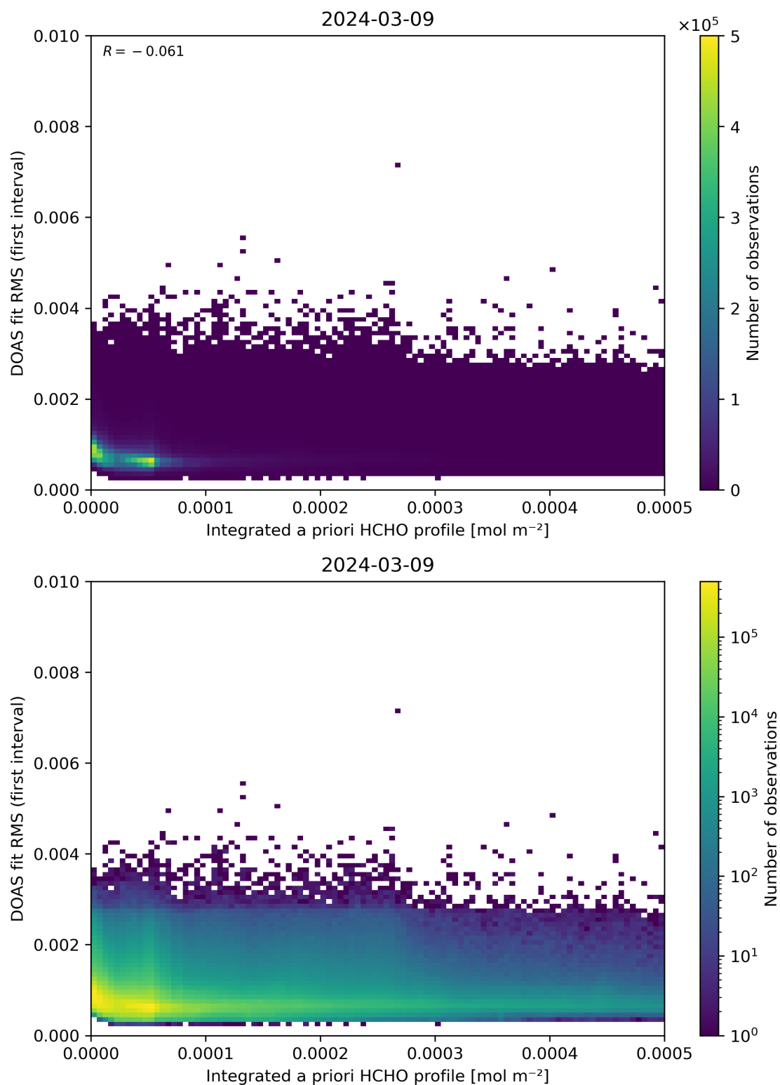
Figure 148: Scatter density plot of “Integrated a priori HCHO profile” against “DOAS fit RMS (first interval)” for 2024-03-09 to 2024-03-10.
