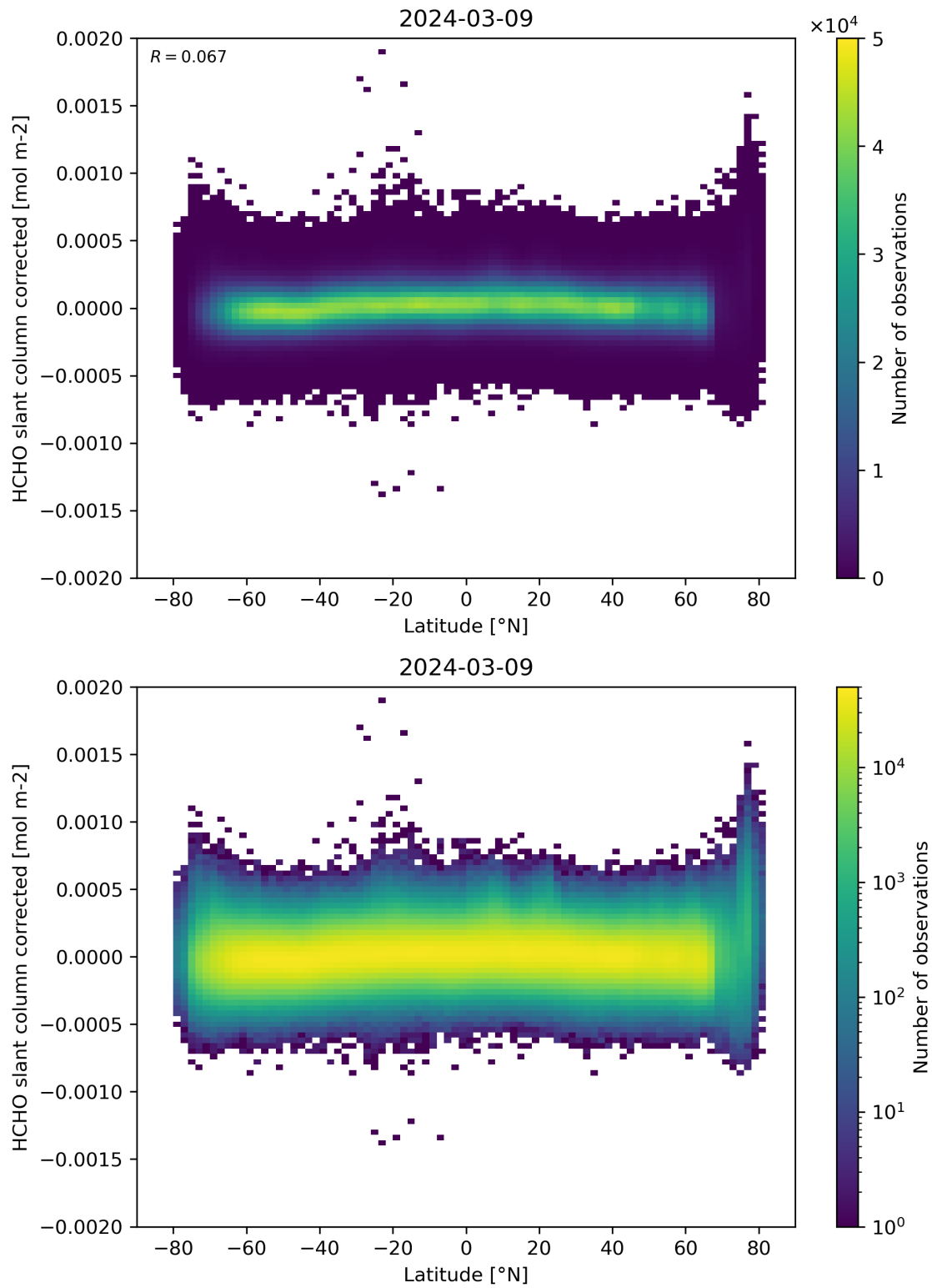
Figure 157: Scatter density plot of “Latitude” against “HCHO slant column corrected” for 2024-03-09 to 2024-03-10.
