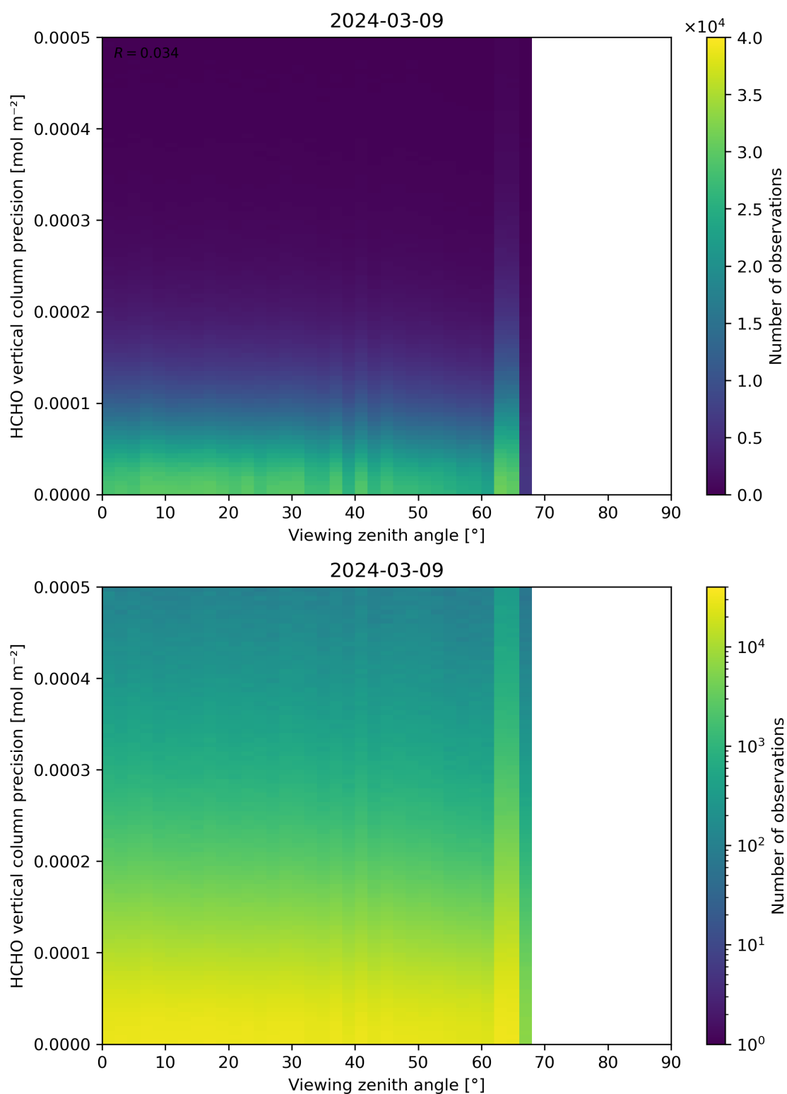
Figure 194: Scatter density plot of “Viewing zenith angle” against “HCHO vertical column precision” for 2024-03-09 to 2024-03-10.
