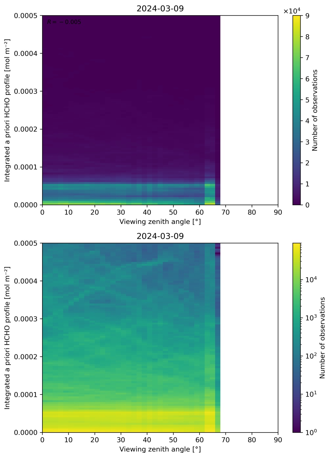
Figure 195: Scatter density plot of “Viewing zenith angle” against “Integrated a priori HCHO profile” for 2024-03-09 to 2024-03-10.
