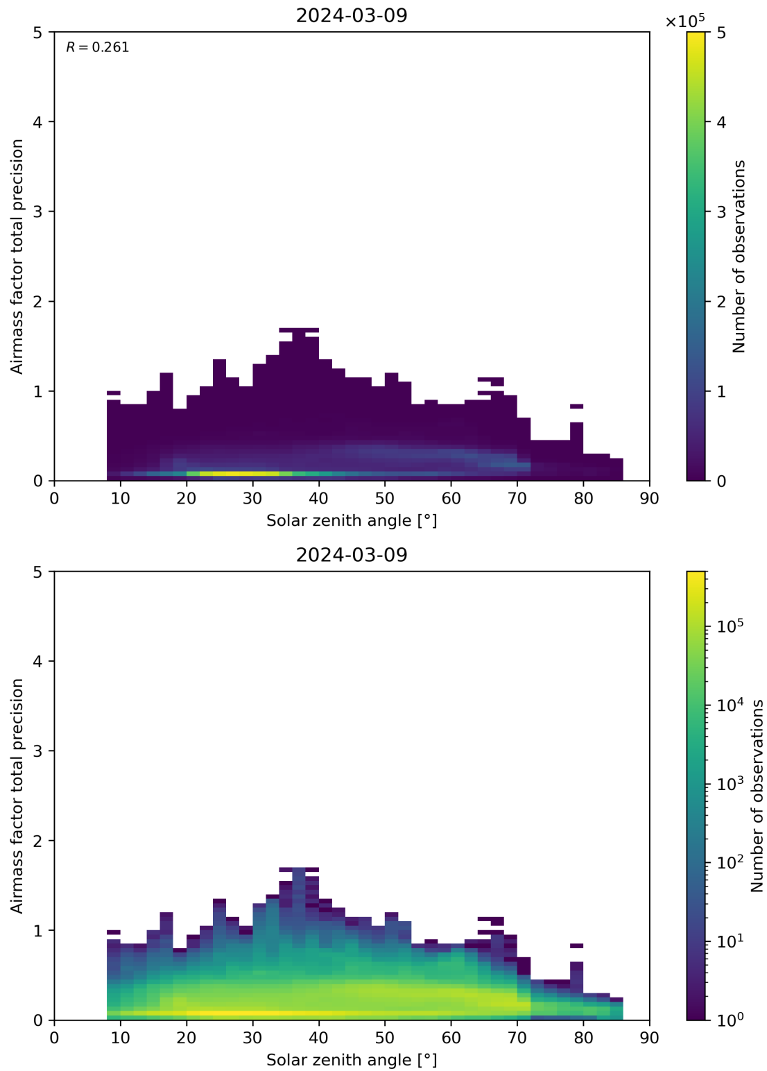
Figure 176: Scatter density plot of “Solar zenith angle” against “Airmass factor total precision” for 2024-03-09 to 2024-03-10.
