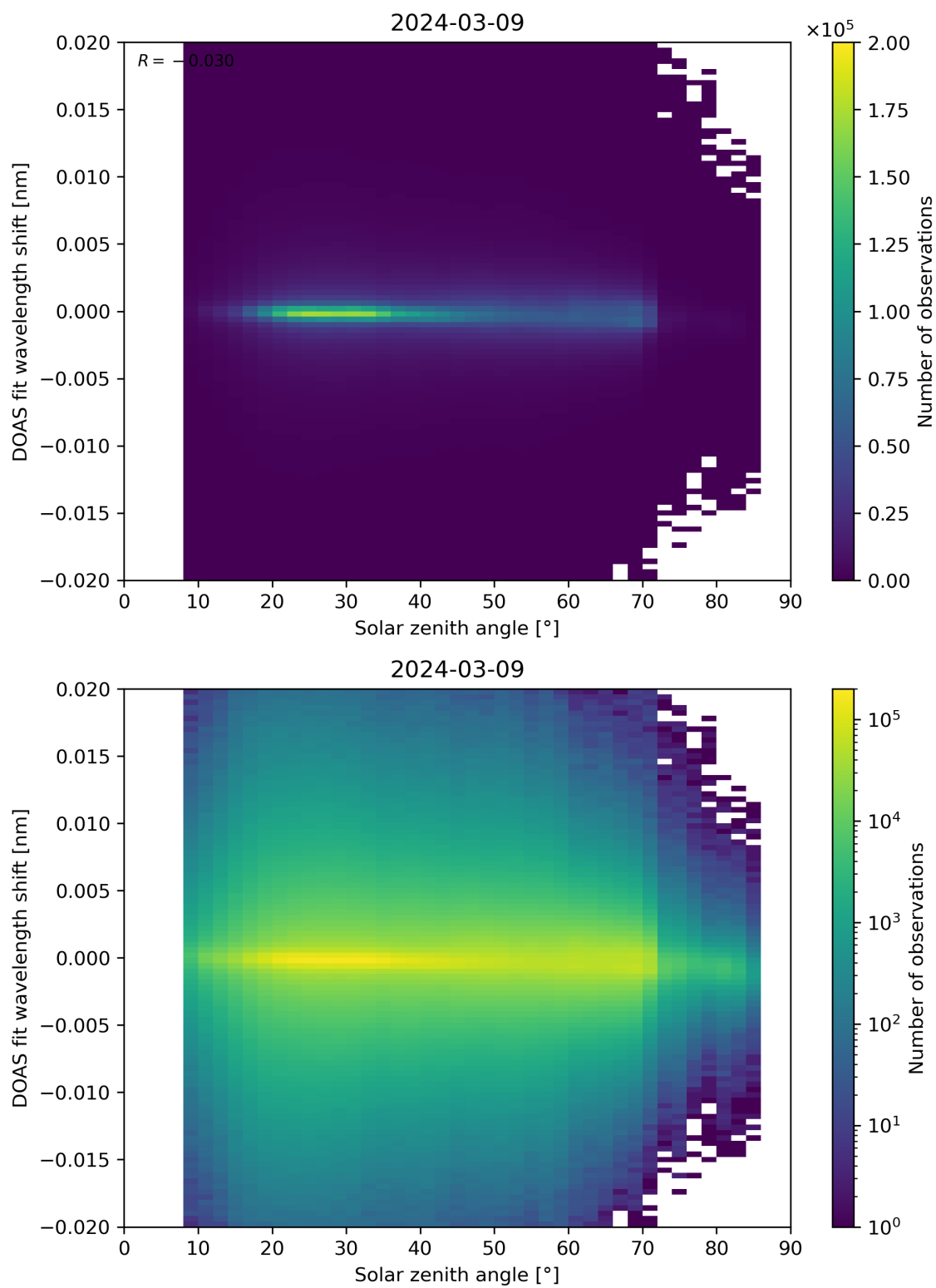
Figure 168: Scatter density plot of “Solar zenith angle” against “DOAS fit wavelength shift” for 2024-03-09 to 2024-03-10.
