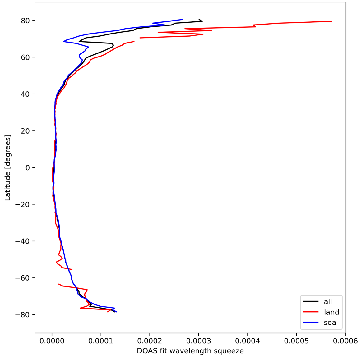
Figure 31: Zonal average of “DOAS fit wavelength squeeze” for 2024-03-09 to 2024-03-10.
