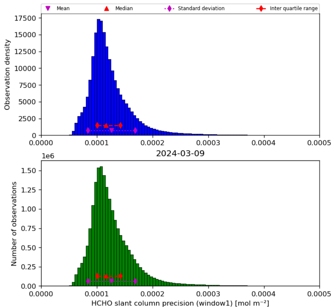
Figure 39: Histogram of “HCHO slant column precision (window1)” for 2024-03-09 to 2024-03-10
