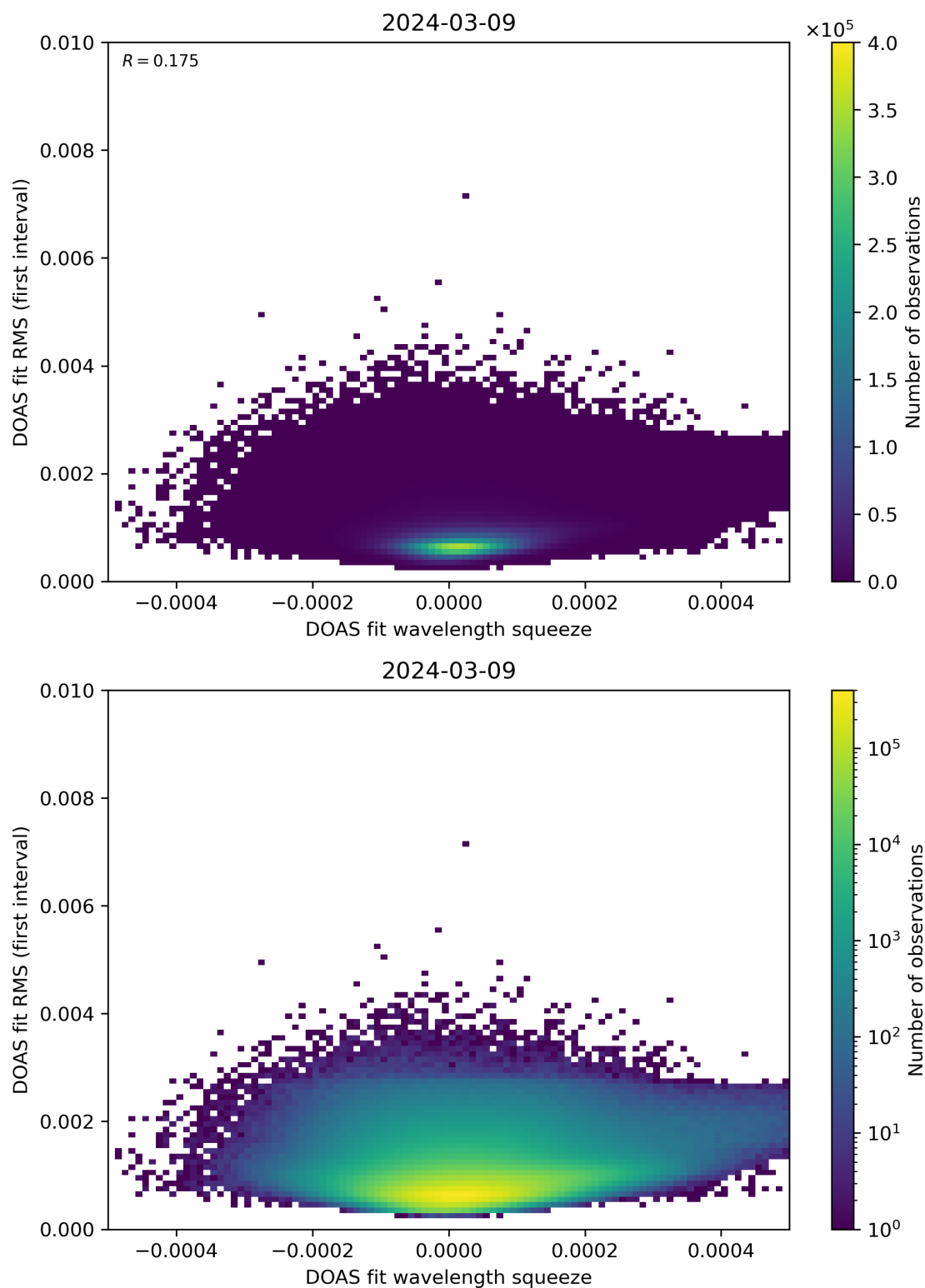
Figure 68: Scatter density plot of “DOAS fit wavelength squeeze” against “DOAS fit RMS (first interval)” for 2024-03-09 to 2024-03-10.
