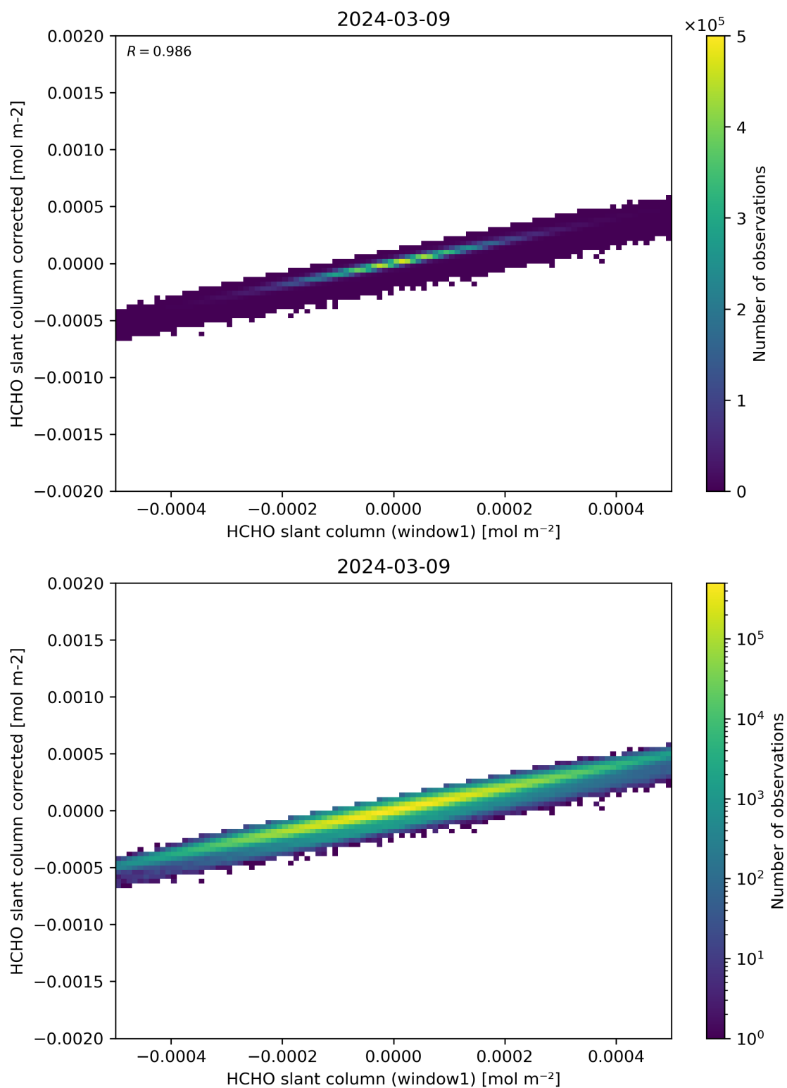
Figure 82: Scatter density plot of “HCHO slant column (window1)” against “HCHO slant column corrected” for 2024-03-09 to 2024-03-10.
