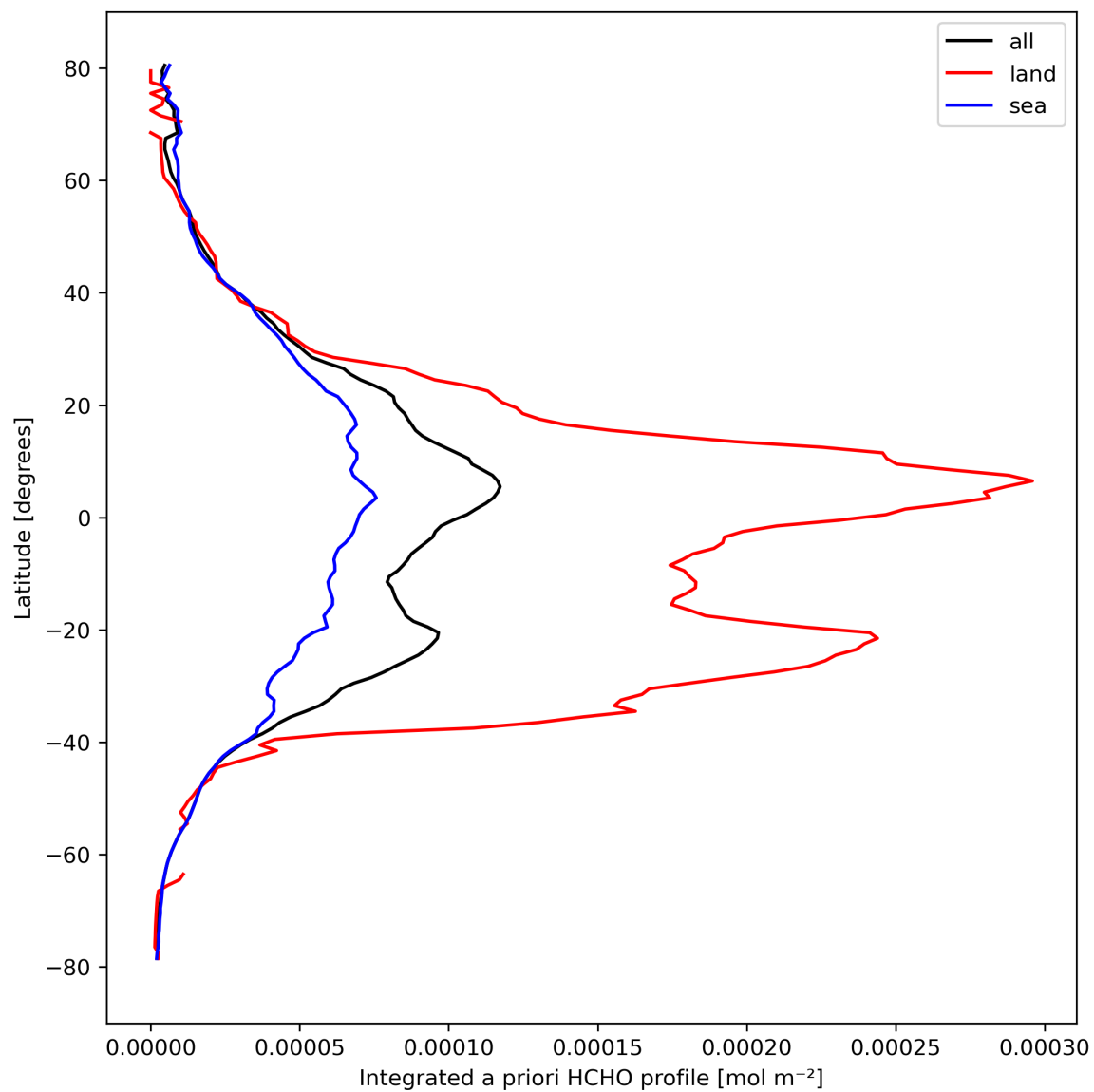
Figure 29: Zonal average of “Integrated a priori HCHO profile” for 2024-03-09 to 2024-03-10.
