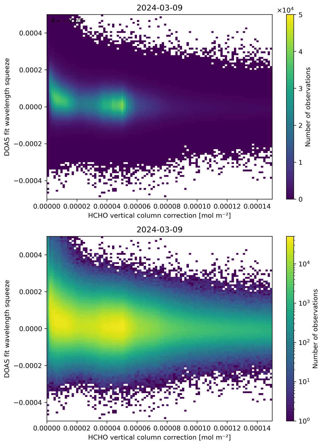
Figure 114: Scatter density plot of “HCHO vertical column correction” against “DOAS fit wavelength squeeze” for 2024-03-09 to 2024-03-10.
