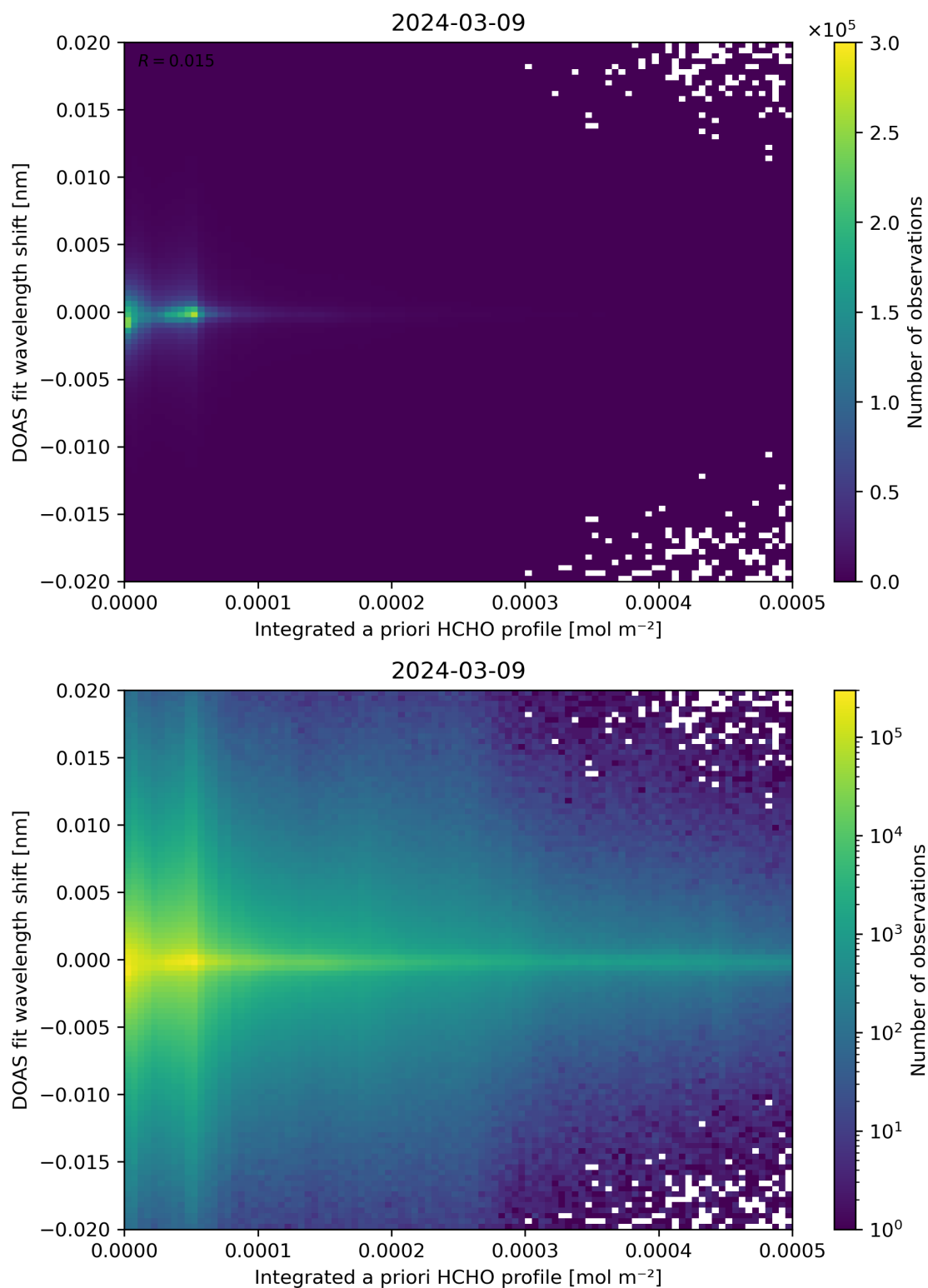
Figure 149: Scatter density plot of “Integrated a priori HCHO profile” against “DOAS fit wavelength shift” for 2024-03-09 to 2024-03-10.
