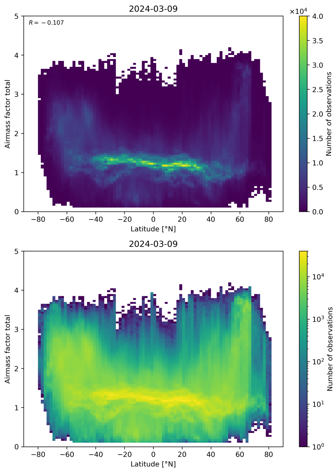
Figure 161: Scatter density plot of “Latitude” against “Airmass factor total” for 2024-03-09 to 2024-03-10.
