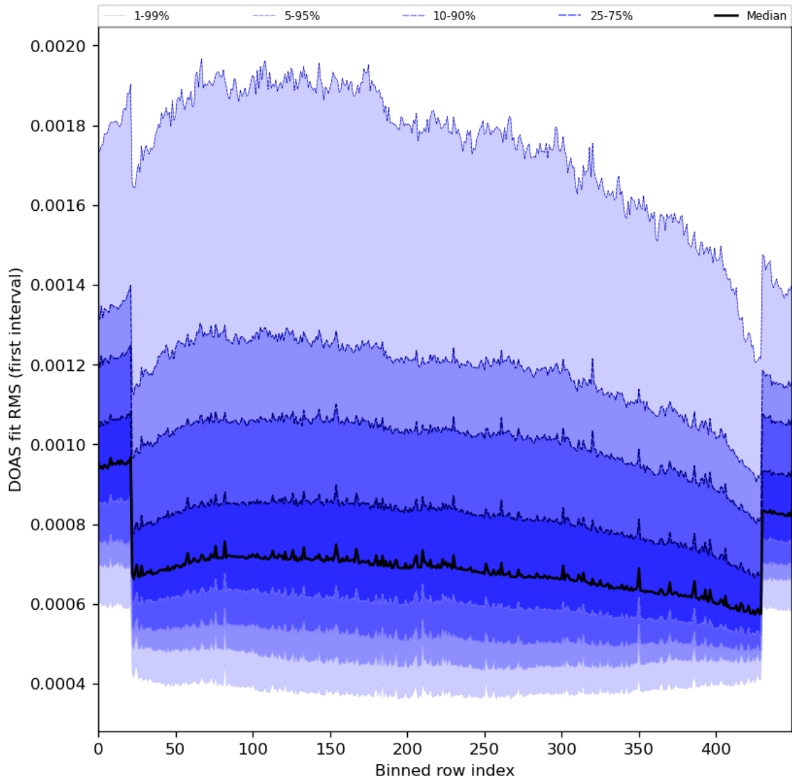
Figure 60: Along track statistics of “DOAS fit RMS (first interval)” for 2024-03-09 to 2024-03-10
