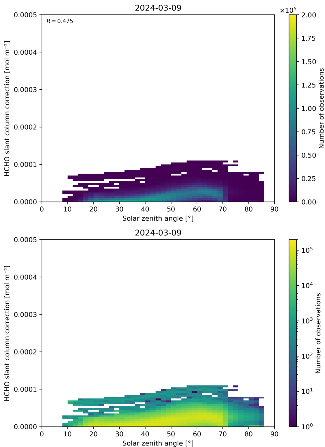
Figure 172: Scatter density plot of “Solar zenith angle” against “HCHO slant column correction” for 2024-03-09 to 2024-03-10.
