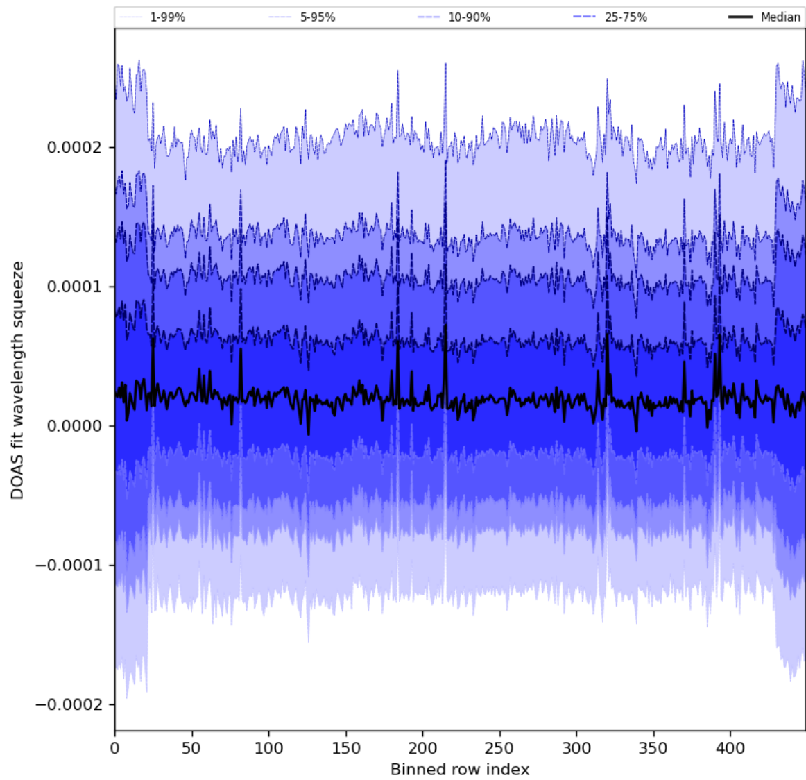
Figure 59: Along track statistics of “DOAS fit wavelength squeeze” for 2024-03-09 to 2024-03-10
