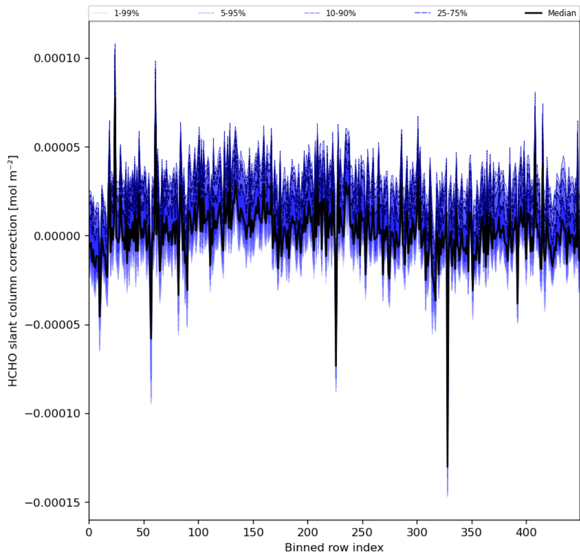
Figure 61: Along track statistics of “HCHO slant column correction” for 2024-03-09 to 2024-03-10
