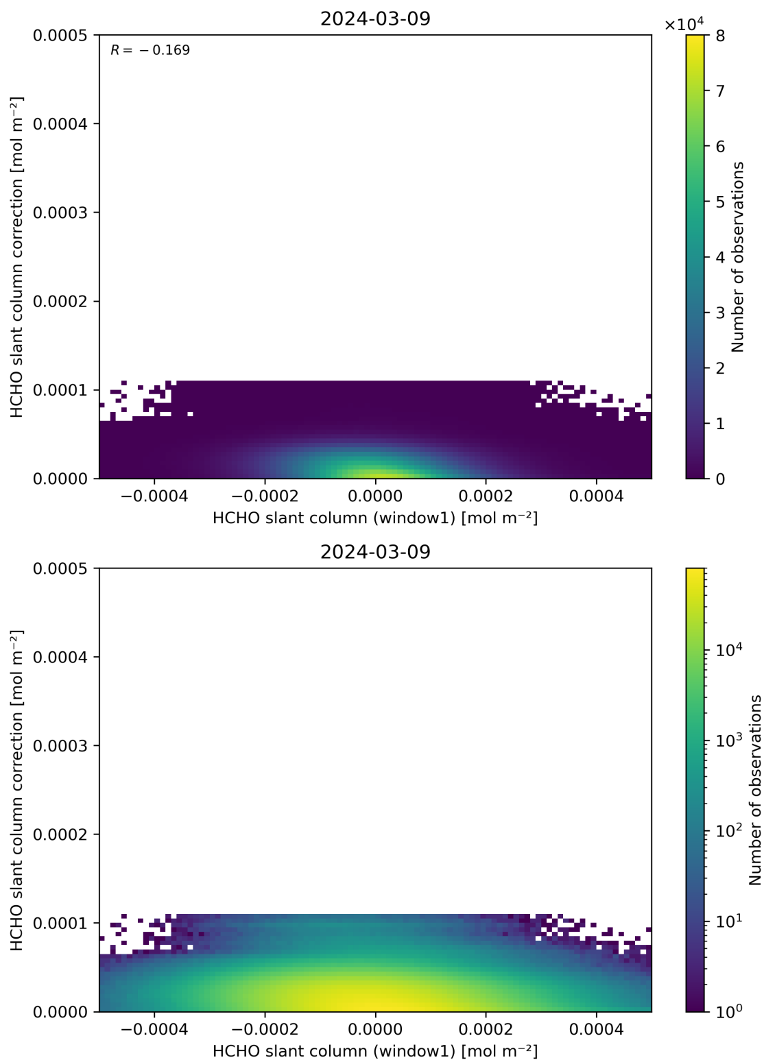
Figure 83: Scatter density plot of “HCHO slant column (window1)” against “HCHO slant column correction” for 2024-03-09 to 2024-03-10.
