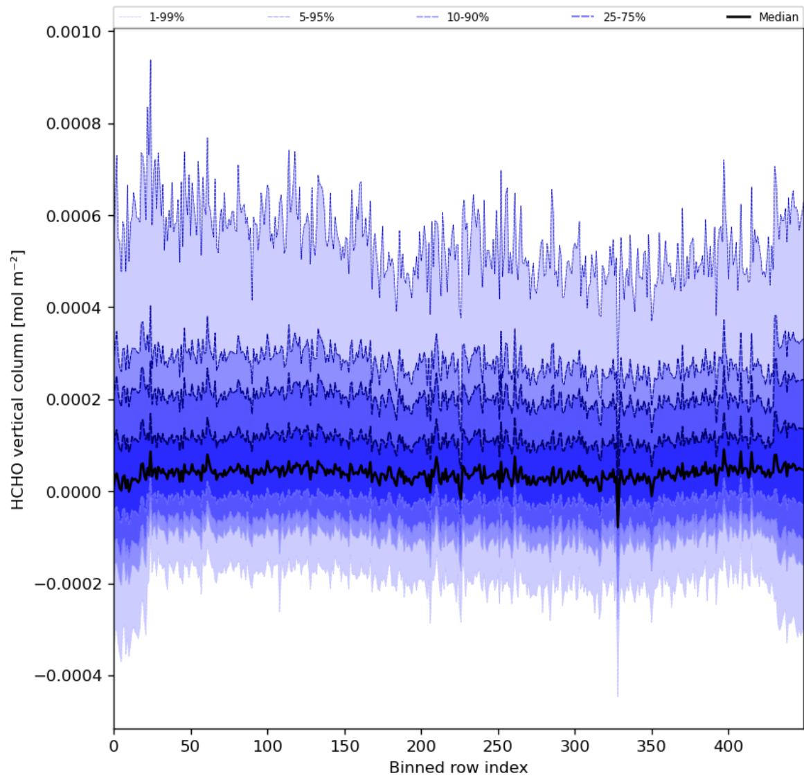
Figure 49: Along track statistics of “HCHO vertical column” for 2024-03-09 to 2024-03-10
