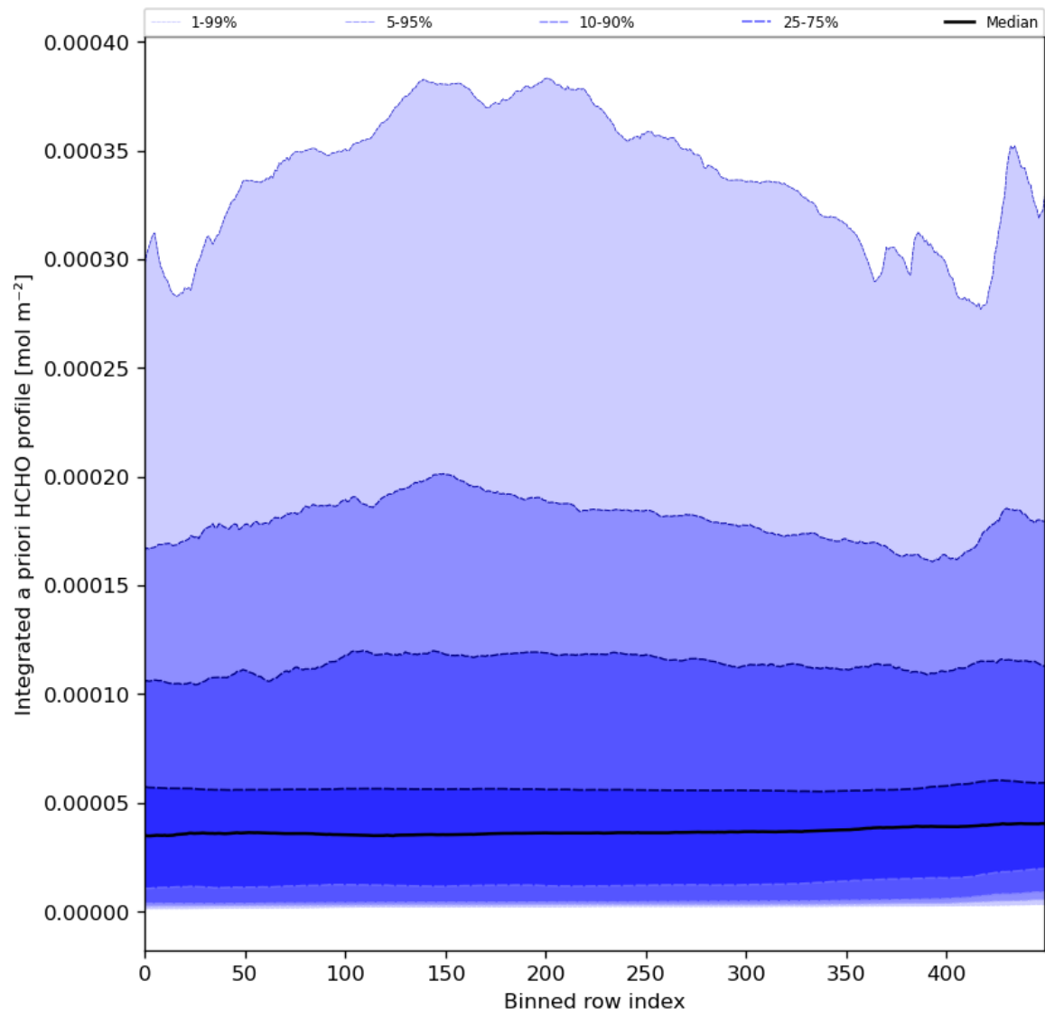
Figure 57: Along track statistics of "Integrated a priori HCHO profile" for 2024-03-09 to 2024-03-10
