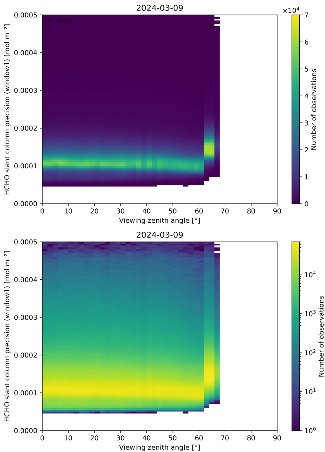
Figure 189: Scatter density plot of “Viewing zenith angle” against “HCHO slant column precision (window1)” for 2024-03-09 to 2024-03-10.
