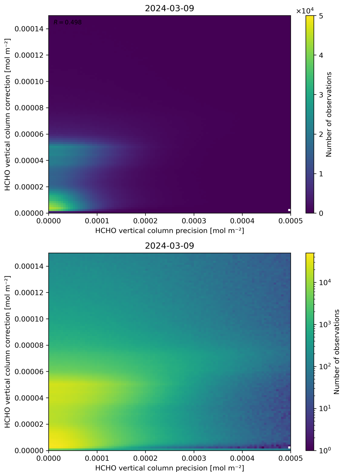
Figure 146: Scatter density plot of “HCHO vertical column precision” against “HCHO vertical column correction” for 2024-03-09 to 2024-03-10.
