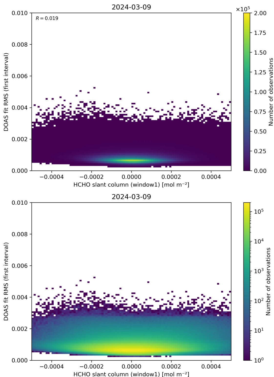
Figure 78: Scatter density plot of “HCHO slant column (window1)” against “DOAS fit RMS (first interval)” for 2024-03-09 to 2024-03-10.
