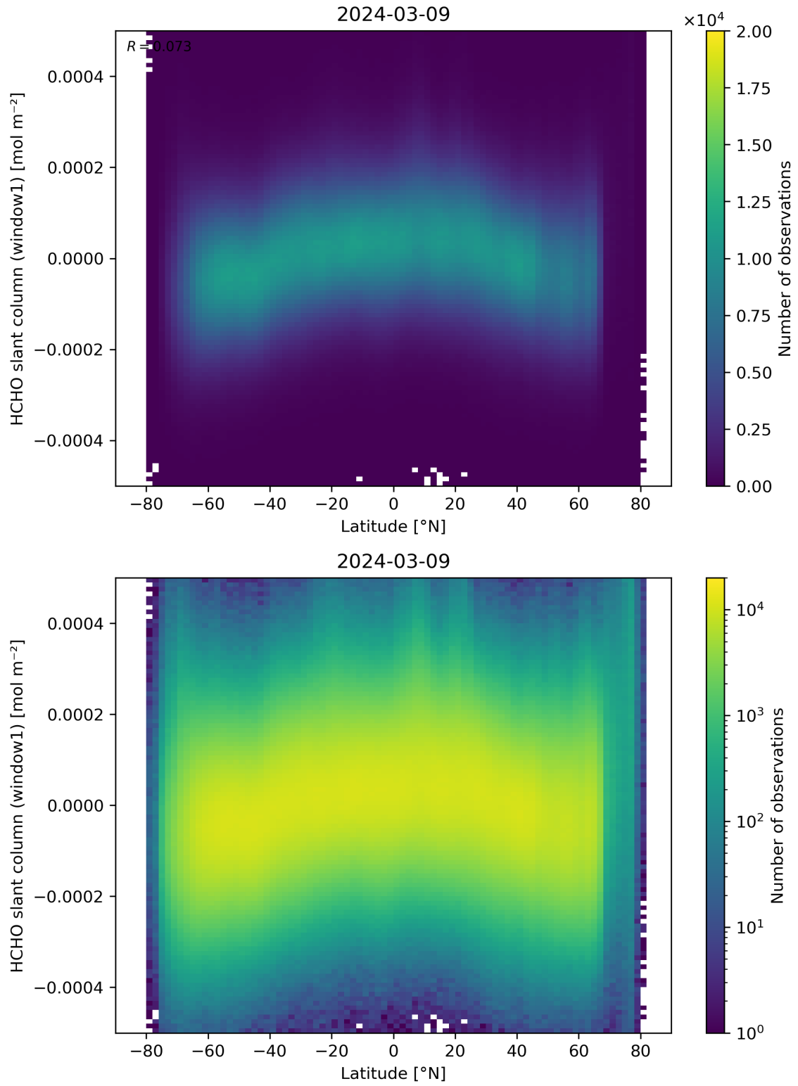
Figure 159: Scatter density plot of “Latitude” against “HCHO slant column (window1)” for 2024-03-09 to 2024-03-10.
