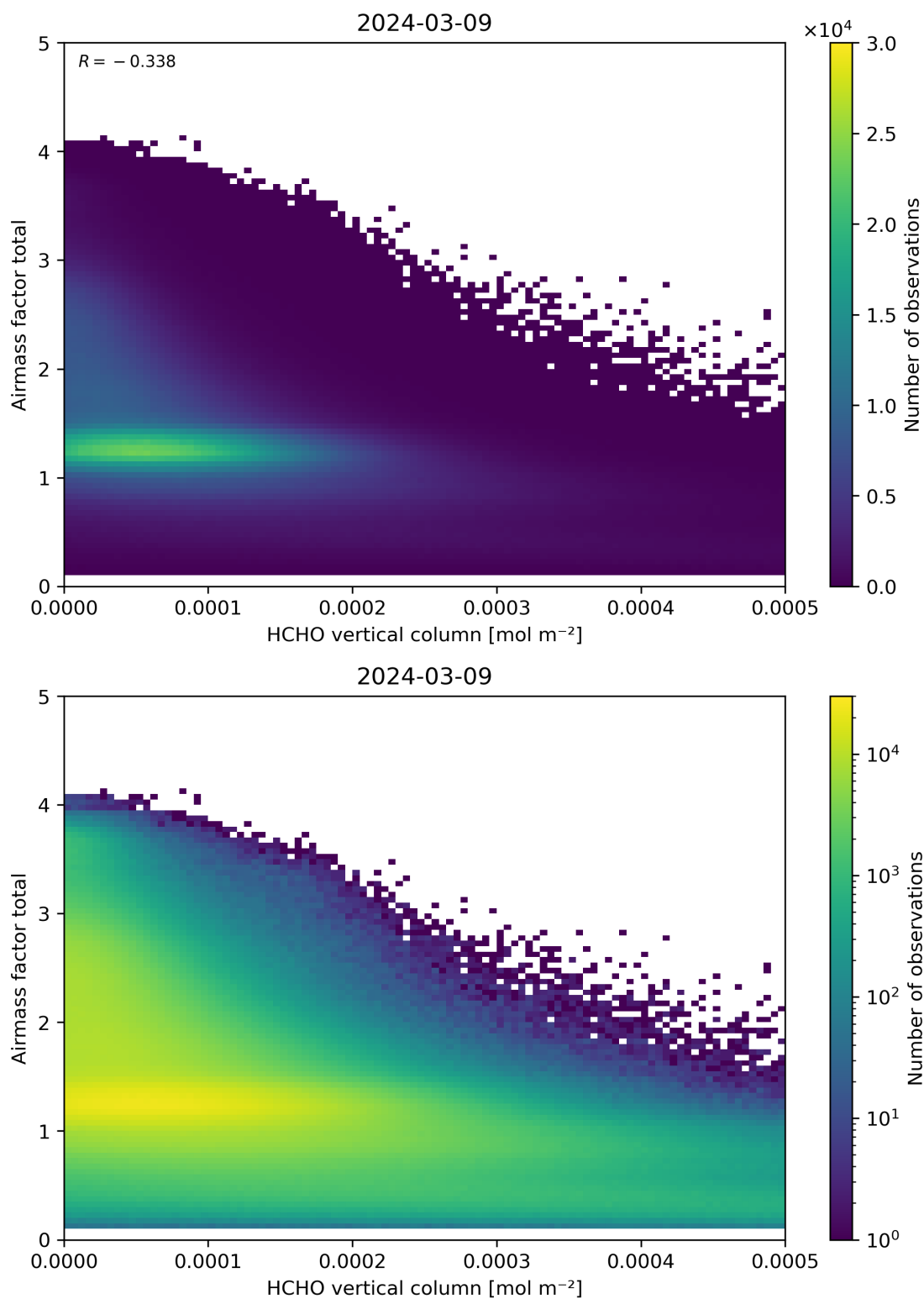
Figure 131: Scatter density plot of “HCHO vertical column” against “Airmass factor total” for 2024-03-09 to 2024-03-10.
