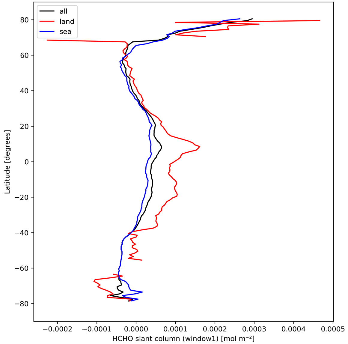
Figure 24: Zonal average of “HCHO slant column (window1)” for 2024-03-09 to 2024-03-10.
