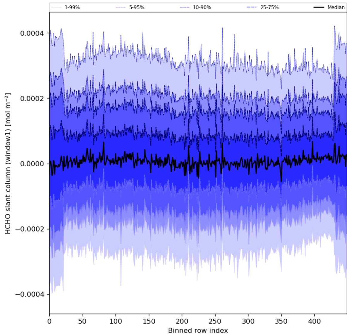
Figure 52: Along track statistics of “HCHO slant column (window1)” for 2024-03-09 to 2024-03-10
