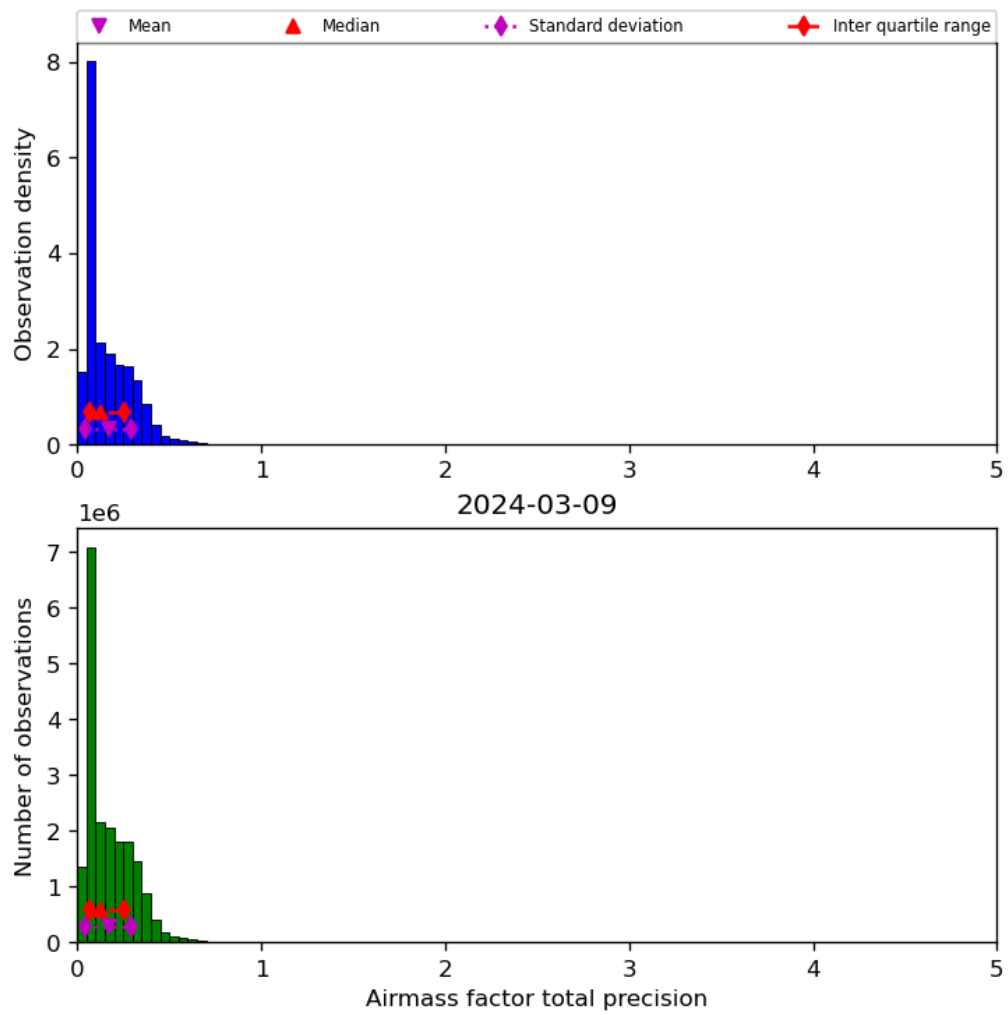
Figure 41: Histogram of “Airmass factor total precision” for 2024-03-09 to 2024-03-10
