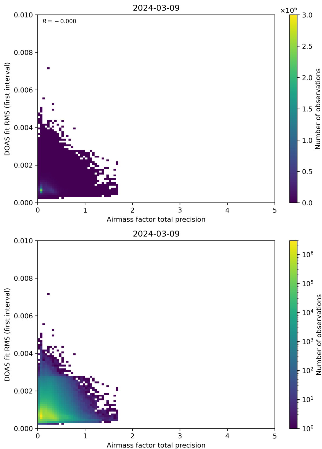
Figure 105: Scatter density plot of “Airmass factor total precision” against “DOAS fit RMS (first interval)” for 2024-03-09 to 2024-03-10.
