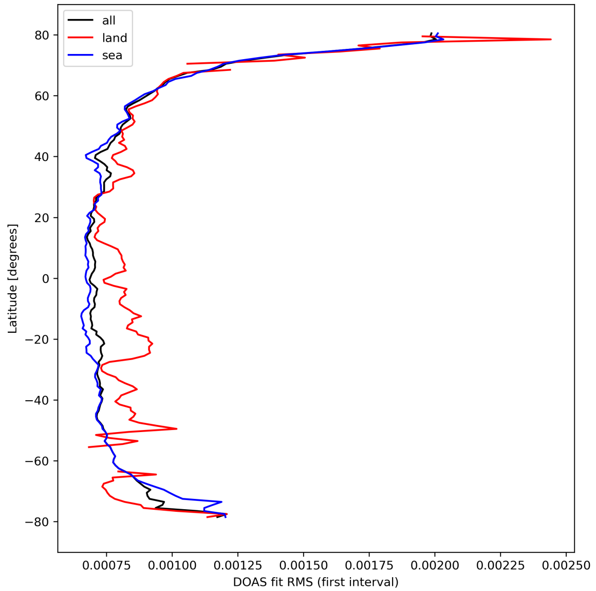
Figure 32: Zonal average of “DOAS fit RMS (first interval)” for 2024-03-09 to 2024-03-10.
