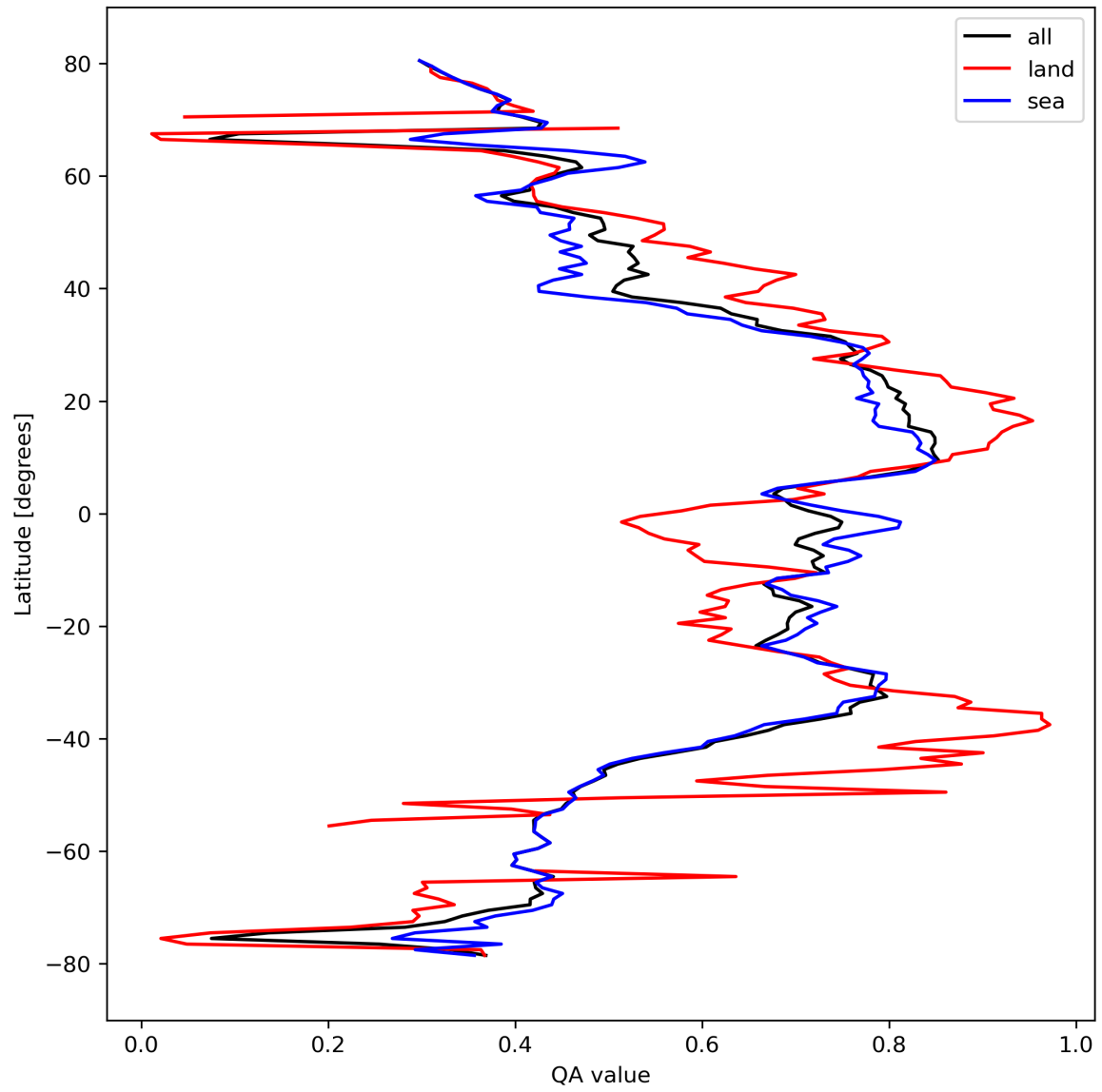
Figure 20: Zonal average of “QA value” for 2024-03-09 to 2024-03-10.
