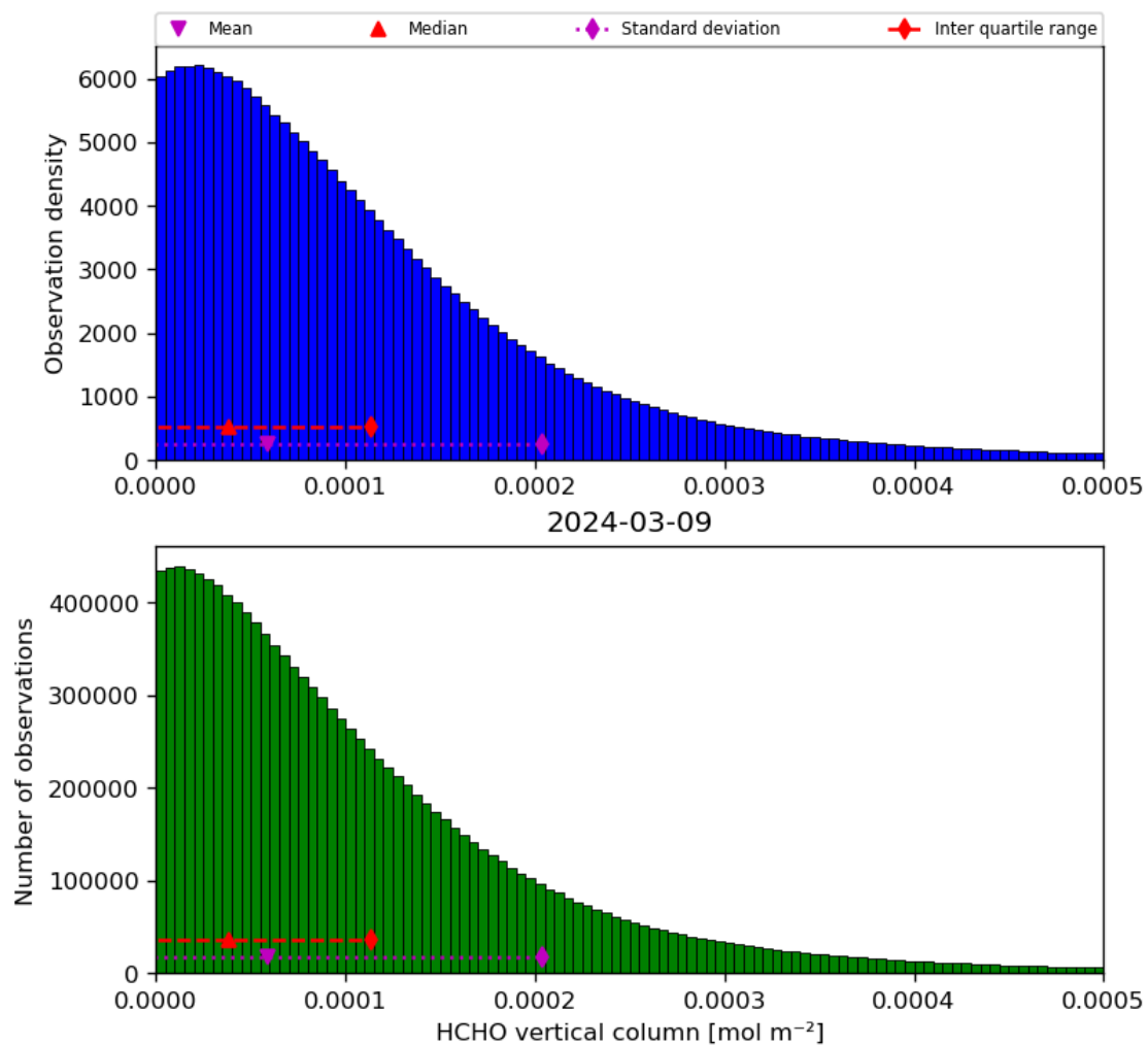
Figure 35: Histogram of “HCHO vertical column” for 2024-03-09 to 2024-03-10
