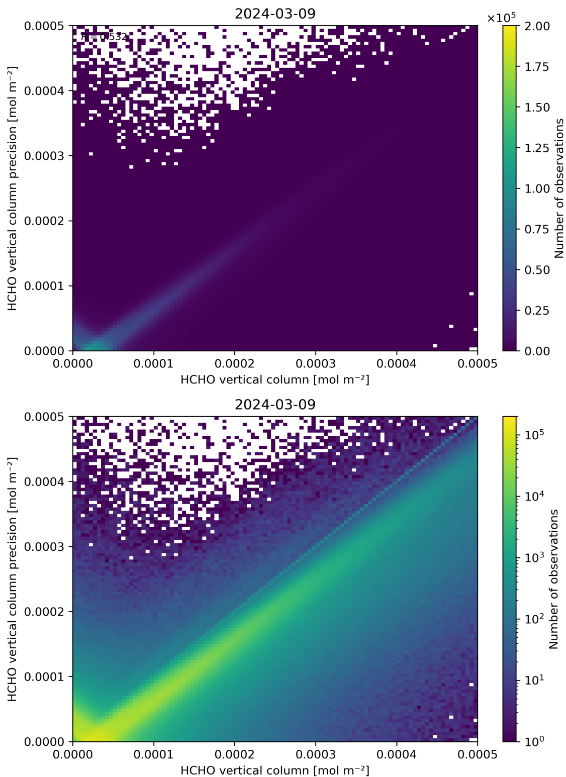
Figure 134: Scatter density plot of “HCHO vertical column” against “HCHO vertical column precision” for 2024-03-09 to 2024-03-10.
