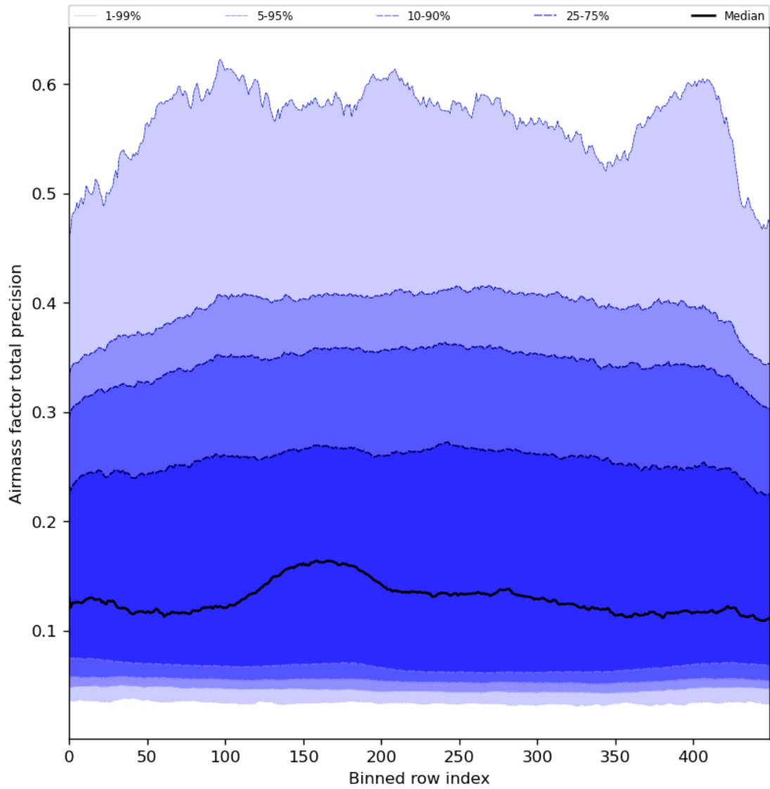
Figure 55: Along track statistics of “Airmass factor total precision” for 2024-03-09 to 2024-03-10
