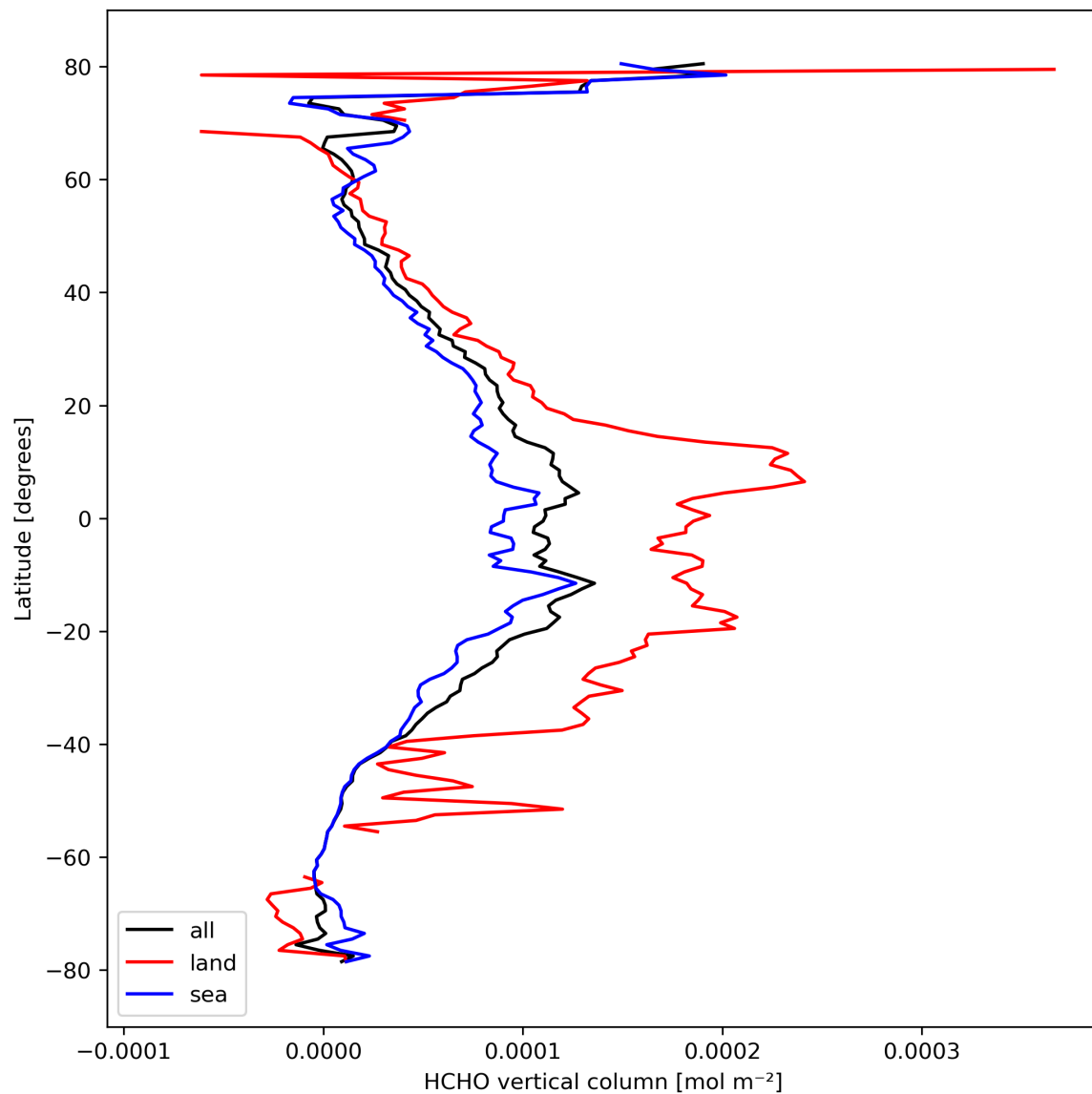
Figure 21: Zonal average of “HCHO vertical column” for 2024-03-09 to 2024-03-10.
