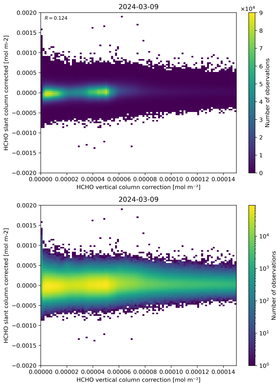
Figure 116: Scatter density plot of “HCHO vertical column correction” against “HCHO slant column corrected” for 2024-03-09 to 2024-03-10.
