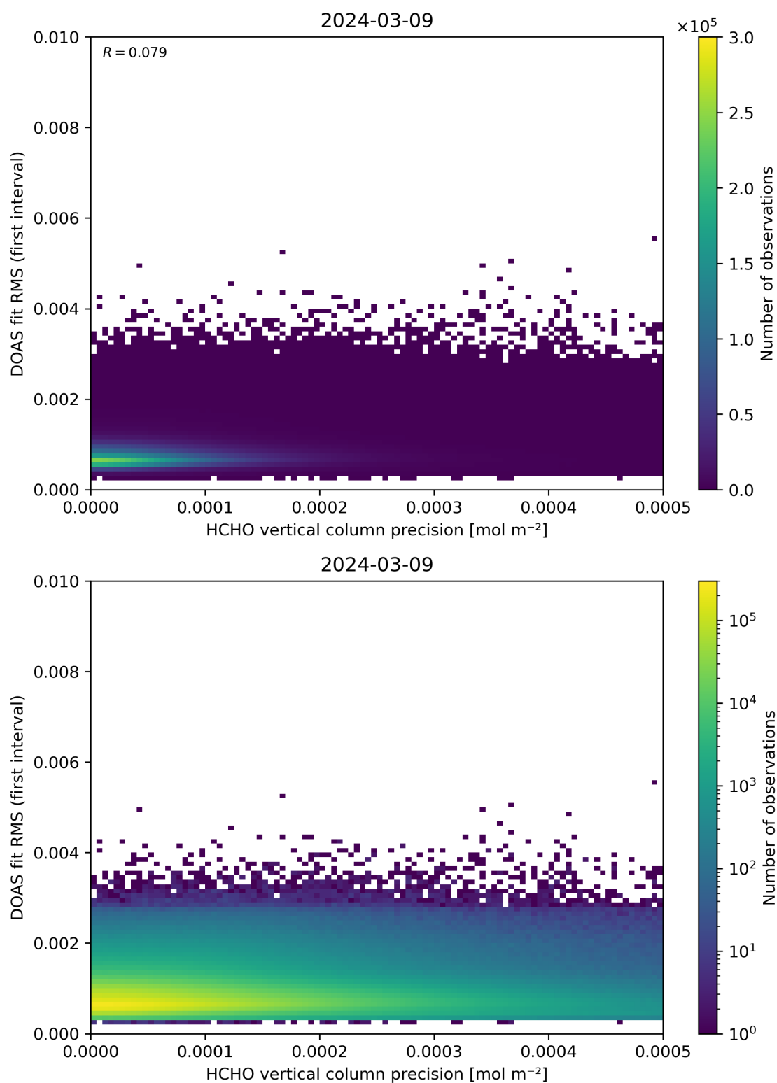
Figure 136: Scatter density plot of “HCHO vertical column precision” against “DOAS fit RMS (first interval)” for 2024-03-09 to 2024-03-10.
