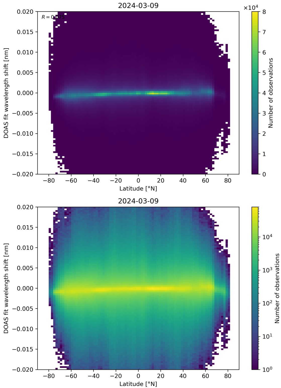
Figure 154: Scatter density plot of “Latitude” against “DOAS fit wavelength shift” for 2024-03-09 to 2024-03-10.
