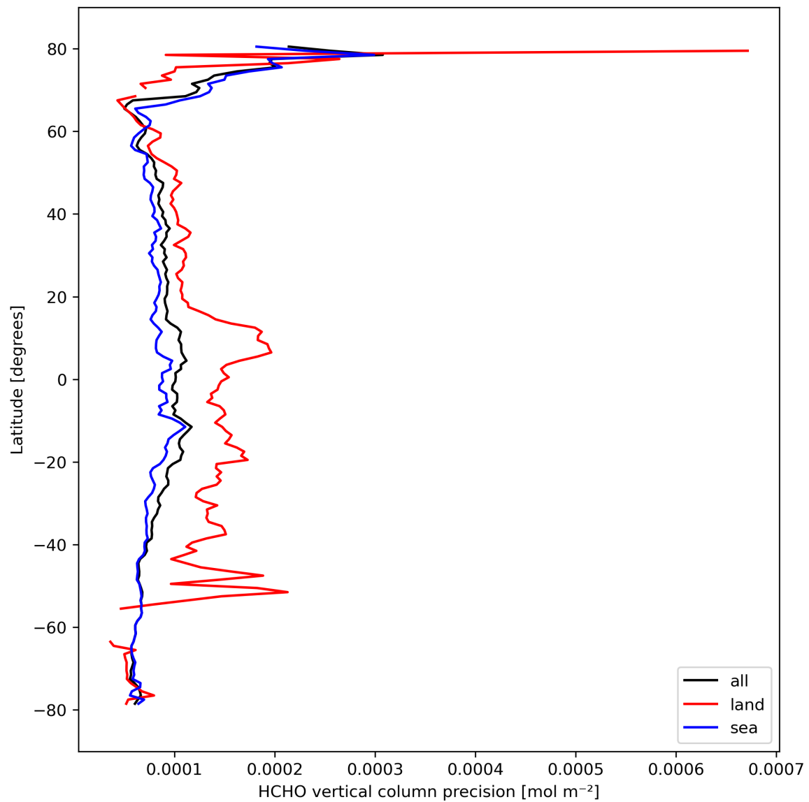
Figure 22: Zonal average of “HCHO vertical column precision” for 2024-03-09 to 2024-03-10.
