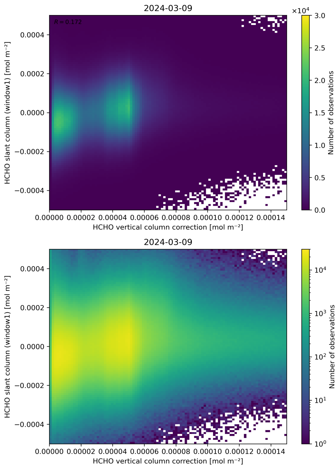
Figure 118: Scatter density plot of “HCHO vertical column correction” against “HCHO slant column (window1)” for 2024-03-09 to 2024-03-10.
