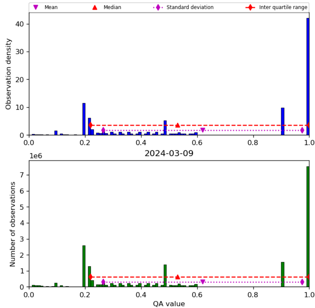
Figure 34: Histogram of “QA value” for 2024-03-09 to 2024-03-10
