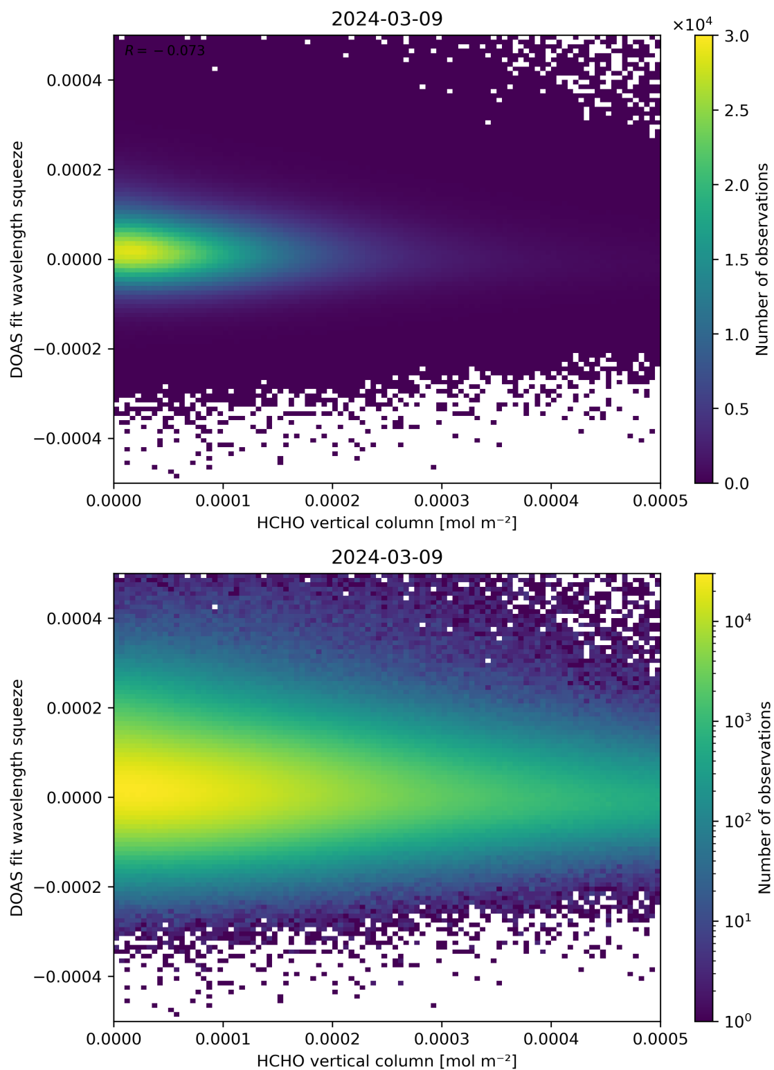
Figure 125: Scatter density plot of “HCHO vertical column” against “DOAS fit wavelength squeeze” for 2024-03-09 to 2024-03-10.
