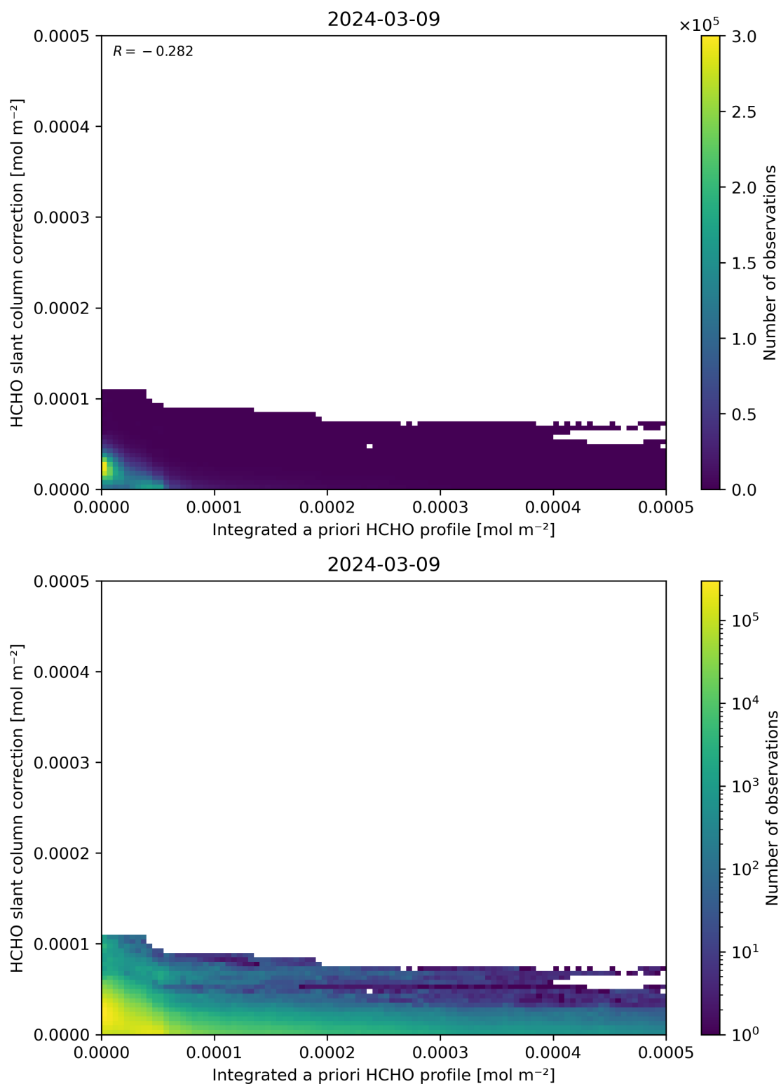
Figure 152: Scatter density plot of “Integrated a priori HCHO profile” against “HCHO slant column correction” for 2024-03-09 to 2024-03-10.
