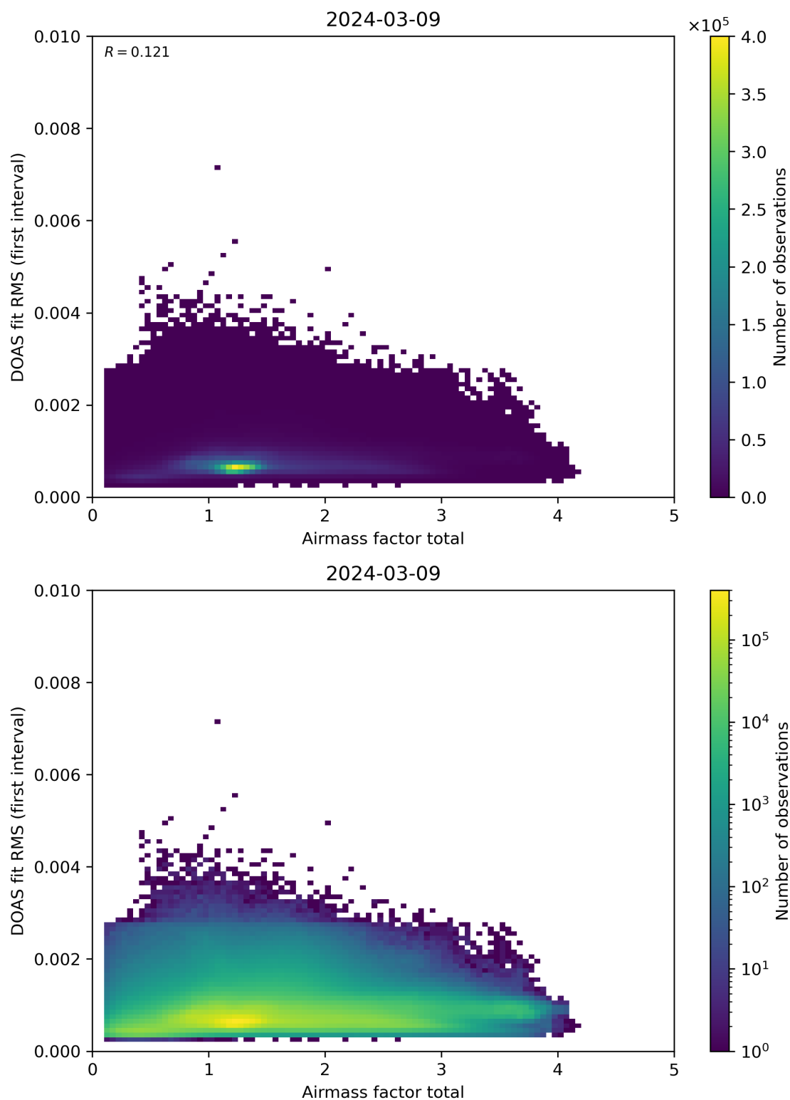
Figure 97: Scatter density plot of “Airmass factor total” against “DOAS fit RMS (first interval)” for 2024-03-09 to 2024-03-10.
