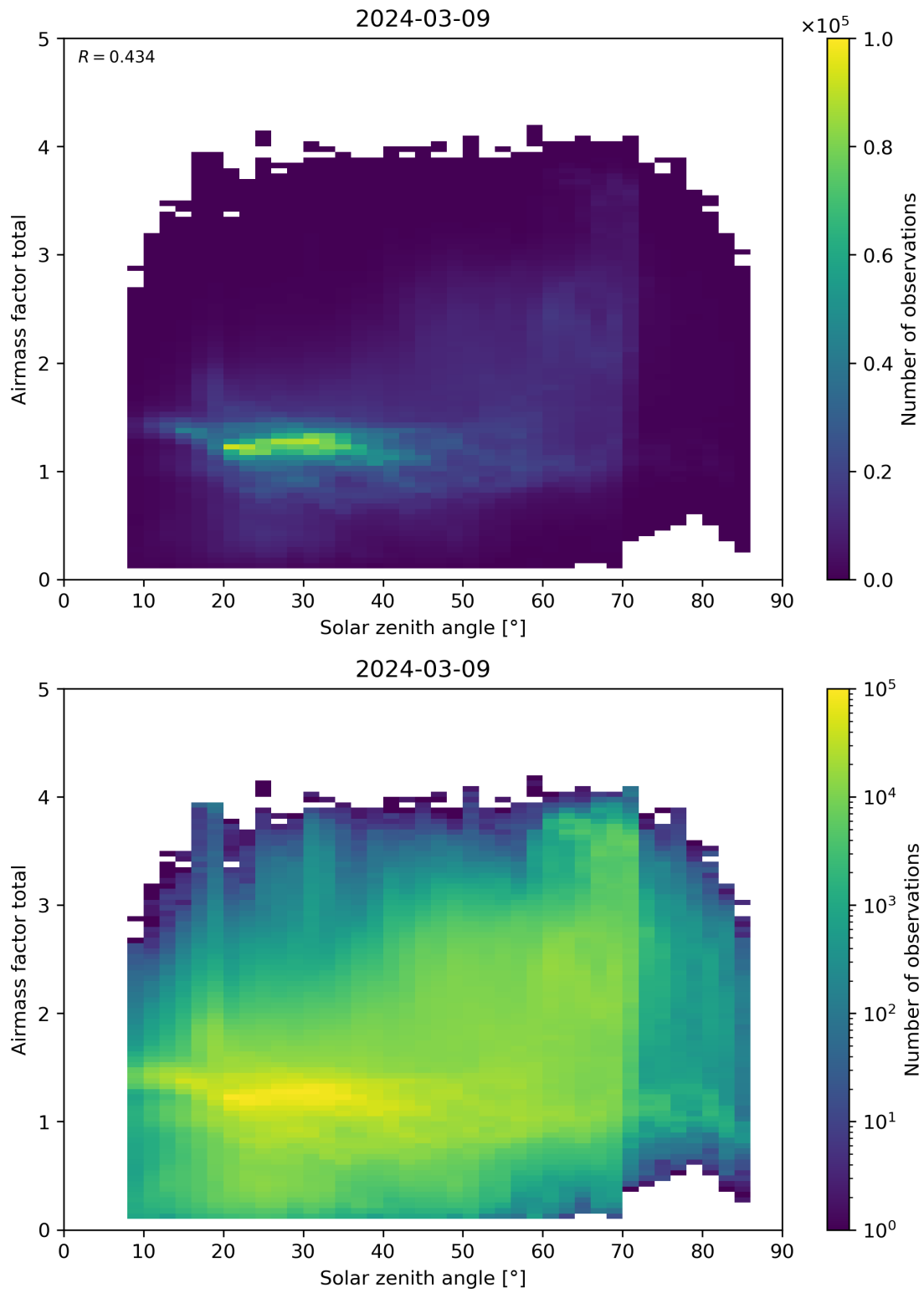
Figure 175: Scatter density plot of “Solar zenith angle” against “Airmass factor total” for 2024-03-09 to 2024-03-10.
