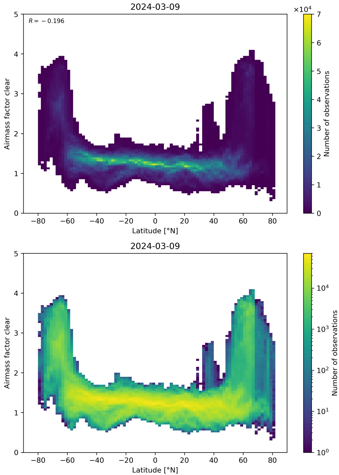
Figure 156: Scatter density plot of “Latitude” against “Airmass factor clear” for 2024-03-09 to 2024-03-10.
