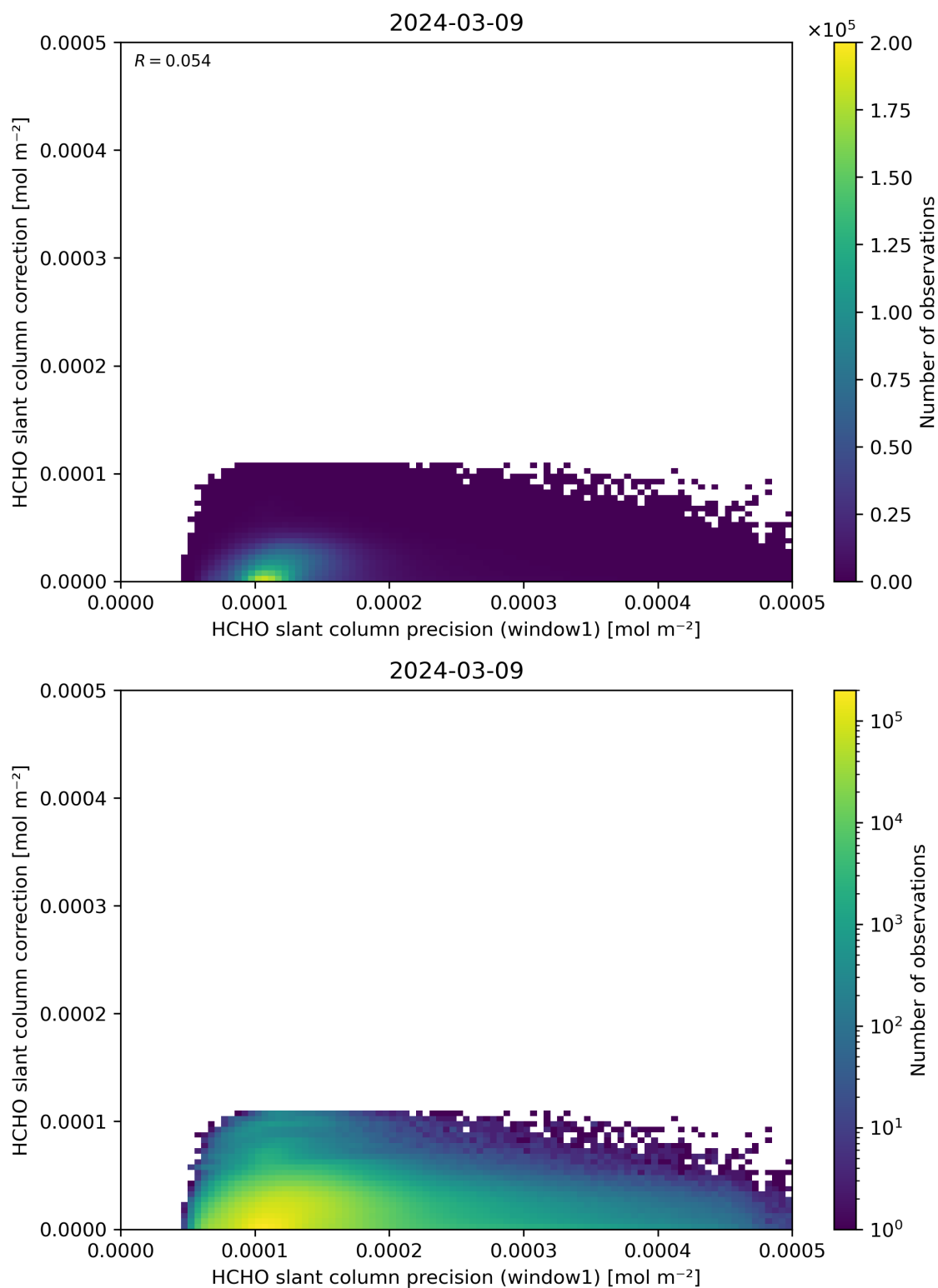
Figure 93: Scatter density plot of “HCHO slant column precision (window1)” against “HCHO slant column correction” for 2024-03-09 to 2024-03-10.
