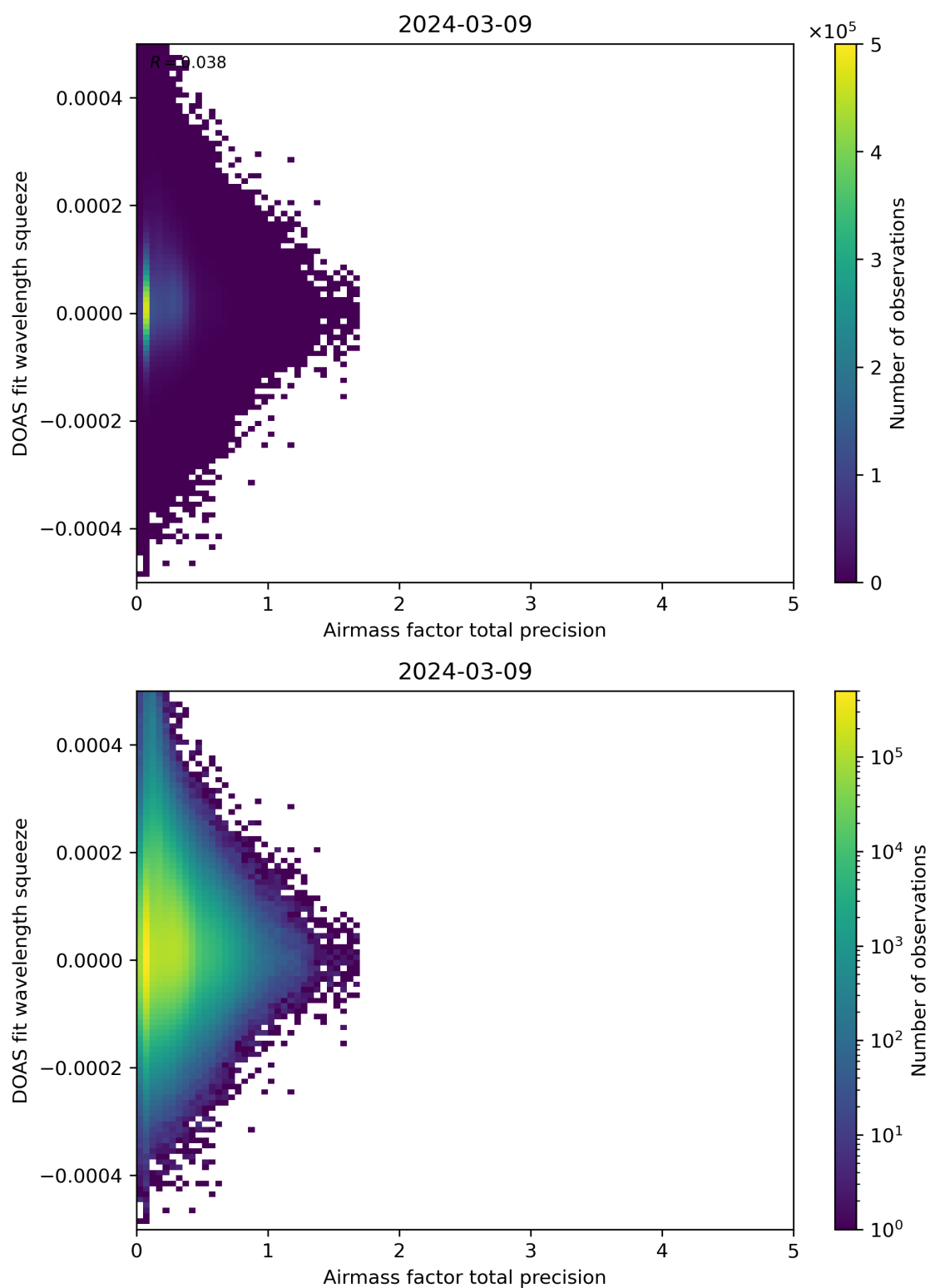
Figure 107: Scatter density plot of “Airmass factor total precision” against “DOAS fit wavelength squeeze” for 2024-03-09 to 2024-03-10.
