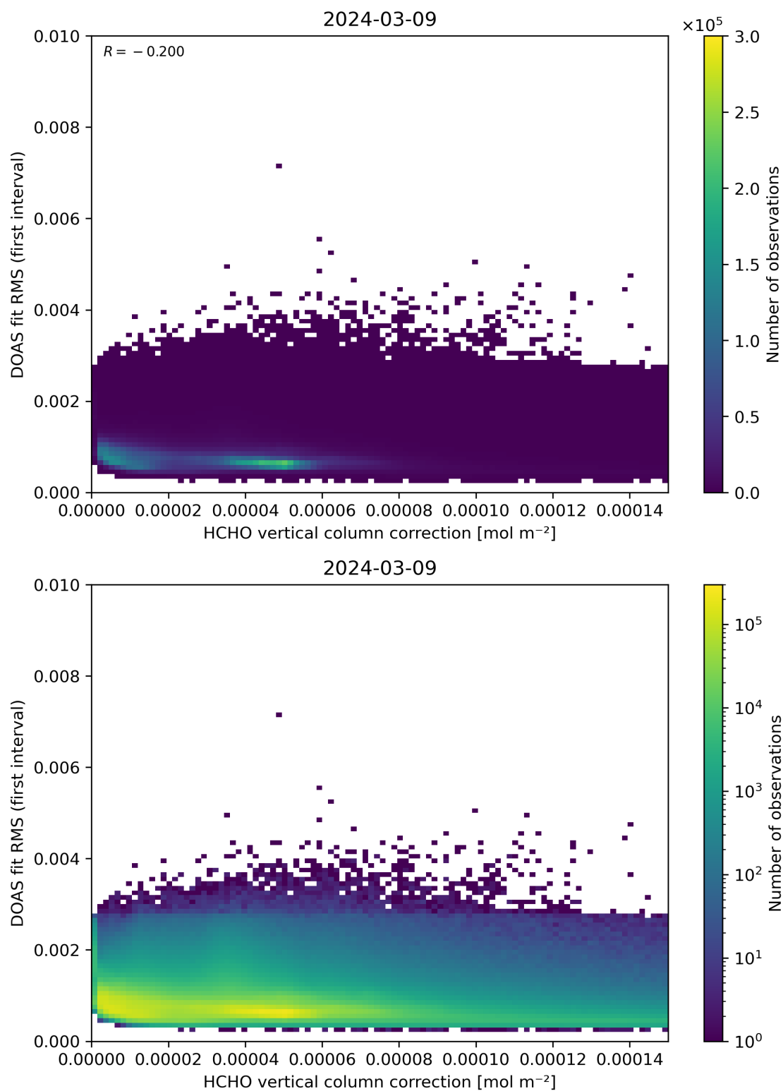
Figure 112: Scatter density plot of “HCHO vertical column correction” against “DOAS fit RMS (first interval)” for 2024-03-09 to 2024-03-10.
