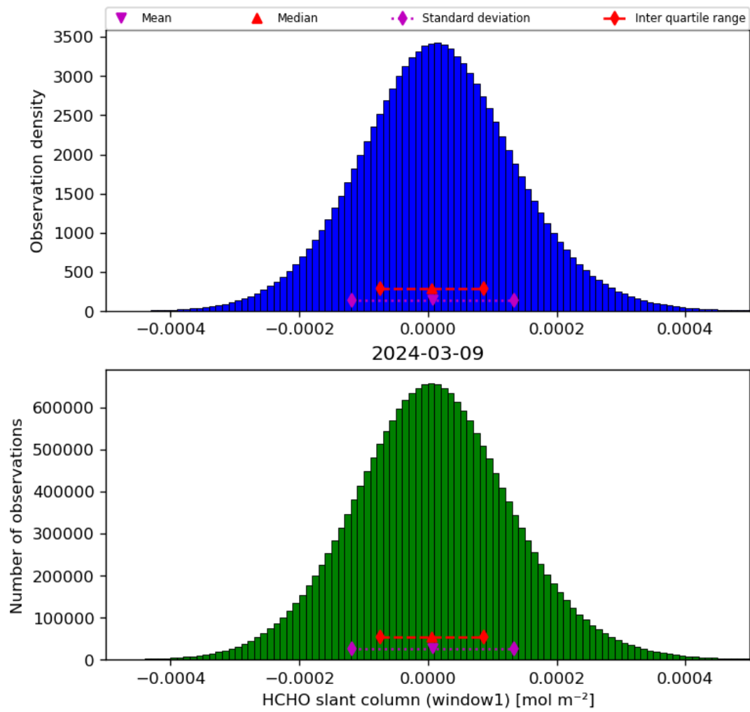
Figure 38: Histogram of “HCHO slant column (window1)” for 2024-03-09 to 2024-03-10
