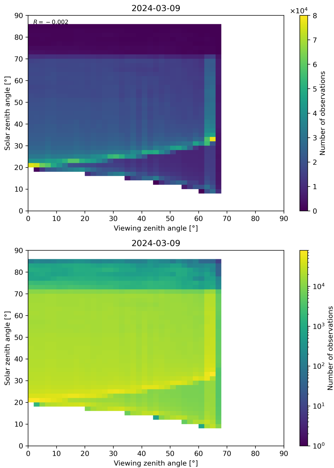
Figure 197: Scatter density plot of “Viewing zenith angle” against “Solar zenith angle” for 2024-03-09 to 2024-03-10.
