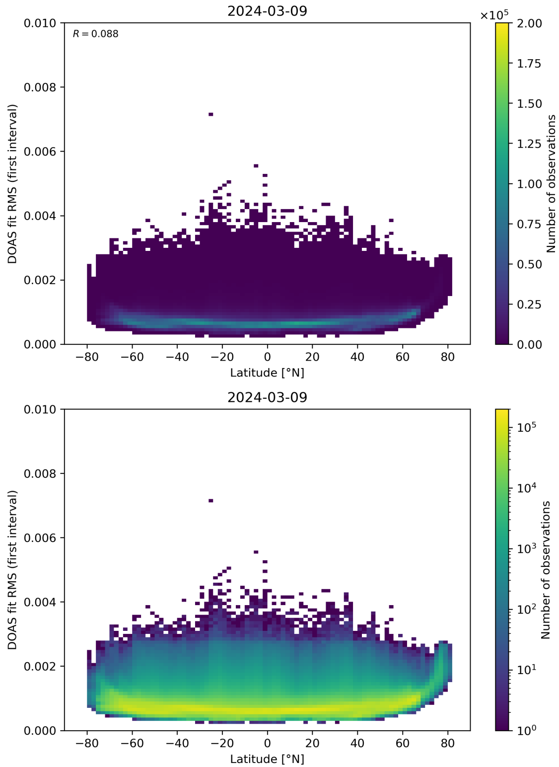
Figure 153: Scatter density plot of “Latitude” against “DOAS fit RMS (first interval)” for 2024-03-09 to 2024-03-10.
