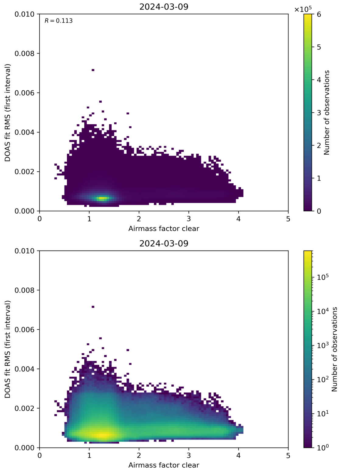
Figure 71: Scatter density plot of “Airmass factor clear” against “DOAS fit RMS (first interval)” for 2024-03-09 to 2024-03-10.
