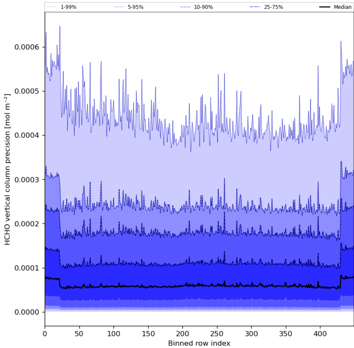
Figure 50: Along track statistics of “HCHO vertical column precision” for 2024-03-09 to 2024-03-10
