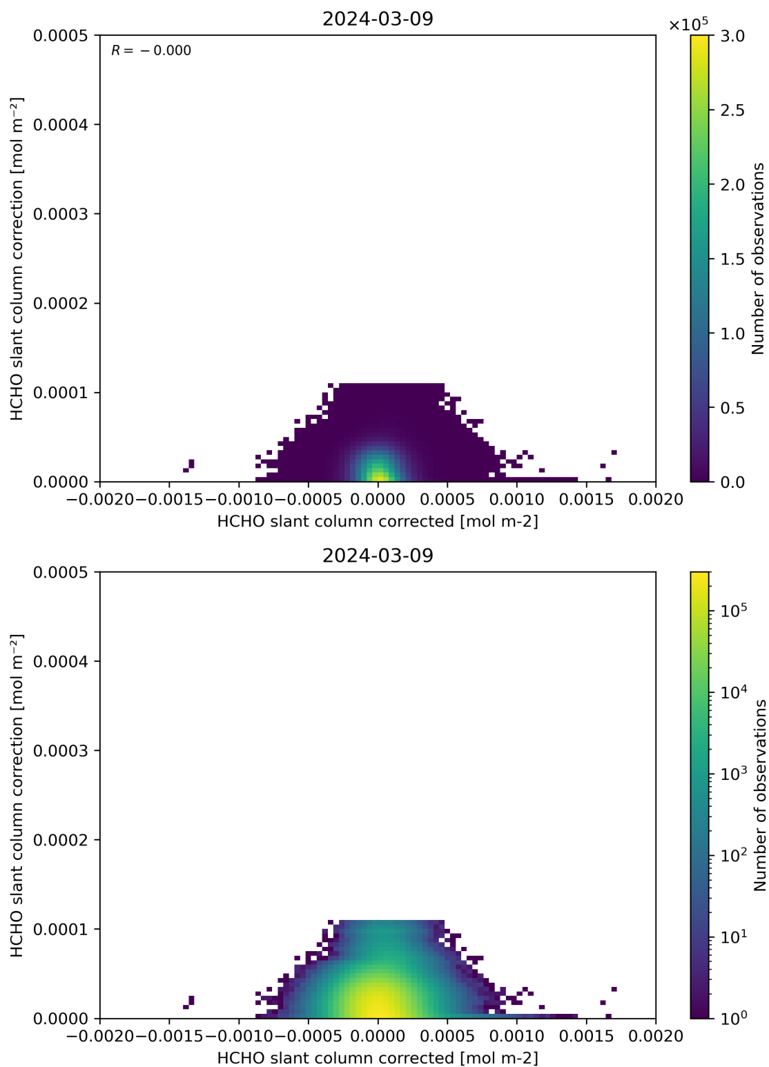
Figure 77: Scatter density plot of “HCHO slant column corrected” against “HCHO slant column correction” for 2024-03-09 to 2024-03-10.
