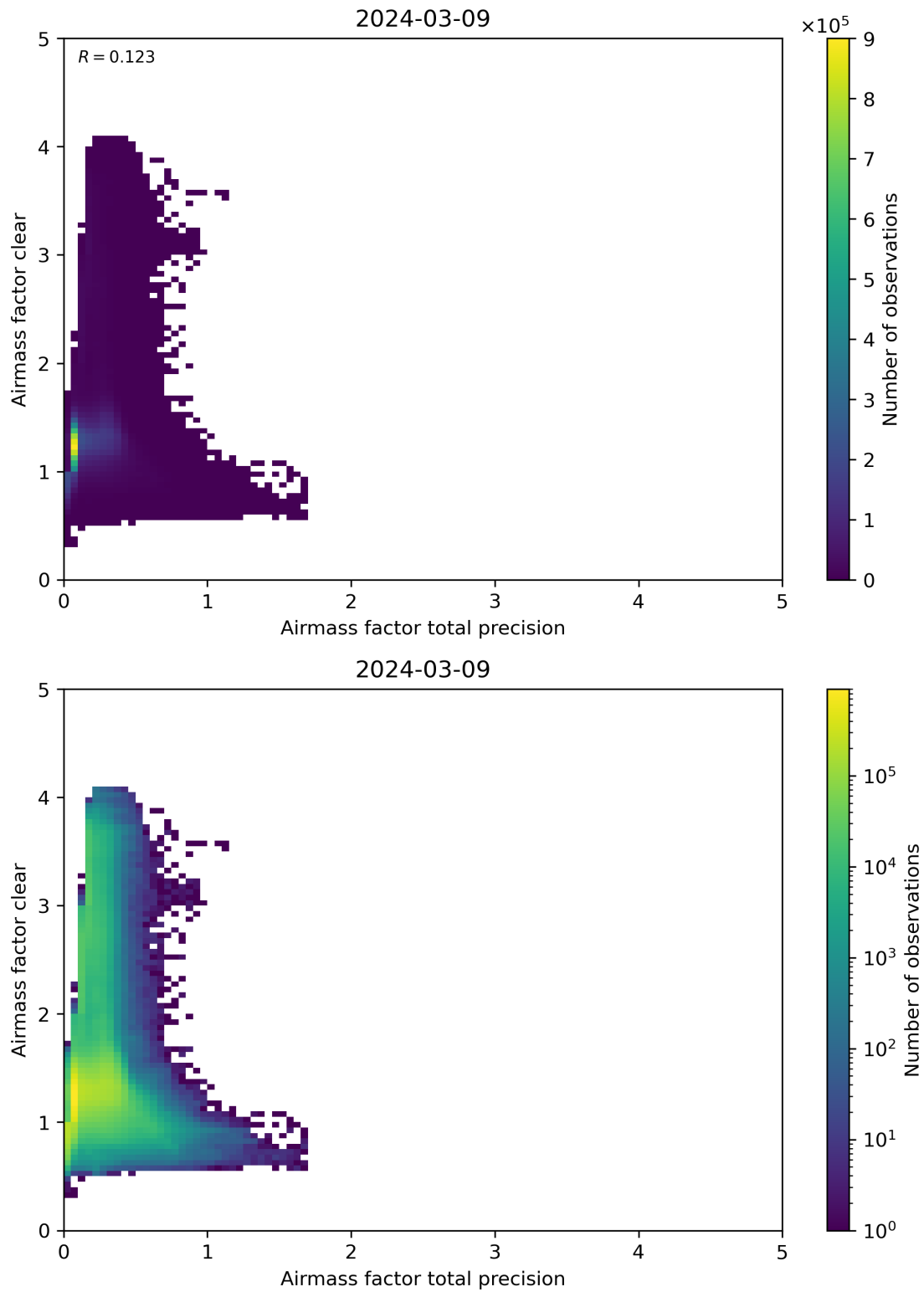
Figure 108: Scatter density plot of “Airmass factor total precision” against “Airmass factor clear” for 2024-03-09 to 2024-03-10.
