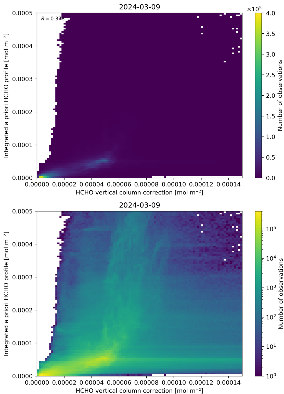
Figure 122: Scatter density plot of “HCHO vertical column correction” against “Integrated a priori HCHO profile” for 2024-03-09 to 2024-03-10.
