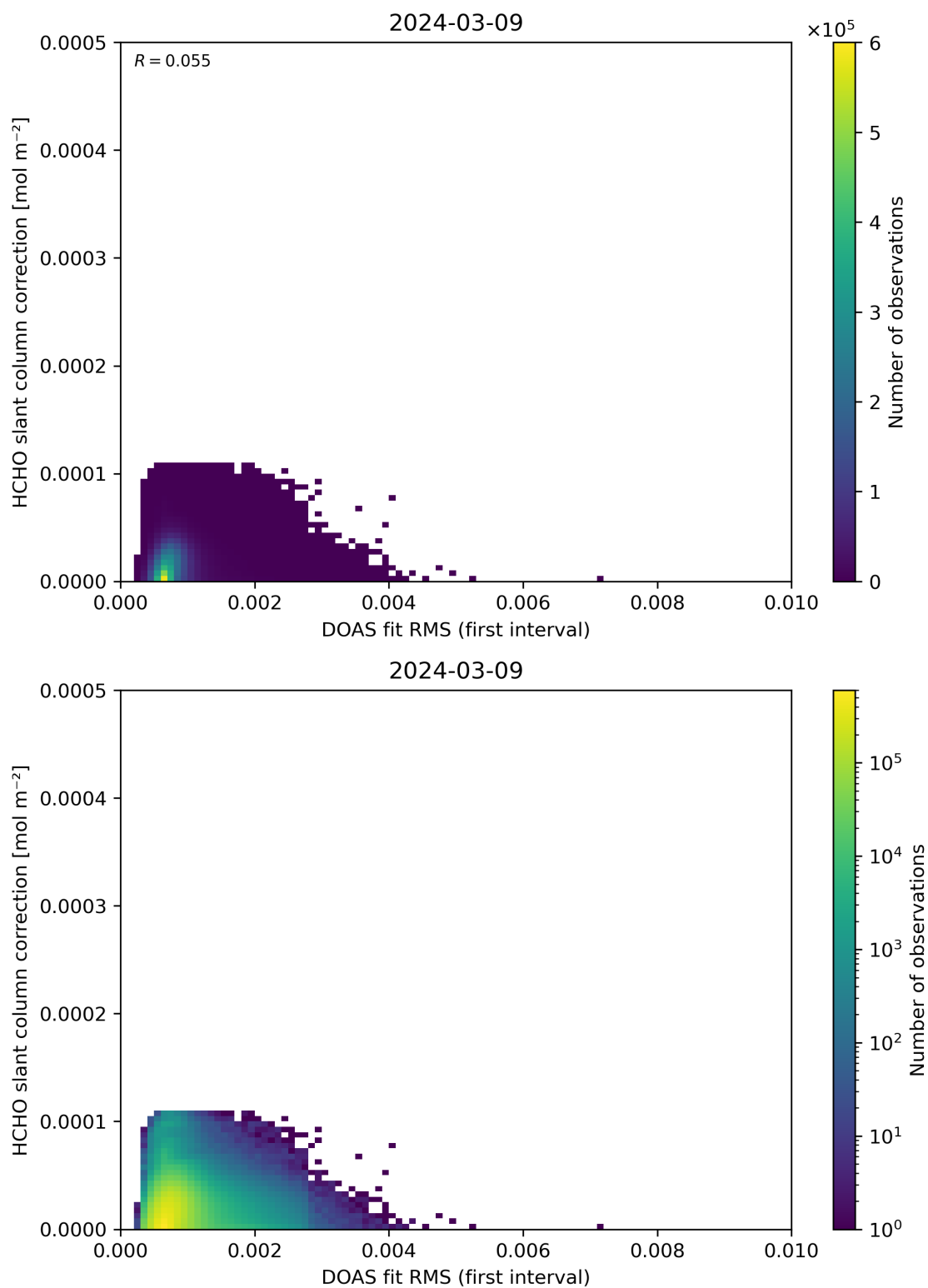
Figure 63: Scatter density plot of “DOAS fit RMS (first interval)” against “HCHO slant column correction” for 2024-03-09 to 2024-03-10.
