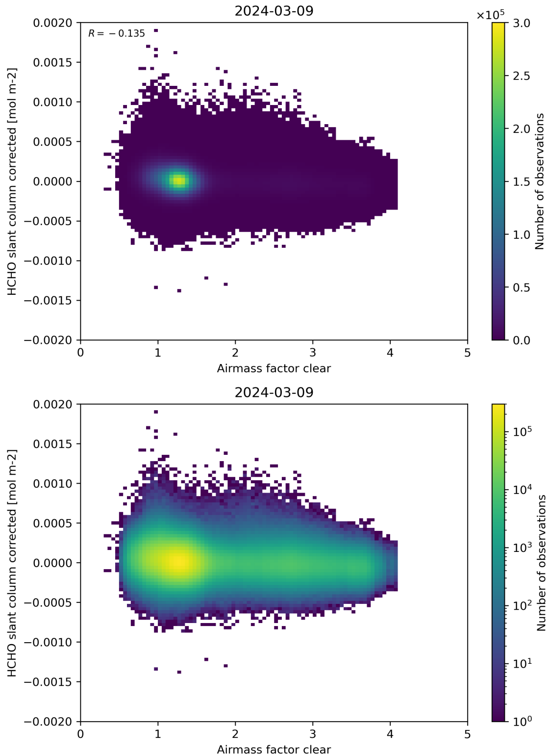
Figure 74: Scatter density plot of “Airmass factor clear” against “HCHO slant column corrected” for 2024-03-09 to 2024-03-10.
