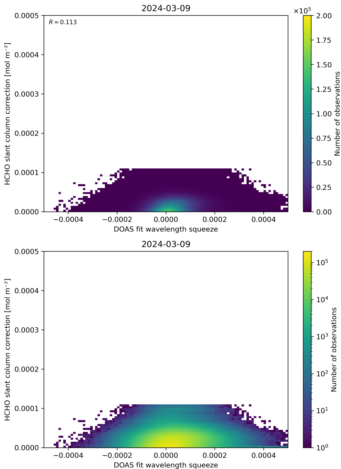
Figure 70: Scatter density plot of “DOAS fit wavelength squeeze” against “HCHO slant column correction” for 2024-03-09 to 2024-03-10.
