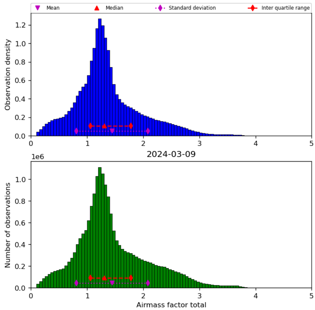
Figure 40: Histogram of “Airmass factor total” for 2024-03-09 to 2024-03-10
