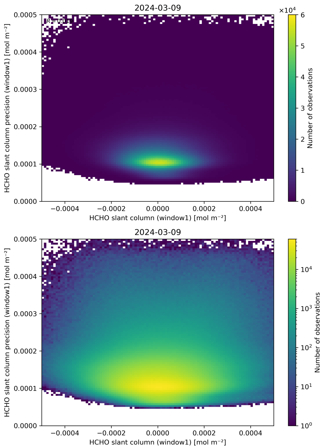
Figure 84: Scatter density plot of “HCHO slant column (window1)” against “HCHO slant column precision (window1)” for 2024-03-09 to 2024-03-10.
