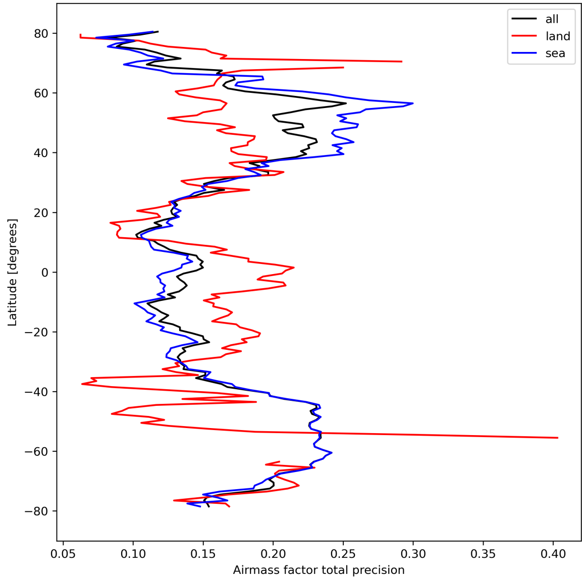
Figure 27: Zonal average of “Airmass factor total precision” for 2024-03-09 to 2024-03-10.
