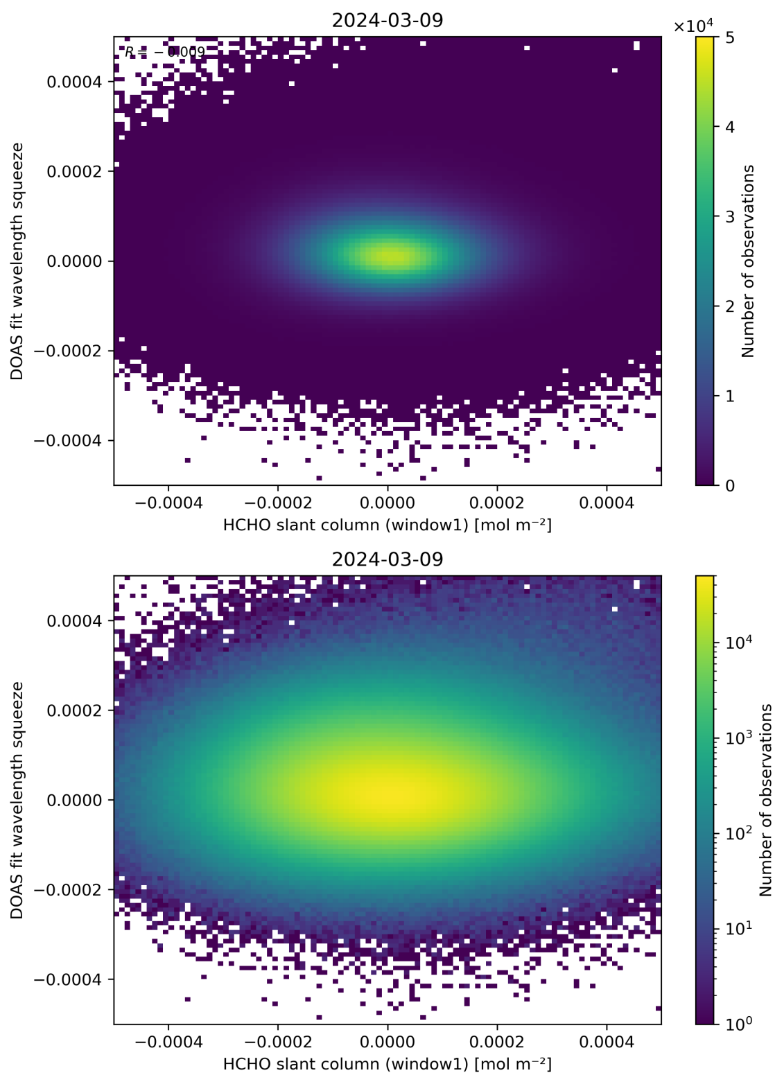
Figure 80: Scatter density plot of “HCHO slant column (window1)” against “DOAS fit wavelength squeeze” for 2024-03-09 to 2024-03-10.
