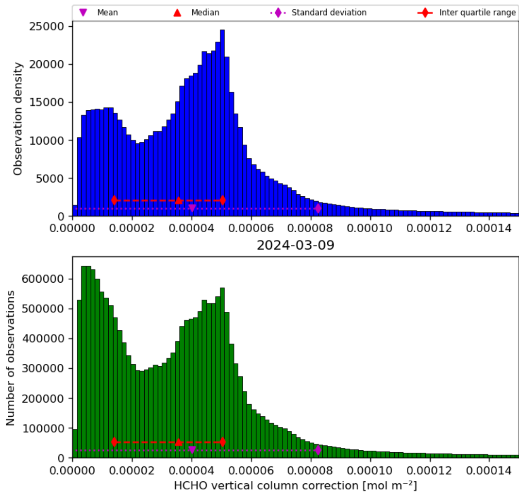
Figure 37: Histogram of “HCHO vertical column correction” for 2024-03-09 to 2024-03-10
