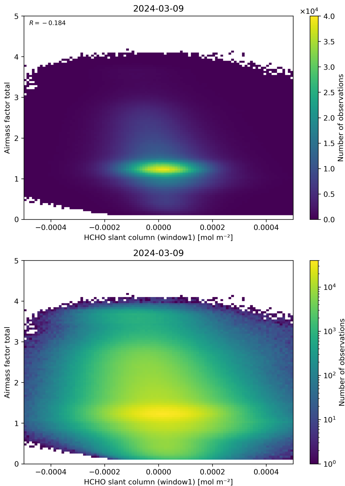
Figure 85: Scatter density plot of “HCHO slant column (window1)” against “Airmass factor total” for 2024-03-09 to 2024-03-10.
