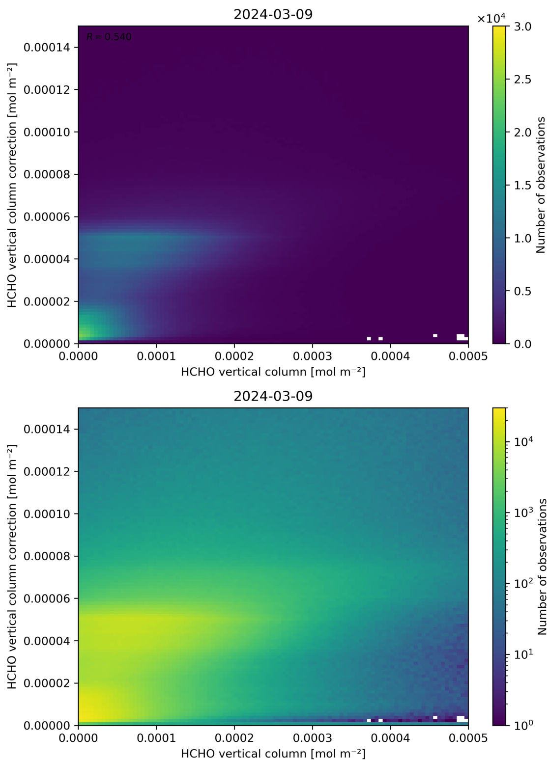
Figure 133: Scatter density plot of “HCHO vertical column” against “HCHO vertical column correction” for 2024-03-09 to 2024-03-10.
