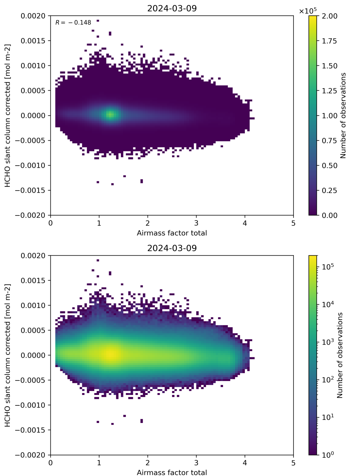
Figure 101: Scatter density plot of “Airmass factor total” against “HCHO slant column corrected” for 2024-03-09 to 2024-03-10.
