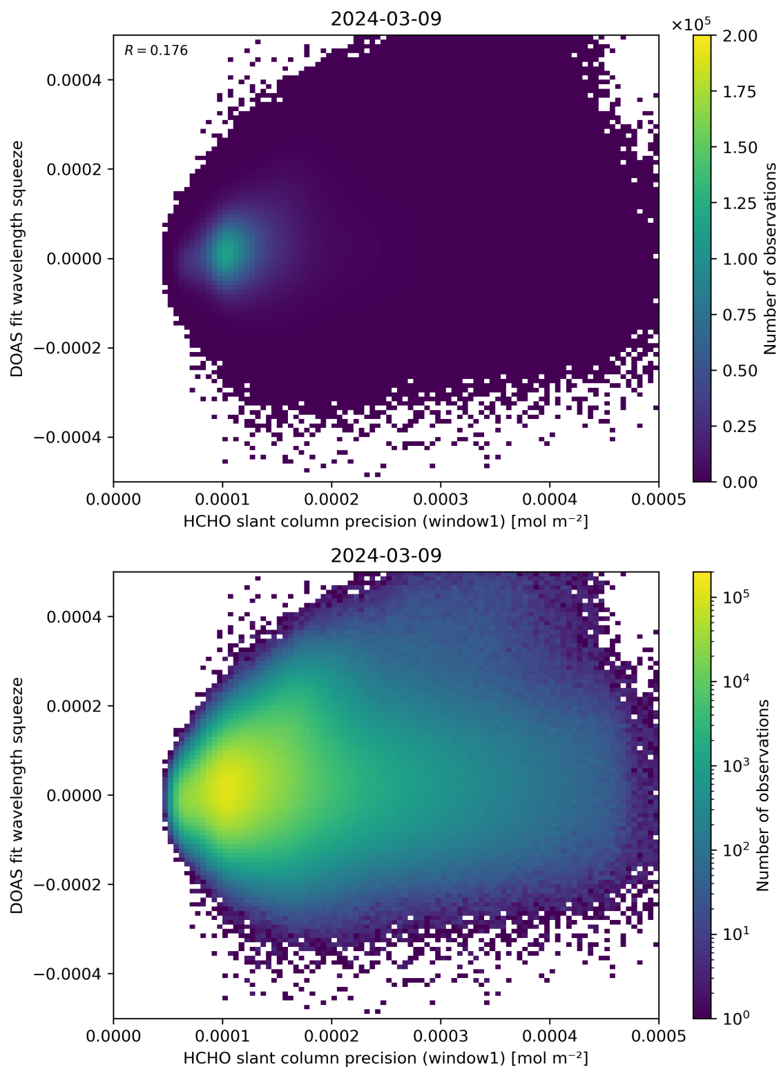
Figure 90: Scatter density plot of “HCHO slant column precision (window1)” against “DOAS fit wavelength squeeze” for 2024-03-09 to 2024-03-10.
