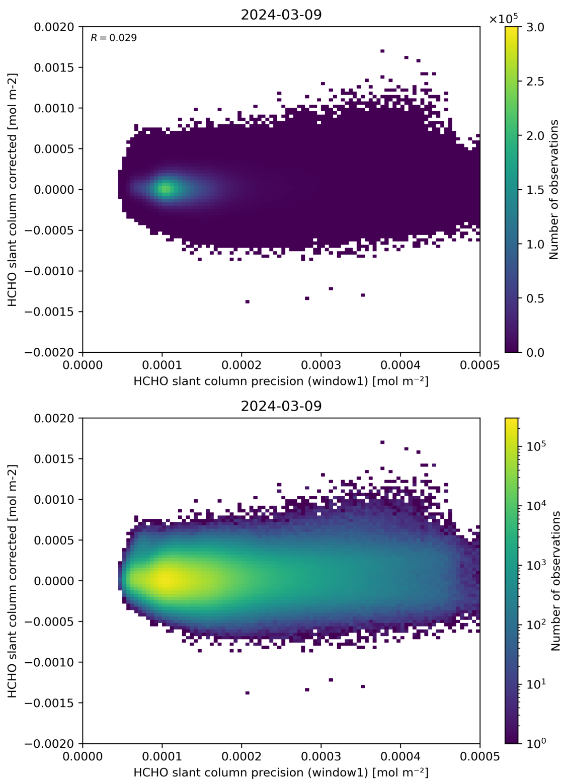
Figure 92: Scatter density plot of “HCHO slant column precision (window1)” against “HCHO slant column corrected” for 2024-03-09 to 2024-03-10.
