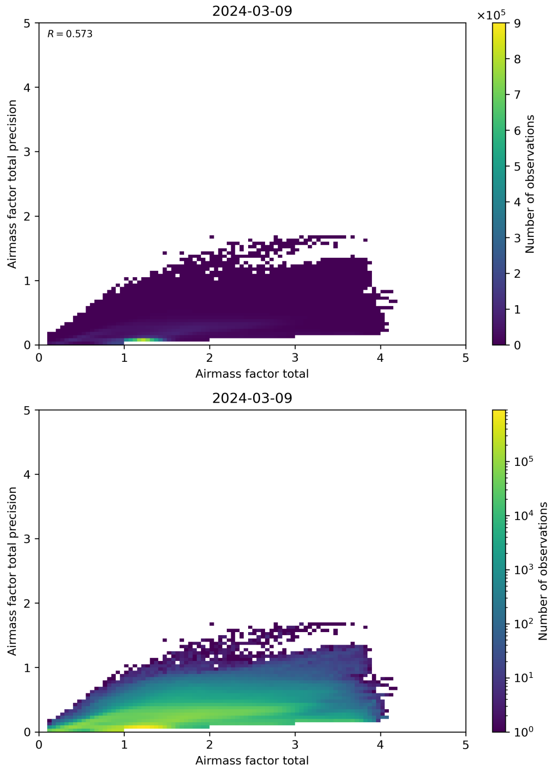
Figure 103: Scatter density plot of “Airmass factor total” against “Airmass factor total precision” for 2024-03-09 to 2024-03-10.
