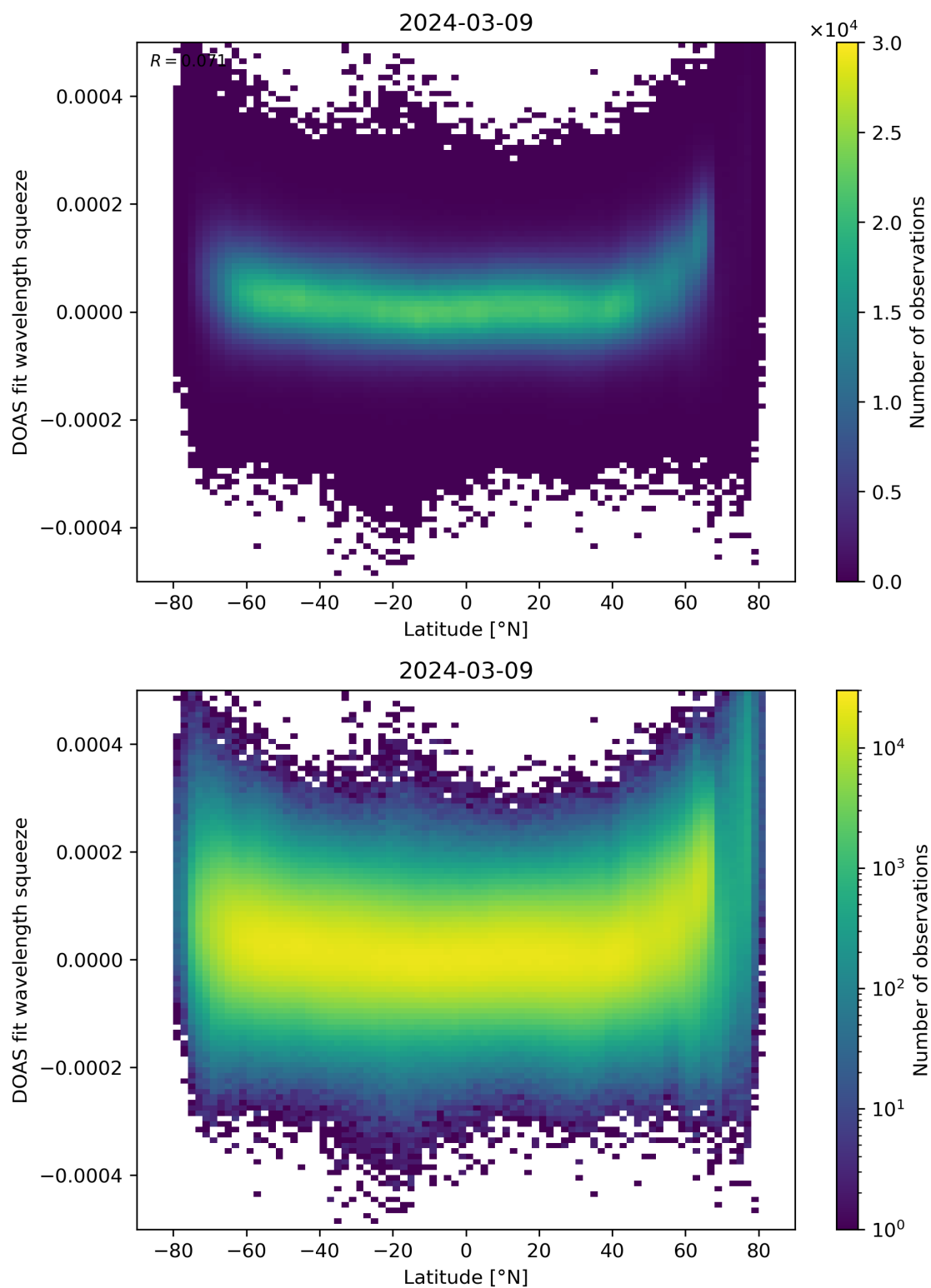
Figure 155: Scatter density plot of “Latitude” against “DOAS fit wavelength squeeze” for 2024-03-09 to 2024-03-10.
