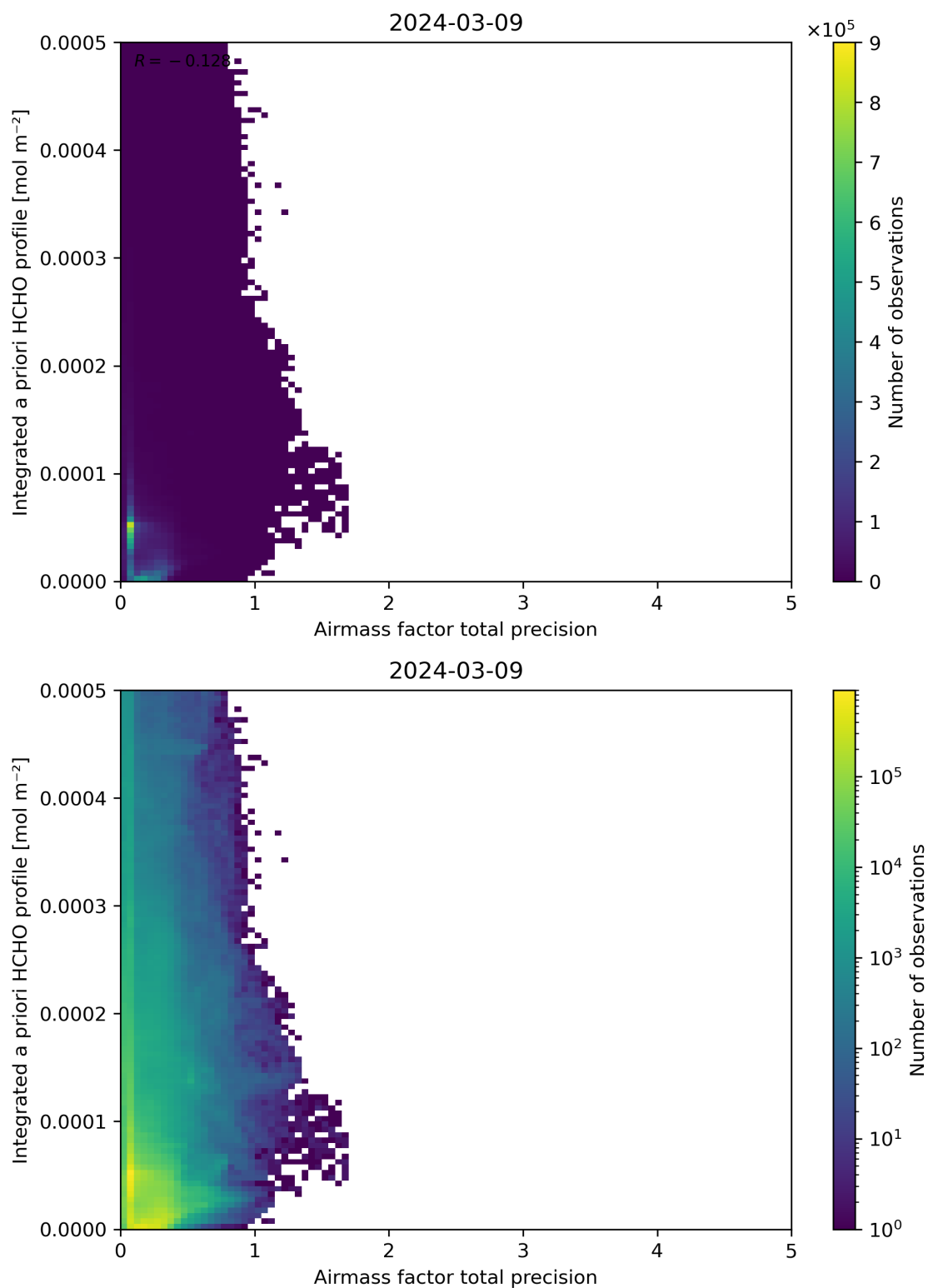
Figure 111: Scatter density plot of “Airmass factor total precision” against “Integrated a priori HCHO profile” for 2024-03-09 to 2024-03-10.
