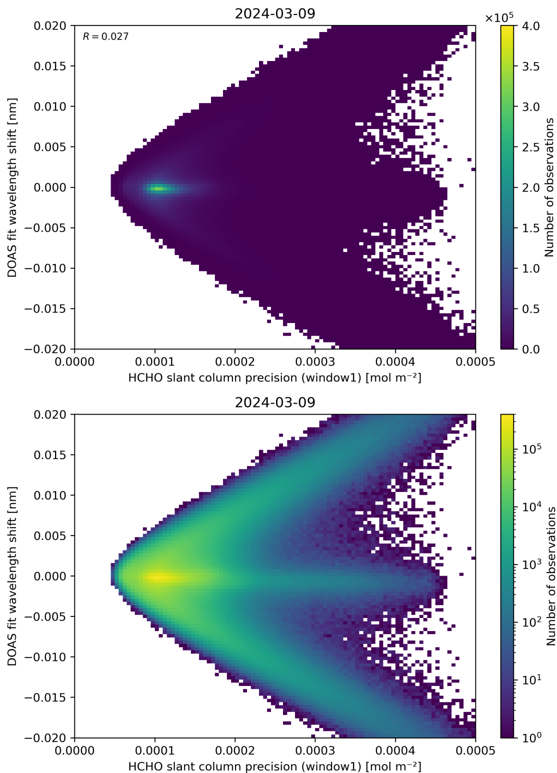
Figure 89: Scatter density plot of “HCHO slant column precision (window1)” against “DOAS fit wavelength shift” for 2024-03-09 to 2024-03-10.
