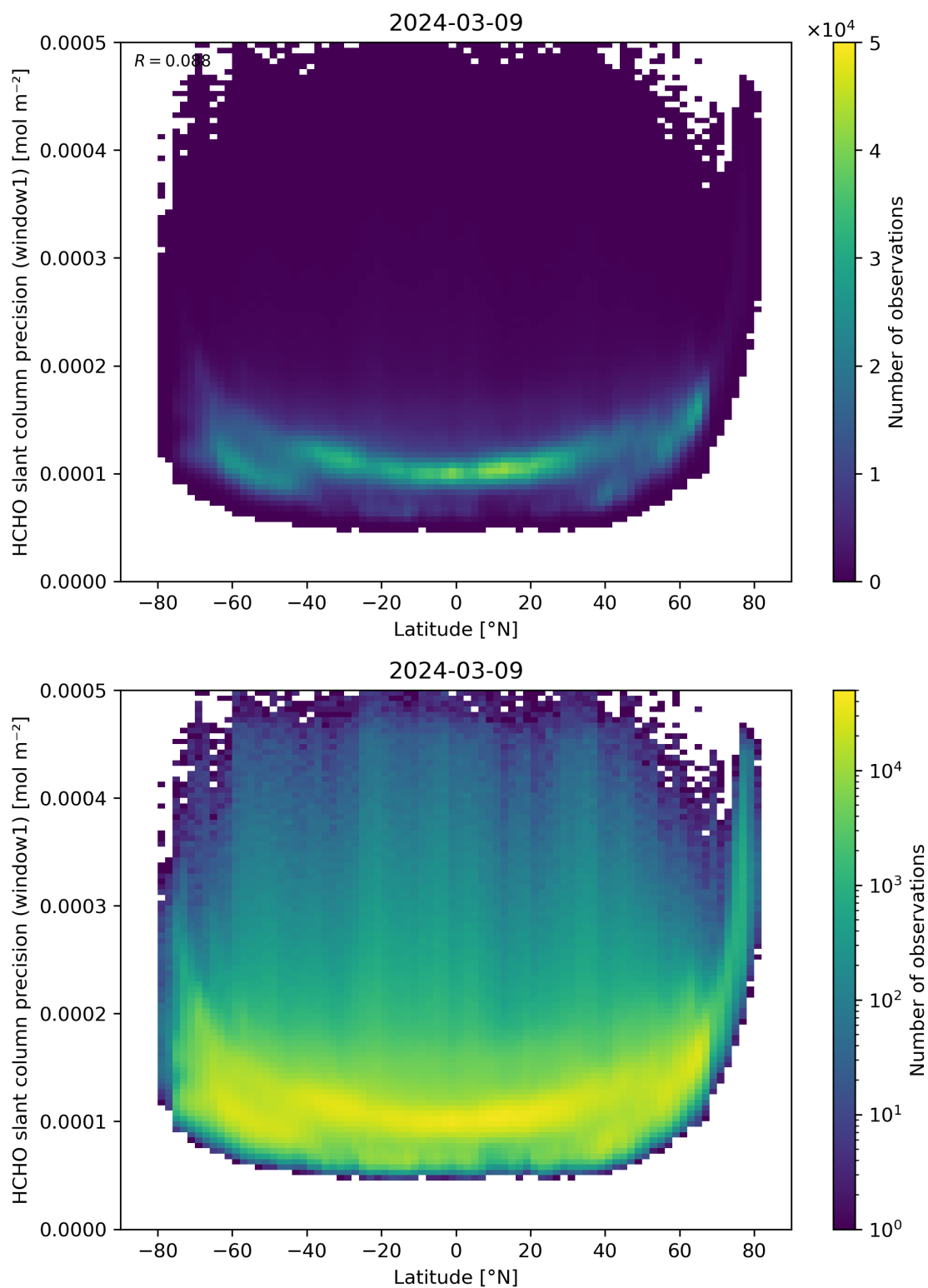
Figure 160: Scatter density plot of “Latitude” against “HCHO slant column precision (window1)” for 2024-03-09 to 2024-03-10.
