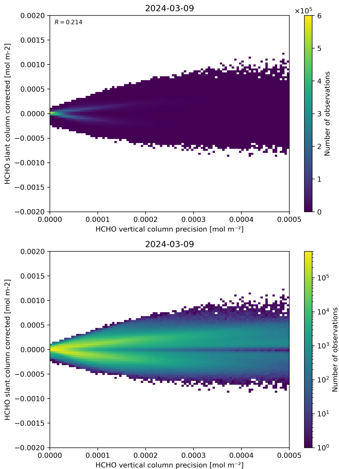
Figure 140: Scatter density plot of “HCHO vertical column precision” against “HCHO slant column corrected” for 2024-03-09 to 2024-03-10.
