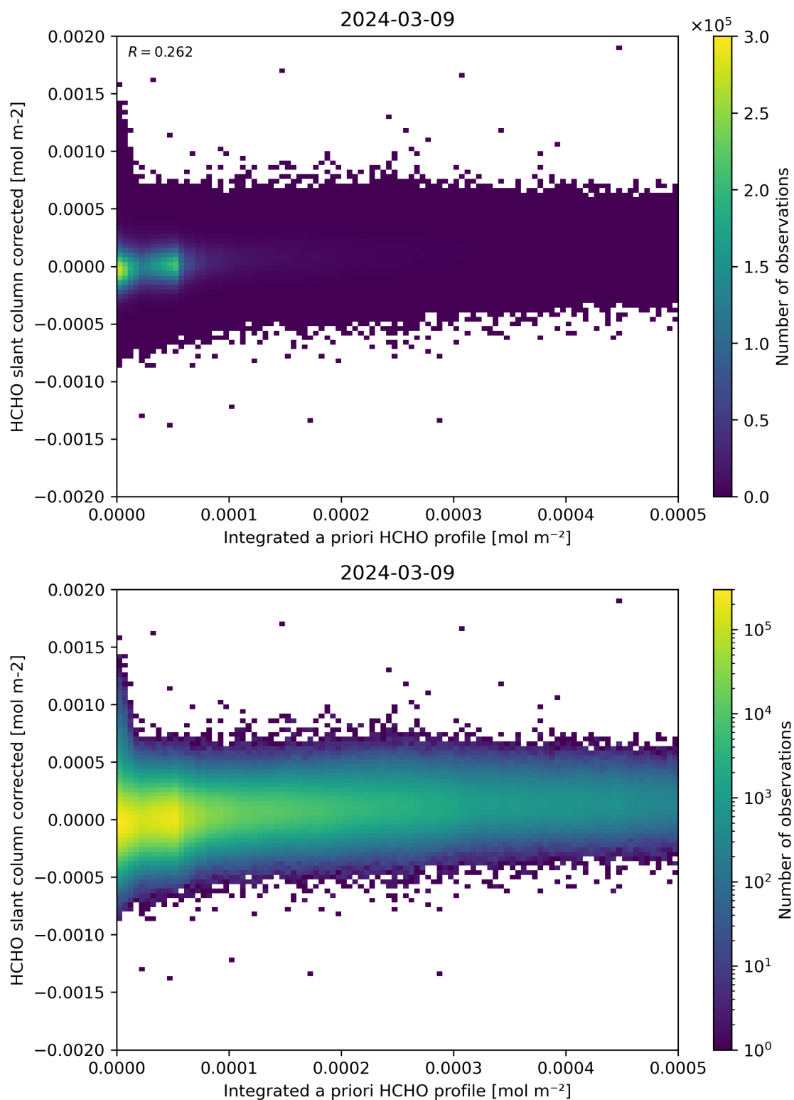
Figure 151: Scatter density plot of “Integrated a priori HCHO profile” against “HCHO slant column corrected” for 2024-03-09 to 2024-03-10.
