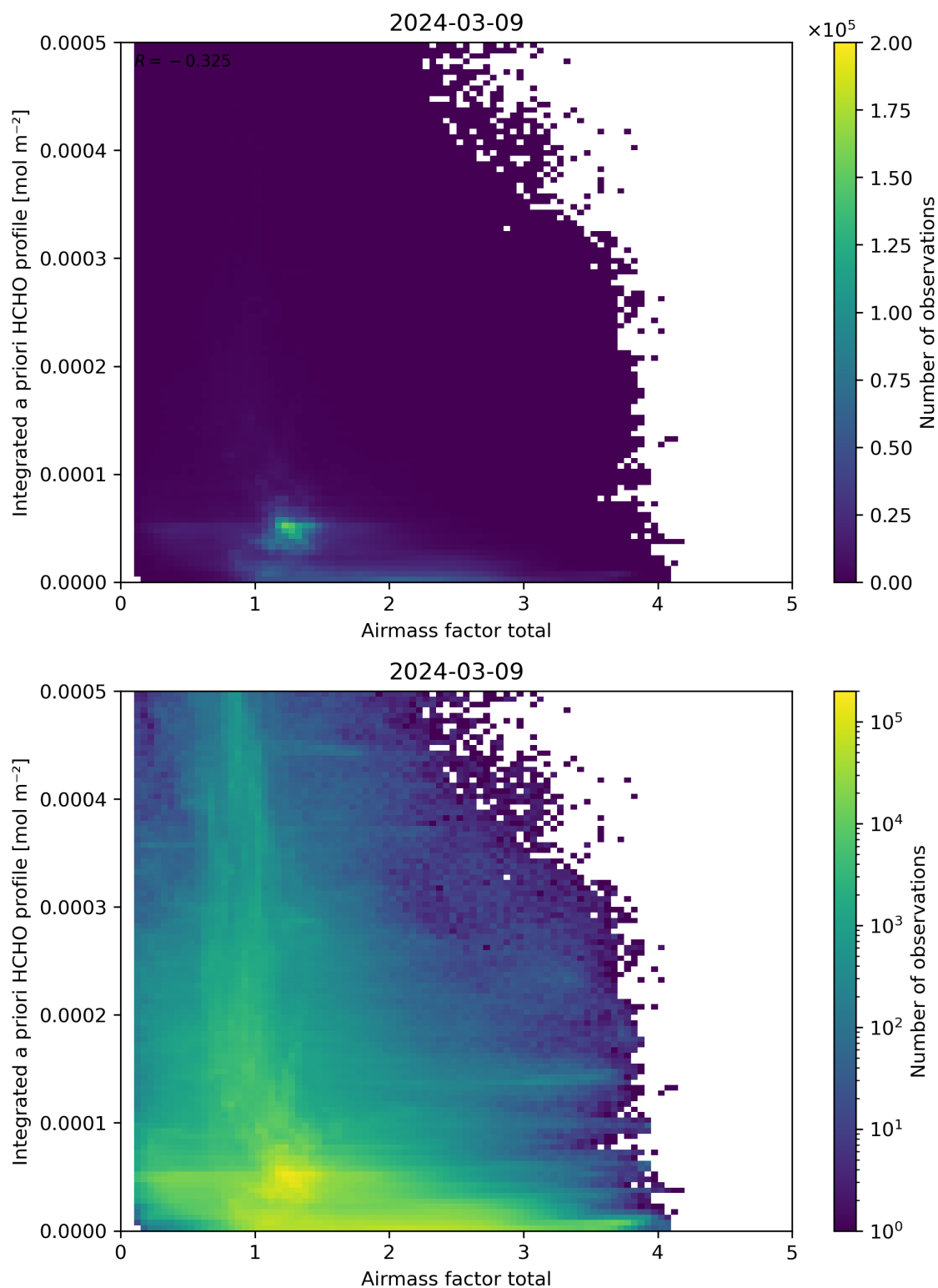
Figure 104: Scatter density plot of “Airmass factor total” against “Integrated a priori HCHO profile” for 2024-03-09 to 2024-03-10.
