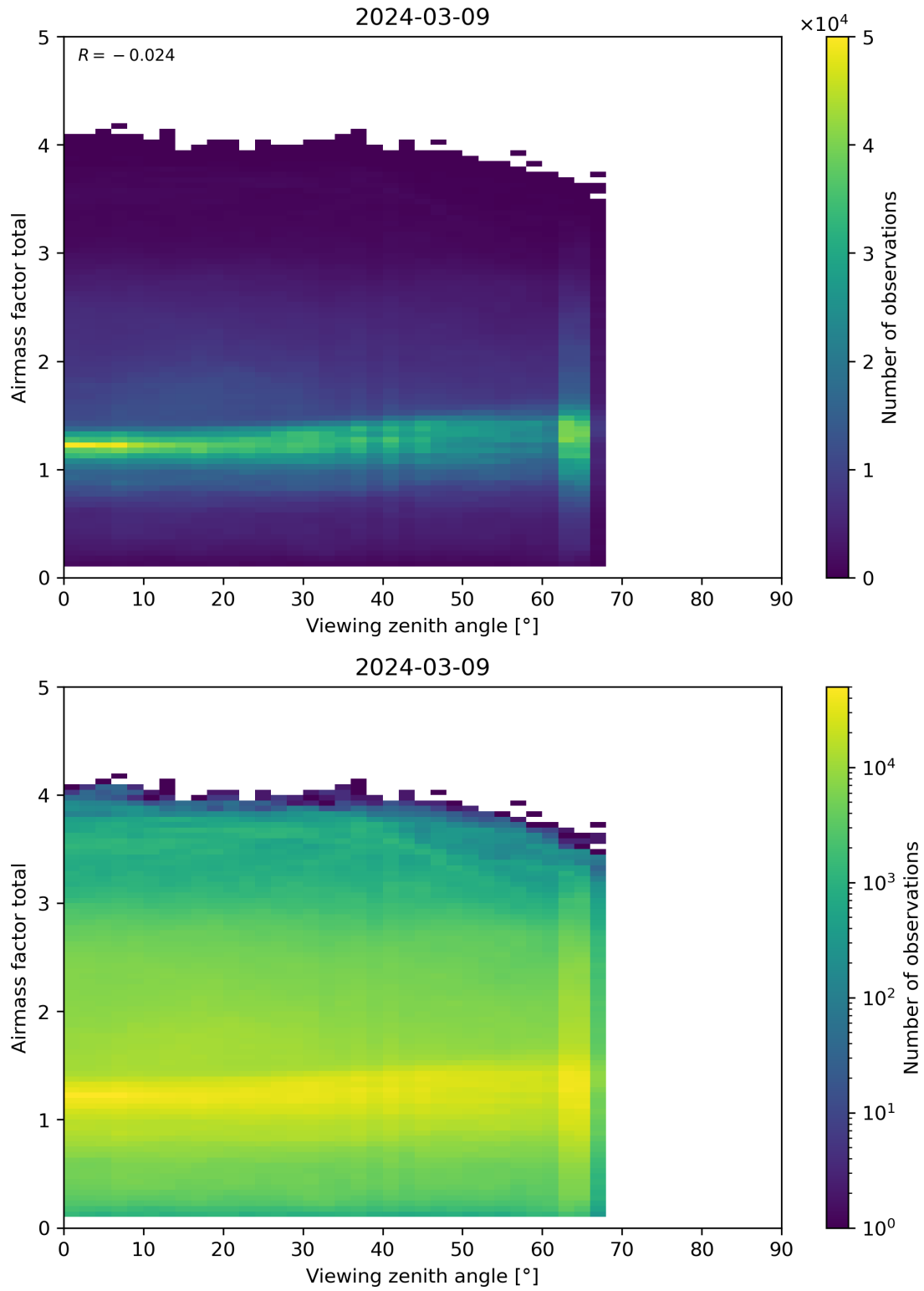
Figure 190: Scatter density plot of “Viewing zenith angle” against “Airmass factor total” for 2024-03-09 to 2024-03-10.
