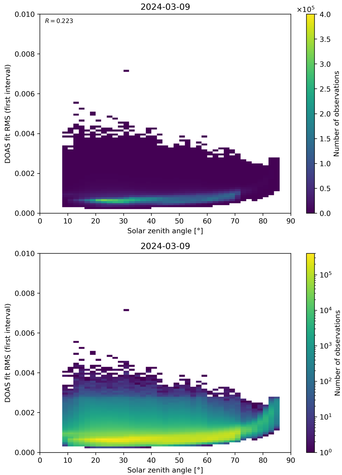
Figure 167: Scatter density plot of “Solar zenith angle” against “DOAS fit RMS (first interval)” for 2024-03-09 to 2024-03-10.
