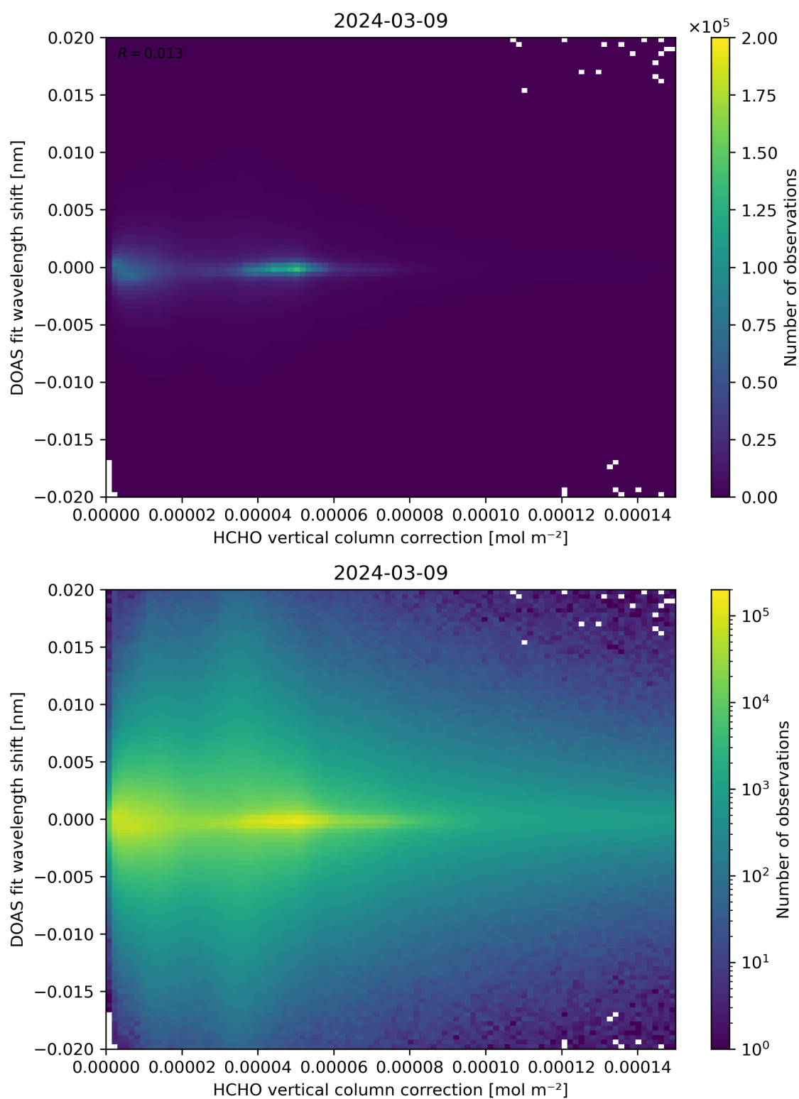
Figure 113: Scatter density plot of “HCHO vertical column correction” against “DOAS fit wavelength shift” for 2024-03-09 to 2024-03-10.
