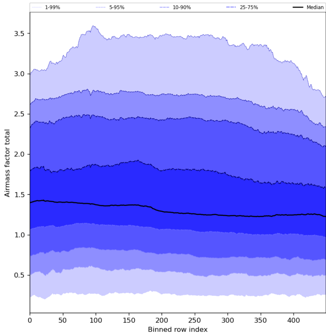
Figure 54: Along track statistics of “Airmass factor total” for 2024-03-09 to 2024-03-10
