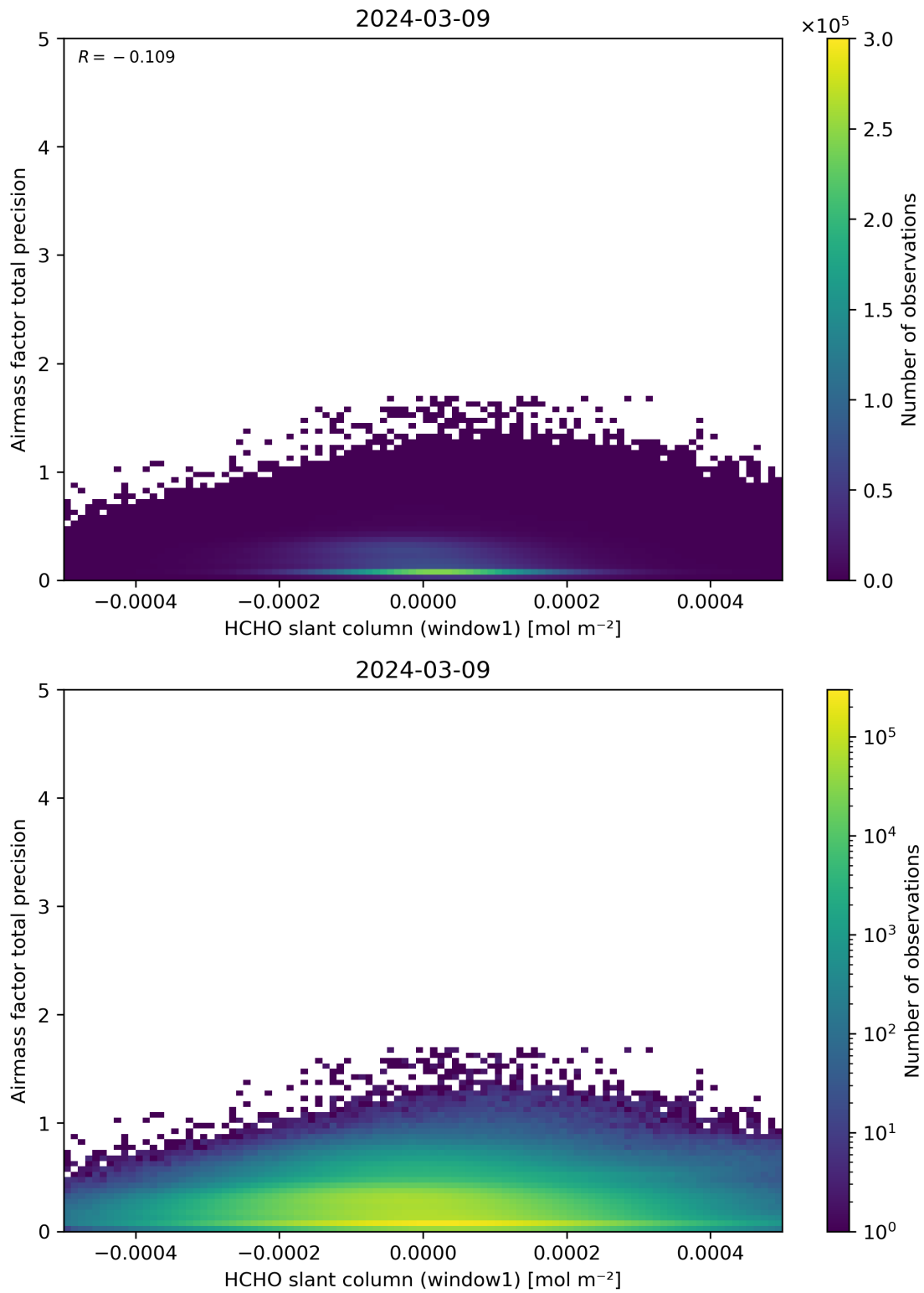
Figure 86: Scatter density plot of “HCHO slant column (window1)” against “Airmass factor total precision” for 2024-03-09 to 2024-03-10.
