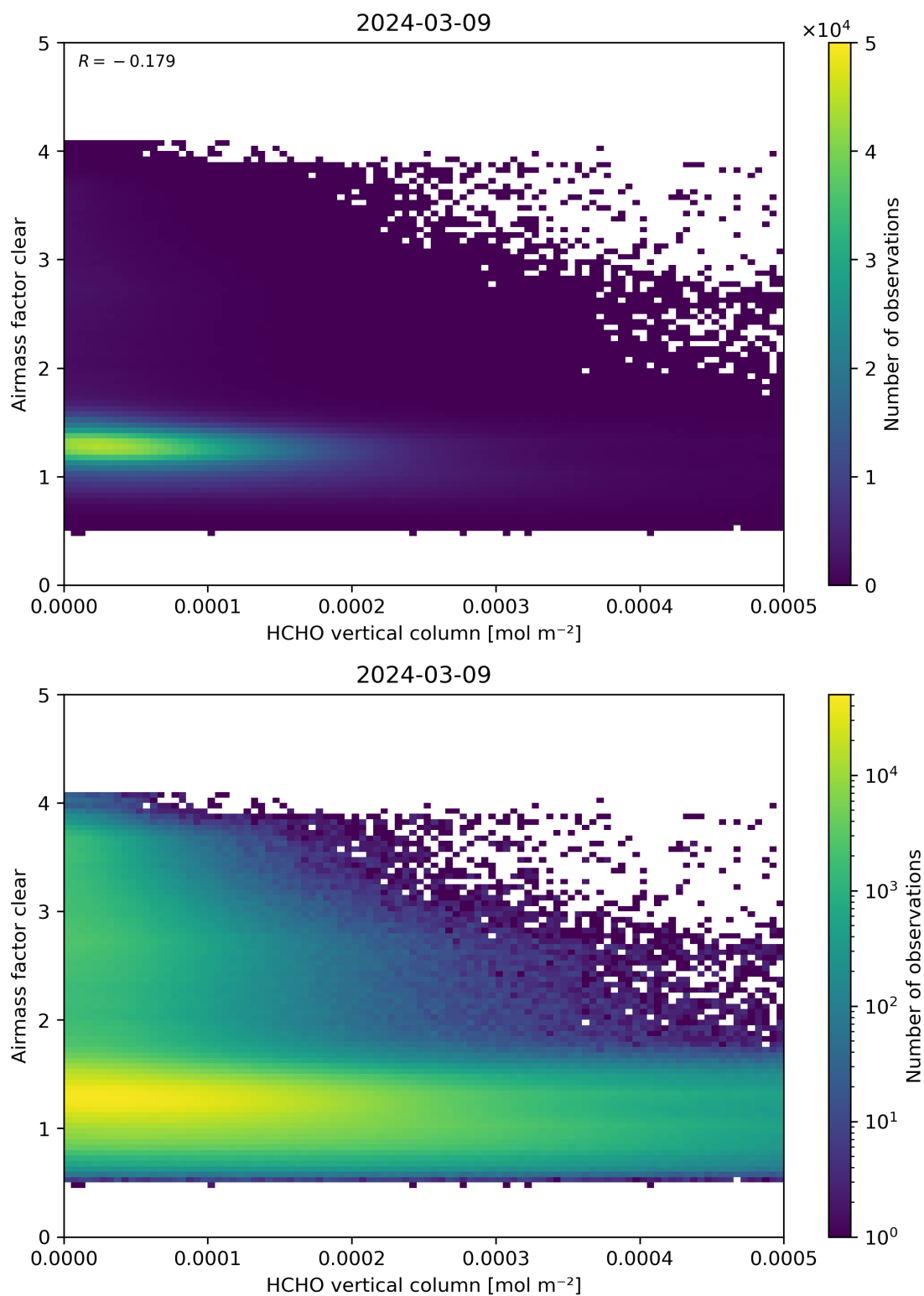
Figure 126: Scatter density plot of “HCHO vertical column” against “Airmass factor clear” for 2024-03-09 to 2024-03-10.
