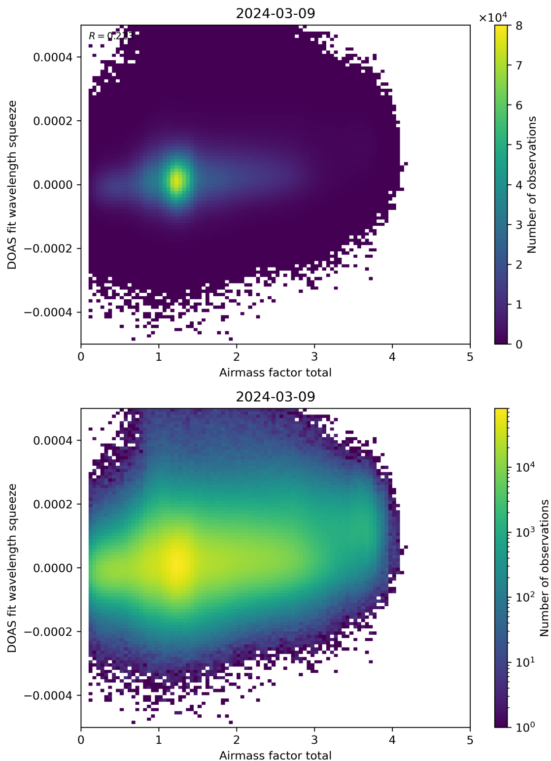
Figure 99: Scatter density plot of “Airmass factor total” against “DOAS fit wavelength squeeze” for 2024-03-09 to 2024-03-10.
