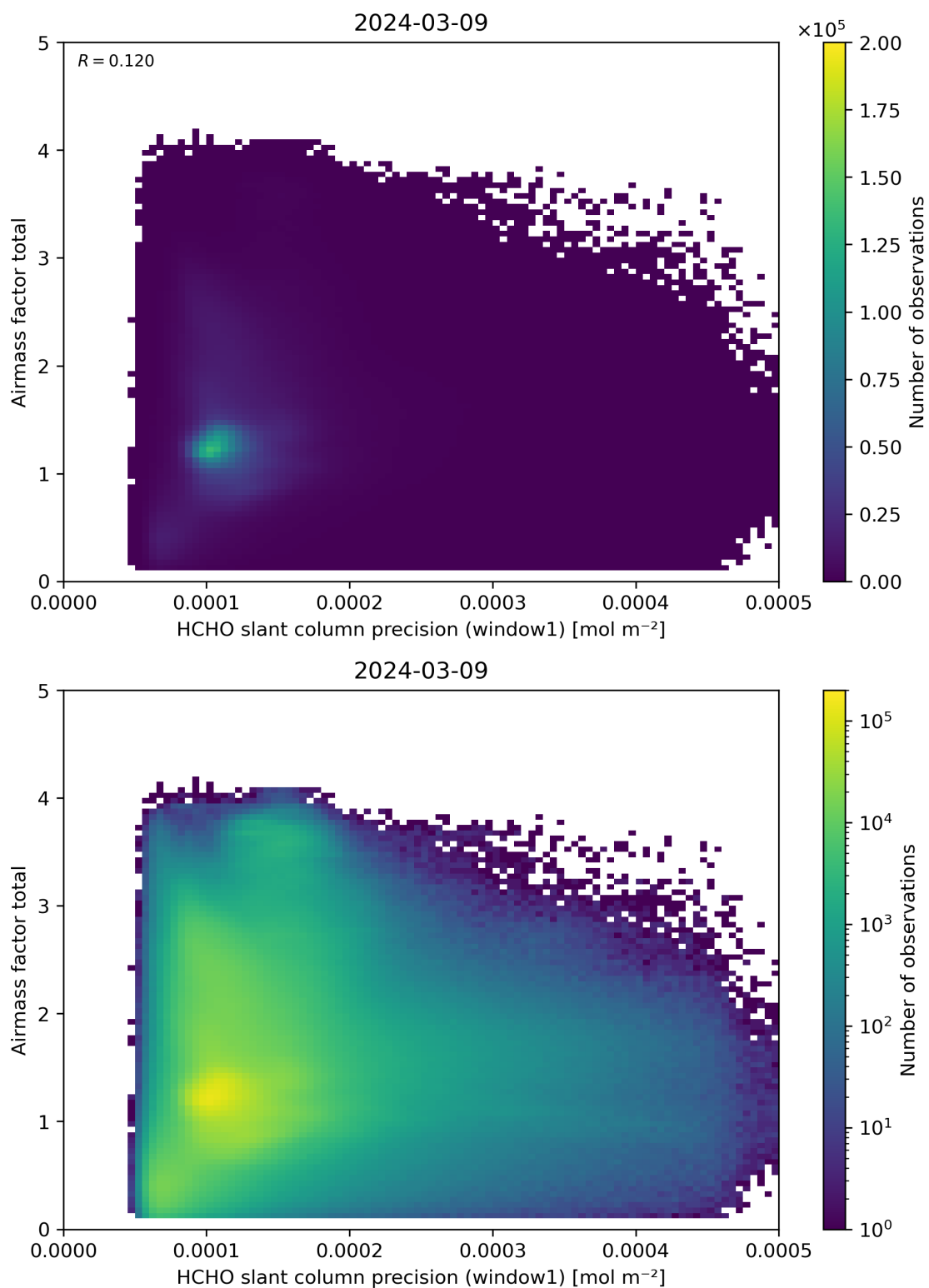
Figure 94: Scatter density plot of “HCHO slant column precision (window1)” against “Airmass factor total” for 2024-03-09 to 2024-03-10.
