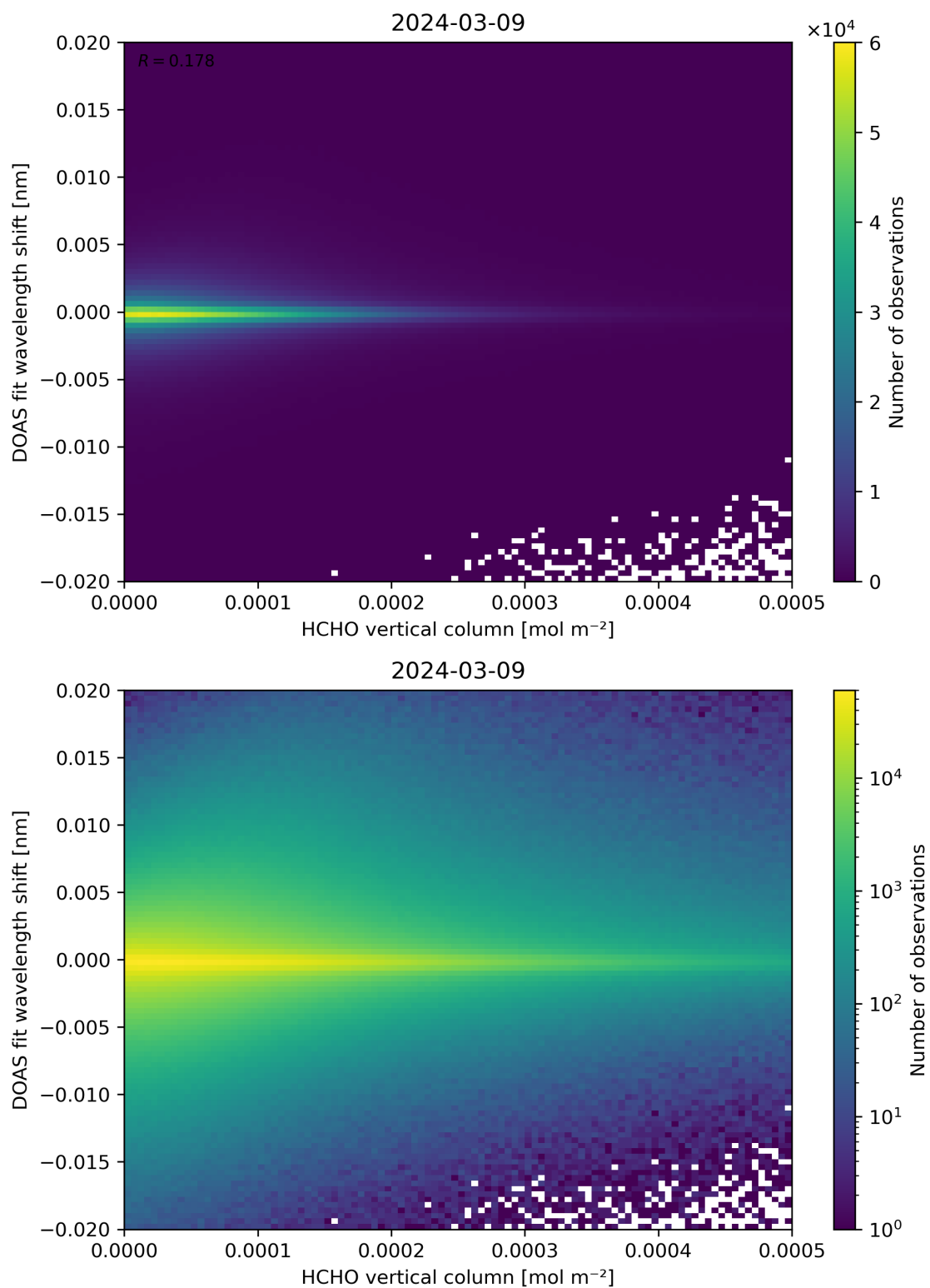
Figure 124: Scatter density plot of “HCHO vertical column” against “DOAS fit wavelength shift” for 2024-03-09 to 2024-03-10.
