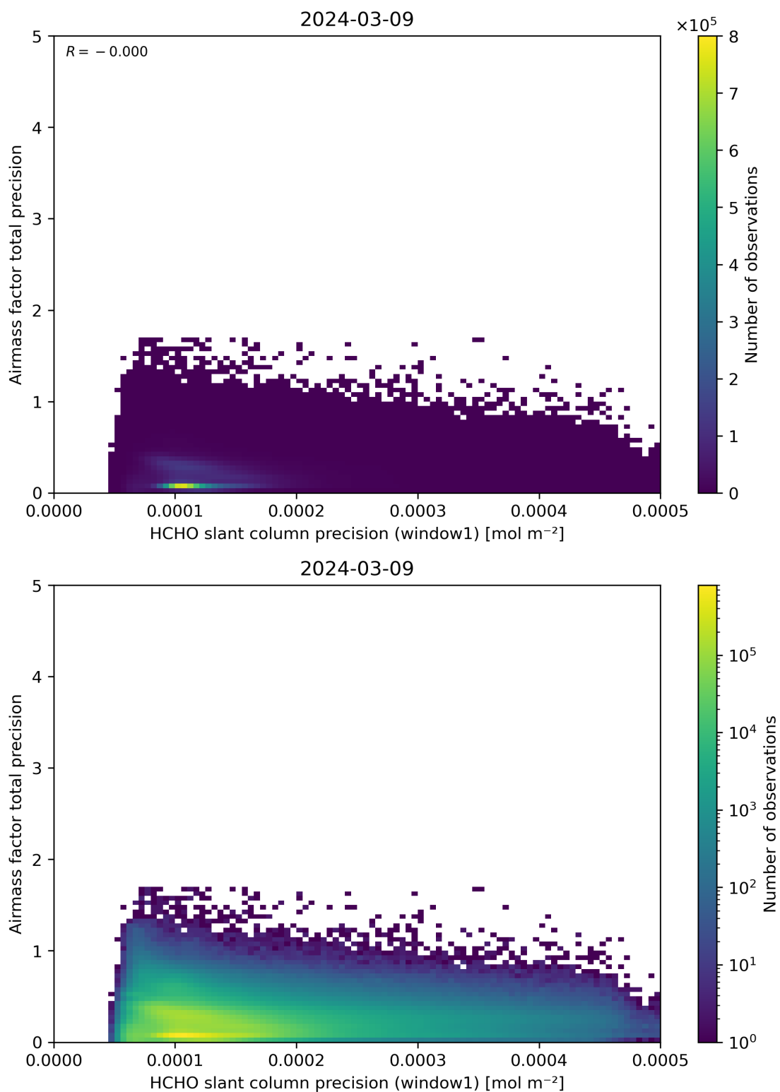
Figure 95: Scatter density plot of “HCHO slant column precision (window1)” against “Airmass factor total precision” for 2024-03-09 to 2024-03-10.
