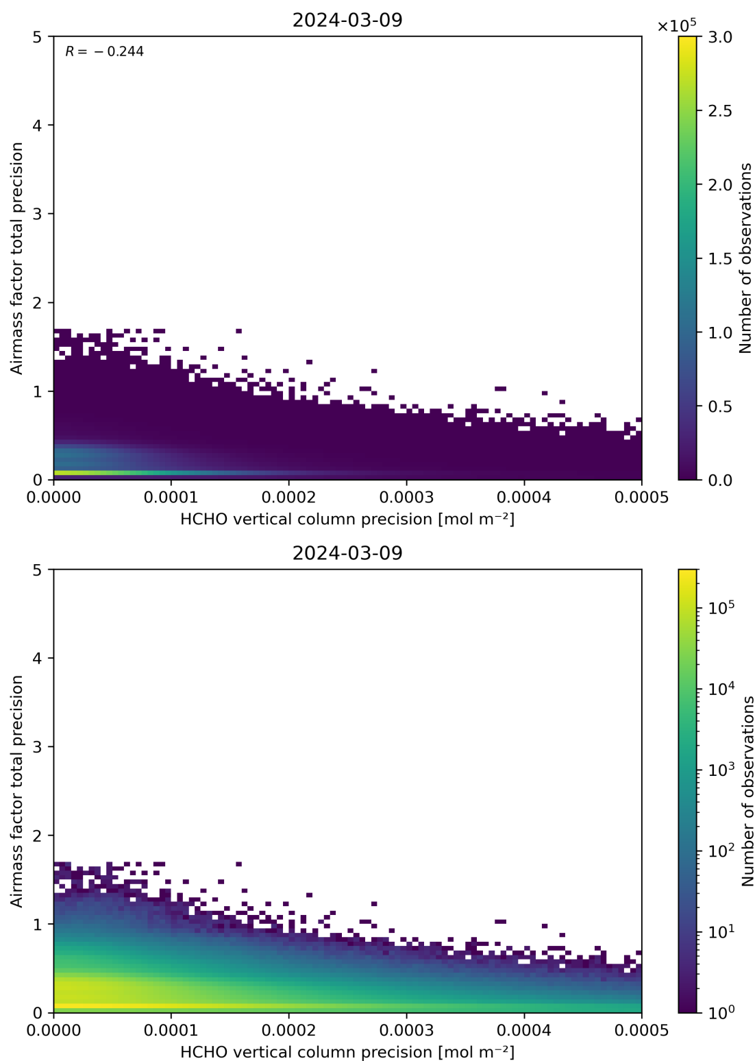
Figure 145: Scatter density plot of “HCHO vertical column precision” against “Airmass factor total precision” for 2024-03-09 to 2024-03-10.
