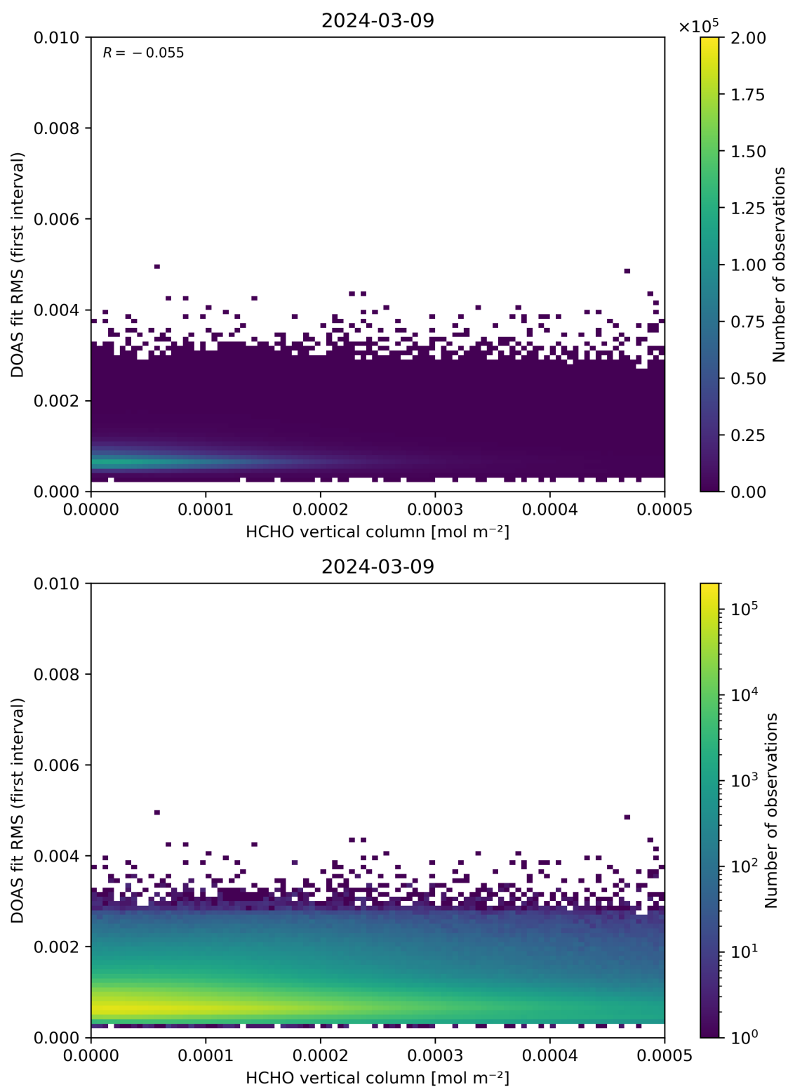
Figure 123: Scatter density plot of “HCHO vertical column” against “DOAS fit RMS (first interval)” for 2024-03-09 to 2024-03-10.
