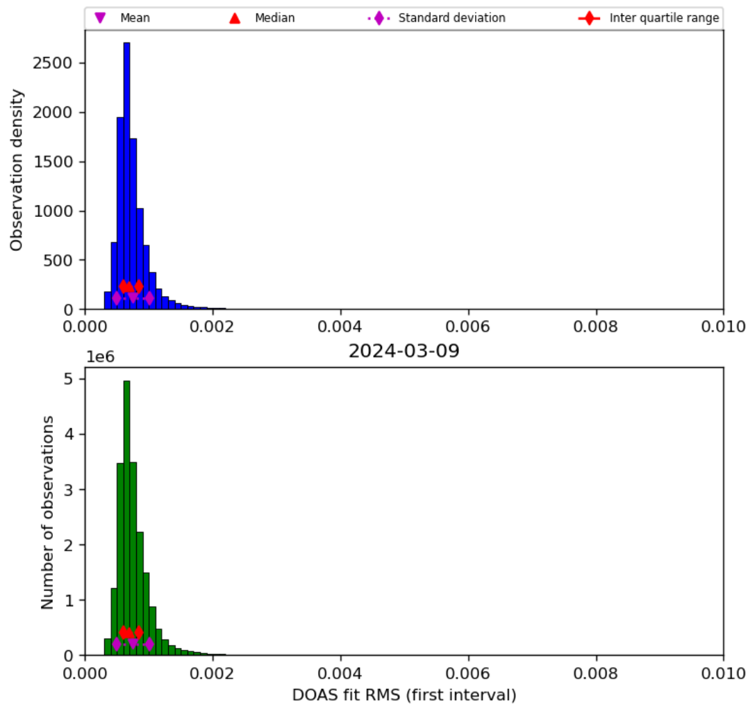
Figure 46: Histogram of “DOAS fit RMS (first interval)” for 2024-03-09 to 2024-03-10
