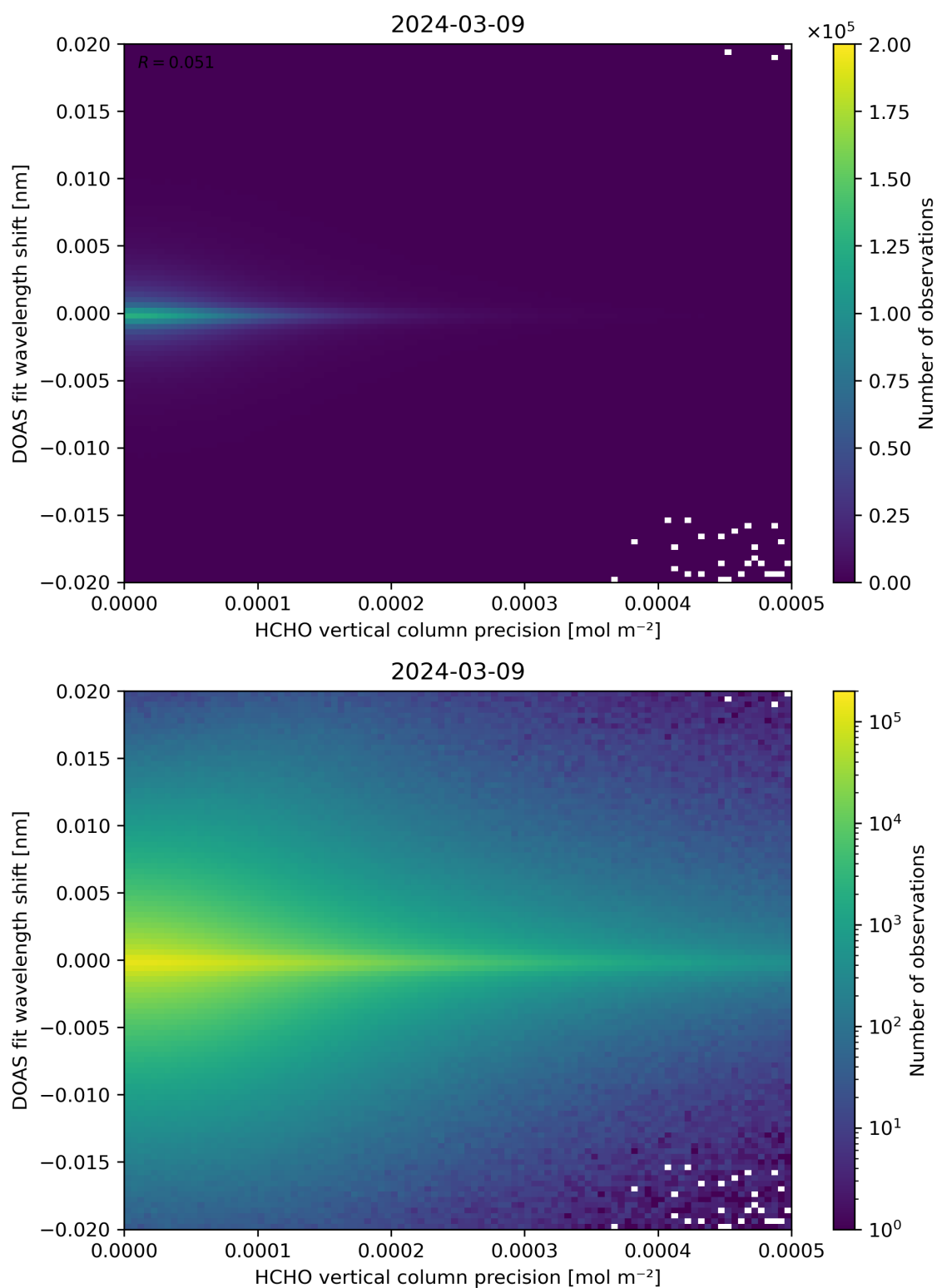
Figure 137: Scatter density plot of “HCHO vertical column precision” against “DOAS fit wavelength shift” for 2024-03-09 to 2024-03-10.
