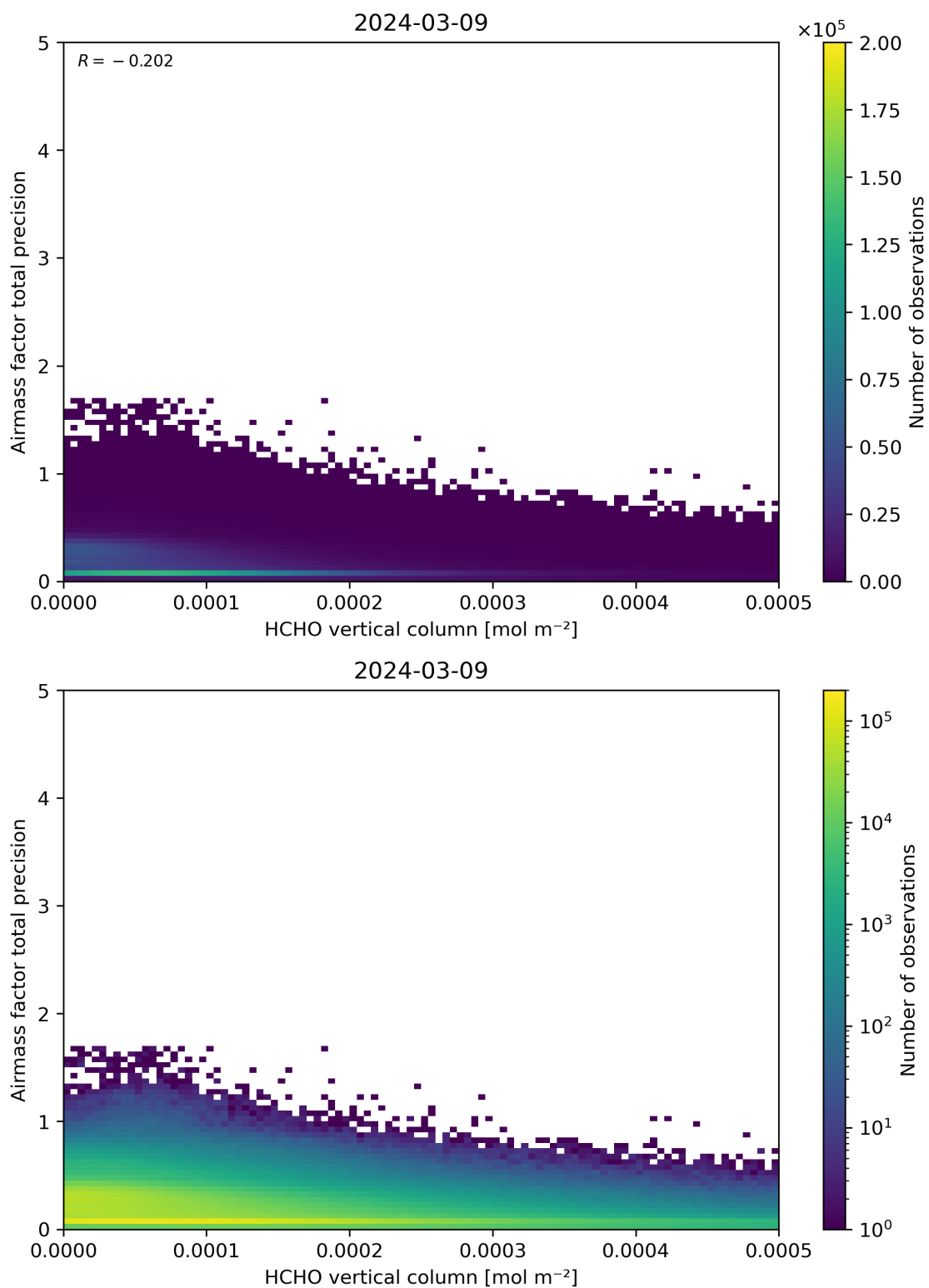
Figure 132: Scatter density plot of “HCHO vertical column” against “Airmass factor total precision” for 2024-03-09 to 2024-03-10.
