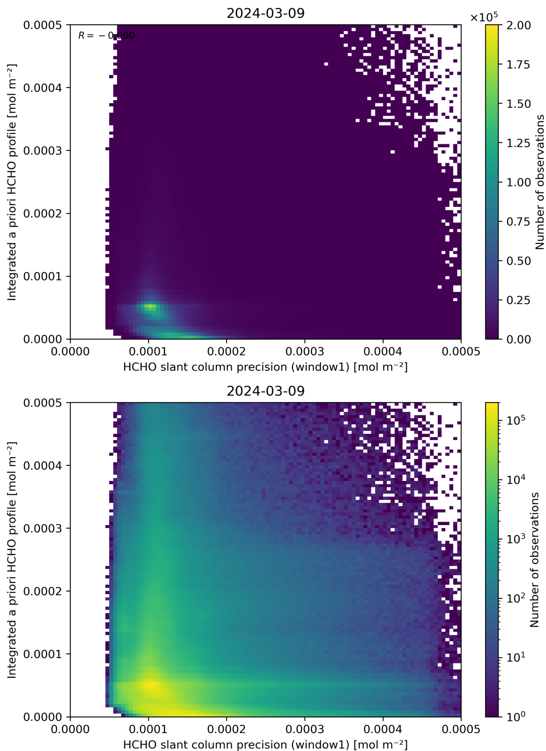
Figure 96: Scatter density plot of “HCHO slant column precision (window1)” against “Integrated a priori HCHO profile” for 2024-03-09 to 2024-03-10.
