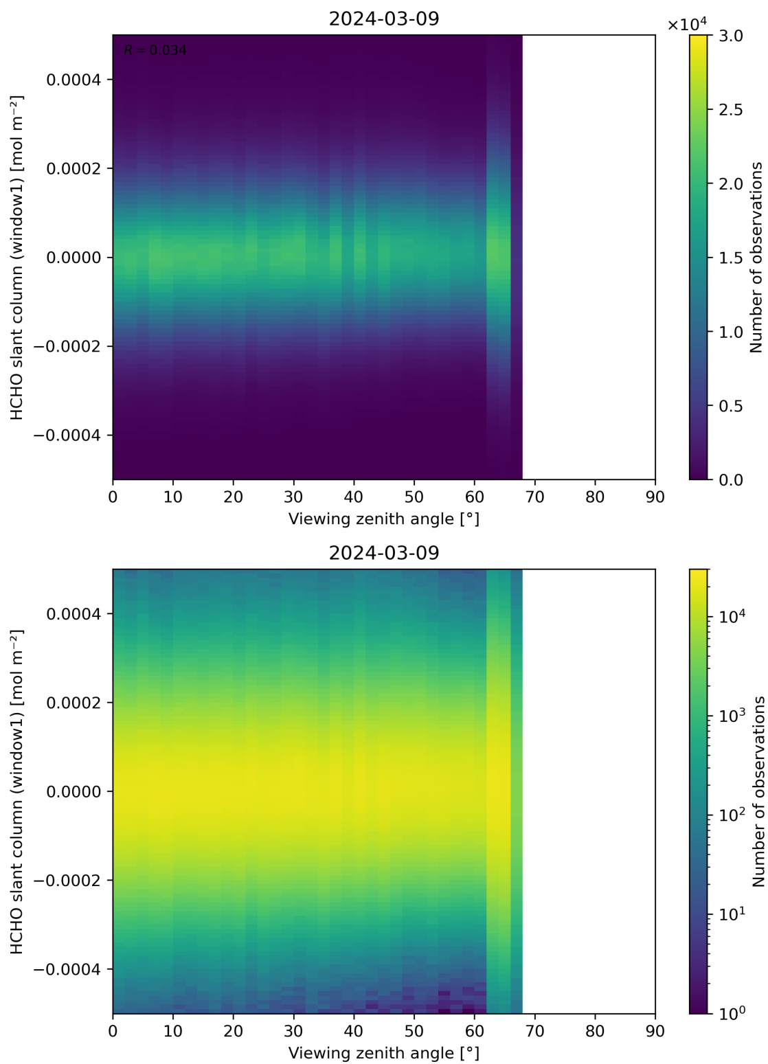
Figure 188: Scatter density plot of “Viewing zenith angle” against “HCHO slant column (window1)” for 2024-03-09 to 2024-03-10.
