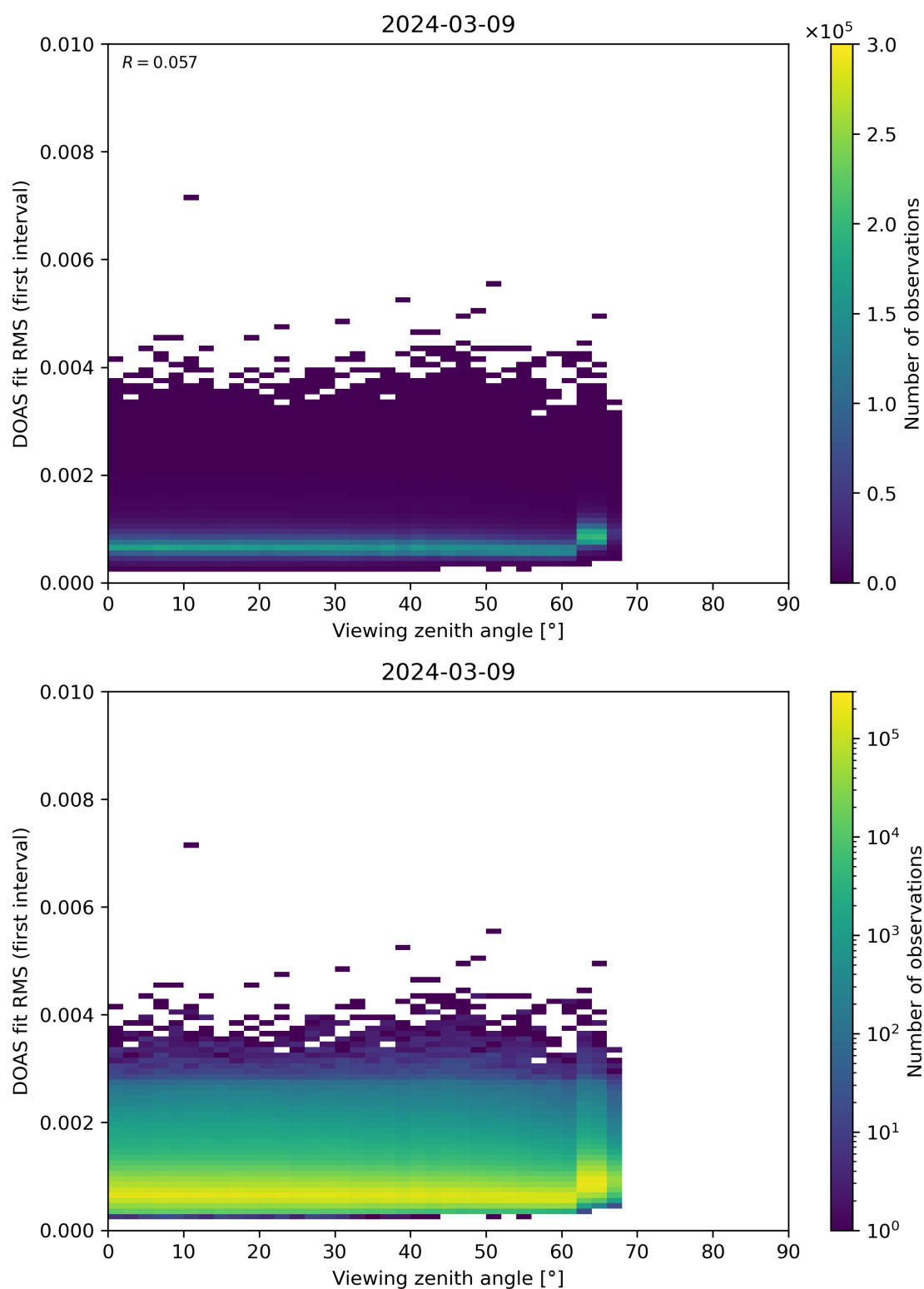
Figure 182: Scatter density plot of “Viewing zenith angle” against “DOAS fit RMS (first interval)” for 2024-03-09 to 2024-03-10.
