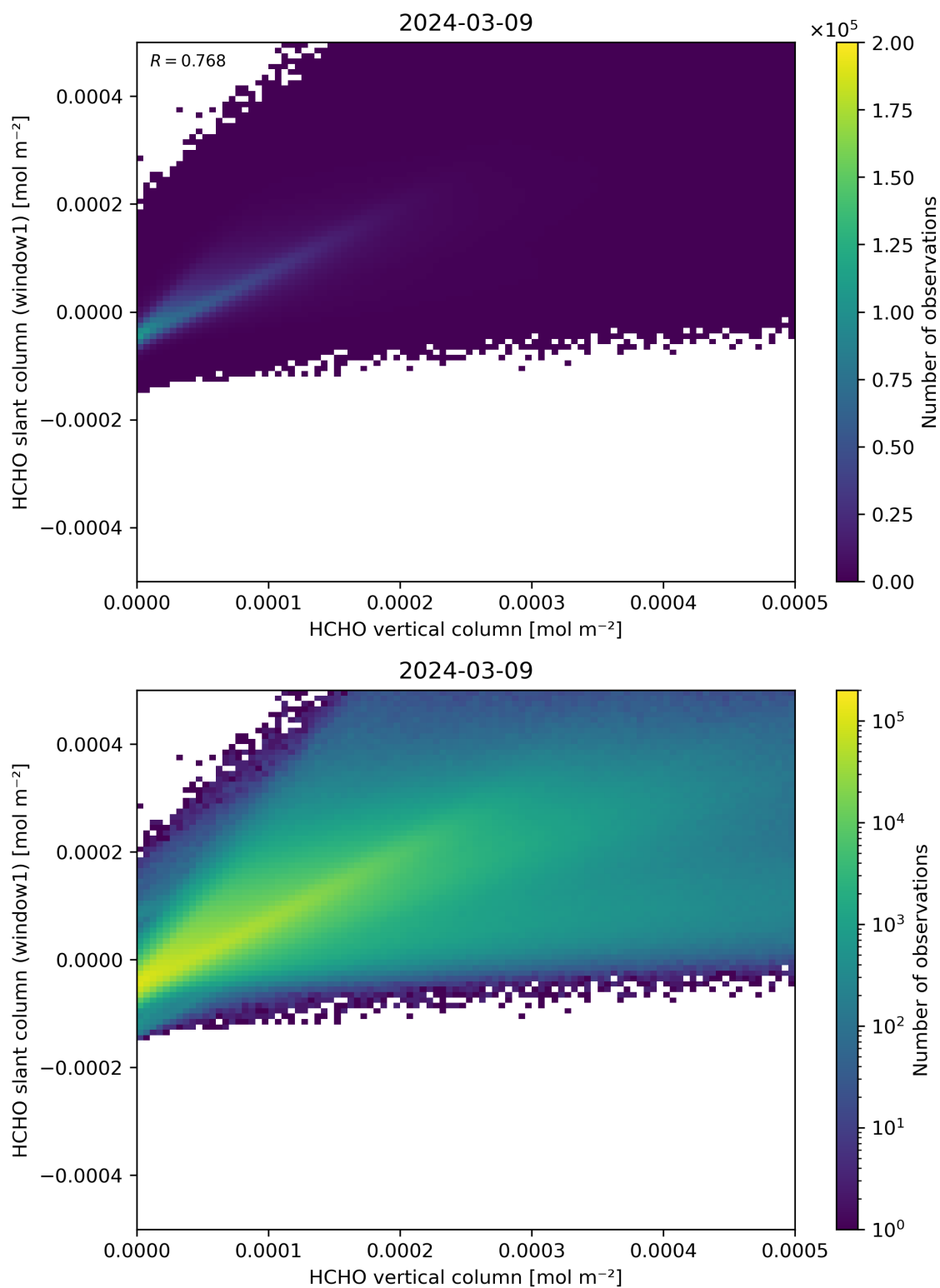
Figure 129: Scatter density plot of “HCHO vertical column” against “HCHO slant column (window1)” for 2024-03-09 to 2024-03-10.
