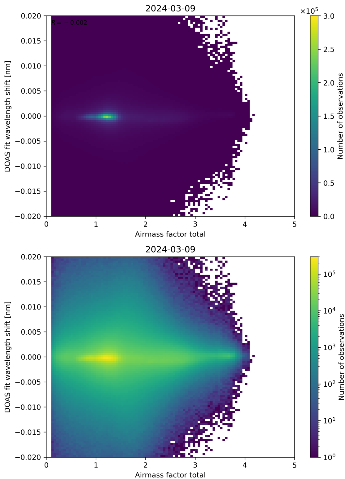
Figure 98: Scatter density plot of “Airmass factor total” against “DOAS fit wavelength shift” for 2024-03-09 to 2024-03-10.
