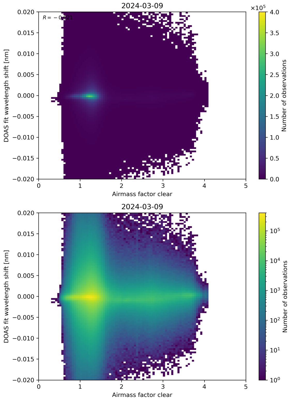
Figure 72: Scatter density plot of “Airmass factor clear” against “DOAS fit wavelength shift” for 2024-03-09 to 2024-03-10.
