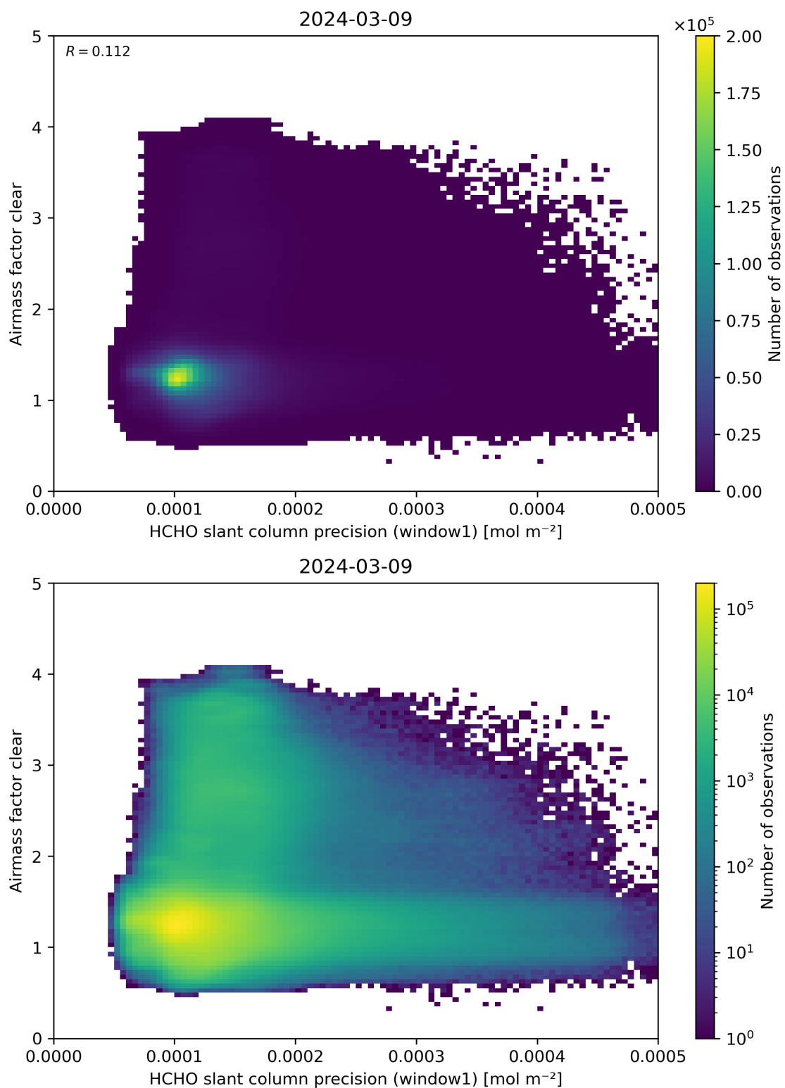
Figure 91: Scatter density plot of “HCHO slant column precision (window1)” against “Airmass factor clear” for 2024-03-09 to 2024-03-10.
