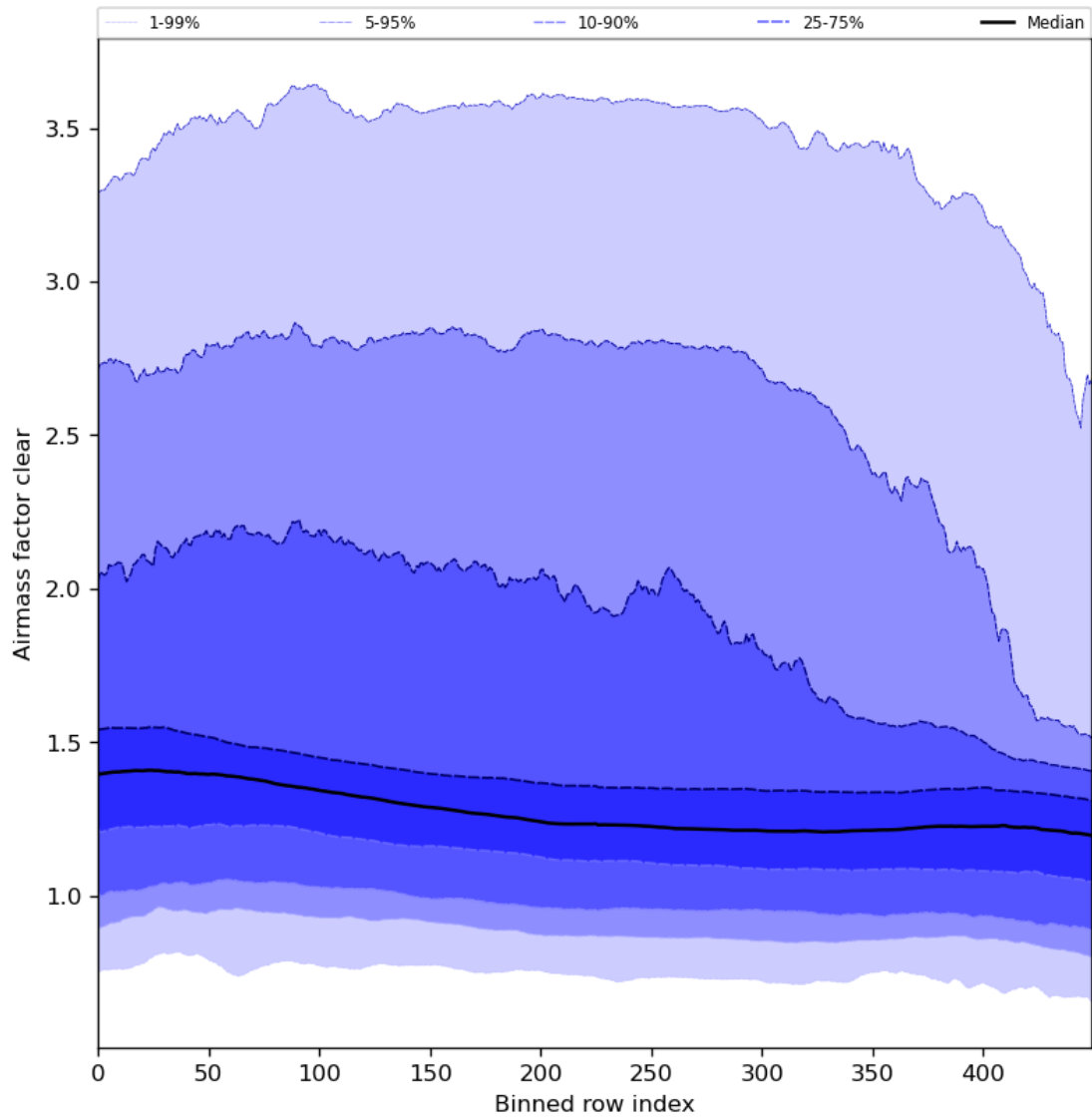
Figure 56: Along track statistics of “Airmass factor clear” for 2024-03-09 to 2024-03-10
