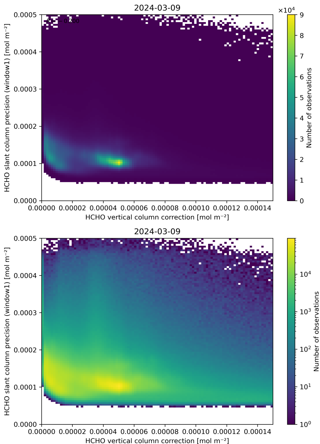
Figure 119: Scatter density plot of “HCHO vertical column correction” against “HCHO slant column precision (window1)” for 2024-03-09 to 2024-03-10.
