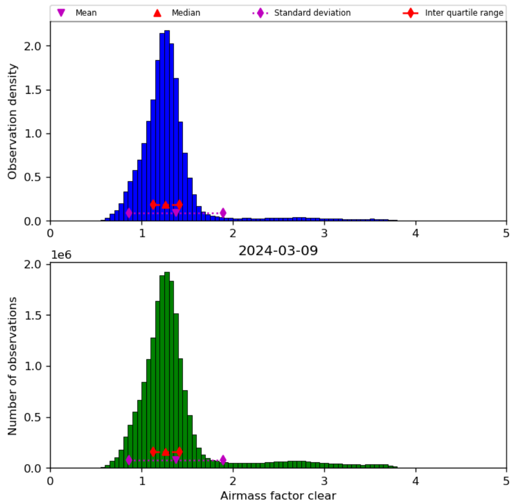
Figure 42: Histogram of “Airmass factor clear” for 2024-03-09 to 2024-03-10
