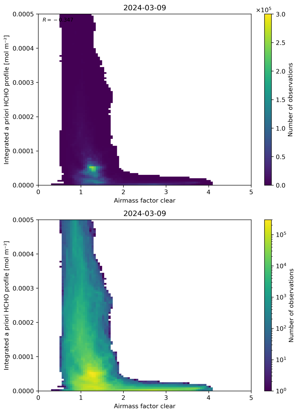
Figure 76: Scatter density plot of “Airmass factor clear” against “Integrated a priori HCHO profile” for 2024-03-09 to 2024-03-10.
