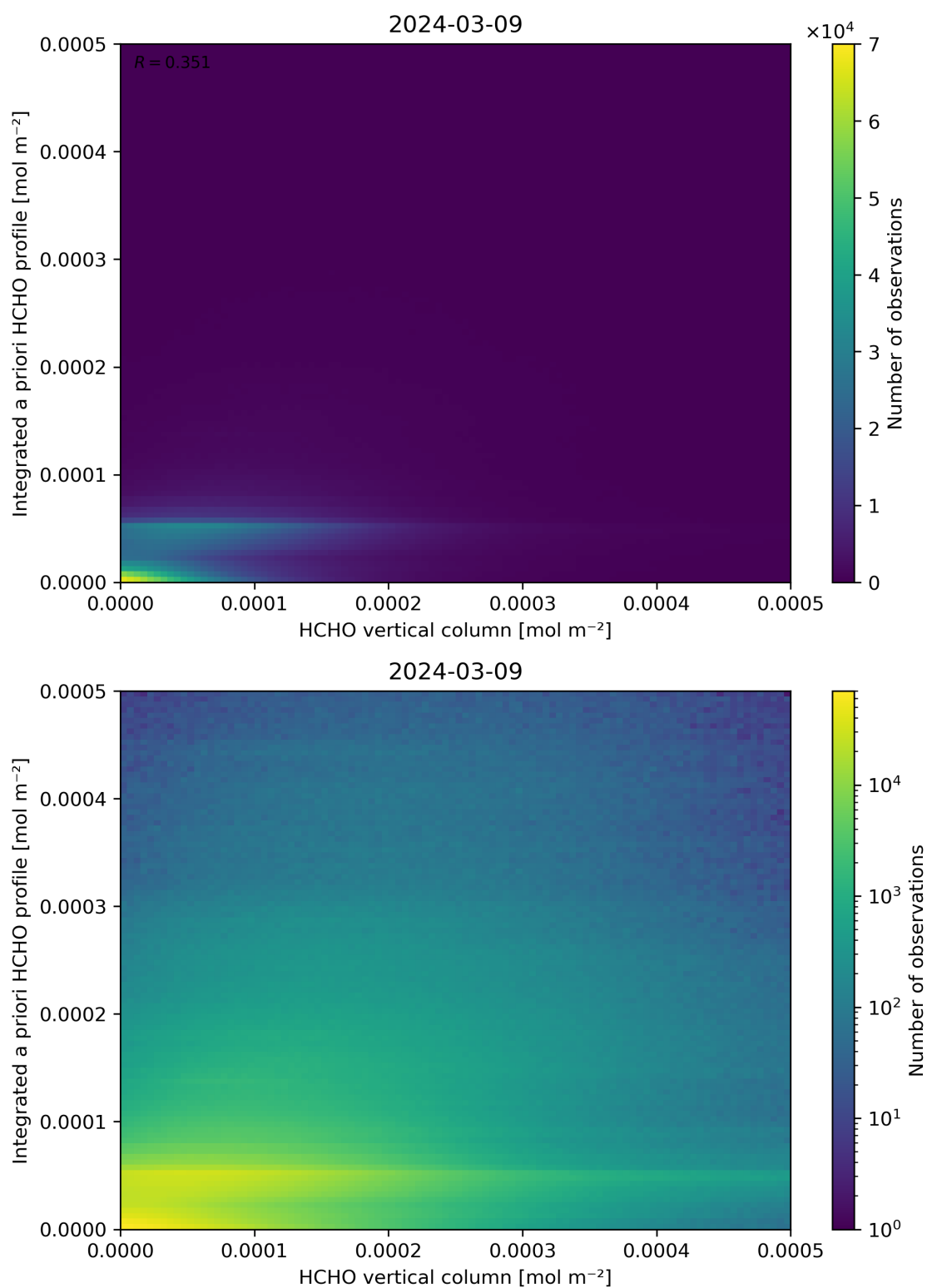
Figure 135: Scatter density plot of “HCHO vertical column” against “Integrated a priori HCHO profile” for 2024-03-09 to 2024-03-10.
