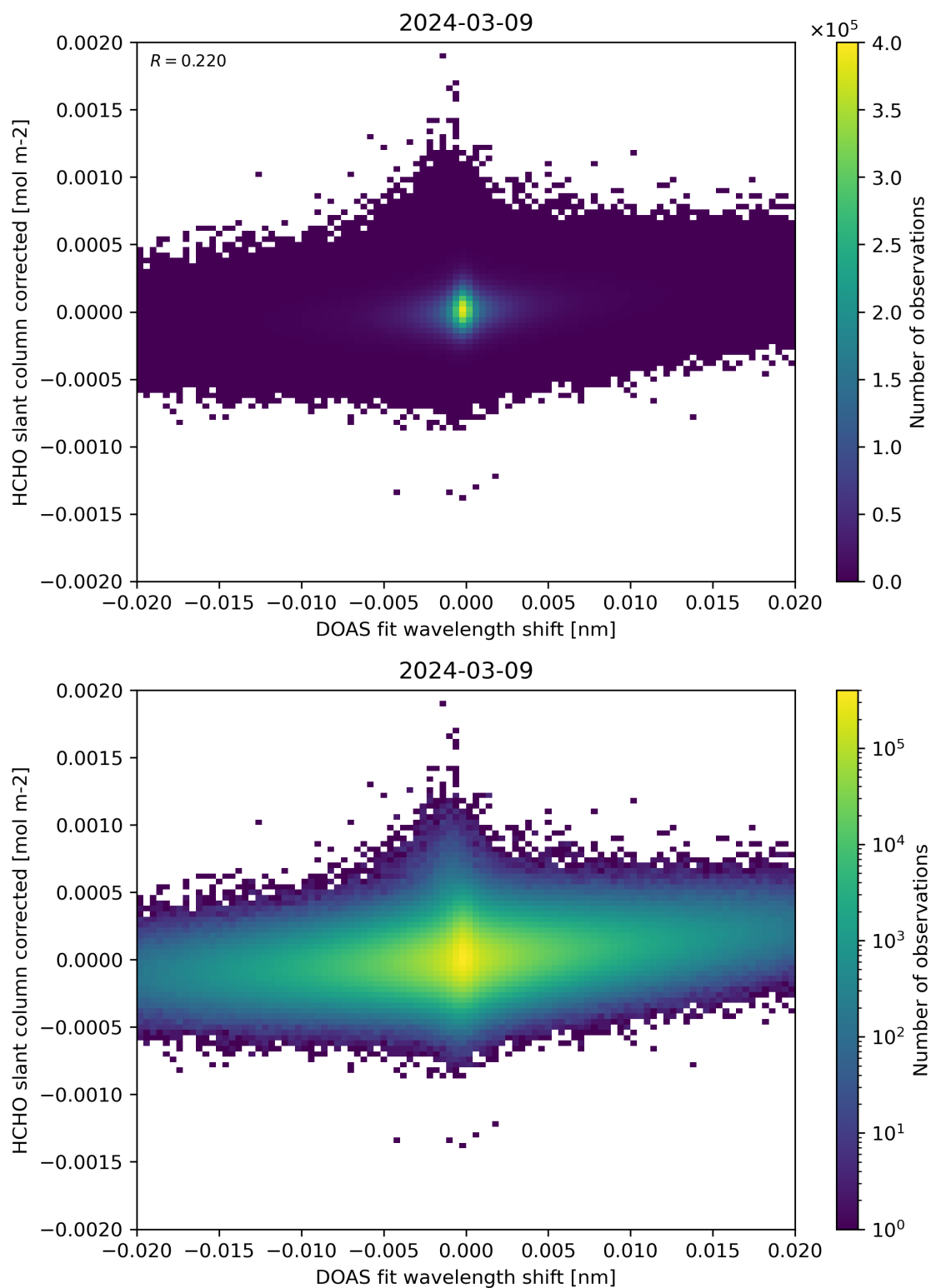
Figure 66: Scatter density plot of “DOAS fit wavelength shift” against “HCHO slant column corrected” for 2024-03-09 to 2024-03-10.
