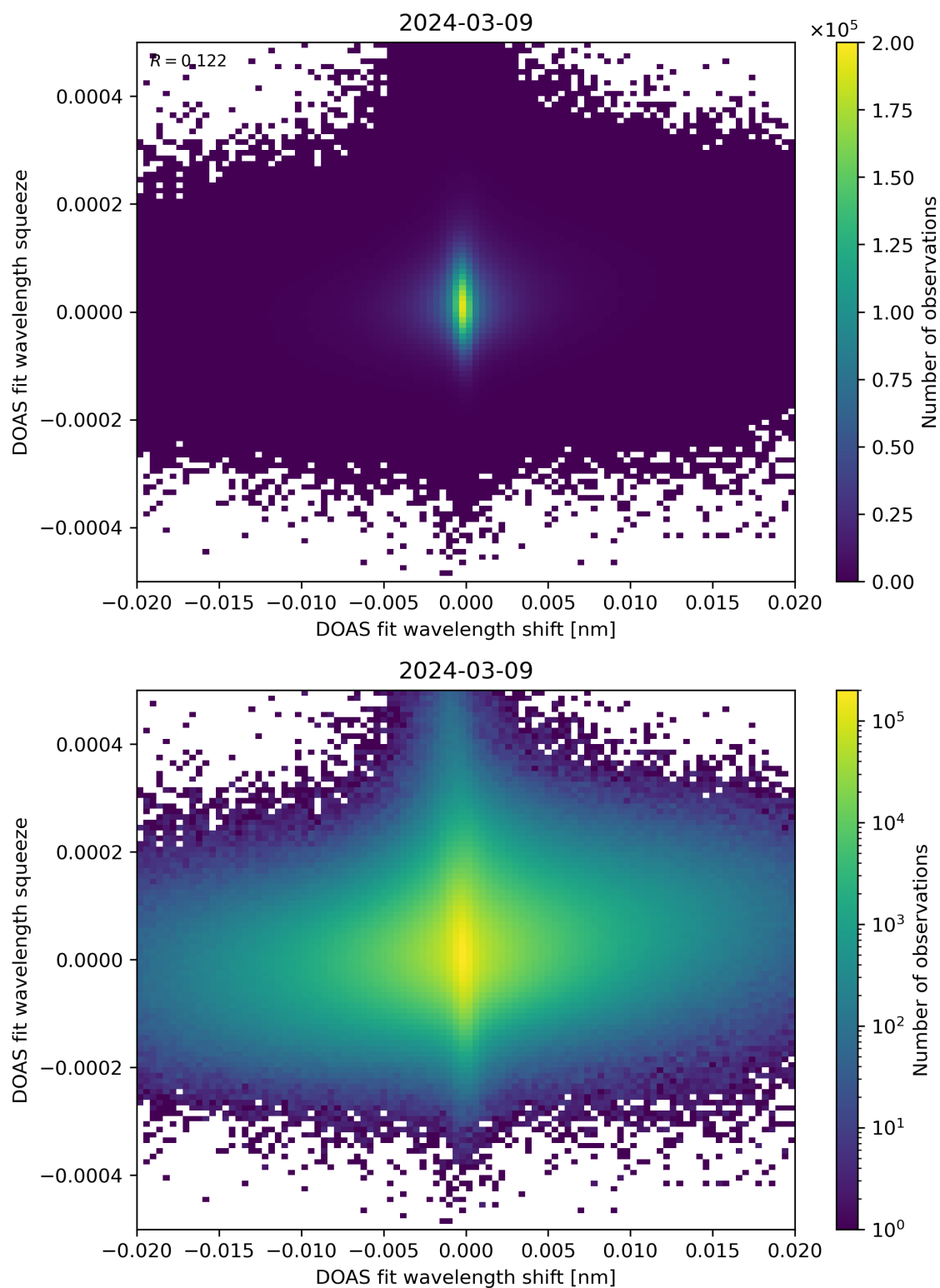
Figure 65: Scatter density plot of “DOAS fit wavelength shift” against “DOAS fit wavelength squeeze” for 2024-03-09 to 2024-03-10.
