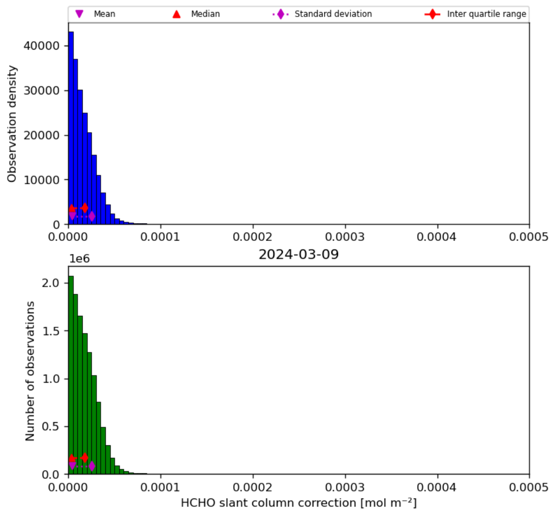
Figure 47: Histogram of “HCHO slant column correction” for 2024-03-09 to 2024-03-10
