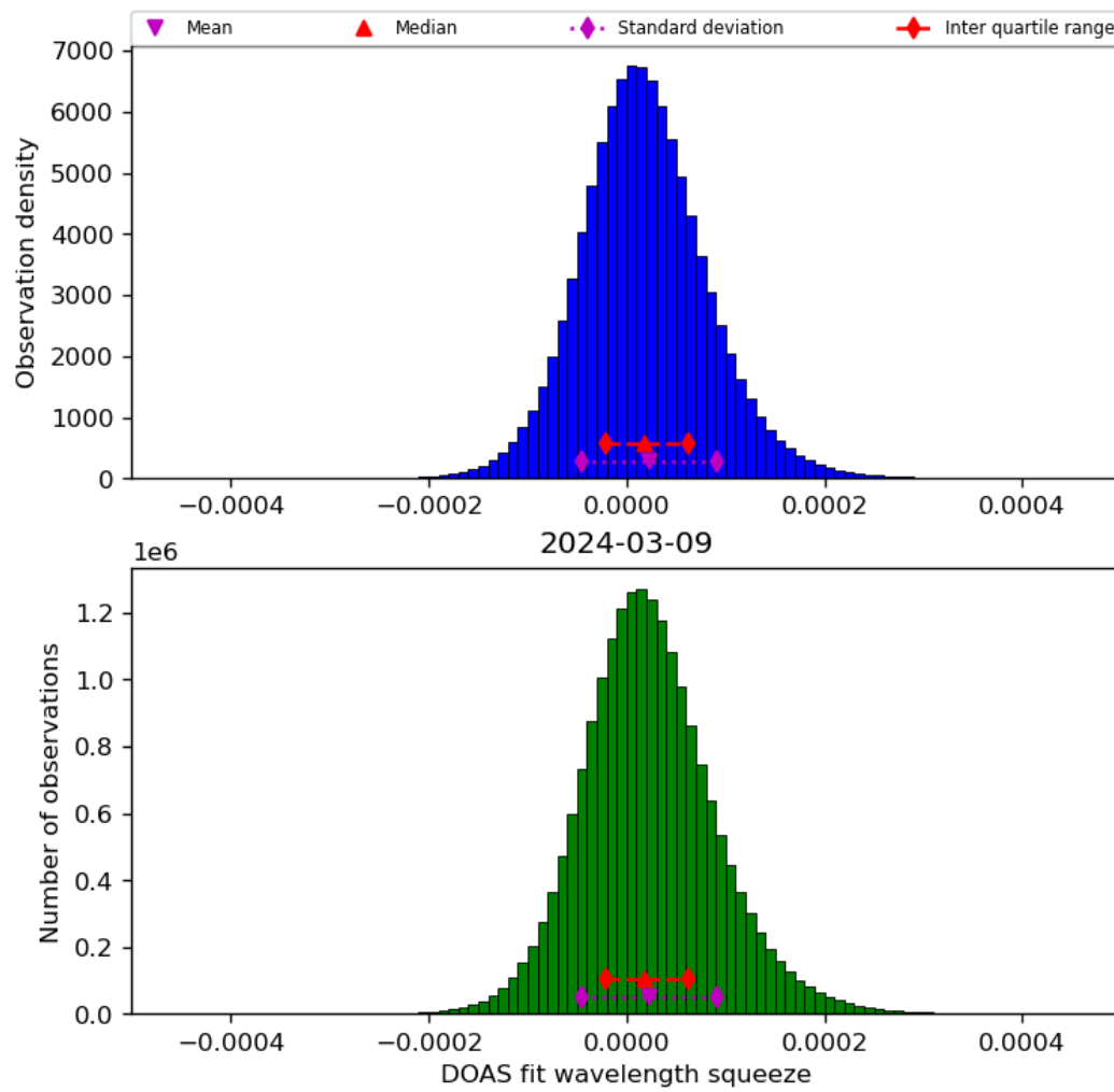
Figure 45: Histogram of “DOAS fit wavelength squeeze” for 2024-03-09 to 2024-03-10
