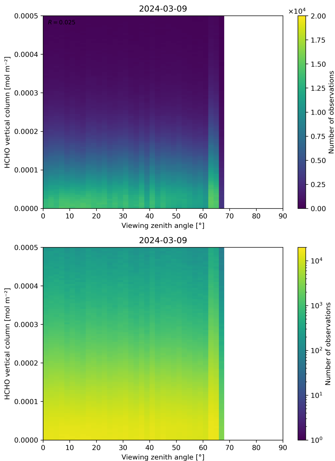
Figure 192: Scatter density plot of “Viewing zenith angle” against “HCHO vertical column” for 2024-03-09 to 2024-03-10.
