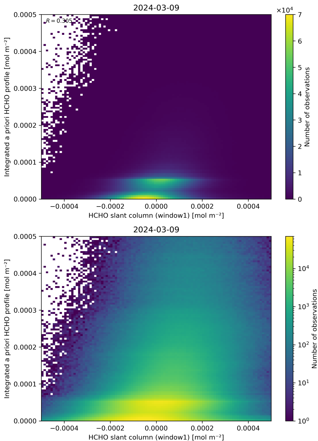
Figure 87: Scatter density plot of “HCHO slant column (window1)” against “Integrated a priori HCHO profile” for 2024-03-09 to 2024-03-10.
