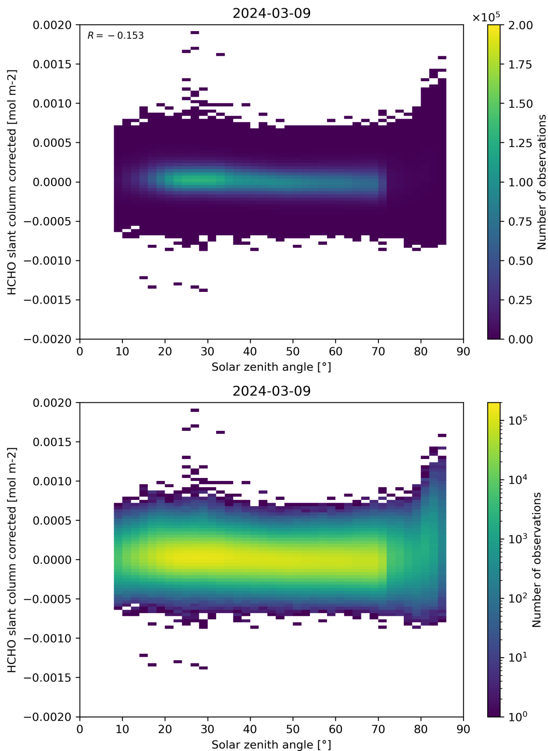
Figure 171: Scatter density plot of “Solar zenith angle” against “HCHO slant column corrected” for 2024-03-09 to 2024-03-10.
