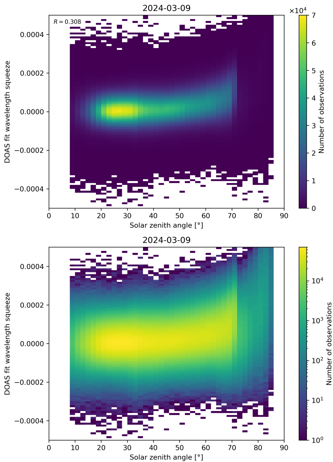
Figure 169: Scatter density plot of “Solar zenith angle” against “DOAS fit wavelength squeeze” for 2024-03-09 to 2024-03-10.
