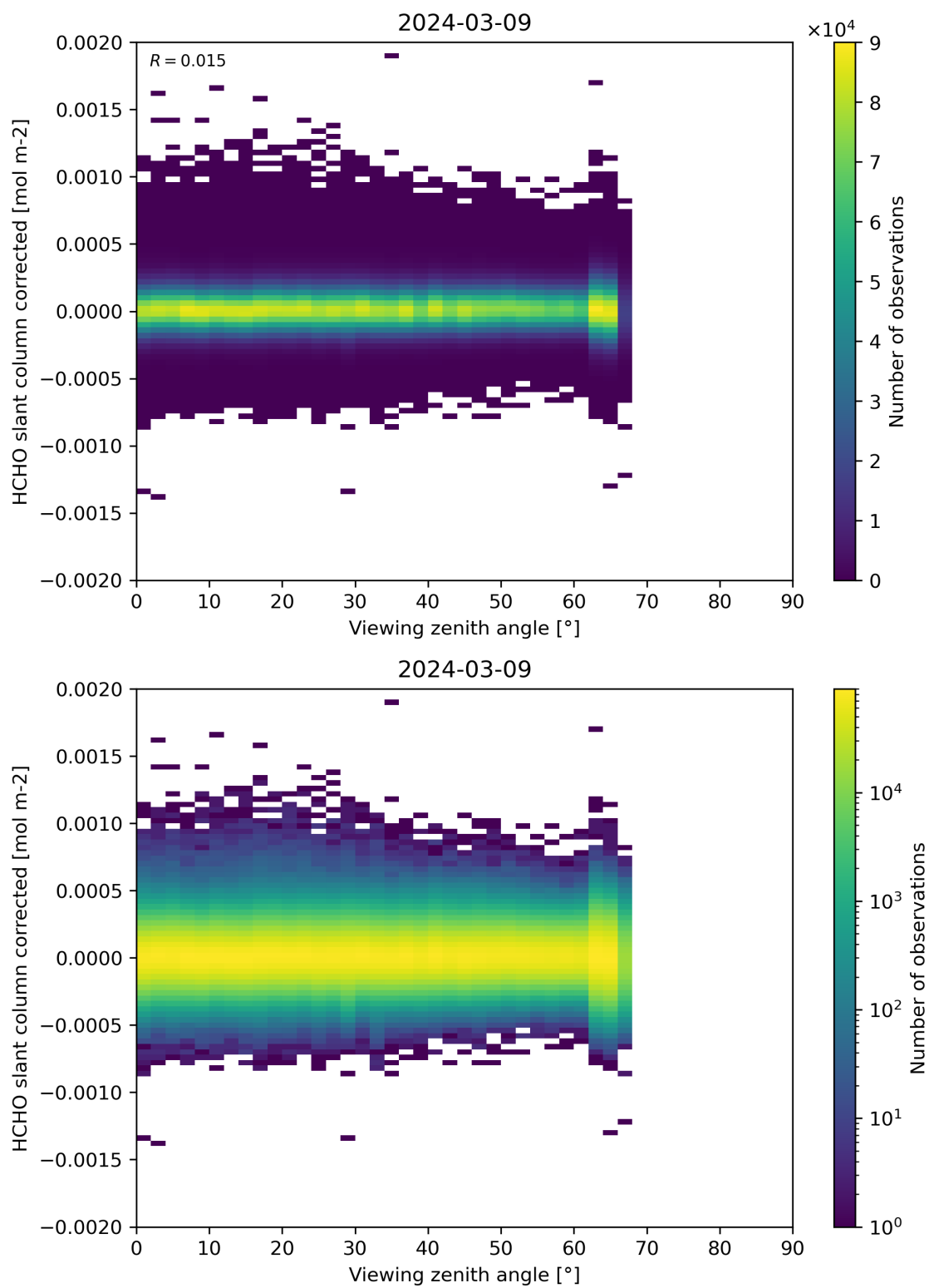
Figure 186: Scatter density plot of “Viewing zenith angle” against “HCHO slant column corrected” for 2024-03-09 to 2024-03-10.
