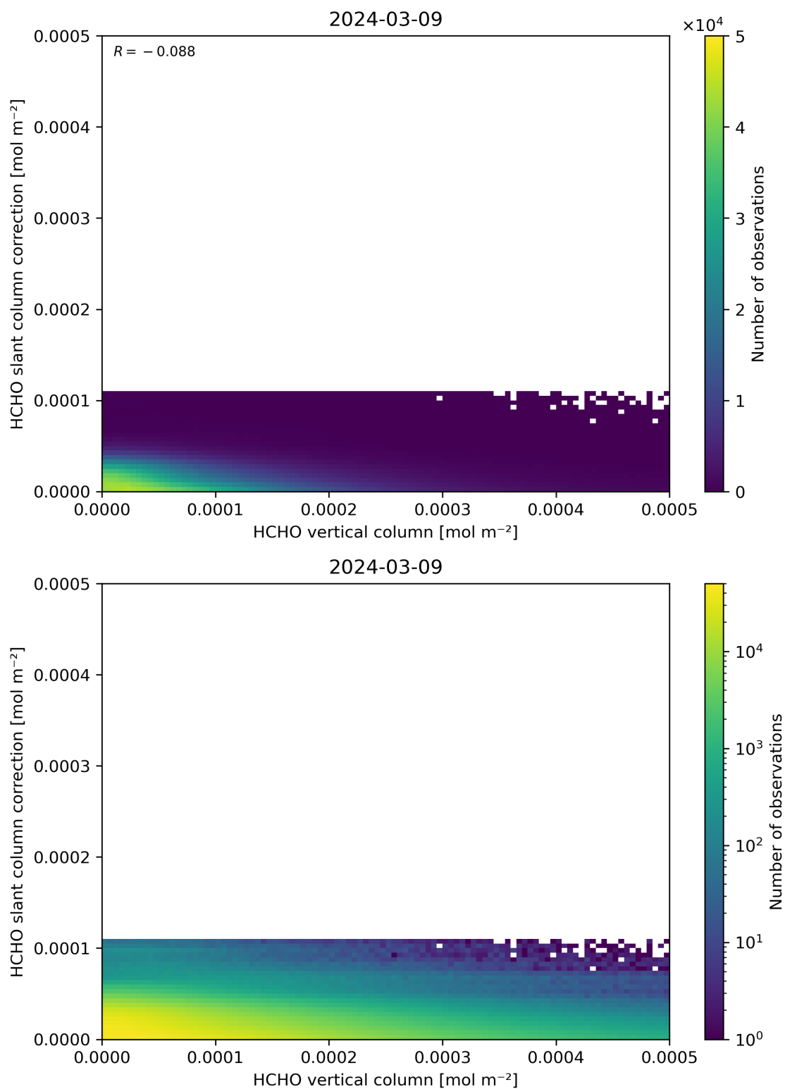
Figure 128: Scatter density plot of “HCHO vertical column” against “HCHO slant column correction” for 2024-03-09 to 2024-03-10.
