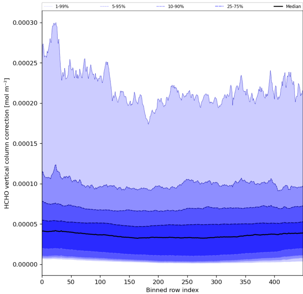
Figure 51: Along track statistics of “HCHO vertical column correction” for 2024-03-09 to 2024-03-10
