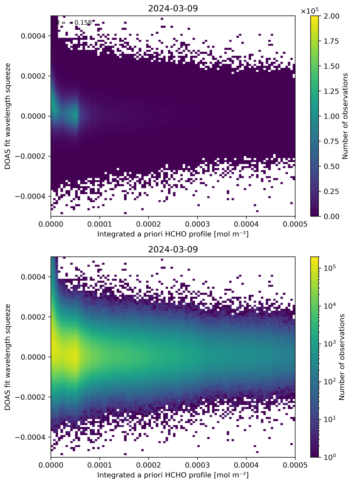
Figure 150: Scatter density plot of “Integrated a priori HCHO profile” against “DOAS fit wavelength squeeze” for 2024-03-09 to 2024-03-10.
