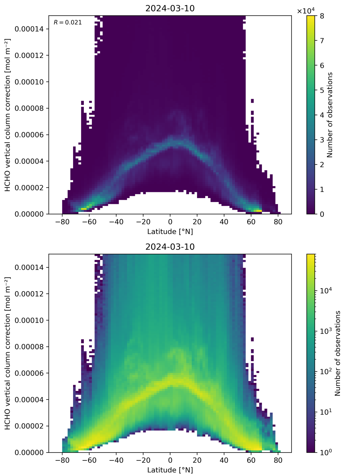
Figure 164: Scatter density plot of “Latitude” against “HCHO vertical column correction” for 2024-03-09 to 2024-03-11.
