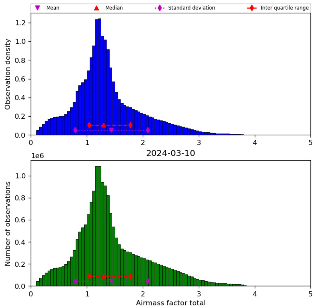
Figure 40: Histogram of “Airmass factor total” for 2024-03-09 to 2024-03-11
