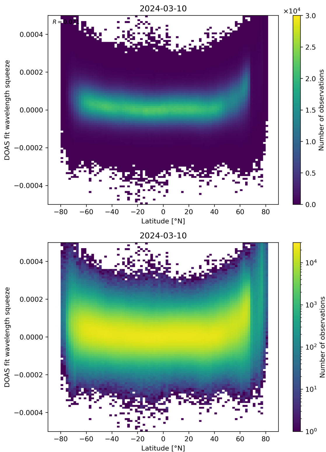
Figure 155: Scatter density plot of “Latitude” against “DOAS fit wavelength squeeze” for 2024-03-09 to 2024-03-11.
