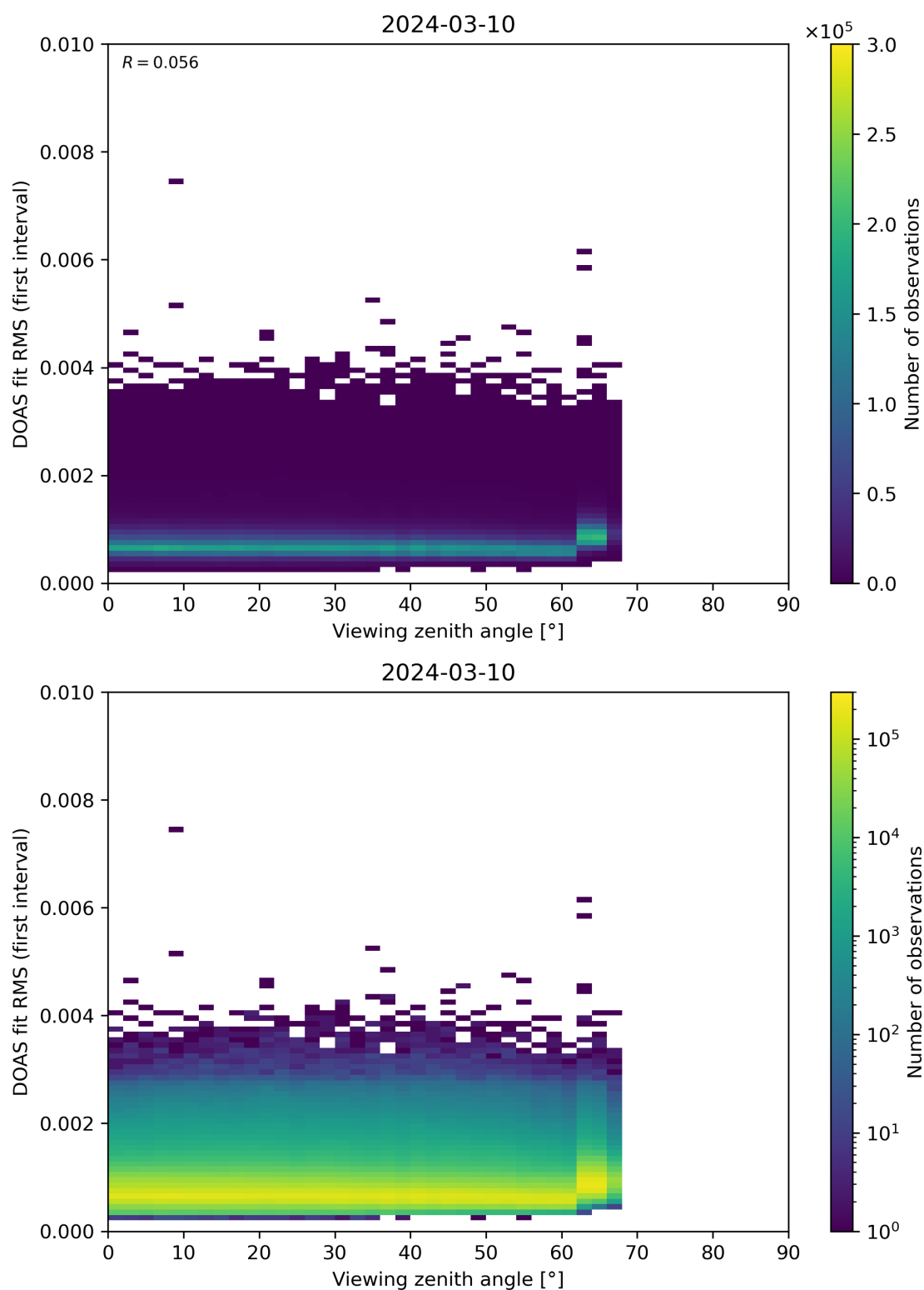
Figure 182: Scatter density plot of “Viewing zenith angle” against “DOAS fit RMS (first interval)” for 2024-03-09 to 2024-03-11.
