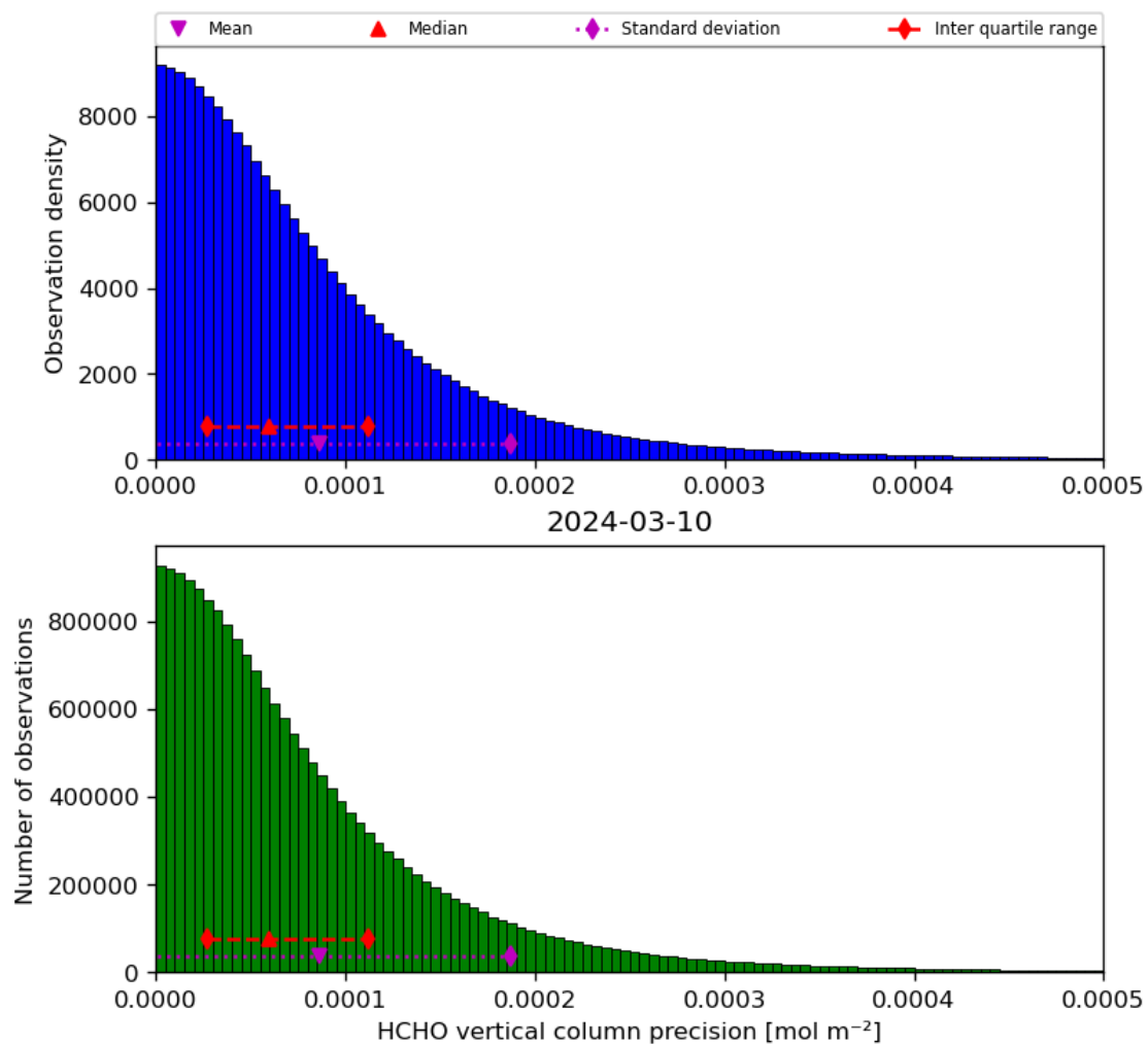
Figure 36: Histogram of “HCHO vertical column precision” for 2024-03-09 to 2024-03-11
