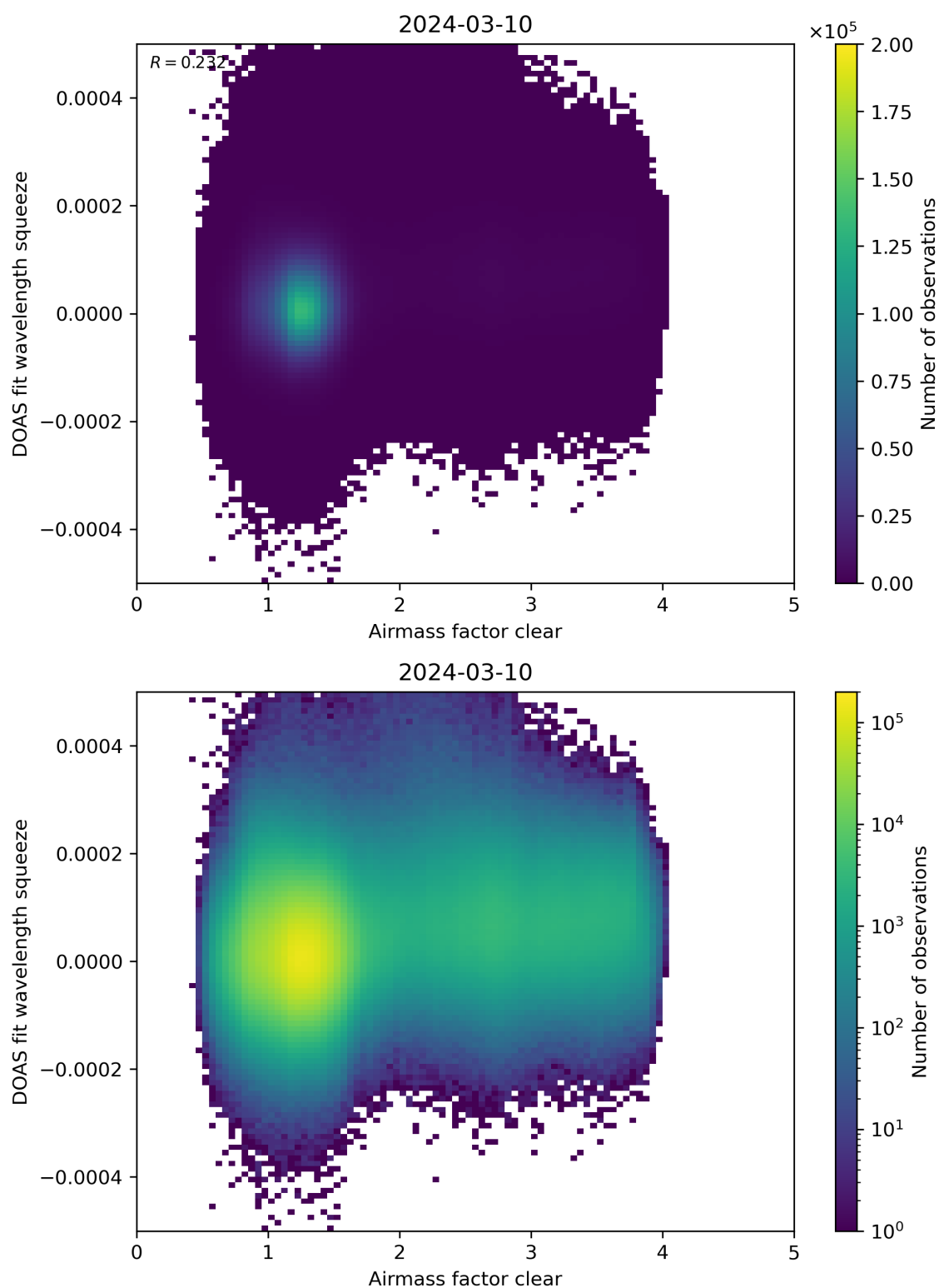
Figure 73: Scatter density plot of “Airmass factor clear” against “DOAS fit wavelength squeeze” for 2024-03-09 to 2024-03-11.
