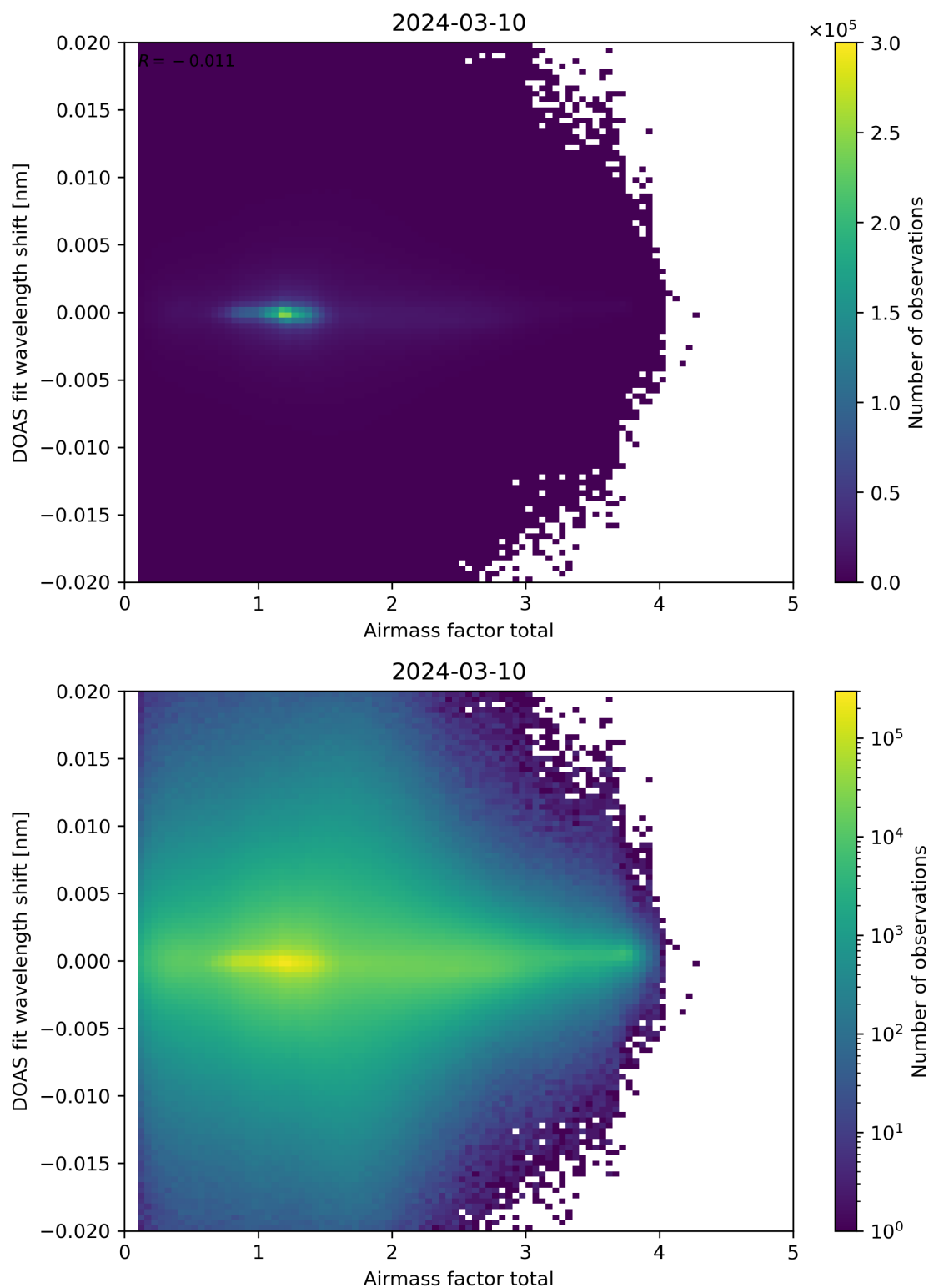
Figure 98: Scatter density plot of “Airmass factor total” against “DOAS fit wavelength shift” for 2024-03-09 to 2024-03-11.
