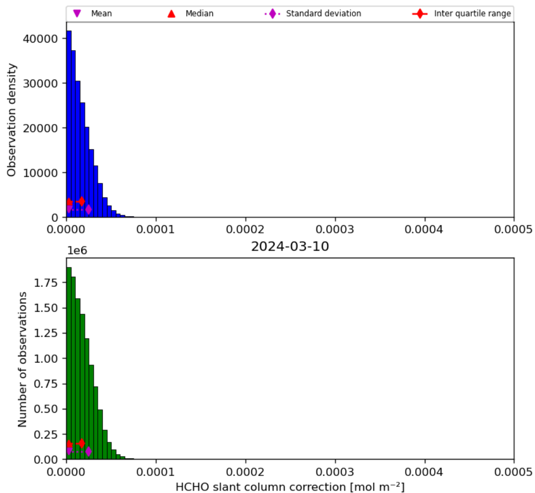
Figure 47: Histogram of “HCHO slant column correction” for 2024-03-09 to 2024-03-11
