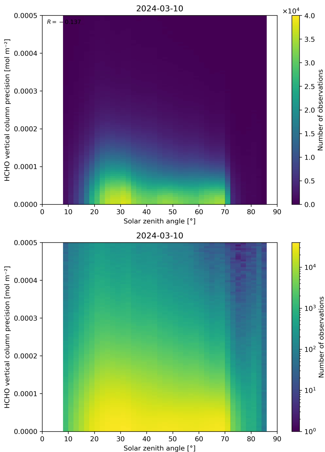
Figure 179: Scatter density plot of “Solar zenith angle” against “HCHO vertical column precision” for 2024-03-09 to 2024-03-11.
