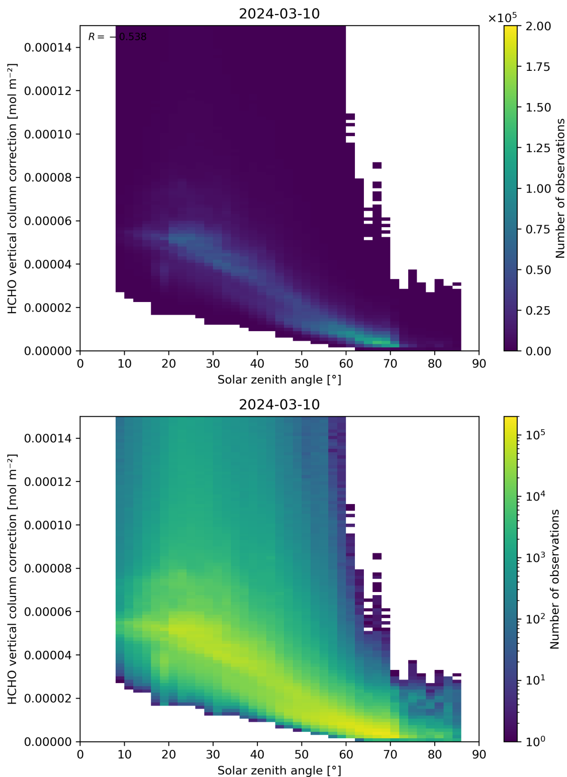
Figure 178: Scatter density plot of “Solar zenith angle” against “HCHO vertical column correction” for 2024-03-09 to 2024-03-11.
