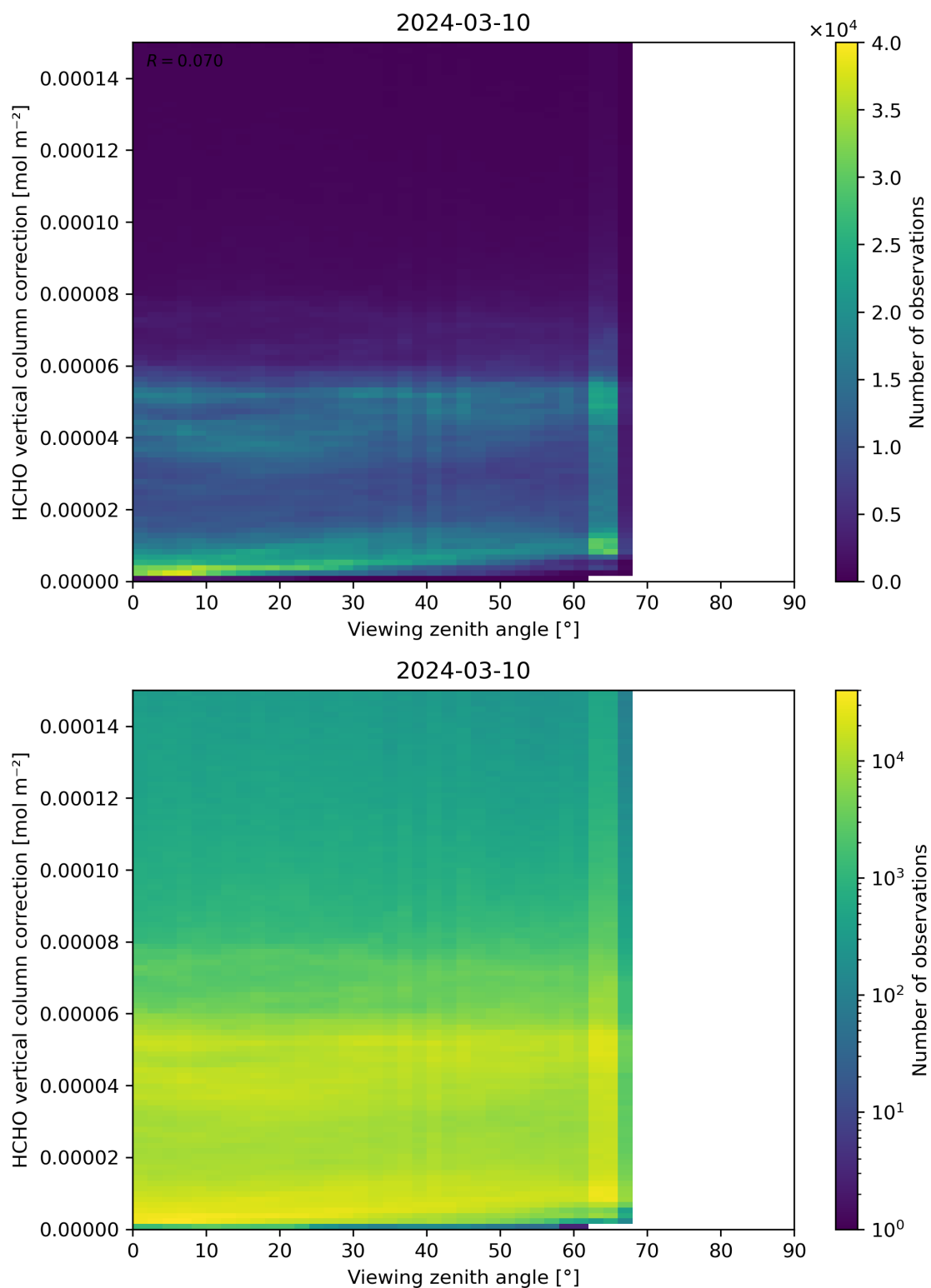
Figure 193: Scatter density plot of “Viewing zenith angle” against “HCHO vertical column correction” for 2024-03-09 to 2024-03-11.
