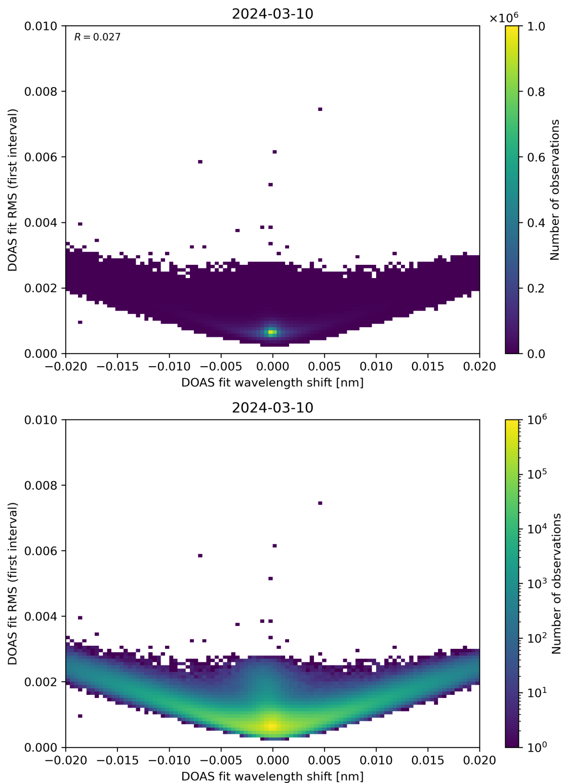
Figure 64: Scatter density plot of “DOAS fit wavelength shift” against “DOAS fit RMS (first interval)” for 2024-03-09 to 2024-03-11.
