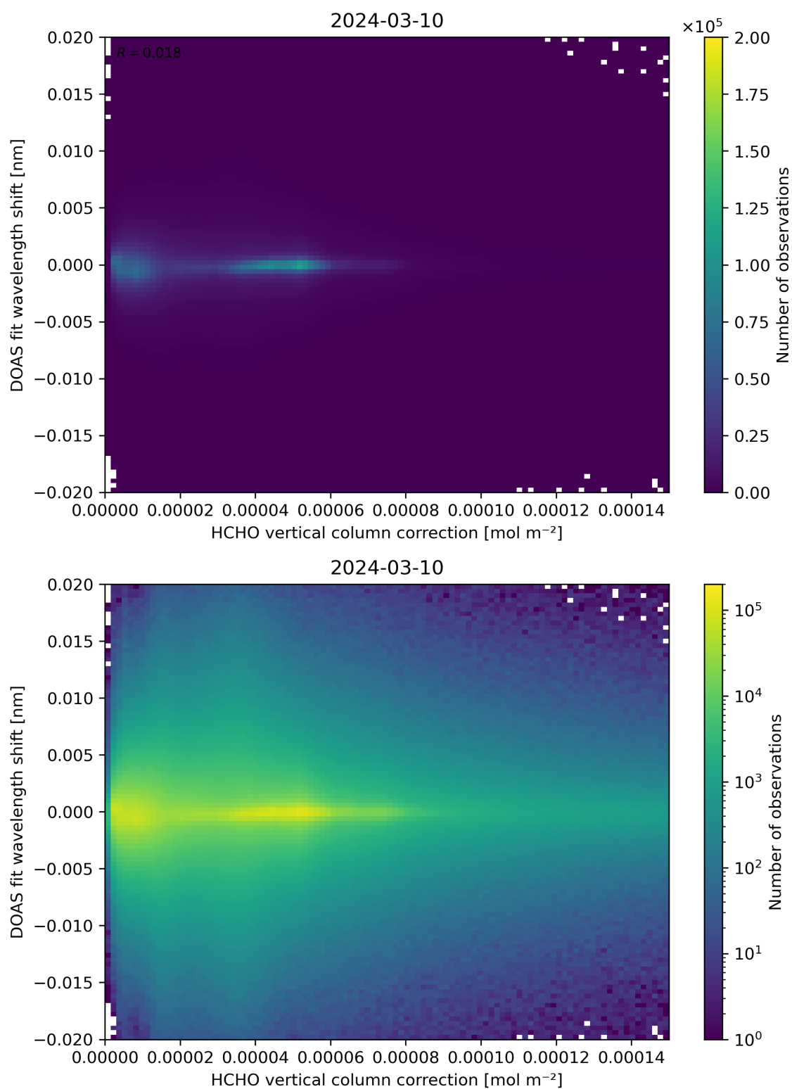
Figure 113: Scatter density plot of “HCHO vertical column correction” against “DOAS fit wavelength shift” for 2024-03-09 to 2024-03-11.
