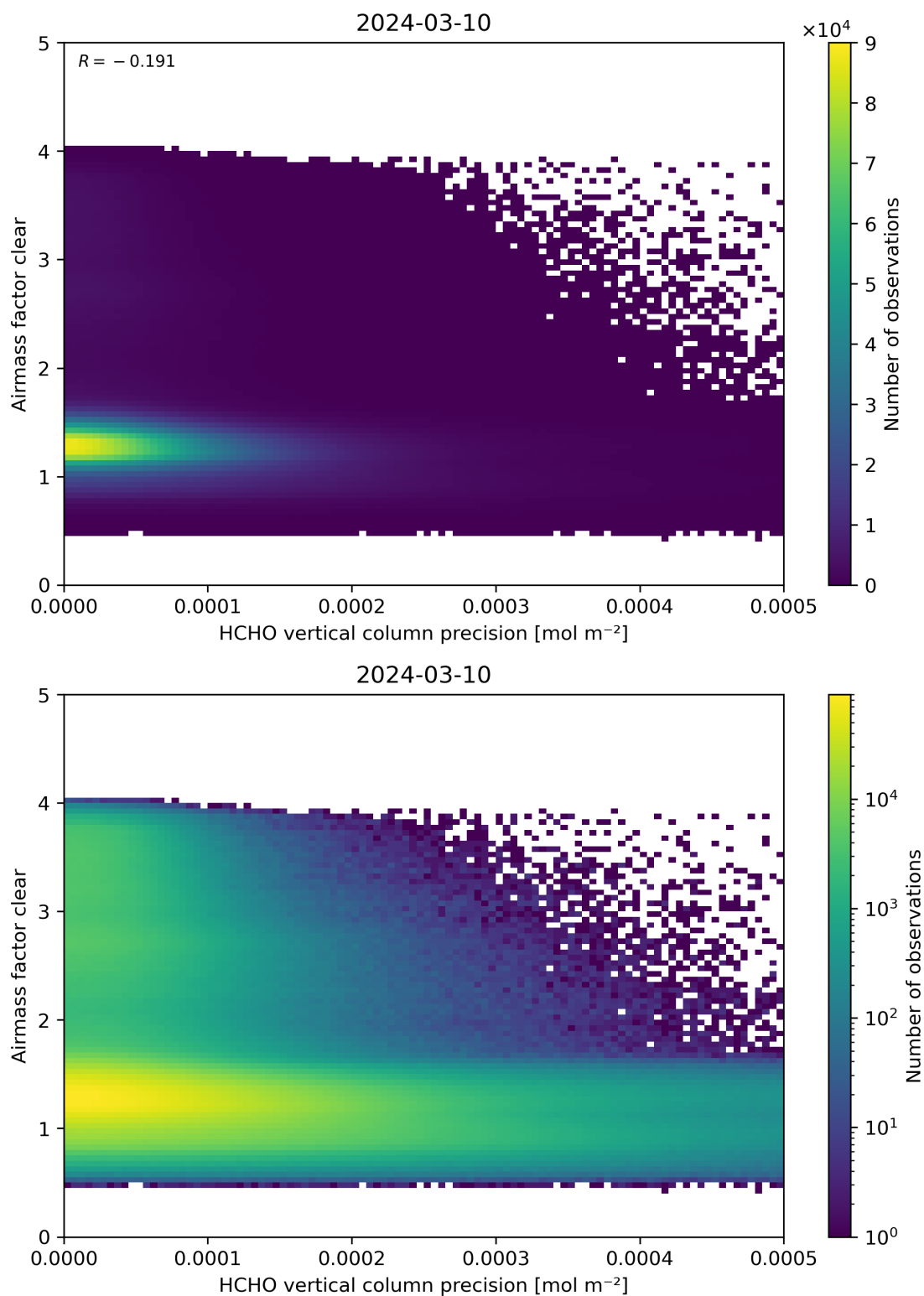
Figure 139: Scatter density plot of “HCHO vertical column precision” against “Airmass factor clear” for 2024-03-09 to 2024-03-11.
