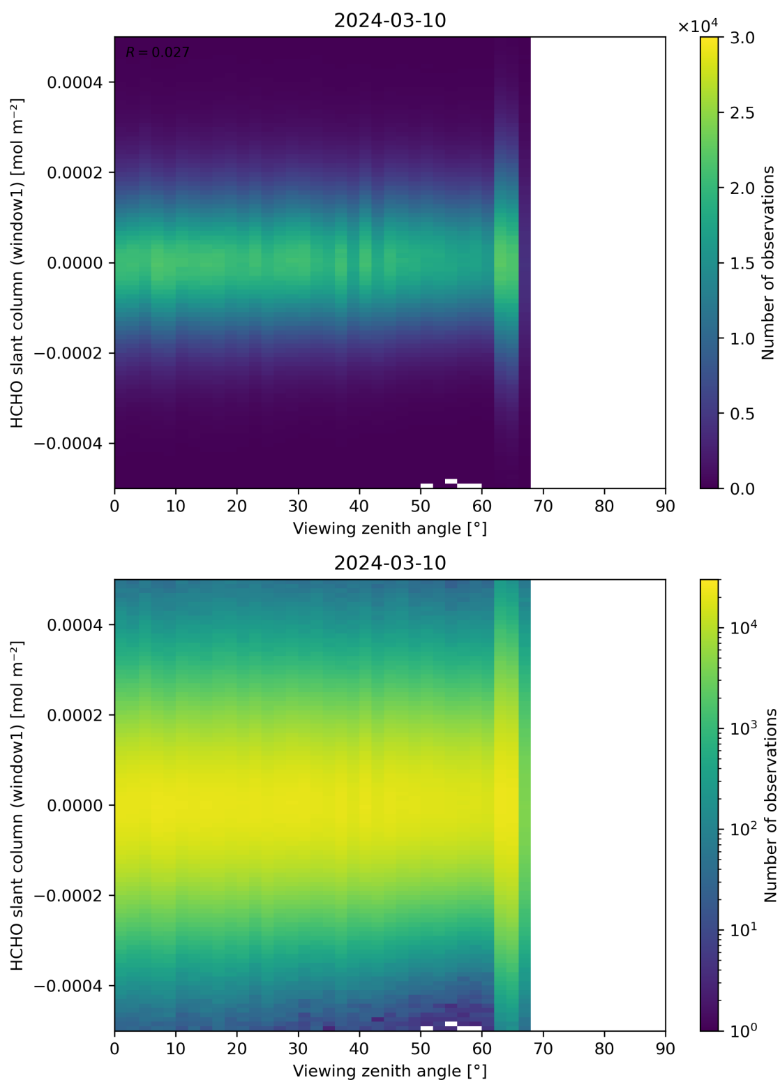
Figure 188: Scatter density plot of “Viewing zenith angle” against “HCHO slant column (window1)” for 2024-03-09 to 2024-03-11.
