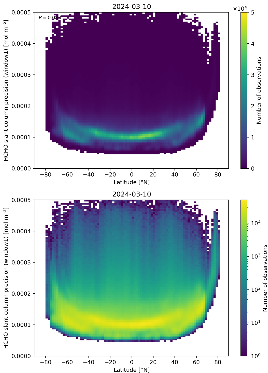
Figure 160: Scatter density plot of “Latitude” against “HCHO slant column precision (window1)” for 2024-03-09 to 2024-03-11.
