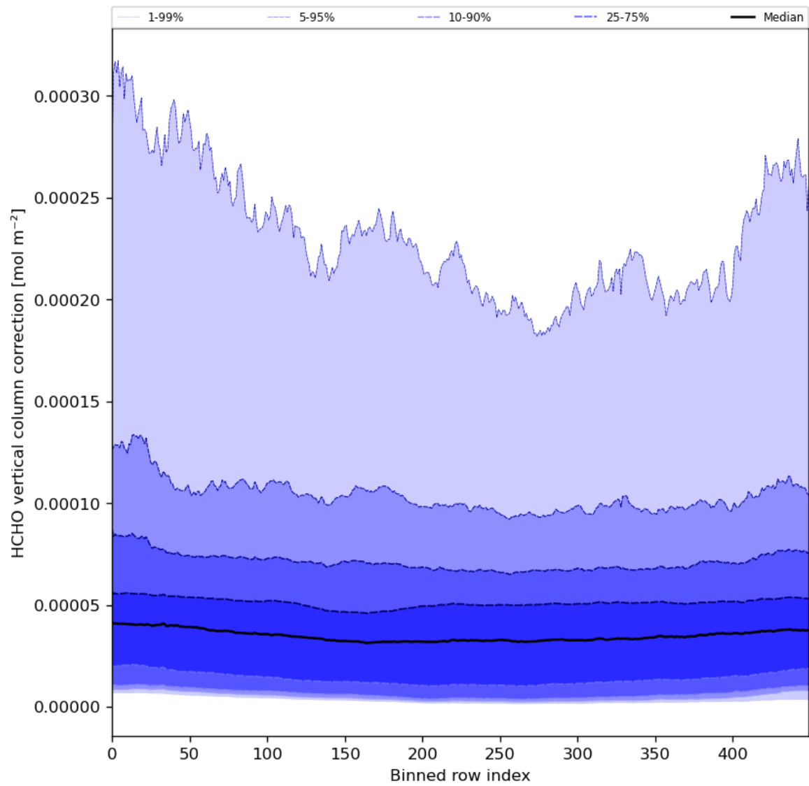
Figure 51: Along track statistics of “HCHO vertical column correction” for 2024-03-09 to 2024-03-11
