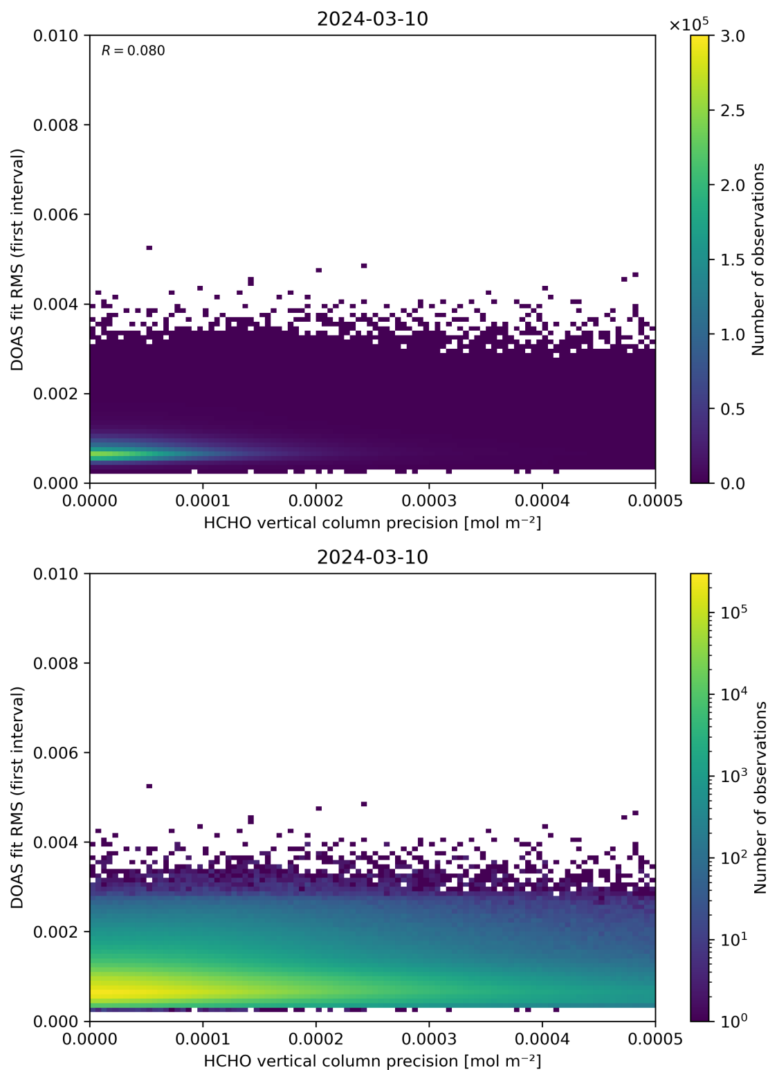
Figure 136: Scatter density plot of “HCHO vertical column precision” against “DOAS fit RMS (first interval)” for 2024-03-09 to 2024-03-11.
