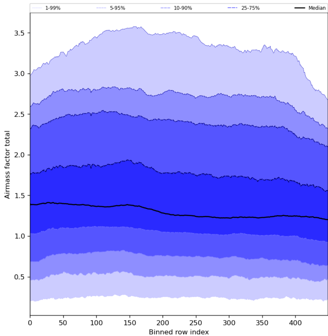
Figure 54: Along track statistics of “Airmass factor total” for 2024-03-09 to 2024-03-11
