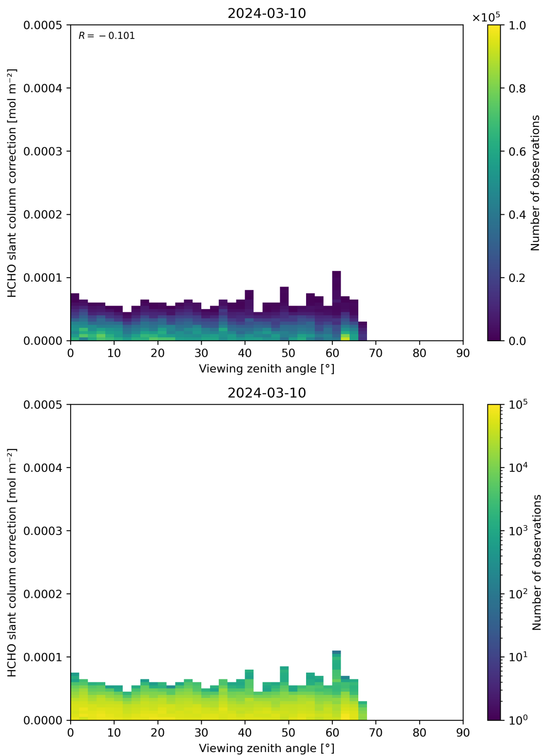
Figure 187: Scatter density plot of “Viewing zenith angle” against “HCHO slant column correction” for 2024-03-09 to 2024-03-11.
