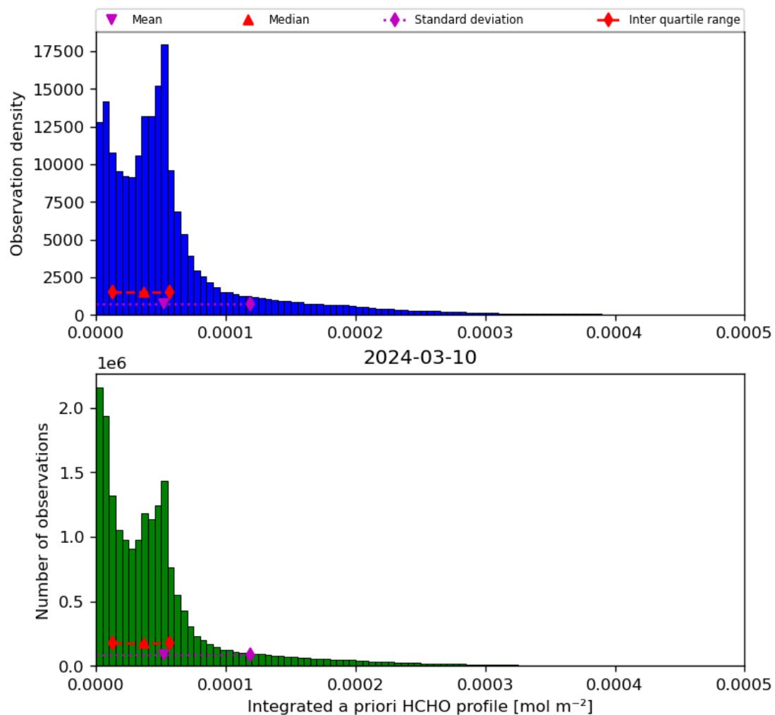
Figure 43: Histogram of “Integrated a priori HCHO profile” for 2024-03-09 to 2024-03-11
