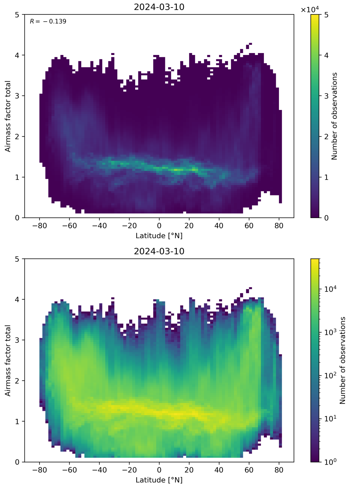
Figure 161: Scatter density plot of “Latitude” against “Airmass factor total” for 2024-03-09 to 2024-03-11.
