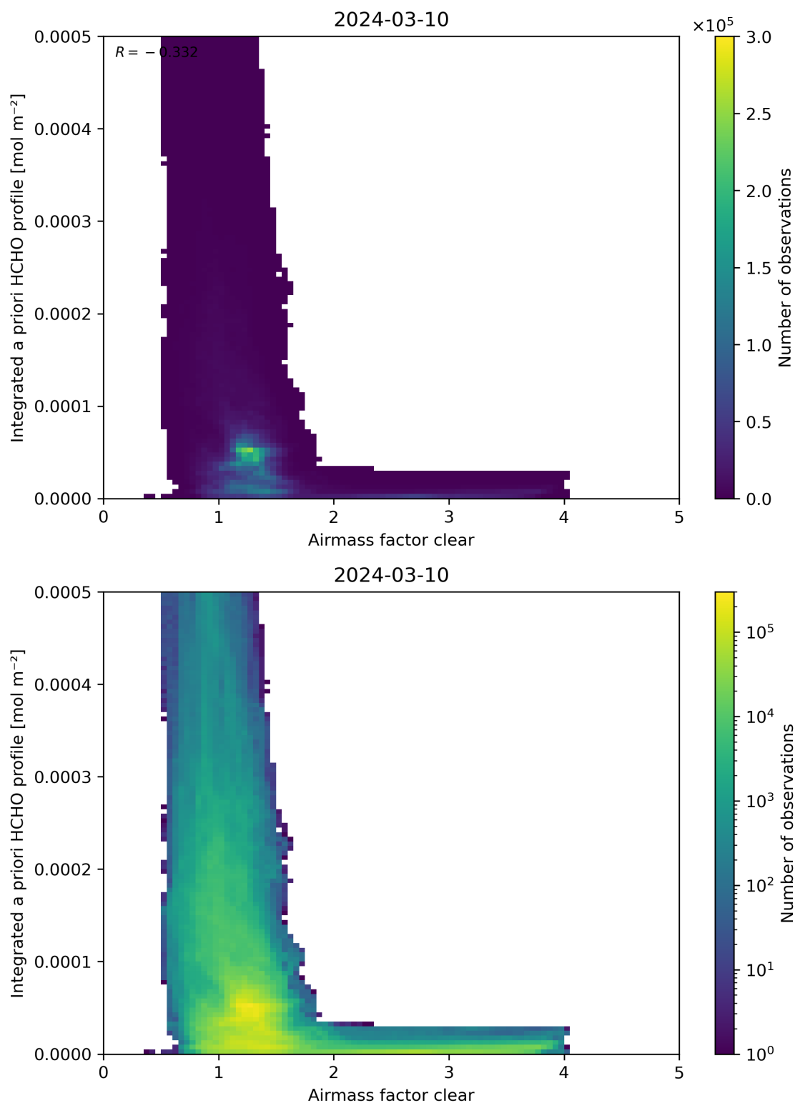
Figure 76: Scatter density plot of “Airmass factor clear” against “Integrated a priori HCHO profile” for 2024-03-09 to 2024-03-11.
