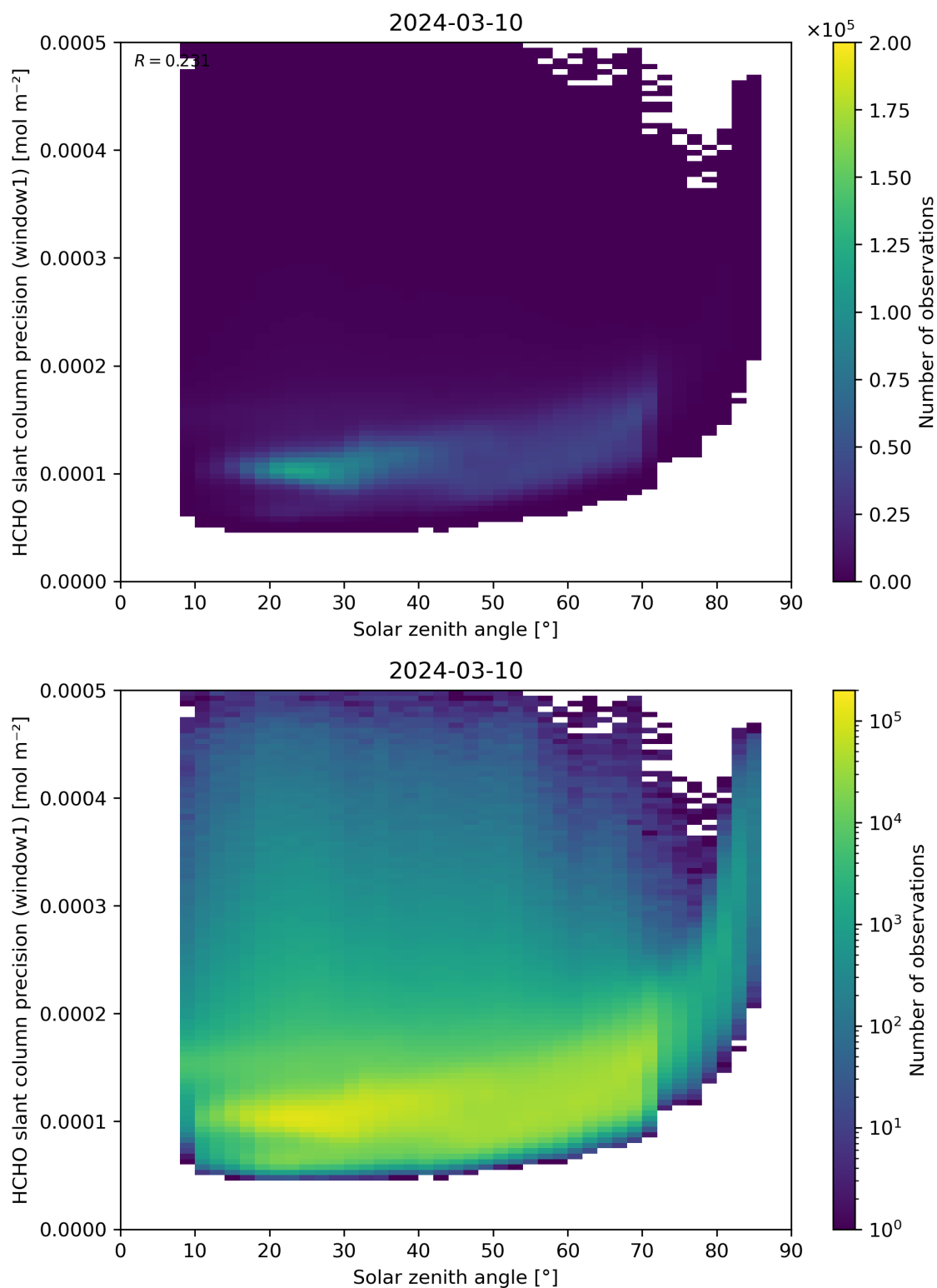
Figure 174: Scatter density plot of “Solar zenith angle” against “HCHO slant column precision (window1)” for 2024-03-09 to 2024-03-11.
