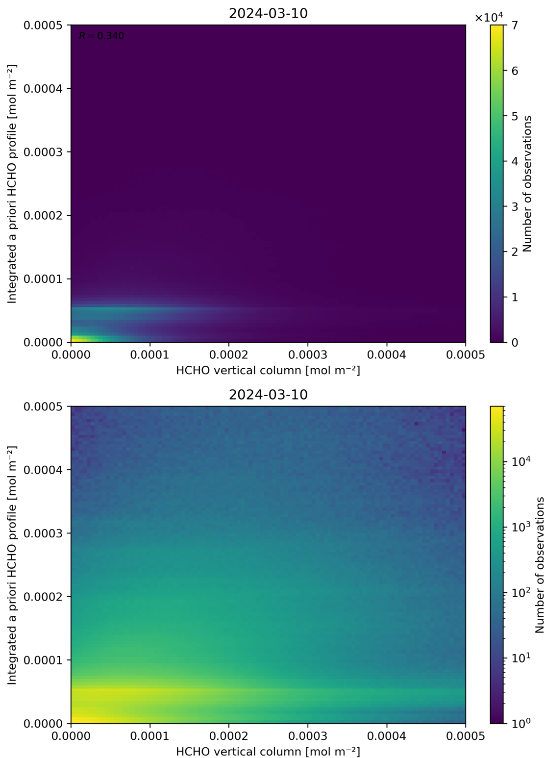
Figure 135: Scatter density plot of “HCHO vertical column” against “Integrated a priori HCHO profile” for 2024-03-09 to 2024-03-11.
