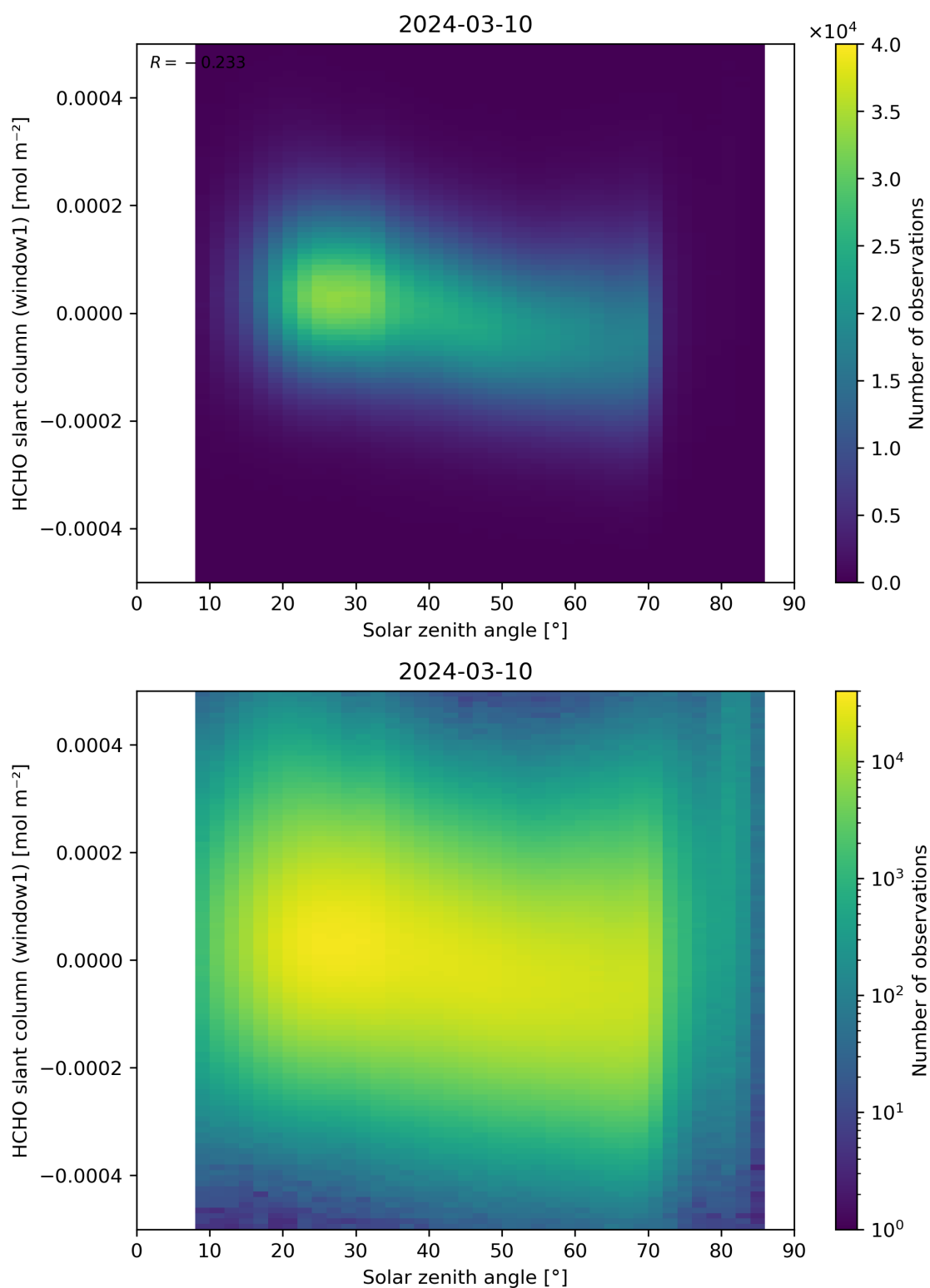
Figure 173: Scatter density plot of “Solar zenith angle” against “HCHO slant column (window1)” for 2024-03-09 to 2024-03-11.
