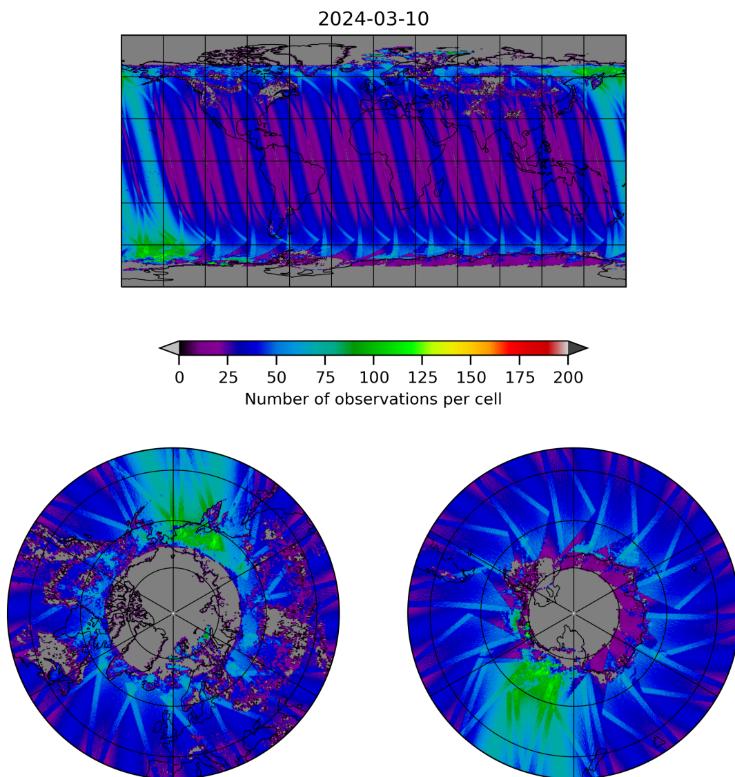
Figure 19: Map of the number of observations for 2024-03-09 to 2024-03-11
