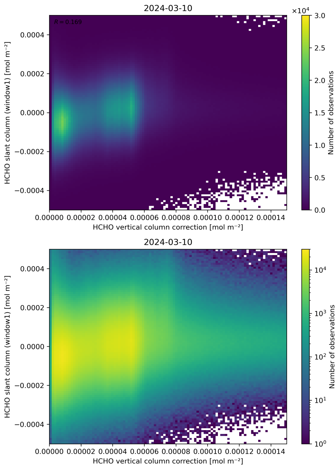
Figure 118: Scatter density plot of “HCHO vertical column correction” against “HCHO slant column (window1)” for 2024-03-09 to 2024-03-11.
