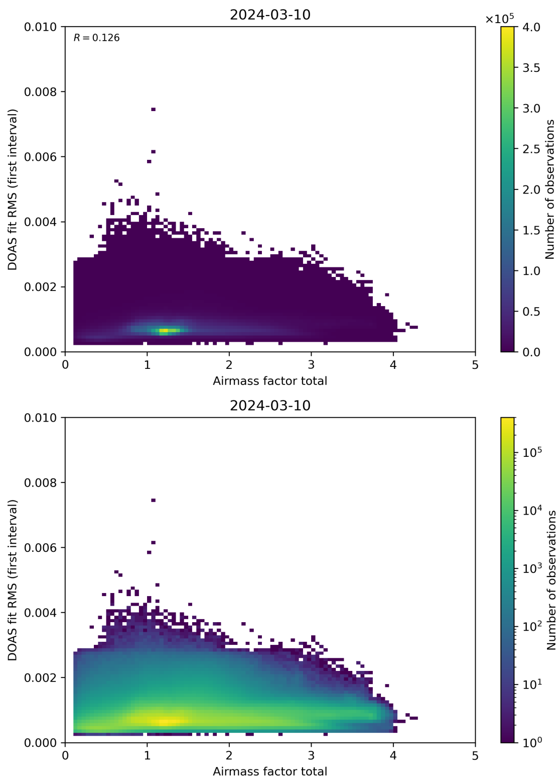
Figure 97: Scatter density plot of “Airmass factor total” against “DOAS fit RMS (first interval)” for 2024-03-09 to 2024-03-11.
