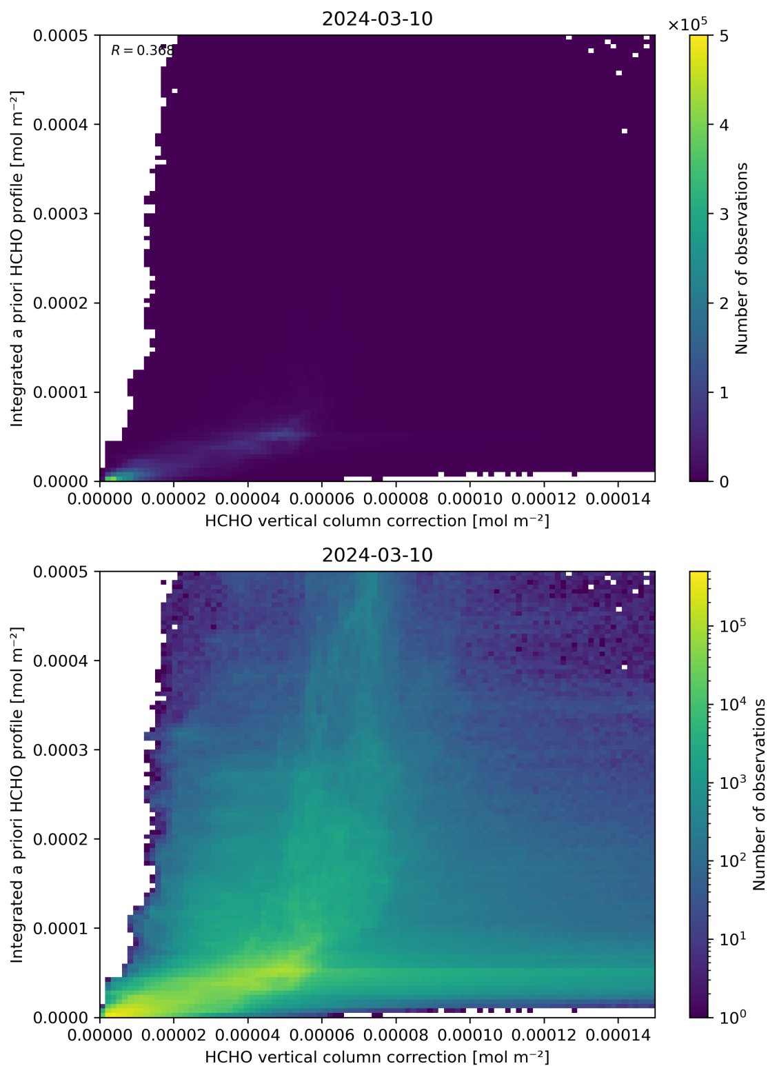
Figure 122: Scatter density plot of “HCHO vertical column correction” against “Integrated a priori HCHO profile” for 2024-03-09 to 2024-03-11.
