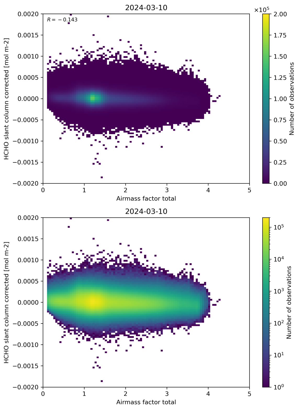
Figure 101: Scatter density plot of “Airmass factor total” against “HCHO slant column corrected” for 2024-03-09 to 2024-03-11.
