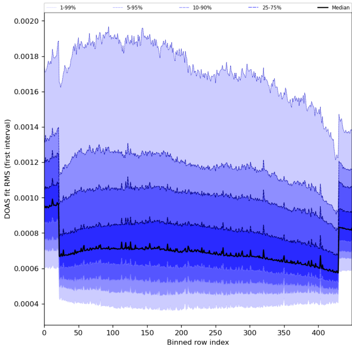
Figure 60: Along track statistics of “DOAS fit RMS (first interval)” for 2024-03-09 to 2024-03-11
