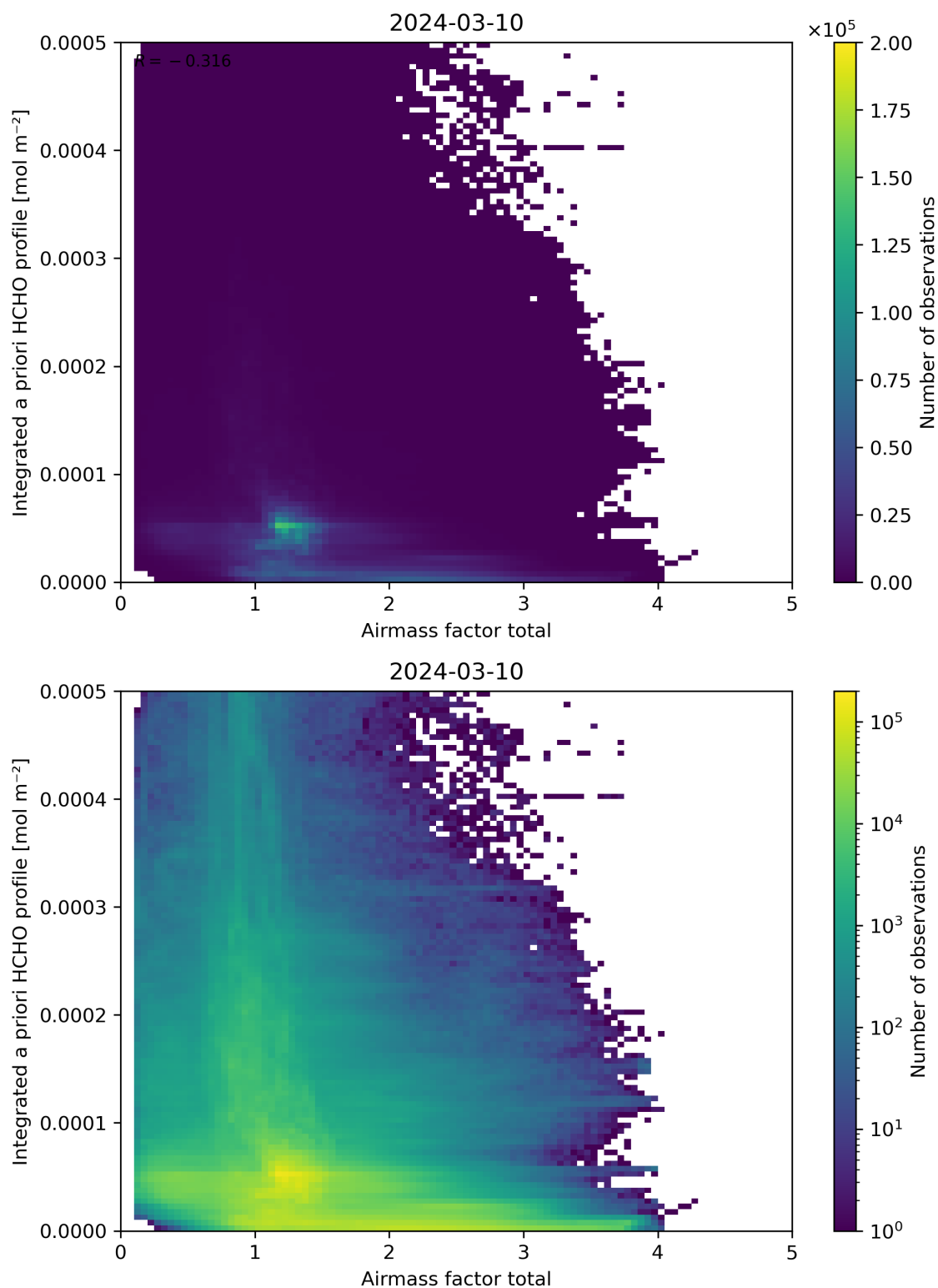
Figure 104: Scatter density plot of “Airmass factor total” against “Integrated a priori HCHO profile” for 2024-03-09 to 2024-03-11.
