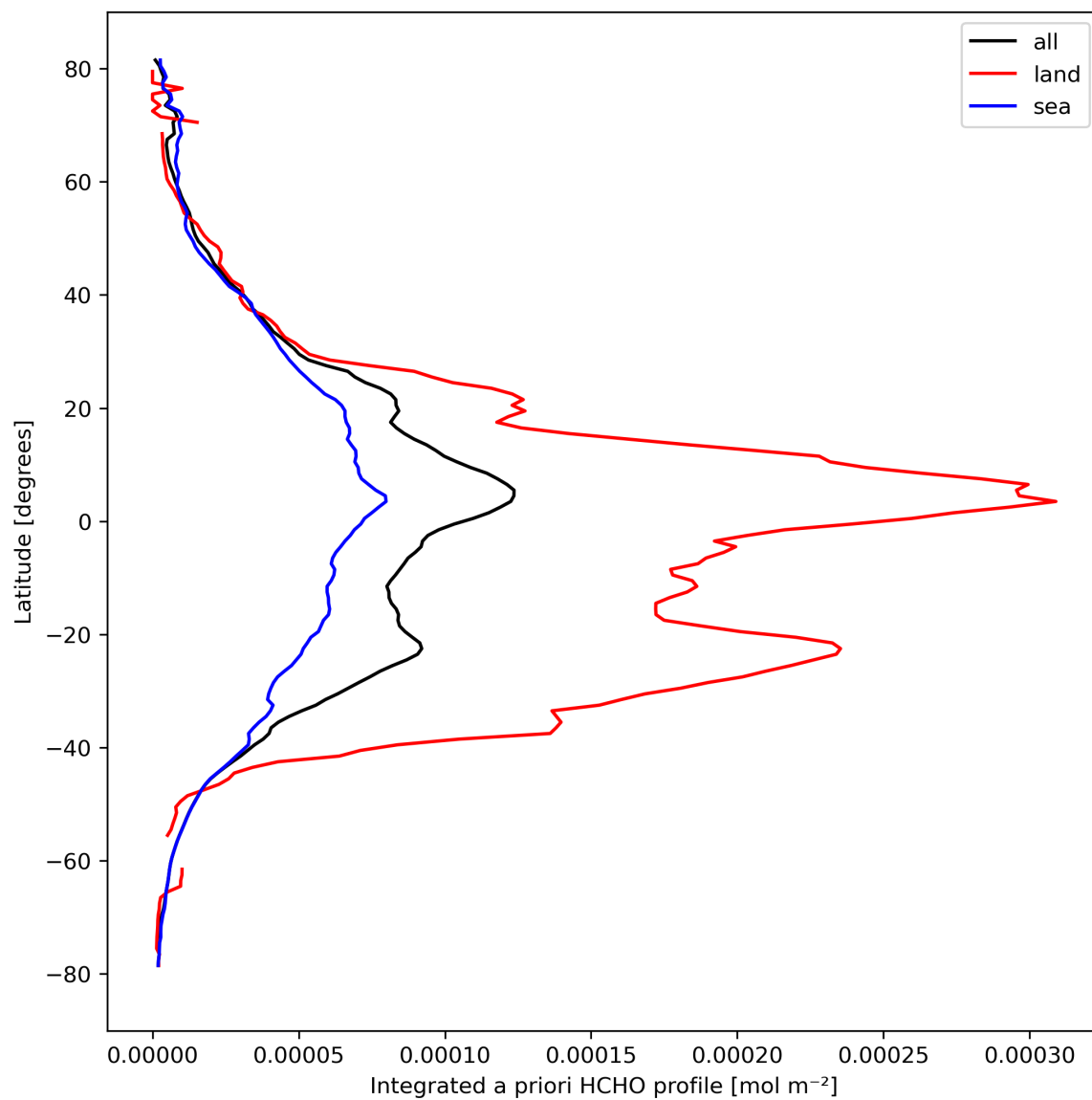
Figure 29: Zonal average of “Integrated a priori HCHO profile” for 2024-03-09 to 2024-03-11.
