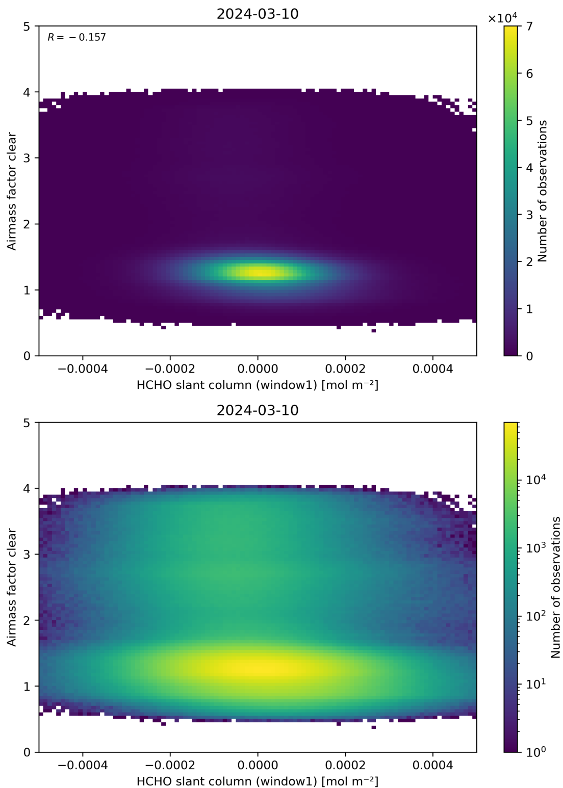
Figure 81: Scatter density plot of “HCHO slant column (window1)” against “Airmass factor clear” for 2024-03-09 to 2024-03-11.
