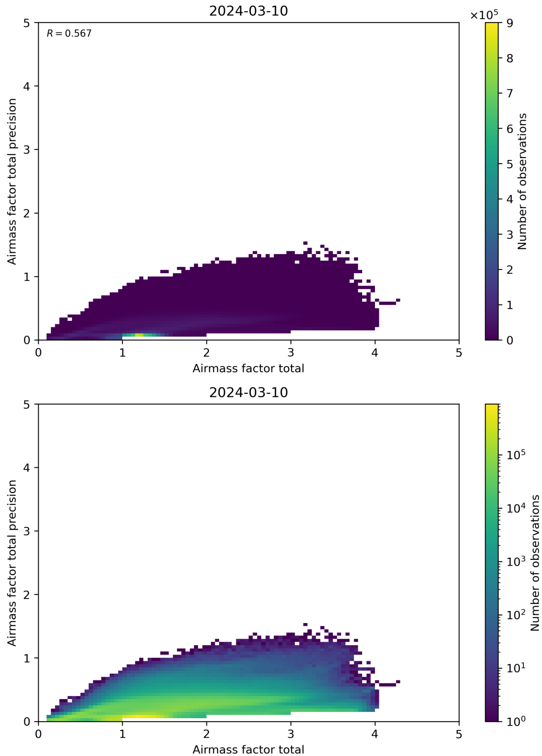
Figure 103: Scatter density plot of “Airmass factor total” against “Airmass factor total precision” for 2024-03-09 to 2024-03-11.
