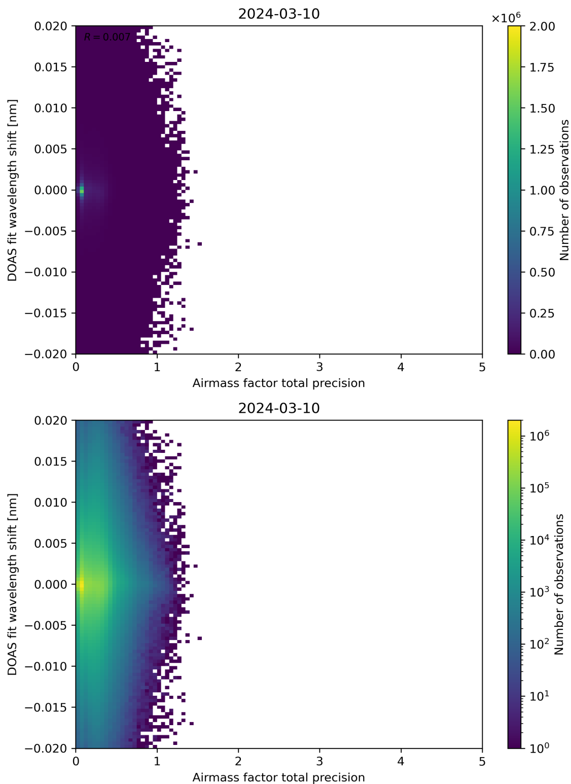
Figure 106: Scatter density plot of “Airmass factor total precision” against “DOAS fit wavelength shift” for 2024-03-09 to 2024-03-11.
