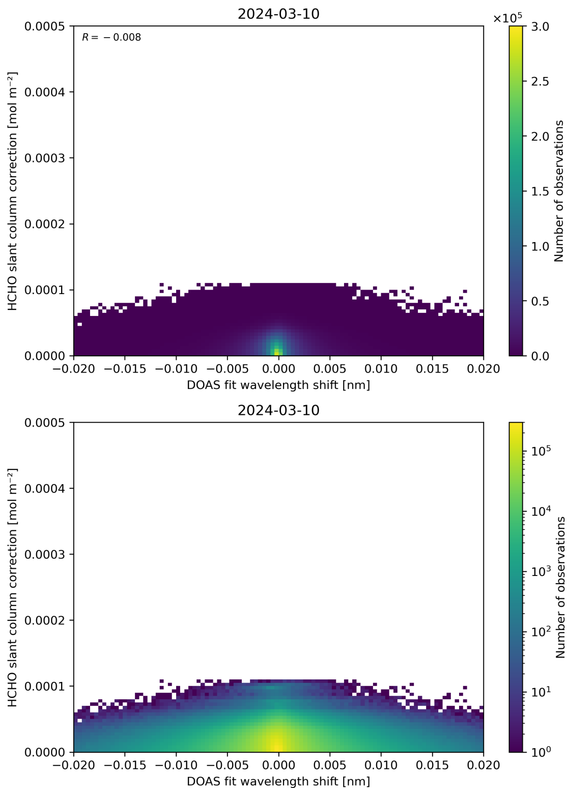
Figure 67: Scatter density plot of “DOAS fit wavelength shift” against “HCHO slant column correction” for 2024-03-09 to 2024-03-11.
