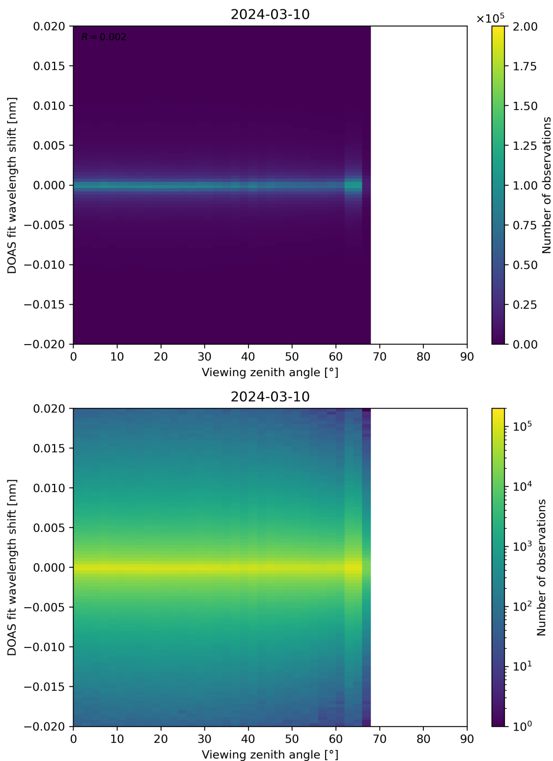
Figure 183: Scatter density plot of “Viewing zenith angle” against “DOAS fit wavelength shift” for 2024-03-09 to 2024-03-11.
