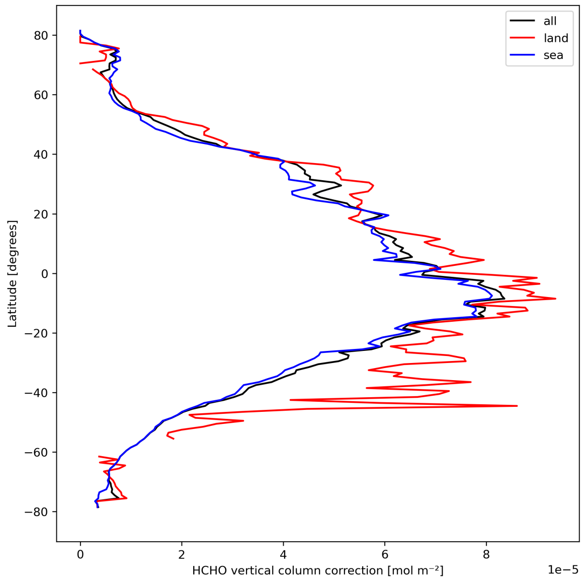
Figure 23: Zonal average of “HCHO vertical column correction” for 2024-03-09 to 2024-03-11.
