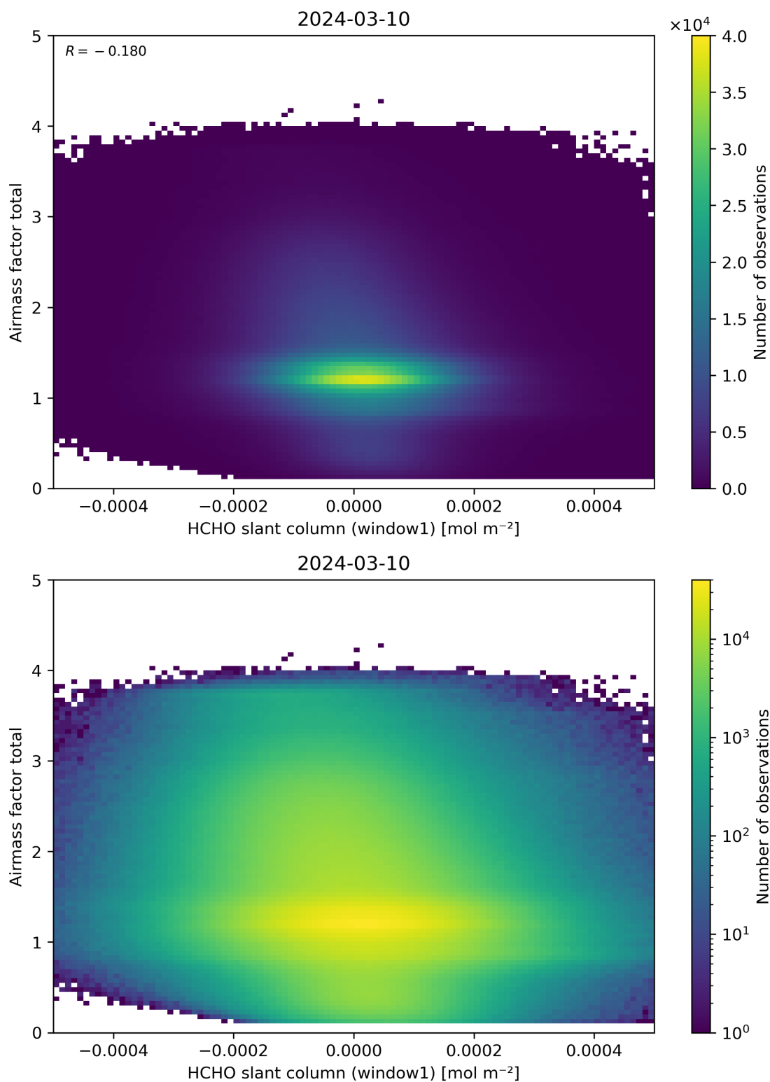
Figure 85: Scatter density plot of “HCHO slant column (window1)” against “Airmass factor total” for 2024-03-09 to 2024-03-11.
