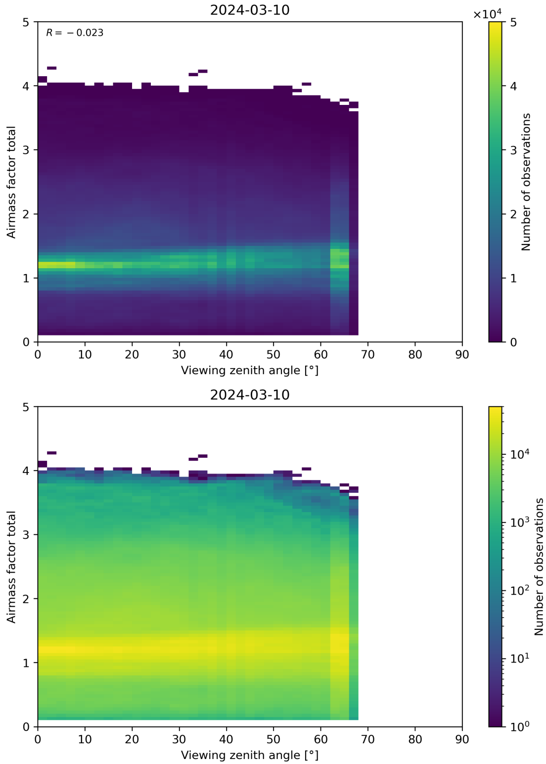
Figure 190: Scatter density plot of “Viewing zenith angle” against “Airmass factor total” for 2024-03-09 to 2024-03-11.
