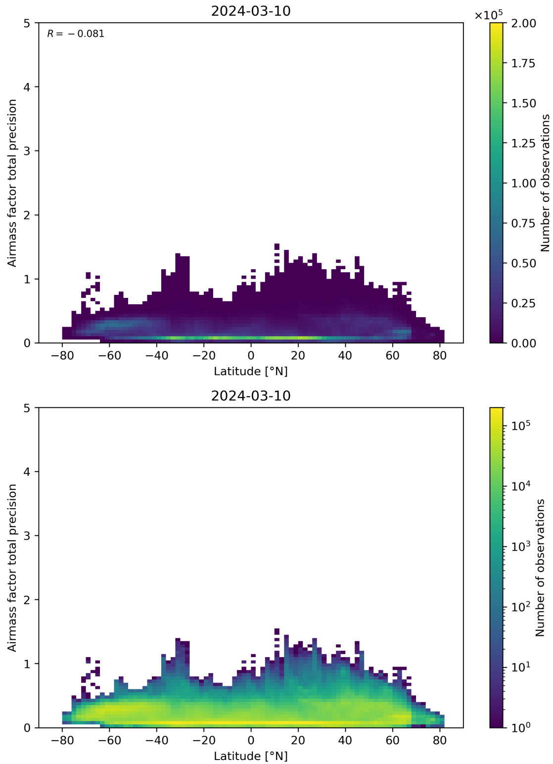
Figure 162: Scatter density plot of “Latitude” against “Airmass factor total precision” for 2024-03-09 to 2024-03-11.
