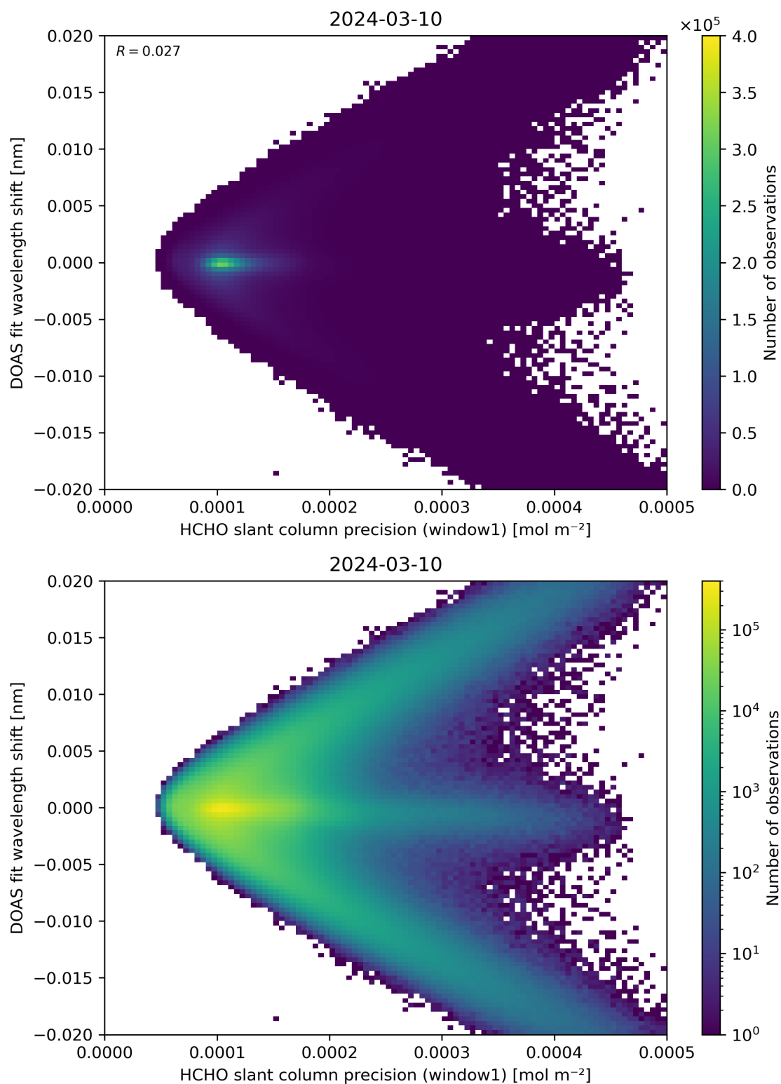
Figure 89: Scatter density plot of “HCHO slant column precision (window1)” against “DOAS fit wavelength shift” for 2024-03-09 to 2024-03-11.
