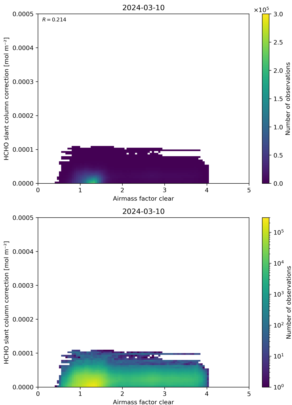
Figure 75: Scatter density plot of “Airmass factor clear” against “HCHO slant column correction” for 2024-03-09 to 2024-03-11.
