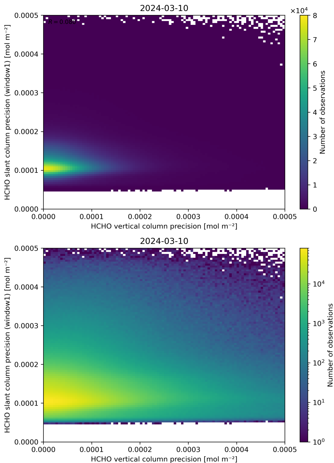
Figure 143: Scatter density plot of “HCHO vertical column precision” against “HCHO slant column precision (window1)” for 2024-03-09 to 2024-03-11.
