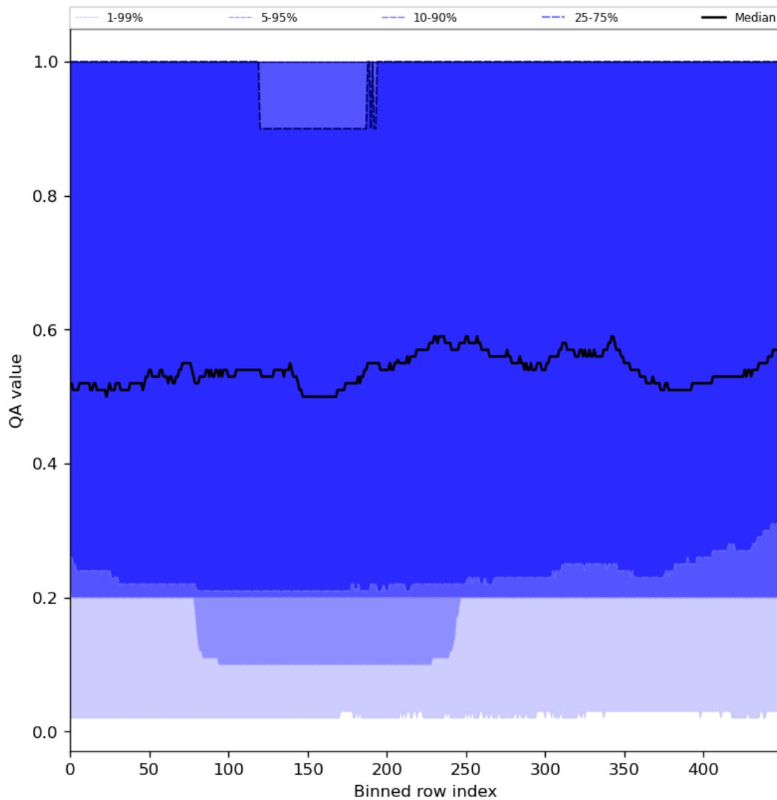
Figure 48: Along track statistics of “QA value” for 2024-03-09 to 2024-03-11
