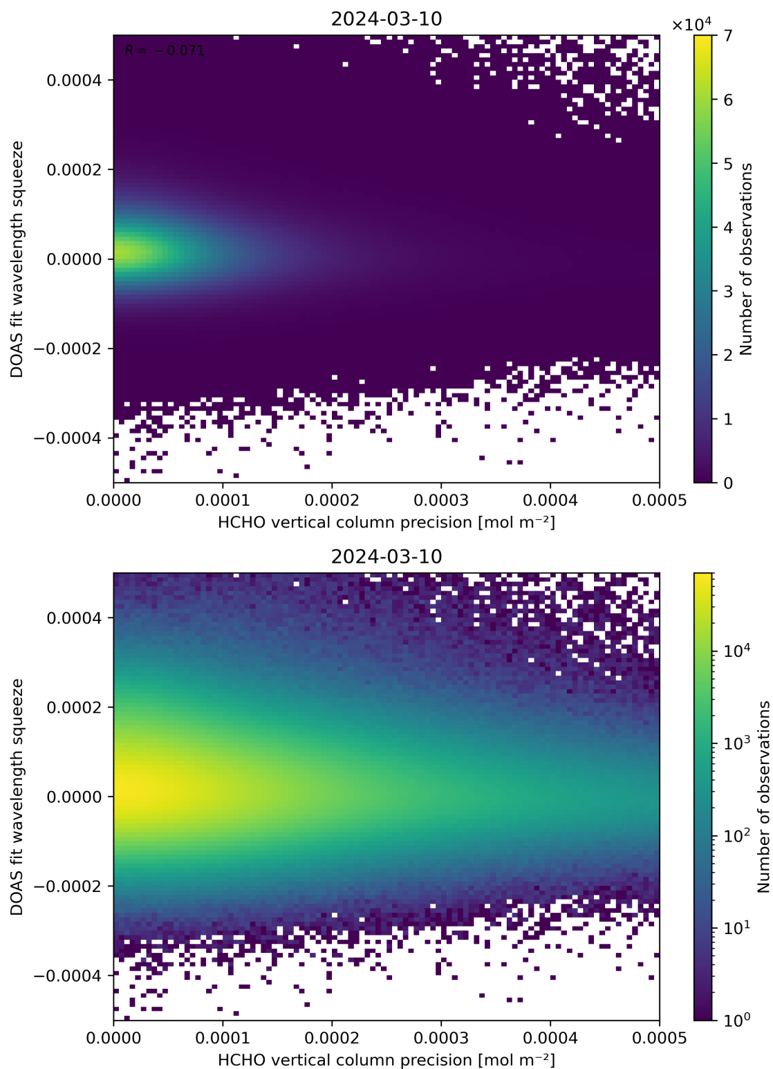
Figure 138: Scatter density plot of “HCHO vertical column precision” against “DOAS fit wavelength squeeze” for 2024-03-09 to 2024-03-11.
