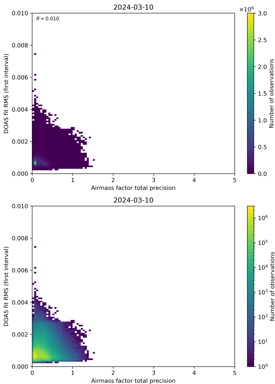
Figure 105: Scatter density plot of “Airmass factor total precision” against “DOAS fit RMS (first interval)” for 2024-03-09 to 2024-03-11.
