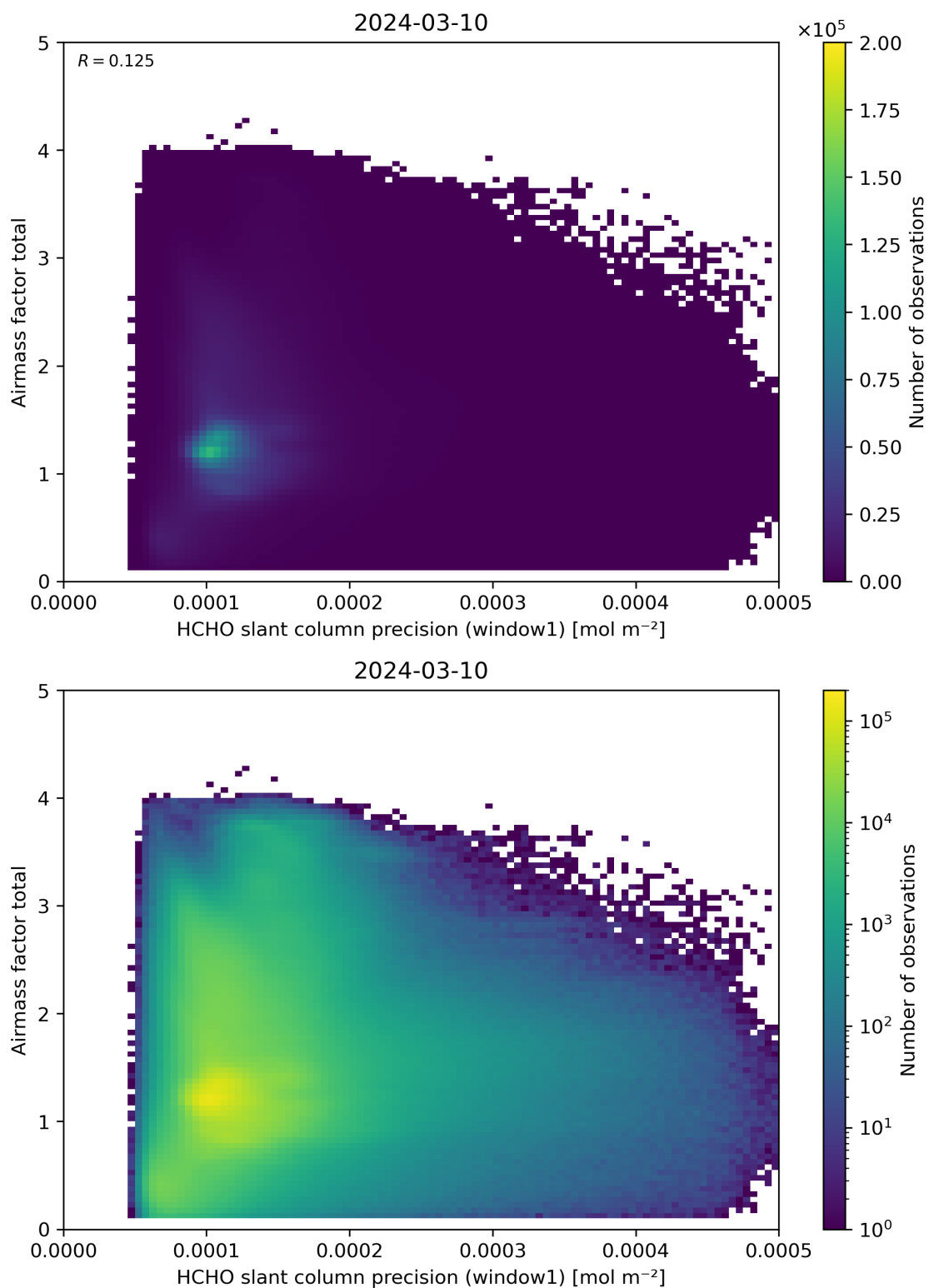
Figure 94: Scatter density plot of “HCHO slant column precision (window1)” against “Airmass factor total” for 2024-03-09 to 2024-03-11.
