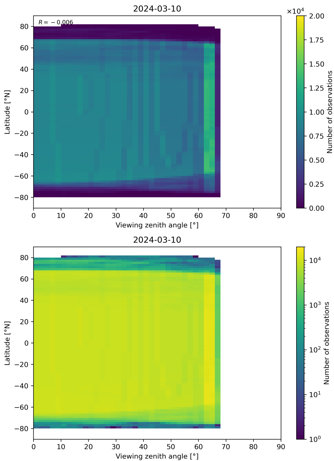
Figure 196: Scatter density plot of “Viewing zenith angle” against “Latitude” for 2024-03-09 to 2024-03-11.
