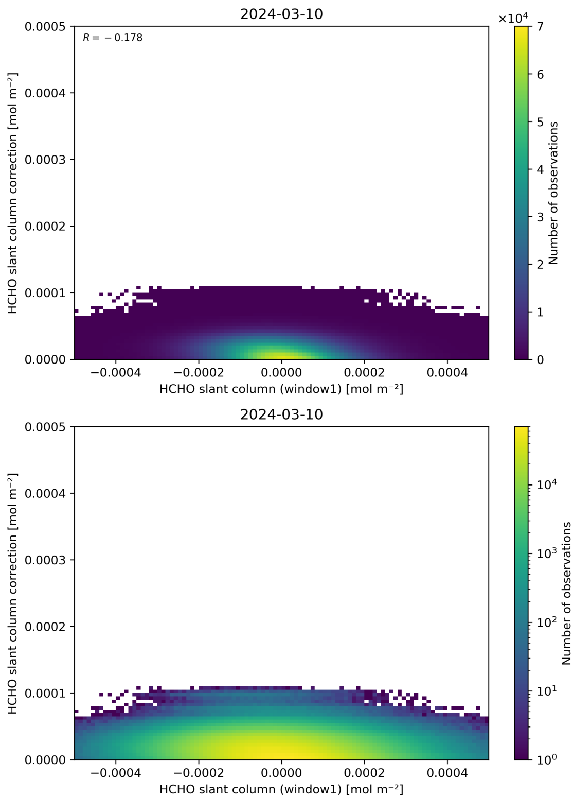
Figure 83: Scatter density plot of “HCHO slant column (window1)” against “HCHO slant column correction” for 2024-03-09 to 2024-03-11.
