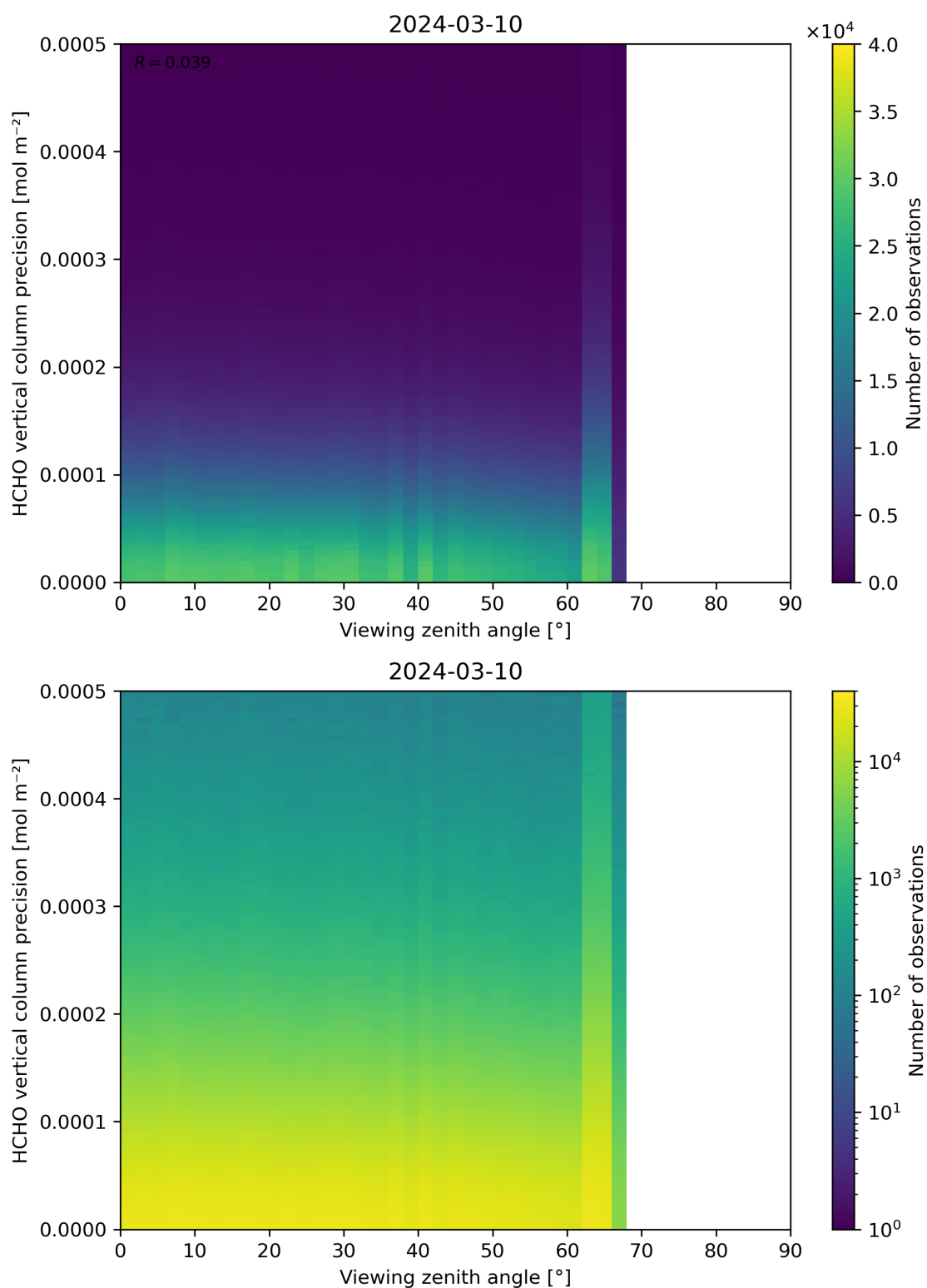
Figure 194: Scatter density plot of “Viewing zenith angle” against “HCHO vertical column precision” for 2024-03-09 to 2024-03-11.
