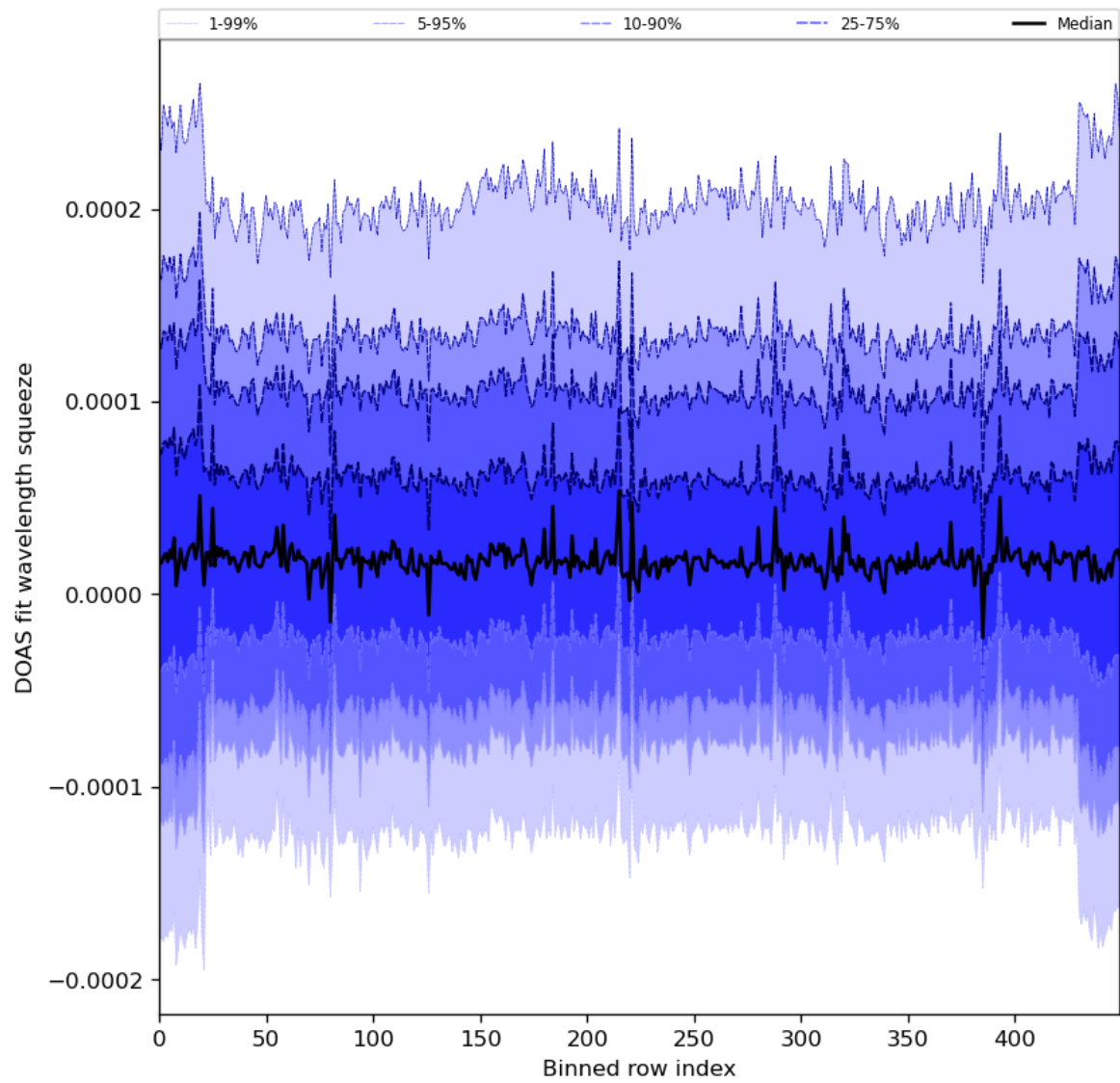
Figure 59: Along track statistics of “DOAS fit wavelength squeeze” for 2024-03-09 to 2024-03-11
