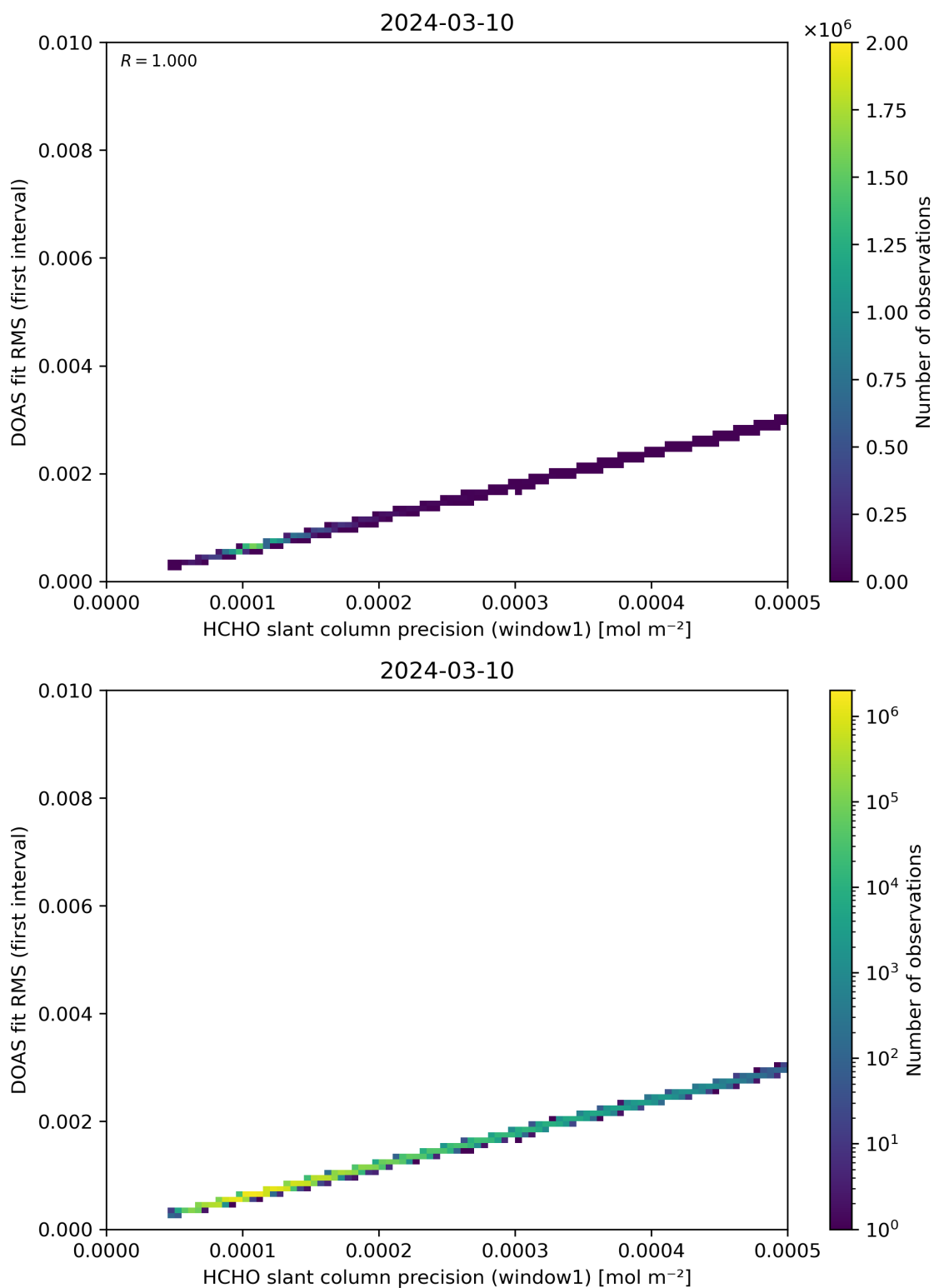
Figure 88: Scatter density plot of “HCHO slant column precision (window1)” against “DOAS fit RMS (first interval)” for 2024-03-09 to 2024-03-11.
