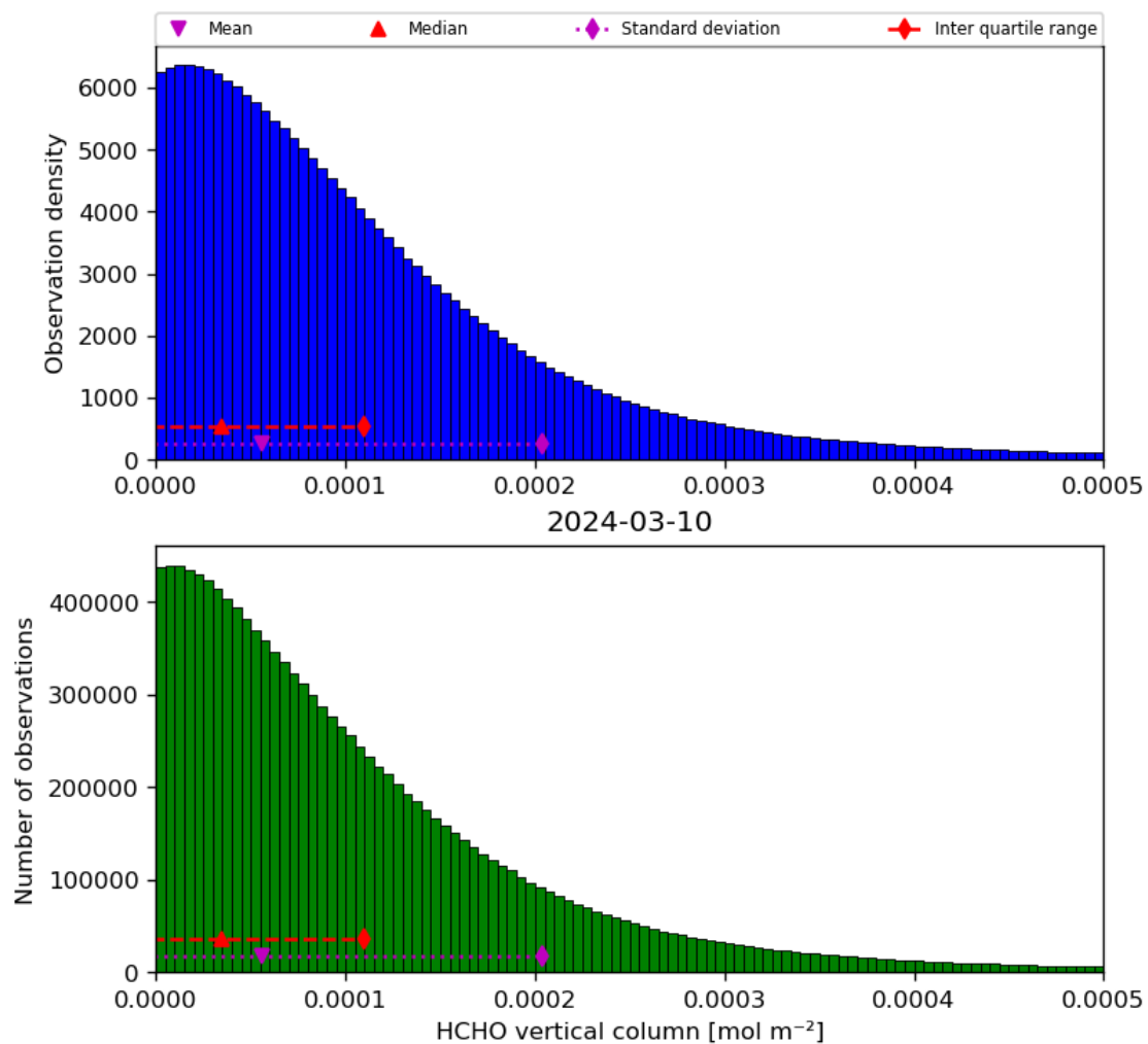
Figure 35: Histogram of “HCHO vertical column” for 2024-03-09 to 2024-03-11
