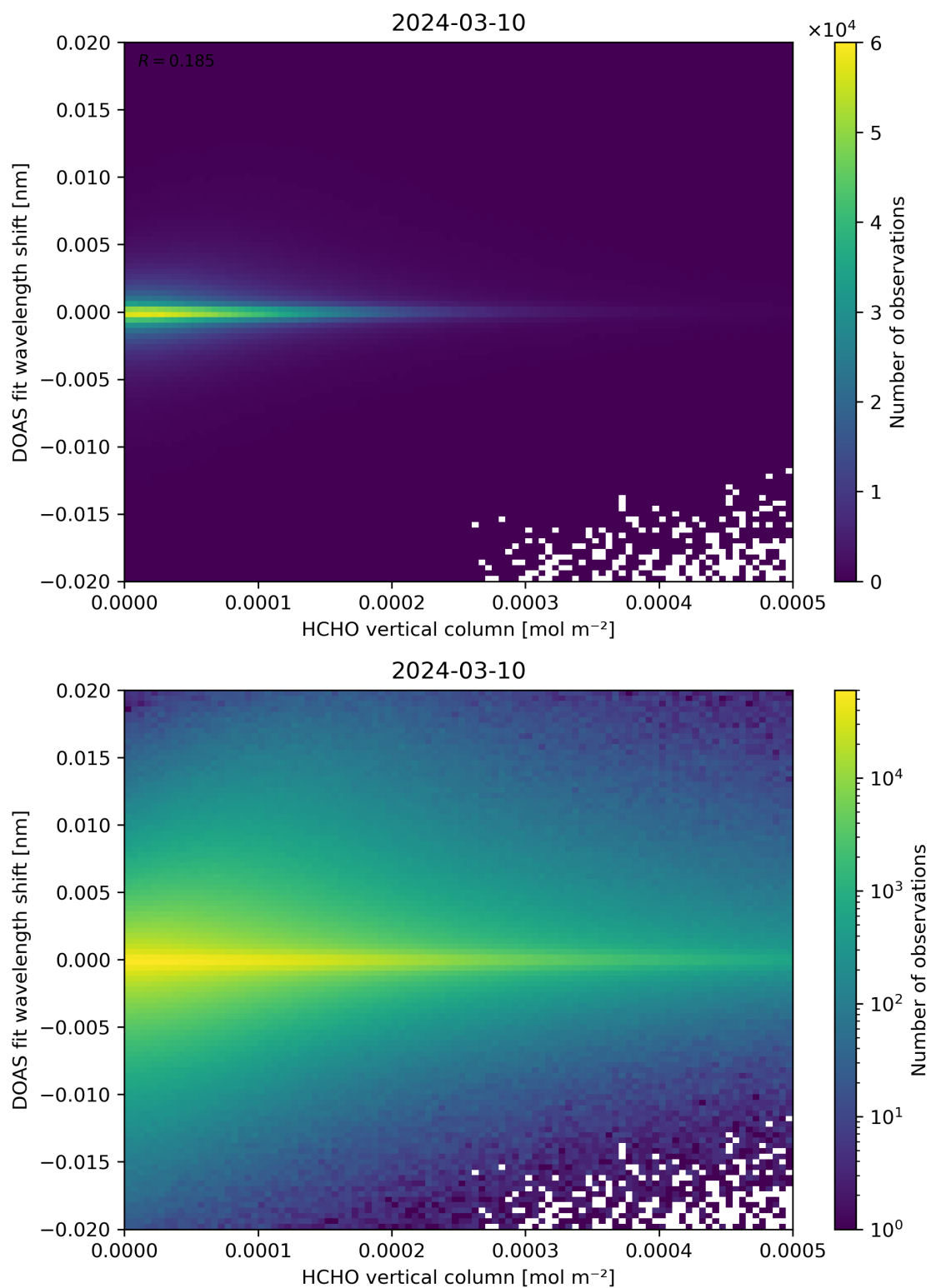
Figure 124: Scatter density plot of “HCHO vertical column” against “DOAS fit wavelength shift” for 2024-03-09 to 2024-03-11.
