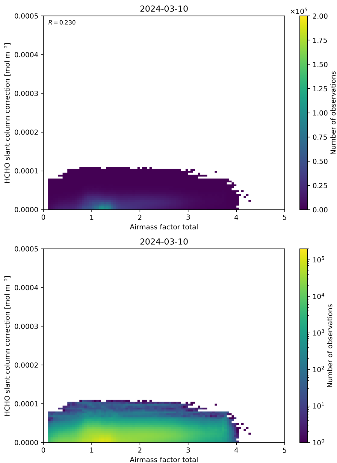
Figure 102: Scatter density plot of “Airmass factor total” against “HCHO slant column correction” for 2024-03-09 to 2024-03-11.
