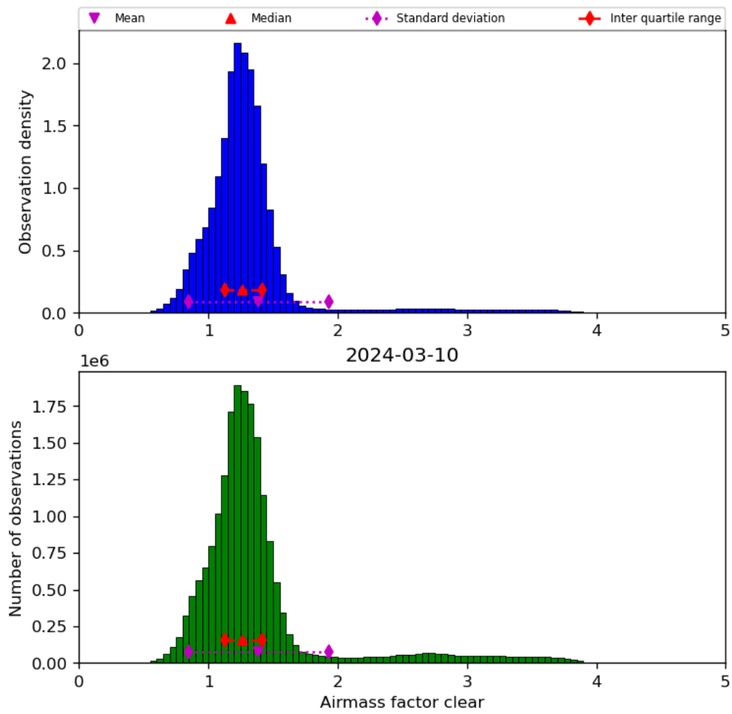
Figure 42: Histogram of “Airmass factor clear” for 2024-03-09 to 2024-03-11
