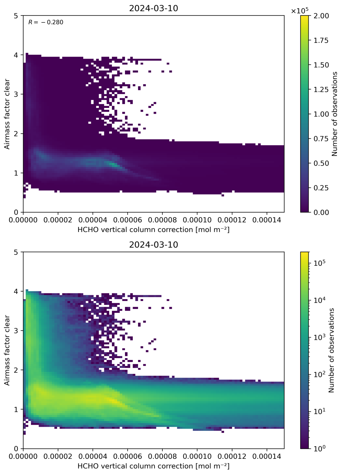
Figure 115: Scatter density plot of “HCHO vertical column correction” against “Airmass factor clear” for 2024-03-09 to 2024-03-11.
