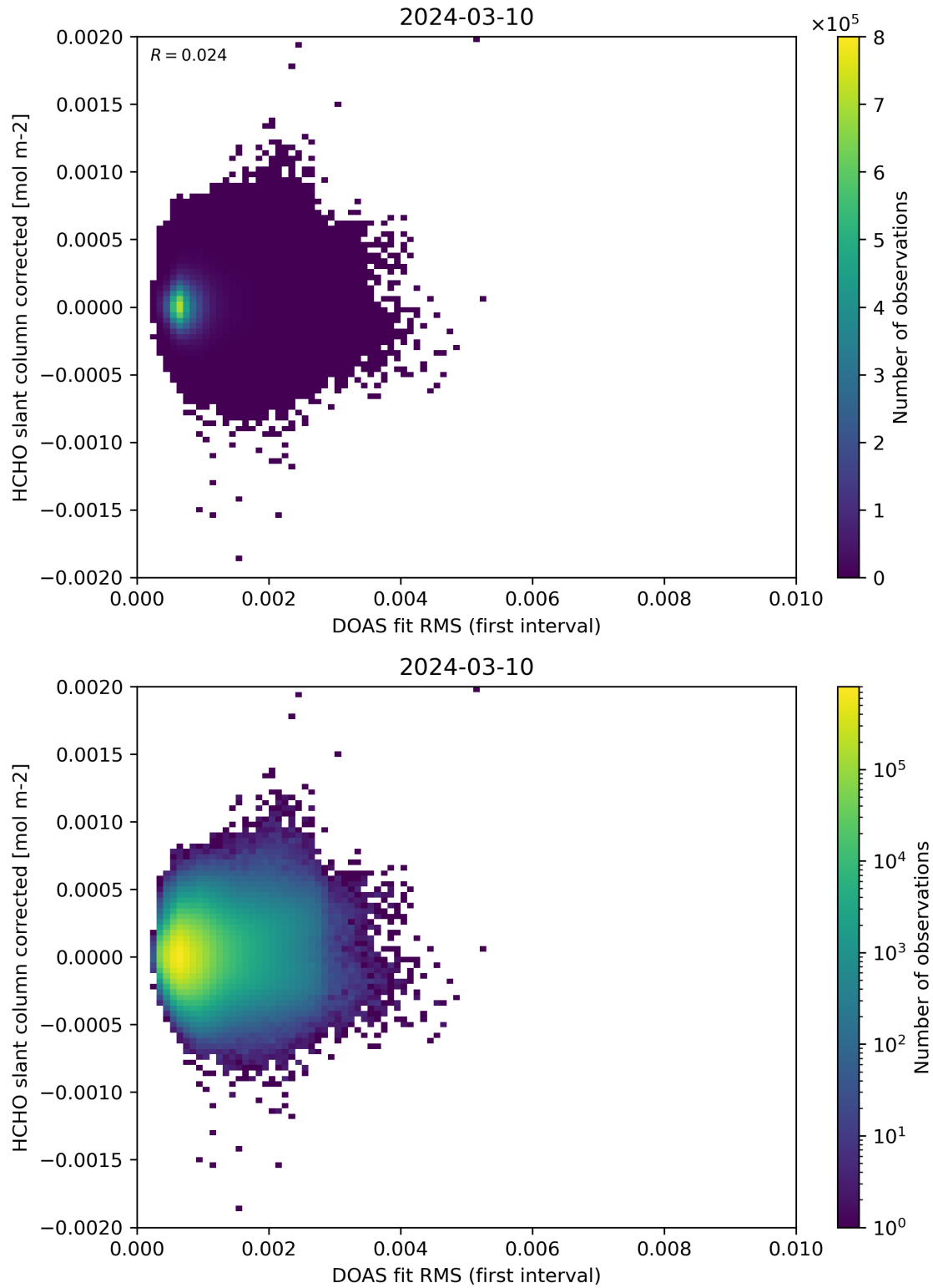
Figure 62: Scatter density plot of “DOAS fit RMS (first interval)” against “HCHO slant column corrected” for 2024-03-09 to 2024-03-11.
