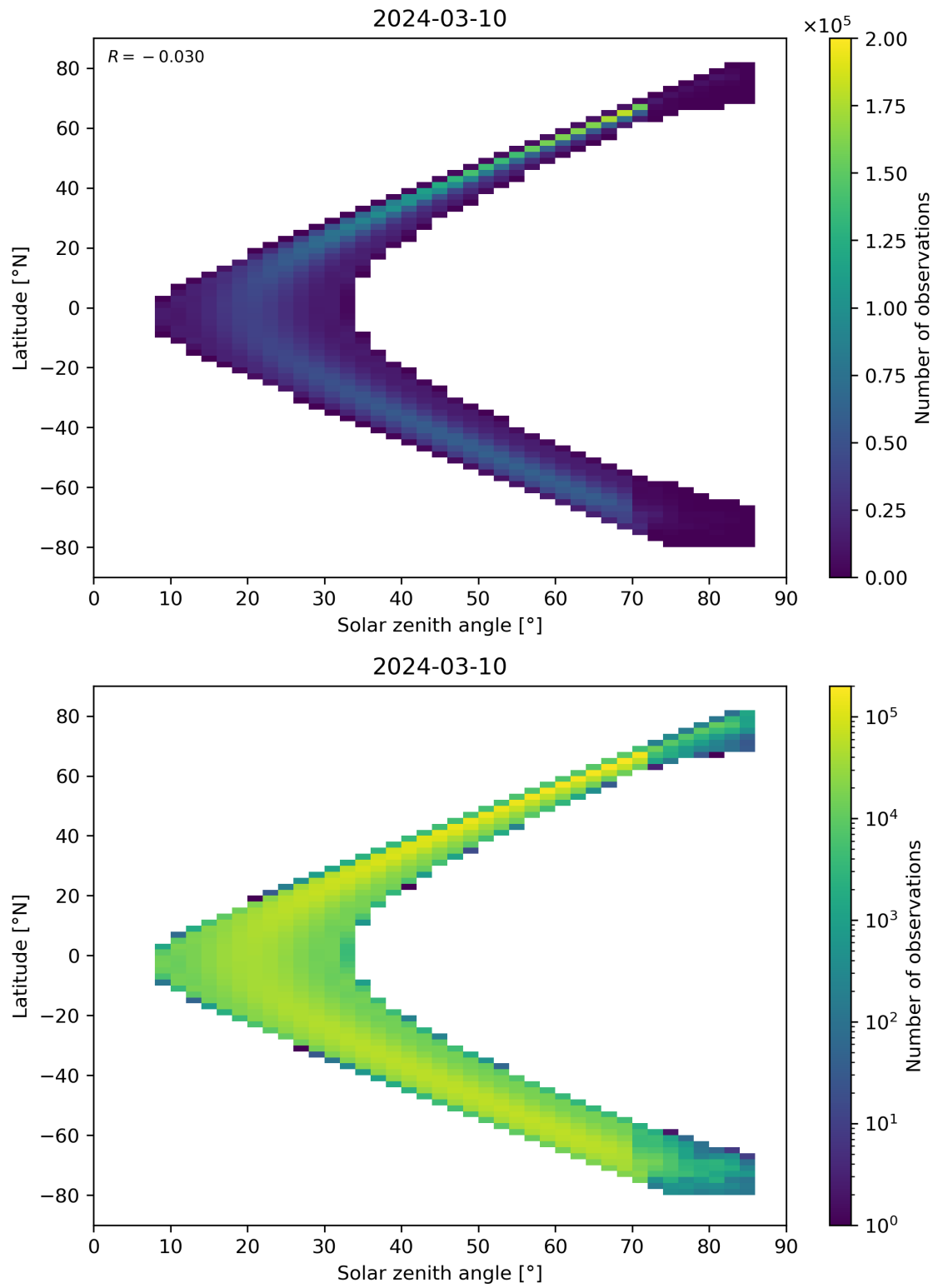
Figure 181: Scatter density plot of “Solar zenith angle” against “Latitude” for 2024-03-09 to 2024-03-11.
