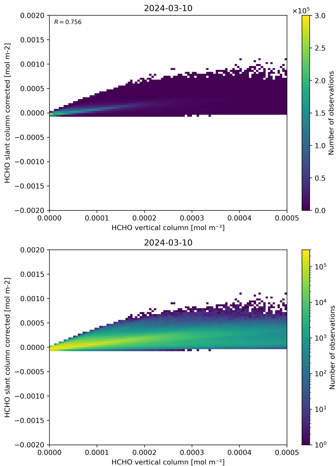
Figure 127: Scatter density plot of “HCHO vertical column” against “HCHO slant column corrected” for 2024-03-09 to 2024-03-11.
