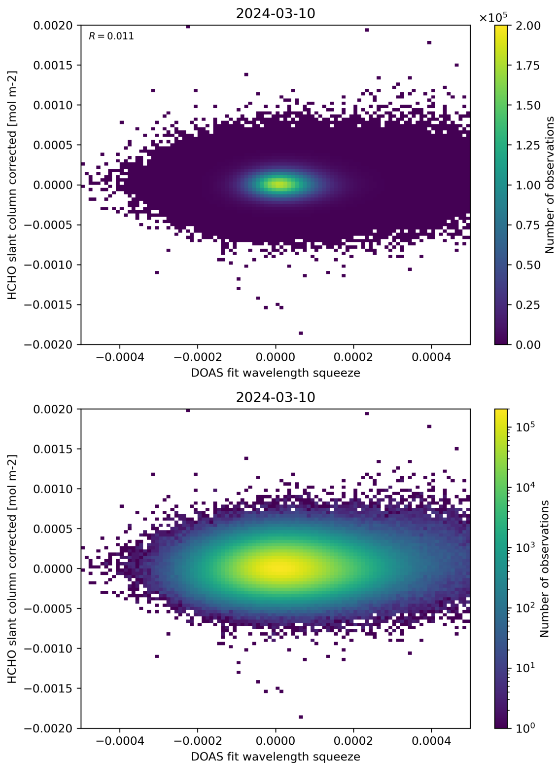
Figure 69: Scatter density plot of “DOAS fit wavelength squeeze” against “HCHO slant column corrected” for 2024-03-09 to 2024-03-11.
