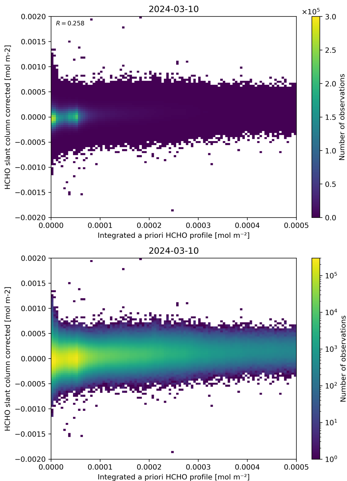
Figure 151: Scatter density plot of “Integrated a priori HCHO profile” against “HCHO slant column corrected” for 2024-03-09 to 2024-03-11.
