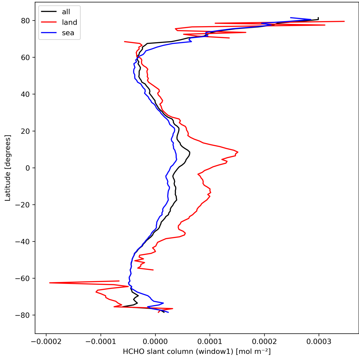
Figure 24: Zonal average of “HCHO slant column (window1)” for 2024-03-09 to 2024-03-11.
