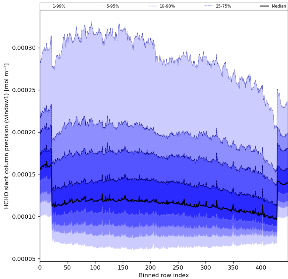
Figure 53: Along track statistics of “HCHO slant column precision (window1)” for 2024-03-09 to 2024-03-11
