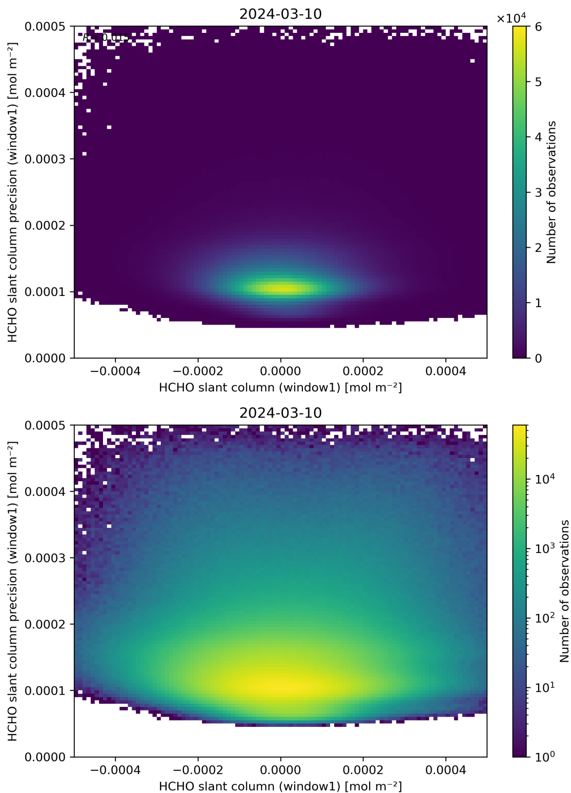
Figure 84: Scatter density plot of “HCHO slant column (window1)” against “HCHO slant column precision (window1)” for 2024-03-09 to 2024-03-11.
