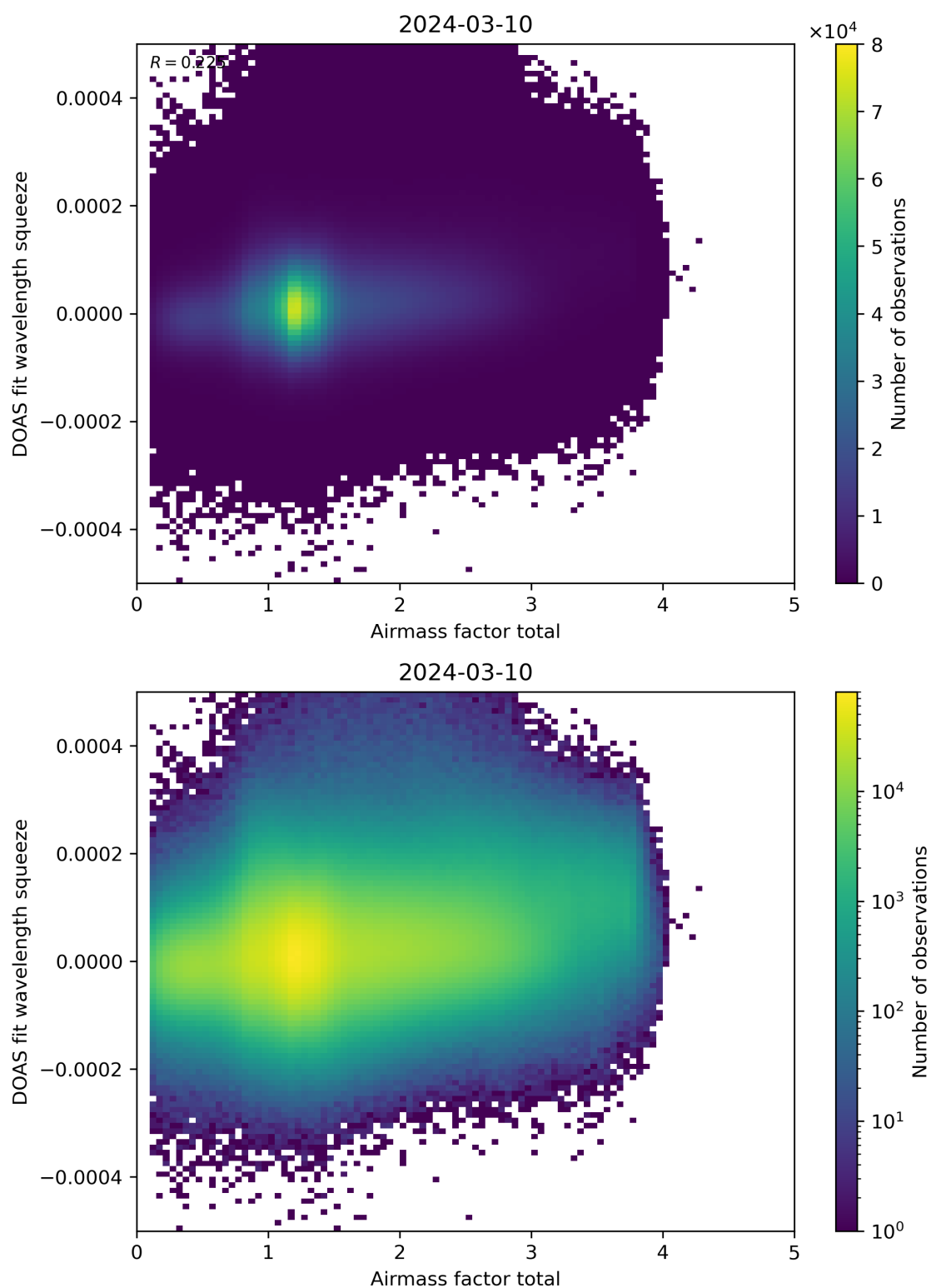
Figure 99: Scatter density plot of “Airmass factor total” against “DOAS fit wavelength squeeze” for 2024-03-09 to 2024-03-11.
