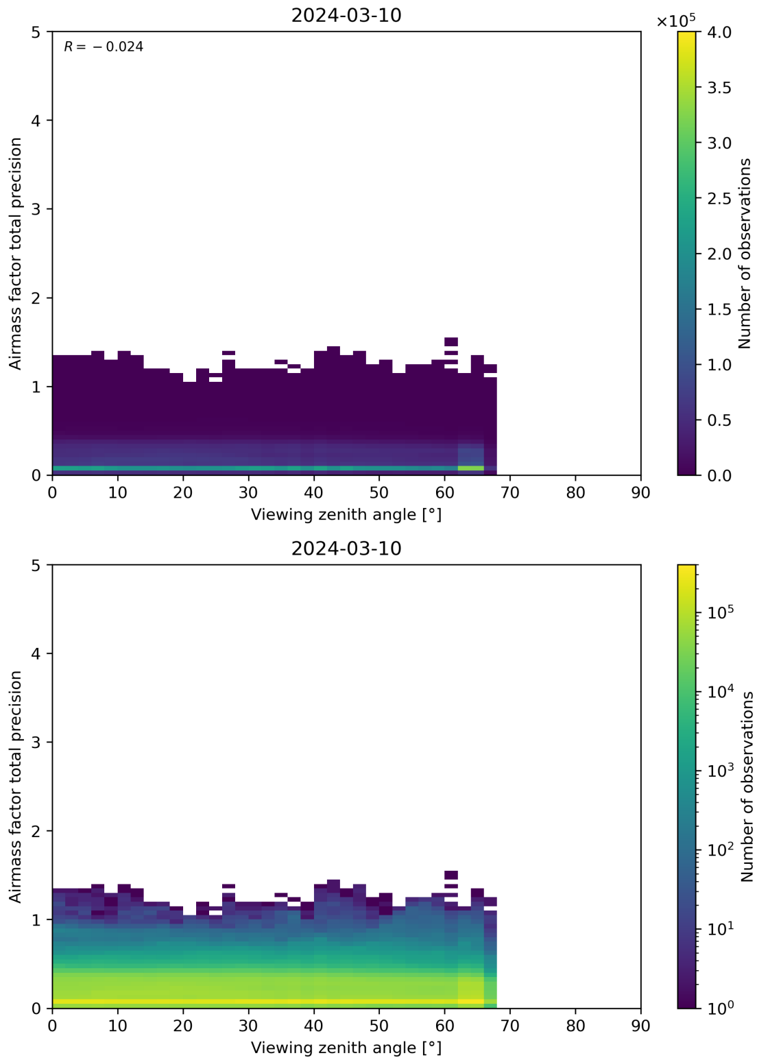
Figure 191: Scatter density plot of “Viewing zenith angle” against “Airmass factor total precision” for 2024-03-09 to 2024-03-11.
