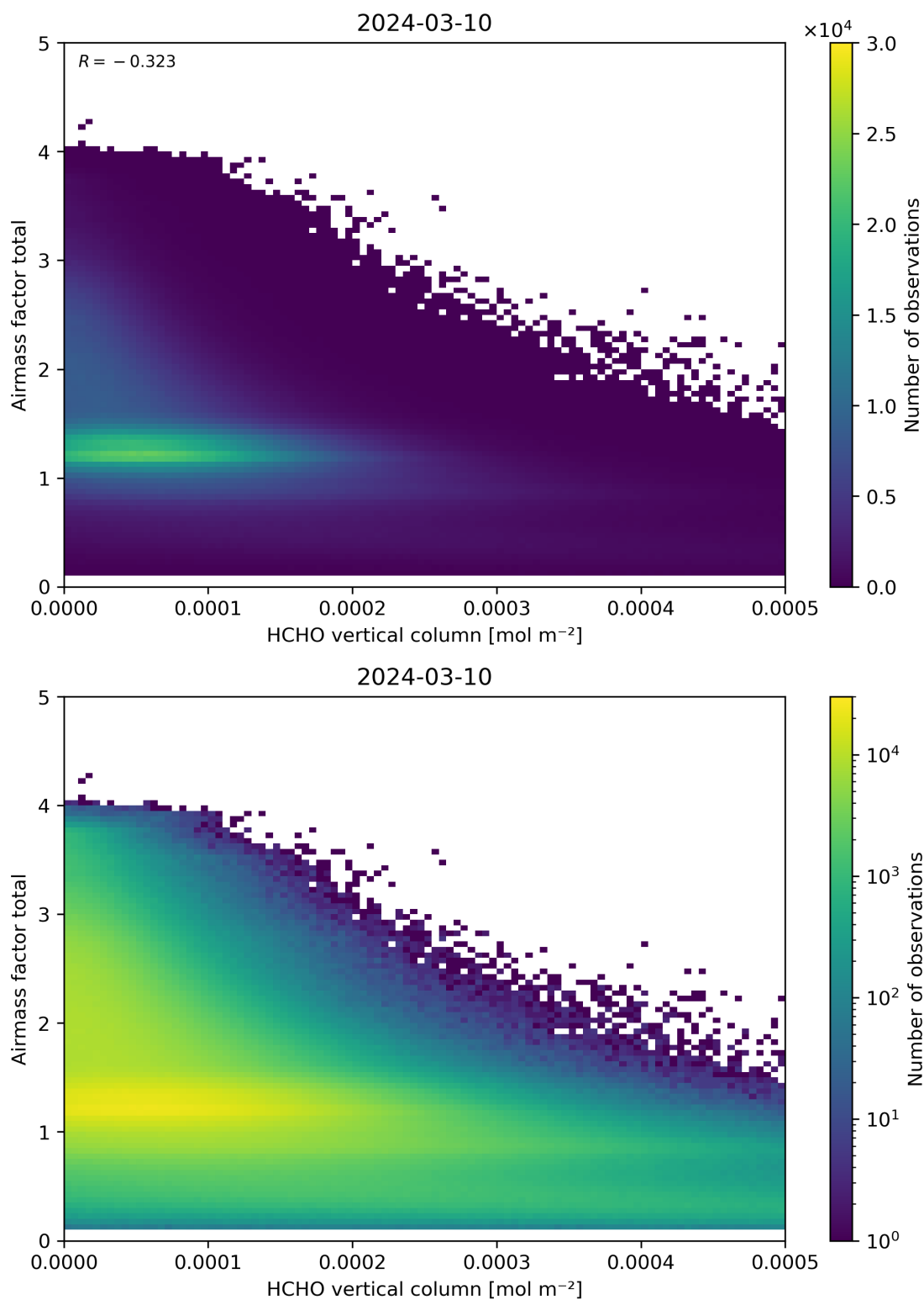
Figure 131: Scatter density plot of “HCHO vertical column” against “Airmass factor total” for 2024-03-09 to 2024-03-11.
