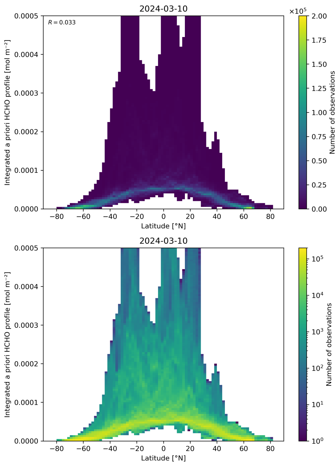
Figure 166: Scatter density plot of “Latitude” against “Integrated a priori HCHO profile” for 2024-03-09 to 2024-03-11.
