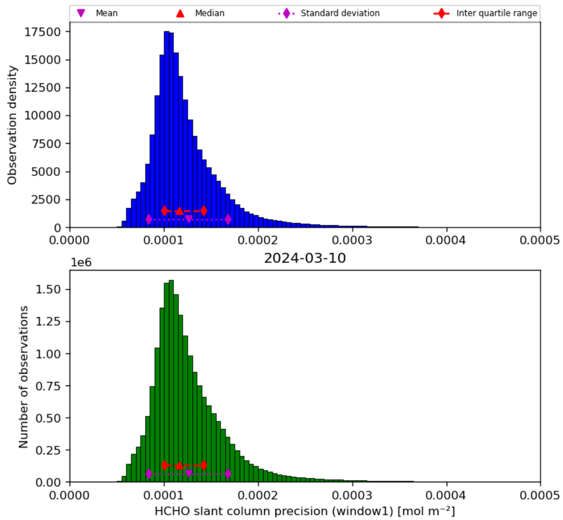
Figure 39: Histogram of “HCHO slant column precision (window1)” for 2024-03-09 to 2024-03-11
