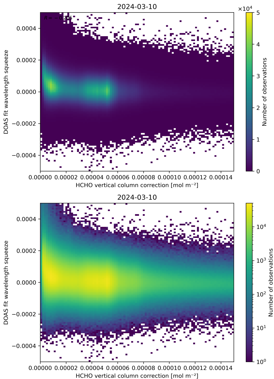
Figure 114: Scatter density plot of “HCHO vertical column correction” against “DOAS fit wavelength squeeze” for 2024-03-09 to 2024-03-11.
