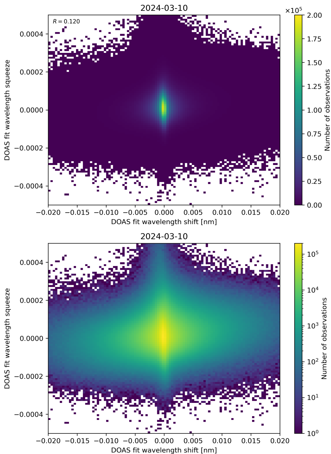
Figure 65: Scatter density plot of “DOAS fit wavelength shift” against “DOAS fit wavelength squeeze” for 2024-03-09 to 2024-03-11.
