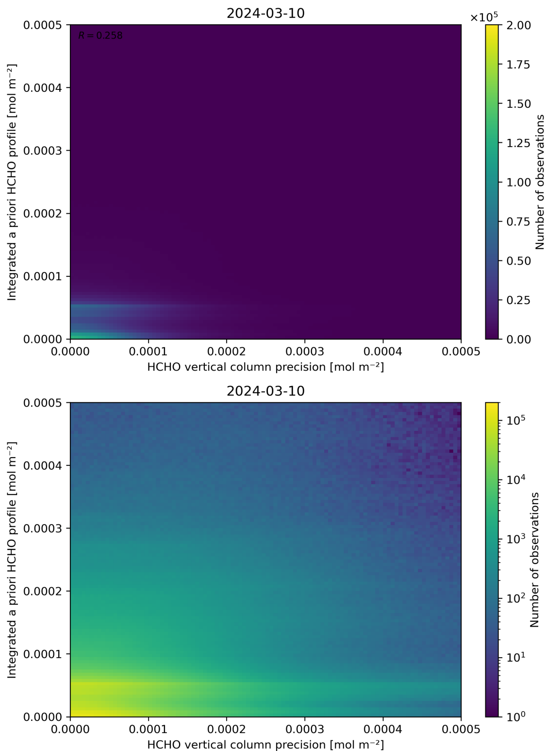
Figure 147: Scatter density plot of “HCHO vertical column precision” against “Integrated a priori HCHO profile” for 2024-03-09 to 2024-03-11.
