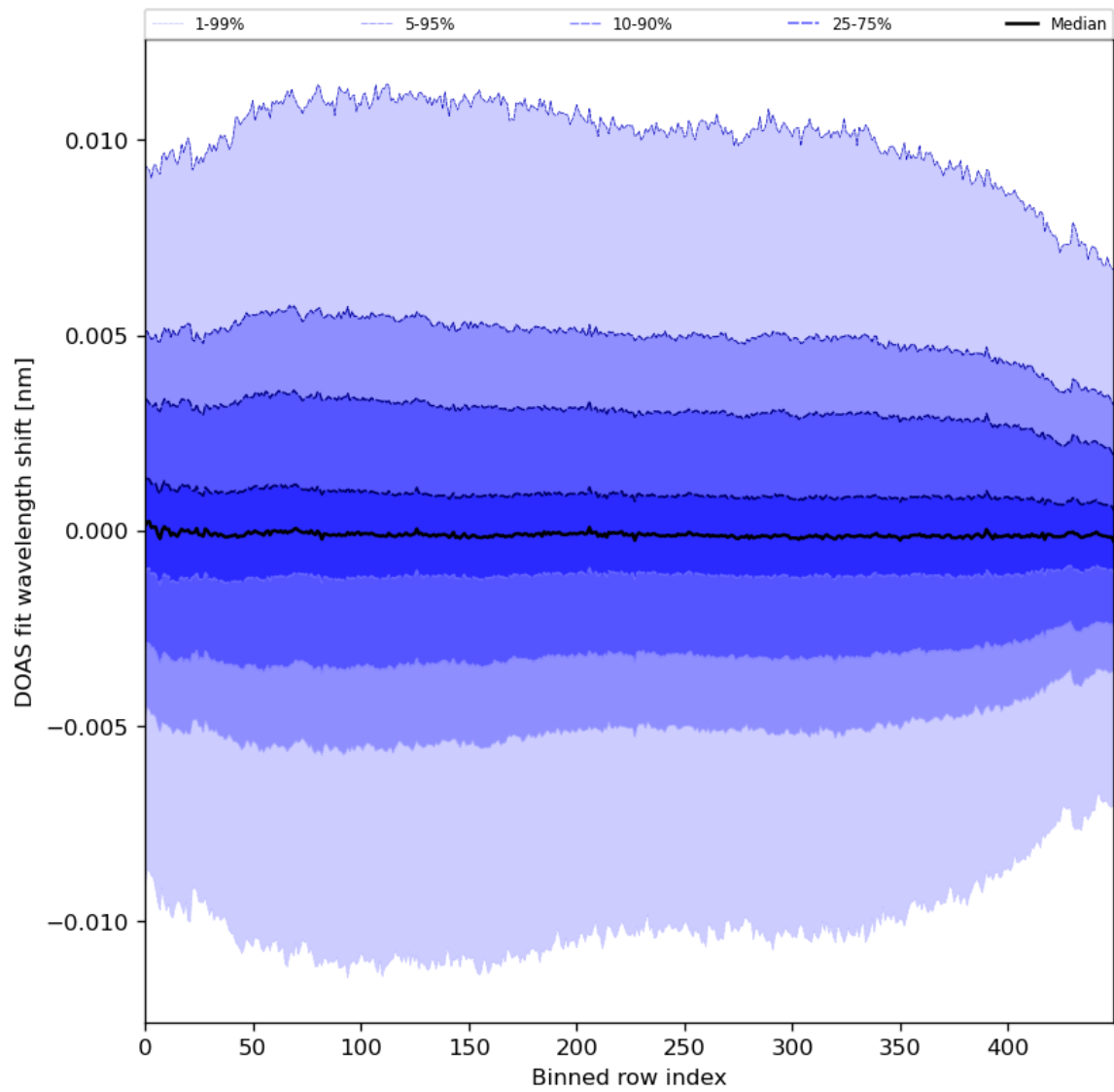
Figure 58: Along track statistics of “DOAS fit wavelength shift” for 2024-03-09 to 2024-03-11
