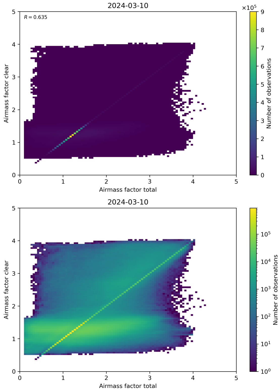
Figure 100: Scatter density plot of “Airmass factor total” against “Airmass factor clear” for 2024-03-09 to 2024-03-11.
