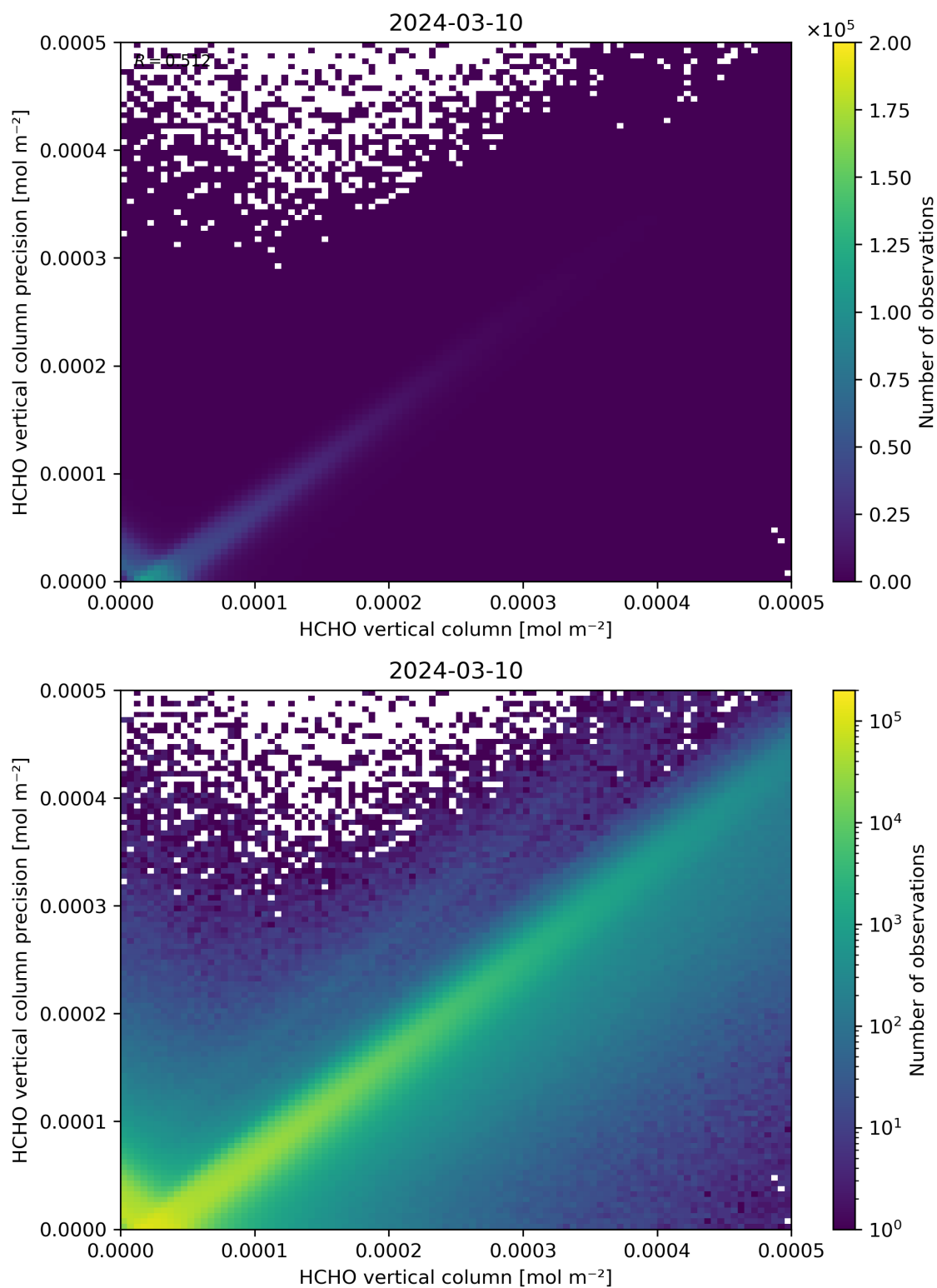
Figure 134: Scatter density plot of “HCHO vertical column” against “HCHO vertical column precision” for 2024-03-09 to 2024-03-11.
