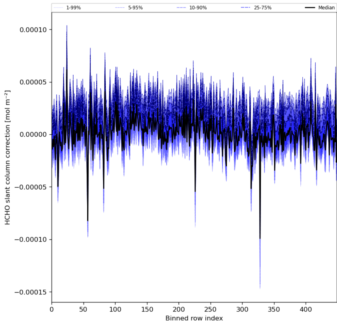
Figure 61: Along track statistics of “HCHO slant column correction” for 2024-03-09 to 2024-03-11
