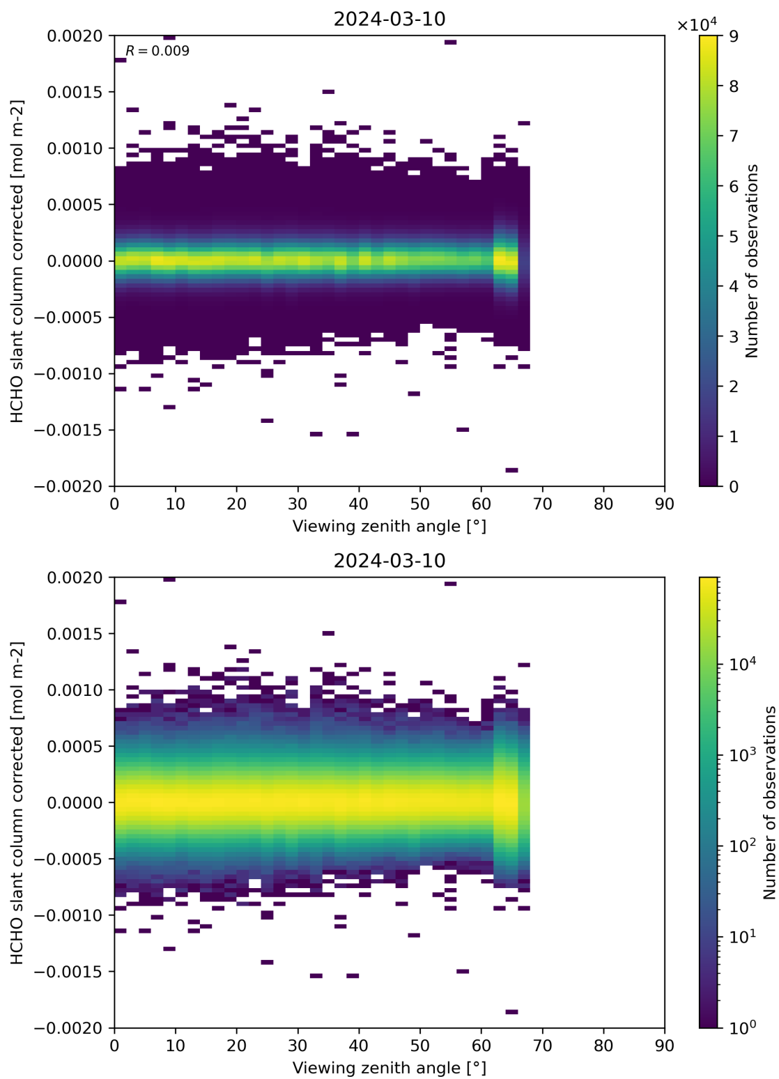
Figure 186: Scatter density plot of “Viewing zenith angle” against “HCHO slant column corrected” for 2024-03-09 to 2024-03-11.
