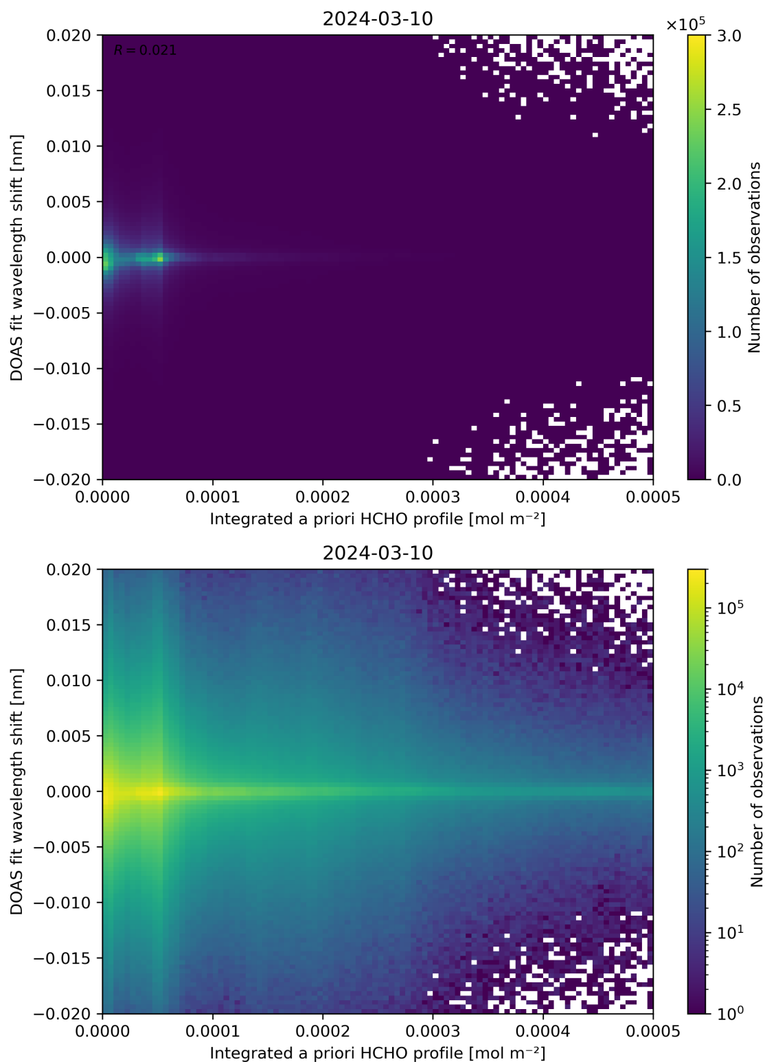
Figure 149: Scatter density plot of “Integrated a priori HCHO profile” against “DOAS fit wavelength shift” for 2024-03-09 to 2024-03-11.
