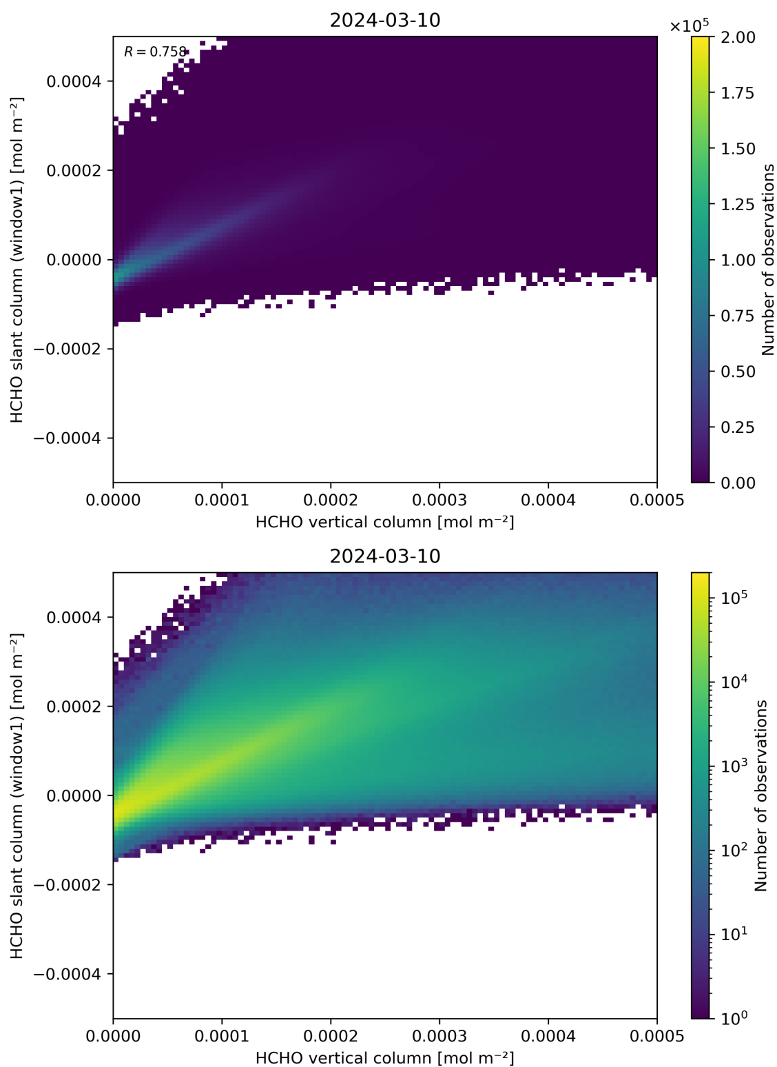
Figure 129: Scatter density plot of “HCHO vertical column” against “HCHO slant column (window1)” for 2024-03-09 to 2024-03-11.
