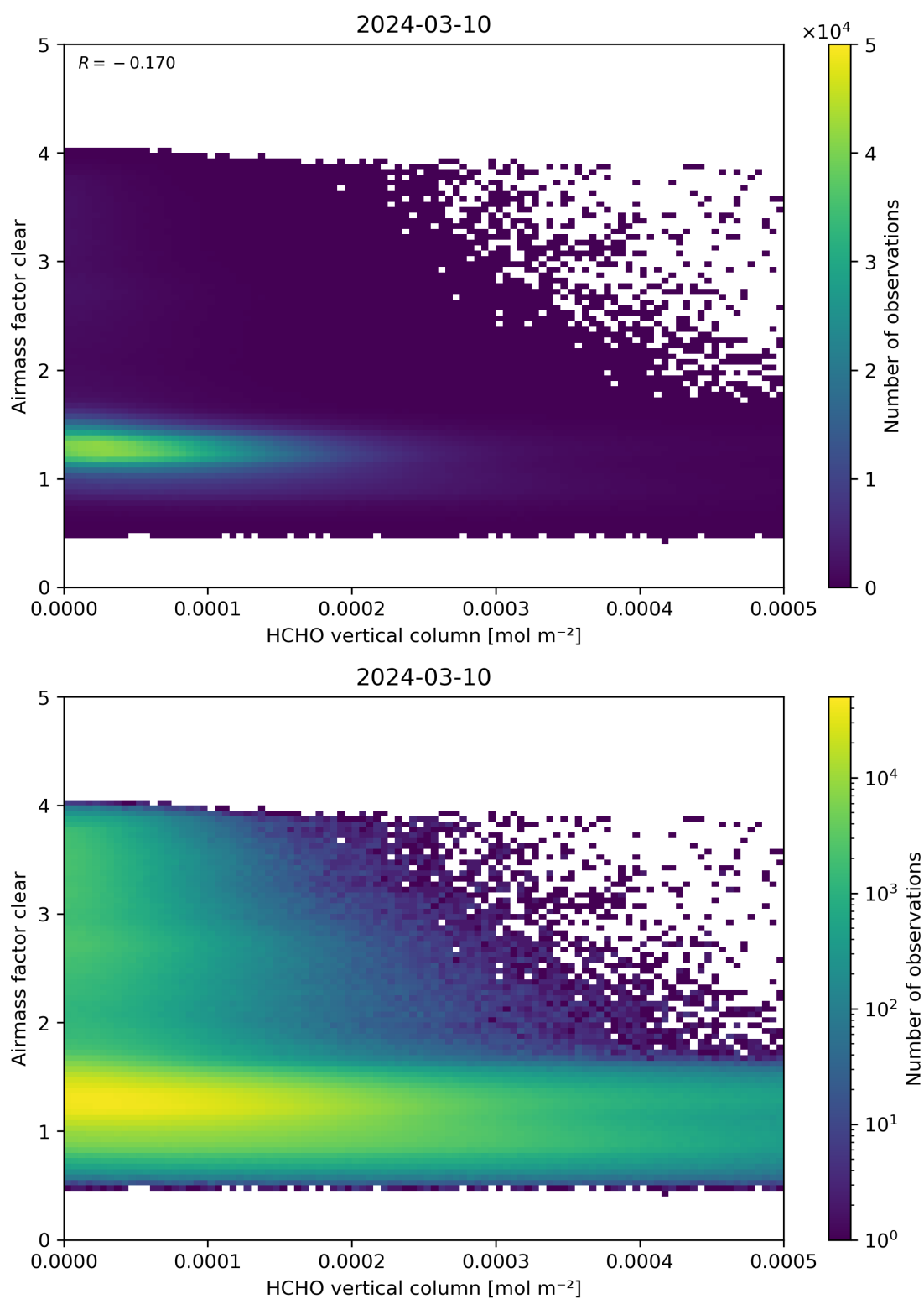
Figure 126: Scatter density plot of “HCHO vertical column” against “Airmass factor clear” for 2024-03-09 to 2024-03-11.
