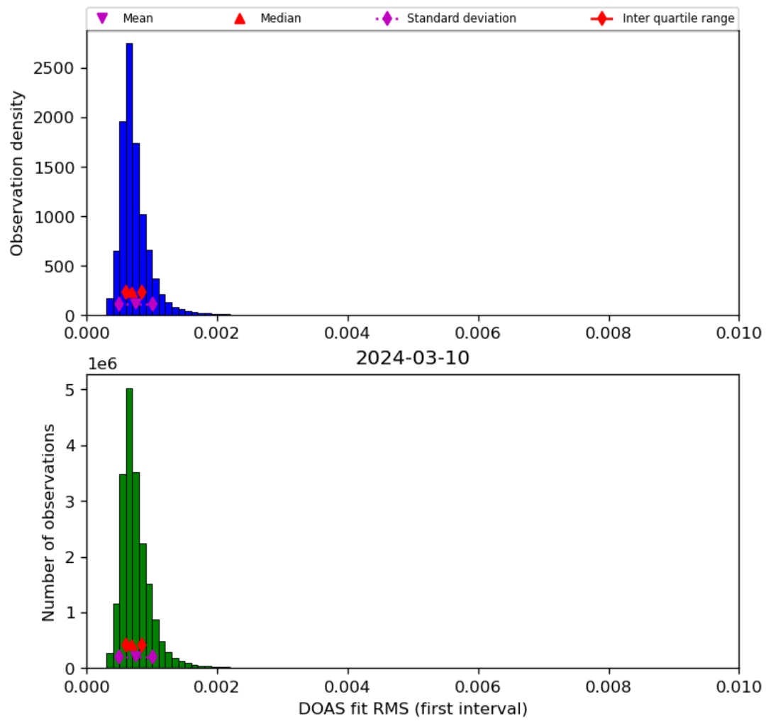
Figure 46: Histogram of “DOAS fit RMS (first interval)” for 2024-03-09 to 2024-03-11
