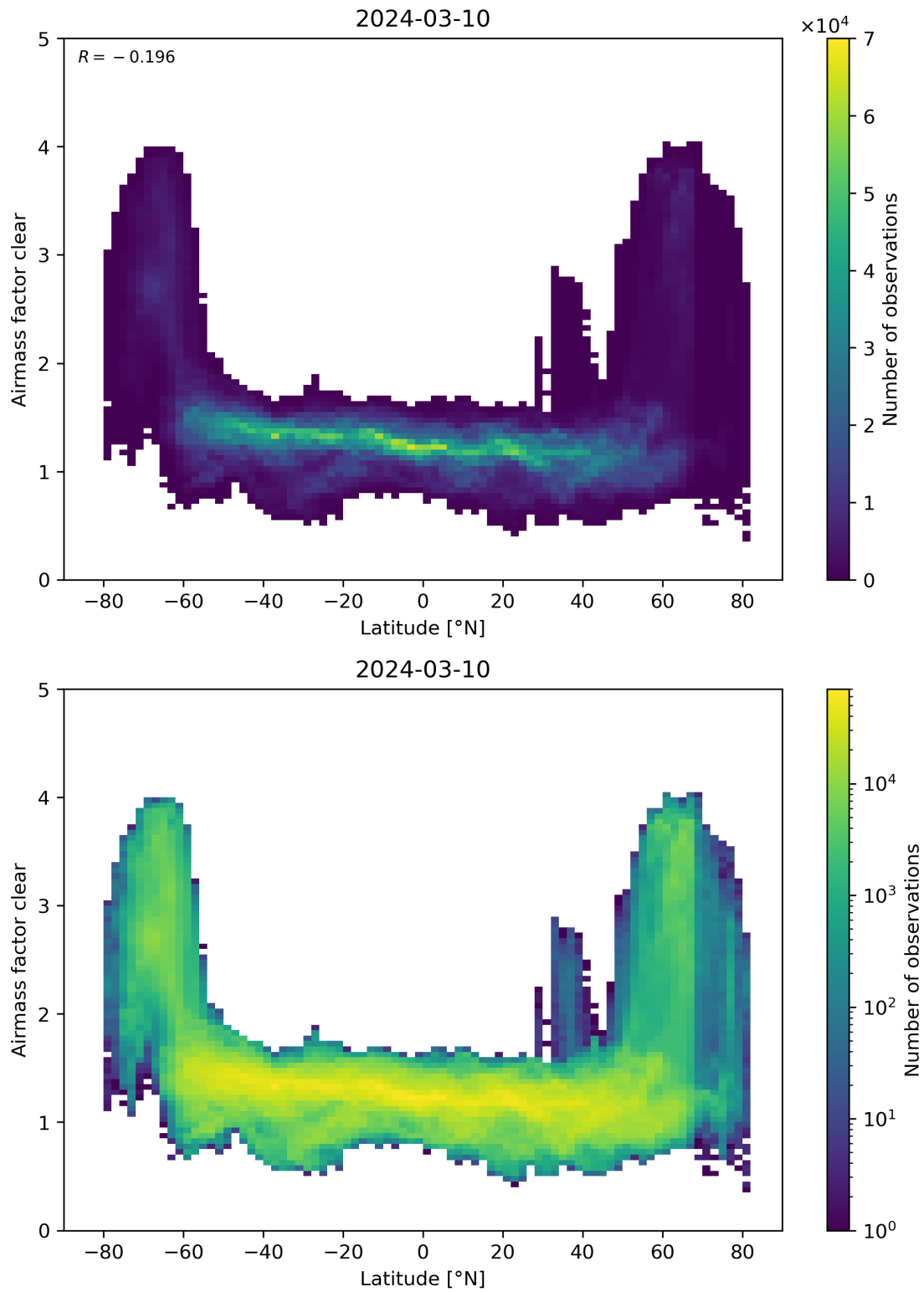
Figure 156: Scatter density plot of “Latitude” against “Airmass factor clear” for 2024-03-09 to 2024-03-11.
