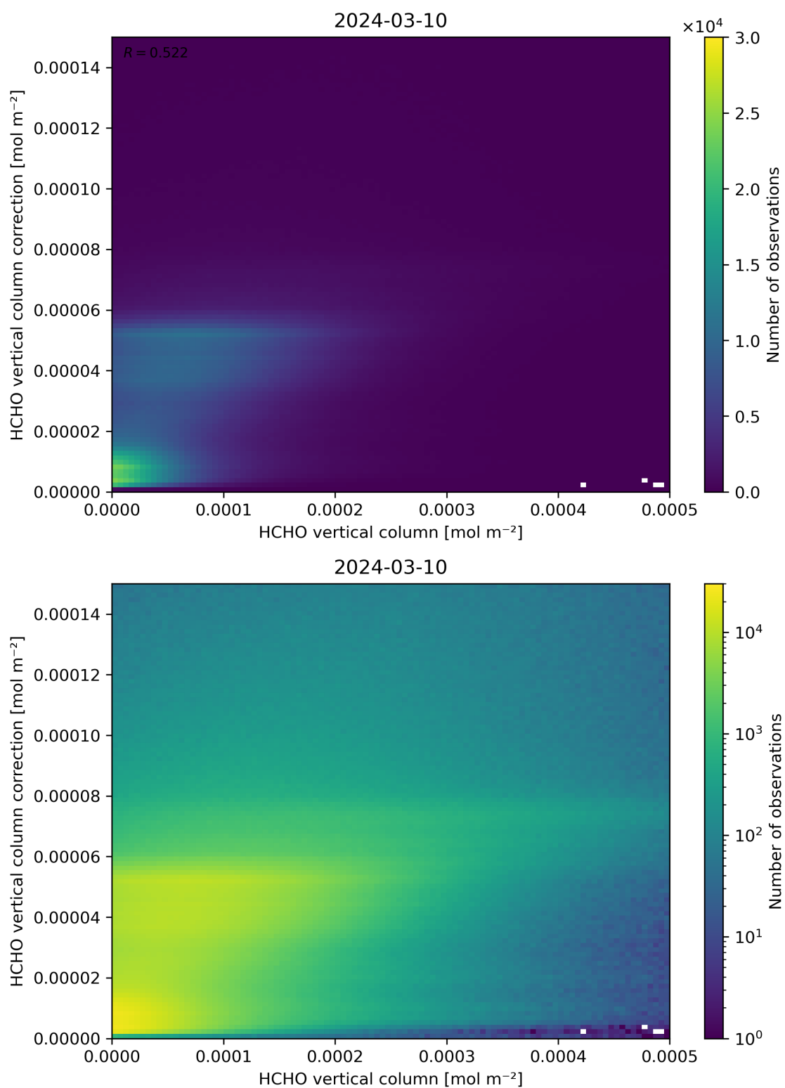
Figure 133: Scatter density plot of “HCHO vertical column” against “HCHO vertical column correction” for 2024-03-09 to 2024-03-11.
