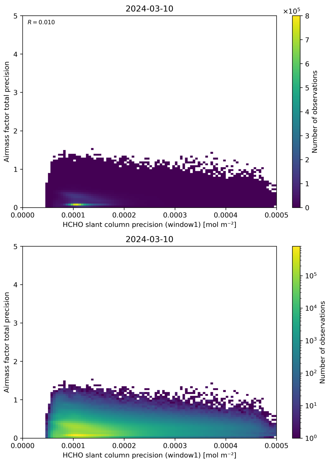
Figure 95: Scatter density plot of “HCHO slant column precision (window1)” against “Airmass factor total precision” for 2024-03-09 to 2024-03-11.
