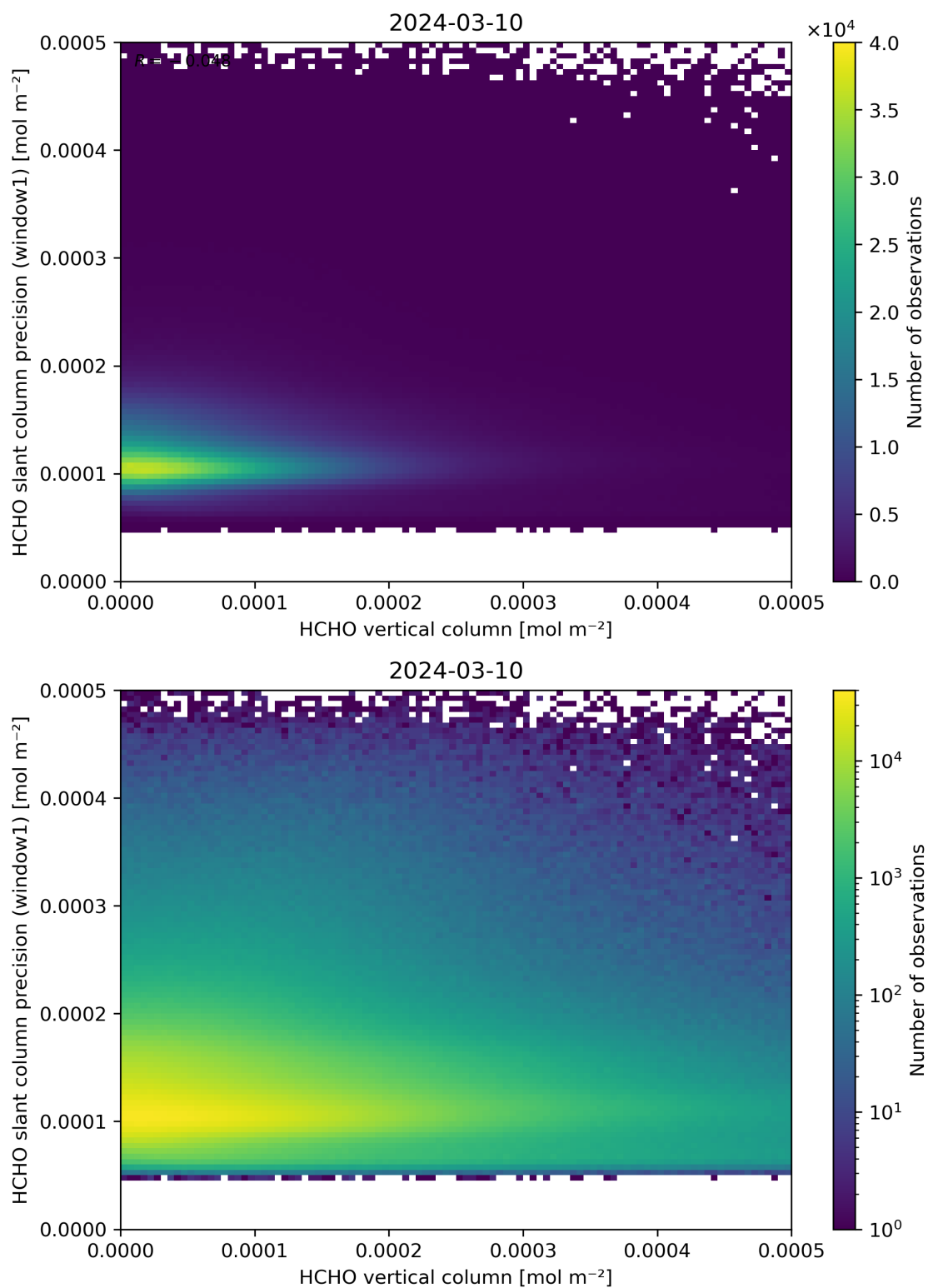
Figure 130: Scatter density plot of “HCHO vertical column” against “HCHO slant column precision (window1)” for 2024-03-09 to 2024-03-11.
