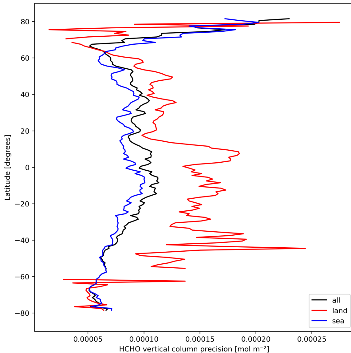
Figure 22: Zonal average of “HCHO vertical column precision” for 2024-03-09 to 2024-03-11.
