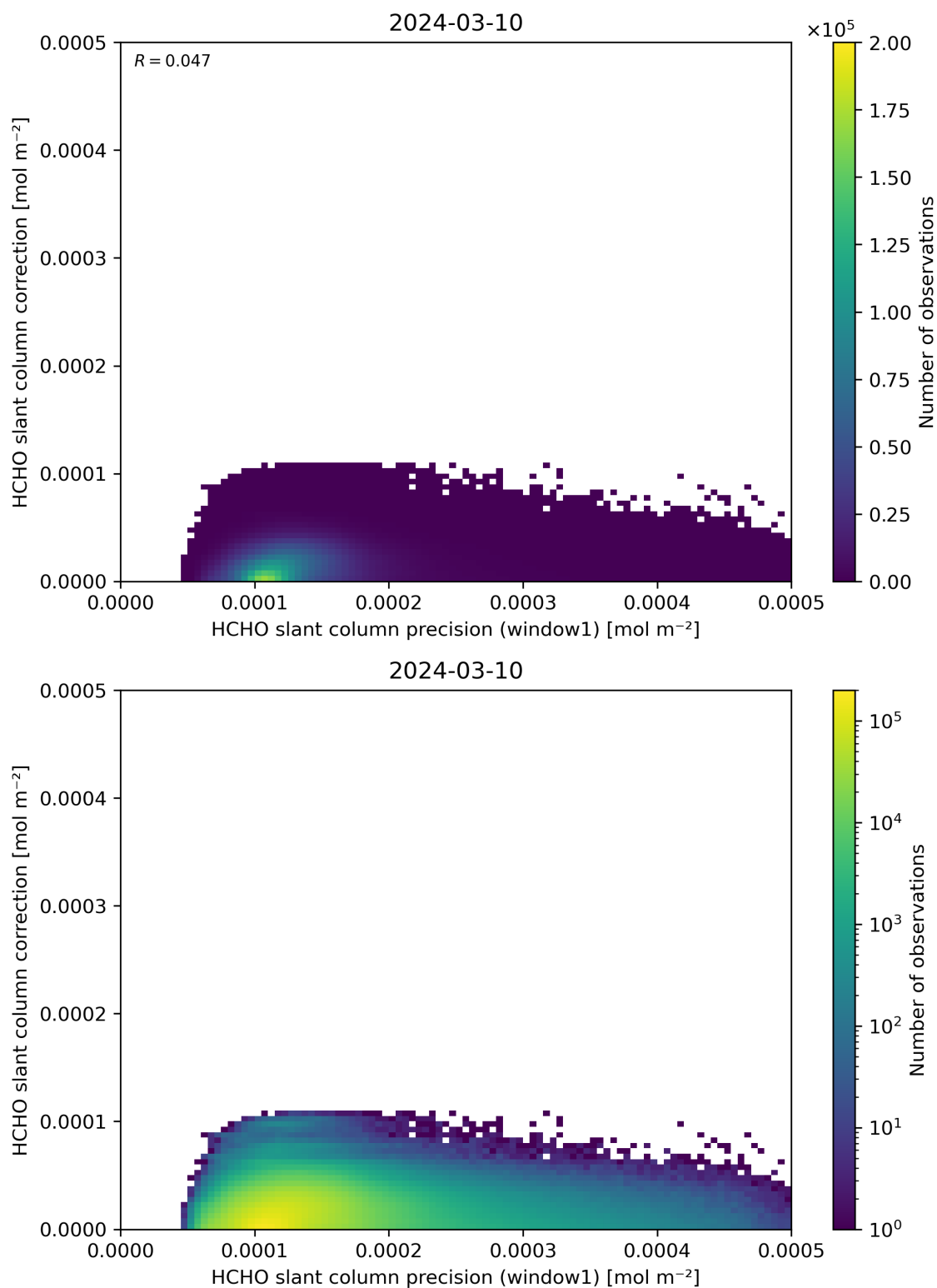
Figure 93: Scatter density plot of “HCHO slant column precision (window1)” against “HCHO slant column correction” for 2024-03-09 to 2024-03-11.
