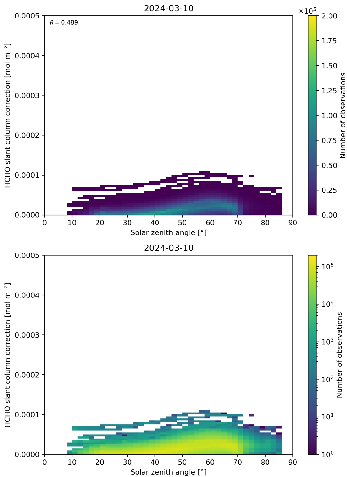
Figure 172: Scatter density plot of “Solar zenith angle” against “HCHO slant column correction” for 2024-03-09 to 2024-03-11.
