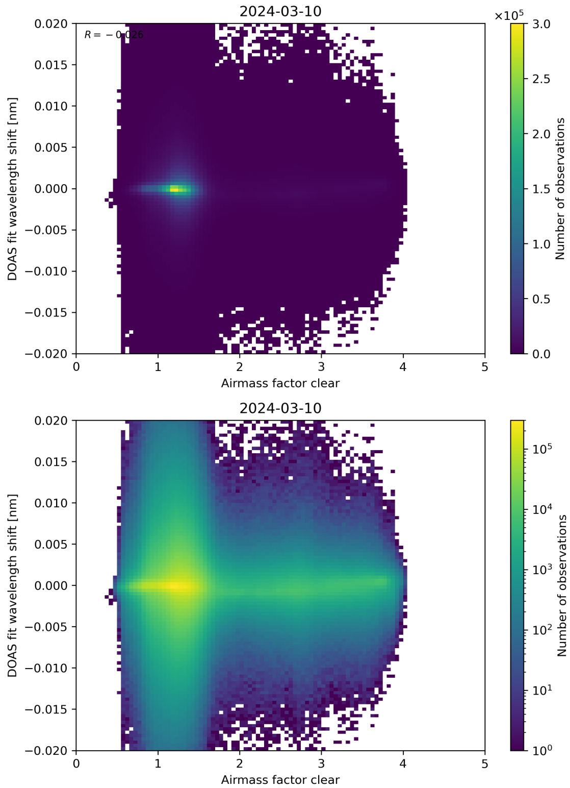
Figure 72: Scatter density plot of “Airmass factor clear” against “DOAS fit wavelength shift” for 2024-03-09 to 2024-03-11.
