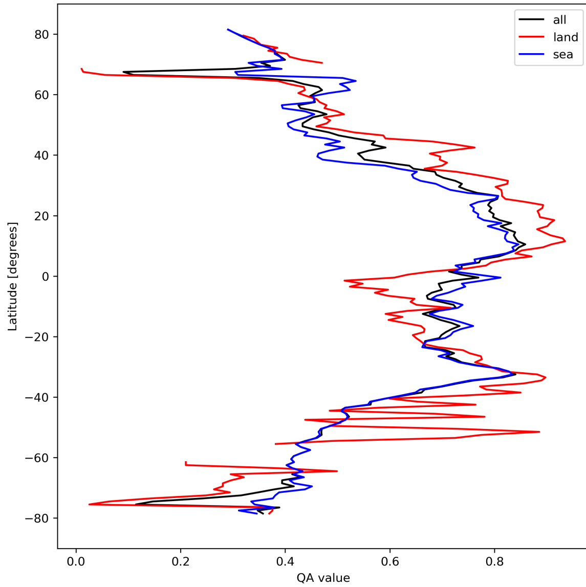
Figure 20: Zonal average of “QA value” for 2024-03-09 to 2024-03-11.
