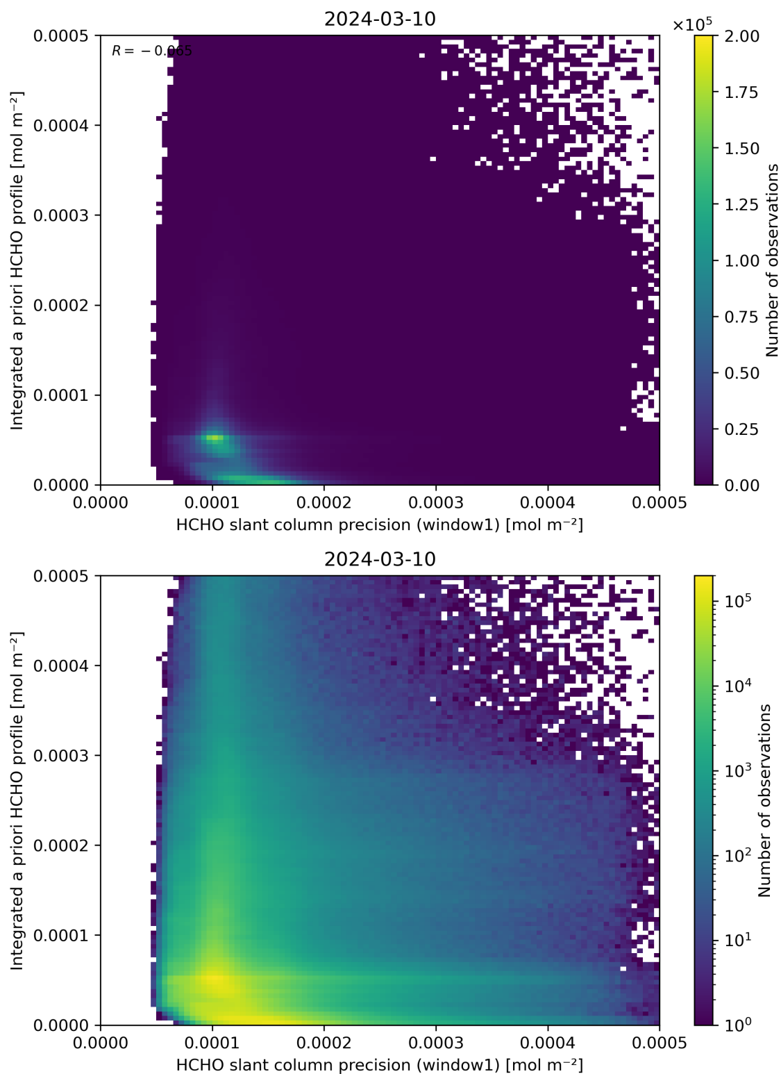
Figure 96: Scatter density plot of “HCHO slant column precision (window1)” against “Integrated a priori HCHO profile” for 2024-03-09 to 2024-03-11.
