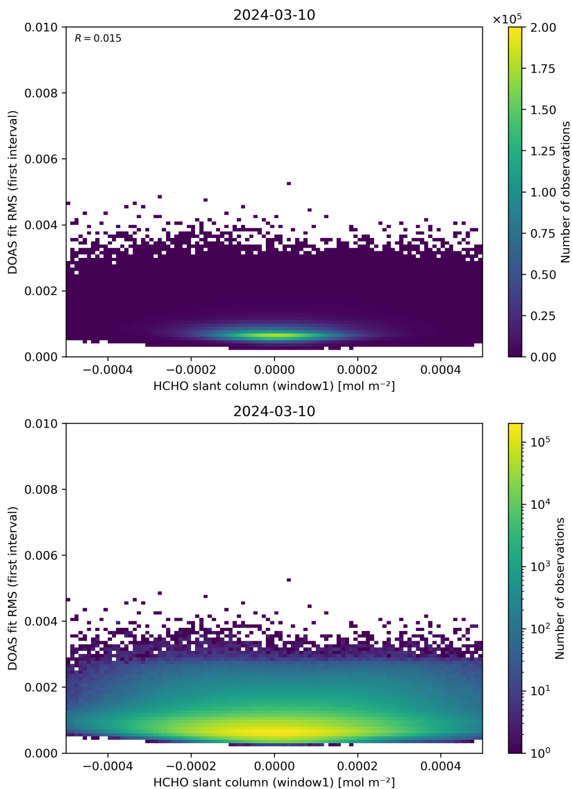
Figure 78: Scatter density plot of “HCHO slant column (window1)” against “DOAS fit RMS (first interval)” for 2024-03-09 to 2024-03-11.
