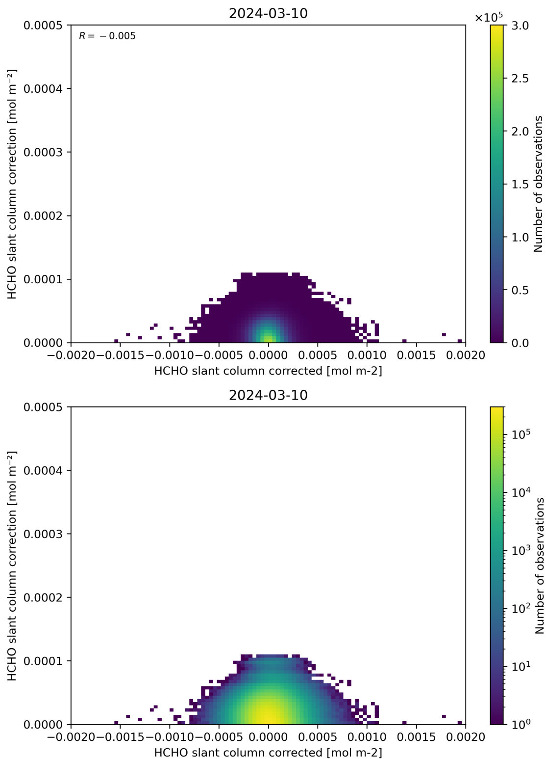
Figure 77: Scatter density plot of “HCHO slant column corrected” against “HCHO slant column correction” for 2024-03-09 to 2024-03-11.
