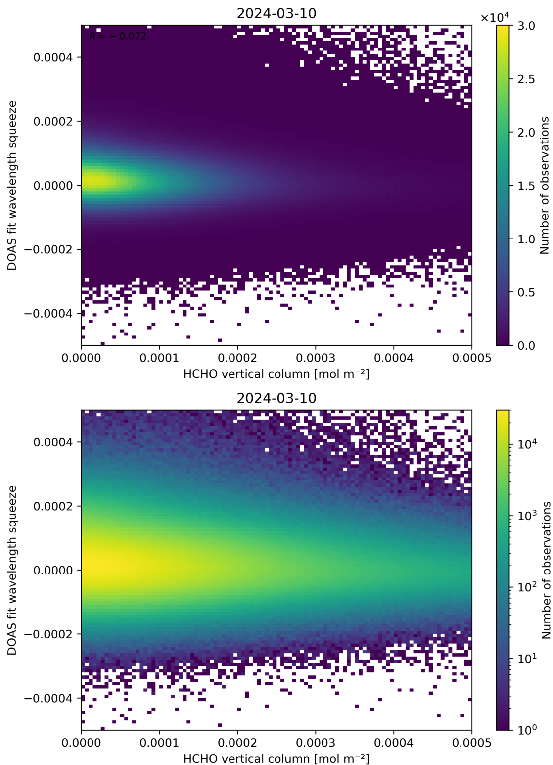
Figure 125: Scatter density plot of “HCHO vertical column” against “DOAS fit wavelength squeeze” for 2024-03-09 to 2024-03-11.
