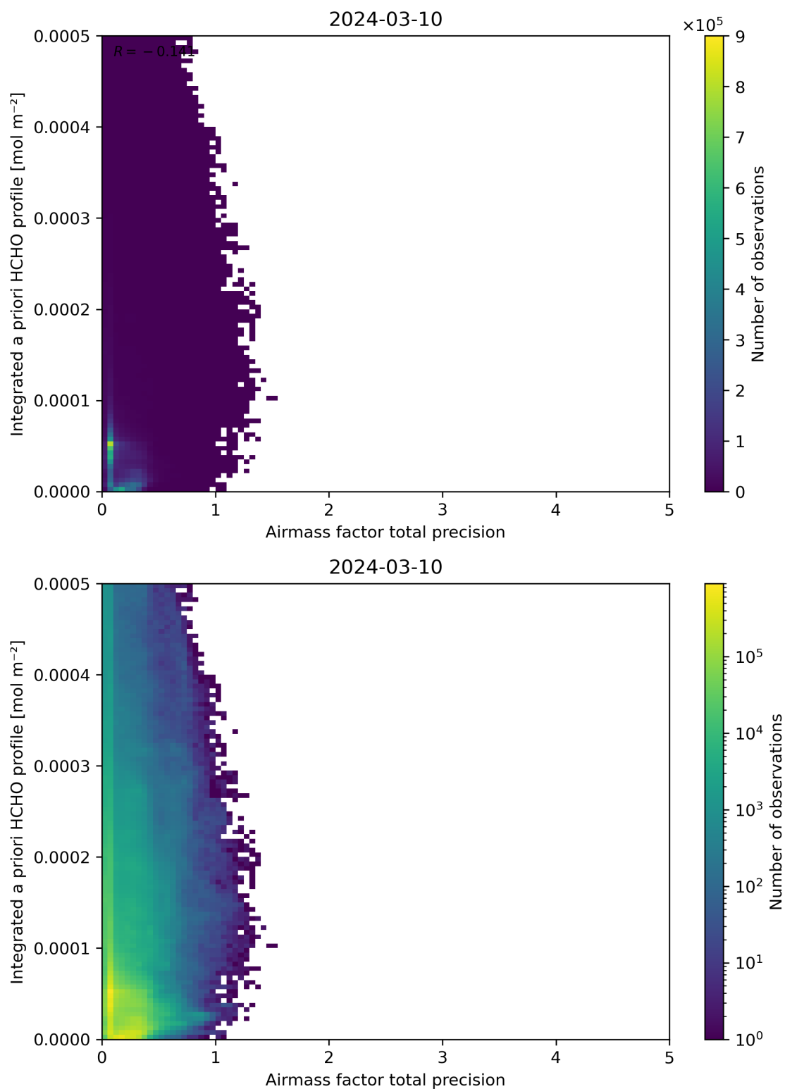
Figure 111: Scatter density plot of “Airmass factor total precision” against “Integrated a priori HCHO profile” for 2024-03-09 to 2024-03-11.
