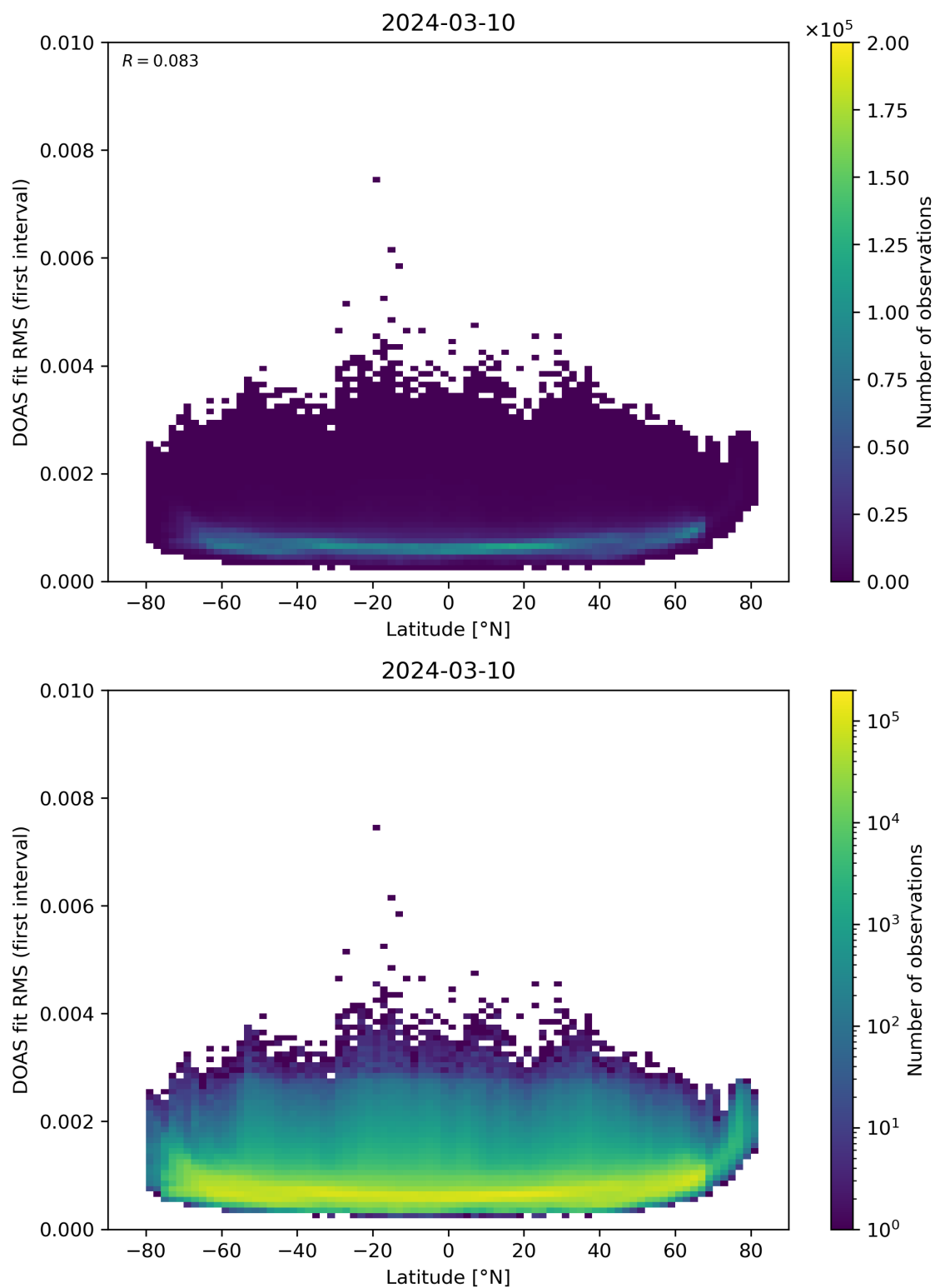
Figure 153: Scatter density plot of “Latitude” against “DOAS fit RMS (first interval)” for 2024-03-09 to 2024-03-11.
