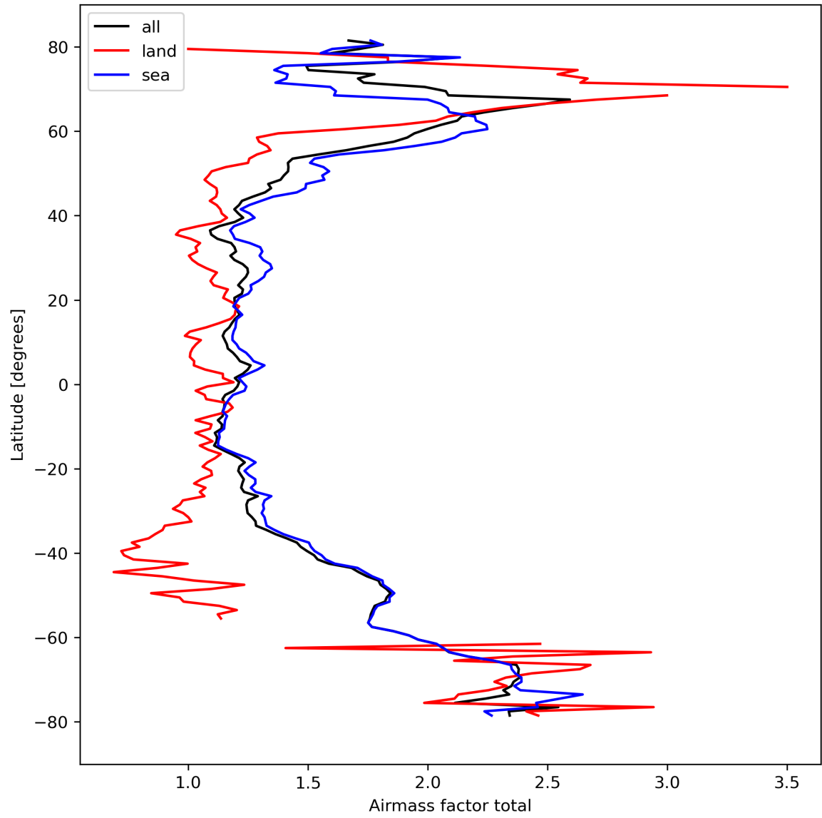
Figure 26: Zonal average of “Airmass factor total” for 2024-03-09 to 2024-03-11.
