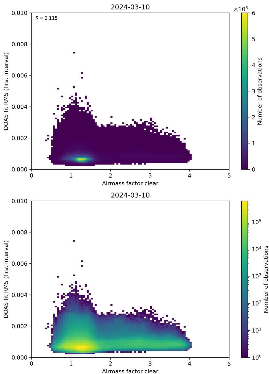
Figure 71: Scatter density plot of “Airmass factor clear” against “DOAS fit RMS (first interval)” for 2024-03-09 to 2024-03-11.
