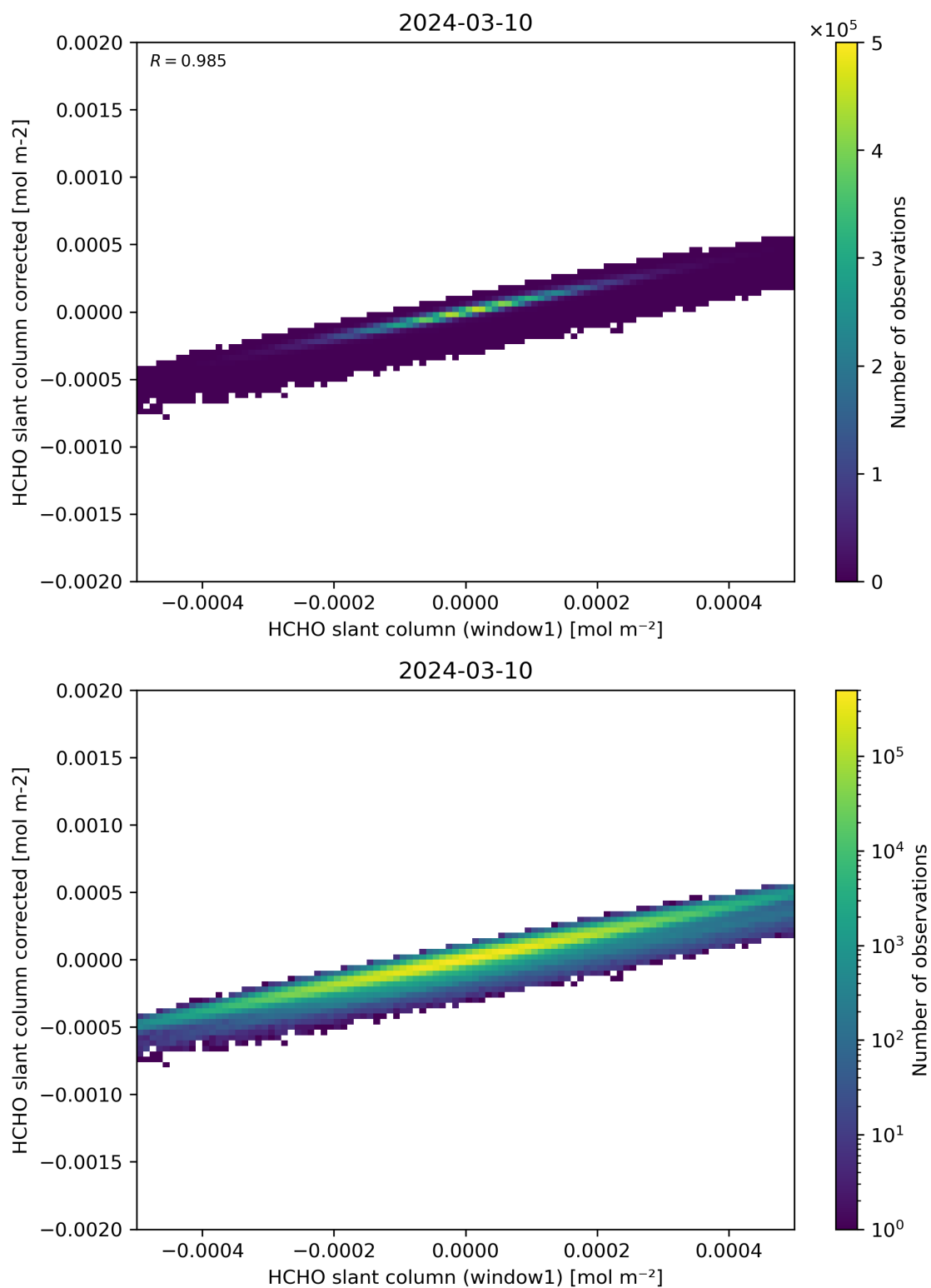
Figure 82: Scatter density plot of “HCHO slant column (window1)” against “HCHO slant column corrected” for 2024-03-09 to 2024-03-11.
