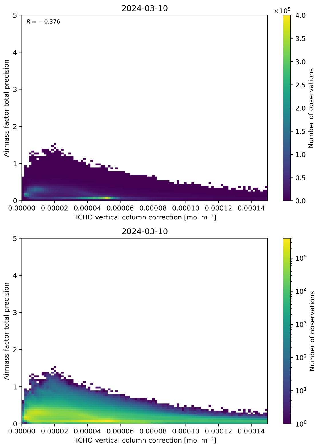
Figure 121: Scatter density plot of “HCHO vertical column correction” against “Airmass factor total precision” for 2024-03-09 to 2024-03-11.
