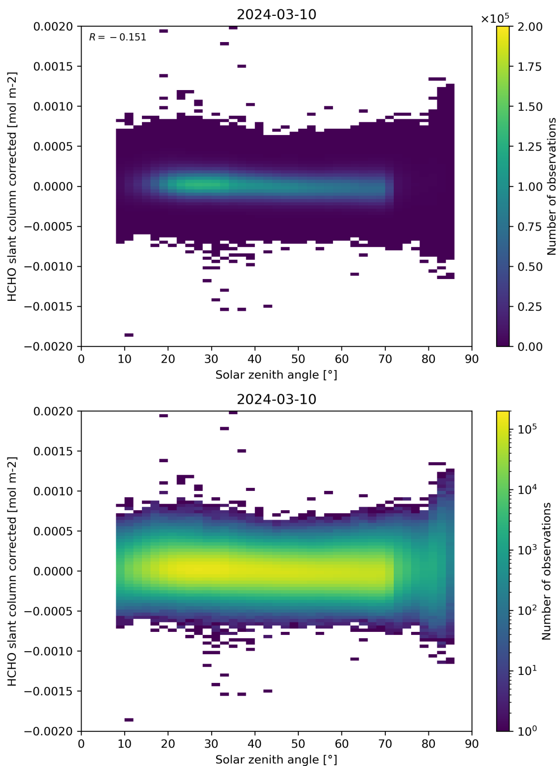
Figure 171: Scatter density plot of “Solar zenith angle” against “HCHO slant column corrected” for 2024-03-09 to 2024-03-11.
