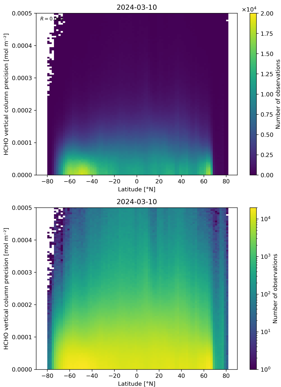
Figure 165: Scatter density plot of “Latitude” against “HCHO vertical column precision” for 2024-03-09 to 2024-03-11.
