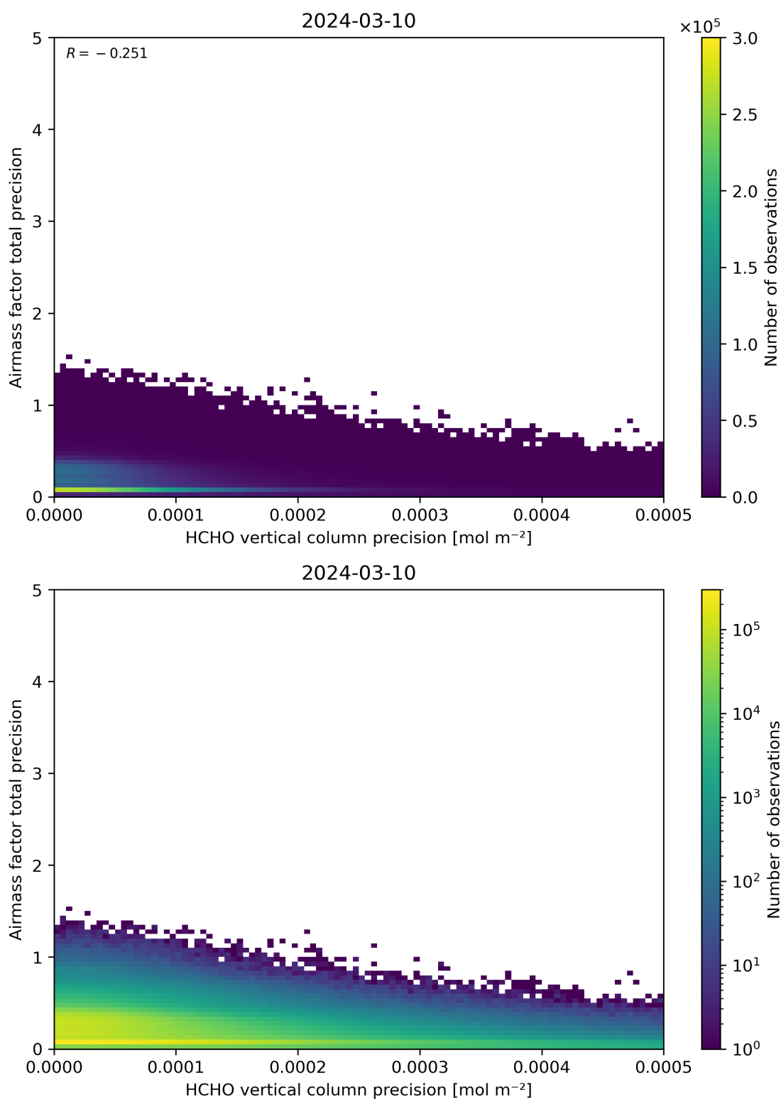
Figure 145: Scatter density plot of “HCHO vertical column precision” against “Airmass factor total precision” for 2024-03-09 to 2024-03-11.
