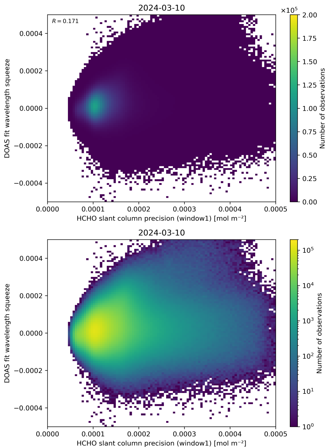
Figure 90: Scatter density plot of “HCHO slant column precision (window1)” against “DOAS fit wavelength squeeze” for 2024-03-09 to 2024-03-11.
