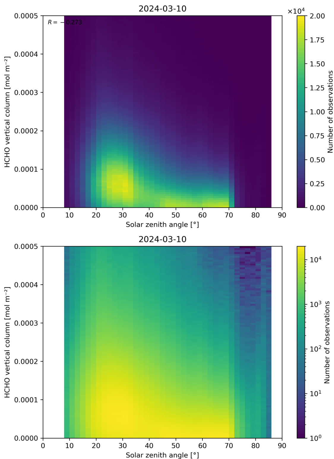
Figure 177: Scatter density plot of “Solar zenith angle” against “HCHO vertical column” for 2024-03-09 to 2024-03-11.
