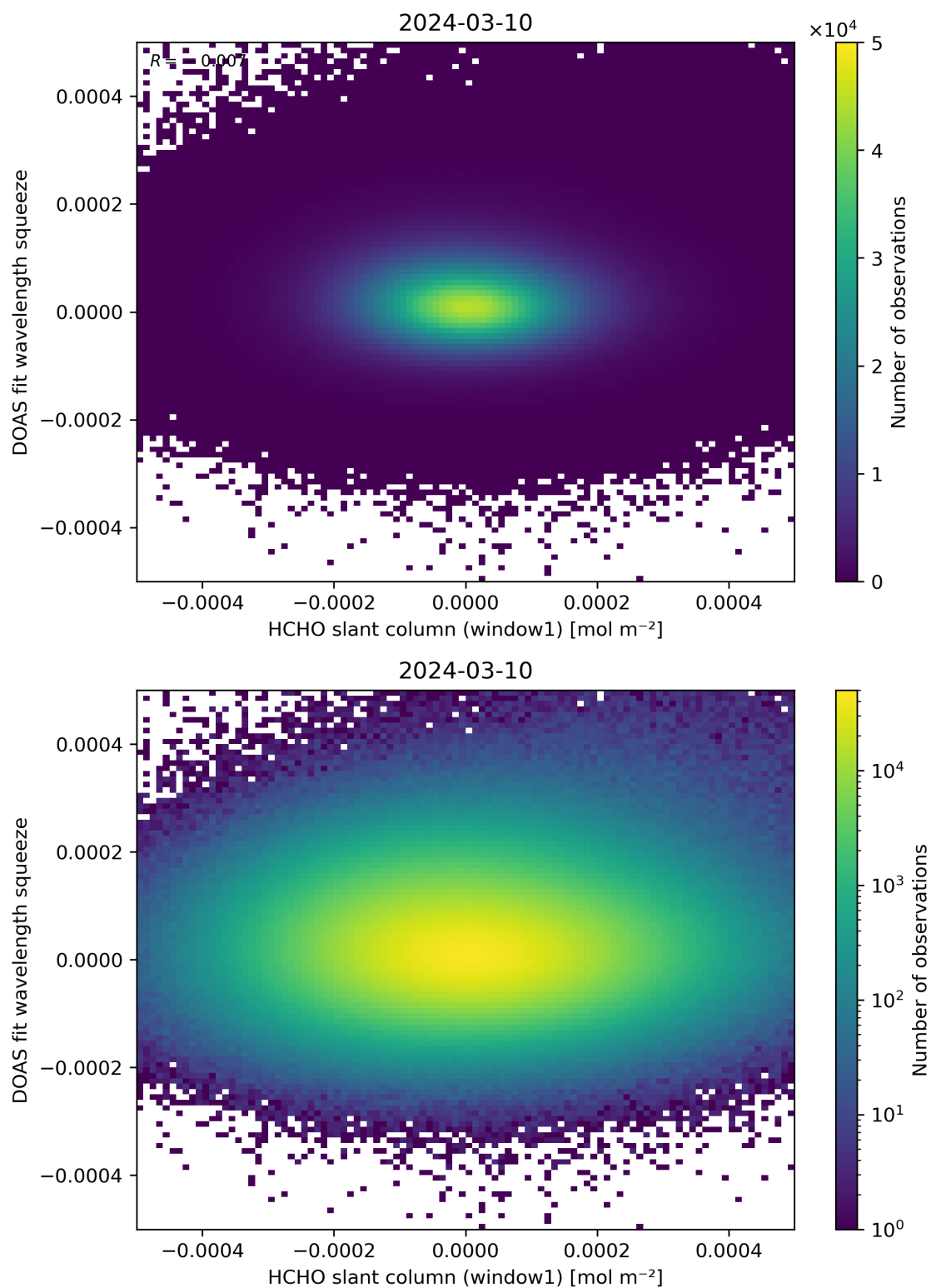
Figure 80: Scatter density plot of “HCHO slant column (window1)” against “DOAS fit wavelength squeeze” for 2024-03-09 to 2024-03-11.
