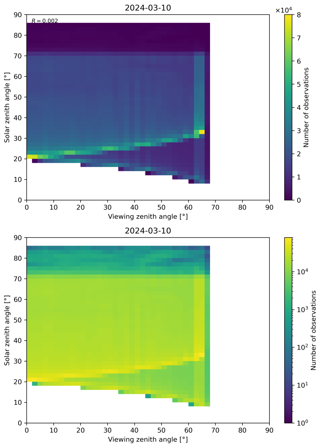
Figure 197: Scatter density plot of “Viewing zenith angle” against “Solar zenith angle” for 2024-03-09 to 2024-03-11.
