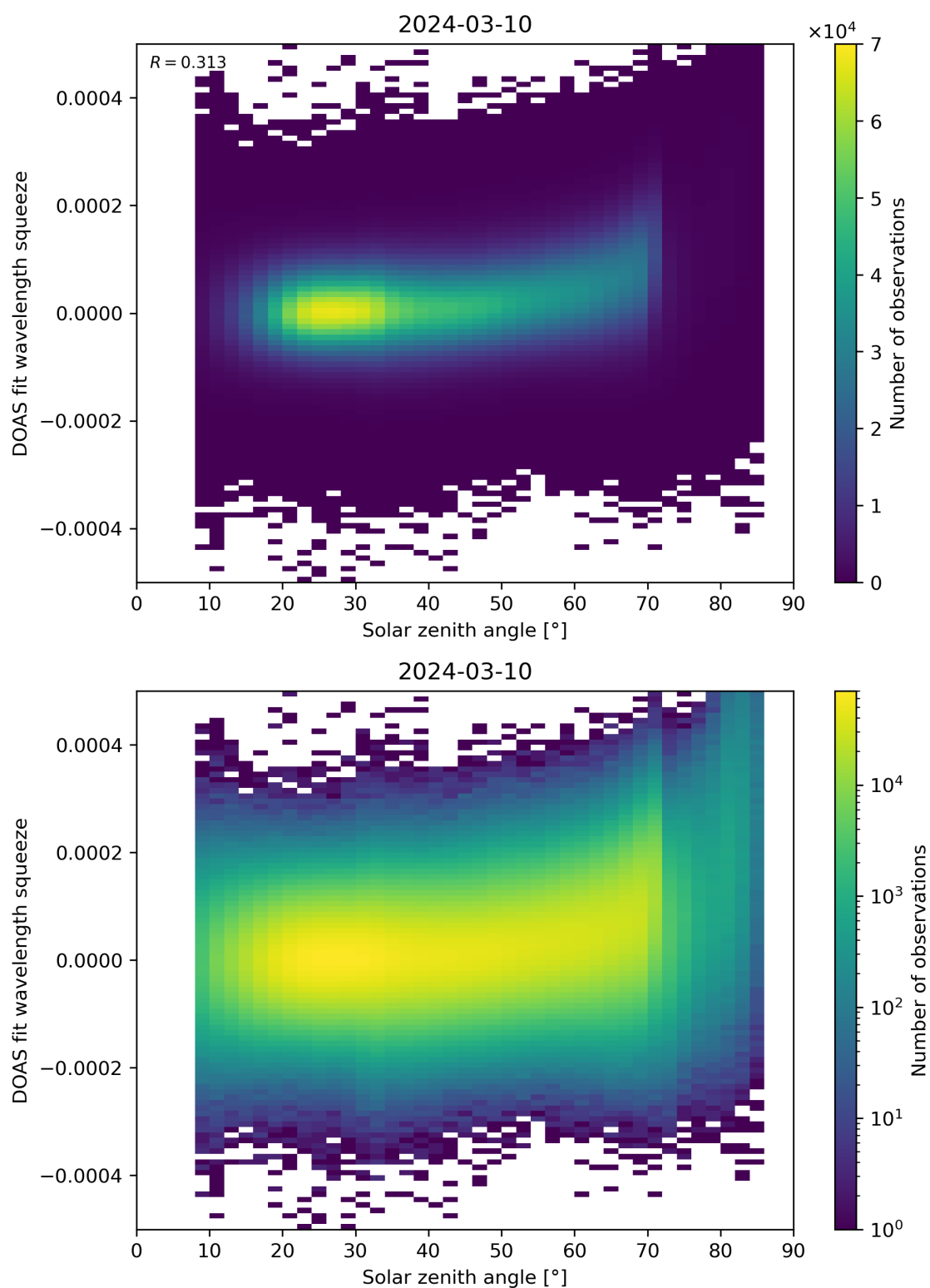
Figure 169: Scatter density plot of “Solar zenith angle” against “DOAS fit wavelength squeeze” for 2024-03-09 to 2024-03-11.
