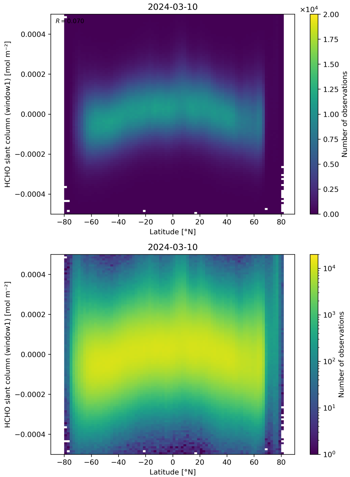
Figure 159: Scatter density plot of “Latitude” against “HCHO slant column (window1)” for 2024-03-09 to 2024-03-11.
