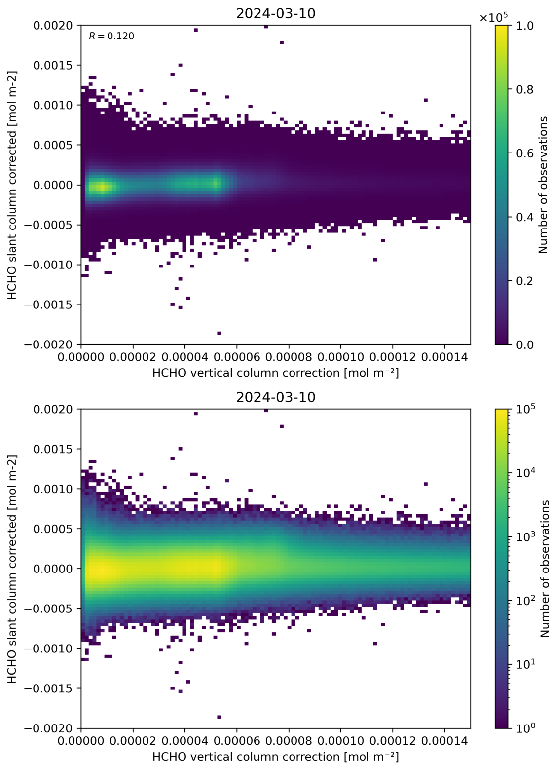
Figure 116: Scatter density plot of “HCHO vertical column correction” against “HCHO slant column corrected” for 2024-03-09 to 2024-03-11.
