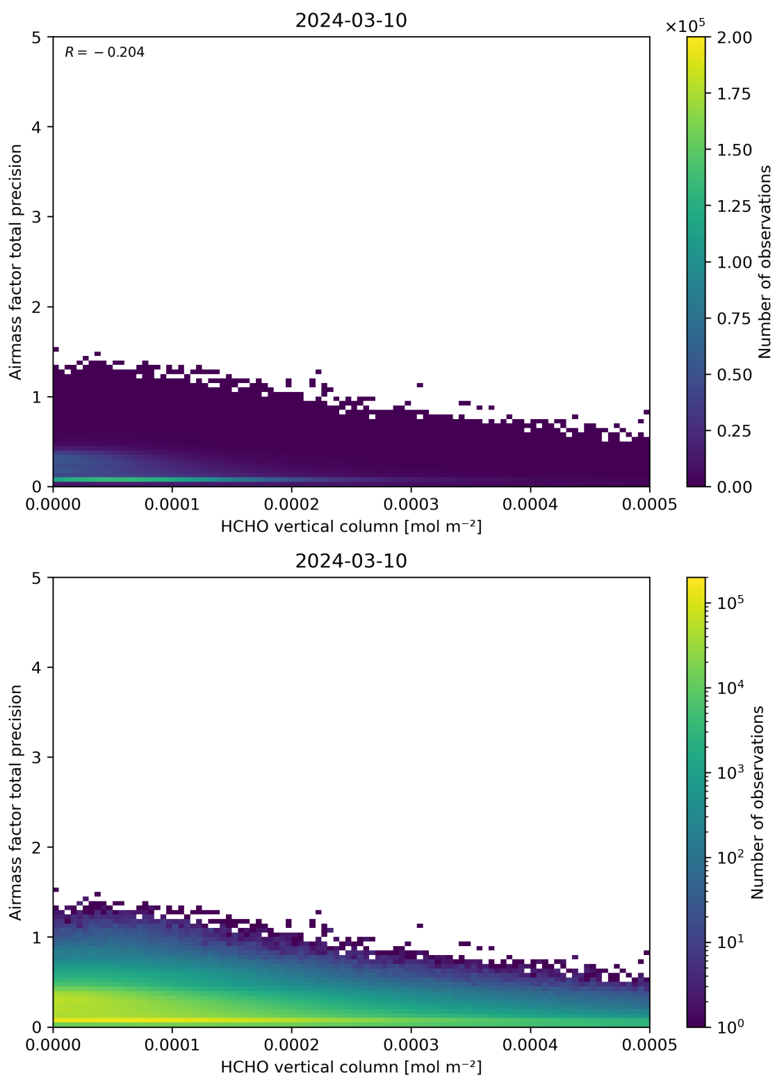
Figure 132: Scatter density plot of “HCHO vertical column” against “Airmass factor total precision” for 2024-03-09 to 2024-03-11.
