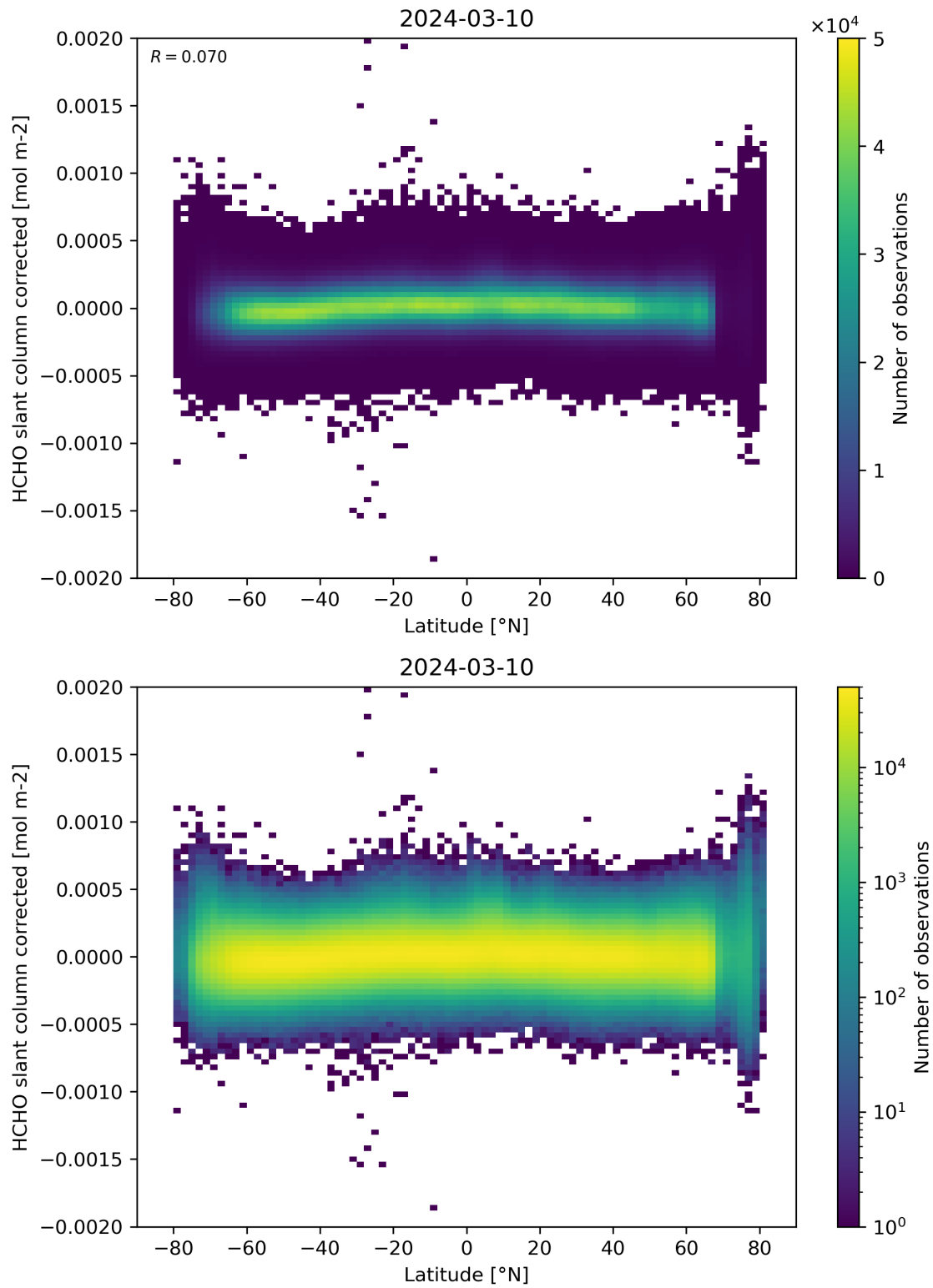
Figure 157: Scatter density plot of “Latitude” against “HCHO slant column corrected” for 2024-03-09 to 2024-03-11.
