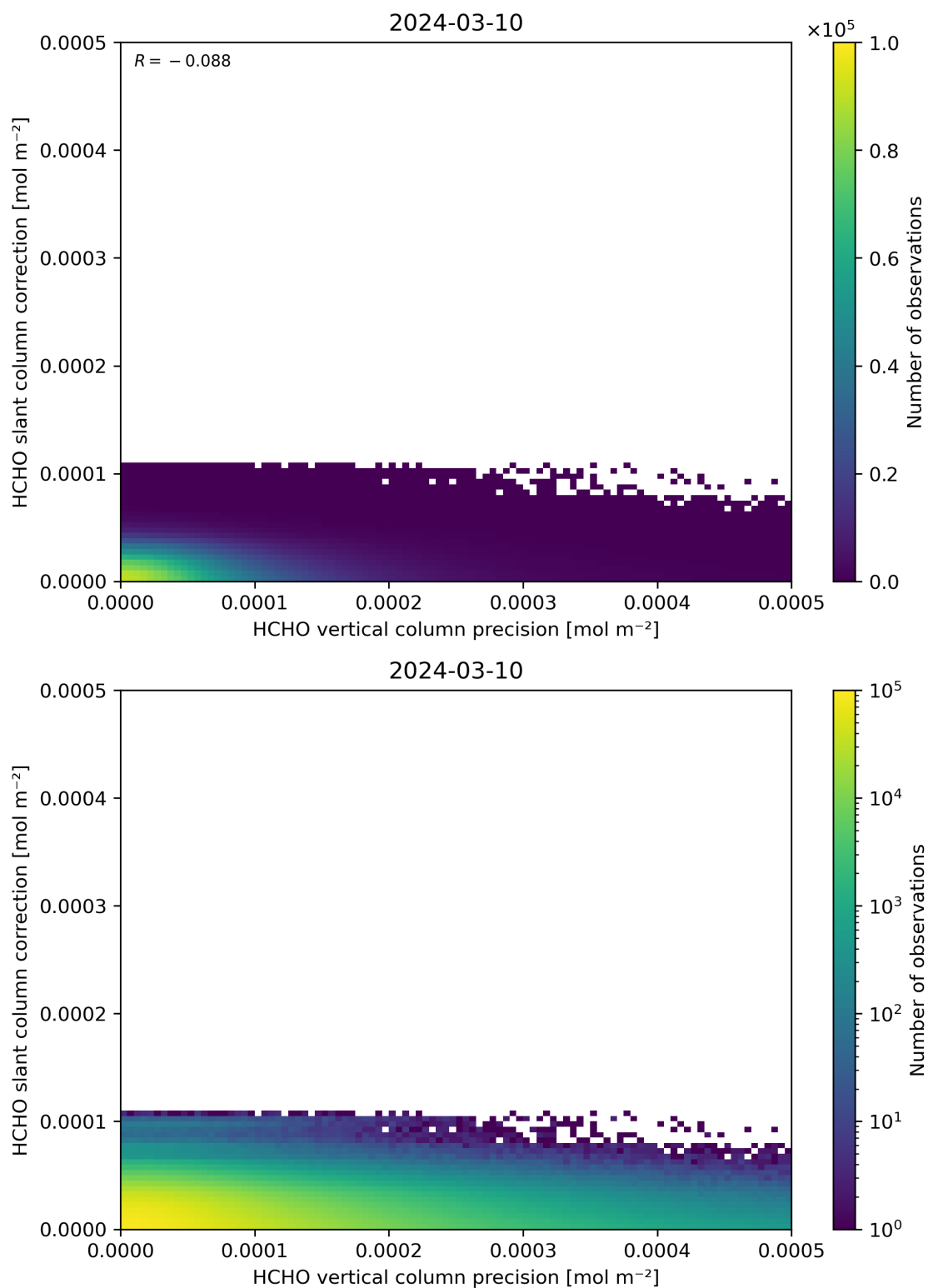
Figure 141: Scatter density plot of “HCHO vertical column precision” against “HCHO slant column correction” for 2024-03-09 to 2024-03-11.
