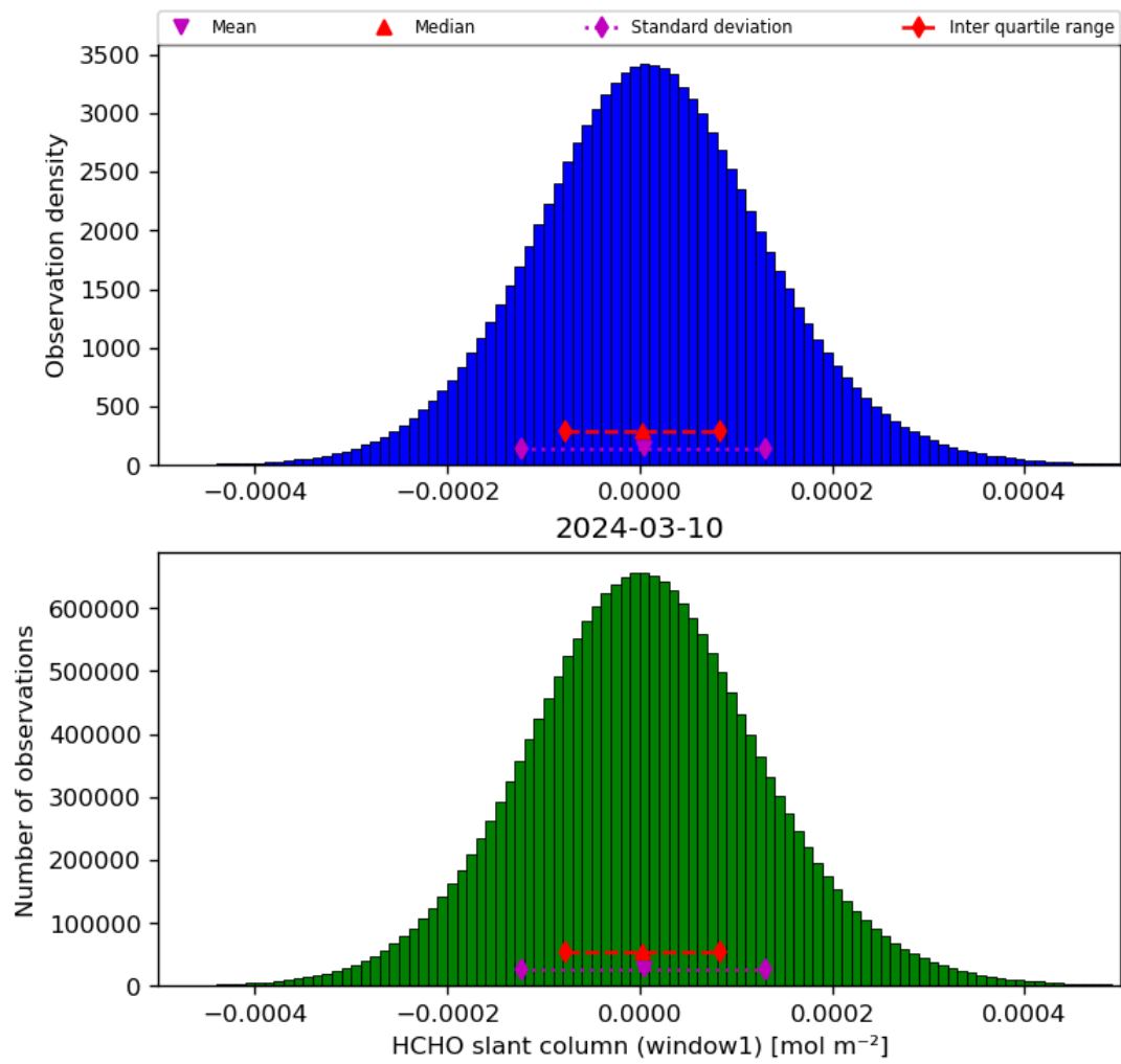
Figure 38: Histogram of “HCHO slant column (window1)” for 2024-03-09 to 2024-03-11
