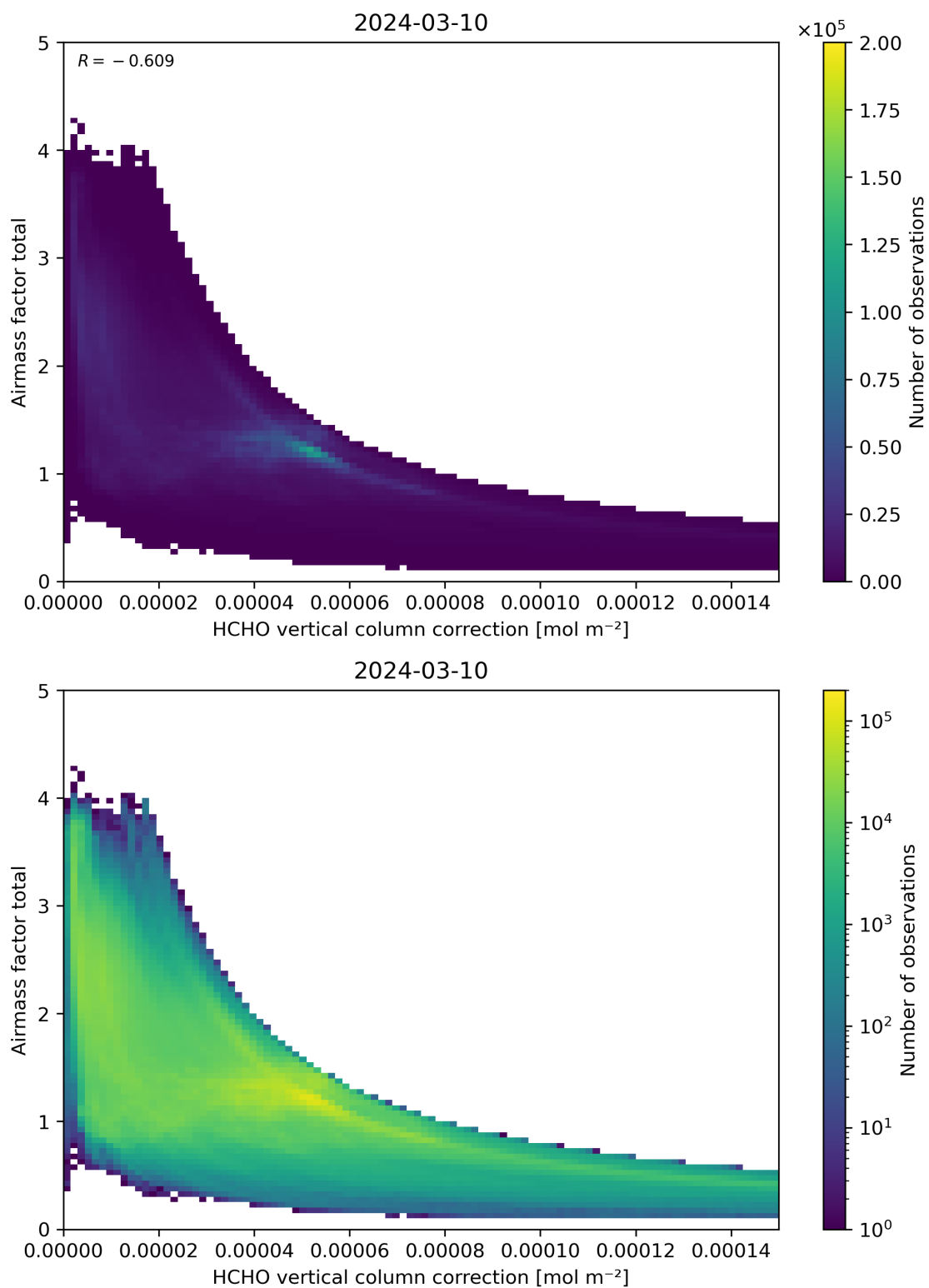
Figure 120: Scatter density plot of “HCHO vertical column correction” against “Airmass factor total” for 2024-03-09 to 2024-03-11.
