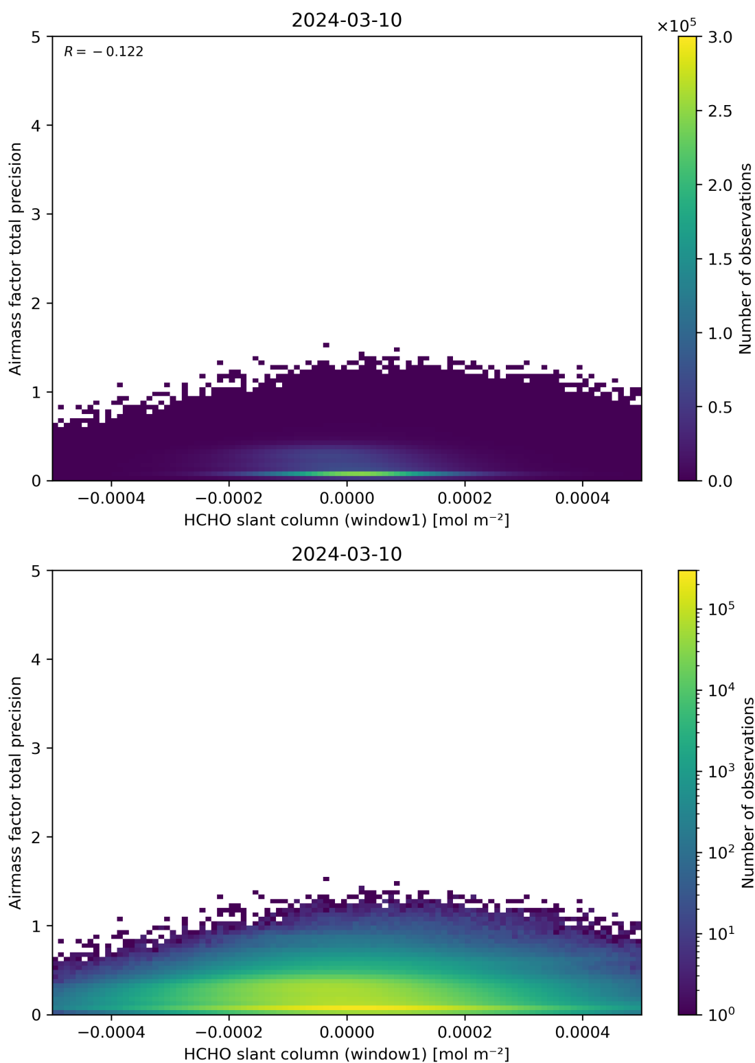
Figure 86: Scatter density plot of “HCHO slant column (window1)” against “Airmass factor total precision” for 2024-03-09 to 2024-03-11.
