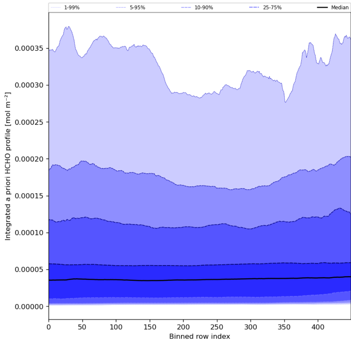
Figure 57: Along track statistics of "Integrated a priori HCHO profile" for 2024-03-09 to 2024-03-11
