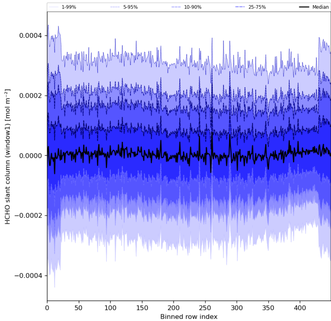
Figure 52: Along track statistics of “HCHO slant column (window1)” for 2024-03-09 to 2024-03-11
