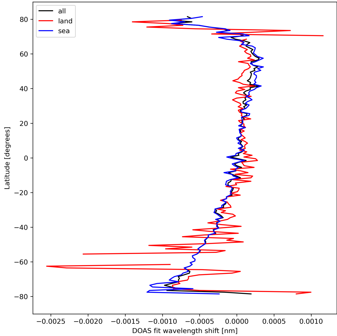
Figure 30: Zonal average of “DOAS fit wavelength shift” for 2024-03-09 to 2024-03-11.
