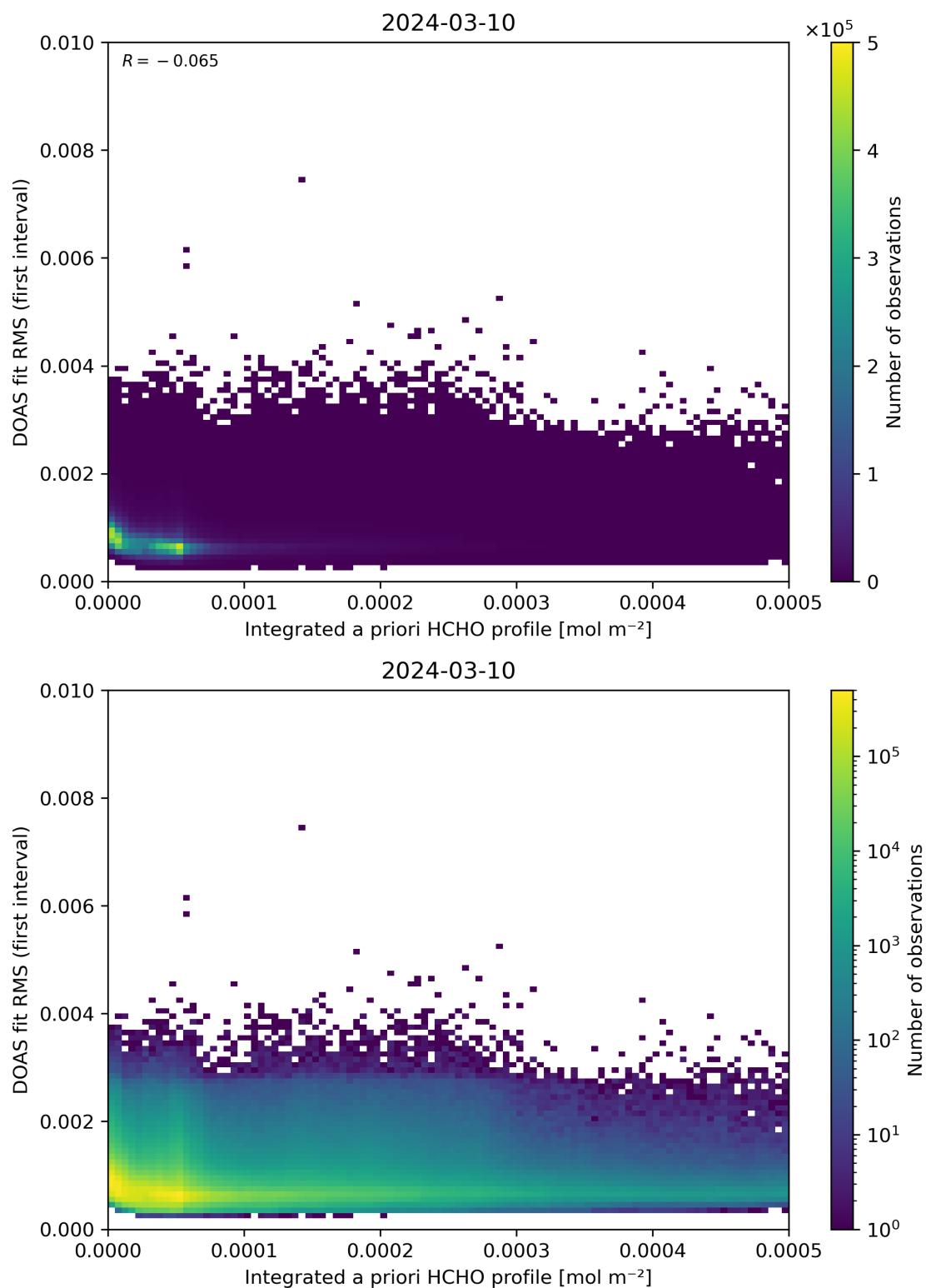
Figure 148: Scatter density plot of “Integrated a priori HCHO profile” against “DOAS fit RMS (first interval)” for 2024-03-09 to 2024-03-11.
