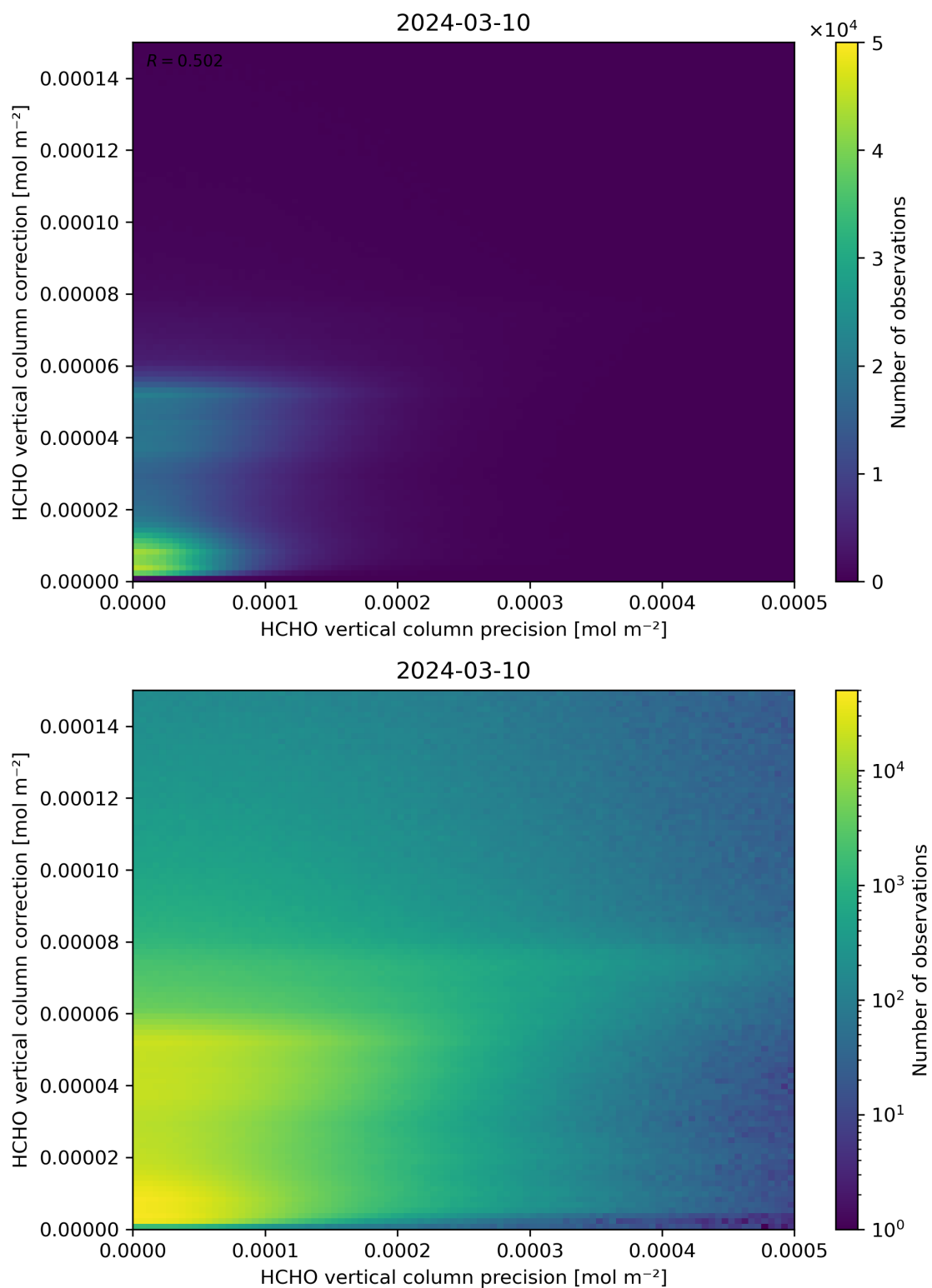
Figure 146: Scatter density plot of “HCHO vertical column precision” against “HCHO vertical column correction” for 2024-03-09 to 2024-03-11.
