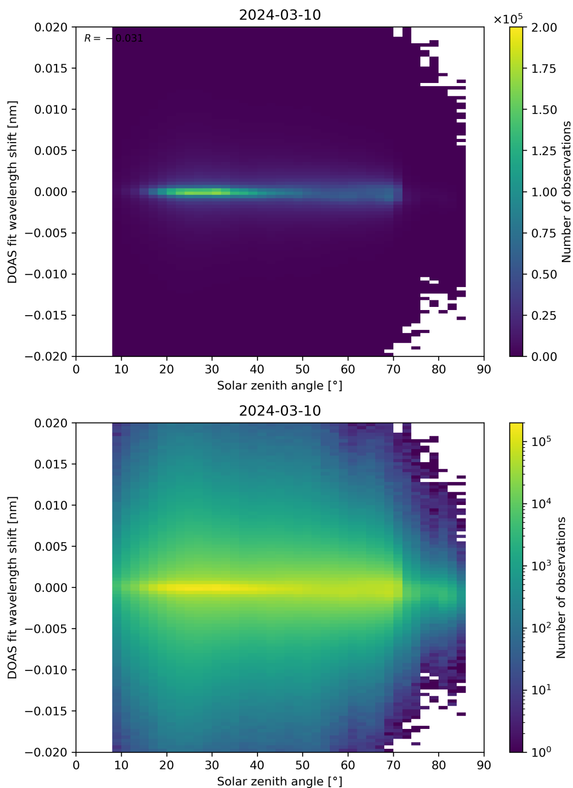
Figure 168: Scatter density plot of “Solar zenith angle” against “DOAS fit wavelength shift” for 2024-03-09 to 2024-03-11.
