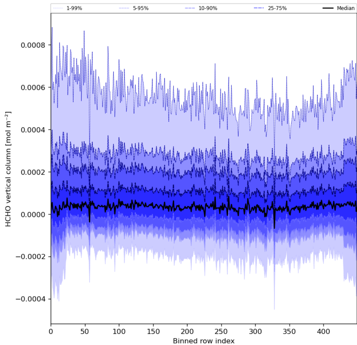
Figure 49: Along track statistics of “HCHO vertical column” for 2024-03-09 to 2024-03-11
