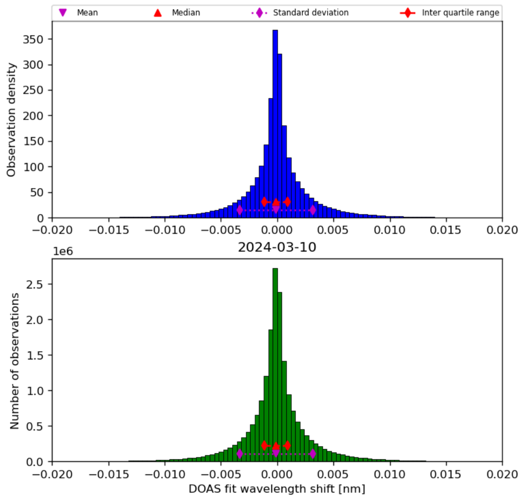
Figure 44: Histogram of “DOAS fit wavelength shift” for 2024-03-09 to 2024-03-11
