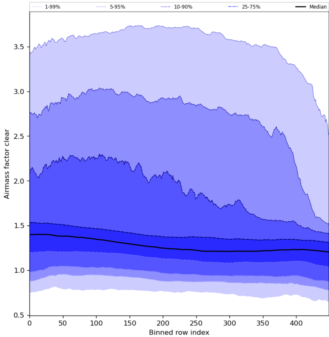
Figure 56: Along track statistics of “Airmass factor clear” for 2024-03-09 to 2024-03-11
