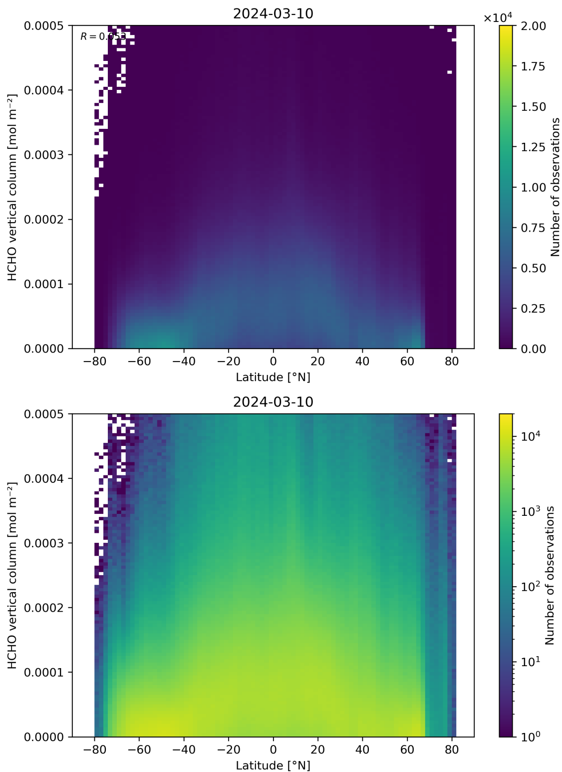
Figure 163: Scatter density plot of “Latitude” against “HCHO vertical column” for 2024-03-09 to 2024-03-11.
