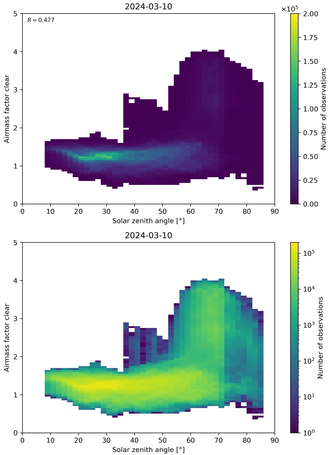
Figure 170: Scatter density plot of “Solar zenith angle” against “Airmass factor clear” for 2024-03-09 to 2024-03-11.
