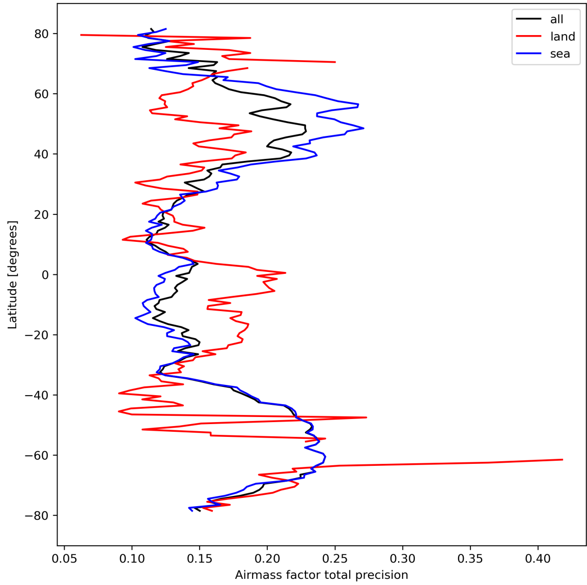
Figure 27: Zonal average of “Airmass factor total precision” for 2024-03-09 to 2024-03-11.
