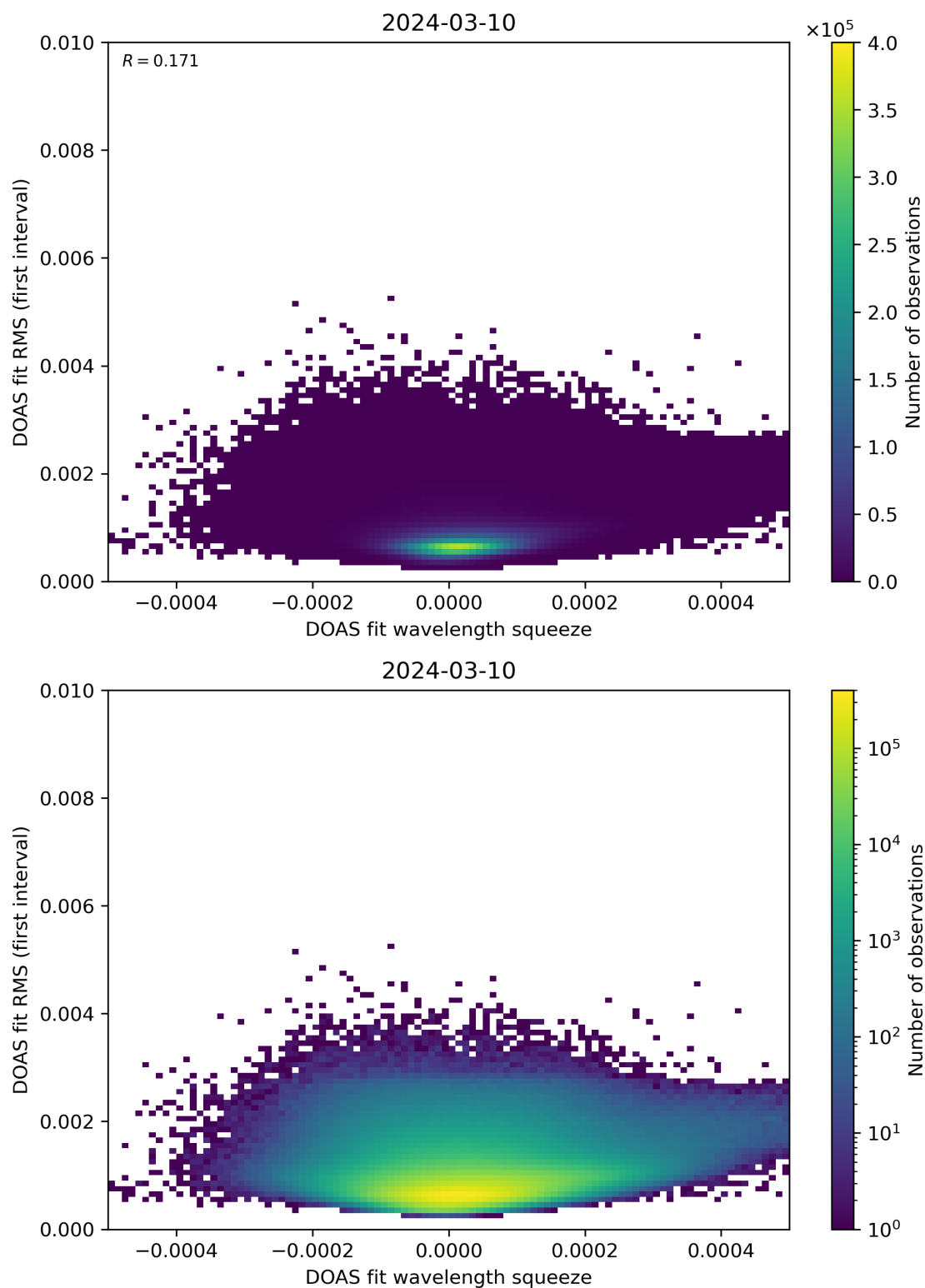
Figure 68: Scatter density plot of “DOAS fit wavelength squeeze” against “DOAS fit RMS (first interval)” for 2024-03-09 to 2024-03-11.
