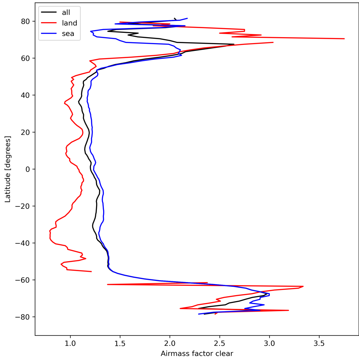
Figure 28: Zonal average of “Airmass factor clear” for 2024-03-09 to 2024-03-11.
