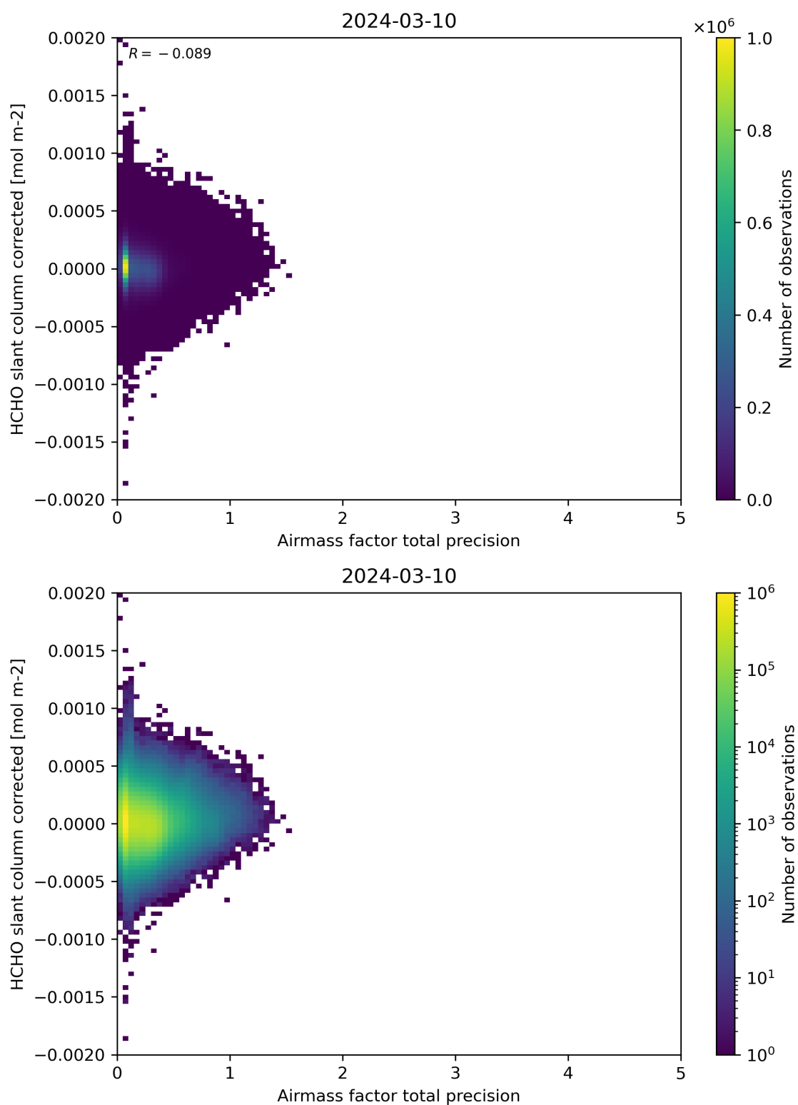
Figure 109: Scatter density plot of “Airmass factor total precision” against “HCHO slant column corrected” for 2024-03-09 to 2024-03-11.
