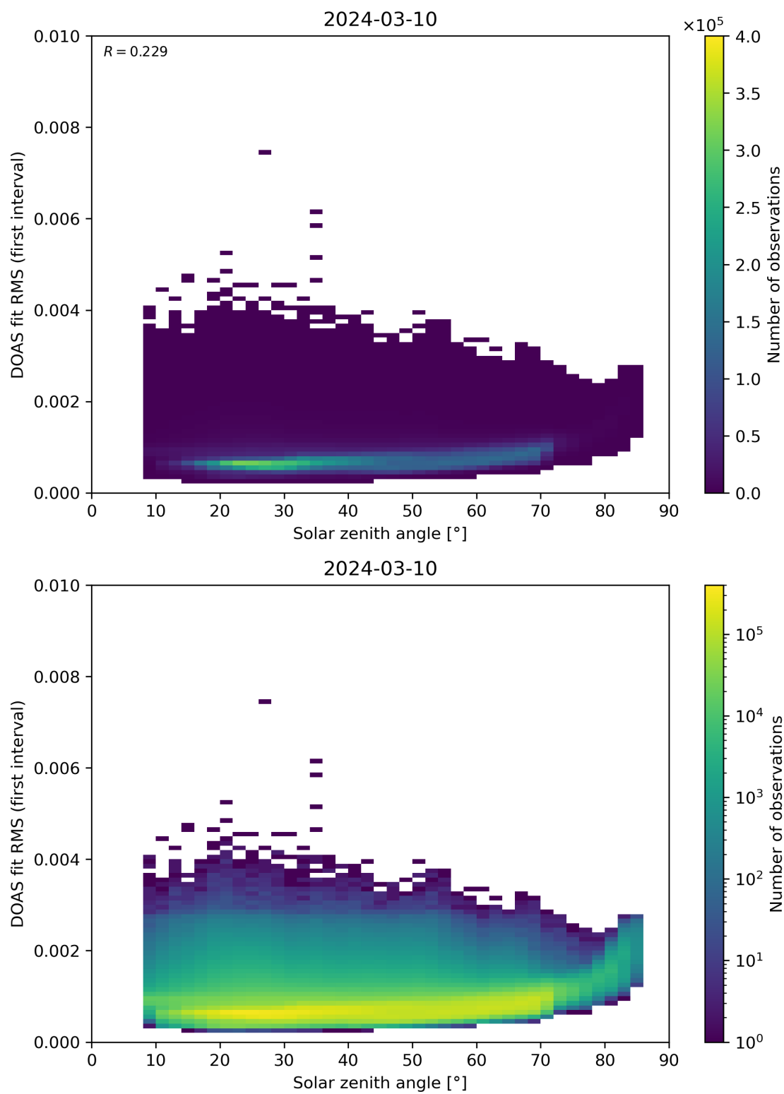
Figure 167: Scatter density plot of “Solar zenith angle” against “DOAS fit RMS (first interval)” for 2024-03-09 to 2024-03-11.
