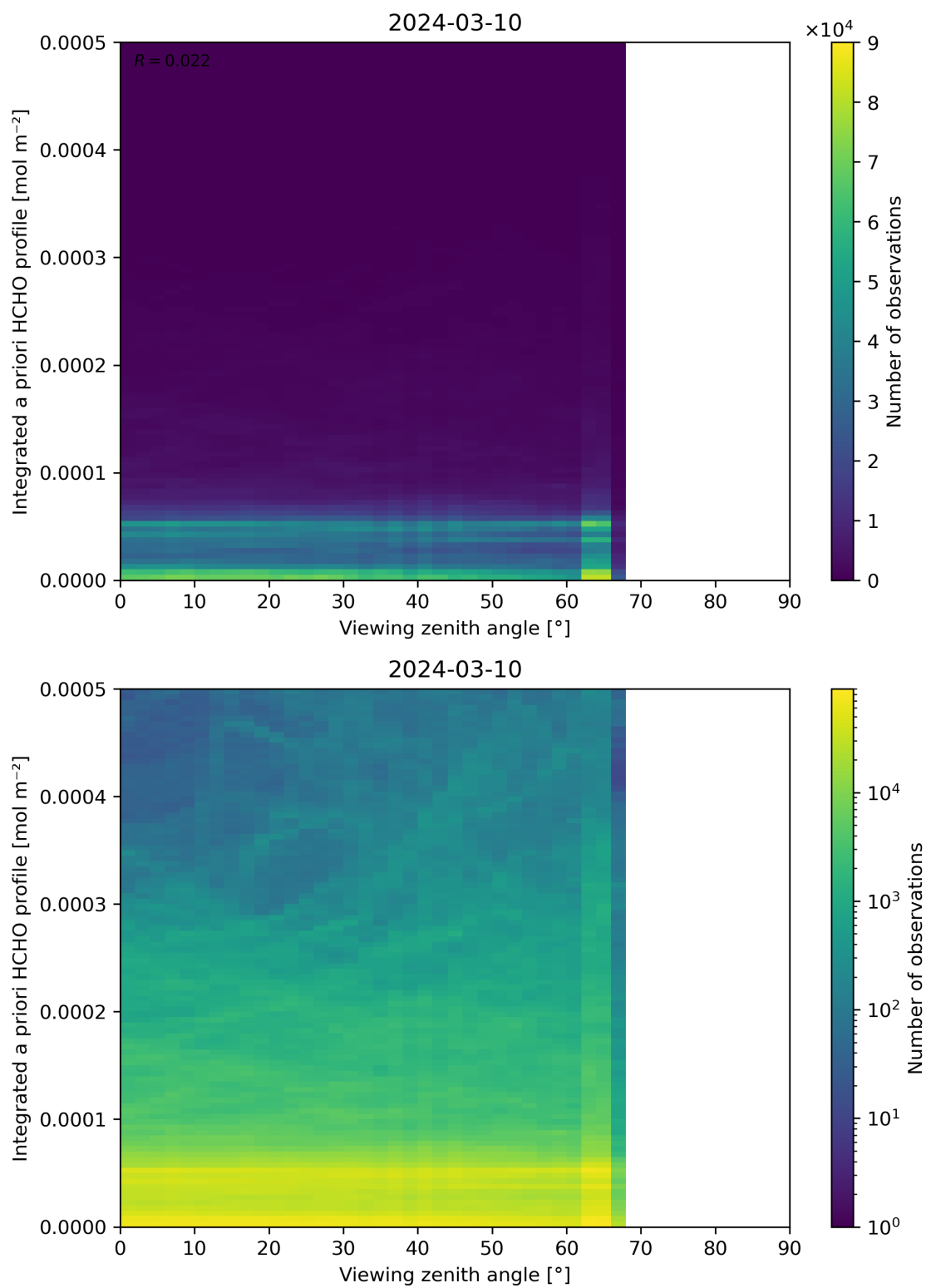
Figure 195: Scatter density plot of “Viewing zenith angle” against “Integrated a priori HCHO profile” for 2024-03-09 to 2024-03-11.
