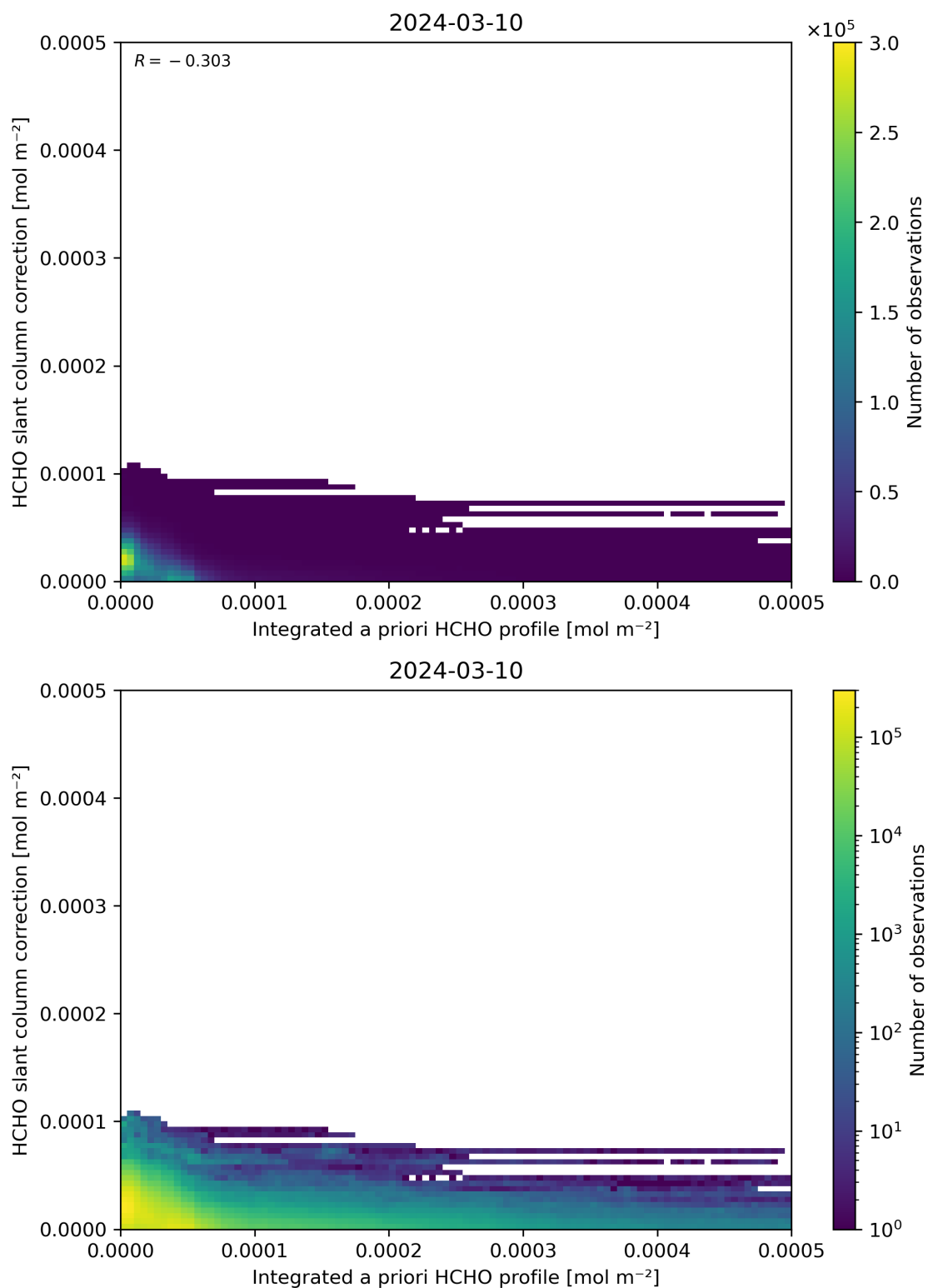
Figure 152: Scatter density plot of “Integrated a priori HCHO profile” against “HCHO slant column correction” for 2024-03-09 to 2024-03-11.
