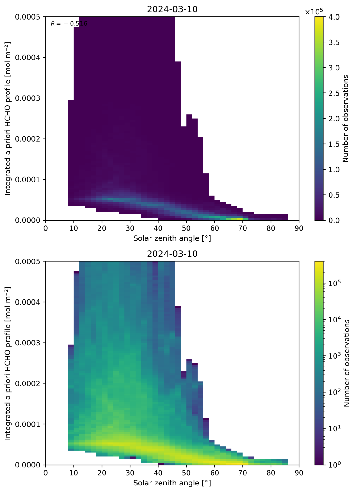
Figure 180: Scatter density plot of “Solar zenith angle” against “Integrated a priori HCHO profile” for 2024-03-09 to 2024-03-11.
