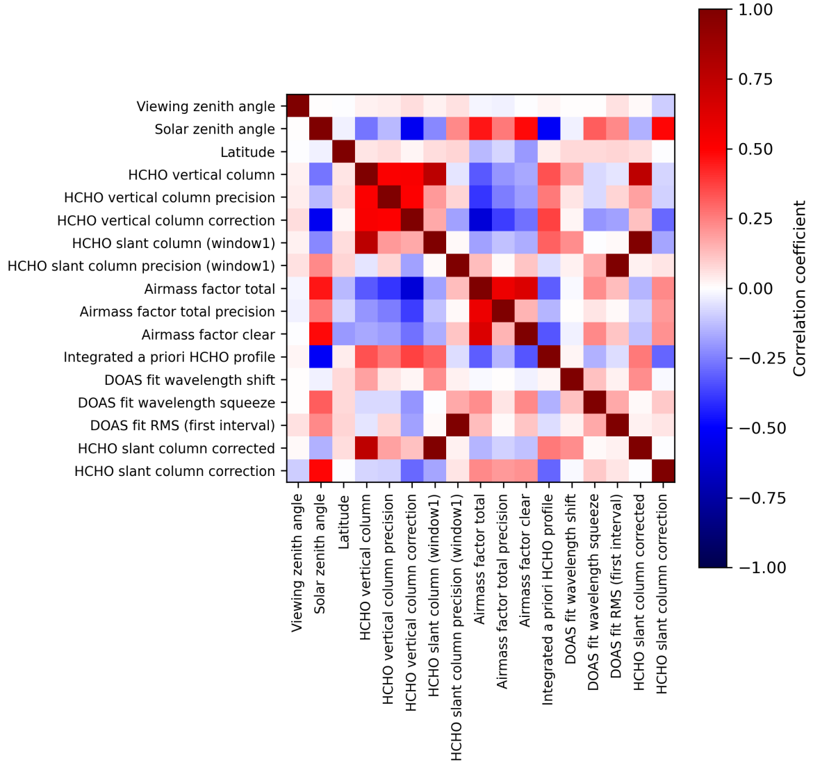
Figure 2: Map of correlation matrix for 2024-03-09 to 2024-03-11.
