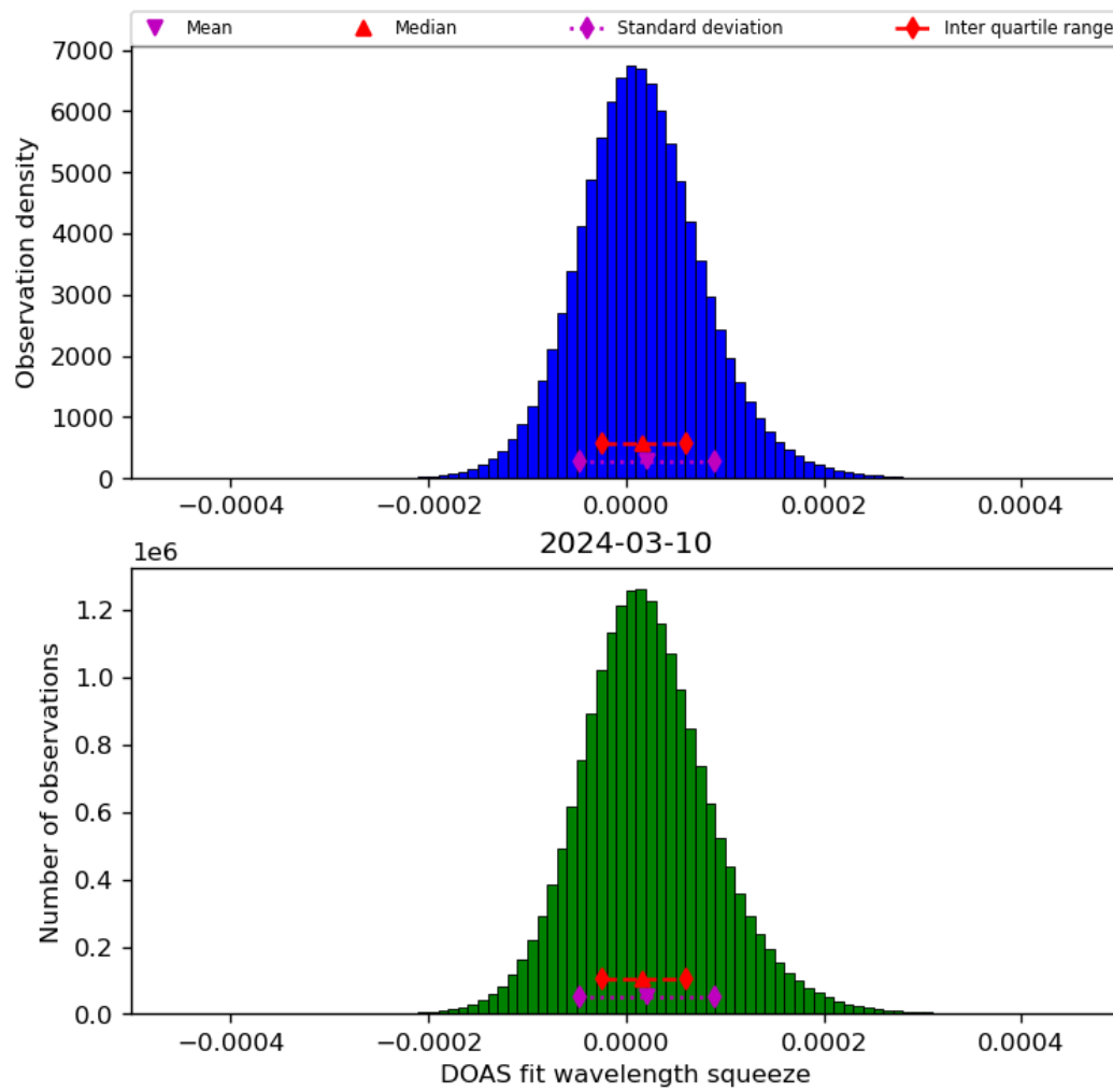
Figure 45: Histogram of “DOAS fit wavelength squeeze” for 2024-03-09 to 2024-03-11
