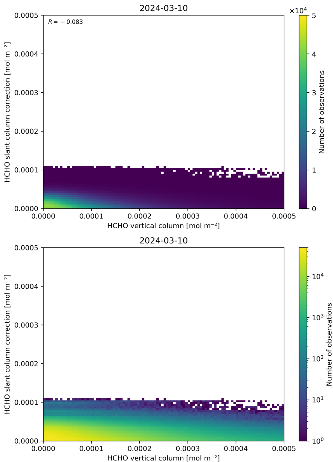
Figure 128: Scatter density plot of “HCHO vertical column” against “HCHO slant column correction” for 2024-03-09 to 2024-03-11.
