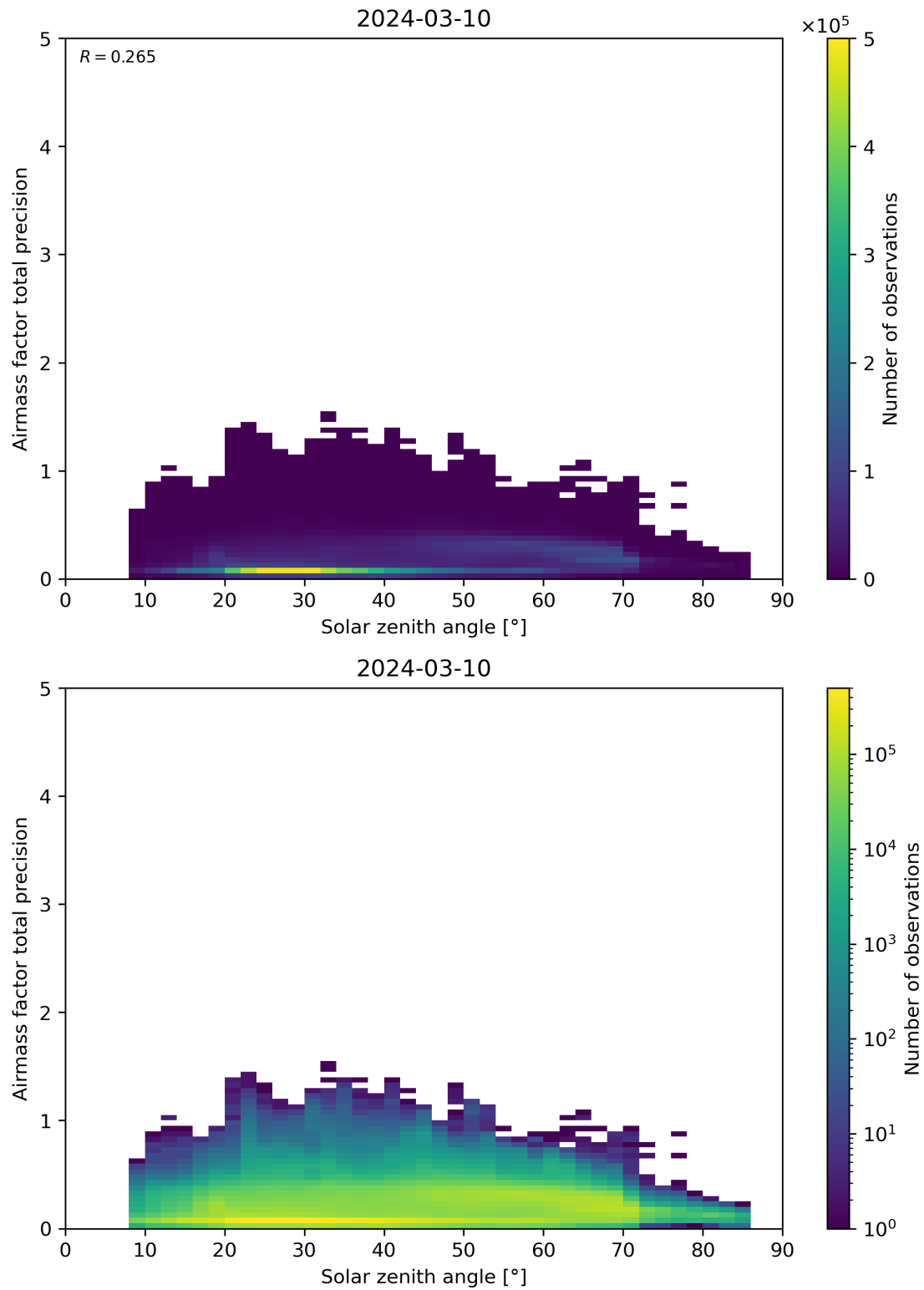
Figure 176: Scatter density plot of “Solar zenith angle” against “Airmass factor total precision” for 2024-03-09 to 2024-03-11.
