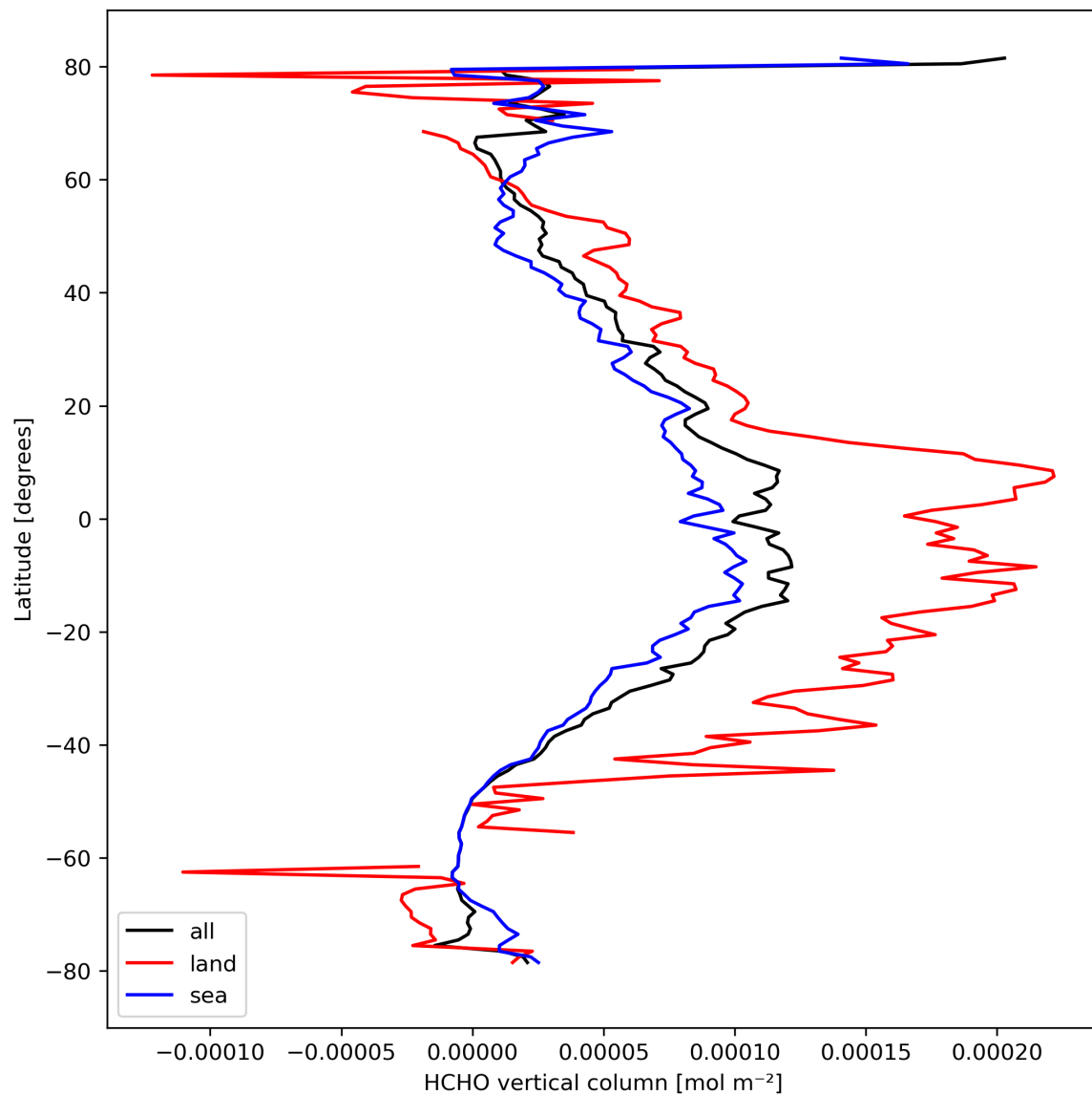
Figure 21: Zonal average of “HCHO vertical column” for 2024-03-09 to 2024-03-11.
