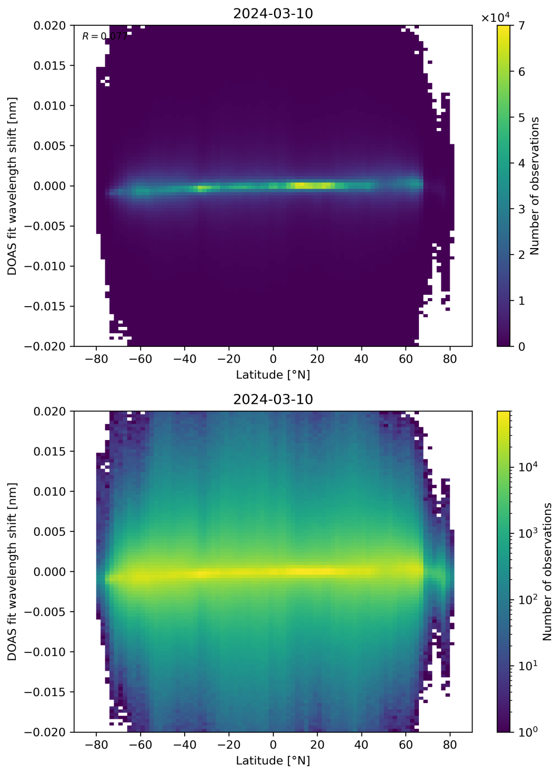
Figure 154: Scatter density plot of “Latitude” against “DOAS fit wavelength shift” for 2024-03-09 to 2024-03-11.
