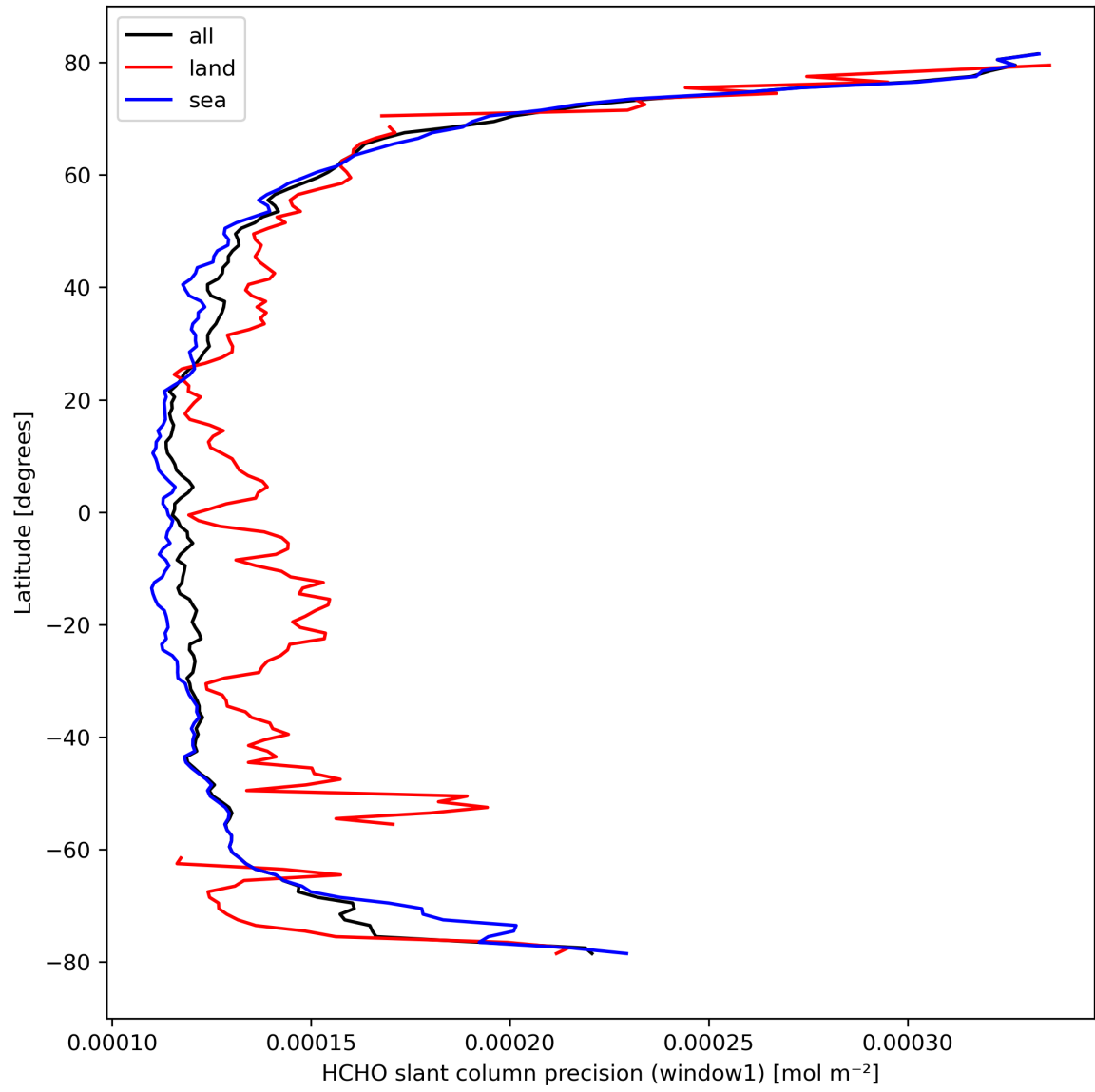
Figure 25: Zonal average of “HCHO slant column precision (window1)” for 2024-03-09 to 2024-03-11.
