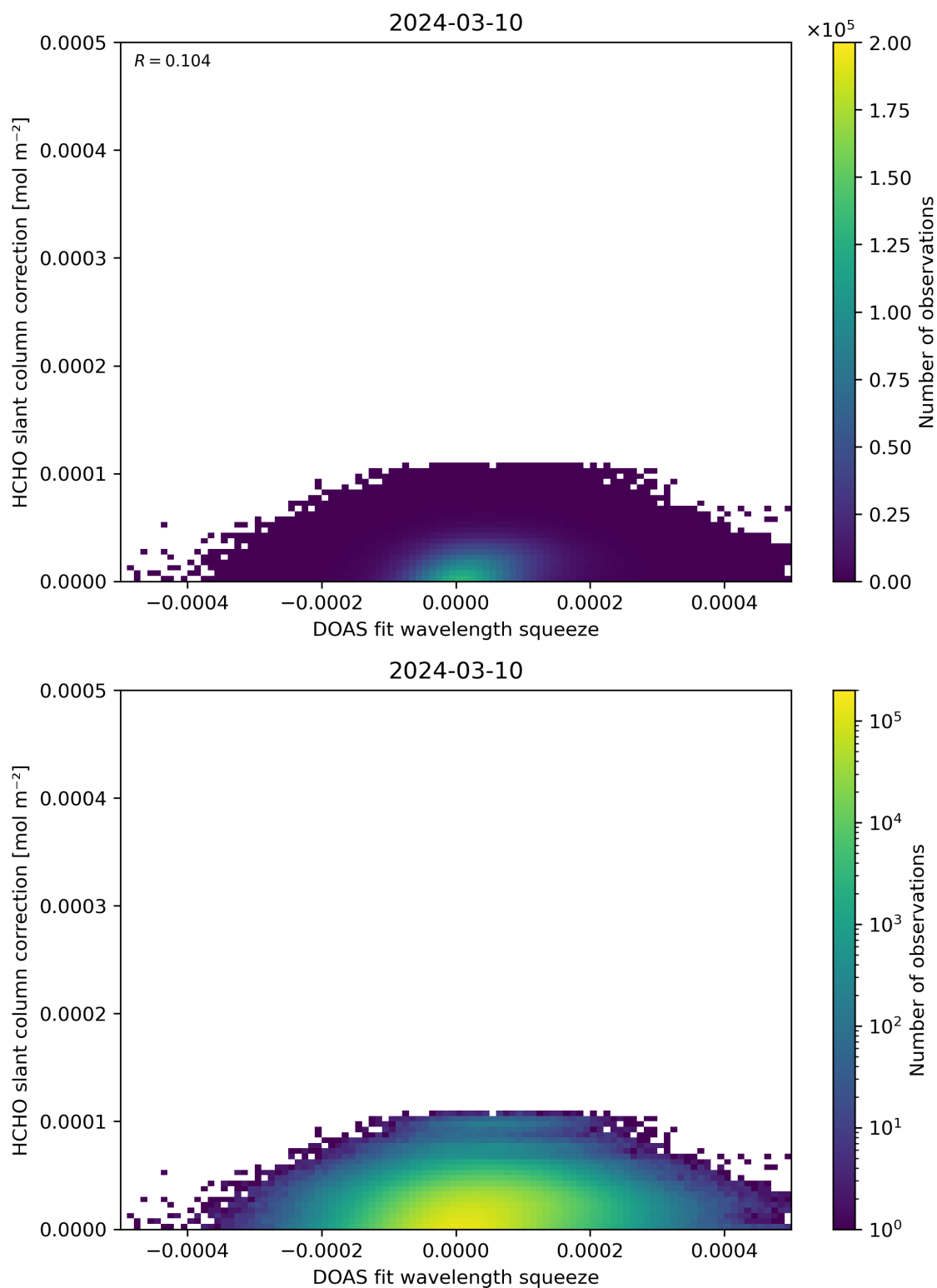
Figure 70: Scatter density plot of “DOAS fit wavelength squeeze” against “HCHO slant column correction” for 2024-03-09 to 2024-03-11.
