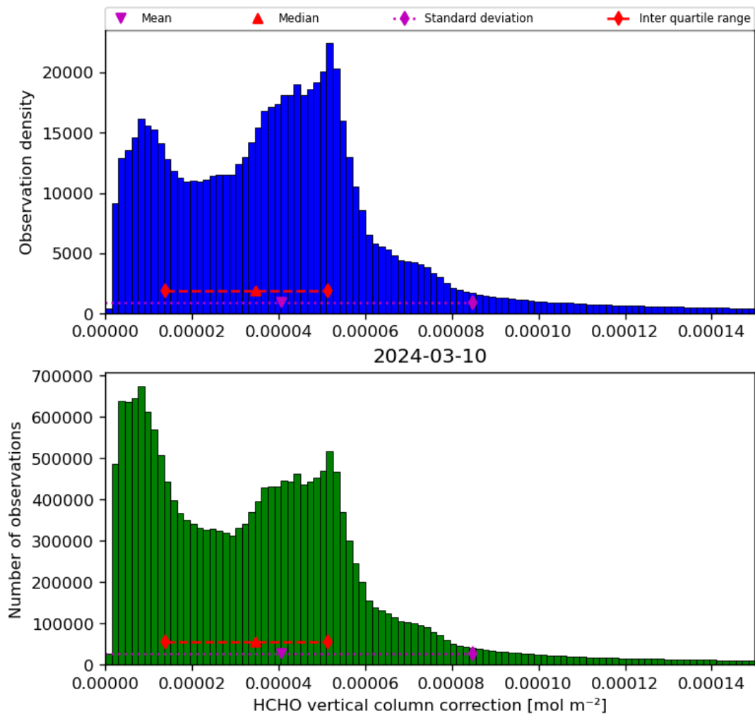
Figure 37: Histogram of “HCHO vertical column correction” for 2024-03-09 to 2024-03-11
