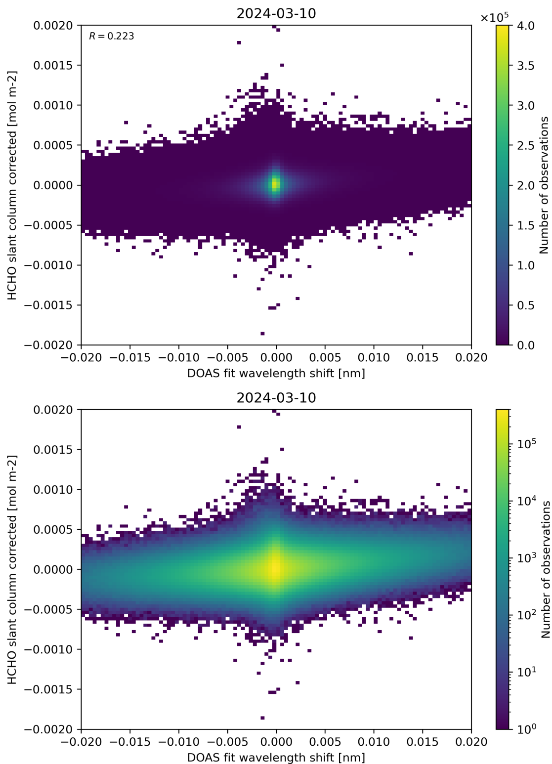
Figure 66: Scatter density plot of “DOAS fit wavelength shift” against “HCHO slant column corrected” for 2024-03-09 to 2024-03-11.
