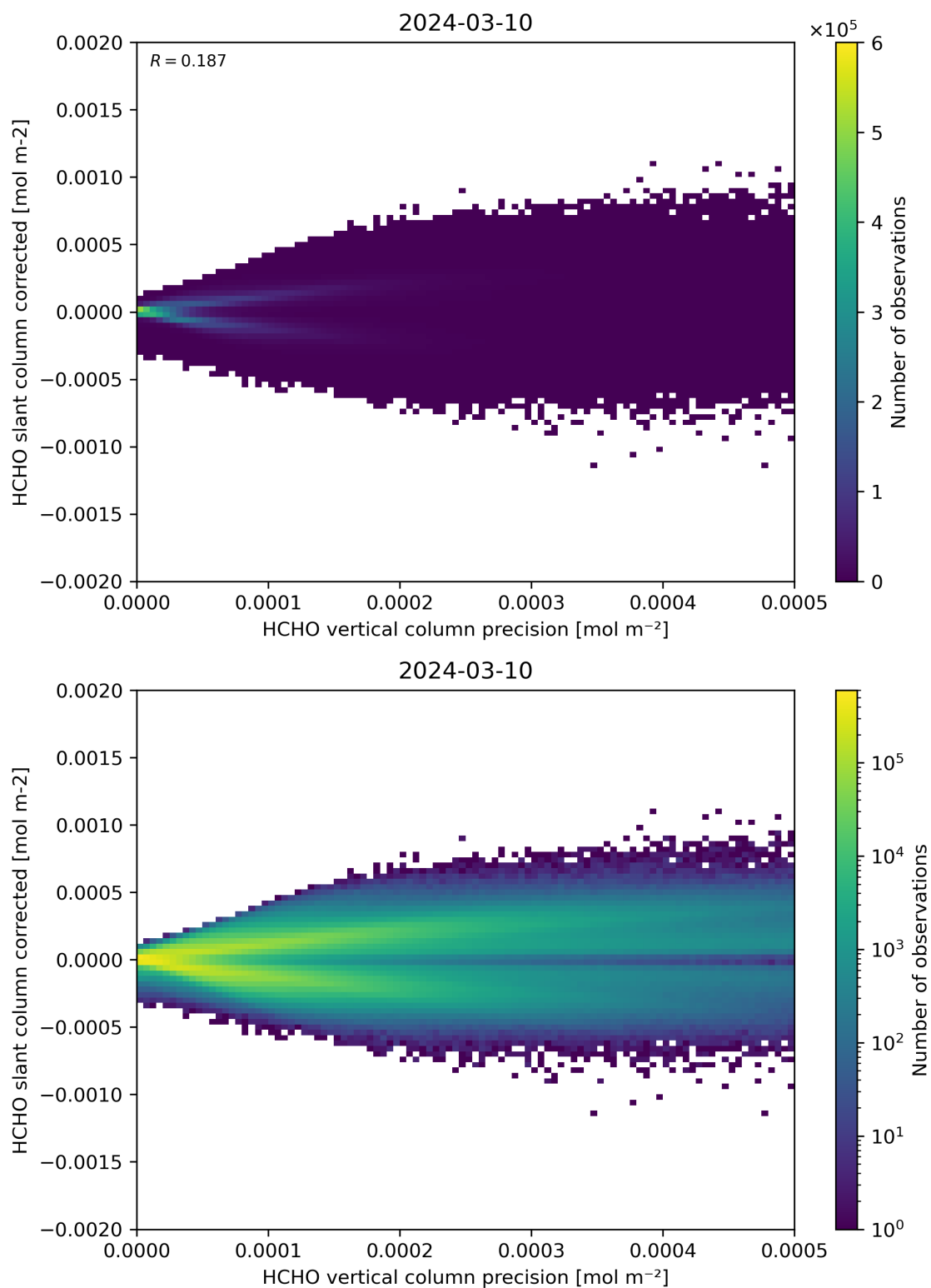
Figure 140: Scatter density plot of “HCHO vertical column precision” against “HCHO slant column corrected” for 2024-03-09 to 2024-03-11.
