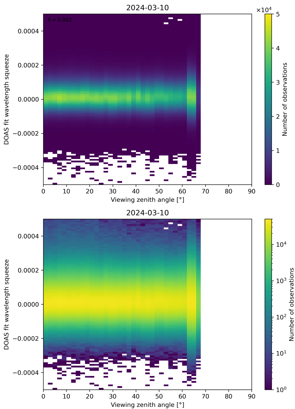
Figure 184: Scatter density plot of “Viewing zenith angle” against “DOAS fit wavelength squeeze” for 2024-03-09 to 2024-03-11.
