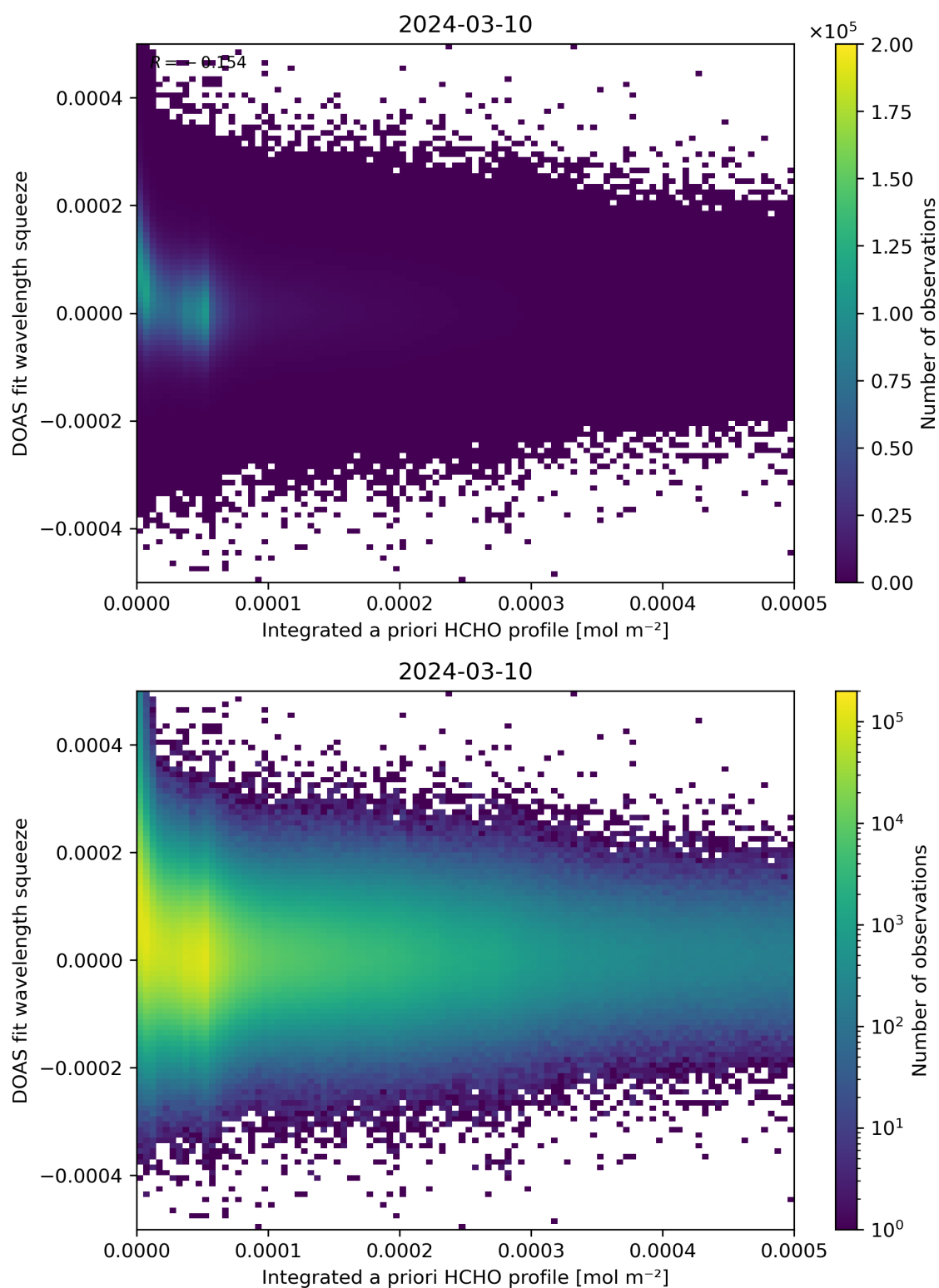
Figure 150: Scatter density plot of “Integrated a priori HCHO profile” against “DOAS fit wavelength squeeze” for 2024-03-09 to 2024-03-11.
