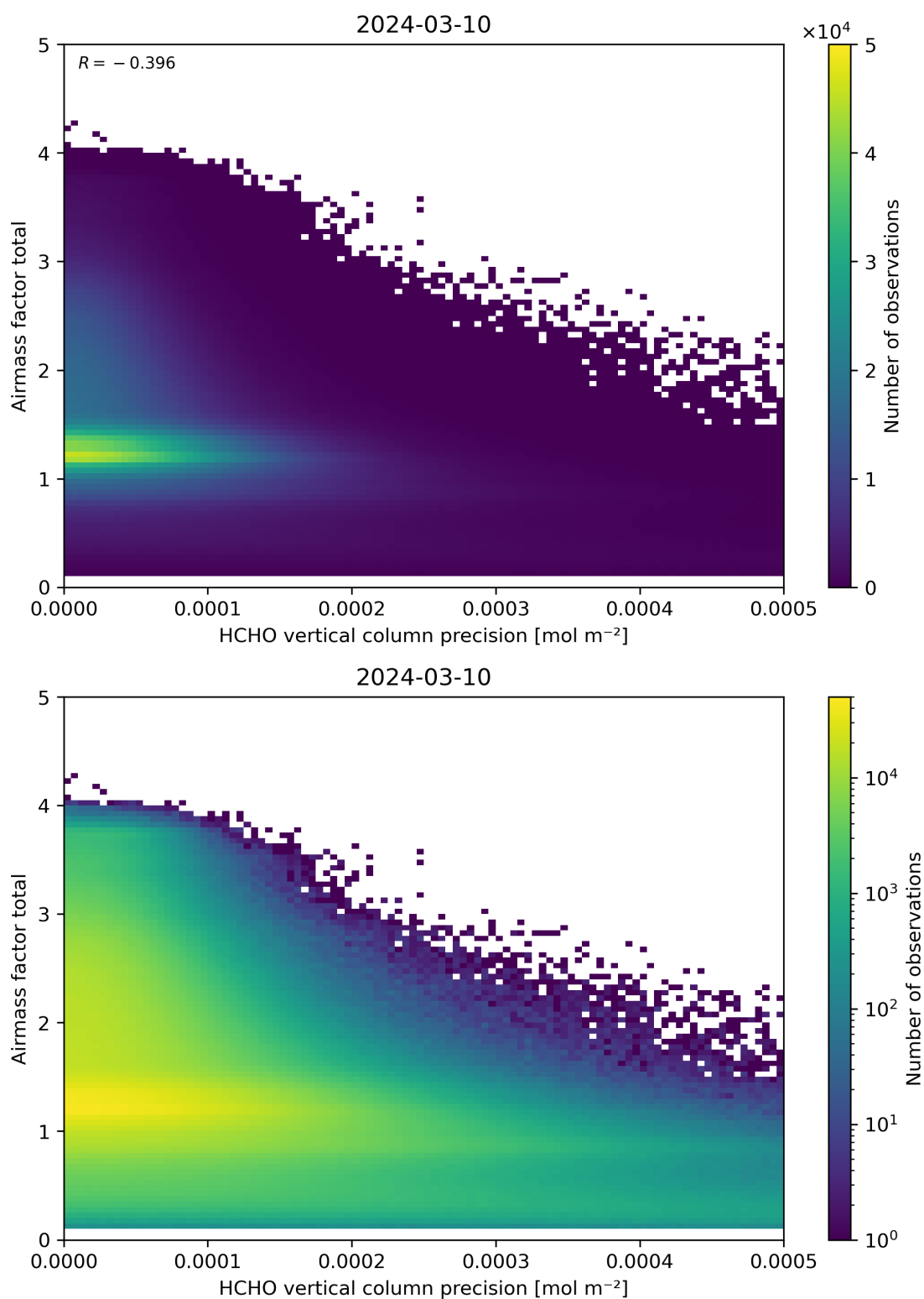
Figure 144: Scatter density plot of “HCHO vertical column precision” against “Airmass factor total” for 2024-03-09 to 2024-03-11.
