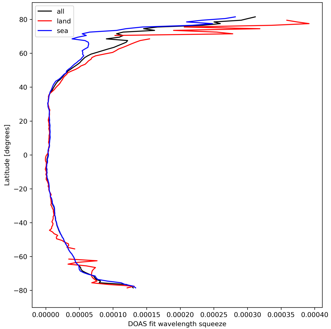
Figure 31: Zonal average of “DOAS fit wavelength squeeze” for 2024-03-09 to 2024-03-11.
