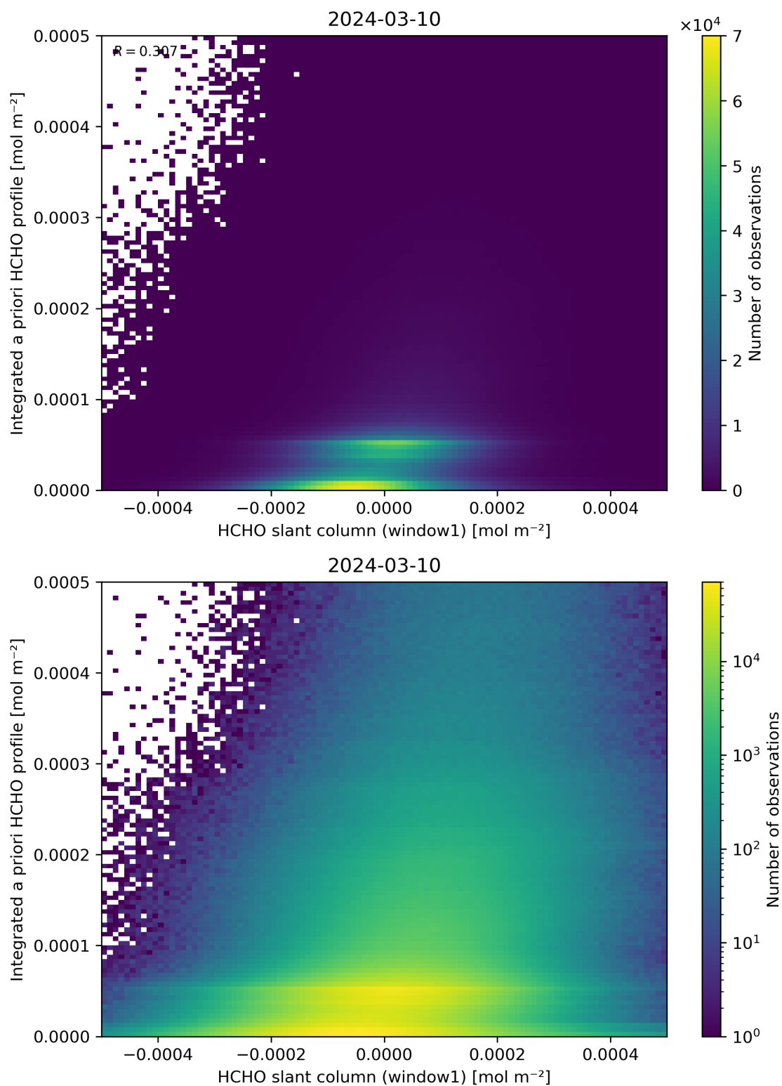
Figure 87: Scatter density plot of “HCHO slant column (window1)” against “Integrated a priori HCHO profile” for 2024-03-09 to 2024-03-11.
