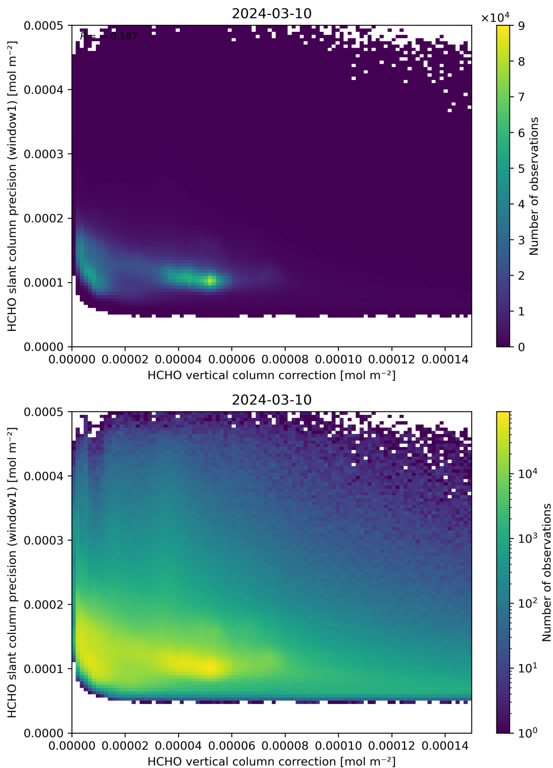
Figure 119: Scatter density plot of “HCHO vertical column correction” against “HCHO slant column precision (window1)” for 2024-03-09 to 2024-03-11.
