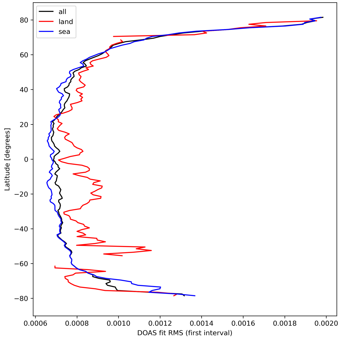
Figure 32: Zonal average of “DOAS fit RMS (first interval)” for 2024-03-09 to 2024-03-11.
