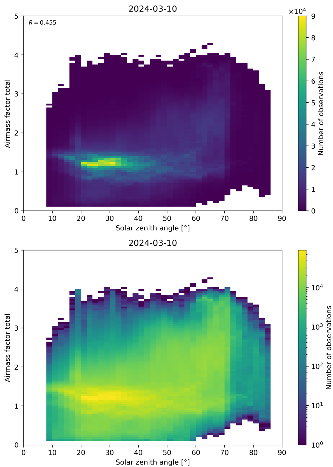
Figure 175: Scatter density plot of “Solar zenith angle” against “Airmass factor total” for 2024-03-09 to 2024-03-11.
