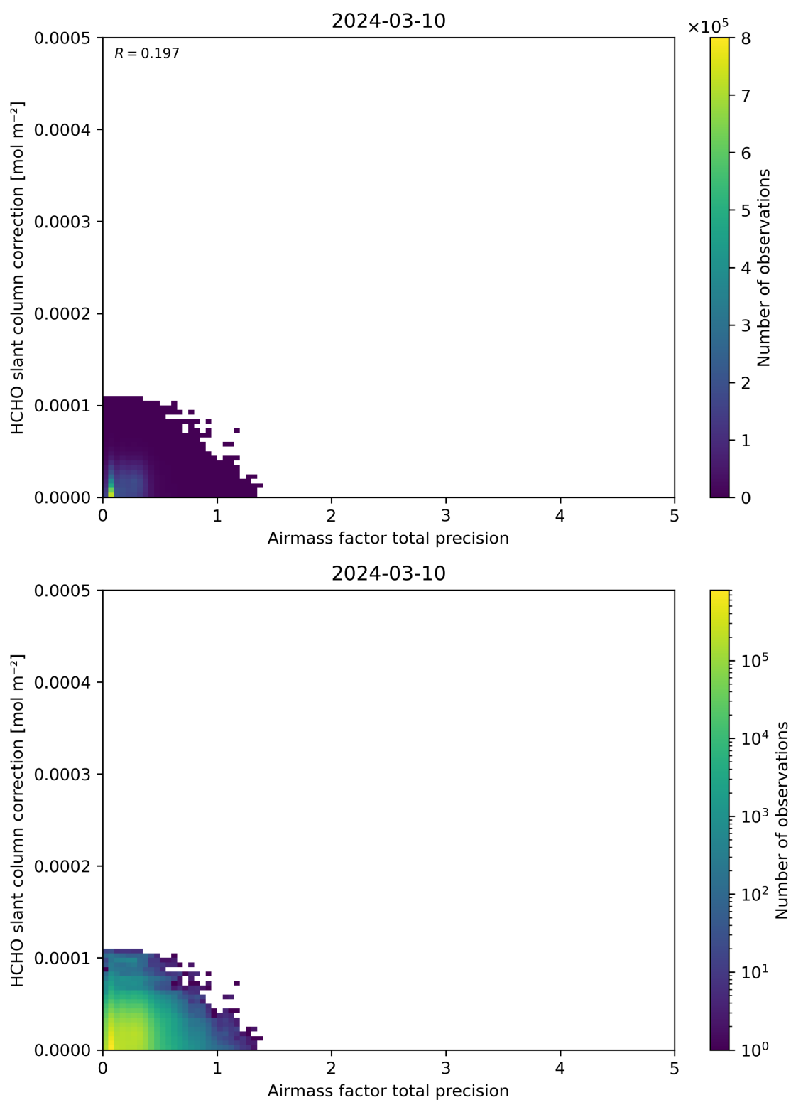
Figure 110: Scatter density plot of “Airmass factor total precision” against “HCHO slant column correction” for 2024-03-09 to 2024-03-11.
