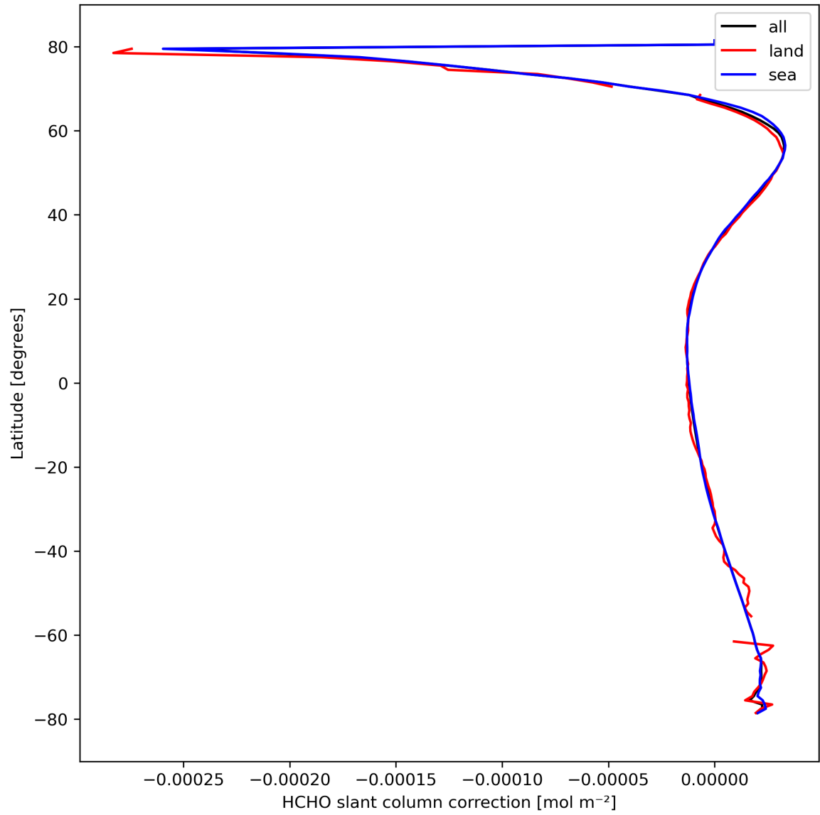
Figure 33: Zonal average of “HCHO slant column correction” for 2024-03-09 to 2024-03-11.
