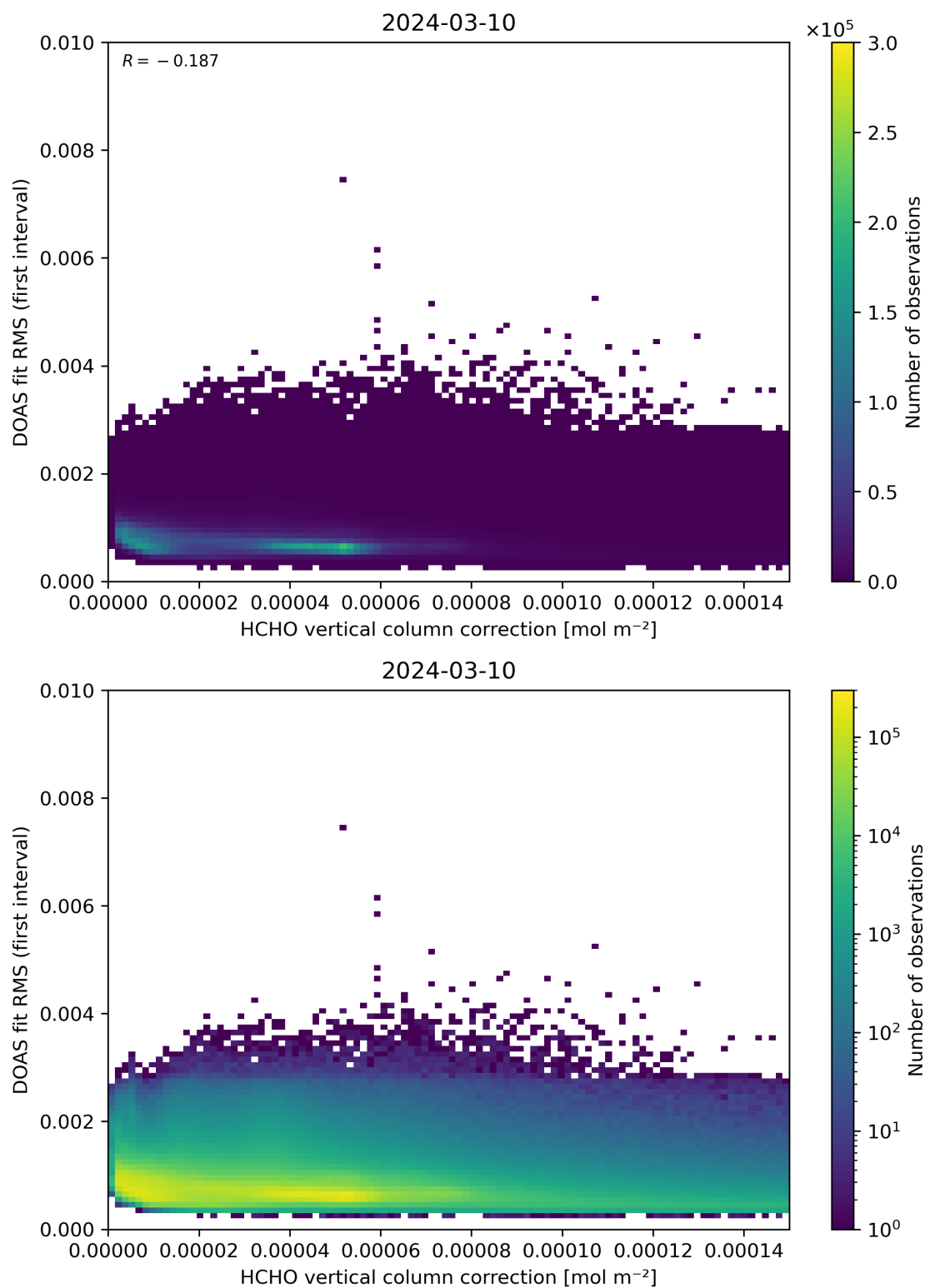
Figure 112: Scatter density plot of “HCHO vertical column correction” against “DOAS fit RMS (first interval)” for 2024-03-09 to 2024-03-11.
