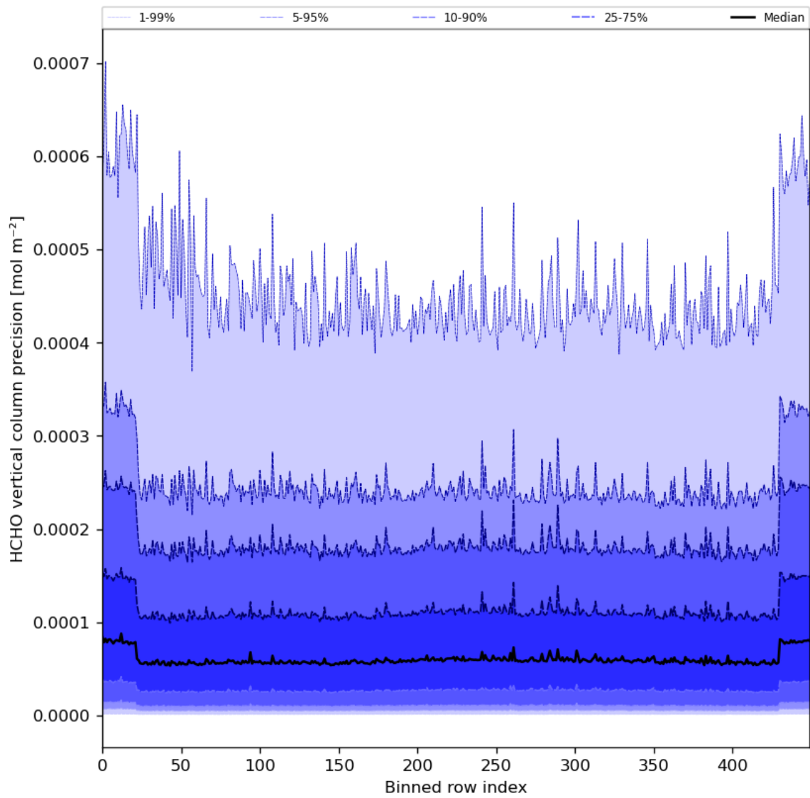
Figure 50: Along track statistics of “HCHO vertical column precision” for 2024-03-09 to 2024-03-11
