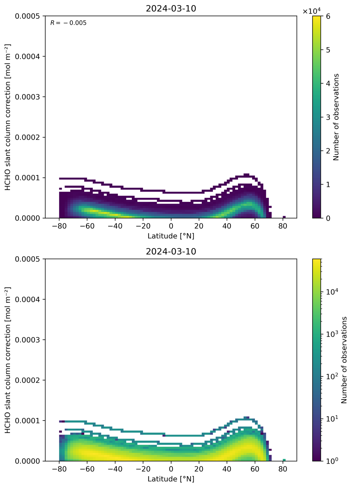
Figure 158: Scatter density plot of “Latitude” against “HCHO slant column correction” for 2024-03-09 to 2024-03-11.
