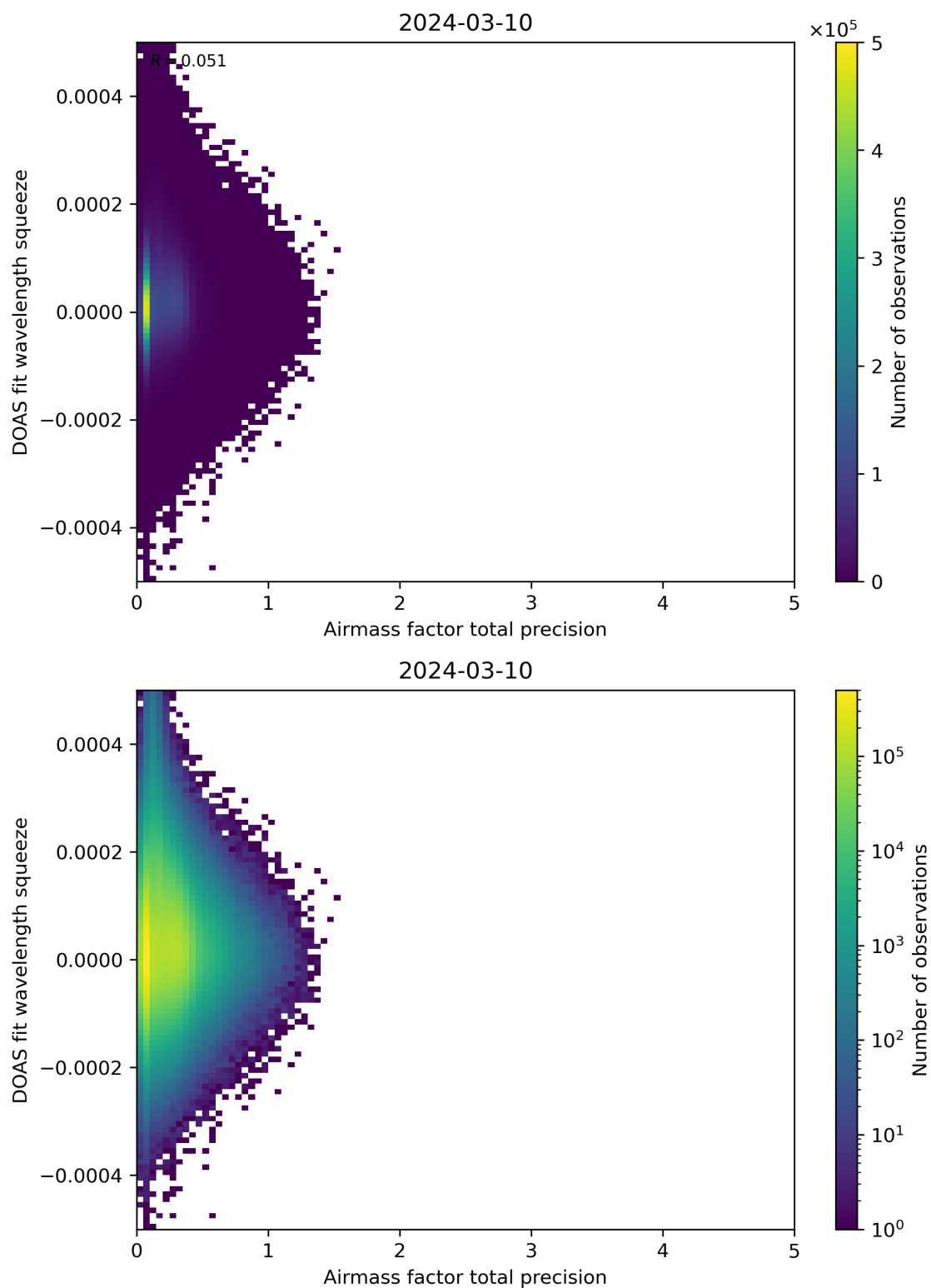
Figure 107: Scatter density plot of “Airmass factor total precision” against “DOAS fit wavelength squeeze” for 2024-03-09 to 2024-03-11.
