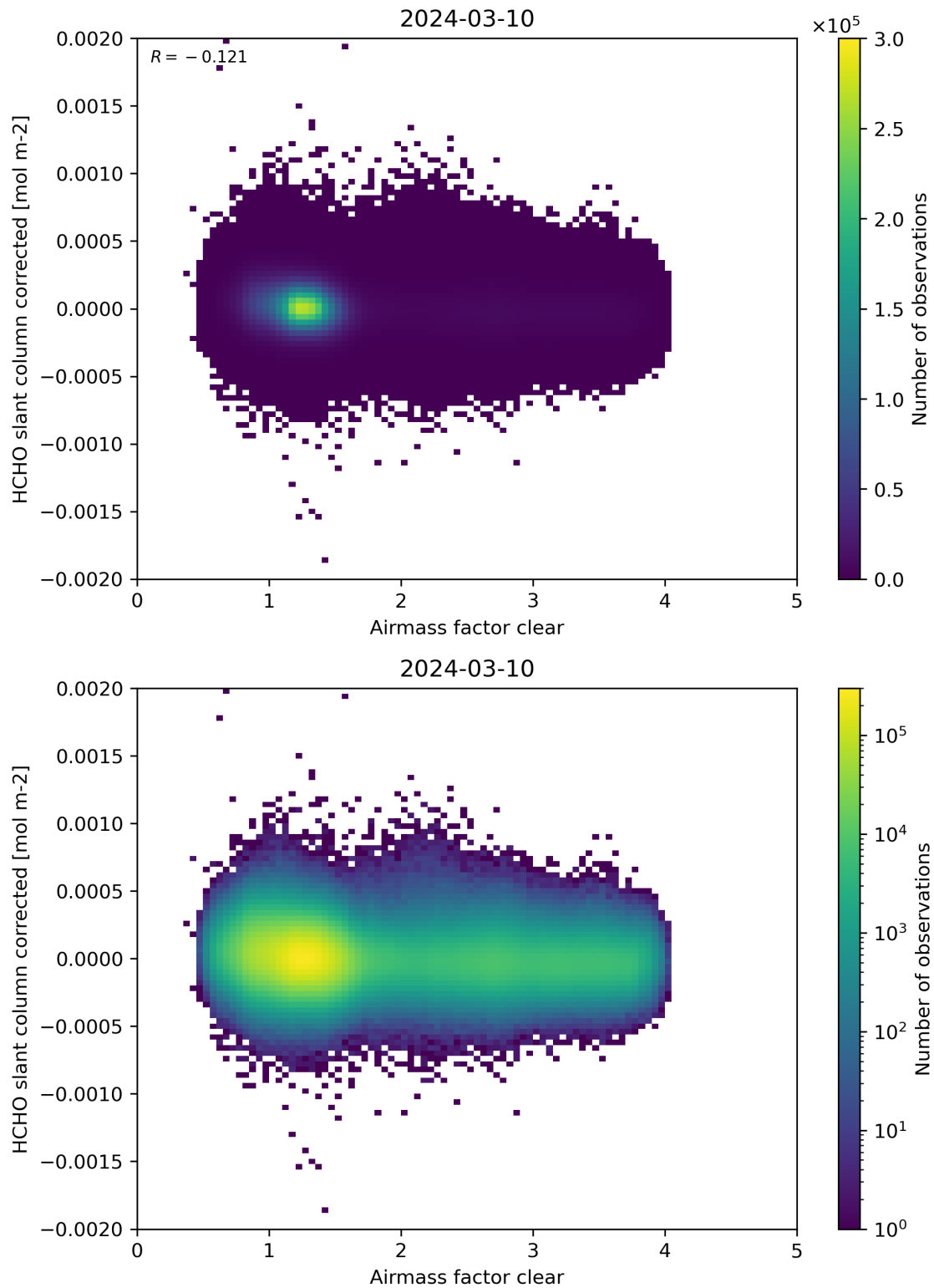
Figure 74: Scatter density plot of “Airmass factor clear” against “HCHO slant column corrected” for 2024-03-09 to 2024-03-11.
