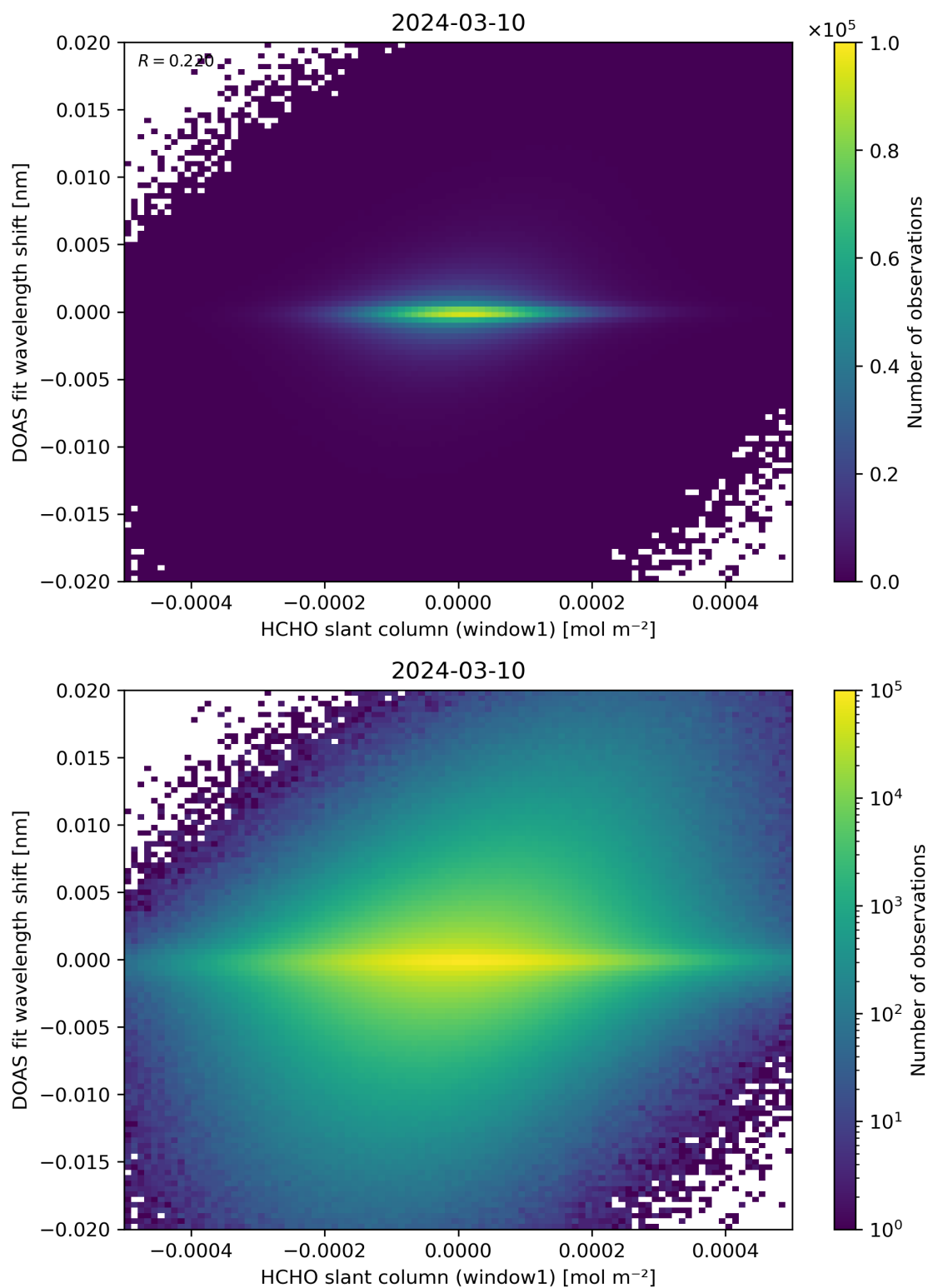
Figure 79: Scatter density plot of “HCHO slant column (window1)” against “DOAS fit wavelength shift” for 2024-03-09 to 2024-03-11.
