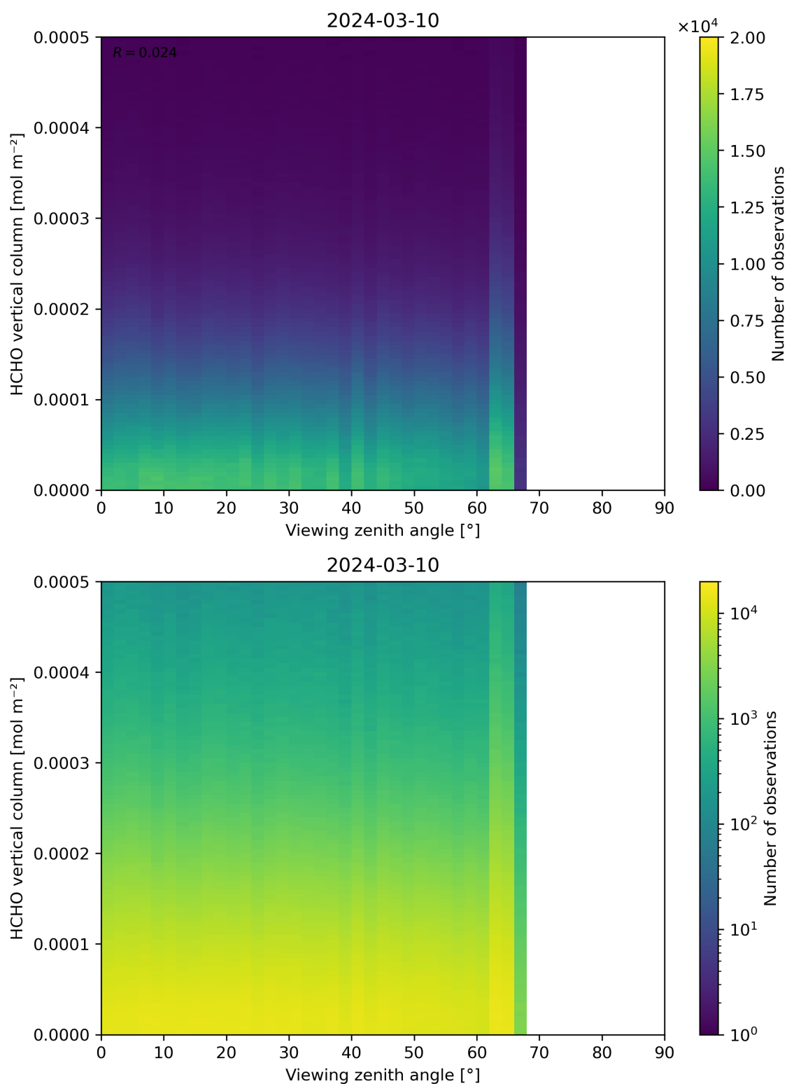
Figure 192: Scatter density plot of “Viewing zenith angle” against “HCHO vertical column” for 2024-03-09 to 2024-03-11.
