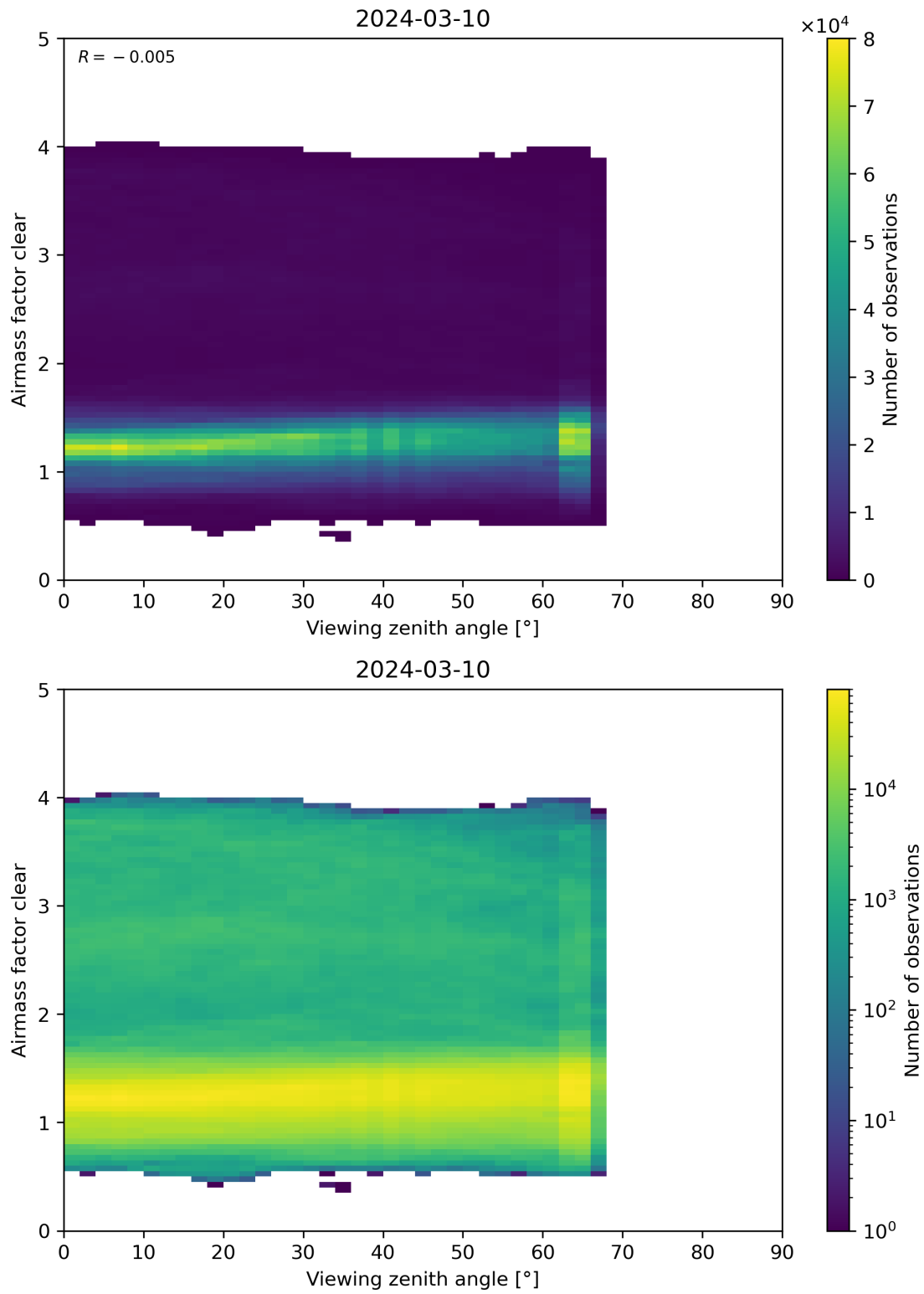
Figure 185: Scatter density plot of “Viewing zenith angle” against “Airmass factor clear” for 2024-03-09 to 2024-03-11.
