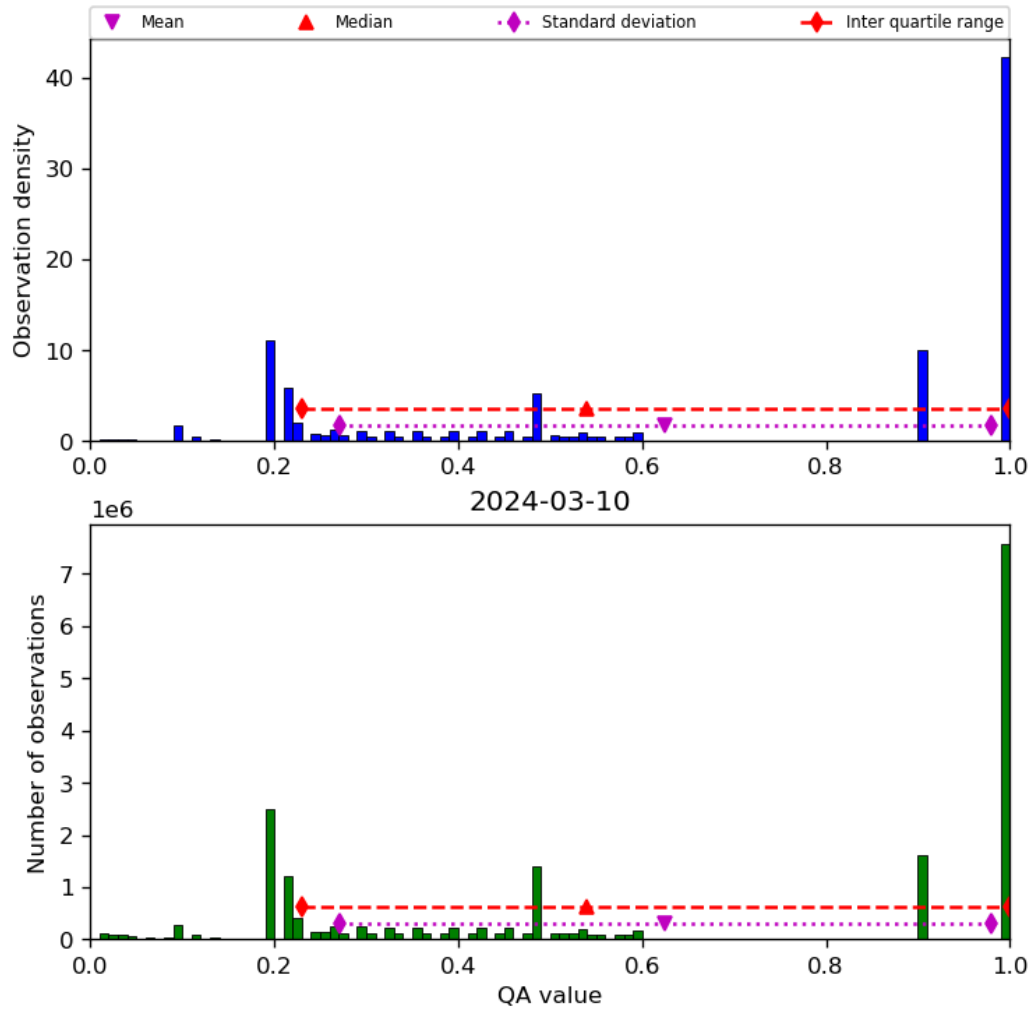
Figure 34: Histogram of “QA value” for 2024-03-09 to 2024-03-11
