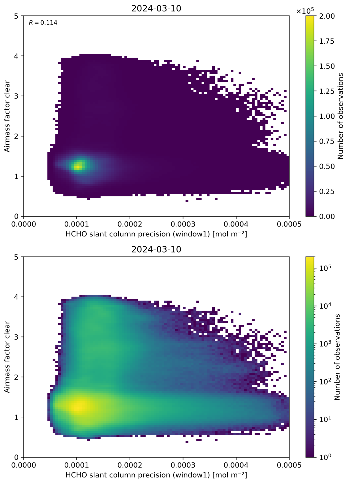
Figure 91: Scatter density plot of “HCHO slant column precision (window1)” against “Airmass factor clear” for 2024-03-09 to 2024-03-11.
