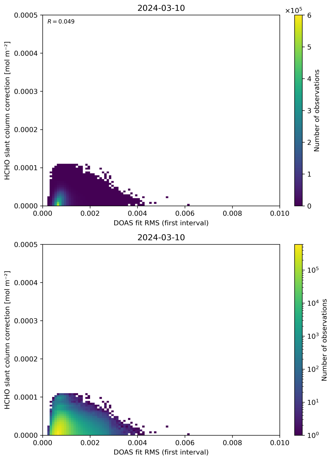
Figure 63: Scatter density plot of “DOAS fit RMS (first interval)” against “HCHO slant column correction” for 2024-03-09 to 2024-03-11.
