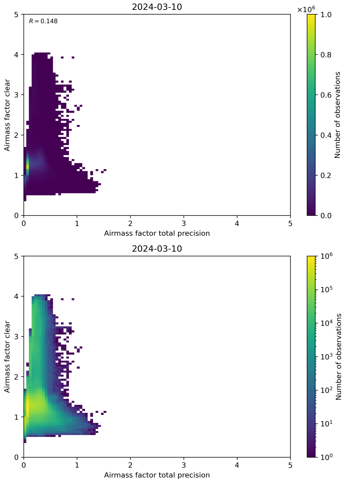
Figure 108: Scatter density plot of “Airmass factor total precision” against “Airmass factor clear” for 2024-03-09 to 2024-03-11.
