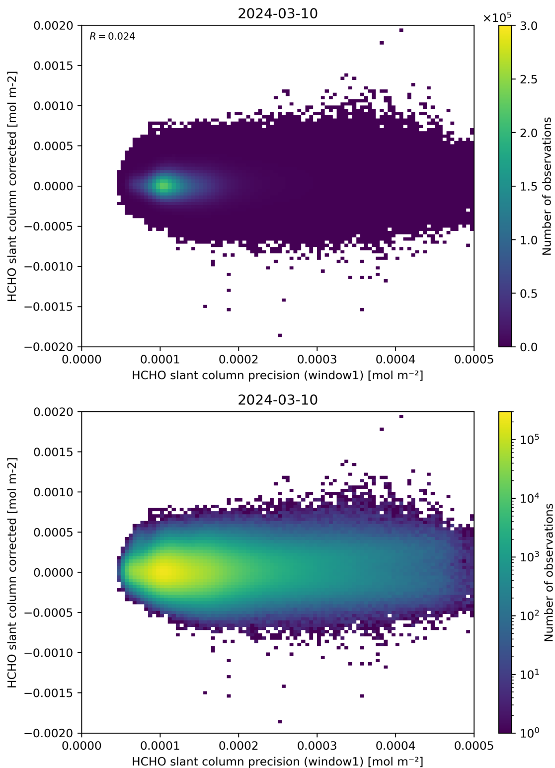
Figure 92: Scatter density plot of “HCHO slant column precision (window1)” against “HCHO slant column corrected” for 2024-03-09 to 2024-03-11.
