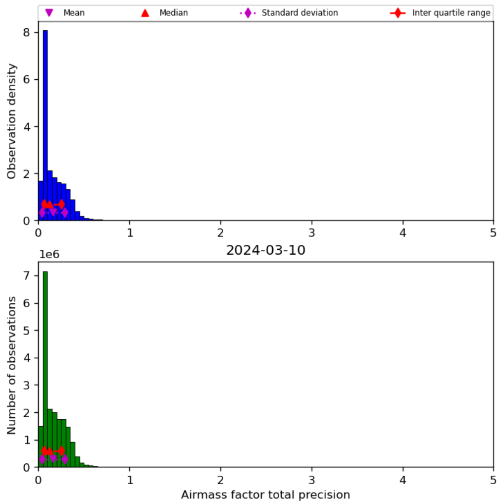
Figure 41: Histogram of “Airmass factor total precision” for 2024-03-09 to 2024-03-11
