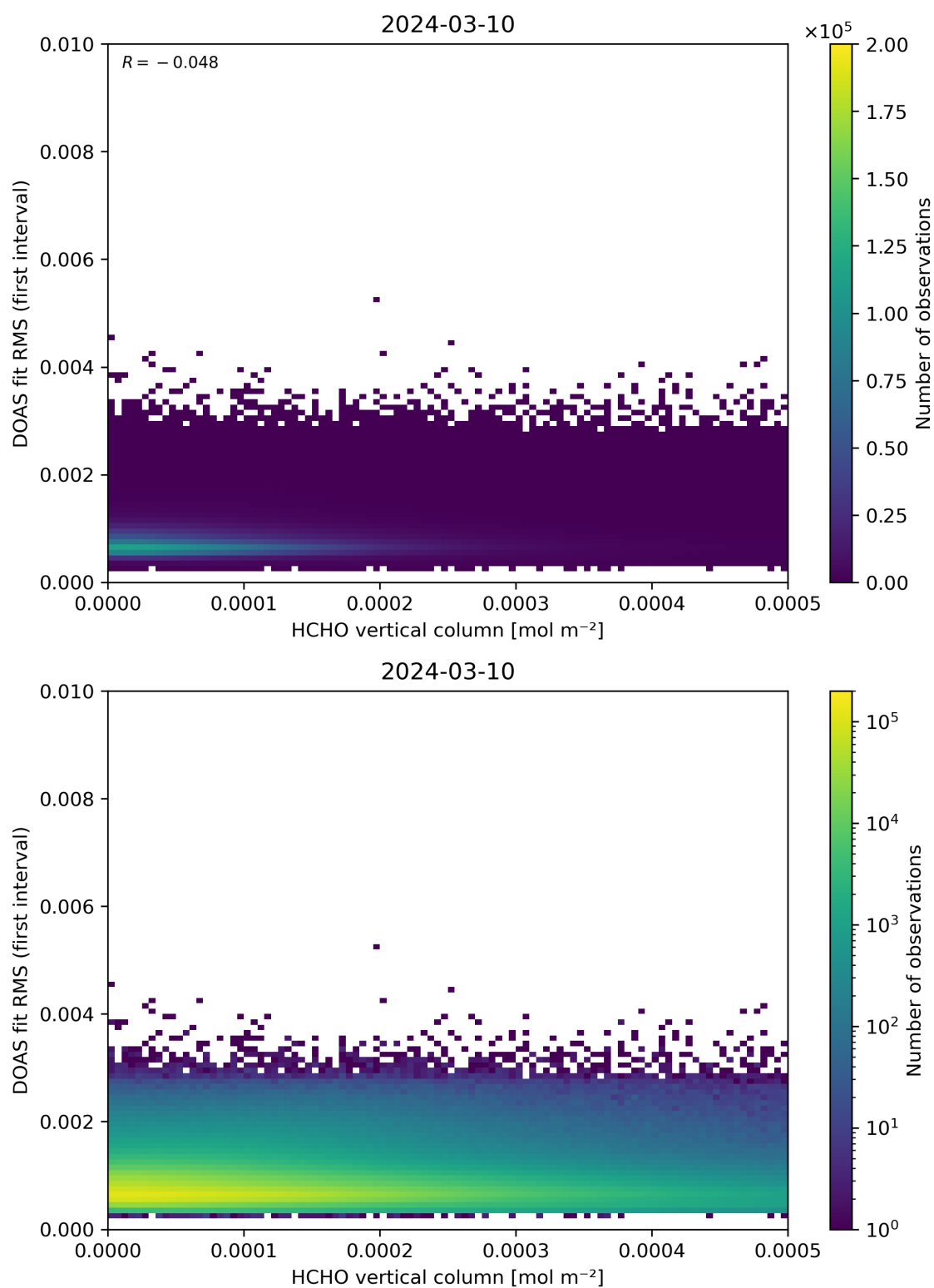
Figure 123: Scatter density plot of “HCHO vertical column” against “DOAS fit RMS (first interval)” for 2024-03-09 to 2024-03-11.
