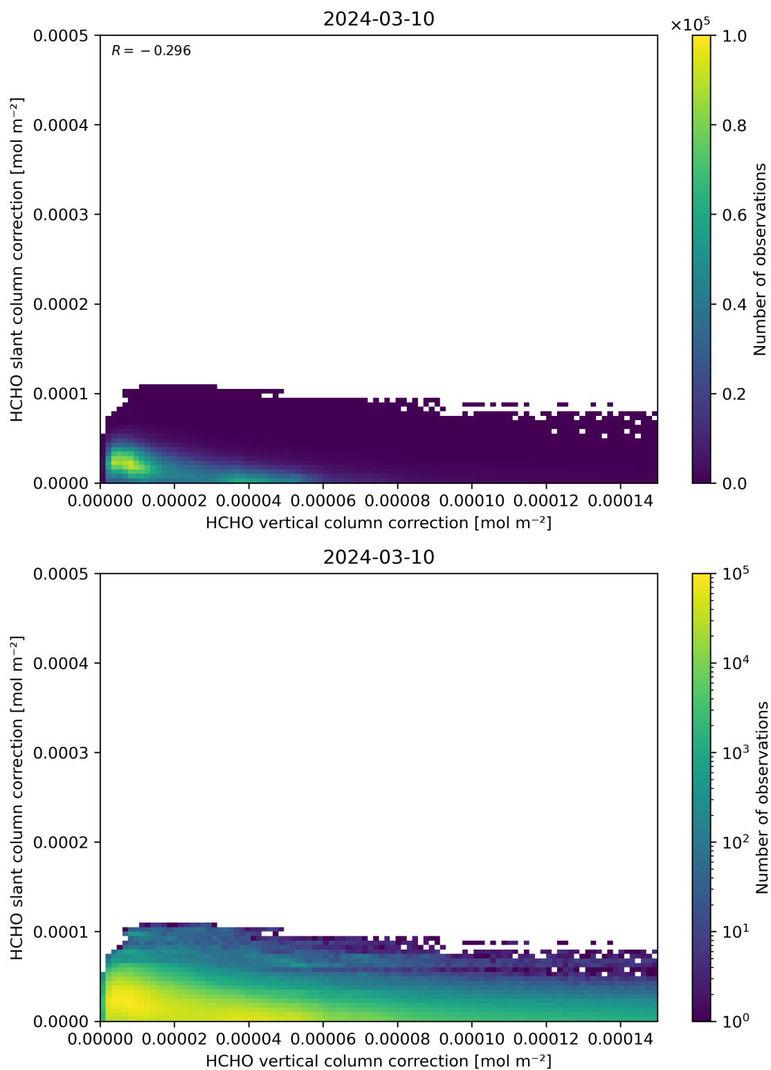
Figure 117: Scatter density plot of “HCHO vertical column correction” against “HCHO slant column correction” for 2024-03-09 to 2024-03-11.
