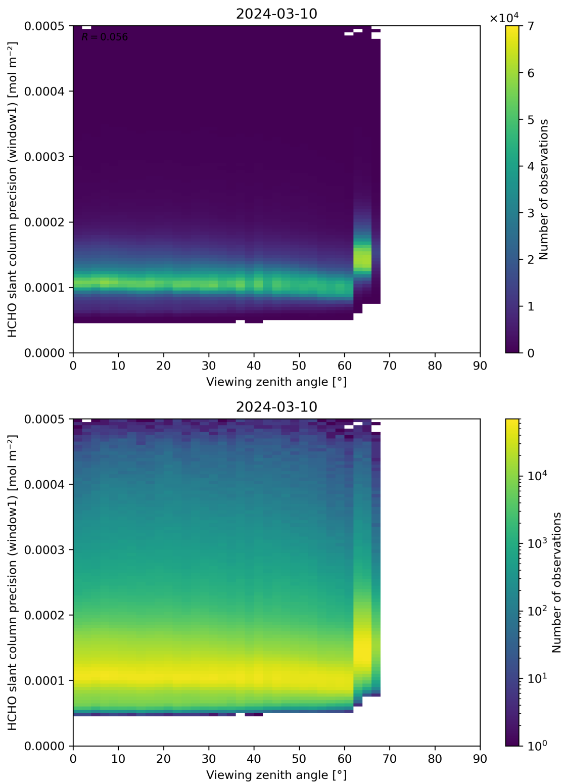
Figure 189: Scatter density plot of “Viewing zenith angle” against “HCHO slant column precision (window1)” for 2024-03-09 to 2024-03-11.
