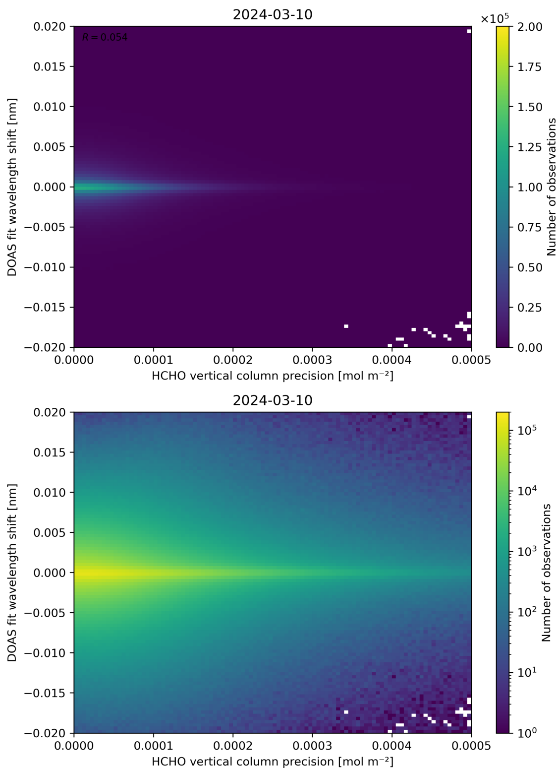
Figure 137: Scatter density plot of “HCHO vertical column precision” against “DOAS fit wavelength shift” for 2024-03-09 to 2024-03-11.
