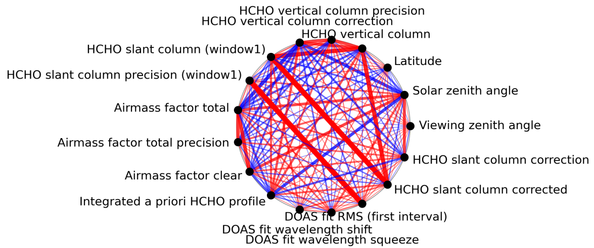
Figure 1: Map of correlation graph for 2024-03-09 to 2024-03-11.
