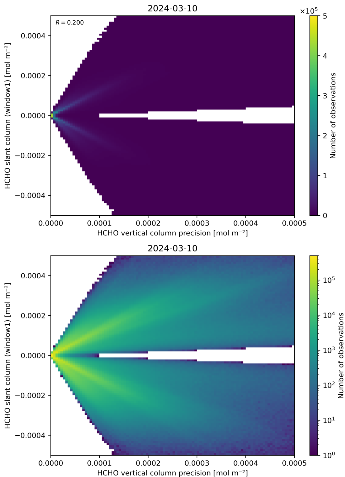
Figure 142: Scatter density plot of “HCHO vertical column precision” against “HCHO slant column (window1)” for 2024-03-09 to 2024-03-11.
