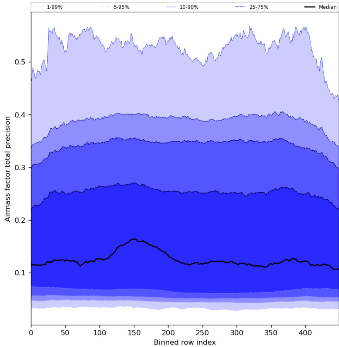
Figure 55: Along track statistics of “Airmass factor total precision” for 2024-03-09 to 2024-03-11
