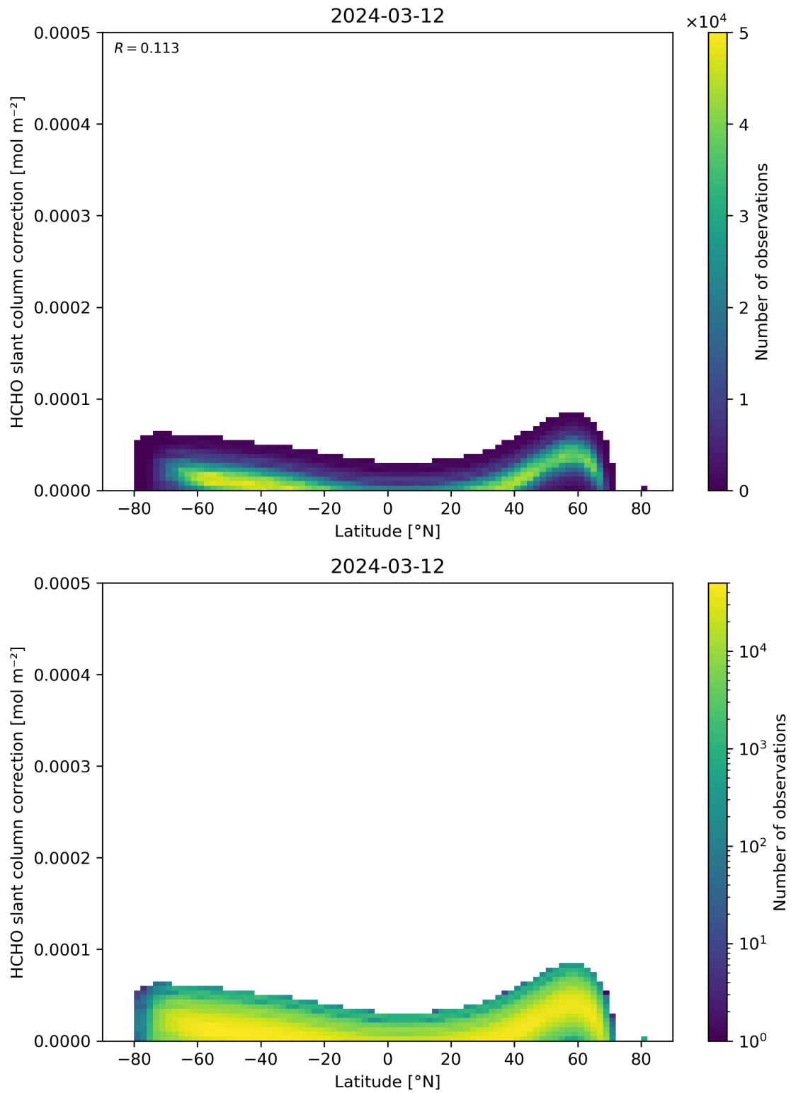
Figure 158: Scatter density plot of “Latitude” against “HCHO slant column correction” for 2024-03-11 to 2024-03-13.
