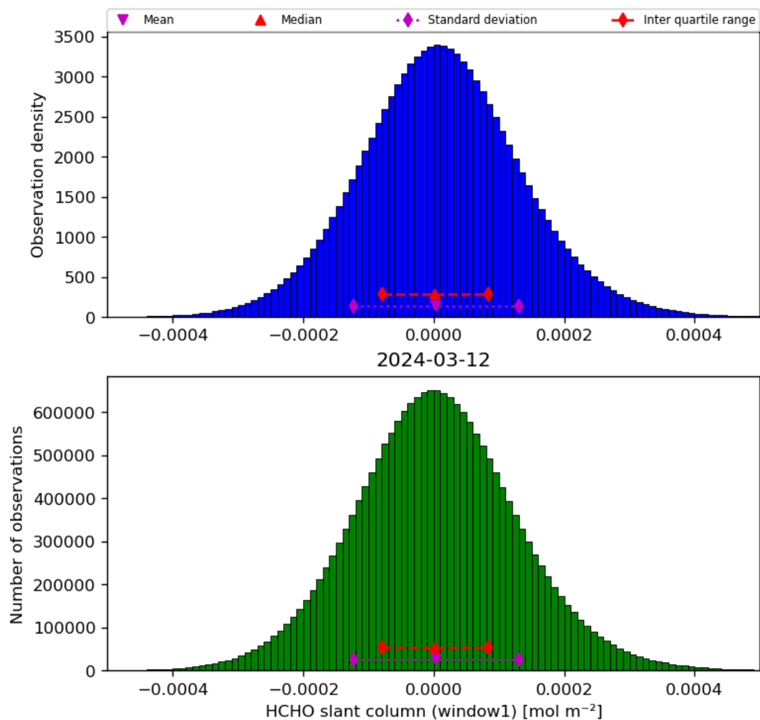
Figure 38: Histogram of “HCHO slant column (window1)” for 2024-03-11 to 2024-03-13
