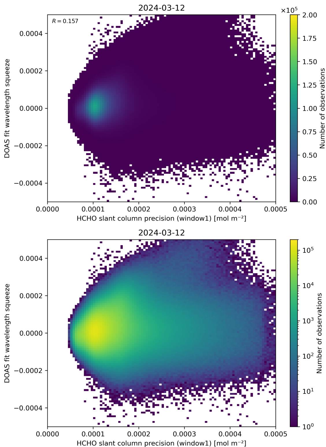
Figure 90: Scatter density plot of “HCHO slant column precision (window1)” against “DOAS fit wavelength squeeze” for 2024-03-11 to 2024-03-13.
