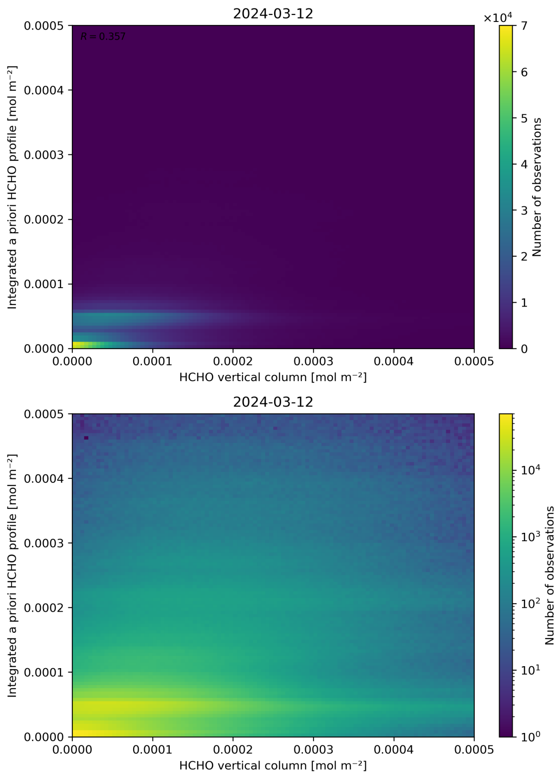
Figure 135: Scatter density plot of “HCHO vertical column” against “Integrated a priori HCHO profile” for 2024-03-11 to 2024-03-13.
