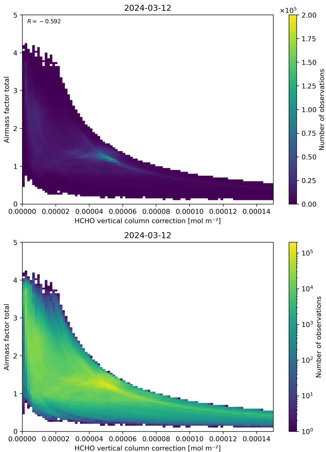
Figure 120: Scatter density plot of “HCHO vertical column correction” against “Airmass factor total” for 2024-03-11 to 2024-03-13.
