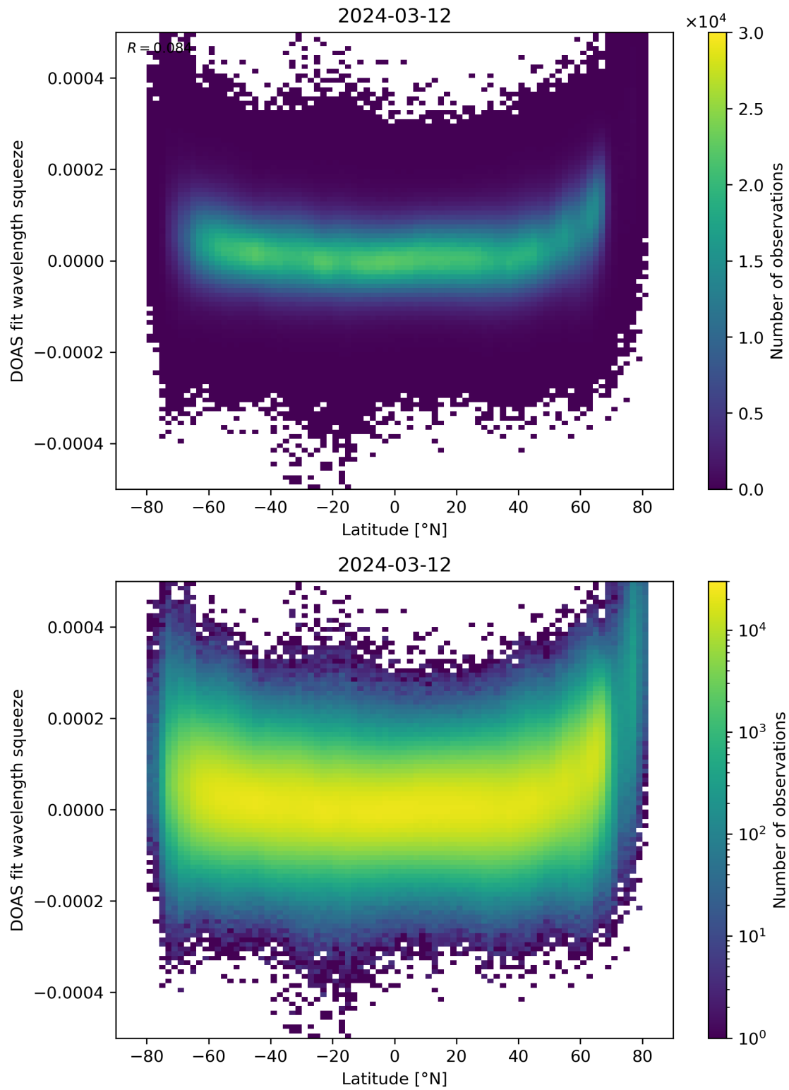
Figure 155: Scatter density plot of “Latitude” against “DOAS fit wavelength squeeze” for 2024-03-11 to 2024-03-13.
