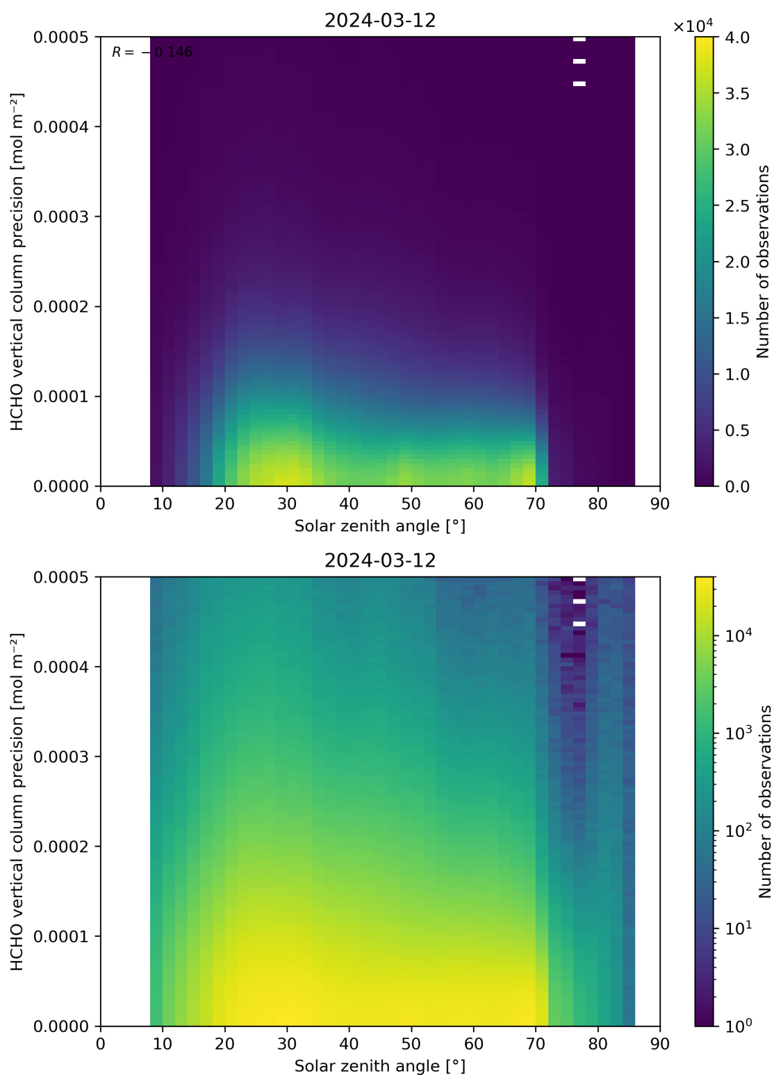
Figure 179: Scatter density plot of “Solar zenith angle” against “HCHO vertical column precision” for 2024-03-11 to 2024-03-13.
