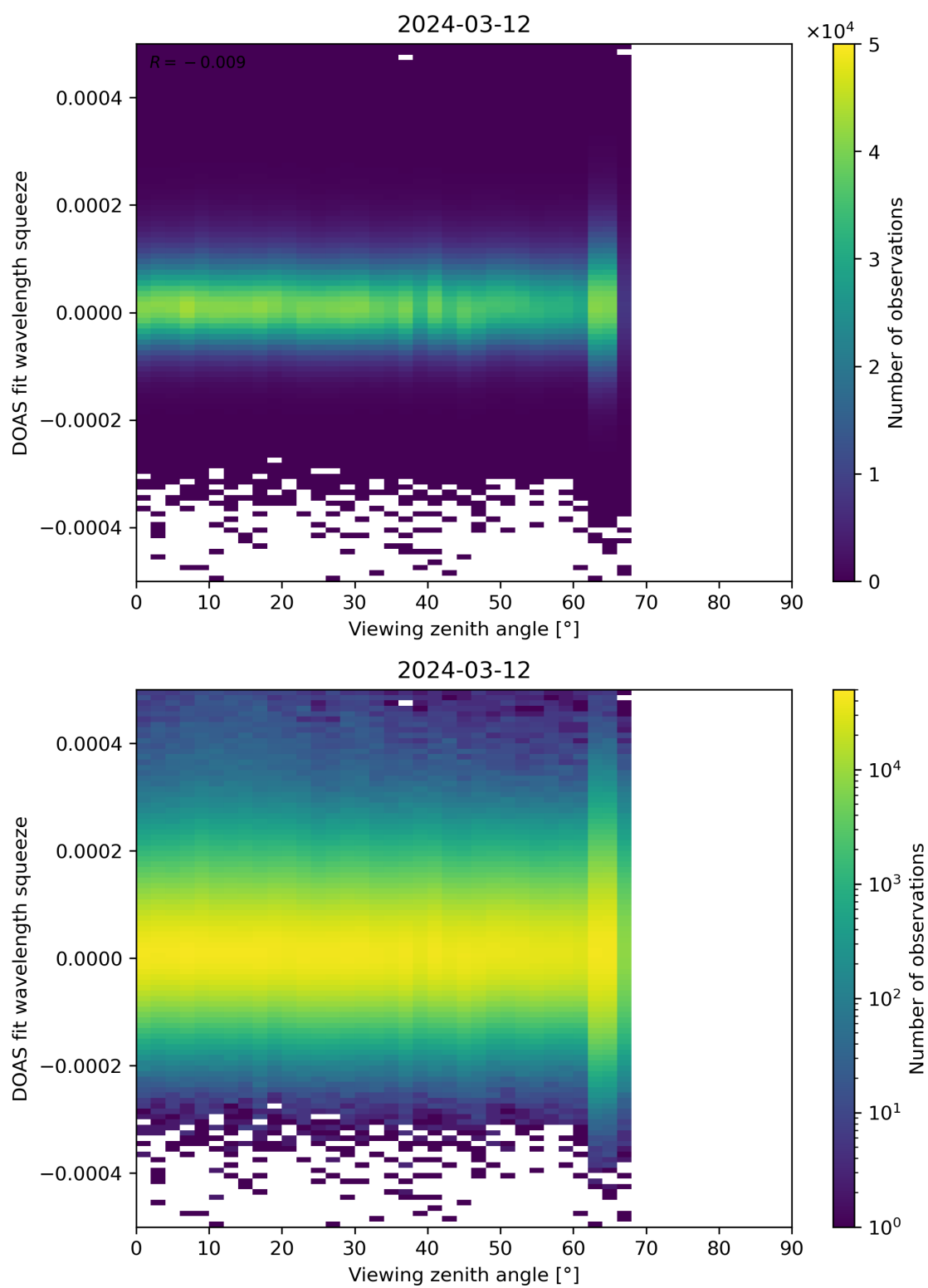
Figure 184: Scatter density plot of “Viewing zenith angle” against “DOAS fit wavelength squeeze” for 2024-03-11 to 2024-03-13.
