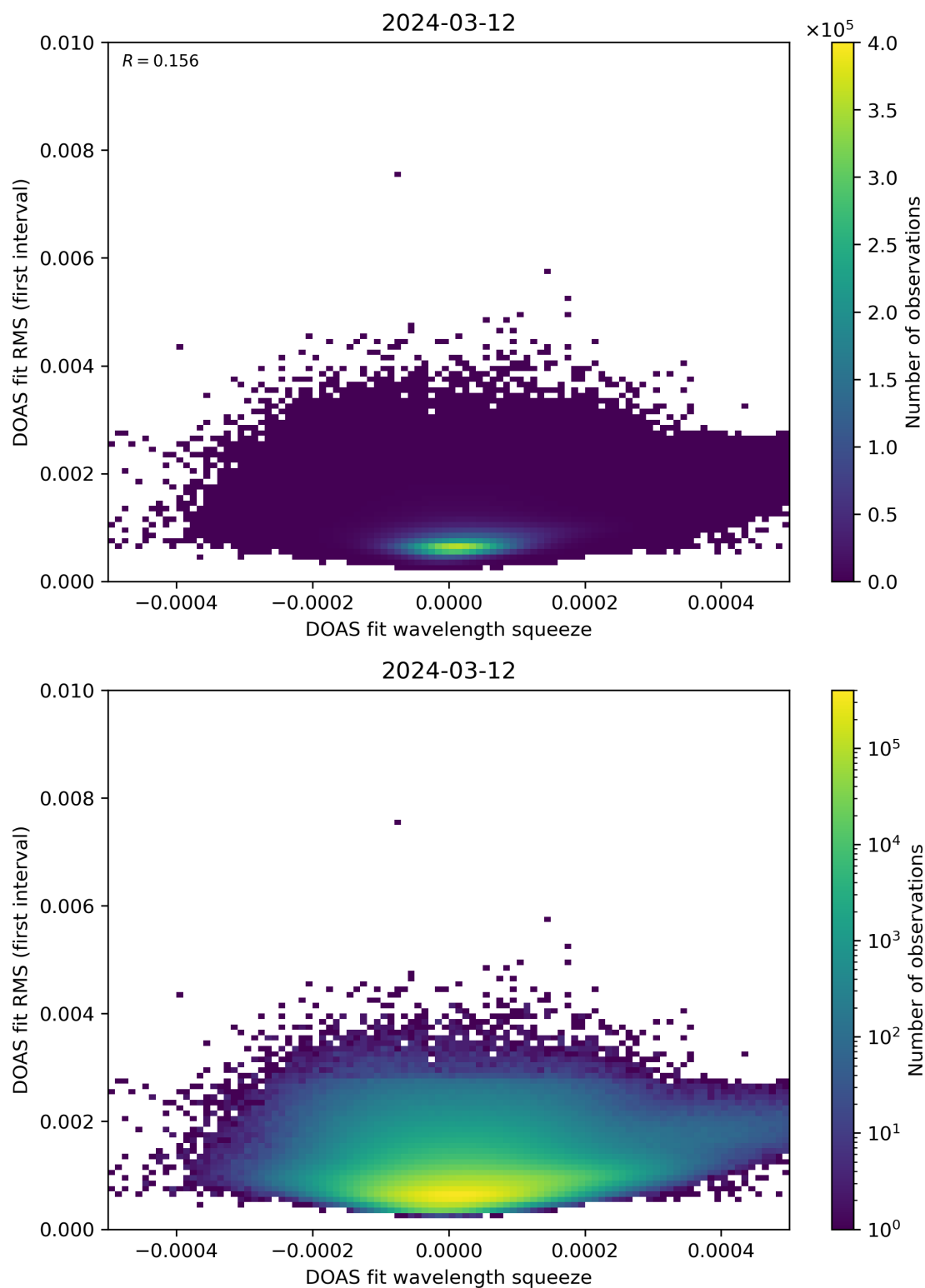
Figure 68: Scatter density plot of “DOAS fit wavelength squeeze” against “DOAS fit RMS (first interval)” for 2024-03-11 to 2024-03-13.
