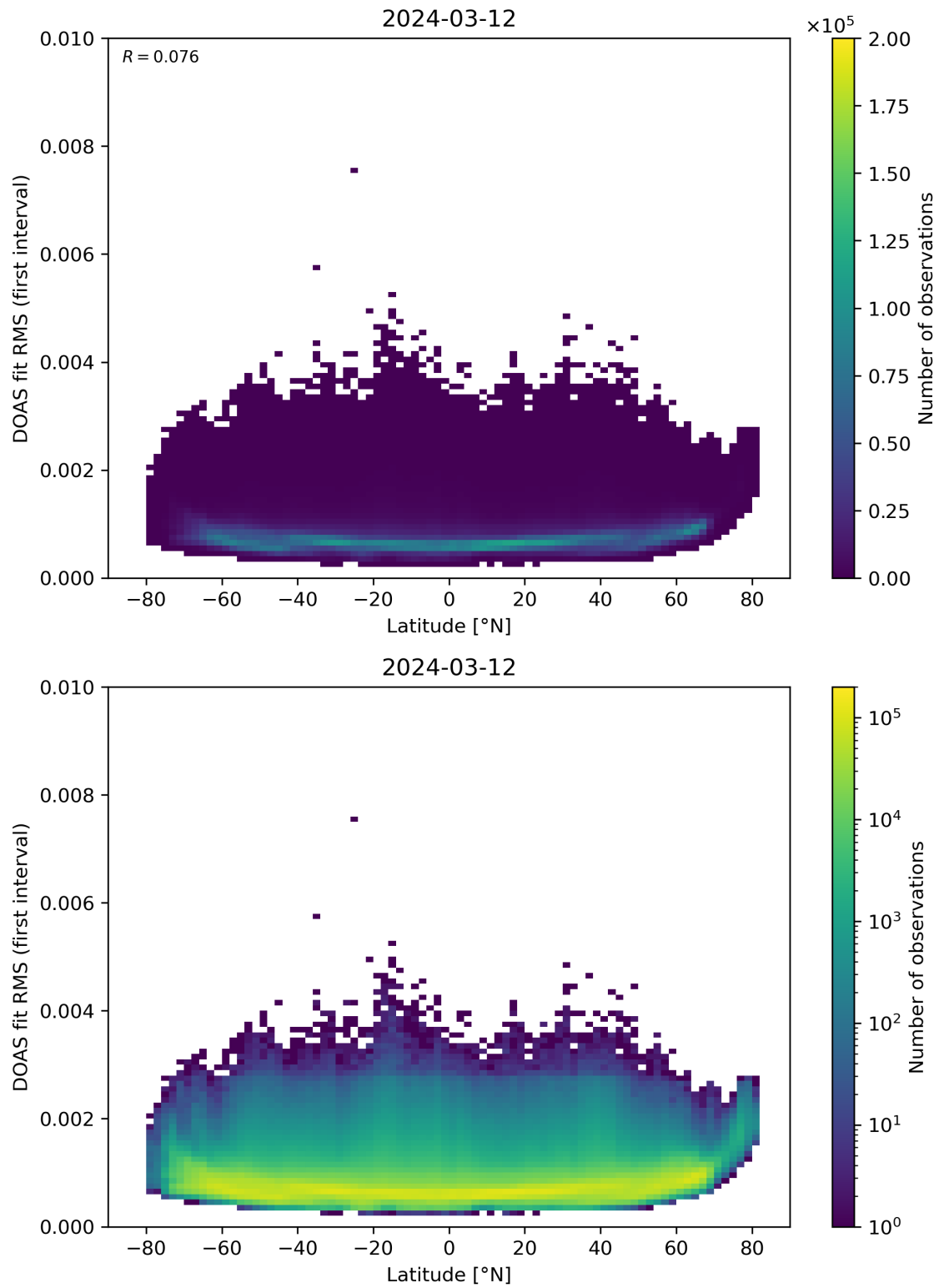
Figure 153: Scatter density plot of “Latitude” against “DOAS fit RMS (first interval)” for 2024-03-11 to 2024-03-13.
