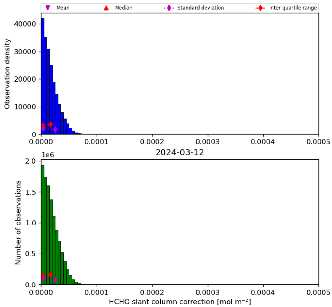
Figure 47: Histogram of “HCHO slant column correction” for 2024-03-11 to 2024-03-13
