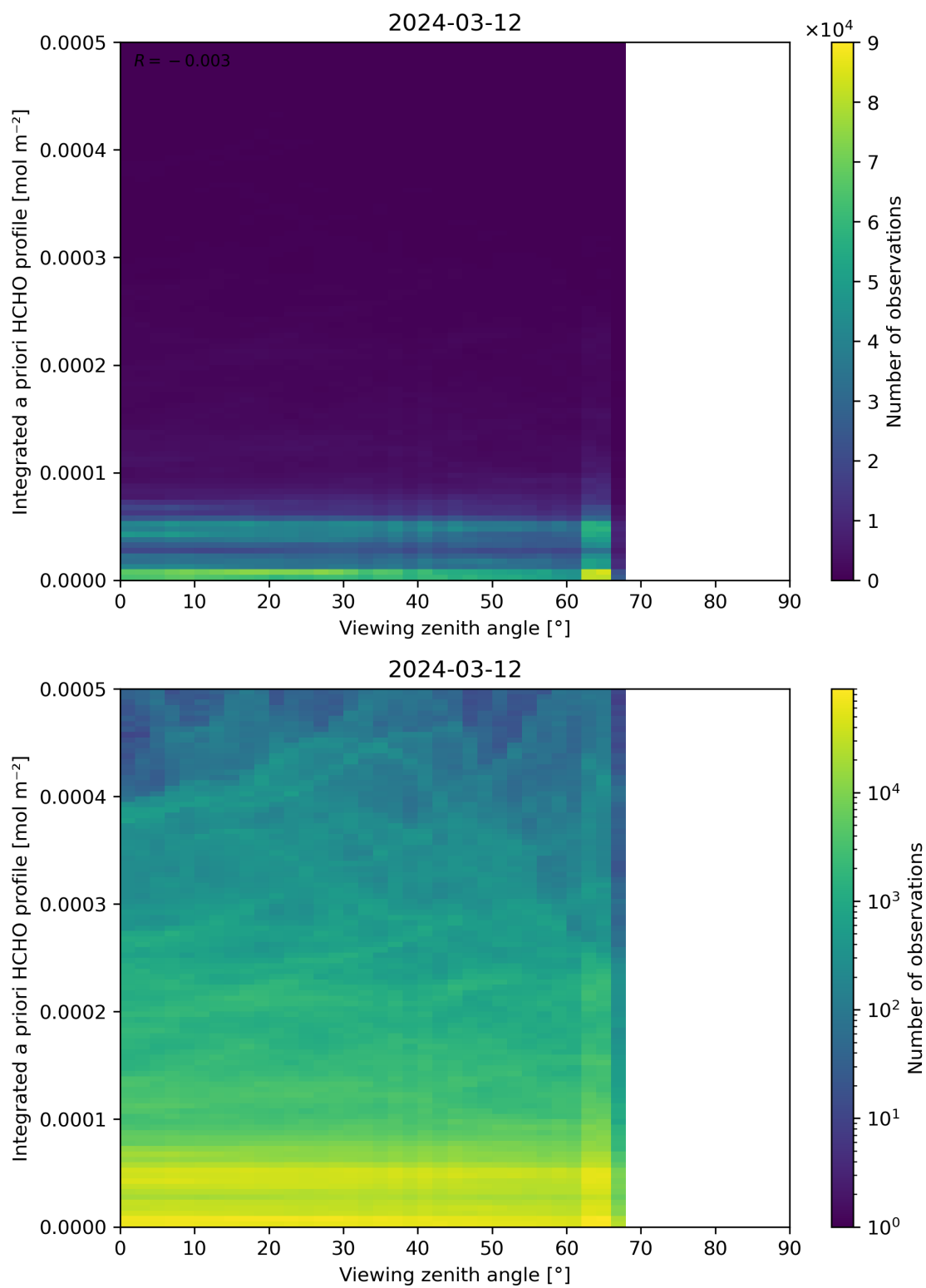
Figure 195: Scatter density plot of “Viewing zenith angle” against “Integrated a priori HCHO profile” for 2024-03-11 to 2024-03-13.
