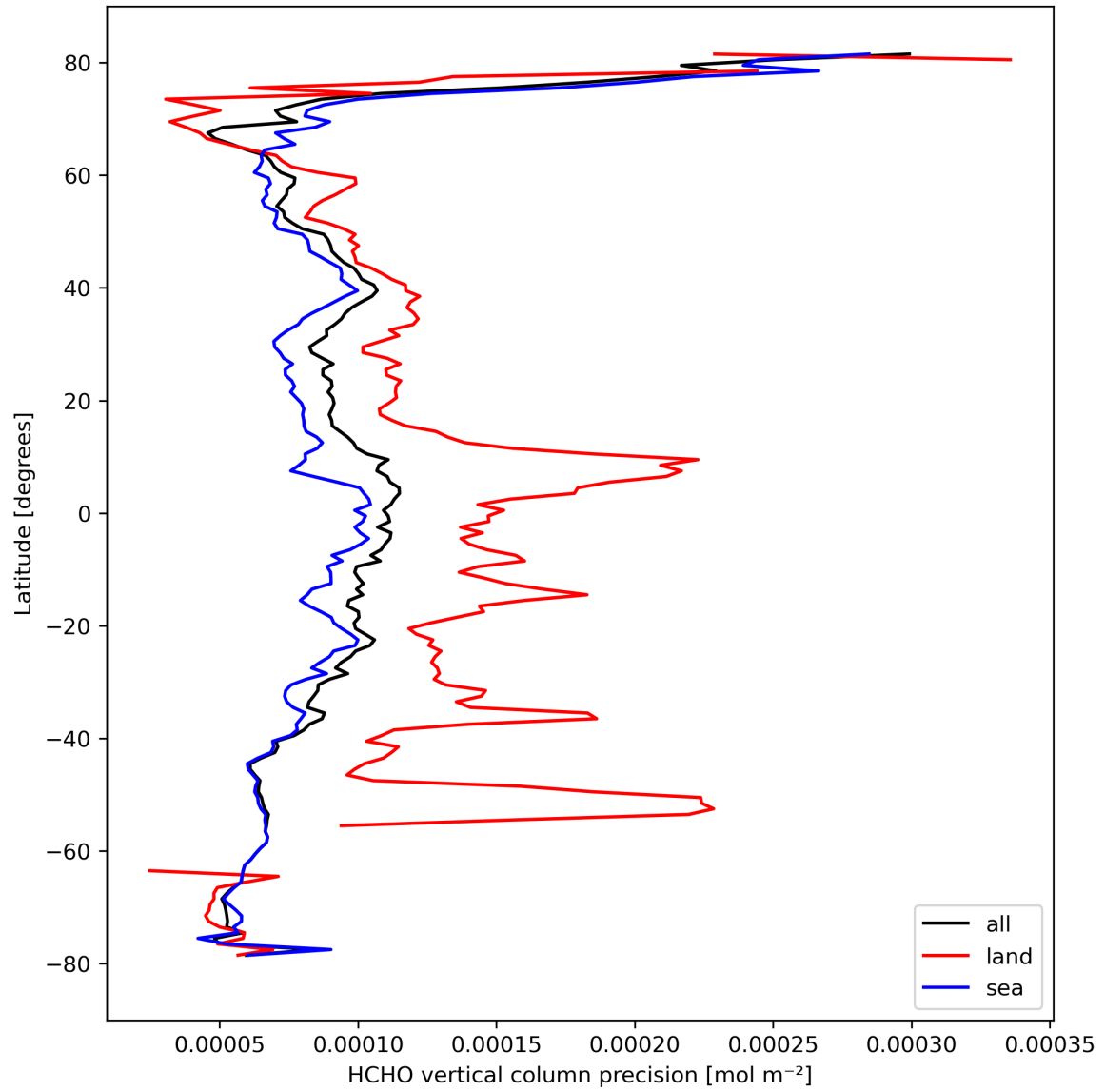
Figure 22: Zonal average of "HCHO vertical column precision" for 2024-03-11 to 2024-03-13.
