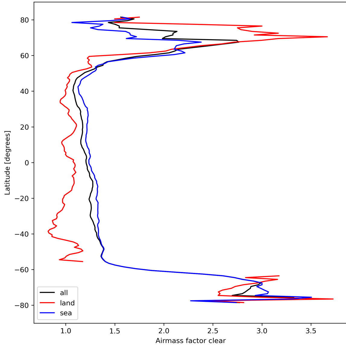
Figure 28: Zonal average of “Airmass factor clear” for 2024-03-11 to 2024-03-13.
