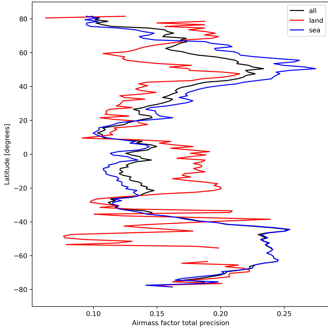
Figure 27: Zonal average of “Airmass factor total precision” for 2024-03-11 to 2024-03-13.
