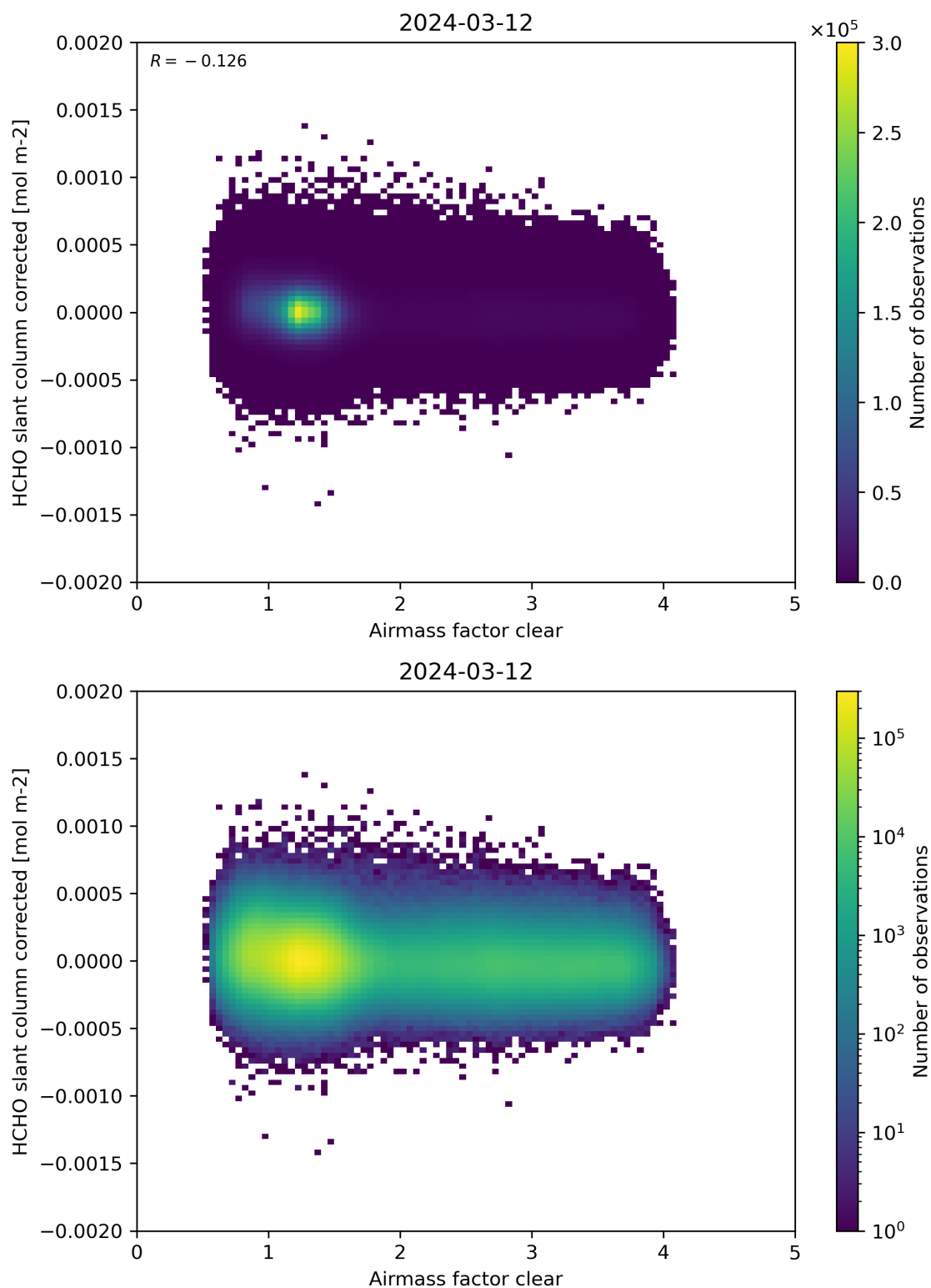
Figure 74: Scatter density plot of “Airmass factor clear” against “HCHO slant column corrected” for 2024-03-11 to 2024-03-13.
