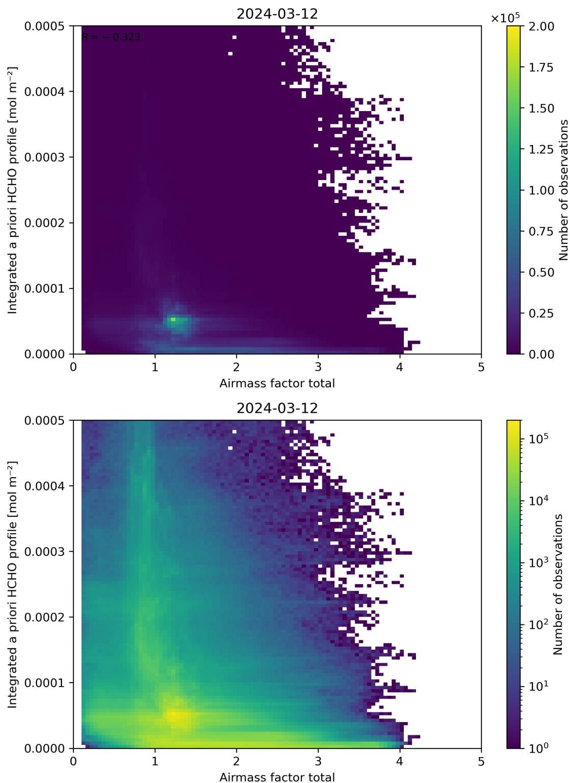
Figure 104: Scatter density plot of “Airmass factor total” against “Integrated a priori HCHO profile” for 2024-03-11 to 2024-03-13.
