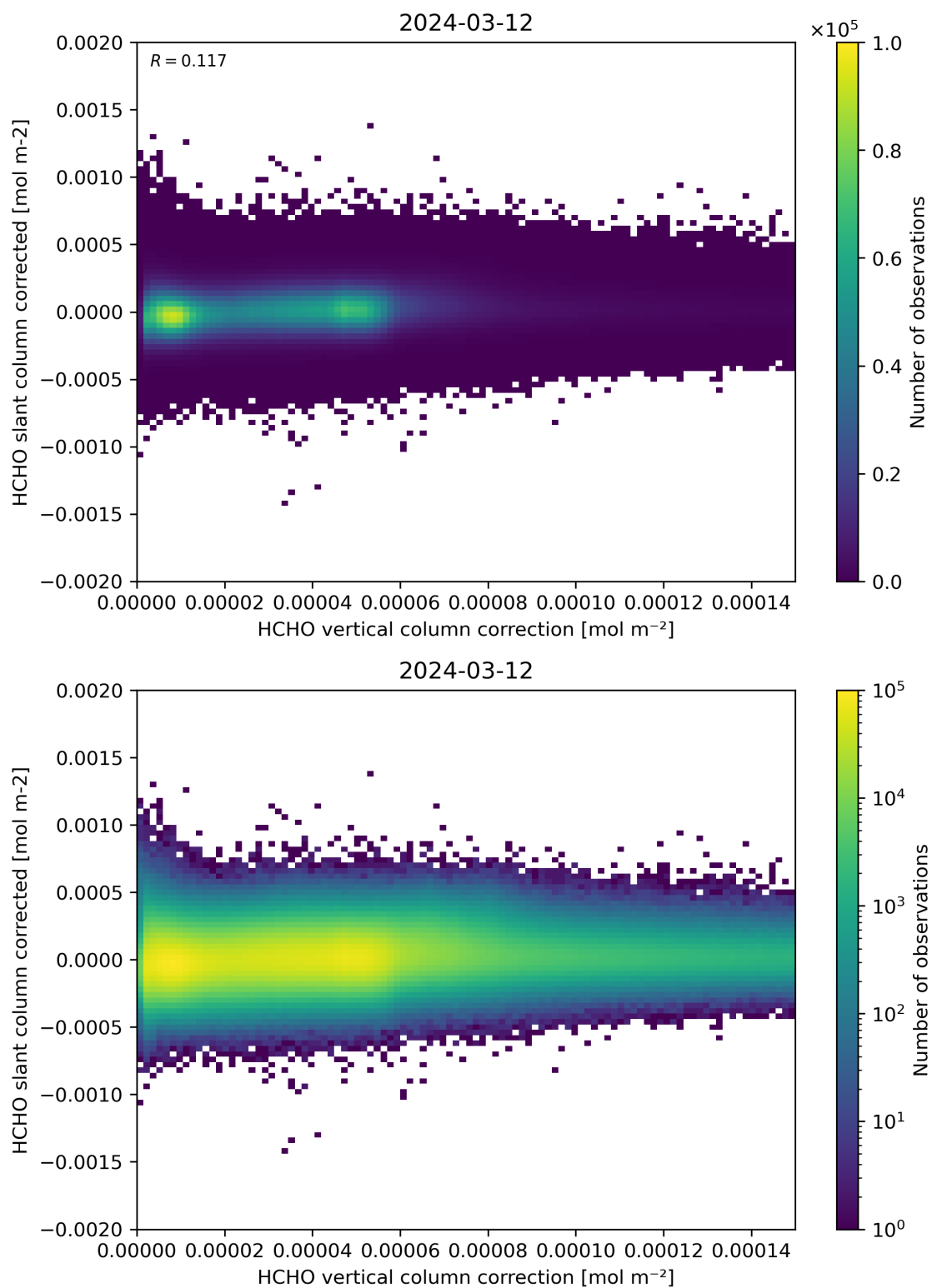
Figure 116: Scatter density plot of “HCHO vertical column correction” against “HCHO slant column corrected” for 2024-03-11 to 2024-03-13.
