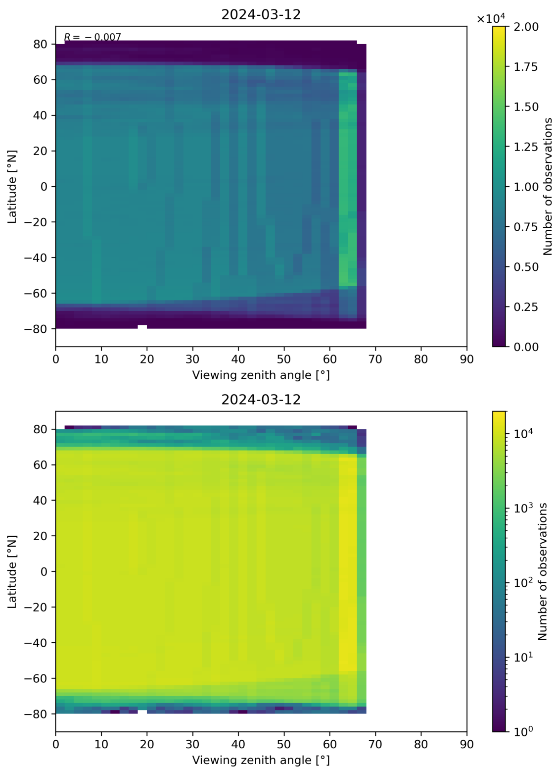
Figure 196: Scatter density plot of “Viewing zenith angle” against “Latitude” for 2024-03-11 to 2024-03-13.
