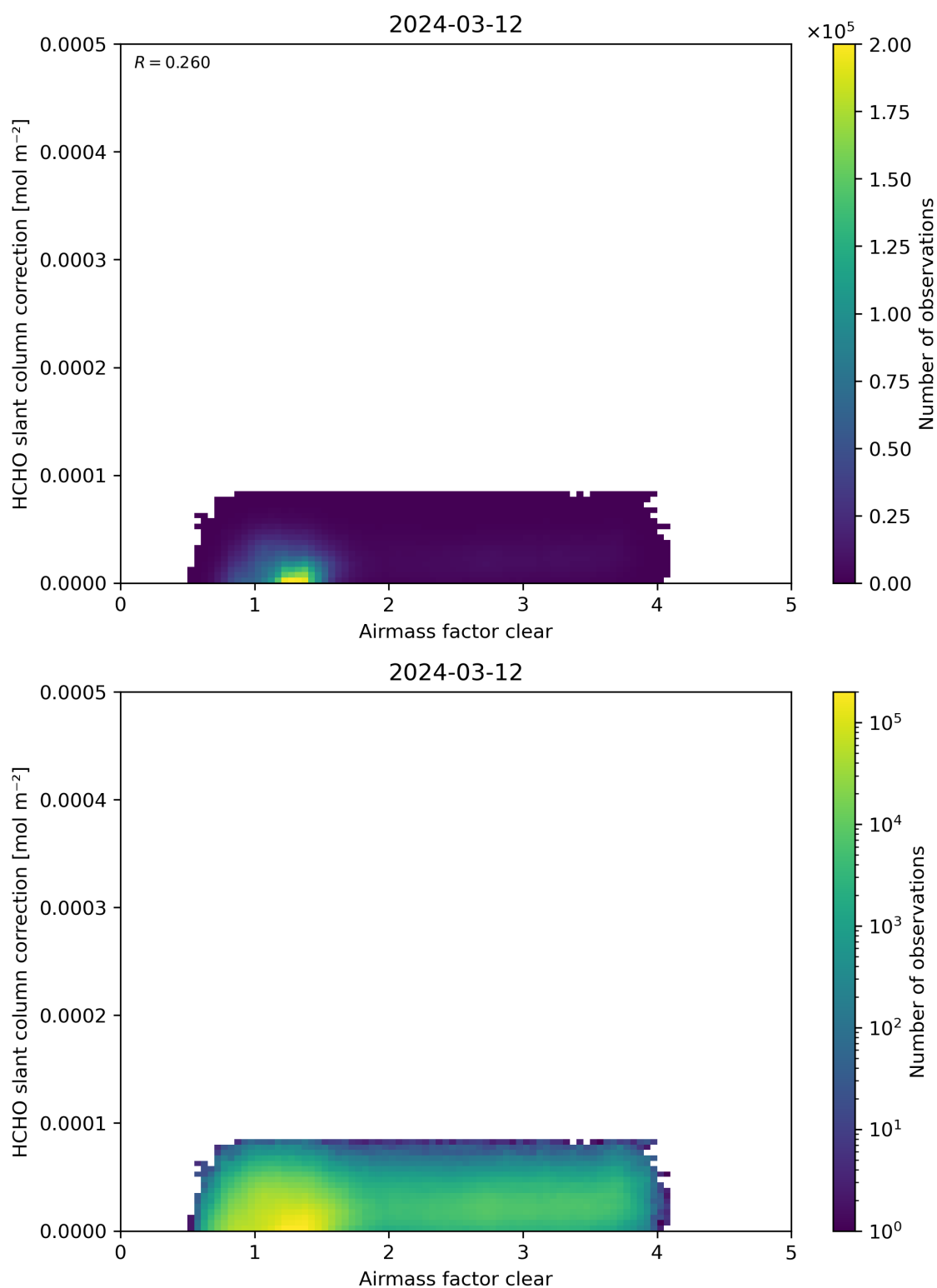
Figure 75: Scatter density plot of “Airmass factor clear” against “HCHO slant column correction” for 2024-03-11 to 2024-03-13.
