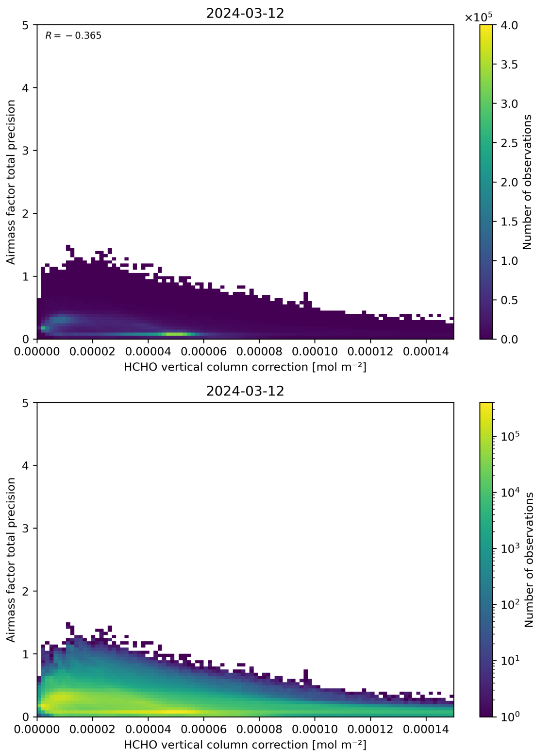
Figure 121: Scatter density plot of “HCHO vertical column correction” against “Airmass factor total precision” for 2024-03-11 to 2024-03-13.
