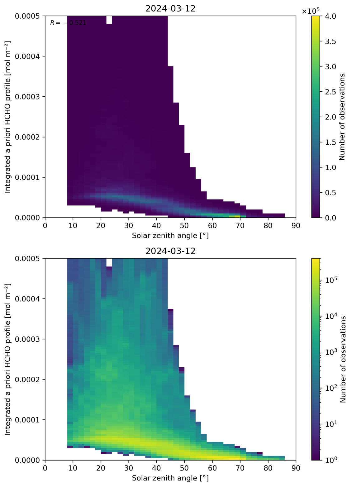
Figure 180: Scatter density plot of “Solar zenith angle” against “Integrated a priori HCHO profile” for 2024-03-11 to 2024-03-13.
