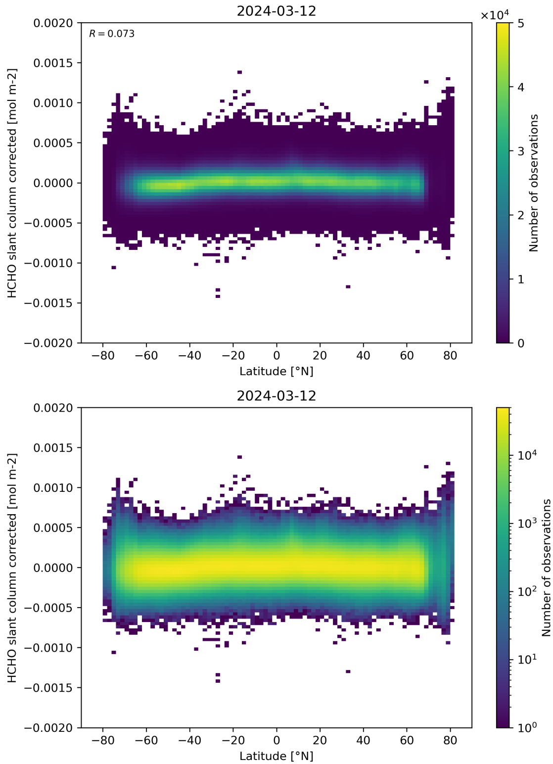
Figure 157: Scatter density plot of “Latitude” against “HCHO slant column corrected” for 2024-03-11 to 2024-03-13.
