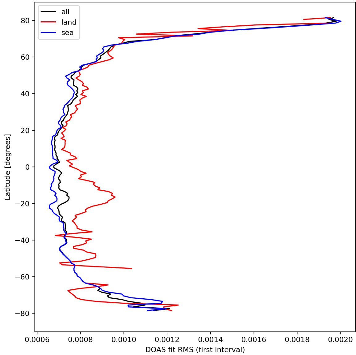
Figure 32: Zonal average of “DOAS fit RMS (first interval)” for 2024-03-11 to 2024-03-13.
