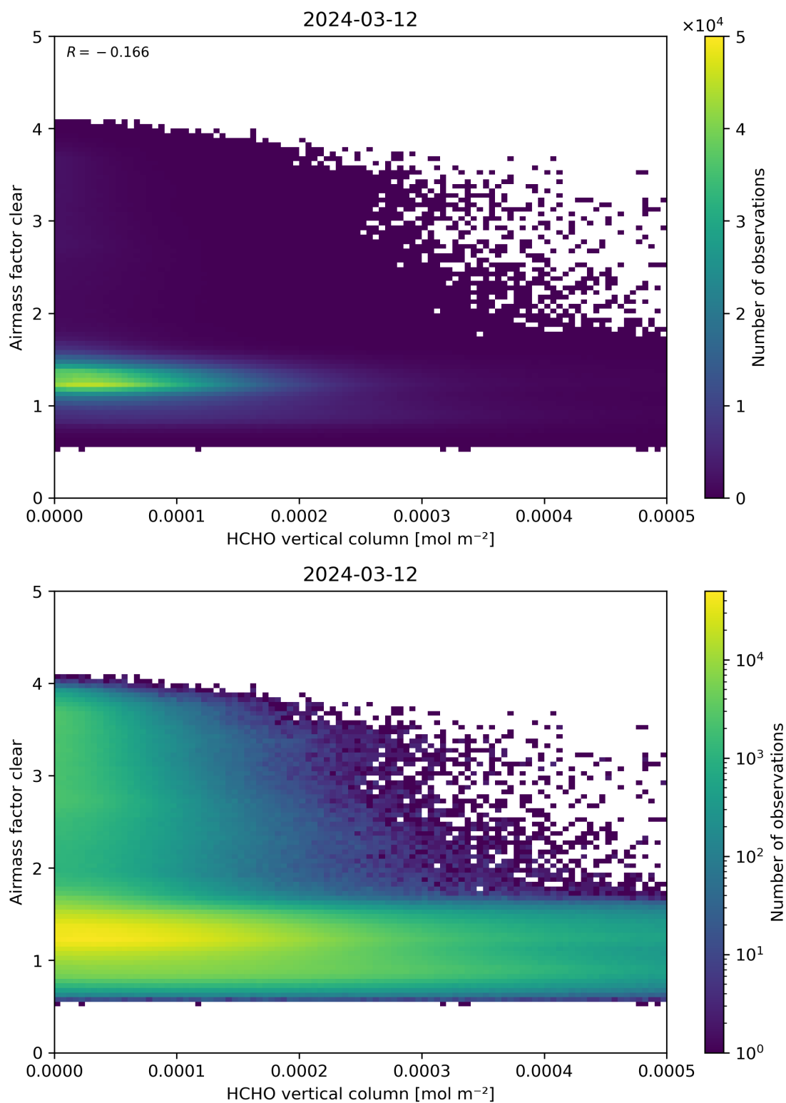
Figure 126: Scatter density plot of “HCHO vertical column” against “Airmass factor clear” for 2024-03-11 to 2024-03-13.
