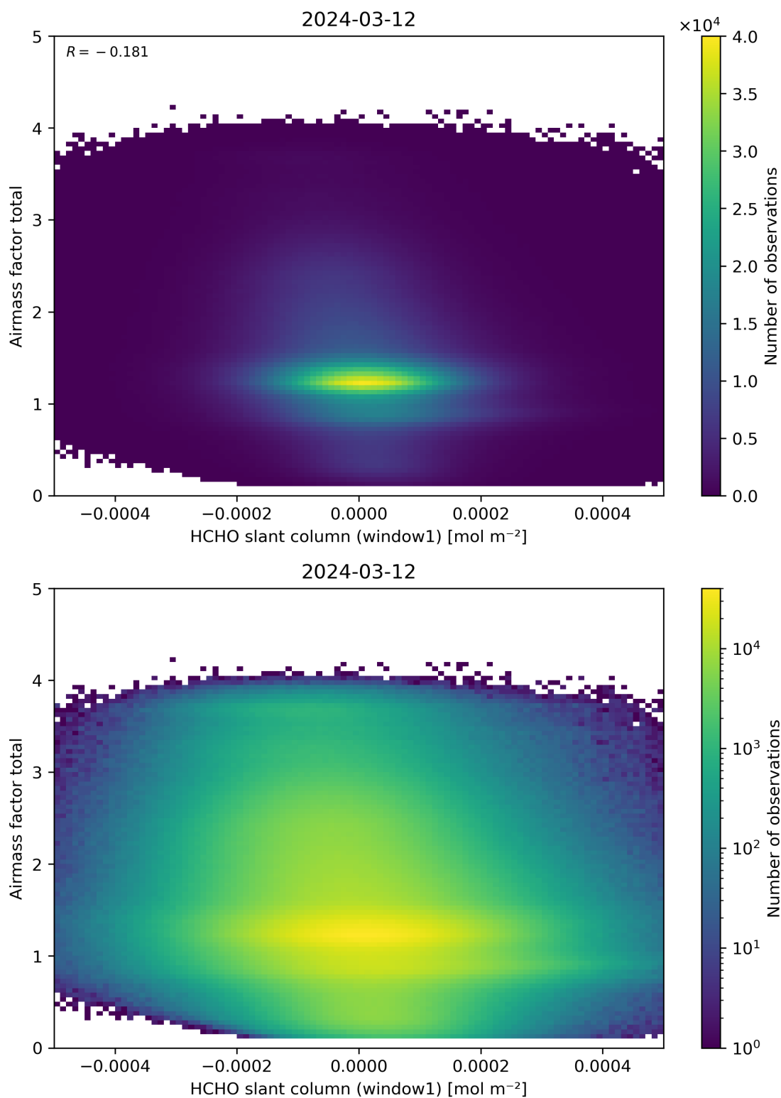
Figure 85: Scatter density plot of “HCHO slant column (window1)” against “Airmass factor total” for 2024-03-11 to 2024-03-13.
