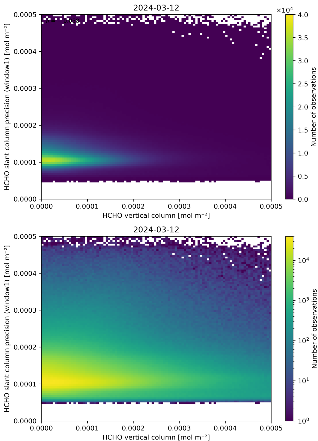
Figure 130: Scatter density plot of “HCHO vertical column” against “HCHO slant column precision (window1)” for 2024-03-11 to 2024-03-13.
