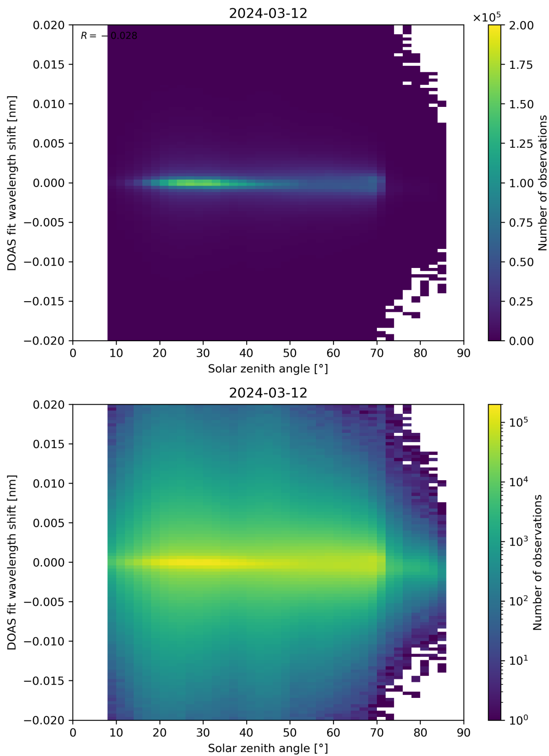
Figure 168: Scatter density plot of “Solar zenith angle” against “DOAS fit wavelength shift” for 2024-03-11 to 2024-03-13.
