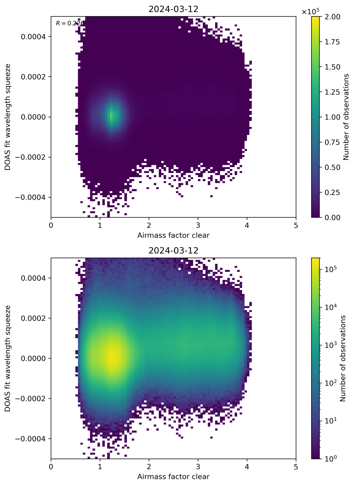
Figure 73: Scatter density plot of “Airmass factor clear” against “DOAS fit wavelength squeeze” for 2024-03-11 to 2024-03-13.
