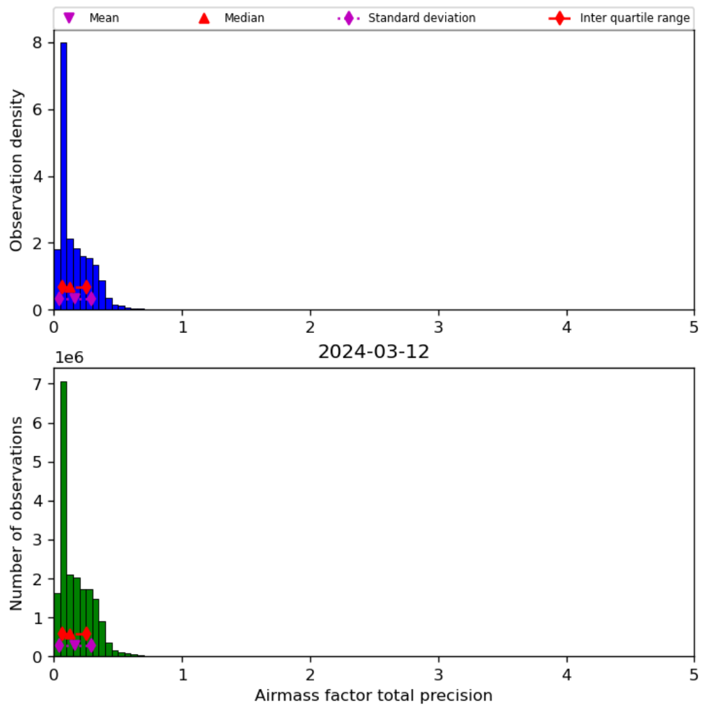
Figure 41: Histogram of “Airmass factor total precision” for 2024-03-11 to 2024-03-13
