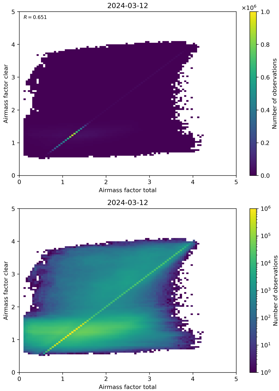
Figure 100: Scatter density plot of “Airmass factor total” against “Airmass factor clear” for 2024-03-11 to 2024-03-13.
