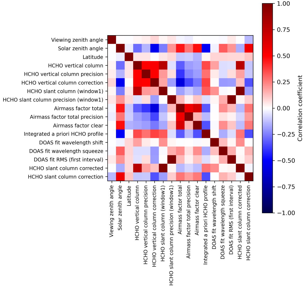
Figure 2: Map of correlation matrix for 2024-03-11 to 2024-03-13.
