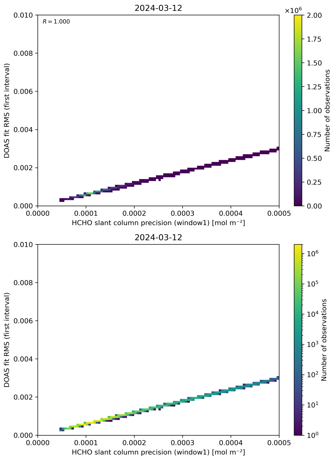
Figure 88: Scatter density plot of “HCHO slant column precision (window1)” against “DOAS fit RMS (first interval)” for 2024-03-11 to 2024-03-13.
