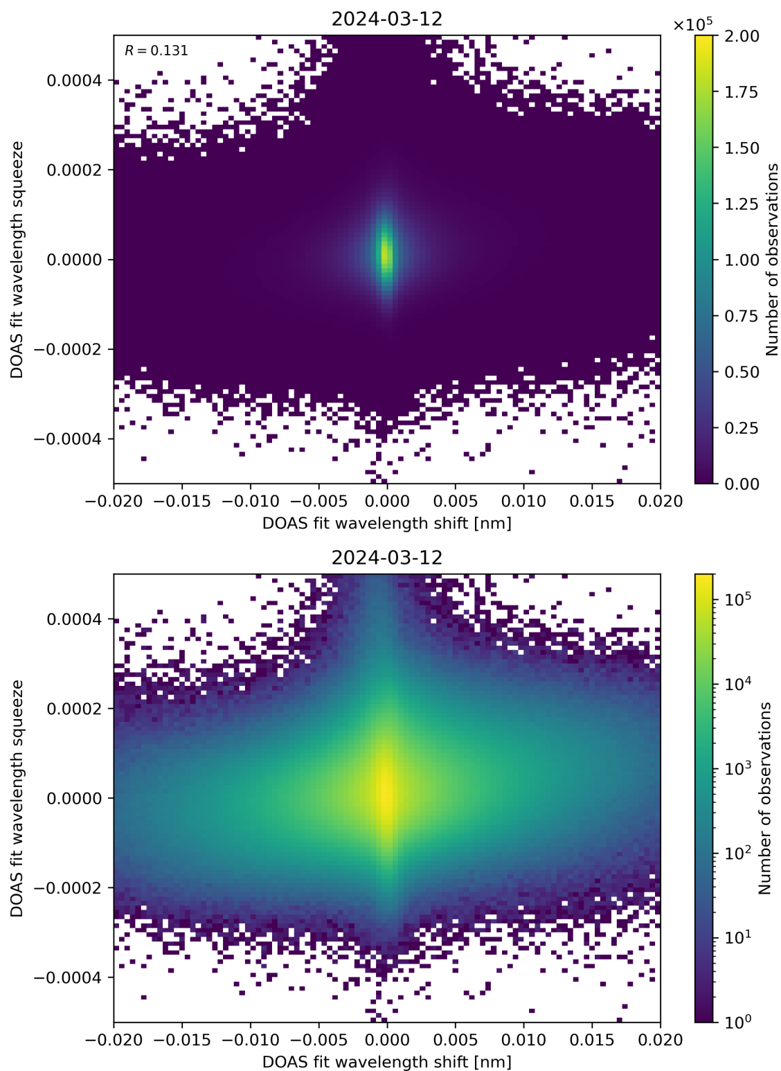
Figure 65: Scatter density plot of “DOAS fit wavelength shift” against “DOAS fit wavelength squeeze” for 2024-03-11 to 2024-03-13.
