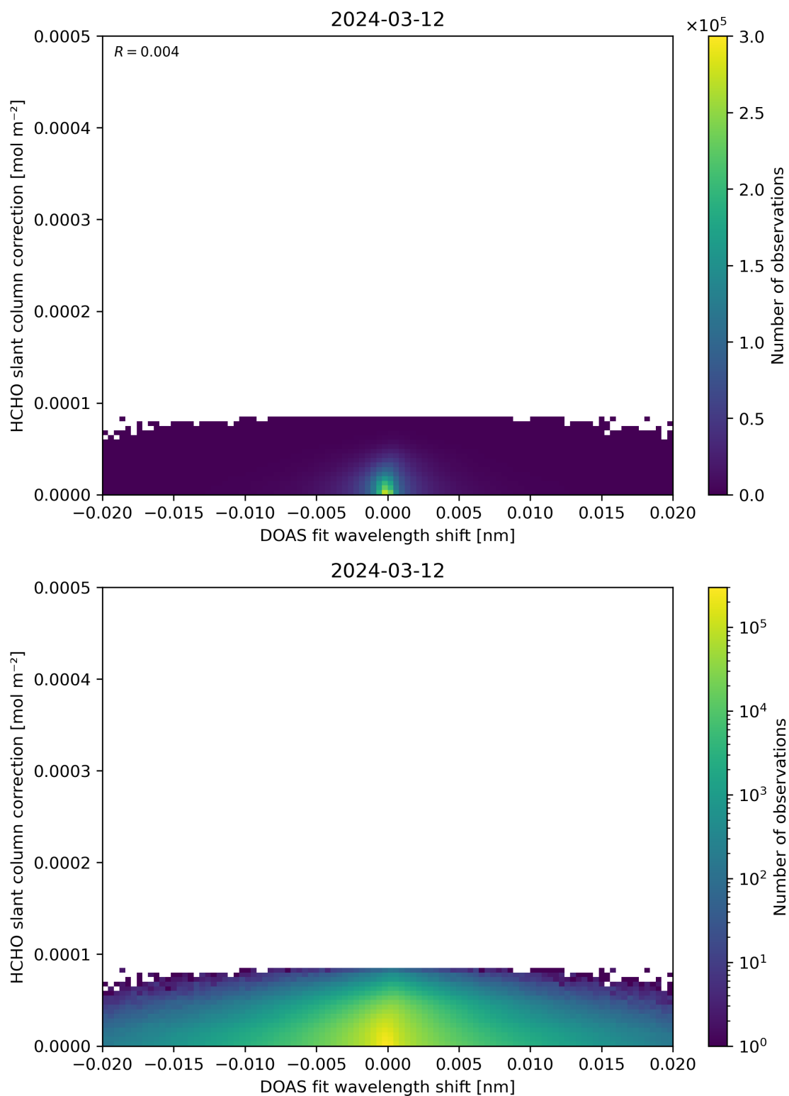
Figure 67: Scatter density plot of “DOAS fit wavelength shift” against “HCHO slant column correction” for 2024-03-11 to 2024-03-13.
