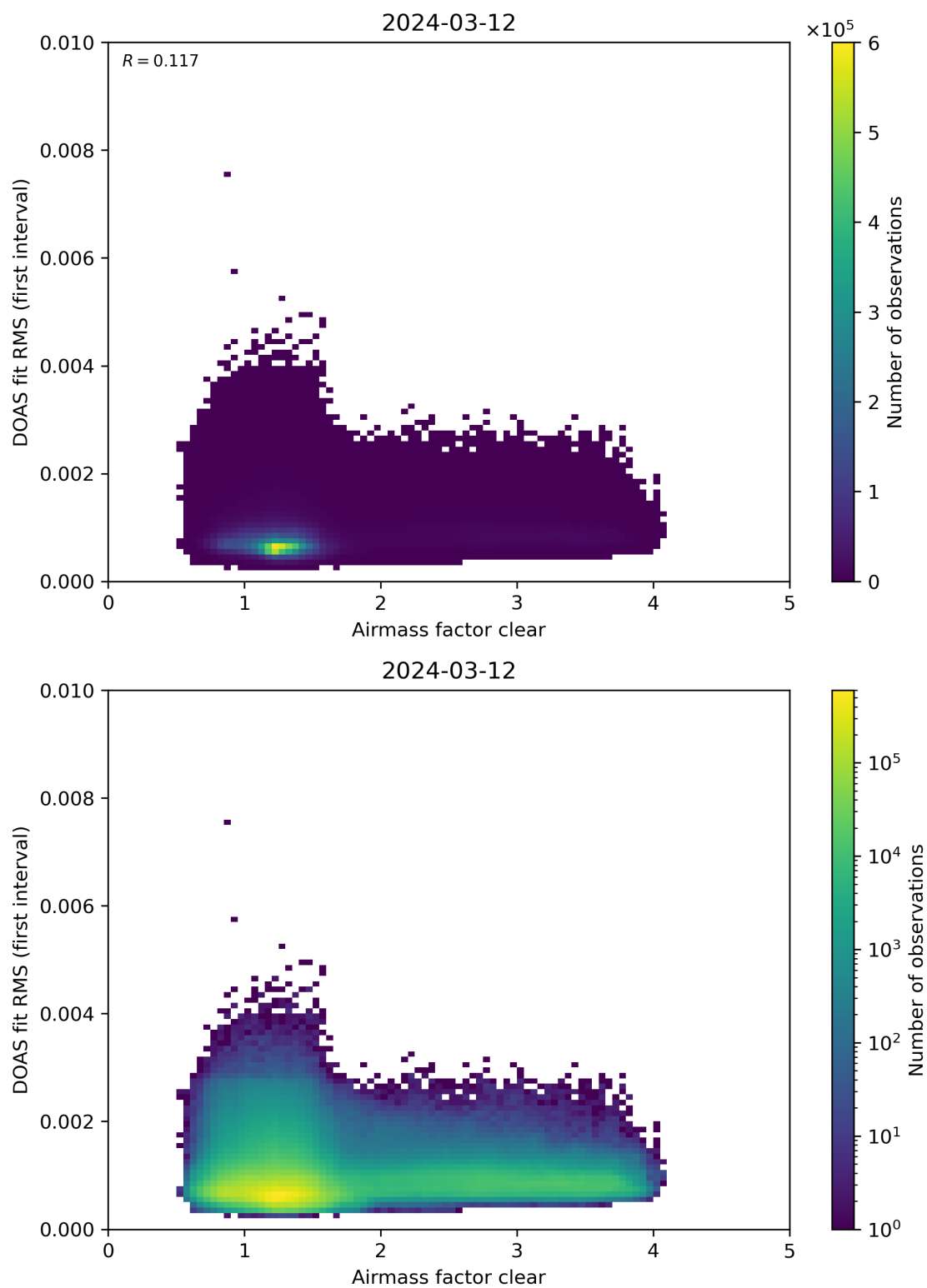
Figure 71: Scatter density plot of “Airmass factor clear” against “DOAS fit RMS (first interval)” for 2024-03-11 to 2024-03-13.
