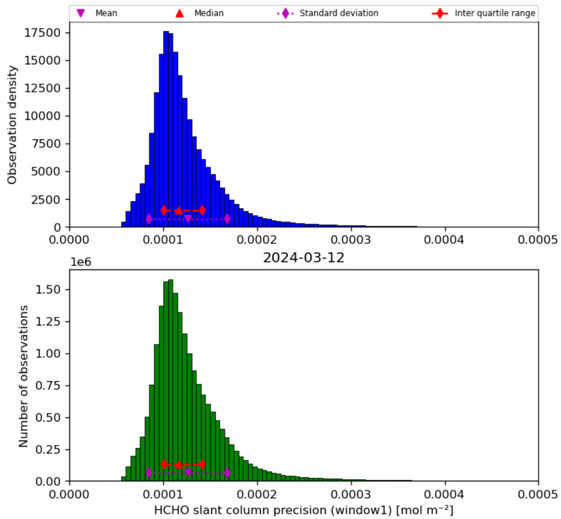
Figure 39: Histogram of “HCHO slant column precision (window1)” for 2024-03-11 to 2024-03-13
