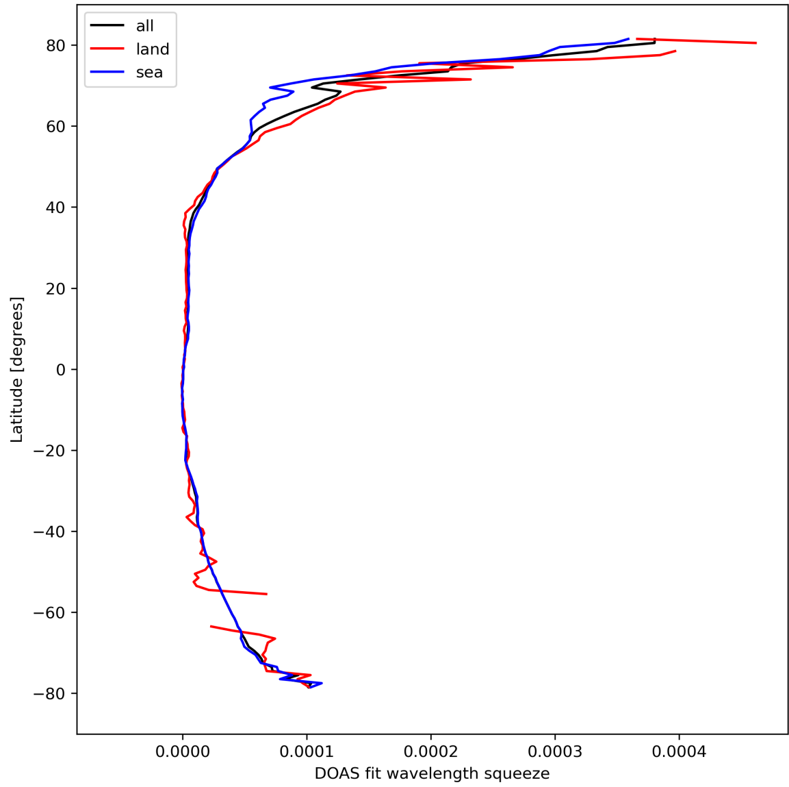
Figure 31: Zonal average of “DOAS fit wavelength squeeze” for 2024-03-11 to 2024-03-13.
