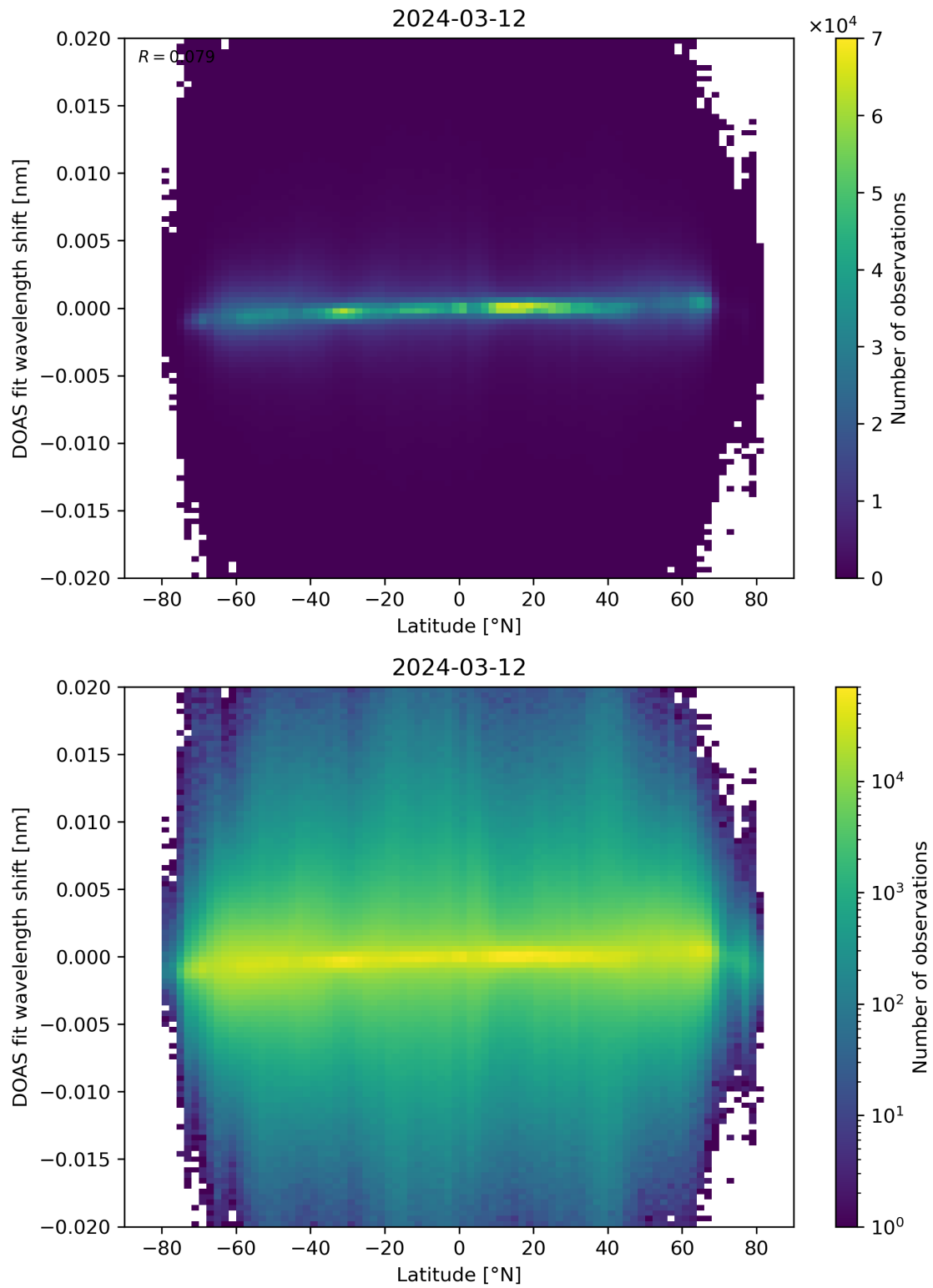
Figure 154: Scatter density plot of “Latitude” against “DOAS fit wavelength shift” for 2024-03-11 to 2024-03-13.
