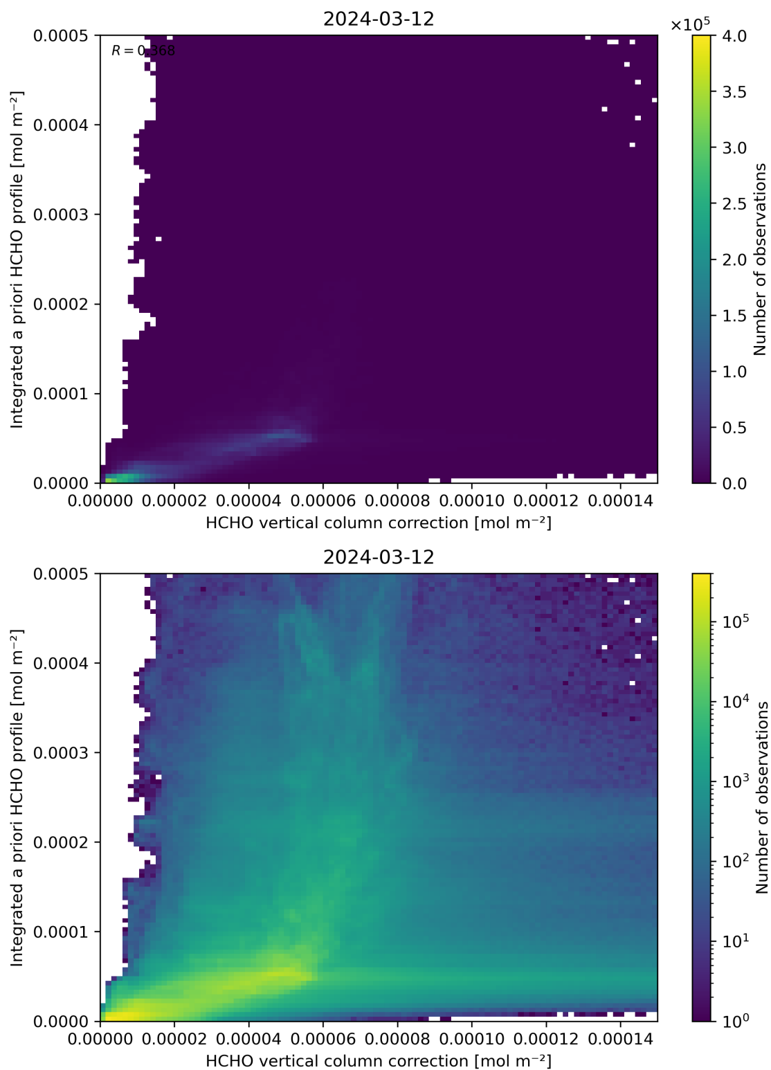
Figure 122: Scatter density plot of “HCHO vertical column correction” against “Integrated a priori HCHO profile” for 2024-03-11 to 2024-03-13.
