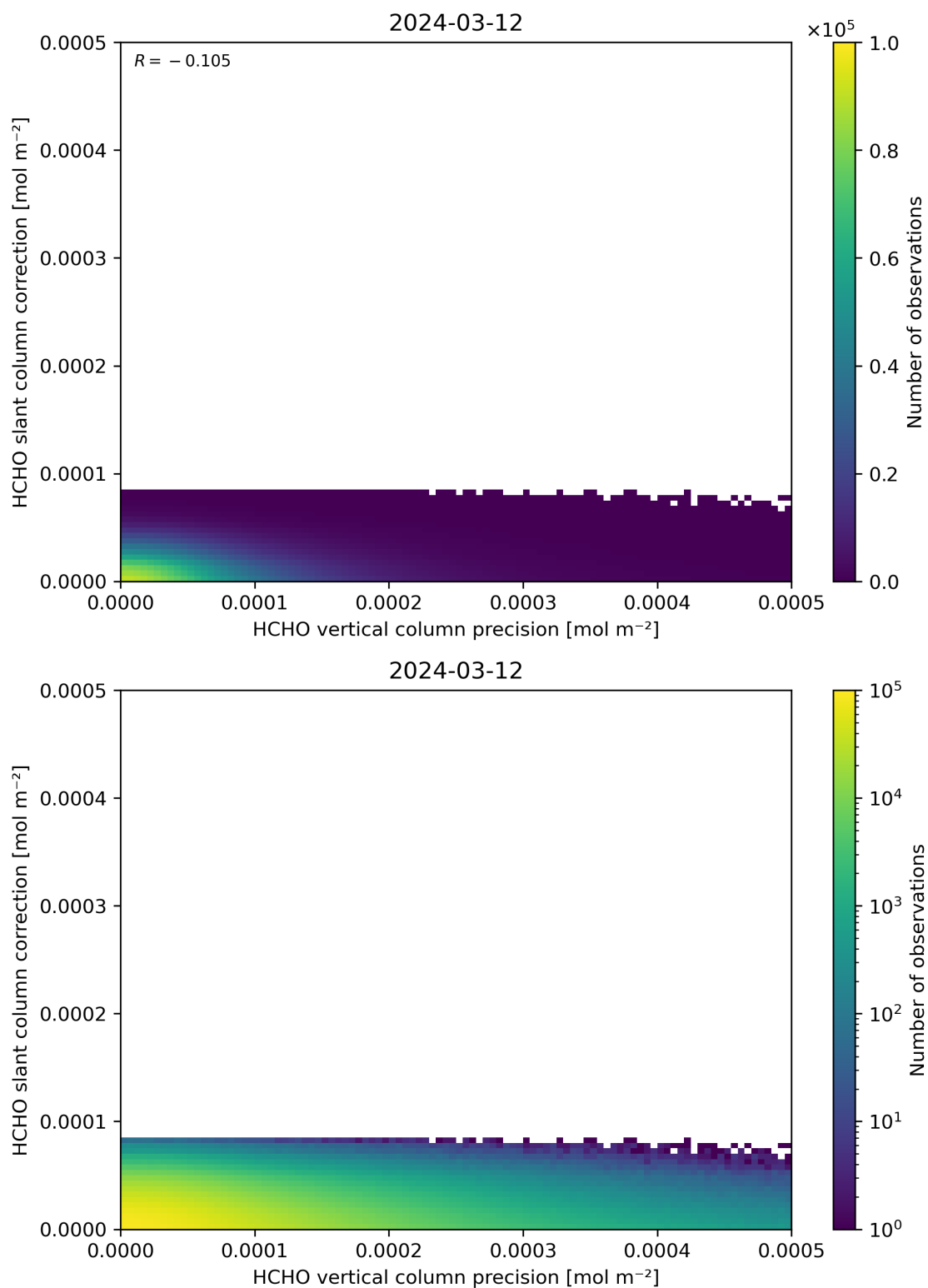
Figure 141: Scatter density plot of “HCHO vertical column precision” against “HCHO slant column correction” for 2024-03-11 to 2024-03-13.
