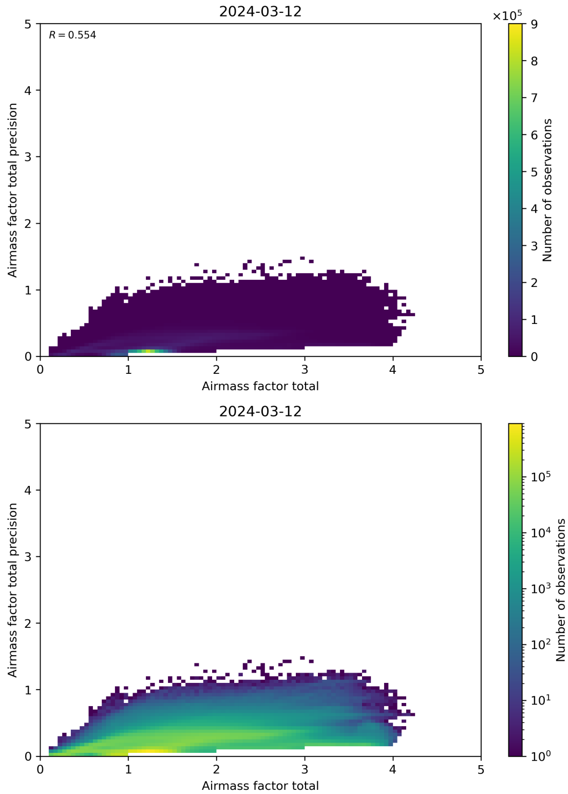
Figure 103: Scatter density plot of “Airmass factor total” against “Airmass factor total precision” for 2024-03-11 to 2024-03-13.
