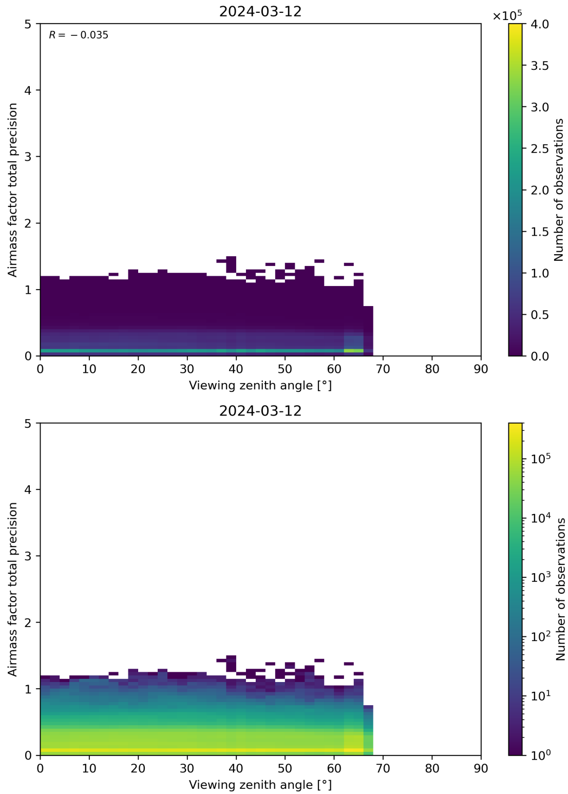
Figure 191: Scatter density plot of “Viewing zenith angle” against “Airmass factor total precision” for 2024-03-11 to 2024-03-13.
