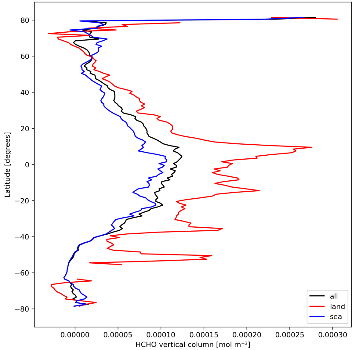
Figure 21: Zonal average of “HCHO vertical column” for 2024-03-11 to 2024-03-13.
