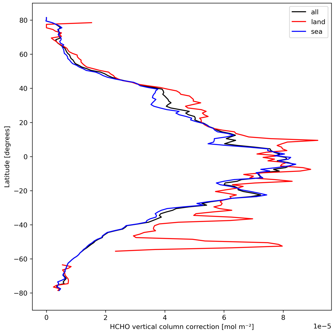
Figure 23: Zonal average of “HCHO vertical column correction” for 2024-03-11 to 2024-03-13.
