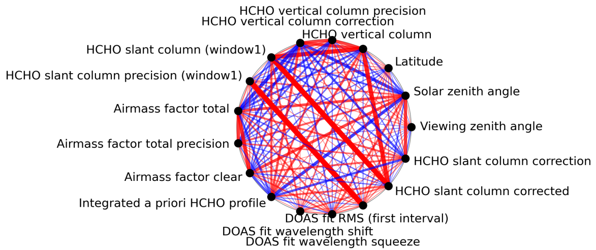
Figure 1: Map of correlation graph for 2024-03-11 to 2024-03-13.
