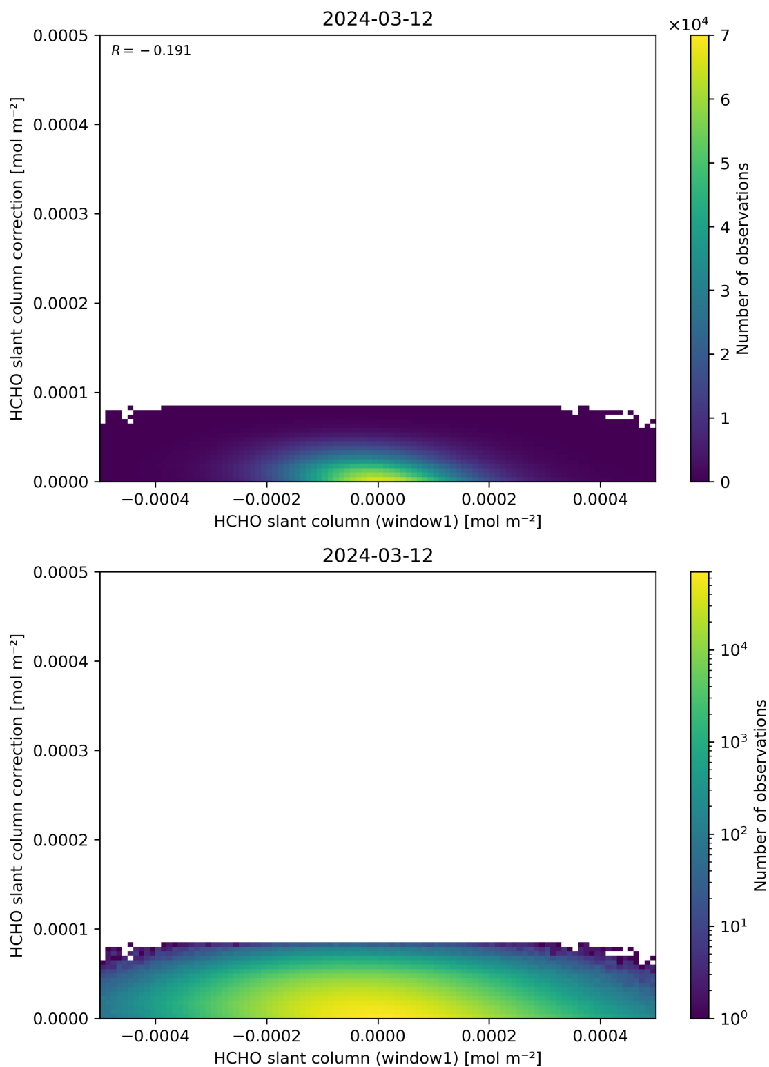
Figure 83: Scatter density plot of “HCHO slant column (window1)” against “HCHO slant column correction” for 2024-03-11 to 2024-03-13.
