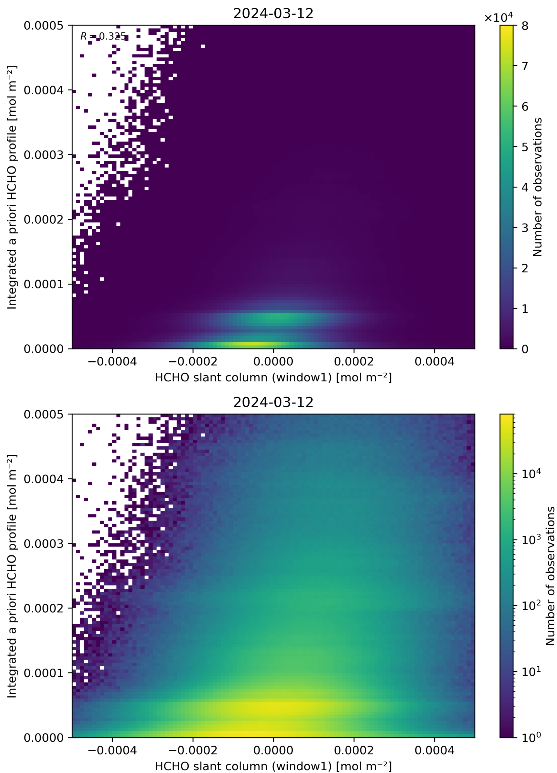
Figure 87: Scatter density plot of “HCHO slant column (window1)” against “Integrated a priori HCHO profile” for 2024-03-11 to 2024-03-13.
