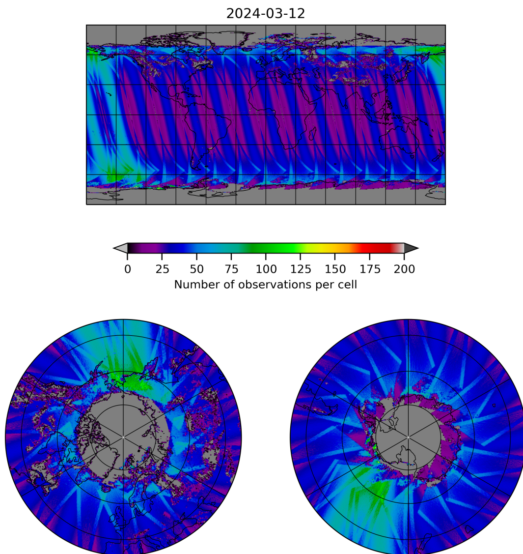
Figure 19: Map of the number of observations for 2024-03-11 to 2024-03-13
