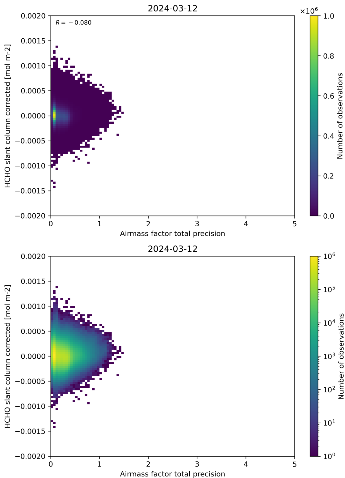
Figure 109: Scatter density plot of “Airmass factor total precision” against “HCHO slant column corrected” for 2024-03-11 to 2024-03-13.
