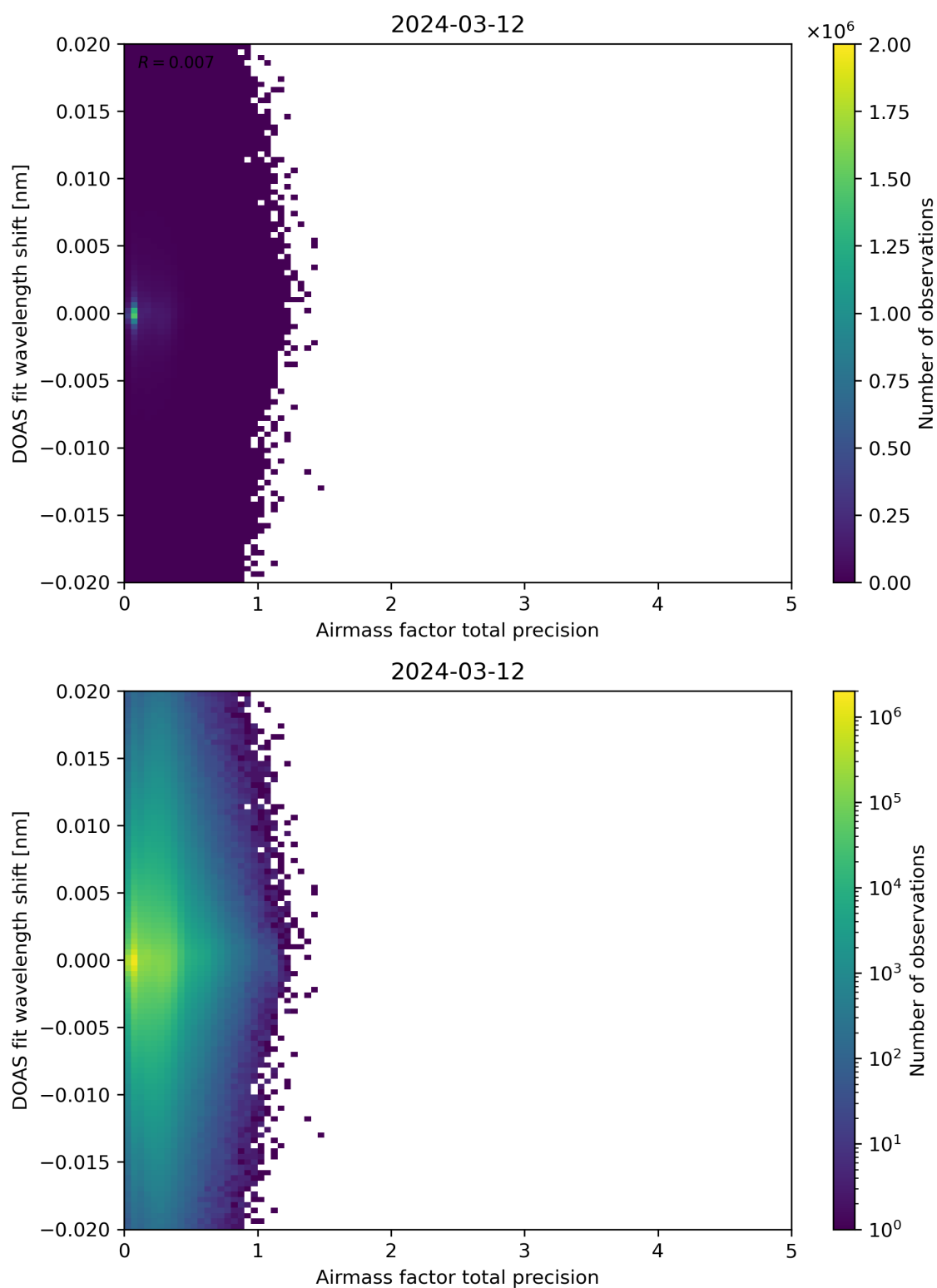
Figure 106: Scatter density plot of “Airmass factor total precision” against “DOAS fit wavelength shift” for 2024-03-11 to 2024-03-13.
