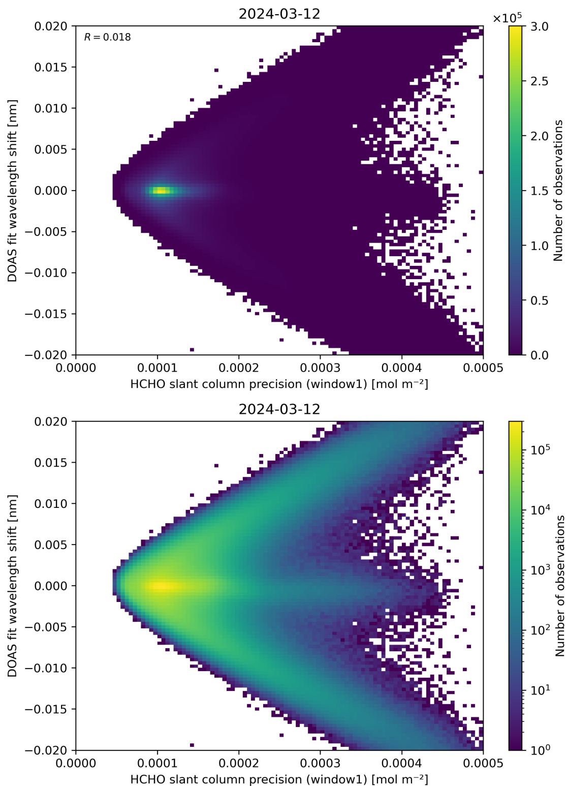
Figure 89: Scatter density plot of “HCHO slant column precision (window1)” against “DOAS fit wavelength shift” for 2024-03-11 to 2024-03-13.
