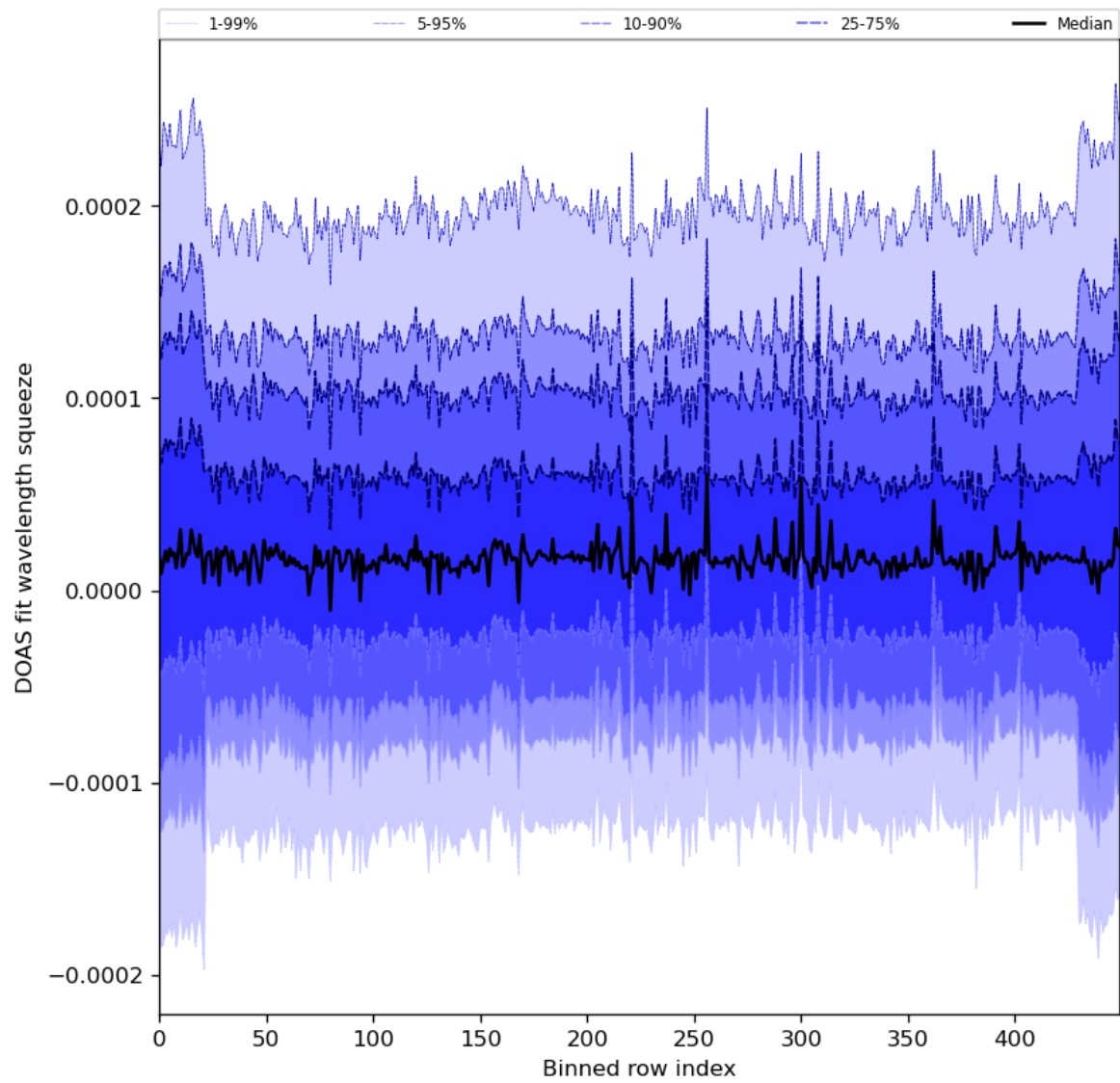
Figure 59: Along track statistics of “DOAS fit wavelength squeeze” for 2024-03-11 to 2024-03-13
