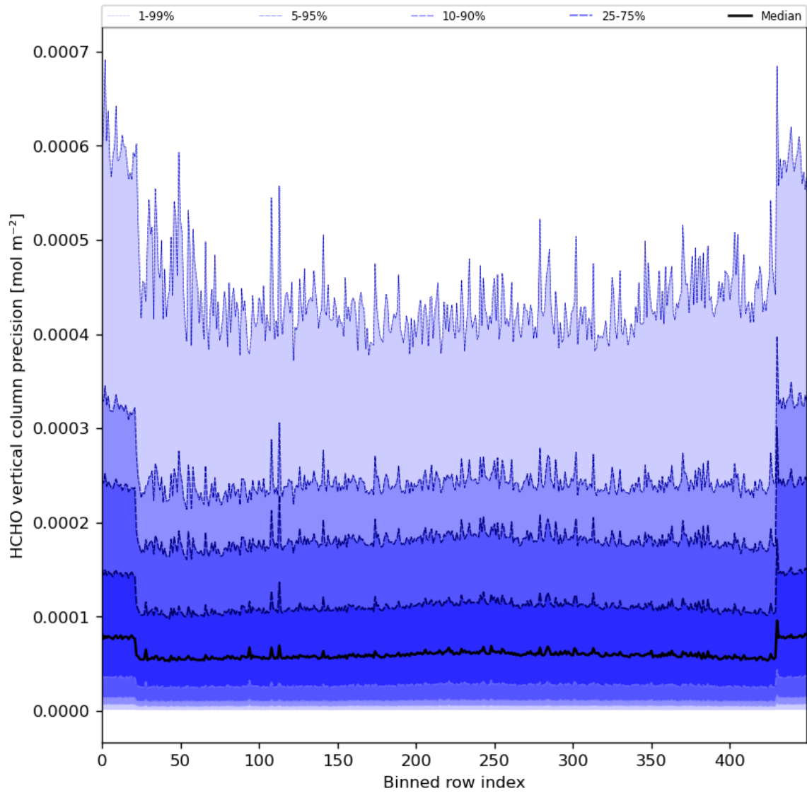
Figure 50: Along track statistics of “HCHO vertical column precision” for 2024-03-11 to 2024-03-13
