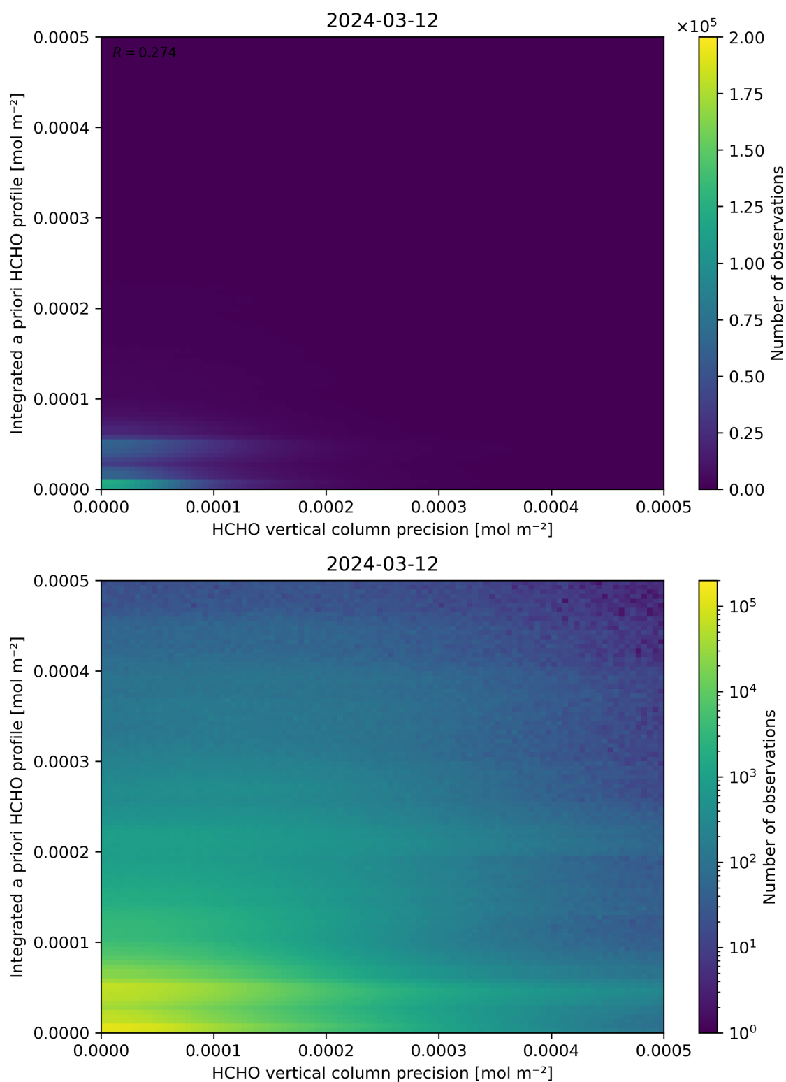
Figure 147: Scatter density plot of “HCHO vertical column precision” against “Integrated a priori HCHO profile” for 2024-03-11 to 2024-03-13.
