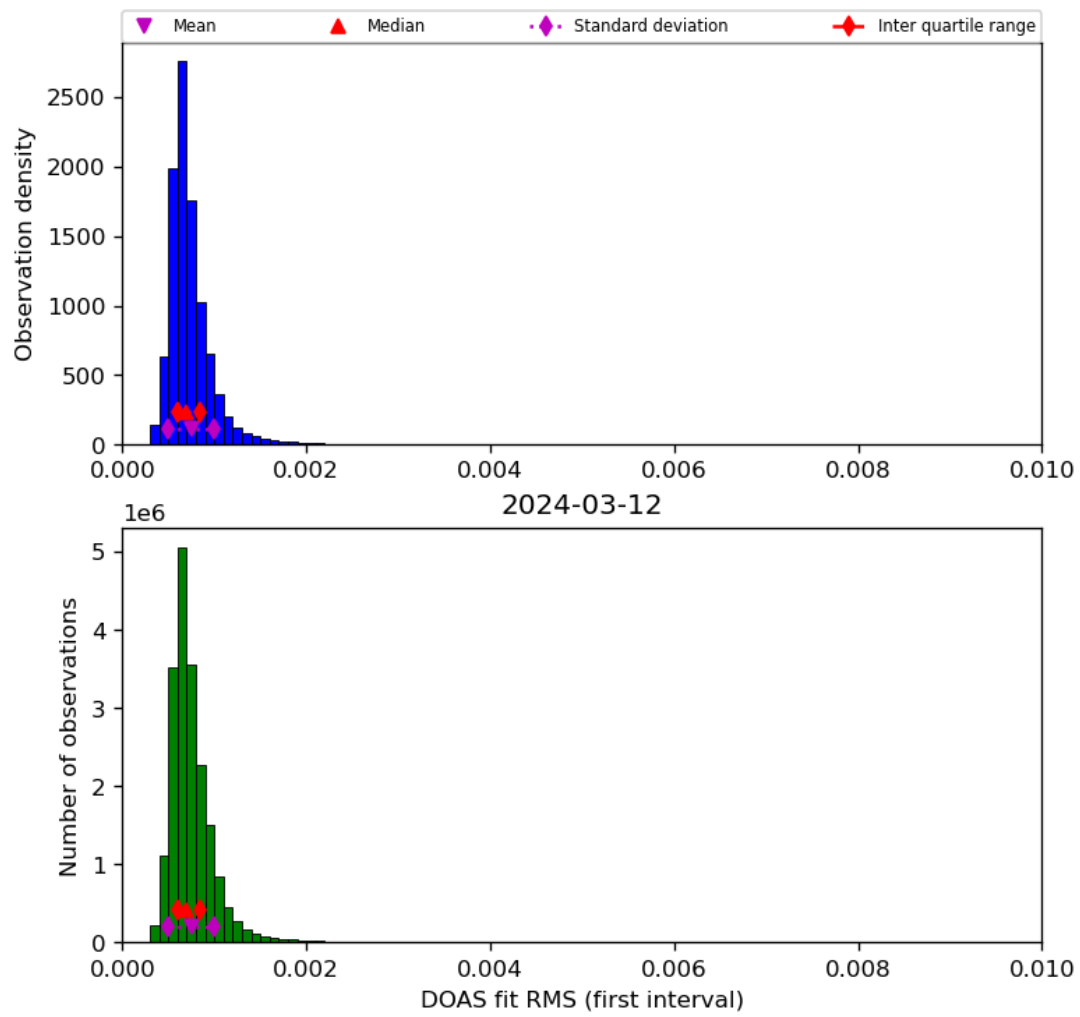
Figure 46: Histogram of “DOAS fit RMS (first interval)” for 2024-03-11 to 2024-03-13
