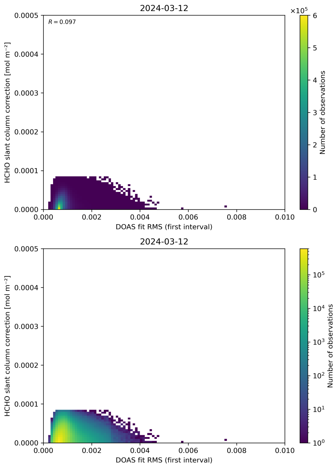
Figure 63: Scatter density plot of “DOAS fit RMS (first interval)” against “HCHO slant column correction” for 2024-03-11 to 2024-03-13.
