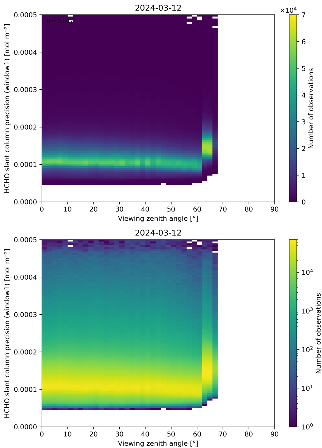
Figure 189: Scatter density plot of “Viewing zenith angle” against “HCHO slant column precision (window1)” for 2024-03-11 to 2024-03-13.
