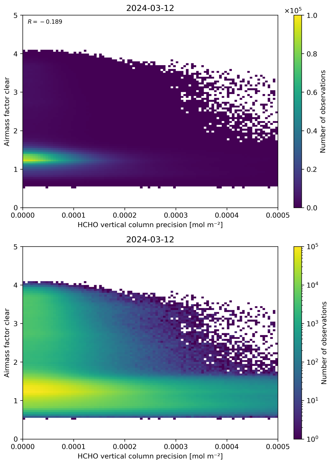
Figure 139: Scatter density plot of “HCHO vertical column precision” against “Airmass factor clear” for 2024-03-11 to 2024-03-13.
