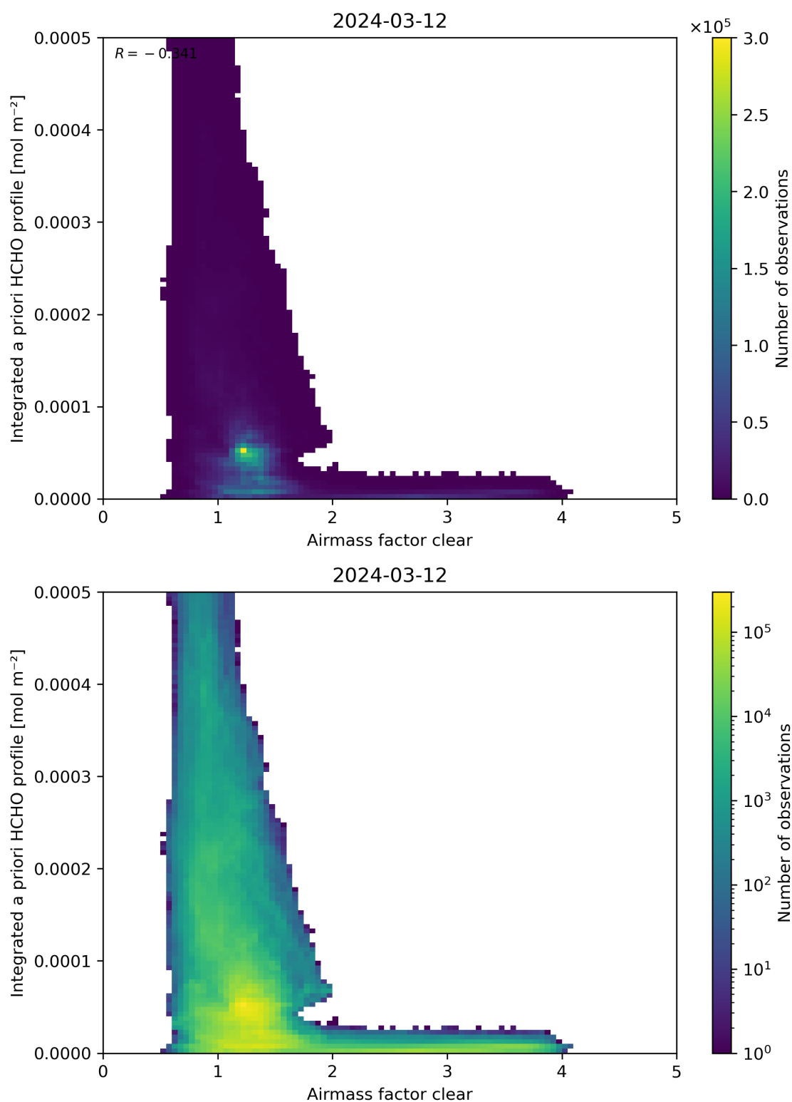
Figure 76: Scatter density plot of “Airmass factor clear” against “Integrated a priori HCHO profile” for 2024-03-11 to 2024-03-13.
