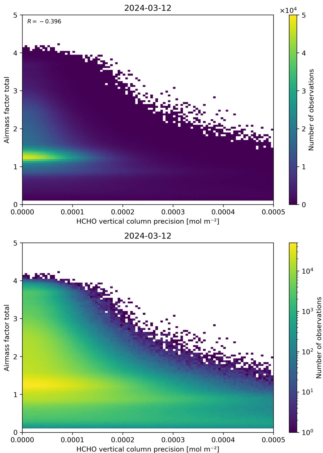
Figure 144: Scatter density plot of “HCHO vertical column precision” against “Airmass factor total” for 2024-03-11 to 2024-03-13.
