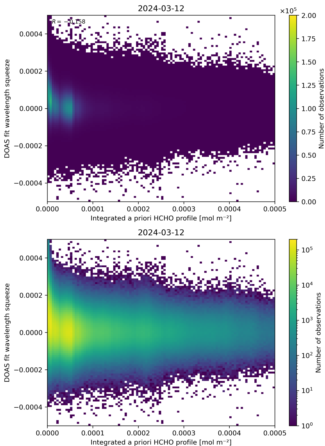
Figure 150: Scatter density plot of “Integrated a priori HCHO profile” against “DOAS fit wavelength squeeze” for 2024-03-11 to 2024-03-13.
