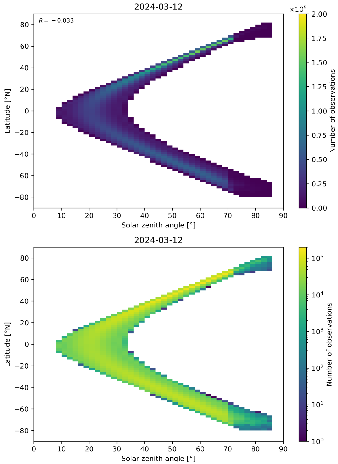
Figure 181: Scatter density plot of “Solar zenith angle” against “Latitude” for 2024-03-11 to 2024-03-13.
