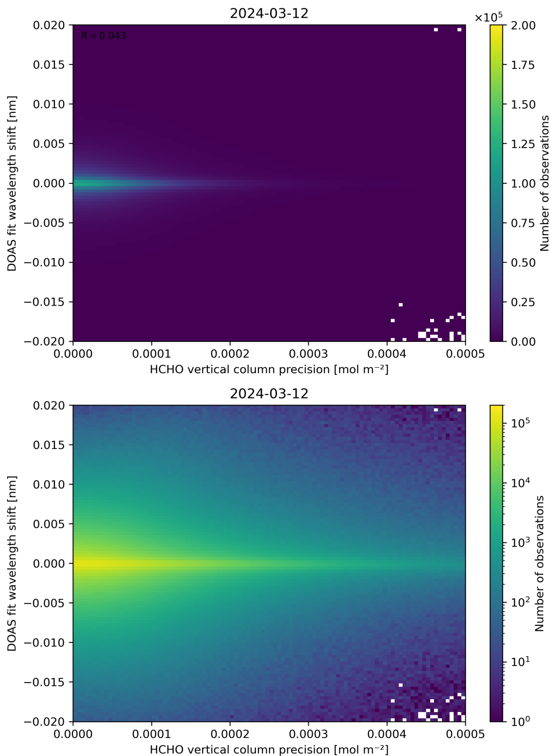
Figure 137: Scatter density plot of “HCHO vertical column precision” against “DOAS fit wavelength shift” for 2024-03-11 to 2024-03-13.
