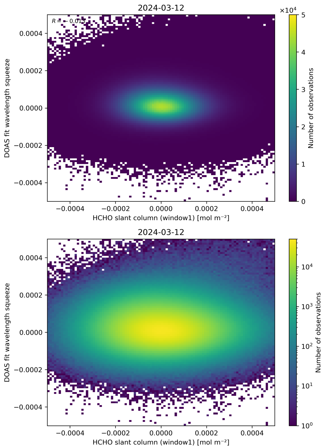
Figure 80: Scatter density plot of “HCHO slant column (window1)” against “DOAS fit wavelength squeeze” for 2024-03-11 to 2024-03-13.
