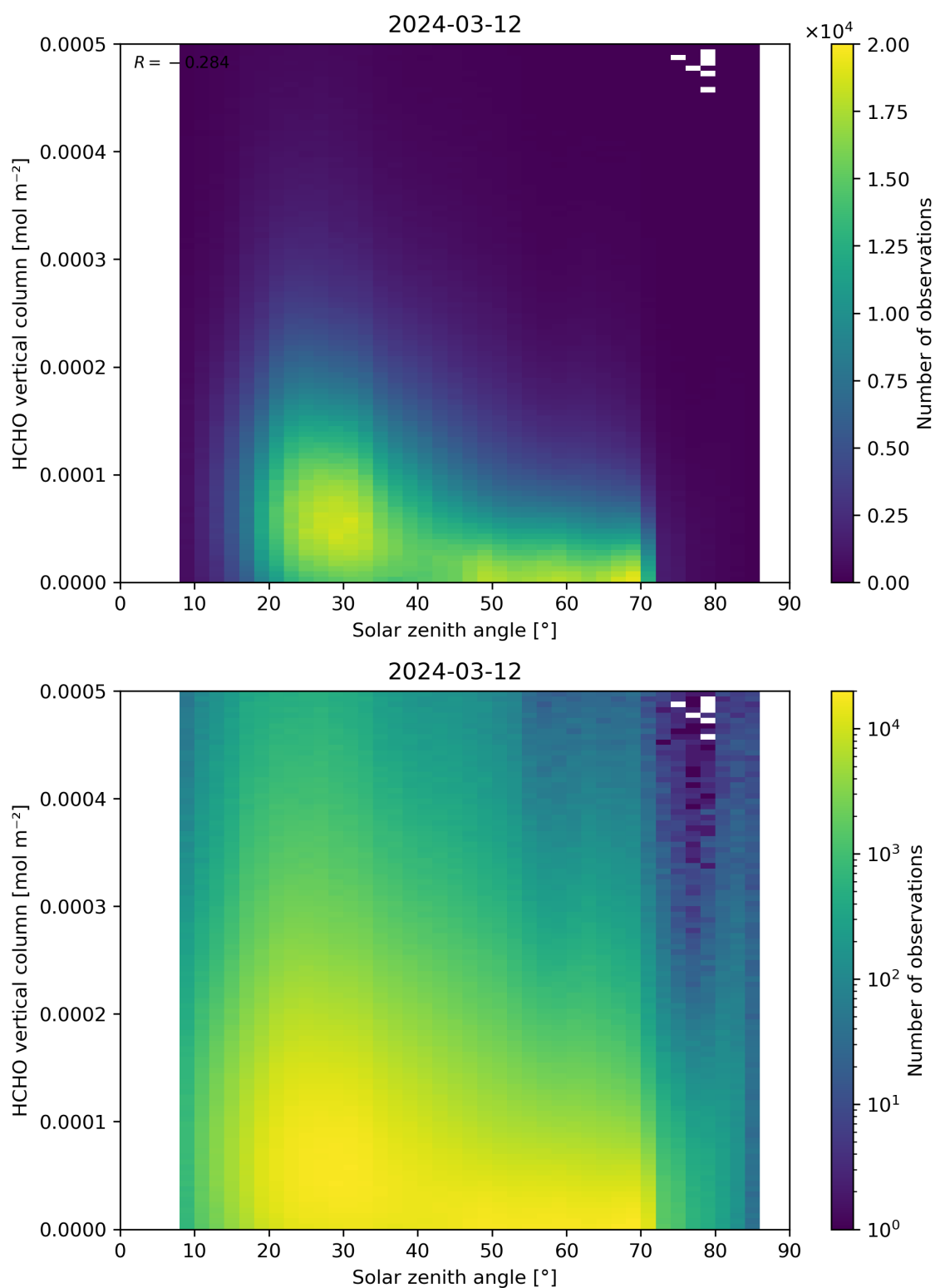
Figure 177: Scatter density plot of “Solar zenith angle” against “HCHO vertical column” for 2024-03-11 to 2024-03-13.
