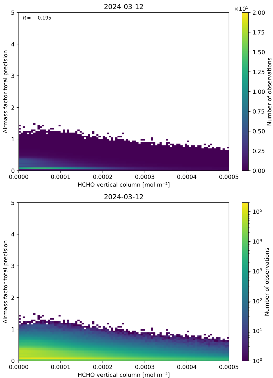
Figure 132: Scatter density plot of “HCHO vertical column” against “Airmass factor total precision” for 2024-03-11 to 2024-03-13.
