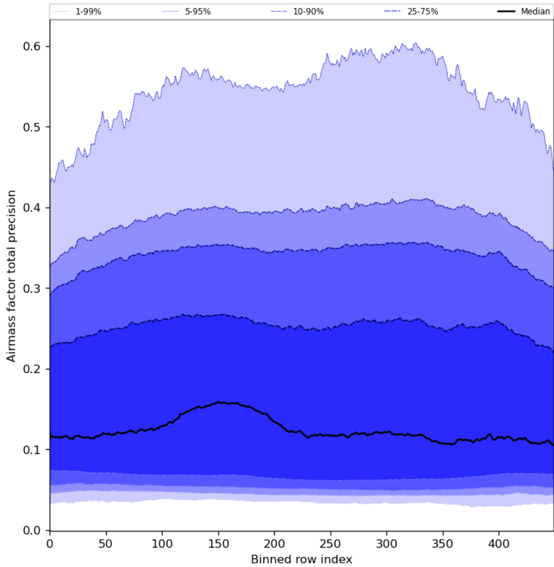
Figure 55: Along track statistics of “Airmass factor total precision” for 2024-03-11 to 2024-03-13
