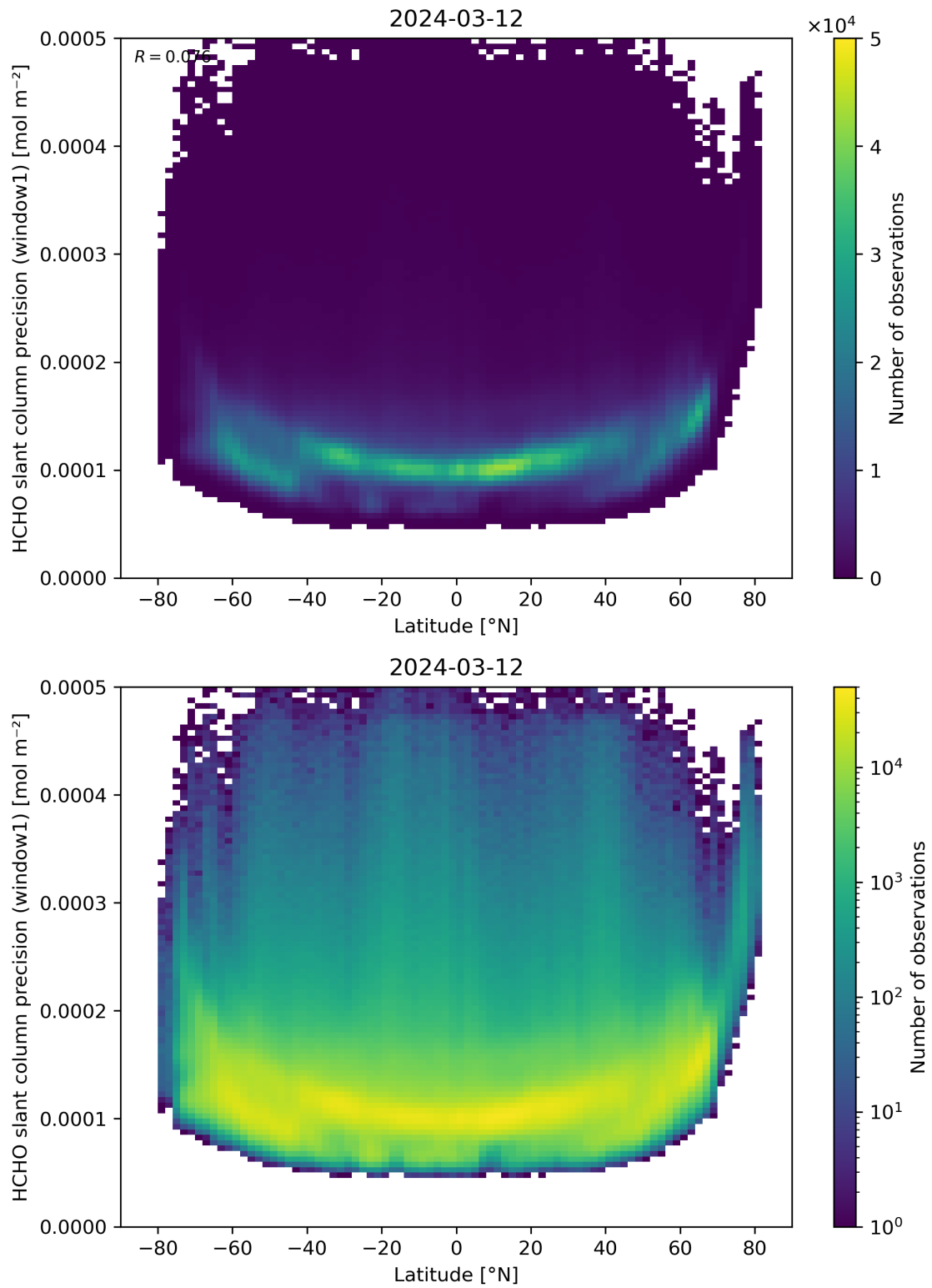
Figure 160: Scatter density plot of “Latitude” against “HCHO slant column precision (window1)” for 2024-03-11 to 2024-03-13.
