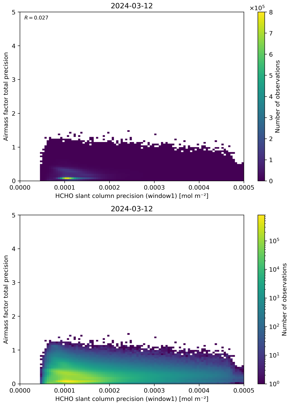
Figure 95: Scatter density plot of “HCHO slant column precision (window1)” against “Airmass factor total precision” for 2024-03-11 to 2024-03-13.
