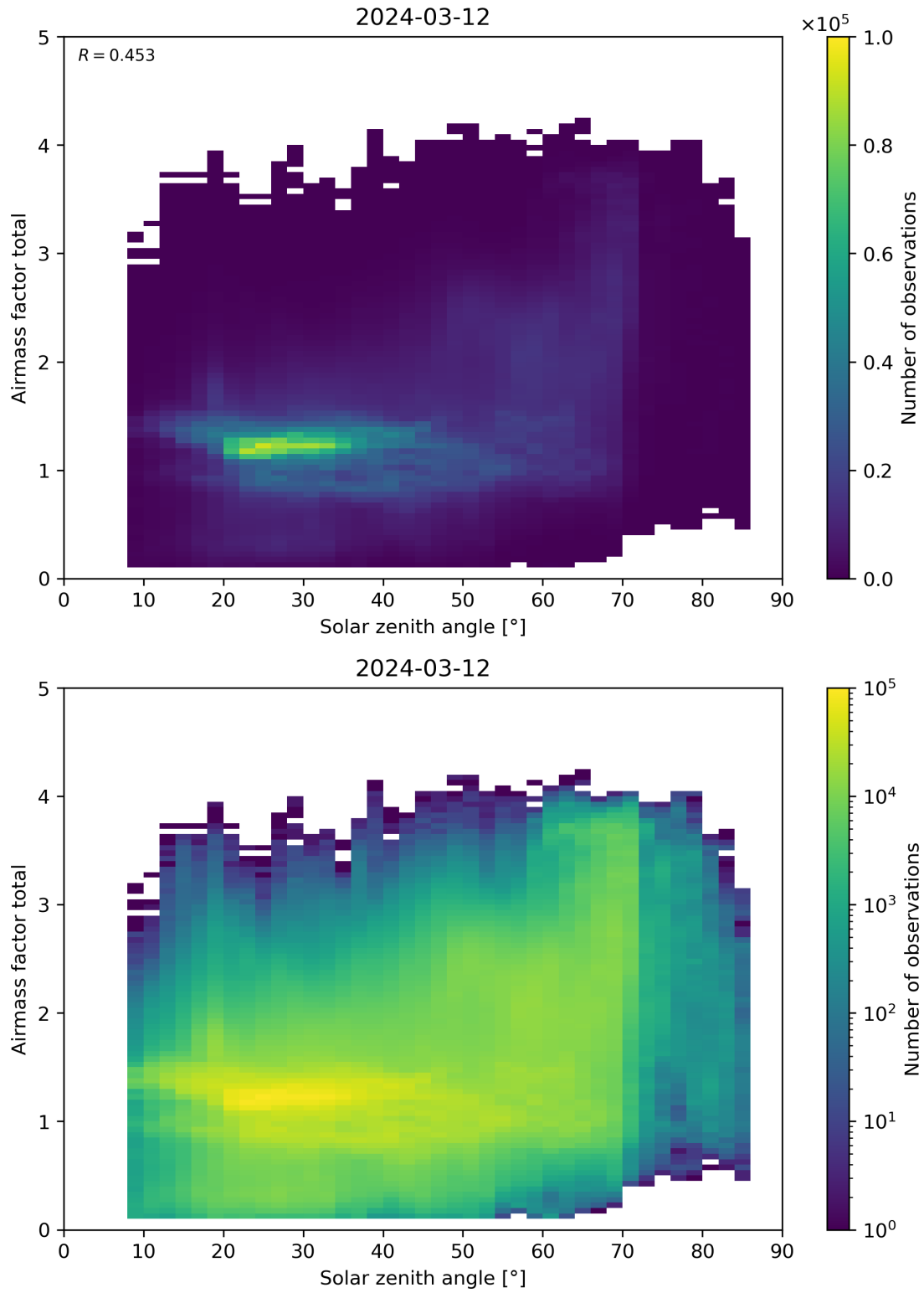
Figure 175: Scatter density plot of “Solar zenith angle” against “Airmass factor total” for 2024-03-11 to 2024-03-13.
