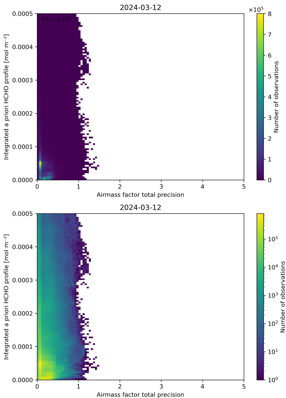
Figure 111: Scatter density plot of “Airmass factor total precision” against “Integrated a priori HCHO profile” for 2024-03-11 to 2024-03-13.
