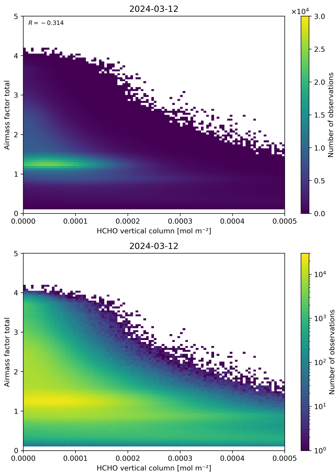
Figure 131: Scatter density plot of “HCHO vertical column” against “Airmass factor total” for 2024-03-11 to 2024-03-13.
