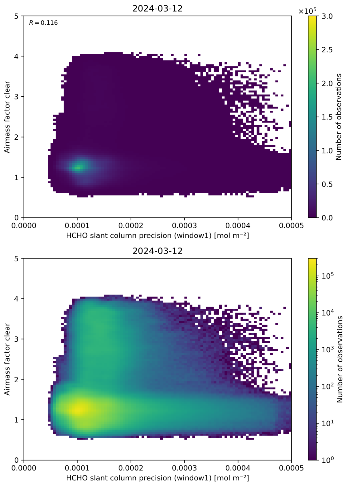
Figure 91: Scatter density plot of “HCHO slant column precision (window1)” against “Airmass factor clear” for 2024-03-11 to 2024-03-13.
