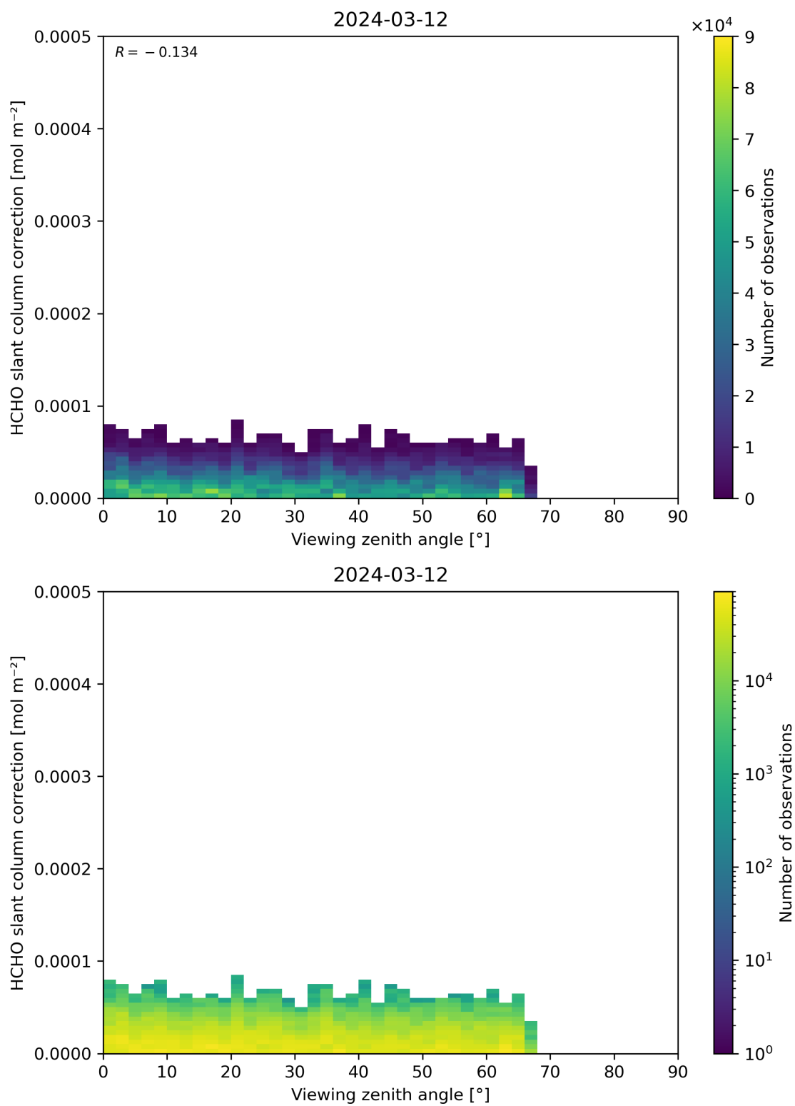
Figure 187: Scatter density plot of “Viewing zenith angle” against “HCHO slant column correction” for 2024-03-11 to 2024-03-13.
