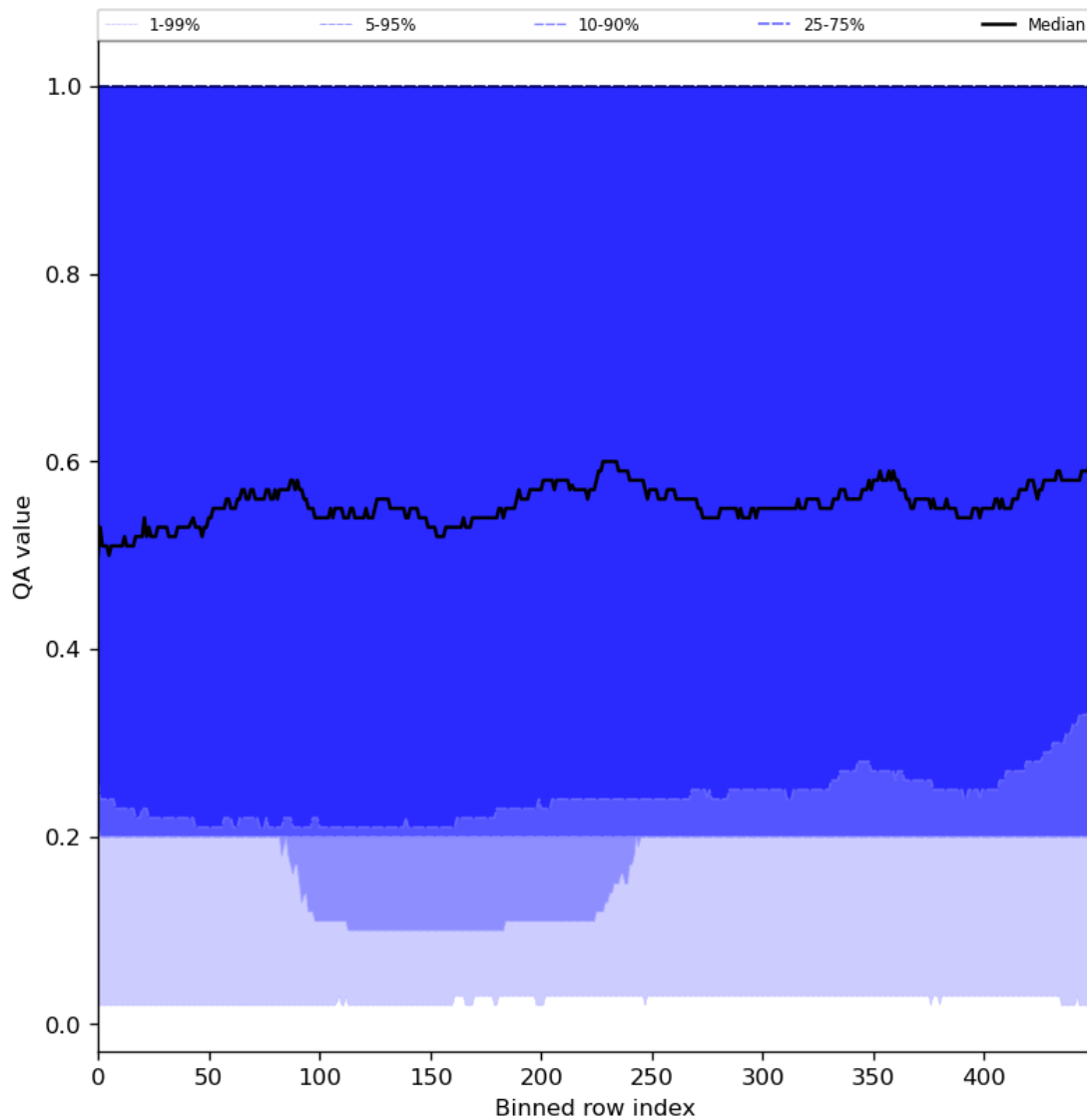
Figure 48: Along track statistics of “QA value” for 2024-03-11 to 2024-03-13
