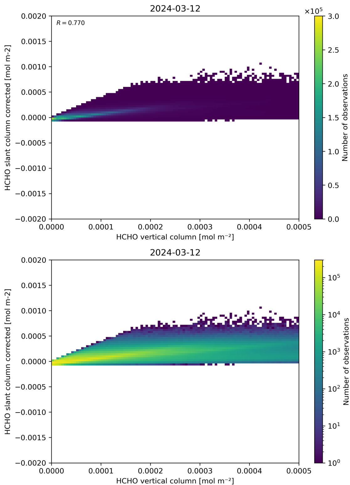
Figure 127: Scatter density plot of “HCHO vertical column” against “HCHO slant column corrected” for 2024-03-11 to 2024-03-13.
