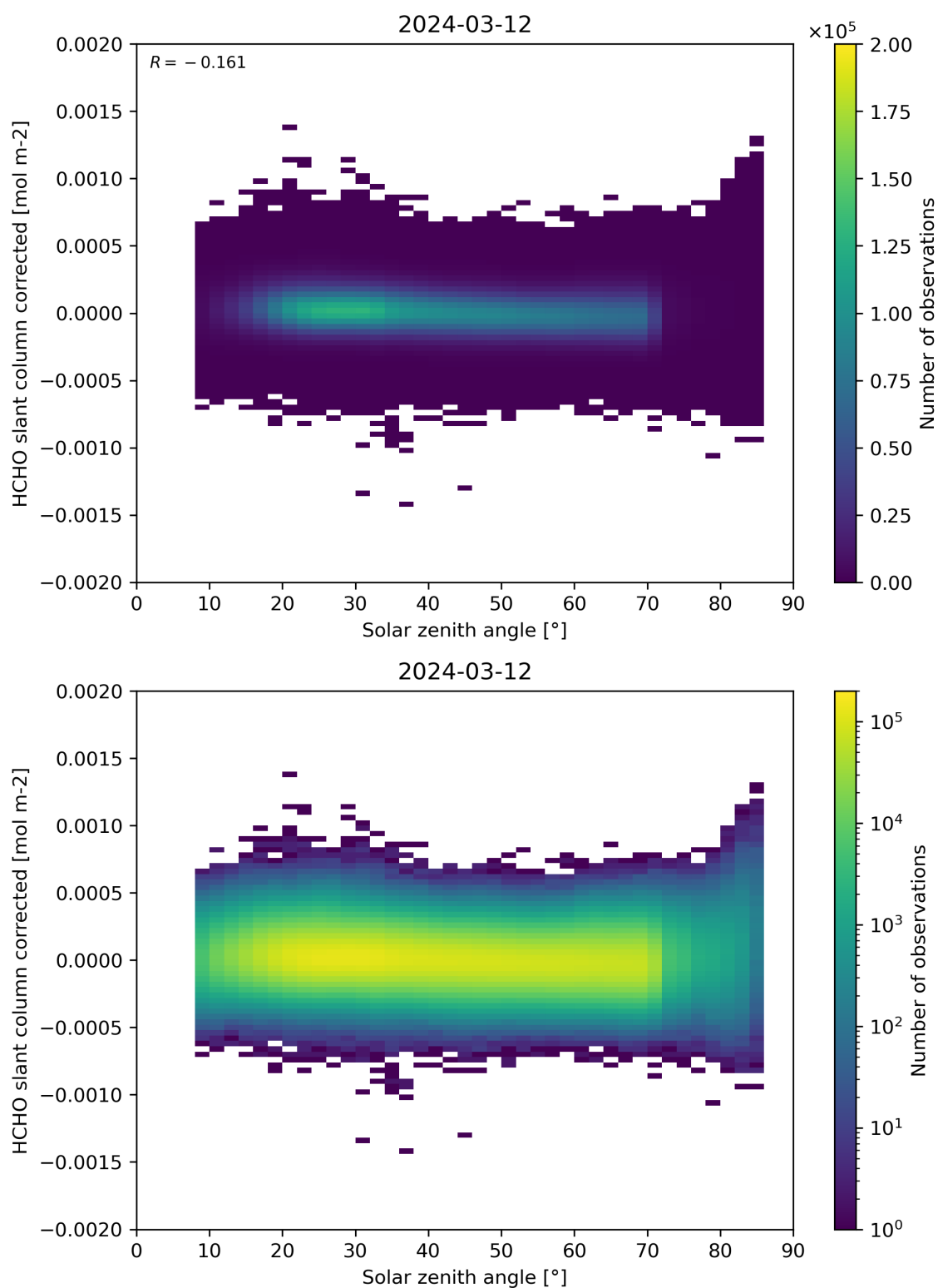
Figure 171: Scatter density plot of “Solar zenith angle” against “HCHO slant column corrected” for 2024-03-11 to 2024-03-13.
