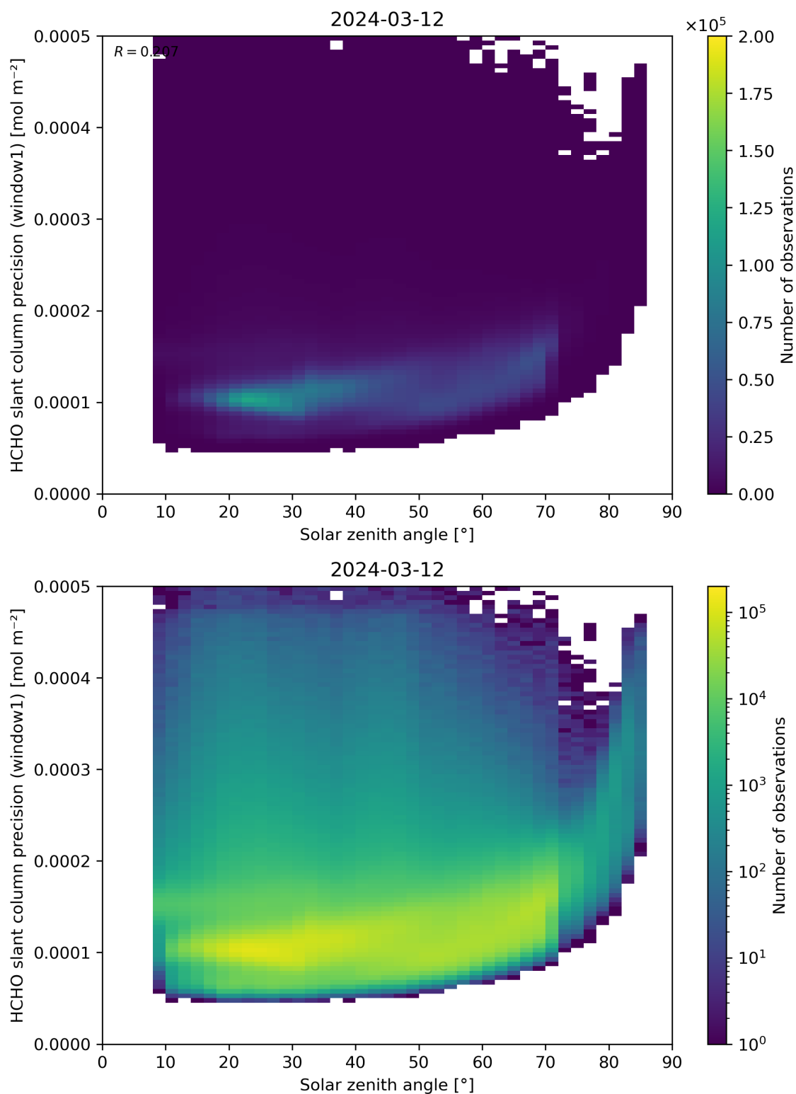
Figure 174: Scatter density plot of “Solar zenith angle” against “HCHO slant column precision (window1)” for 2024-03-11 to 2024-03-13.
