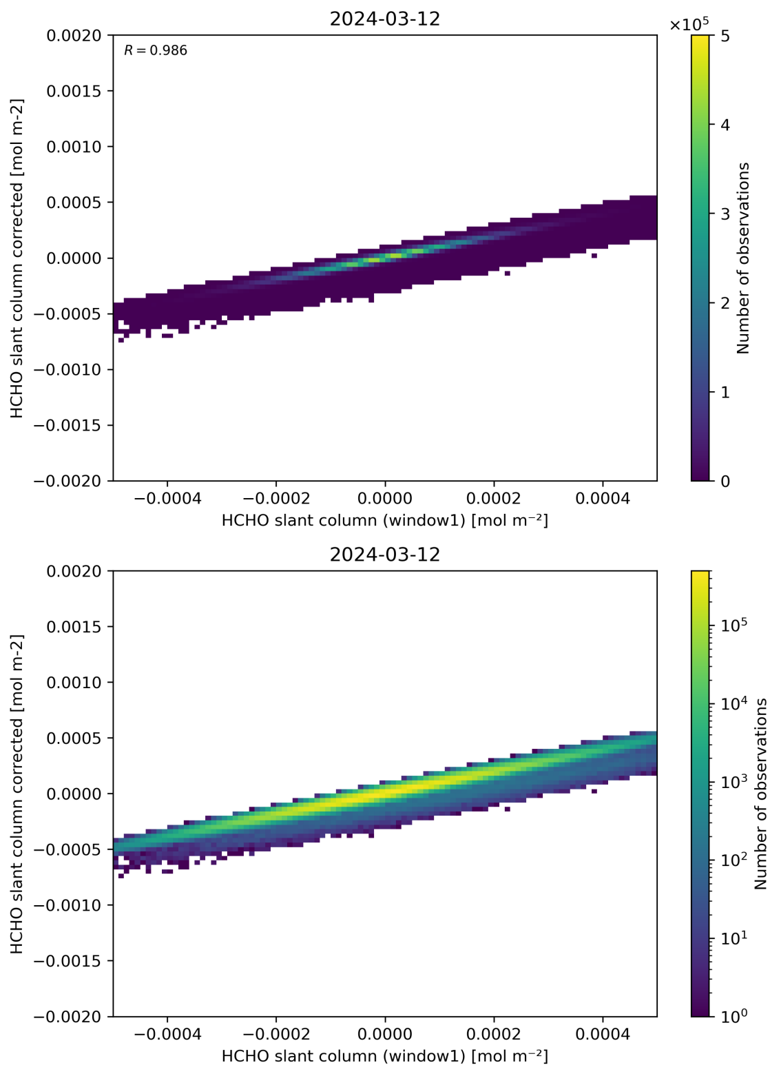
Figure 82: Scatter density plot of “HCHO slant column (window1)” against “HCHO slant column corrected” for 2024-03-11 to 2024-03-13.
