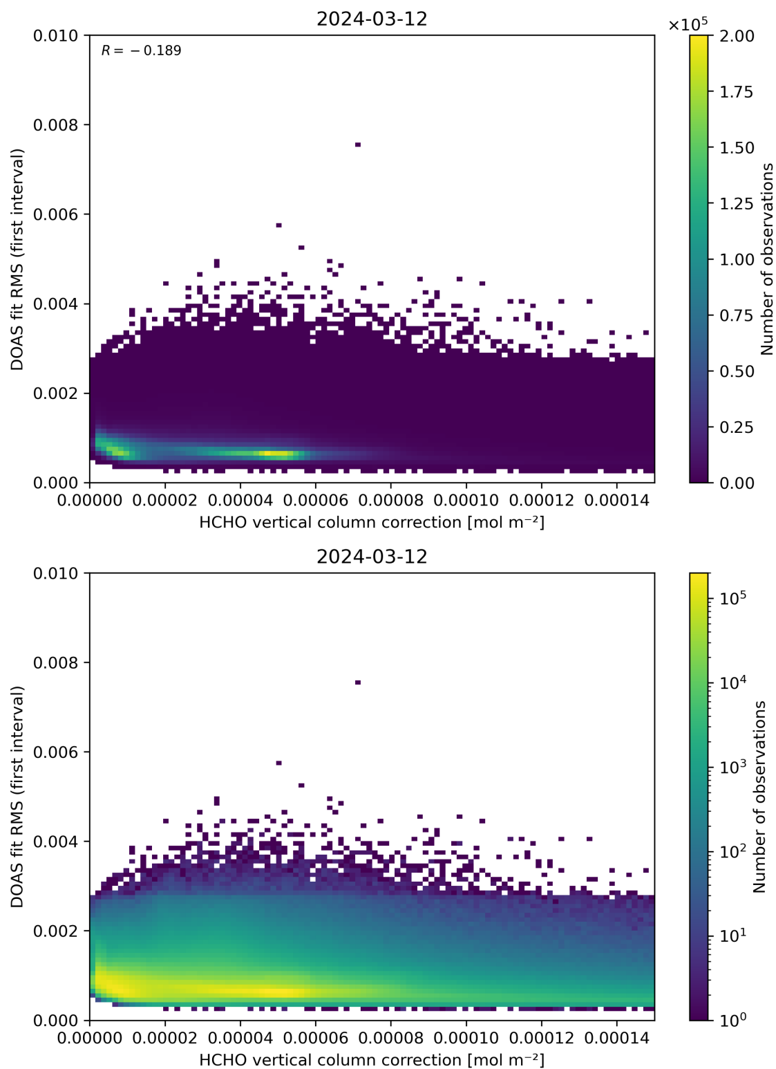
Figure 112: Scatter density plot of “HCHO vertical column correction” against “DOAS fit RMS (first interval)” for 2024-03-11 to 2024-03-13.
