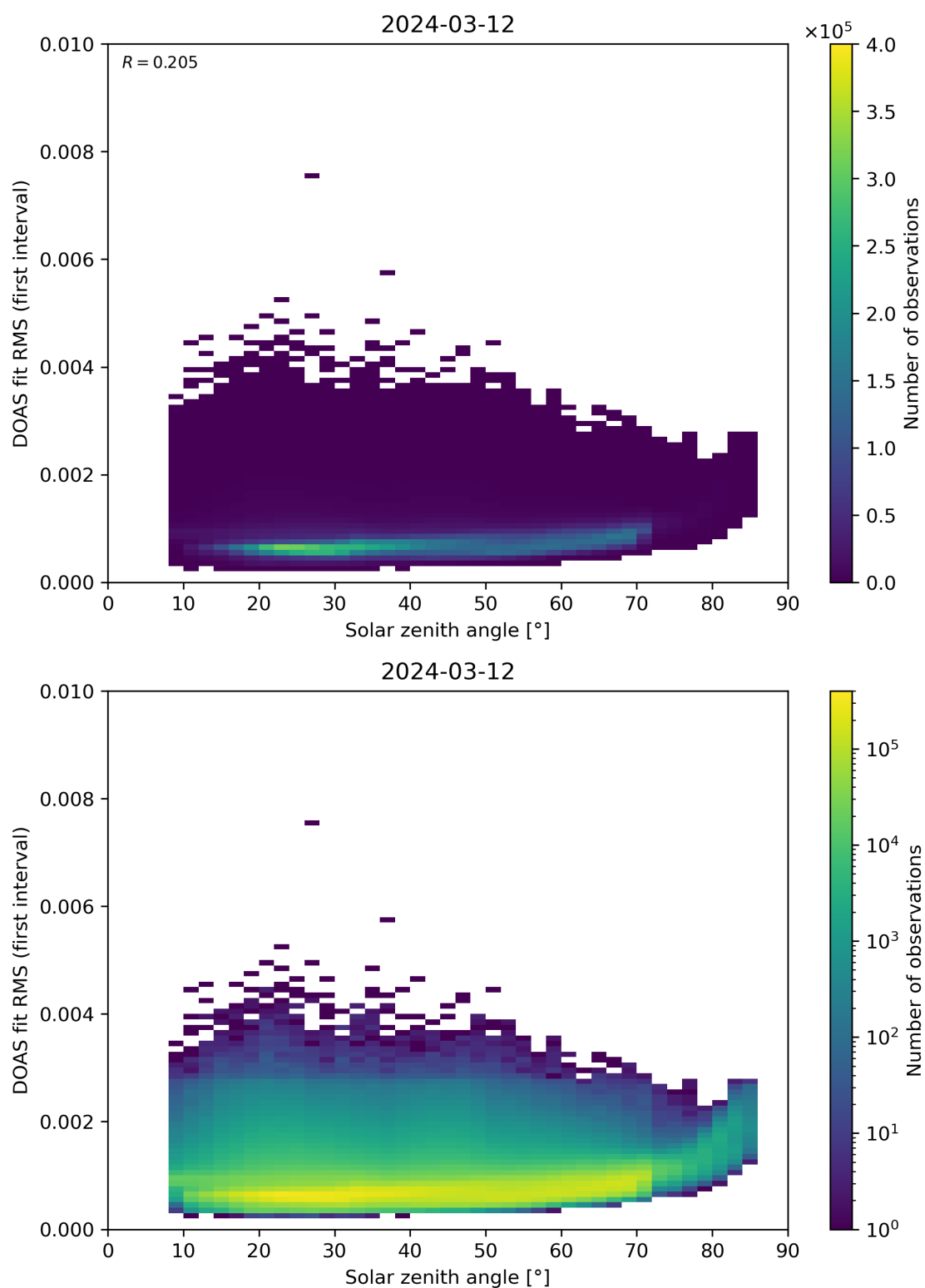
Figure 167: Scatter density plot of “Solar zenith angle” against “DOAS fit RMS (first interval)” for 2024-03-11 to 2024-03-13.
