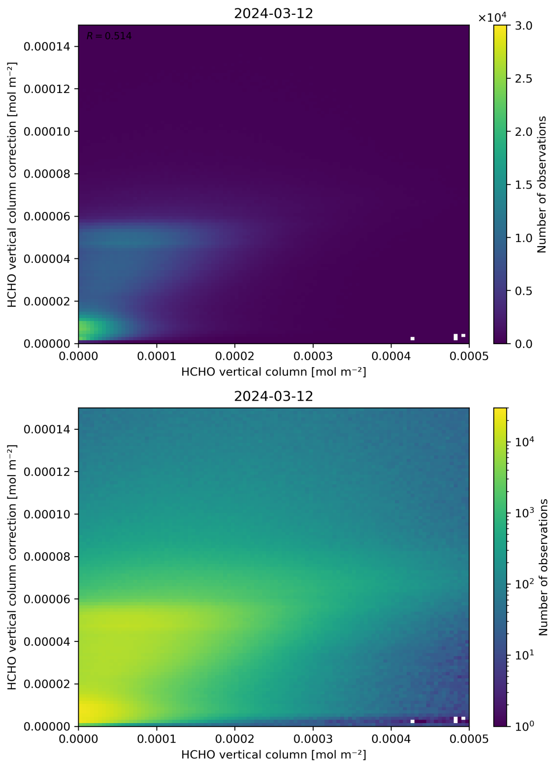
Figure 133: Scatter density plot of “HCHO vertical column” against “HCHO vertical column correction” for 2024-03-11 to 2024-03-13.
