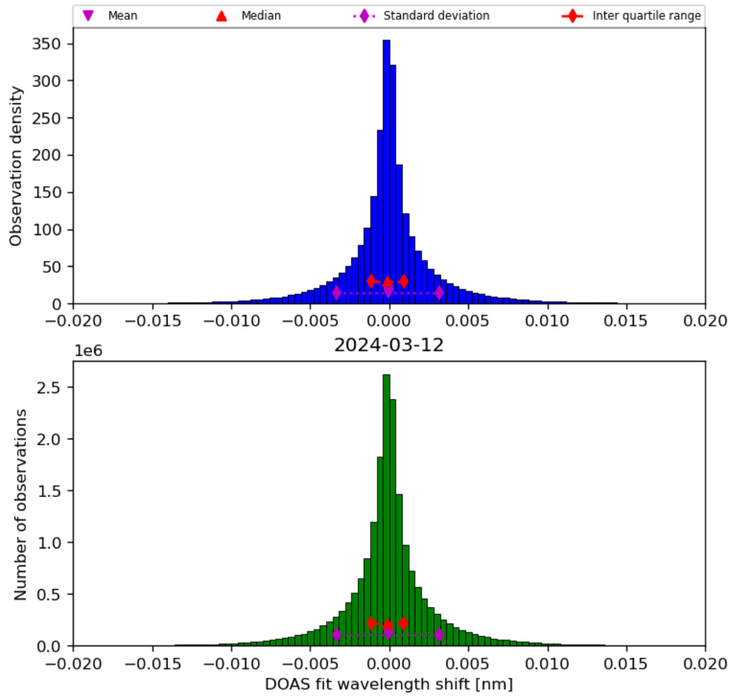
Figure 44: Histogram of “DOAS fit wavelength shift” for 2024-03-11 to 2024-03-13
