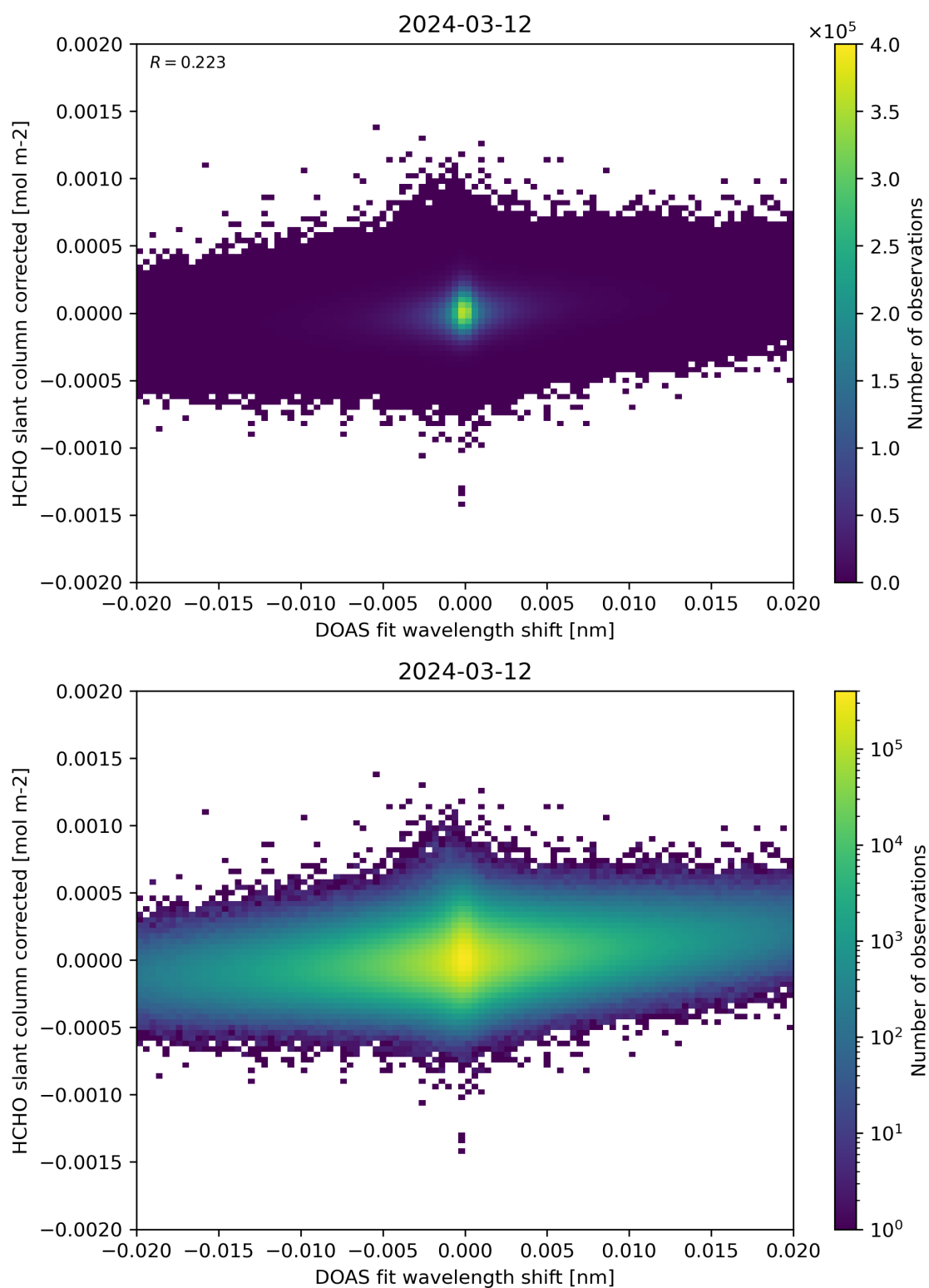
Figure 66: Scatter density plot of “DOAS fit wavelength shift” against “HCHO slant column corrected” for 2024-03-11 to 2024-03-13.
