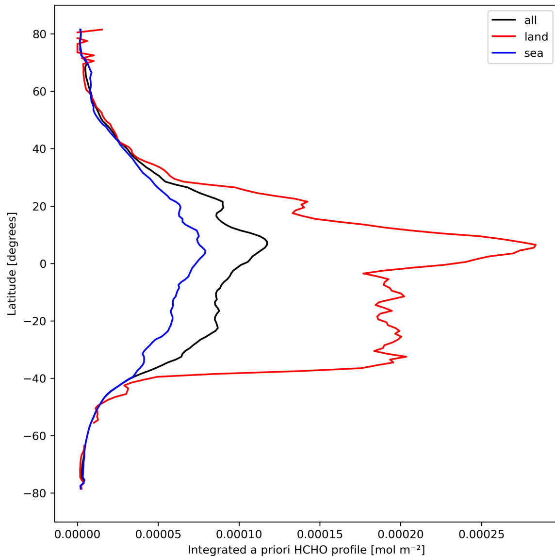
Figure 29: Zonal average of “Integrated a priori HCHO profile” for 2024-03-11 to 2024-03-13.
