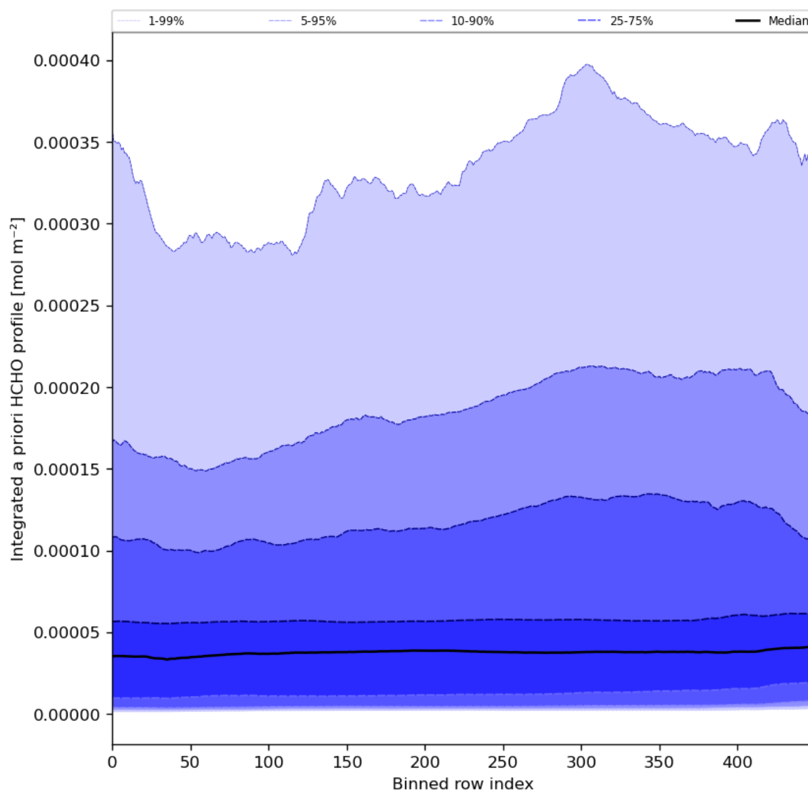
Figure 57: Along track statistics of “Integrated a priori HCHO profile” for 2024-03-11 to 2024-03-13
