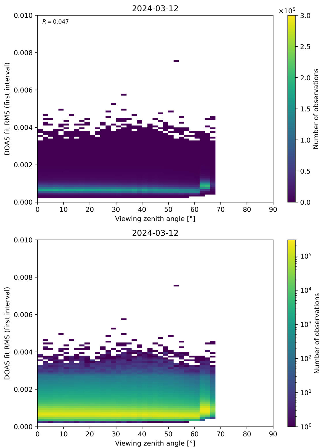
Figure 182: Scatter density plot of “Viewing zenith angle” against “DOAS fit RMS (first interval)” for 2024-03-11 to 2024-03-13.
