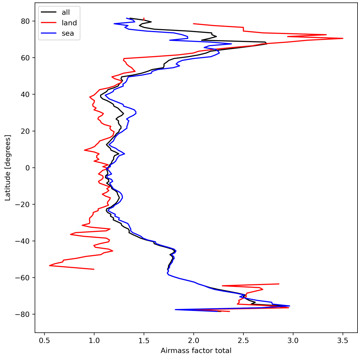
Figure 26: Zonal average of “Airmass factor total” for 2024-03-11 to 2024-03-13.
