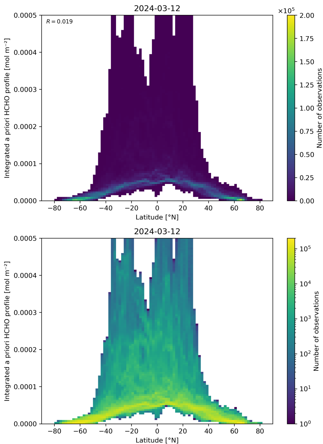
Figure 166: Scatter density plot of “Latitude” against “Integrated a priori HCHO profile” for 2024-03-11 to 2024-03-13.
