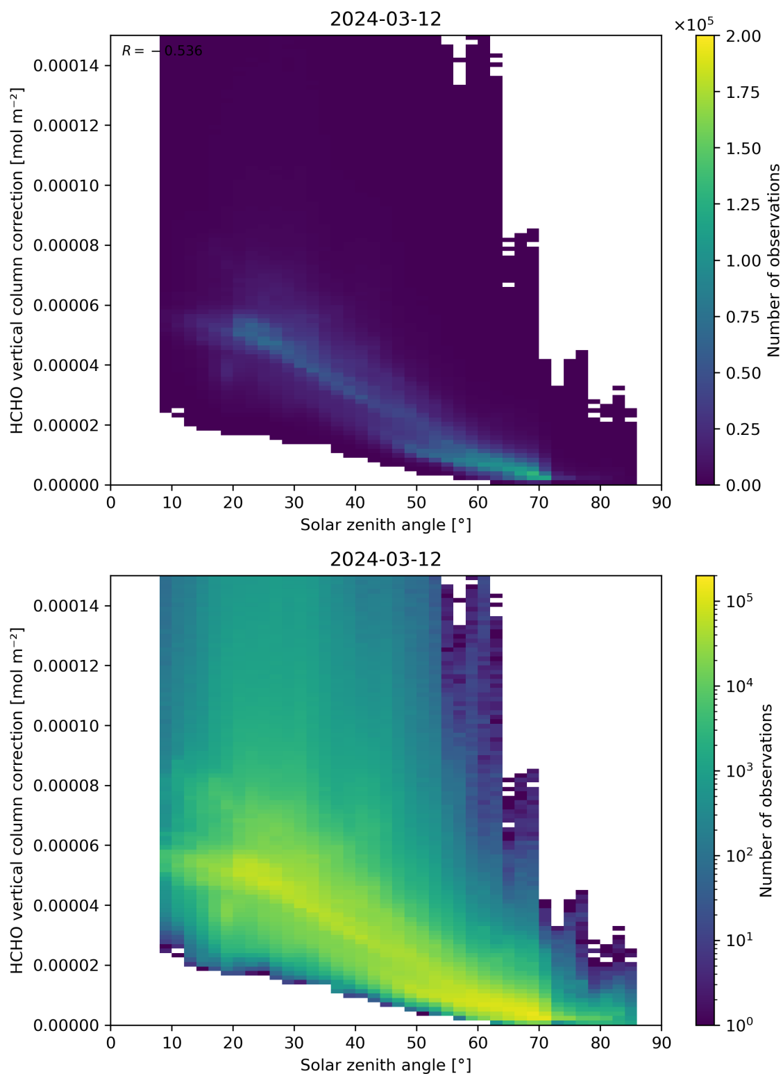
Figure 178: Scatter density plot of “Solar zenith angle” against “HCHO vertical column correction” for 2024-03-11 to 2024-03-13.
