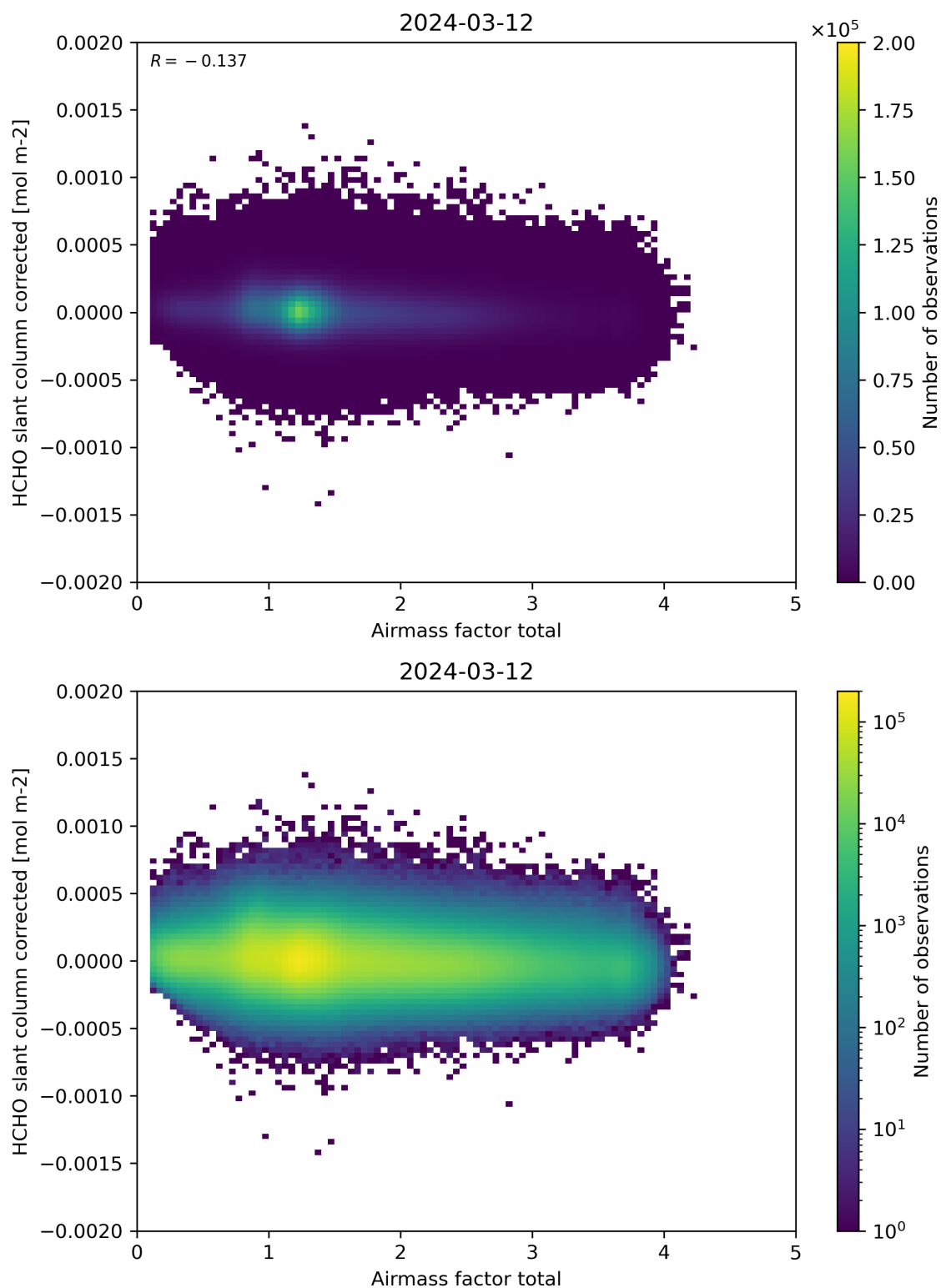
Figure 101: Scatter density plot of “Airmass factor total” against “HCHO slant column corrected” for 2024-03-11 to 2024-03-13.
