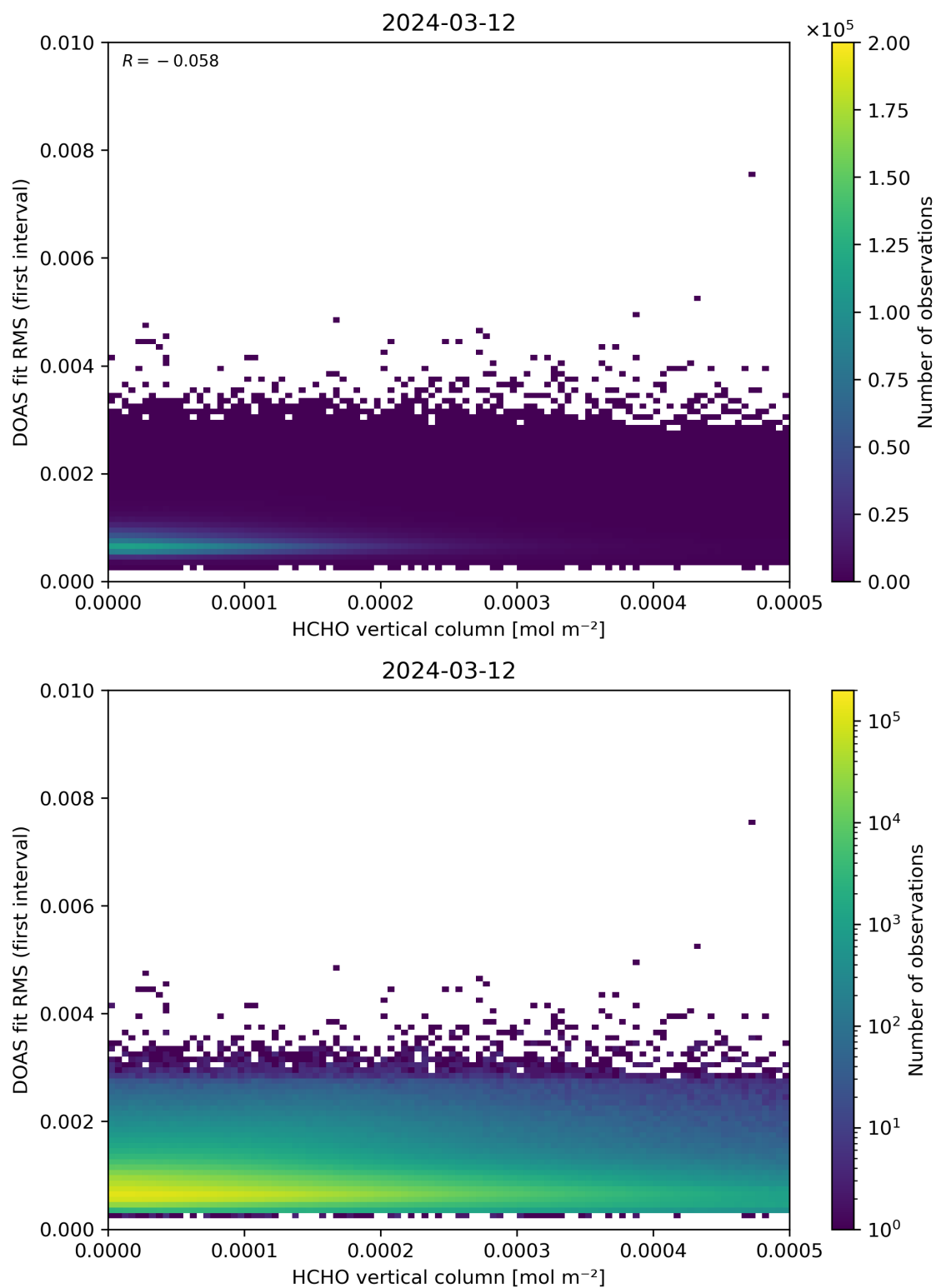
Figure 123: Scatter density plot of “HCHO vertical column” against “DOAS fit RMS (first interval)” for 2024-03-11 to 2024-03-13.
