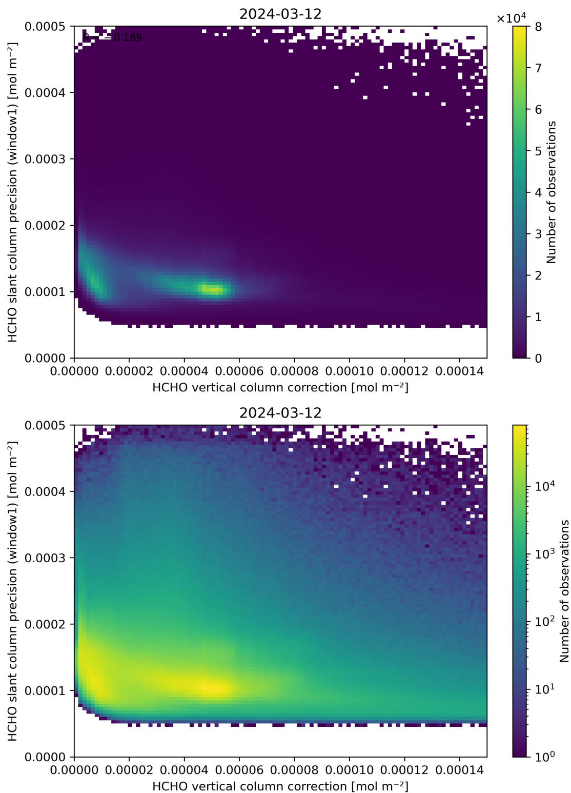
Figure 119: Scatter density plot of “HCHO vertical column correction” against “HCHO slant column precision (window1)” for 2024-03-11 to 2024-03-13.
