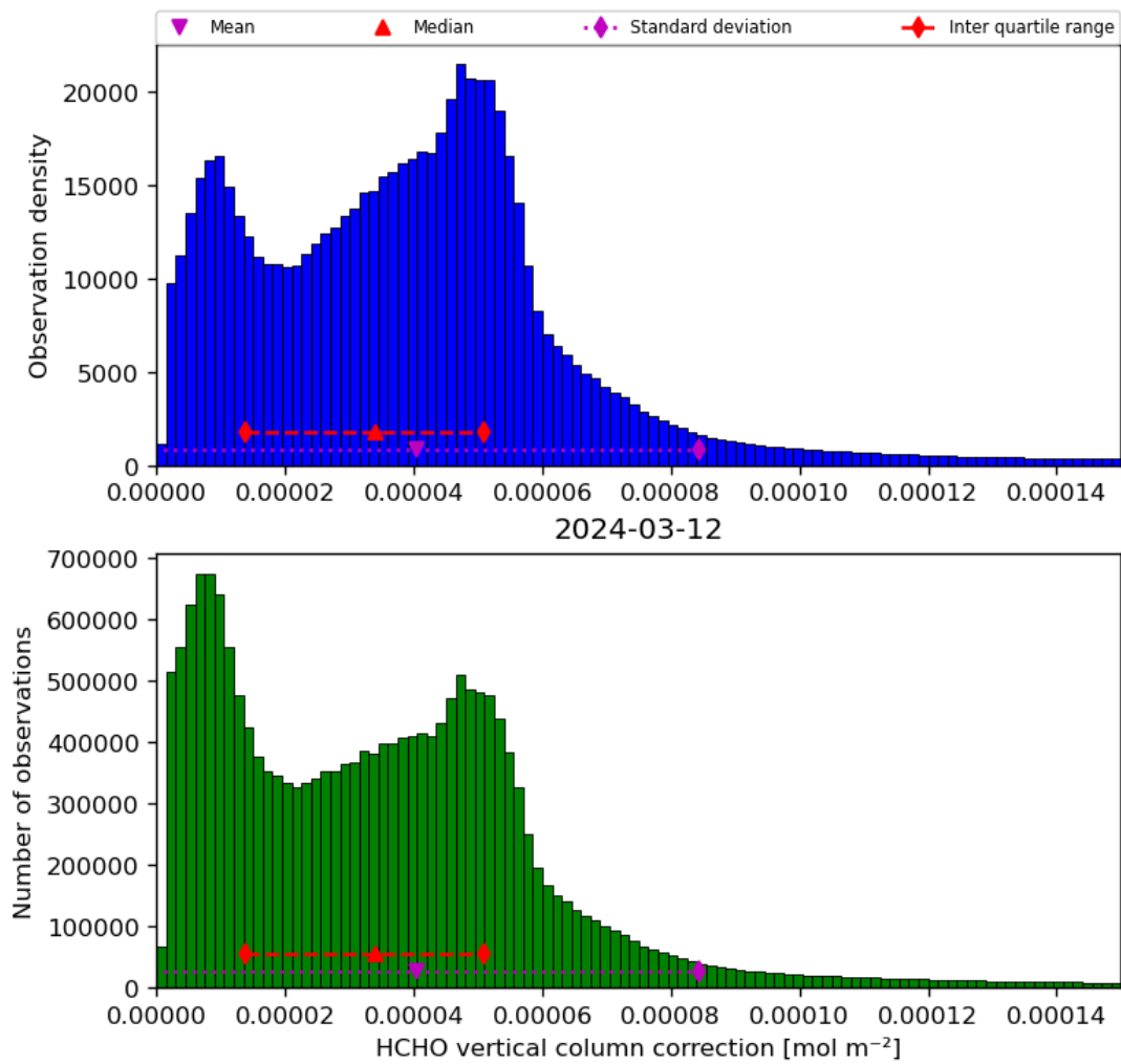
Figure 37: Histogram of “HCHO vertical column correction” for 2024-03-11 to 2024-03-13
