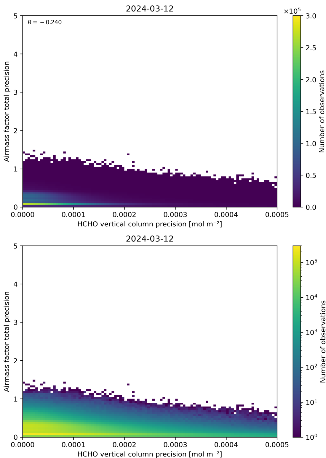
Figure 145: Scatter density plot of “HCHO vertical column precision” against “Airmass factor total precision” for 2024-03-11 to 2024-03-13.
