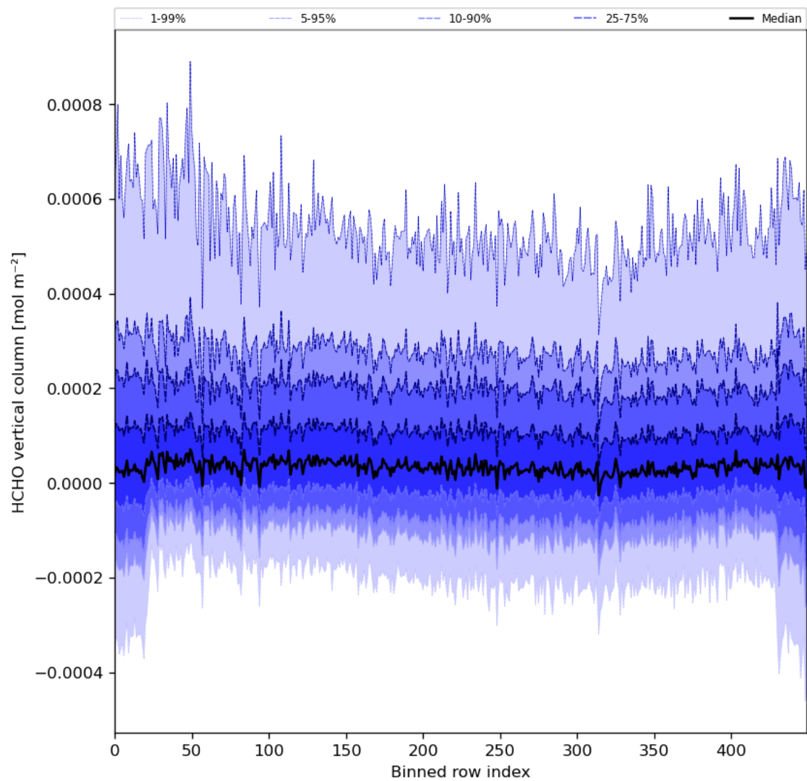
Figure 49: Along track statistics of “HCHO vertical column” for 2024-03-11 to 2024-03-13
