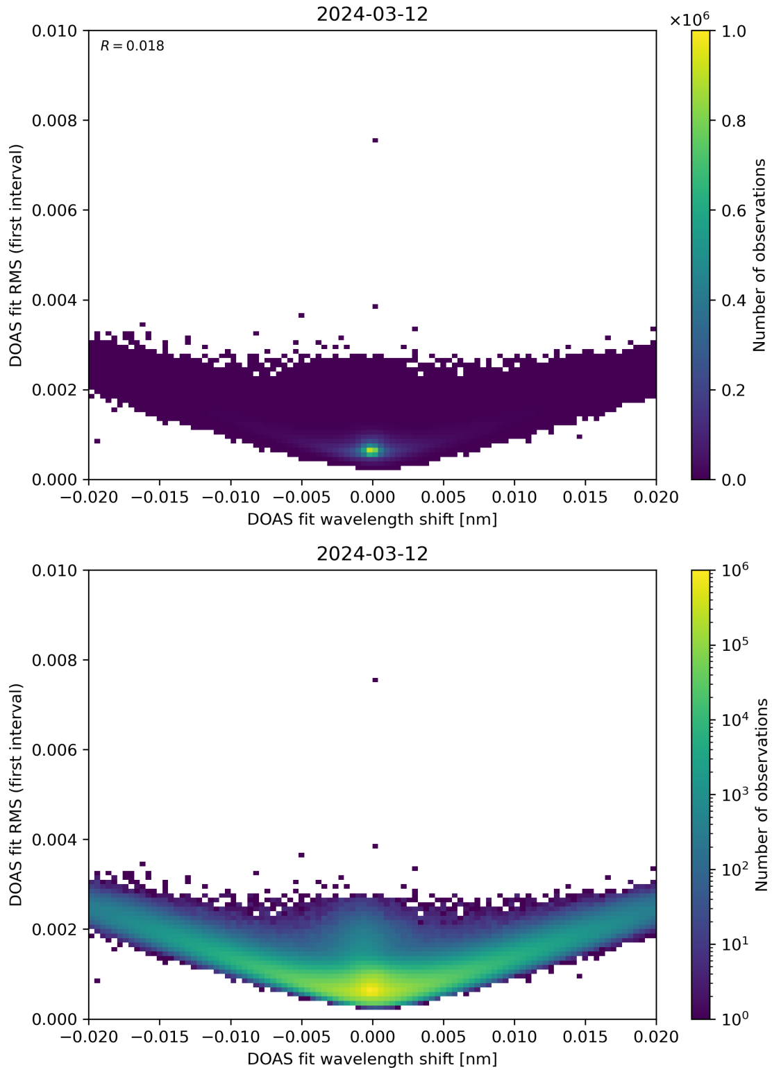
Figure 64: Scatter density plot of “DOAS fit wavelength shift” against “DOAS fit RMS (first interval)” for 2024-03-11 to 2024-03-13.
