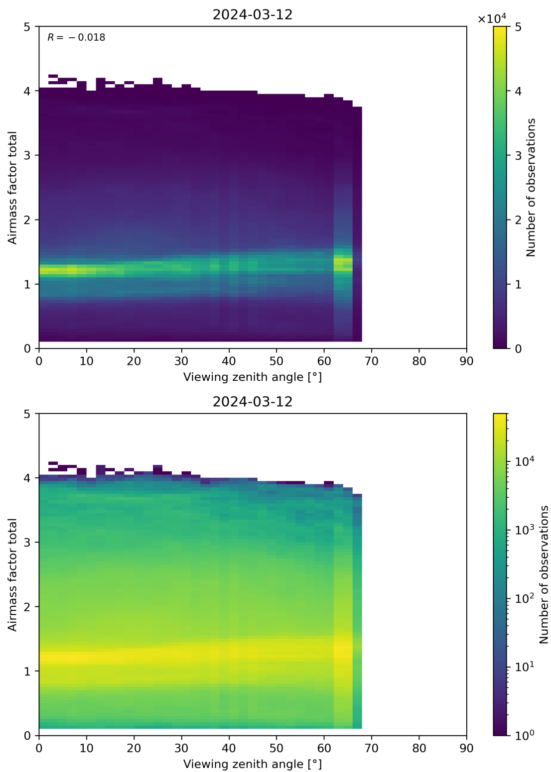
Figure 190: Scatter density plot of “Viewing zenith angle” against “Airmass factor total” for 2024-03-11 to 2024-03-13.
