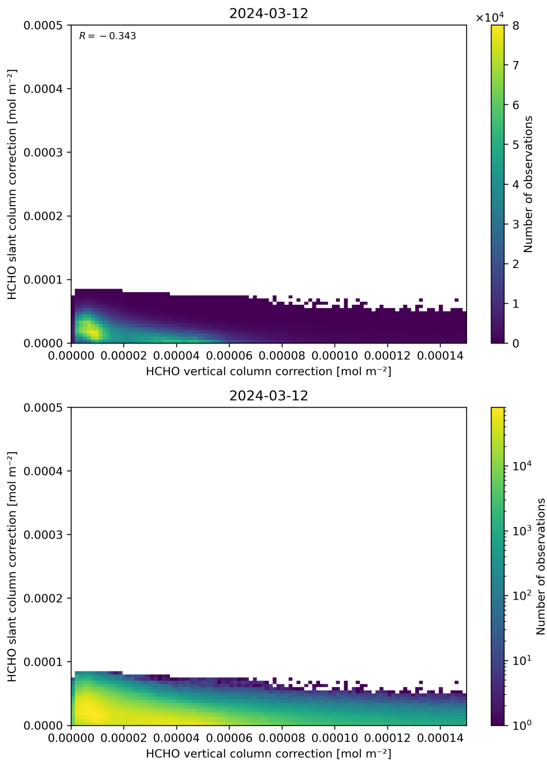
Figure 117: Scatter density plot of “HCHO vertical column correction” against “HCHO slant column correction” for 2024-03-11 to 2024-03-13.
