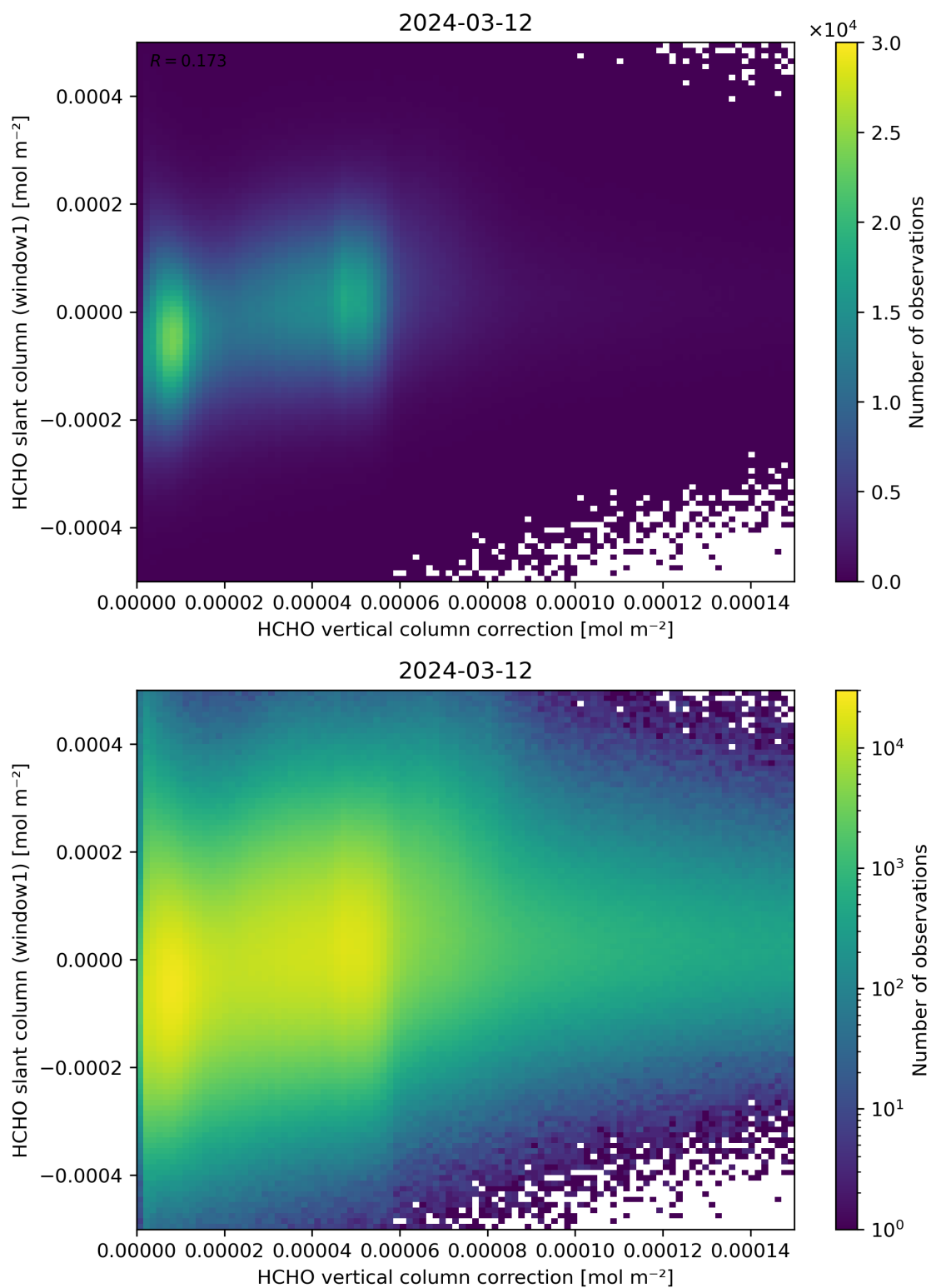
Figure 118: Scatter density plot of “HCHO vertical column correction” against “HCHO slant column (window1)” for 2024-03-11 to 2024-03-13.
