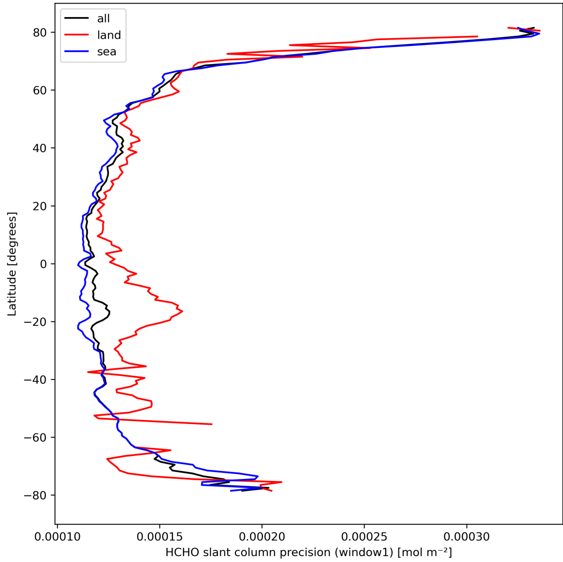
Figure 25: Zonal average of “HCHO slant column precision (window1)” for 2024-03-11 to 2024-03-13.
