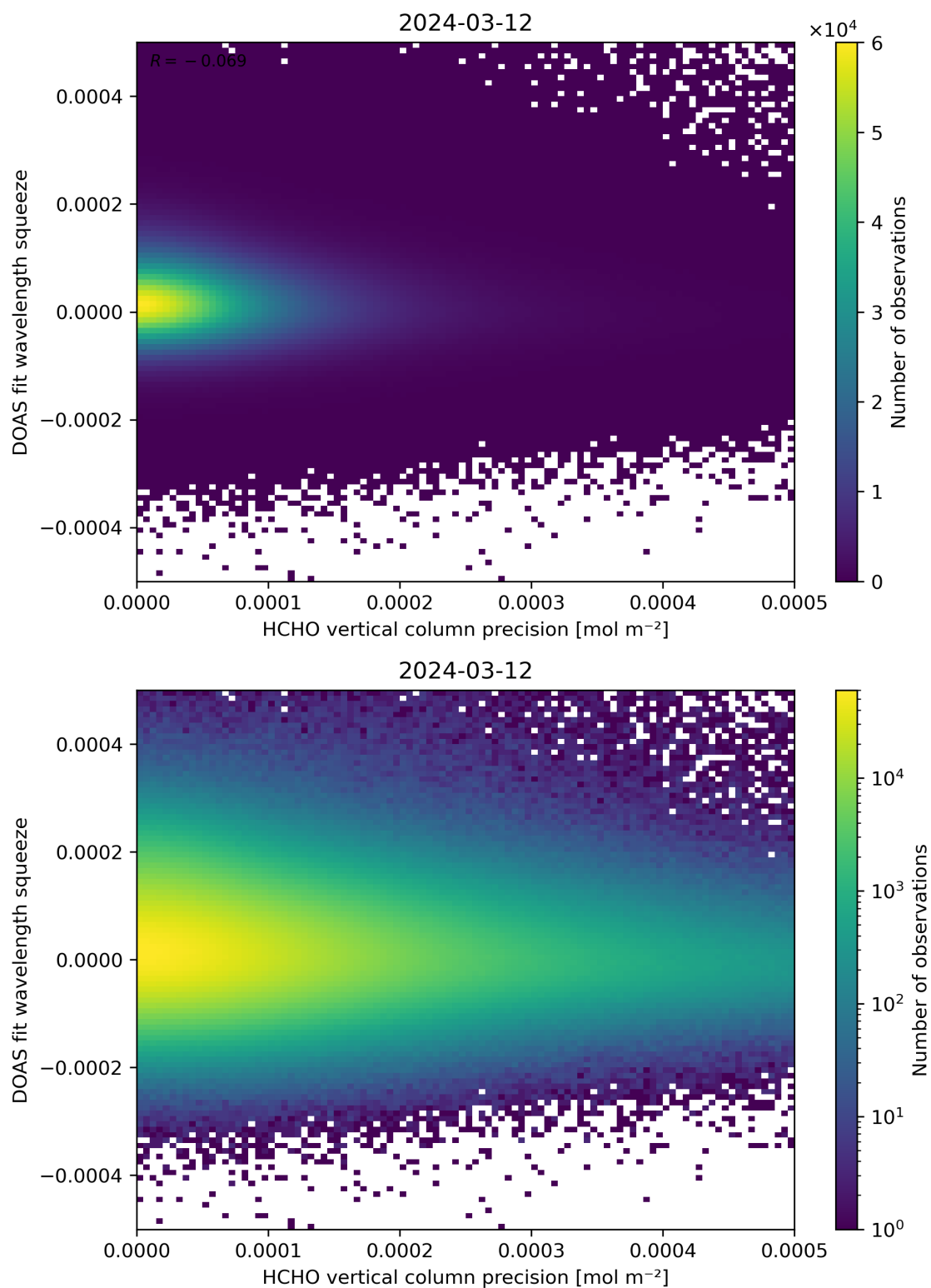
Figure 138: Scatter density plot of “HCHO vertical column precision” against “DOAS fit wavelength squeeze” for 2024-03-11 to 2024-03-13.
