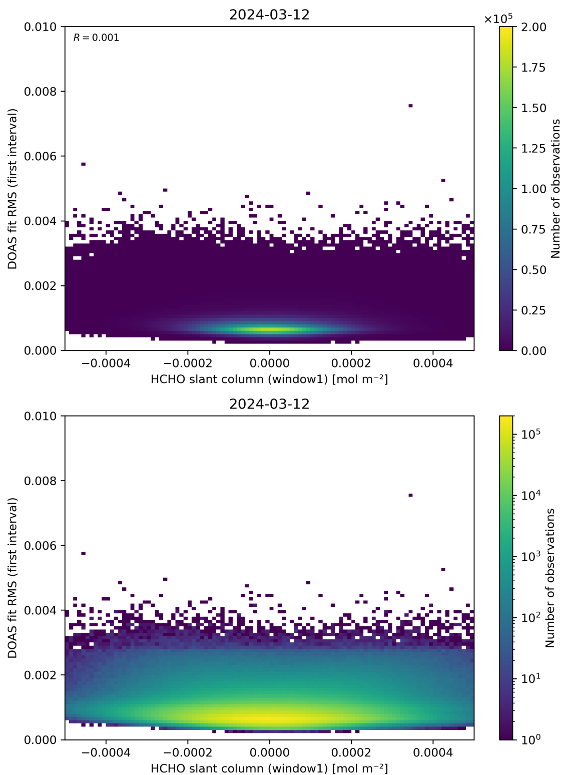
Figure 78: Scatter density plot of “HCHO slant column (window1)” against “DOAS fit RMS (first interval)” for 2024-03-11 to 2024-03-13.
