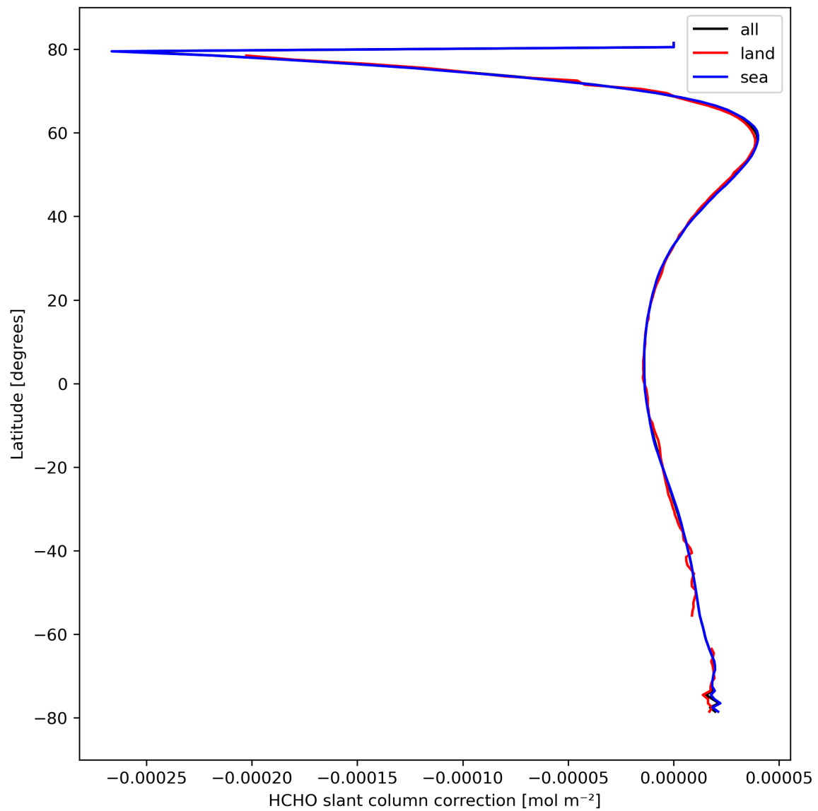
Figure 33: Zonal average of “HCHO slant column correction” for 2024-03-11 to 2024-03-13.
