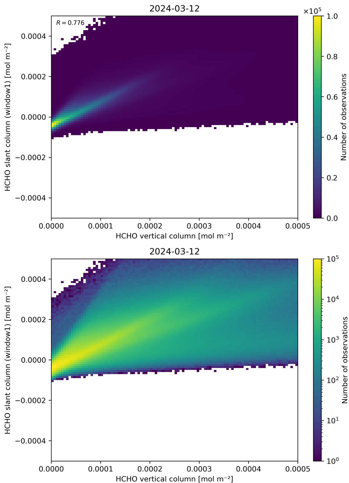
Figure 129: Scatter density plot of “HCHO vertical column” against “HCHO slant column (window1)” for 2024-03-11 to 2024-03-13.
