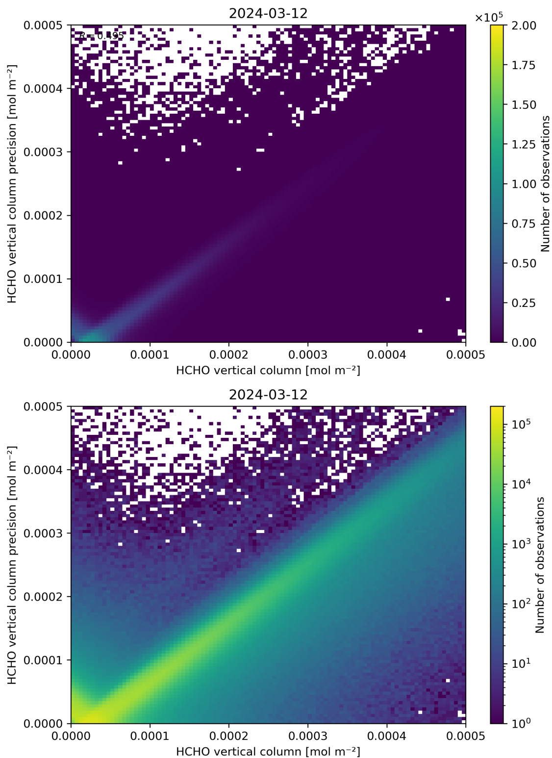
Figure 134: Scatter density plot of “HCHO vertical column” against “HCHO vertical column precision” for 2024-03-11 to 2024-03-13.
