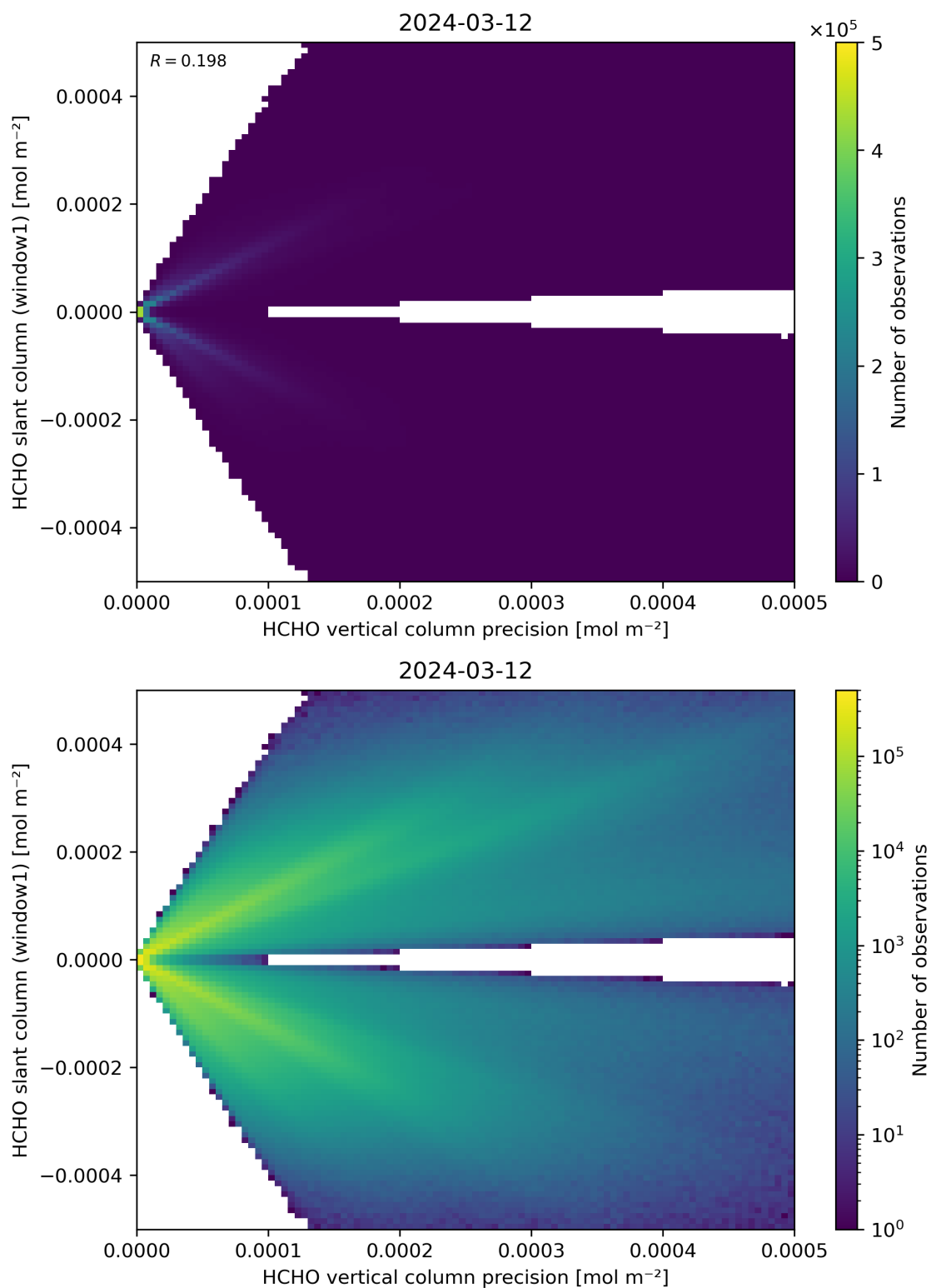
Figure 142: Scatter density plot of “HCHO vertical column precision” against “HCHO slant column (window1)” for 2024-03-11 to 2024-03-13.
