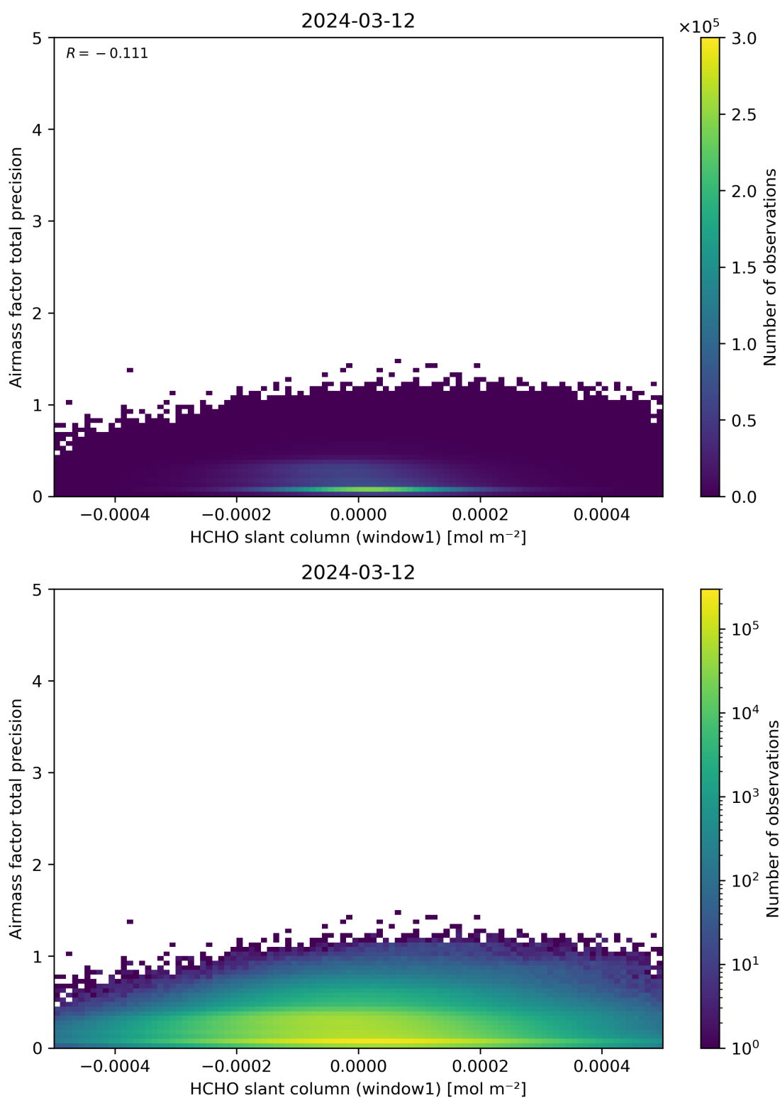
Figure 86: Scatter density plot of “HCHO slant column (window1)” against “Airmass factor total precision” for 2024-03-11 to 2024-03-13.
