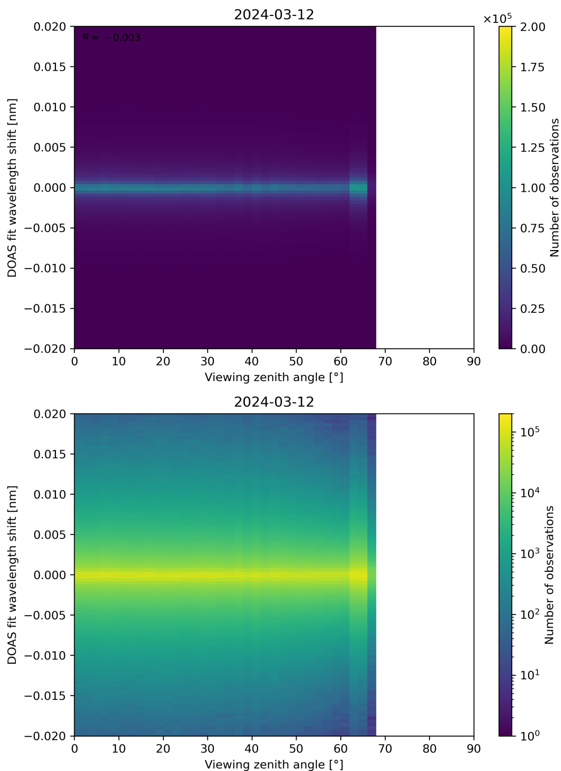
Figure 183: Scatter density plot of “Viewing zenith angle” against “DOAS fit wavelength shift” for 2024-03-11 to 2024-03-13.
