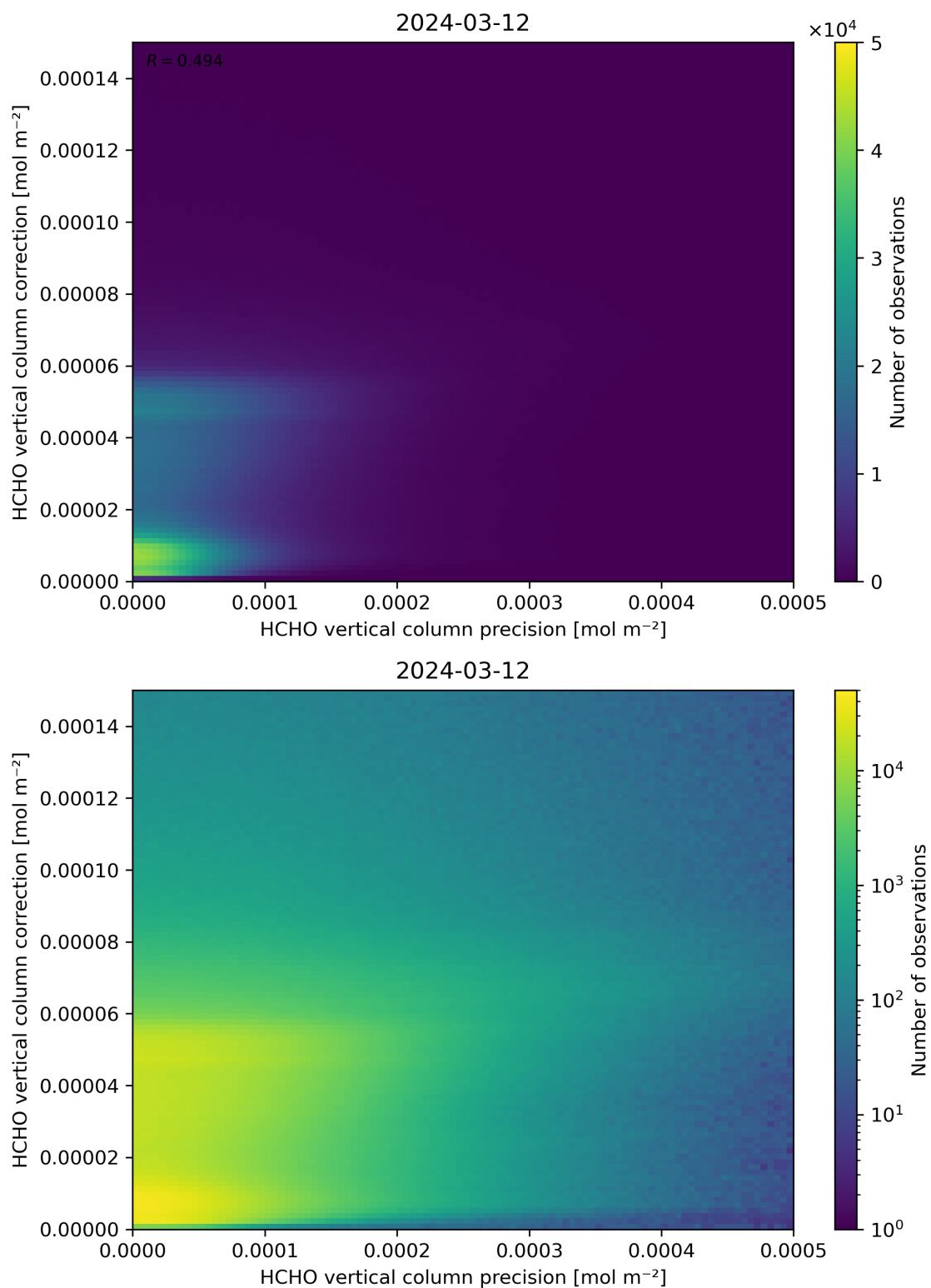
Figure 146: Scatter density plot of “HCHO vertical column precision” against “HCHO vertical column correction” for 2024-03-11 to 2024-03-13.
