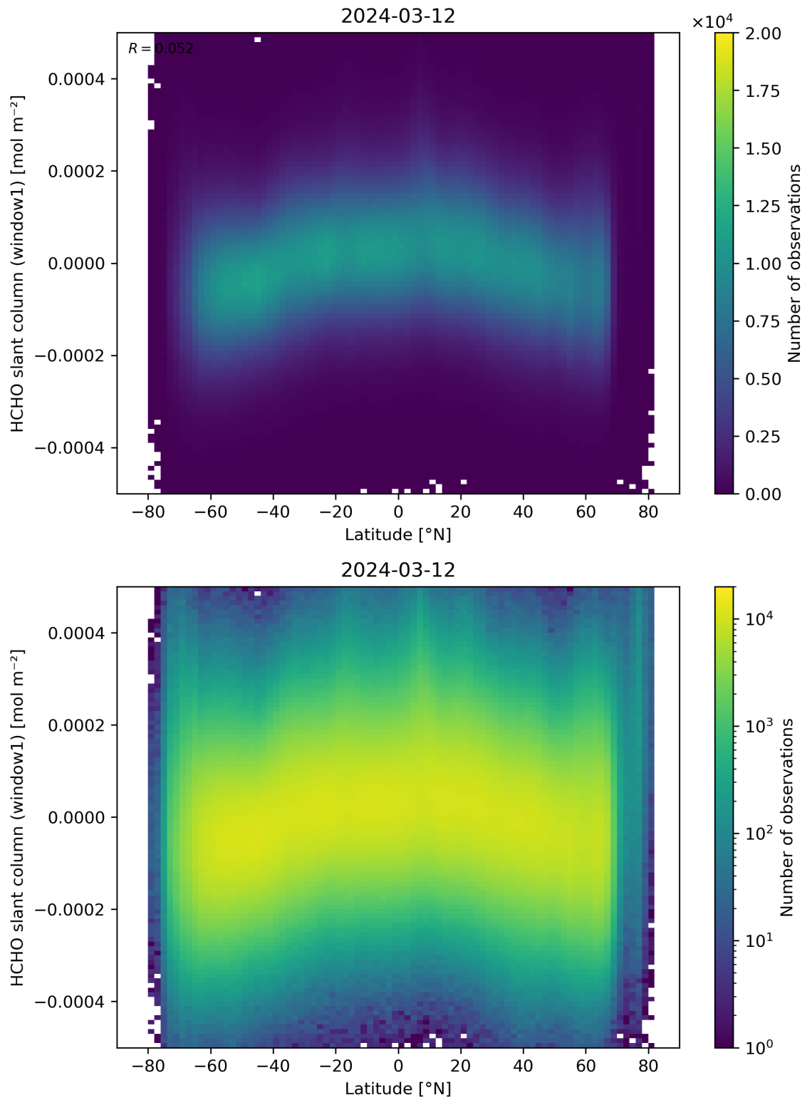
Figure 159: Scatter density plot of “Latitude” against “HCHO slant column (window1)” for 2024-03-11 to 2024-03-13.
