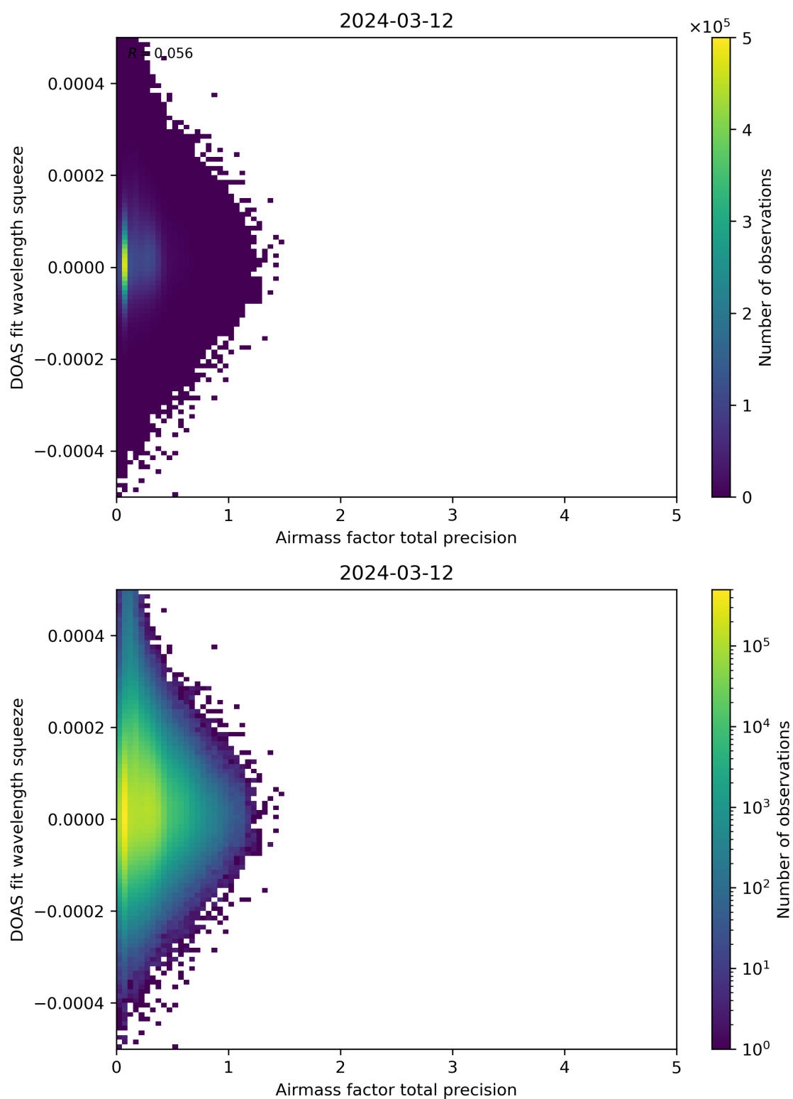
Figure 107: Scatter density plot of “Airmass factor total precision” against “DOAS fit wavelength squeeze” for 2024-03-11 to 2024-03-13.
