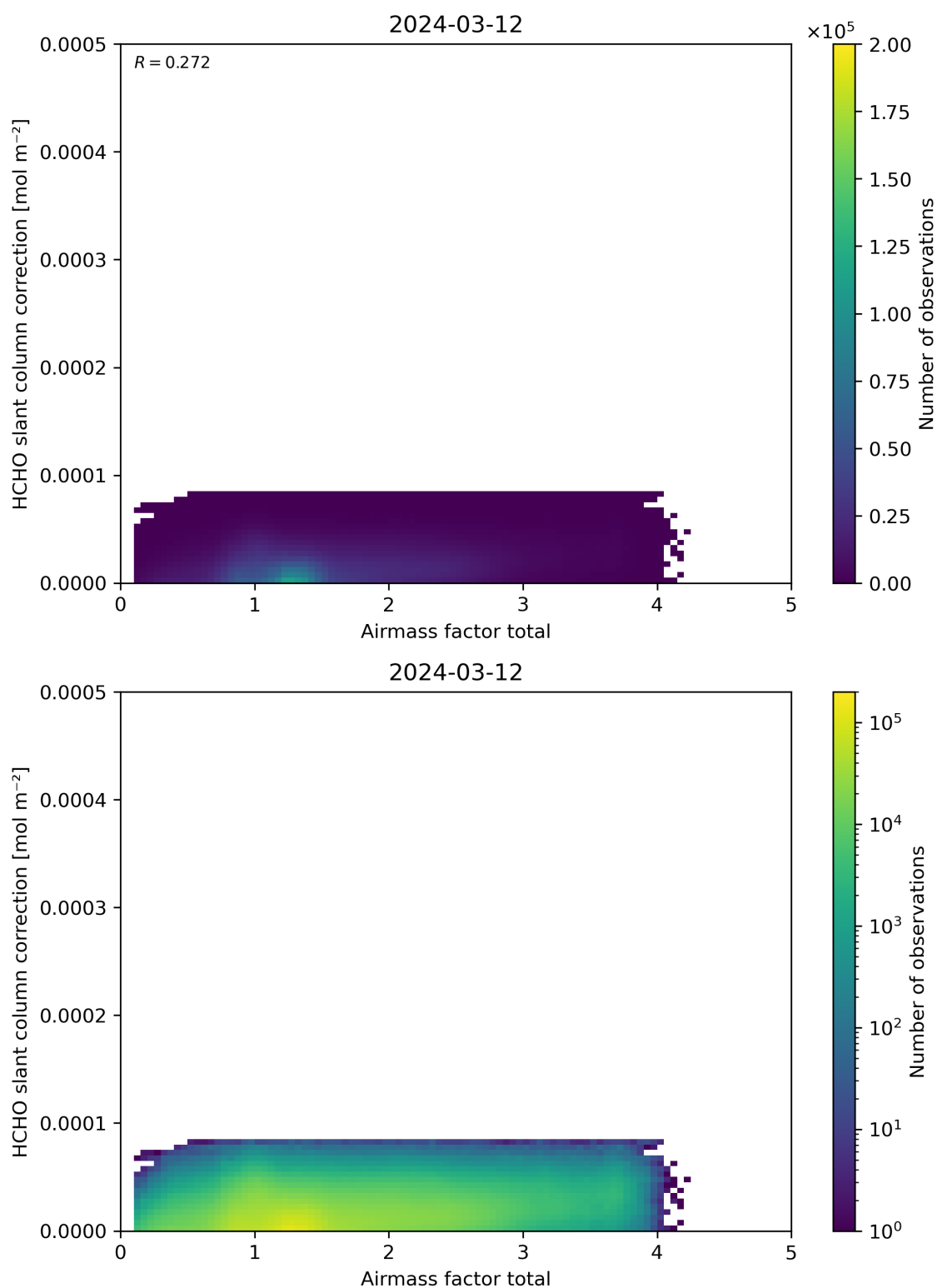
Figure 102: Scatter density plot of “Airmass factor total” against “HCHO slant column correction” for 2024-03-11 to 2024-03-13.
