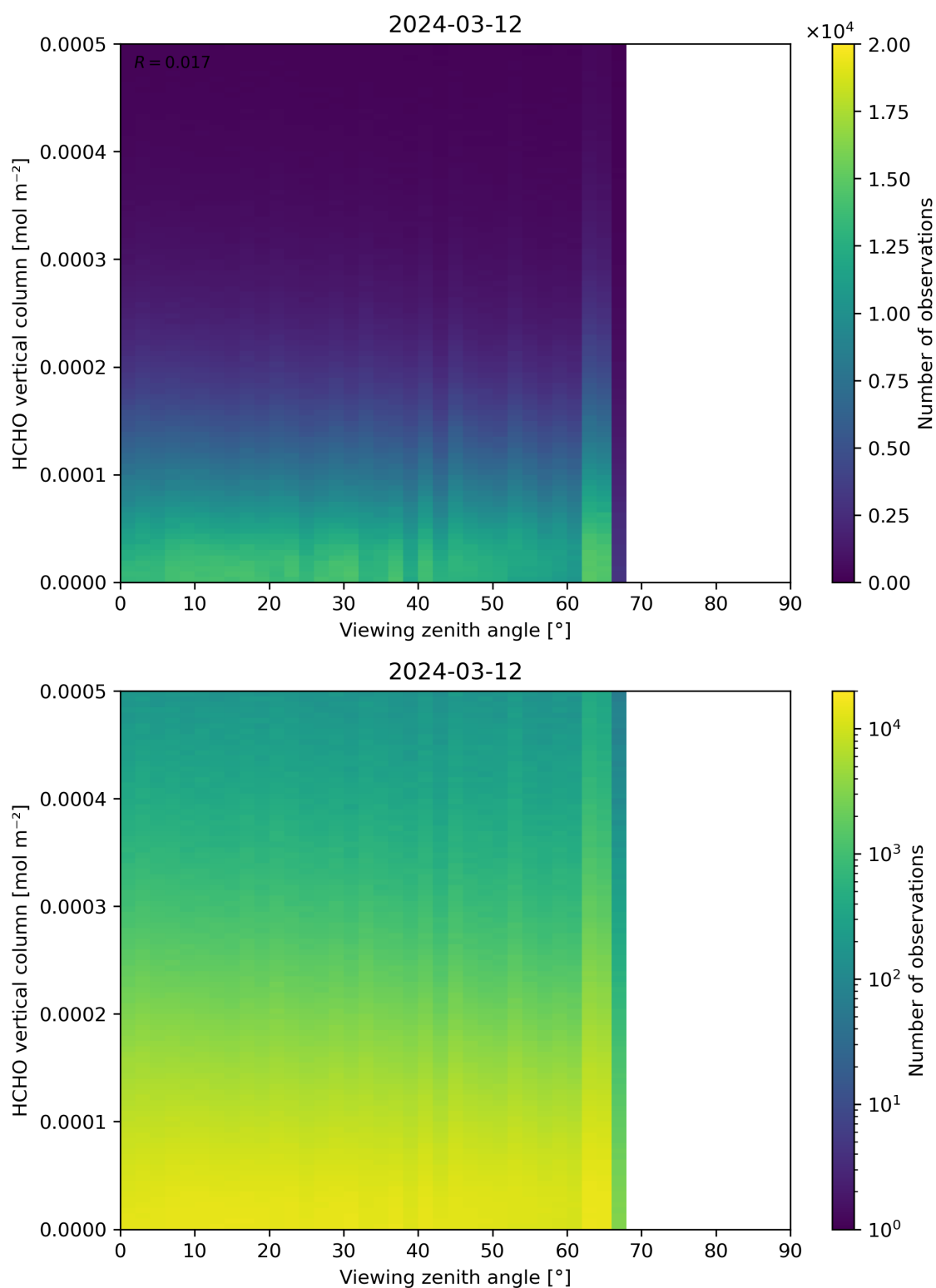
Figure 192: Scatter density plot of “Viewing zenith angle” against “HCHO vertical column” for 2024-03-11 to 2024-03-13.
