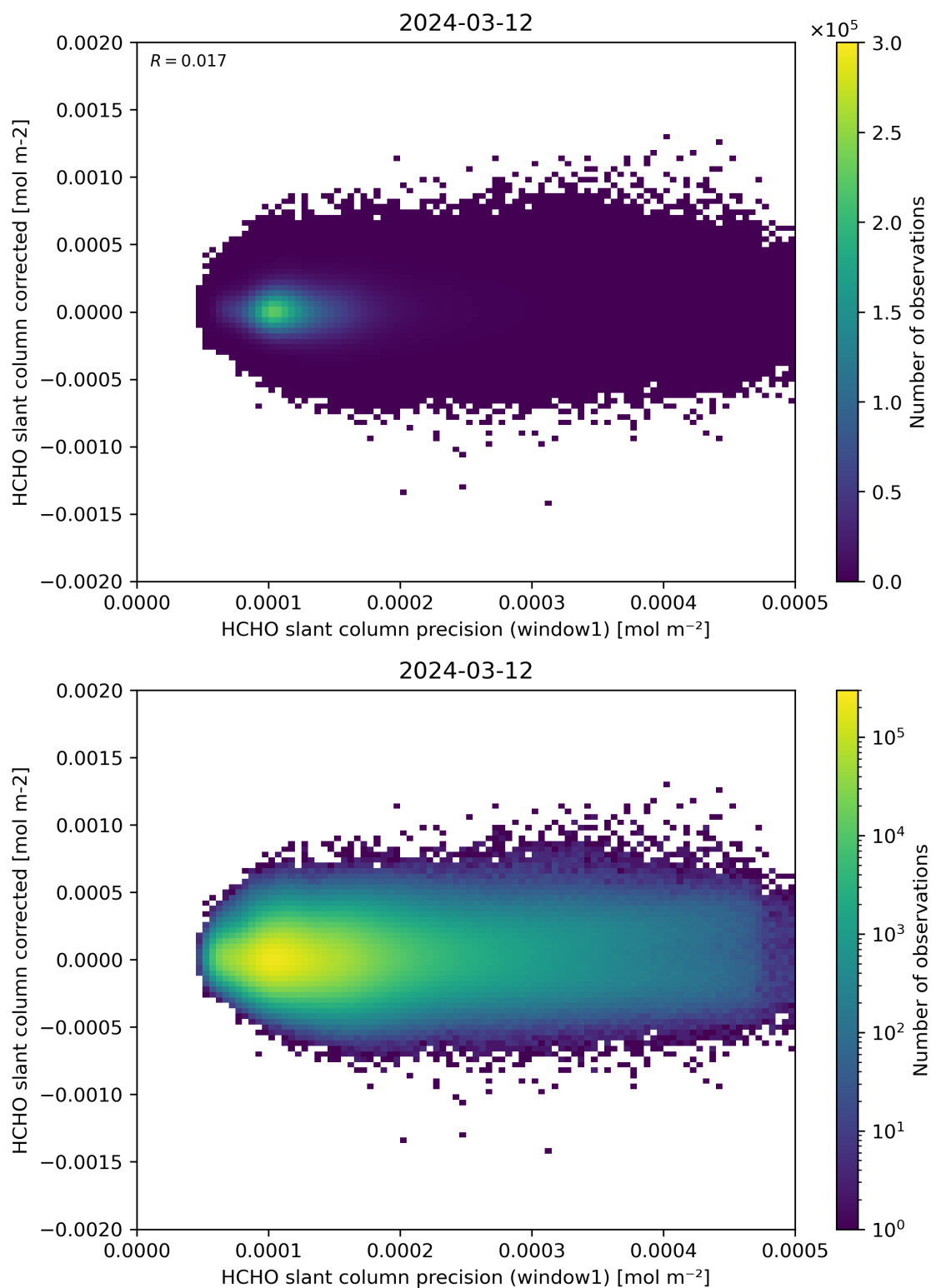
Figure 92: Scatter density plot of “HCHO slant column precision (window1)” against “HCHO slant column corrected” for 2024-03-11 to 2024-03-13.
