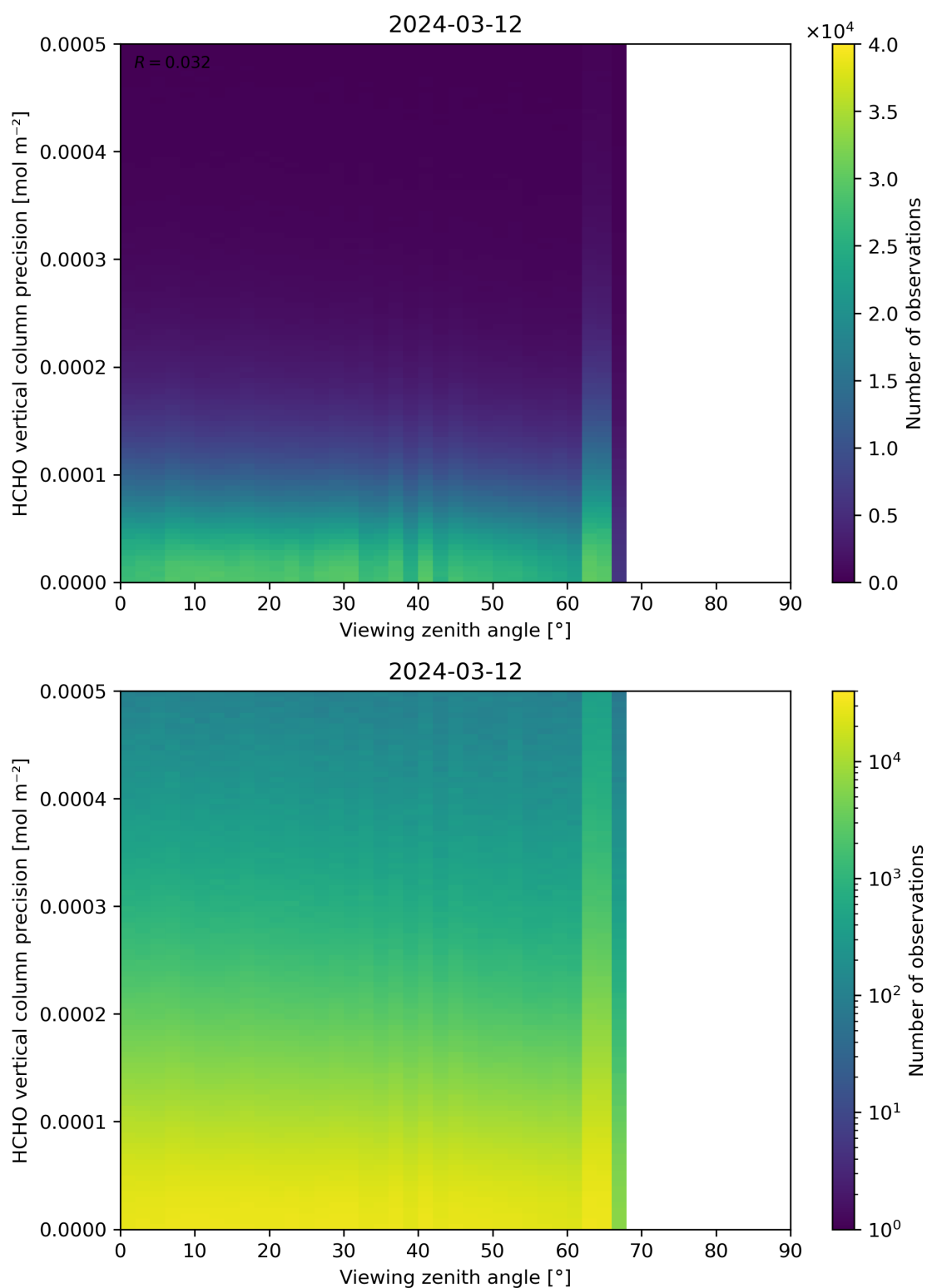
Figure 194: Scatter density plot of “Viewing zenith angle” against “HCHO vertical column precision” for 2024-03-11 to 2024-03-13.
