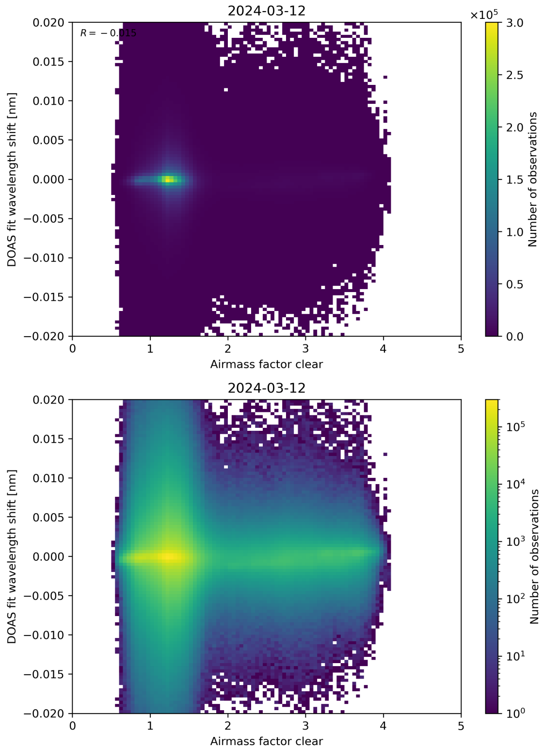
Figure 72: Scatter density plot of “Airmass factor clear” against “DOAS fit wavelength shift” for 2024-03-11 to 2024-03-13.
