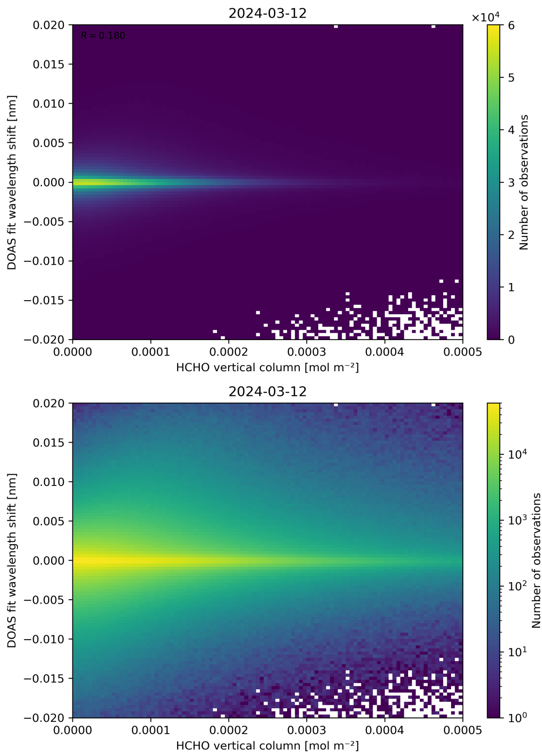
Figure 124: Scatter density plot of “HCHO vertical column” against “DOAS fit wavelength shift” for 2024-03-11 to 2024-03-13.
