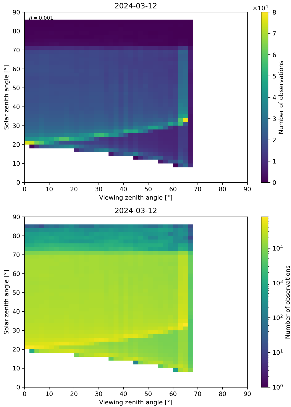
Figure 197: Scatter density plot of “Viewing zenith angle” against “Solar zenith angle” for 2024-03-11 to 2024-03-13.
