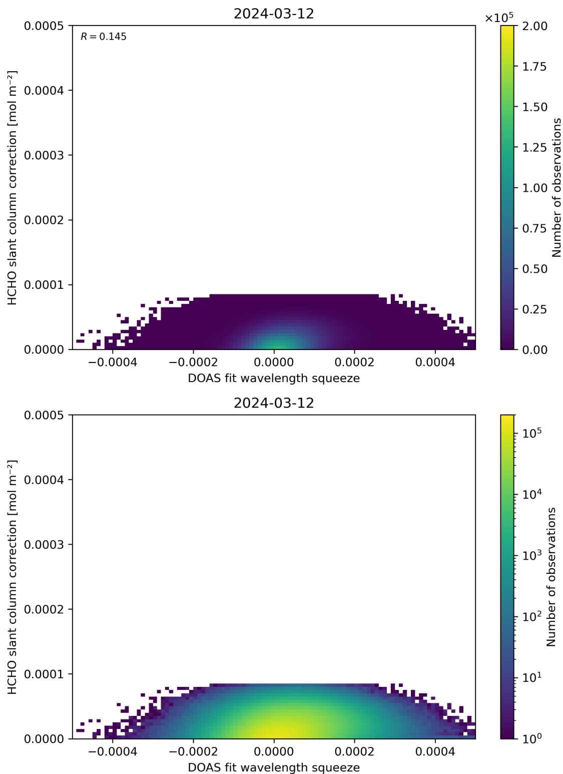
Figure 70: Scatter density plot of “DOAS fit wavelength squeeze” against “HCHO slant column correction” for 2024-03-11 to 2024-03-13.
