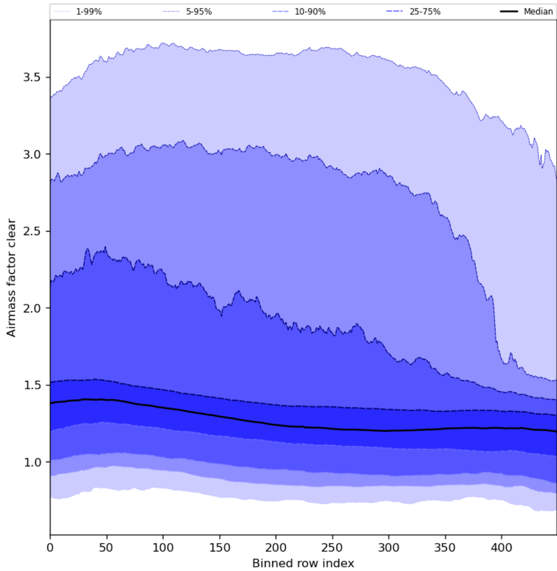
Figure 56: Along track statistics of “Airmass factor clear” for 2024-03-11 to 2024-03-13
