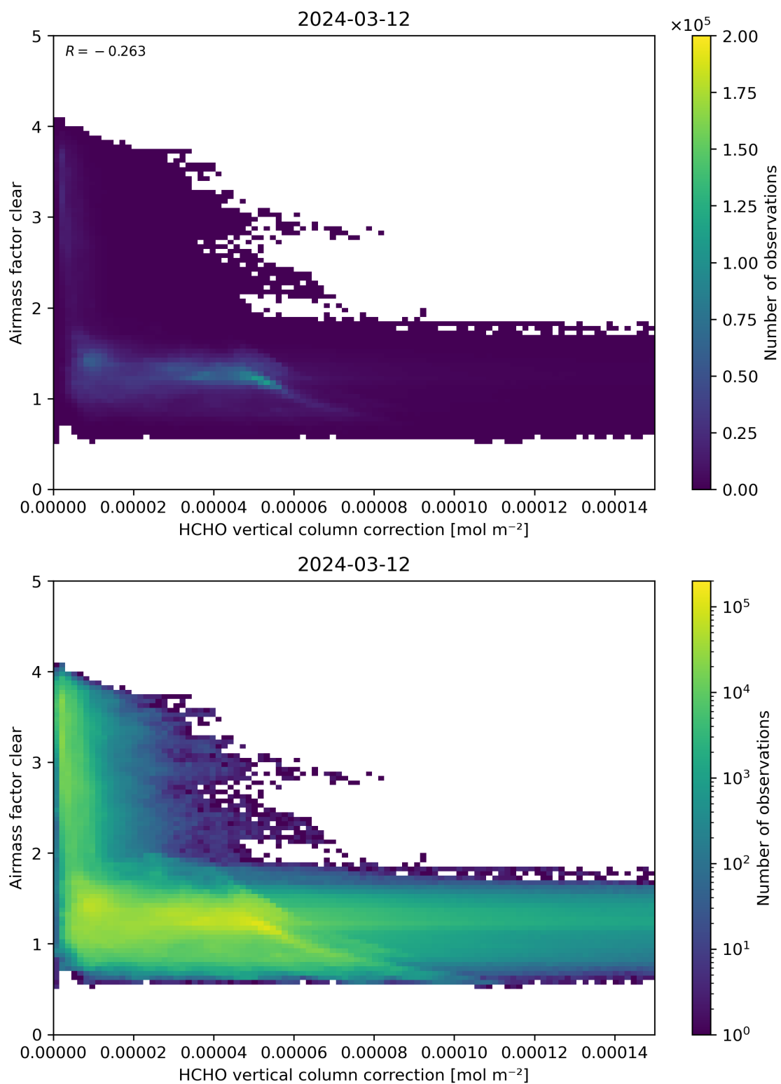
Figure 115: Scatter density plot of “HCHO vertical column correction” against “Airmass factor clear” for 2024-03-11 to 2024-03-13.
