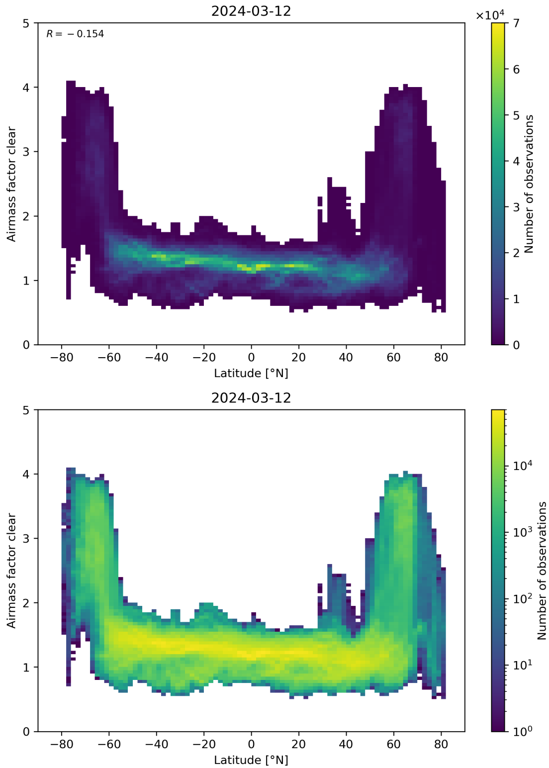
Figure 156: Scatter density plot of “Latitude” against “Airmass factor clear” for 2024-03-11 to 2024-03-13.
