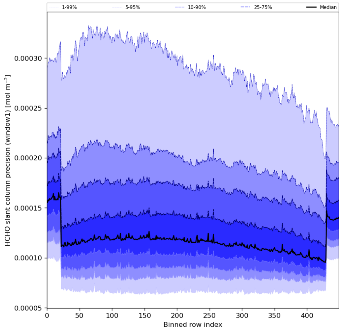
Figure 53: Along track statistics of “HCHO slant column precision (window1)” for 2024-03-11 to 2024-03-13
