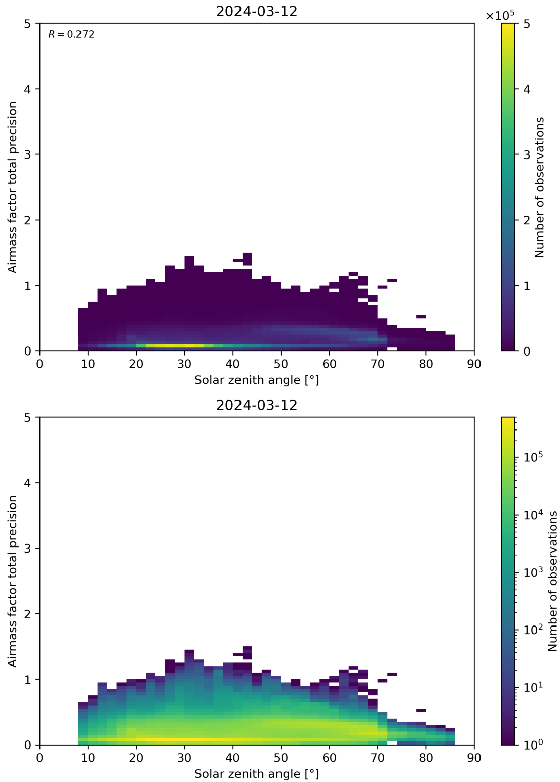
Figure 176: Scatter density plot of “Solar zenith angle” against “Airmass factor total precision” for 2024-03-11 to 2024-03-13.
