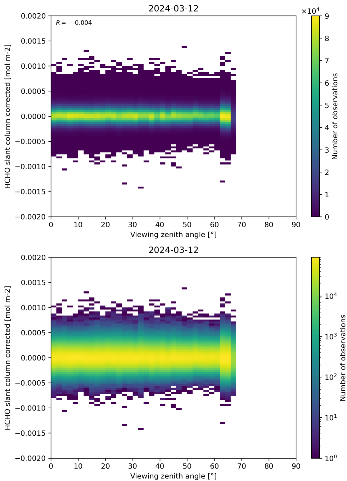
Figure 186: Scatter density plot of “Viewing zenith angle” against “HCHO slant column corrected” for 2024-03-11 to 2024-03-13.
