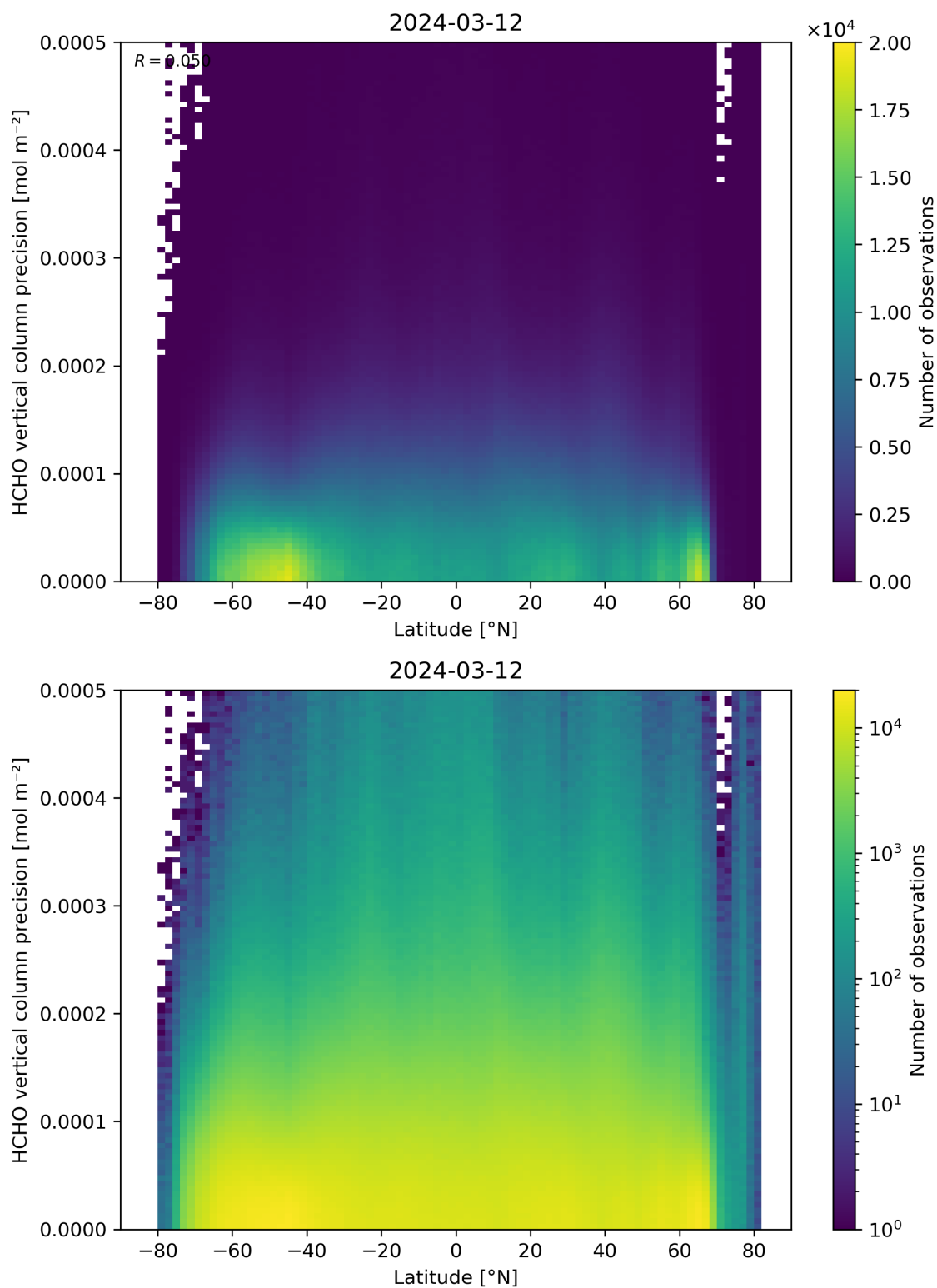
Figure 165: Scatter density plot of “Latitude” against “HCHO vertical column precision” for 2024-03-11 to 2024-03-13.
