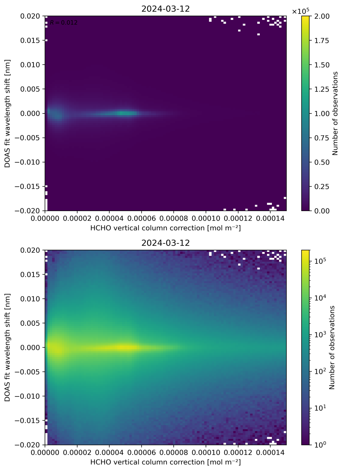
Figure 113: Scatter density plot of “HCHO vertical column correction” against “DOAS fit wavelength shift” for 2024-03-11 to 2024-03-13.
