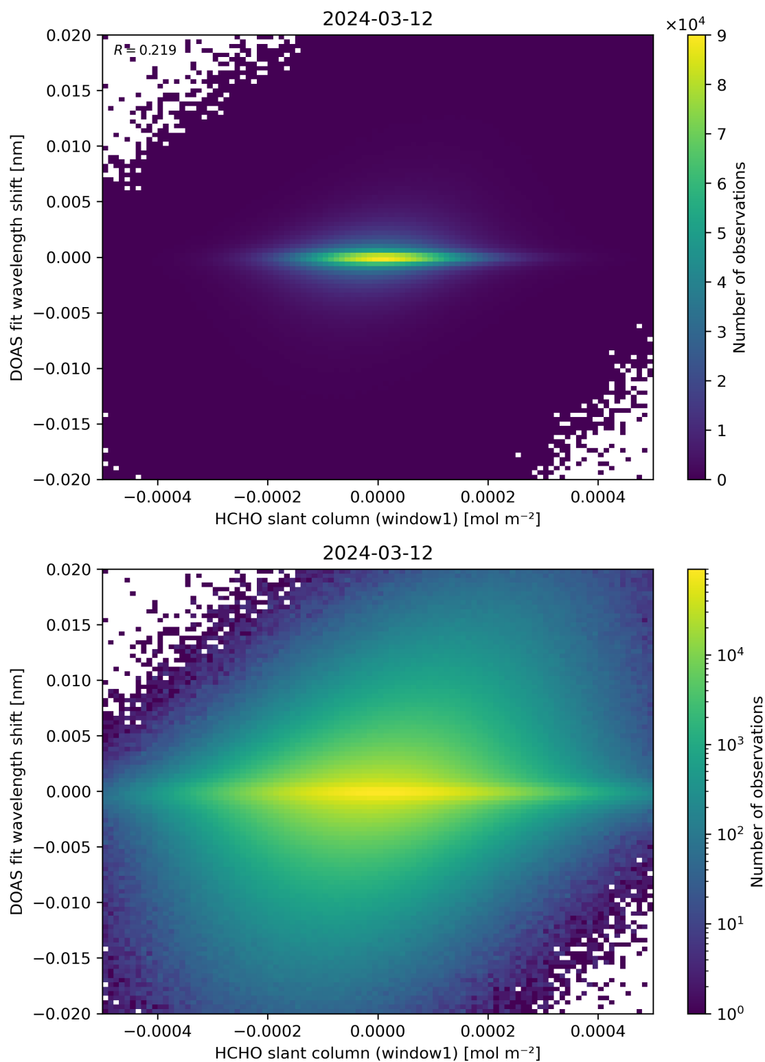
Figure 79: Scatter density plot of “HCHO slant column (window1)” against “DOAS fit wavelength shift” for 2024-03-11 to 2024-03-13.
