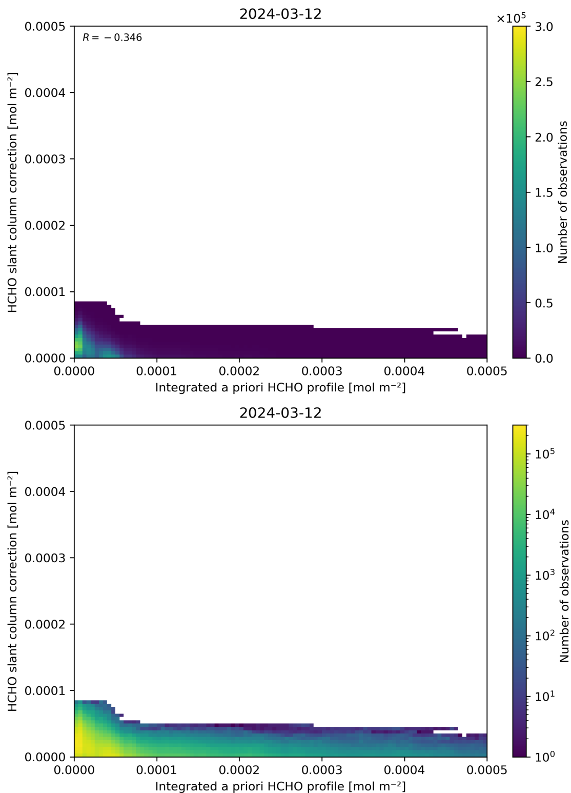
Figure 152: Scatter density plot of “Integrated a priori HCHO profile” against “HCHO slant column correction” for 2024-03-11 to 2024-03-13.
