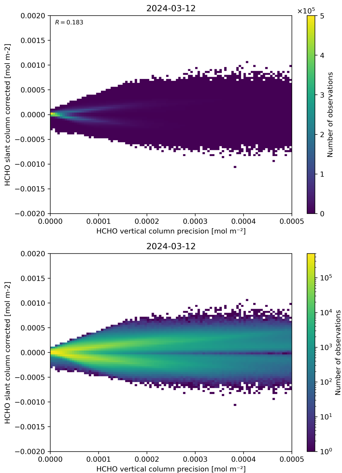
Figure 140: Scatter density plot of “HCHO vertical column precision” against “HCHO slant column corrected” for 2024-03-11 to 2024-03-13.
