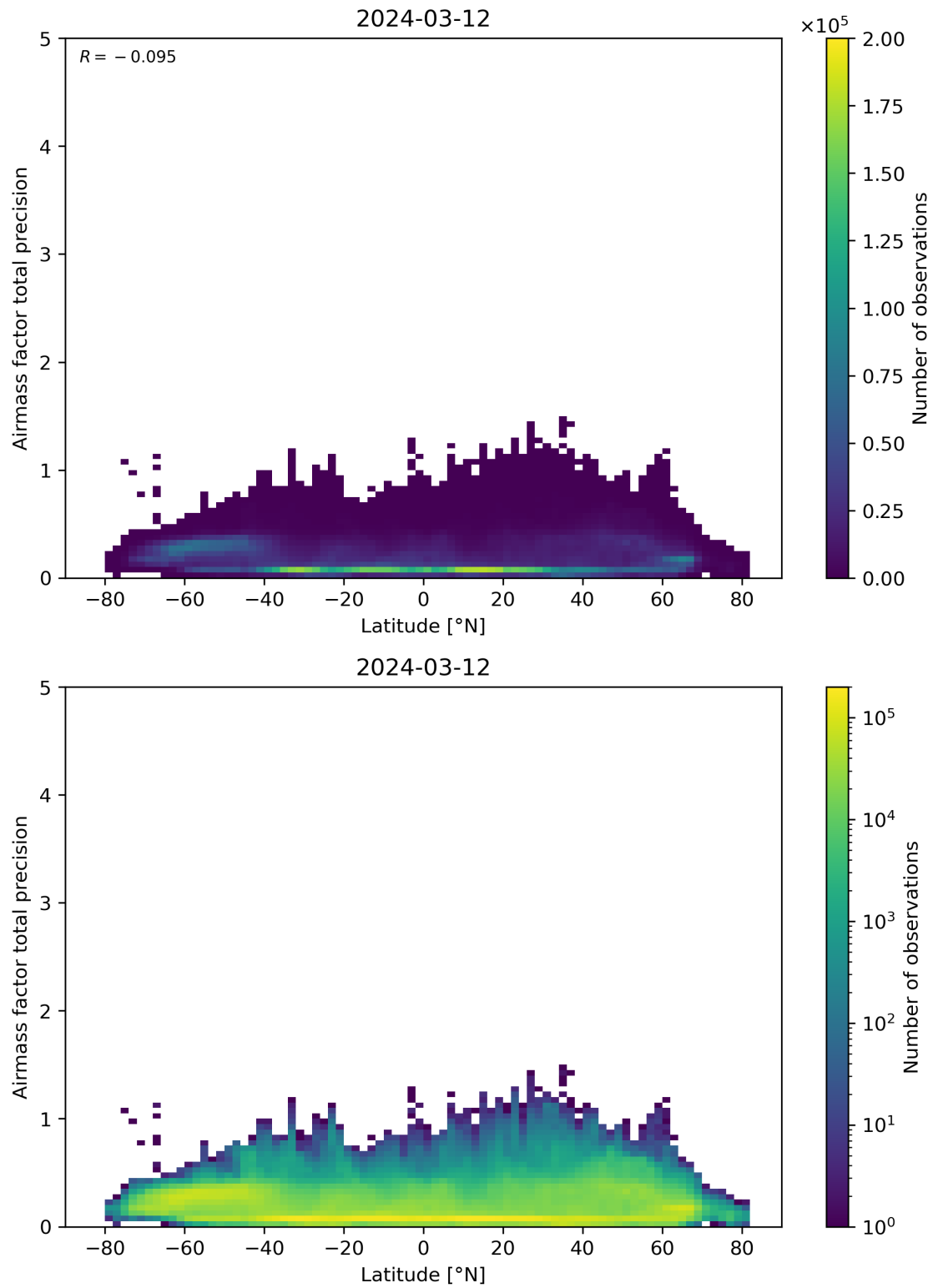
Figure 162: Scatter density plot of “Latitude” against “Airmass factor total precision” for 2024-03-11 to 2024-03-13.
