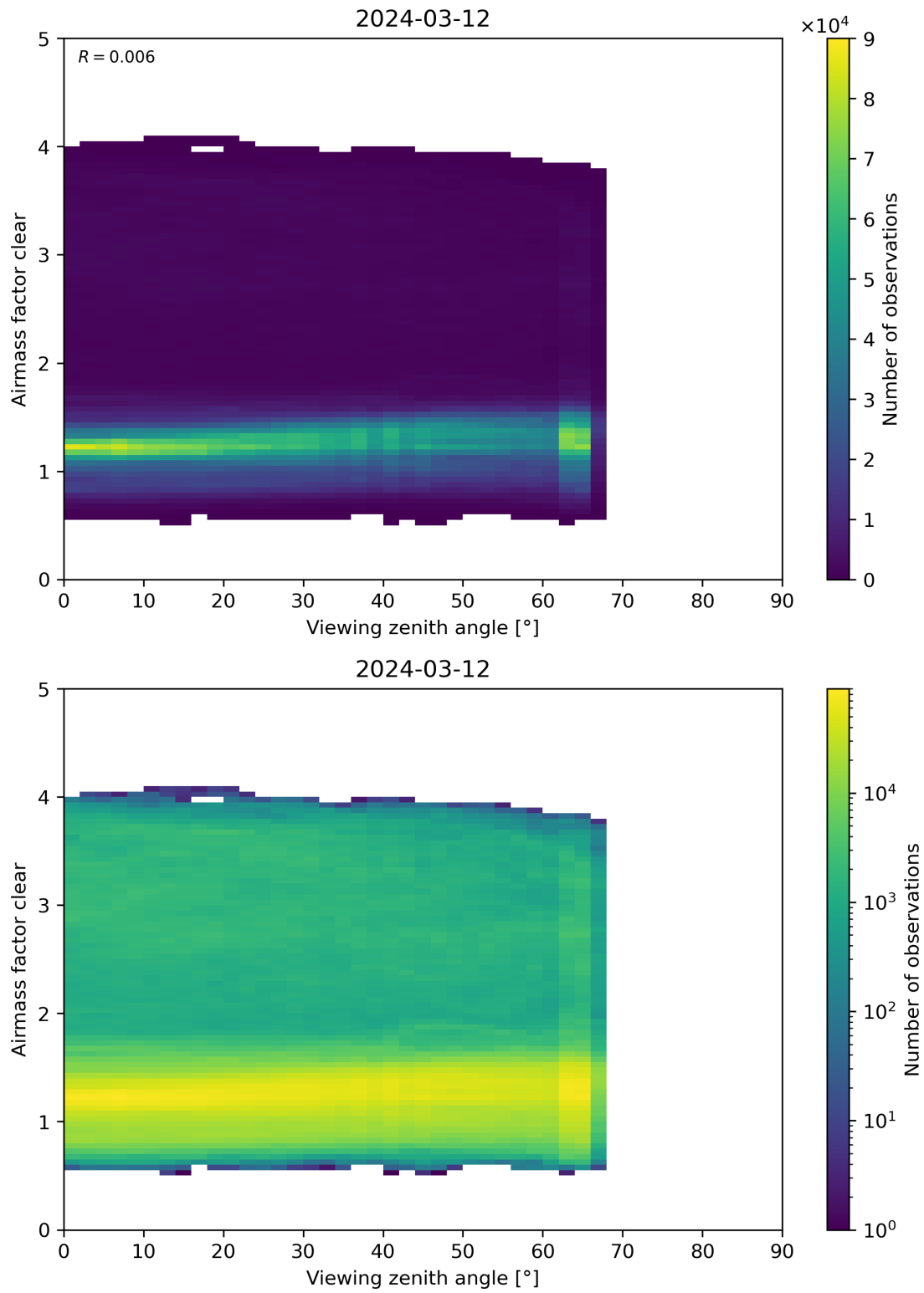
Figure 185: Scatter density plot of “Viewing zenith angle” against “Airmass factor clear” for 2024-03-11 to 2024-03-13.
