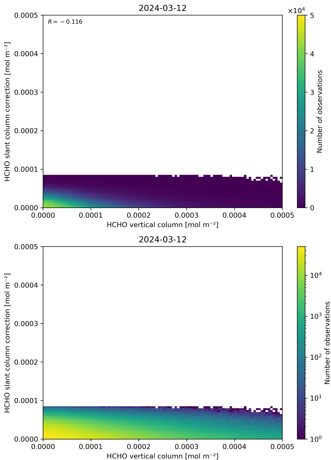
Figure 128: Scatter density plot of “HCHO vertical column” against “HCHO slant column correction” for 2024-03-11 to 2024-03-13.
