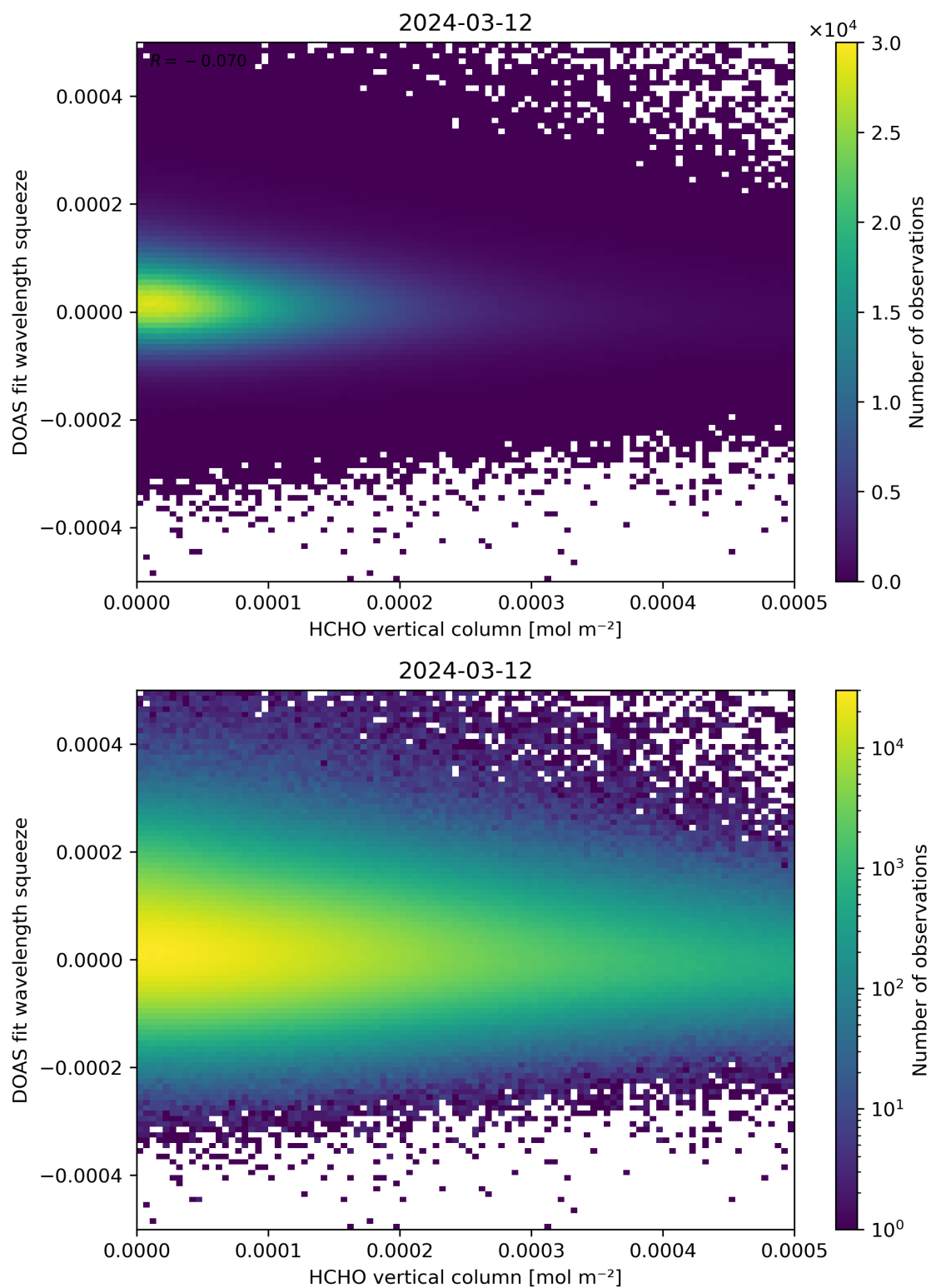
Figure 125: Scatter density plot of “HCHO vertical column” against “DOAS fit wavelength squeeze” for 2024-03-11 to 2024-03-13.
