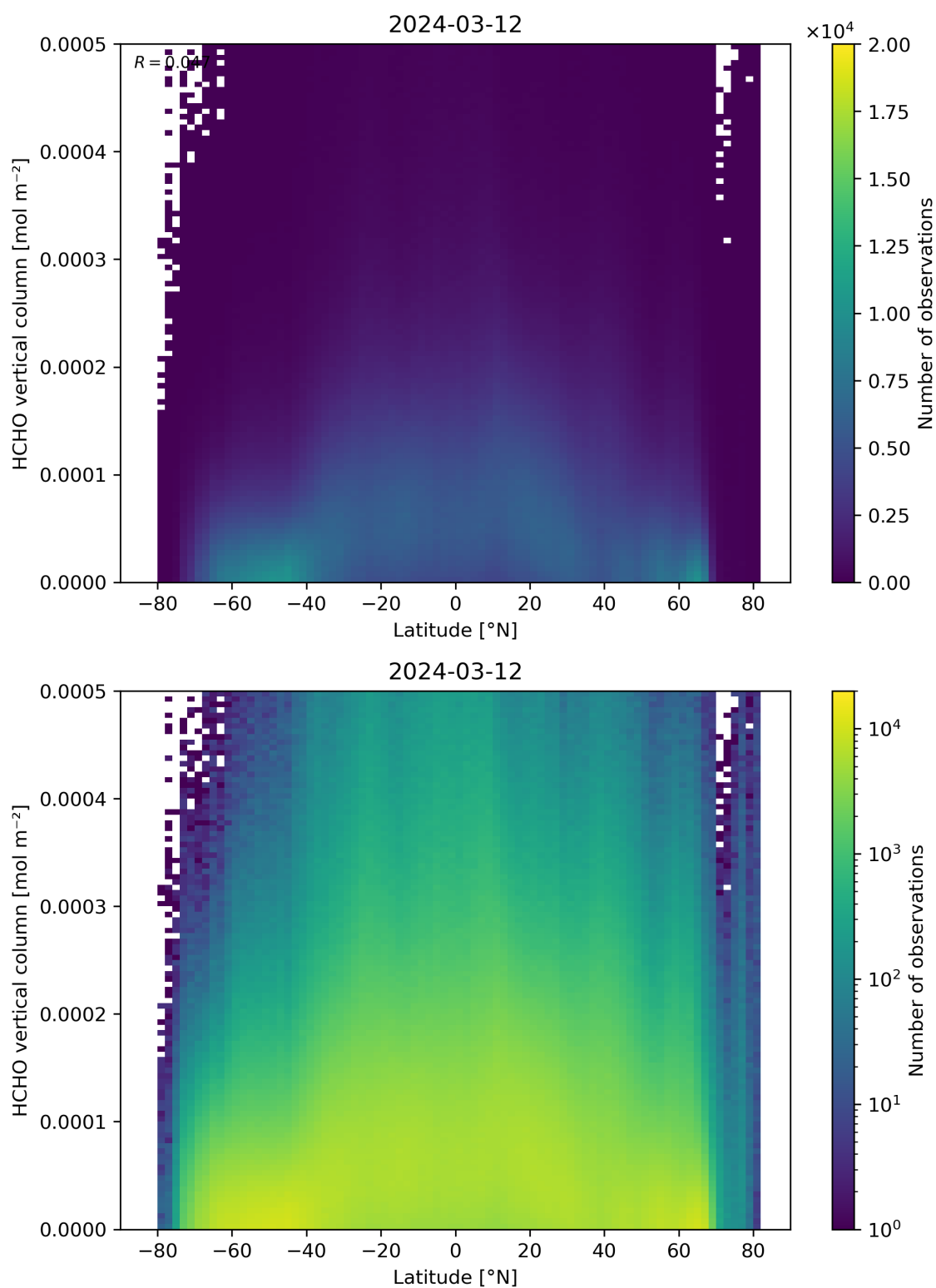
Figure 163: Scatter density plot of “Latitude” against “HCHO vertical column” for 2024-03-11 to 2024-03-13.
