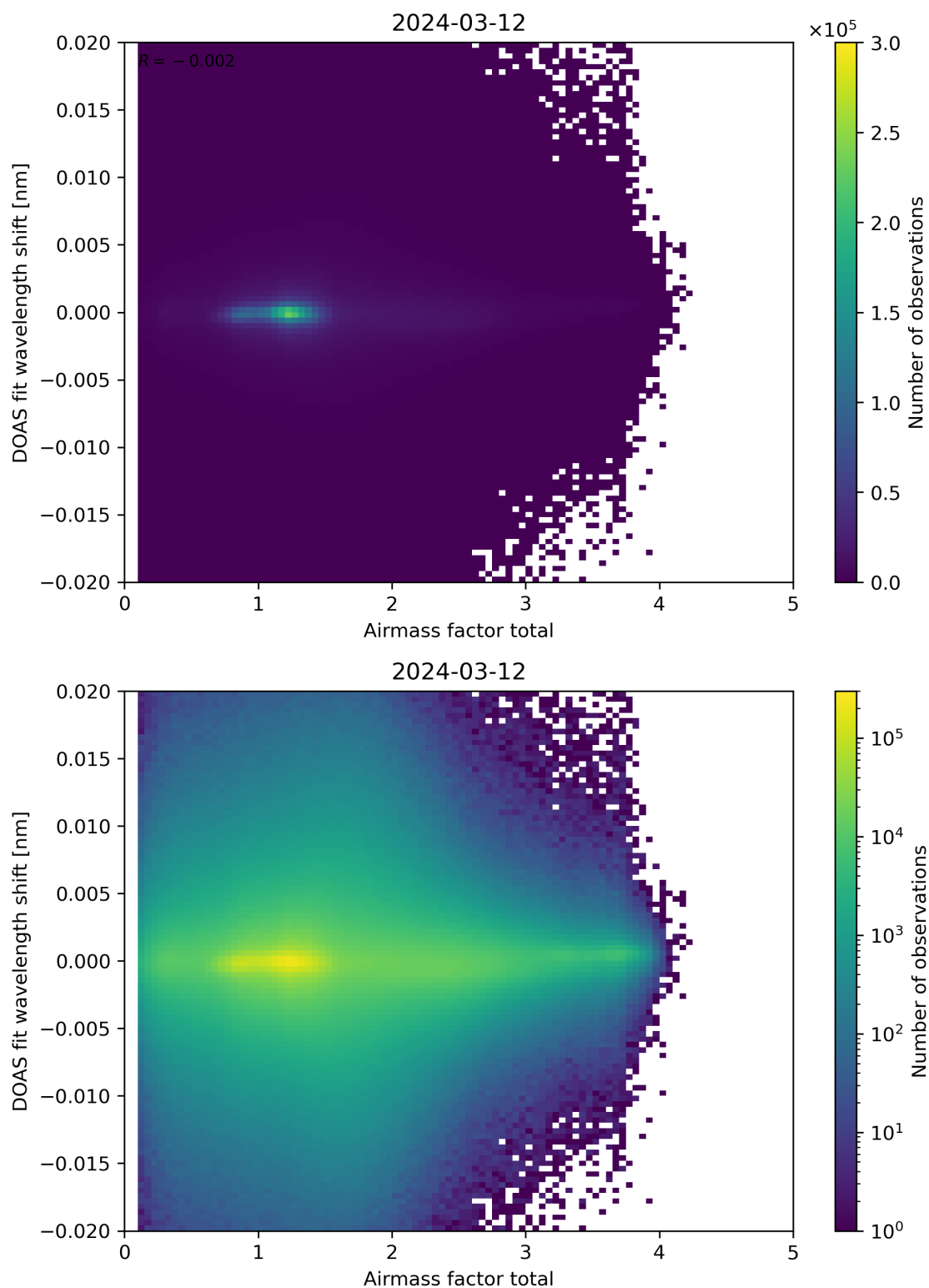
Figure 98: Scatter density plot of “Airmass factor total” against “DOAS fit wavelength shift” for 2024-03-11 to 2024-03-13.
