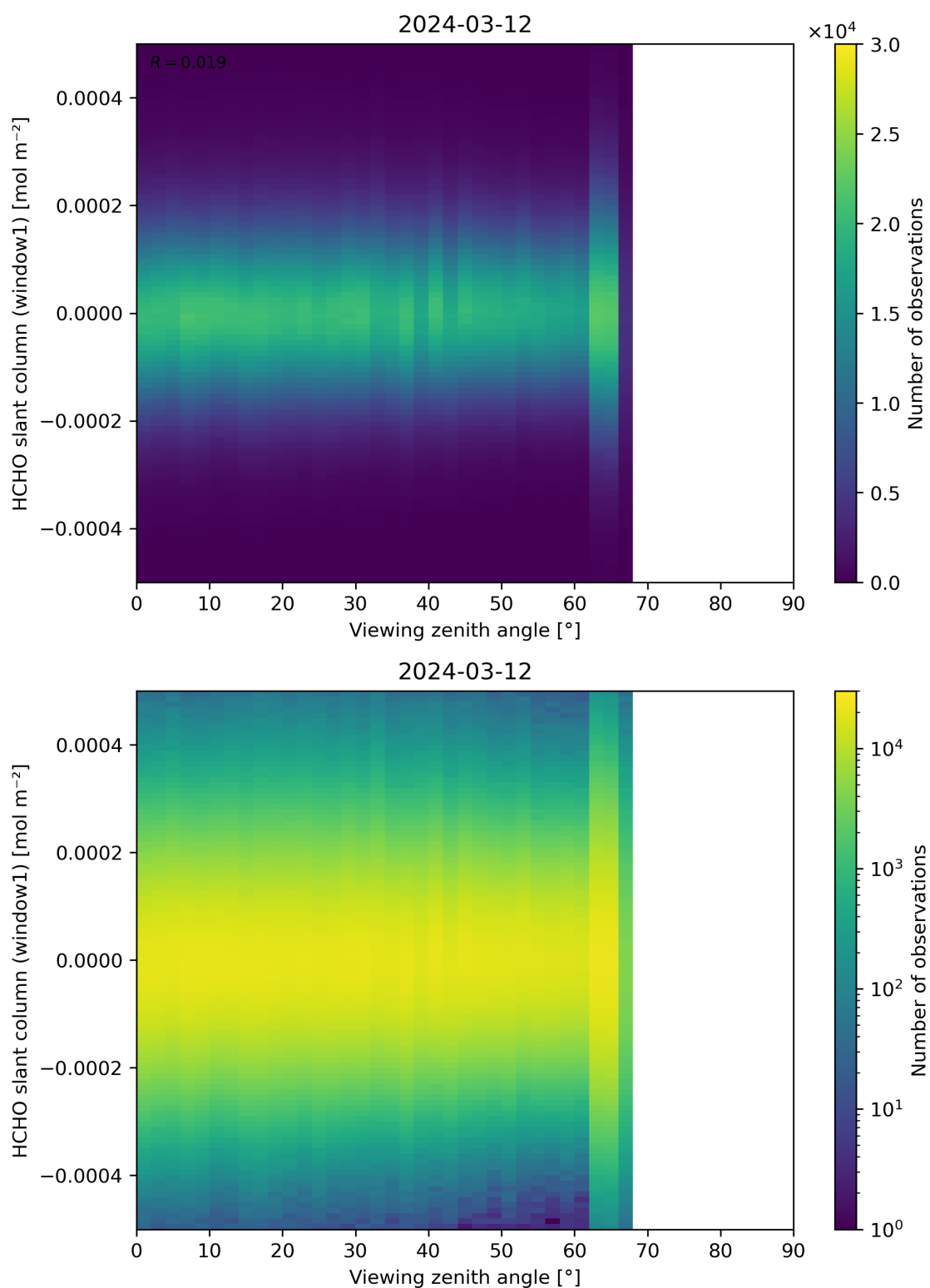
Figure 188: Scatter density plot of “Viewing zenith angle” against “HCHO slant column (window1)” for 2024-03-11 to 2024-03-13.
