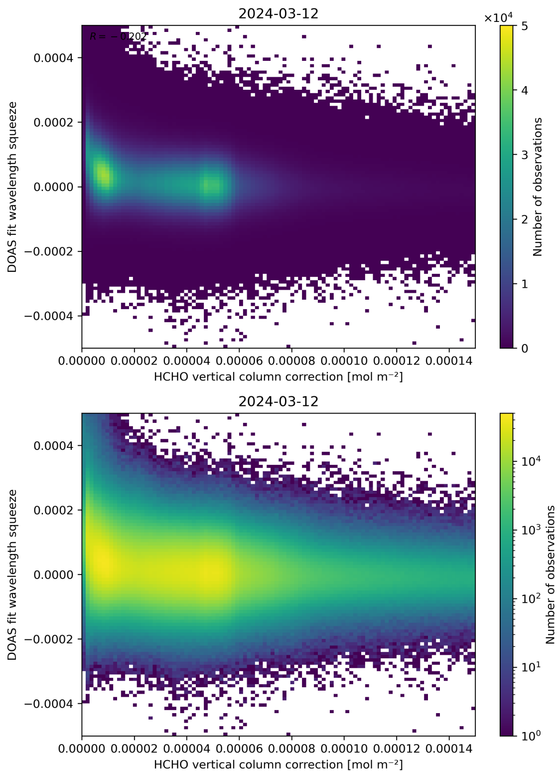
Figure 114: Scatter density plot of “HCHO vertical column correction” against “DOAS fit wavelength squeeze” for 2024-03-11 to 2024-03-13.
