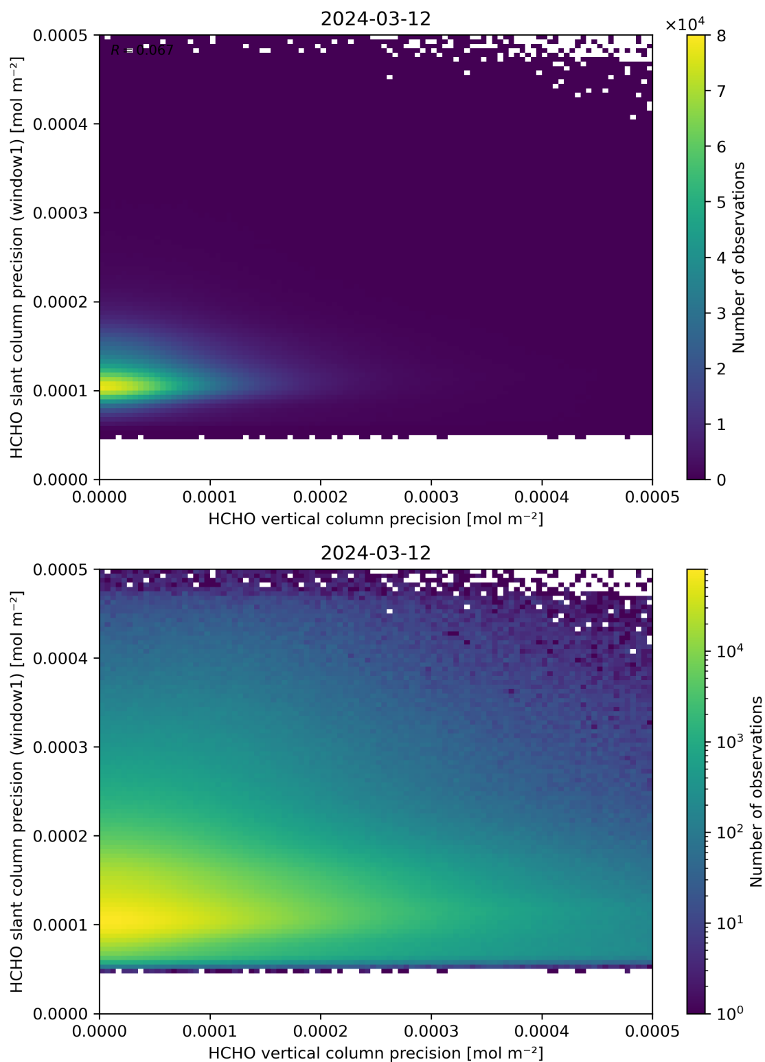
Figure 143: Scatter density plot of “HCHO vertical column precision” against “HCHO slant column precision (window1)” for 2024-03-11 to 2024-03-13.
