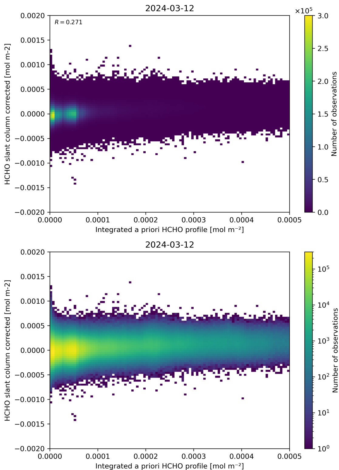
Figure 151: Scatter density plot of “Integrated a priori HCHO profile” against “HCHO slant column corrected” for 2024-03-11 to 2024-03-13.
