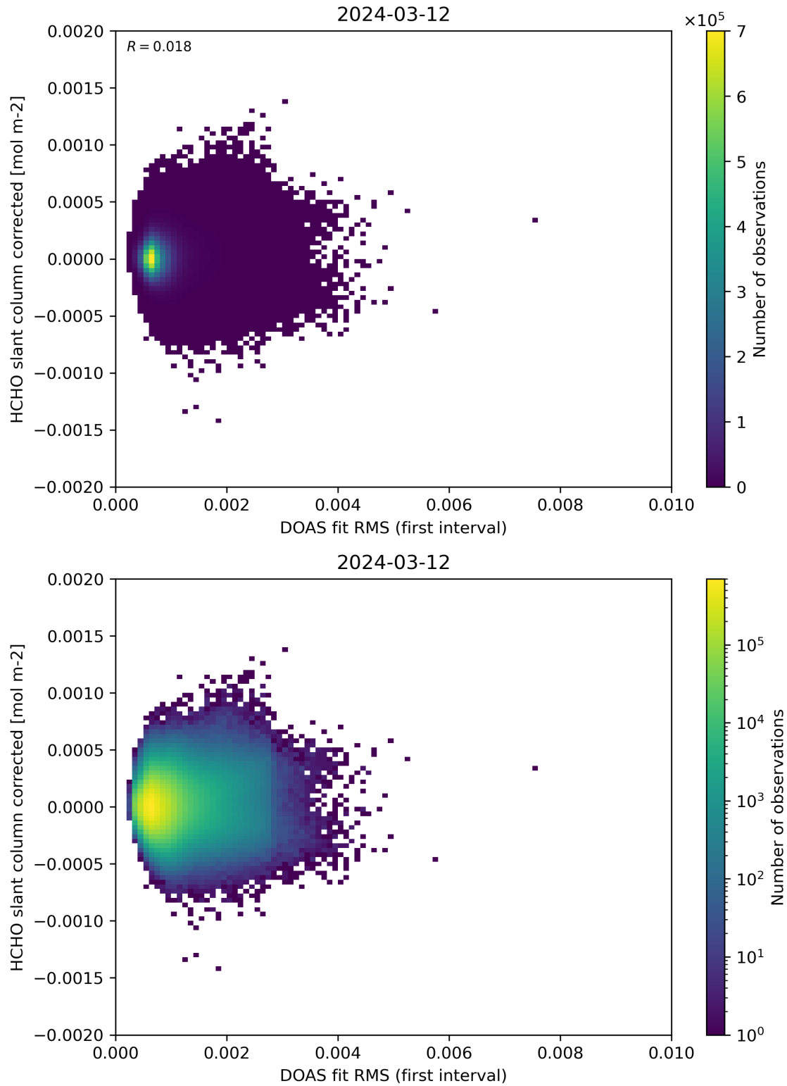
Figure 62: Scatter density plot of “DOAS fit RMS (first interval)” against “HCHO slant column corrected” for 2024-03-11 to 2024-03-13.
