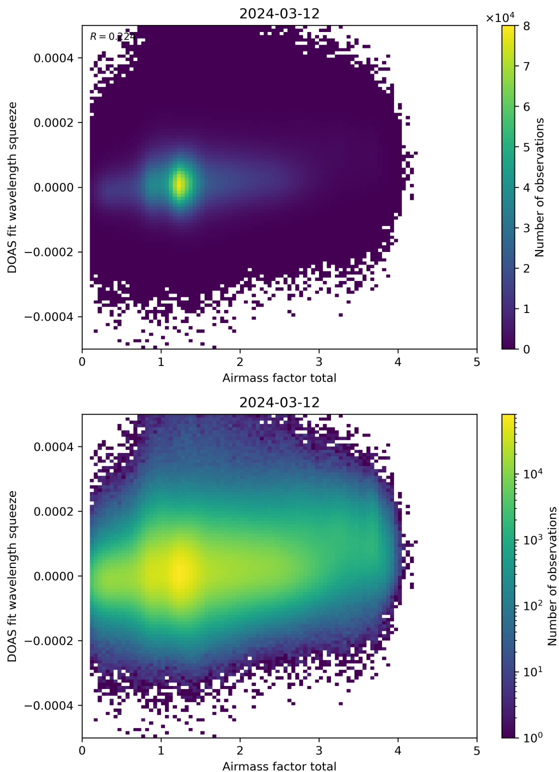
Figure 99: Scatter density plot of “Airmass factor total” against “DOAS fit wavelength squeeze” for 2024-03-11 to 2024-03-13.
