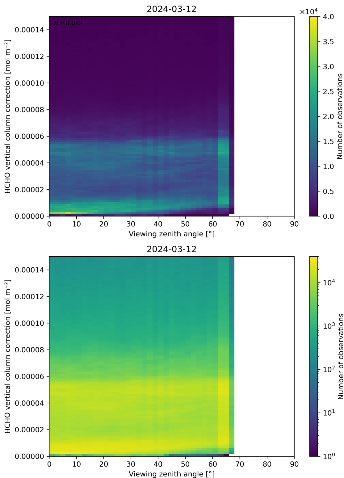
Figure 193: Scatter density plot of “Viewing zenith angle” against “HCHO vertical column correction” for 2024-03-11 to 2024-03-13.
