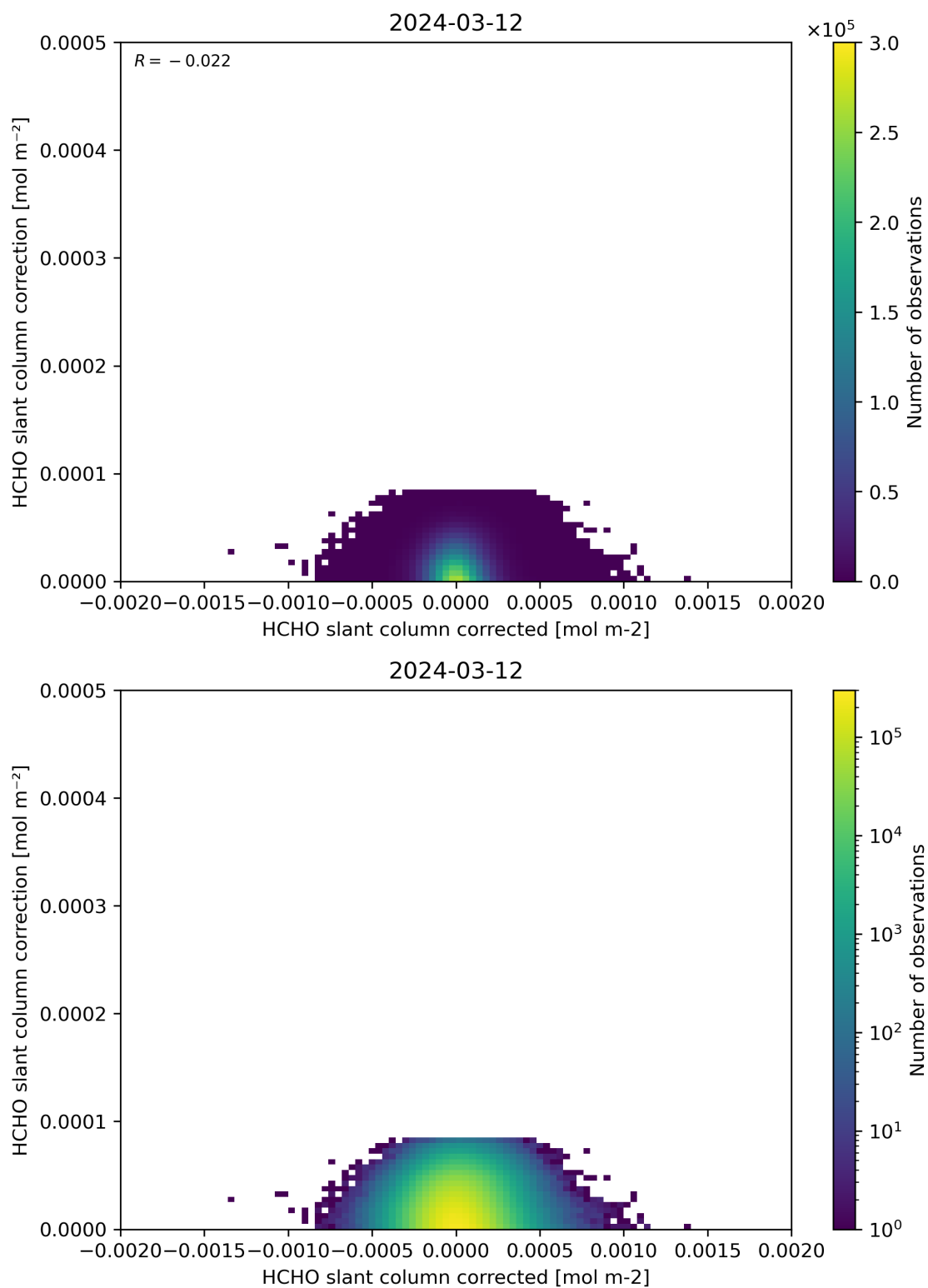
Figure 77: Scatter density plot of “HCHO slant column corrected” against “HCHO slant column correction” for 2024-03-11 to 2024-03-13.
