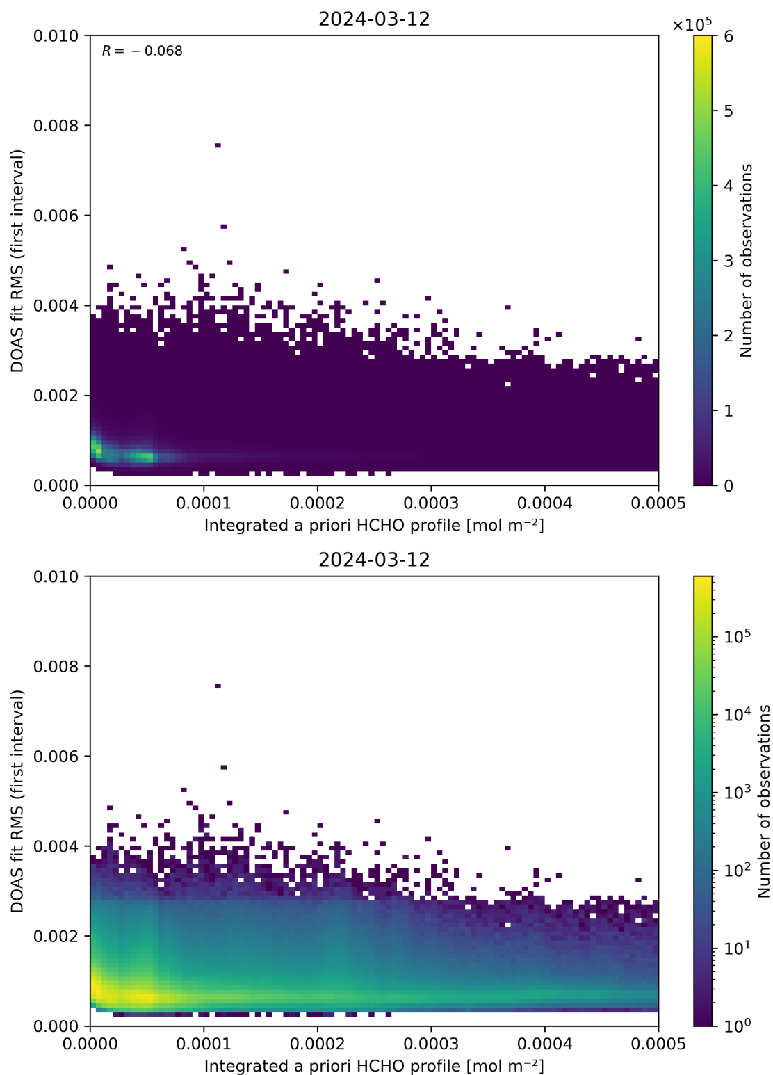
Figure 148: Scatter density plot of “Integrated a priori HCHO profile” against “DOAS fit RMS (first interval)” for 2024-03-11 to 2024-03-13.
