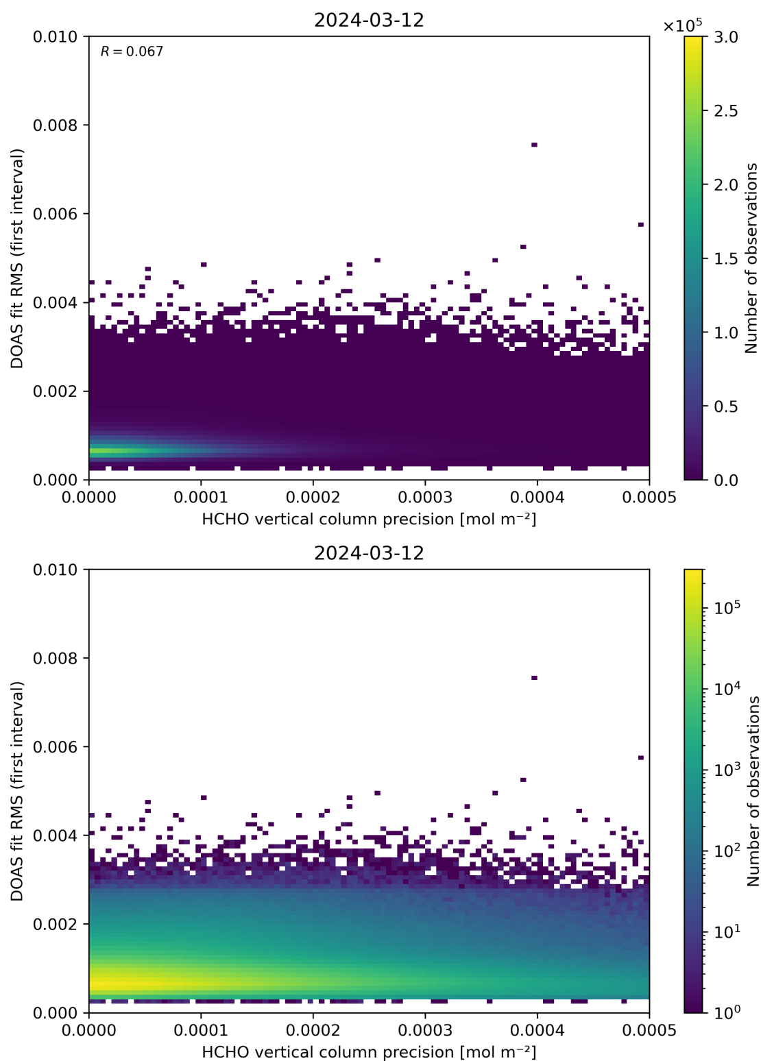
Figure 136: Scatter density plot of “HCHO vertical column precision” against “DOAS fit RMS (first interval)” for 2024-03-11 to 2024-03-13.
