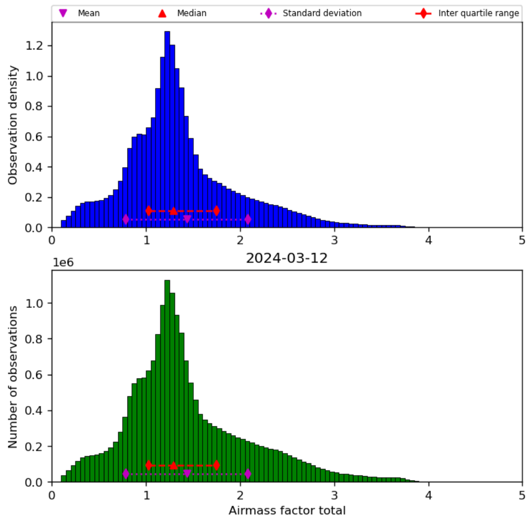
Figure 40: Histogram of “Airmass factor total” for 2024-03-11 to 2024-03-13
