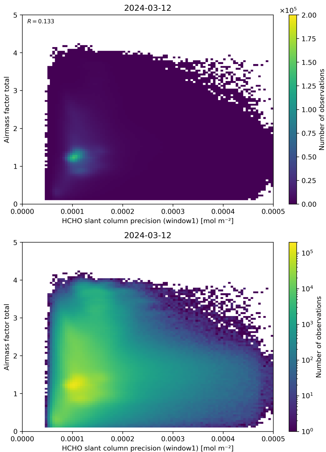
Figure 94: Scatter density plot of “HCHO slant column precision (window1)” against “Airmass factor total” for 2024-03-11 to 2024-03-13.
