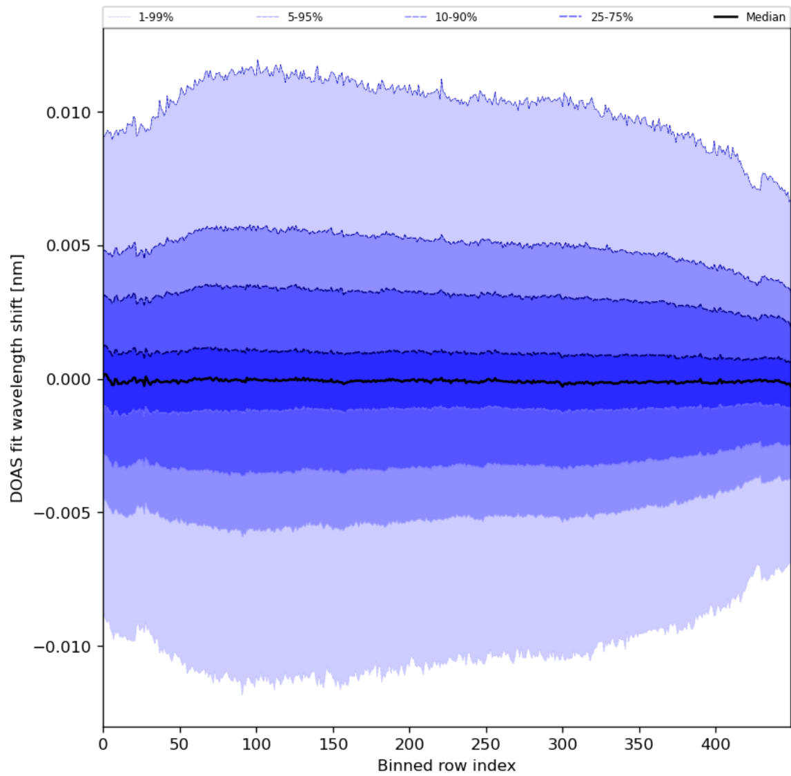
Figure 58: Along track statistics of “DOAS fit wavelength shift” for 2024-03-11 to 2024-03-13
