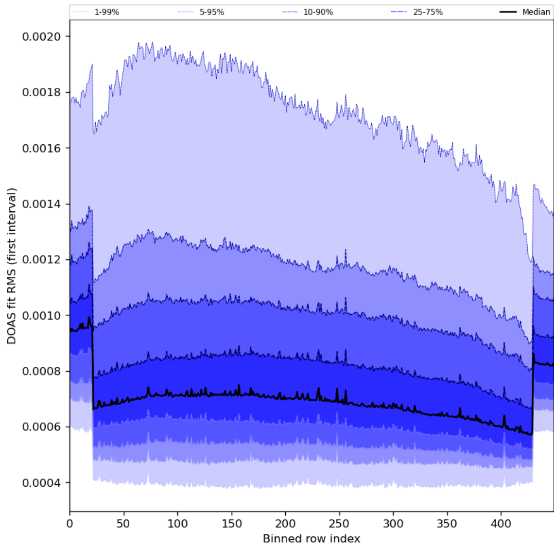
Figure 60: Along track statistics of “DOAS fit RMS (first interval)” for 2024-03-11 to 2024-03-13
