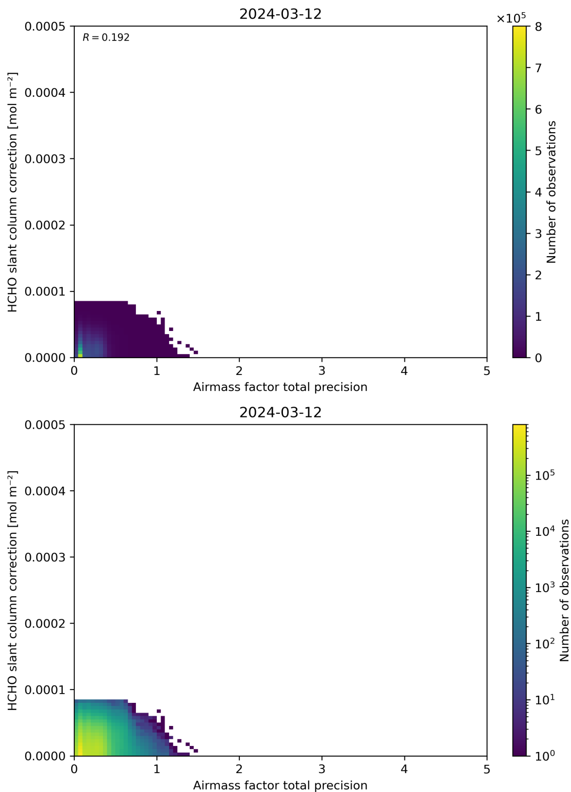
Figure 110: Scatter density plot of “Airmass factor total precision” against “HCHO slant column correction” for 2024-03-11 to 2024-03-13.
