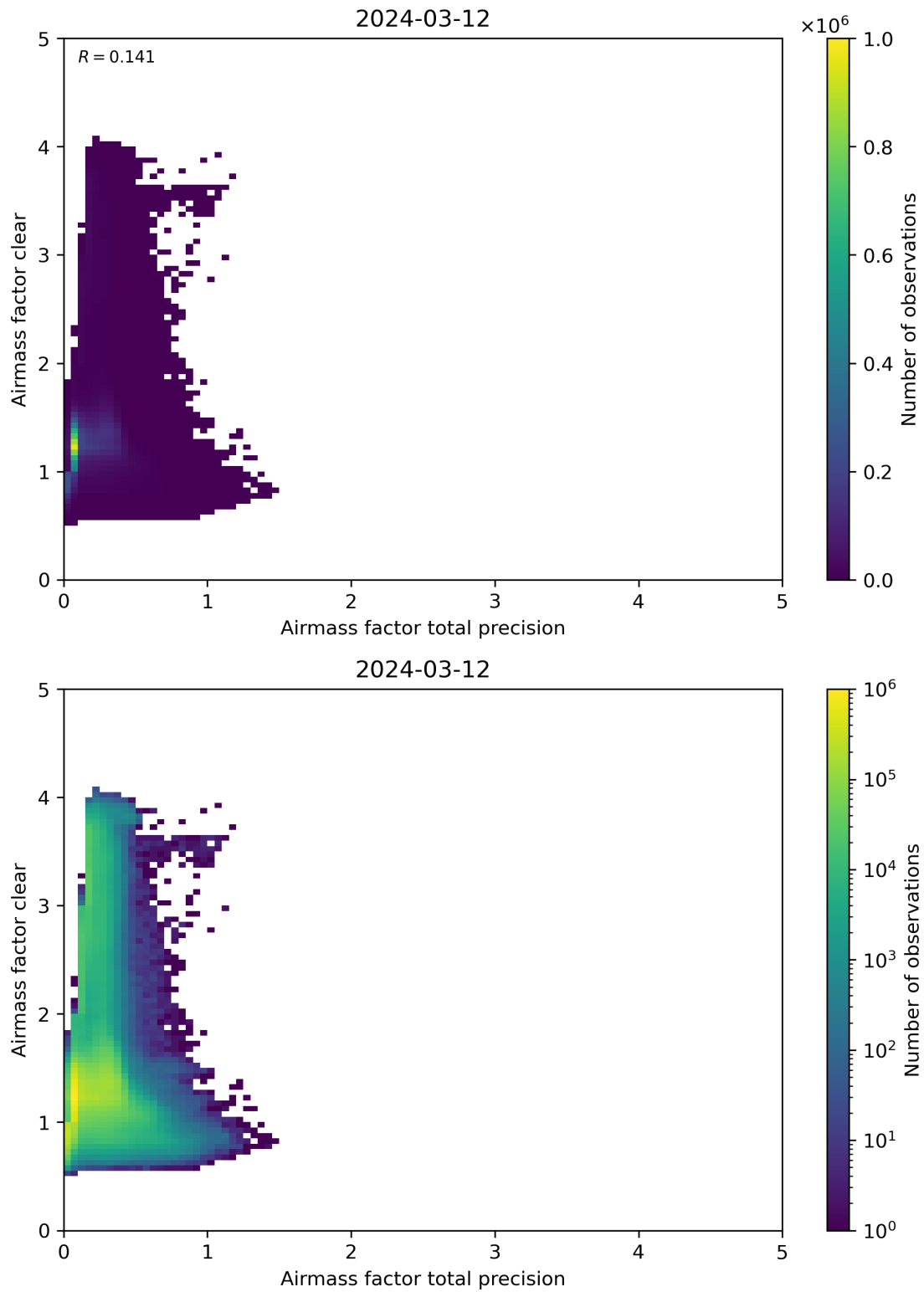
Figure 108: Scatter density plot of “Airmass factor total precision” against “Airmass factor clear” for 2024-03-11 to 2024-03-13.
