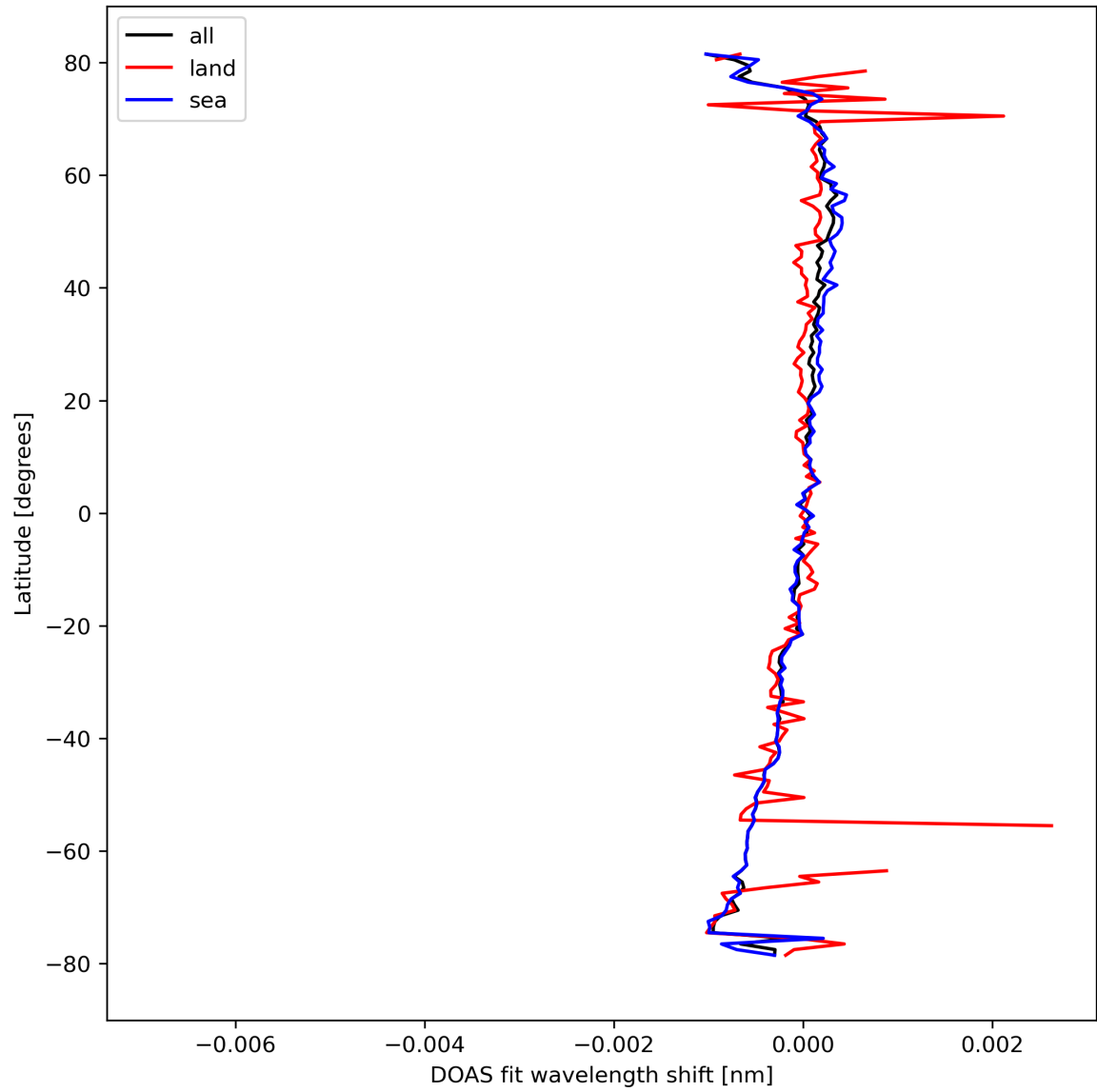
Figure 30: Zonal average of “DOAS fit wavelength shift” for 2024-03-11 to 2024-03-13.
