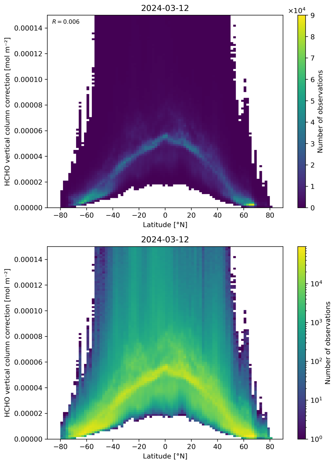
Figure 164: Scatter density plot of “Latitude” against “HCHO vertical column correction” for 2024-03-11 to 2024-03-13.
