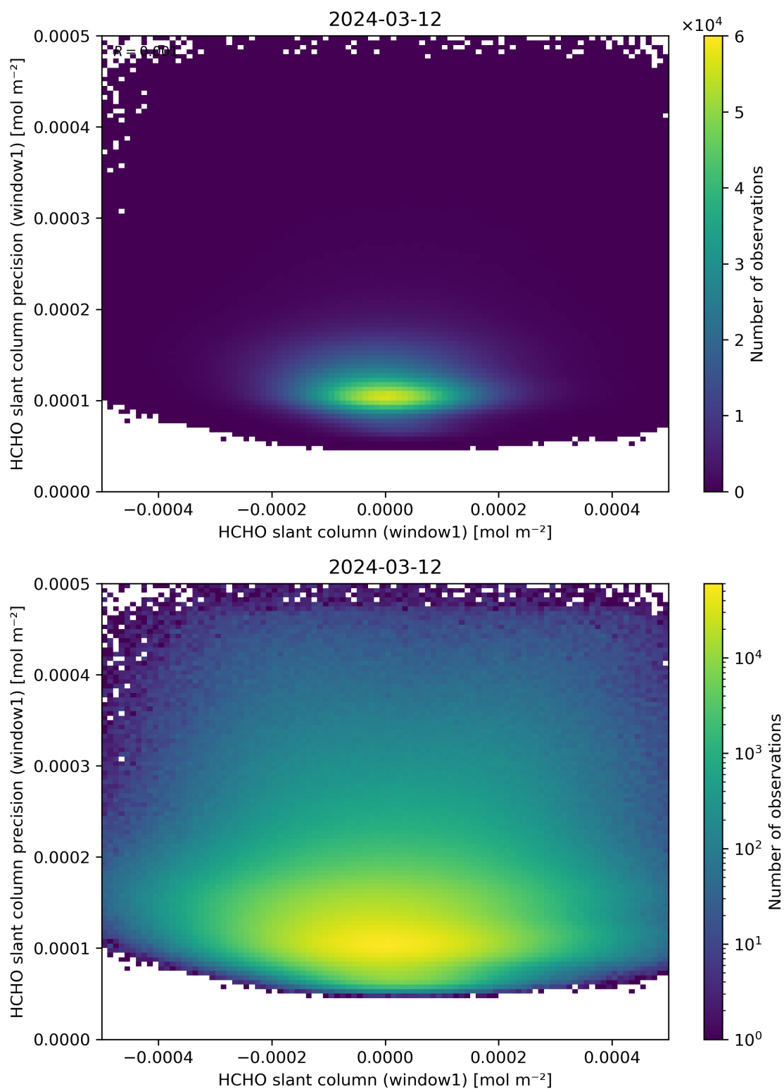
Figure 84: Scatter density plot of “HCHO slant column (window1)” against “HCHO slant column precision (window1)” for 2024-03-11 to 2024-03-13.
