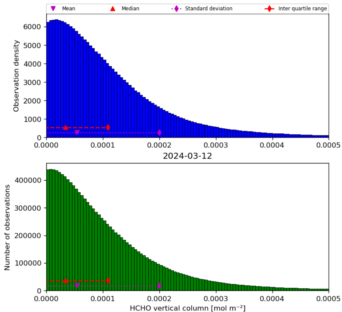
Figure 35: Histogram of “HCHO vertical column” for 2024-03-11 to 2024-03-13
