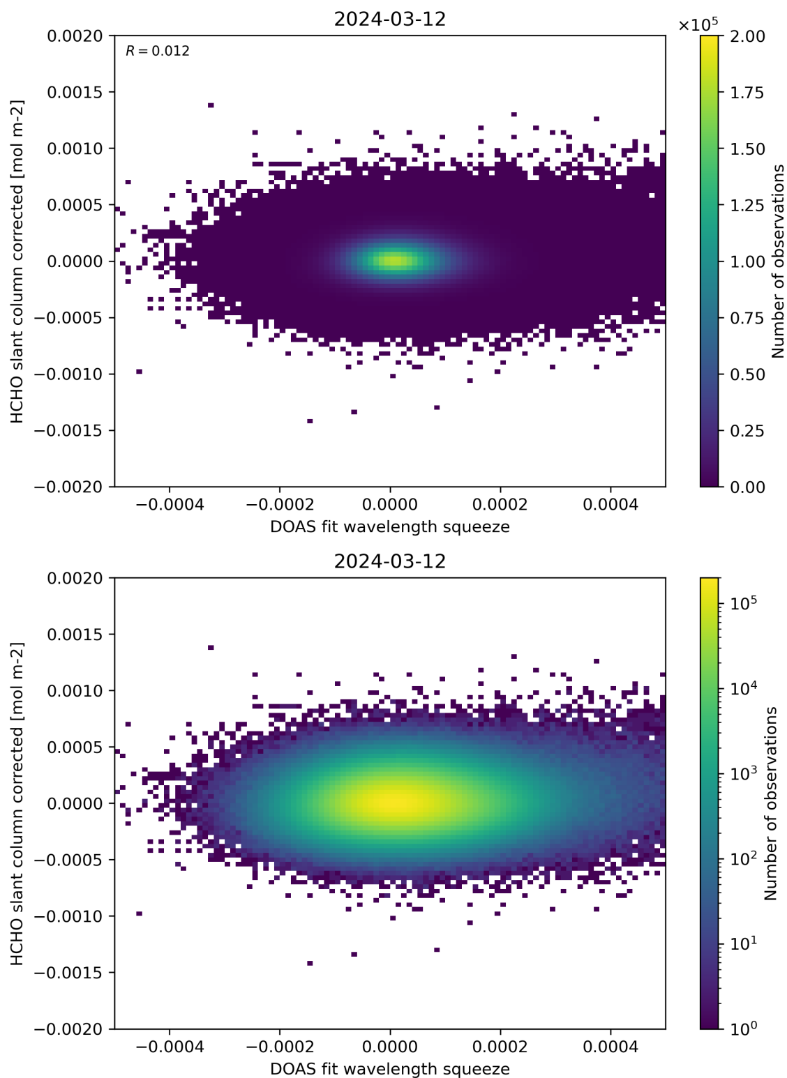
Figure 69: Scatter density plot of “DOAS fit wavelength squeeze” against “HCHO slant column corrected” for 2024-03-11 to 2024-03-13.
