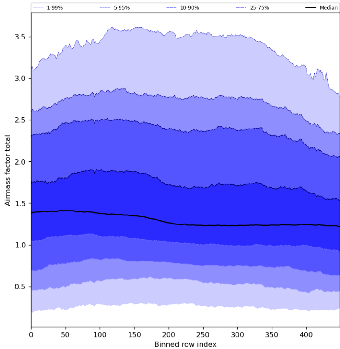
Figure 54: Along track statistics of “Airmass factor total” for 2024-03-11 to 2024-03-13
