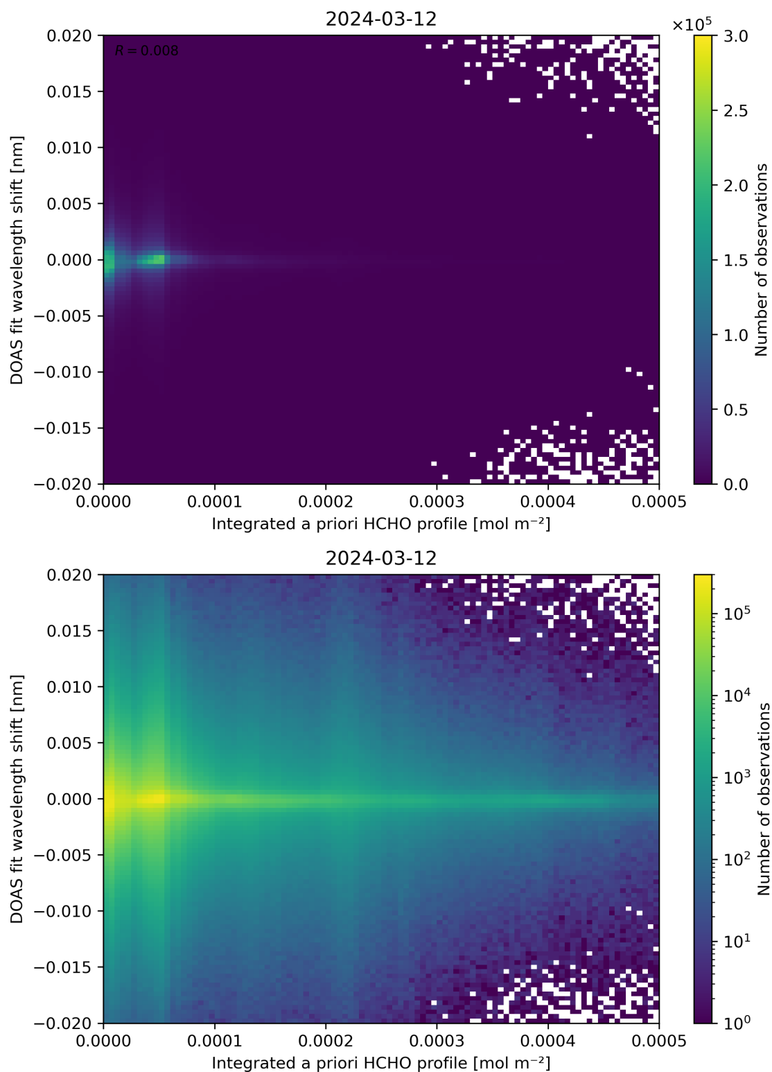
Figure 149: Scatter density plot of “Integrated a priori HCHO profile” against “DOAS fit wavelength shift” for 2024-03-11 to 2024-03-13.
