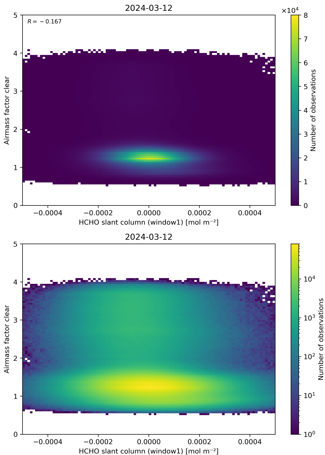
Figure 81: Scatter density plot of “HCHO slant column (window1)” against “Airmass factor clear” for 2024-03-11 to 2024-03-13.
