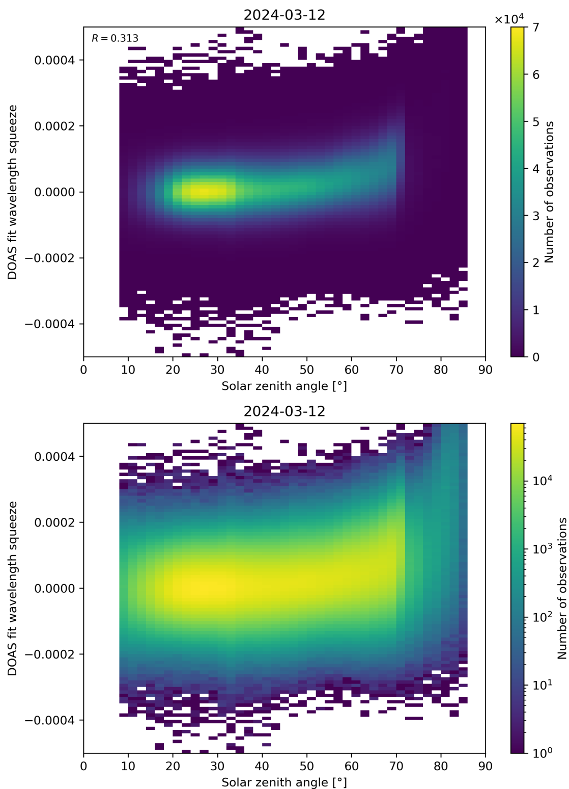
Figure 169: Scatter density plot of “Solar zenith angle” against “DOAS fit wavelength squeeze” for 2024-03-11 to 2024-03-13.
