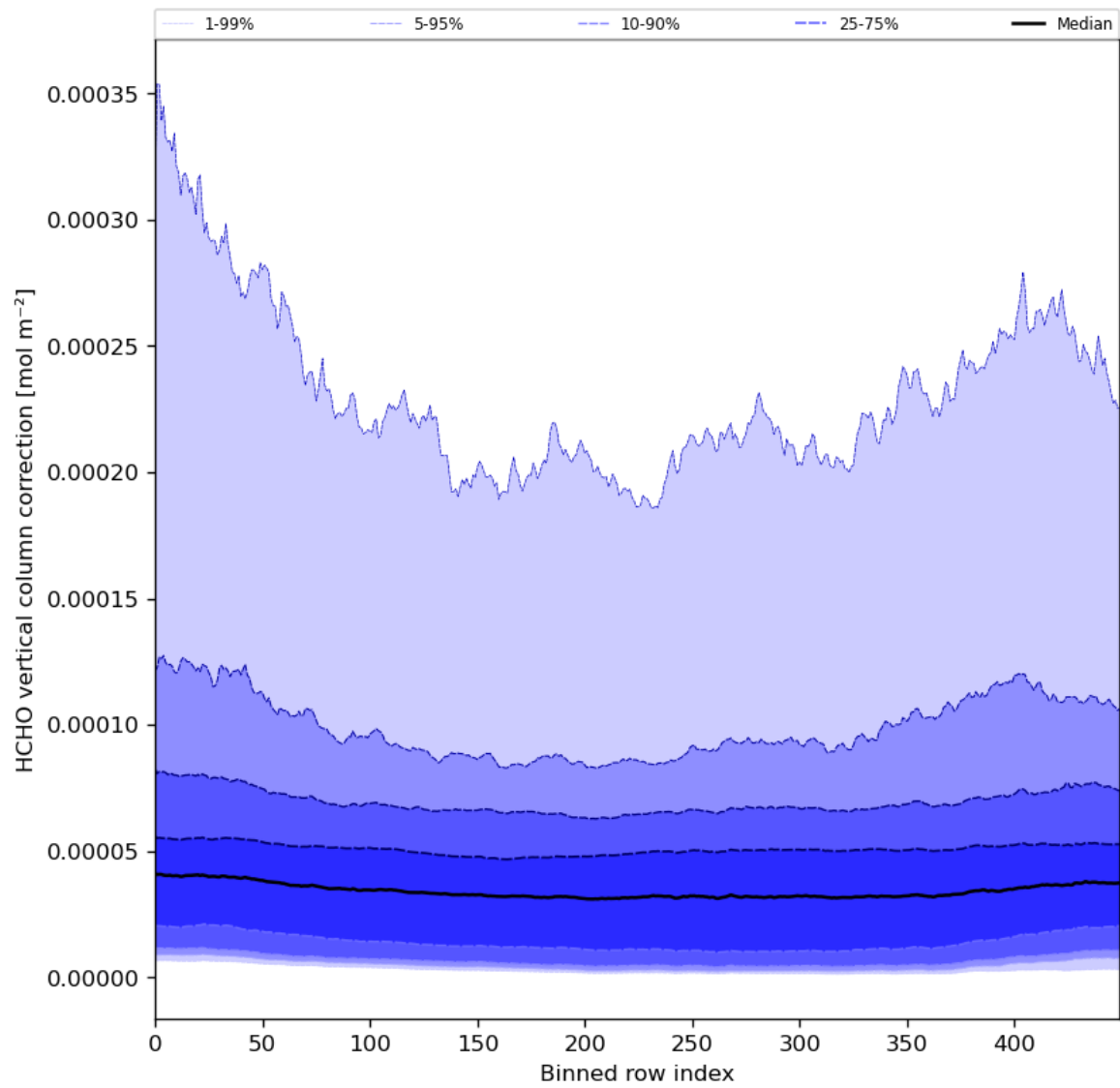
Figure 51: Along track statistics of “HCHO vertical column correction” for 2024-03-11 to 2024-03-13
