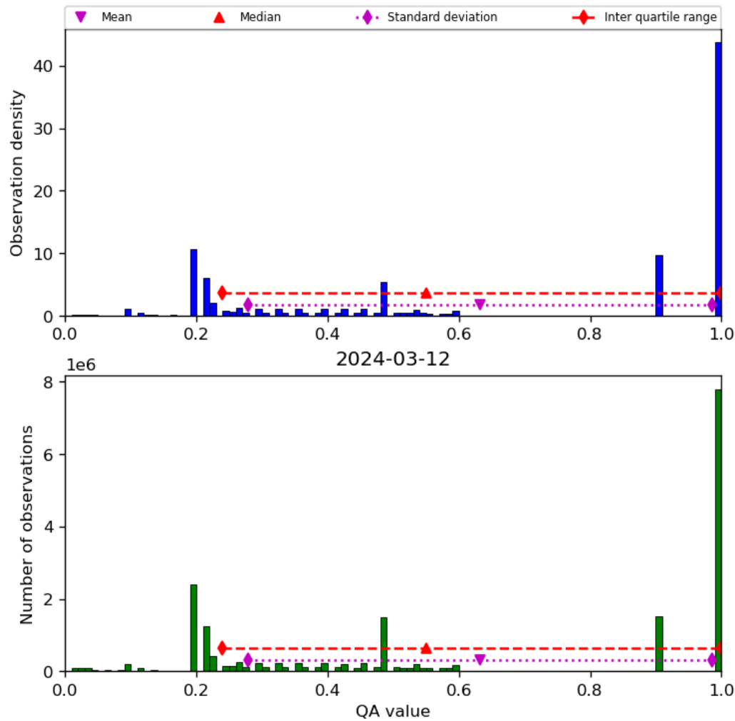
Figure 34: Histogram of “QA value” for 2024-03-11 to 2024-03-13
