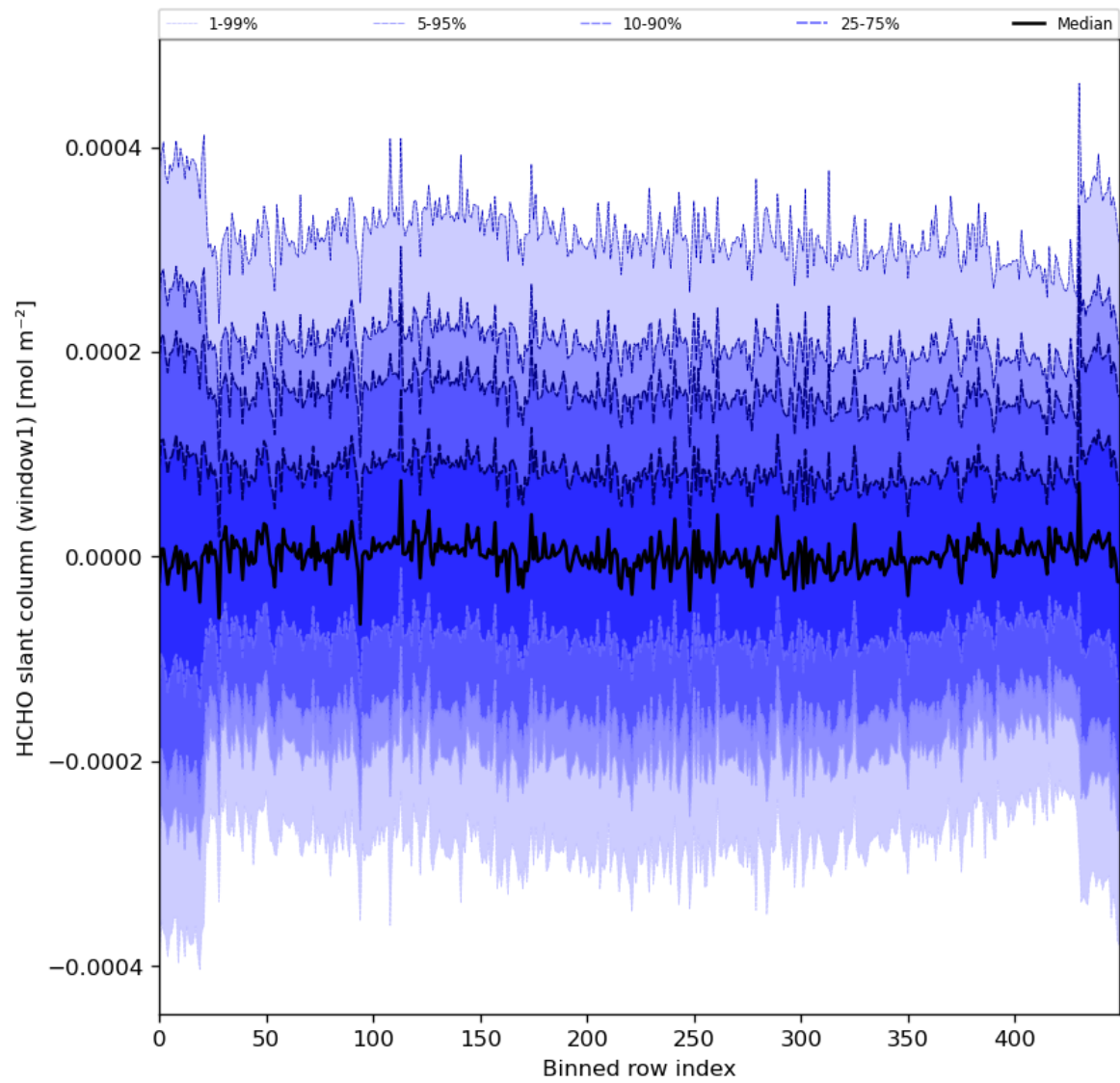
Figure 52: Along track statistics of “HCHO slant column (window1)” for 2024-03-11 to 2024-03-13
