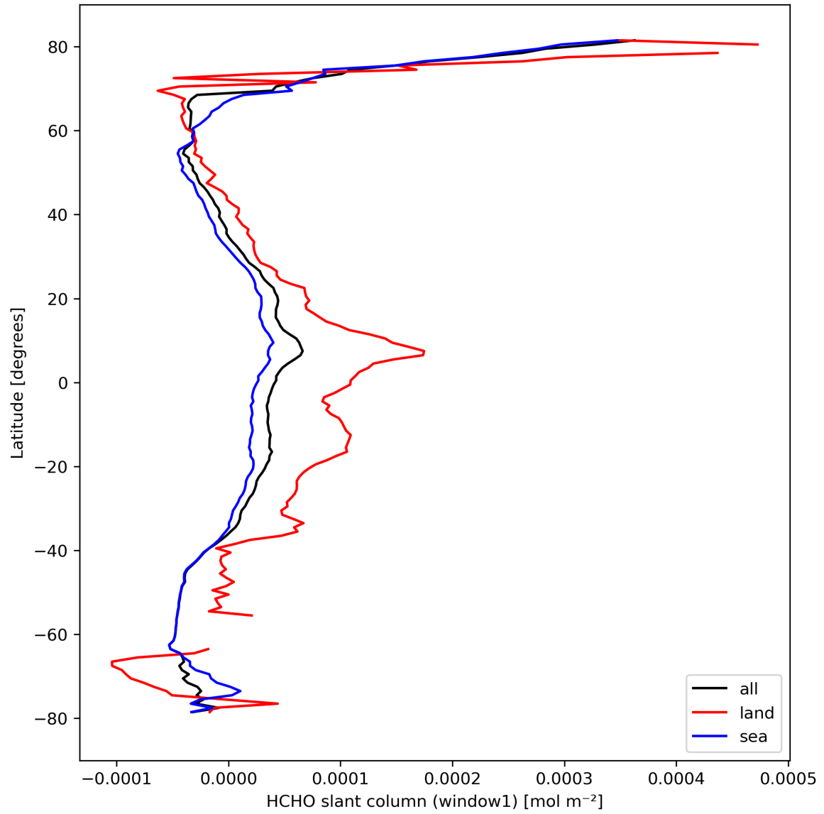
Figure 24: Zonal average of “HCHO slant column (window1)” for 2024-03-11 to 2024-03-13.
