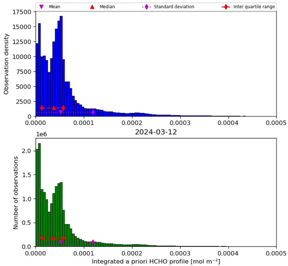
Figure 43: Histogram of “Integrated a priori HCHO profile” for 2024-03-11 to 2024-03-13
