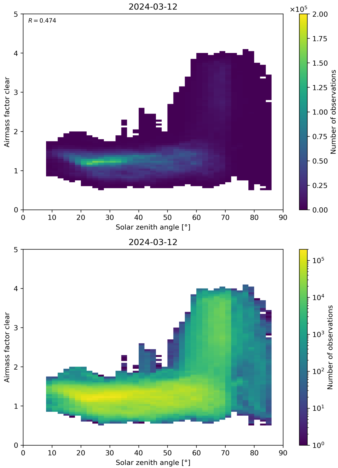
Figure 170: Scatter density plot of “Solar zenith angle” against “Airmass factor clear” for 2024-03-11 to 2024-03-13.
