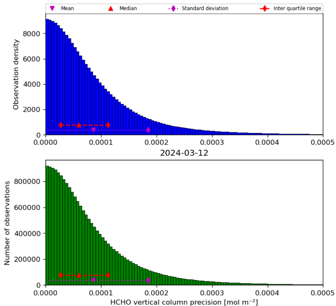
Figure 36: Histogram of “HCHO vertical column precision” for 2024-03-11 to 2024-03-13
