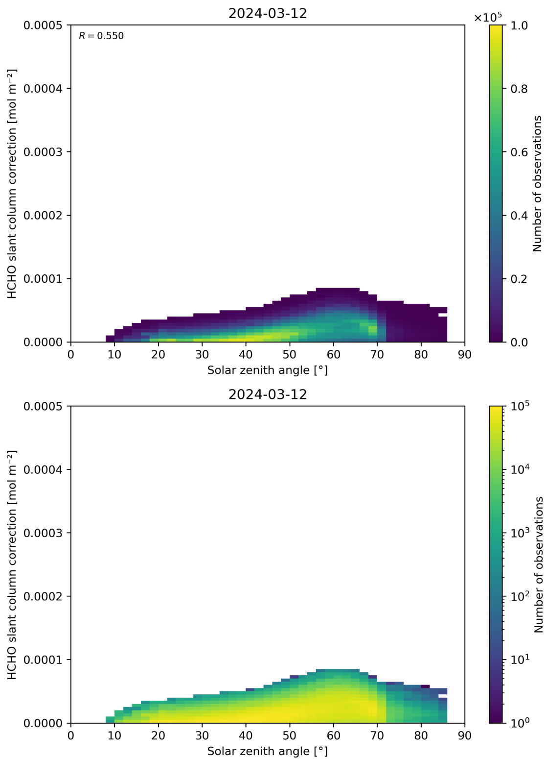
Figure 172: Scatter density plot of “Solar zenith angle” against “HCHO slant column correction” for 2024-03-11 to 2024-03-13.
