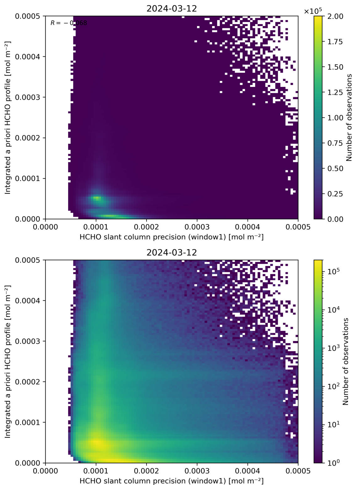
Figure 96: Scatter density plot of “HCHO slant column precision (window1)” against “Integrated a priori HCHO profile” for 2024-03-11 to 2024-03-13.
