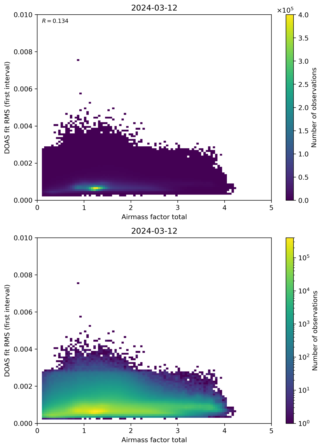
Figure 97: Scatter density plot of “Airmass factor total” against “DOAS fit RMS (first interval)” for 2024-03-11 to 2024-03-13.
