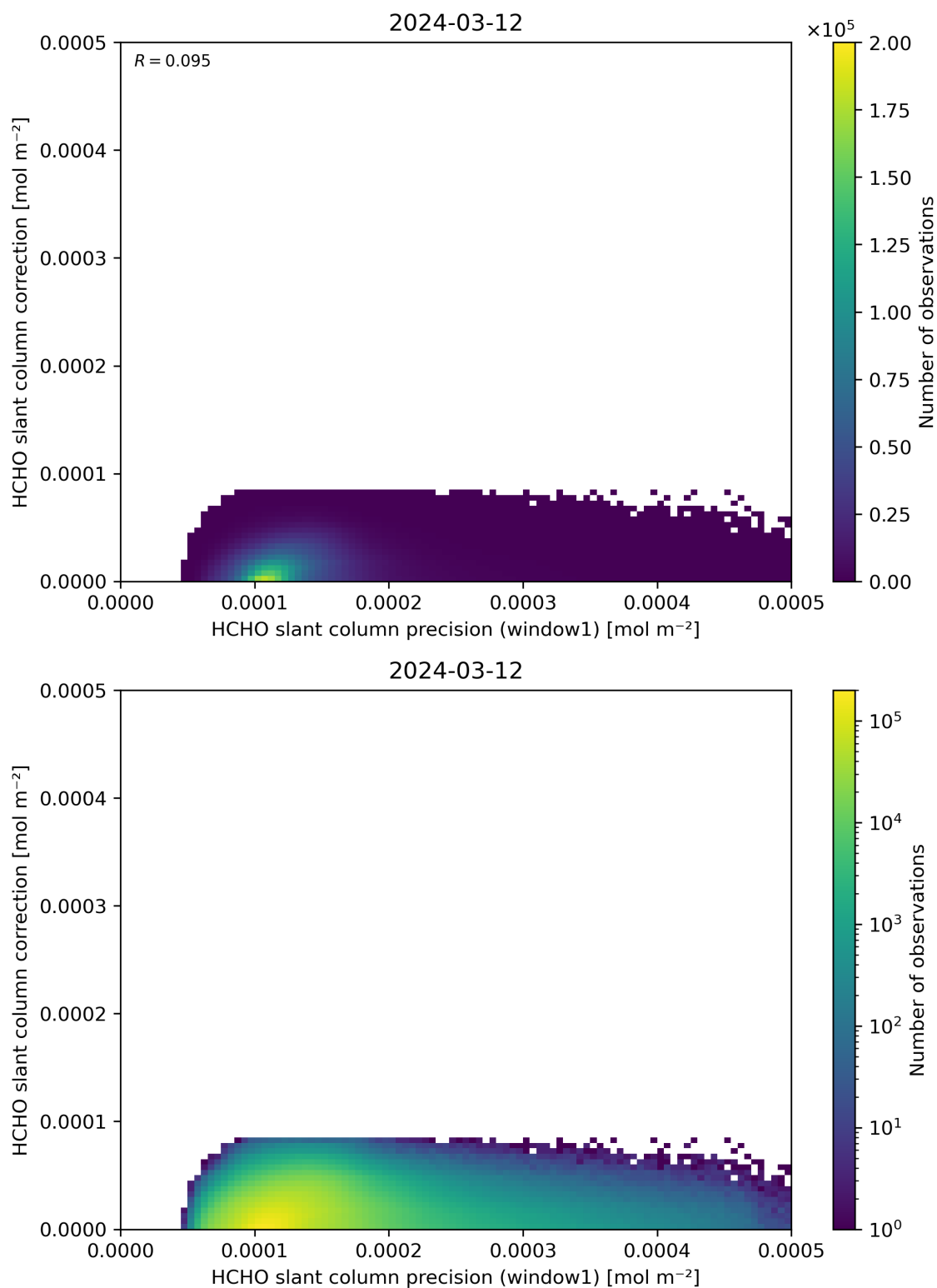
Figure 93: Scatter density plot of “HCHO slant column precision (window1)” against “HCHO slant column correction” for 2024-03-11 to 2024-03-13.
