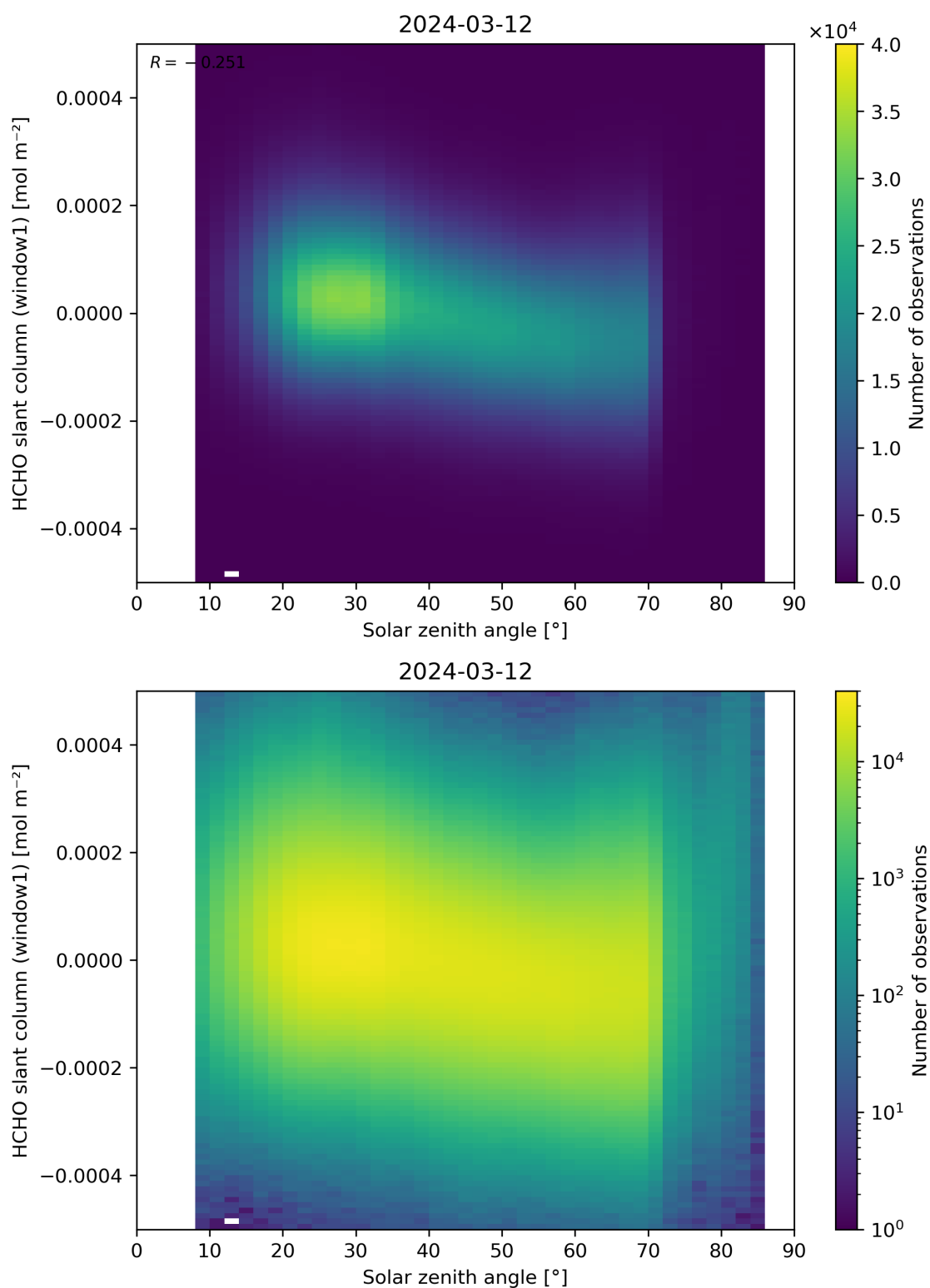
Figure 173: Scatter density plot of “Solar zenith angle” against “HCHO slant column (window1)” for 2024-03-11 to 2024-03-13.
