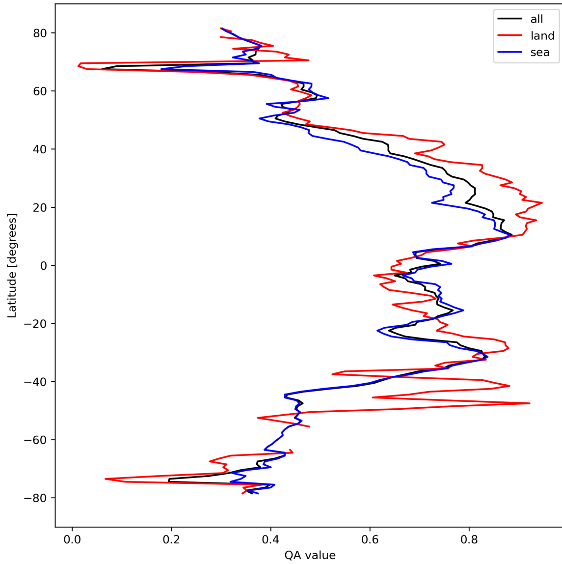
Figure 20: Zonal average of “QA value” for 2024-03-11 to 2024-03-13.
