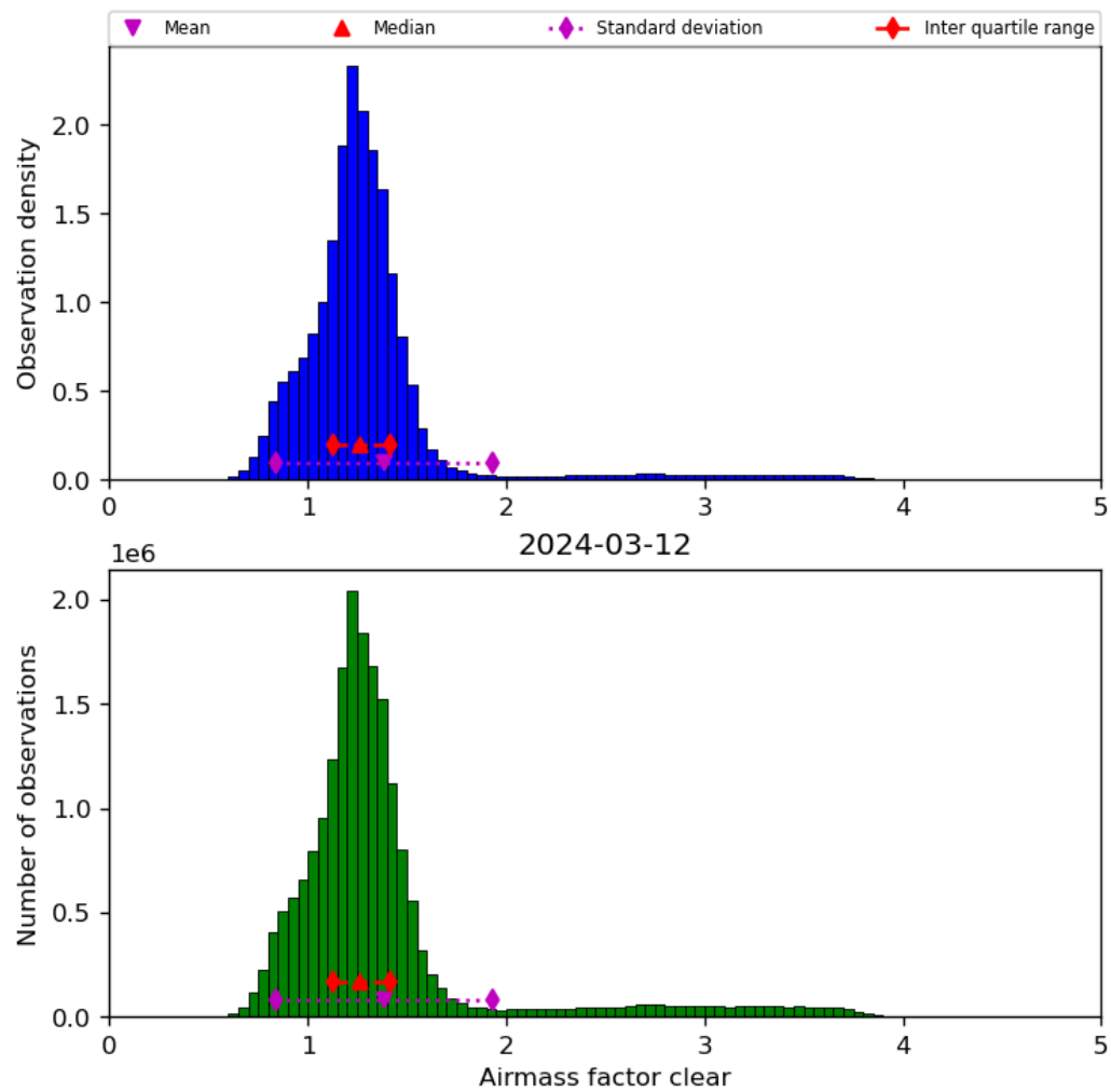
Figure 42: Histogram of “Airmass factor clear” for 2024-03-11 to 2024-03-13
