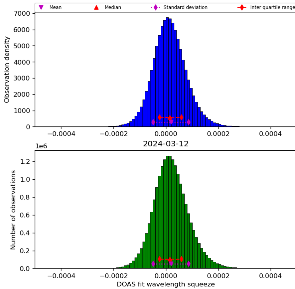
Figure 45: Histogram of “DOAS fit wavelength squeeze” for 2024-03-11 to 2024-03-13
