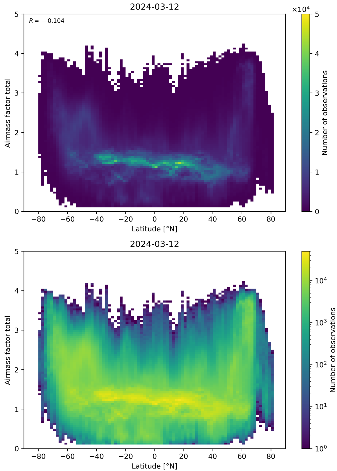
Figure 161: Scatter density plot of “Latitude” against “Airmass factor total” for 2024-03-11 to 2024-03-13.
