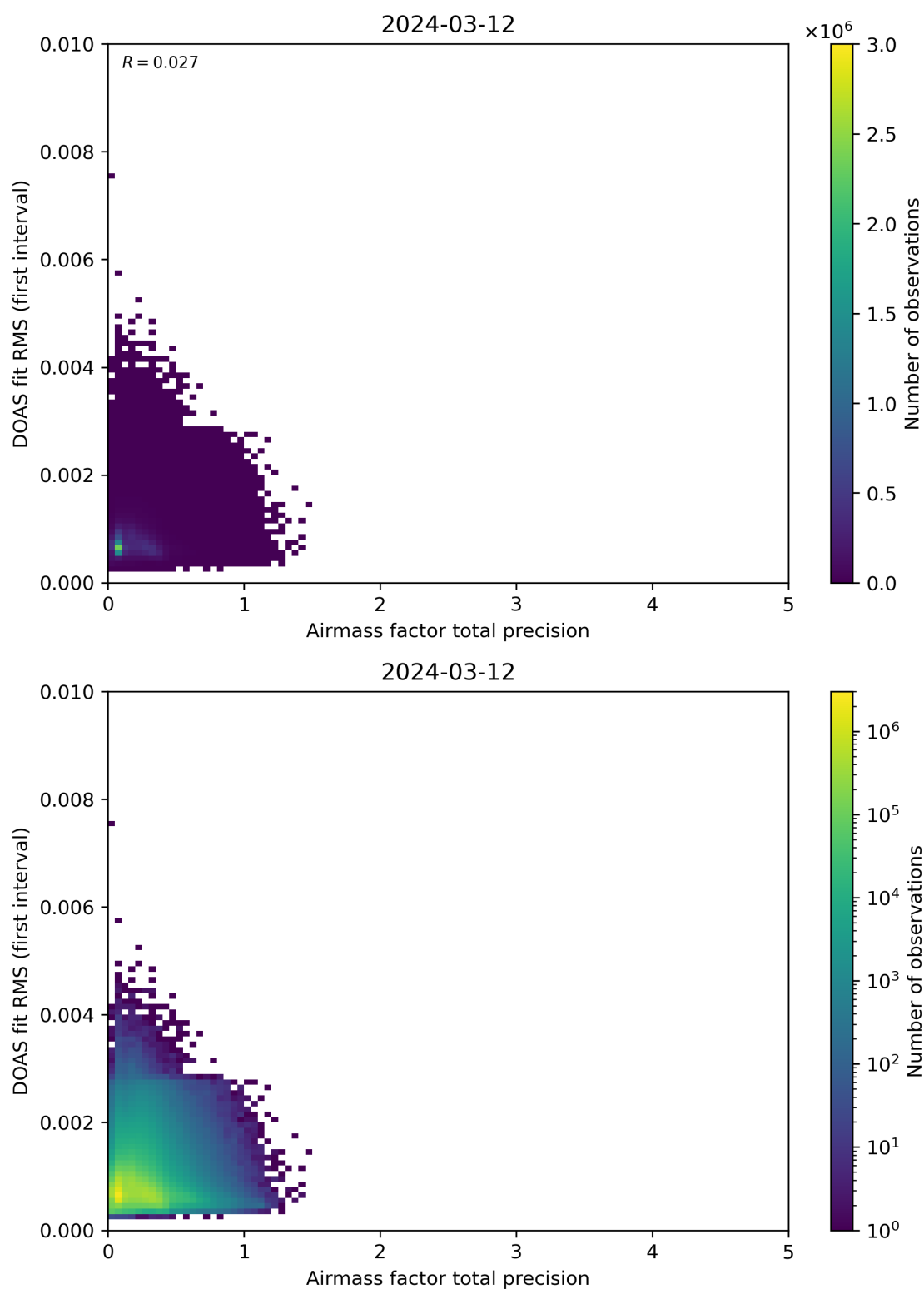
Figure 105: Scatter density plot of “Airmass factor total precision” against “DOAS fit RMS (first interval)” for 2024-03-11 to 2024-03-13.
