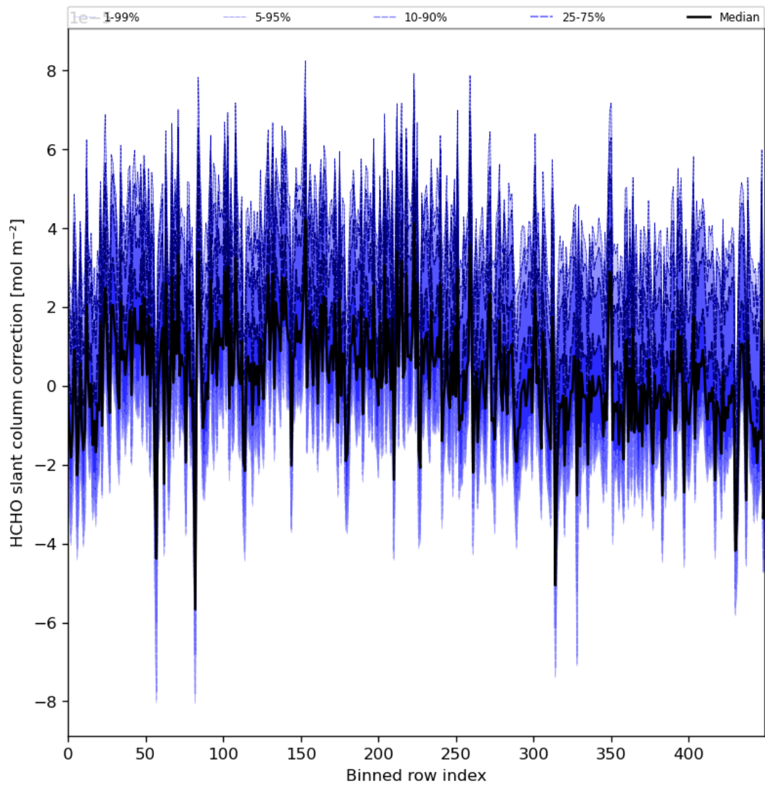
Figure 61: Along track statistics of “HCHO slant column correction” for 2024-03-11 to 2024-03-13
