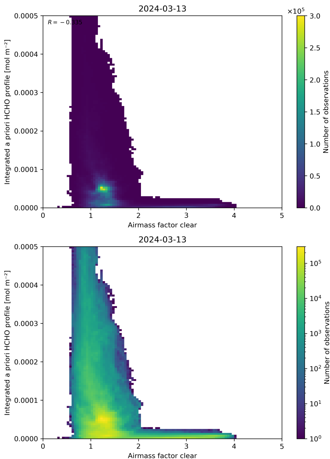
Figure 76: Scatter density plot of “Airmass factor clear” against “Integrated a priori HCHO profile” for 2024-03-12 to 2024-03-14.
