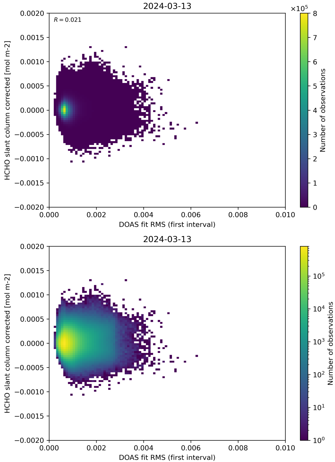
Figure 62: Scatter density plot of “DOAS fit RMS (first interval)” against “HCHO slant column corrected” for 2024-03-12 to 2024-03-14.
