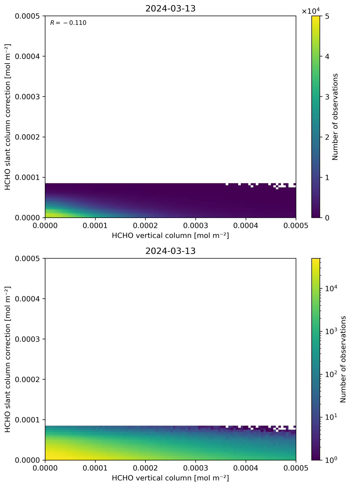
Figure 128: Scatter density plot of “HCHO vertical column” against “HCHO slant column correction” for 2024-03-12 to 2024-03-14.
