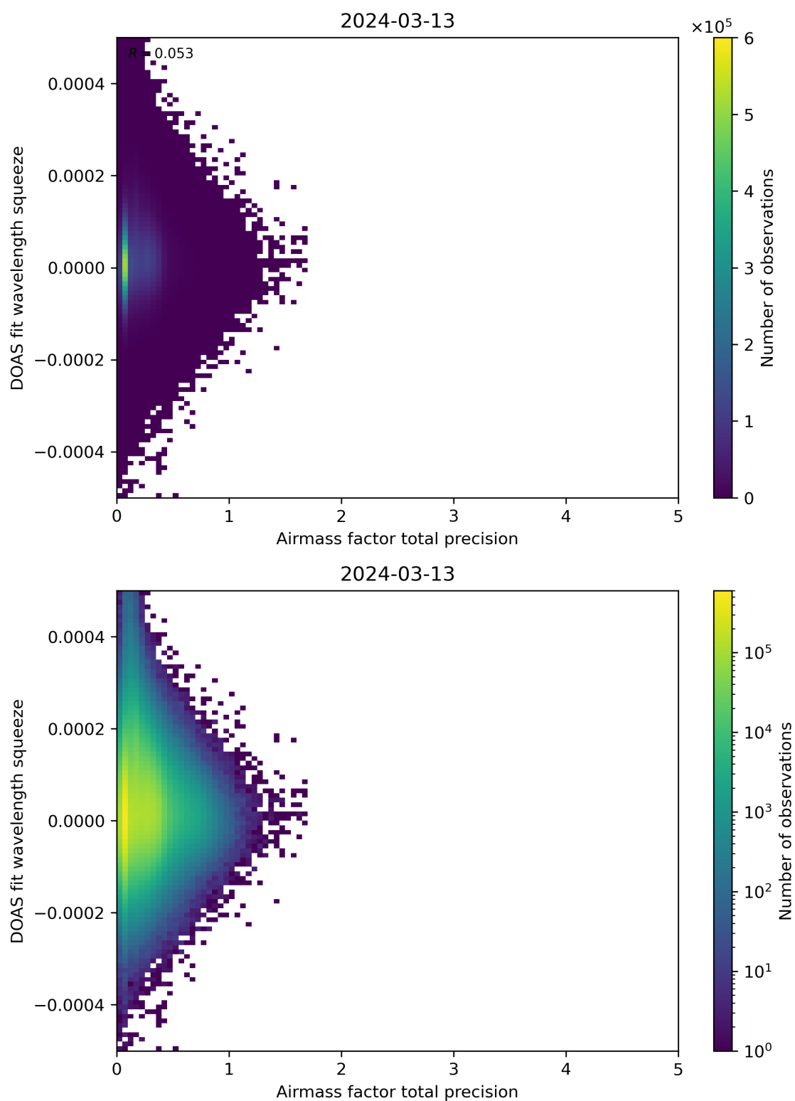
Figure 107: Scatter density plot of “Airmass factor total precision” against “DOAS fit wavelength squeeze” for 2024-03-12 to 2024-03-14.
