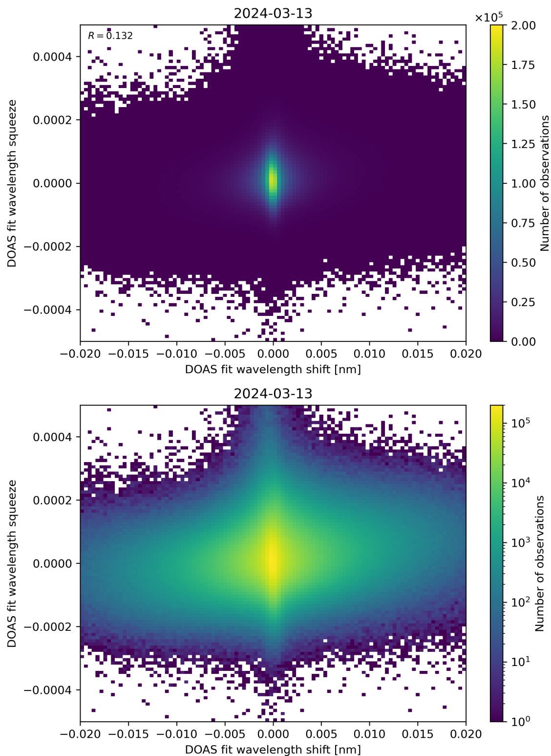
Figure 65: Scatter density plot of “DOAS fit wavelength shift” against “DOAS fit wavelength squeeze” for 2024-03-12 to 2024-03-14.
