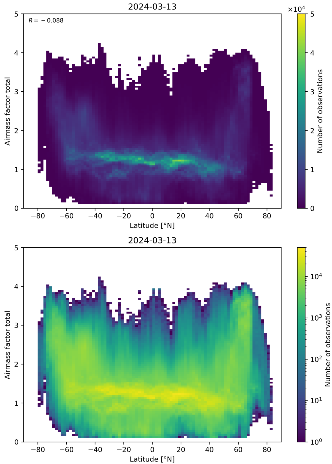
Figure 161: Scatter density plot of “Latitude” against “Airmass factor total” for 2024-03-12 to 2024-03-14.
