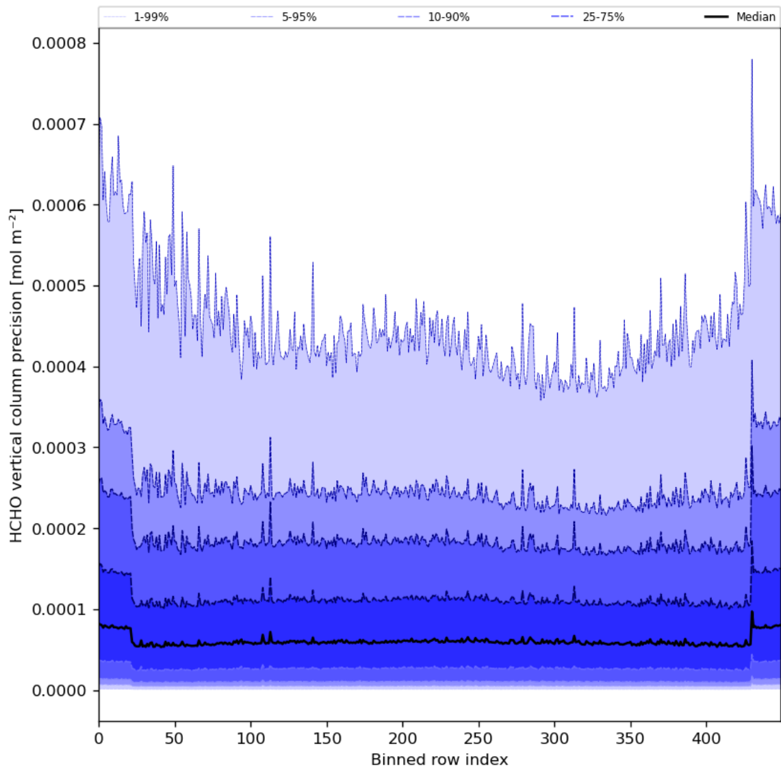
Figure 50: Along track statistics of “HCHO vertical column precision” for 2024-03-12 to 2024-03-14
