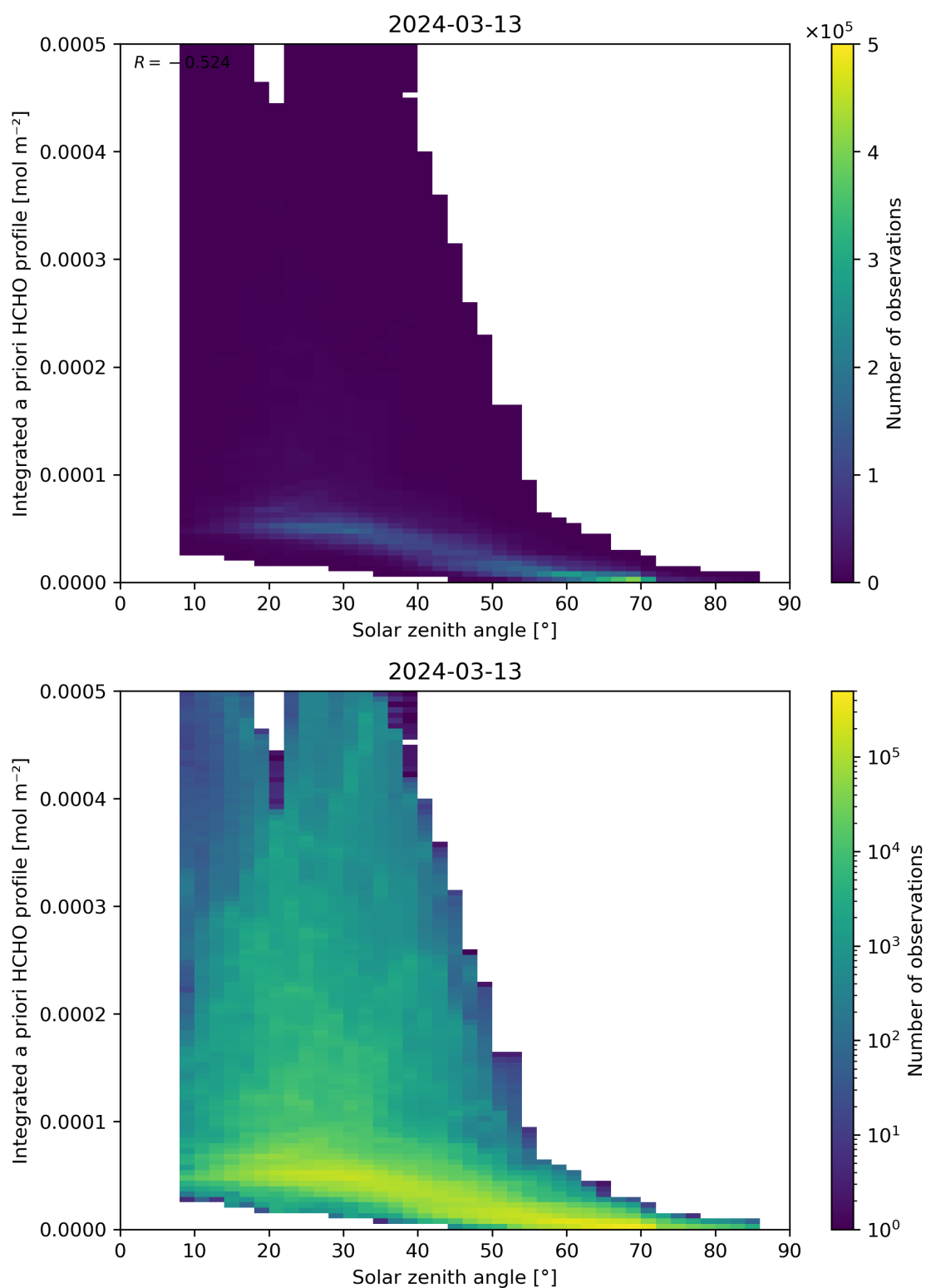
Figure 180: Scatter density plot of “Solar zenith angle” against “Integrated a priori HCHO profile” for 2024-03-12 to 2024-03-14.
