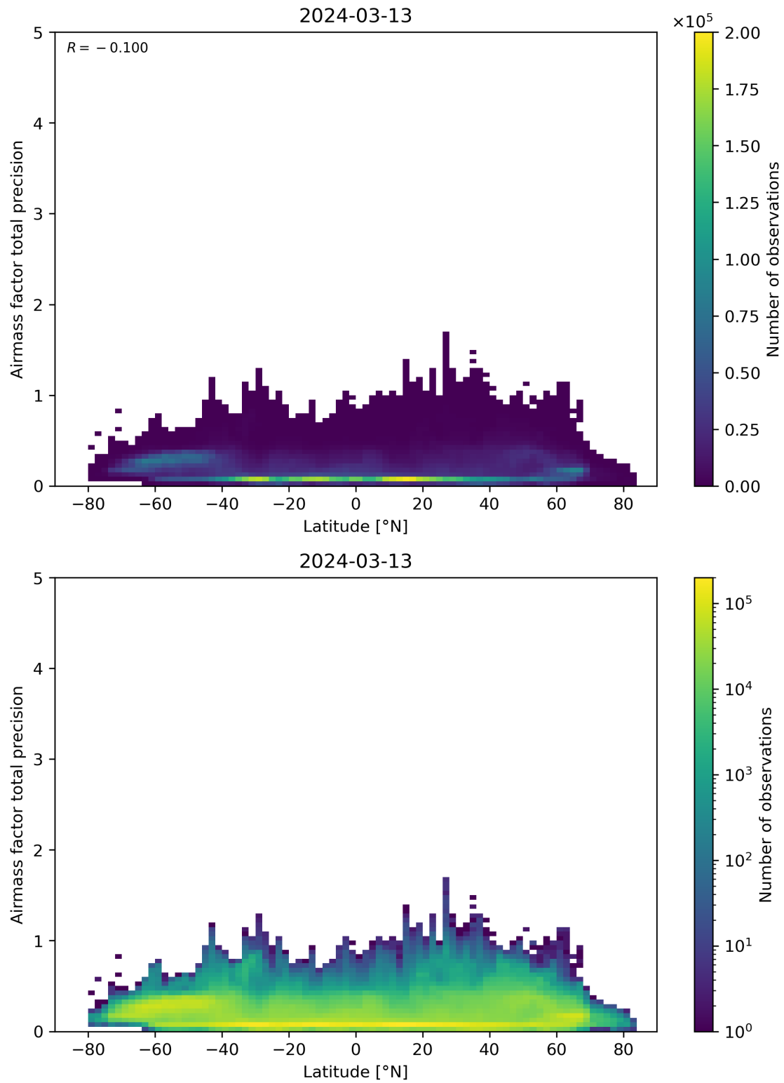
Figure 162: Scatter density plot of “Latitude” against “Airmass factor total precision” for 2024-03-12 to 2024-03-14.
