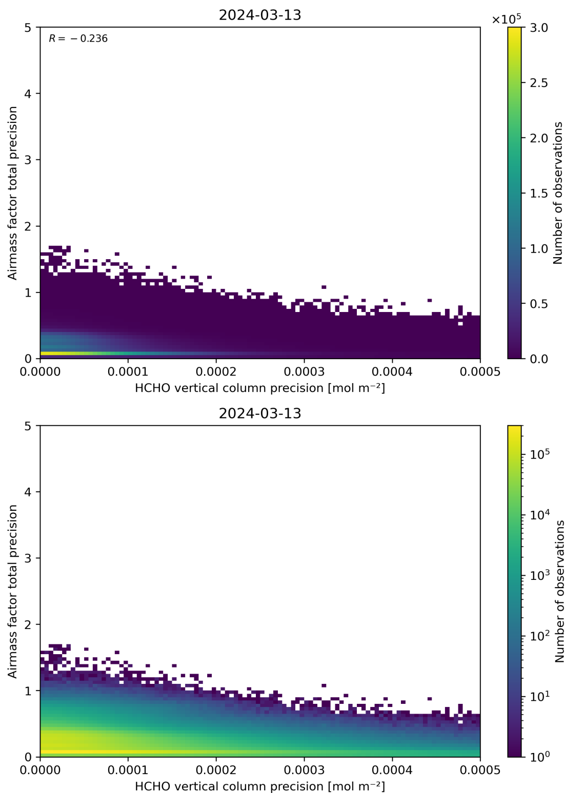
Figure 145: Scatter density plot of “HCHO vertical column precision” against “Airmass factor total precision” for 2024-03-12 to 2024-03-14.
