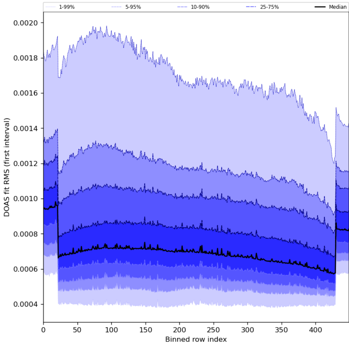
Figure 60: Along track statistics of “DOAS fit RMS (first interval)” for 2024-03-12 to 2024-03-14
