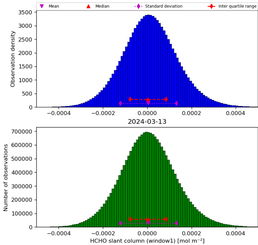
Figure 38: Histogram of “HCHO slant column (window1)” for 2024-03-12 to 2024-03-14
