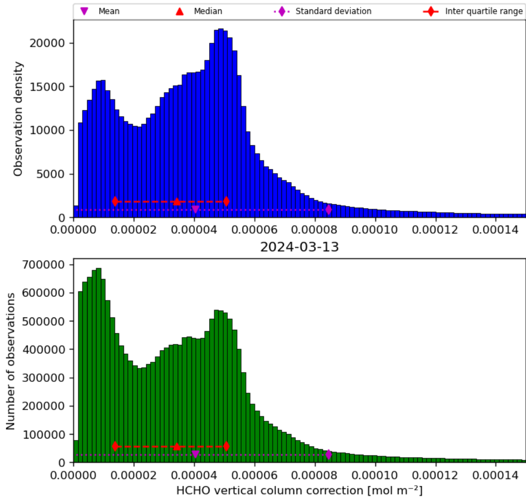
Figure 37: Histogram of “HCHO vertical column correction” for 2024-03-12 to 2024-03-14
