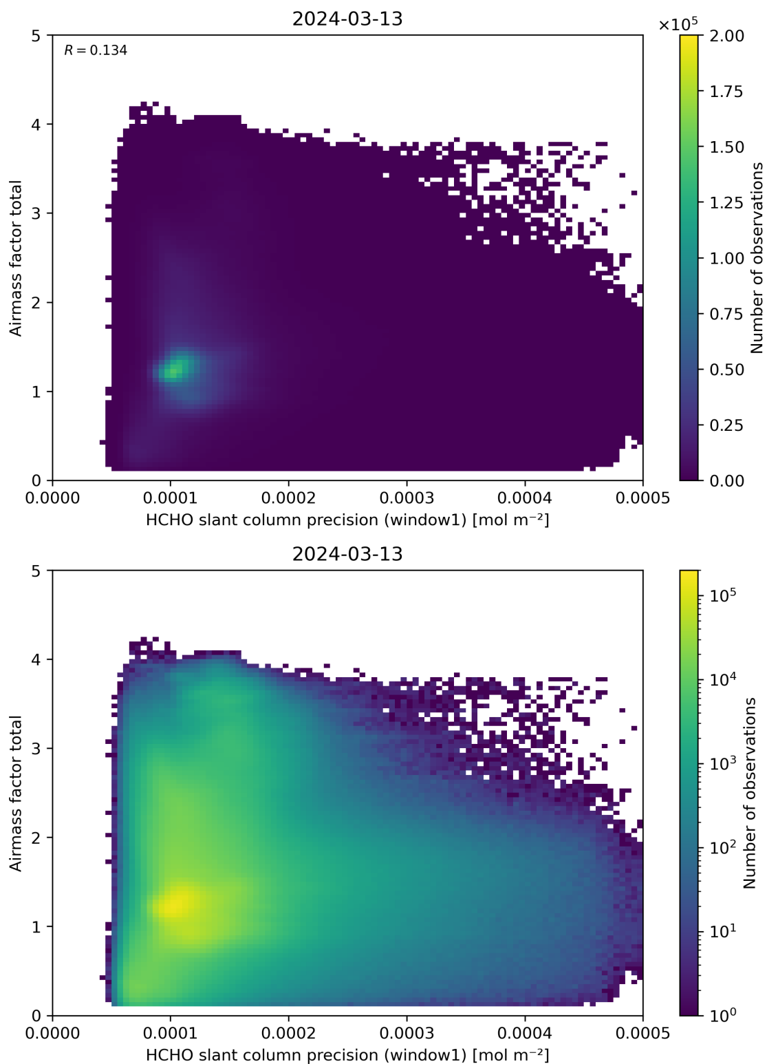
Figure 94: Scatter density plot of “HCHO slant column precision (window1)” against “Airmass factor total” for 2024-03-12 to 2024-03-14.
