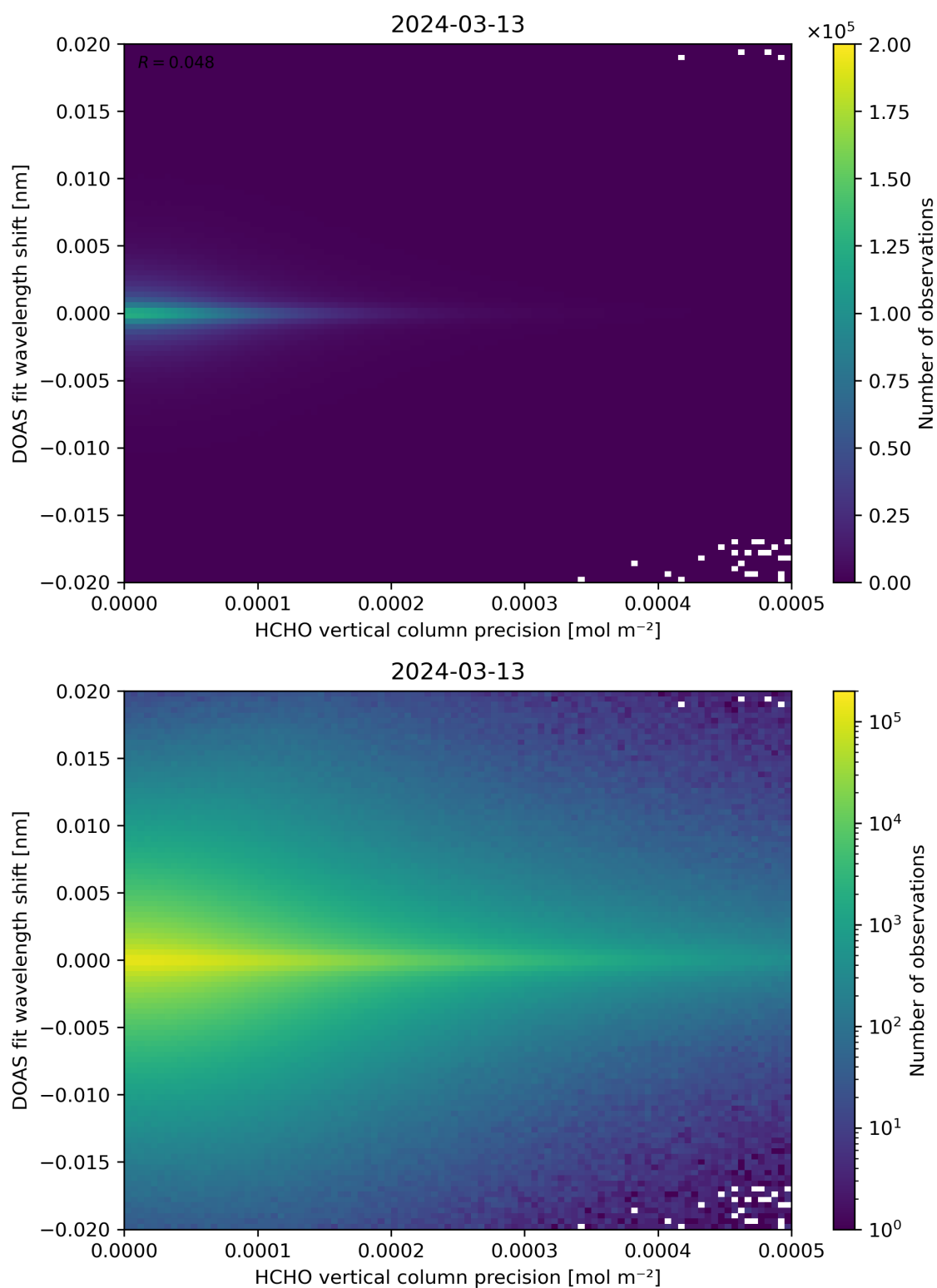
Figure 137: Scatter density plot of “HCHO vertical column precision” against “DOAS fit wavelength shift” for 2024-03-12 to 2024-03-14.
