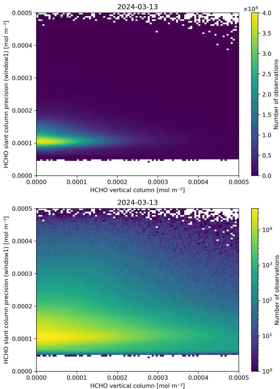
Figure 130: Scatter density plot of “HCHO vertical column” against “HCHO slant column precision (window1)” for 2024-03-12 to 2024-03-14.
