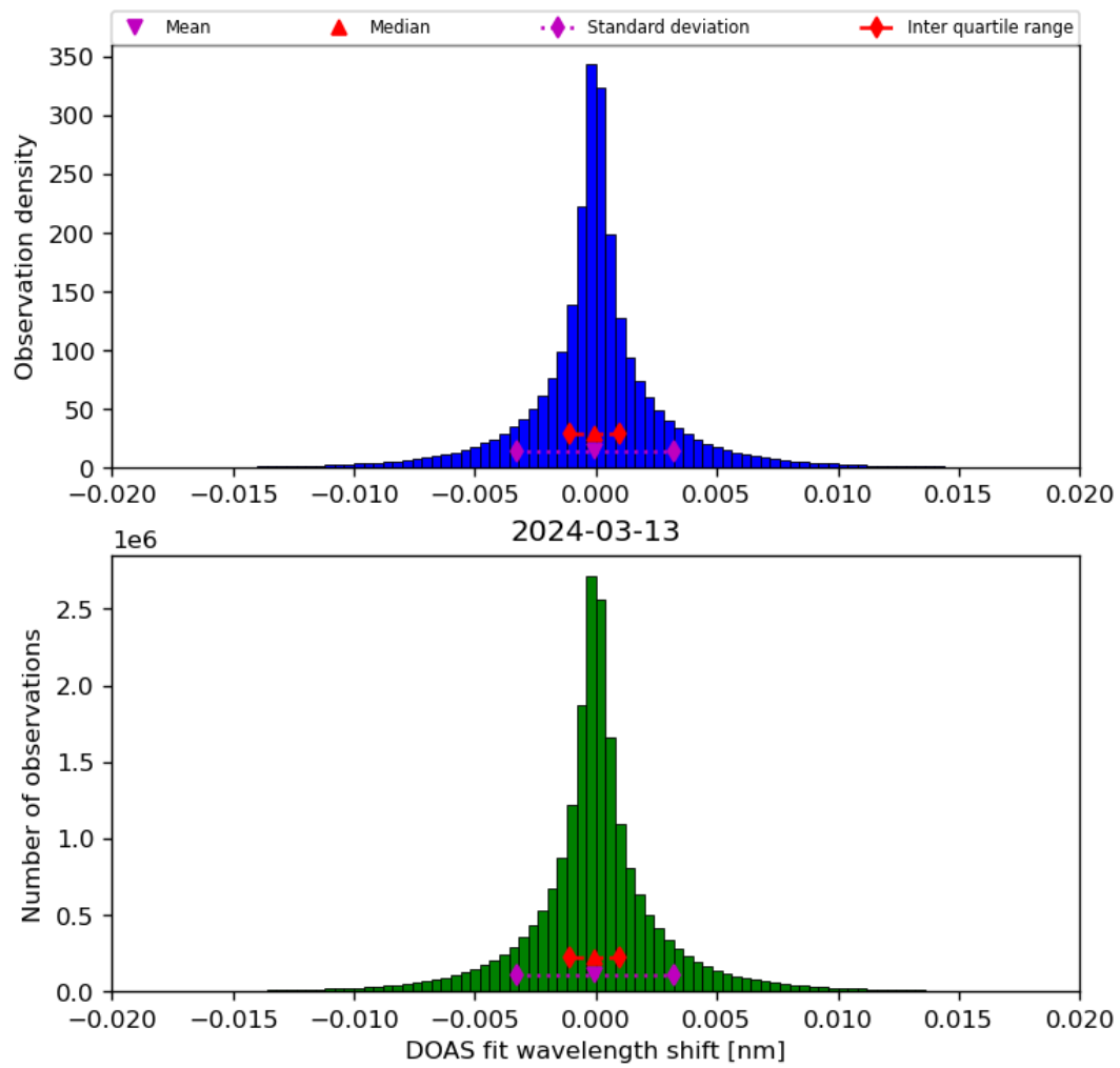
Figure 44: Histogram of “DOAS fit wavelength shift” for 2024-03-12 to 2024-03-14
