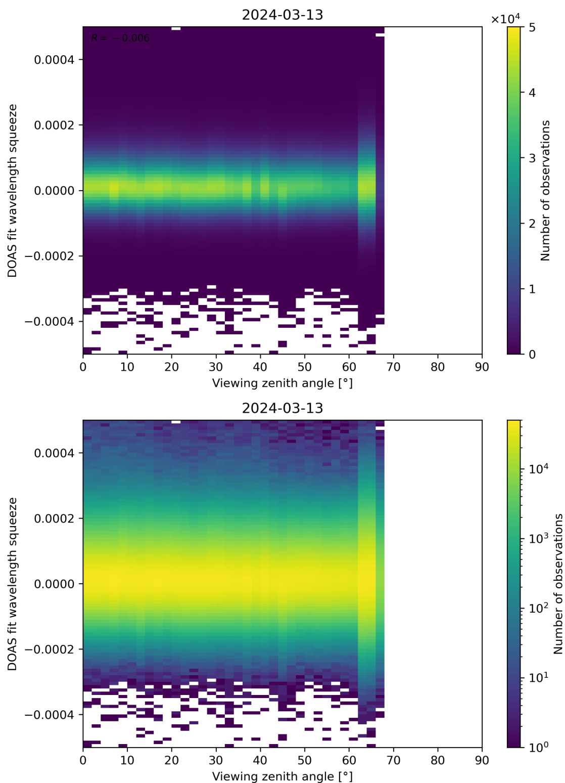
Figure 184: Scatter density plot of “Viewing zenith angle” against “DOAS fit wavelength squeeze” for 2024-03-12 to 2024-03-14.
