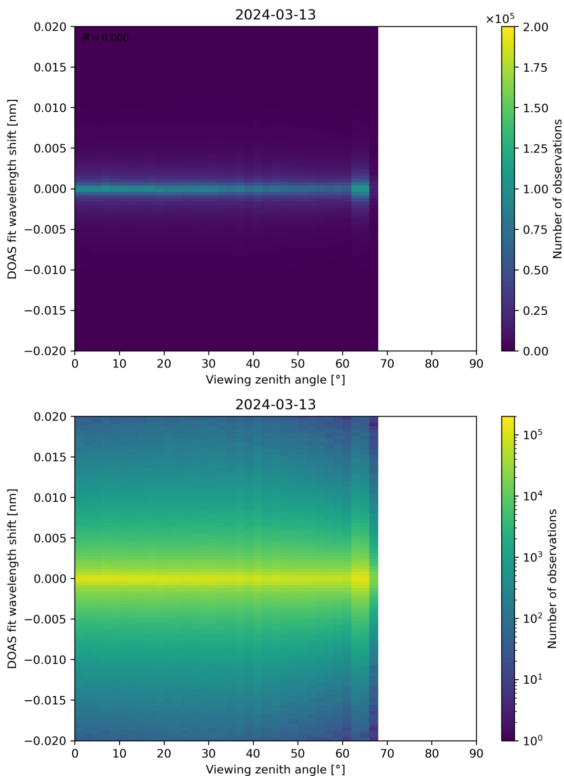
Figure 183: Scatter density plot of “Viewing zenith angle” against “DOAS fit wavelength shift” for 2024-03-12 to 2024-03-14.
