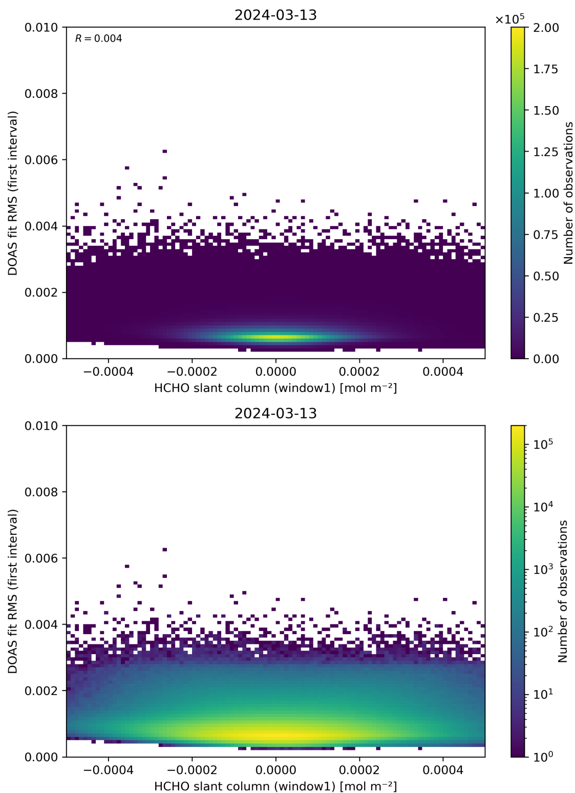
Figure 78: Scatter density plot of “HCHO slant column (window1)” against “DOAS fit RMS (first interval)” for 2024-03-12 to 2024-03-14.
