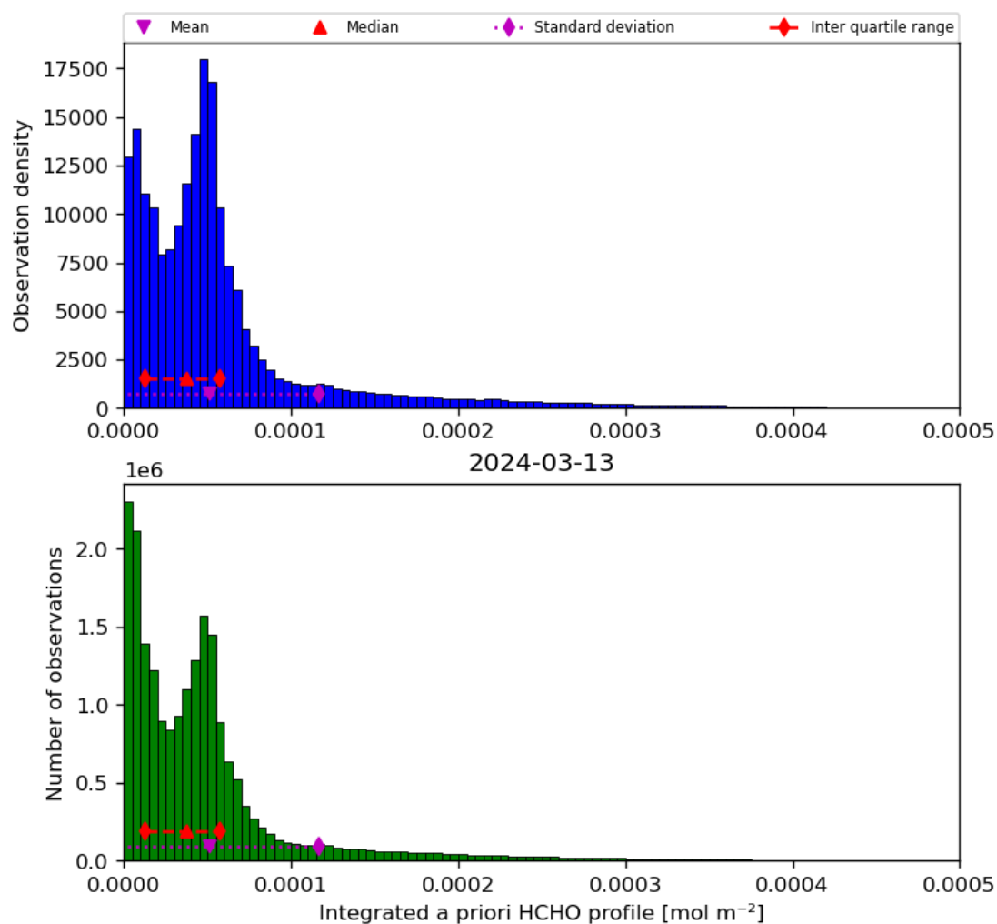
Figure 43: Histogram of “Integrated a priori HCHO profile” for 2024-03-12 to 2024-03-14
