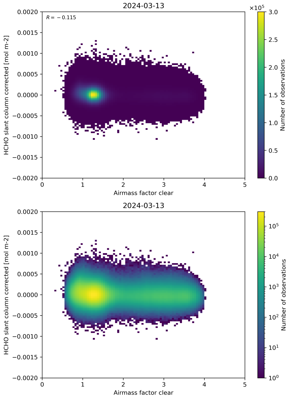
Figure 74: Scatter density plot of “Airmass factor clear” against “HCHO slant column corrected” for 2024-03-12 to 2024-03-14.
