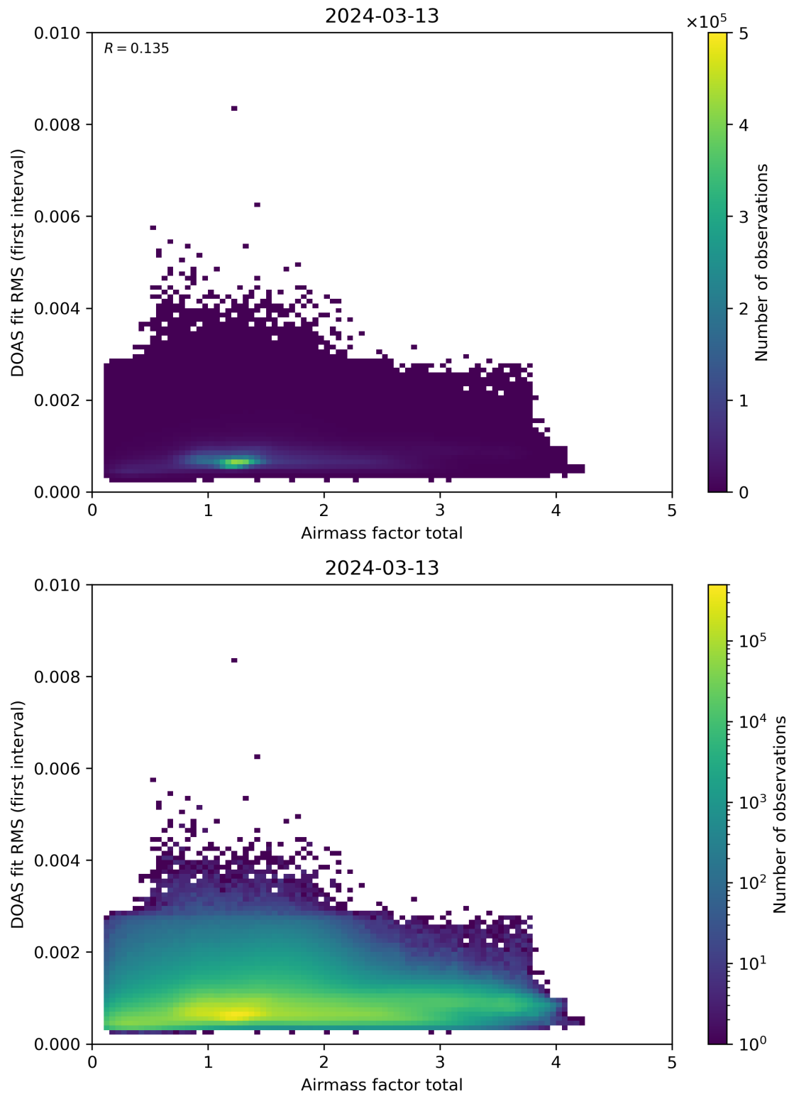
Figure 97: Scatter density plot of “Airmass factor total” against “DOAS fit RMS (first interval)” for 2024-03-12 to 2024-03-14.
