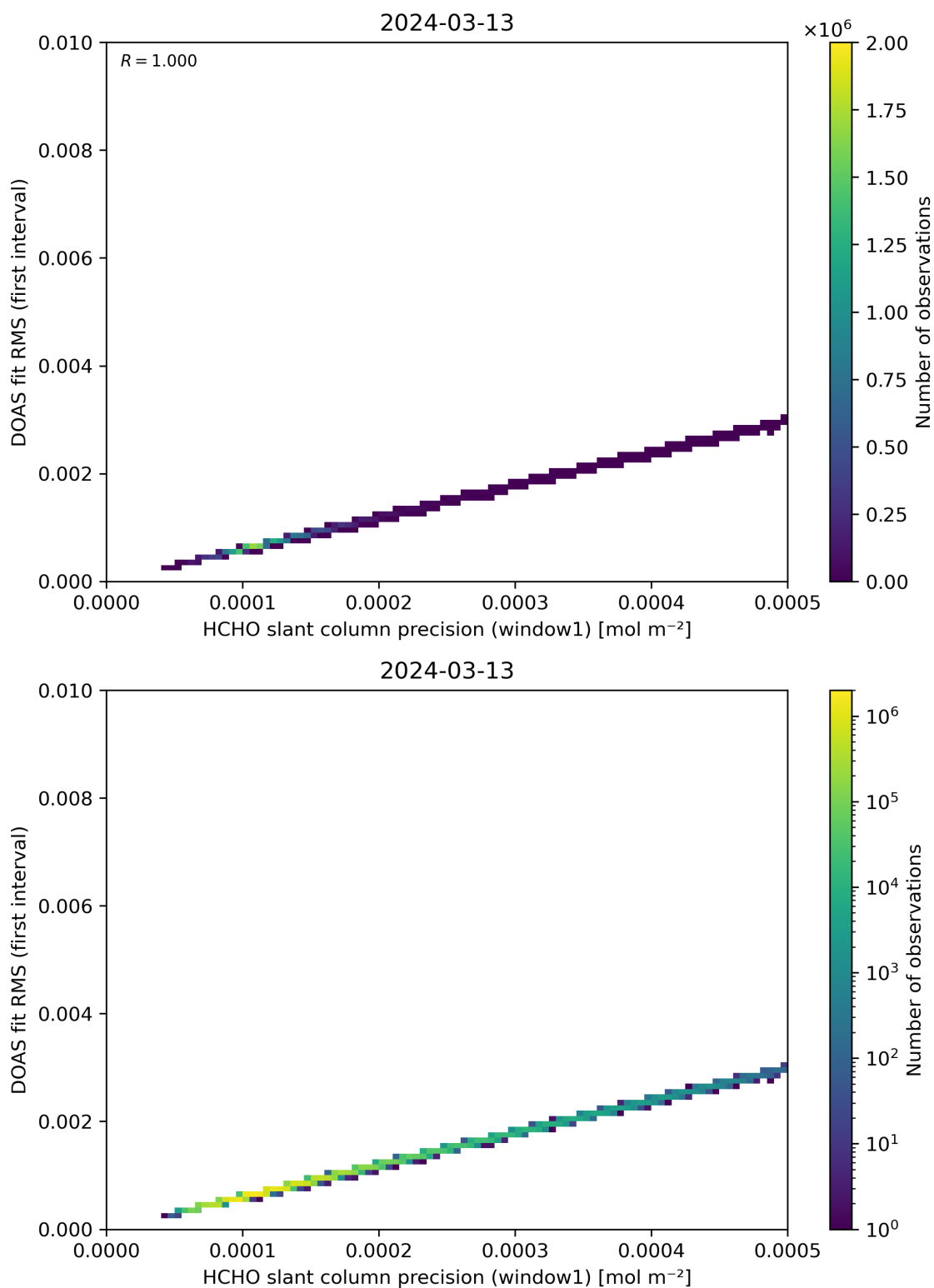
Figure 88: Scatter density plot of “HCHO slant column precision (window1)” against “DOAS fit RMS (first interval)” for 2024-03-12 to 2024-03-14.
