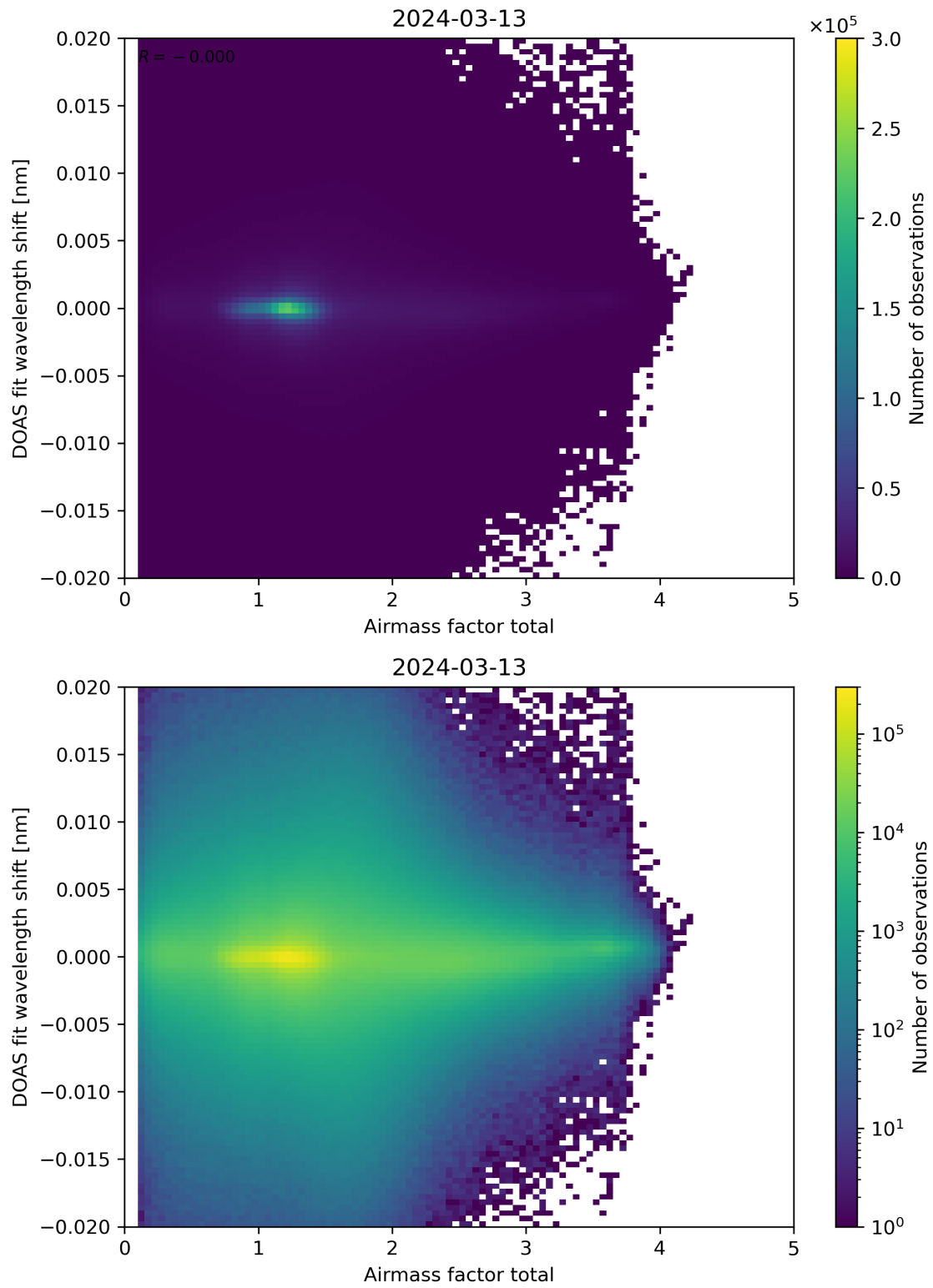
Figure 98: Scatter density plot of “Airmass factor total” against “DOAS fit wavelength shift” for 2024-03-12 to 2024-03-14.
