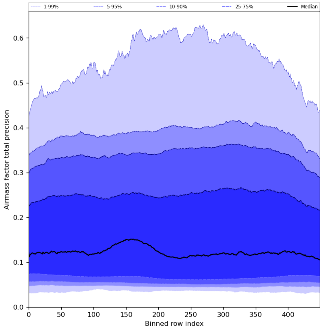
Figure 55: Along track statistics of “Airmass factor total precision” for 2024-03-12 to 2024-03-14
