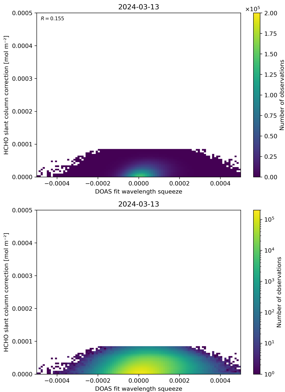
Figure 70: Scatter density plot of “DOAS fit wavelength squeeze” against “HCHO slant column correction” for 2024-03-12 to 2024-03-14.
