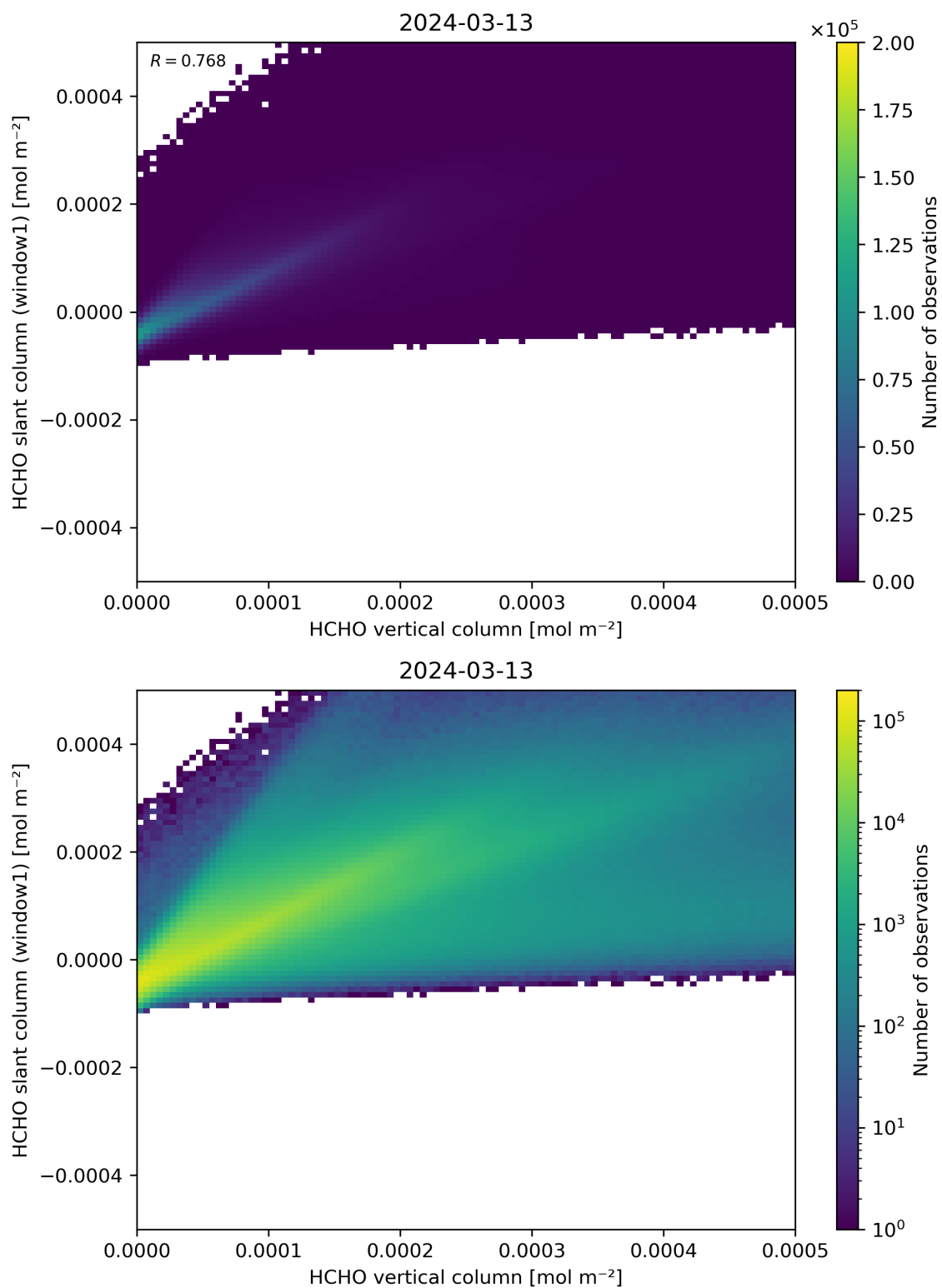
Figure 129: Scatter density plot of “HCHO vertical column” against “HCHO slant column (window1)” for 2024-03-12 to 2024-03-14.
