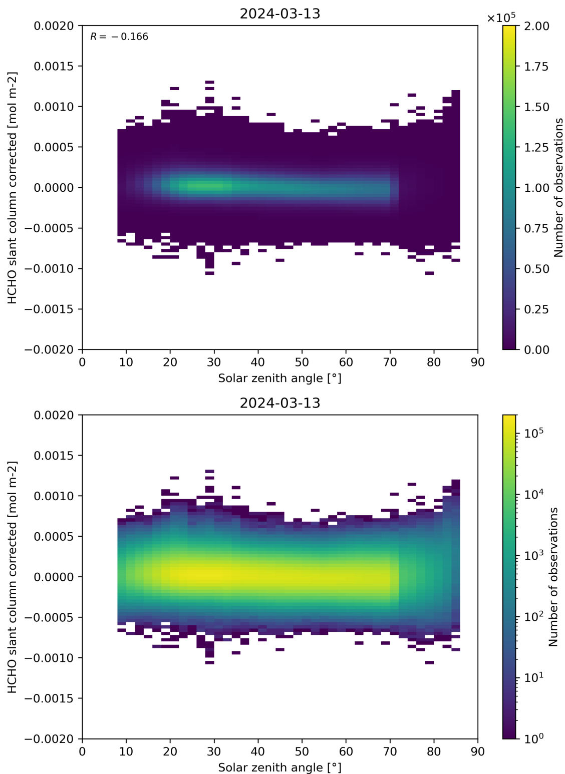
Figure 171: Scatter density plot of “Solar zenith angle” against “HCHO slant column corrected” for 2024-03-12 to 2024-03-14.
