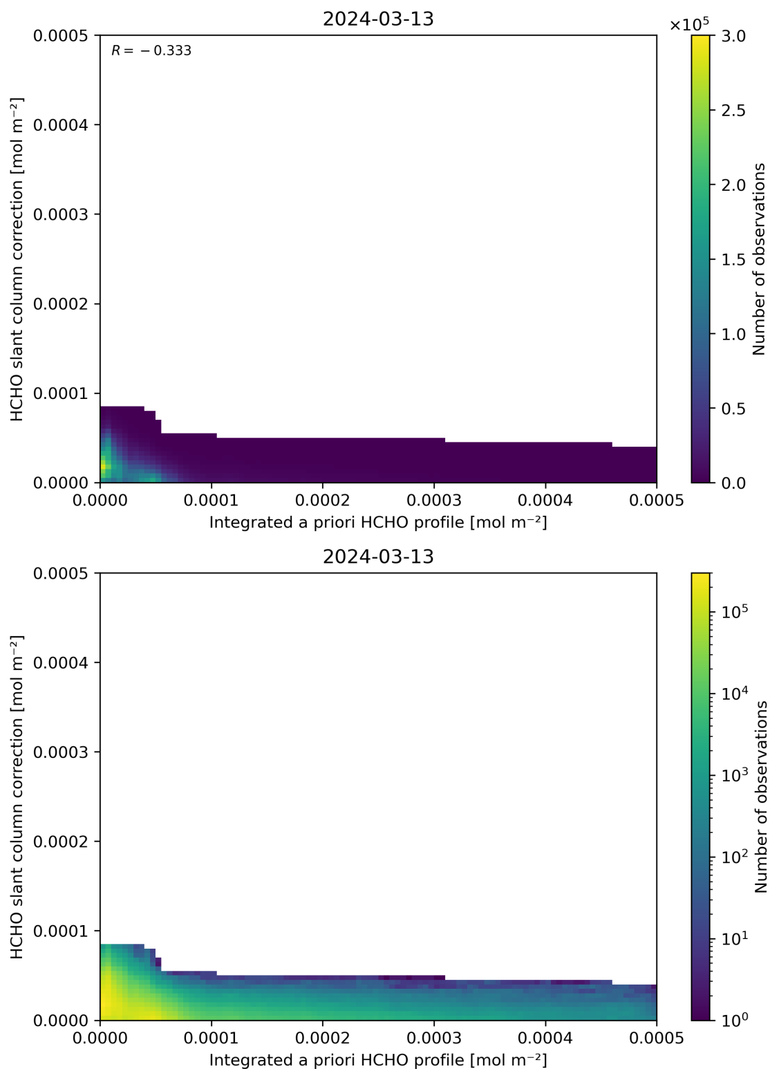
Figure 152: Scatter density plot of “Integrated a priori HCHO profile” against “HCHO slant column correction” for 2024-03-12 to 2024-03-14.
