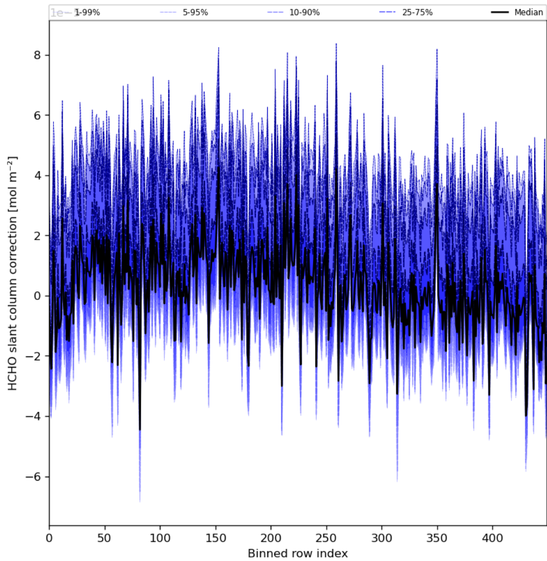
Figure 61: Along track statistics of “HCHO slant column correction” for 2024-03-12 to 2024-03-14
