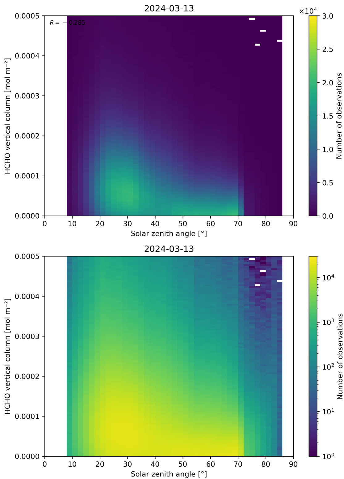
Figure 177: Scatter density plot of “Solar zenith angle” against “HCHO vertical column” for 2024-03-12 to 2024-03-14.
