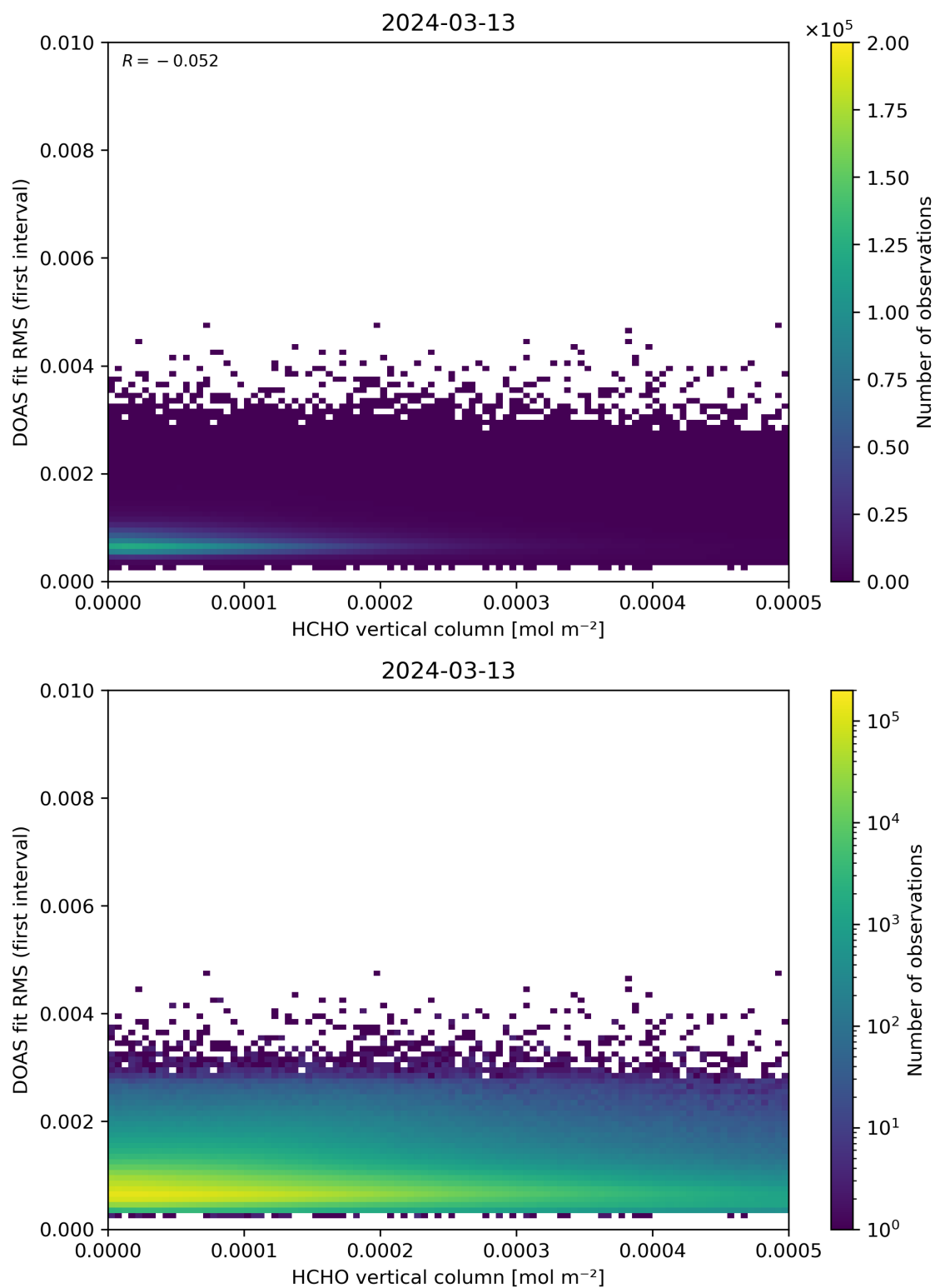
Figure 123: Scatter density plot of “HCHO vertical column” against “DOAS fit RMS (first interval)” for 2024-03-12 to 2024-03-14.
