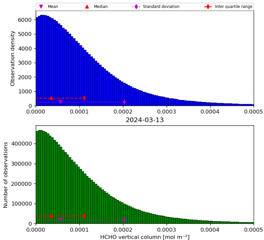
Figure 35: Histogram of “HCHO vertical column” for 2024-03-12 to 2024-03-14
