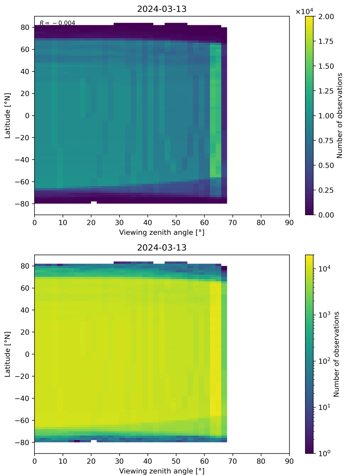
Figure 196: Scatter density plot of “Viewing zenith angle” against “Latitude” for 2024-03-12 to 2024-03-14.
