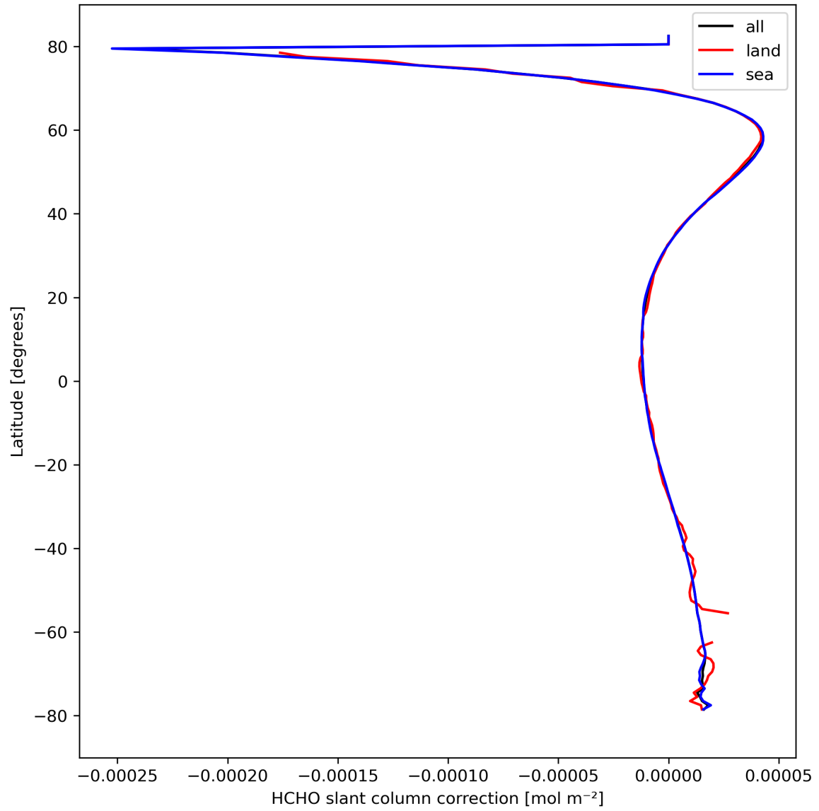
Figure 33: Zonal average of "HCHO slant column correction" for 2024-03-12 to 2024-03-14.
