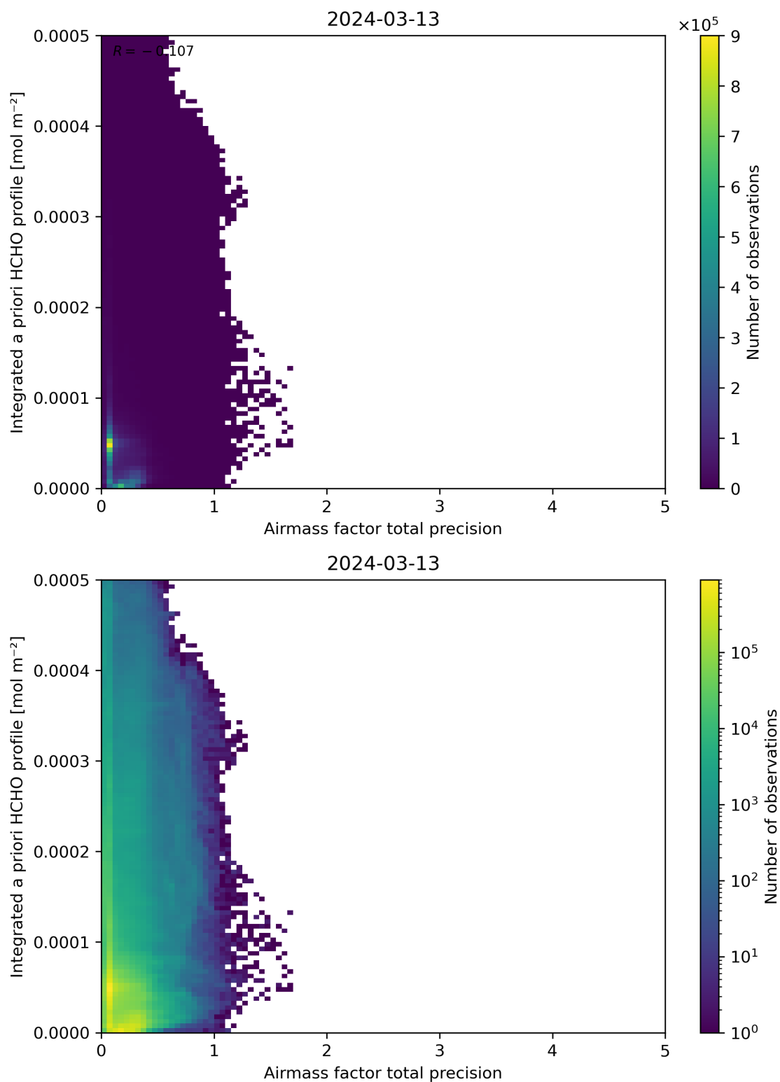
Figure 111: Scatter density plot of “Airmass factor total precision” against “Integrated a priori HCHO profile” for 2024-03-12 to 2024-03-14.
