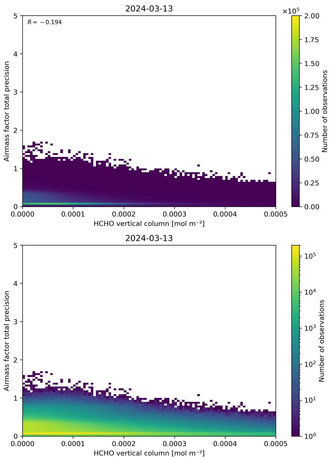
Figure 132: Scatter density plot of “HCHO vertical column” against “Airmass factor total precision” for 2024-03-12 to 2024-03-14.
