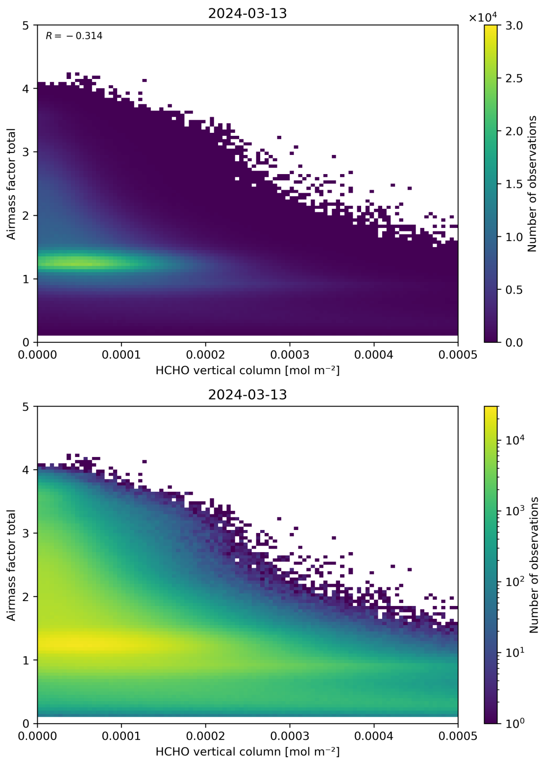
Figure 131: Scatter density plot of “HCHO vertical column” against “Airmass factor total” for 2024-03-12 to 2024-03-14.
