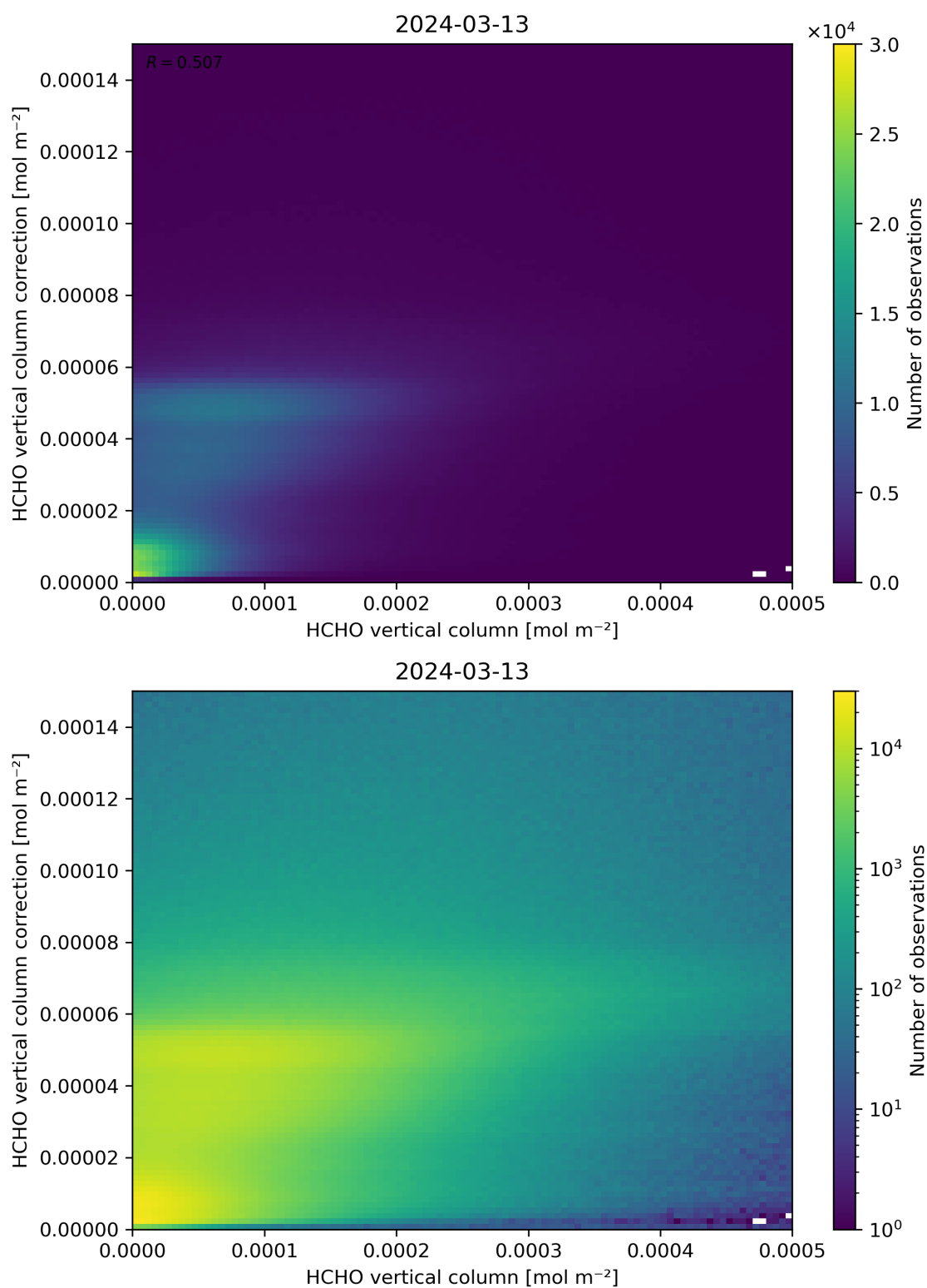
Figure 133: Scatter density plot of “HCHO vertical column” against “HCHO vertical column correction” for 2024-03-12 to 2024-03-14.
