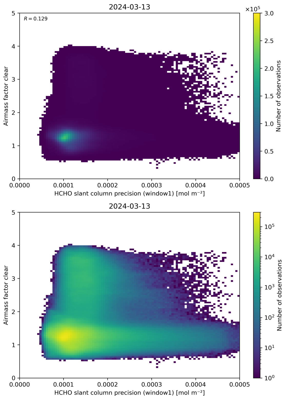
Figure 91: Scatter density plot of “HCHO slant column precision (window1)” against “Airmass factor clear” for 2024-03-12 to 2024-03-14.
