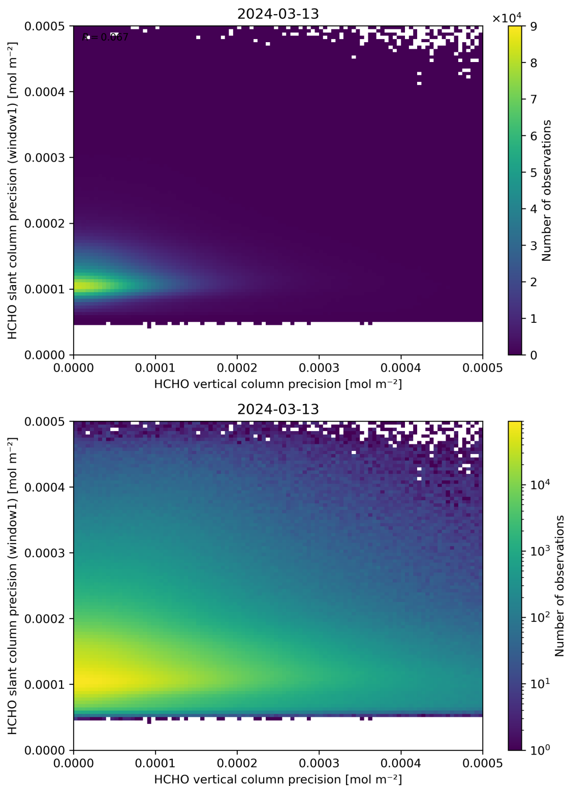
Figure 143: Scatter density plot of “HCHO vertical column precision” against “HCHO slant column precision (window1)” for 2024-03-12 to 2024-03-14.
