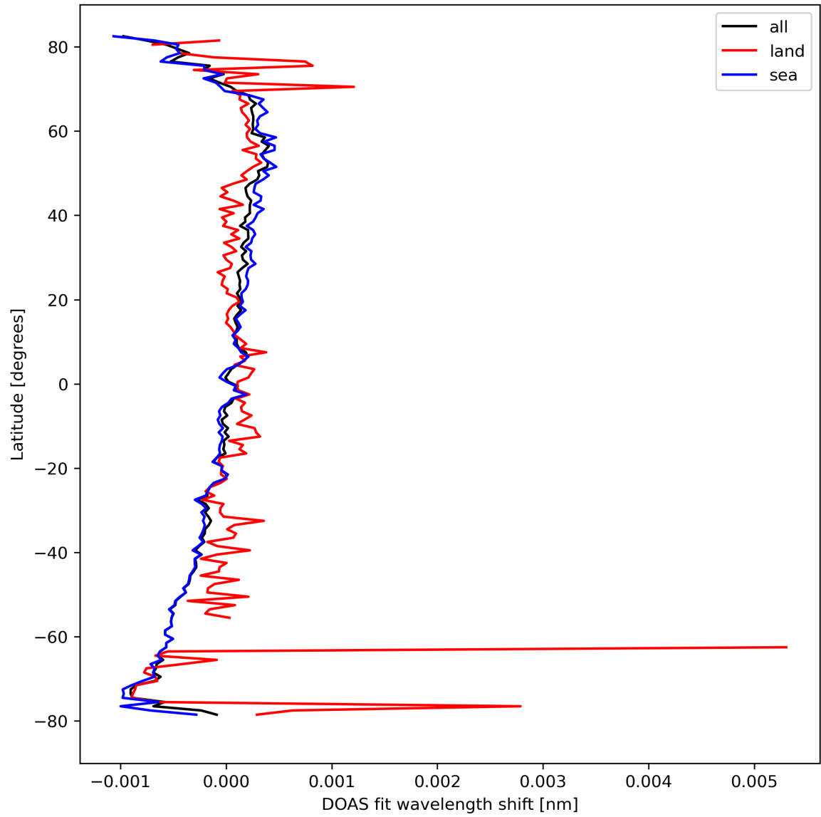
Figure 30: Zonal average of "DOAS fit wavelength shift" for 2024-03-12 to 2024-03-14.
