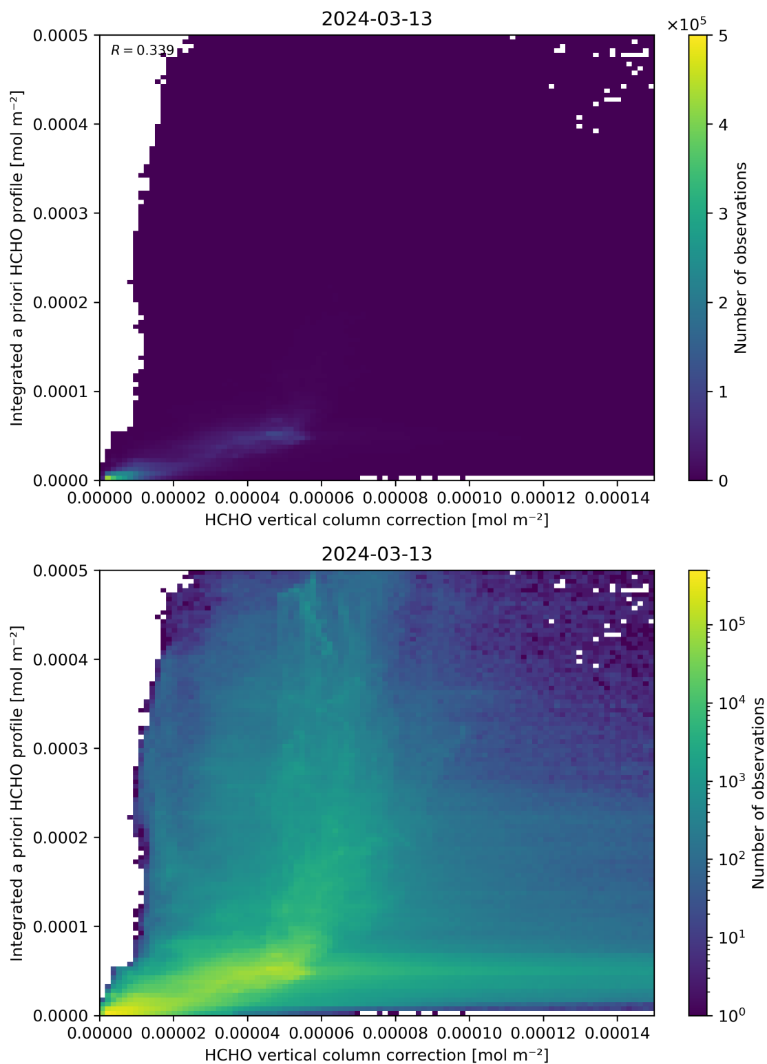
Figure 122: Scatter density plot of “HCHO vertical column correction” against “Integrated a priori HCHO profile” for 2024-03-12 to 2024-03-14.
