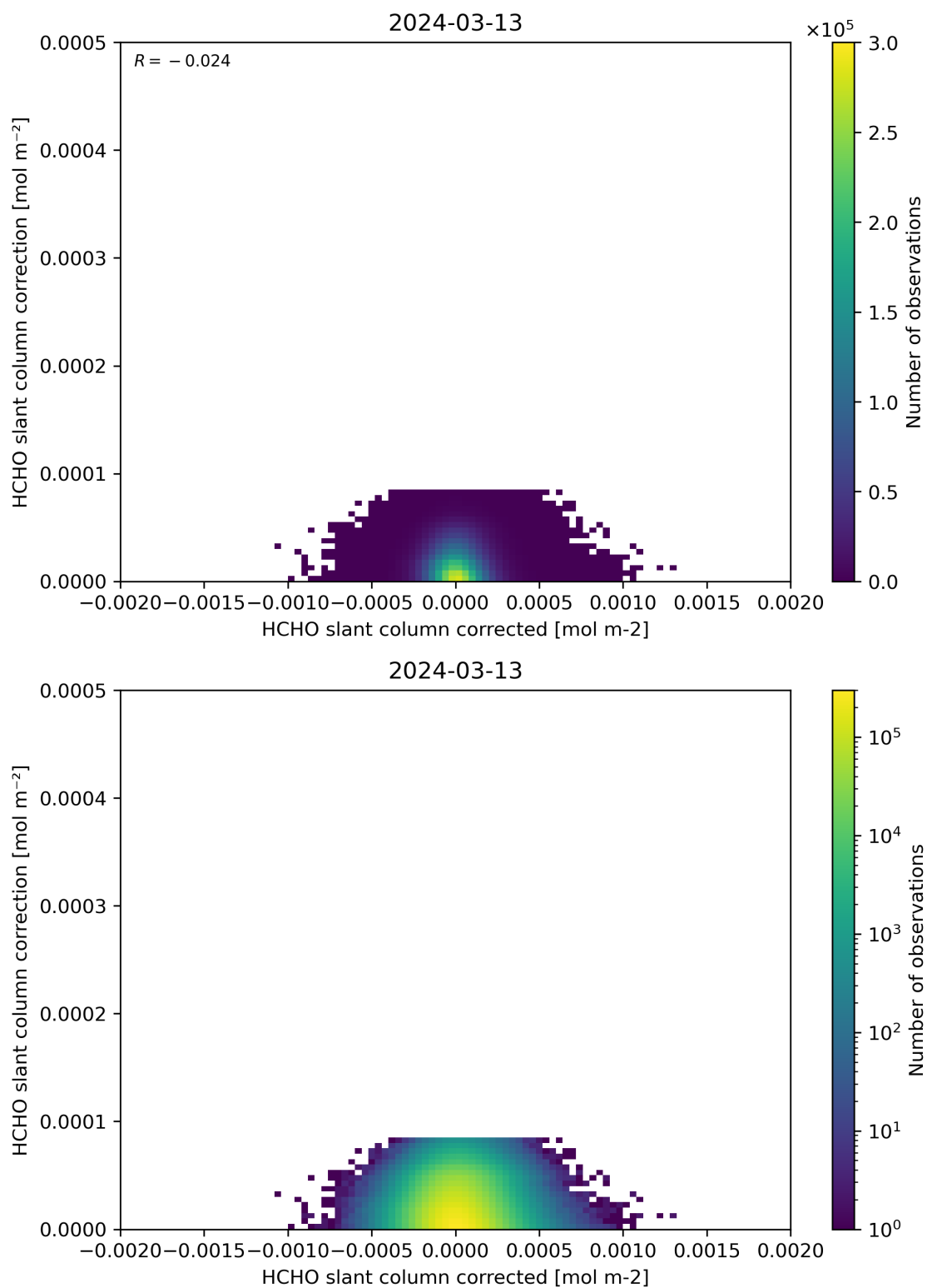
Figure 77: Scatter density plot of “HCHO slant column corrected” against “HCHO slant column correction” for 2024-03-12 to 2024-03-14.
