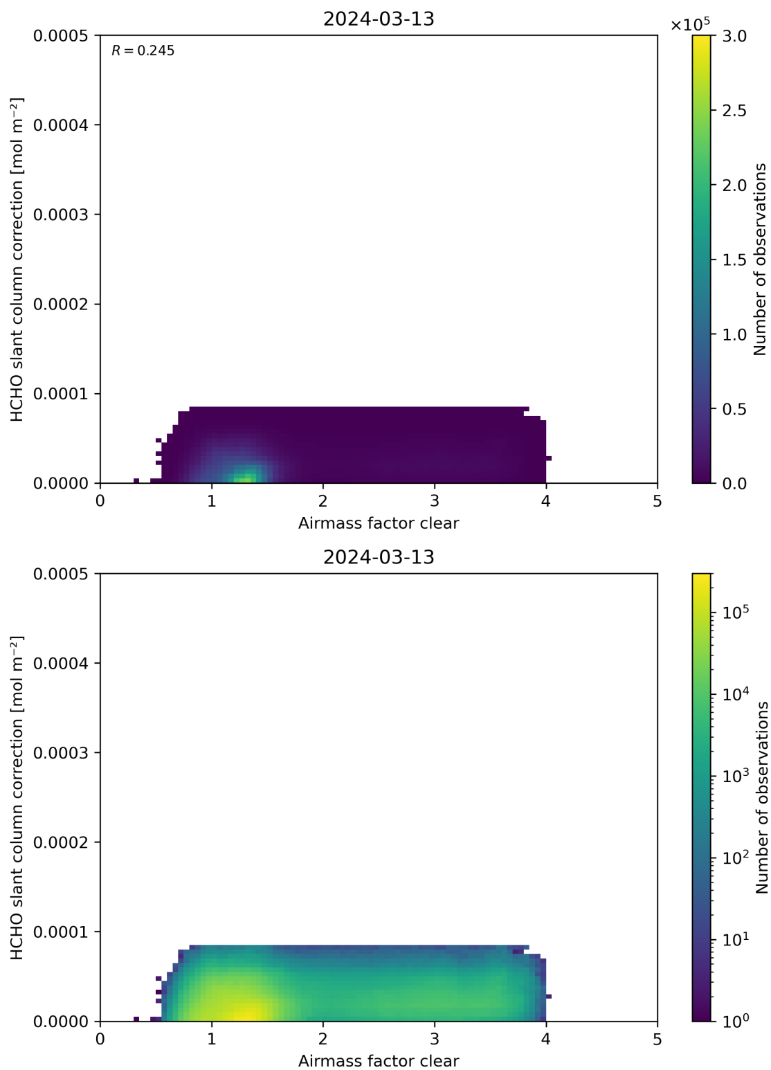
Figure 75: Scatter density plot of “Airmass factor clear” against “HCHO slant column correction” for 2024-03-12 to 2024-03-14.
