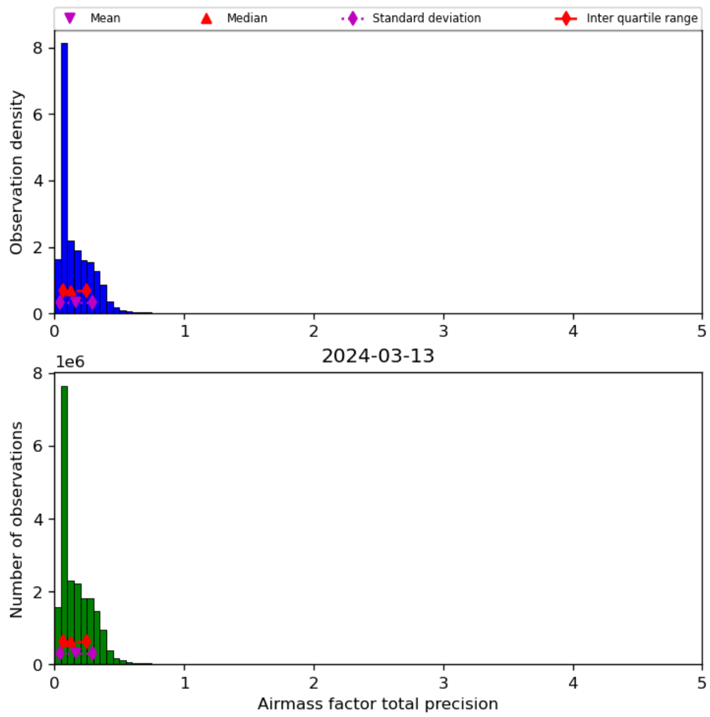
Figure 41: Histogram of “Airmass factor total precision” for 2024-03-12 to 2024-03-14
