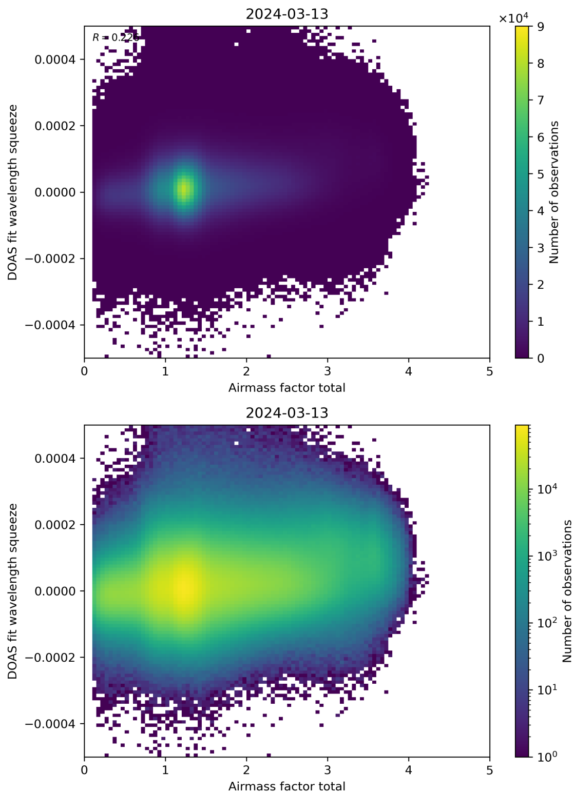
Figure 99: Scatter density plot of “Airmass factor total” against “DOAS fit wavelength squeeze” for 2024-03-12 to 2024-03-14.
