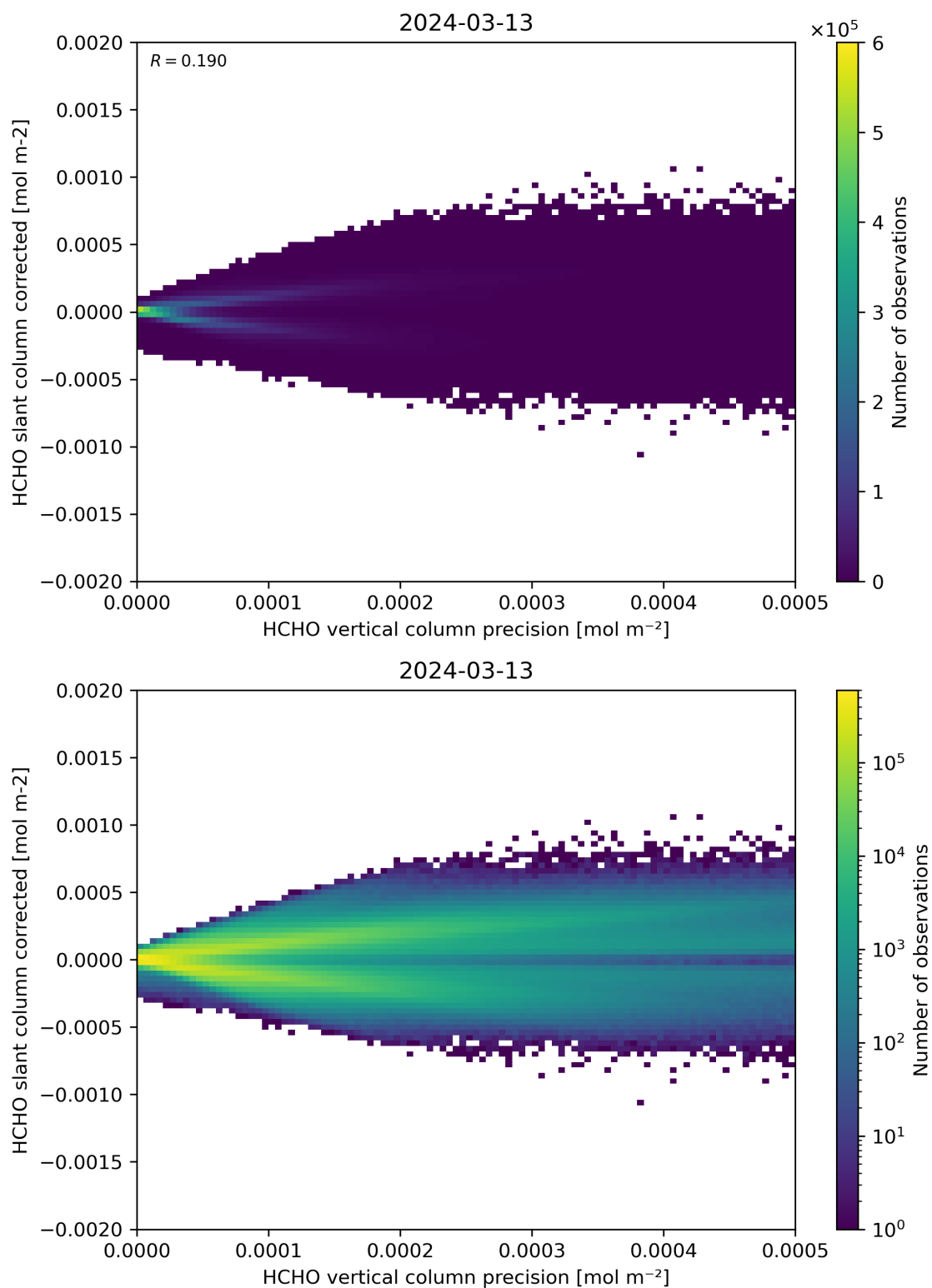
Figure 140: Scatter density plot of “HCHO vertical column precision” against “HCHO slant column corrected” for 2024-03-12 to 2024-03-14.
