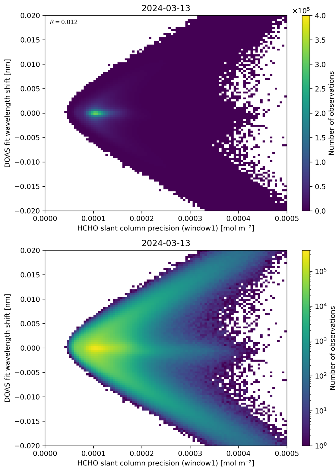
Figure 89: Scatter density plot of “HCHO slant column precision (window1)” against “DOAS fit wavelength shift” for 2024-03-12 to 2024-03-14.
