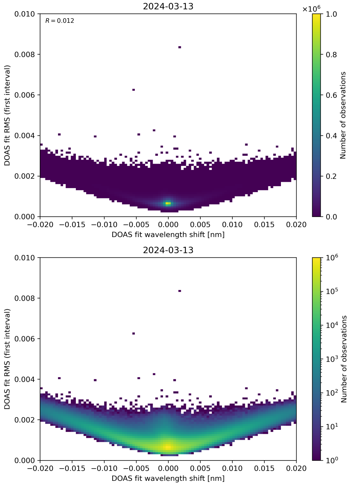
Figure 64: Scatter density plot of “DOAS fit wavelength shift” against “DOAS fit RMS (first interval)” for 2024-03-12 to 2024-03-14.
