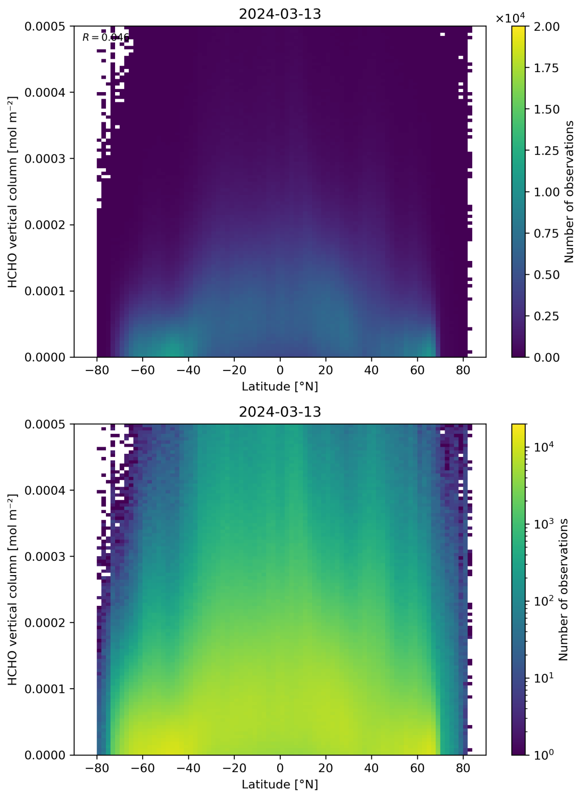
Figure 163: Scatter density plot of “Latitude” against “HCHO vertical column” for 2024-03-12 to 2024-03-14.
