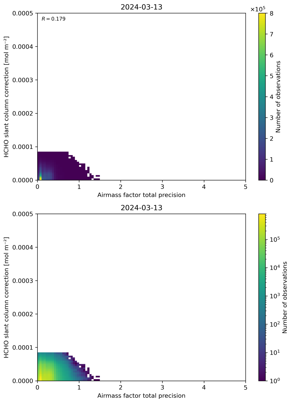
Figure 110: Scatter density plot of “Airmass factor total precision” against “HCHO slant column correction” for 2024-03-12 to 2024-03-14.
