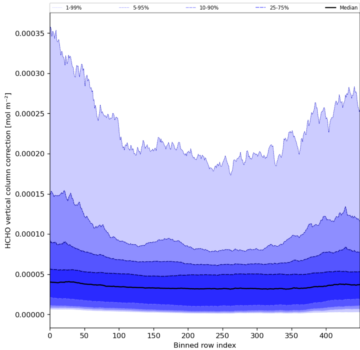
Figure 51: Along track statistics of “HCHO vertical column correction” for 2024-03-12 to 2024-03-14
