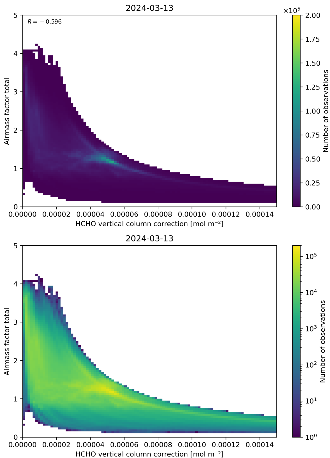
Figure 120: Scatter density plot of “HCHO vertical column correction” against “Airmass factor total” for 2024-03-12 to 2024-03-14.
