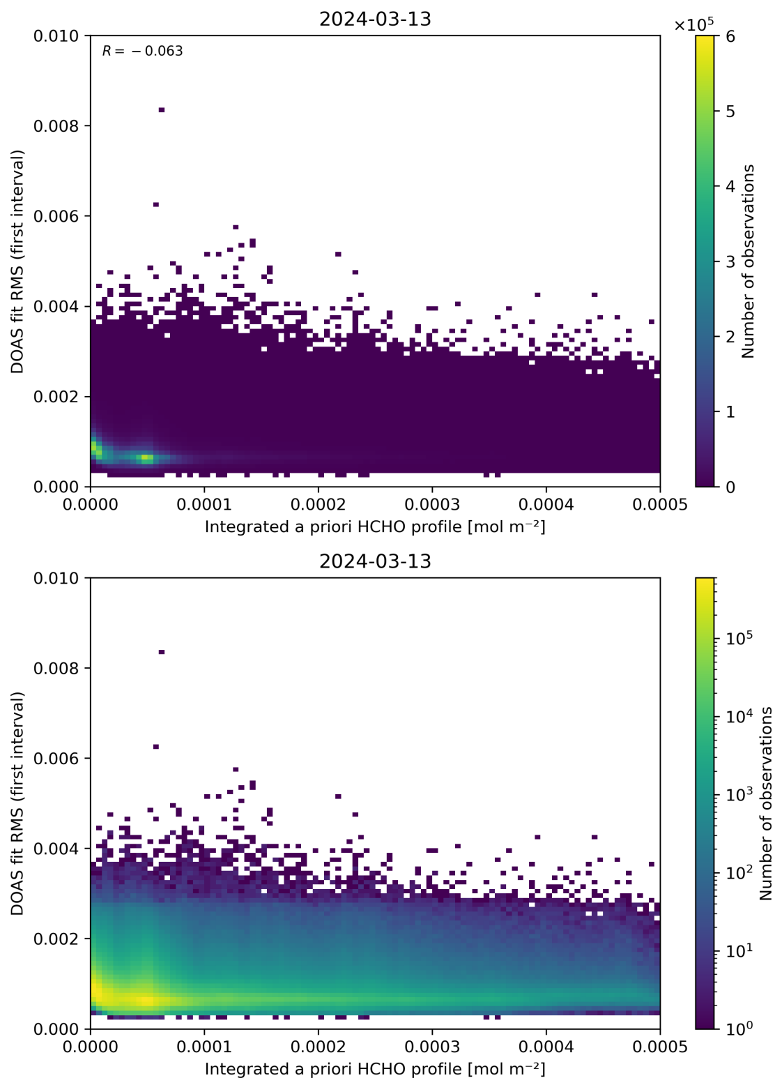
Figure 148: Scatter density plot of “Integrated a priori HCHO profile” against “DOAS fit RMS (first interval)” for 2024-03-12 to 2024-03-14.
