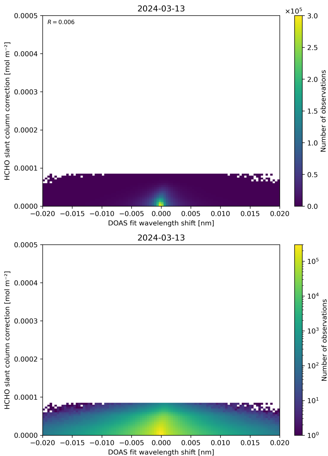
Figure 67: Scatter density plot of “DOAS fit wavelength shift” against “HCHO slant column correction” for 2024-03-12 to 2024-03-14.
