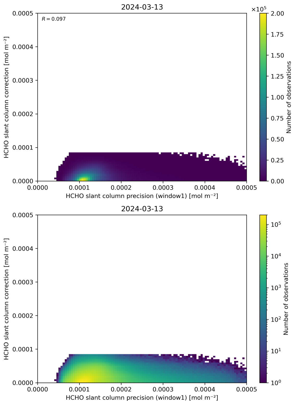
Figure 93: Scatter density plot of “HCHO slant column precision (window1)” against “HCHO slant column correction” for 2024-03-12 to 2024-03-14.
