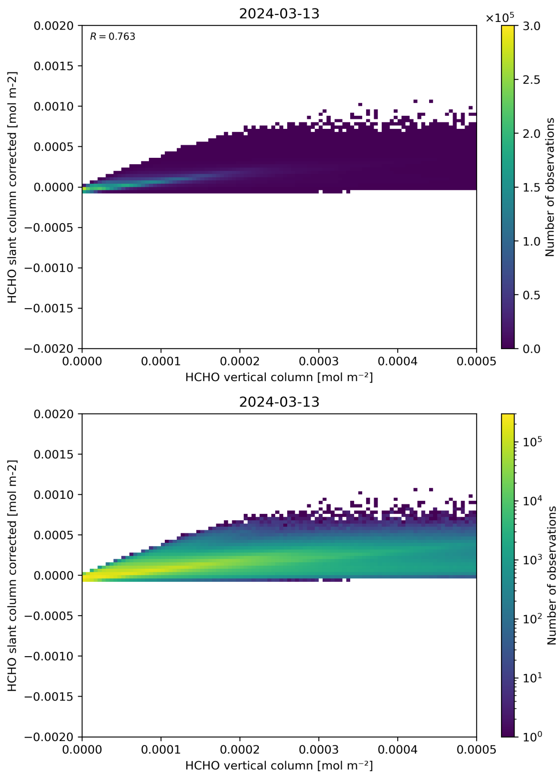
Figure 127: Scatter density plot of “HCHO vertical column” against “HCHO slant column corrected” for 2024-03-12 to 2024-03-14.
