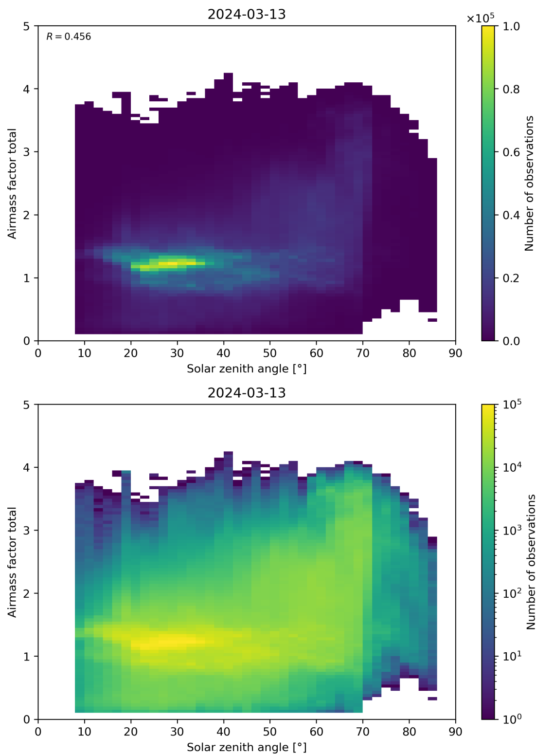
Figure 175: Scatter density plot of “Solar zenith angle” against “Airmass factor total” for 2024-03-12 to 2024-03-14.
