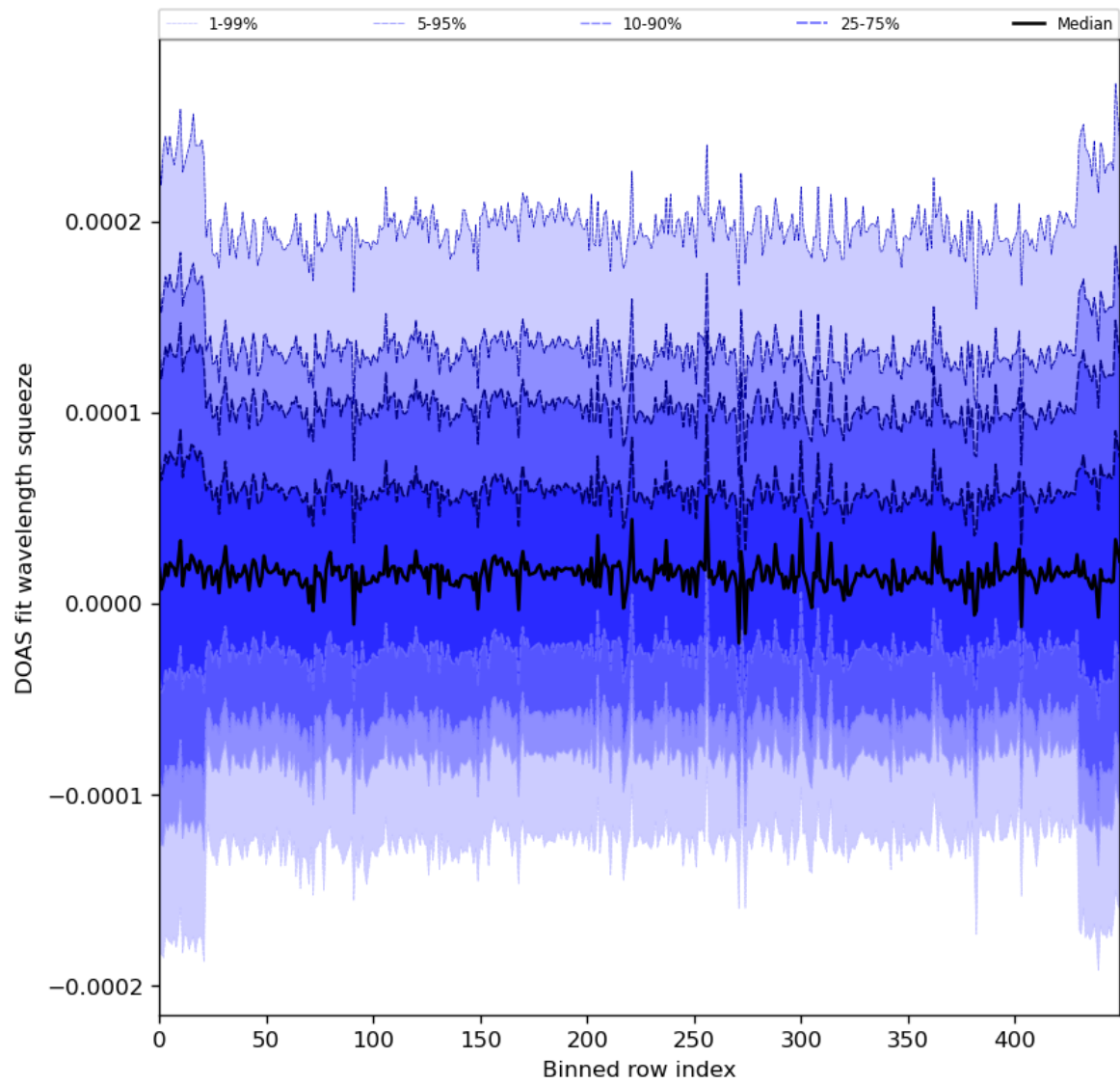
Figure 59: Along track statistics of “DOAS fit wavelength squeeze” for 2024-03-12 to 2024-03-14
