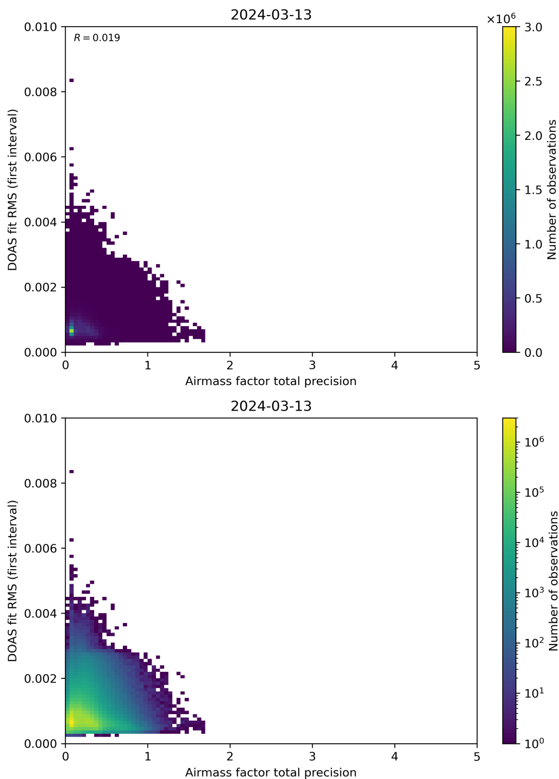
Figure 105: Scatter density plot of “Airmass factor total precision” against “DOAS fit RMS (first interval)” for 2024-03-12 to 2024-03-14.
