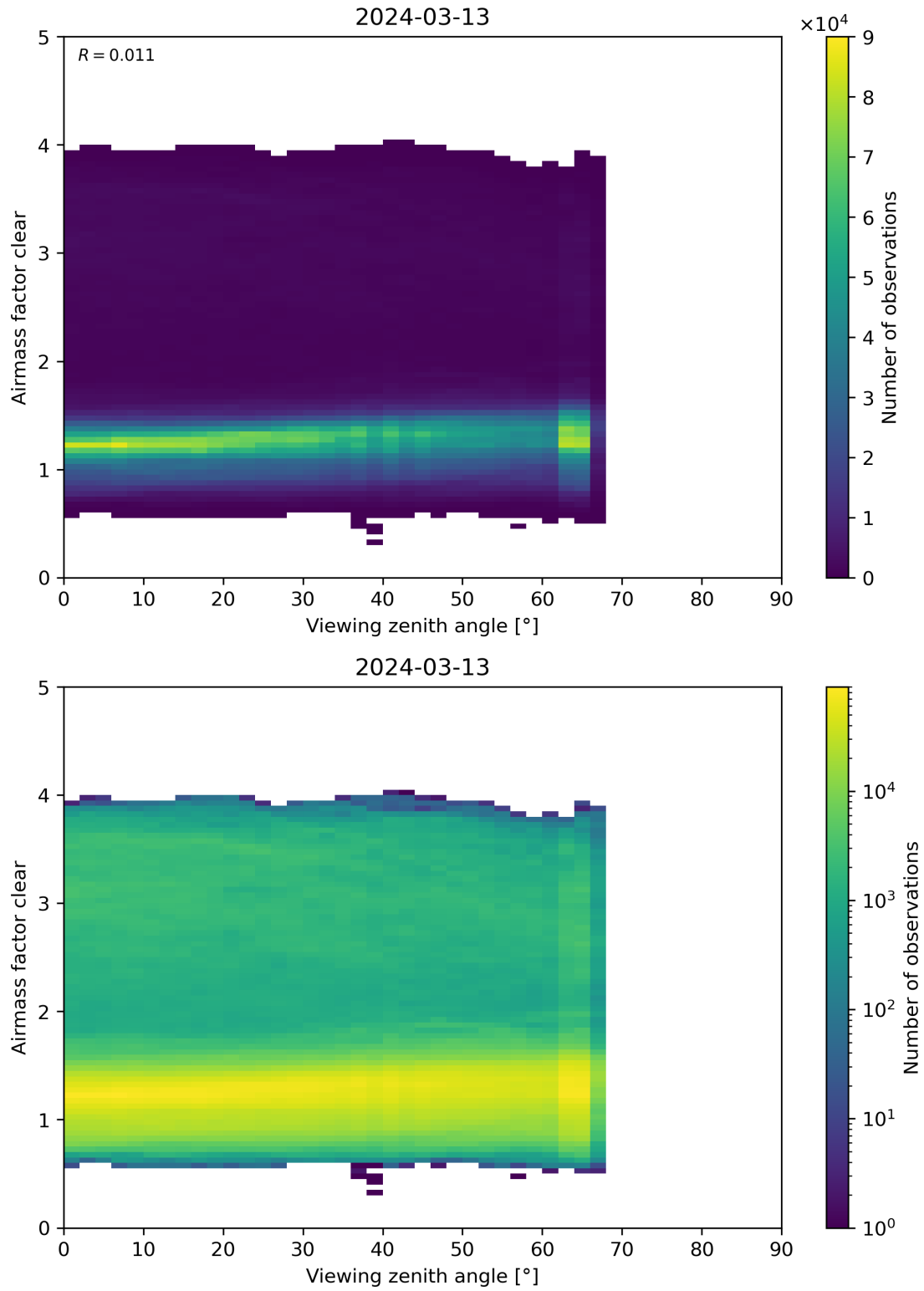
Figure 185: Scatter density plot of “Viewing zenith angle” against “Airmass factor clear” for 2024-03-12 to 2024-03-14.
