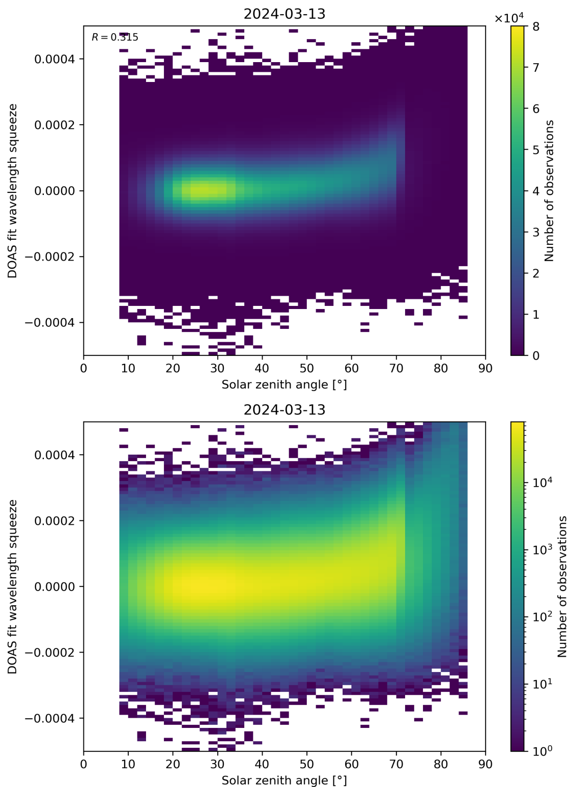
Figure 169: Scatter density plot of “Solar zenith angle” against “DOAS fit wavelength squeeze” for 2024-03-12 to 2024-03-14.
