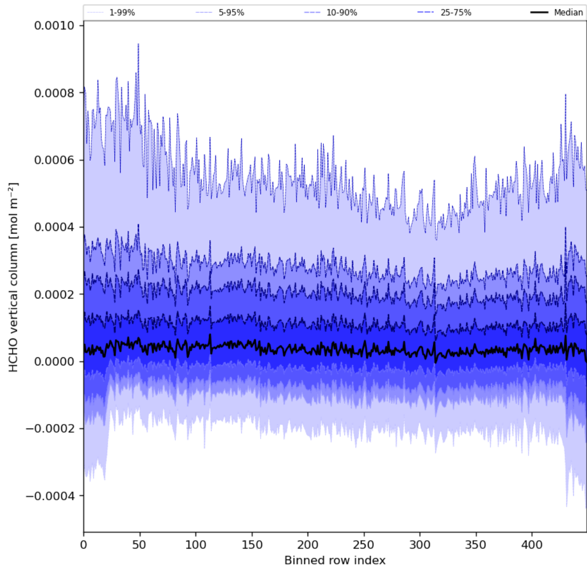
Figure 49: Along track statistics of “HCHO vertical column” for 2024-03-12 to 2024-03-14
