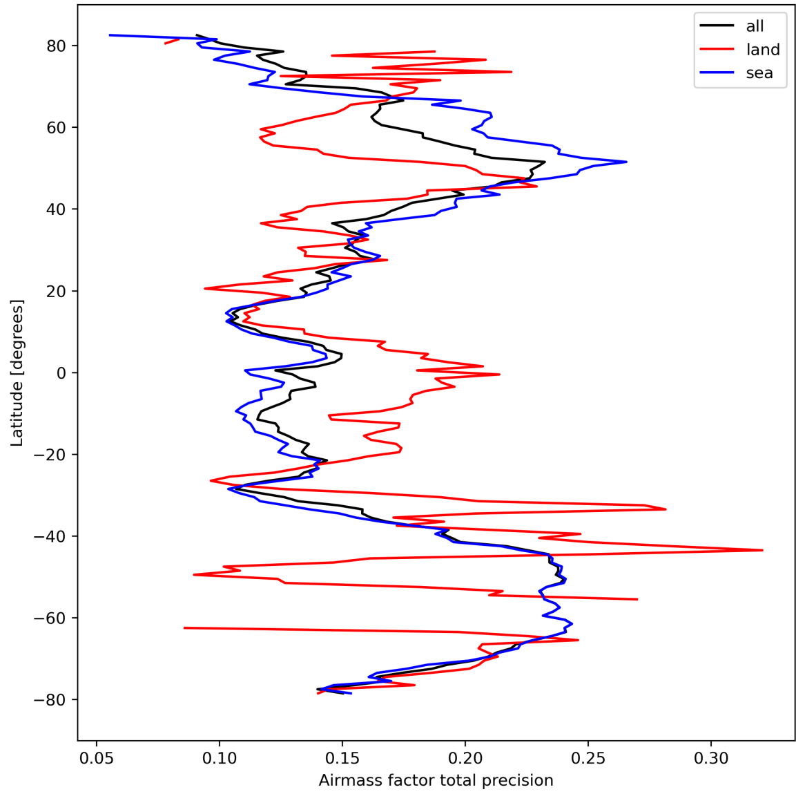
Figure 27: Zonal average of “Airmass factor total precision” for 2024-03-12 to 2024-03-14.
