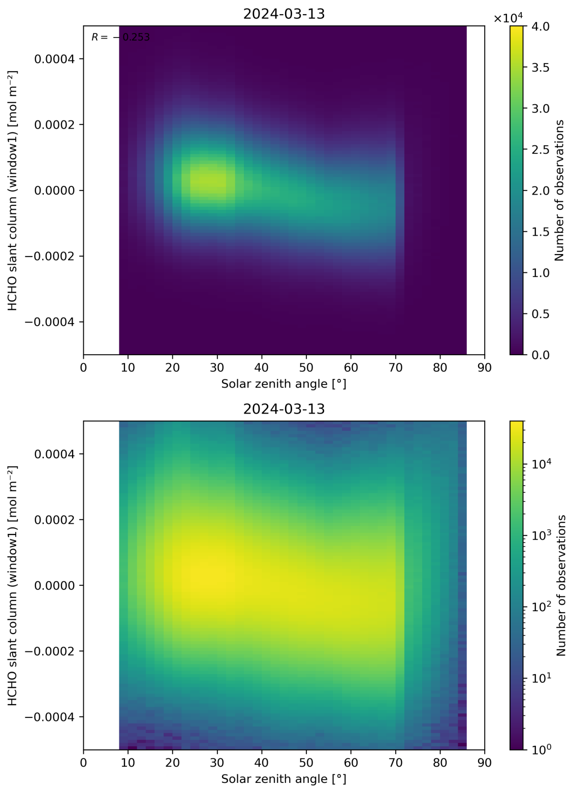
Figure 173: Scatter density plot of “Solar zenith angle” against “HCHO slant column (window1)” for 2024-03-12 to 2024-03-14.
