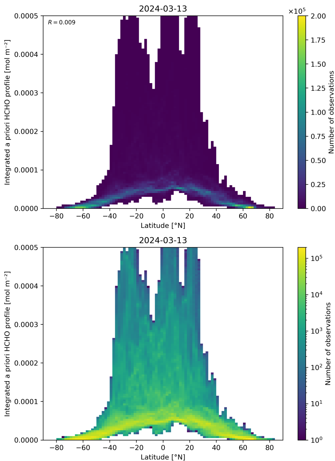
Figure 166: Scatter density plot of “Latitude” against “Integrated a priori HCHO profile” for 2024-03-12 to 2024-03-14.
