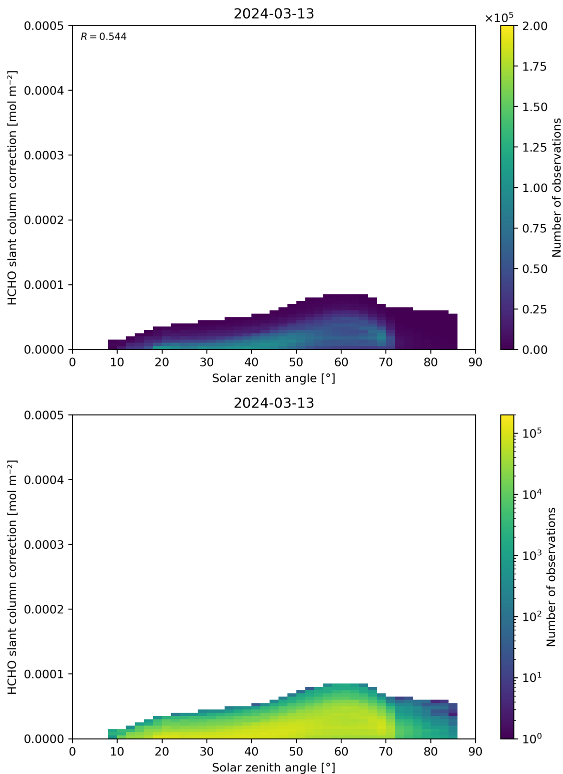
Figure 172: Scatter density plot of “Solar zenith angle” against “HCHO slant column correction” for 2024-03-12 to 2024-03-14.
