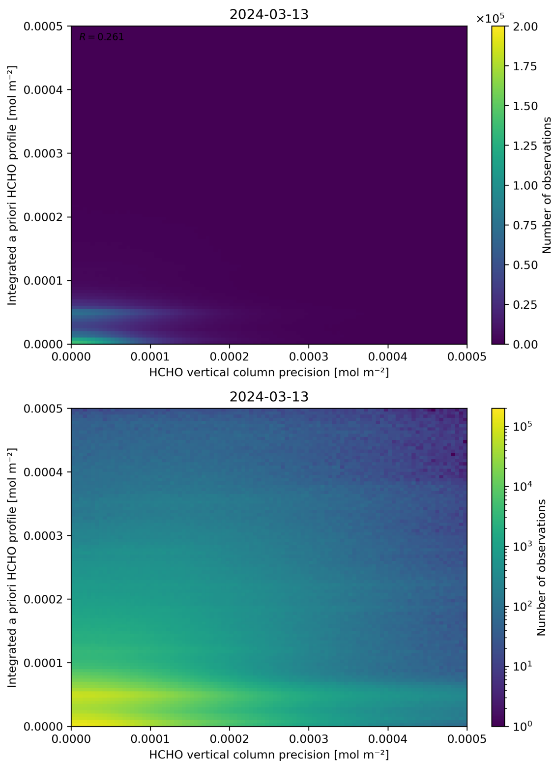
Figure 147: Scatter density plot of “HCHO vertical column precision” against “Integrated a priori HCHO profile” for 2024-03-12 to 2024-03-14.
