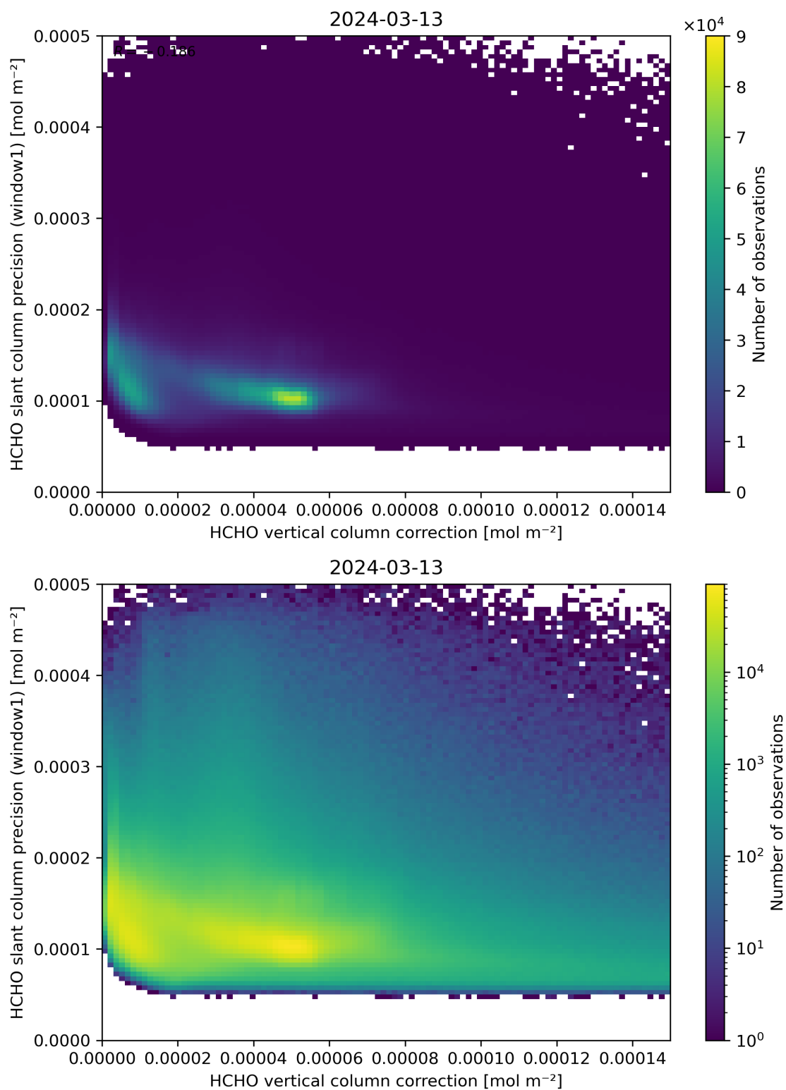
Figure 119: Scatter density plot of “HCHO vertical column correction” against “HCHO slant column precision (window1)” for 2024-03-12 to 2024-03-14.
