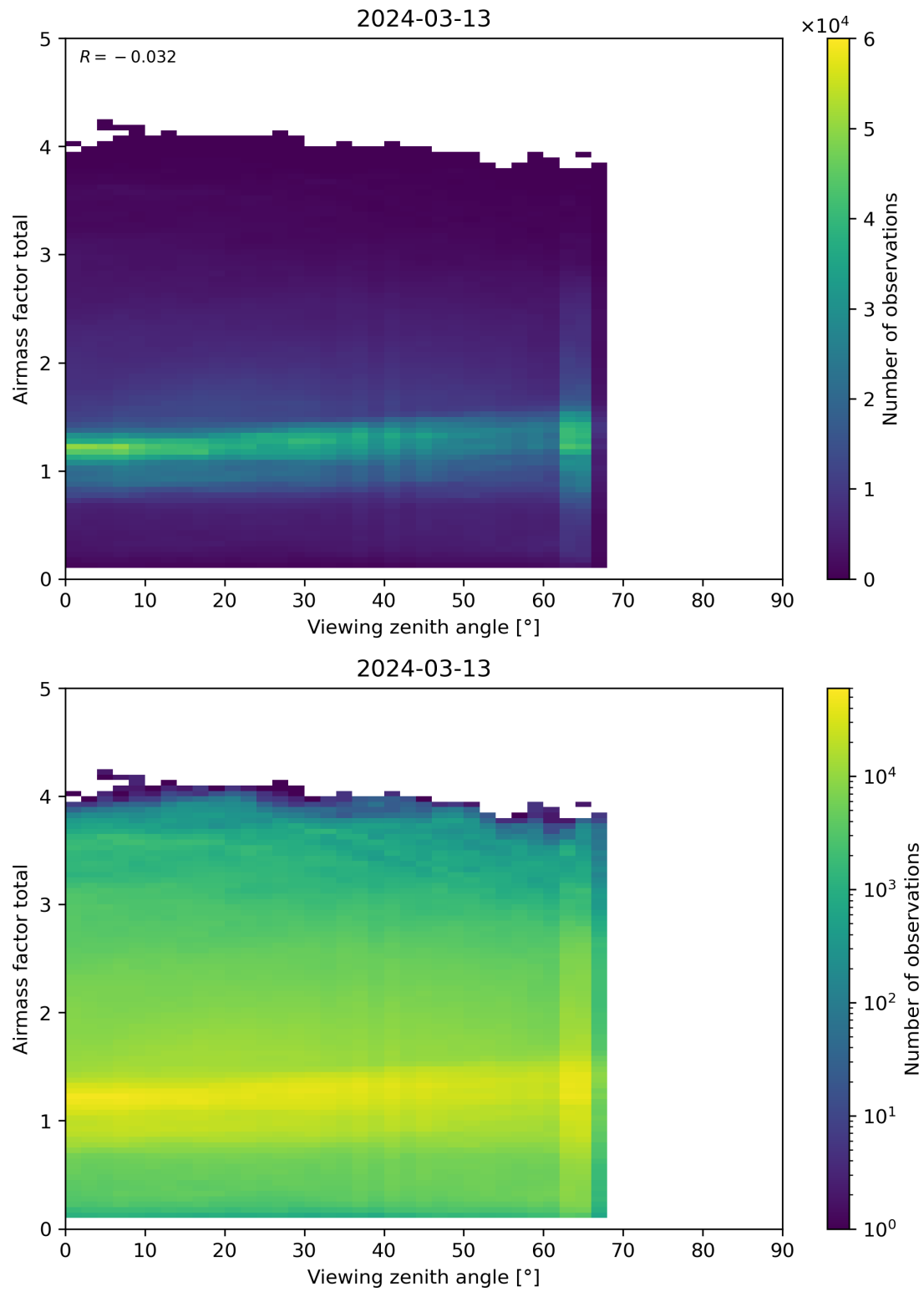
Figure 190: Scatter density plot of “Viewing zenith angle” against “Airmass factor total” for 2024-03-12 to 2024-03-14.
