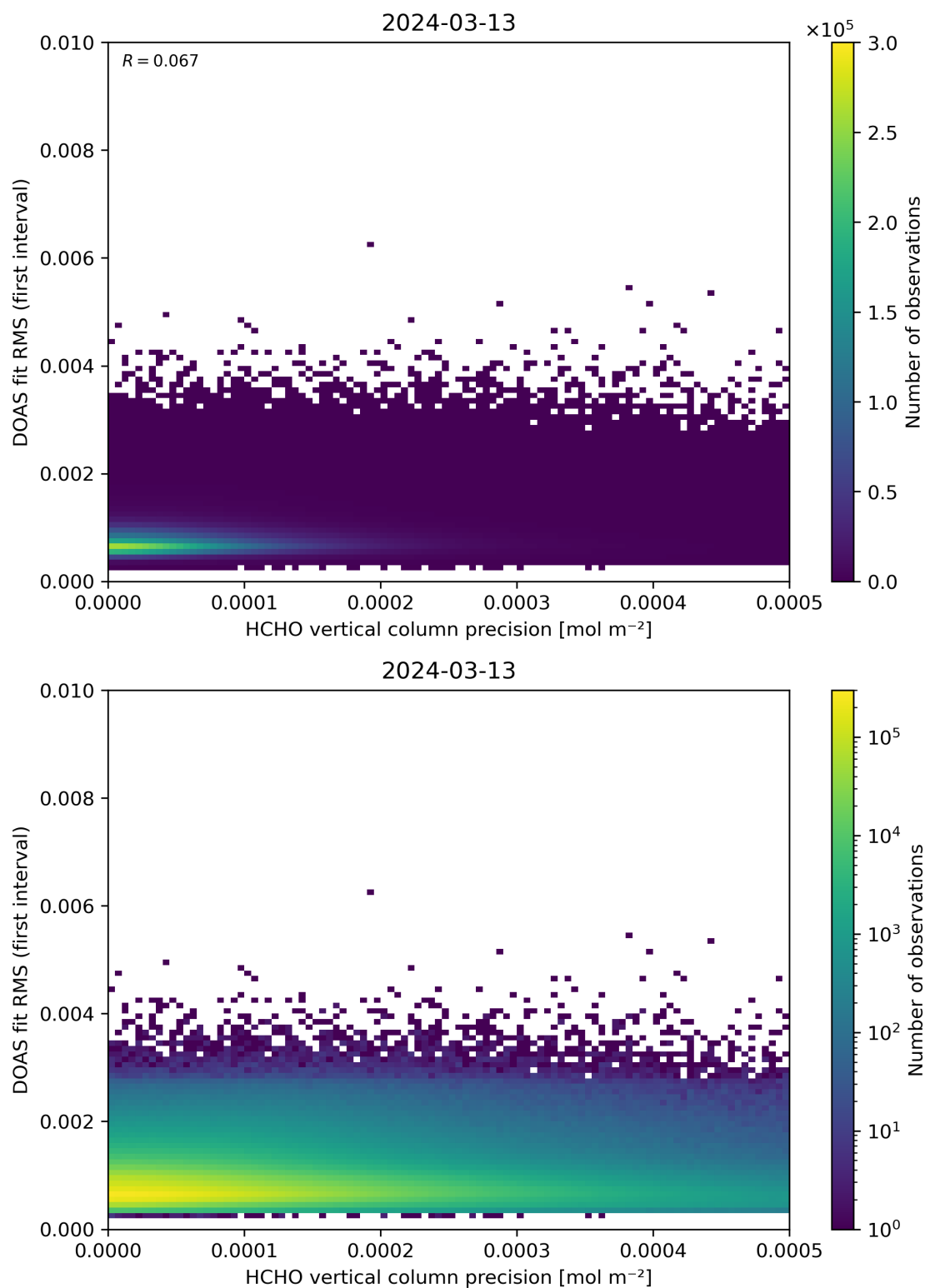
Figure 136: Scatter density plot of “HCHO vertical column precision” against “DOAS fit RMS (first interval)” for 2024-03-12 to 2024-03-14.
