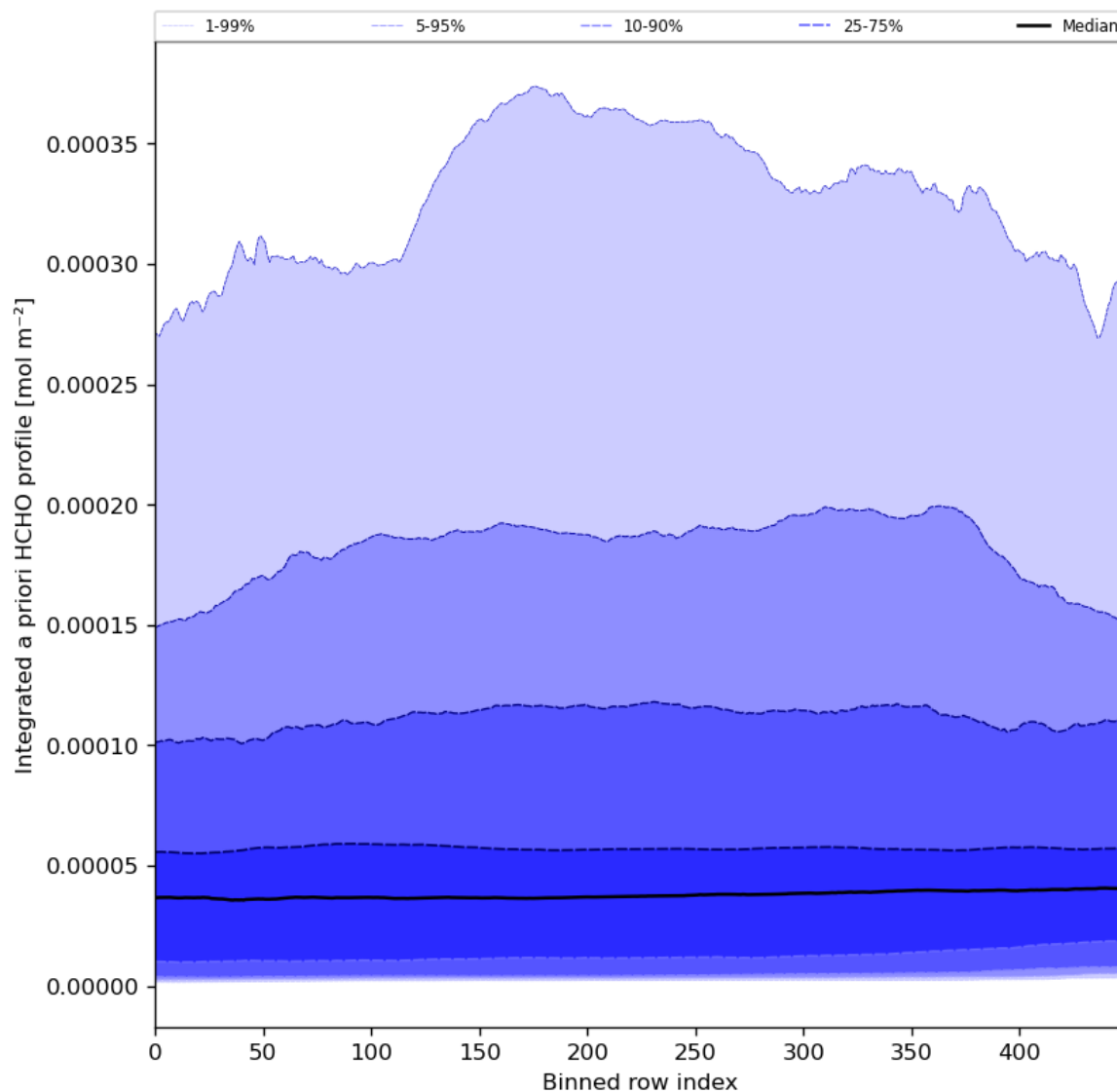
Figure 57: Along track statistics of “Integrated a priori HCHO profile” for 2024-03-12 to 2024-03-14
