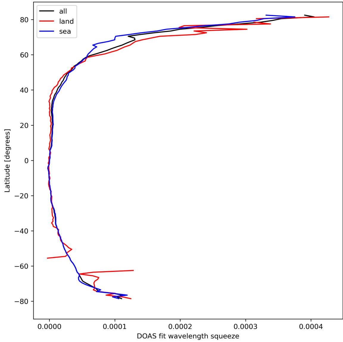
Figure 31: Zonal average of “DOAS fit wavelength squeeze” for 2024-03-12 to 2024-03-14.
