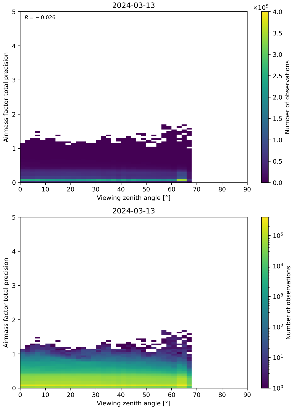
Figure 191: Scatter density plot of “Viewing zenith angle” against “Airmass factor total precision” for 2024-03-12 to 2024-03-14.
