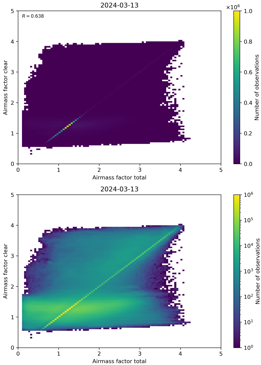
Figure 100: Scatter density plot of “Airmass factor total” against “Airmass factor clear” for 2024-03-12 to 2024-03-14.
