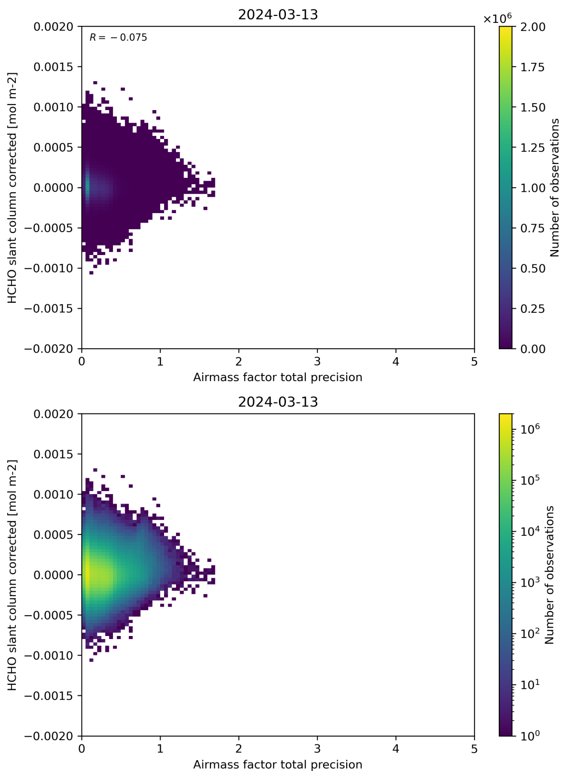
Figure 109: Scatter density plot of “Airmass factor total precision” against “HCHO slant column corrected” for 2024-03-12 to 2024-03-14.
