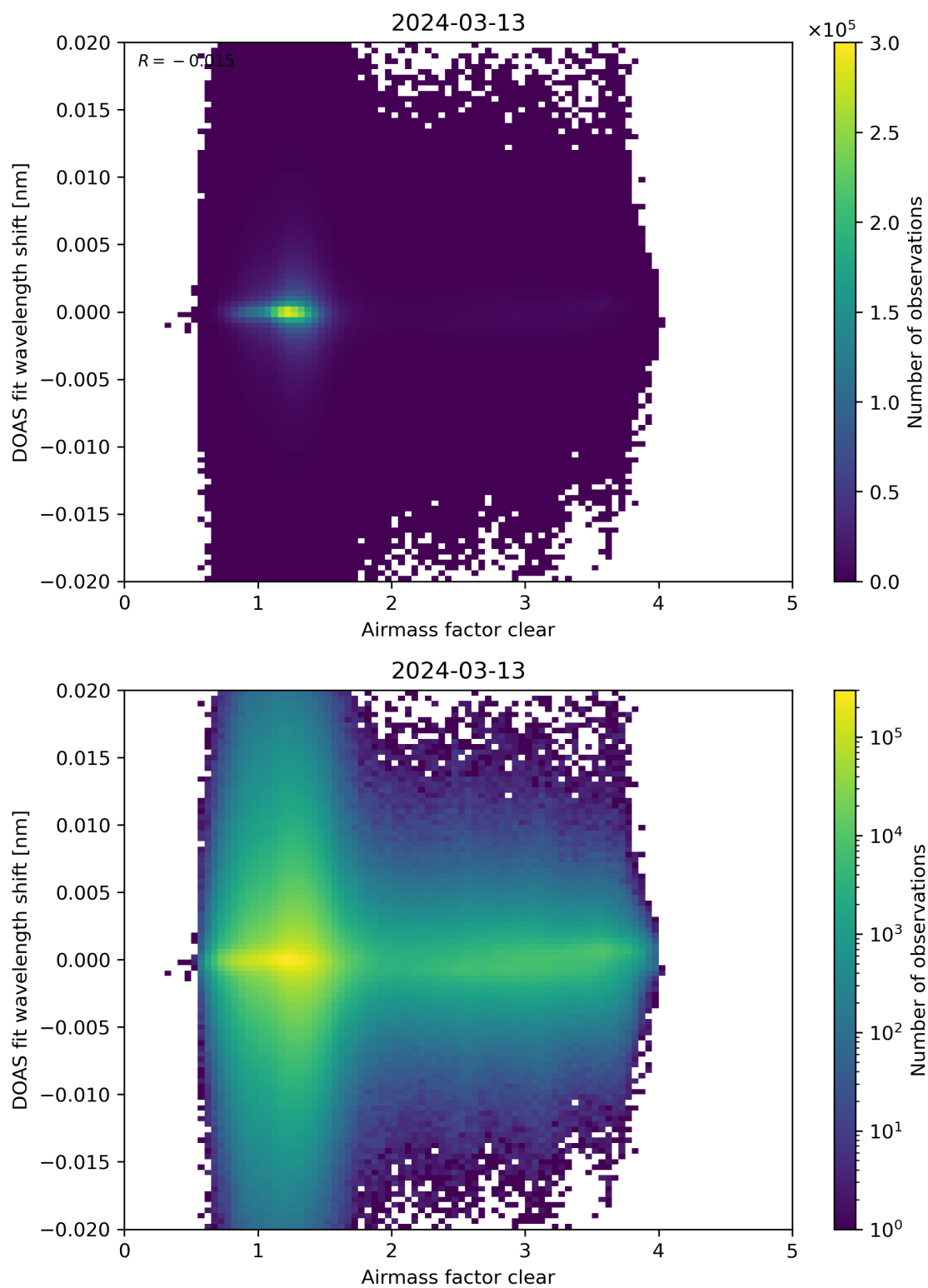
Figure 72: Scatter density plot of “Airmass factor clear” against “DOAS fit wavelength shift” for 2024-03-12 to 2024-03-14.
