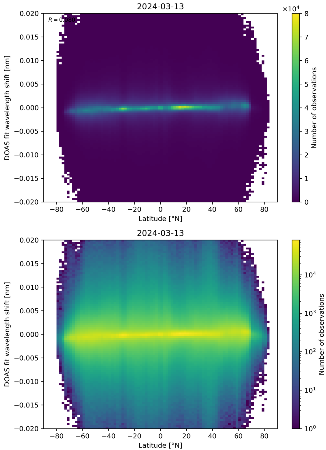
Figure 154: Scatter density plot of “Latitude” against “DOAS fit wavelength shift” for 2024-03-12 to 2024-03-14.
