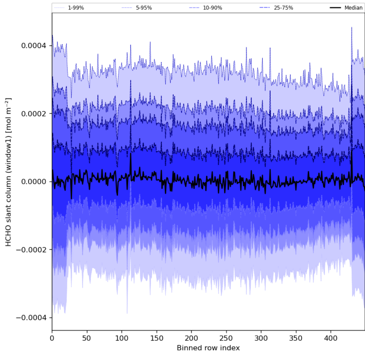
Figure 52: Along track statistics of “HCHO slant column (window1)” for 2024-03-12 to 2024-03-14
