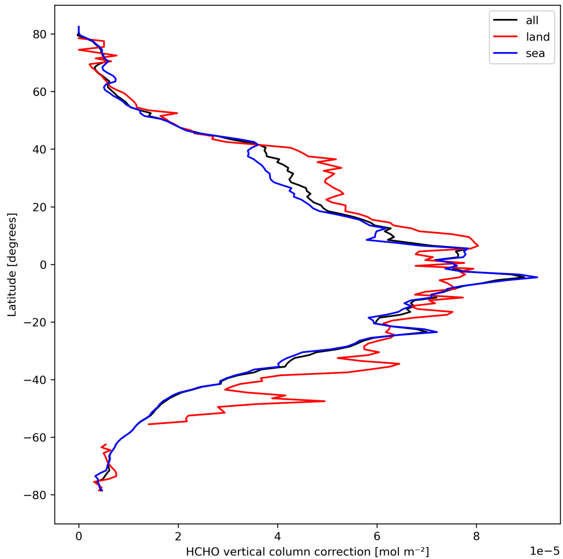
Figure 23: Zonal average of “HCHO vertical column correction” for 2024-03-12 to 2024-03-14.
