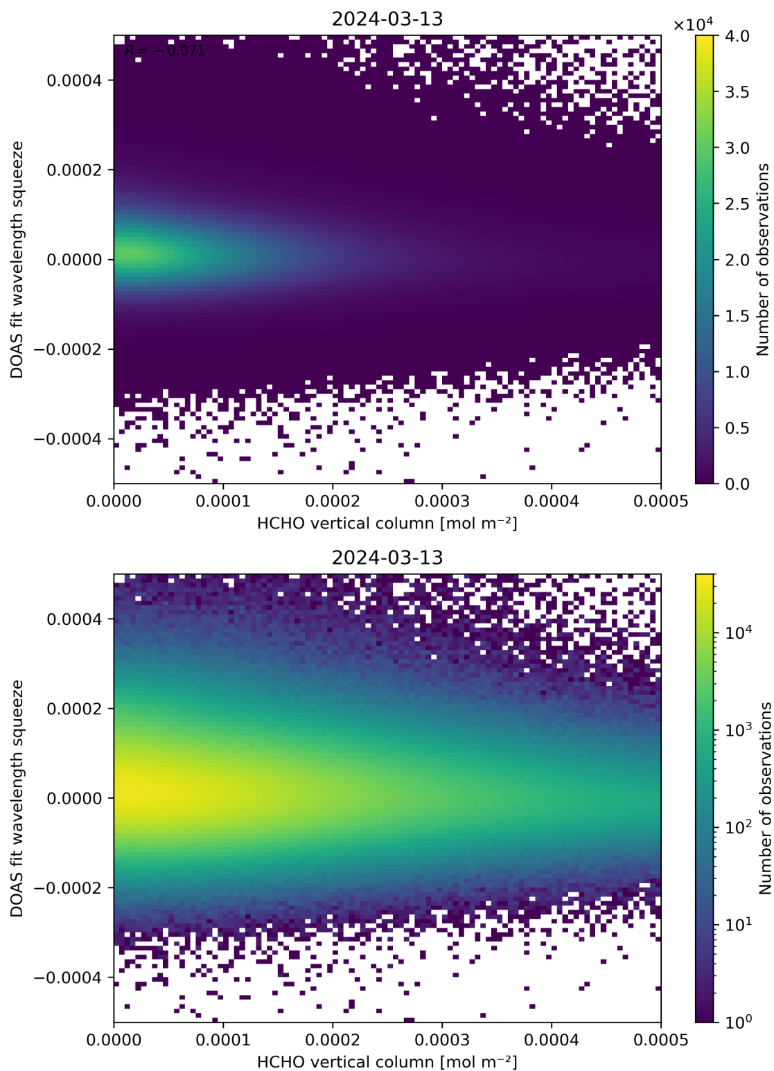
Figure 125: Scatter density plot of “HCHO vertical column” against “DOAS fit wavelength squeeze” for 2024-03-12 to 2024-03-14.
