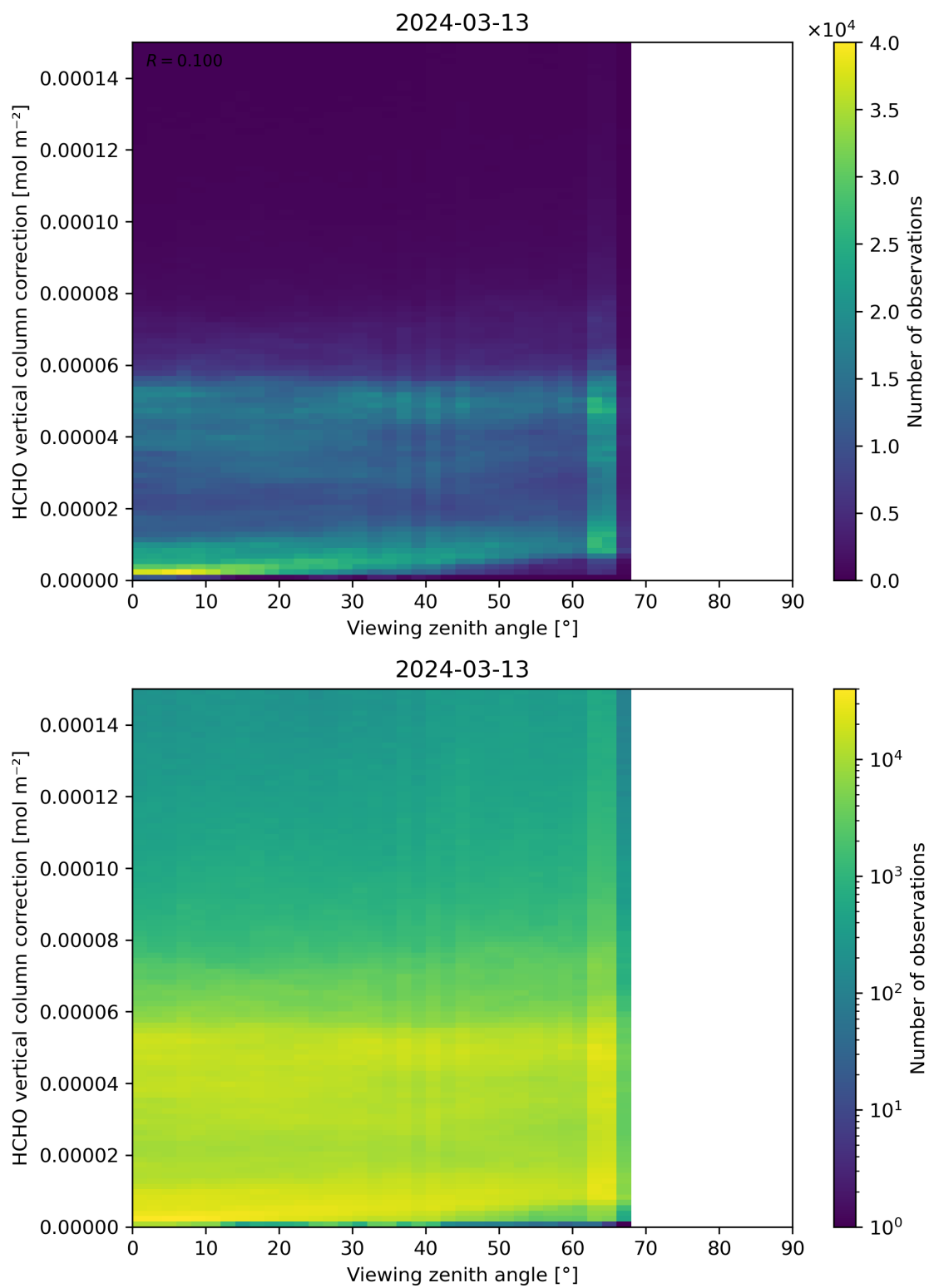
Figure 193: Scatter density plot of “Viewing zenith angle” against “HCHO vertical column correction” for 2024-03-12 to 2024-03-14.
