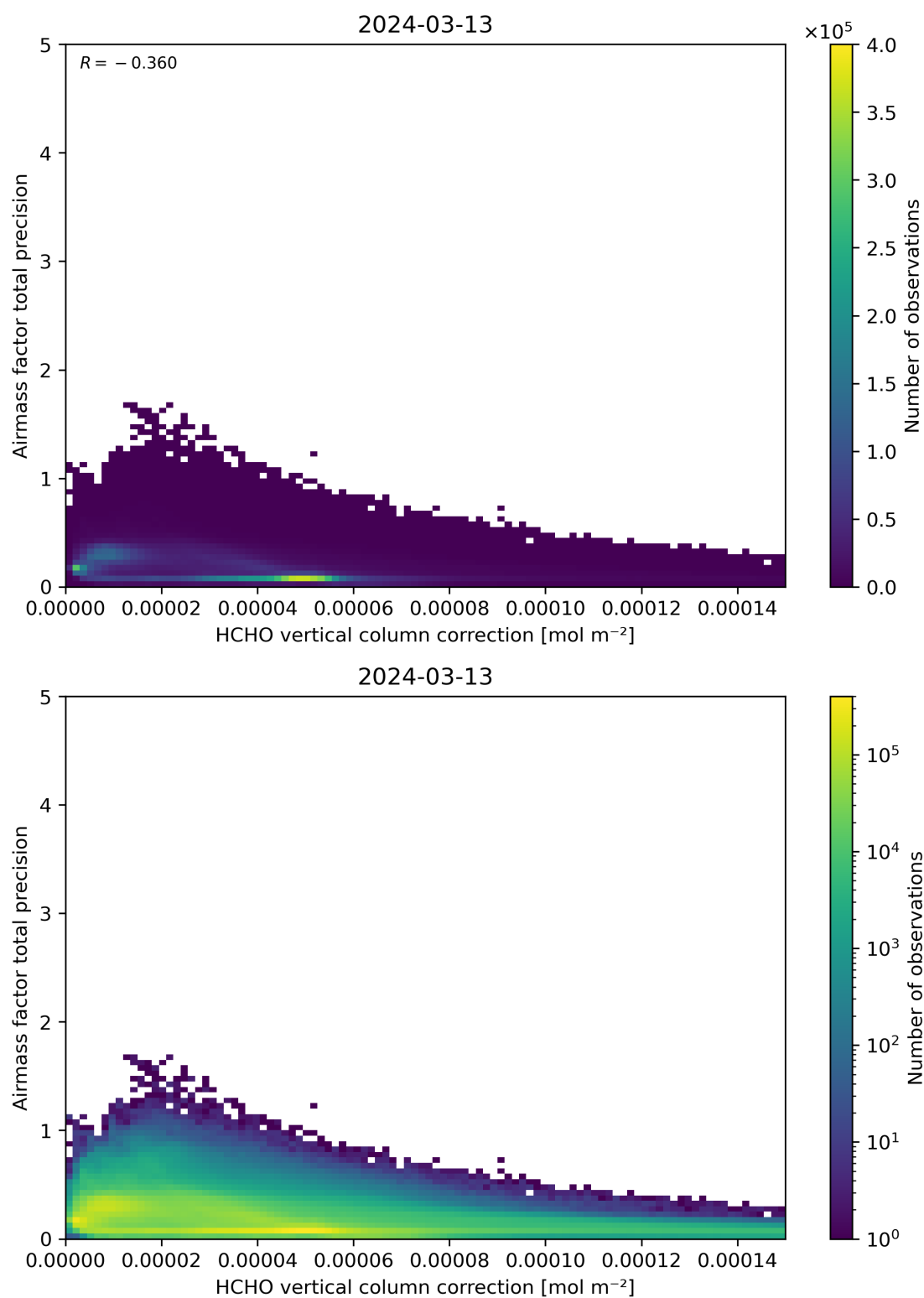
Figure 121: Scatter density plot of “HCHO vertical column correction” against “Airmass factor total precision” for 2024-03-12 to 2024-03-14.
