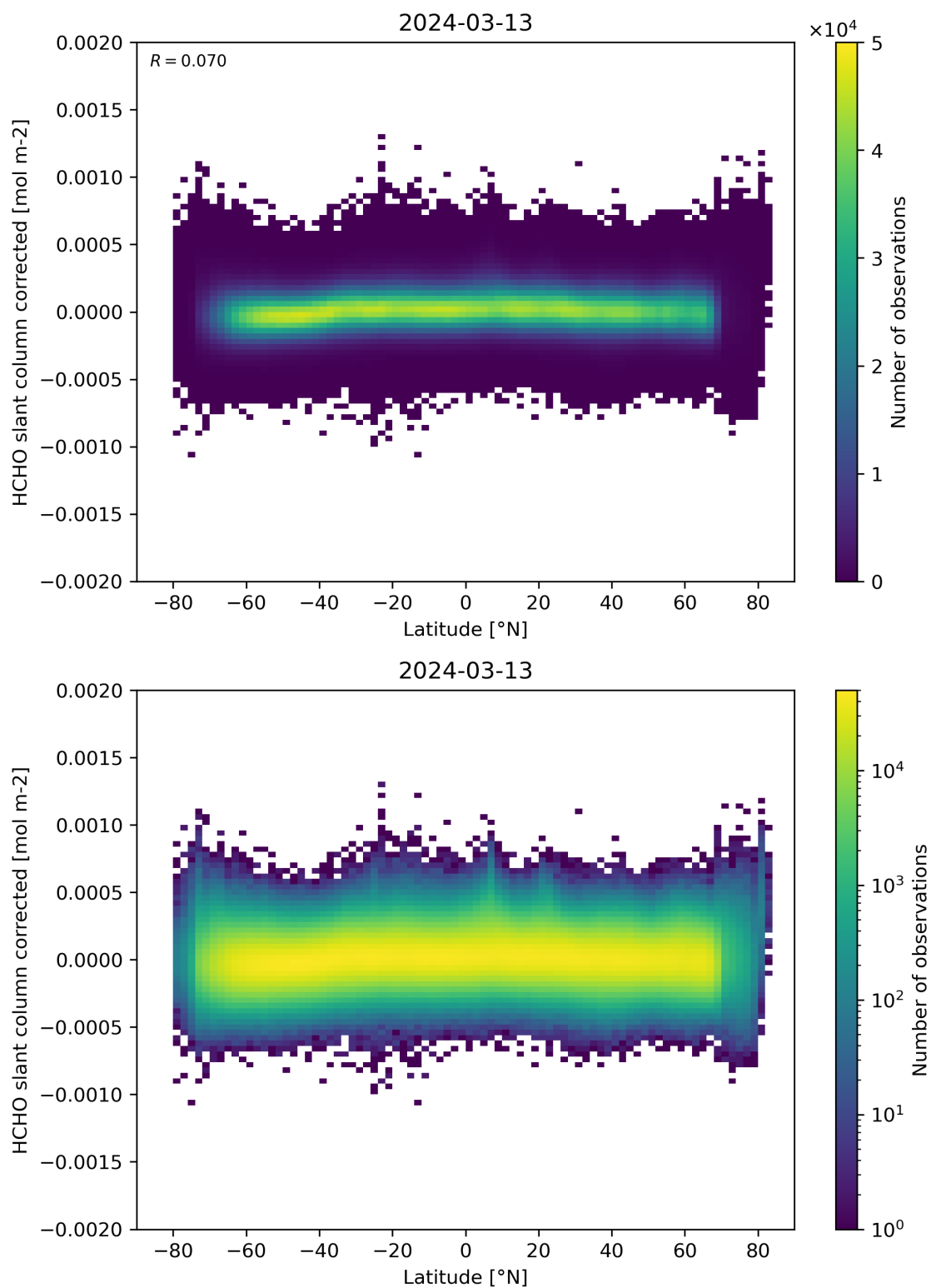
Figure 157: Scatter density plot of “Latitude” against “HCHO slant column corrected” for 2024-03-12 to 2024-03-14.
