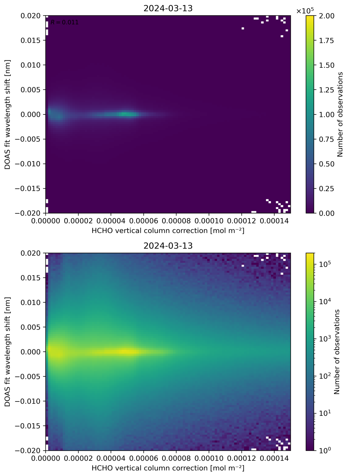
Figure 113: Scatter density plot of “HCHO vertical column correction” against “DOAS fit wavelength shift” for 2024-03-12 to 2024-03-14.
