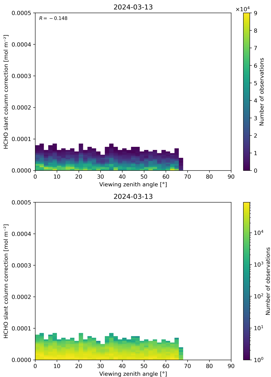
Figure 187: Scatter density plot of “Viewing zenith angle” against “HCHO slant column correction” for 2024-03-12 to 2024-03-14.
