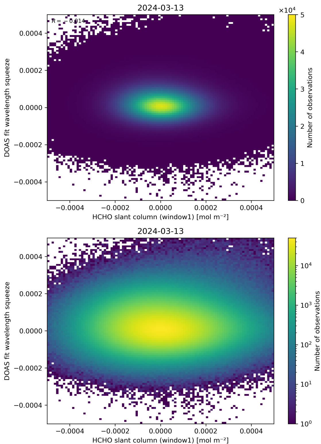
Figure 80: Scatter density plot of “HCHO slant column (window1)” against “DOAS fit wavelength squeeze” for 2024-03-12 to 2024-03-14.
