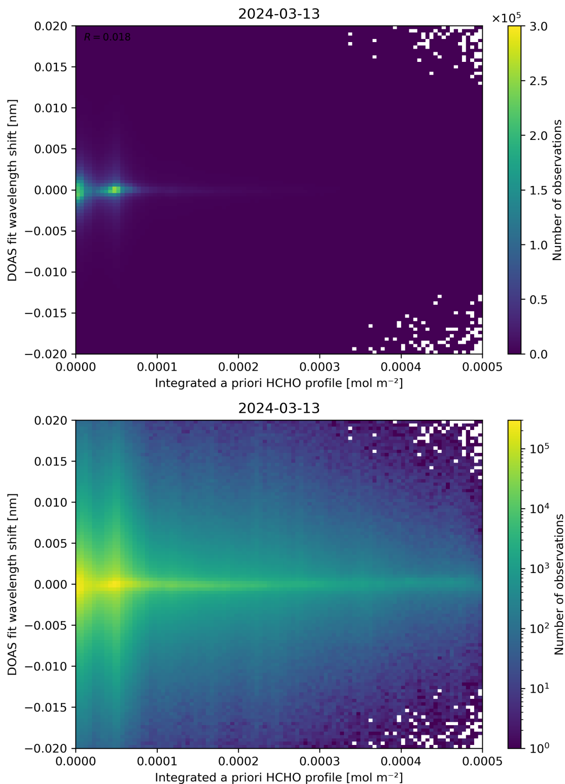
Figure 149: Scatter density plot of “Integrated a priori HCHO profile” against “DOAS fit wavelength shift” for 2024-03-12 to 2024-03-14.
