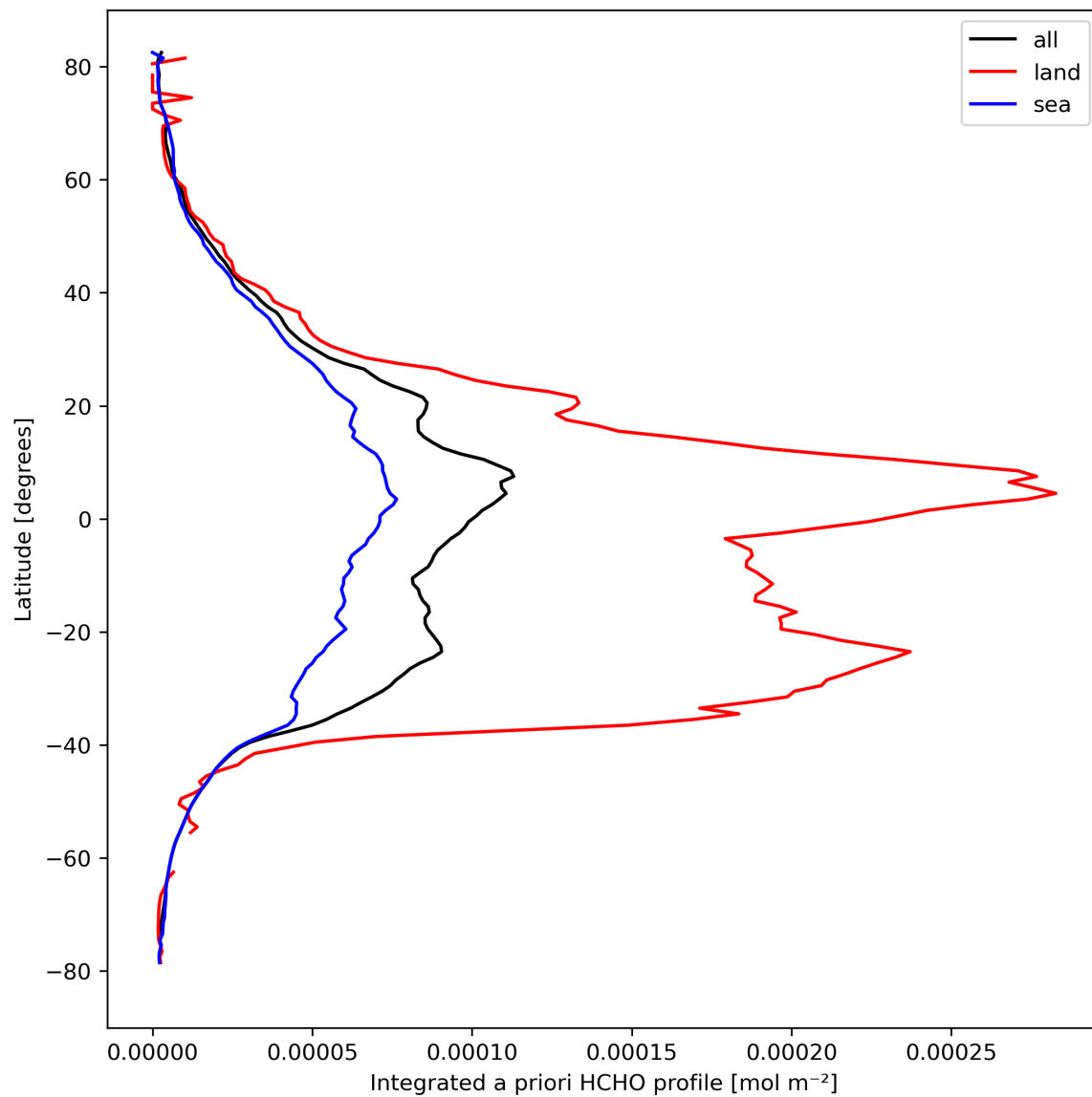
Figure 29: Zonal average of “Integrated a priori HCHO profile” for 2024-03-12 to 2024-03-14.
