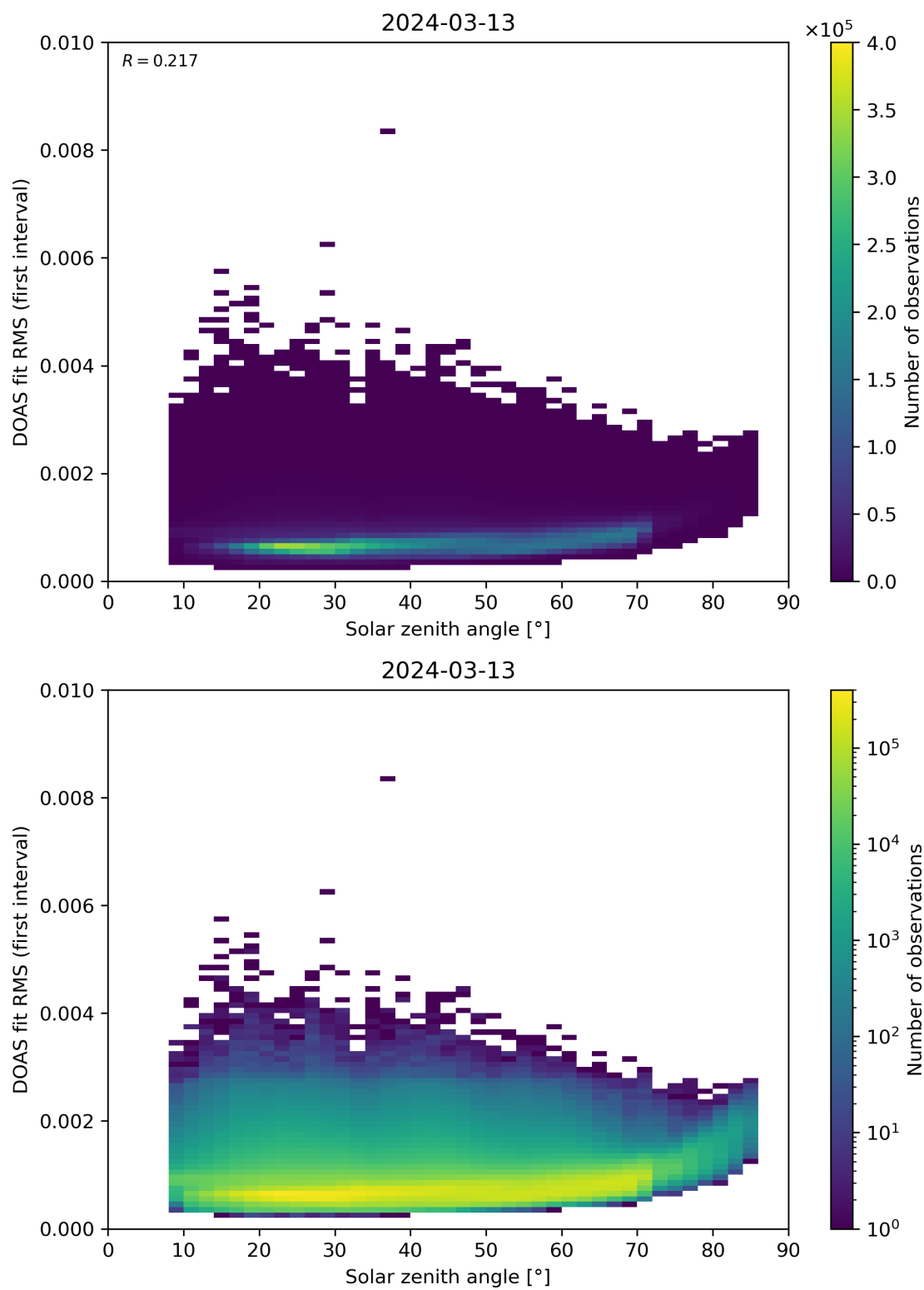
Figure 167: Scatter density plot of “Solar zenith angle” against “DOAS fit RMS (first interval)” for 2024-03-12 to 2024-03-14.
