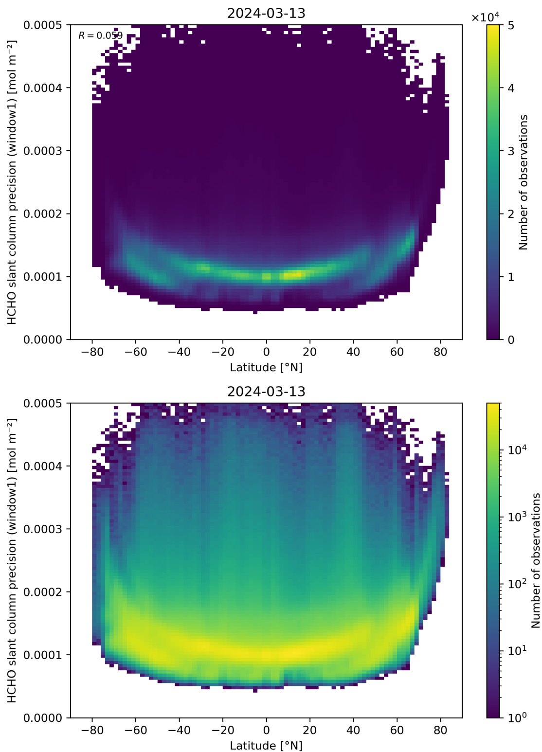
Figure 160: Scatter density plot of “Latitude” against “HCHO slant column precision (window1)” for 2024-03-12 to 2024-03-14.
