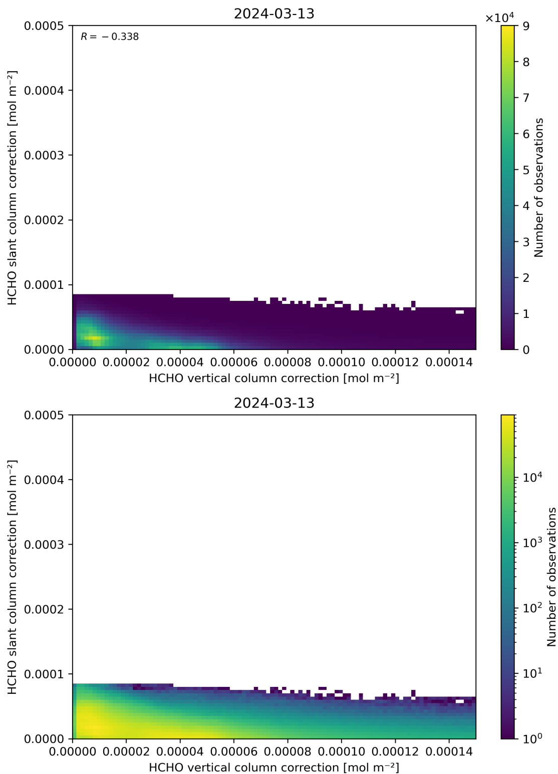
Figure 117: Scatter density plot of “HCHO vertical column correction” against “HCHO slant column correction” for 2024-03-12 to 2024-03-14.
