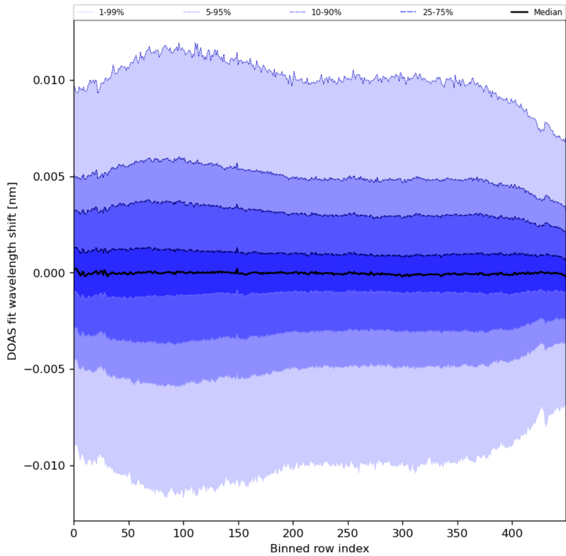
Figure 58: Along track statistics of “DOAS fit wavelength shift” for 2024-03-12 to 2024-03-14
