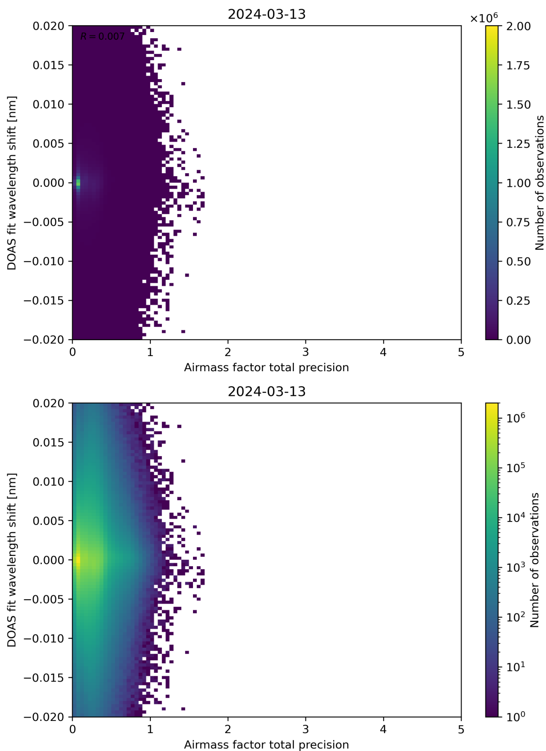
Figure 106: Scatter density plot of “Airmass factor total precision” against “DOAS fit wavelength shift” for 2024-03-12 to 2024-03-14.
