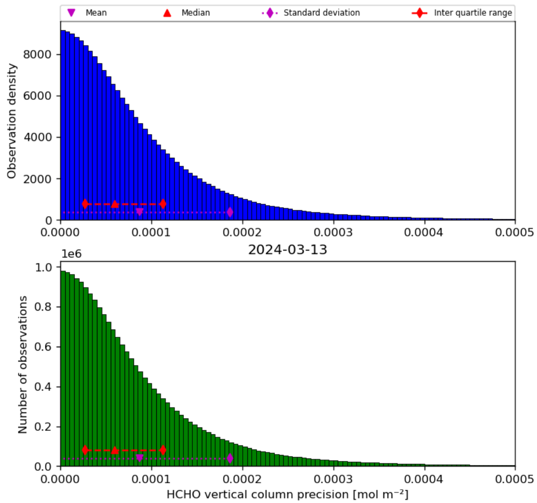
Figure 36: Histogram of “HCHO vertical column precision” for 2024-03-12 to 2024-03-14
