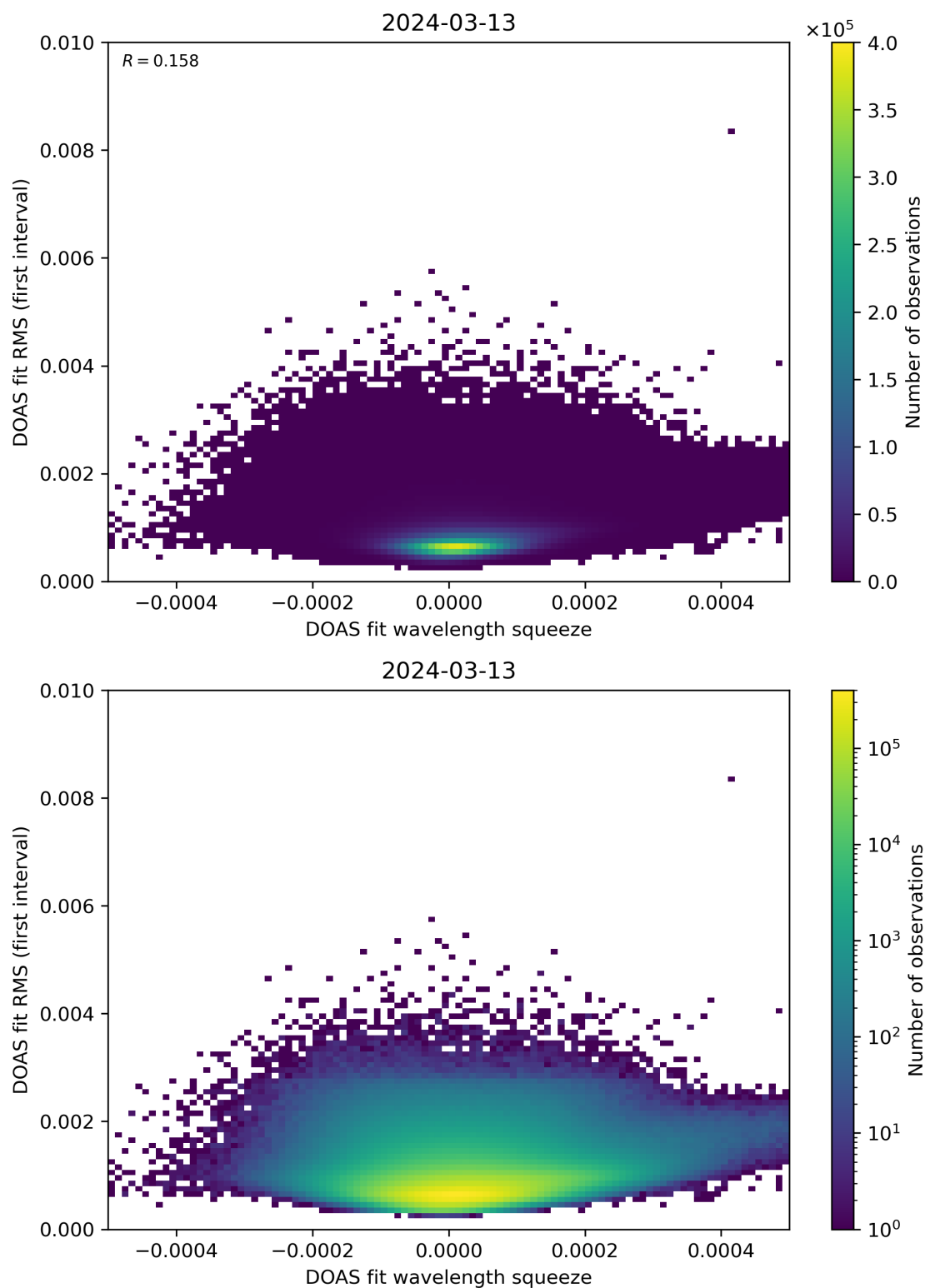
Figure 68: Scatter density plot of “DOAS fit wavelength squeeze” against “DOAS fit RMS (first interval)” for 2024-03-12 to 2024-03-14.
