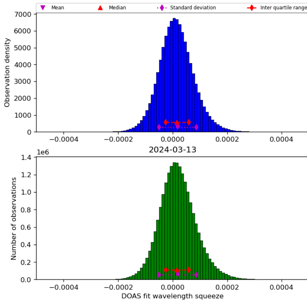
Figure 45: Histogram of “DOAS fit wavelength squeeze” for 2024-03-12 to 2024-03-14
