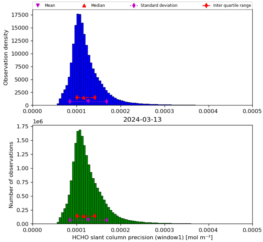
Figure 39: Histogram of “HCHO slant column precision (window1)” for 2024-03-12 to 2024-03-14
