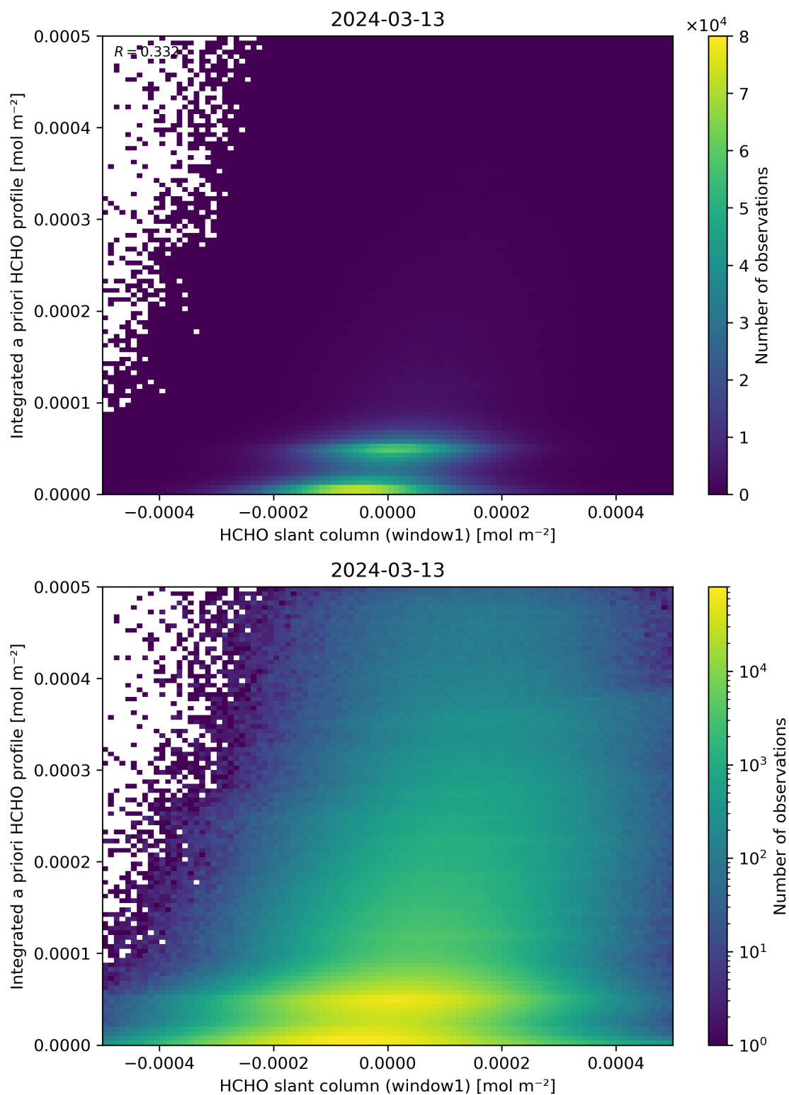
Figure 87: Scatter density plot of “HCHO slant column (window1)” against “Integrated a priori HCHO profile” for 2024-03-12 to 2024-03-14.
