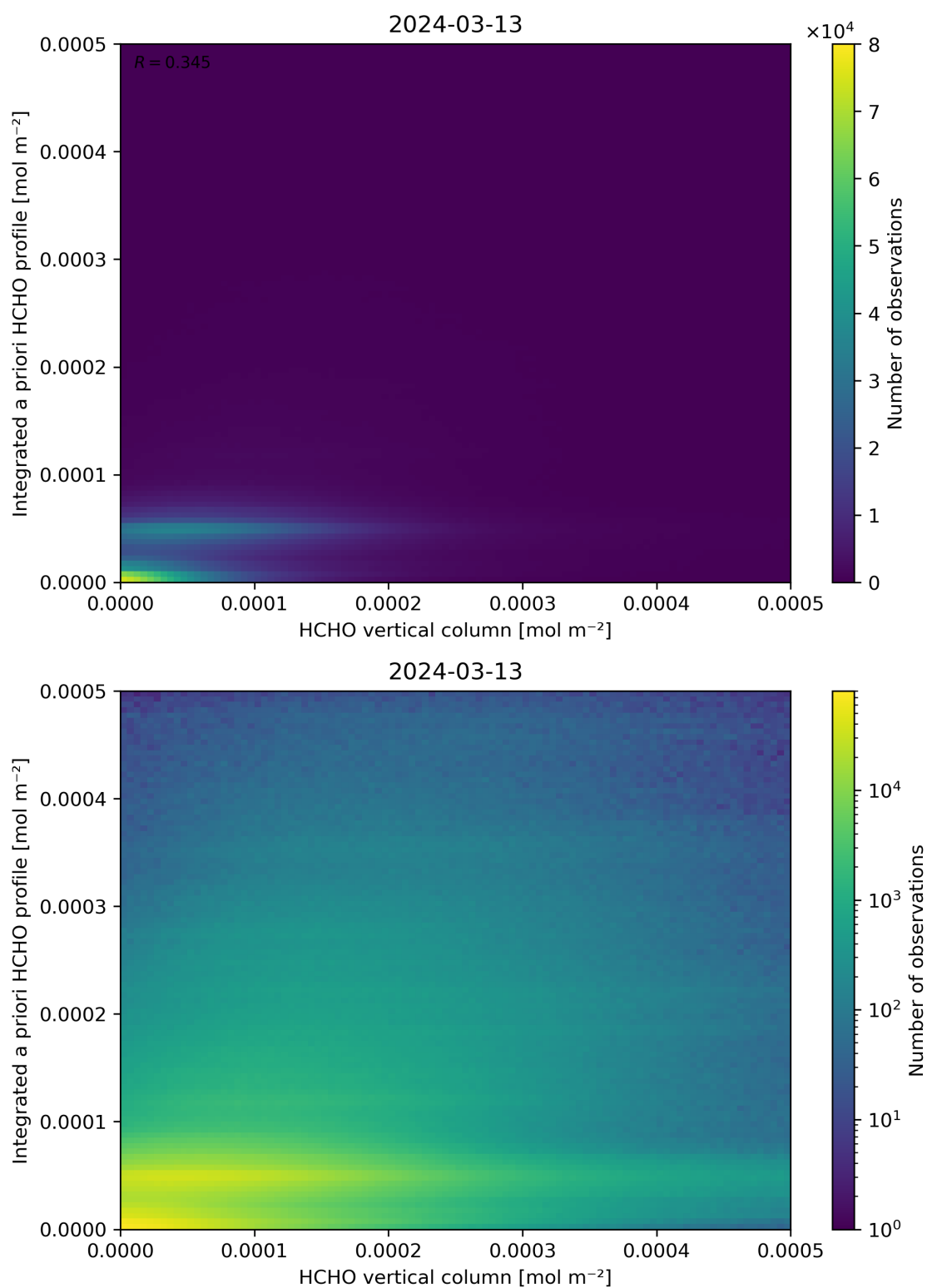
Figure 135: Scatter density plot of “HCHO vertical column” against “Integrated a priori HCHO profile” for 2024-03-12 to 2024-03-14.
