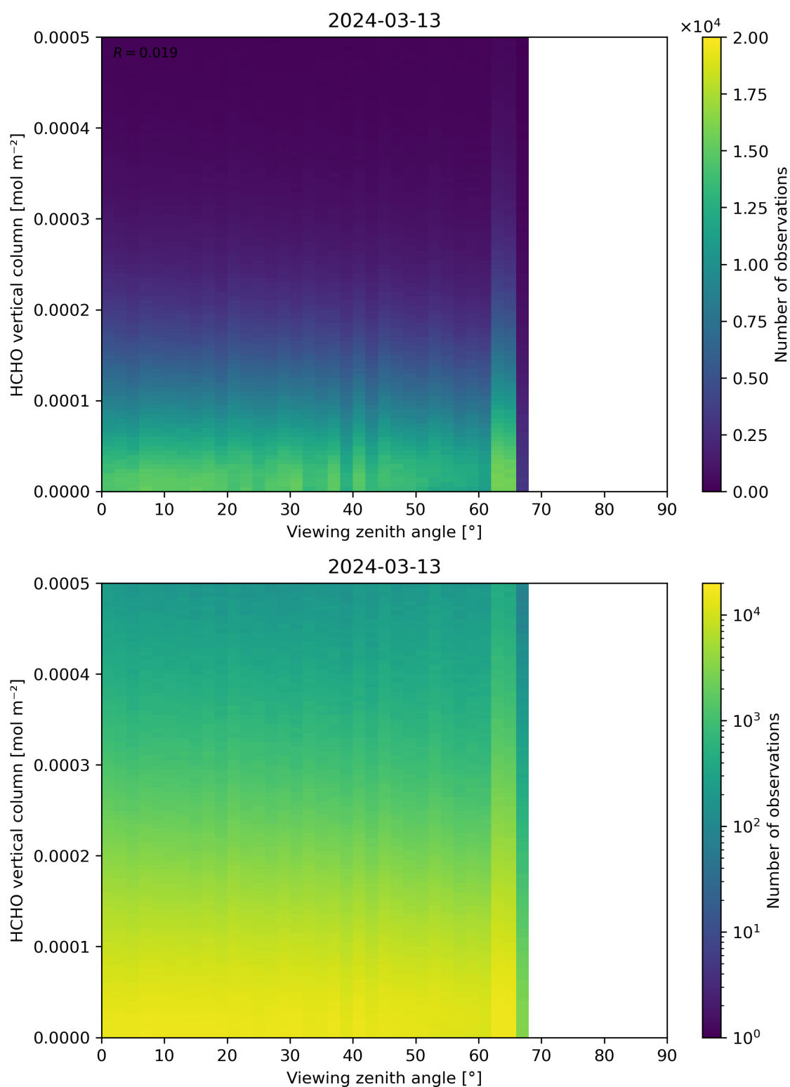
Figure 192: Scatter density plot of “Viewing zenith angle” against “HCHO vertical column” for 2024-03-12 to 2024-03-14.
