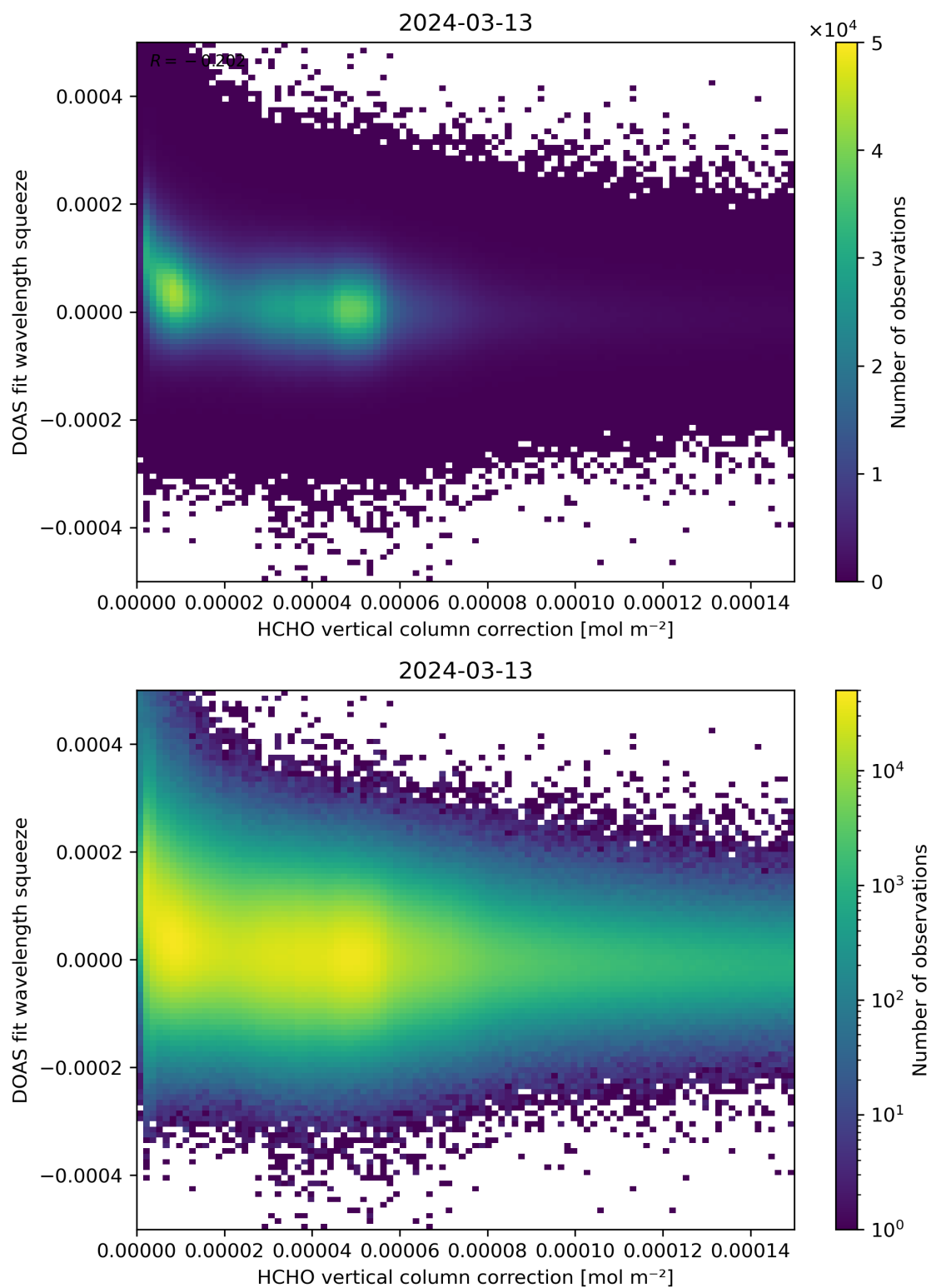
Figure 114: Scatter density plot of “HCHO vertical column correction” against “DOAS fit wavelength squeeze” for 2024-03-12 to 2024-03-14.
