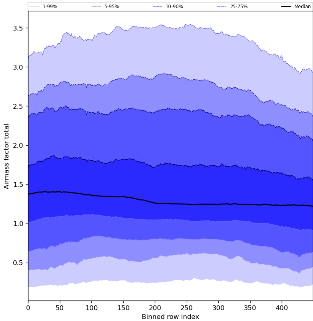
Figure 54: Along track statistics of “Airmass factor total” for 2024-03-12 to 2024-03-14
