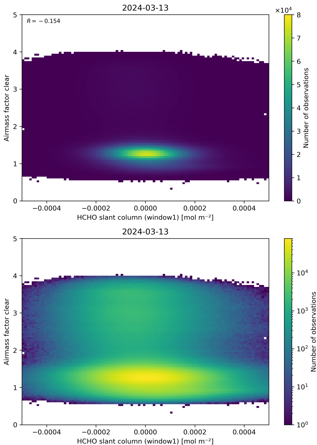
Figure 81: Scatter density plot of “HCHO slant column (window1)” against “Airmass factor clear” for 2024-03-12 to 2024-03-14.
