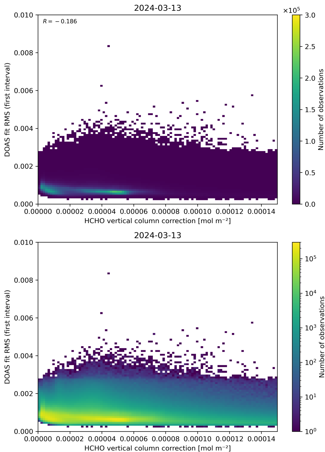
Figure 112: Scatter density plot of “HCHO vertical column correction” against “DOAS fit RMS (first interval)” for 2024-03-12 to 2024-03-14.
