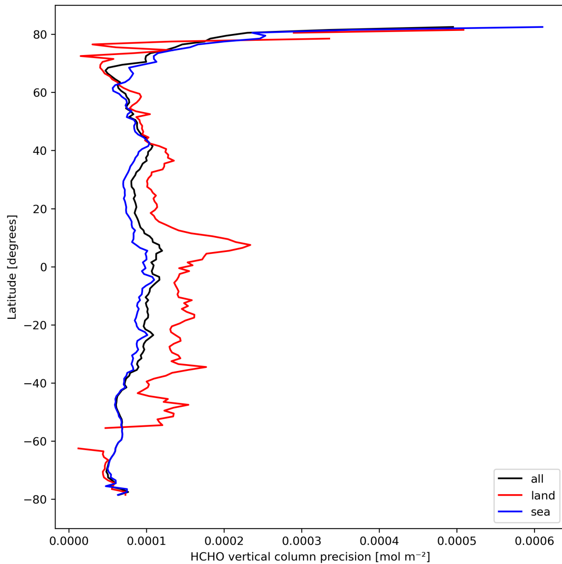
Figure 22: Zonal average of “HCHO vertical column precision” for 2024-03-12 to 2024-03-14.
