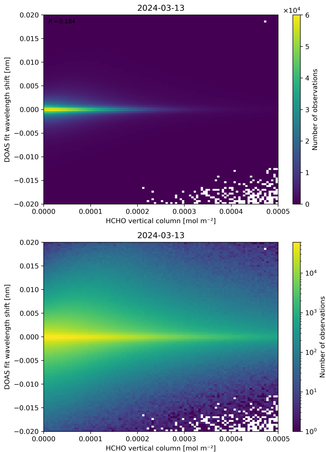
Figure 124: Scatter density plot of “HCHO vertical column” against “DOAS fit wavelength shift” for 2024-03-12 to 2024-03-14.
