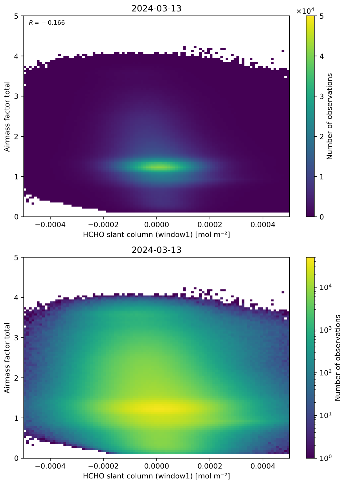
Figure 85: Scatter density plot of “HCHO slant column (window1)” against “Airmass factor total” for 2024-03-12 to 2024-03-14.
