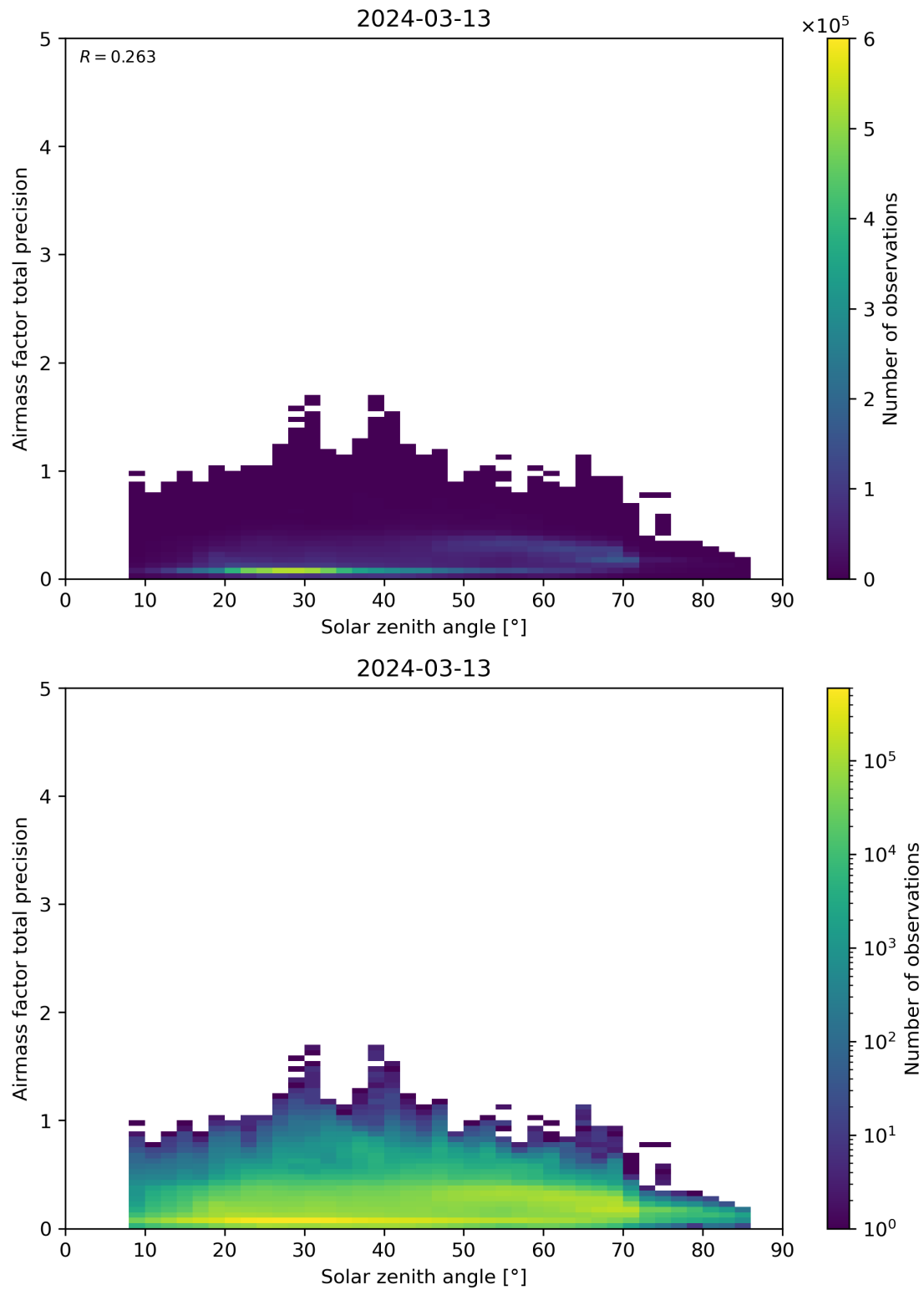
Figure 176: Scatter density plot of “Solar zenith angle” against “Airmass factor total precision” for 2024-03-12 to 2024-03-14.
