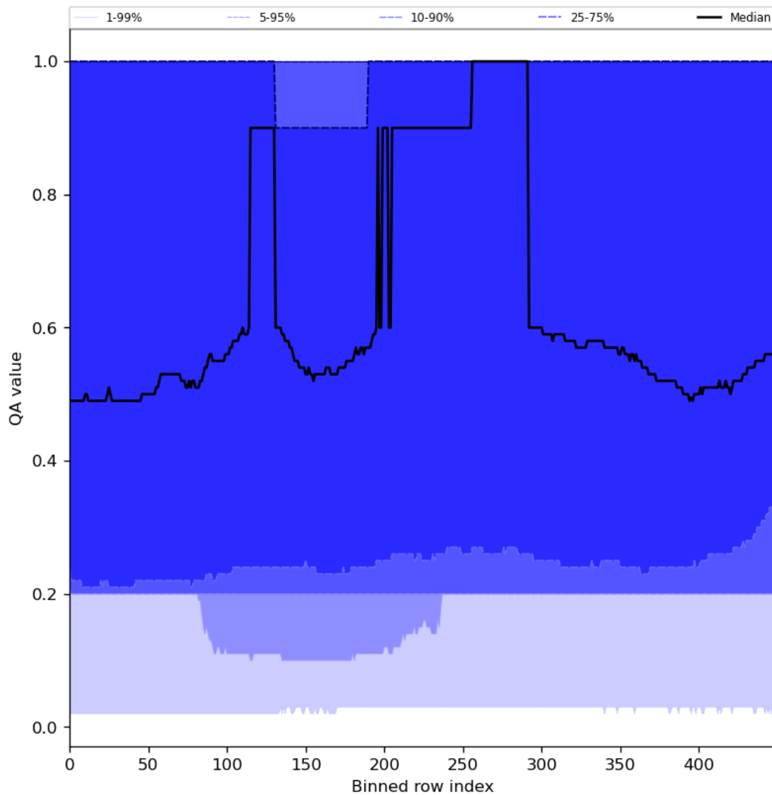
Figure 48: Along track statistics of “QA value” for 2024-03-12 to 2024-03-14
