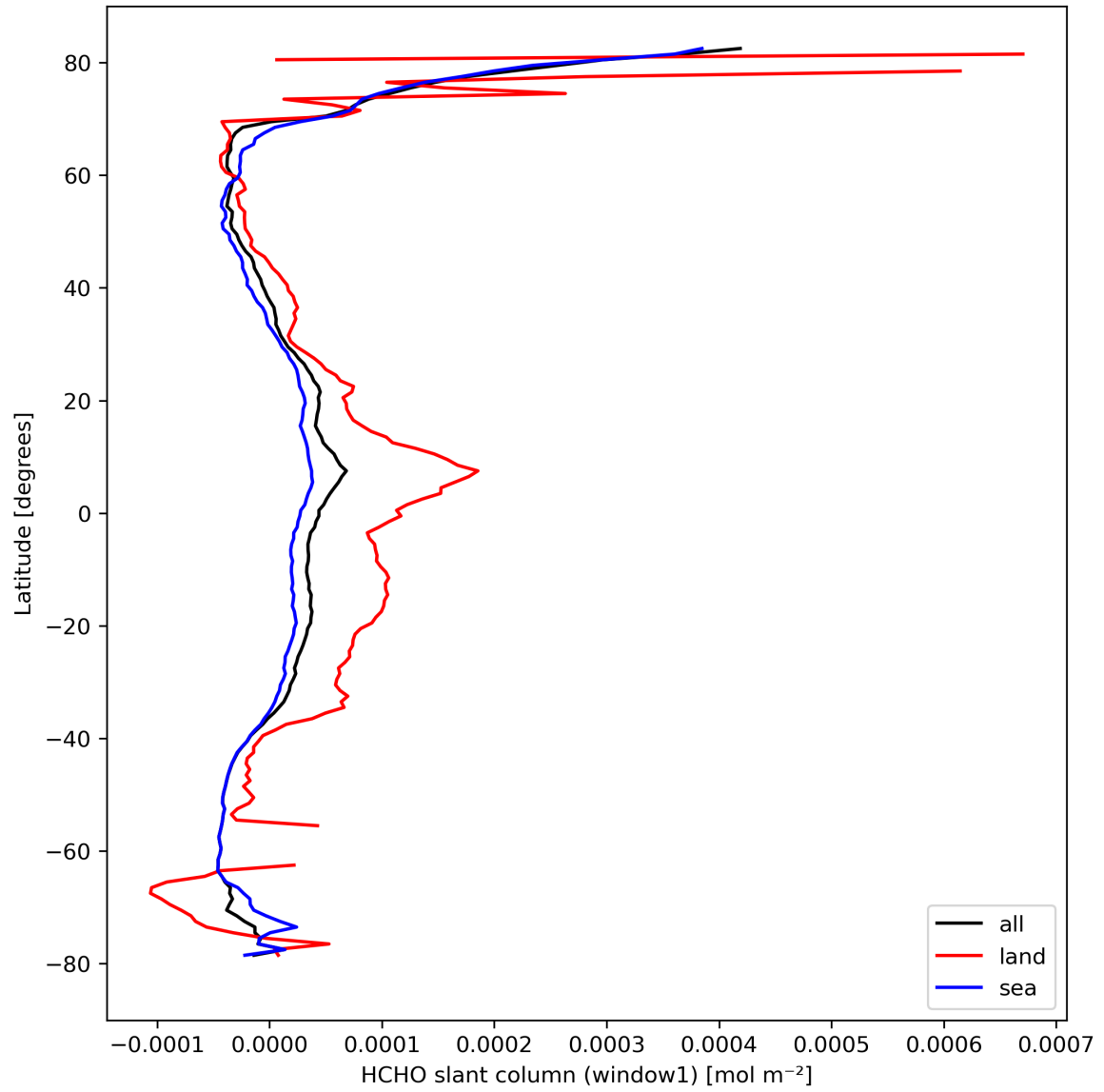
Figure 24: Zonal average of “HCHO slant column (window1)” for 2024-03-12 to 2024-03-14.
