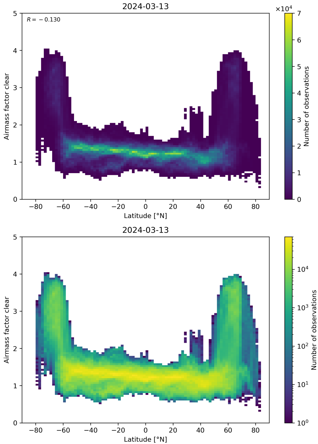
Figure 156: Scatter density plot of “Latitude” against “Airmass factor clear” for 2024-03-12 to 2024-03-14.
