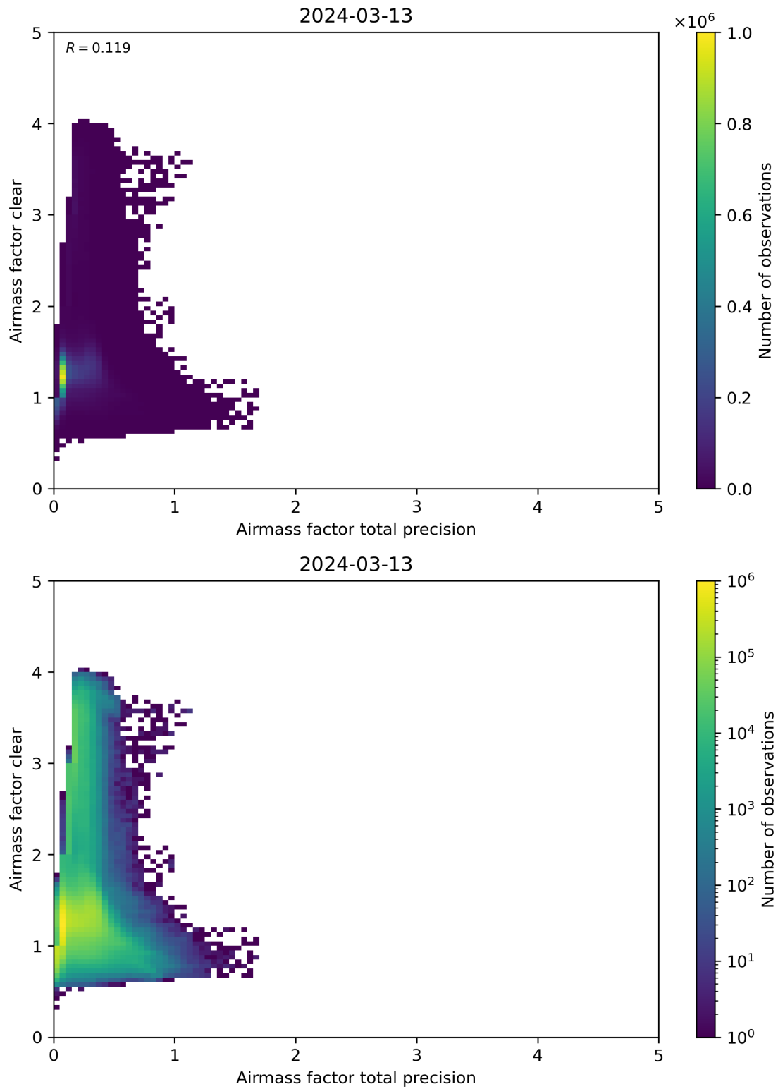
Figure 108: Scatter density plot of “Airmass factor total precision” against “Airmass factor clear” for 2024-03-12 to 2024-03-14.
