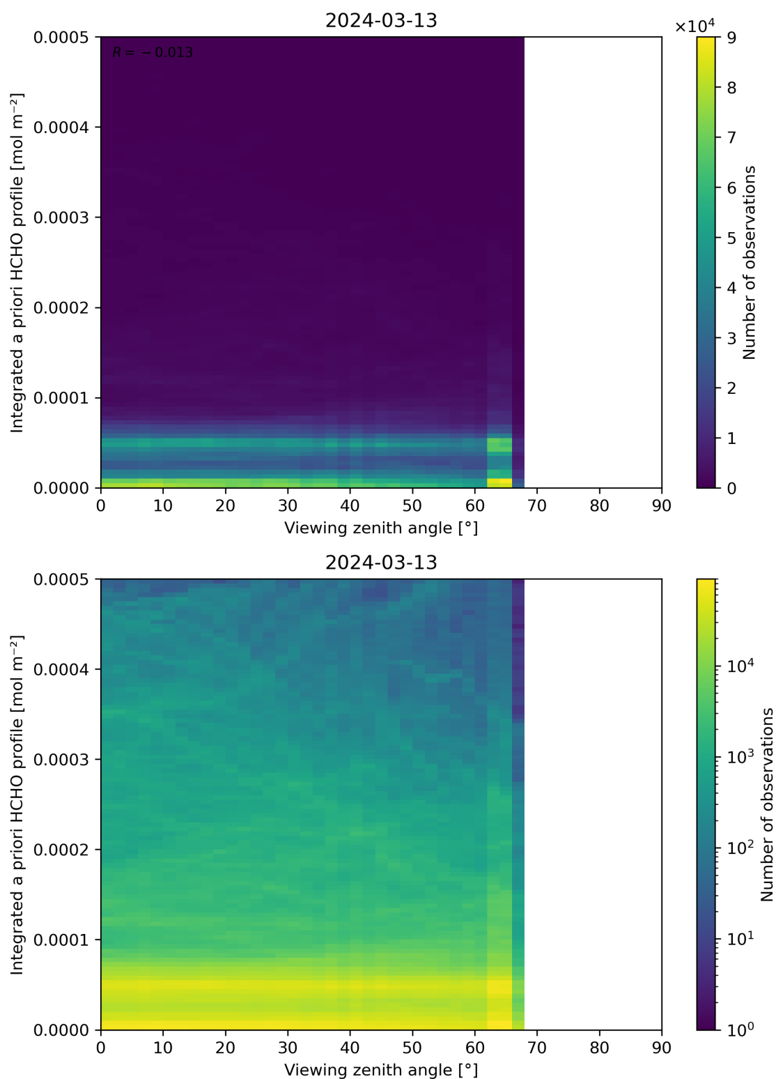
Figure 195: Scatter density plot of “Viewing zenith angle” against “Integrated a priori HCHO profile” for 2024-03-12 to 2024-03-14.
