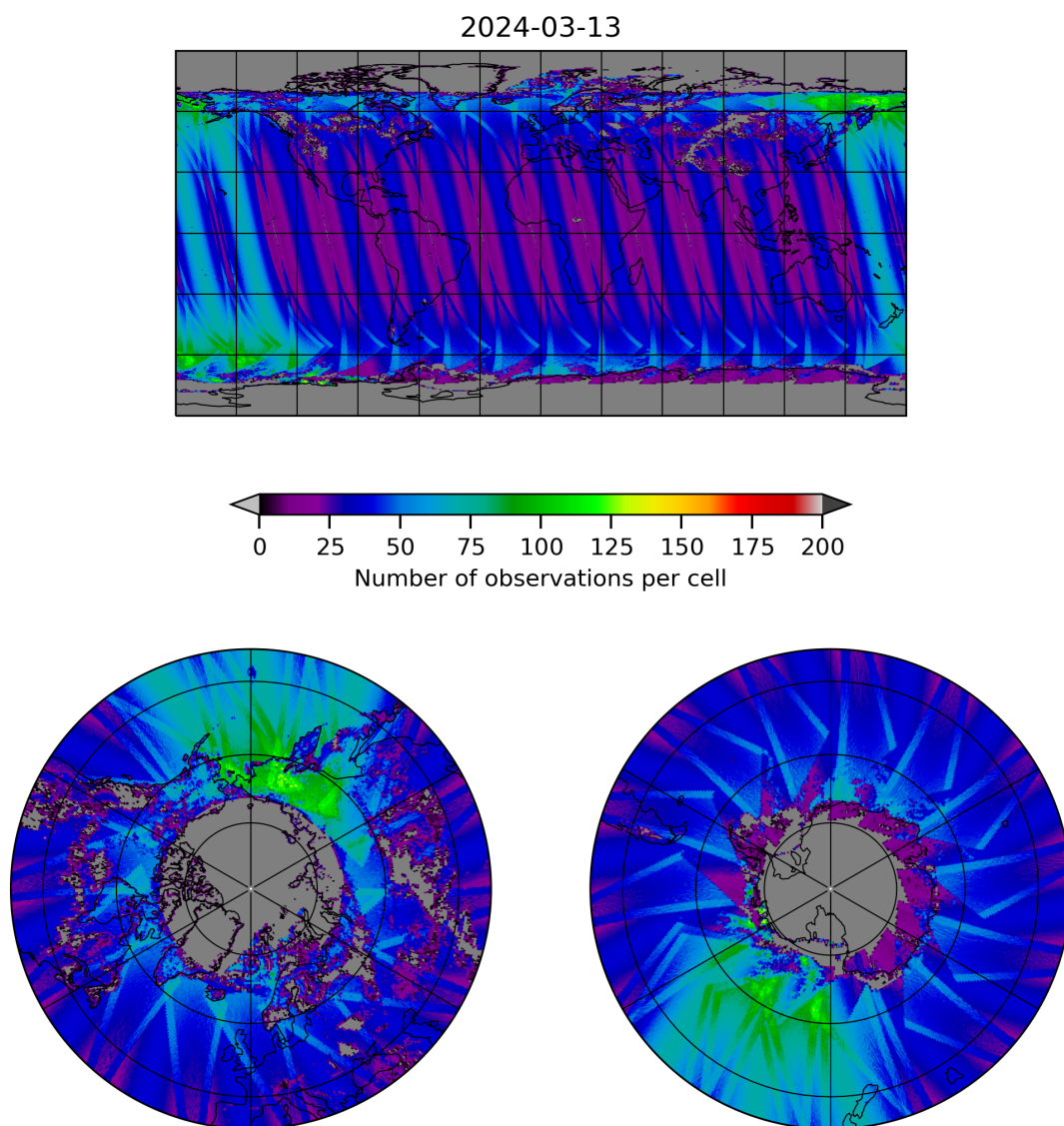
Figure 19: Map of the number of observations for 2024-03-12 to 2024-03-14
