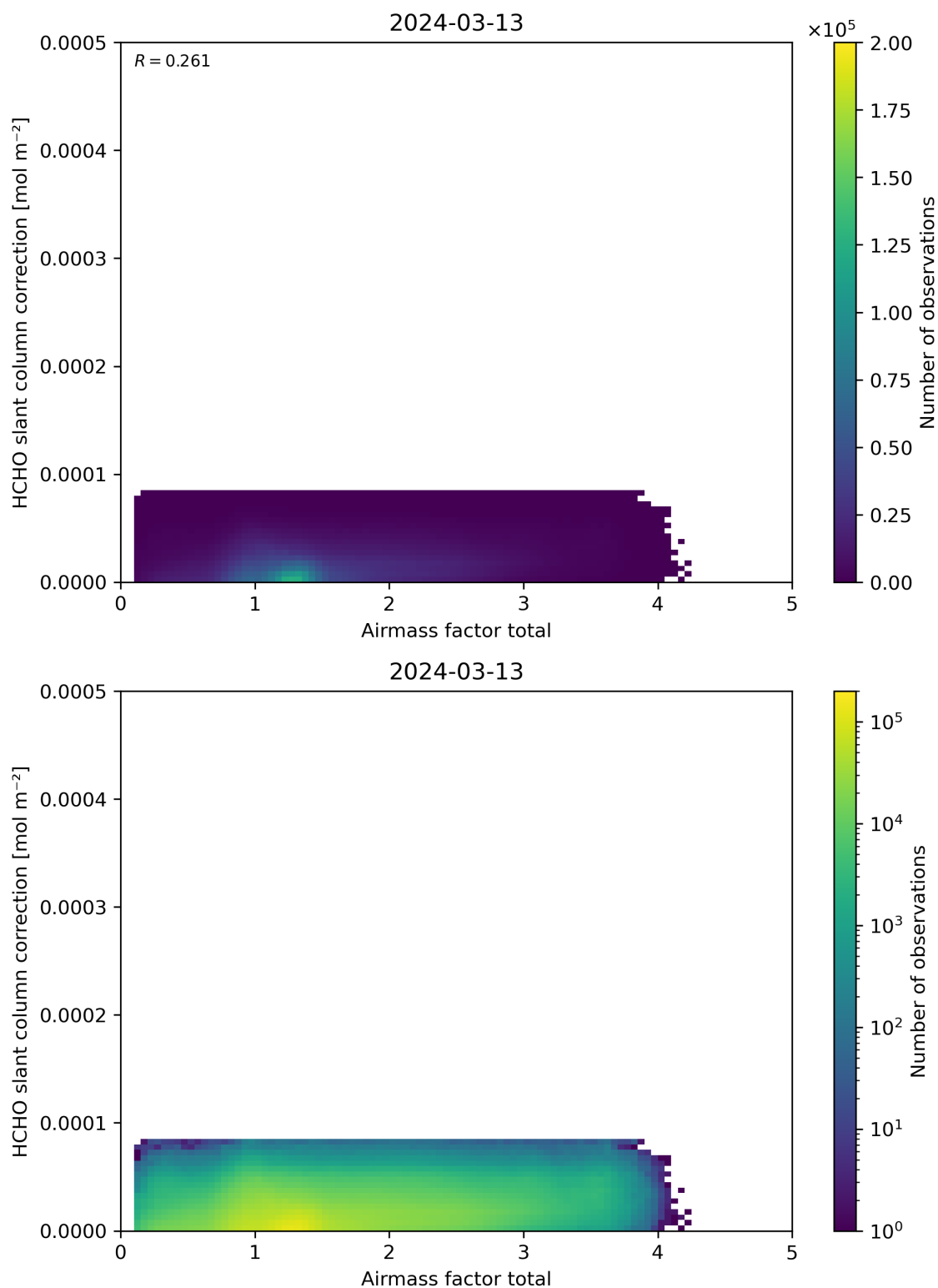
Figure 102: Scatter density plot of “Airmass factor total” against “HCHO slant column correction” for 2024-03-12 to 2024-03-14.
