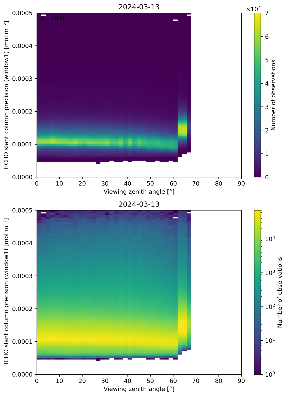
Figure 189: Scatter density plot of “Viewing zenith angle” against “HCHO slant column precision (window1)” for 2024-03-12 to 2024-03-14.
