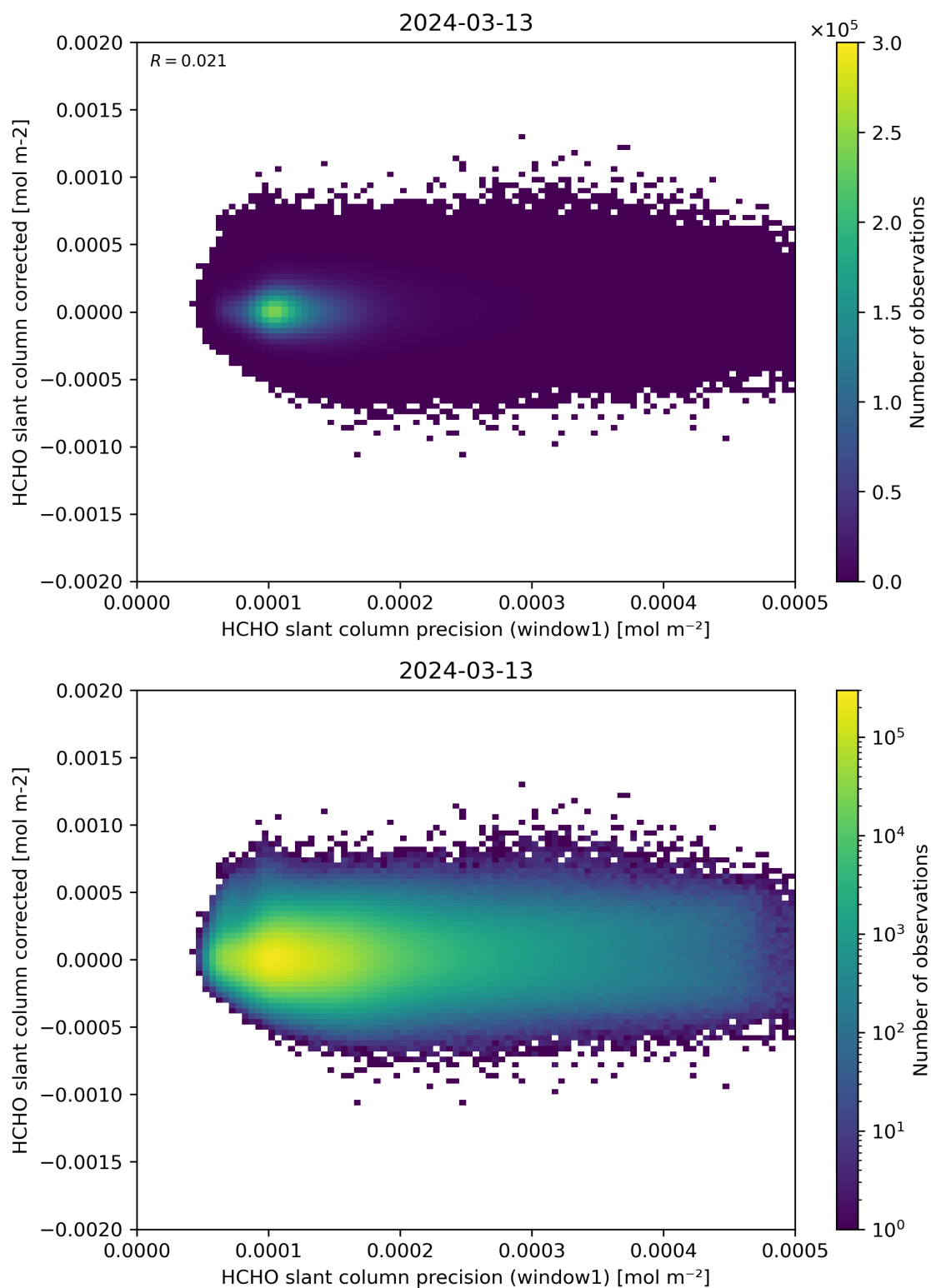
Figure 92: Scatter density plot of “HCHO slant column precision (window1)” against “HCHO slant column corrected” for 2024-03-12 to 2024-03-14.
