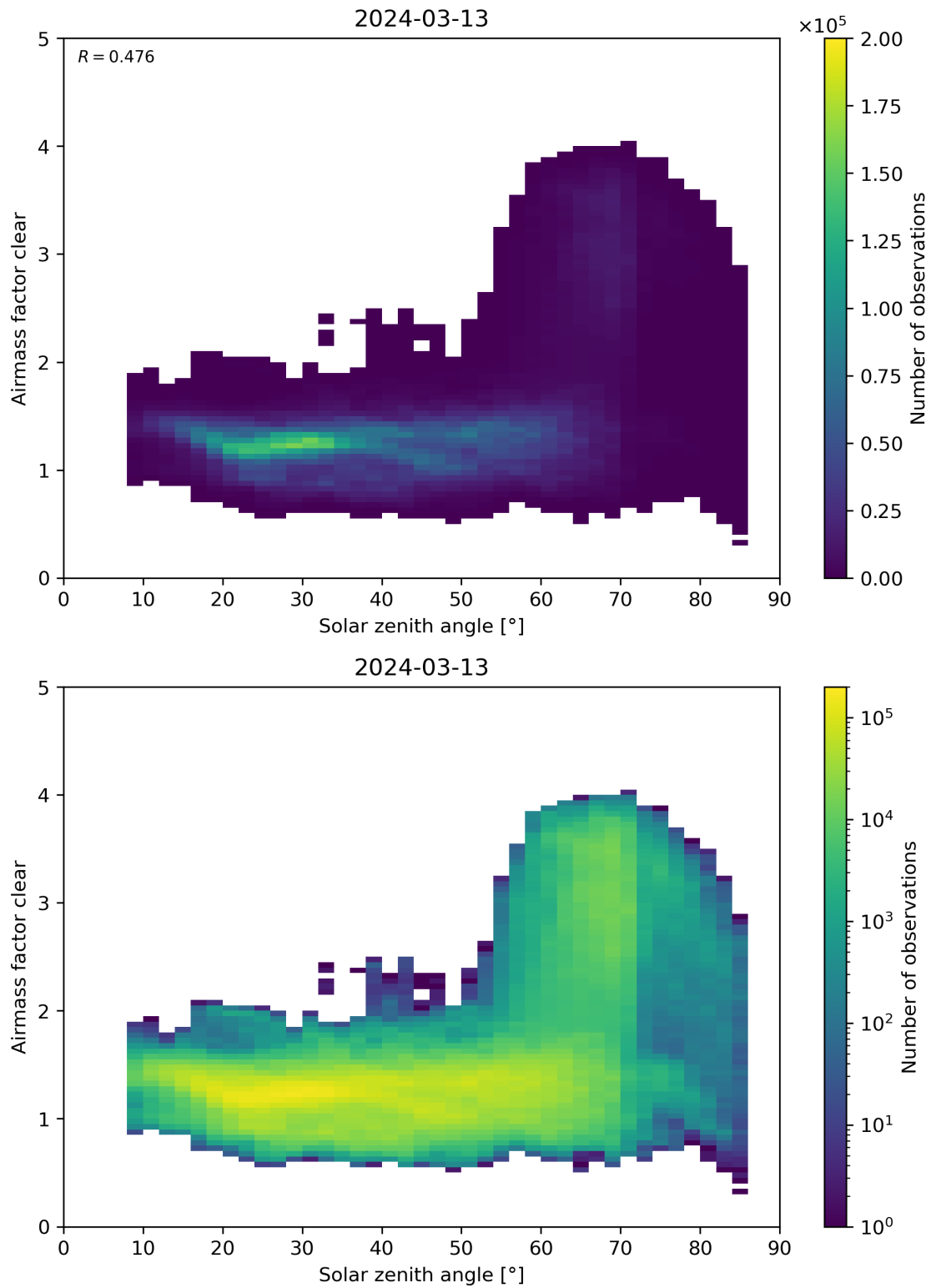
Figure 170: Scatter density plot of “Solar zenith angle” against “Airmass factor clear” for 2024-03-12 to 2024-03-14.
