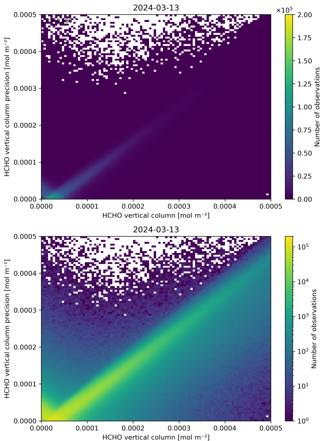
Figure 134: Scatter density plot of “HCHO vertical column” against “HCHO vertical column precision” for 2024-03-12 to 2024-03-14.
