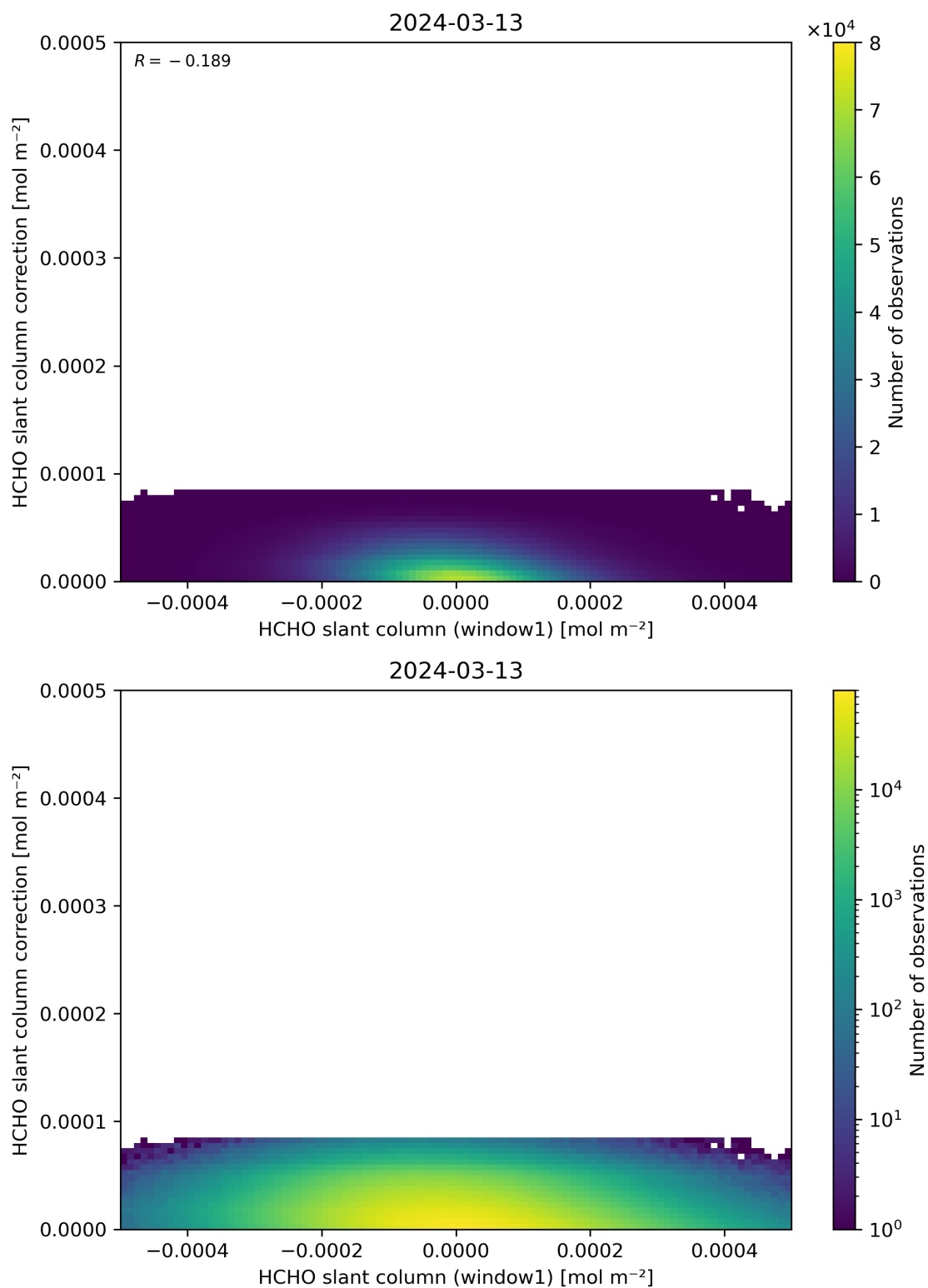
Figure 83: Scatter density plot of “HCHO slant column (window1)” against “HCHO slant column correction” for 2024-03-12 to 2024-03-14.
