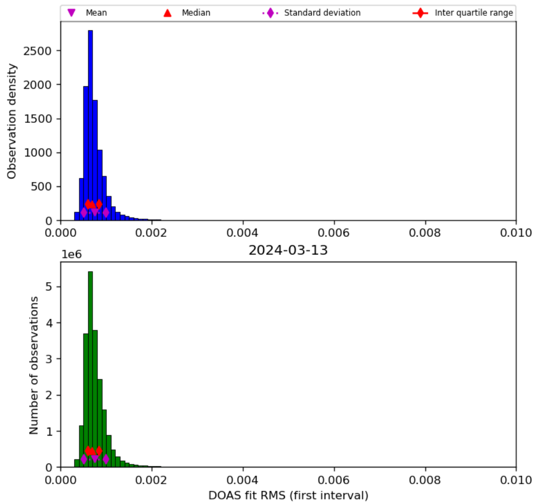
Figure 46: Histogram of “DOAS fit RMS (first interval)” for 2024-03-12 to 2024-03-14
