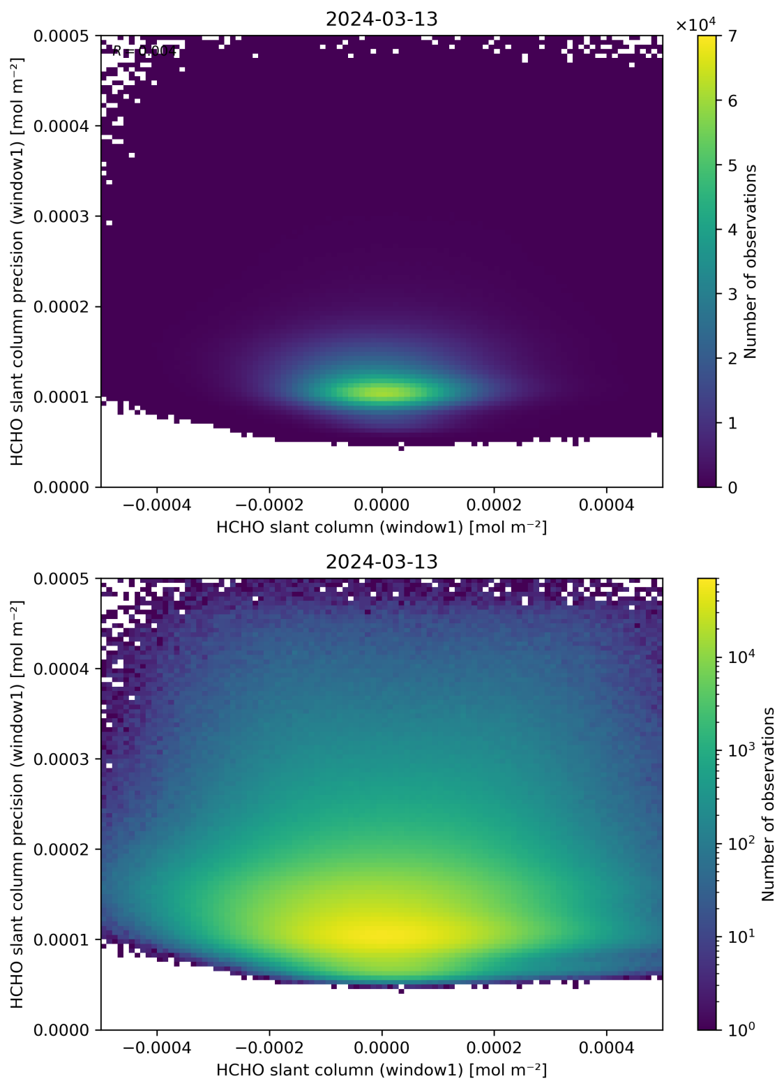
Figure 84: Scatter density plot of “HCHO slant column (window1)” against “HCHO slant column precision (window1)” for 2024-03-12 to 2024-03-14.
