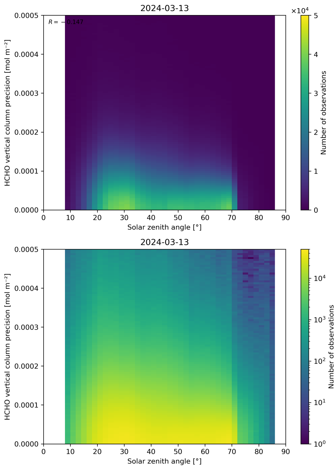
Figure 179: Scatter density plot of “Solar zenith angle” against “HCHO vertical column precision” for 2024-03-12 to 2024-03-14.
