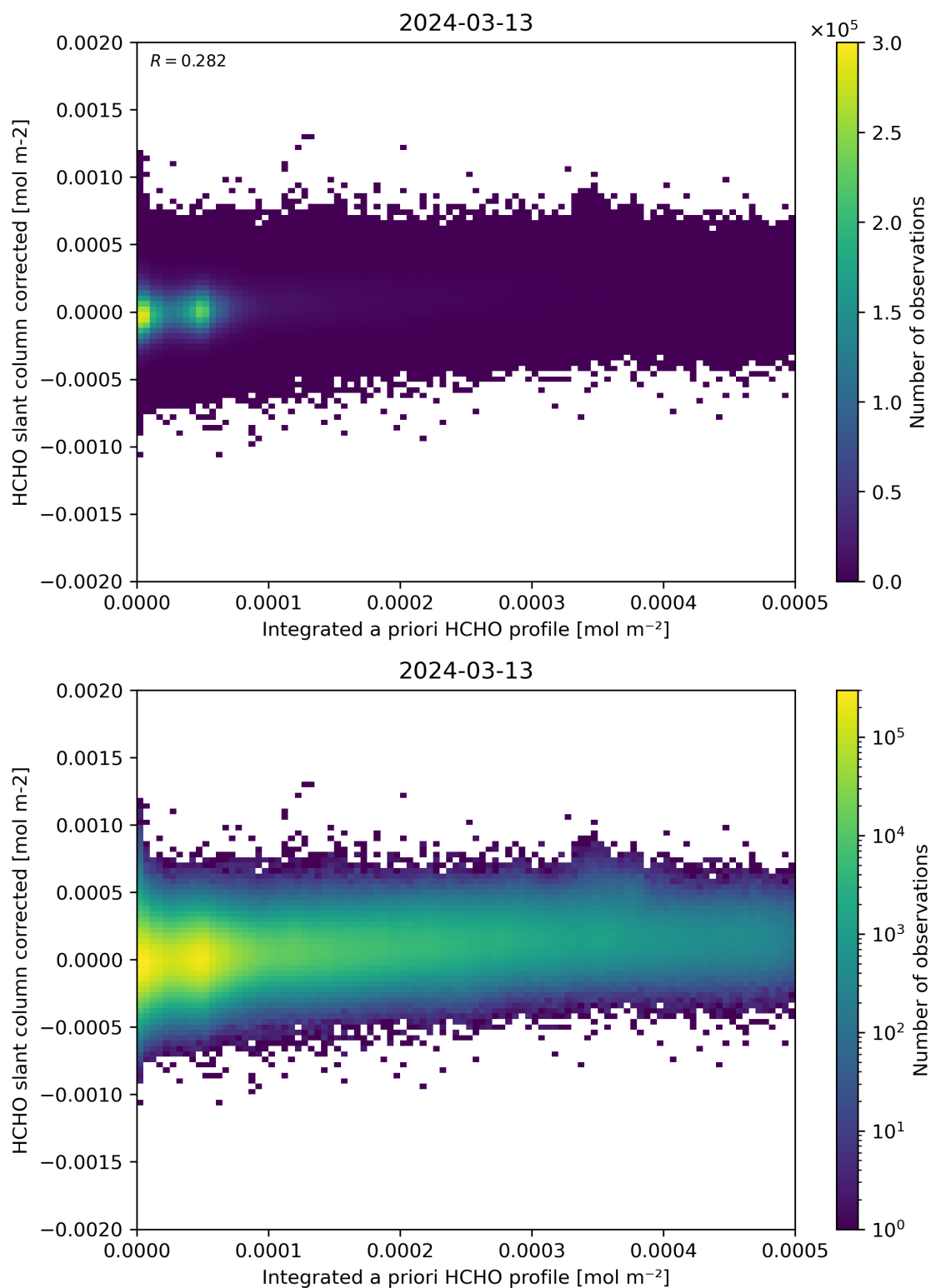
Figure 151: Scatter density plot of “Integrated a priori HCHO profile” against “HCHO slant column corrected” for 2024-03-12 to 2024-03-14.
