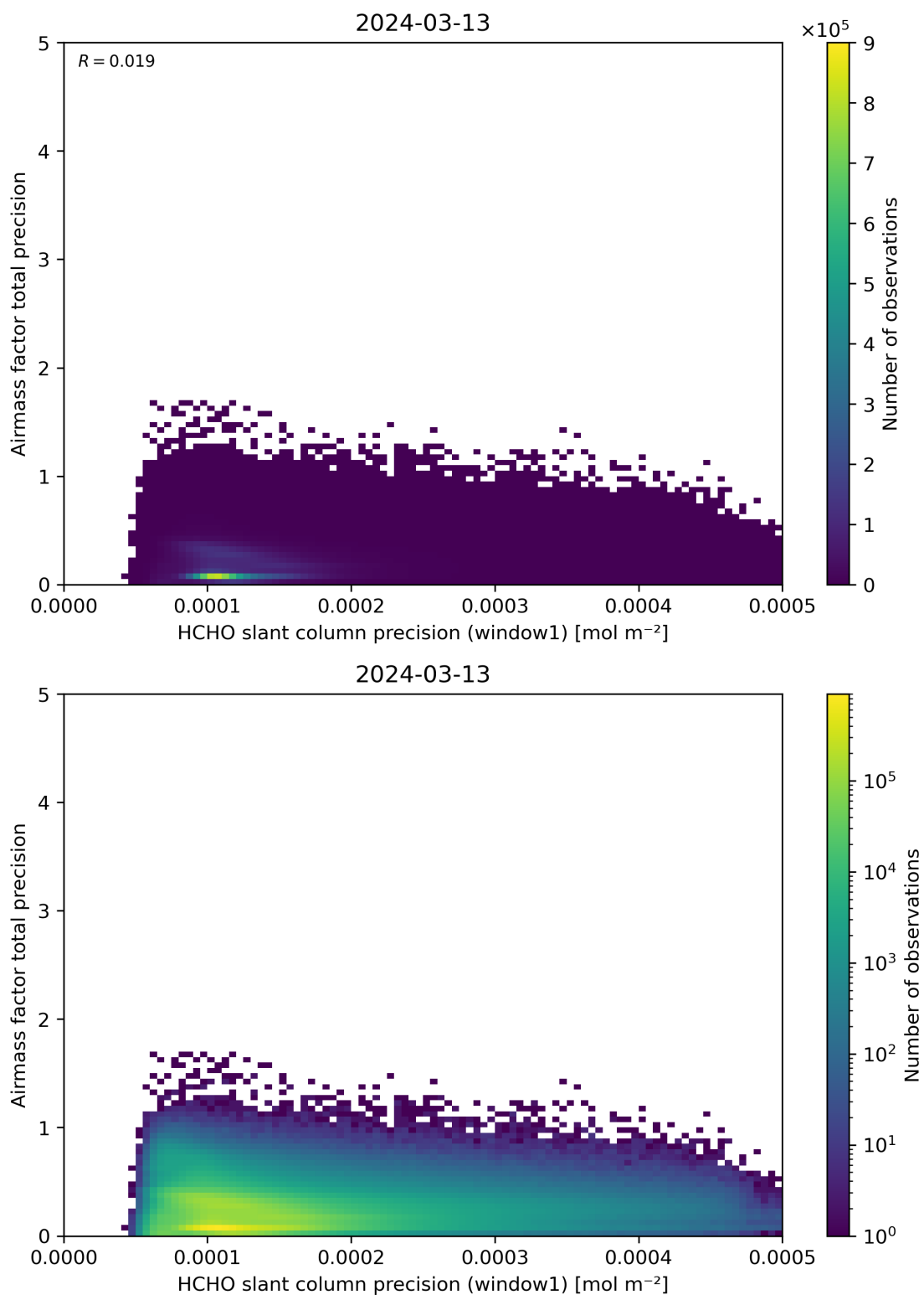
Figure 95: Scatter density plot of “HCHO slant column precision (window1)” against “Airmass factor total precision” for 2024-03-12 to 2024-03-14.
