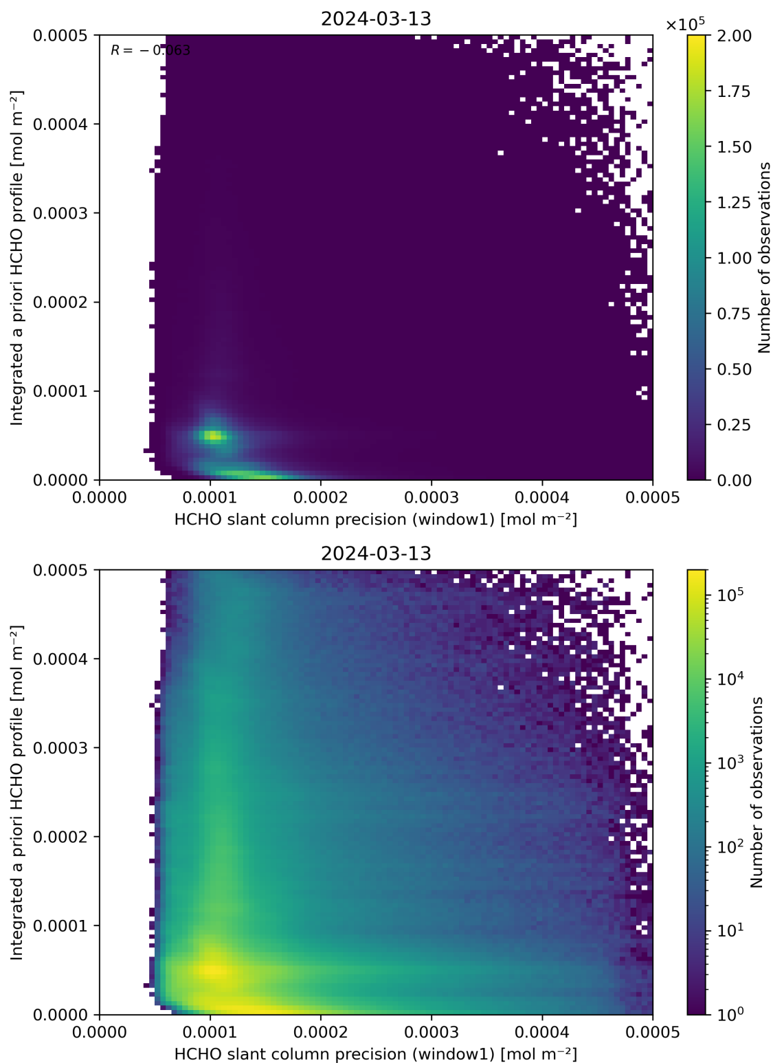
Figure 96: Scatter density plot of “HCHO slant column precision (window1)” against “Integrated a priori HCHO profile” for 2024-03-12 to 2024-03-14.
