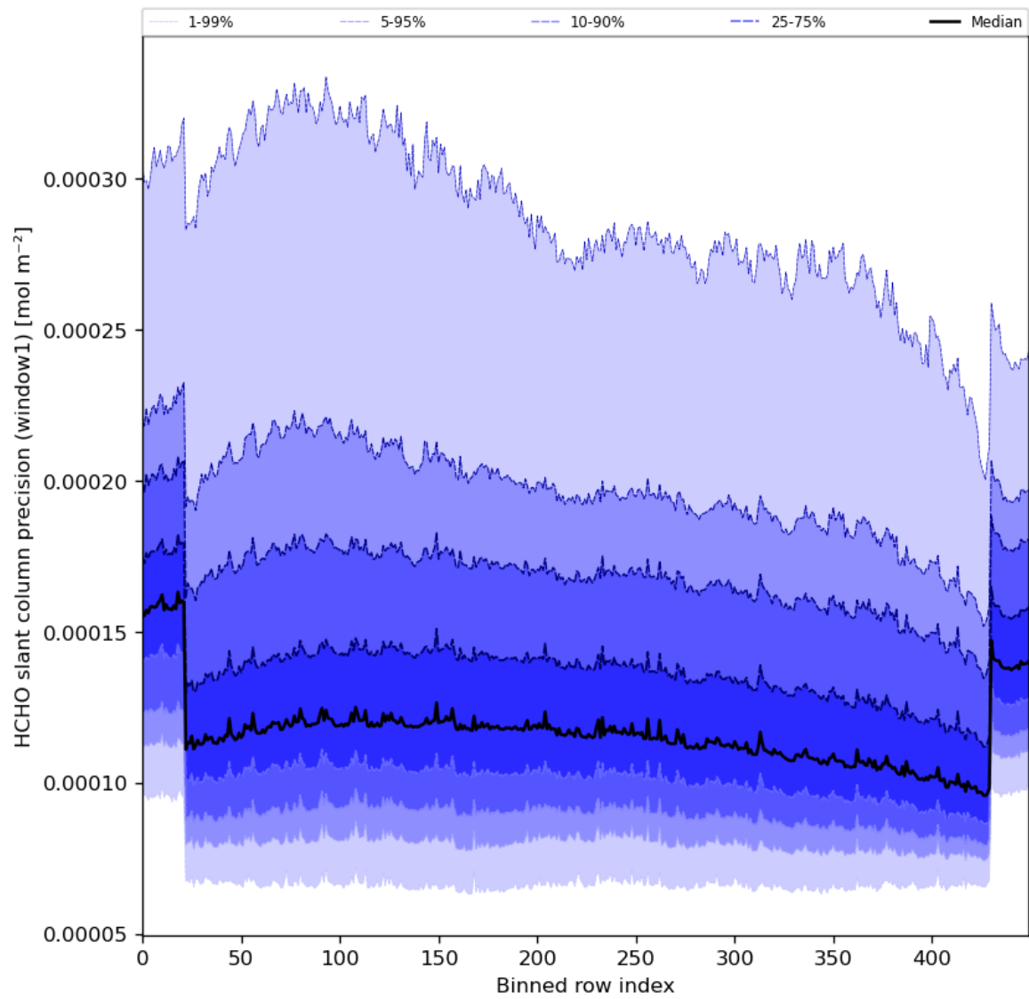
Figure 53: Along track statistics of “HCHO slant column precision (window1)” for 2024-03-12 to 2024-03-14
