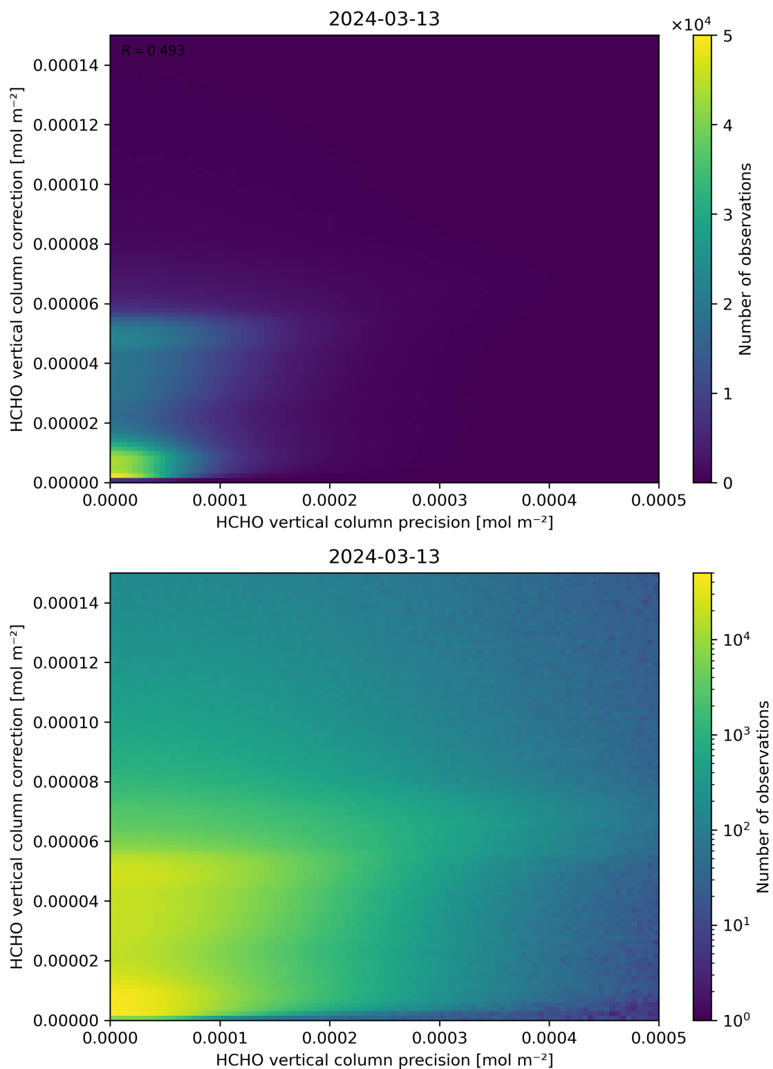
Figure 146: Scatter density plot of “HCHO vertical column precision” against “HCHO vertical column correction” for 2024-03-12 to 2024-03-14.
