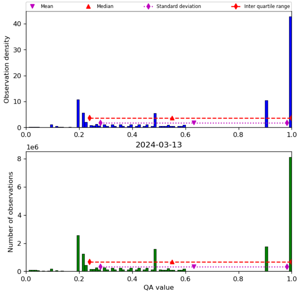
Figure 34: Histogram of “QA value” for 2024-03-12 to 2024-03-14
