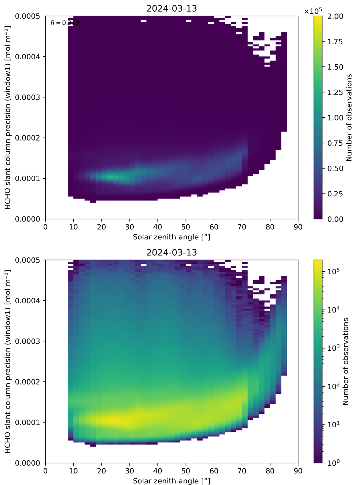
Figure 174: Scatter density plot of “Solar zenith angle” against “HCHO slant column precision (window1)” for 2024-03-12 to 2024-03-14.
