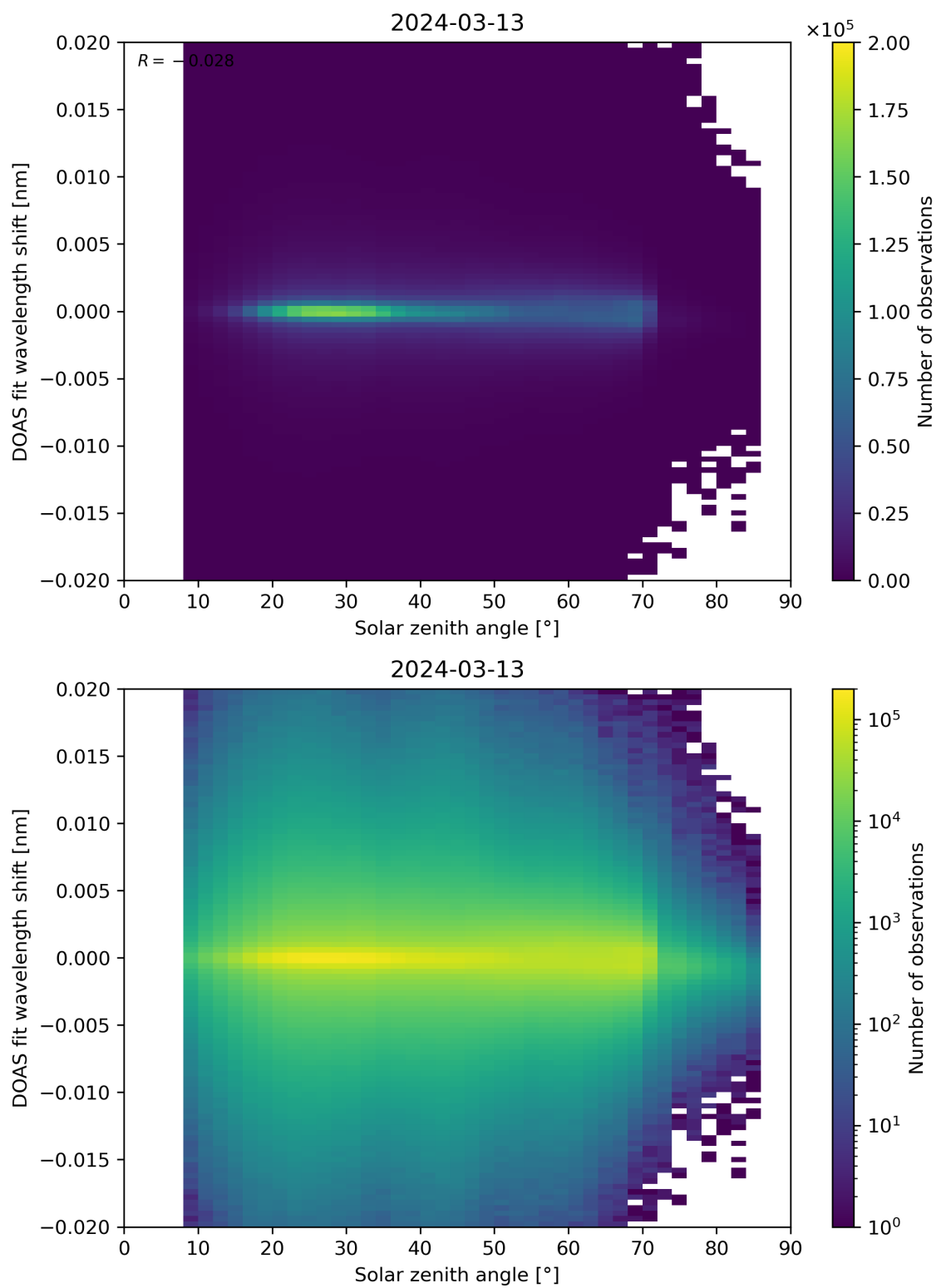
Figure 168: Scatter density plot of “Solar zenith angle” against “DOAS fit wavelength shift” for 2024-03-12 to 2024-03-14.
