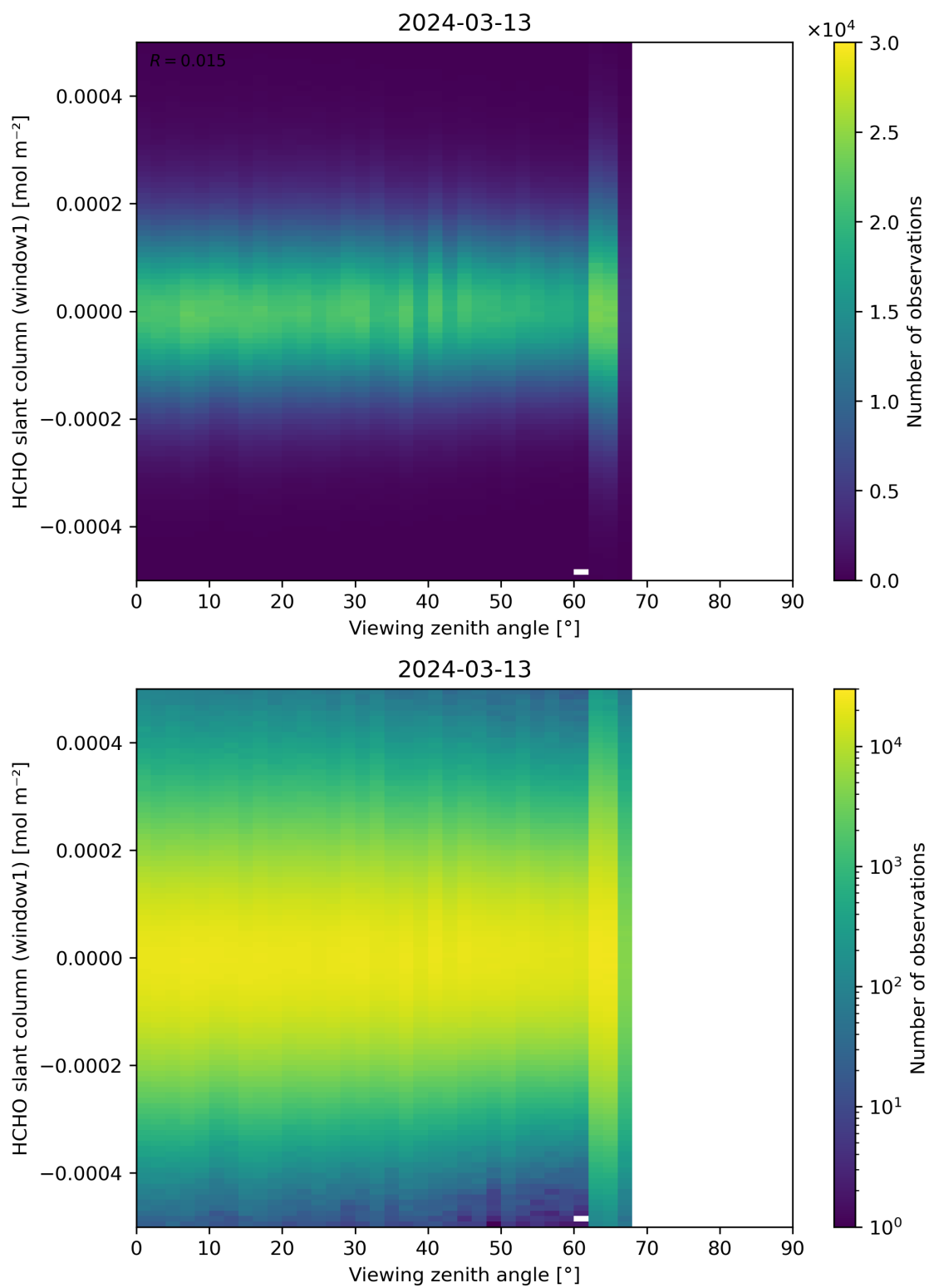
Figure 188: Scatter density plot of “Viewing zenith angle” against “HCHO slant column (window1)” for 2024-03-12 to 2024-03-14.
