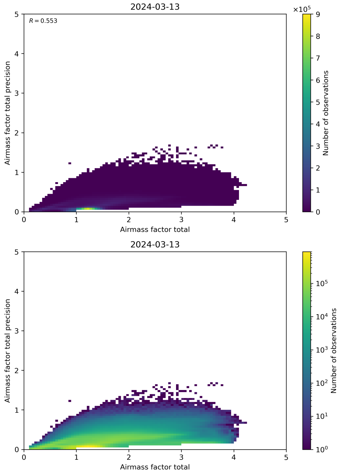
Figure 103: Scatter density plot of “Airmass factor total” against “Airmass factor total precision” for 2024-03-12 to 2024-03-14.
