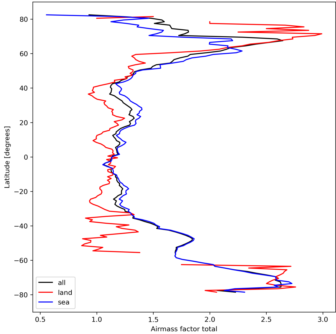
Figure 26: Zonal average of “Airmass factor total” for 2024-03-12 to 2024-03-14.
