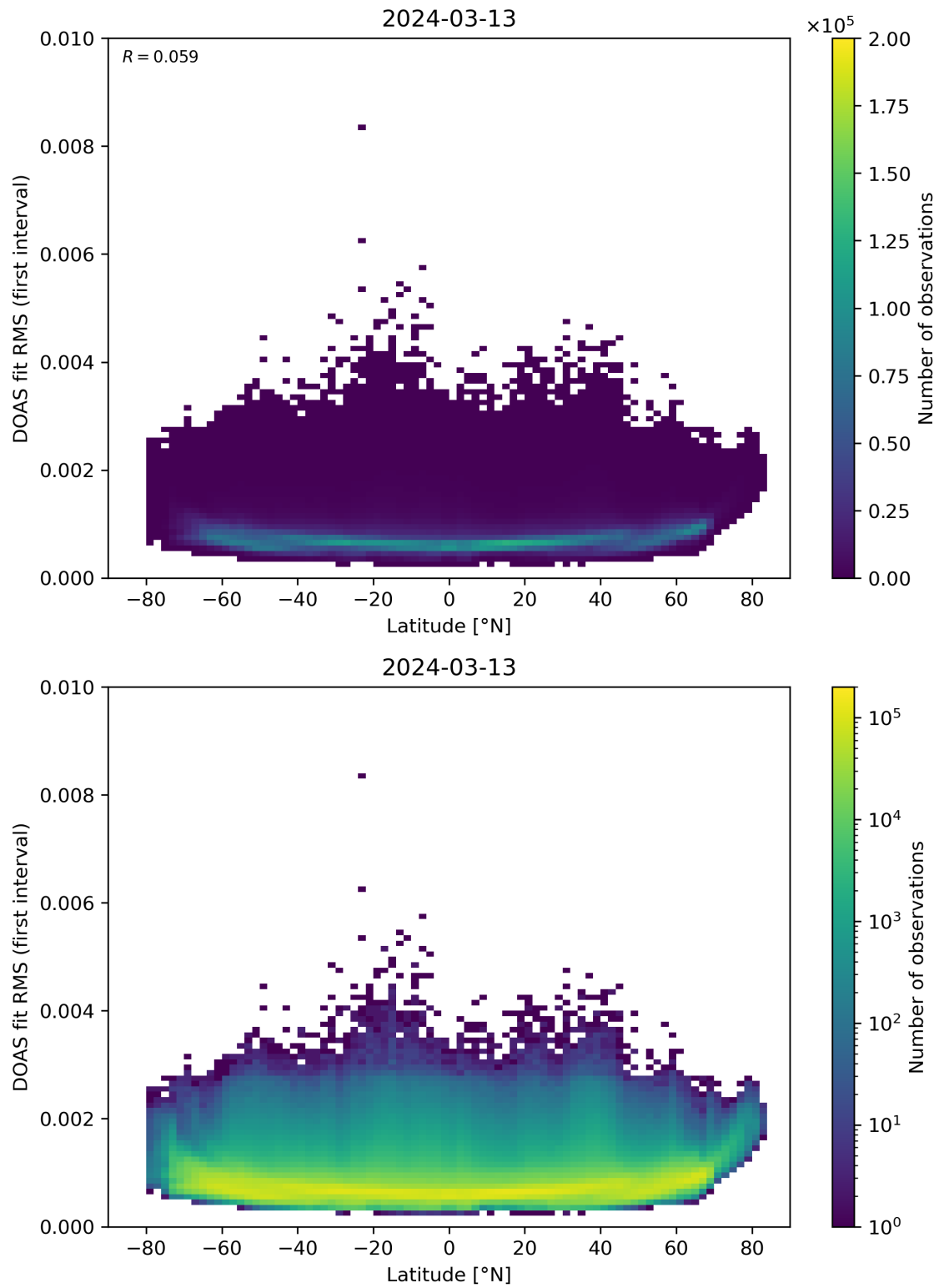
Figure 153: Scatter density plot of “Latitude” against “DOAS fit RMS (first interval)” for 2024-03-12 to 2024-03-14.
