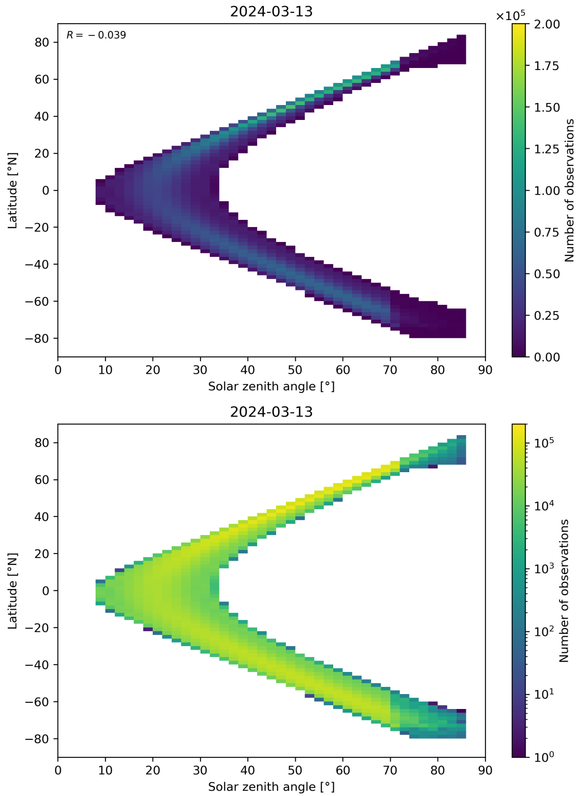
Figure 181: Scatter density plot of “Solar zenith angle” against “Latitude” for 2024-03-12 to 2024-03-14.
