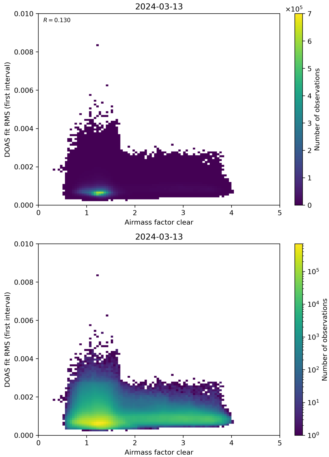
Figure 71: Scatter density plot of “Airmass factor clear” against “DOAS fit RMS (first interval)” for 2024-03-12 to 2024-03-14.
