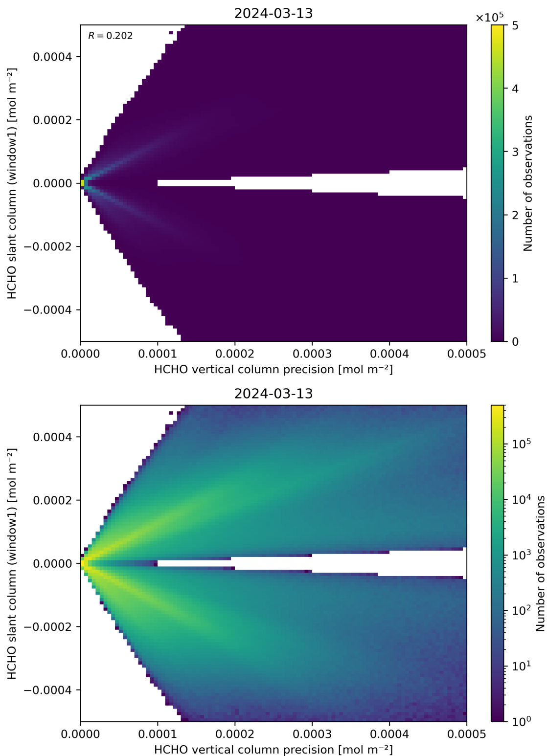
Figure 142: Scatter density plot of “HCHO vertical column precision” against “HCHO slant column (window1)” for 2024-03-12 to 2024-03-14.
