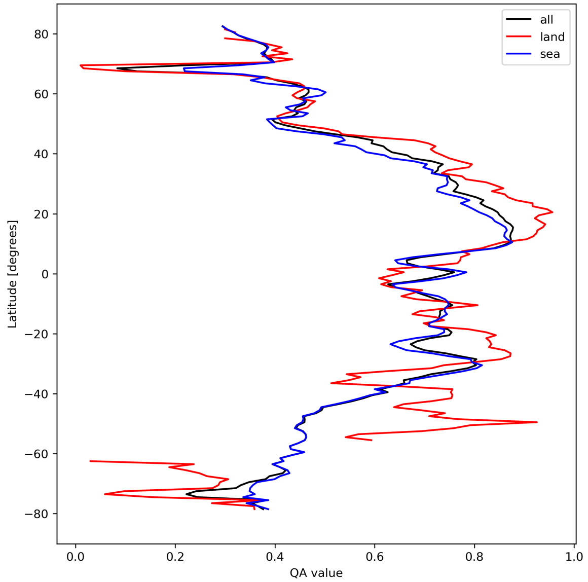
Figure 20: Zonal average of “QA value” for 2024-03-12 to 2024-03-14.
