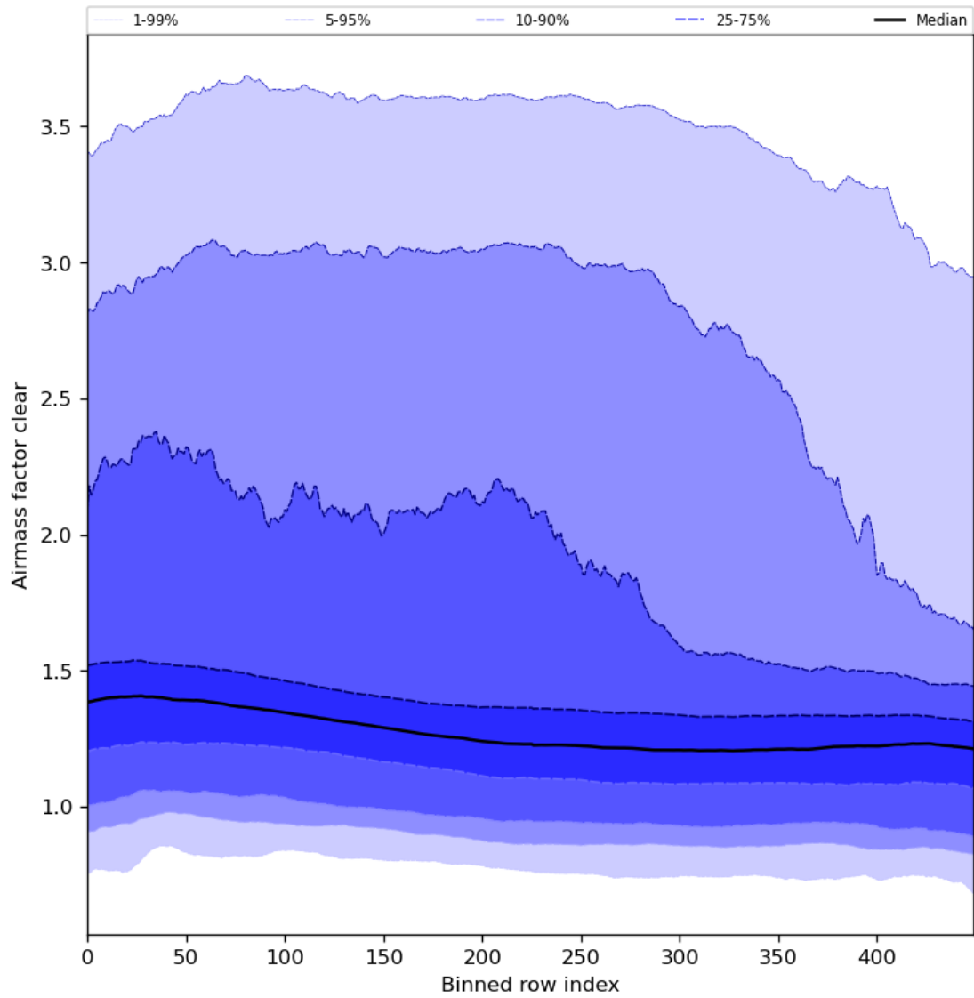
Figure 56: Along track statistics of “Airmass factor clear” for 2024-03-12 to 2024-03-14
