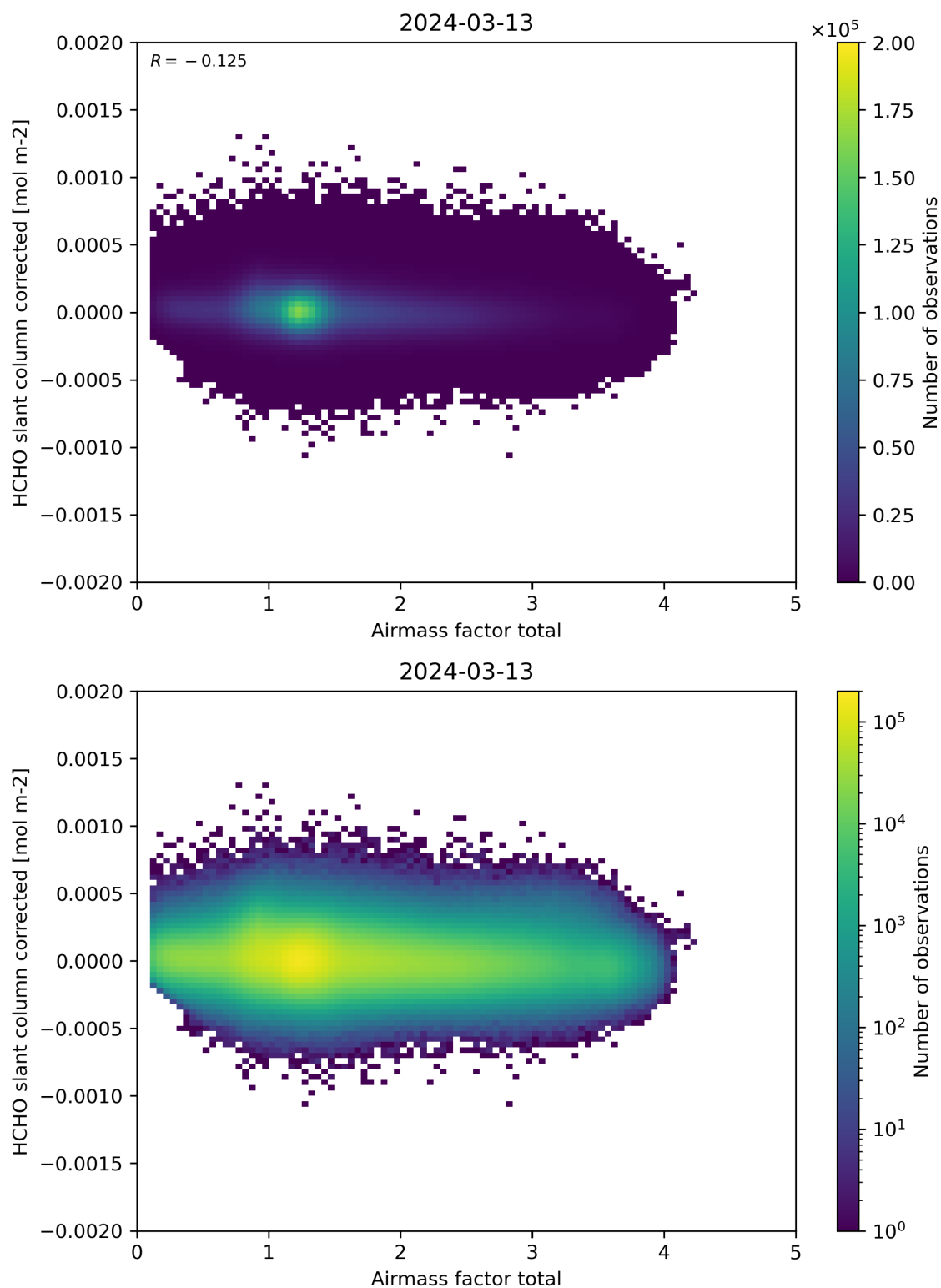
Figure 101: Scatter density plot of “Airmass factor total” against “HCHO slant column corrected” for 2024-03-12 to 2024-03-14.
