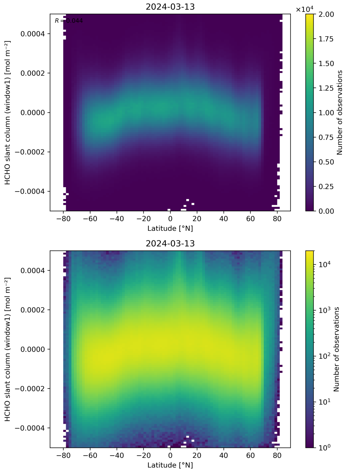
Figure 159: Scatter density plot of “Latitude” against “HCHO slant column (window1)” for 2024-03-12 to 2024-03-14.
