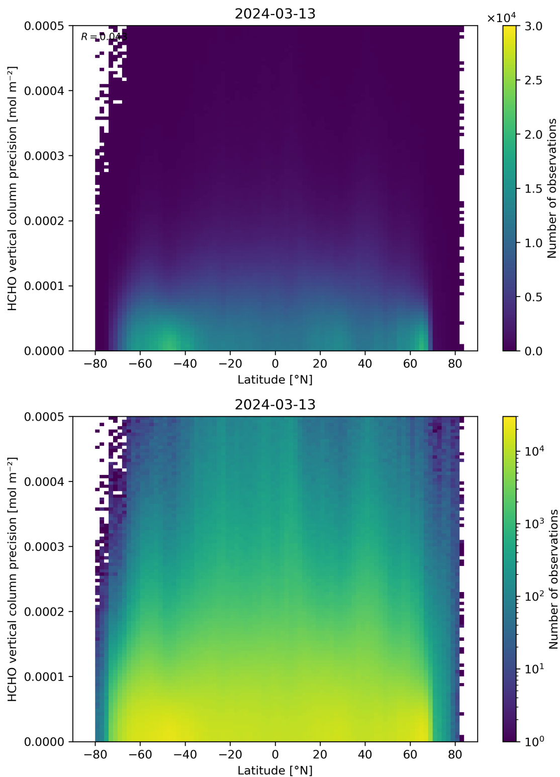
Figure 165: Scatter density plot of “Latitude” against “HCHO vertical column precision” for 2024-03-12 to 2024-03-14.
