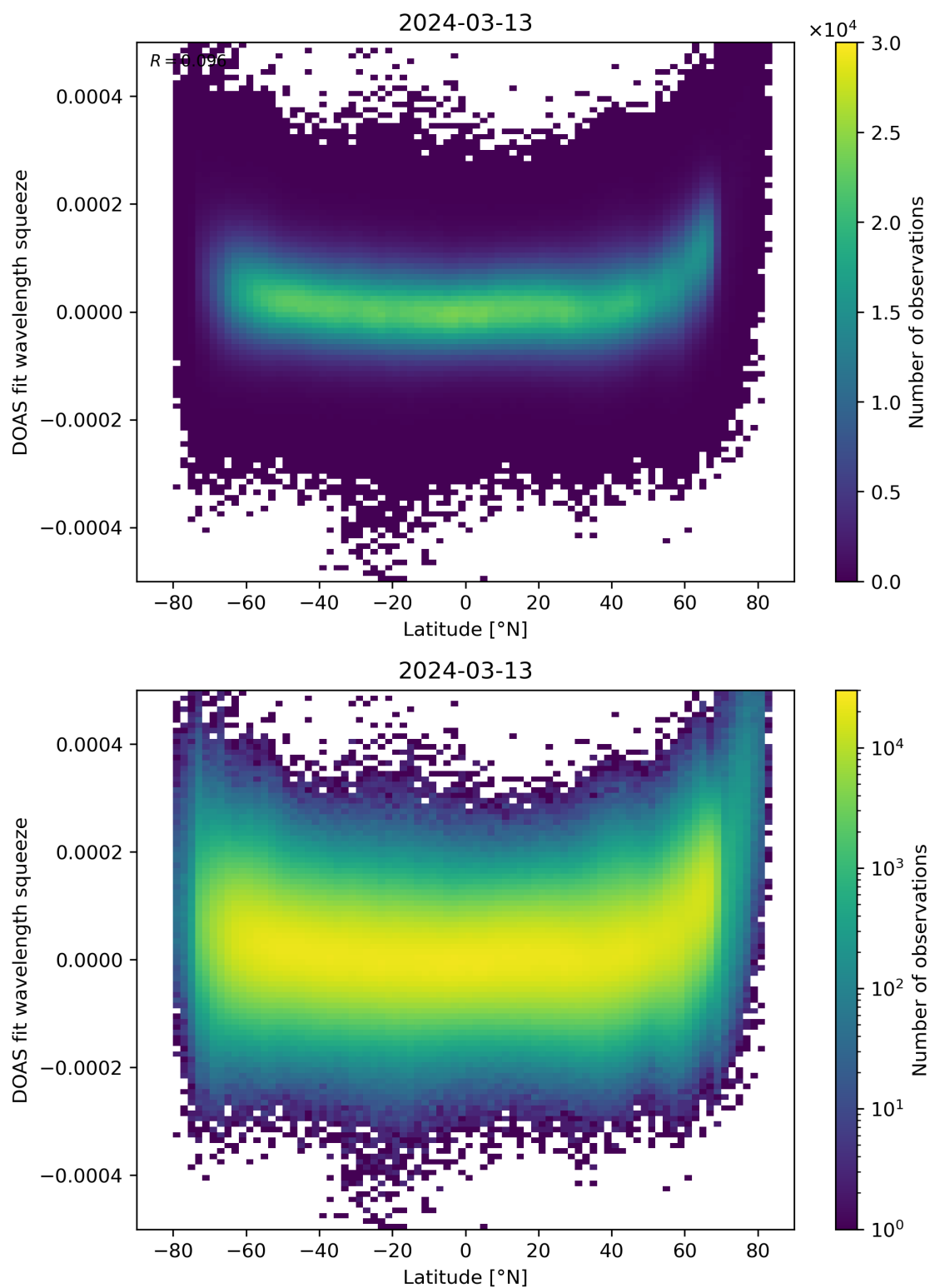
Figure 155: Scatter density plot of “Latitude” against “DOAS fit wavelength squeeze” for 2024-03-12 to 2024-03-14.
