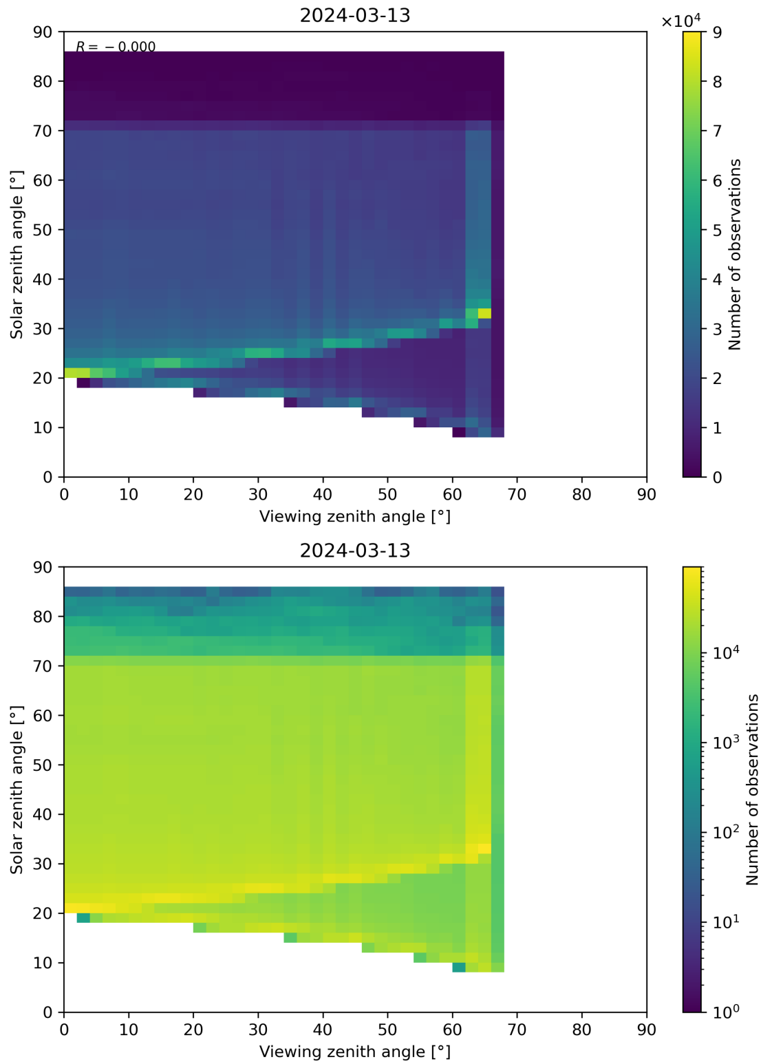
Figure 197: Scatter density plot of “Viewing zenith angle” against “Solar zenith angle” for 2024-03-12 to 2024-03-14.
