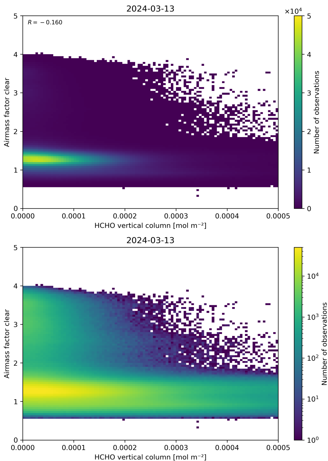
Figure 126: Scatter density plot of “HCHO vertical column” against “Airmass factor clear” for 2024-03-12 to 2024-03-14.
