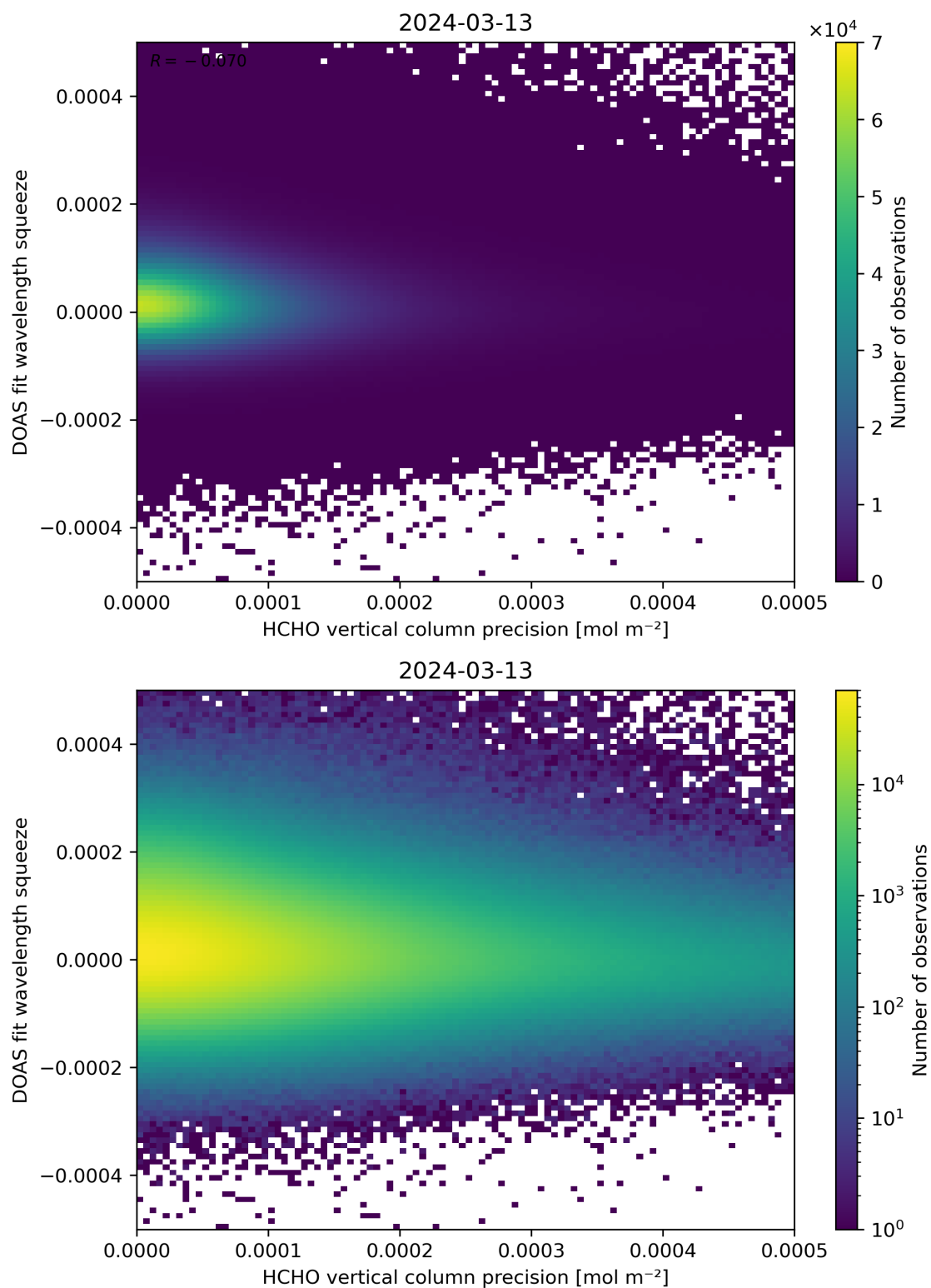
Figure 138: Scatter density plot of “HCHO vertical column precision” against “DOAS fit wavelength squeeze” for 2024-03-12 to 2024-03-14.
