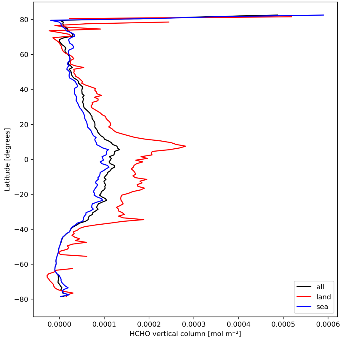
Figure 21: Zonal average of “HCHO vertical column” for 2024-03-12 to 2024-03-14.
