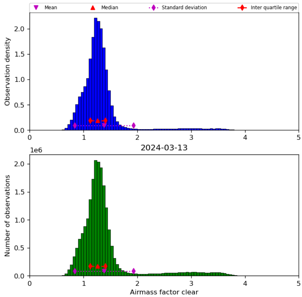
Figure 42: Histogram of “Airmass factor clear” for 2024-03-12 to 2024-03-14
