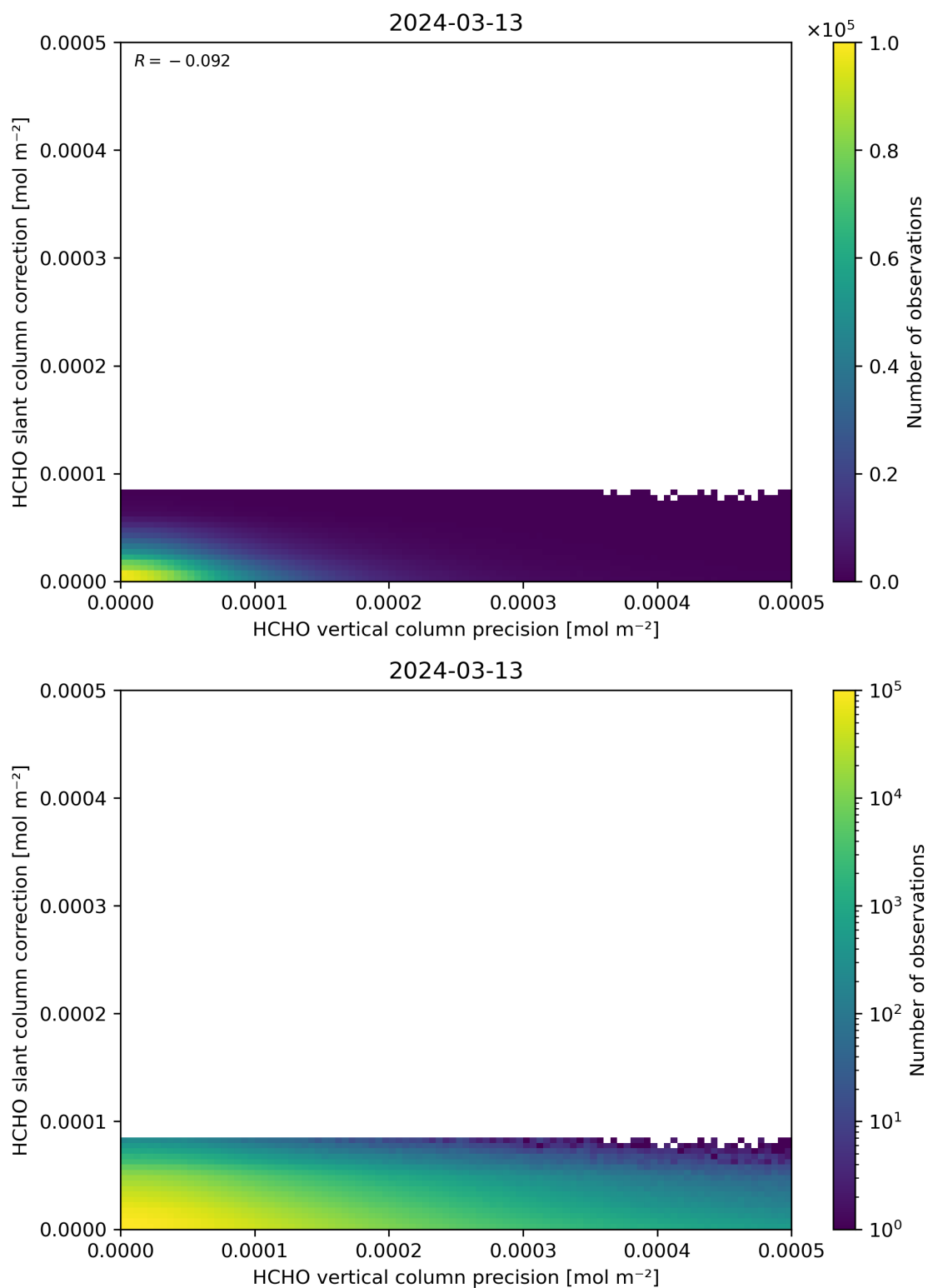
Figure 141: Scatter density plot of “HCHO vertical column precision” against “HCHO slant column correction” for 2024-03-12 to 2024-03-14.
