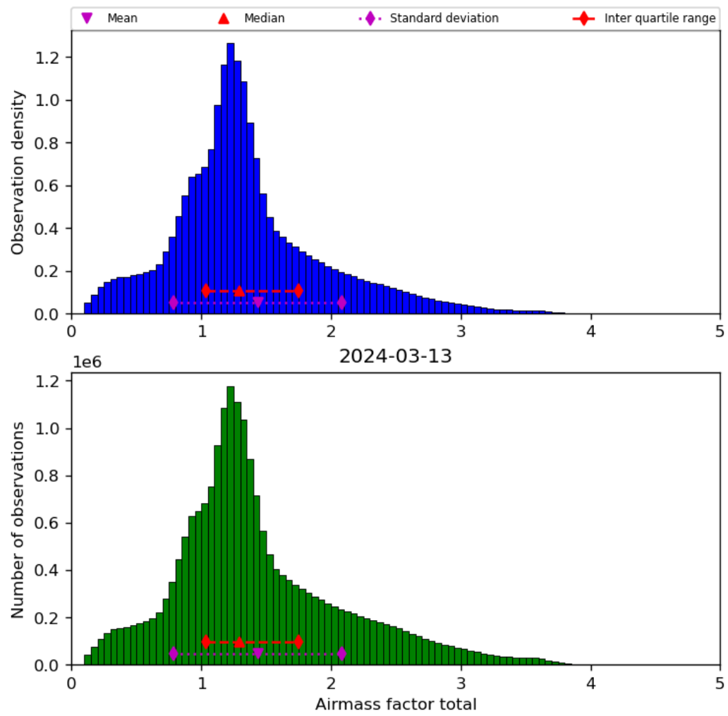
Figure 40: Histogram of “Airmass factor total” for 2024-03-12 to 2024-03-14
