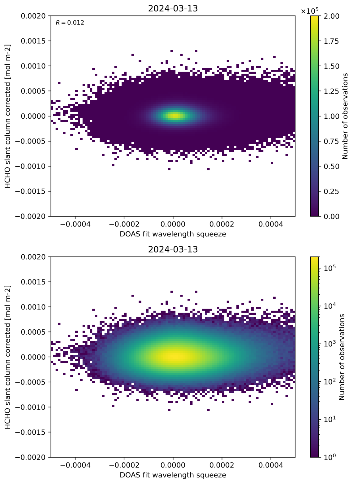
Figure 69: Scatter density plot of “DOAS fit wavelength squeeze” against “HCHO slant column corrected” for 2024-03-12 to 2024-03-14.
