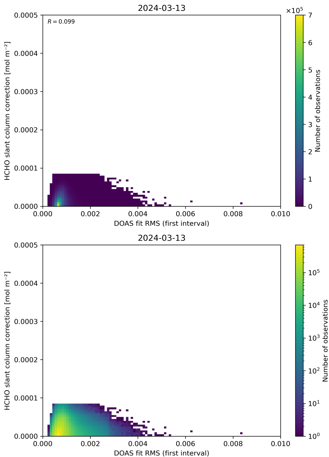
Figure 63: Scatter density plot of “DOAS fit RMS (first interval)” against “HCHO slant column correction” for 2024-03-12 to 2024-03-14.
