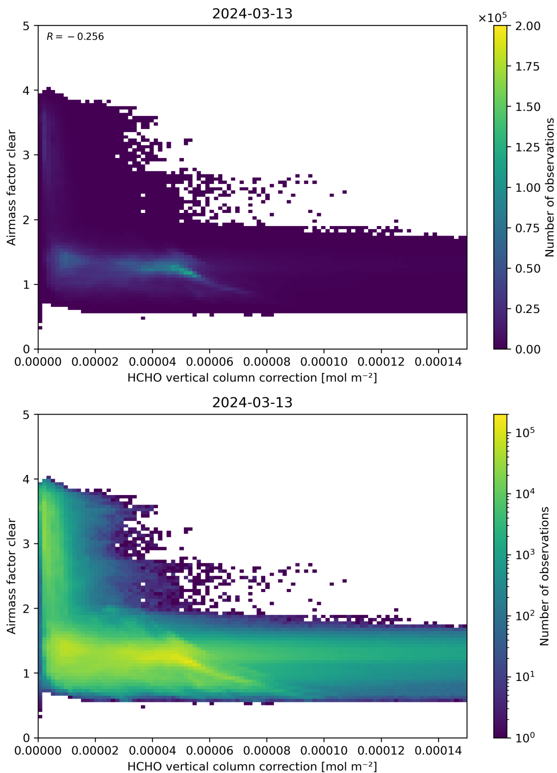
Figure 115: Scatter density plot of “HCHO vertical column correction” against “Airmass factor clear” for 2024-03-12 to 2024-03-14.
