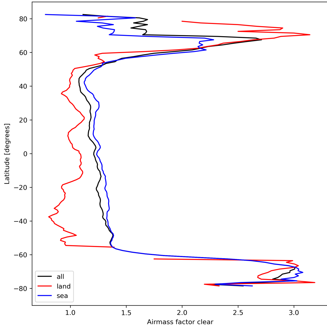
Figure 28: Zonal average of “Airmass factor clear” for 2024-03-12 to 2024-03-14.
