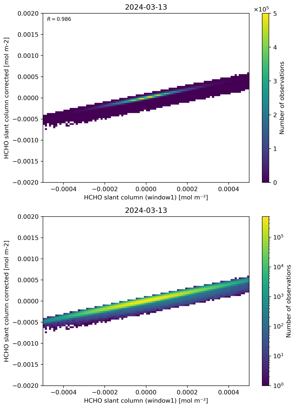
Figure 82: Scatter density plot of “HCHO slant column (window1)” against “HCHO slant column corrected” for 2024-03-12 to 2024-03-14.
