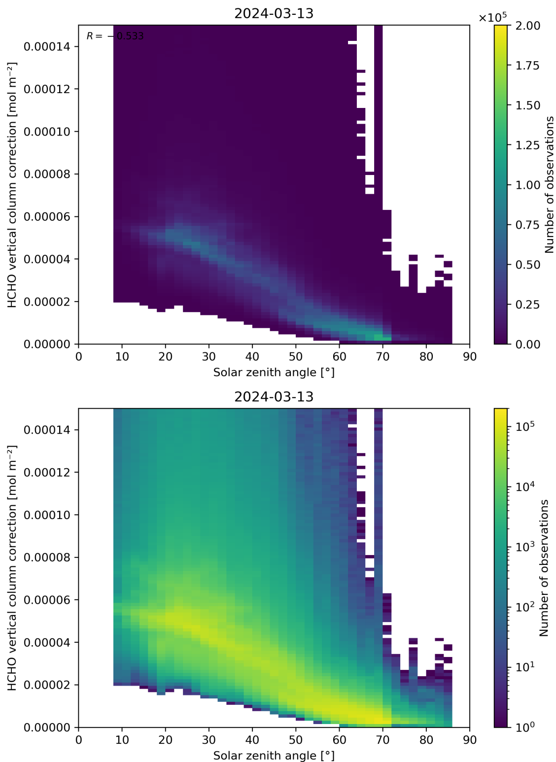
Figure 178: Scatter density plot of “Solar zenith angle” against “HCHO vertical column correction” for 2024-03-12 to 2024-03-14.
