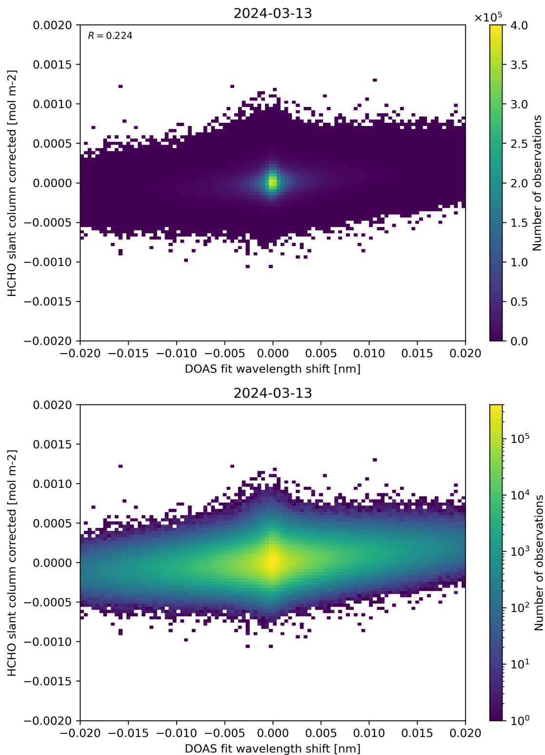
Figure 66: Scatter density plot of “DOAS fit wavelength shift” against “HCHO slant column corrected” for 2024-03-12 to 2024-03-14.
