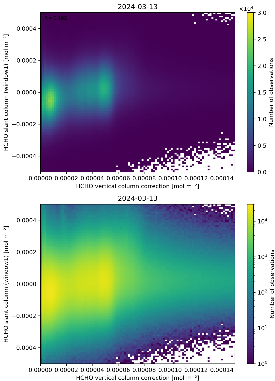
Figure 118: Scatter density plot of “HCHO vertical column correction” against “HCHO slant column (window1)” for 2024-03-12 to 2024-03-14.
