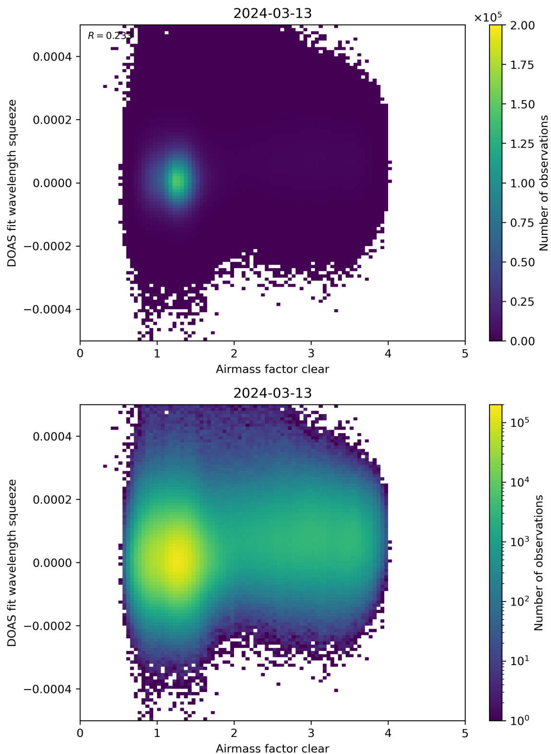
Figure 73: Scatter density plot of “Airmass factor clear” against “DOAS fit wavelength squeeze” for 2024-03-12 to 2024-03-14.
