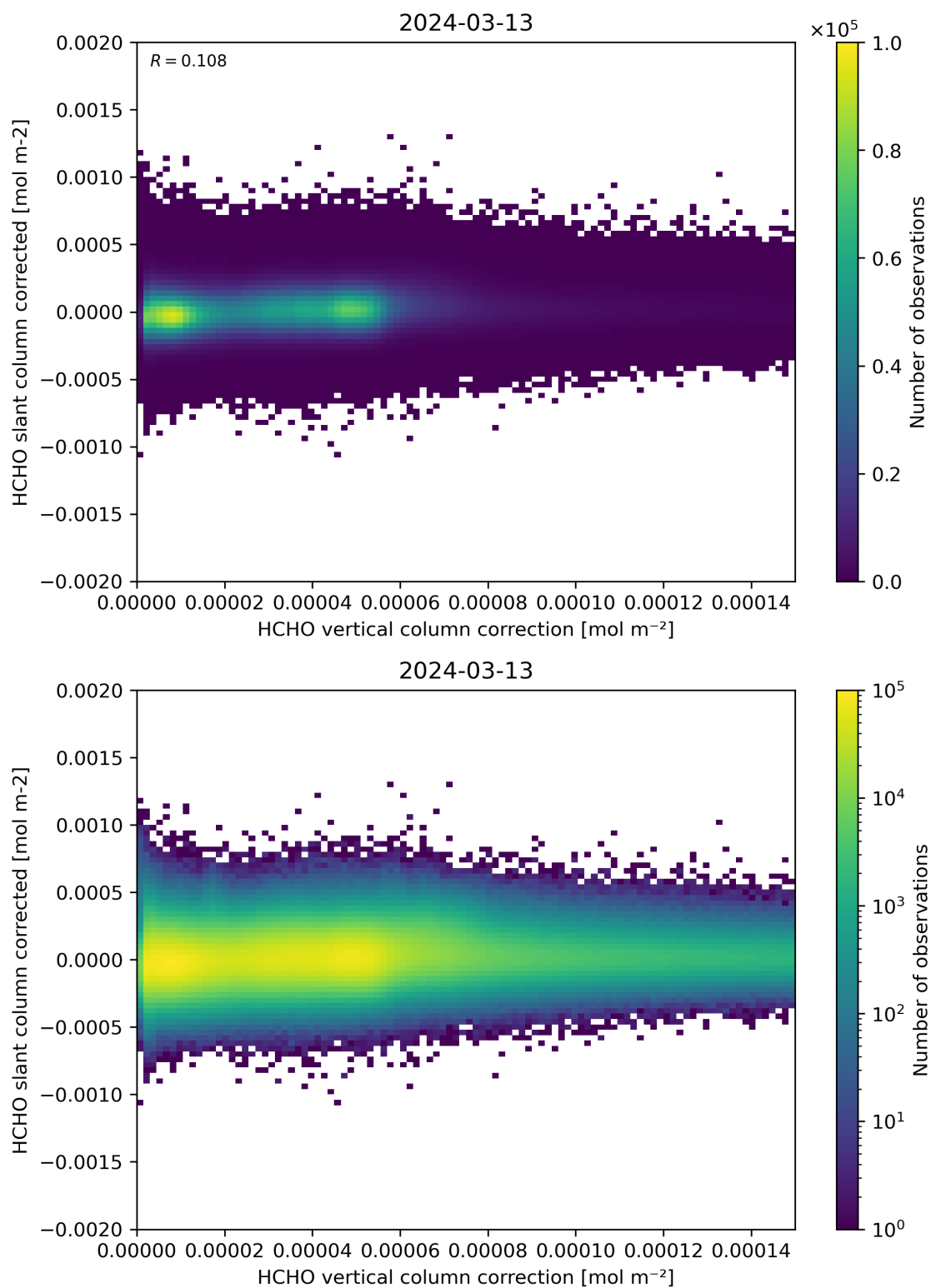
Figure 116: Scatter density plot of “HCHO vertical column correction” against “HCHO slant column corrected” for 2024-03-12 to 2024-03-14.
