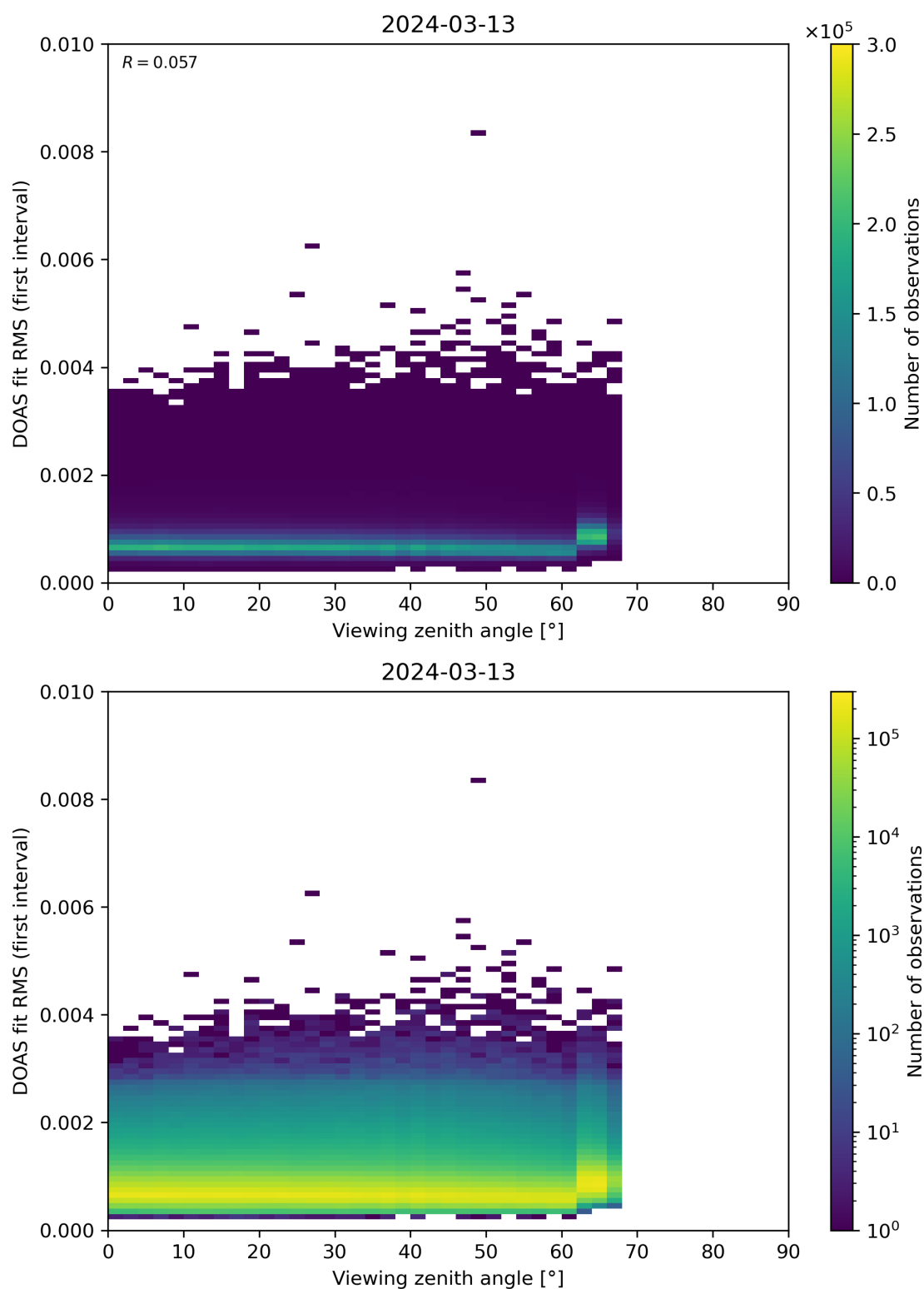
Figure 182: Scatter density plot of “Viewing zenith angle” against “DOAS fit RMS (first interval)” for 2024-03-12 to 2024-03-14.
