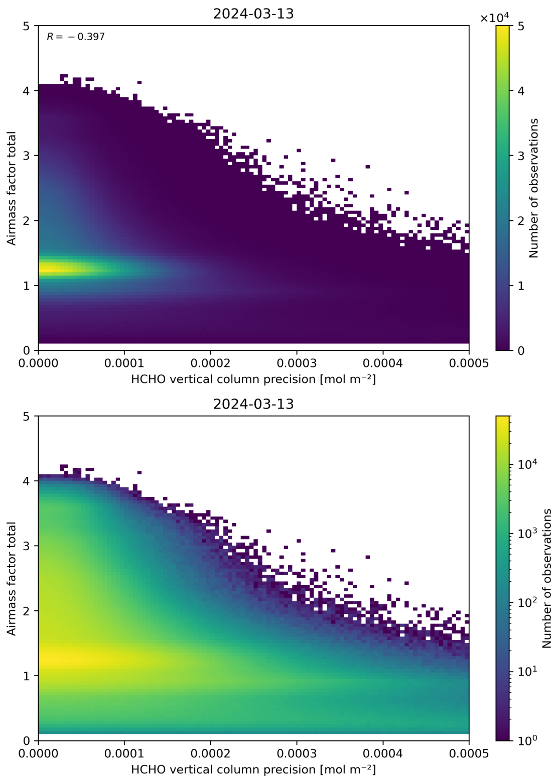
Figure 144: Scatter density plot of “HCHO vertical column precision” against “Airmass factor total” for 2024-03-12 to 2024-03-14.
