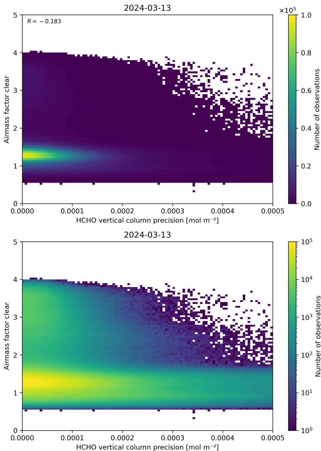
Figure 139: Scatter density plot of “HCHO vertical column precision” against “Airmass factor clear” for 2024-03-12 to 2024-03-14.
