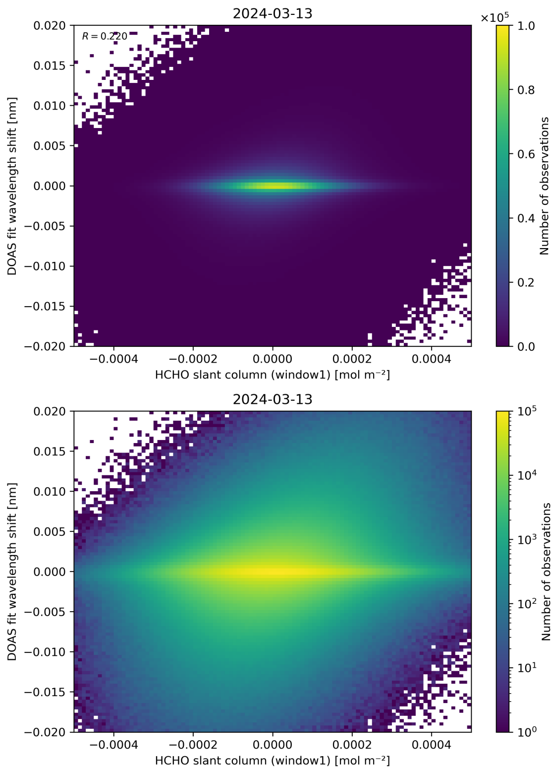
Figure 79: Scatter density plot of “HCHO slant column (window1)” against “DOAS fit wavelength shift” for 2024-03-12 to 2024-03-14.
