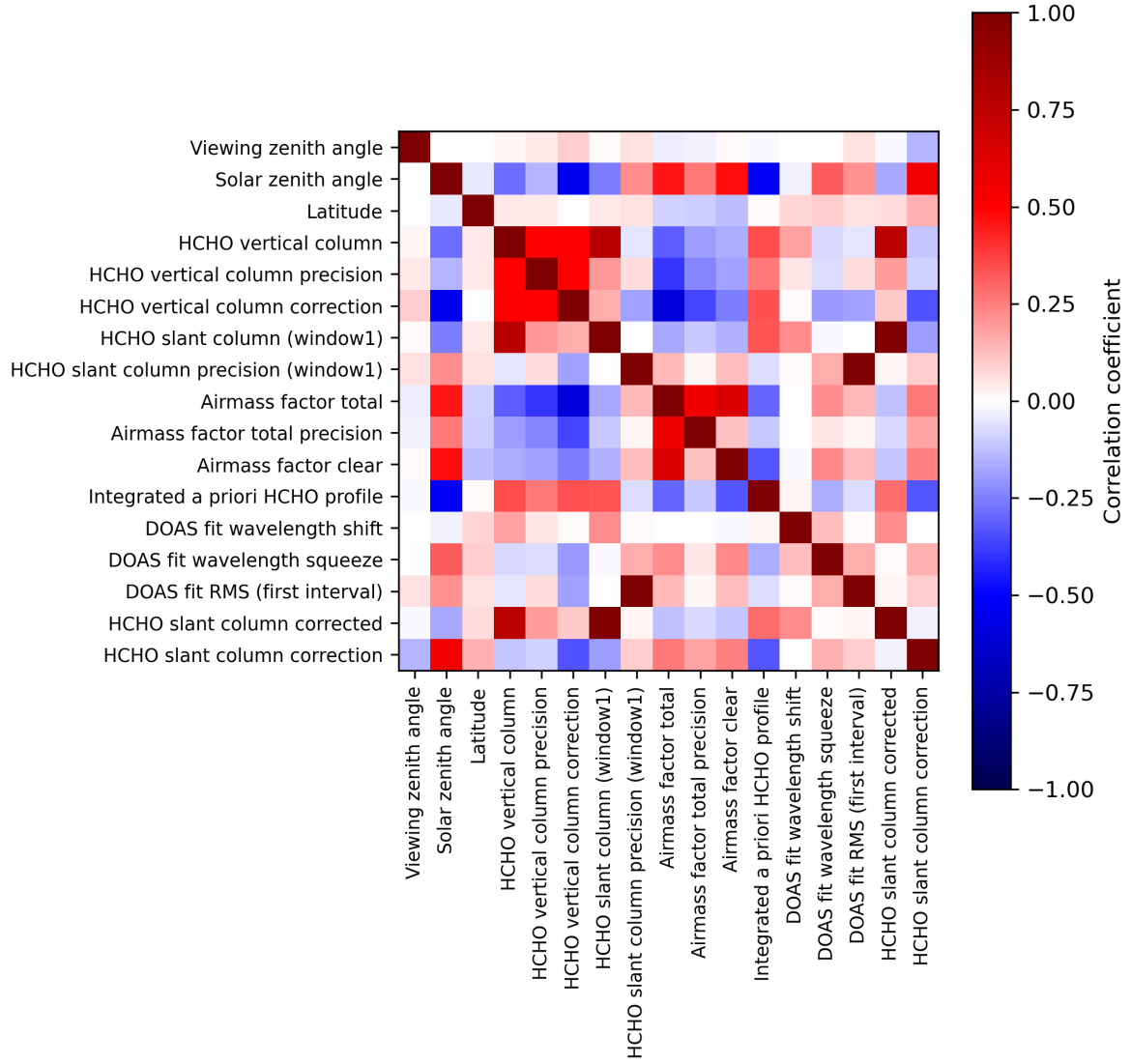
Figure 2: Map of correlation matrix for 2024-03-12 to 2024-03-14.
