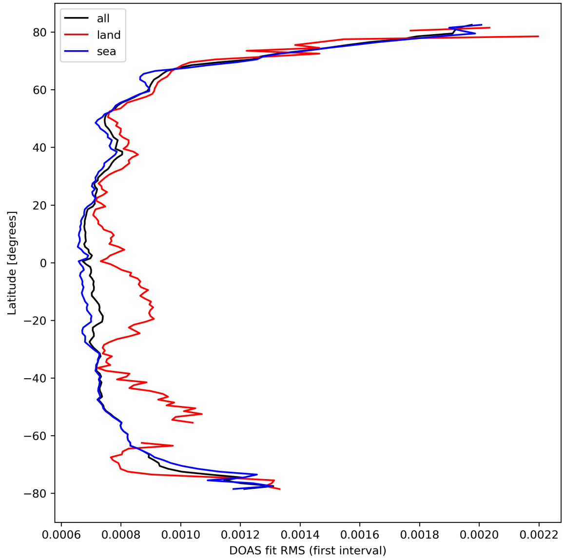
Figure 32: Zonal average of “DOAS fit RMS (first interval)” for 2024-03-12 to 2024-03-14.
