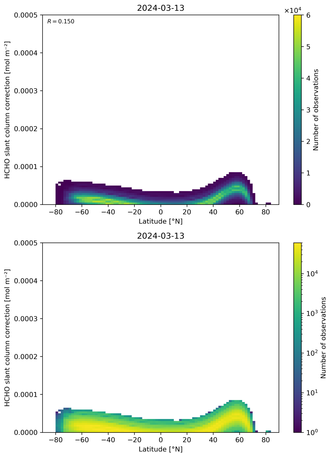
Figure 158: Scatter density plot of “Latitude” against “HCHO slant column correction” for 2024-03-12 to 2024-03-14.
