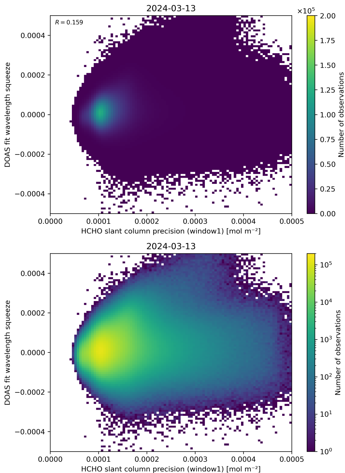
Figure 90: Scatter density plot of “HCHO slant column precision (window1)” against “DOAS fit wavelength squeeze” for 2024-03-12 to 2024-03-14.
