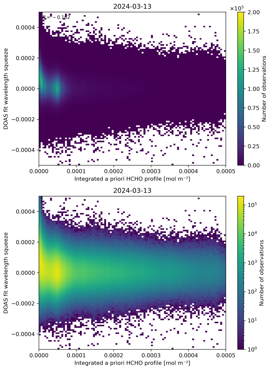
Figure 150: Scatter density plot of “Integrated a priori HCHO profile” against “DOAS fit wavelength squeeze” for 2024-03-12 to 2024-03-14.
