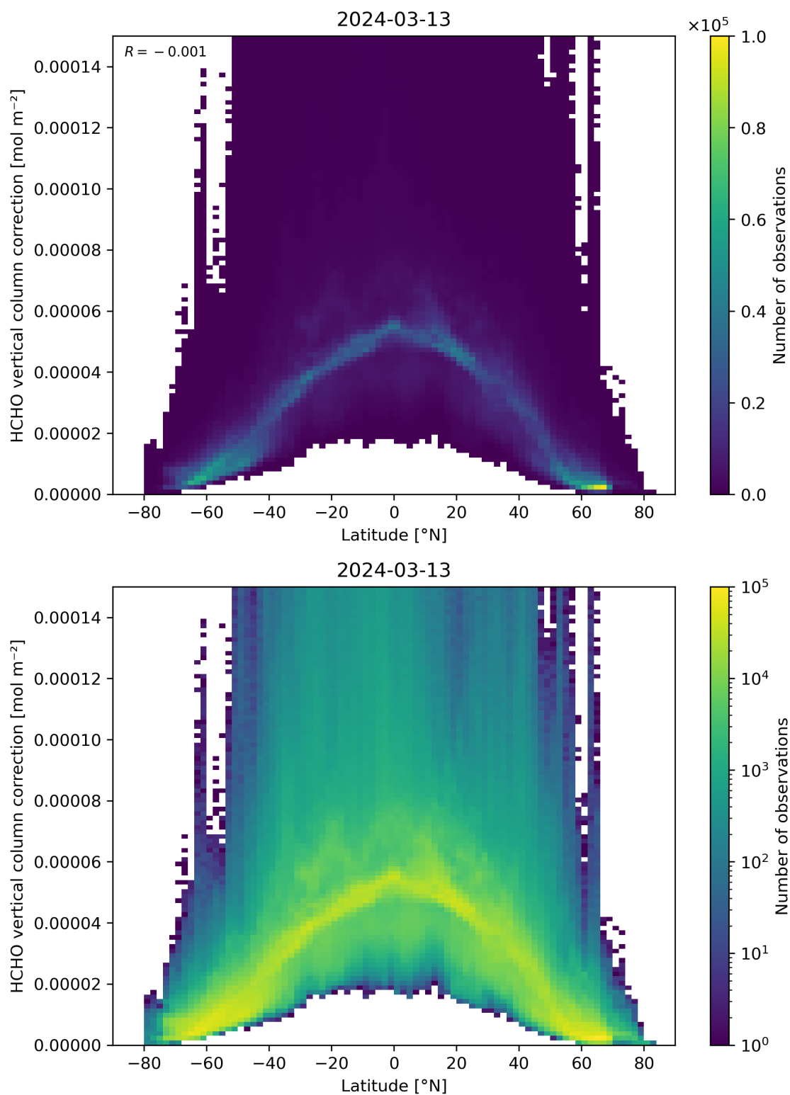
Figure 164: Scatter density plot of “Latitude” against “HCHO vertical column correction” for 2024-03-12 to 2024-03-14.
