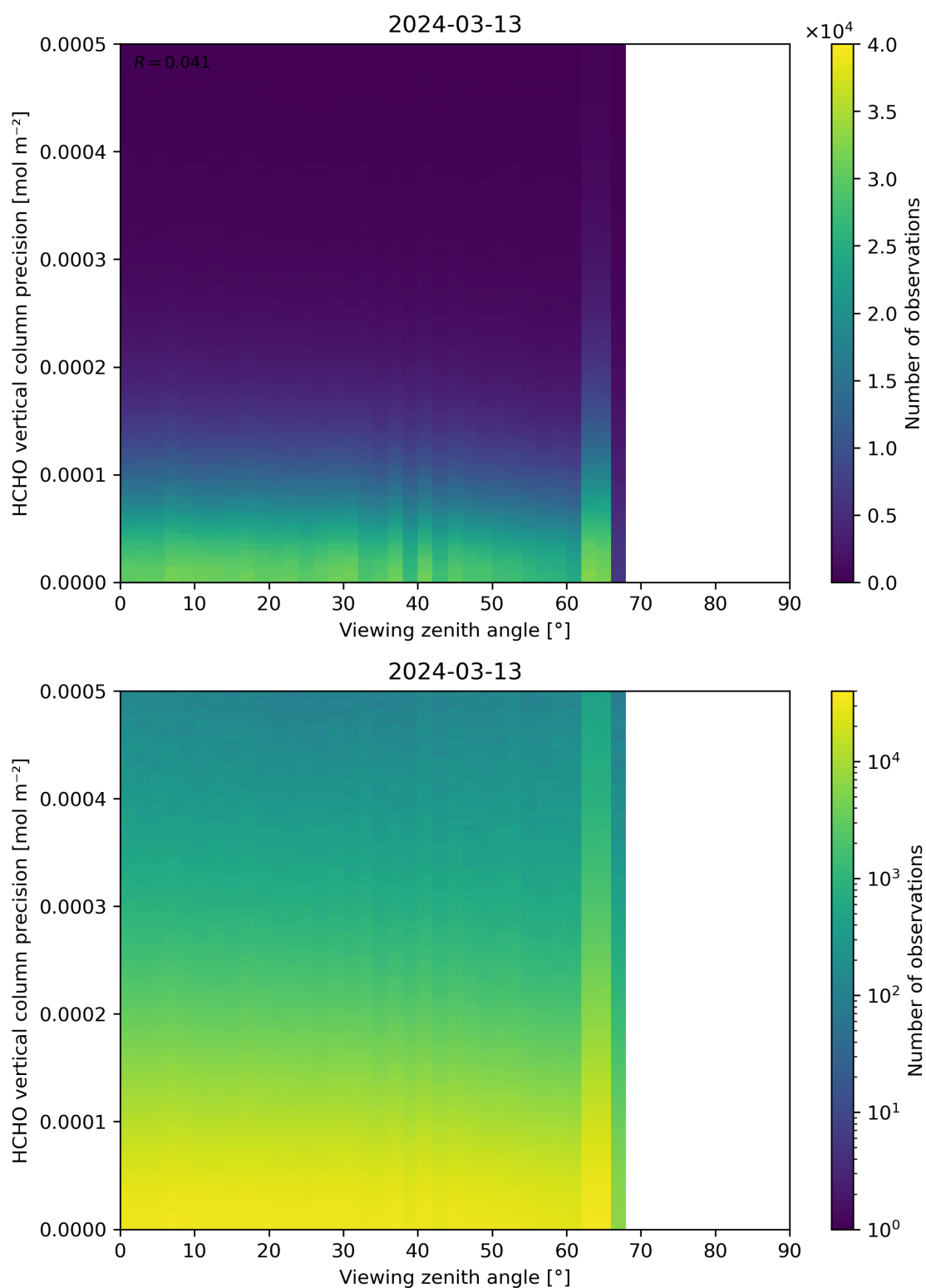
Figure 194: Scatter density plot of “Viewing zenith angle” against “HCHO vertical column precision” for 2024-03-12 to 2024-03-14.
