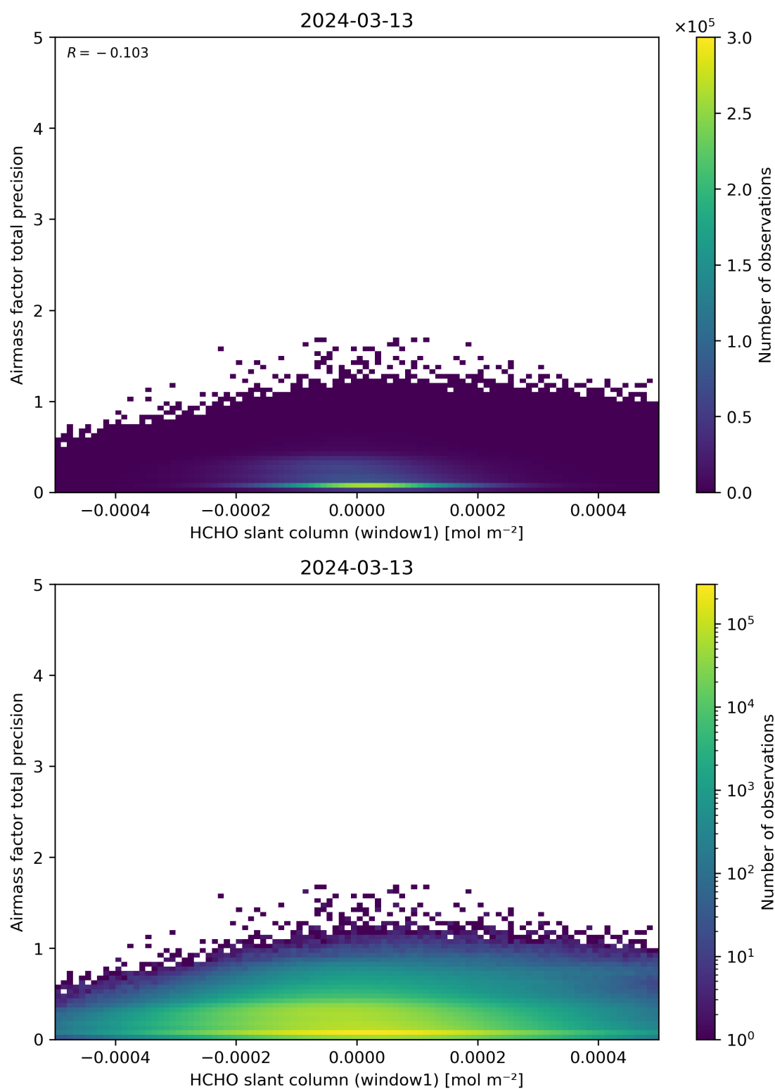
Figure 86: Scatter density plot of “HCHO slant column (window1)” against “Airmass factor total precision” for 2024-03-12 to 2024-03-14.
