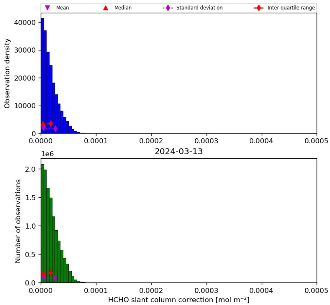
Figure 47: Histogram of “HCHO slant column correction” for 2024-03-12 to 2024-03-14
