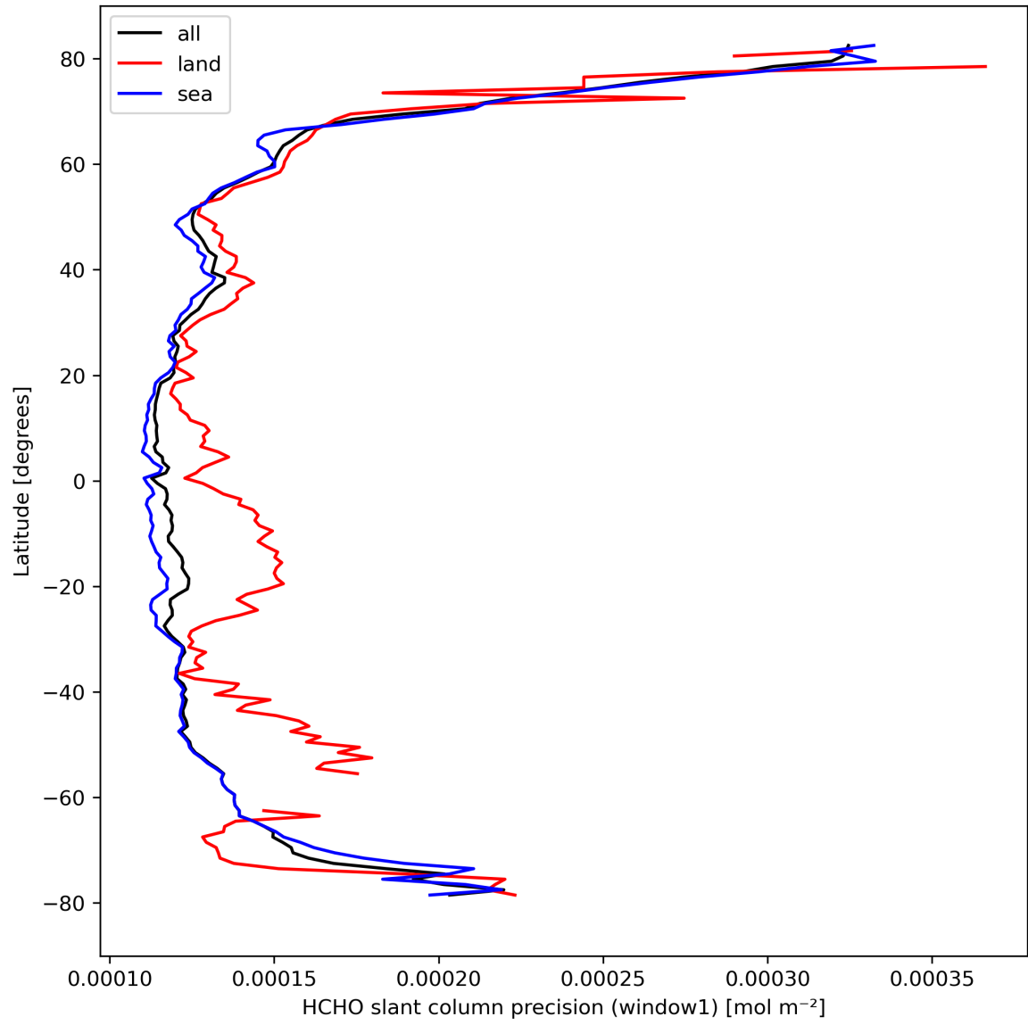
Figure 25: Zonal average of “HCHO slant column precision (window1)” for 2024-03-12 to 2024-03-14.
