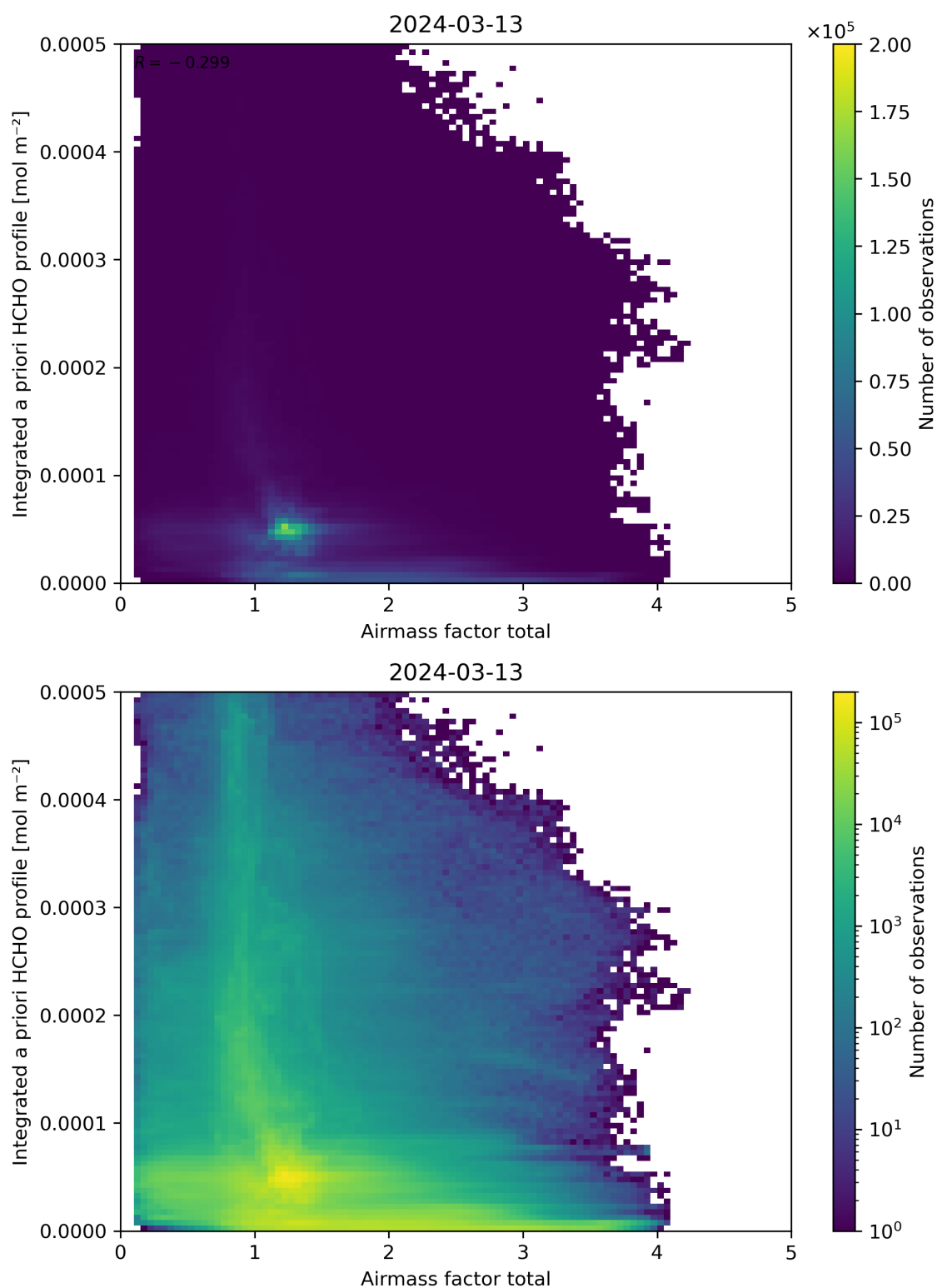
Figure 104: Scatter density plot of “Airmass factor total” against “Integrated a priori HCHO profile” for 2024-03-12 to 2024-03-14.
