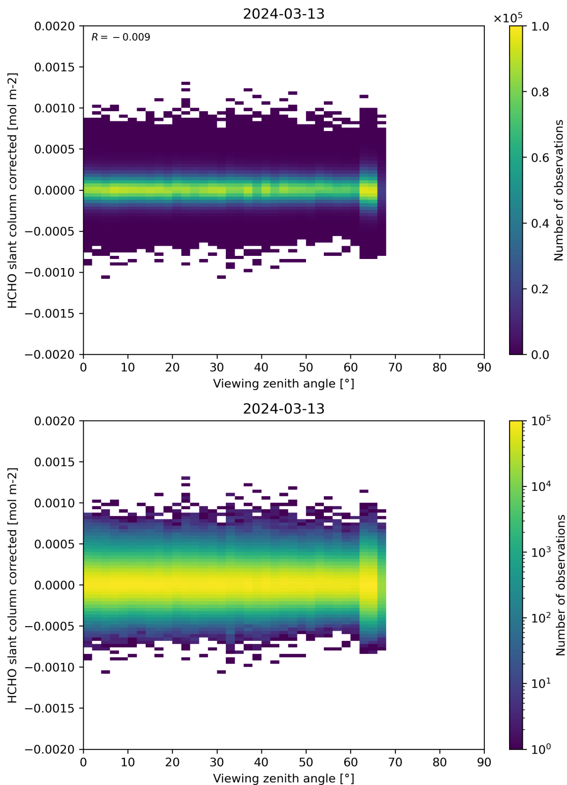
Figure 186: Scatter density plot of “Viewing zenith angle” against “HCHO slant column corrected” for 2024-03-12 to 2024-03-14.
