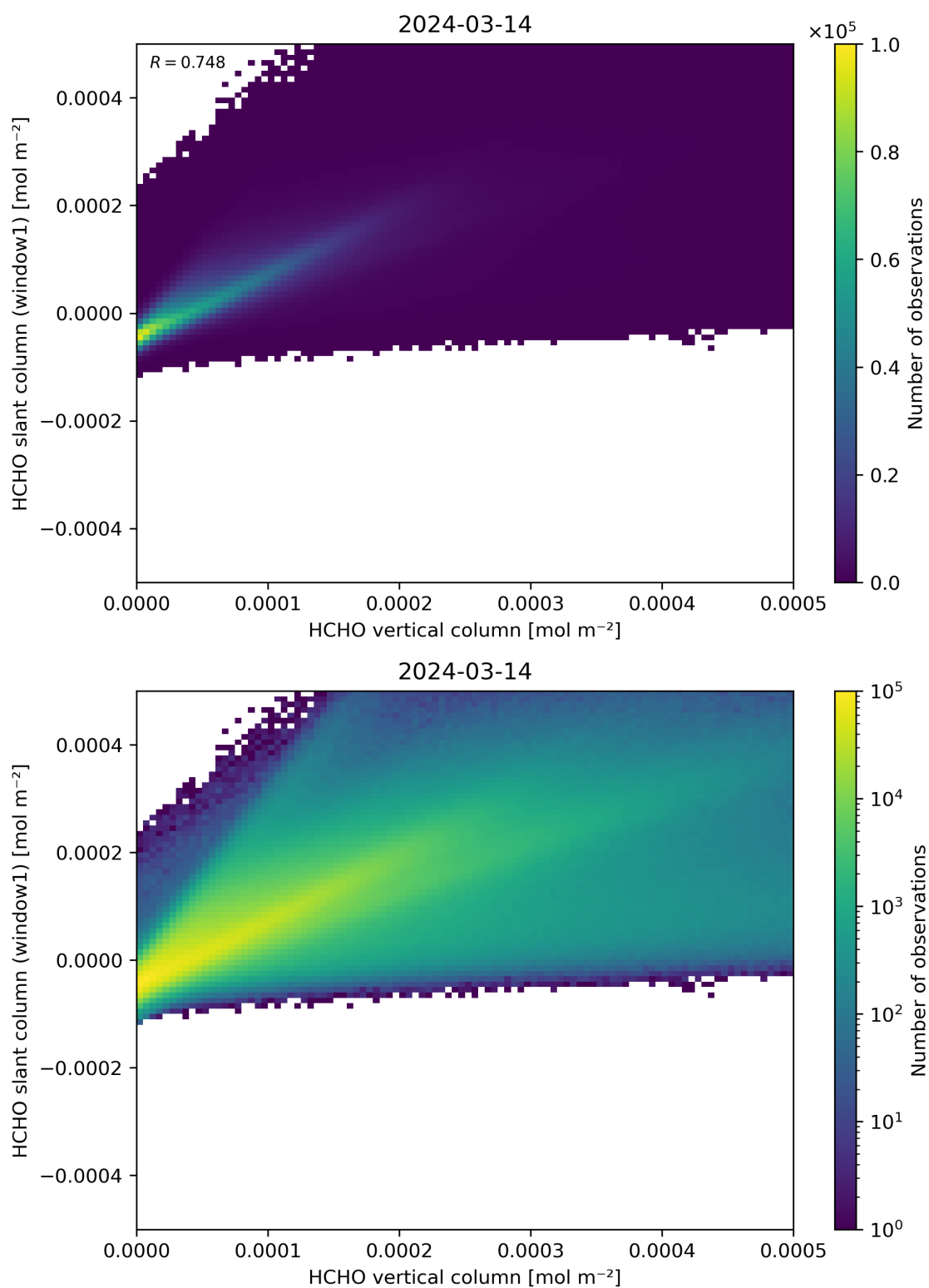
Figure 129: Scatter density plot of “HCHO vertical column” against “HCHO slant column (window1)” for 2024-03-14 to 2024-03-15.
