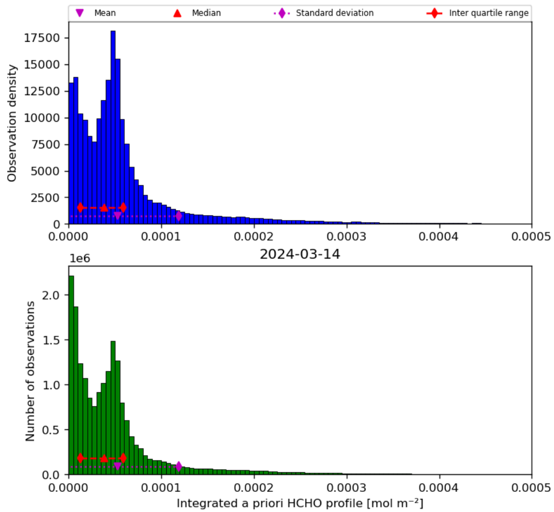
Figure 43: Histogram of “Integrated a priori HCHO profile” for 2024-03-14 to 2024-03-15
