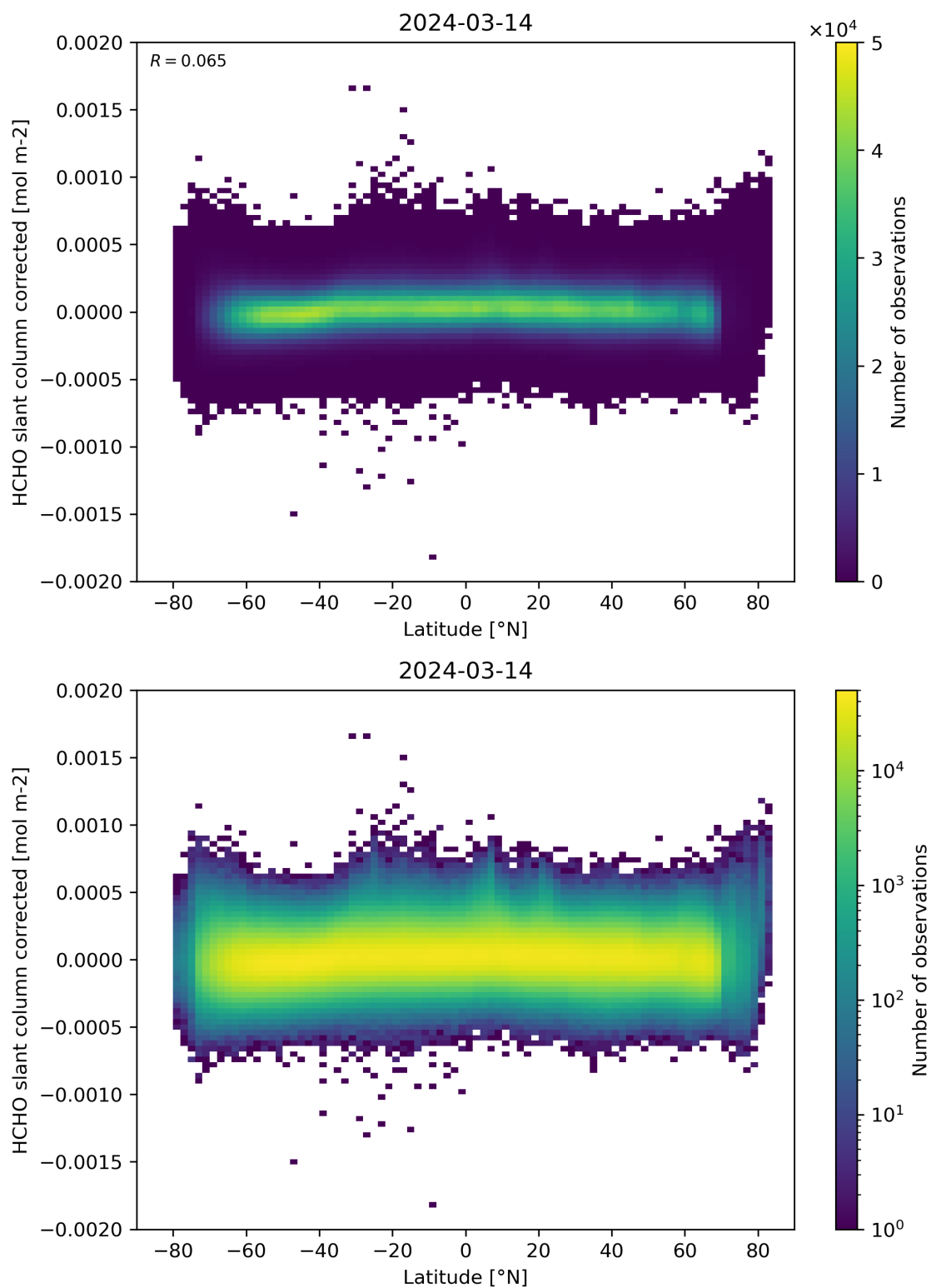
Figure 157: Scatter density plot of “Latitude” against “HCHO slant column corrected” for 2024-03-14 to 2024-03-15.
