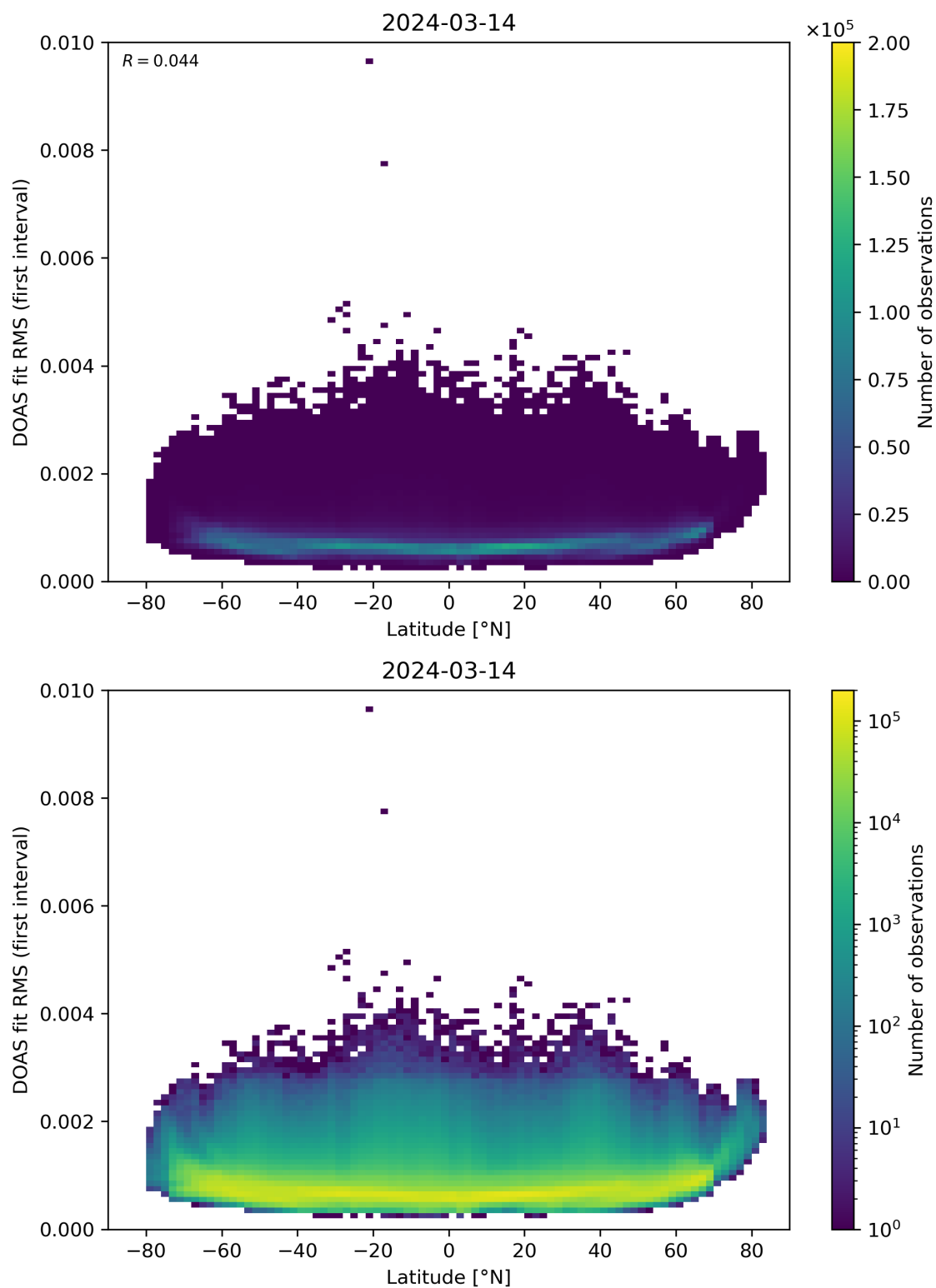
Figure 153: Scatter density plot of “Latitude” against “DOAS fit RMS (first interval)” for 2024-03-14 to 2024-03-15.
