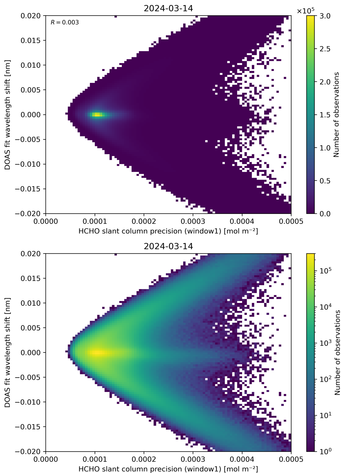
Figure 89: Scatter density plot of “HCHO slant column precision (window1)” against “DOAS fit wavelength shift” for 2024-03-14 to 2024-03-15.
