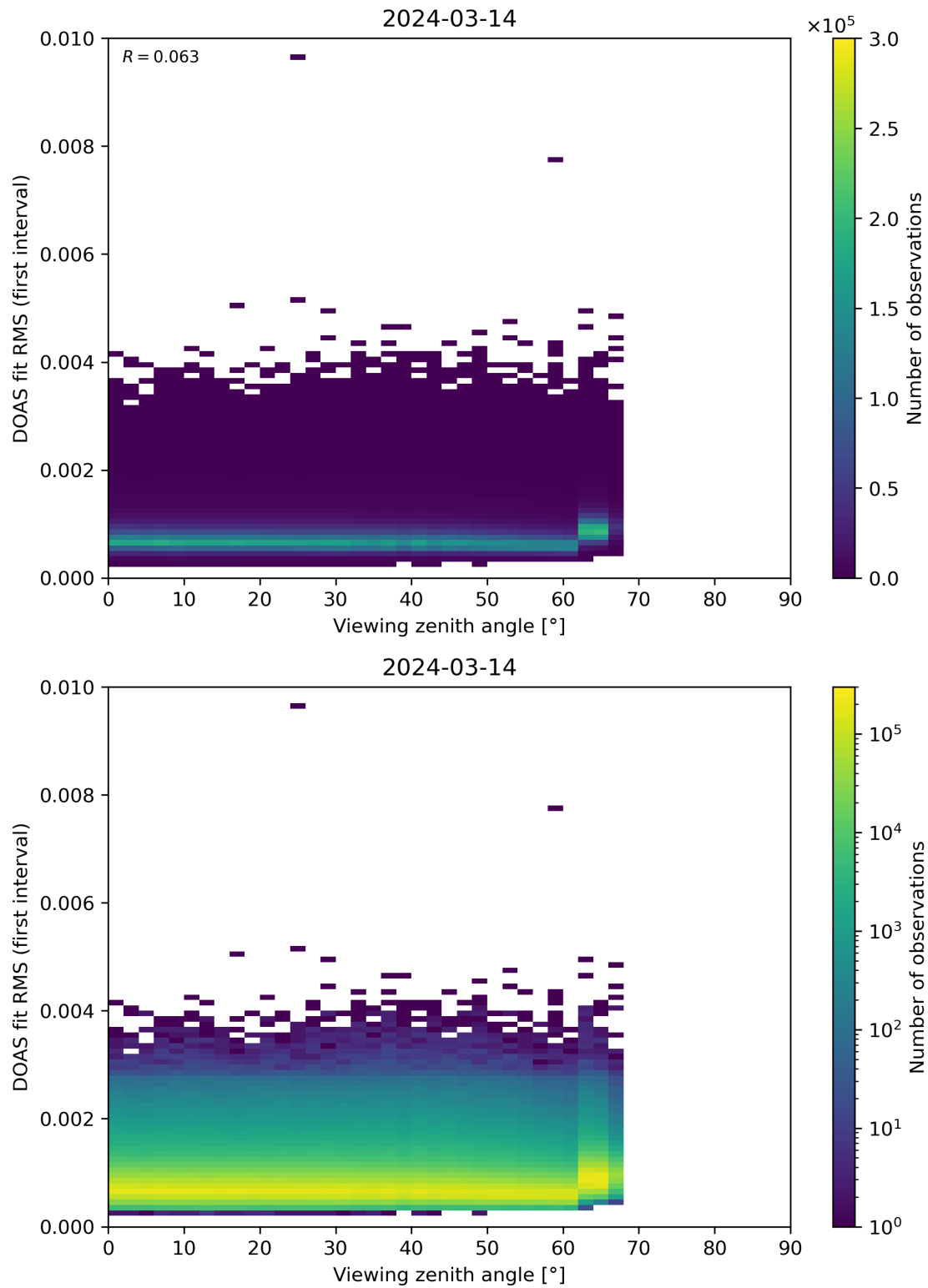
Figure 182: Scatter density plot of “Viewing zenith angle” against “DOAS fit RMS (first interval)” for 2024-03-14 to 2024-03-15.
