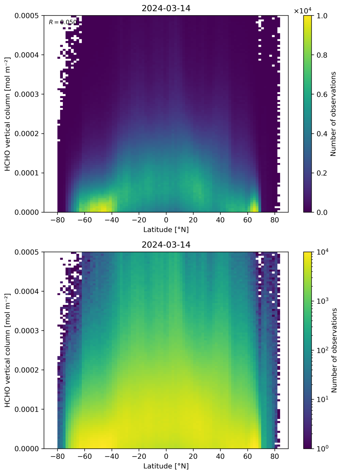
Figure 163: Scatter density plot of “Latitude” against “HCHO vertical column” for 2024-03-14 to 2024-03-15.
