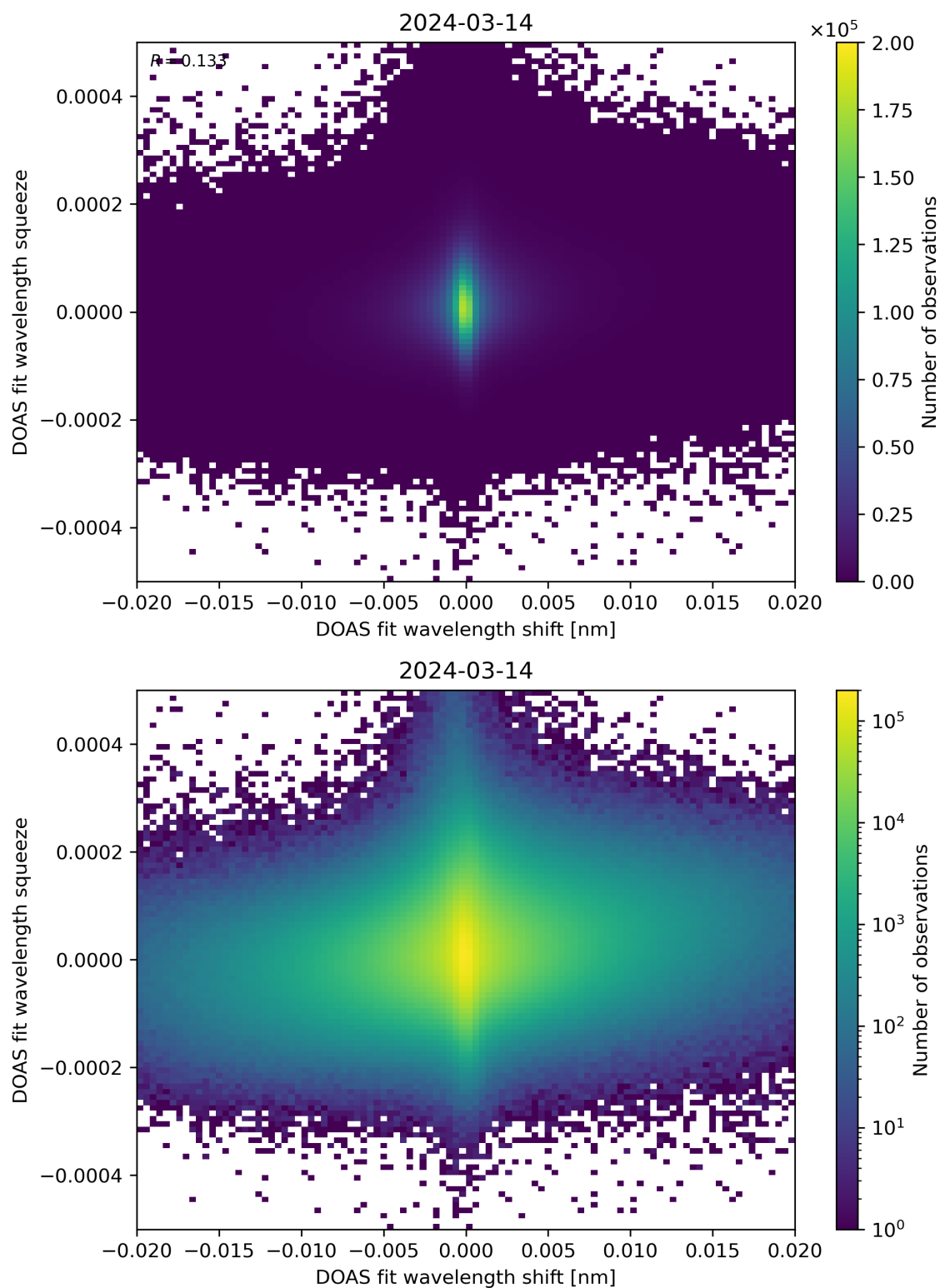
Figure 65: Scatter density plot of “DOAS fit wavelength shift” against “DOAS fit wavelength squeeze” for 2024-03-14 to 2024-03-15.
