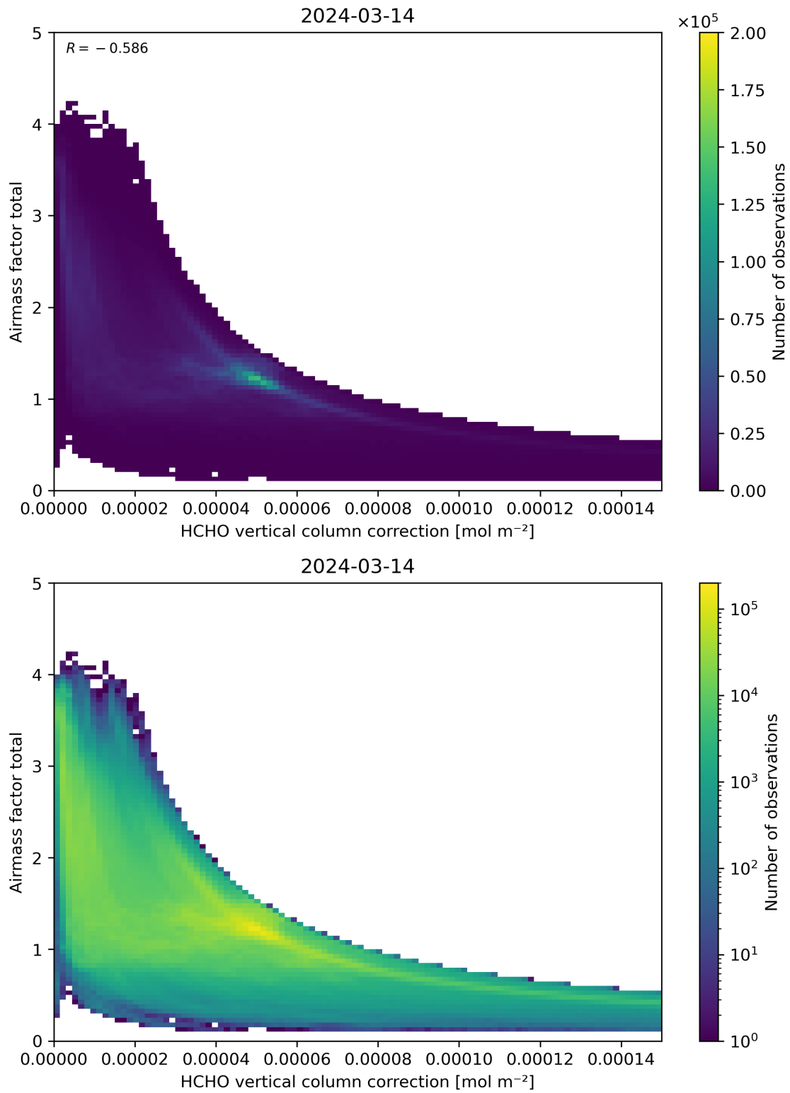
Figure 120: Scatter density plot of “HCHO vertical column correction” against “Airmass factor total” for 2024-03-14 to 2024-03-15.
