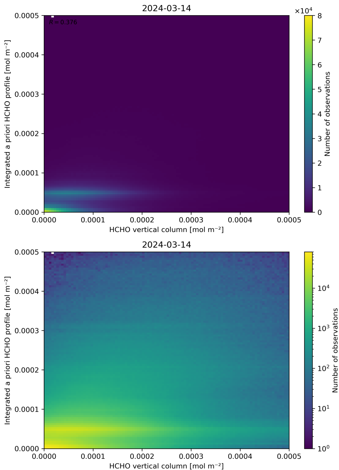
Figure 135: Scatter density plot of “HCHO vertical column” against “Integrated a priori HCHO profile” for 2024-03-14 to 2024-03-15.
