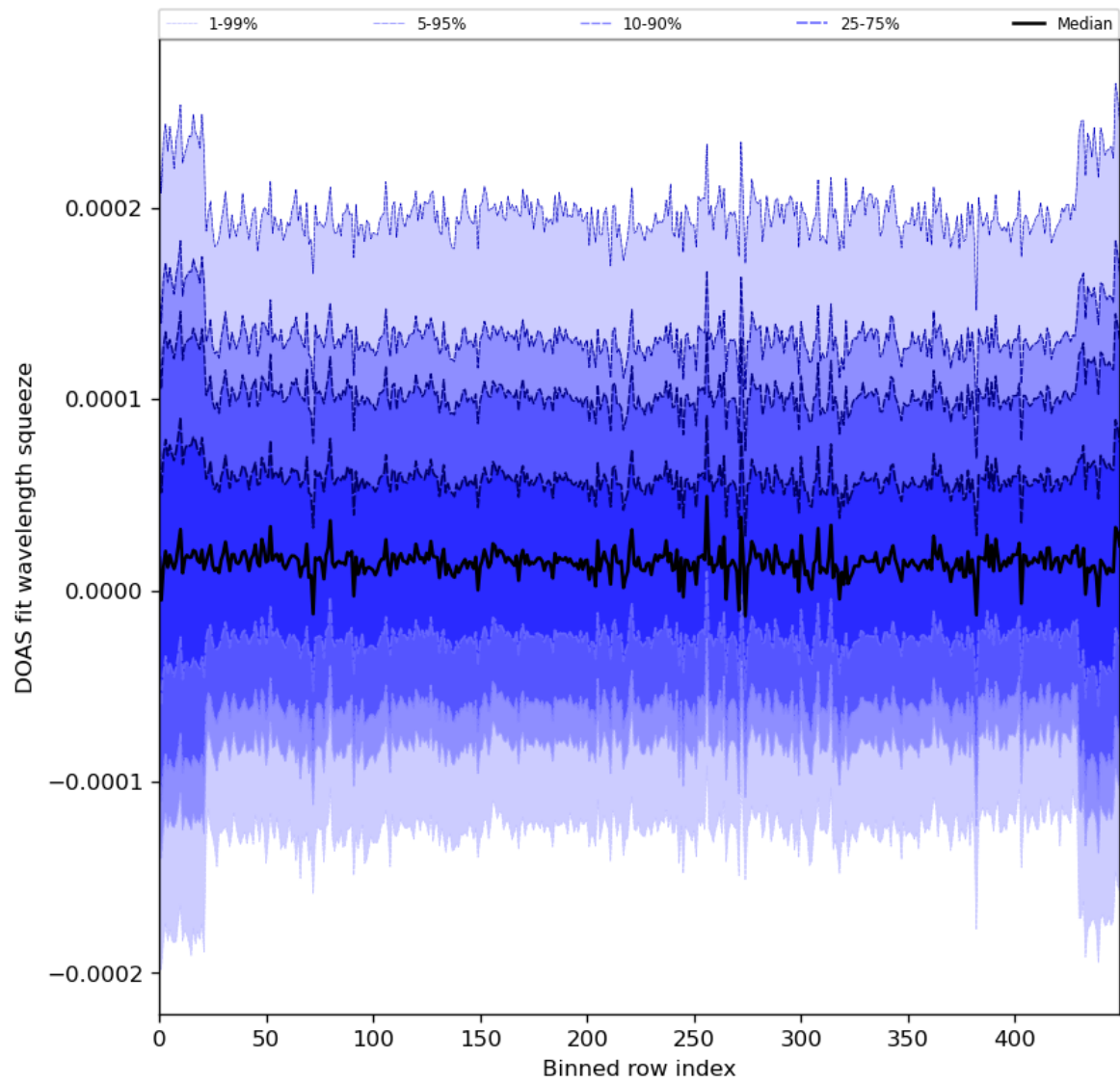
Figure 59: Along track statistics of “DOAS fit wavelength squeeze” for 2024-03-14 to 2024-03-15
