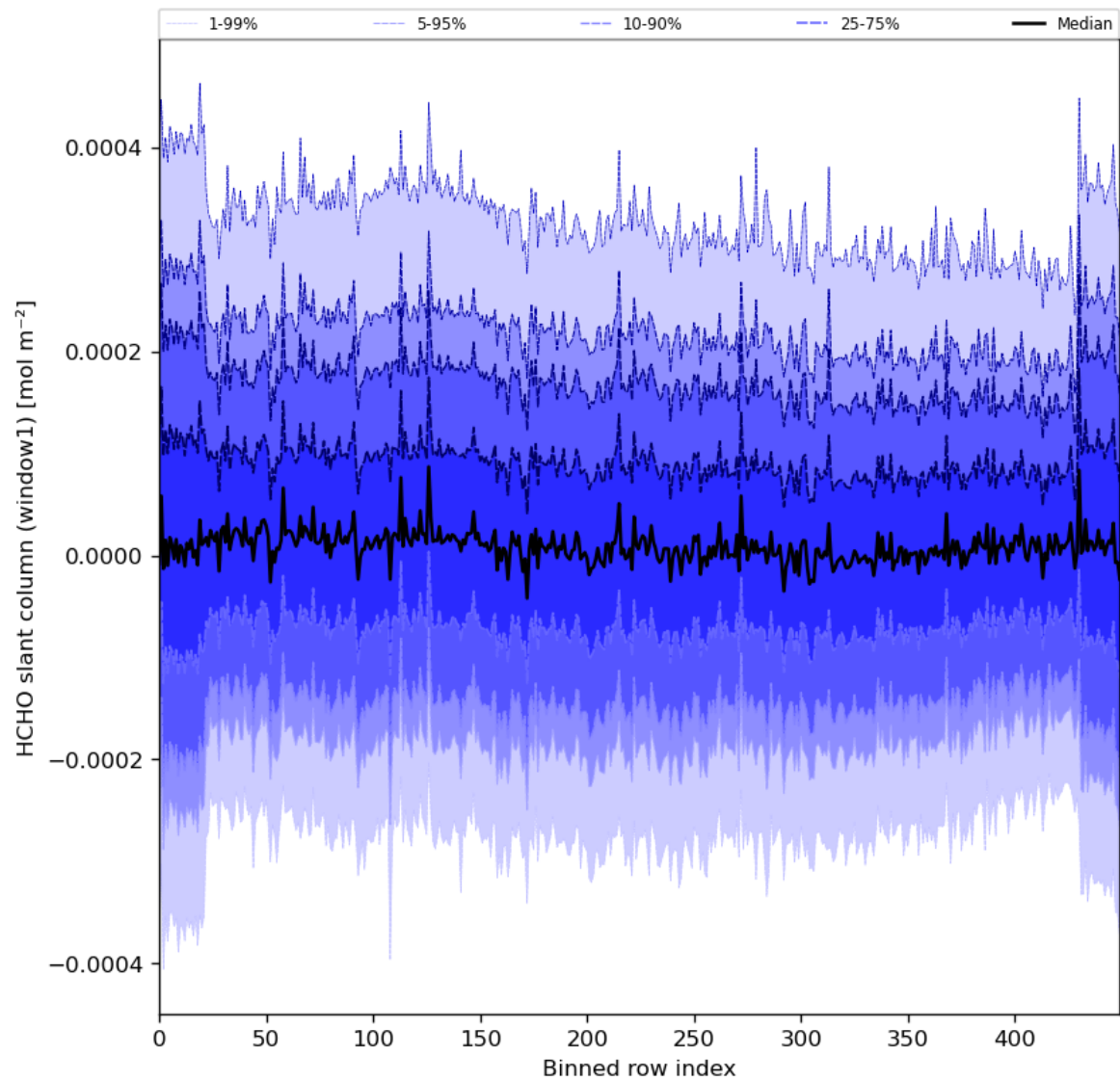
Figure 52: Along track statistics of “HCHO slant column (window1)” for 2024-03-14 to 2024-03-15
