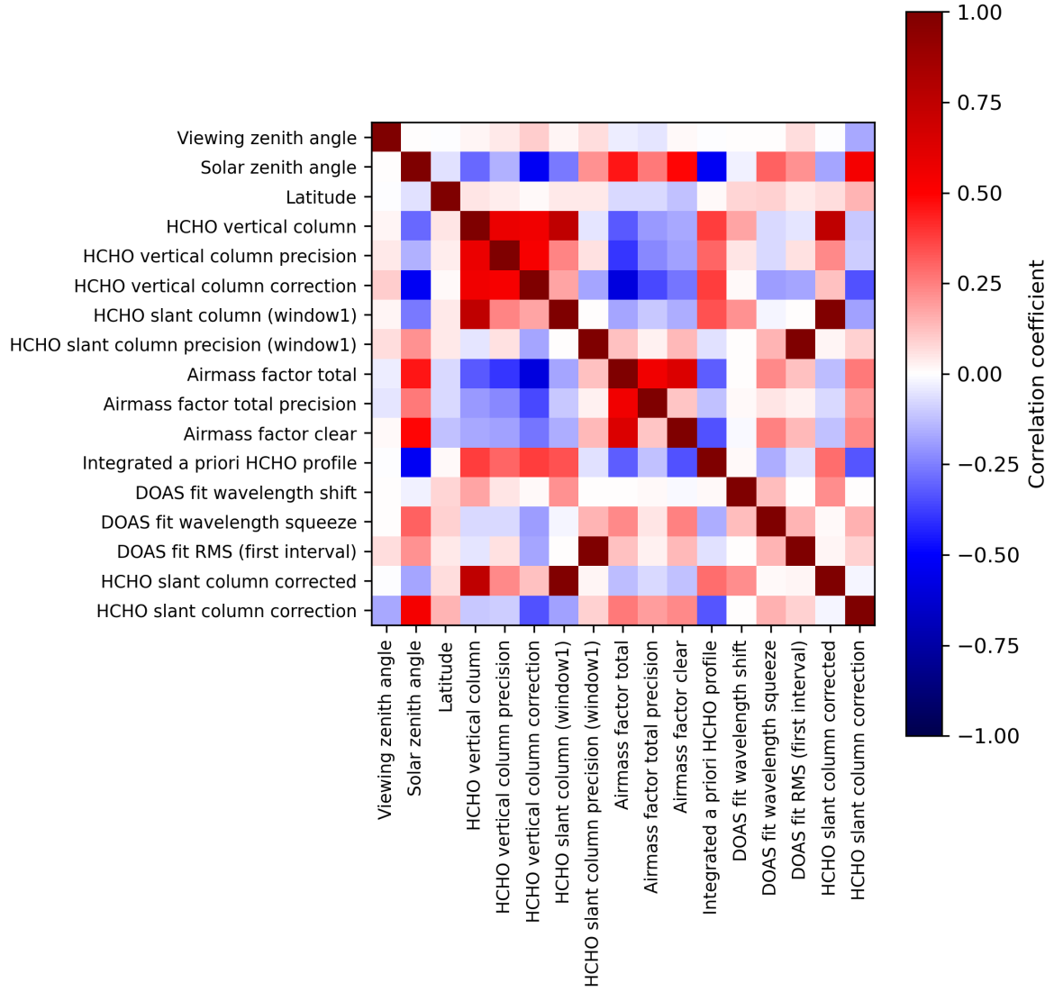
Figure 2: Map of correlation matrix for 2024-03-14 to 2024-03-15.
