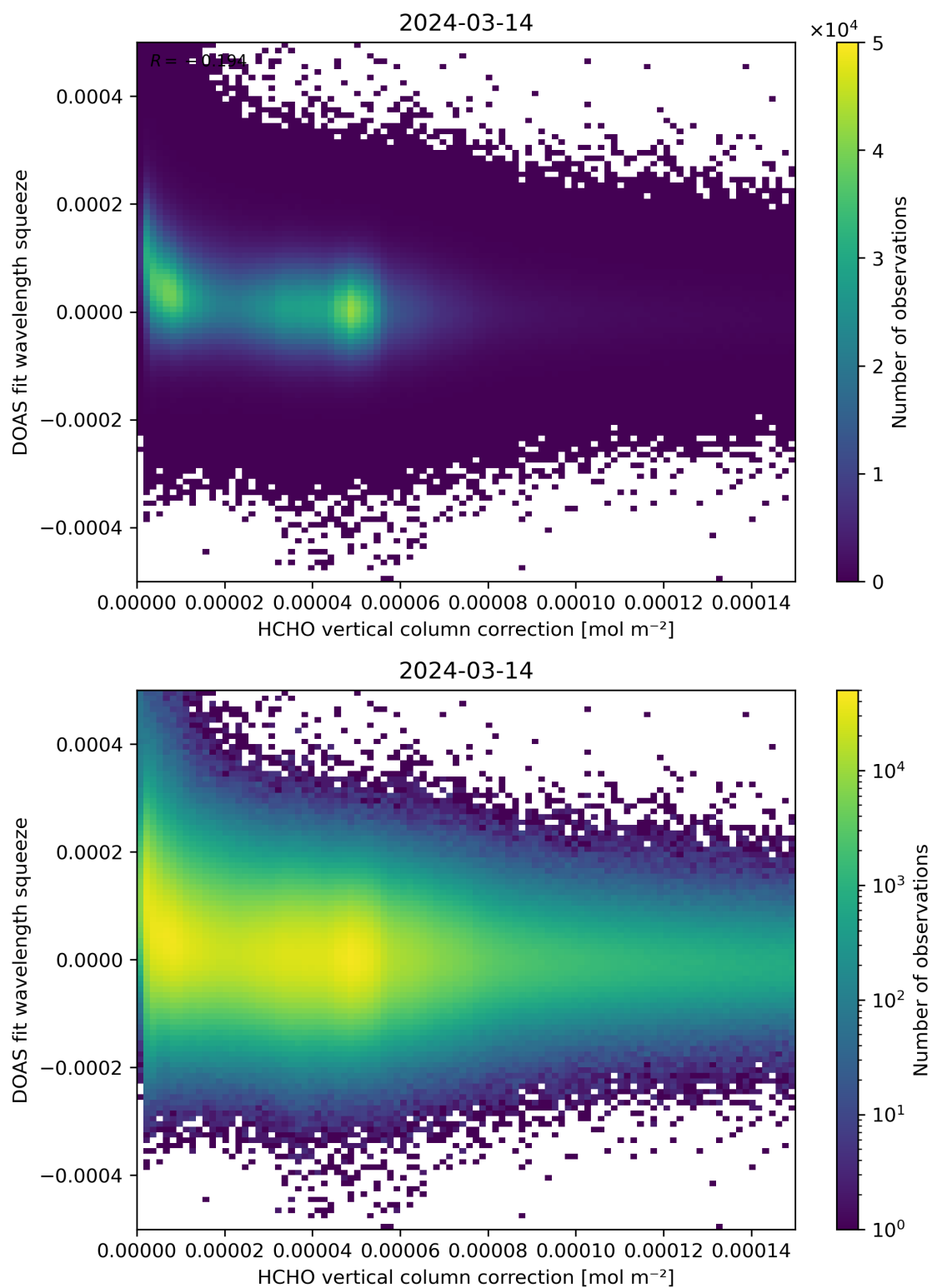
Figure 114: Scatter density plot of “HCHO vertical column correction” against “DOAS fit wavelength squeeze” for 2024-03-14 to 2024-03-15.
