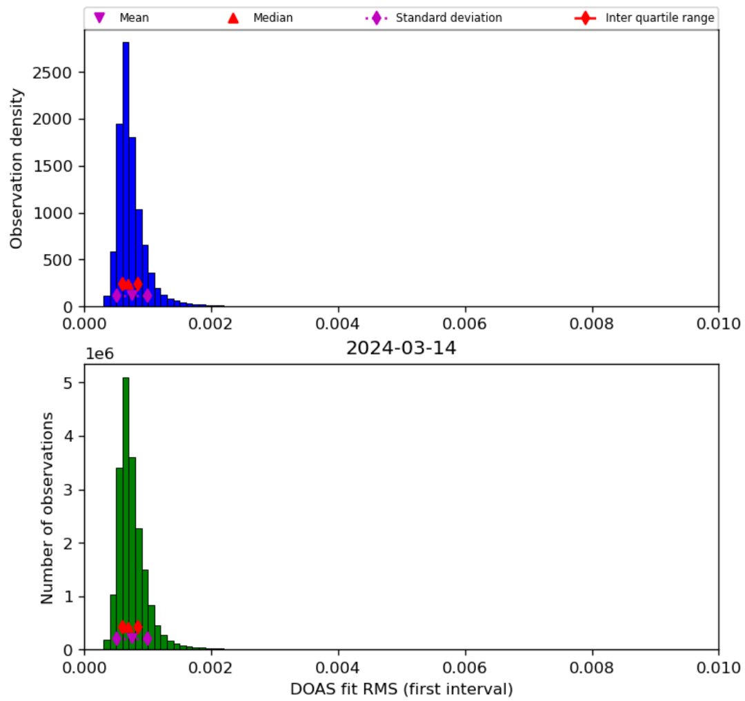
Figure 46: Histogram of “DOAS fit RMS (first interval)” for 2024-03-14 to 2024-03-15
