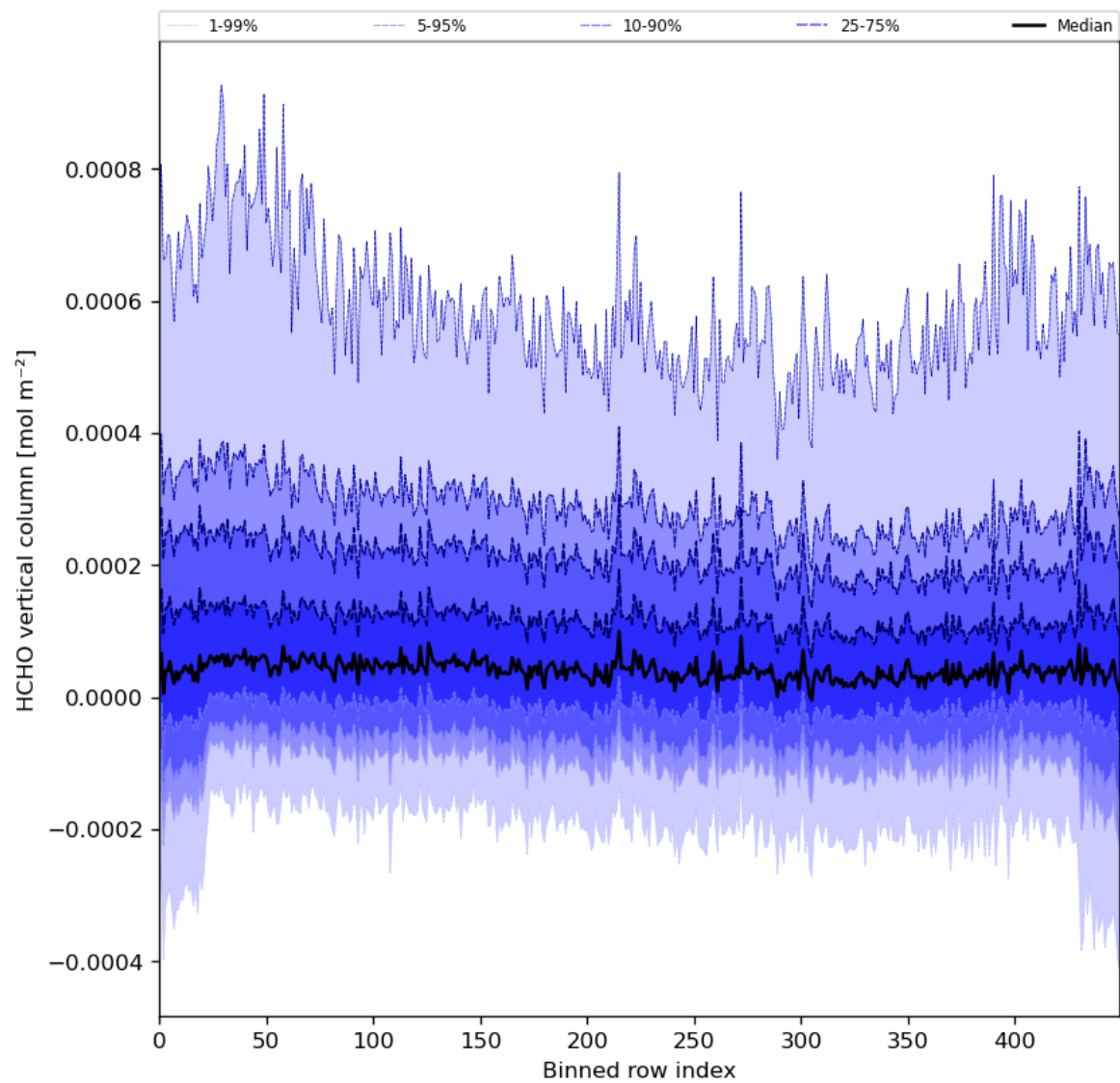
Figure 49: Along track statistics of “HCHO vertical column” for 2024-03-14 to 2024-03-15
