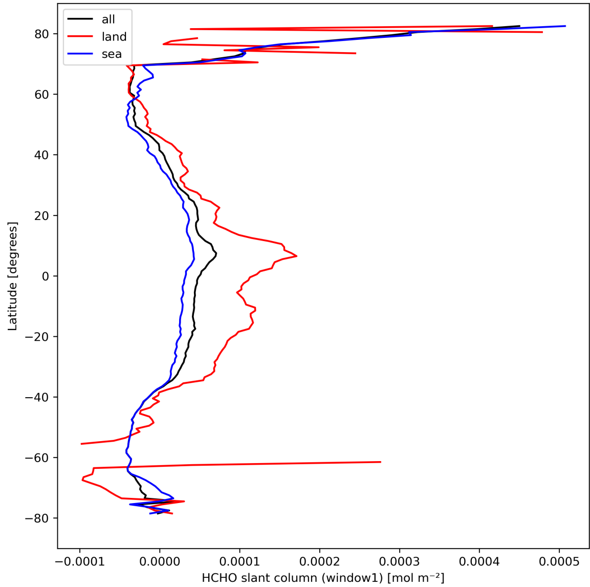
Figure 24: Zonal average of “HCHO slant column (window1)” for 2024-03-14 to 2024-03-15.
