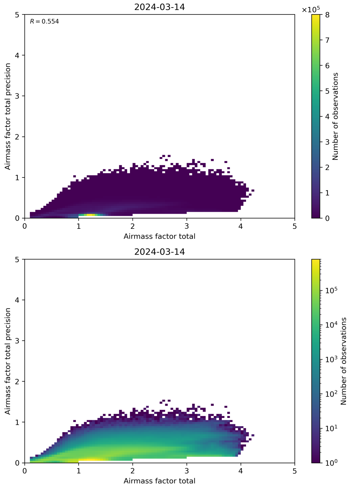
Figure 103: Scatter density plot of “Airmass factor total” against “Airmass factor total precision” for 2024-03-14 to 2024-03-15.
