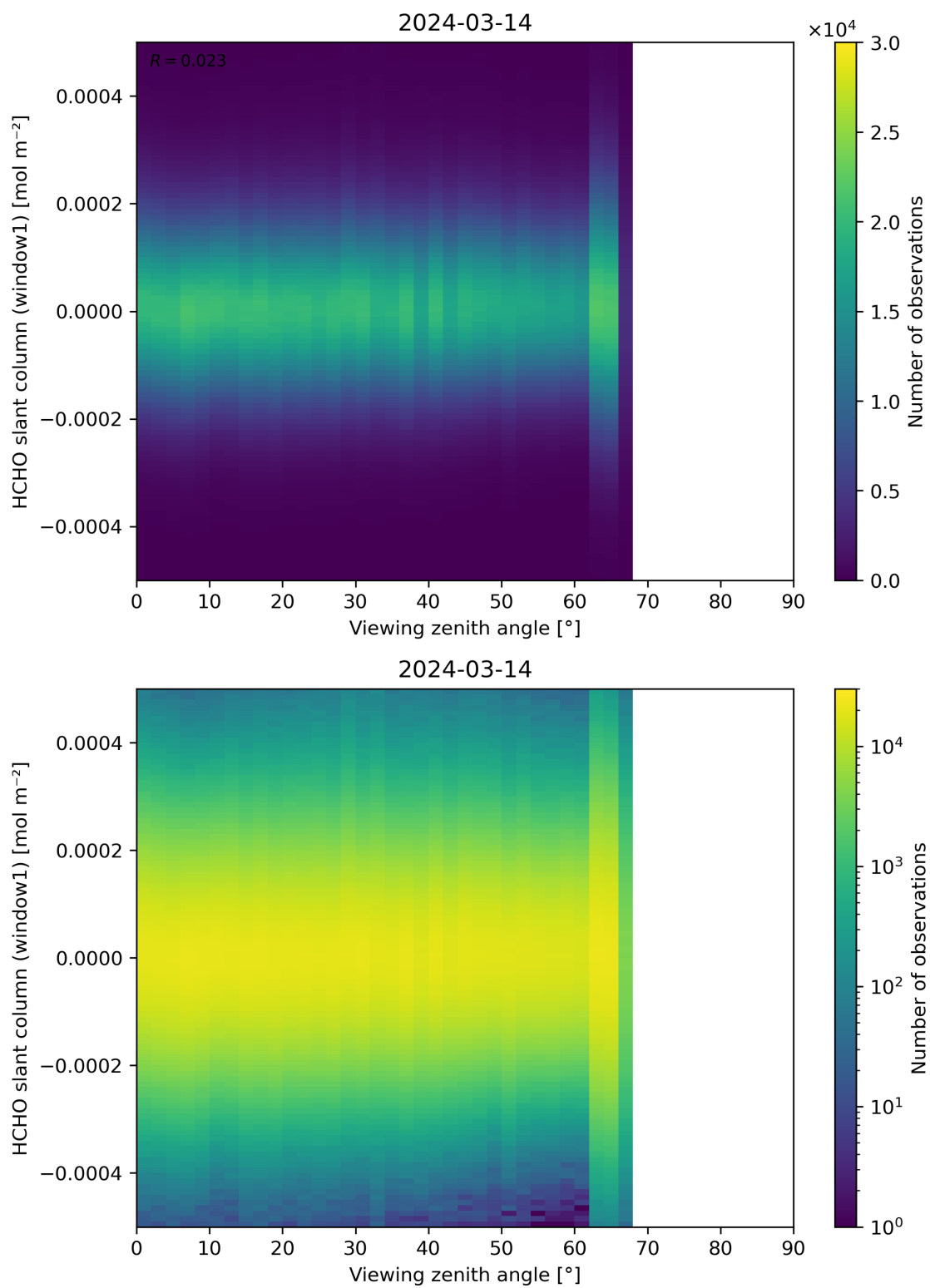
Figure 188: Scatter density plot of “Viewing zenith angle” against “HCHO slant column (window1)” for 2024-03-14 to 2024-03-15.
