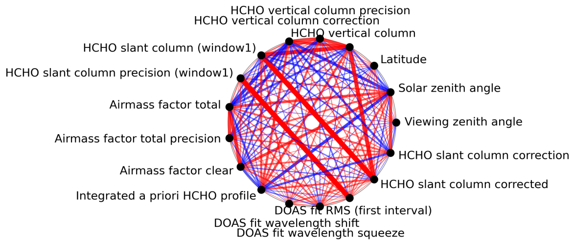
Figure 1: Map of correlation graph for 2024-03-14 to 2024-03-15.
