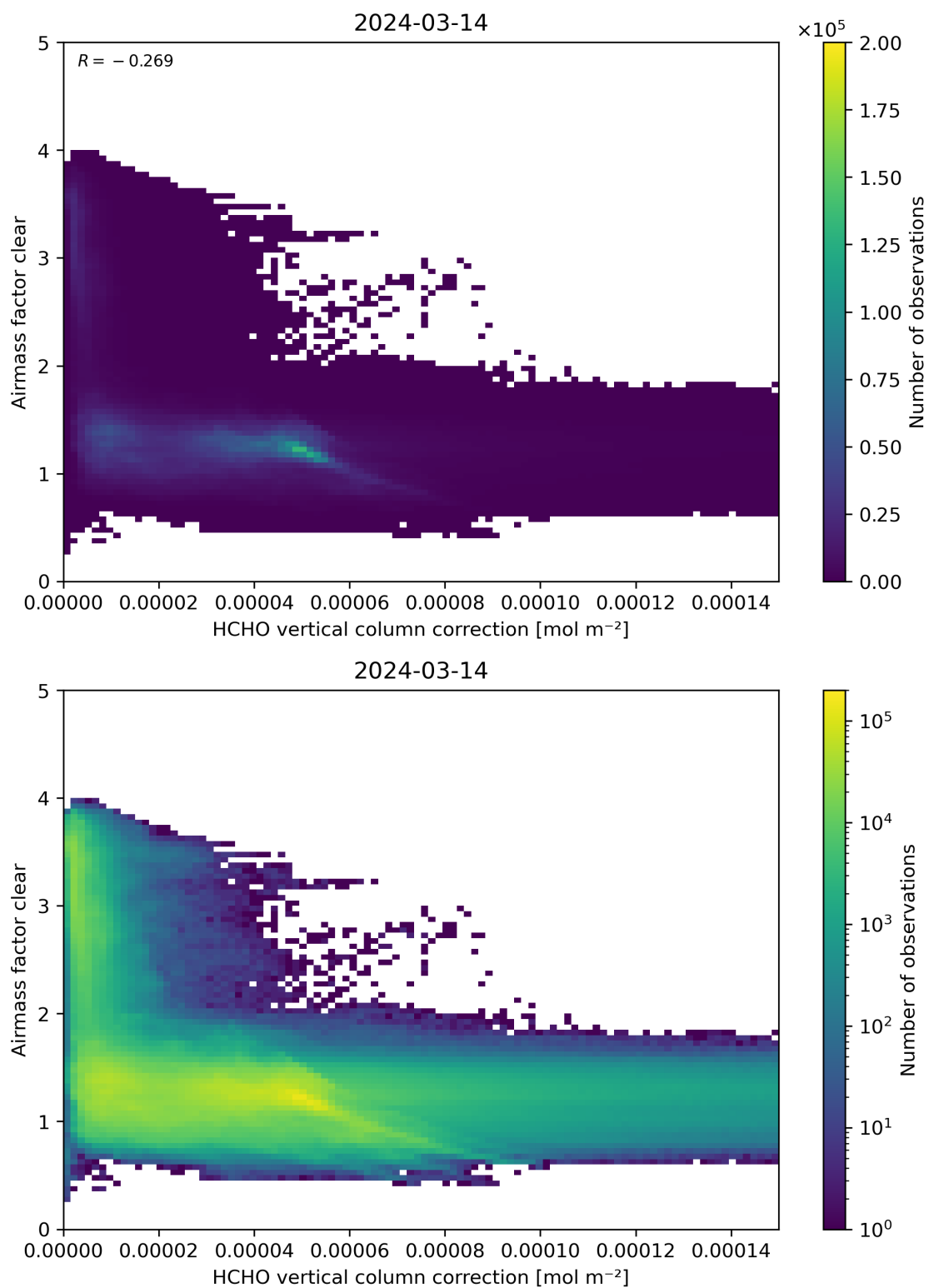
Figure 115: Scatter density plot of “HCHO vertical column correction” against “Airmass factor clear” for 2024-03-14 to 2024-03-15.
