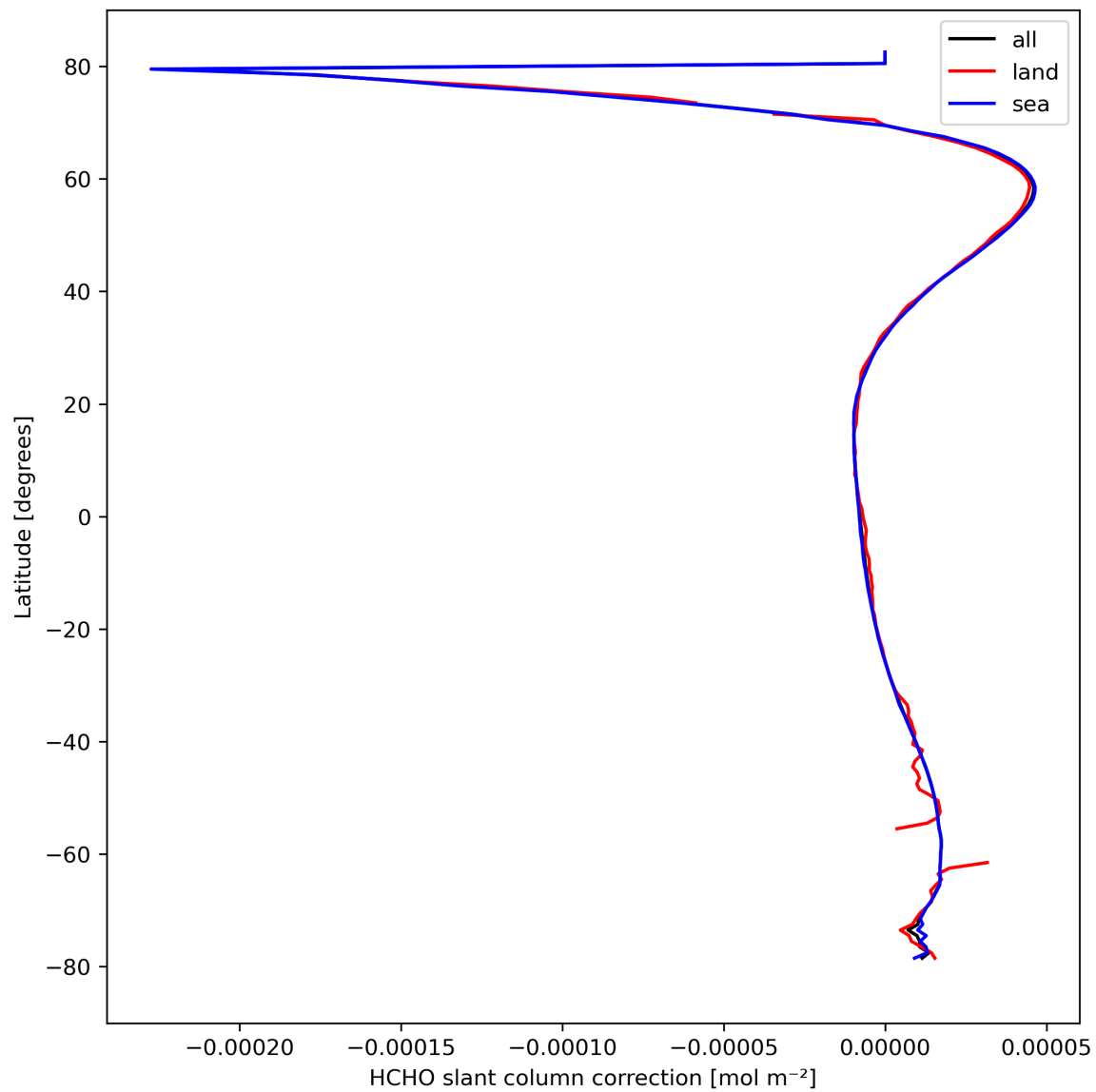
Figure 33: Zonal average of “HCHO slant column correction” for 2024-03-14 to 2024-03-15.
