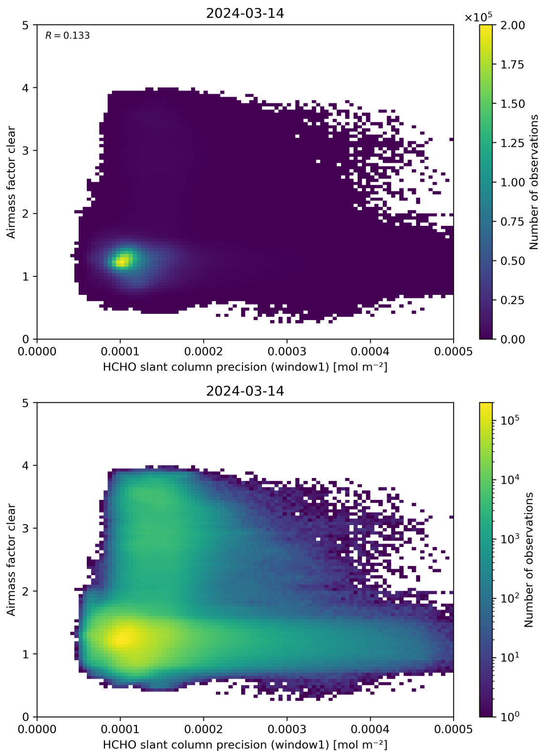
Figure 91: Scatter density plot of “HCHO slant column precision (window1)” against “Airmass factor clear” for 2024-03-14 to 2024-03-15.
