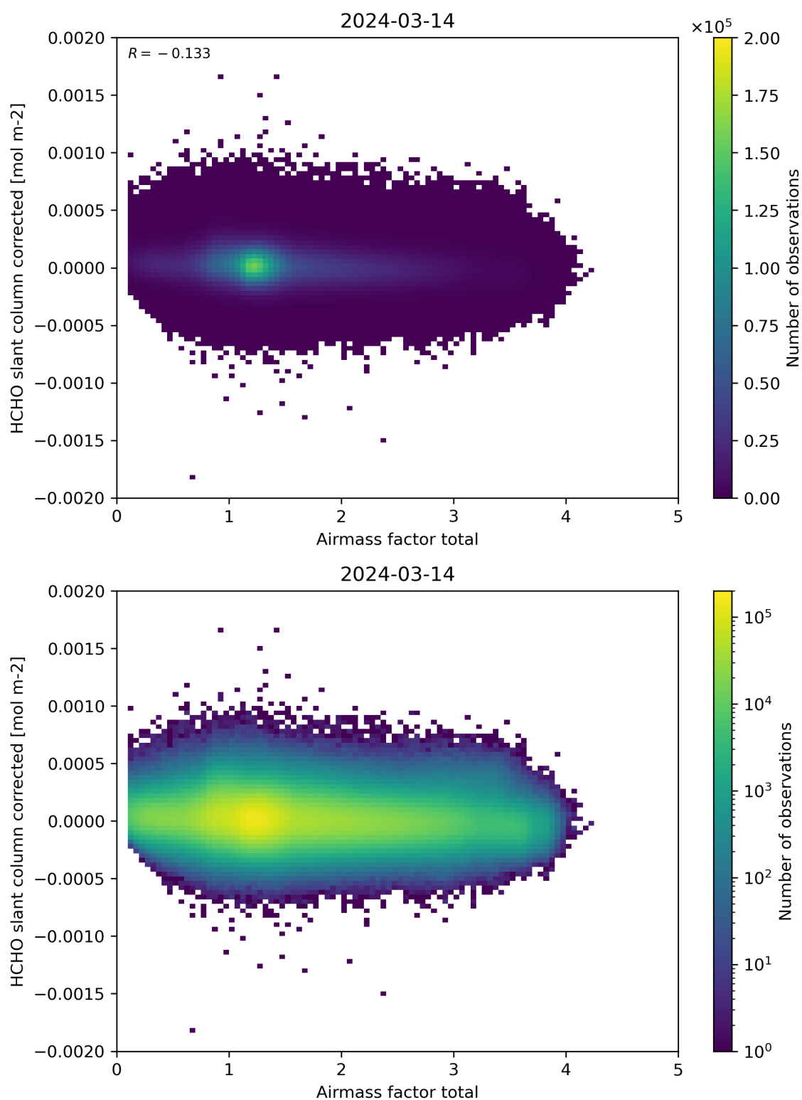
Figure 101: Scatter density plot of “Airmass factor total” against “HCHO slant column corrected” for 2024-03-14 to 2024-03-15.
