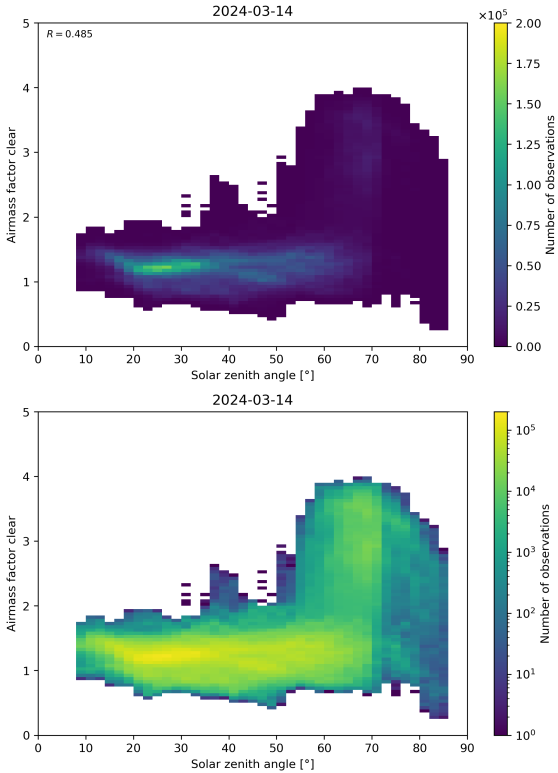
Figure 170: Scatter density plot of “Solar zenith angle” against “Airmass factor clear” for 2024-03-14 to 2024-03-15.
