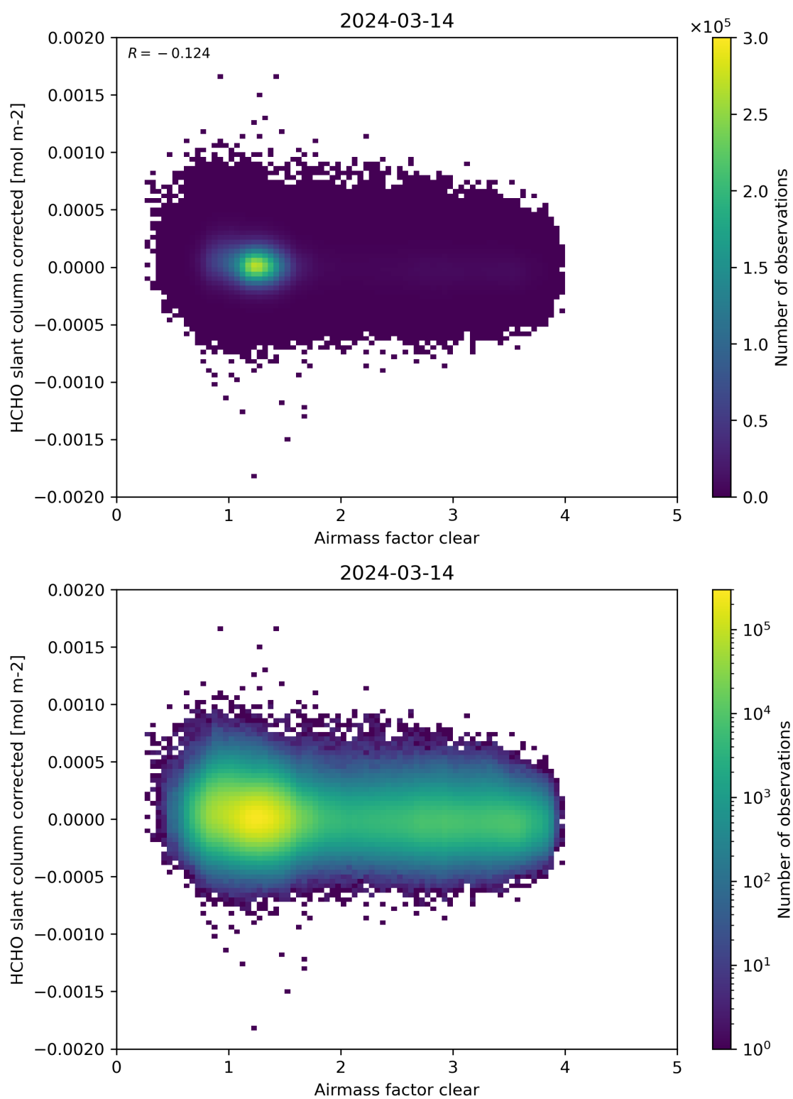
Figure 74: Scatter density plot of “Airmass factor clear” against “HCHO slant column corrected” for 2024-03-14 to 2024-03-15.
