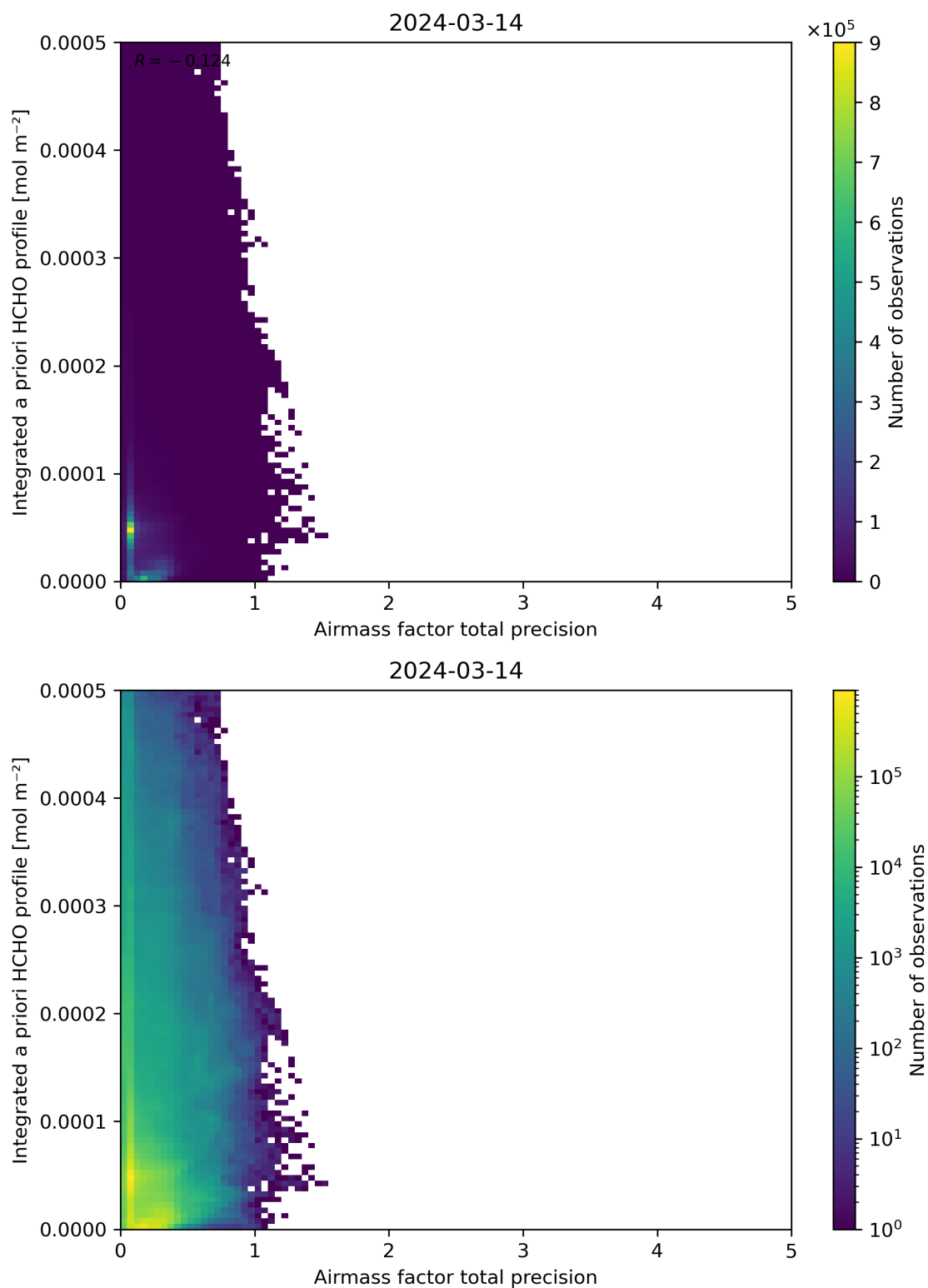
Figure 111: Scatter density plot of “Airmass factor total precision” against “Integrated a priori HCHO profile” for 2024-03-14 to 2024-03-15.
