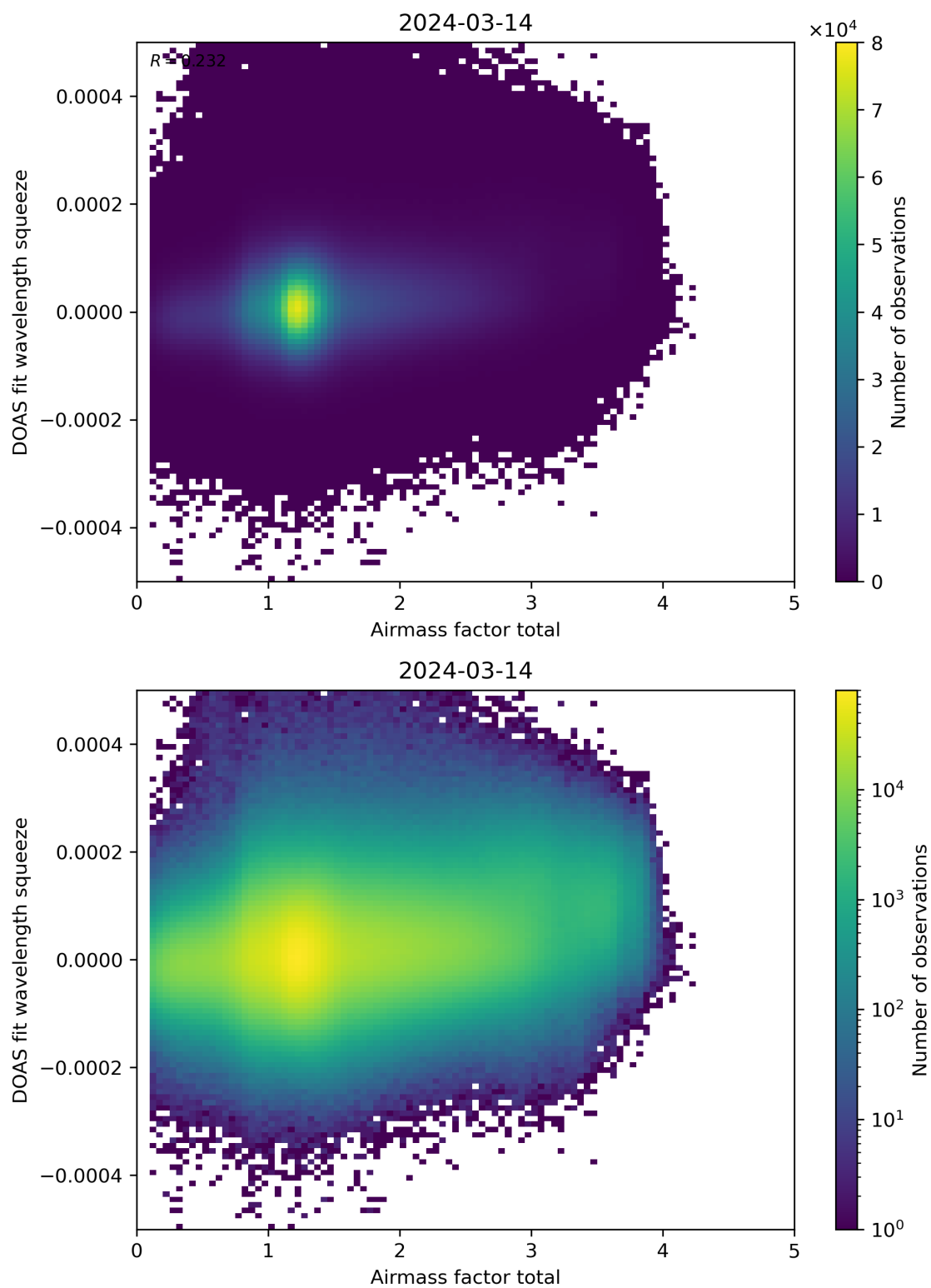
Figure 99: Scatter density plot of “Airmass factor total” against “DOAS fit wavelength squeeze” for 2024-03-14 to 2024-03-15.
