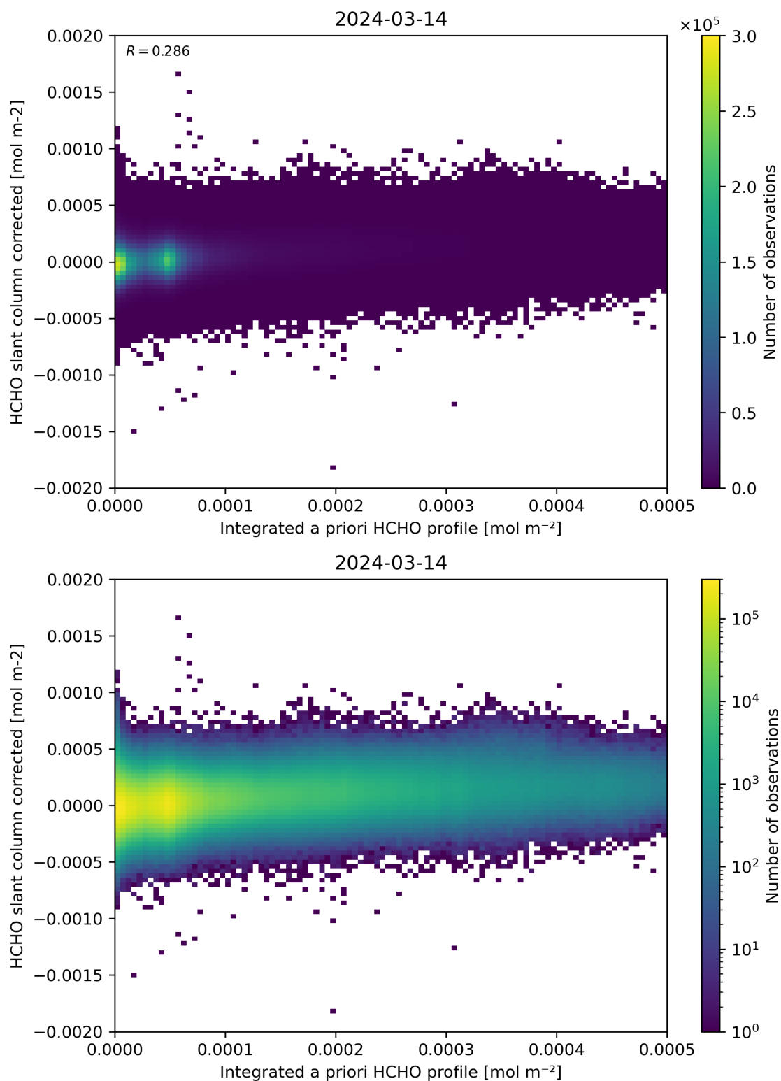
Figure 151: Scatter density plot of “Integrated a priori HCHO profile” against “HCHO slant column corrected” for 2024-03-14 to 2024-03-15.
