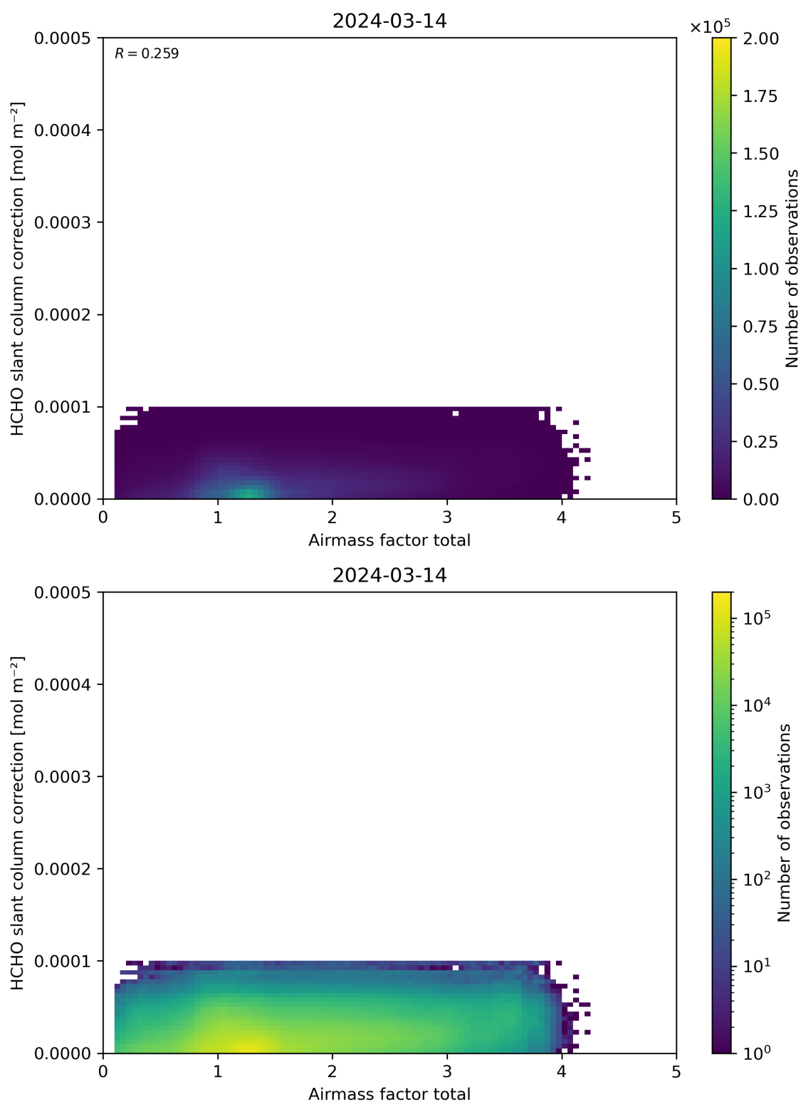
Figure 102: Scatter density plot of “Airmass factor total” against “HCHO slant column correction” for 2024-03-14 to 2024-03-15.
