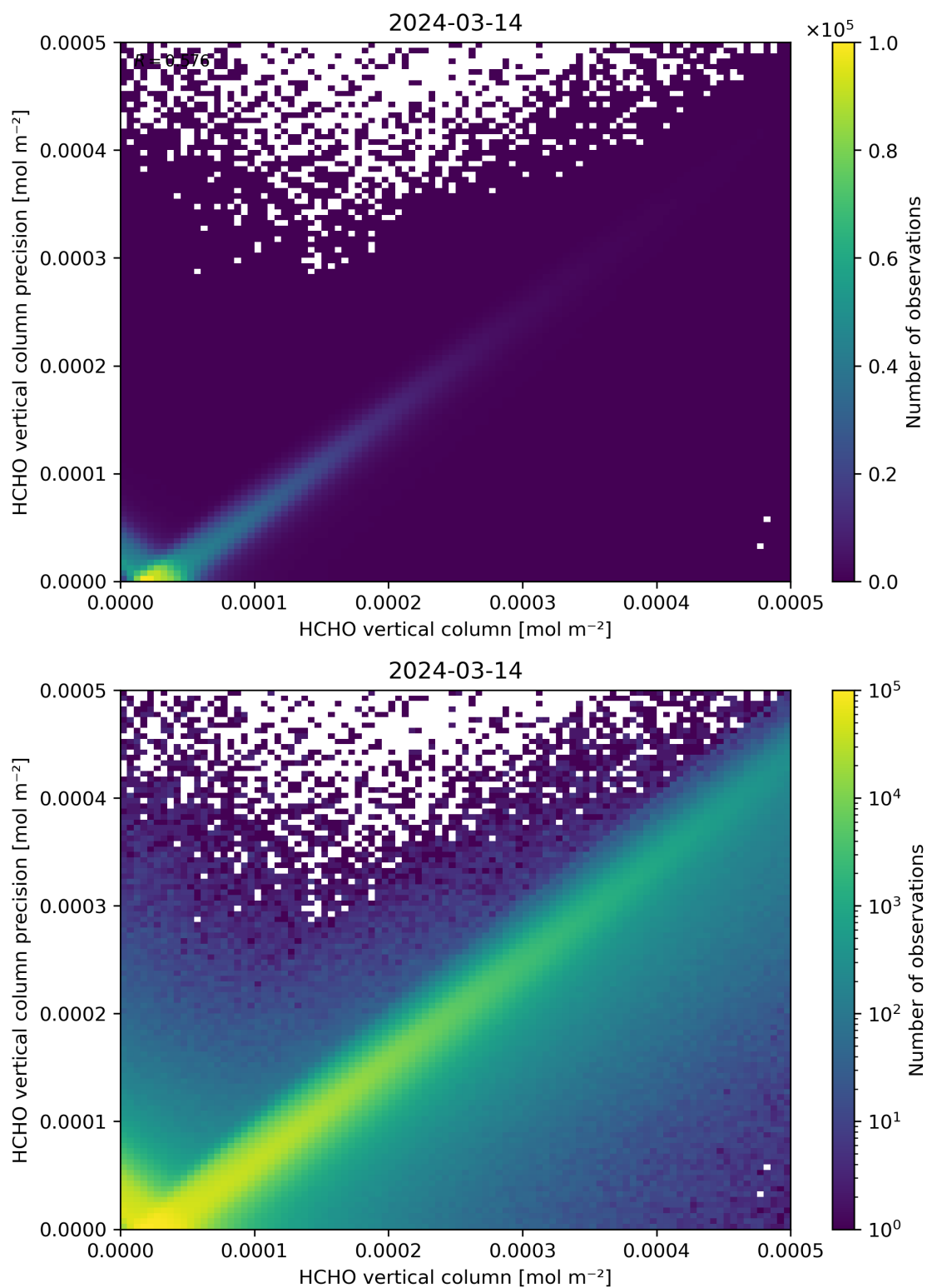
Figure 134: Scatter density plot of “HCHO vertical column” against “HCHO vertical column precision” for 2024-03-14 to 2024-03-15.
