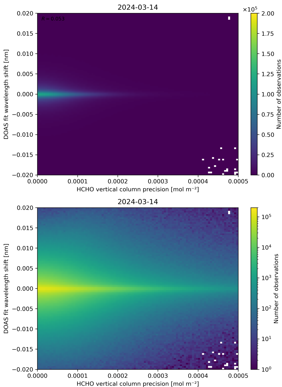
Figure 137: Scatter density plot of “HCHO vertical column precision” against “DOAS fit wavelength shift” for 2024-03-14 to 2024-03-15.
