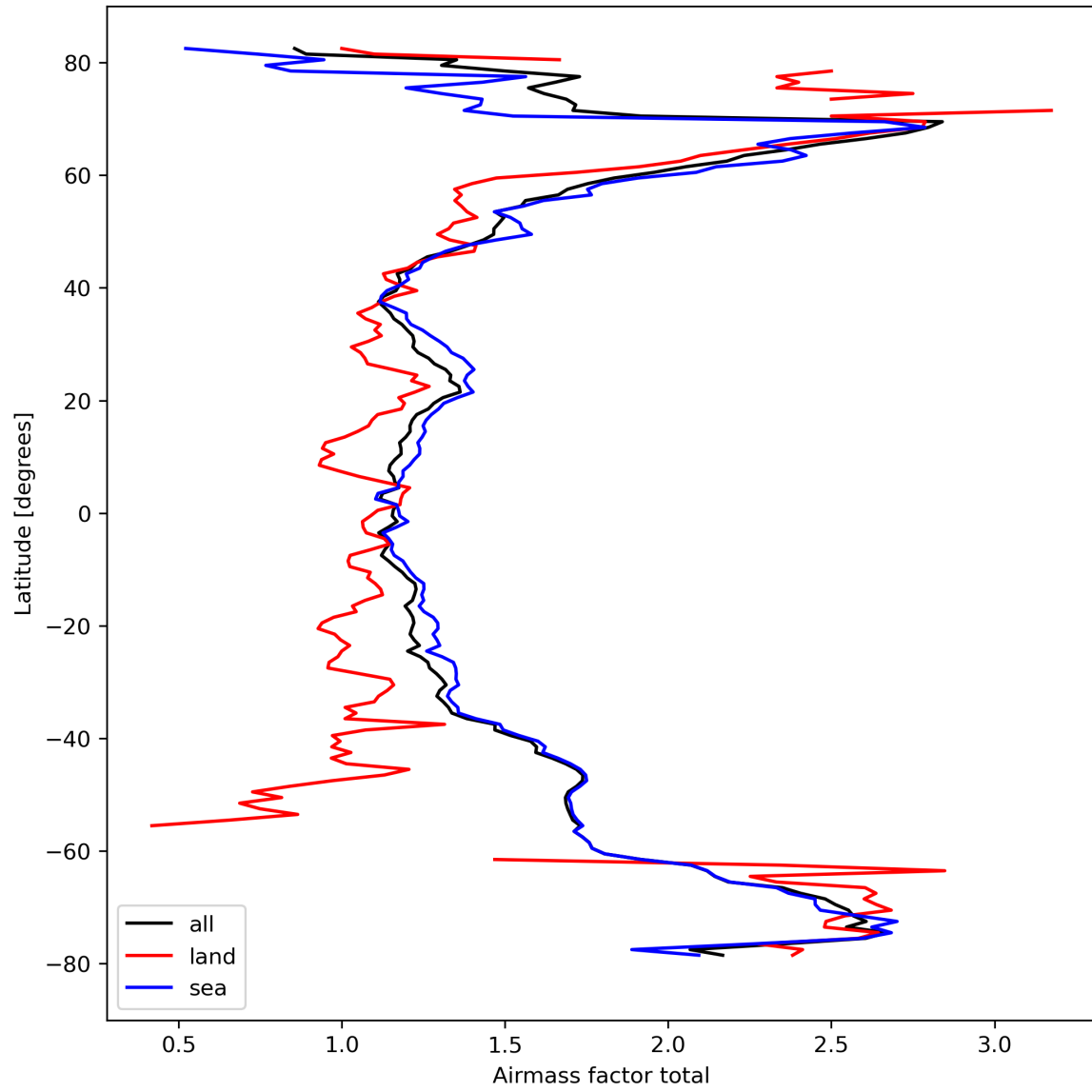
Figure 26: Zonal average of “Airmass factor total” for 2024-03-14 to 2024-03-15.
