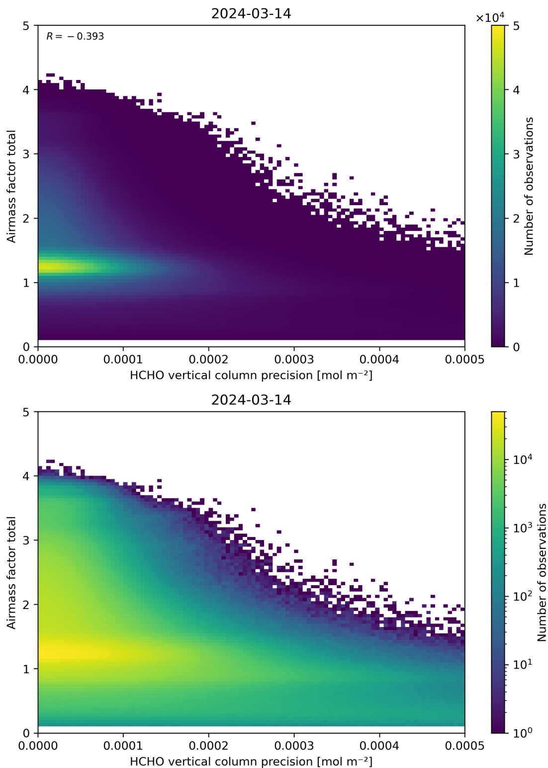
Figure 144: Scatter density plot of “HCHO vertical column precision” against “Airmass factor total” for 2024-03-14 to 2024-03-15.
