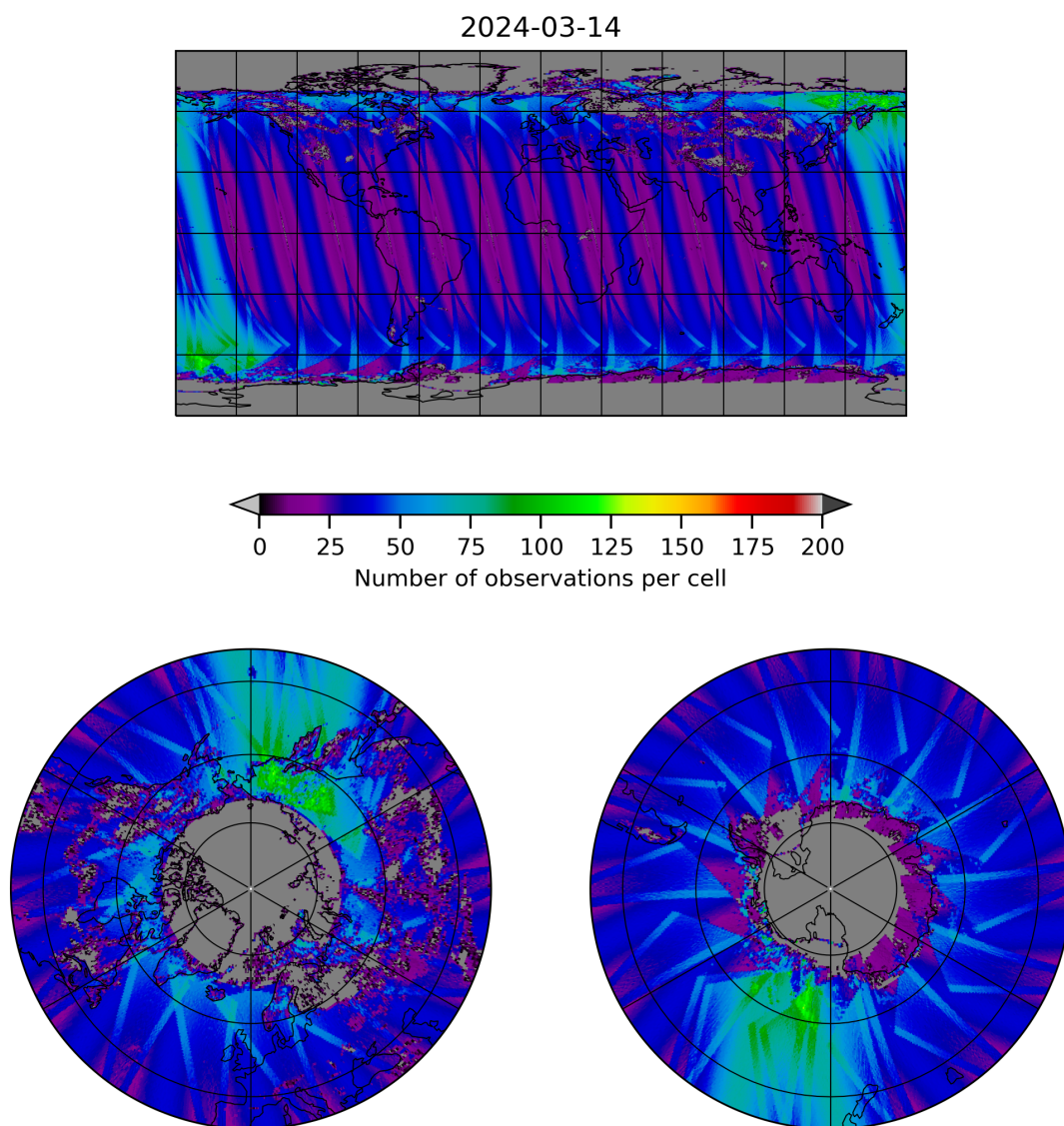
Figure 19: Map of the number of observations for 2024-03-14 to 2024-03-15
