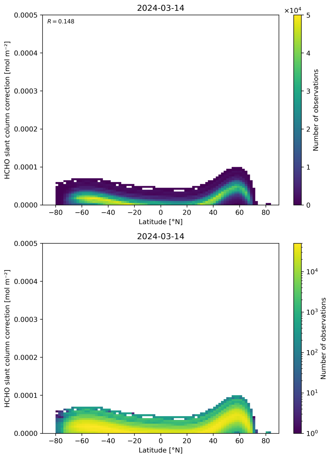
Figure 158: Scatter density plot of “Latitude” against “HCHO slant column correction” for 2024-03-14 to 2024-03-15.
