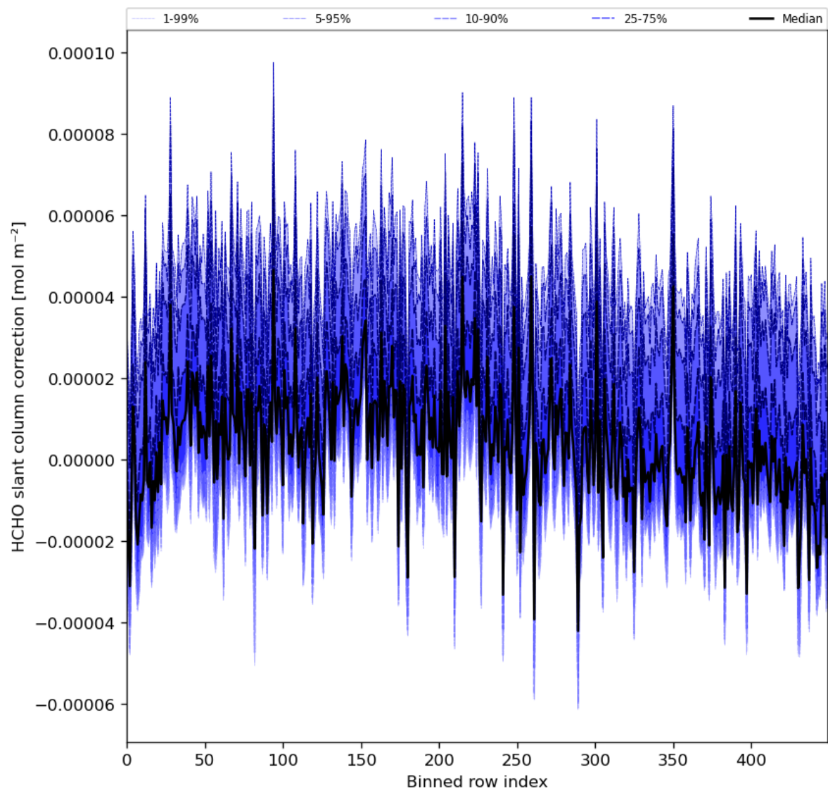
Figure 61: Along track statistics of “HCHO slant column correction” for 2024-03-14 to 2024-03-15
