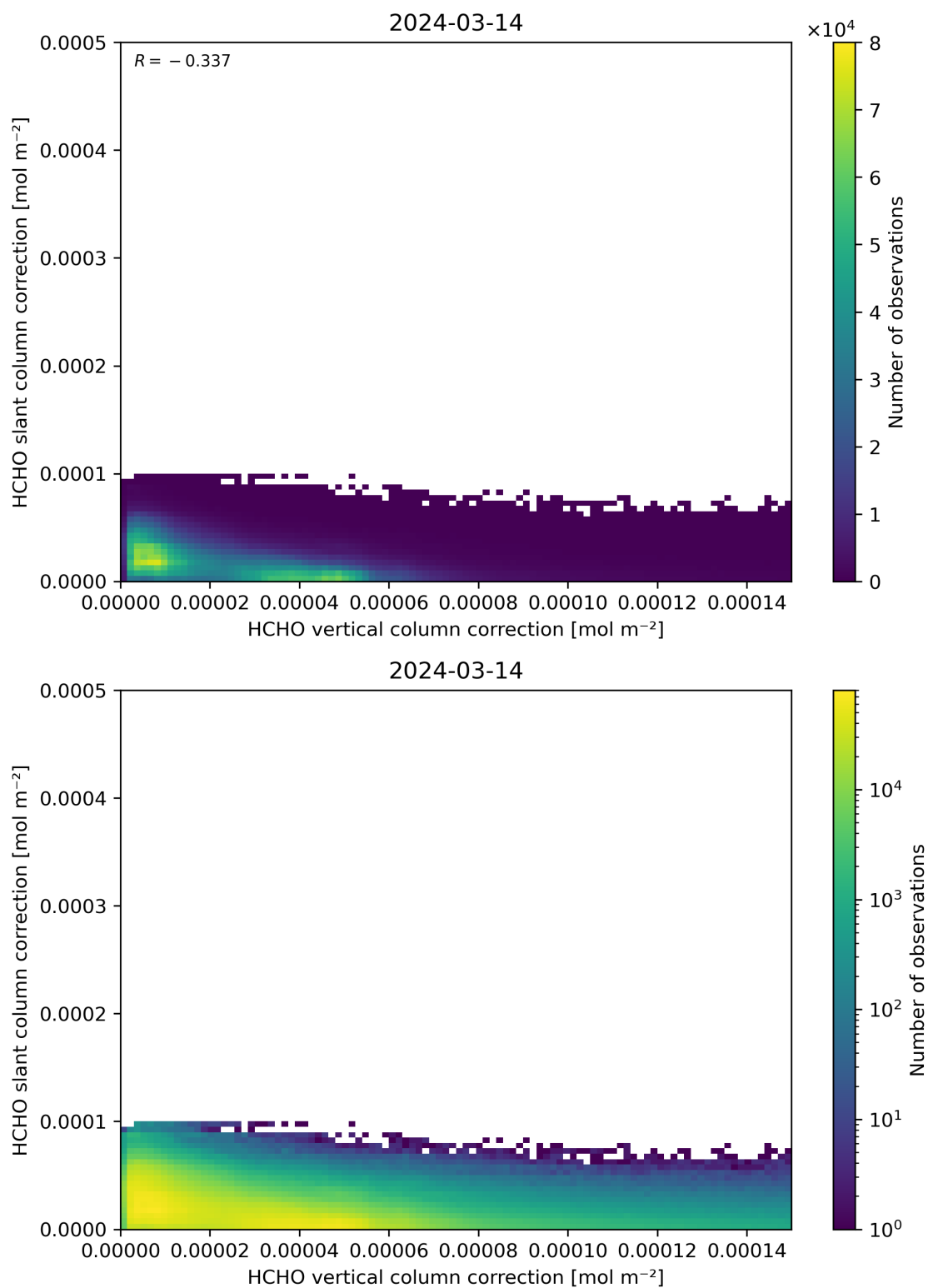
Figure 117: Scatter density plot of “HCHO vertical column correction” against “HCHO slant column correction” for 2024-03-14 to 2024-03-15.
