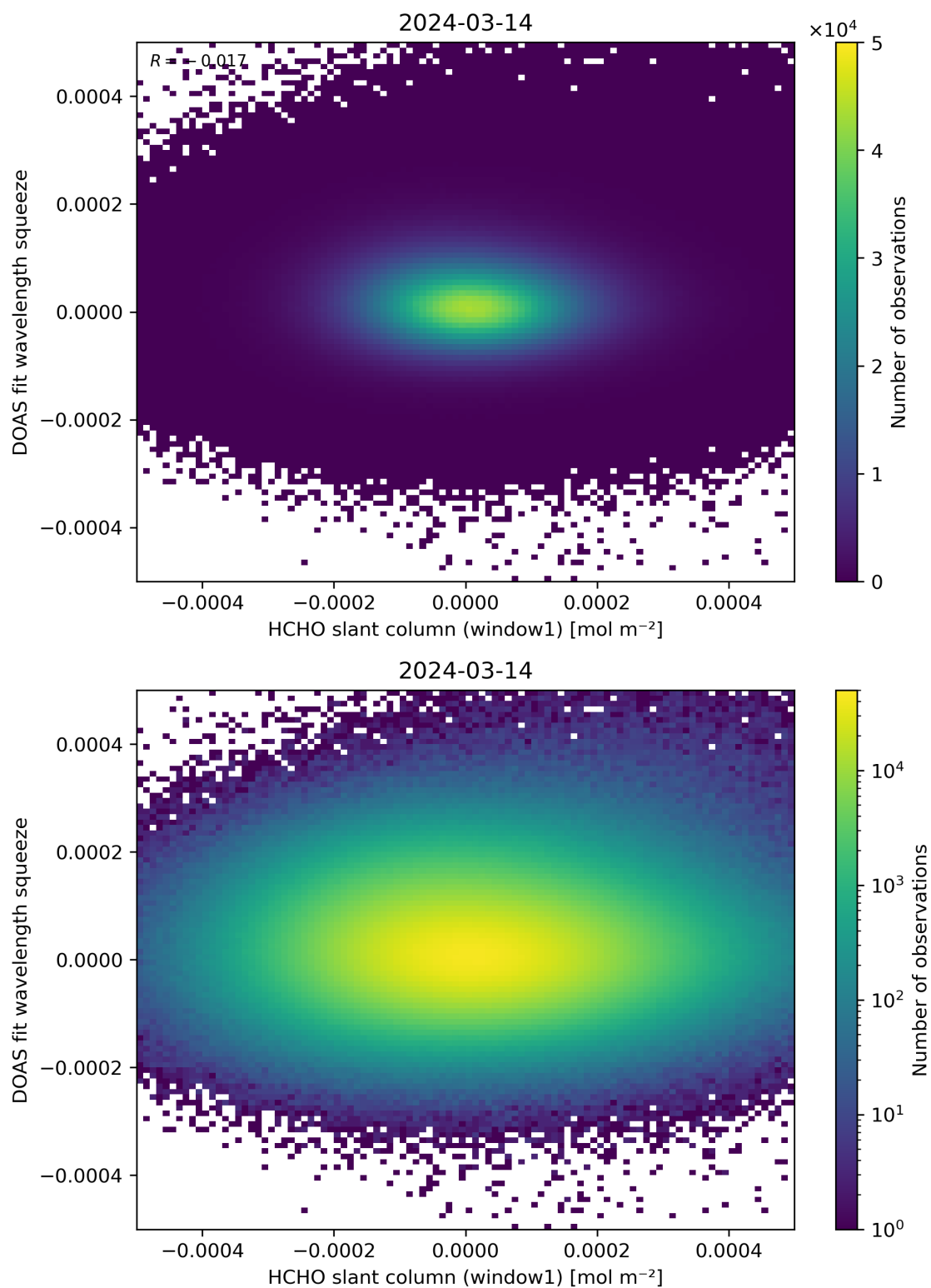
Figure 80: Scatter density plot of “HCHO slant column (window1)” against “DOAS fit wavelength squeeze” for 2024-03-14 to 2024-03-15.
