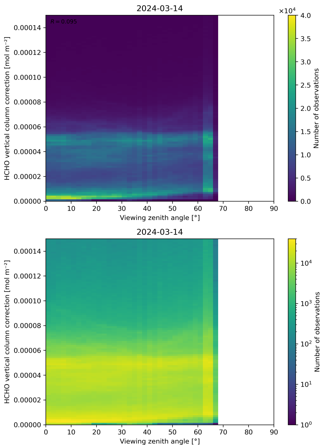
Figure 193: Scatter density plot of “Viewing zenith angle” against “HCHO vertical column correction” for 2024-03-14 to 2024-03-15.
