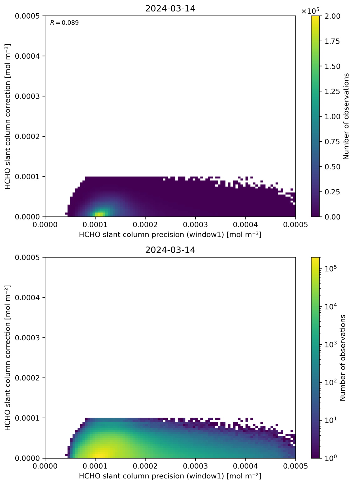
Figure 93: Scatter density plot of “HCHO slant column precision (window1)” against “HCHO slant column correction” for 2024-03-14 to 2024-03-15.
