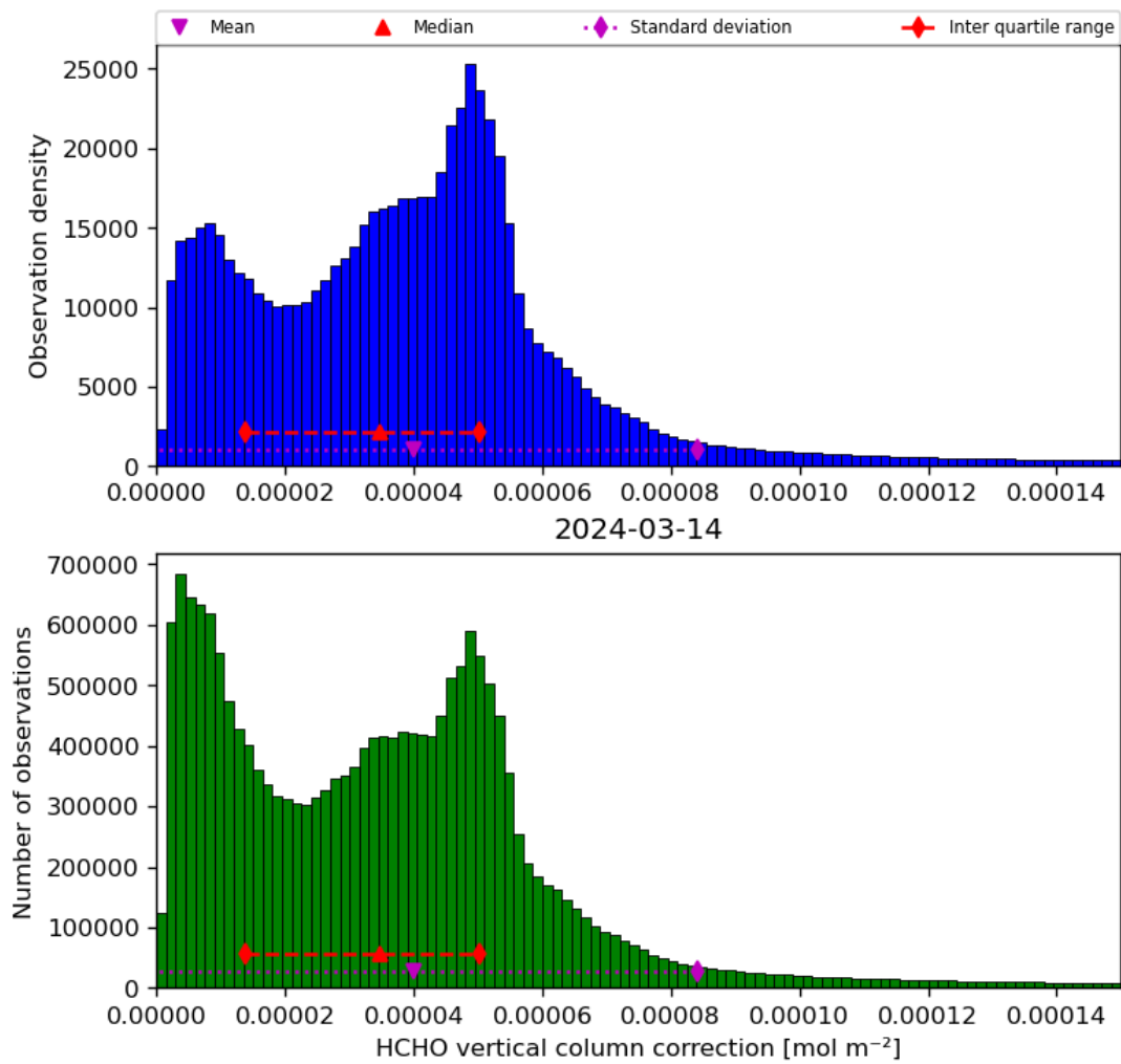
Figure 37: Histogram of “HCHO vertical column correction” for 2024-03-14 to 2024-03-15
