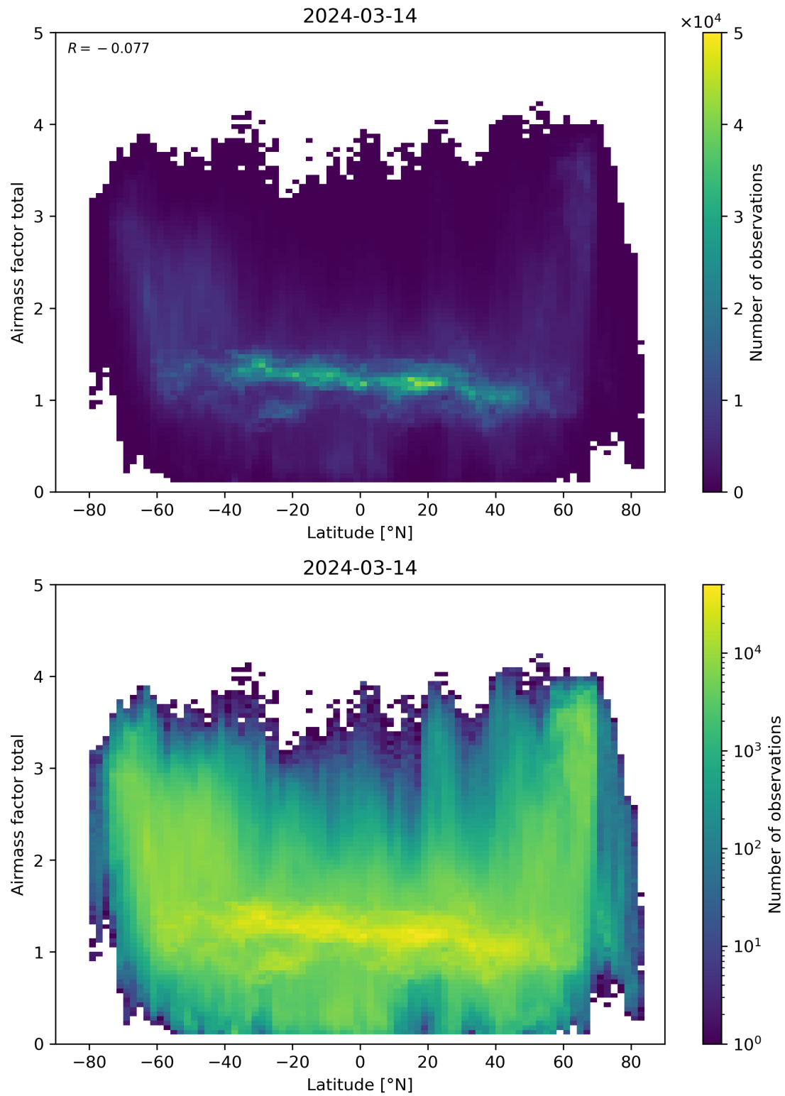
Figure 161: Scatter density plot of “Latitude” against “Airmass factor total” for 2024-03-14 to 2024-03-15.
