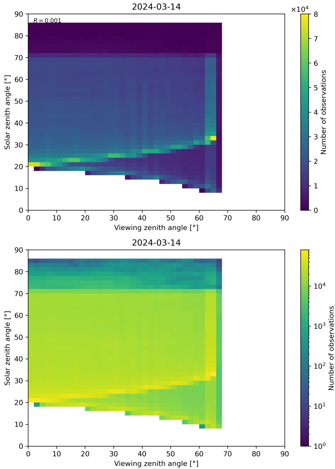
Figure 197: Scatter density plot of “Viewing zenith angle” against “Solar zenith angle” for 2024-03-14 to 2024-03-15.
