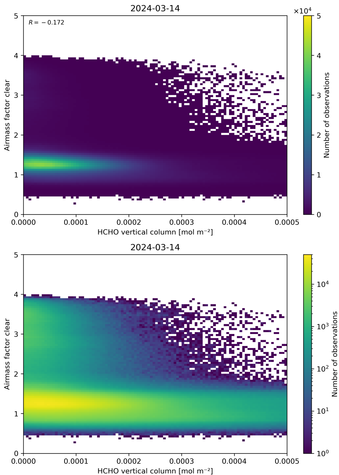
Figure 126: Scatter density plot of “HCHO vertical column” against “Airmass factor clear” for 2024-03-14 to 2024-03-15.
