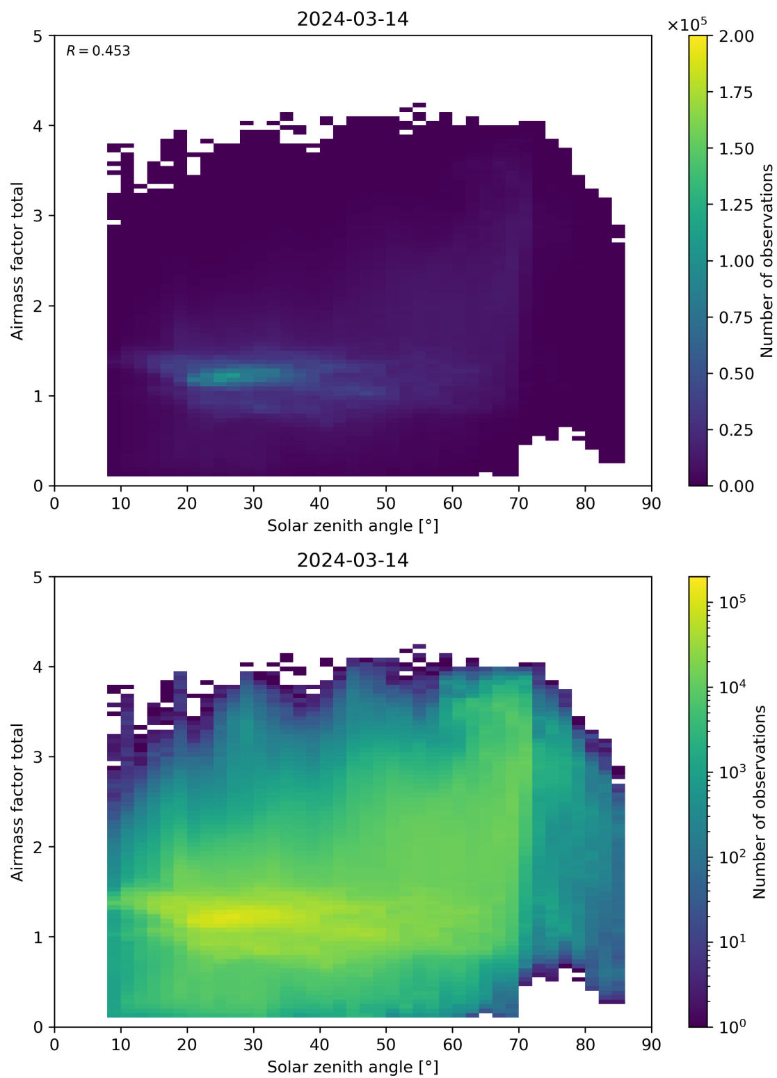
Figure 175: Scatter density plot of “Solar zenith angle” against “Airmass factor total” for 2024-03-14 to 2024-03-15.
