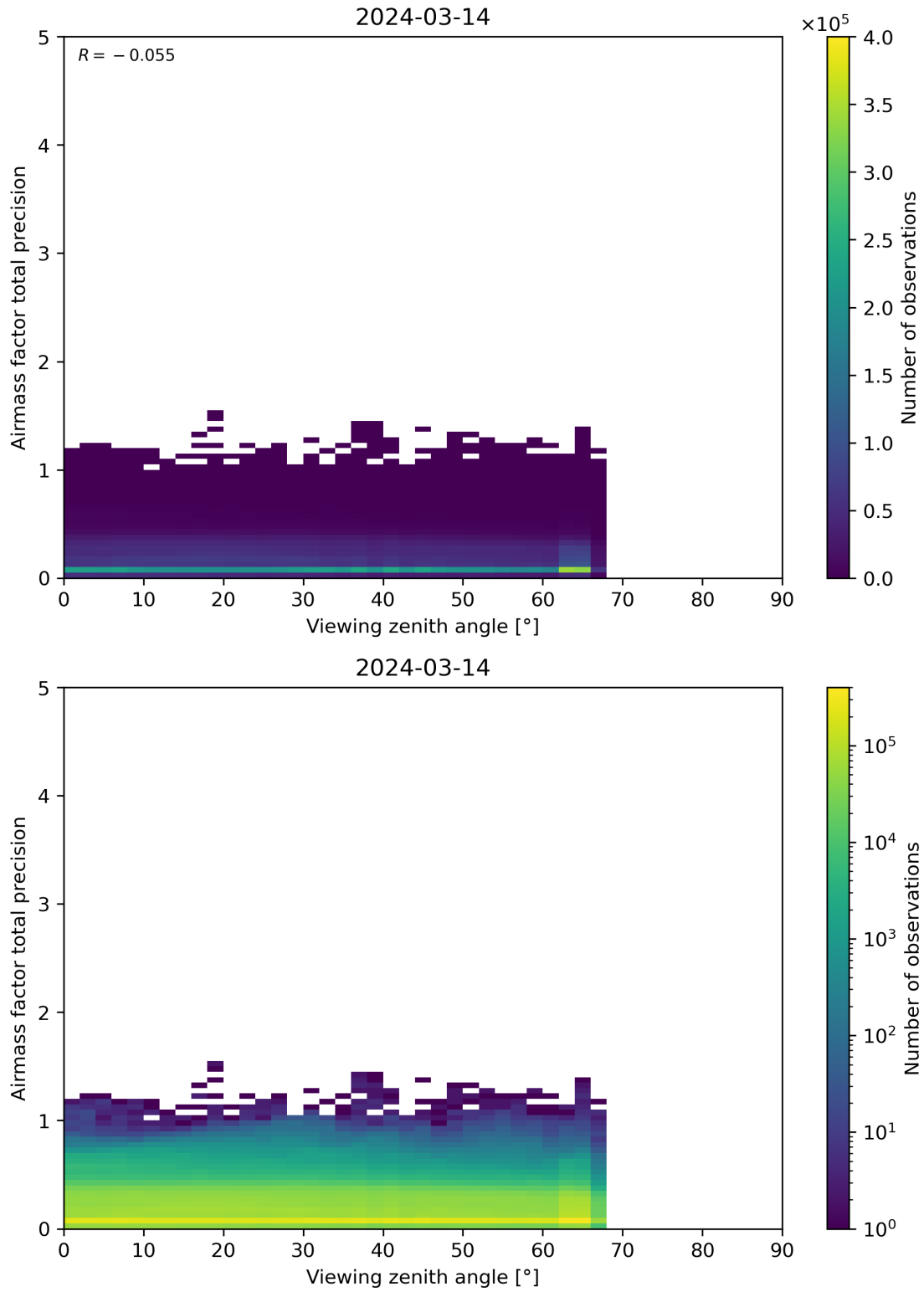
Figure 191: Scatter density plot of “Viewing zenith angle” against “Airmass factor total precision” for 2024-03-14 to 2024-03-15.
