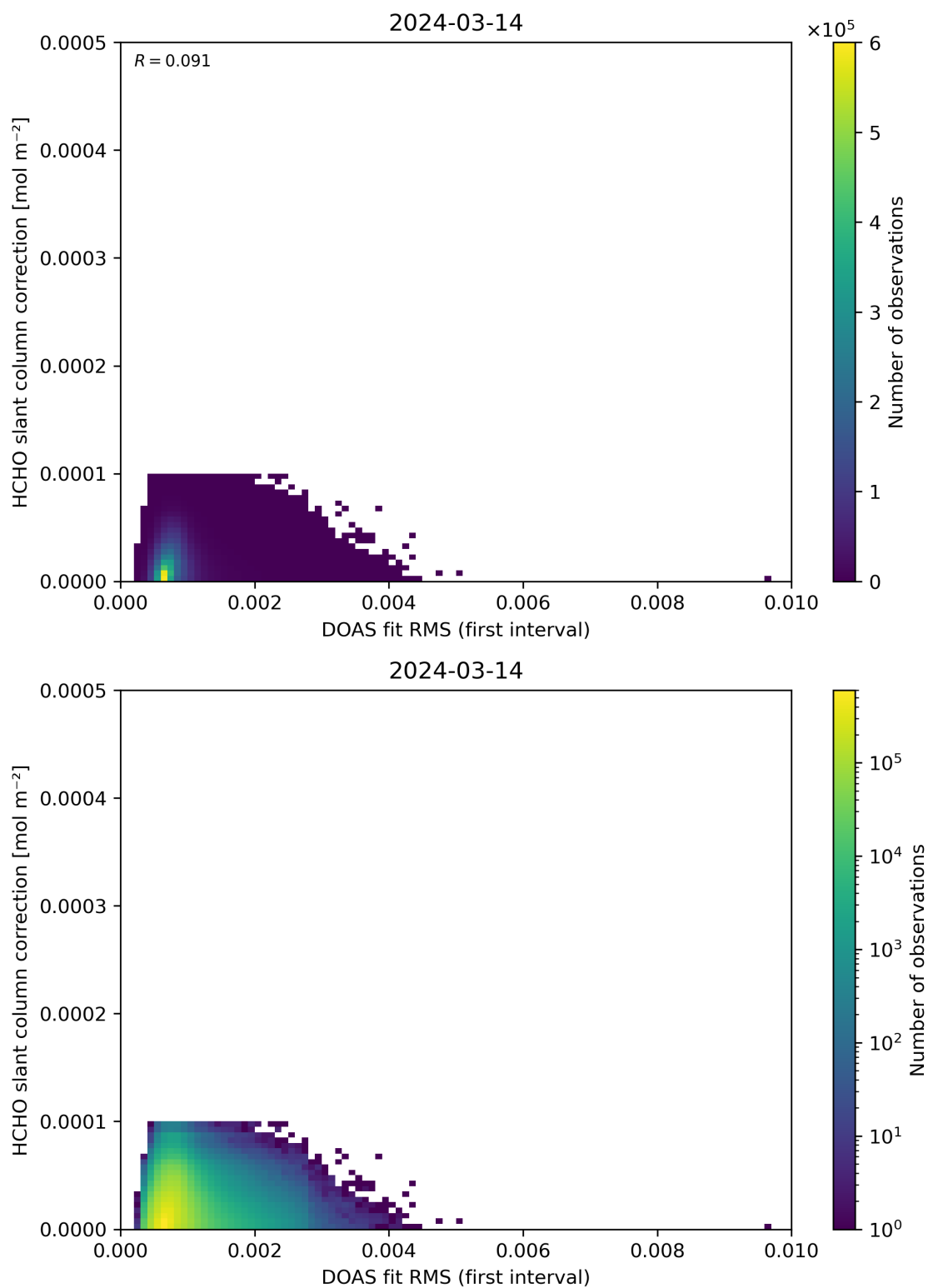
Figure 63: Scatter density plot of “DOAS fit RMS (first interval)” against “HCHO slant column correction” for 2024-03-14 to 2024-03-15.
