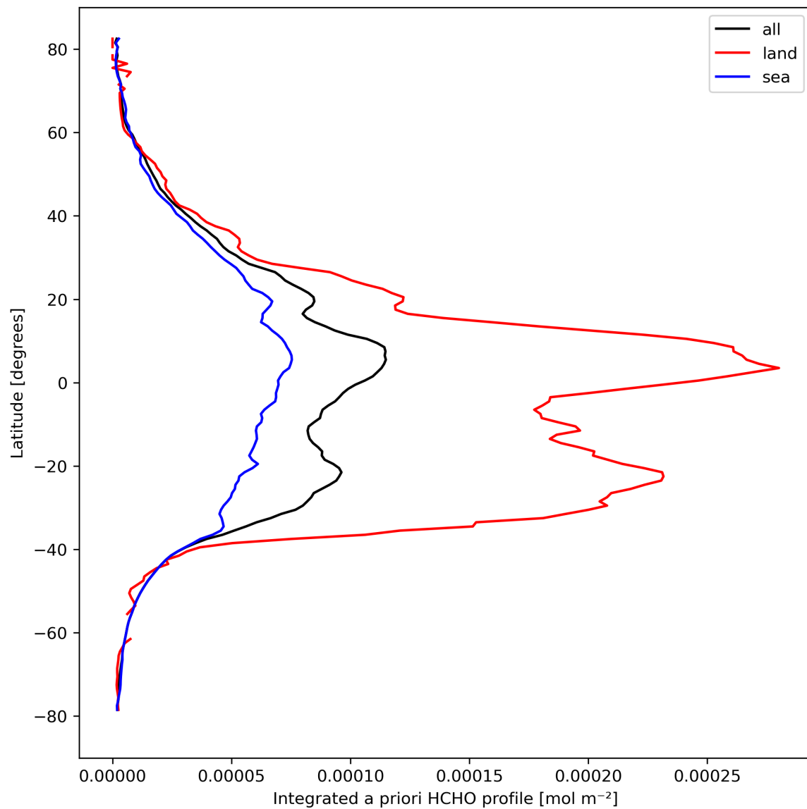
Figure 29: Zonal average of “Integrated a priori HCHO profile” for 2024-03-14 to 2024-03-15.
