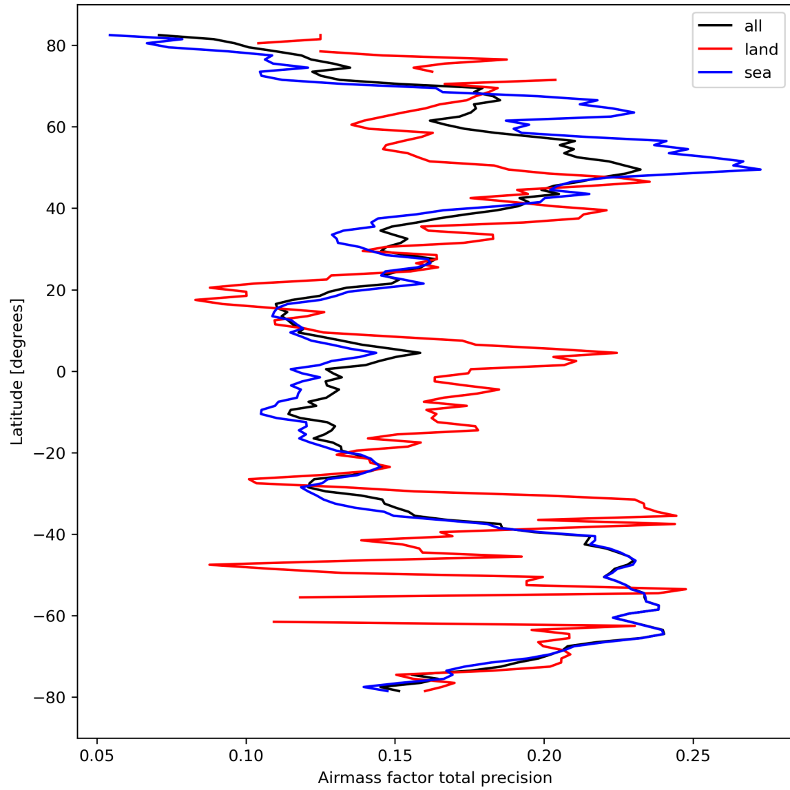
Figure 27: Zonal average of “Airmass factor total precision” for 2024-03-14 to 2024-03-15.
