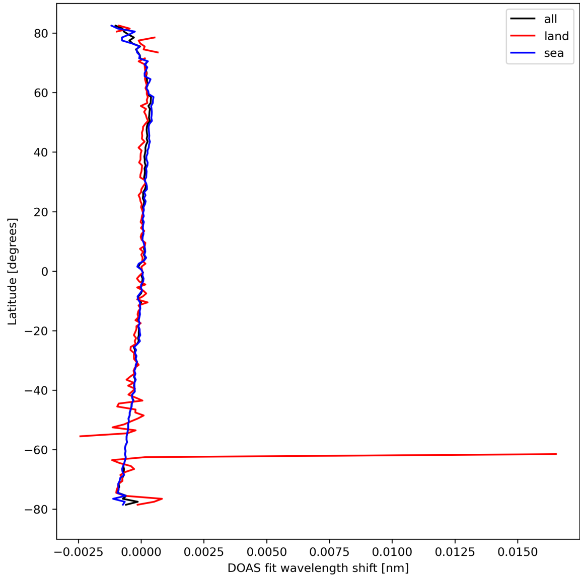
Figure 30: Zonal average of “DOAS fit wavelength shift” for 2024-03-14 to 2024-03-15.
