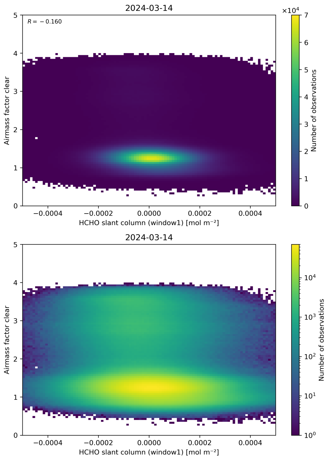
Figure 81: Scatter density plot of “HCHO slant column (window1)” against “Airmass factor clear” for 2024-03-14 to 2024-03-15.
