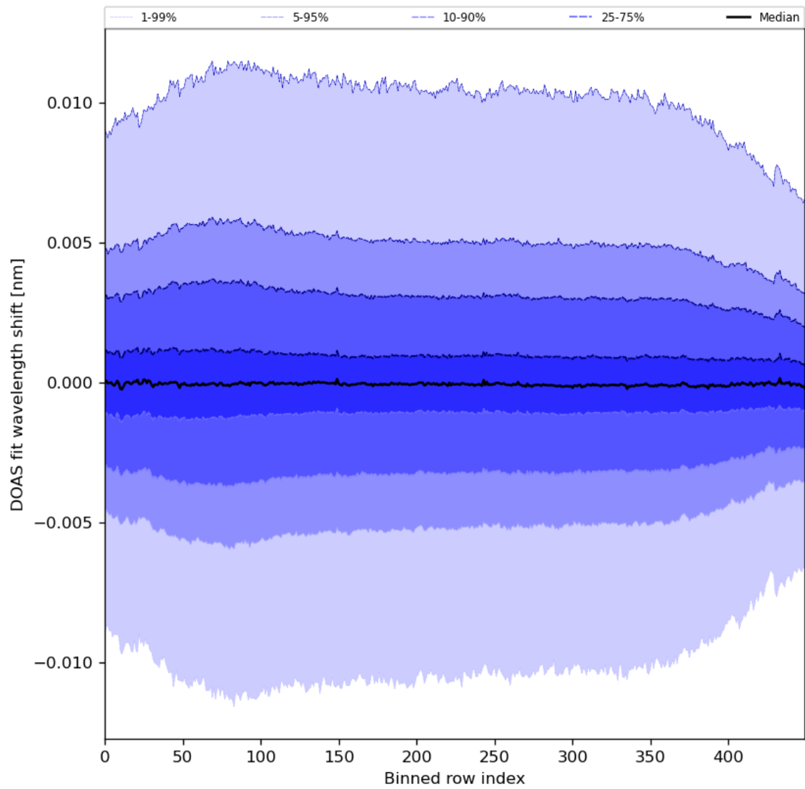
Figure 58: Along track statistics of “DOAS fit wavelength shift” for 2024-03-14 to 2024-03-15
