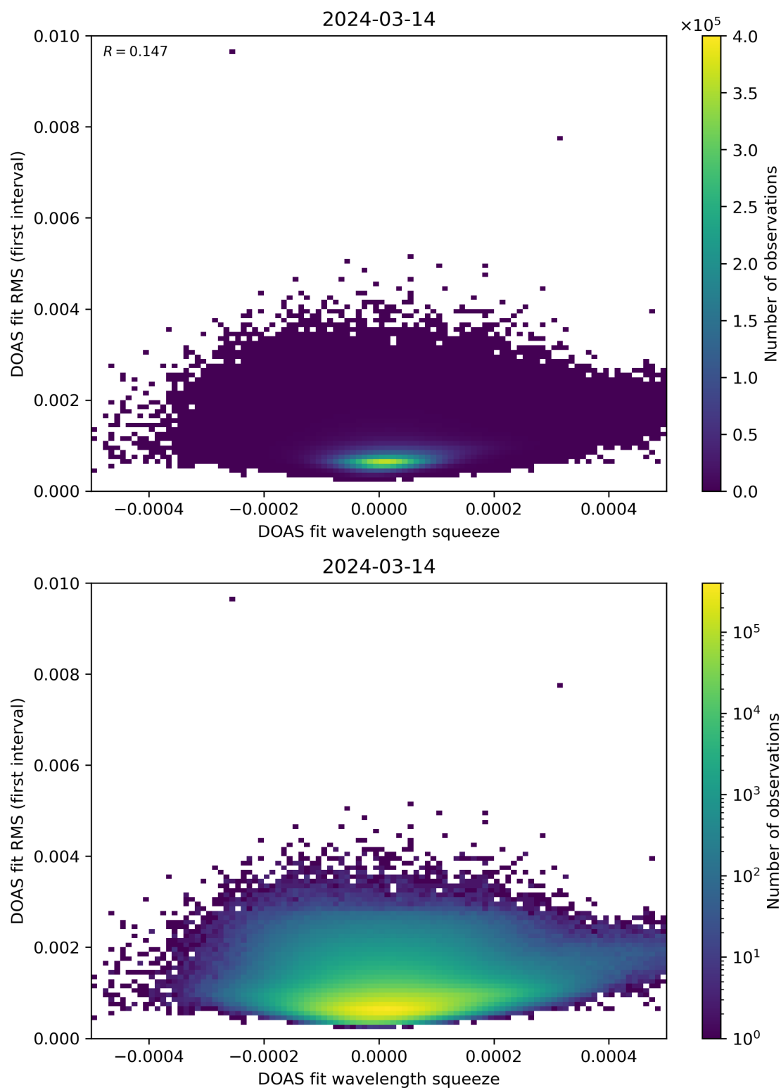
Figure 68: Scatter density plot of “DOAS fit wavelength squeeze” against “DOAS fit RMS (first interval)” for 2024-03-14 to 2024-03-15.
