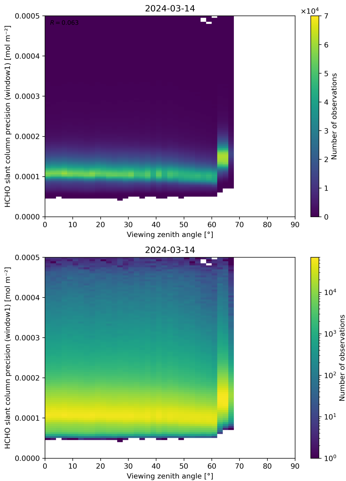
Figure 189: Scatter density plot of “Viewing zenith angle” against “HCHO slant column precision (window1)” for 2024-03-14 to 2024-03-15.
