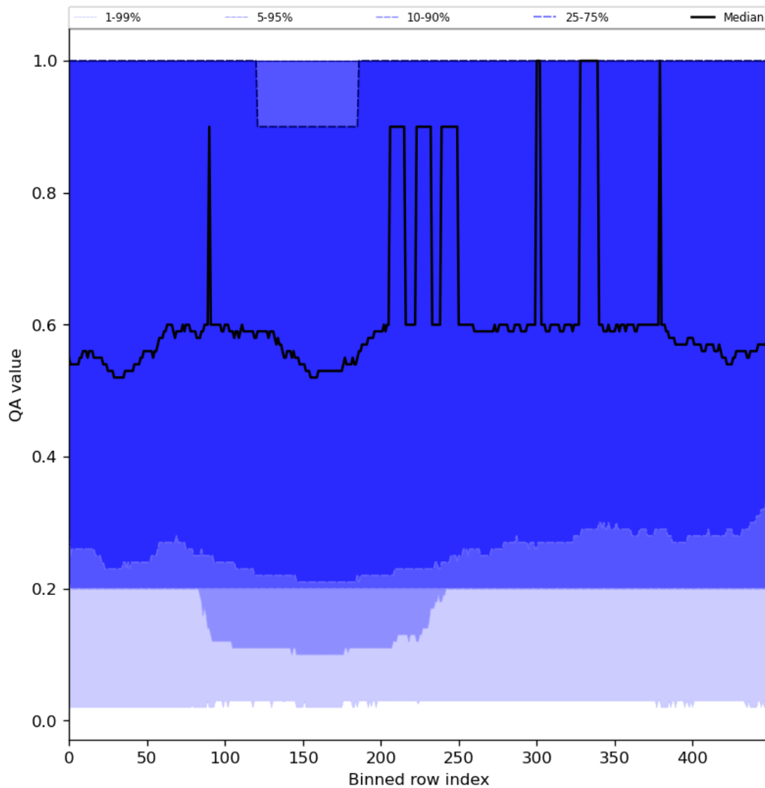
Figure 48: Along track statistics of “QA value” for 2024-03-14 to 2024-03-15
