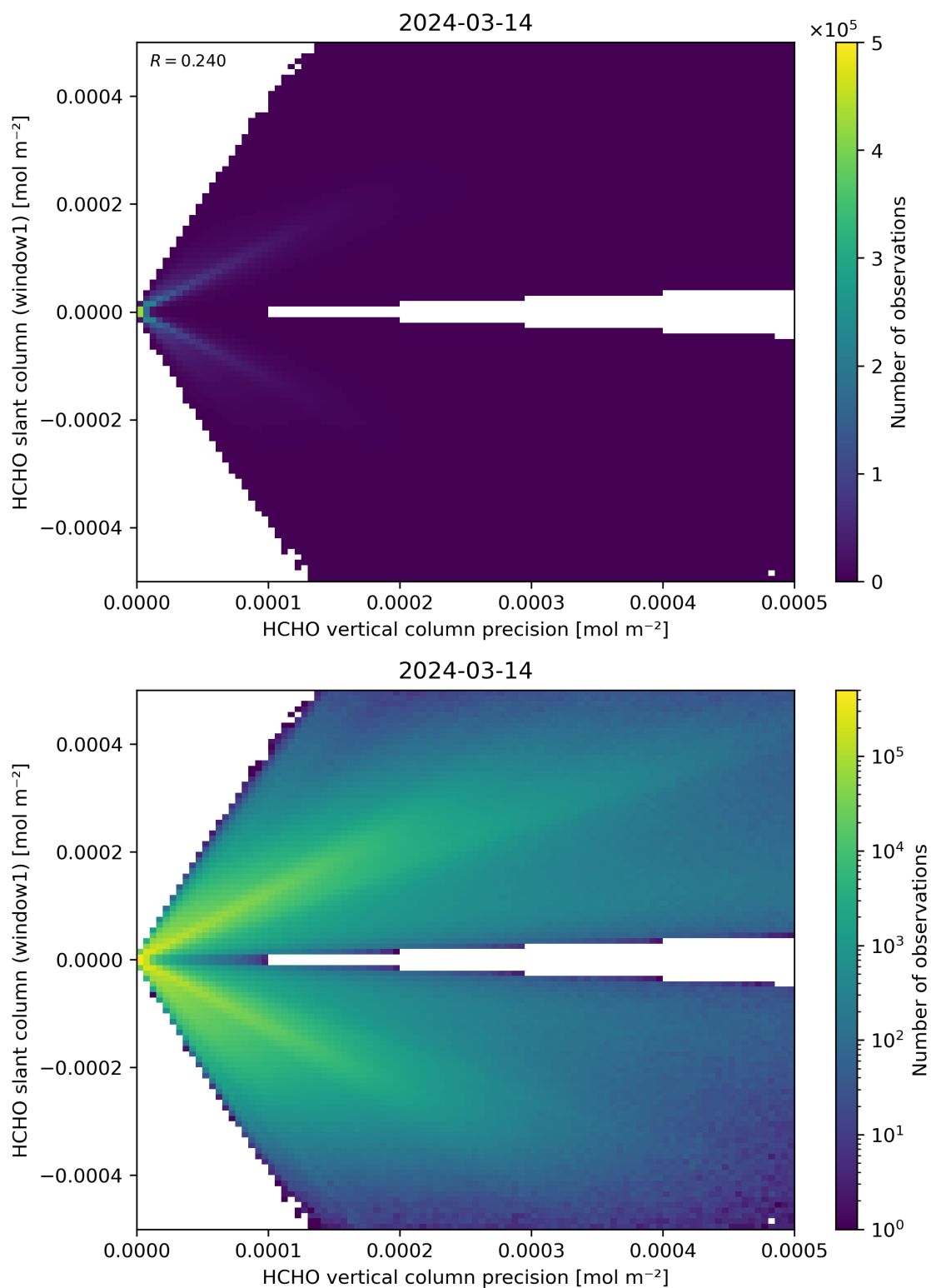
Figure 142: Scatter density plot of “HCHO vertical column precision” against “HCHO slant column (window1)” for 2024-03-14 to 2024-03-15.
