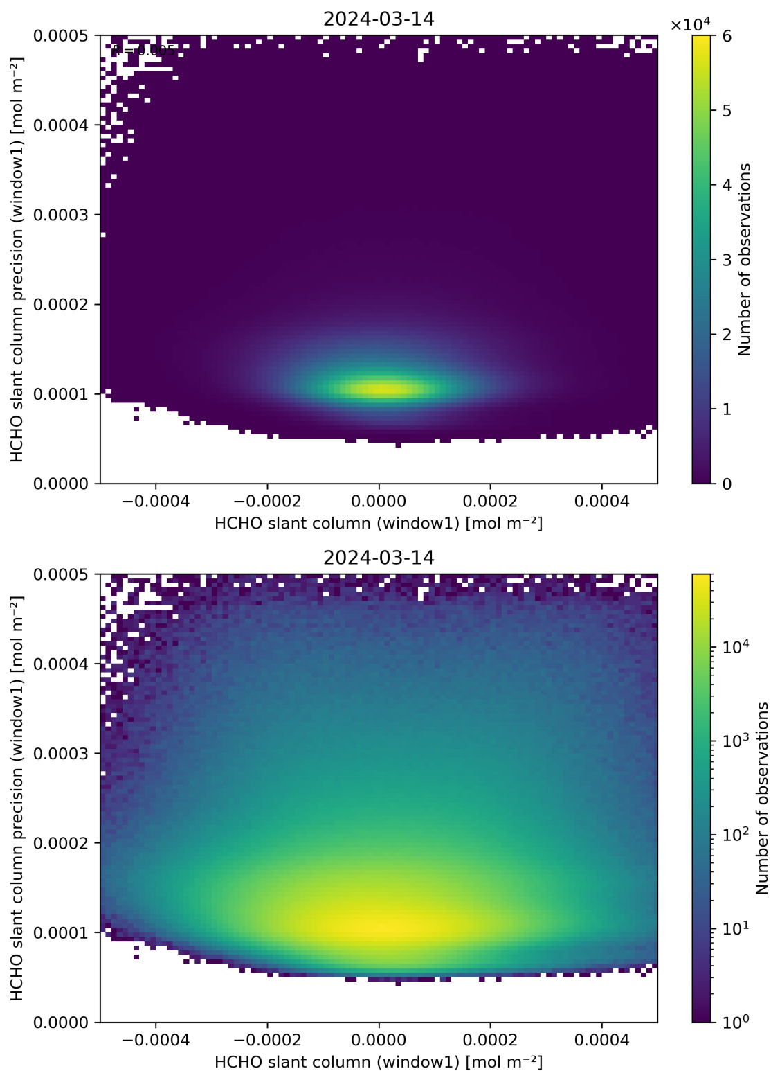
Figure 84: Scatter density plot of “HCHO slant column (window1)” against “HCHO slant column precision (window1)” for 2024-03-14 to 2024-03-15.
