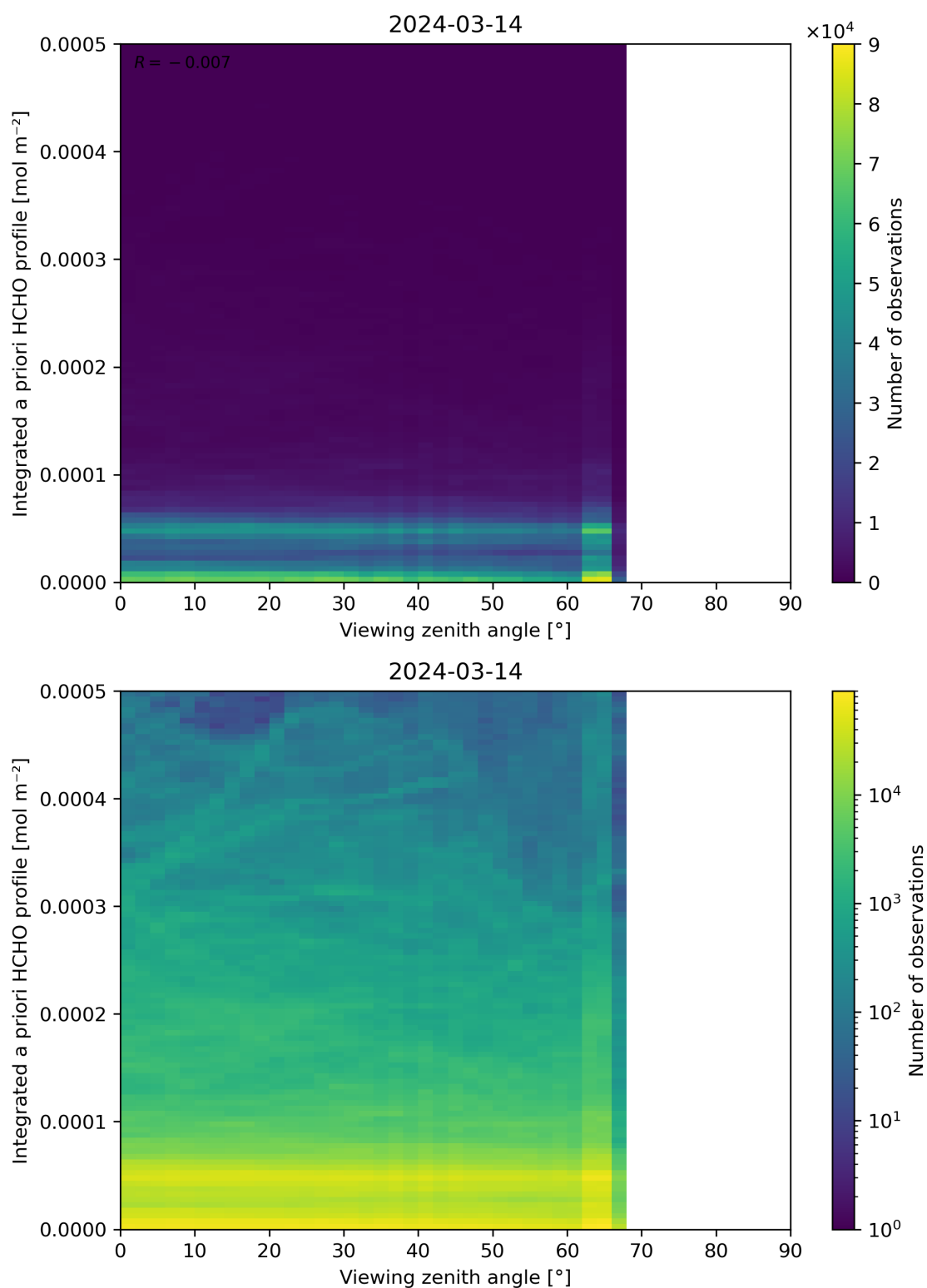
Figure 195: Scatter density plot of “Viewing zenith angle” against “Integrated a priori HCHO profile” for 2024-03-14 to 2024-03-15.
