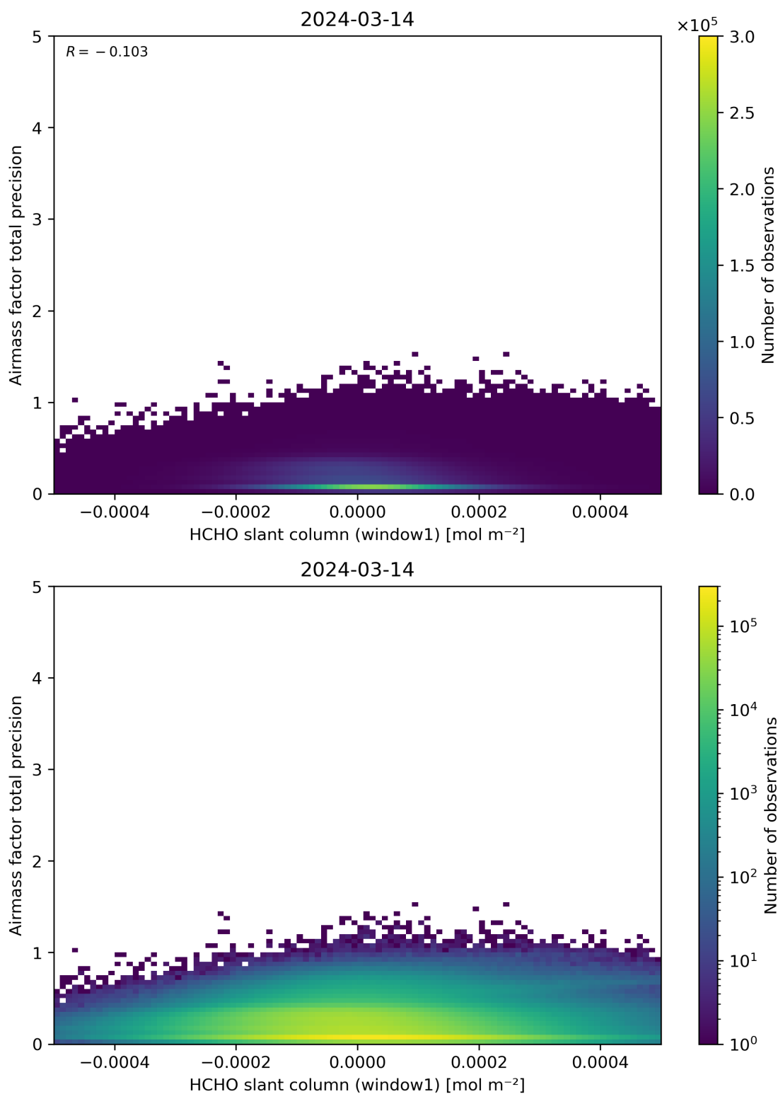
Figure 86: Scatter density plot of “HCHO slant column (window1)” against “Airmass factor total precision” for 2024-03-14 to 2024-03-15.
