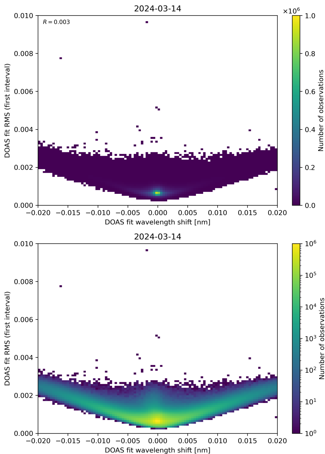
Figure 64: Scatter density plot of “DOAS fit wavelength shift” against “DOAS fit RMS (first interval)” for 2024-03-14 to 2024-03-15.
