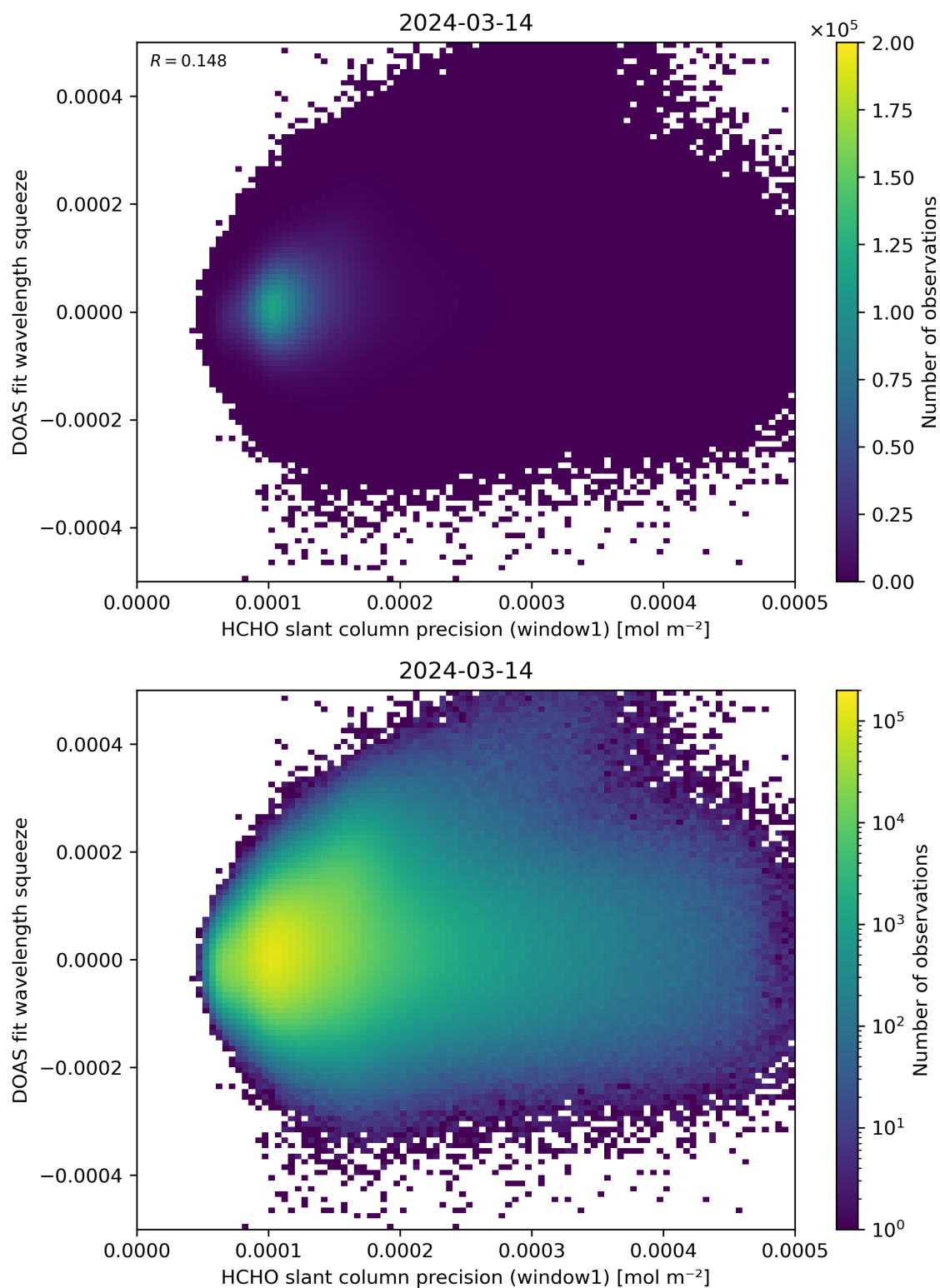
Figure 90: Scatter density plot of “HCHO slant column precision (window1)” against “DOAS fit wavelength squeeze” for 2024-03-14 to 2024-03-15.
