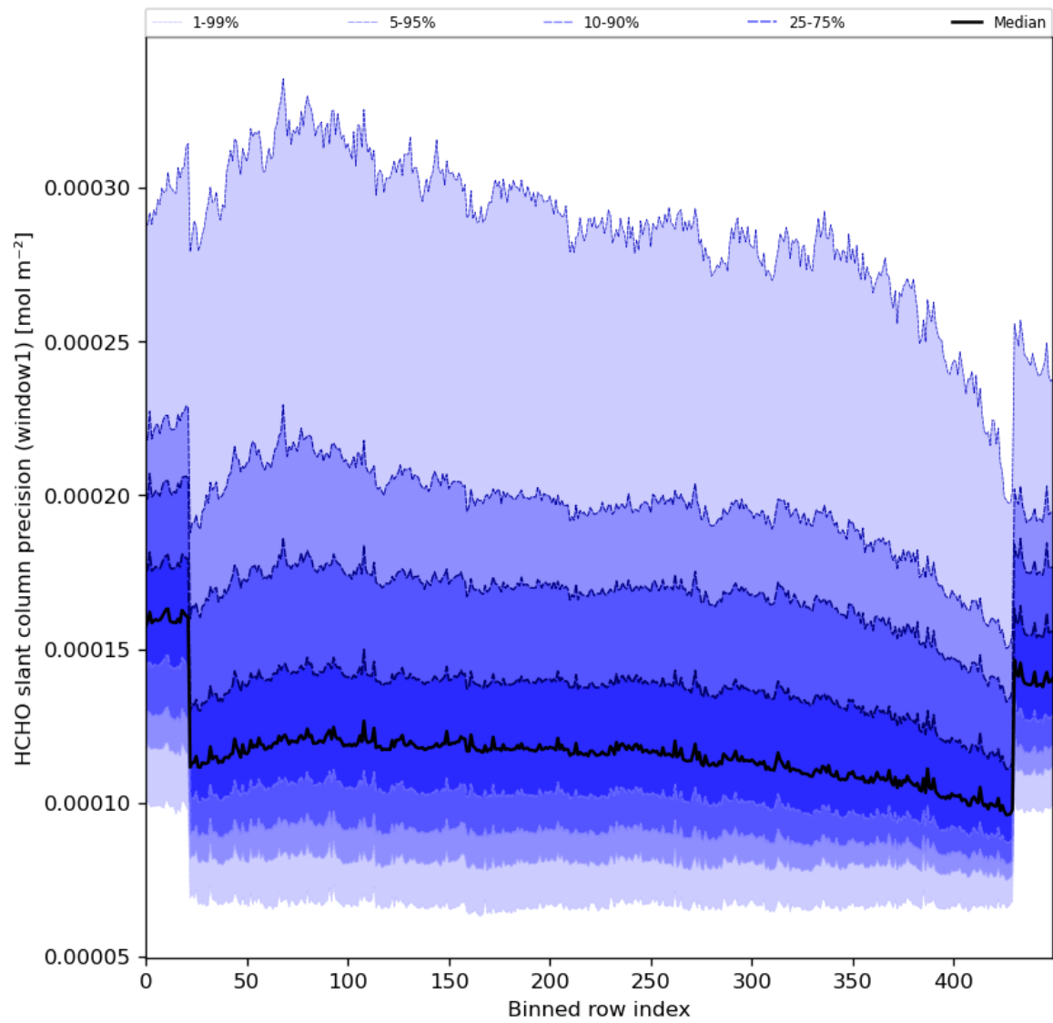
Figure 53: Along track statistics of “HCHO slant column precision (window1)” for 2024-03-14 to 2024-03-15
