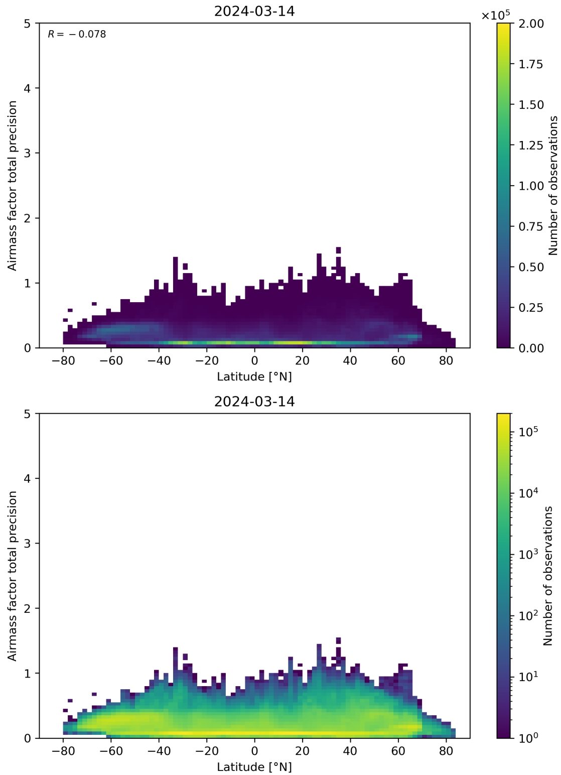
Figure 162: Scatter density plot of “Latitude” against “Airmass factor total precision” for 2024-03-14 to 2024-03-15.
