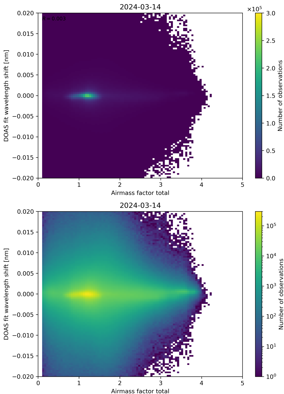
Figure 98: Scatter density plot of “Airmass factor total” against “DOAS fit wavelength shift” for 2024-03-14 to 2024-03-15.
