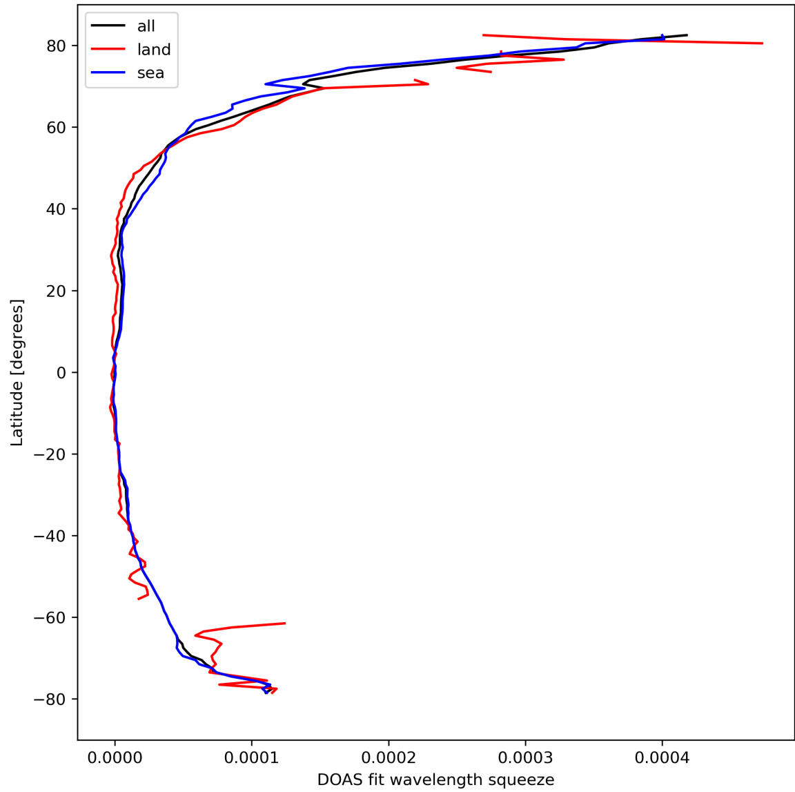
Figure 31: Zonal average of “DOAS fit wavelength squeeze” for 2024-03-14 to 2024-03-15.
