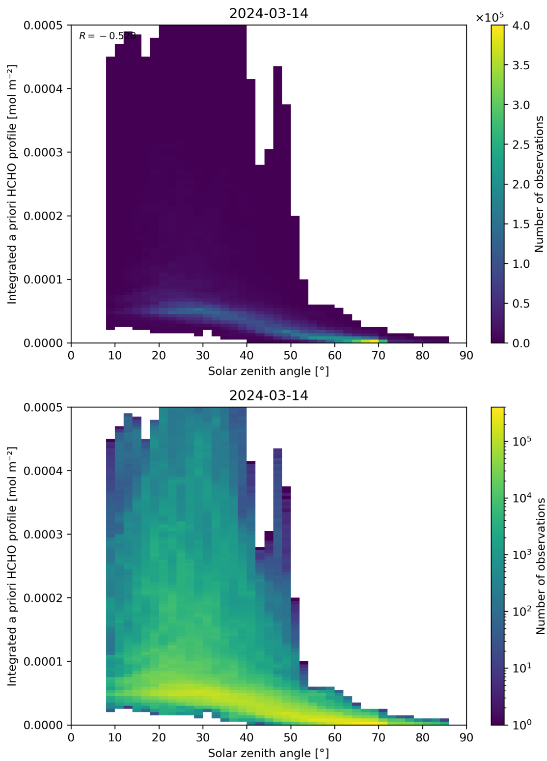
Figure 180: Scatter density plot of “Solar zenith angle” against “Integrated a priori HCHO profile” for 2024-03-14 to 2024-03-15.
