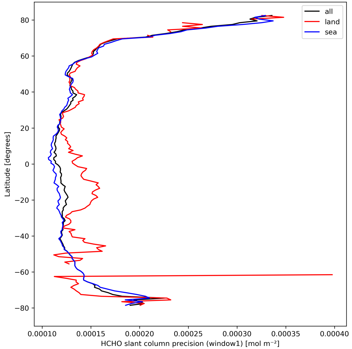
Figure 25: Zonal average of “HCHO slant column precision (window1)” for 2024-03-14 to 2024-03-15.
