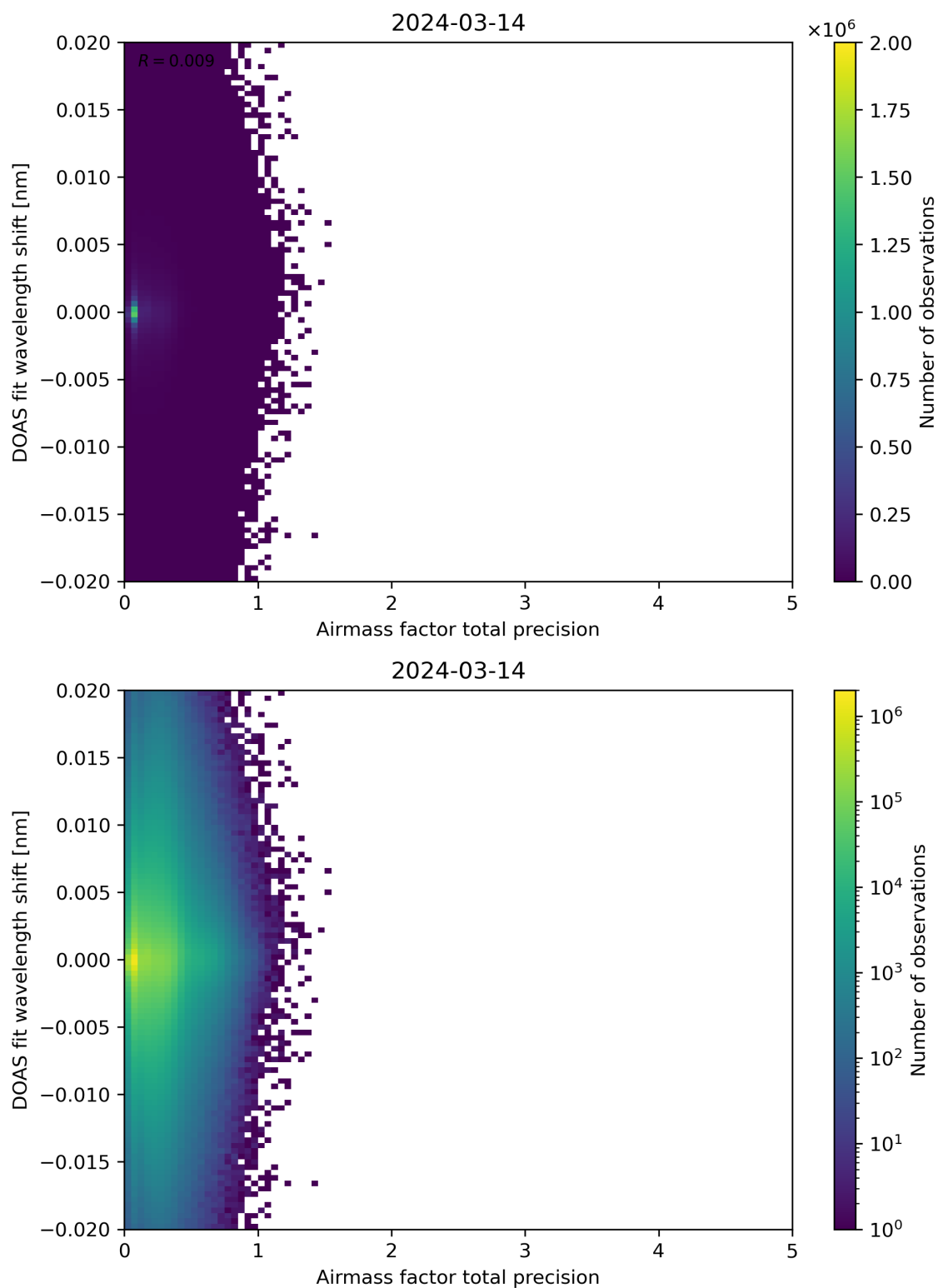
Figure 106: Scatter density plot of “Airmass factor total precision” against “DOAS fit wavelength shift” for 2024-03-14 to 2024-03-15.
