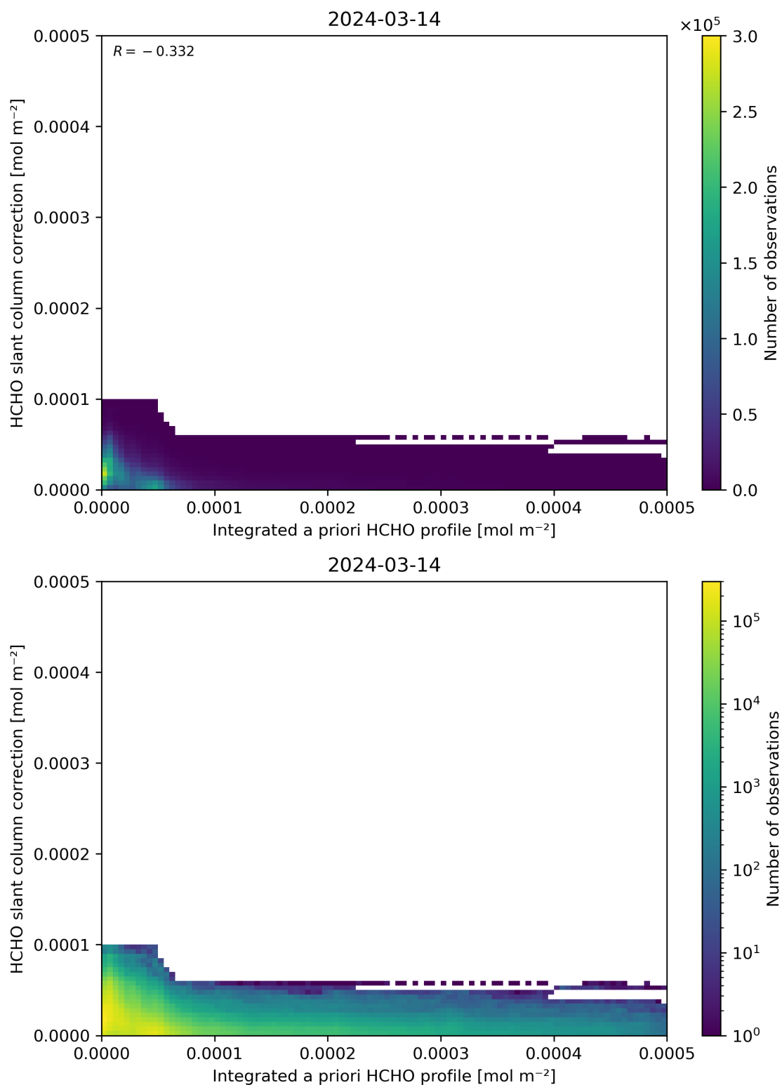
Figure 152: Scatter density plot of “Integrated a priori HCHO profile” against “HCHO slant column correction” for 2024-03-14 to 2024-03-15.
