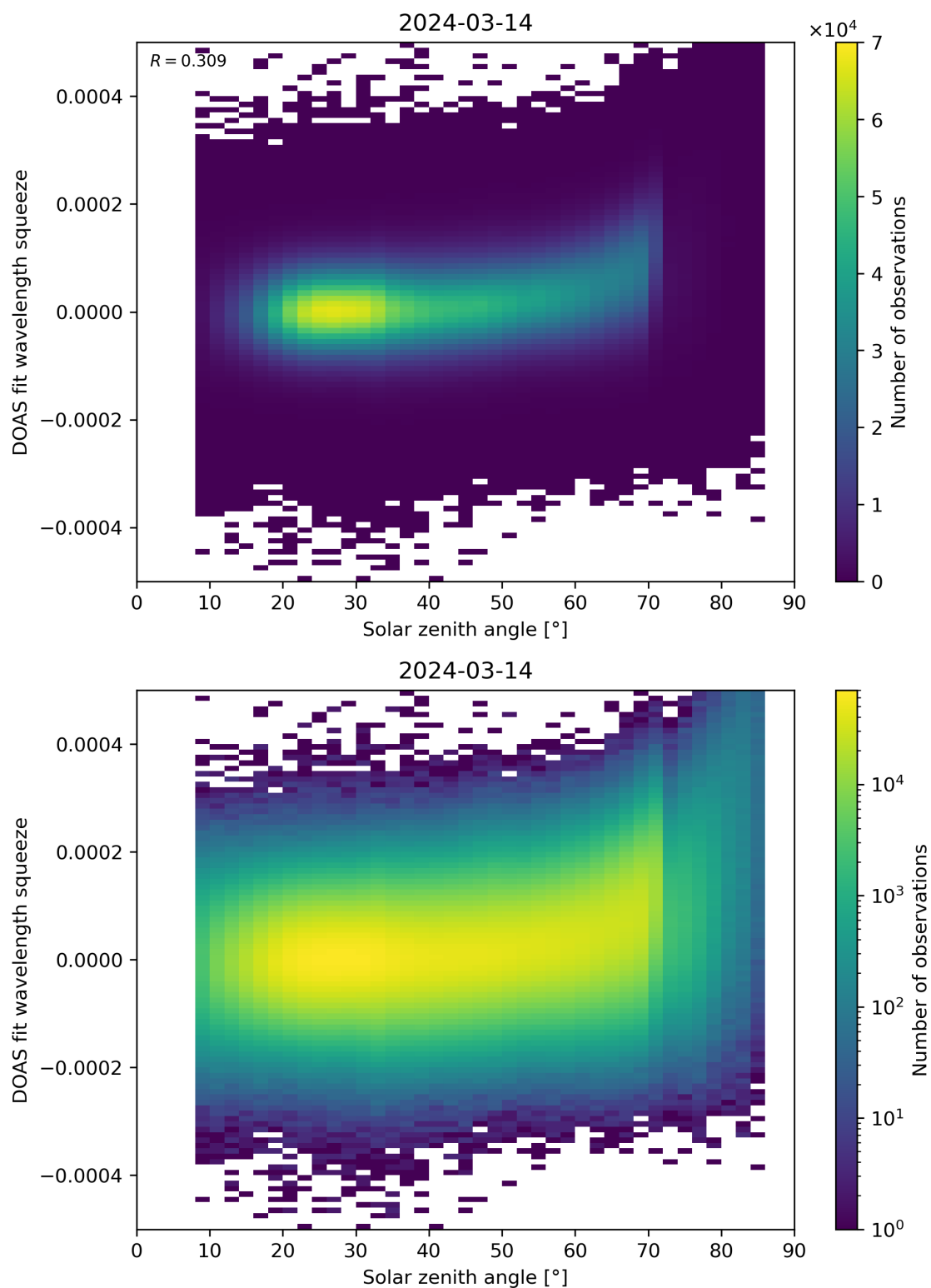
Figure 169: Scatter density plot of “Solar zenith angle” against “DOAS fit wavelength squeeze” for 2024-03-14 to 2024-03-15.
