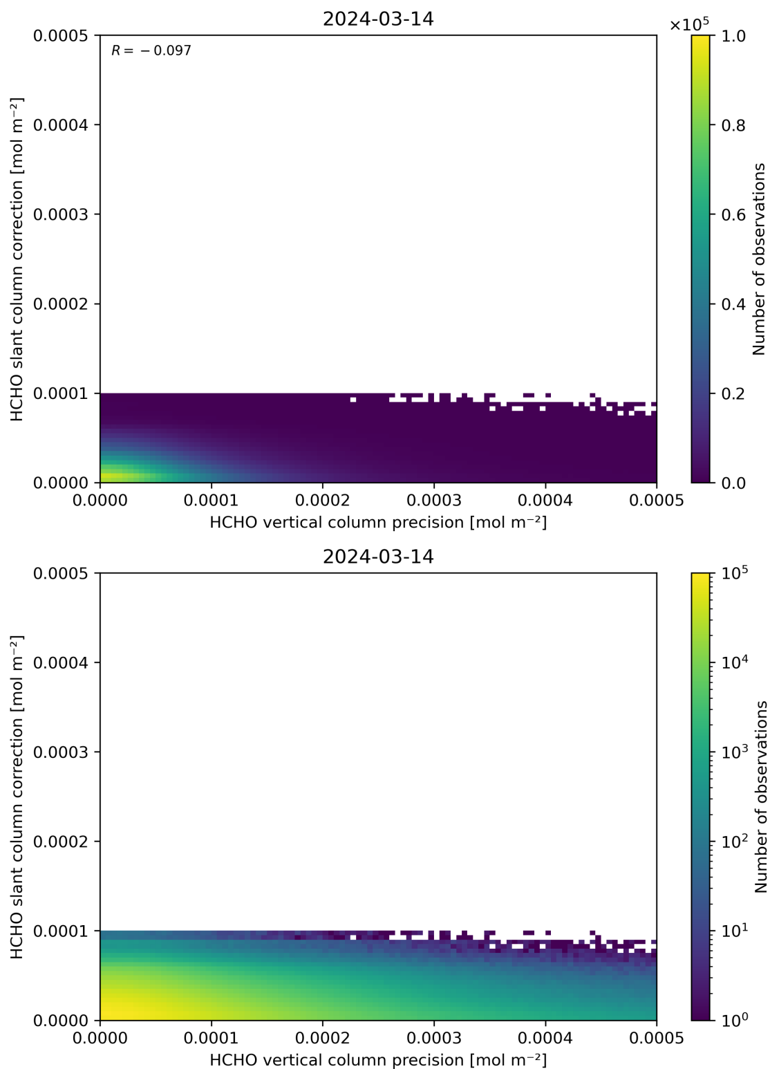
Figure 141: Scatter density plot of “HCHO vertical column precision” against “HCHO slant column correction” for 2024-03-14 to 2024-03-15.
