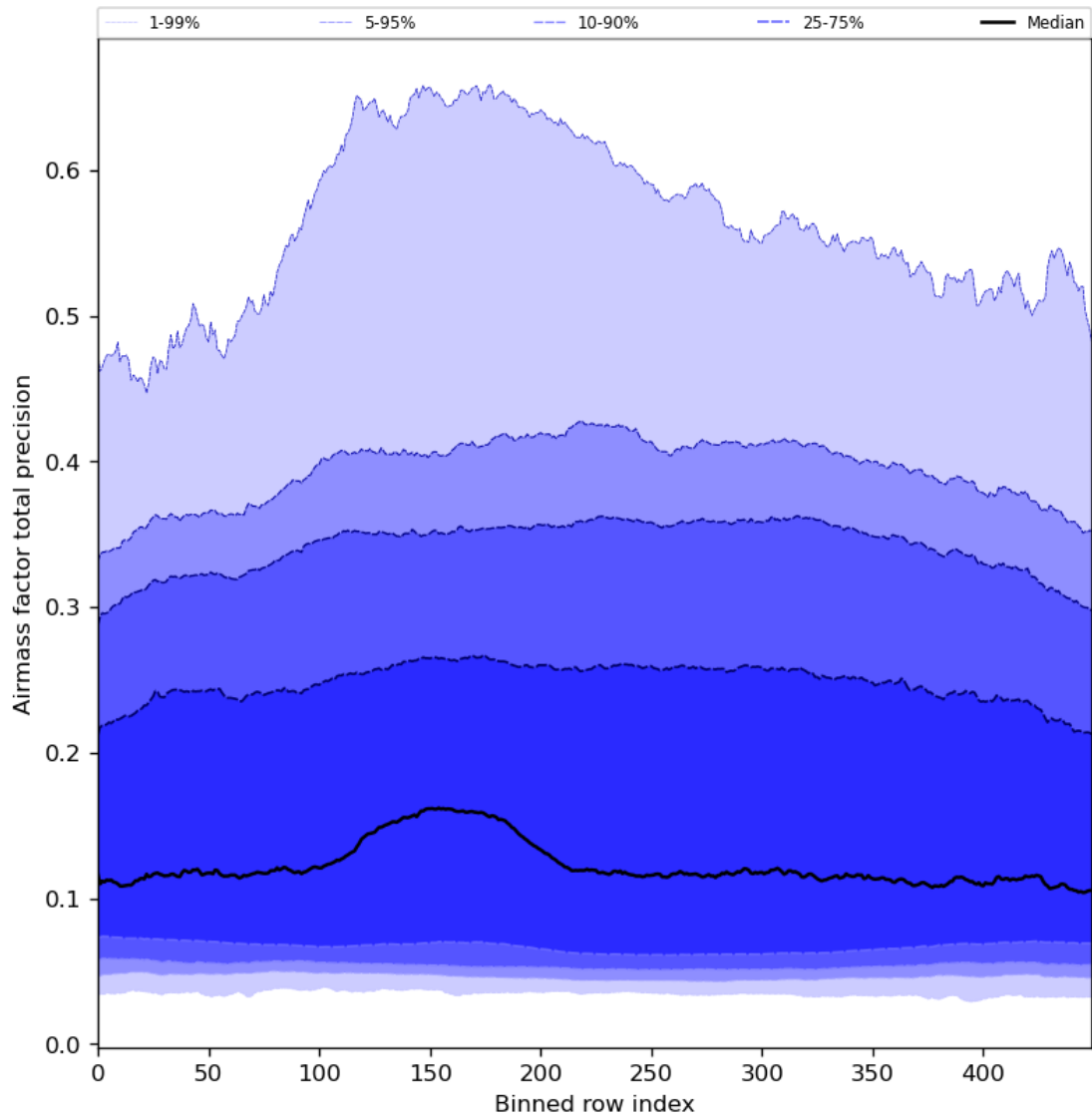
Figure 55: Along track statistics of “Airmass factor total precision” for 2024-03-14 to 2024-03-15
