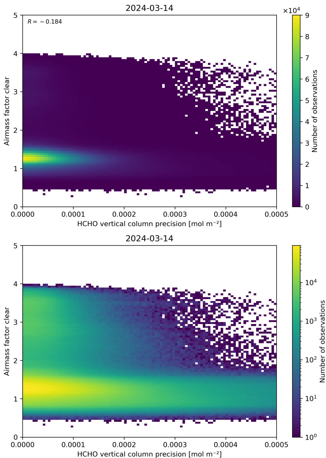
Figure 139: Scatter density plot of “HCHO vertical column precision” against “Airmass factor clear” for 2024-03-14 to 2024-03-15.
