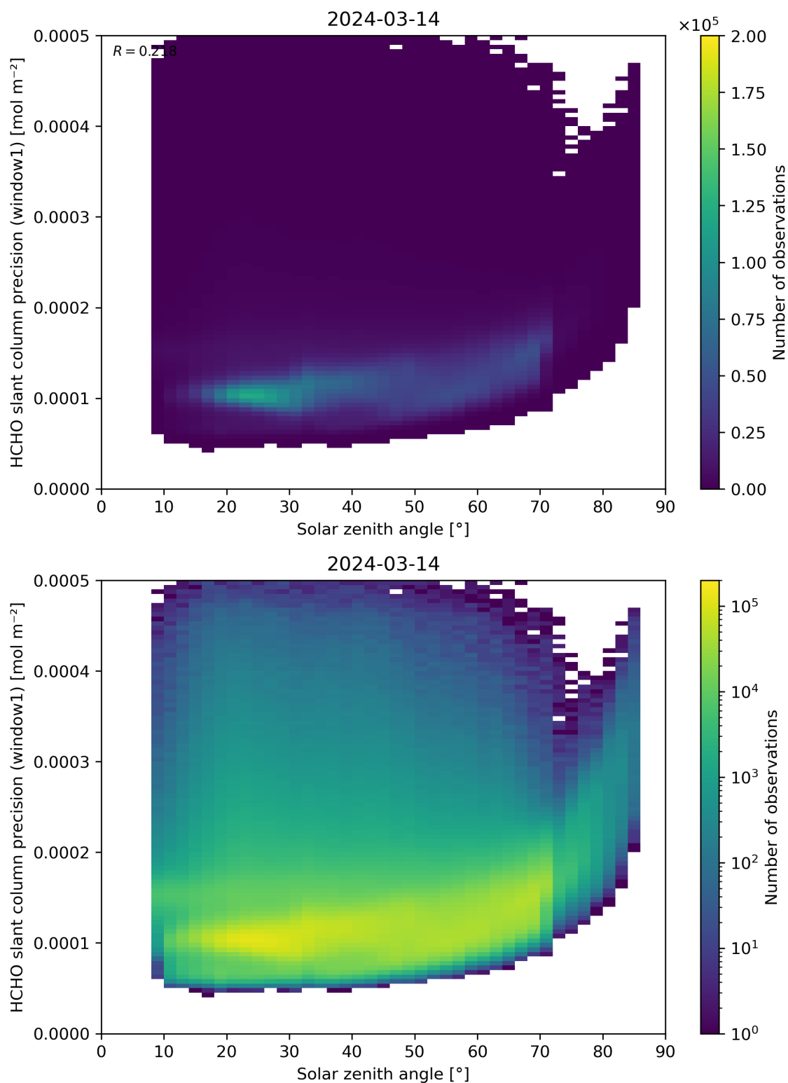
Figure 174: Scatter density plot of “Solar zenith angle” against “HCHO slant column precision (window1)” for 2024-03-14 to 2024-03-15.
