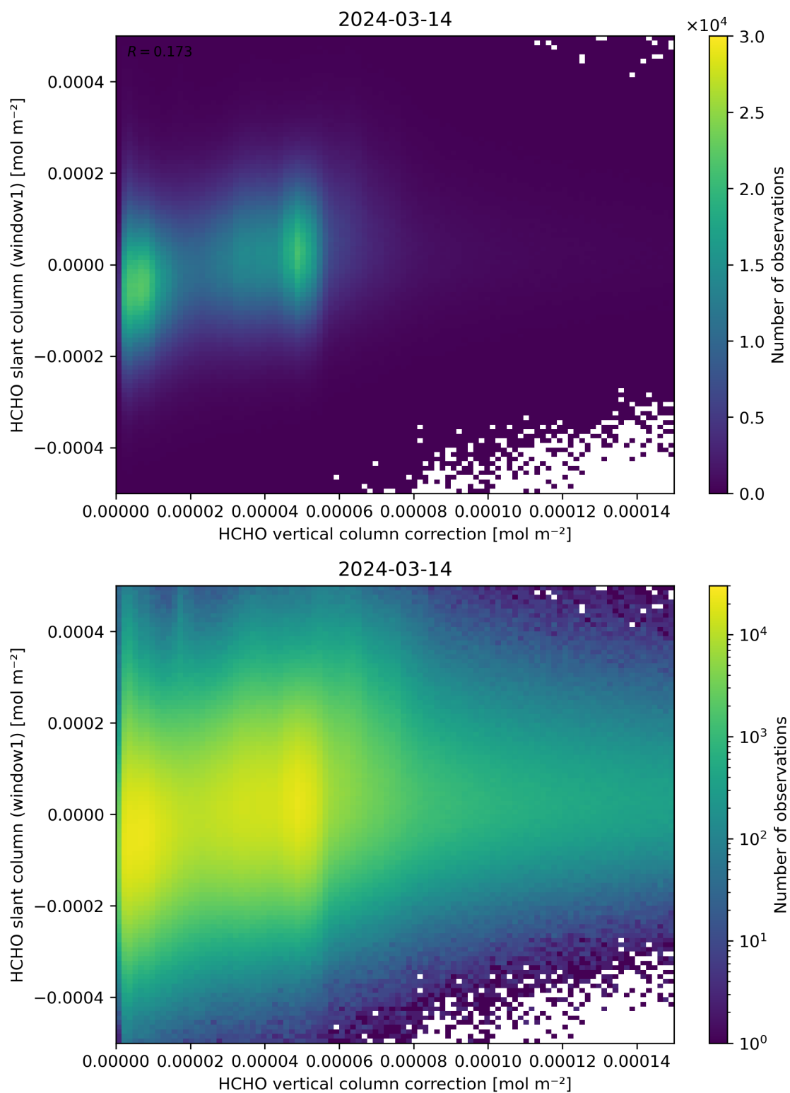
Figure 118: Scatter density plot of “HCHO vertical column correction” against “HCHO slant column (window1)” for 2024-03-14 to 2024-03-15.
