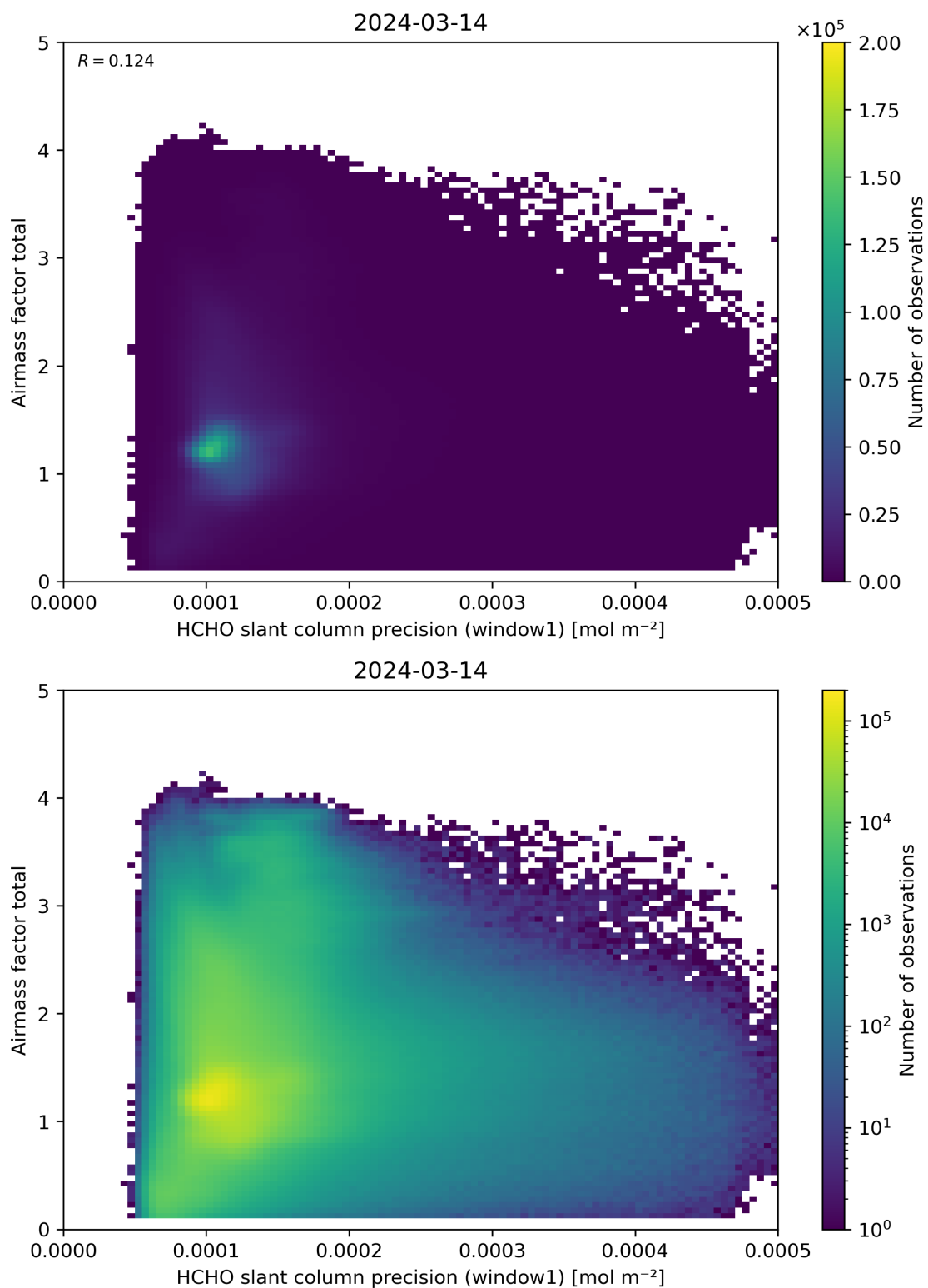
Figure 94: Scatter density plot of “HCHO slant column precision (window1)” against “Airmass factor total” for 2024-03-14 to 2024-03-15.
