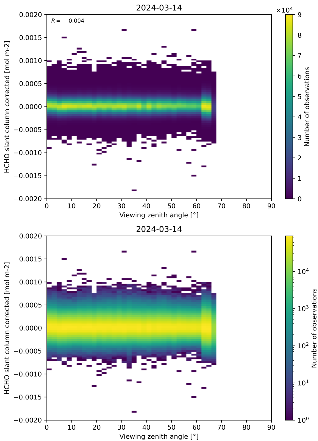
Figure 186: Scatter density plot of “Viewing zenith angle” against “HCHO slant column corrected” for 2024-03-14 to 2024-03-15.
