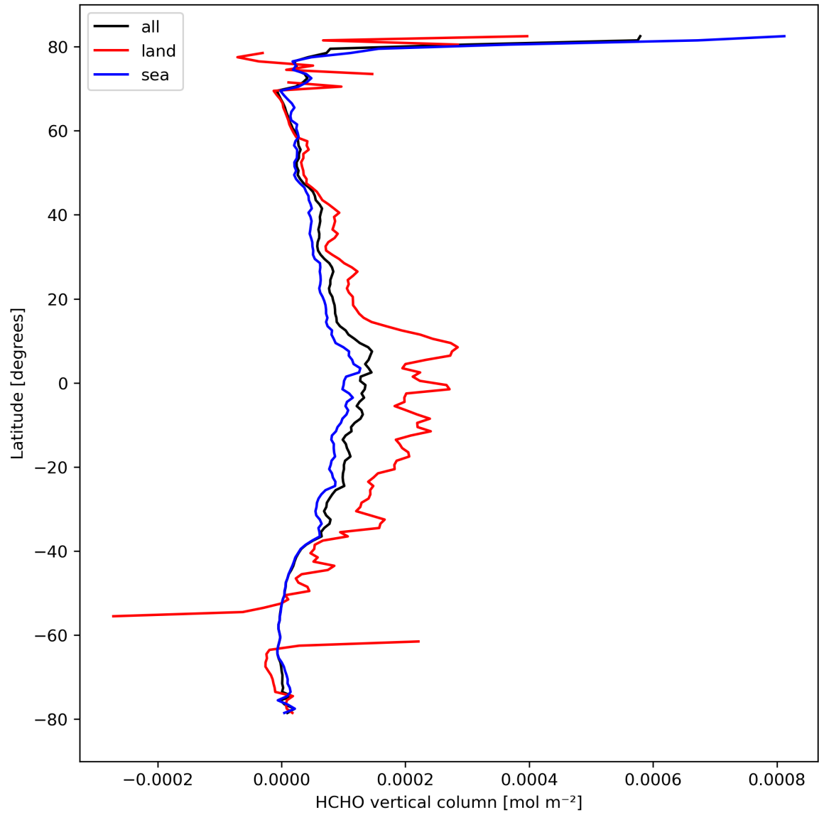
Figure 21: Zonal average of “HCHO vertical column” for 2024-03-14 to 2024-03-15.
