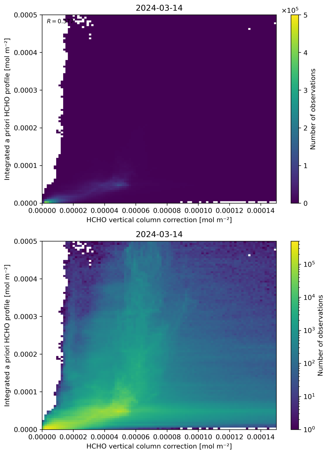
Figure 122: Scatter density plot of “HCHO vertical column correction” against “Integrated a priori HCHO profile” for 2024-03-14 to 2024-03-15.
