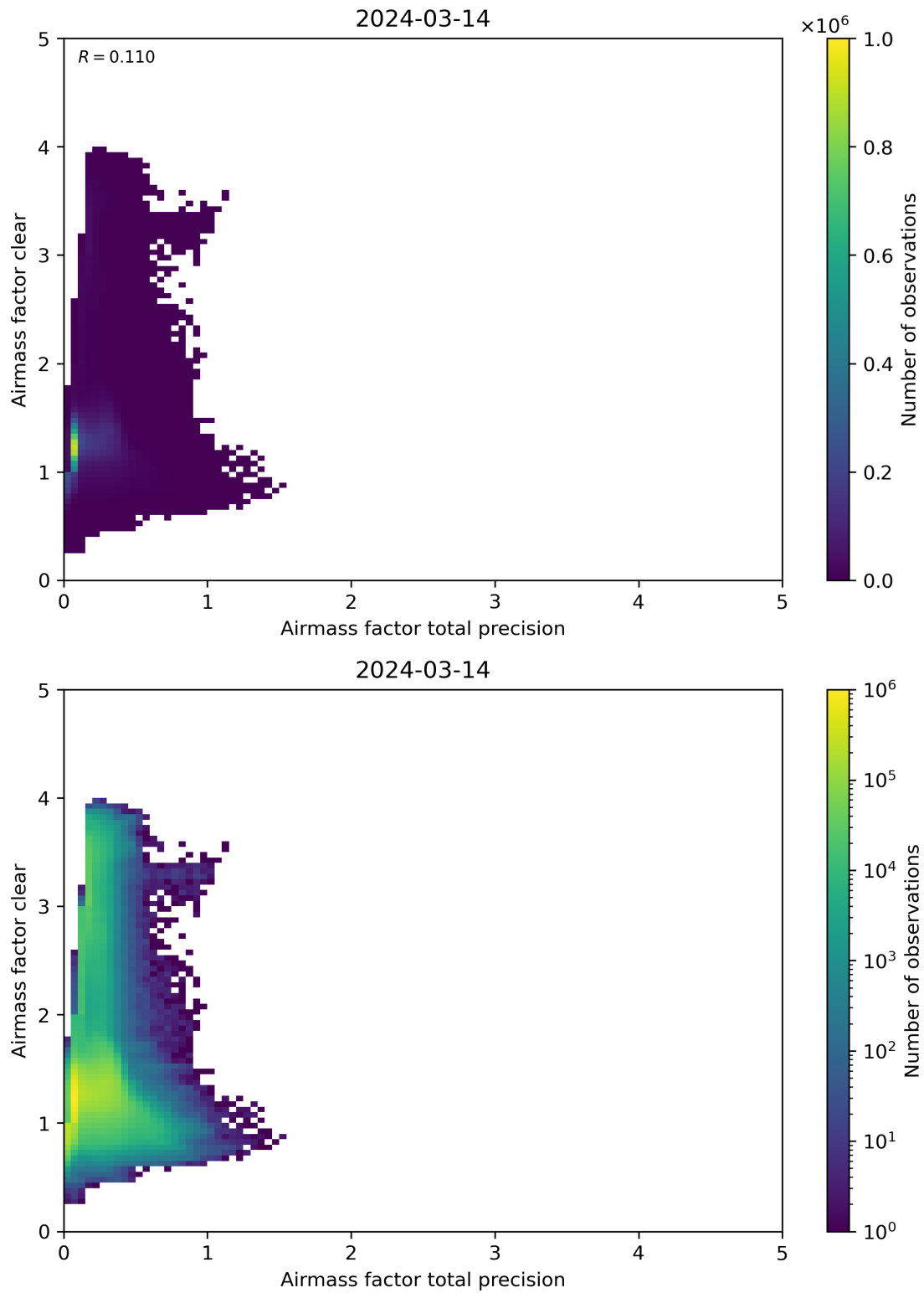
Figure 108: Scatter density plot of “Airmass factor total precision” against “Airmass factor clear” for 2024-03-14 to 2024-03-15.
