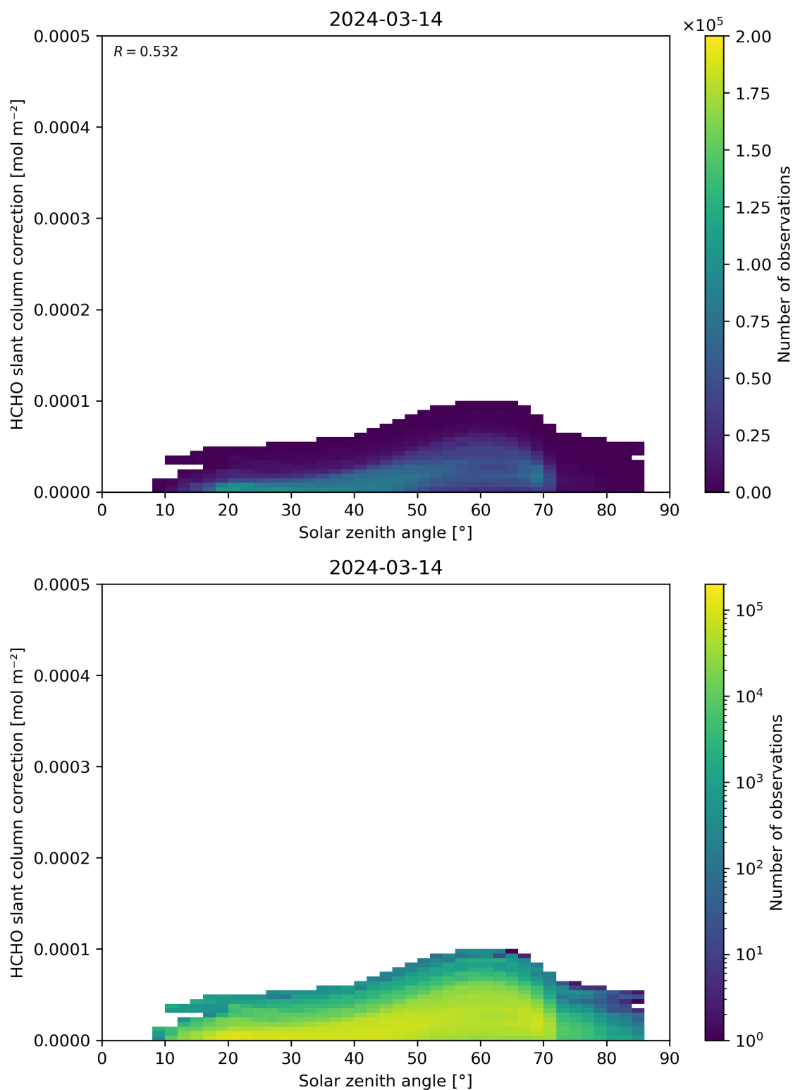
Figure 172: Scatter density plot of “Solar zenith angle” against “HCHO slant column correction” for 2024-03-14 to 2024-03-15.
