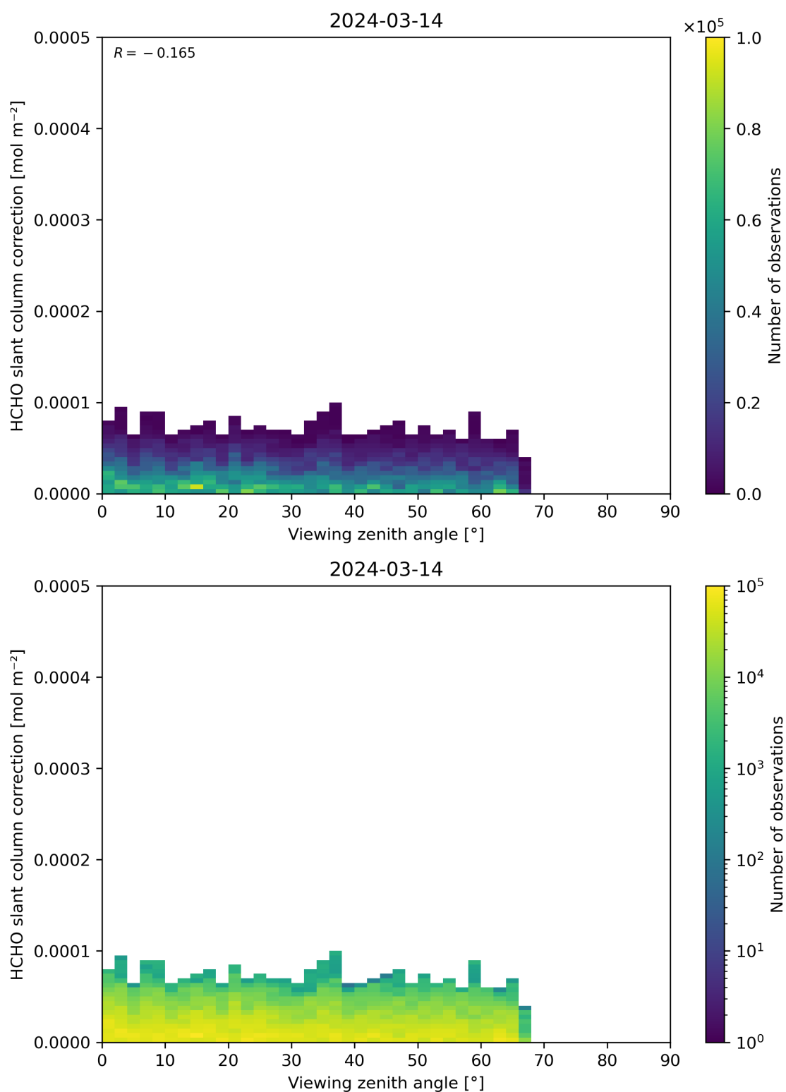
Figure 187: Scatter density plot of “Viewing zenith angle” against “HCHO slant column correction” for 2024-03-14 to 2024-03-15.
