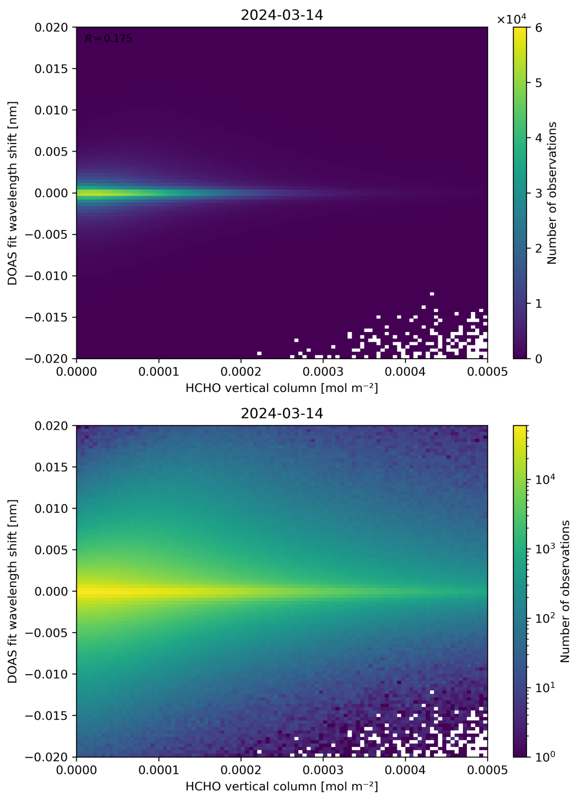
Figure 124: Scatter density plot of “HCHO vertical column” against “DOAS fit wavelength shift” for 2024-03-14 to 2024-03-15.
