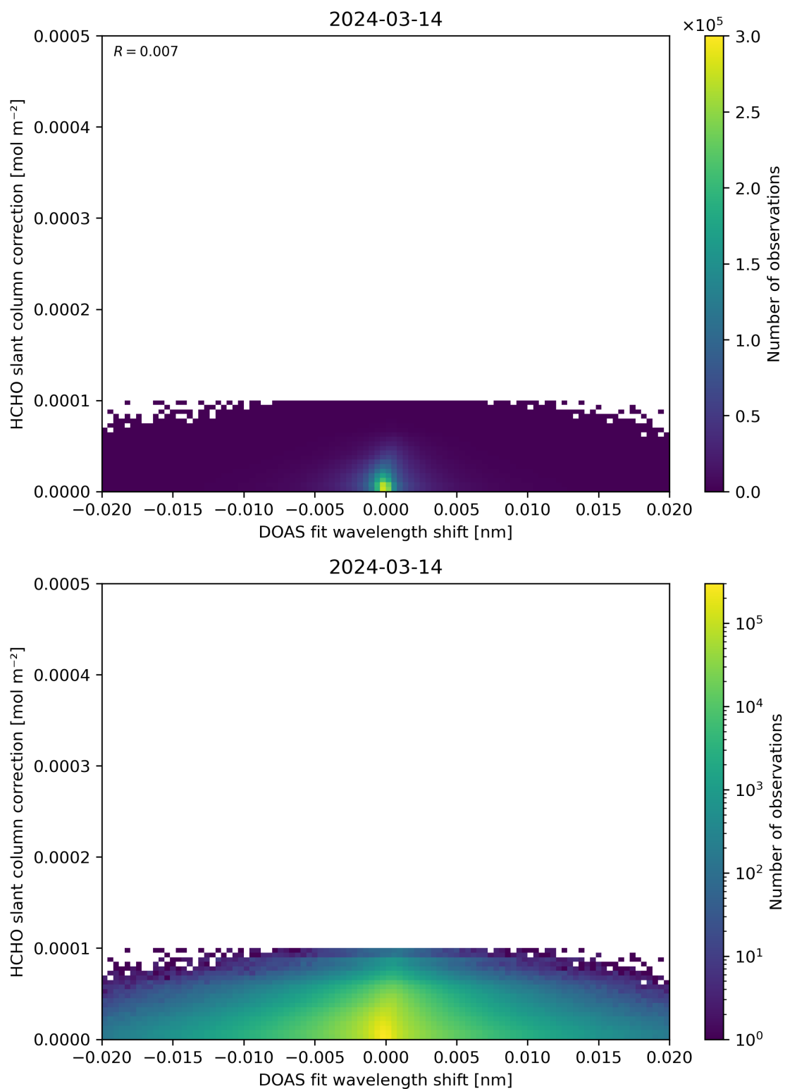
Figure 67: Scatter density plot of “DOAS fit wavelength shift” against “HCHO slant column correction” for 2024-03-14 to 2024-03-15.
