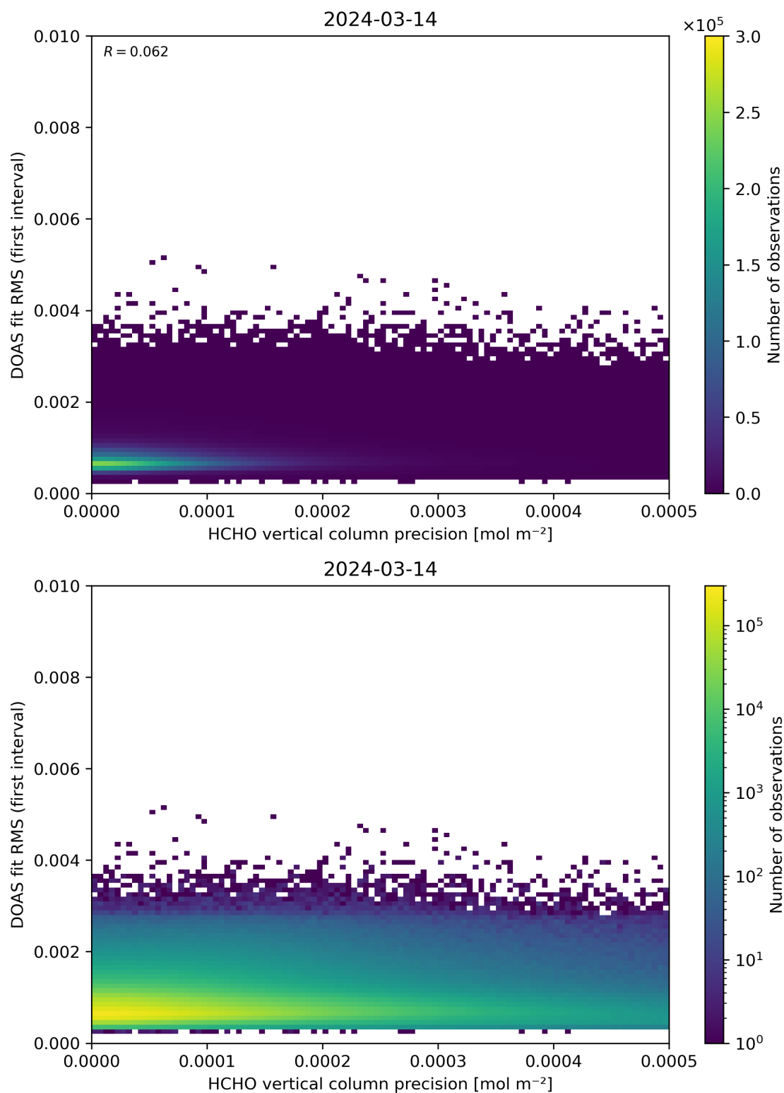
Figure 136: Scatter density plot of “HCHO vertical column precision” against “DOAS fit RMS (first interval)” for 2024-03-14 to 2024-03-15.
