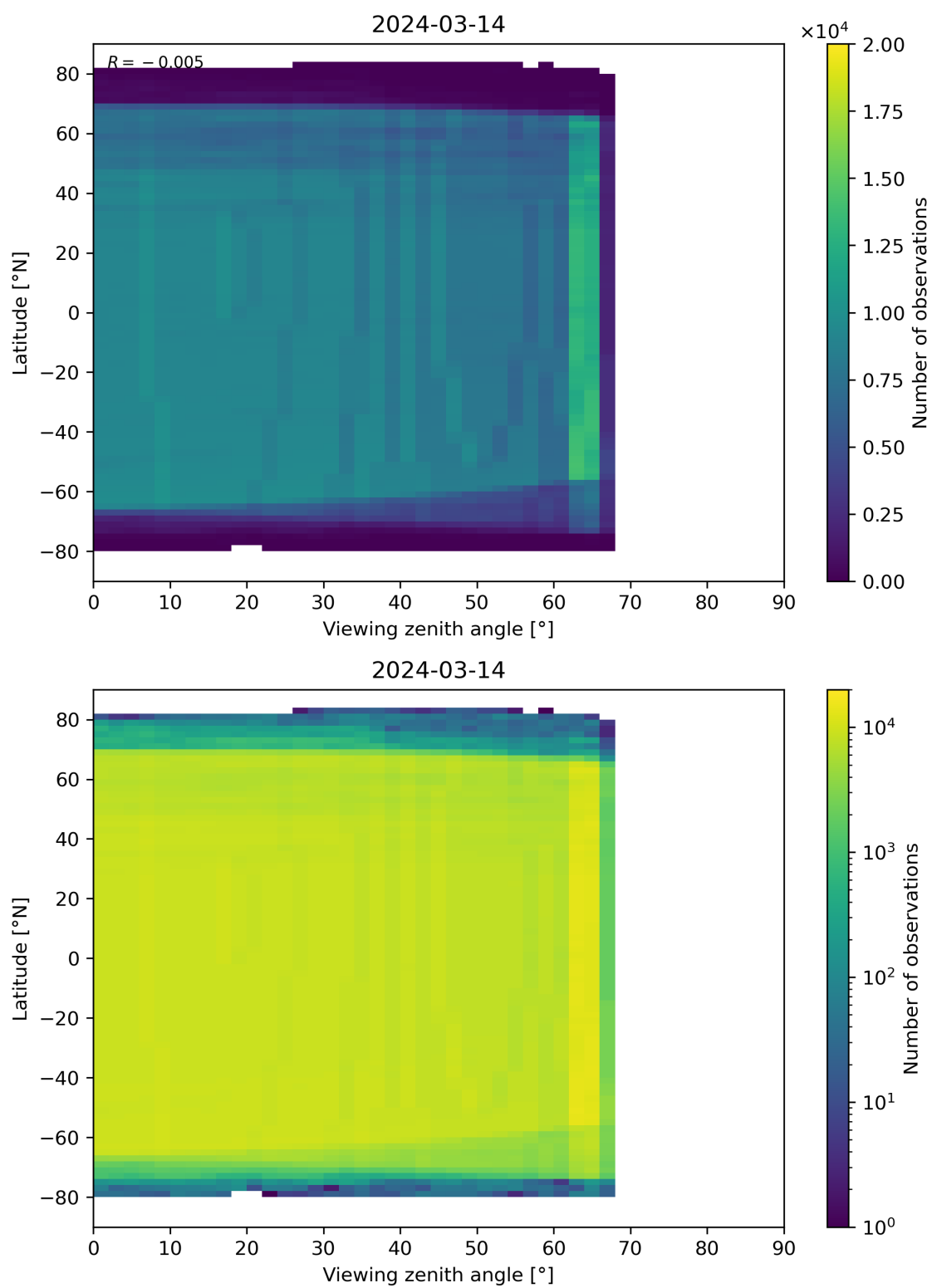
Figure 196: Scatter density plot of “Viewing zenith angle” against “Latitude” for 2024-03-14 to 2024-03-15.
