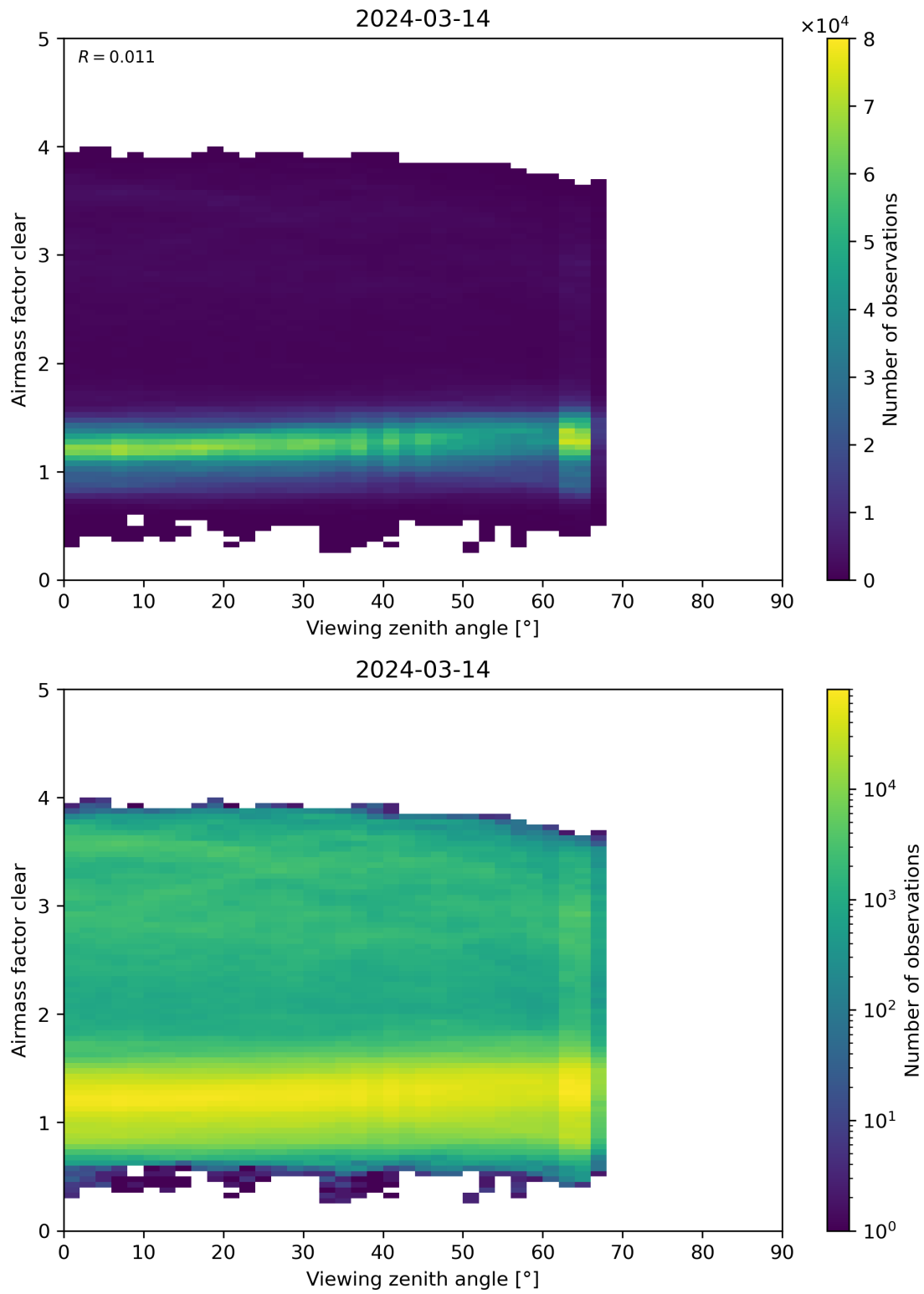
Figure 185: Scatter density plot of “Viewing zenith angle” against “Airmass factor clear” for 2024-03-14 to 2024-03-15.
