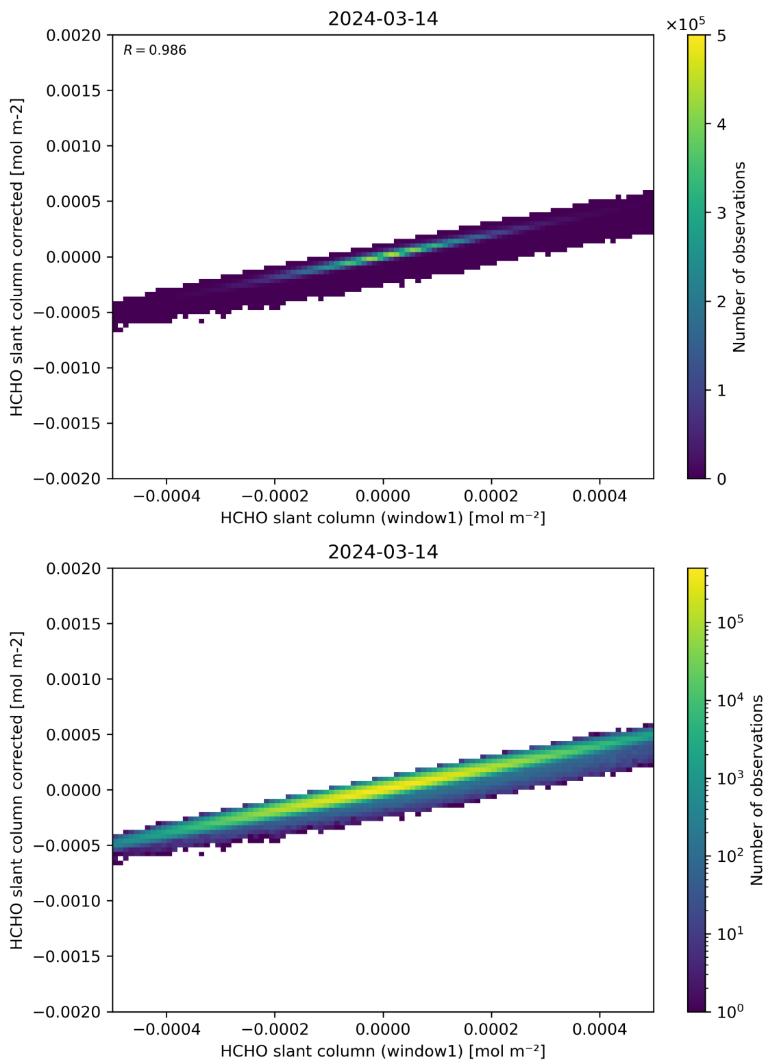
Figure 82: Scatter density plot of “HCHO slant column (window1)” against “HCHO slant column corrected” for 2024-03-14 to 2024-03-15.
