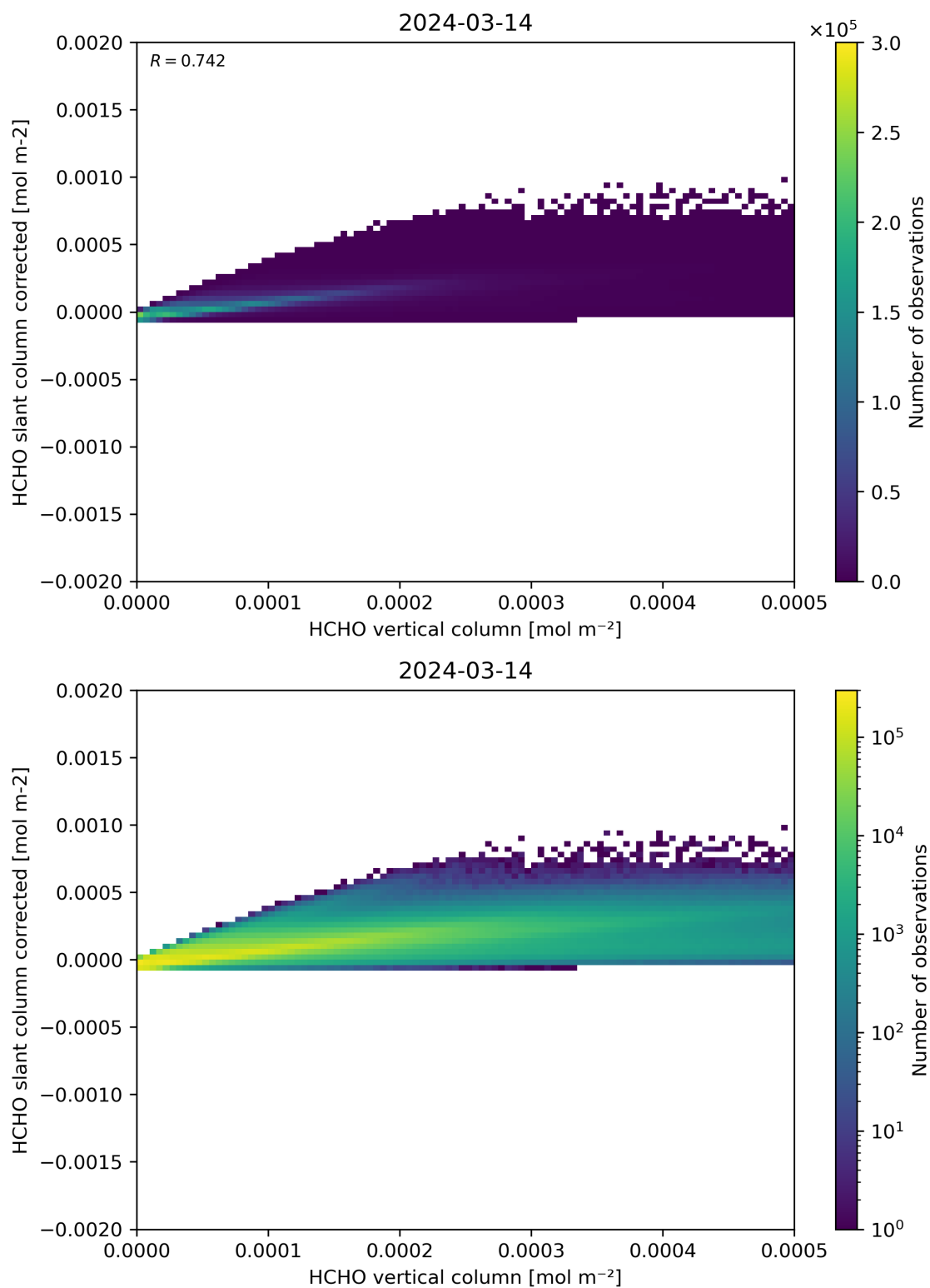
Figure 127: Scatter density plot of “HCHO vertical column” against “HCHO slant column corrected” for 2024-03-14 to 2024-03-15.
