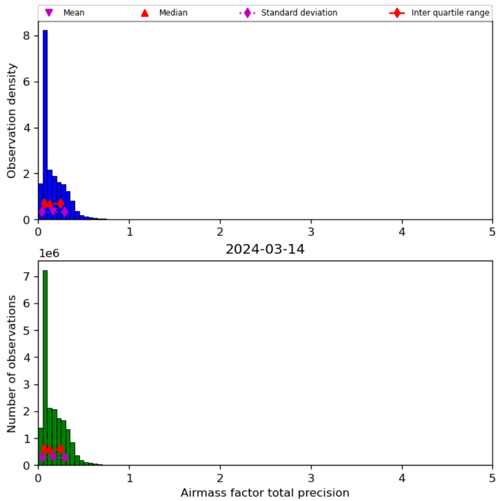
Figure 41: Histogram of “Airmass factor total precision” for 2024-03-14 to 2024-03-15
