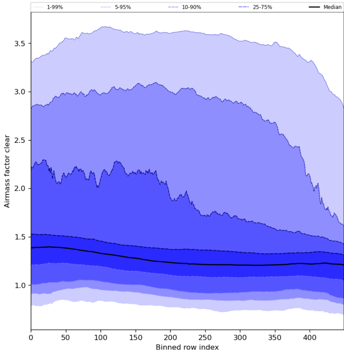
Figure 56: Along track statistics of “Airmass factor clear” for 2024-03-14 to 2024-03-15
