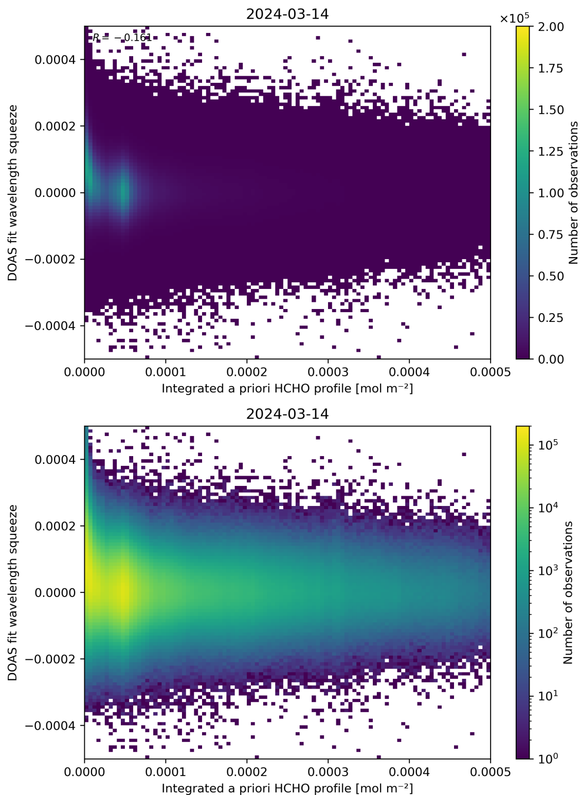
Figure 150: Scatter density plot of “Integrated a priori HCHO profile” against “DOAS fit wavelength squeeze” for 2024-03-14 to 2024-03-15.
