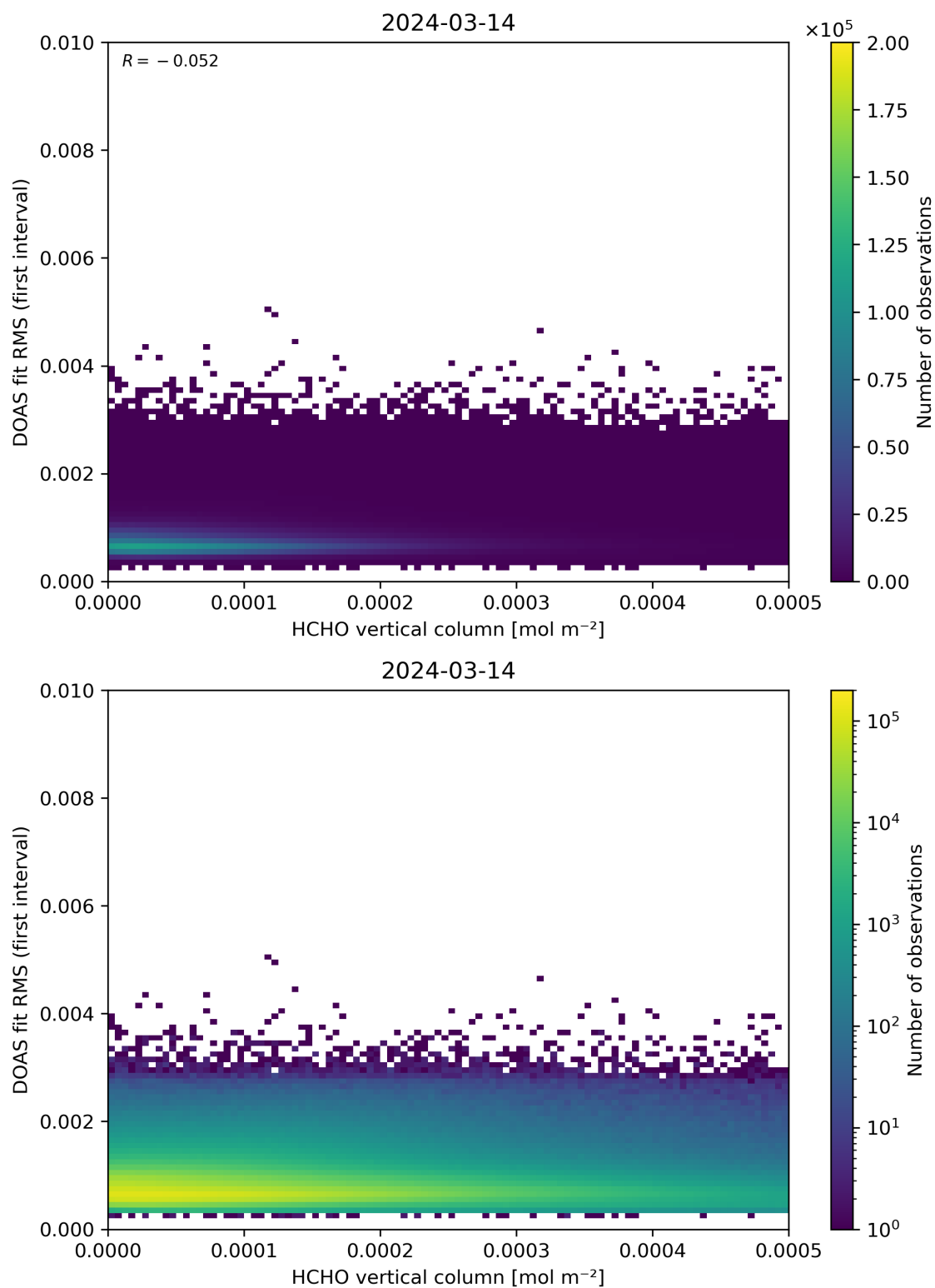
Figure 123: Scatter density plot of “HCHO vertical column” against “DOAS fit RMS (first interval)” for 2024-03-14 to 2024-03-15.
