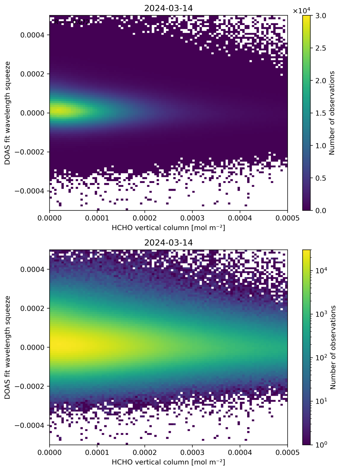
Figure 125: Scatter density plot of “HCHO vertical column” against “DOAS fit wavelength squeeze” for 2024-03-14 to 2024-03-15.
