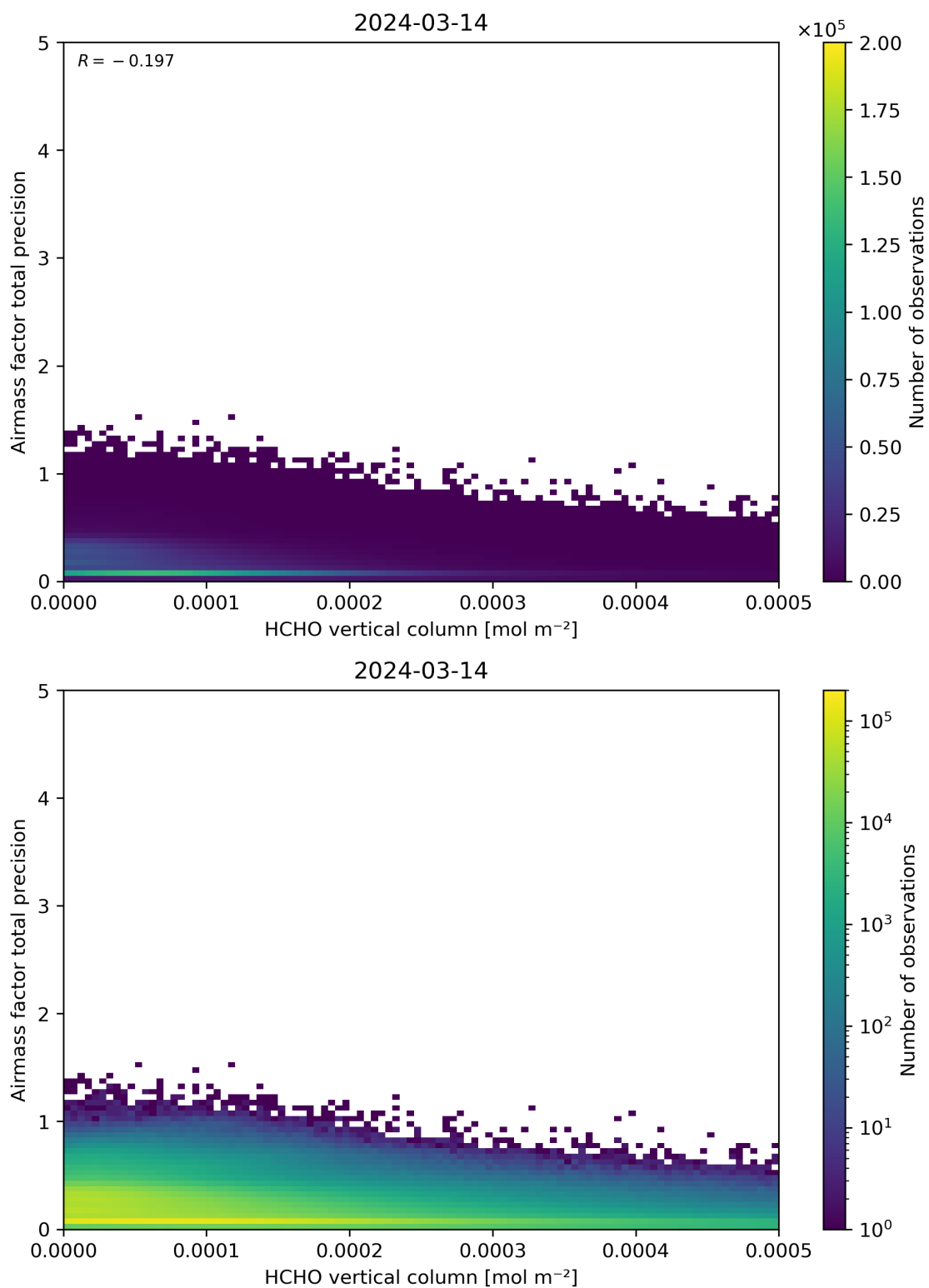
Figure 132: Scatter density plot of “HCHO vertical column” against “Airmass factor total precision” for 2024-03-14 to 2024-03-15.
