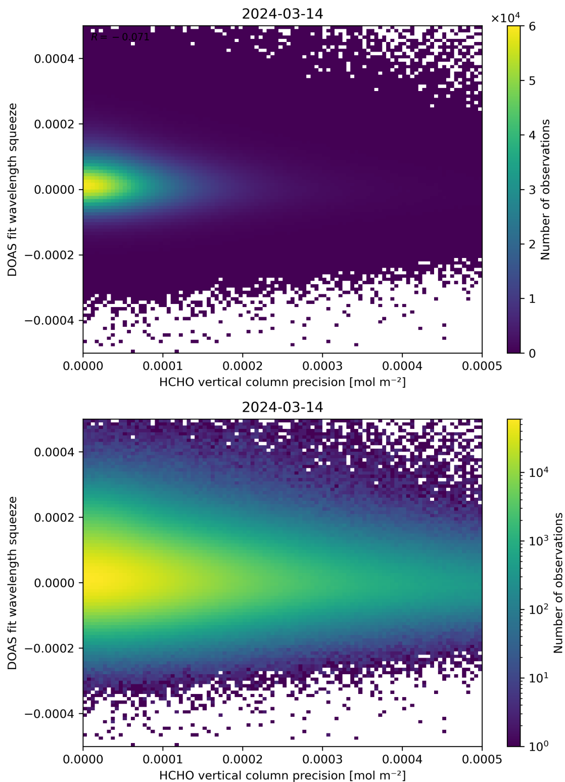
Figure 138: Scatter density plot of “HCHO vertical column precision” against “DOAS fit wavelength squeeze” for 2024-03-14 to 2024-03-15.
