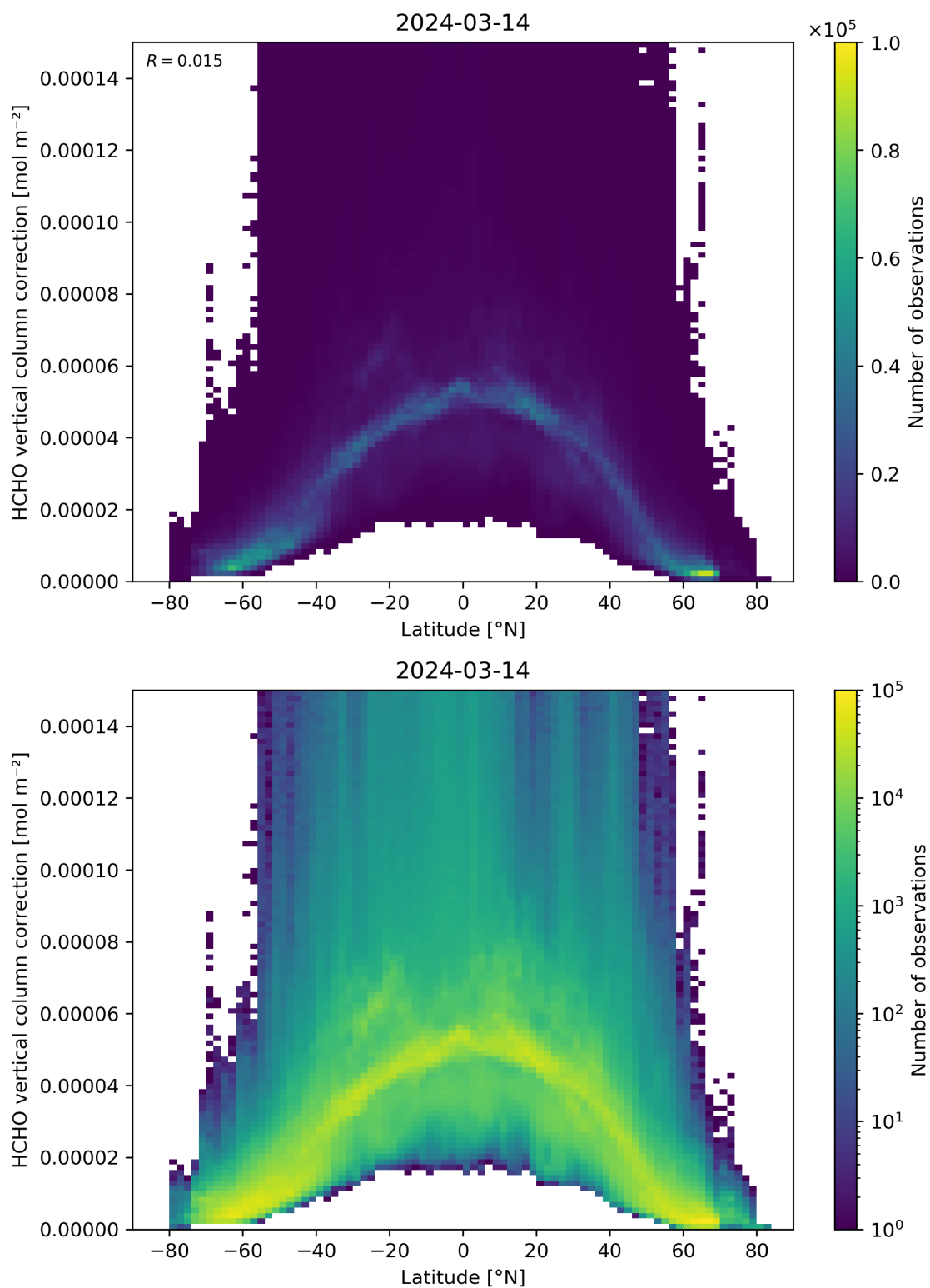
Figure 164: Scatter density plot of “Latitude” against “HCHO vertical column correction” for 2024-03-14 to 2024-03-15.
