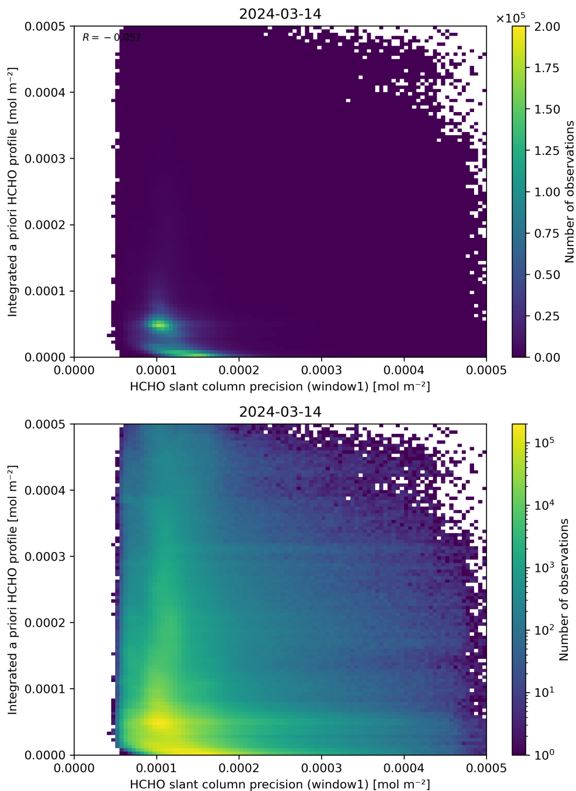
Figure 96: Scatter density plot of “HCHO slant column precision (window1)” against “Integrated a priori HCHO profile” for 2024-03-14 to 2024-03-15.
