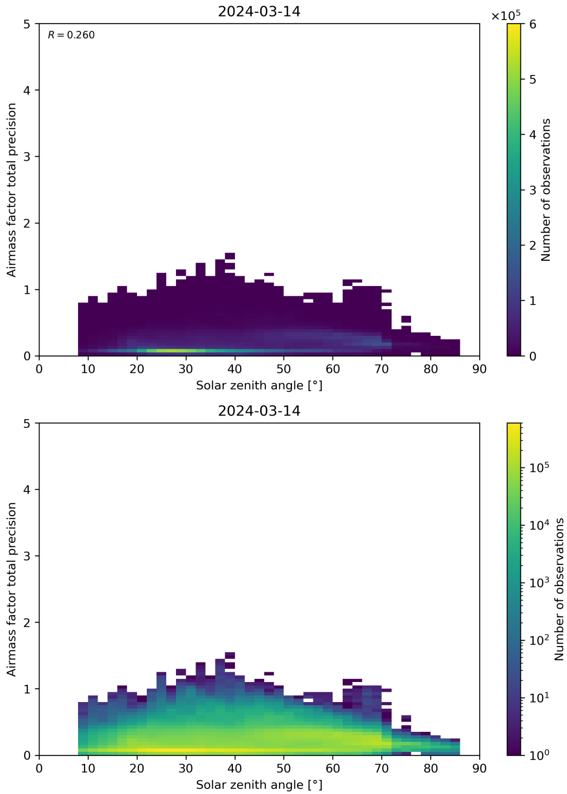
Figure 176: Scatter density plot of “Solar zenith angle” against “Airmass factor total precision” for 2024-03-14 to 2024-03-15.
