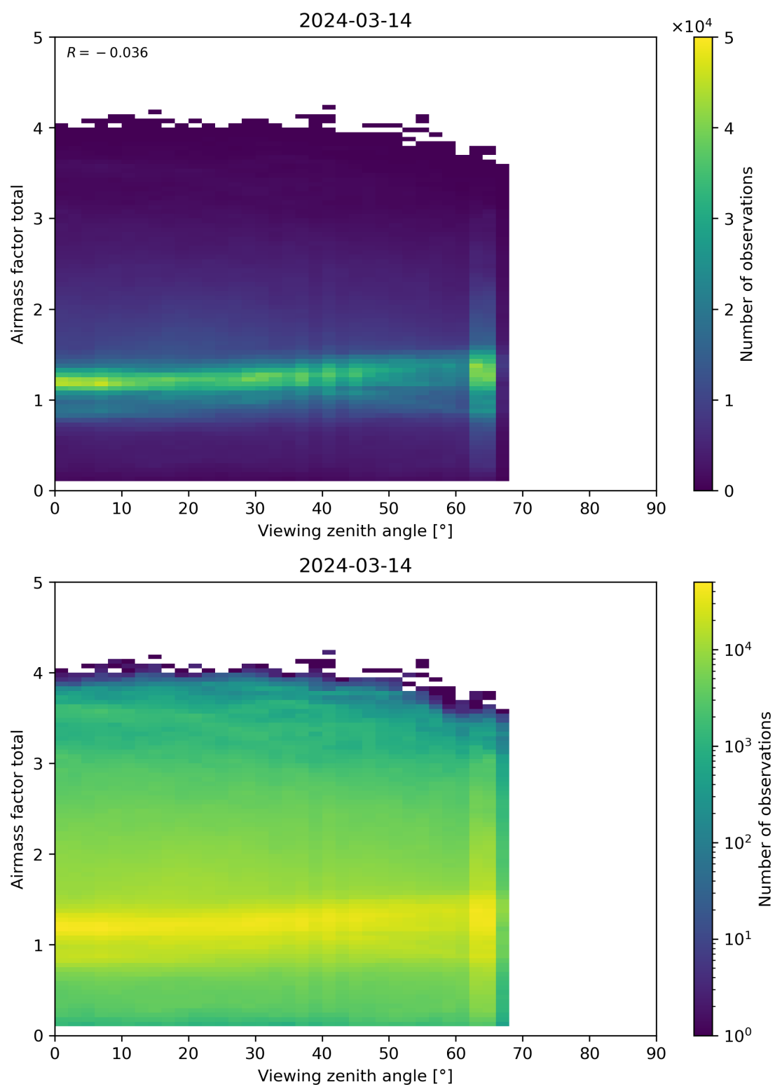
Figure 190: Scatter density plot of “Viewing zenith angle” against “Airmass factor total” for 2024-03-14 to 2024-03-15.
