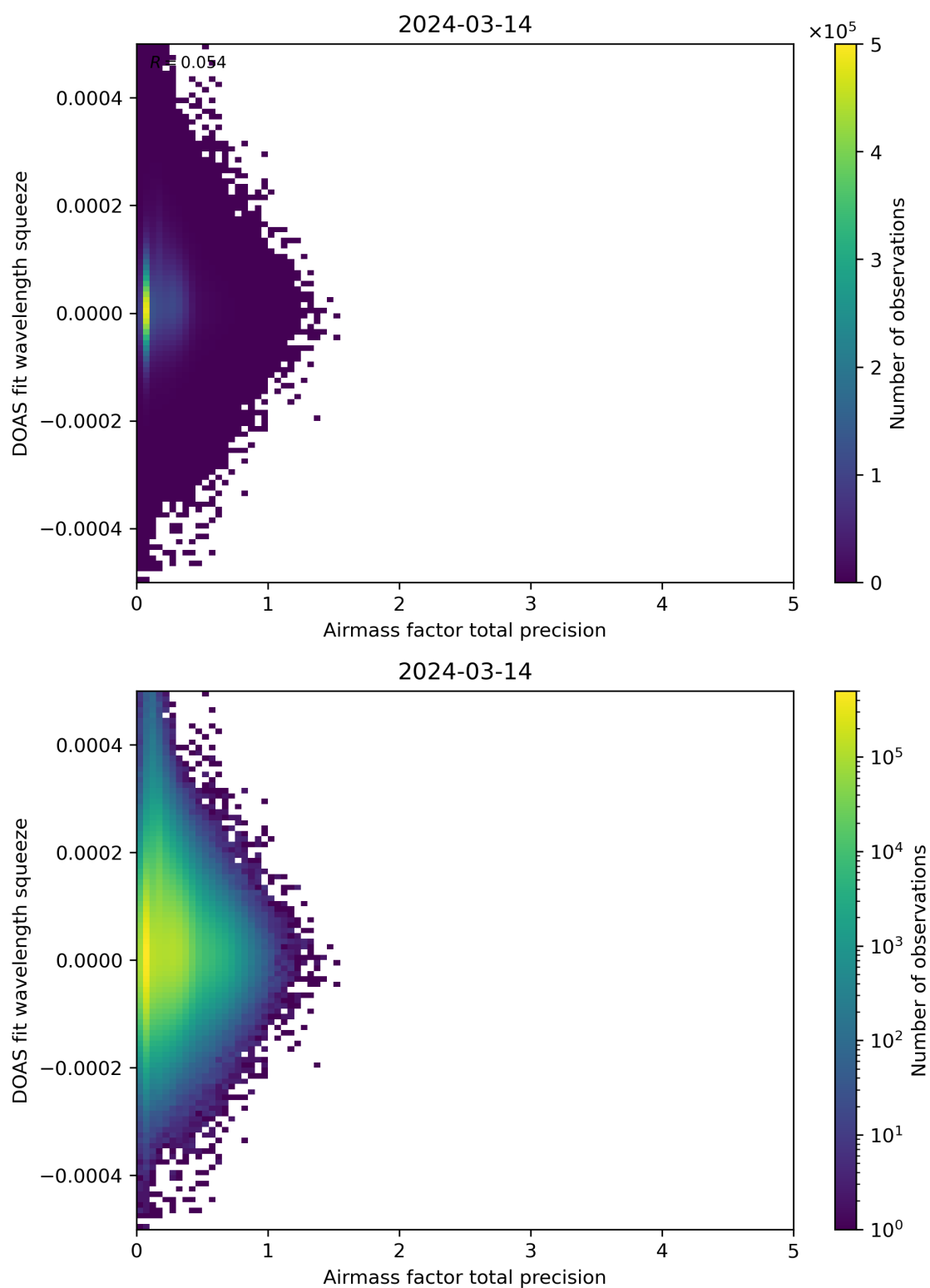
Figure 107: Scatter density plot of “Airmass factor total precision” against “DOAS fit wavelength squeeze” for 2024-03-14 to 2024-03-15.
