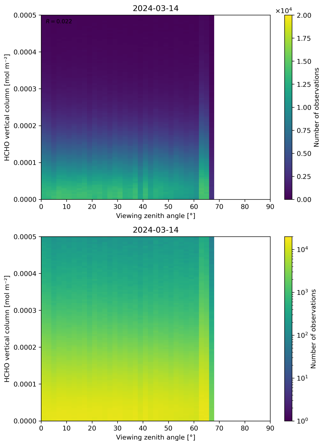
Figure 192: Scatter density plot of “Viewing zenith angle” against “HCHO vertical column” for 2024-03-14 to 2024-03-15.
