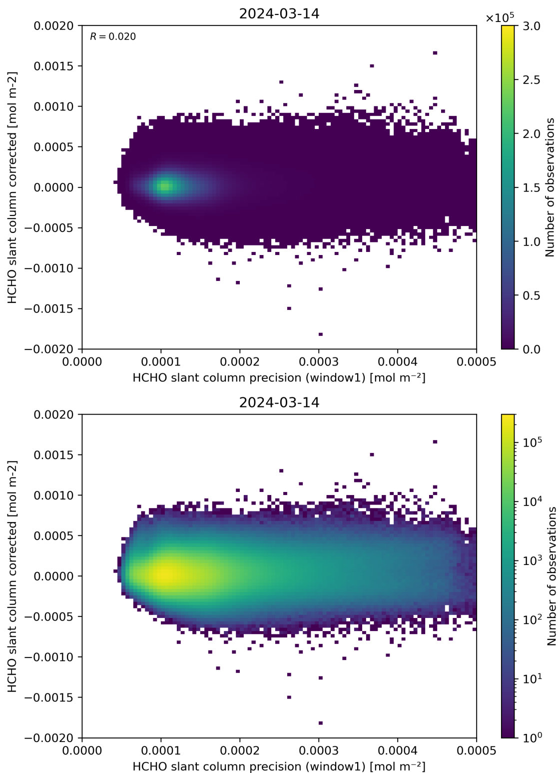
Figure 92: Scatter density plot of “HCHO slant column precision (window1)” against “HCHO slant column corrected” for 2024-03-14 to 2024-03-15.
