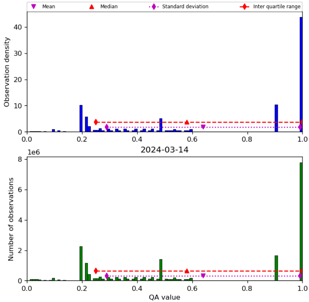
Figure 34: Histogram of “QA value” for 2024-03-14 to 2024-03-15
