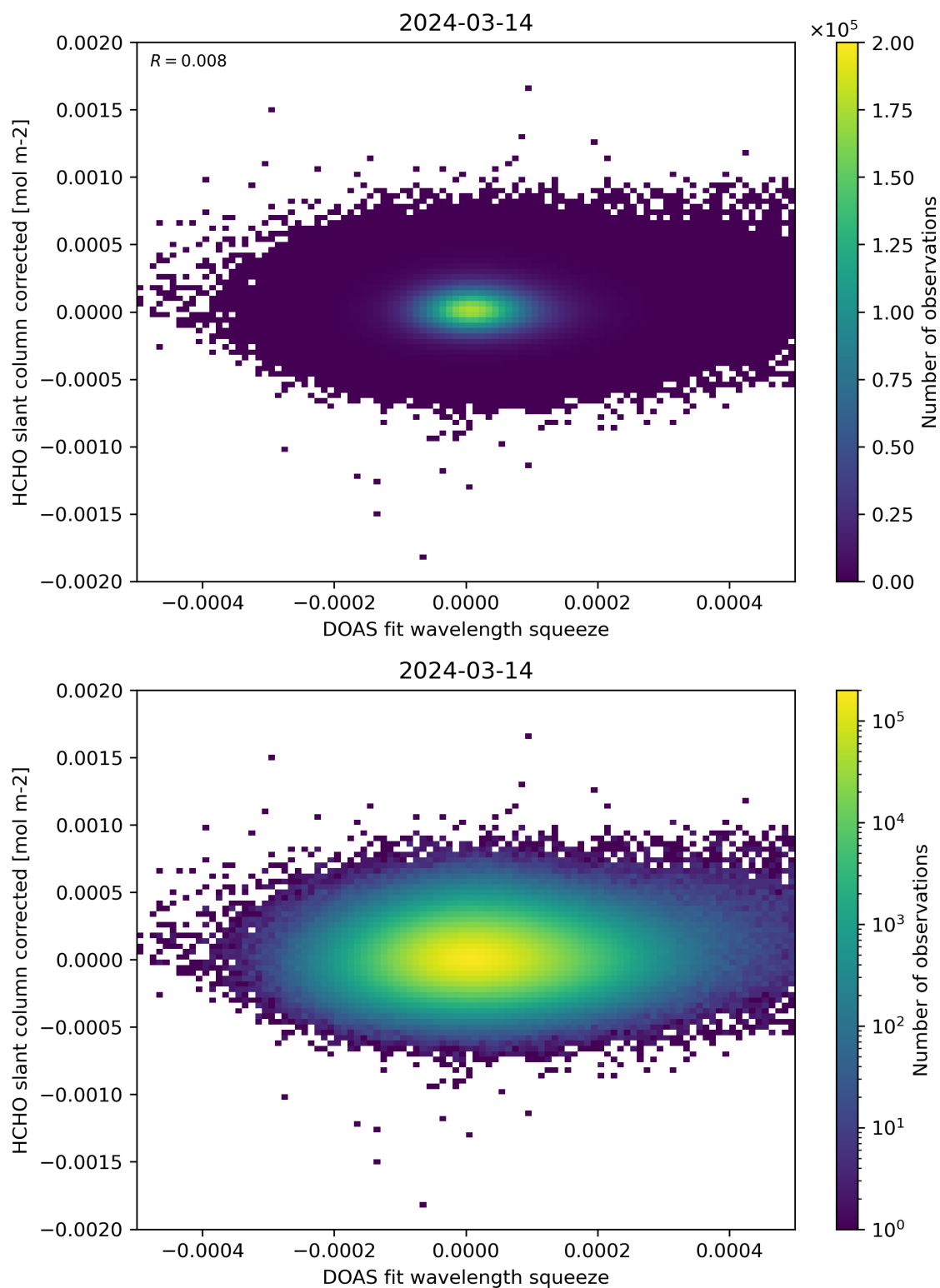
Figure 69: Scatter density plot of “DOAS fit wavelength squeeze” against “HCHO slant column corrected” for 2024-03-14 to 2024-03-15.
