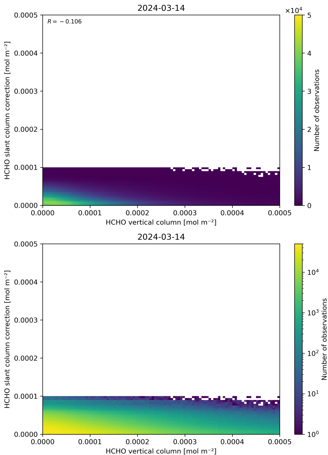
Figure 128: Scatter density plot of “HCHO vertical column” against “HCHO slant column correction” for 2024-03-14 to 2024-03-15.
