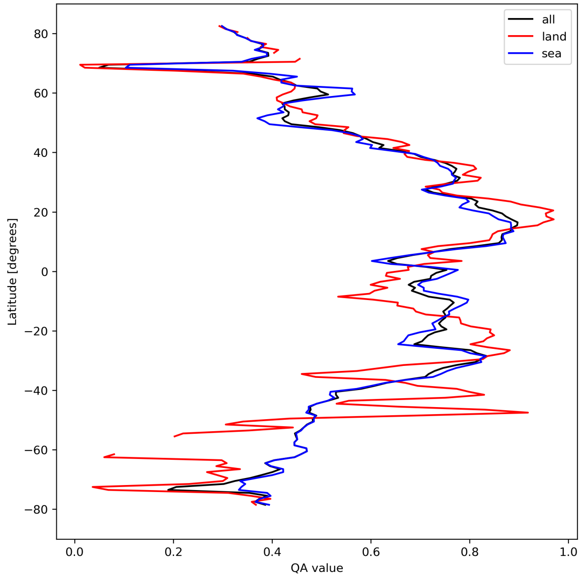
Figure 20: Zonal average of “QA value” for 2024-03-14 to 2024-03-15.
