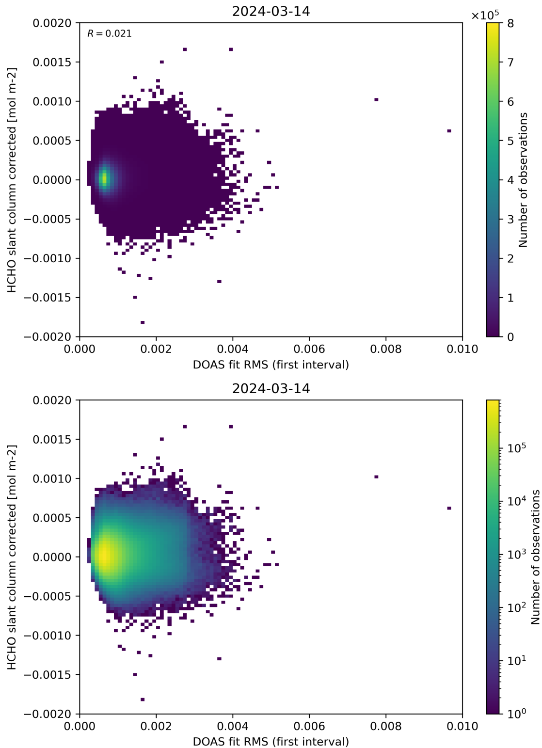
Figure 62: Scatter density plot of “DOAS fit RMS (first interval)” against “HCHO slant column corrected” for 2024-03-14 to 2024-03-15.
