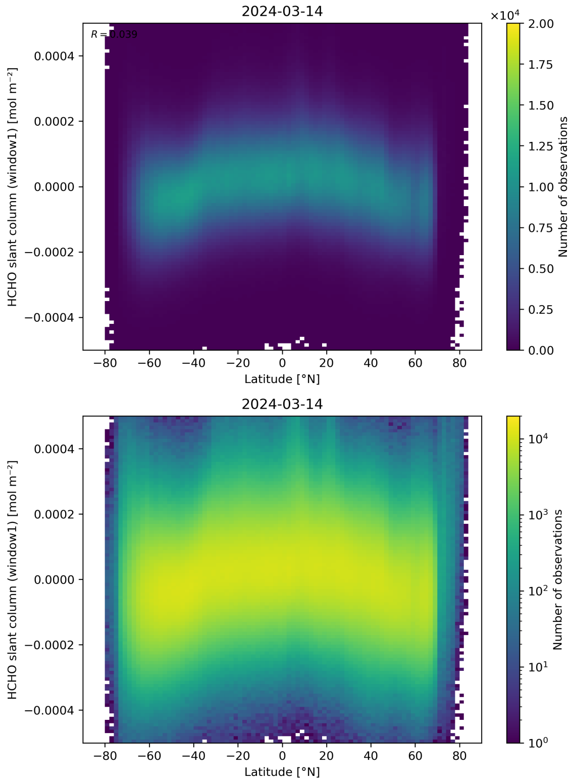
Figure 159: Scatter density plot of “Latitude” against “HCHO slant column (window1)” for 2024-03-14 to 2024-03-15.
