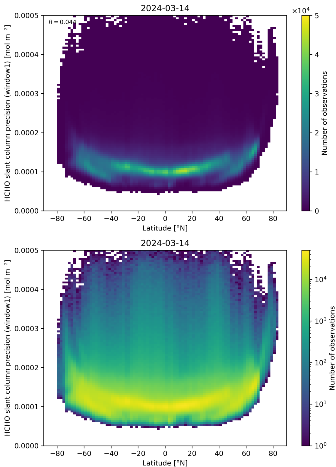
Figure 160: Scatter density plot of “Latitude” against “HCHO slant column precision (window1)” for 2024-03-14 to 2024-03-15.
