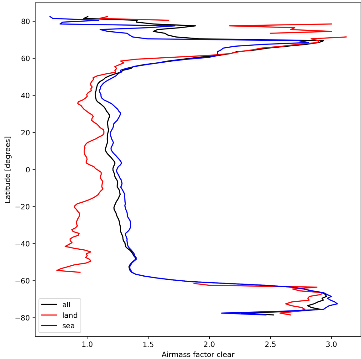
Figure 28: Zonal average of “Airmass factor clear” for 2024-03-14 to 2024-03-15.
