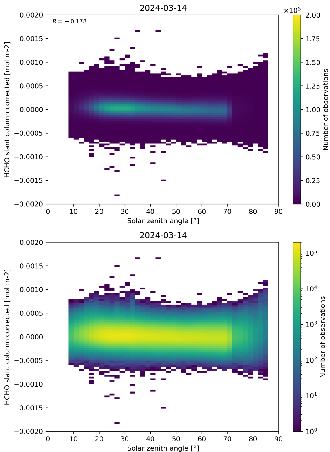
Figure 171: Scatter density plot of “Solar zenith angle” against “HCHO slant column corrected” for 2024-03-14 to 2024-03-15.
