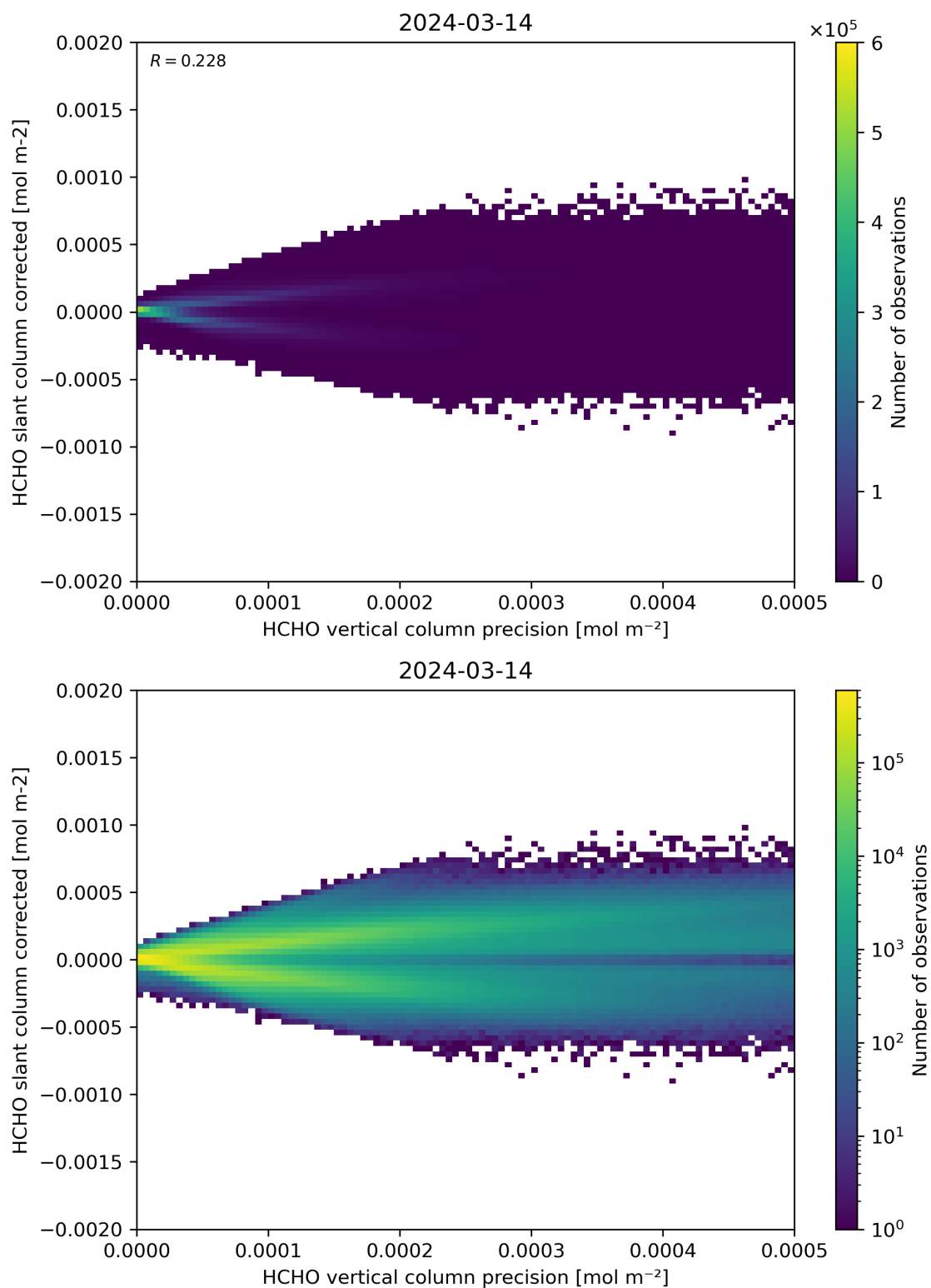
Figure 140: Scatter density plot of “HCHO vertical column precision” against “HCHO slant column corrected” for 2024-03-14 to 2024-03-15.
