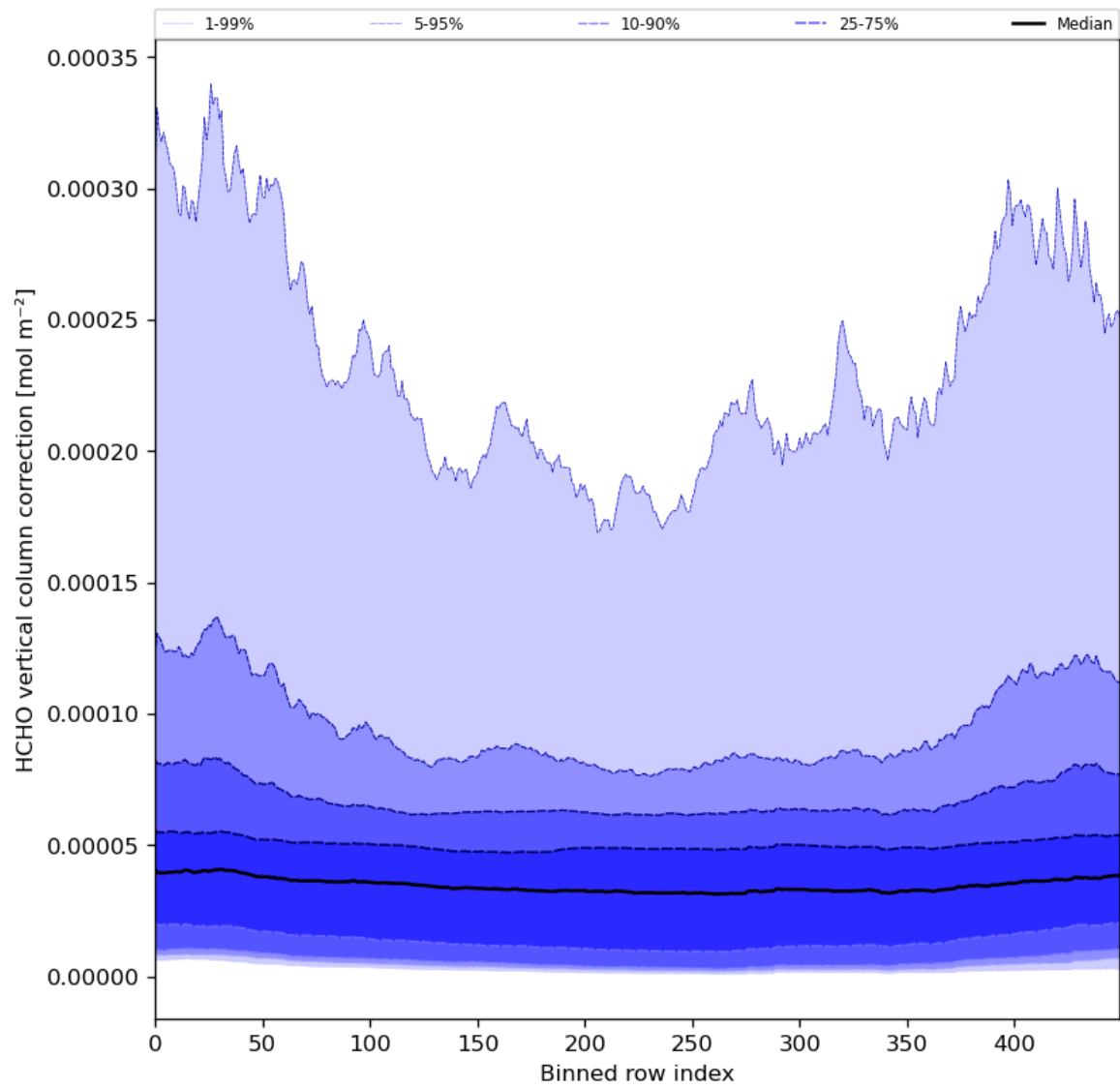
Figure 51: Along track statistics of “HCHO vertical column correction” for 2024-03-14 to 2024-03-15
