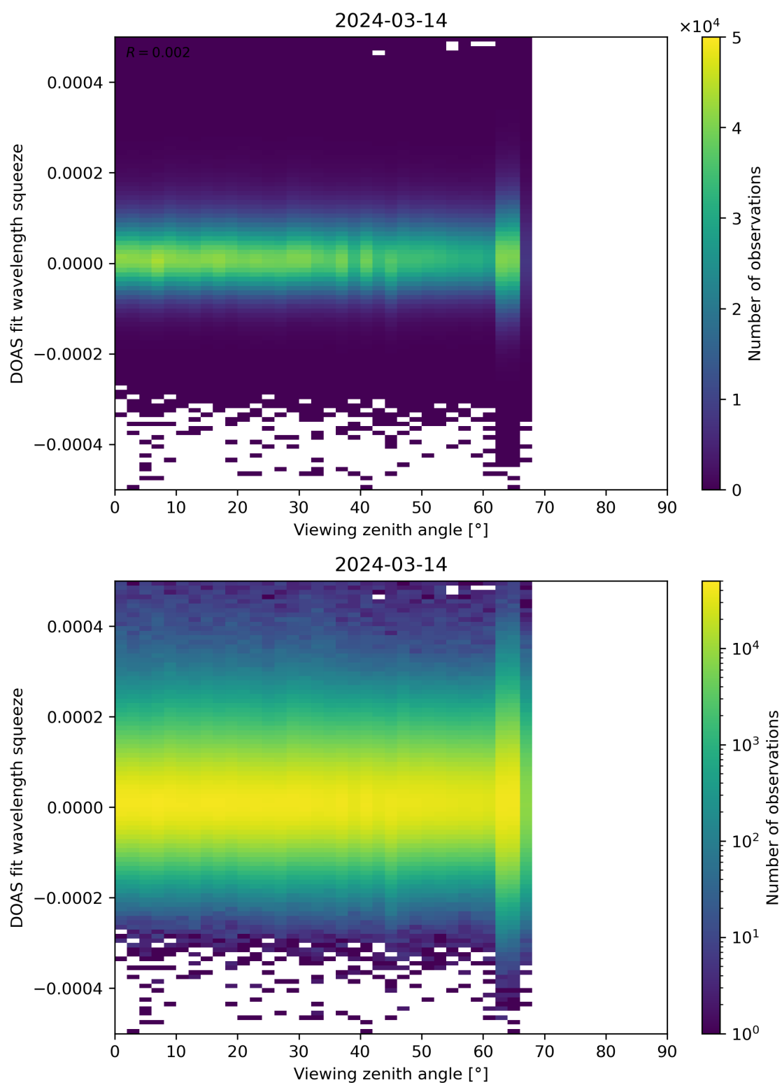
Figure 184: Scatter density plot of “Viewing zenith angle” against “DOAS fit wavelength squeeze” for 2024-03-14 to 2024-03-15.
