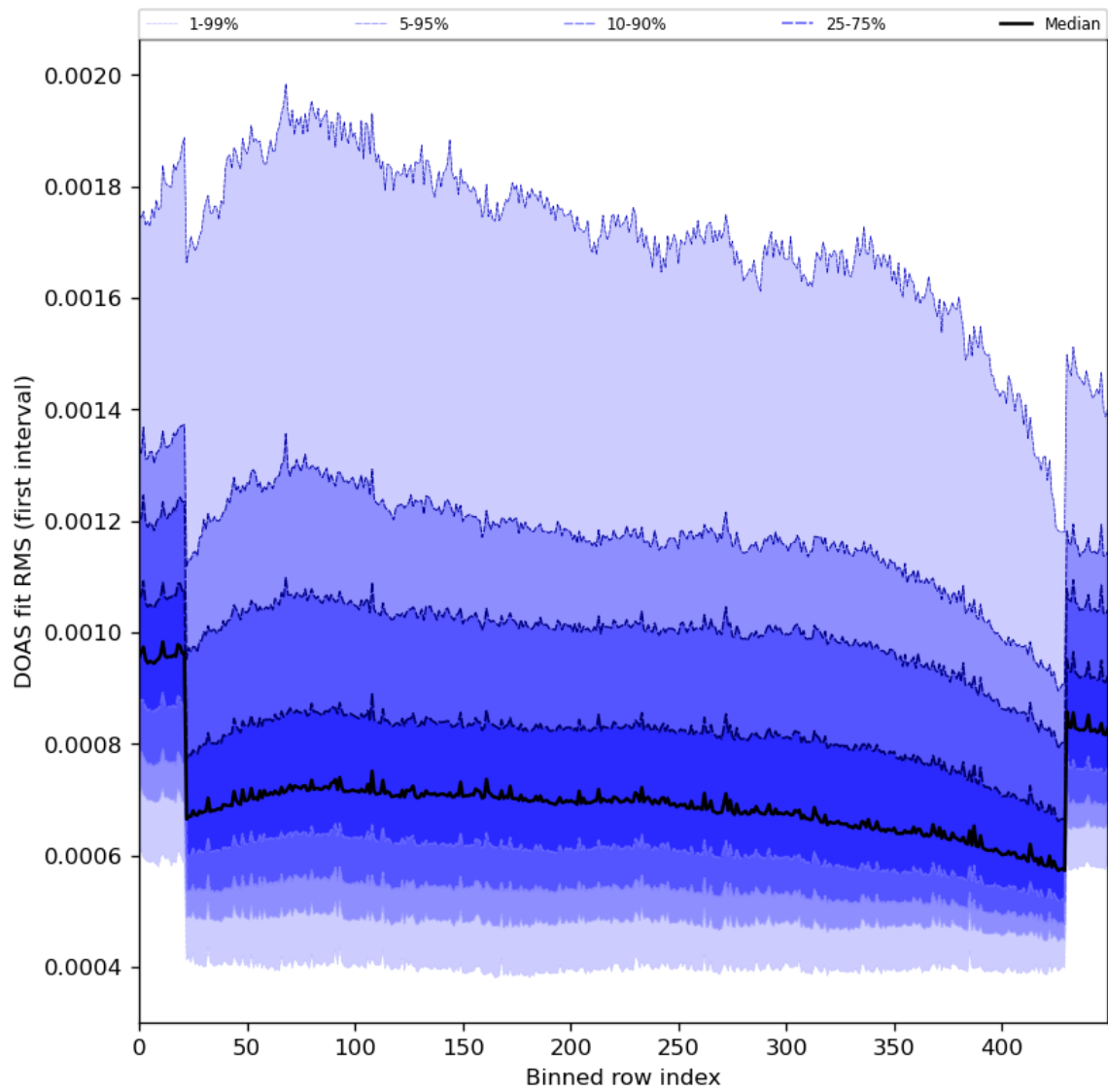
Figure 60: Along track statistics of “DOAS fit RMS (first interval)” for 2024-03-14 to 2024-03-15
