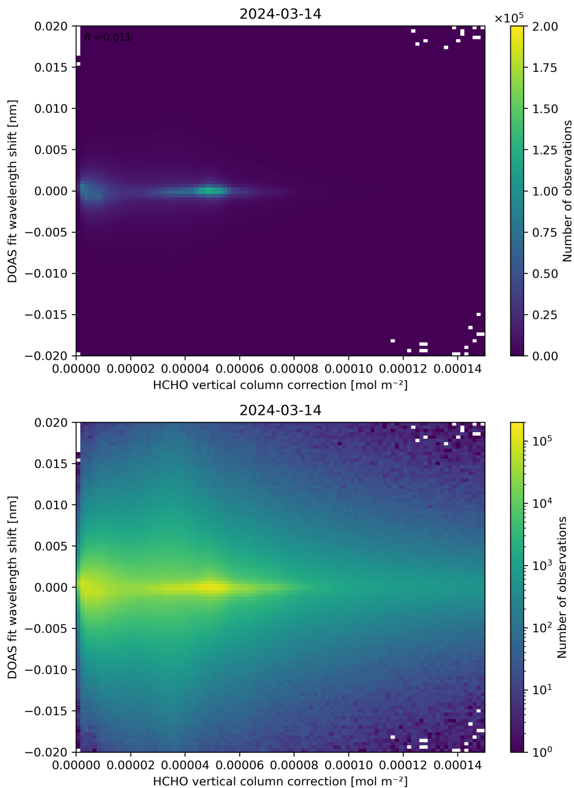
Figure 113: Scatter density plot of “HCHO vertical column correction” against “DOAS fit wavelength shift” for 2024-03-14 to 2024-03-15.
