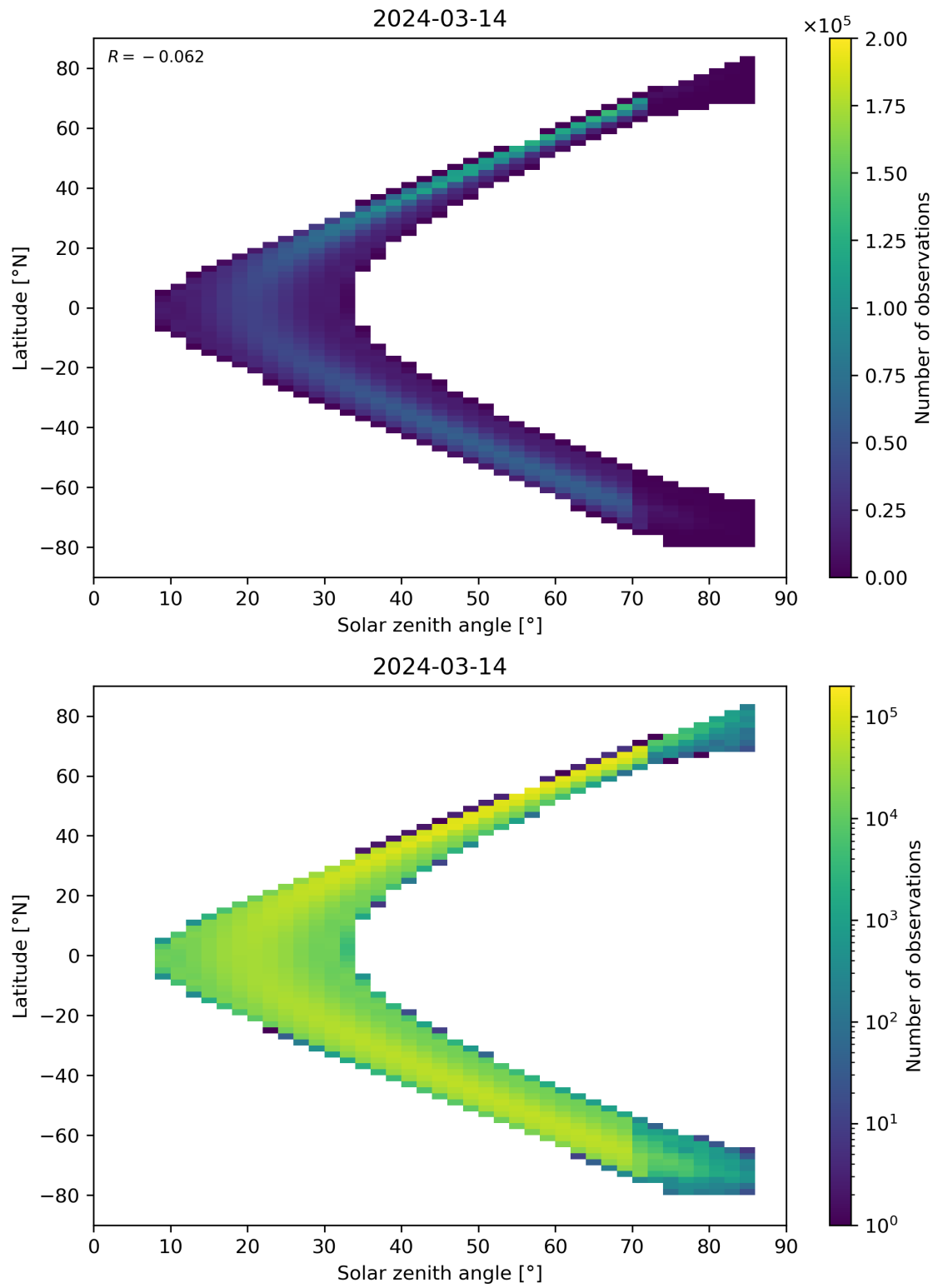
Figure 181: Scatter density plot of “Solar zenith angle” against “Latitude” for 2024-03-14 to 2024-03-15.
