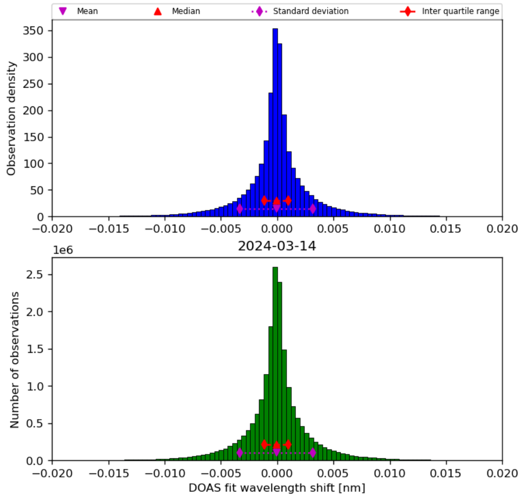
Figure 44: Histogram of “DOAS fit wavelength shift” for 2024-03-14 to 2024-03-15
