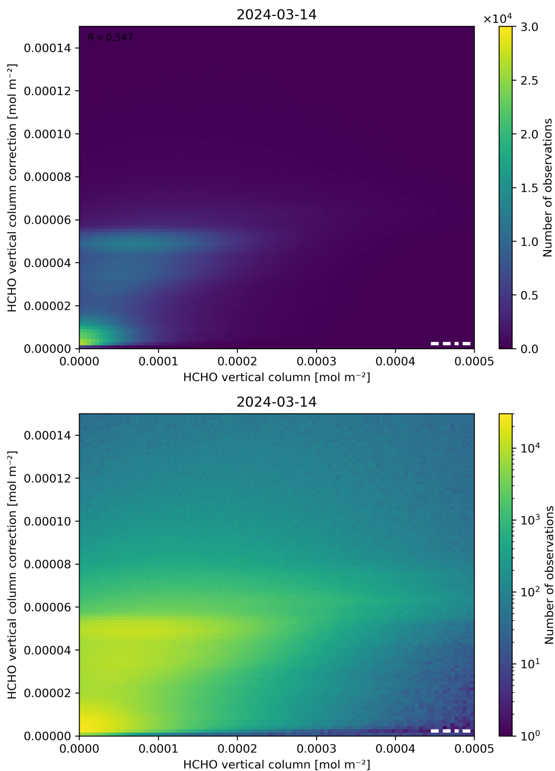
Figure 133: Scatter density plot of “HCHO vertical column” against “HCHO vertical column correction” for 2024-03-14 to 2024-03-15.
