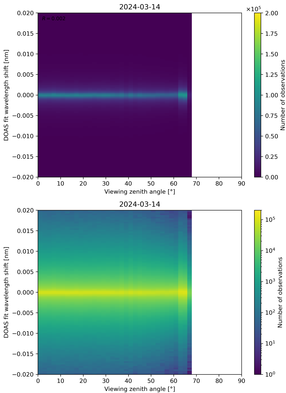
Figure 183: Scatter density plot of “Viewing zenith angle” against “DOAS fit wavelength shift” for 2024-03-14 to 2024-03-15.
