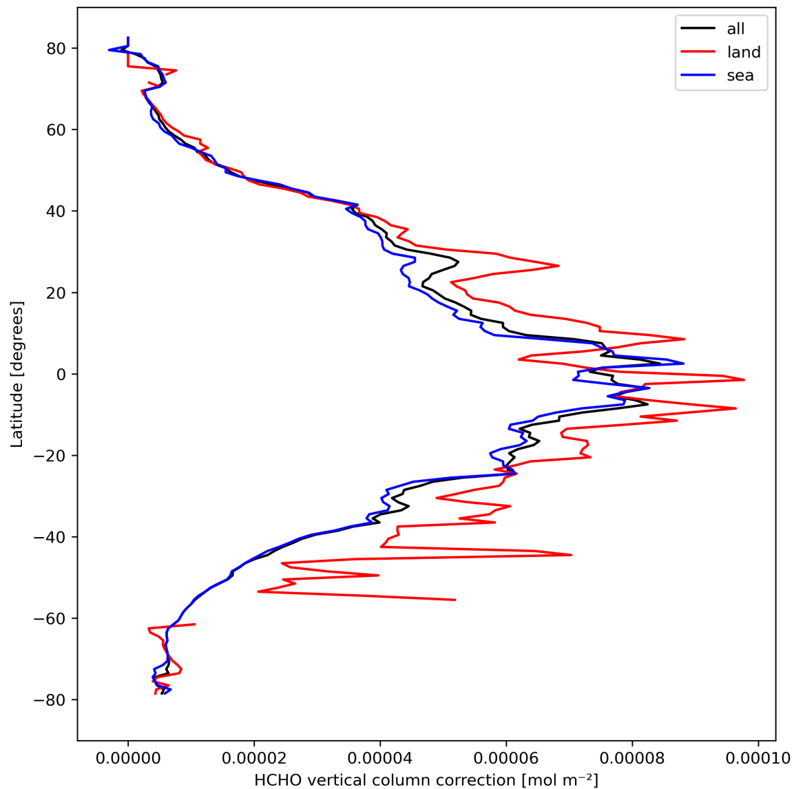
Figure 23: Zonal average of “HCHO vertical column correction” for 2024-03-14 to 2024-03-15.
