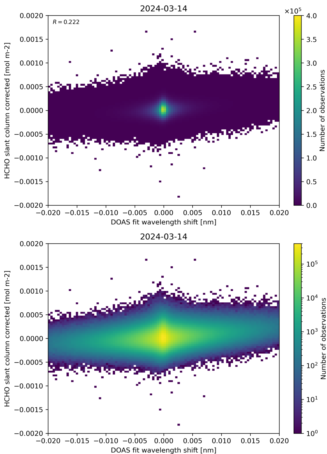
Figure 66: Scatter density plot of “DOAS fit wavelength shift” against “HCHO slant column corrected” for 2024-03-14 to 2024-03-15.
