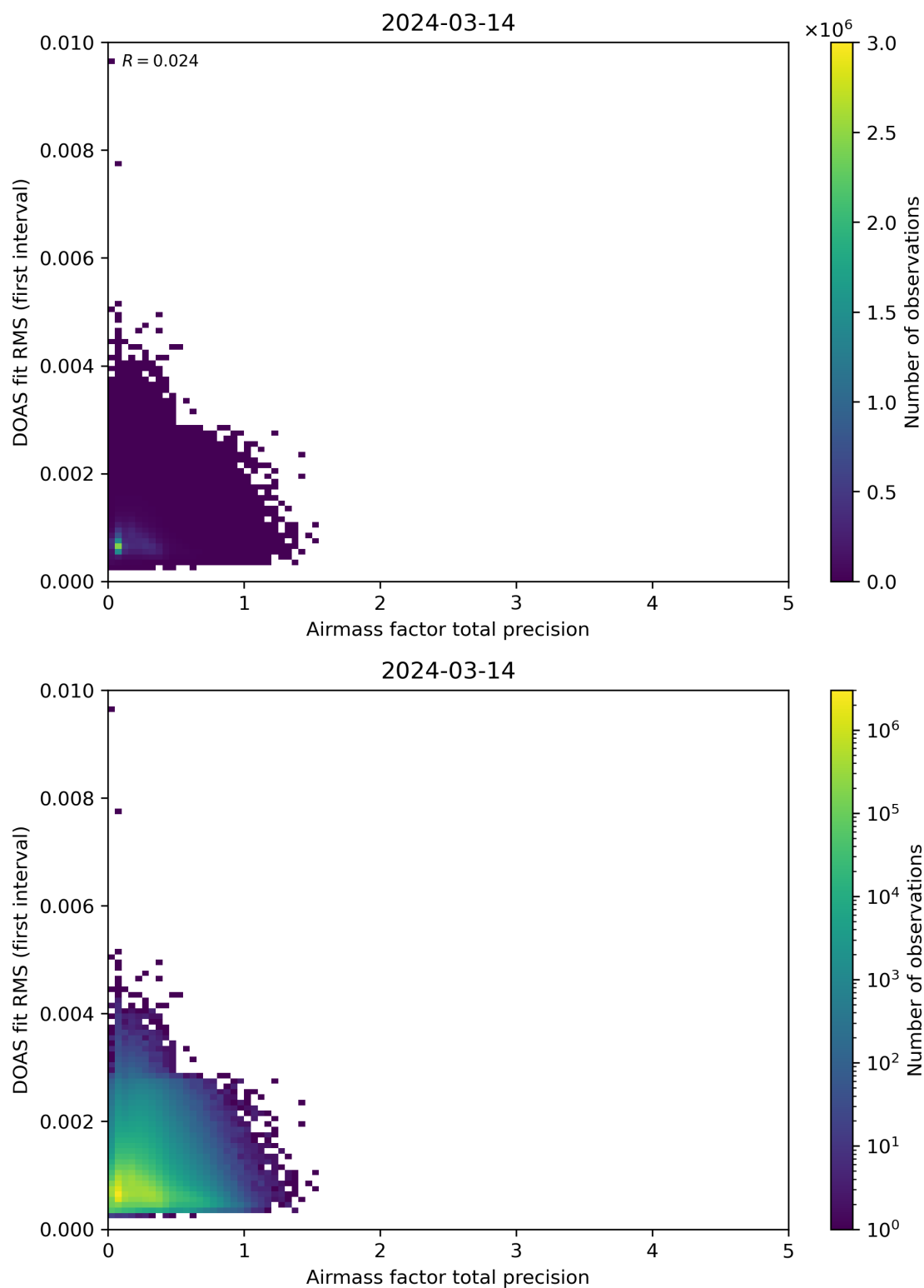
Figure 105: Scatter density plot of “Airmass factor total precision” against “DOAS fit RMS (first interval)” for 2024-03-14 to 2024-03-15.
