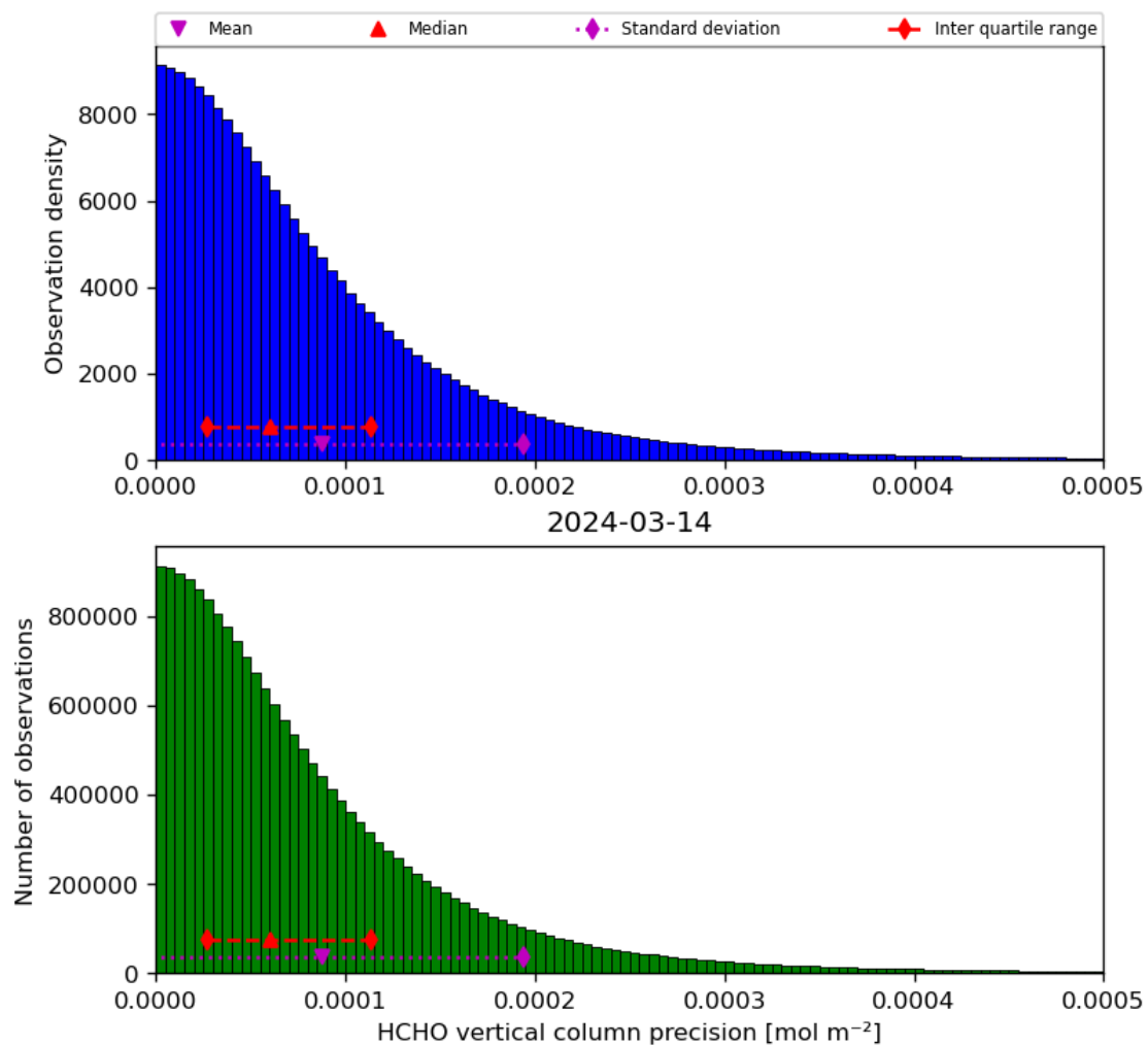
Figure 36: Histogram of “HCHO vertical column precision” for 2024-03-14 to 2024-03-15
