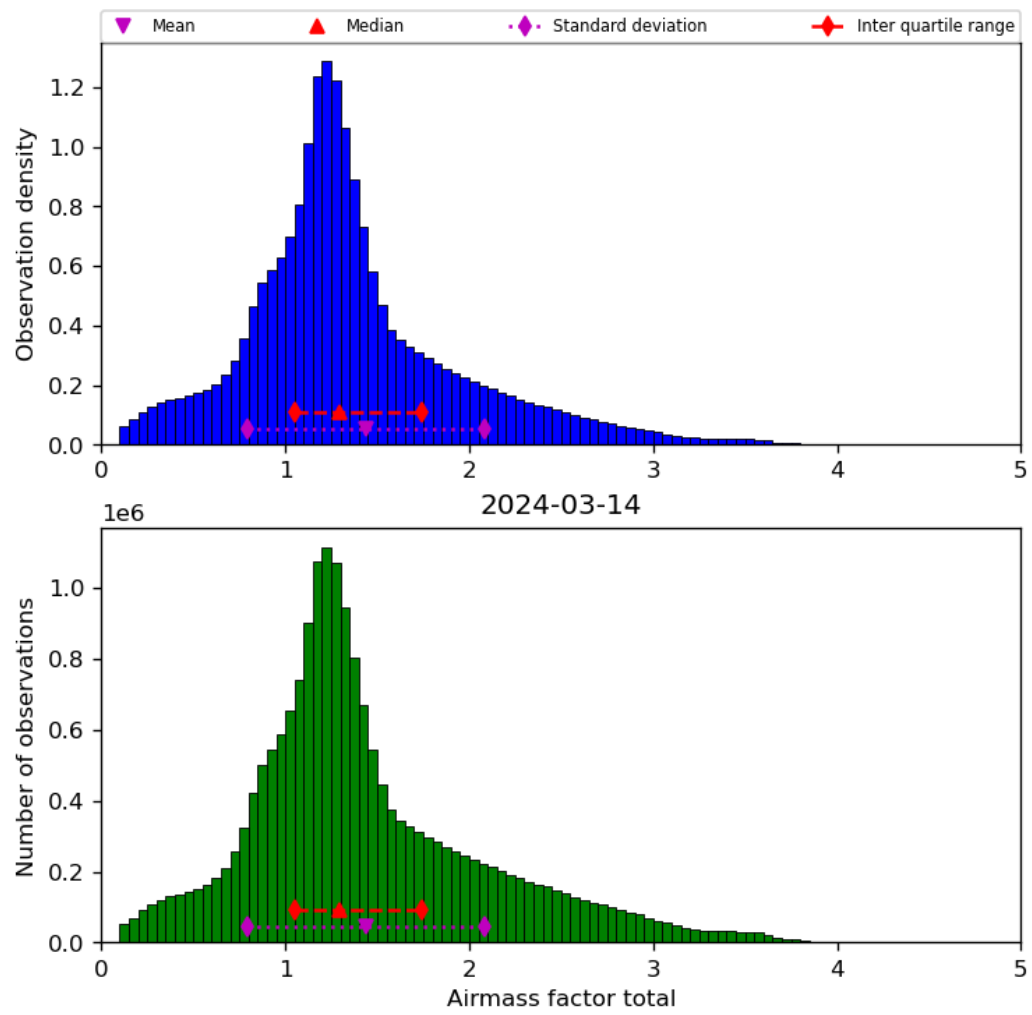
Figure 40: Histogram of “Airmass factor total” for 2024-03-14 to 2024-03-15
