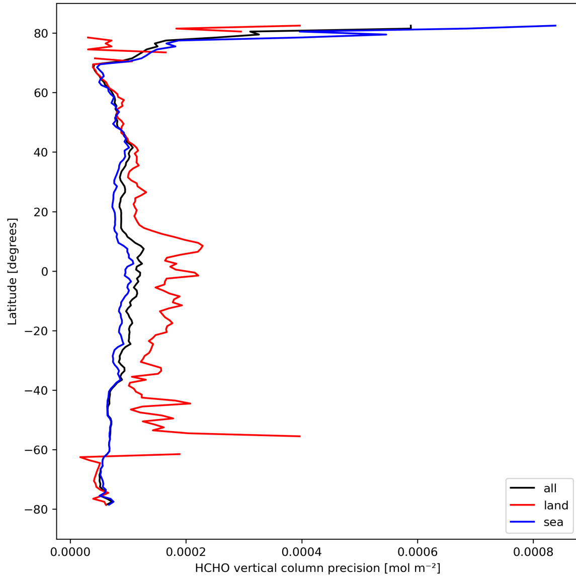
Figure 22: Zonal average of “HCHO vertical column precision” for 2024-03-14 to 2024-03-15.
