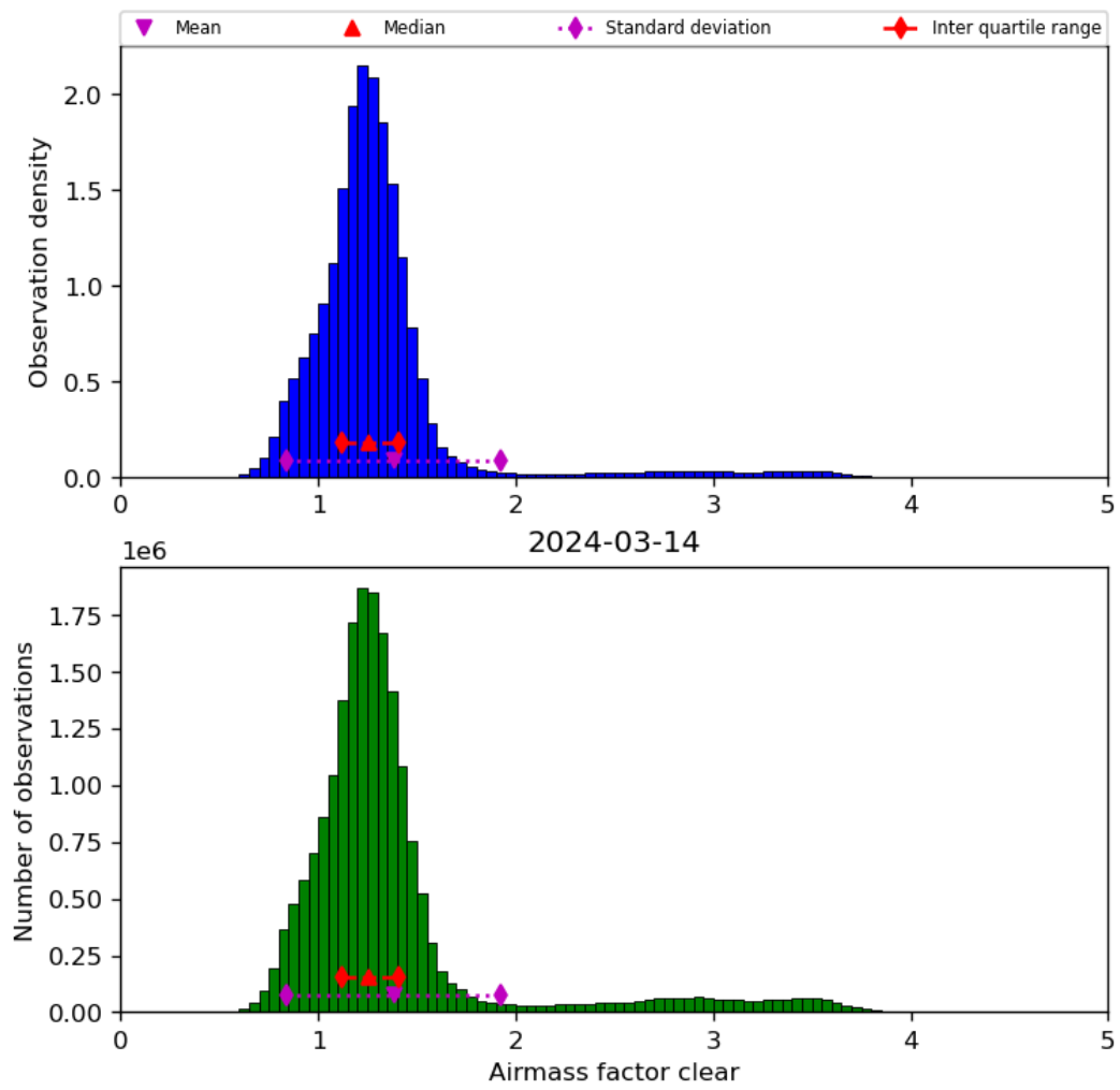
Figure 42: Histogram of “Airmass factor clear” for 2024-03-14 to 2024-03-15
