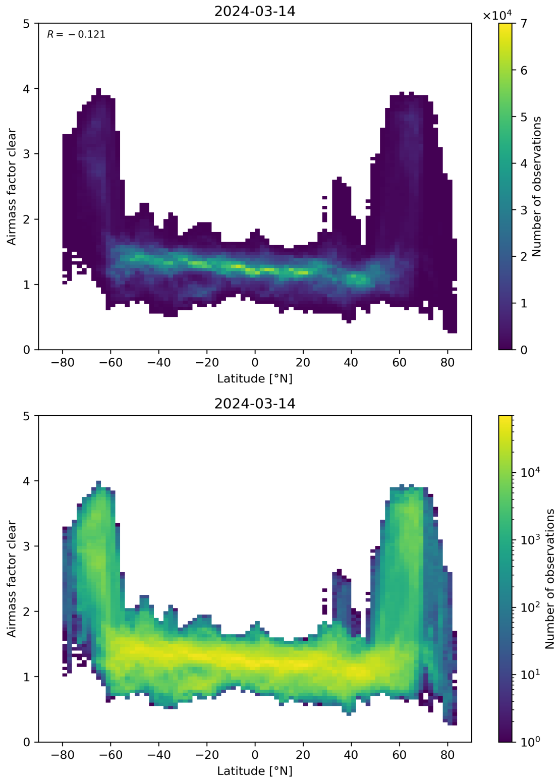
Figure 156: Scatter density plot of “Latitude” against “Airmass factor clear” for 2024-03-14 to 2024-03-15.
