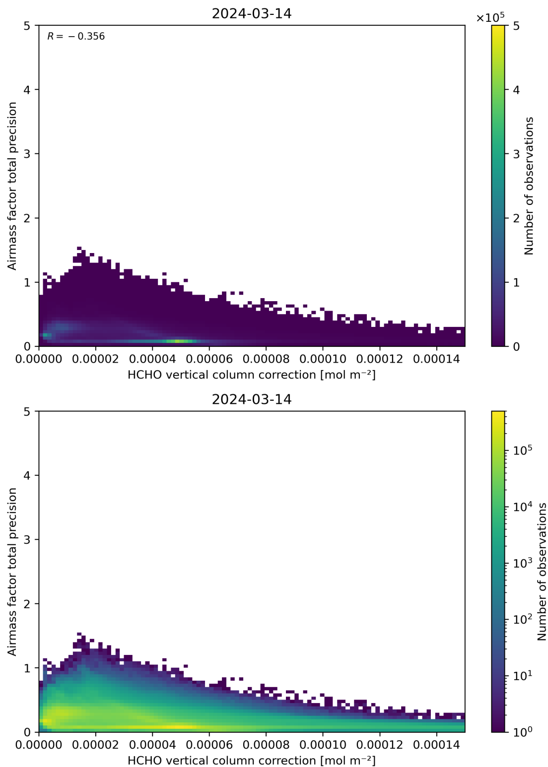
Figure 121: Scatter density plot of “HCHO vertical column correction” against “Airmass factor total precision” for 2024-03-14 to 2024-03-15.
