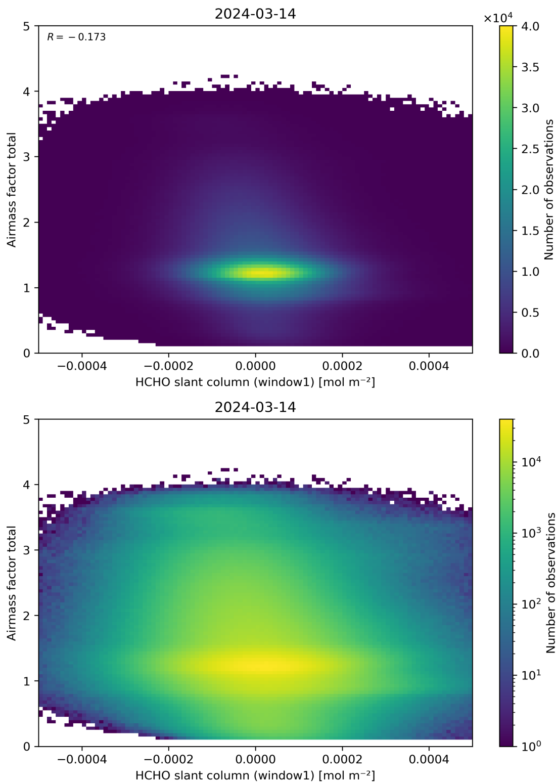
Figure 85: Scatter density plot of “HCHO slant column (window1)” against “Airmass factor total” for 2024-03-14 to 2024-03-15.
