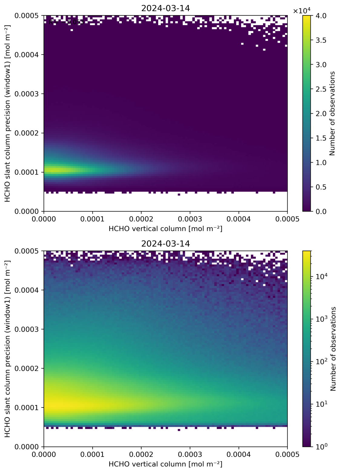
Figure 130: Scatter density plot of “HCHO vertical column” against “HCHO slant column precision (window1)” for 2024-03-14 to 2024-03-15.
