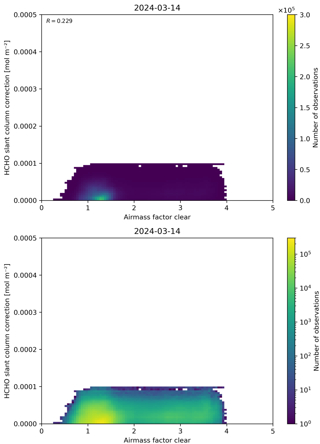
Figure 75: Scatter density plot of “Airmass factor clear” against “HCHO slant column correction” for 2024-03-14 to 2024-03-15.
