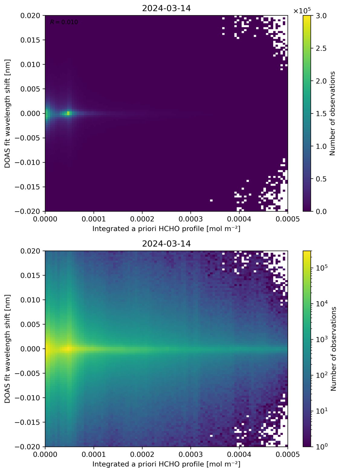
Figure 149: Scatter density plot of “Integrated a priori HCHO profile” against “DOAS fit wavelength shift” for 2024-03-14 to 2024-03-15.
