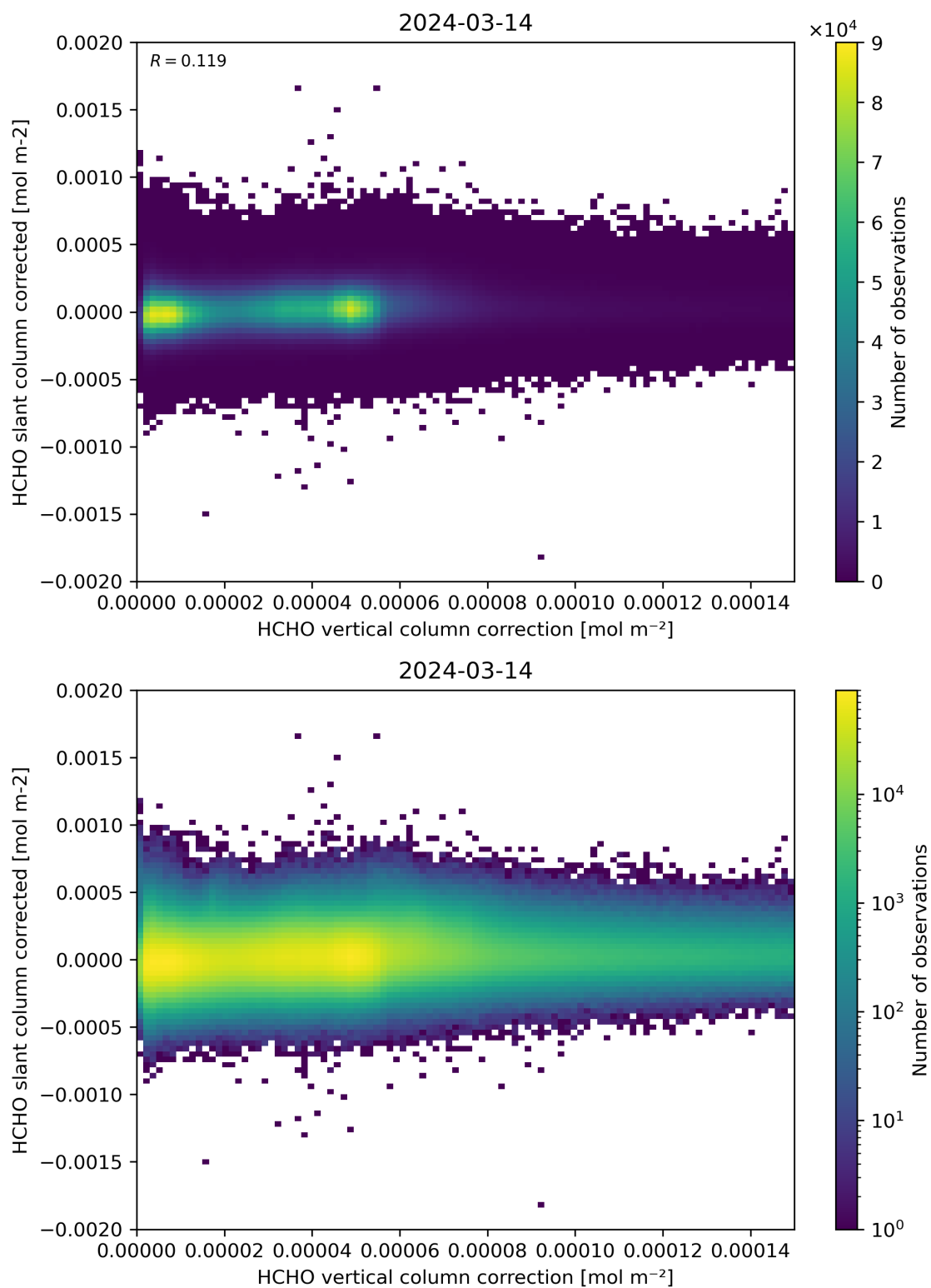
Figure 116: Scatter density plot of “HCHO vertical column correction” against “HCHO slant column corrected” for 2024-03-14 to 2024-03-15.
