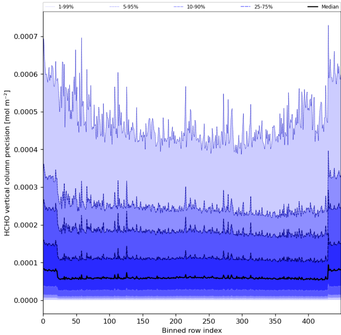
Figure 50: Along track statistics of “HCHO vertical column precision” for 2024-03-14 to 2024-03-15
