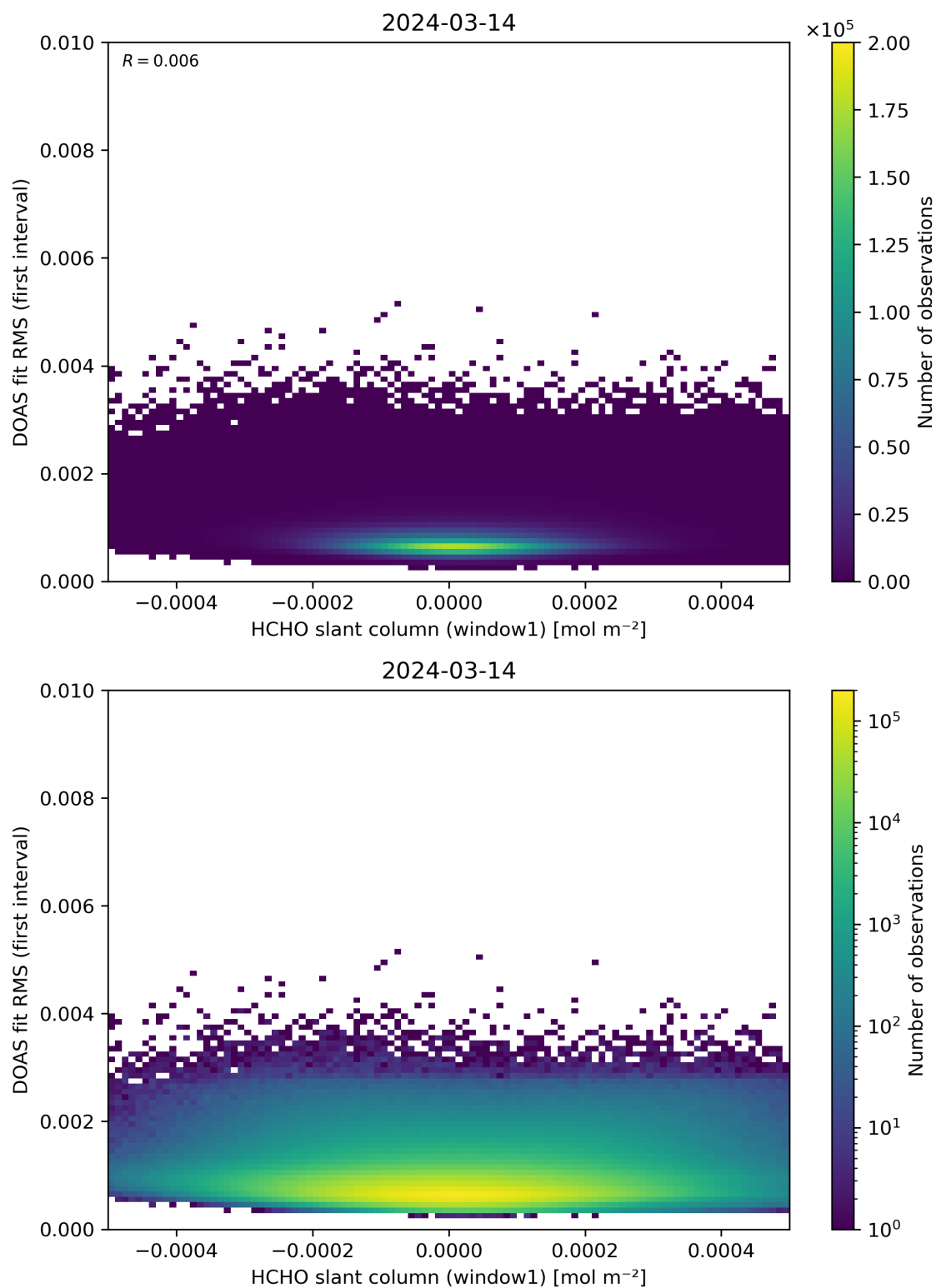
Figure 78: Scatter density plot of “HCHO slant column (window1)” against “DOAS fit RMS (first interval)” for 2024-03-14 to 2024-03-15.
