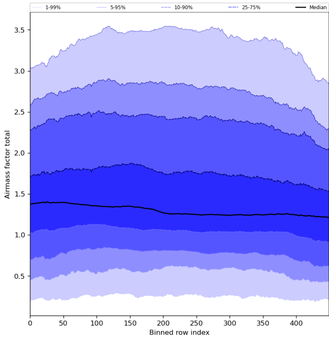
Figure 54: Along track statistics of “Airmass factor total” for 2024-03-14 to 2024-03-15
