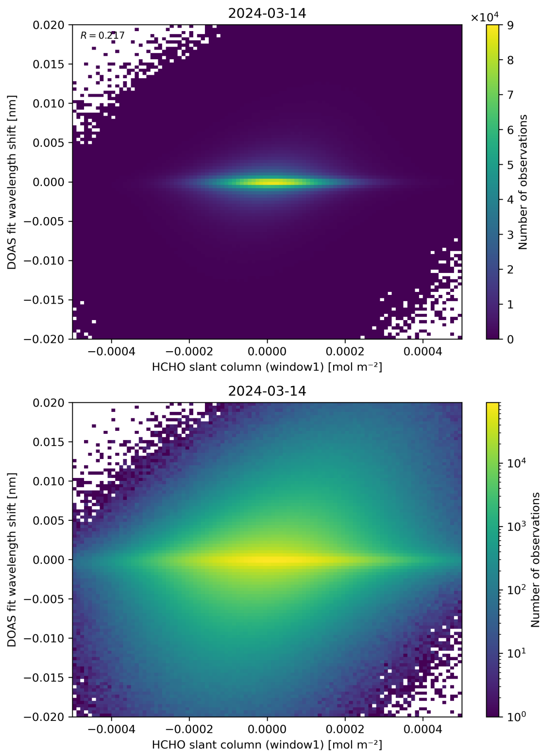
Figure 79: Scatter density plot of “HCHO slant column (window1)” against “DOAS fit wavelength shift” for 2024-03-14 to 2024-03-15.
