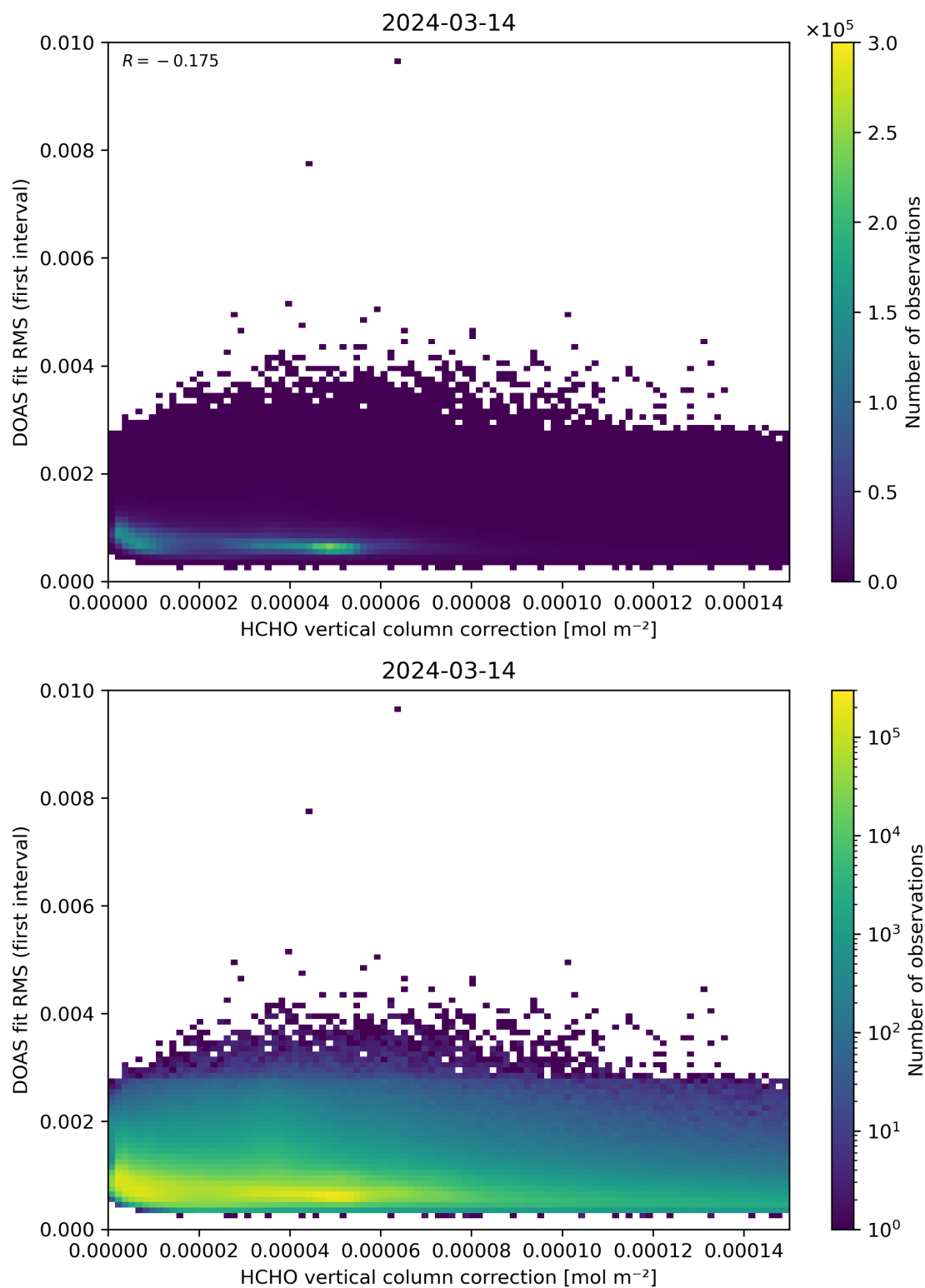
Figure 112: Scatter density plot of “HCHO vertical column correction” against “DOAS fit RMS (first interval)” for 2024-03-14 to 2024-03-15.
