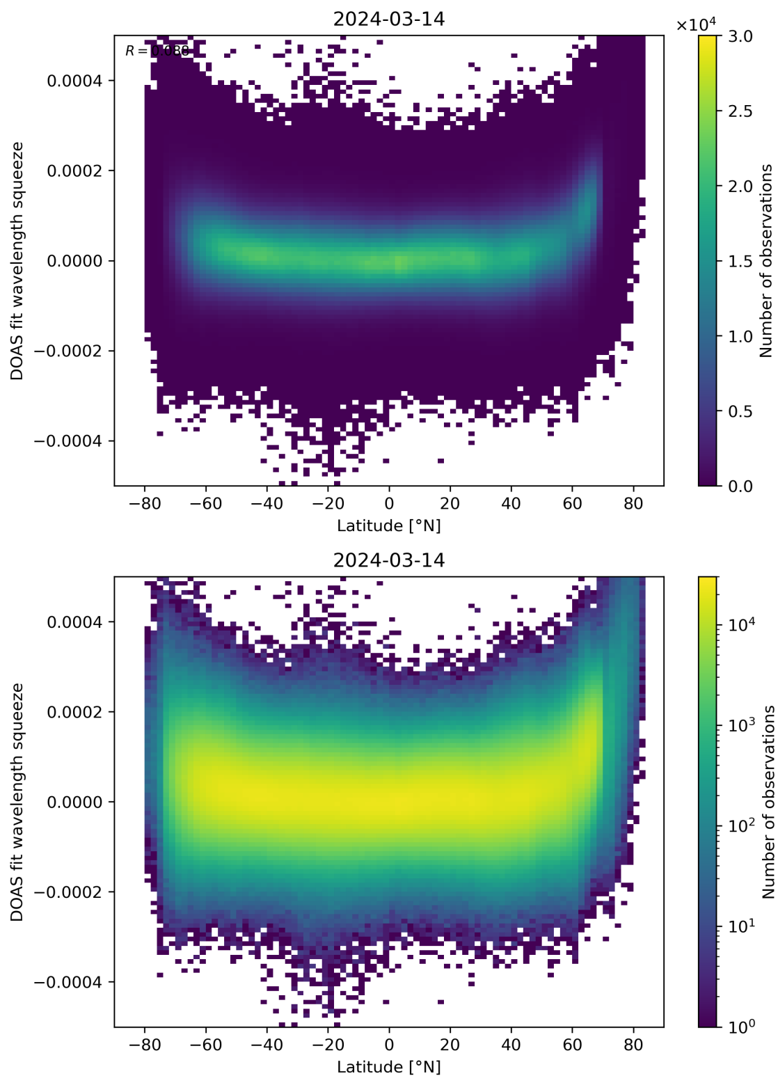
Figure 155: Scatter density plot of “Latitude” against “DOAS fit wavelength squeeze” for 2024-03-14 to 2024-03-15.
