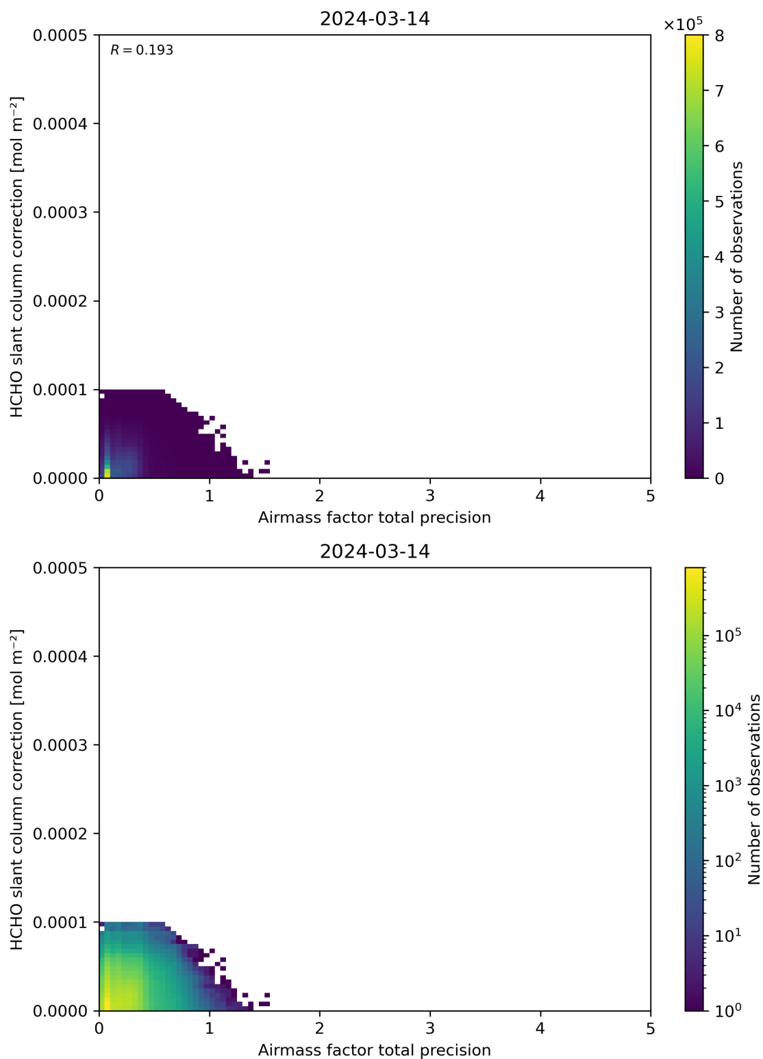
Figure 110: Scatter density plot of “Airmass factor total precision” against “HCHO slant column correction” for 2024-03-14 to 2024-03-15.
