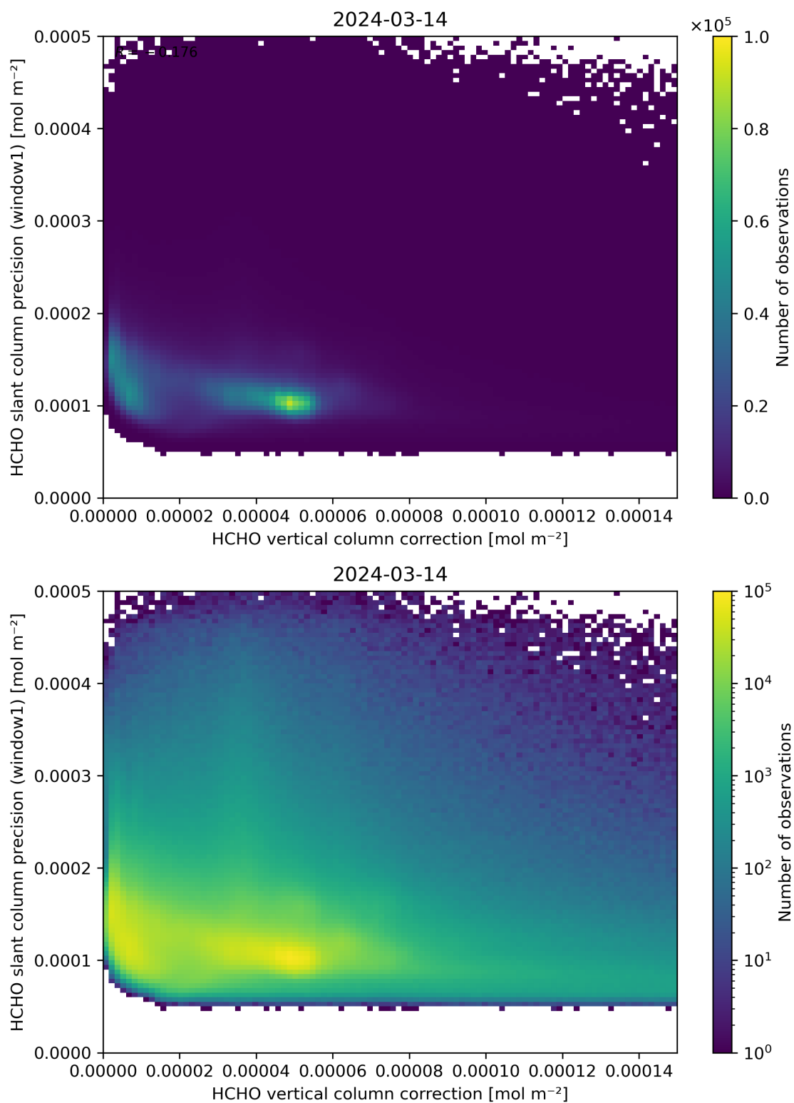
Figure 119: Scatter density plot of “HCHO vertical column correction” against “HCHO slant column precision (window1)” for 2024-03-14 to 2024-03-15.
