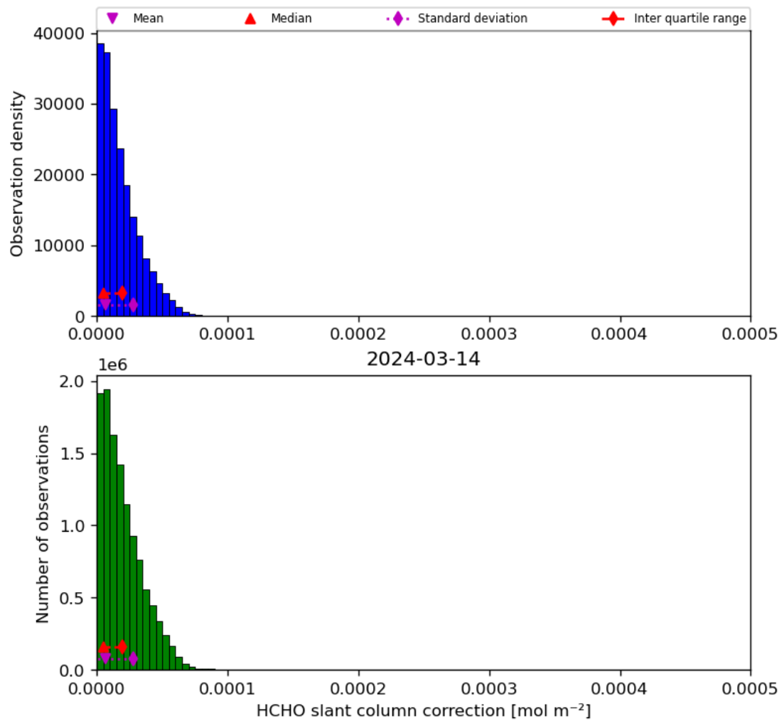
Figure 47: Histogram of “HCHO slant column correction” for 2024-03-14 to 2024-03-15
