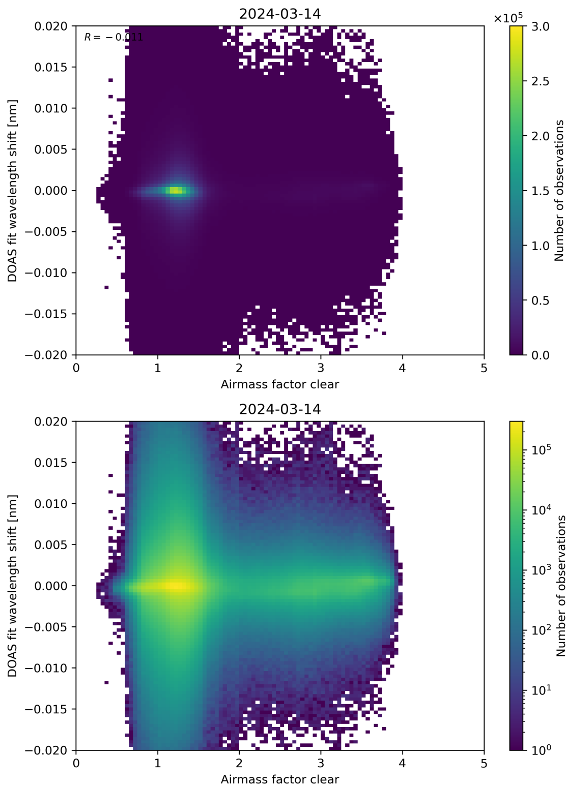
Figure 72: Scatter density plot of “Airmass factor clear” against “DOAS fit wavelength shift” for 2024-03-14 to 2024-03-15.
