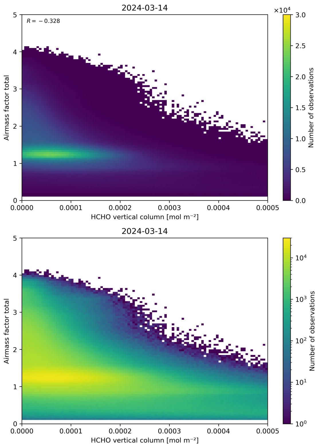
Figure 131: Scatter density plot of “HCHO vertical column” against “Airmass factor total” for 2024-03-14 to 2024-03-15.
