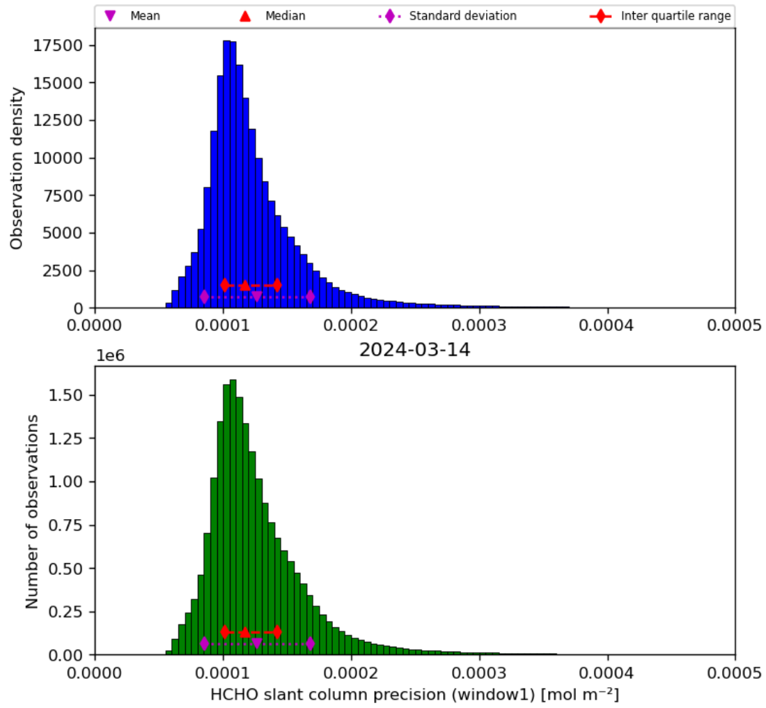
Figure 39: Histogram of “HCHO slant column precision (window1)” for 2024-03-14 to 2024-03-15
