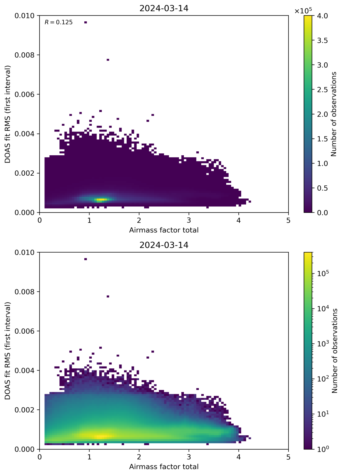
Figure 97: Scatter density plot of “Airmass factor total” against “DOAS fit RMS (first interval)” for 2024-03-14 to 2024-03-15.
