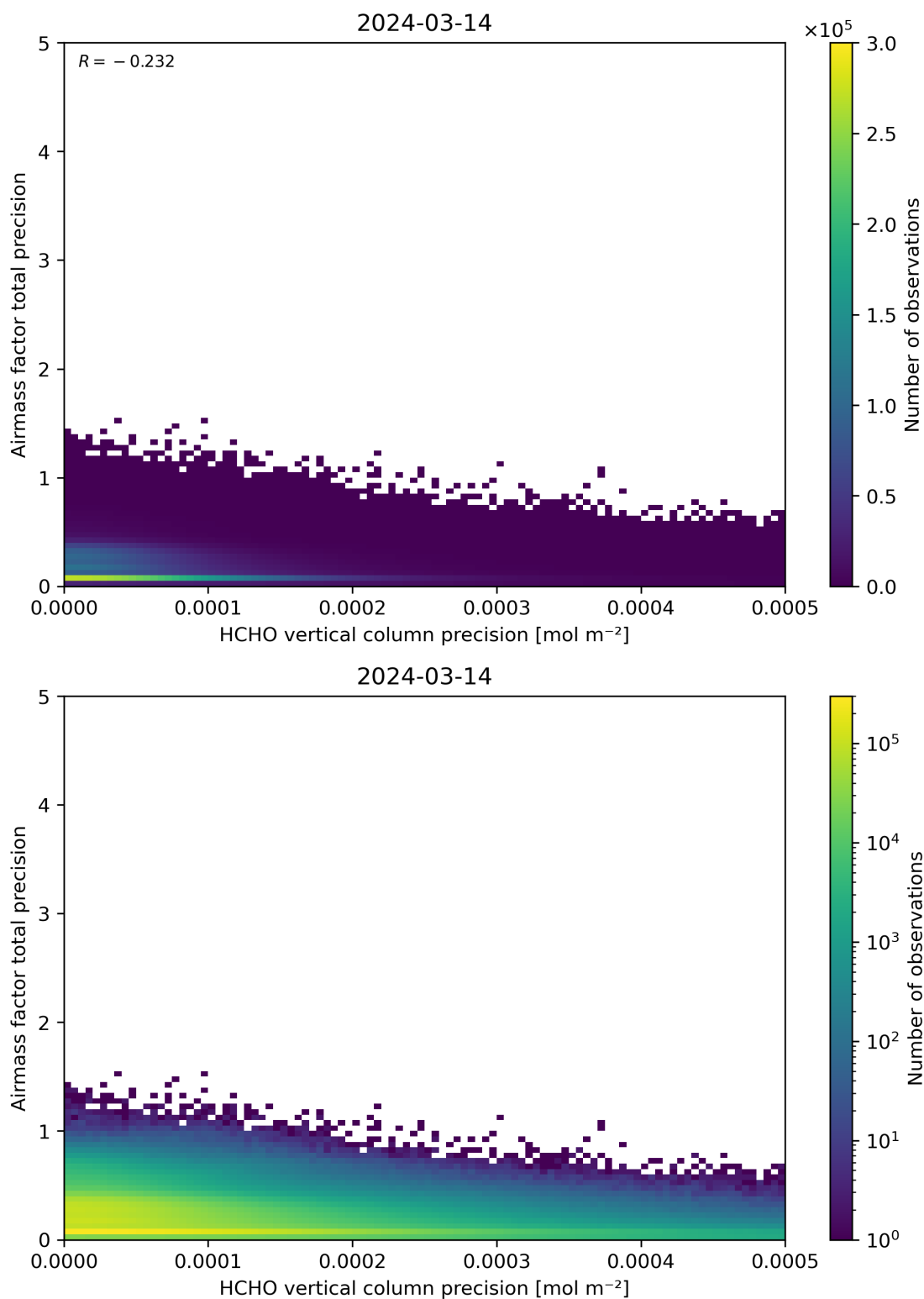
Figure 145: Scatter density plot of “HCHO vertical column precision” against “Airmass factor total precision” for 2024-03-14 to 2024-03-15.
