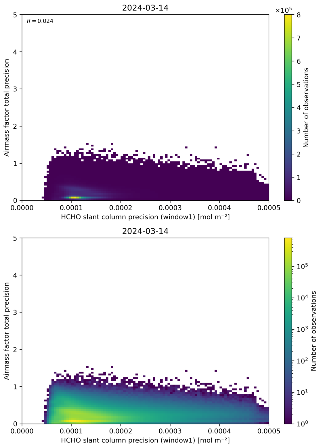
Figure 95: Scatter density plot of “HCHO slant column precision (window1)” against “Airmass factor total precision” for 2024-03-14 to 2024-03-15.
