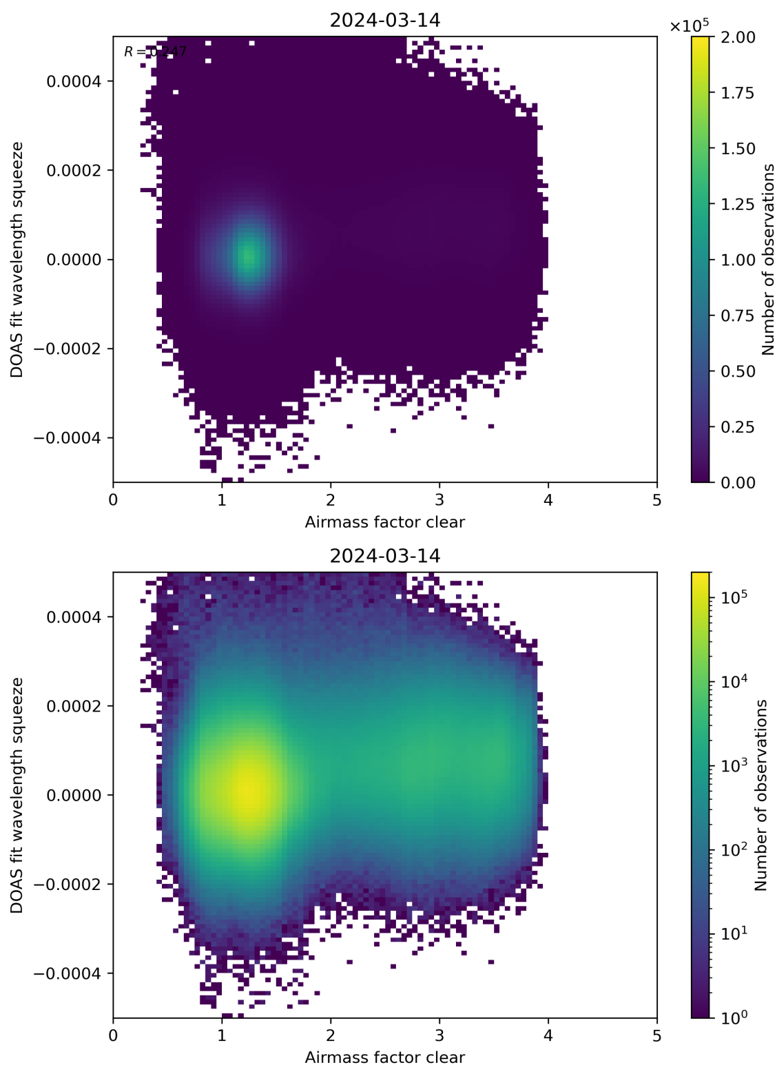
Figure 73: Scatter density plot of “Airmass factor clear” against “DOAS fit wavelength squeeze” for 2024-03-14 to 2024-03-15.
