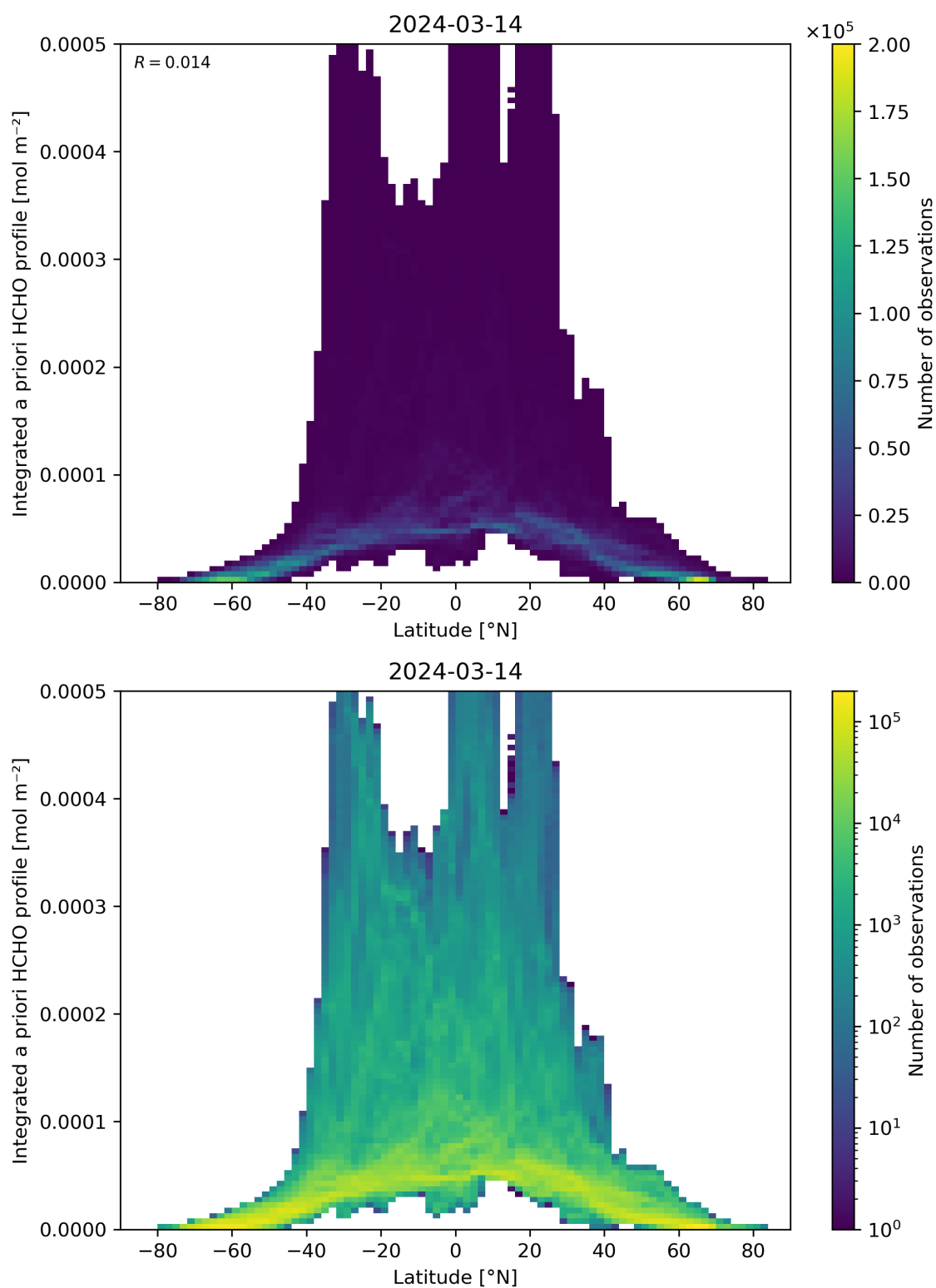
Figure 166: Scatter density plot of “Latitude” against “Integrated a priori HCHO profile” for 2024-03-14 to 2024-03-15.
