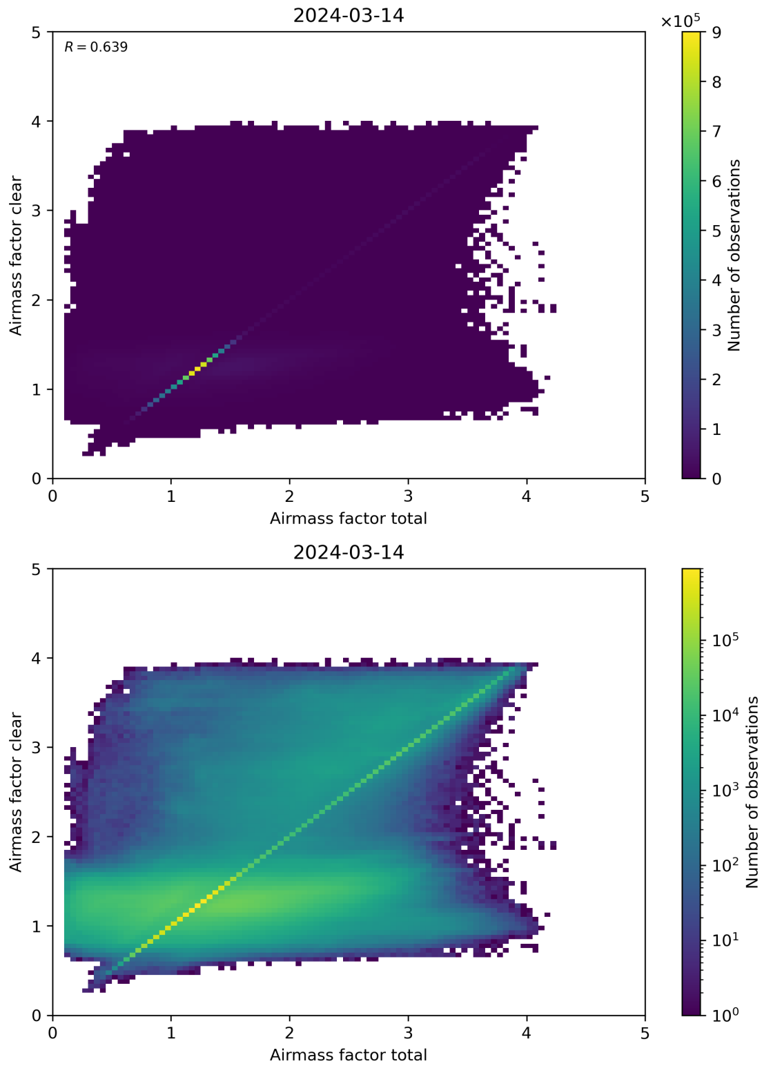
Figure 100: Scatter density plot of “Airmass factor total” against “Airmass factor clear” for 2024-03-14 to 2024-03-15.
