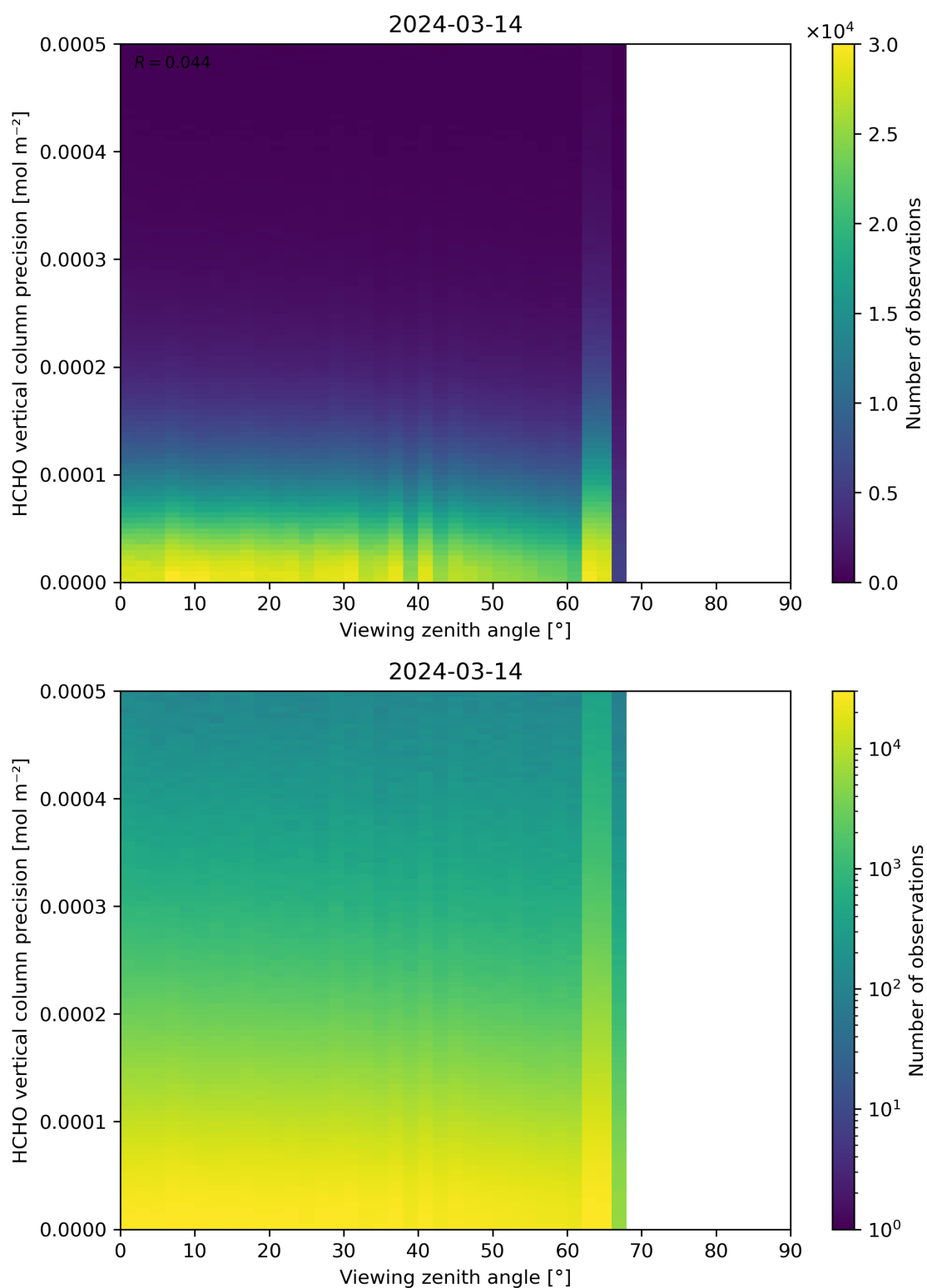
Figure 194: Scatter density plot of “Viewing zenith angle” against “HCHO vertical column precision” for 2024-03-14 to 2024-03-15.
