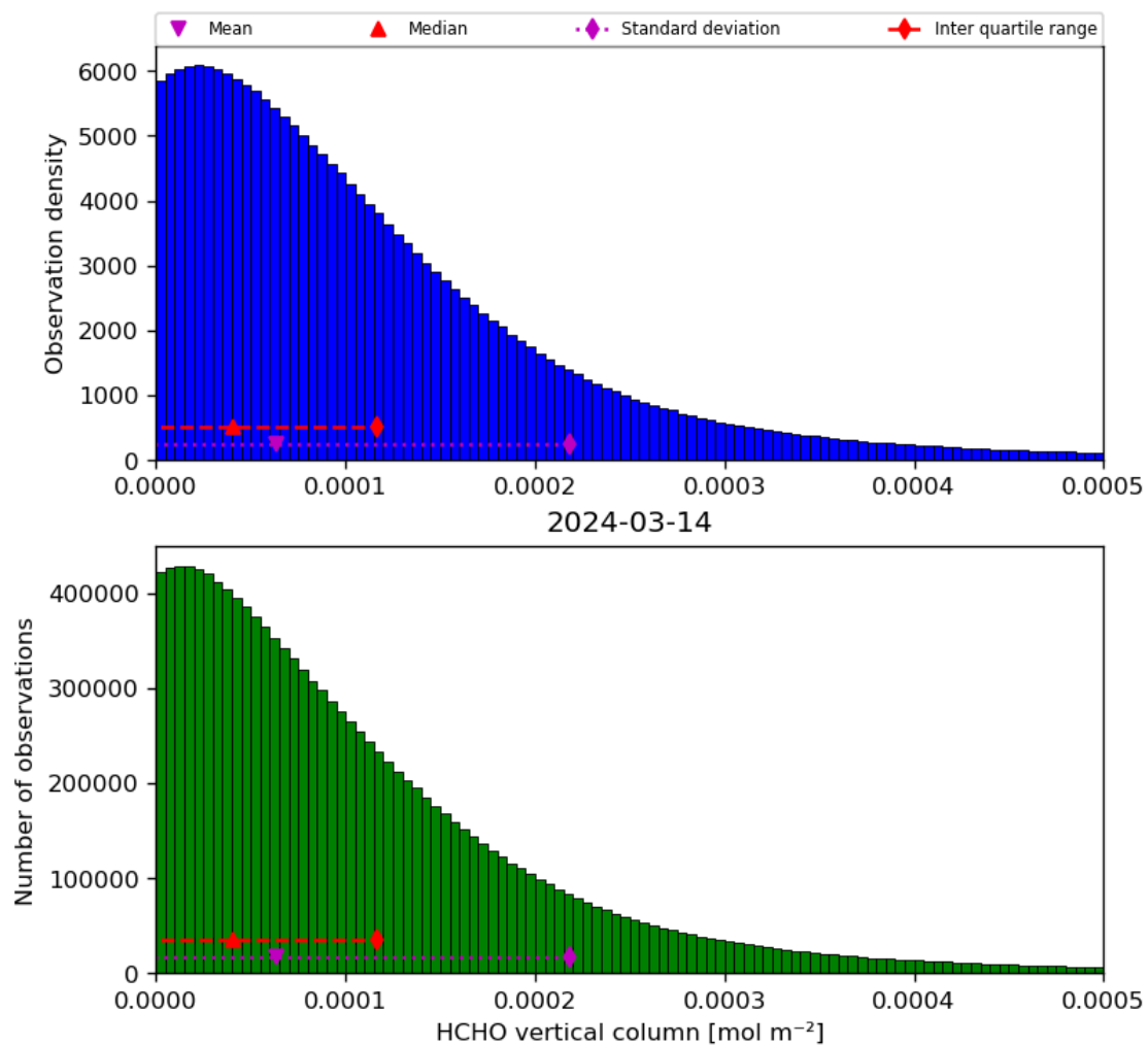
Figure 35: Histogram of “HCHO vertical column” for 2024-03-14 to 2024-03-15
