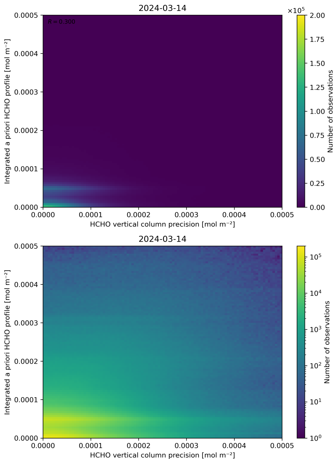
Figure 147: Scatter density plot of “HCHO vertical column precision” against “Integrated a priori HCHO profile” for 2024-03-14 to 2024-03-15.
