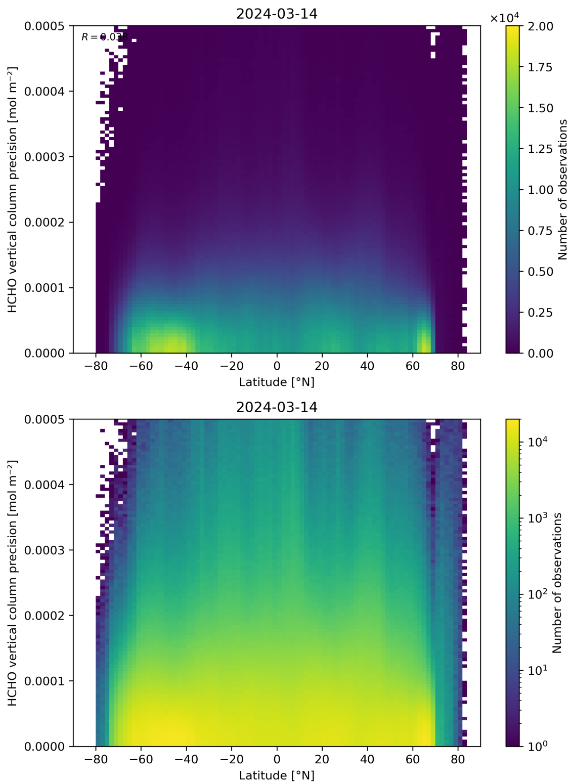
Figure 165: Scatter density plot of “Latitude” against “HCHO vertical column precision” for 2024-03-14 to 2024-03-15.
