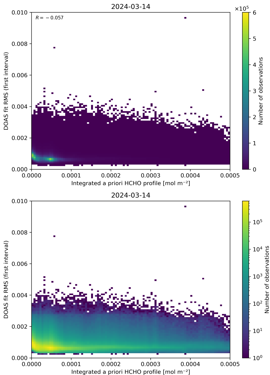
Figure 148: Scatter density plot of “Integrated a priori HCHO profile” against “DOAS fit RMS (first interval)” for 2024-03-14 to 2024-03-15.
