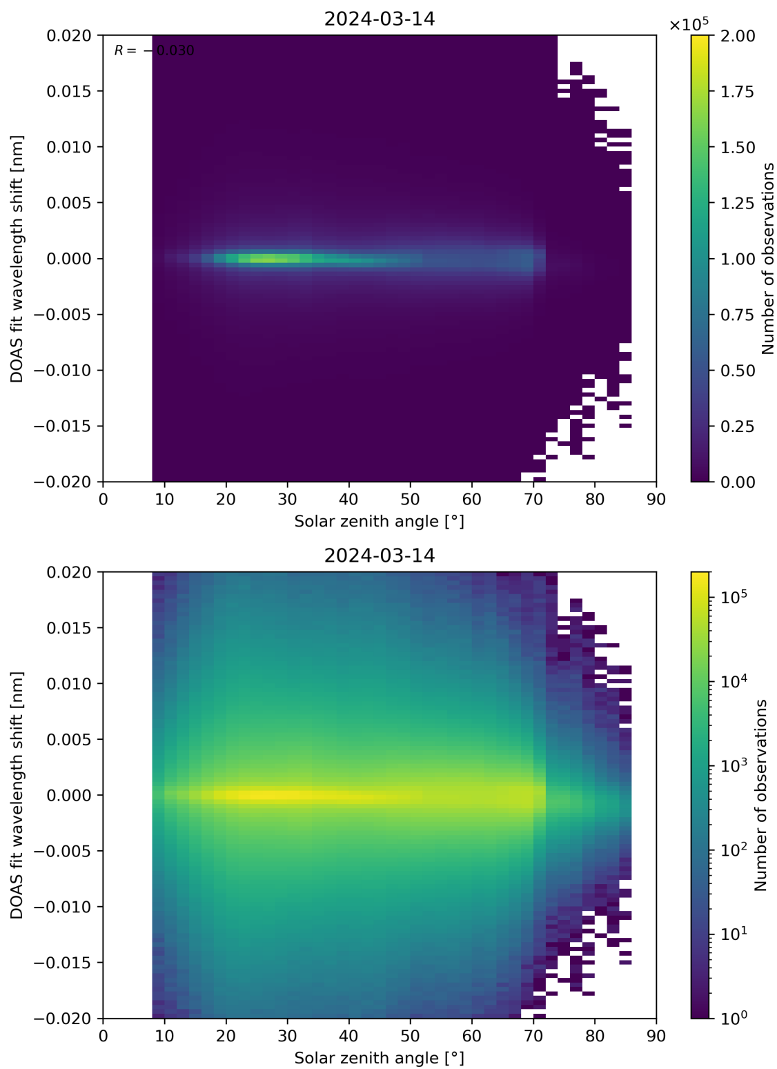
Figure 168: Scatter density plot of “Solar zenith angle” against “DOAS fit wavelength shift” for 2024-03-14 to 2024-03-15.
