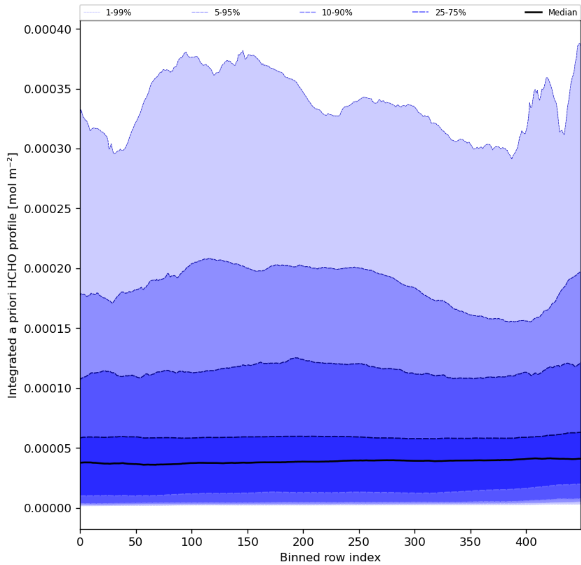
Figure 57: Along track statistics of “Integrated a priori HCHO profile” for 2024-03-14 to 2024-03-15
