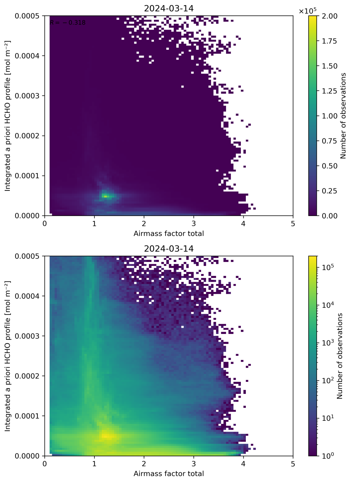
Figure 104: Scatter density plot of “Airmass factor total” against “Integrated a priori HCHO profile” for 2024-03-14 to 2024-03-15.
