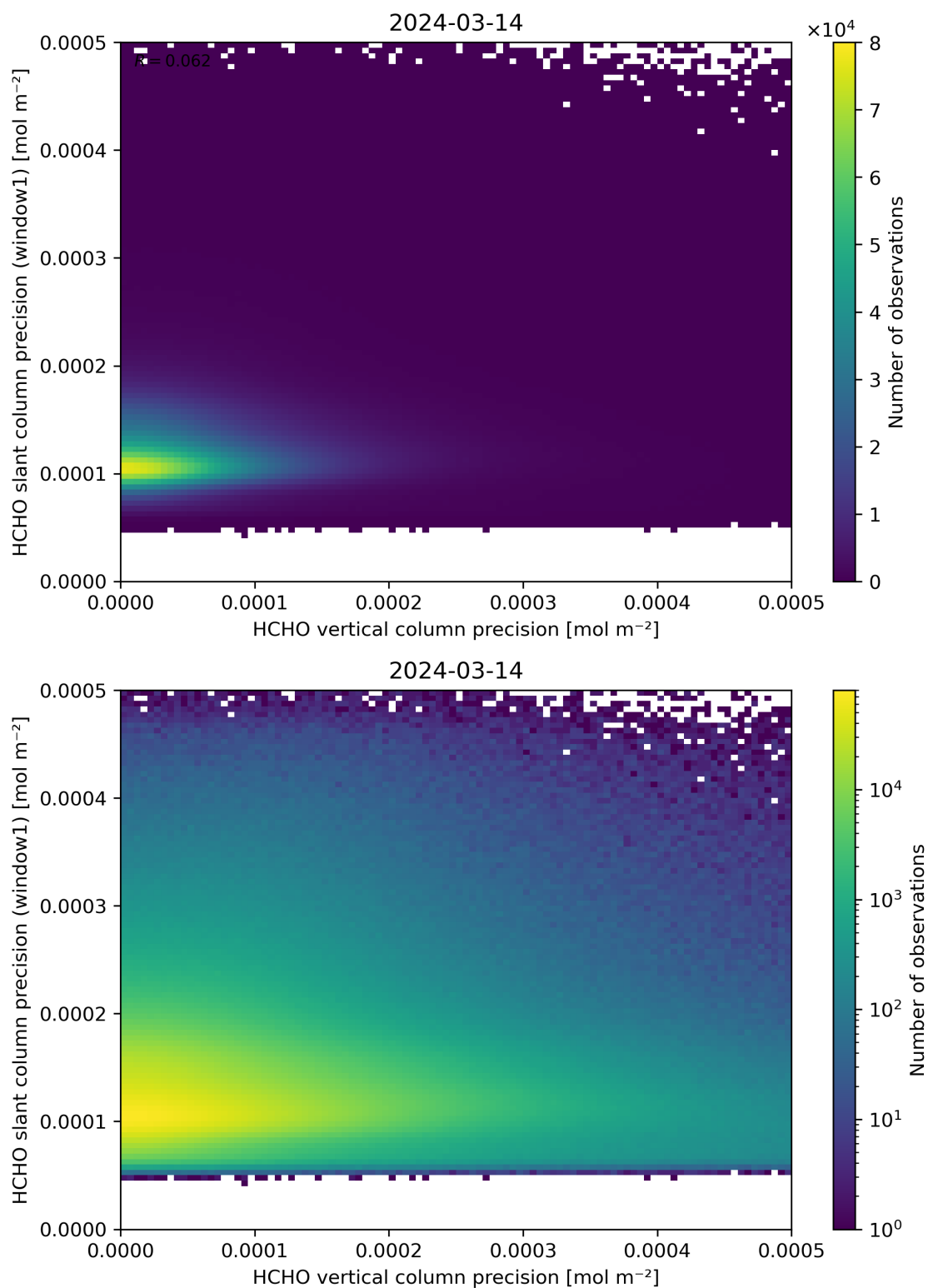
Figure 143: Scatter density plot of “HCHO vertical column precision” against “HCHO slant column precision (window1)” for 2024-03-14 to 2024-03-15.
