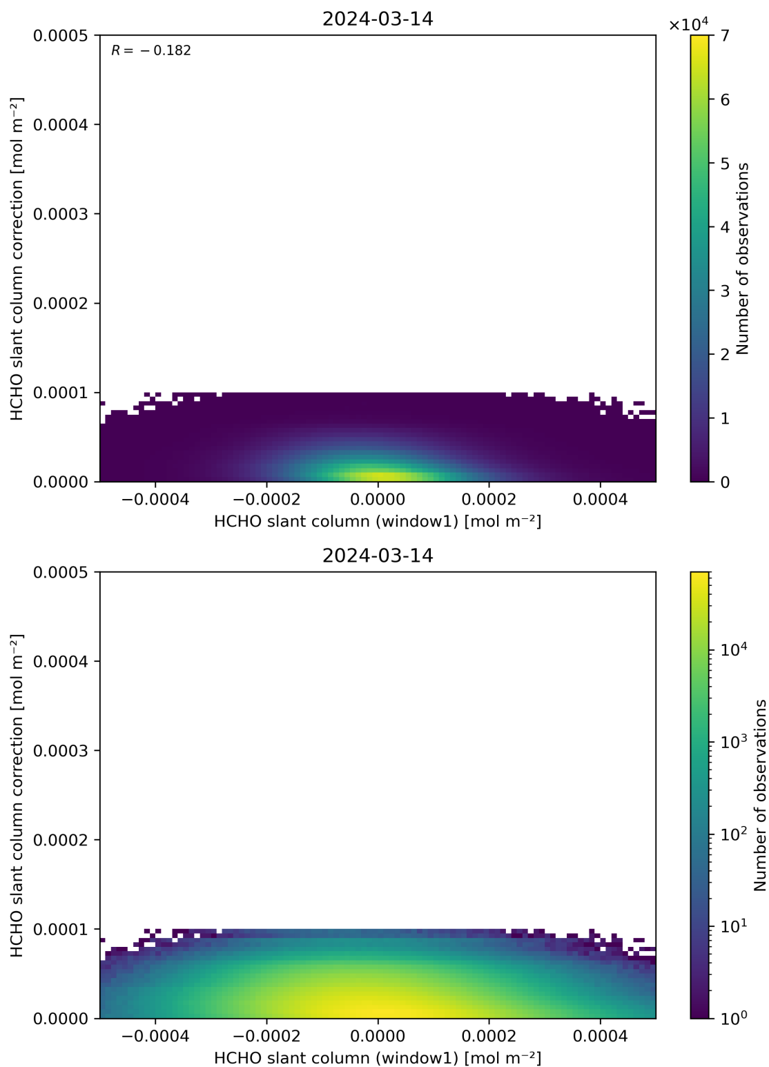
Figure 83: Scatter density plot of “HCHO slant column (window1)” against “HCHO slant column correction” for 2024-03-14 to 2024-03-15.
