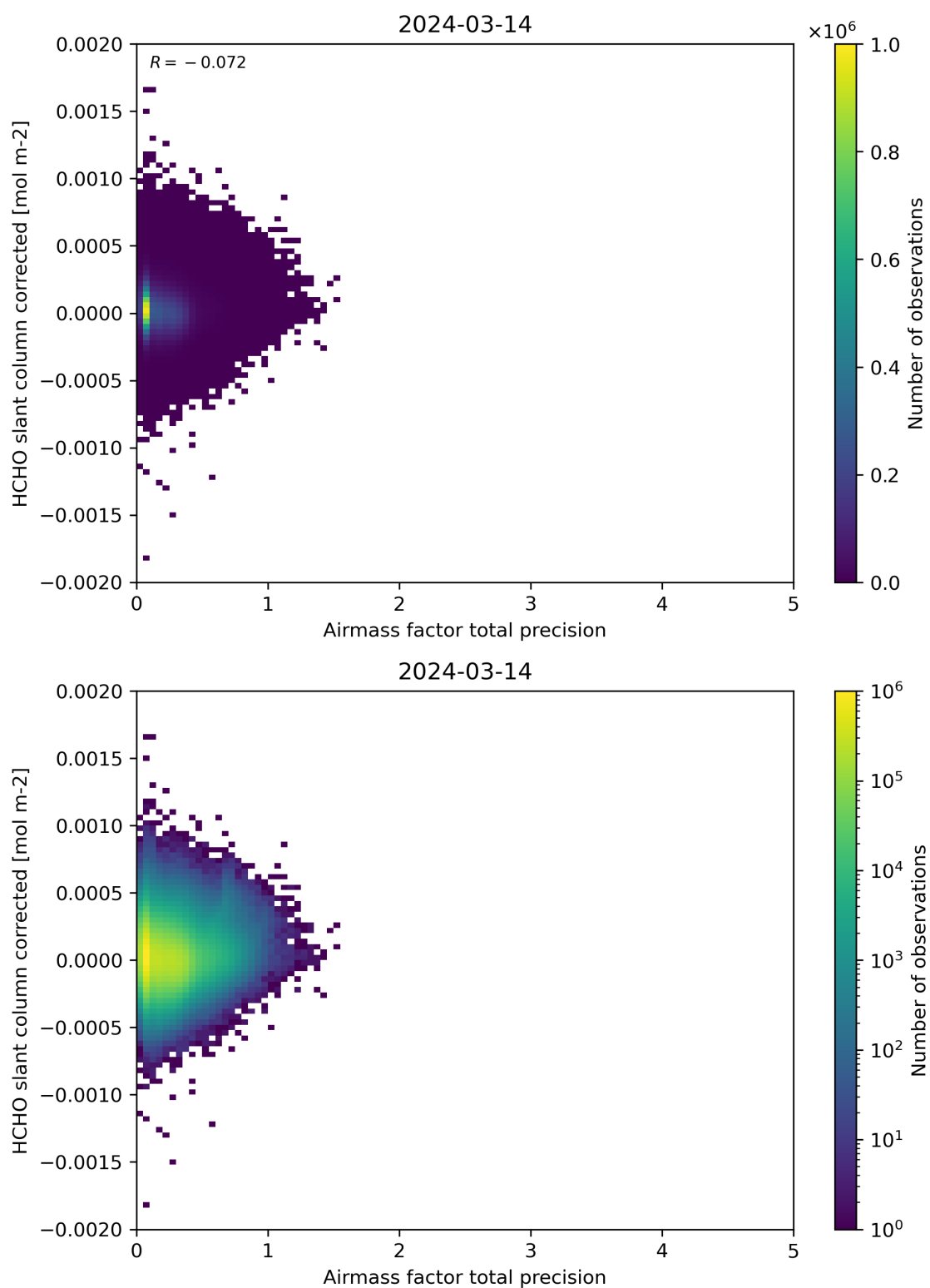
Figure 109: Scatter density plot of “Airmass factor total precision” against “HCHO slant column corrected” for 2024-03-14 to 2024-03-15.
