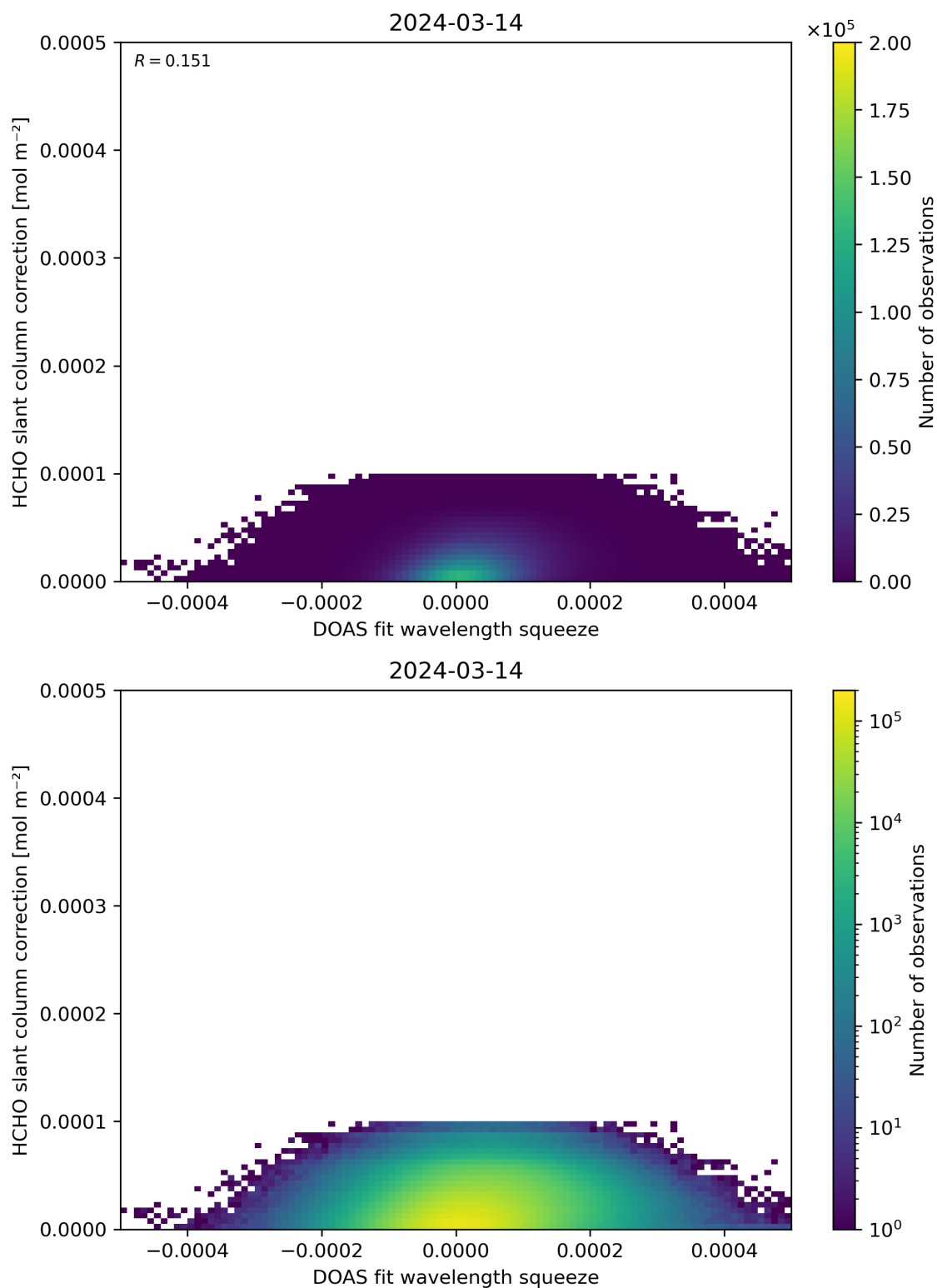
Figure 70: Scatter density plot of “DOAS fit wavelength squeeze” against “HCHO slant column correction” for 2024-03-14 to 2024-03-15.
