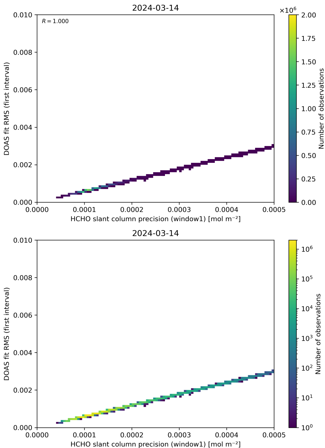
Figure 88: Scatter density plot of “HCHO slant column precision (window1)” against “DOAS fit RMS (first interval)” for 2024-03-14 to 2024-03-15.
