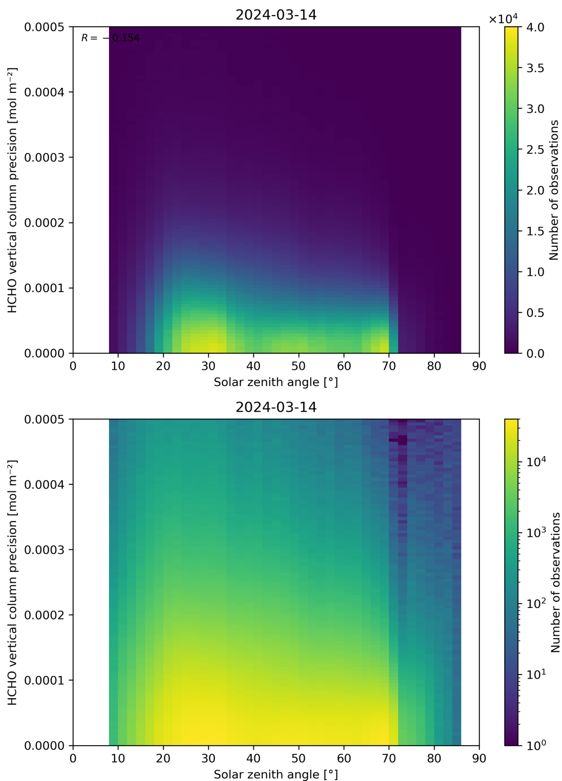
Figure 179: Scatter density plot of “Solar zenith angle” against “HCHO vertical column precision” for 2024-03-14 to 2024-03-15.
