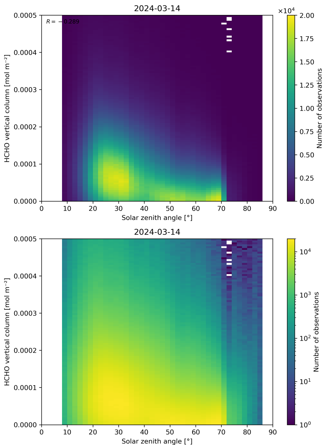
Figure 177: Scatter density plot of “Solar zenith angle” against “HCHO vertical column” for 2024-03-14 to 2024-03-15.
