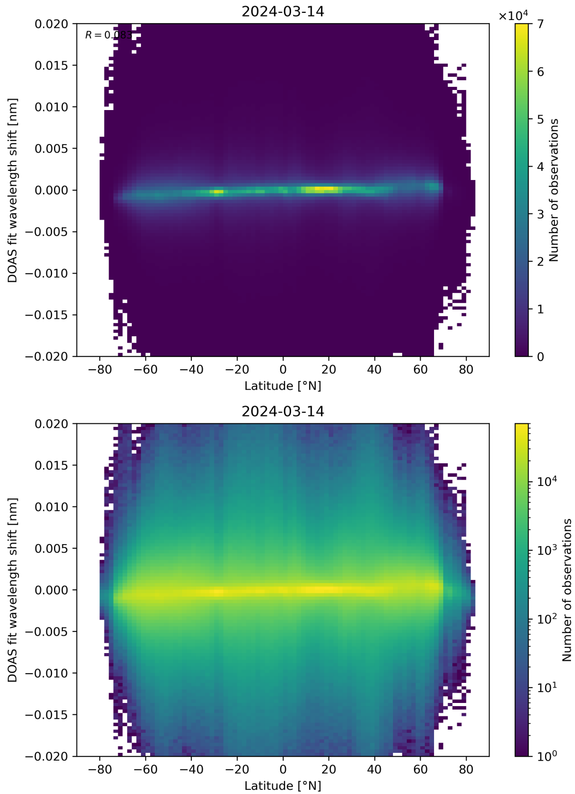
Figure 154: Scatter density plot of “Latitude” against “DOAS fit wavelength shift” for 2024-03-14 to 2024-03-15.
