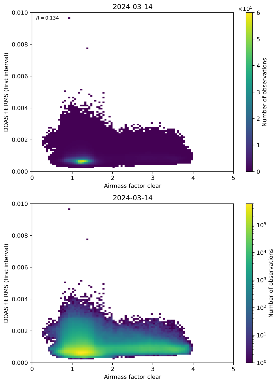
Figure 71: Scatter density plot of “Airmass factor clear” against “DOAS fit RMS (first interval)” for 2024-03-14 to 2024-03-15.
