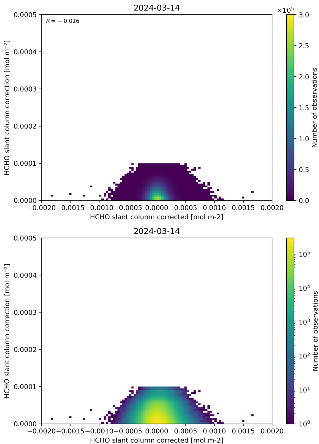
Figure 77: Scatter density plot of “HCHO slant column corrected” against “HCHO slant column correction” for 2024-03-14 to 2024-03-15.
