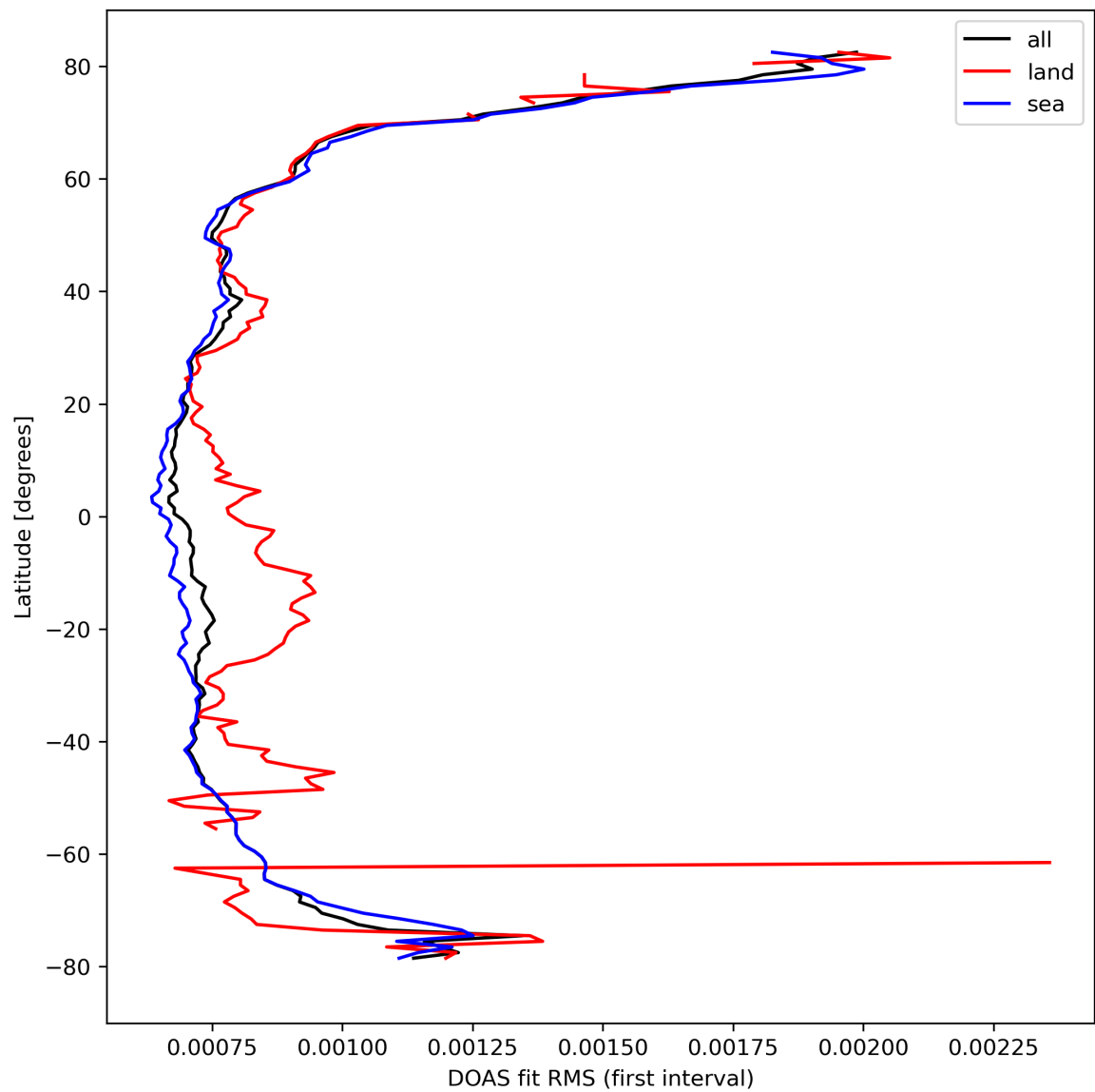
Figure 32: Zonal average of “DOAS fit RMS (first interval)” for 2024-03-14 to 2024-03-15.
