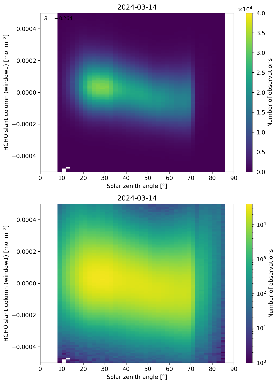
Figure 173: Scatter density plot of “Solar zenith angle” against “HCHO slant column (window1)” for 2024-03-14 to 2024-03-15.
