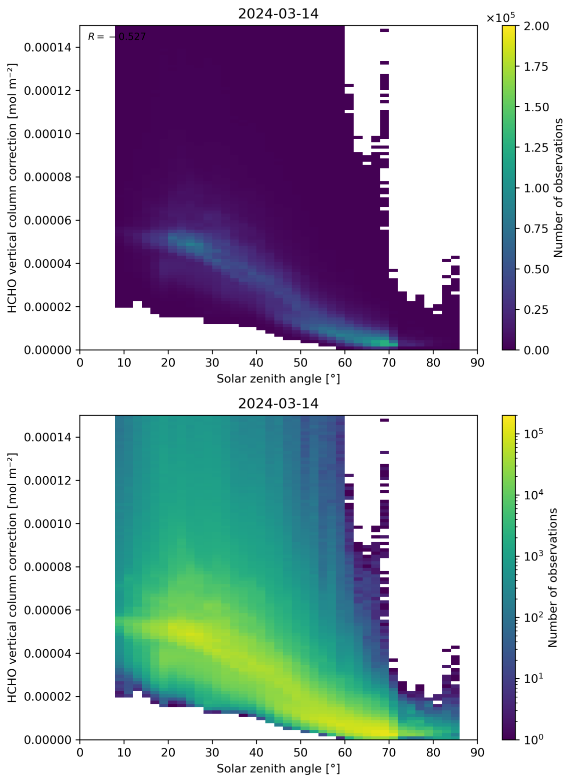
Figure 178: Scatter density plot of “Solar zenith angle” against “HCHO vertical column correction” for 2024-03-14 to 2024-03-15.
