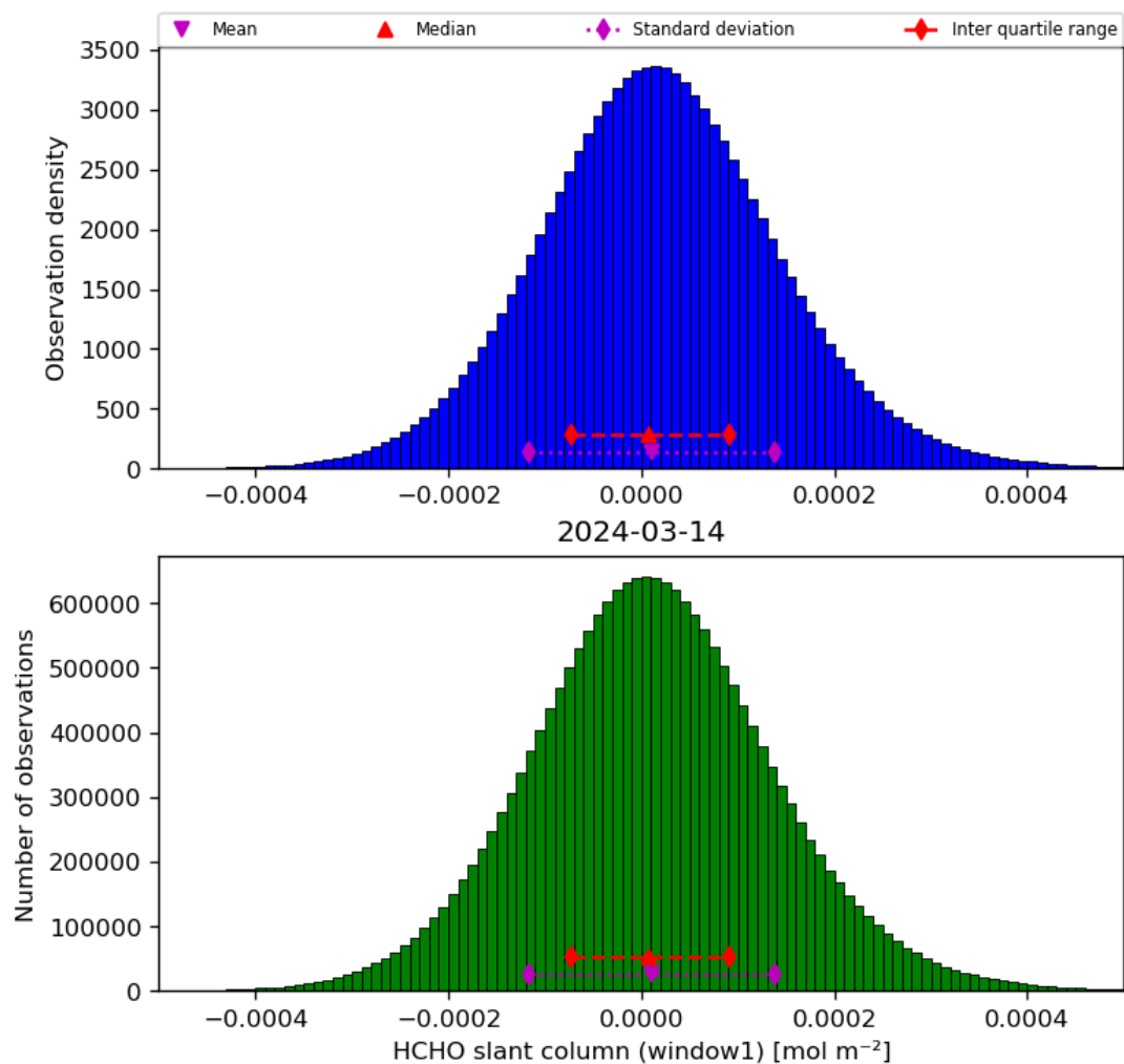
Figure 38: Histogram of “HCHO slant column (window1)” for 2024-03-14 to 2024-03-15
