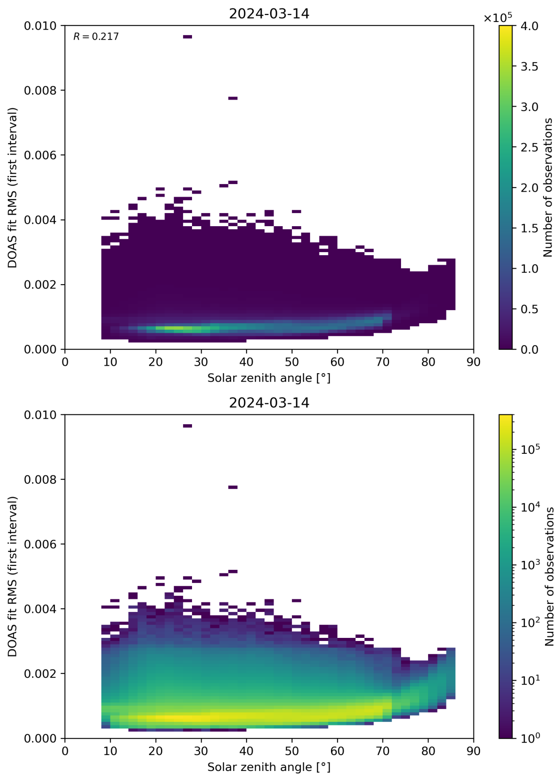
Figure 167: Scatter density plot of “Solar zenith angle” against “DOAS fit RMS (first interval)” for 2024-03-14 to 2024-03-15.
