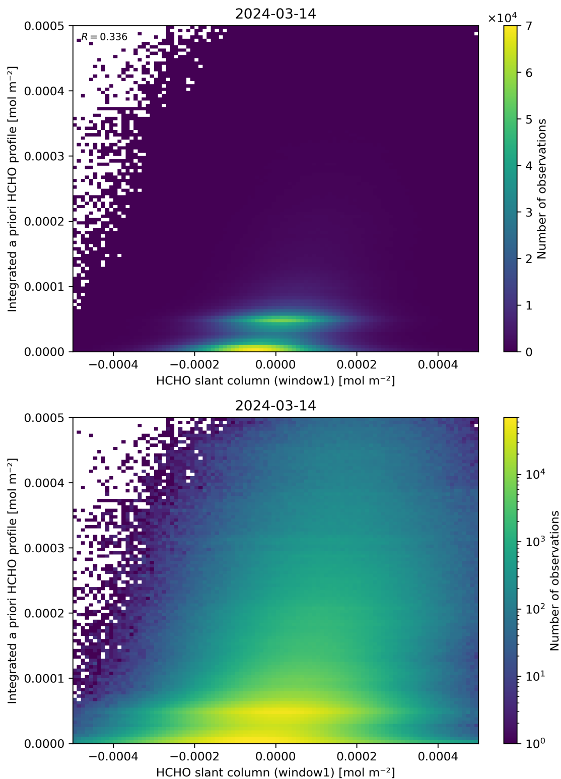
Figure 87: Scatter density plot of “HCHO slant column (window1)” against “Integrated a priori HCHO profile” for 2024-03-14 to 2024-03-15.
