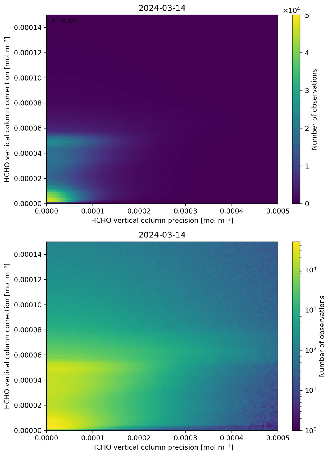
Figure 146: Scatter density plot of “HCHO vertical column precision” against “HCHO vertical column correction” for 2024-03-14 to 2024-03-15.
