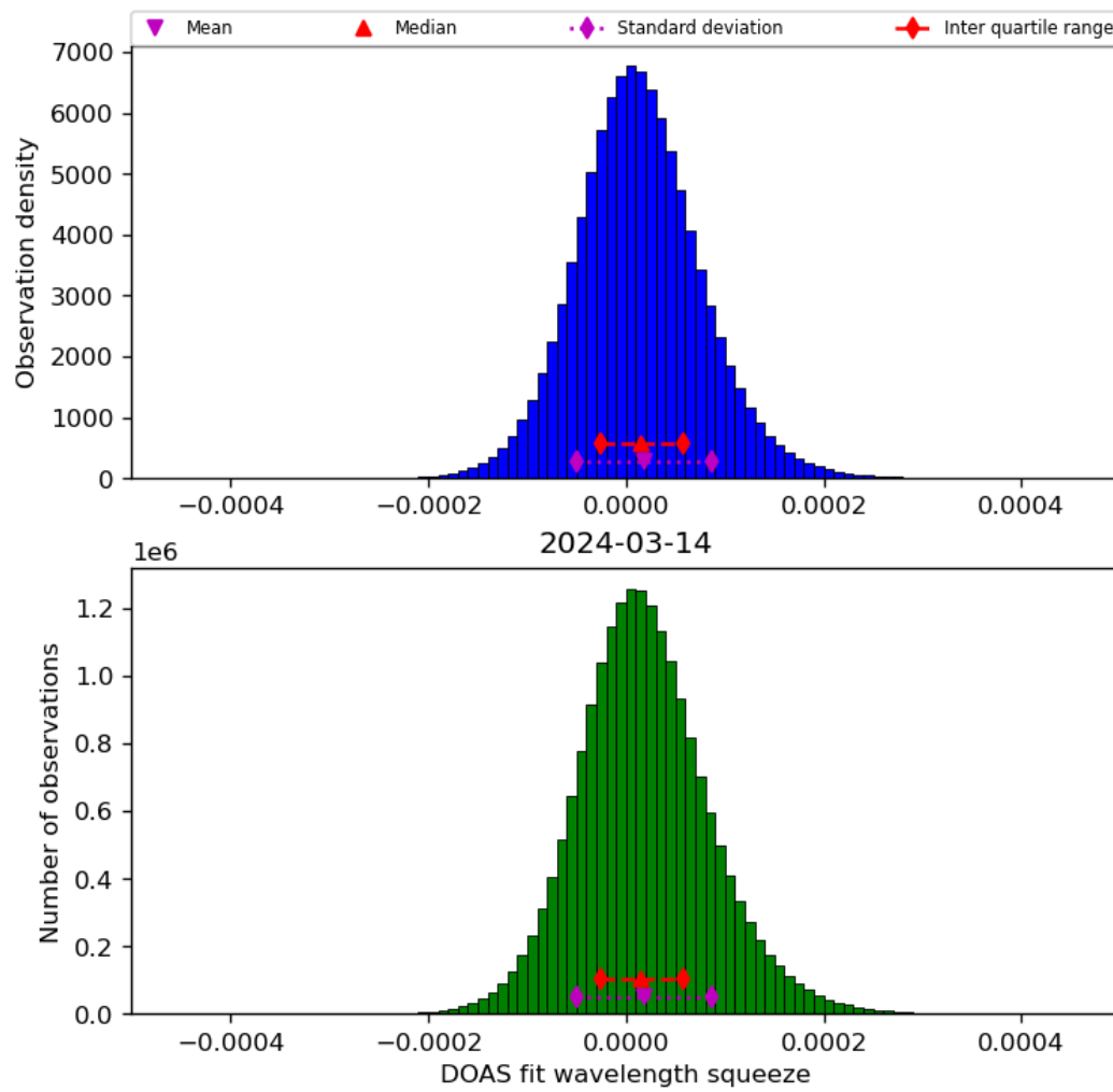
Figure 45: Histogram of “DOAS fit wavelength squeeze” for 2024-03-14 to 2024-03-15
