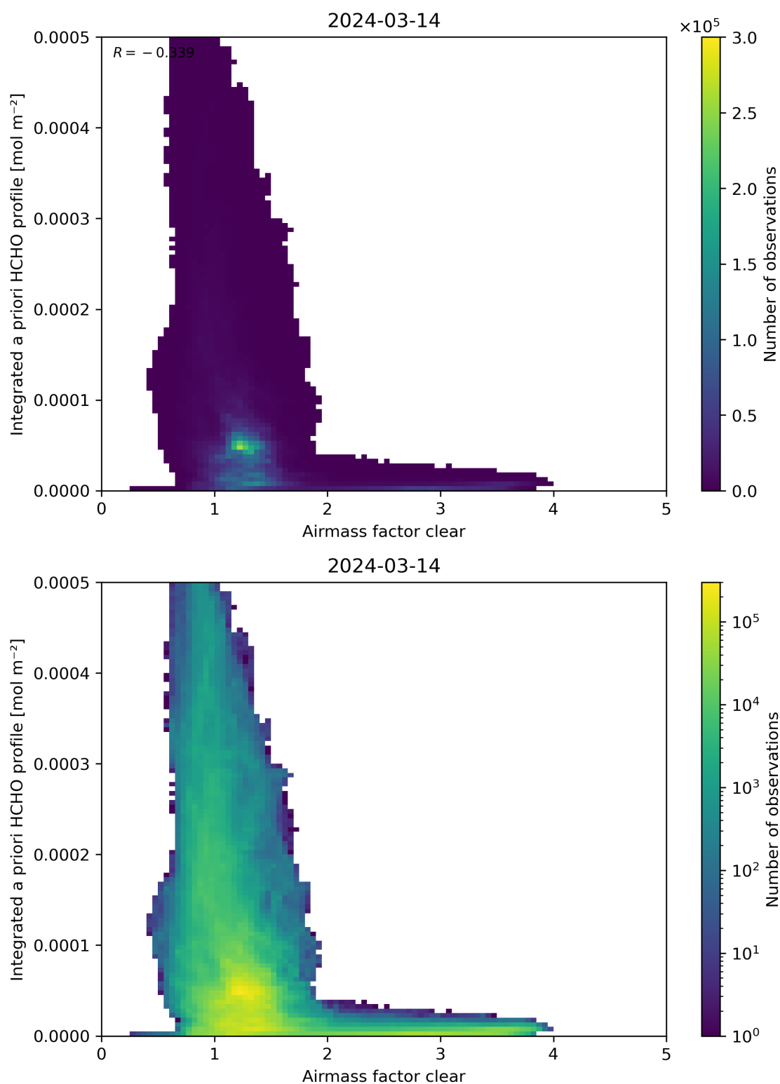
Figure 76: Scatter density plot of “Airmass factor clear” against “Integrated a priori HCHO profile” for 2024-03-14 to 2024-03-15.
