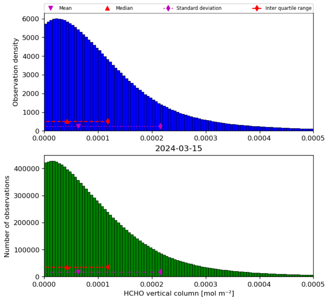
Figure 35: Histogram of “HCHO vertical column” for 2024-03-14 to 2024-03-16
