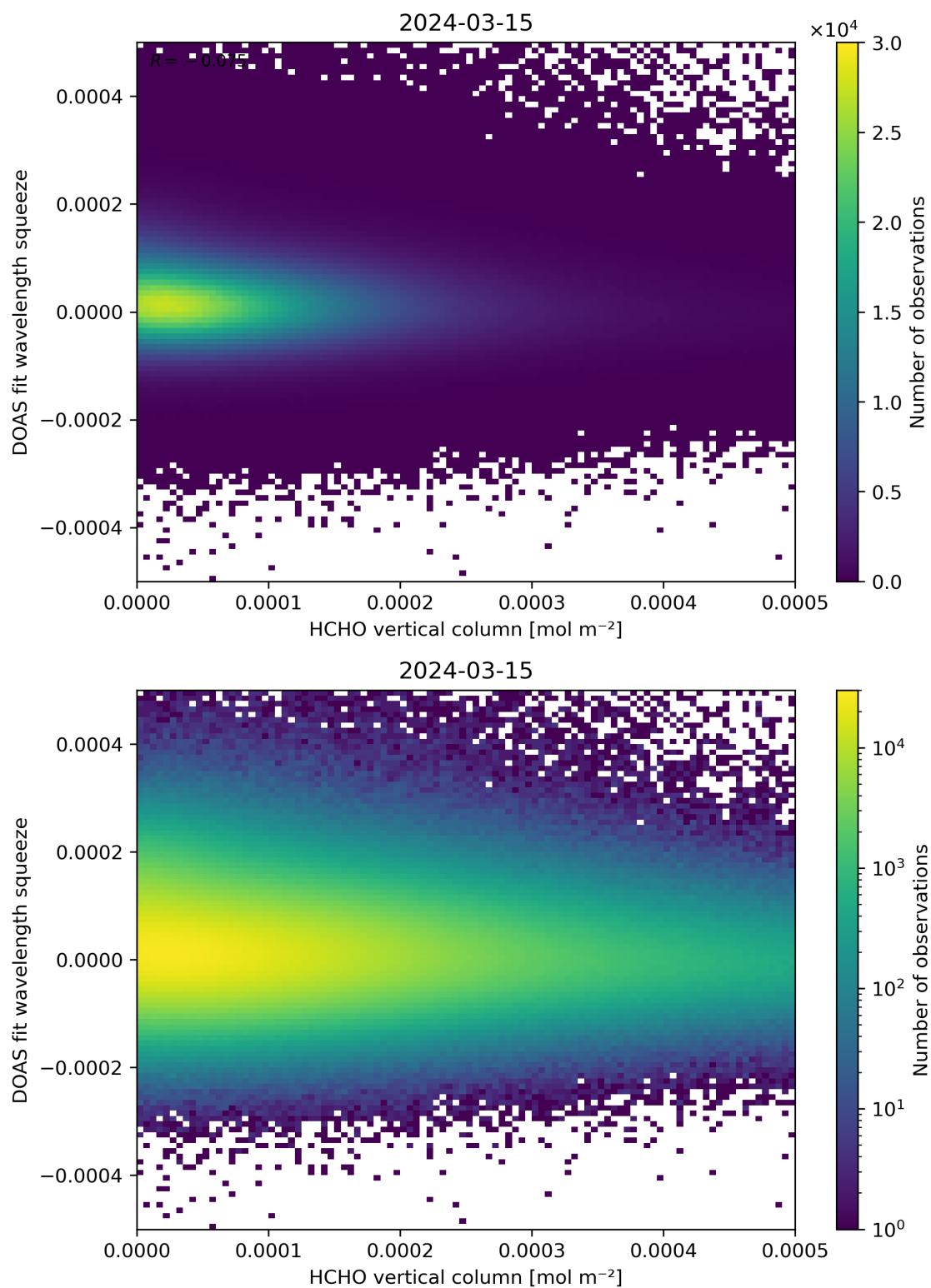
Figure 125: Scatter density plot of “HCHO vertical column” against “DOAS fit wavelength squeeze” for 2024-03-14 to 2024-03-16.
