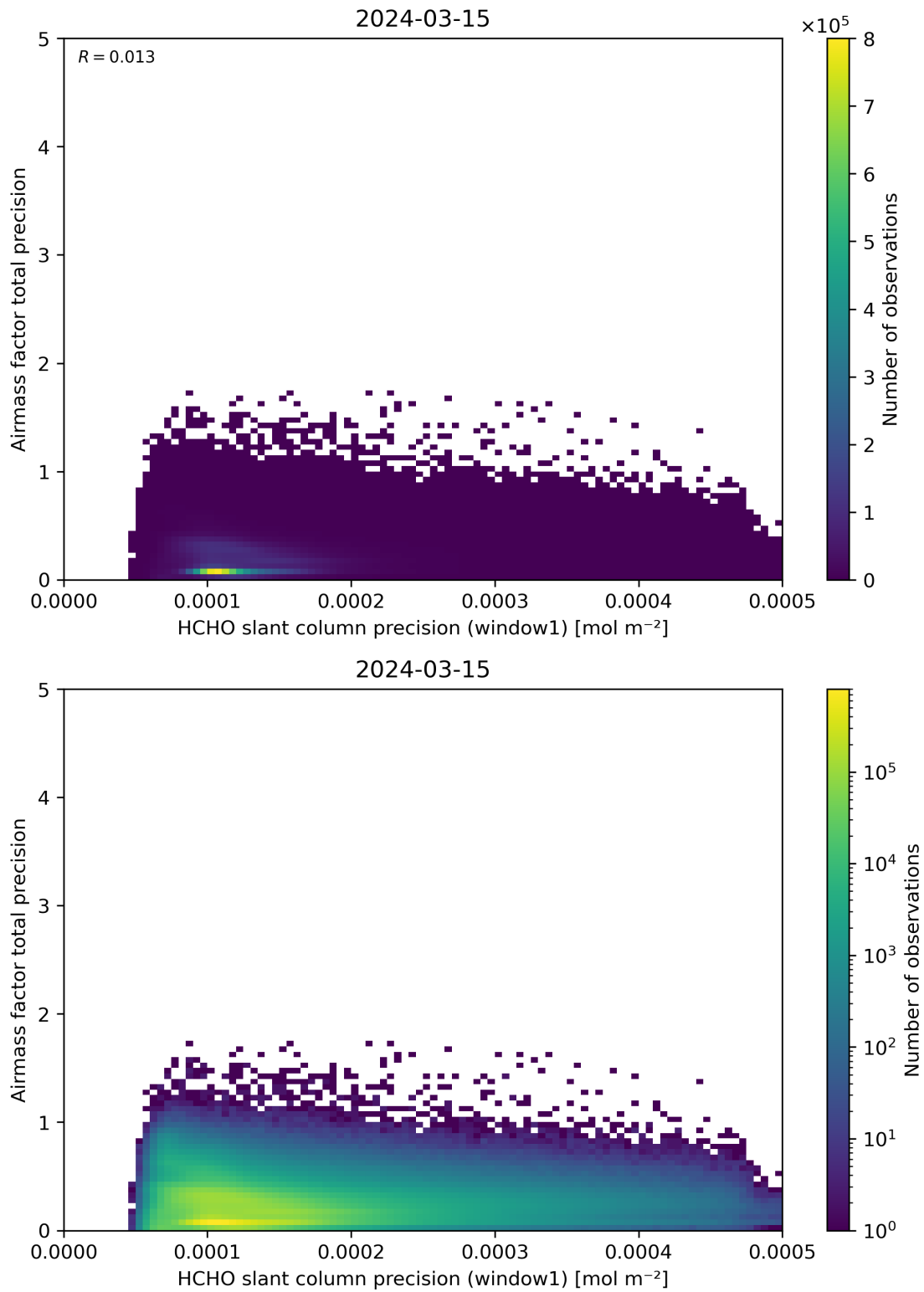
Figure 95: Scatter density plot of “HCHO slant column precision (window1)” against “Airmass factor total precision” for 2024-03-14 to 2024-03-16.
