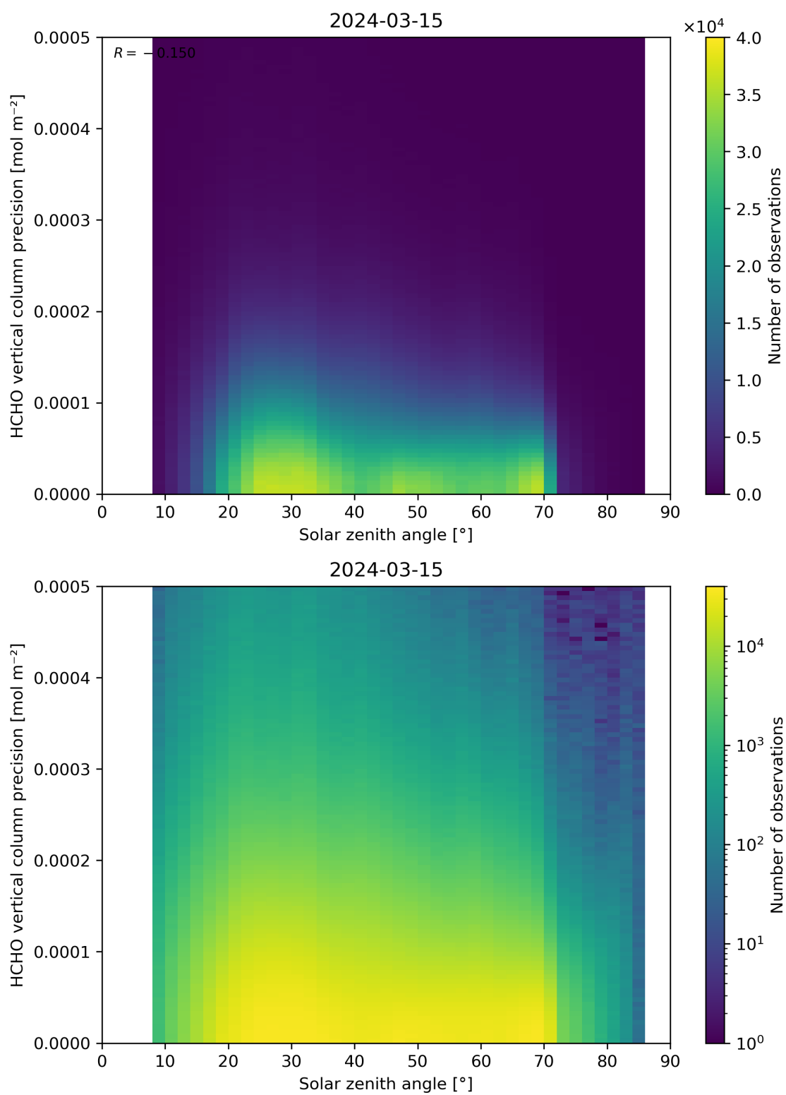
Figure 179: Scatter density plot of “Solar zenith angle” against “HCHO vertical column precision” for 2024-03-14 to 2024-03-16.
