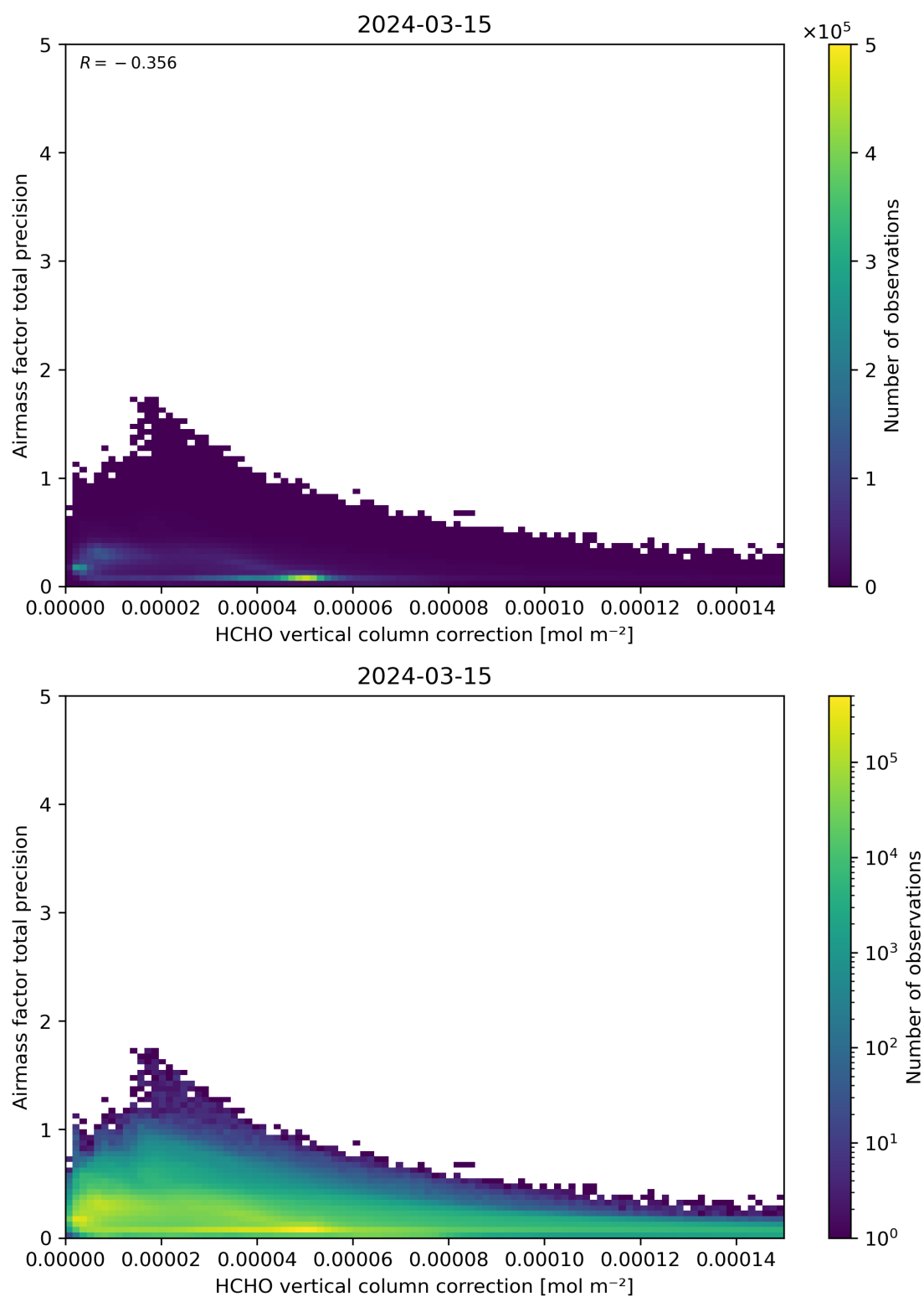
Figure 121: Scatter density plot of “HCHO vertical column correction” against “Airmass factor total precision” for 2024-03-14 to 2024-03-16.
