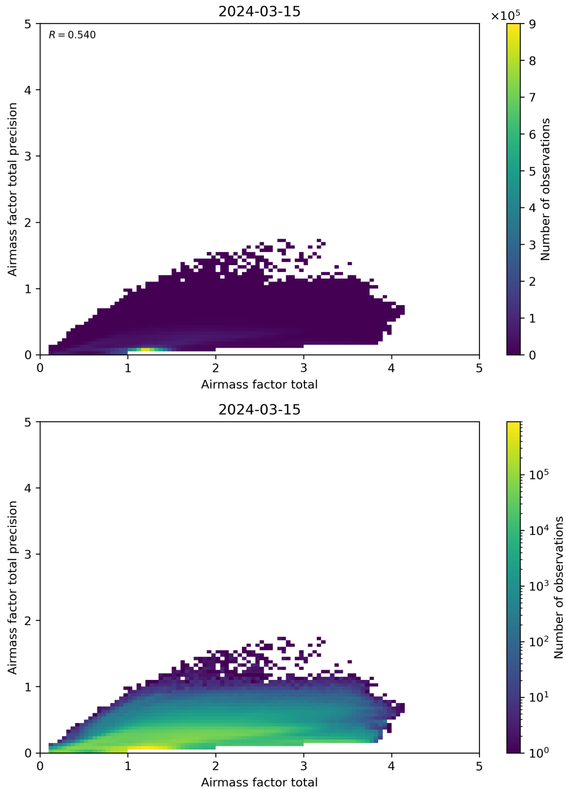
Figure 103: Scatter density plot of “Airmass factor total” against “Airmass factor total precision” for 2024-03-14 to 2024-03-16.
