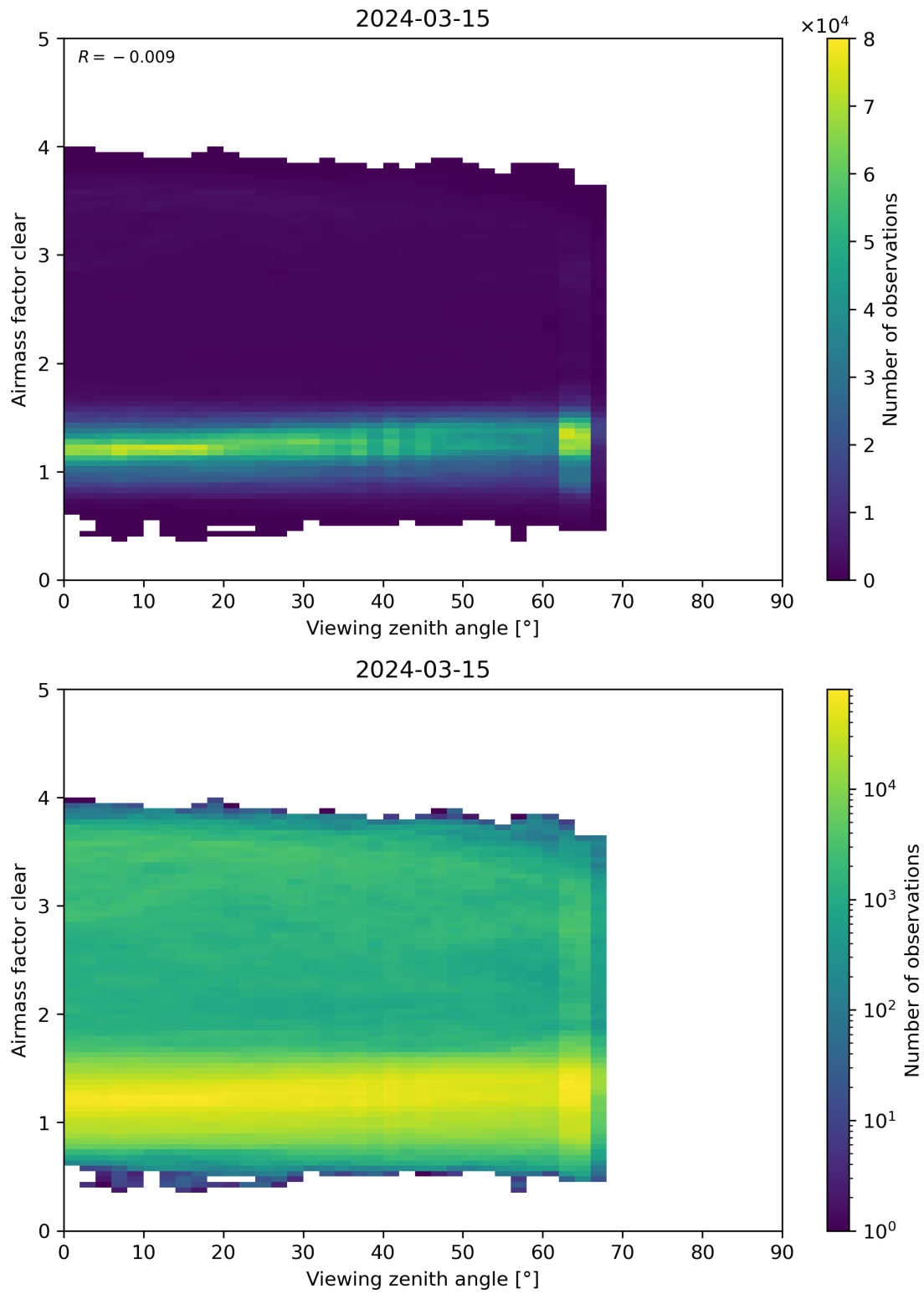
Figure 185: Scatter density plot of “Viewing zenith angle” against “Airmass factor clear” for 2024-03-14 to 2024-03-16.
