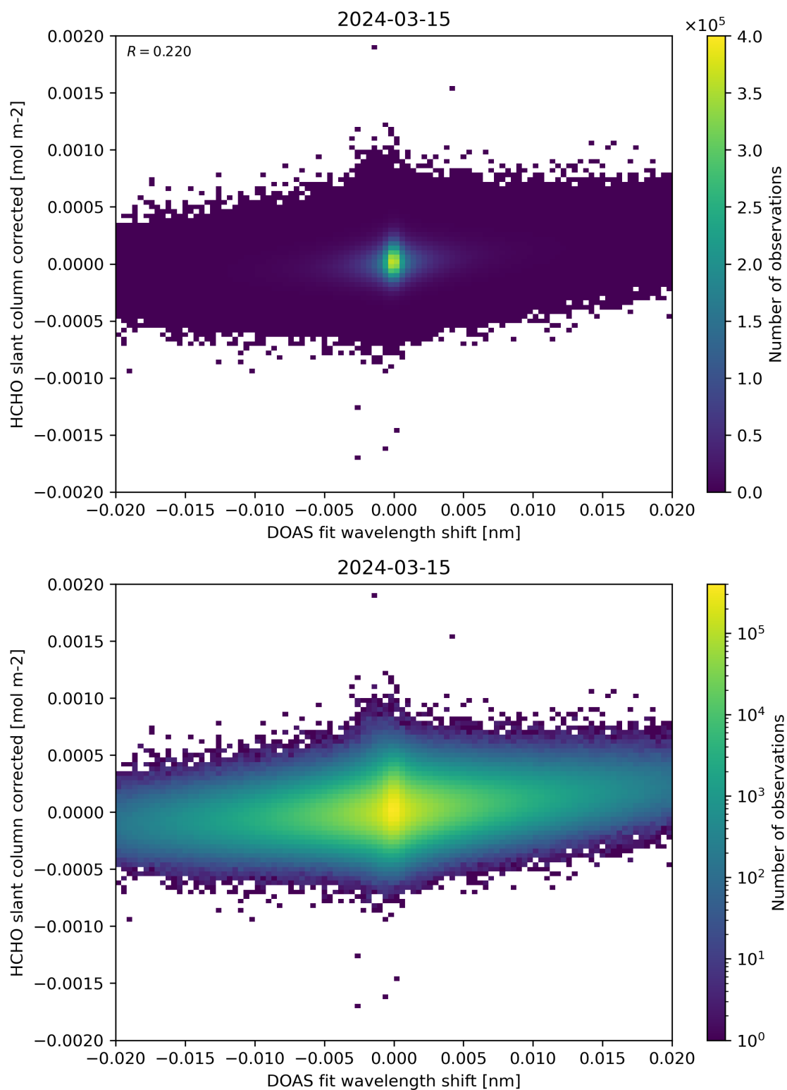
Figure 66: Scatter density plot of “DOAS fit wavelength shift” against “HCHO slant column corrected” for 2024-03-14 to 2024-03-16.
