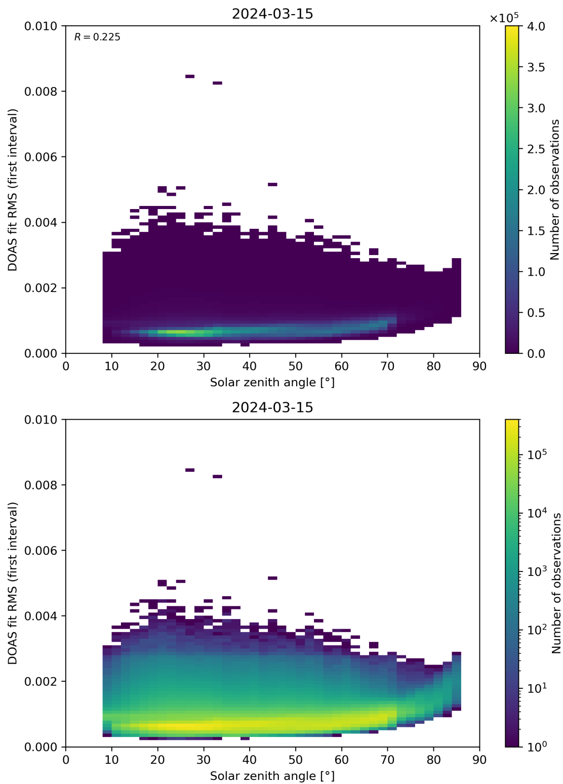
Figure 167: Scatter density plot of “Solar zenith angle” against “DOAS fit RMS (first interval)” for 2024-03-14 to 2024-03-16.
