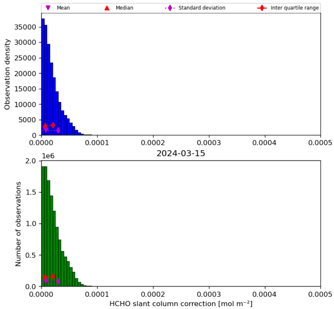
Figure 47: Histogram of “HCHO slant column correction” for 2024-03-14 to 2024-03-16
