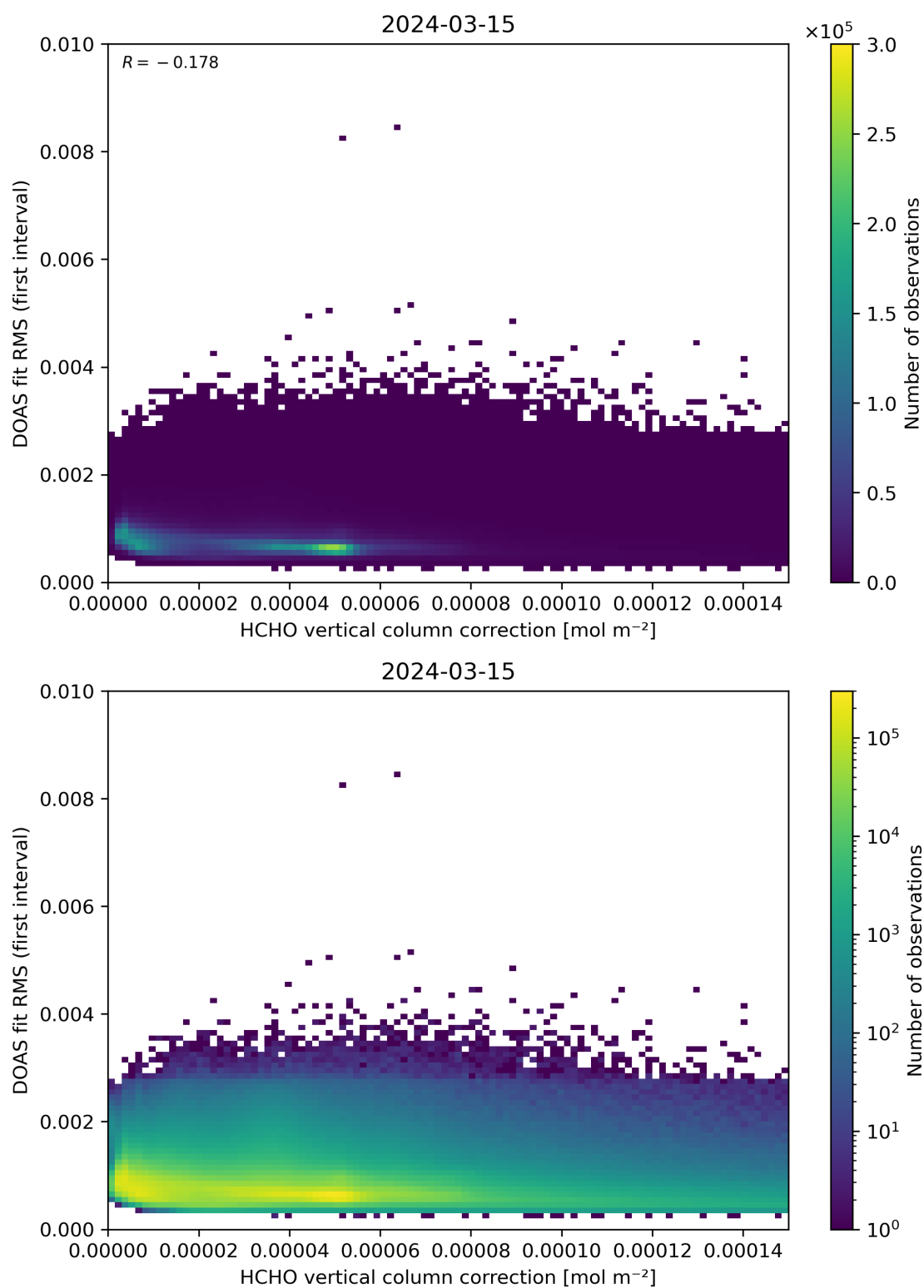
Figure 112: Scatter density plot of “HCHO vertical column correction” against “DOAS fit RMS (first interval)” for 2024-03-14 to 2024-03-16.
