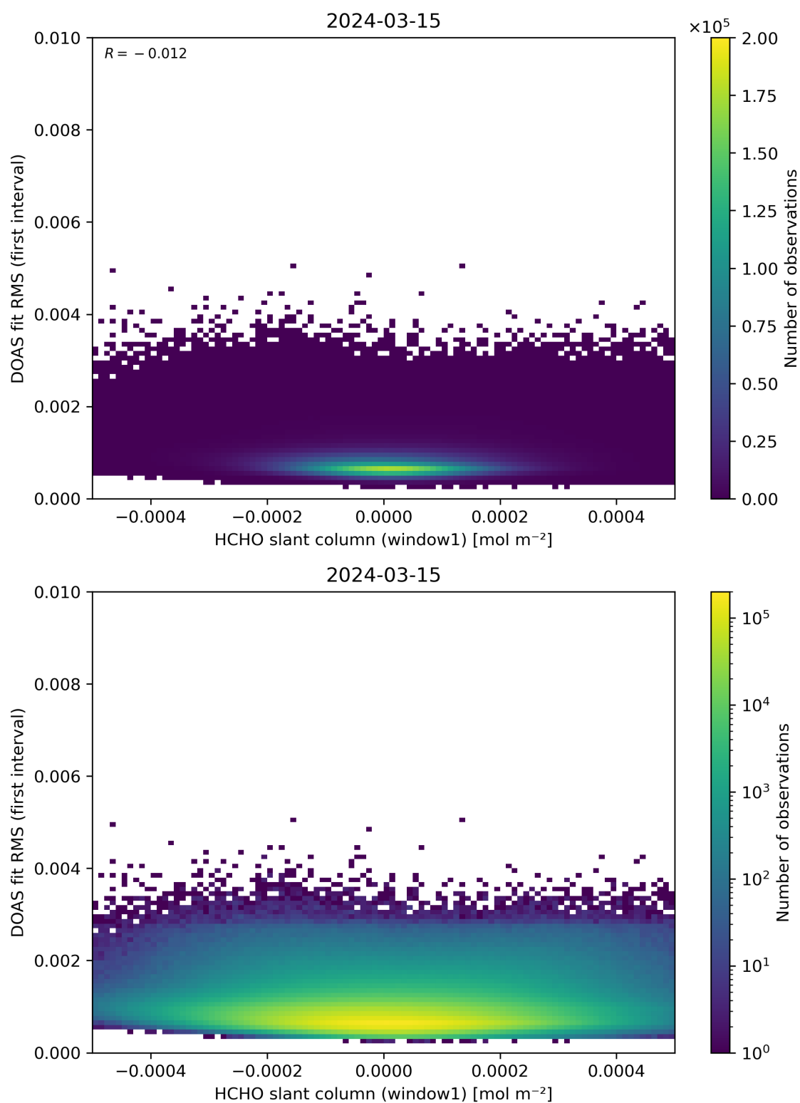
Figure 78: Scatter density plot of “HCHO slant column (window1)” against “DOAS fit RMS (first interval)” for 2024-03-14 to 2024-03-16.
