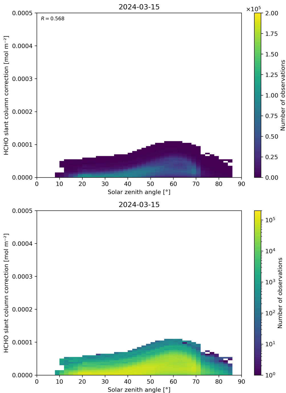
Figure 172: Scatter density plot of “Solar zenith angle” against “HCHO slant column correction” for 2024-03-14 to 2024-03-16.
