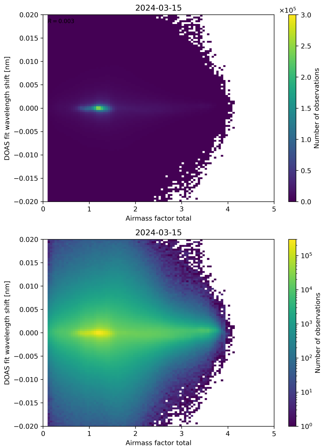
Figure 98: Scatter density plot of “Airmass factor total” against “DOAS fit wavelength shift” for 2024-03-14 to 2024-03-16.
