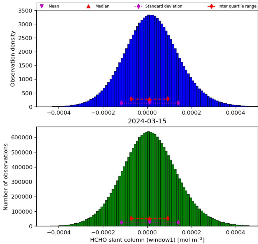
Figure 38: Histogram of “HCHO slant column (window1)” for 2024-03-14 to 2024-03-16
