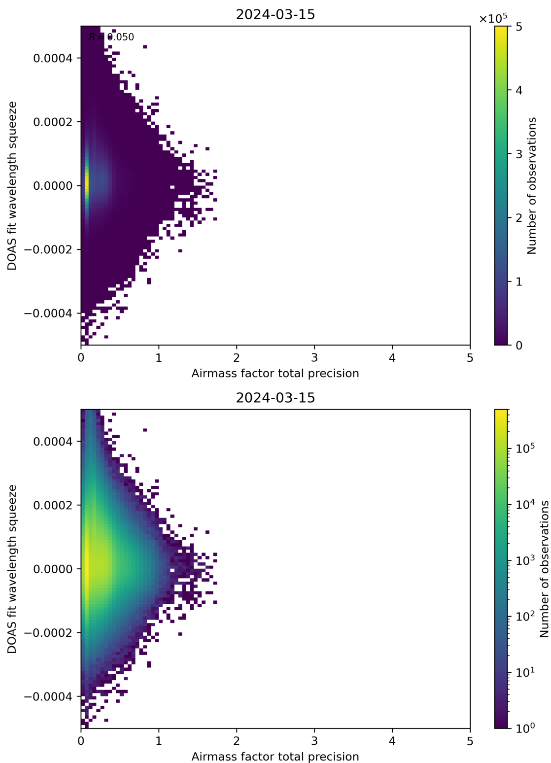
Figure 107: Scatter density plot of “Airmass factor total precision” against “DOAS fit wavelength squeeze” for 2024-03-14 to 2024-03-16.
