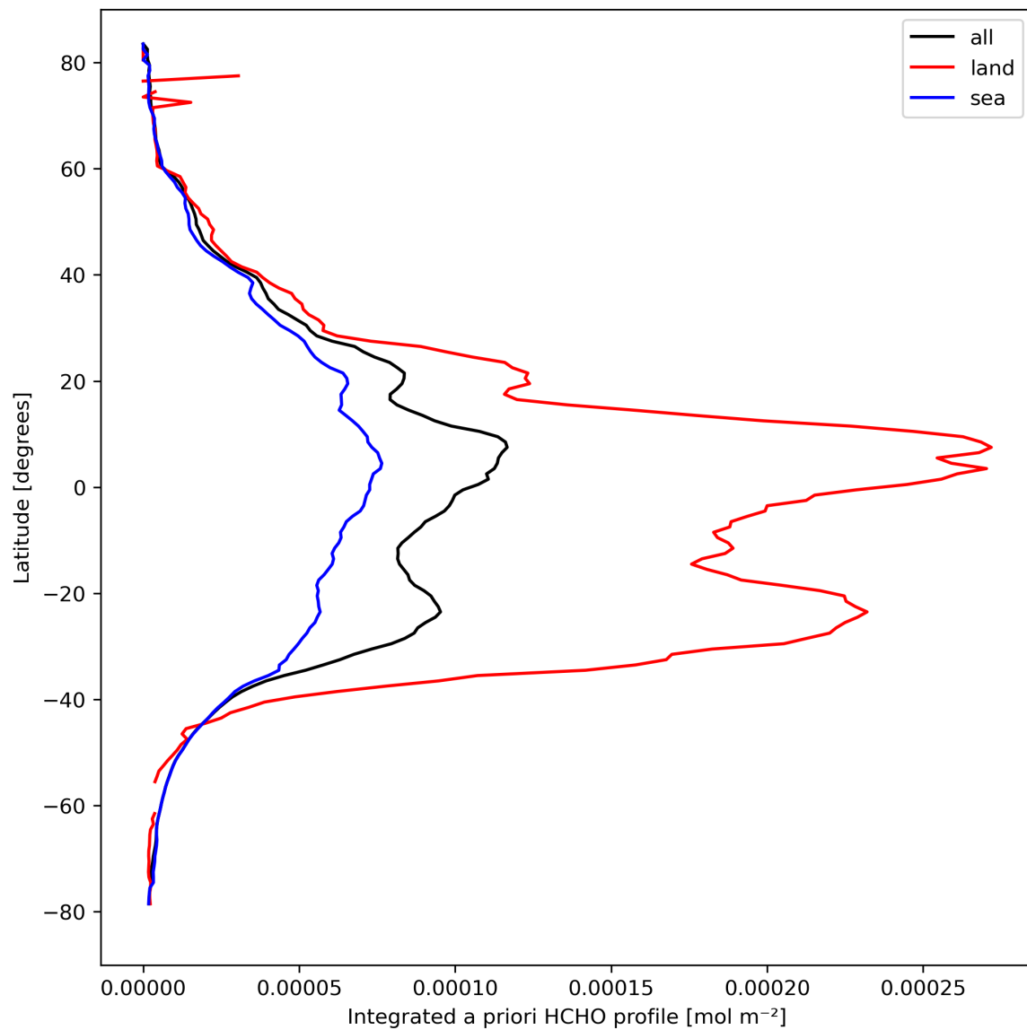
Figure 29: Zonal average of “Integrated a priori HCHO profile” for 2024-03-14 to 2024-03-16.
