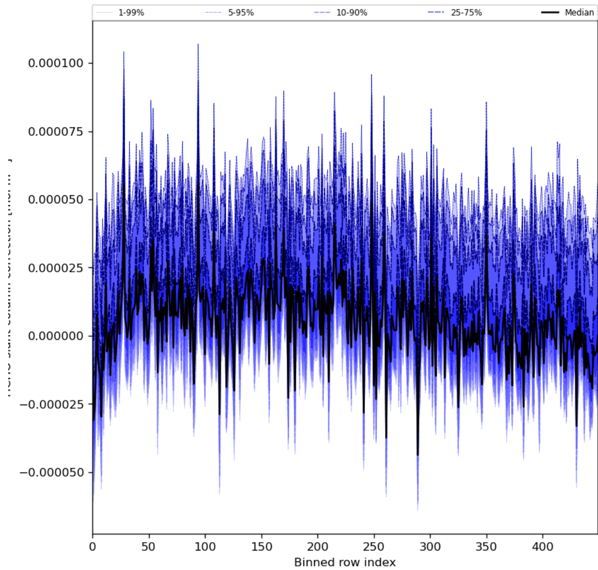
Figure 61: Along track statistics of “HCHO slant column correction” for 2024-03-14 to 2024-03-16
