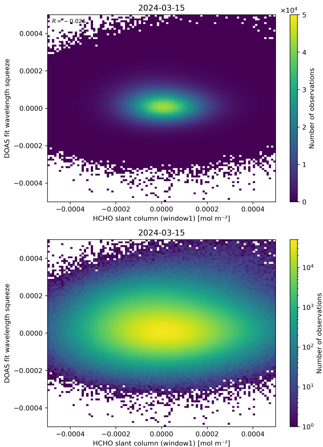
Figure 80: Scatter density plot of “HCHO slant column (window1)” against “DOAS fit wavelength squeeze” for 2024-03-14 to 2024-03-16.
