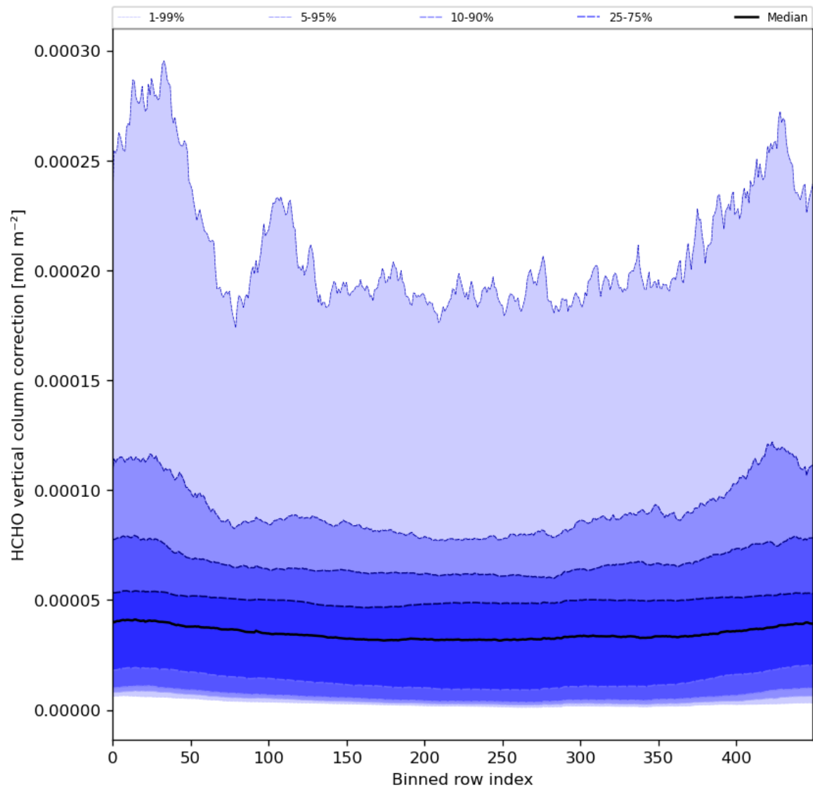
Figure 51: Along track statistics of “HCHO vertical column correction” for 2024-03-14 to 2024-03-16
