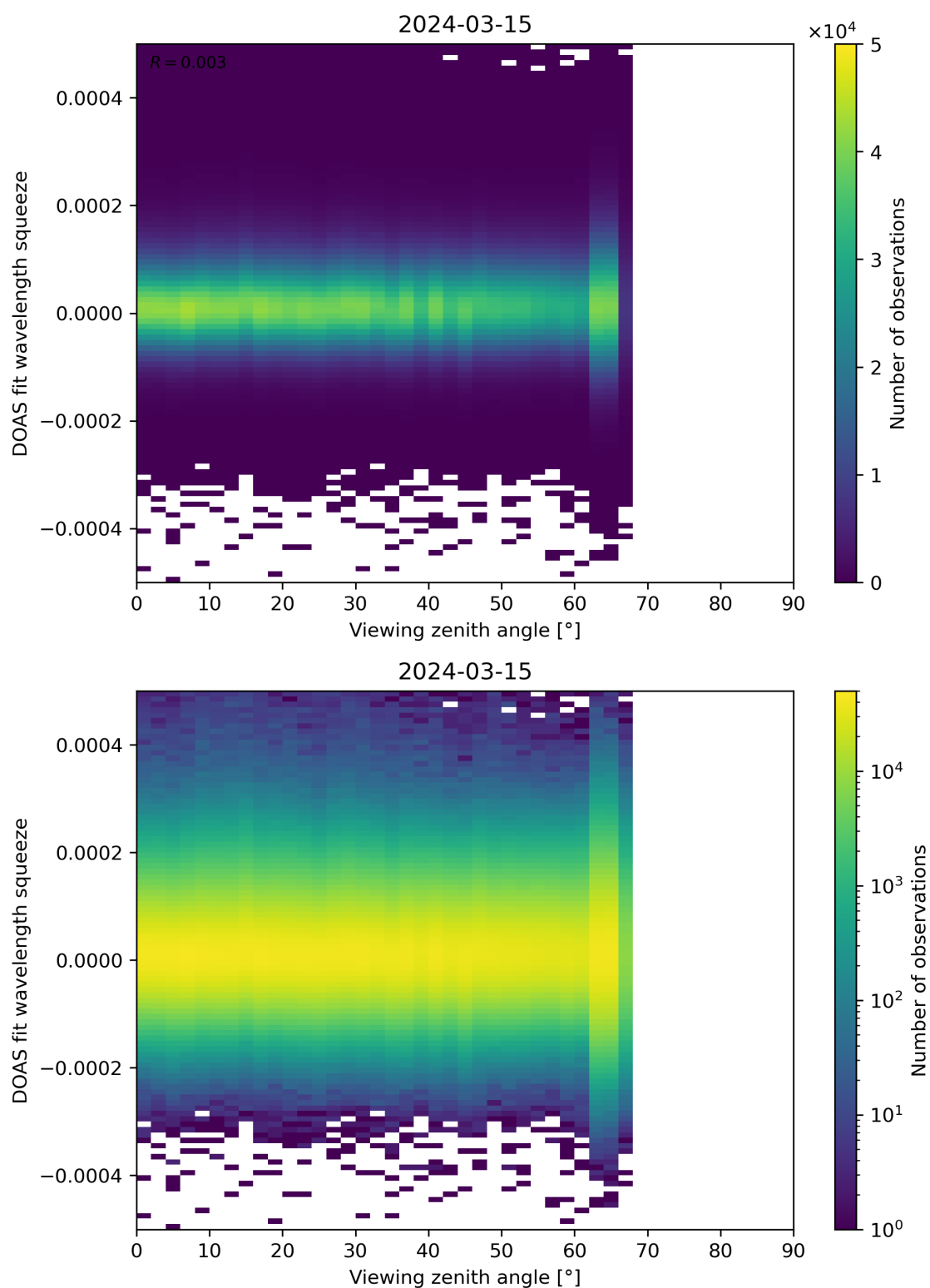
Figure 184: Scatter density plot of “Viewing zenith angle” against “DOAS fit wavelength squeeze” for 2024-03-14 to 2024-03-16.
