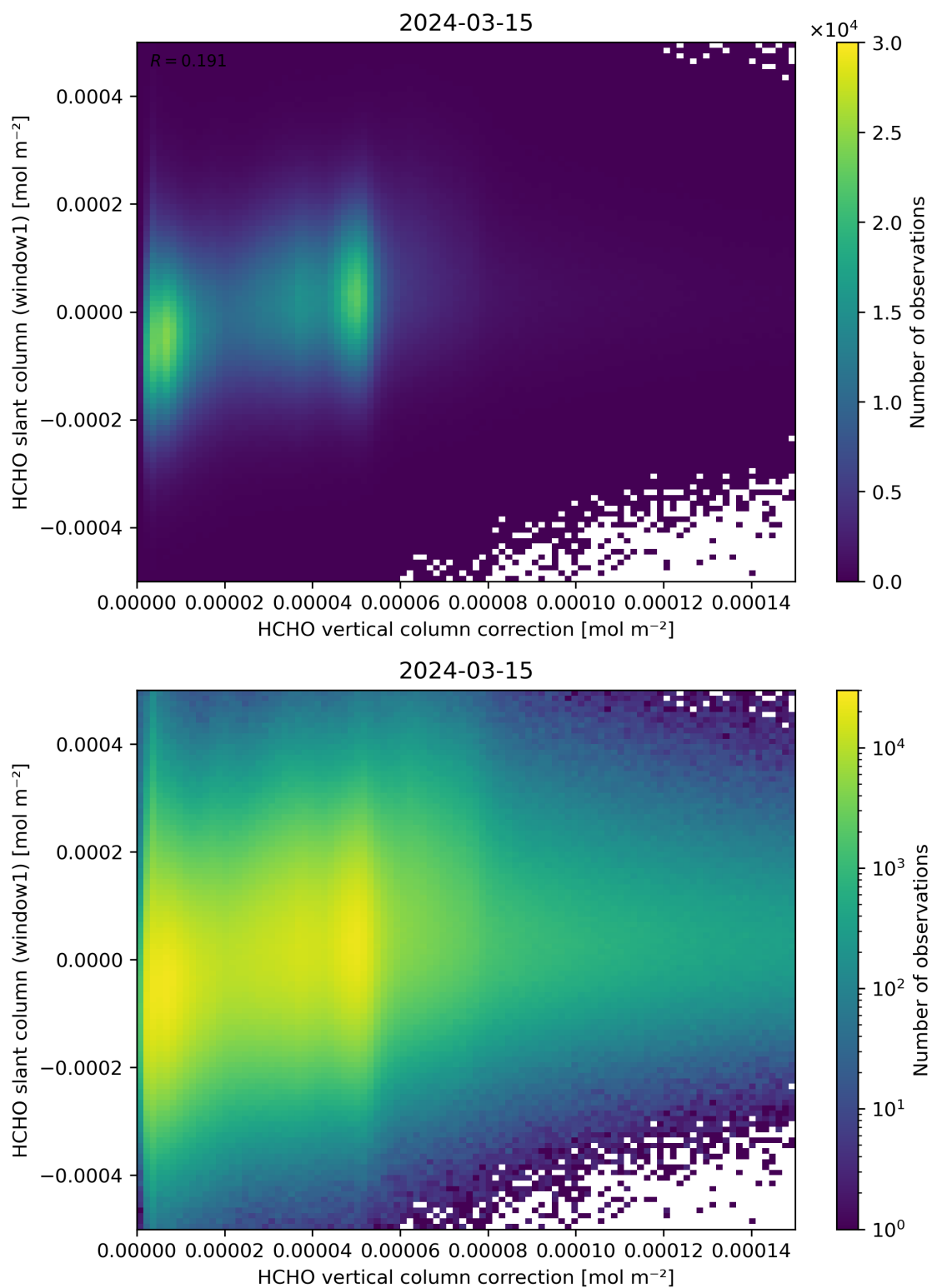
Figure 118: Scatter density plot of “HCHO vertical column correction” against “HCHO slant column (window1)” for 2024-03-14 to 2024-03-16.
