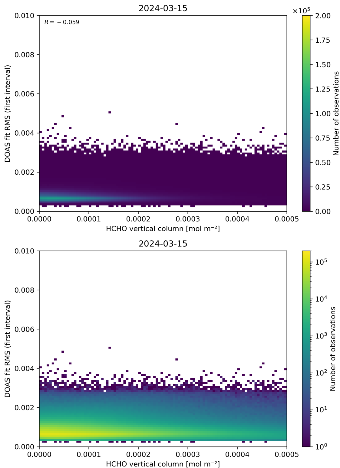
Figure 123: Scatter density plot of “HCHO vertical column” against “DOAS fit RMS (first interval)” for 2024-03-14 to 2024-03-16.
