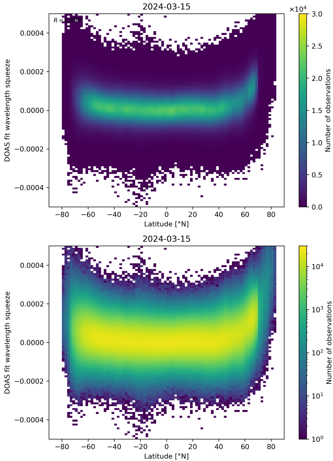
Figure 155: Scatter density plot of “Latitude” against “DOAS fit wavelength squeeze” for 2024-03-14 to 2024-03-16.
