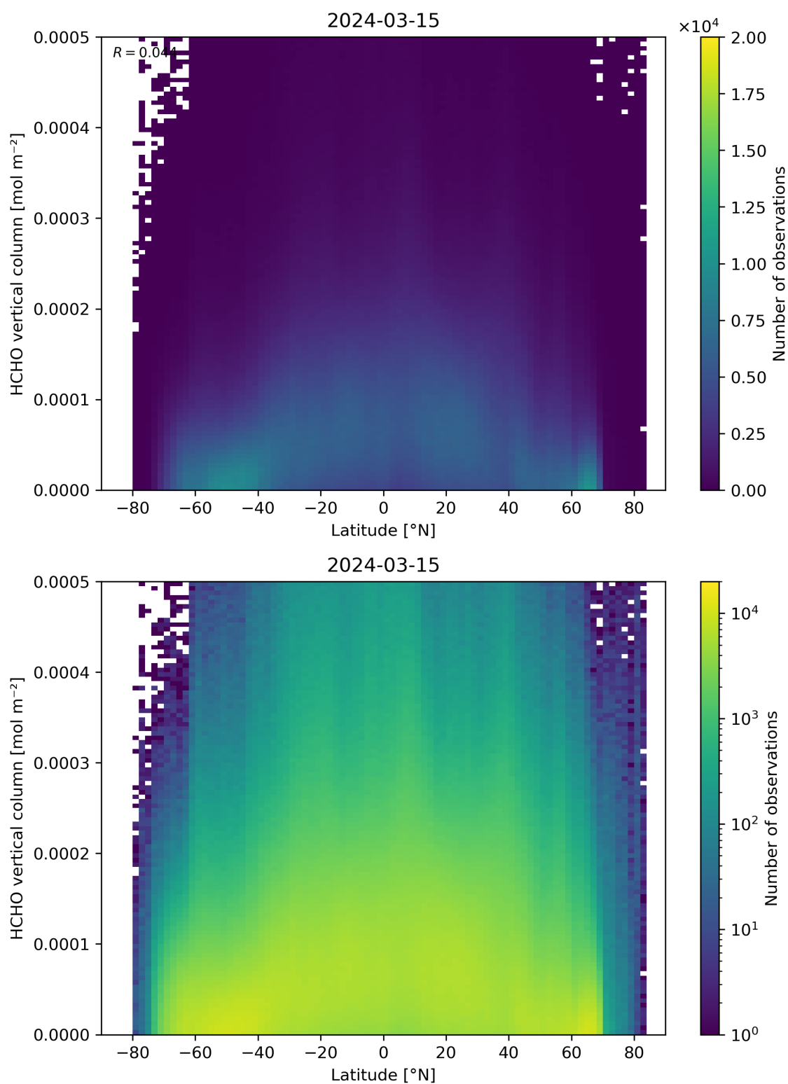
Figure 163: Scatter density plot of “Latitude” against “HCHO vertical column” for 2024-03-14 to 2024-03-16.
