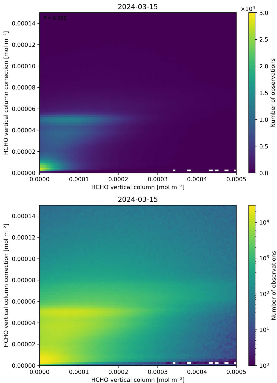
Figure 133: Scatter density plot of “HCHO vertical column” against “HCHO vertical column correction” for 2024-03-14 to 2024-03-16.
