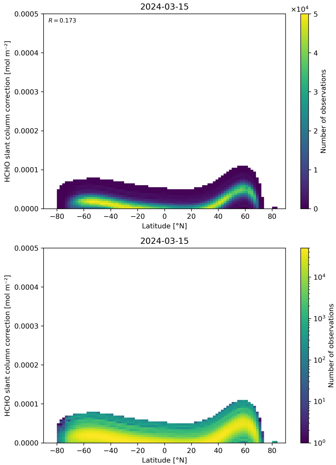
Figure 158: Scatter density plot of “Latitude” against “HCHO slant column correction” for 2024-03-14 to 2024-03-16.
