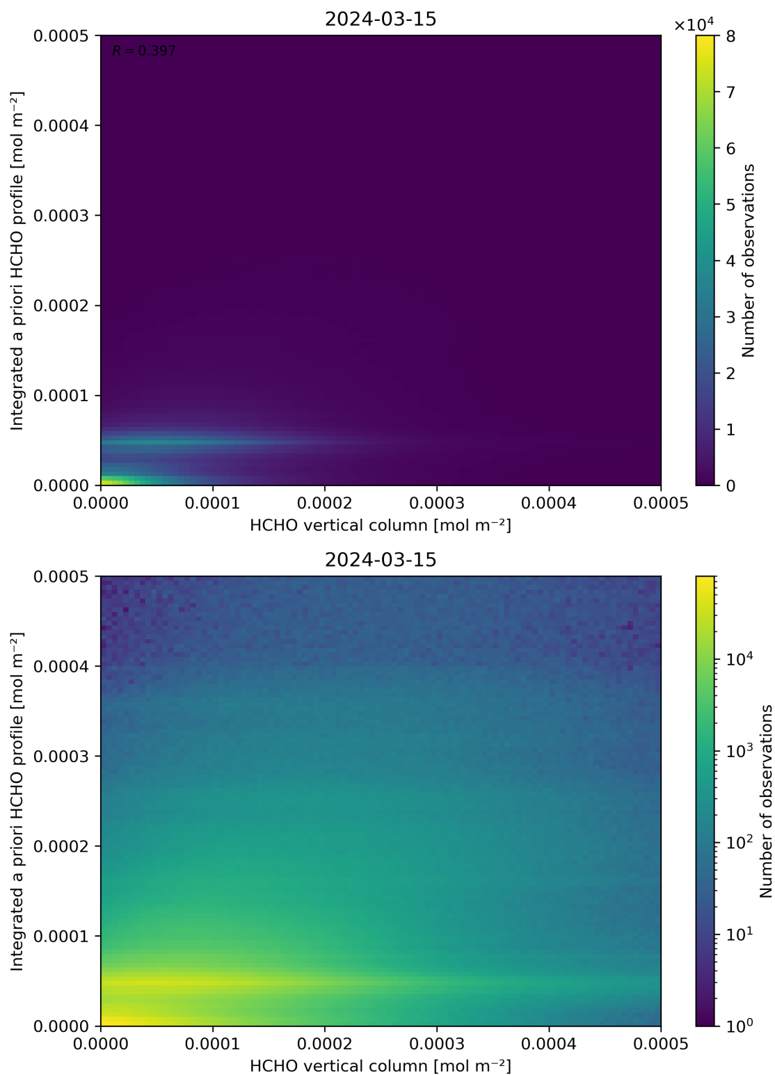
Figure 135: Scatter density plot of “HCHO vertical column” against “Integrated a priori HCHO profile” for 2024-03-14 to 2024-03-16.
