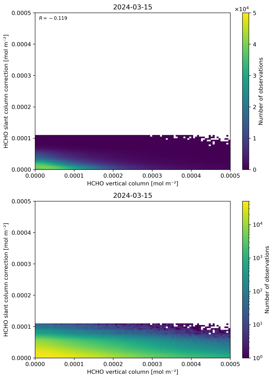
Figure 128: Scatter density plot of “HCHO vertical column” against “HCHO slant column correction” for 2024-03-14 to 2024-03-16.
