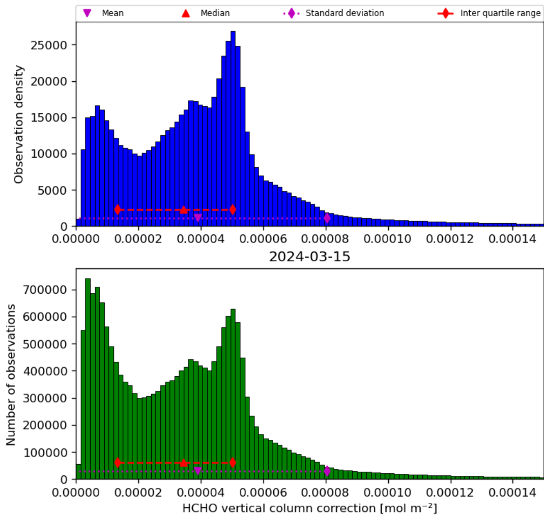
Figure 37: Histogram of “HCHO vertical column correction” for 2024-03-14 to 2024-03-16
