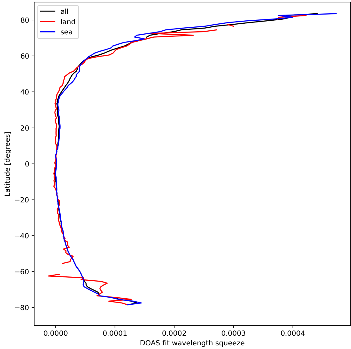
Figure 31: Zonal average of “DOAS fit wavelength squeeze” for 2024-03-14 to 2024-03-16.
