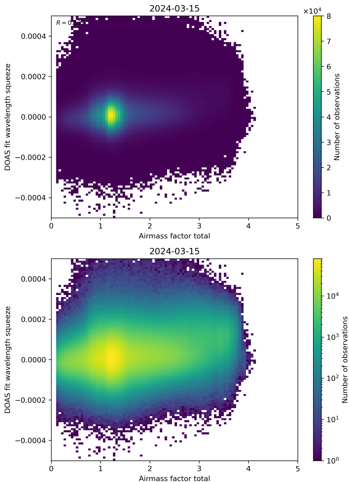
Figure 99: Scatter density plot of “Airmass factor total” against “DOAS fit wavelength squeeze” for 2024-03-14 to 2024-03-16.
