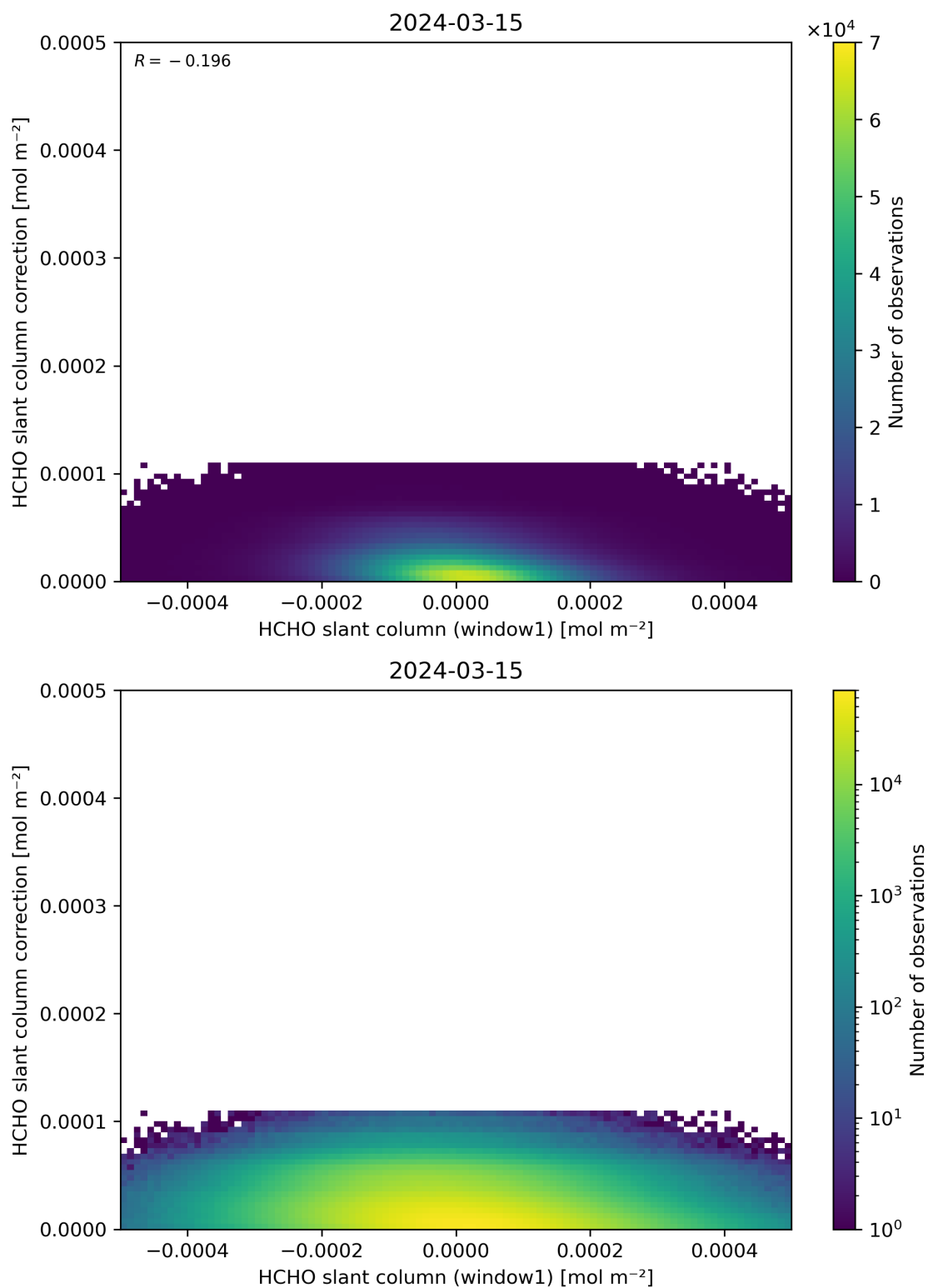
Figure 83: Scatter density plot of “HCHO slant column (window1)” against “HCHO slant column correction” for 2024-03-14 to 2024-03-16.
