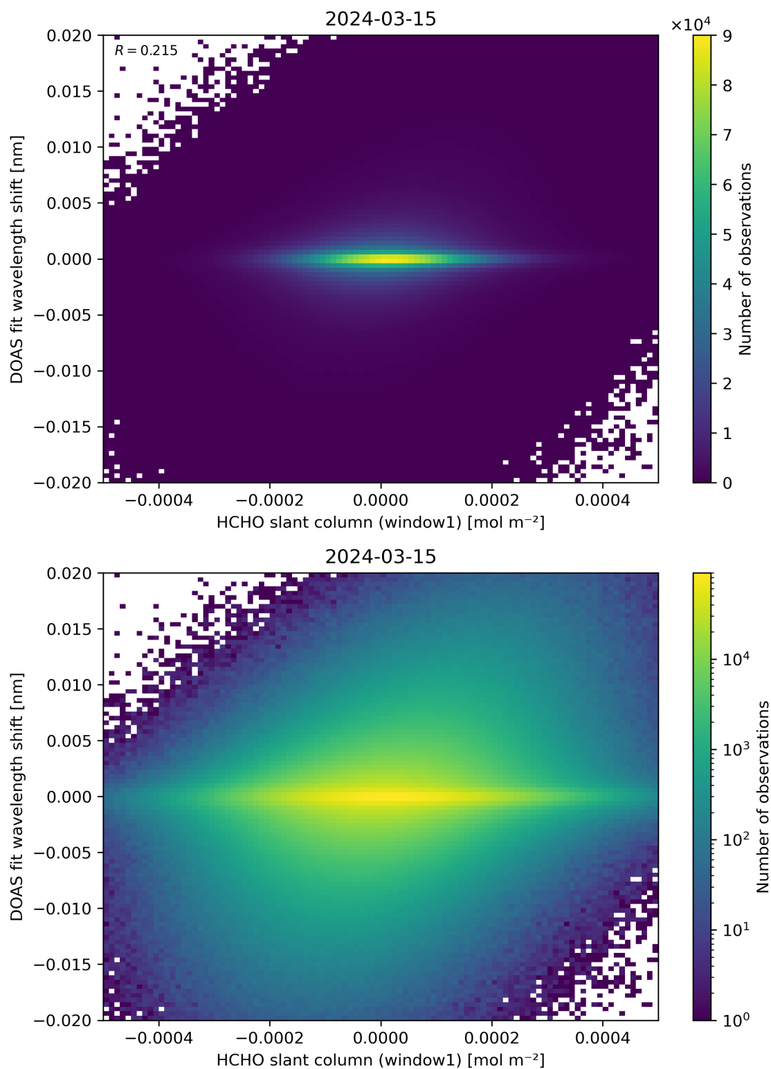
Figure 79: Scatter density plot of “HCHO slant column (window1)” against “DOAS fit wavelength shift” for 2024-03-14 to 2024-03-16.
