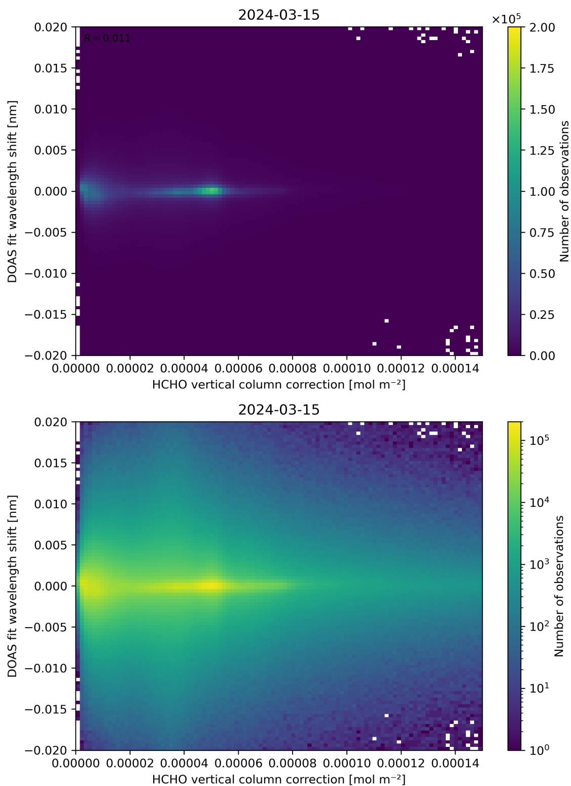
Figure 113: Scatter density plot of “HCHO vertical column correction” against “DOAS fit wavelength shift” for 2024-03-14 to 2024-03-16.
