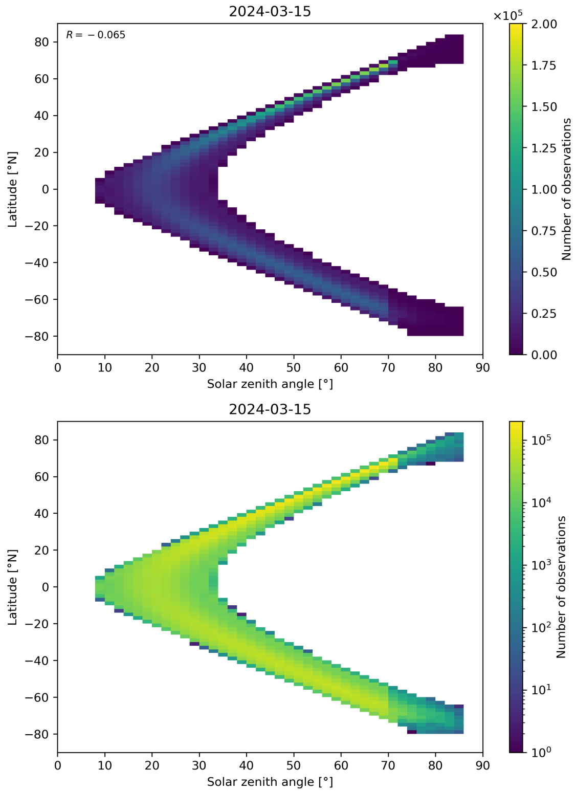
Figure 181: Scatter density plot of “Solar zenith angle” against “Latitude” for 2024-03-14 to 2024-03-16.
