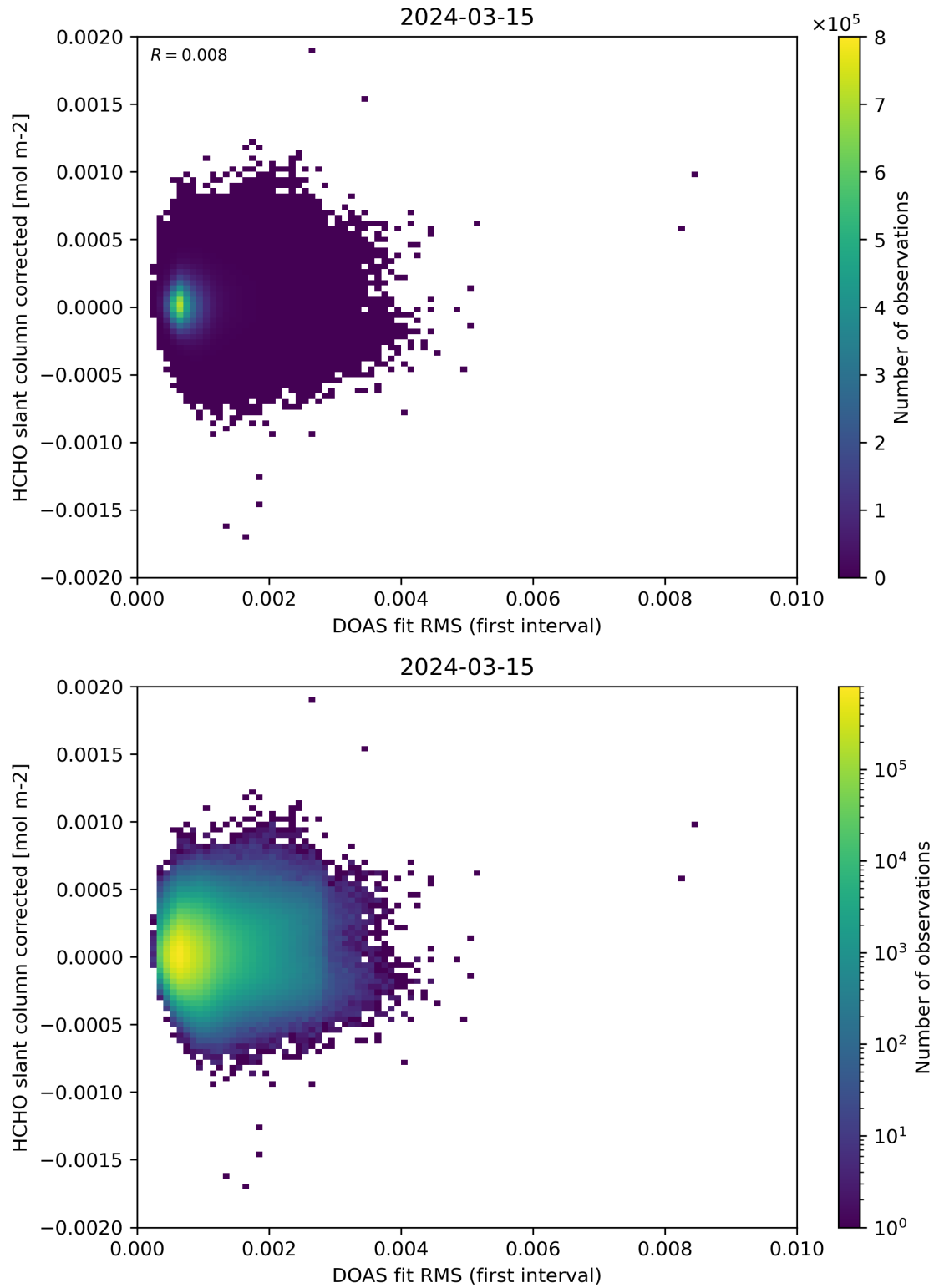
Figure 62: Scatter density plot of “DOAS fit RMS (first interval)” against “HCHO slant column corrected” for 2024-03-14 to 2024-03-16.
