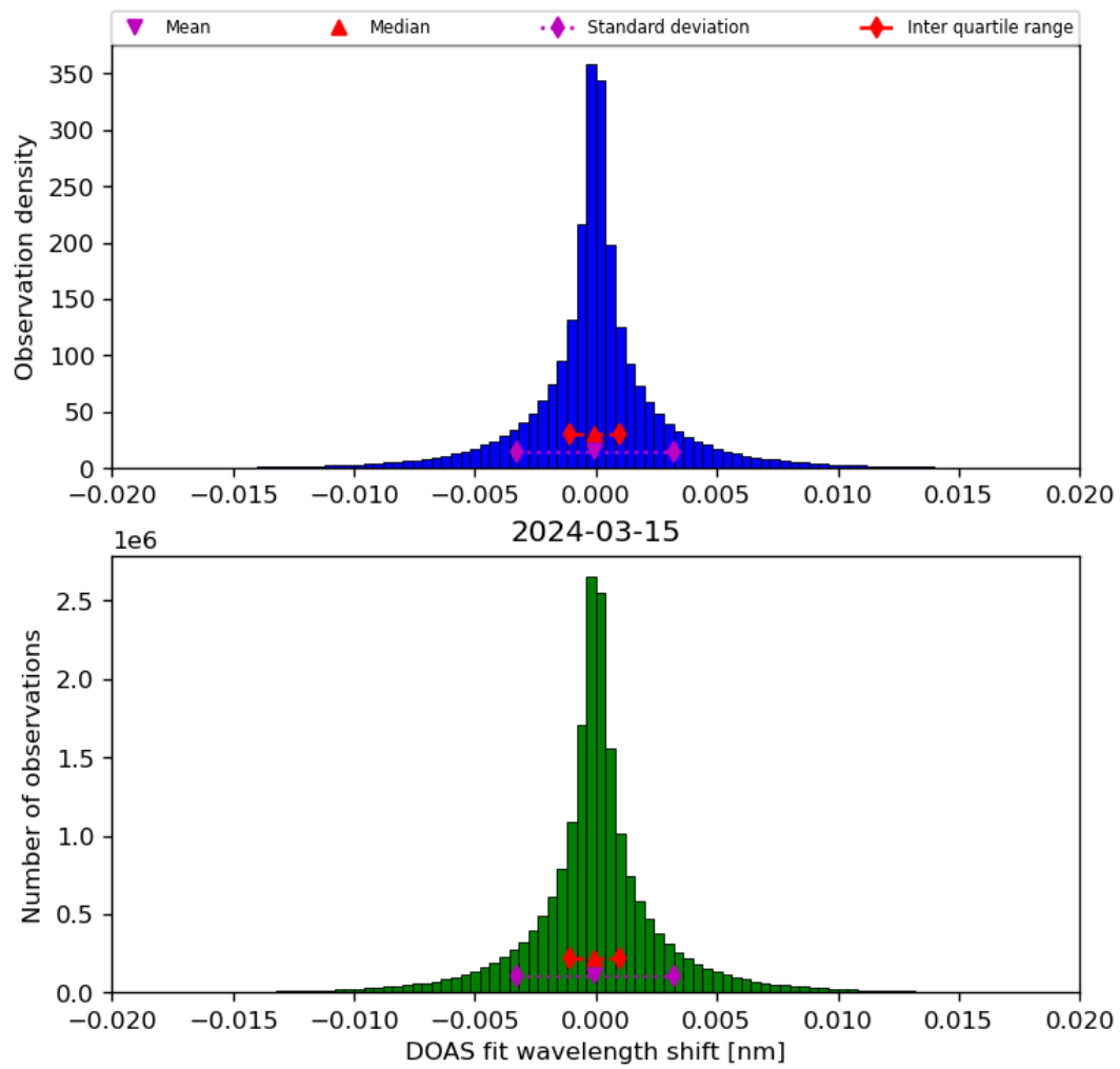
Figure 44: Histogram of “DOAS fit wavelength shift” for 2024-03-14 to 2024-03-16
