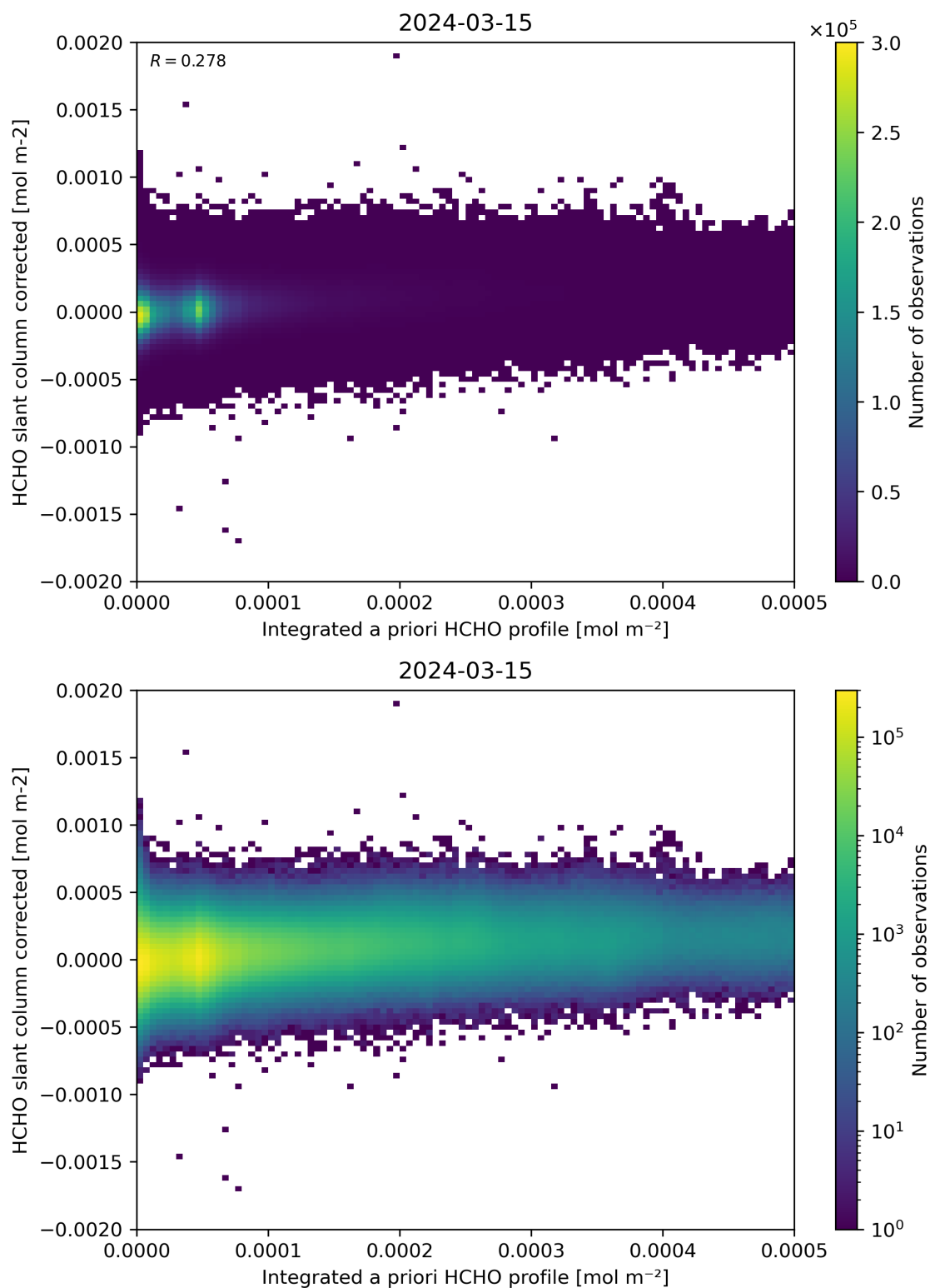
Figure 151: Scatter density plot of “Integrated a priori HCHO profile” against “HCHO slant column corrected” for 2024-03-14 to 2024-03-16.
