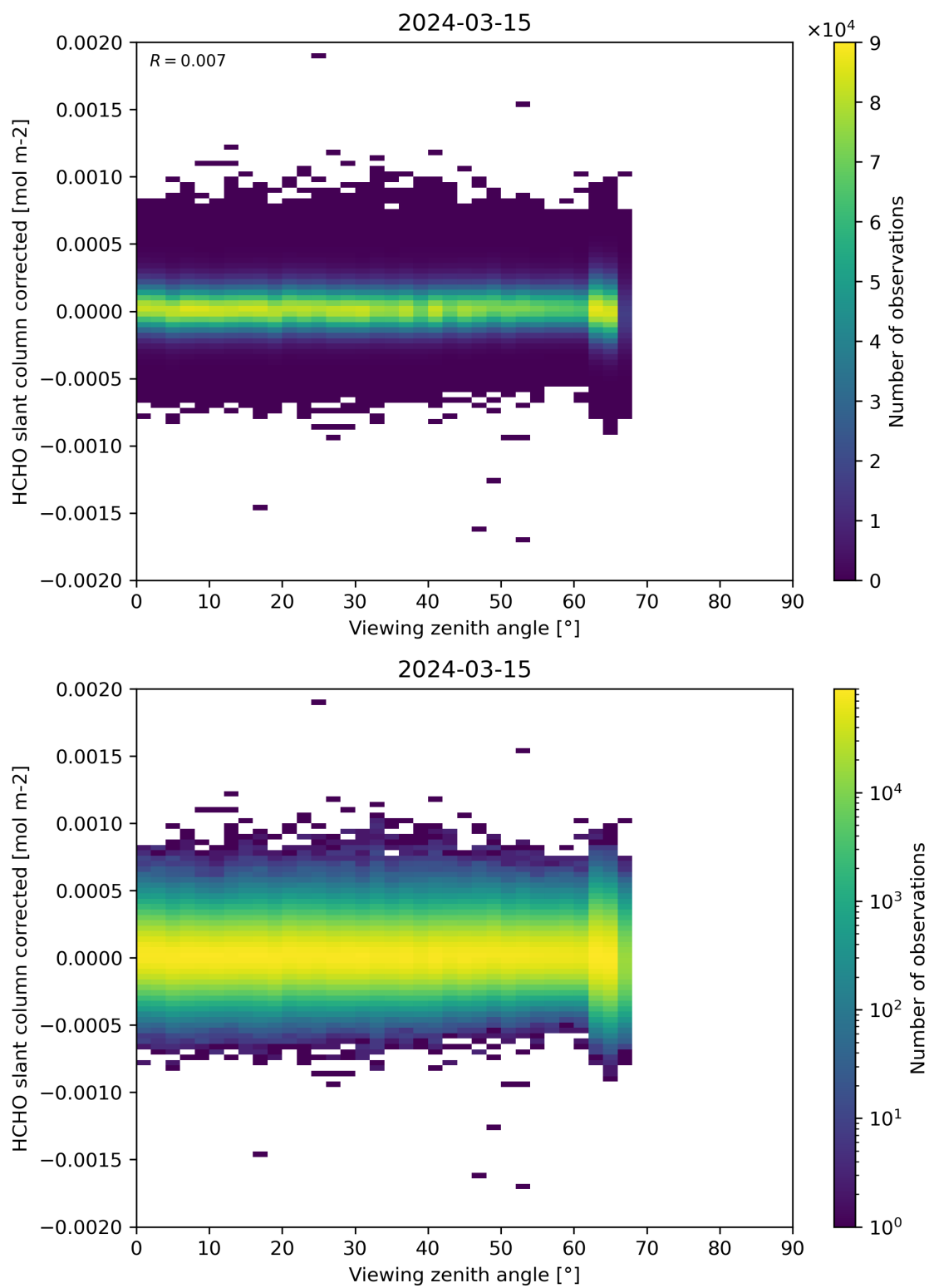
Figure 186: Scatter density plot of “Viewing zenith angle” against “HCHO slant column corrected” for 2024-03-14 to 2024-03-16.
