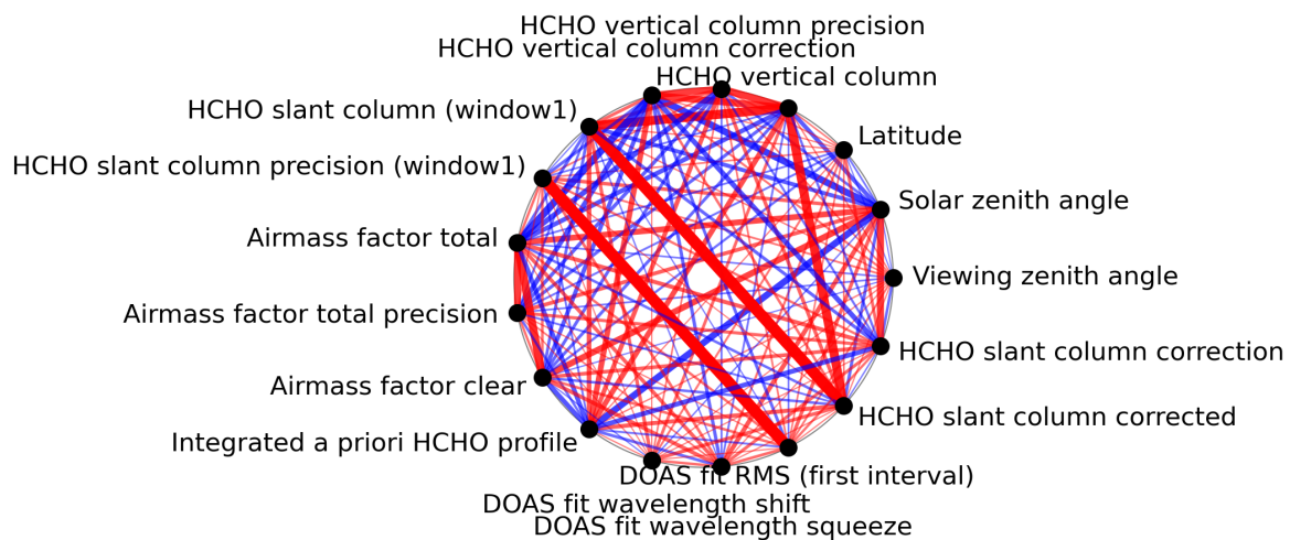
Figure 1: Map of correlation graph for 2024-03-14 to 2024-03-16.
