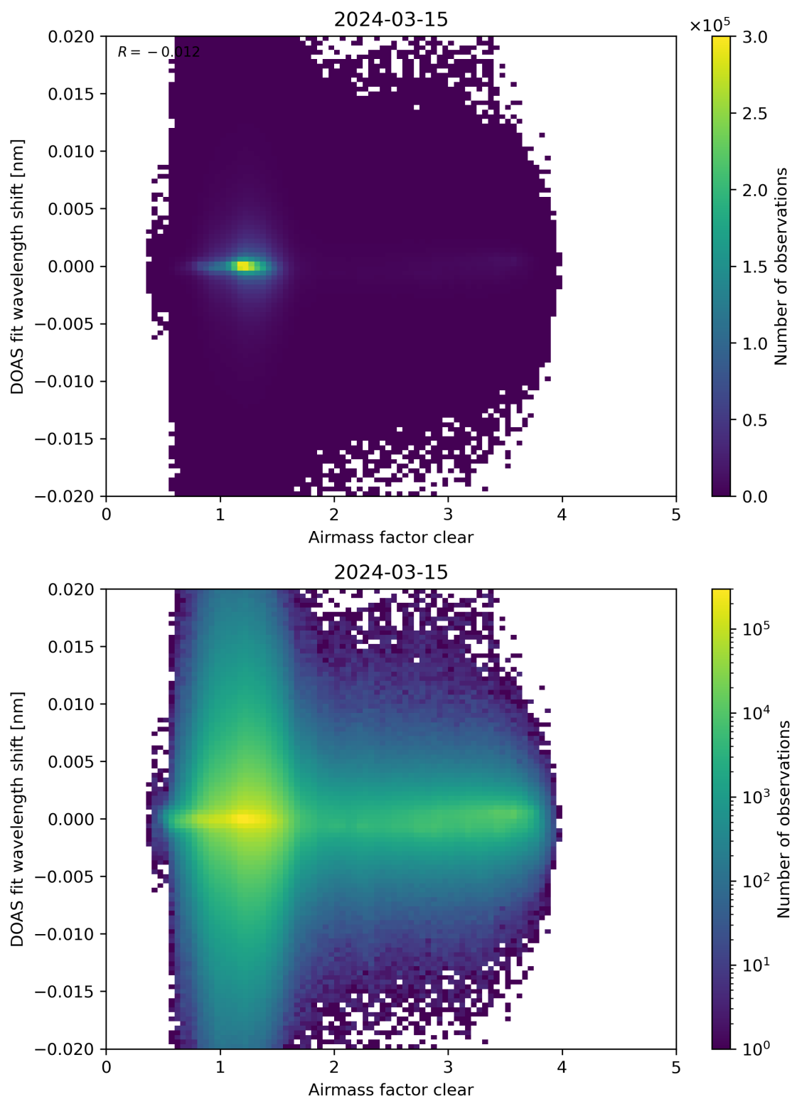
Figure 72: Scatter density plot of “Airmass factor clear” against “DOAS fit wavelength shift” for 2024-03-14 to 2024-03-16.
