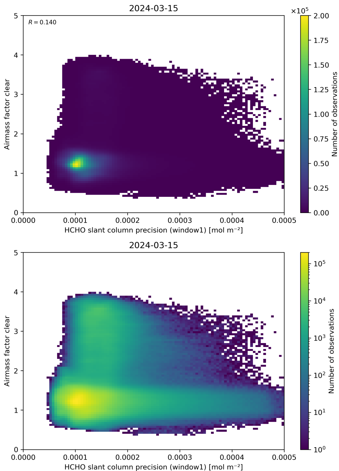
Figure 91: Scatter density plot of “HCHO slant column precision (window1)” against “Airmass factor clear” for 2024-03-14 to 2024-03-16.
