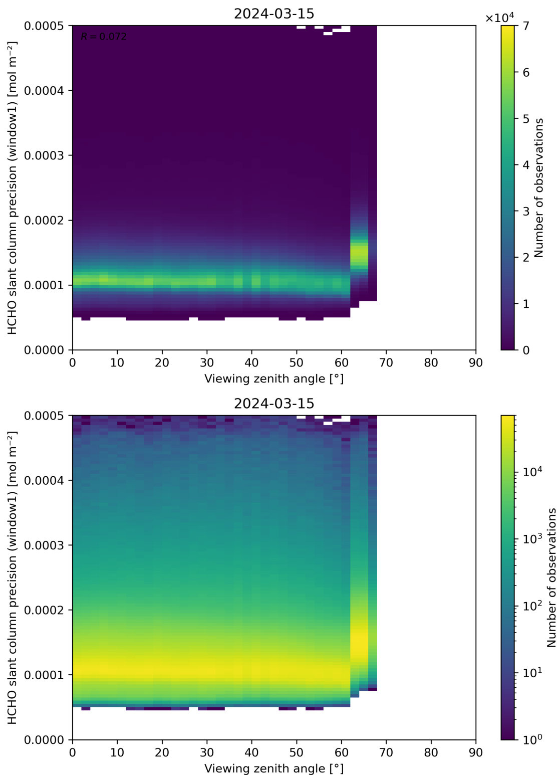
Figure 189: Scatter density plot of “Viewing zenith angle” against “HCHO slant column precision (window1)” for 2024-03-14 to 2024-03-16.
