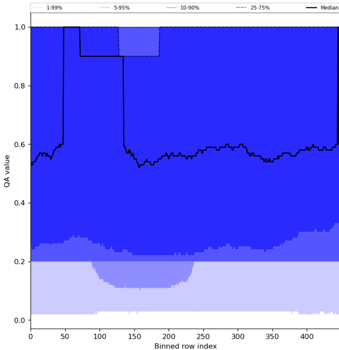
Figure 48: Along track statistics of “QA value” for 2024-03-14 to 2024-03-16
