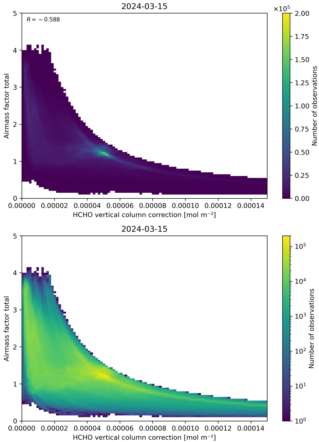
Figure 120: Scatter density plot of “HCHO vertical column correction” against “Airmass factor total” for 2024-03-14 to 2024-03-16.
