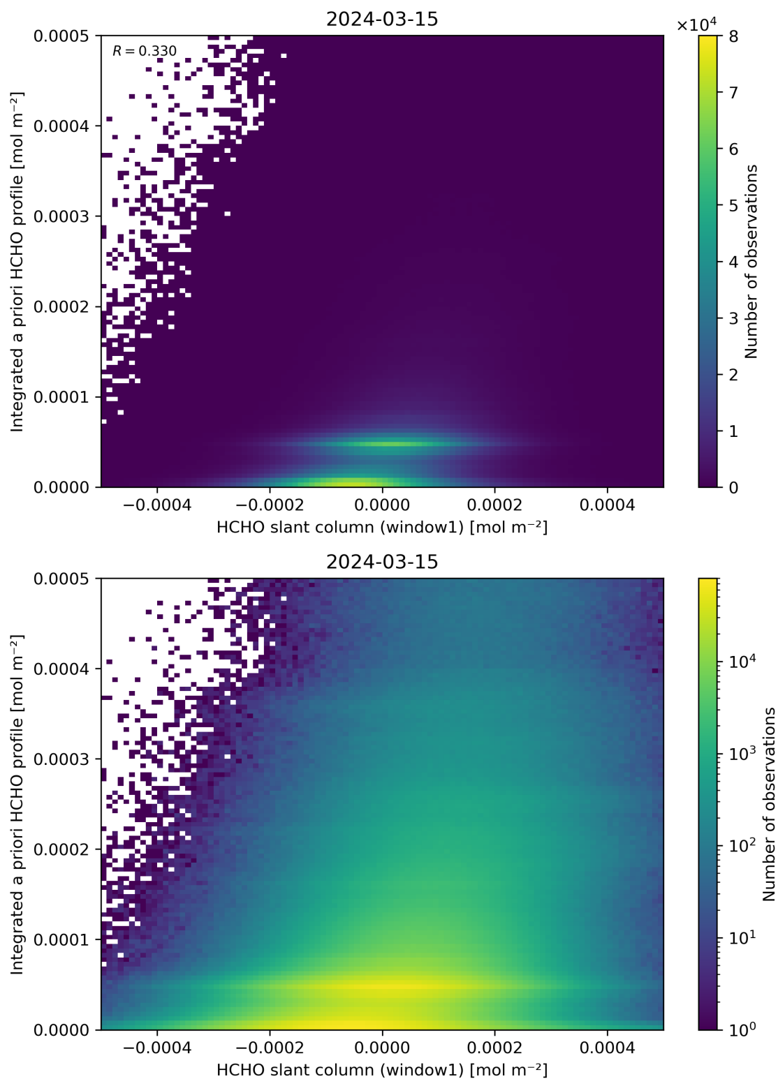
Figure 87: Scatter density plot of “HCHO slant column (window1)” against “Integrated a priori HCHO profile” for 2024-03-14 to 2024-03-16.
