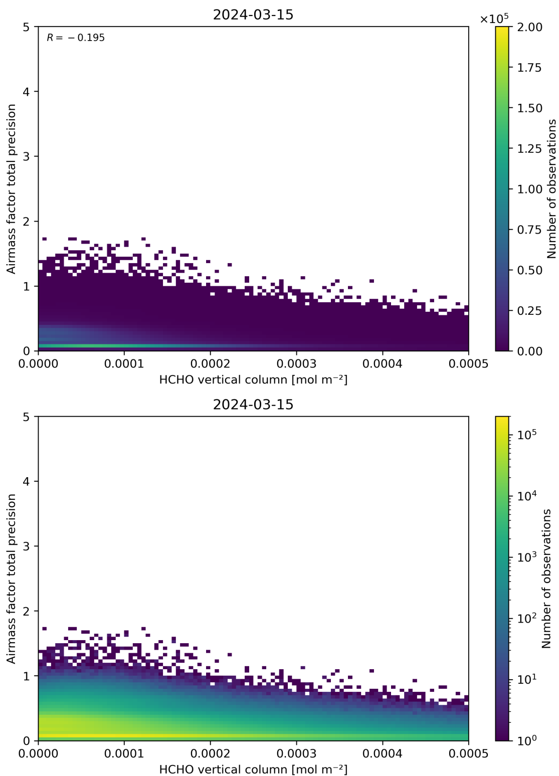
Figure 132: Scatter density plot of “HCHO vertical column” against “Airmass factor total precision” for 2024-03-14 to 2024-03-16.
