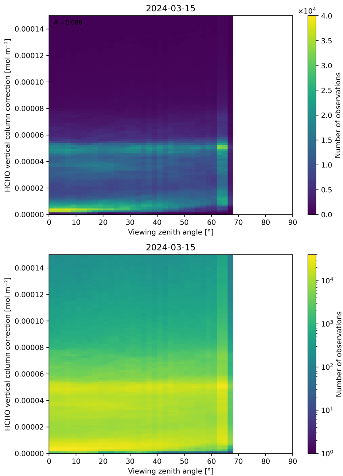
Figure 193: Scatter density plot of “Viewing zenith angle” against “HCHO vertical column correction” for 2024-03-14 to 2024-03-16.
