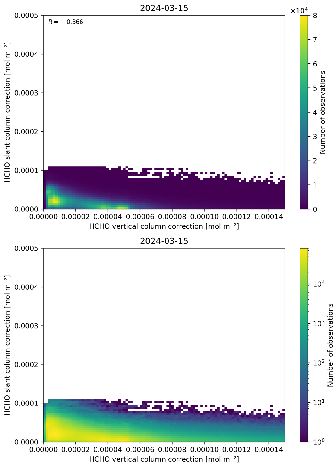
Figure 117: Scatter density plot of “HCHO vertical column correction” against “HCHO slant column correction” for 2024-03-14 to 2024-03-16.
