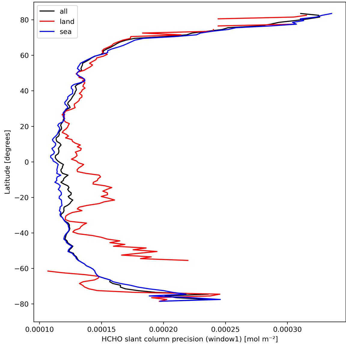
Figure 25: Zonal average of “HCHO slant column precision (window1)” for 2024-03-14 to 2024-03-16.
