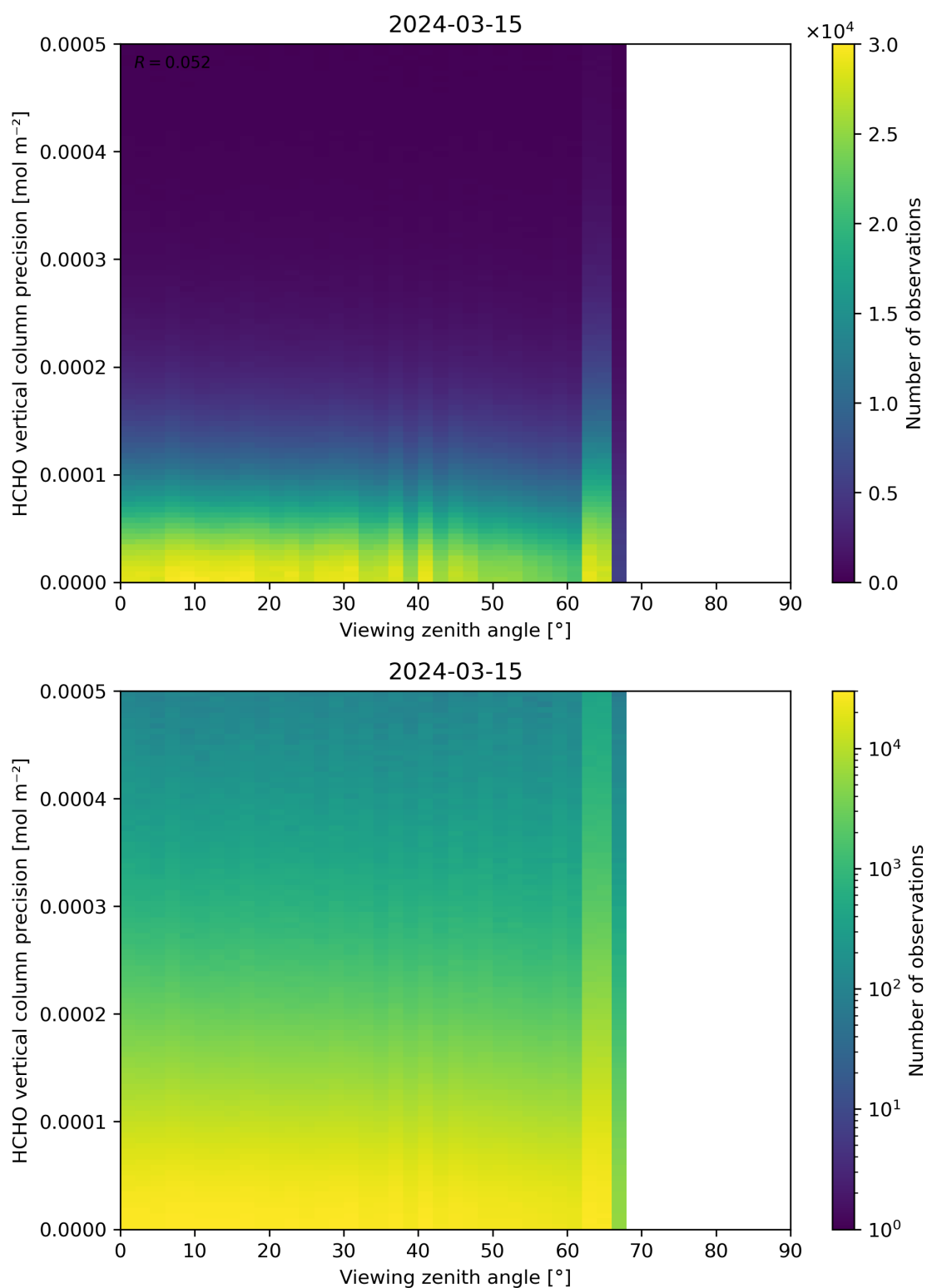
Figure 194: Scatter density plot of “Viewing zenith angle” against “HCHO vertical column precision” for 2024-03-14 to 2024-03-16.
