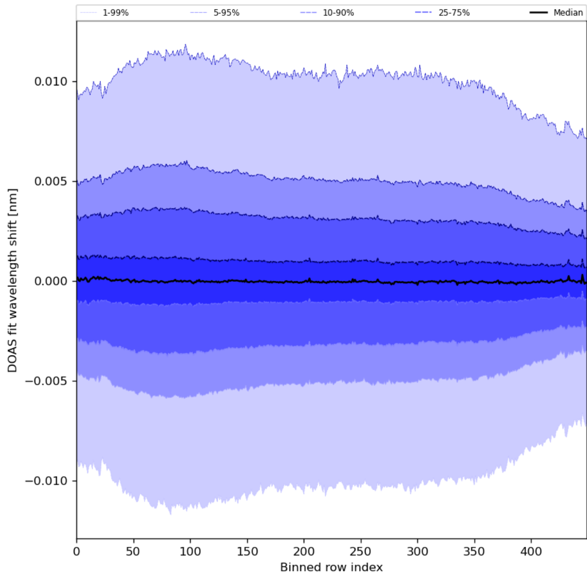
Figure 58: Along track statistics of “DOAS fit wavelength shift” for 2024-03-14 to 2024-03-16
