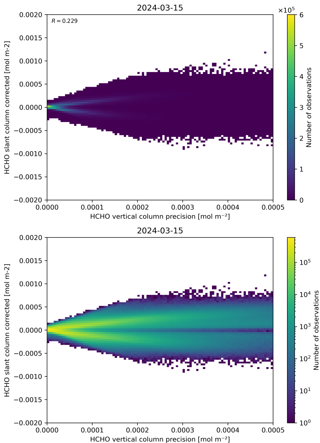
Figure 140: Scatter density plot of “HCHO vertical column precision” against “HCHO slant column corrected” for 2024-03-14 to 2024-03-16.
