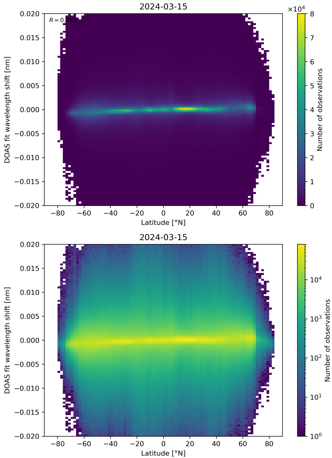
Figure 154: Scatter density plot of “Latitude” against “DOAS fit wavelength shift” for 2024-03-14 to 2024-03-16.
