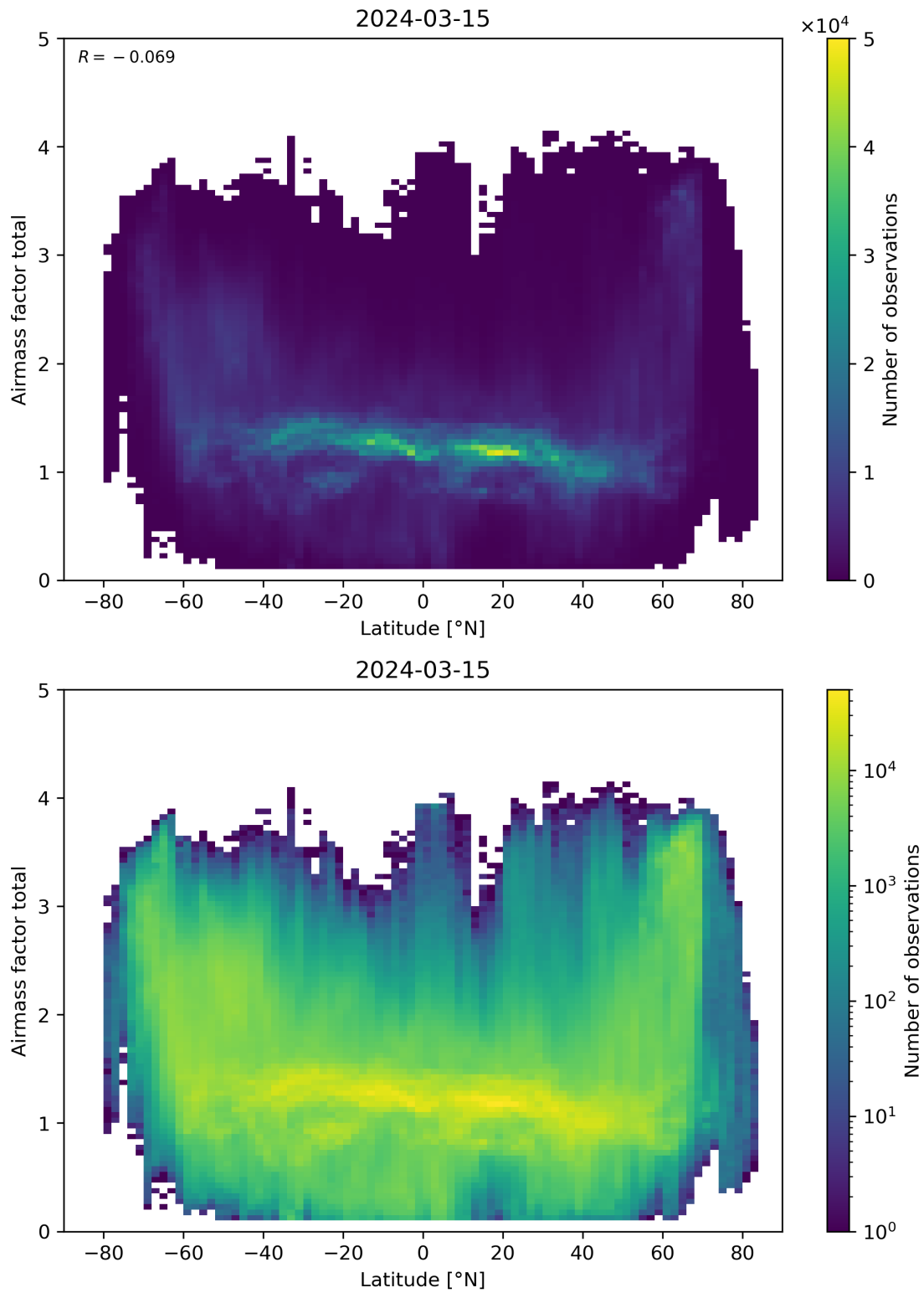
Figure 161: Scatter density plot of “Latitude” against “Airmass factor total” for 2024-03-14 to 2024-03-16.
