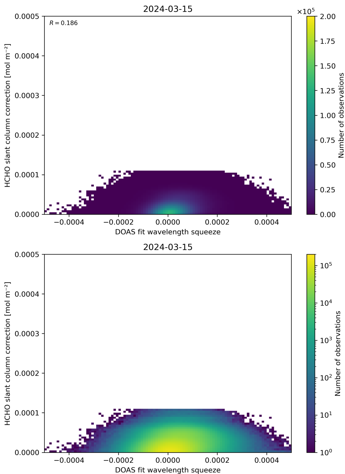
Figure 70: Scatter density plot of “DOAS fit wavelength squeeze” against “HCHO slant column correction” for 2024-03-14 to 2024-03-16.
