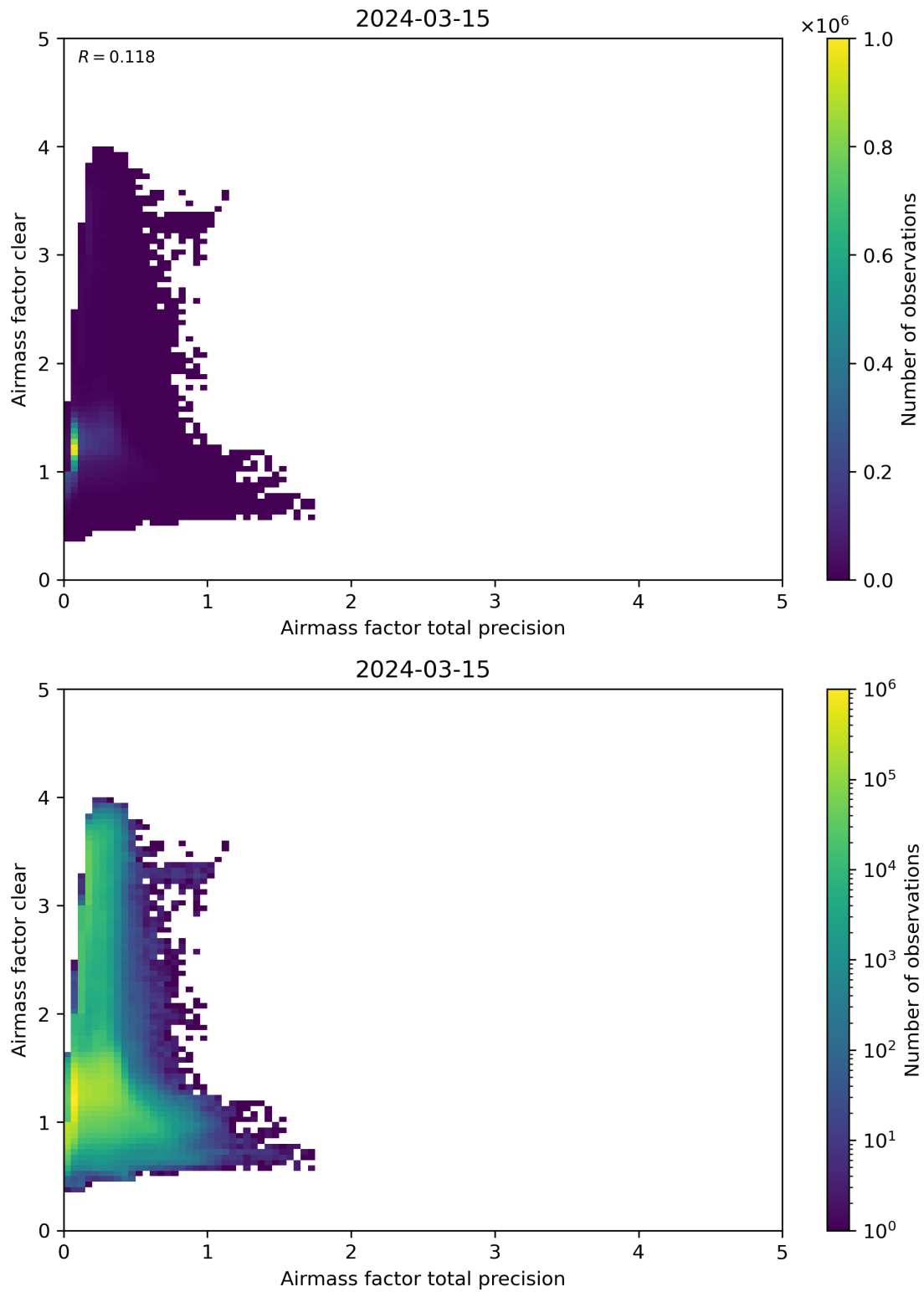
Figure 108: Scatter density plot of “Airmass factor total precision” against “Airmass factor clear” for 2024-03-14 to 2024-03-16.
