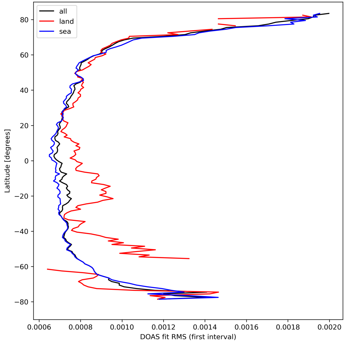
Figure 32: Zonal average of "DOAS fit RMS (first interval)" for 2024-03-14 to 2024-03-16.
