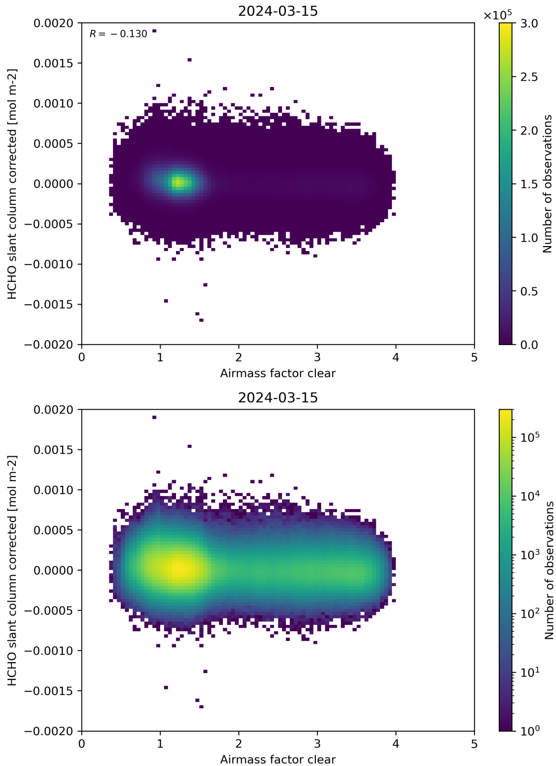
Figure 74: Scatter density plot of “Airmass factor clear” against “HCHO slant column corrected” for 2024-03-14 to 2024-03-16.
