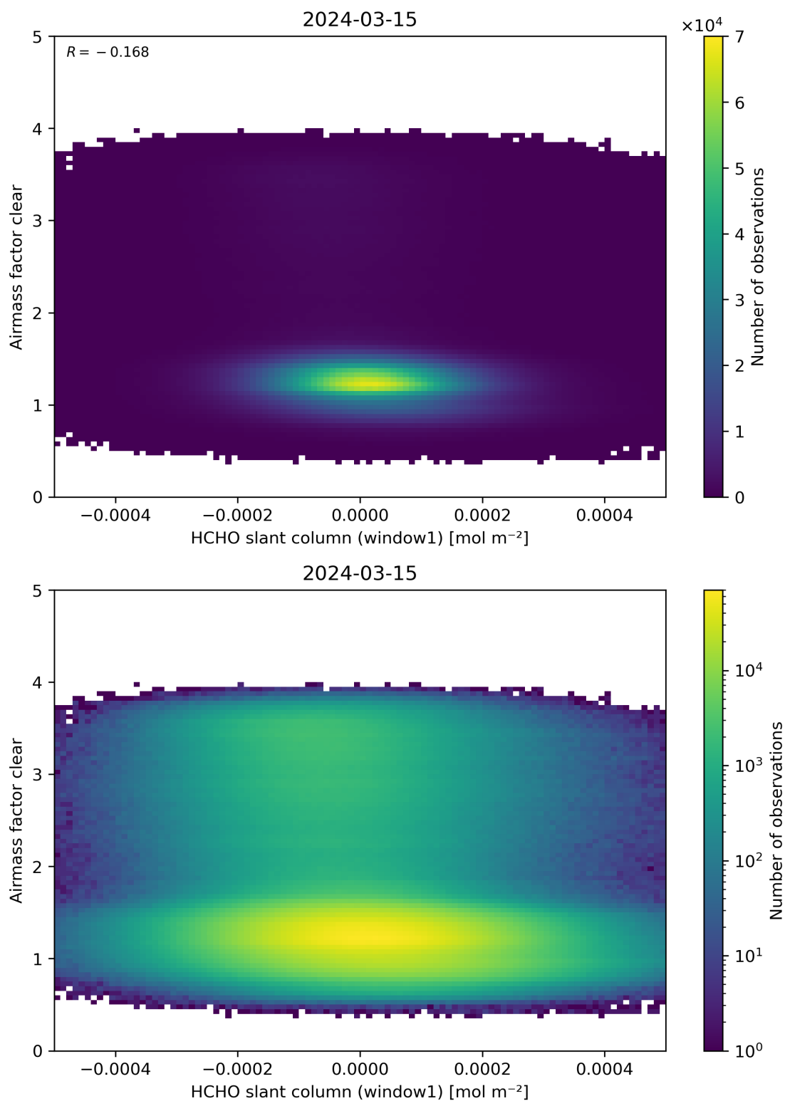
Figure 81: Scatter density plot of “HCHO slant column (window1)” against “Airmass factor clear” for 2024-03-14 to 2024-03-16.
