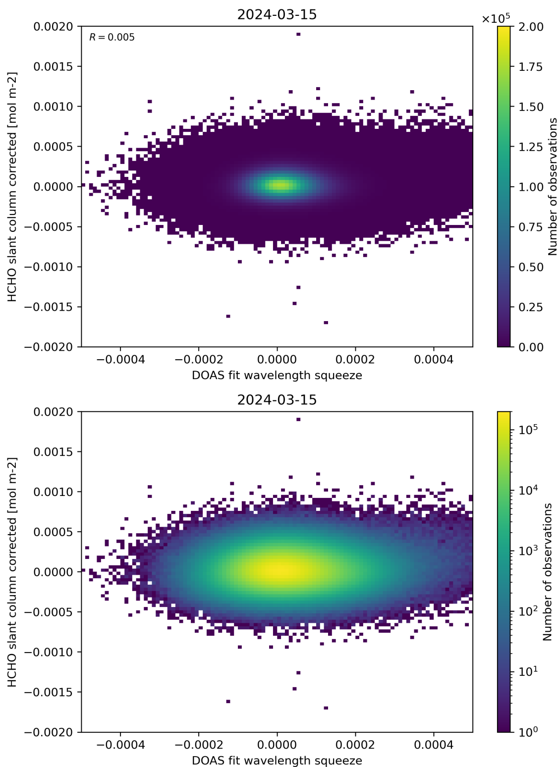
Figure 69: Scatter density plot of “DOAS fit wavelength squeeze” against “HCHO slant column corrected” for 2024-03-14 to 2024-03-16.
