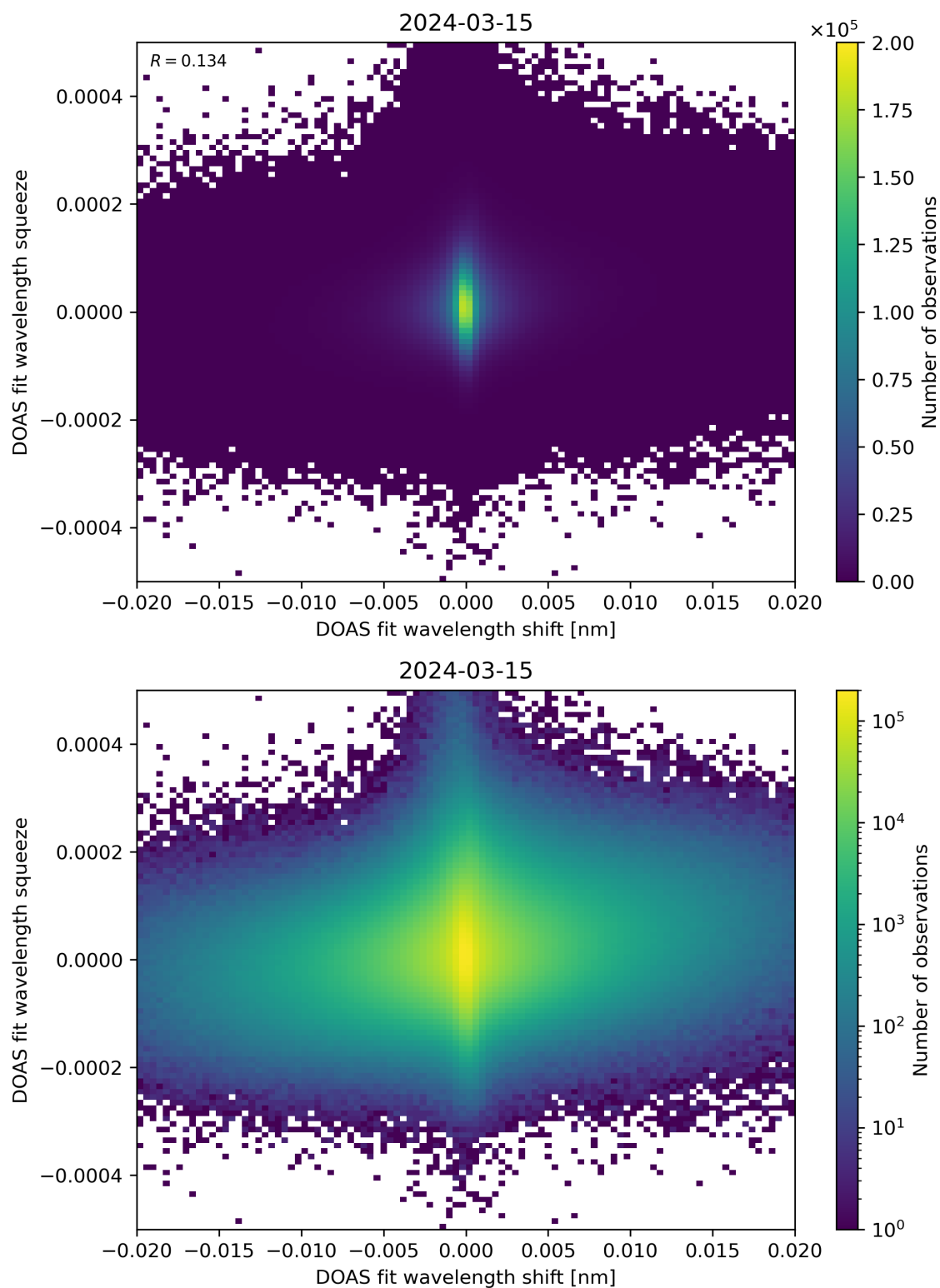
Figure 65: Scatter density plot of “DOAS fit wavelength shift” against “DOAS fit wavelength squeeze” for 2024-03-14 to 2024-03-16.
