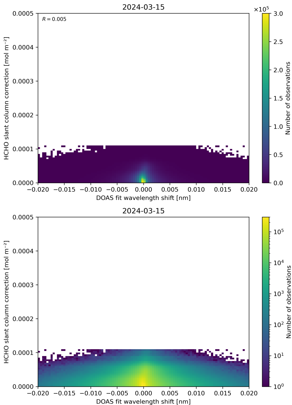
Figure 67: Scatter density plot of “DOAS fit wavelength shift” against “HCHO slant column correction” for 2024-03-14 to 2024-03-16.
