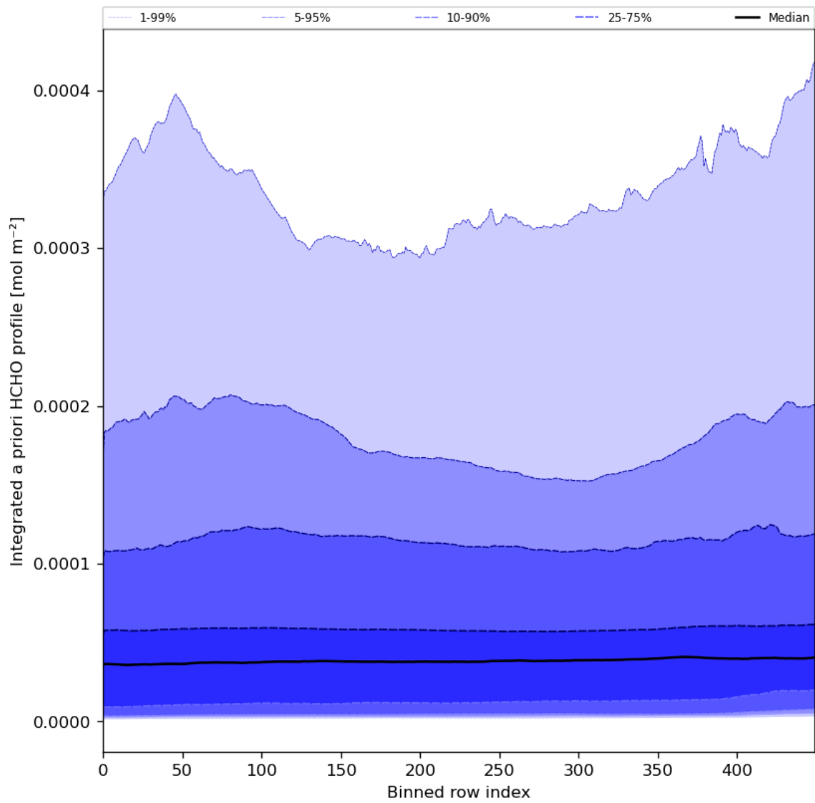
Figure 57: Along track statistics of “Integrated a priori HCHO profile” for 2024-03-14 to 2024-03-16
