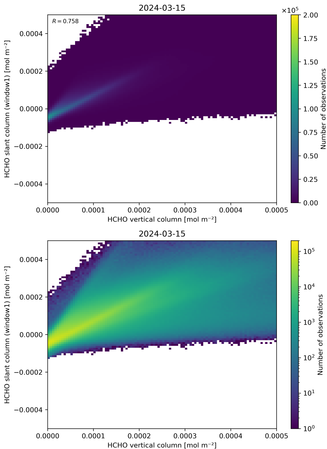
Figure 129: Scatter density plot of “HCHO vertical column” against “HCHO slant column (window1)” for 2024-03-14 to 2024-03-16.
