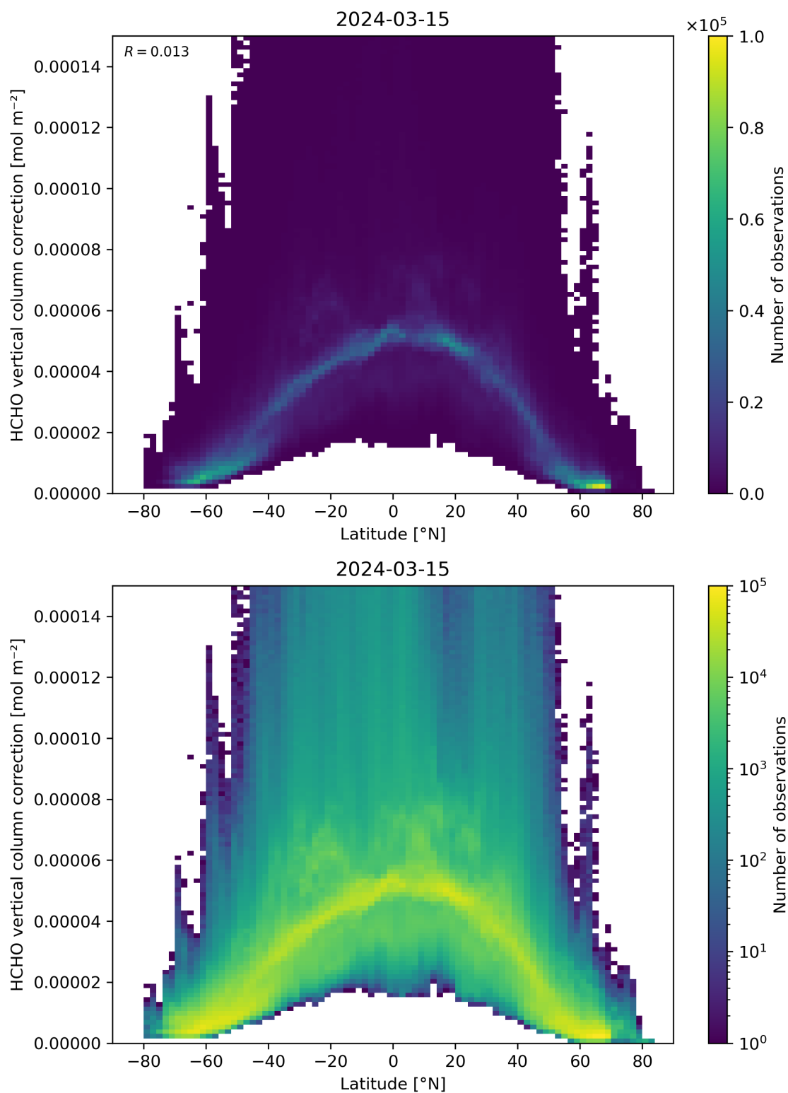
Figure 164: Scatter density plot of “Latitude” against “HCHO vertical column correction” for 2024-03-14 to 2024-03-16.
