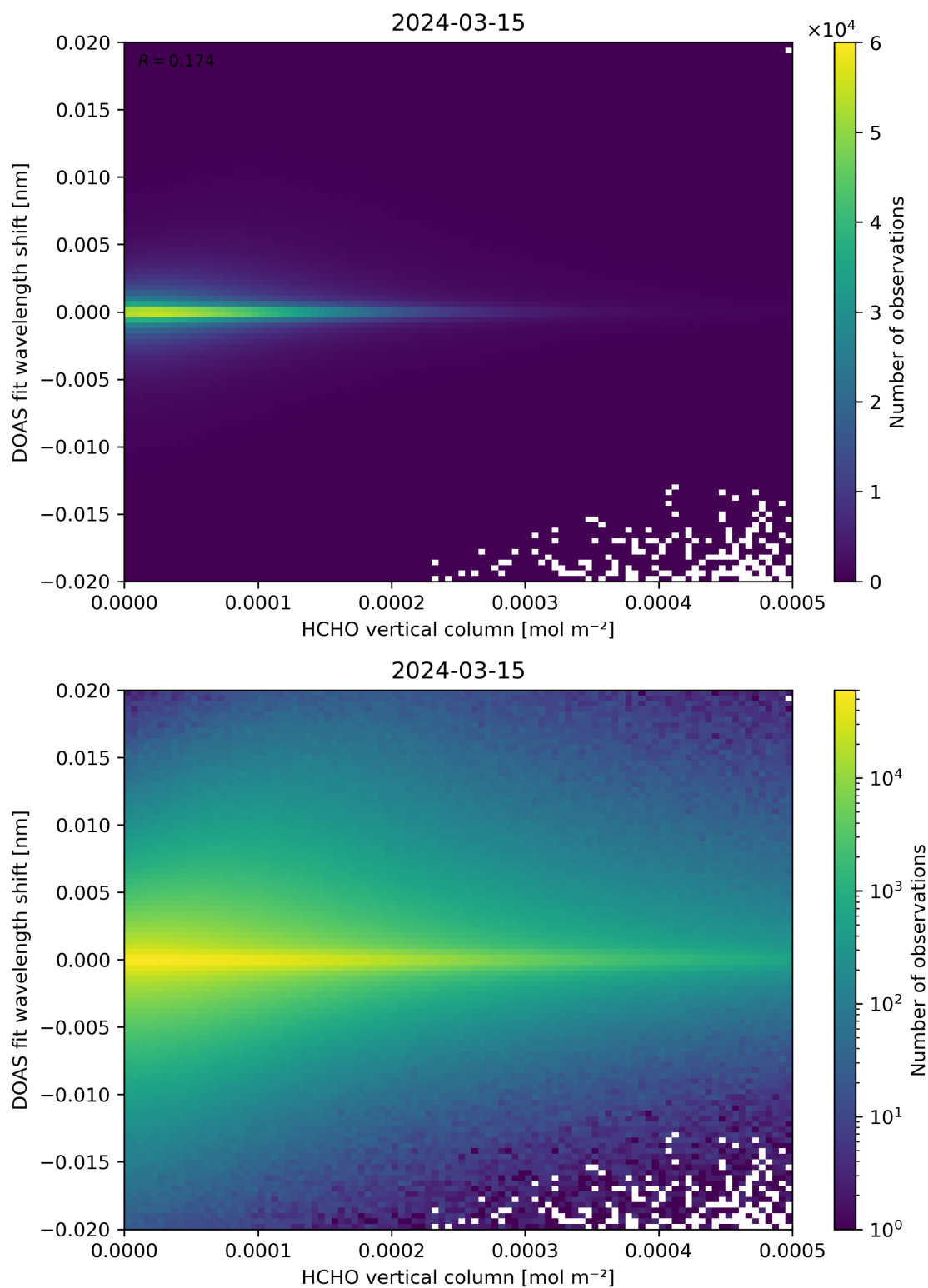
Figure 124: Scatter density plot of “HCHO vertical column” against “DOAS fit wavelength shift” for 2024-03-14 to 2024-03-16.
