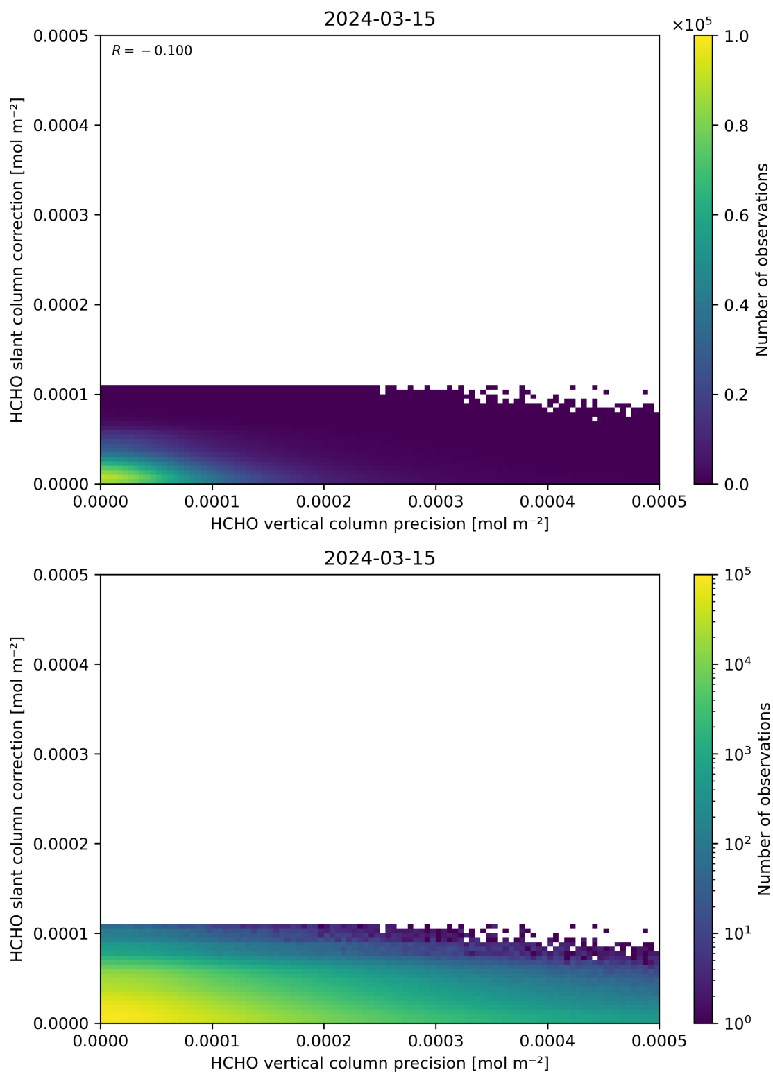
Figure 141: Scatter density plot of “HCHO vertical column precision” against “HCHO slant column correction” for 2024-03-14 to 2024-03-16.
