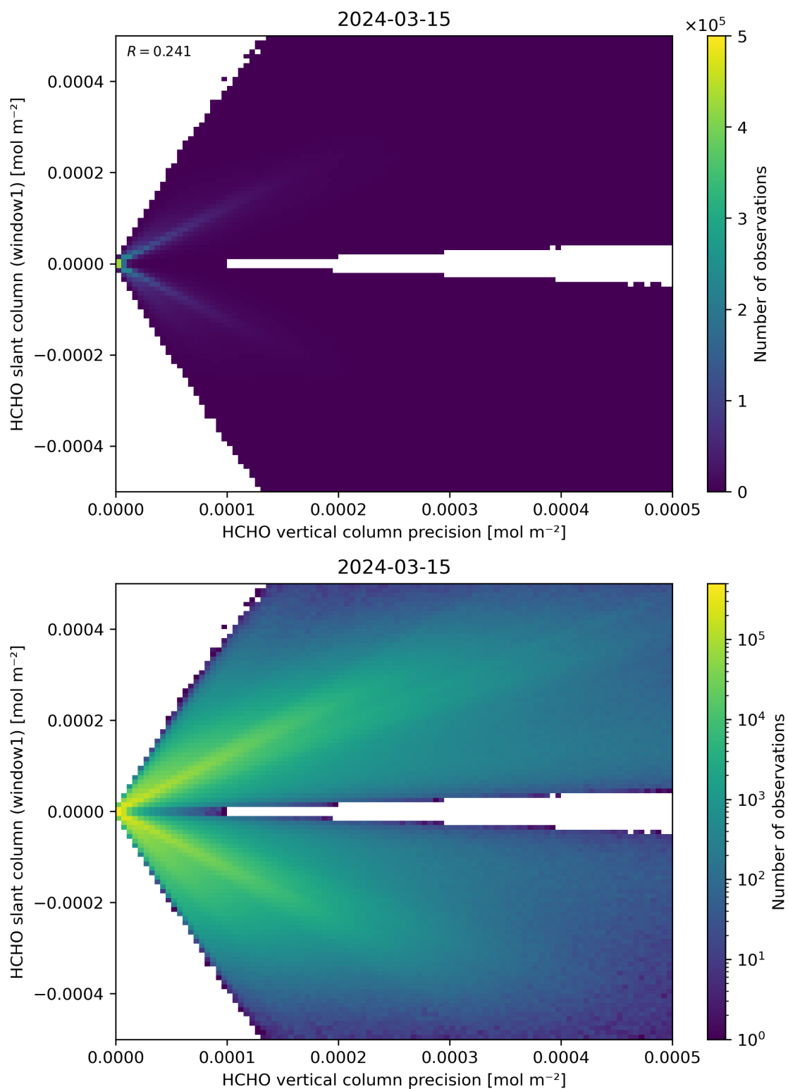
Figure 142: Scatter density plot of “HCHO vertical column precision” against “HCHO slant column (window1)” for 2024-03-14 to 2024-03-16.
