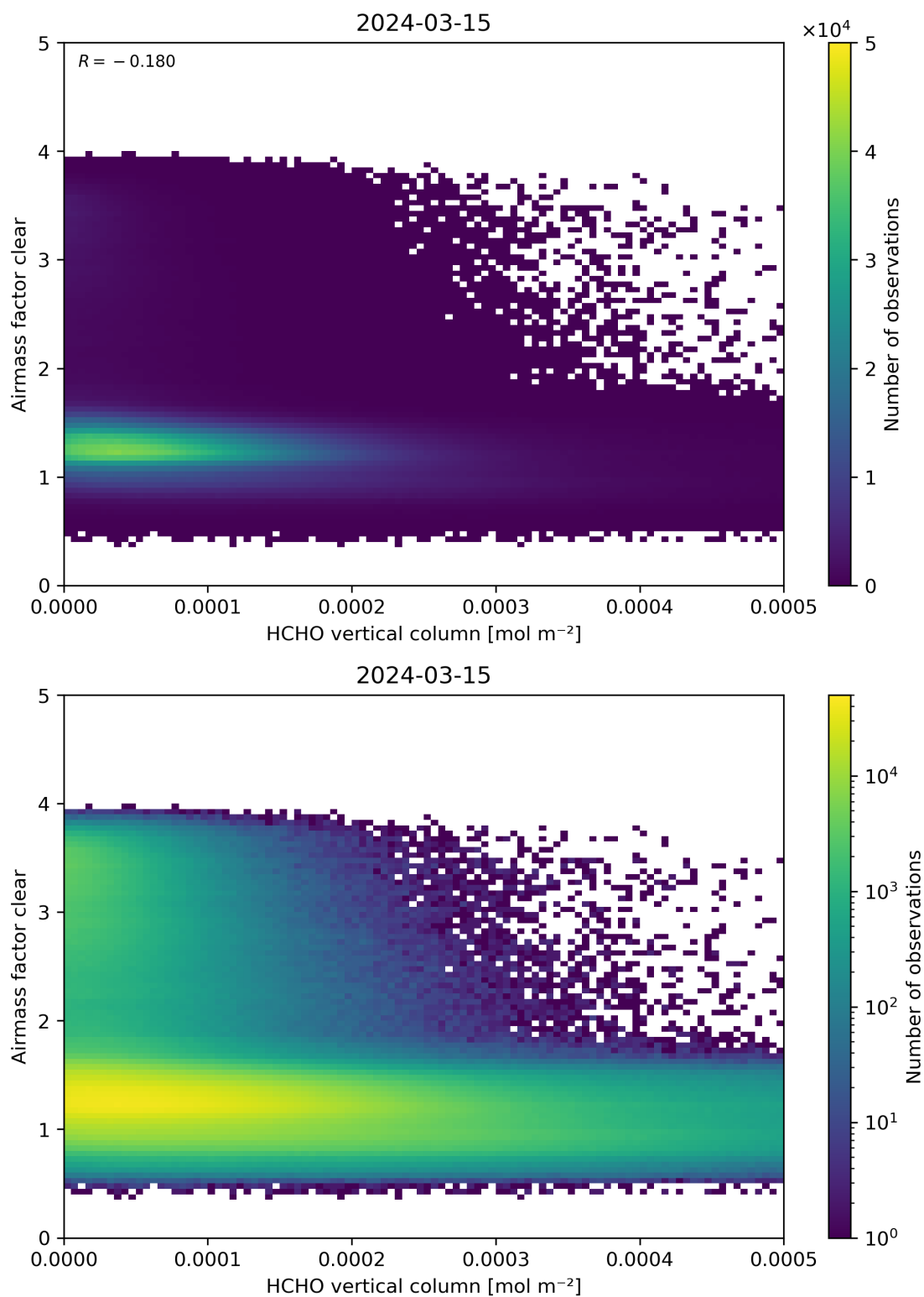
Figure 126: Scatter density plot of “HCHO vertical column” against “Airmass factor clear” for 2024-03-14 to 2024-03-16.
