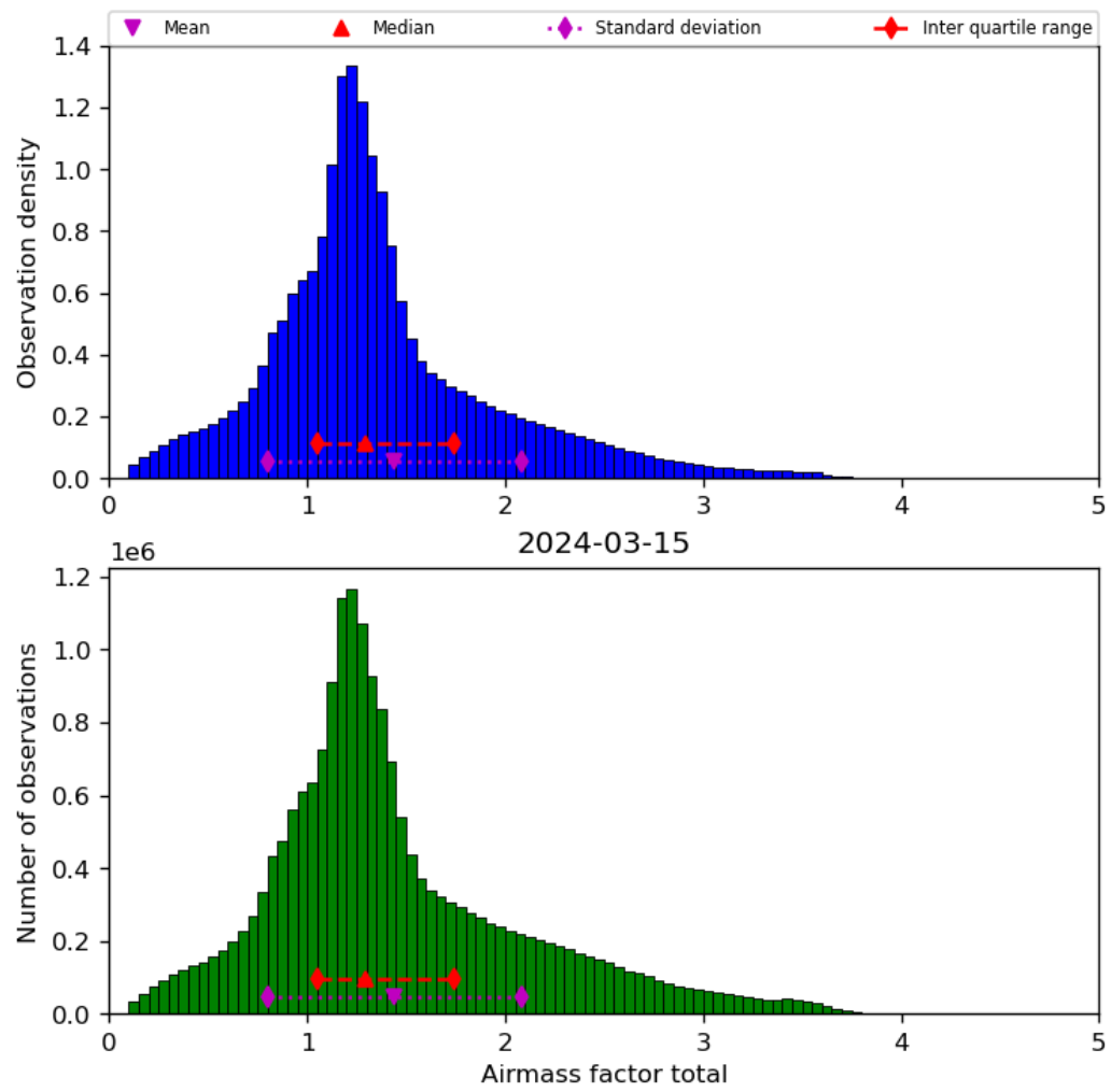
Figure 40: Histogram of “Airmass factor total” for 2024-03-14 to 2024-03-16
