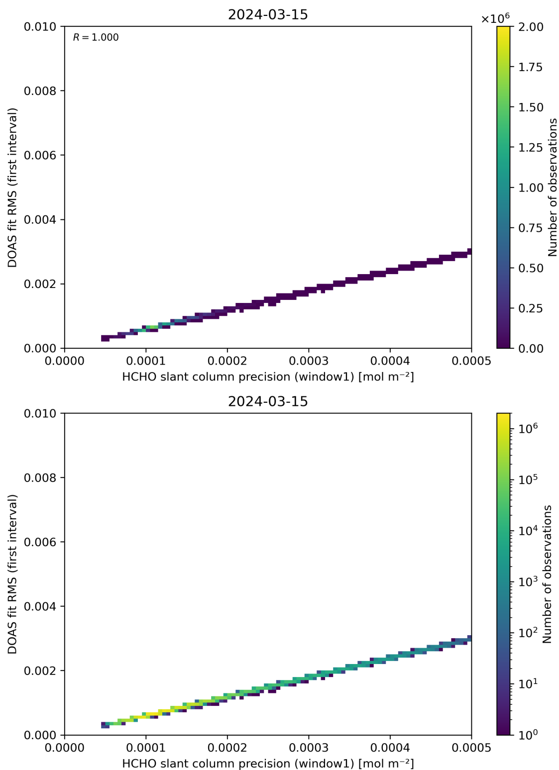
Figure 88: Scatter density plot of “HCHO slant column precision (window1)” against “DOAS fit RMS (first interval)” for 2024-03-14 to 2024-03-16.
