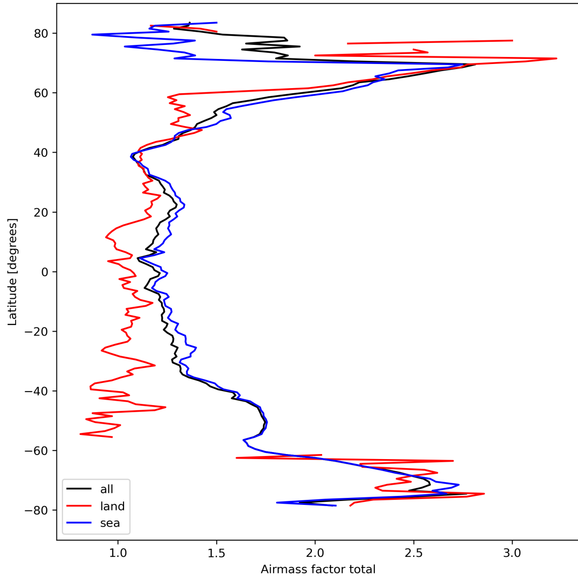
Figure 26: Zonal average of “Airmass factor total” for 2024-03-14 to 2024-03-16.
