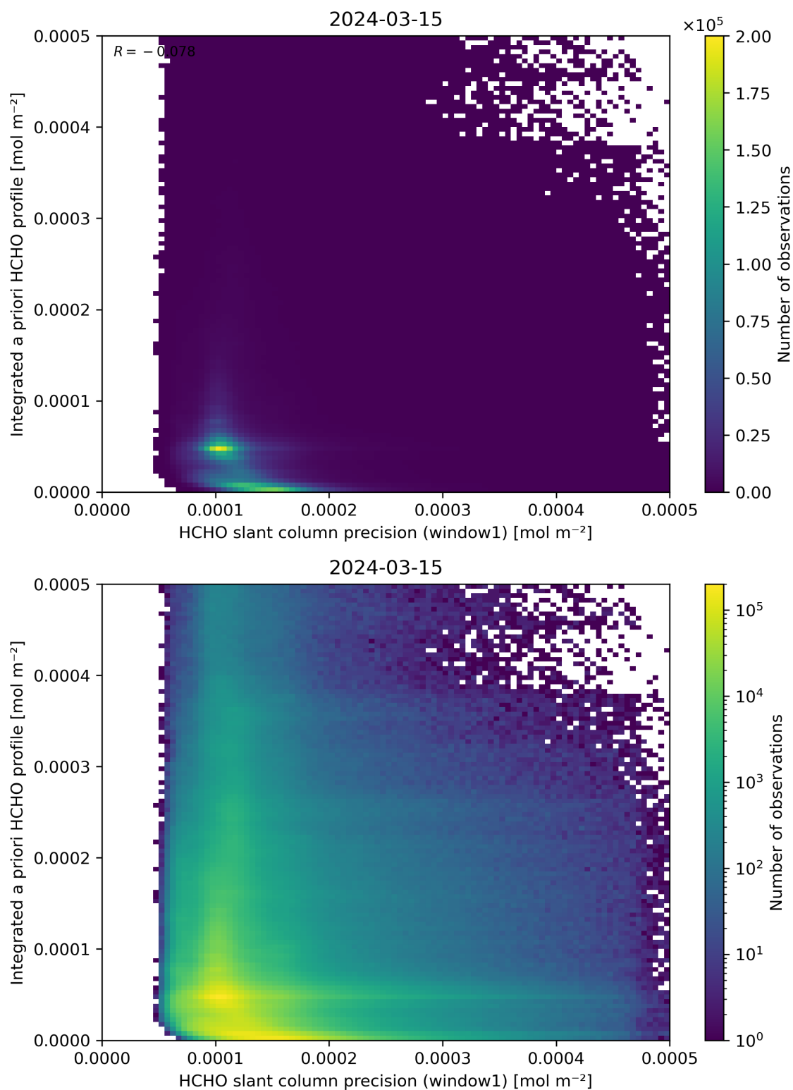
Figure 96: Scatter density plot of “HCHO slant column precision (window1)” against “Integrated a priori HCHO profile” for 2024-03-14 to 2024-03-16.
