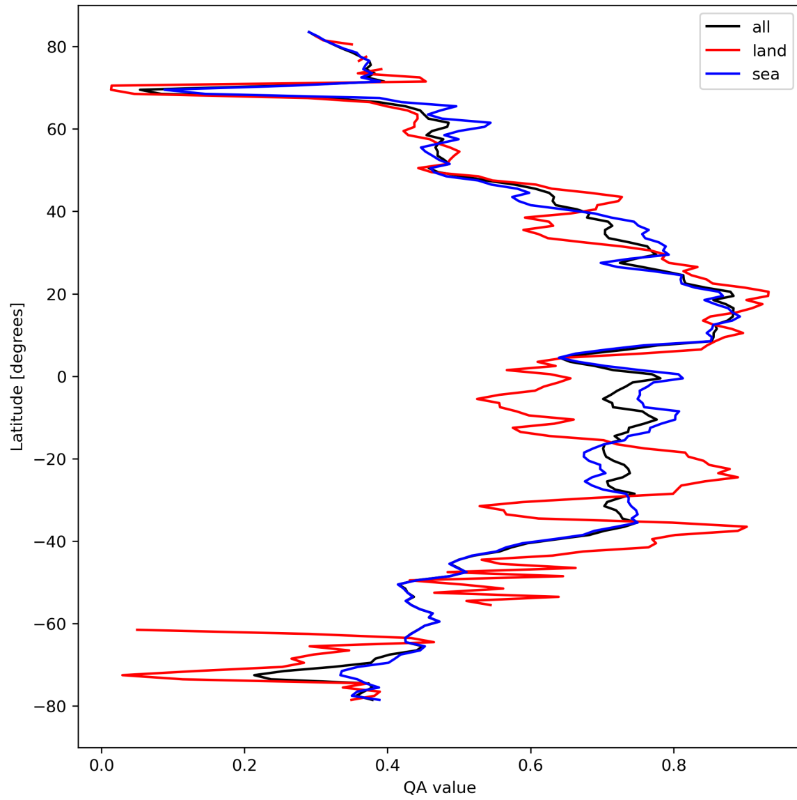
Figure 20: Zonal average of “QA value” for 2024-03-14 to 2024-03-16.
