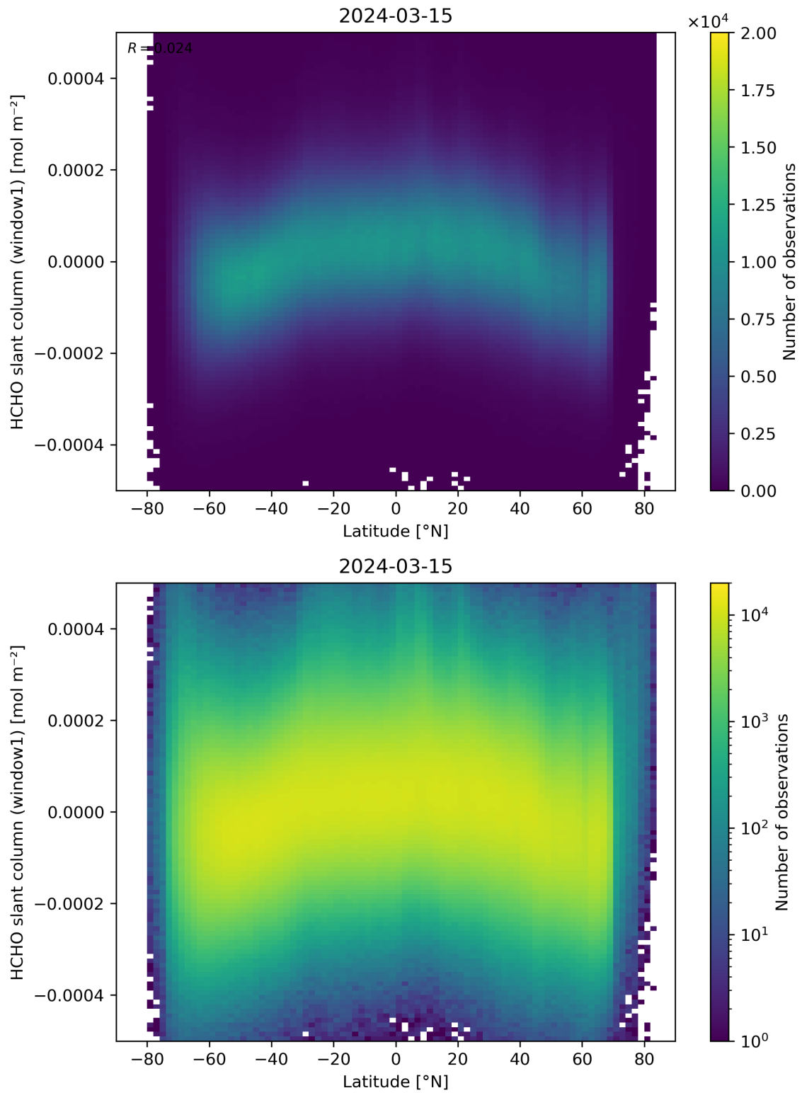
Figure 159: Scatter density plot of “Latitude” against “HCHO slant column (window1)” for 2024-03-14 to 2024-03-16.
