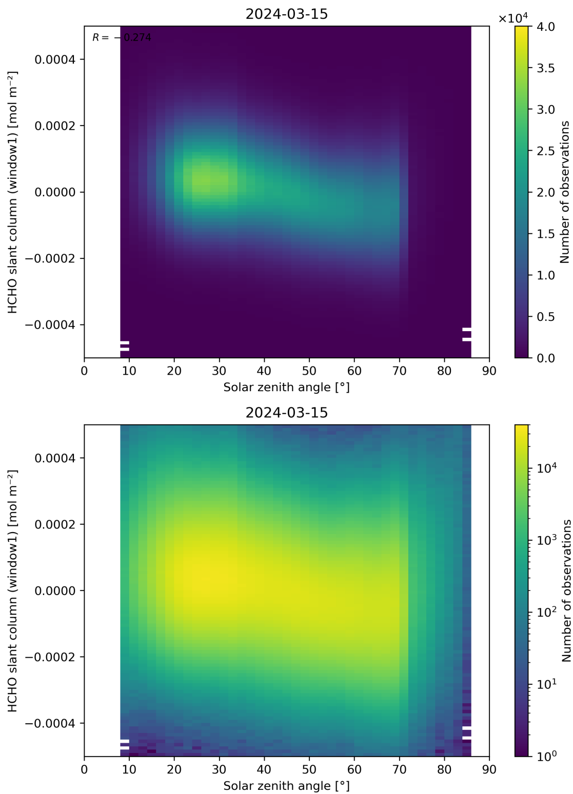
Figure 173: Scatter density plot of “Solar zenith angle” against “HCHO slant column (window1)” for 2024-03-14 to 2024-03-16.
