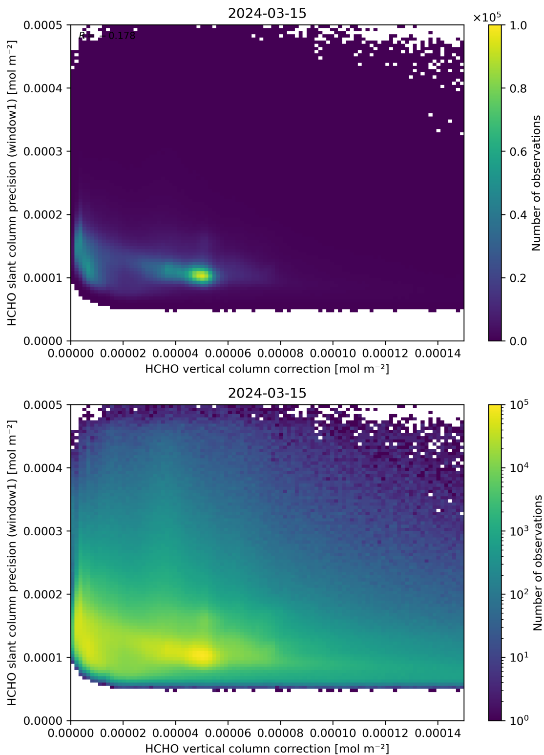
Figure 119: Scatter density plot of “HCHO vertical column correction” against “HCHO slant column precision (window1)” for 2024-03-14 to 2024-03-16.
