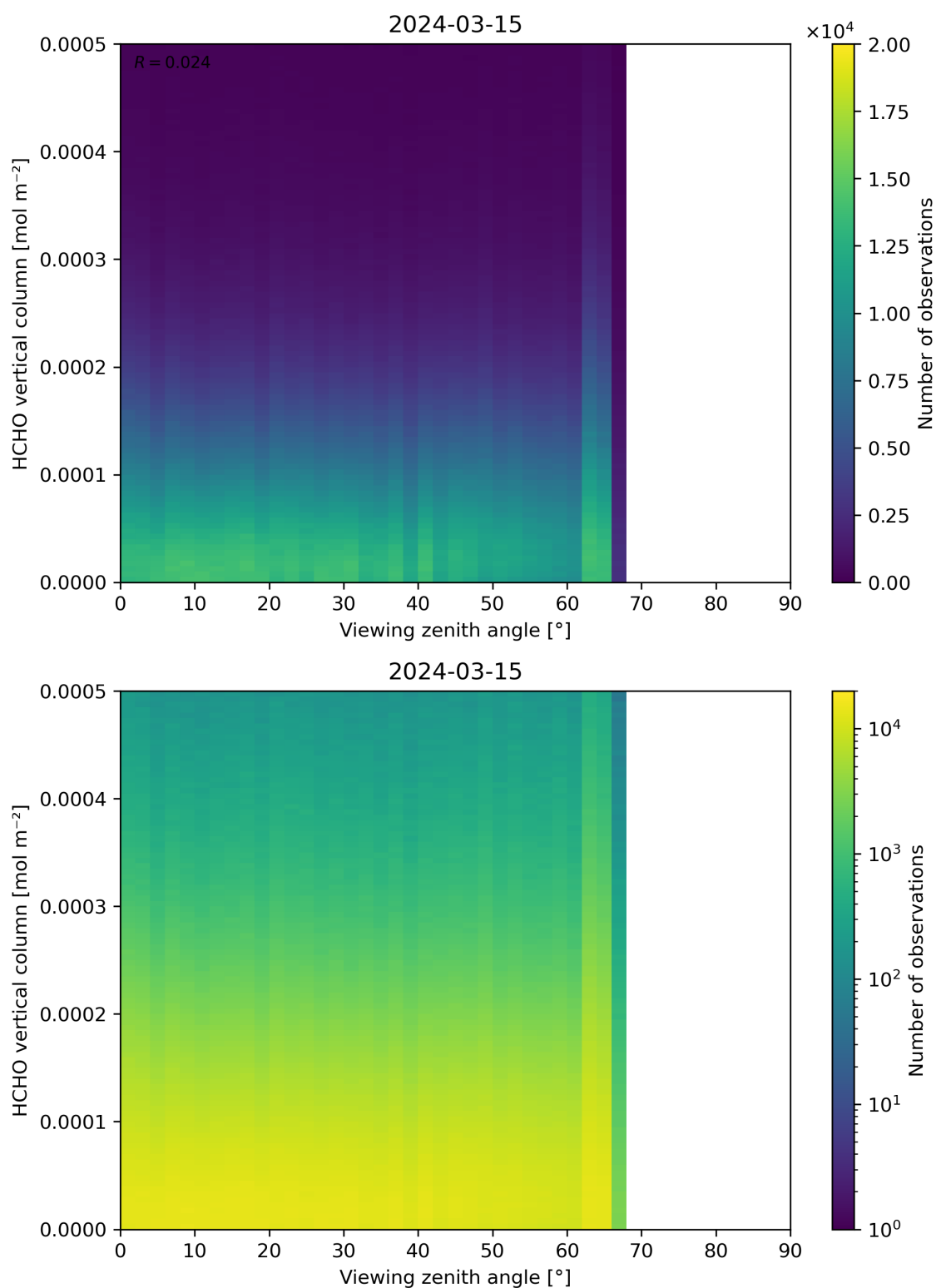
Figure 192: Scatter density plot of “Viewing zenith angle” against “HCHO vertical column” for 2024-03-14 to 2024-03-16.
