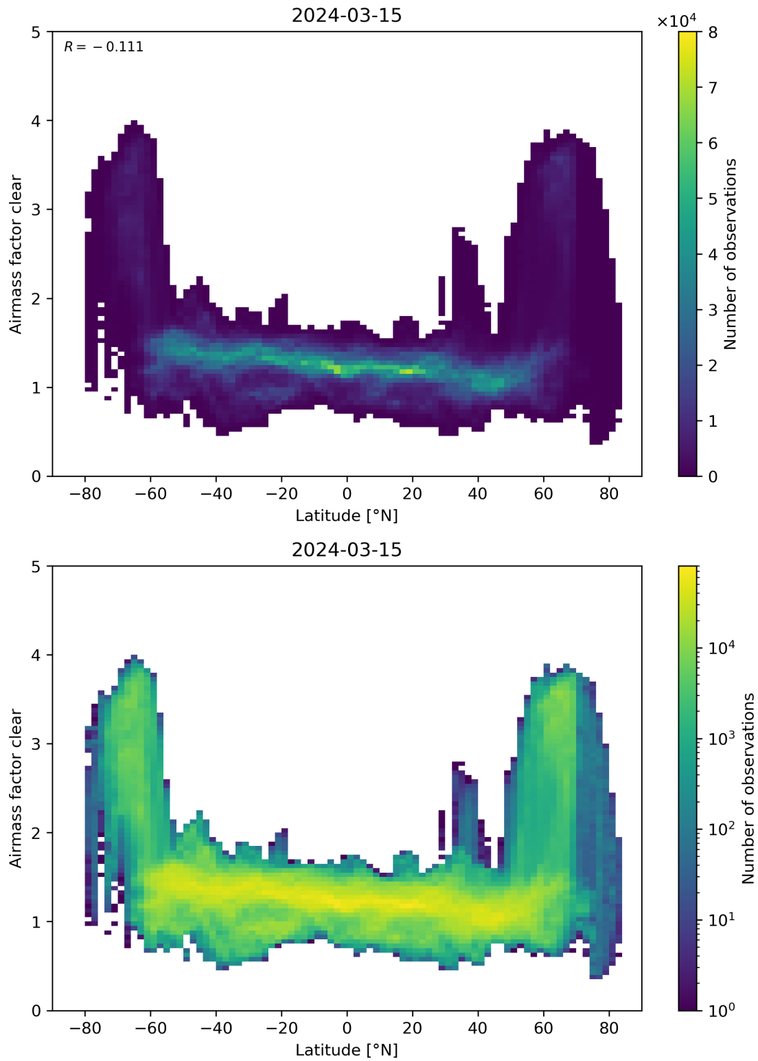
Figure 156: Scatter density plot of “Latitude” against “Airmass factor clear” for 2024-03-14 to 2024-03-16.
