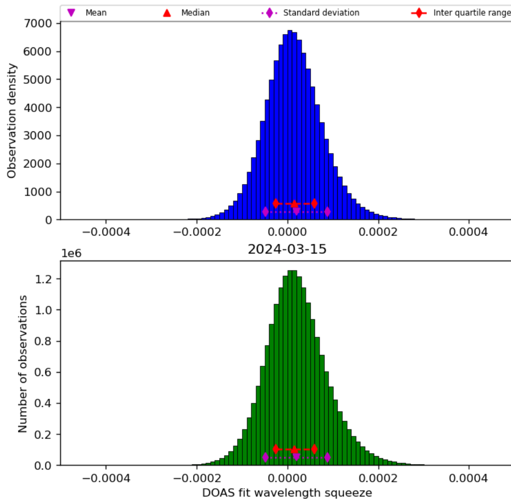
Figure 45: Histogram of “DOAS fit wavelength squeeze” for 2024-03-14 to 2024-03-16
