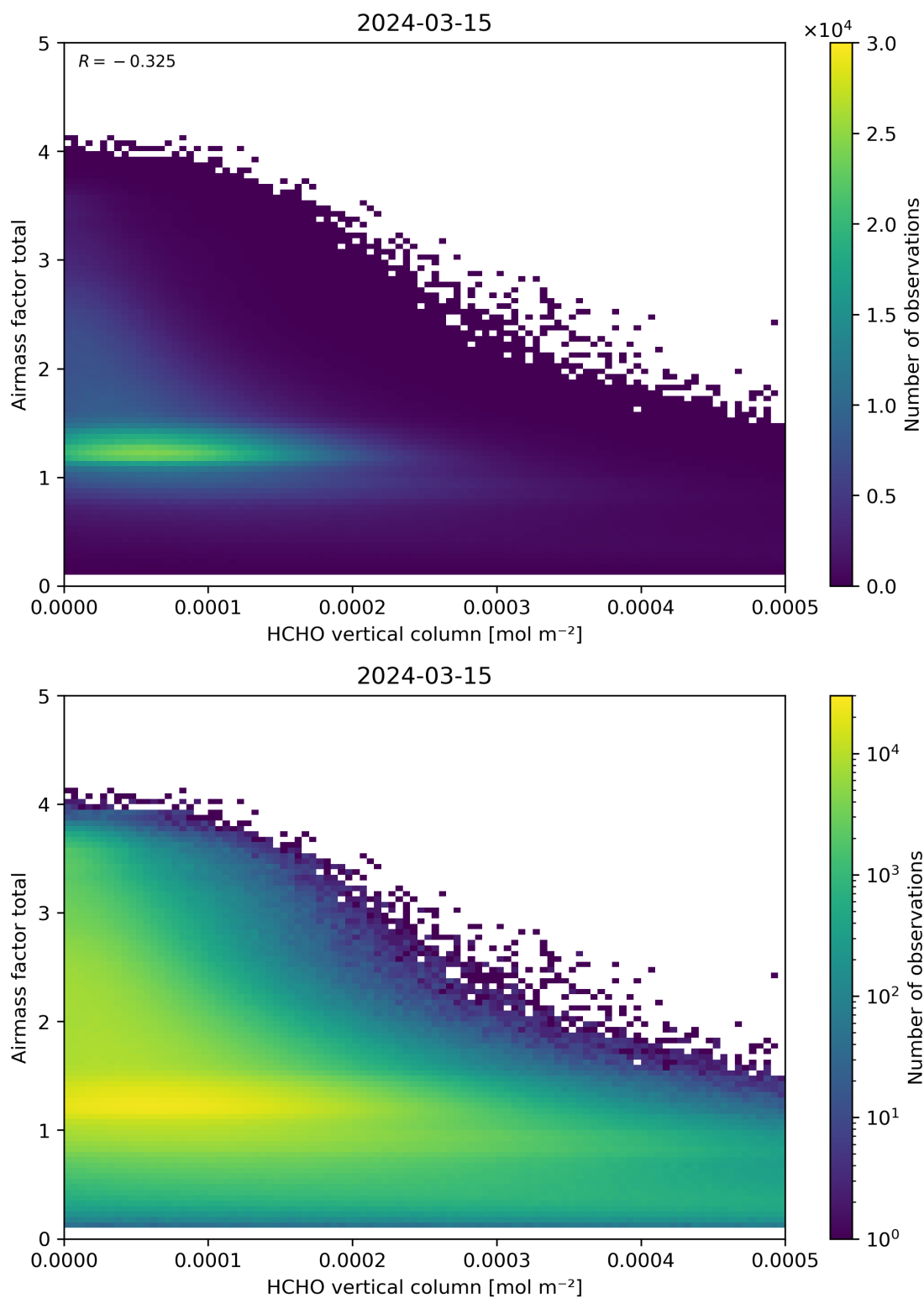
Figure 131: Scatter density plot of “HCHO vertical column” against “Airmass factor total” for 2024-03-14 to 2024-03-16.
