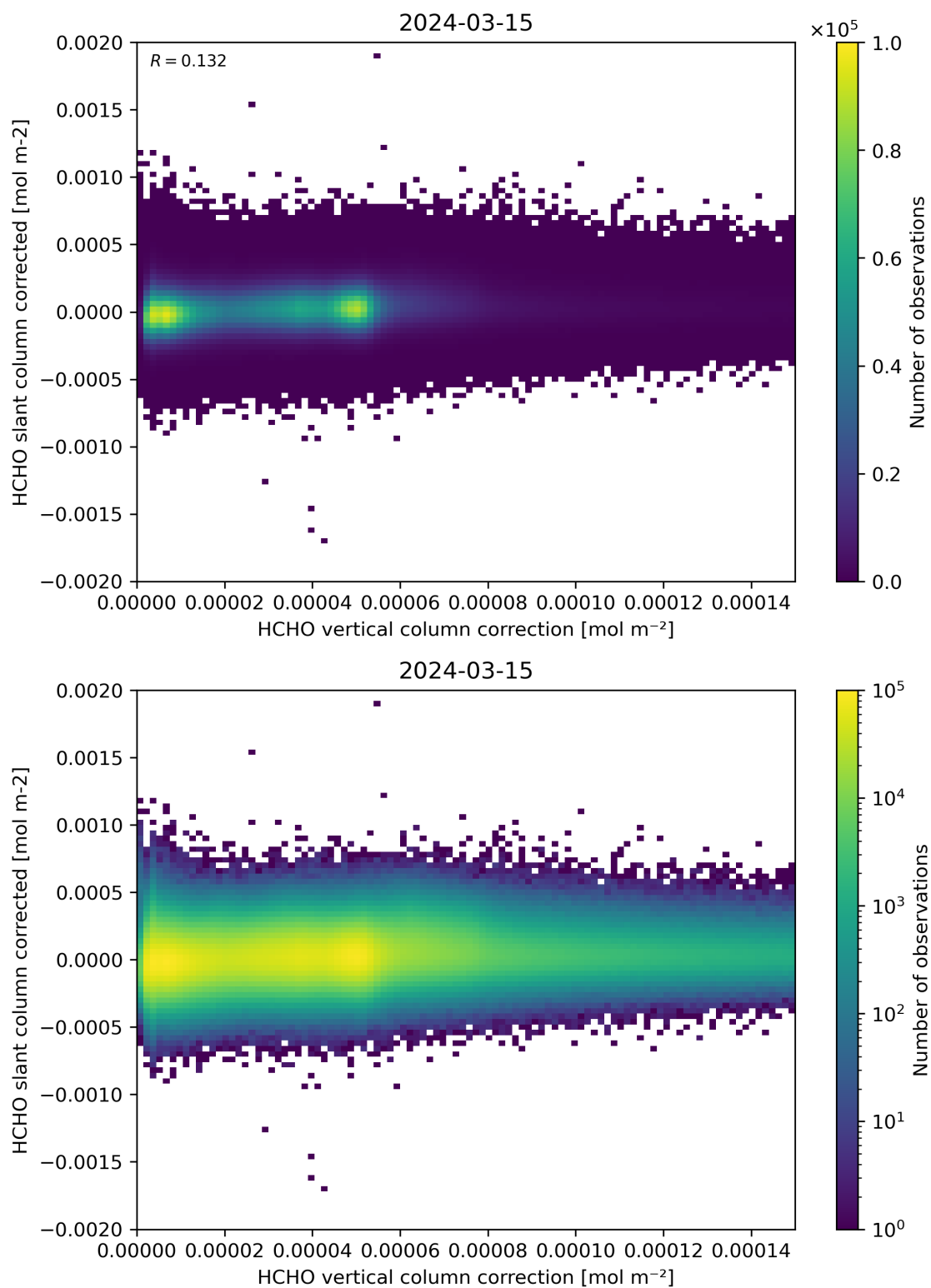
Figure 116: Scatter density plot of “HCHO vertical column correction” against “HCHO slant column corrected” for 2024-03-14 to 2024-03-16.
