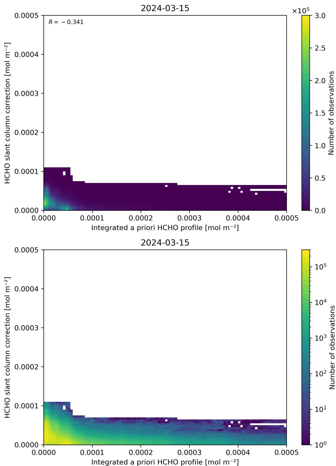
Figure 152: Scatter density plot of “Integrated a priori HCHO profile” against “HCHO slant column correction” for 2024-03-14 to 2024-03-16.
