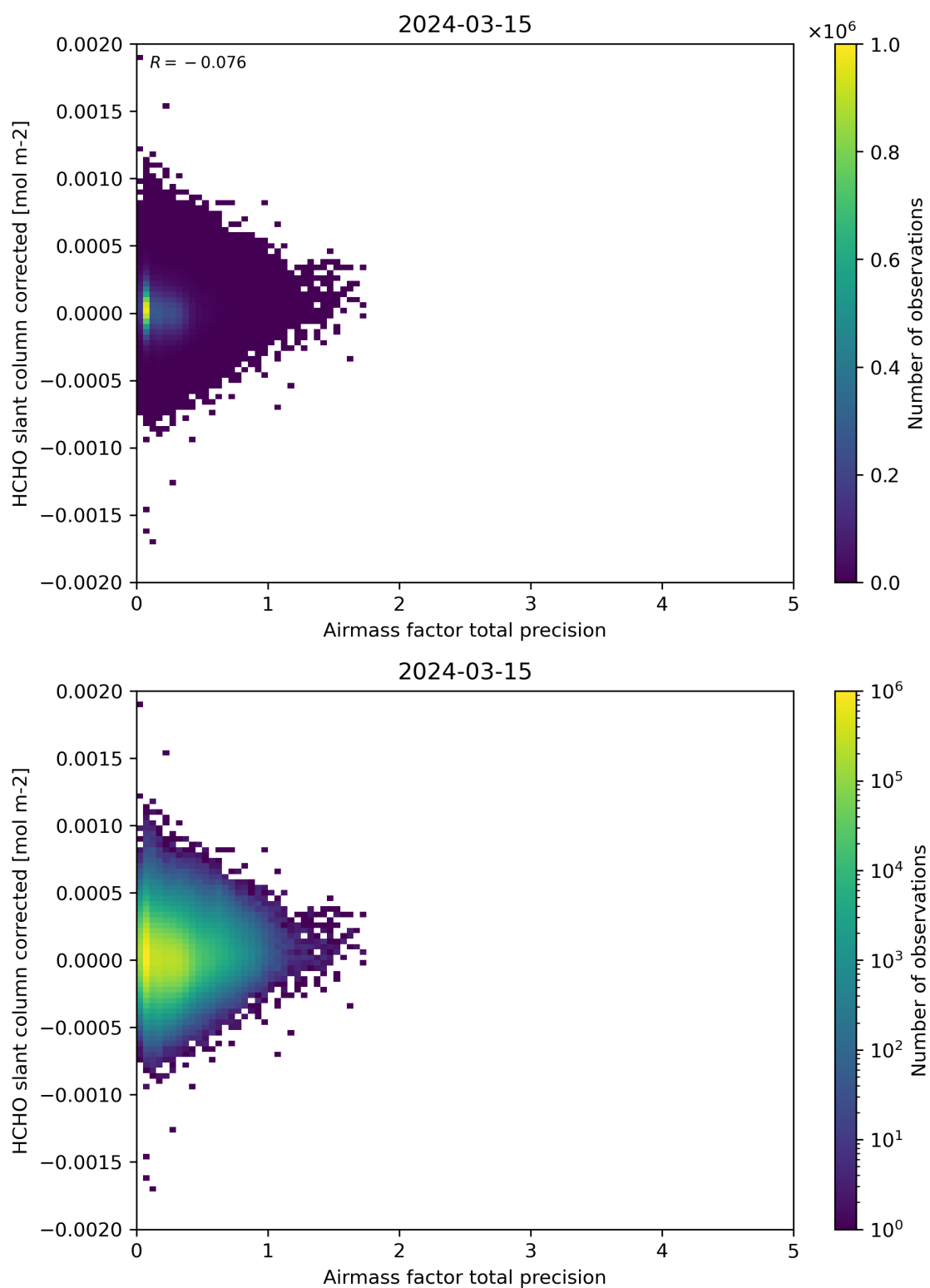
Figure 109: Scatter density plot of “Airmass factor total precision” against “HCHO slant column corrected” for 2024-03-14 to 2024-03-16.
