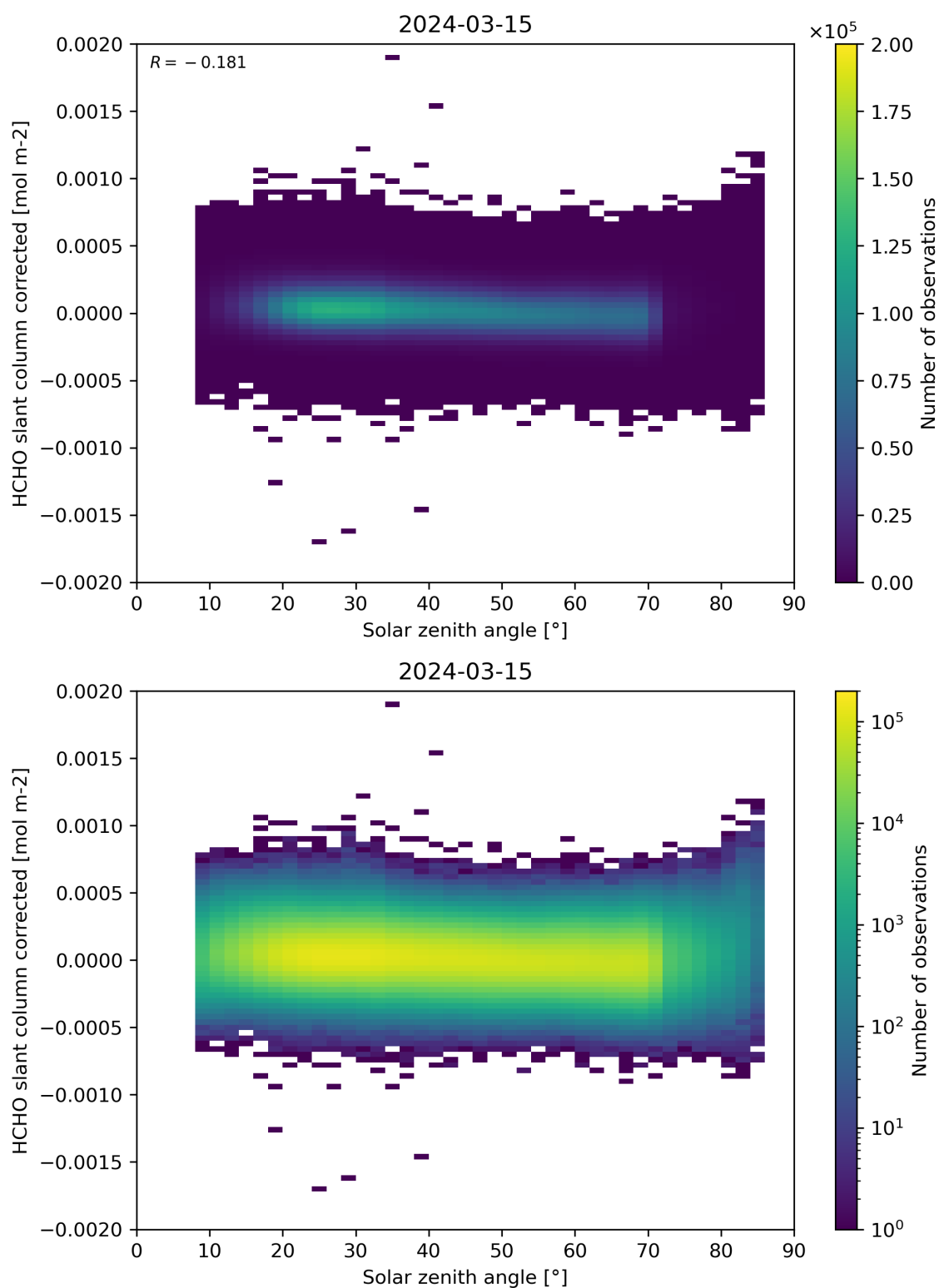
Figure 171: Scatter density plot of “Solar zenith angle” against “HCHO slant column corrected” for 2024-03-14 to 2024-03-16.
