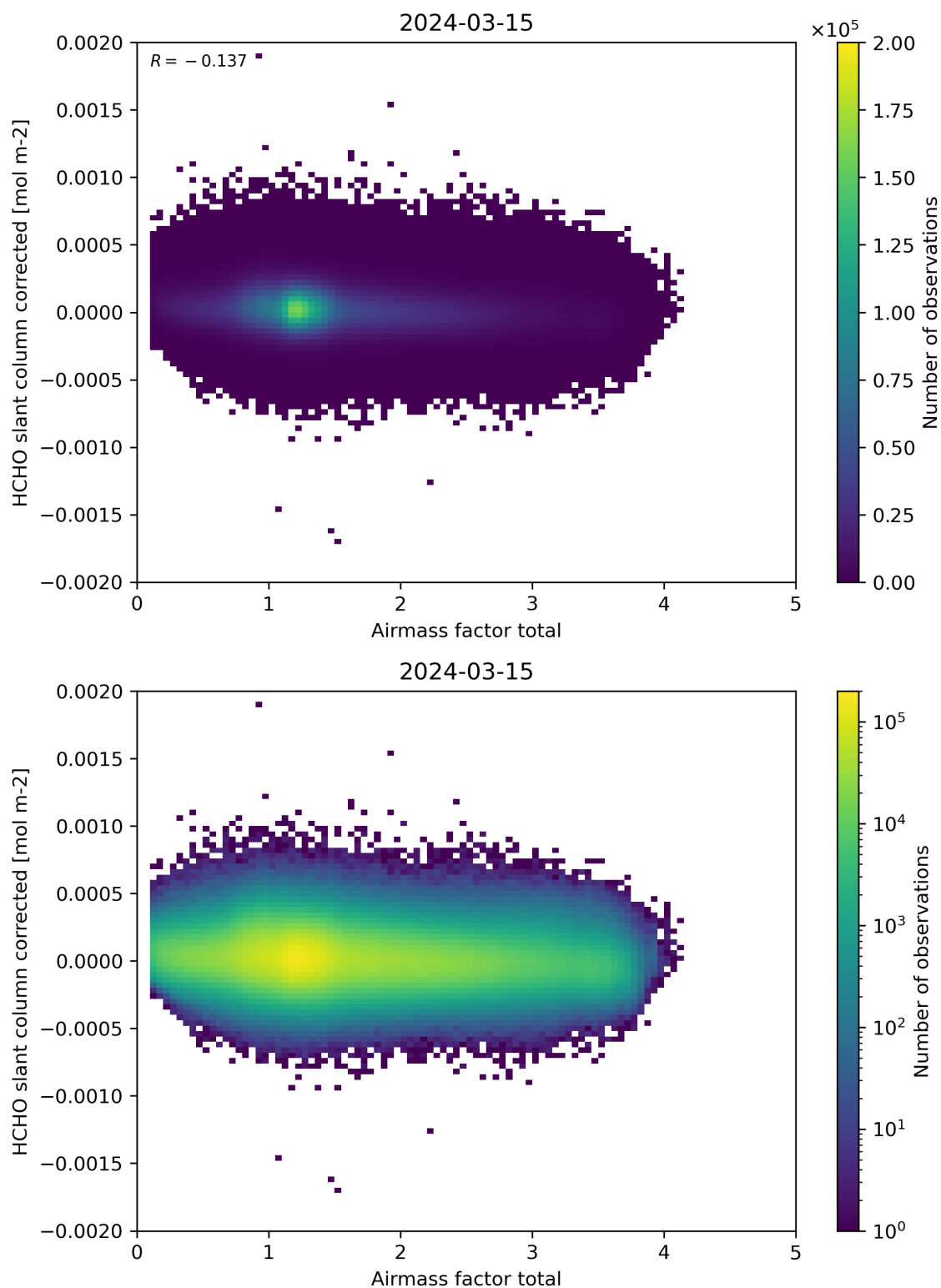
Figure 101: Scatter density plot of “Airmass factor total” against “HCHO slant column corrected” for 2024-03-14 to 2024-03-16.
