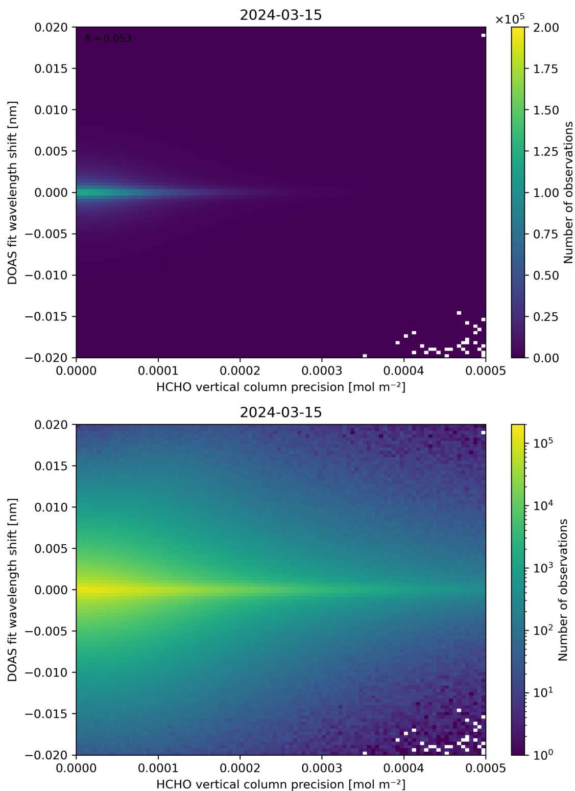
Figure 137: Scatter density plot of “HCHO vertical column precision” against “DOAS fit wavelength shift” for 2024-03-14 to 2024-03-16.
