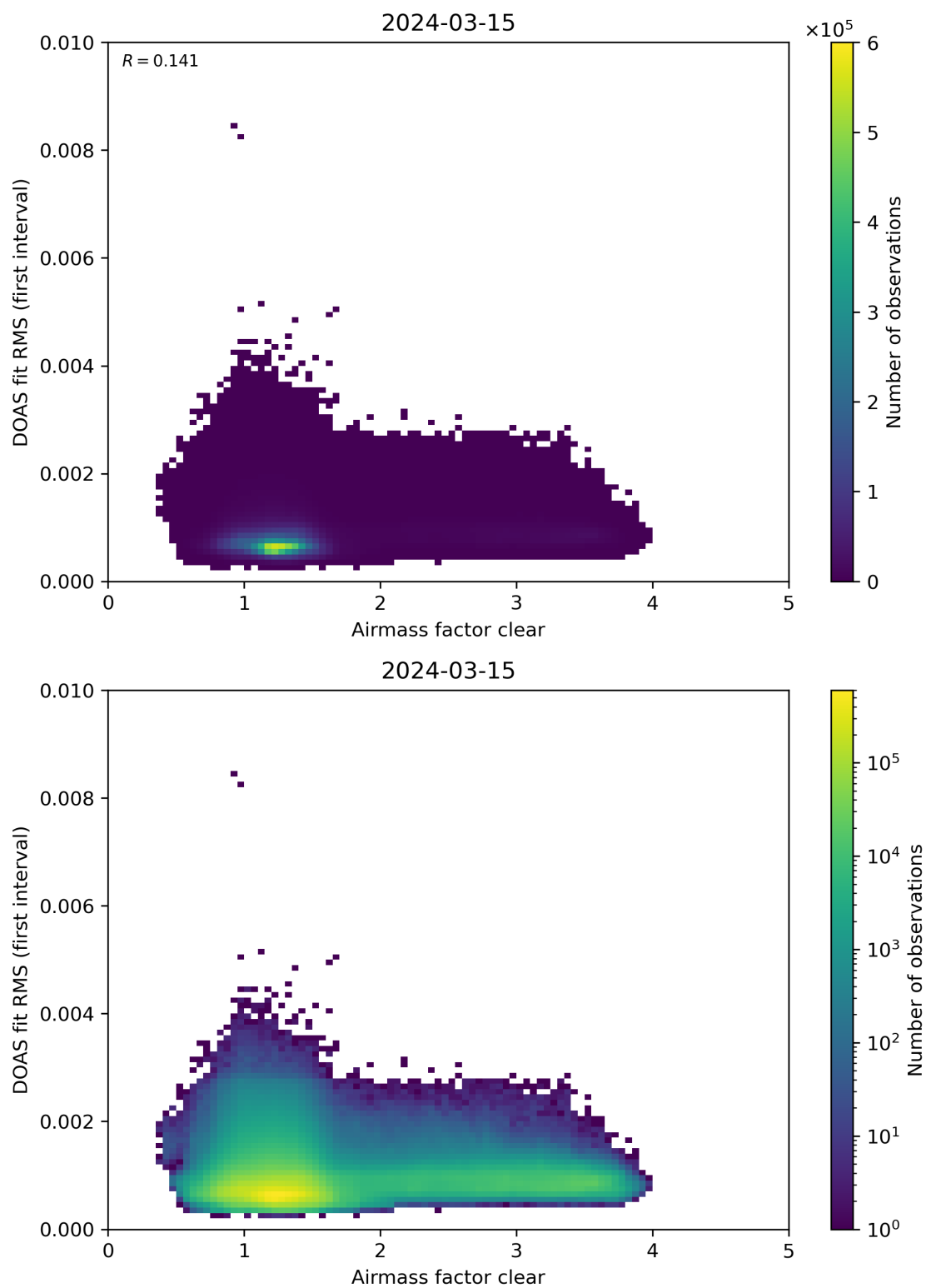
Figure 71: Scatter density plot of “Airmass factor clear” against “DOAS fit RMS (first interval)” for 2024-03-14 to 2024-03-16.
