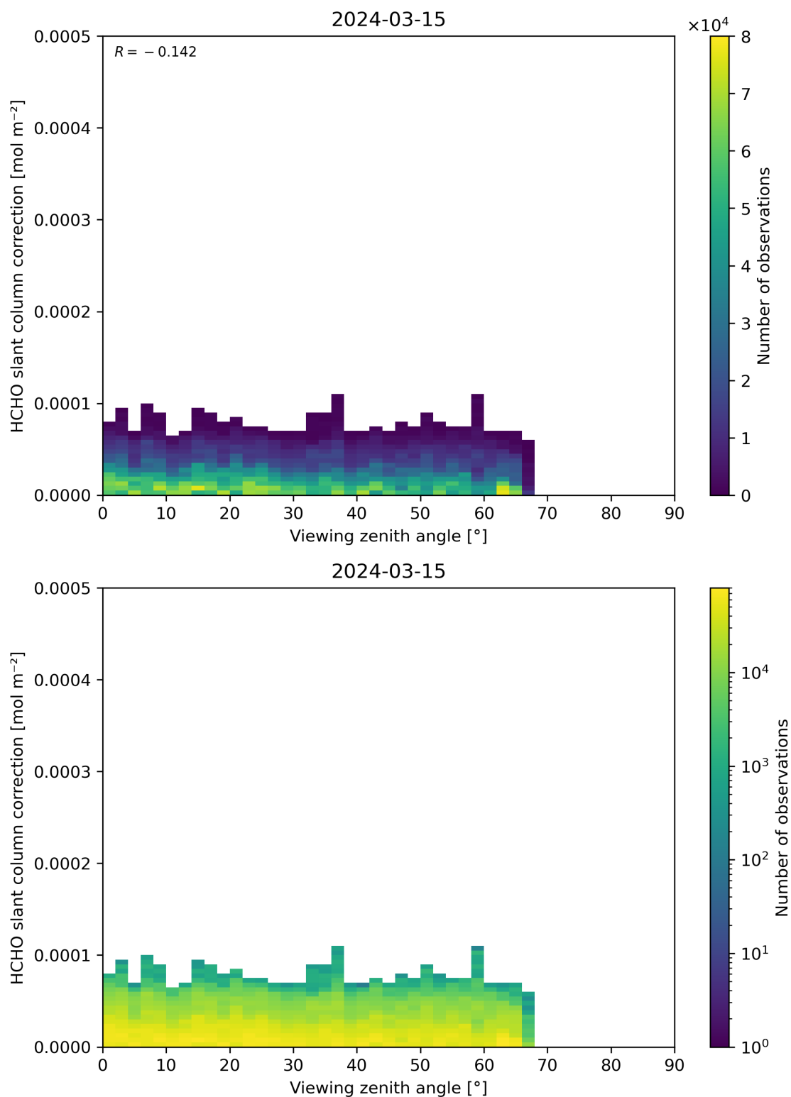
Figure 187: Scatter density plot of “Viewing zenith angle” against “HCHO slant column correction” for 2024-03-14 to 2024-03-16.
