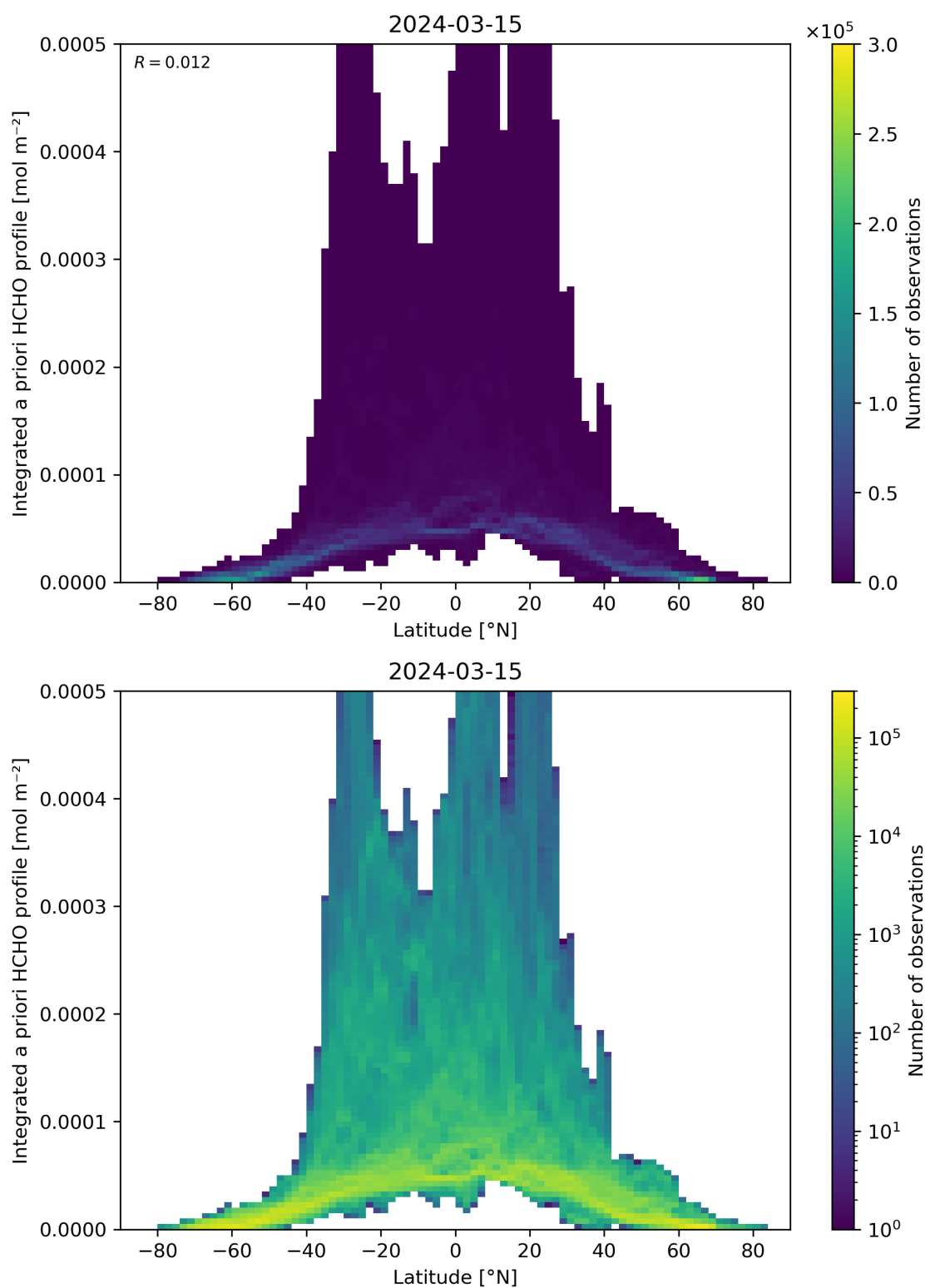
Figure 166: Scatter density plot of “Latitude” against “Integrated a priori HCHO profile” for 2024-03-14 to 2024-03-16.
