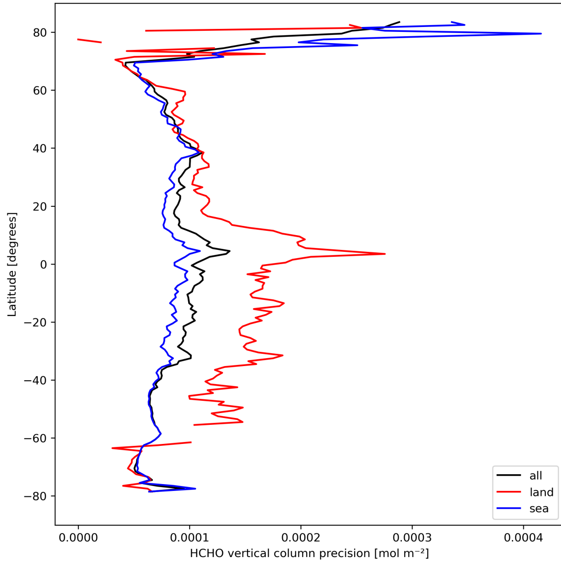
Figure 22: Zonal average of “HCHO vertical column precision” for 2024-03-14 to 2024-03-16.
