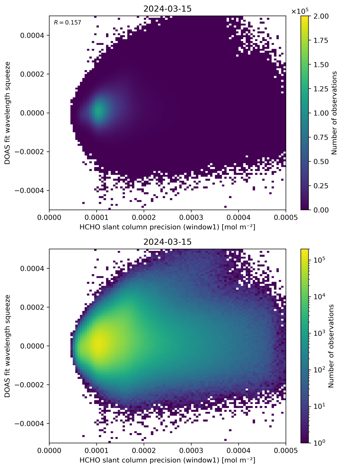
Figure 90: Scatter density plot of “HCHO slant column precision (window1)” against “DOAS fit wavelength squeeze” for 2024-03-14 to 2024-03-16.
