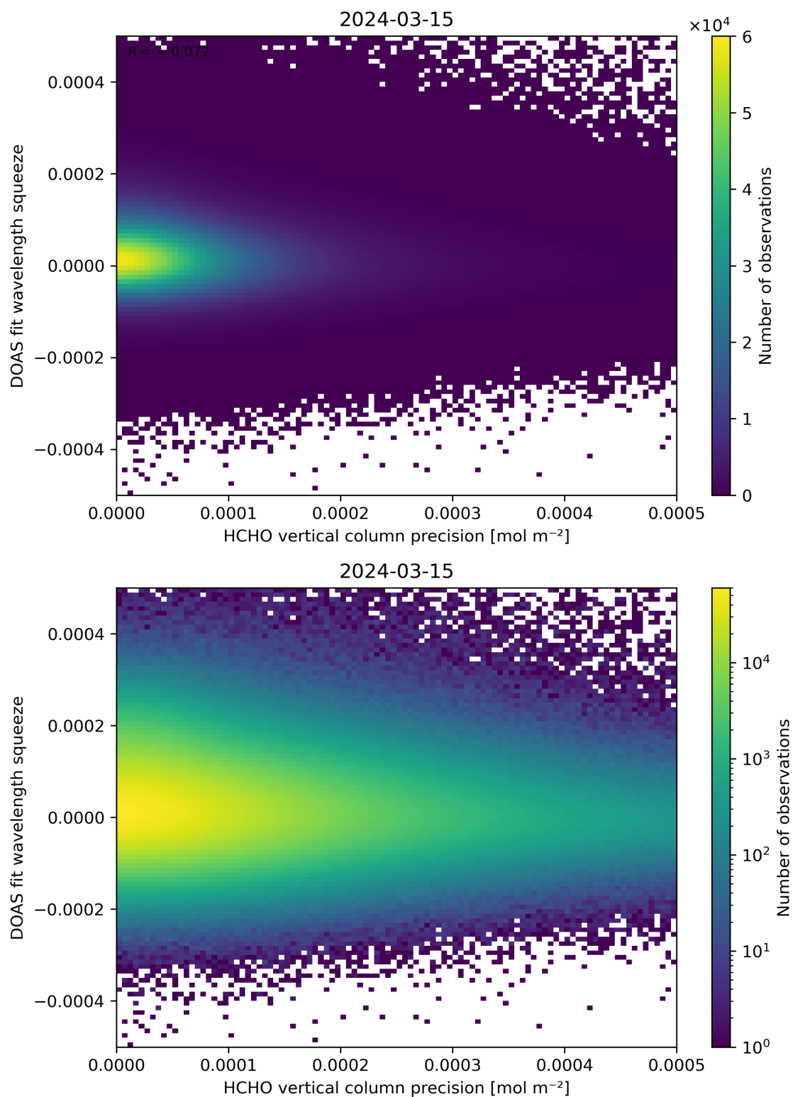
Figure 138: Scatter density plot of “HCHO vertical column precision” against “DOAS fit wavelength squeeze” for 2024-03-14 to 2024-03-16.
