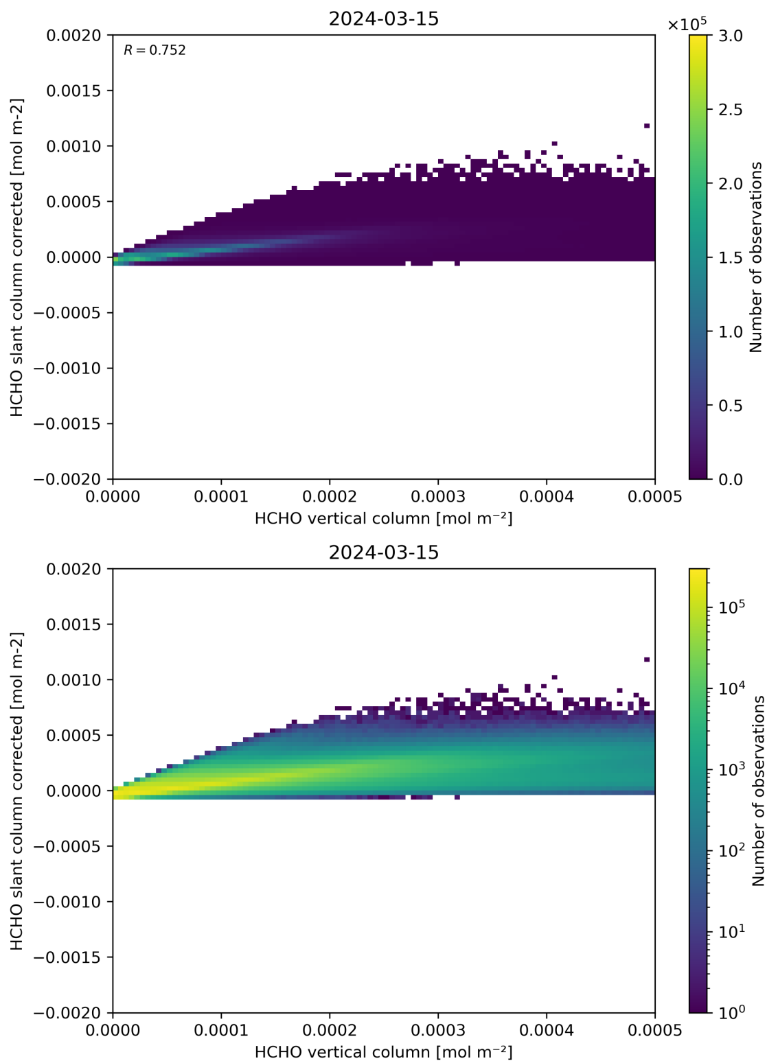
Figure 127: Scatter density plot of “HCHO vertical column” against “HCHO slant column corrected” for 2024-03-14 to 2024-03-16.
