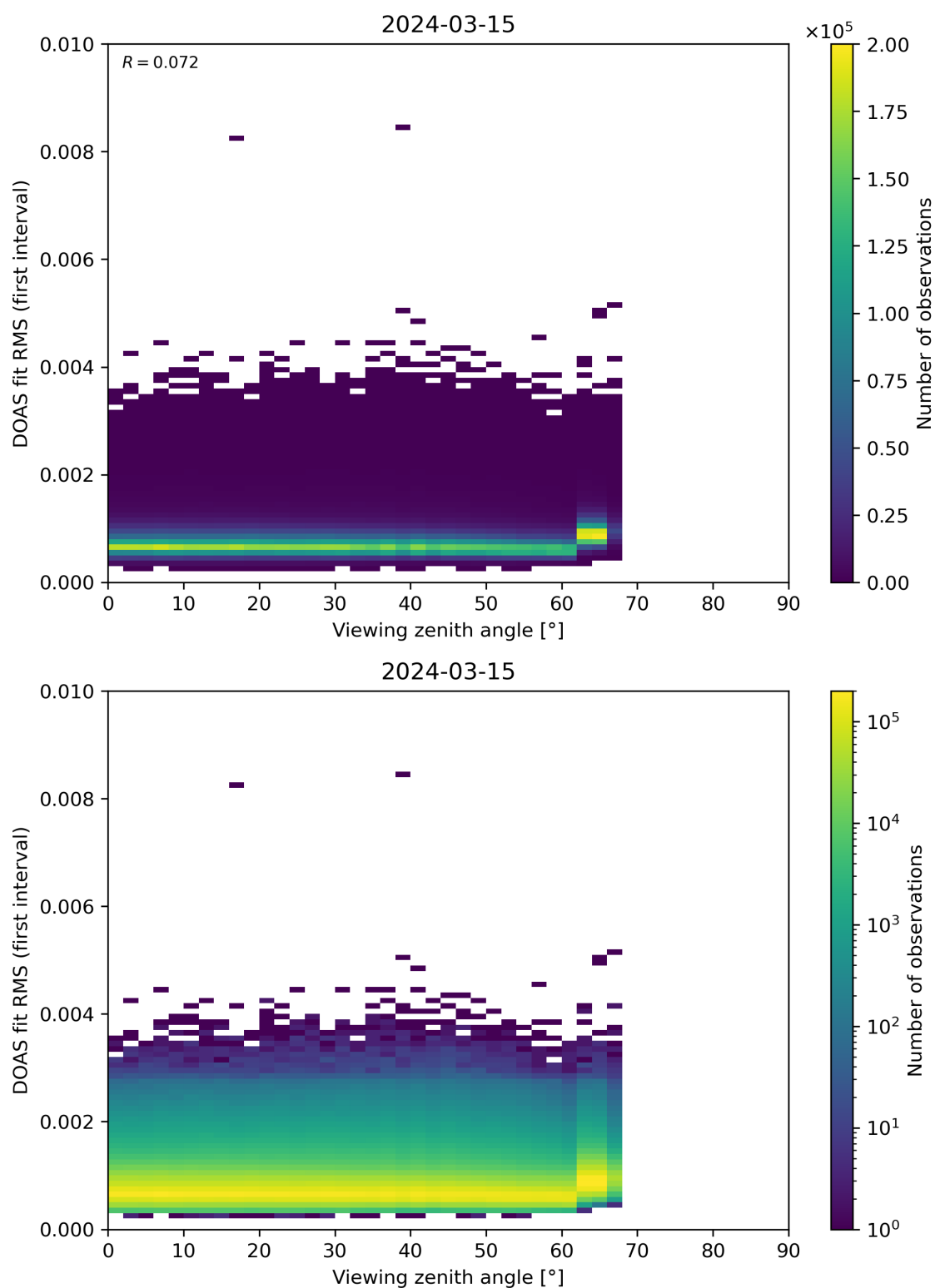
Figure 182: Scatter density plot of “Viewing zenith angle” against “DOAS fit RMS (first interval)” for 2024-03-14 to 2024-03-16.
