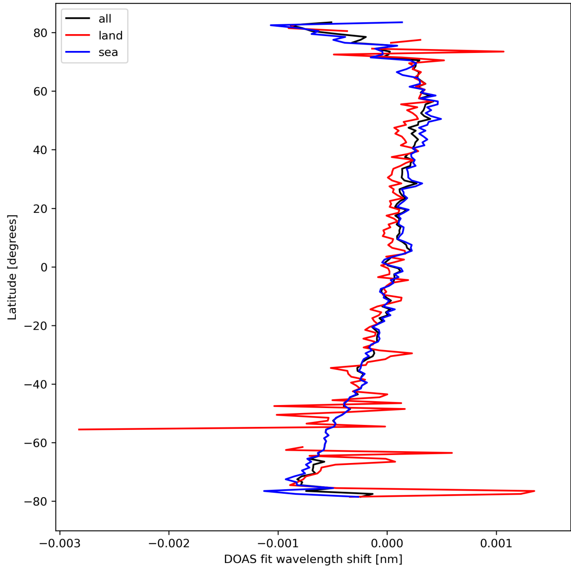
Figure 30: Zonal average of "DOAS fit wavelength shift" for 2024-03-14 to 2024-03-16.
