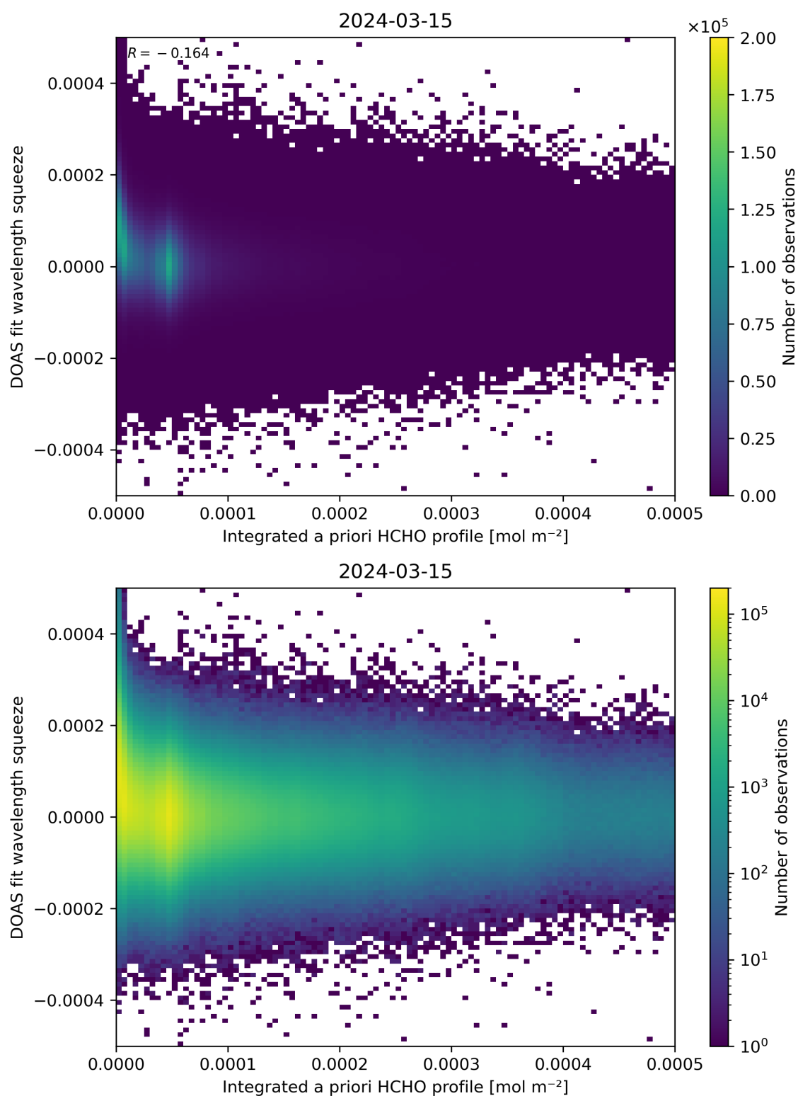
Figure 150: Scatter density plot of “Integrated a priori HCHO profile” against “DOAS fit wavelength squeeze” for 2024-03-14 to 2024-03-16.
