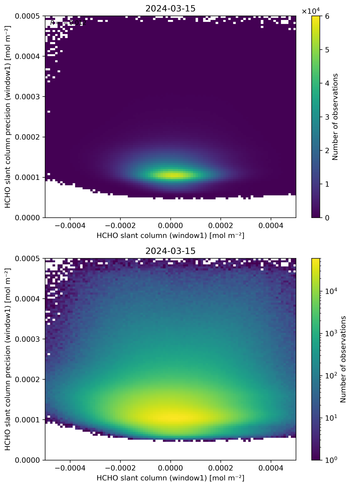
Figure 84: Scatter density plot of “HCHO slant column (window1)” against “HCHO slant column precision (window1)” for 2024-03-14 to 2024-03-16.
