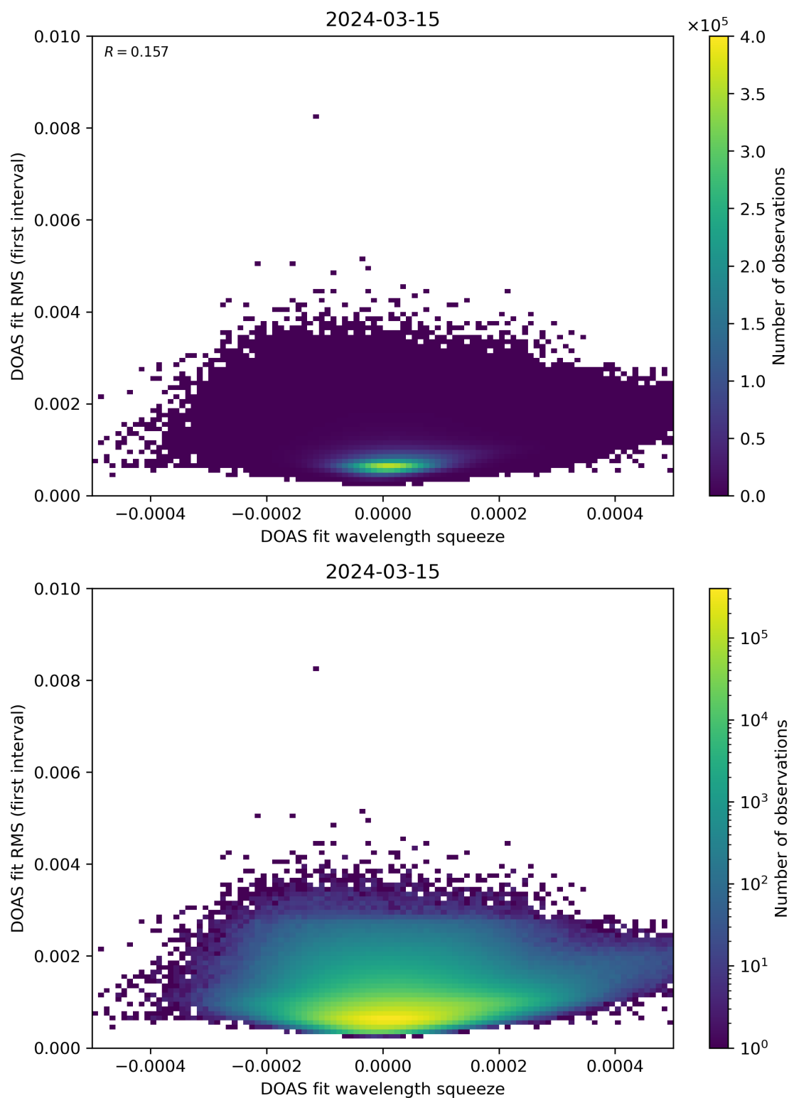
Figure 68: Scatter density plot of “DOAS fit wavelength squeeze” against “DOAS fit RMS (first interval)” for 2024-03-14 to 2024-03-16.
