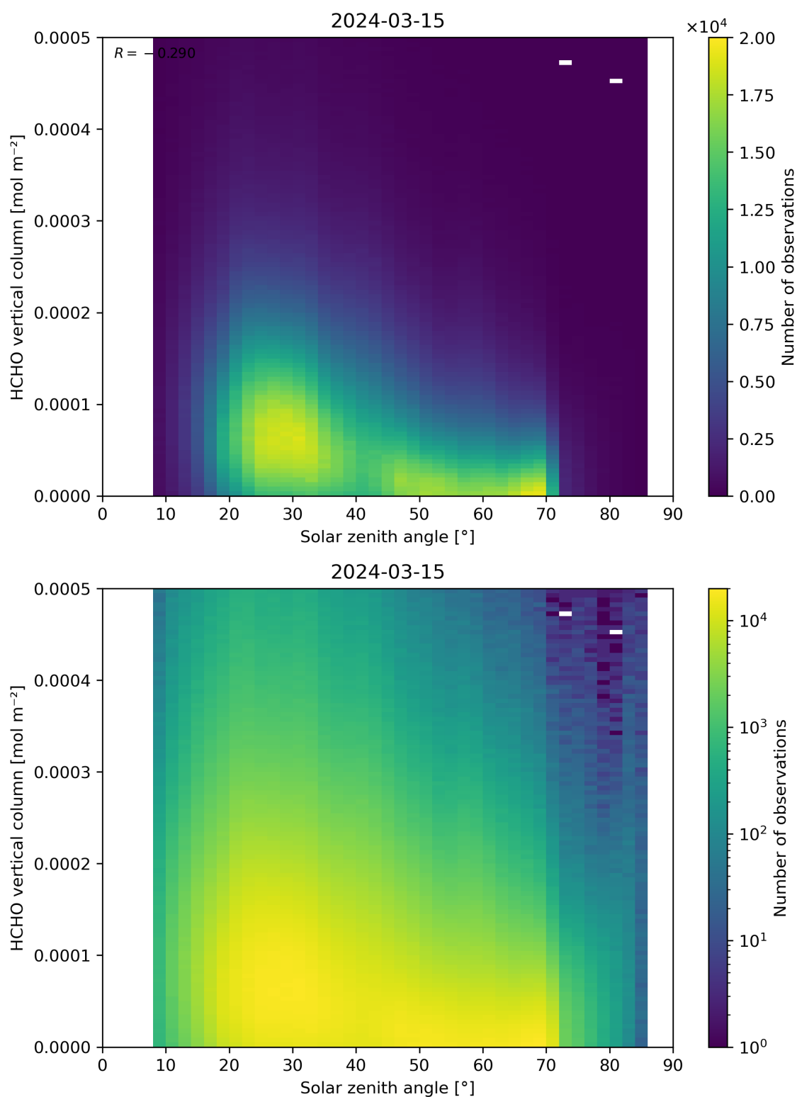
Figure 177: Scatter density plot of “Solar zenith angle” against “HCHO vertical column” for 2024-03-14 to 2024-03-16.
