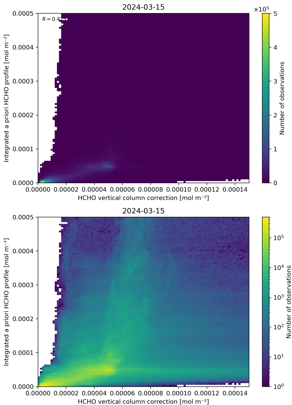
Figure 122: Scatter density plot of “HCHO vertical column correction” against “Integrated a priori HCHO profile” for 2024-03-14 to 2024-03-16.
