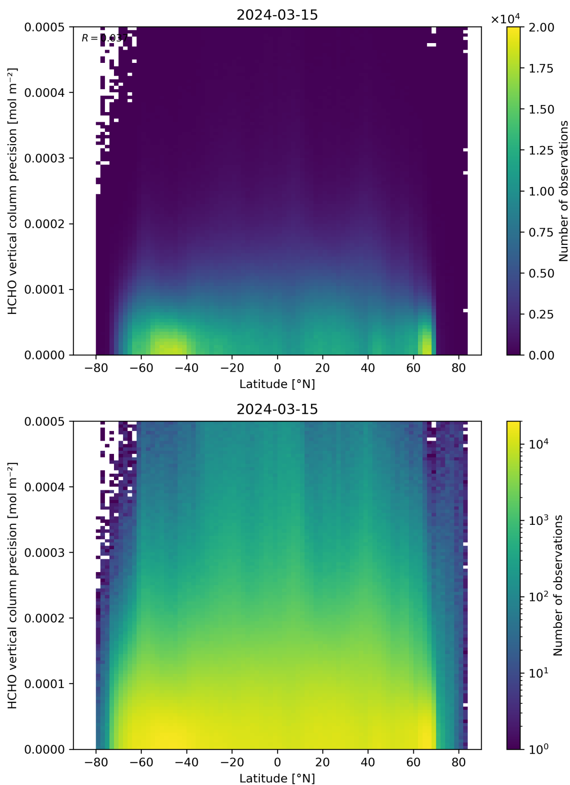
Figure 165: Scatter density plot of “Latitude” against “HCHO vertical column precision” for 2024-03-14 to 2024-03-16.
