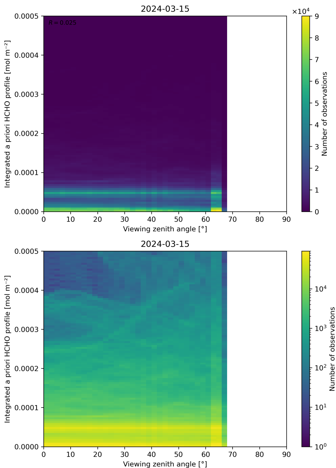
Figure 195: Scatter density plot of “Viewing zenith angle” against “Integrated a priori HCHO profile” for 2024-03-14 to 2024-03-16.
