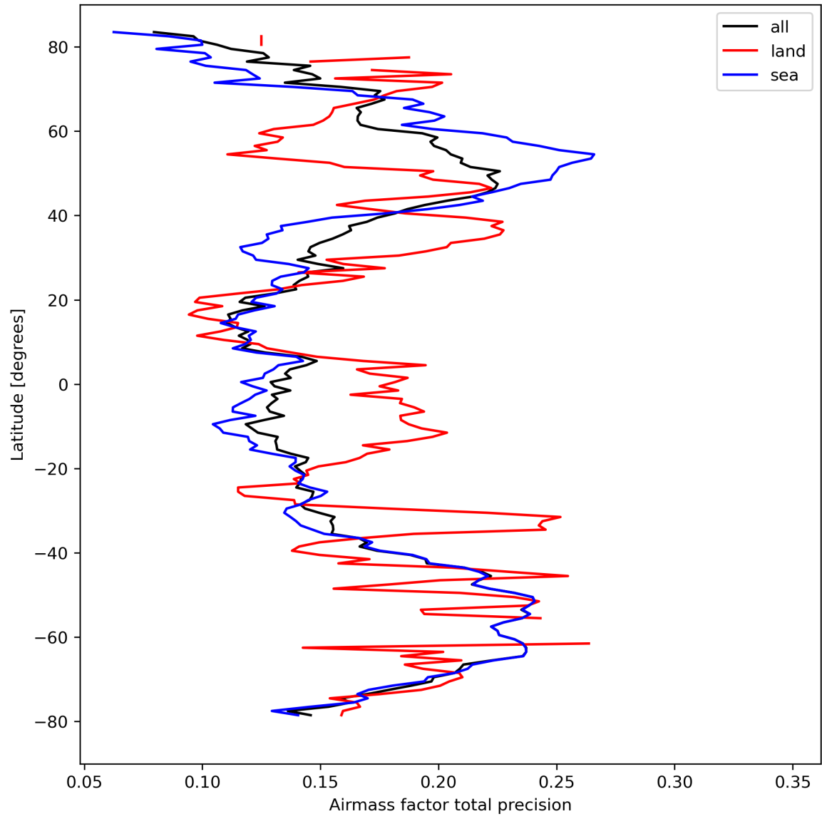
Figure 27: Zonal average of “Airmass factor total precision” for 2024-03-14 to 2024-03-16.
