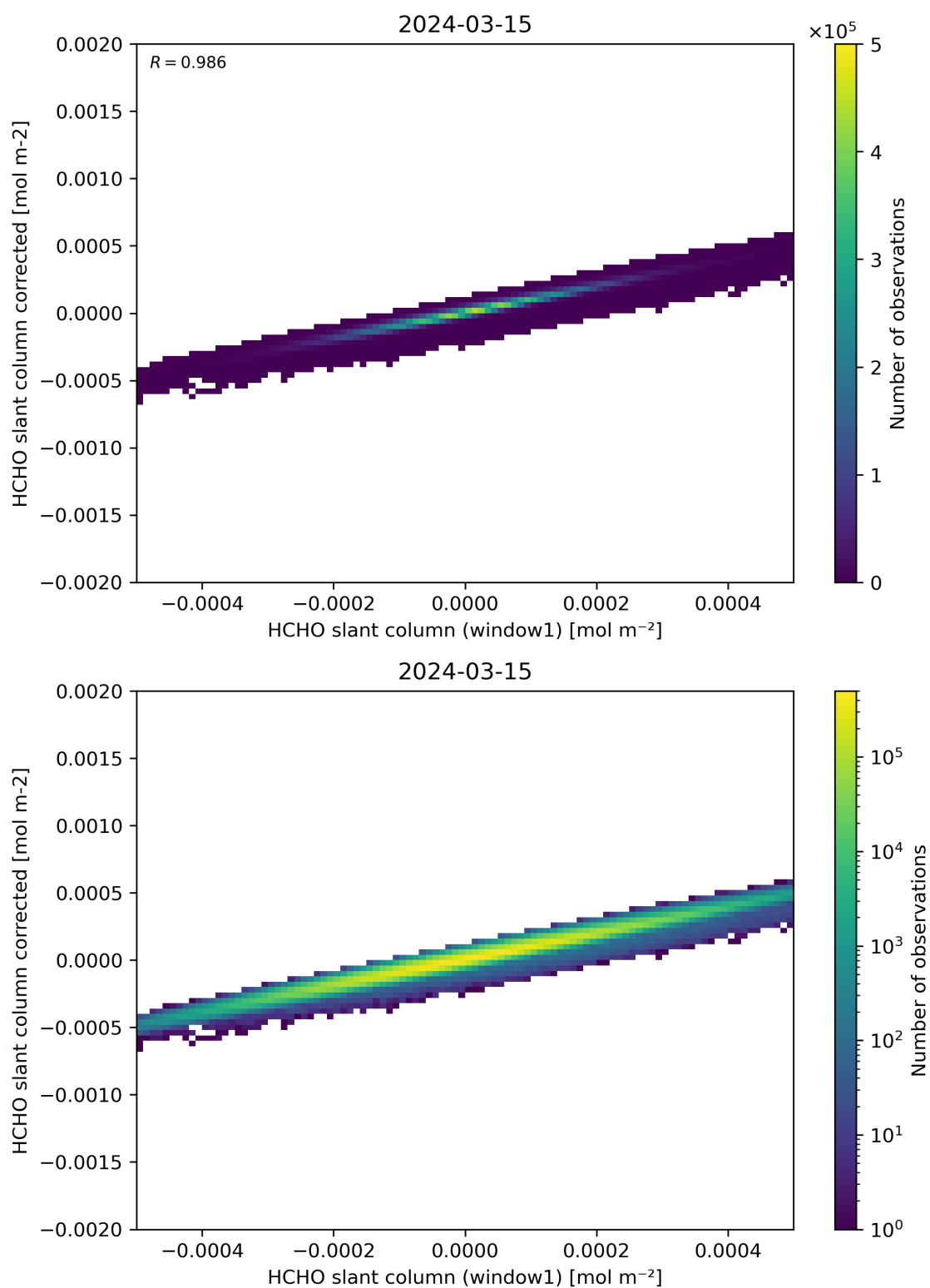
Figure 82: Scatter density plot of “HCHO slant column (window1)” against “HCHO slant column corrected” for 2024-03-14 to 2024-03-16.
