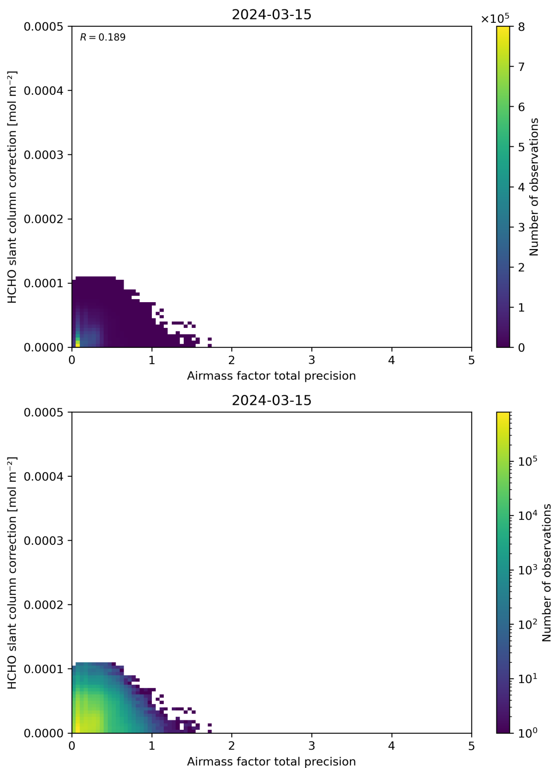
Figure 110: Scatter density plot of “Airmass factor total precision” against “HCHO slant column correction” for 2024-03-14 to 2024-03-16.
