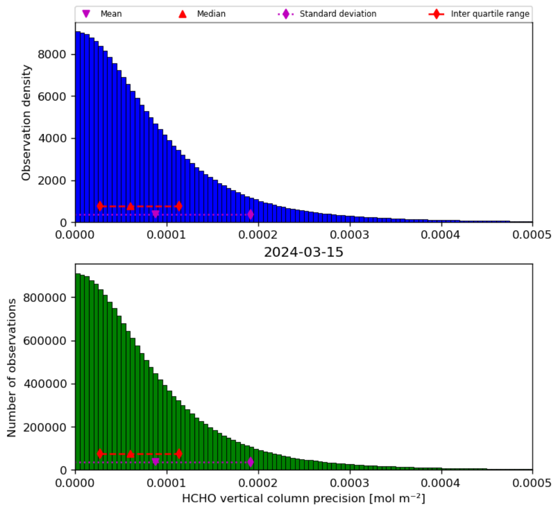
Figure 36: Histogram of “HCHO vertical column precision” for 2024-03-14 to 2024-03-16
