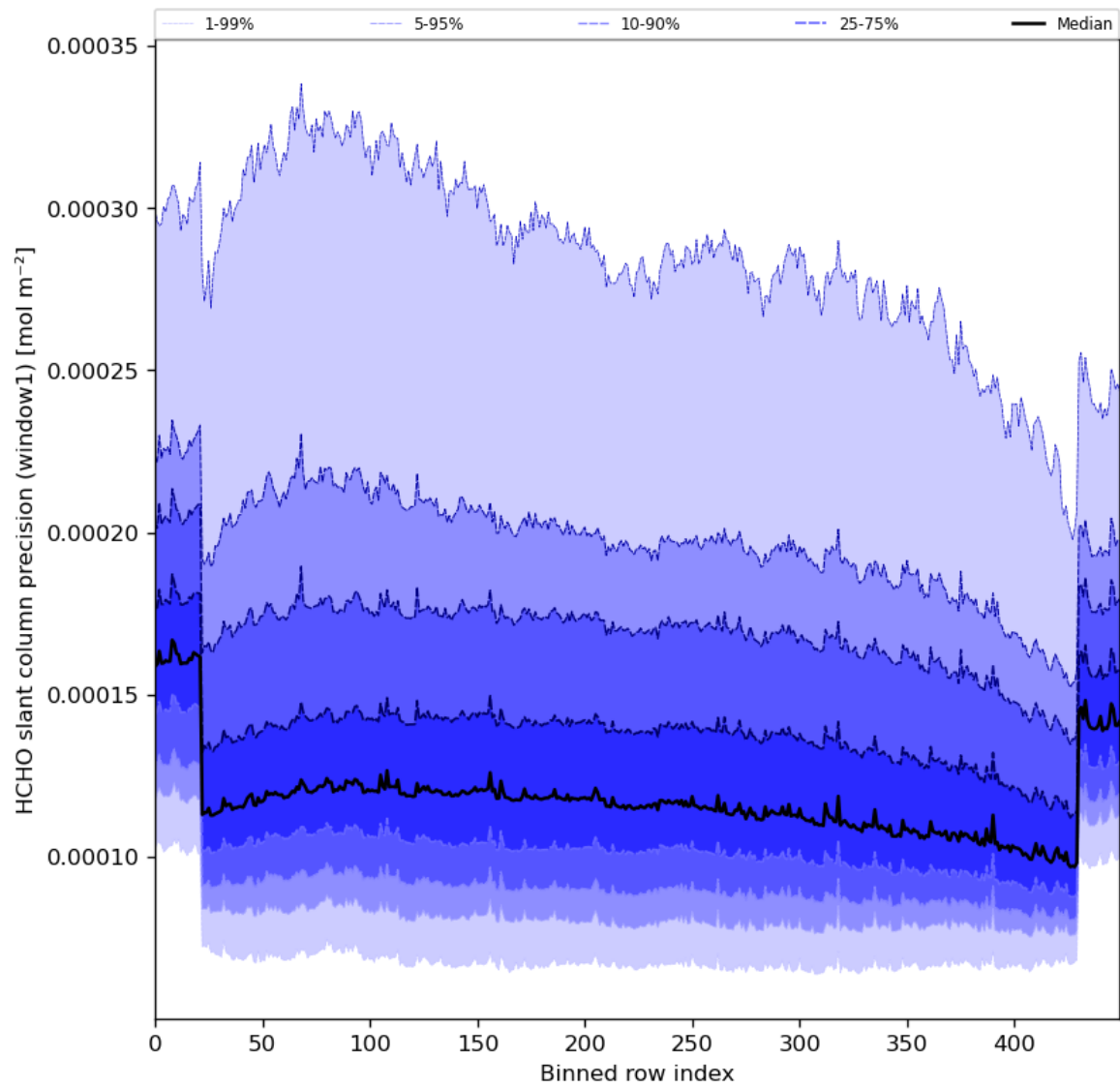
Figure 53: Along track statistics of “HCHO slant column precision (window1)” for 2024-03-14 to 2024-03-16
