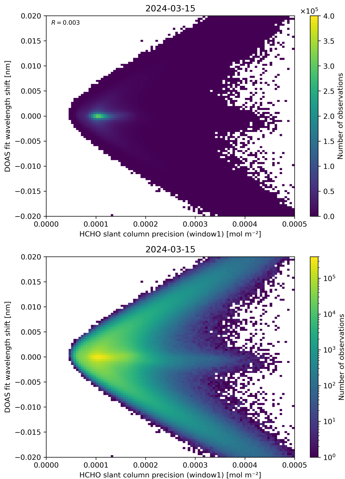
Figure 89: Scatter density plot of “HCHO slant column precision (window1)” against “DOAS fit wavelength shift” for 2024-03-14 to 2024-03-16.
