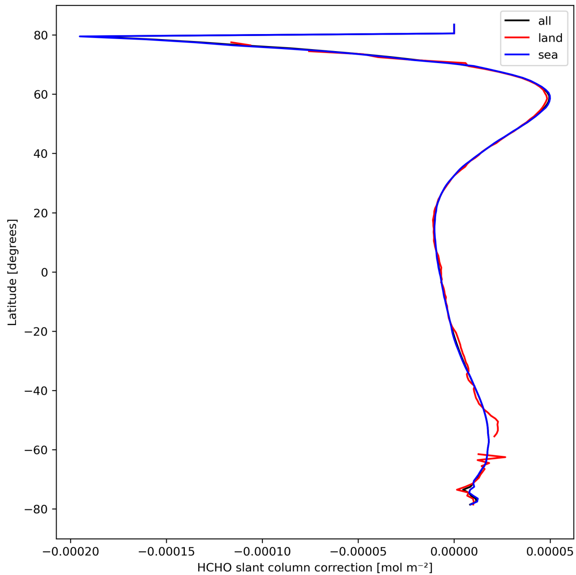
Figure 33: Zonal average of “HCHO slant column correction” for 2024-03-14 to 2024-03-16.
