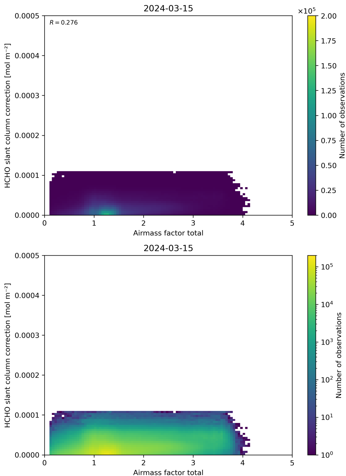
Figure 102: Scatter density plot of “Airmass factor total” against “HCHO slant column correction” for 2024-03-14 to 2024-03-16.
