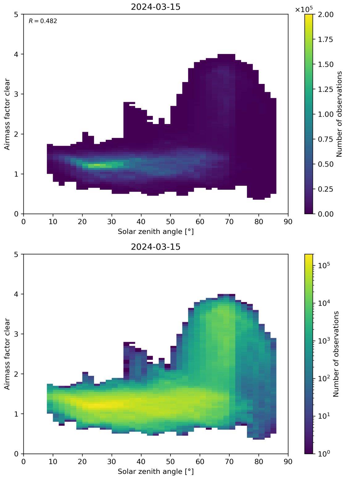
Figure 170: Scatter density plot of “Solar zenith angle” against “Airmass factor clear” for 2024-03-14 to 2024-03-16.
