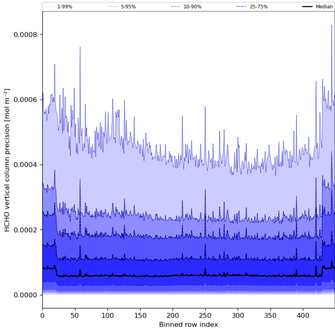
Figure 50: Along track statistics of “HCHO vertical column precision” for 2024-03-14 to 2024-03-16
