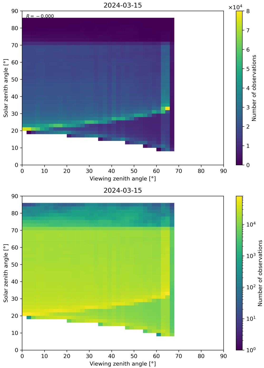
Figure 197: Scatter density plot of “Viewing zenith angle” against “Solar zenith angle” for 2024-03-14 to 2024-03-16.
