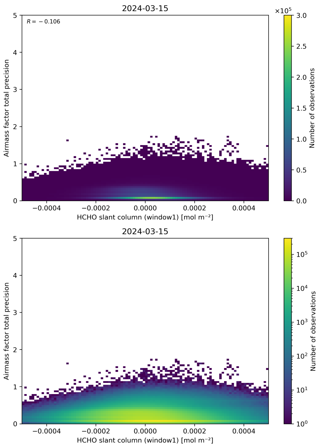
Figure 86: Scatter density plot of “HCHO slant column (window1)” against “Airmass factor total precision” for 2024-03-14 to 2024-03-16.
