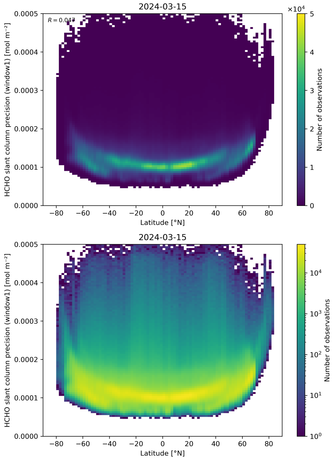
Figure 160: Scatter density plot of “Latitude” against “HCHO slant column precision (window1)” for 2024-03-14 to 2024-03-16.
