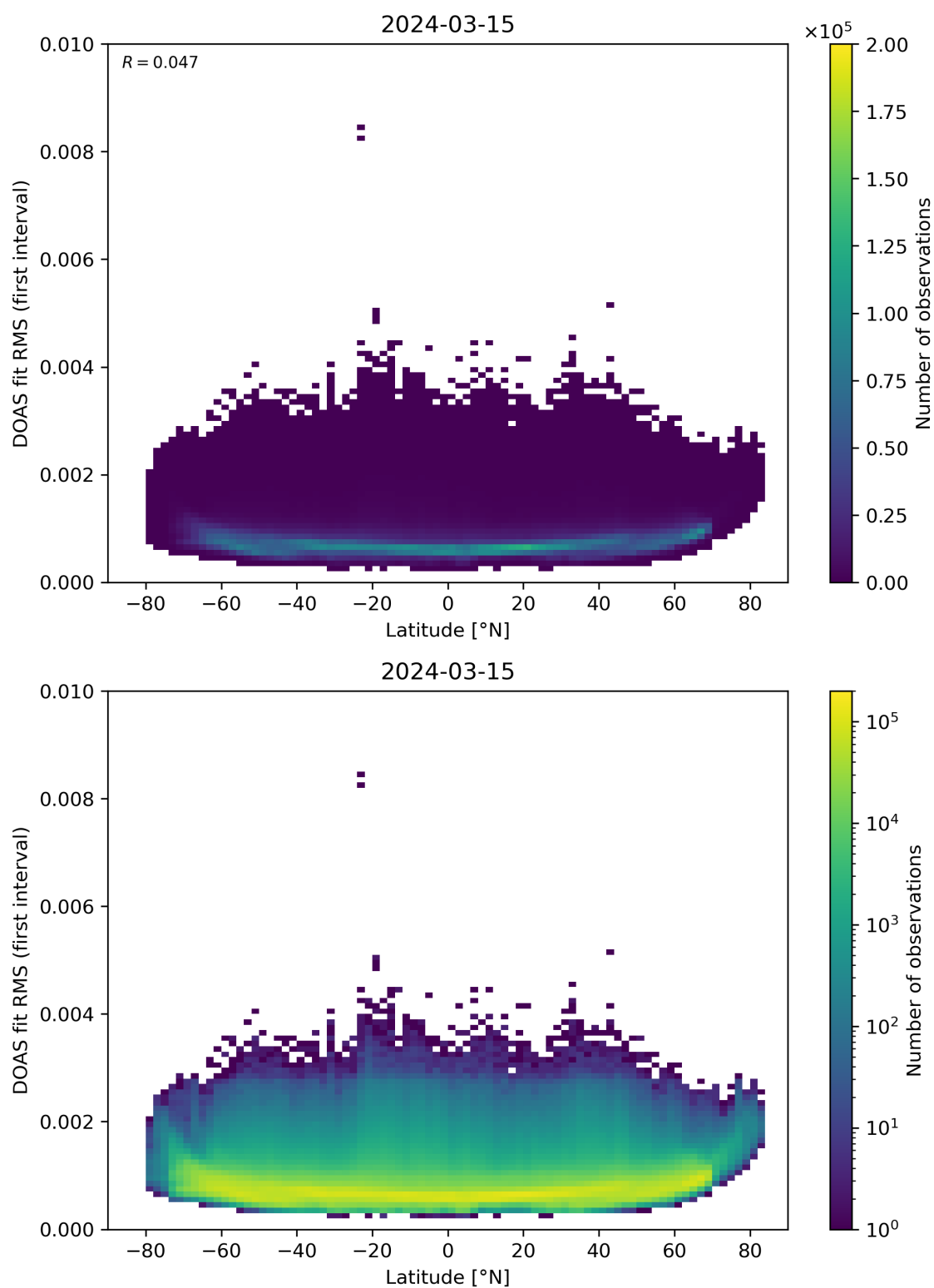
Figure 153: Scatter density plot of “Latitude” against “DOAS fit RMS (first interval)” for 2024-03-14 to 2024-03-16.
