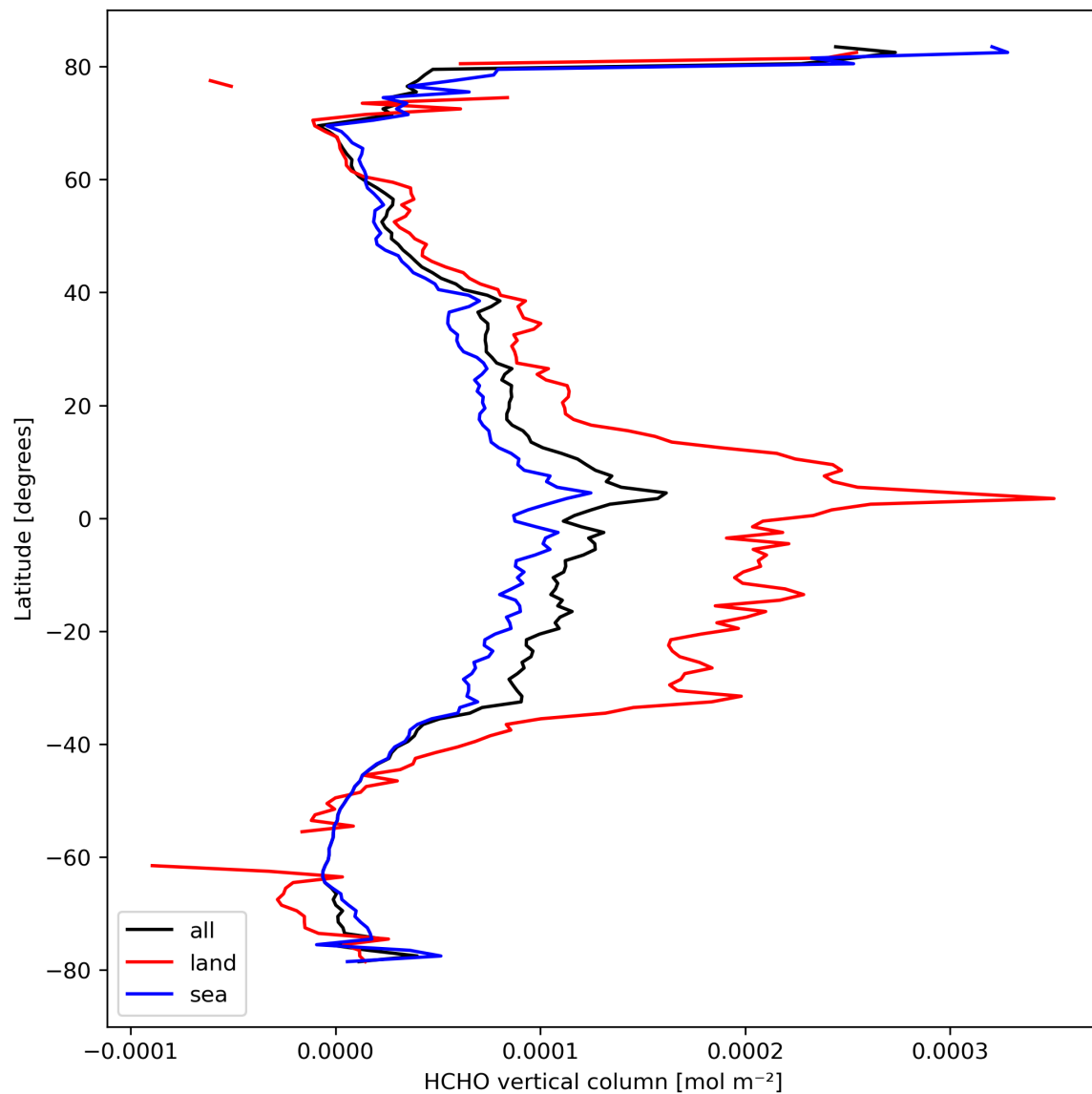
Figure 21: Zonal average of “HCHO vertical column” for 2024-03-14 to 2024-03-16.
