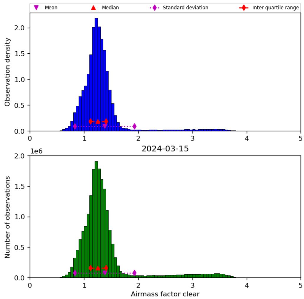
Figure 42: Histogram of “Airmass factor clear” for 2024-03-14 to 2024-03-16
