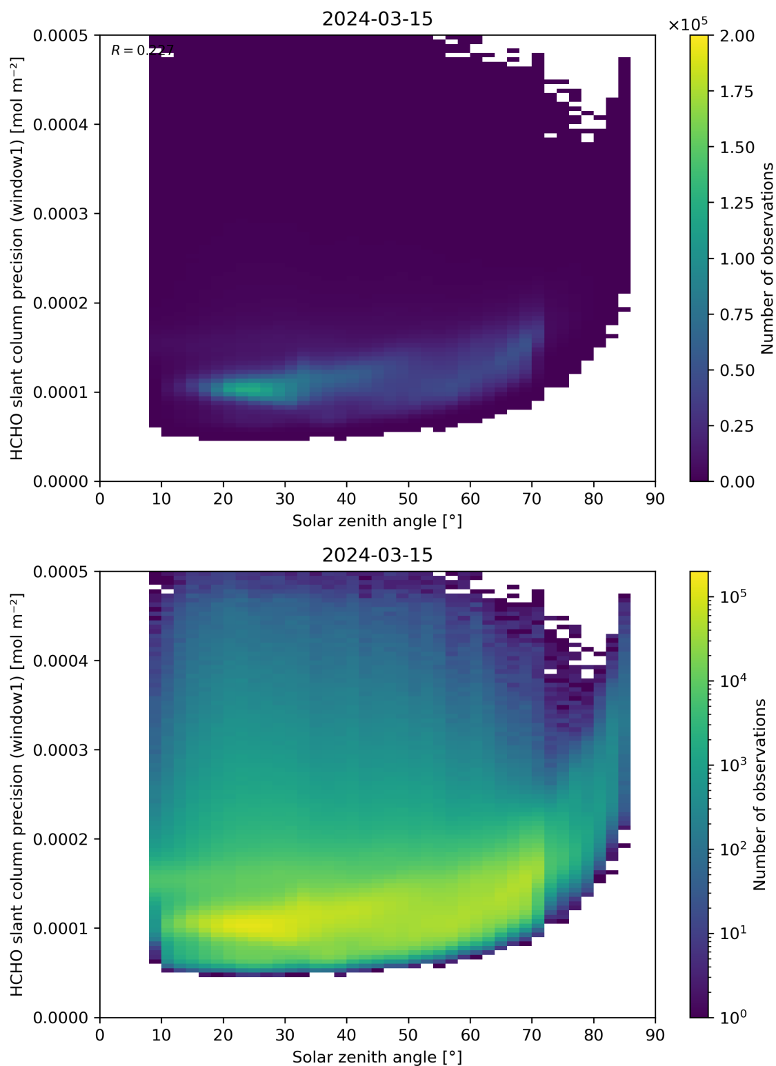
Figure 174: Scatter density plot of “Solar zenith angle” against “HCHO slant column precision (window1)” for 2024-03-14 to 2024-03-16.
