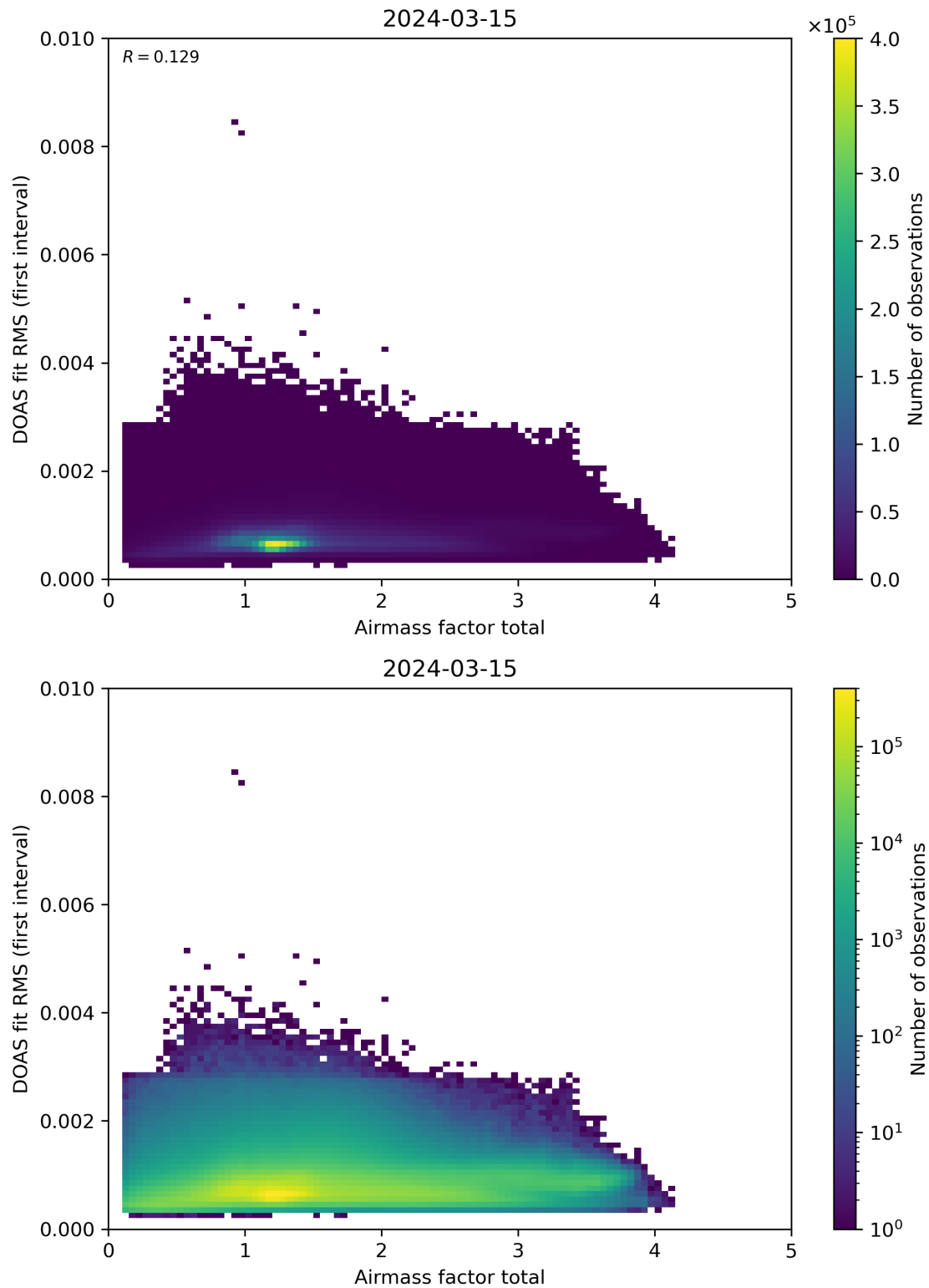
Figure 97: Scatter density plot of “Airmass factor total” against “DOAS fit RMS (first interval)” for 2024-03-14 to 2024-03-16.
