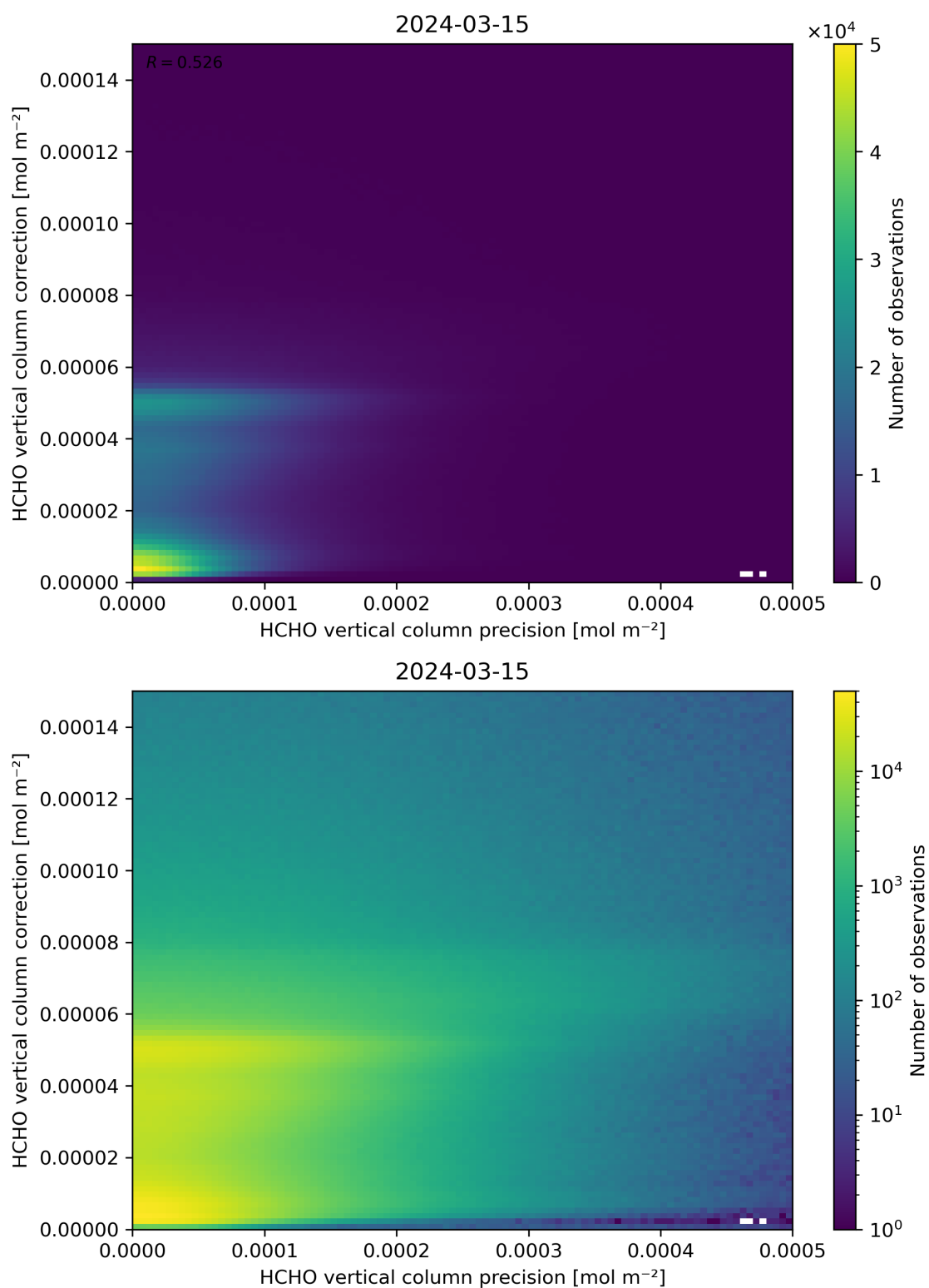
Figure 146: Scatter density plot of “HCHO vertical column precision” against “HCHO vertical column correction” for 2024-03-14 to 2024-03-16.
