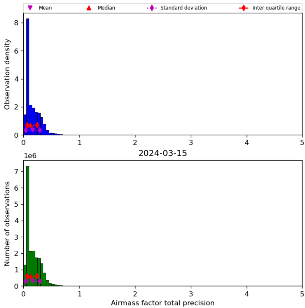
Figure 41: Histogram of “Airmass factor total precision” for 2024-03-14 to 2024-03-16
