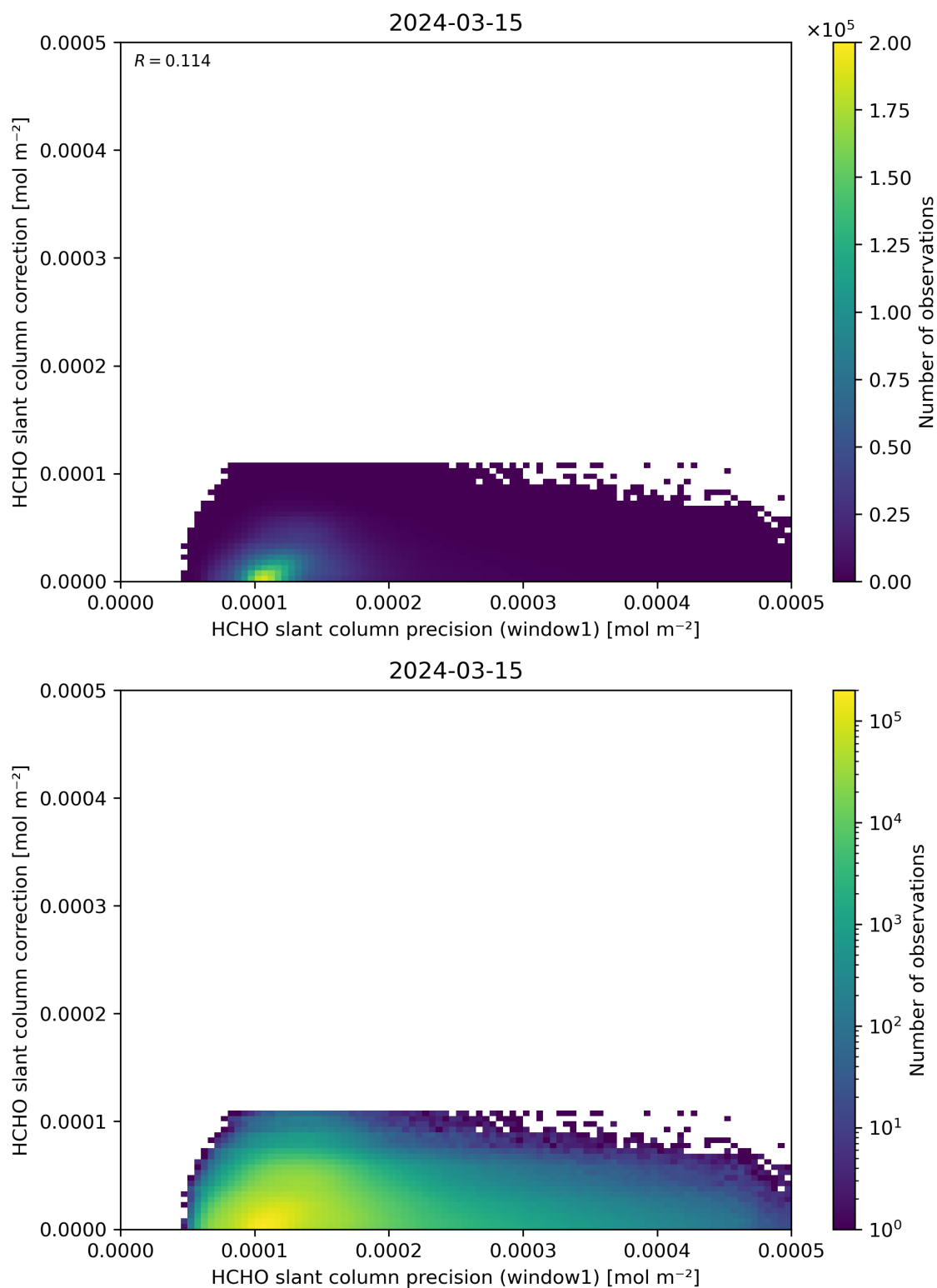
Figure 93: Scatter density plot of “HCHO slant column precision (window1)” against “HCHO slant column correction” for 2024-03-14 to 2024-03-16.
