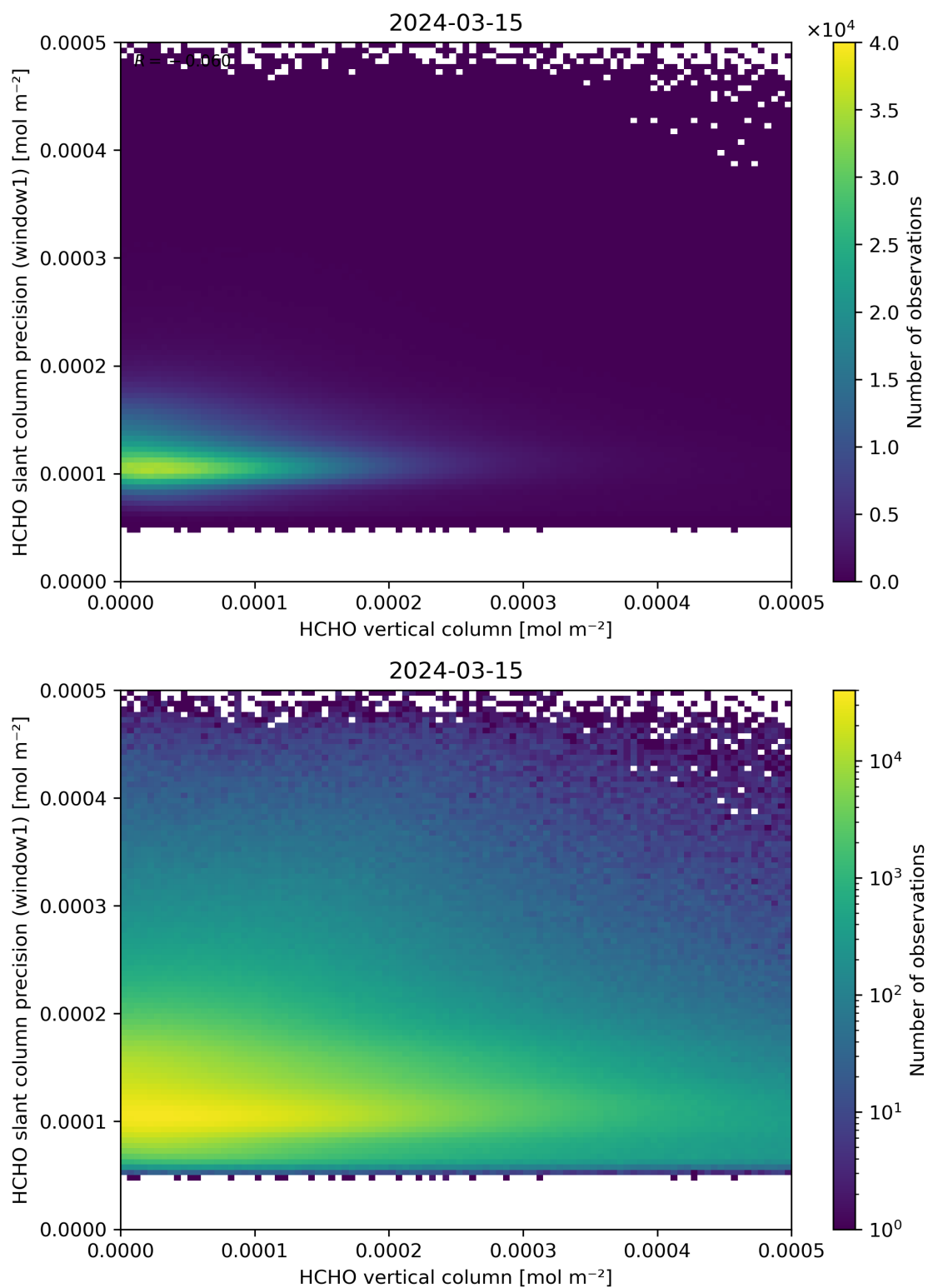
Figure 130: Scatter density plot of “HCHO vertical column” against “HCHO slant column precision (window1)” for 2024-03-14 to 2024-03-16.
