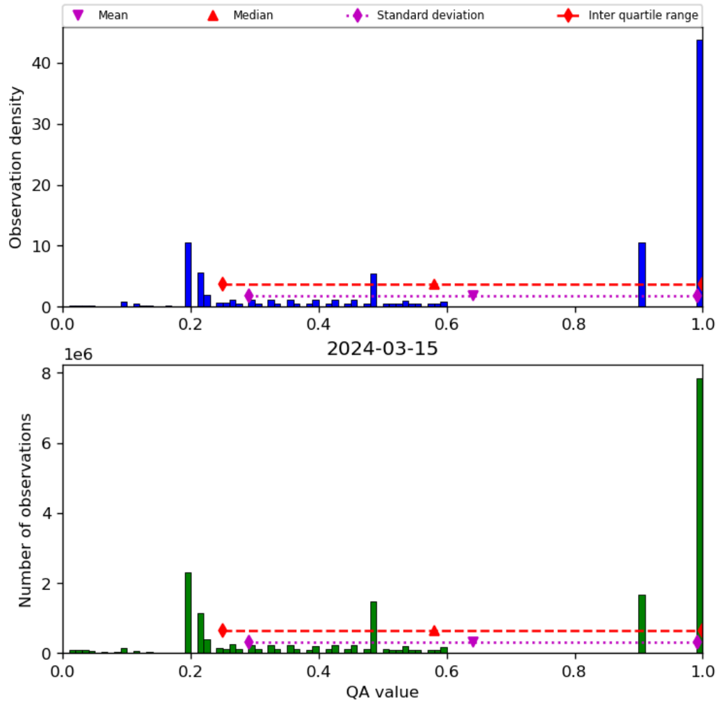
Figure 34: Histogram of “QA value” for 2024-03-14 to 2024-03-16
