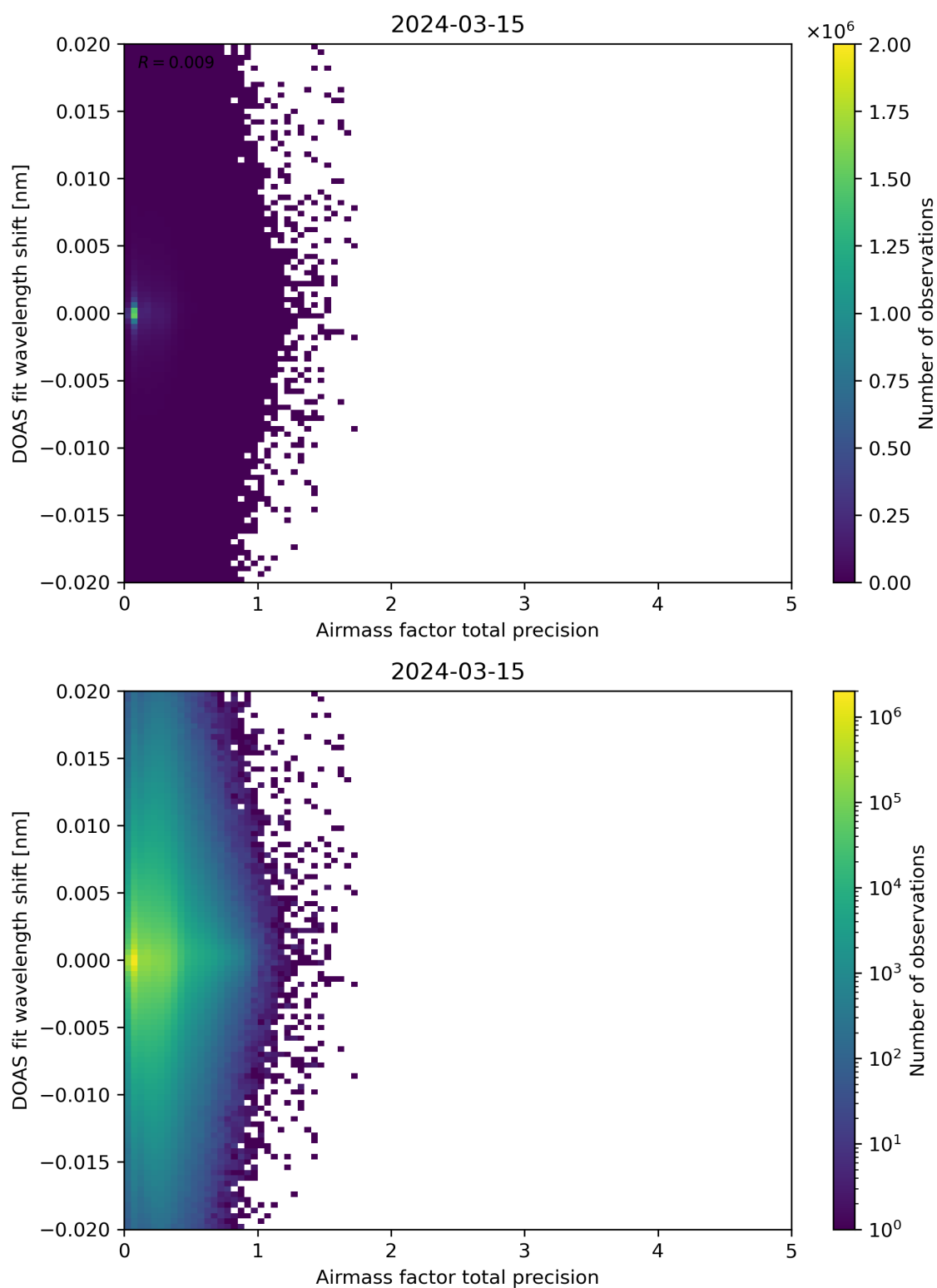
Figure 106: Scatter density plot of “Airmass factor total precision” against “DOAS fit wavelength shift” for 2024-03-14 to 2024-03-16.
