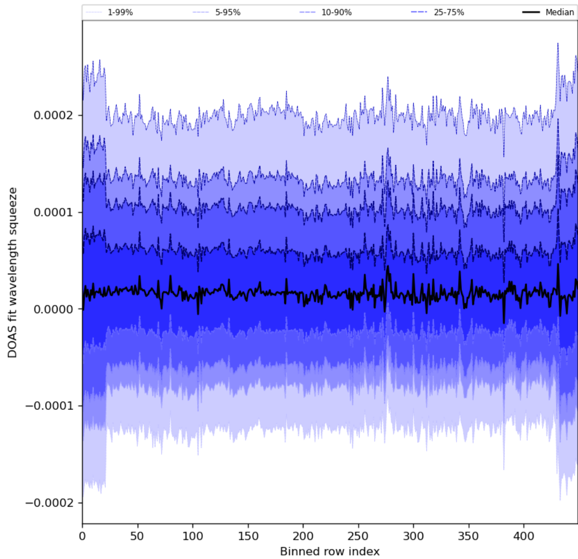
Figure 59: Along track statistics of “DOAS fit wavelength squeeze” for 2024-03-14 to 2024-03-16
