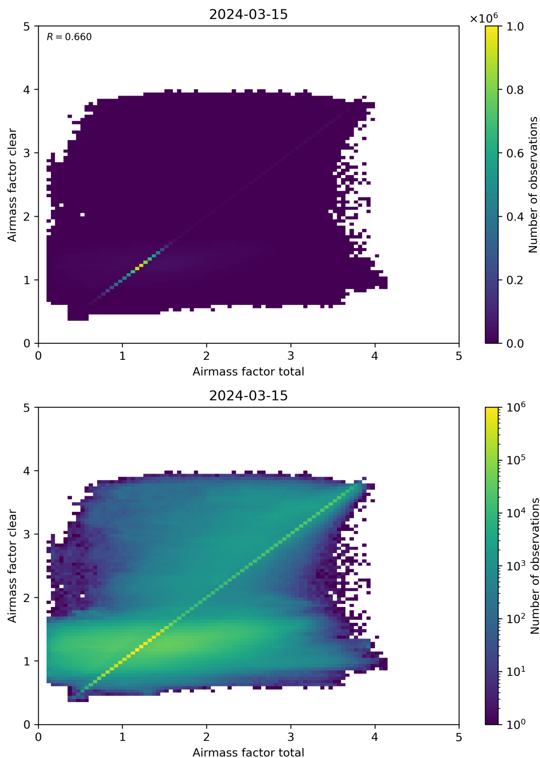
Figure 100: Scatter density plot of “Airmass factor total” against “Airmass factor clear” for 2024-03-14 to 2024-03-16.
