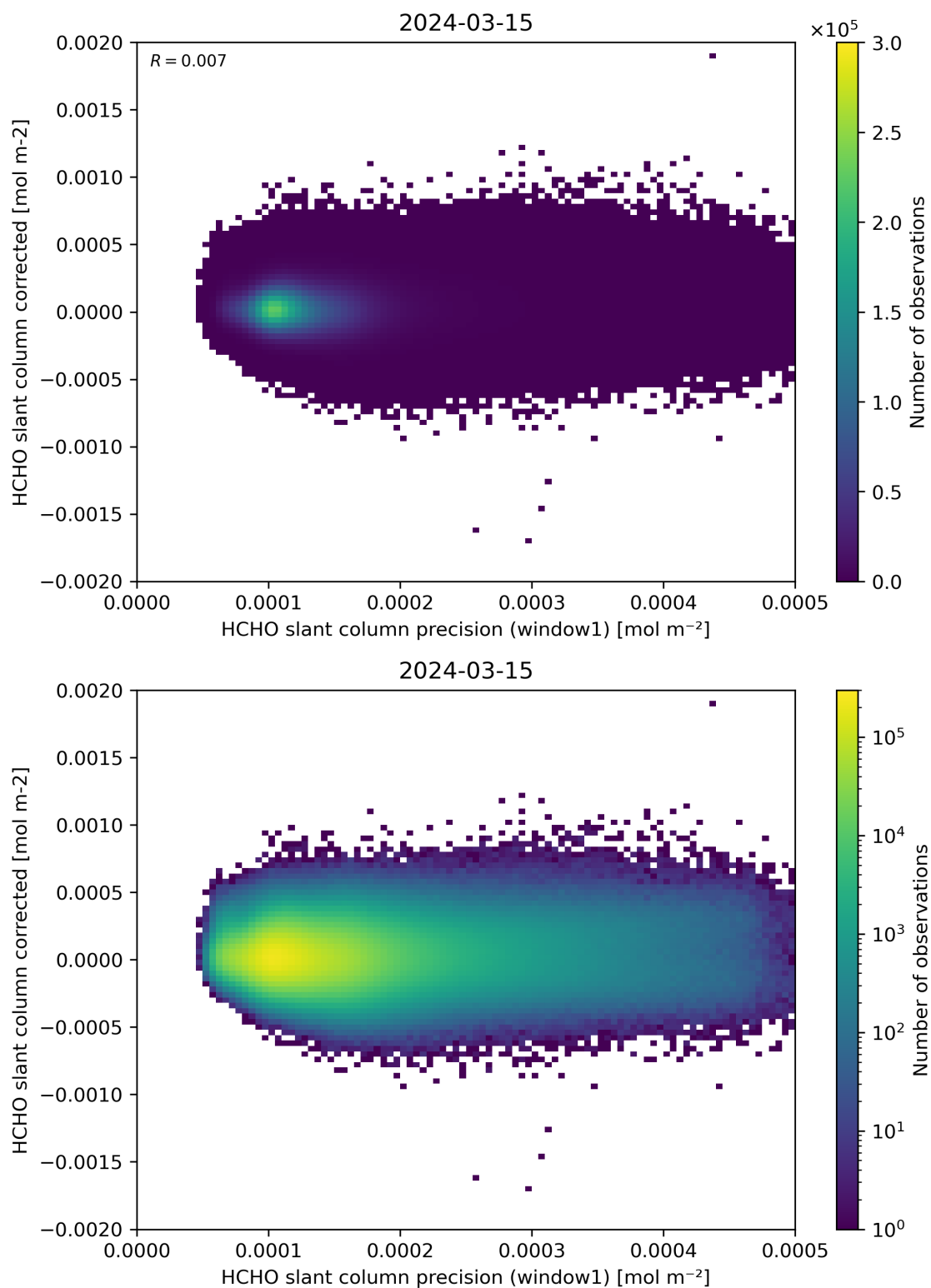
Figure 92: Scatter density plot of “HCHO slant column precision (window1)” against “HCHO slant column corrected” for 2024-03-14 to 2024-03-16.
