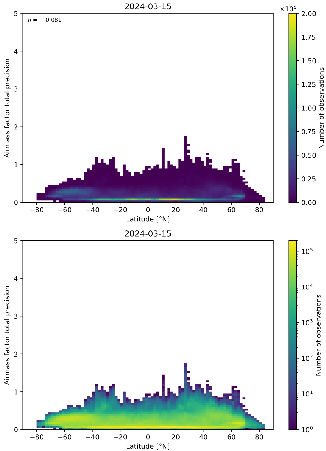
Figure 162: Scatter density plot of “Latitude” against “Airmass factor total precision” for 2024-03-14 to 2024-03-16.
