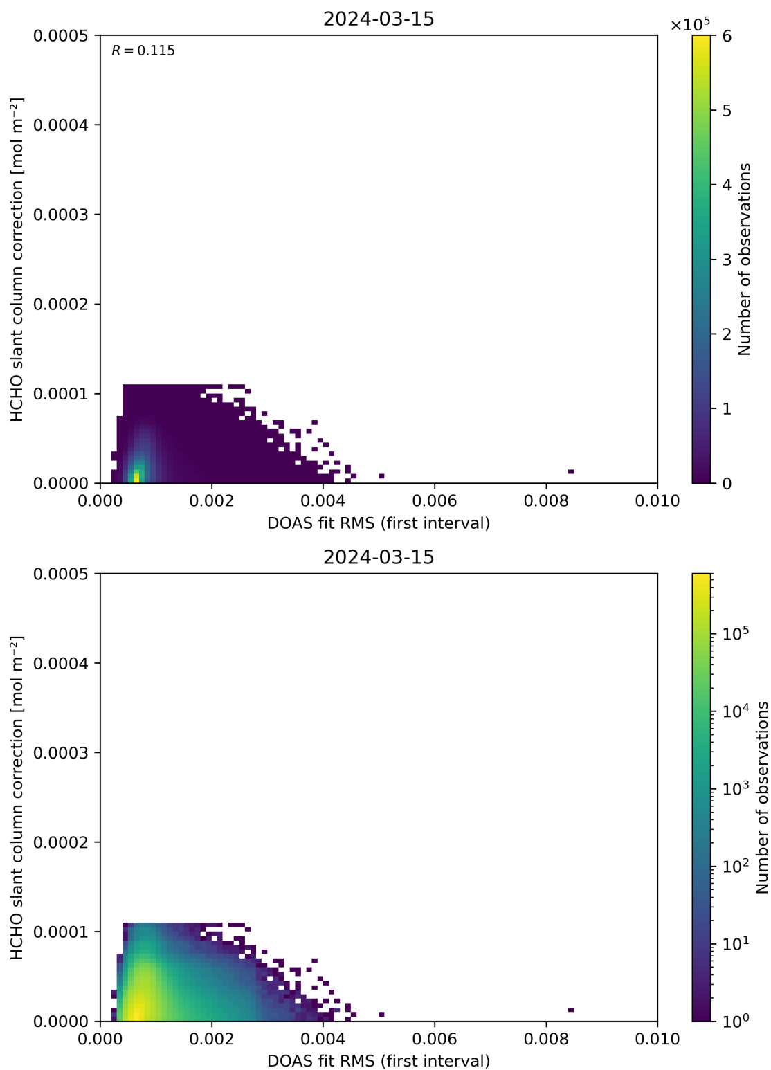
Figure 63: Scatter density plot of “DOAS fit RMS (first interval)” against “HCHO slant column correction” for 2024-03-14 to 2024-03-16.
