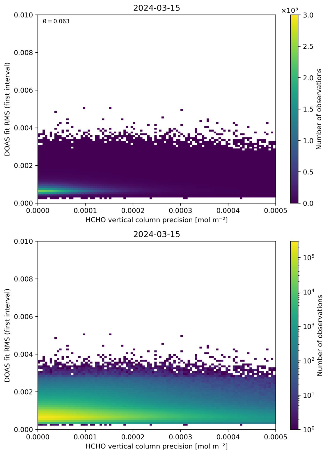
Figure 136: Scatter density plot of “HCHO vertical column precision” against “DOAS fit RMS (first interval)” for 2024-03-14 to 2024-03-16.
