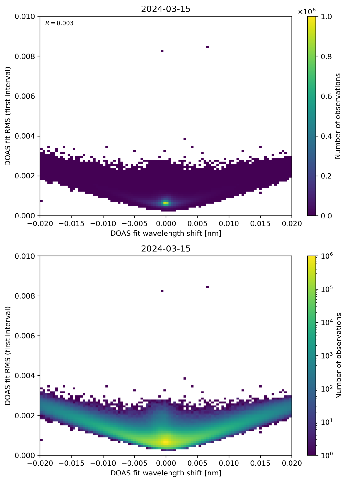
Figure 64: Scatter density plot of “DOAS fit wavelength shift” against “DOAS fit RMS (first interval)” for 2024-03-14 to 2024-03-16.
