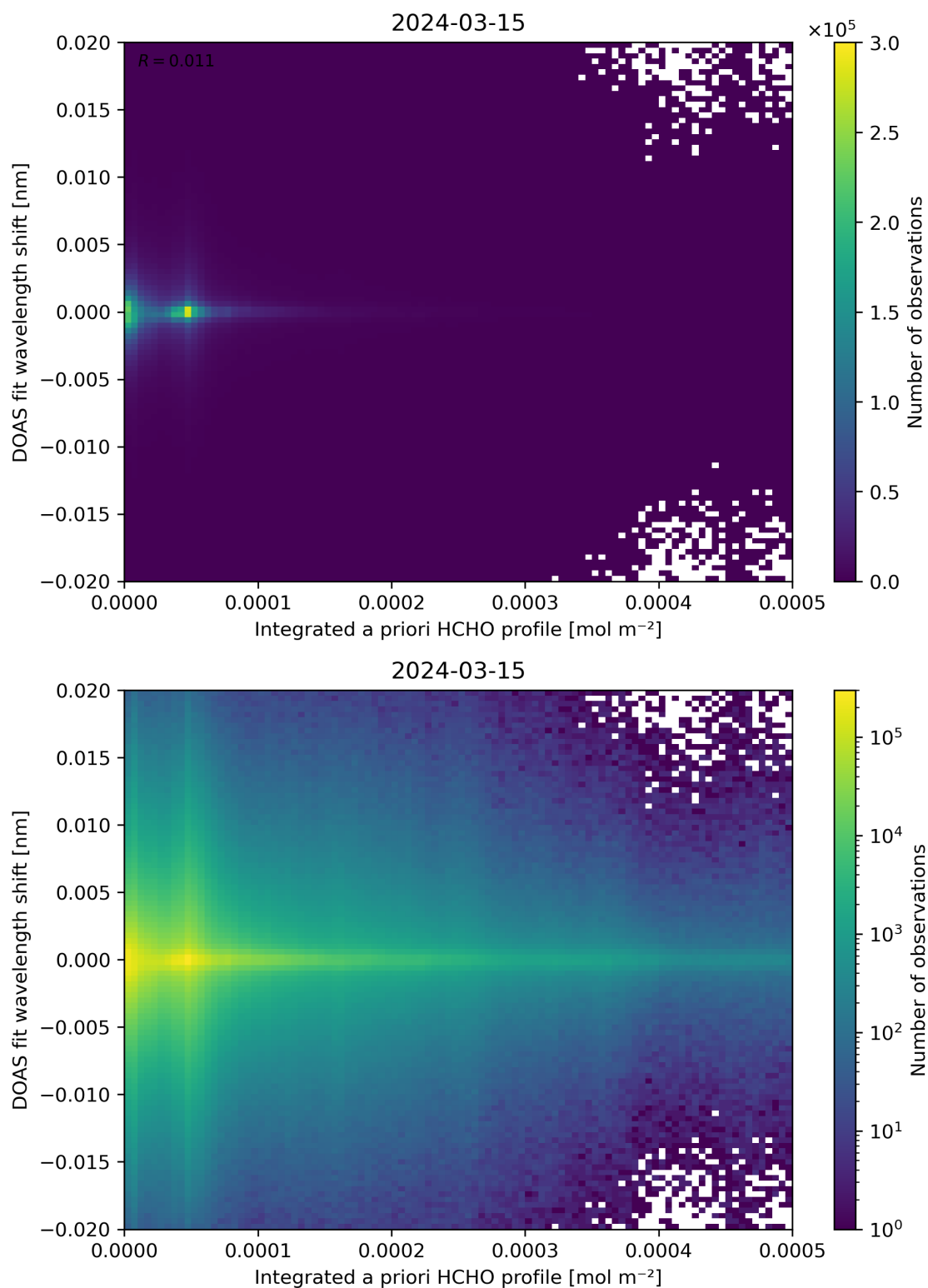
Figure 149: Scatter density plot of “Integrated a priori HCHO profile” against “DOAS fit wavelength shift” for 2024-03-14 to 2024-03-16.
