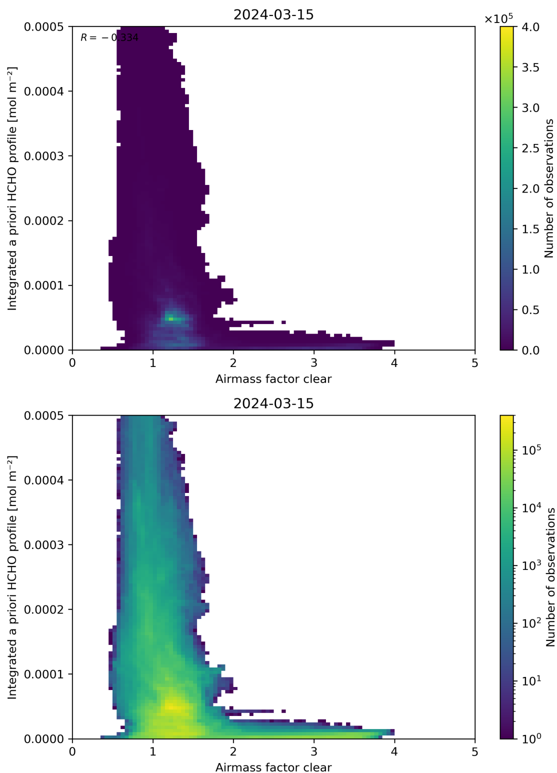
Figure 76: Scatter density plot of “Airmass factor clear” against “Integrated a priori HCHO profile” for 2024-03-14 to 2024-03-16.
