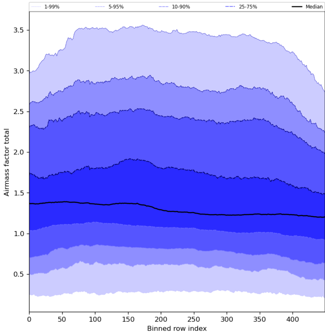
Figure 54: Along track statistics of “Airmass factor total” for 2024-03-14 to 2024-03-16
