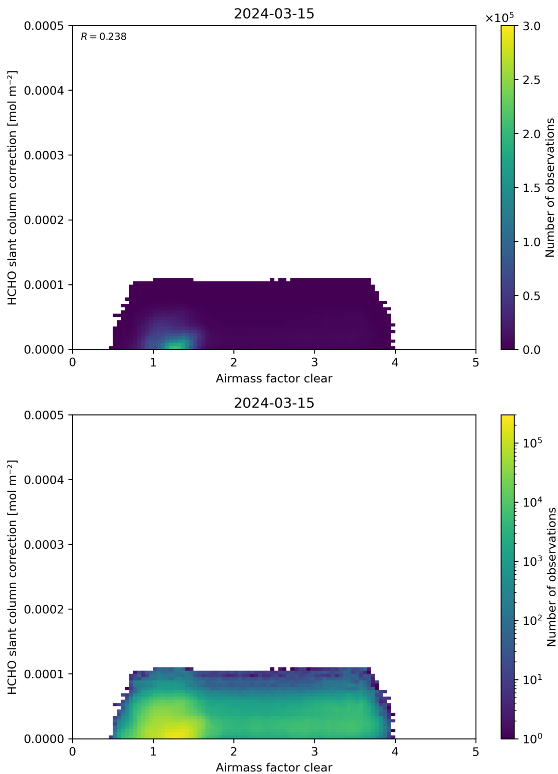
Figure 75: Scatter density plot of “Airmass factor clear” against “HCHO slant column correction” for 2024-03-14 to 2024-03-16.
