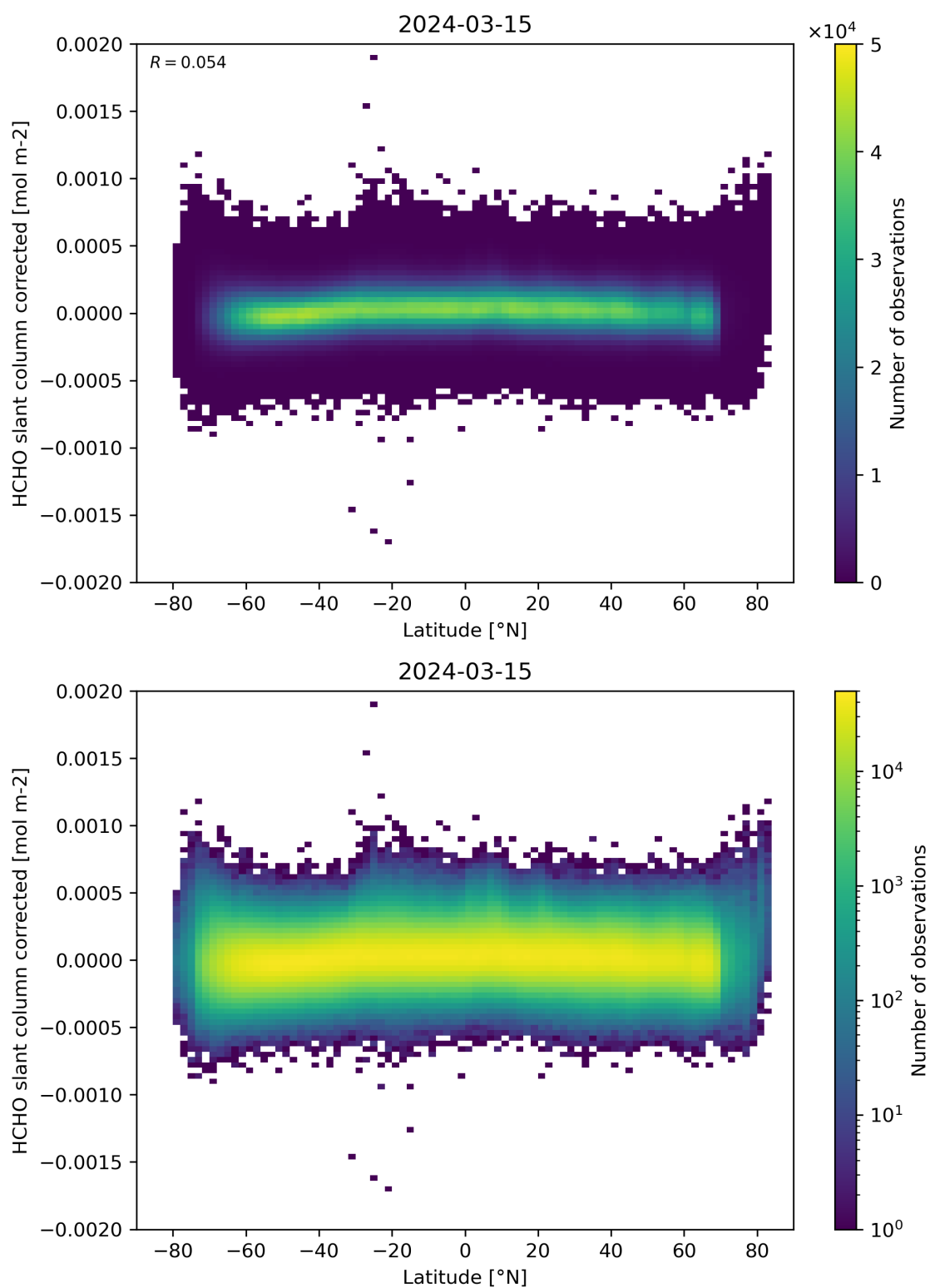
Figure 157: Scatter density plot of “Latitude” against “HCHO slant column corrected” for 2024-03-14 to 2024-03-16.
