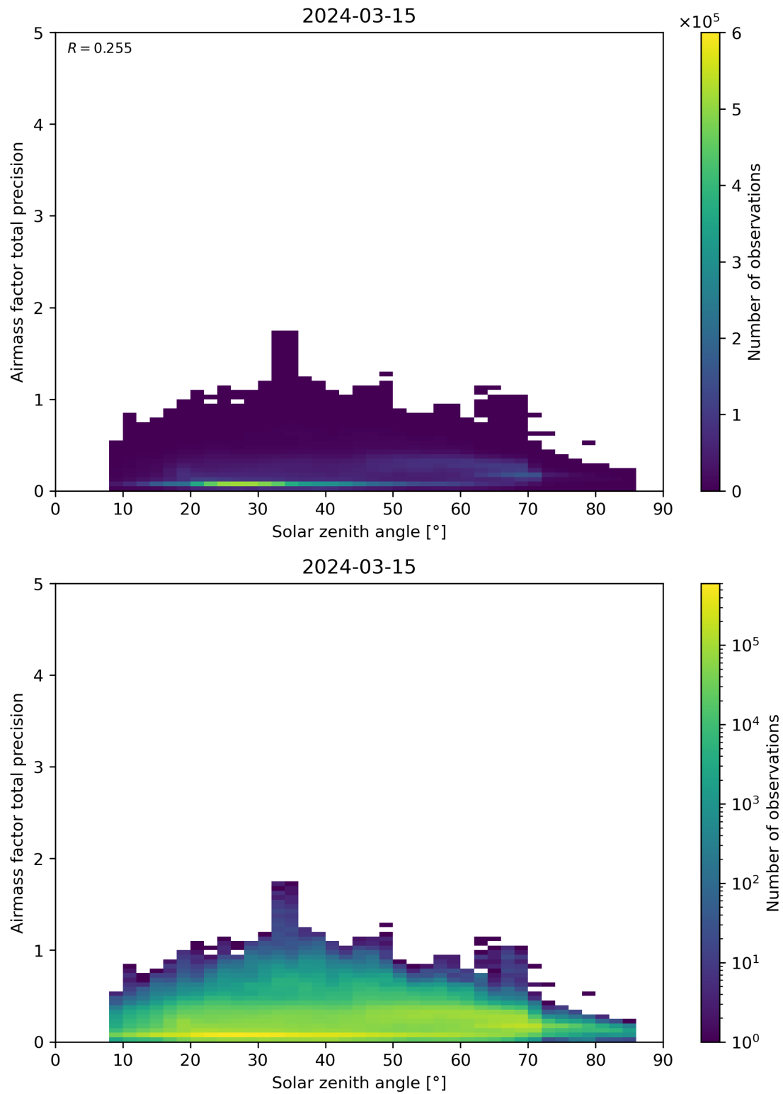
Figure 176: Scatter density plot of “Solar zenith angle” against “Airmass factor total precision” for 2024-03-14 to 2024-03-16.
