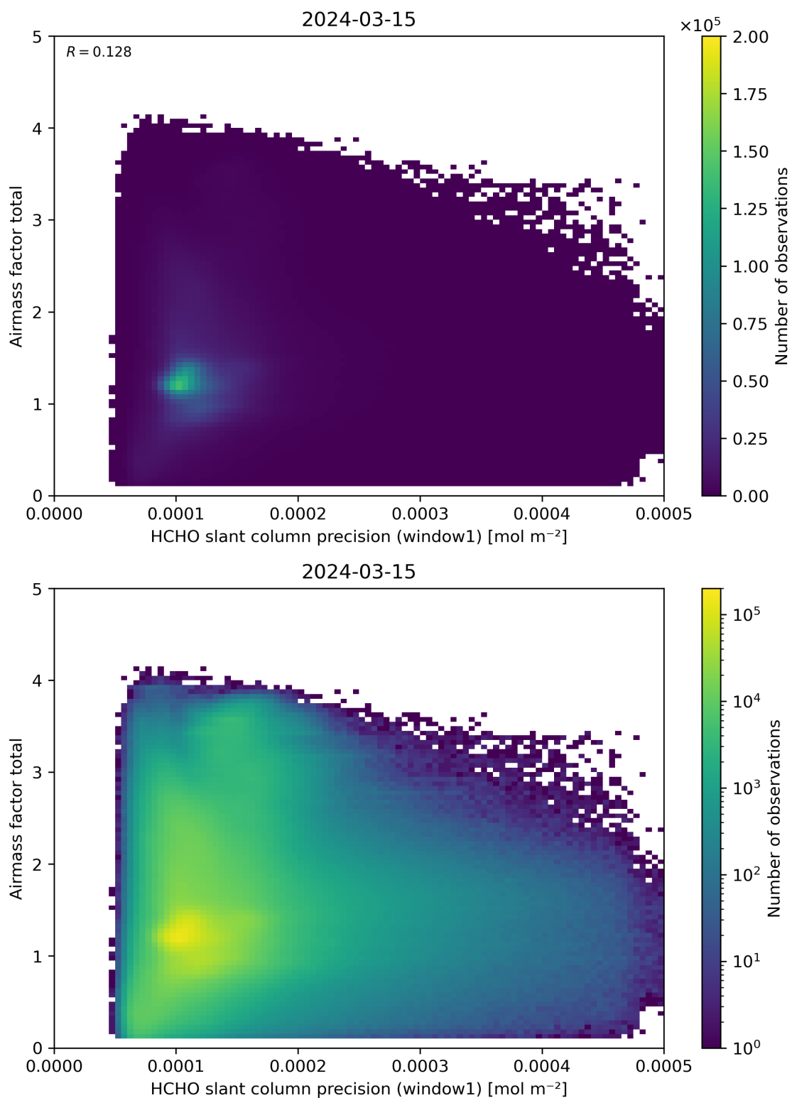
Figure 94: Scatter density plot of “HCHO slant column precision (window1)” against “Airmass factor total” for 2024-03-14 to 2024-03-16.
