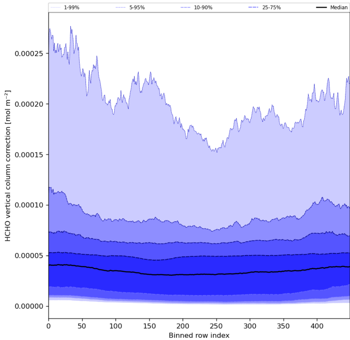
Figure 51: Along track statistics of “HCHO vertical column correction” for 2024-03-15 to 2024-03-17
