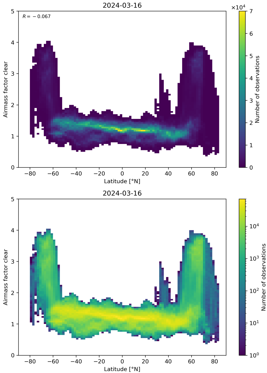
Figure 156: Scatter density plot of “Latitude” against “Airmass factor clear” for 2024-03-15 to 2024-03-17.
