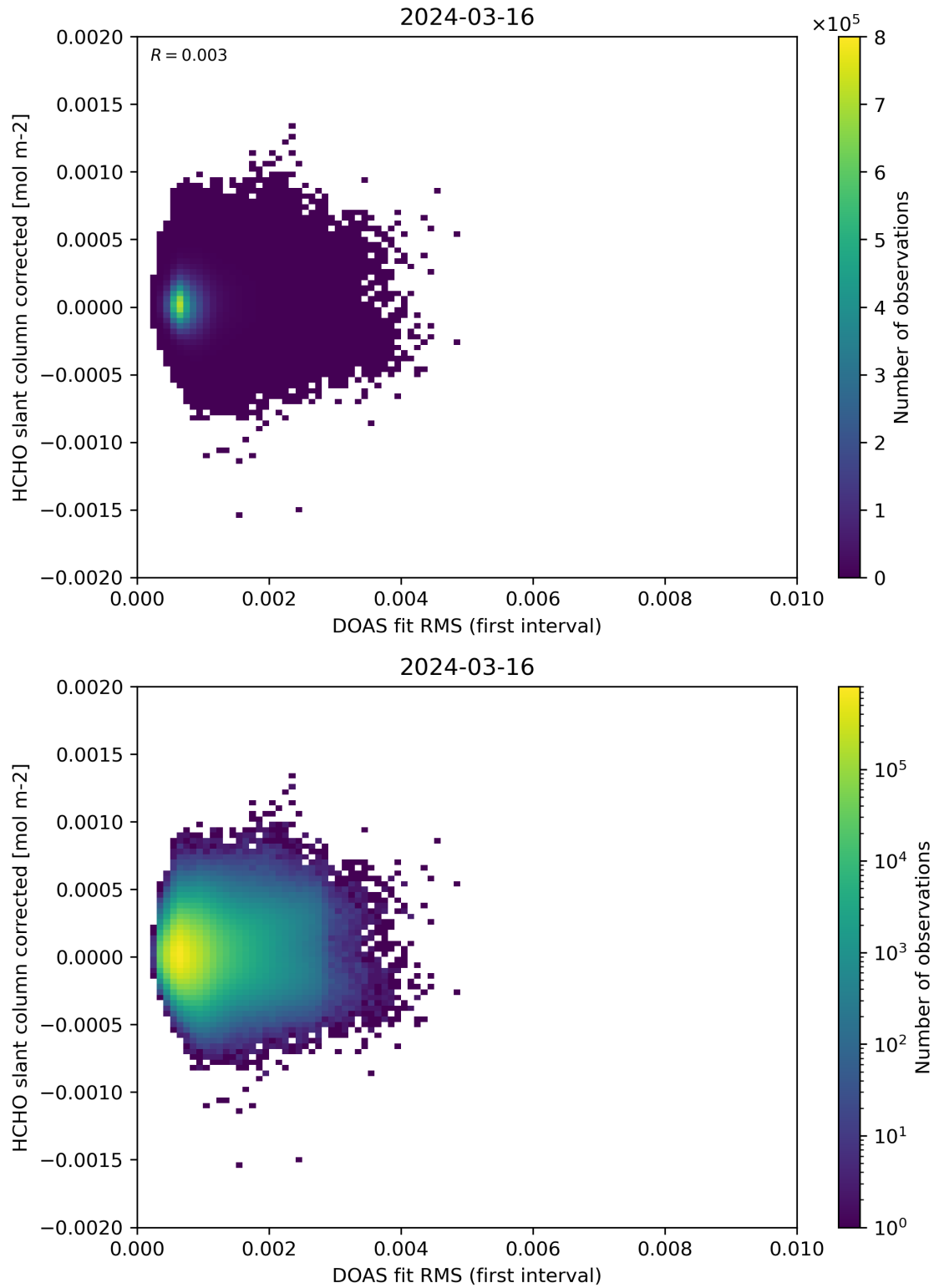
Figure 62: Scatter density plot of “DOAS fit RMS (first interval)” against “HCHO slant column corrected” for 2024-03-15 to 2024-03-17.
