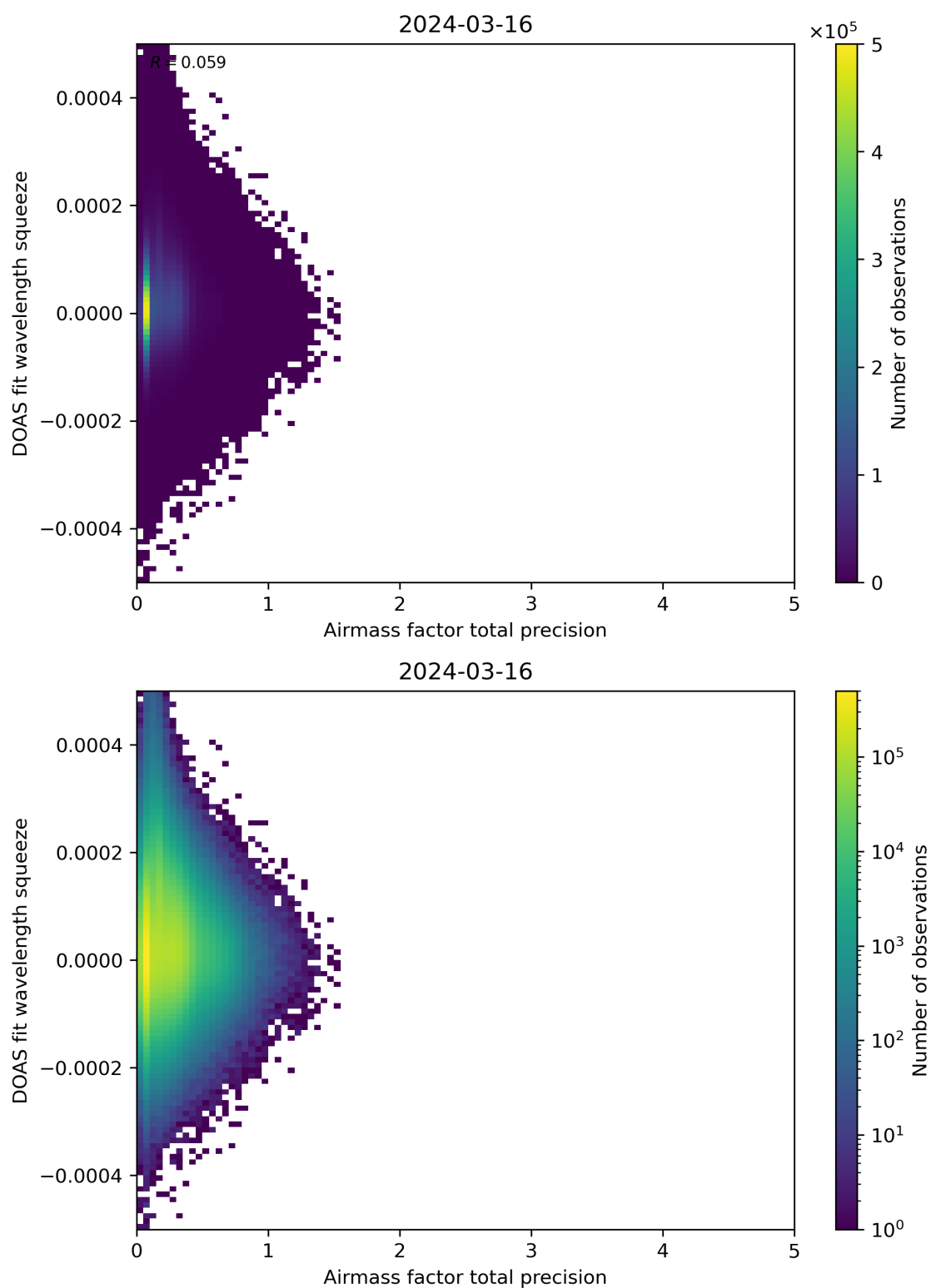
Figure 107: Scatter density plot of “Airmass factor total precision” against “DOAS fit wavelength squeeze” for 2024-03-15 to 2024-03-17.
