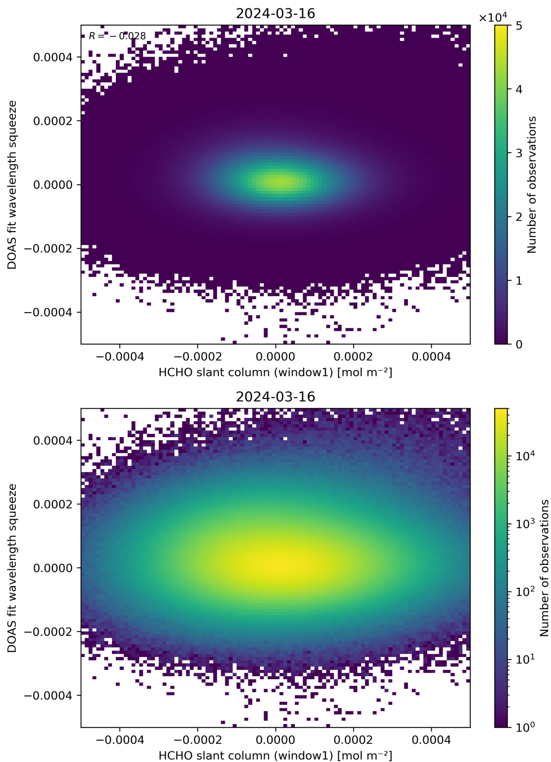
Figure 80: Scatter density plot of “HCHO slant column (window1)” against “DOAS fit wavelength squeeze” for 2024-03-15 to 2024-03-17.
