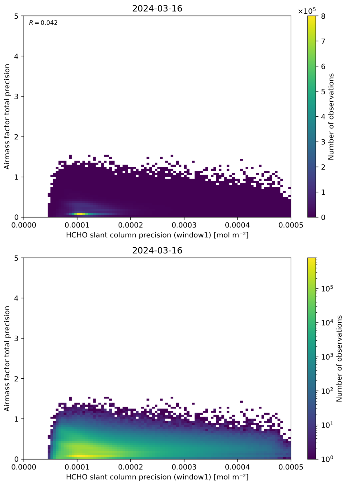
Figure 95: Scatter density plot of “HCHO slant column precision (window1)” against “Airmass factor total precision” for 2024-03-15 to 2024-03-17.
