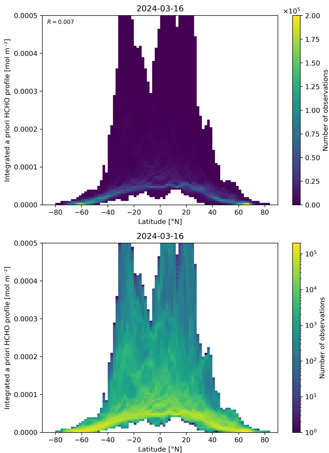
Figure 166: Scatter density plot of “Latitude” against “Integrated a priori HCHO profile” for 2024-03-15 to 2024-03-17.
