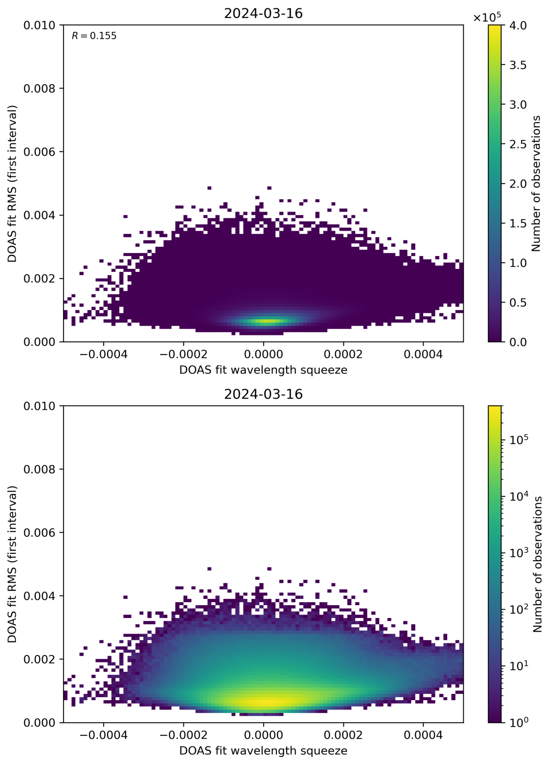
Figure 68: Scatter density plot of “DOAS fit wavelength squeeze” against “DOAS fit RMS (first interval)” for 2024-03-15 to 2024-03-17.
