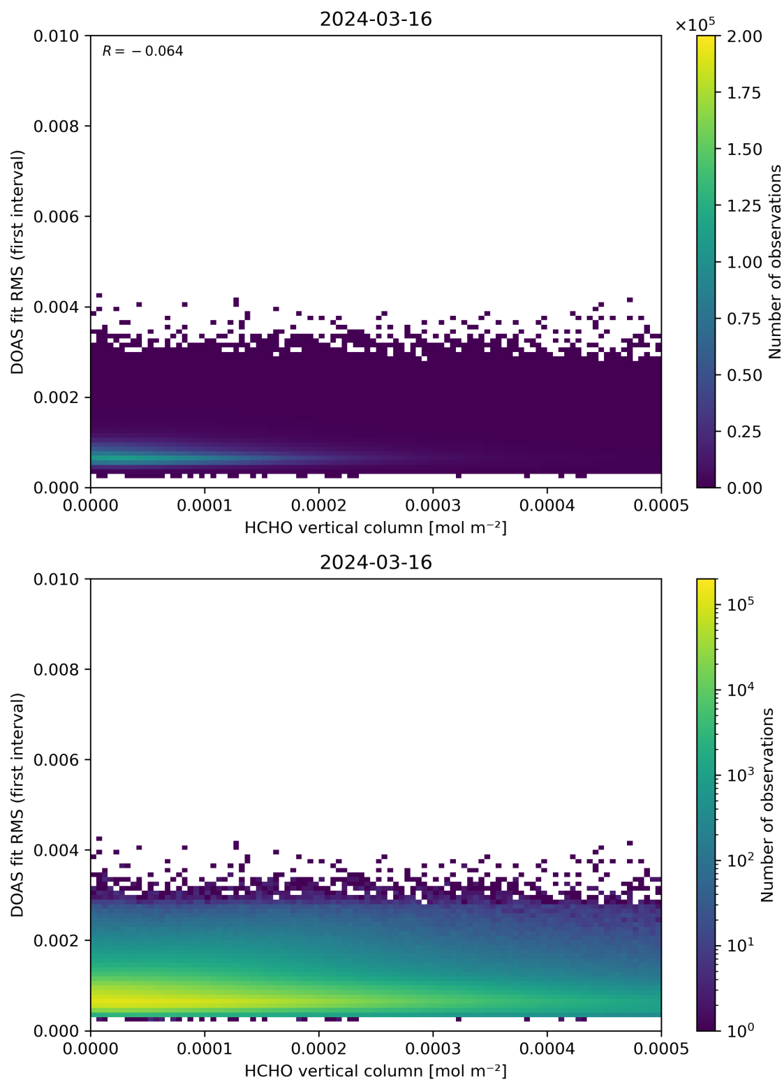
Figure 123: Scatter density plot of “HCHO vertical column” against “DOAS fit RMS (first interval)” for 2024-03-15 to 2024-03-17.
