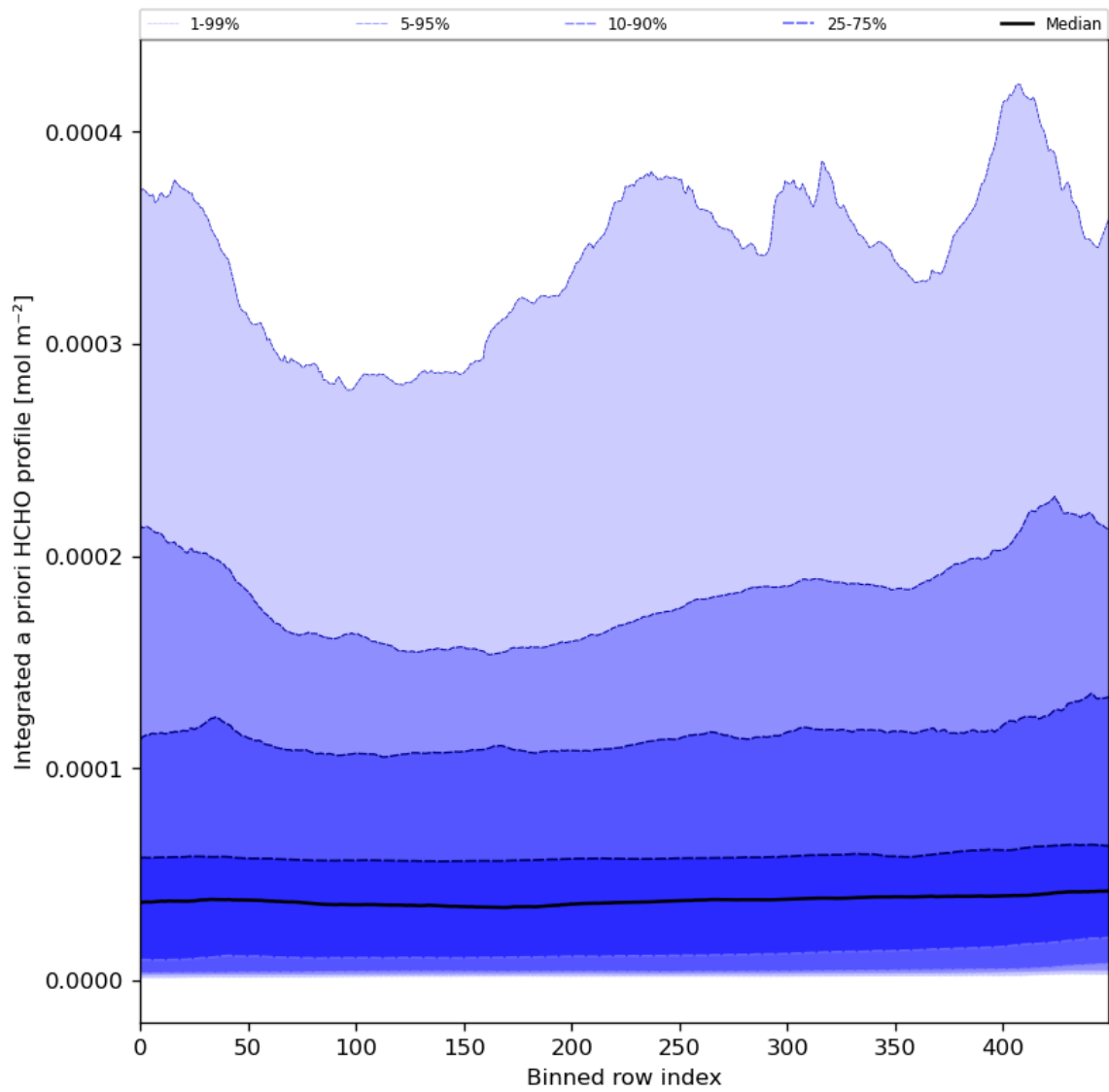
Figure 57: Along track statistics of "Integrated a priori HCHO profile" for 2024-03-15 to 2024-03-17
