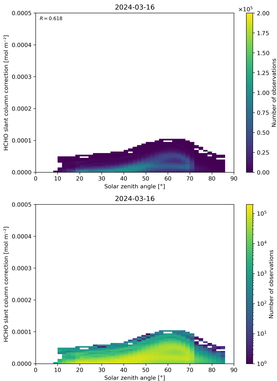
Figure 172: Scatter density plot of “Solar zenith angle” against “HCHO slant column correction” for 2024-03-15 to 2024-03-17.
