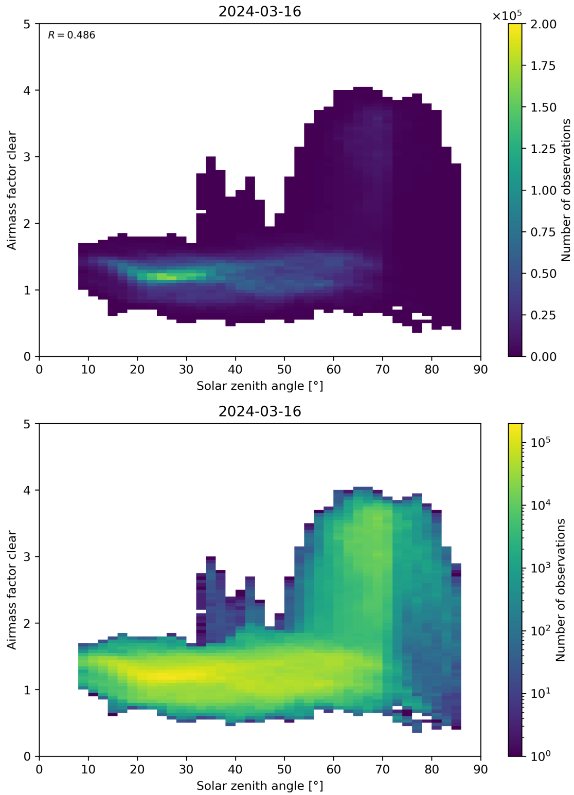
Figure 170: Scatter density plot of “Solar zenith angle” against “Airmass factor clear” for 2024-03-15 to 2024-03-17.
