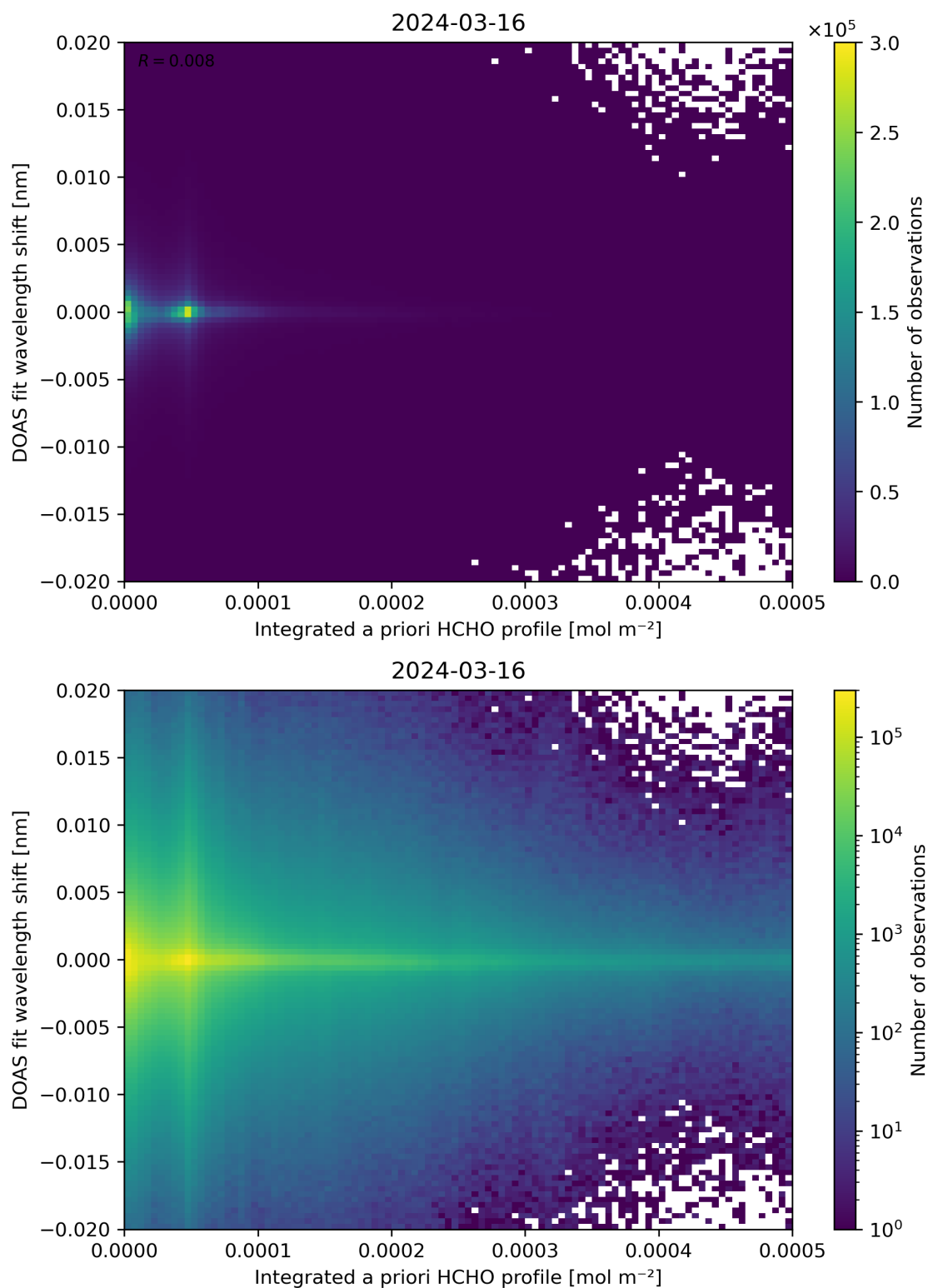
Figure 149: Scatter density plot of “Integrated a priori HCHO profile” against “DOAS fit wavelength shift” for 2024-03-15 to 2024-03-17.
