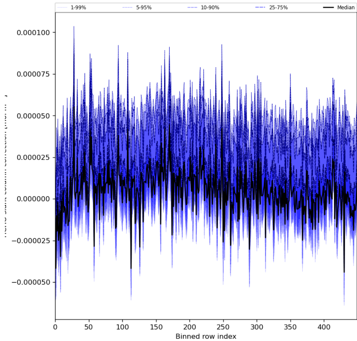
Figure 61: Along track statistics of “HCHO slant column correction” for 2024-03-15 to 2024-03-17
