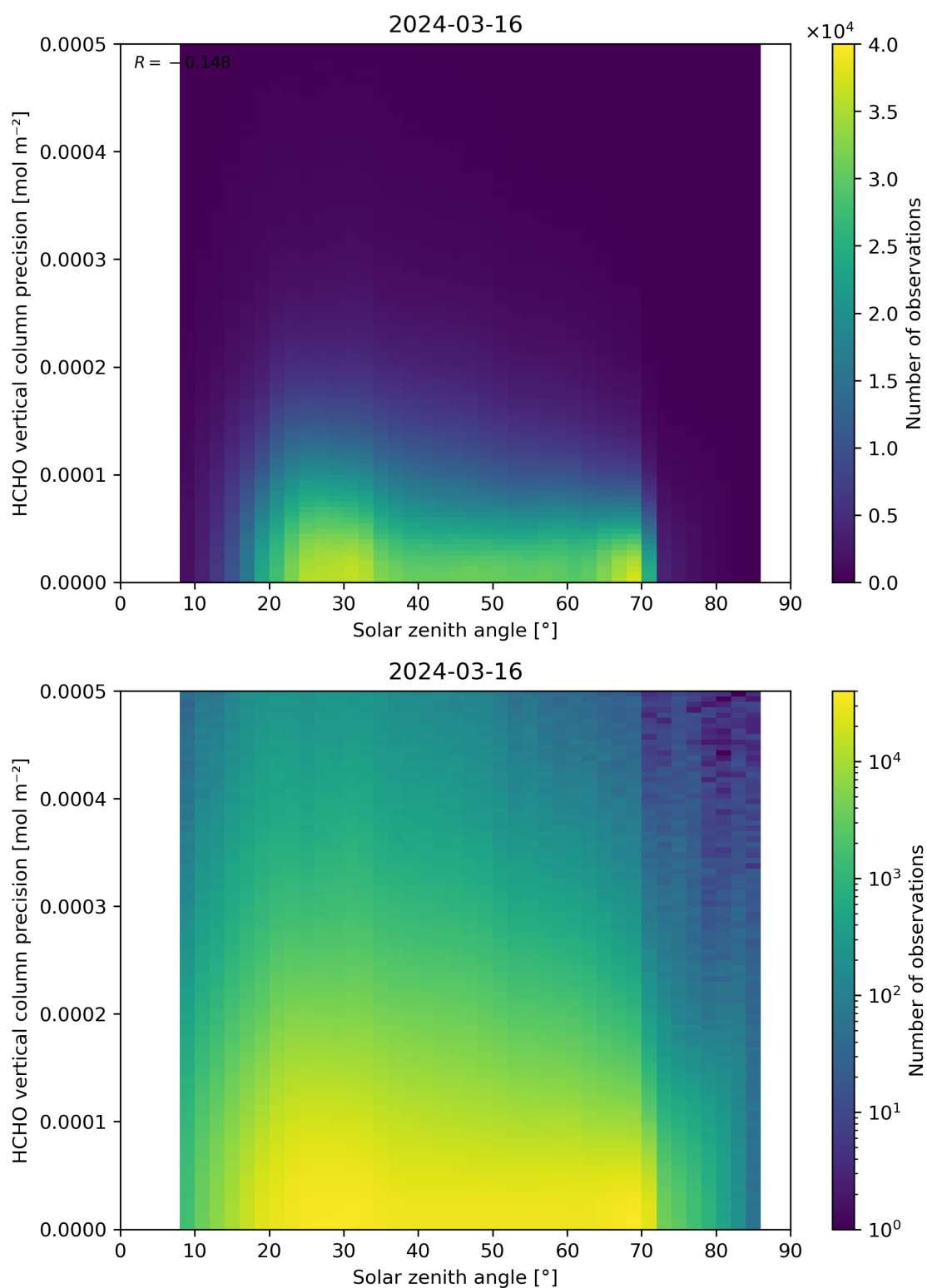
Figure 179: Scatter density plot of “Solar zenith angle” against “HCHO vertical column precision” for 2024-03-15 to 2024-03-17.
