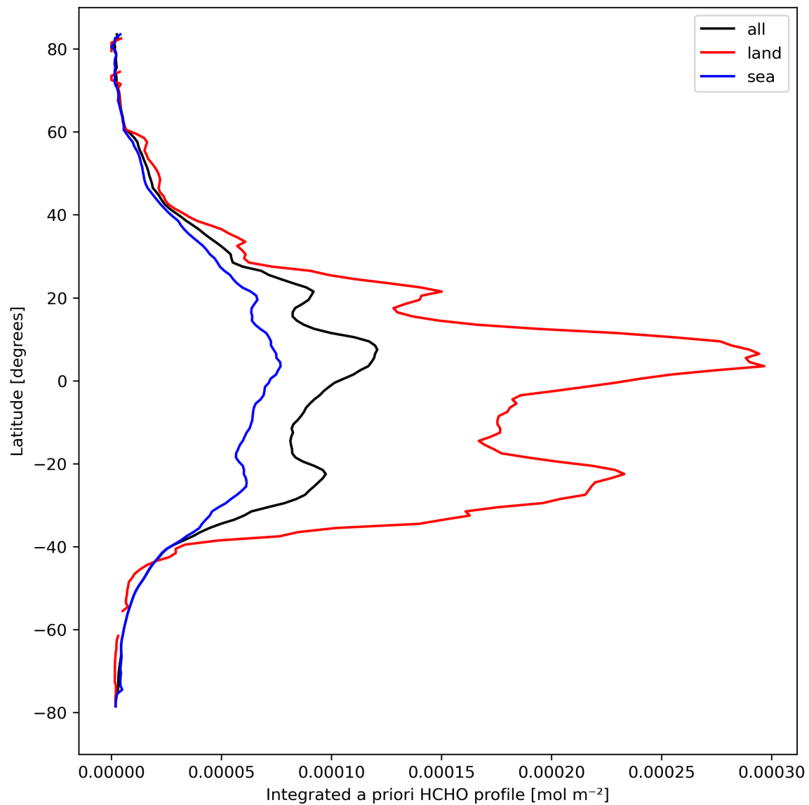
Figure 29: Zonal average of “Integrated a priori HCHO profile” for 2024-03-15 to 2024-03-17.
