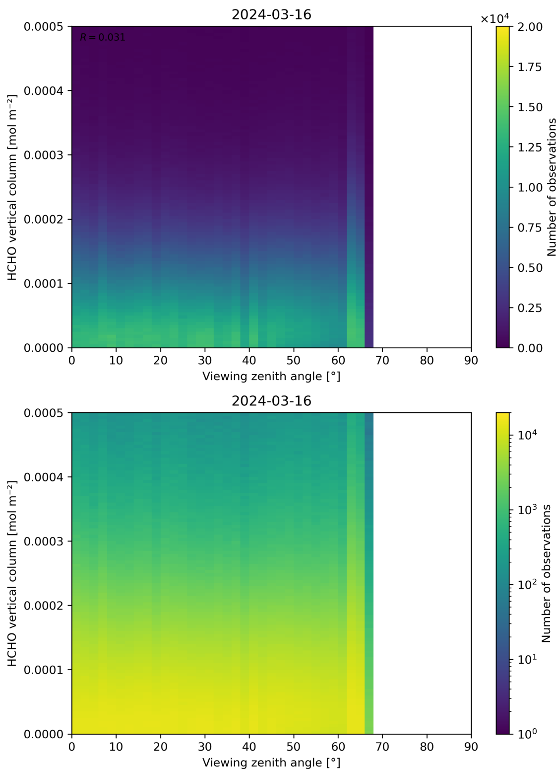
Figure 192: Scatter density plot of “Viewing zenith angle” against “HCHO vertical column” for 2024-03-15 to 2024-03-17.
