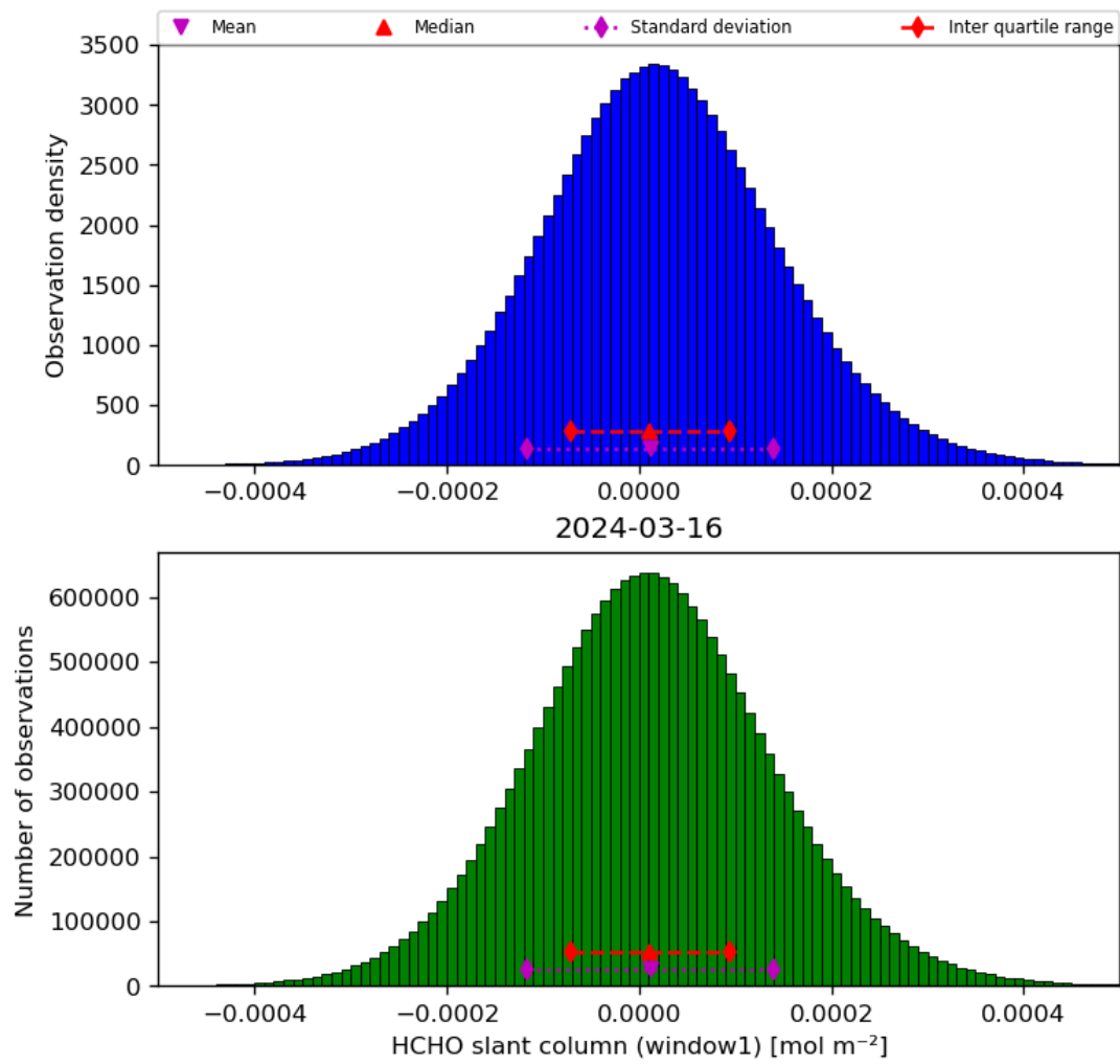
Figure 38: Histogram of “HCHO slant column (window1)” for 2024-03-15 to 2024-03-17
