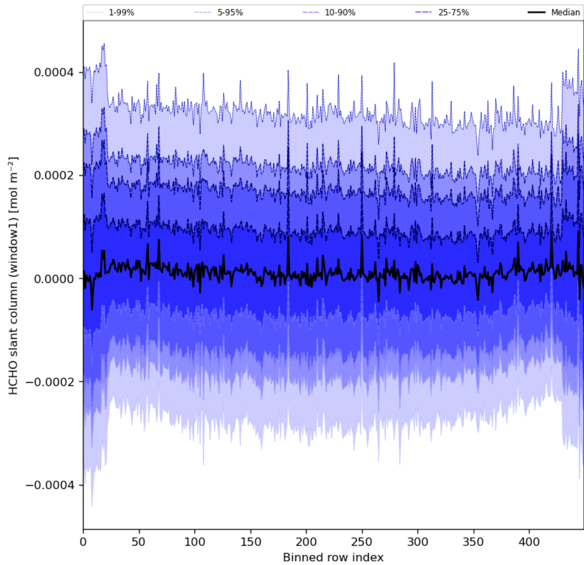
Figure 52: Along track statistics of “HCHO slant column (window1)” for 2024-03-15 to 2024-03-17
