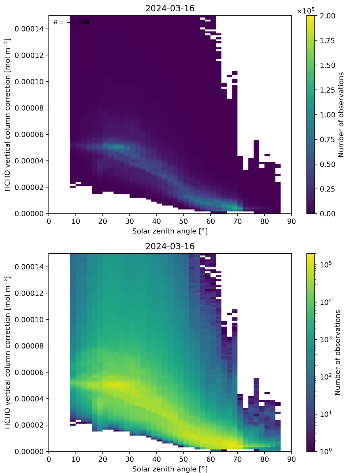
Figure 178: Scatter density plot of “Solar zenith angle” against “HCHO vertical column correction” for 2024-03-15 to 2024-03-17.
