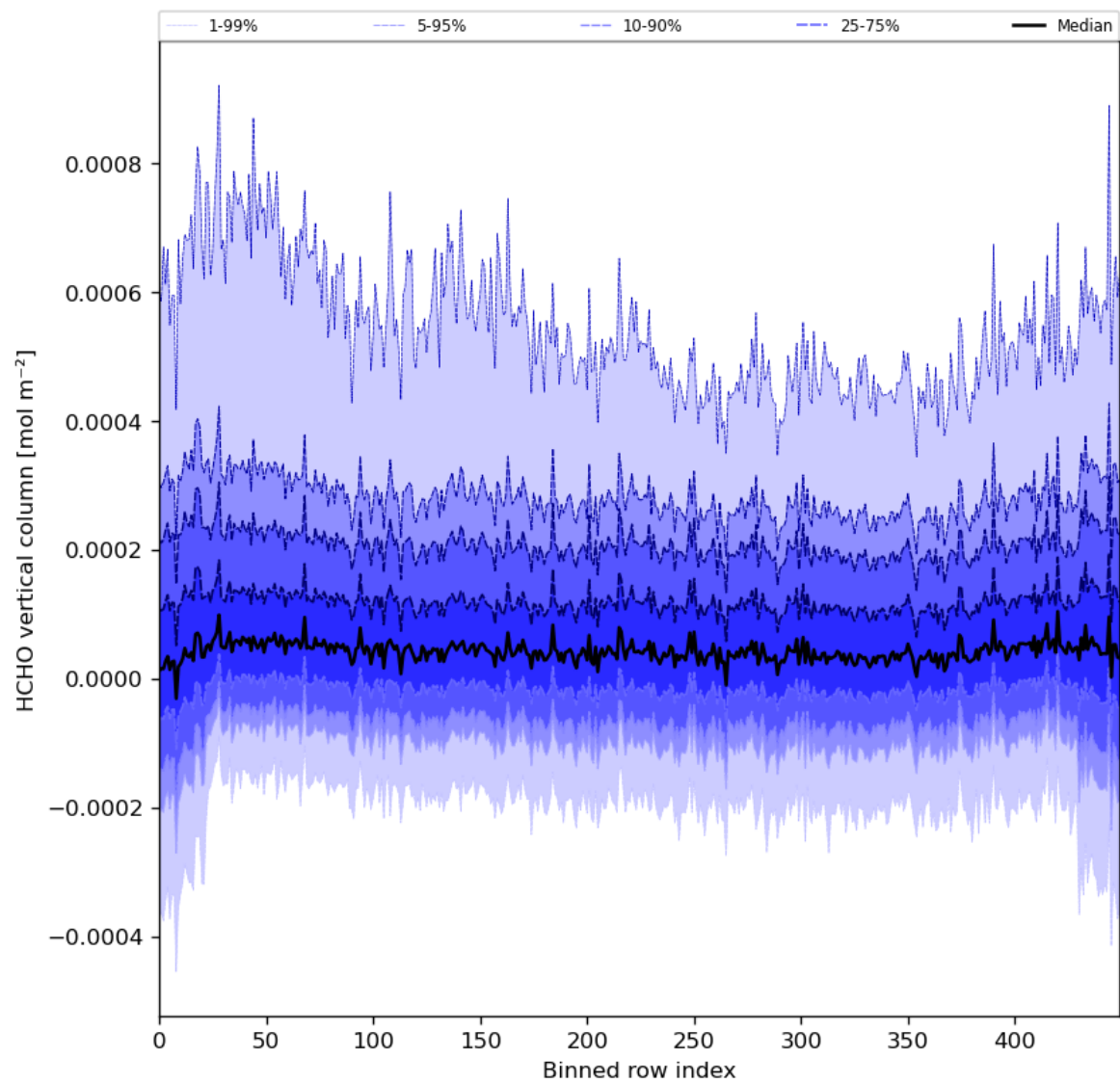
Figure 49: Along track statistics of “HCHO vertical column” for 2024-03-15 to 2024-03-17
