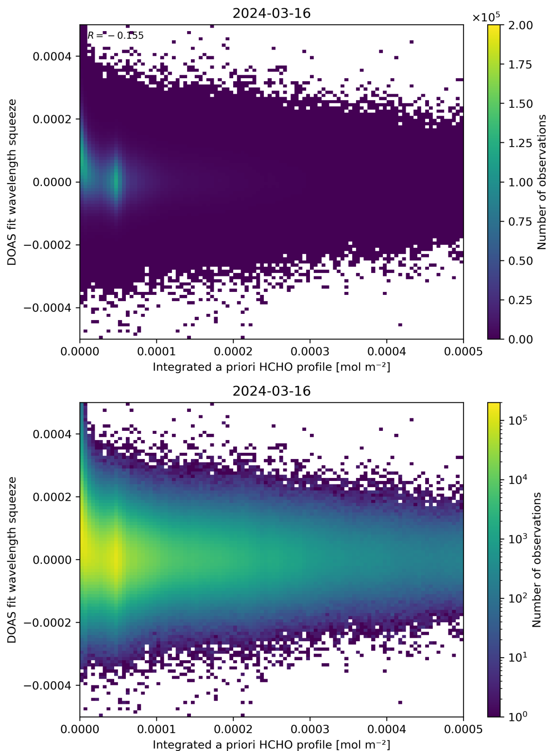
Figure 150: Scatter density plot of “Integrated a priori HCHO profile” against “DOAS fit wavelength squeeze” for 2024-03-15 to 2024-03-17.
