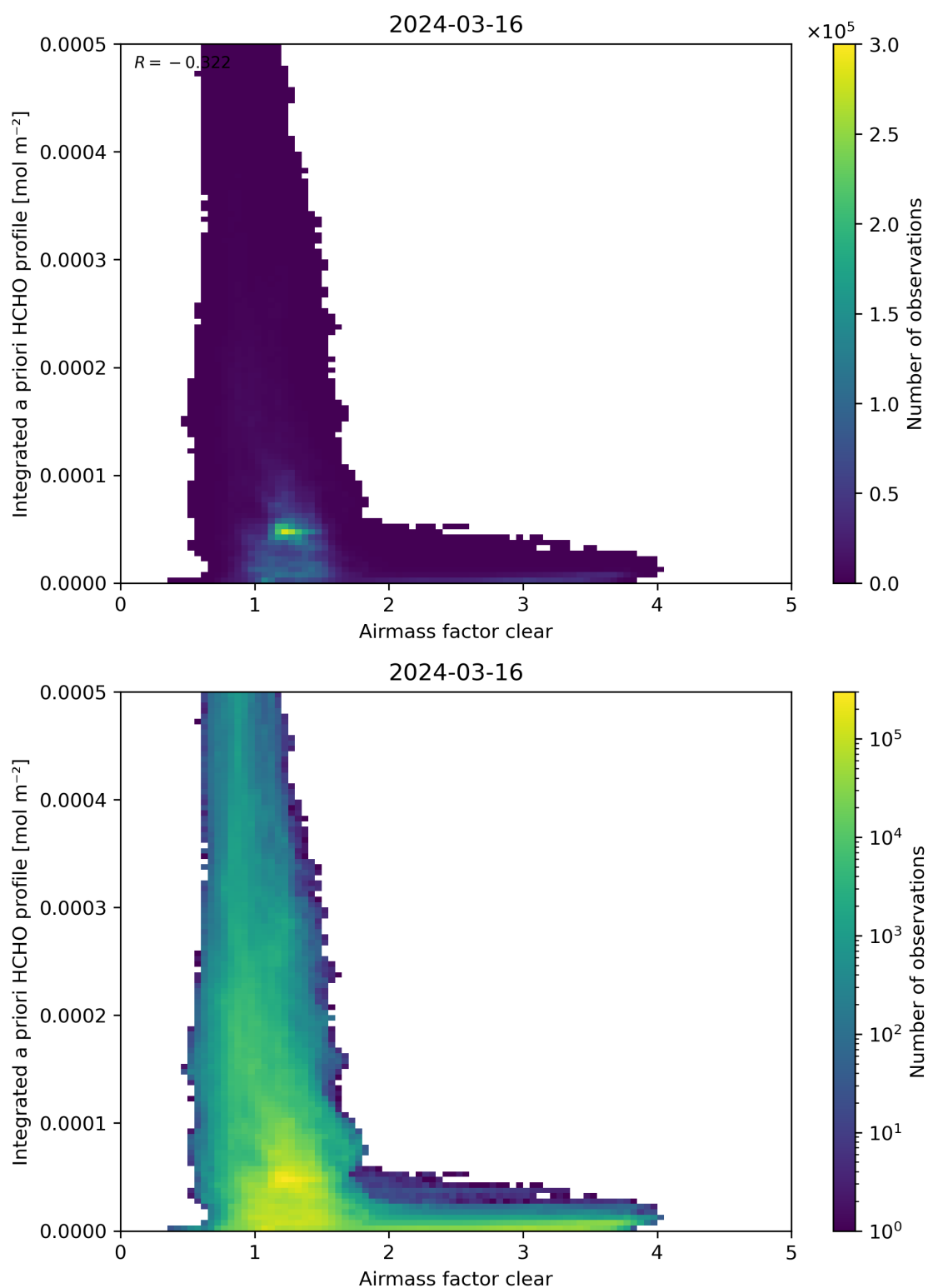
Figure 76: Scatter density plot of “Airmass factor clear” against “Integrated a priori HCHO profile” for 2024-03-15 to 2024-03-17.
