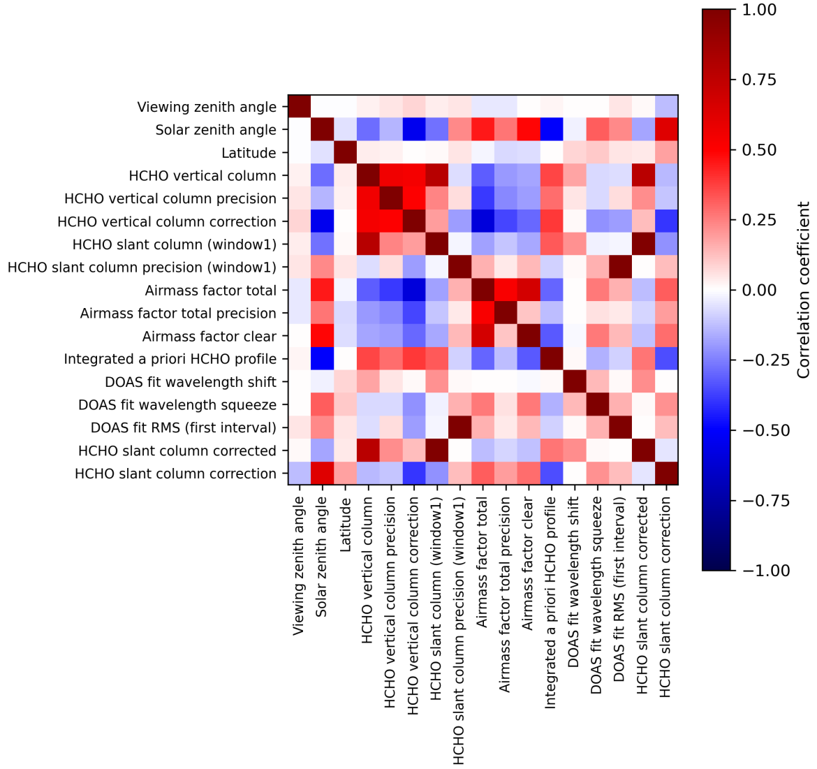
Figure 2: Map of correlation matrix for 2024-03-15 to 2024-03-17.
