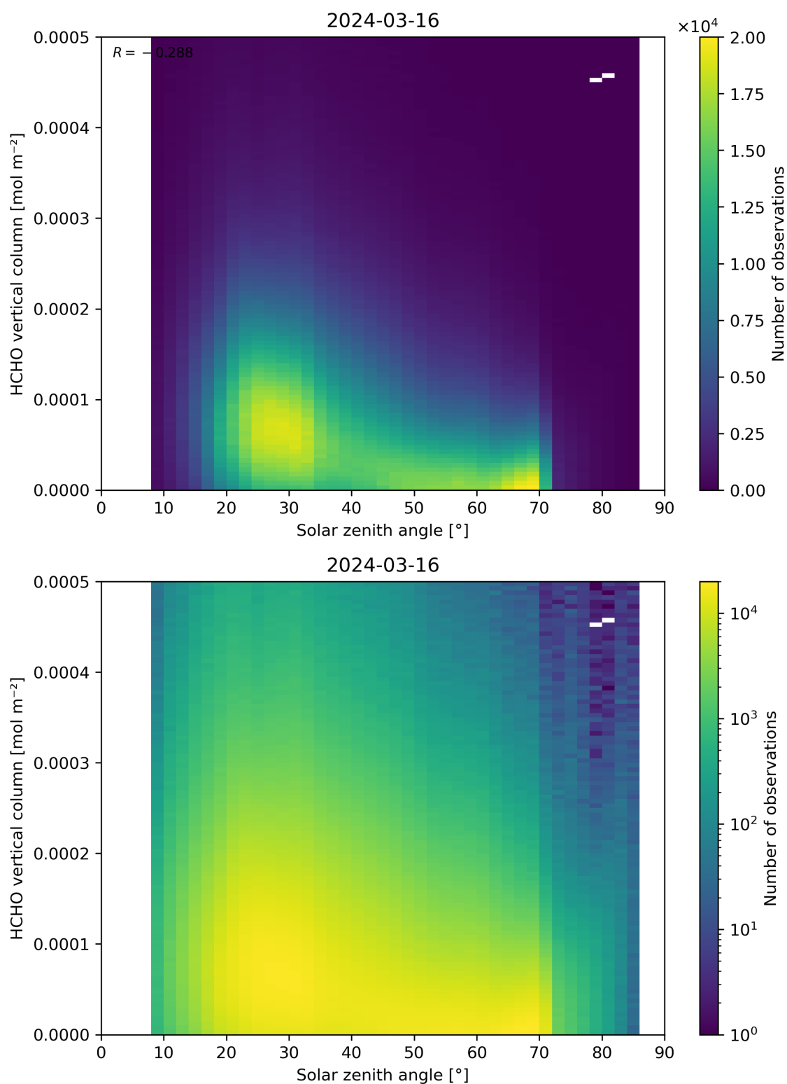
Figure 177: Scatter density plot of “Solar zenith angle” against “HCHO vertical column” for 2024-03-15 to 2024-03-17.
