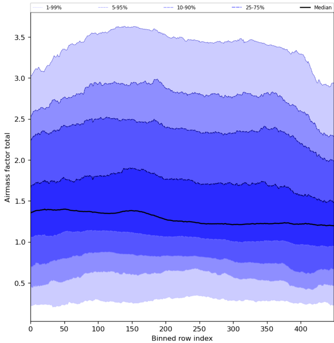
Figure 54: Along track statistics of “Airmass factor total” for 2024-03-15 to 2024-03-17
