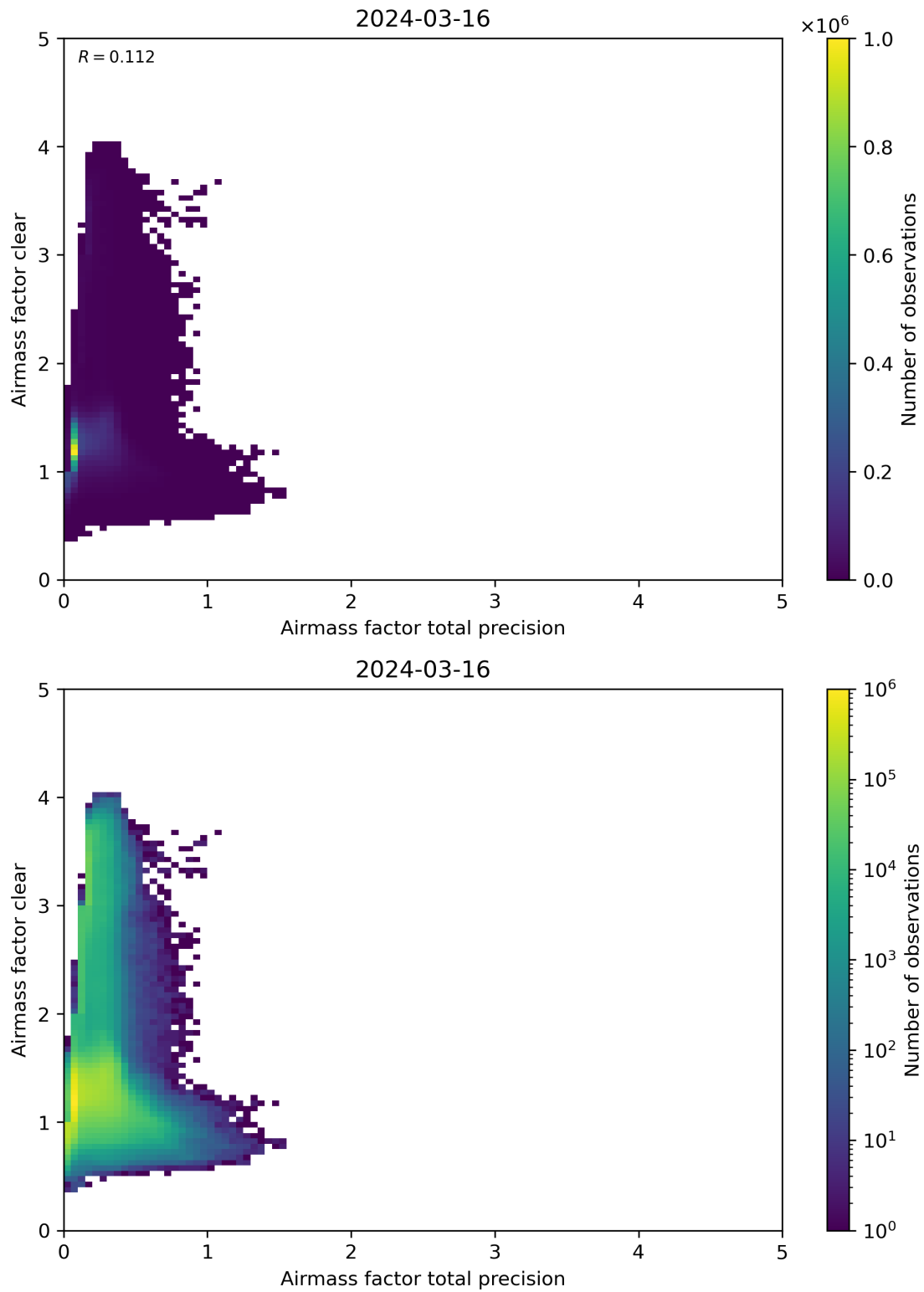
Figure 108: Scatter density plot of “Airmass factor total precision” against “Airmass factor clear” for 2024-03-15 to 2024-03-17.
