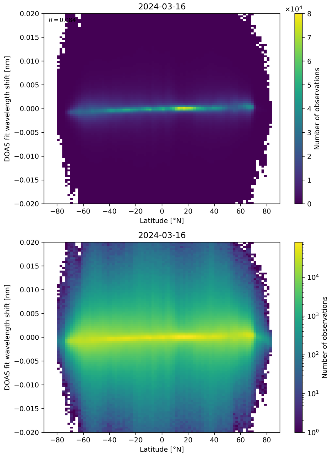
Figure 154: Scatter density plot of “Latitude” against “DOAS fit wavelength shift” for 2024-03-15 to 2024-03-17.
