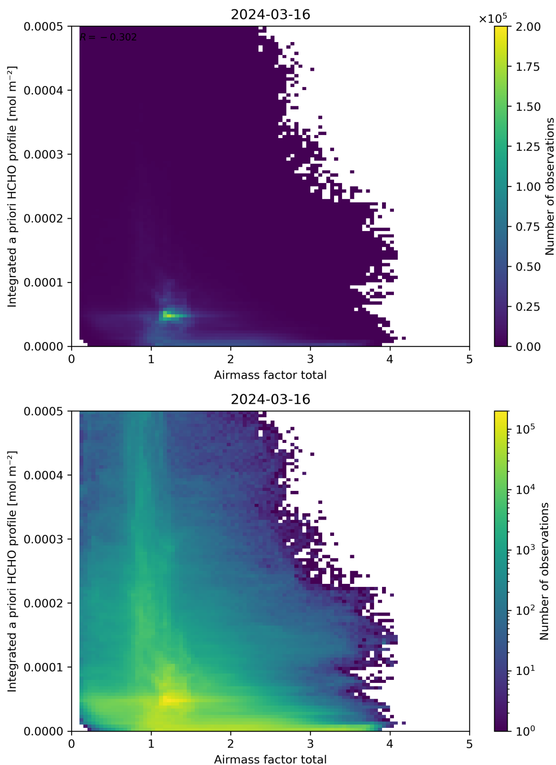
Figure 104: Scatter density plot of “Air mass factor total” against “Integrated a priori HCHO profile” for 2024-03-15 to 2024-03-17.
