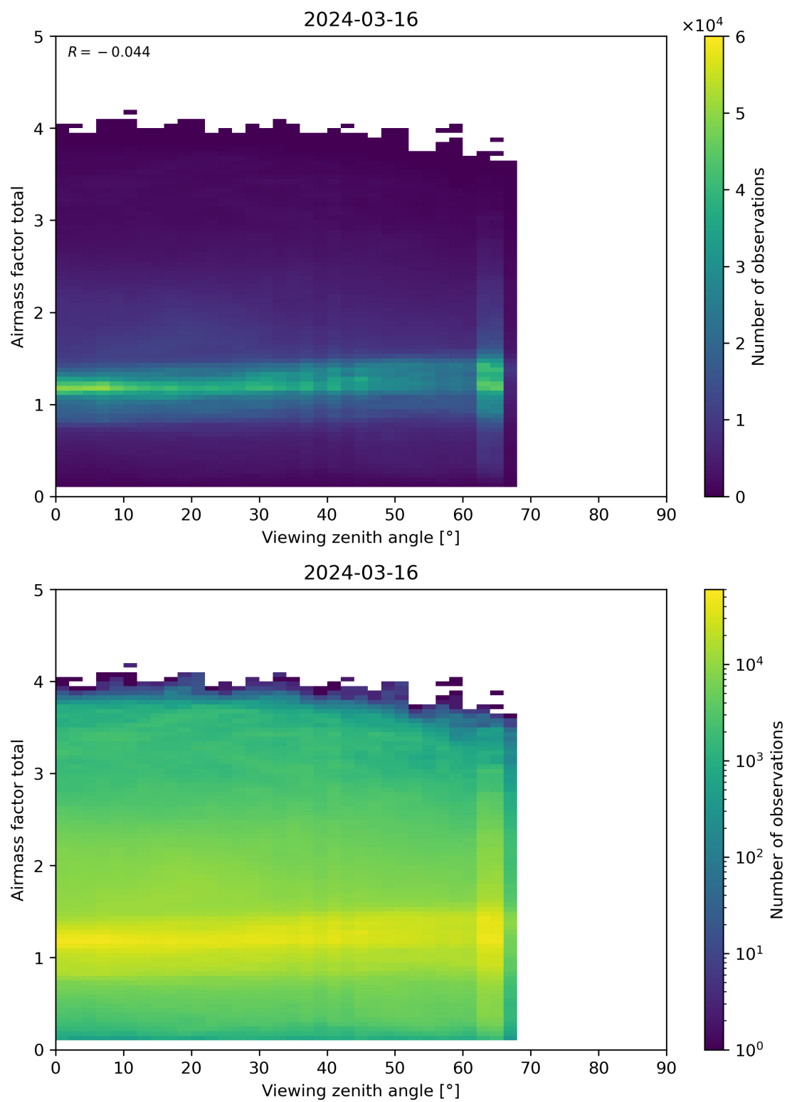
Figure 190: Scatter density plot of “Viewing zenith angle” against “Airmass factor total” for 2024-03-15 to 2024-03-17.
