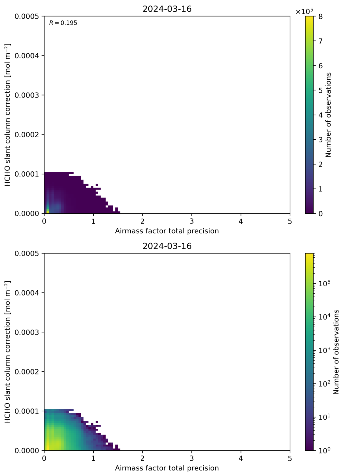
Figure 110: Scatter density plot of “Airmass factor total precision” against “HCHO slant column correction” for 2024-03-15 to 2024-03-17.
