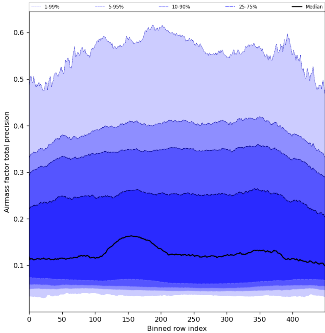
Figure 55: Along track statistics of “Airmass factor total precision” for 2024-03-15 to 2024-03-17
