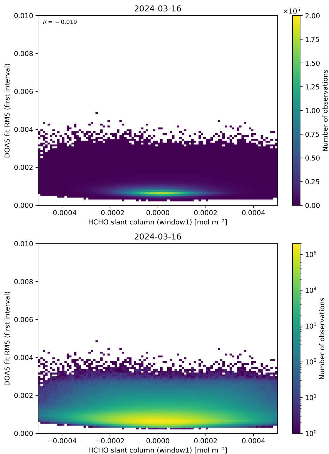
Figure 78: Scatter density plot of “HCHO slant column (window1)” against “DOAS fit RMS (first interval)” for 2024-03-15 to 2024-03-17.
