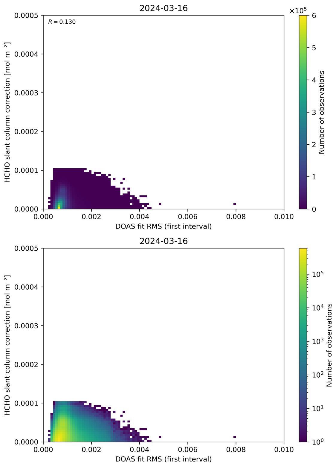
Figure 63: Scatter density plot of “DOAS fit RMS (first interval)” against “HCHO slant column correction” for 2024-03-15 to 2024-03-17.
