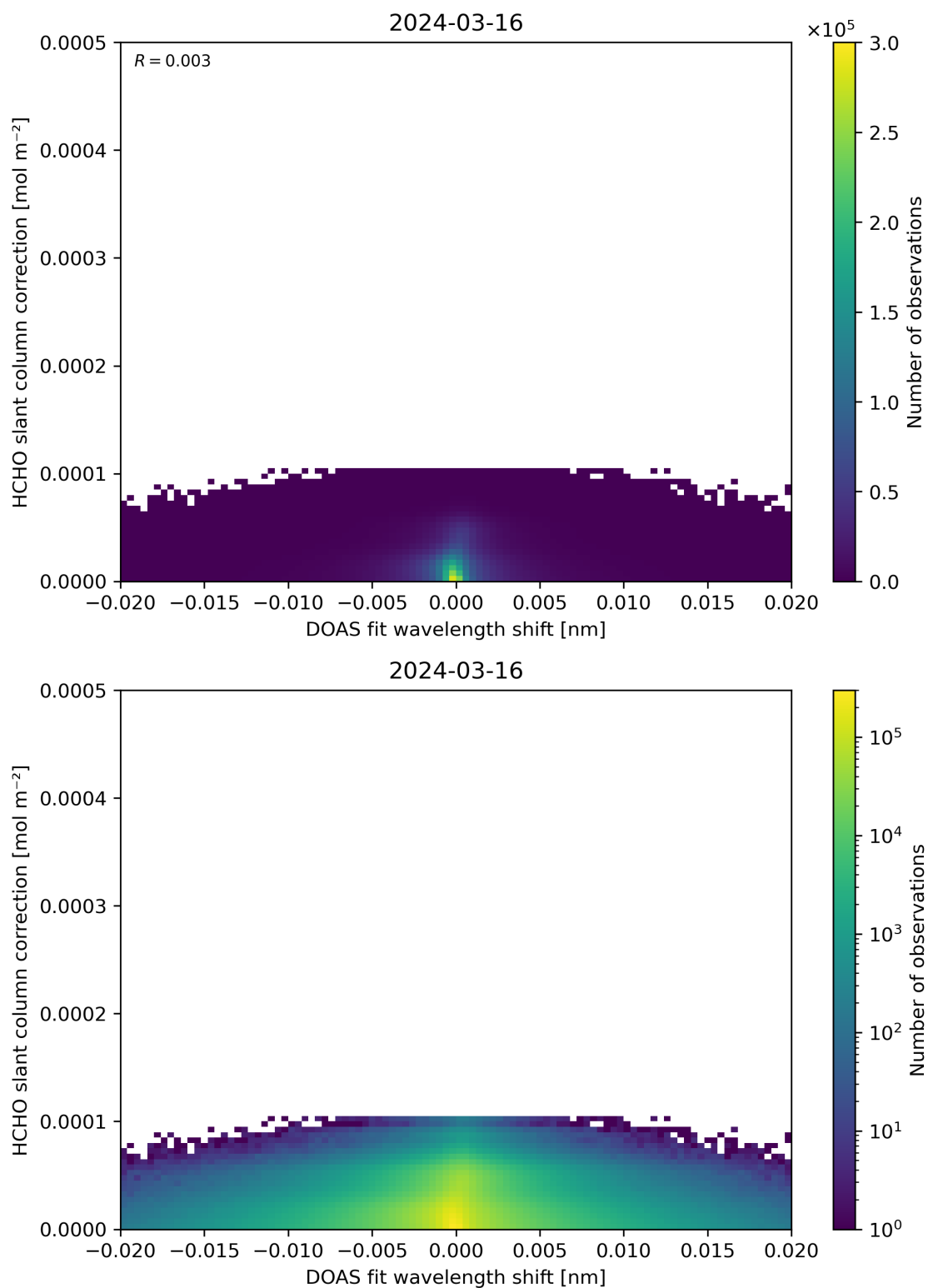
Figure 67: Scatter density plot of “DOAS fit wavelength shift” against “HCHO slant column correction” for 2024-03-15 to 2024-03-17.
