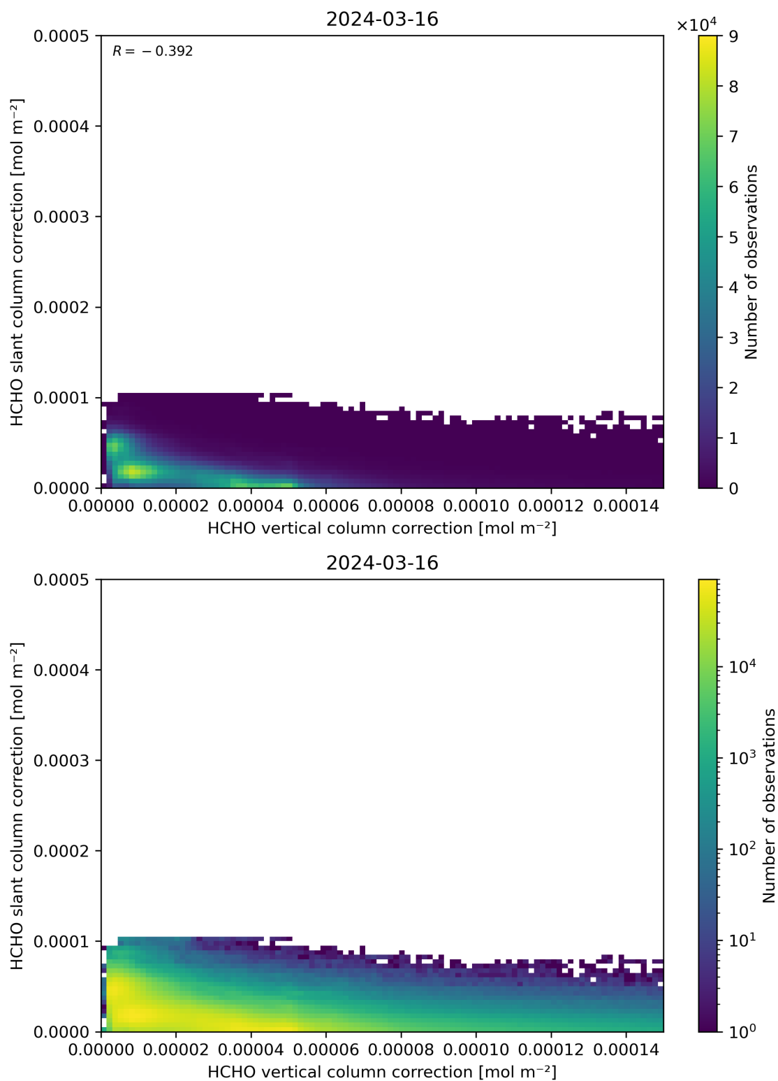
Figure 117: Scatter density plot of “HCHO vertical column correction” against “HCHO slant column correction” for 2024-03-15 to 2024-03-17.
