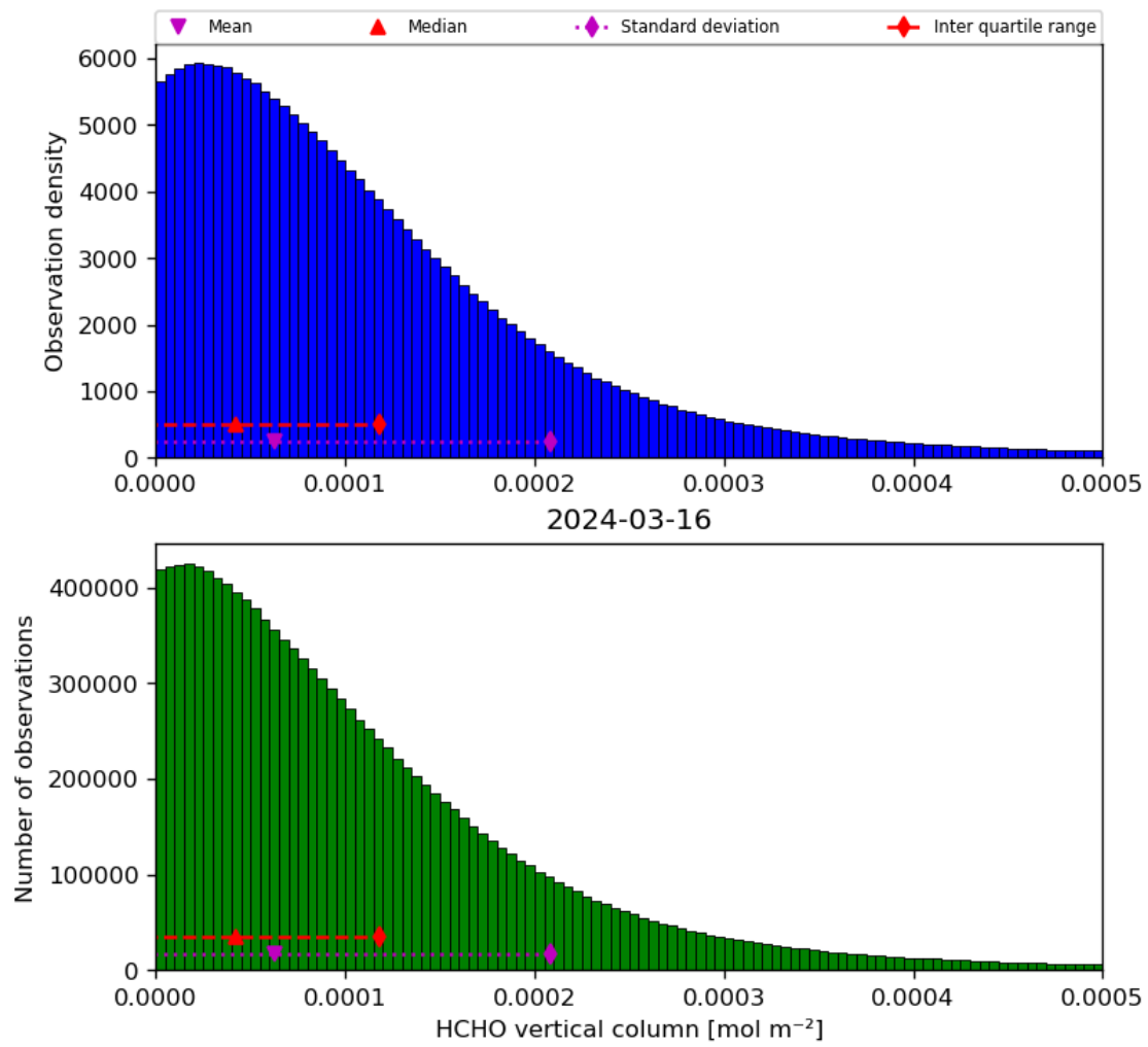
Figure 35: Histogram of “HCHO vertical column” for 2024-03-15 to 2024-03-17
