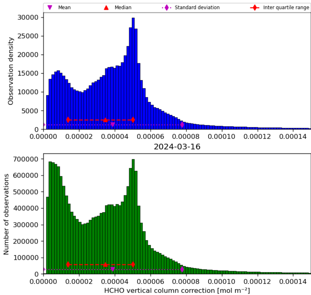
Figure 37: Histogram of “HCHO vertical column correction” for 2024-03-15 to 2024-03-17
