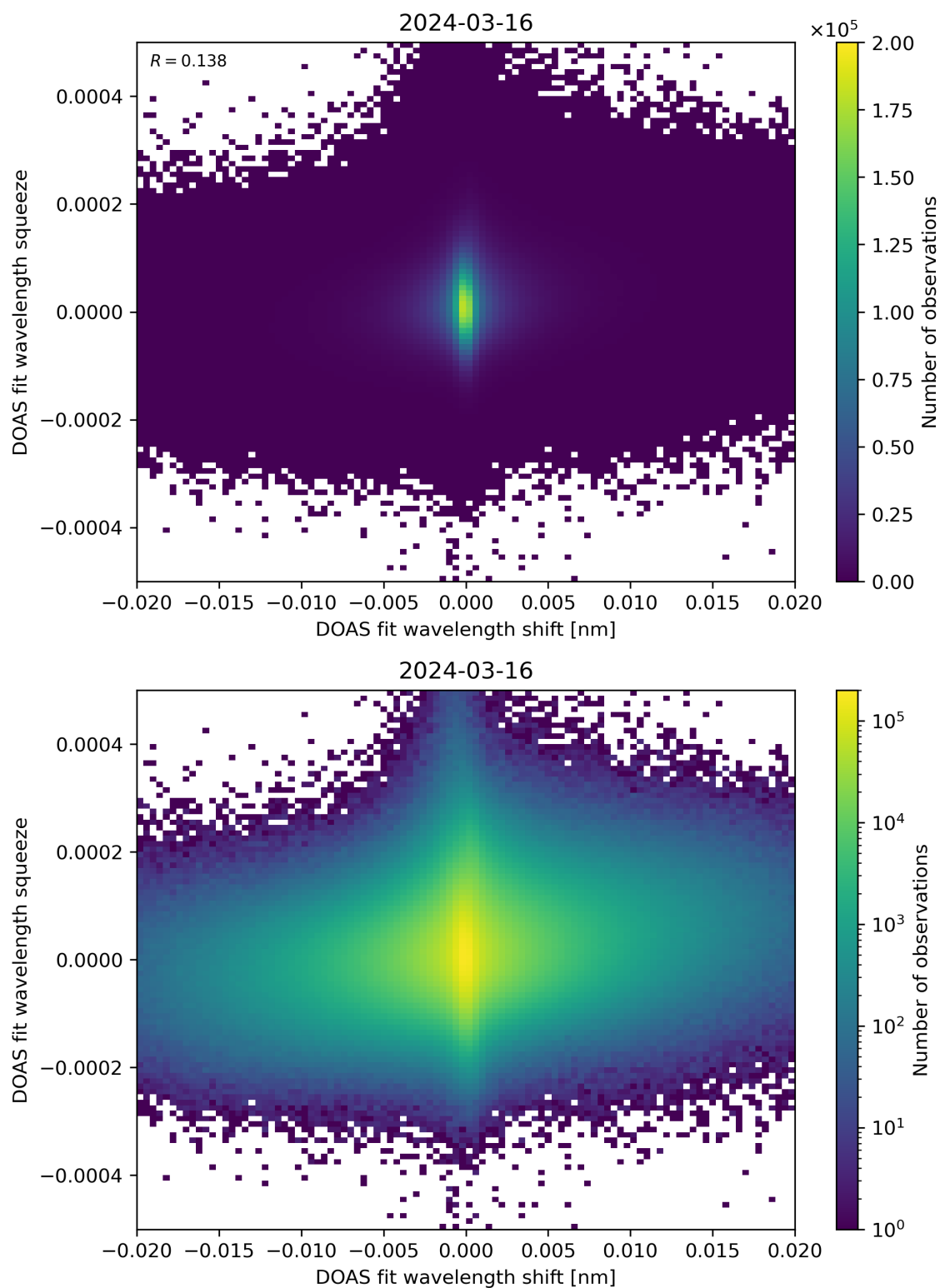
Figure 65: Scatter density plot of “DOAS fit wavelength shift” against “DOAS fit wavelength squeeze” for 2024-03-15 to 2024-03-17.
