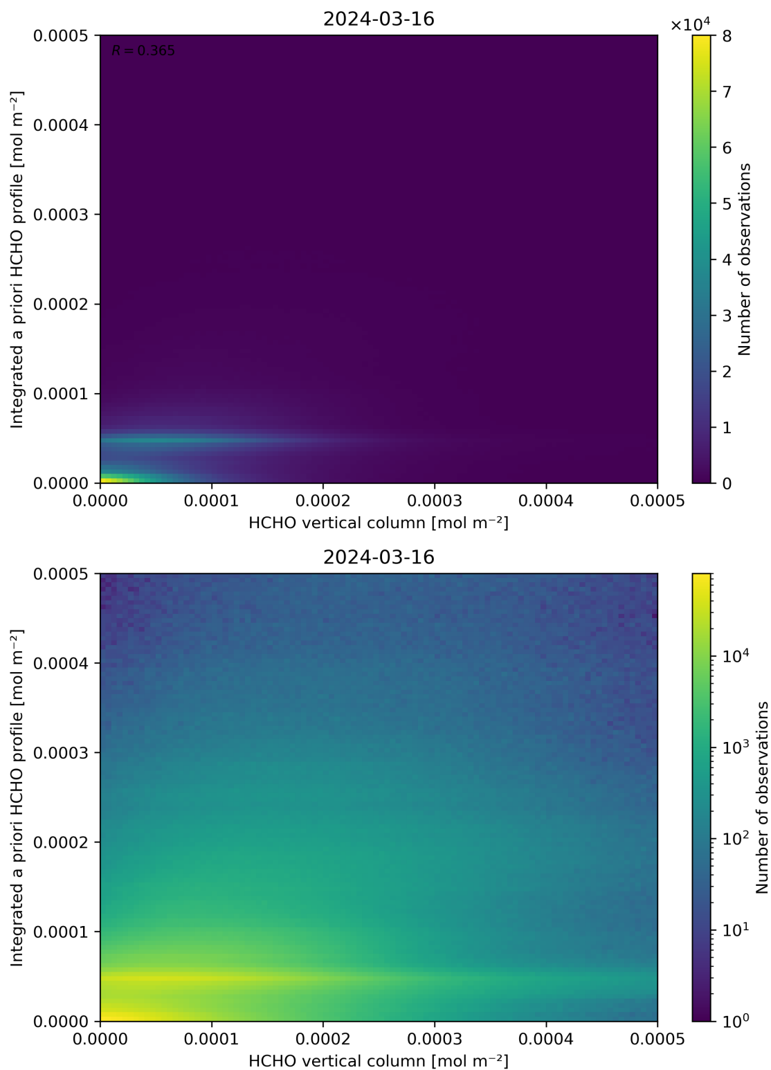
Figure 135: Scatter density plot of “HCHO vertical column” against “Integrated a priori HCHO profile” for 2024-03-15 to 2024-03-17.
