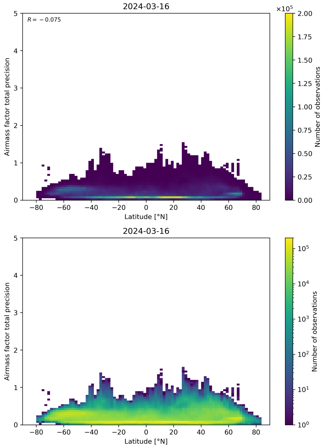
Figure 162: Scatter density plot of “Latitude” against “Airmass factor total precision” for 2024-03-15 to 2024-03-17.
