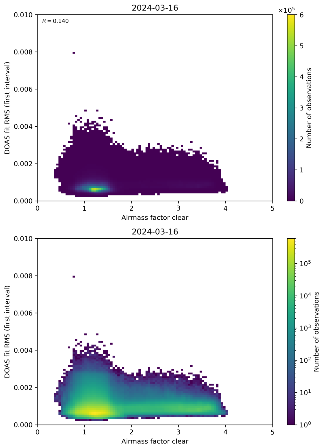
Figure 71: Scatter density plot of “Airmass factor clear” against “DOAS fit RMS (first interval)” for 2024-03-15 to 2024-03-17.
