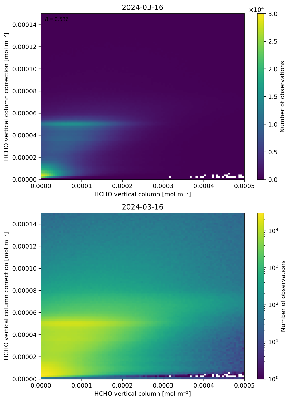
Figure 133: Scatter density plot of “HCHO vertical column” against “HCHO vertical column correction” for 2024-03-15 to 2024-03-17.
