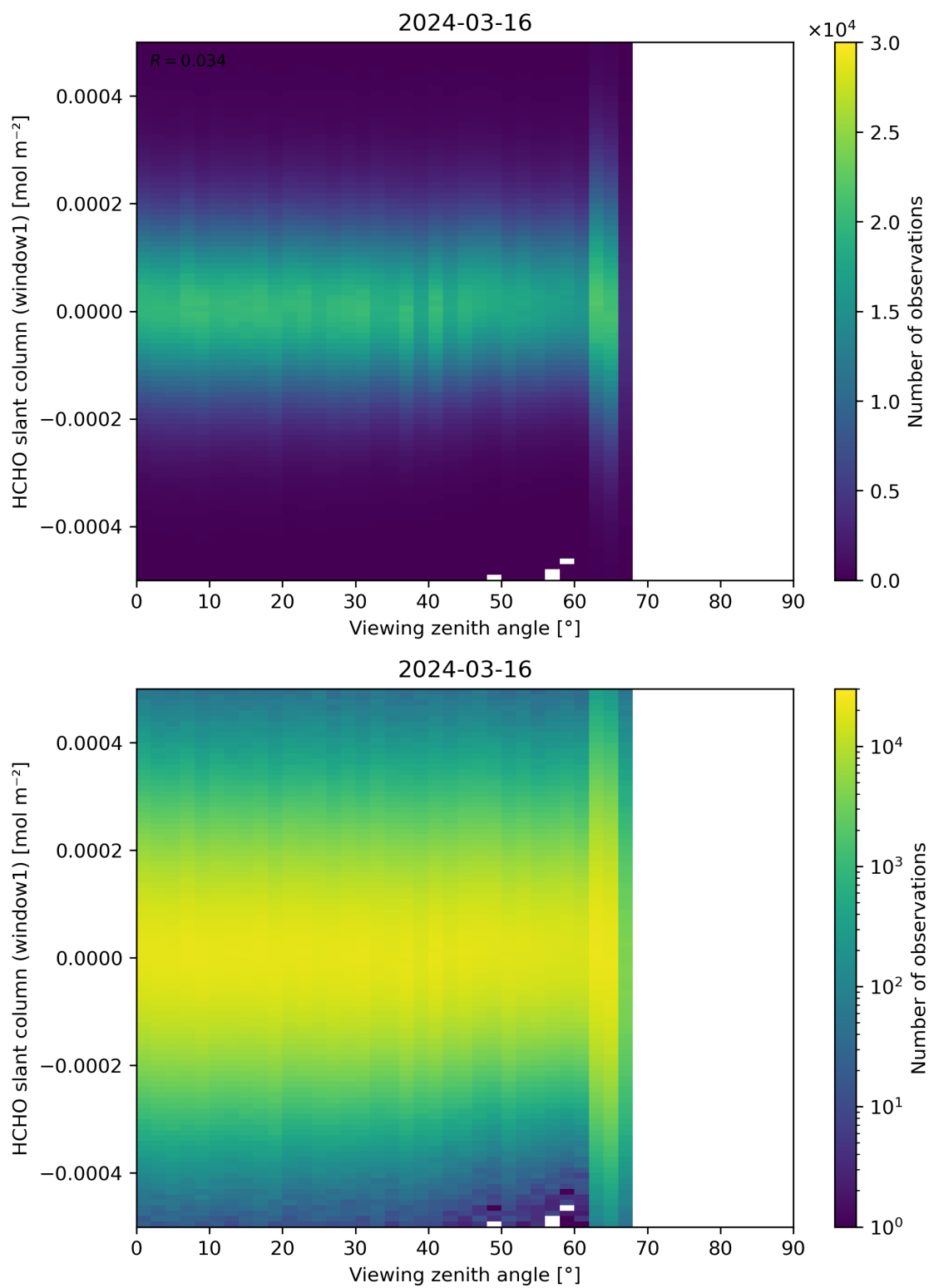
Figure 188: Scatter density plot of “Viewing zenith angle” against “HCHO slant column (window1)” for 2024-03-15 to 2024-03-17.
