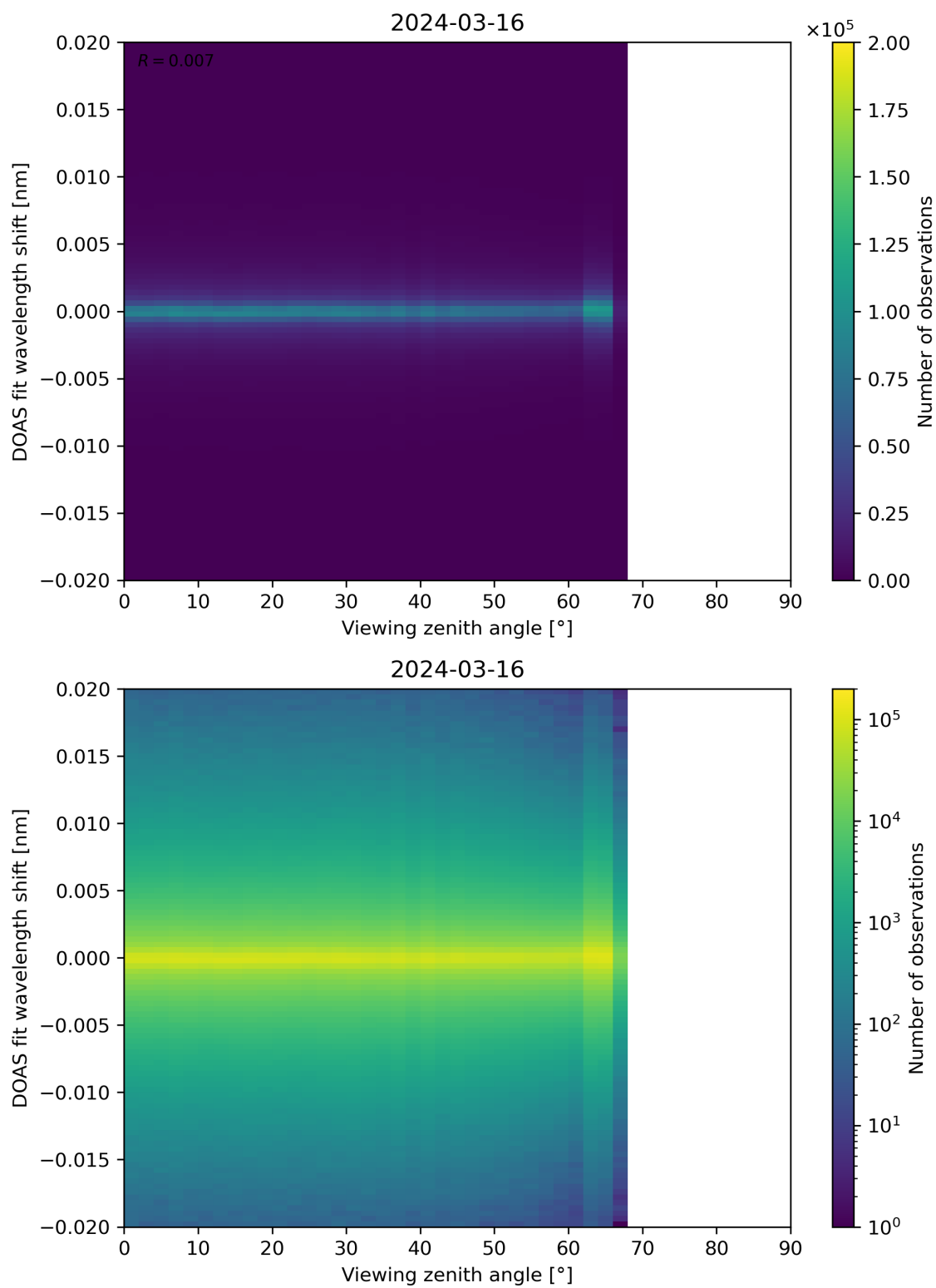
Figure 183: Scatter density plot of “Viewing zenith angle” against “DOAS fit wavelength shift” for 2024-03-15 to 2024-03-17.
