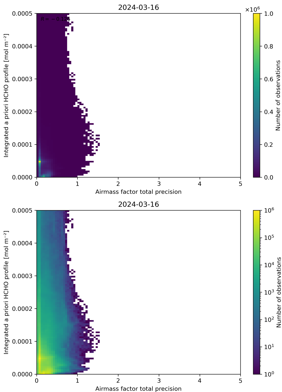
Figure 111: Scatter density plot of “Airmass factor total precision” against “Integrated a priori HCHO profile” for 2024-03-15 to 2024-03-17.
