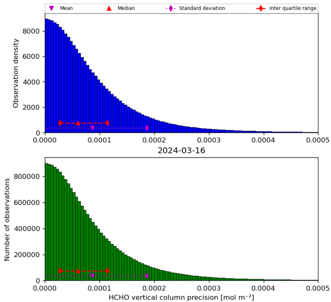
Figure 36: Histogram of “HCHO vertical column precision” for 2024-03-15 to 2024-03-17
