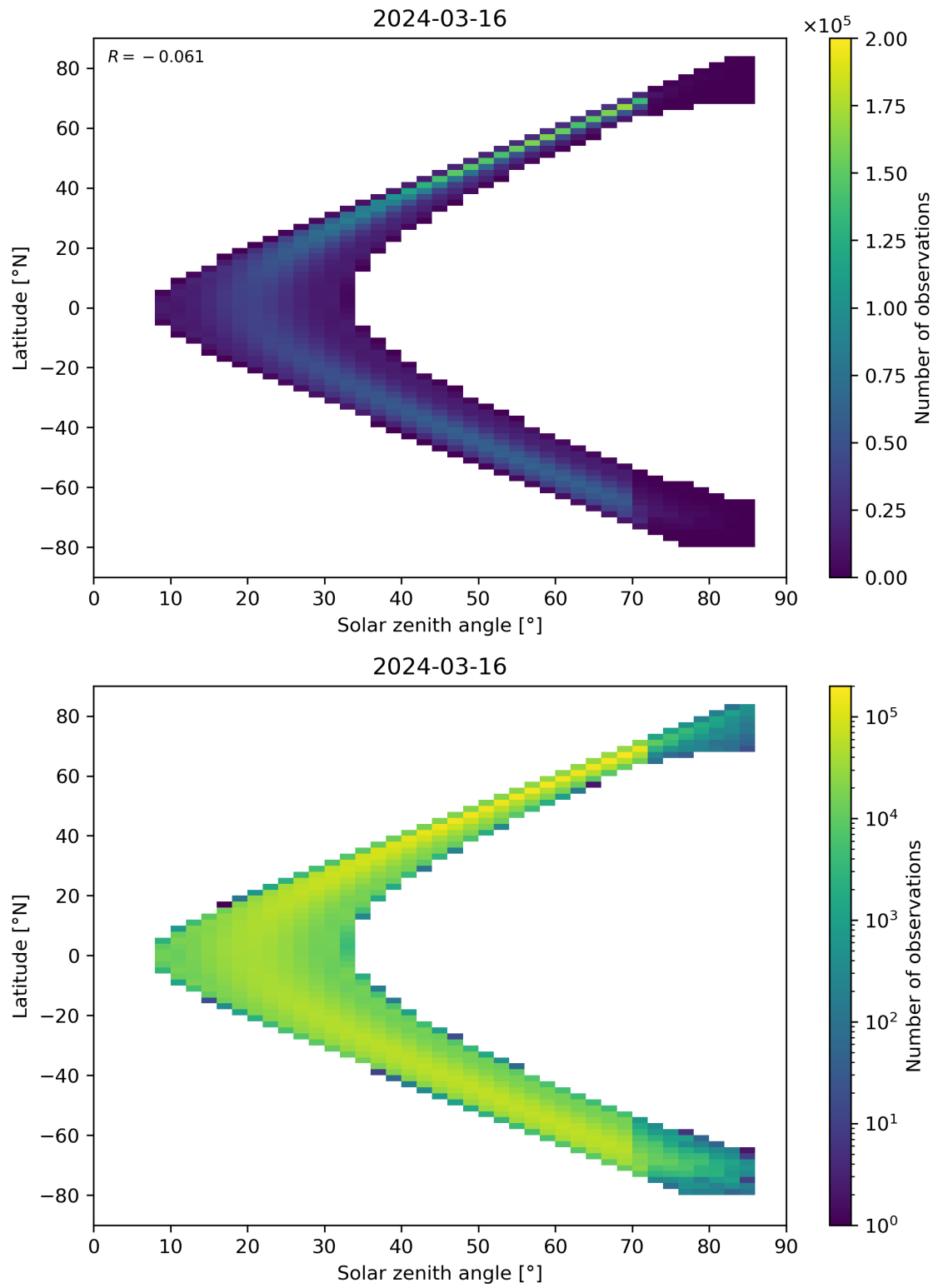
Figure 181: Scatter density plot of “Solar zenith angle” against “Latitude” for 2024-03-15 to 2024-03-17.
