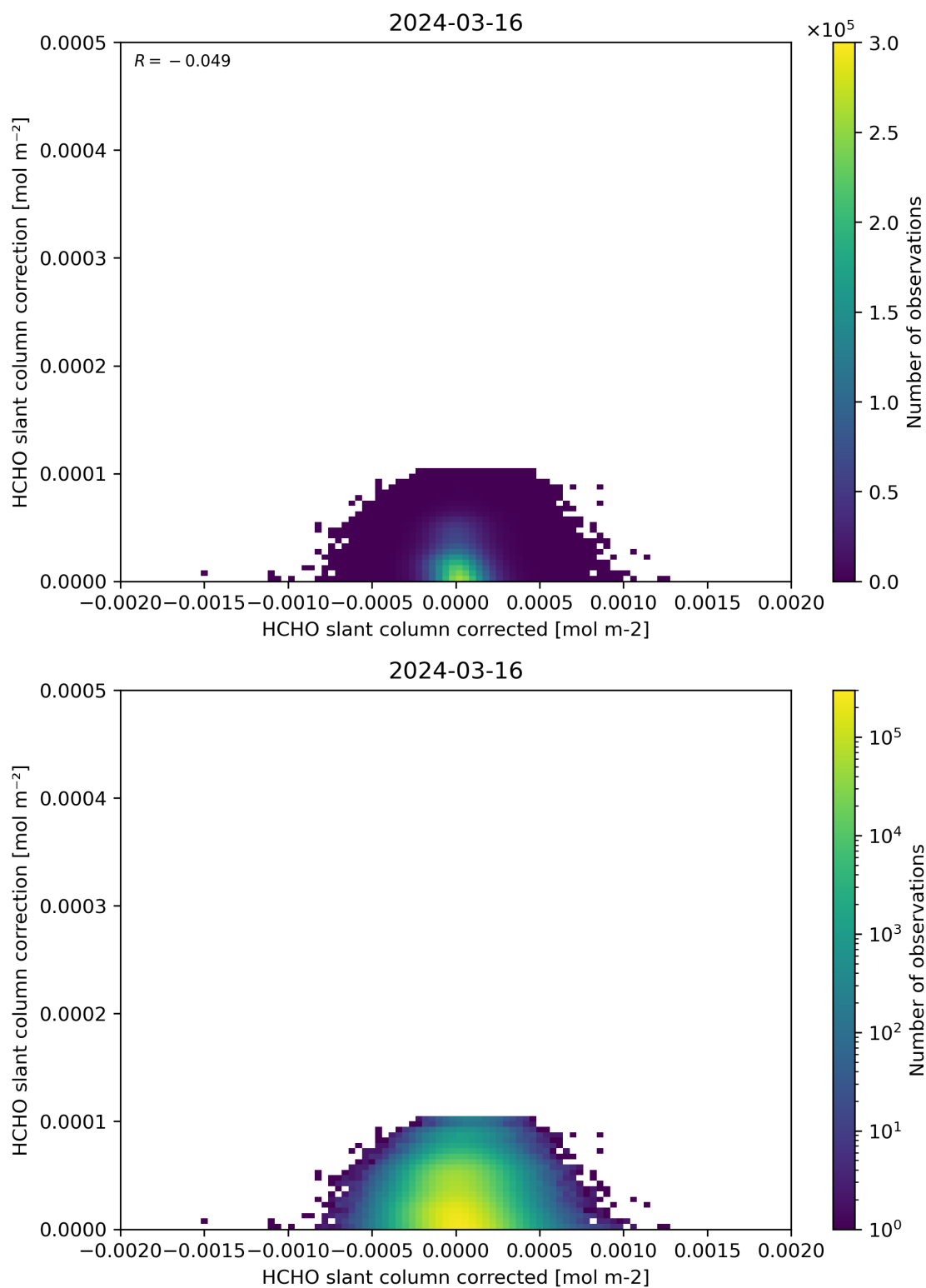
Figure 77: Scatter density plot of “HCHO slant column corrected” against “HCHO slant column correction” for 2024-03-15 to 2024-03-17.
