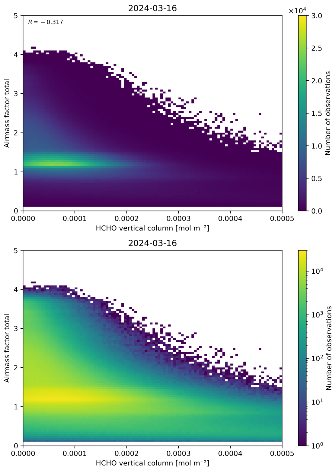
Figure 131: Scatter density plot of “HCHO vertical column” against “Airmass factor total” for 2024-03-15 to 2024-03-17.
