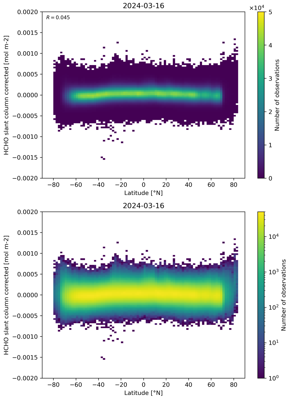
Figure 157: Scatter density plot of “Latitude” against “HCHO slant column corrected” for 2024-03-15 to 2024-03-17.
