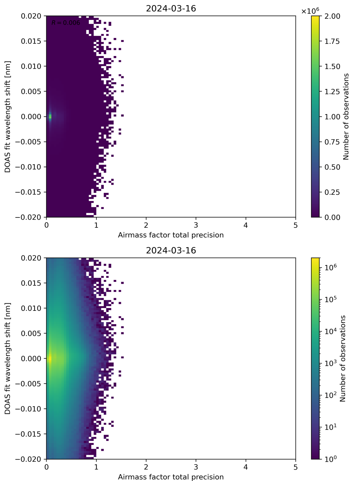
Figure 106: Scatter density plot of “Airmass factor total precision” against “DOAS fit wavelength shift” for 2024-03-15 to 2024-03-17.
