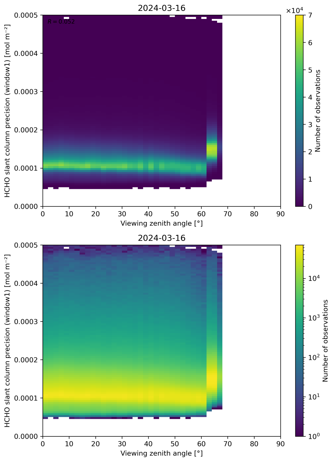
Figure 189: Scatter density plot of “Viewing zenith angle” against “HCHO slant column precision (window1)” for 2024-03-15 to 2024-03-17.
