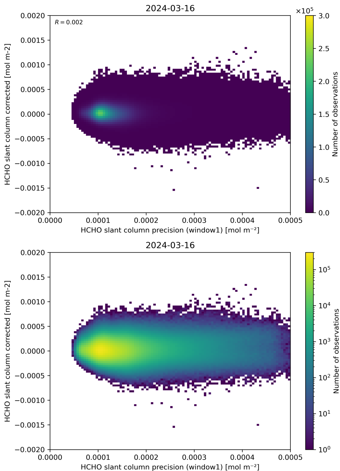
Figure 92: Scatter density plot of “HCHO slant column precision (window1)” against “HCHO slant column corrected” for 2024-03-15 to 2024-03-17.
