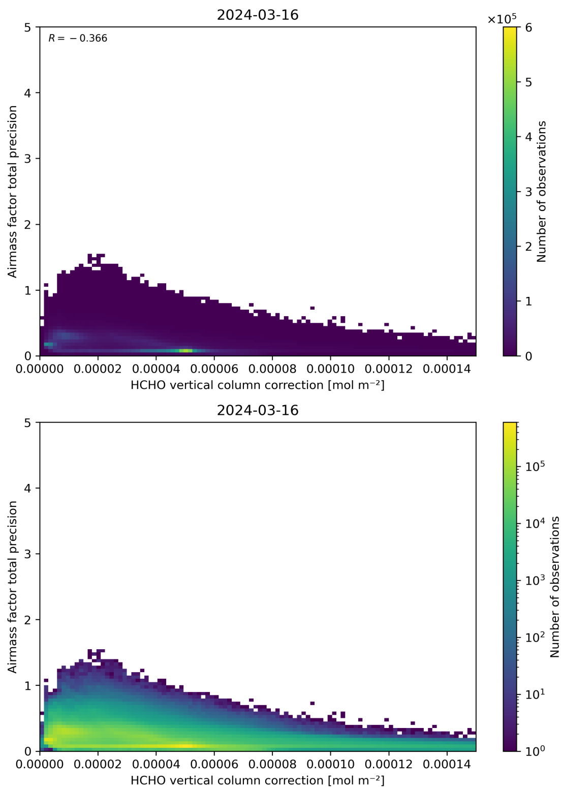
Figure 121: Scatter density plot of “HCHO vertical column correction” against “Airmass factor total precision” for 2024-03-15 to 2024-03-17.
