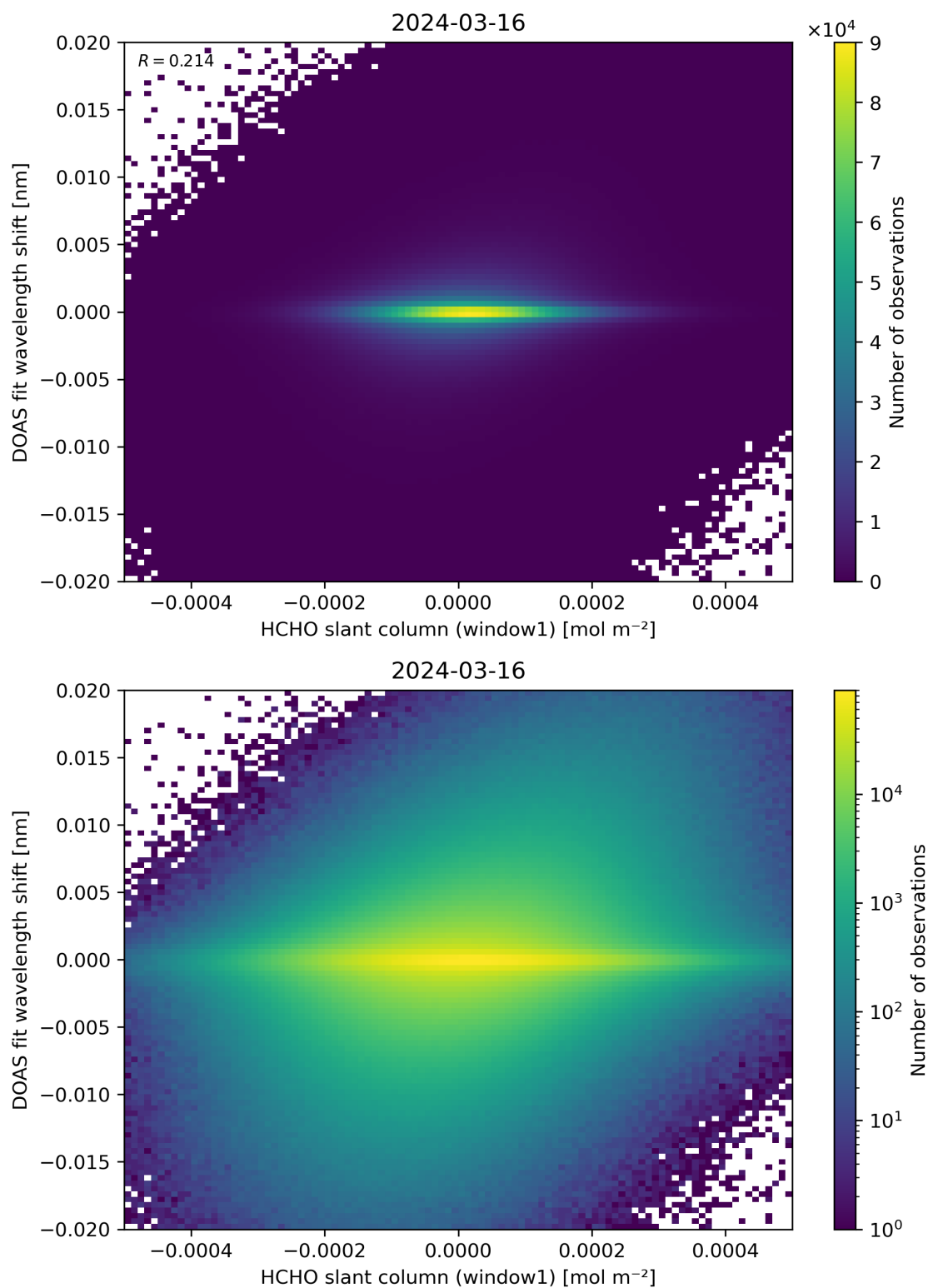
Figure 79: Scatter density plot of “HCHO slant column (window1)” against “DOAS fit wavelength shift” for 2024-03-15 to 2024-03-17.
