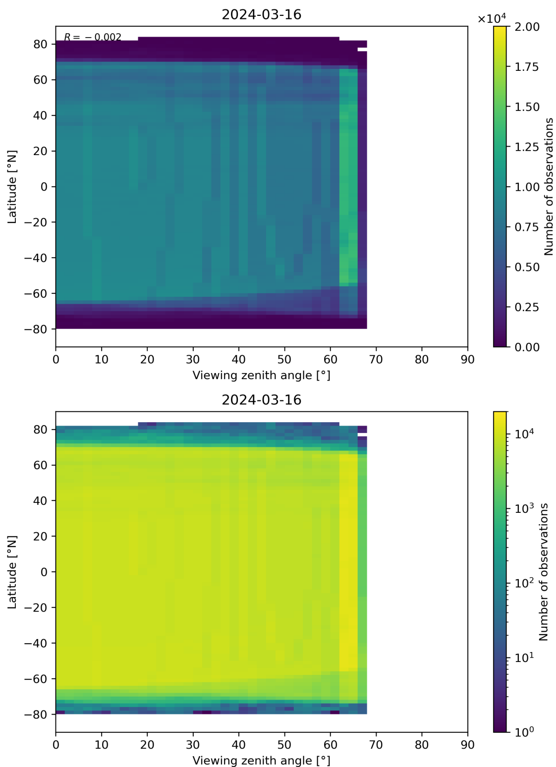
Figure 196: Scatter density plot of “Viewing zenith angle” against “Latitude” for 2024-03-15 to 2024-03-17.
