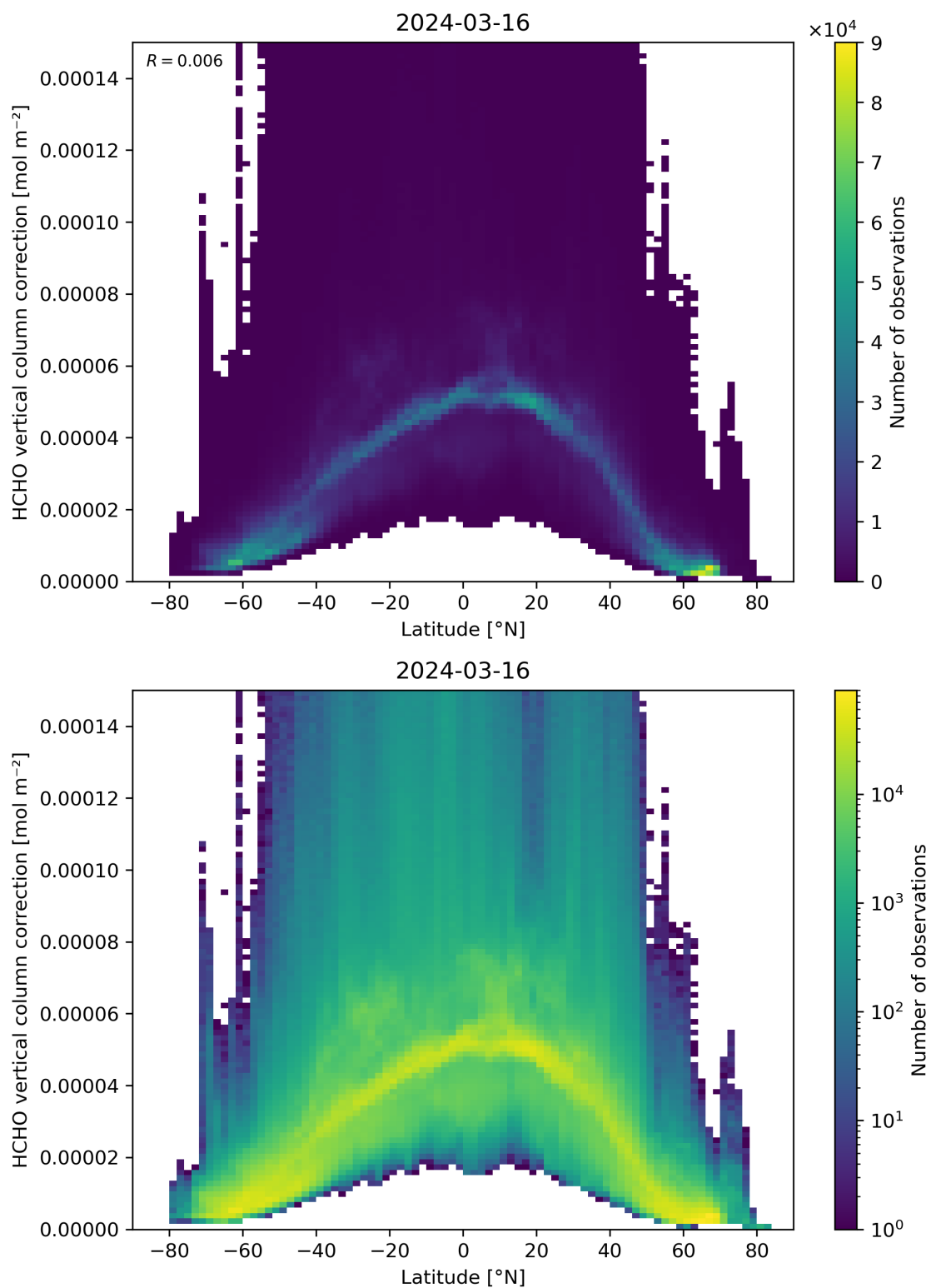
Figure 164: Scatter density plot of “Latitude” against “HCHO vertical column correction” for 2024-03-15 to 2024-03-17.
