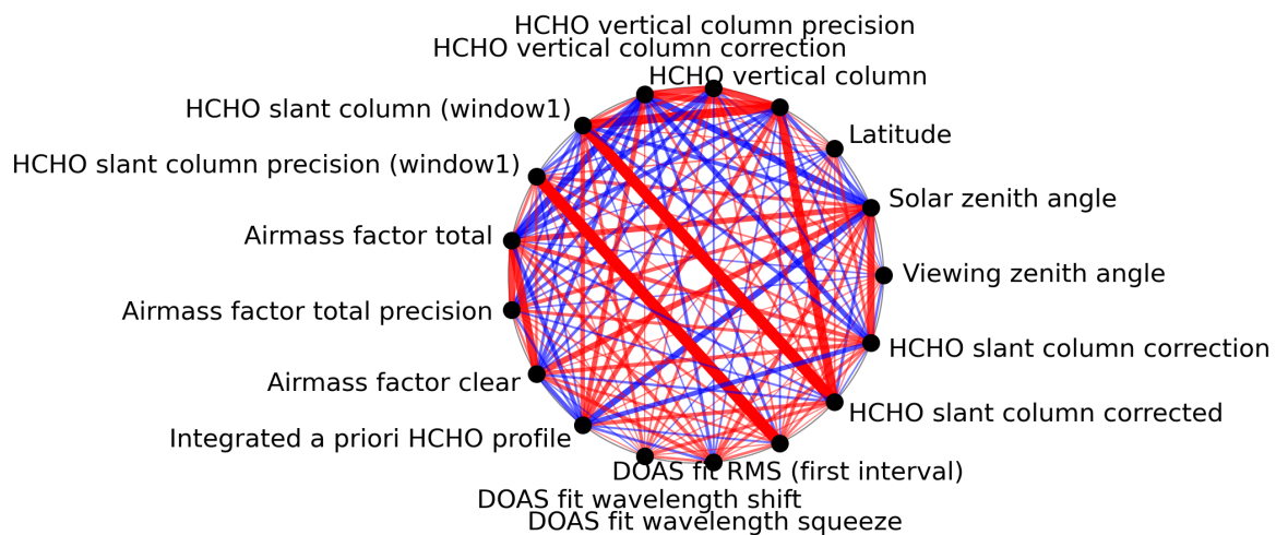
Figure 1: Map of correlation graph for 2024-03-15 to 2024-03-17.
