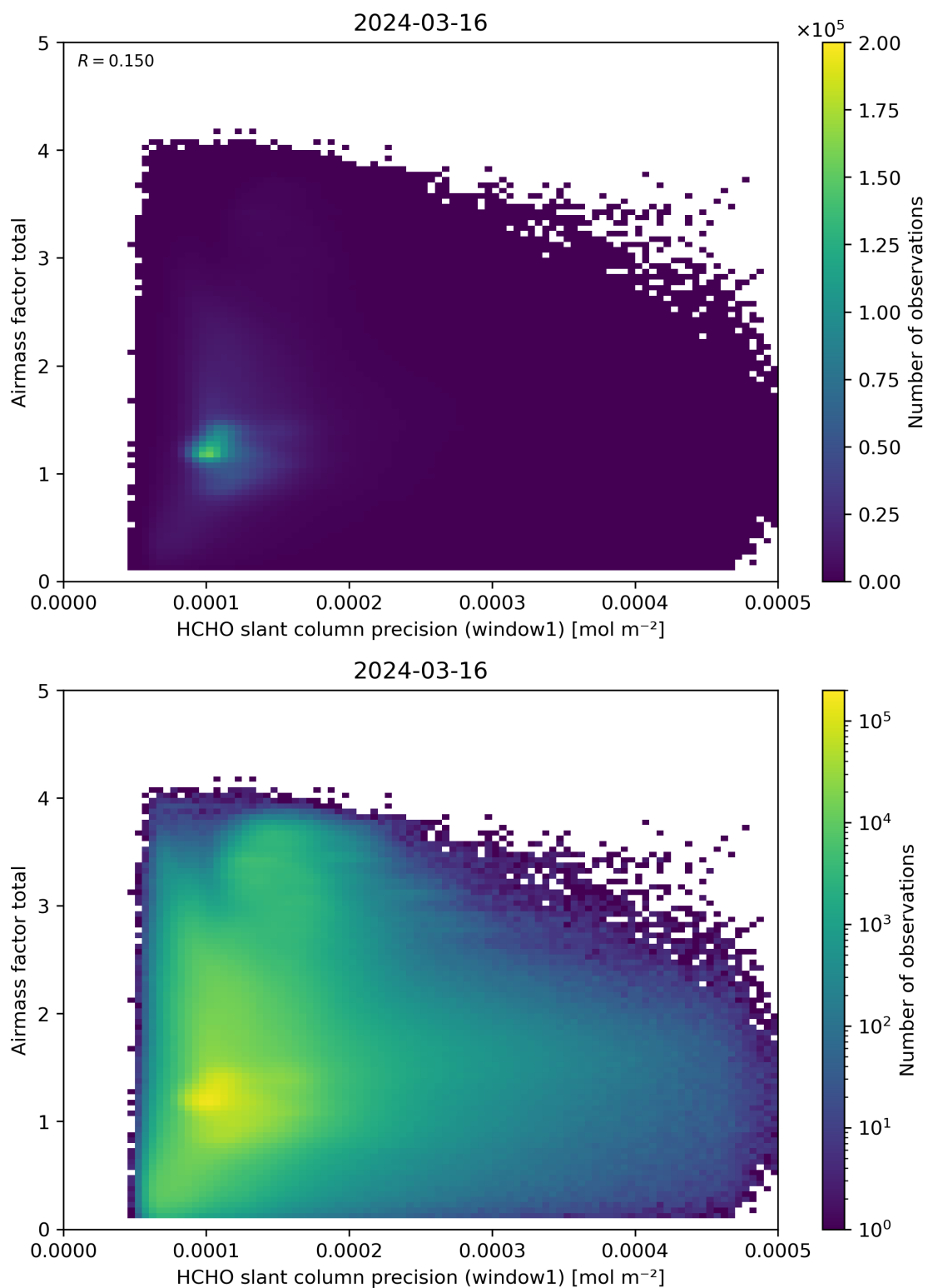
Figure 94: Scatter density plot of “HCHO slant column precision (window1)” against “Airmass factor total” for 2024-03-15 to 2024-03-17.
