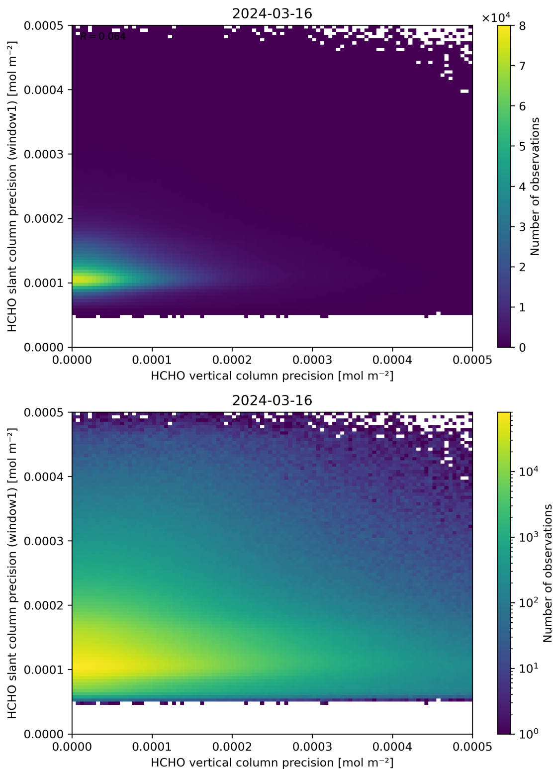
Figure 143: Scatter density plot of “HCHO vertical column precision” against “HCHO slant column precision (window1)” for 2024-03-15 to 2024-03-17.
