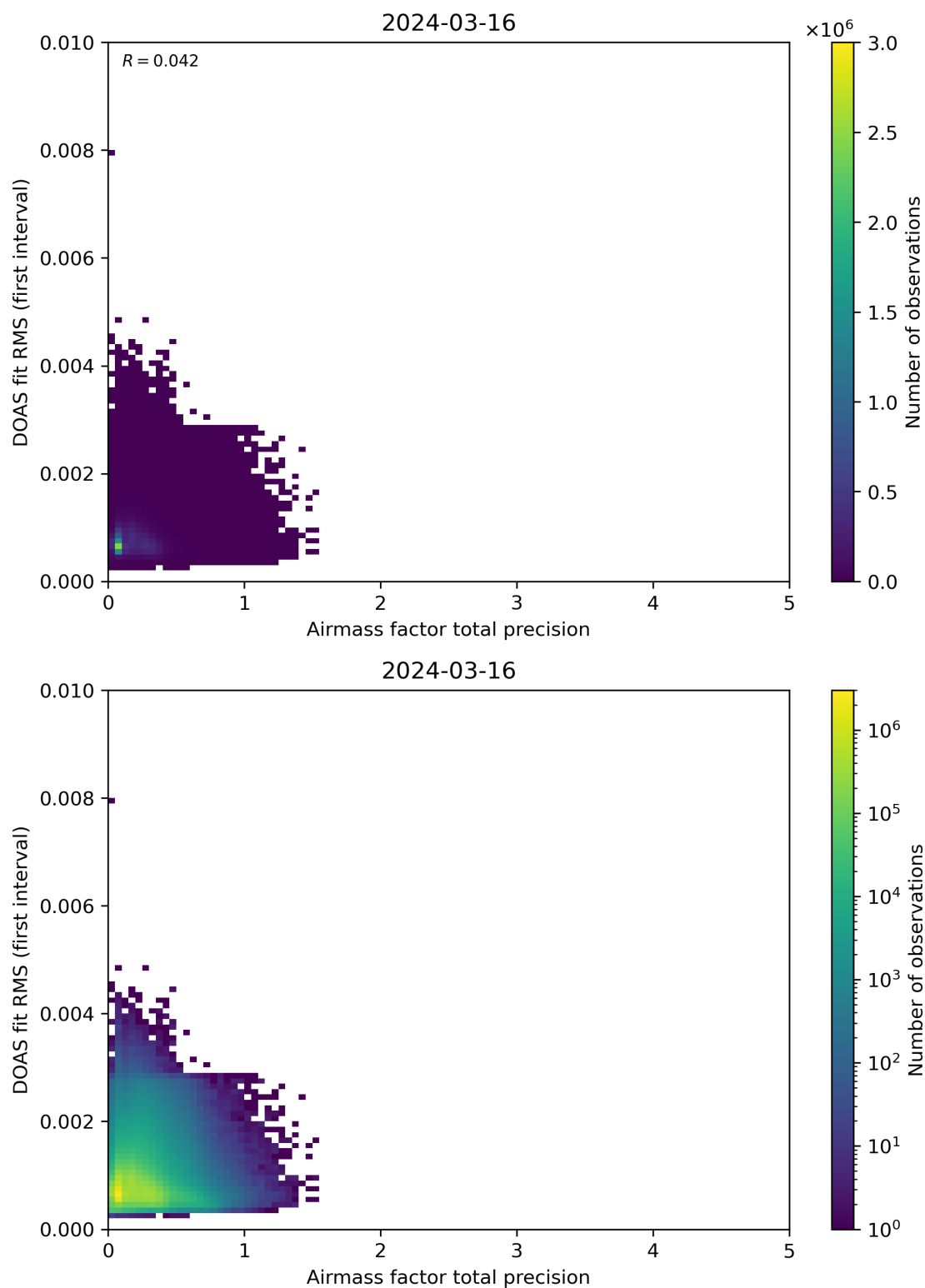
Figure 105: Scatter density plot of “Airmass factor total precision” against “DOAS fit RMS (first interval)” for 2024-03-15 to 2024-03-17.
