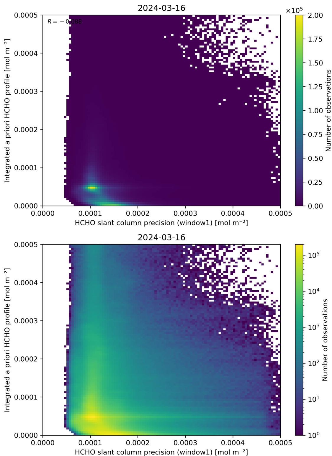
Figure 96: Scatter density plot of “HCHO slant column precision (window1)” against “Integrated a priori HCHO profile” for 2024-03-15 to 2024-03-17.
