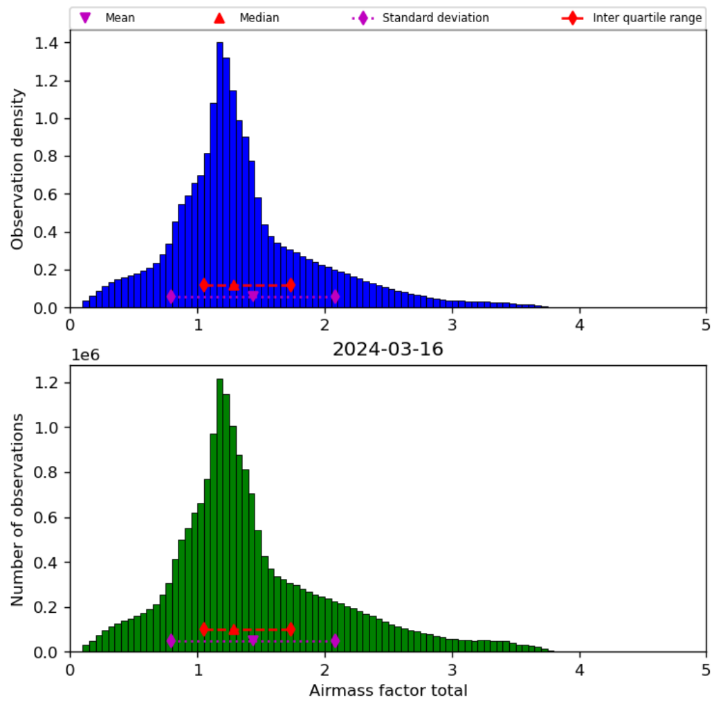
Figure 40: Histogram of “Airmass factor total” for 2024-03-15 to 2024-03-17
