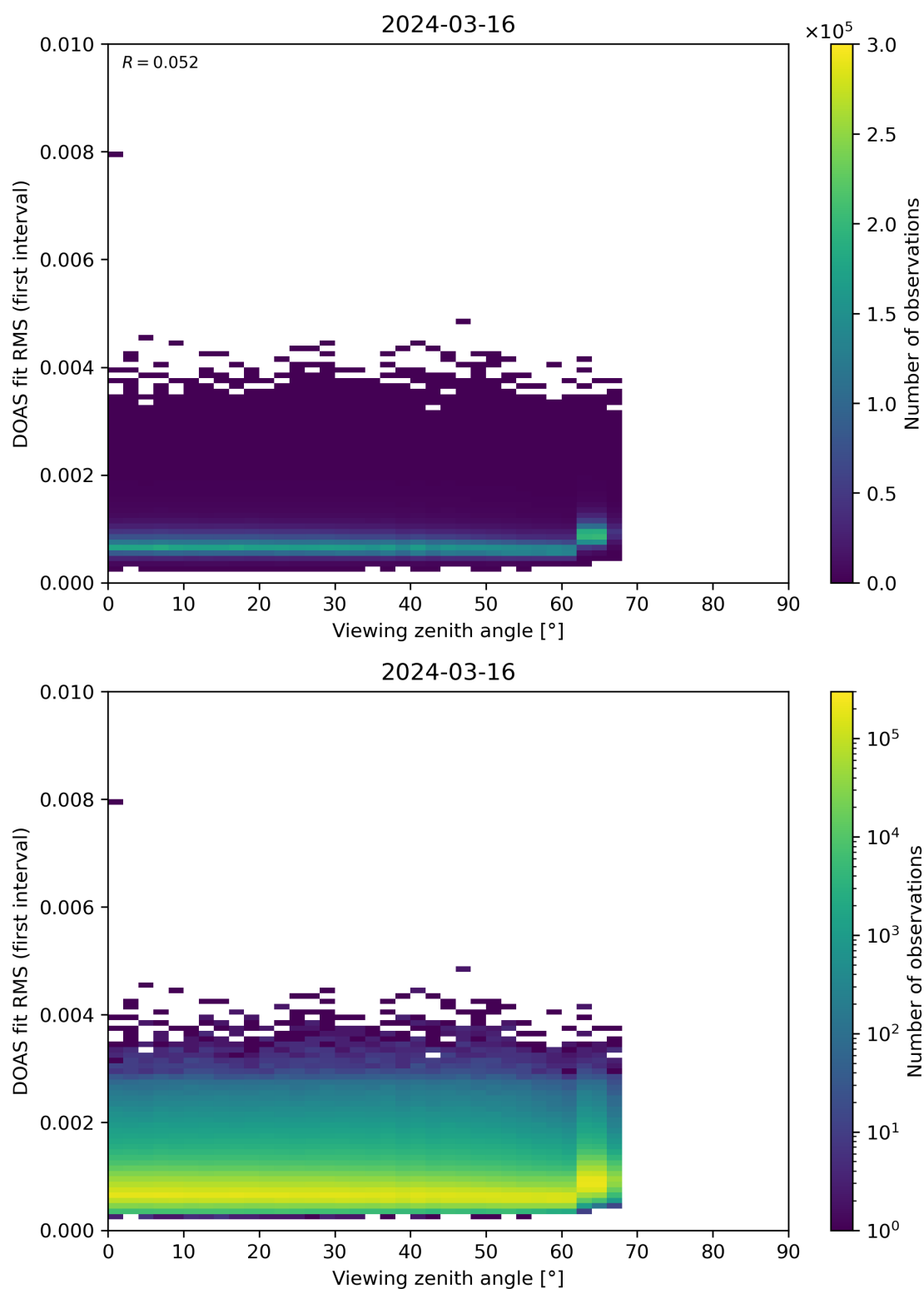
Figure 182: Scatter density plot of “Viewing zenith angle” against “DOAS fit RMS (first interval)” for 2024-03-15 to 2024-03-17.
