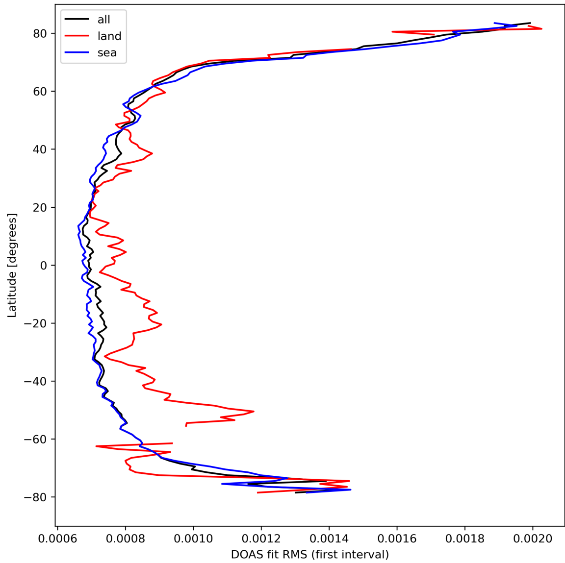
Figure 32: Zonal average of “DOAS fit RMS (first interval)” for 2024-03-15 to 2024-03-17.
