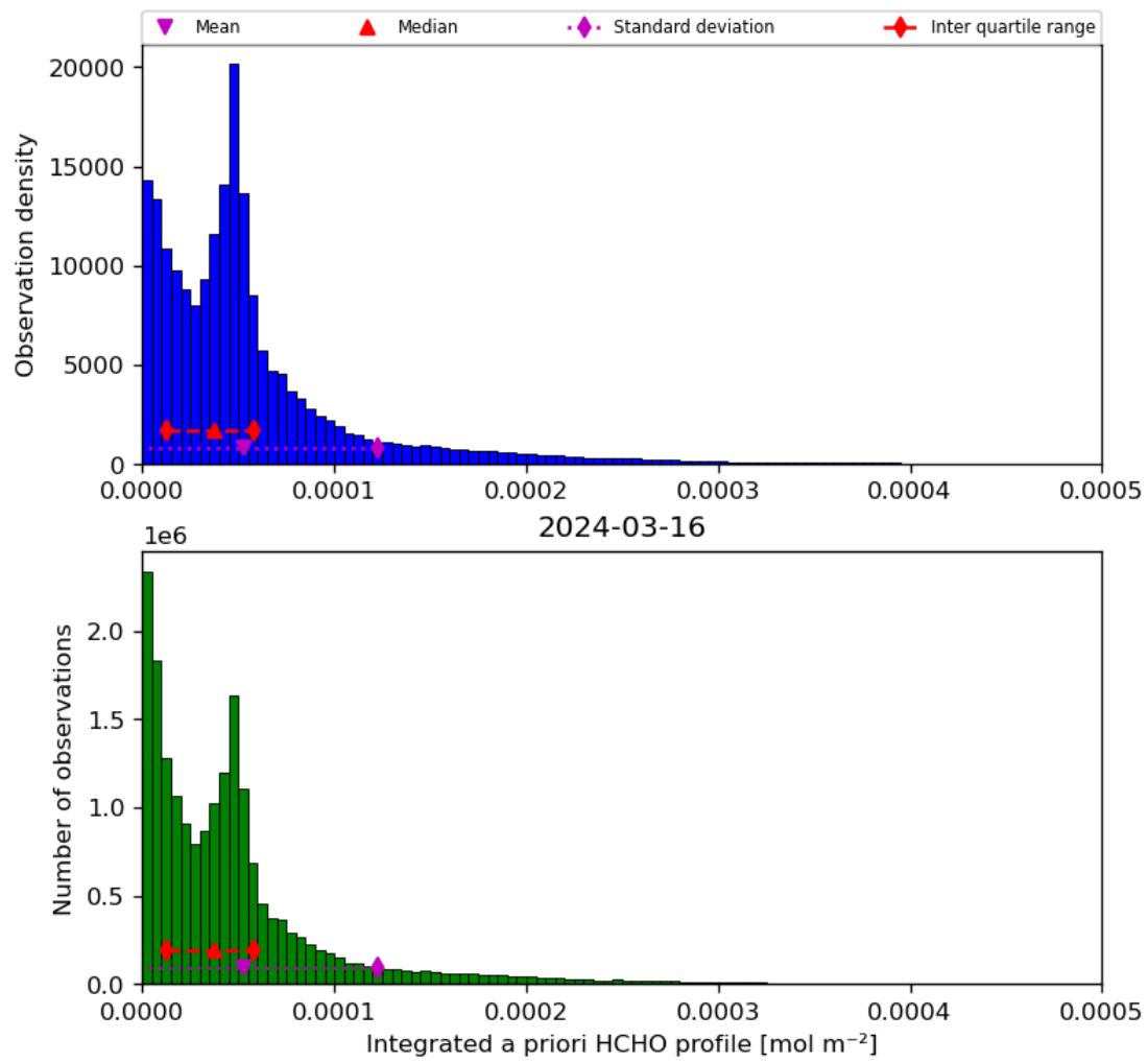
Figure 43: Histogram of “Integrated a priori HCHO profile” for 2024-03-15 to 2024-03-17
