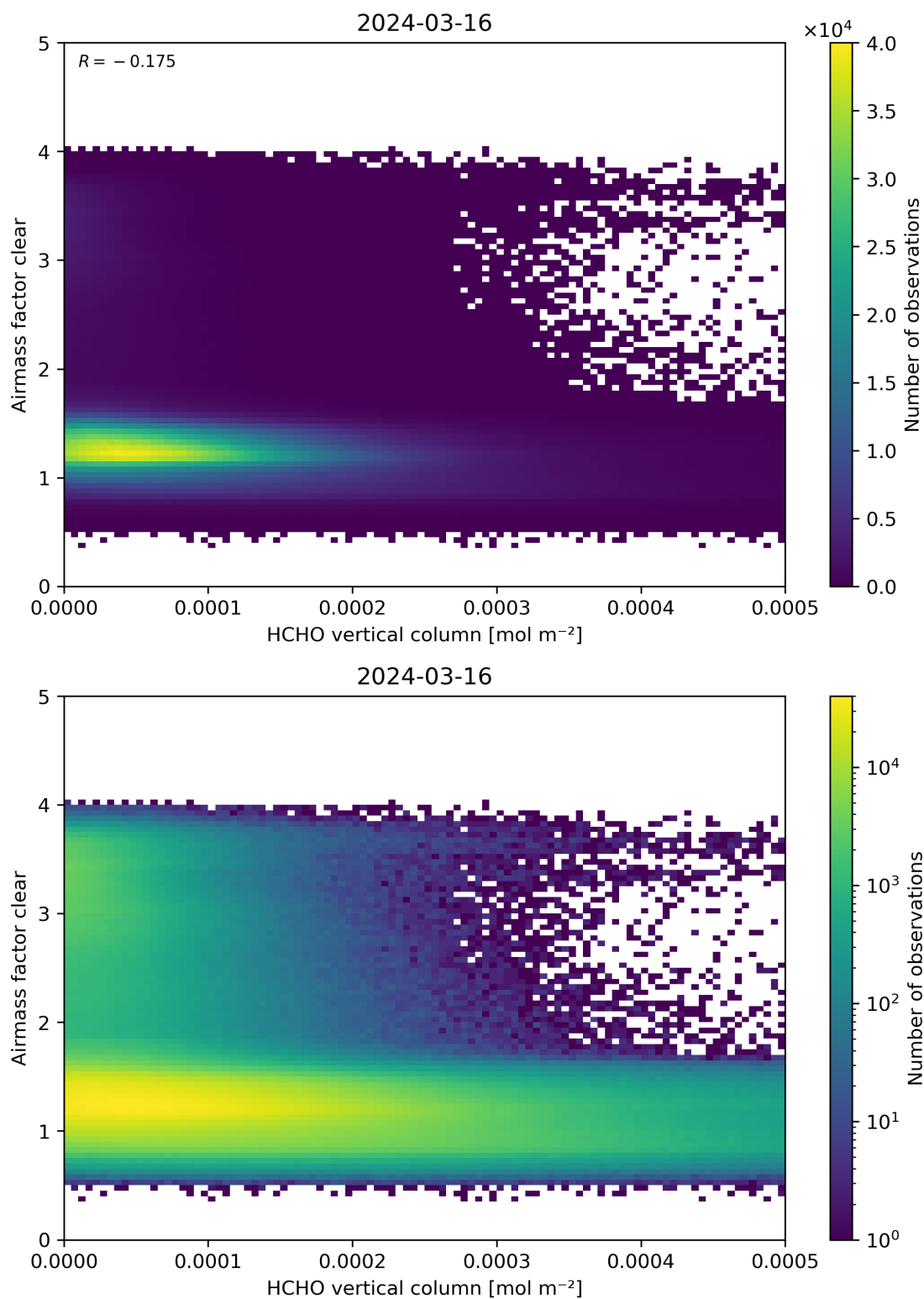
Figure 126: Scatter density plot of “HCHO vertical column” against “Airmass factor clear” for 2024-03-15 to 2024-03-17.
