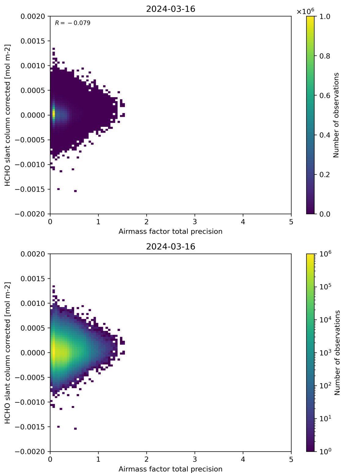
Figure 109: Scatter density plot of “Airmass factor total precision” against “HCHO slant column corrected” for 2024-03-15 to 2024-03-17.
