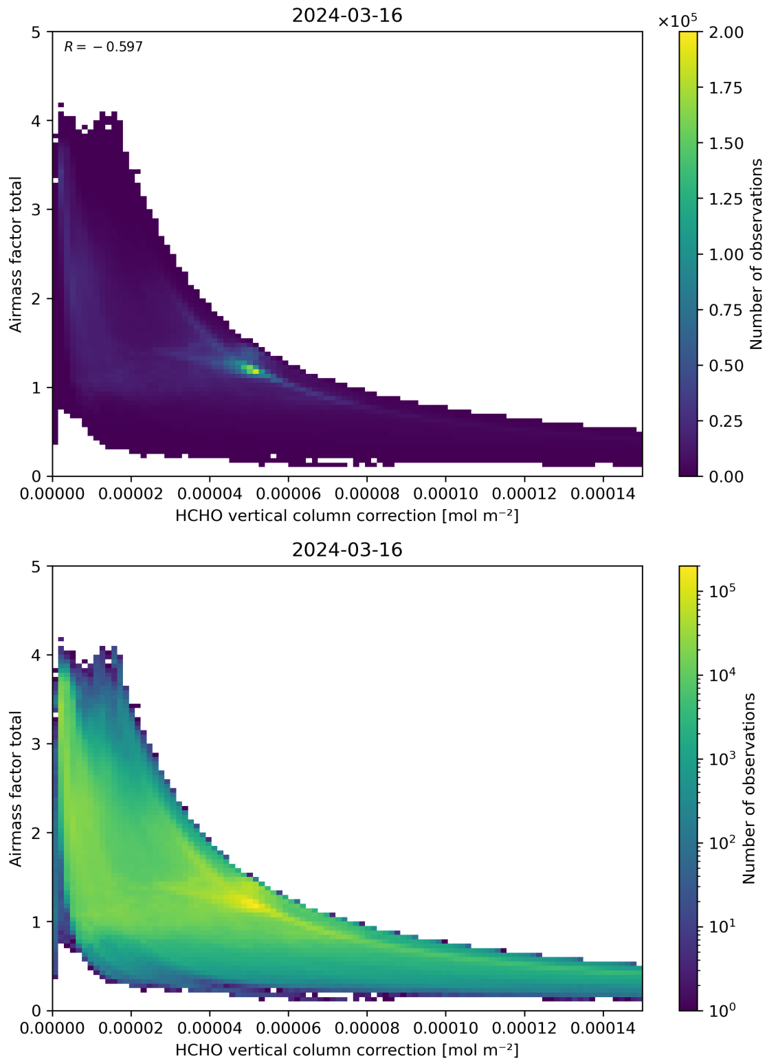
Figure 120: Scatter density plot of “HCHO vertical column correction” against “Airmass factor total” for 2024-03-15 to 2024-03-17.
