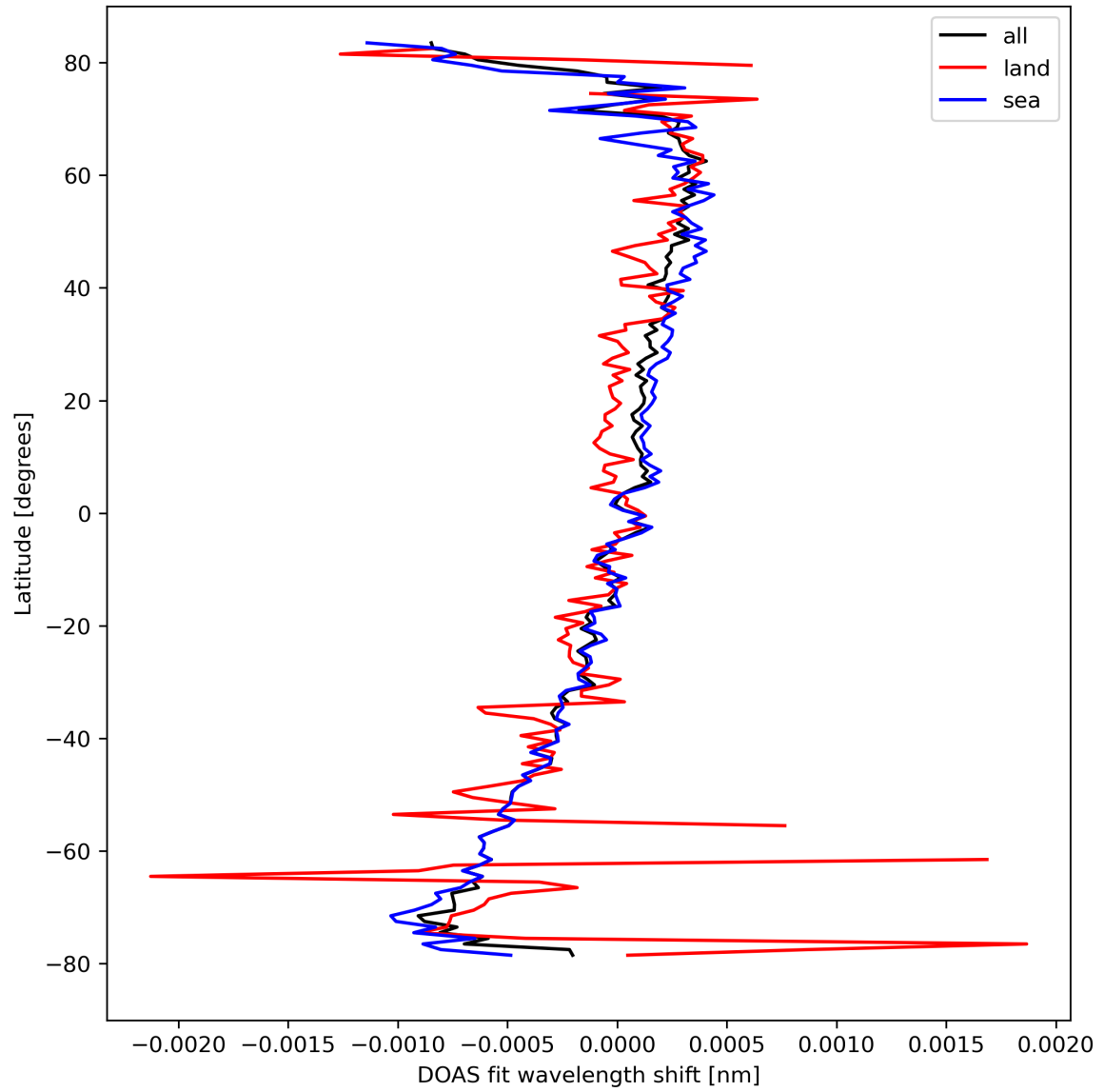
Figure 30: Zonal average of "DOAS fit wavelength shift" for 2024-03-15 to 2024-03-17.
