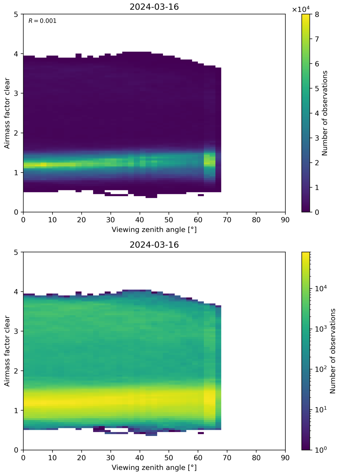
Figure 185: Scatter density plot of “Viewing zenith angle” against “Airmass factor clear” for 2024-03-15 to 2024-03-17.
