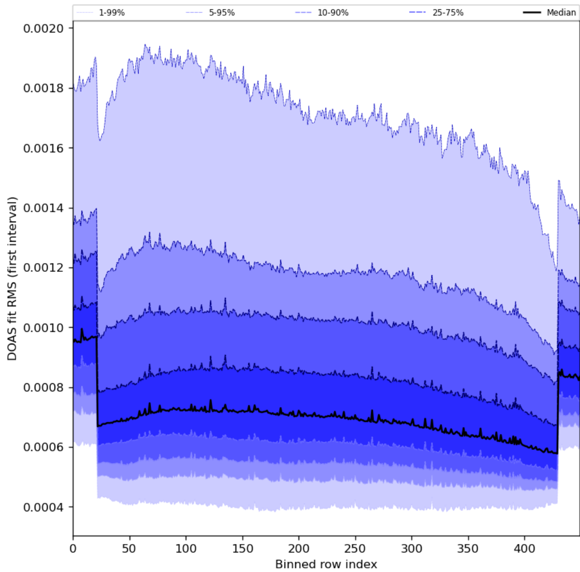
Figure 60: Along track statistics of “DOAS fit RMS (first interval)” for 2024-03-15 to 2024-03-17
