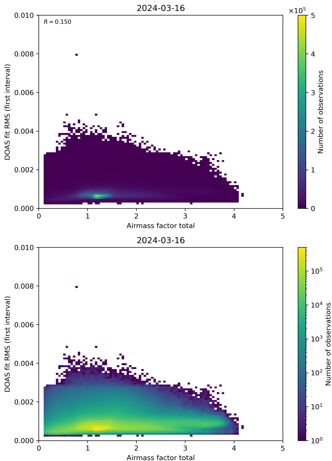
Figure 97: Scatter density plot of “Airmass factor total” against “DOAS fit RMS (first interval)” for 2024-03-15 to 2024-03-17.
