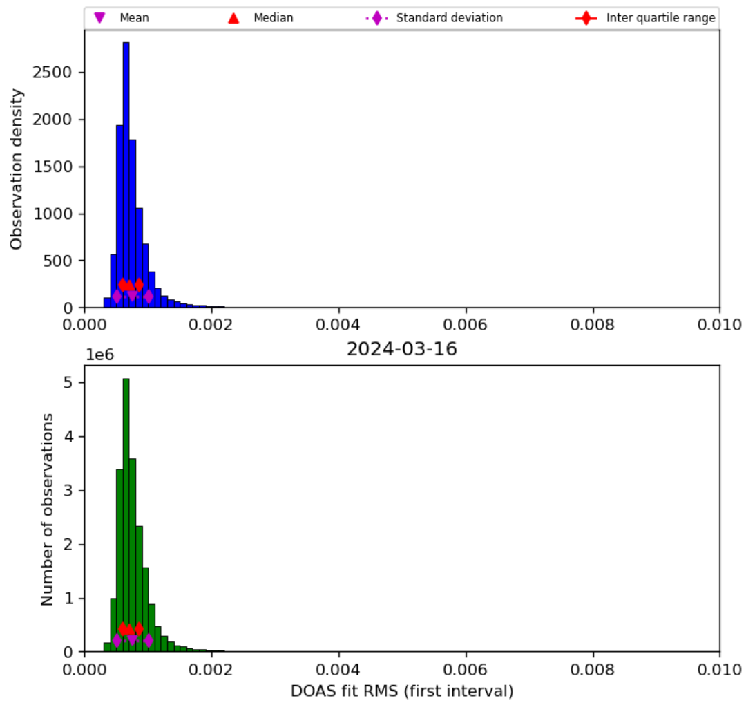
Figure 46: Histogram of “DOAS fit RMS (first interval)” for 2024-03-15 to 2024-03-17
