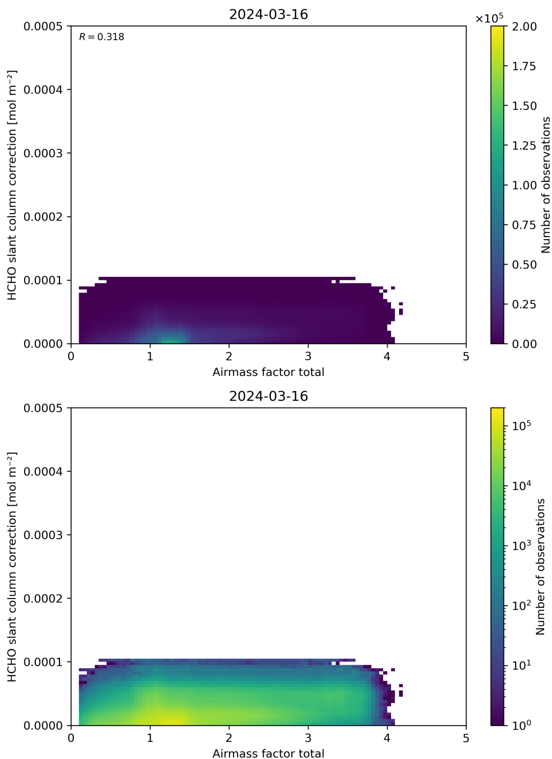
Figure 102: Scatter density plot of “Airmass factor total” against “HCHO slant column correction” for 2024-03-15 to 2024-03-17.
