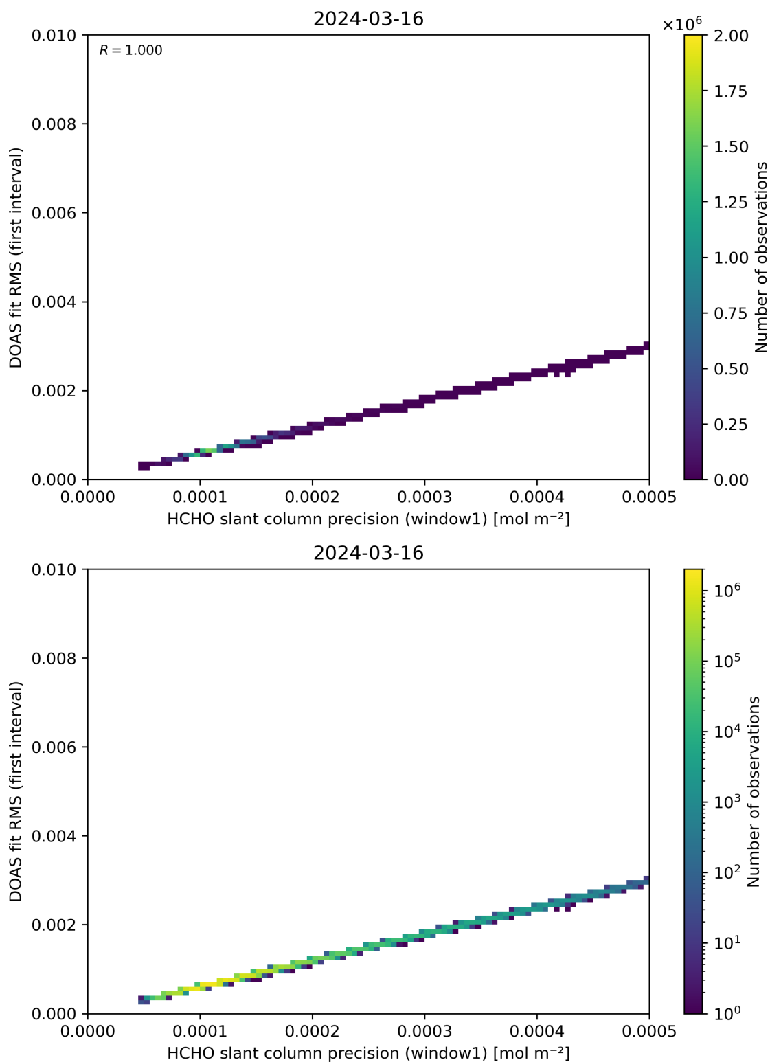
Figure 88: Scatter density plot of “HCHO slant column precision (window1)” against “DOAS fit RMS (first interval)” for 2024-03-15 to 2024-03-17.
