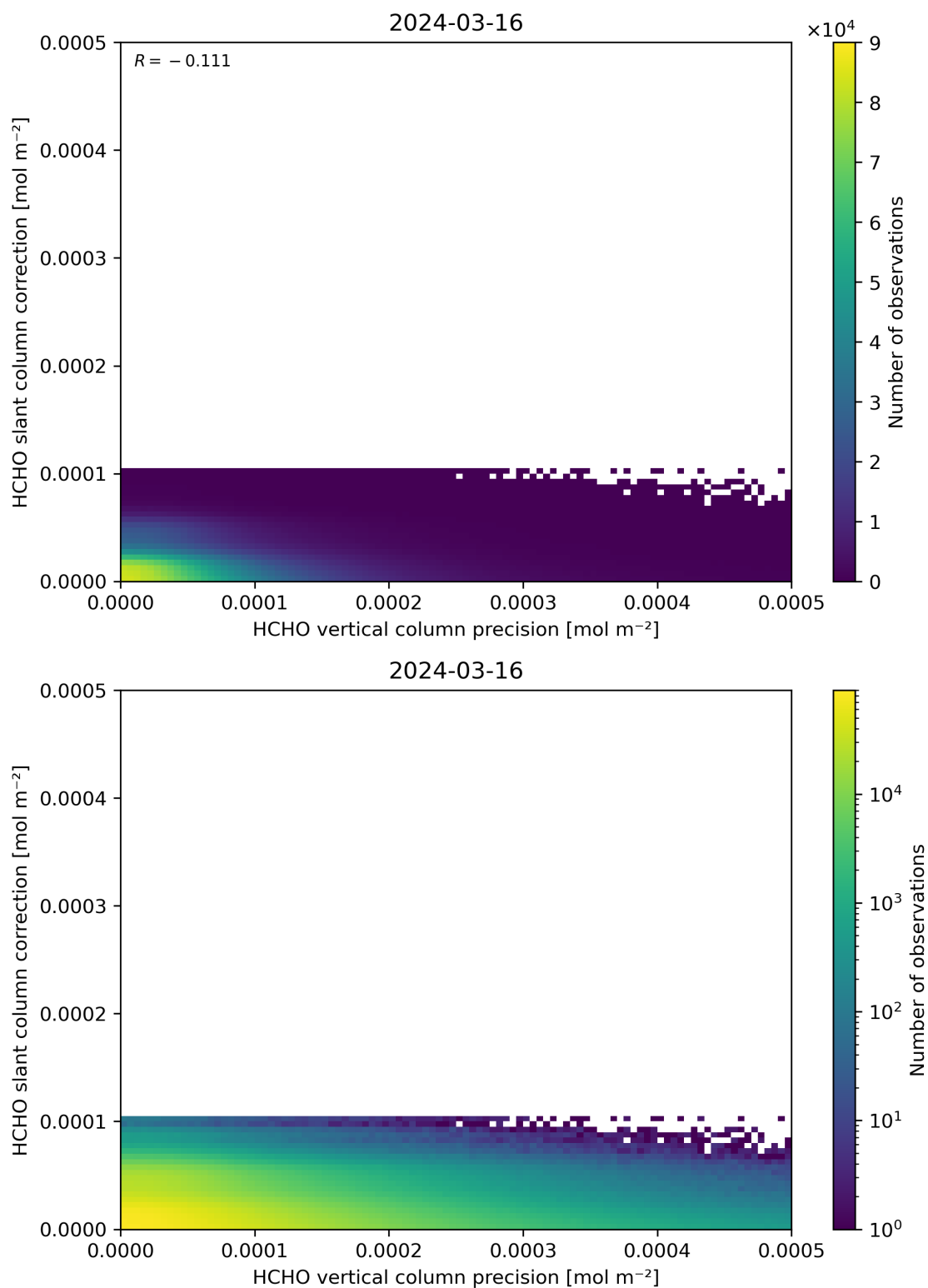
Figure 141: Scatter density plot of “HCHO vertical column precision” against “HCHO slant column correction” for 2024-03-15 to 2024-03-17.
