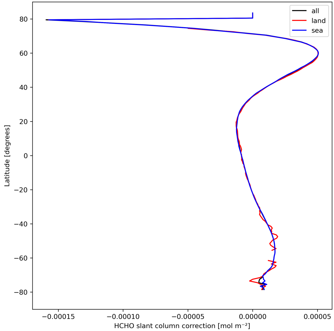
Figure 33: Zonal average of “HCHO slant column correction” for 2024-03-15 to 2024-03-17.
