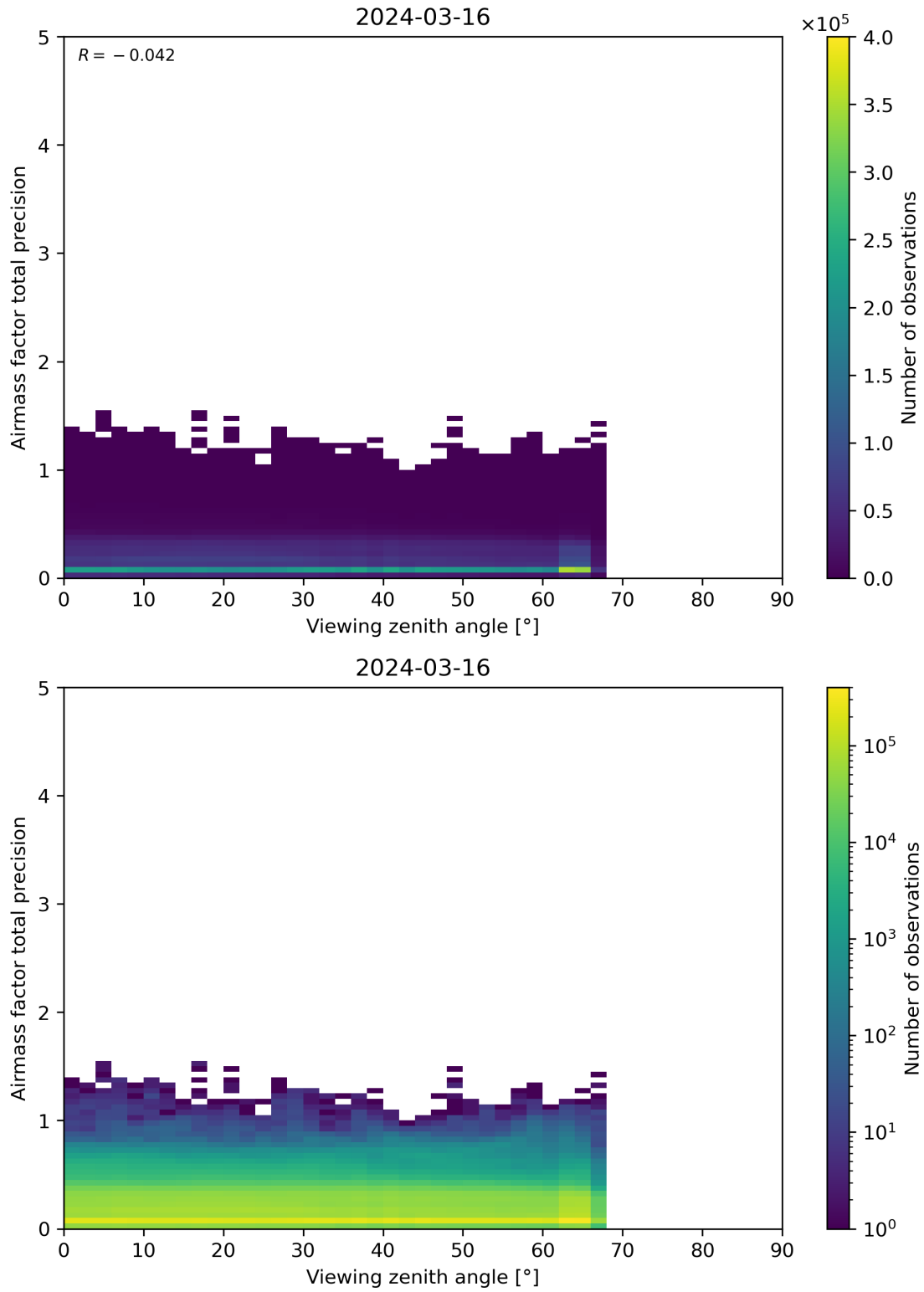
Figure 191: Scatter density plot of “Viewing zenith angle” against “Airmass factor total precision” for 2024-03-15 to 2024-03-17.
