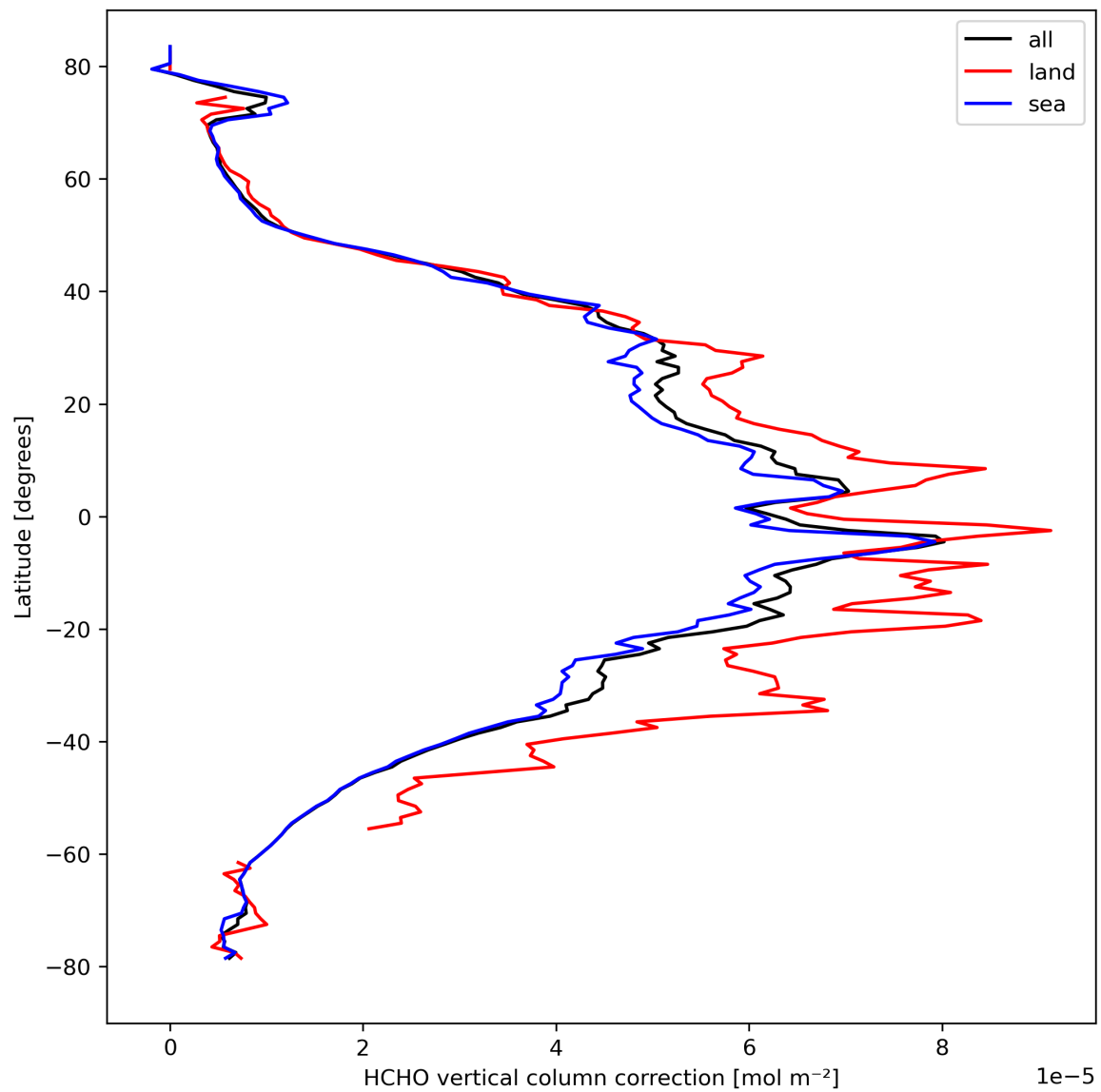
Figure 23: Zonal average of “HCHO vertical column correction” for 2024-03-15 to 2024-03-17.
