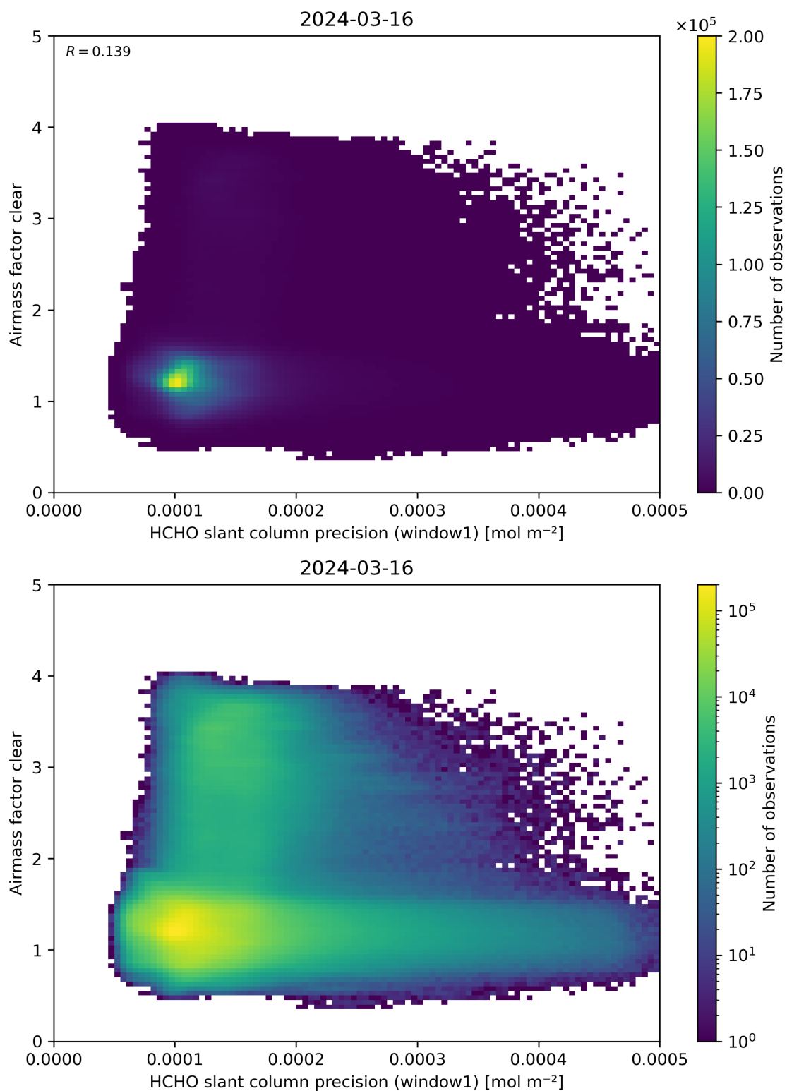
Figure 91: Scatter density plot of “HCHO slant column precision (window1)” against “Airmass factor clear” for 2024-03-15 to 2024-03-17.
