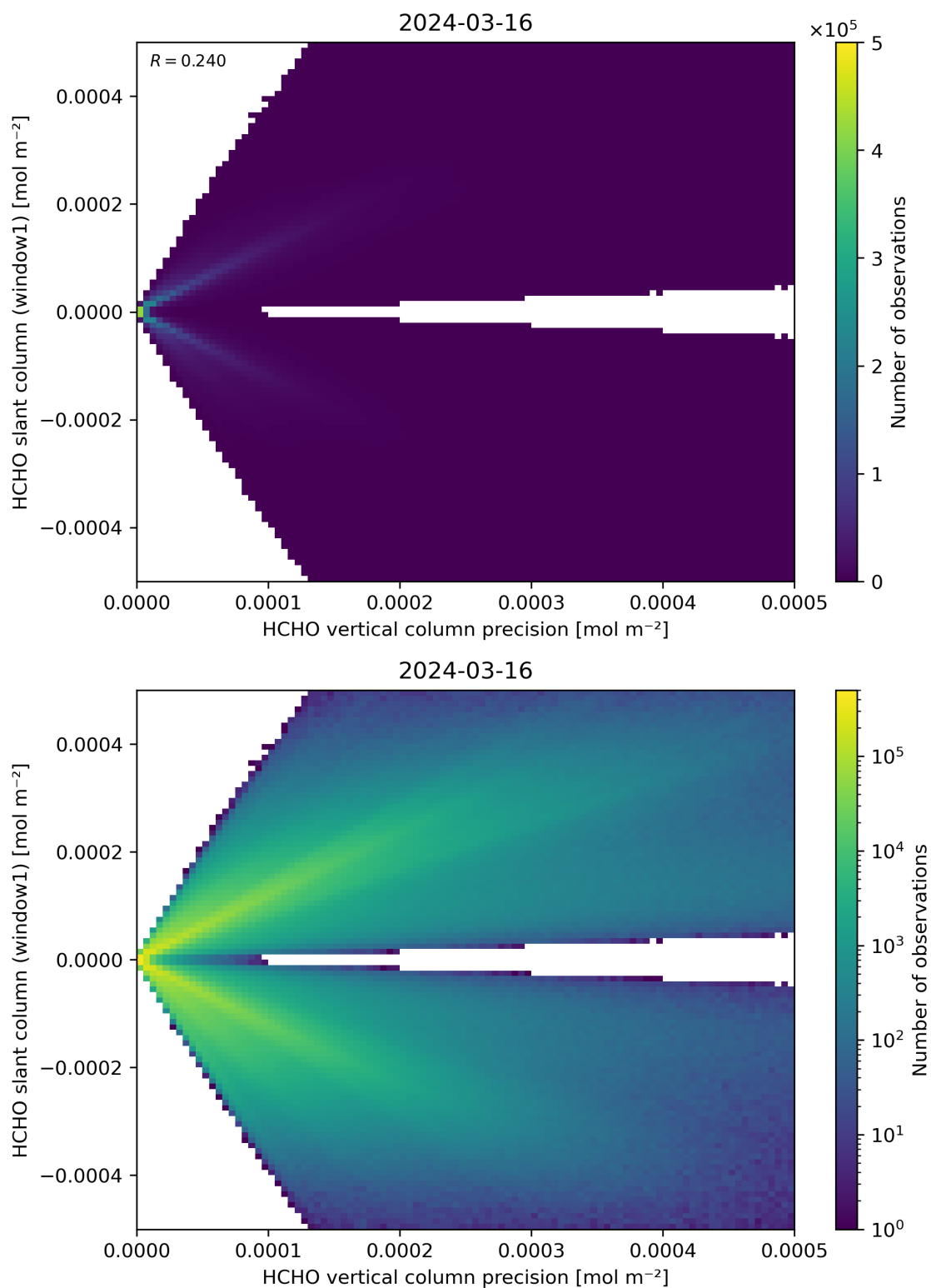
Figure 142: Scatter density plot of “HCHO vertical column precision” against “HCHO slant column (window1)” for 2024-03-15 to 2024-03-17.
