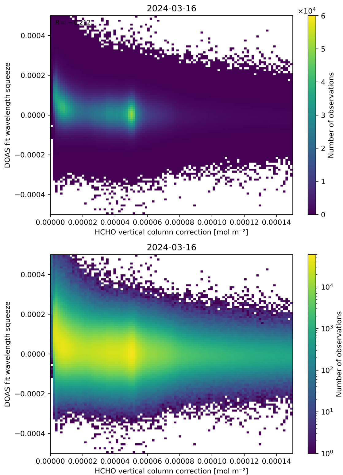
Figure 114: Scatter density plot of “HCHO vertical column correction” against “DOAS fit wavelength squeeze” for 2024-03-15 to 2024-03-17.
