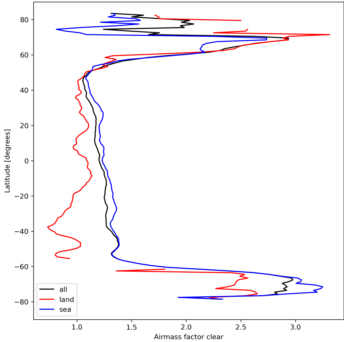
Figure 28: Zonal average of “Airmass factor clear” for 2024-03-15 to 2024-03-17.
