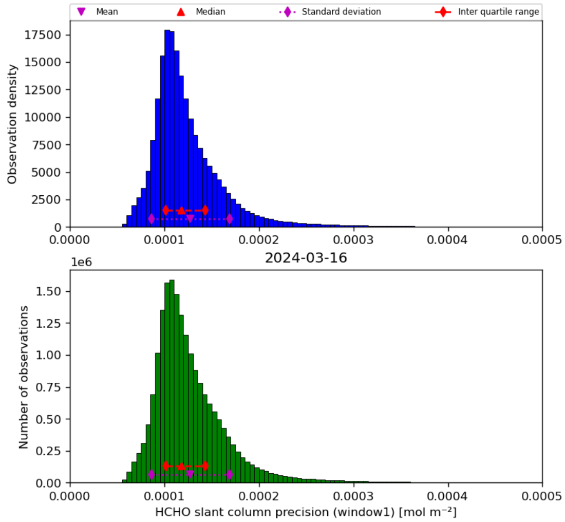
Figure 39: Histogram of “HCHO slant column precision (window1)” for 2024-03-15 to 2024-03-17
