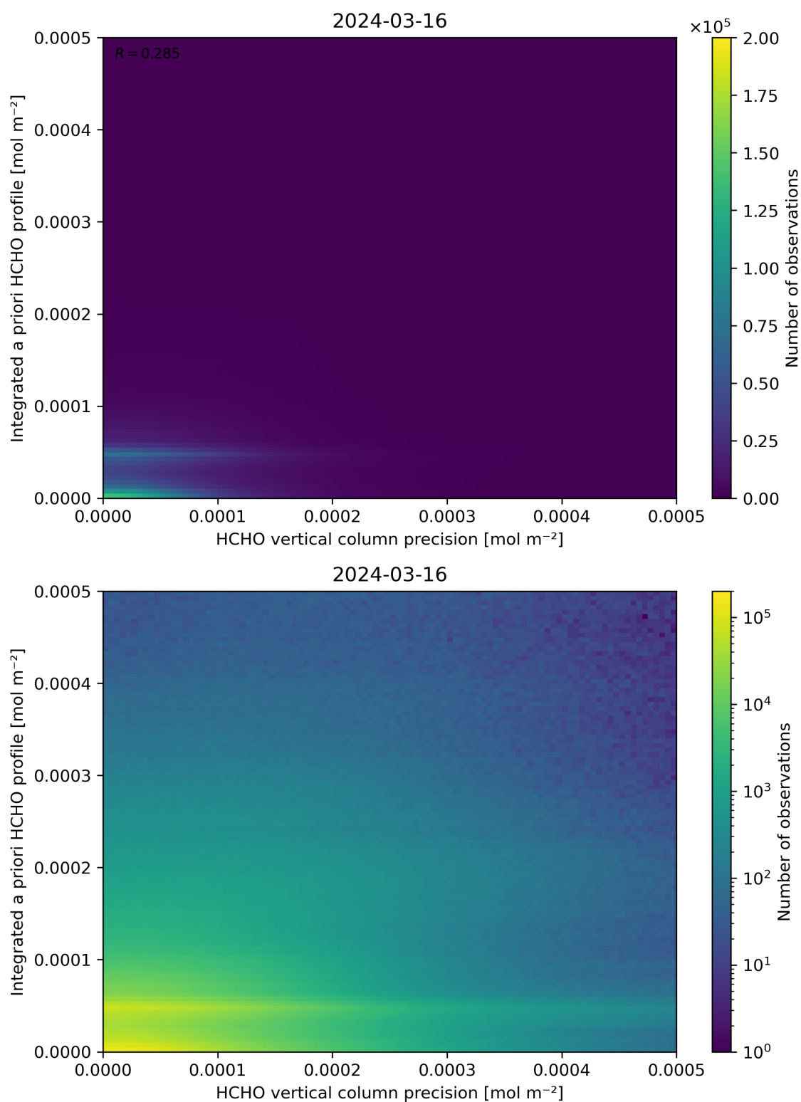
Figure 147: Scatter density plot of “HCHO vertical column precision” against “Integrated a priori HCHO profile” for 2024-03-15 to 2024-03-17.
