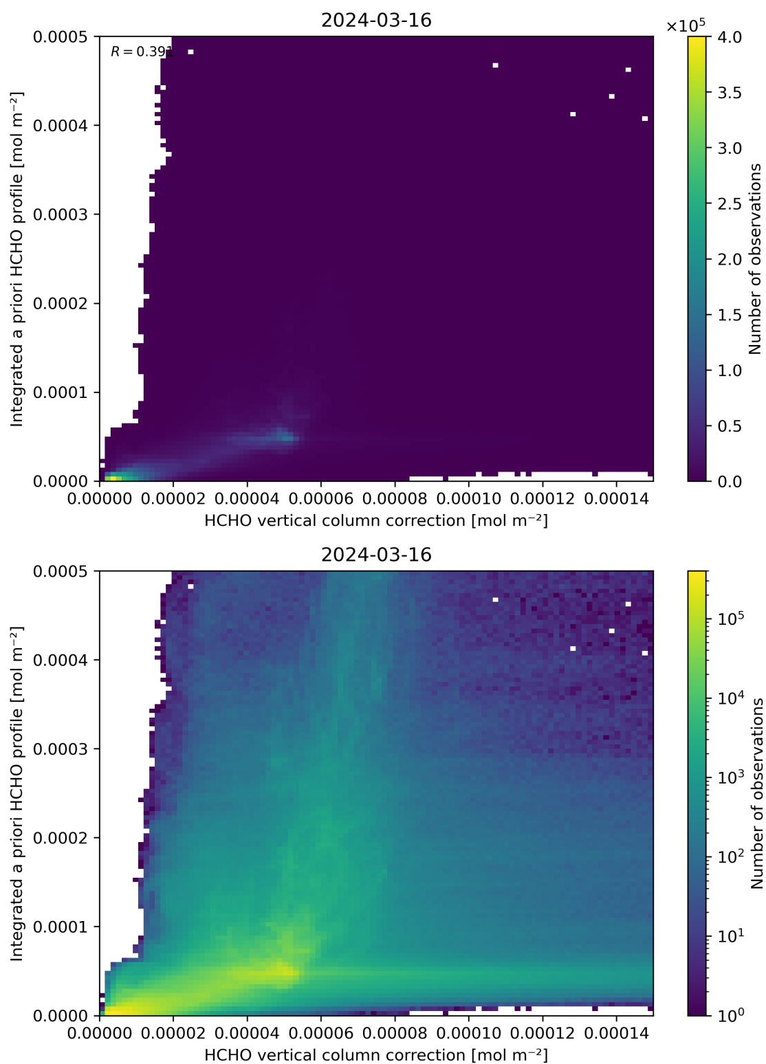
Figure 122: Scatter density plot of “HCHO vertical column correction” against “Integrated a priori HCHO profile” for 2024-03-15 to 2024-03-17.
