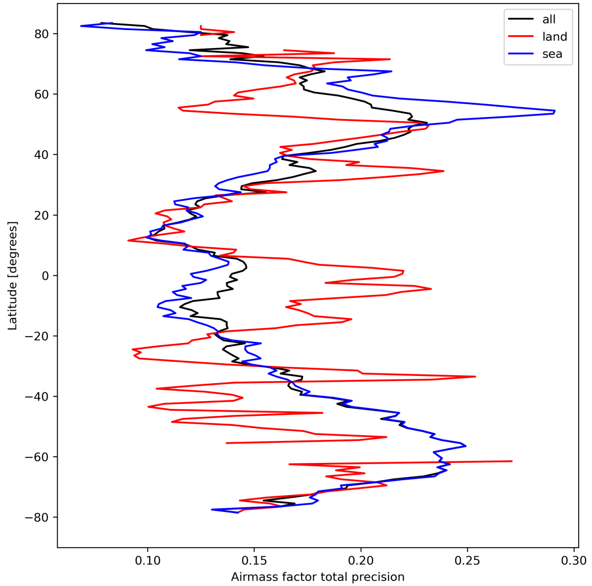
Figure 27: Zonal average of “Airmass factor total precision” for 2024-03-15 to 2024-03-17.
