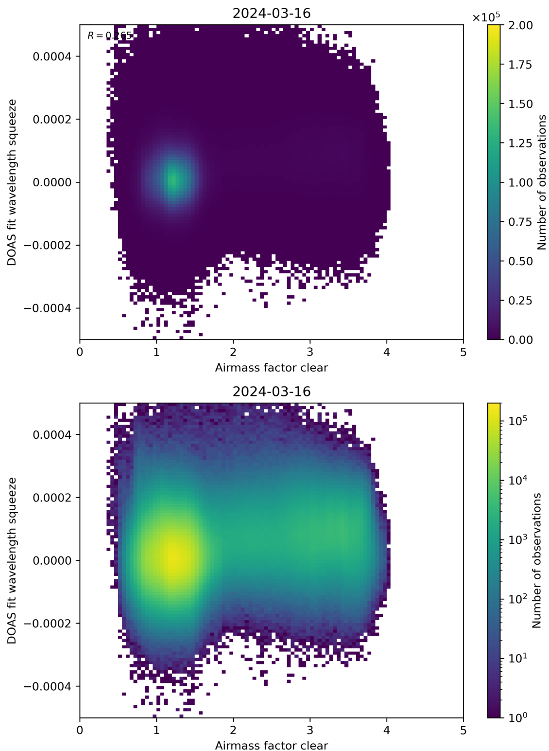
Figure 73: Scatter density plot of “Airmass factor clear” against “DOAS fit wavelength squeeze” for 2024-03-15 to 2024-03-17.
