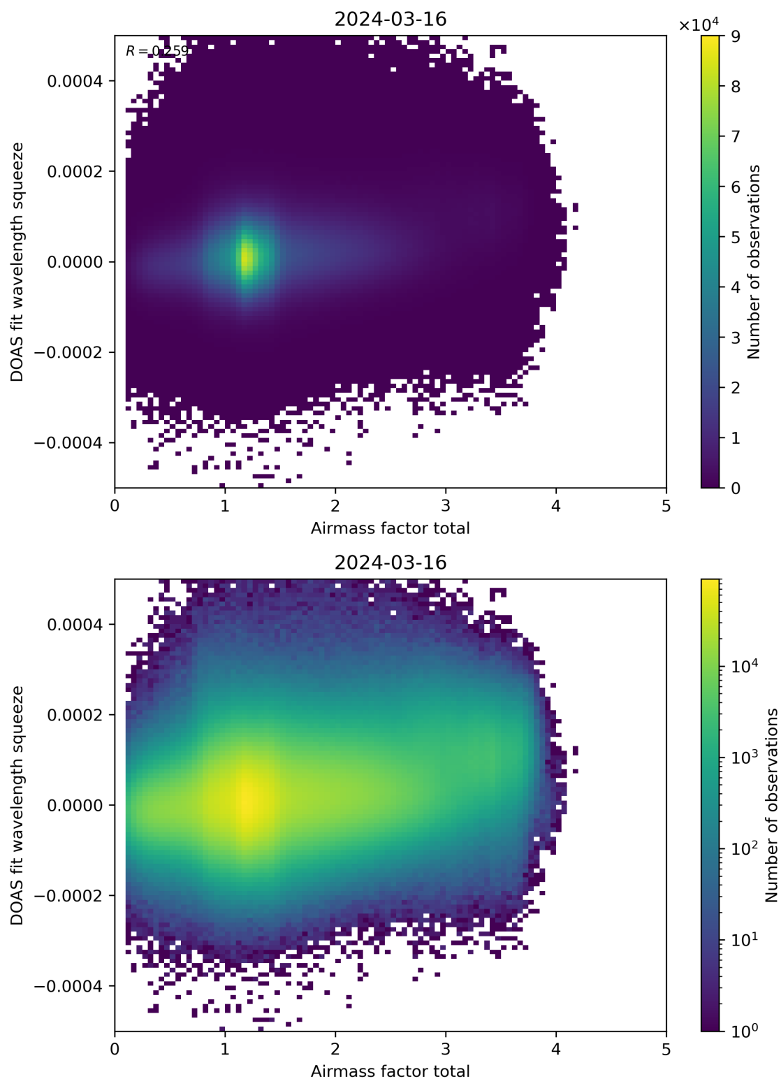
Figure 99: Scatter density plot of “Airmass factor total” against “DOAS fit wavelength squeeze” for 2024-03-15 to 2024-03-17.
