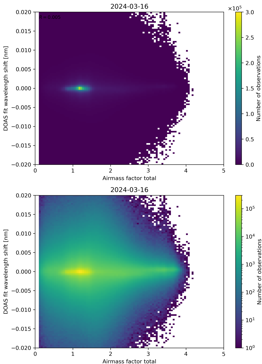
Figure 98: Scatter density plot of “Airmass factor total” against “DOAS fit wavelength shift” for 2024-03-15 to 2024-03-17.
