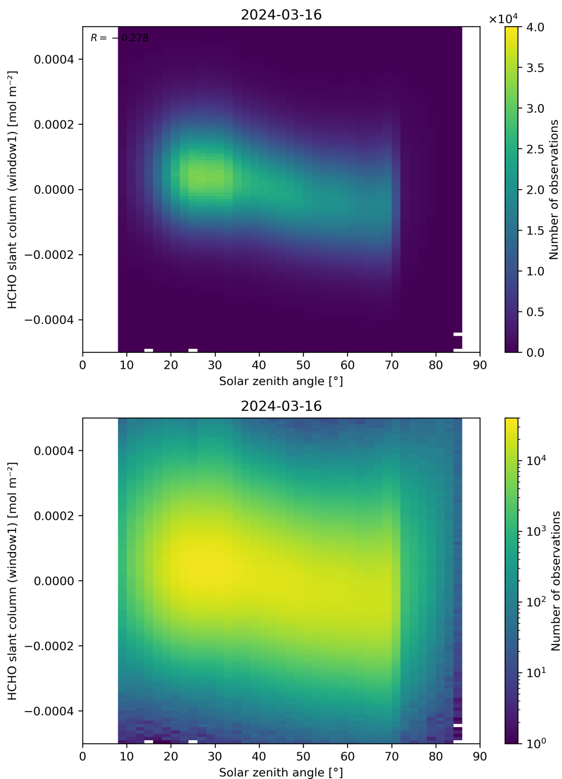
Figure 173: Scatter density plot of “Solar zenith angle” against “HCHO slant column (window1)” for 2024-03-15 to 2024-03-17.
