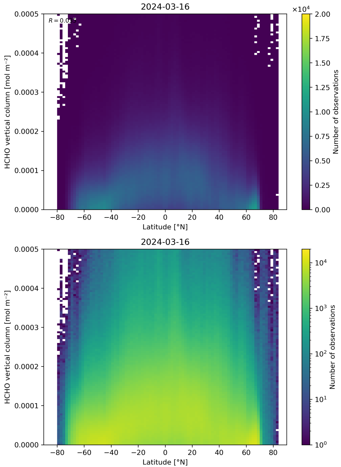
Figure 163: Scatter density plot of “Latitude” against “HCHO vertical column” for 2024-03-15 to 2024-03-17.
