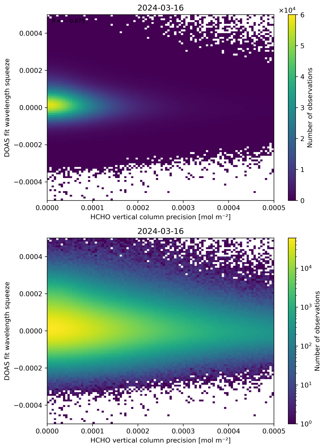
Figure 138: Scatter density plot of “HCHO vertical column precision” against “DOAS fit wavelength squeeze” for 2024-03-15 to 2024-03-17.
