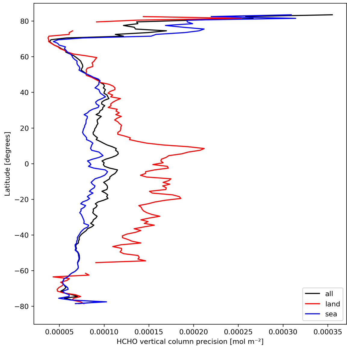
Figure 22: Zonal average of “HCHO vertical column precision” for 2024-03-15 to 2024-03-17.
