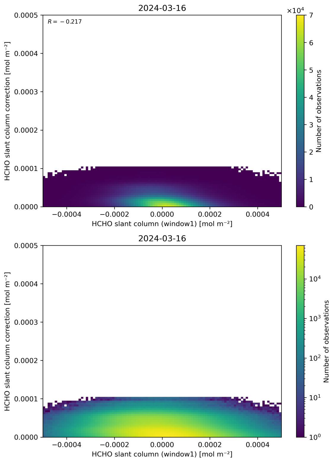
Figure 83: Scatter density plot of “HCHO slant column (window1)” against “HCHO slant column correction” for 2024-03-15 to 2024-03-17.
