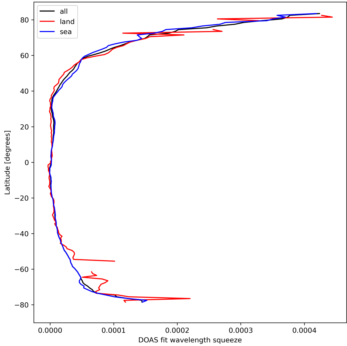
Figure 31: Zonal average of “DOAS fit wavelength squeeze” for 2024-03-15 to 2024-03-17.
