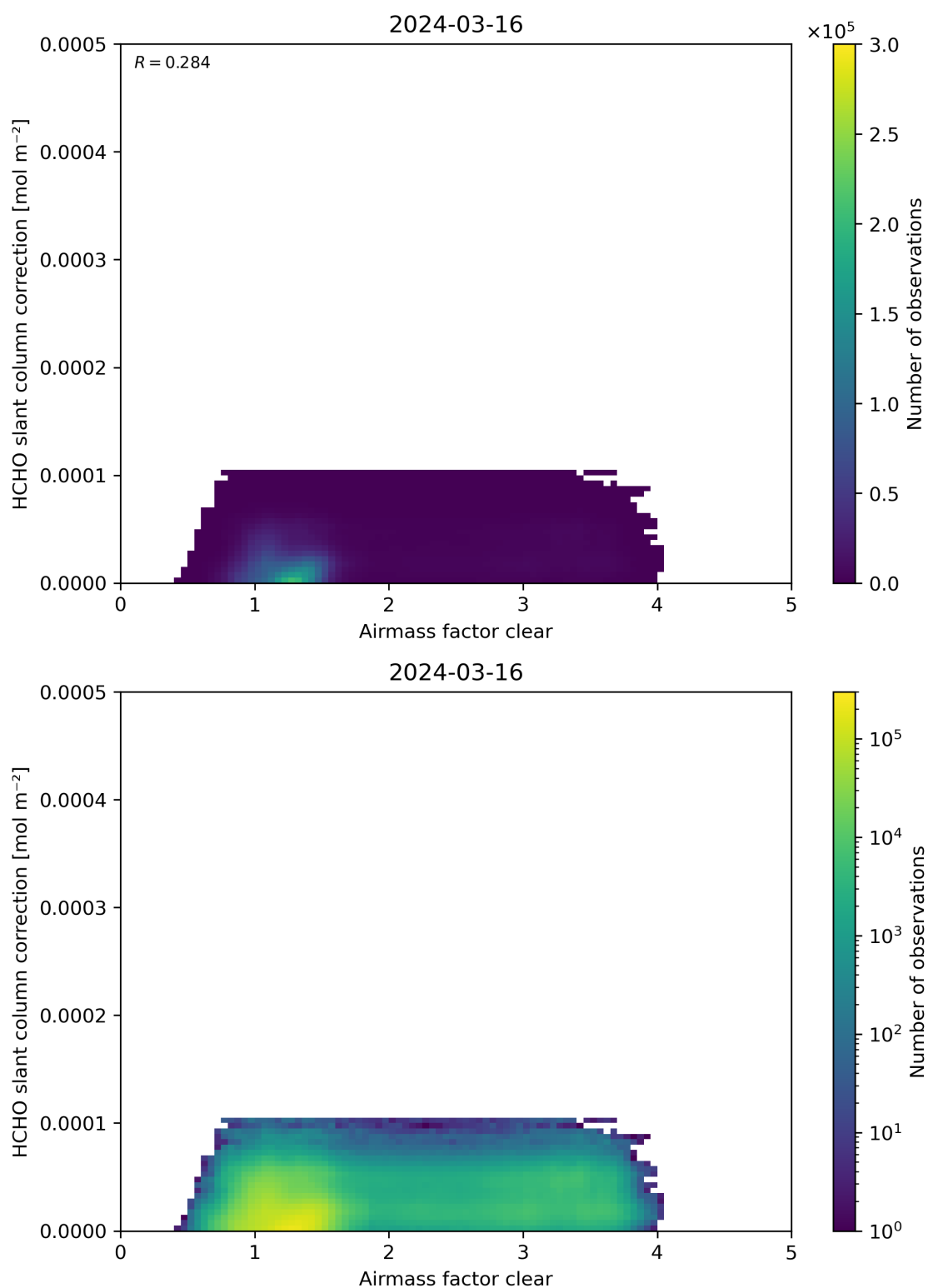
Figure 75: Scatter density plot of “Airmass factor clear” against “HCHO slant column correction” for 2024-03-15 to 2024-03-17.
