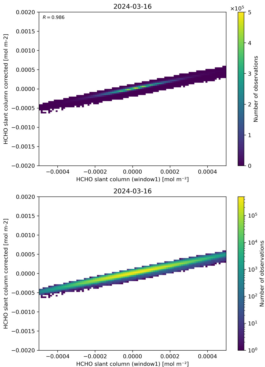
Figure 82: Scatter density plot of “HCHO slant column (window1)” against “HCHO slant column corrected” for 2024-03-15 to 2024-03-17.
