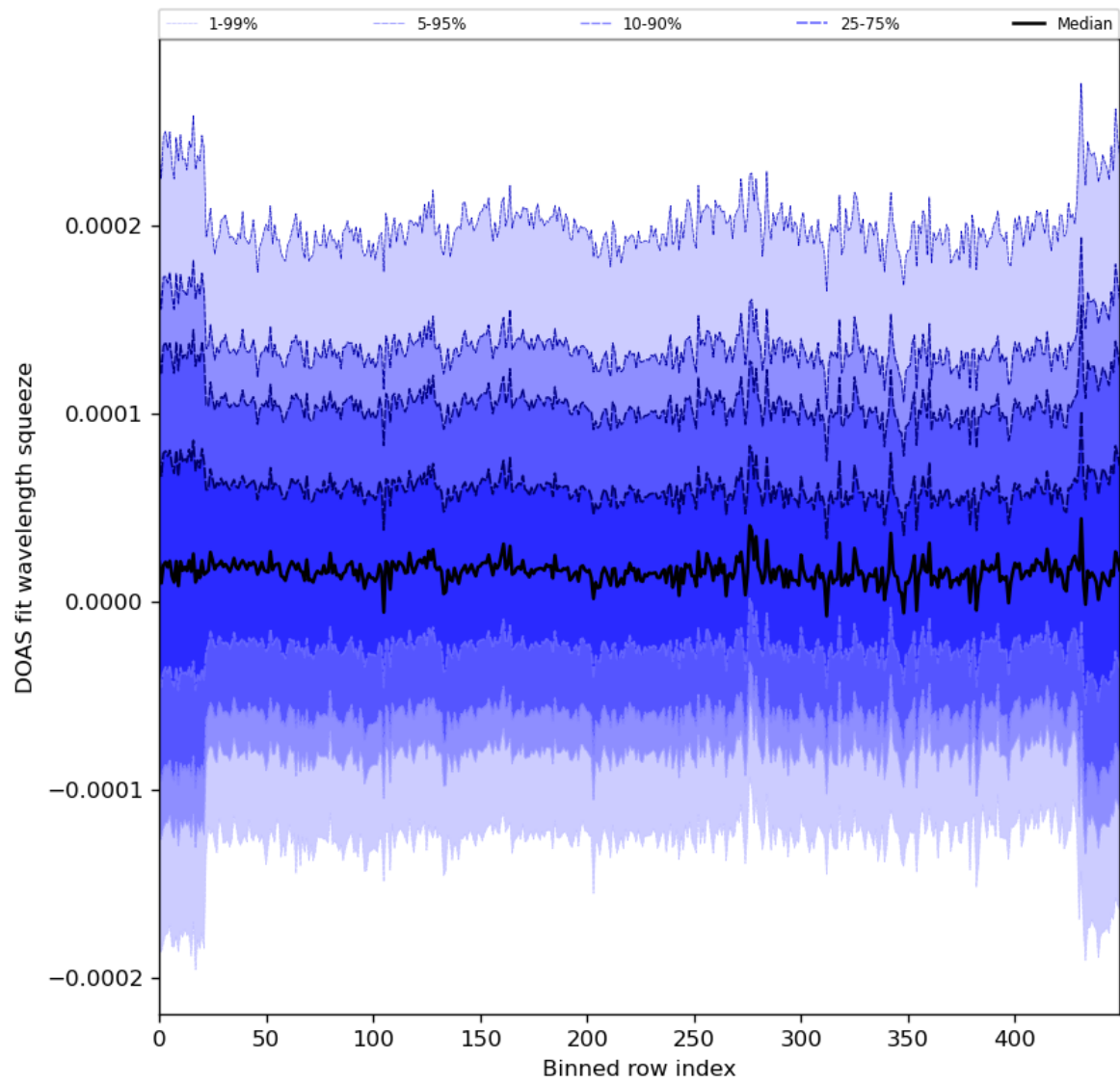
Figure 59: Along track statistics of “DOAS fit wavelength squeeze” for 2024-03-15 to 2024-03-17
