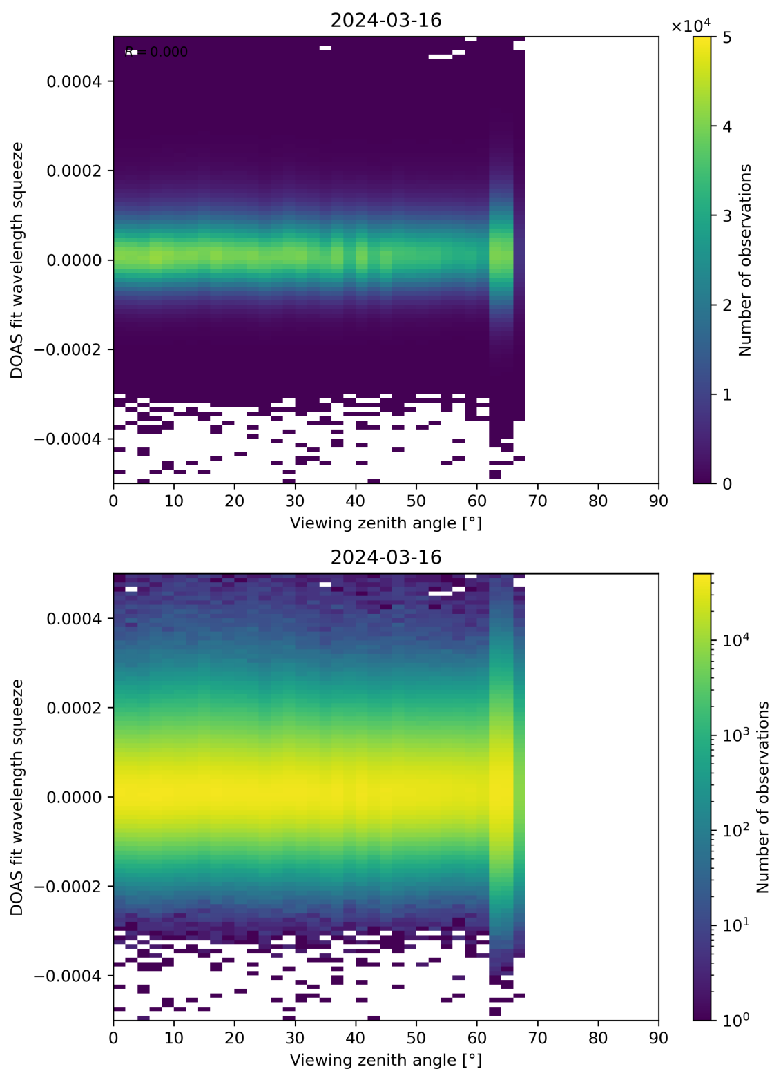
Figure 184: Scatter density plot of “Viewing zenith angle” against “DOAS fit wavelength squeeze” for 2024-03-15 to 2024-03-17.
