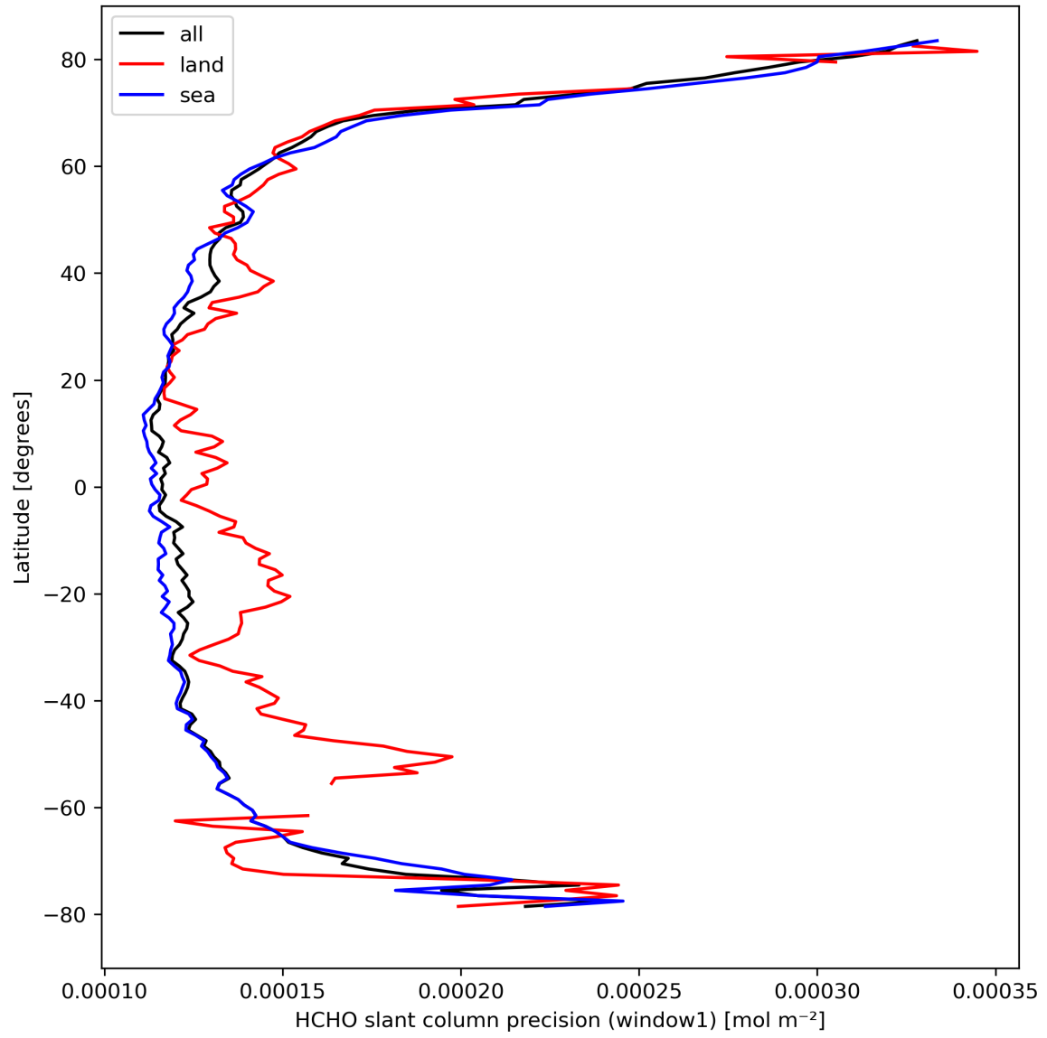
Figure 25: Zonal average of “HCHO slant column precision (window1)” for 2024-03-15 to 2024-03-17.
