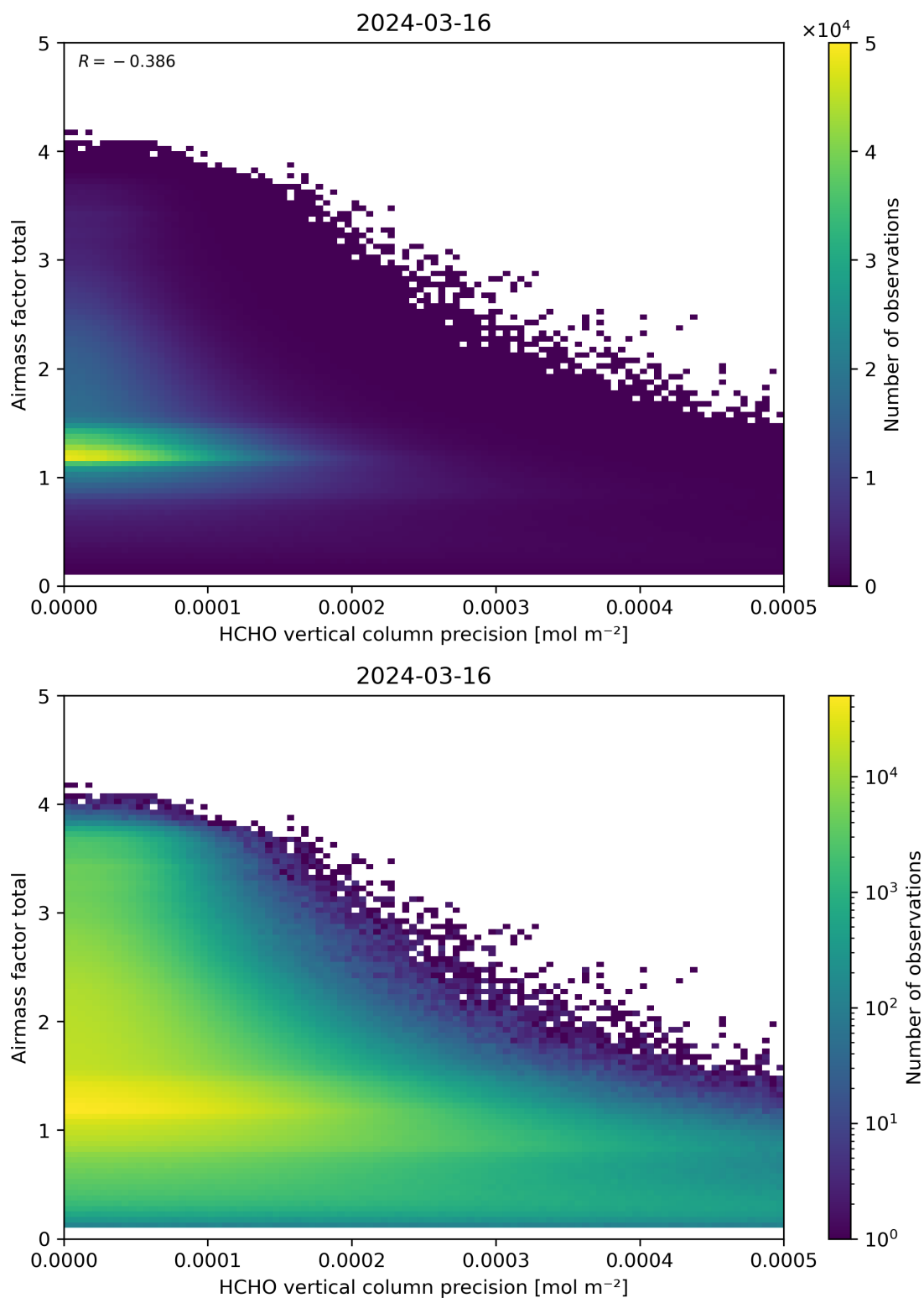
Figure 144: Scatter density plot of “HCHO vertical column precision” against “Airmass factor total” for 2024-03-15 to 2024-03-17.
