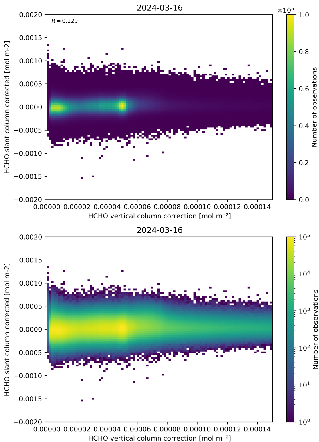
Figure 116: Scatter density plot of “HCHO vertical column correction” against “HCHO slant column corrected” for 2024-03-15 to 2024-03-17.
