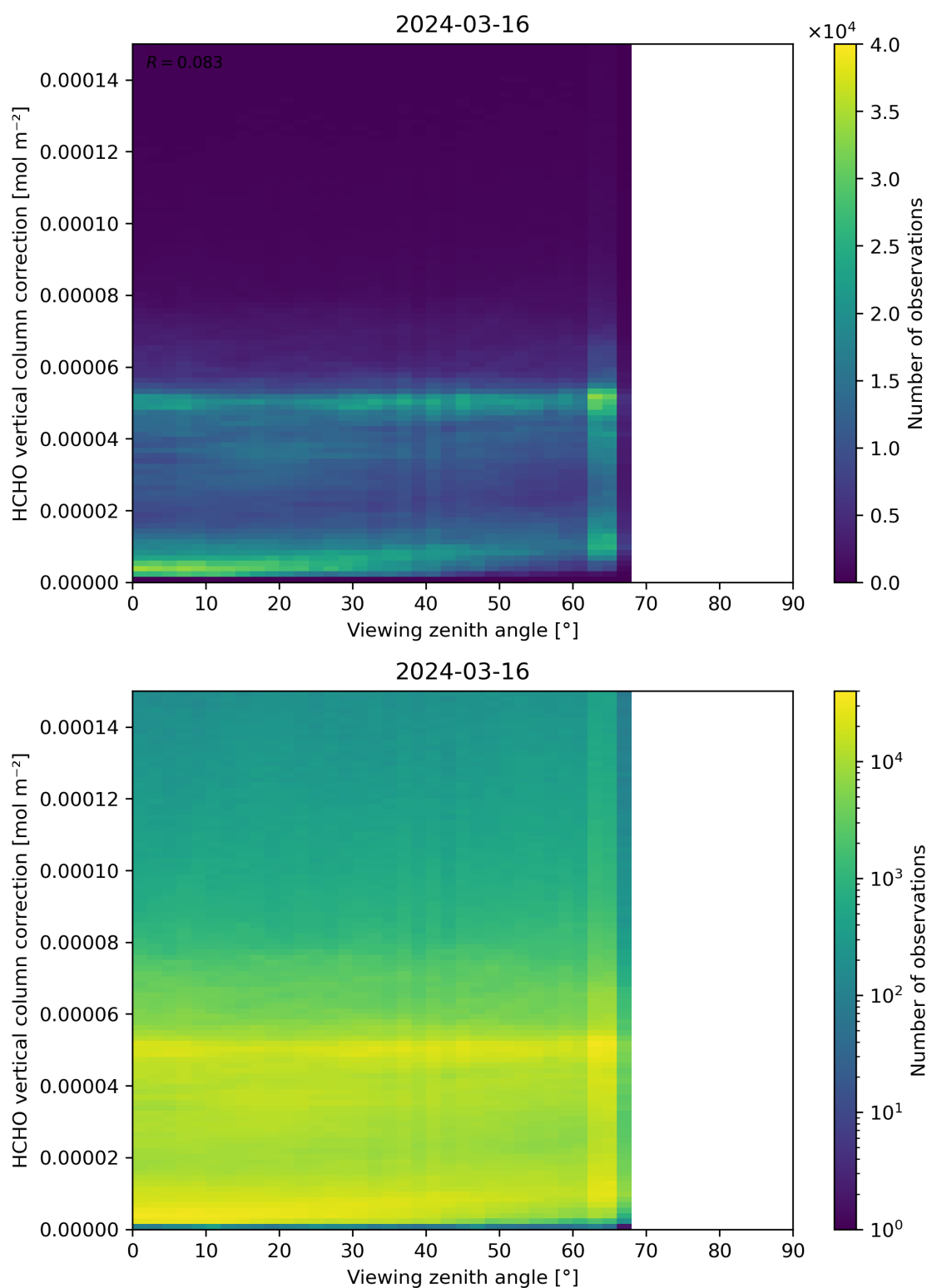
Figure 193: Scatter density plot of “Viewing zenith angle” against “HCHO vertical column correction” for 2024-03-15 to 2024-03-17.
