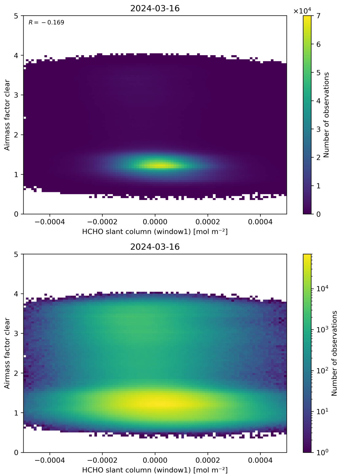
Figure 81: Scatter density plot of “HCHO slant column (window1)” against “Airmass factor clear” for 2024-03-15 to 2024-03-17.
