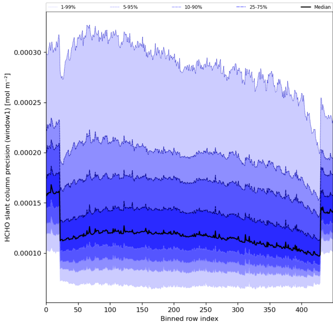
Figure 53: Along track statistics of “HCHO slant column precision (window1)” for 2024-03-15 to 2024-03-17
