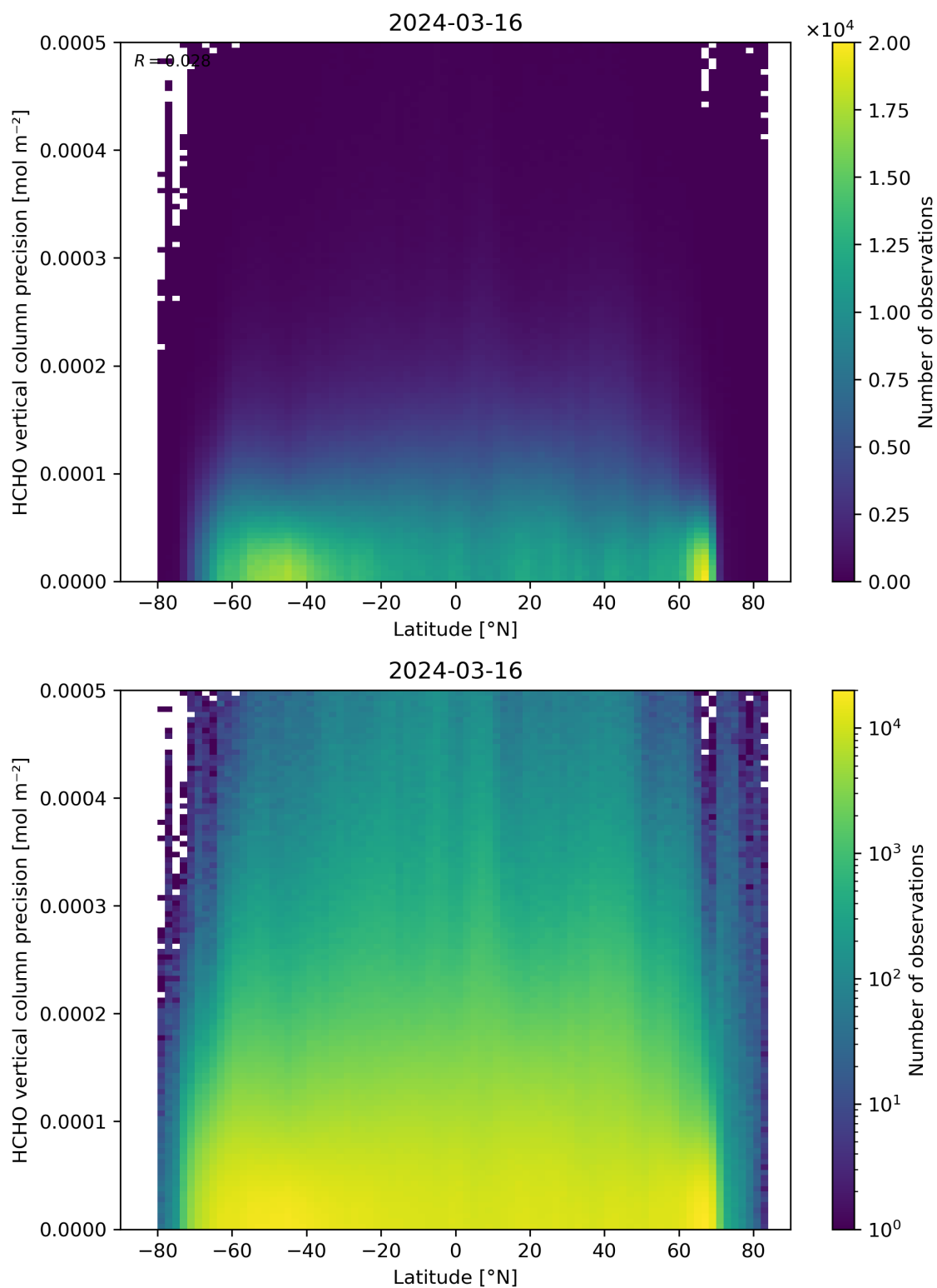
Figure 165: Scatter density plot of “Latitude” against “HCHO vertical column precision” for 2024-03-15 to 2024-03-17.
