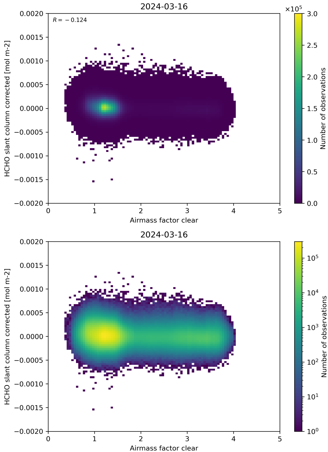
Figure 74: Scatter density plot of “Airmass factor clear” against “HCHO slant column corrected” for 2024-03-15 to 2024-03-17.
