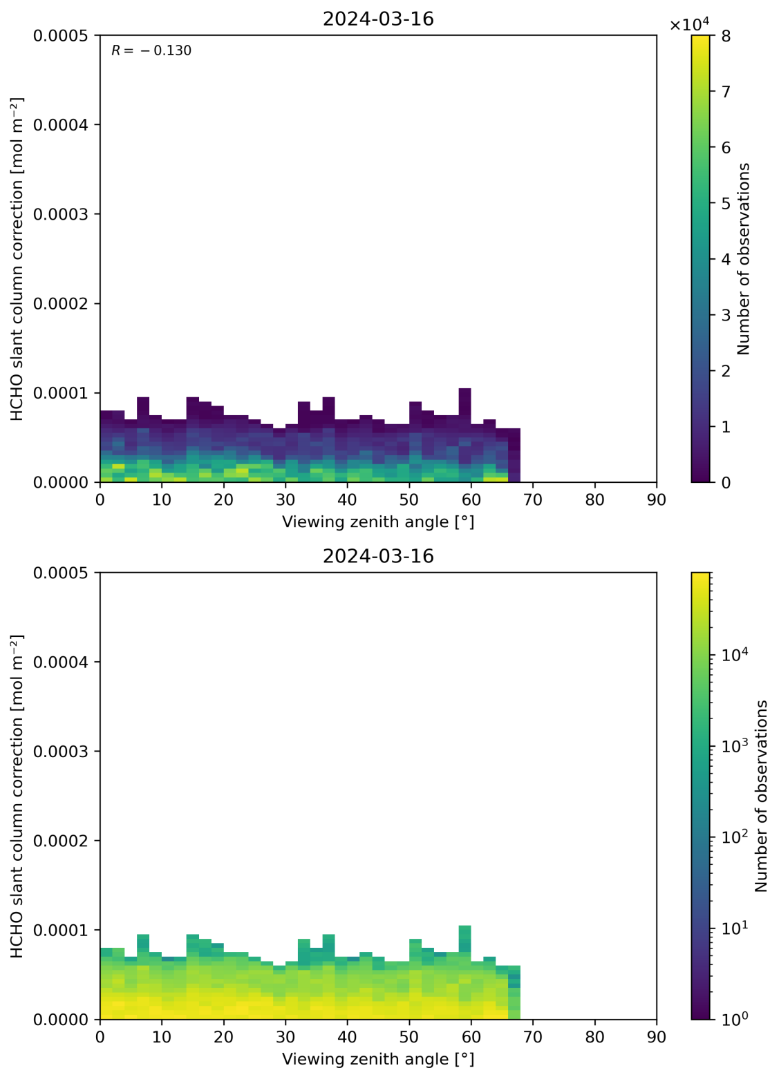
Figure 187: Scatter density plot of “Viewing zenith angle” against “HCHO slant column correction” for 2024-03-15 to 2024-03-17.
