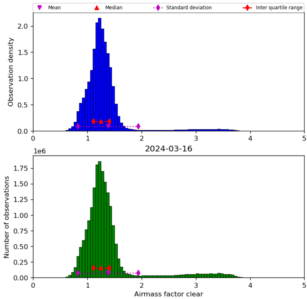
Figure 42: Histogram of “Airmass factor clear” for 2024-03-15 to 2024-03-17
