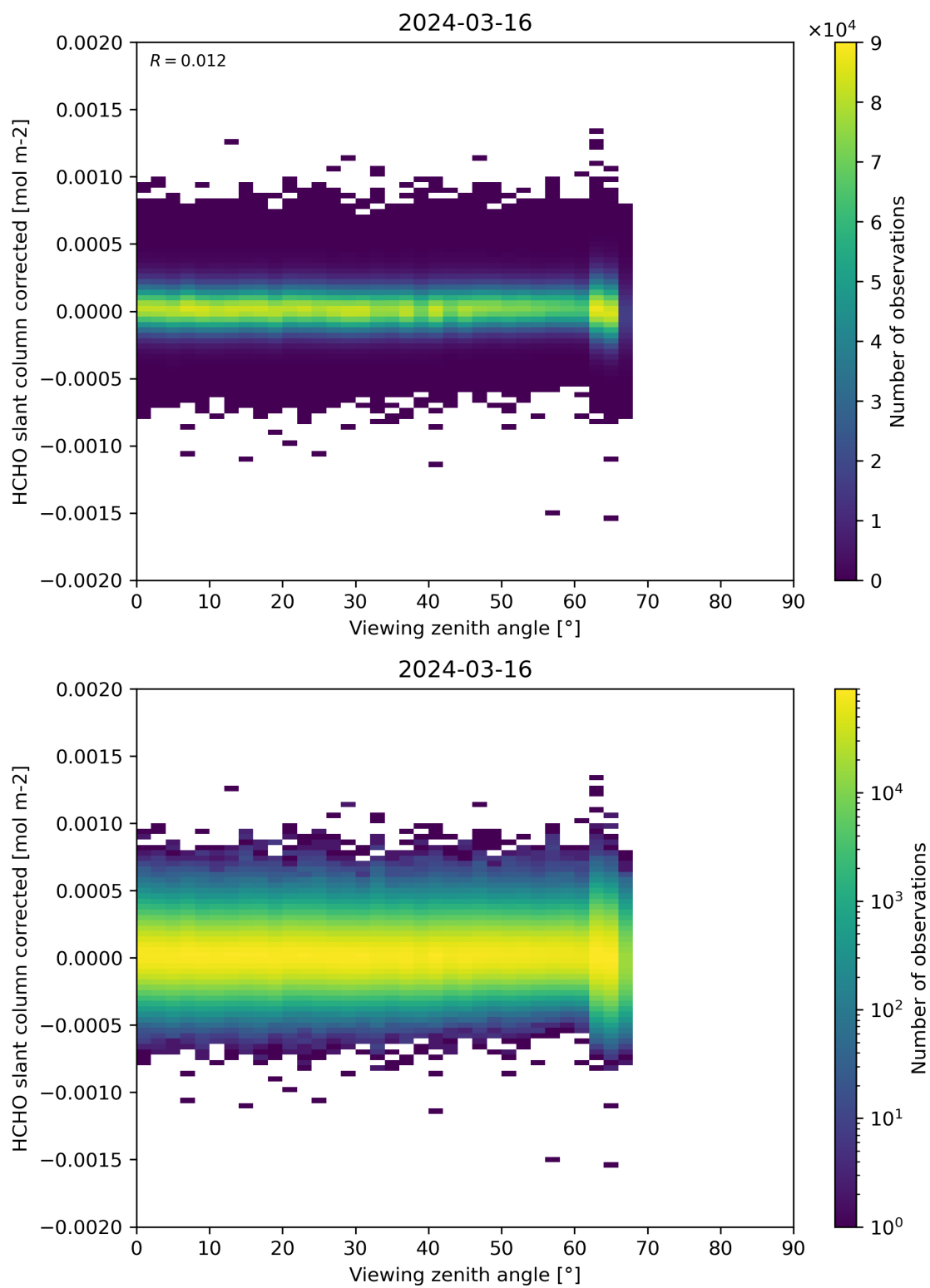
Figure 186: Scatter density plot of “Viewing zenith angle” against “HCHO slant column corrected” for 2024-03-15 to 2024-03-17.
