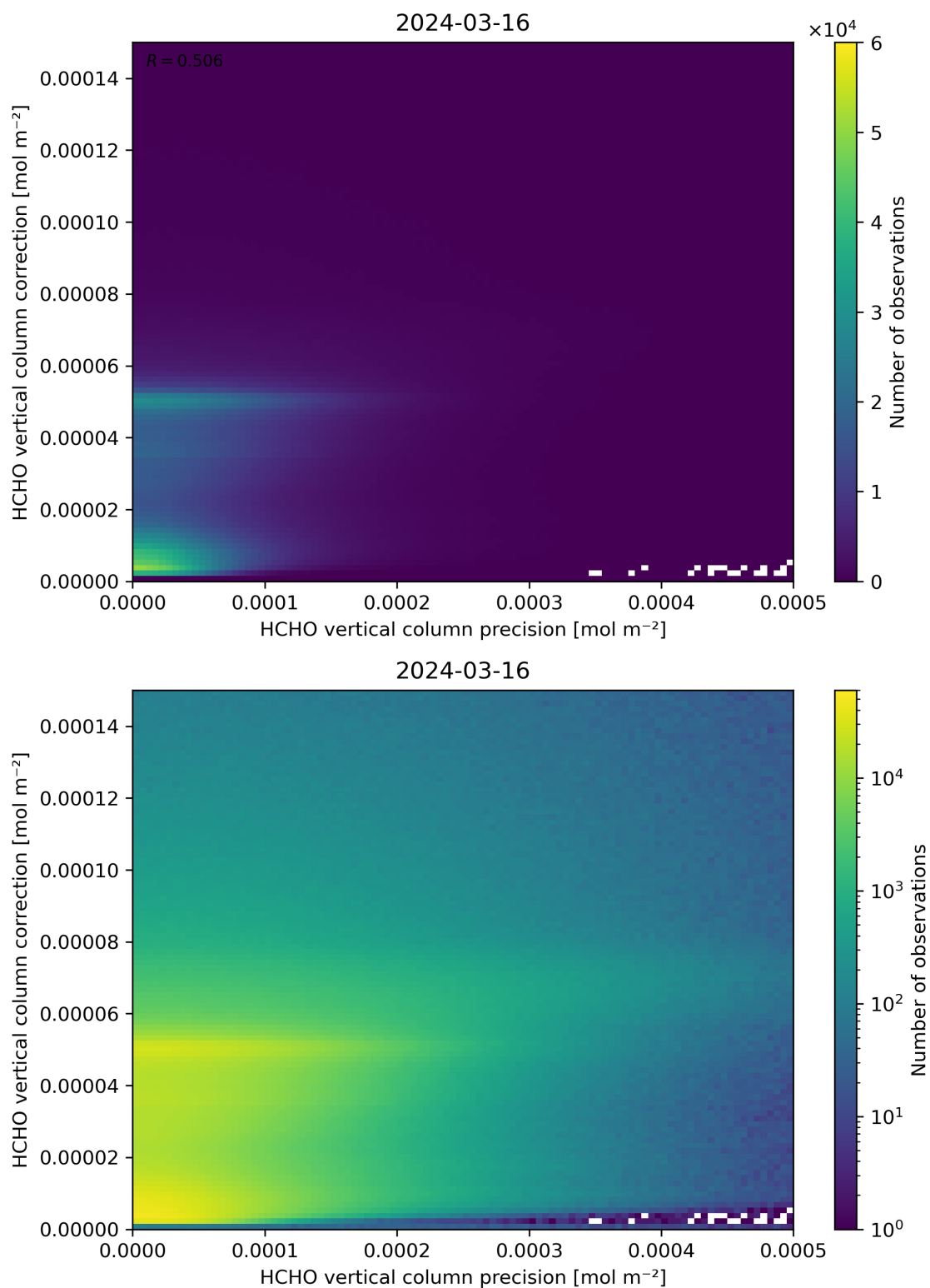
Figure 146: Scatter density plot of “HCHO vertical column precision” against “HCHO vertical column correction” for 2024-03-15 to 2024-03-17.
