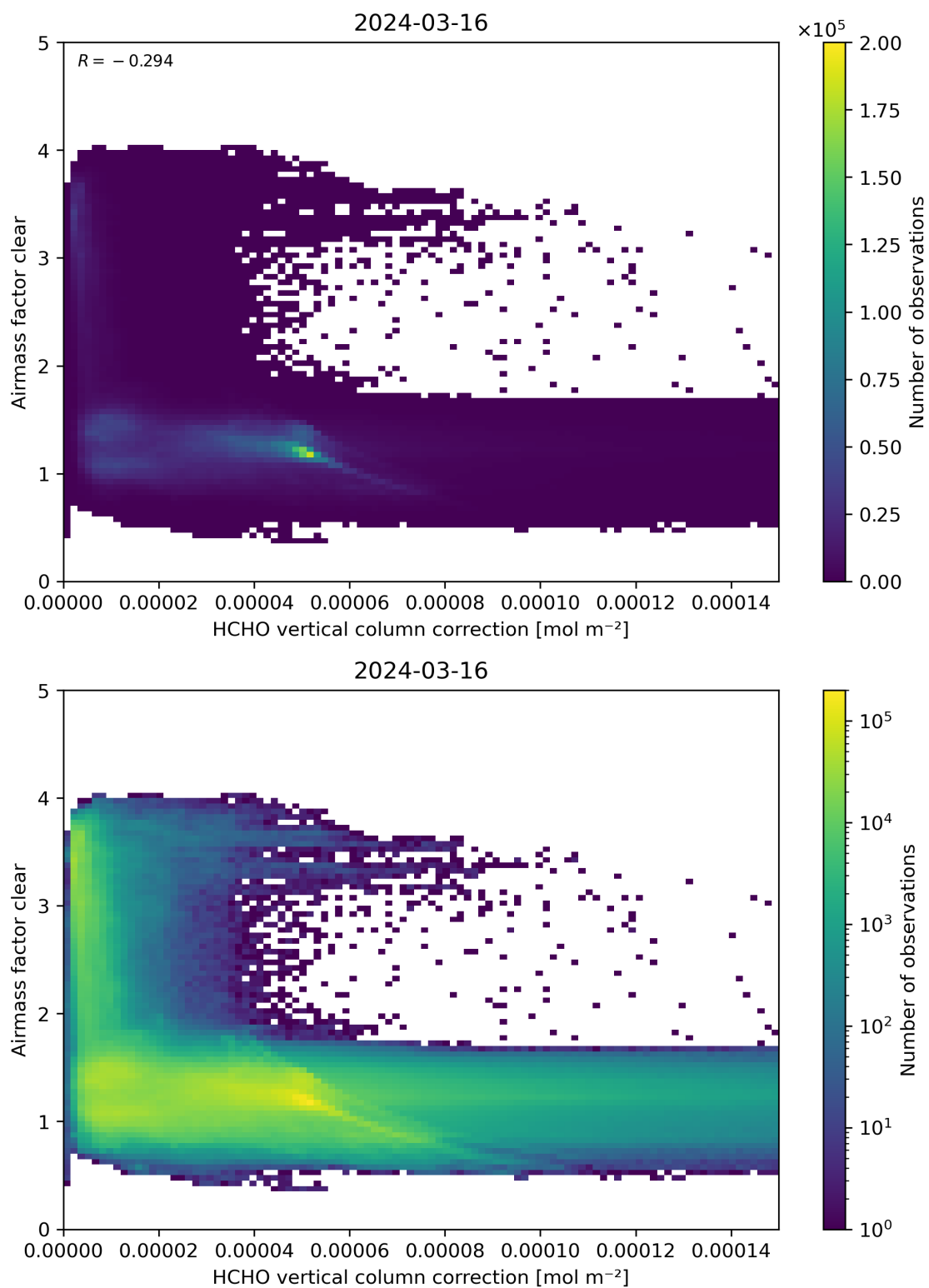
Figure 115: Scatter density plot of “HCHO vertical column correction” against “Airmass factor clear” for 2024-03-15 to 2024-03-17.
