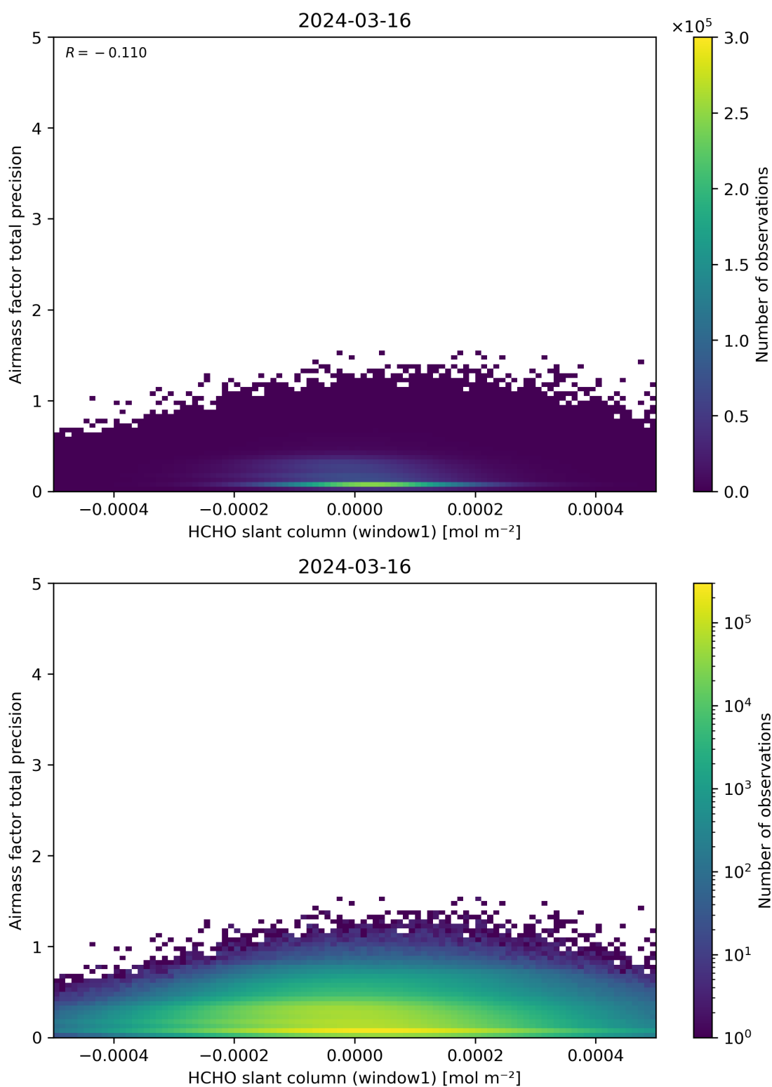
Figure 86: Scatter density plot of “HCHO slant column (window1)” against “Airmass factor total precision” for 2024-03-15 to 2024-03-17.
