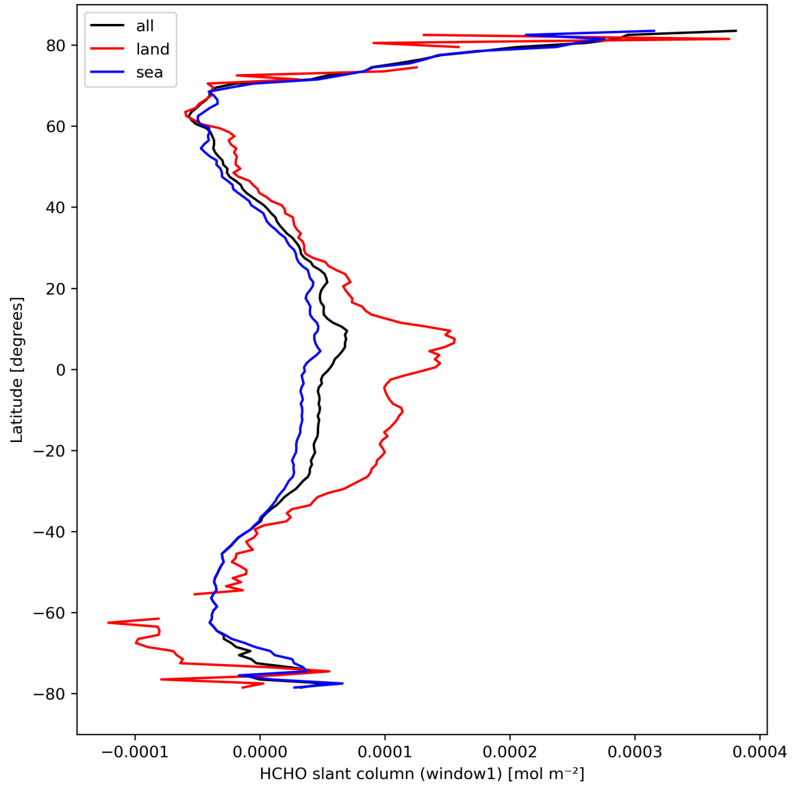
Figure 24: Zonal average of “HCHO slant column (window1)” for 2024-03-15 to 2024-03-17.
