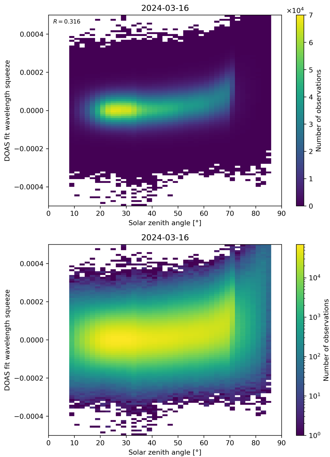
Figure 169: Scatter density plot of “Solar zenith angle” against “DOAS fit wavelength squeeze” for 2024-03-15 to 2024-03-17.
