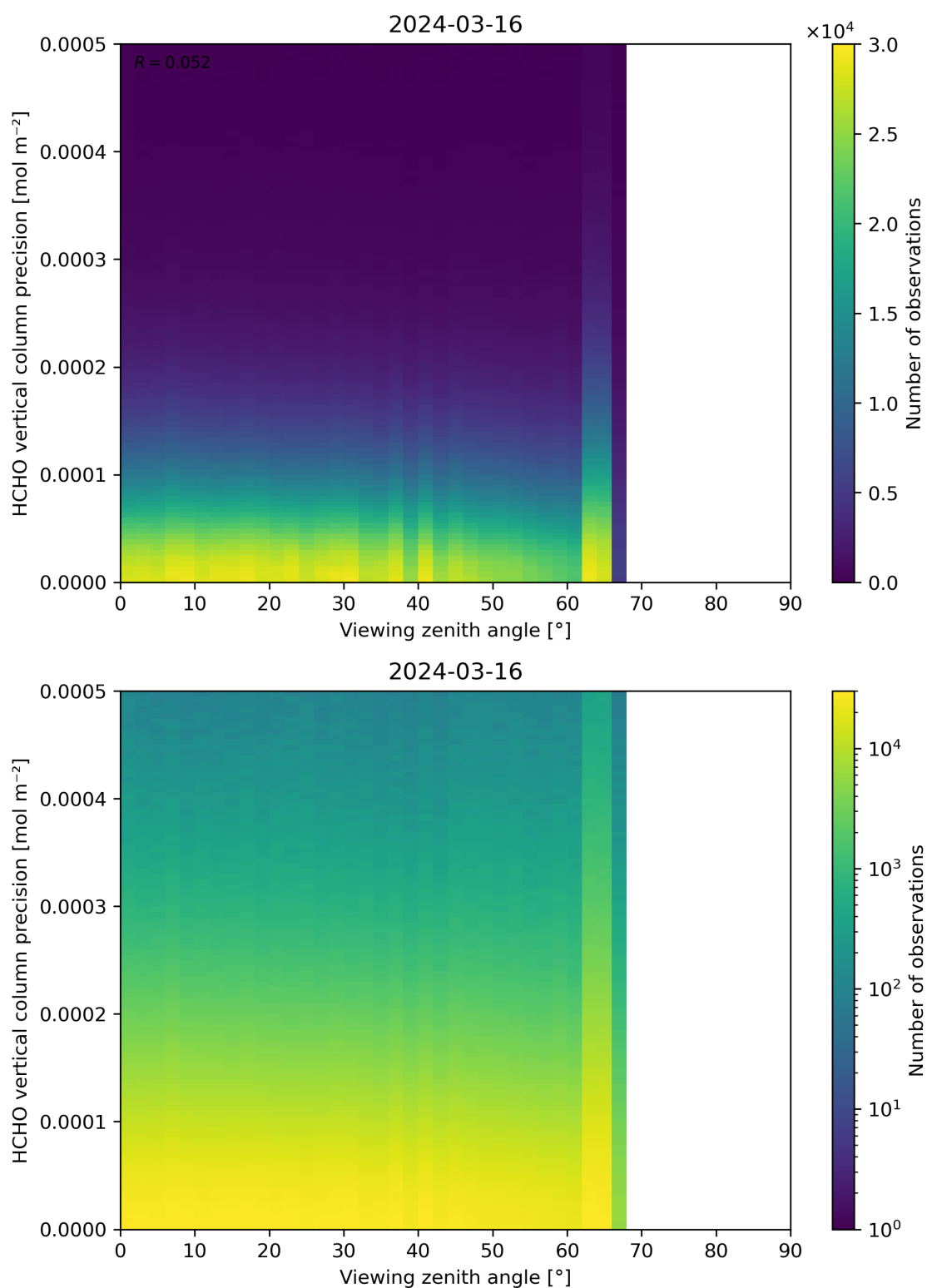
Figure 194: Scatter density plot of “Viewing zenith angle” against “HCHO vertical column precision” for 2024-03-15 to 2024-03-17.
