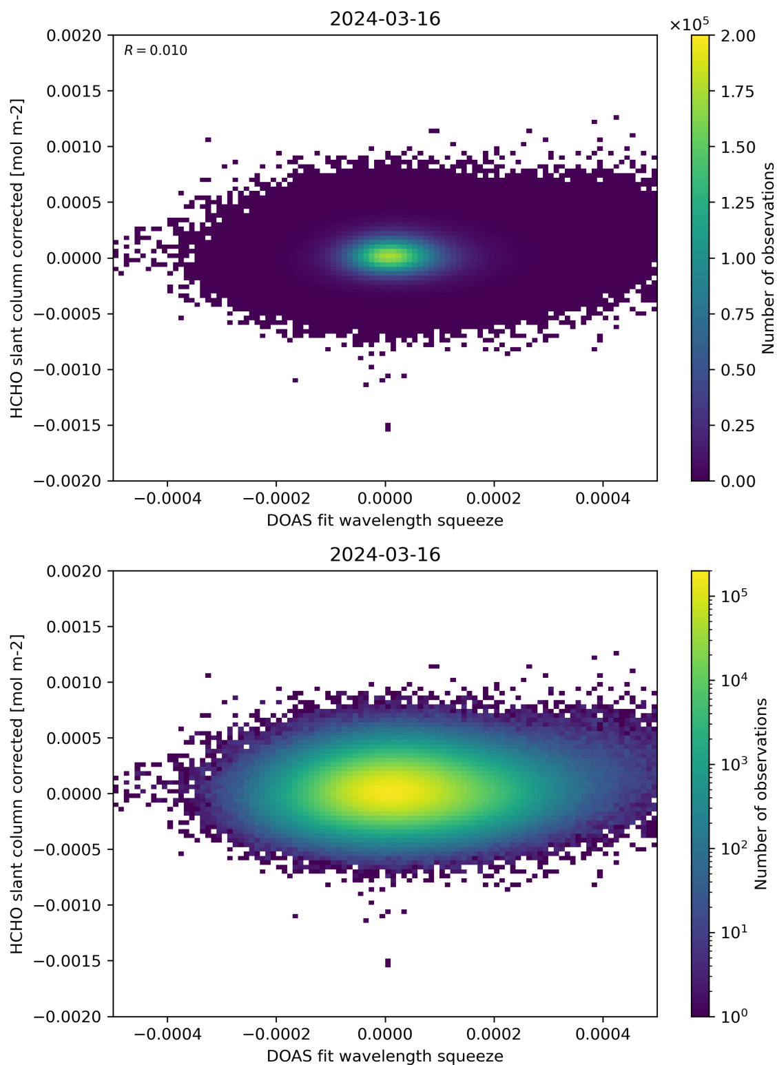
Figure 69: Scatter density plot of “DOAS fit wavelength squeeze” against “HCHO slant column corrected” for 2024-03-15 to 2024-03-17.
