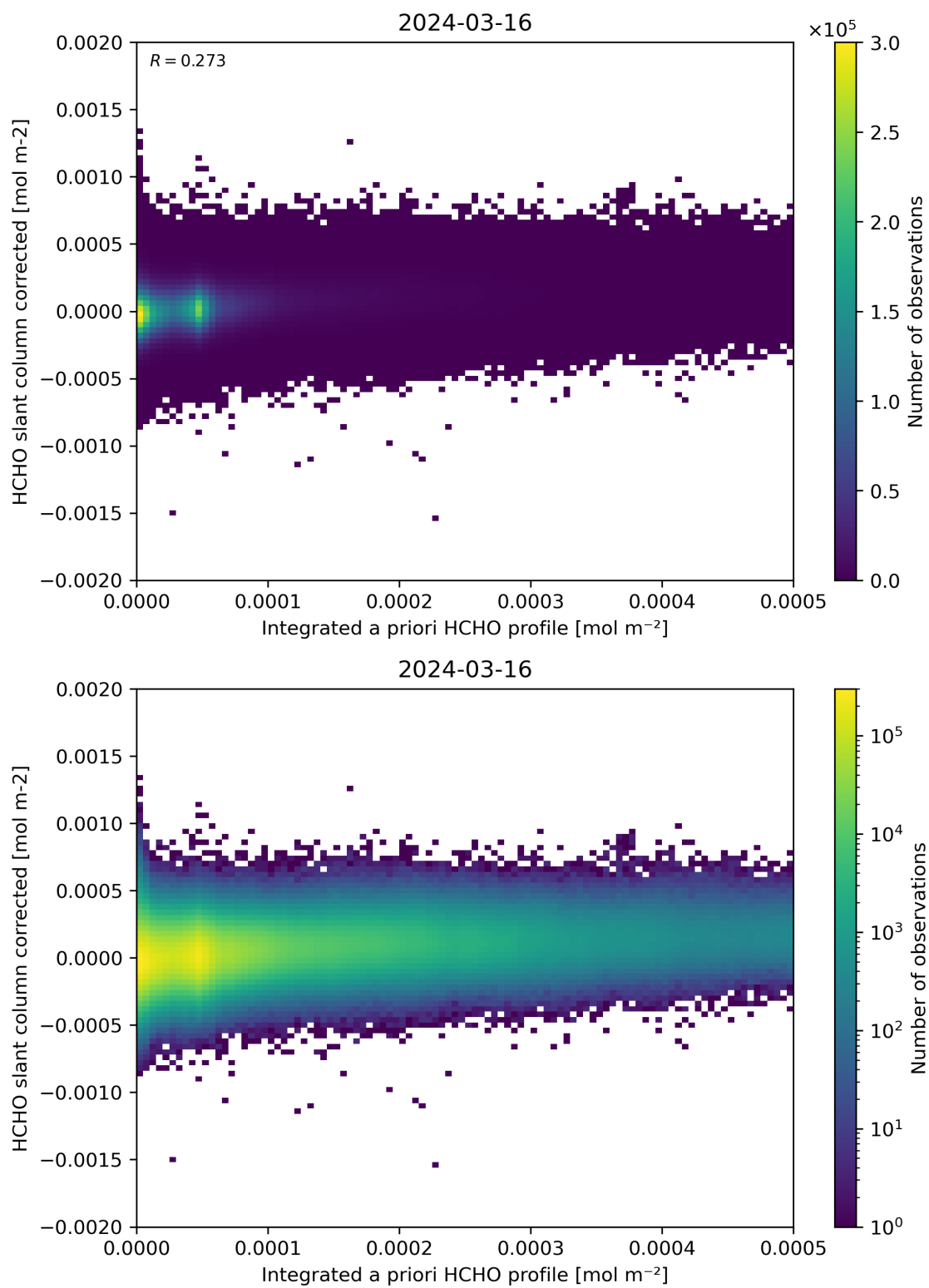
Figure 151: Scatter density plot of “Integrated a priori HCHO profile” against “HCHO slant column corrected” for 2024-03-15 to 2024-03-17.
