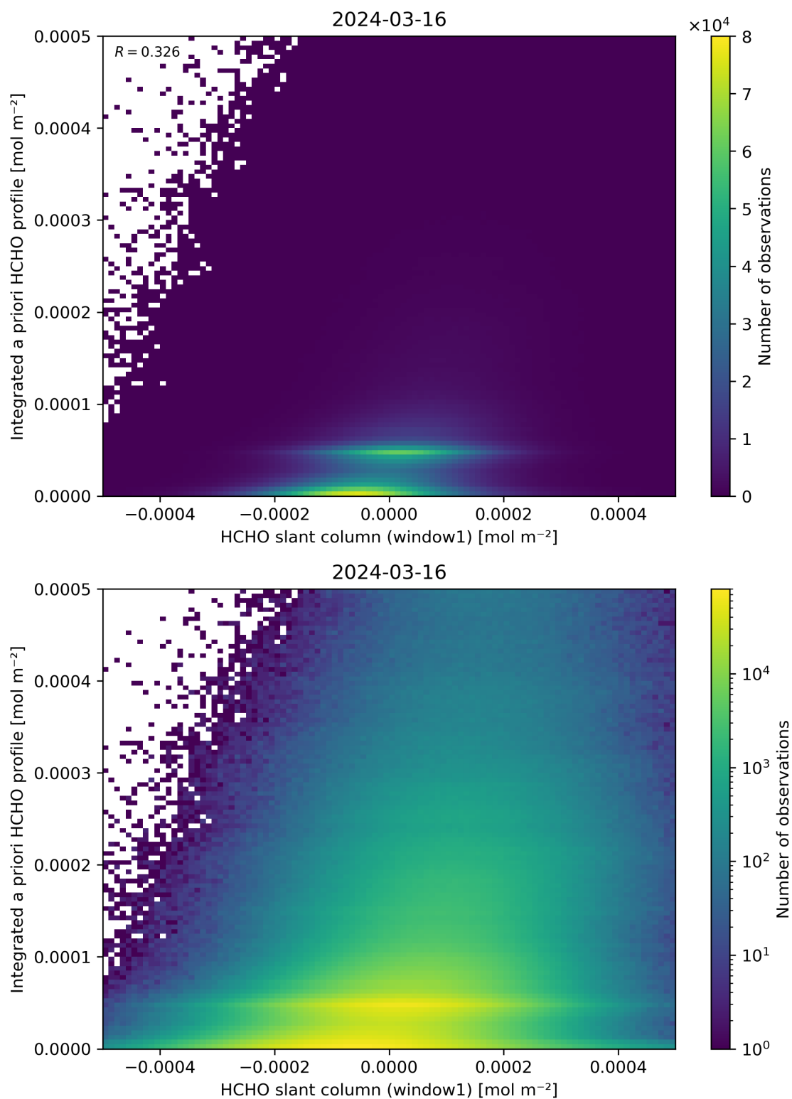
Figure 87: Scatter density plot of “HCHO slant column (window1)” against “Integrated a priori HCHO profile” for 2024-03-15 to 2024-03-17.
