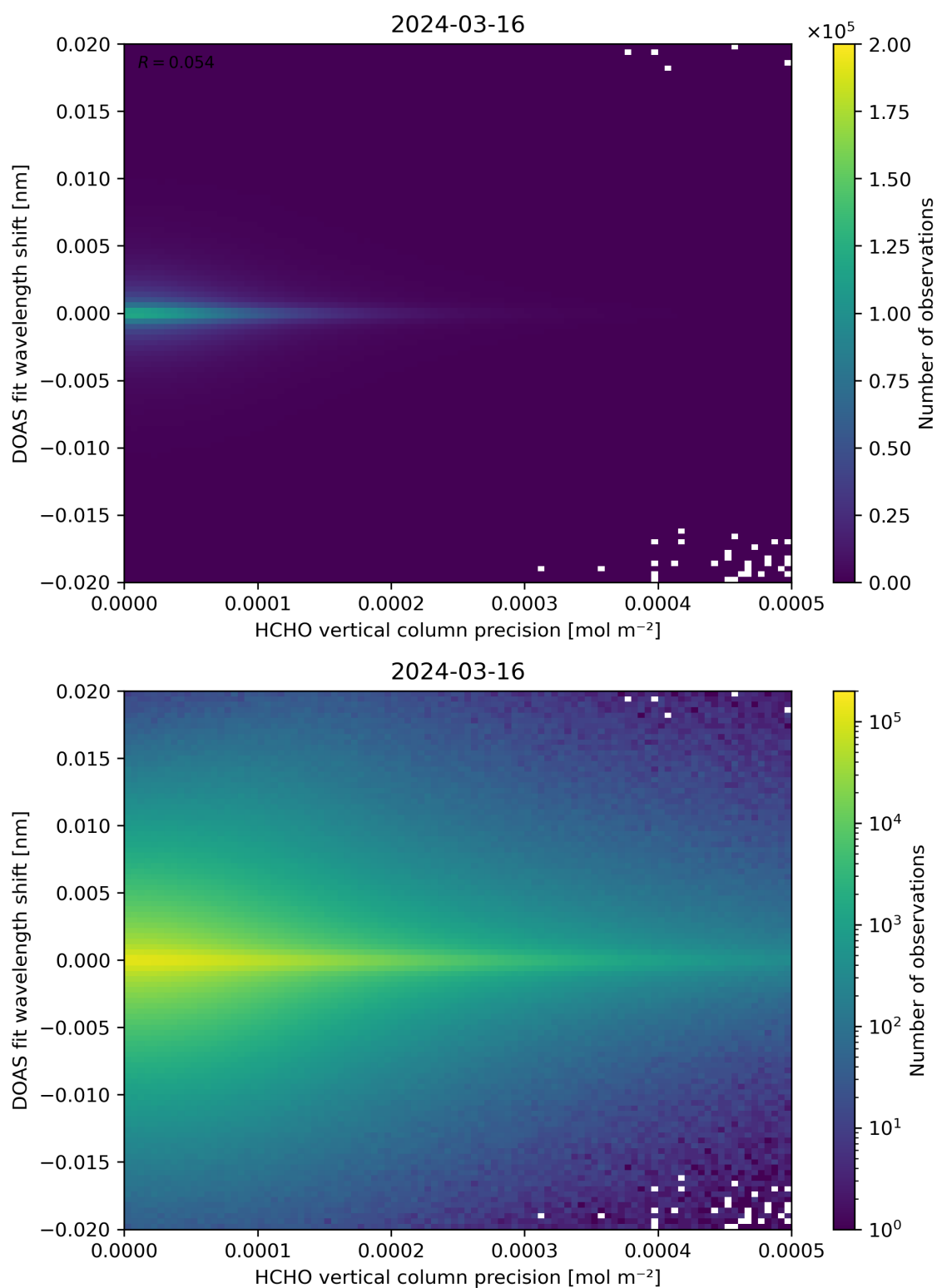
Figure 137: Scatter density plot of “HCHO vertical column precision” against “DOAS fit wavelength shift” for 2024-03-15 to 2024-03-17.
