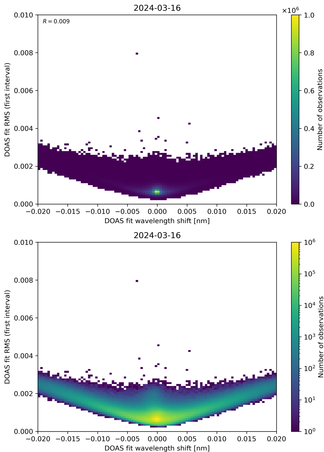
Figure 64: Scatter density plot of “DOAS fit wavelength shift” against “DOAS fit RMS (first interval)” for 2024-03-15 to 2024-03-17.
