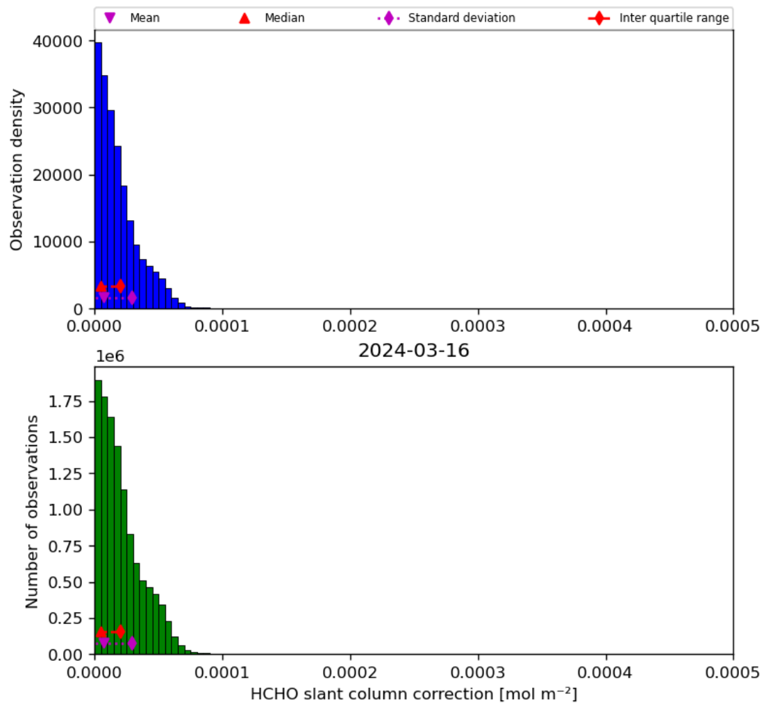
Figure 47: Histogram of “HCHO slant column correction” for 2024-03-15 to 2024-03-17
