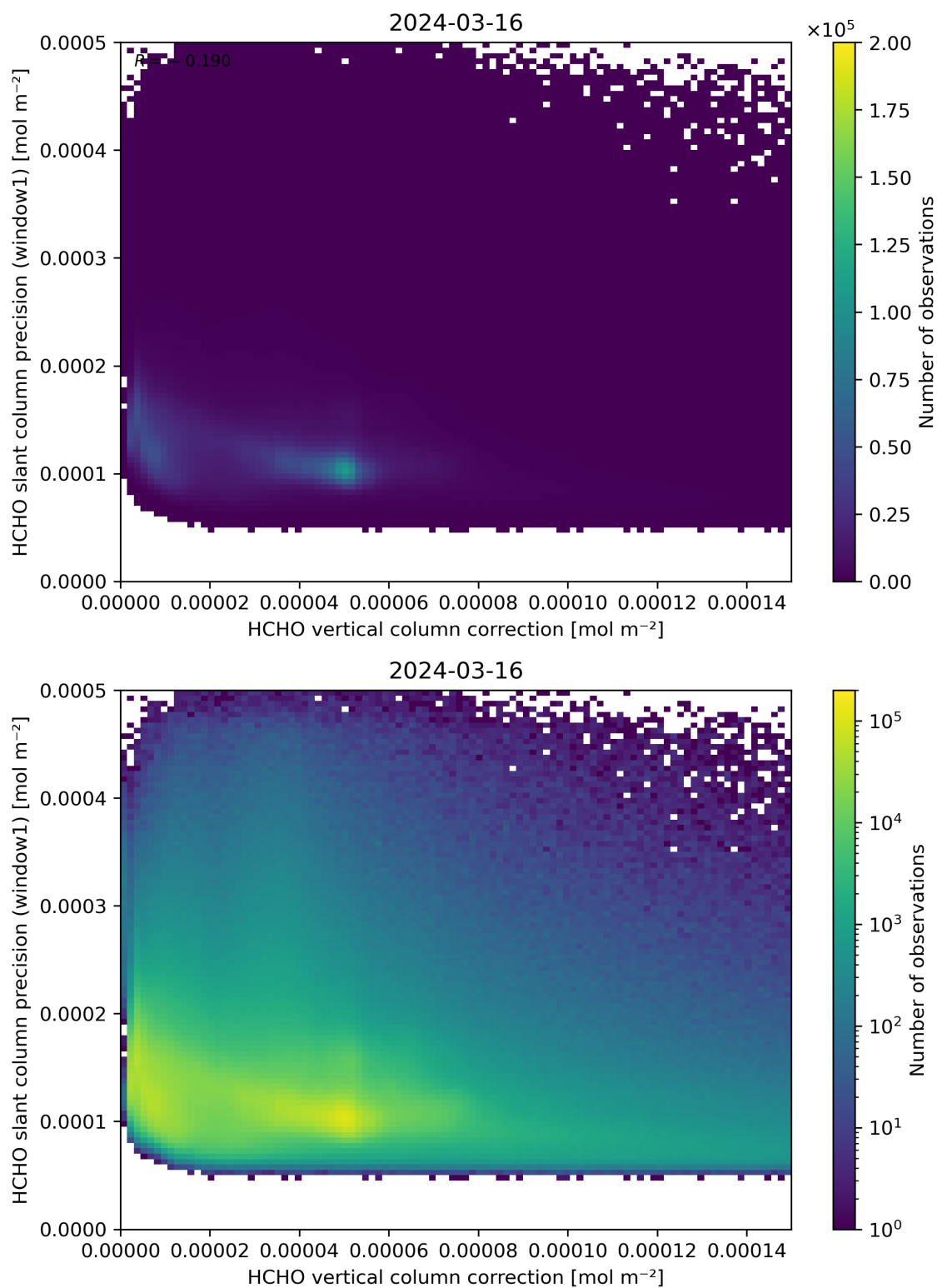
Figure 119: Scatter density plot of “HCHO vertical column correction” against “HCHO slant column precision (window1)” for 2024-03-15 to 2024-03-17.
