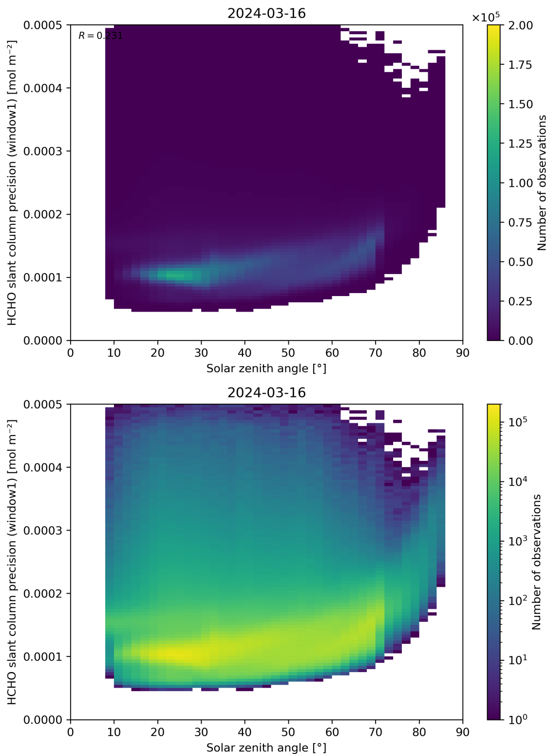
Figure 174: Scatter density plot of “Solar zenith angle” against “HCHO slant column precision (window1)” for 2024-03-15 to 2024-03-17.
