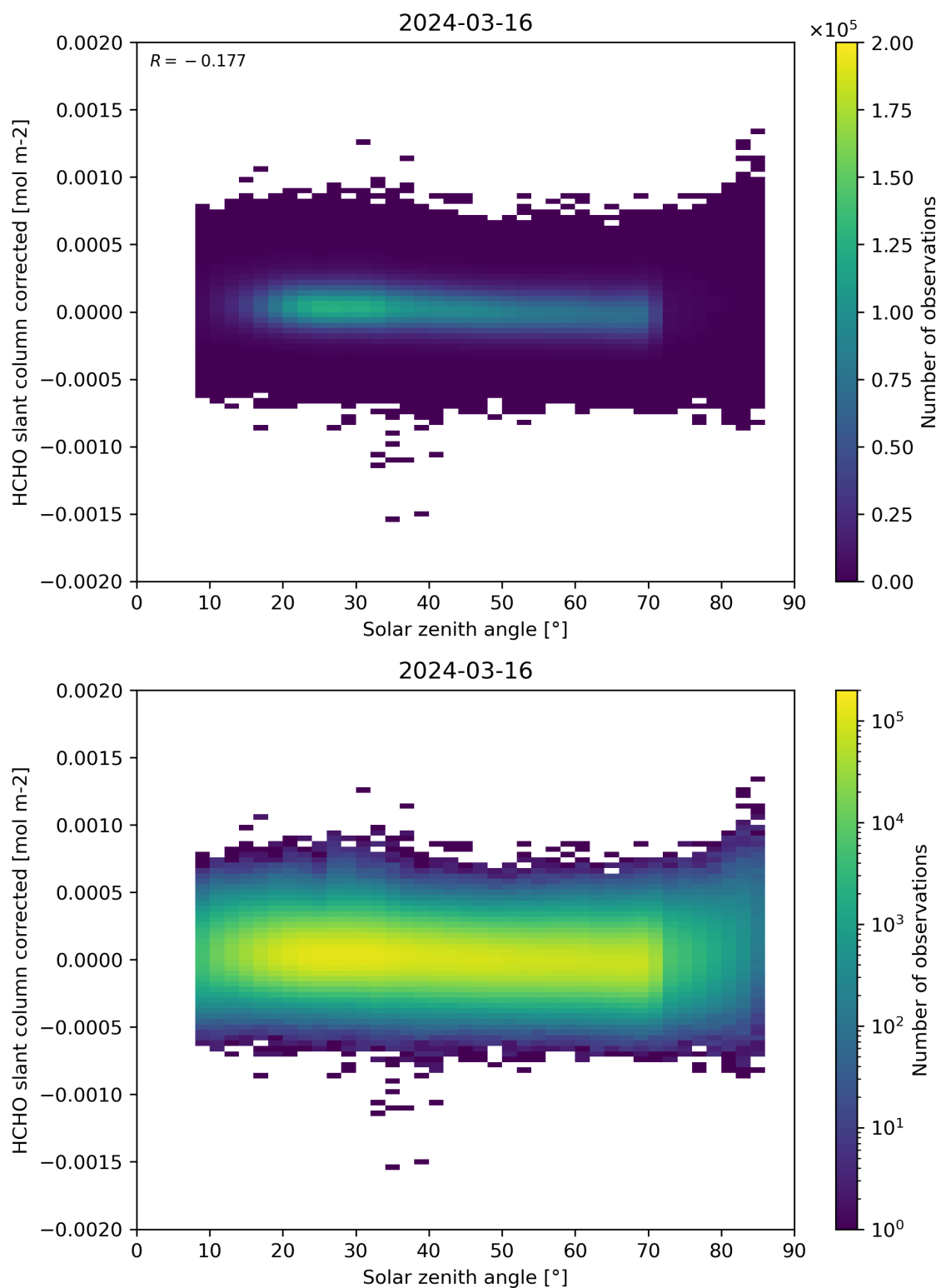
Figure 171: Scatter density plot of “Solar zenith angle” against “HCHO slant column corrected” for 2024-03-15 to 2024-03-17.
