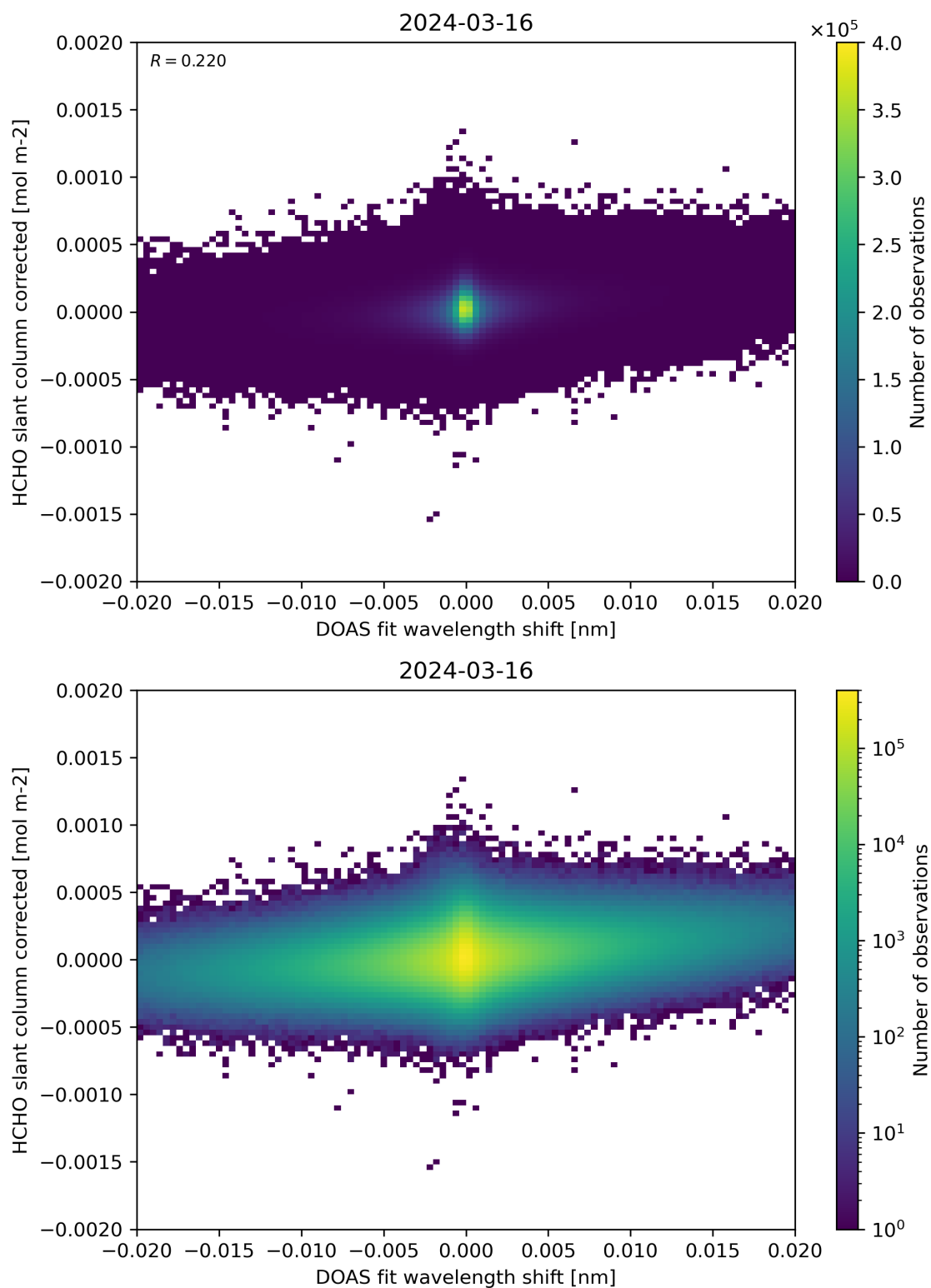
Figure 66: Scatter density plot of “DOAS fit wavelength shift” against “HCHO slant column corrected” for 2024-03-15 to 2024-03-17.
