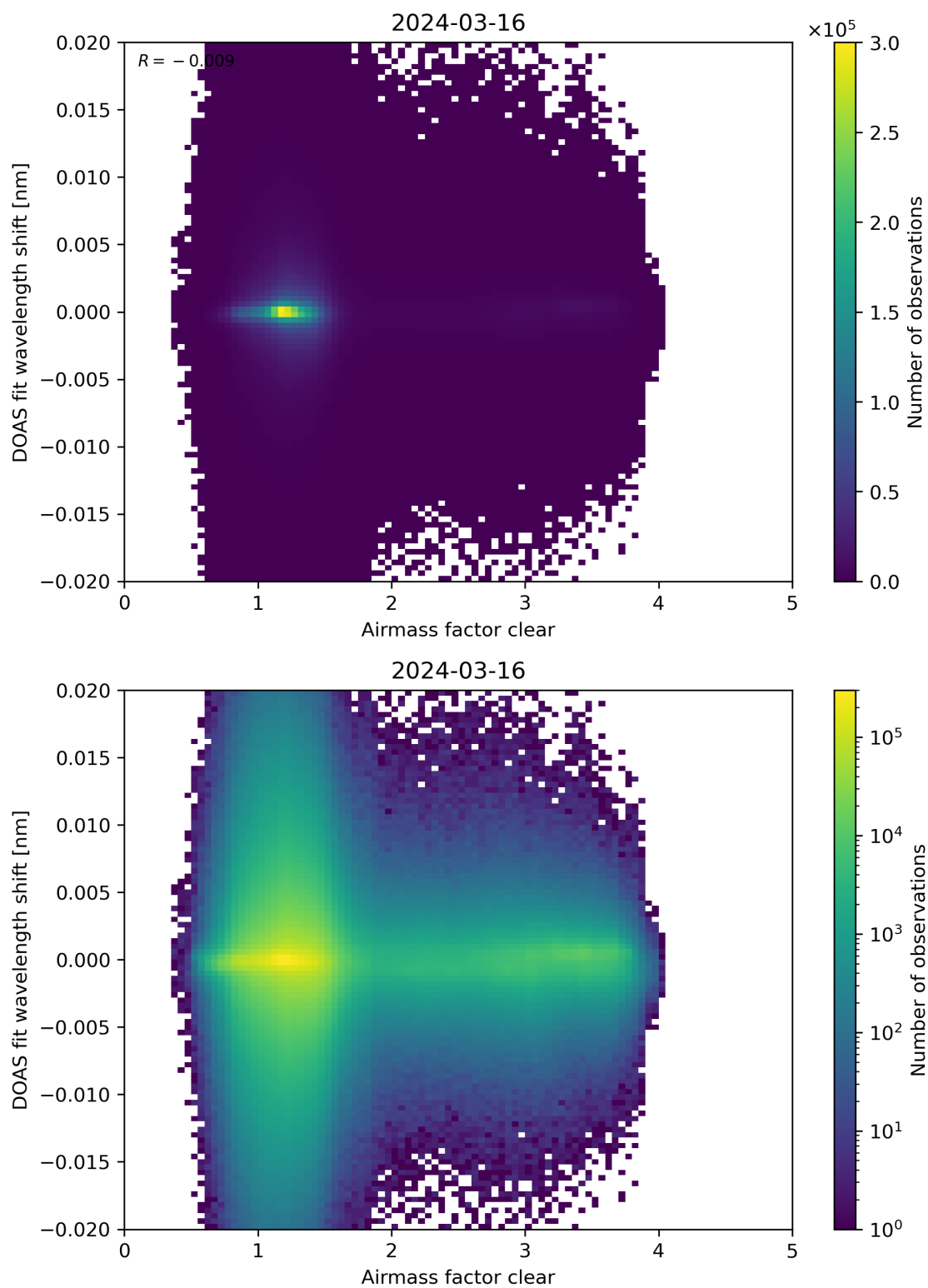
Figure 72: Scatter density plot of “Airmass factor clear” against “DOAS fit wavelength shift” for 2024-03-15 to 2024-03-17.
