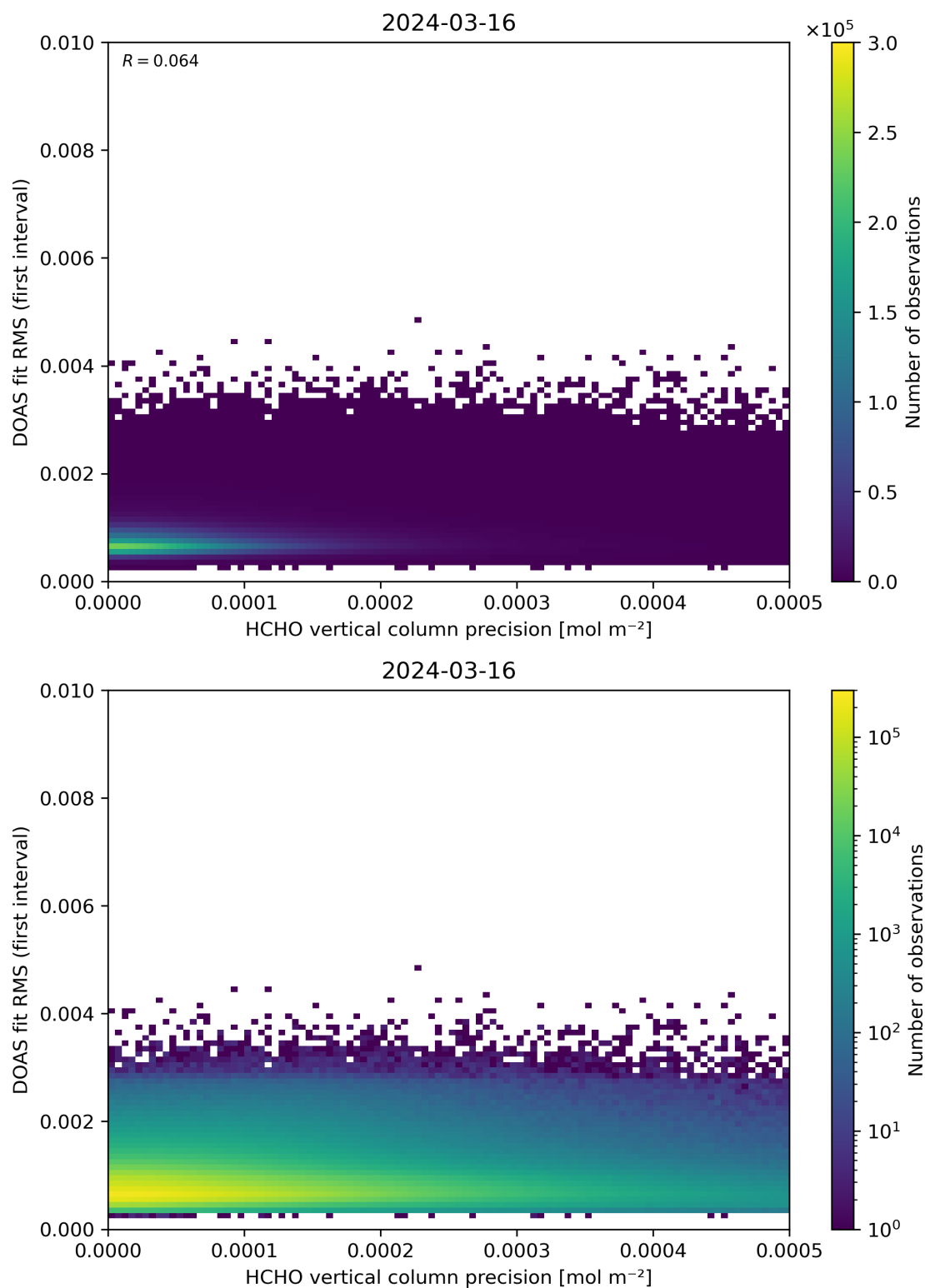
Figure 136: Scatter density plot of “HCHO vertical column precision” against “DOAS fit RMS (first interval)” for 2024-03-15 to 2024-03-17.
