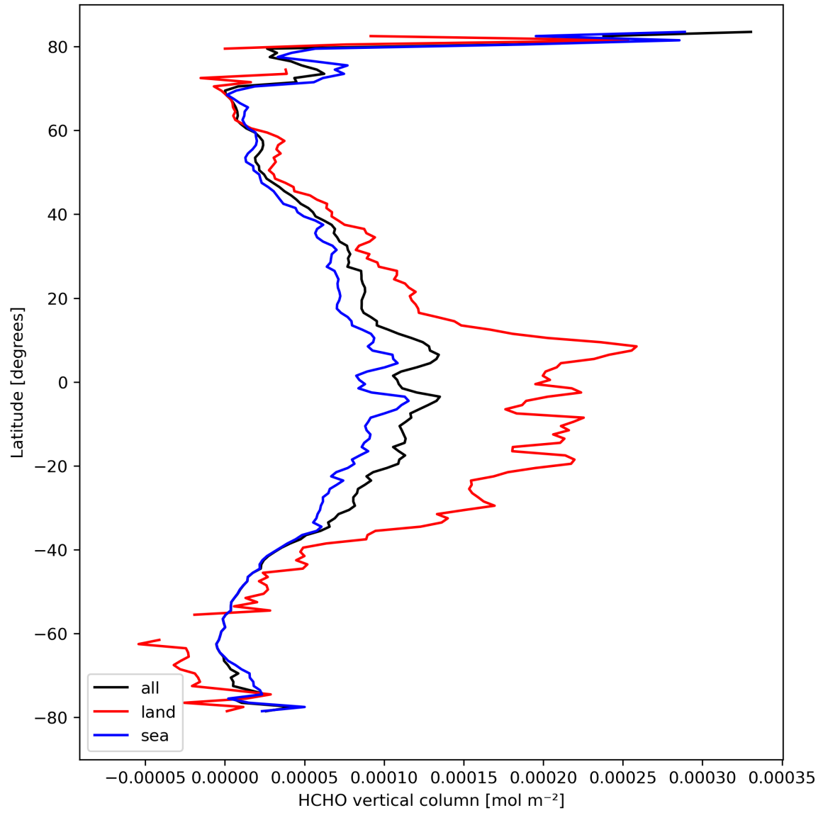
Figure 21: Zonal average of “HCHO vertical column” for 2024-03-15 to 2024-03-17.
