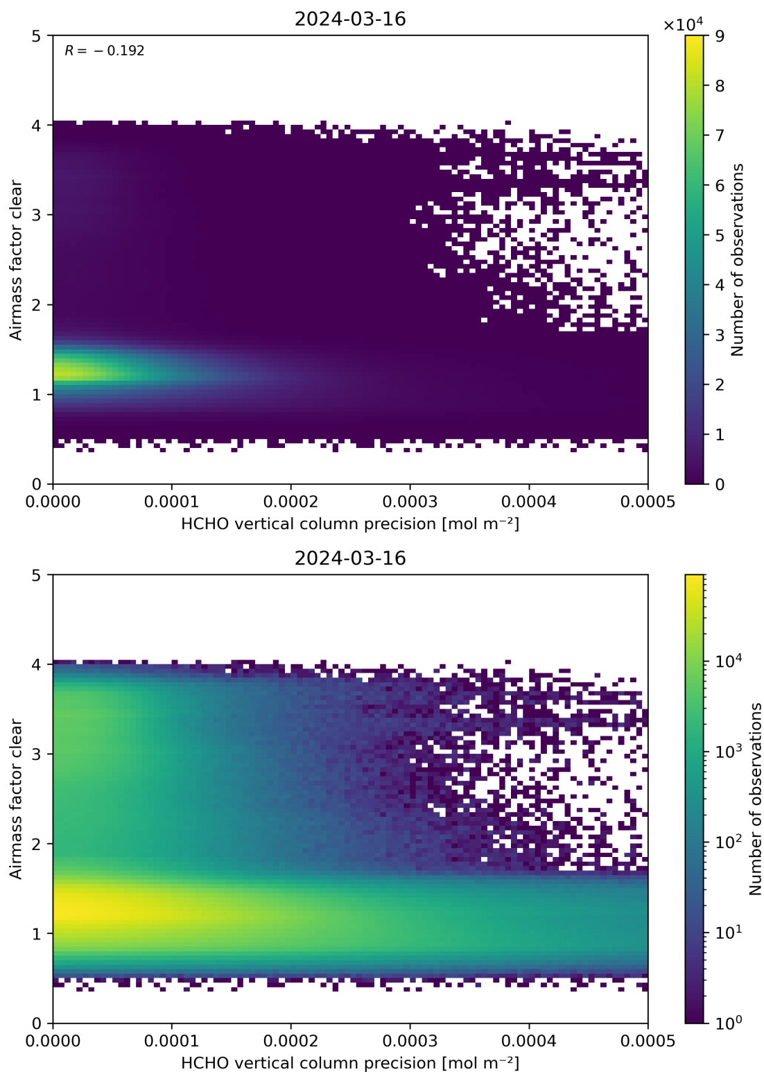
Figure 139: Scatter density plot of “HCHO vertical column precision” against “Airmass factor clear” for 2024-03-15 to 2024-03-17.
