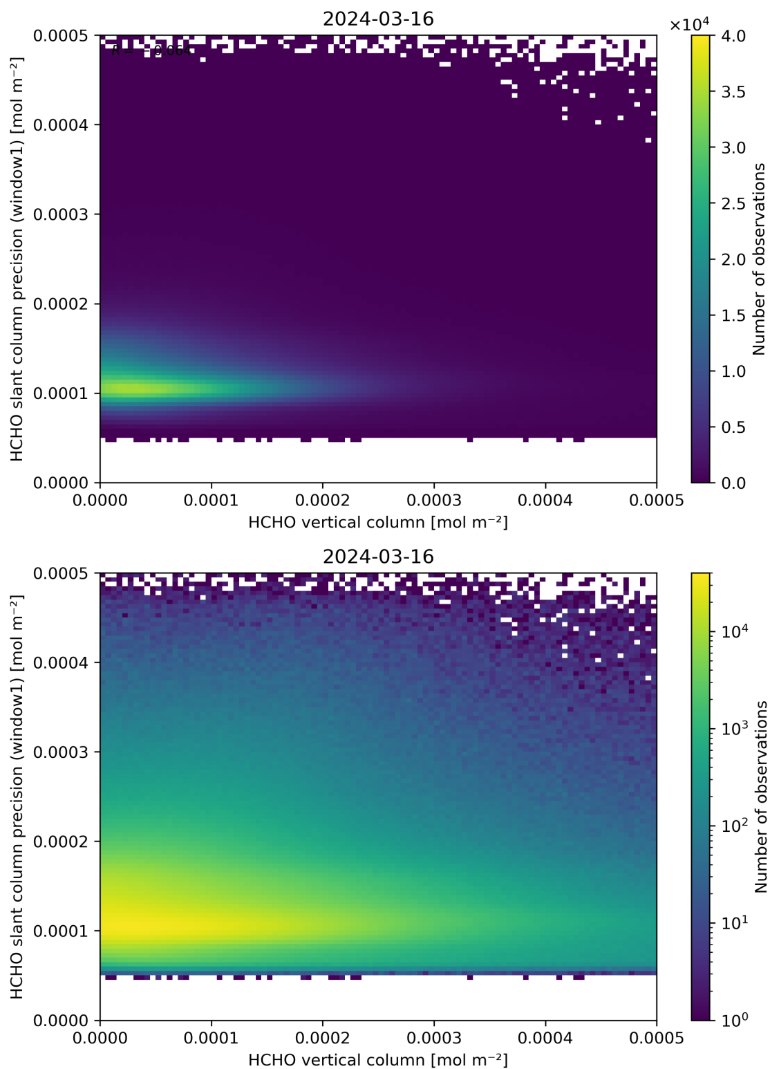
Figure 130: Scatter density plot of “HCHO vertical column” against “HCHO slant column precision (window1)” for 2024-03-15 to 2024-03-17.
