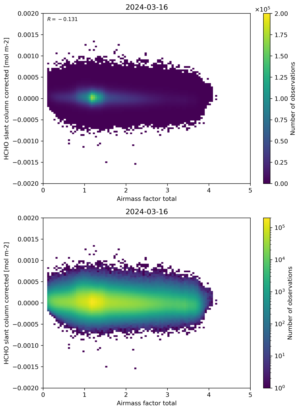
Figure 101: Scatter density plot of “Airmass factor total” against “HCHO slant column corrected” for 2024-03-15 to 2024-03-17.
