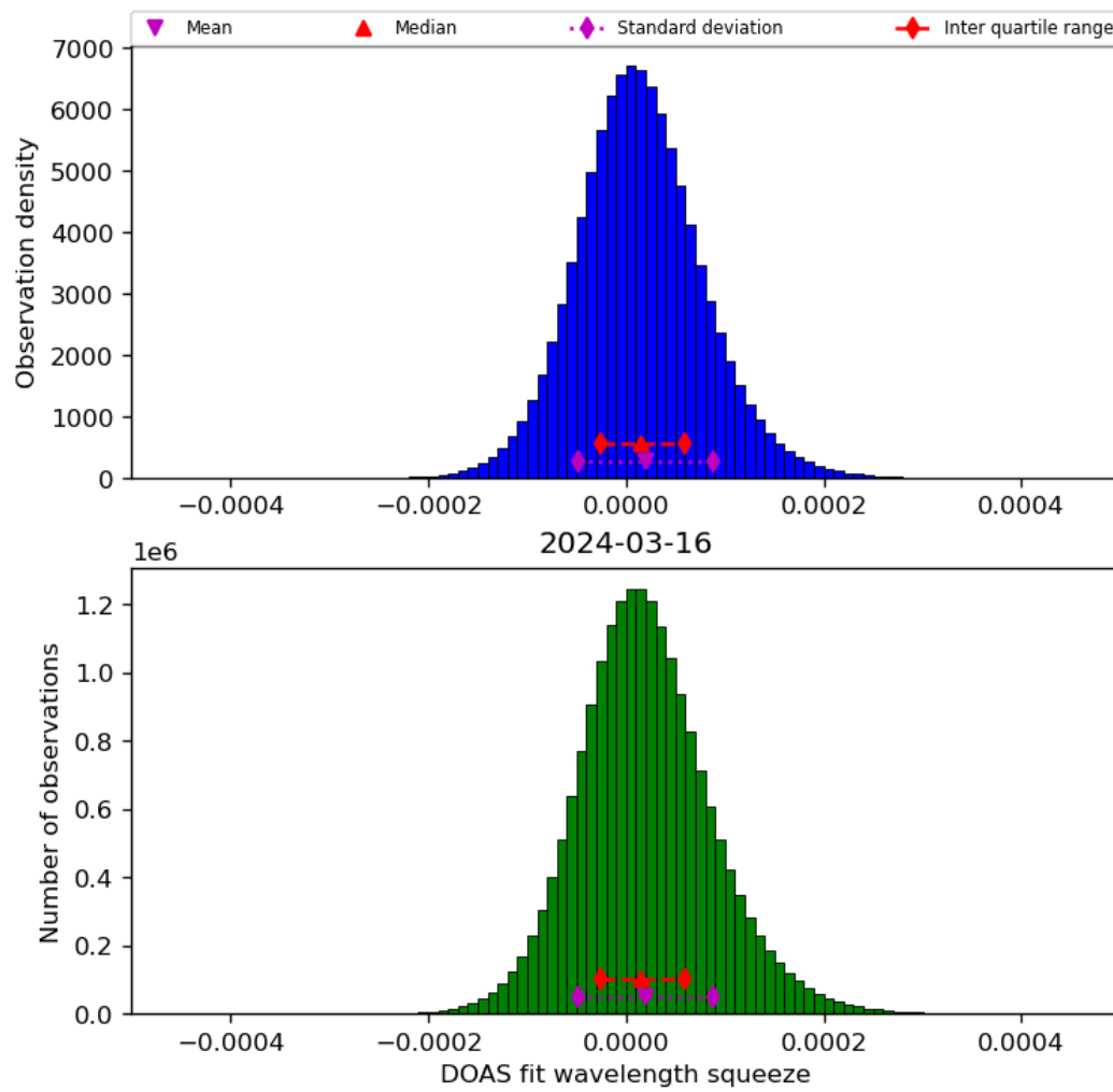
Figure 45: Histogram of “DOAS fit wavelength squeeze” for 2024-03-15 to 2024-03-17
