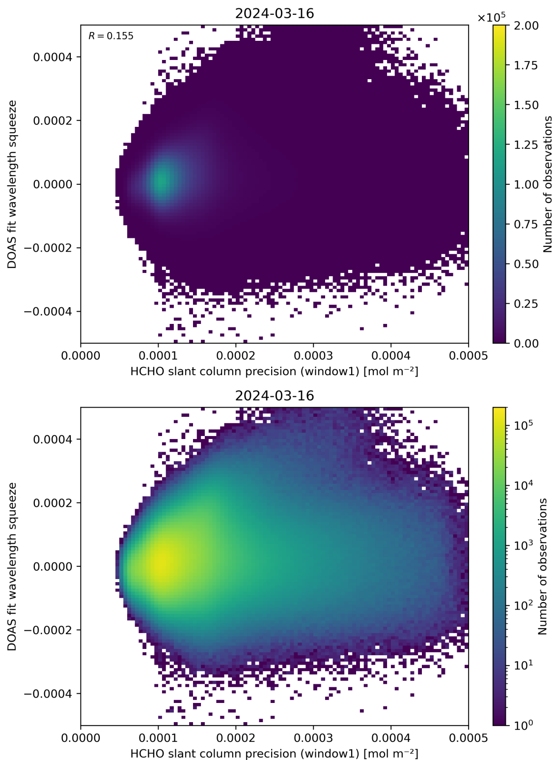
Figure 90: Scatter density plot of “HCHO slant column precision (window1)” against “DOAS fit wavelength squeeze” for 2024-03-15 to 2024-03-17.
