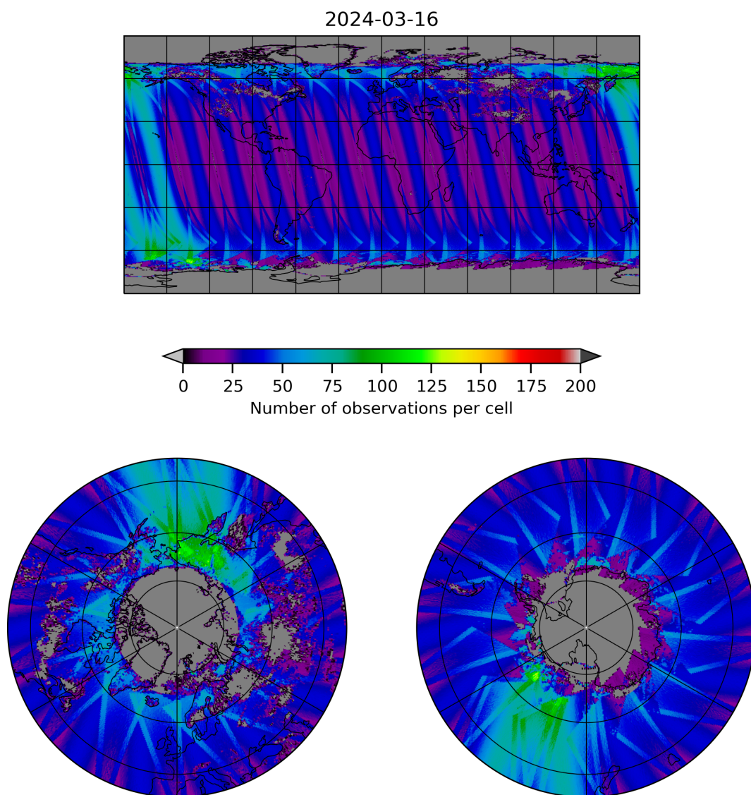
Figure 19: Map of the number of observations for 2024-03-15 to 2024-03-17
