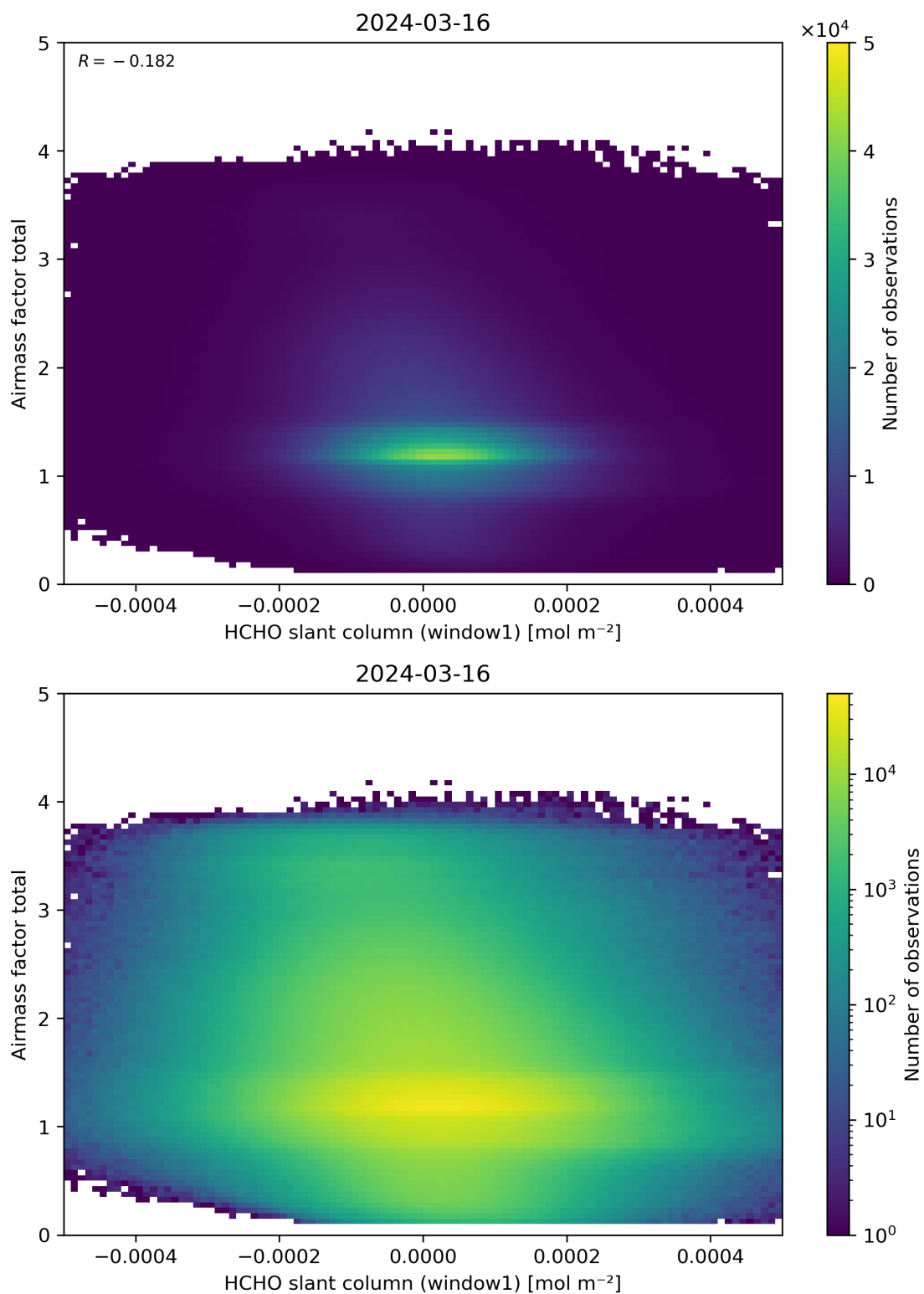
Figure 85: Scatter density plot of “HCHO slant column (window1)” against “Airmass factor total” for 2024-03-15 to 2024-03-17.
