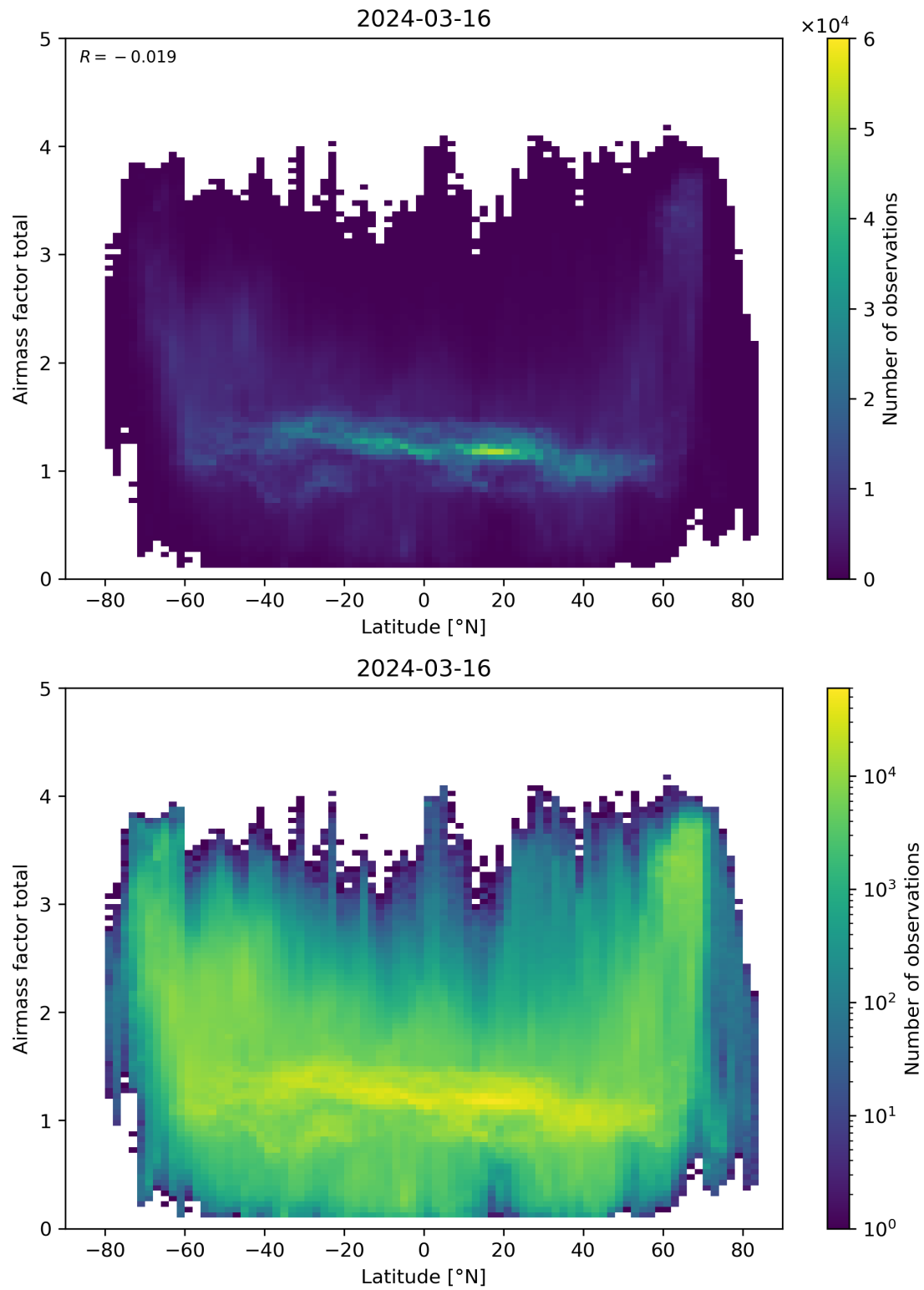
Figure 161: Scatter density plot of “Latitude” against “Airmass factor total” for 2024-03-15 to 2024-03-17.
