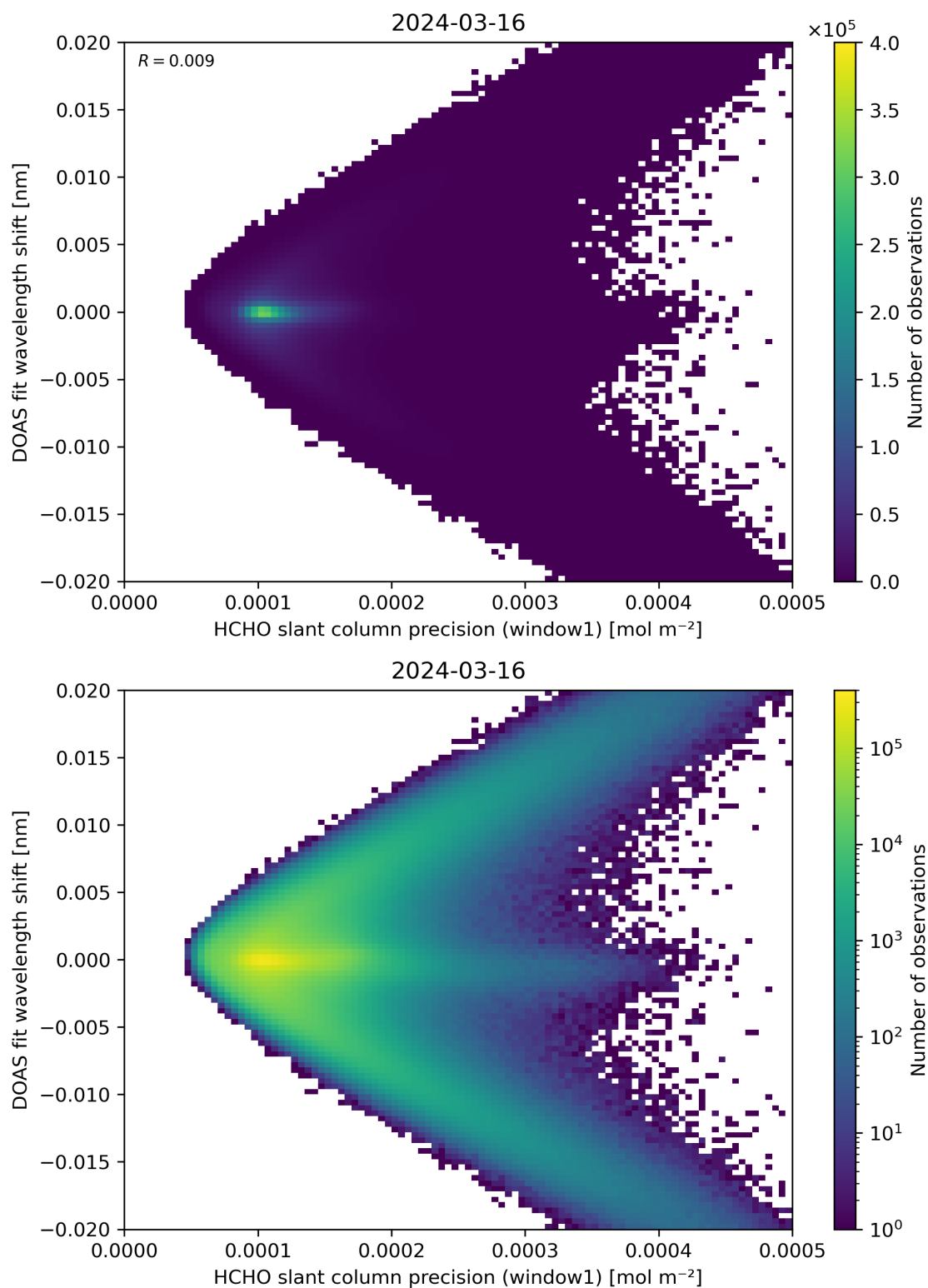
Figure 89: Scatter density plot of “HCHO slant column precision (window1)” against “DOAS fit wavelength shift” for 2024-03-15 to 2024-03-17.
