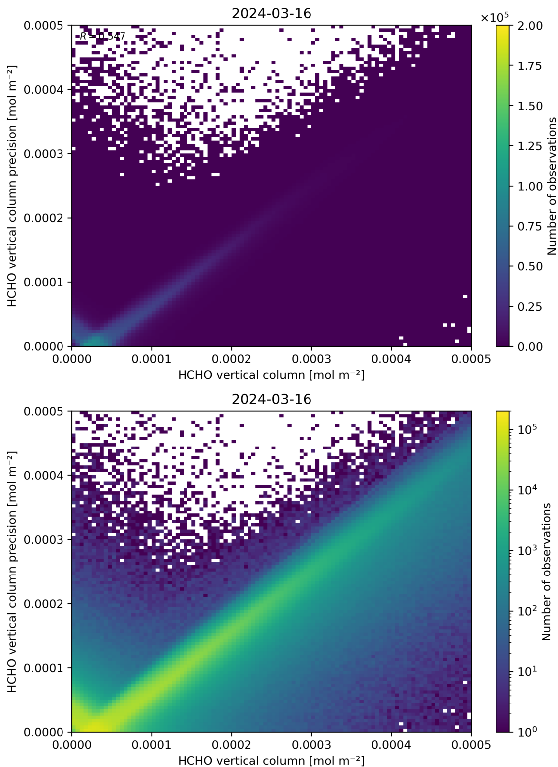
Figure 134: Scatter density plot of “HCHO vertical column” against “HCHO vertical column precision” for 2024-03-15 to 2024-03-17.
