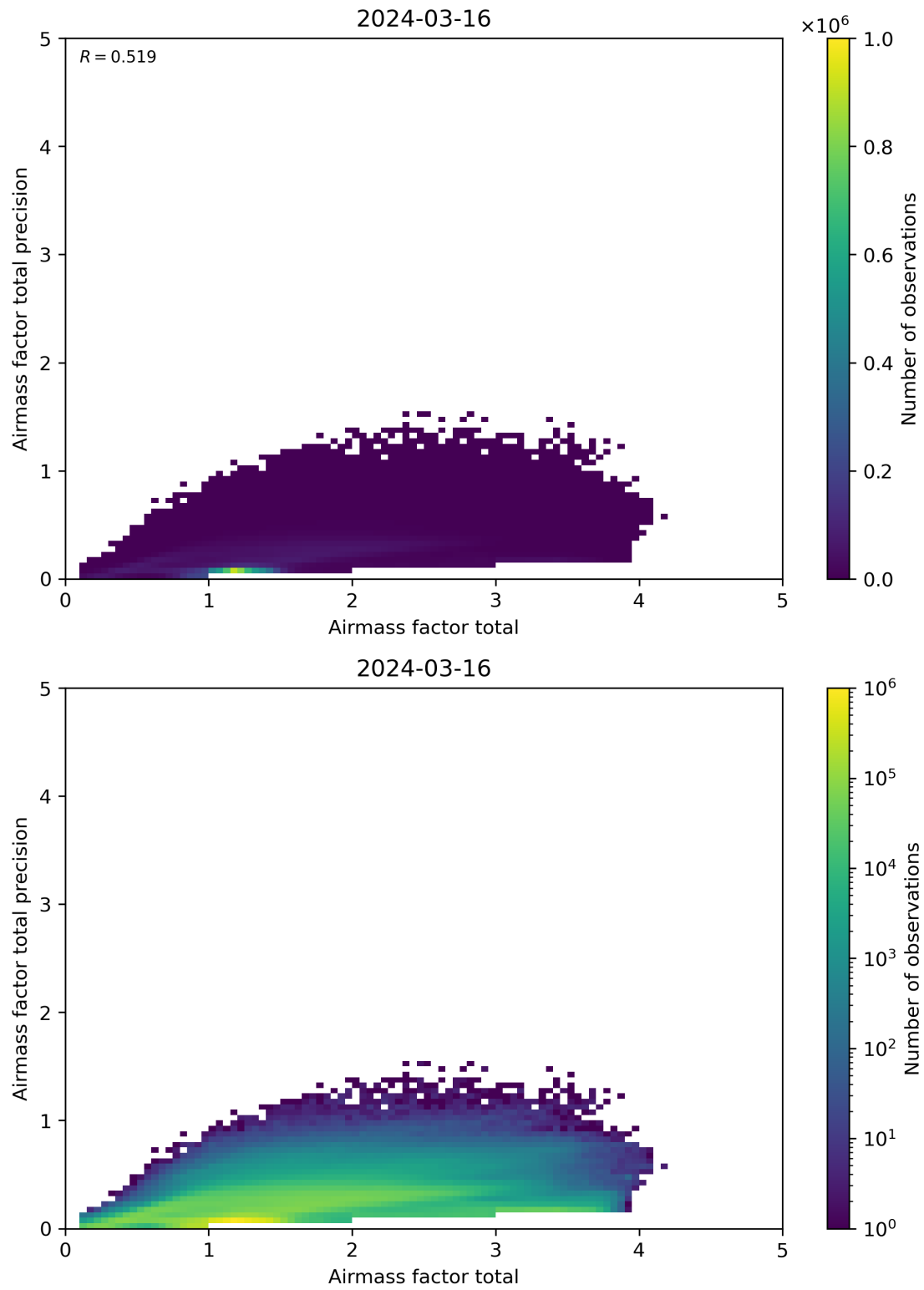
Figure 103: Scatter density plot of “Airmass factor total” against “Airmass factor total precision” for 2024-03-15 to 2024-03-17.
