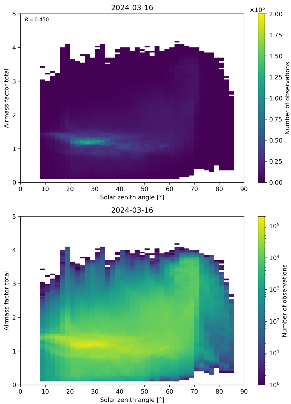
Figure 175: Scatter density plot of “Solar zenith angle” against “Airmass factor total” for 2024-03-15 to 2024-03-17.
