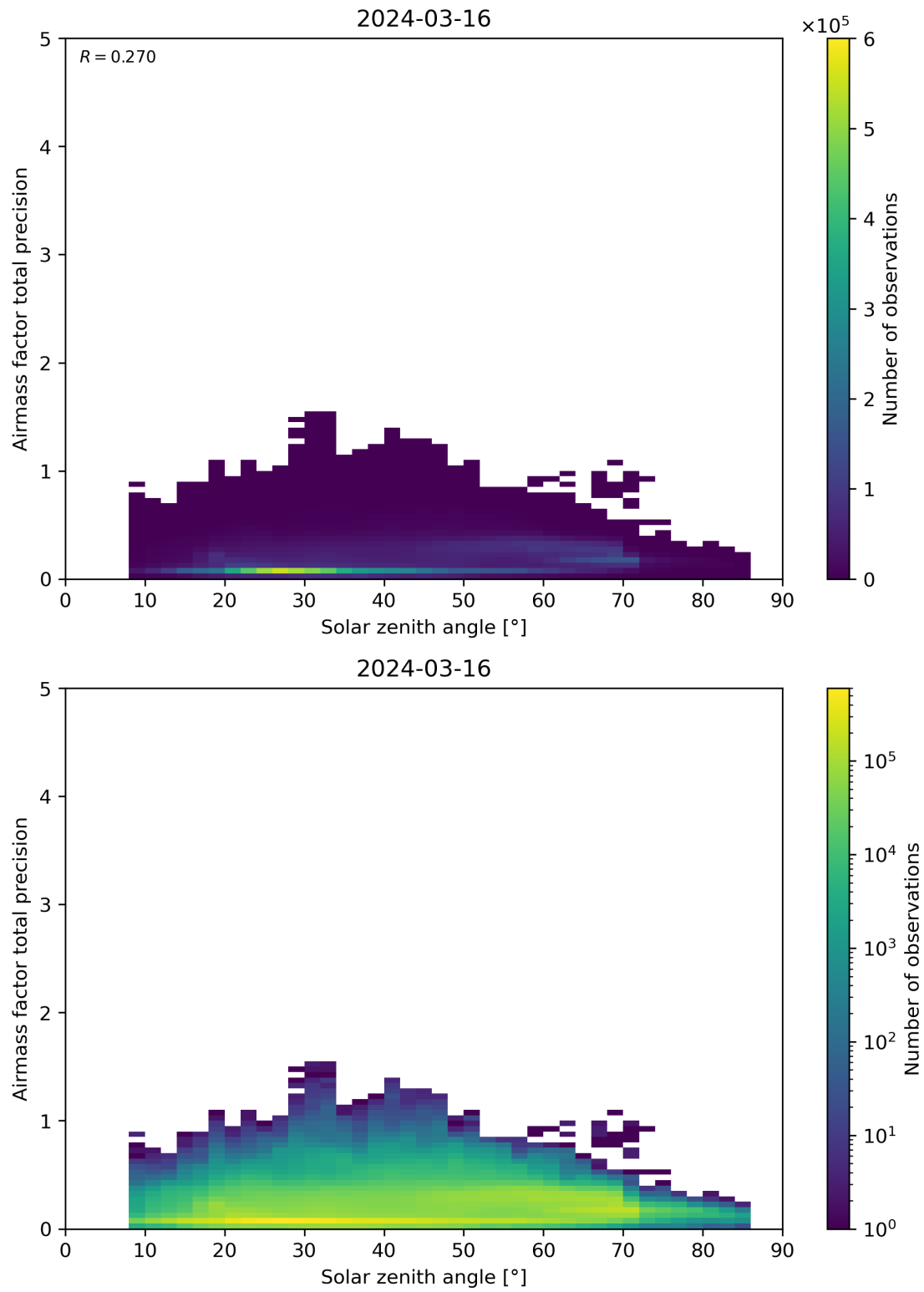
Figure 176: Scatter density plot of “Solar zenith angle” against “Airmass factor total precision” for 2024-03-15 to 2024-03-17.
