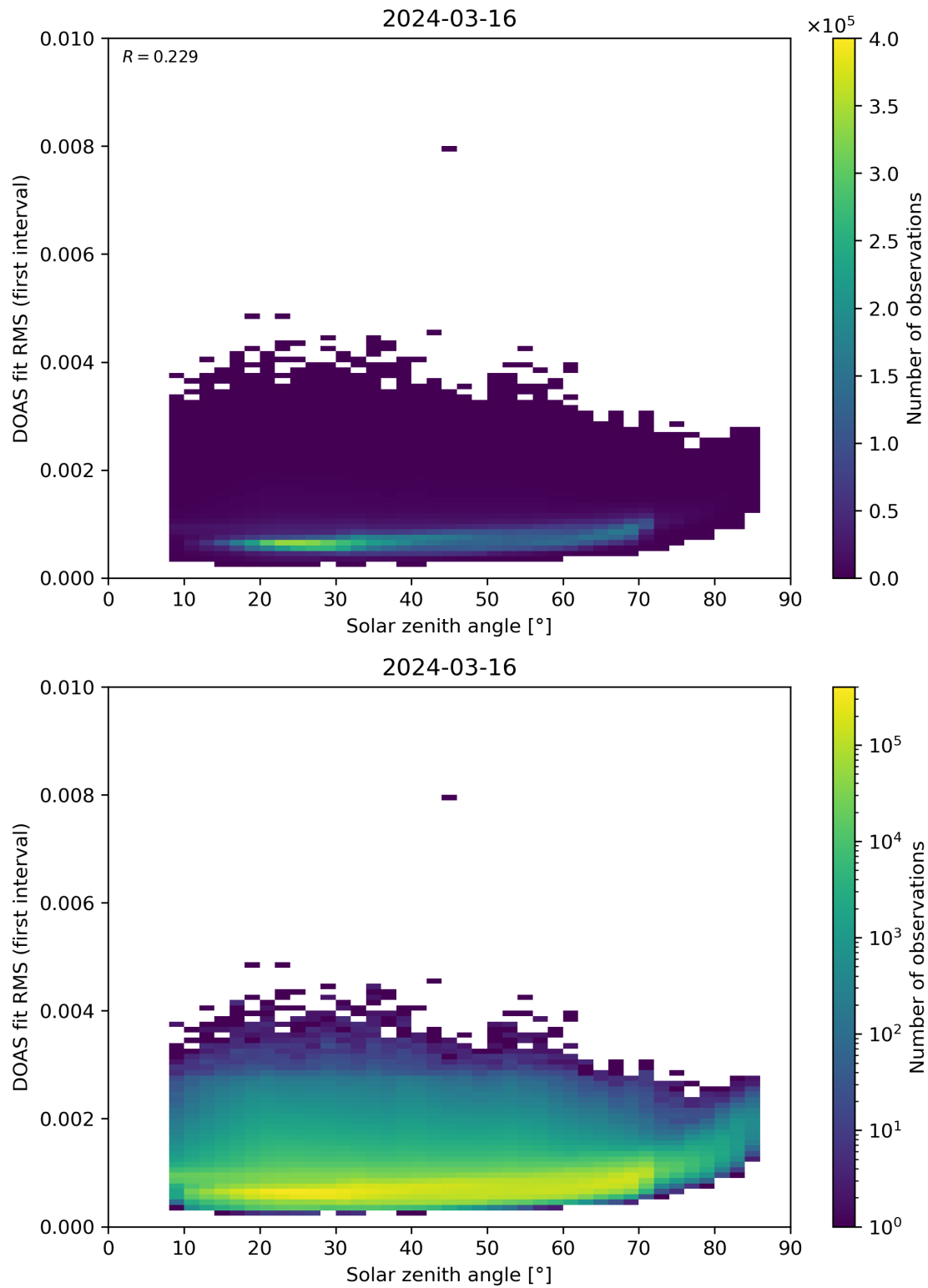
Figure 167: Scatter density plot of “Solar zenith angle” against “DOAS fit RMS (first interval)” for 2024-03-15 to 2024-03-17.
