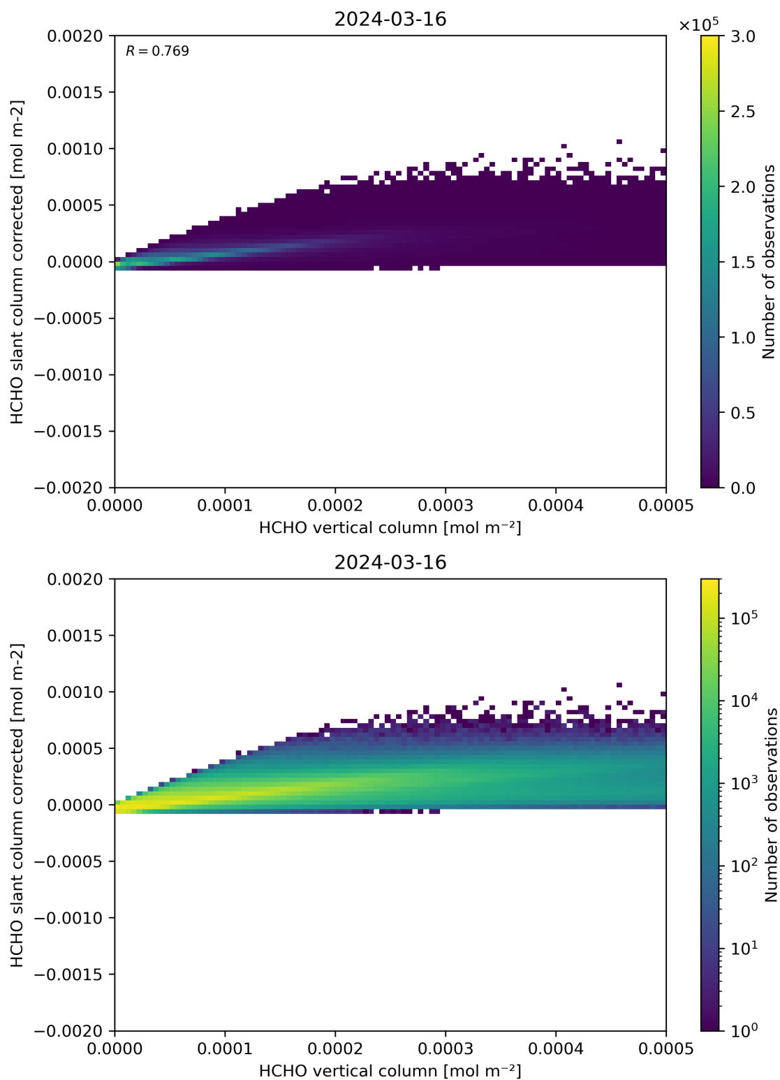
Figure 127: Scatter density plot of “HCHO vertical column” against “HCHO slant column corrected” for 2024-03-15 to 2024-03-17.
