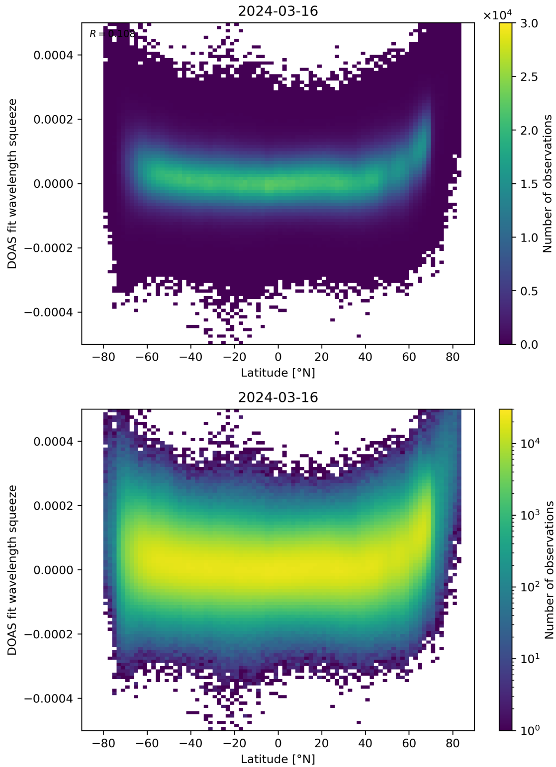
Figure 155: Scatter density plot of “Latitude” against “DOAS fit wavelength squeeze” for 2024-03-15 to 2024-03-17.
