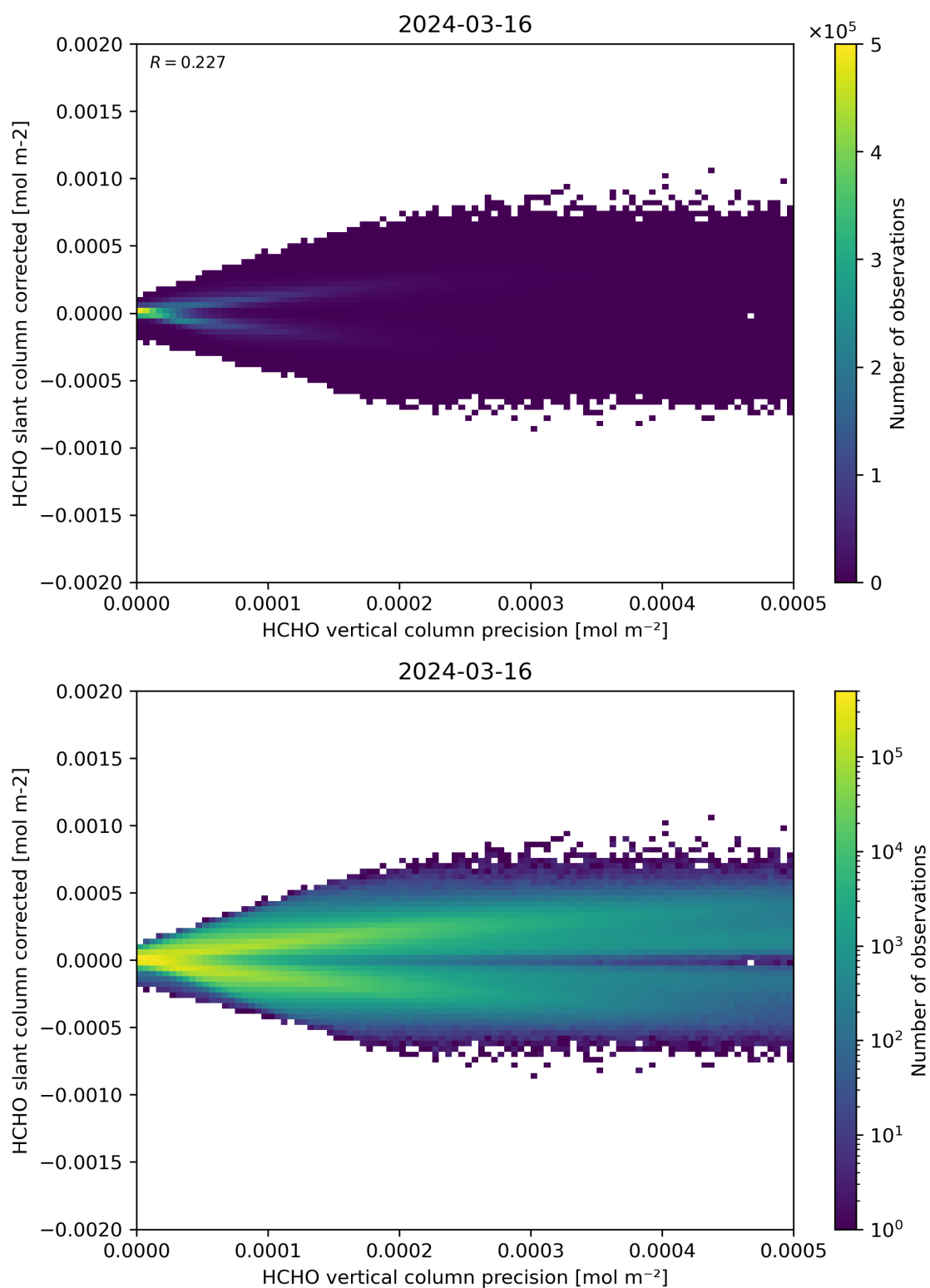
Figure 140: Scatter density plot of “HCHO vertical column precision” against “HCHO slant column corrected” for 2024-03-15 to 2024-03-17.
