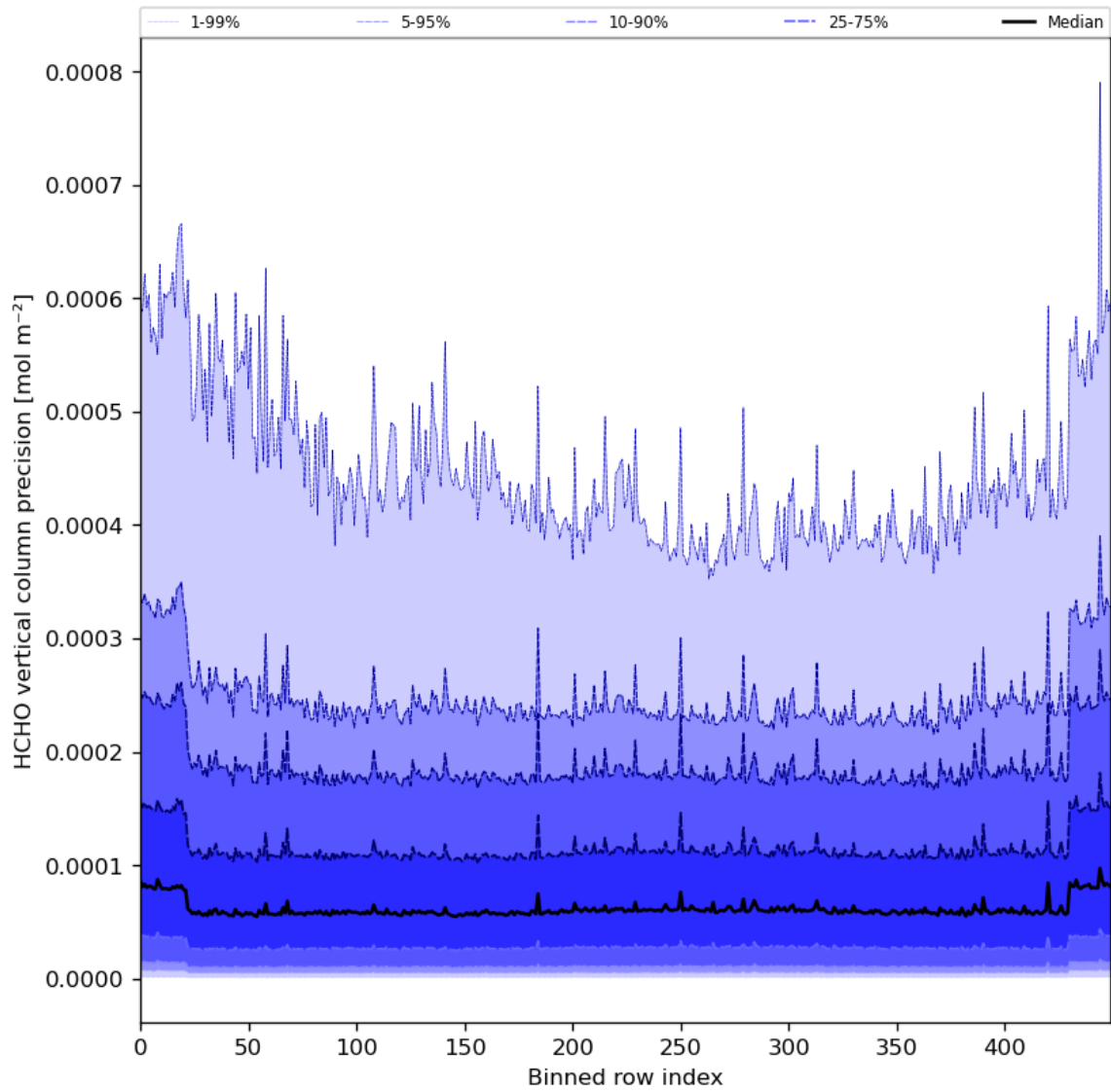
Figure 50: Along track statistics of “HCHO vertical column precision” for 2024-03-15 to 2024-03-17
