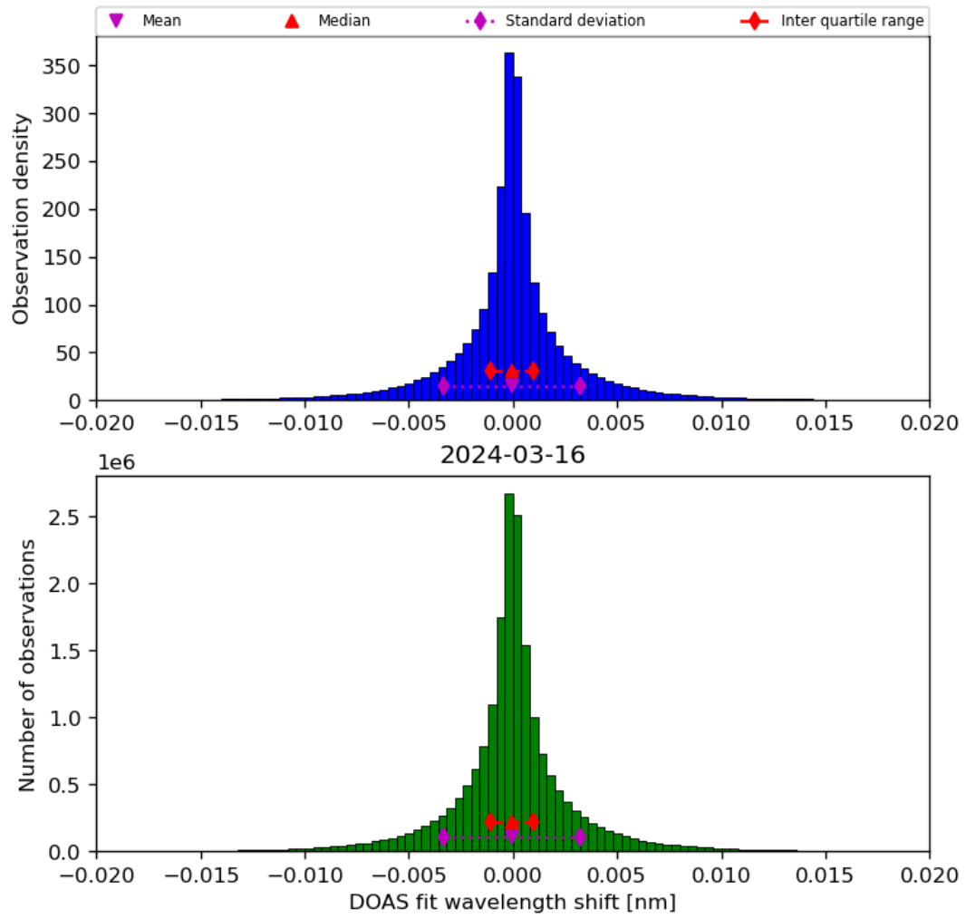
Figure 44: Histogram of “DOAS fit wavelength shift” for 2024-03-15 to 2024-03-17
