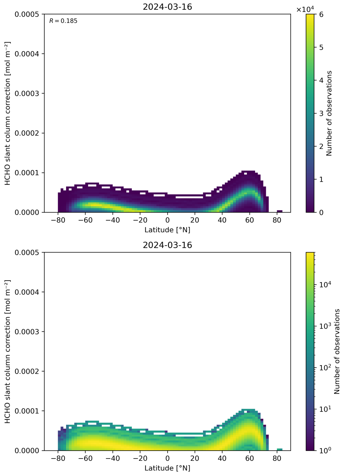
Figure 158: Scatter density plot of “Latitude” against “HCHO slant column correction” for 2024-03-15 to 2024-03-17.
