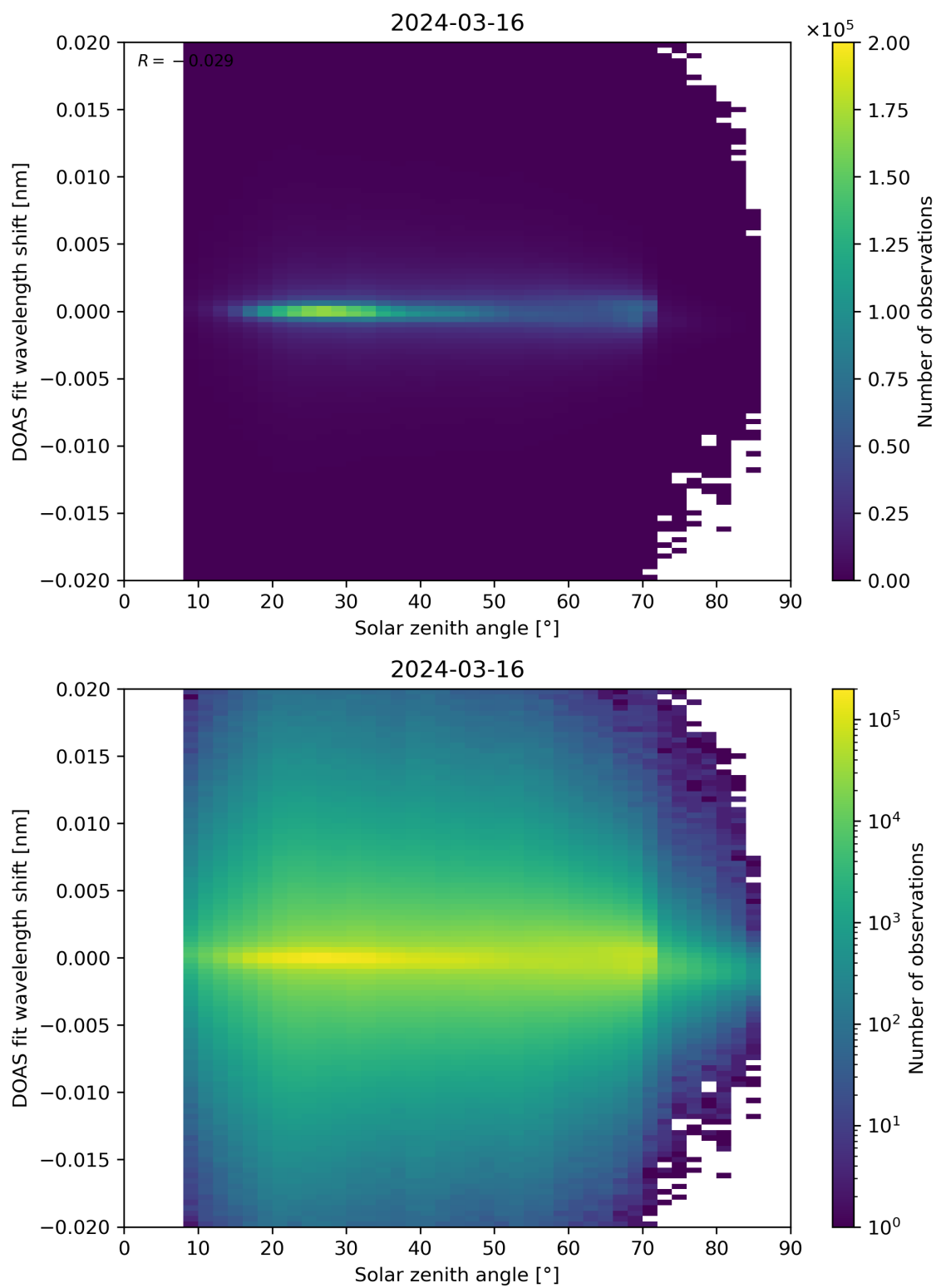
Figure 168: Scatter density plot of “Solar zenith angle” against “DOAS fit wavelength shift” for 2024-03-15 to 2024-03-17.
