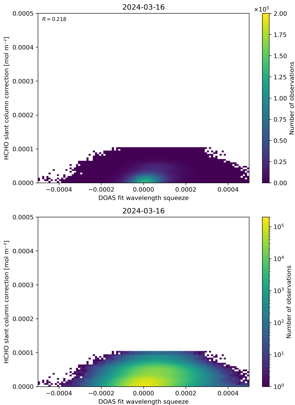
Figure 70: Scatter density plot of “DOAS fit wavelength squeeze” against “HCHO slant column correction” for 2024-03-15 to 2024-03-17.
