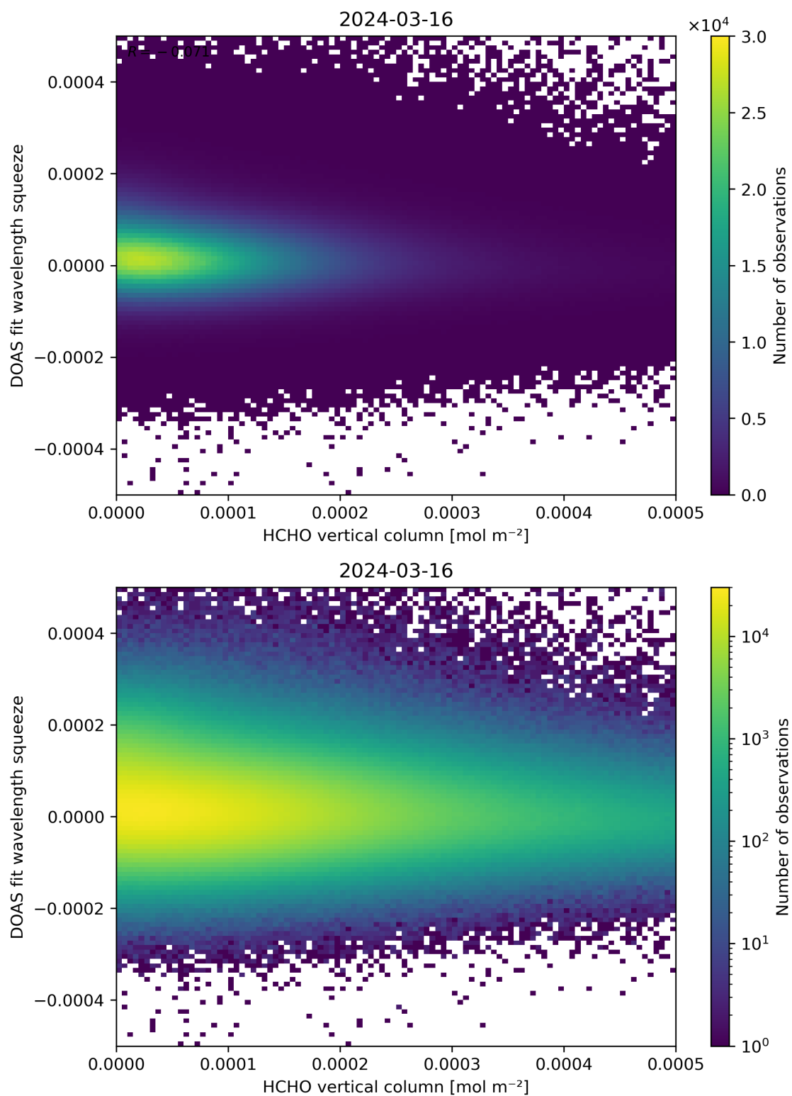
Figure 125: Scatter density plot of “HCHO vertical column” against “DOAS fit wavelength squeeze” for 2024-03-15 to 2024-03-17.
