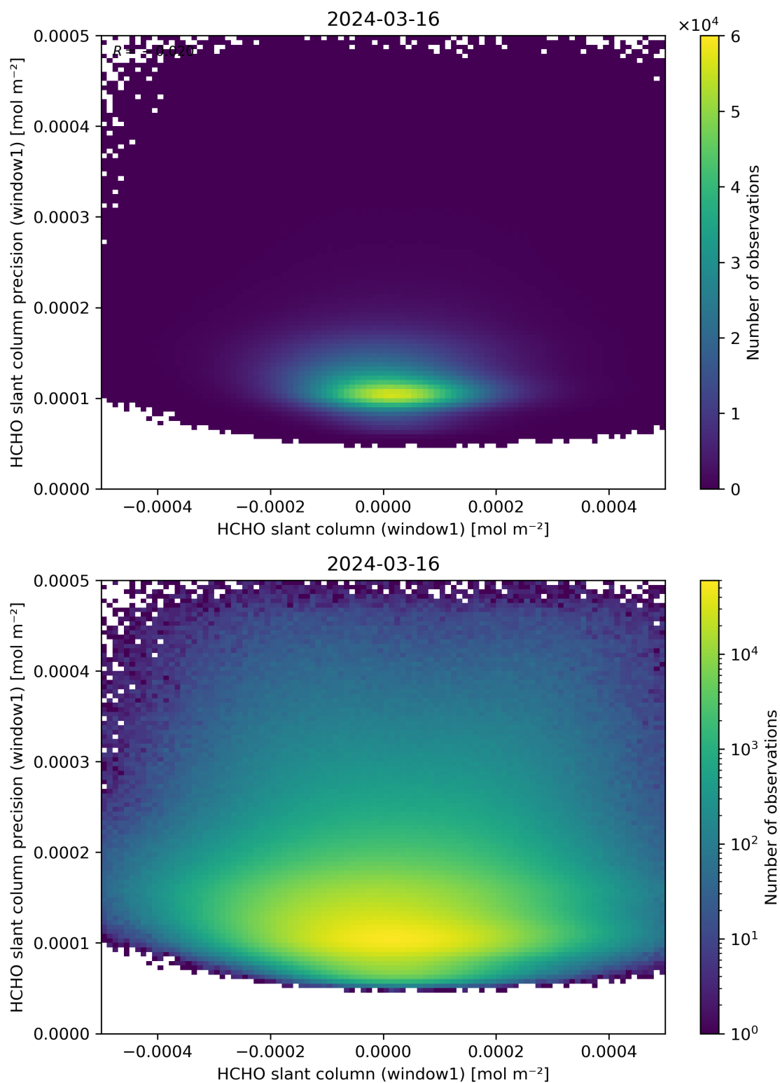
Figure 84: Scatter density plot of “HCHO slant column (window1)” against “HCHO slant column precision (window1)” for 2024-03-15 to 2024-03-17.
