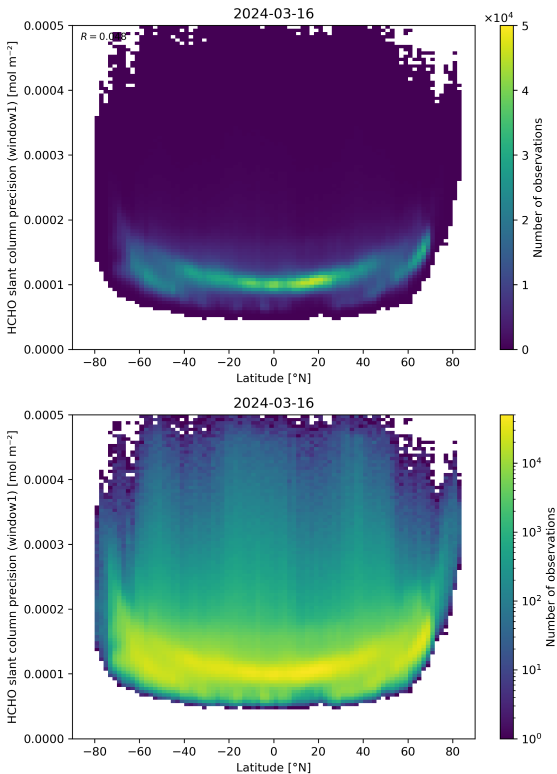
Figure 160: Scatter density plot of “Latitude” against “HCHO slant column precision (window1)” for 2024-03-15 to 2024-03-17.
