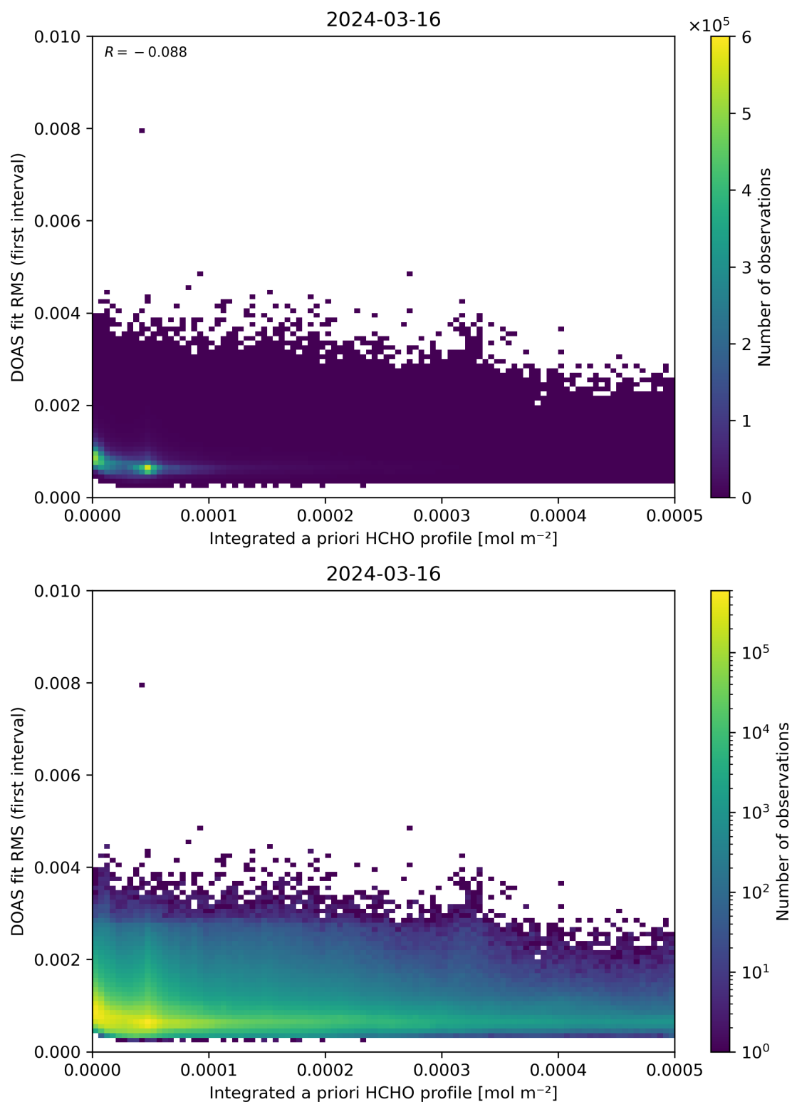
Figure 148: Scatter density plot of “Integrated a priori HCHO profile” against “DOAS fit RMS (first interval)” for 2024-03-15 to 2024-03-17.
