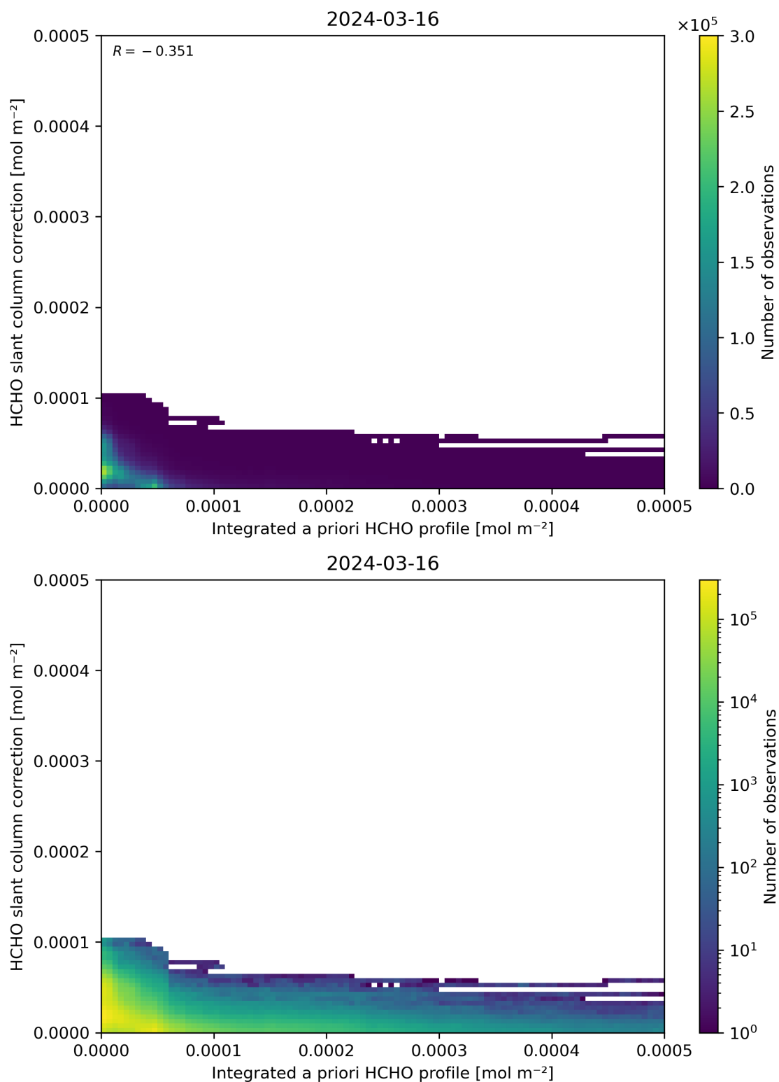
Figure 152: Scatter density plot of “Integrated a priori HCHO profile” against “HCHO slant column correction” for 2024-03-15 to 2024-03-17.
