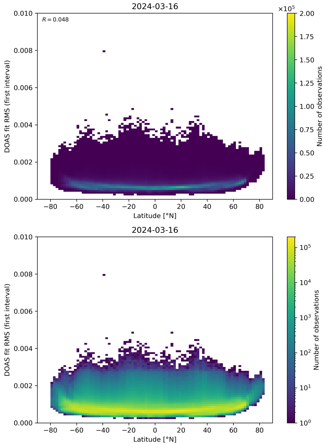
Figure 153: Scatter density plot of “Latitude” against “DOAS fit RMS (first interval)” for 2024-03-15 to 2024-03-17.
