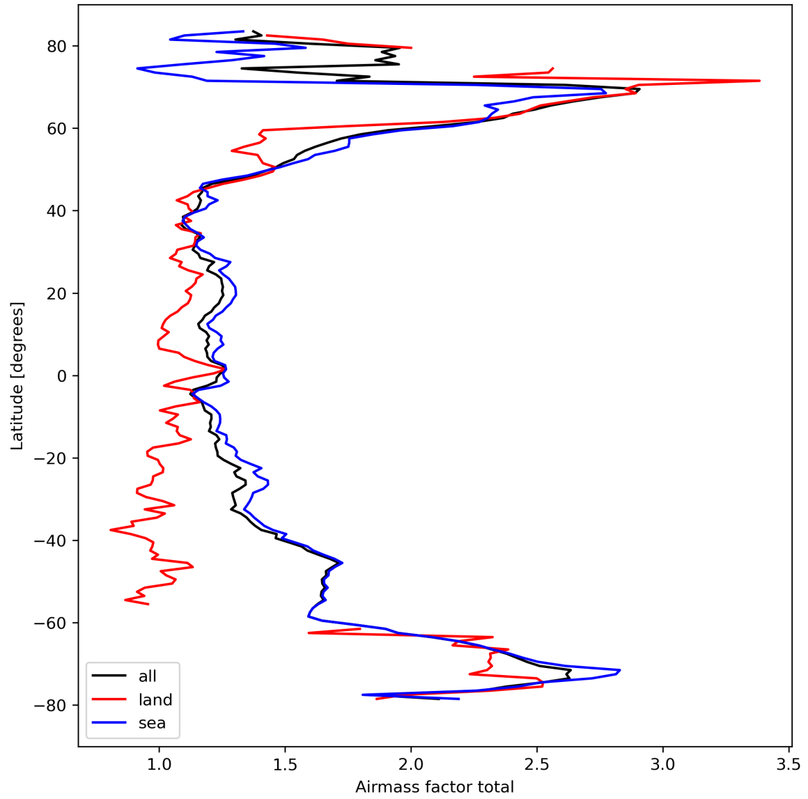
Figure 26: Zonal average of “Airmass factor total” for 2024-03-15 to 2024-03-17.
