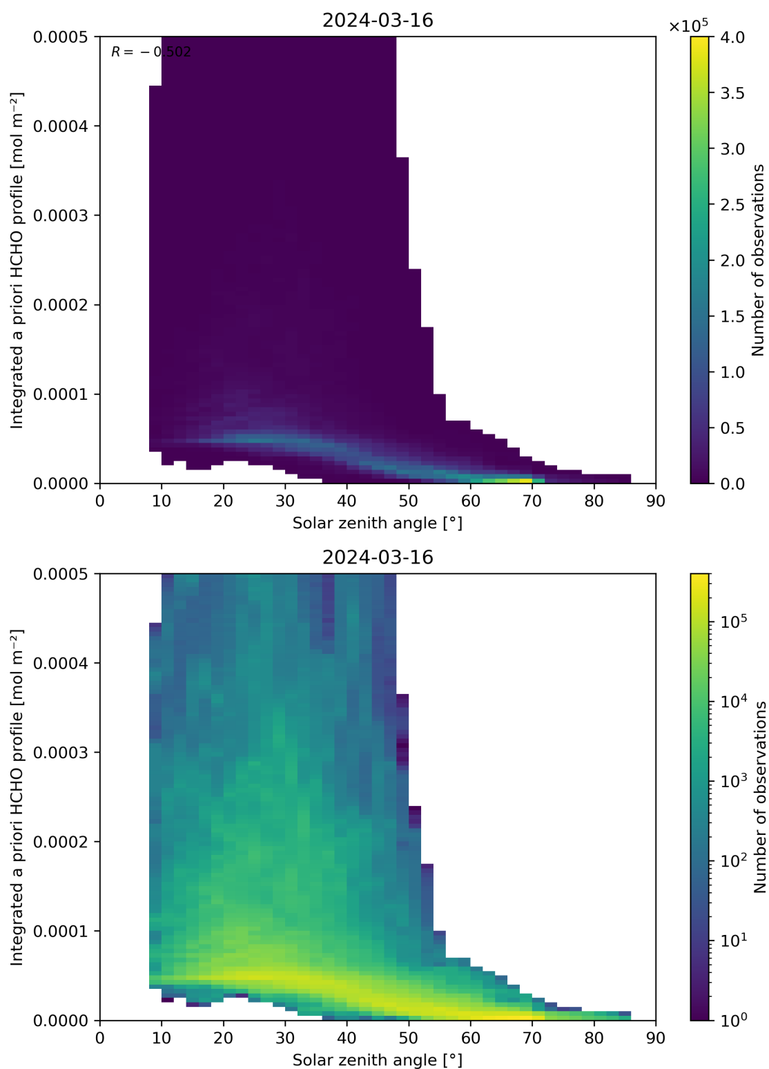
Figure 180: Scatter density plot of “Solar zenith angle” against “Integrated a priori HCHO profile” for 2024-03-15 to 2024-03-17.
