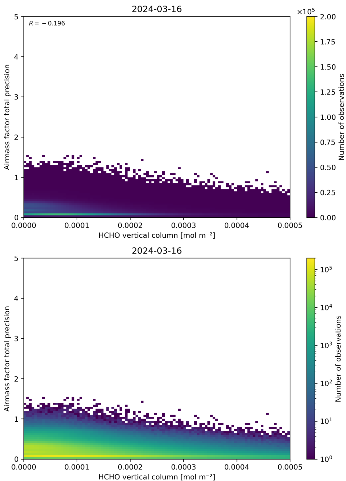
Figure 132: Scatter density plot of “HCHO vertical column” against “Airmass factor total precision” for 2024-03-15 to 2024-03-17.
