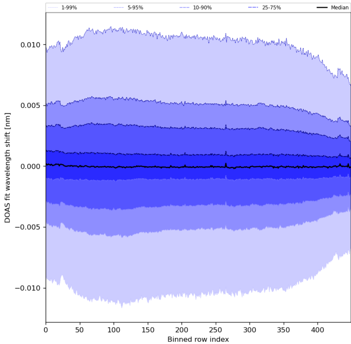
Figure 58: Along track statistics of “DOAS fit wavelength shift” for 2024-03-15 to 2024-03-17
