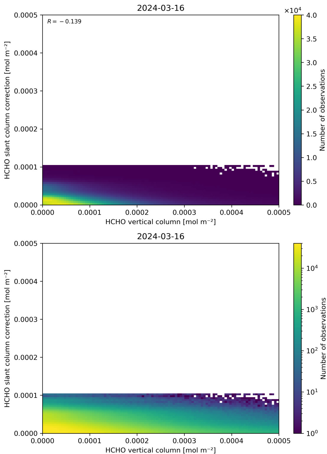
Figure 128: Scatter density plot of “HCHO vertical column” against “HCHO slant column correction” for 2024-03-15 to 2024-03-17.
