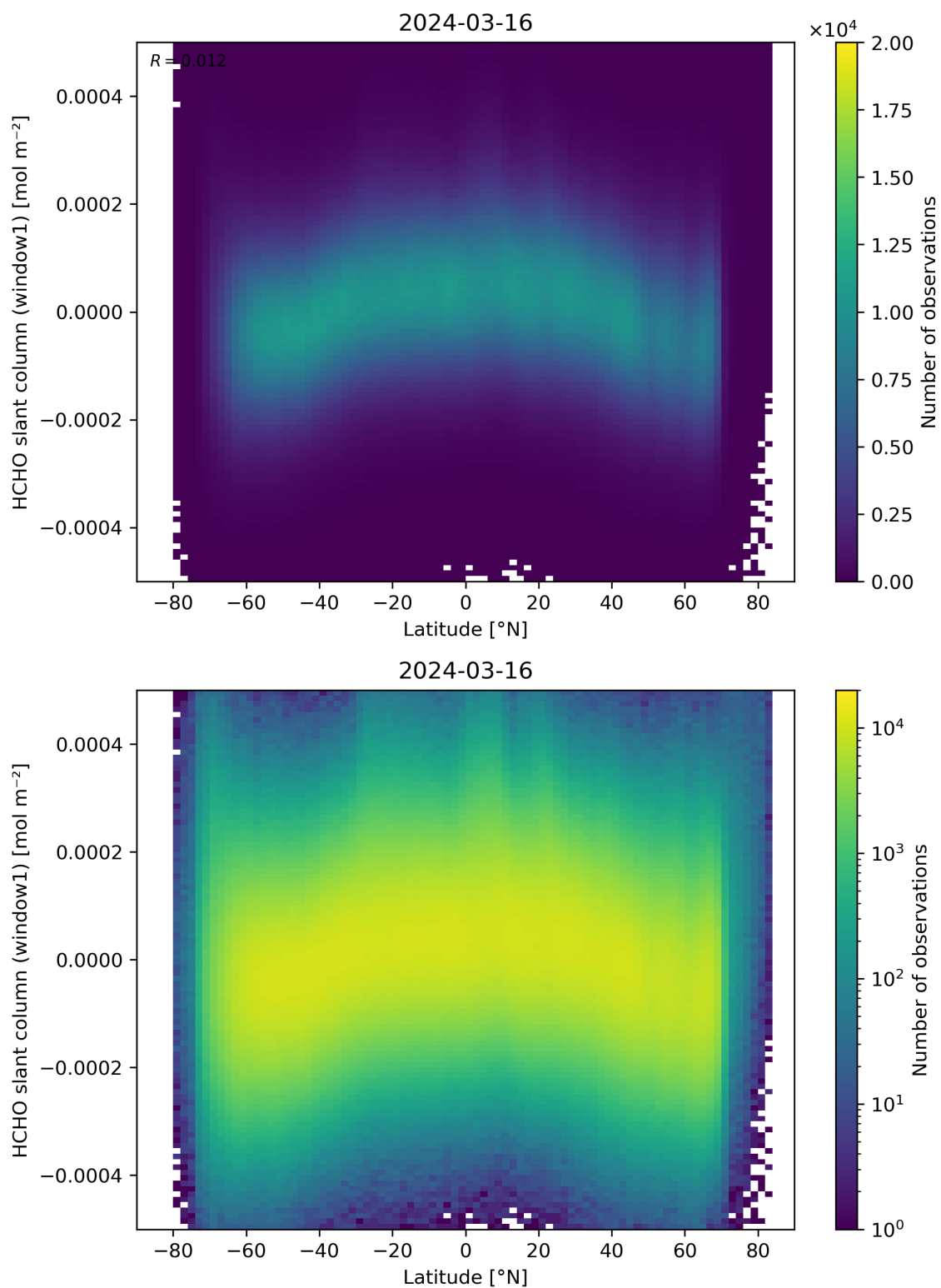
Figure 159: Scatter density plot of “Latitude” against “HCHO slant column (window1)” for 2024-03-15 to 2024-03-17.
