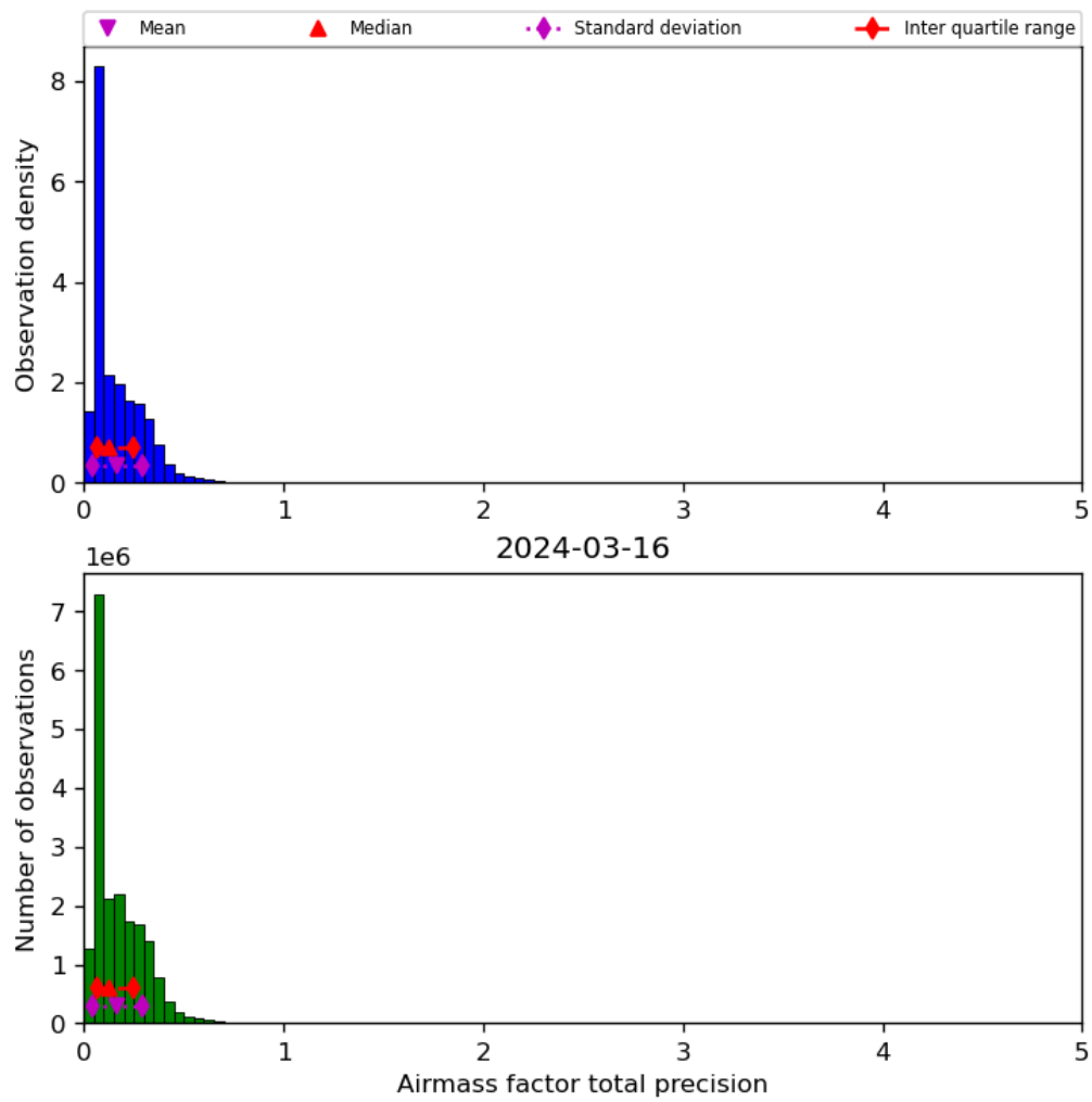
Figure 41: Histogram of “Airmass factor total precision” for 2024-03-15 to 2024-03-17
