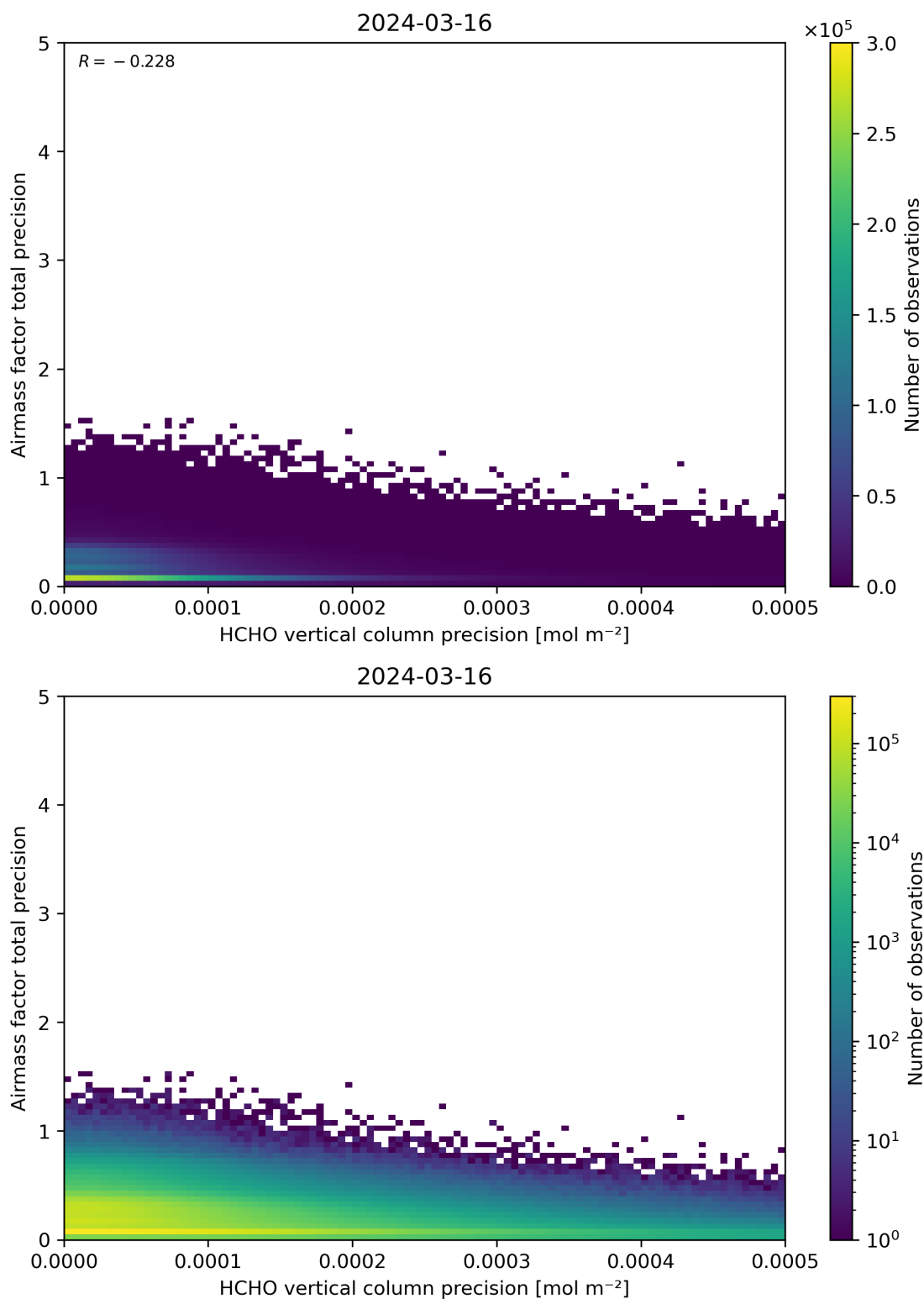
Figure 145: Scatter density plot of “HCHO vertical column precision” against “Airmass factor total precision” for 2024-03-15 to 2024-03-17.
