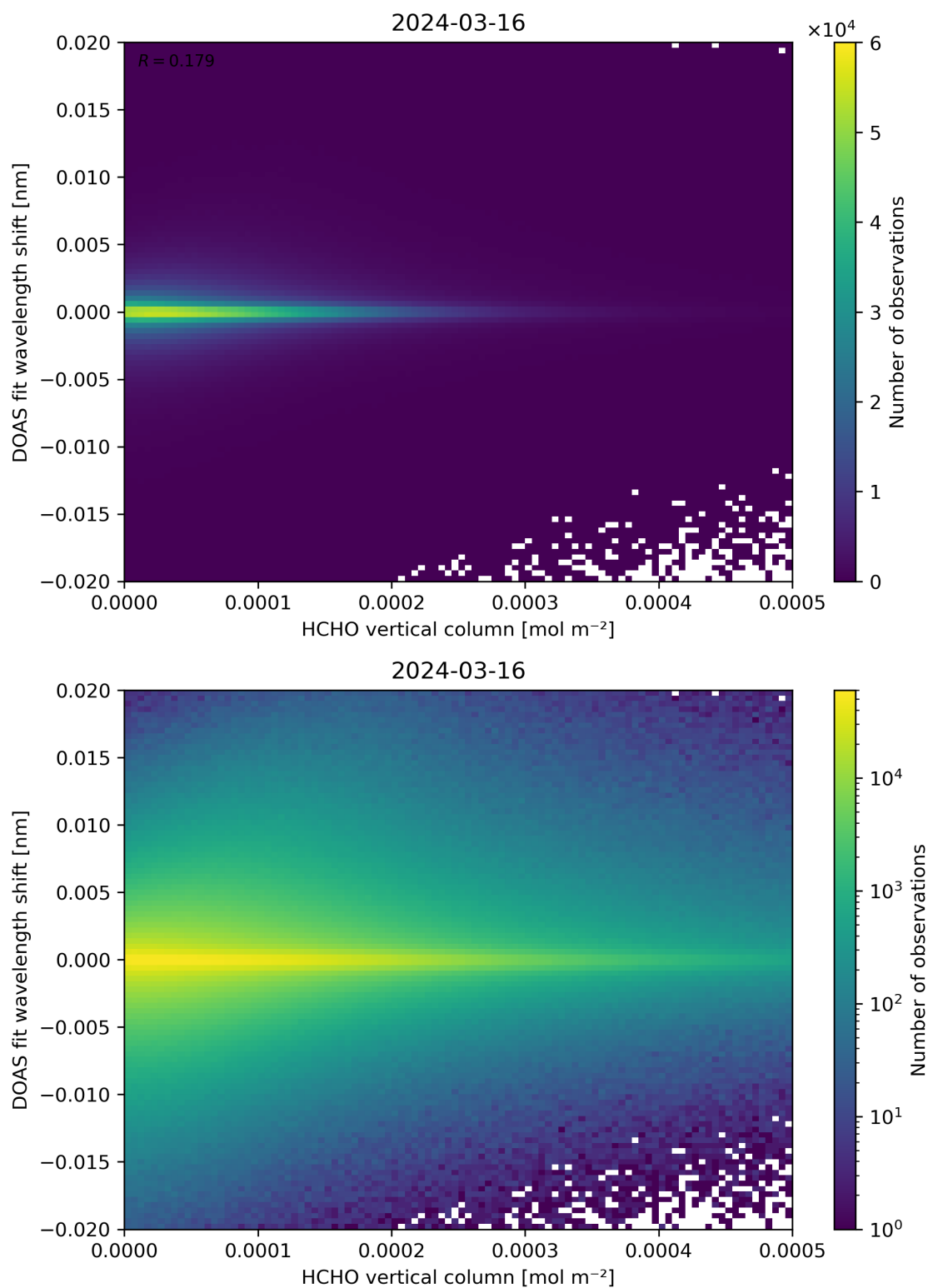
Figure 124: Scatter density plot of “HCHO vertical column” against “DOAS fit wavelength shift” for 2024-03-15 to 2024-03-17.
