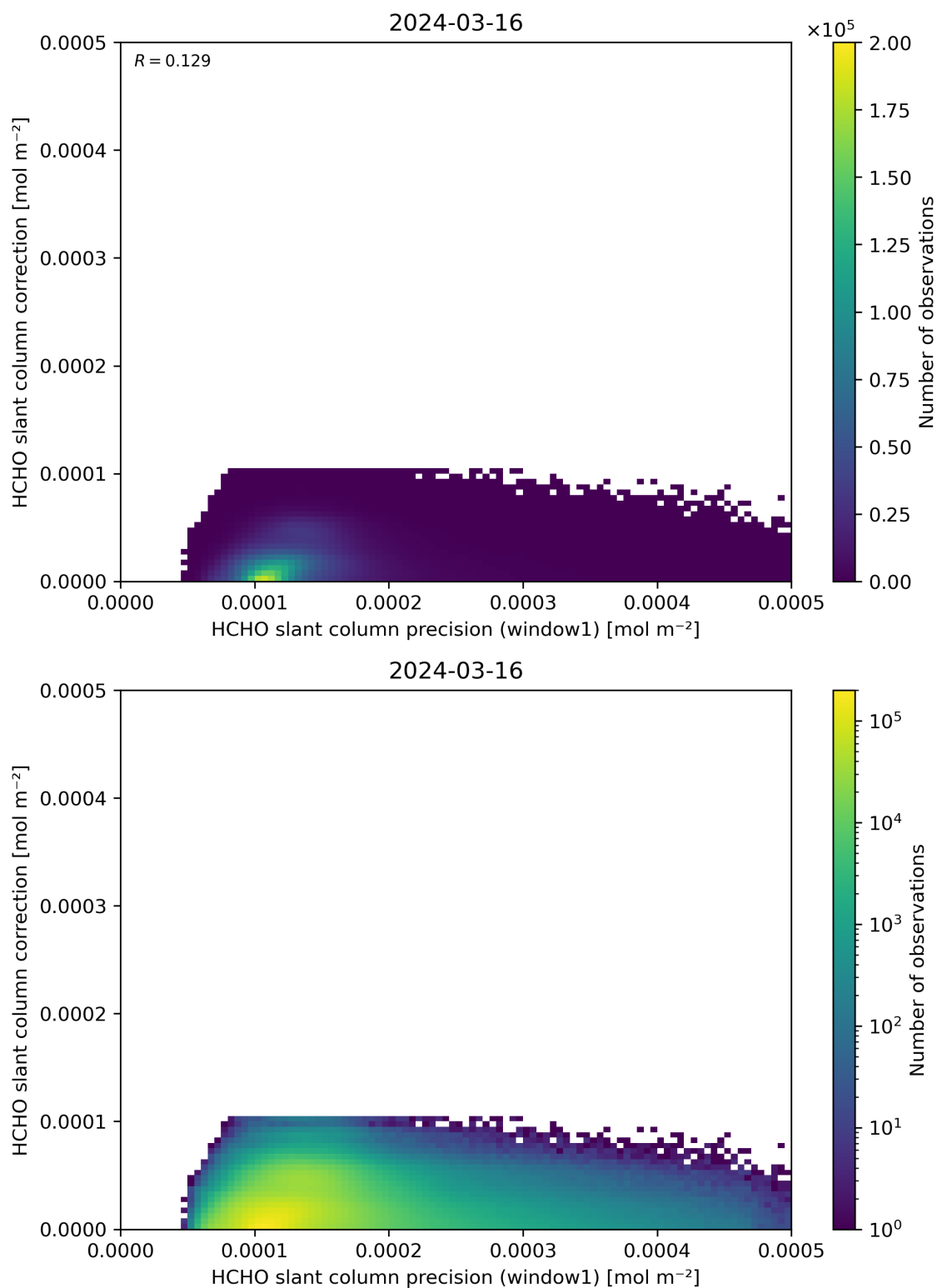
Figure 93: Scatter density plot of “HCHO slant column precision (window1)” against “HCHO slant column correction” for 2024-03-15 to 2024-03-17.
