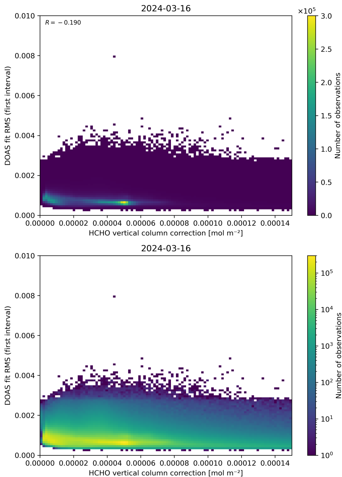
Figure 112: Scatter density plot of “HCHO vertical column correction” against “DOAS fit RMS (first interval)” for 2024-03-15 to 2024-03-17.
