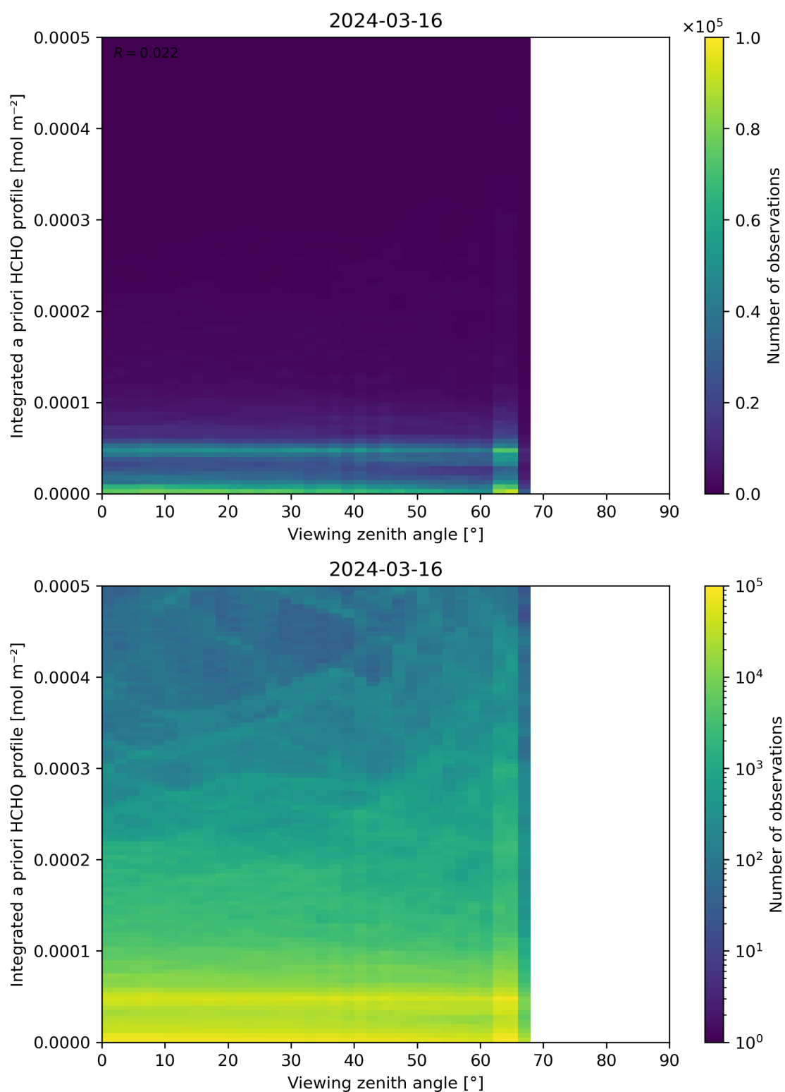
Figure 195: Scatter density plot of “Viewing zenith angle” against “Integrated a priori HCHO profile” for 2024-03-15 to 2024-03-17.
