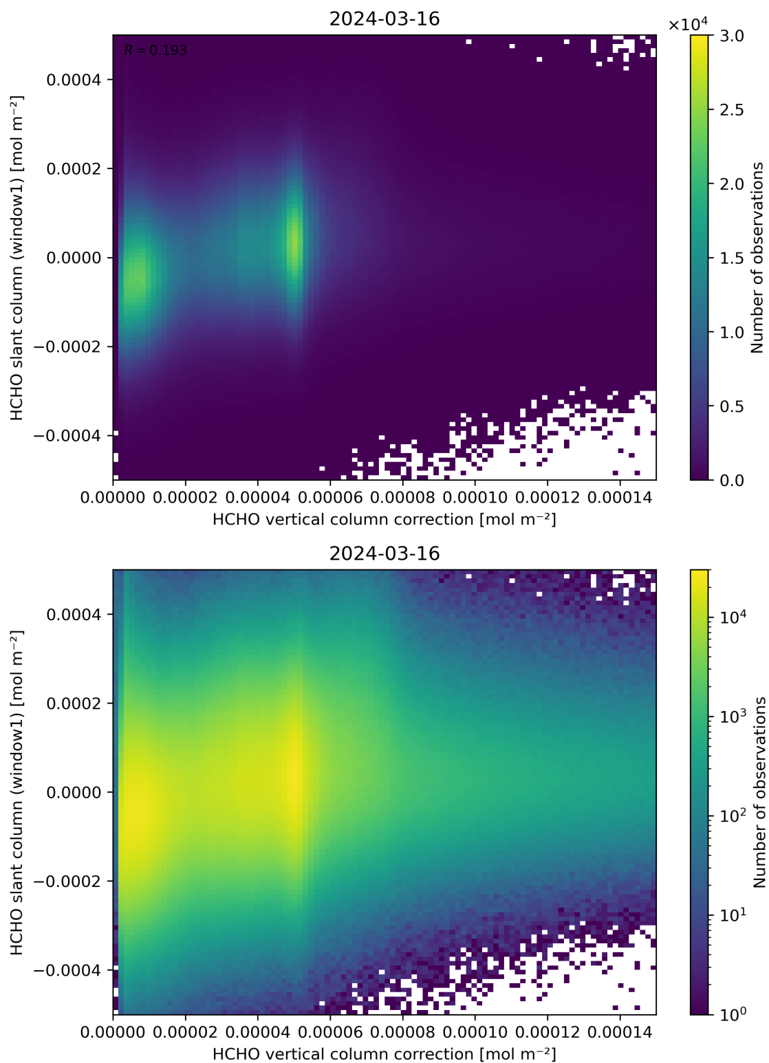
Figure 118: Scatter density plot of “HCHO vertical column correction” against “HCHO slant column (window1)” for 2024-03-15 to 2024-03-17.
