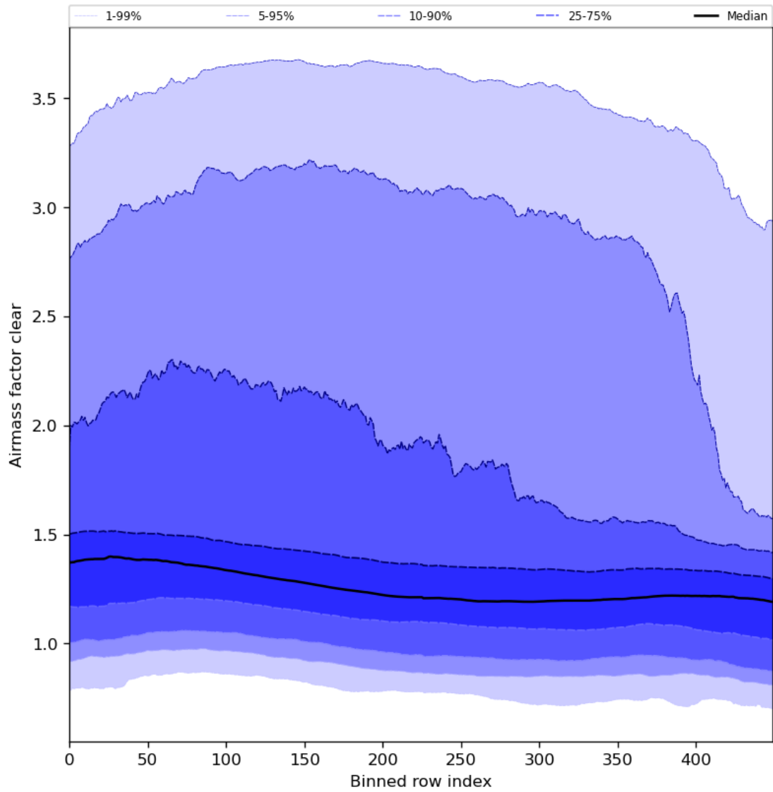
Figure 56: Along track statistics of “Airmass factor clear” for 2024-03-15 to 2024-03-17
