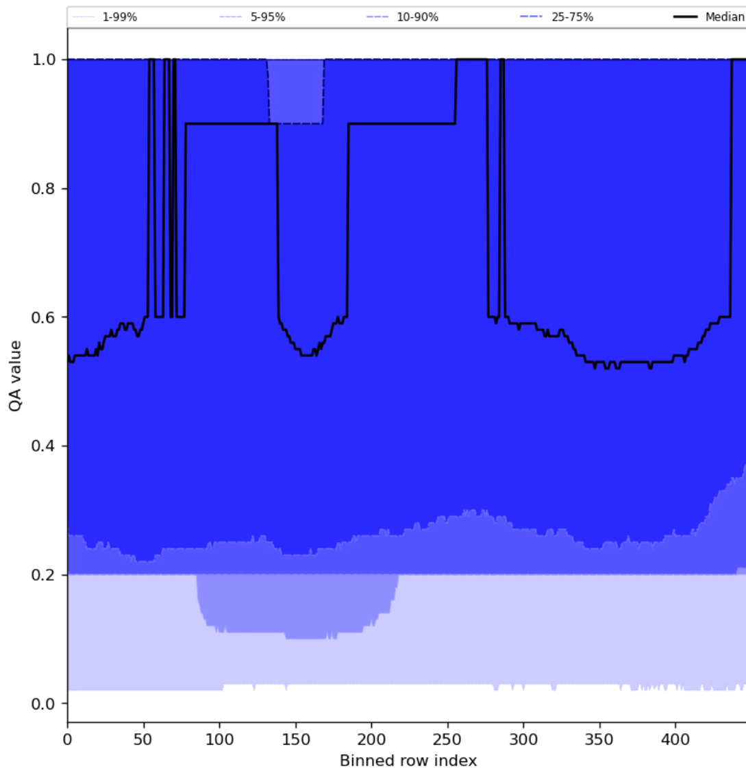
Figure 48: Along track statistics of “QA value” for 2024-03-15 to 2024-03-17
