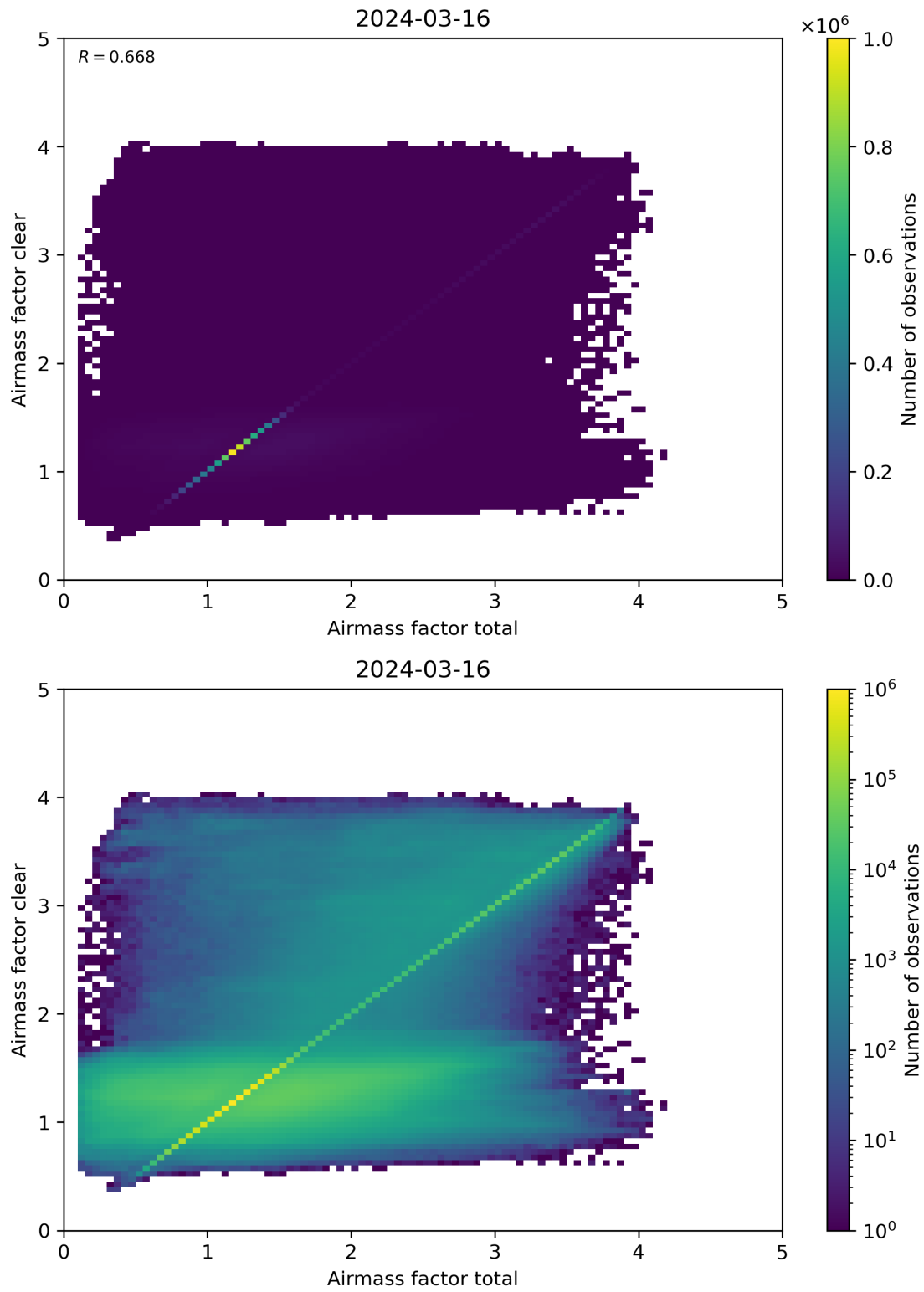
Figure 100: Scatter density plot of “Airmass factor total” against “Airmass factor clear” for 2024-03-15 to 2024-03-17.
