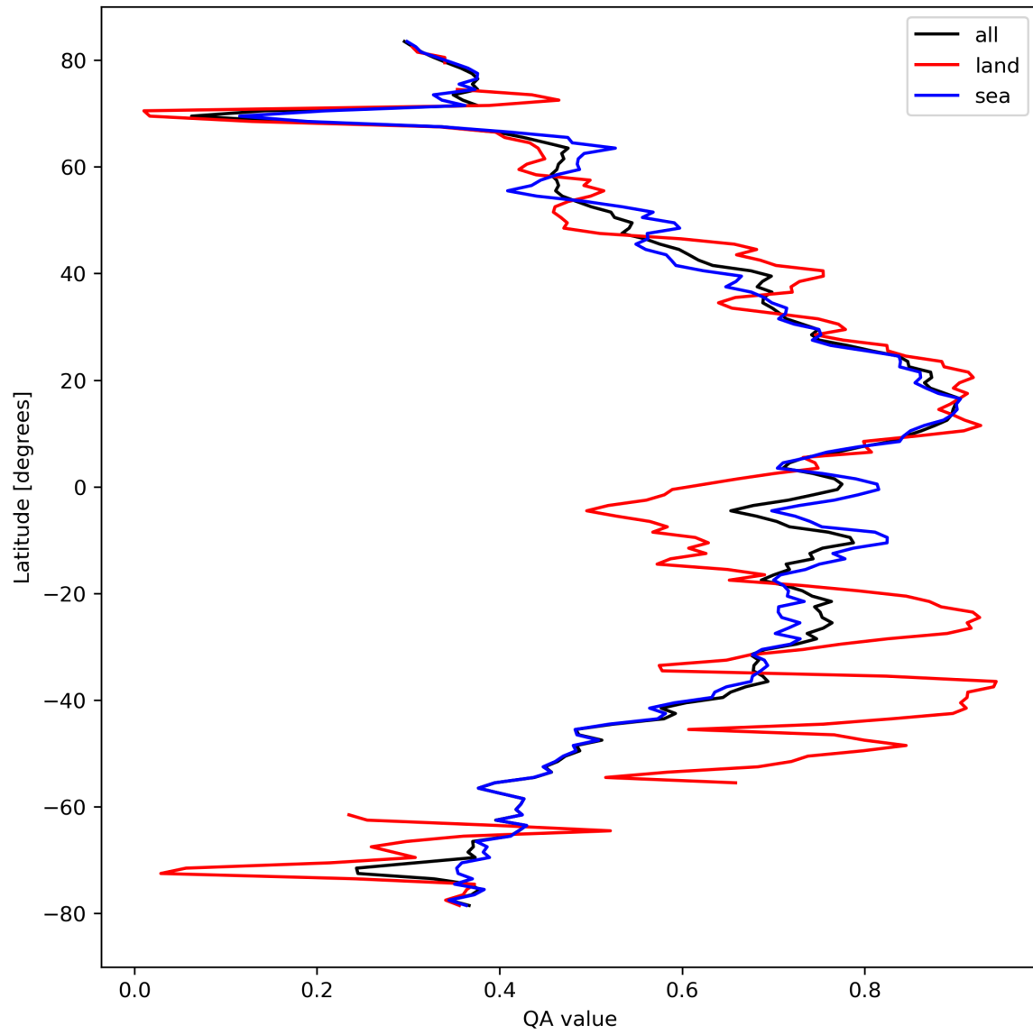
Figure 20: Zonal average of “QA value” for 2024-03-15 to 2024-03-17.
