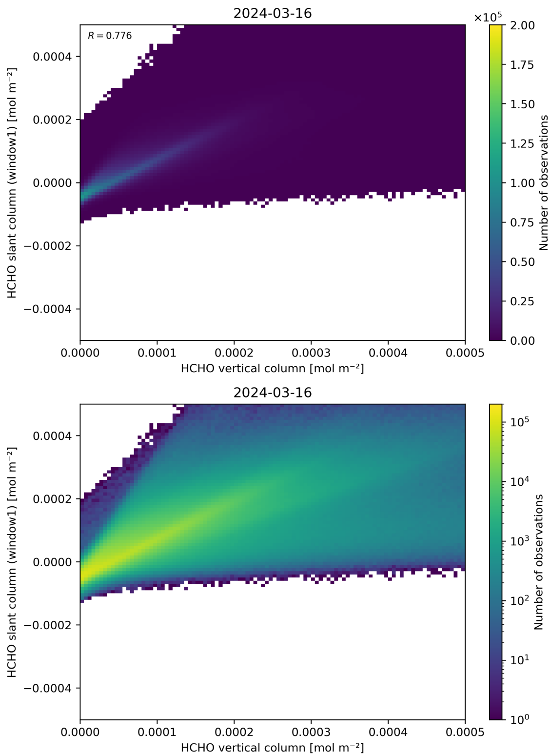
Figure 129: Scatter density plot of “HCHO vertical column” against “HCHO slant column (window1)” for 2024-03-15 to 2024-03-17.
