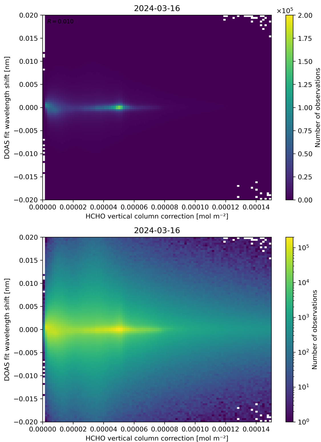
Figure 113: Scatter density plot of “HCHO vertical column correction” against “DOAS fit wavelength shift” for 2024-03-15 to 2024-03-17.
