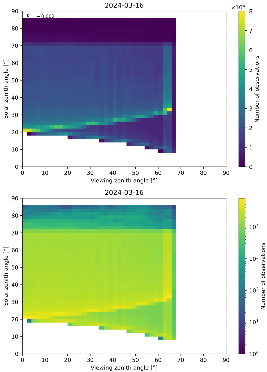
Figure 197: Scatter density plot of “Viewing zenith angle” against “Solar zenith angle” for 2024-03-15 to 2024-03-17.
