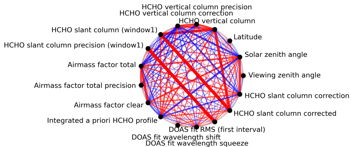
Figure 1: Map of correlation graph for 2024-03-16 to 2024-03-18.
