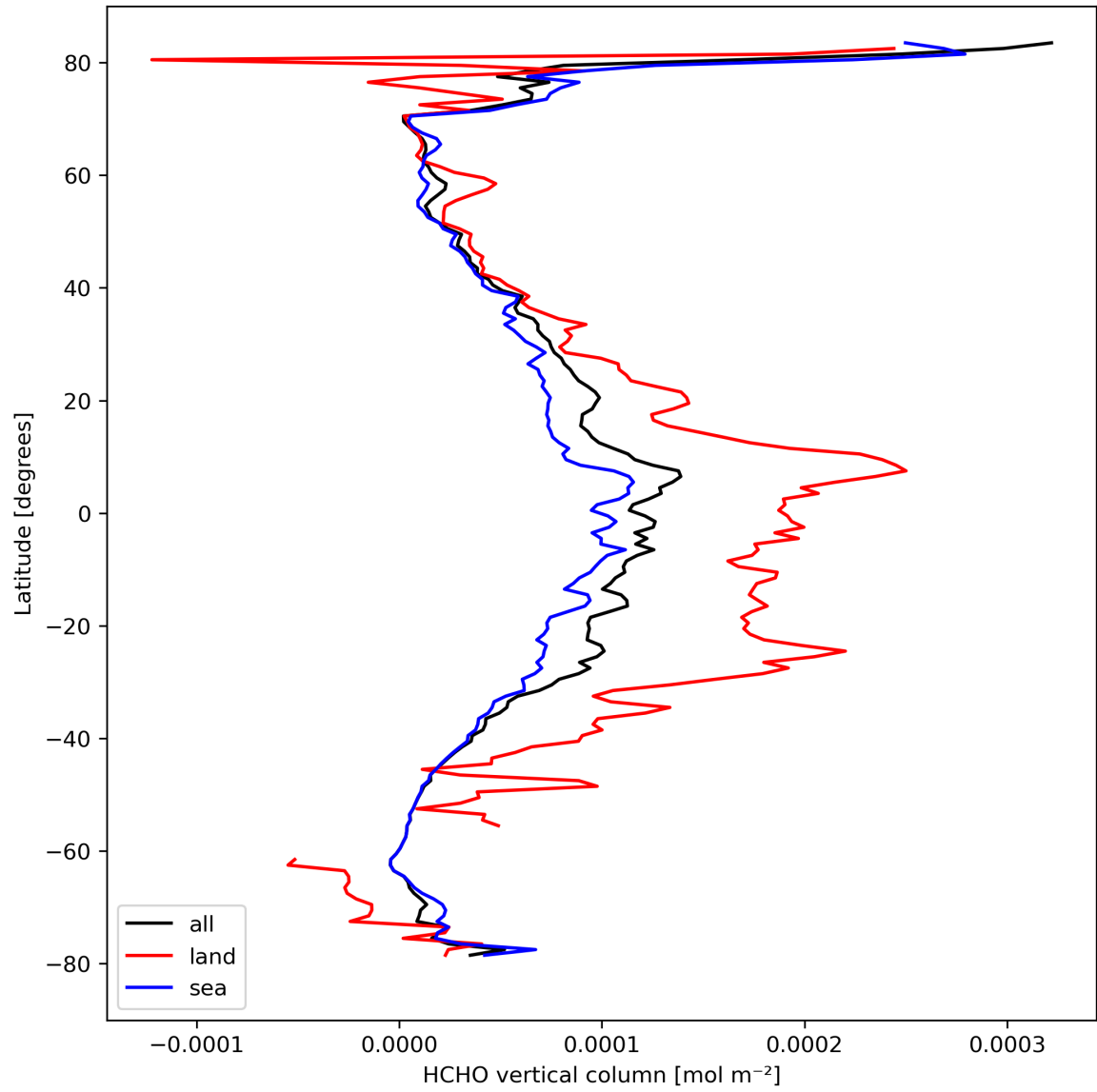
Figure 21: Zonal average of “HCHO vertical column” for 2024-03-16 to 2024-03-18.
