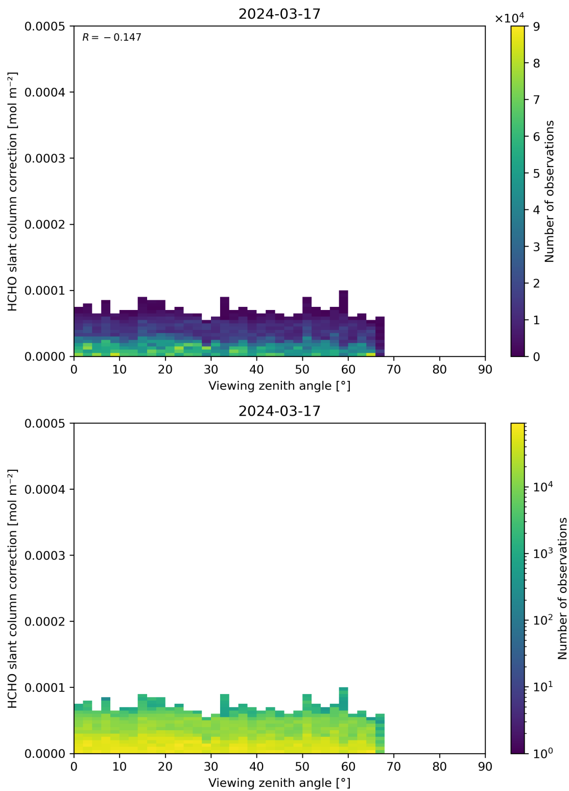
Figure 187: Scatter density plot of “Viewing zenith angle” against “HCHO slant column correction” for 2024-03-16 to 2024-03-18.
