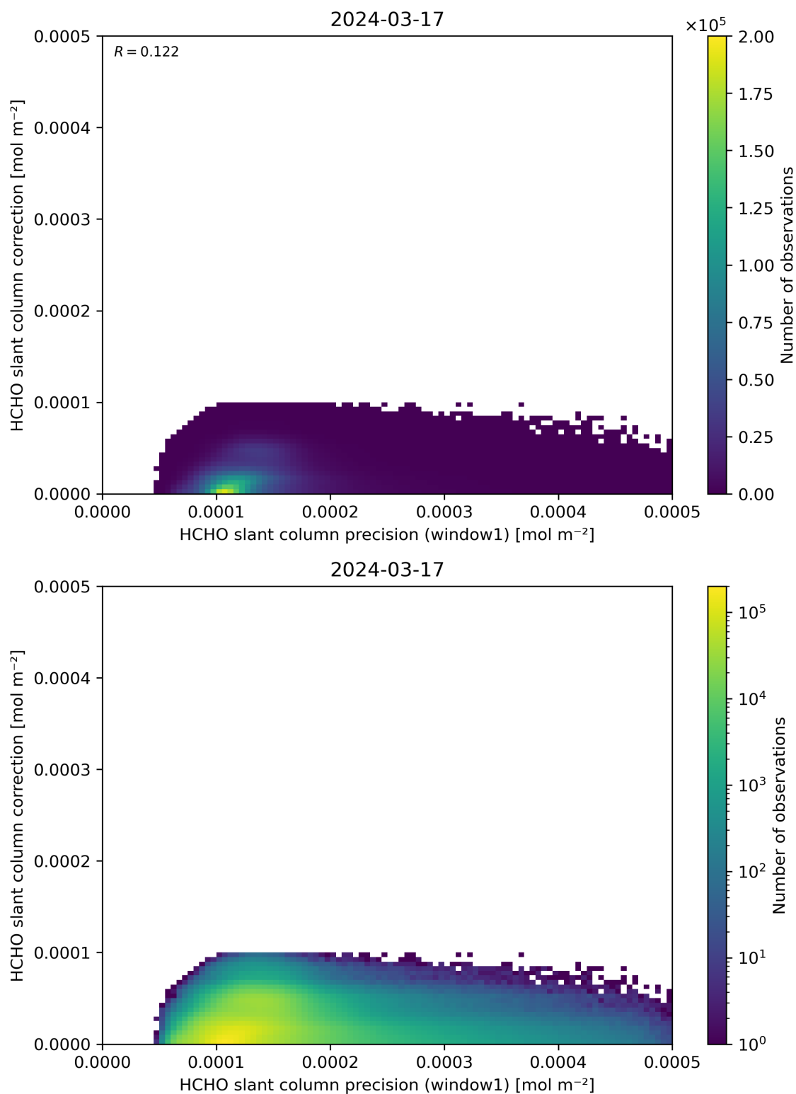
Figure 93: Scatter density plot of “HCHO slant column precision (window1)” against “HCHO slant column correction” for 2024-03-16 to 2024-03-18.
