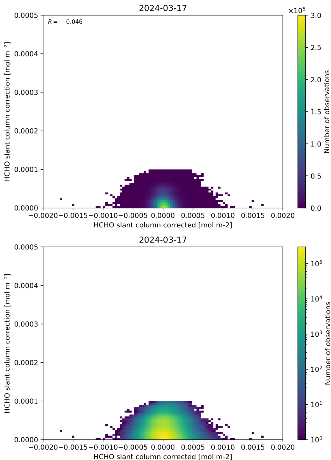
Figure 77: Scatter density plot of “HCHO slant column corrected” against “HCHO slant column correction” for 2024-03-16 to 2024-03-18.
