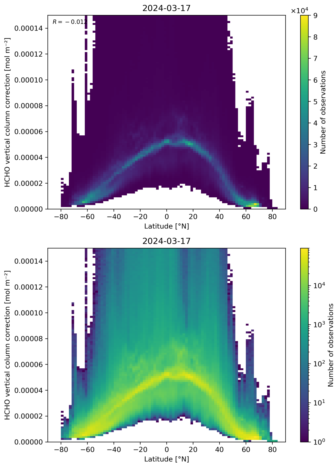
Figure 164: Scatter density plot of “Latitude” against “HCHO vertical column correction” for 2024-03-16 to 2024-03-18.
