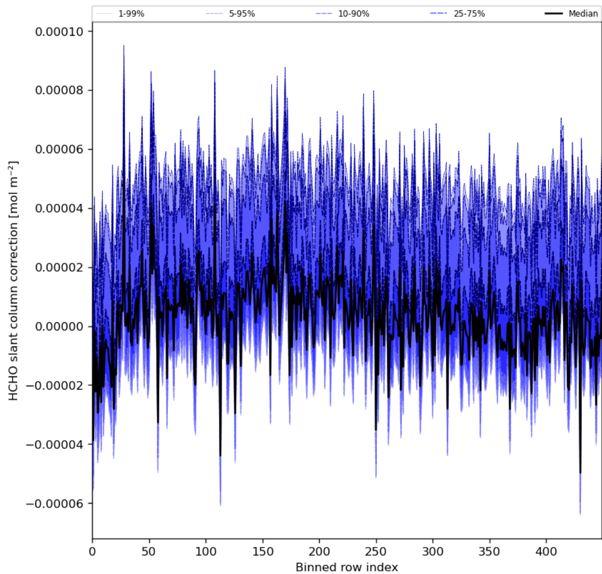
Figure 61: Along track statistics of “HCHO slant column correction” for 2024-03-16 to 2024-03-18
