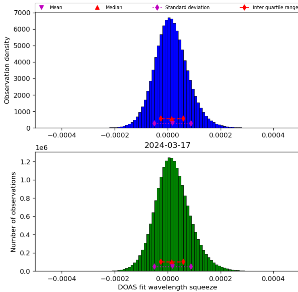
Figure 45: Histogram of “DOAS fit wavelength squeeze” for 2024-03-16 to 2024-03-18
