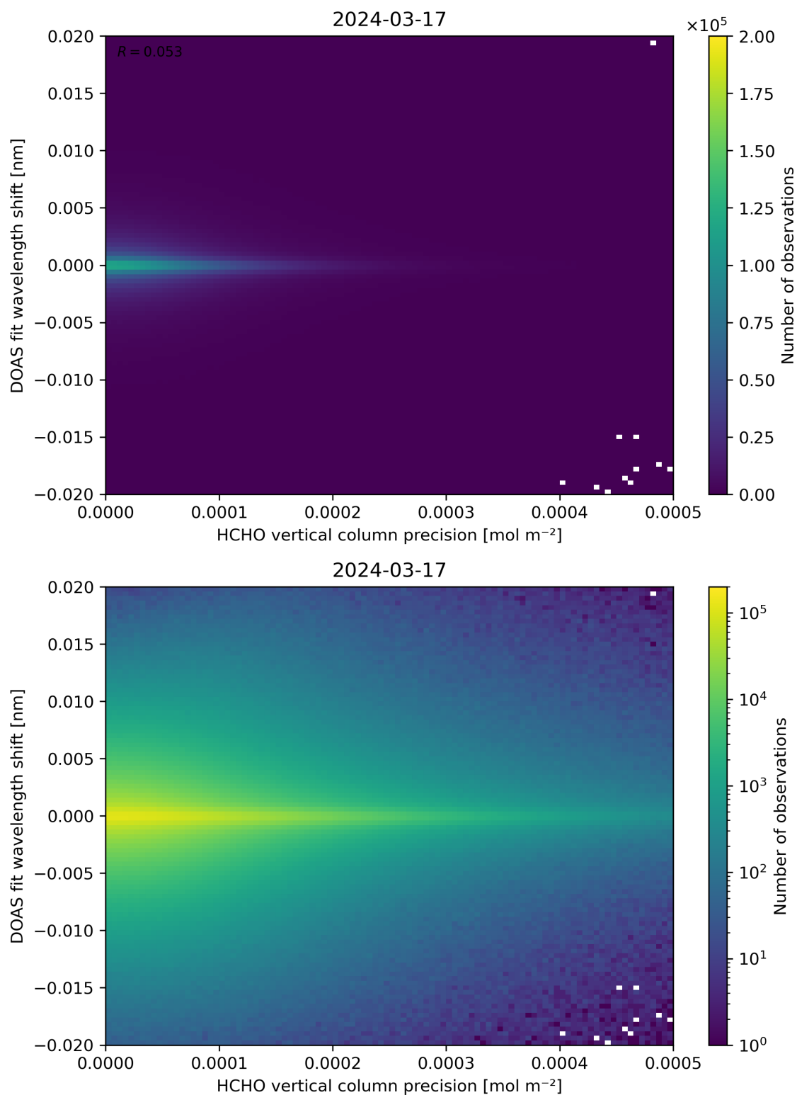
Figure 137: Scatter density plot of “HCHO vertical column precision” against “DOAS fit wavelength shift” for 2024-03-16 to 2024-03-18.
