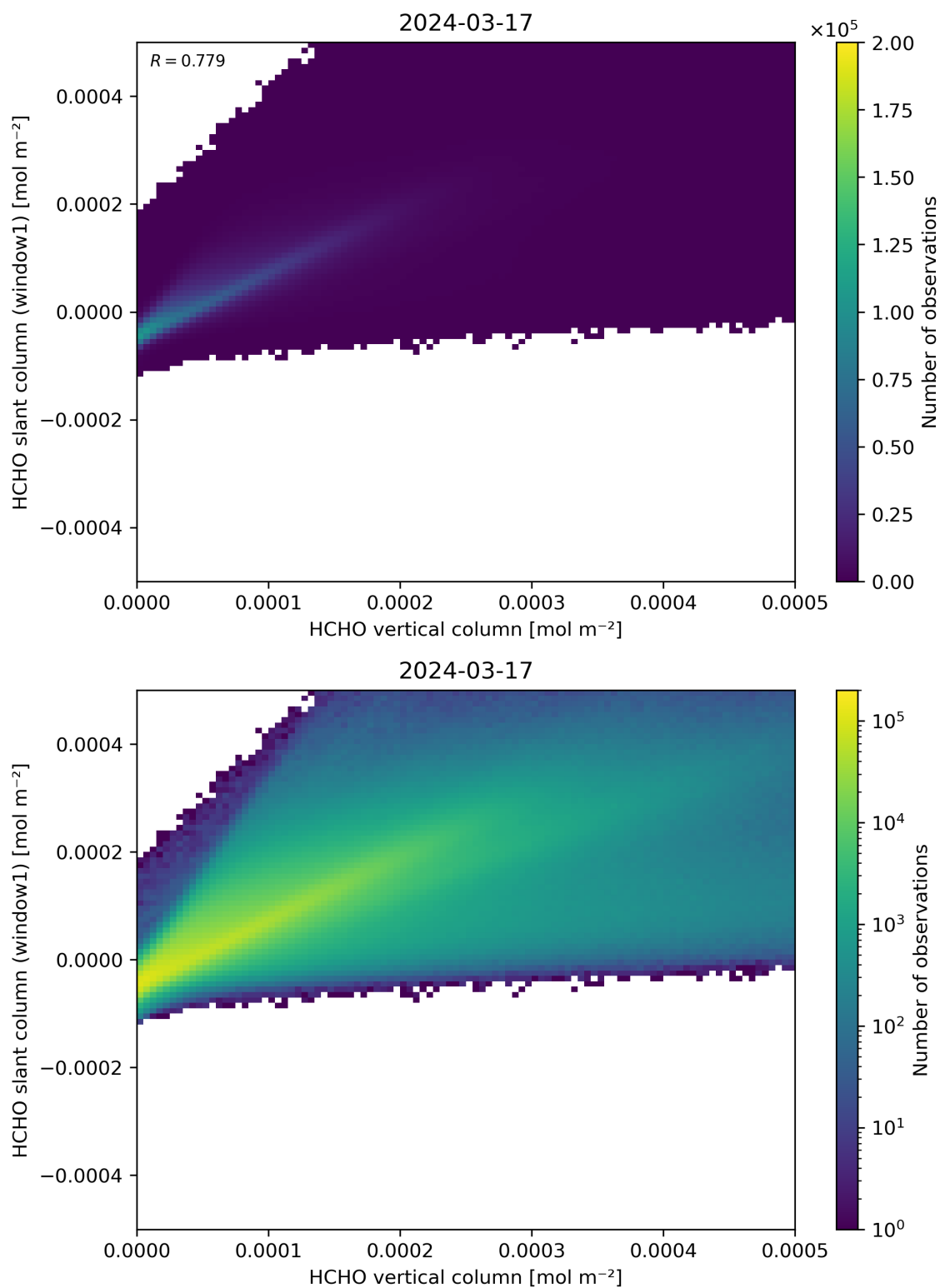
Figure 129: Scatter density plot of “HCHO vertical column” against “HCHO slant column (window1)” for 2024-03-16 to 2024-03-18.
