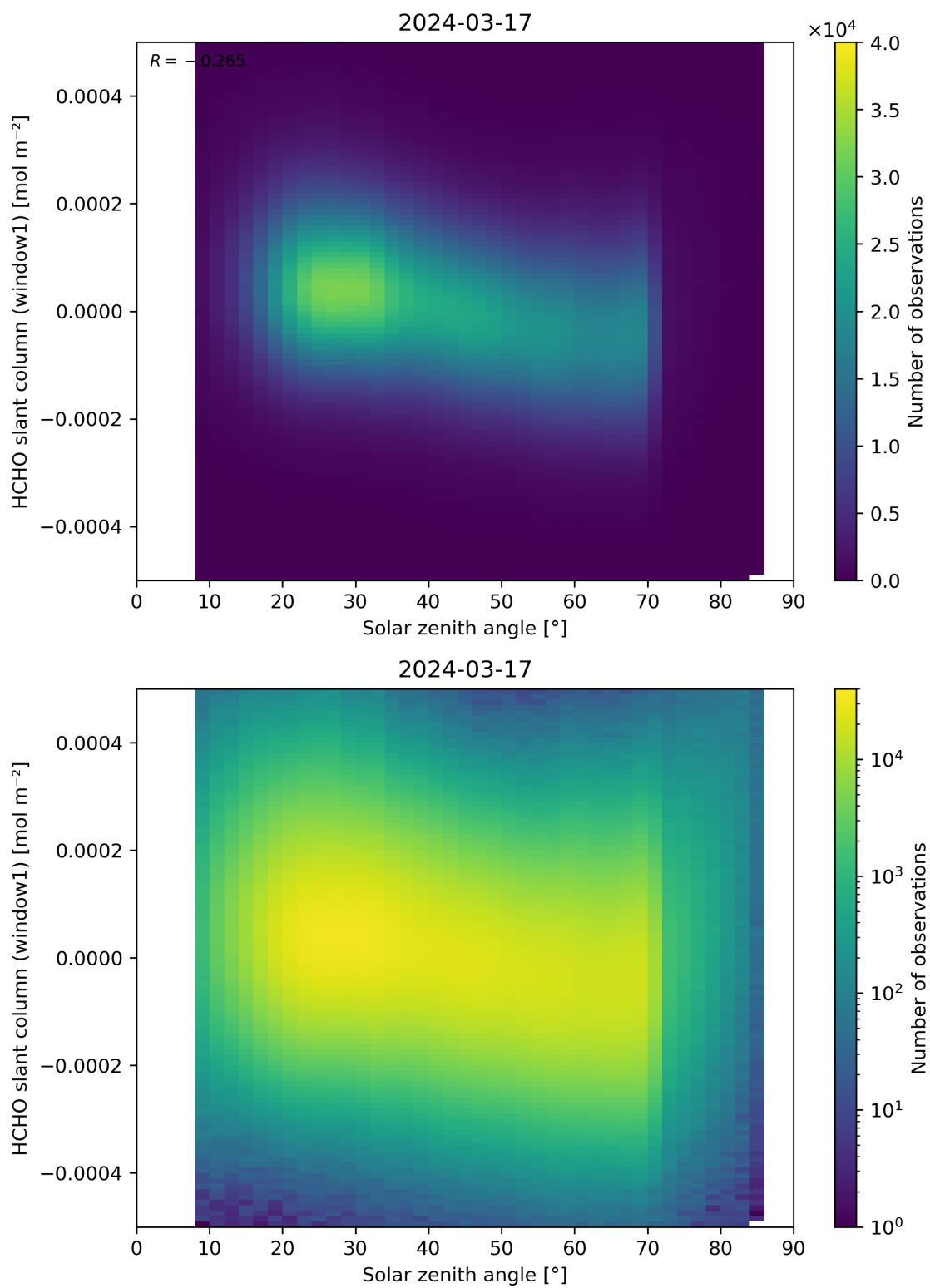
Figure 173: Scatter density plot of “Solar zenith angle” against “HCHO slant column (window1)” for 2024-03-16 to 2024-03-18.
