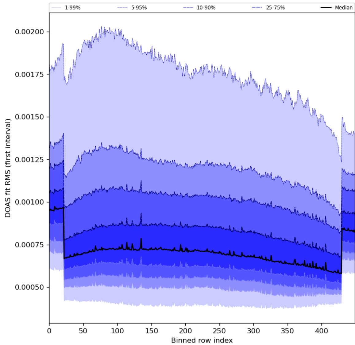
Figure 60: Along track statistics of “DOAS fit RMS (first interval)” for 2024-03-16 to 2024-03-18
