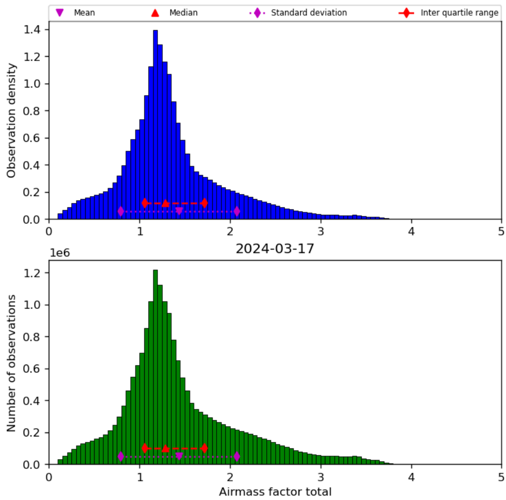
Figure 40: Histogram of “Airmass factor total” for 2024-03-16 to 2024-03-18
