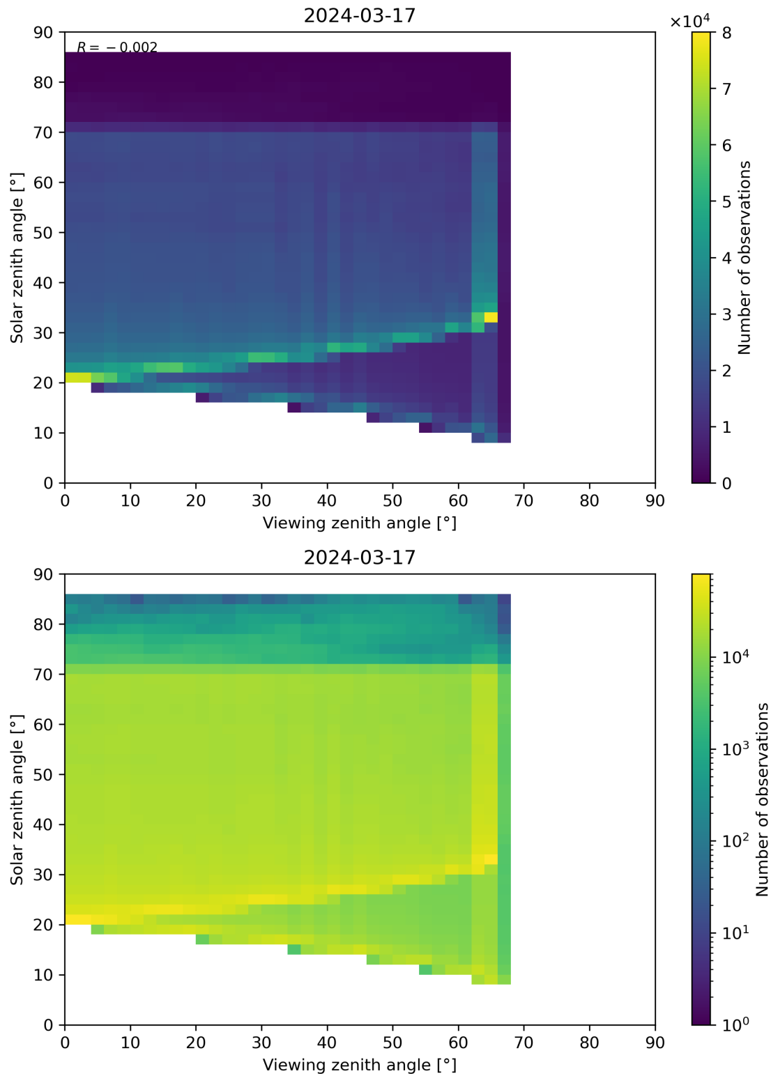
Figure 197: Scatter density plot of “Viewing zenith angle” against “Solar zenith angle” for 2024-03-16 to 2024-03-18.
