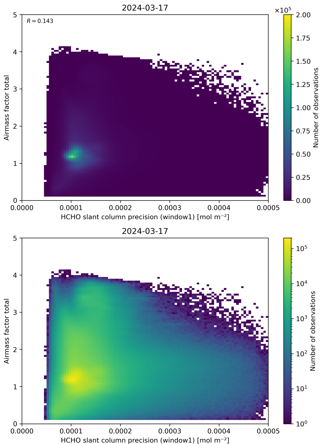
Figure 94: Scatter density plot of “HCHO slant column precision (window1)” against “Airmass factor total” for 2024-03-16 to 2024-03-18.
