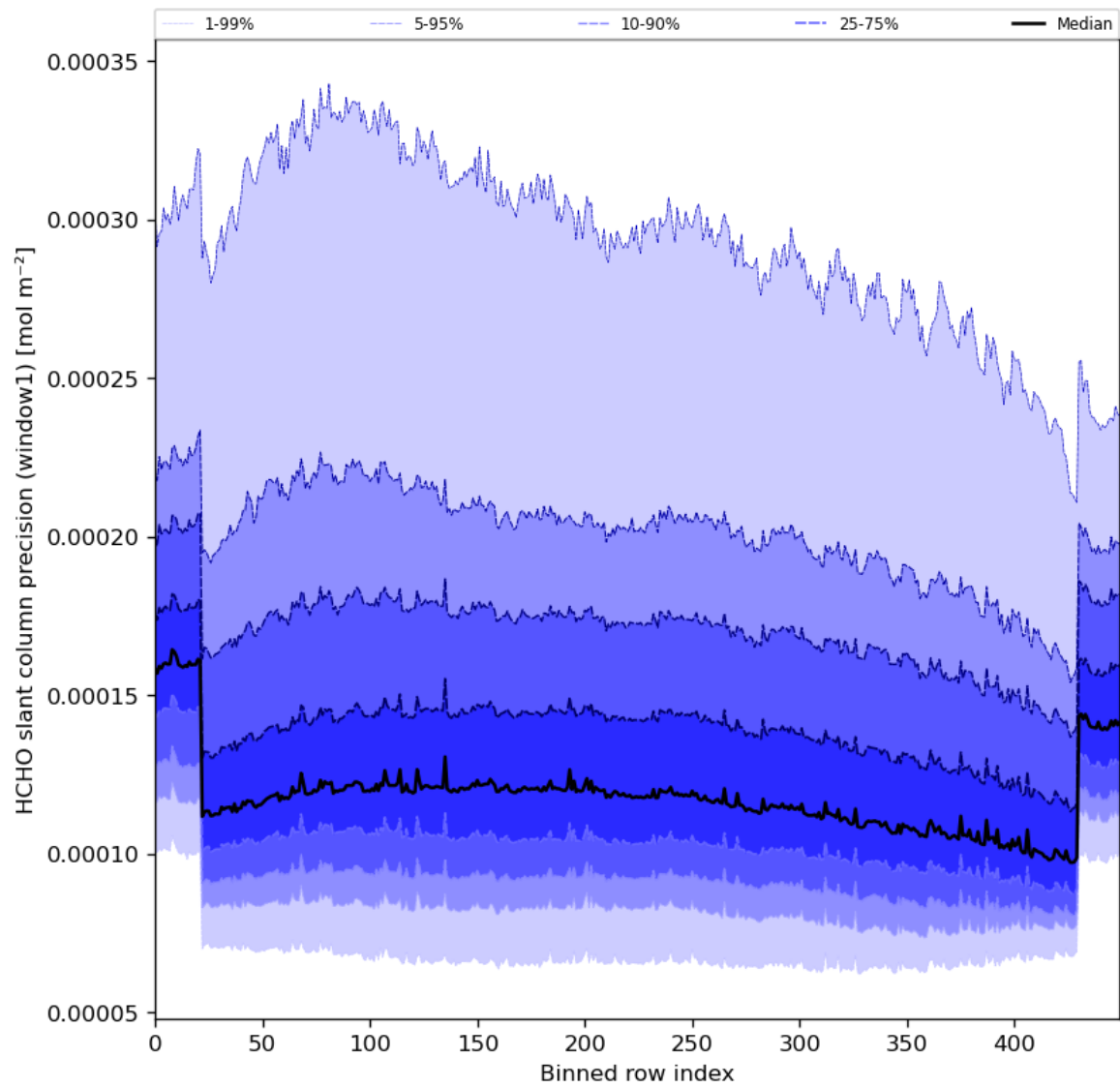
Figure 53: Along track statistics of “HCHO slant column precision (window1)” for 2024-03-16 to 2024-03-18
