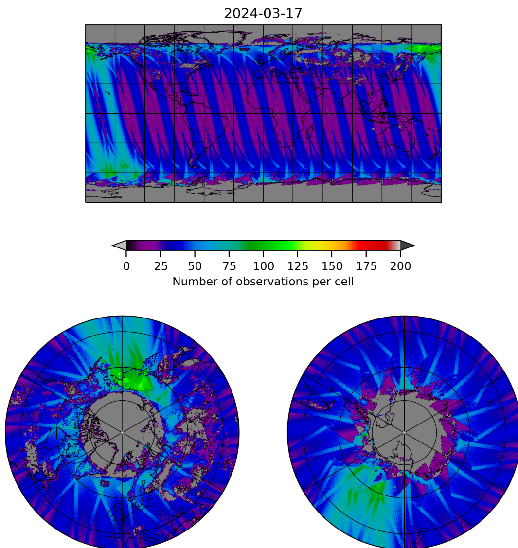
Figure 19: Map of the number of observations for 2024-03-16 to 2024-03-18
