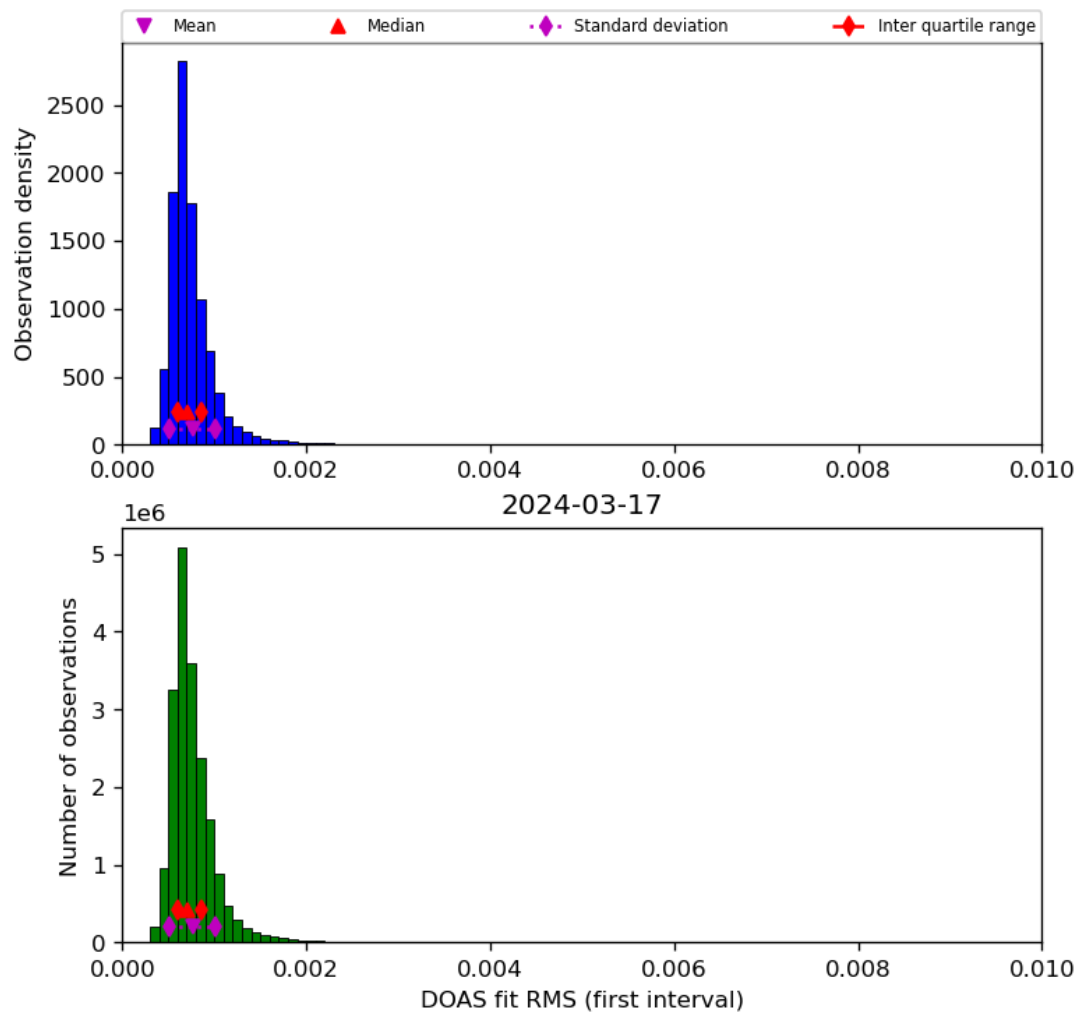
Figure 46: Histogram of “DOAS fit RMS (first interval)” for 2024-03-16 to 2024-03-18
