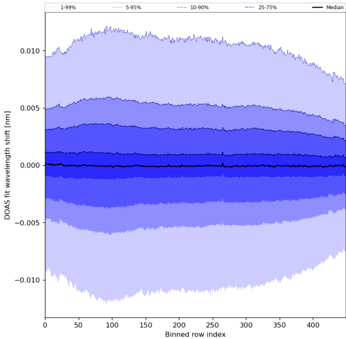
Figure 58: Along track statistics of “DOAS fit wavelength shift” for 2024-03-16 to 2024-03-18
