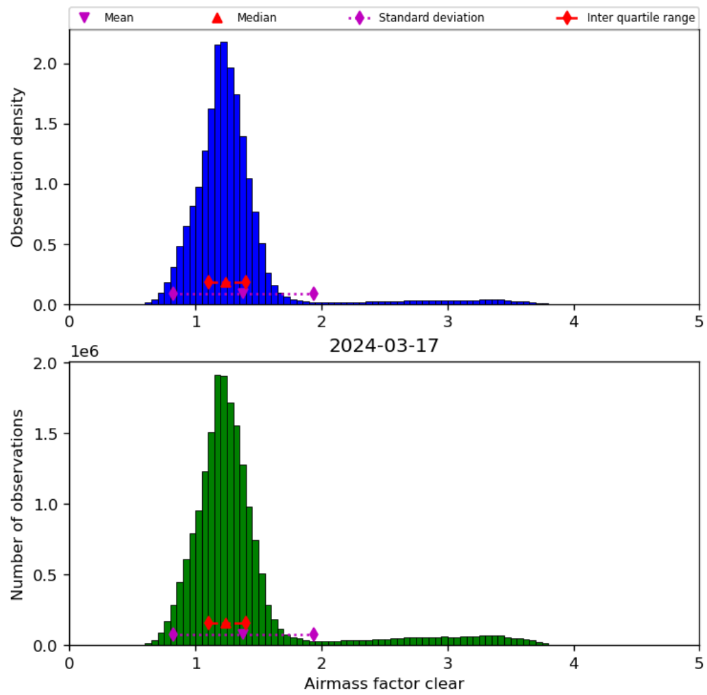
Figure 42: Histogram of “Airmass factor clear” for 2024-03-16 to 2024-03-18
