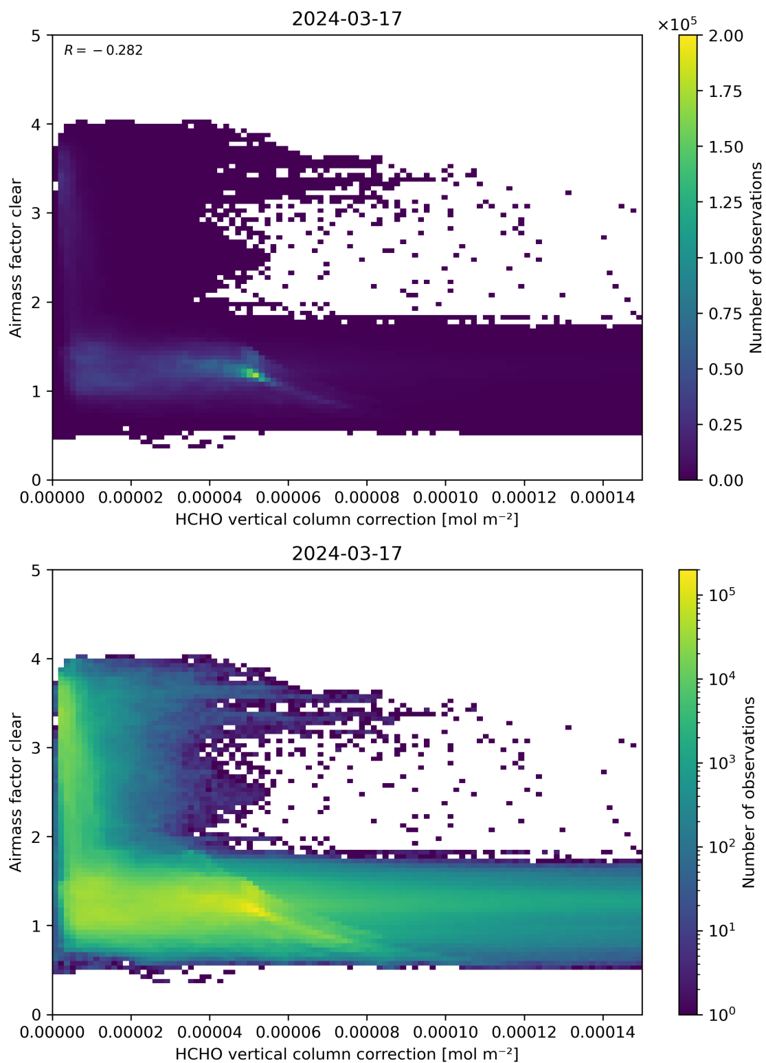
Figure 115: Scatter density plot of “HCHO vertical column correction” against “Airmass factor clear” for 2024-03-16 to 2024-03-18.
