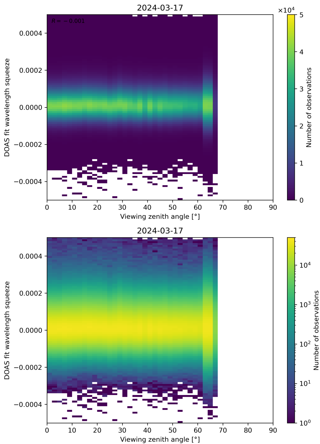
Figure 184: Scatter density plot of “Viewing zenith angle” against “DOAS fit wavelength squeeze” for 2024-03-16 to 2024-03-18.
