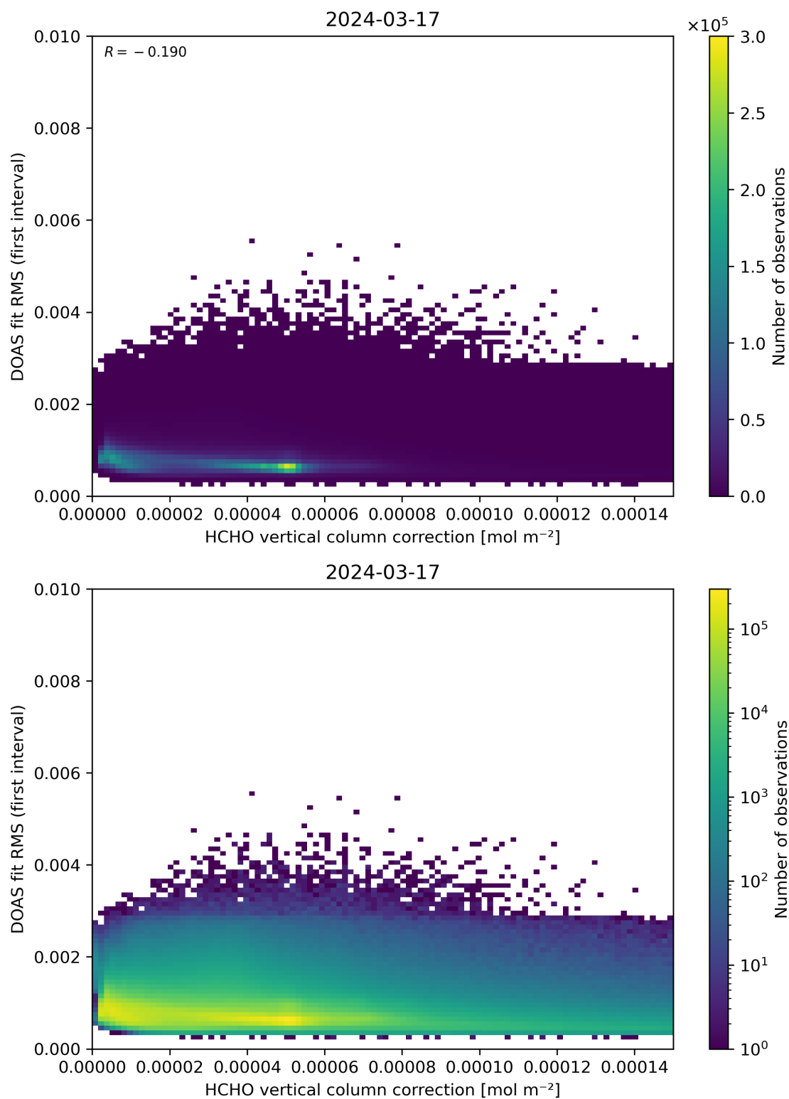
Figure 112: Scatter density plot of “HCHO vertical column correction” against “DOAS fit RMS (first interval)” for 2024-03-16 to 2024-03-18.
