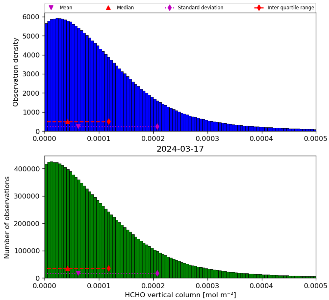
Figure 35: Histogram of “HCHO vertical column” for 2024-03-16 to 2024-03-18
