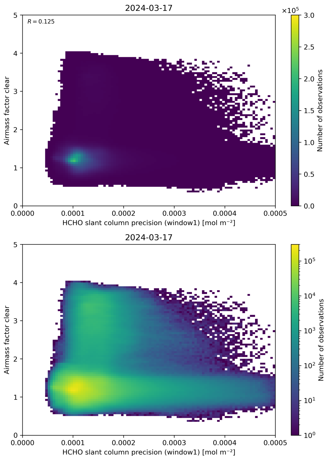
Figure 91: Scatter density plot of “HCHO slant column precision (window1)” against “Airmass factor clear” for 2024-03-16 to 2024-03-18.
