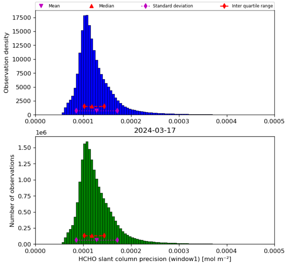
Figure 39: Histogram of “HCHO slant column precision (window1)” for 2024-03-16 to 2024-03-18
