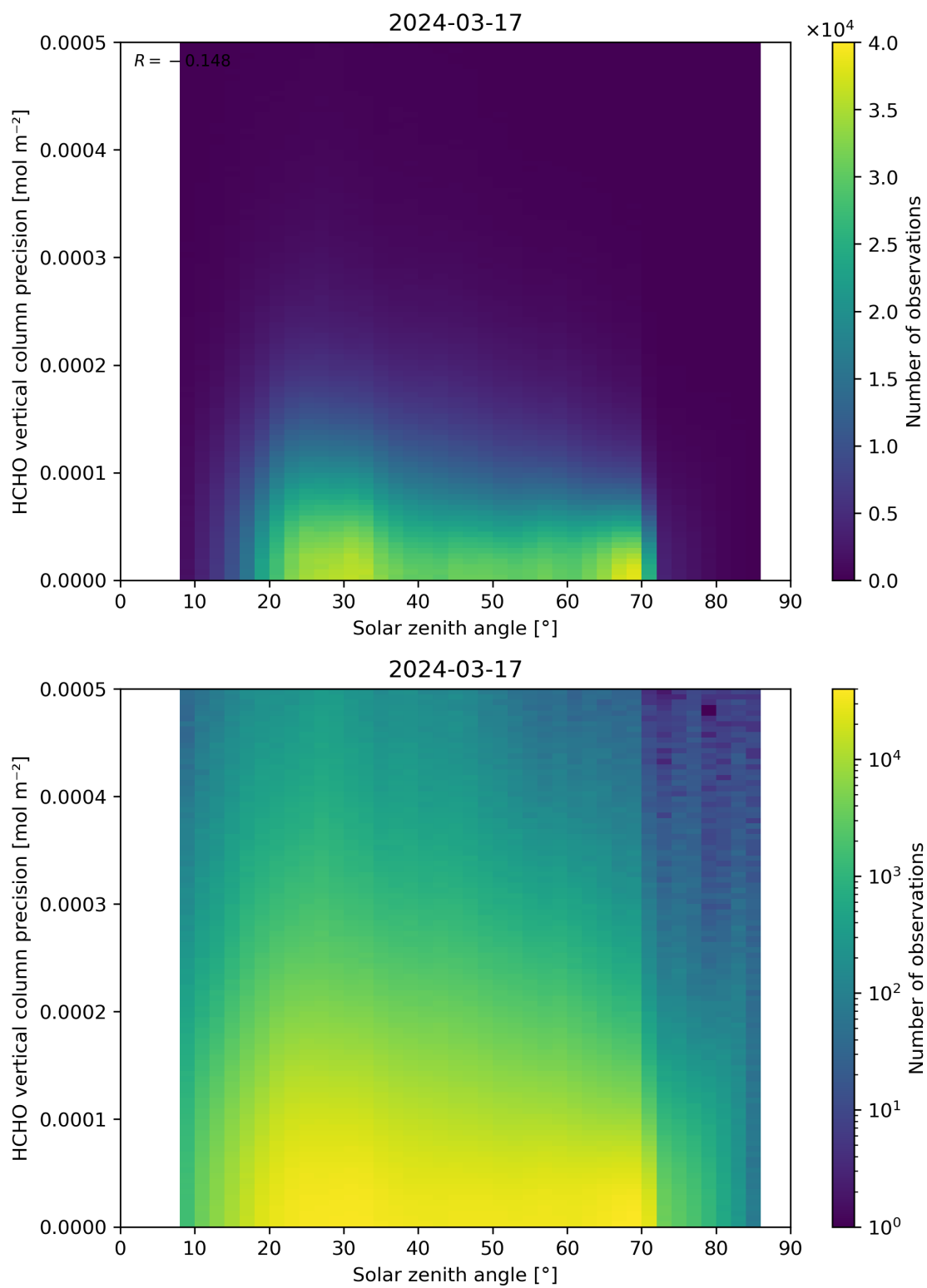
Figure 179: Scatter density plot of “Solar zenith angle” against “HCHO vertical column precision” for 2024-03-16 to 2024-03-18.
