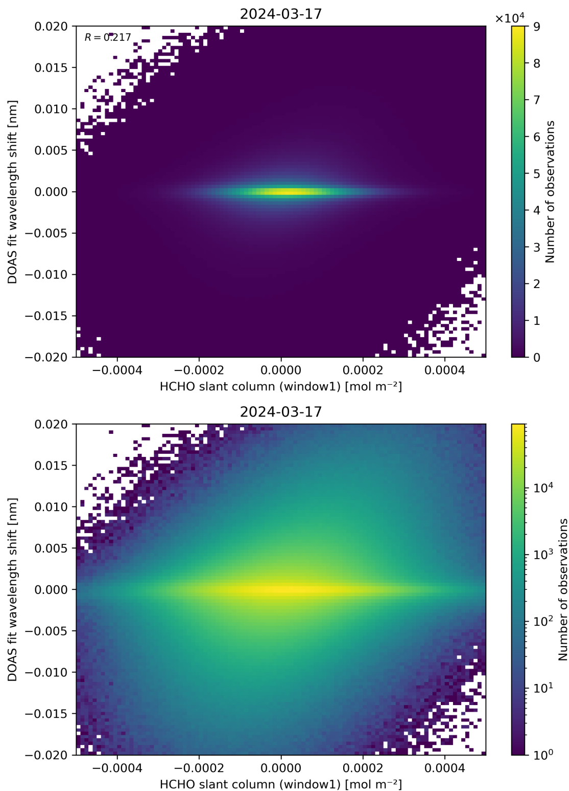
Figure 79: Scatter density plot of “HCHO slant column (window1)” against “DOAS fit wavelength shift” for 2024-03-16 to 2024-03-18.
