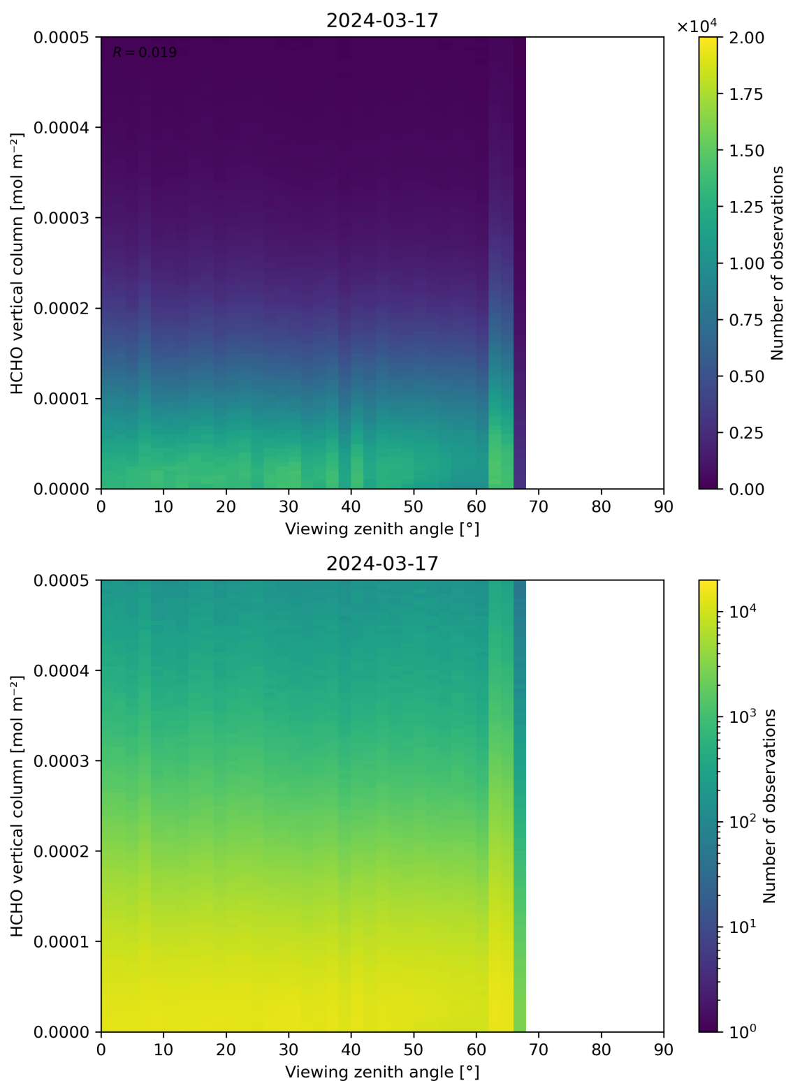
Figure 192: Scatter density plot of “Viewing zenith angle” against “HCHO vertical column” for 2024-03-16 to 2024-03-18.
