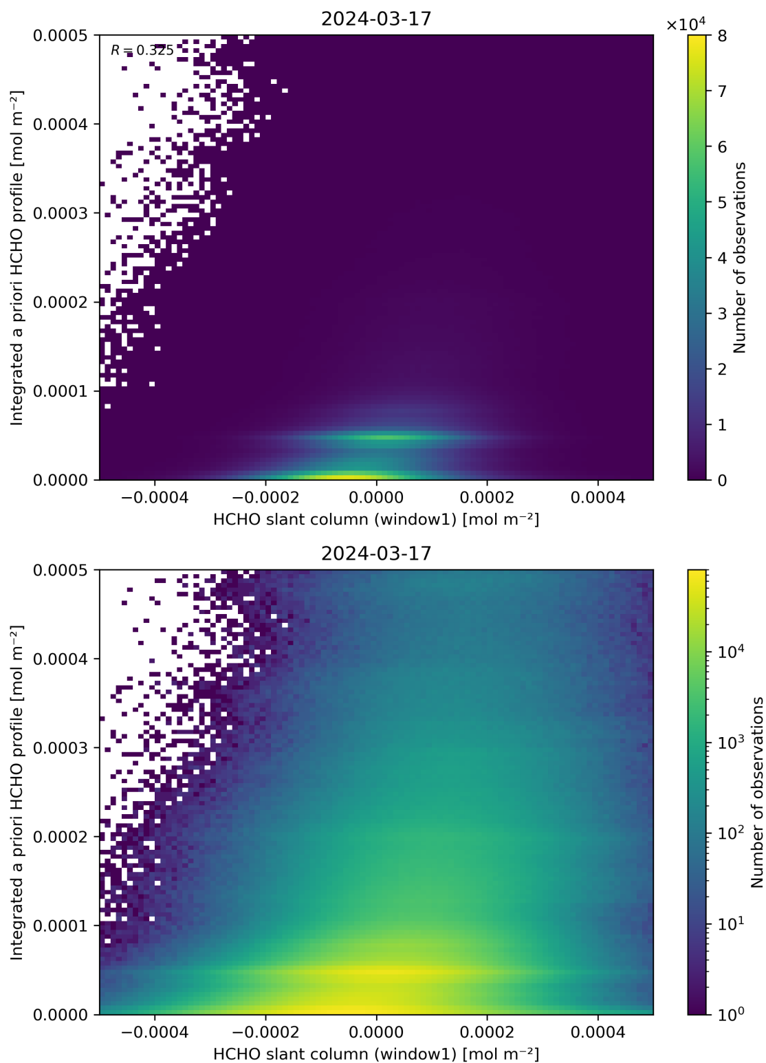
Figure 87: Scatter density plot of “HCHO slant column (window1)” against “Integrated a priori HCHO profile” for 2024-03-16 to 2024-03-18.
