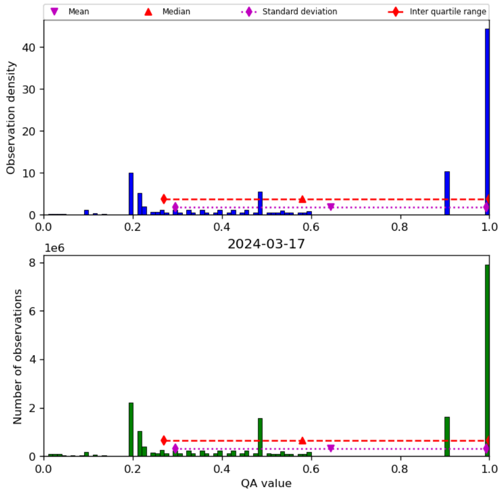
Figure 34: Histogram of “QA value” for 2024-03-16 to 2024-03-18
