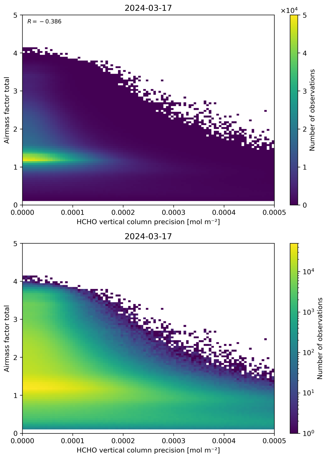
Figure 144: Scatter density plot of “HCHO vertical column precision” against “Airmass factor total” for 2024-03-16 to 2024-03-18.
