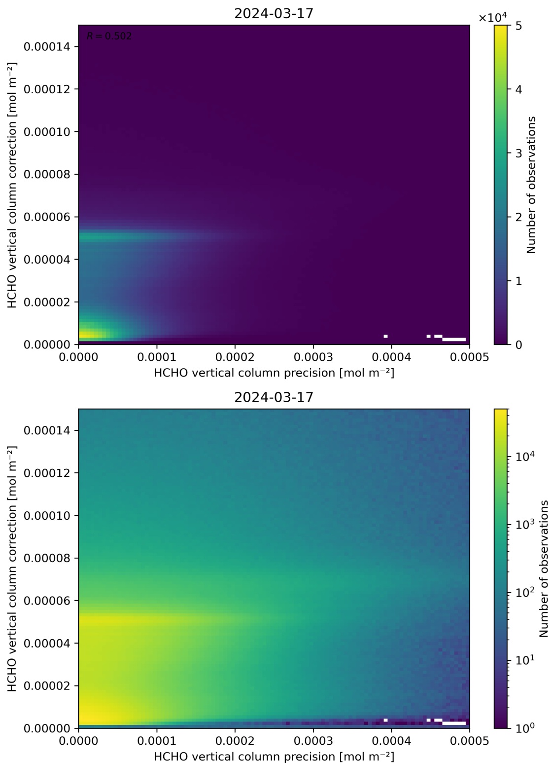
Figure 146: Scatter density plot of “HCHO vertical column precision” against “HCHO vertical column correction” for 2024-03-16 to 2024-03-18.
