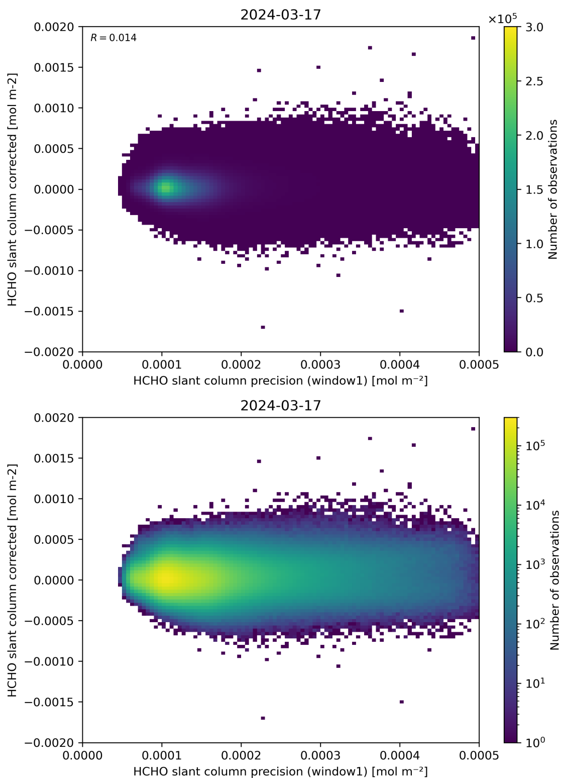
Figure 92: Scatter density plot of “HCHO slant column precision (window1)” against “HCHO slant column corrected” for 2024-03-16 to 2024-03-18.
