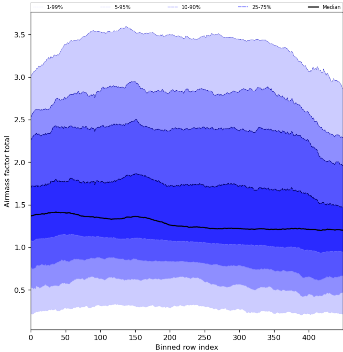
Figure 54: Along track statistics of “Airmass factor total” for 2024-03-16 to 2024-03-18
