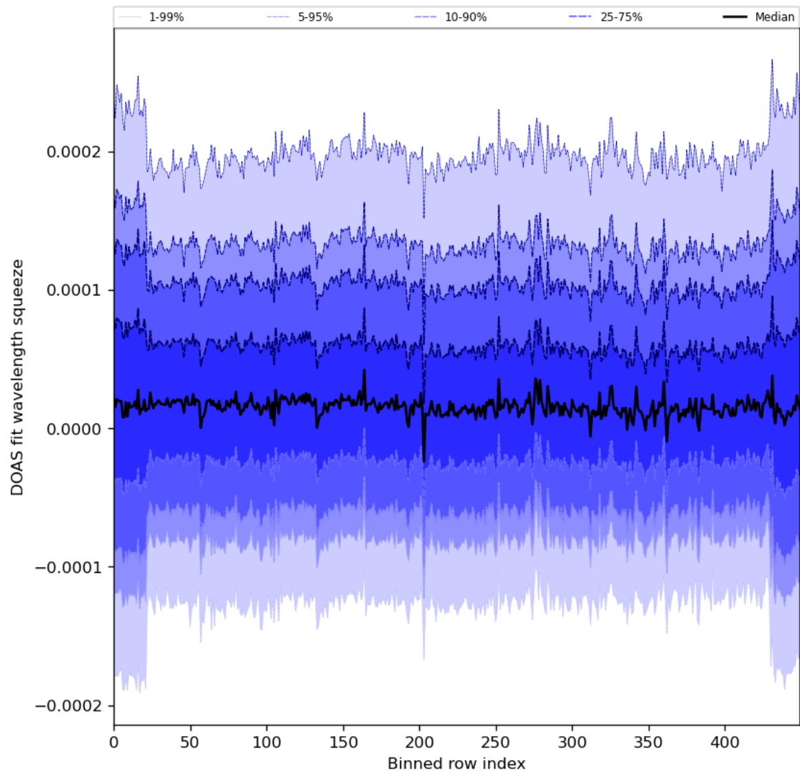
Figure 59: Along track statistics of “DOAS fit wavelength squeeze” for 2024-03-16 to 2024-03-18
