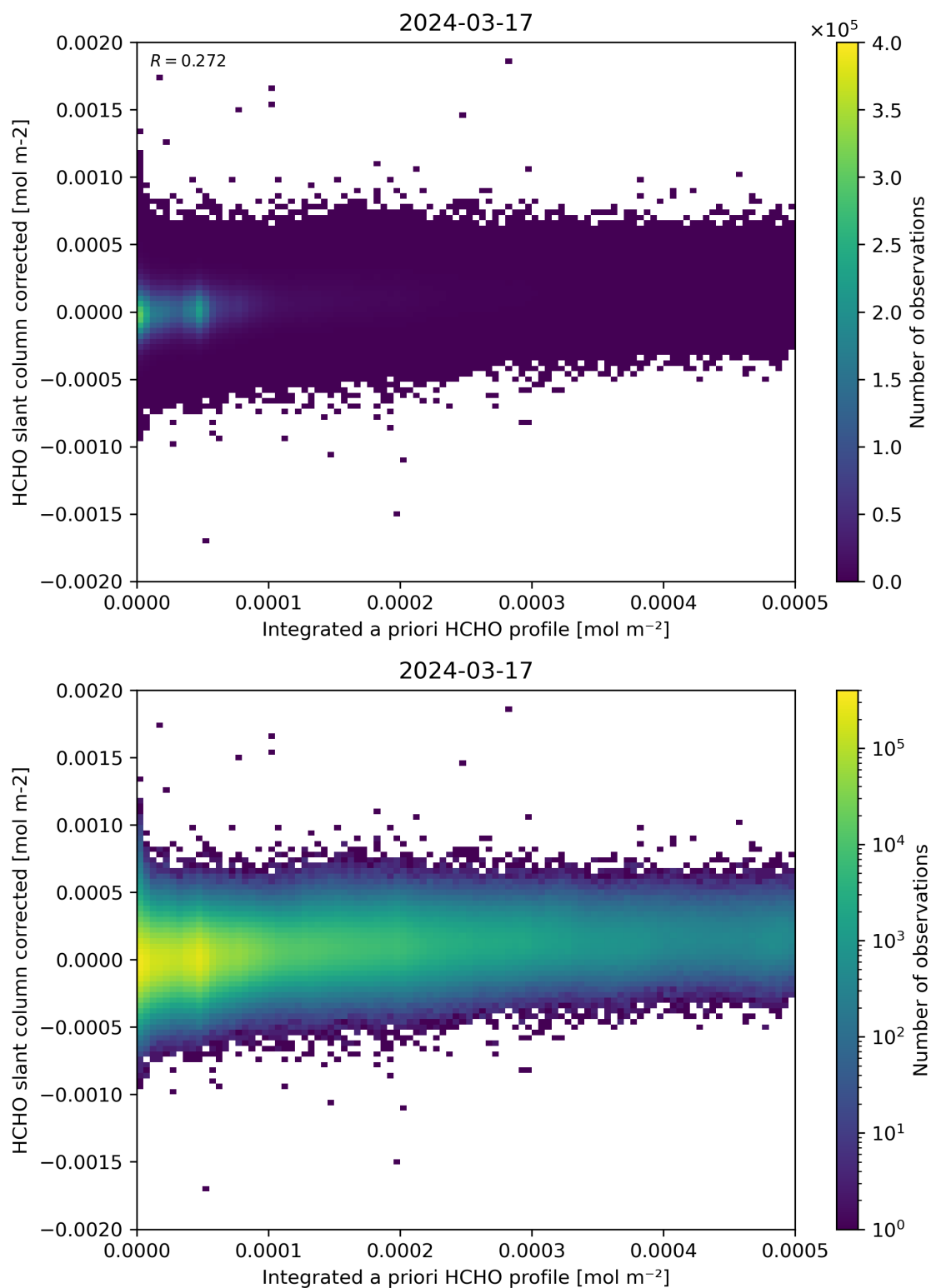
Figure 151: Scatter density plot of “Integrated a priori HCHO profile” against “HCHO slant column corrected” for 2024-03-16 to 2024-03-18.
