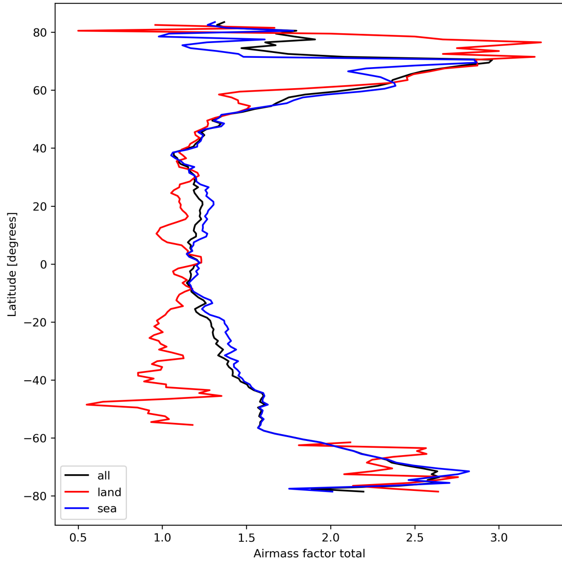
Figure 26: Zonal average of “Airmass factor total” for 2024-03-16 to 2024-03-18.
