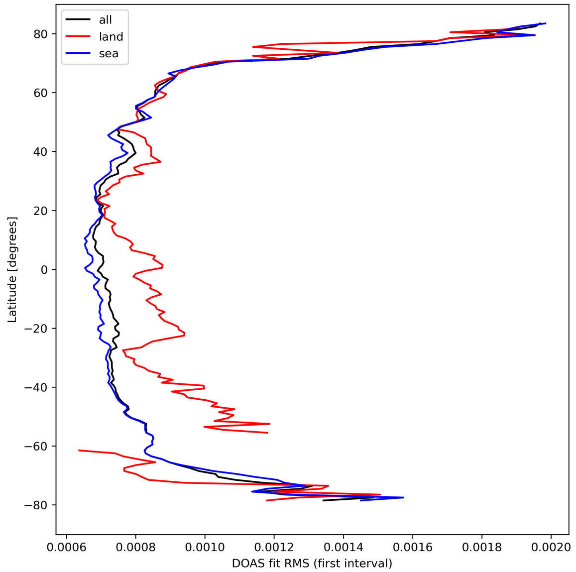
Figure 32: Zonal average of “DOAS fit RMS (first interval)” for 2024-03-16 to 2024-03-18.
