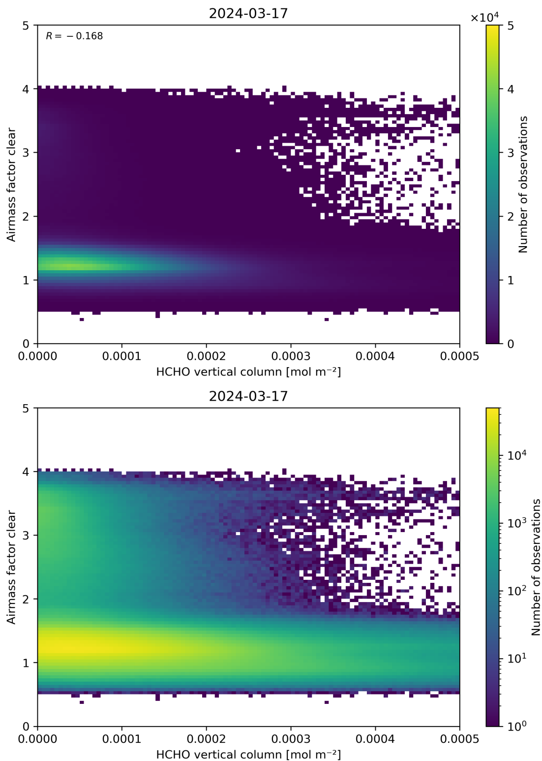
Figure 126: Scatter density plot of “HCHO vertical column” against “Airmass factor clear” for 2024-03-16 to 2024-03-18.
