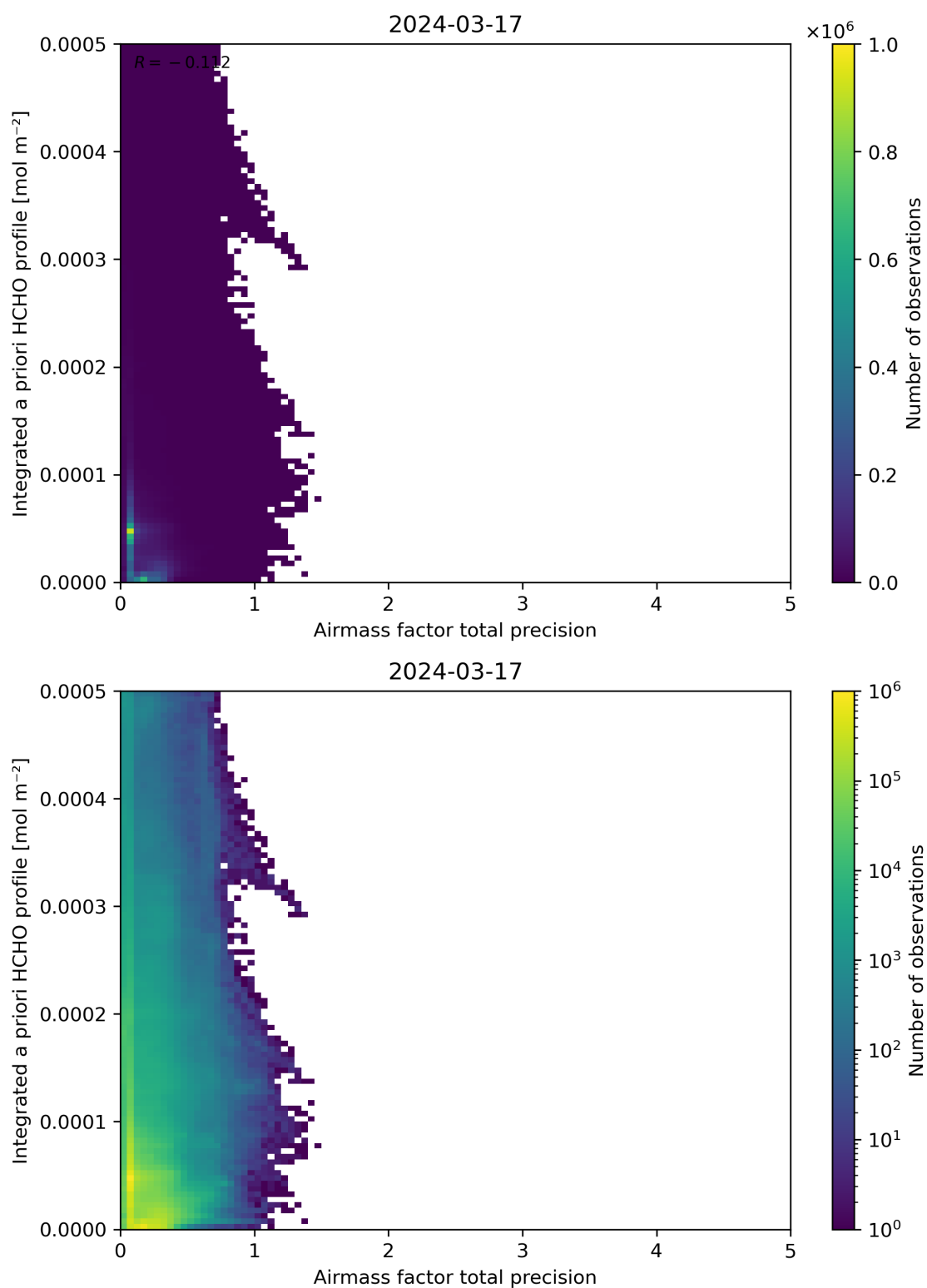
Figure 111: Scatter density plot of “Airmass factor total precision” against “Integrated a priori HCHO profile” for 2024-03-16 to 2024-03-18.
