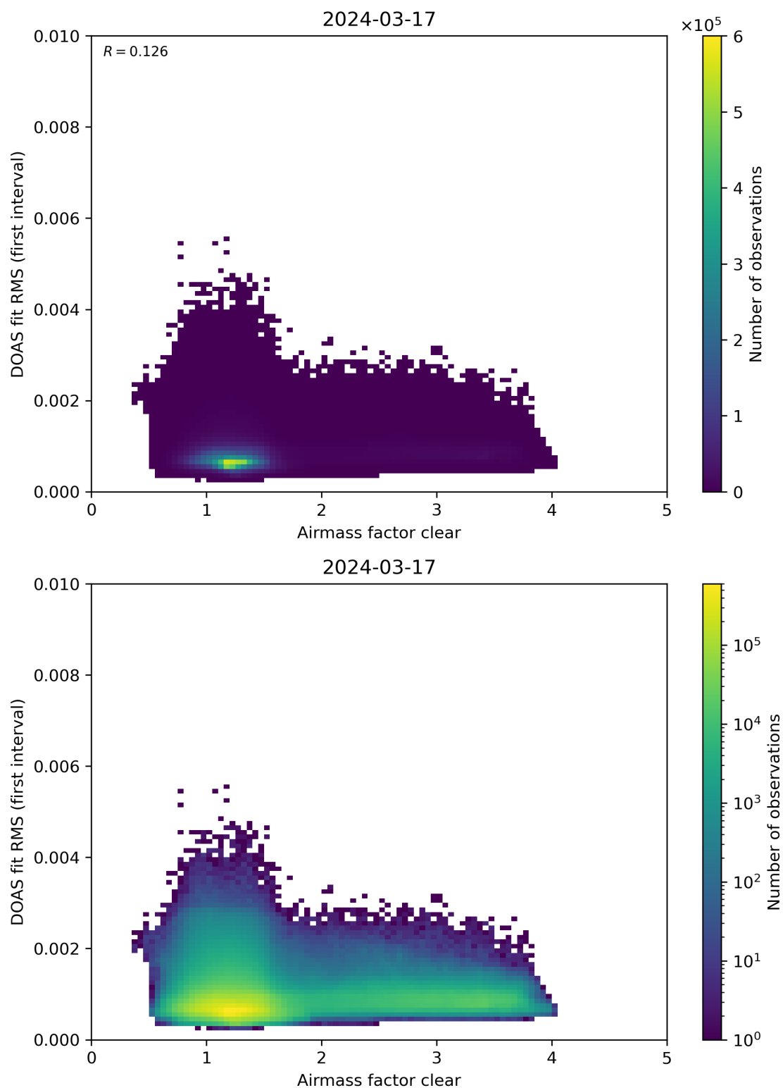
Figure 71: Scatter density plot of “Airmass factor clear” against “DOAS fit RMS (first interval)” for 2024-03-16 to 2024-03-18.
