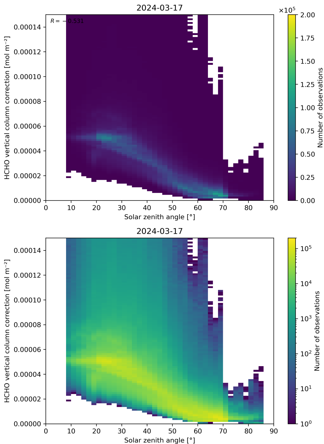
Figure 178: Scatter density plot of “Solar zenith angle” against “HCHO vertical column correction” for 2024-03-16 to 2024-03-18.
