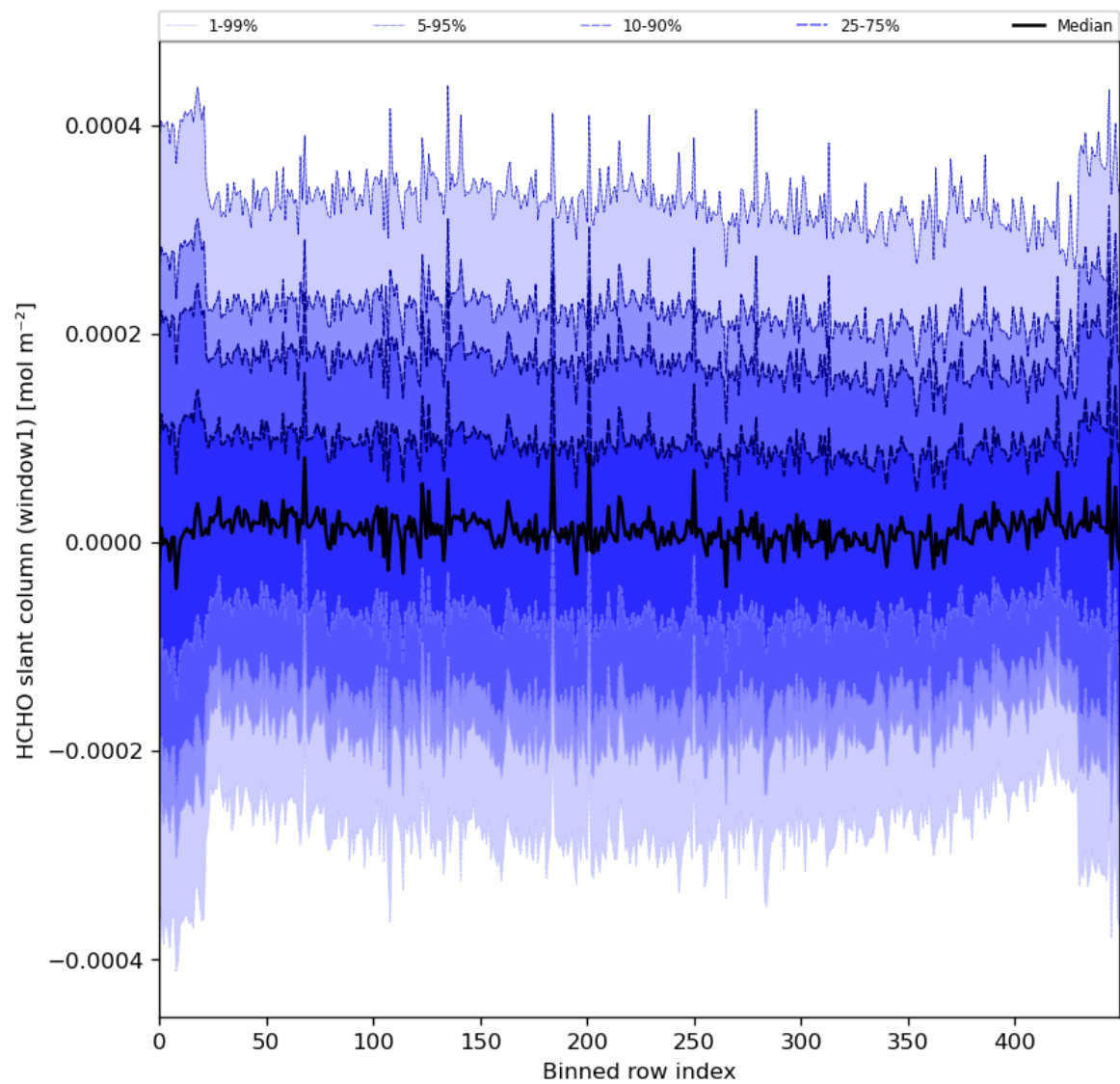
Figure 52: Along track statistics of “HCHO slant column (window1)” for 2024-03-16 to 2024-03-18
