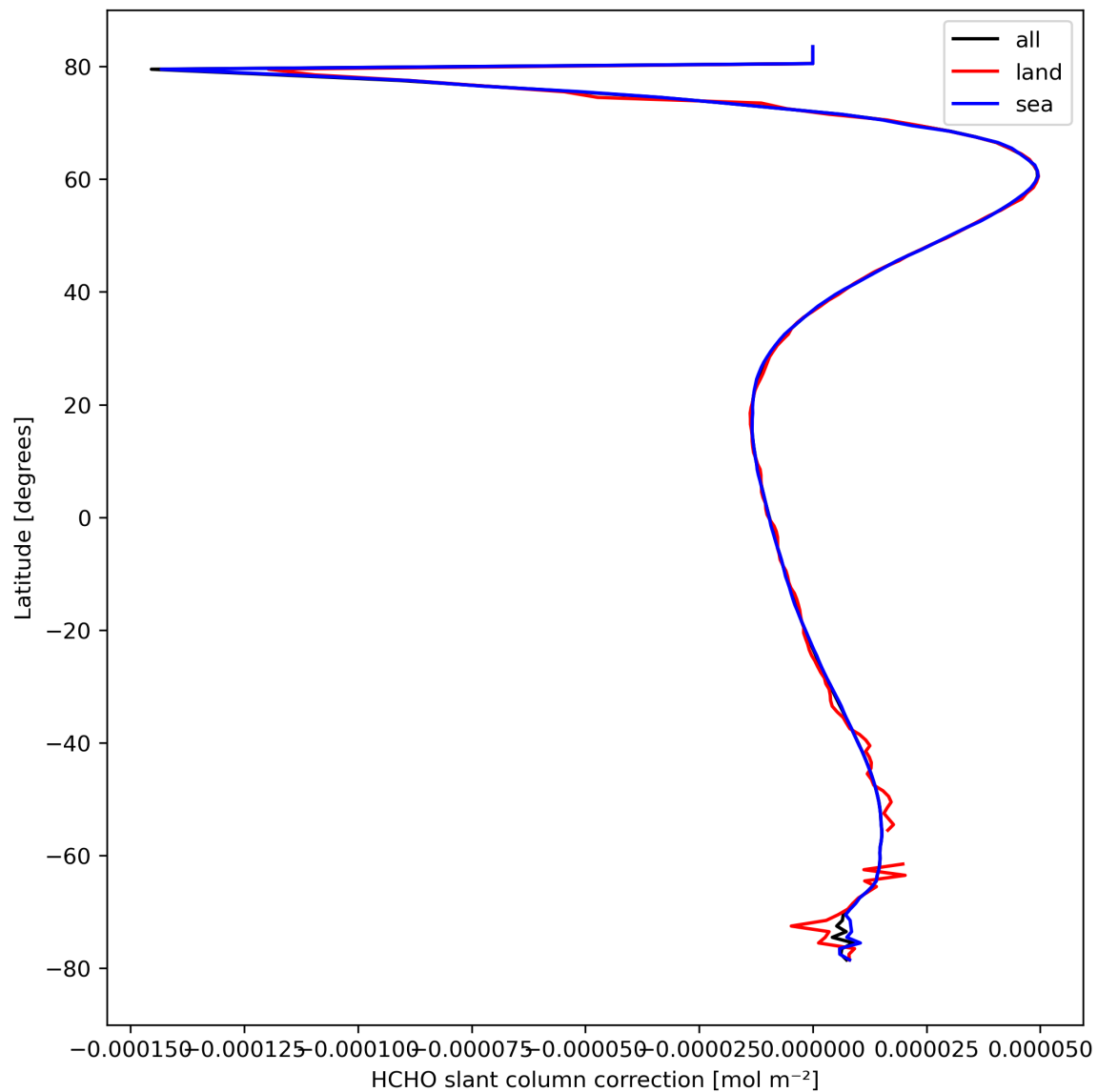
Figure 33: Zonal average of “HCHO slant column correction” for 2024-03-16 to 2024-03-18.
