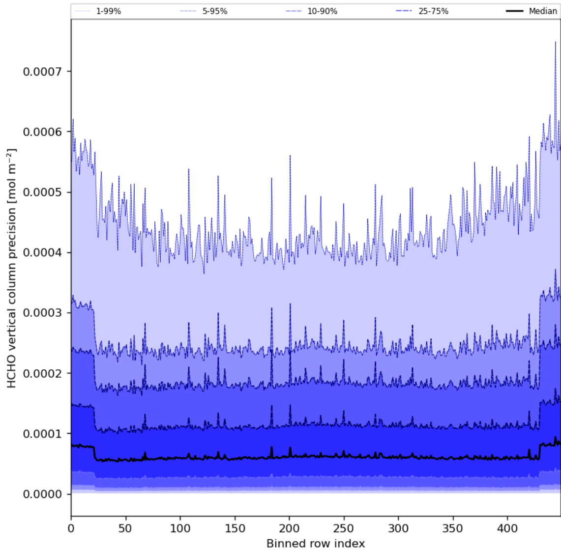
Figure 50: Along track statistics of “HCHO vertical column precision” for 2024-03-16 to 2024-03-18
