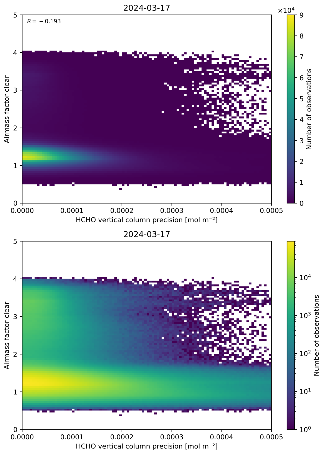
Figure 139: Scatter density plot of “HCHO vertical column precision” against “Airmass factor clear” for 2024-03-16 to 2024-03-18.
