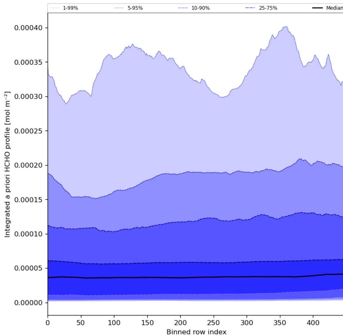
Figure 57: Along track statistics of "Integrated a priori HCHO profile" for 2024-03-16 to 2024-03-18
