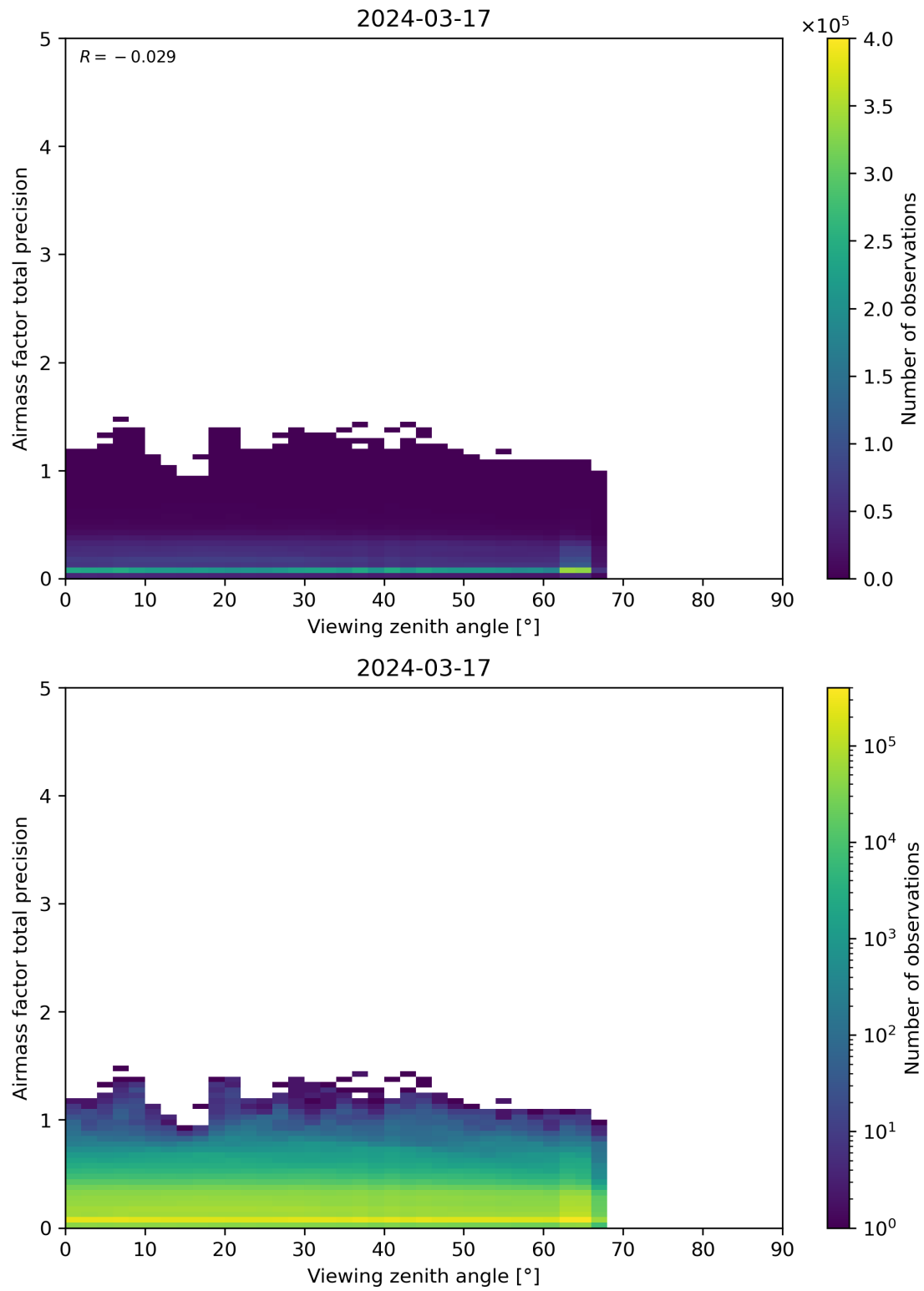
Figure 191: Scatter density plot of “Viewing zenith angle” against “Airmass factor total precision” for 2024-03-16 to 2024-03-18.
