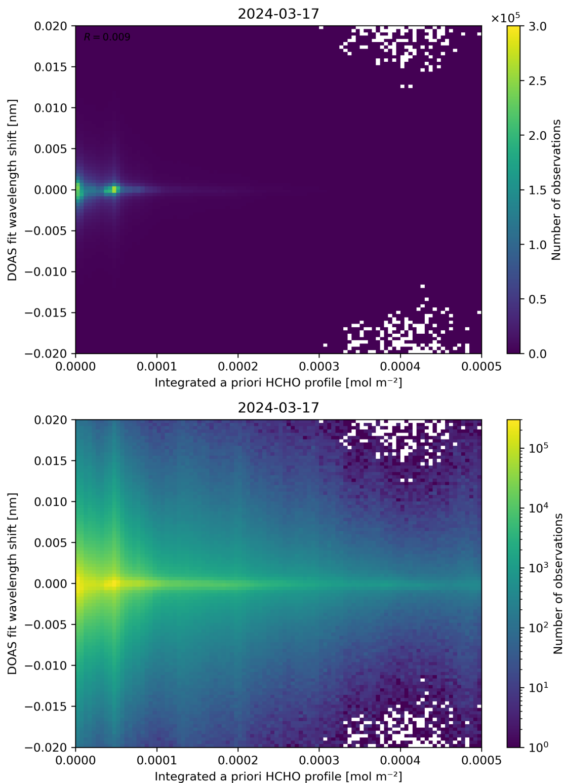
Figure 149: Scatter density plot of “Integrated a priori HCHO profile” against “DOAS fit wavelength shift” for 2024-03-16 to 2024-03-18.
