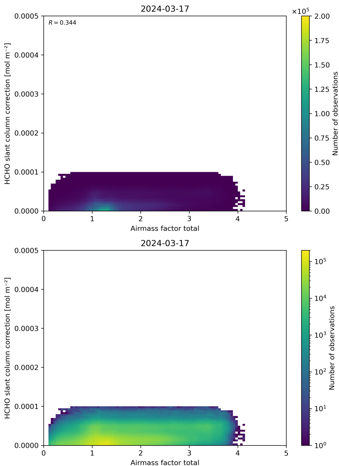
Figure 102: Scatter density plot of “Airmass factor total” against “HCHO slant column correction” for 2024-03-16 to 2024-03-18.
