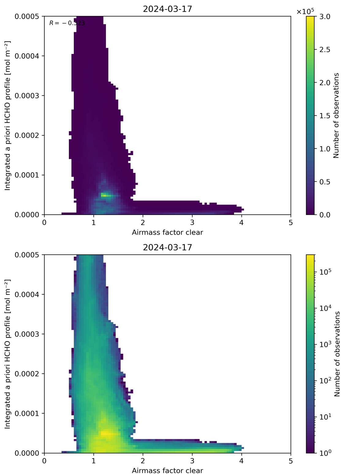
Figure 76: Scatter density plot of “Airmass factor clear” against “Integrated a priori HCHO profile” for 2024-03-16 to 2024-03-18.
