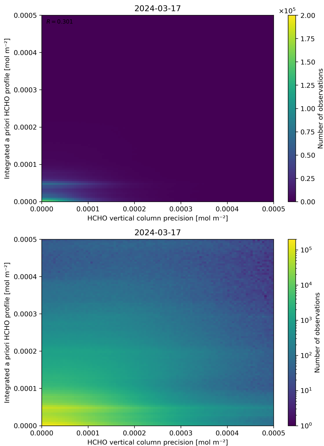
Figure 147: Scatter density plot of “HCHO vertical column precision” against “Integrated a priori HCHO profile” for 2024-03-16 to 2024-03-18.
