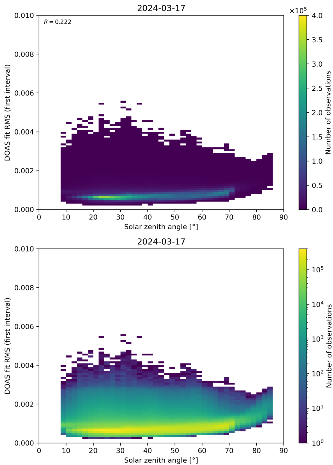
Figure 167: Scatter density plot of “Solar zenith angle” against “DOAS fit RMS (first interval)” for 2024-03-16 to 2024-03-18.
