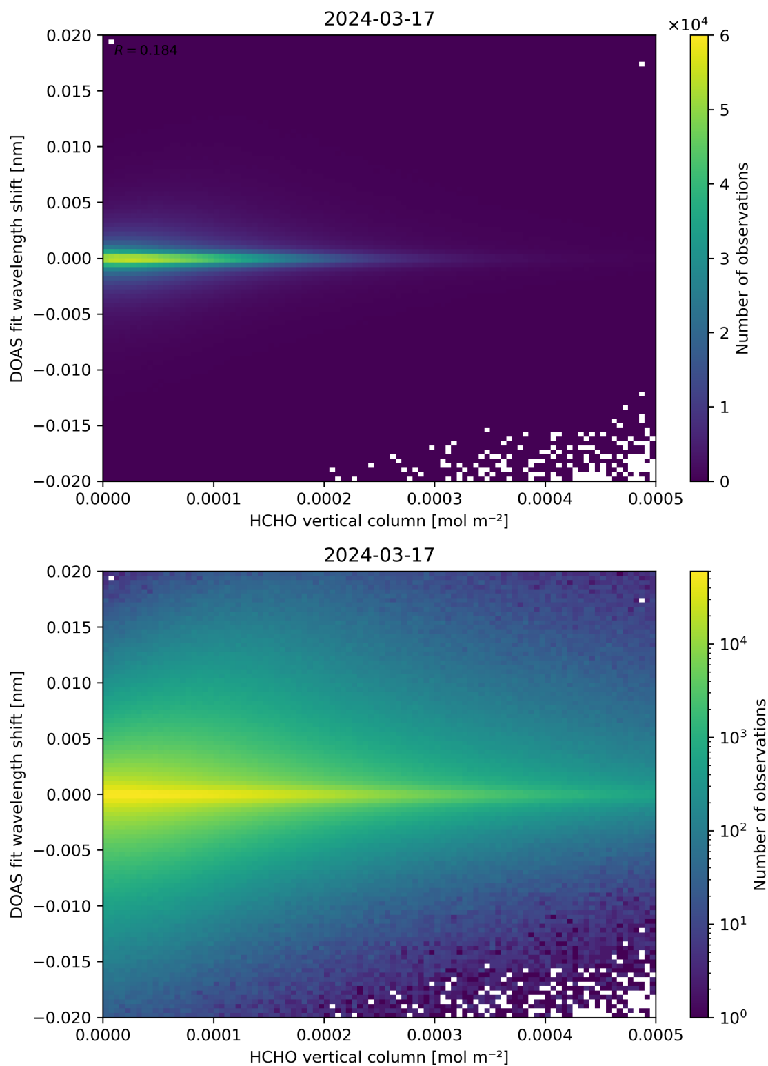
Figure 124: Scatter density plot of “HCHO vertical column” against “DOAS fit wavelength shift” for 2024-03-16 to 2024-03-18.
