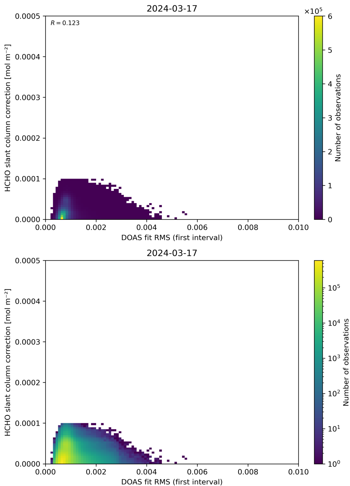
Figure 63: Scatter density plot of “DOAS fit RMS (first interval)” against “HCHO slant column correction” for 2024-03-16 to 2024-03-18.
