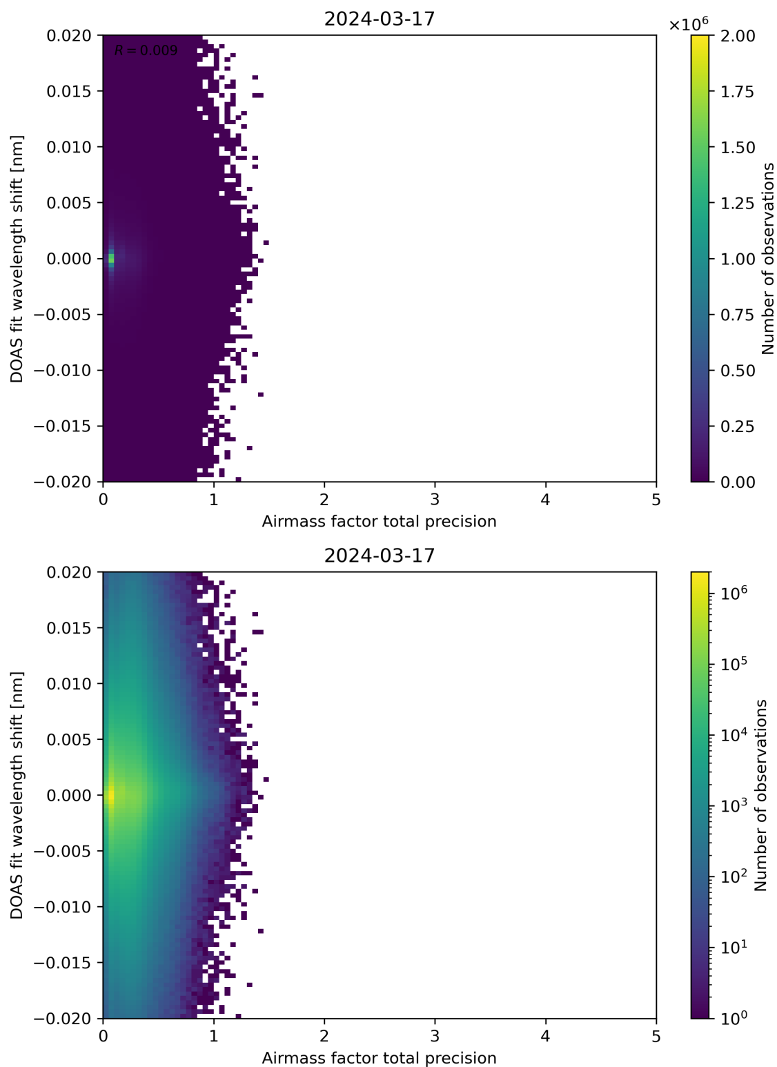
Figure 106: Scatter density plot of “Airmass factor total precision” against “DOAS fit wavelength shift” for 2024-03-16 to 2024-03-18.
