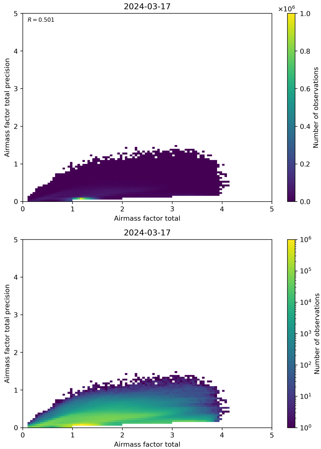
Figure 103: Scatter density plot of “Airmass factor total” against “Airmass factor total precision” for 2024-03-16 to 2024-03-18.
