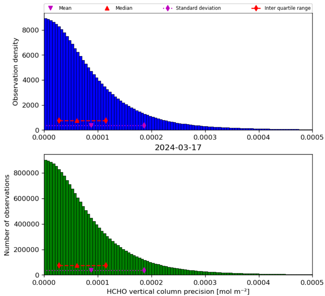
Figure 36: Histogram of “HCHO vertical column precision” for 2024-03-16 to 2024-03-18
