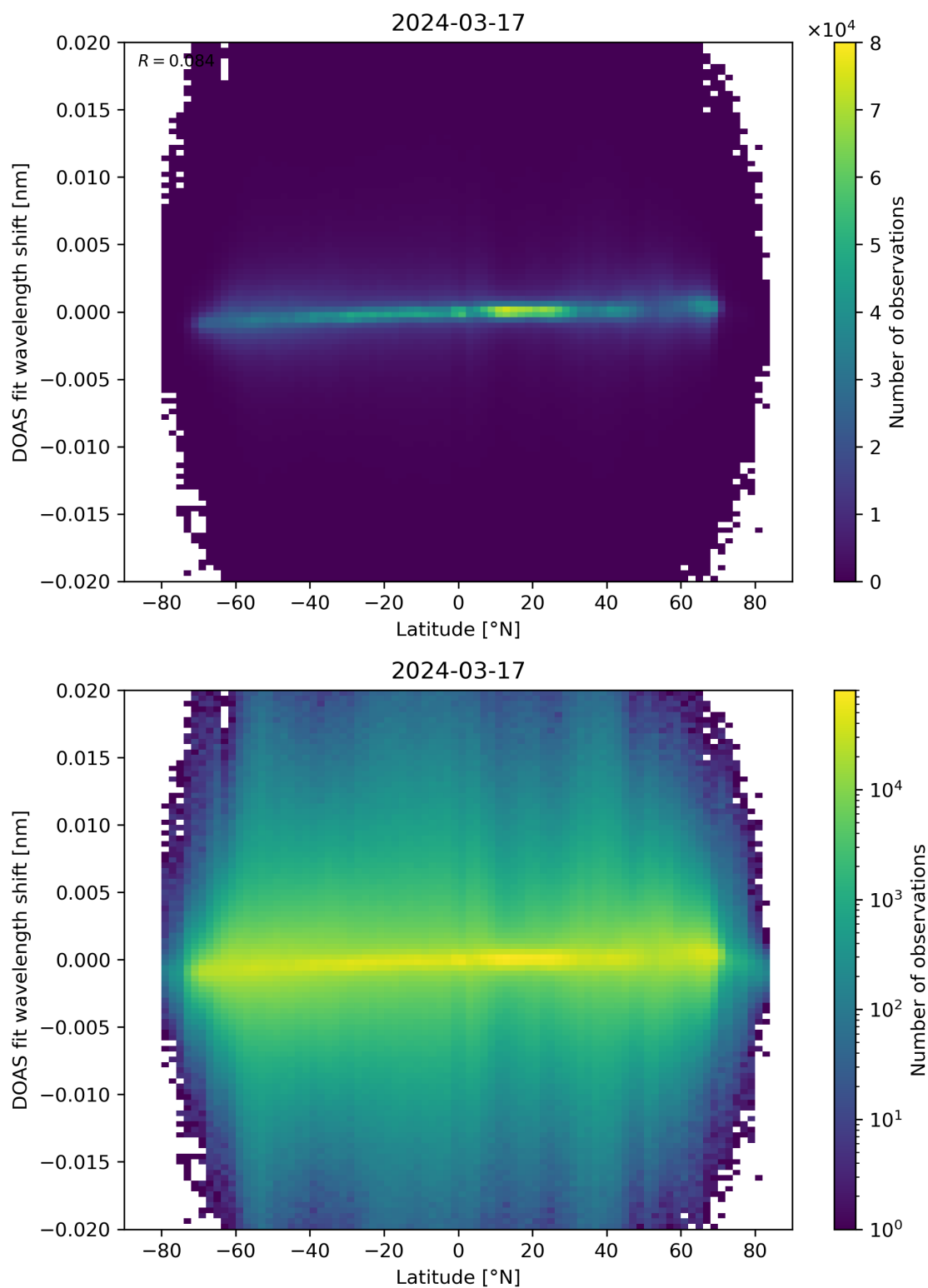
Figure 154: Scatter density plot of “Latitude” against “DOAS fit wavelength shift” for 2024-03-16 to 2024-03-18.
