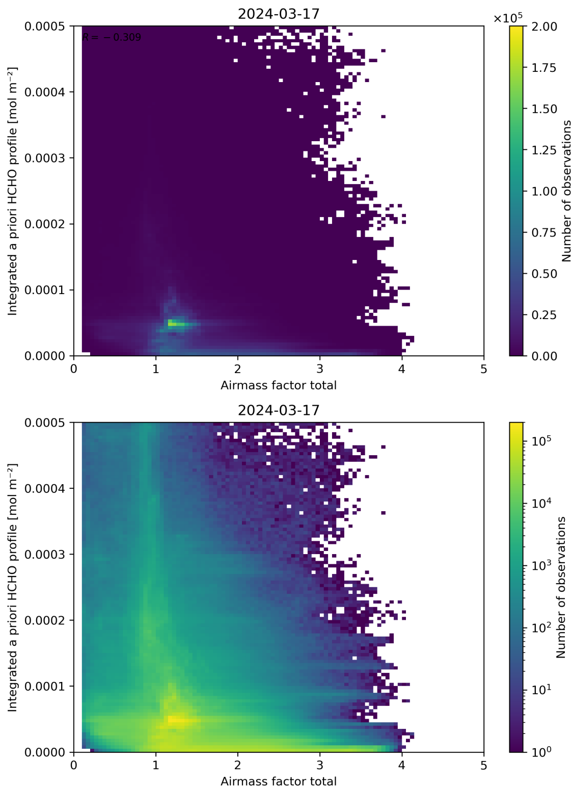
Figure 104: Scatter density plot of “Airmass factor total” against “Integrated a priori HCHO profile” for 2024-03-16 to 2024-03-18.
