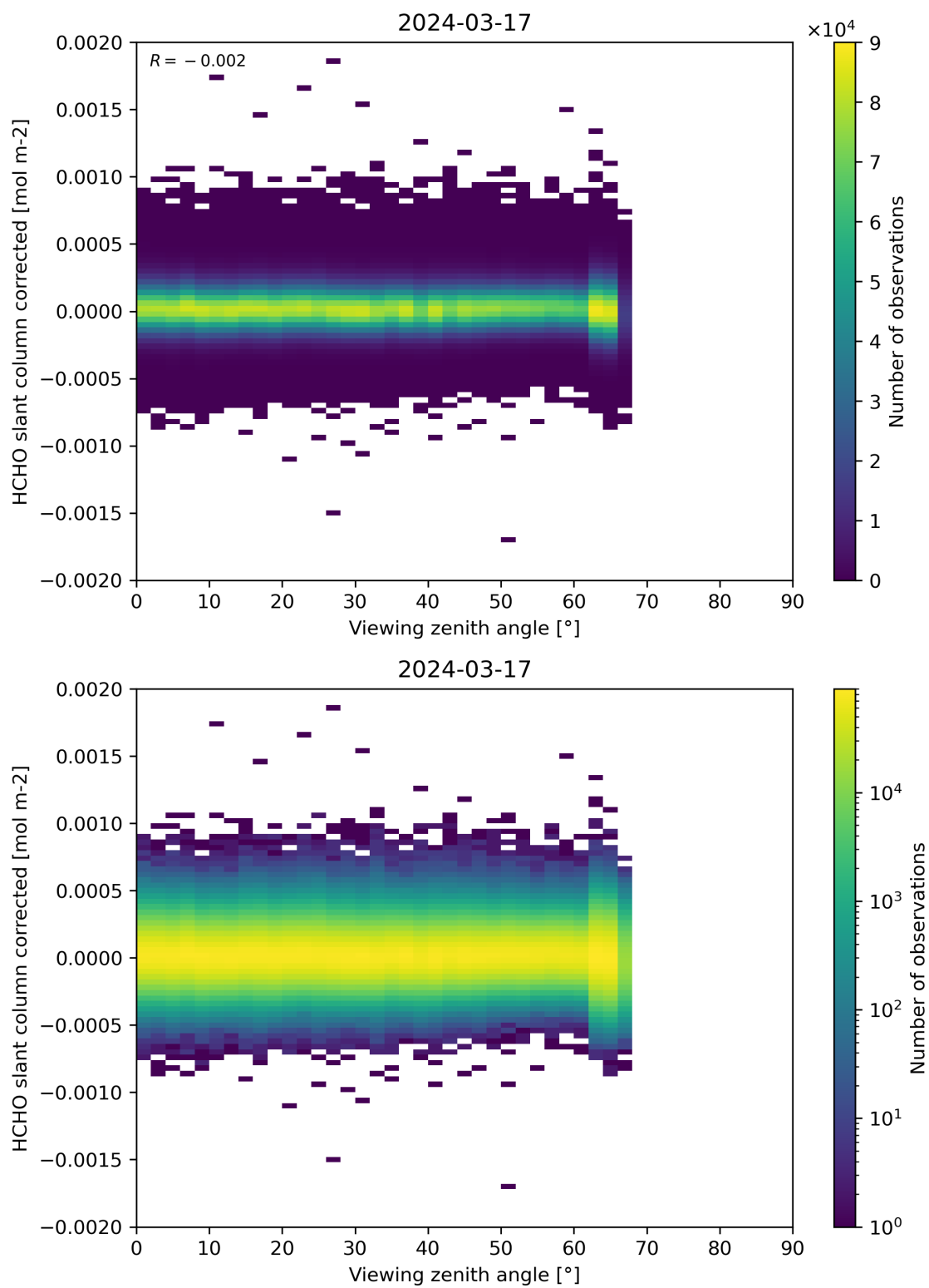
Figure 186: Scatter density plot of “Viewing zenith angle” against “HCHO slant column corrected” for 2024-03-16 to 2024-03-18.
