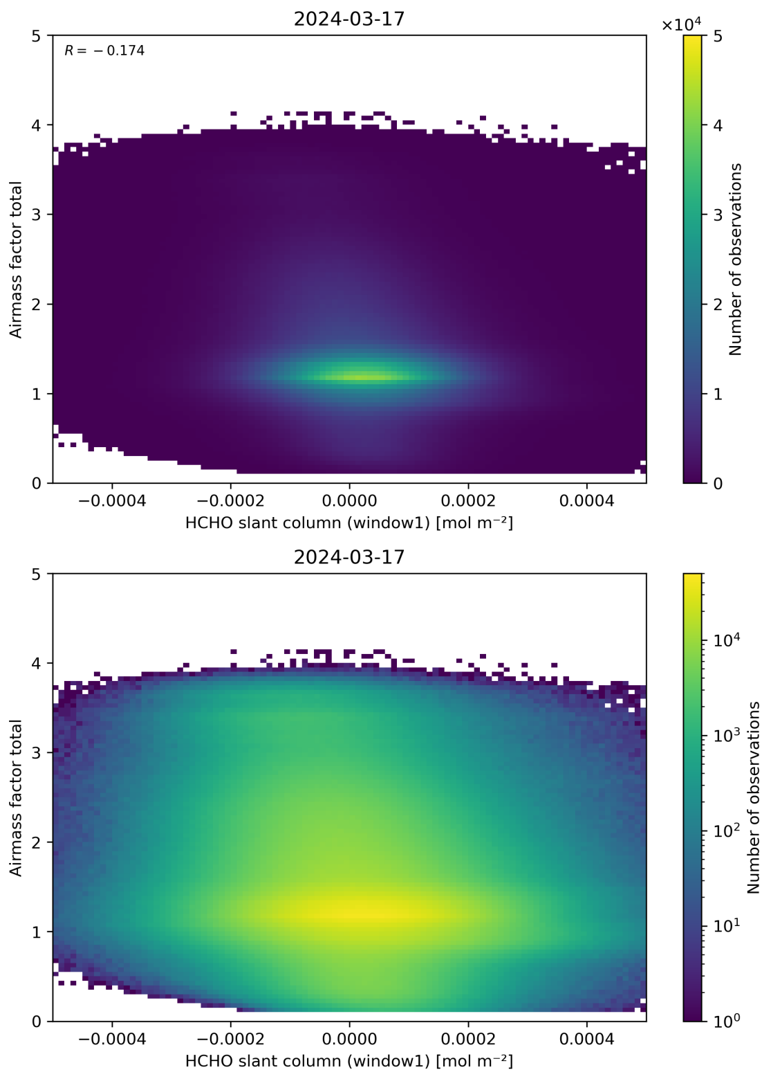
Figure 85: Scatter density plot of “HCHO slant column (window1)” against “Airmass factor total” for 2024-03-16 to 2024-03-18.
