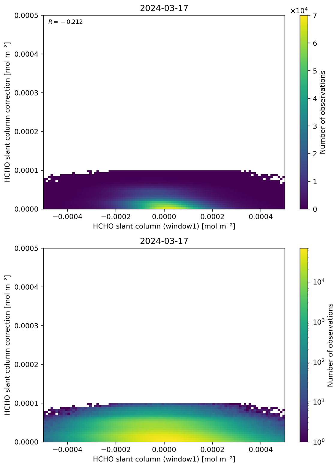
Figure 83: Scatter density plot of “HCHO slant column (window1)” against “HCHO slant column correction” for 2024-03-16 to 2024-03-18.
