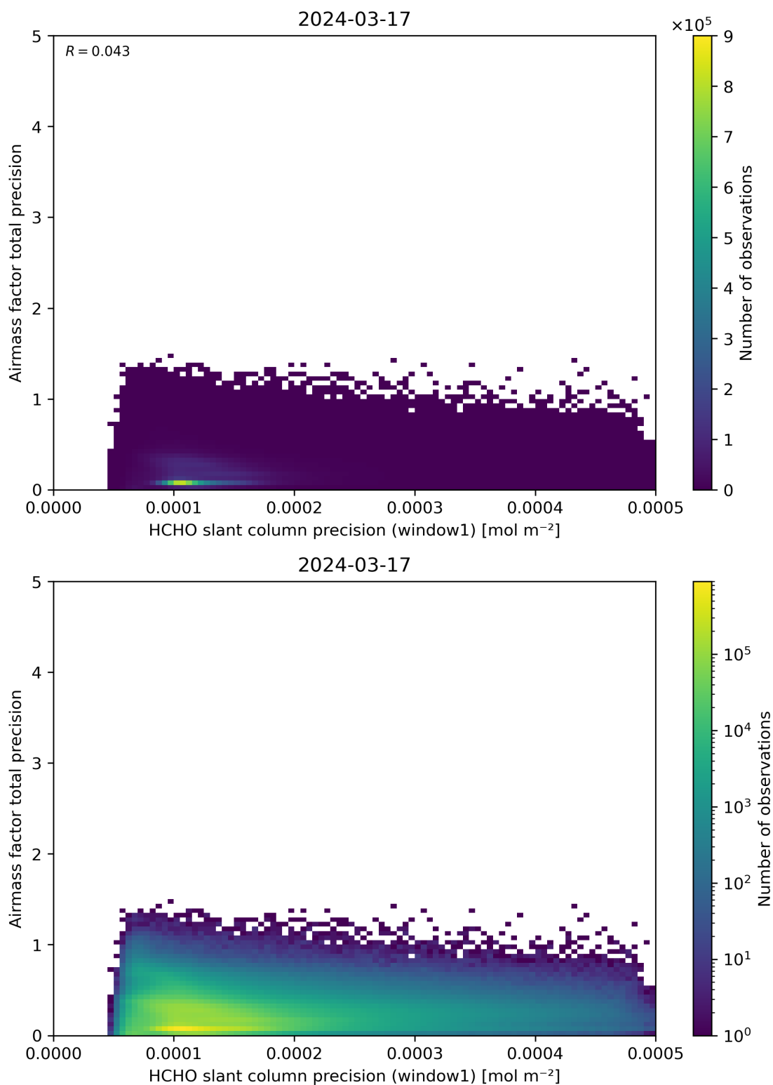
Figure 95: Scatter density plot of “HCHO slant column precision (window1)” against “Airmass factor total precision” for 2024-03-16 to 2024-03-18.
