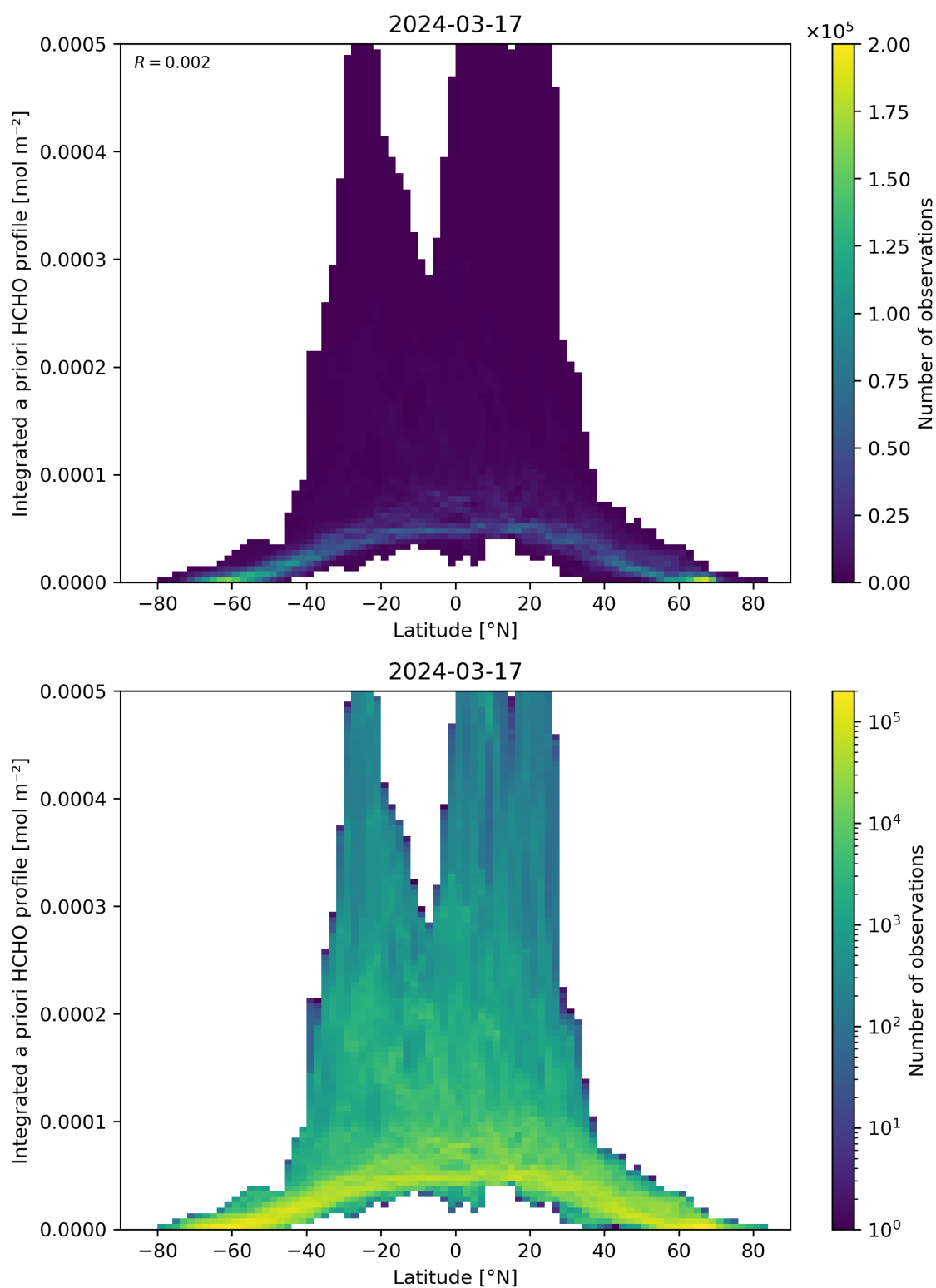
Figure 166: Scatter density plot of “Latitude” against “Integrated a priori HCHO profile” for 2024-03-16 to 2024-03-18.
