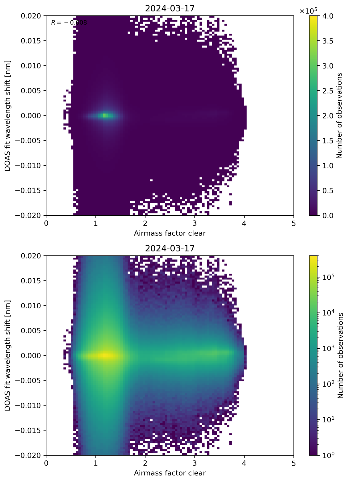
Figure 72: Scatter density plot of “Airmass factor clear” against “DOAS fit wavelength shift” for 2024-03-16 to 2024-03-18.
