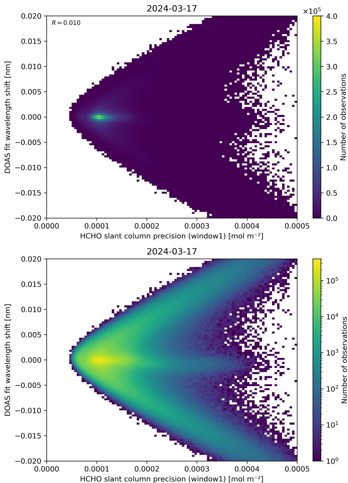
Figure 89: Scatter density plot of “HCHO slant column precision (window1)” against “DOAS fit wavelength shift” for 2024-03-16 to 2024-03-18.
