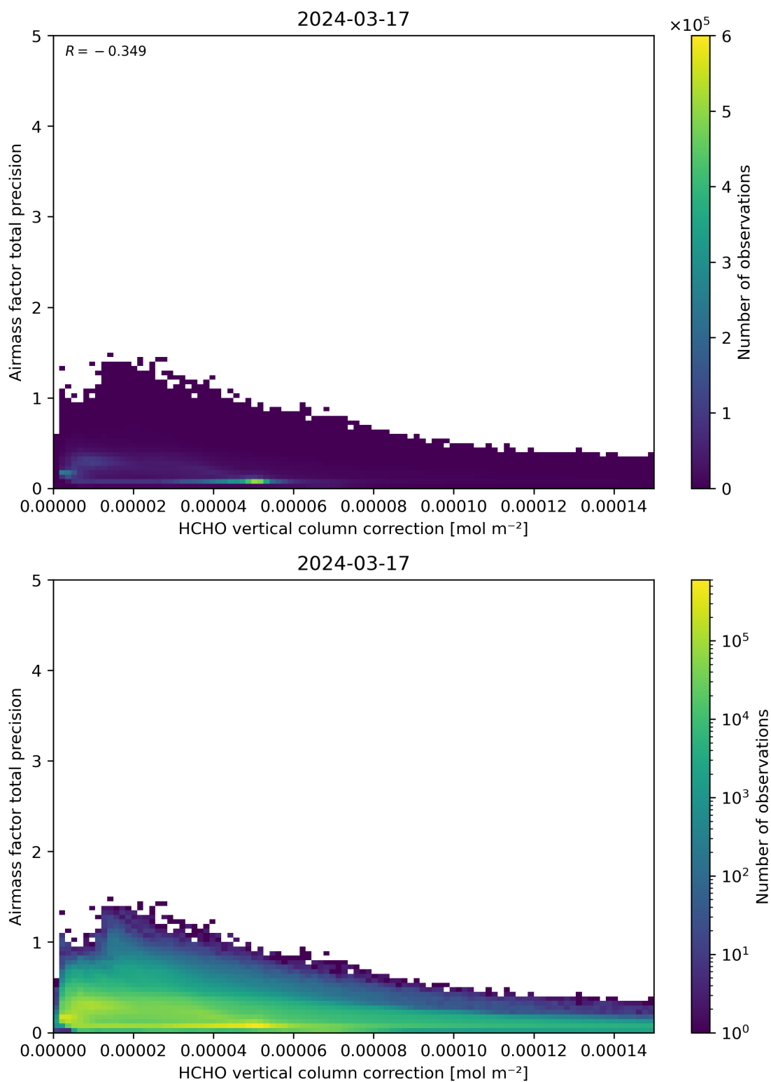
Figure 121: Scatter density plot of “HCHO vertical column correction” against “Airmass factor total precision” for 2024-03-16 to 2024-03-18.
