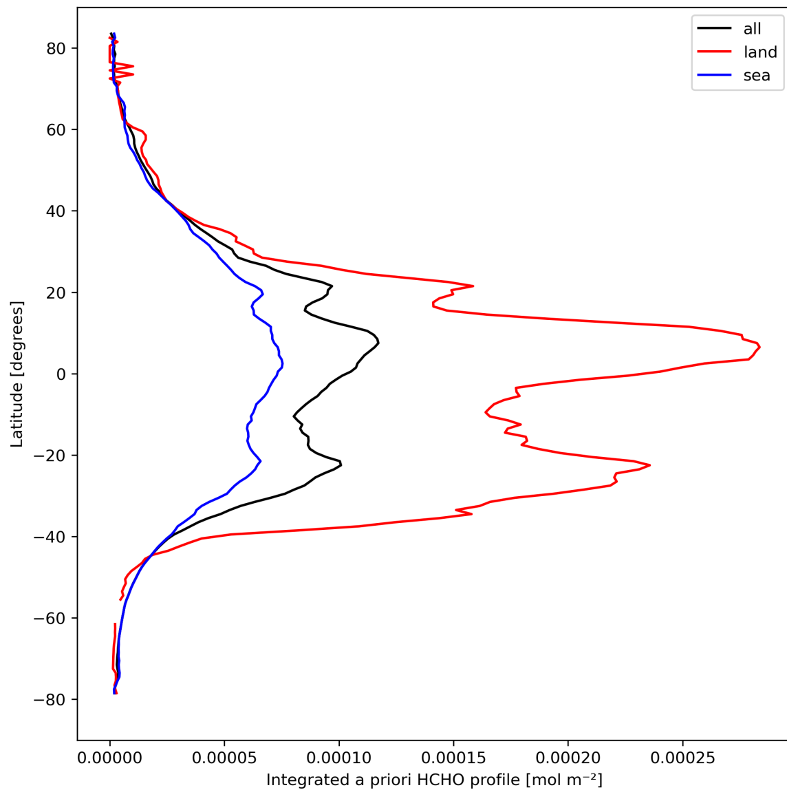
Figure 29: Zonal average of “Integrated a priori HCHO profile” for 2024-03-16 to 2024-03-18.
