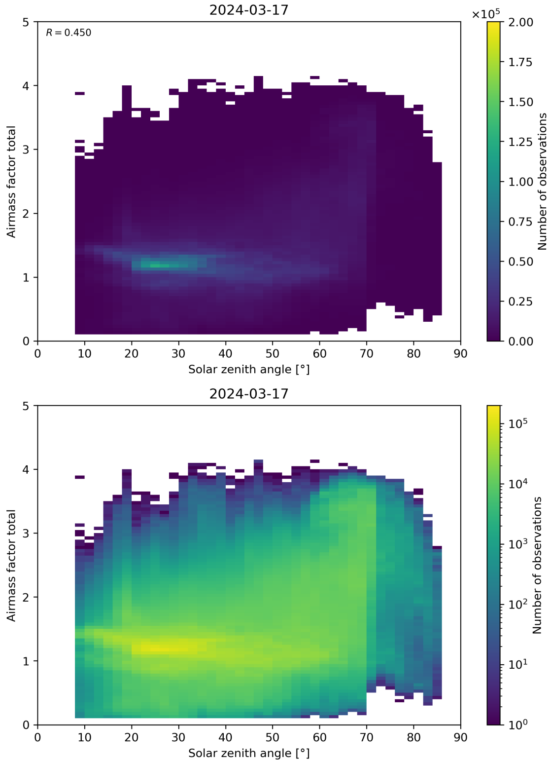
Figure 175: Scatter density plot of “Solar zenith angle” against “Airmass factor total” for 2024-03-16 to 2024-03-18.
