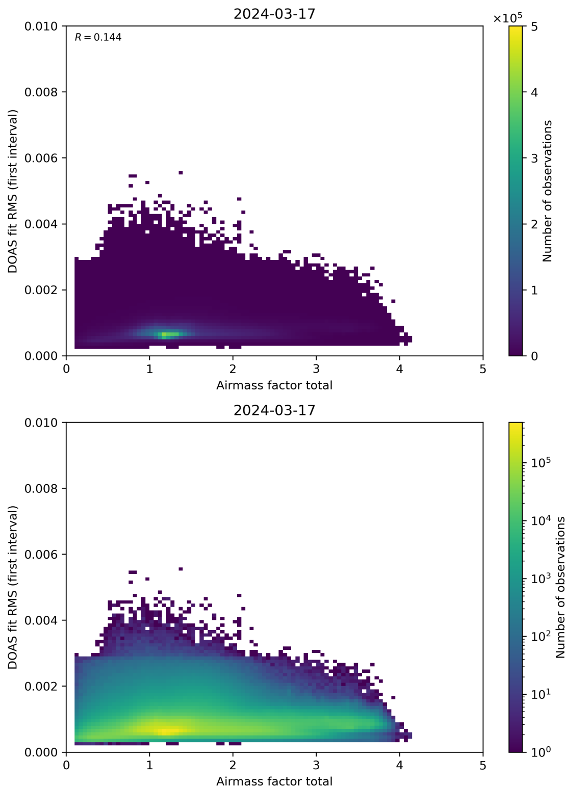
Figure 97: Scatter density plot of “Airmass factor total” against “DOAS fit RMS (first interval)” for 2024-03-16 to 2024-03-18.
