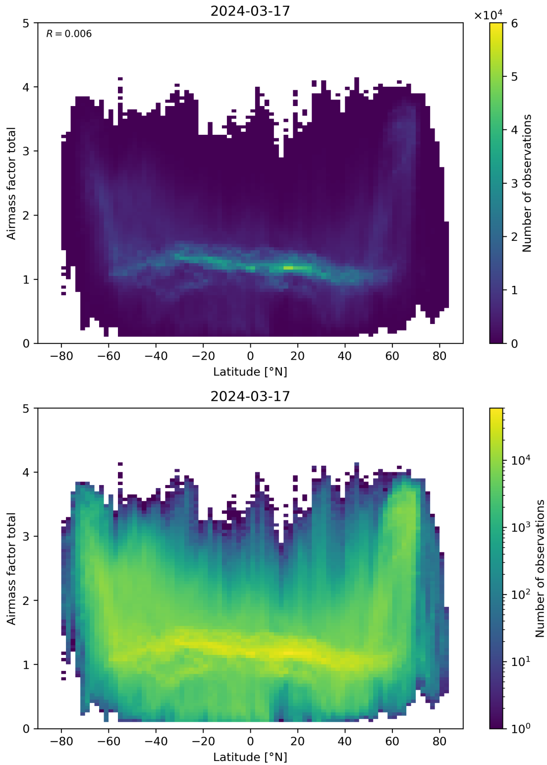
Figure 161: Scatter density plot of “Latitude” against “Airmass factor total” for 2024-03-16 to 2024-03-18.
