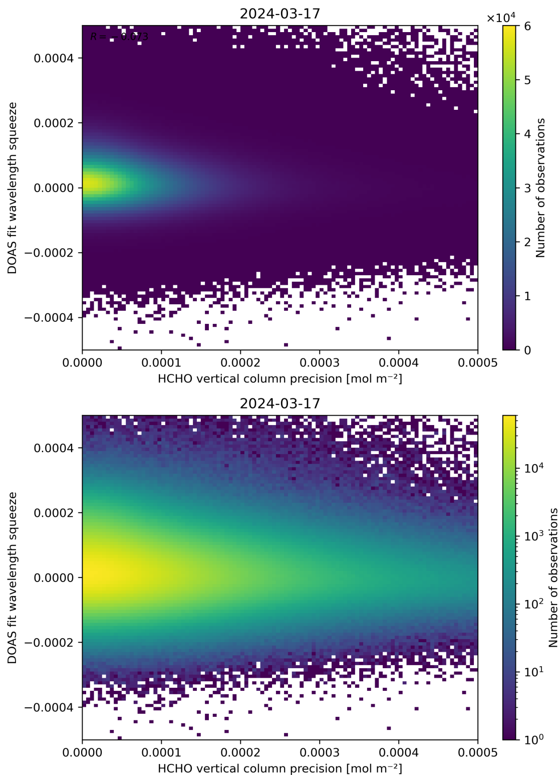
Figure 138: Scatter density plot of “HCHO vertical column precision” against “DOAS fit wavelength squeeze” for 2024-03-16 to 2024-03-18.
