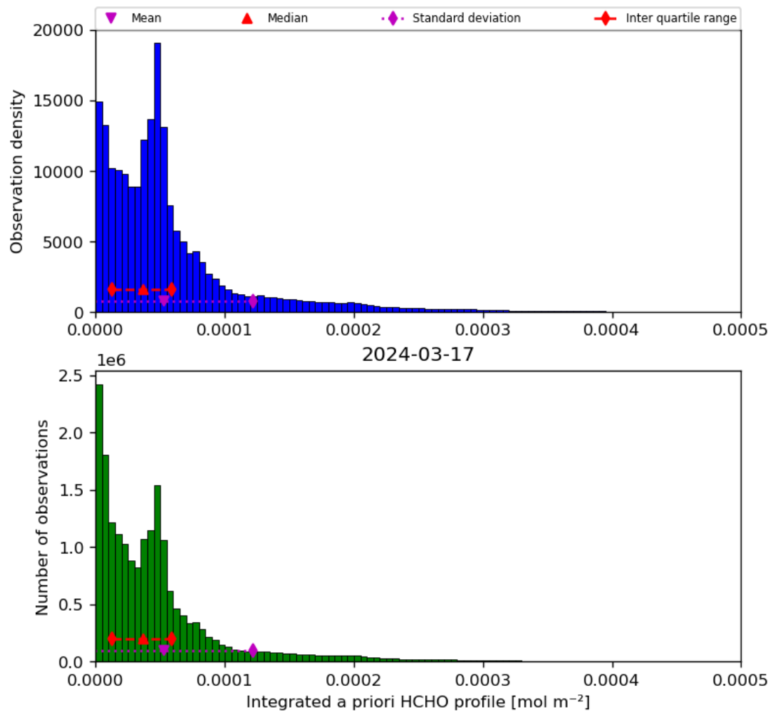
Figure 43: Histogram of “Integrated a priori HCHO profile” for 2024-03-16 to 2024-03-18
