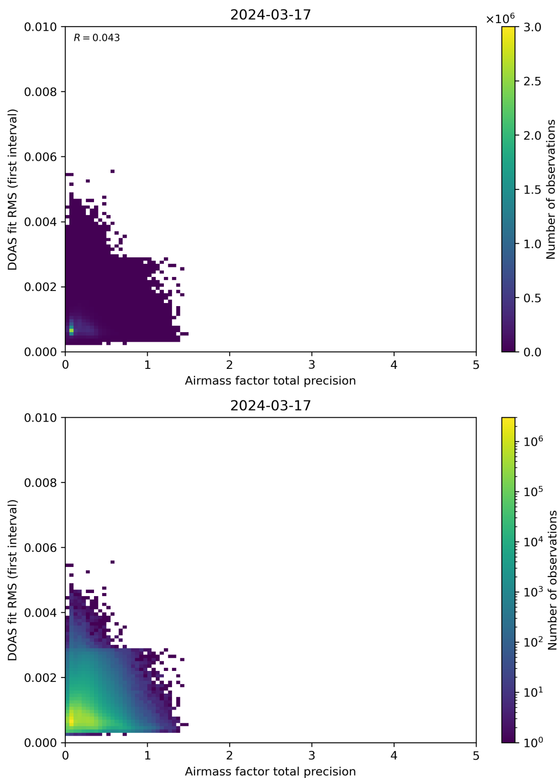
Figure 105: Scatter density plot of “Airmass factor total precision” against “DOAS fit RMS (first interval)” for 2024-03-16 to 2024-03-18.
