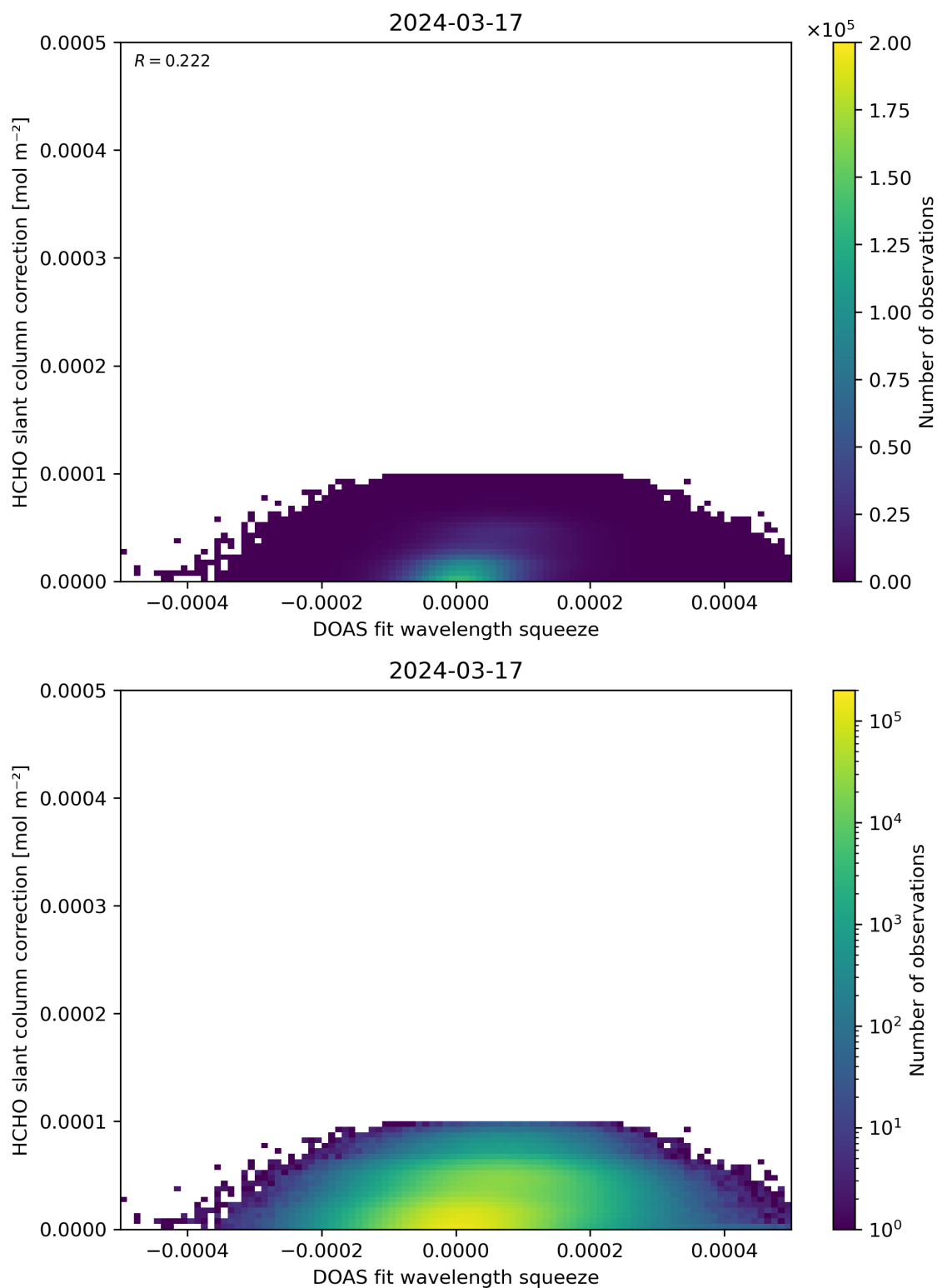
Figure 70: Scatter density plot of “DOAS fit wavelength squeeze” against “HCHO slant column correction” for 2024-03-16 to 2024-03-18.
