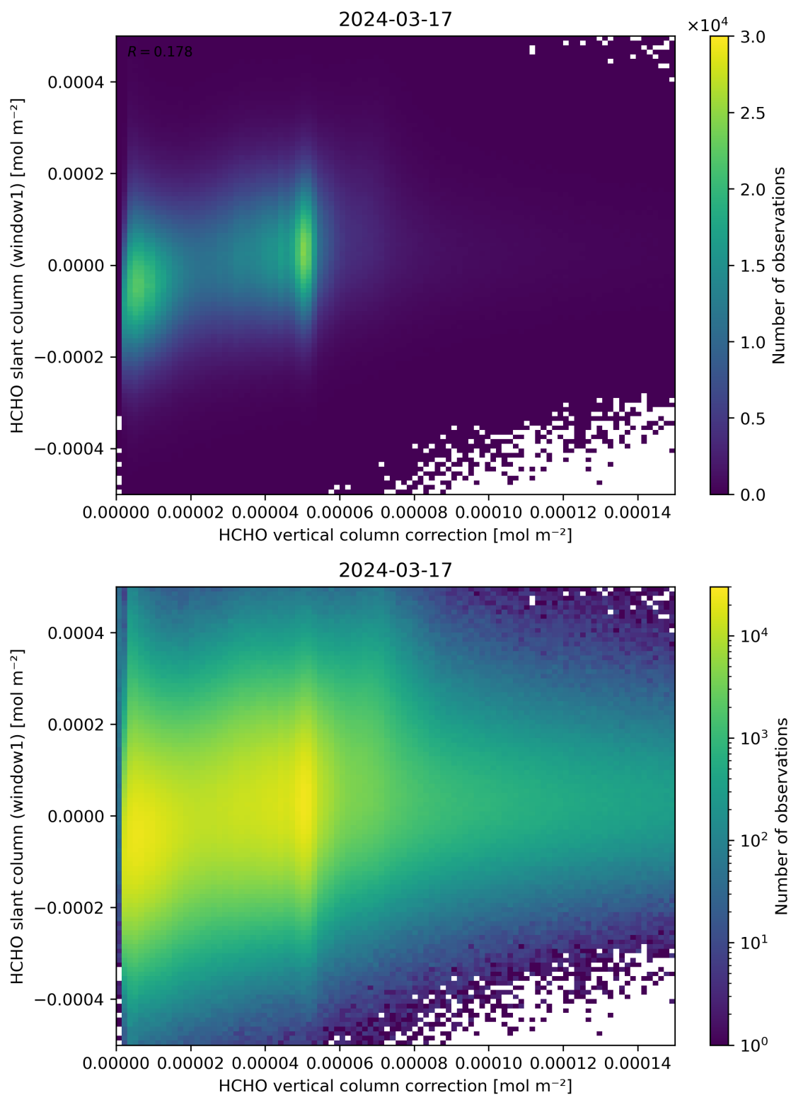
Figure 118: Scatter density plot of “HCHO vertical column correction” against “HCHO slant column (window1)” for 2024-03-16 to 2024-03-18.
