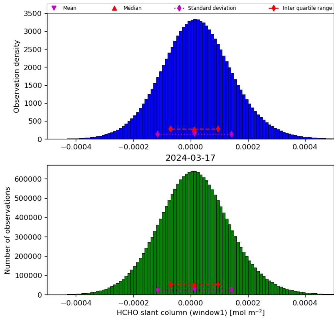
Figure 38: Histogram of “HCHO slant column (window1)” for 2024-03-16 to 2024-03-18
