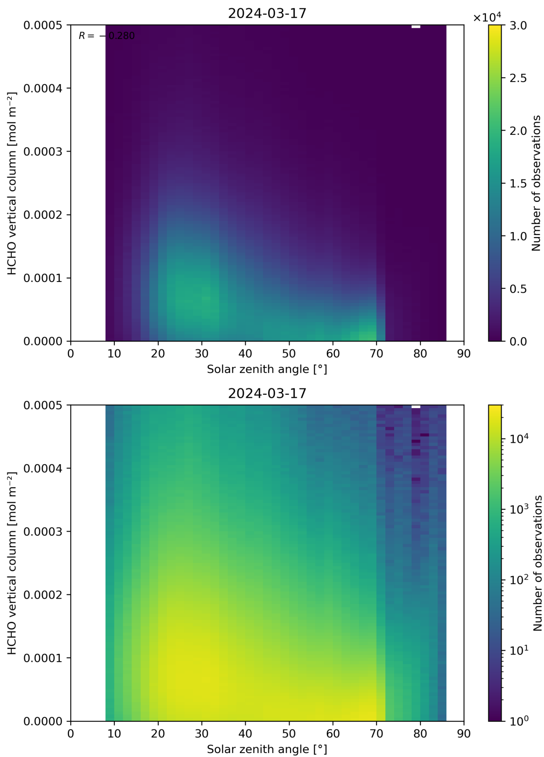
Figure 177: Scatter density plot of “Solar zenith angle” against “HCHO vertical column” for 2024-03-16 to 2024-03-18.
