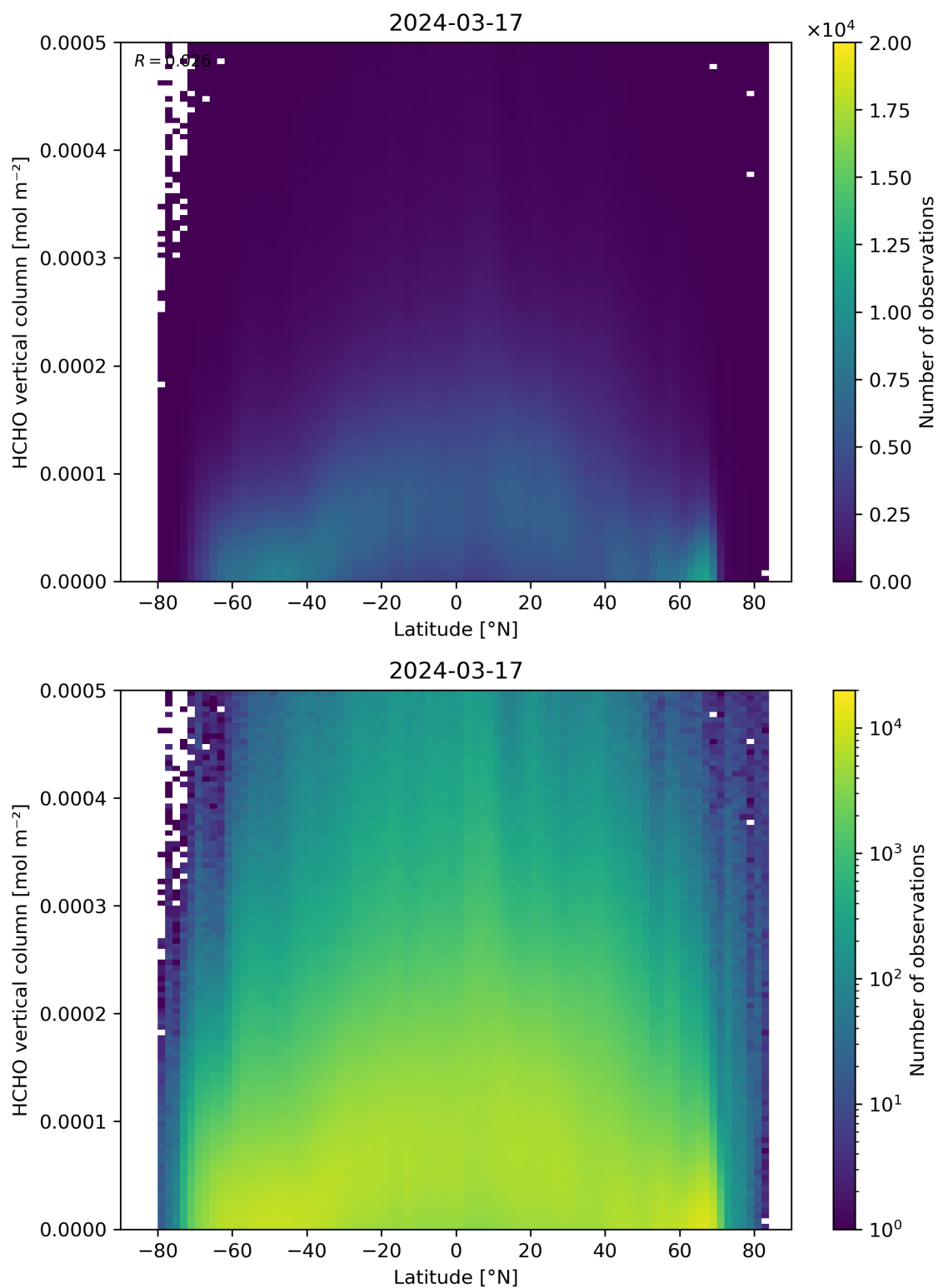
Figure 163: Scatter density plot of “Latitude” against “HCHO vertical column” for 2024-03-16 to 2024-03-18.
