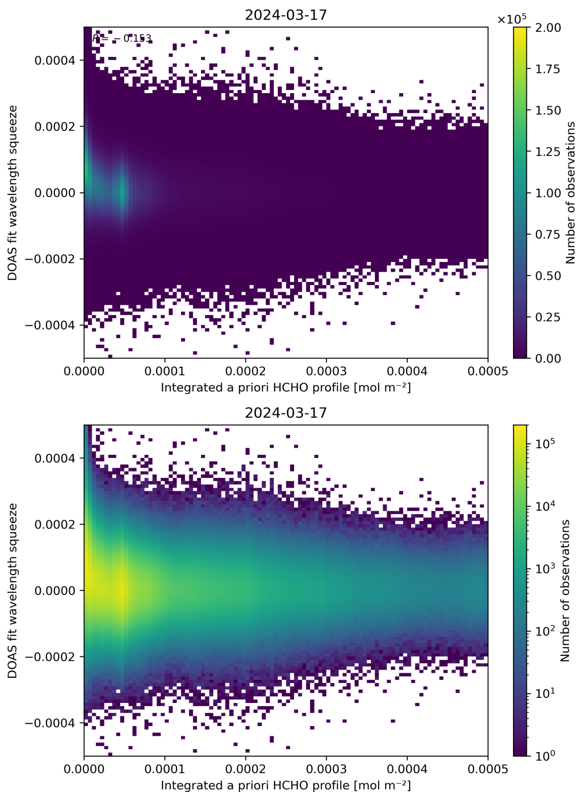
Figure 150: Scatter density plot of “Integrated a priori HCHO profile” against “DOAS fit wavelength squeeze” for 2024-03-16 to 2024-03-18.
