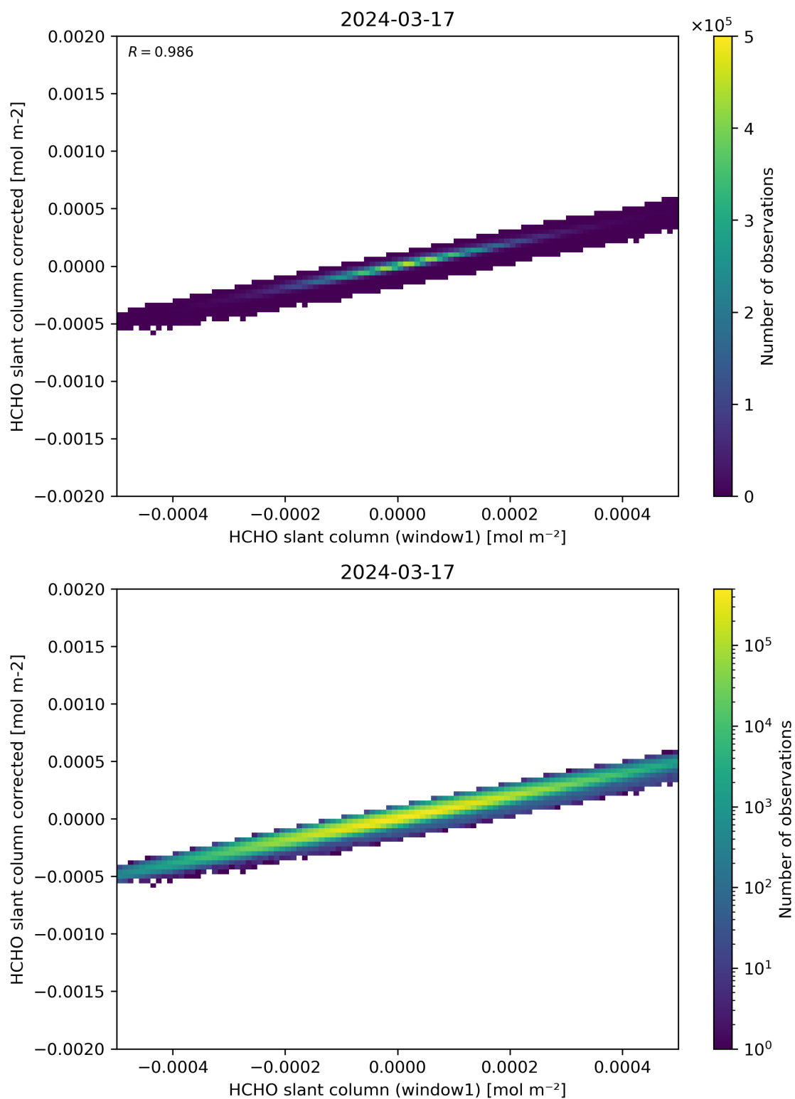
Figure 82: Scatter density plot of “HCHO slant column (window1)” against “HCHO slant column corrected” for 2024-03-16 to 2024-03-18.
