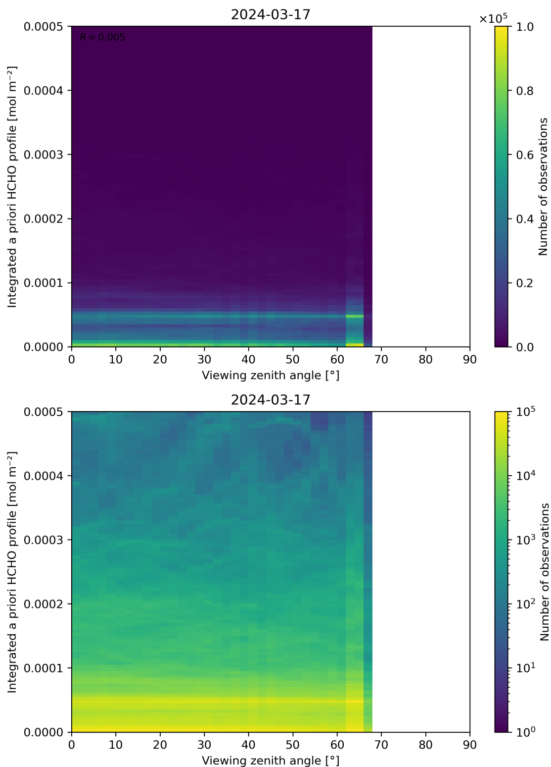
Figure 195: Scatter density plot of “Viewing zenith angle” against “Integrated a priori HCHO profile” for 2024-03-16 to 2024-03-18.
