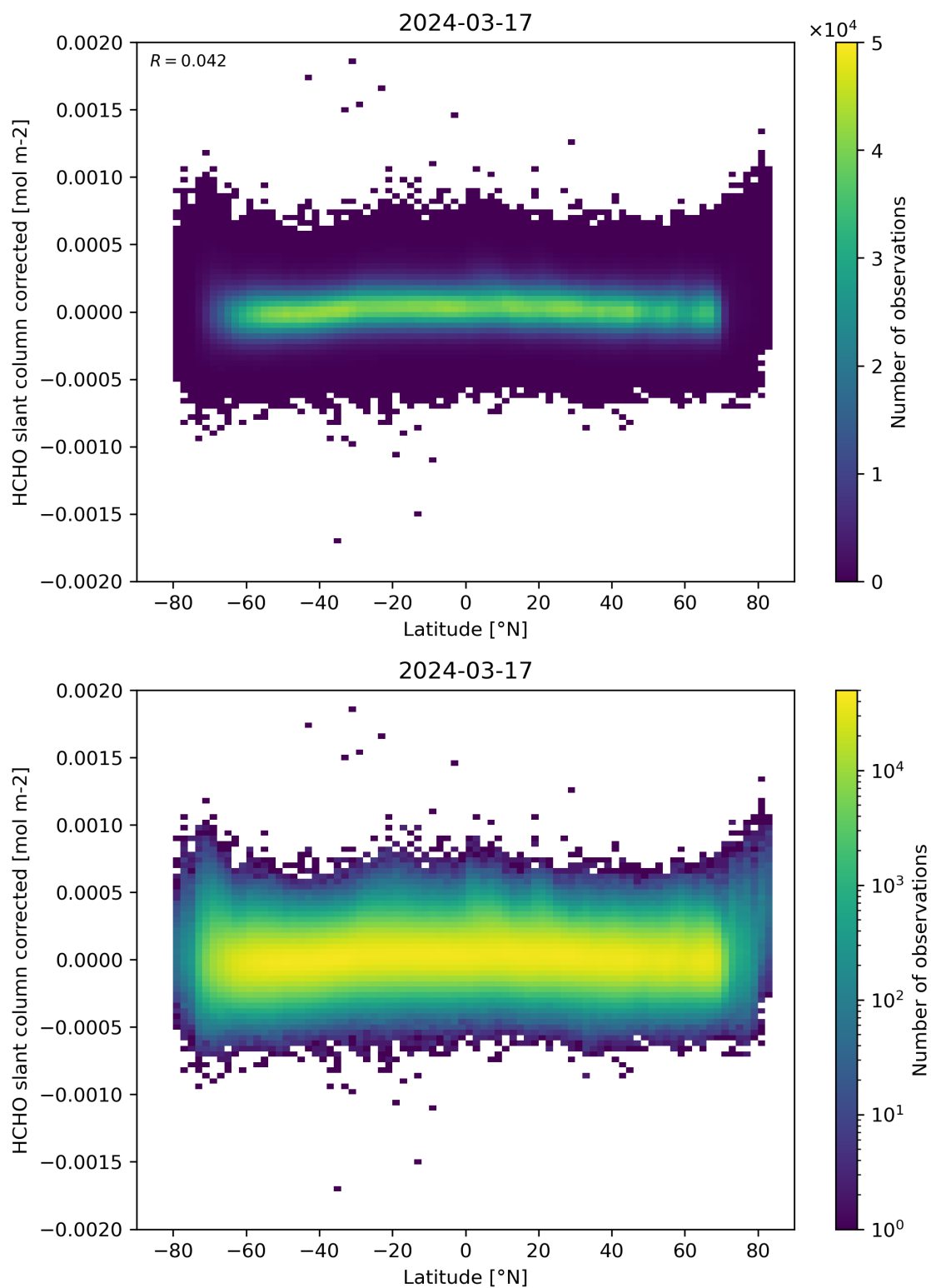
Figure 157: Scatter density plot of “Latitude” against “HCHO slant column corrected” for 2024-03-16 to 2024-03-18.
