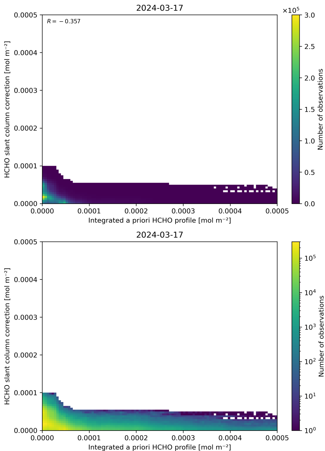
Figure 152: Scatter density plot of “Integrated a priori HCHO profile” against “HCHO slant column correction” for 2024-03-16 to 2024-03-18.
