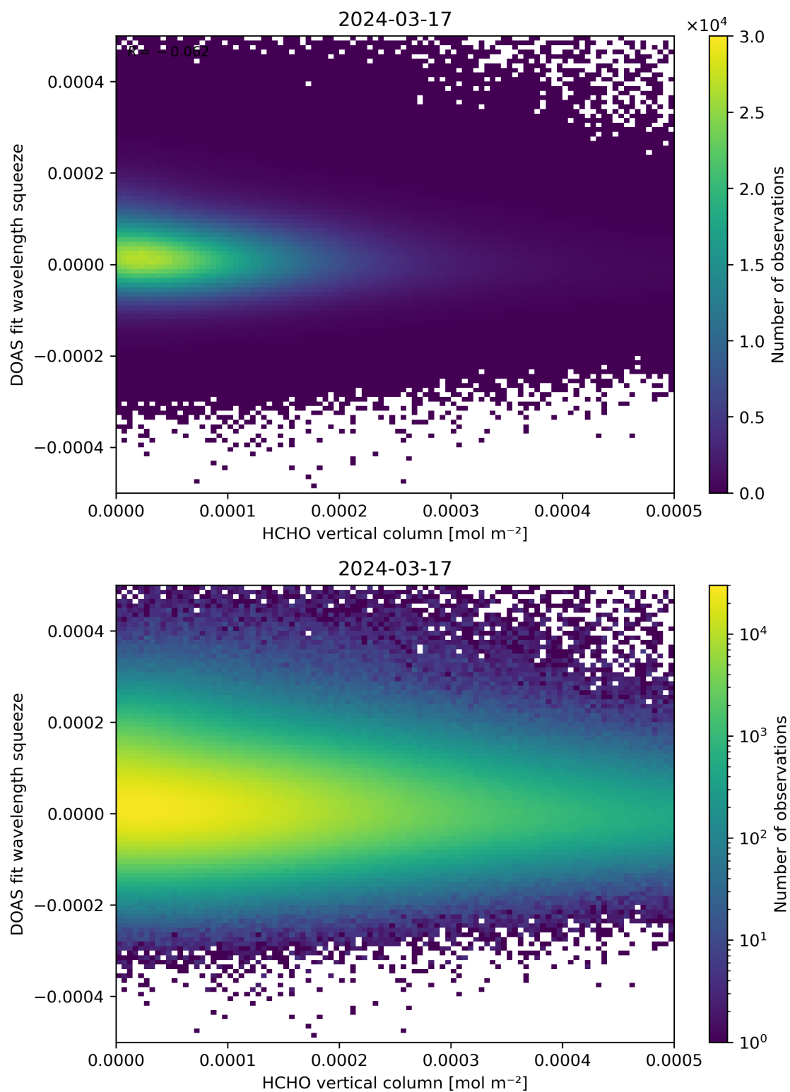
Figure 125: Scatter density plot of “HCHO vertical column” against “DOAS fit wavelength squeeze” for 2024-03-16 to 2024-03-18.
