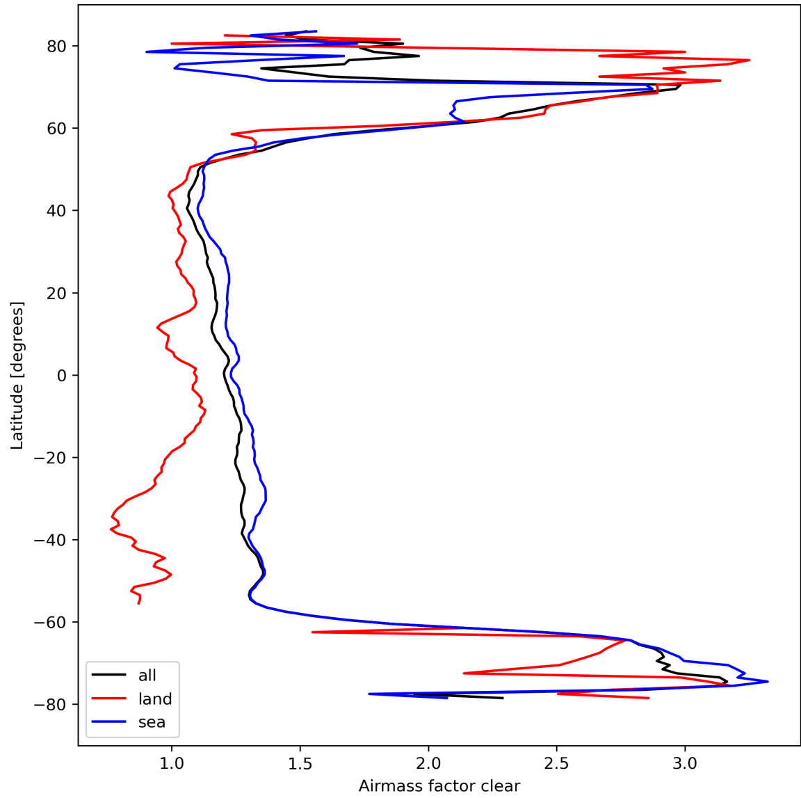
Figure 28: Zonal average of “Airmass factor clear” for 2024-03-16 to 2024-03-18.
