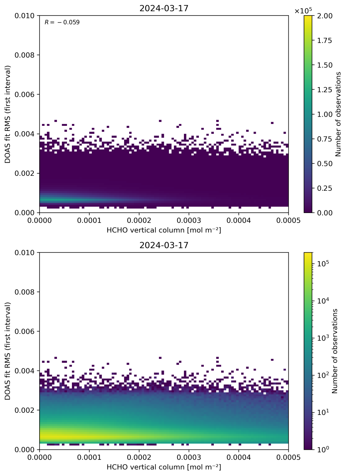
Figure 123: Scatter density plot of “HCHO vertical column” against “DOAS fit RMS (first interval)” for 2024-03-16 to 2024-03-18.
