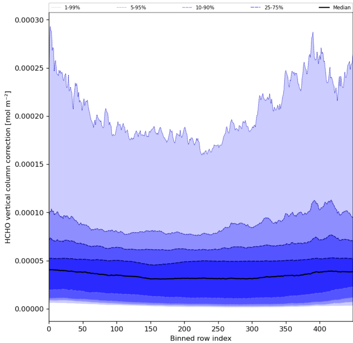
Figure 51: Along track statistics of “HCHO vertical column correction” for 2024-03-16 to 2024-03-18
