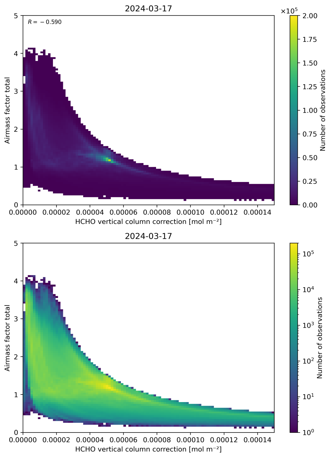
Figure 120: Scatter density plot of “HCHO vertical column correction” against “Airmass factor total” for 2024-03-16 to 2024-03-18.
