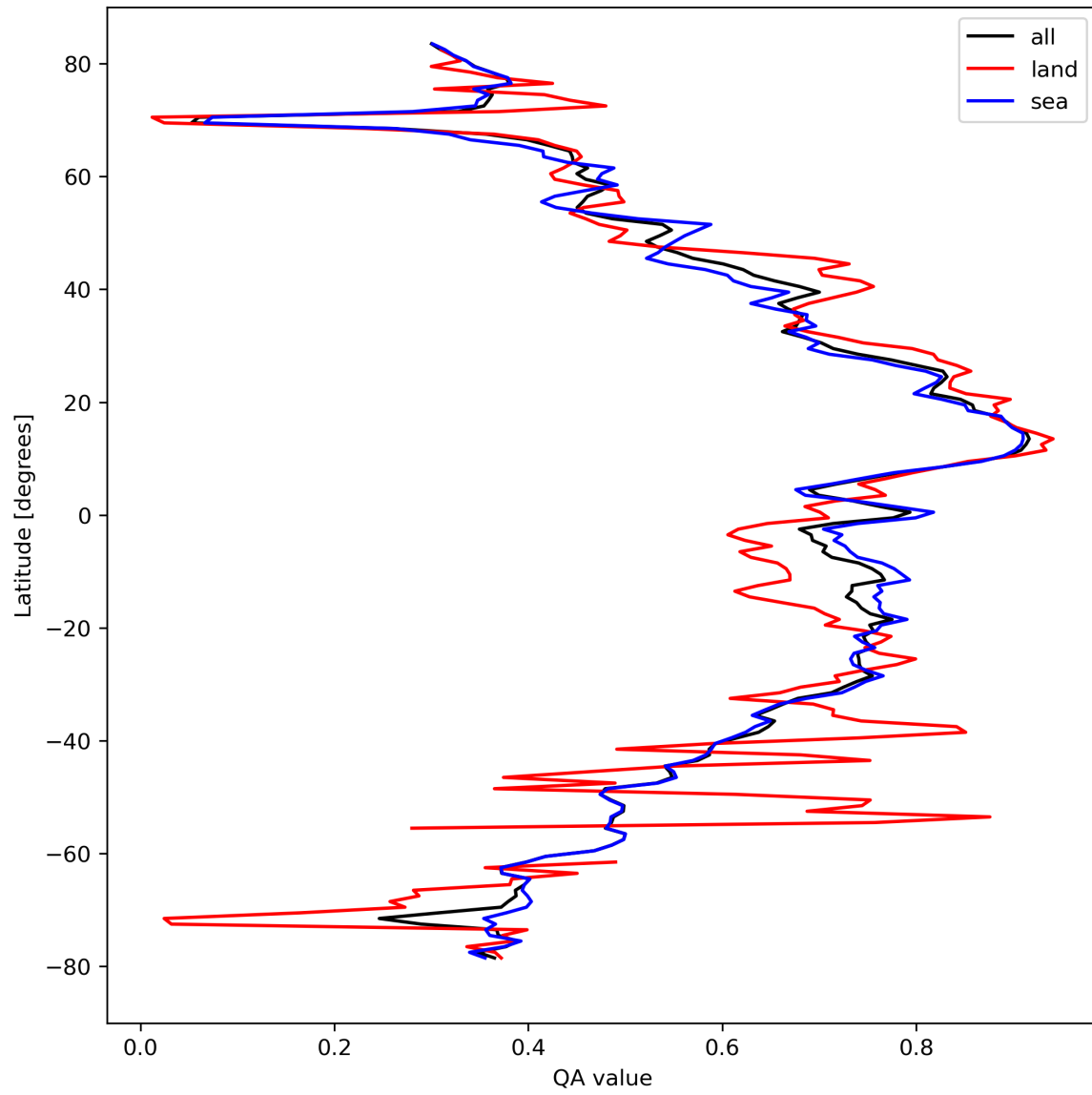
Figure 20: Zonal average of “QA value” for 2024-03-16 to 2024-03-18.
