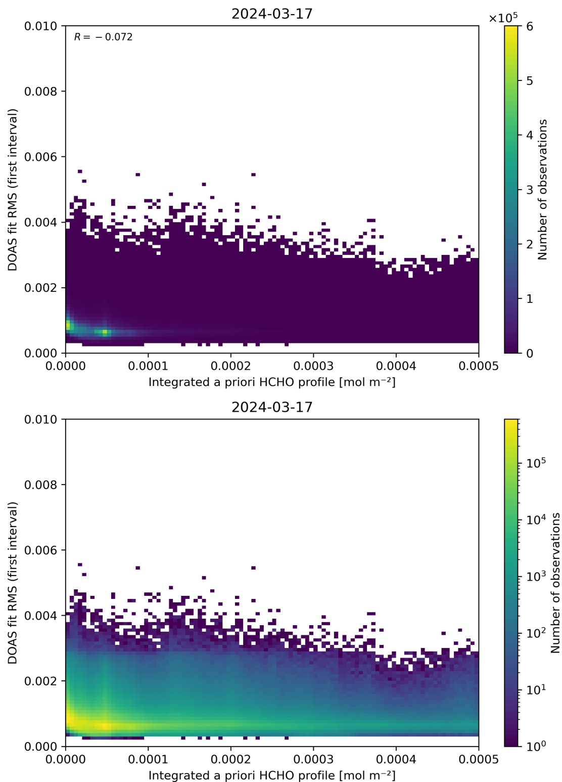
Figure 148: Scatter density plot of “Integrated a priori HCHO profile” against “DOAS fit RMS (first interval)” for 2024-03-16 to 2024-03-18.
