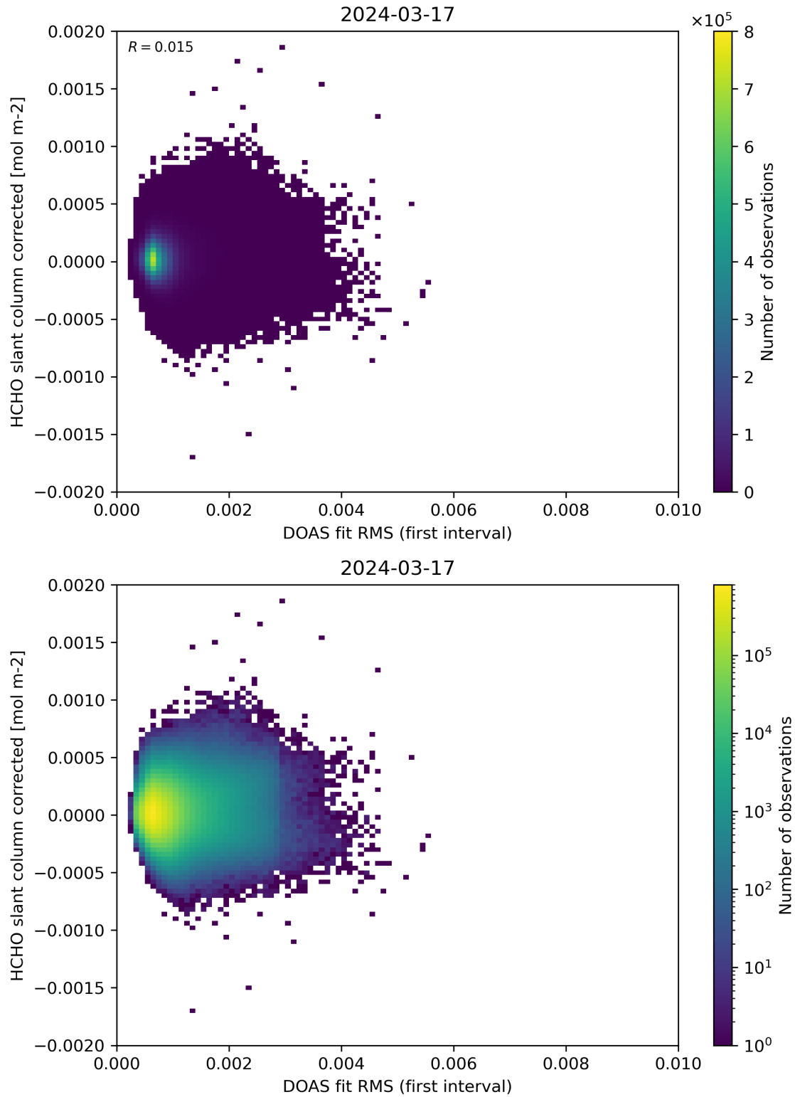
Figure 62: Scatter density plot of “DOAS fit RMS (first interval)” against “HCHO slant column corrected” for 2024-03-16 to 2024-03-18.
