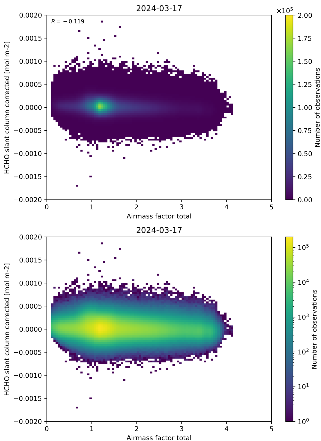
Figure 101: Scatter density plot of “Airmass factor total” against “HCHO slant column corrected” for 2024-03-16 to 2024-03-18.
