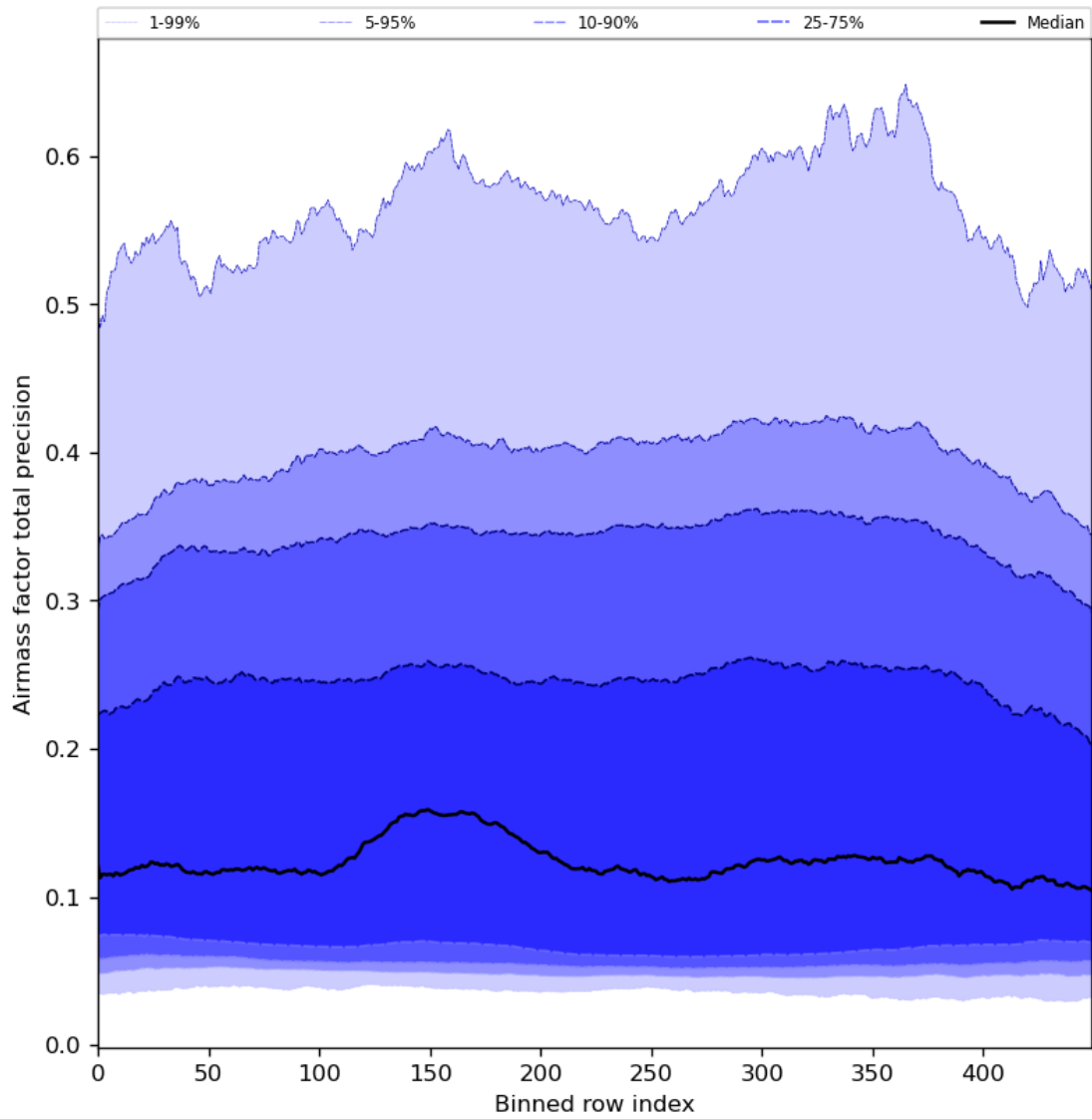
Figure 55: Along track statistics of “Airmass factor total precision” for 2024-03-16 to 2024-03-18
