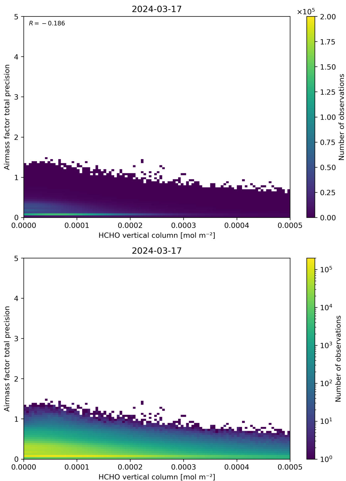
Figure 132: Scatter density plot of “HCHO vertical column” against “Airmass factor total precision” for 2024-03-16 to 2024-03-18.
