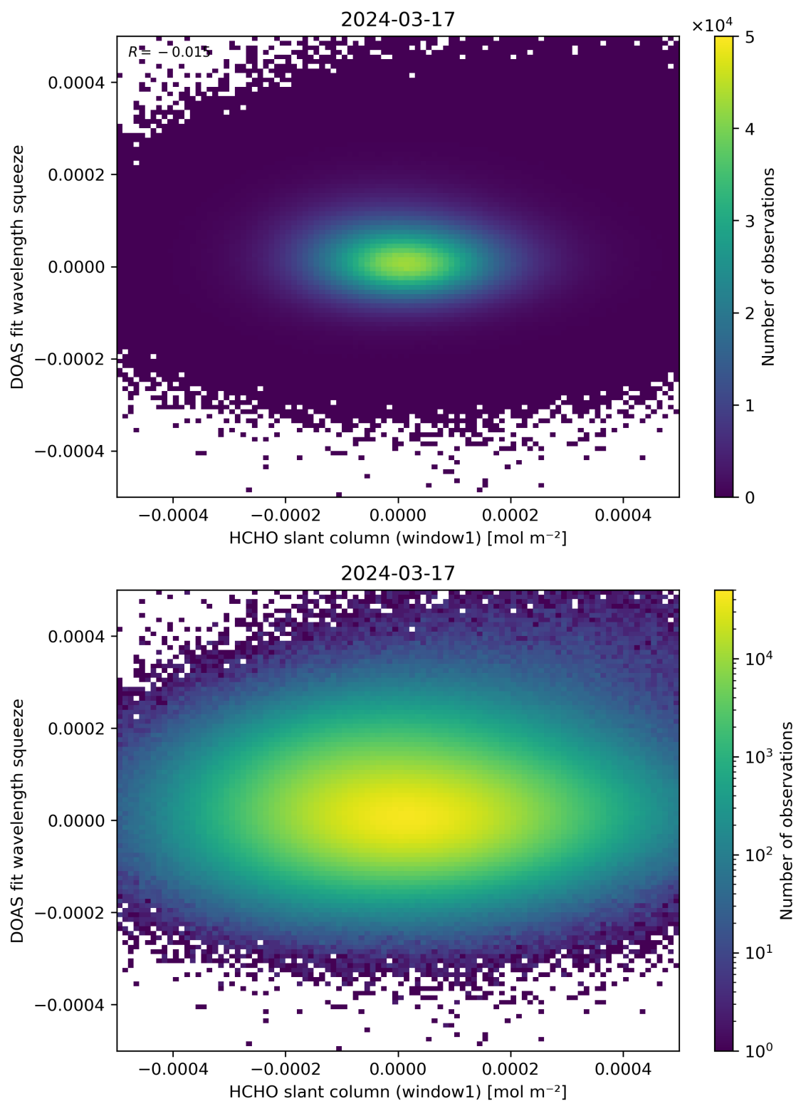
Figure 80: Scatter density plot of “HCHO slant column (window1)” against “DOAS fit wavelength squeeze” for 2024-03-16 to 2024-03-18.
