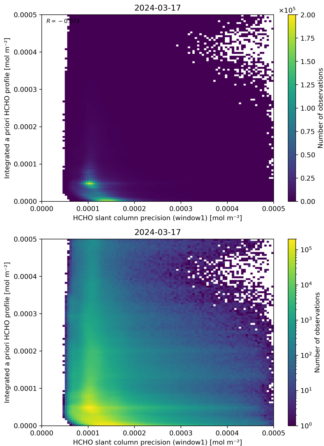
Figure 96: Scatter density plot of “HCHO slant column precision (window1)” against “Integrated a priori HCHO profile” for 2024-03-16 to 2024-03-18.
