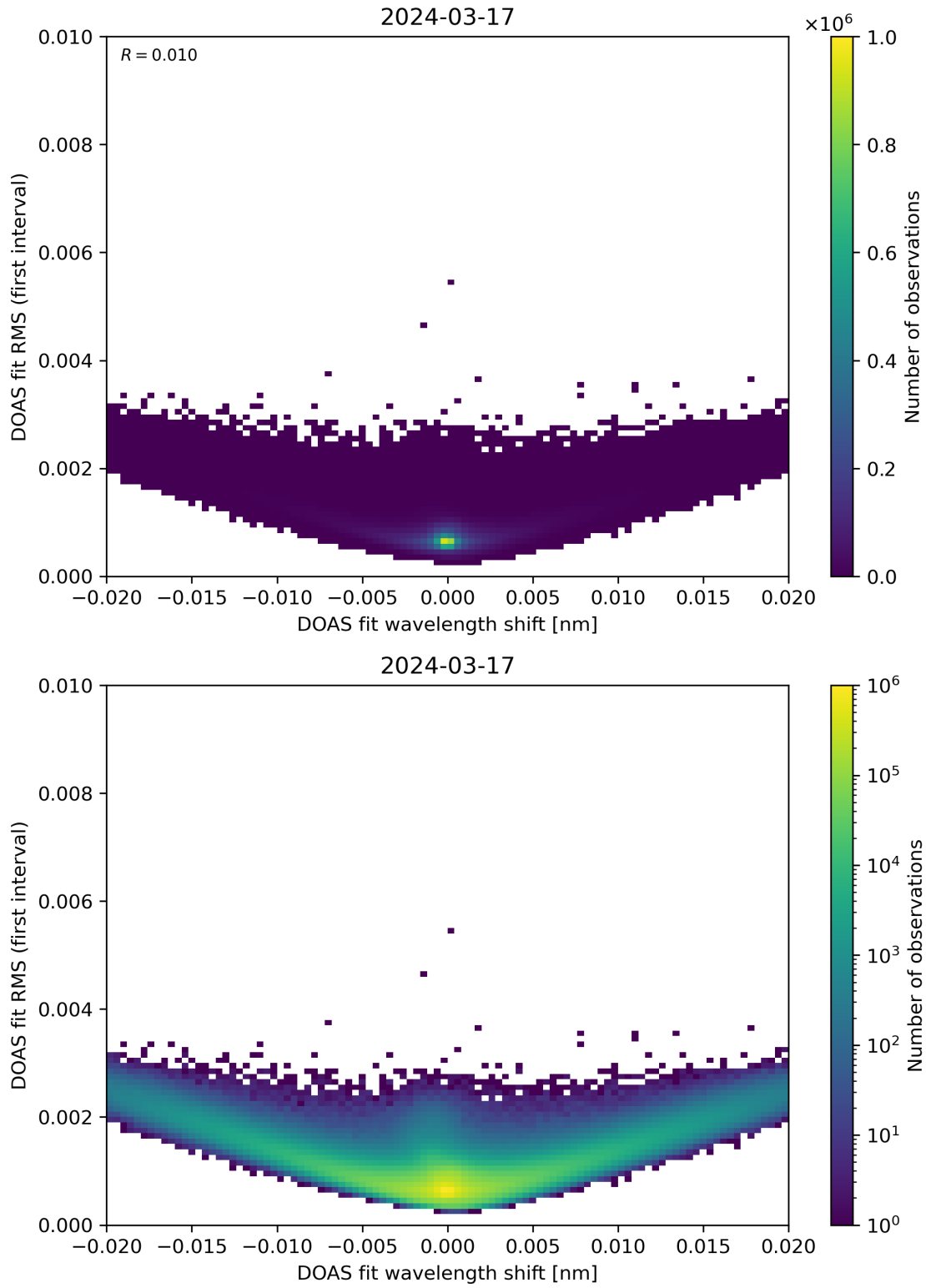
Figure 64: Scatter density plot of “DOAS fit wavelength shift” against “DOAS fit RMS (first interval)” for 2024-03-16 to 2024-03-18.
