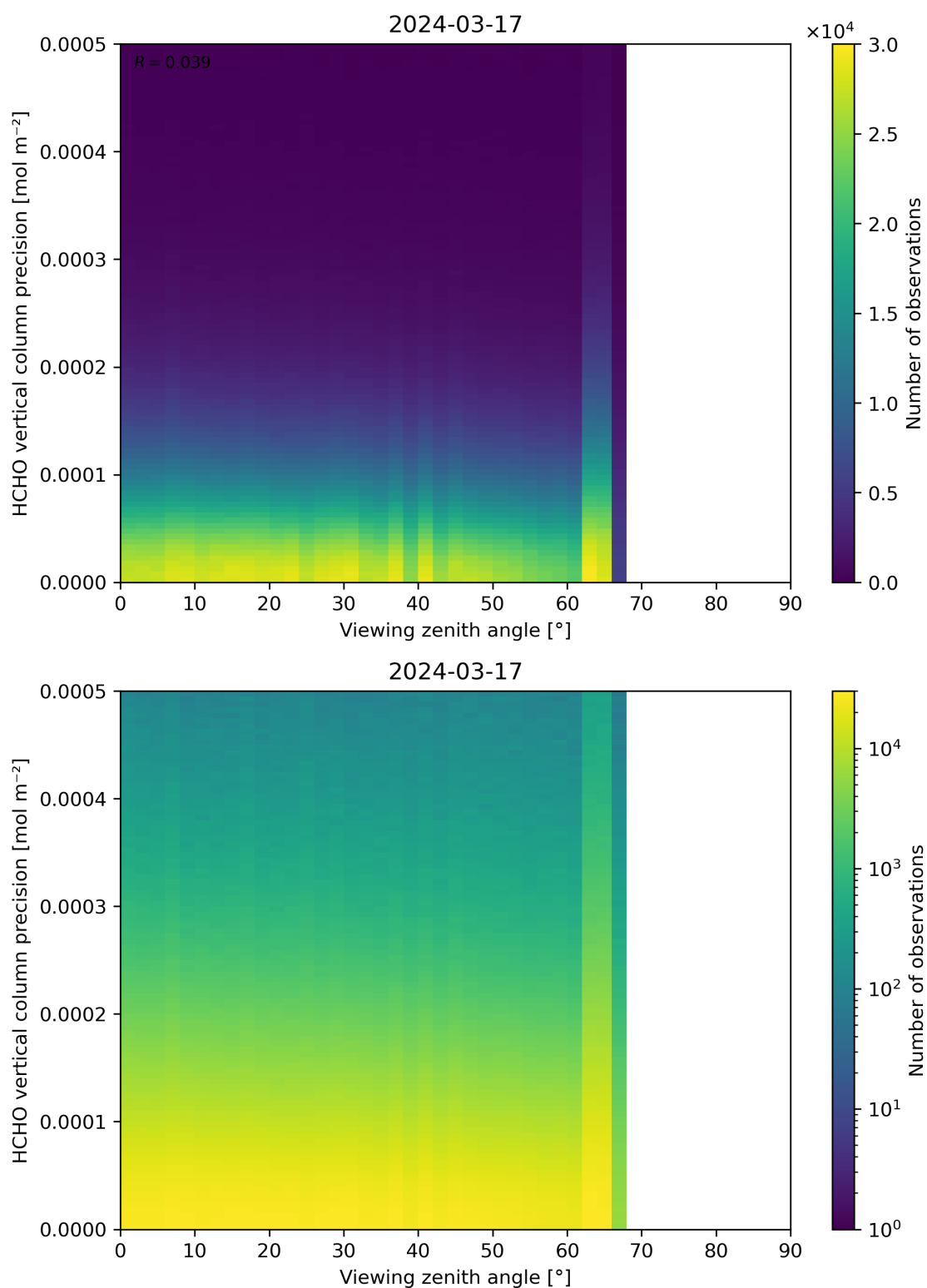
Figure 194: Scatter density plot of “Viewing zenith angle” against “HCHO vertical column precision” for 2024-03-16 to 2024-03-18.
