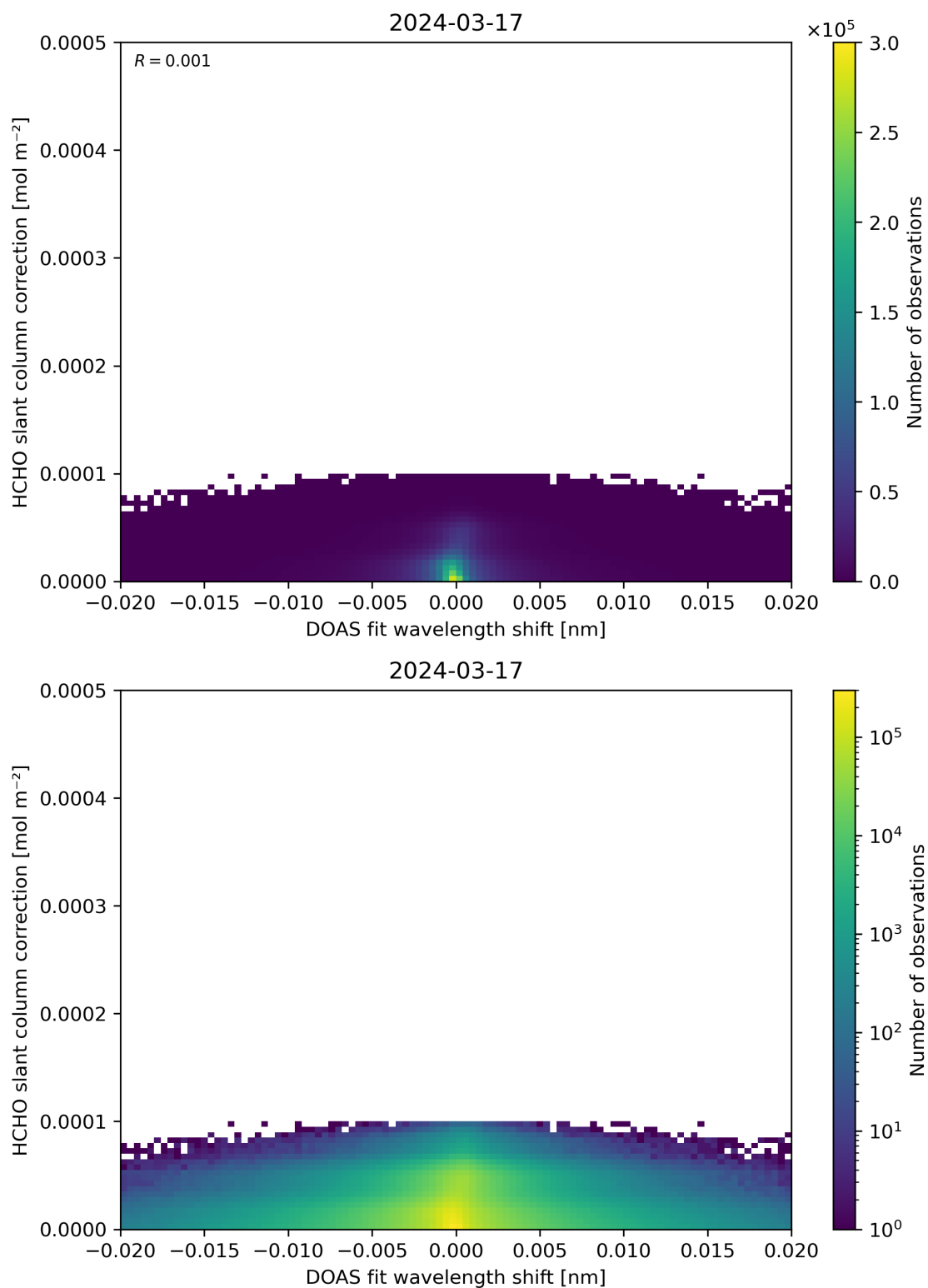
Figure 67: Scatter density plot of “DOAS fit wavelength shift” against “HCHO slant column correction” for 2024-03-16 to 2024-03-18.
