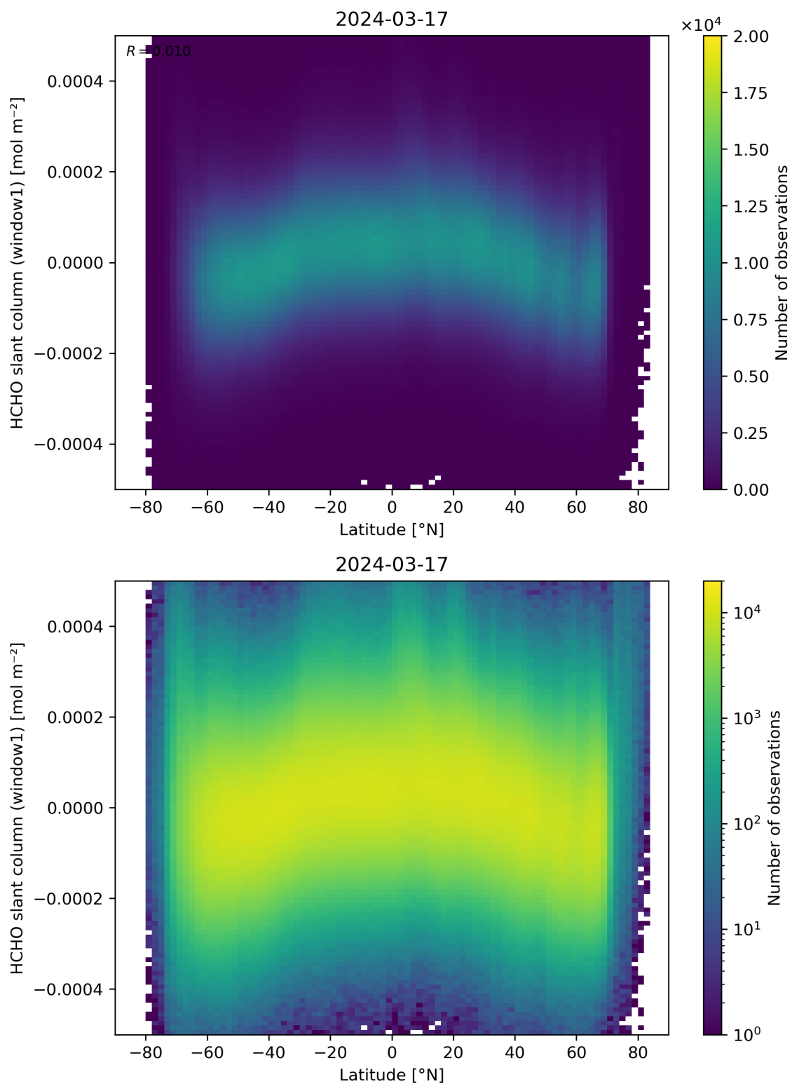
Figure 159: Scatter density plot of “Latitude” against “HCHO slant column (window1)” for 2024-03-16 to 2024-03-18.
