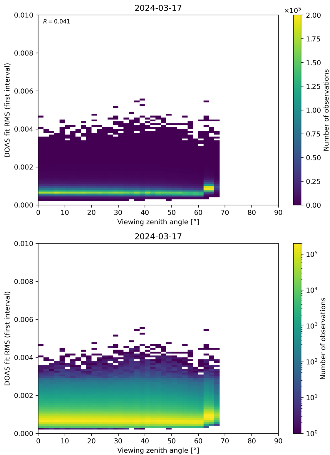
Figure 182: Scatter density plot of “Viewing zenith angle” against “DOAS fit RMS (first interval)” for 2024-03-16 to 2024-03-18.
