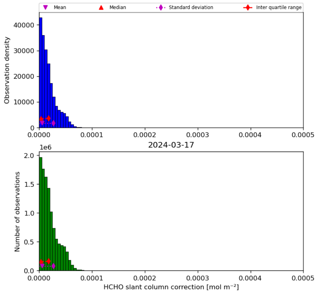
Figure 47: Histogram of “HCHO slant column correction” for 2024-03-16 to 2024-03-18
