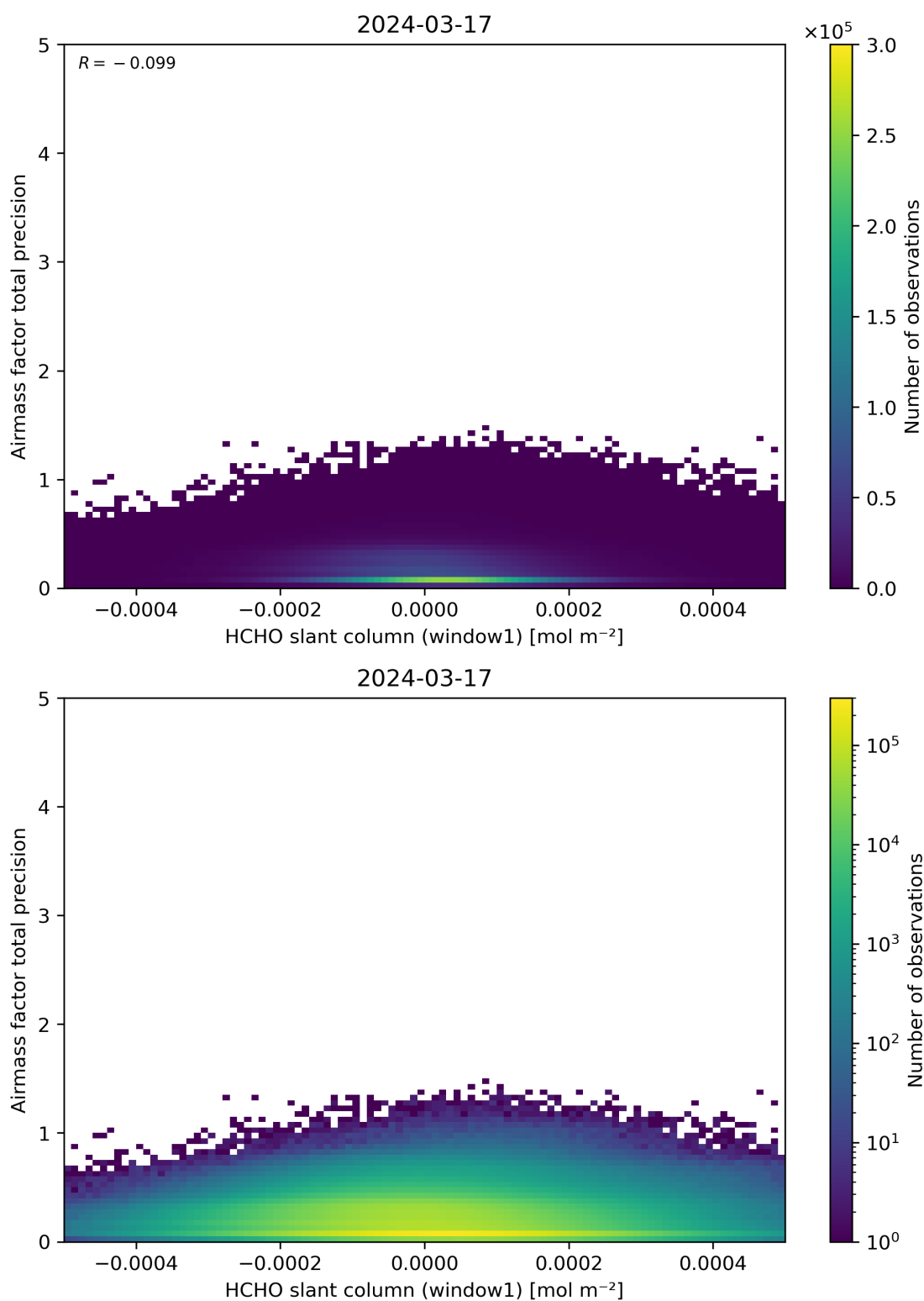
Figure 86: Scatter density plot of “HCHO slant column (window1)” against “Airmass factor total precision” for 2024-03-16 to 2024-03-18.
