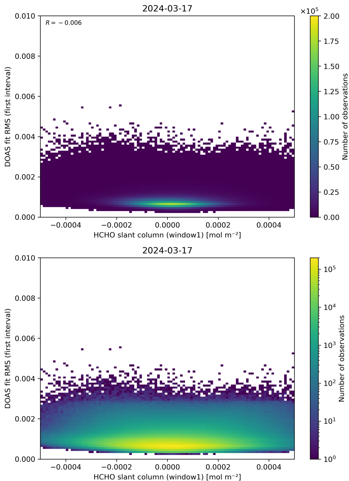
Figure 78: Scatter density plot of “HCHO slant column (window1)” against “DOAS fit RMS (first interval)” for 2024-03-16 to 2024-03-18.
