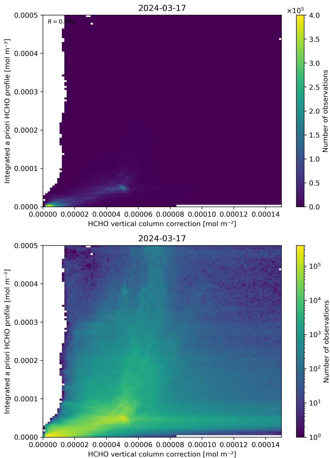
Figure 122: Scatter density plot of “HCHO vertical column correction” against “Integrated a priori HCHO profile” for 2024-03-16 to 2024-03-18.
