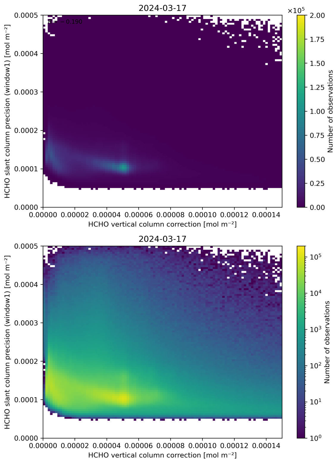
Figure 119: Scatter density plot of “HCHO vertical column correction” against “HCHO slant column precision (window1)” for 2024-03-16 to 2024-03-18.
