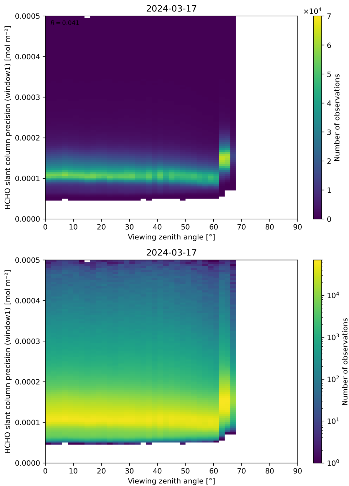
Figure 189: Scatter density plot of “Viewing zenith angle” against “HCHO slant column precision (window1)” for 2024-03-16 to 2024-03-18.
