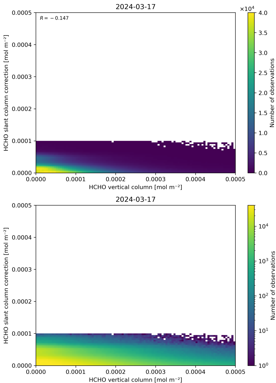
Figure 128: Scatter density plot of “HCHO vertical column” against “HCHO slant column correction” for 2024-03-16 to 2024-03-18.
