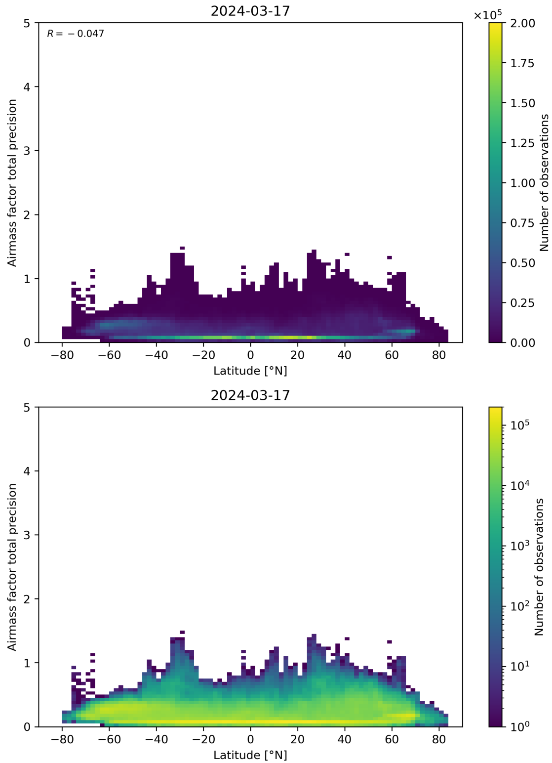
Figure 162: Scatter density plot of “Latitude” against “Airmass factor total precision” for 2024-03-16 to 2024-03-18.
