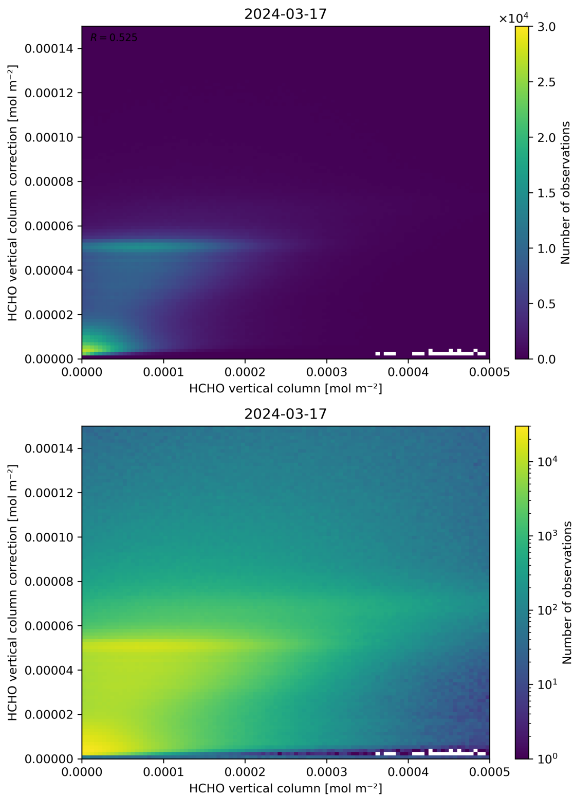
Figure 133: Scatter density plot of “HCHO vertical column” against “HCHO vertical column correction” for 2024-03-16 to 2024-03-18.
