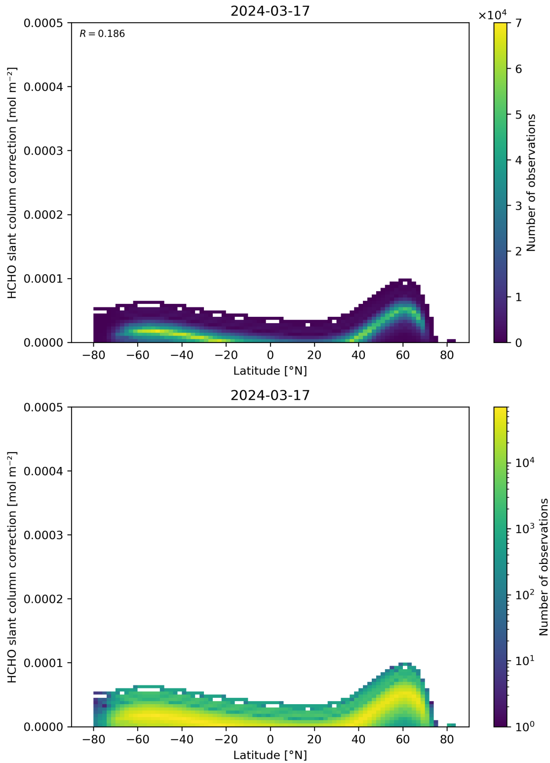
Figure 158: Scatter density plot of “Latitude” against “HCHO slant column correction” for 2024-03-16 to 2024-03-18.
