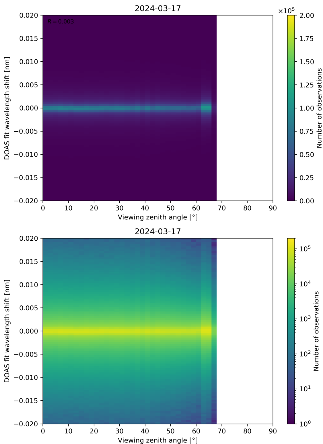
Figure 183: Scatter density plot of “Viewing zenith angle” against “DOAS fit wavelength shift” for 2024-03-16 to 2024-03-18.
