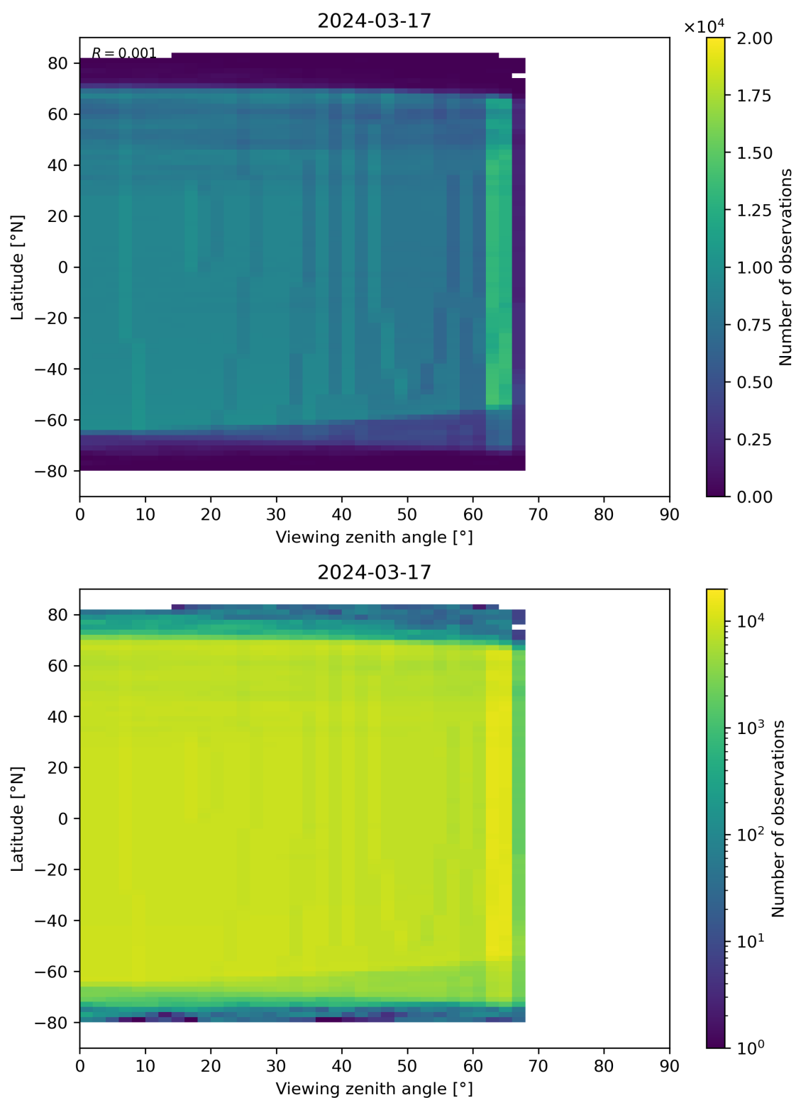
Figure 196: Scatter density plot of “Viewing zenith angle” against “Latitude” for 2024-03-16 to 2024-03-18.
