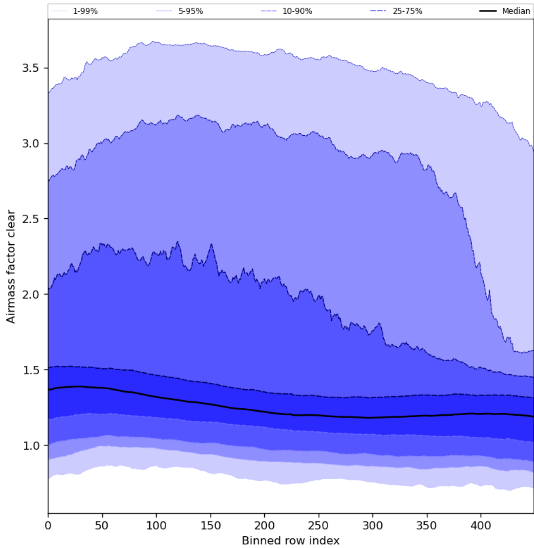
Figure 56: Along track statistics of “Airmass factor clear” for 2024-03-16 to 2024-03-18
