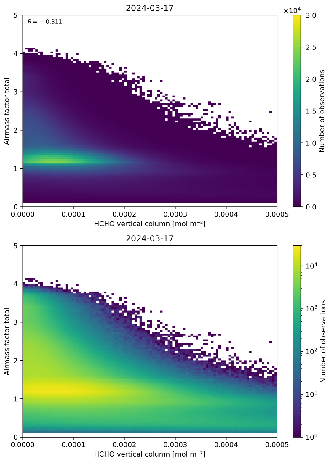
Figure 131: Scatter density plot of “HCHO vertical column” against “Airmass factor total” for 2024-03-16 to 2024-03-18.
