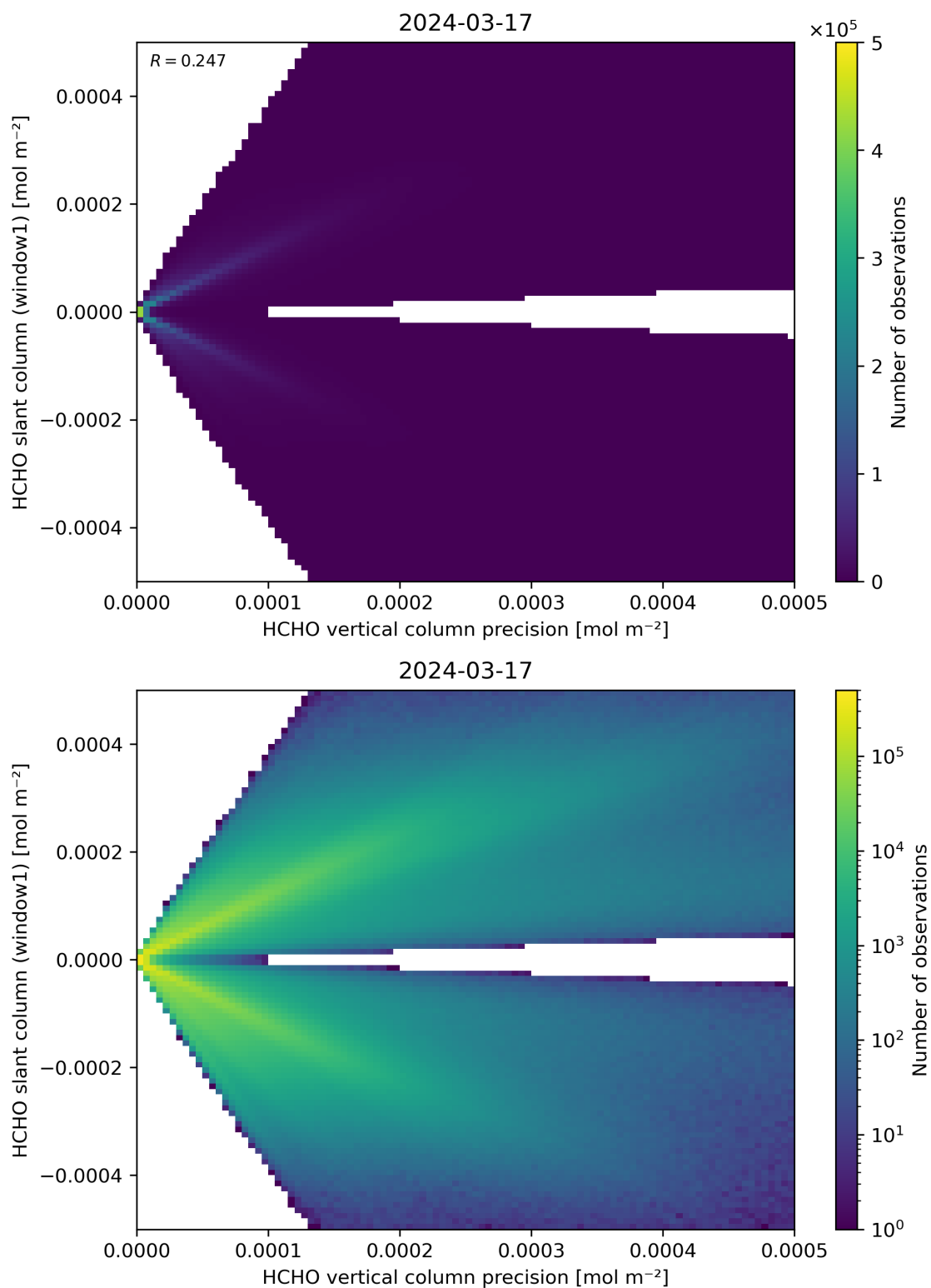
Figure 142: Scatter density plot of “HCHO vertical column precision” against “HCHO slant column (window1)” for 2024-03-16 to 2024-03-18.
