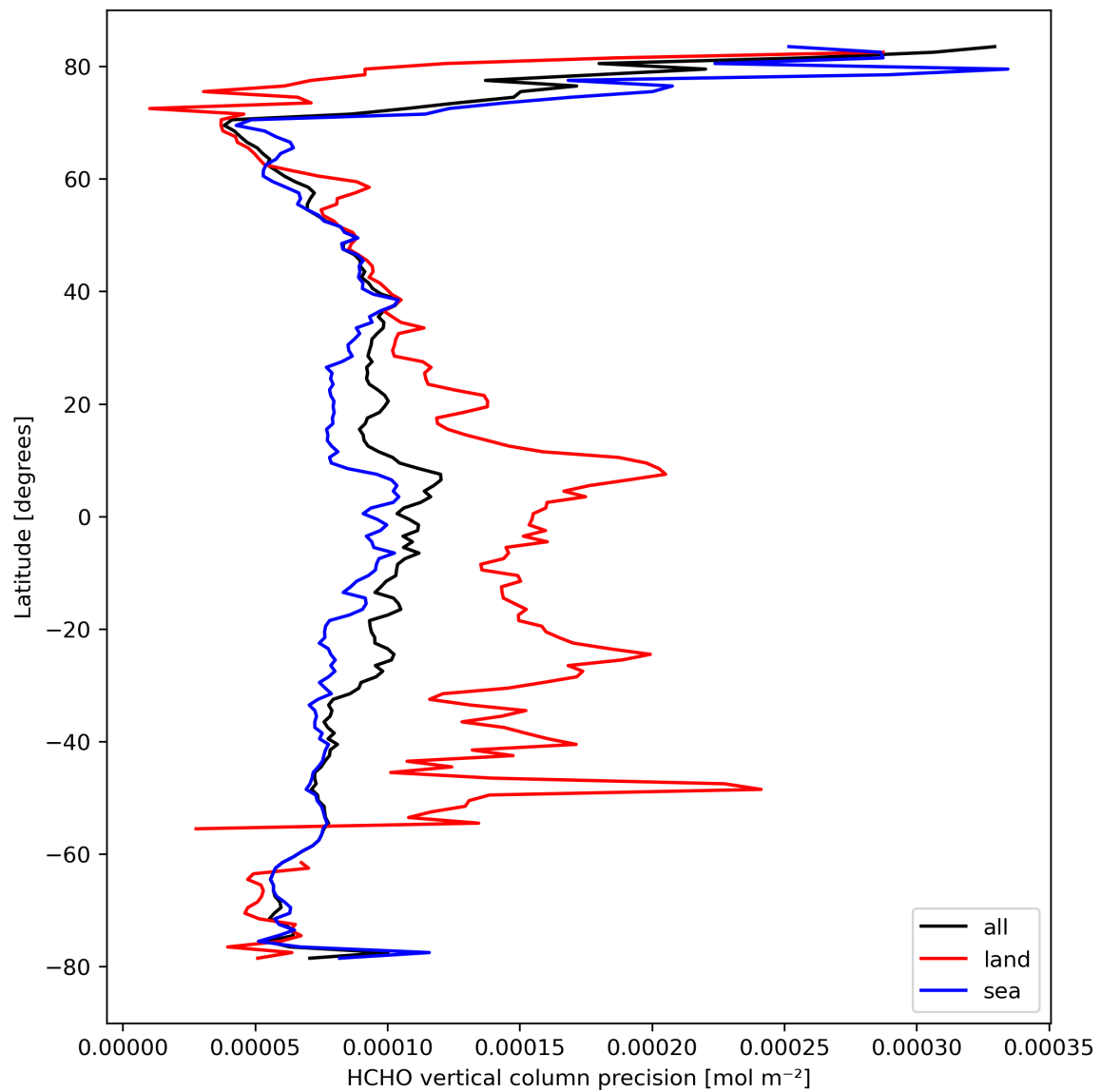
Figure 22: Zonal average of “HCHO vertical column precision” for 2024-03-16 to 2024-03-18.
