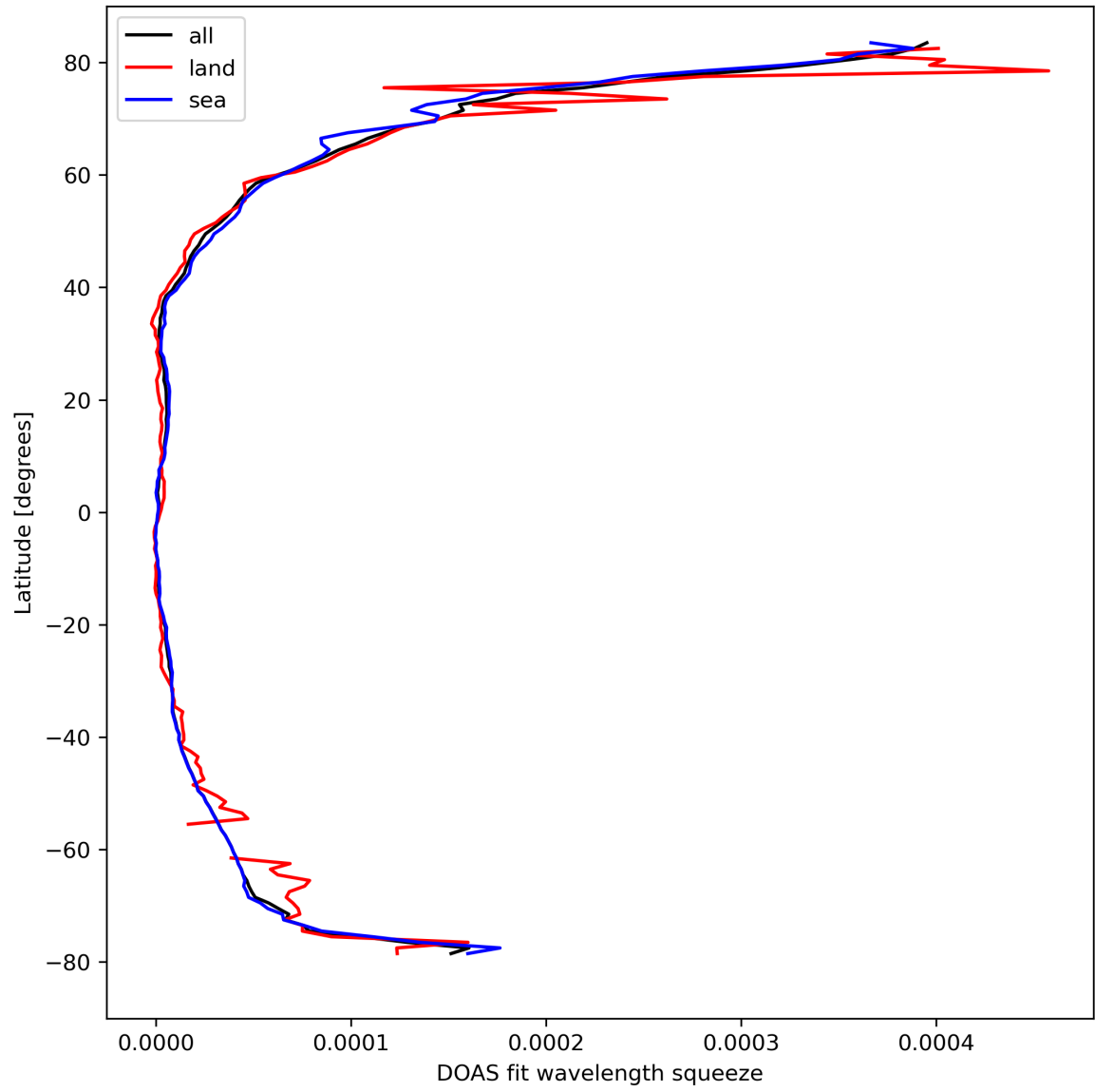
Figure 31: Zonal average of “DOAS fit wavelength squeeze” for 2024-03-16 to 2024-03-18.
