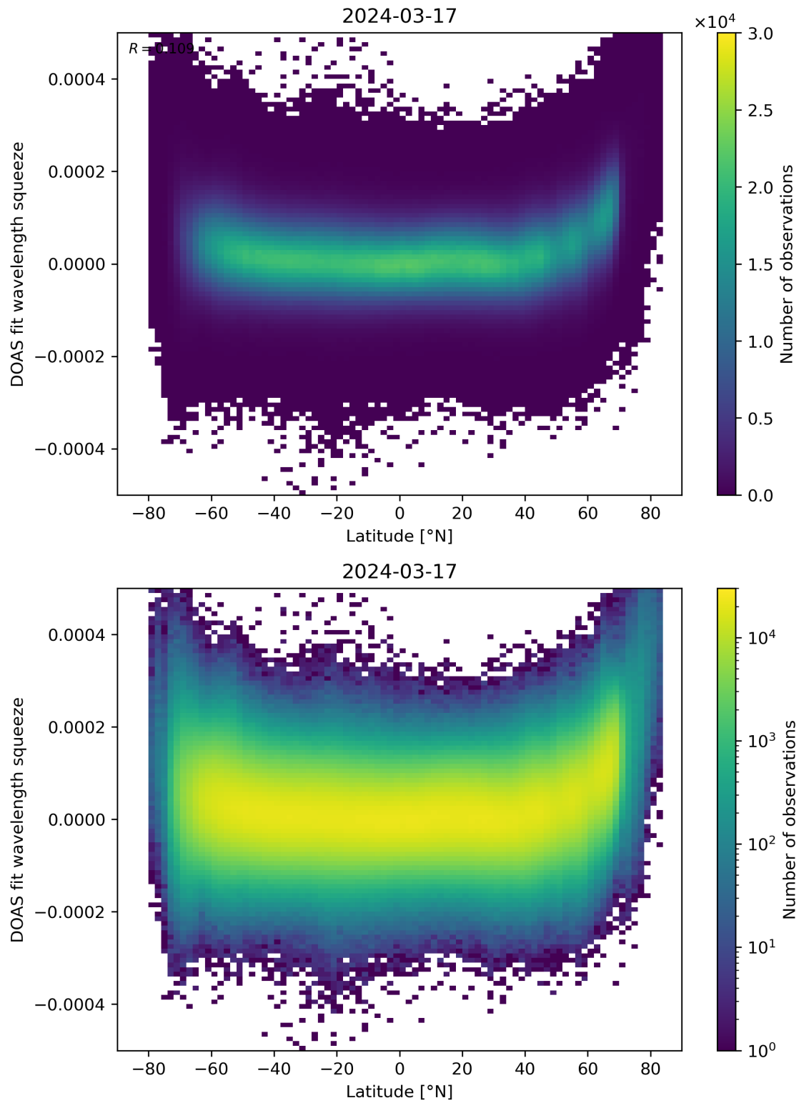
Figure 155: Scatter density plot of “Latitude” against “DOAS fit wavelength squeeze” for 2024-03-16 to 2024-03-18.
