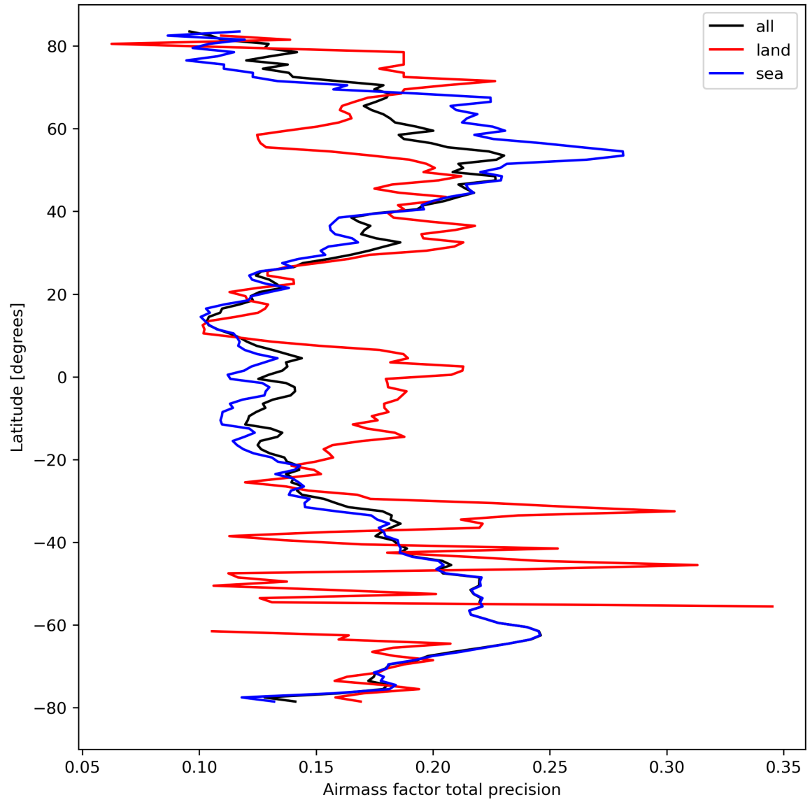
Figure 27: Zonal average of “Airmass factor total precision” for 2024-03-16 to 2024-03-18.
