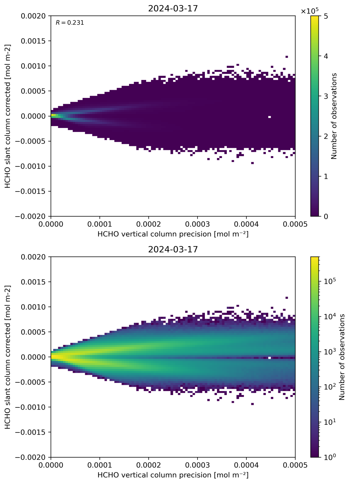
Figure 140: Scatter density plot of “HCHO vertical column precision” against “HCHO slant column corrected” for 2024-03-16 to 2024-03-18.
