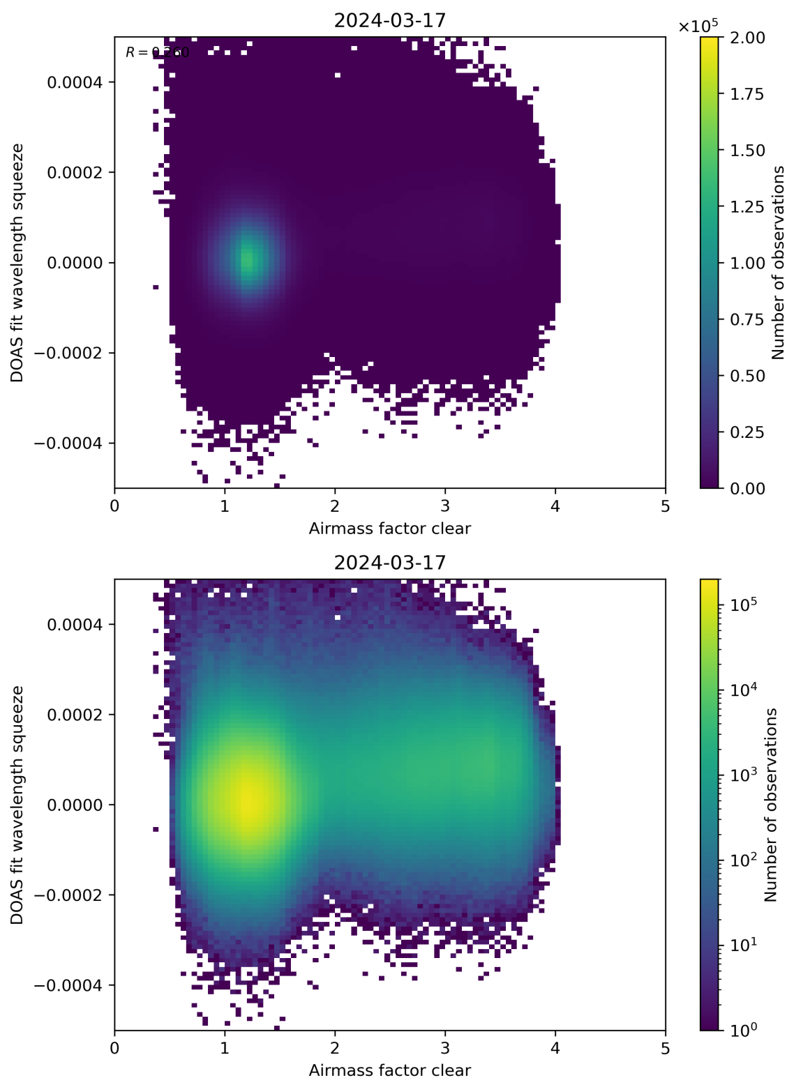
Figure 73: Scatter density plot of “Airmass factor clear” against “DOAS fit wavelength squeeze” for 2024-03-16 to 2024-03-18.
