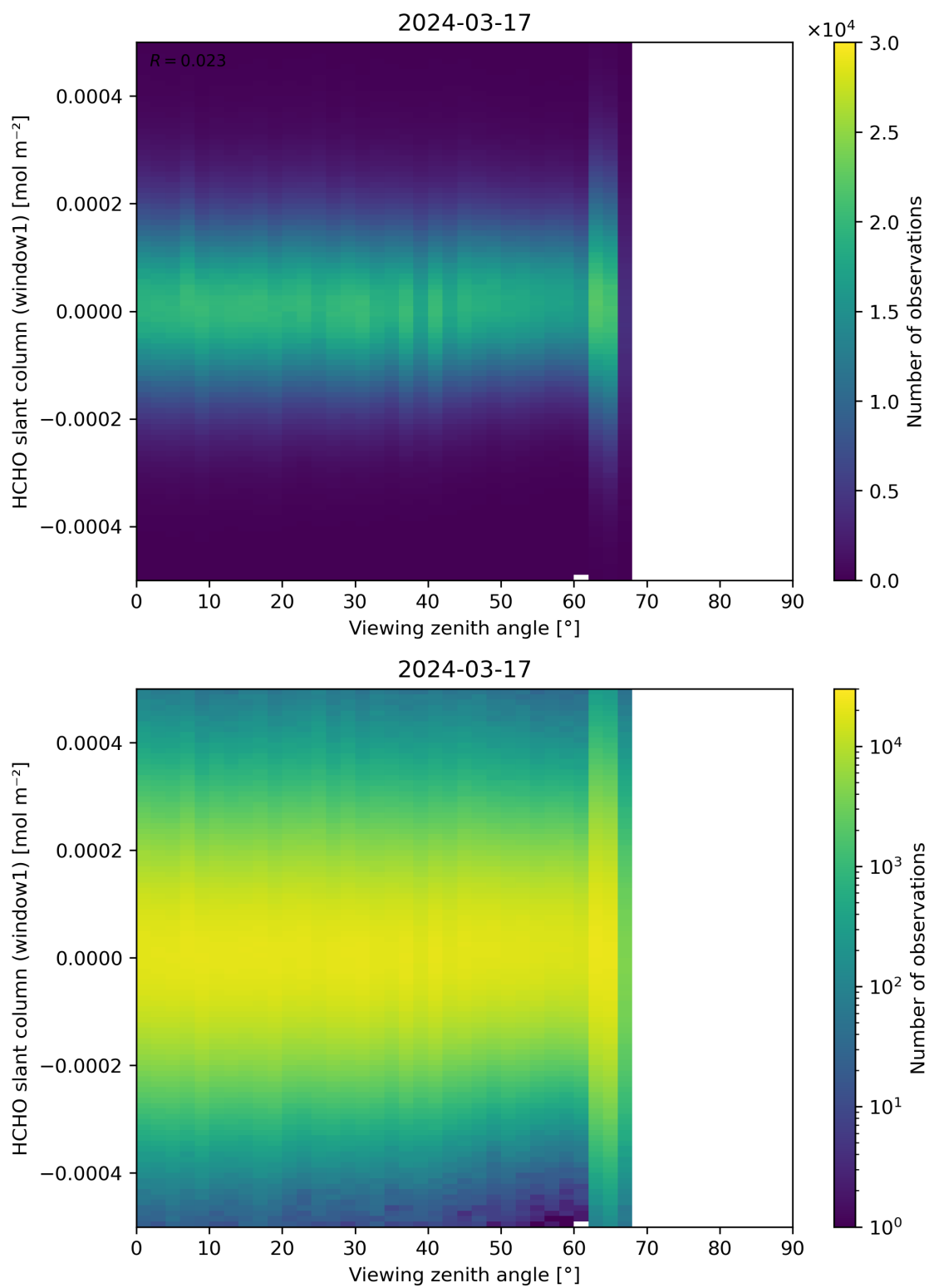
Figure 188: Scatter density plot of “Viewing zenith angle” against “HCHO slant column (window1)” for 2024-03-16 to 2024-03-18.
