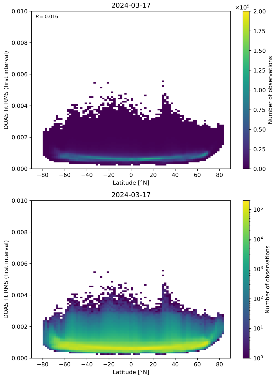
Figure 153: Scatter density plot of “Latitude” against “DOAS fit RMS (first interval)” for 2024-03-16 to 2024-03-18.
