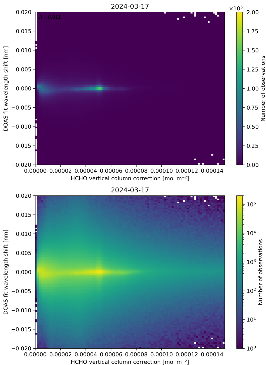
Figure 113: Scatter density plot of “HCHO vertical column correction” against “DOAS fit wavelength shift” for 2024-03-16 to 2024-03-18.
