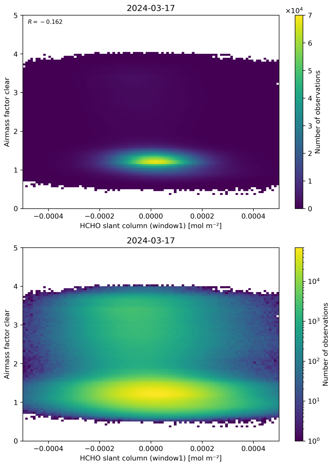
Figure 81: Scatter density plot of “HCHO slant column (window1)” against “Airmass factor clear” for 2024-03-16 to 2024-03-18.
