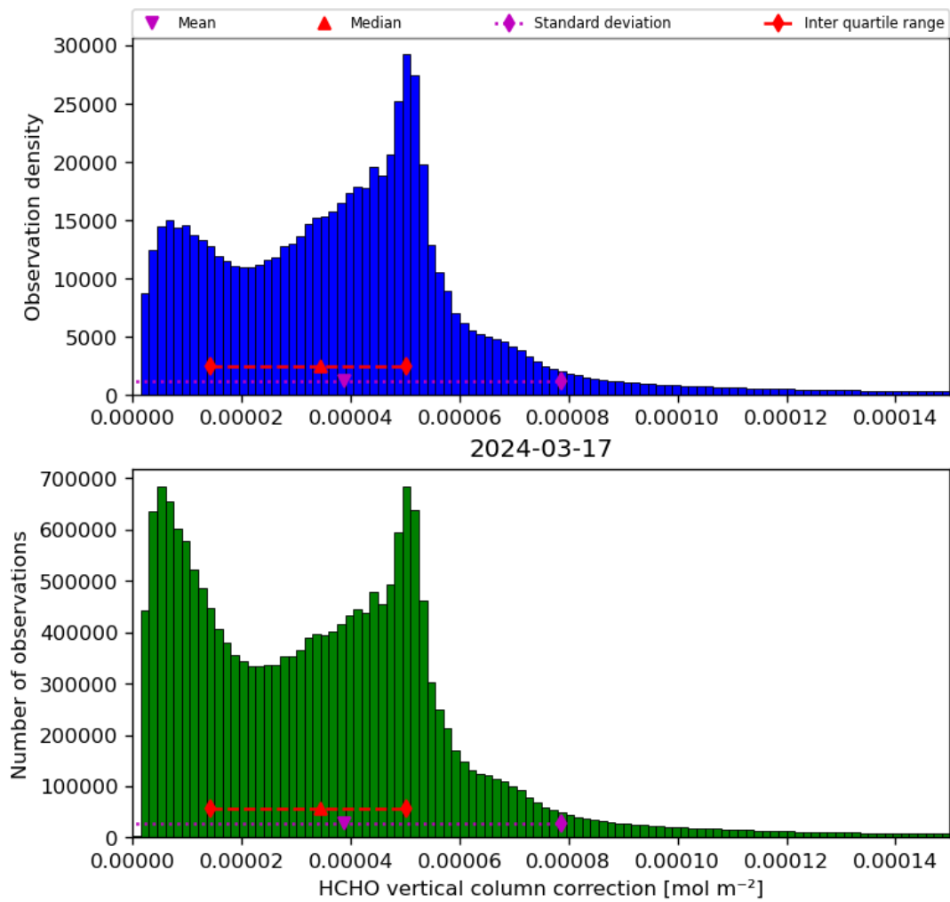
Figure 37: Histogram of “HCHO vertical column correction” for 2024-03-16 to 2024-03-18
