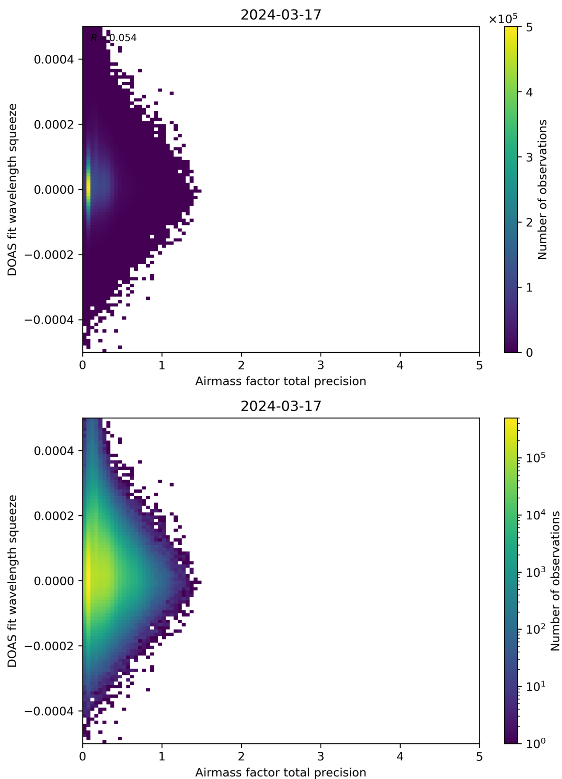
Figure 107: Scatter density plot of “Airmass factor total precision” against “DOAS fit wavelength squeeze” for 2024-03-16 to 2024-03-18.
