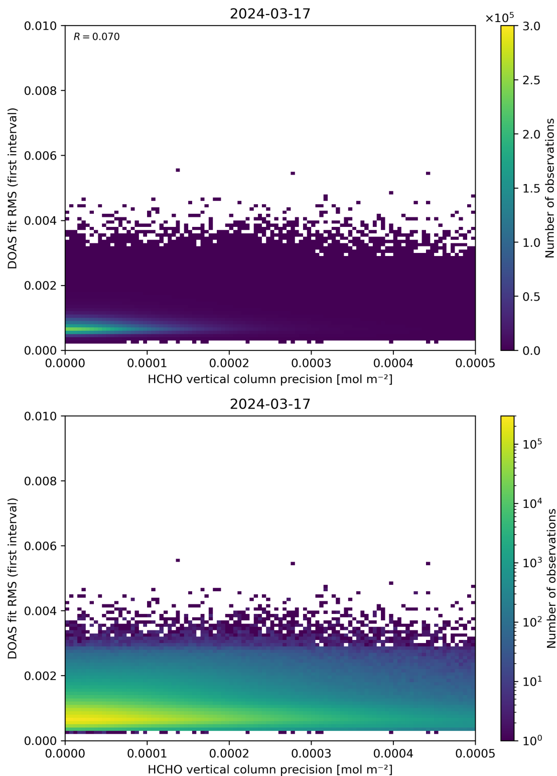
Figure 136: Scatter density plot of “HCHO vertical column precision” against “DOAS fit RMS (first interval)” for 2024-03-16 to 2024-03-18.
