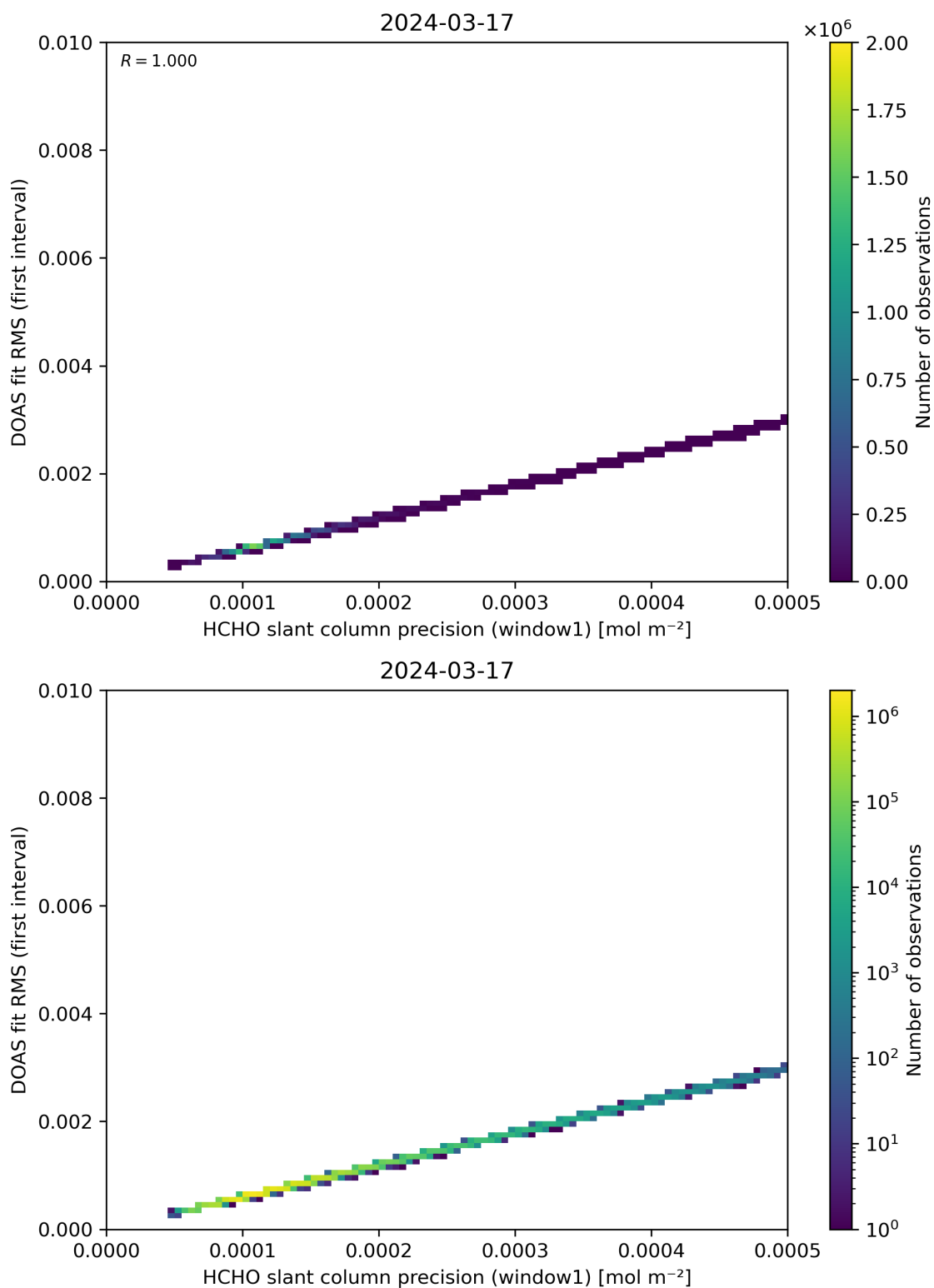
Figure 88: Scatter density plot of “HCHO slant column precision (window1)” against “DOAS fit RMS (first interval)” for 2024-03-16 to 2024-03-18.
