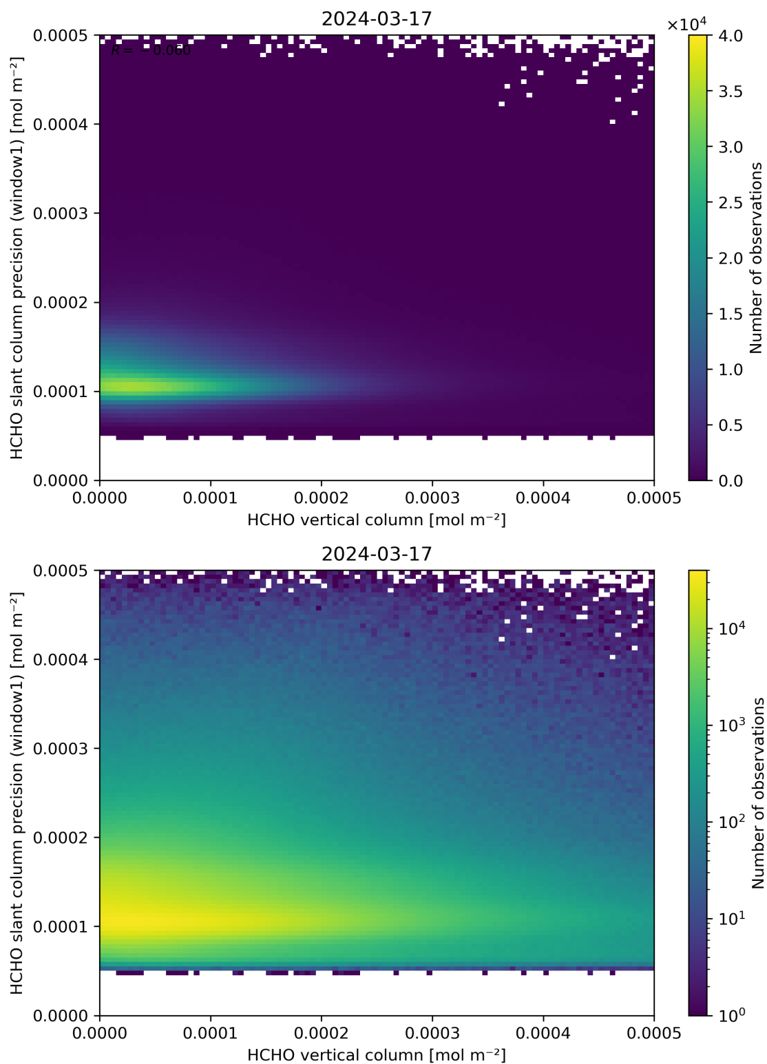
Figure 130: Scatter density plot of “HCHO vertical column” against “HCHO slant column precision (window1)” for 2024-03-16 to 2024-03-18.
