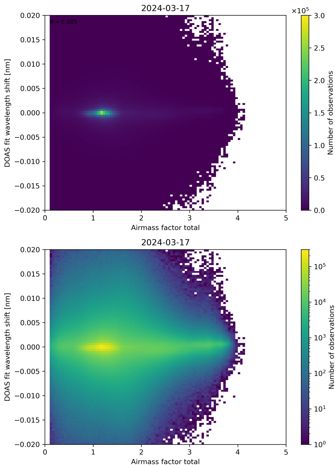
Figure 98: Scatter density plot of “Airmass factor total” against “DOAS fit wavelength shift” for 2024-03-16 to 2024-03-18.
