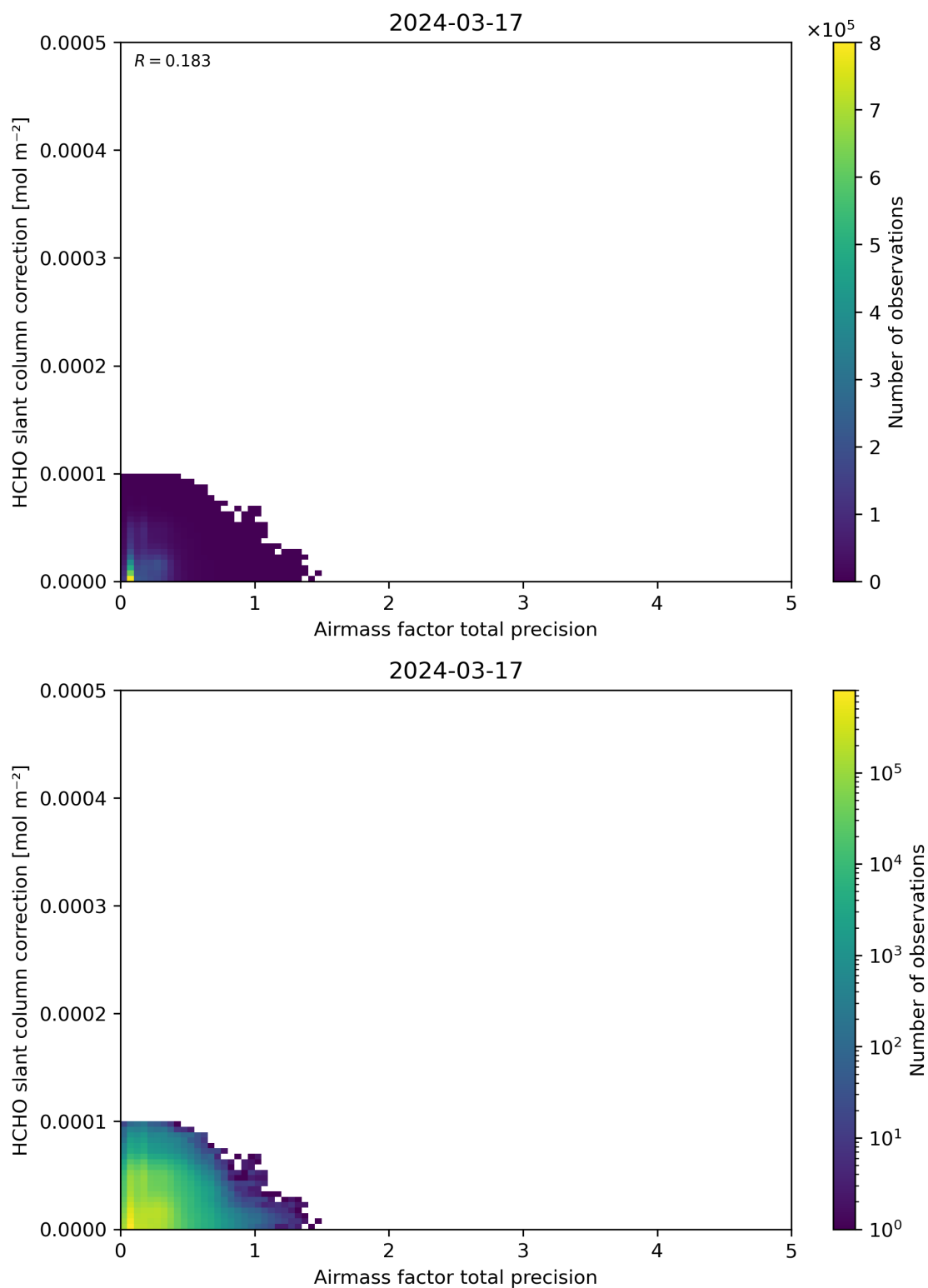
Figure 110: Scatter density plot of “Airmass factor total precision” against “HCHO slant column correction” for 2024-03-16 to 2024-03-18.
