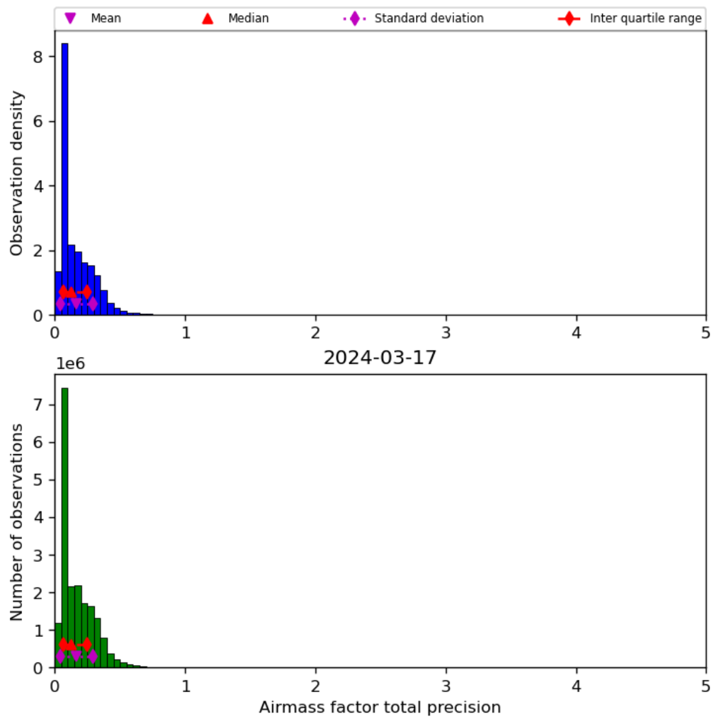
Figure 41: Histogram of "Airmass factor total precision" for 2024-03-16 to 2024-03-18
