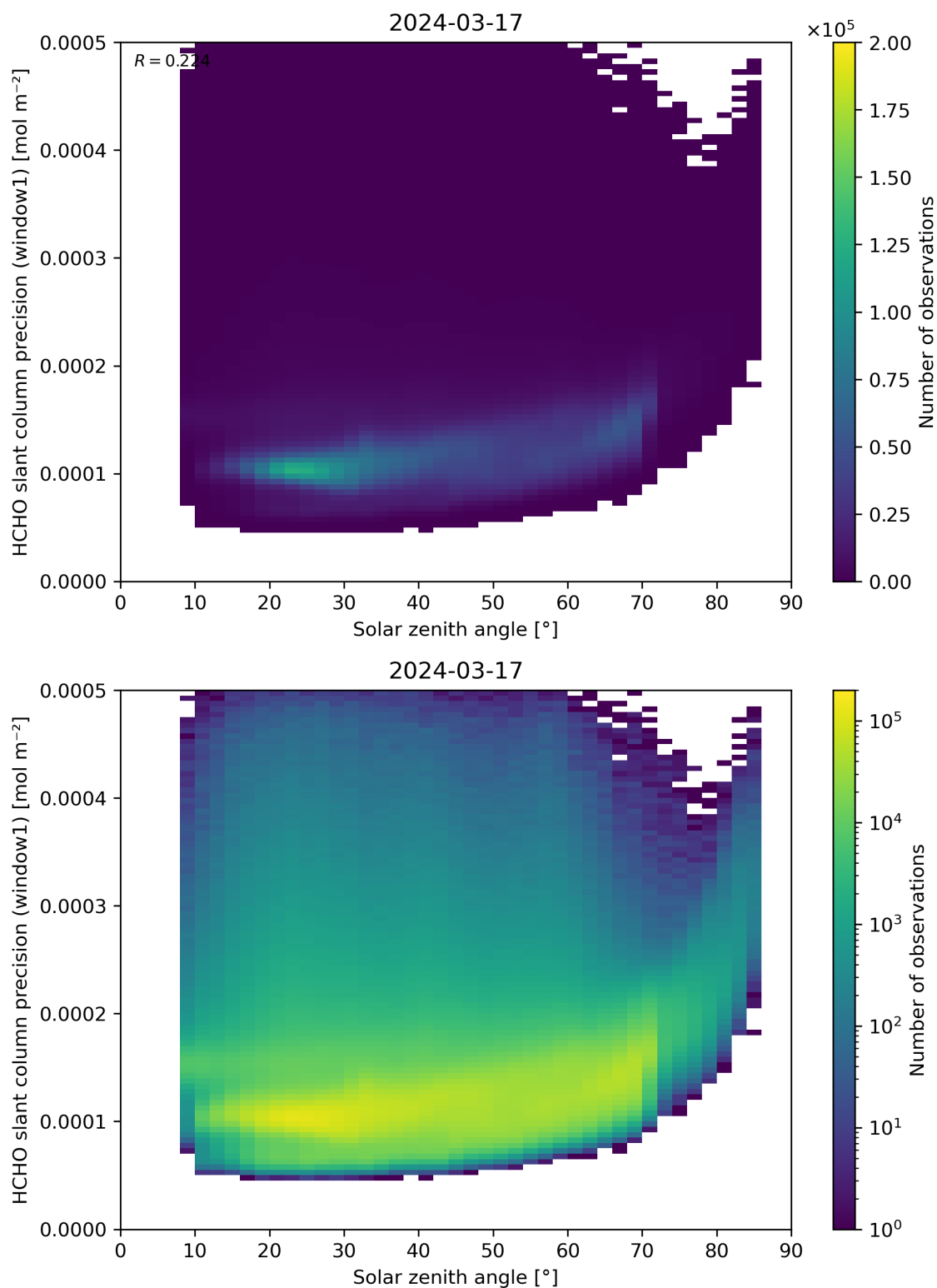
Figure 174: Scatter density plot of “Solar zenith angle” against “HCHO slant column precision (window1)” for 2024-03-16 to 2024-03-18.
