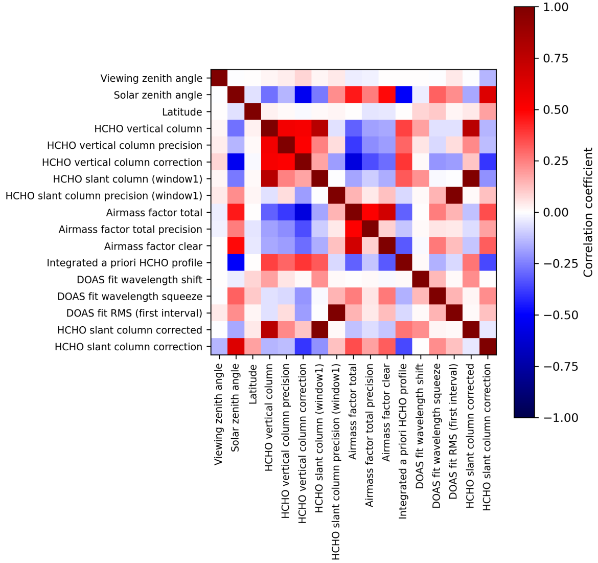
Figure 2: Map of correlation matrix for 2024-03-16 to 2024-03-18.
