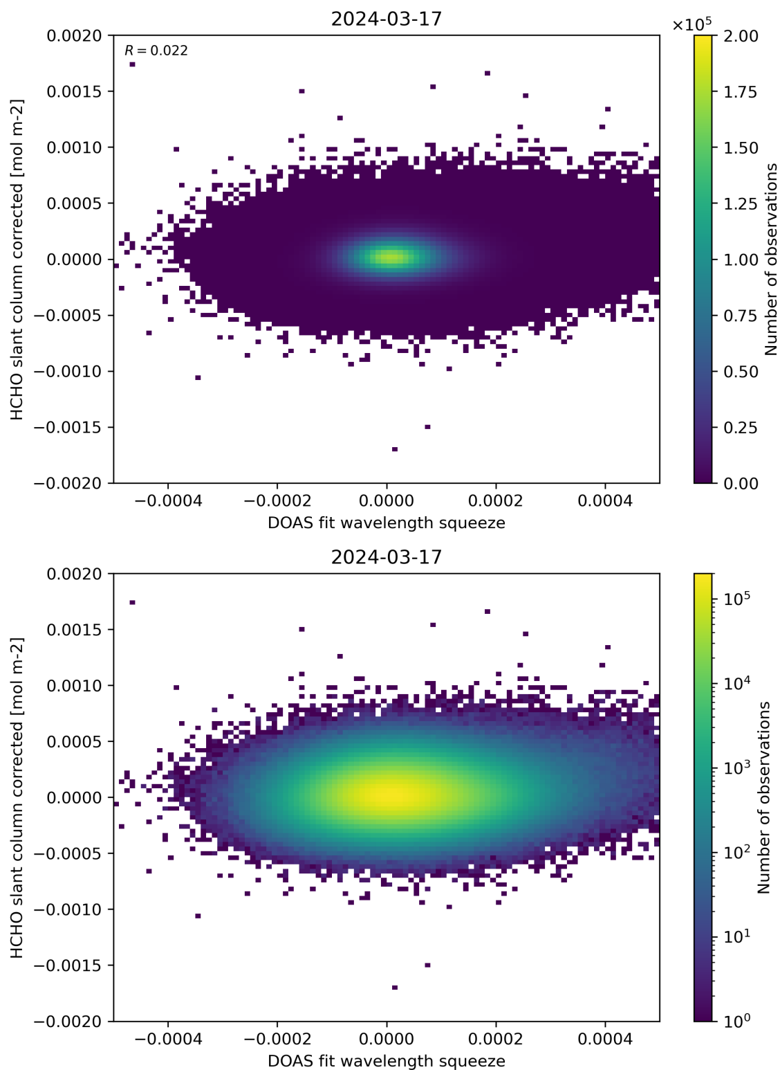
Figure 69: Scatter density plot of “DOAS fit wavelength squeeze” against “HCHO slant column corrected” for 2024-03-16 to 2024-03-18.
