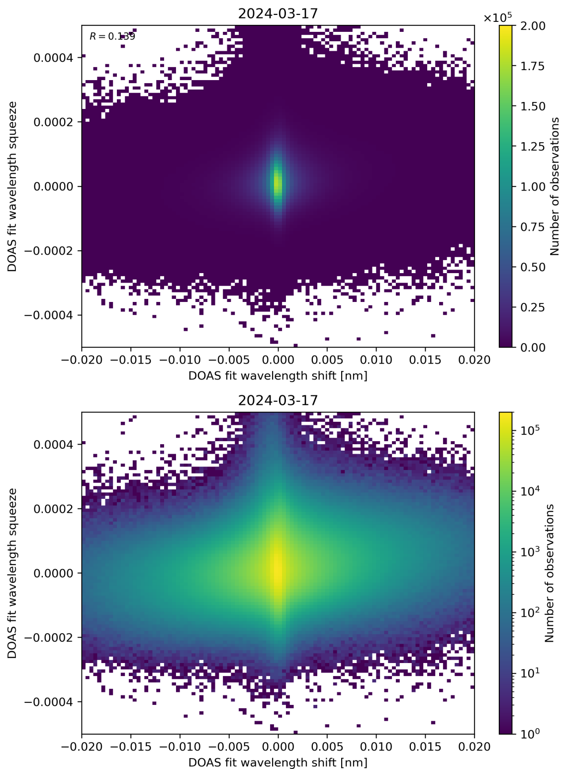
Figure 65: Scatter density plot of “DOAS fit wavelength shift” against “DOAS fit wavelength squeeze” for 2024-03-16 to 2024-03-18.
