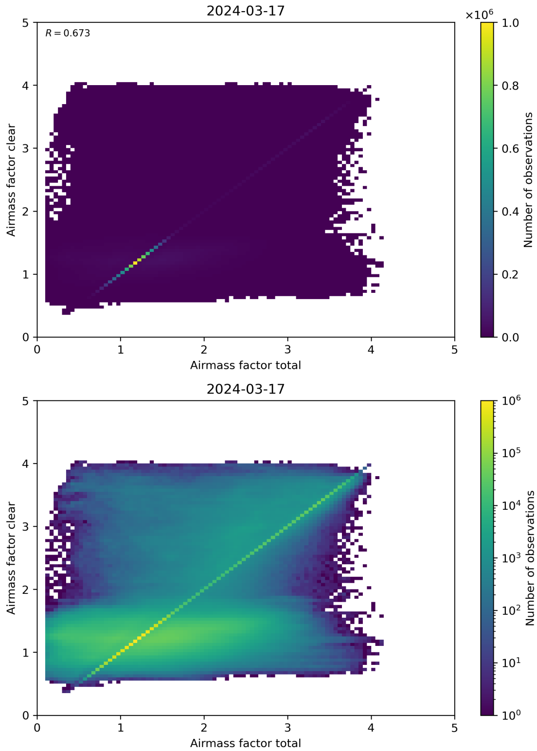
Figure 100: Scatter density plot of “Airmass factor total” against “Airmass factor clear” for 2024-03-16 to 2024-03-18.
