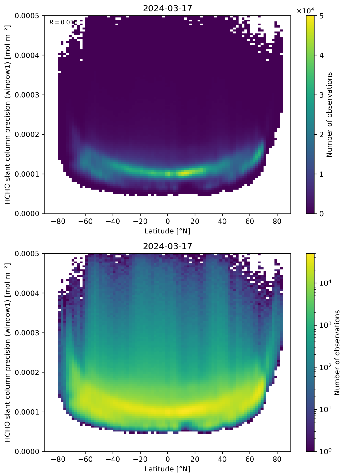
Figure 160: Scatter density plot of “Latitude” against “HCHO slant column precision (window1)” for 2024-03-16 to 2024-03-18.
