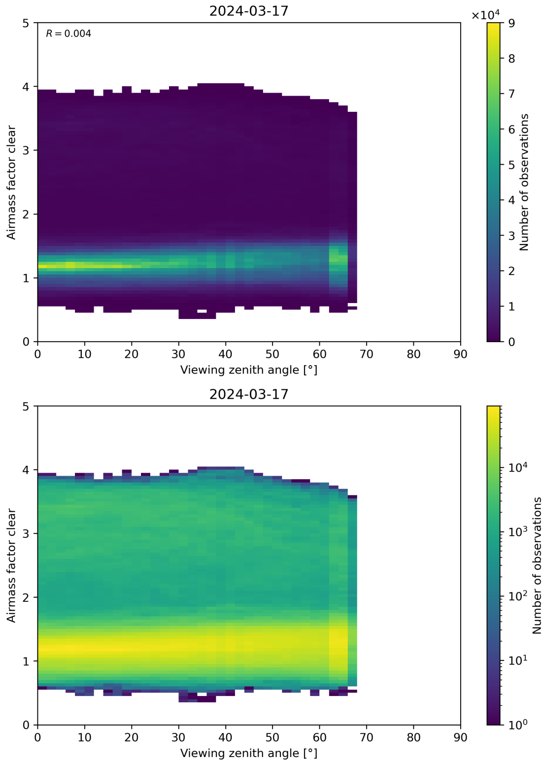
Figure 185: Scatter density plot of “Viewing zenith angle” against “Airmass factor clear” for 2024-03-16 to 2024-03-18.
