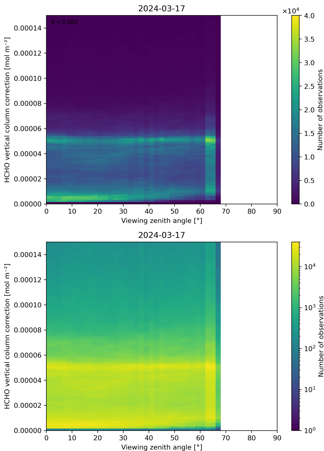
Figure 193: Scatter density plot of “Viewing zenith angle” against “HCHO vertical column correction” for 2024-03-16 to 2024-03-18.
