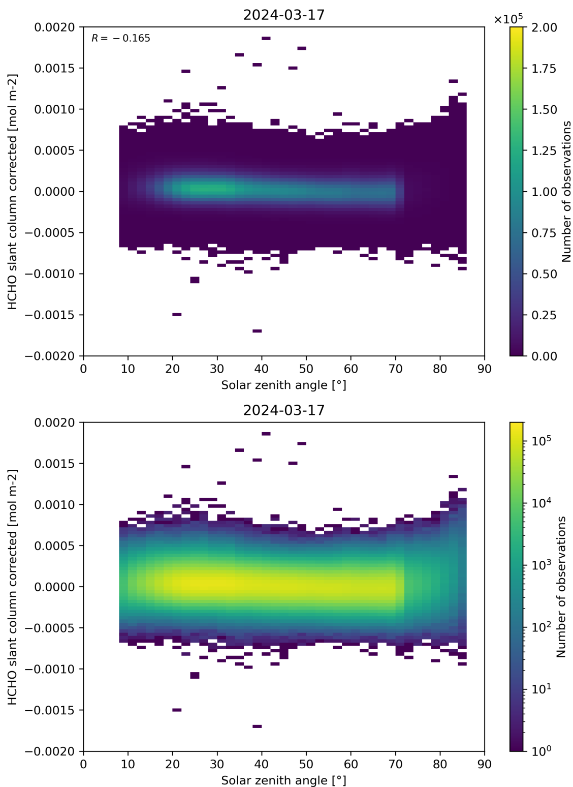
Figure 171: Scatter density plot of “Solar zenith angle” against “HCHO slant column corrected” for 2024-03-16 to 2024-03-18.
