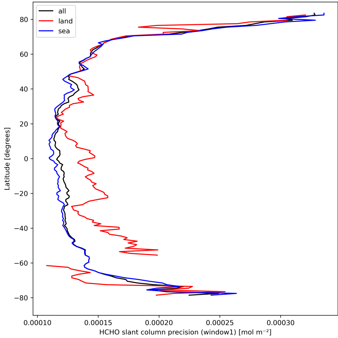
Figure 25: Zonal average of “HCHO slant column precision (window1)” for 2024-03-16 to 2024-03-18.
