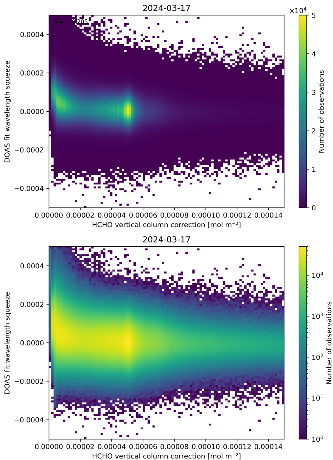
Figure 114: Scatter density plot of “HCHO vertical column correction” against “DOAS fit wavelength squeeze” for 2024-03-16 to 2024-03-18.
