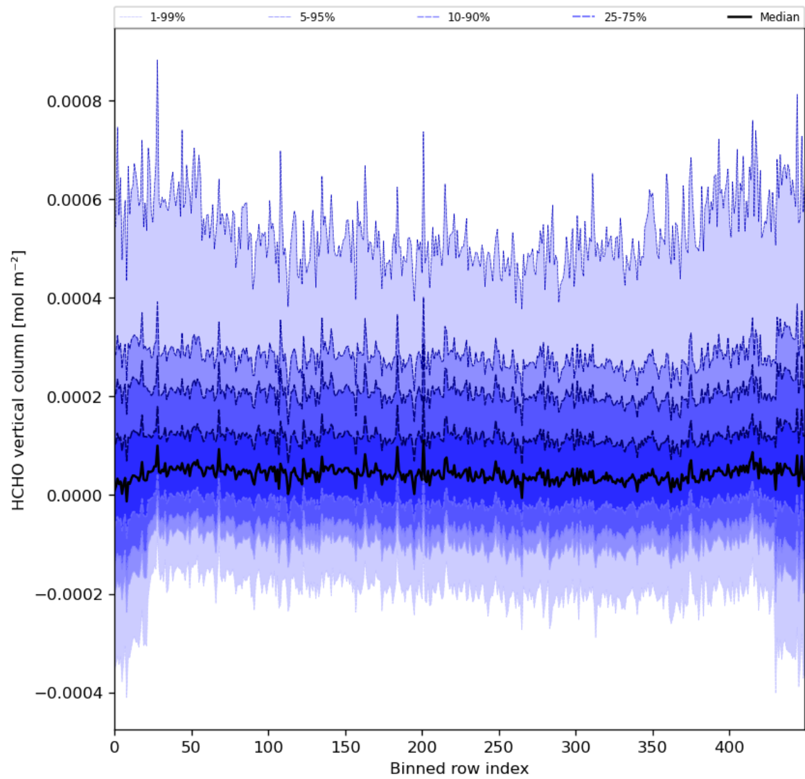
Figure 49: Along track statistics of “HCHO vertical column” for 2024-03-16 to 2024-03-18
