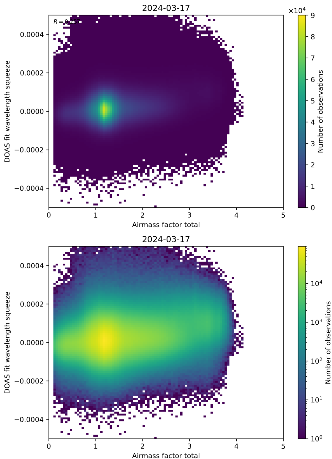
Figure 99: Scatter density plot of “Airmass factor total” against “DOAS fit wavelength squeeze” for 2024-03-16 to 2024-03-18.
