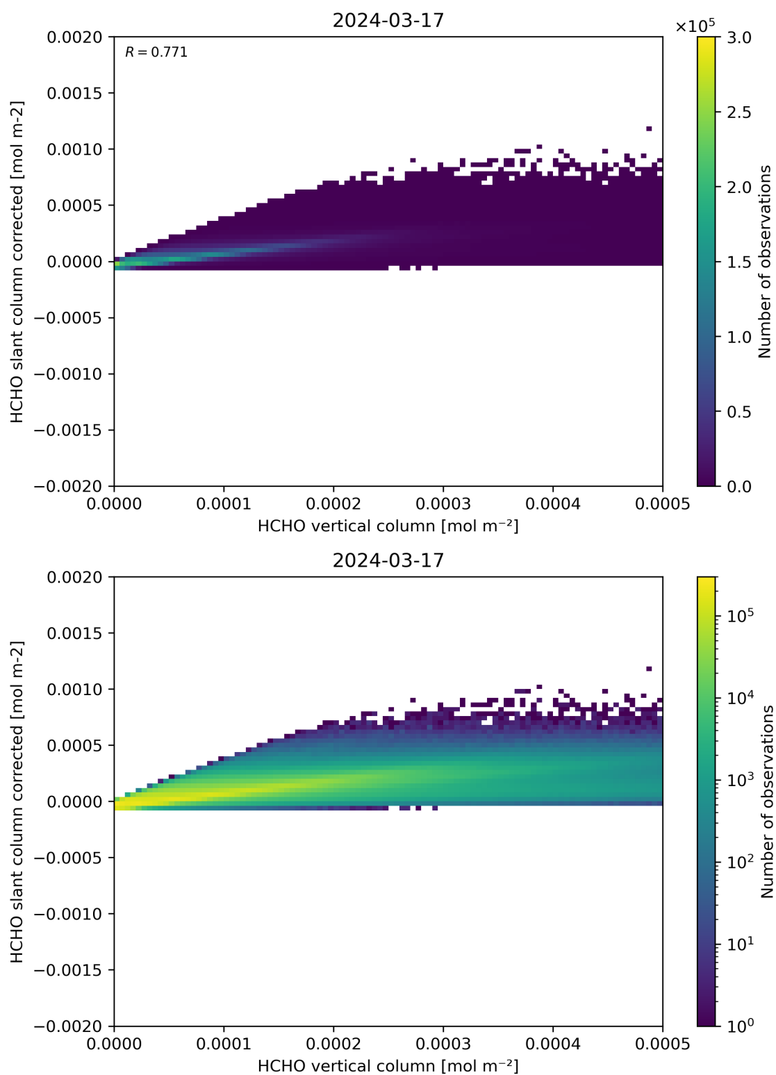
Figure 127: Scatter density plot of “HCHO vertical column” against “HCHO slant column corrected” for 2024-03-16 to 2024-03-18.
