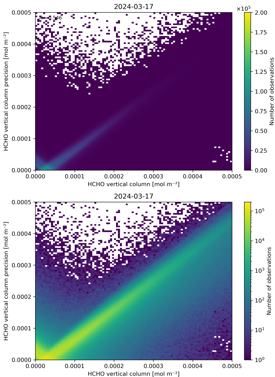
Figure 134: Scatter density plot of “HCHO vertical column” against “HCHO vertical column precision” for 2024-03-16 to 2024-03-18.
