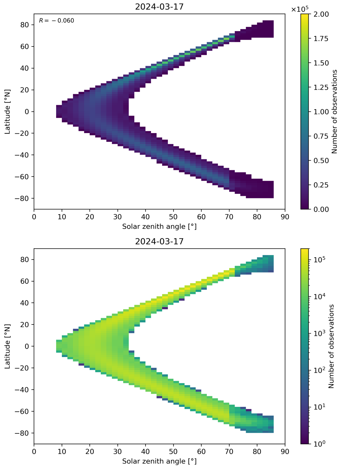
Figure 181: Scatter density plot of “Solar zenith angle” against “Latitude” for 2024-03-16 to 2024-03-18.
