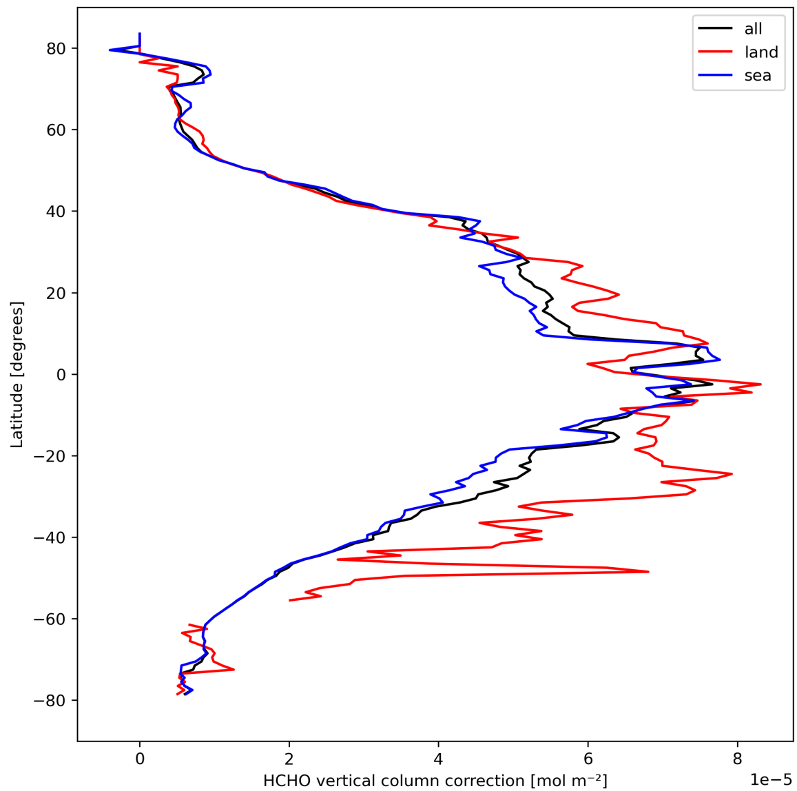
Figure 23: Zonal average of “HCHO vertical column correction” for 2024-03-16 to 2024-03-18.
