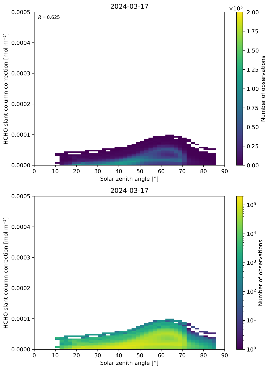
Figure 172: Scatter density plot of “Solar zenith angle” against “HCHO slant column correction” for 2024-03-16 to 2024-03-18.
