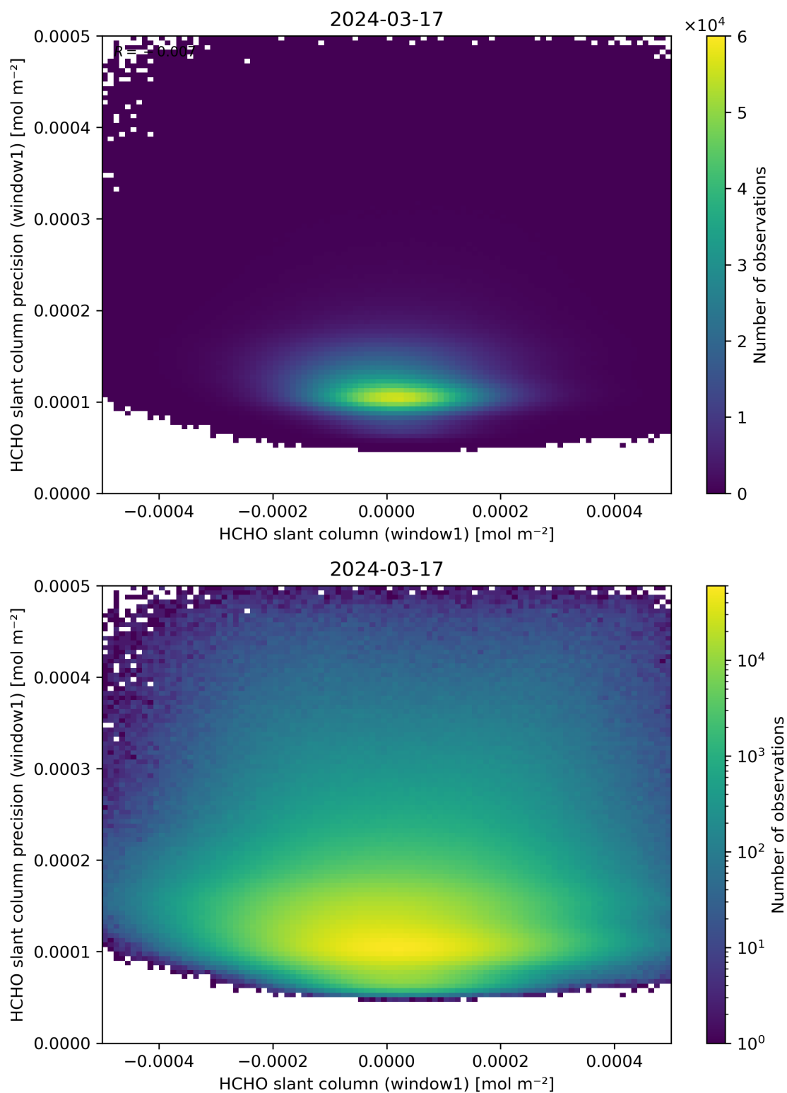
Figure 84: Scatter density plot of “HCHO slant column (window1)” against “HCHO slant column precision (window1)” for 2024-03-16 to 2024-03-18.
