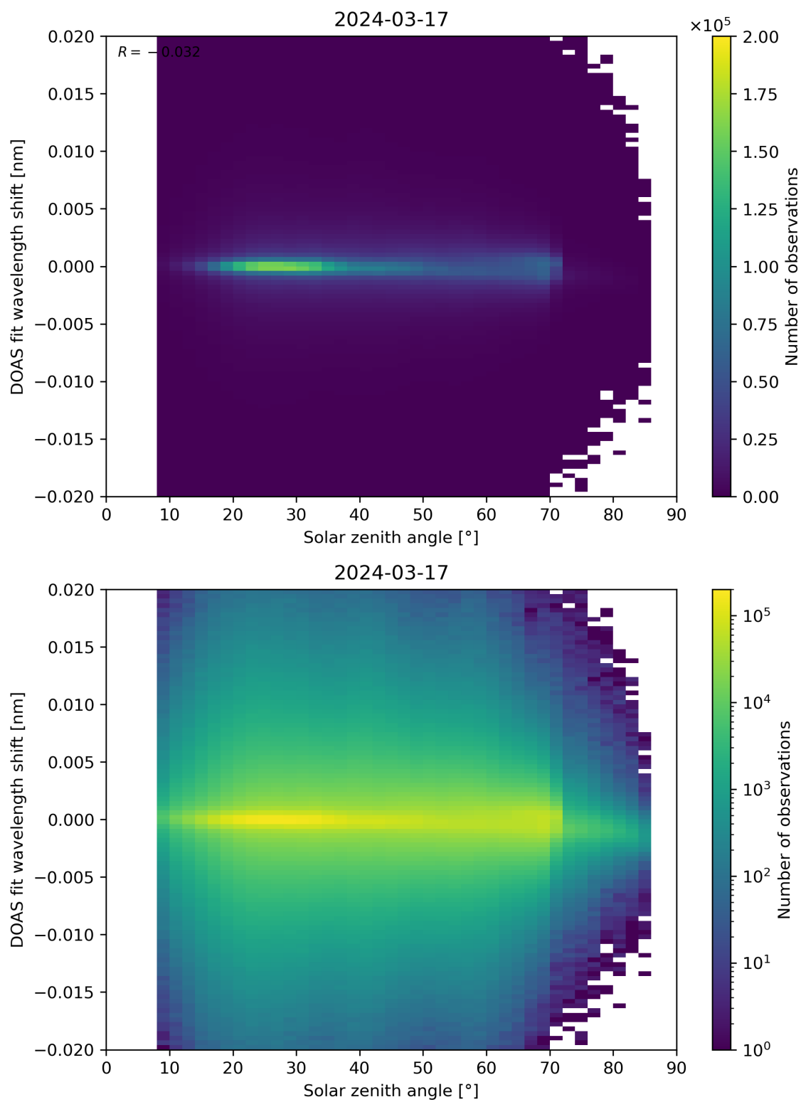
Figure 168: Scatter density plot of “Solar zenith angle” against “DOAS fit wavelength shift” for 2024-03-16 to 2024-03-18.
