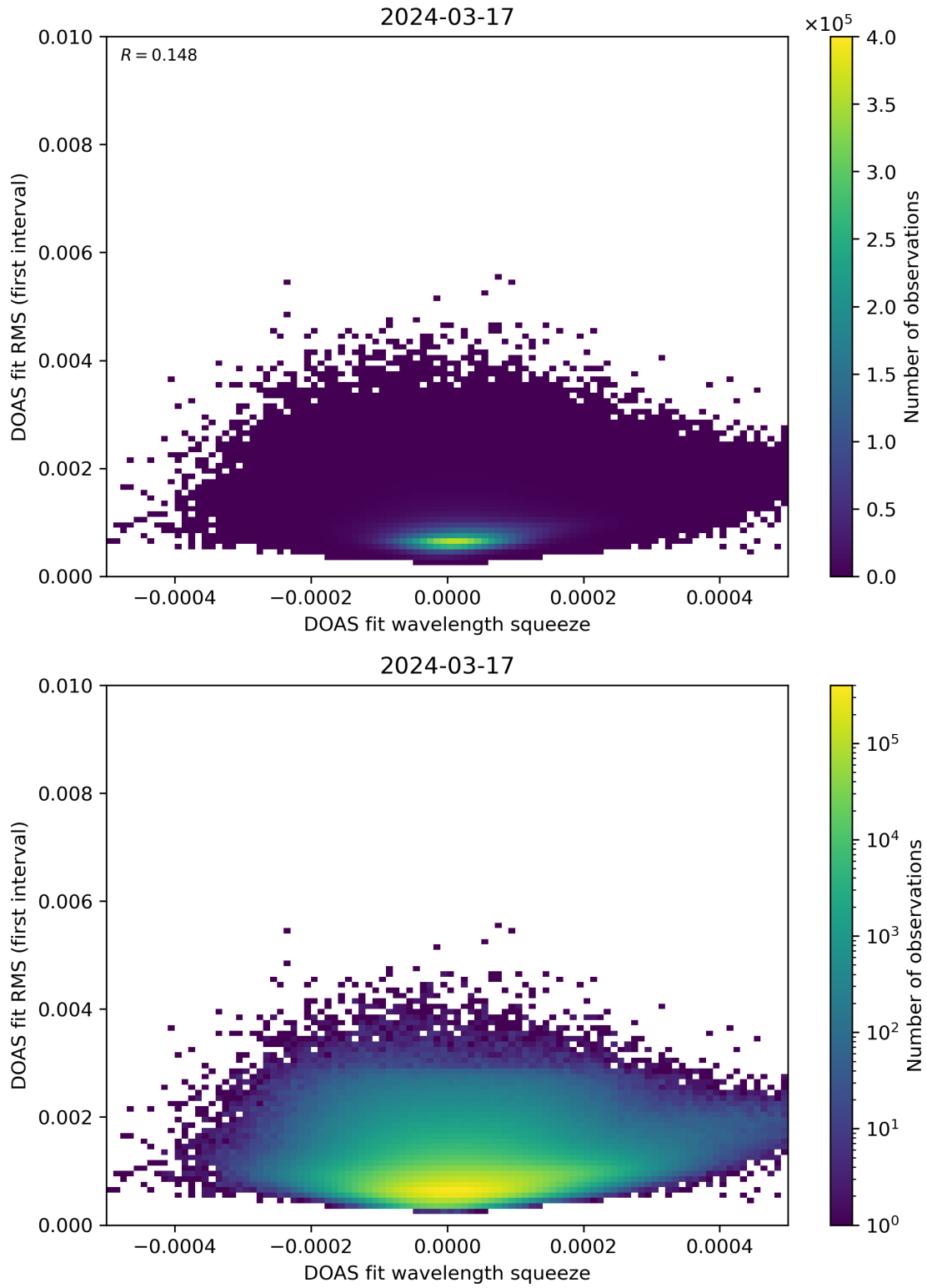
Figure 68: Scatter density plot of “DOAS fit wavelength squeeze” against “DOAS fit RMS (first interval)” for 2024-03-16 to 2024-03-18.
