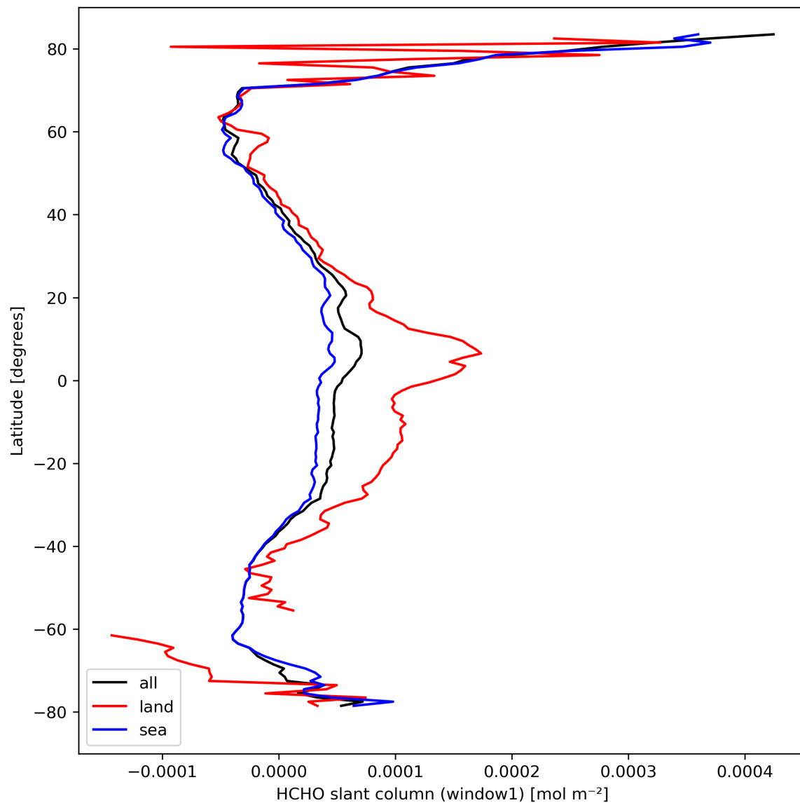
Figure 24: Zonal average of “HCHO slant column (window1)” for 2024-03-16 to 2024-03-18.
