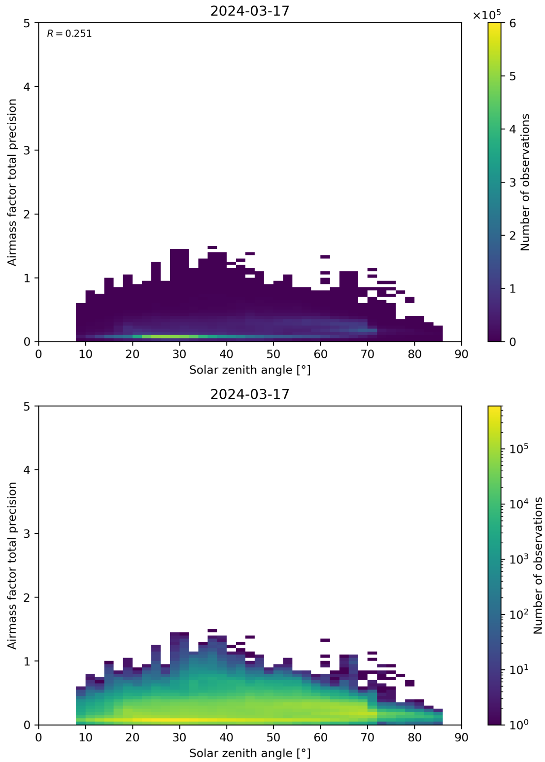
Figure 176: Scatter density plot of “Solar zenith angle” against “Airmass factor total precision” for 2024-03-16 to 2024-03-18.
