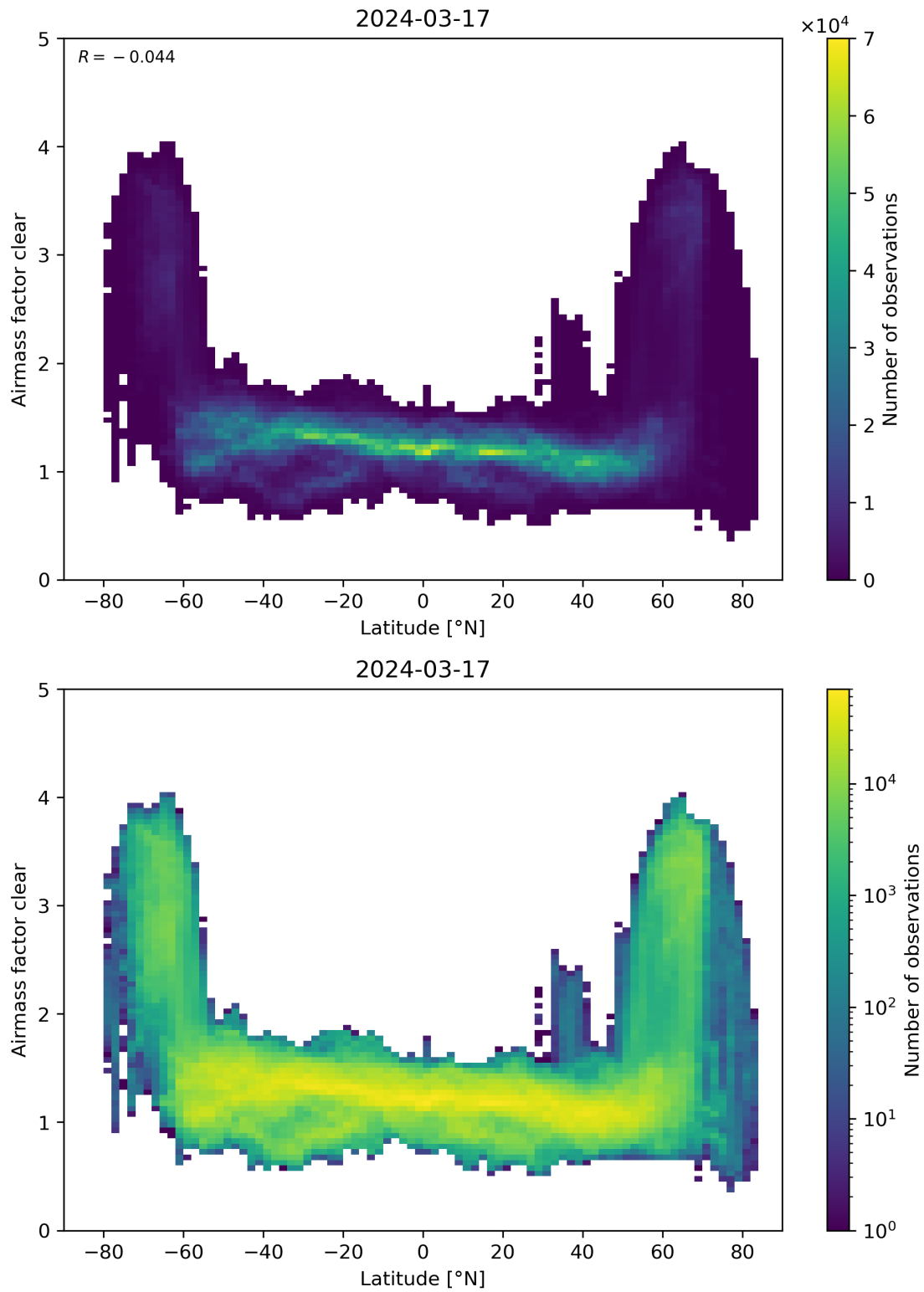
Figure 156: Scatter density plot of “Latitude” against “Airmass factor clear” for 2024-03-16 to 2024-03-18.
