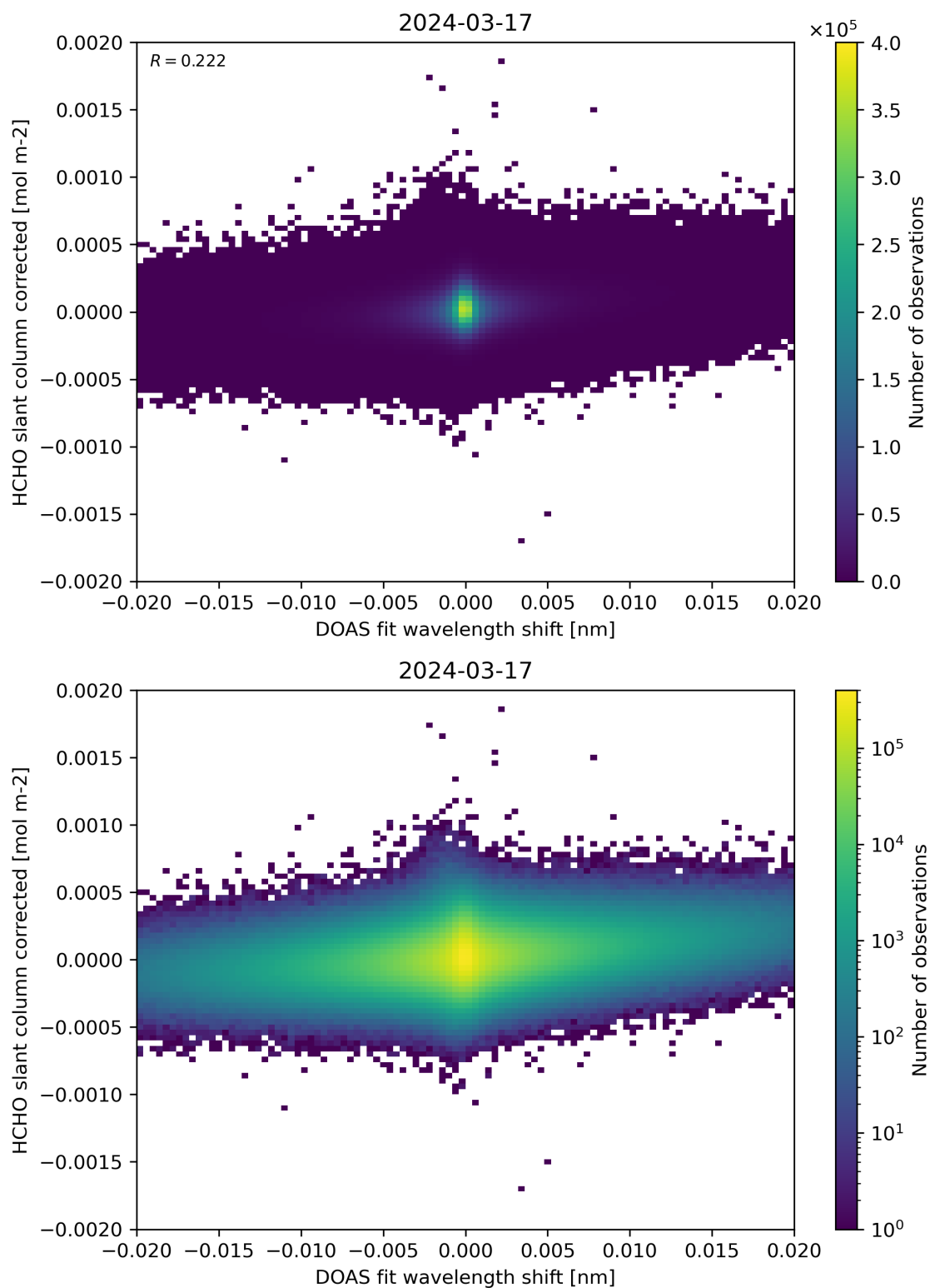
Figure 66: Scatter density plot of “DOAS fit wavelength shift” against “HCHO slant column corrected” for 2024-03-16 to 2024-03-18.
