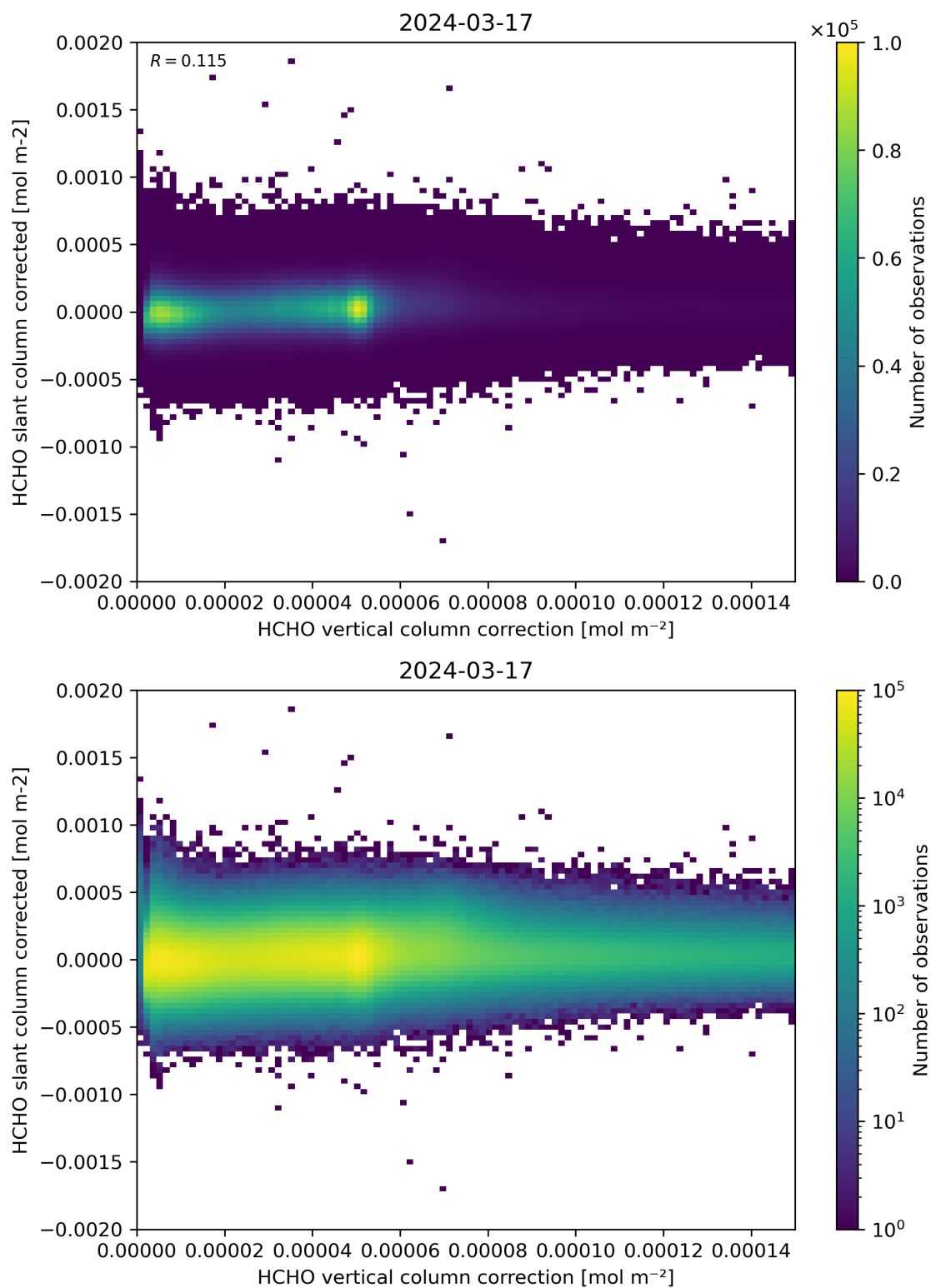
Figure 116: Scatter density plot of “HCHO vertical column correction” against “HCHO slant column corrected” for 2024-03-16 to 2024-03-18.
