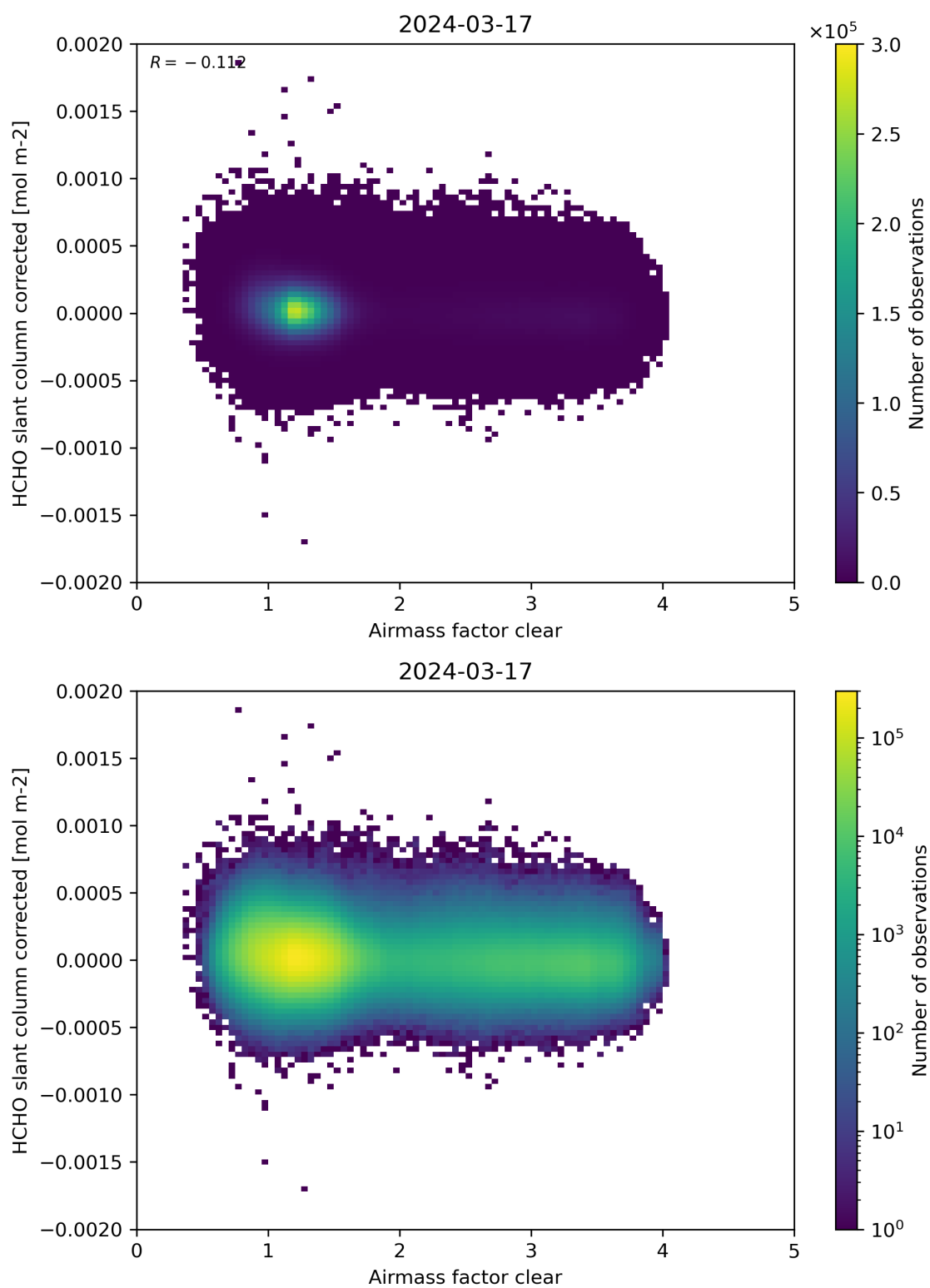
Figure 74: Scatter density plot of “Airmass factor clear” against “HCHO slant column corrected” for 2024-03-16 to 2024-03-18.
