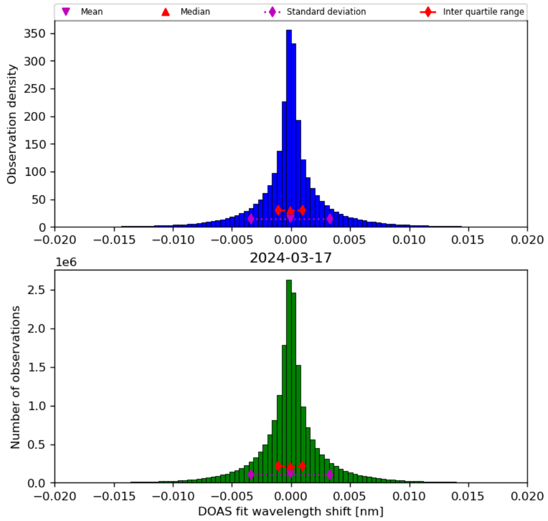
Figure 44: Histogram of “DOAS fit wavelength shift” for 2024-03-16 to 2024-03-18
