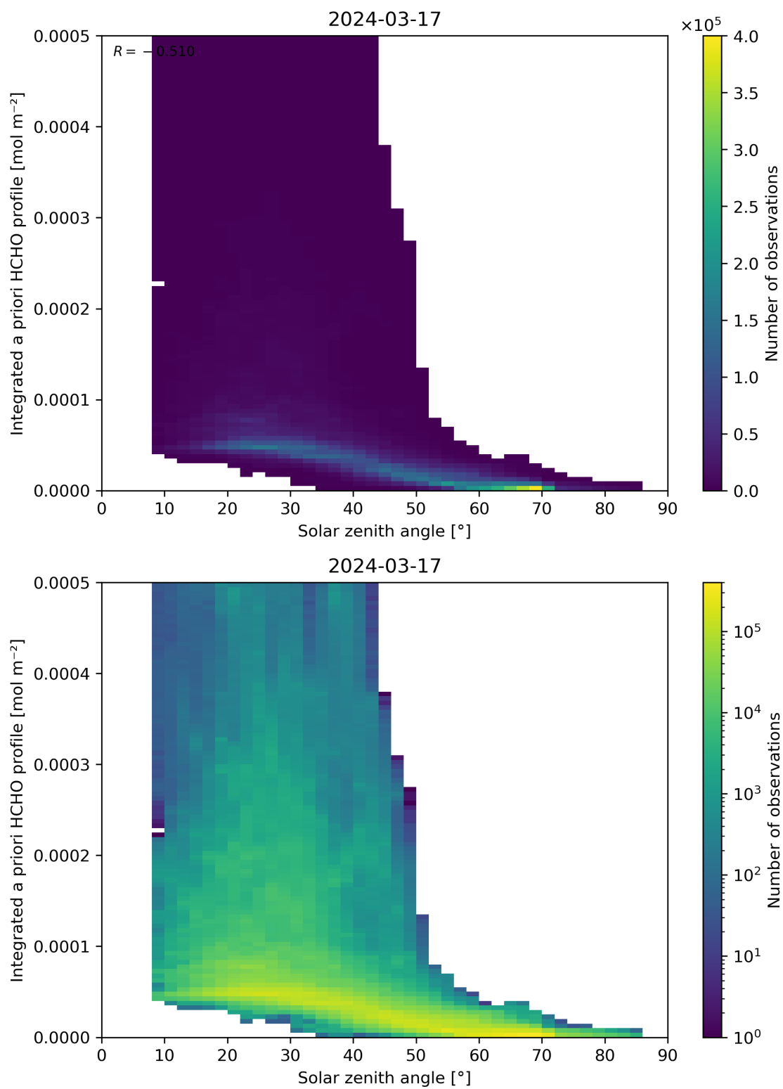
Figure 180: Scatter density plot of “Solar zenith angle” against “Integrated a priori HCHO profile” for 2024-03-16 to 2024-03-18.
