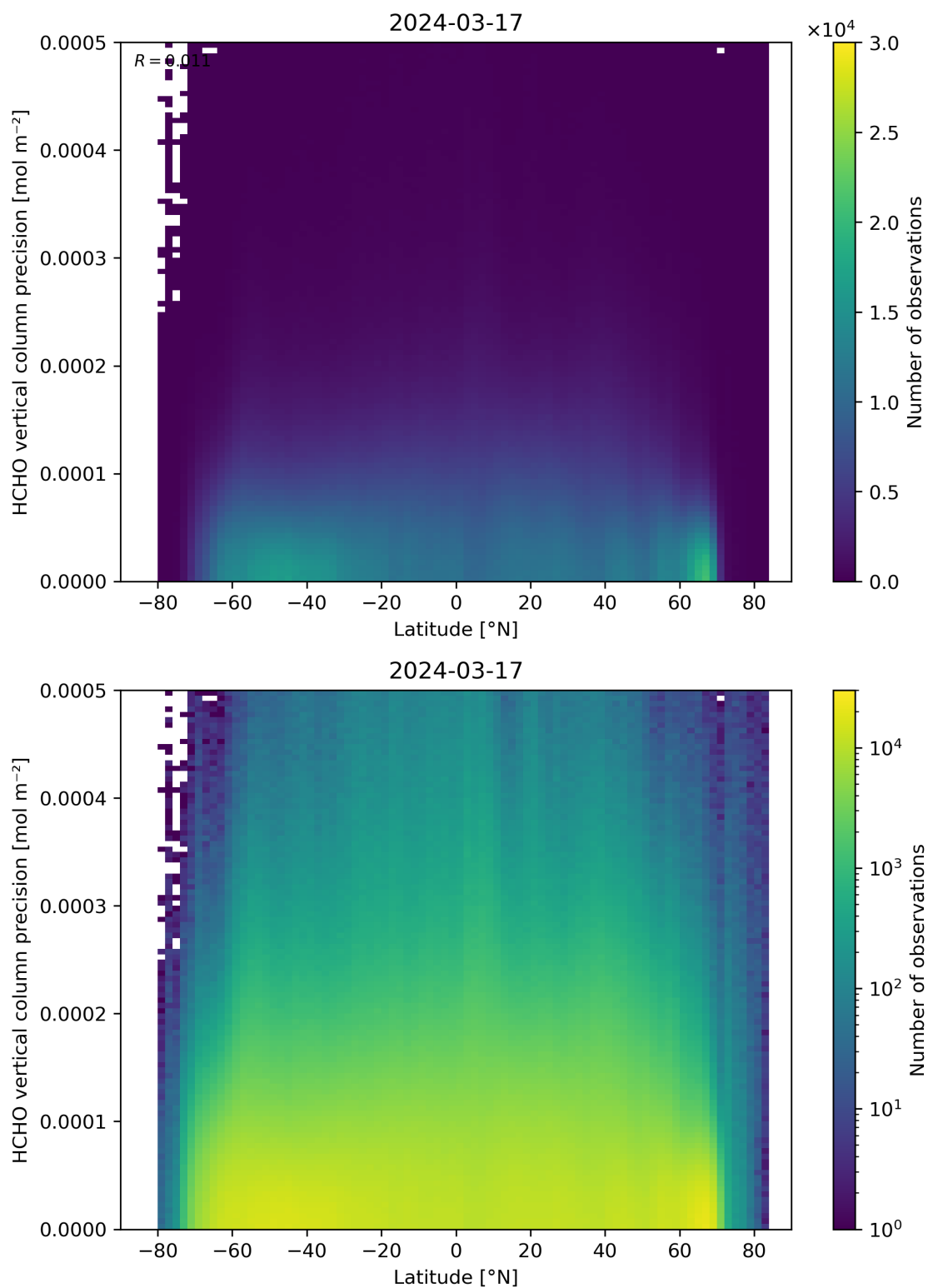
Figure 165: Scatter density plot of “Latitude” against “HCHO vertical column precision” for 2024-03-16 to 2024-03-18.
