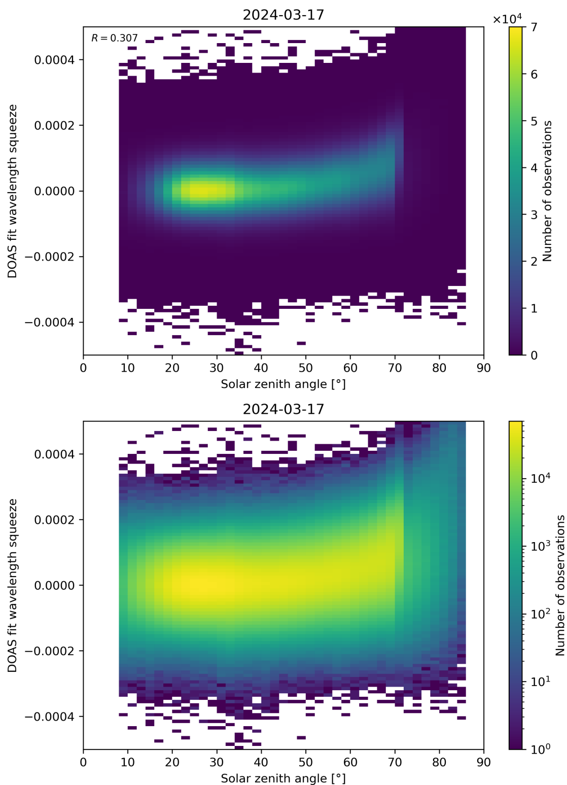
Figure 169: Scatter density plot of “Solar zenith angle” against “DOAS fit wavelength squeeze” for 2024-03-16 to 2024-03-18.
