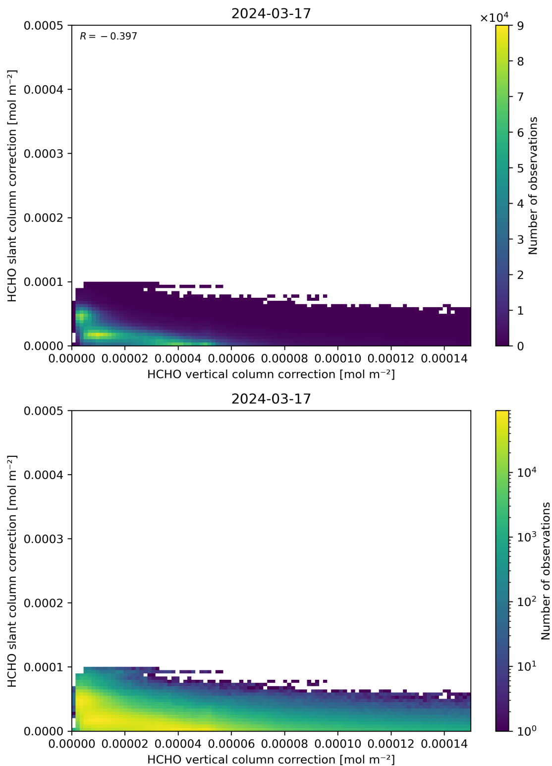
Figure 117: Scatter density plot of “HCHO vertical column correction” against “HCHO slant column correction” for 2024-03-16 to 2024-03-18.
