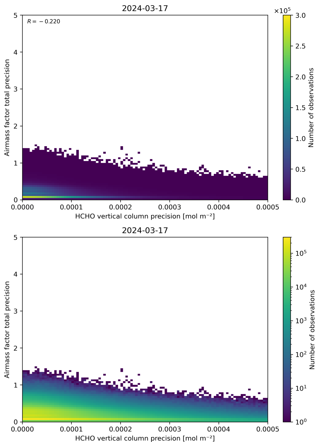
Figure 145: Scatter density plot of “HCHO vertical column precision” against “Airmass factor total precision” for 2024-03-16 to 2024-03-18.
