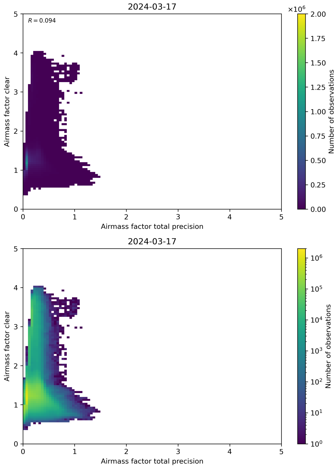
Figure 108: Scatter density plot of “Airmass factor total precision” against “Airmass factor clear” for 2024-03-16 to 2024-03-18.
