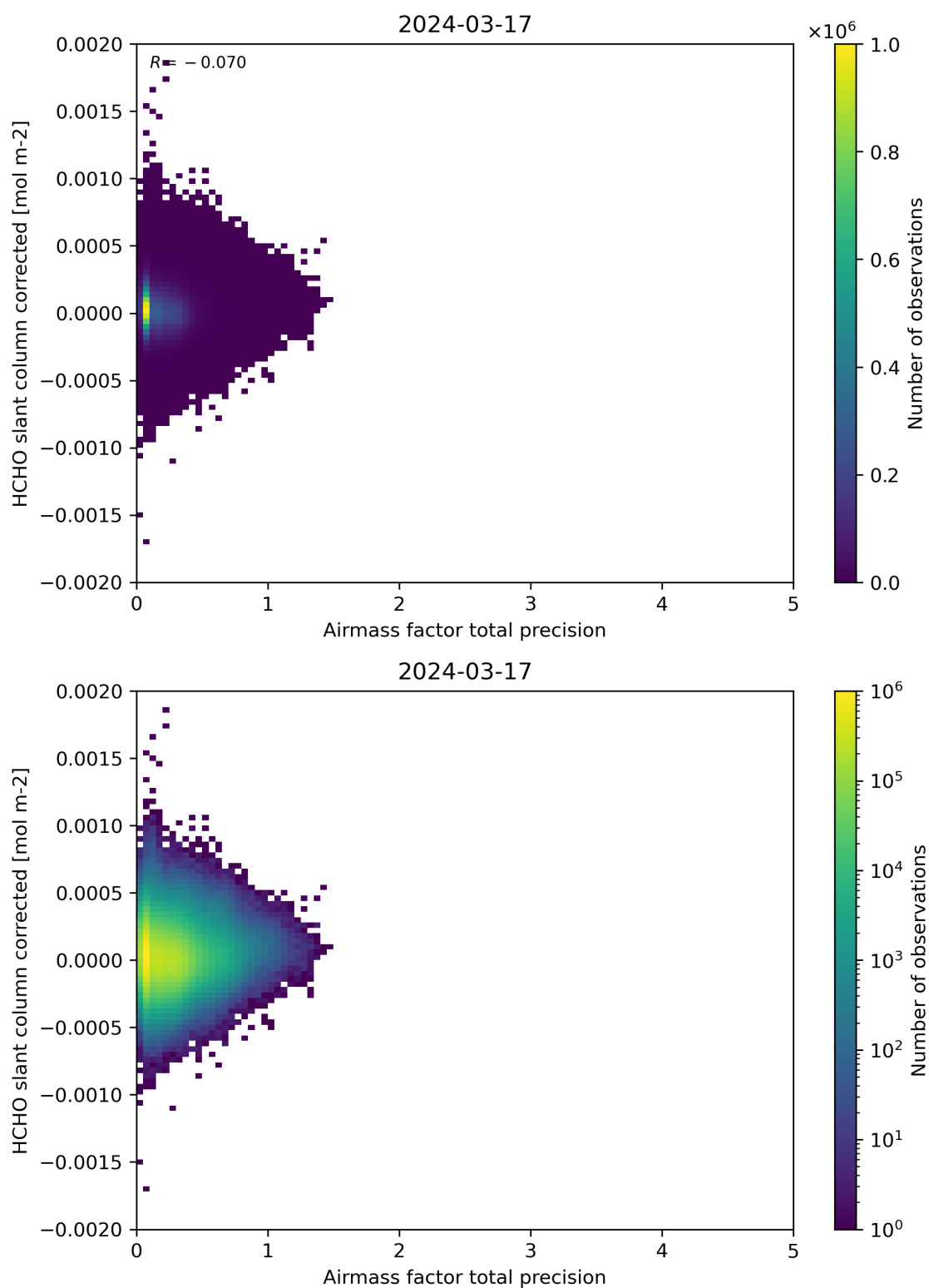
Figure 109: Scatter density plot of “Airmass factor total precision” against “HCHO slant column corrected” for 2024-03-16 to 2024-03-18.
