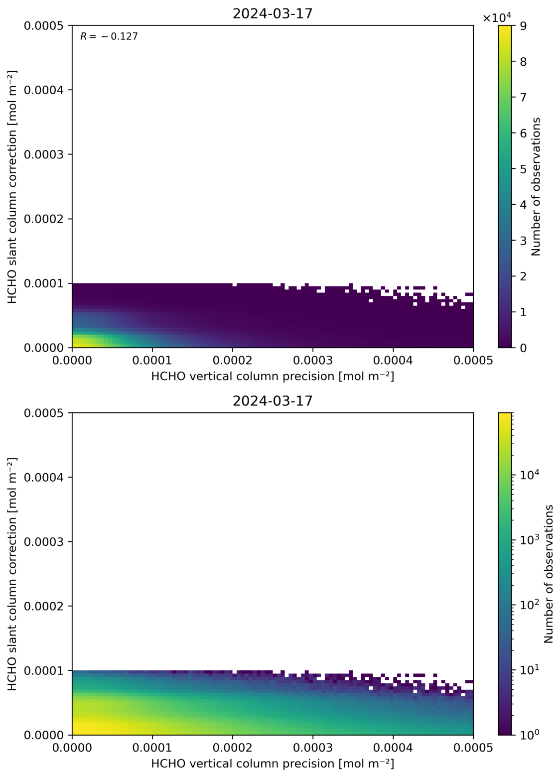
Figure 141: Scatter density plot of “HCHO vertical column precision” against “HCHO slant column correction” for 2024-03-16 to 2024-03-18.
