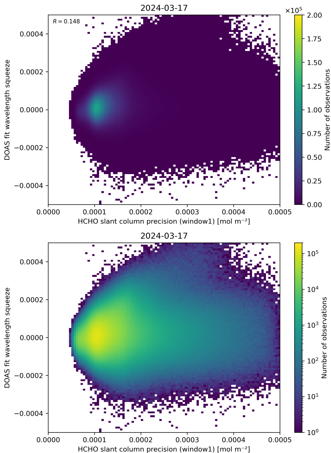
Figure 90: Scatter density plot of “HCHO slant column precision (window1)” against “DOAS fit wavelength squeeze” for 2024-03-16 to 2024-03-18.
