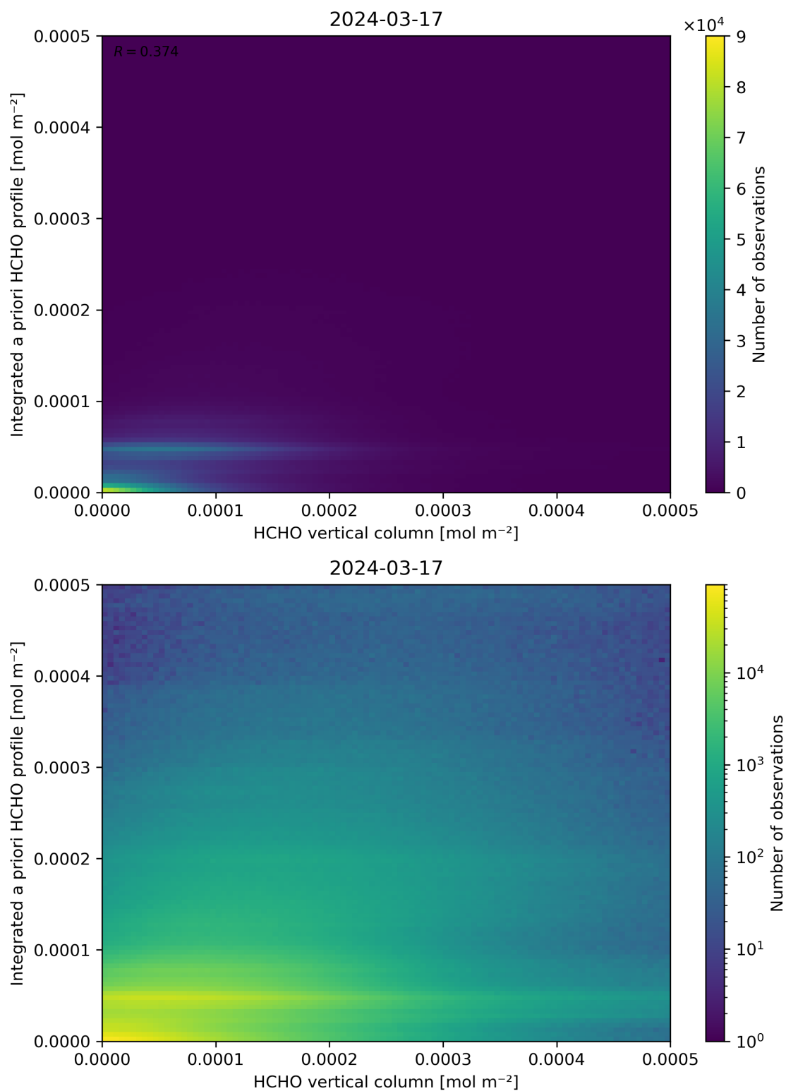
Figure 135: Scatter density plot of “HCHO vertical column” against “Integrated a priori HCHO profile” for 2024-03-16 to 2024-03-18.
