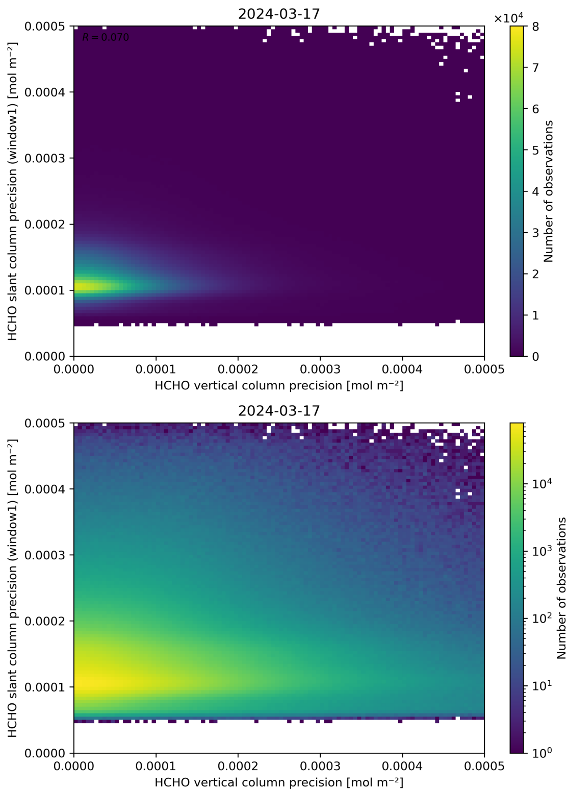
Figure 143: Scatter density plot of “HCHO vertical column precision” against “HCHO slant column precision (window1)” for 2024-03-16 to 2024-03-18.
