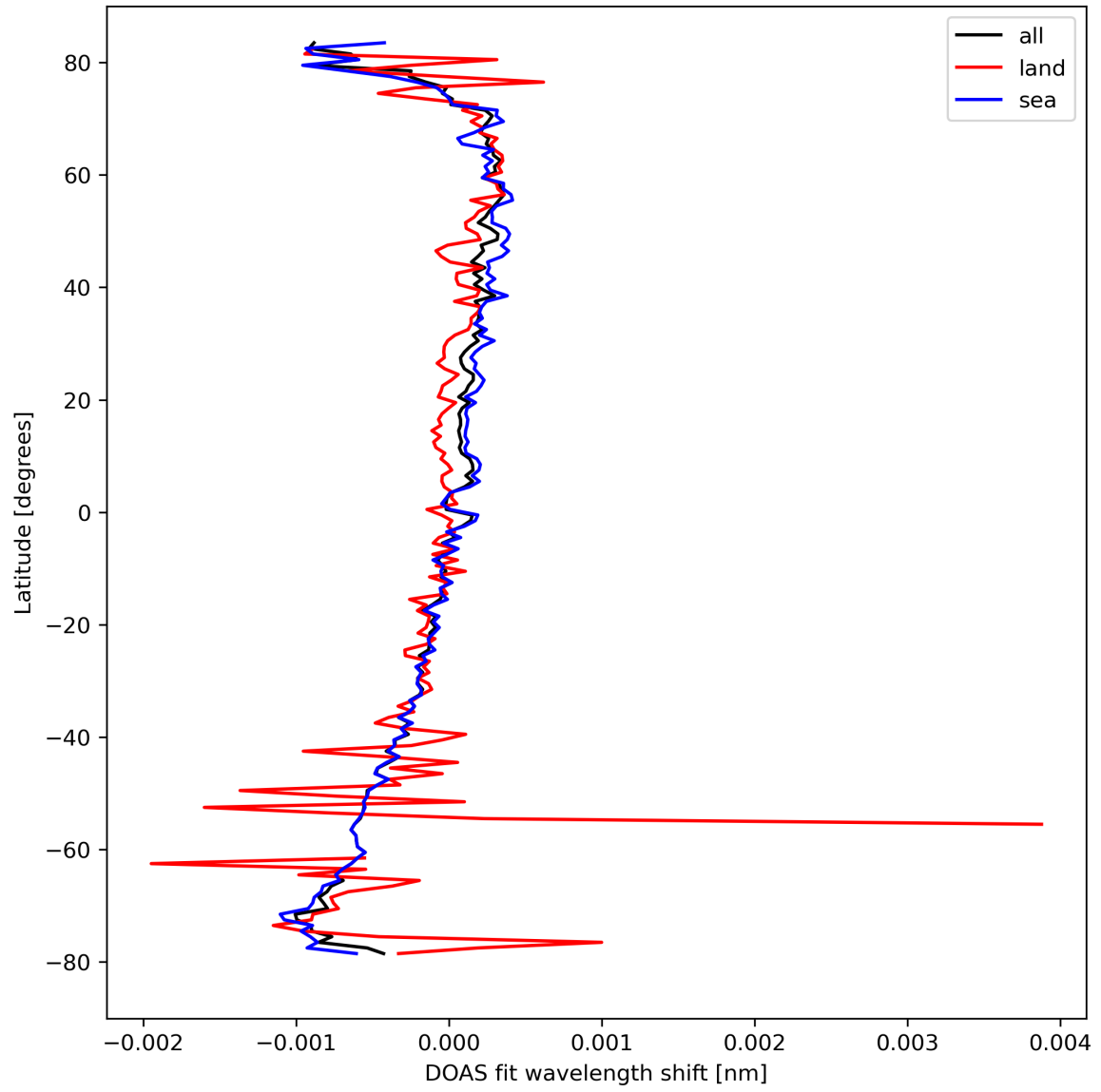
Figure 30: Zonal average of “DOAS fit wavelength shift” for 2024-03-16 to 2024-03-18.
