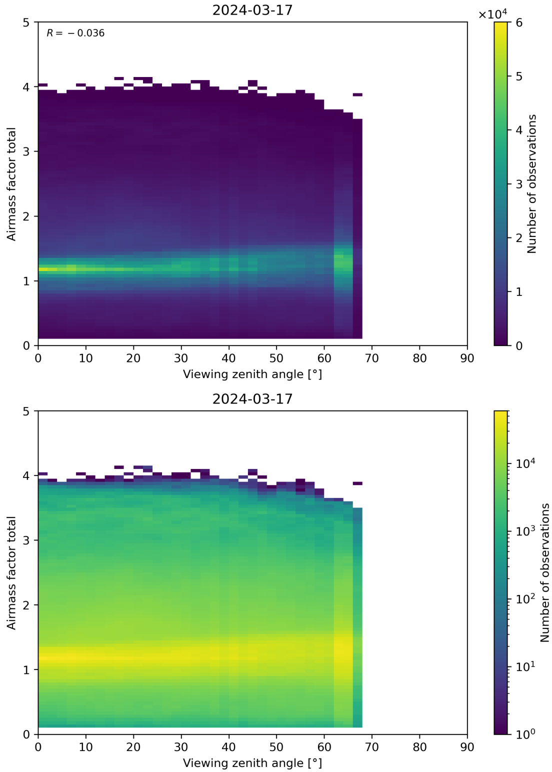
Figure 190: Scatter density plot of “Viewing zenith angle” against “Airmass factor total” for 2024-03-16 to 2024-03-18.
