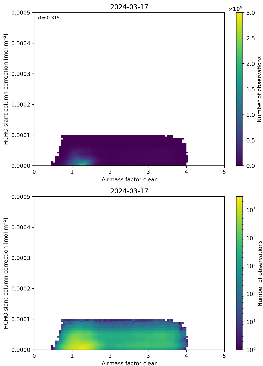
Figure 75: Scatter density plot of “Airmass factor clear” against “HCHO slant column correction” for 2024-03-16 to 2024-03-18.
