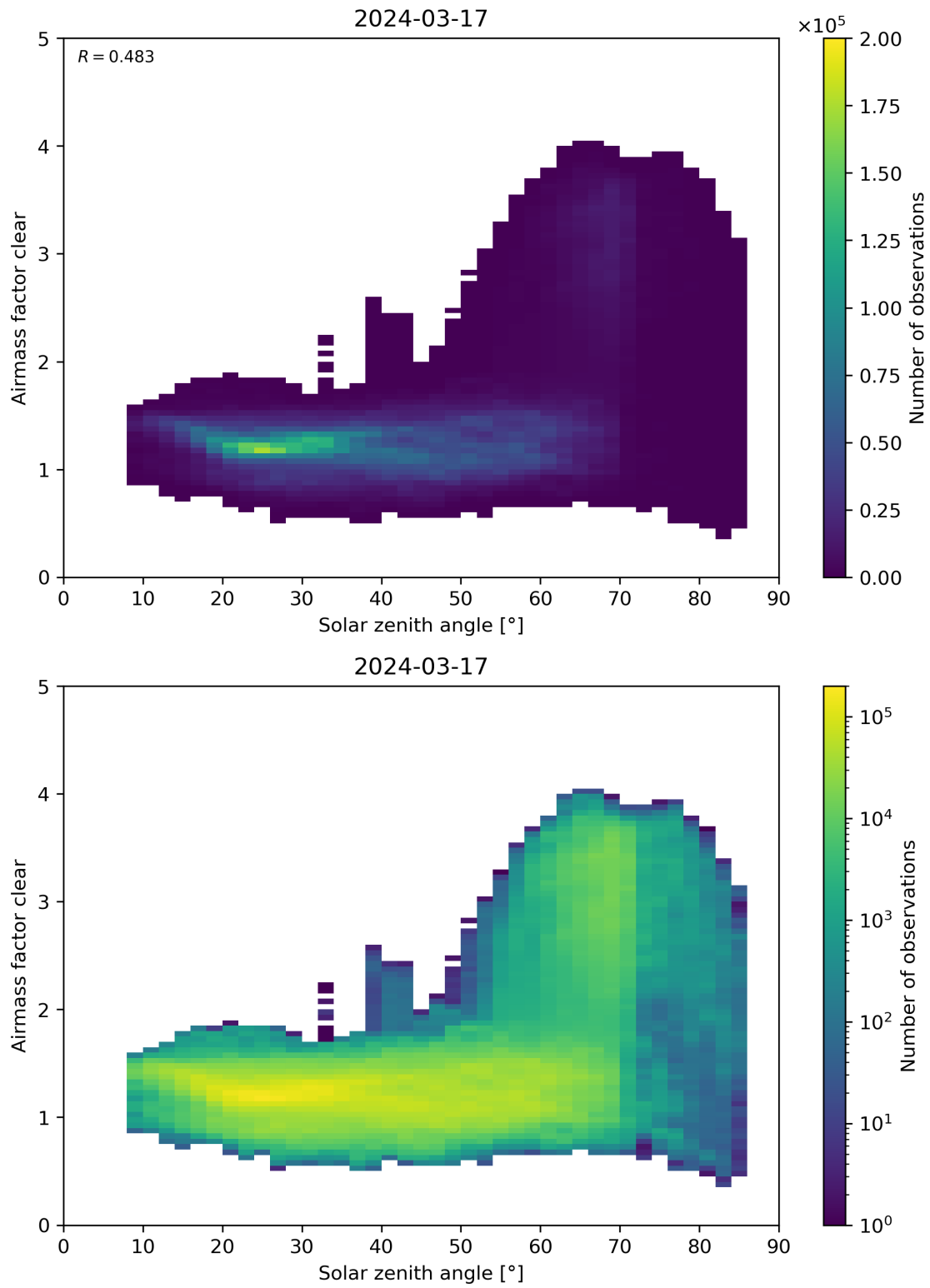
Figure 170: Scatter density plot of “Solar zenith angle” against “Airmass factor clear” for 2024-03-16 to 2024-03-18.
