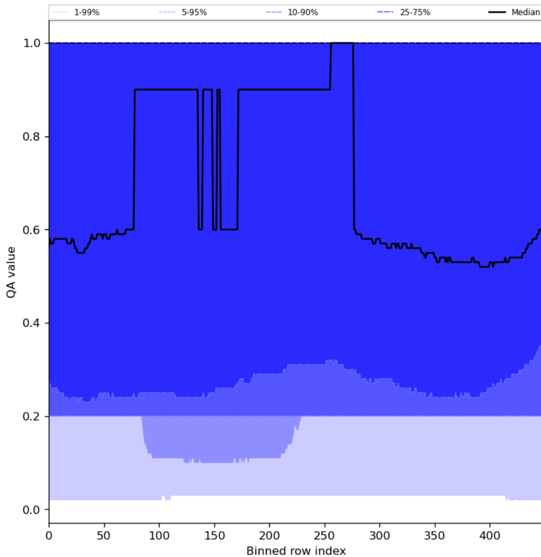
Figure 48: Along track statistics of “QA value” for 2024-03-16 to 2024-03-18
