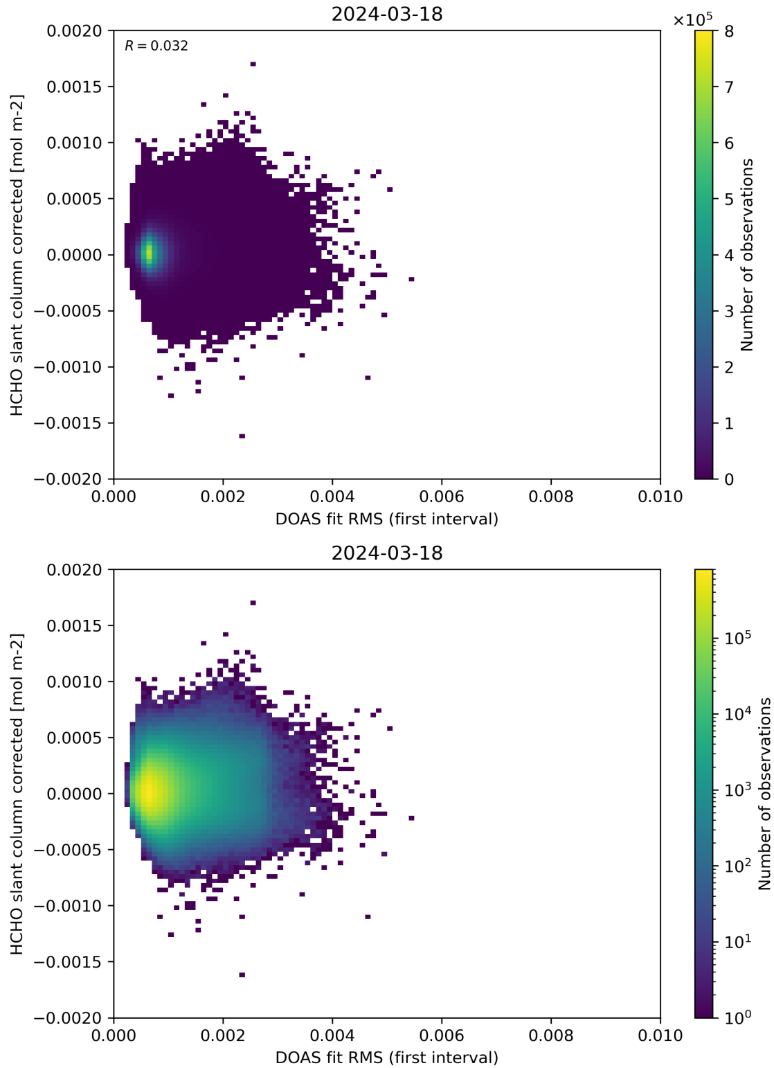
Figure 62: Scatter density plot of “DOAS fit RMS (first interval)” against “HCHO slant column corrected” for 2024-03-17 to 2024-03-19.
