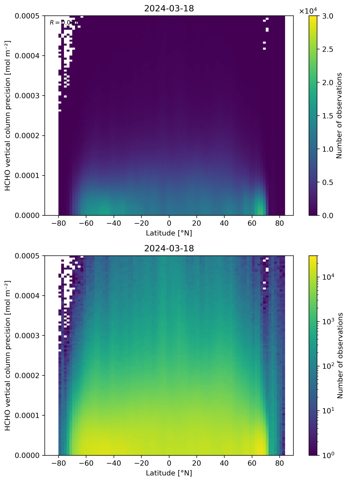
Figure 165: Scatter density plot of “Latitude” against “HCHO vertical column precision” for 2024-03-17 to 2024-03-19.
