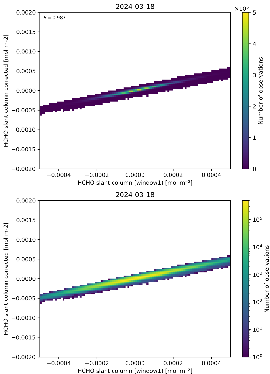
Figure 82: Scatter density plot of “HCHO slant column (window1)” against “HCHO slant column corrected” for 2024-03-17 to 2024-03-19.
