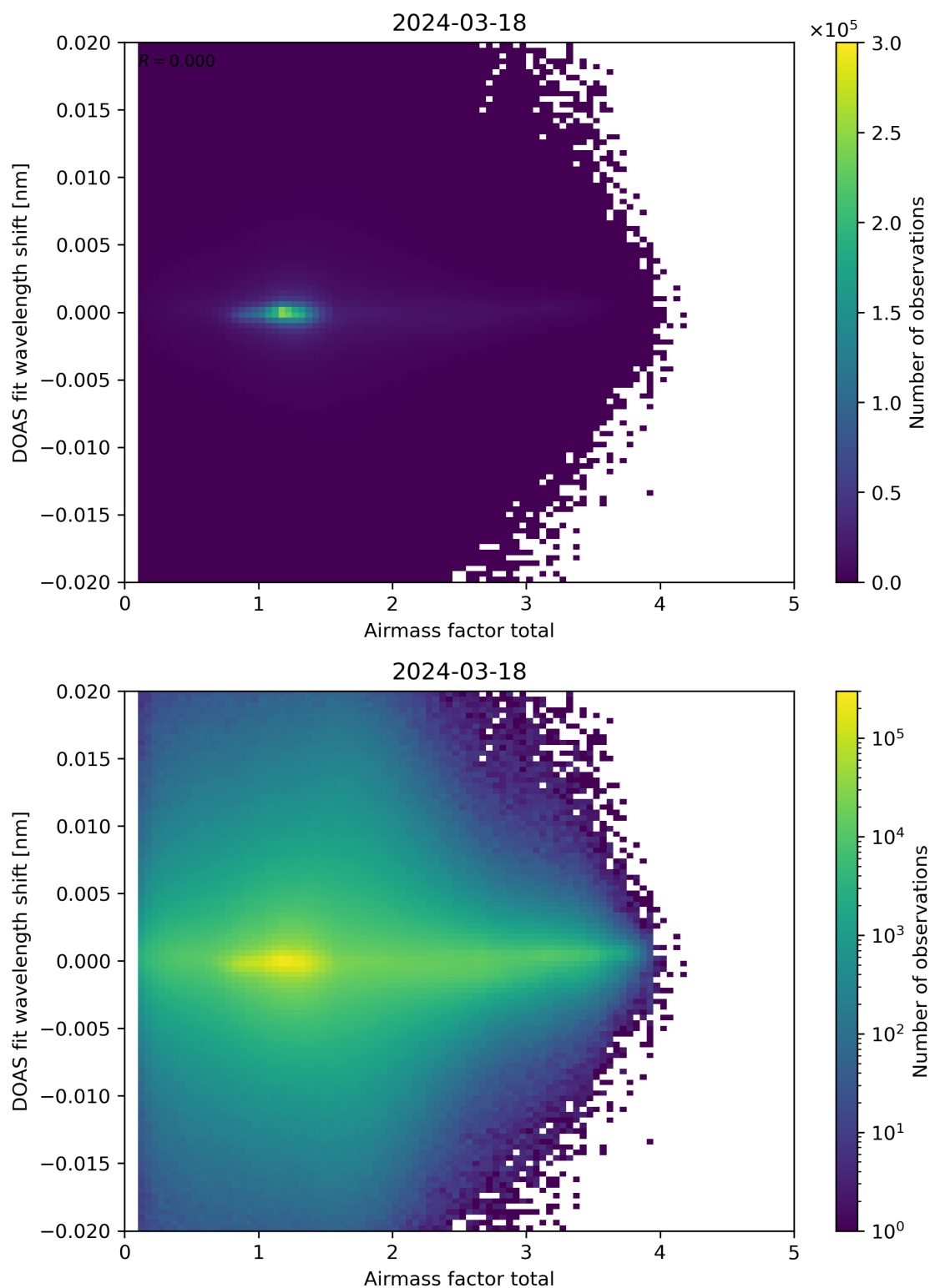
Figure 98: Scatter density plot of “Airmass factor total” against “DOAS fit wavelength shift” for 2024-03-17 to 2024-03-19.
