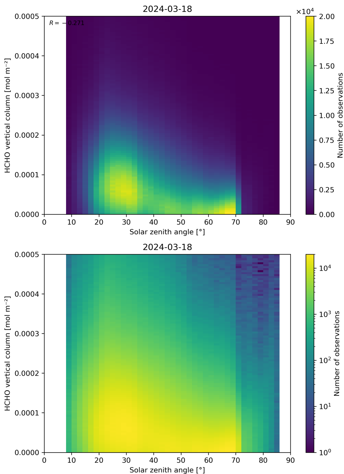
Figure 177: Scatter density plot of “Solar zenith angle” against “HCHO vertical column” for 2024-03-17 to 2024-03-19.
