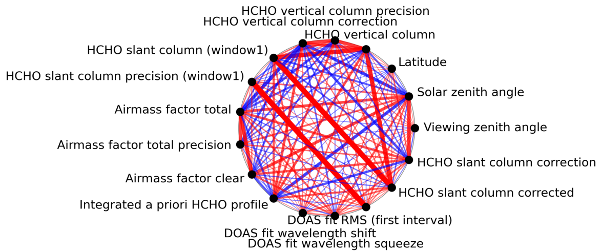
Figure 1: Map of correlation graph for 2024-03-17 to 2024-03-19.
