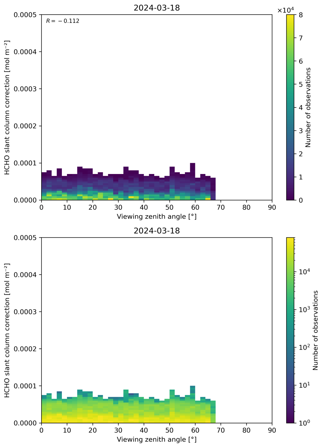
Figure 187: Scatter density plot of “Viewing zenith angle” against “HCHO slant column correction” for 2024-03-17 to 2024-03-19.
