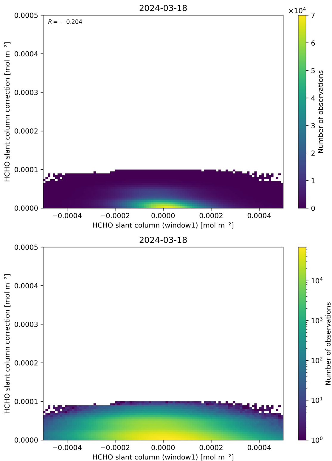
Figure 83: Scatter density plot of “HCHO slant column (window1)” against “HCHO slant column correction” for 2024-03-17 to 2024-03-19.
