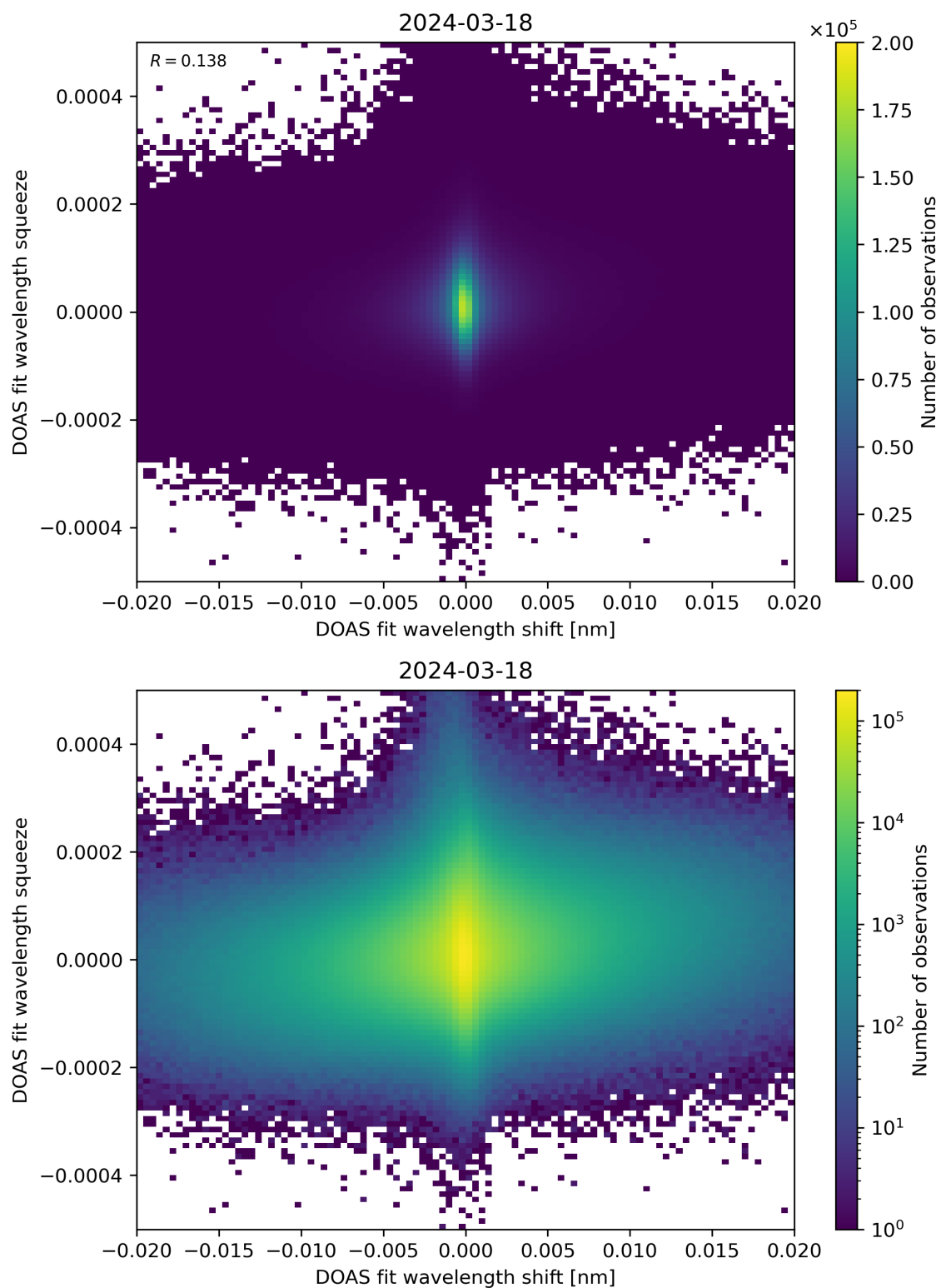
Figure 65: Scatter density plot of “DOAS fit wavelength shift” against “DOAS fit wavelength squeeze” for 2024-03-17 to 2024-03-19.
