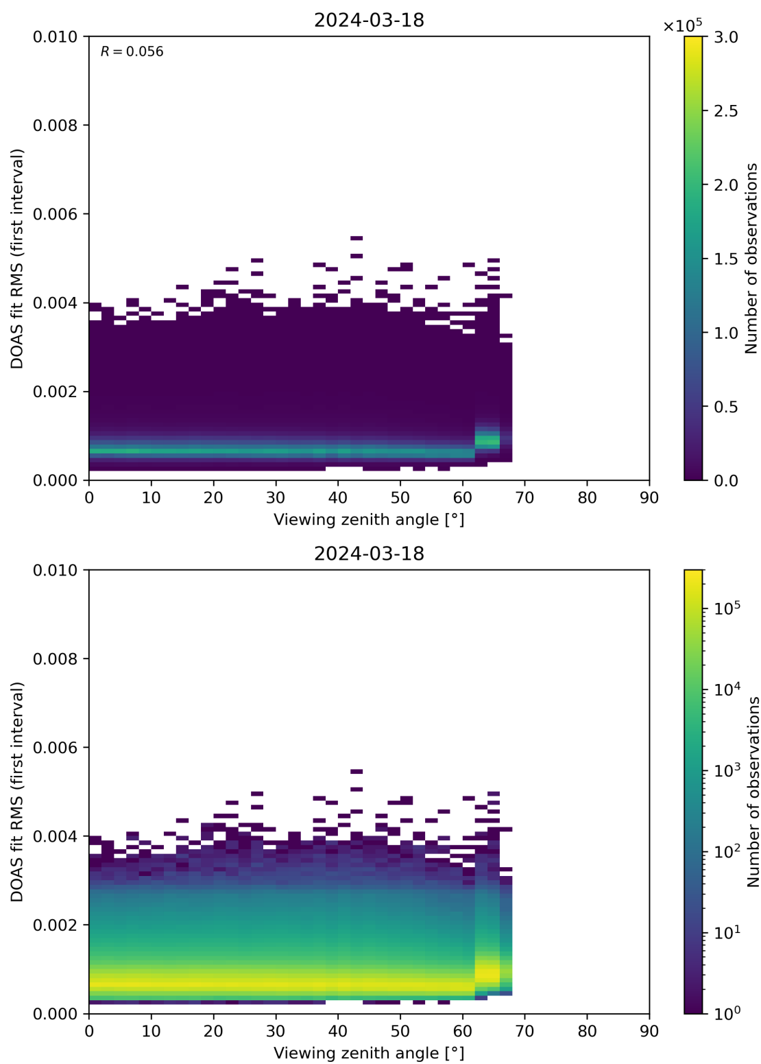
Figure 182: Scatter density plot of “Viewing zenith angle” against “DOAS fit RMS (first interval)” for 2024-03-17 to 2024-03-19.
