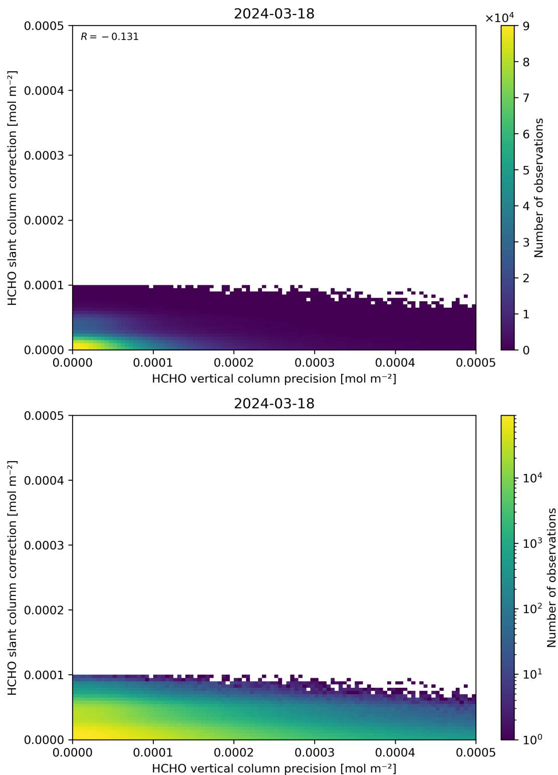
Figure 141: Scatter density plot of “HCHO vertical column precision” against “HCHO slant column correction” for 2024-03-17 to 2024-03-19.
