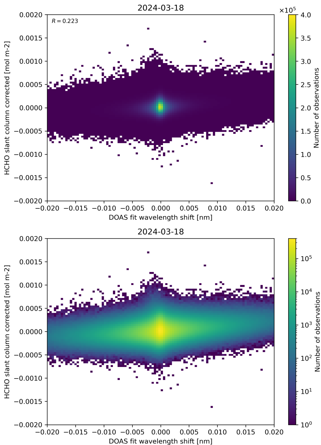
Figure 66: Scatter density plot of “DOAS fit wavelength shift” against “HCHO slant column corrected” for 2024-03-17 to 2024-03-19.
