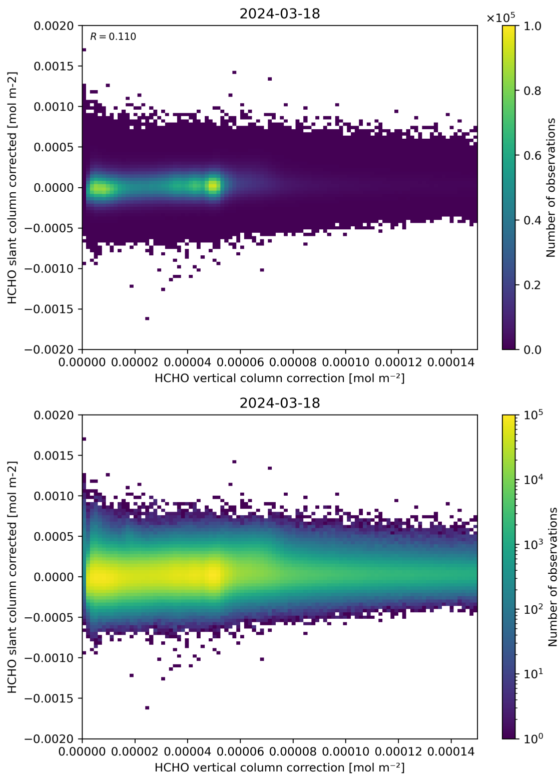
Figure 116: Scatter density plot of “HCHO vertical column correction” against “HCHO slant column corrected” for 2024-03-17 to 2024-03-19.
