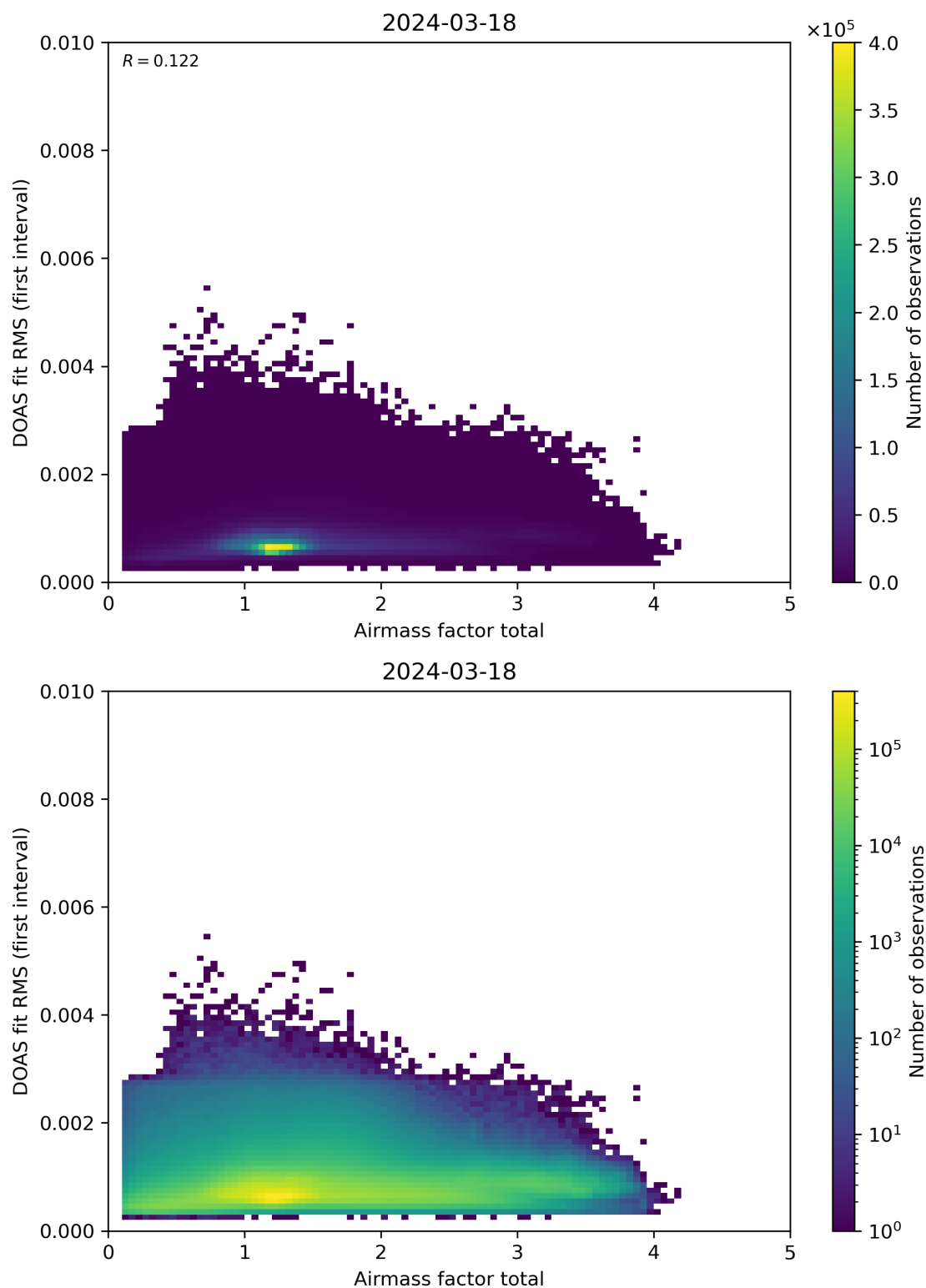
Figure 97: Scatter density plot of “Airmass factor total” against “DOAS fit RMS (first interval)” for 2024-03-17 to 2024-03-19.
