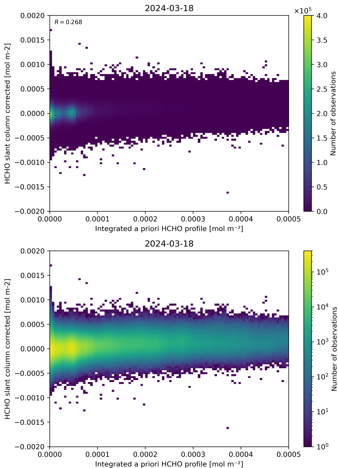
Figure 151: Scatter density plot of “Integrated a priori HCHO profile” against “HCHO slant column corrected” for 2024-03-17 to 2024-03-19.
