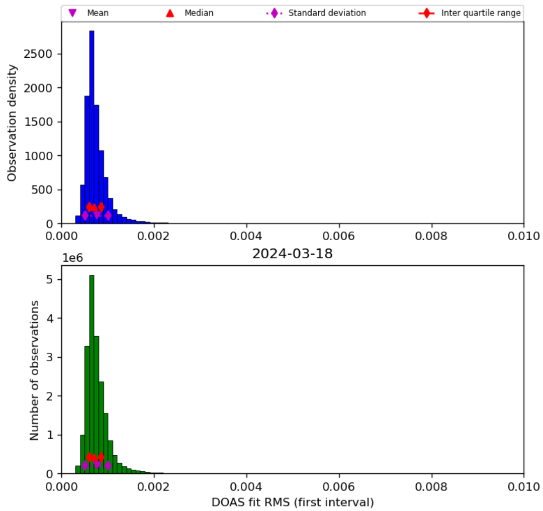
Figure 46: Histogram of “DOAS fit RMS (first interval)” for 2024-03-17 to 2024-03-19
