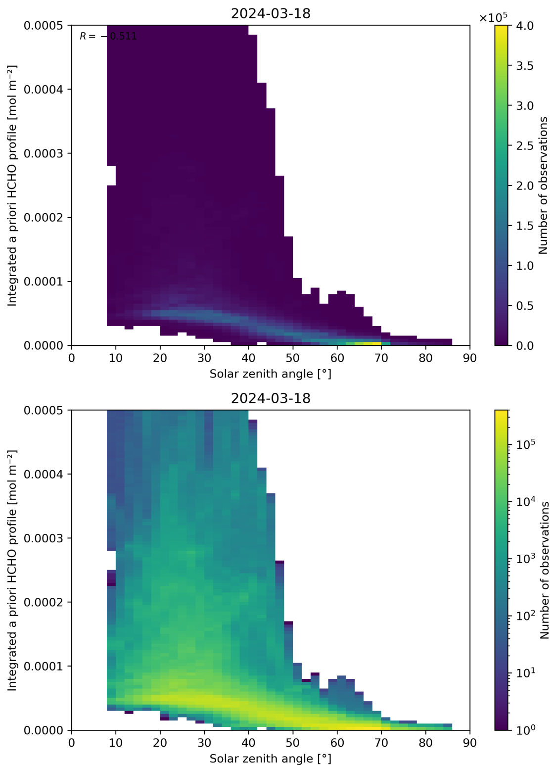
Figure 180: Scatter density plot of “Solar zenith angle” against “Integrated a priori HCHO profile” for 2024-03-17 to 2024-03-19.
