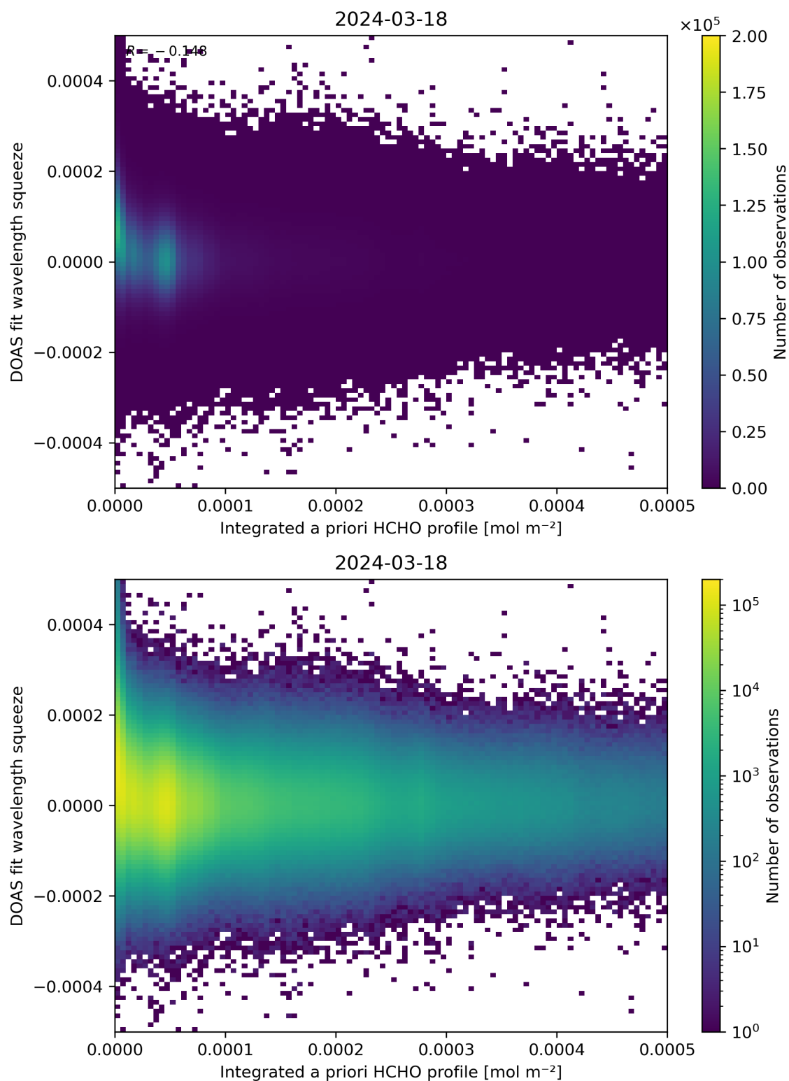
Figure 150: Scatter density plot of “Integrated a priori HCHO profile” against “DOAS fit wavelength squeeze” for 2024-03-17 to 2024-03-19.
