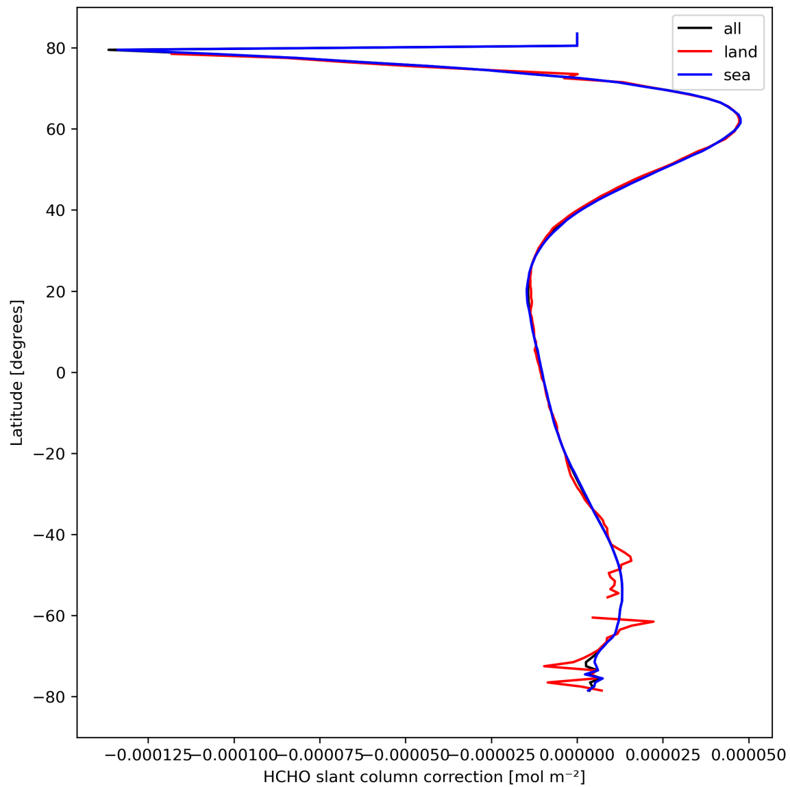
Figure 33: Zonal average of “HCHO slant column correction” for 2024-03-17 to 2024-03-19.
