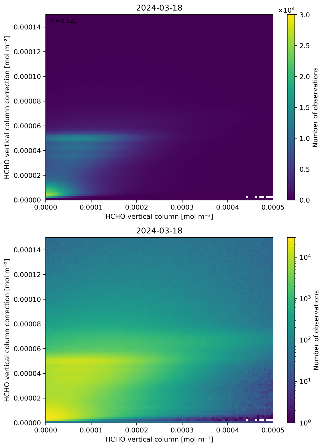
Figure 133: Scatter density plot of “HCHO vertical column” against “HCHO vertical column correction” for 2024-03-17 to 2024-03-19.
