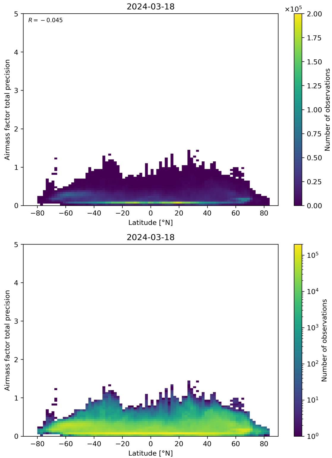
Figure 162: Scatter density plot of “Latitude” against “Airmass factor total precision” for 2024-03-17 to 2024-03-19.
