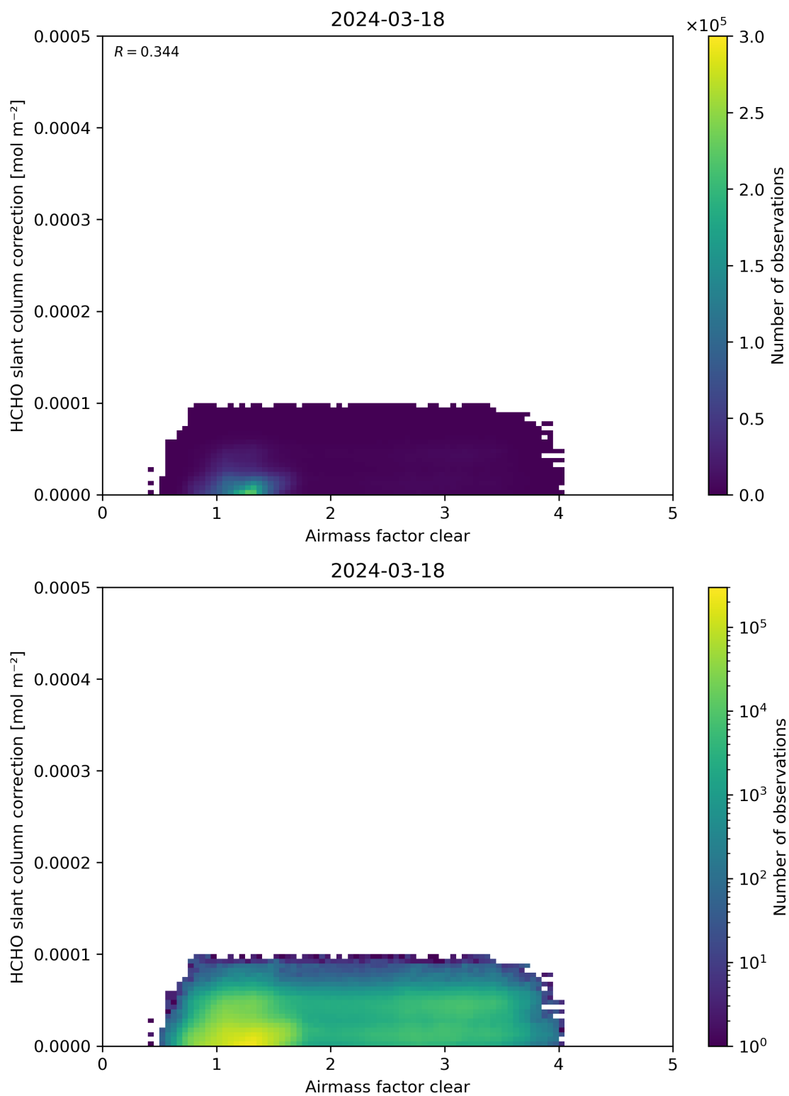
Figure 75: Scatter density plot of “Airmass factor clear” against “HCHO slant column correction” for 2024-03-17 to 2024-03-19.
