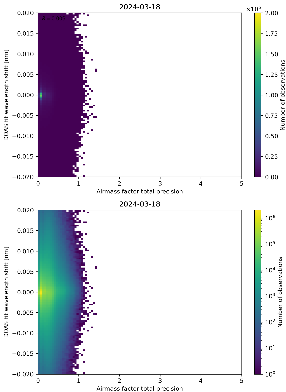
Figure 106: Scatter density plot of “Airmass factor total precision” against “DOAS fit wavelength shift” for 2024-03-17 to 2024-03-19.
