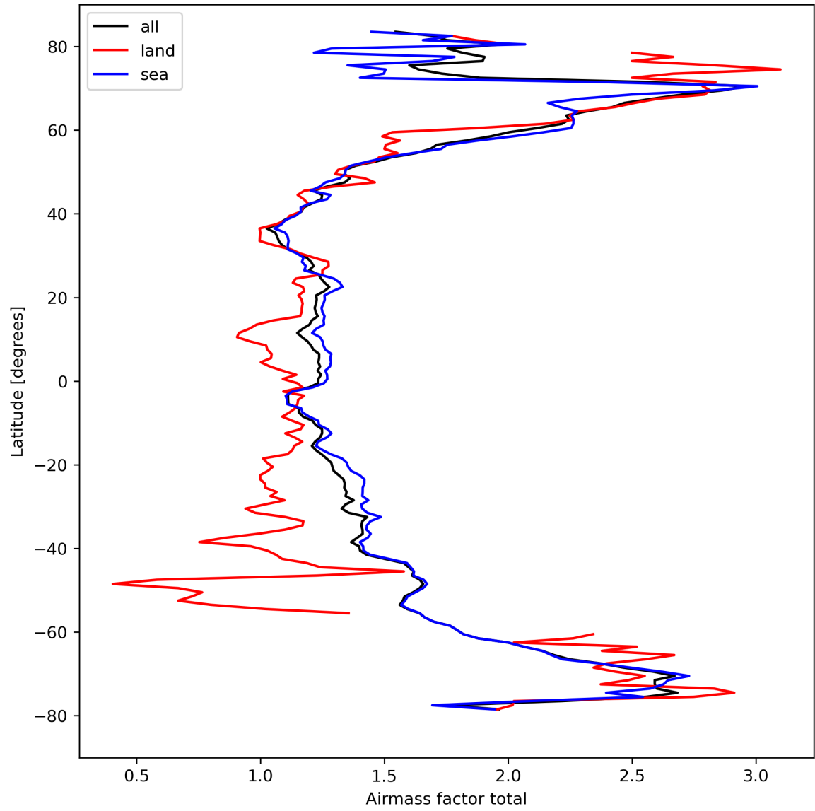
Figure 26: Zonal average of “Airmass factor total” for 2024-03-17 to 2024-03-19.
