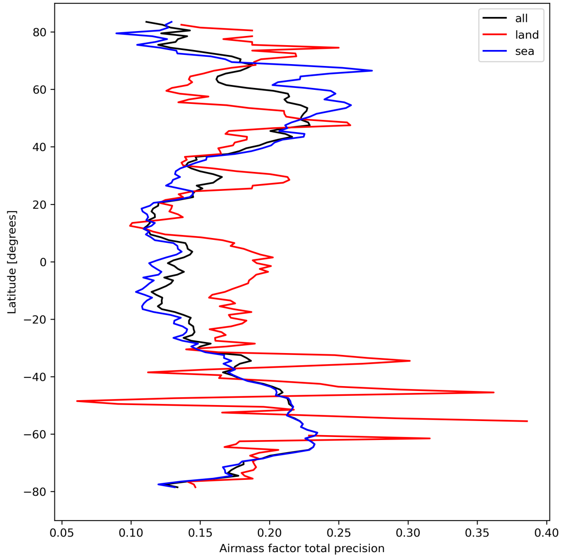
Figure 27: Zonal average of “Airmass factor total precision” for 2024-03-17 to 2024-03-19.
