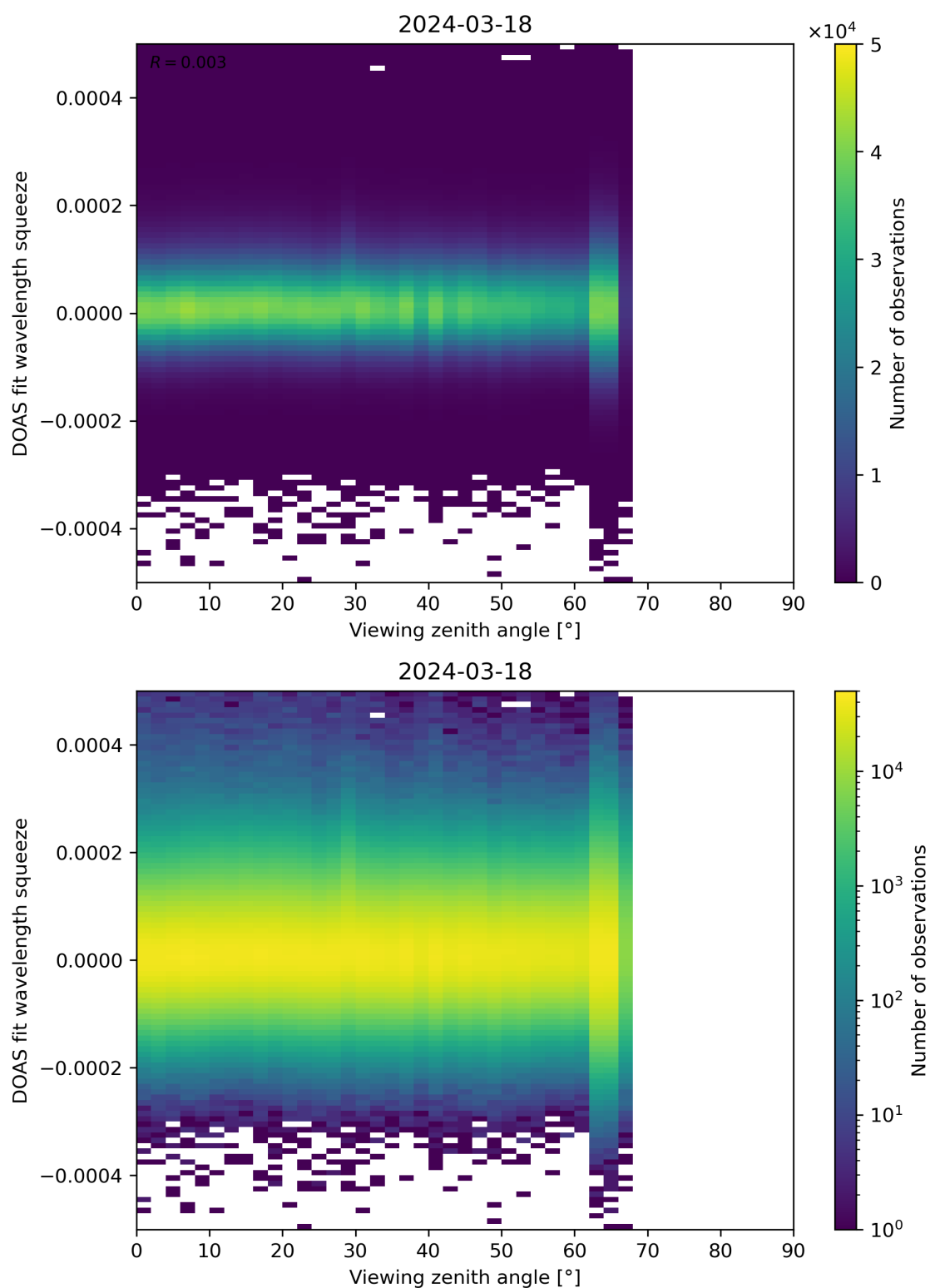
Figure 184: Scatter density plot of “Viewing zenith angle” against “DOAS fit wavelength squeeze” for 2024-03-17 to 2024-03-19.
