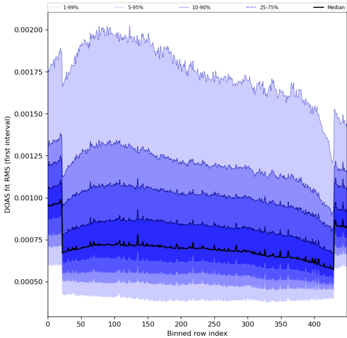
Figure 60: Along track statistics of “DOAS fit RMS (first interval)” for 2024-03-17 to 2024-03-19
