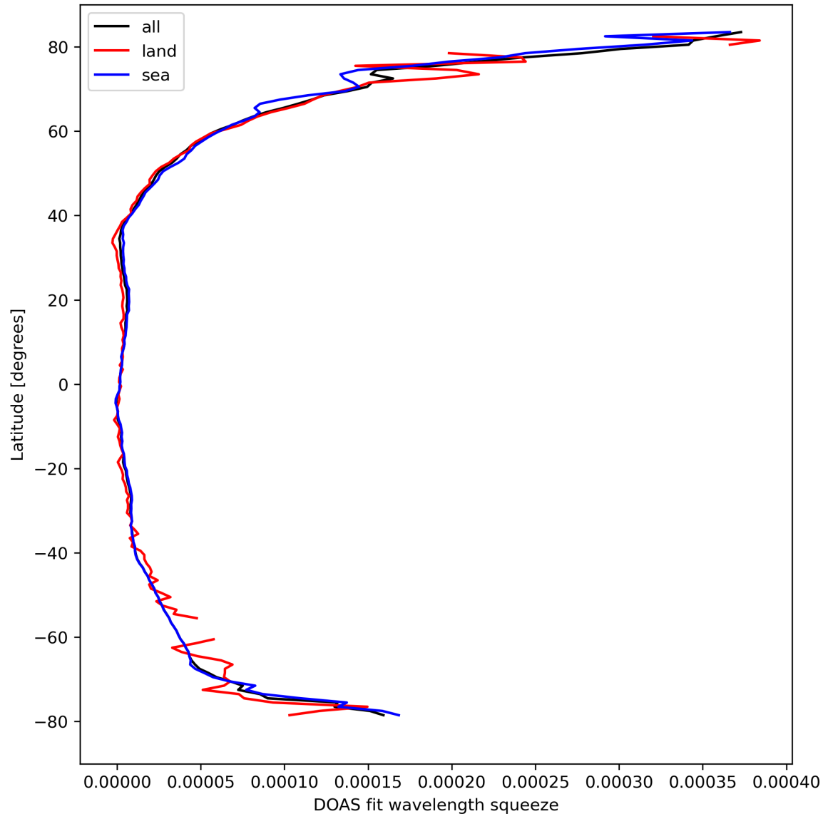
Figure 31: Zonal average of “DOAS fit wavelength squeeze” for 2024-03-17 to 2024-03-19.
