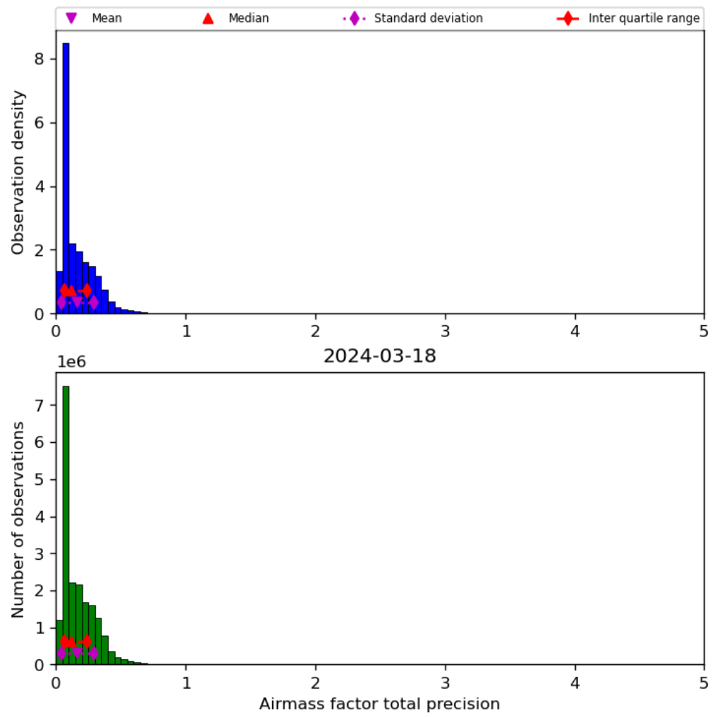
Figure 41: Histogram of “Airmass factor total precision” for 2024-03-17 to 2024-03-19
