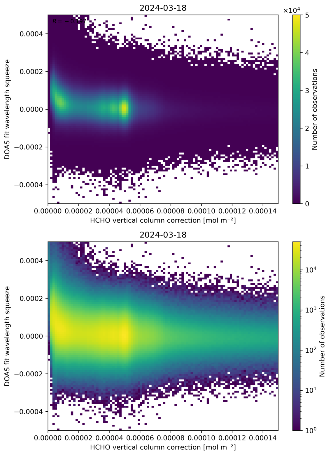
Figure 114: Scatter density plot of “HCHO vertical column correction” against “DOAS fit wavelength squeeze” for 2024-03-17 to 2024-03-19.
