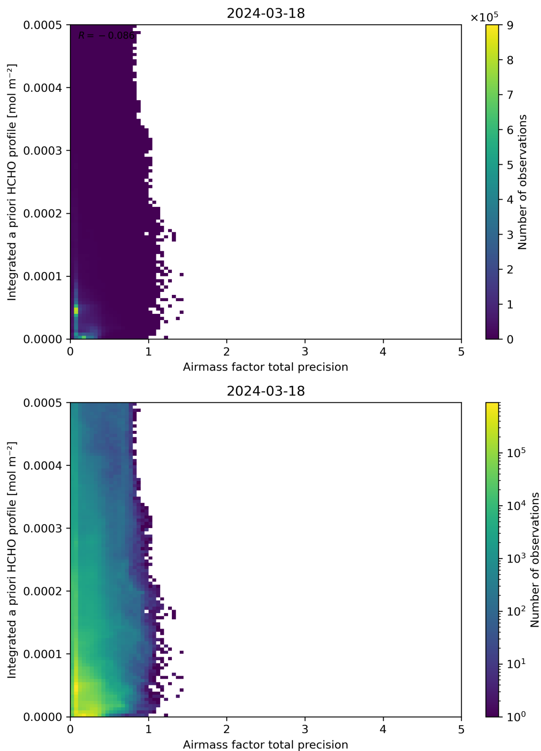
Figure 111: Scatter density plot of “Airmass factor total precision” against “Integrated a priori HCHO profile” for 2024-03-17 to 2024-03-19.
