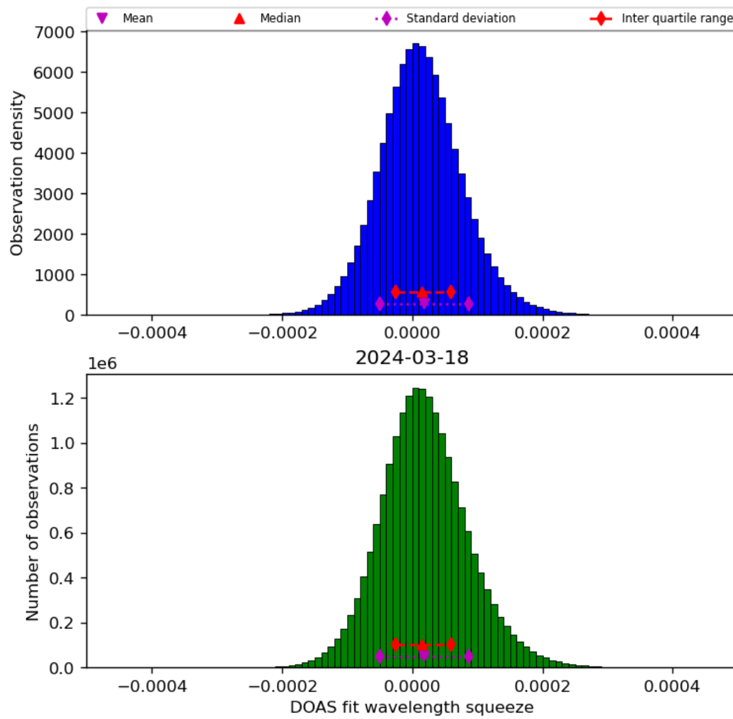
Figure 45: Histogram of “DOAS fit wavelength squeeze” for 2024-03-17 to 2024-03-19
