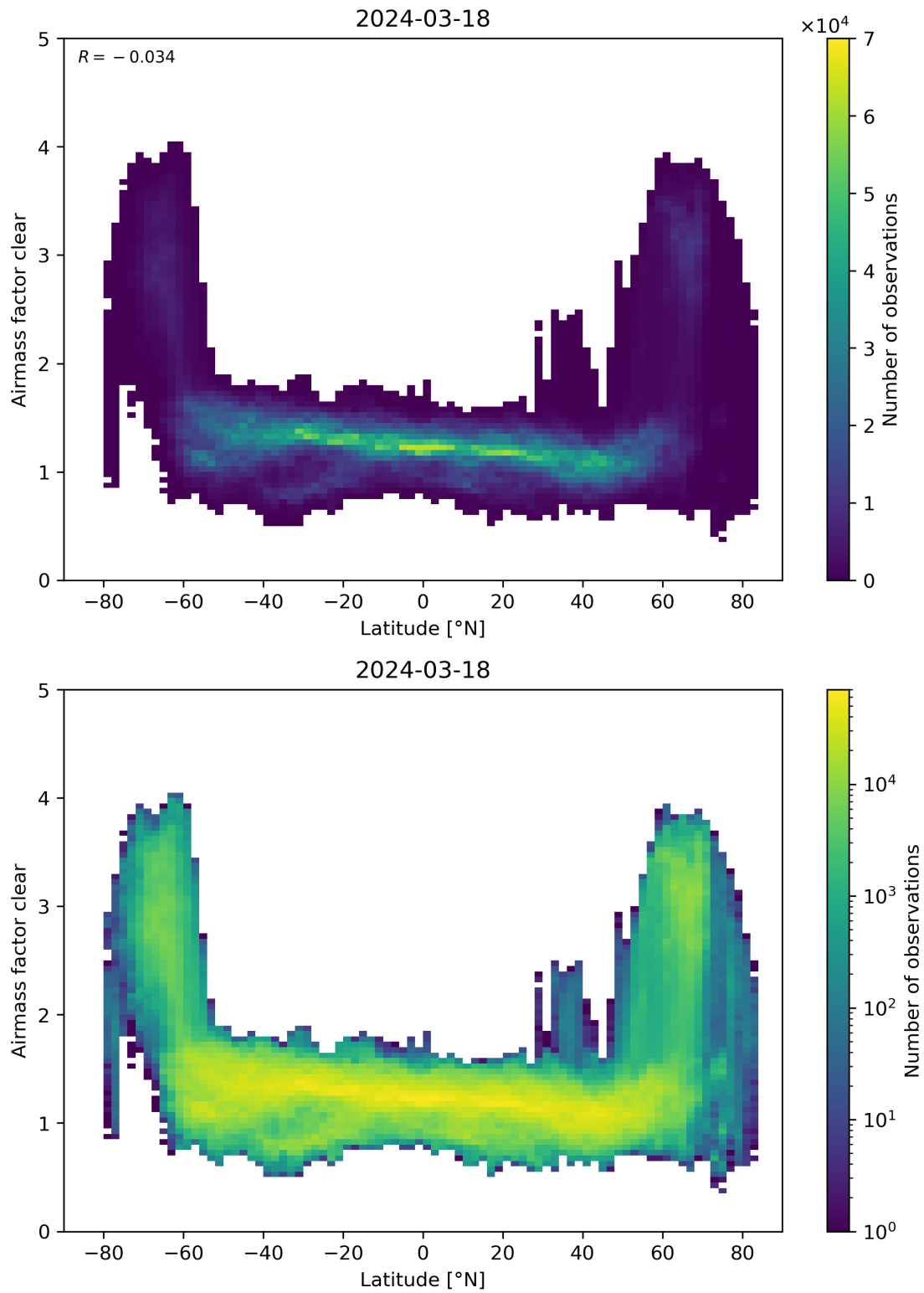
Figure 156: Scatter density plot of “Latitude” against “Airmass factor clear” for 2024-03-17 to 2024-03-19.
