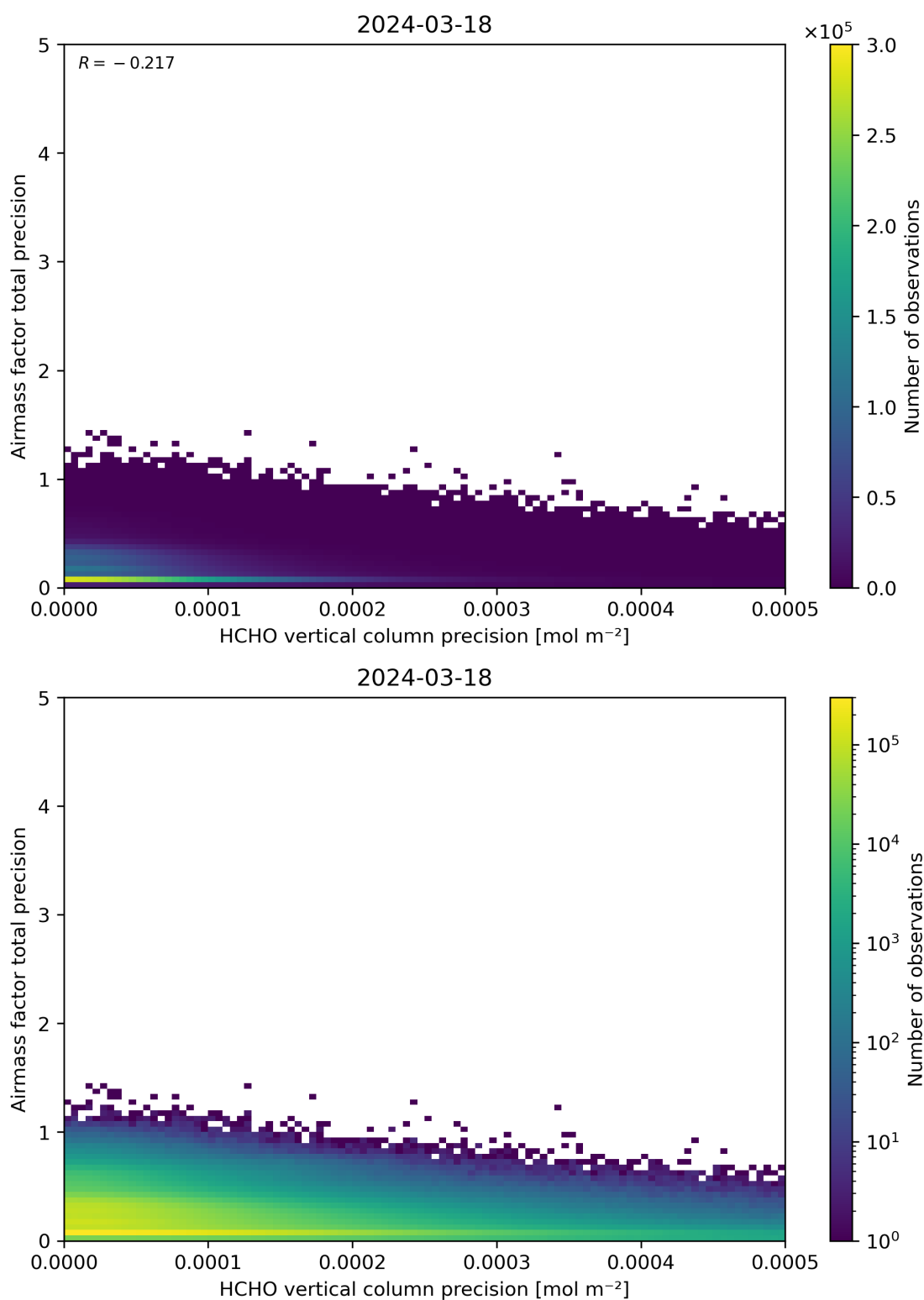
Figure 145: Scatter density plot of “HCHO vertical column precision” against “Airmass factor total precision” for 2024-03-17 to 2024-03-19.
