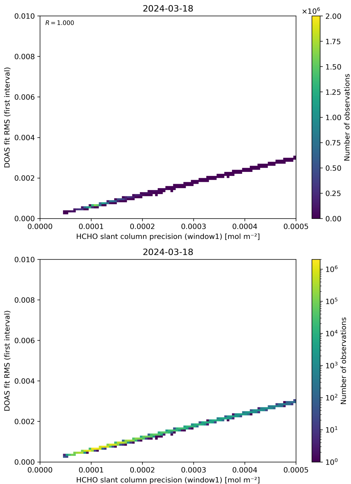
Figure 88: Scatter density plot of “HCHO slant column precision (window1)” against “DOAS fit RMS (first interval)” for 2024-03-17 to 2024-03-19.
