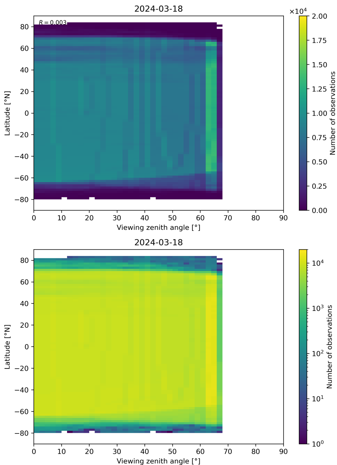
Figure 196: Scatter density plot of “Viewing zenith angle” against “Latitude” for 2024-03-17 to 2024-03-19.
