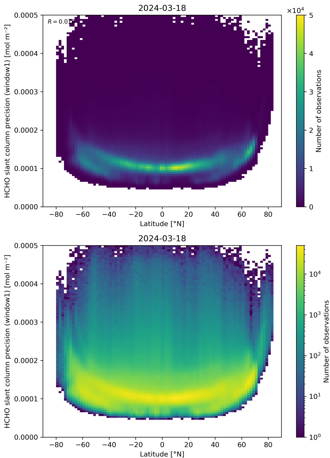
Figure 160: Scatter density plot of “Latitude” against “HCHO slant column precision (window1)” for 2024-03-17 to 2024-03-19.
