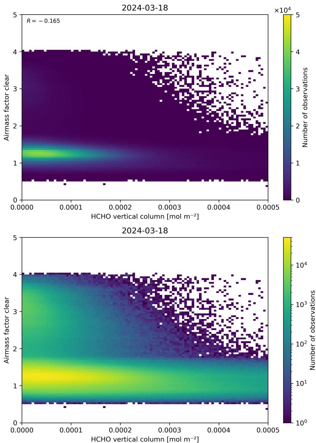
Figure 126: Scatter density plot of “HCHO vertical column” against “Airmass factor clear” for 2024-03-17 to 2024-03-19.
