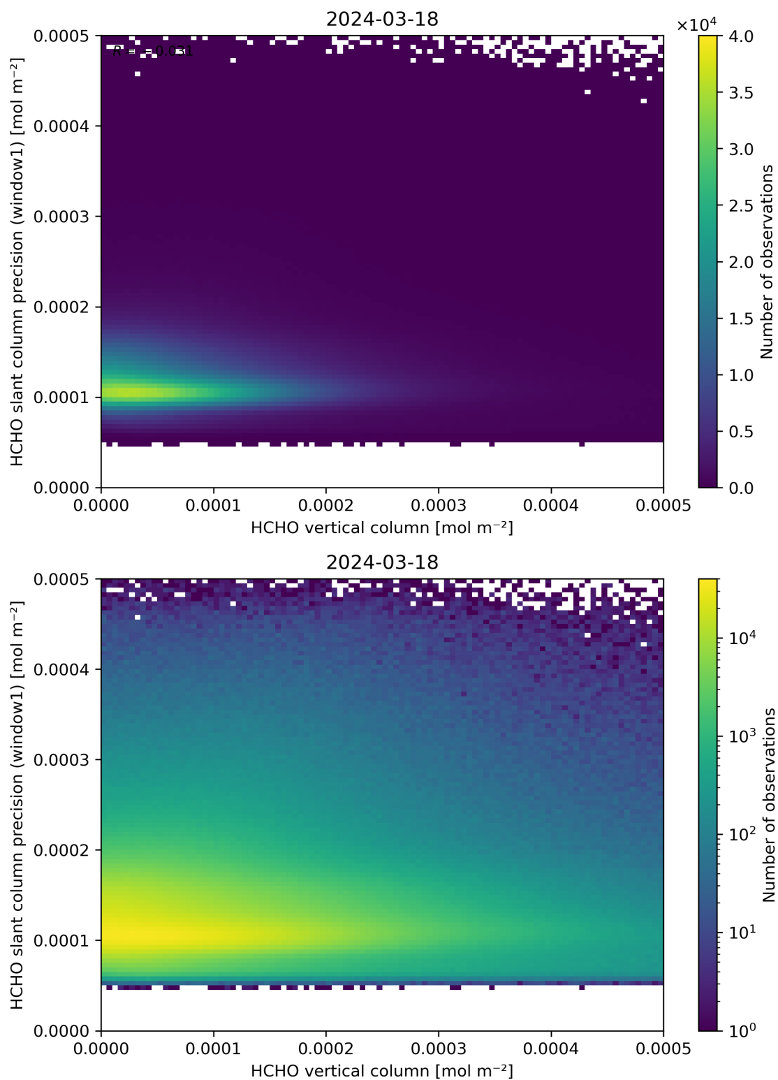
Figure 130: Scatter density plot of “HCHO vertical column” against “HCHO slant column precision (window1)” for 2024-03-17 to 2024-03-19.
