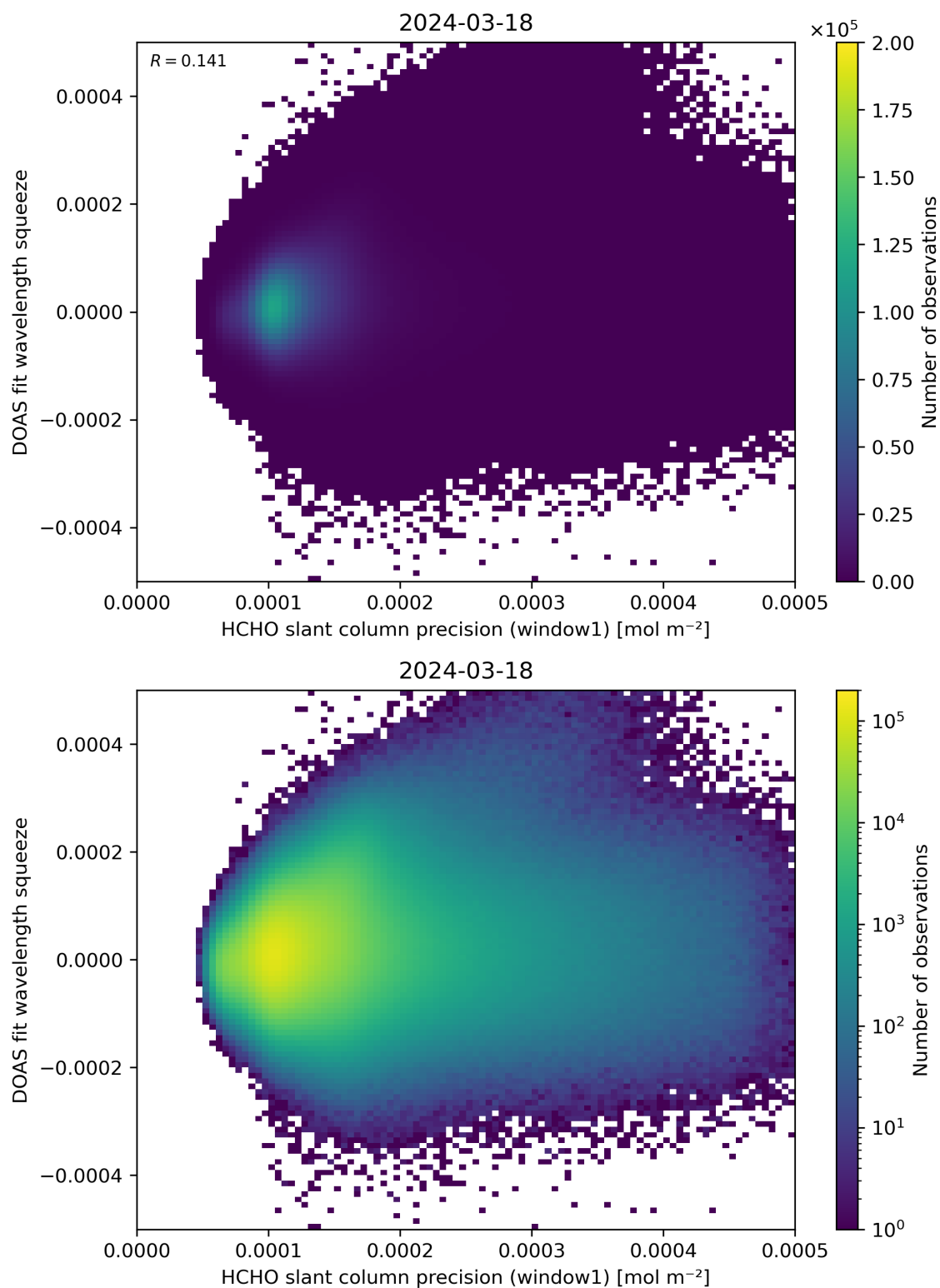
Figure 90: Scatter density plot of “HCHO slant column precision (window1)” against “DOAS fit wavelength squeeze” for 2024-03-17 to 2024-03-19.
