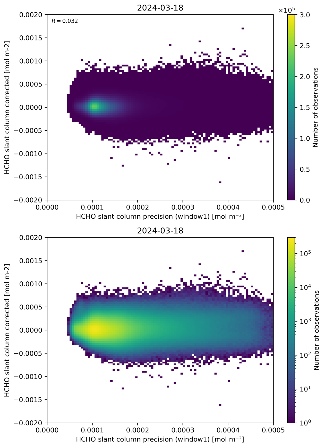
Figure 92: Scatter density plot of “HCHO slant column precision (window1)” against “HCHO slant column corrected” for 2024-03-17 to 2024-03-19.
