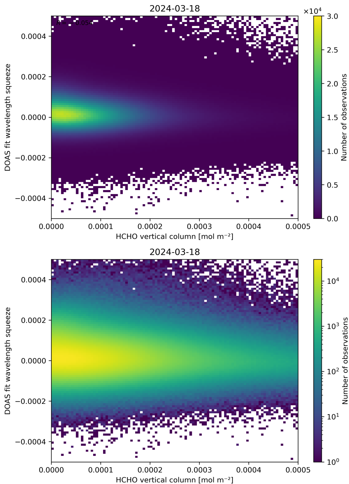
Figure 125: Scatter density plot of “HCHO vertical column” against “DOAS fit wavelength squeeze” for 2024-03-17 to 2024-03-19.
