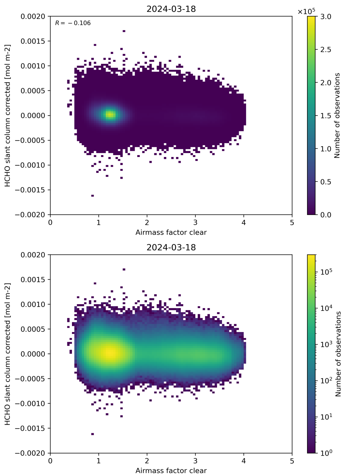
Figure 74: Scatter density plot of “Airmass factor clear” against “HCHO slant column corrected” for 2024-03-17 to 2024-03-19.
