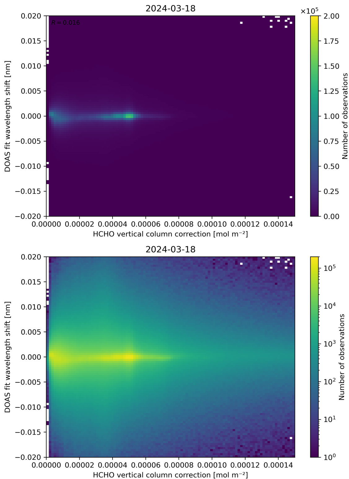
Figure 113: Scatter density plot of “HCHO vertical column correction” against “DOAS fit wavelength shift” for 2024-03-17 to 2024-03-19.
