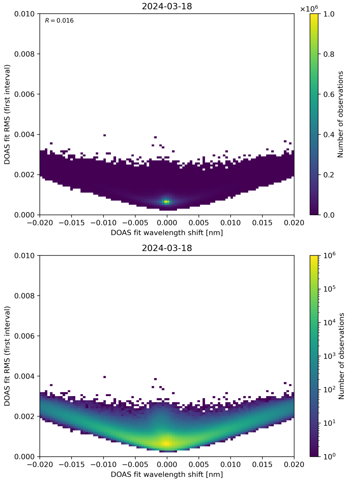
Figure 64: Scatter density plot of “DOAS fit wavelength shift” against “DOAS fit RMS (first interval)” for 2024-03-17 to 2024-03-19.
