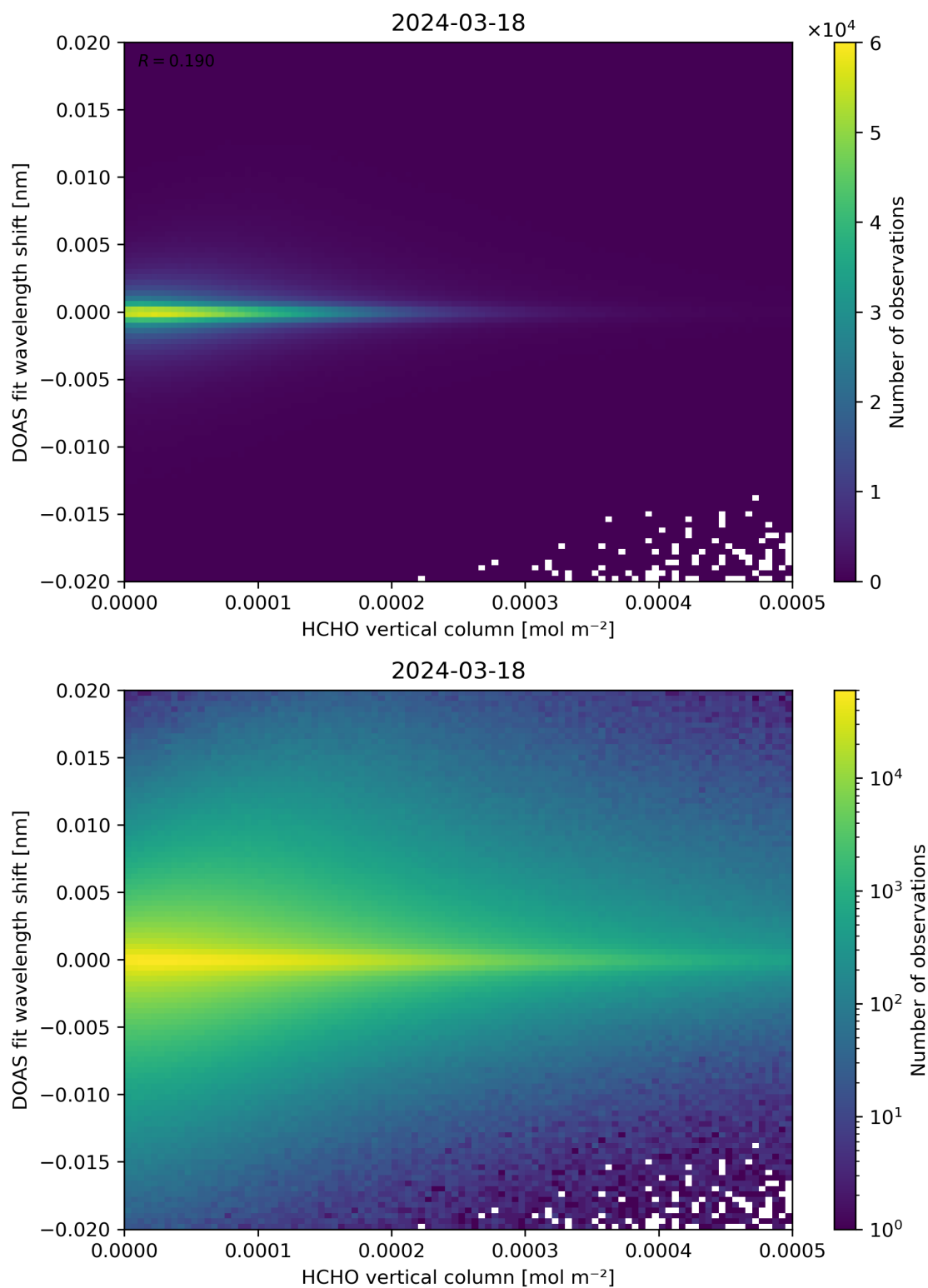
Figure 124: Scatter density plot of “HCHO vertical column” against “DOAS fit wavelength shift” for 2024-03-17 to 2024-03-19.
