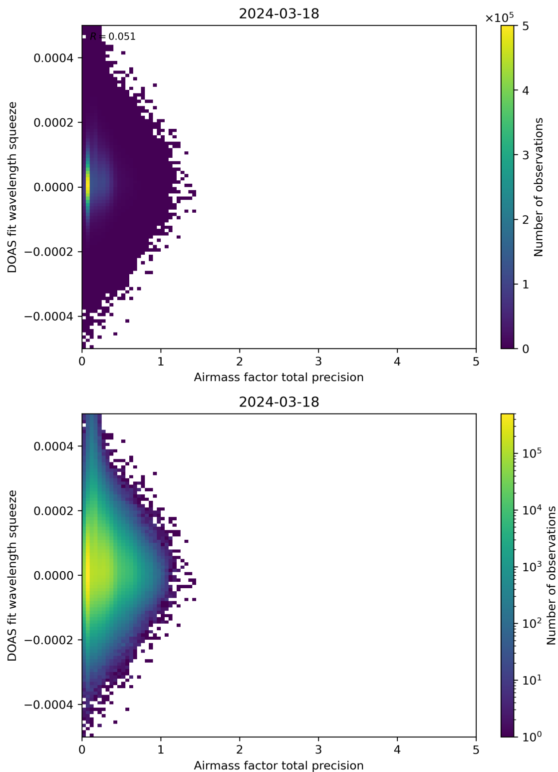
Figure 107: Scatter density plot of “Airmass factor total precision” against “DOAS fit wavelength squeeze” for 2024-03-17 to 2024-03-19.
