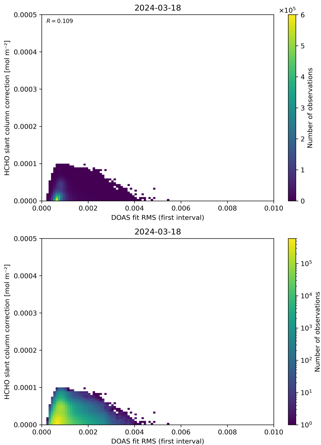
Figure 63: Scatter density plot of “DOAS fit RMS (first interval)” against “HCHO slant column correction” for 2024-03-17 to 2024-03-19.
