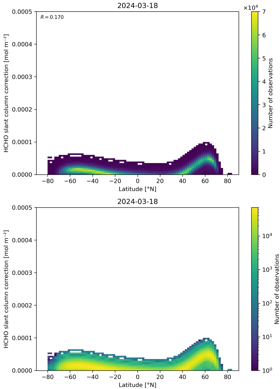
Figure 158: Scatter density plot of “Latitude” against “HCHO slant column correction” for 2024-03-17 to 2024-03-19.
