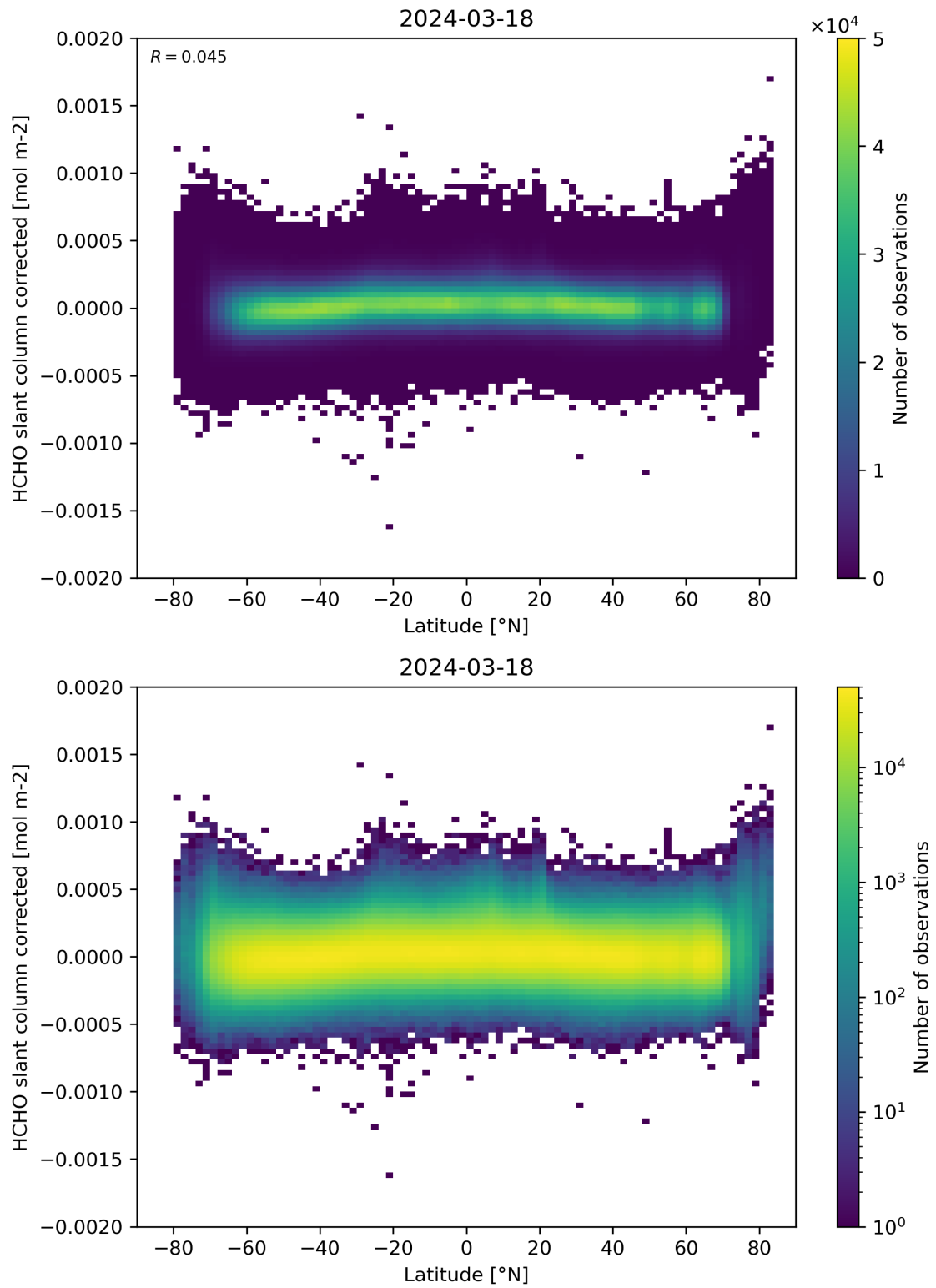
Figure 157: Scatter density plot of “Latitude” against “HCHO slant column corrected” for 2024-03-17 to 2024-03-19.
