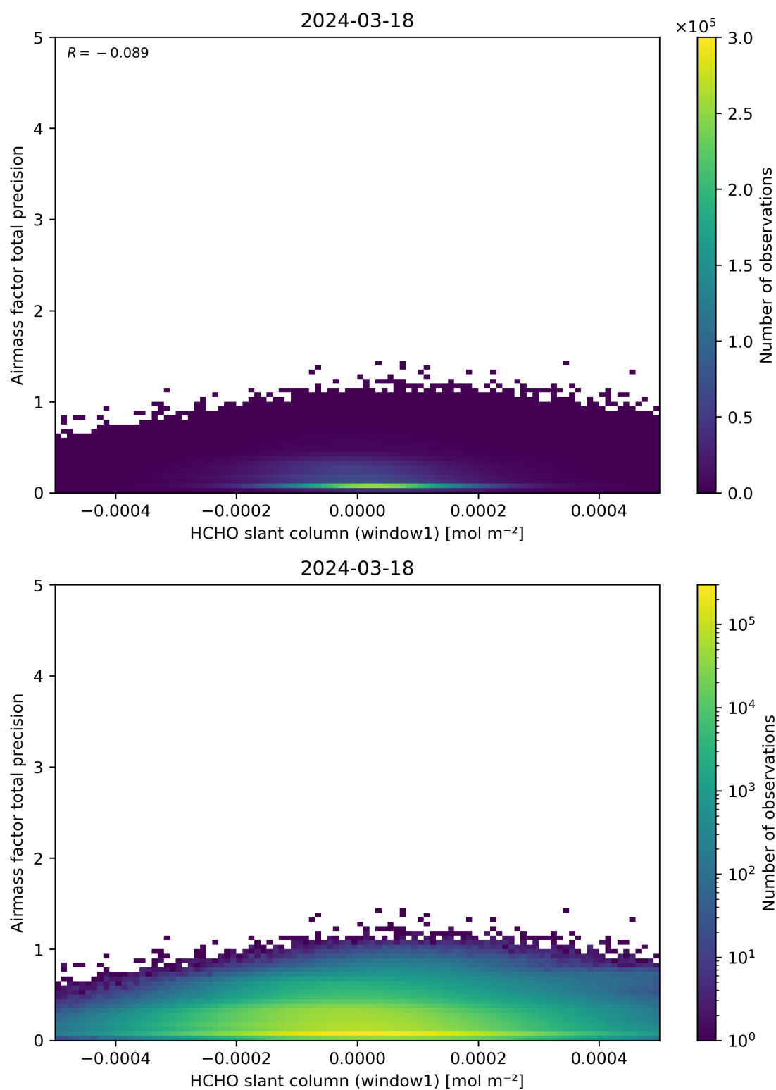
Figure 86: Scatter density plot of “HCHO slant column (window1)” against “Airmass factor total precision” for 2024-03-17 to 2024-03-19.
