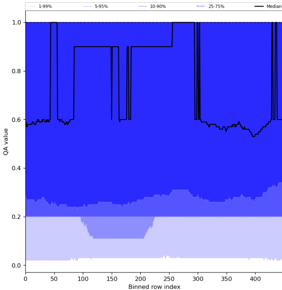
Figure 48: Along track statistics of “QA value” for 2024-03-17 to 2024-03-19
