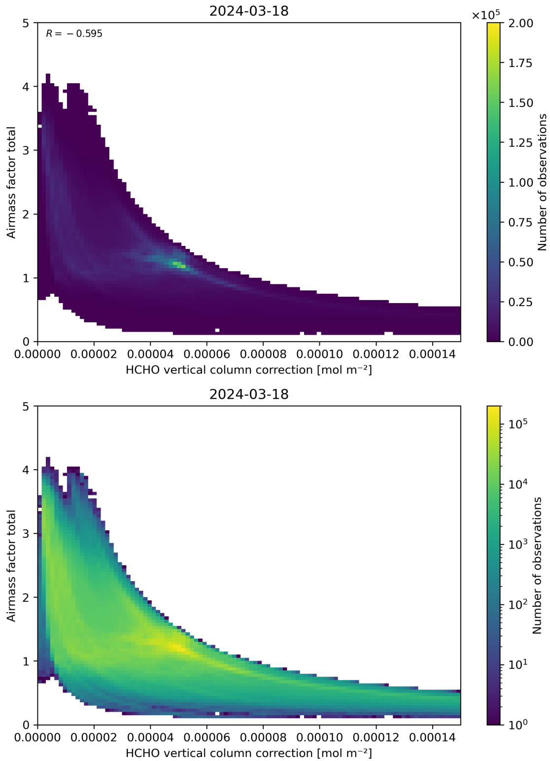
Figure 120: Scatter density plot of “HCHO vertical column correction” against “Airmass factor total” for 2024-03-17 to 2024-03-19.
