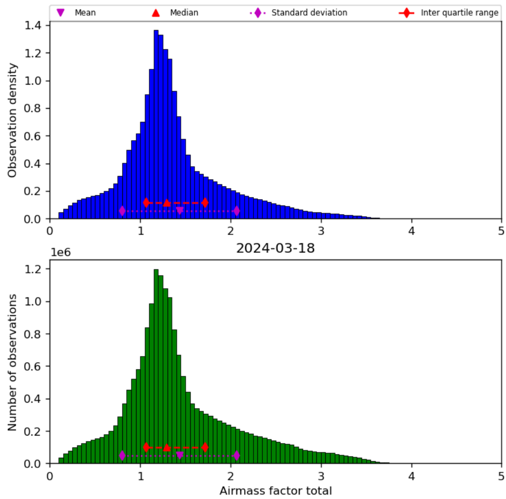
Figure 40: Histogram of “Airmass factor total” for 2024-03-17 to 2024-03-19
