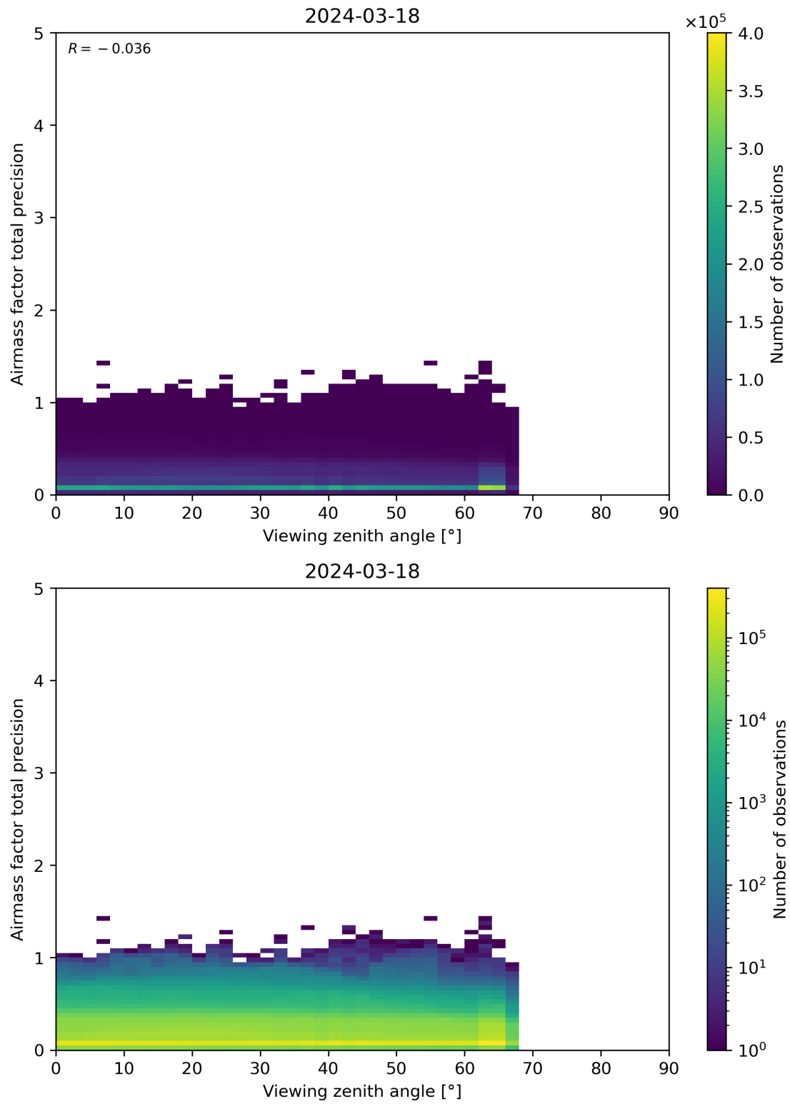
Figure 191: Scatter density plot of “Viewing zenith angle” against “Airmass factor total precision” for 2024-03-17 to 2024-03-19.
