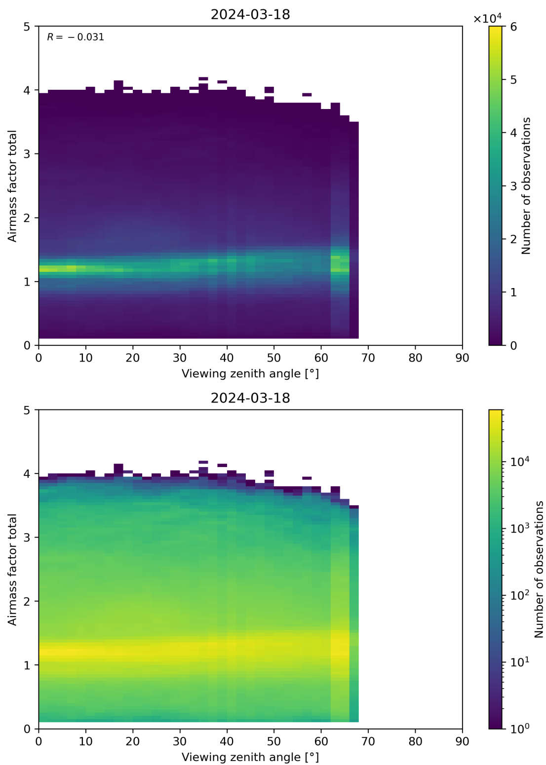
Figure 190: Scatter density plot of “Viewing zenith angle” against “Airmass factor total” for 2024-03-17 to 2024-03-19.
