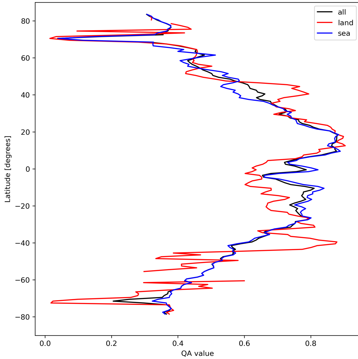
Figure 20: Zonal average of “QA value” for 2024-03-17 to 2024-03-19.
