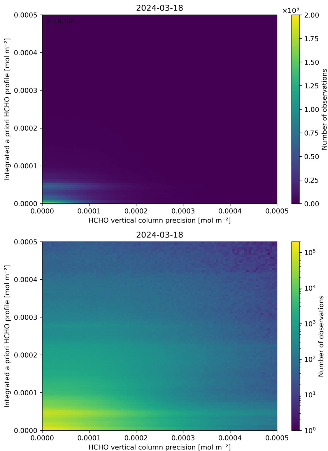
Figure 147: Scatter density plot of “HCHO vertical column precision” against “Integrated a priori HCHO profile” for 2024-03-17 to 2024-03-19.
