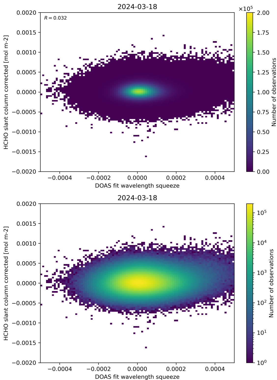
Figure 69: Scatter density plot of “DOAS fit wavelength squeeze” against “HCHO slant column corrected” for 2024-03-17 to 2024-03-19.
