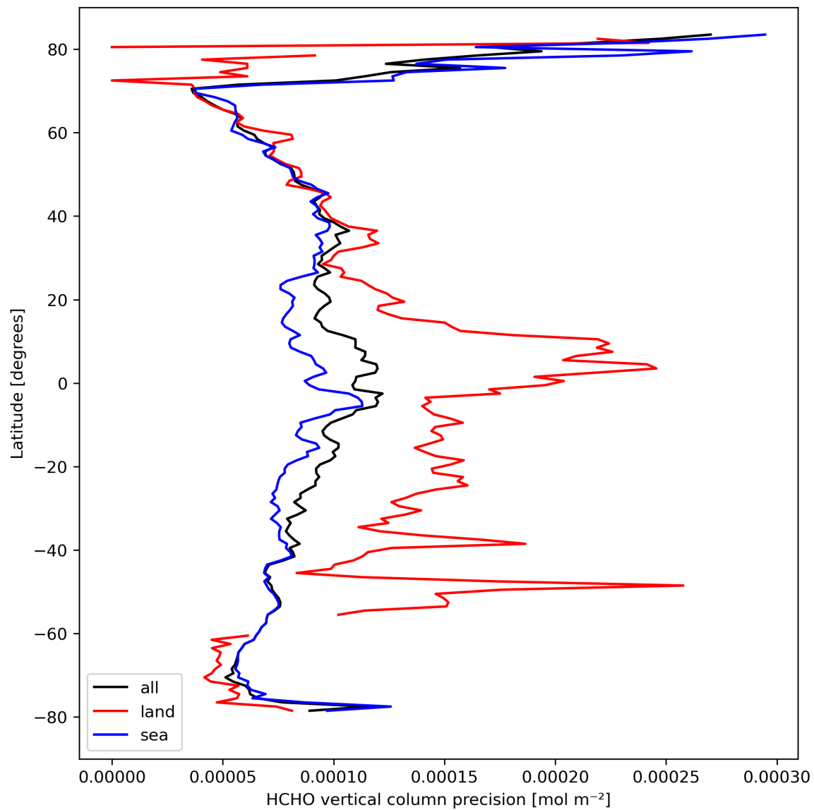
Figure 22: Zonal average of “HCHO vertical column precision” for 2024-03-17 to 2024-03-19.
