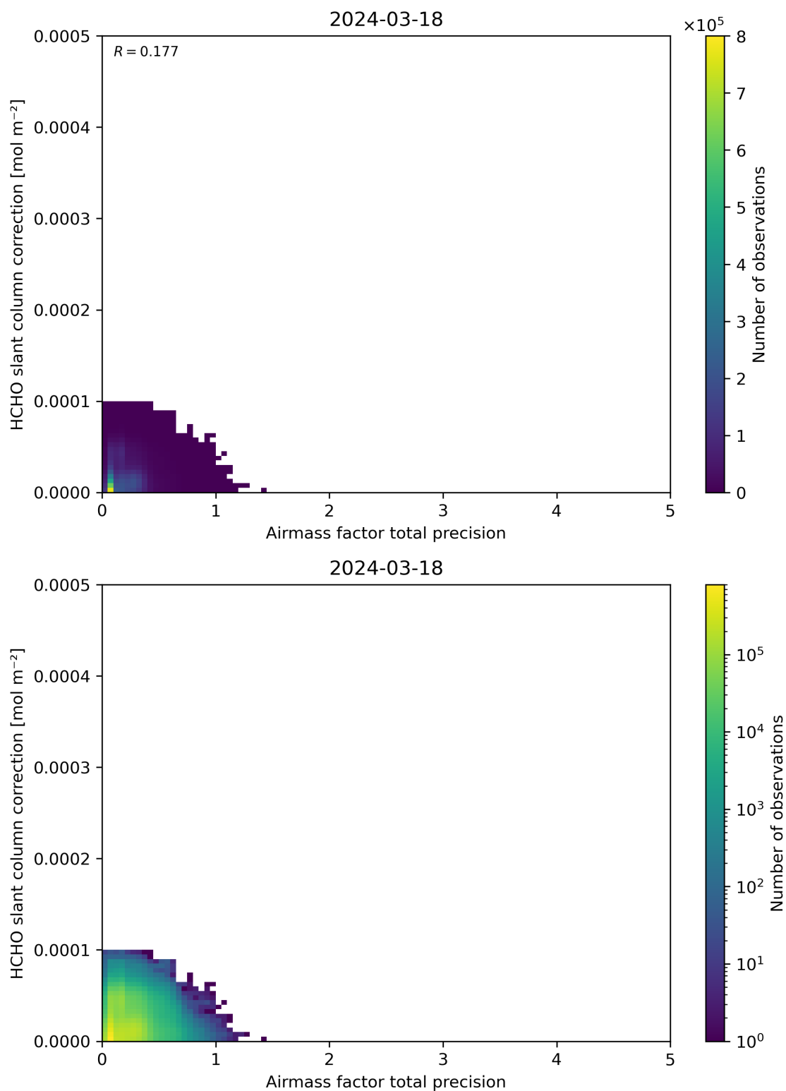
Figure 110: Scatter density plot of “Airmass factor total precision” against “HCHO slant column correction” for 2024-03-17 to 2024-03-19.
