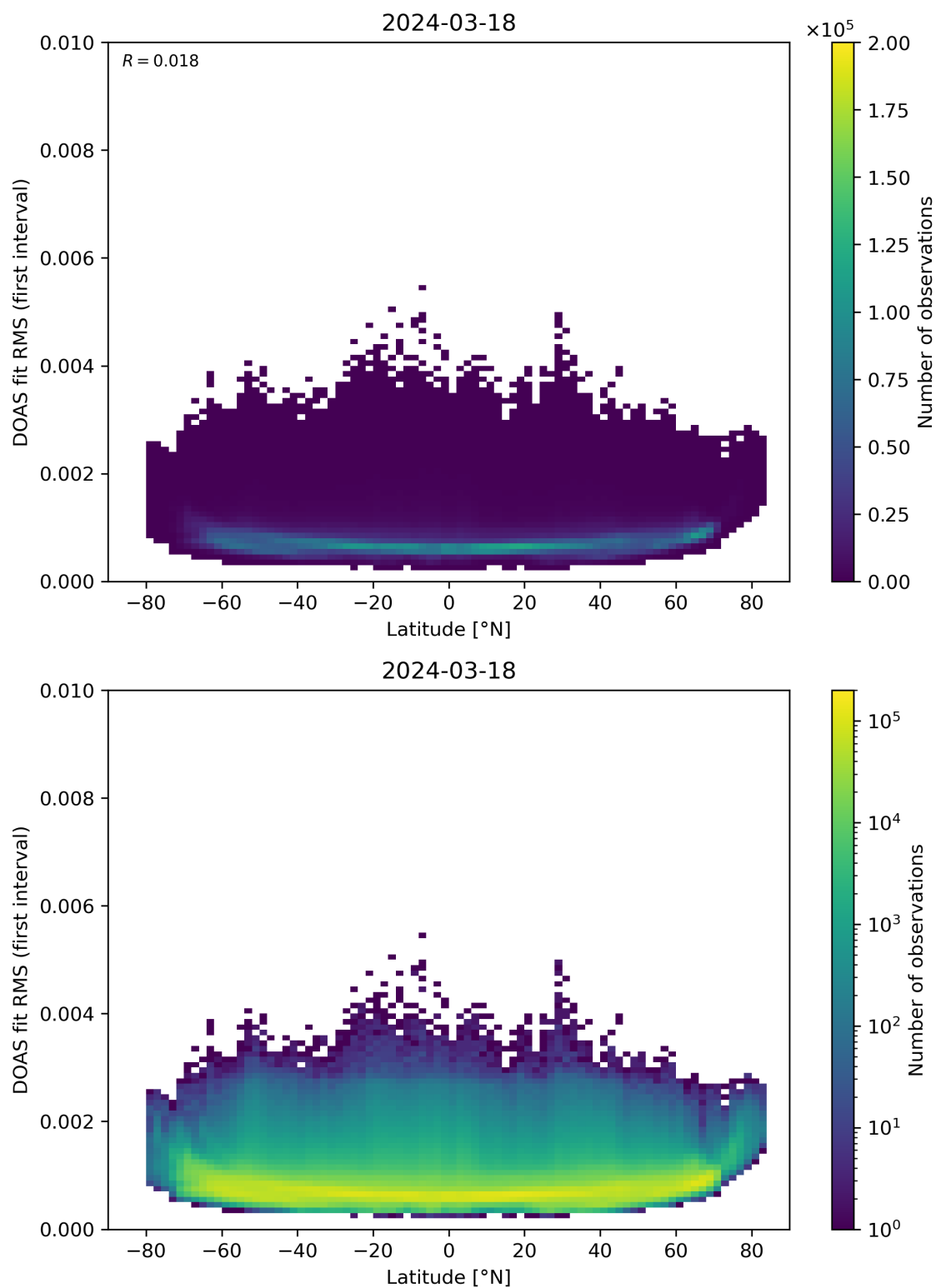
Figure 153: Scatter density plot of “Latitude” against “DOAS fit RMS (first interval)” for 2024-03-17 to 2024-03-19.
