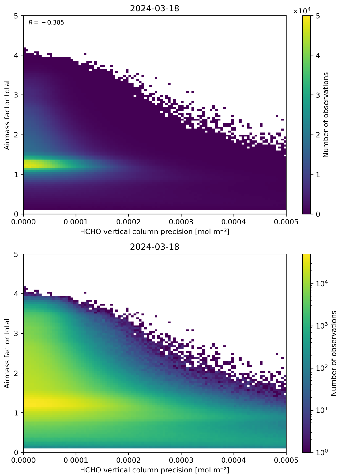
Figure 144: Scatter density plot of “HCHO vertical column precision” against “Airmass factor total” for 2024-03-17 to 2024-03-19.
