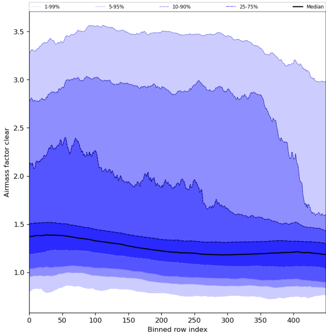
Figure 56: Along track statistics of “Airmass factor clear” for 2024-03-17 to 2024-03-19
