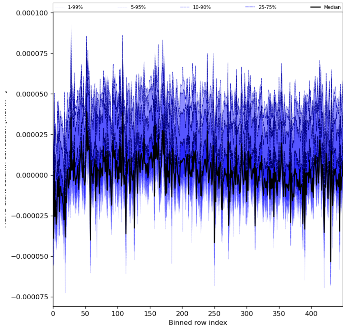
Figure 61: Along track statistics of “HCHO slant column correction” for 2024-03-17 to 2024-03-19
