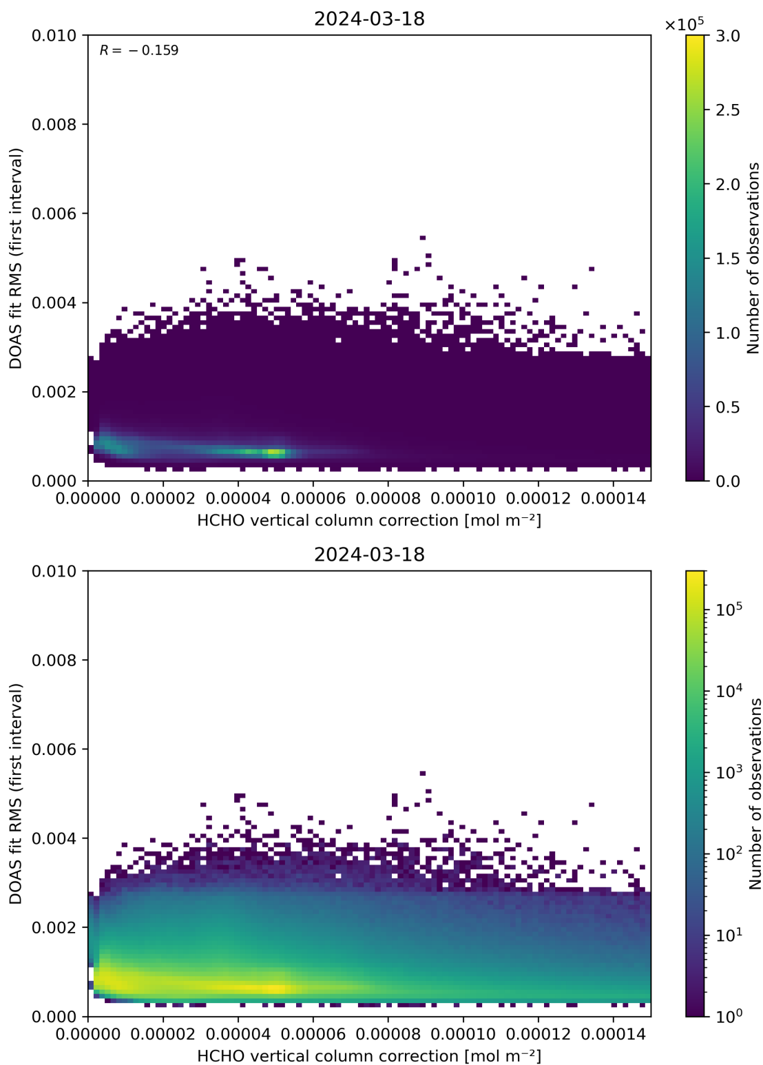
Figure 112: Scatter density plot of “HCHO vertical column correction” against “DOAS fit RMS (first interval)” for 2024-03-17 to 2024-03-19.
