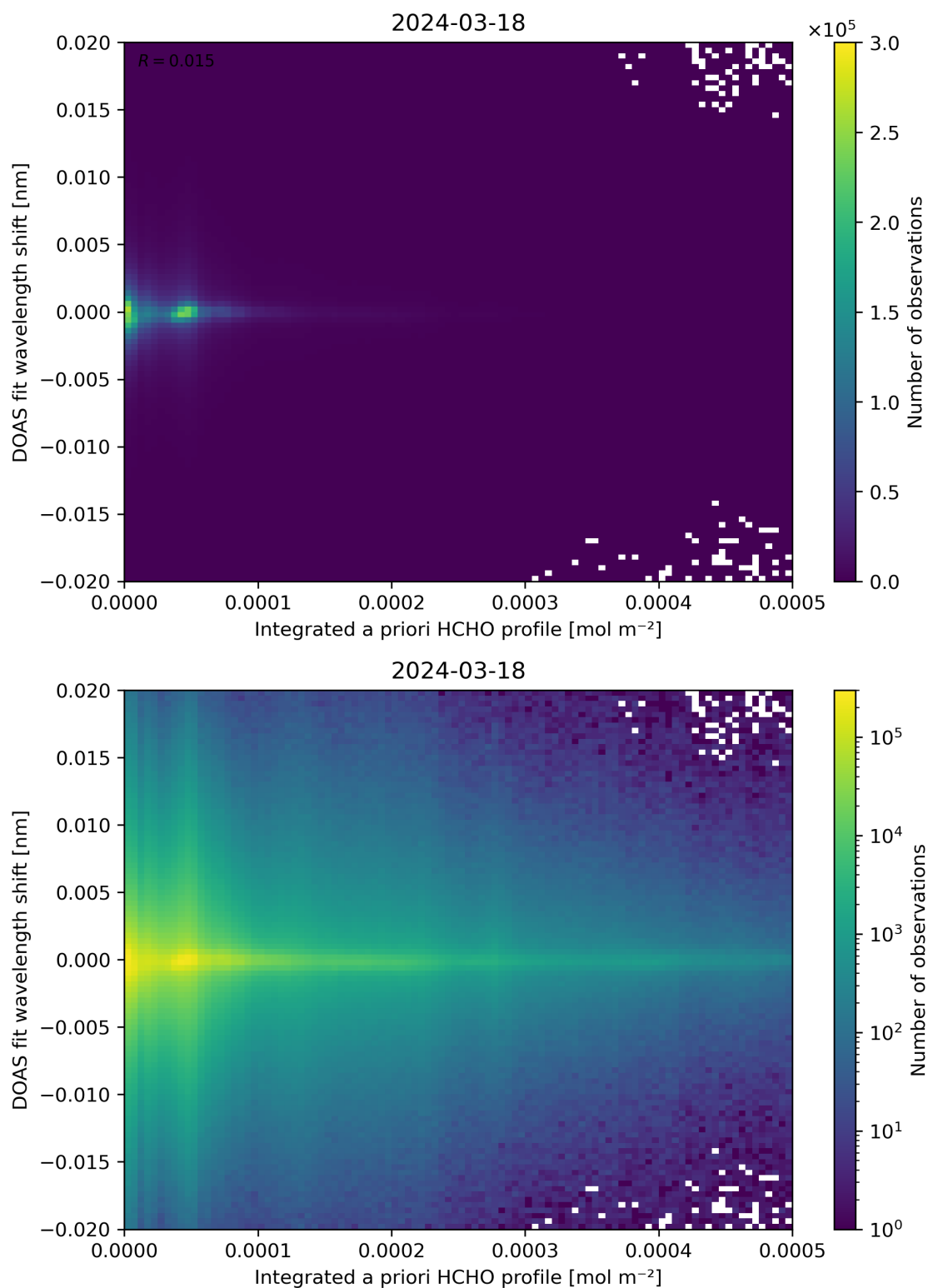
Figure 149: Scatter density plot of “Integrated a priori HCHO profile” against “DOAS fit wavelength shift” for 2024-03-17 to 2024-03-19.
