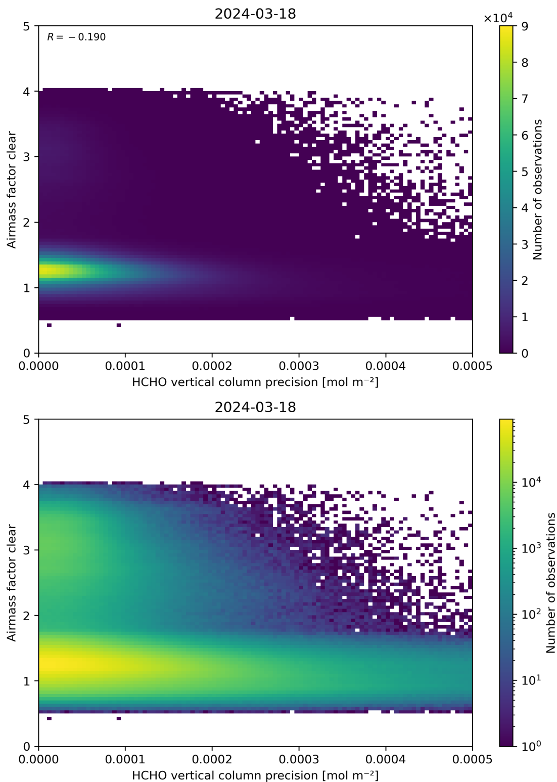
Figure 139: Scatter density plot of “HCHO vertical column precision” against “Airmass factor clear” for 2024-03-17 to 2024-03-19.
