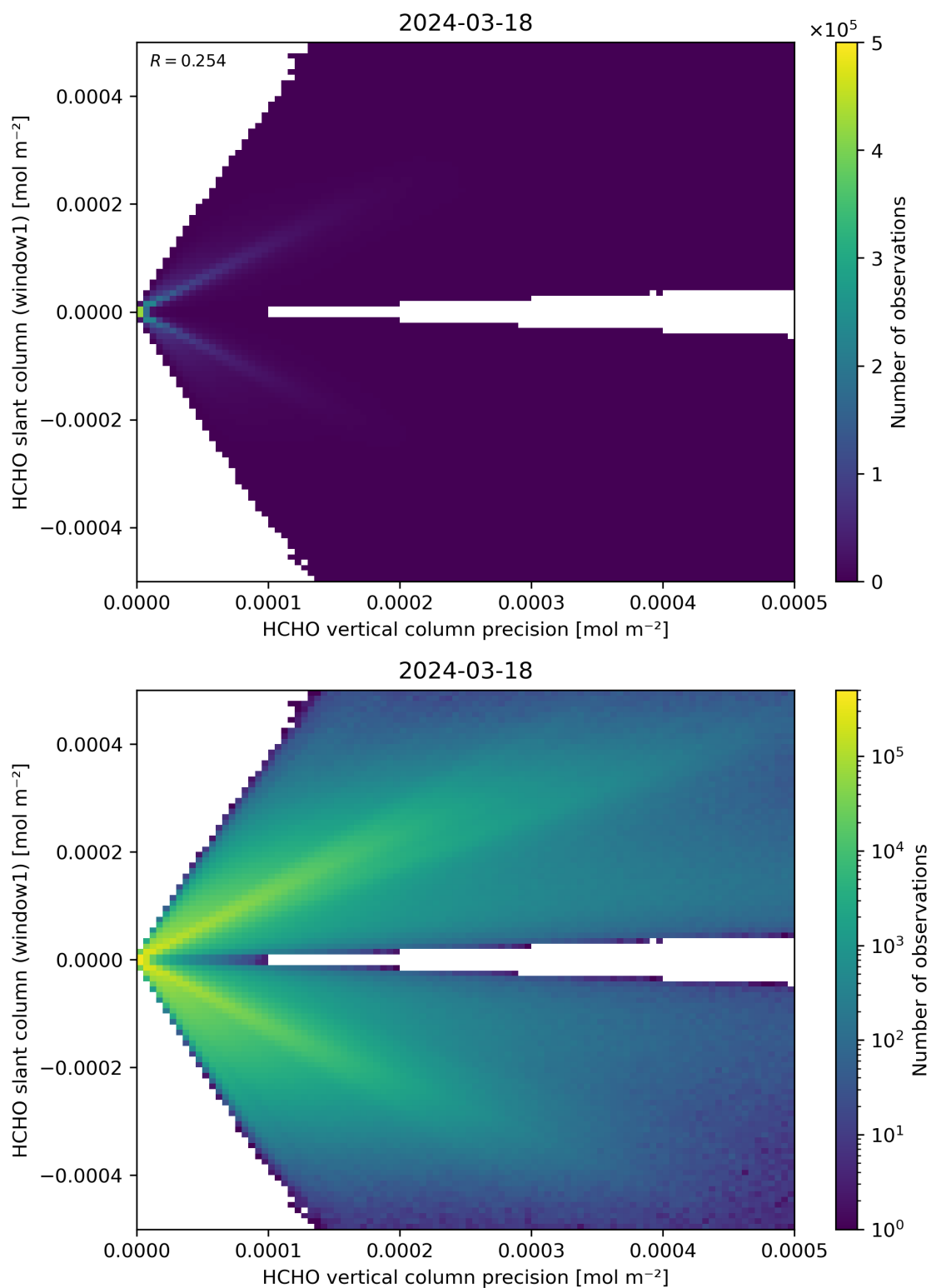
Figure 142: Scatter density plot of “HCHO vertical column precision” against “HCHO slant column (window1)” for 2024-03-17 to 2024-03-19.
