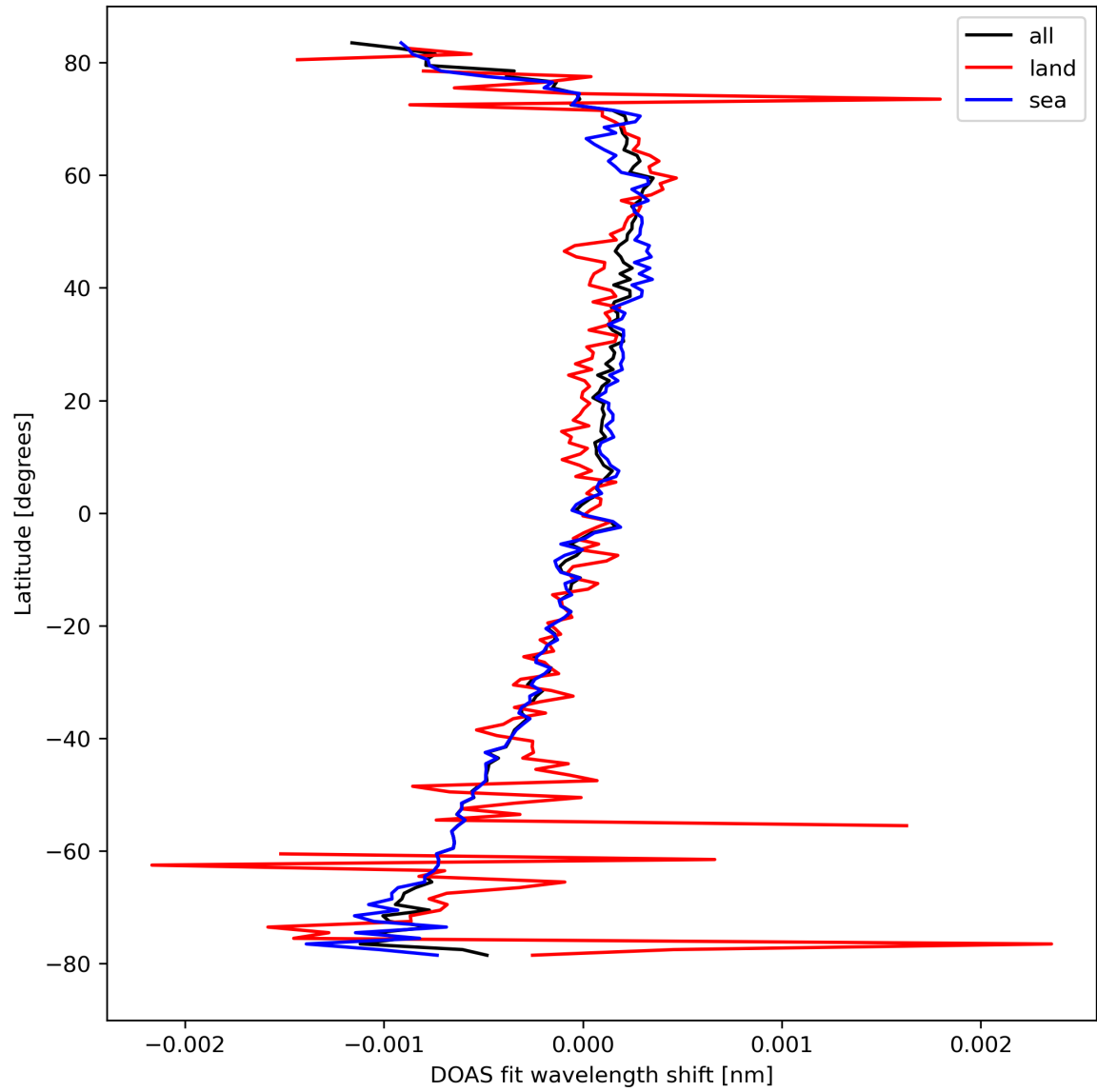
Figure 30: Zonal average of “DOAS fit wavelength shift” for 2024-03-17 to 2024-03-19.
