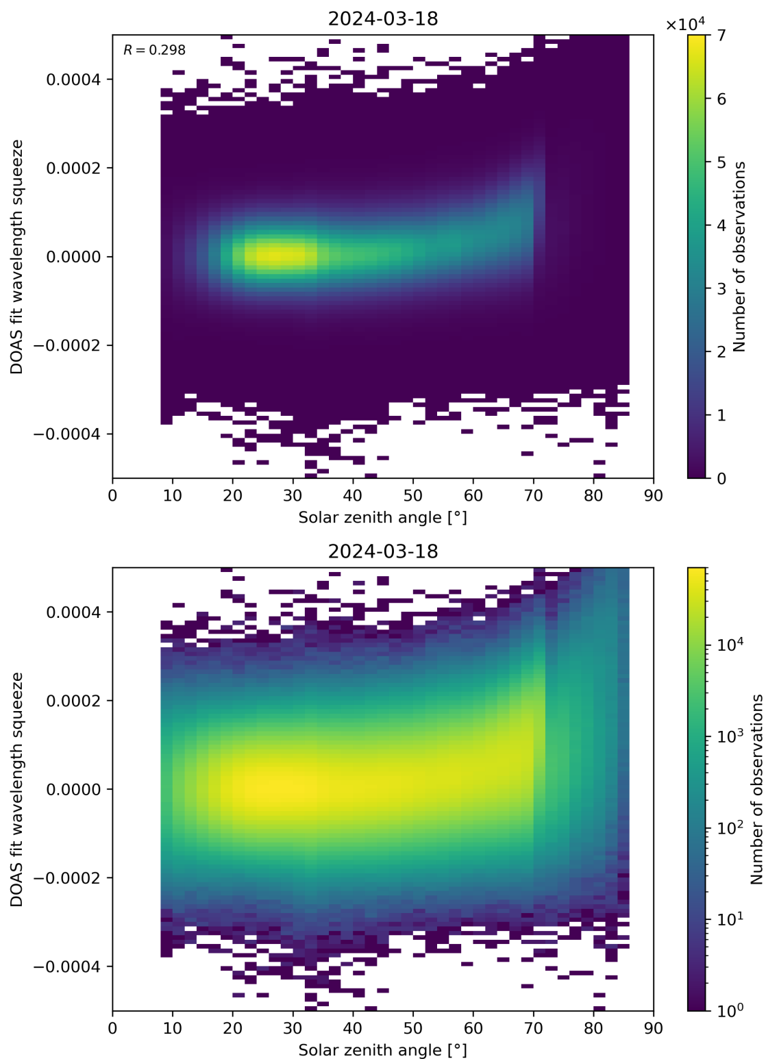
Figure 169: Scatter density plot of “Solar zenith angle” against “DOAS fit wavelength squeeze” for 2024-03-17 to 2024-03-19.
