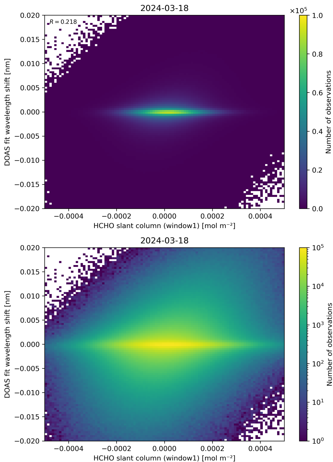
Figure 79: Scatter density plot of “HCHO slant column (window1)” against “DOAS fit wavelength shift” for 2024-03-17 to 2024-03-19.
