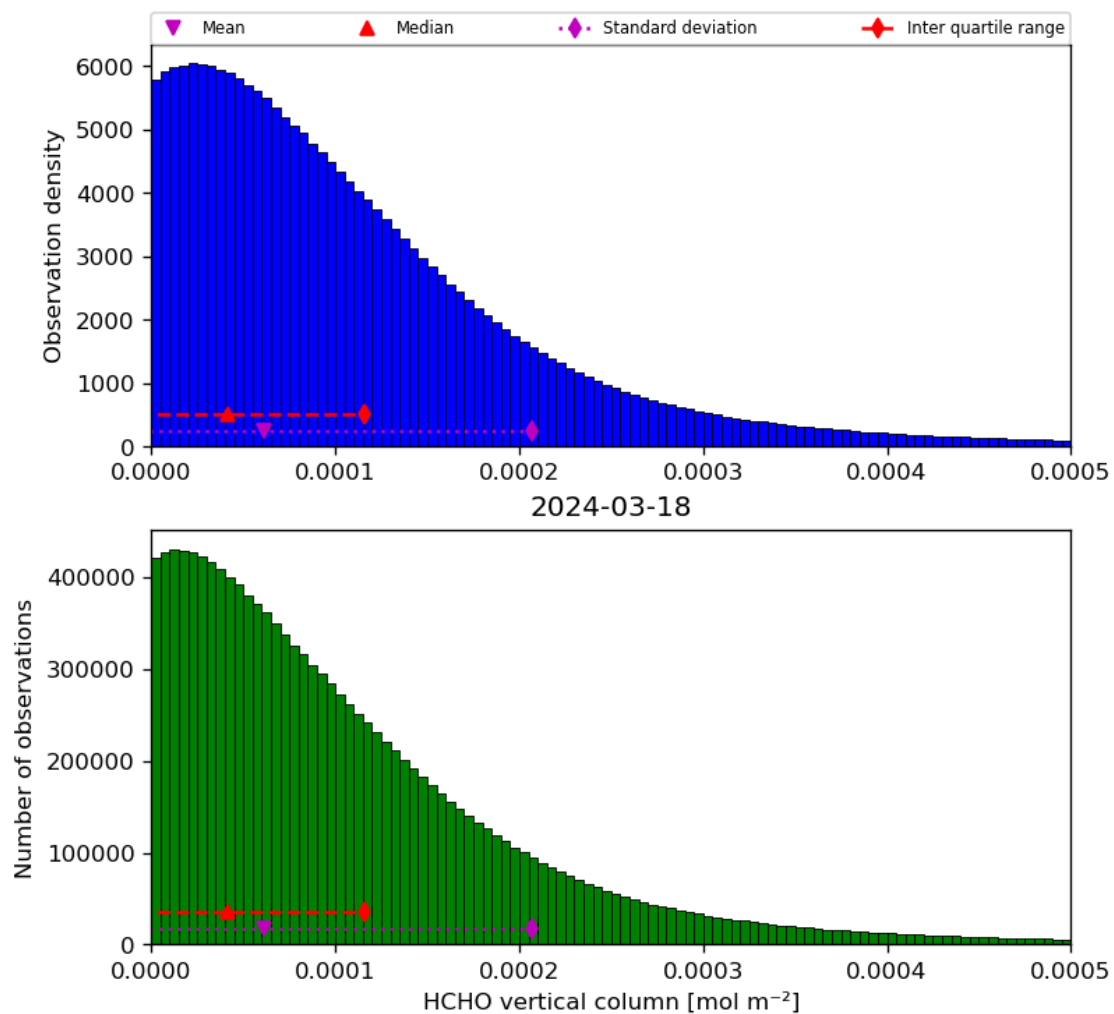
Figure 35: Histogram of “HCHO vertical column” for 2024-03-17 to 2024-03-19
