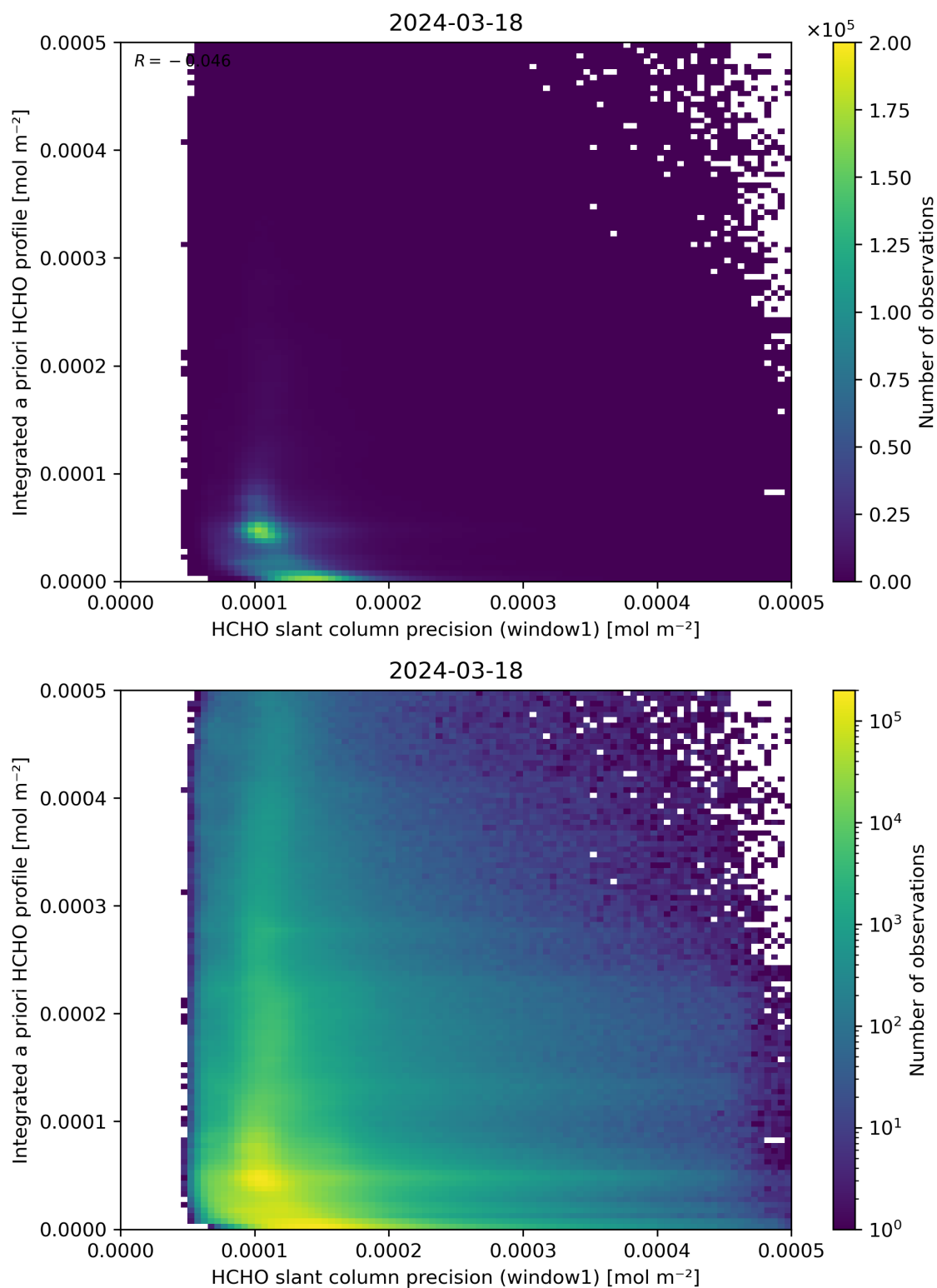
Figure 96: Scatter density plot of “HCHO slant column precision (window1)” against “Integrated a priori HCHO profile” for 2024-03-17 to 2024-03-19.
