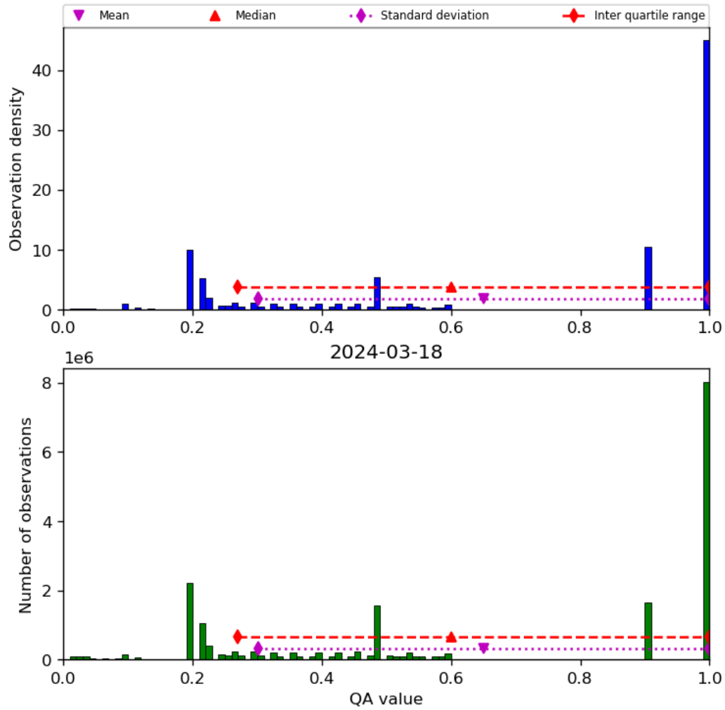
Figure 34: Histogram of “QA value” for 2024-03-17 to 2024-03-19
