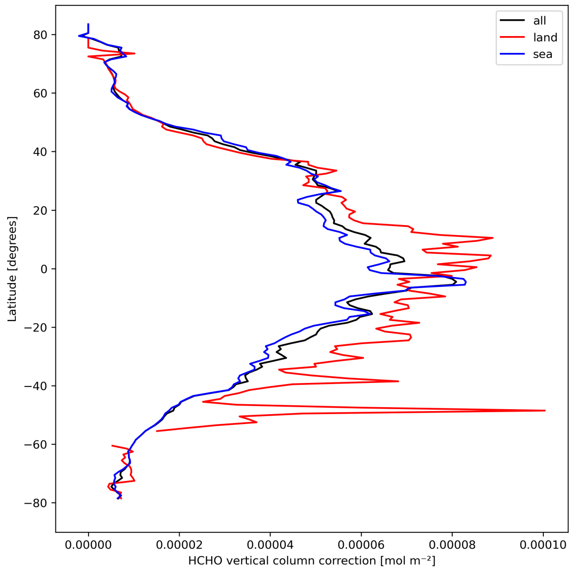
Figure 23: Zonal average of “HCHO vertical column correction” for 2024-03-17 to 2024-03-19.
