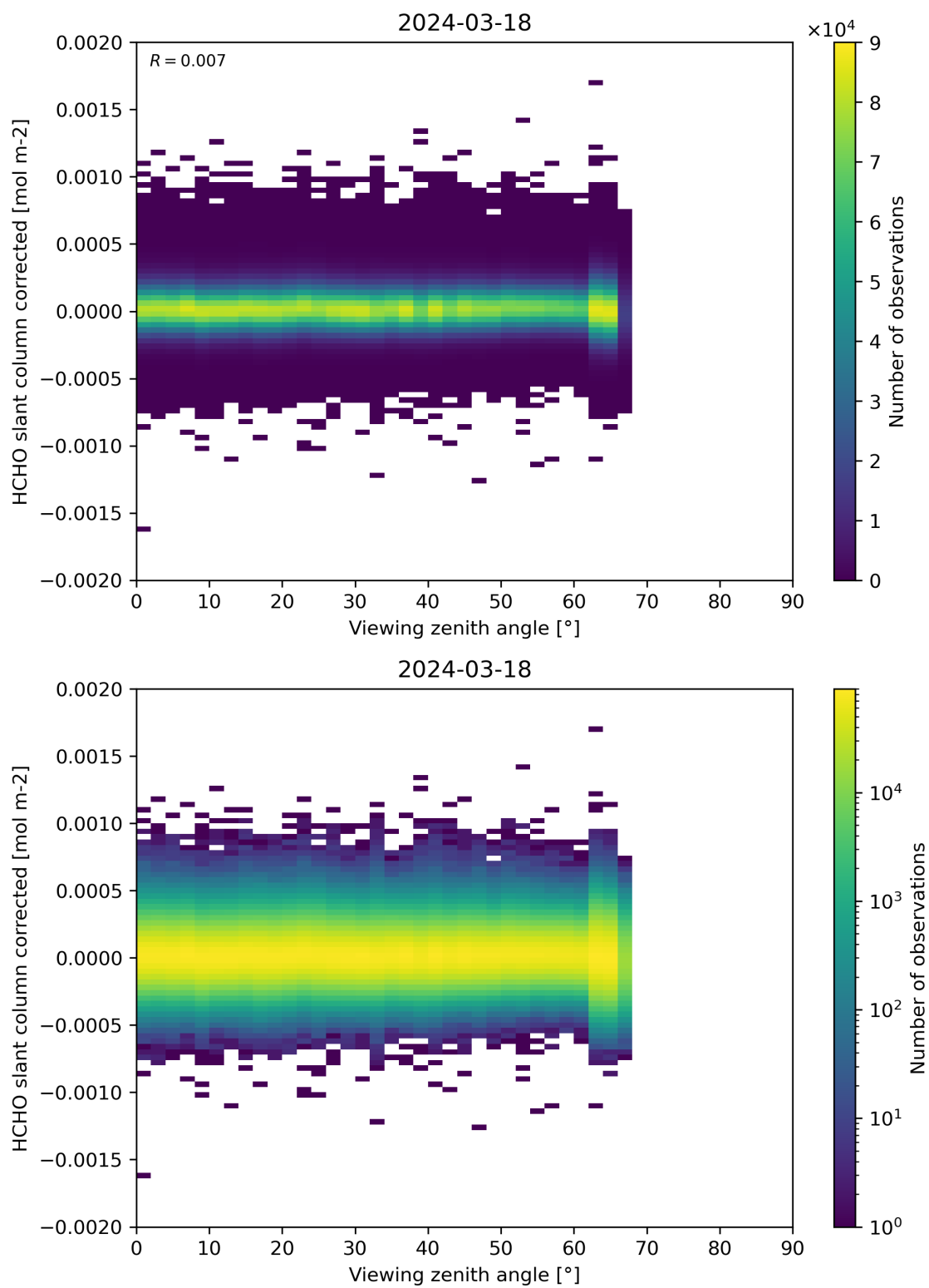
Figure 186: Scatter density plot of “Viewing zenith angle” against “HCHO slant column corrected” for 2024-03-17 to 2024-03-19.
