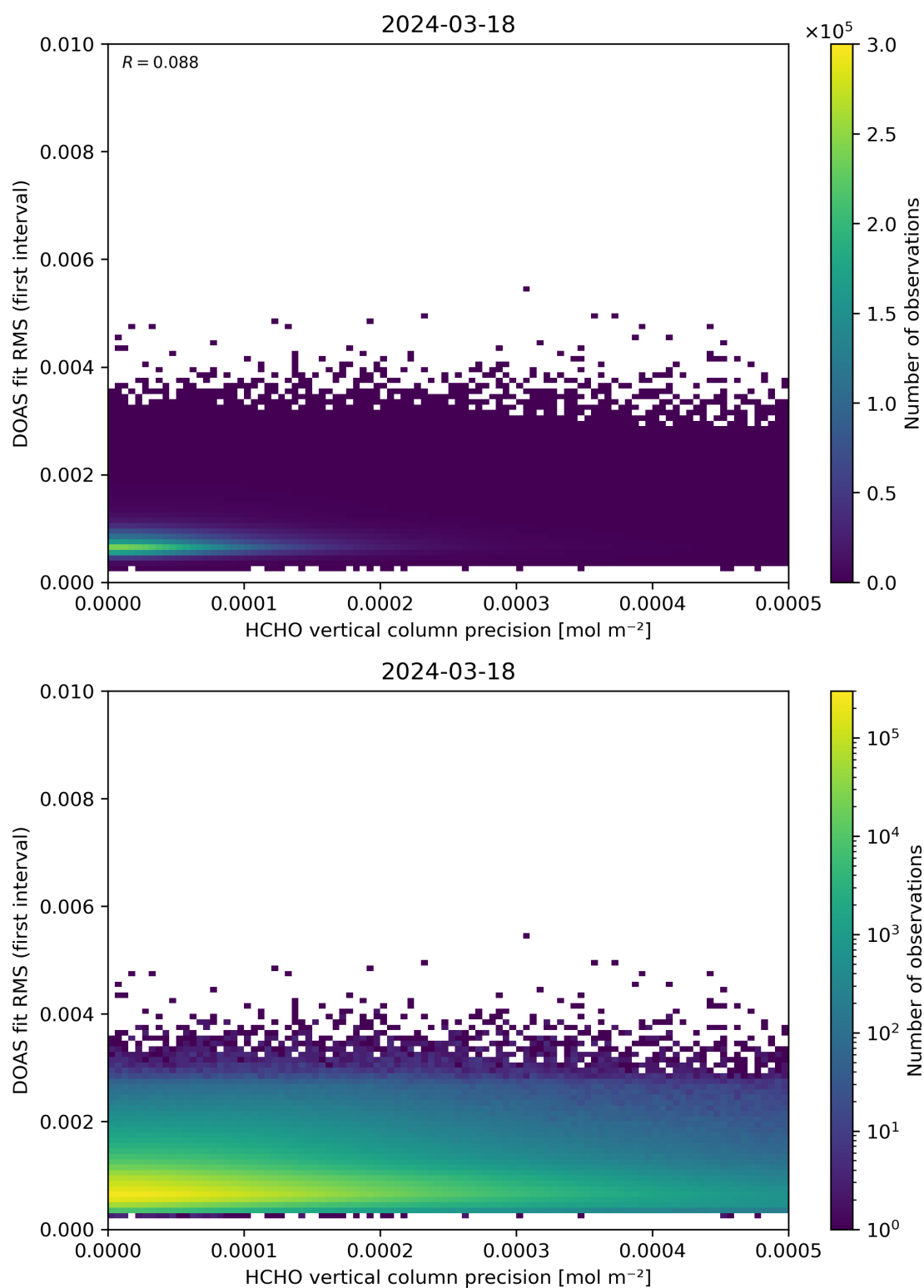
Figure 136: Scatter density plot of “HCHO vertical column precision” against “DOAS fit RMS (first interval)” for 2024-03-17 to 2024-03-19.
