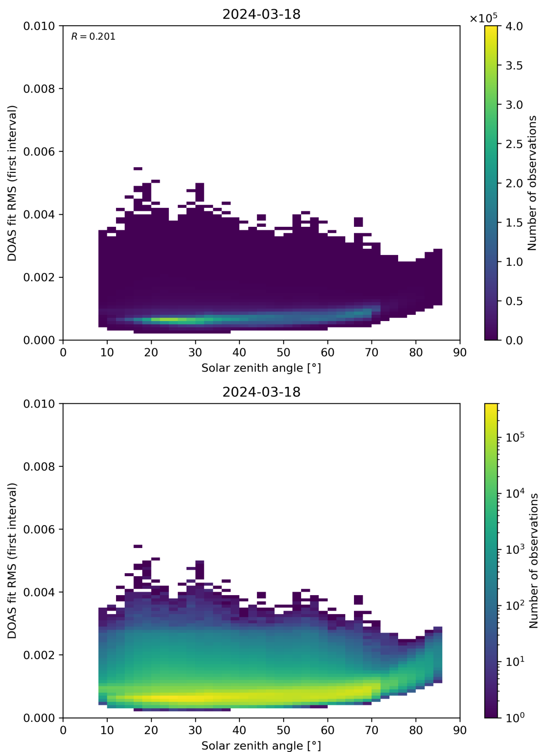
Figure 167: Scatter density plot of “Solar zenith angle” against “DOAS fit RMS (first interval)” for 2024-03-17 to 2024-03-19.
