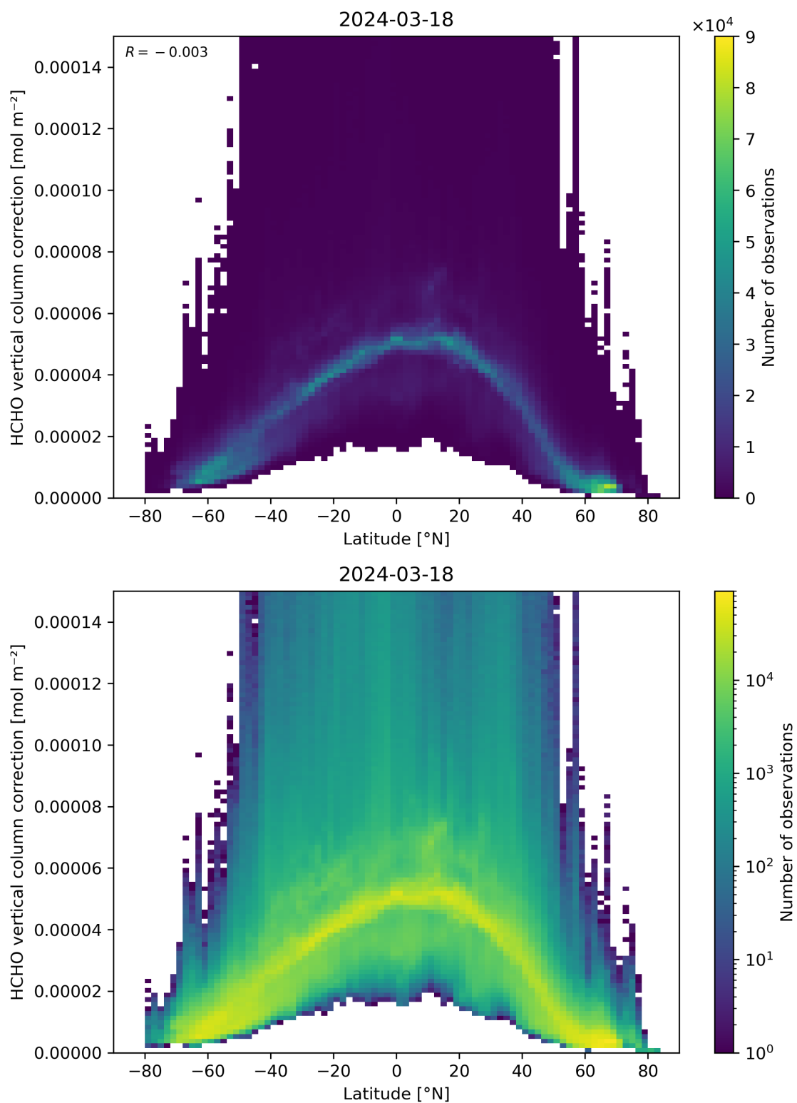
Figure 164: Scatter density plot of “Latitude” against “HCHO vertical column correction” for 2024-03-17 to 2024-03-19.
