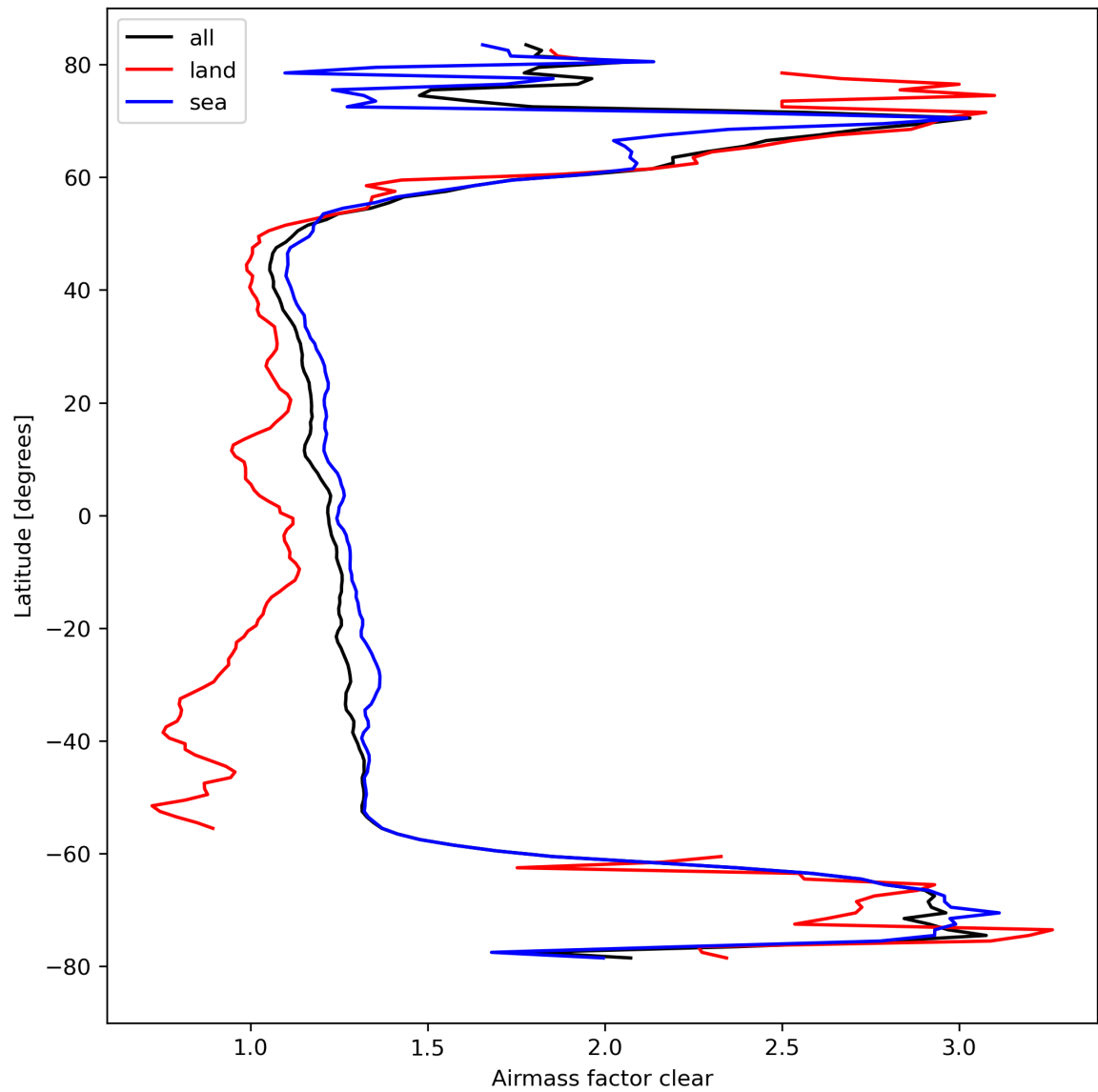
Figure 28: Zonal average of “Airmass factor clear” for 2024-03-17 to 2024-03-19.
