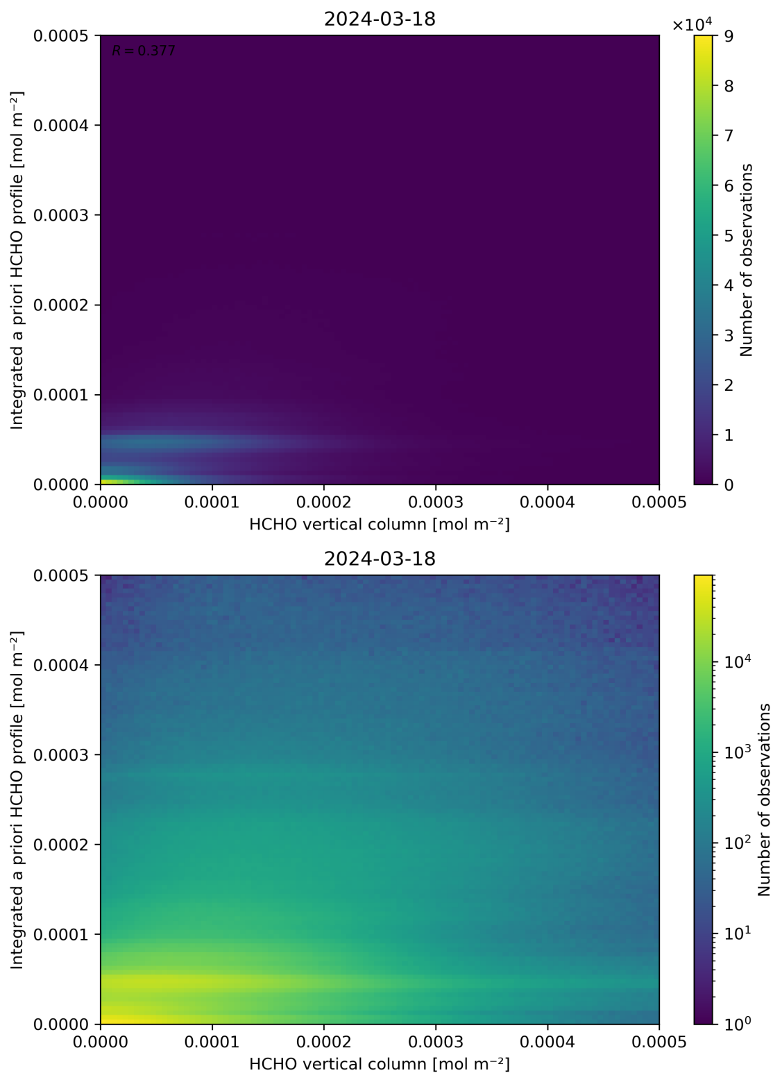
Figure 135: Scatter density plot of “HCHO vertical column” against “Integrated a priori HCHO profile” for 2024-03-17 to 2024-03-19.
