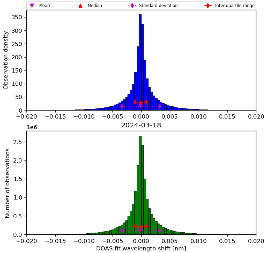
Figure 44: Histogram of “DOAS fit wavelength shift” for 2024-03-17 to 2024-03-19
