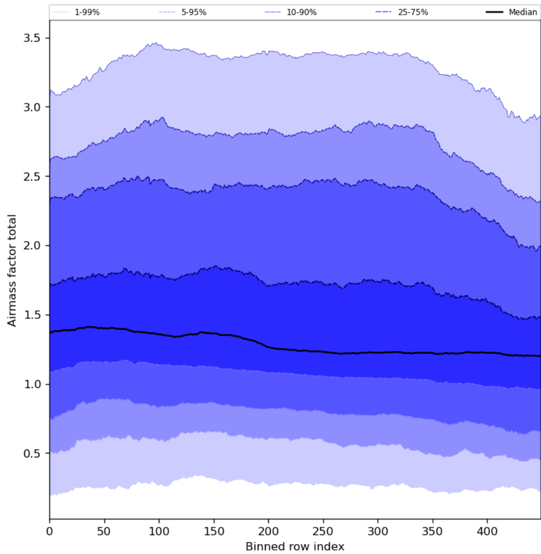
Figure 54: Along track statistics of “Airmass factor total” for 2024-03-17 to 2024-03-19
