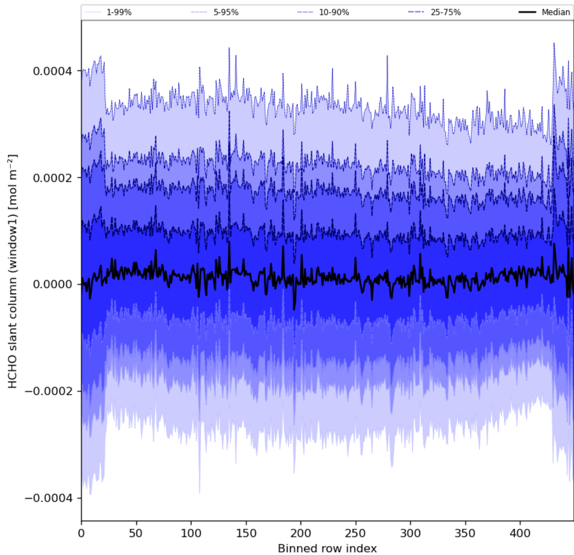
Figure 52: Along track statistics of "HCHO slant column (window1)" for 2024-03-17 to 2024-03-19
