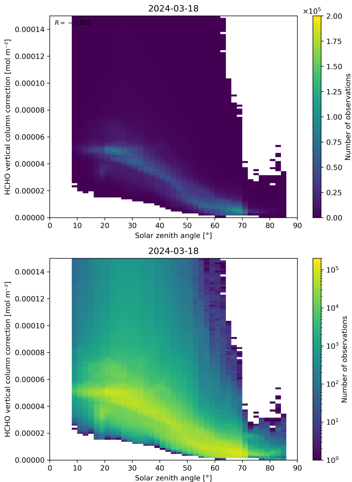
Figure 178: Scatter density plot of “Solar zenith angle” against “HCHO vertical column correction” for 2024-03-17 to 2024-03-19.
