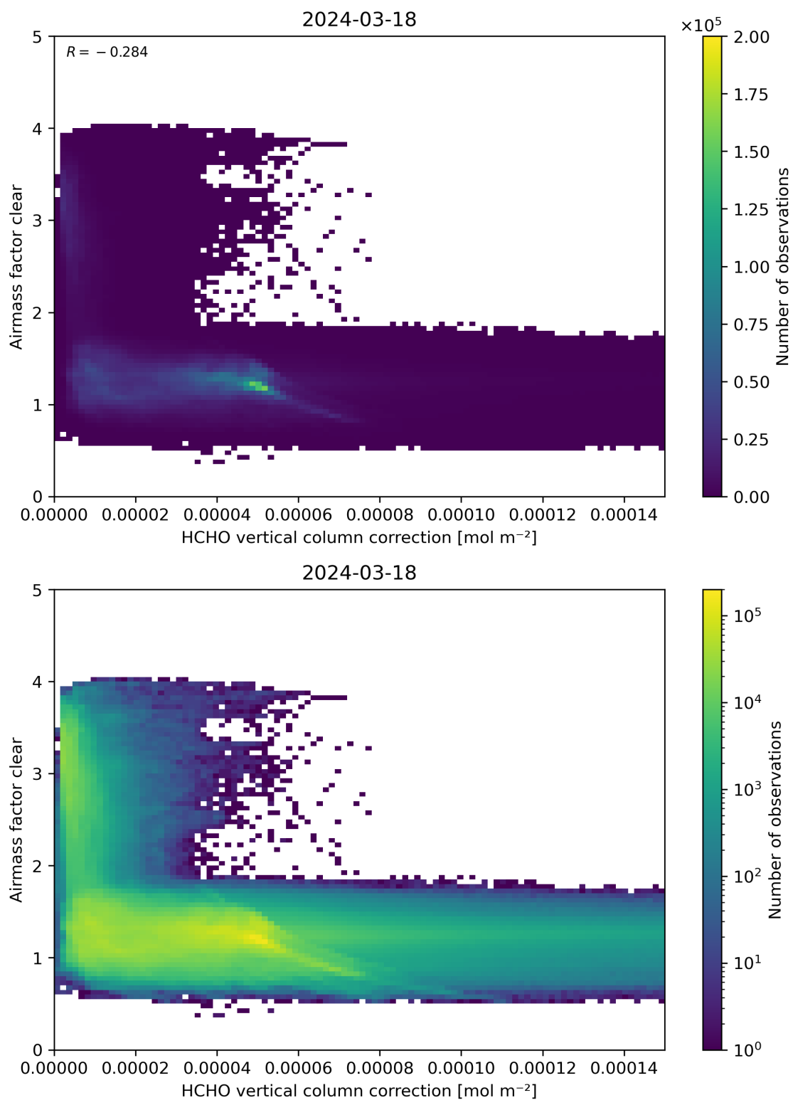
Figure 115: Scatter density plot of “HCHO vertical column correction” against “Airmass factor clear” for 2024-03-17 to 2024-03-19.
