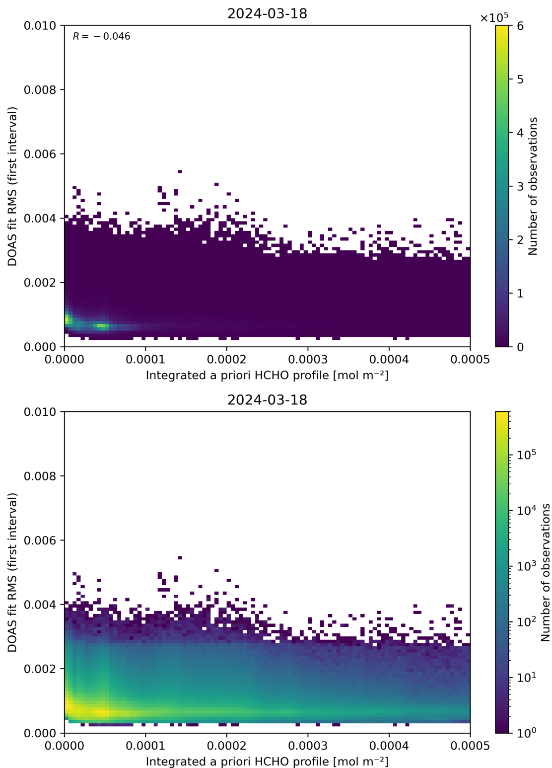
Figure 148: Scatter density plot of “Integrated a priori HCHO profile” against “DOAS fit RMS (first interval)” for 2024-03-17 to 2024-03-19.
