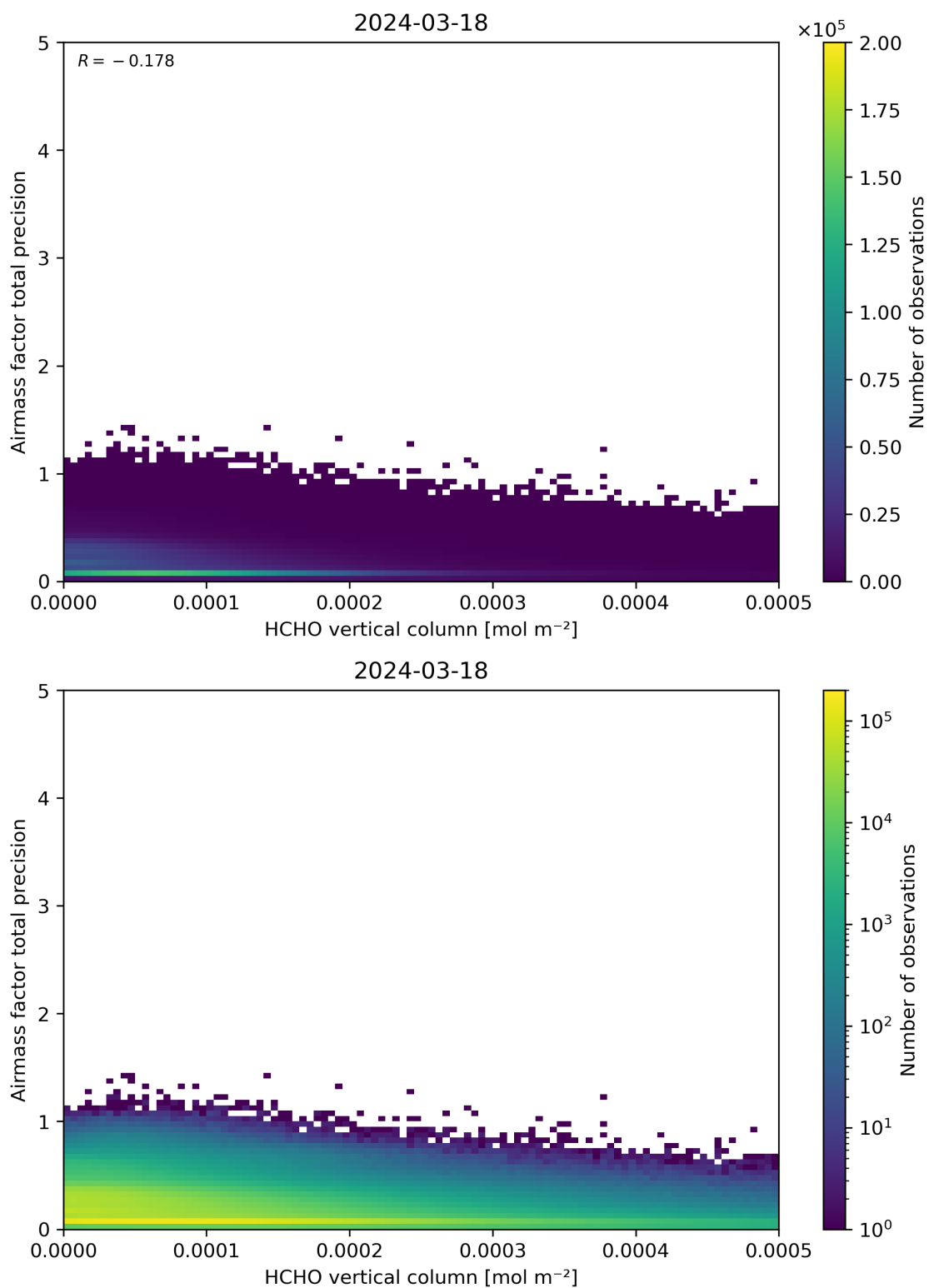
Figure 132: Scatter density plot of “HCHO vertical column” against “Airmass factor total precision” for 2024-03-17 to 2024-03-19.
