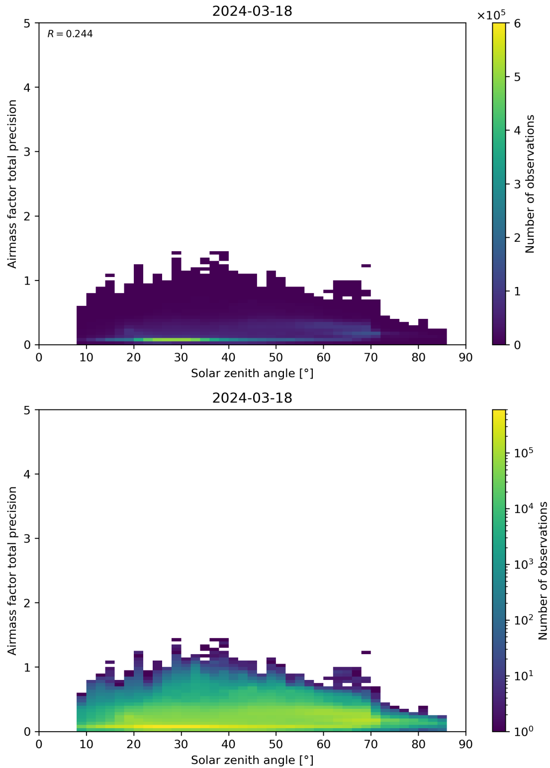
Figure 176: Scatter density plot of “Solar zenith angle” against “Airmass factor total precision” for 2024-03-17 to 2024-03-19.
