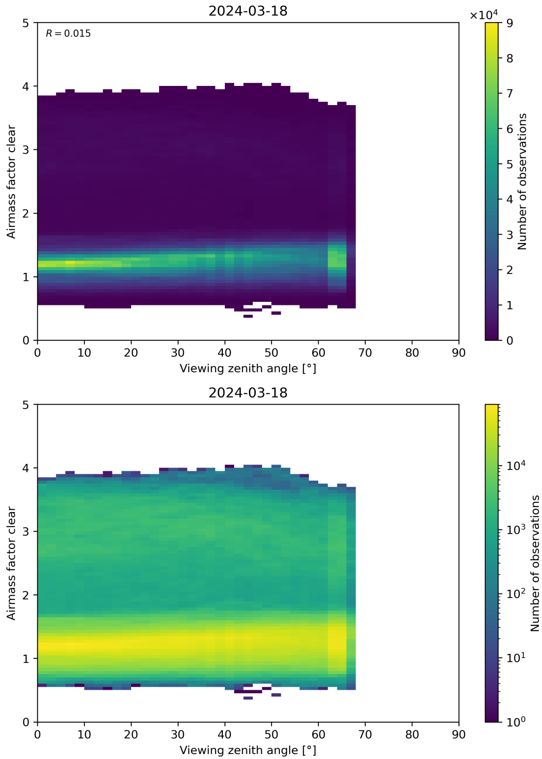
Figure 185: Scatter density plot of “Viewing zenith angle” against “Airmass factor clear” for 2024-03-17 to 2024-03-19.
