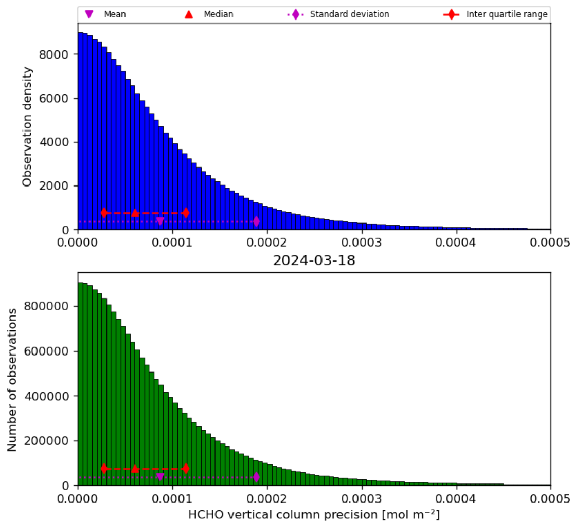
Figure 36: Histogram of “HCHO vertical column precision” for 2024-03-17 to 2024-03-19
