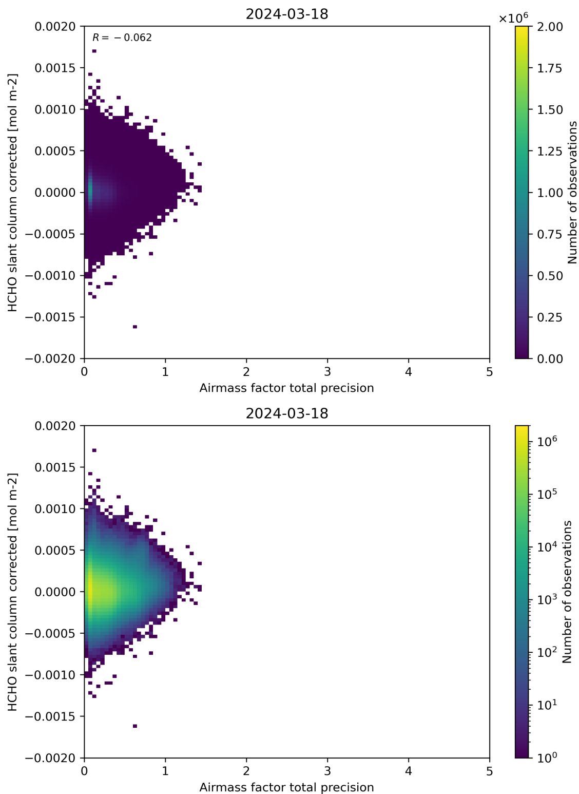
Figure 109: Scatter density plot of “Airmass factor total precision” against “HCHO slant column corrected” for 2024-03-17 to 2024-03-19.
