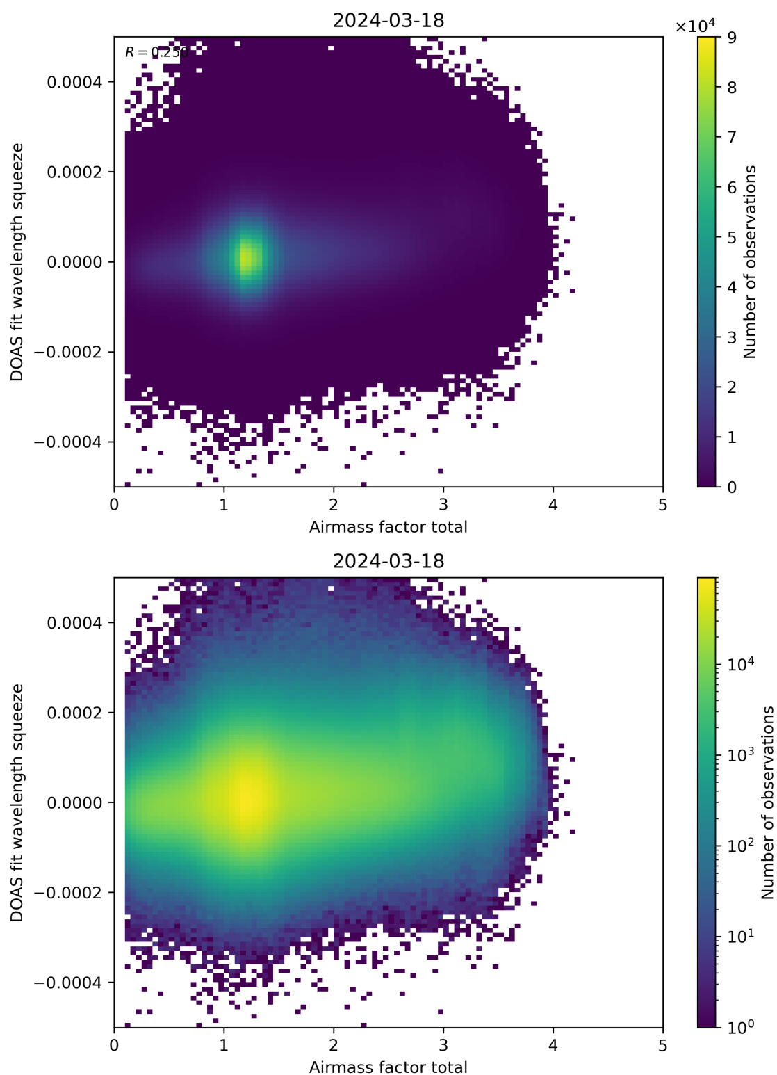
Figure 99: Scatter density plot of “Airmass factor total” against “DOAS fit wavelength squeeze” for 2024-03-17 to 2024-03-19.
