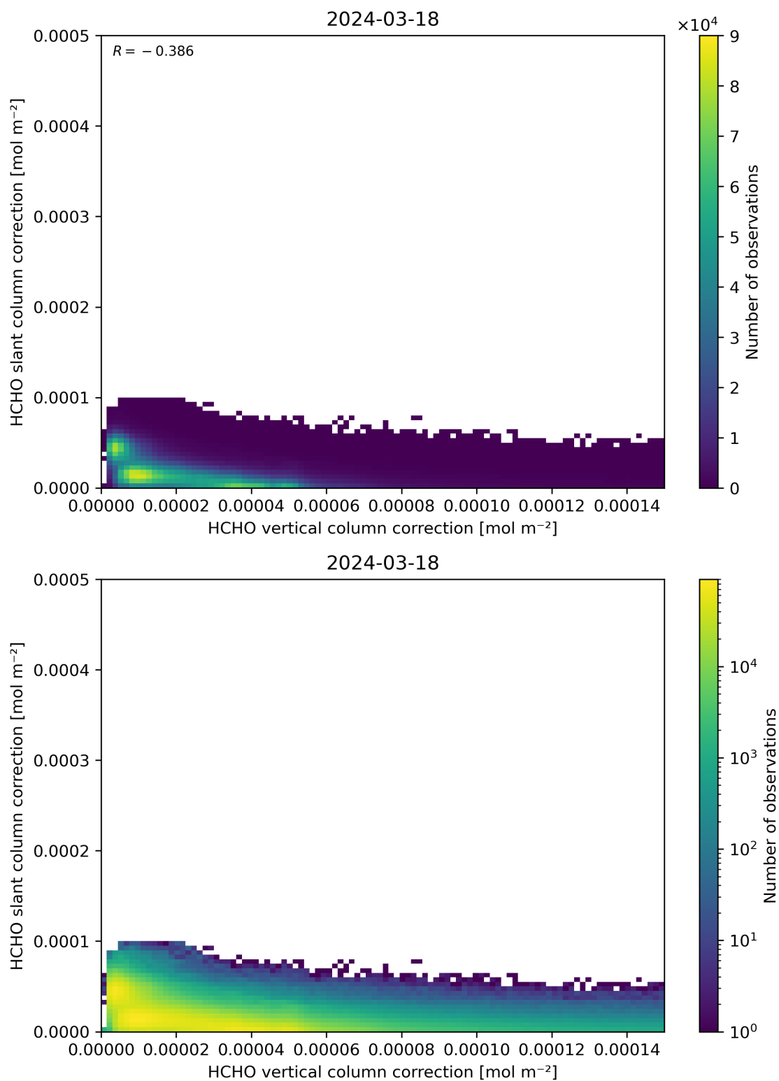
Figure 117: Scatter density plot of “HCHO vertical column correction” against “HCHO slant column correction” for 2024-03-17 to 2024-03-19.
