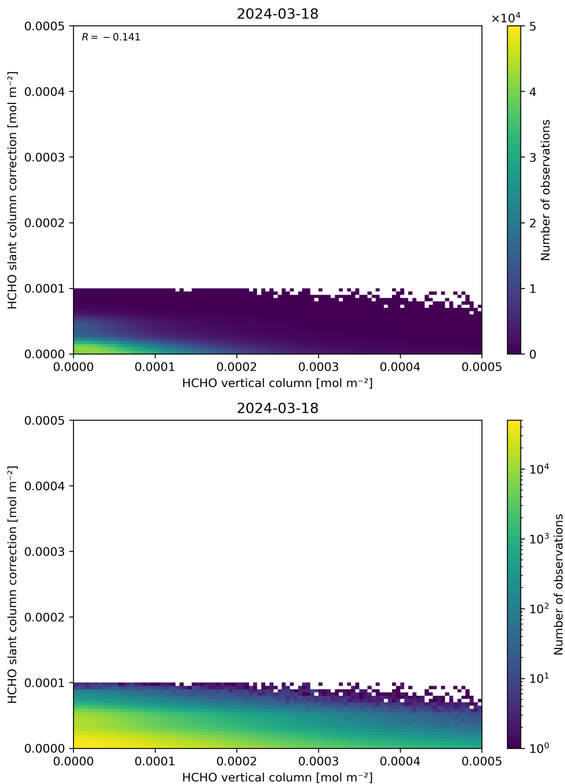
Figure 128: Scatter density plot of “HCHO vertical column” against “HCHO slant column correction” for 2024-03-17 to 2024-03-19.
