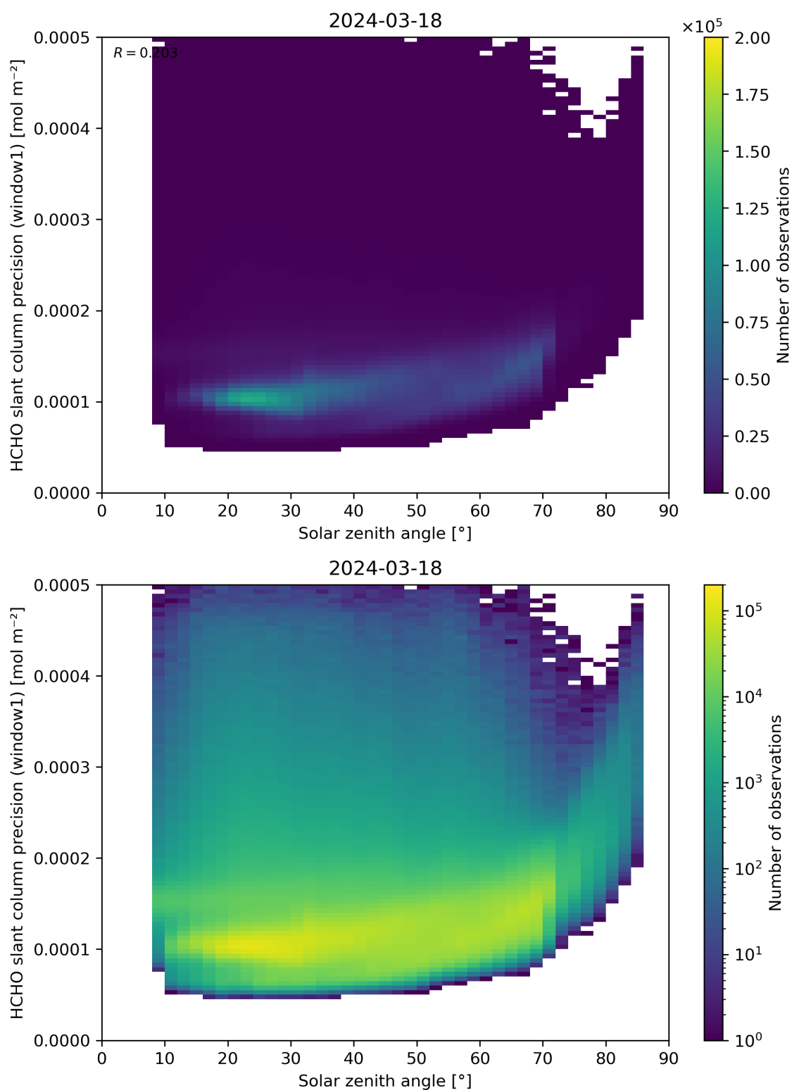
Figure 174: Scatter density plot of “Solar zenith angle” against “HCHO slant column precision (window1)” for 2024-03-17 to 2024-03-19.
