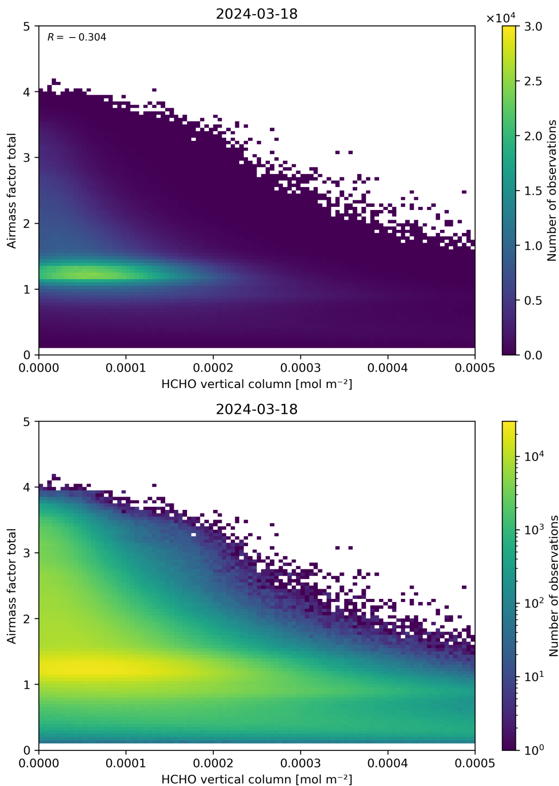
Figure 131: Scatter density plot of “HCHO vertical column” against “Airmass factor total” for 2024-03-17 to 2024-03-19.
