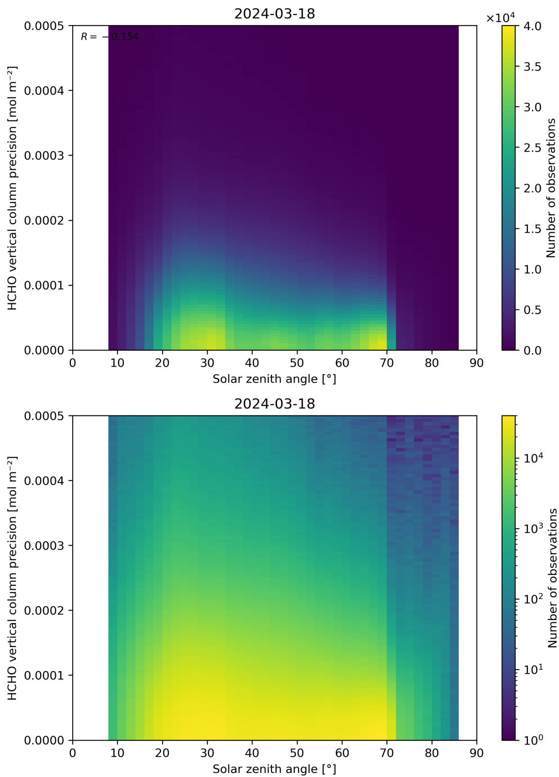
Figure 179: Scatter density plot of “Solar zenith angle” against “HCHO vertical column precision” for 2024-03-17 to 2024-03-19.
