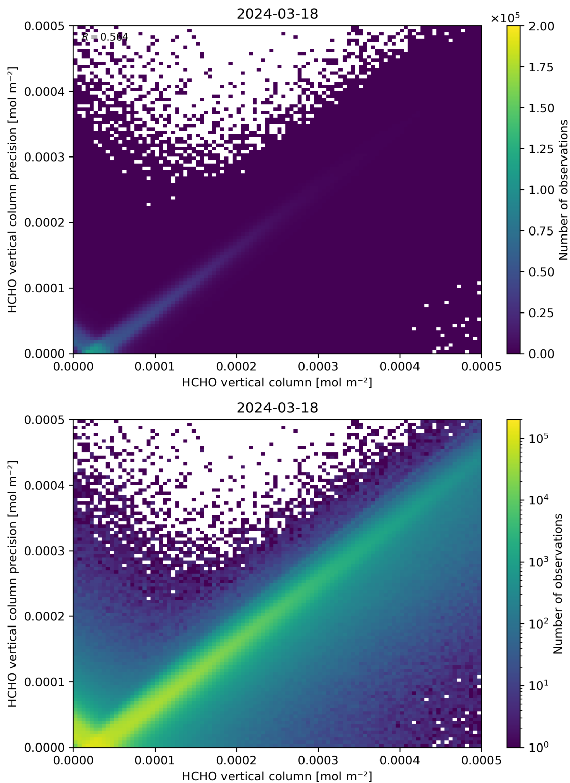
Figure 134: Scatter density plot of “HCHO vertical column” against “HCHO vertical column precision” for 2024-03-17 to 2024-03-19.
