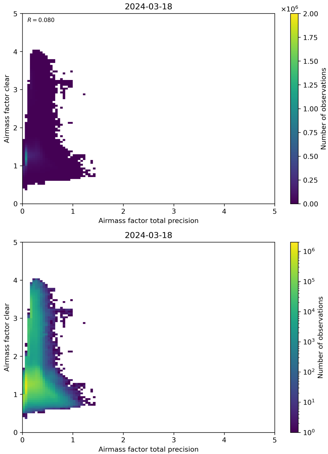
Figure 108: Scatter density plot of “Airmass factor total precision” against “Airmass factor clear” for 2024-03-17 to 2024-03-19.
