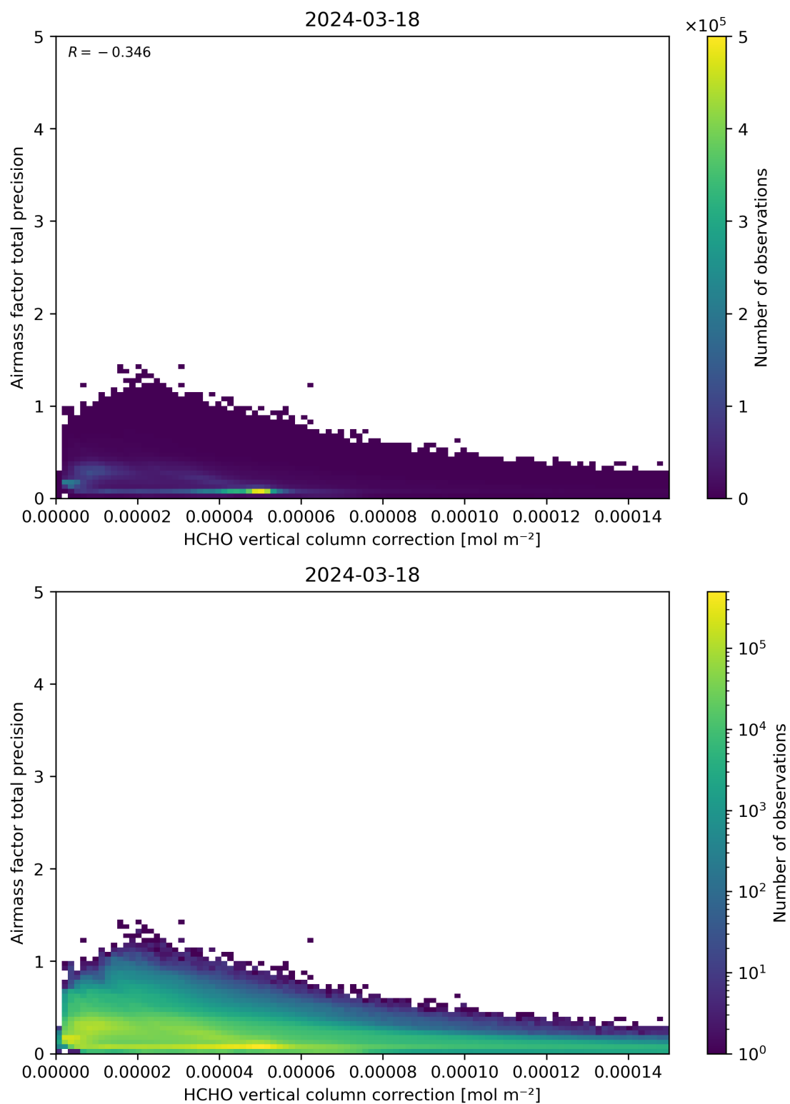
Figure 121: Scatter density plot of “HCHO vertical column correction” against “Airmass factor total precision” for 2024-03-17 to 2024-03-19.
