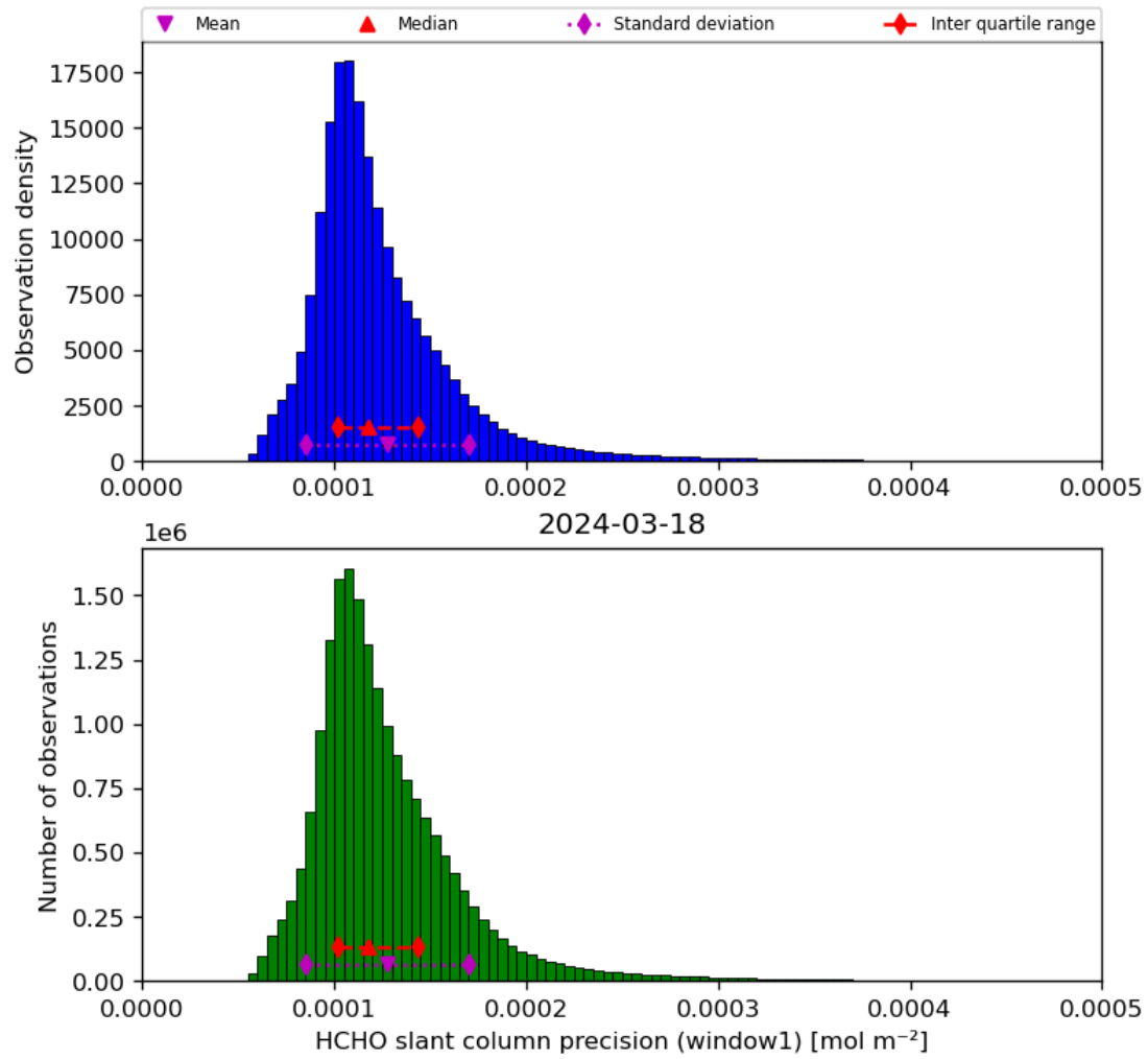
Figure 39: Histogram of “HCHO slant column precision (window1)” for 2024-03-17 to 2024-03-19
