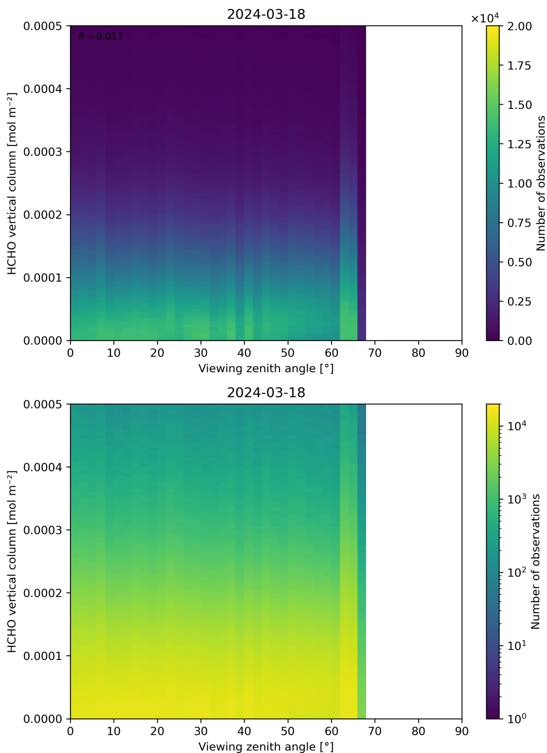
Figure 192: Scatter density plot of “Viewing zenith angle” against “HCHO vertical column” for 2024-03-17 to 2024-03-19.
