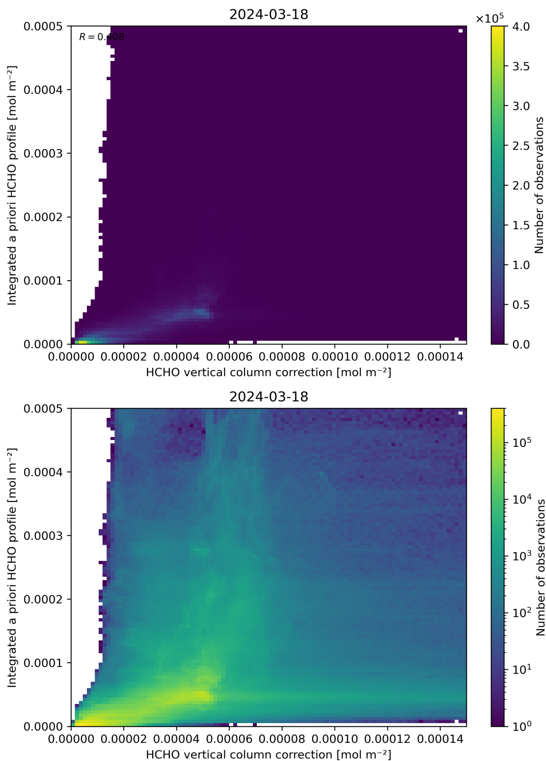
Figure 122: Scatter density plot of “HCHO vertical column correction” against “Integrated a priori HCHO profile” for 2024-03-17 to 2024-03-19.
