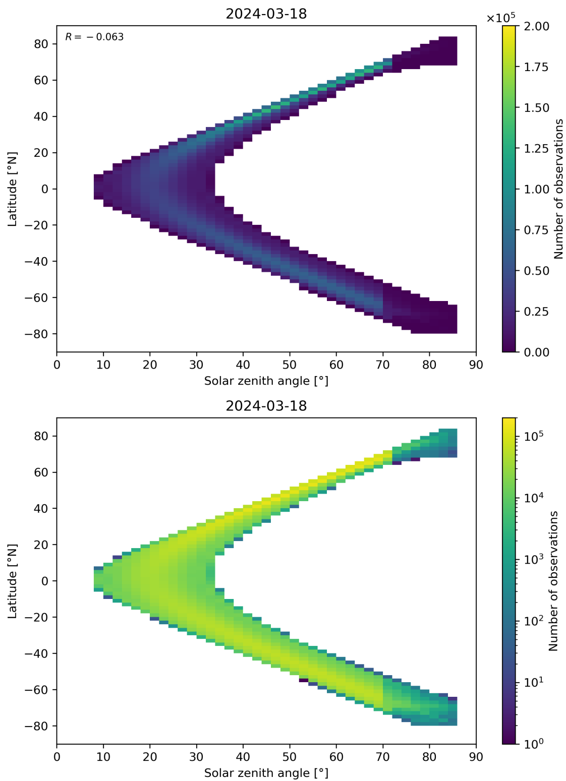
Figure 181: Scatter density plot of “Solar zenith angle” against “Latitude” for 2024-03-17 to 2024-03-19.
