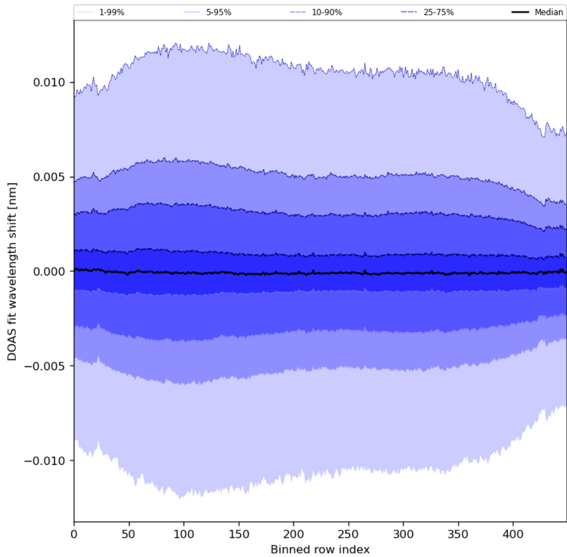
Figure 58: Along track statistics of “DOAS fit wavelength shift” for 2024-03-17 to 2024-03-19
