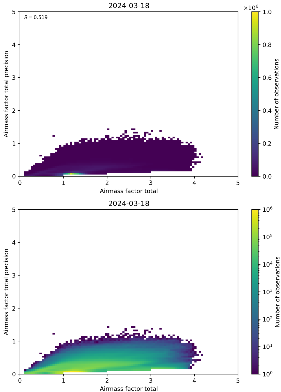
Figure 103: Scatter density plot of “Airmass factor total” against “Airmass factor total precision” for 2024-03-17 to 2024-03-19.
