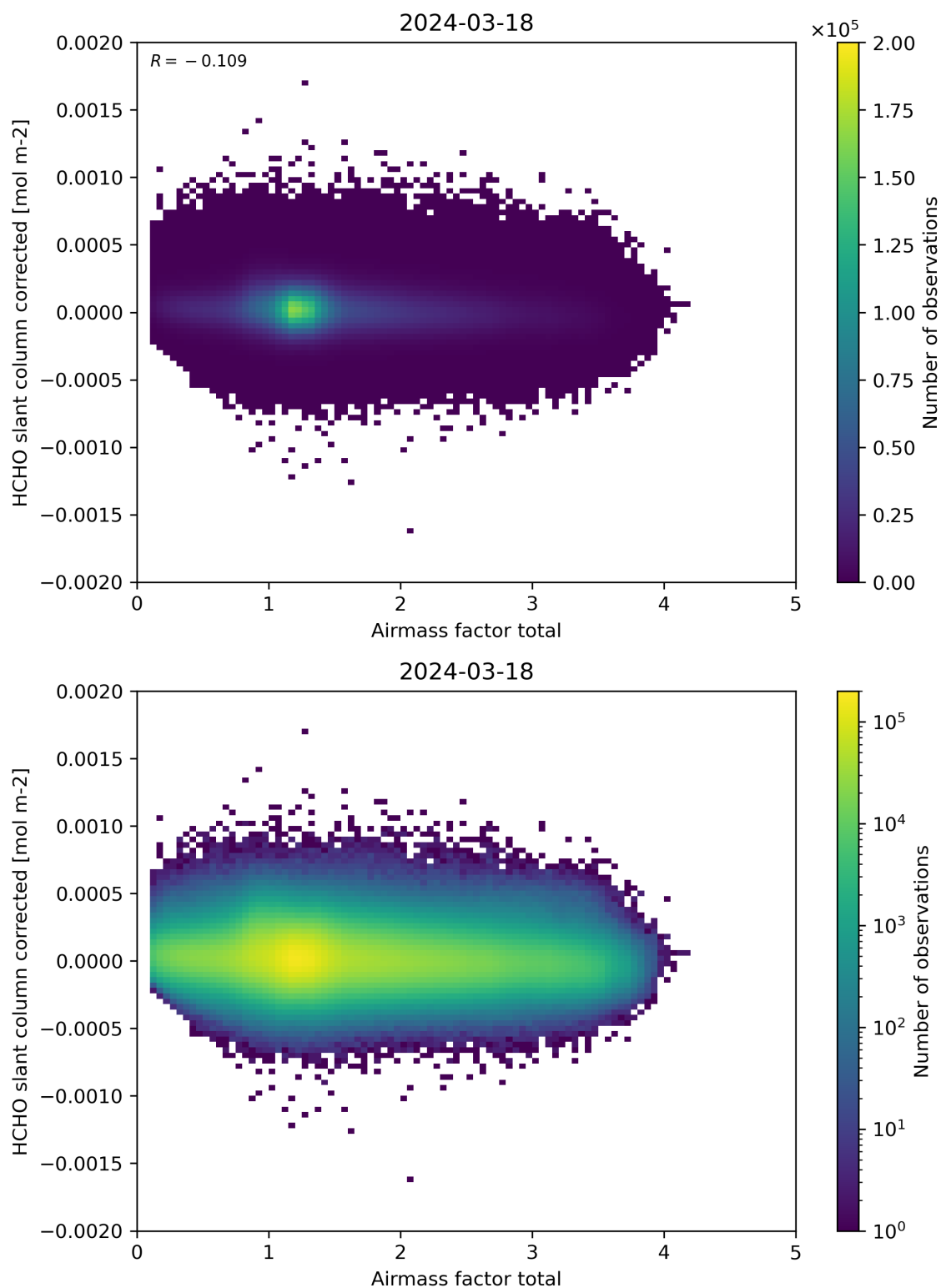
Figure 101: Scatter density plot of “Airmass factor total” against “HCHO slant column corrected” for 2024-03-17 to 2024-03-19.
