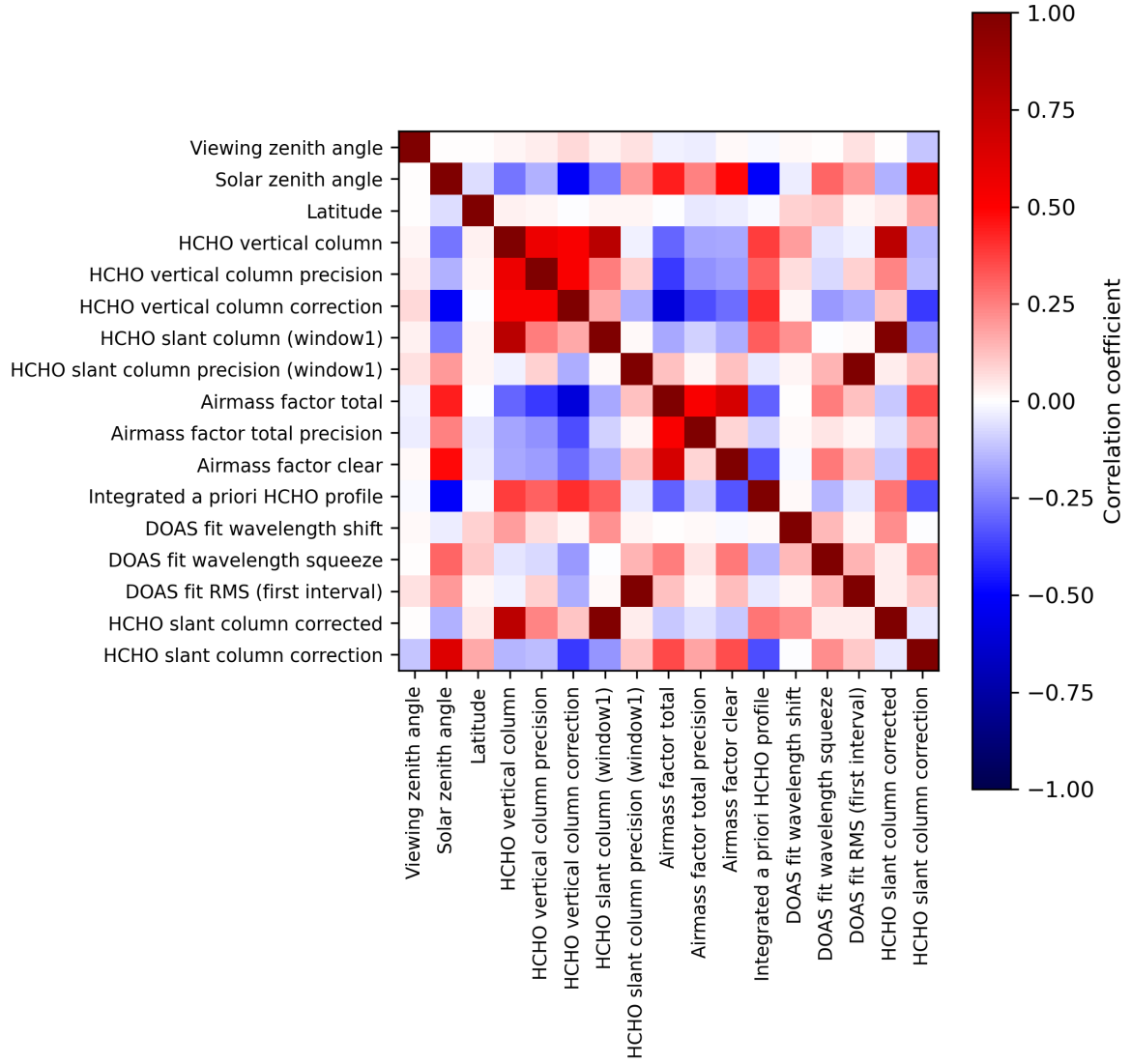
Figure 2: Map of correlation matrix for 2024-03-17 to 2024-03-19.
