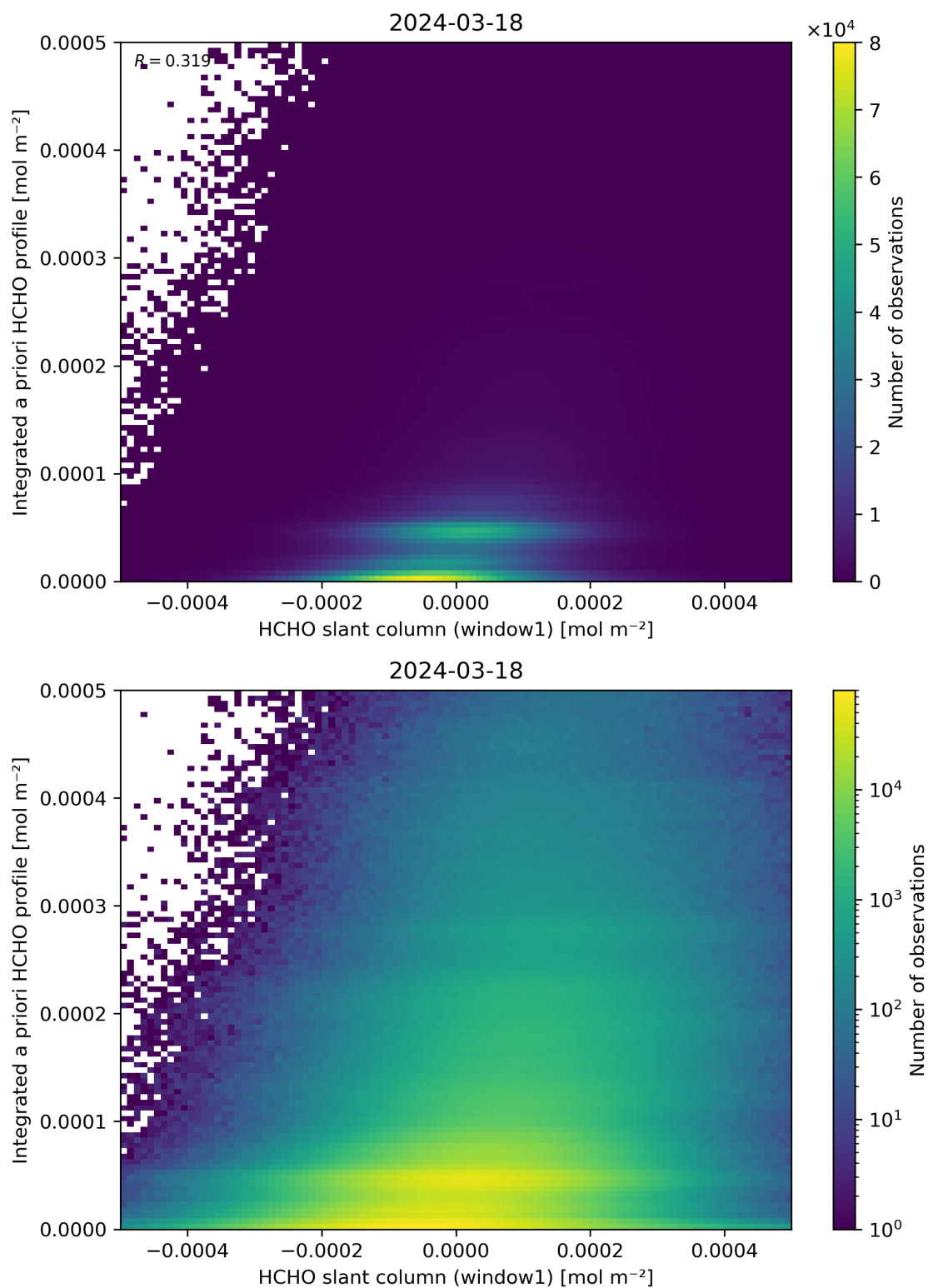
Figure 87: Scatter density plot of “HCHO slant column (window1)” against “Integrated a priori HCHO profile” for 2024-03-17 to 2024-03-19.
