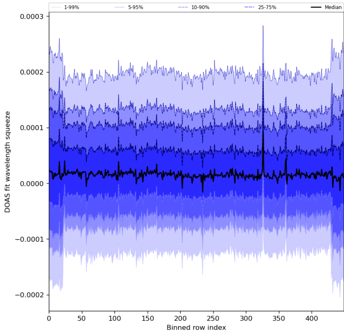
Figure 59: Along track statistics of “DOAS fit wavelength squeeze” for 2024-03-17 to 2024-03-19
