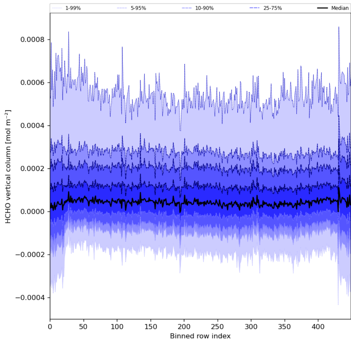
Figure 49: Along track statistics of “HCHO vertical column” for 2024-03-17 to 2024-03-19
