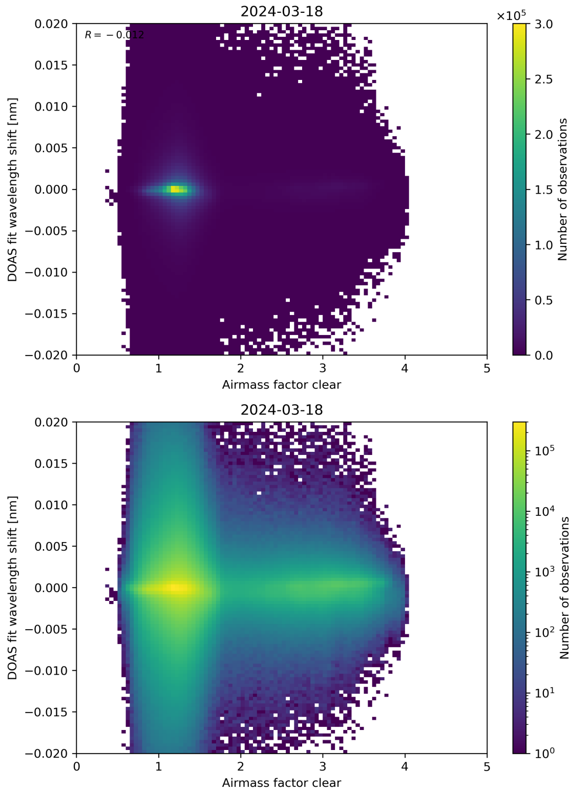
Figure 72: Scatter density plot of “Airmass factor clear” against “DOAS fit wavelength shift” for 2024-03-17 to 2024-03-19.
