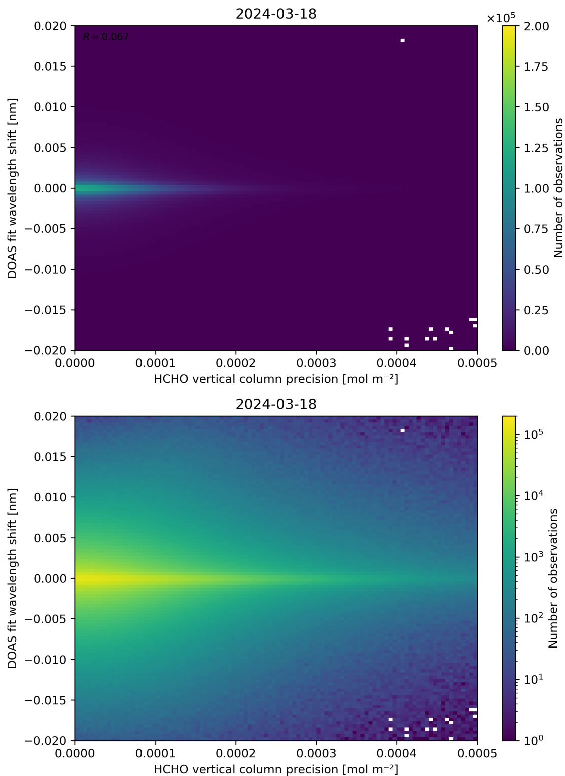
Figure 137: Scatter density plot of “HCHO vertical column precision” against “DOAS fit wavelength shift” for 2024-03-17 to 2024-03-19.
