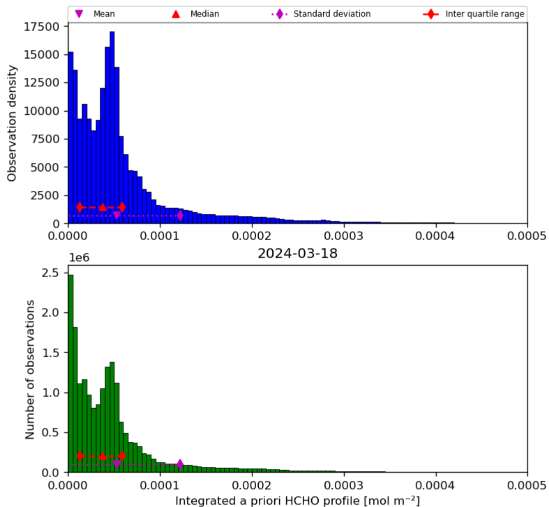
Figure 43: Histogram of “Integrated a priori HCHO profile” for 2024-03-17 to 2024-03-19
