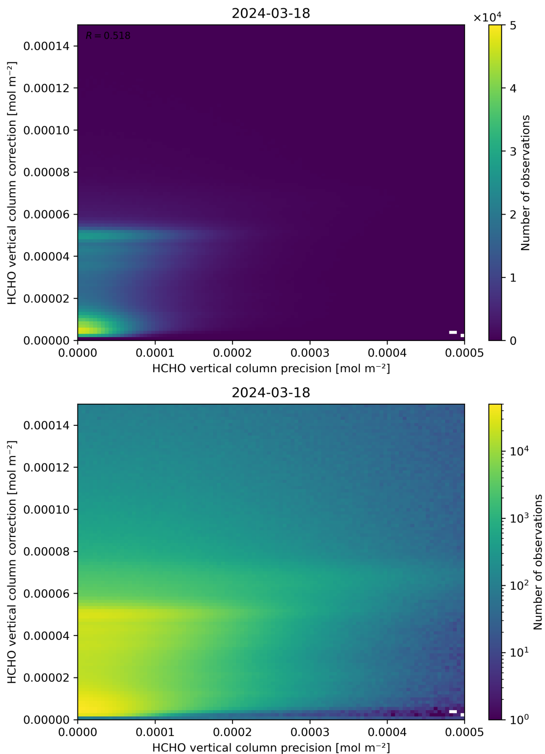
Figure 146: Scatter density plot of “HCHO vertical column precision” against “HCHO vertical column correction” for 2024-03-17 to 2024-03-19.
