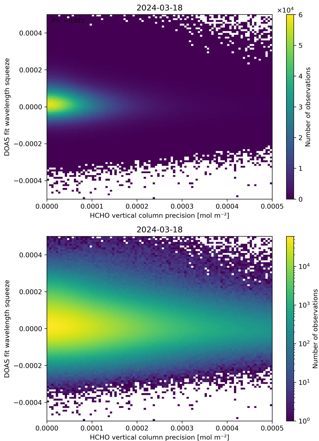
Figure 138: Scatter density plot of “HCHO vertical column precision” against “DOAS fit wavelength squeeze” for 2024-03-17 to 2024-03-19.
