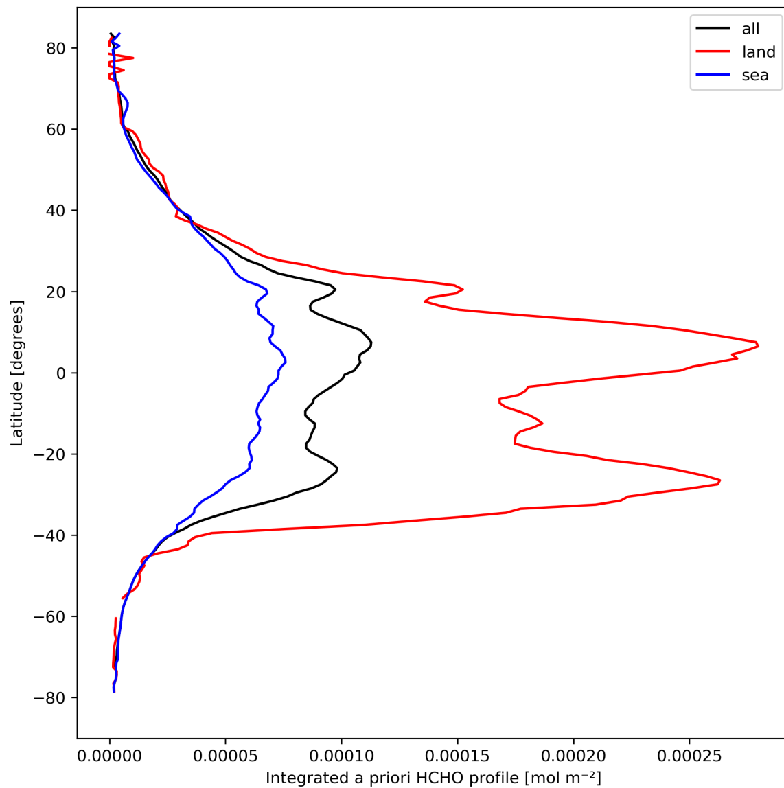
Figure 29: Zonal average of “Integrated a priori HCHO profile” for 2024-03-17 to 2024-03-19.
