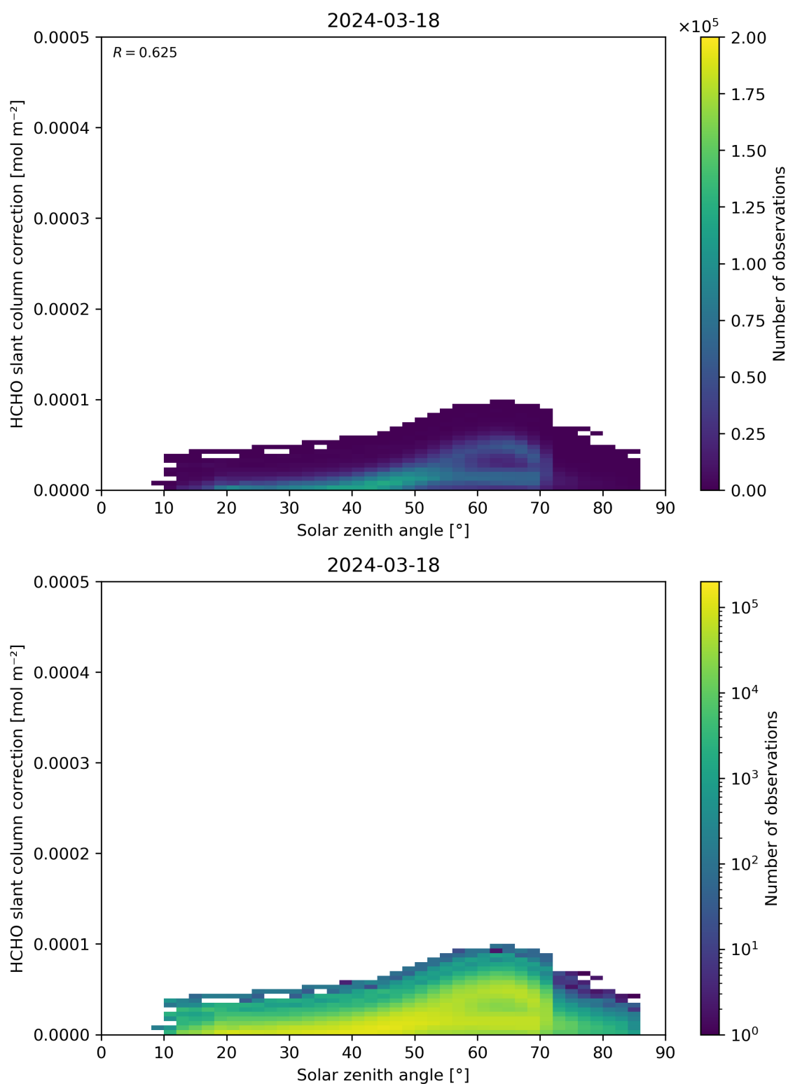
Figure 172: Scatter density plot of “Solar zenith angle” against “HCHO slant column correction” for 2024-03-17 to 2024-03-19.
