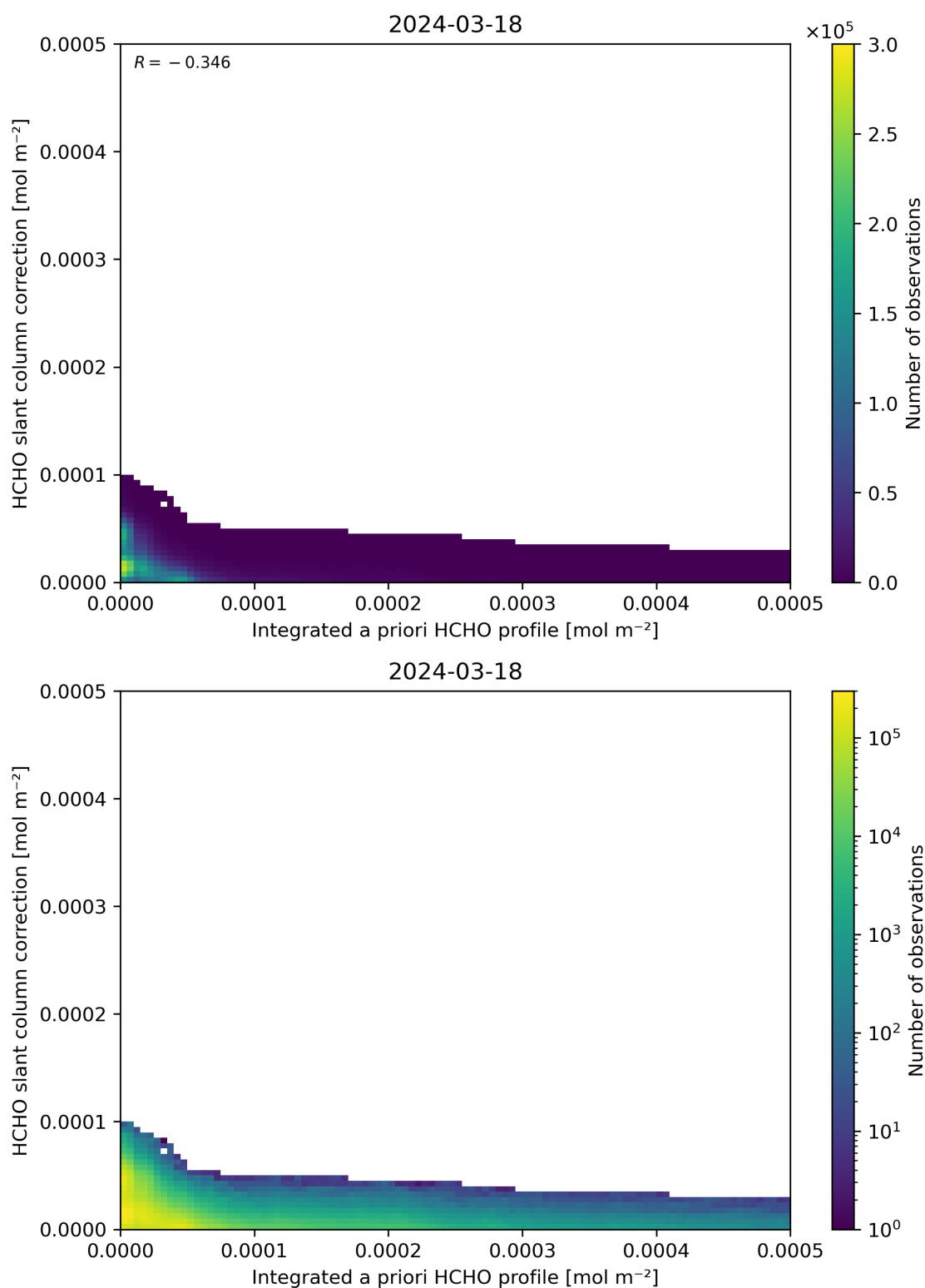
Figure 152: Scatter density plot of “Integrated a priori HCHO profile” against “HCHO slant column correction” for 2024-03-17 to 2024-03-19.
