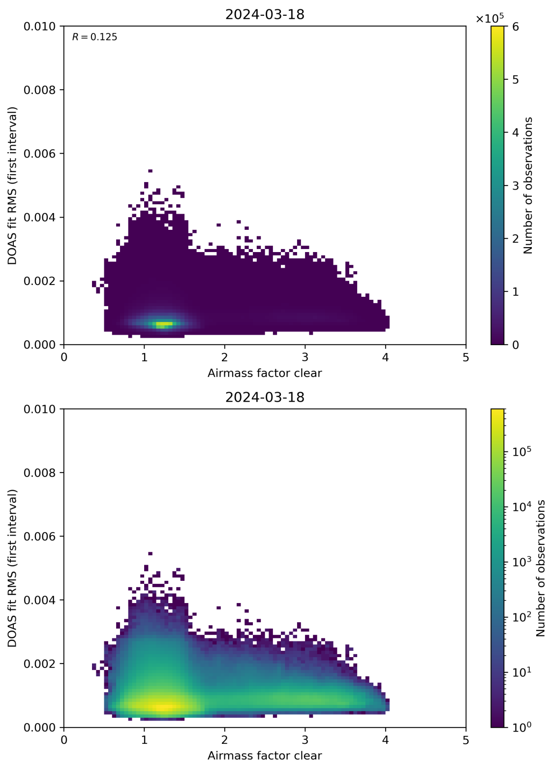
Figure 71: Scatter density plot of “Airmass factor clear” against “DOAS fit RMS (first interval)” for 2024-03-17 to 2024-03-19.
