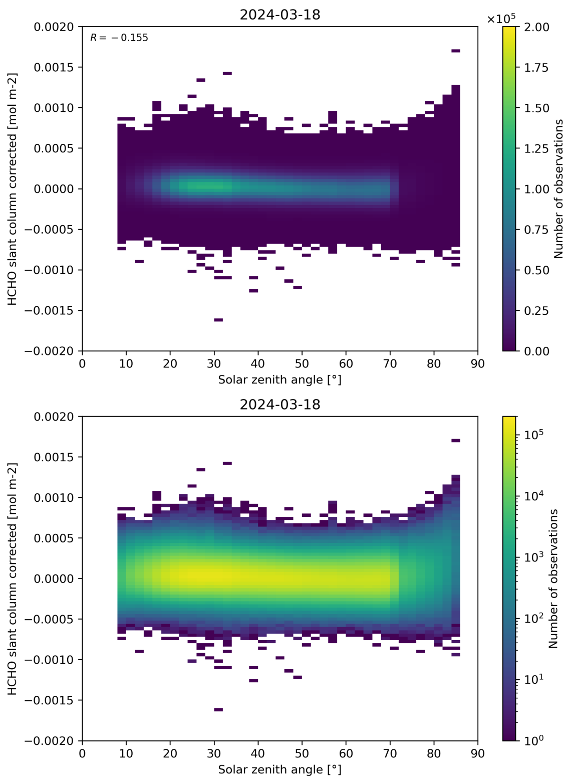
Figure 171: Scatter density plot of “Solar zenith angle” against “HCHO slant column corrected” for 2024-03-17 to 2024-03-19.
