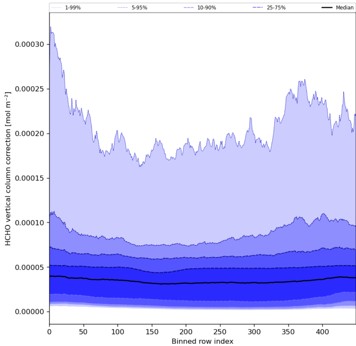
Figure 51: Along track statistics of “HCHO vertical column correction” for 2024-03-17 to 2024-03-19
