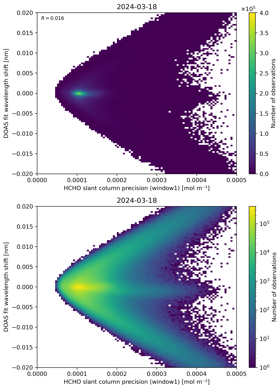
Figure 89: Scatter density plot of “HCHO slant column precision (window1)” against “DOAS fit wavelength shift” for 2024-03-17 to 2024-03-19.
