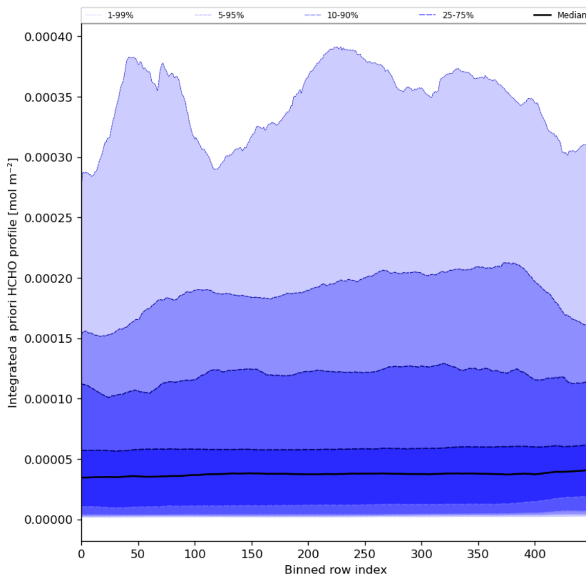
Figure 57: Along track statistics of "Integrated a priori HCHO profile" for 2024-03-17 to 2024-03-19
