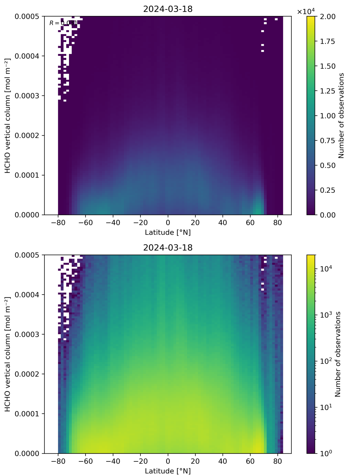
Figure 163: Scatter density plot of “Latitude” against “HCHO vertical column” for 2024-03-17 to 2024-03-19.
