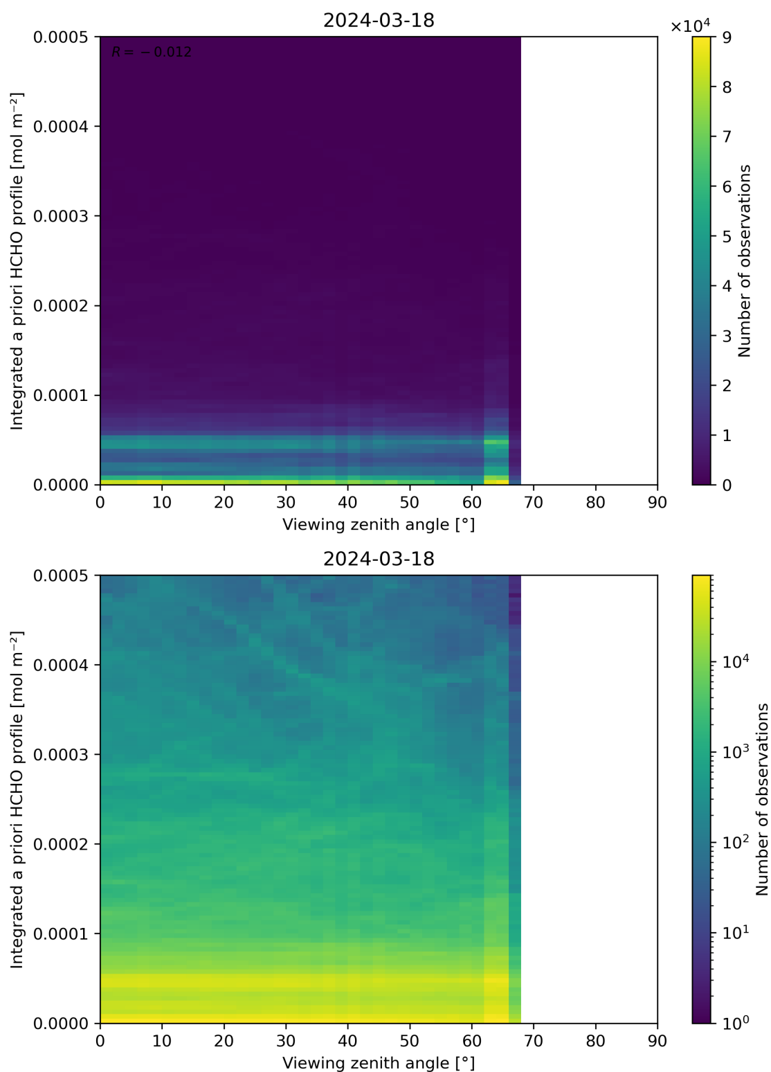
Figure 195: Scatter density plot of “Viewing zenith angle” against “Integrated a priori HCHO profile” for 2024-03-17 to 2024-03-19.
