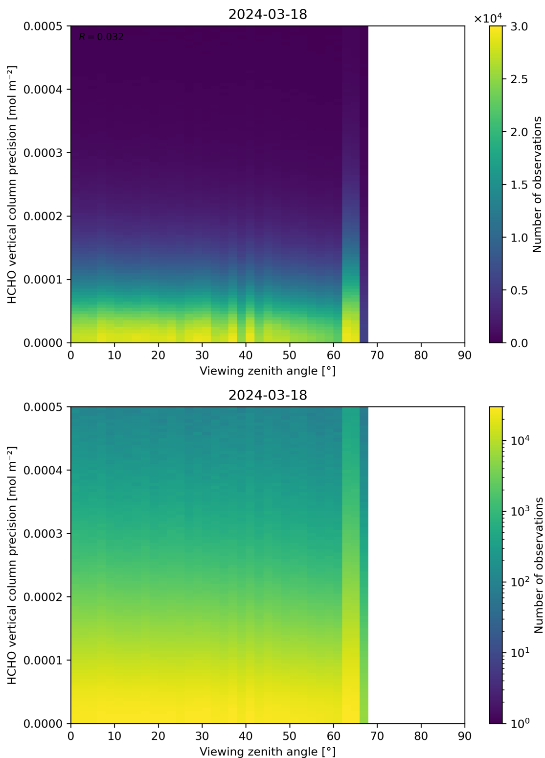
Figure 194: Scatter density plot of “Viewing zenith angle” against “HCHO vertical column precision” for 2024-03-17 to 2024-03-19.
