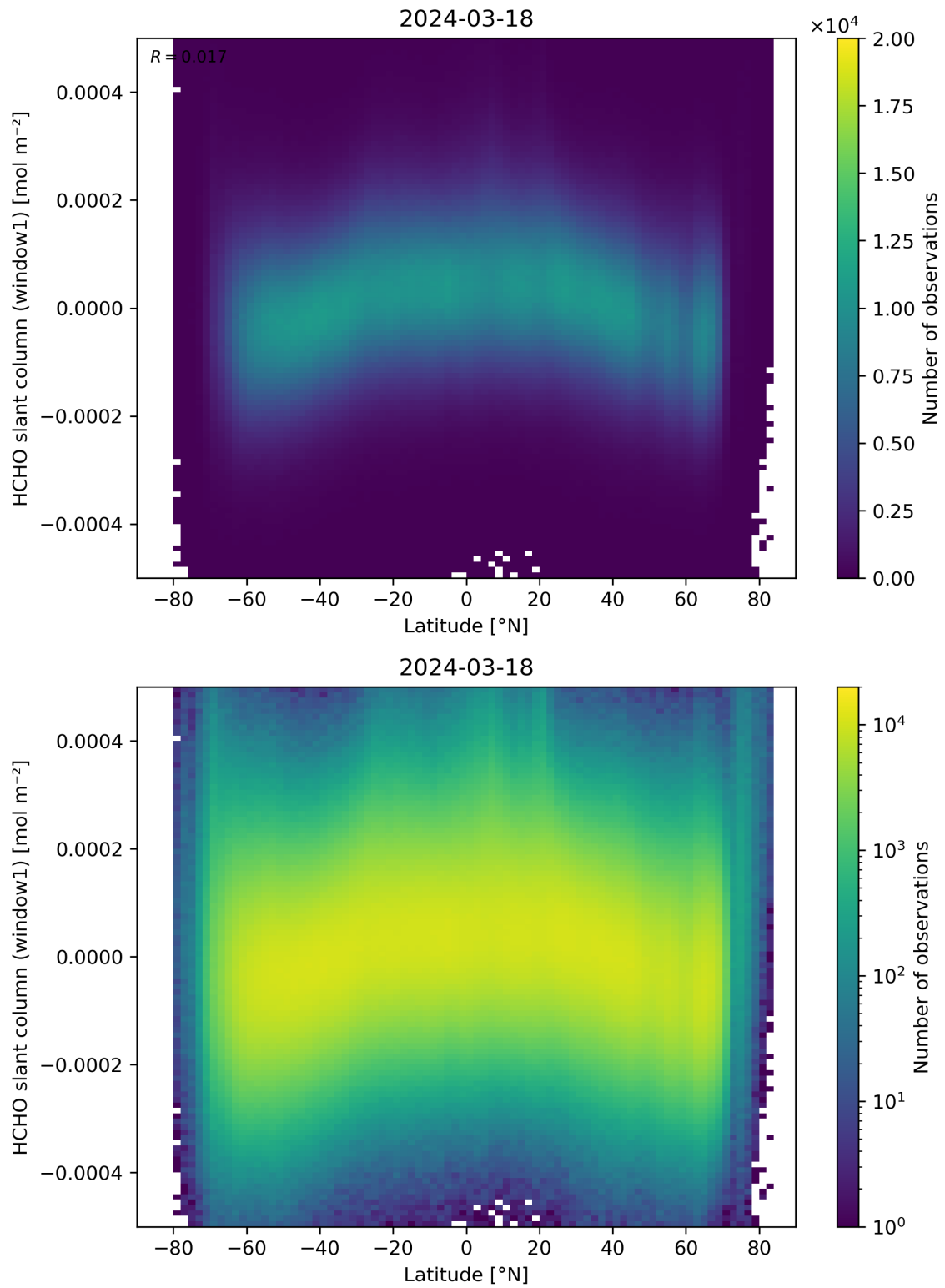
Figure 159: Scatter density plot of “Latitude” against “HCHO slant column (window1)” for 2024-03-17 to 2024-03-19.
