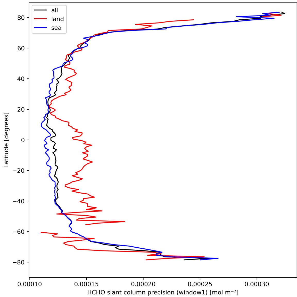
Figure 25: Zonal average of “HCHO slant column precision (window1)” for 2024-03-17 to 2024-03-19.
