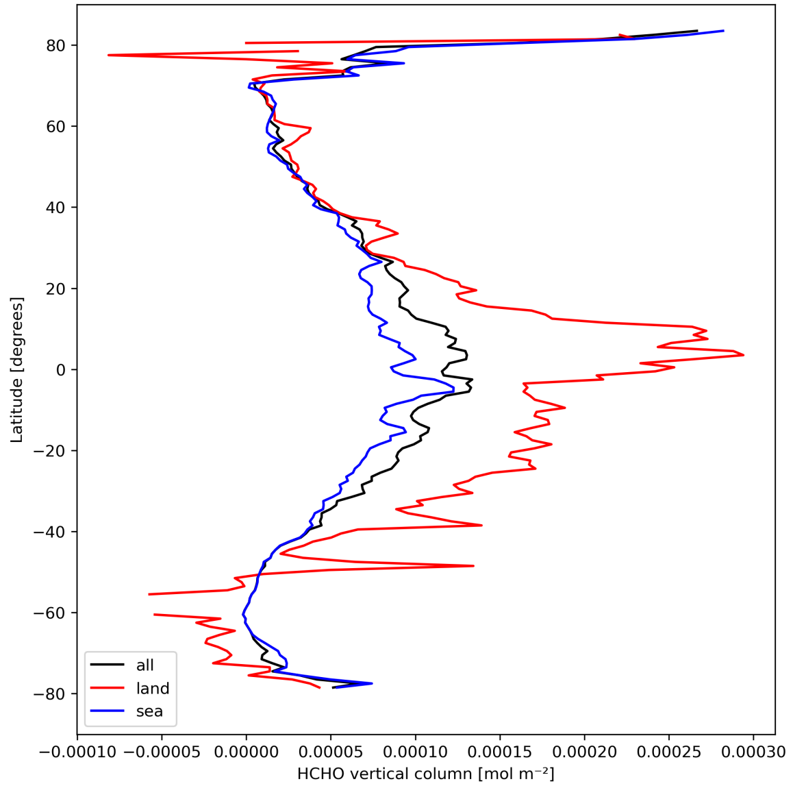
Figure 21: Zonal average of “HCHO vertical column” for 2024-03-17 to 2024-03-19.
