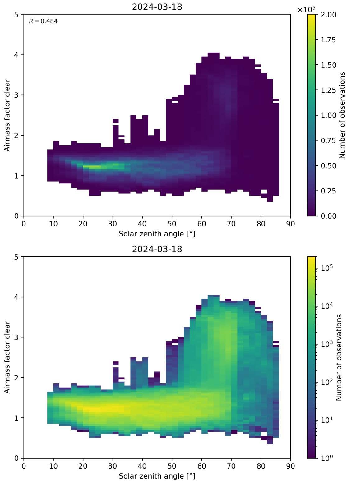
Figure 170: Scatter density plot of “Solar zenith angle” against “Airmass factor clear” for 2024-03-17 to 2024-03-19.
