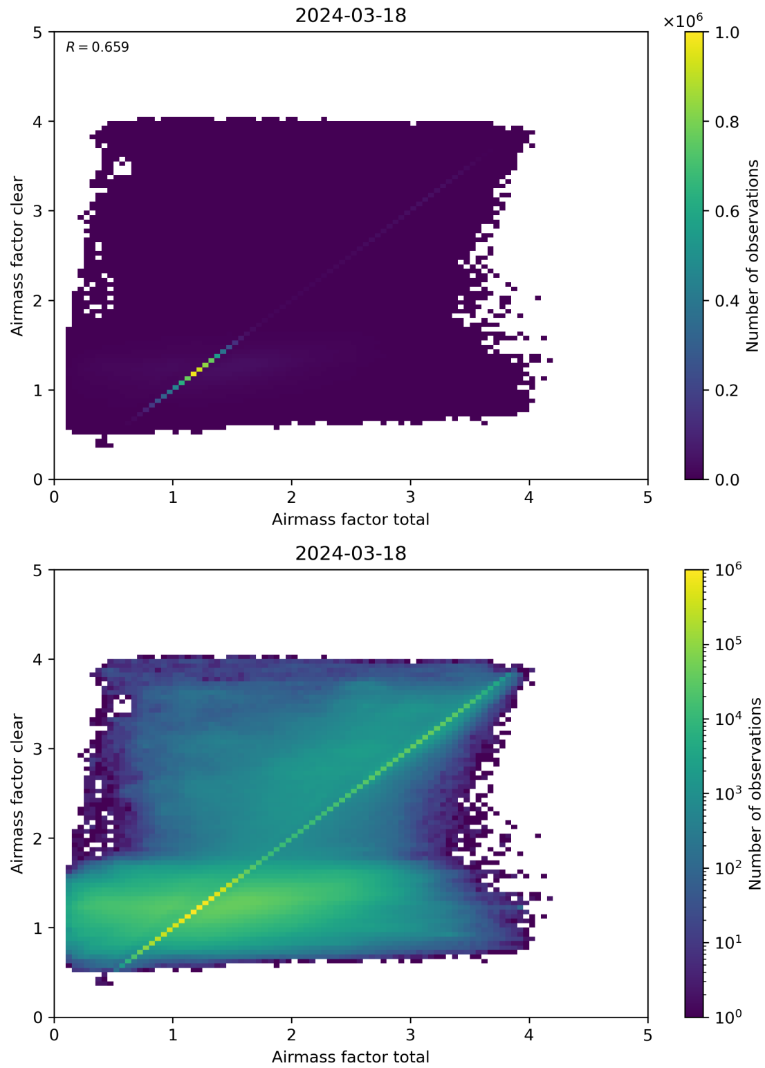
Figure 100: Scatter density plot of “Airmass factor total” against “Airmass factor clear” for 2024-03-17 to 2024-03-19.
