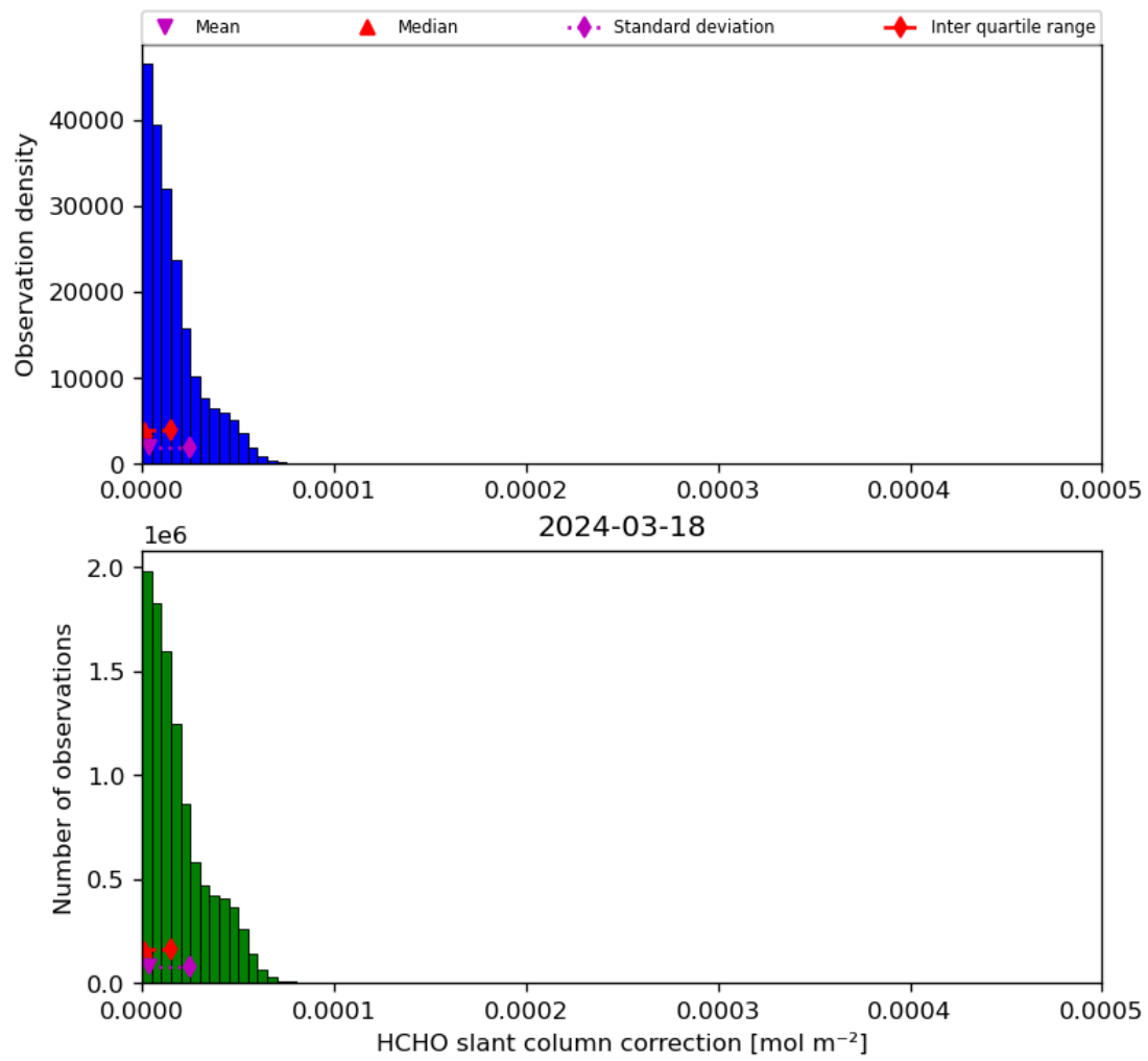
Figure 47: Histogram of “HCHO slant column correction” for 2024-03-17 to 2024-03-19
