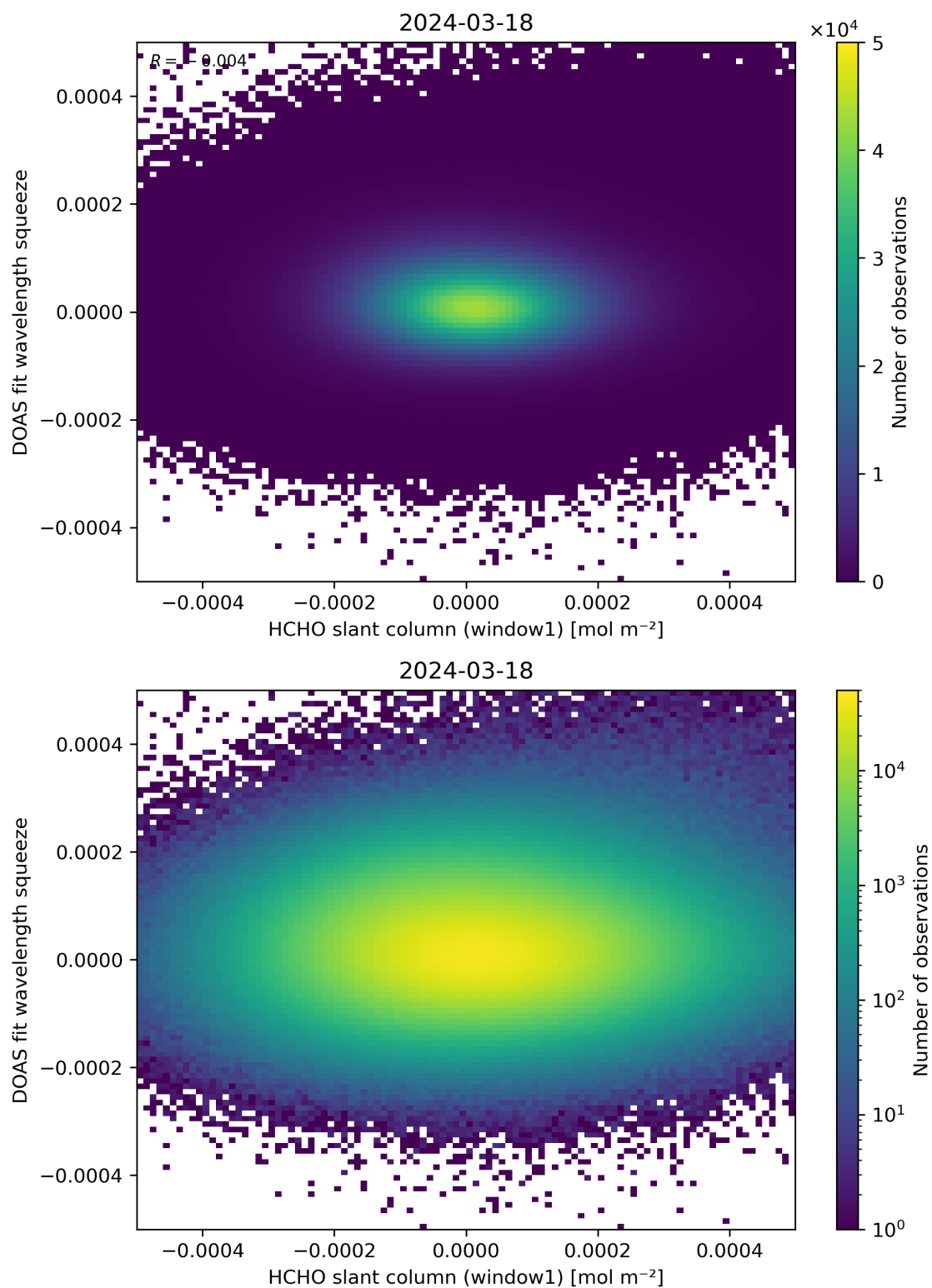
Figure 80: Scatter density plot of “HCHO slant column (window1)” against “DOAS fit wavelength squeeze” for 2024-03-17 to 2024-03-19.
