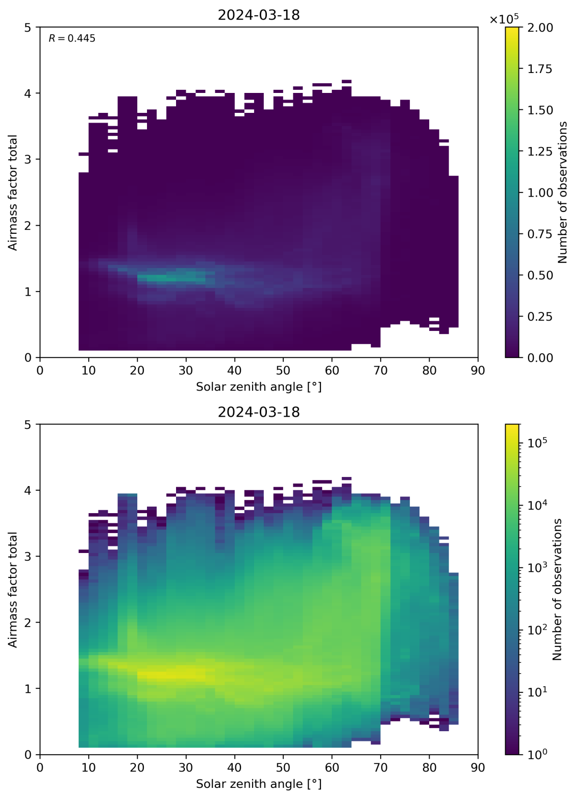
Figure 175: Scatter density plot of “Solar zenith angle” against “Airmass factor total” for 2024-03-17 to 2024-03-19.
