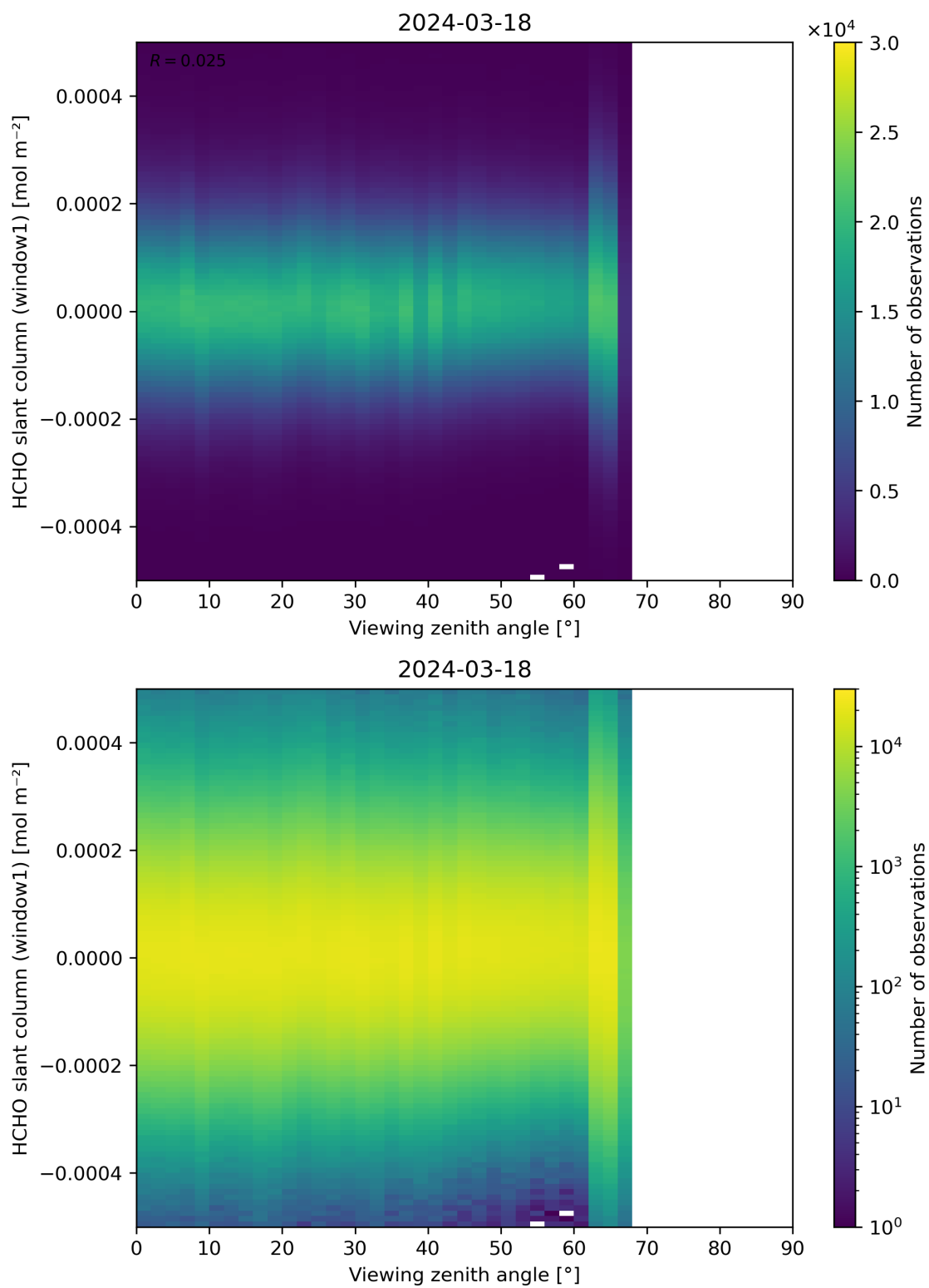
Figure 188: Scatter density plot of “Viewing zenith angle” against “HCHO slant column (window1)” for 2024-03-17 to 2024-03-19.
