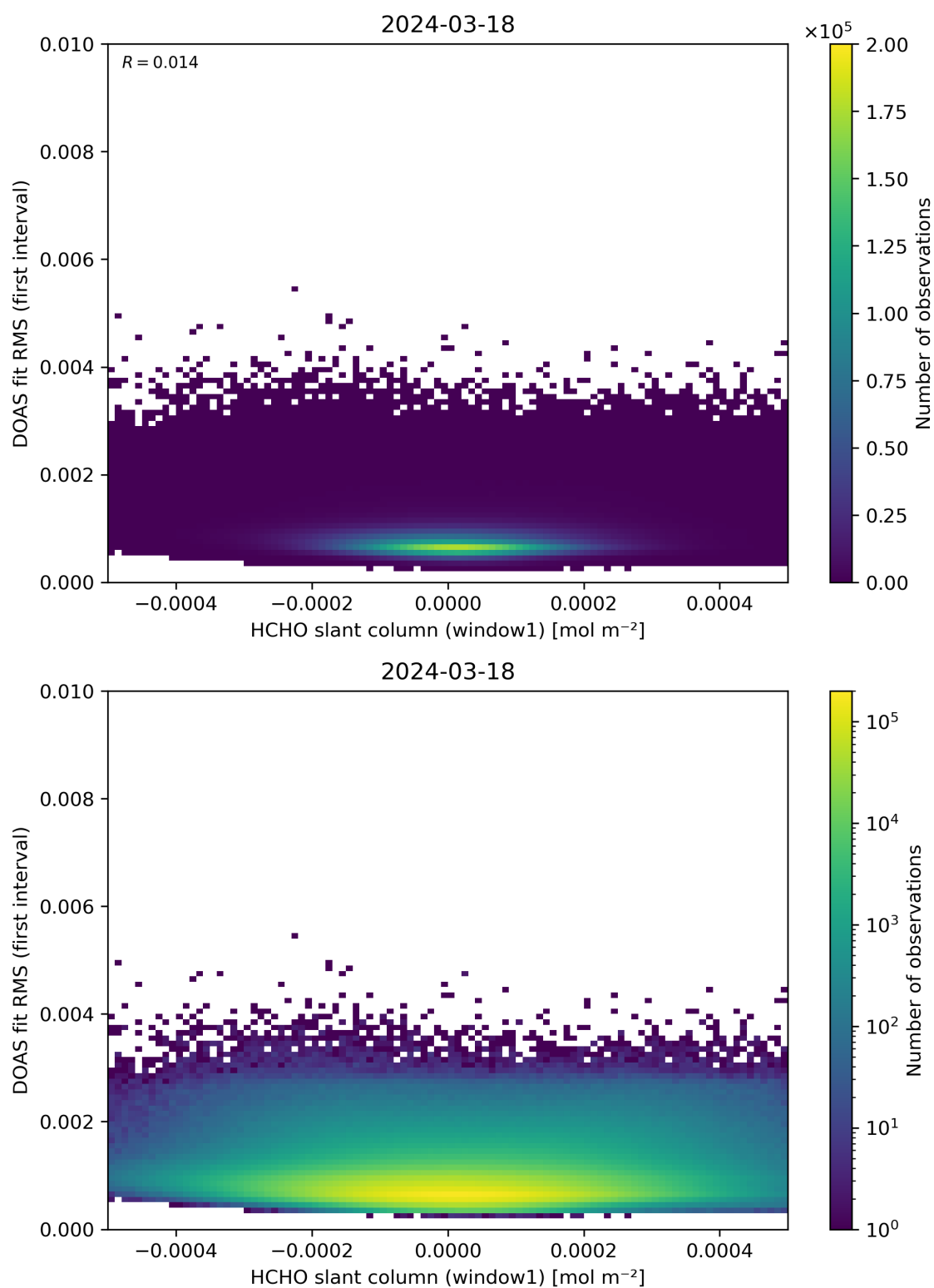
Figure 78: Scatter density plot of “HCHO slant column (window1)” against “DOAS fit RMS (first interval)” for 2024-03-17 to 2024-03-19.
