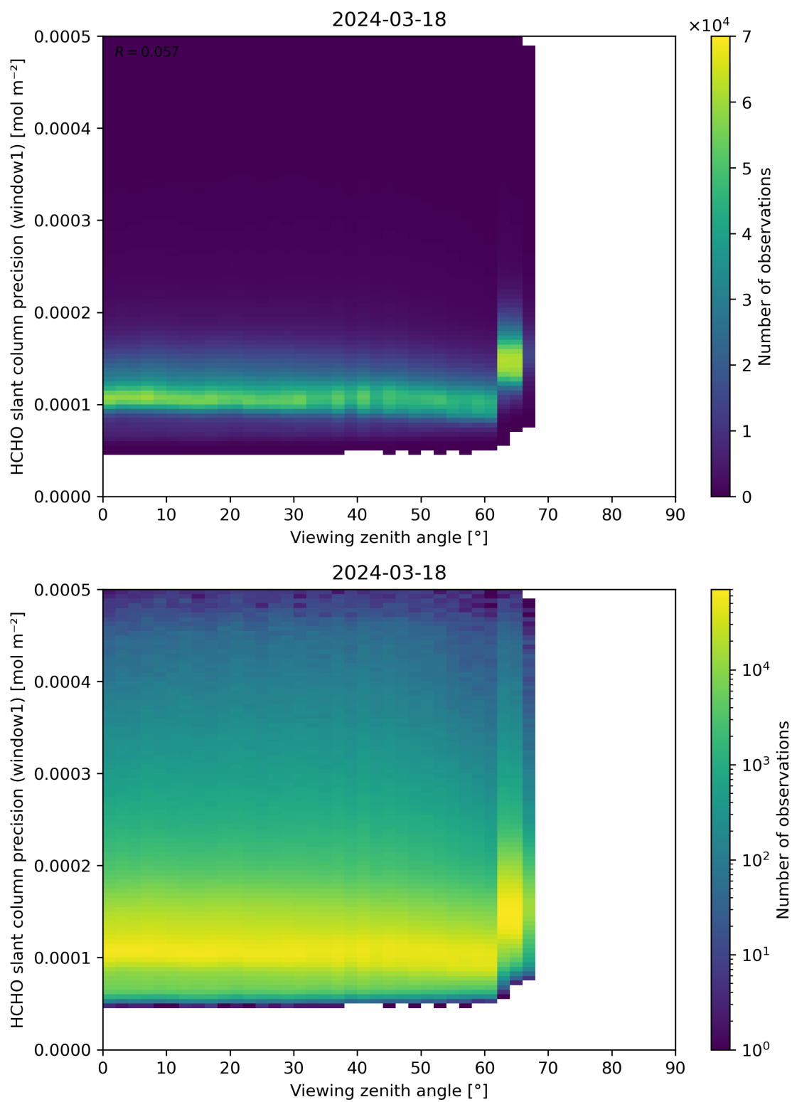
Figure 189: Scatter density plot of “Viewing zenith angle” against “HCHO slant column precision (window1)” for 2024-03-17 to 2024-03-19.
