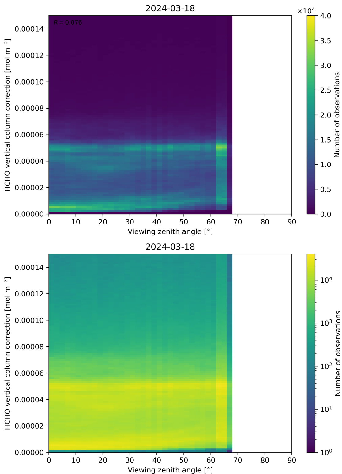
Figure 193: Scatter density plot of “Viewing zenith angle” against “HCHO vertical column correction” for 2024-03-17 to 2024-03-19.
