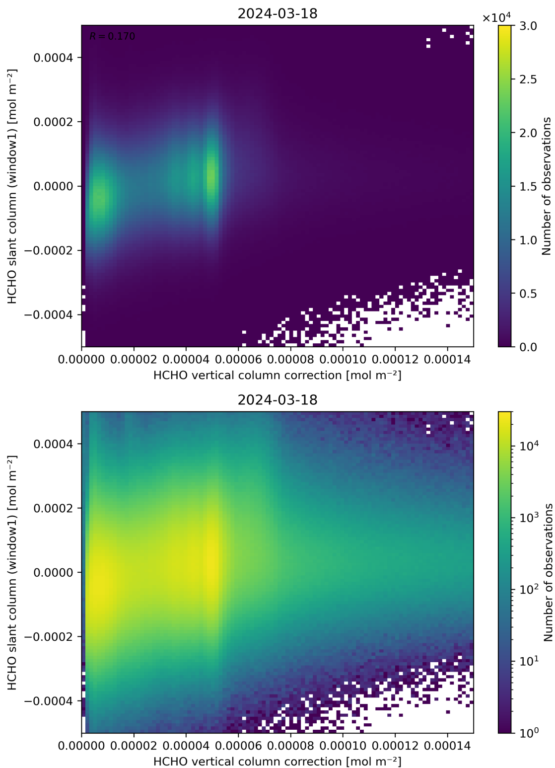
Figure 118: Scatter density plot of “HCHO vertical column correction” against “HCHO slant column (window1)” for 2024-03-17 to 2024-03-19.
