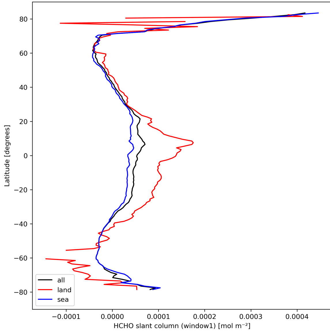
Figure 24: Zonal average of “HCHO slant column (window1)” for 2024-03-17 to 2024-03-19.
