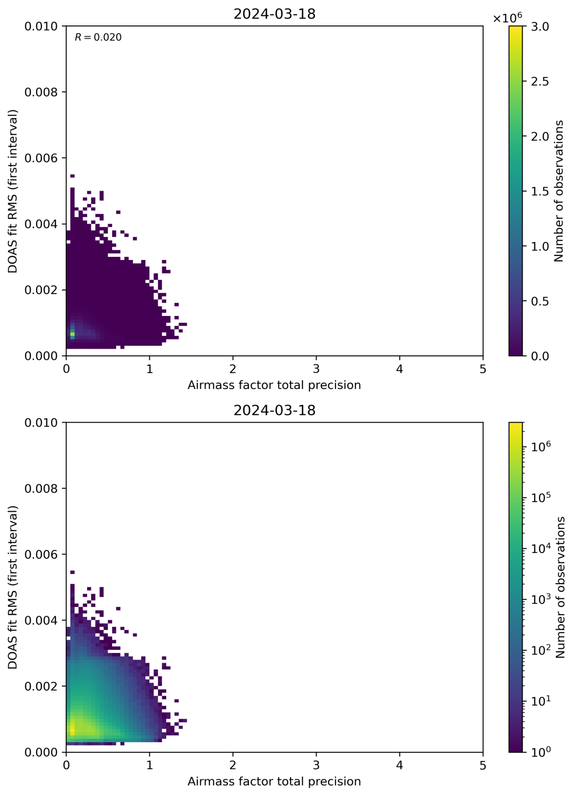
Figure 105: Scatter density plot of “Airmass factor total precision” against “DOAS fit RMS (first interval)” for 2024-03-17 to 2024-03-19.
