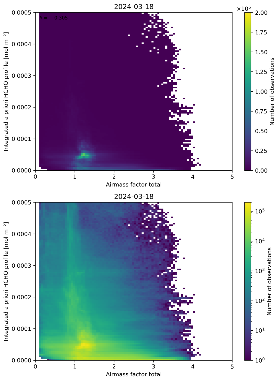
Figure 104: Scatter density plot of “Air mass factor total” against “Integrated a priori HCHO profile” for 2024-03-17 to 2024-03-19.
