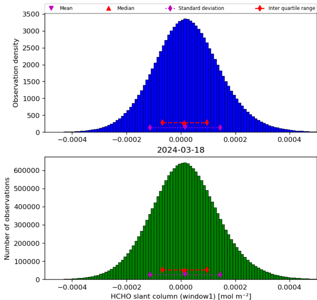
Figure 38: Histogram of “HCHO slant column (window1)” for 2024-03-17 to 2024-03-19
