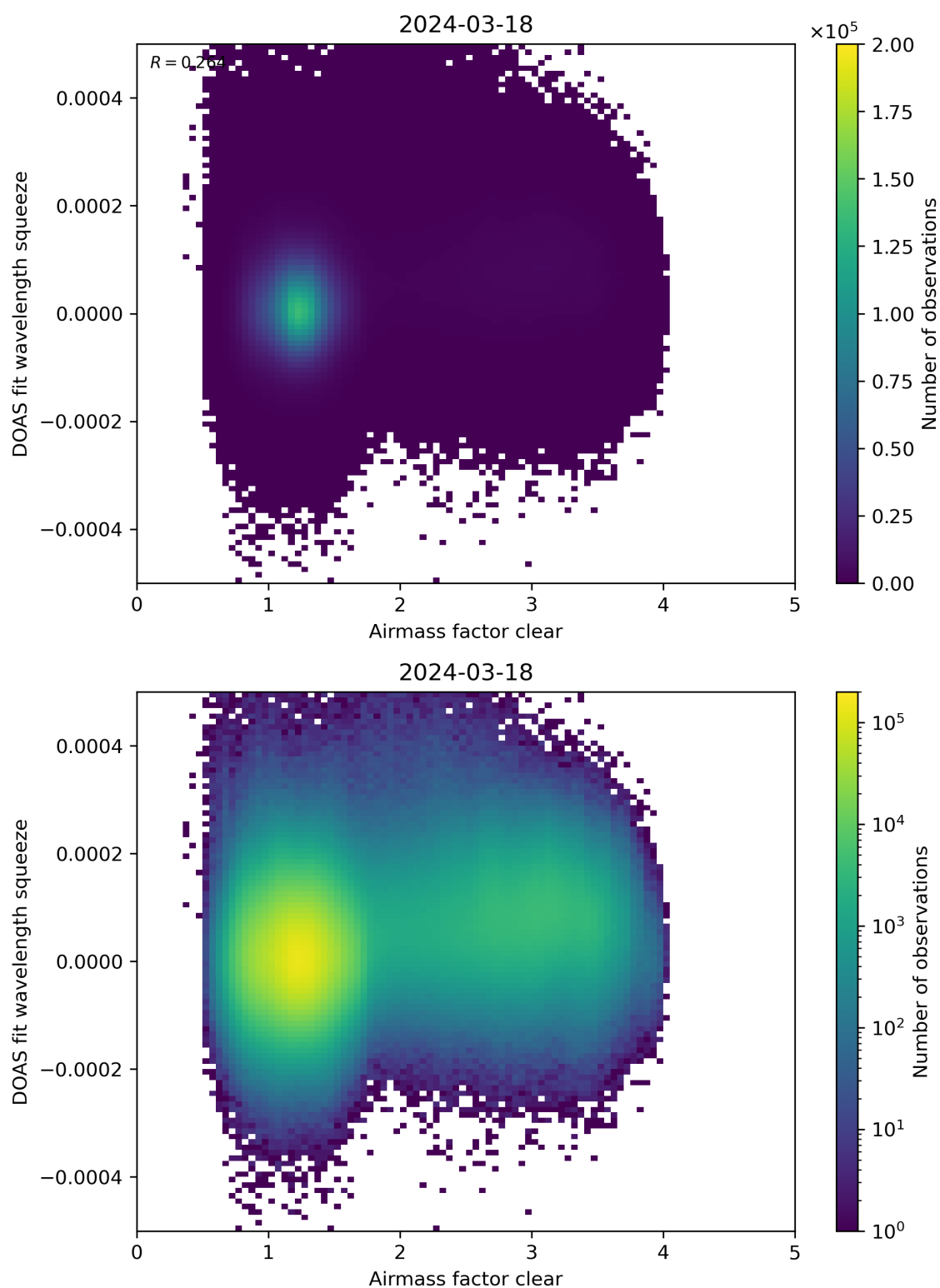
Figure 73: Scatter density plot of “Airmass factor clear” against “DOAS fit wavelength squeeze” for 2024-03-17 to 2024-03-19.
