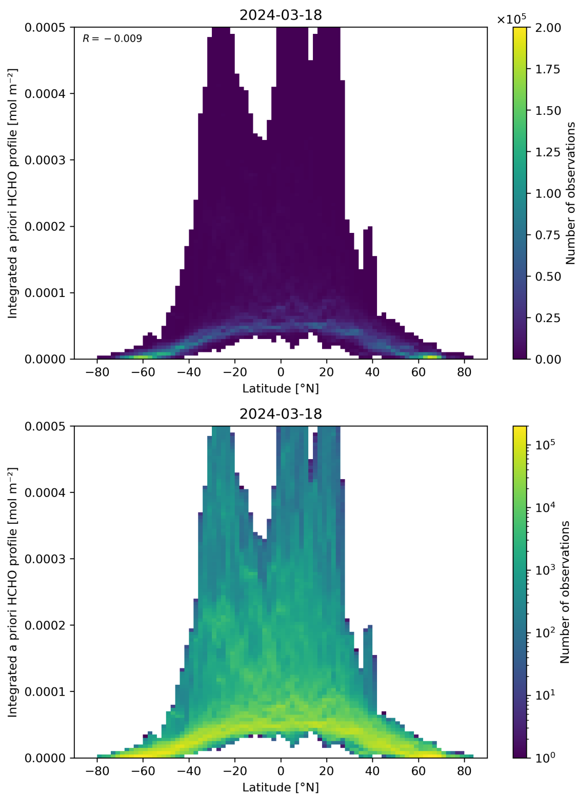
Figure 166: Scatter density plot of “Latitude” against “Integrated a priori HCHO profile” for 2024-03-17 to 2024-03-19.
