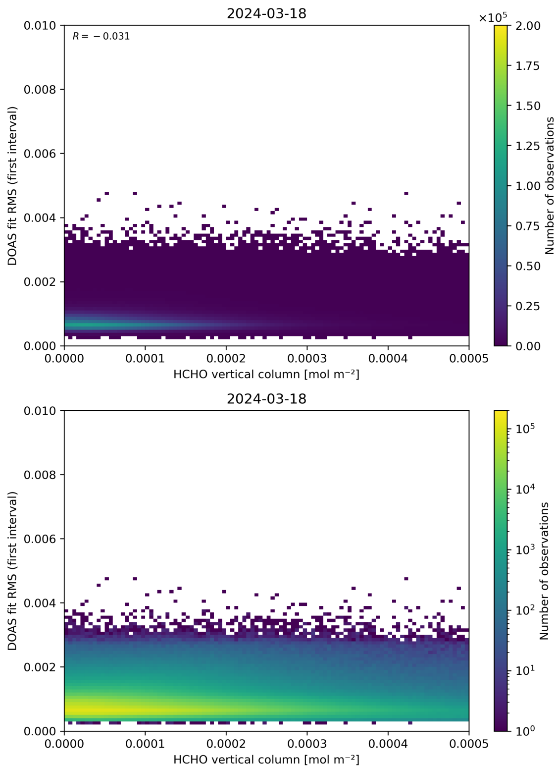
Figure 123: Scatter density plot of “HCHO vertical column” against “DOAS fit RMS (first interval)” for 2024-03-17 to 2024-03-19.
