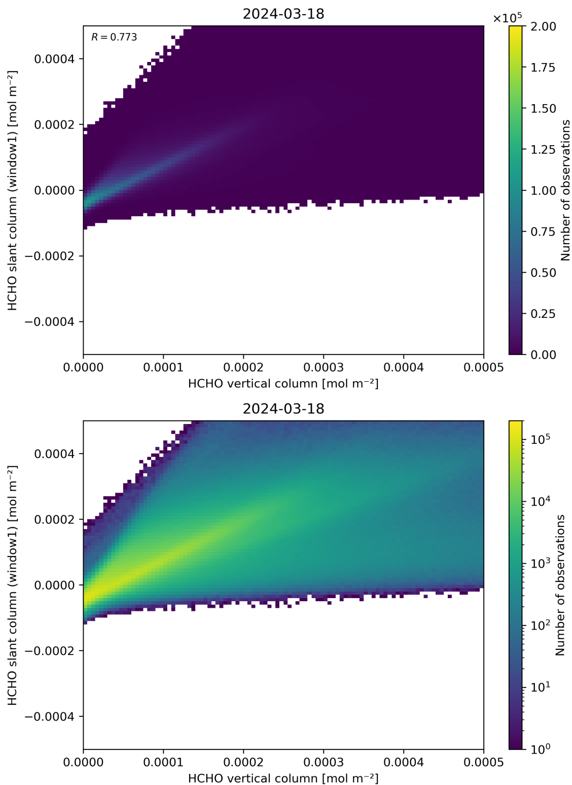
Figure 129: Scatter density plot of “HCHO vertical column” against “HCHO slant column (window1)” for 2024-03-17 to 2024-03-19.
