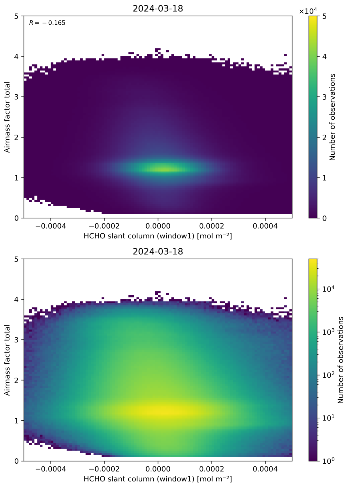
Figure 85: Scatter density plot of “HCHO slant column (window1)” against “Airmass factor total” for 2024-03-17 to 2024-03-19.
