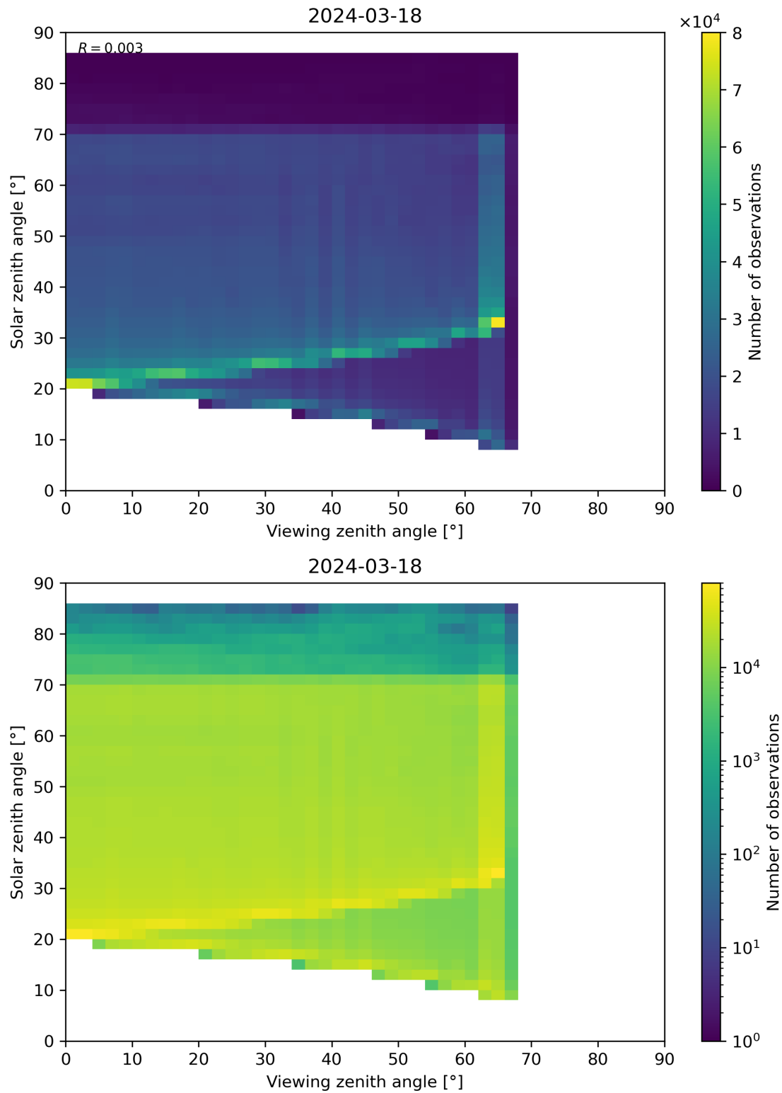
Figure 197: Scatter density plot of “Viewing zenith angle” against “Solar zenith angle” for 2024-03-17 to 2024-03-19.
