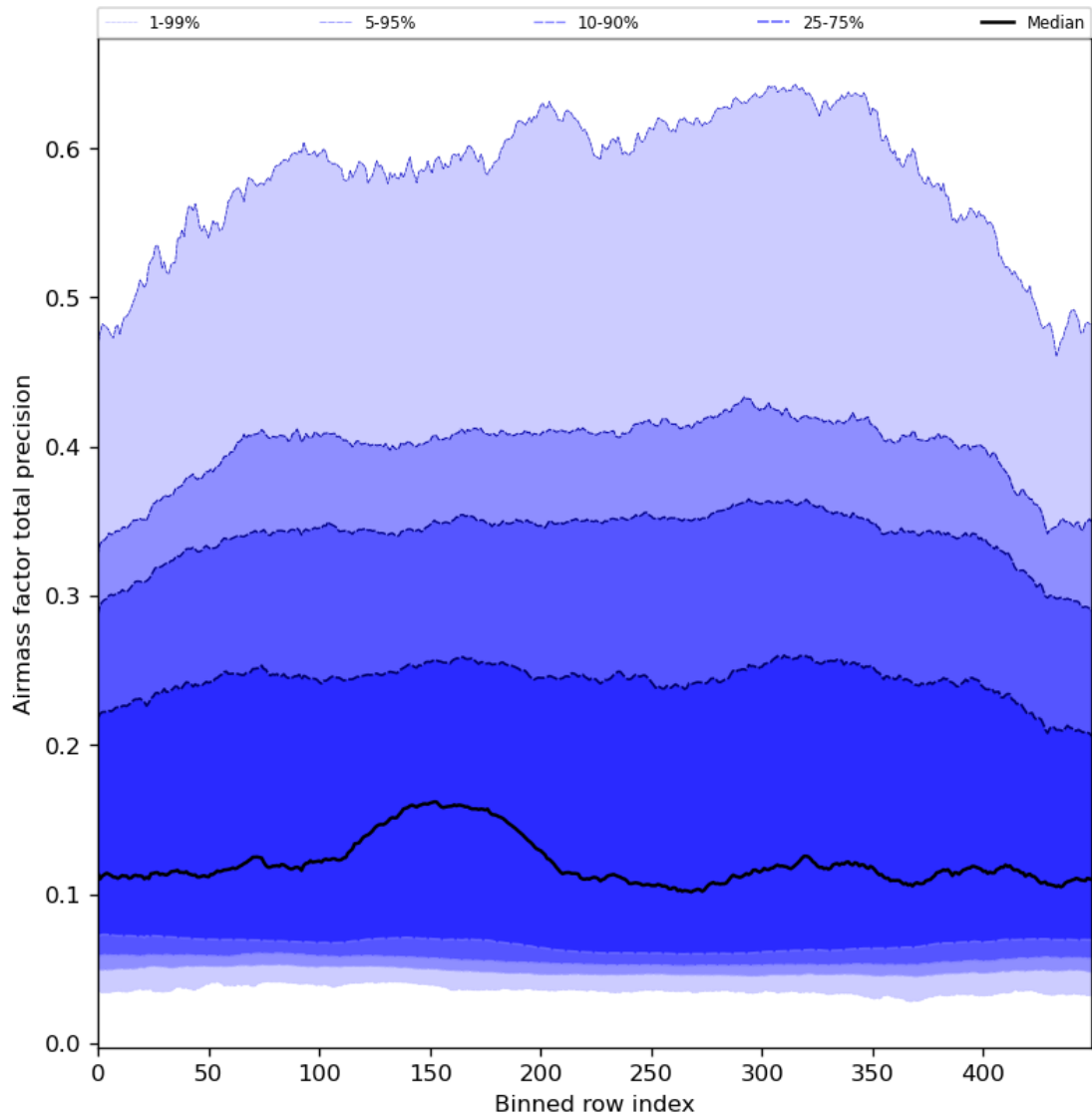
Figure 55: Along track statistics of “Airmass factor total precision” for 2024-03-17 to 2024-03-19
