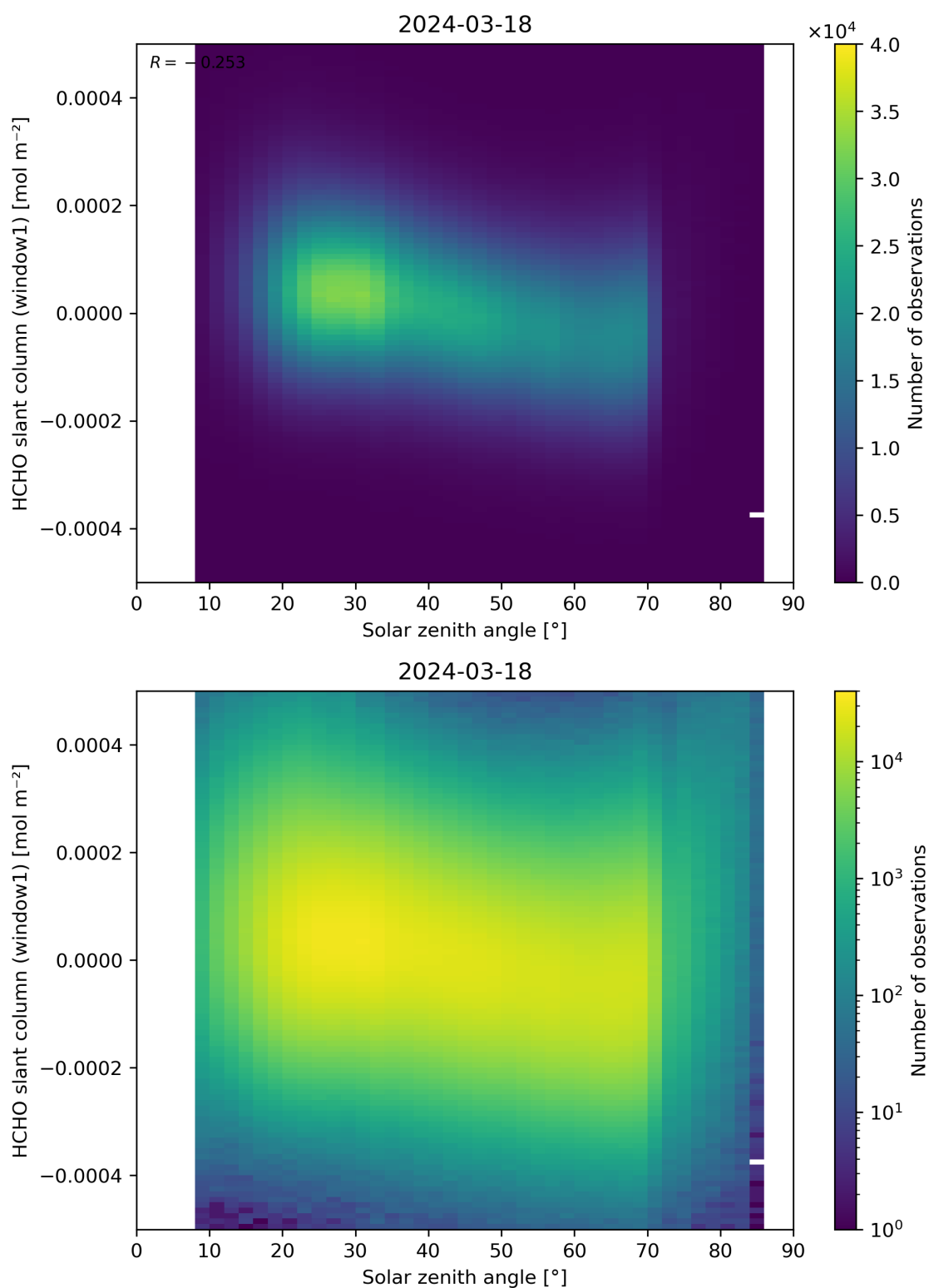
Figure 173: Scatter density plot of “Solar zenith angle” against “HCHO slant column (window1)” for 2024-03-17 to 2024-03-19.
