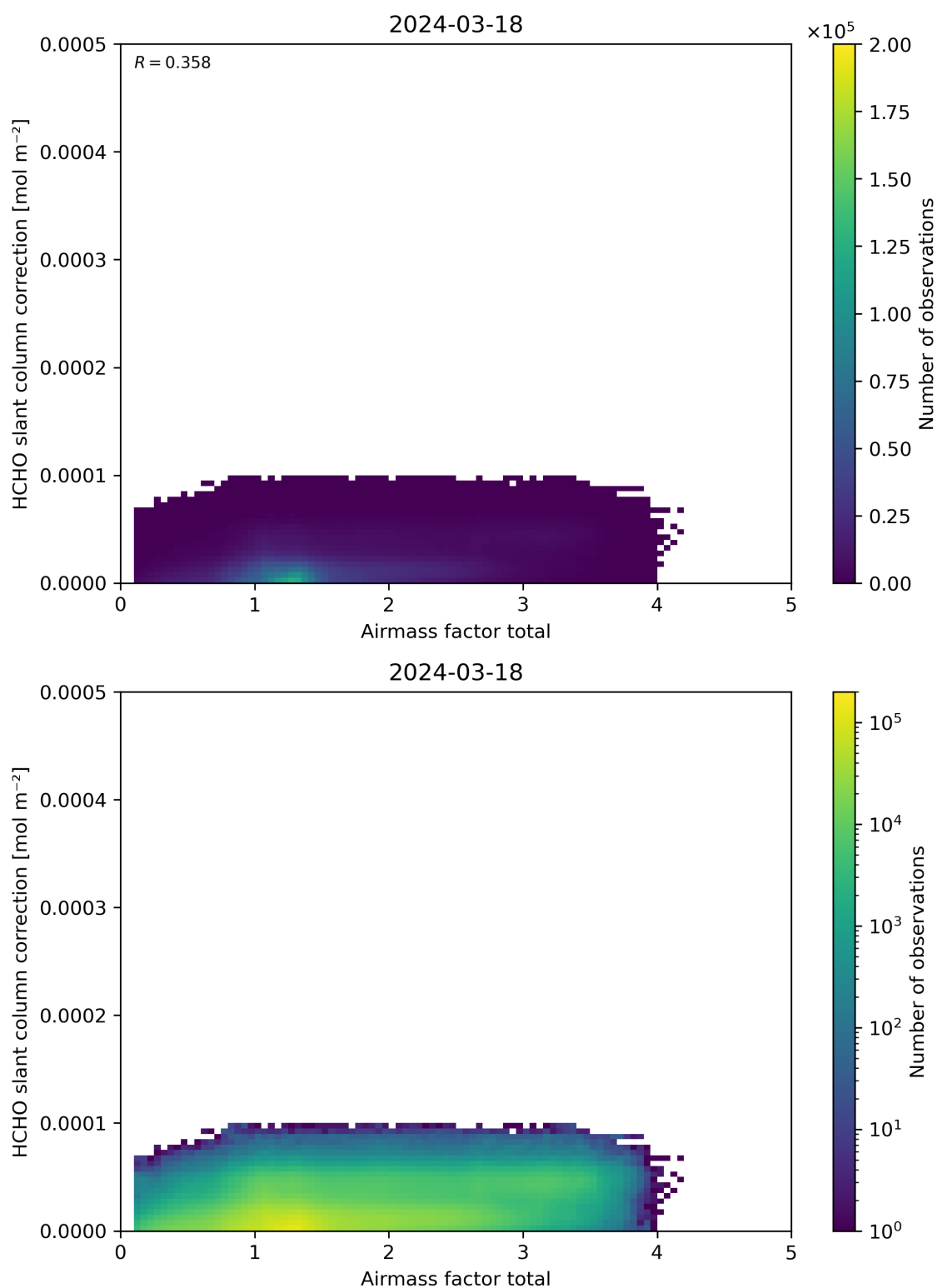
Figure 102: Scatter density plot of “Airmass factor total” against “HCHO slant column correction” for 2024-03-17 to 2024-03-19.
