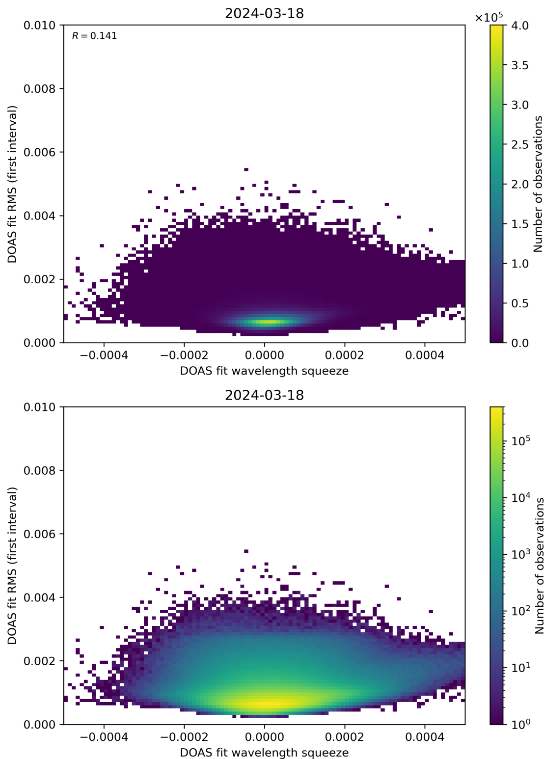
Figure 68: Scatter density plot of “DOAS fit wavelength squeeze” against “DOAS fit RMS (first interval)” for 2024-03-17 to 2024-03-19.
