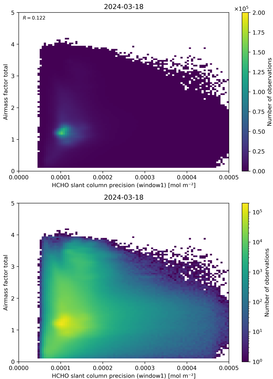
Figure 94: Scatter density plot of “HCHO slant column precision (window1)” against “Airmass factor total” for 2024-03-17 to 2024-03-19.
