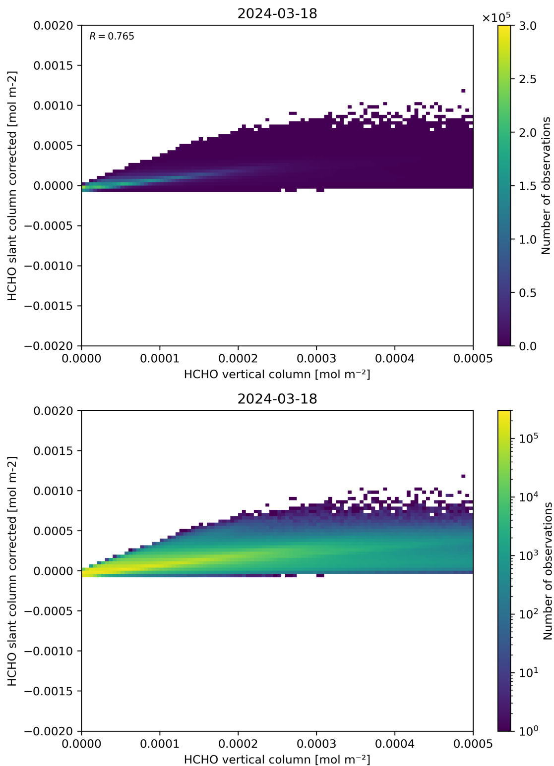
Figure 127: Scatter density plot of “HCHO vertical column” against “HCHO slant column corrected” for 2024-03-17 to 2024-03-19.
