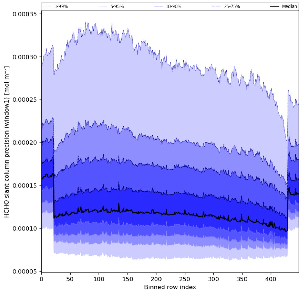
Figure 53: Along track statistics of “HCHO slant column precision (window1)” for 2024-03-17 to 2024-03-19
