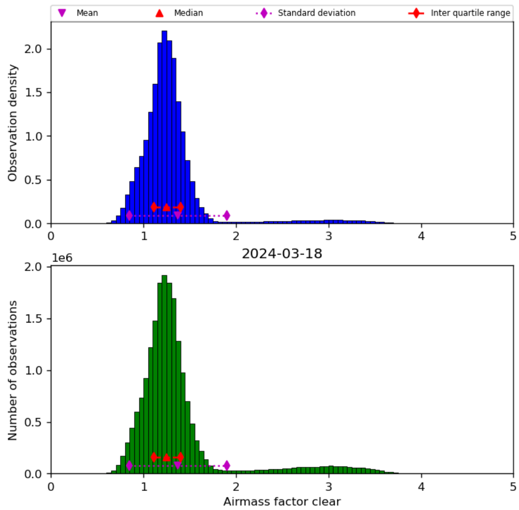
Figure 42: Histogram of “Airmass factor clear” for 2024-03-17 to 2024-03-19
