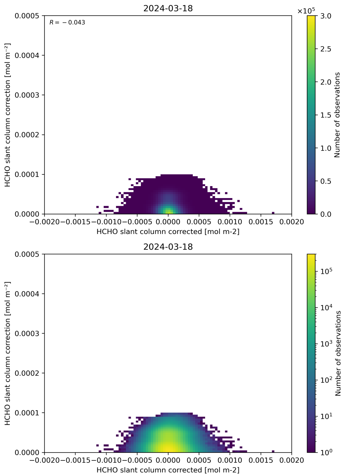
Figure 77: Scatter density plot of “HCHO slant column corrected” against “HCHO slant column correction” for 2024-03-17 to 2024-03-19.
