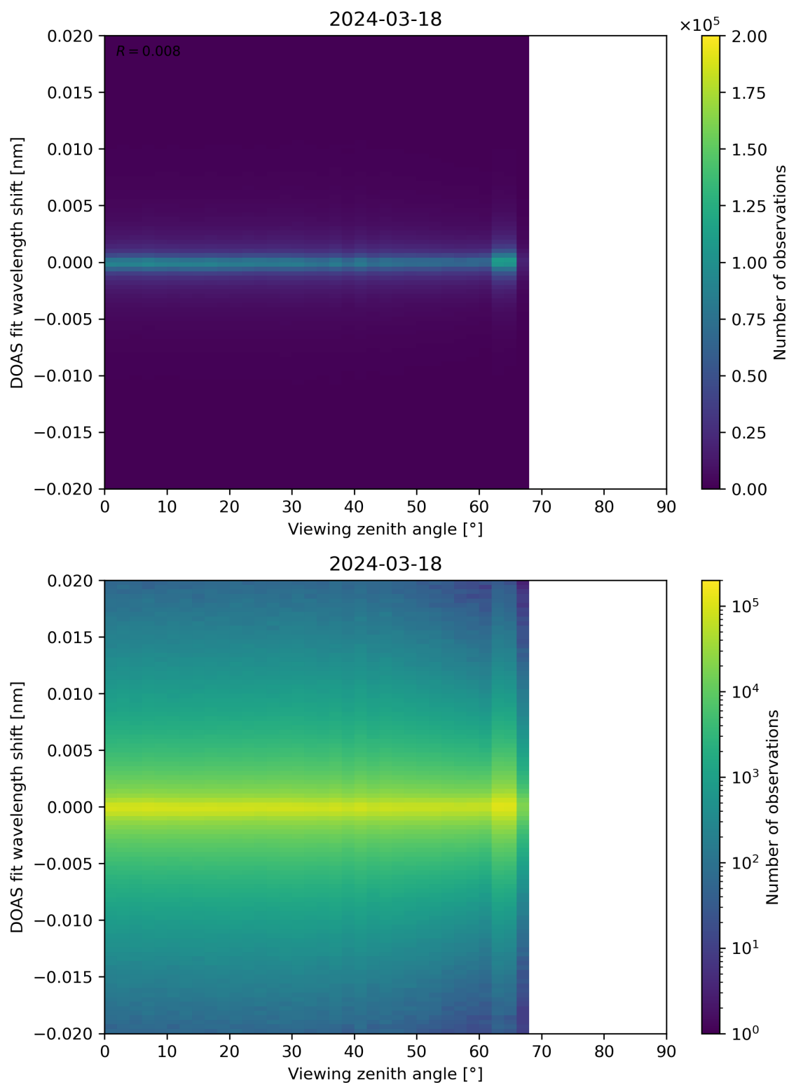
Figure 183: Scatter density plot of “Viewing zenith angle” against “DOAS fit wavelength shift” for 2024-03-17 to 2024-03-19.
