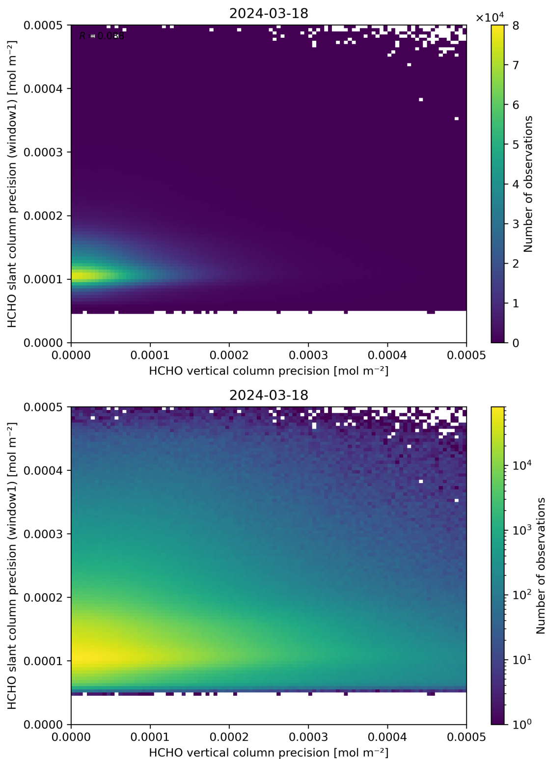
Figure 143: Scatter density plot of “HCHO vertical column precision” against “HCHO slant column precision (window1)” for 2024-03-17 to 2024-03-19.
