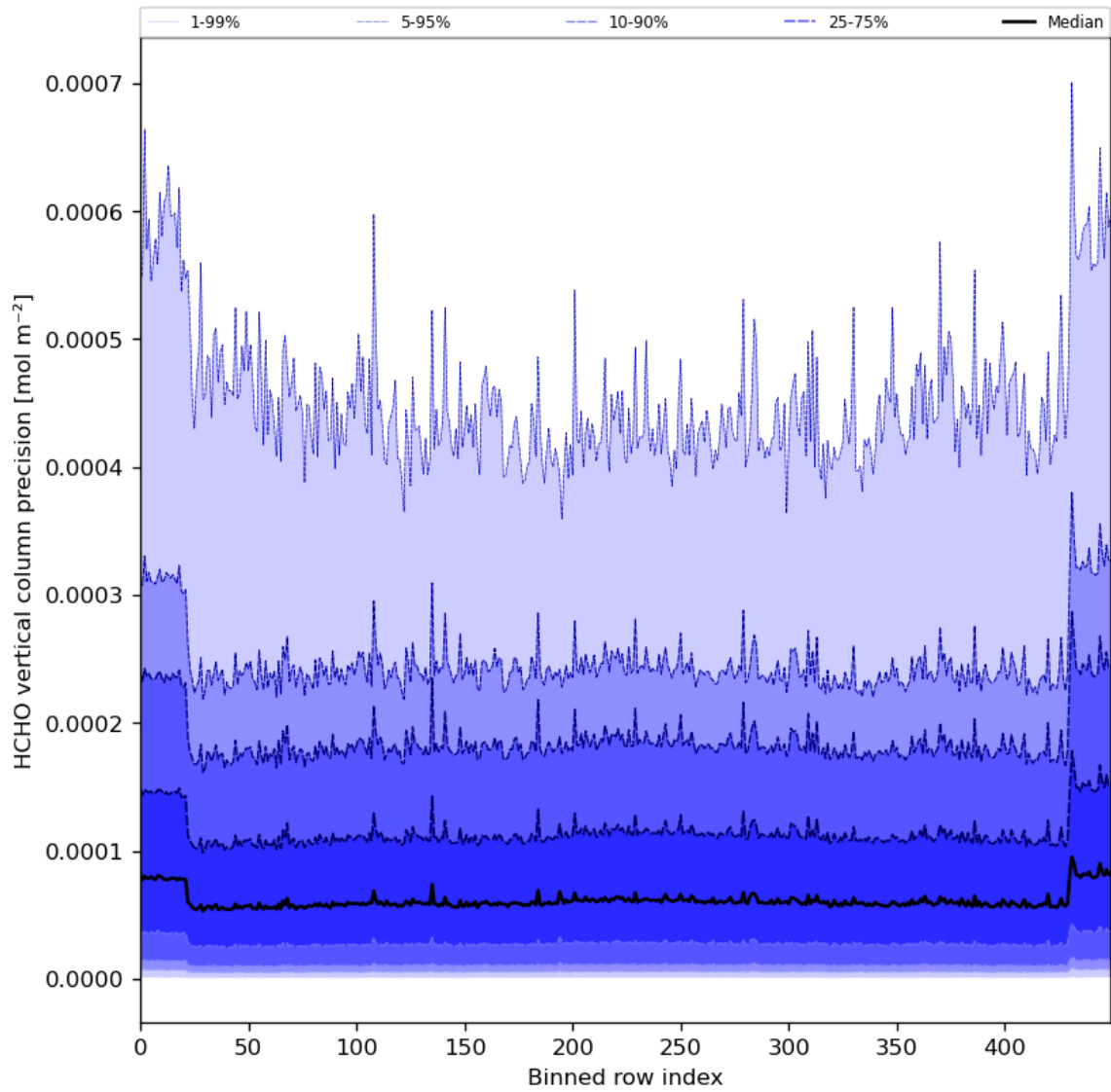
Figure 50: Along track statistics of “HCHO vertical column precision” for 2024-03-17 to 2024-03-19
