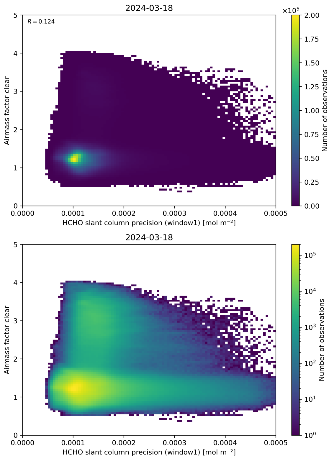
Figure 91: Scatter density plot of “HCHO slant column precision (window1)” against “Airmass factor clear” for 2024-03-17 to 2024-03-19.
