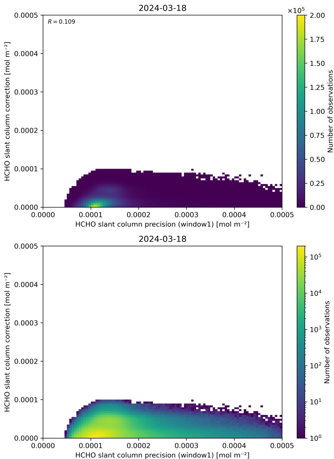
Figure 93: Scatter density plot of “HCHO slant column precision (window1)” against “HCHO slant column correction” for 2024-03-17 to 2024-03-19.
