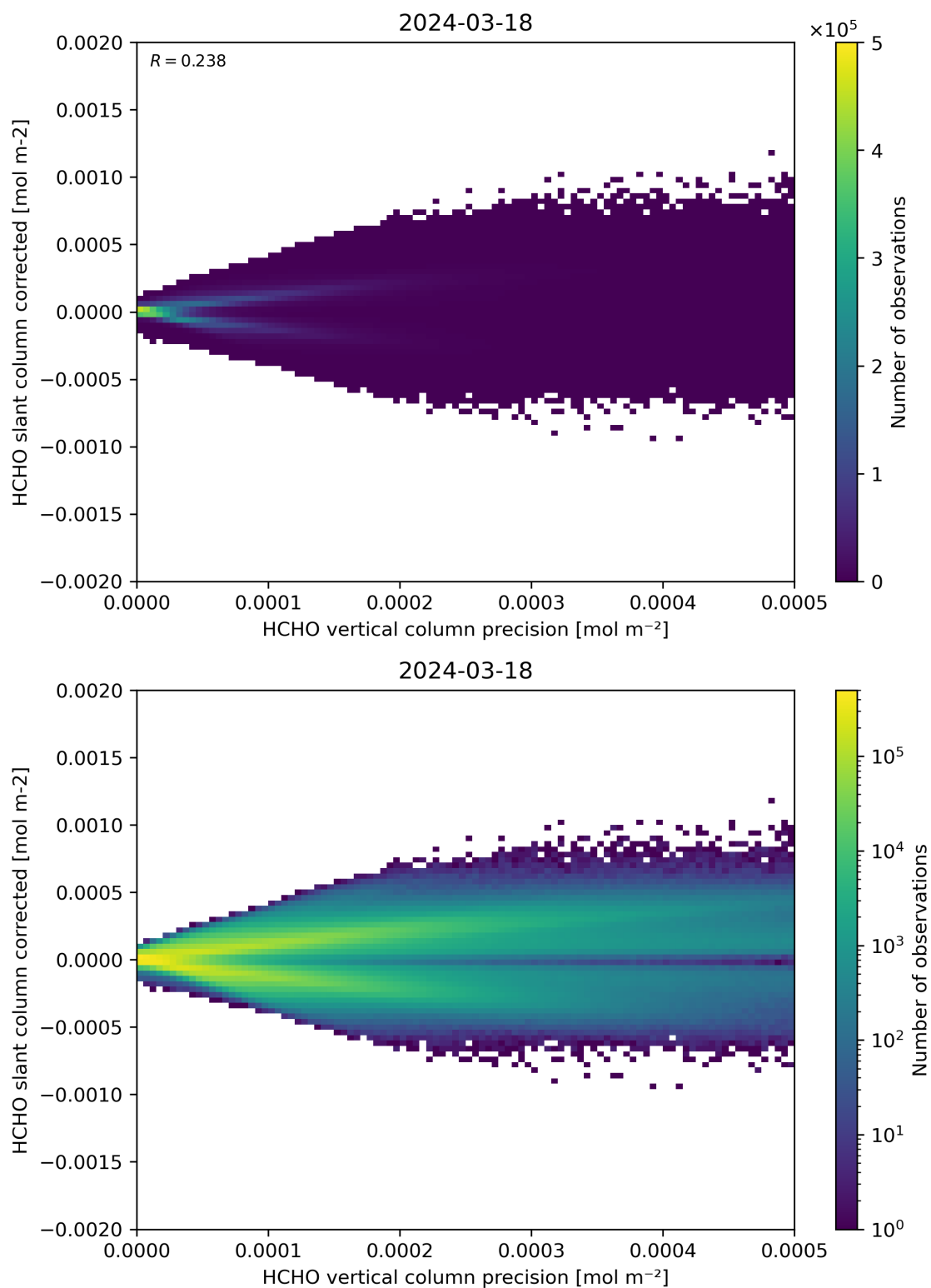
Figure 140: Scatter density plot of “HCHO vertical column precision” against “HCHO slant column corrected” for 2024-03-17 to 2024-03-19.
