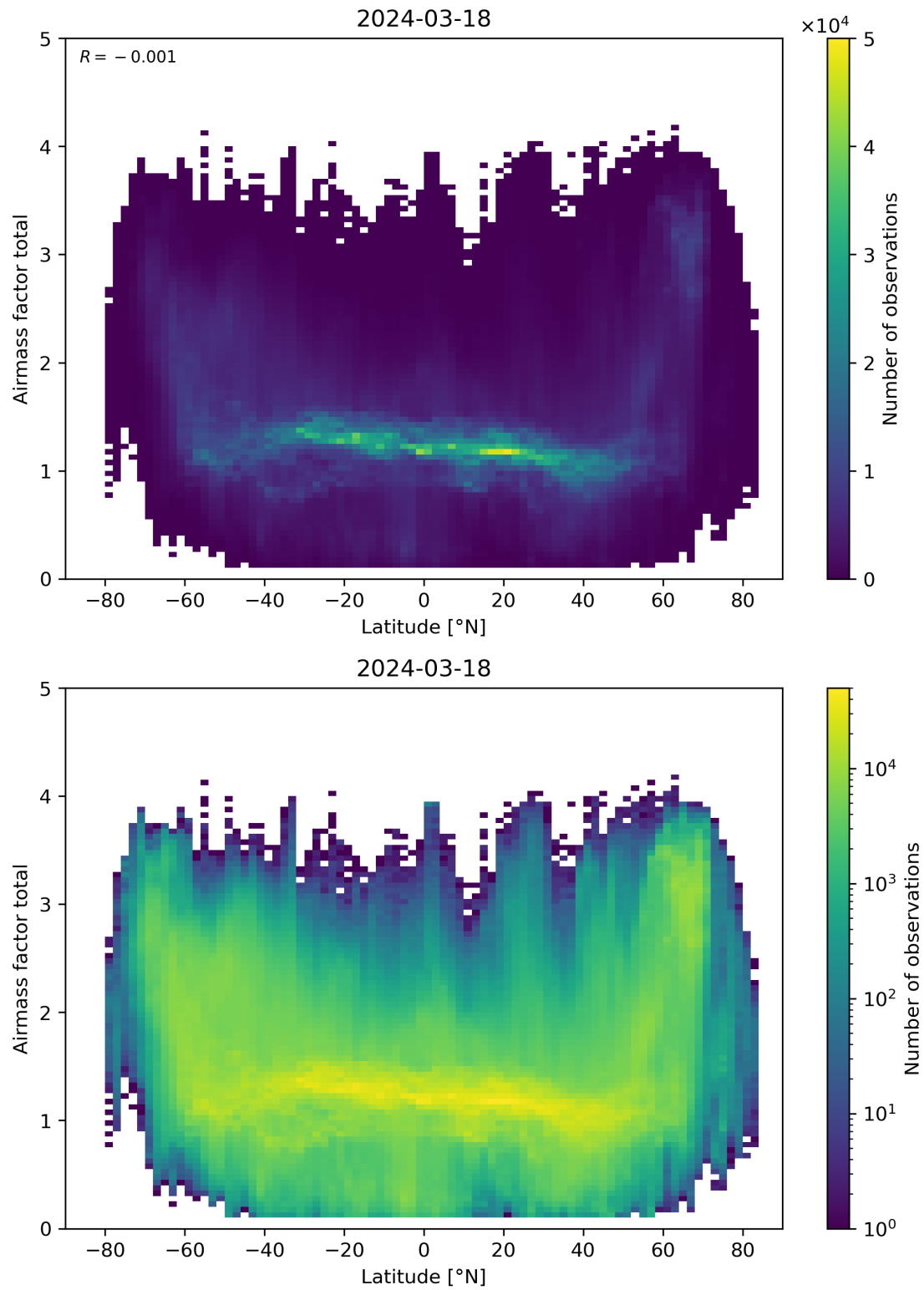
Figure 161: Scatter density plot of “Latitude” against “Airmass factor total” for 2024-03-17 to 2024-03-19.
