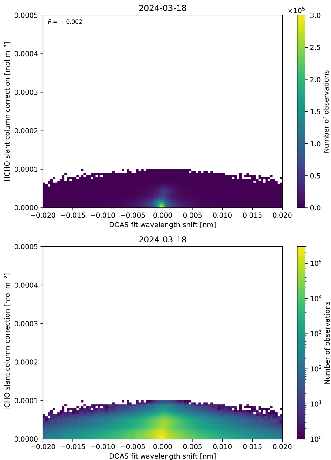
Figure 67: Scatter density plot of “DOAS fit wavelength shift” against “HCHO slant column correction” for 2024-03-17 to 2024-03-19.
