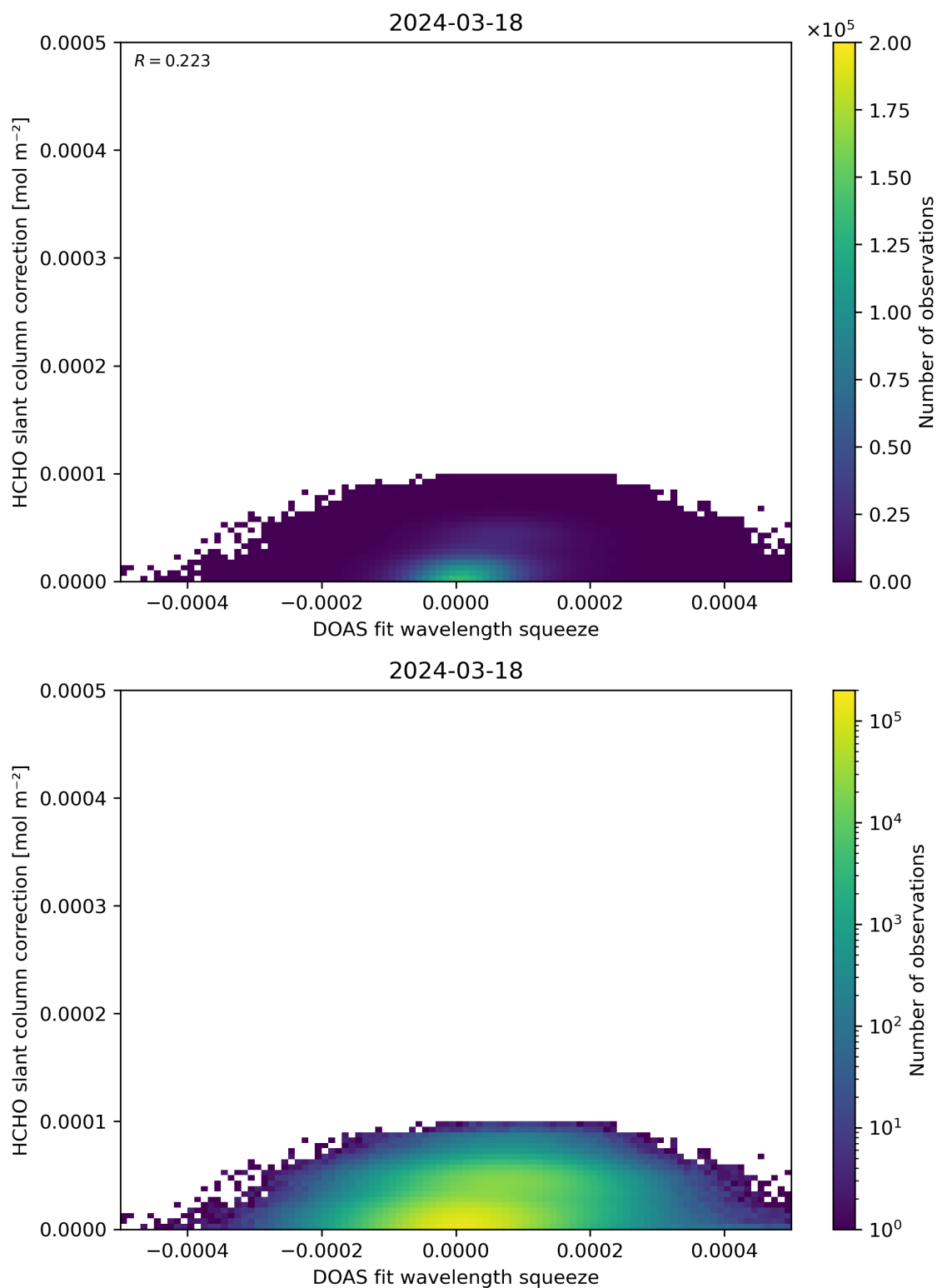
Figure 70: Scatter density plot of “DOAS fit wavelength squeeze” against “HCHO slant column correction” for 2024-03-17 to 2024-03-19.
