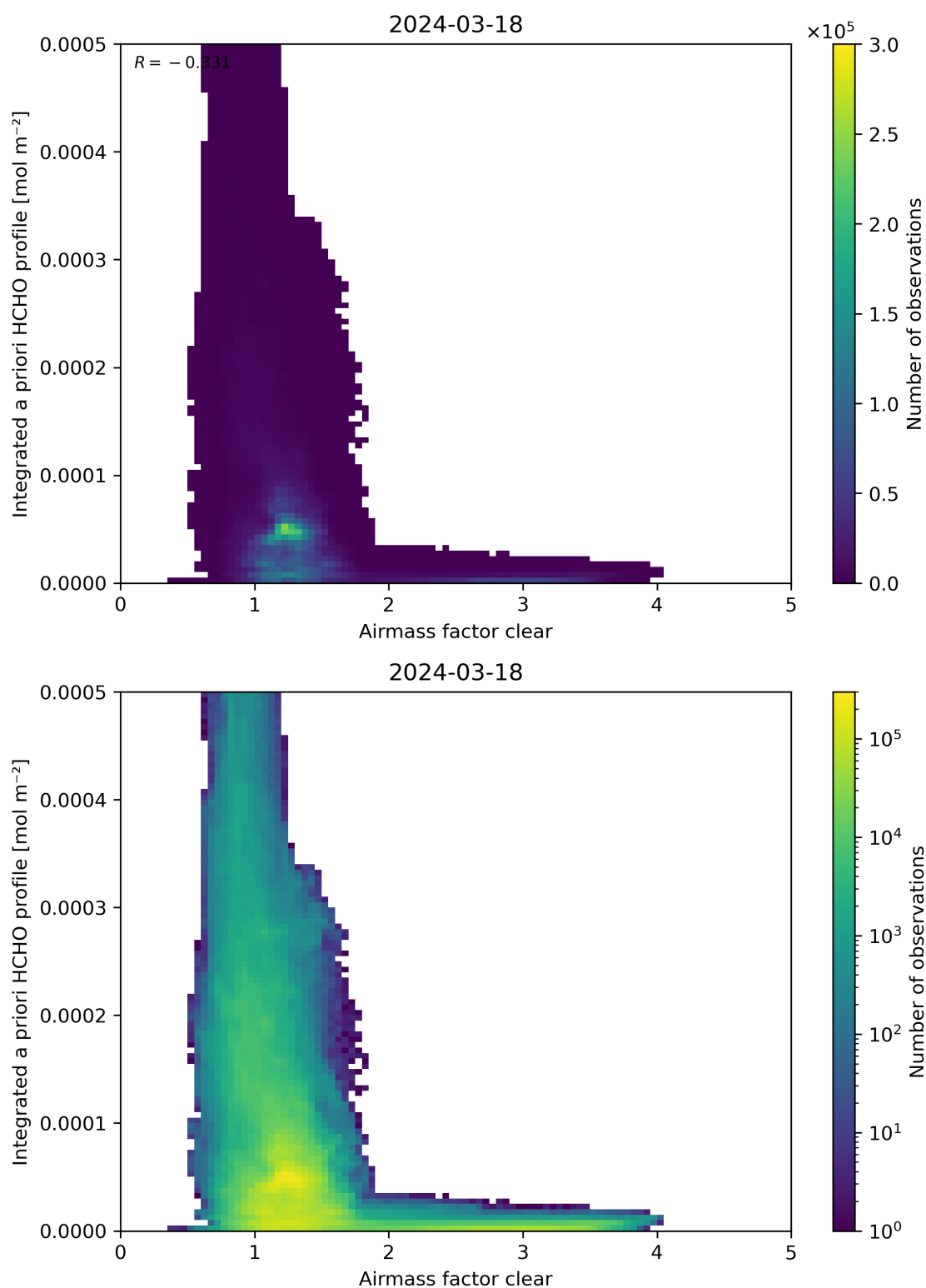
Figure 76: Scatter density plot of “Airmass factor clear” against “Integrated a priori HCHO profile” for 2024-03-17 to 2024-03-19.
