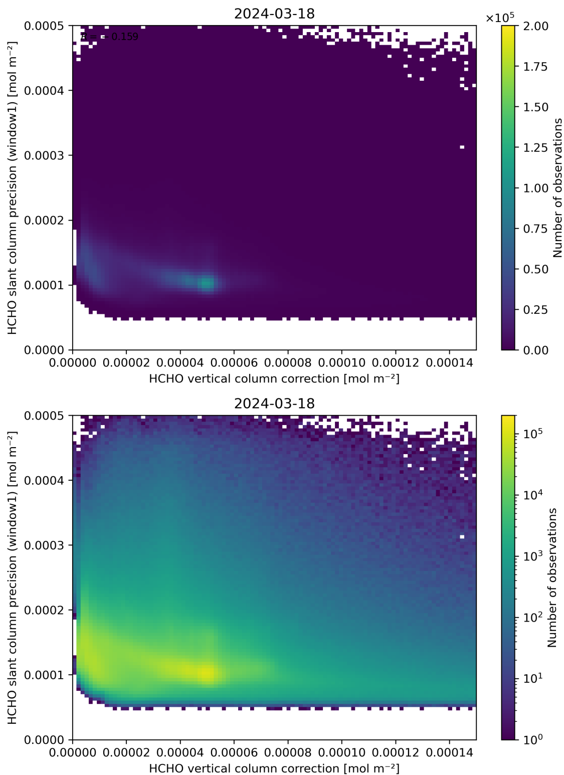
Figure 119: Scatter density plot of “HCHO vertical column correction” against “HCHO slant column precision (window1)” for 2024-03-17 to 2024-03-19.
