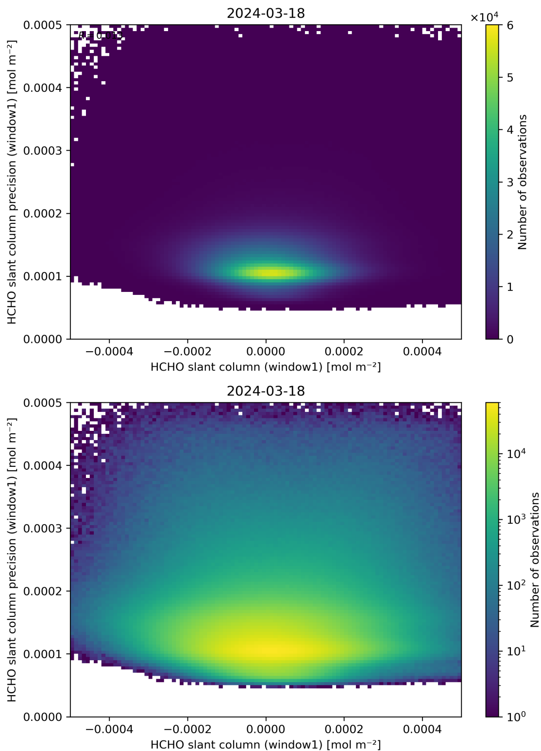
Figure 84: Scatter density plot of “HCHO slant column (window1)” against “HCHO slant column precision (window1)” for 2024-03-17 to 2024-03-19.
