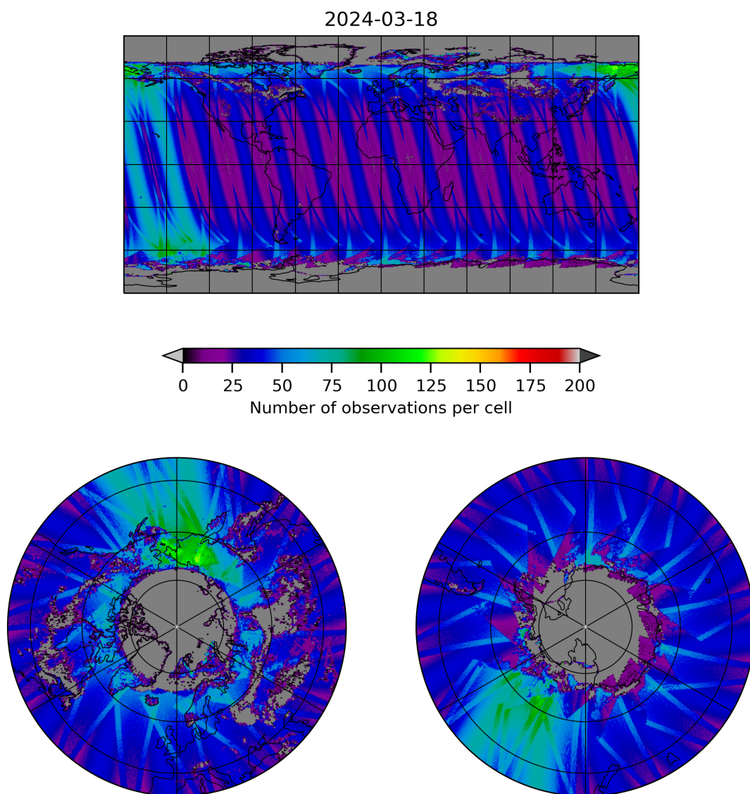
Figure 19: Map of the number of observations for 2024-03-17 to 2024-03-19
