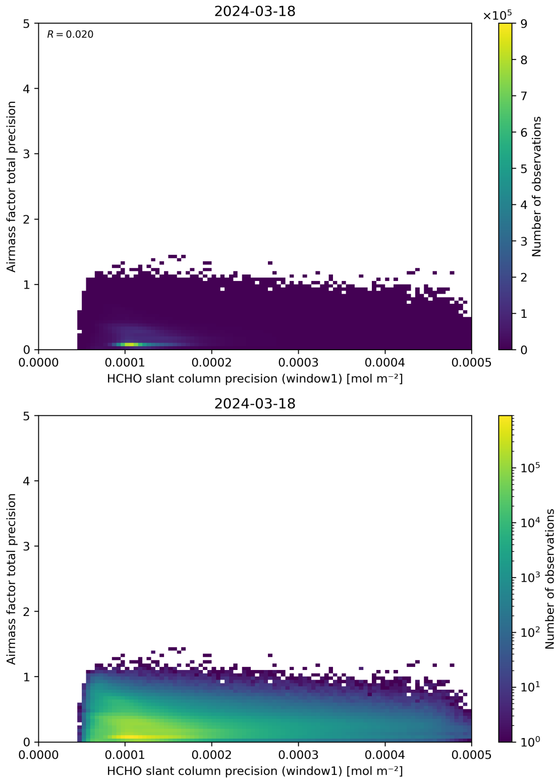
Figure 95: Scatter density plot of “HCHO slant column precision (window1)” against “Airmass factor total precision” for 2024-03-17 to 2024-03-19.
