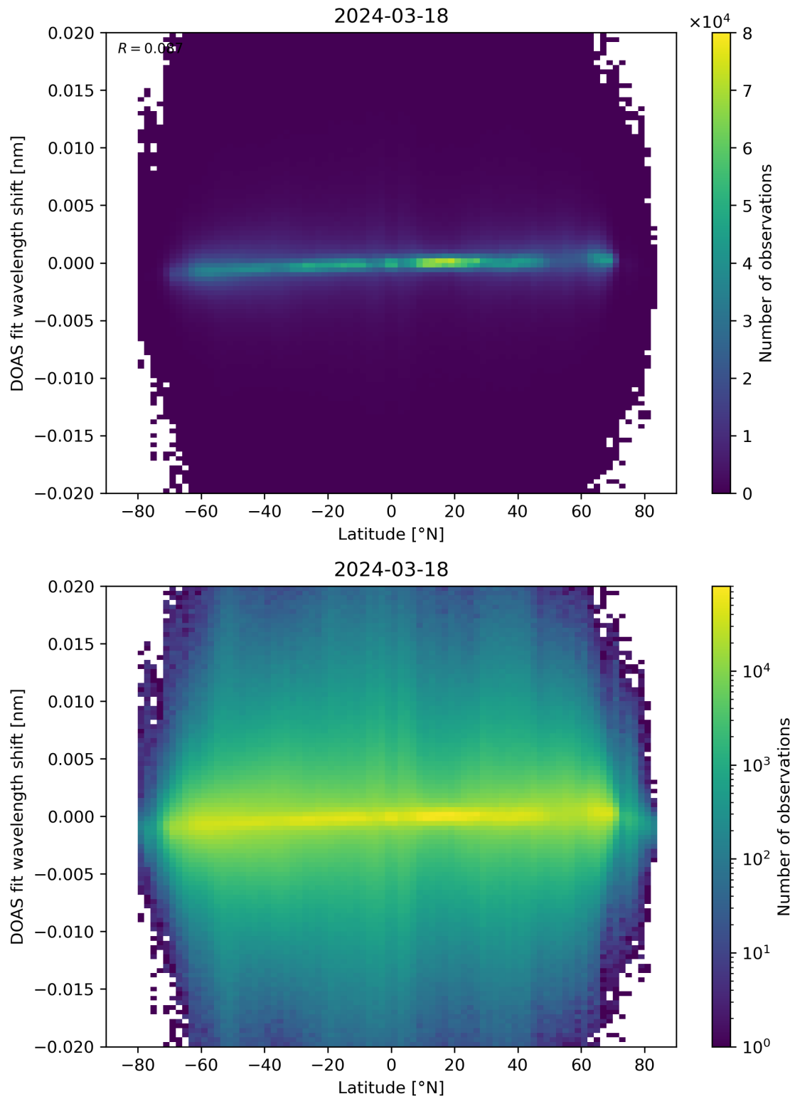
Figure 154: Scatter density plot of “Latitude” against “DOAS fit wavelength shift” for 2024-03-17 to 2024-03-19.
