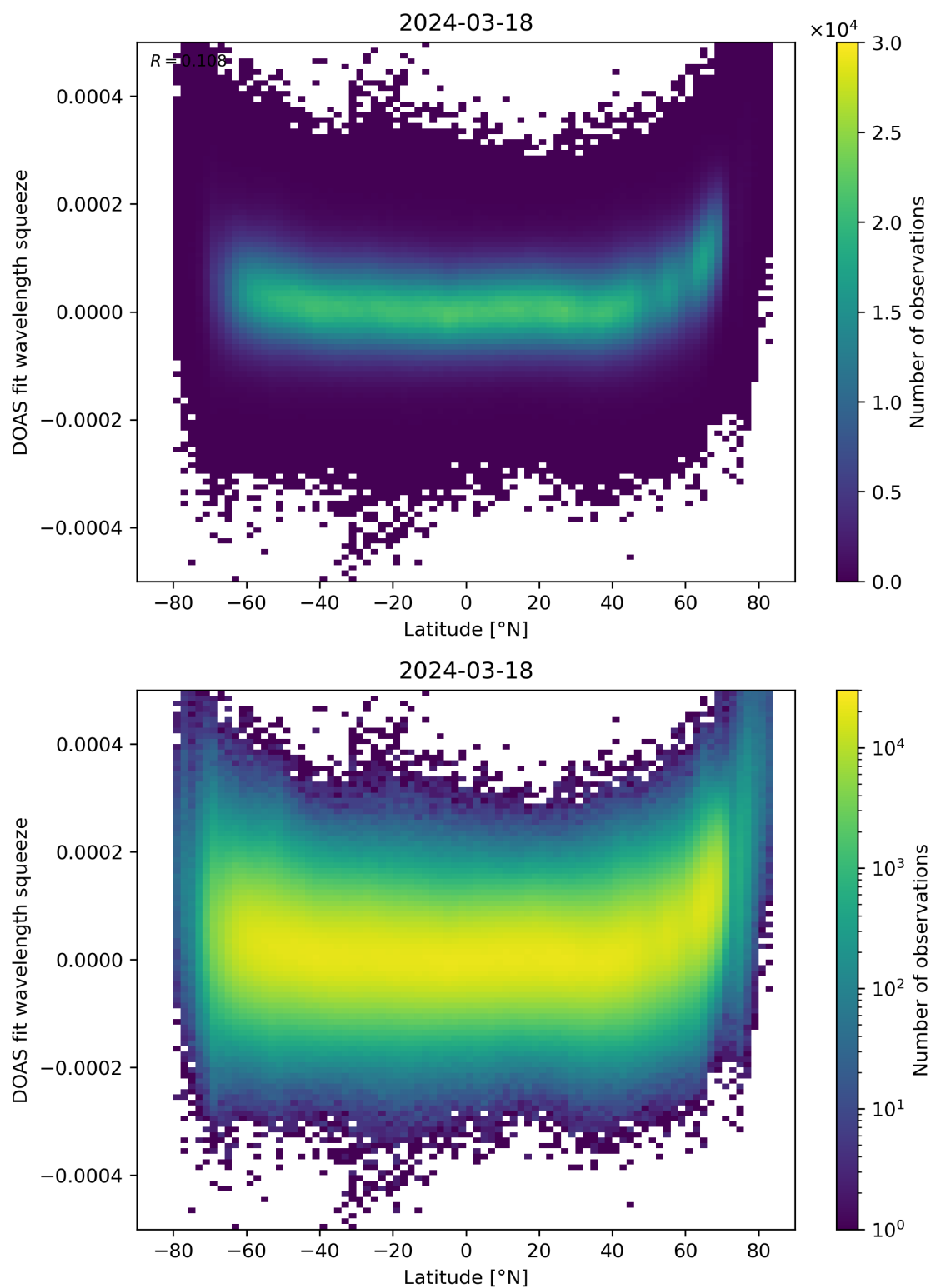
Figure 155: Scatter density plot of “Latitude” against “DOAS fit wavelength squeeze” for 2024-03-17 to 2024-03-19.
