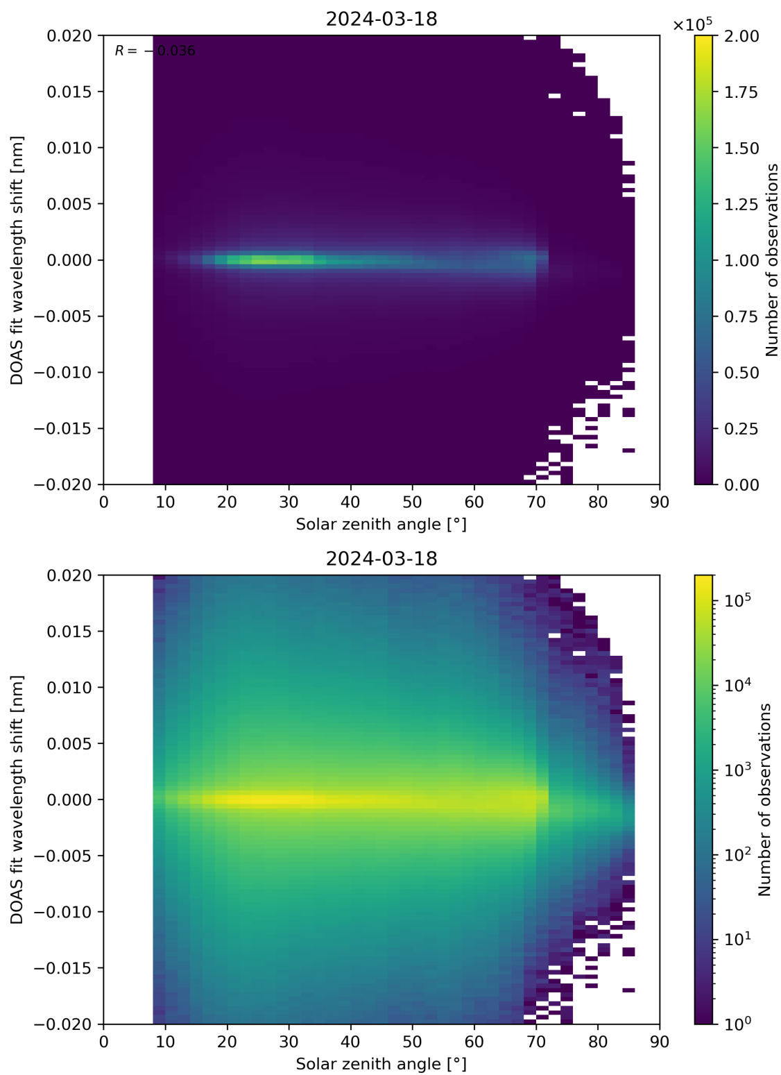
Figure 168: Scatter density plot of “Solar zenith angle” against “DOAS fit wavelength shift” for 2024-03-17 to 2024-03-19.
