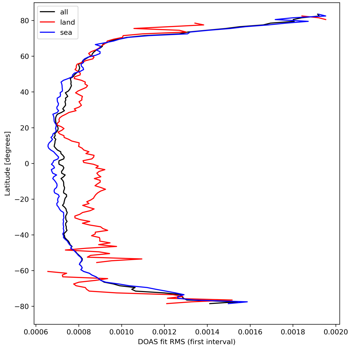
Figure 32: Zonal average of “DOAS fit RMS (first interval)” for 2024-03-17 to 2024-03-19.
