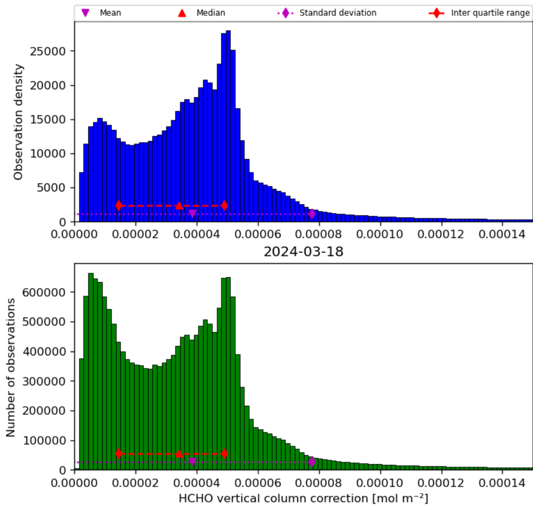
Figure 37: Histogram of “HCHO vertical column correction” for 2024-03-17 to 2024-03-19
