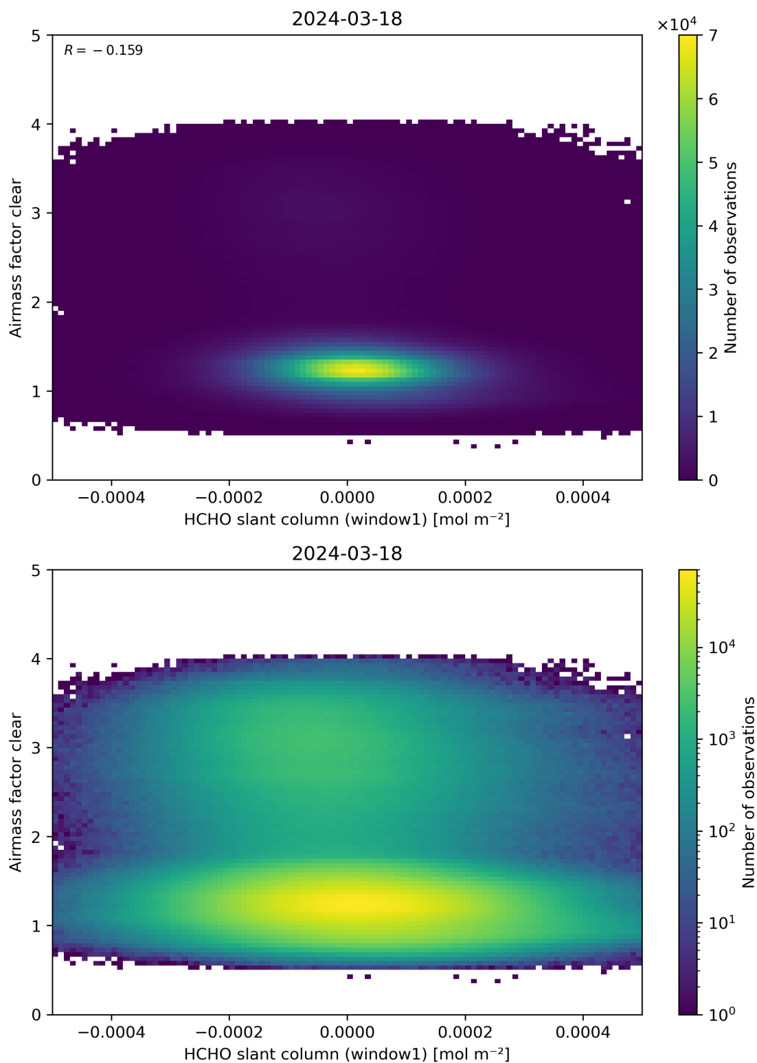
Figure 81: Scatter density plot of “HCHO slant column (window1)” against “Airmass factor clear” for 2024-03-17 to 2024-03-19.
