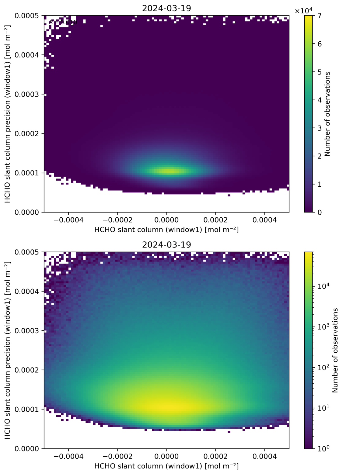
Figure 84: Scatter density plot of “HCHO slant column (window1)” against “HCHO slant column precision (window1)” for 2024-03-18 to 2024-03-20.
