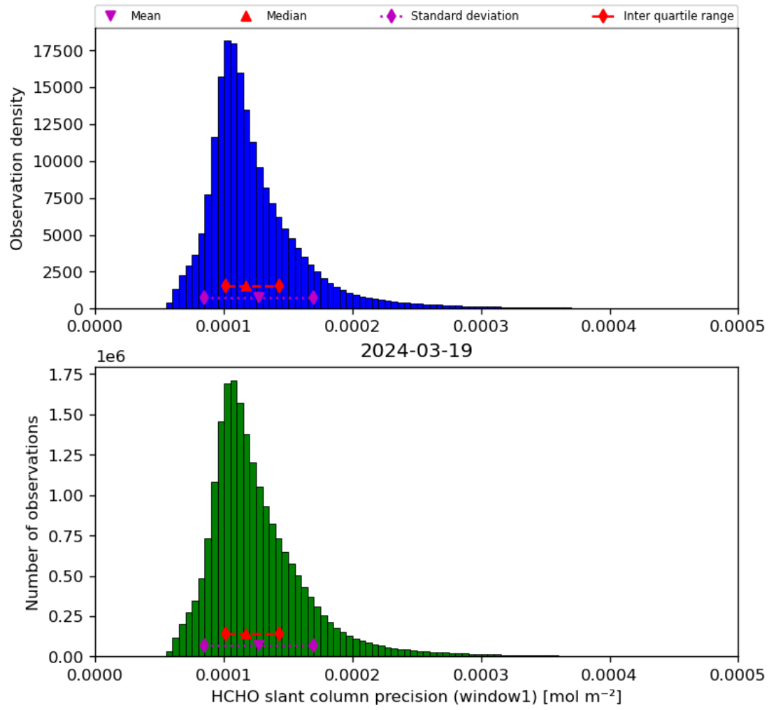
Figure 39: Histogram of “HCHO slant column precision (window1)” for 2024-03-18 to 2024-03-20
