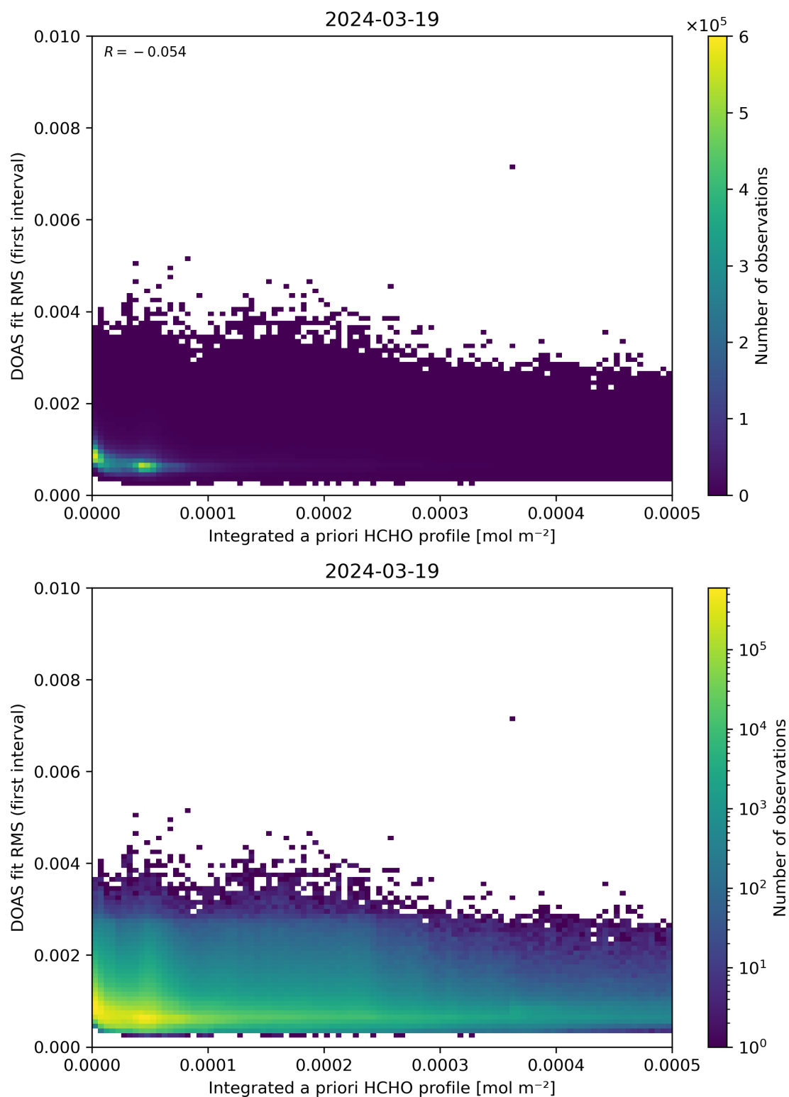
Figure 148: Scatter density plot of “Integrated a priori HCHO profile” against “DOAS fit RMS (first interval)” for 2024-03-18 to 2024-03-20.
