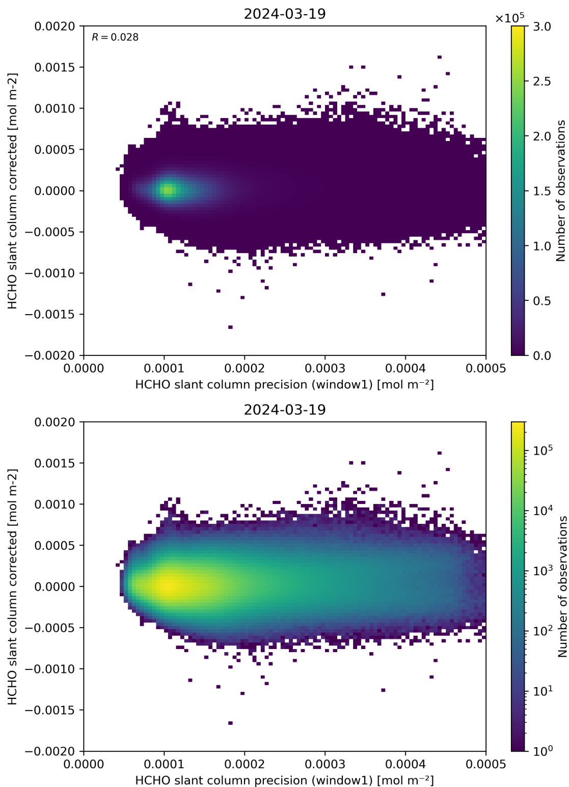
Figure 92: Scatter density plot of “HCHO slant column precision (window1)” against “HCHO slant column corrected” for 2024-03-18 to 2024-03-20.
