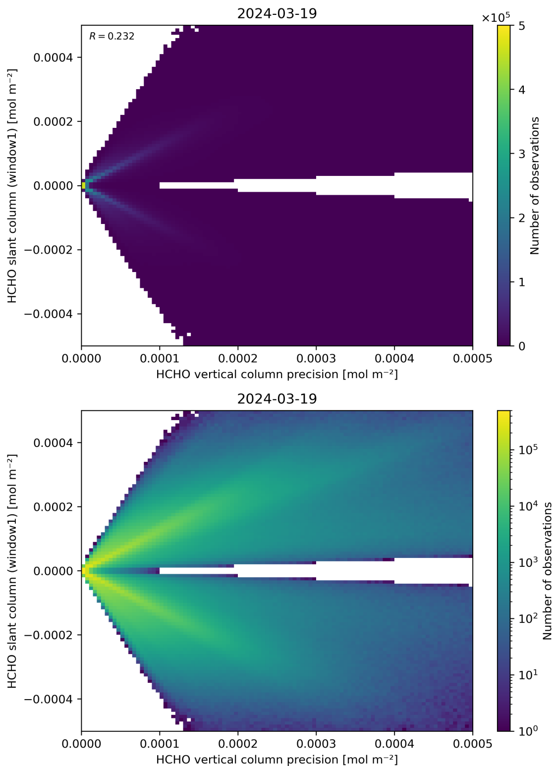
Figure 142: Scatter density plot of “HCHO vertical column precision” against “HCHO slant column (window1)” for 2024-03-18 to 2024-03-20.
