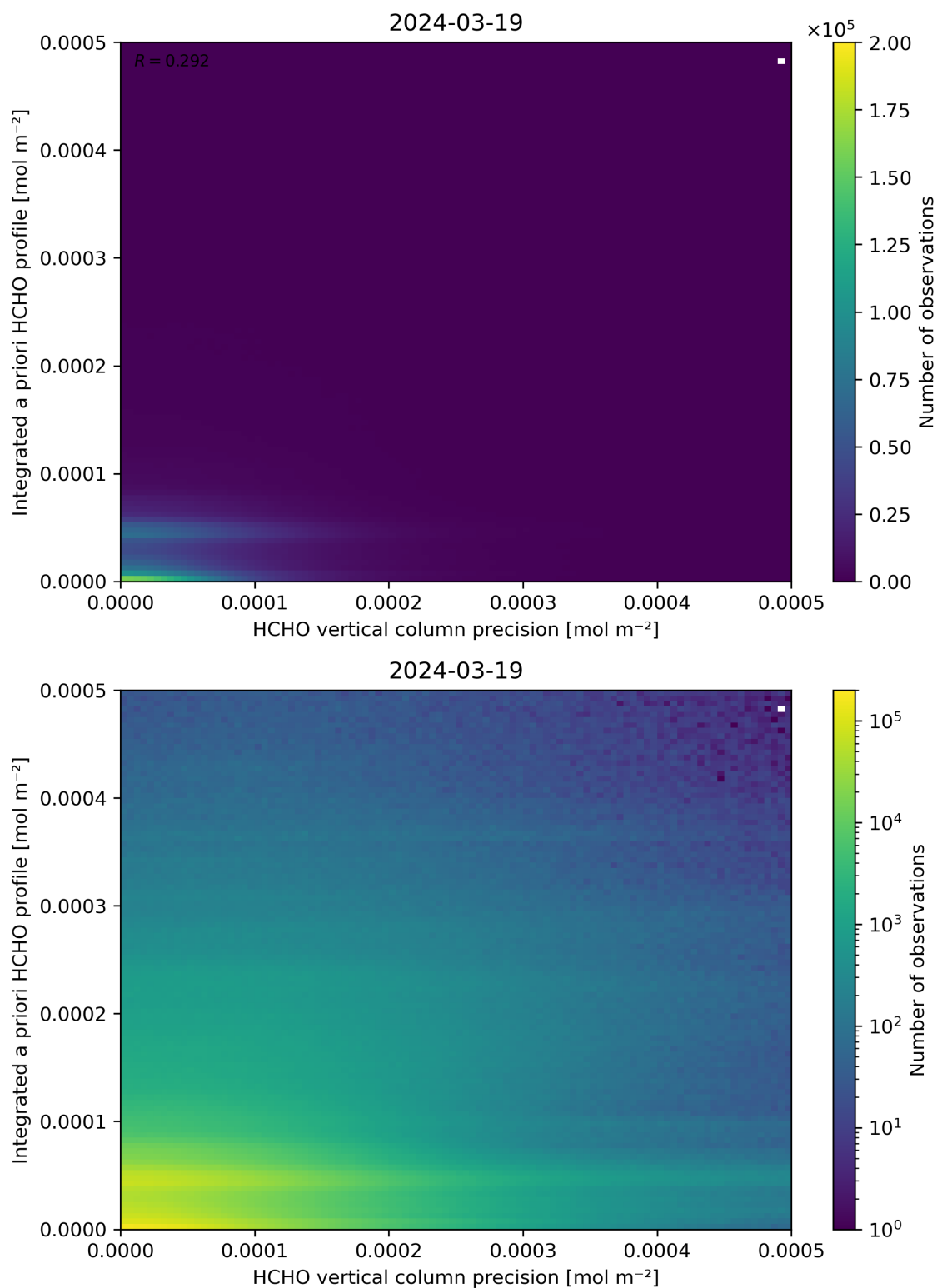
Figure 147: Scatter density plot of “HCHO vertical column precision” against “Integrated a priori HCHO profile” for 2024-03-18 to 2024-03-20.
