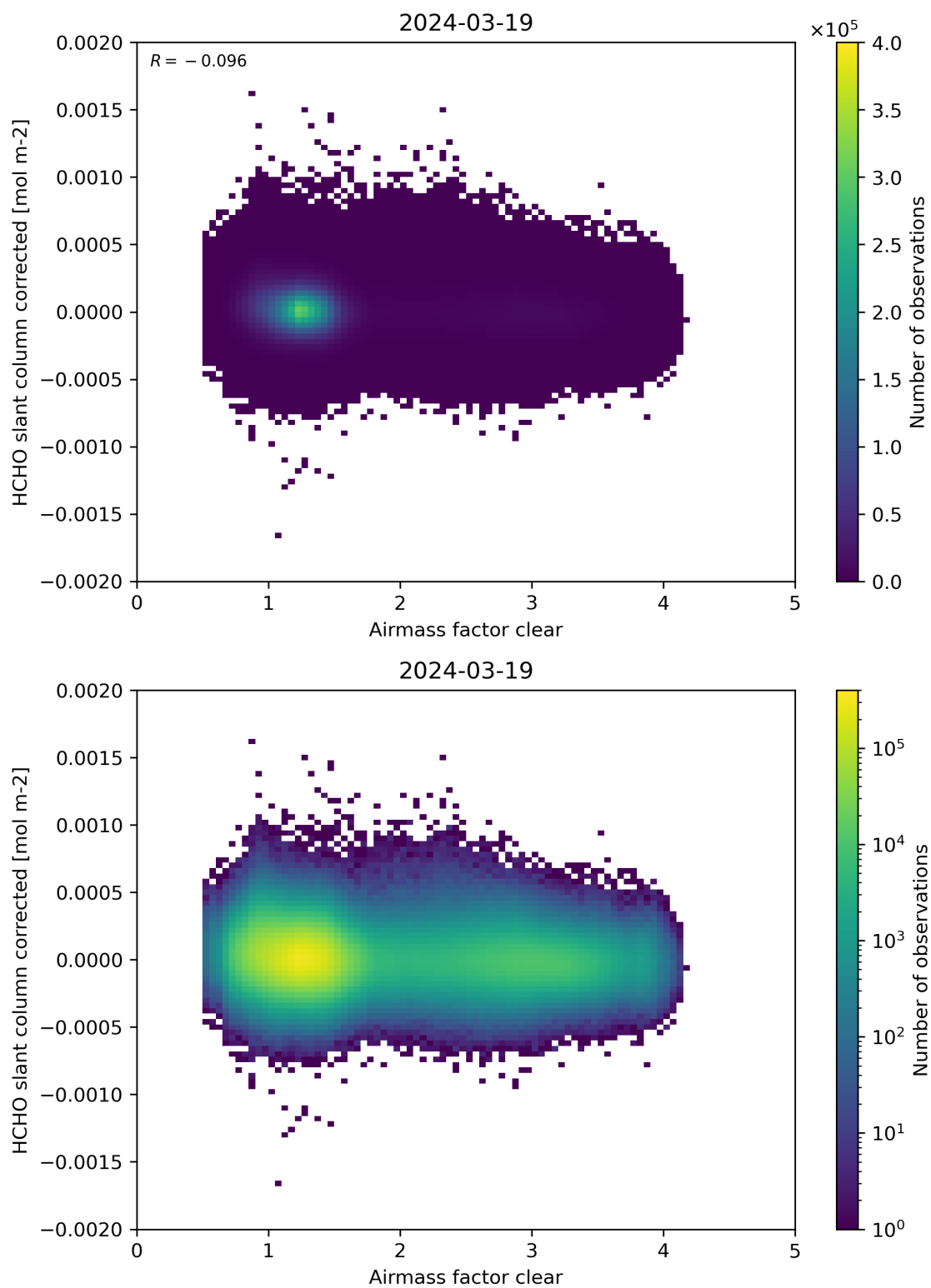
Figure 74: Scatter density plot of “Airmass factor clear” against “HCHO slant column corrected” for 2024-03-18 to 2024-03-20.
