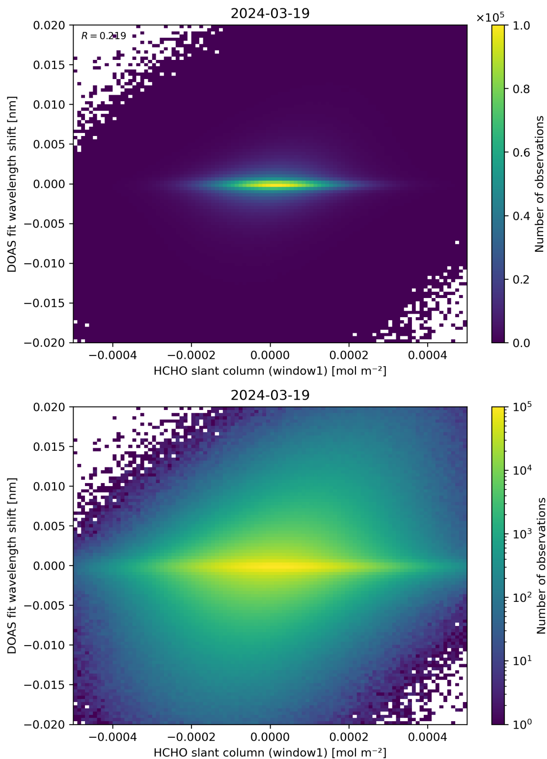
Figure 79: Scatter density plot of “HCHO slant column (window1)” against “DOAS fit wavelength shift” for 2024-03-18 to 2024-03-20.
