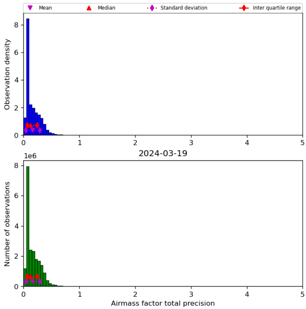
Figure 41: Histogram of “Airmass factor total precision” for 2024-03-18 to 2024-03-20
