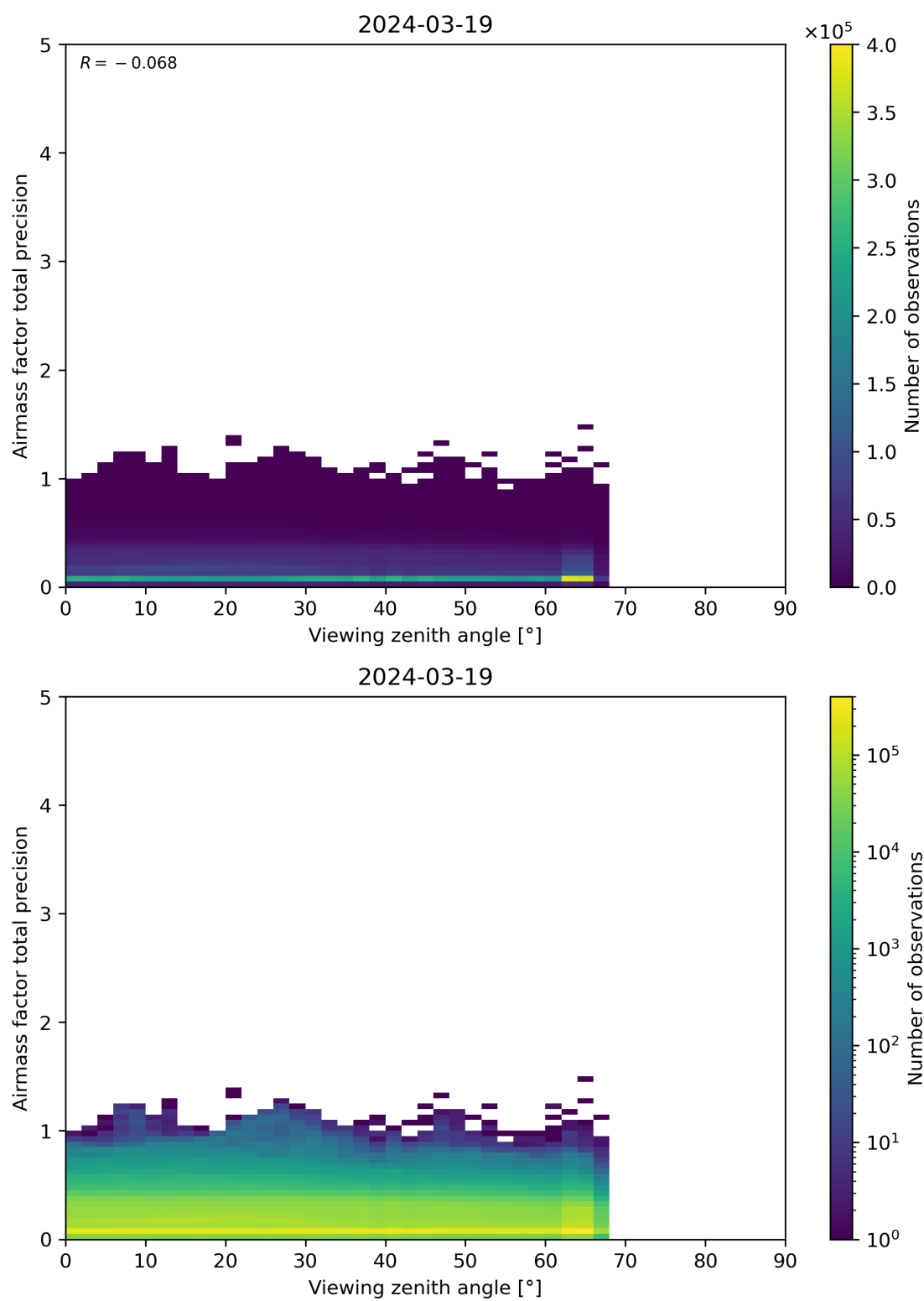
Figure 191: Scatter density plot of “Viewing zenith angle” against “Airmass factor total precision” for 2024-03-18 to 2024-03-20.
