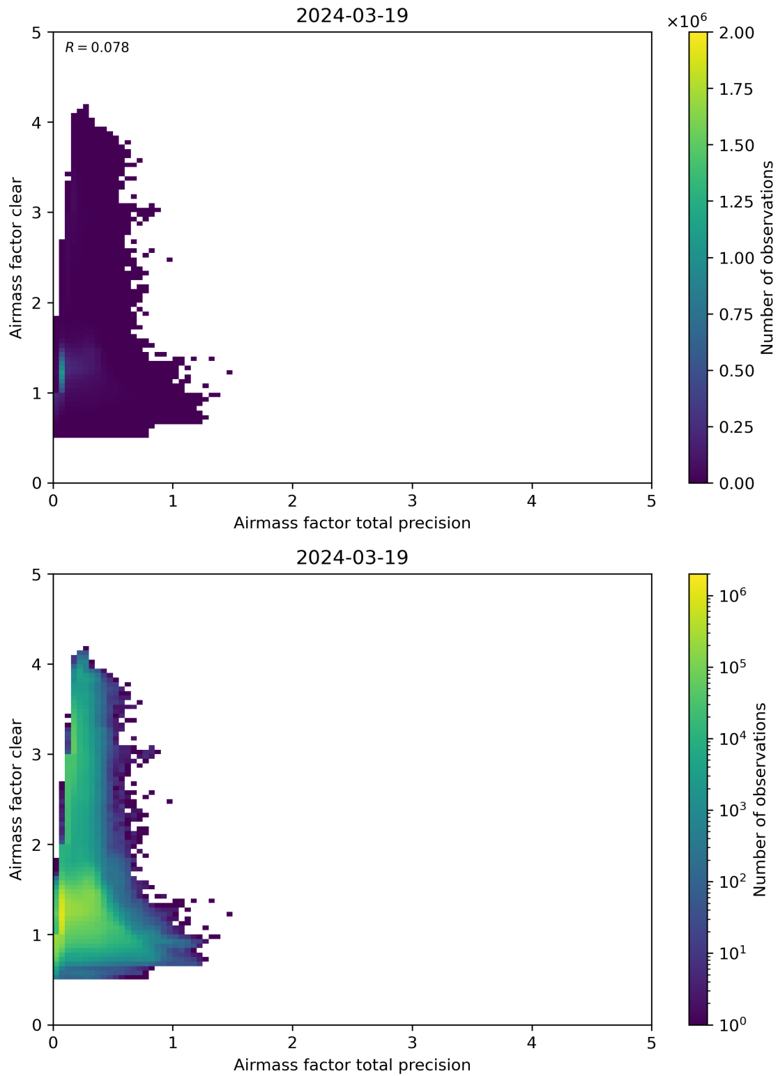
Figure 108: Scatter density plot of “Airmass factor total precision” against “Airmass factor clear” for 2024-03-18 to 2024-03-20.
