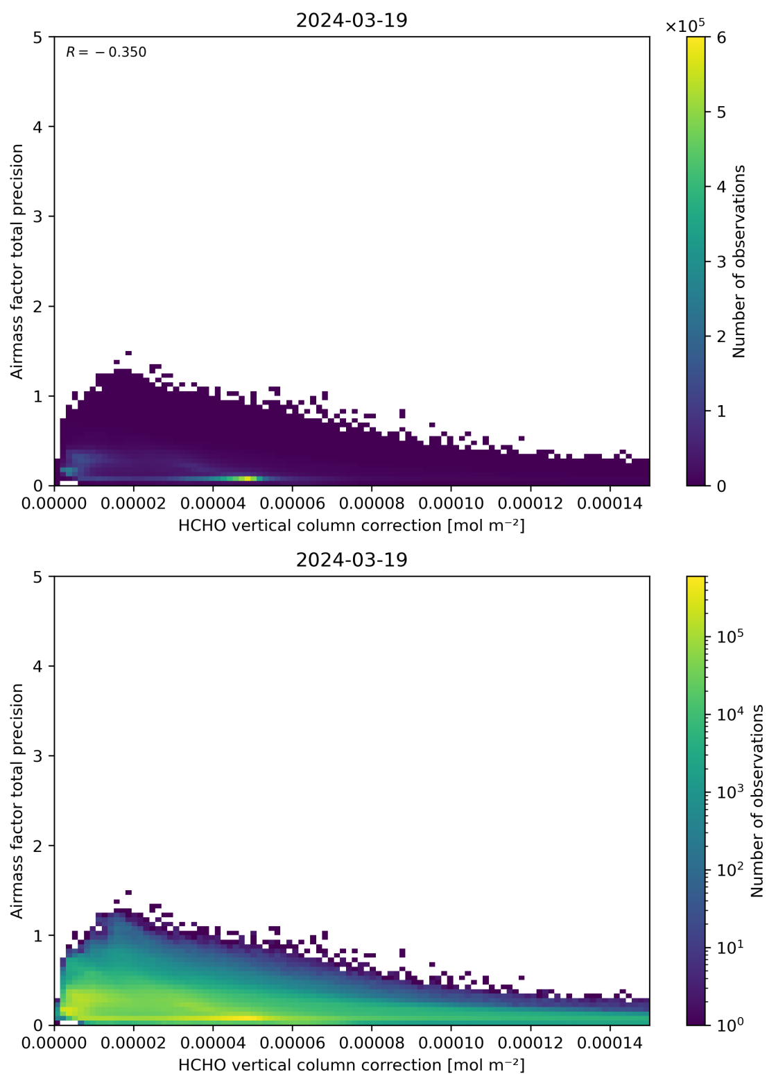
Figure 121: Scatter density plot of “HCHO vertical column correction” against “Airmass factor total precision” for 2024-03-18 to 2024-03-20.
