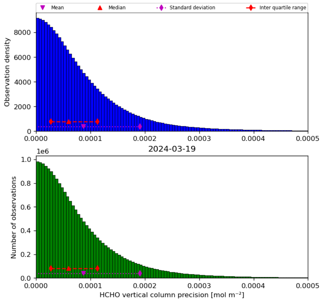
Figure 36: Histogram of “HCHO vertical column precision” for 2024-03-18 to 2024-03-20
