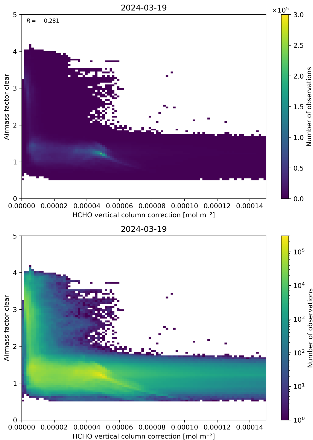
Figure 115: Scatter density plot of “HCHO vertical column correction” against “Airmass factor clear” for 2024-03-18 to 2024-03-20.
