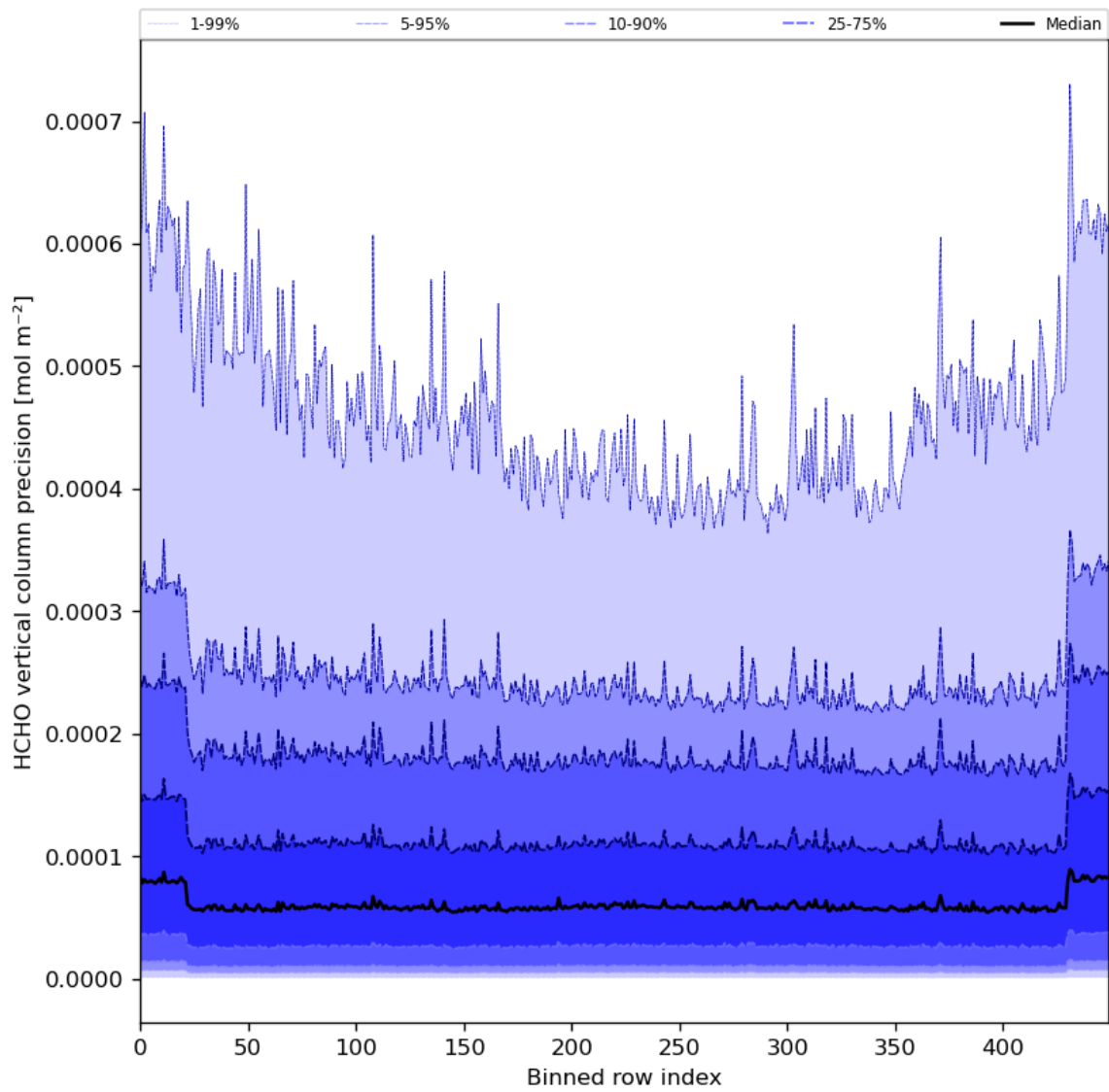
Figure 50: Along track statistics of “HCHO vertical column precision” for 2024-03-18 to 2024-03-20
