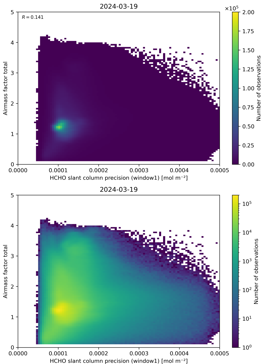
Figure 94: Scatter density plot of “HCHO slant column precision (window1)” against “Airmass factor total” for 2024-03-18 to 2024-03-20.
