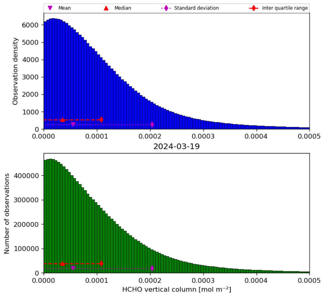
Figure 35: Histogram of “HCHO vertical column” for 2024-03-18 to 2024-03-20
