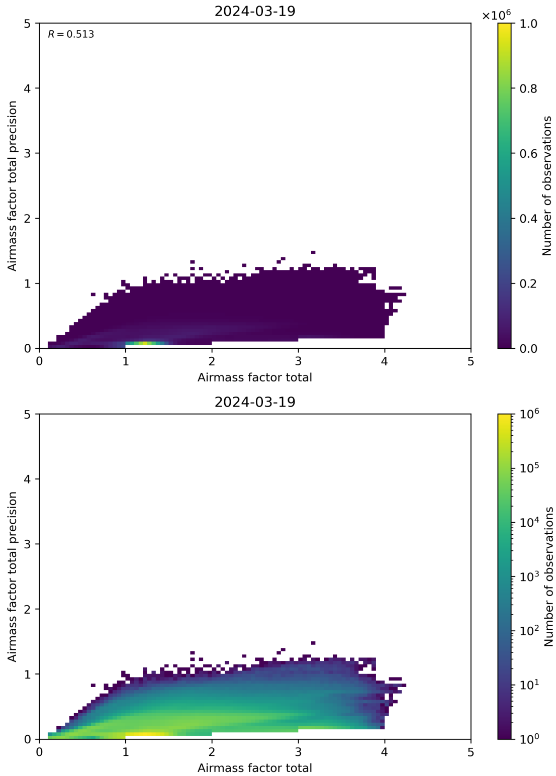
Figure 103: Scatter density plot of “Airmass factor total” against “Airmass factor total precision” for 2024-03-18 to 2024-03-20.
