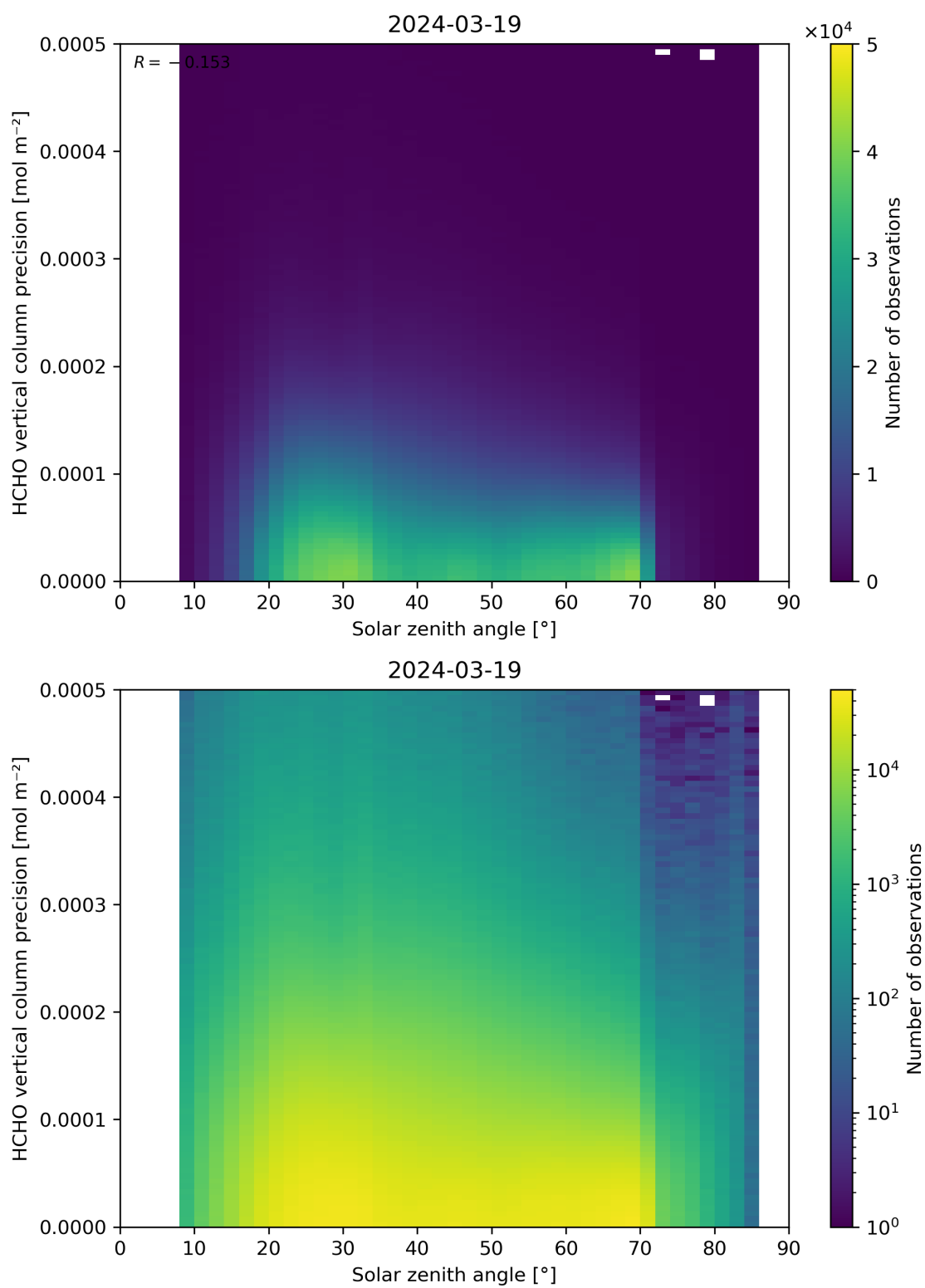
Figure 179: Scatter density plot of “Solar zenith angle” against “HCHO vertical column precision” for 2024-03-18 to 2024-03-20.
