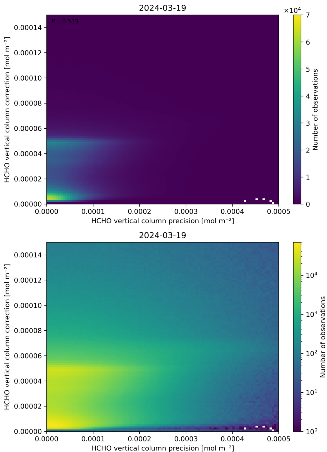
Figure 146: Scatter density plot of “HCHO vertical column precision” against “HCHO vertical column correction” for 2024-03-18 to 2024-03-20.
