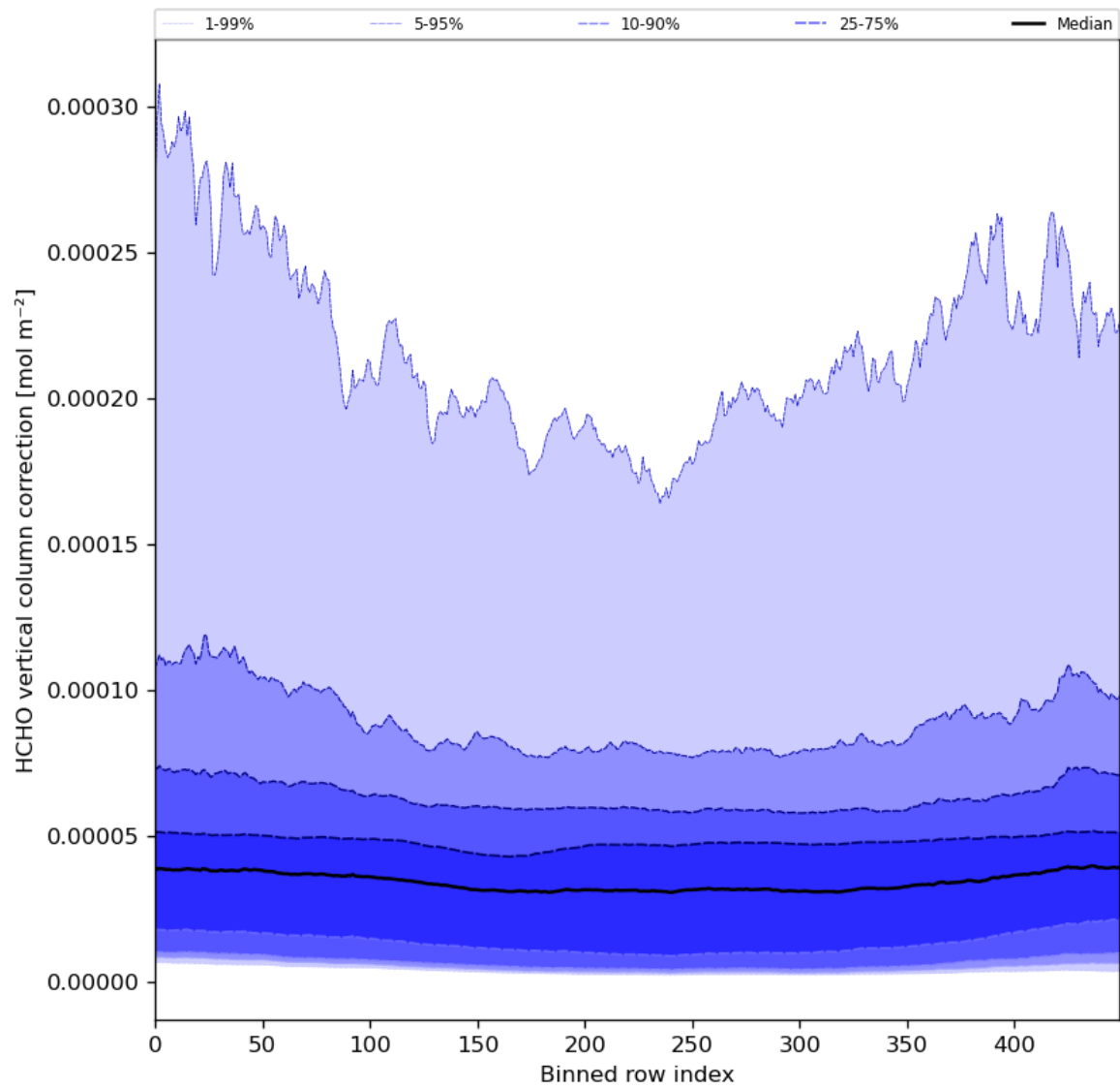
Figure 51: Along track statistics of “HCHO vertical column correction” for 2024-03-18 to 2024-03-20
