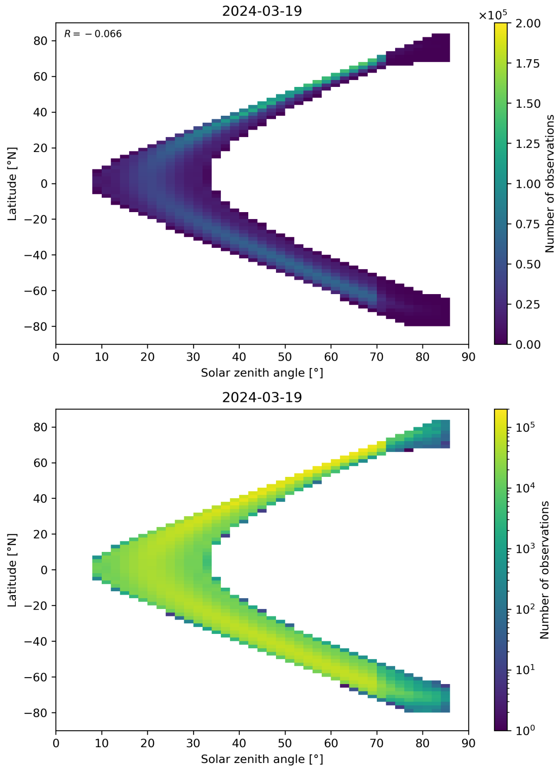
Figure 181: Scatter density plot of “Solar zenith angle” against “Latitude” for 2024-03-18 to 2024-03-20.
