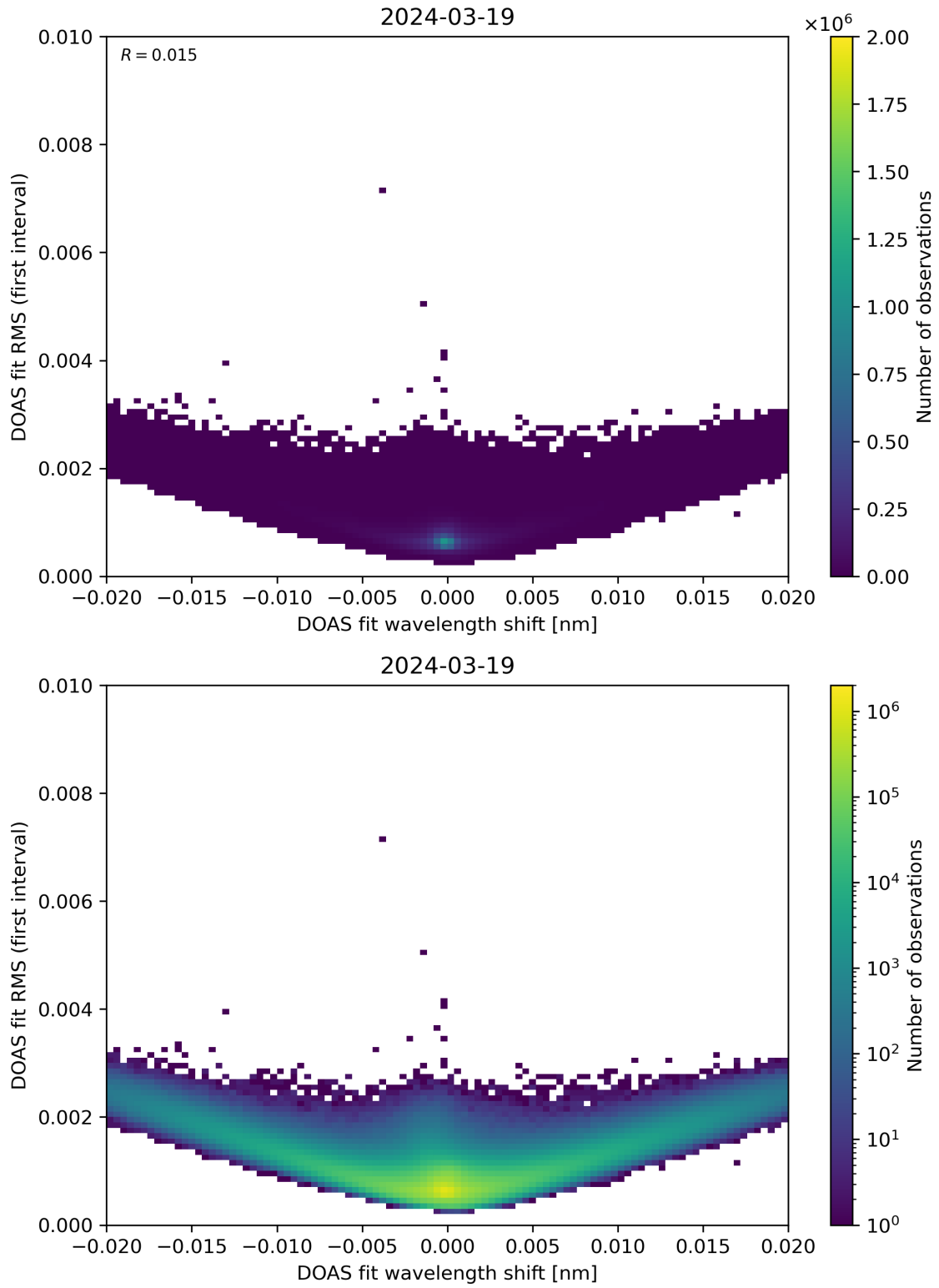
Figure 64: Scatter density plot of “DOAS fit wavelength shift” against “DOAS fit RMS (first interval)” for 2024-03-18 to 2024-03-20.
