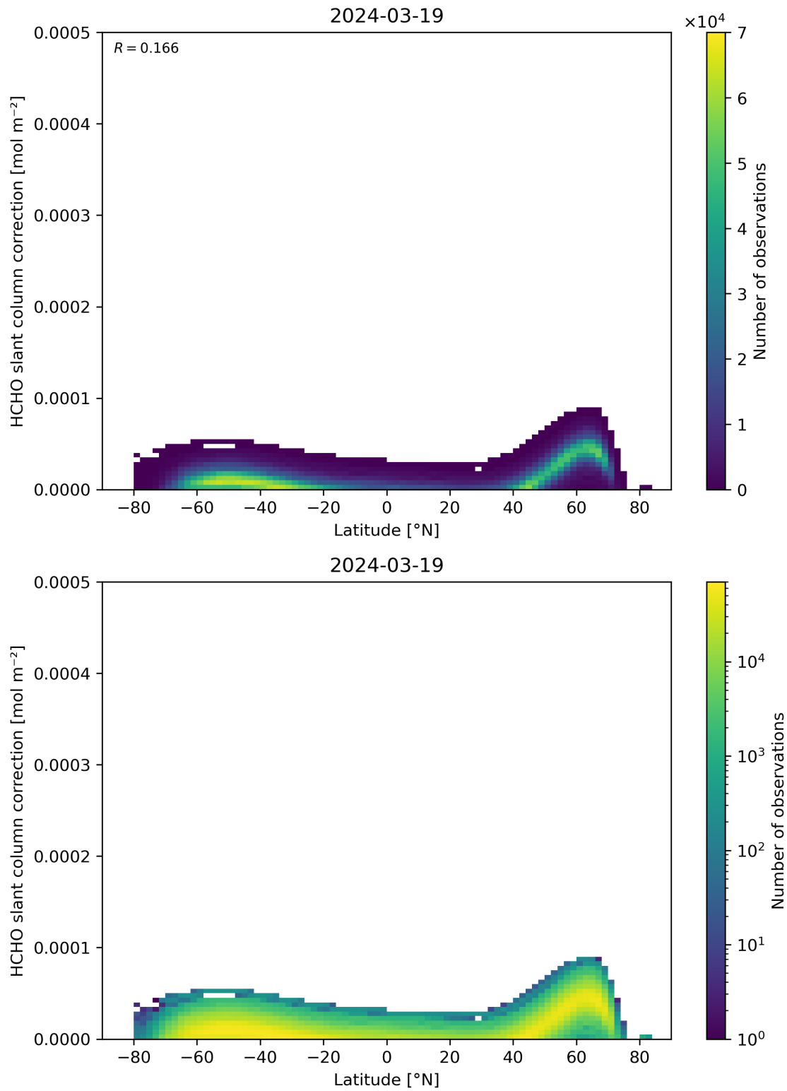
Figure 158: Scatter density plot of “Latitude” against “HCHO slant column correction” for 2024-03-18 to 2024-03-20.
