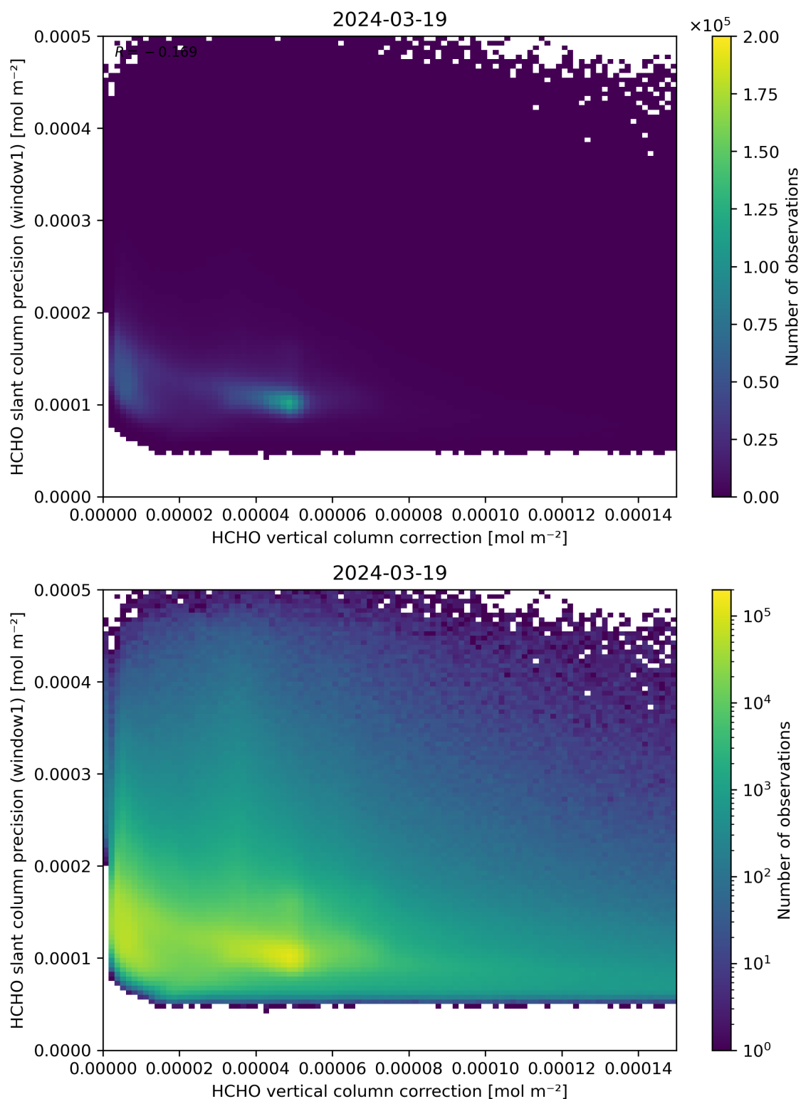
Figure 119: Scatter density plot of “HCHO vertical column correction” against “HCHO slant column precision (window1)” for 2024-03-18 to 2024-03-20.
