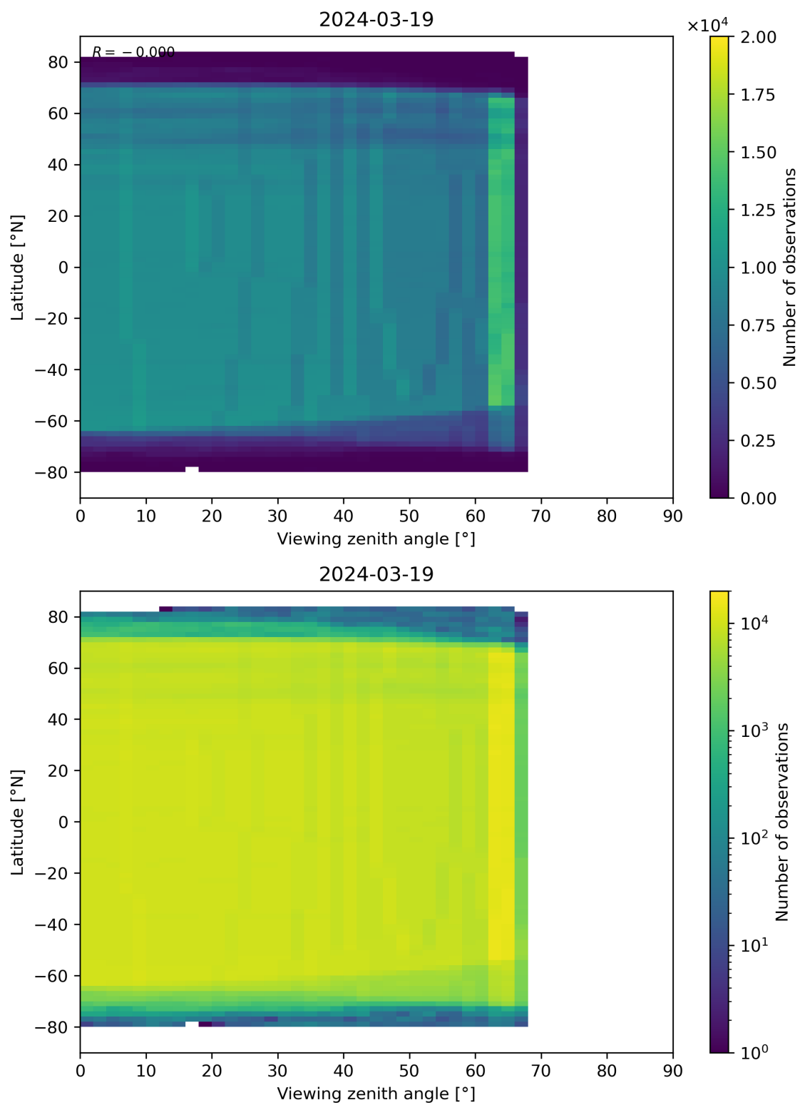
Figure 196: Scatter density plot of “Viewing zenith angle” against “Latitude” for 2024-03-18 to 2024-03-20.
