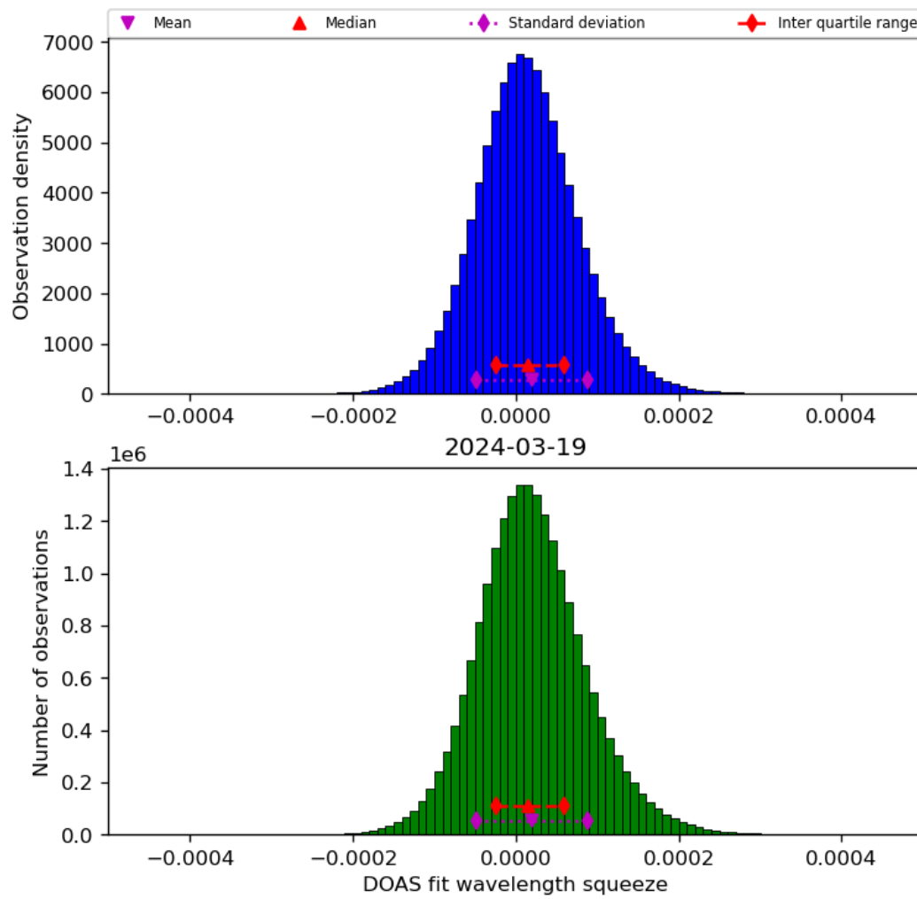
Figure 45: Histogram of “DOAS fit wavelength squeeze” for 2024-03-18 to 2024-03-20
