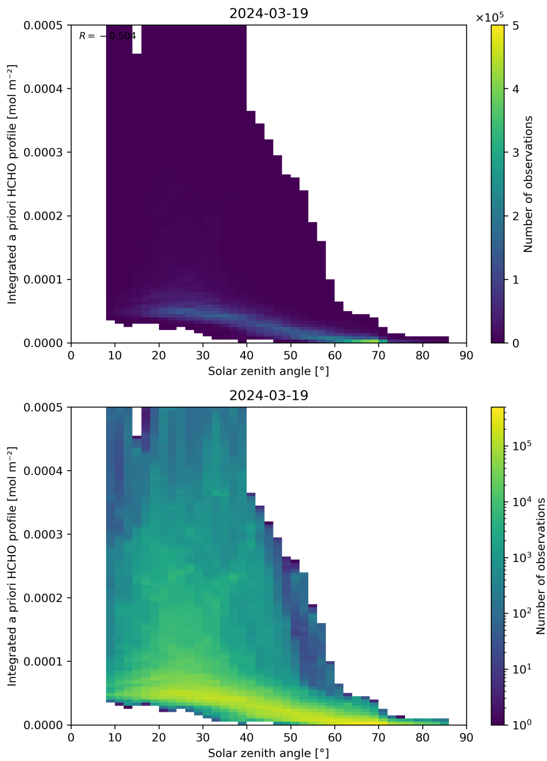
Figure 180: Scatter density plot of “Solar zenith angle” against “Integrated a priori HCHO profile” for 2024-03-18 to 2024-03-20.
