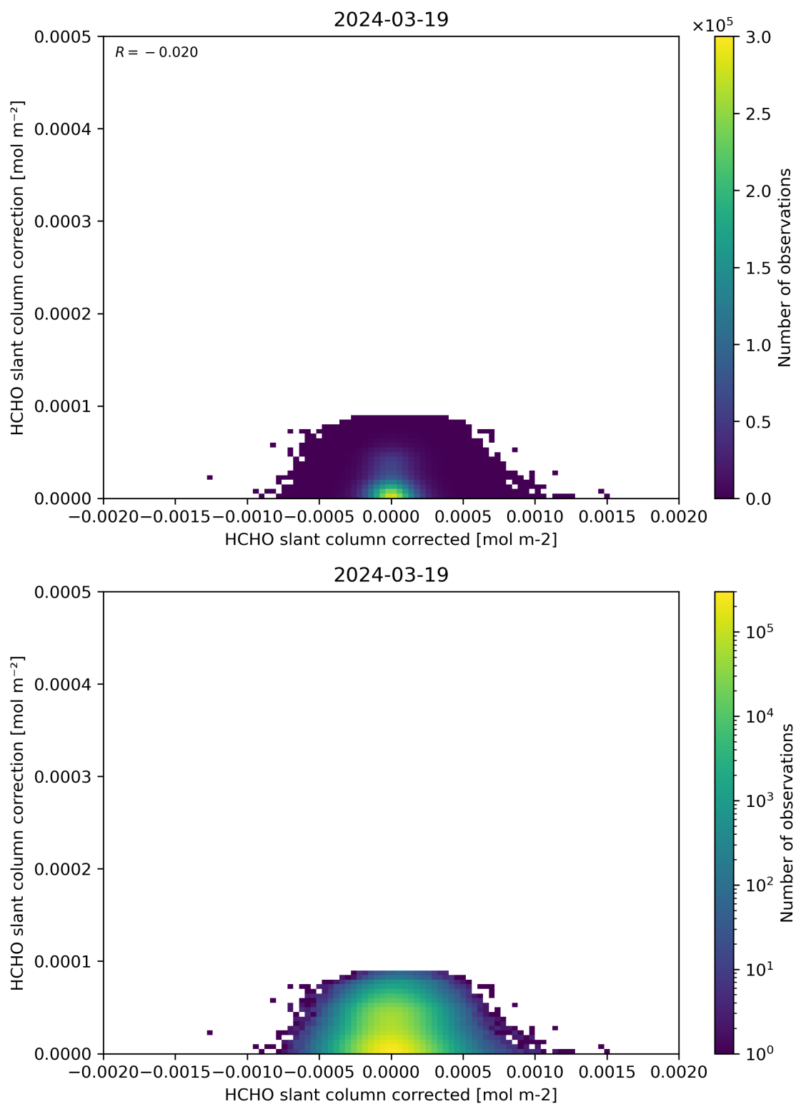
Figure 77: Scatter density plot of “HCHO slant column corrected” against “HCHO slant column correction” for 2024-03-18 to 2024-03-20.
