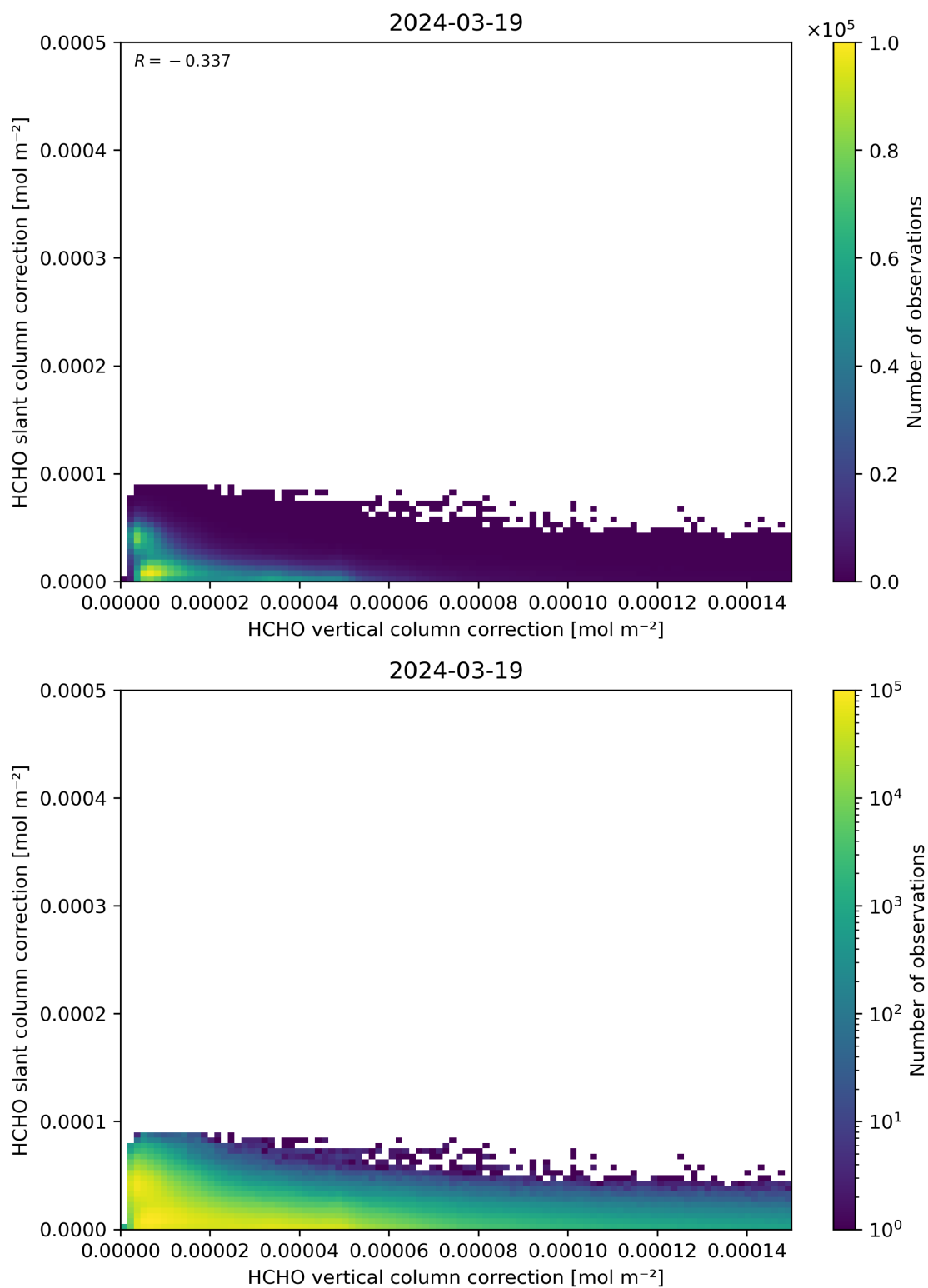
Figure 117: Scatter density plot of “HCHO vertical column correction” against “HCHO slant column correction” for 2024-03-18 to 2024-03-20.
