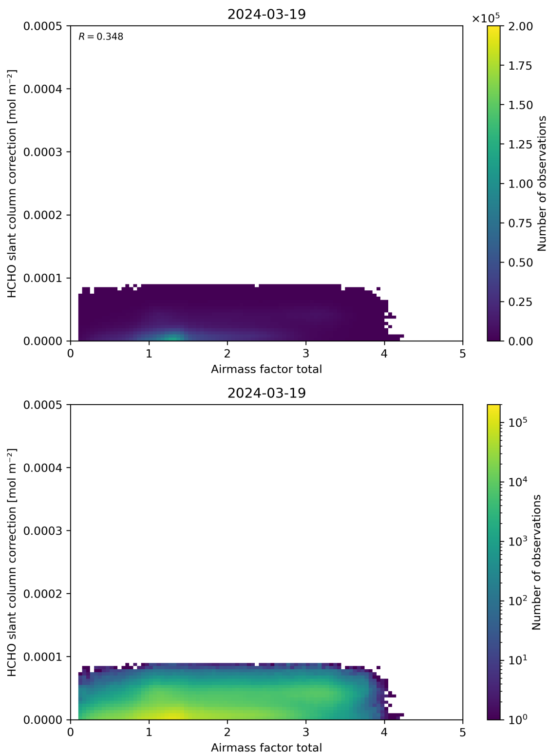
Figure 102: Scatter density plot of “Airmass factor total” against “HCHO slant column correction” for 2024-03-18 to 2024-03-20.
