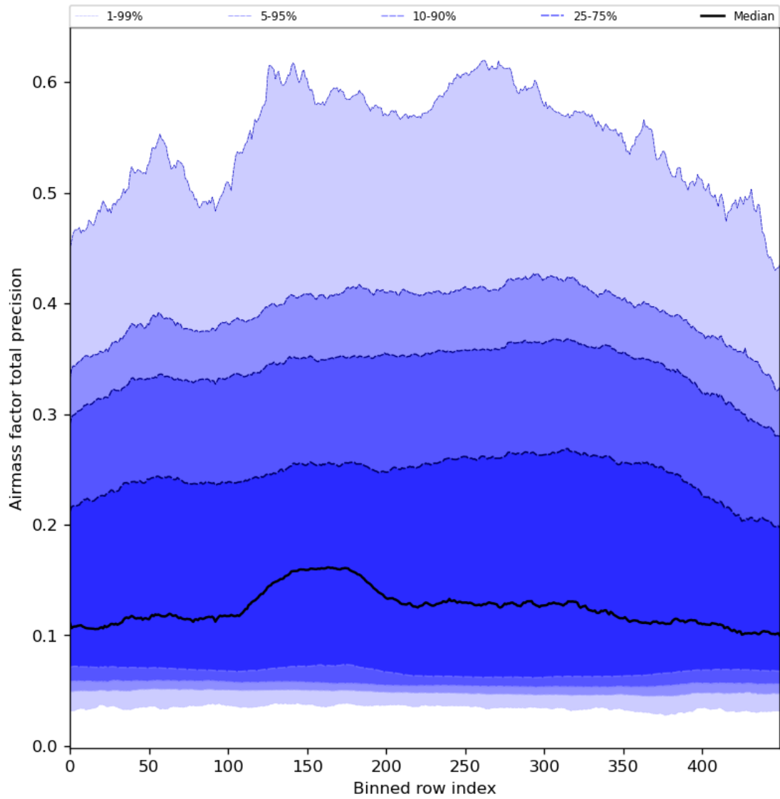
Figure 55: Along track statistics of “Airmass factor total precision” for 2024-03-18 to 2024-03-20
