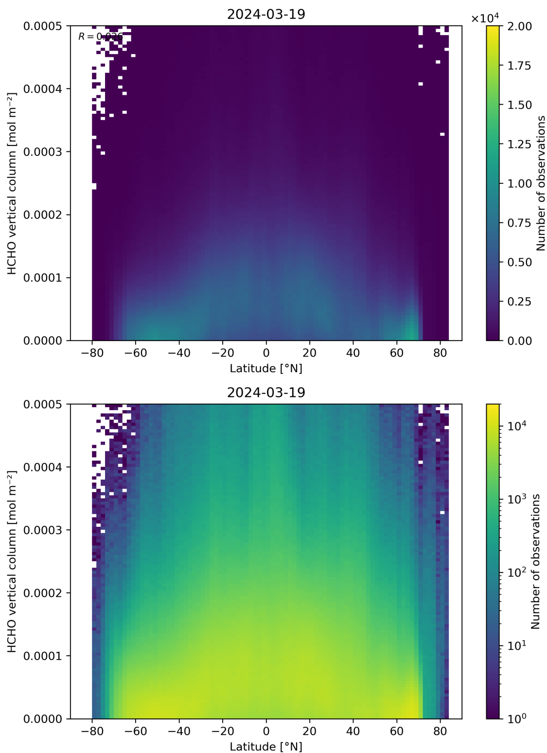
Figure 163: Scatter density plot of “Latitude” against “HCHO vertical column” for 2024-03-18 to 2024-03-20.
