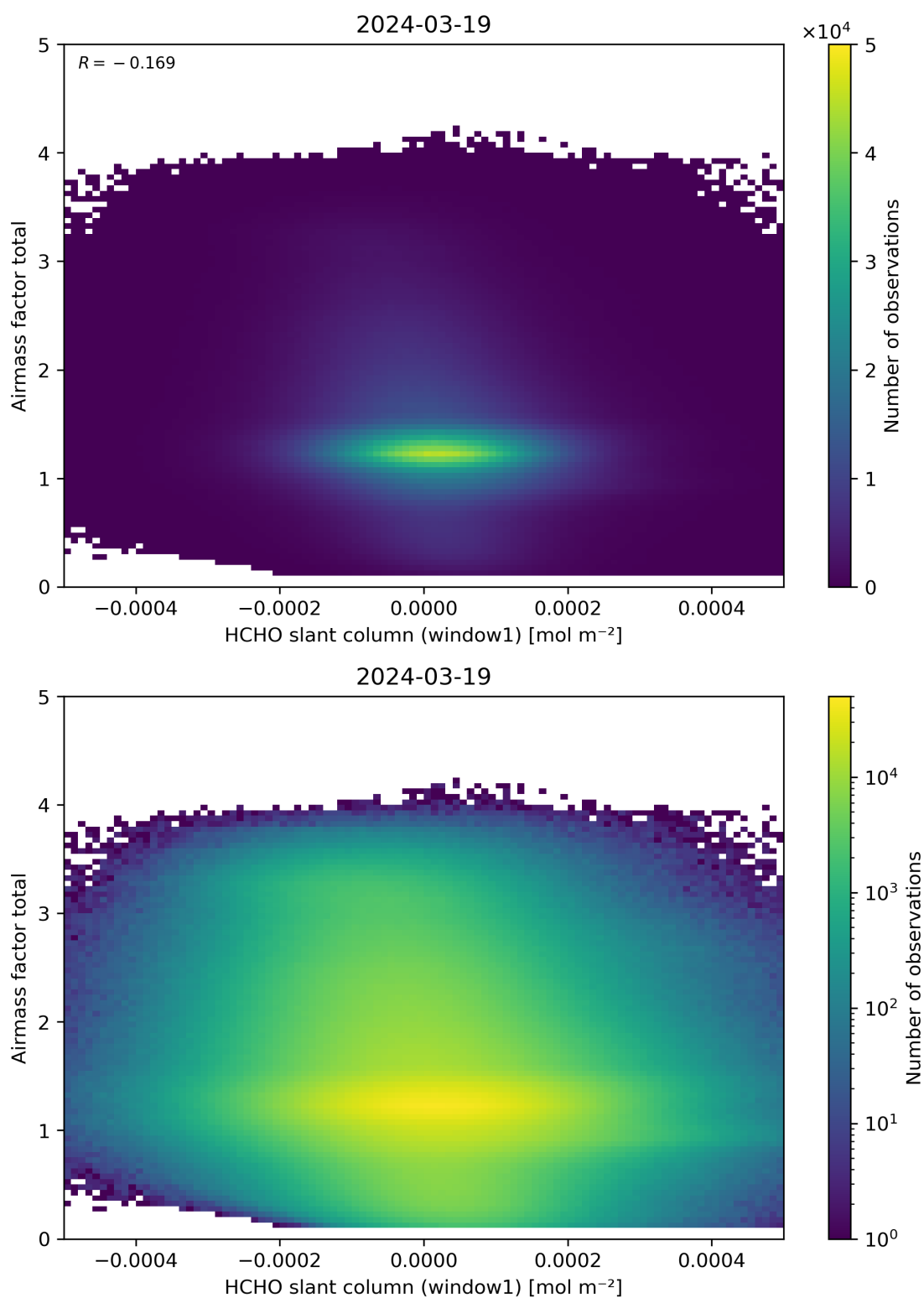
Figure 85: Scatter density plot of “HCHO slant column (window1)” against “Airmass factor total” for 2024-03-18 to 2024-03-20.
