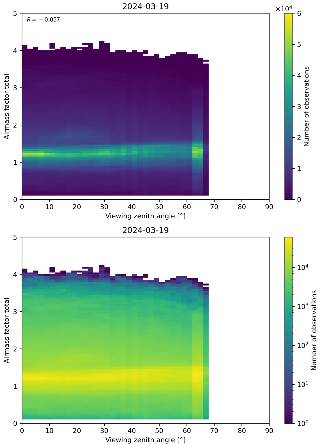
Figure 190: Scatter density plot of “Viewing zenith angle” against “Airmass factor total” for 2024-03-18 to 2024-03-20.
