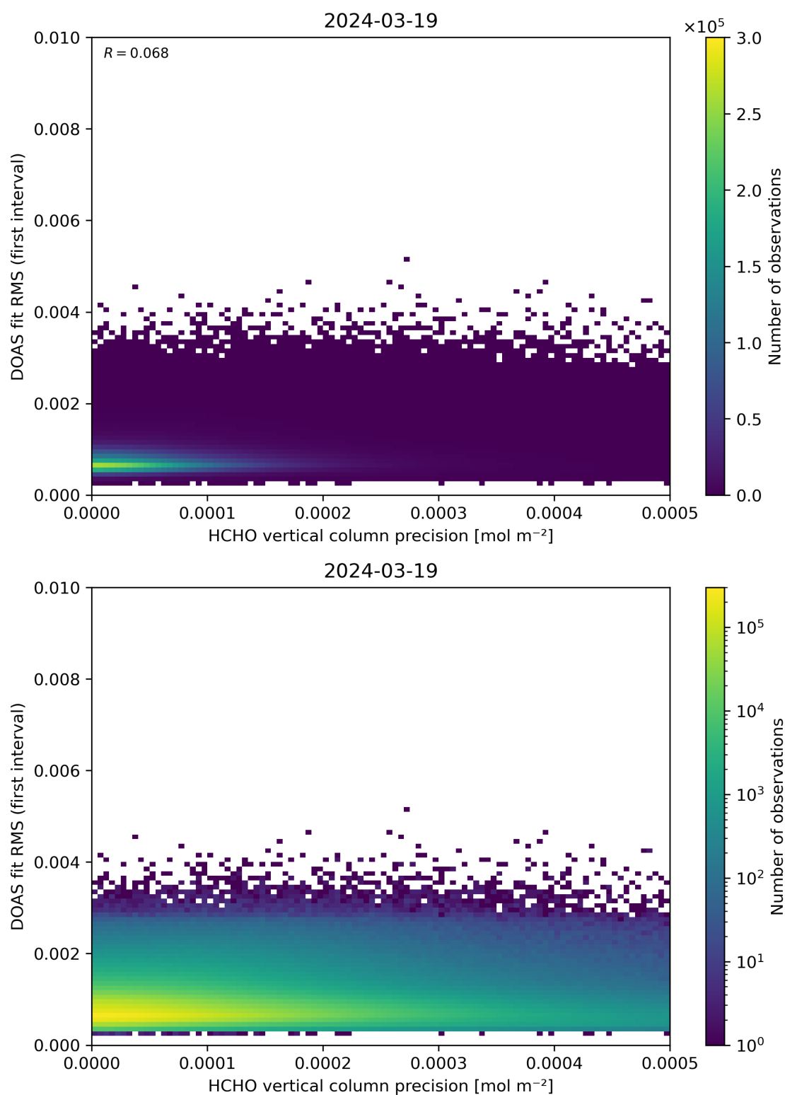
Figure 136: Scatter density plot of “HCHO vertical column precision” against “DOAS fit RMS (first interval)” for 2024-03-18 to 2024-03-20.
