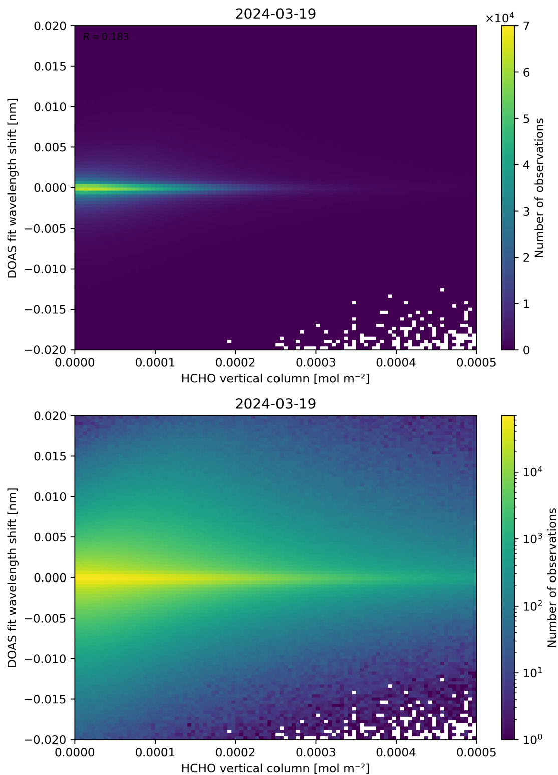
Figure 124: Scatter density plot of “HCHO vertical column” against “DOAS fit wavelength shift” for 2024-03-18 to 2024-03-20.
