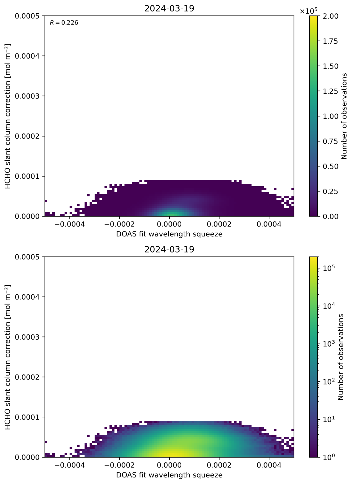
Figure 70: Scatter density plot of “DOAS fit wavelength squeeze” against “HCHO slant column correction” for 2024-03-18 to 2024-03-20.
