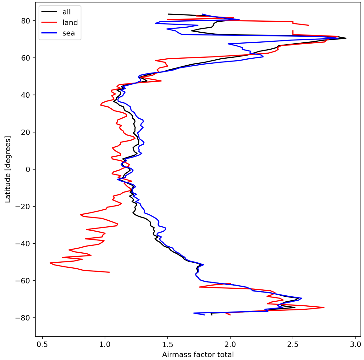
Figure 26: Zonal average of “Airmass factor total” for 2024-03-18 to 2024-03-20.
