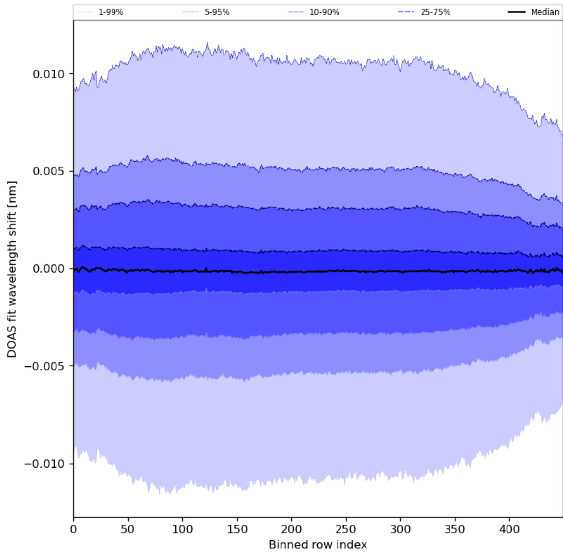
Figure 58: Along track statistics of “DOAS fit wavelength shift” for 2024-03-18 to 2024-03-20
