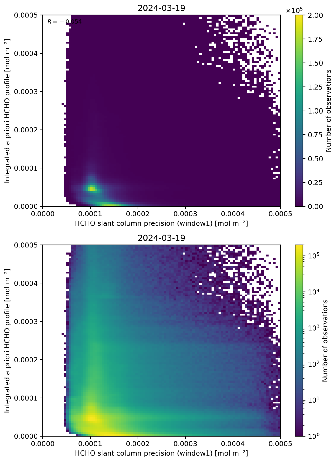
Figure 96: Scatter density plot of “HCHO slant column precision (window1)” against “Integrated a priori HCHO profile” for 2024-03-18 to 2024-03-20.
