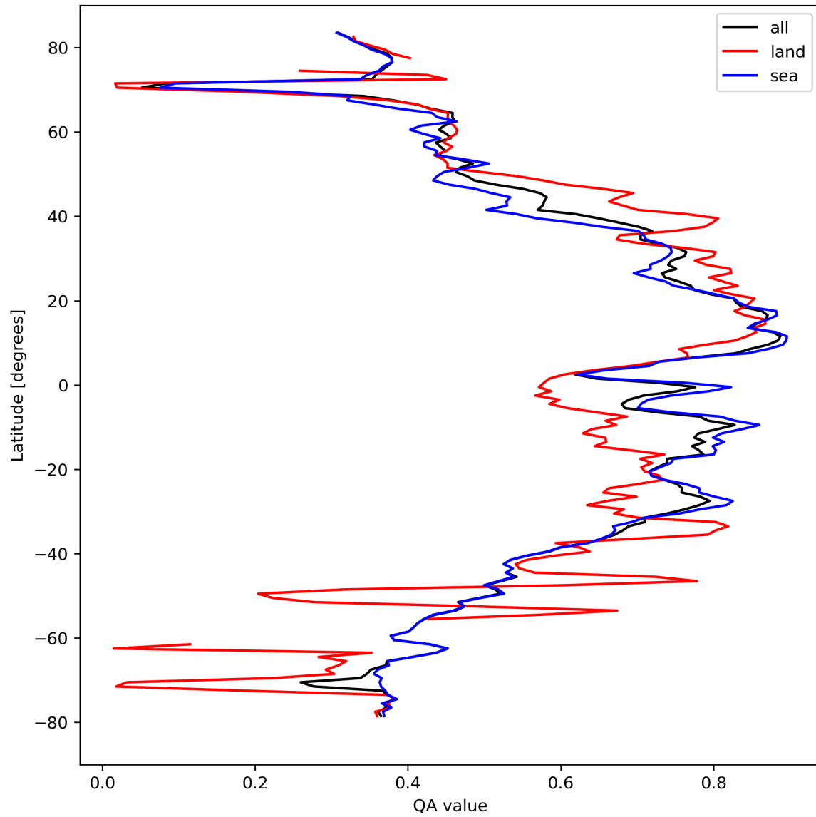
Figure 20: Zonal average of “QA value” for 2024-03-18 to 2024-03-20.
