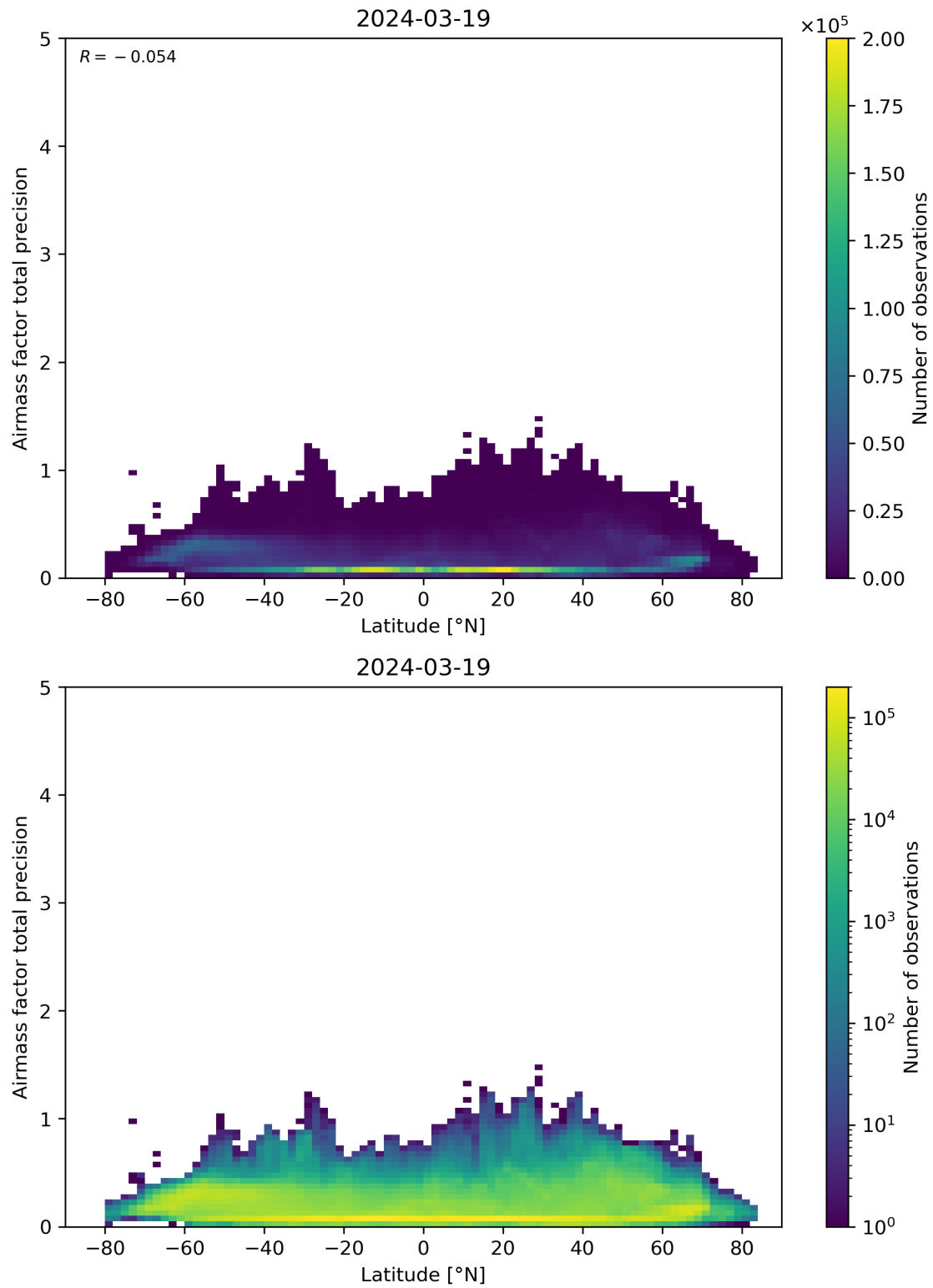
Figure 162: Scatter density plot of “Latitude” against “Airmass factor total precision” for 2024-03-18 to 2024-03-20.
