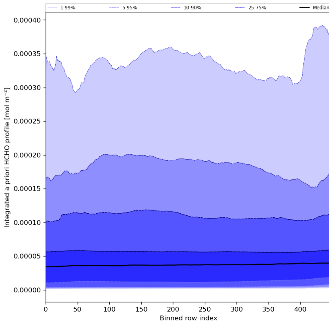
Figure 57: Along track statistics of “Integrated a priori HCHO profile” for 2024-03-18 to 2024-03-20
