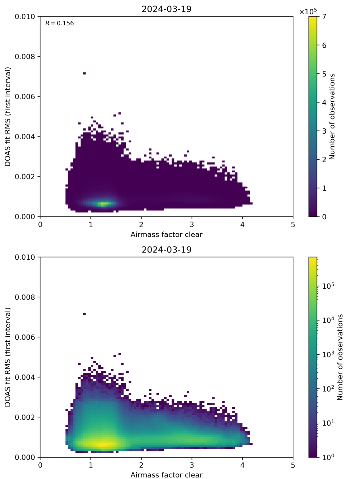
Figure 71: Scatter density plot of “Airmass factor clear” against “DOAS fit RMS (first interval)” for 2024-03-18 to 2024-03-20.
