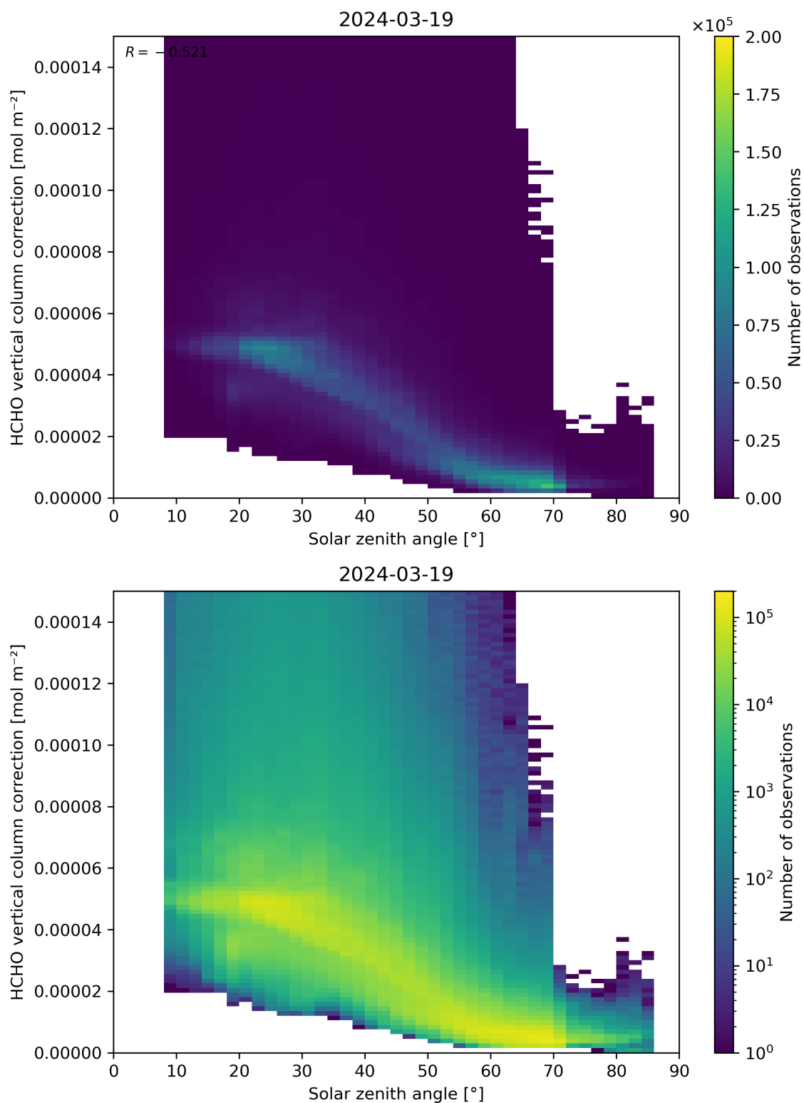
Figure 178: Scatter density plot of “Solar zenith angle” against “HCHO vertical column correction” for 2024-03-18 to 2024-03-20.
