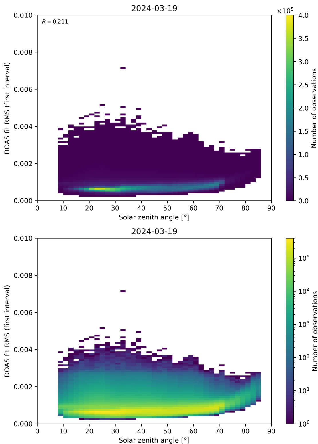
Figure 167: Scatter density plot of “Solar zenith angle” against “DOAS fit RMS (first interval)” for 2024-03-18 to 2024-03-20.
