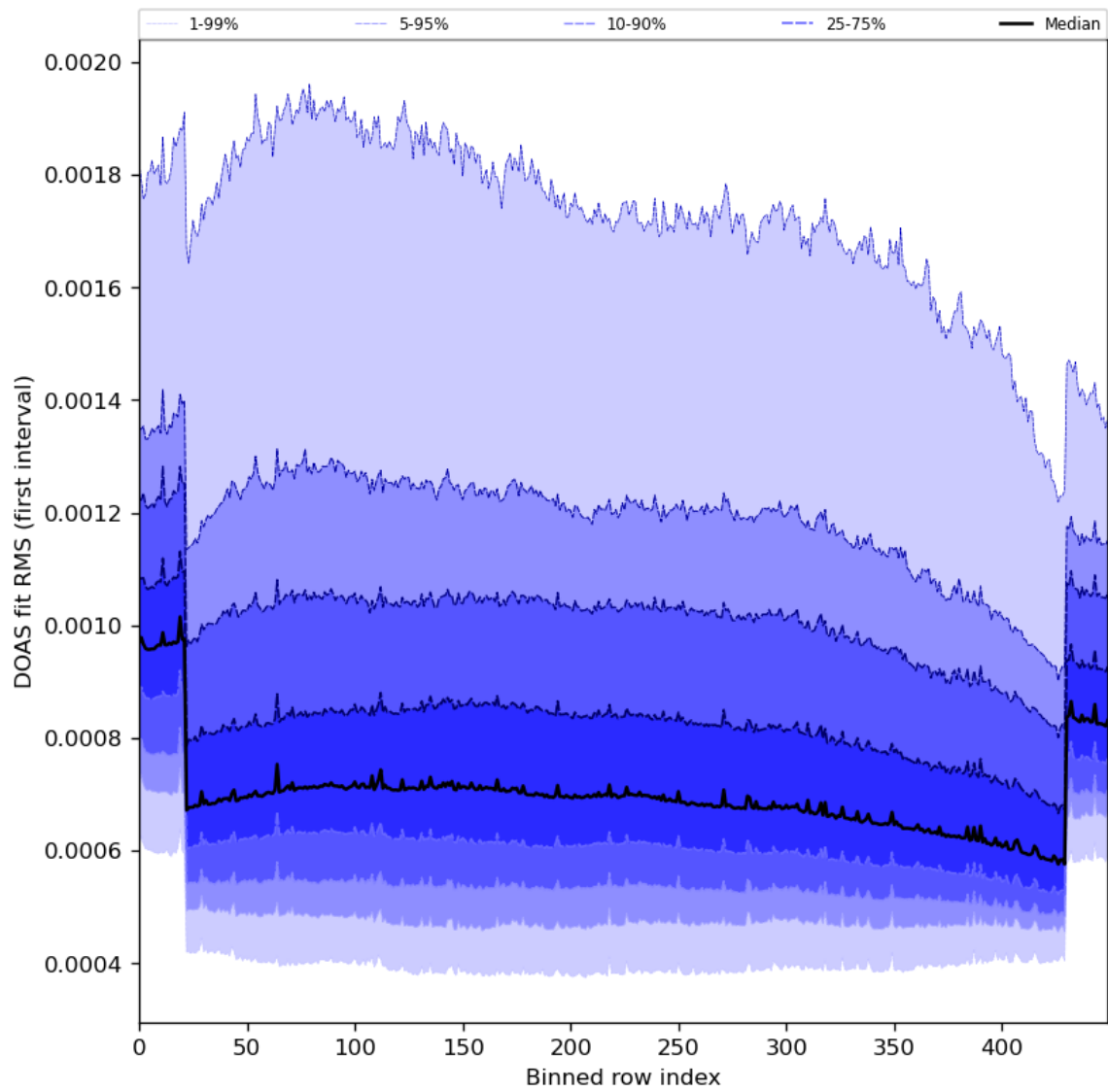
Figure 60: Along track statistics of “DOAS fit RMS (first interval)” for 2024-03-18 to 2024-03-20
