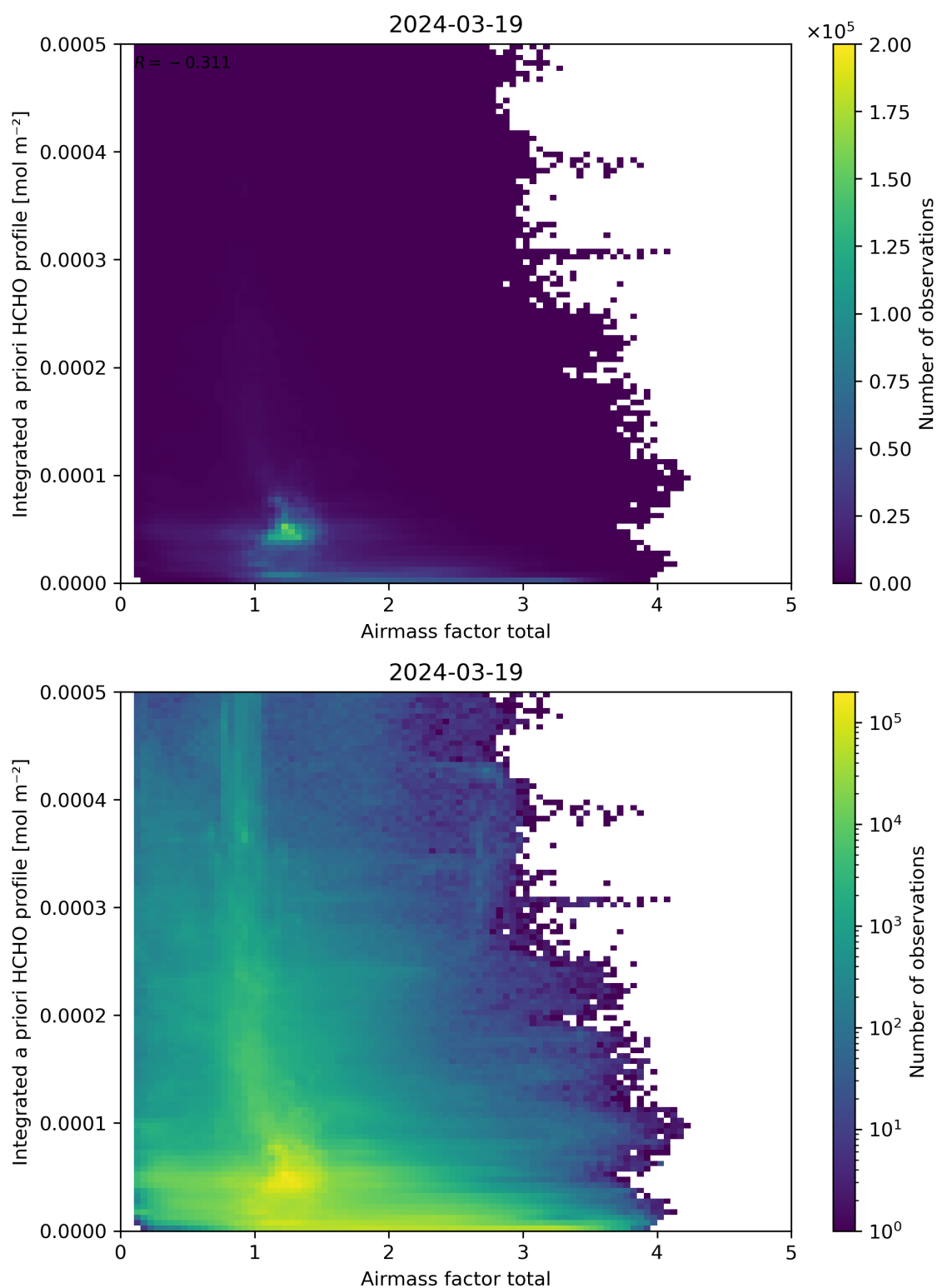
Figure 104: Scatter density plot of “Airmass factor total” against “Integrated a priori HCHO profile” for 2024-03-18 to 2024-03-20.
