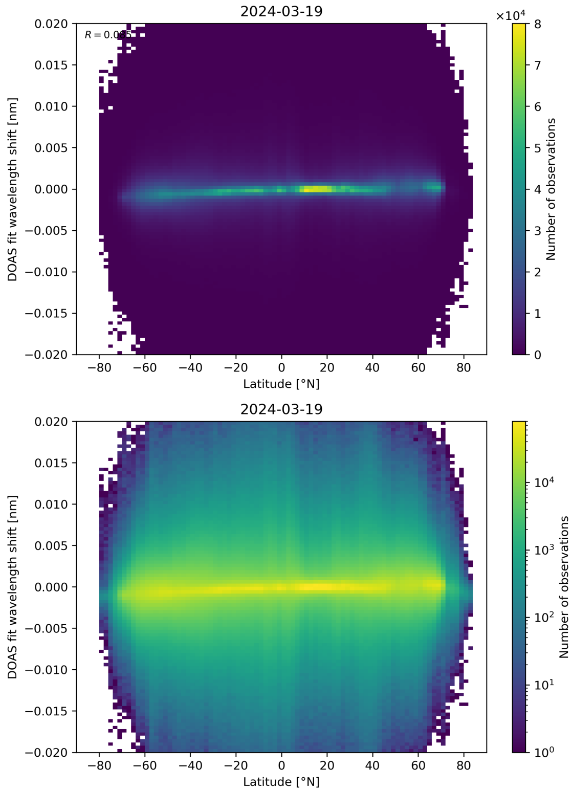
Figure 154: Scatter density plot of “Latitude” against “DOAS fit wavelength shift” for 2024-03-18 to 2024-03-20.
