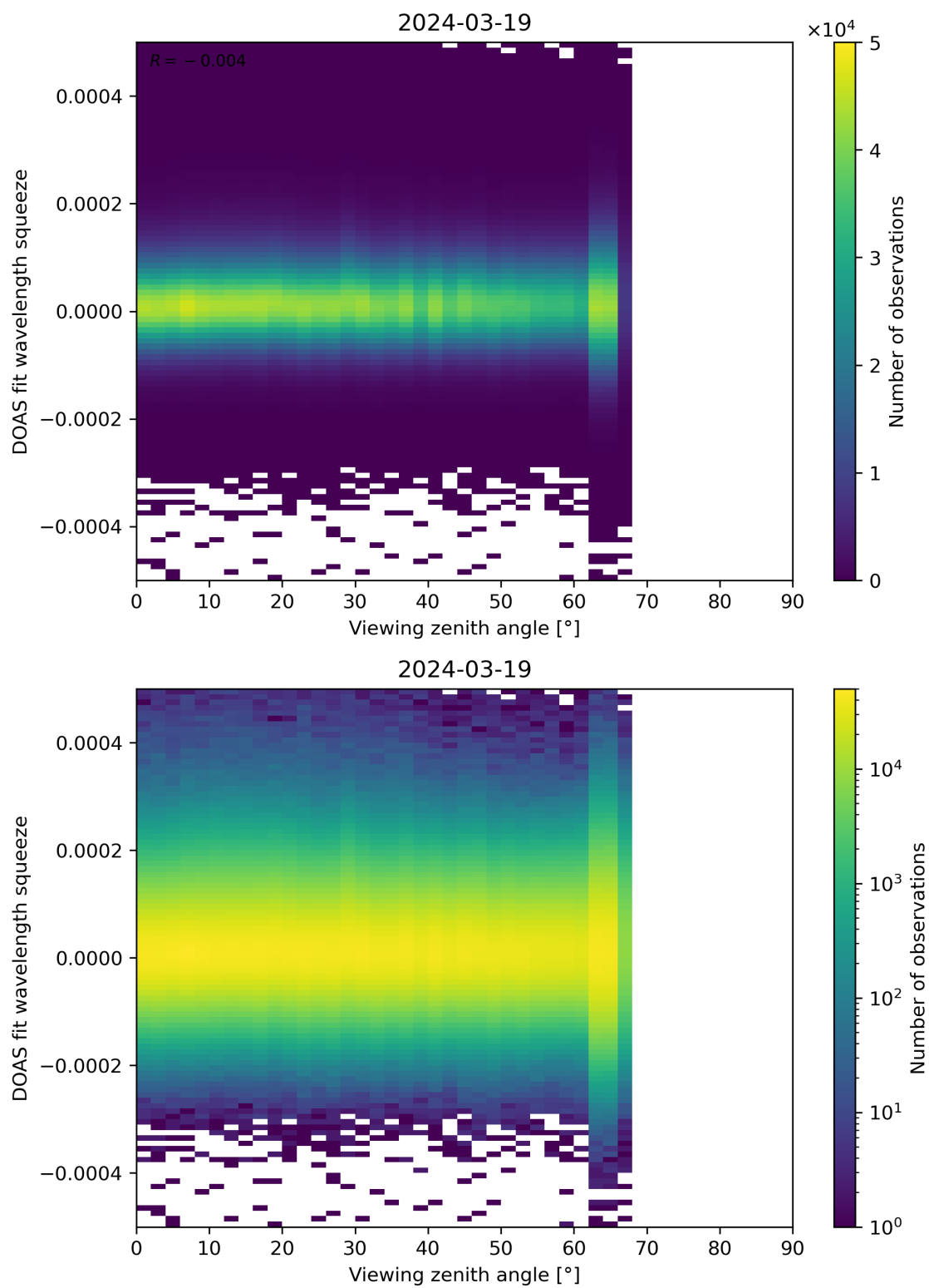
Figure 184: Scatter density plot of “Viewing zenith angle” against “DOAS fit wavelength squeeze” for 2024-03-18 to 2024-03-20.
