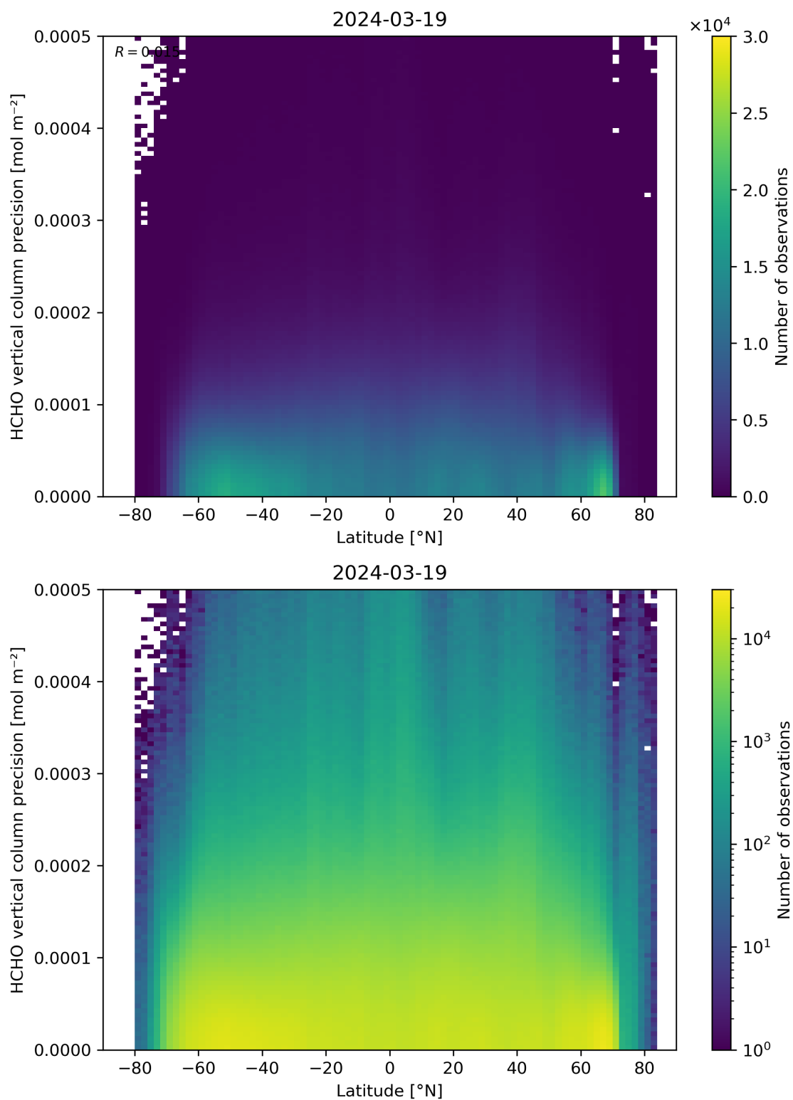
Figure 165: Scatter density plot of “Latitude” against “HCHO vertical column precision” for 2024-03-18 to 2024-03-20.
