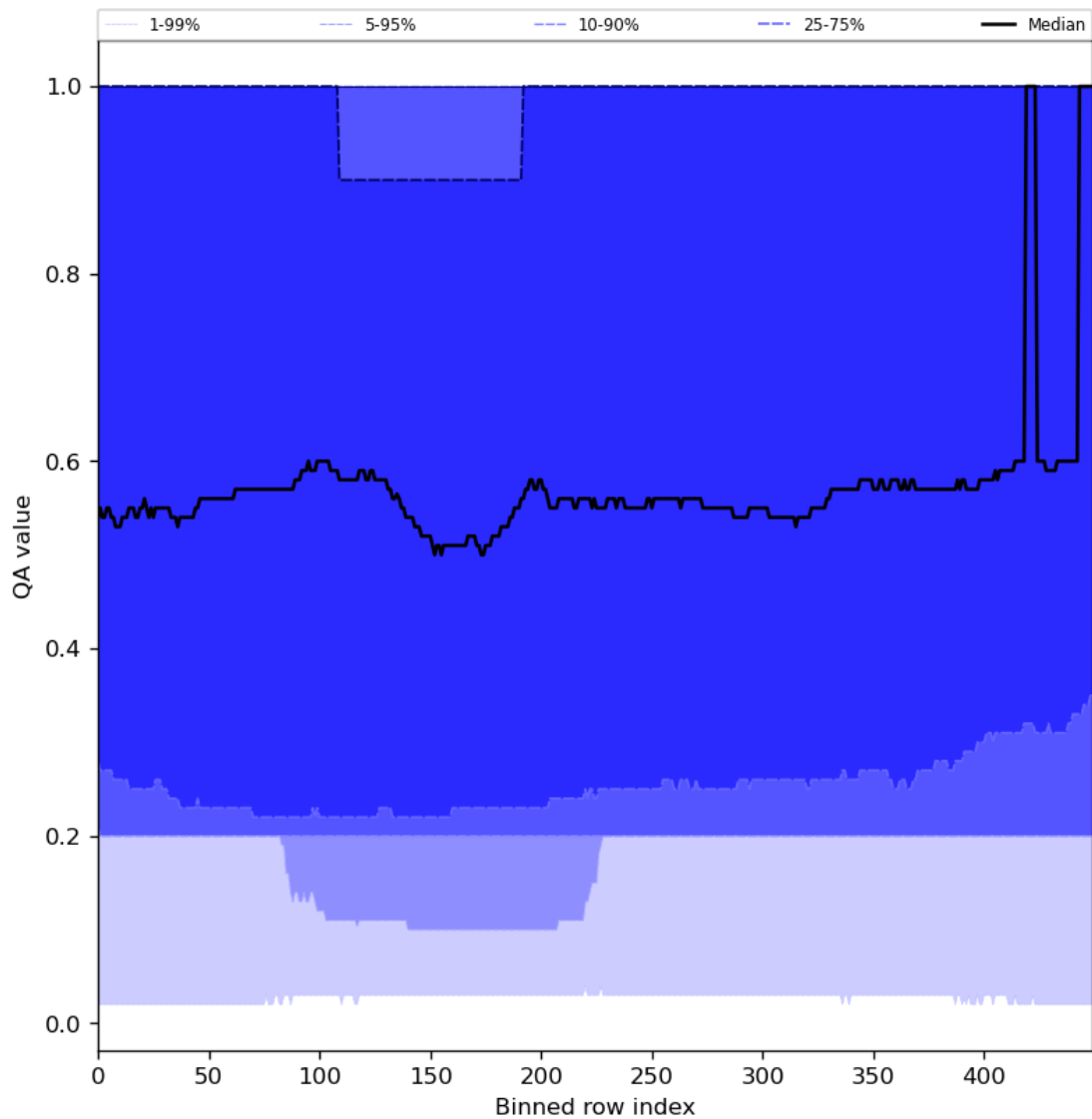
Figure 48: Along track statistics of “QA value” for 2024-03-18 to 2024-03-20
