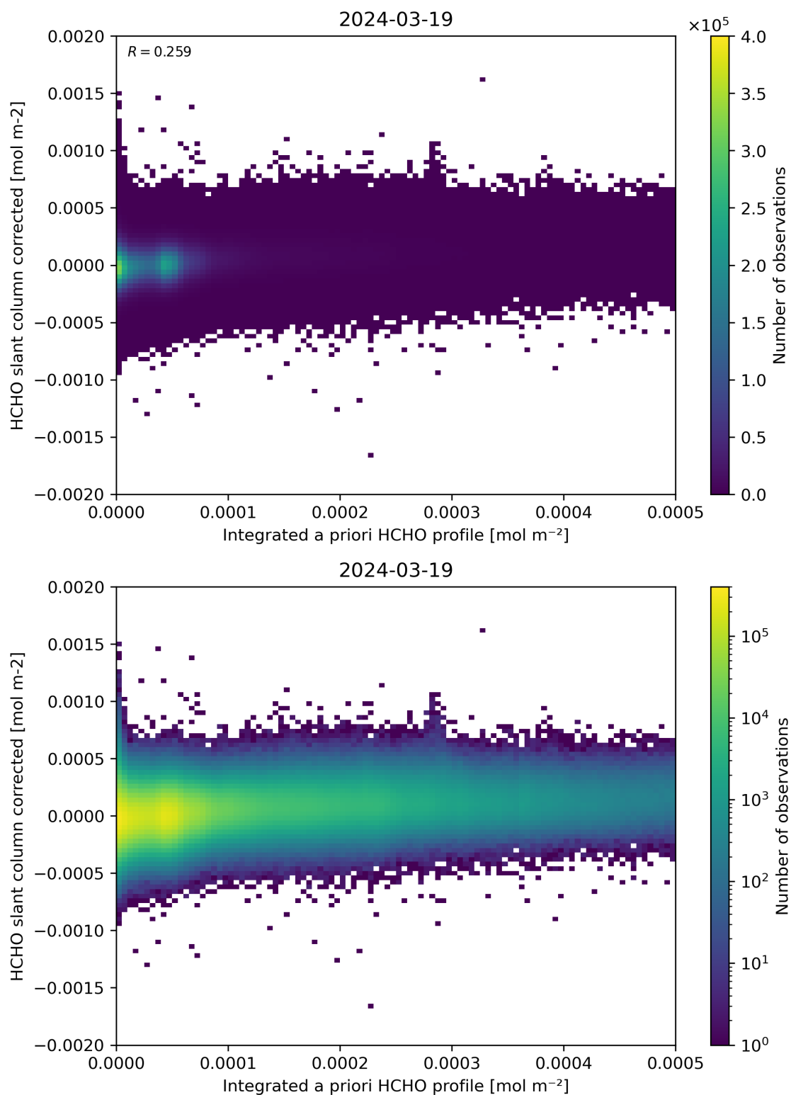
Figure 151: Scatter density plot of “Integrated a priori HCHO profile” against “HCHO slant column corrected” for 2024-03-18 to 2024-03-20.
