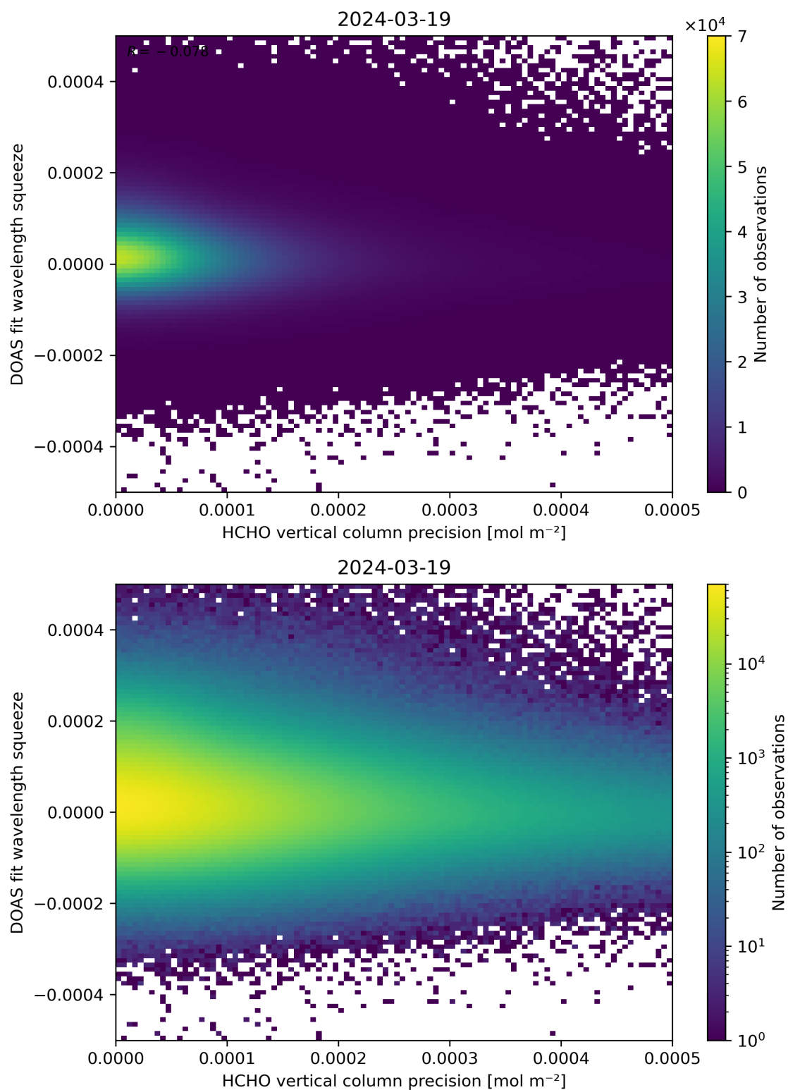
Figure 138: Scatter density plot of “HCHO vertical column precision” against “DOAS fit wavelength squeeze” for 2024-03-18 to 2024-03-20.
