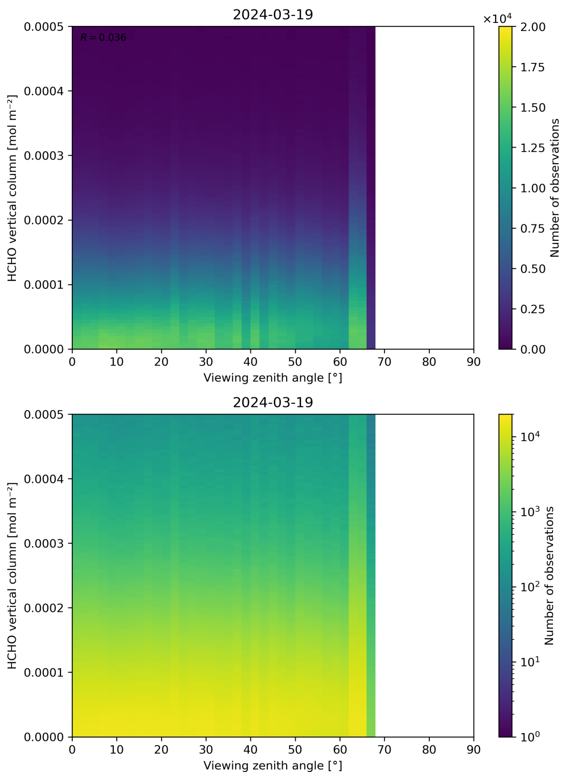
Figure 192: Scatter density plot of “Viewing zenith angle” against “HCHO vertical column” for 2024-03-18 to 2024-03-20.
