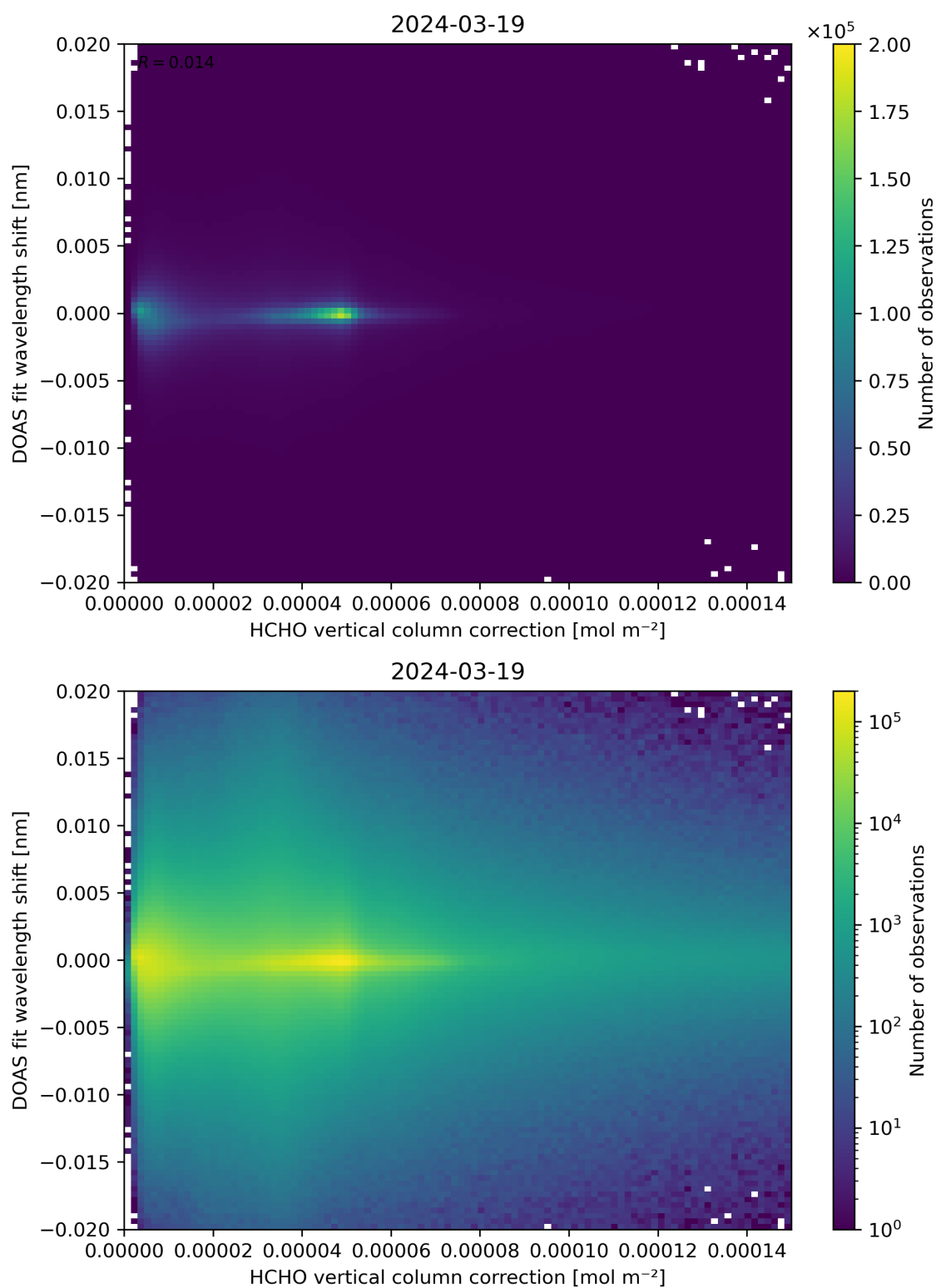
Figure 113: Scatter density plot of “HCHO vertical column correction” against “DOAS fit wavelength shift” for 2024-03-18 to 2024-03-20.
