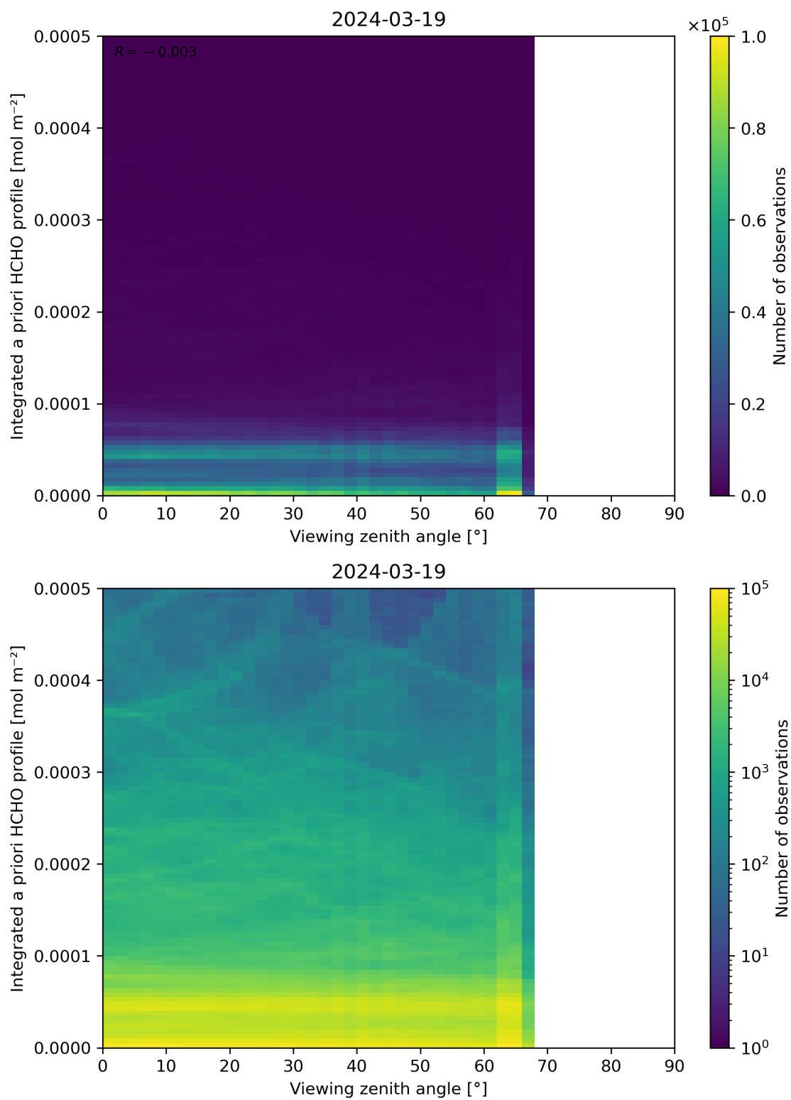
Figure 195: Scatter density plot of “Viewing zenith angle” against “Integrated a priori HCHO profile” for 2024-03-18 to 2024-03-20.
