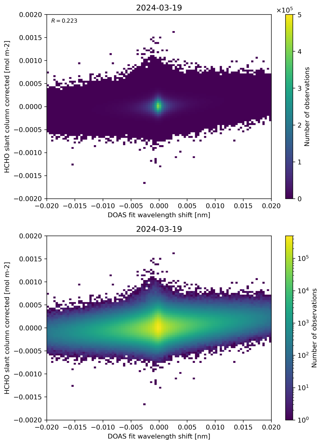
Figure 66: Scatter density plot of “DOAS fit wavelength shift” against “HCHO slant column corrected” for 2024-03-18 to 2024-03-20.
