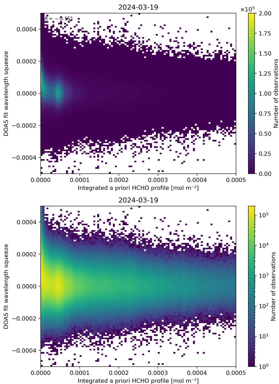
Figure 150: Scatter density plot of “Integrated a priori HCHO profile” against “DOAS fit wavelength squeeze” for 2024-03-18 to 2024-03-20.
