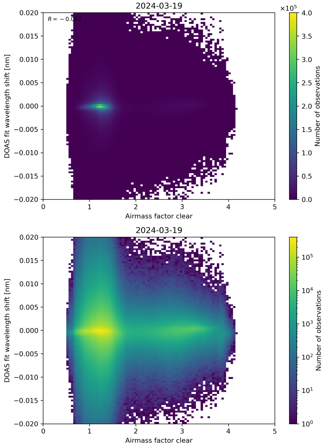
Figure 72: Scatter density plot of “Airmass factor clear” against “DOAS fit wavelength shift” for 2024-03-18 to 2024-03-20.
