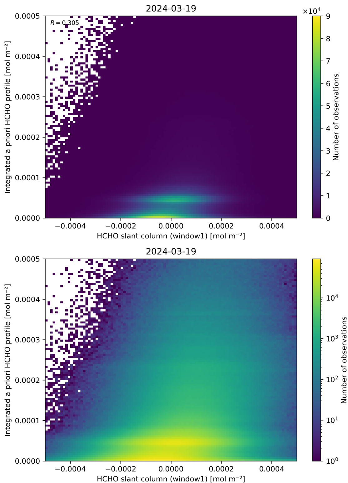
Figure 87: Scatter density plot of “HCHO slant column (window1)” against “Integrated a priori HCHO profile” for 2024-03-18 to 2024-03-20.
