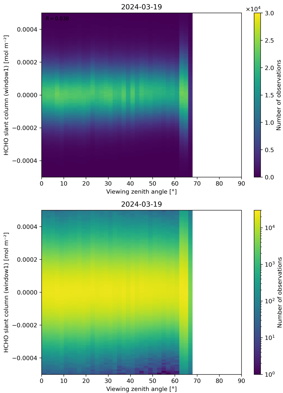
Figure 188: Scatter density plot of “Viewing zenith angle” against “HCHO slant column (window1)” for 2024-03-18 to 2024-03-20.
