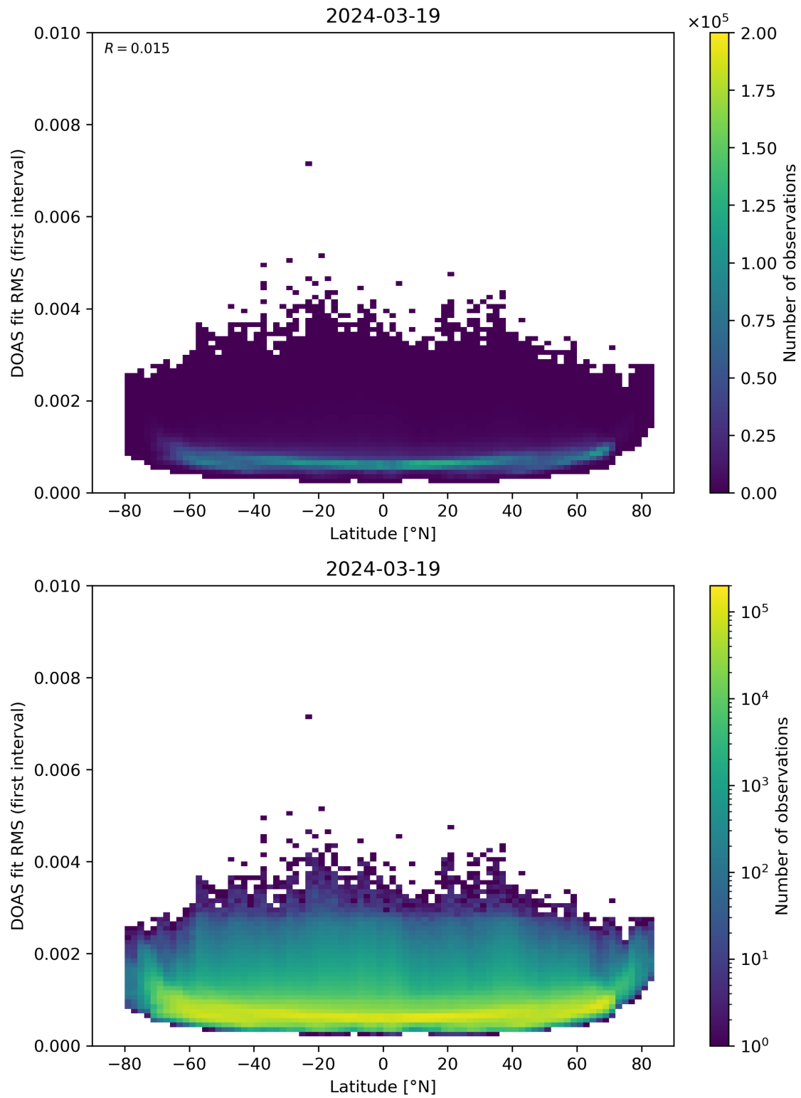
Figure 153: Scatter density plot of “Latitude” against “DOAS fit RMS (first interval)” for 2024-03-18 to 2024-03-20.
