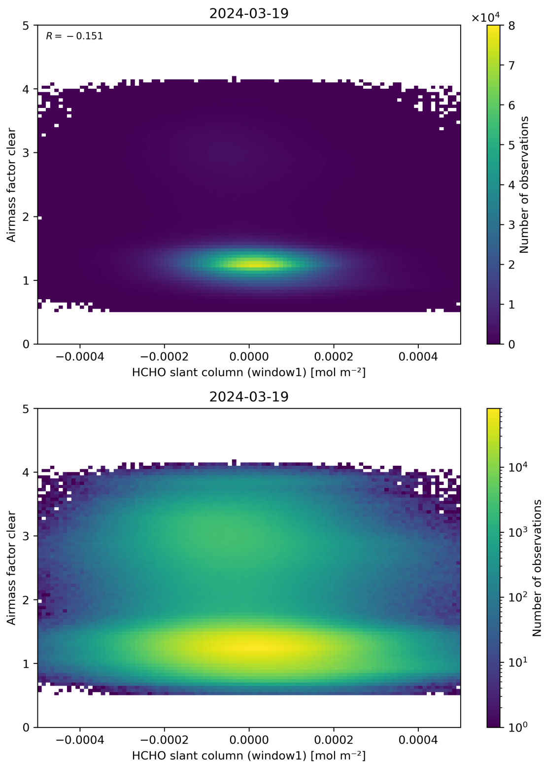
Figure 81: Scatter density plot of “HCHO slant column (window1)” against “Airmass factor clear” for 2024-03-18 to 2024-03-20.
