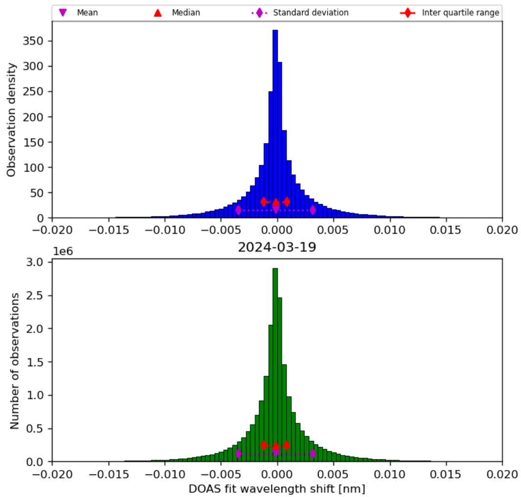
Figure 44: Histogram of “DOAS fit wavelength shift” for 2024-03-18 to 2024-03-20
