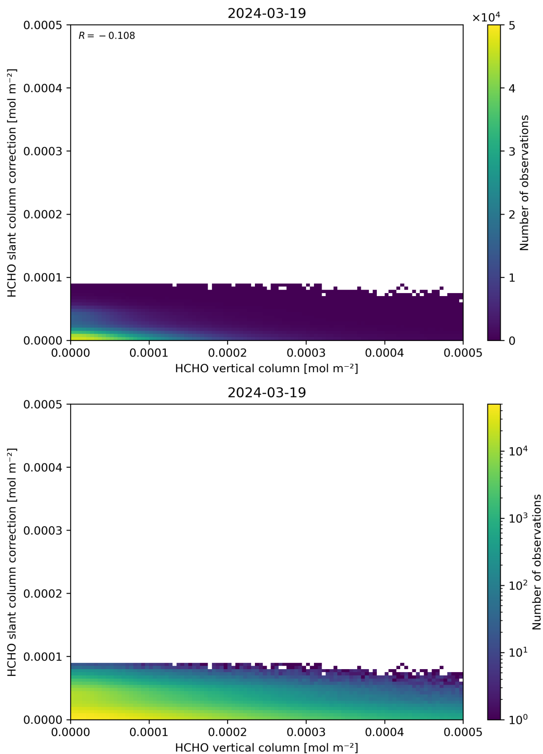
Figure 128: Scatter density plot of “HCHO vertical column” against “HCHO slant column correction” for 2024-03-18 to 2024-03-20.
