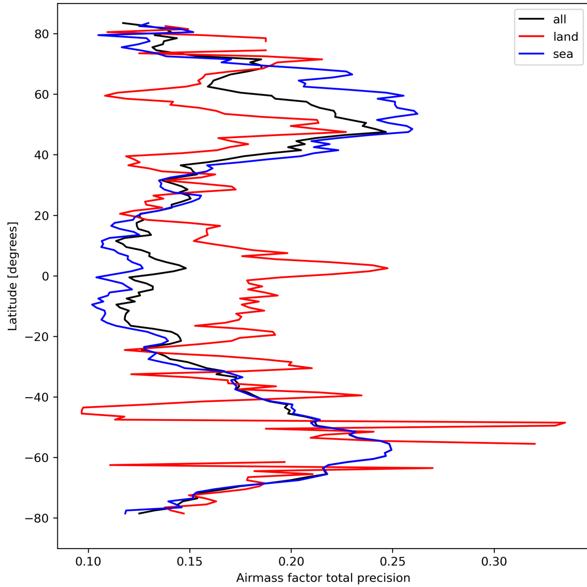
Figure 27: Zonal average of “Airmass factor total precision” for 2024-03-18 to 2024-03-20.
