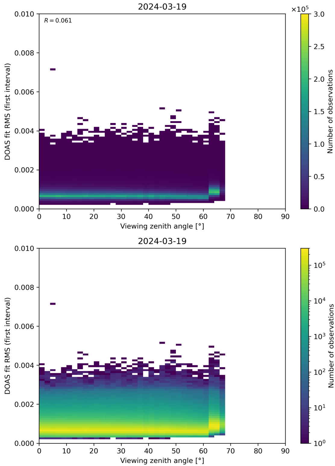
Figure 182: Scatter density plot of “Viewing zenith angle” against “DOAS fit RMS (first interval)” for 2024-03-18 to 2024-03-20.
