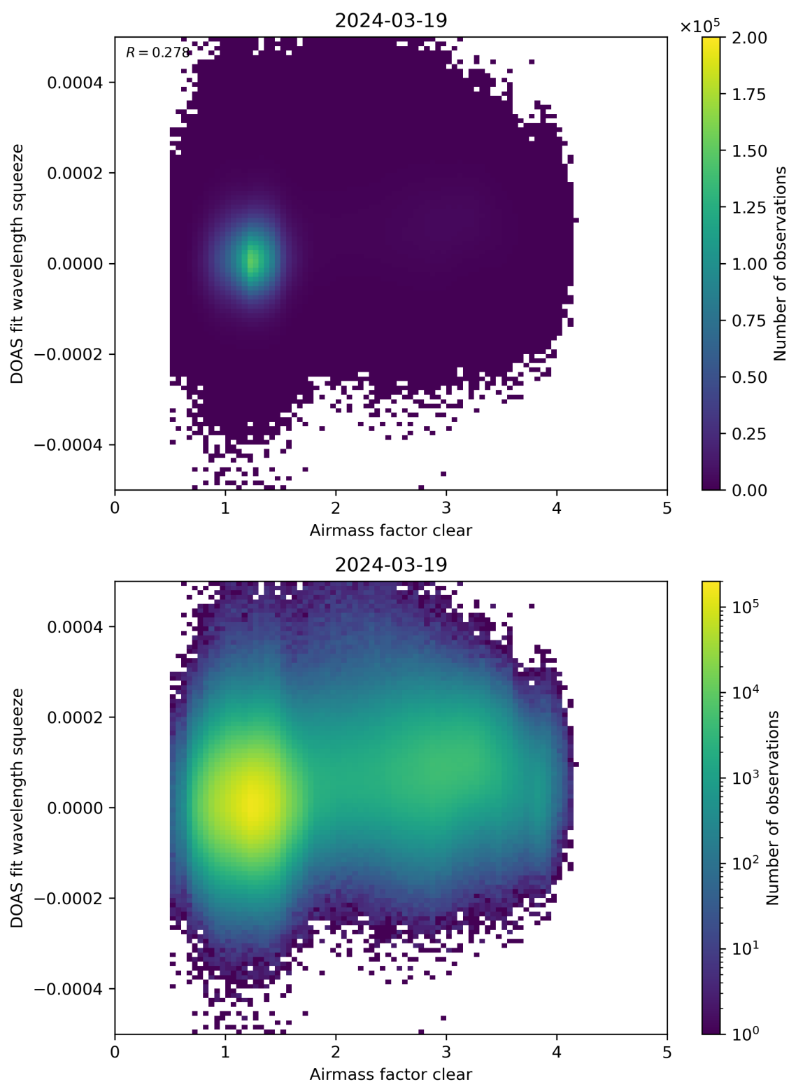
Figure 73: Scatter density plot of “Airmass factor clear” against “DOAS fit wavelength squeeze” for 2024-03-18 to 2024-03-20.
