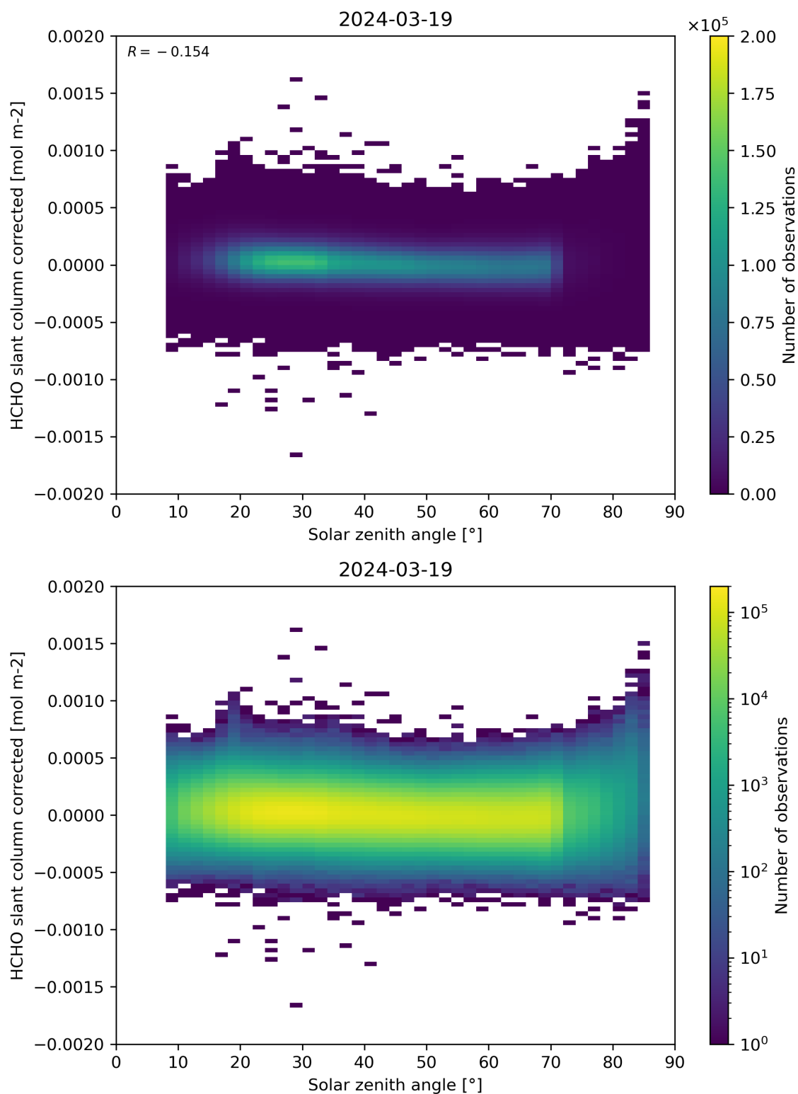
Figure 171: Scatter density plot of “Solar zenith angle” against “HCHO slant column corrected” for 2024-03-18 to 2024-03-20.
