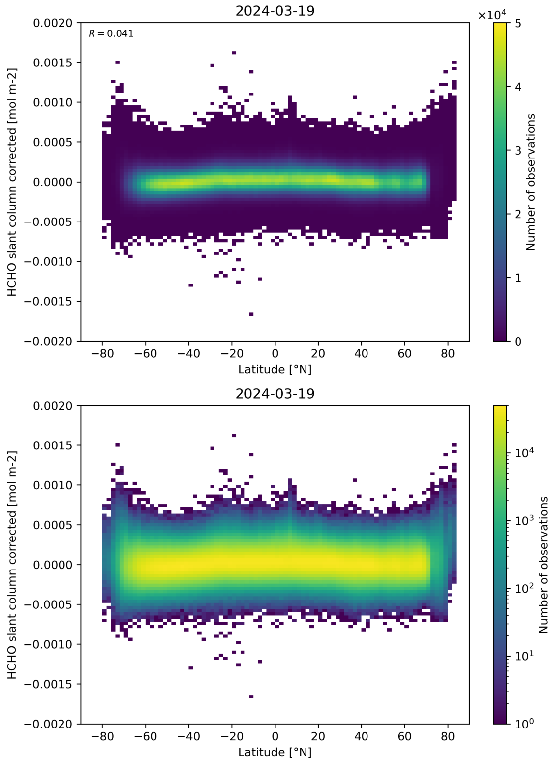
Figure 157: Scatter density plot of “Latitude” against “HCHO slant column corrected” for 2024-03-18 to 2024-03-20.
