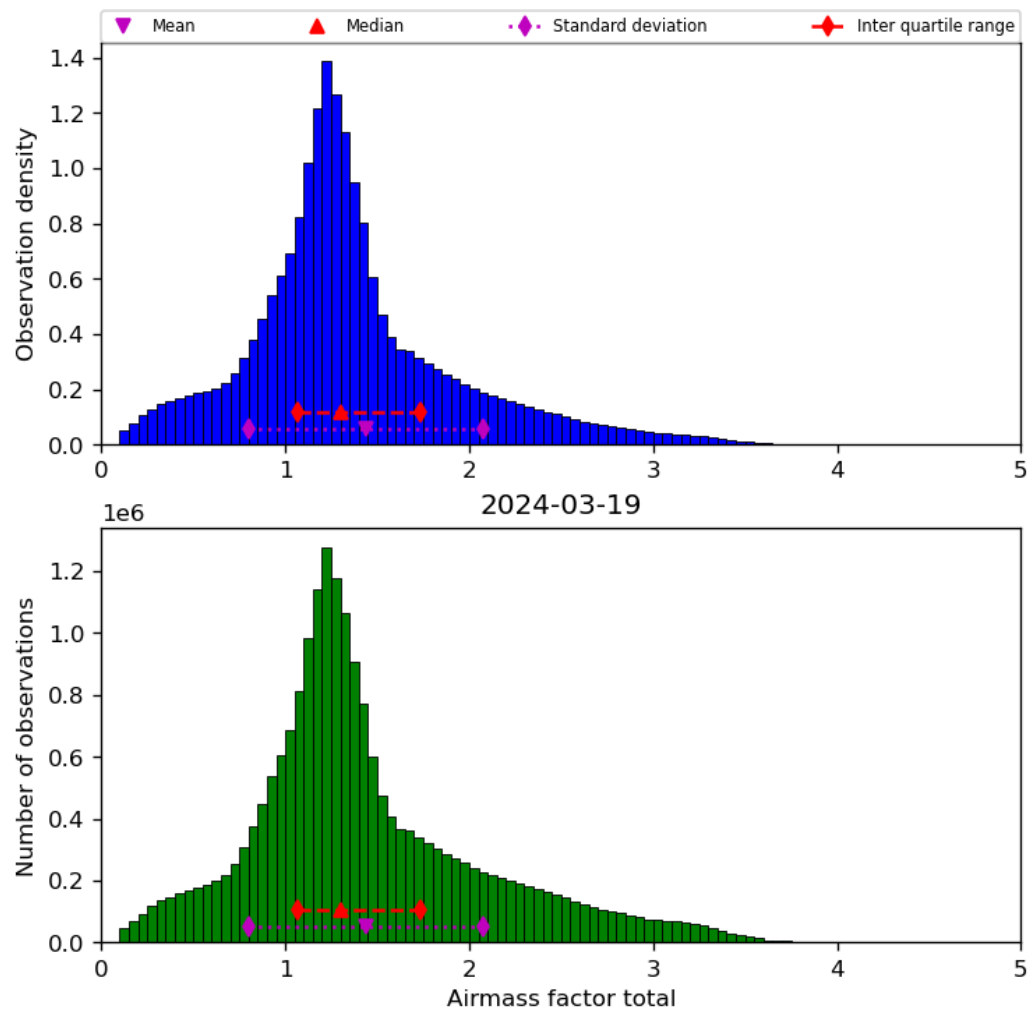
Figure 40: Histogram of “Airmass factor total” for 2024-03-18 to 2024-03-20
