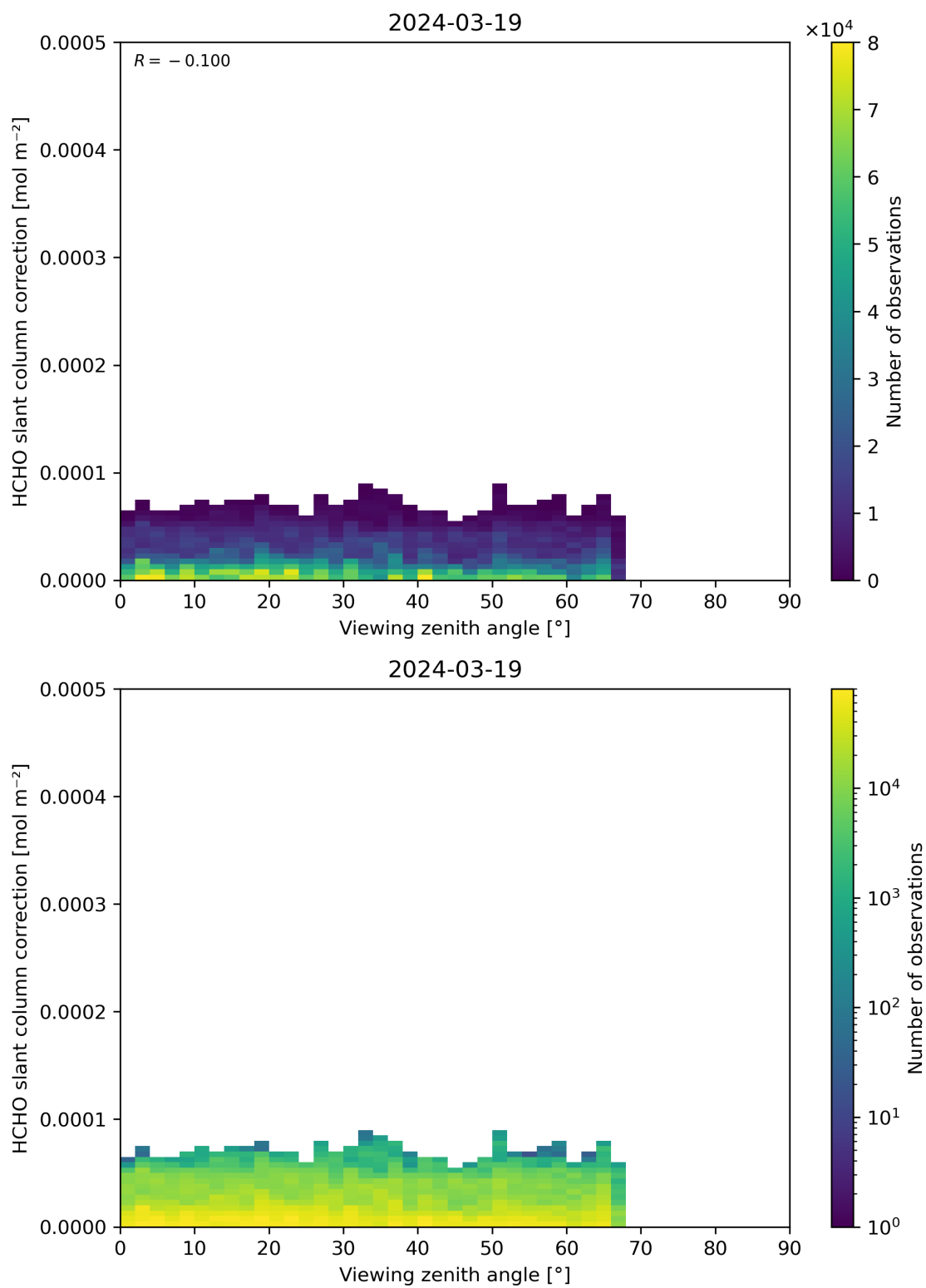
Figure 187: Scatter density plot of “Viewing zenith angle” against “HCHO slant column correction” for 2024-03-18 to 2024-03-20.
