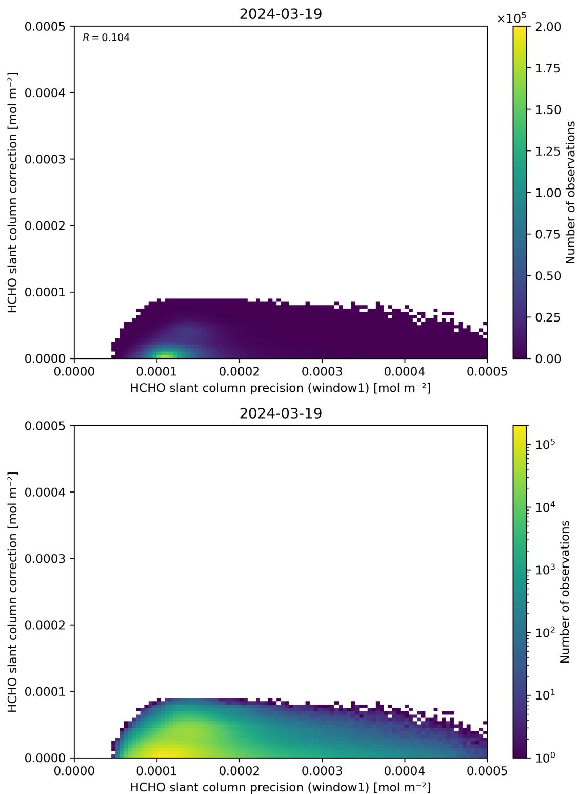
Figure 93: Scatter density plot of “HCHO slant column precision (window1)” against “HCHO slant column correction” for 2024-03-18 to 2024-03-20.
