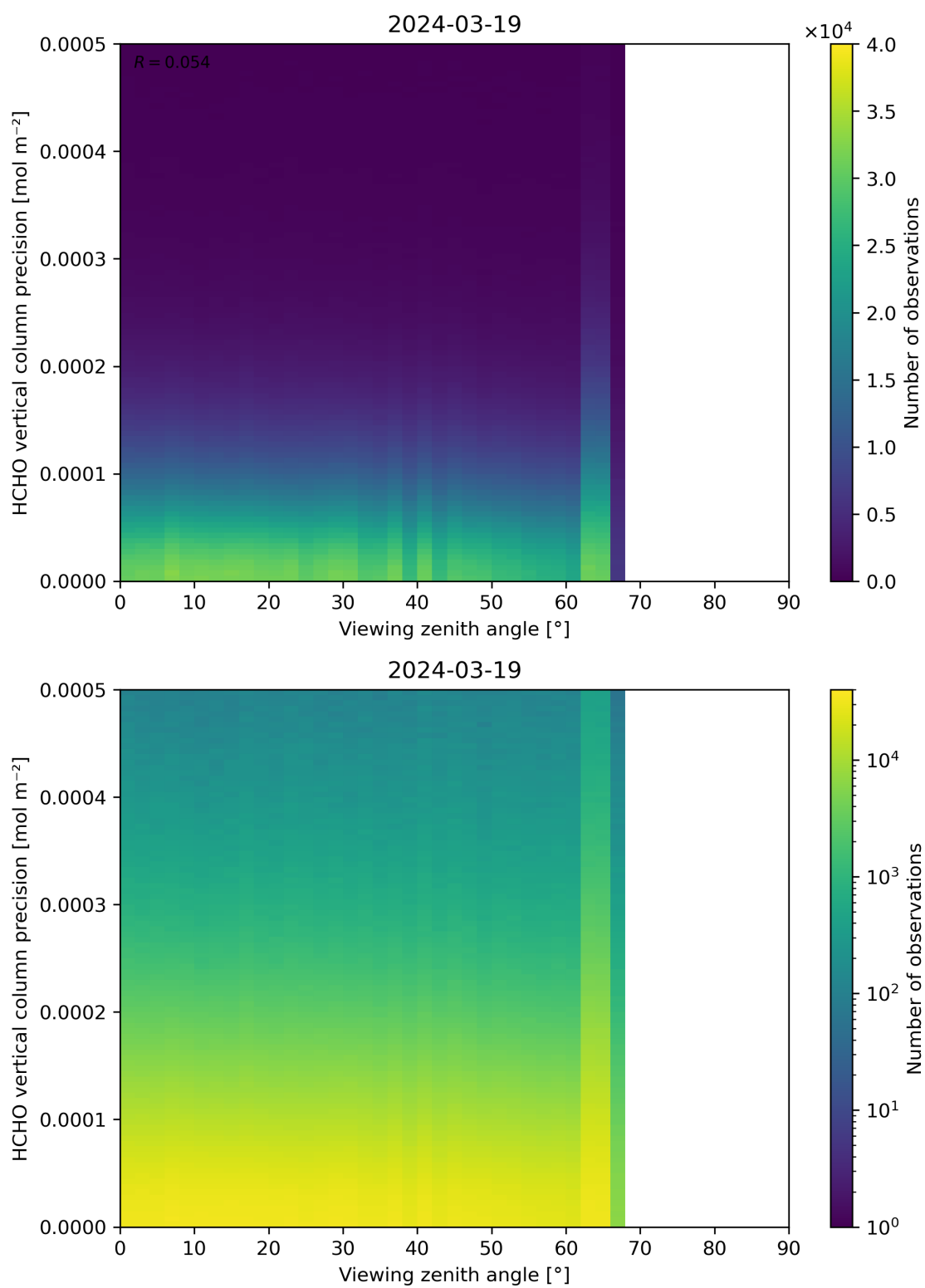
Figure 194: Scatter density plot of “Viewing zenith angle” against “HCHO vertical column precision” for 2024-03-18 to 2024-03-20.
