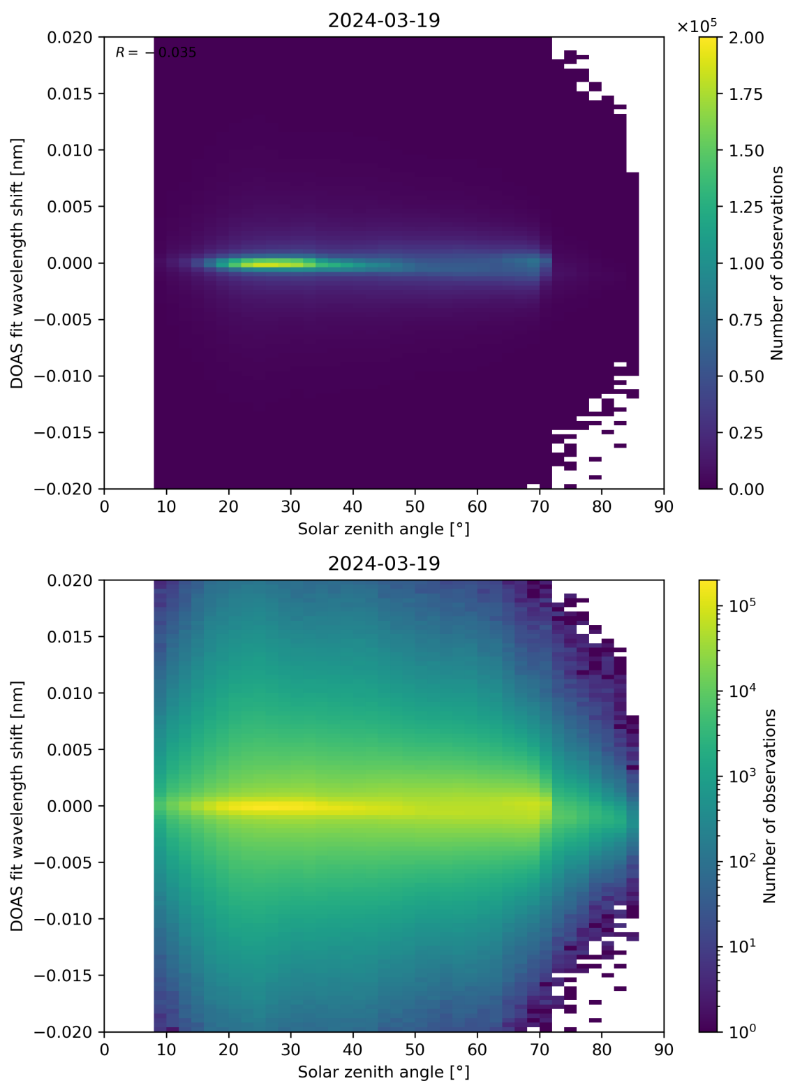
Figure 168: Scatter density plot of “Solar zenith angle” against “DOAS fit wavelength shift” for 2024-03-18 to 2024-03-20.
