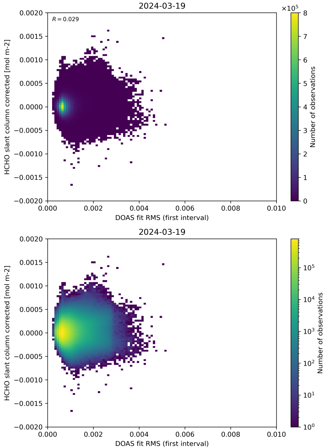
Figure 62: Scatter density plot of “DOAS fit RMS (first interval)” against “HCHO slant column corrected” for 2024-03-18 to 2024-03-20.
