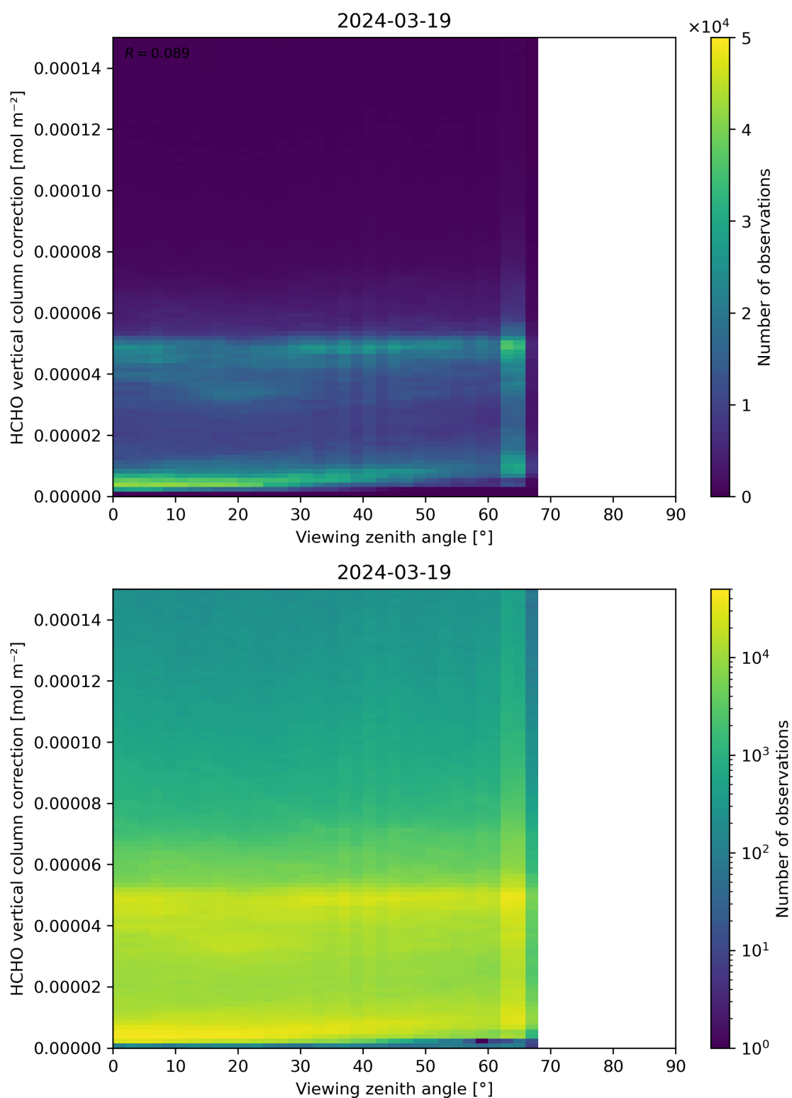
Figure 193: Scatter density plot of “Viewing zenith angle” against “HCHO vertical column correction” for 2024-03-18 to 2024-03-20.
