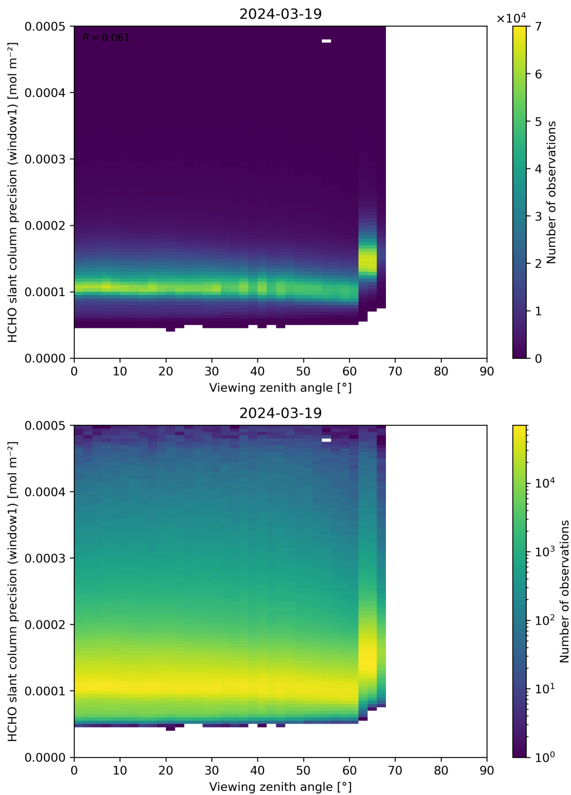
Figure 189: Scatter density plot of “Viewing zenith angle” against “HCHO slant column precision (window1)” for 2024-03-18 to 2024-03-20.
