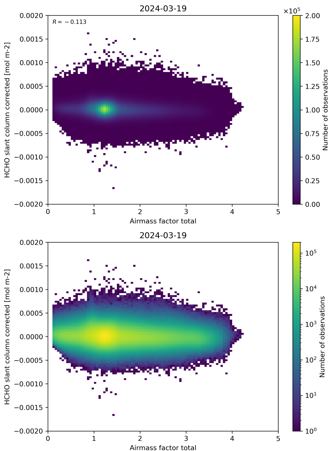
Figure 101: Scatter density plot of “Airmass factor total” against “HCHO slant column corrected” for 2024-03-18 to 2024-03-20.
