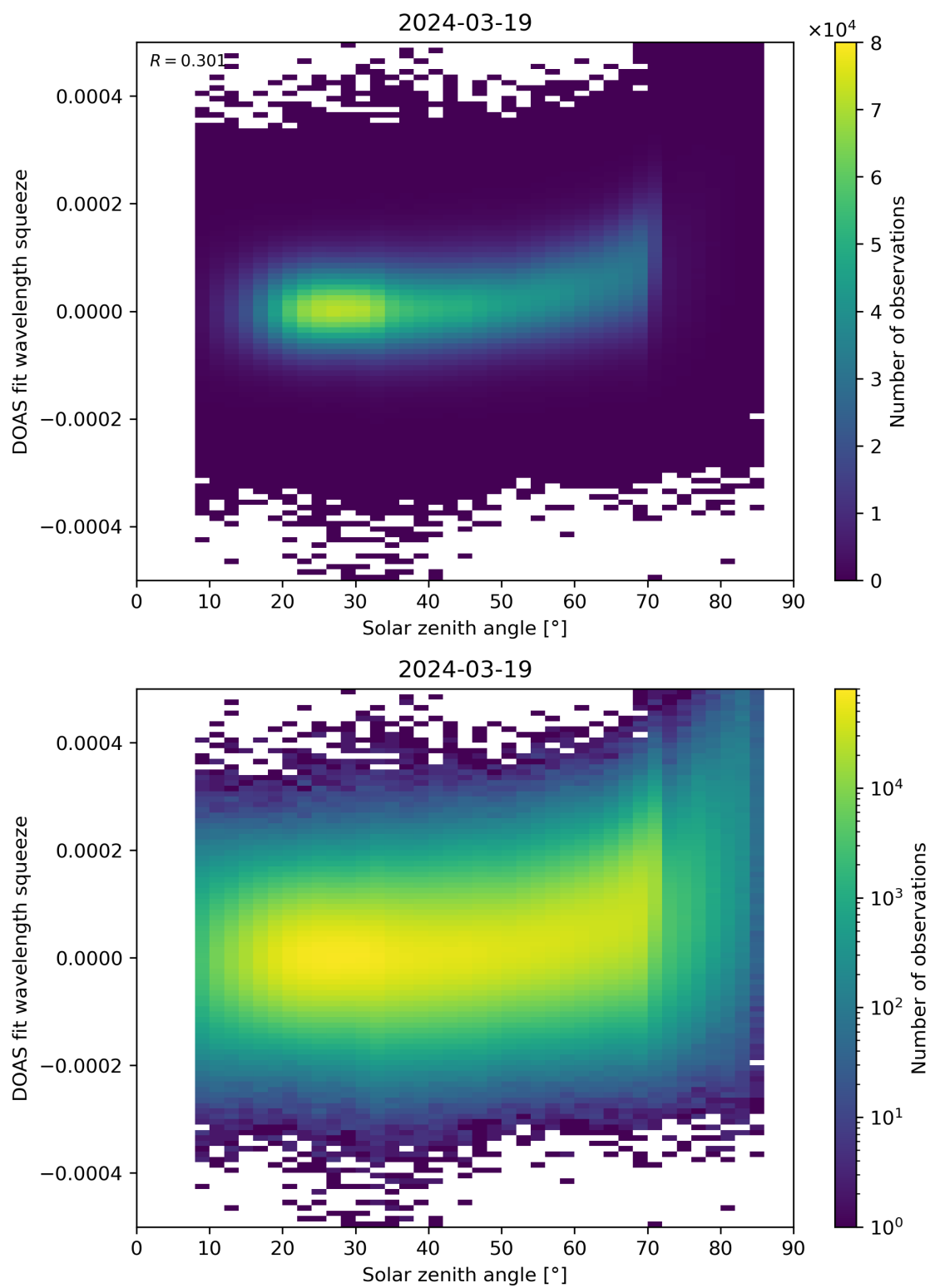
Figure 169: Scatter density plot of “Solar zenith angle” against “DOAS fit wavelength squeeze” for 2024-03-18 to 2024-03-20.
