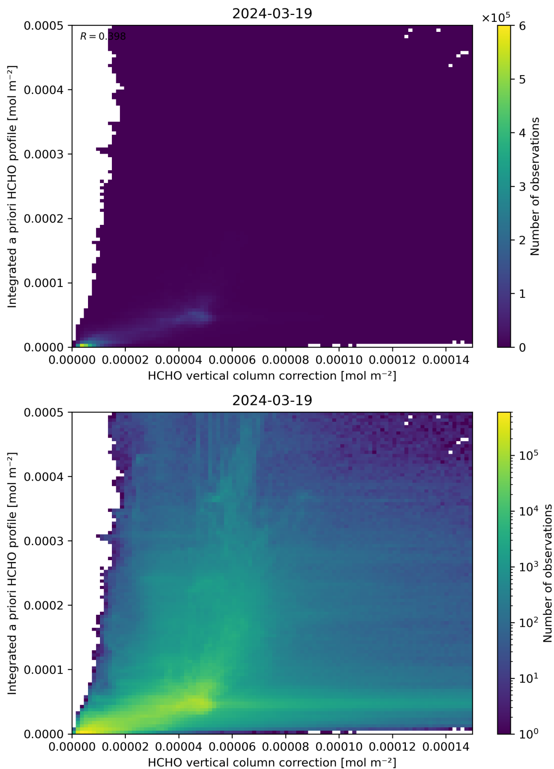
Figure 122: Scatter density plot of “HCHO vertical column correction” against “Integrated a priori HCHO profile” for 2024-03-18 to 2024-03-20.
