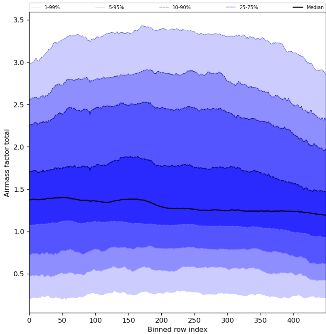
Figure 54: Along track statistics of “Airmass factor total” for 2024-03-18 to 2024-03-20
