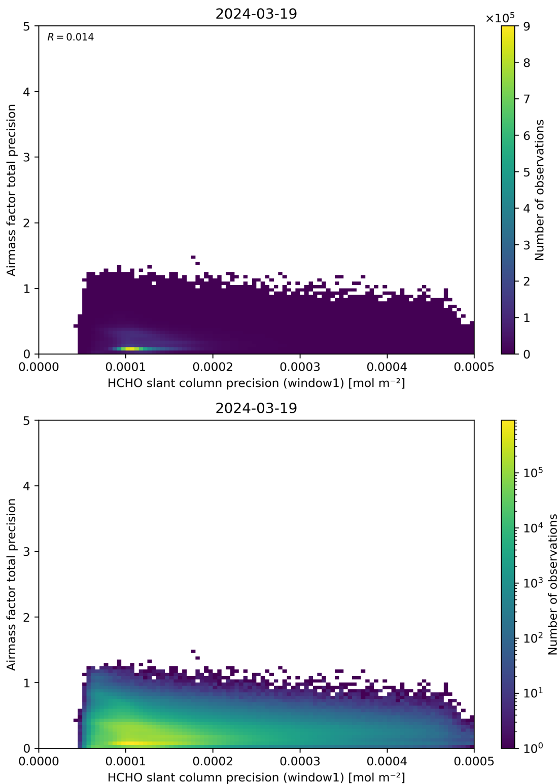
Figure 95: Scatter density plot of “HCHO slant column precision (window1)” against “Airmass factor total precision” for 2024-03-18 to 2024-03-20.
