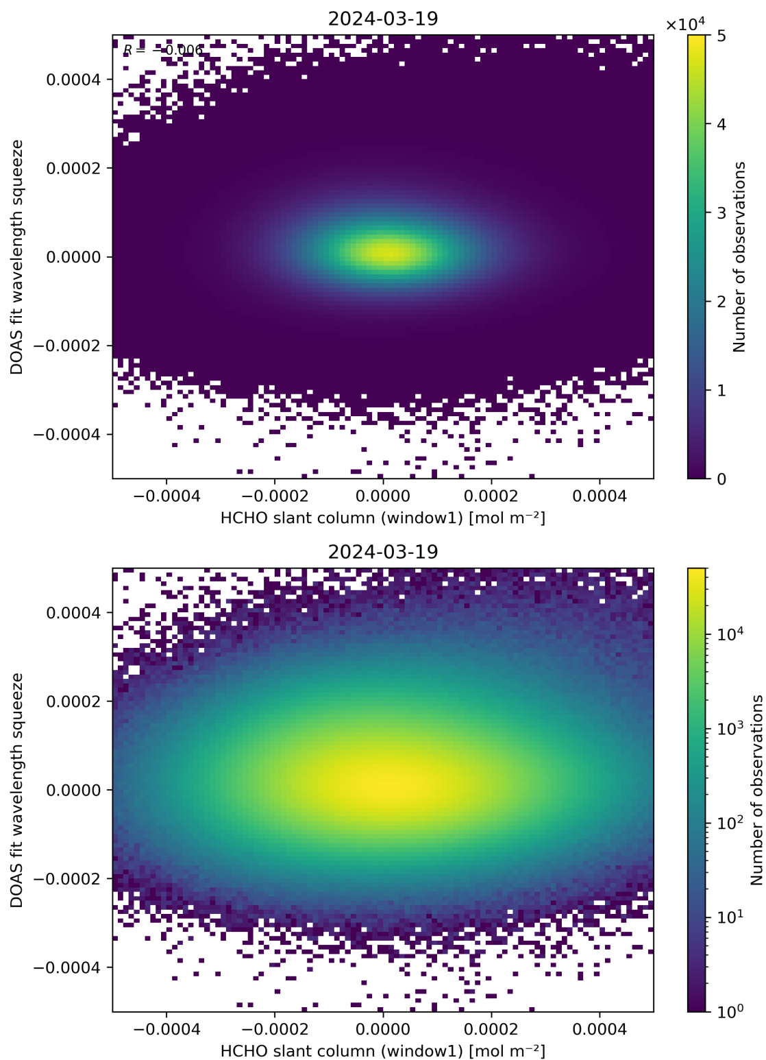
Figure 80: Scatter density plot of “HCHO slant column (window1)” against “DOAS fit wavelength squeeze” for 2024-03-18 to 2024-03-20.
