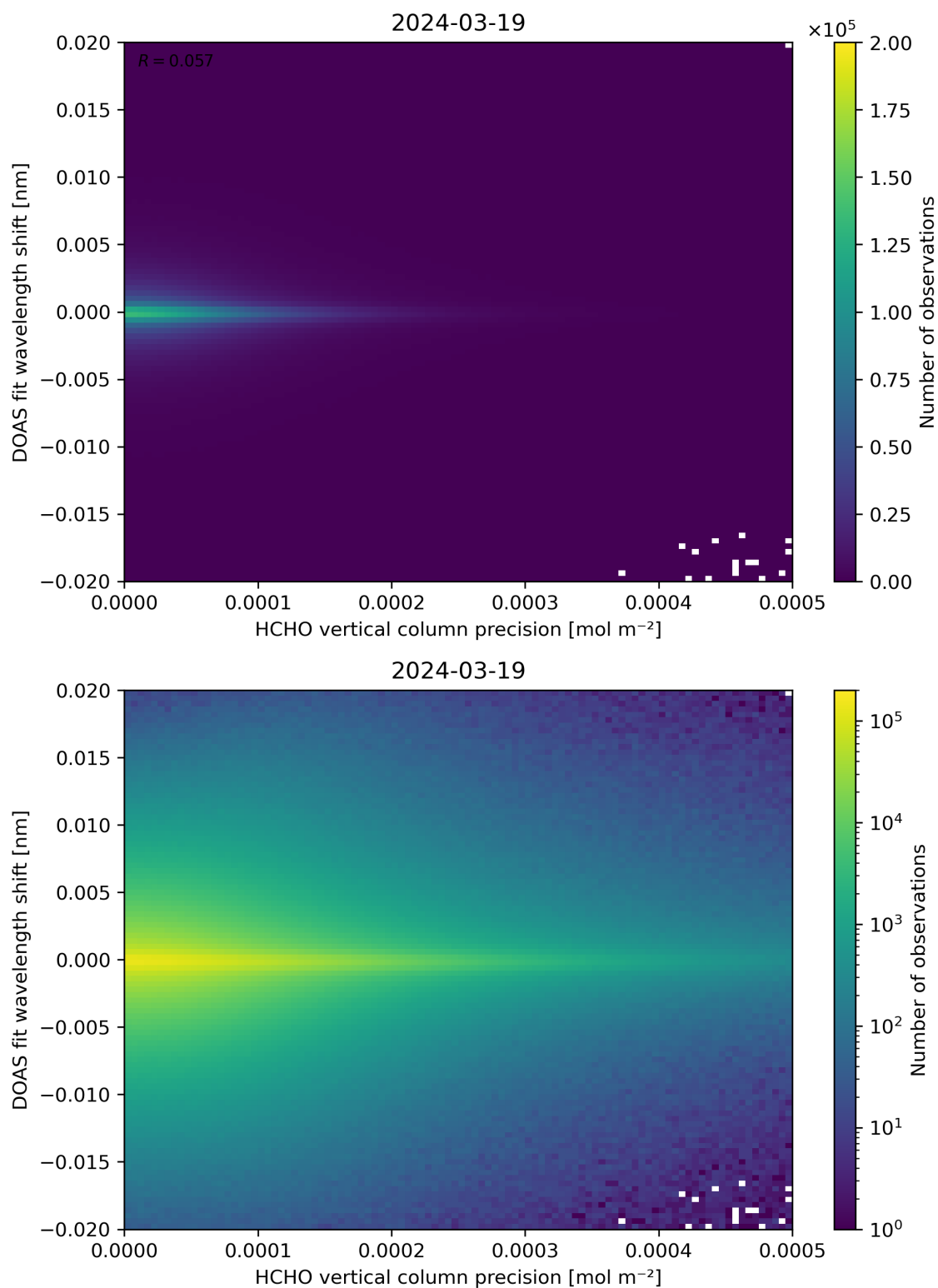
Figure 137: Scatter density plot of “HCHO vertical column precision” against “DOAS fit wavelength shift” for 2024-03-18 to 2024-03-20.
