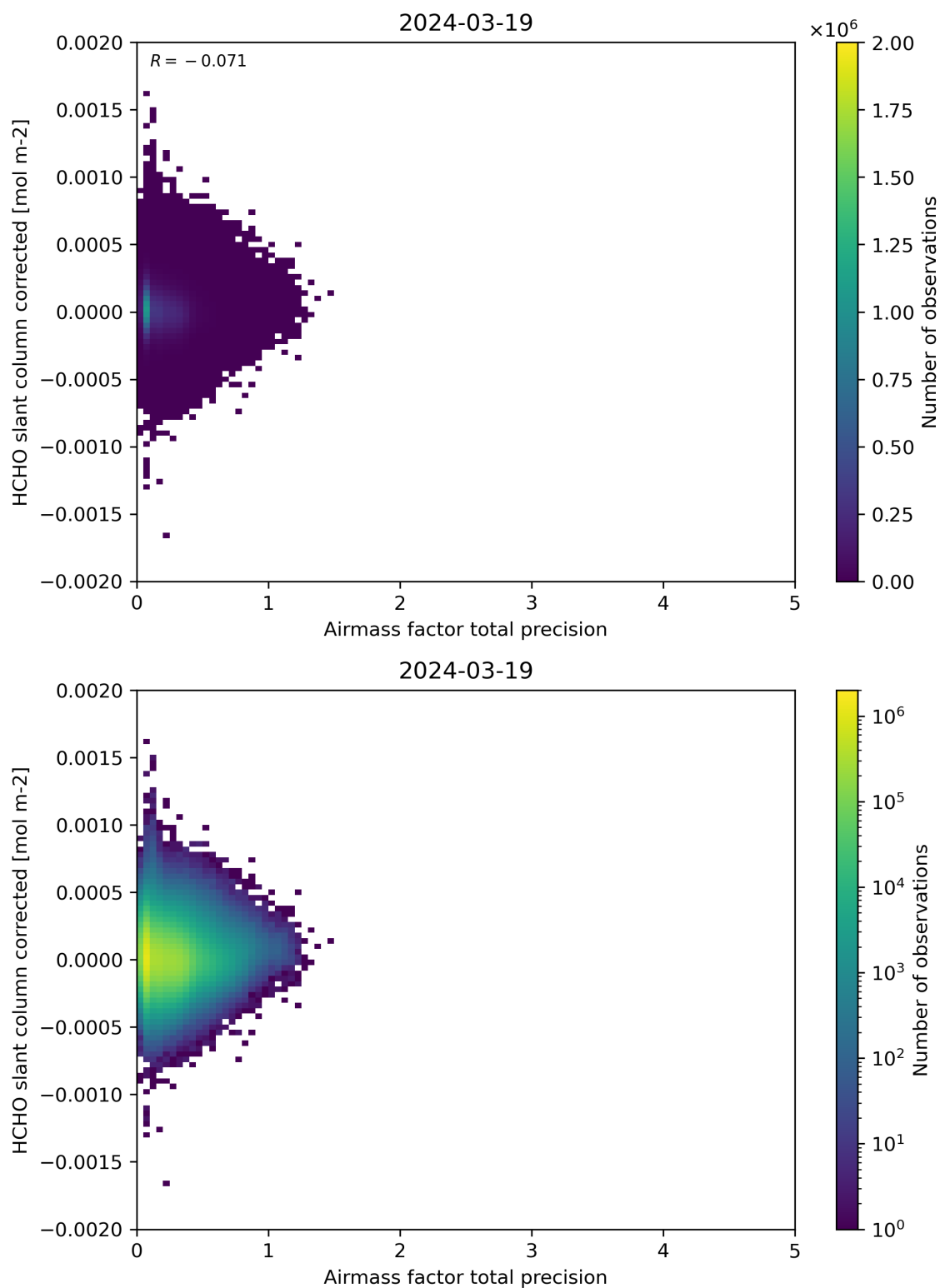
Figure 109: Scatter density plot of “Airmass factor total precision” against “HCHO slant column corrected” for 2024-03-18 to 2024-03-20.
