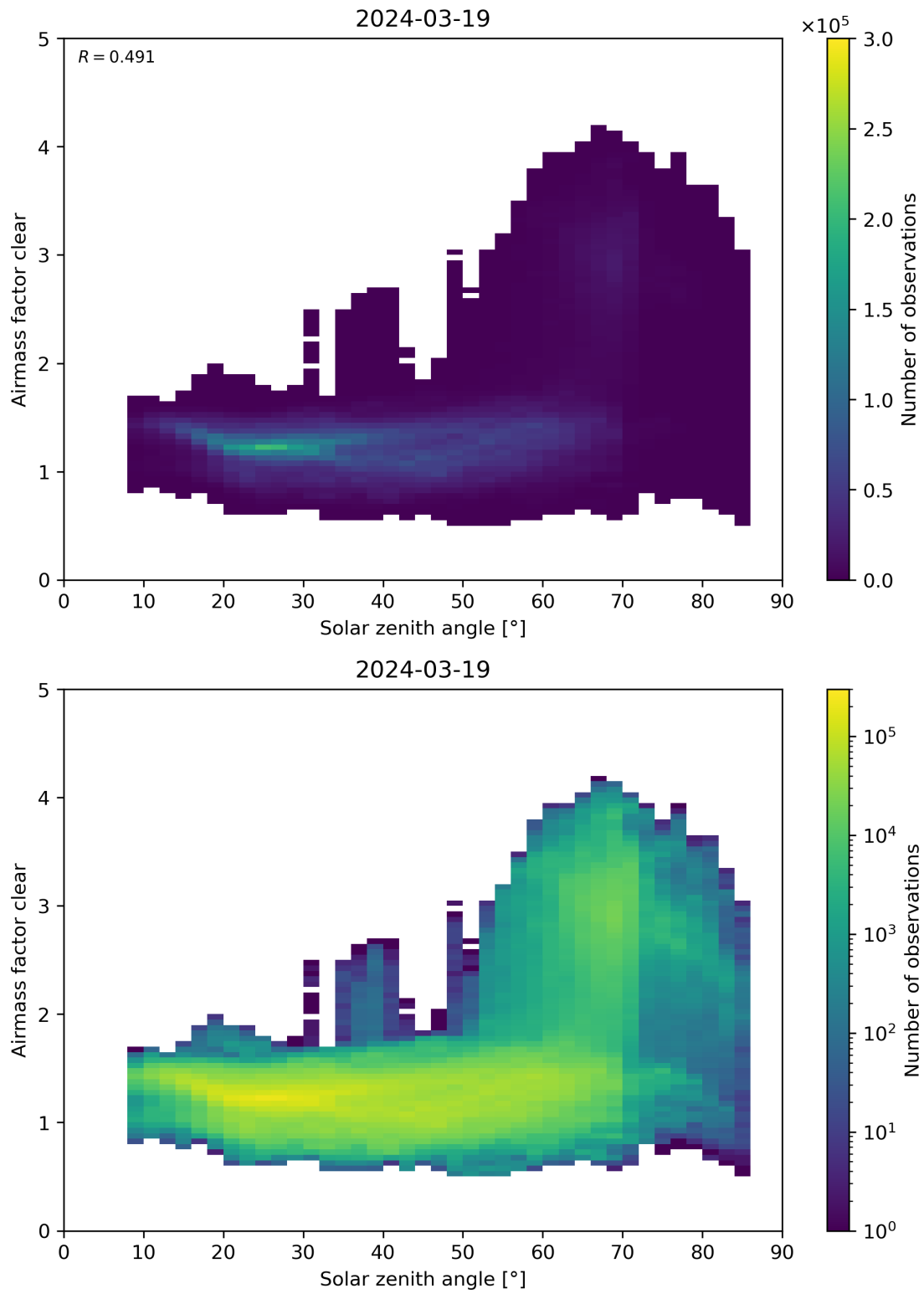
Figure 170: Scatter density plot of “Solar zenith angle” against “Airmass factor clear” for 2024-03-18 to 2024-03-20.
