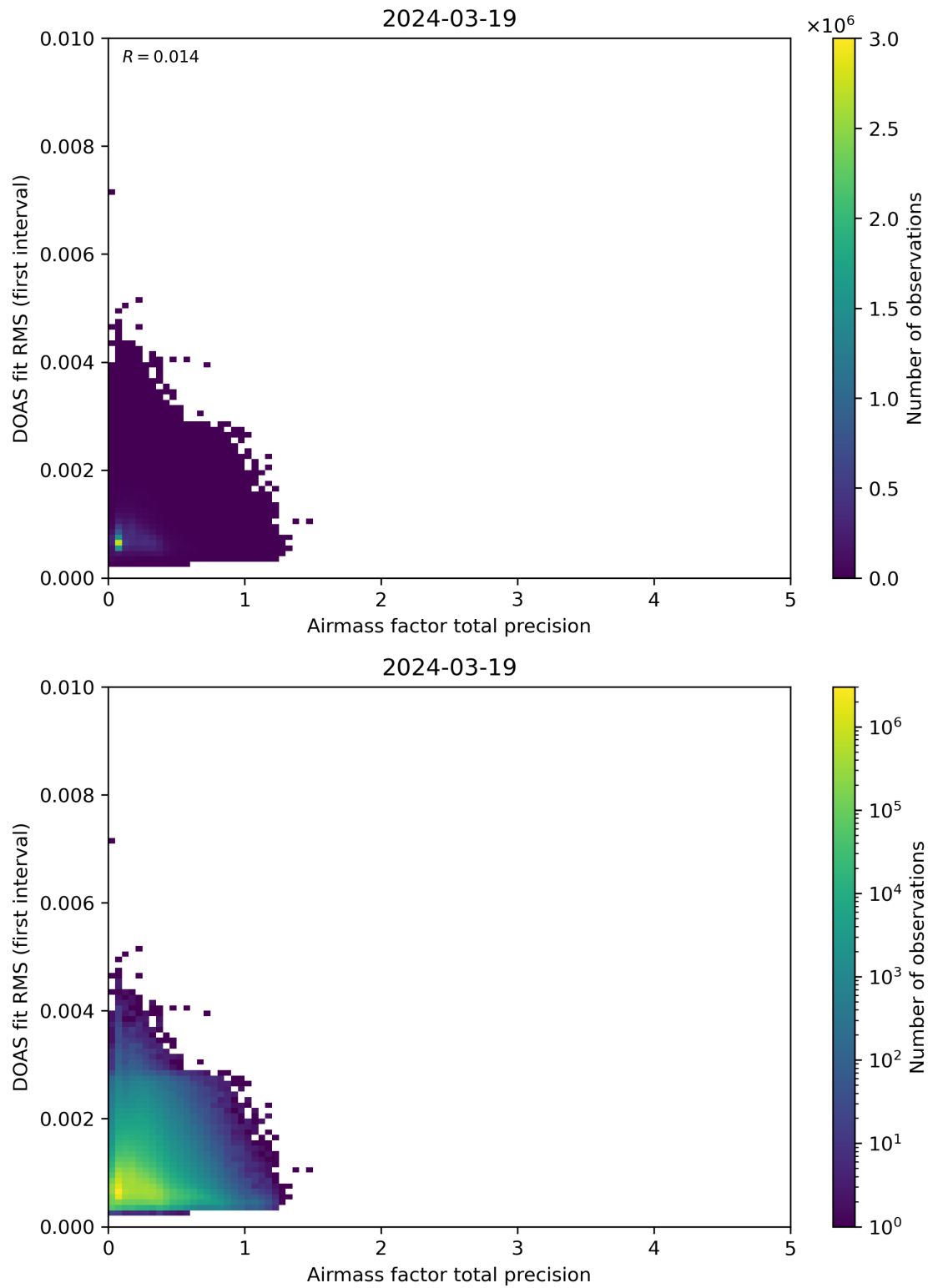
Figure 105: Scatter density plot of “Airmass factor total precision” against “DOAS fit RMS (first interval)” for 2024-03-18 to 2024-03-20.
