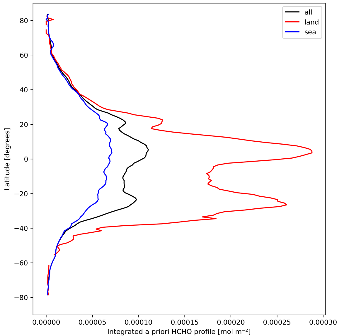
Figure 29: Zonal average of “Integrated a priori HCHO profile” for 2024-03-18 to 2024-03-20.
