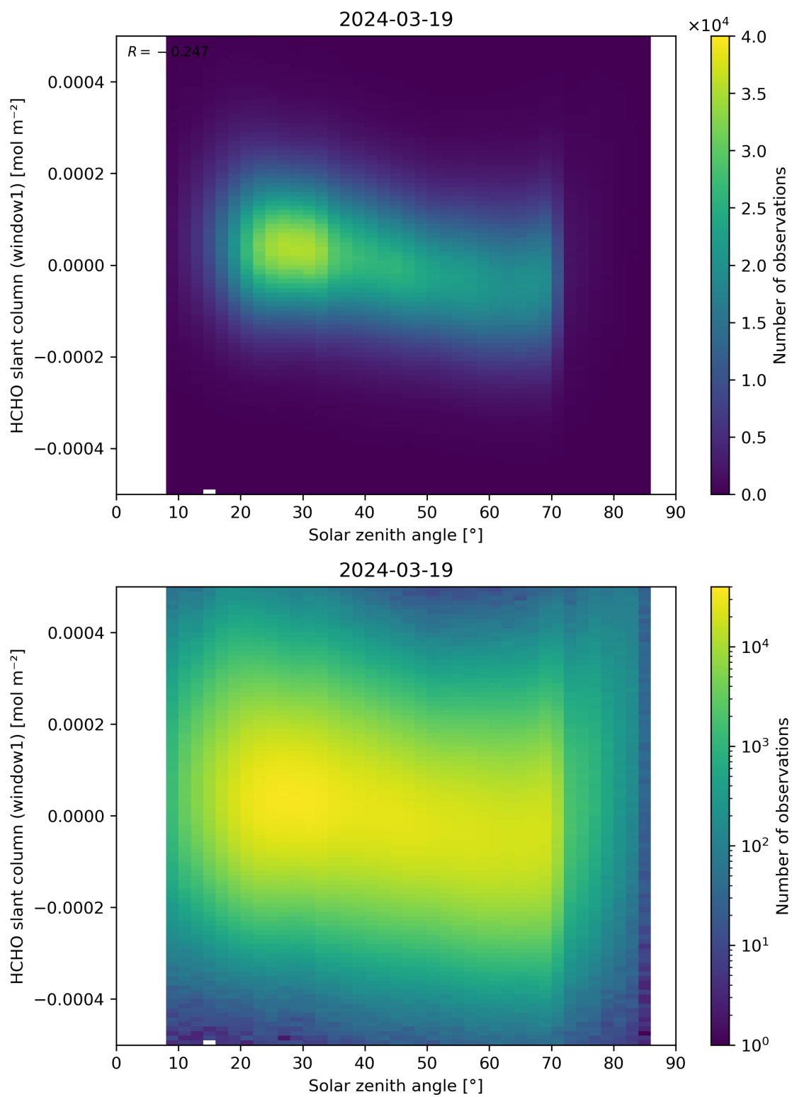
Figure 173: Scatter density plot of “Solar zenith angle” against “HCHO slant column (window1)” for 2024-03-18 to 2024-03-20.
