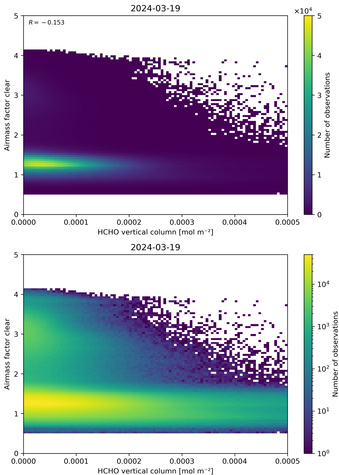
Figure 126: Scatter density plot of “HCHO vertical column” against “Airmass factor clear” for 2024-03-18 to 2024-03-20.
