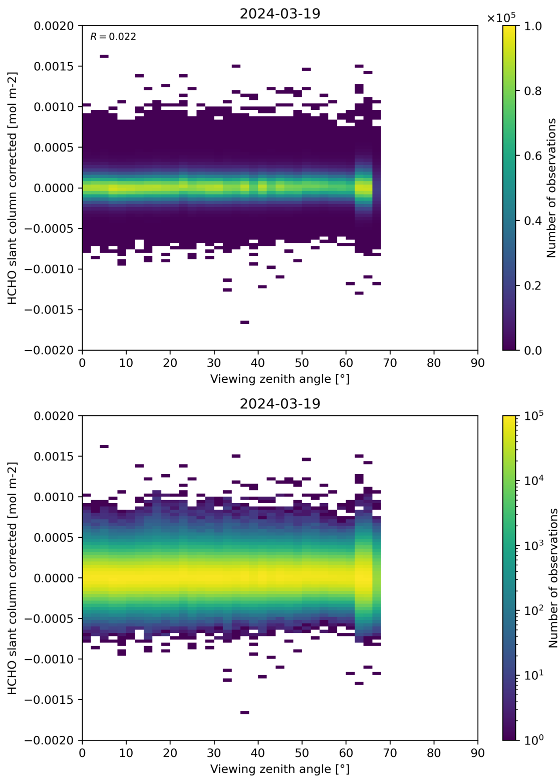
Figure 186: Scatter density plot of “Viewing zenith angle” against “HCHO slant column corrected” for 2024-03-18 to 2024-03-20.
