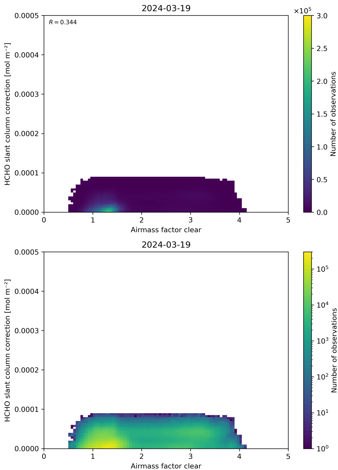
Figure 75: Scatter density plot of “Airmass factor clear” against “HCHO slant column correction” for 2024-03-18 to 2024-03-20.
