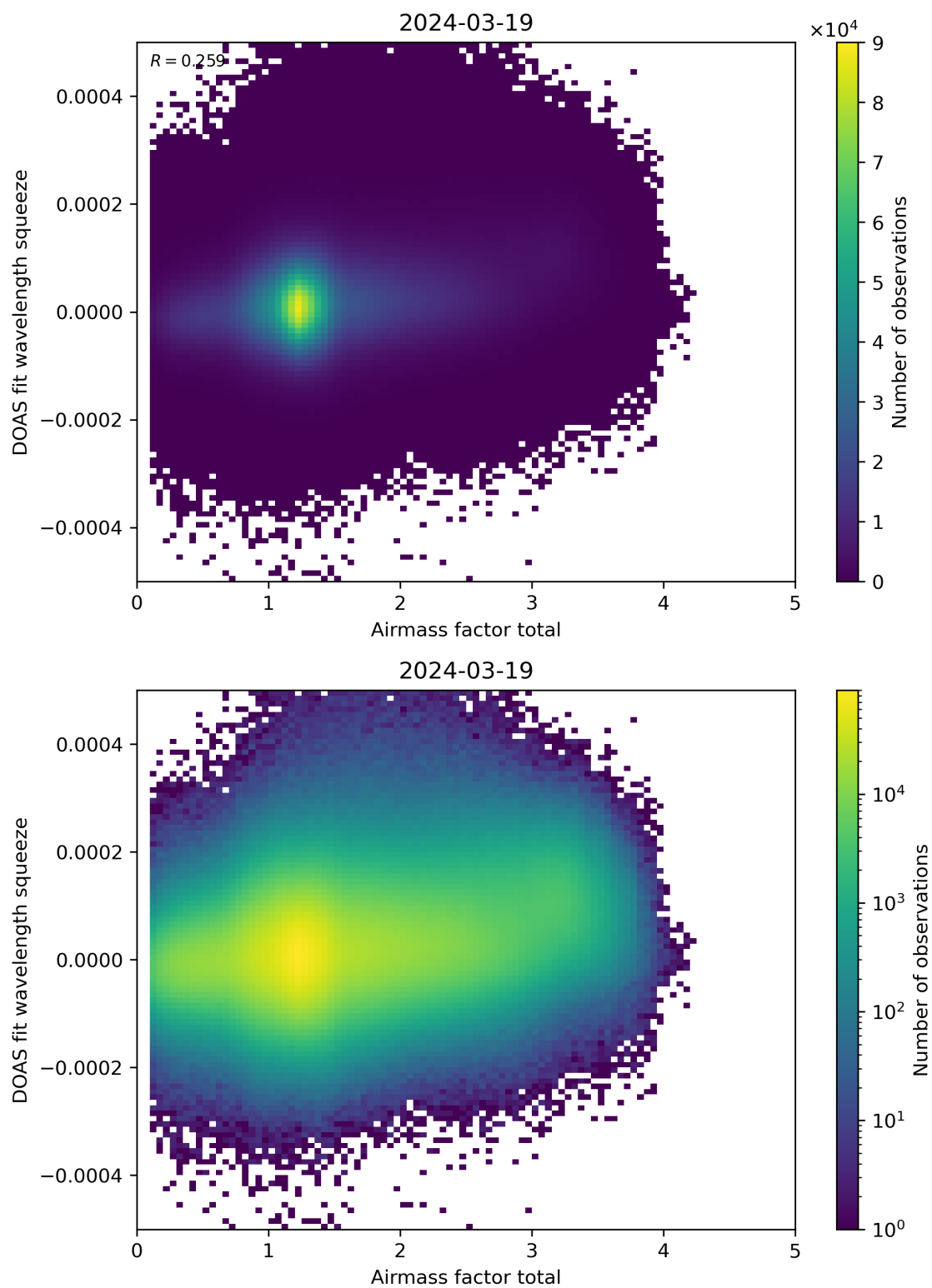
Figure 99: Scatter density plot of “Airmass factor total” against “DOAS fit wavelength squeeze” for 2024-03-18 to 2024-03-20.
