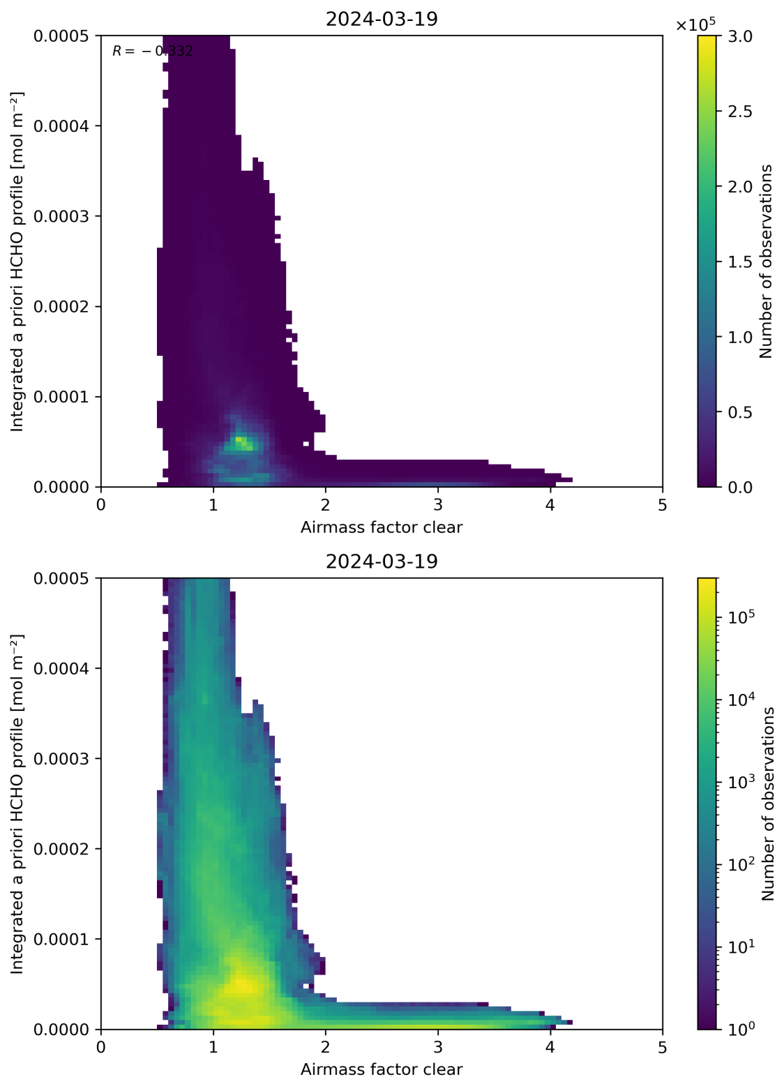
Figure 76: Scatter density plot of “Airmass factor clear” against “Integrated a priori HCHO profile” for 2024-03-18 to 2024-03-20.
