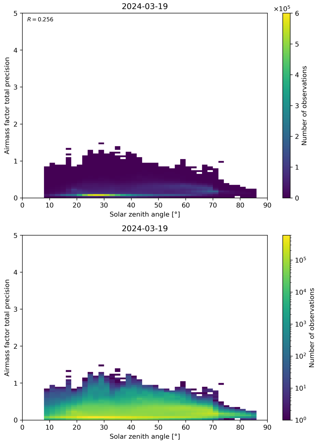
Figure 176: Scatter density plot of “Solar zenith angle” against “Airmass factor total precision” for 2024-03-18 to 2024-03-20.
