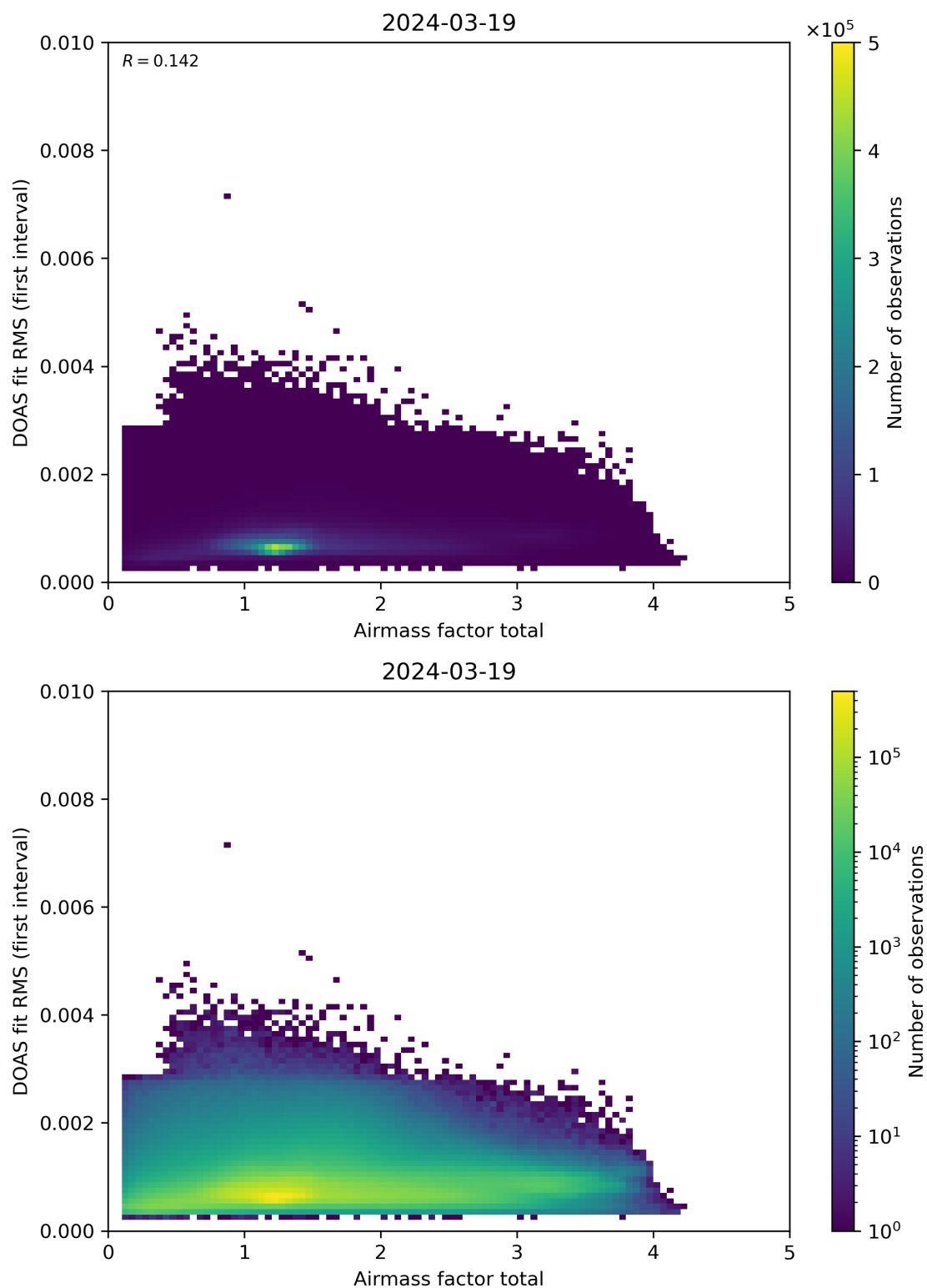
Figure 97: Scatter density plot of “Airmass factor total” against “DOAS fit RMS (first interval)” for 2024-03-18 to 2024-03-20.
