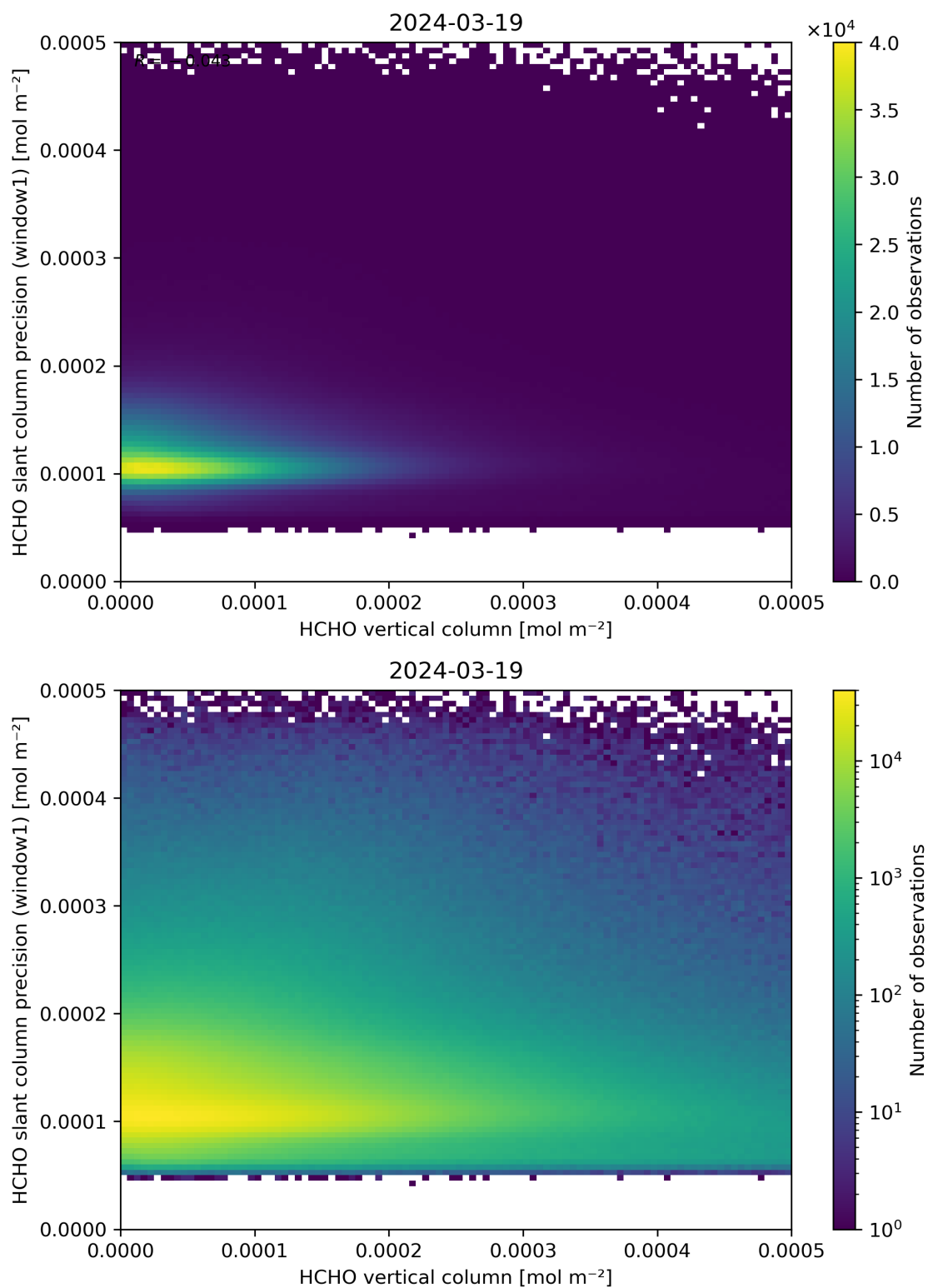
Figure 130: Scatter density plot of “HCHO vertical column” against “HCHO slant column precision (window1)” for 2024-03-18 to 2024-03-20.
