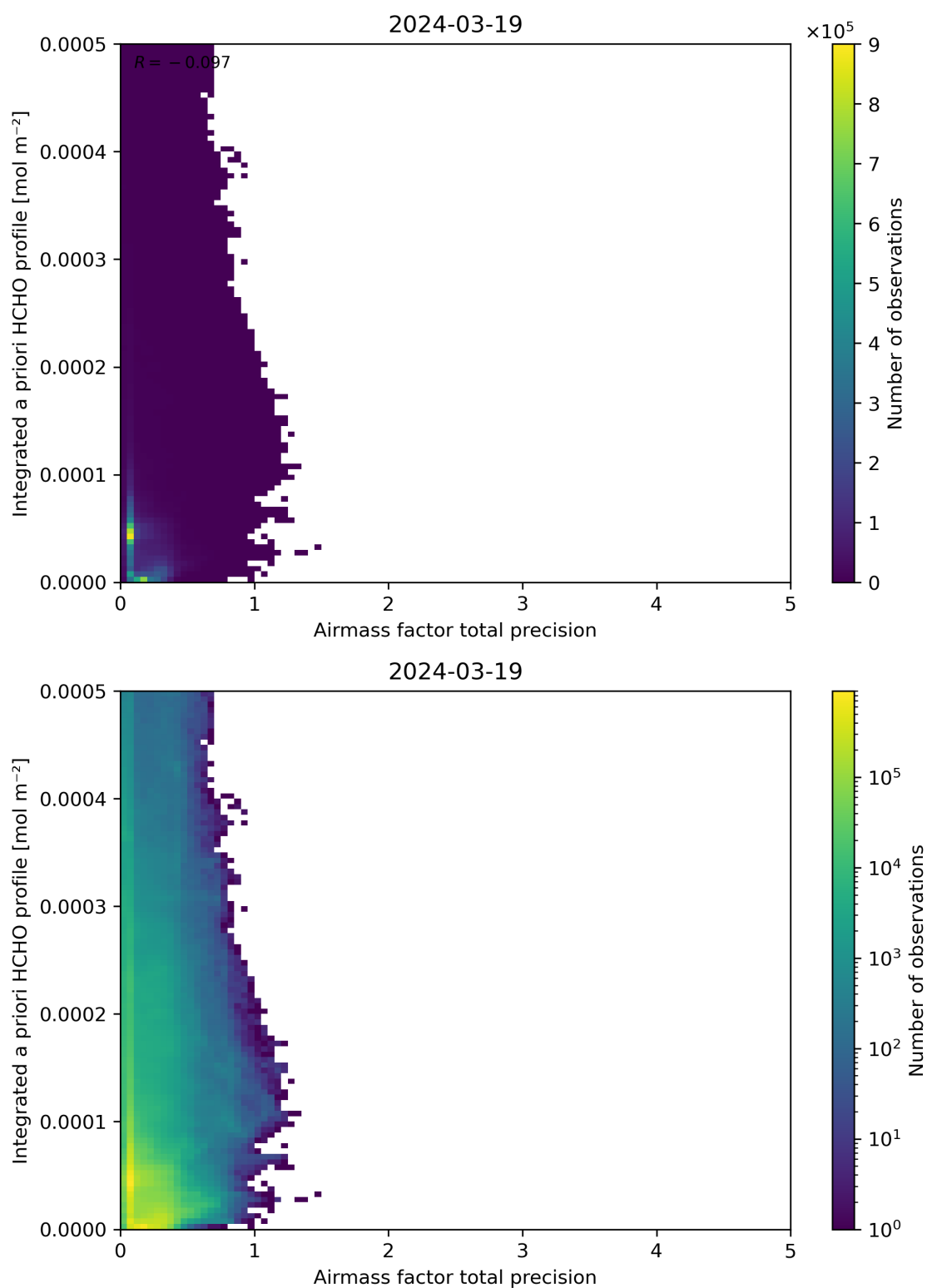
Figure 111: Scatter density plot of “Airmass factor total precision” against “Integrated a priori HCHO profile” for 2024-03-18 to 2024-03-20.
