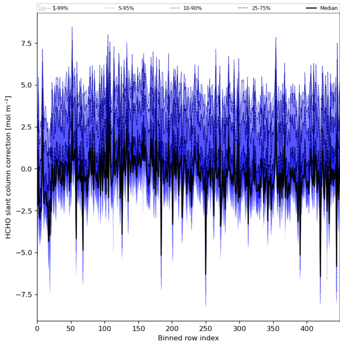
Figure 61: Along track statistics of “HCHO slant column correction” for 2024-03-18 to 2024-03-20
