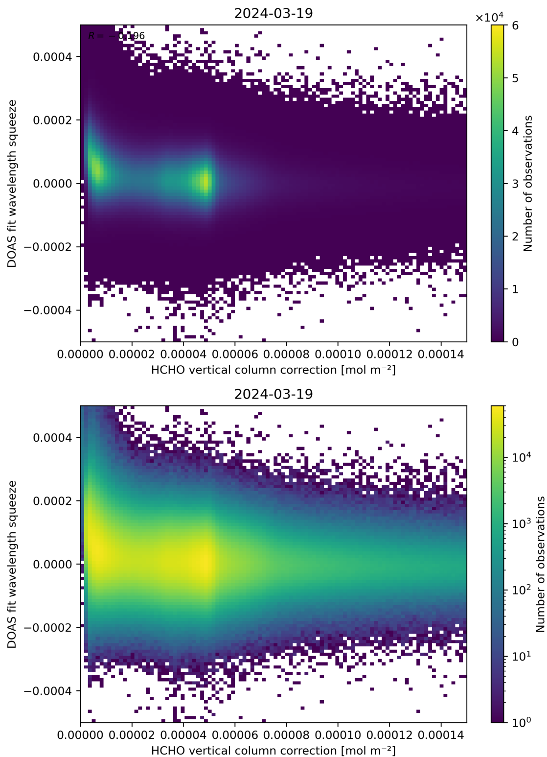
Figure 114: Scatter density plot of “HCHO vertical column correction” against “DOAS fit wavelength squeeze” for 2024-03-18 to 2024-03-20.
