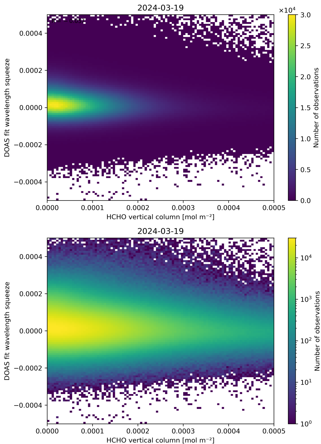
Figure 125: Scatter density plot of “HCHO vertical column” against “DOAS fit wavelength squeeze” for 2024-03-18 to 2024-03-20.
