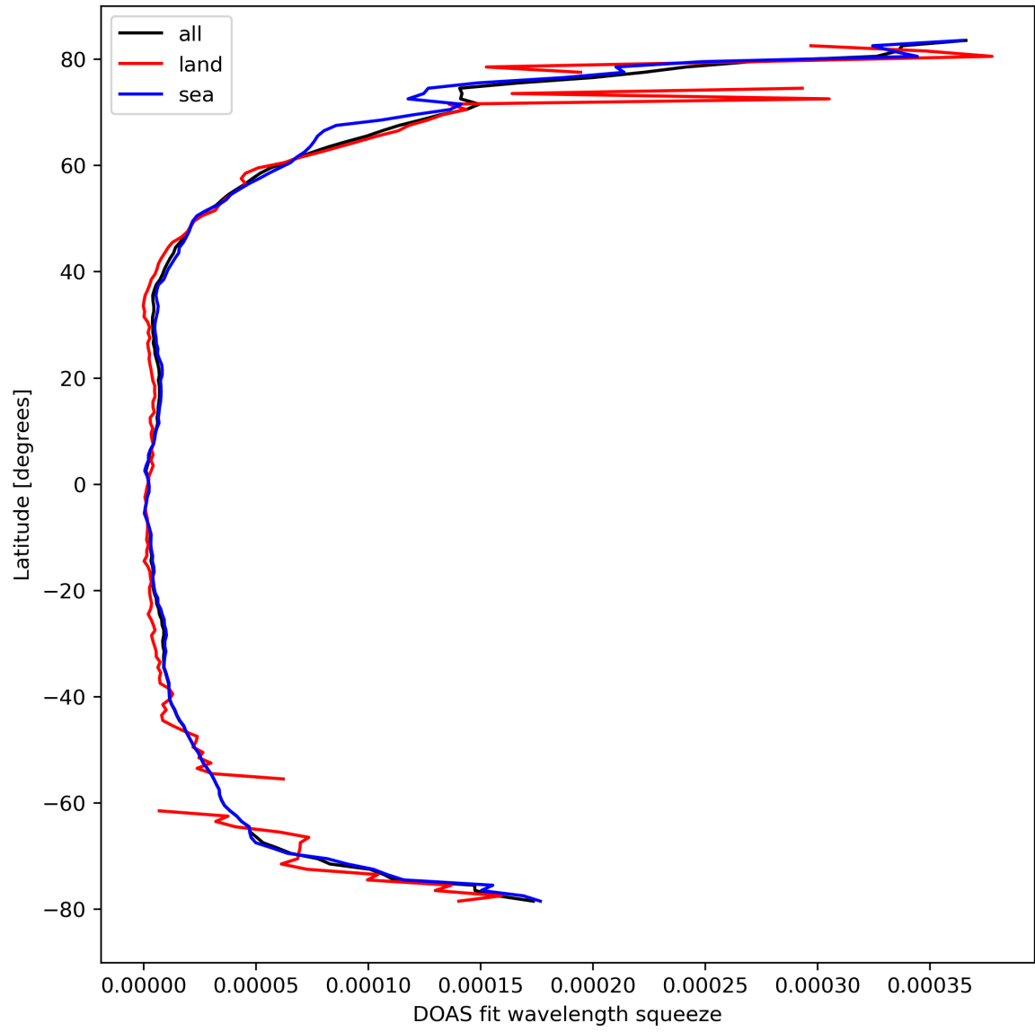
Figure 31: Zonal average of “DOAS fit wavelength squeeze” for 2024-03-18 to 2024-03-20.
