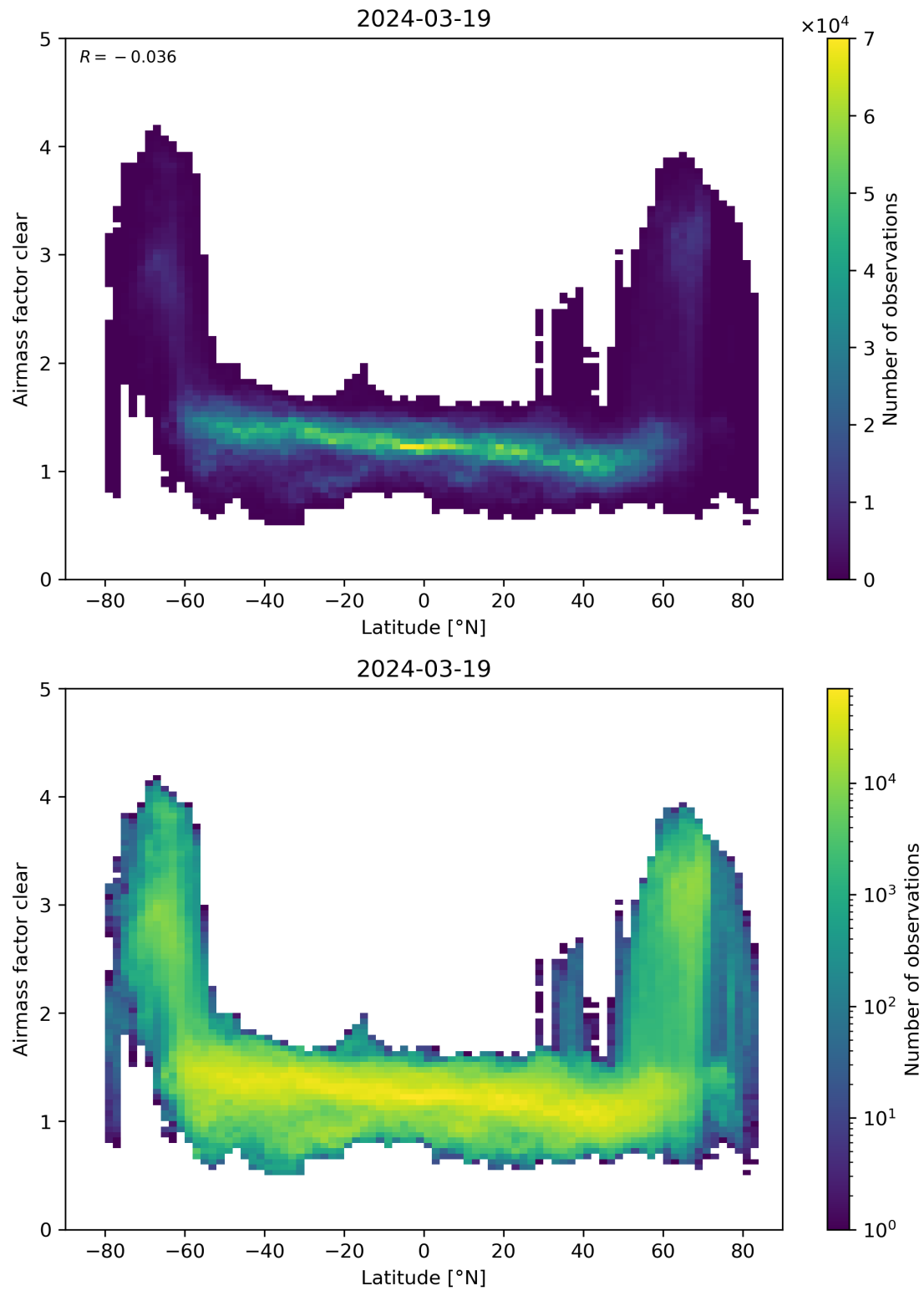
Figure 156: Scatter density plot of “Latitude” against “Airmass factor clear” for 2024-03-18 to 2024-03-20.
