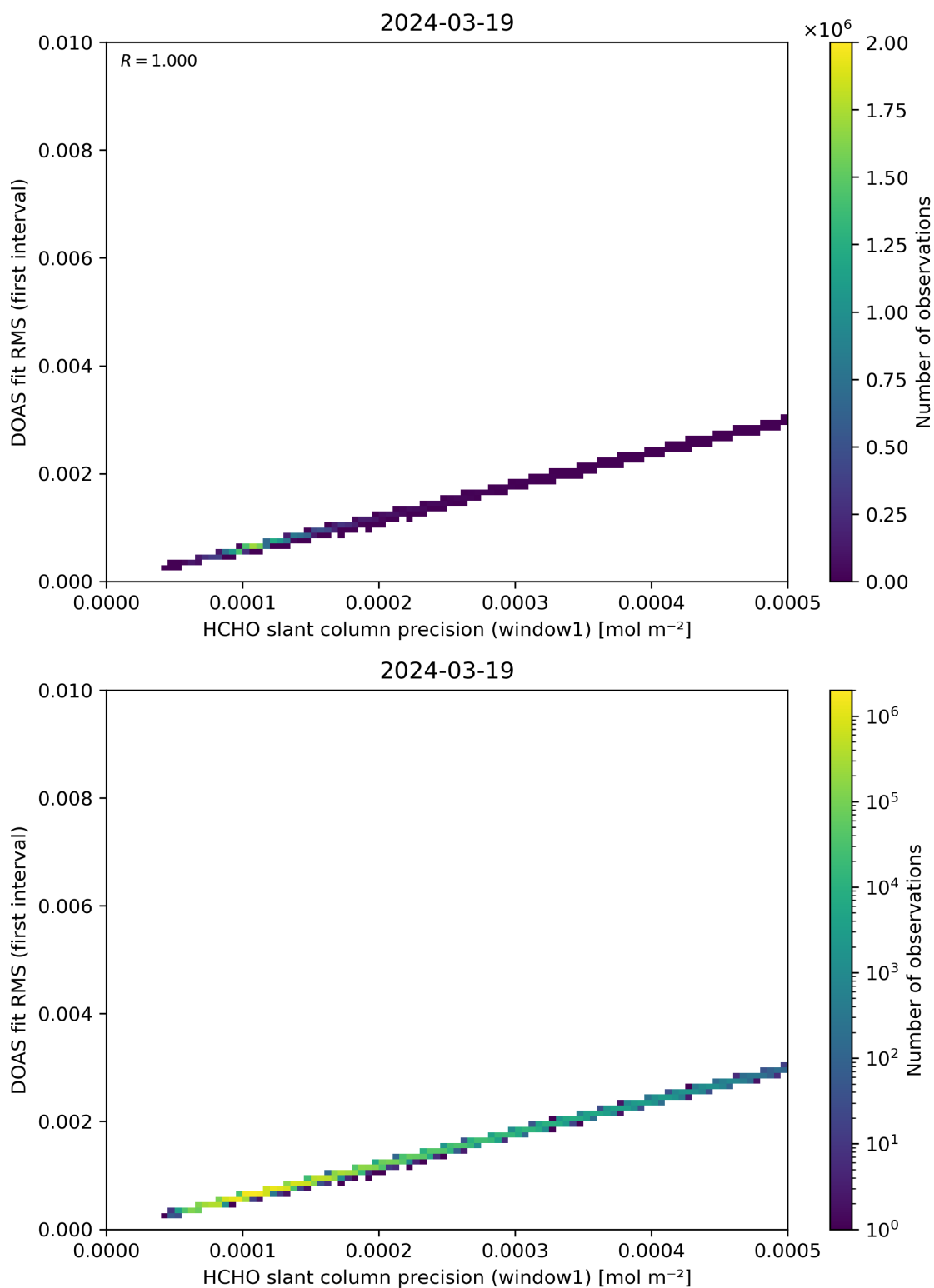
Figure 88: Scatter density plot of “HCHO slant column precision (window1)” against “DOAS fit RMS (first interval)” for 2024-03-18 to 2024-03-20.
