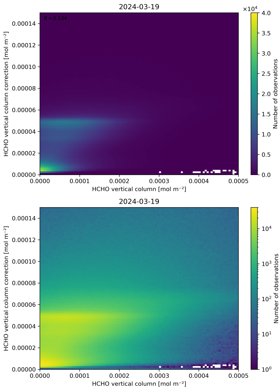
Figure 133: Scatter density plot of “HCHO vertical column” against “HCHO vertical column correction” for 2024-03-18 to 2024-03-20.
