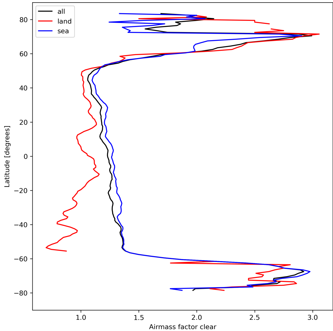
Figure 28: Zonal average of “Airmass factor clear” for 2024-03-18 to 2024-03-20.
