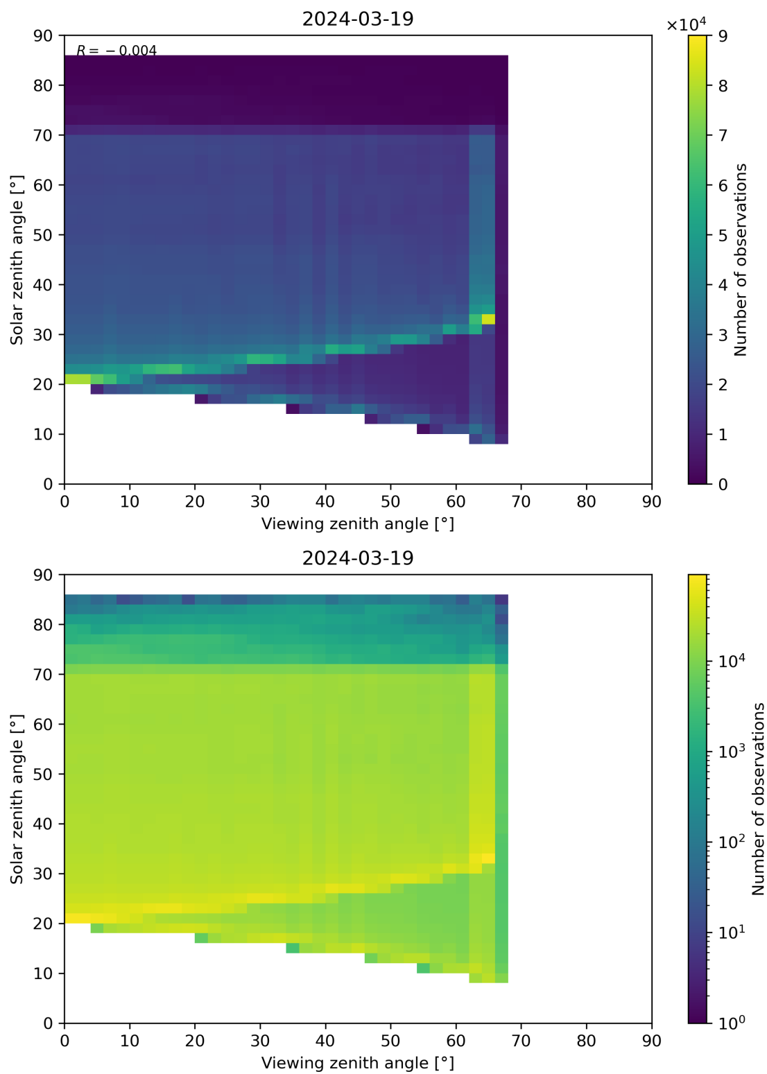
Figure 197: Scatter density plot of “Viewing zenith angle” against “Solar zenith angle” for 2024-03-18 to 2024-03-20.
