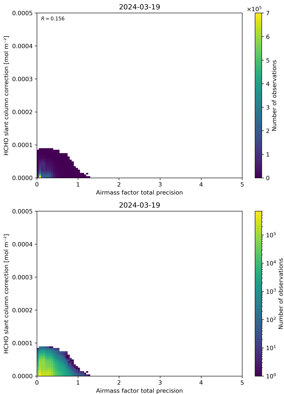
Figure 110: Scatter density plot of “Airmass factor total precision” against “HCHO slant column correction” for 2024-03-18 to 2024-03-20.
