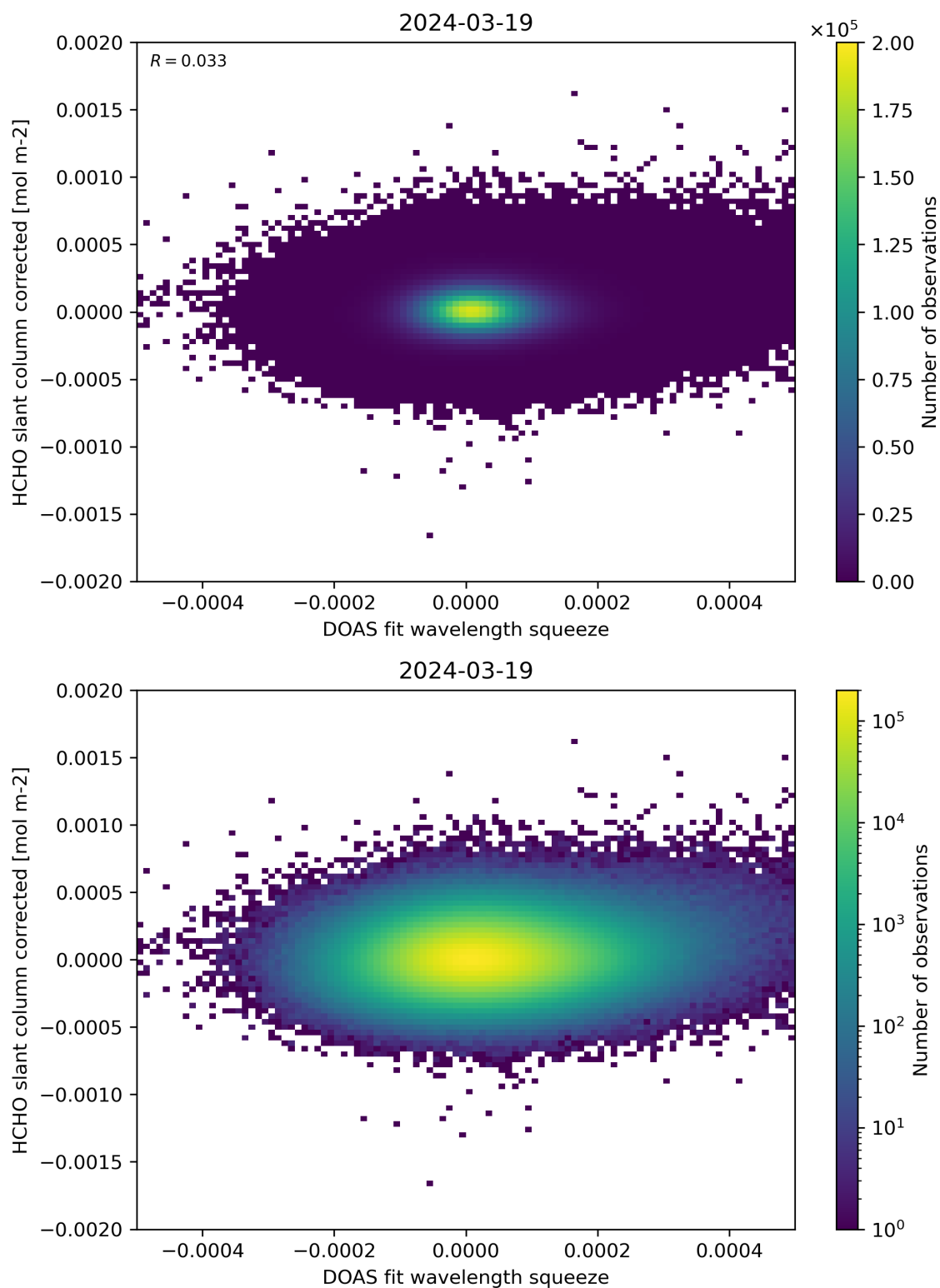
Figure 69: Scatter density plot of “DOAS fit wavelength squeeze” against “HCHO slant column corrected” for 2024-03-18 to 2024-03-20.
