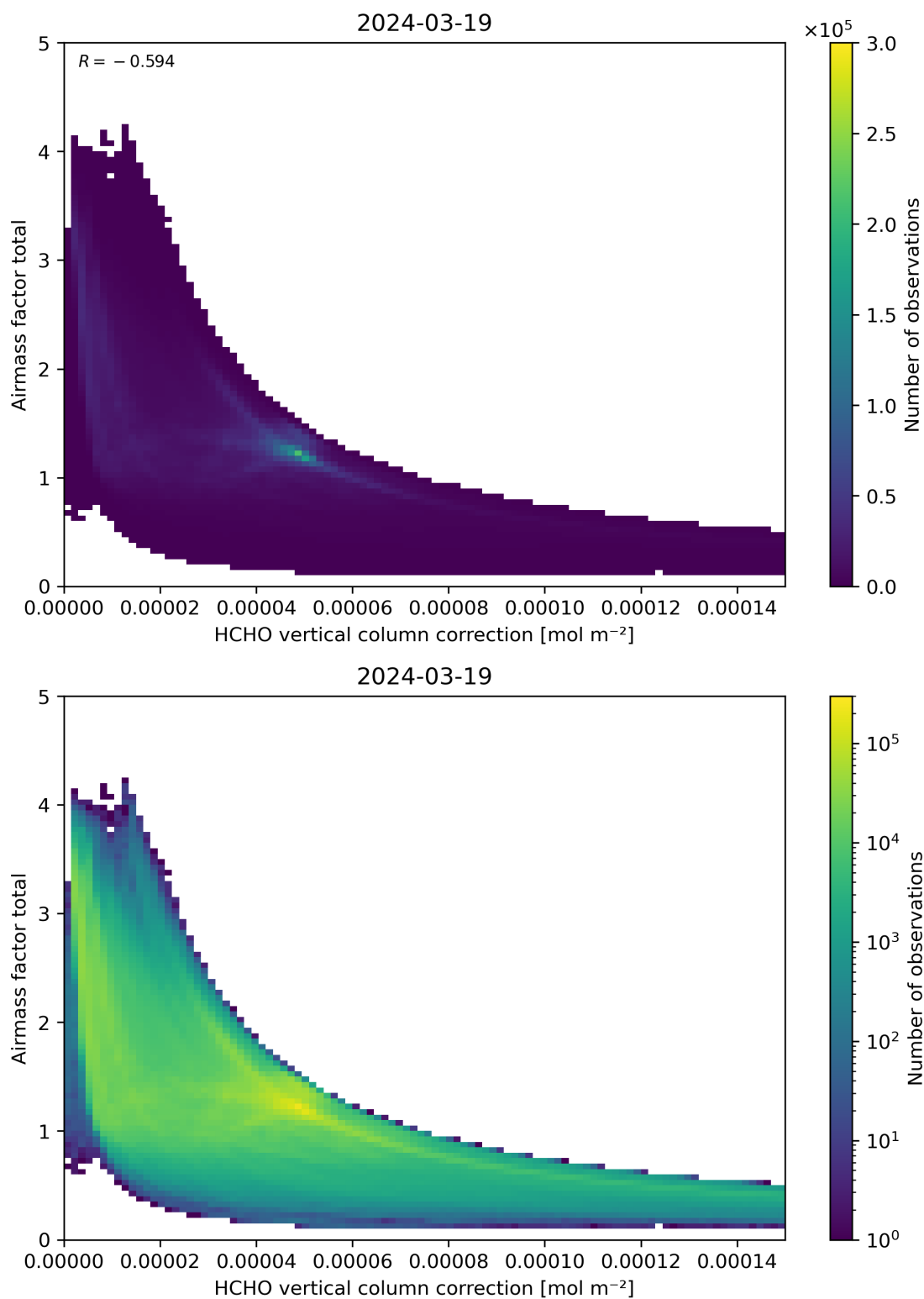
Figure 120: Scatter density plot of “HCHO vertical column correction” against “Airmass factor total” for 2024-03-18 to 2024-03-20.
