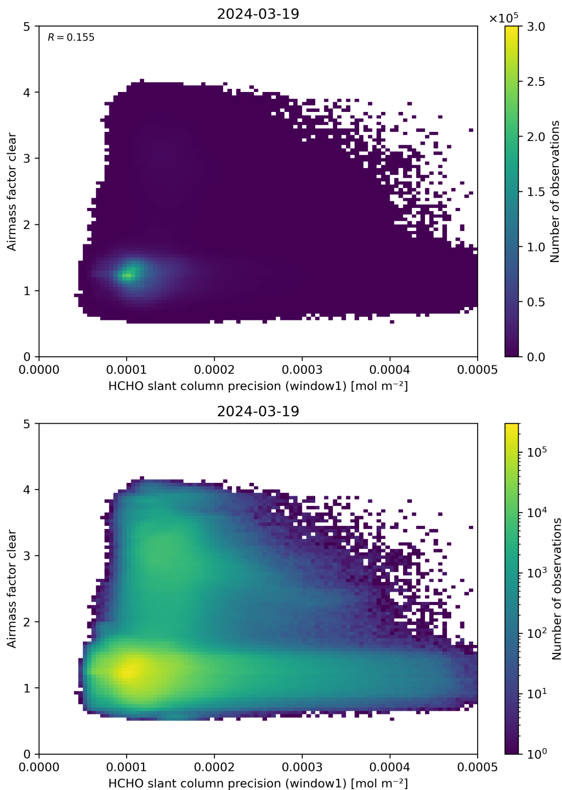
Figure 91: Scatter density plot of “HCHO slant column precision (window1)” against “Airmass factor clear” for 2024-03-18 to 2024-03-20.
