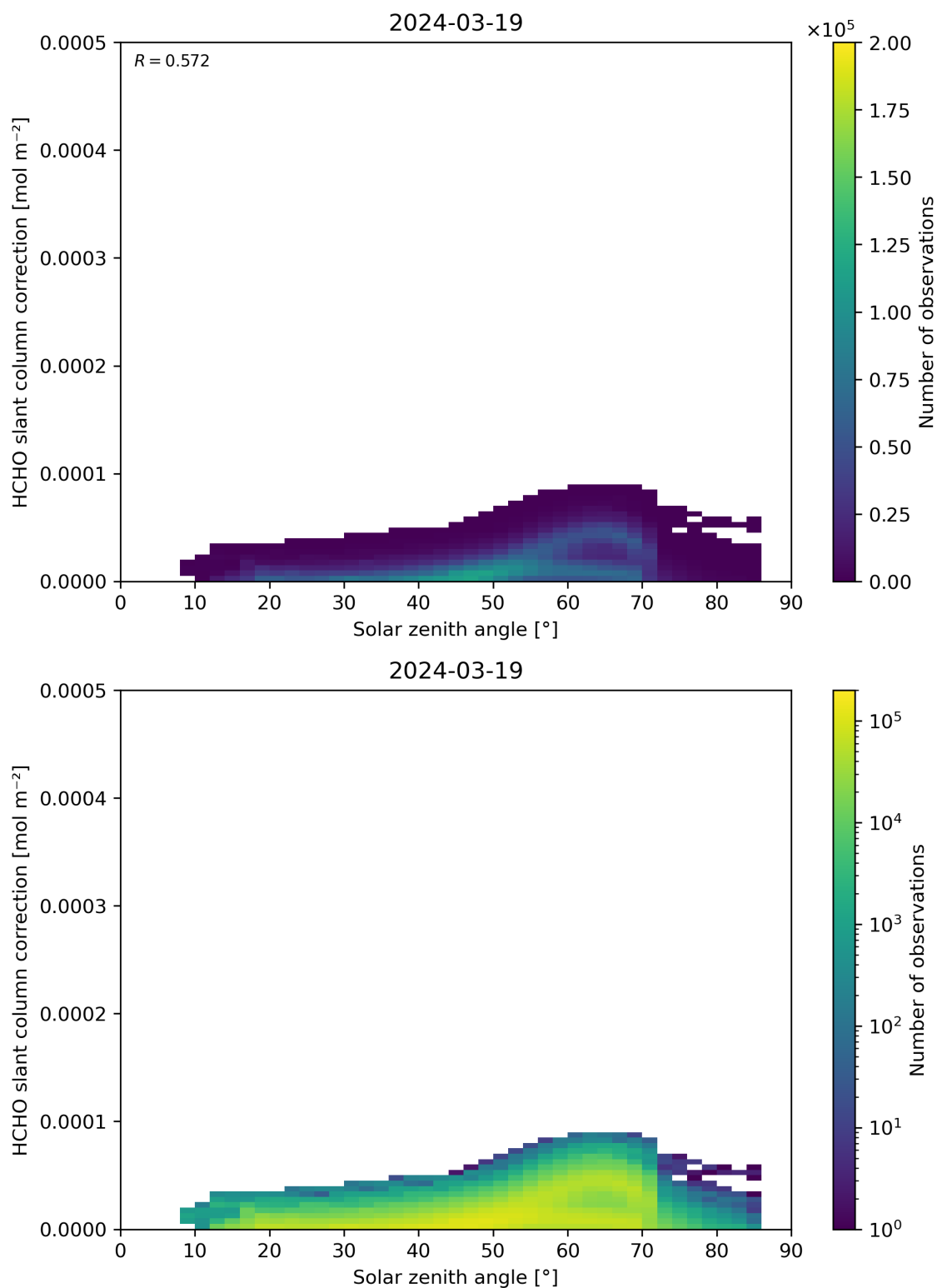
Figure 172: Scatter density plot of “Solar zenith angle” against “HCHO slant column correction” for 2024-03-18 to 2024-03-20.
