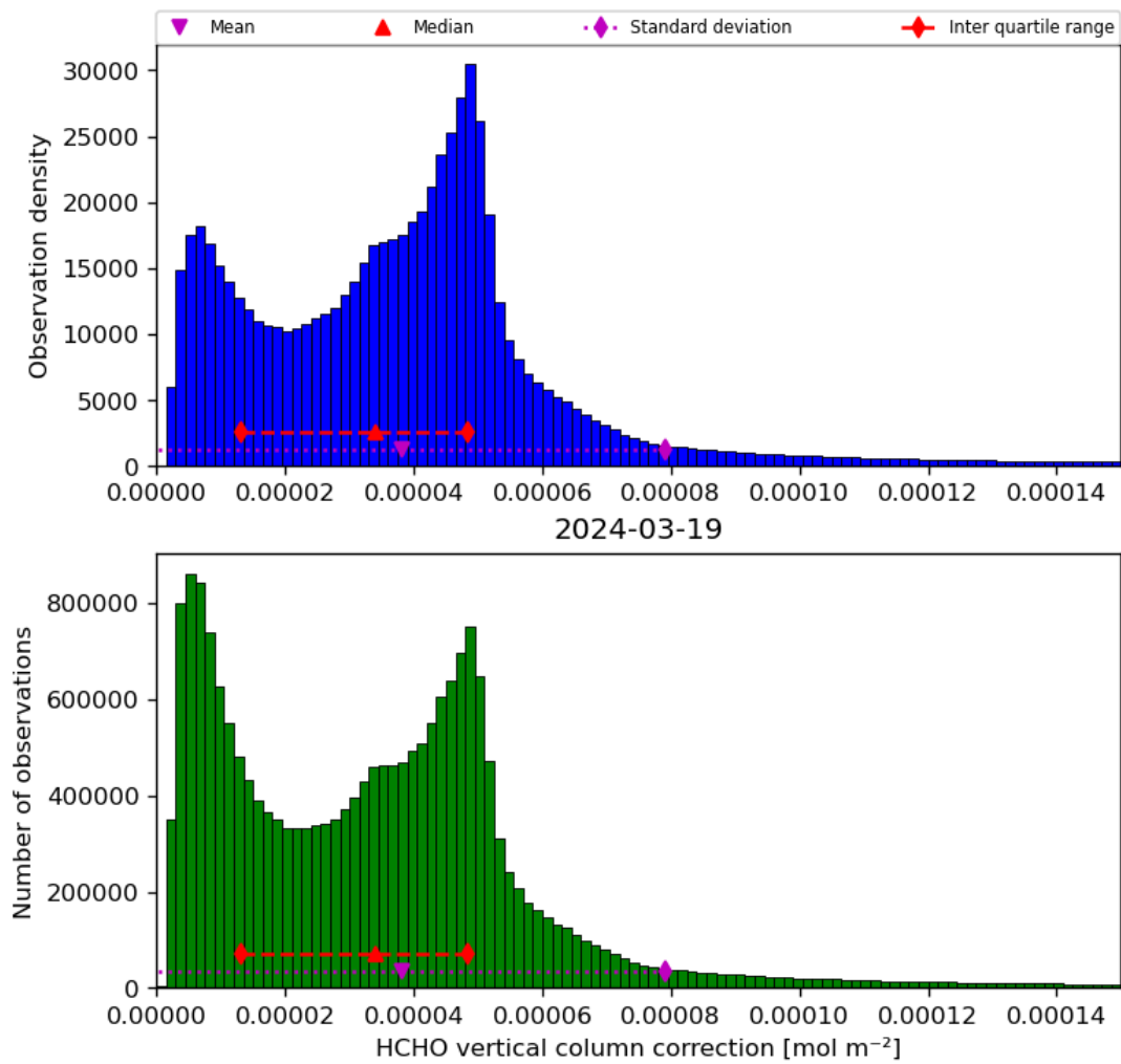
Figure 37: Histogram of “HCHO vertical column correction” for 2024-03-18 to 2024-03-20
