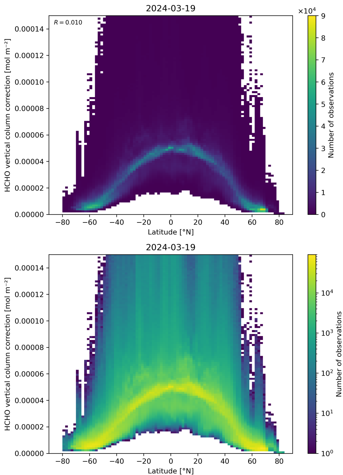
Figure 164: Scatter density plot of “Latitude” against “HCHO vertical column correction” for 2024-03-18 to 2024-03-20.
