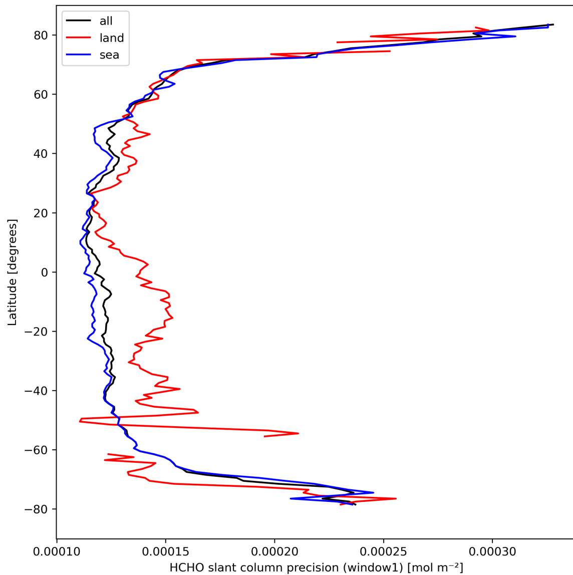
Figure 25: Zonal average of “HCHO slant column precision (window1)” for 2024-03-18 to 2024-03-20.
