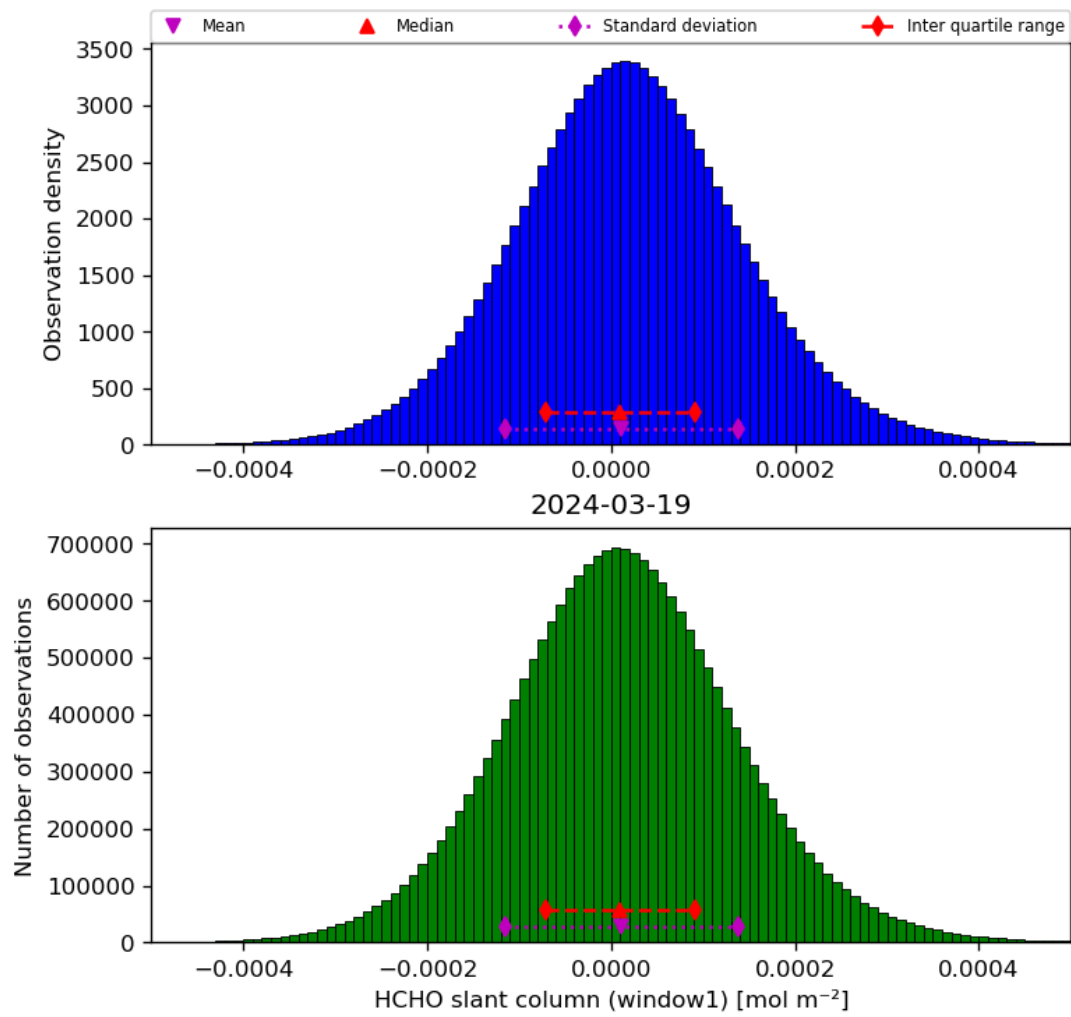
Figure 38: Histogram of “HCHO slant column (window1)” for 2024-03-18 to 2024-03-20
