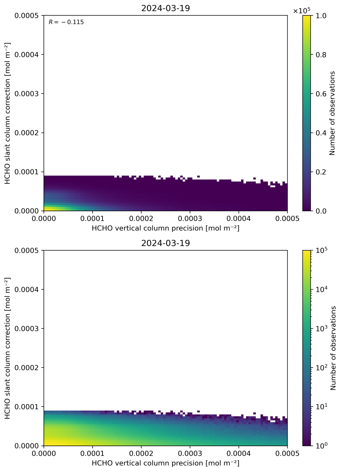
Figure 141: Scatter density plot of “HCHO vertical column precision” against “HCHO slant column correction” for 2024-03-18 to 2024-03-20.
