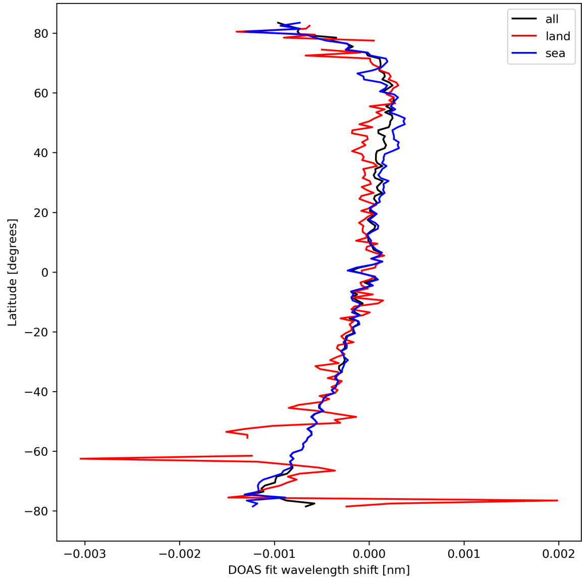
Figure 30: Zonal average of “DOAS fit wavelength shift” for 2024-03-18 to 2024-03-20.
