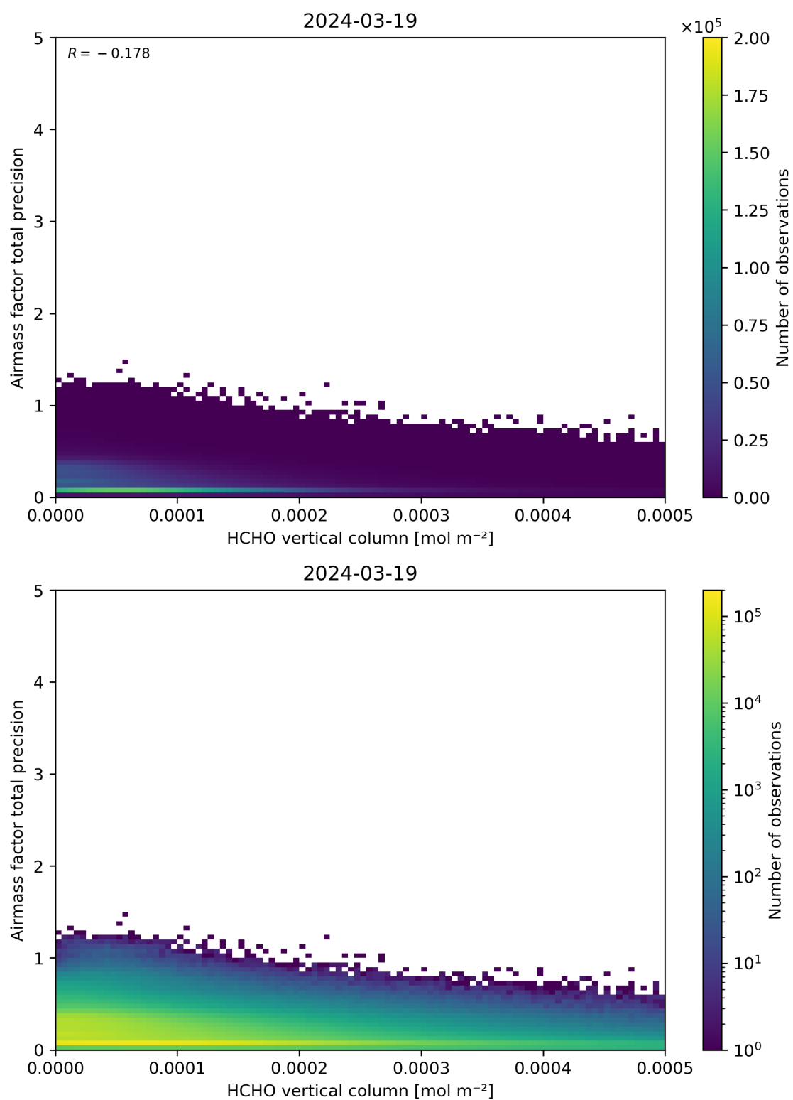
Figure 132: Scatter density plot of “HCHO vertical column” against “Airmass factor total precision” for 2024-03-18 to 2024-03-20.
