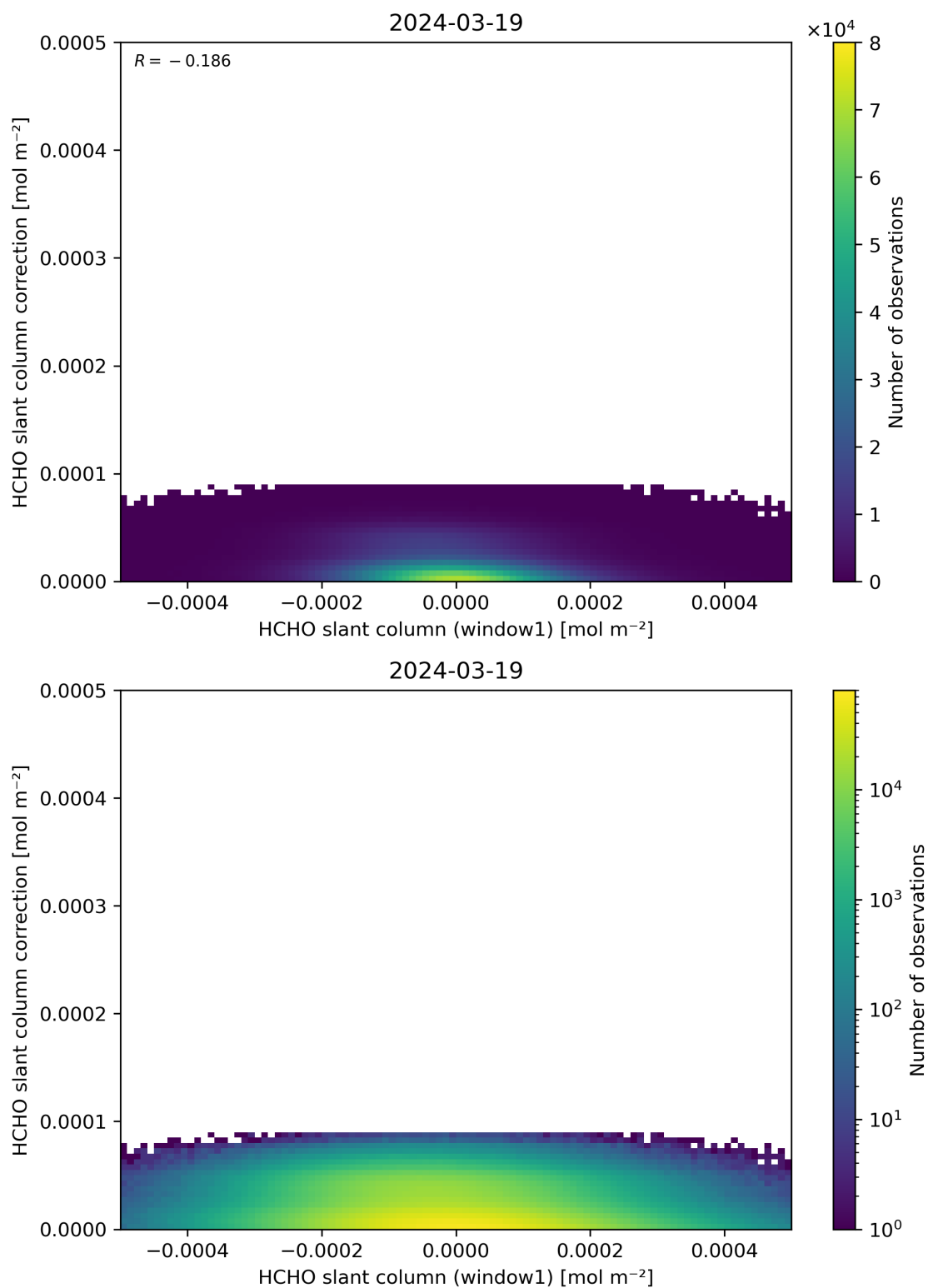
Figure 83: Scatter density plot of “HCHO slant column (window1)” against “HCHO slant column correction” for 2024-03-18 to 2024-03-20.
