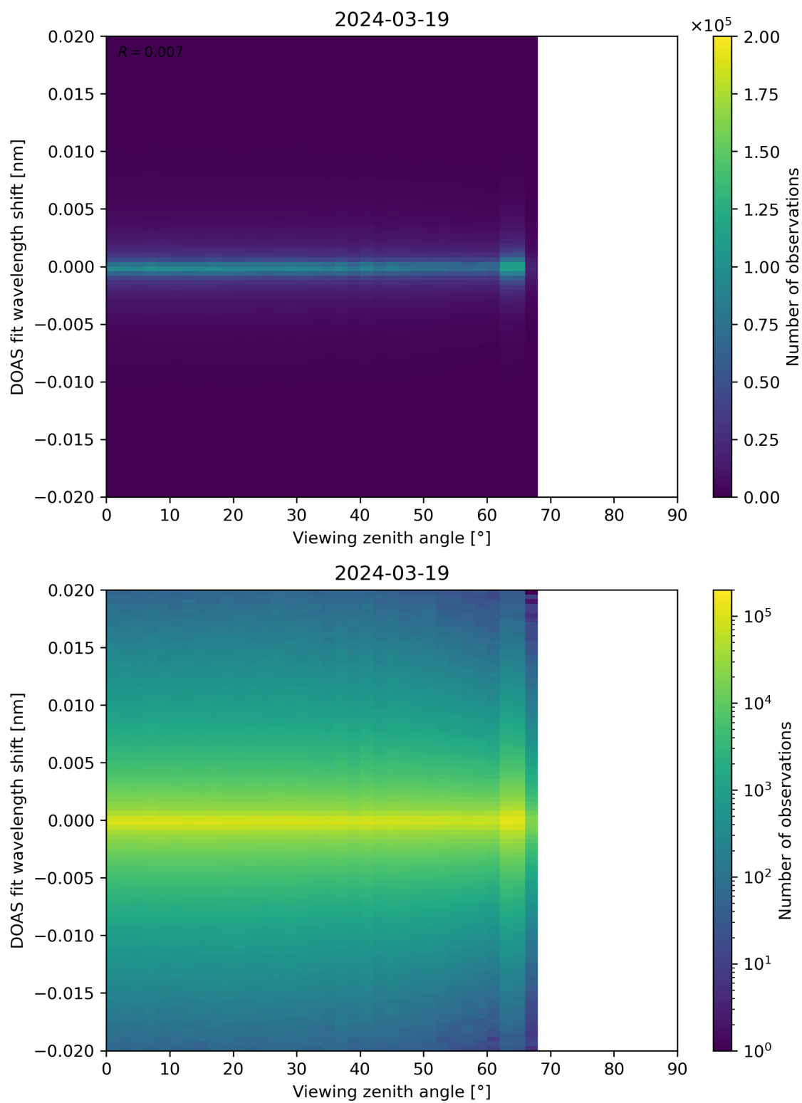
Figure 183: Scatter density plot of “Viewing zenith angle” against “DOAS fit wavelength shift” for 2024-03-18 to 2024-03-20.
