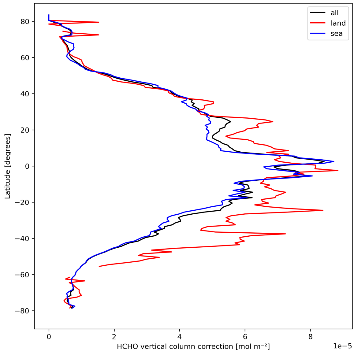
Figure 23: Zonal average of “HCHO vertical column correction” for 2024-03-18 to 2024-03-20.
