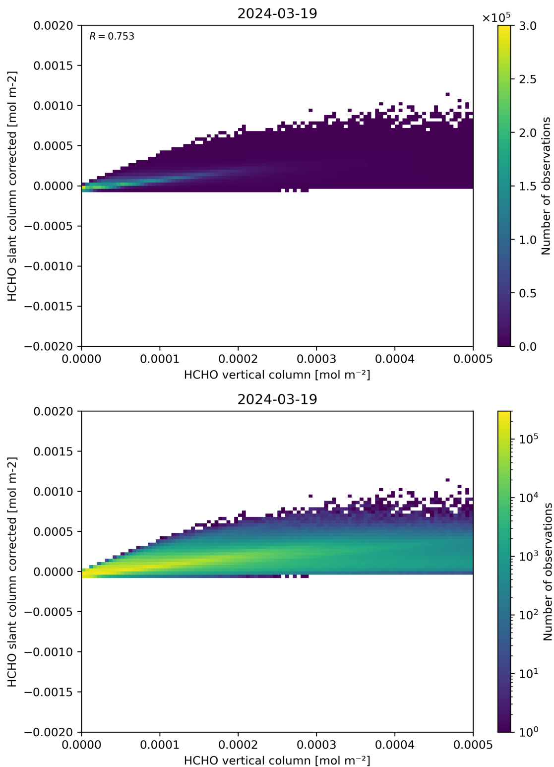
Figure 127: Scatter density plot of “HCHO vertical column” against “HCHO slant column corrected” for 2024-03-18 to 2024-03-20.
