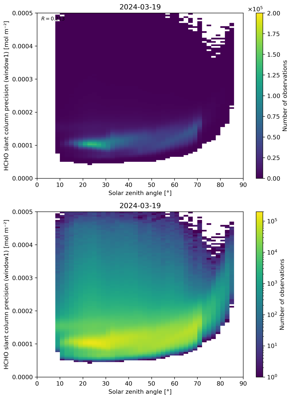
Figure 174: Scatter density plot of “Solar zenith angle” against “HCHO slant column precision (window1)” for 2024-03-18 to 2024-03-20.
