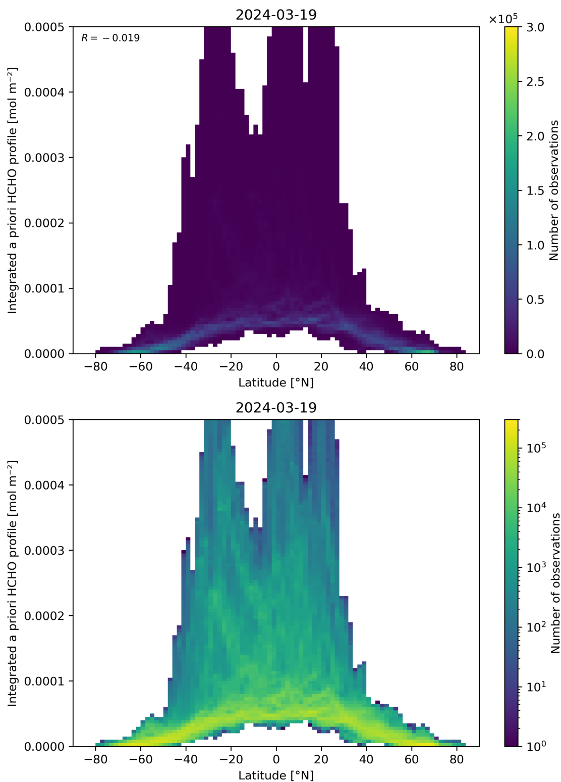
Figure 166: Scatter density plot of “Latitude” against “Integrated a priori HCHO profile” for 2024-03-18 to 2024-03-20.
