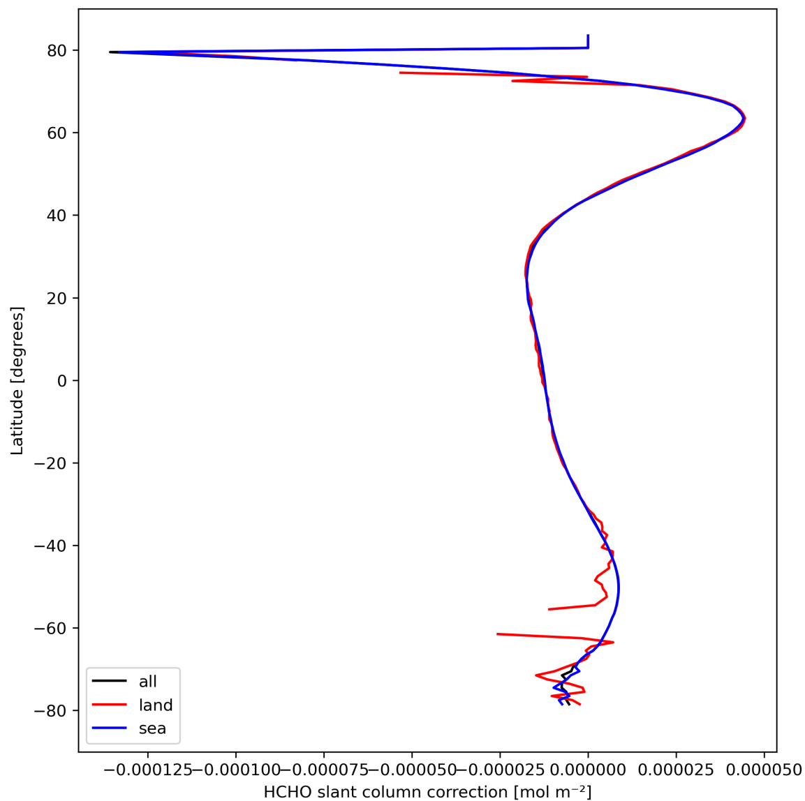
Figure 33: Zonal average of “HCHO slant column correction” for 2024-03-18 to 2024-03-20.
