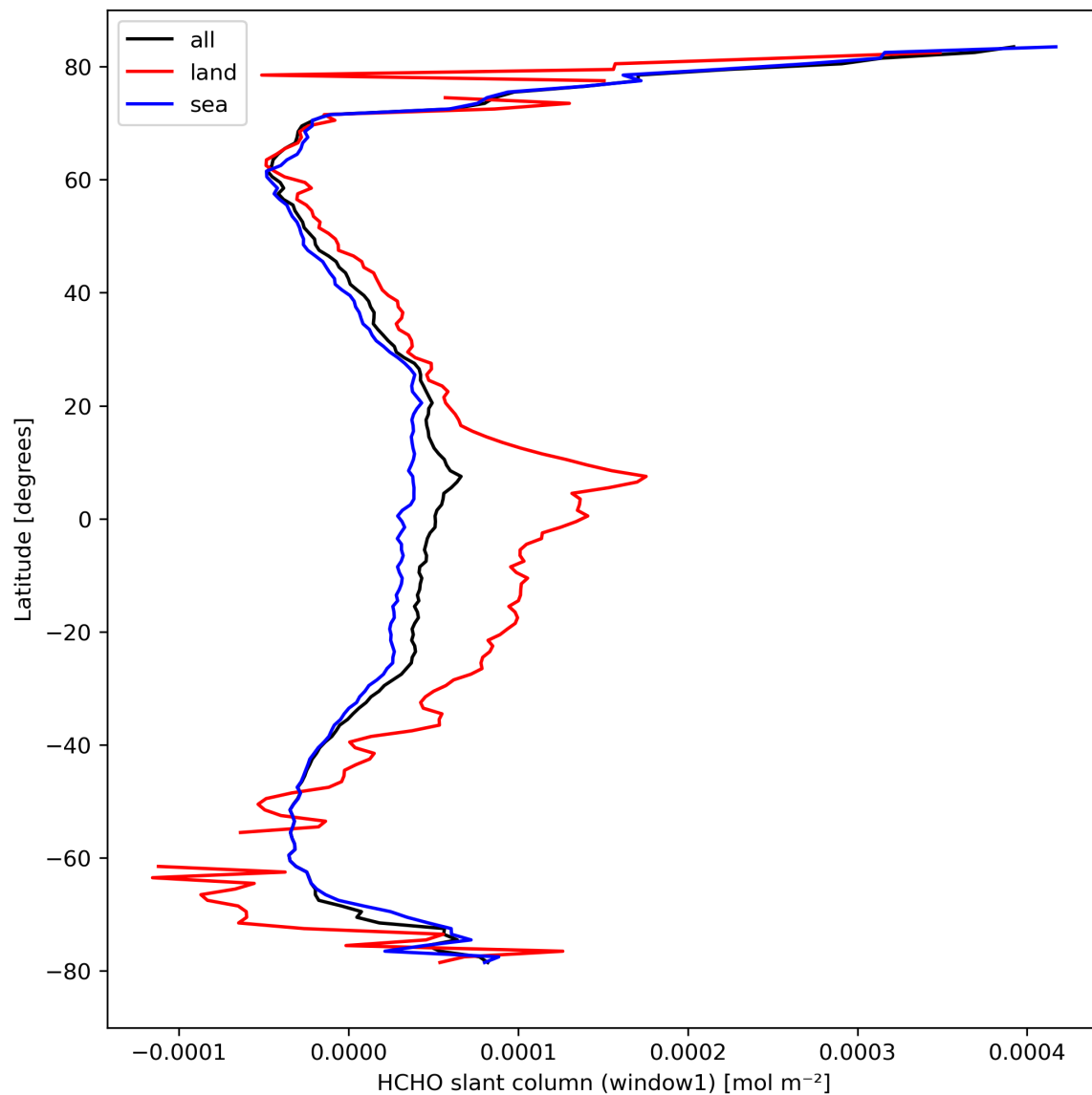
Figure 24: Zonal average of “HCHO slant column (window1)” for 2024-03-18 to 2024-03-20.
