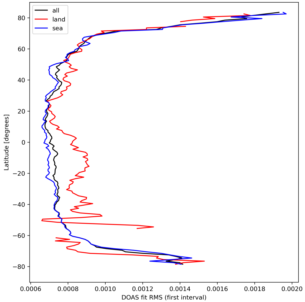
Figure 32: Zonal average of "DOAS fit RMS (first interval)" for 2024-03-18 to 2024-03-20.
