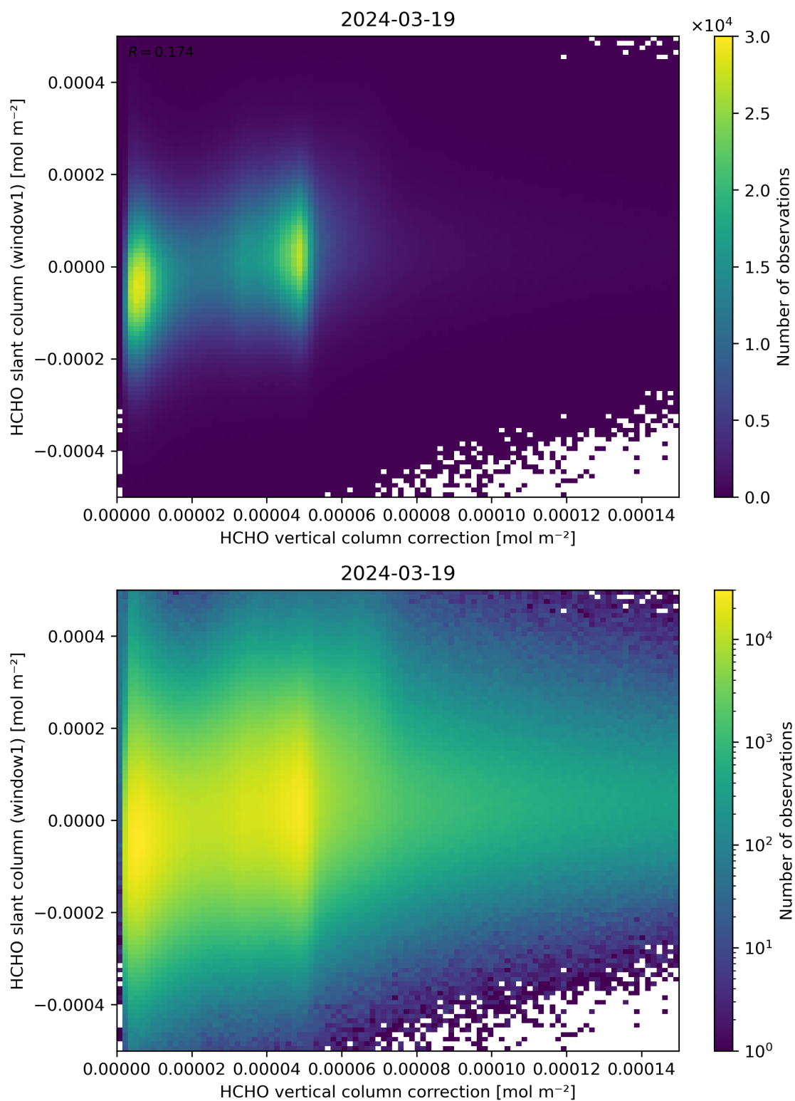
Figure 118: Scatter density plot of “HCHO vertical column correction” against “HCHO slant column (window1)” for 2024-03-18 to 2024-03-20.
