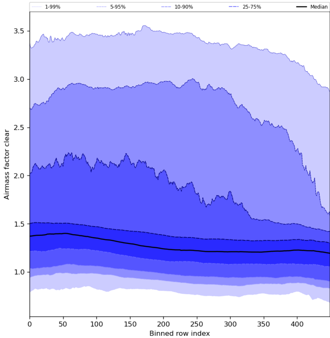
Figure 56: Along track statistics of “Airmass factor clear” for 2024-03-18 to 2024-03-20
