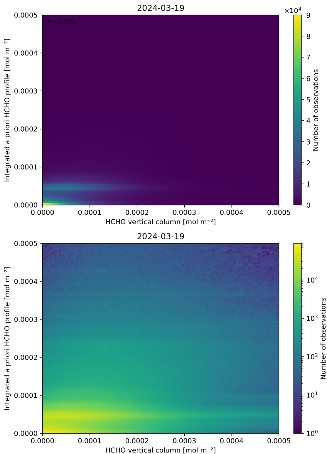
Figure 135: Scatter density plot of “HCHO vertical column” against “Integrated a priori HCHO profile” for 2024-03-18 to 2024-03-20.
