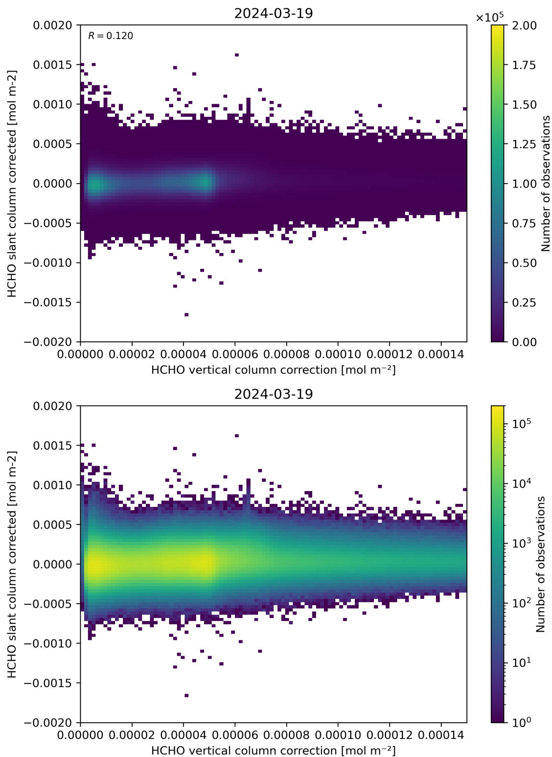
Figure 116: Scatter density plot of “HCHO vertical column correction” against “HCHO slant column corrected” for 2024-03-18 to 2024-03-20.
