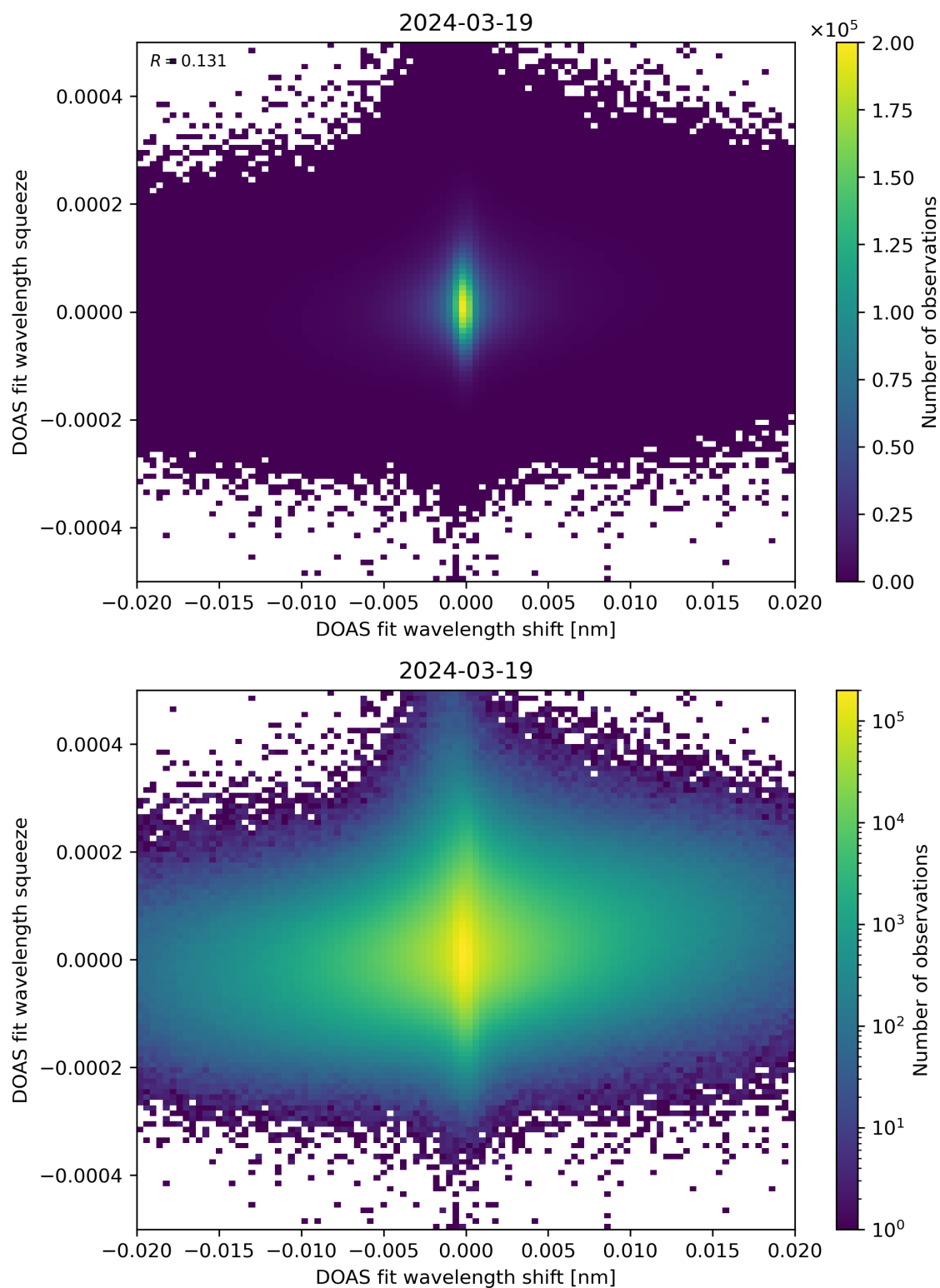
Figure 65: Scatter density plot of “DOAS fit wavelength shift” against “DOAS fit wavelength squeeze” for 2024-03-18 to 2024-03-20.
