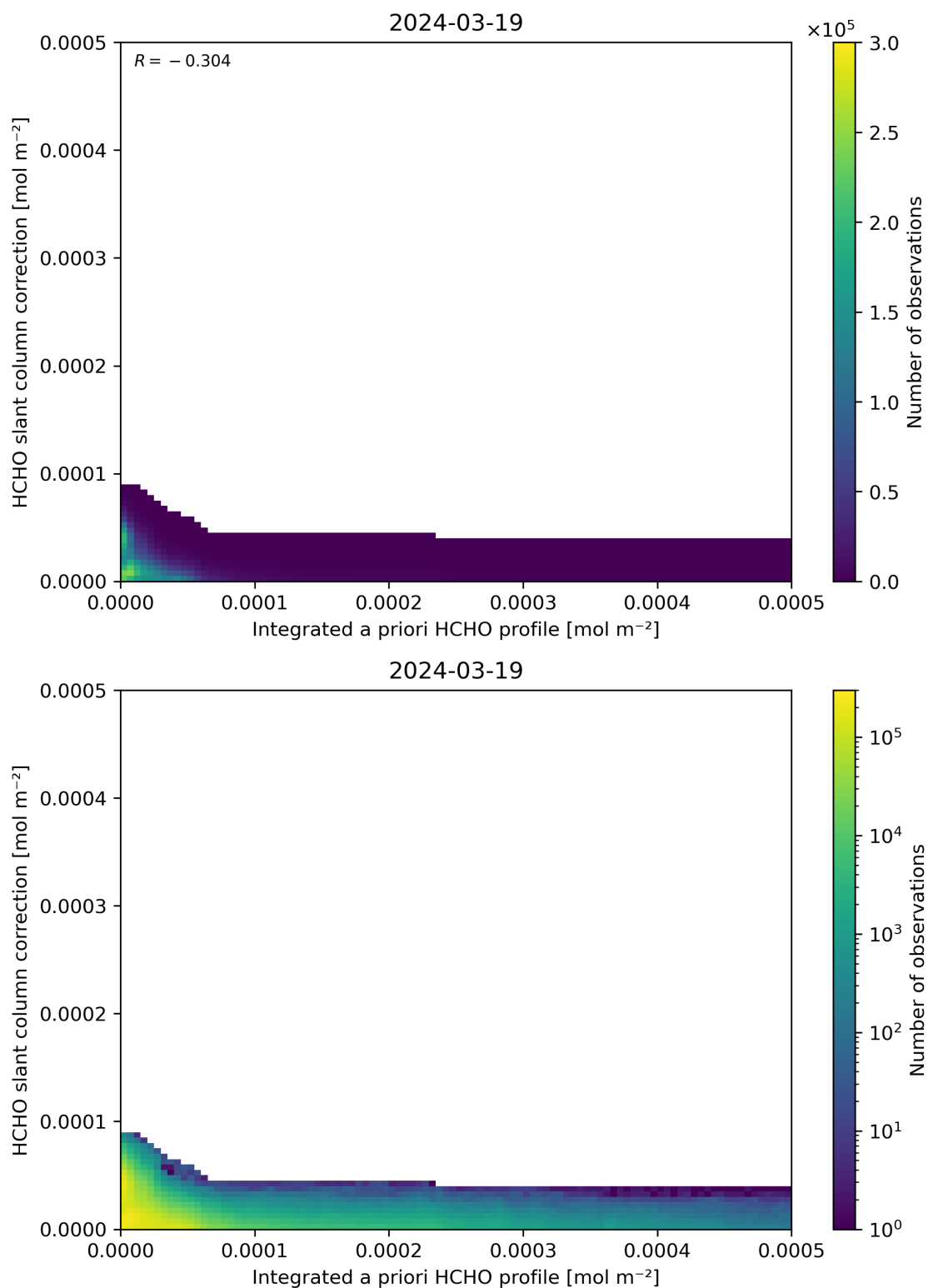
Figure 152: Scatter density plot of “Integrated a priori HCHO profile” against “HCHO slant column correction” for 2024-03-18 to 2024-03-20.
