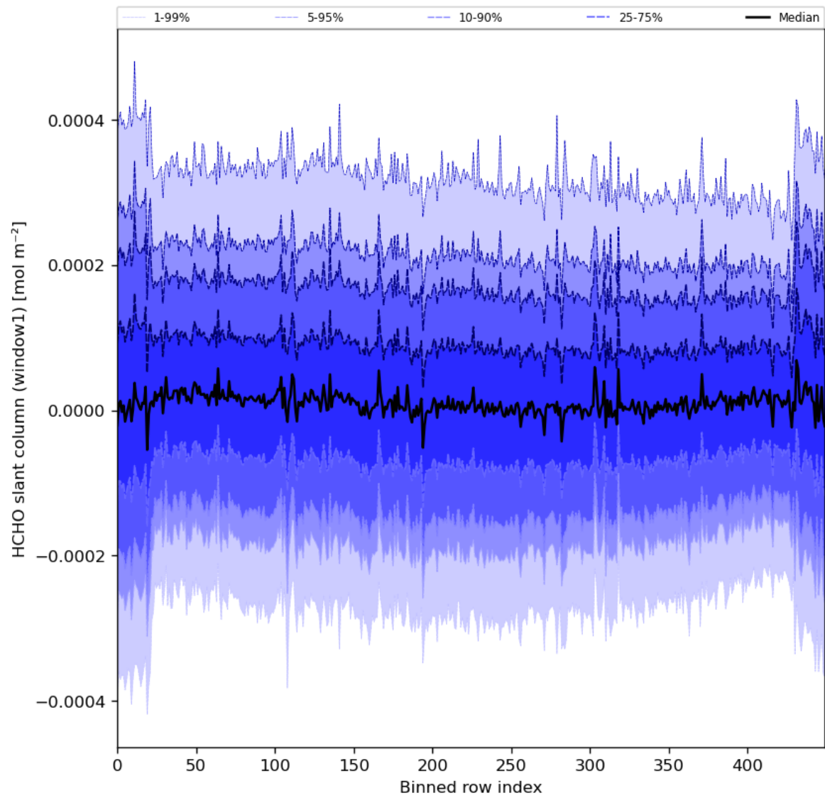
Figure 52: Along track statistics of “HCHO slant column (window1)” for 2024-03-18 to 2024-03-20
