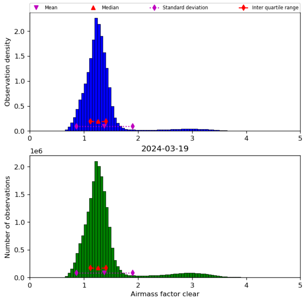
Figure 42: Histogram of “Airmass factor clear” for 2024-03-18 to 2024-03-20
