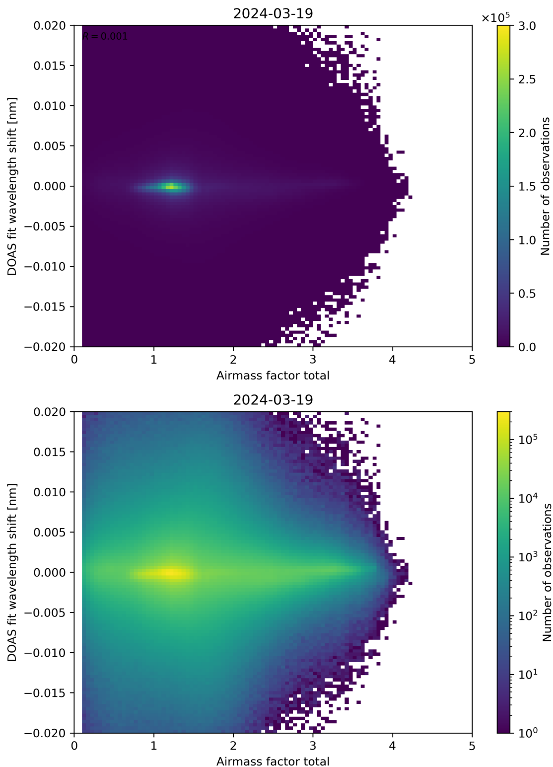
Figure 98: Scatter density plot of “Airmass factor total” against “DOAS fit wavelength shift” for 2024-03-18 to 2024-03-20.
