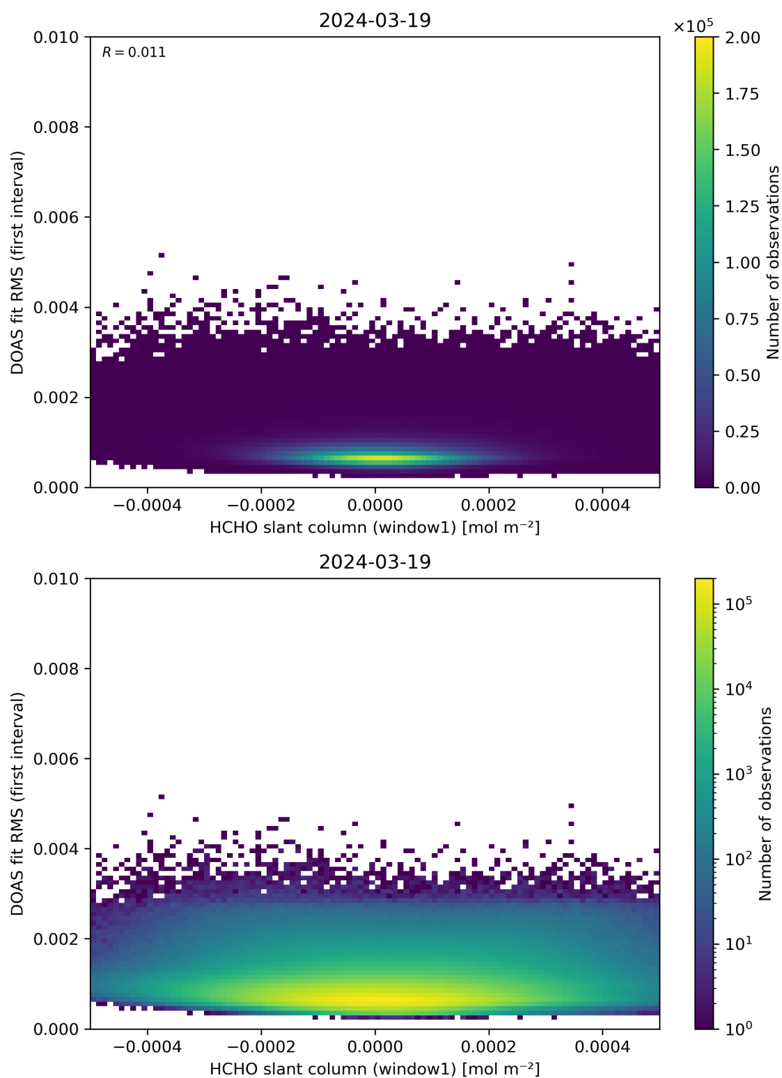
Figure 78: Scatter density plot of “HCHO slant column (window1)” against “DOAS fit RMS (first interval)” for 2024-03-18 to 2024-03-20.
