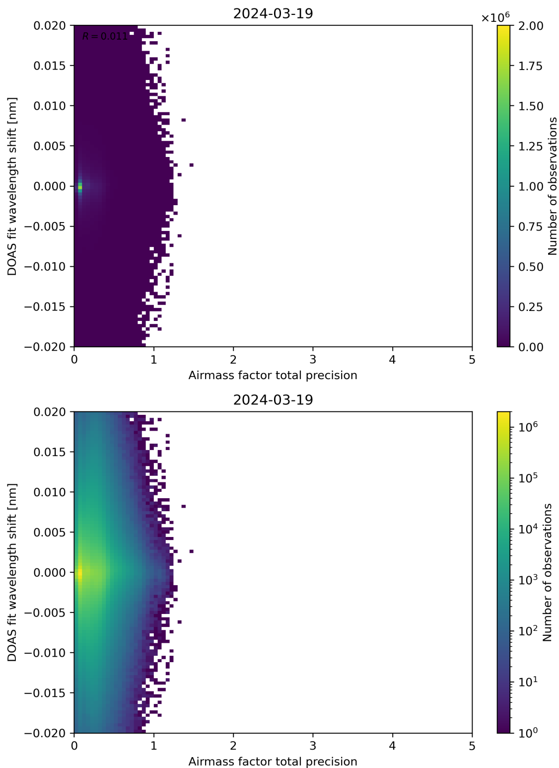
Figure 106: Scatter density plot of “Airmass factor total precision” against “DOAS fit wavelength shift” for 2024-03-18 to 2024-03-20.
