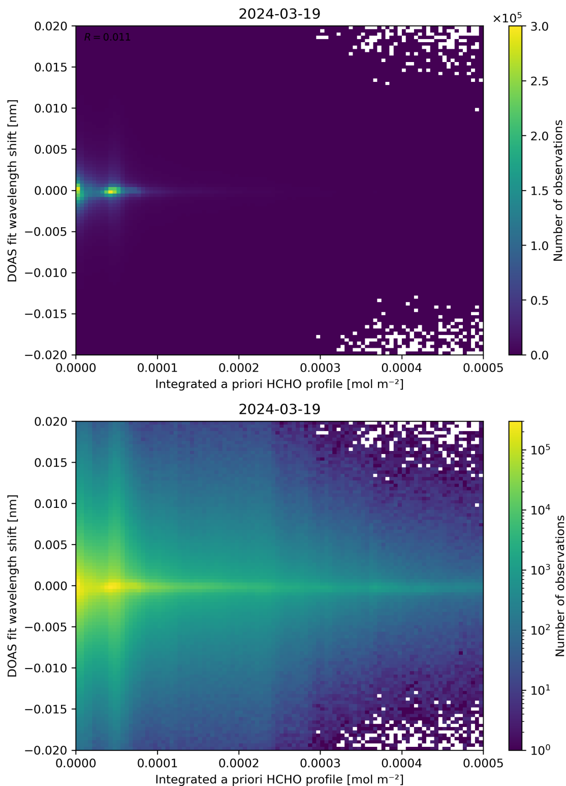
Figure 149: Scatter density plot of “Integrated a priori HCHO profile” against “DOAS fit wavelength shift” for 2024-03-18 to 2024-03-20.
