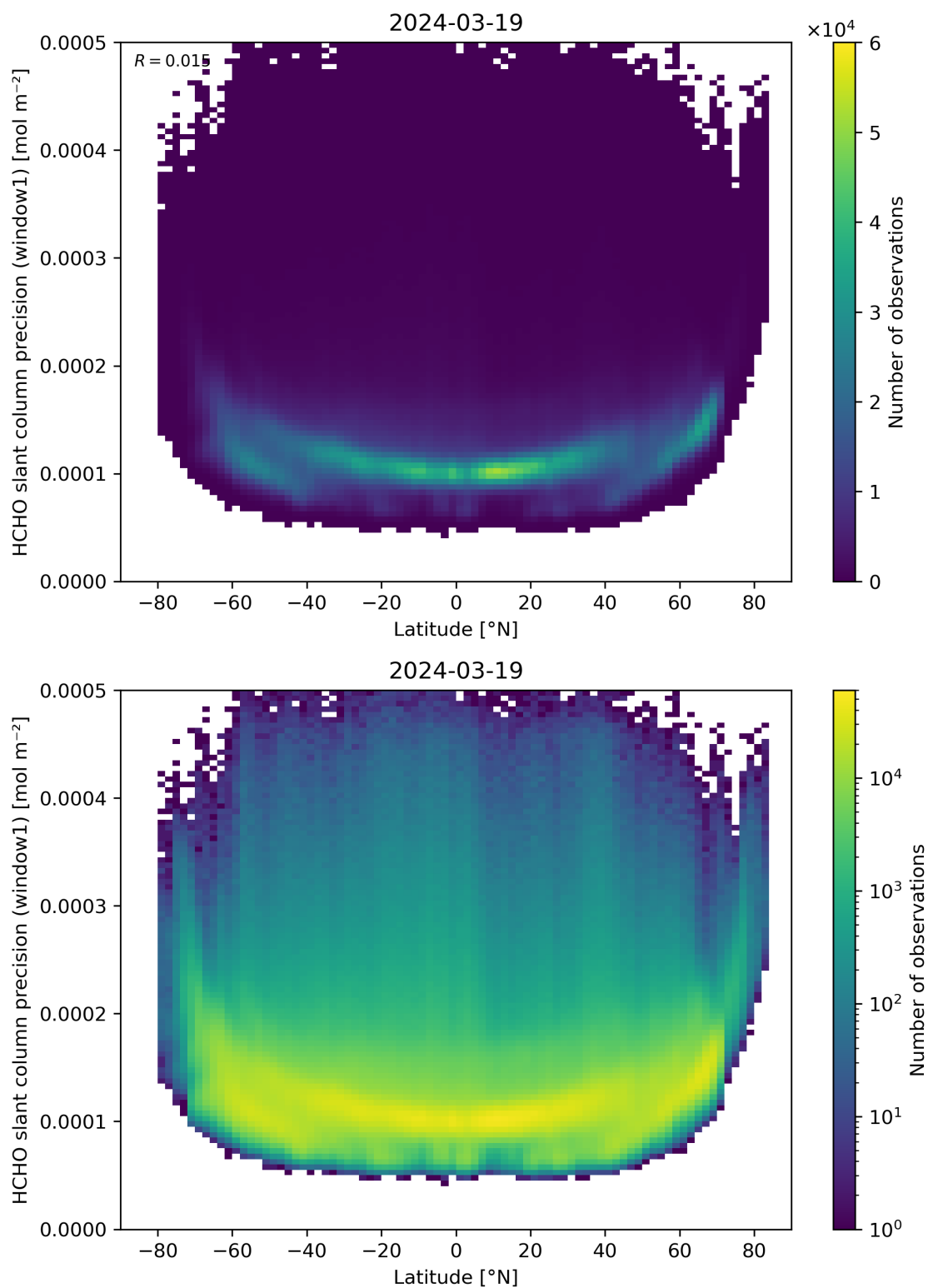
Figure 160: Scatter density plot of “Latitude” against “HCHO slant column precision (window1)” for 2024-03-18 to 2024-03-20.
