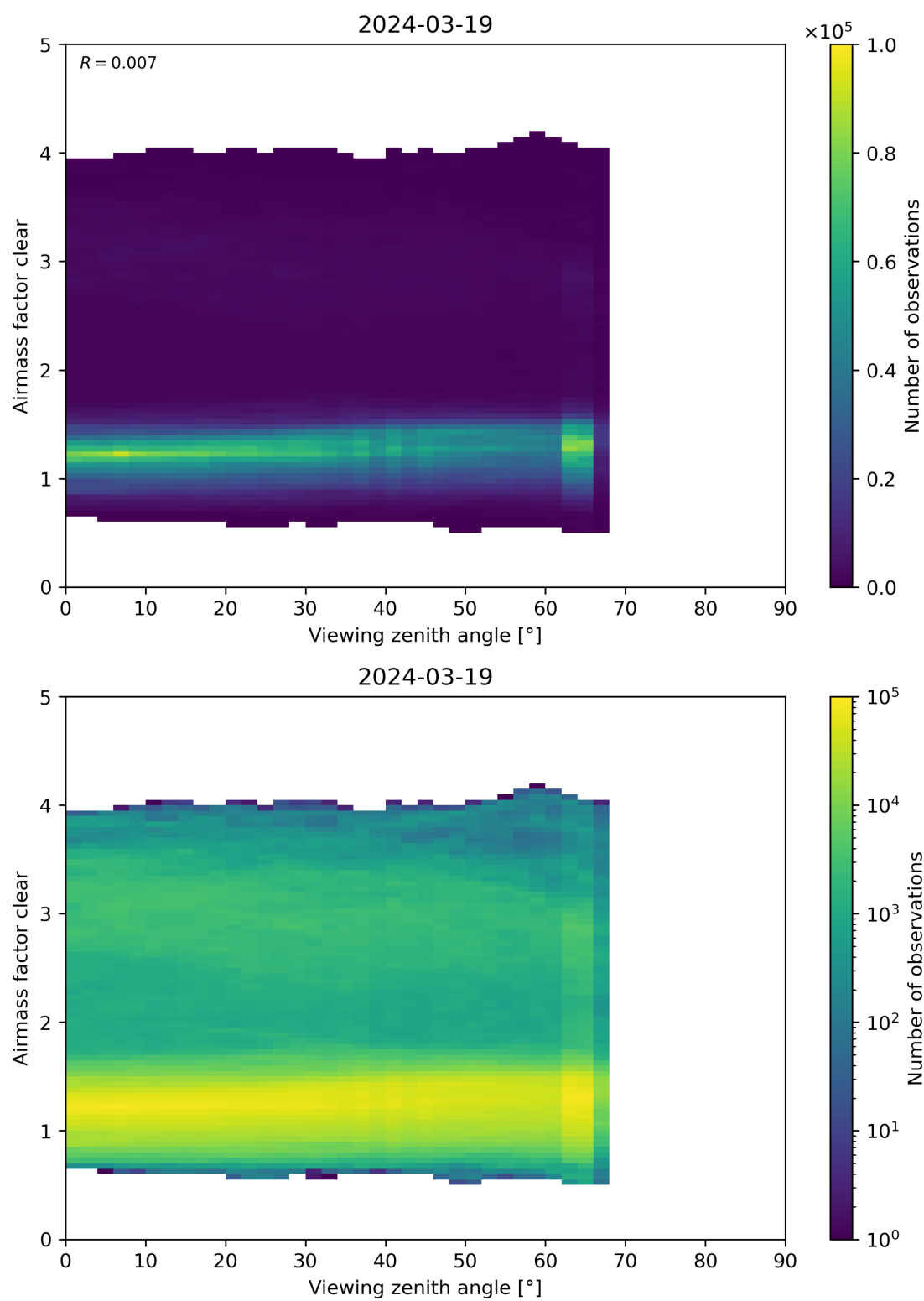
Figure 185: Scatter density plot of “Viewing zenith angle” against “Airmass factor clear” for 2024-03-18 to 2024-03-20.
