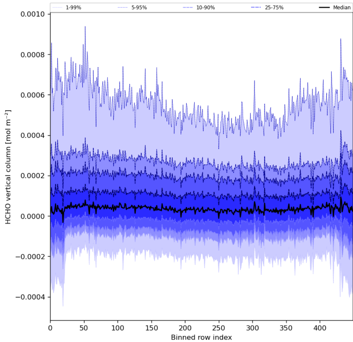
Figure 49: Along track statistics of “HCHO vertical column” for 2024-03-18 to 2024-03-20
