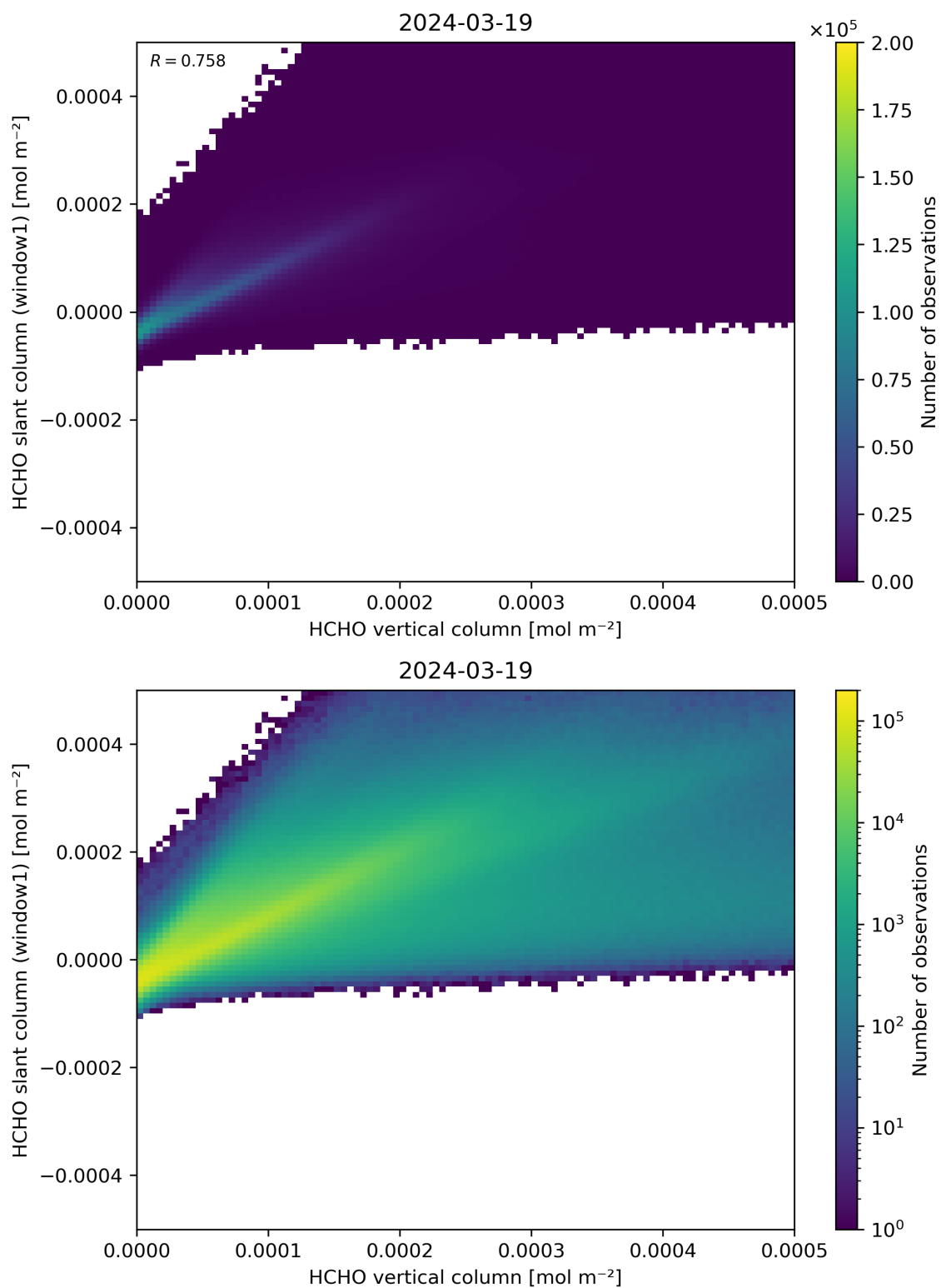
Figure 129: Scatter density plot of “HCHO vertical column” against “HCHO slant column (window1)” for 2024-03-18 to 2024-03-20.
