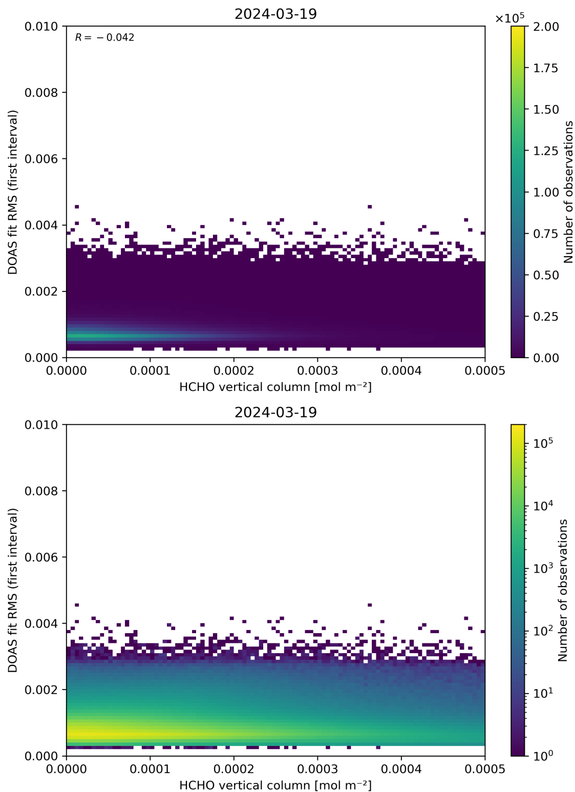
Figure 123: Scatter density plot of “HCHO vertical column” against “DOAS fit RMS (first interval)” for 2024-03-18 to 2024-03-20.
