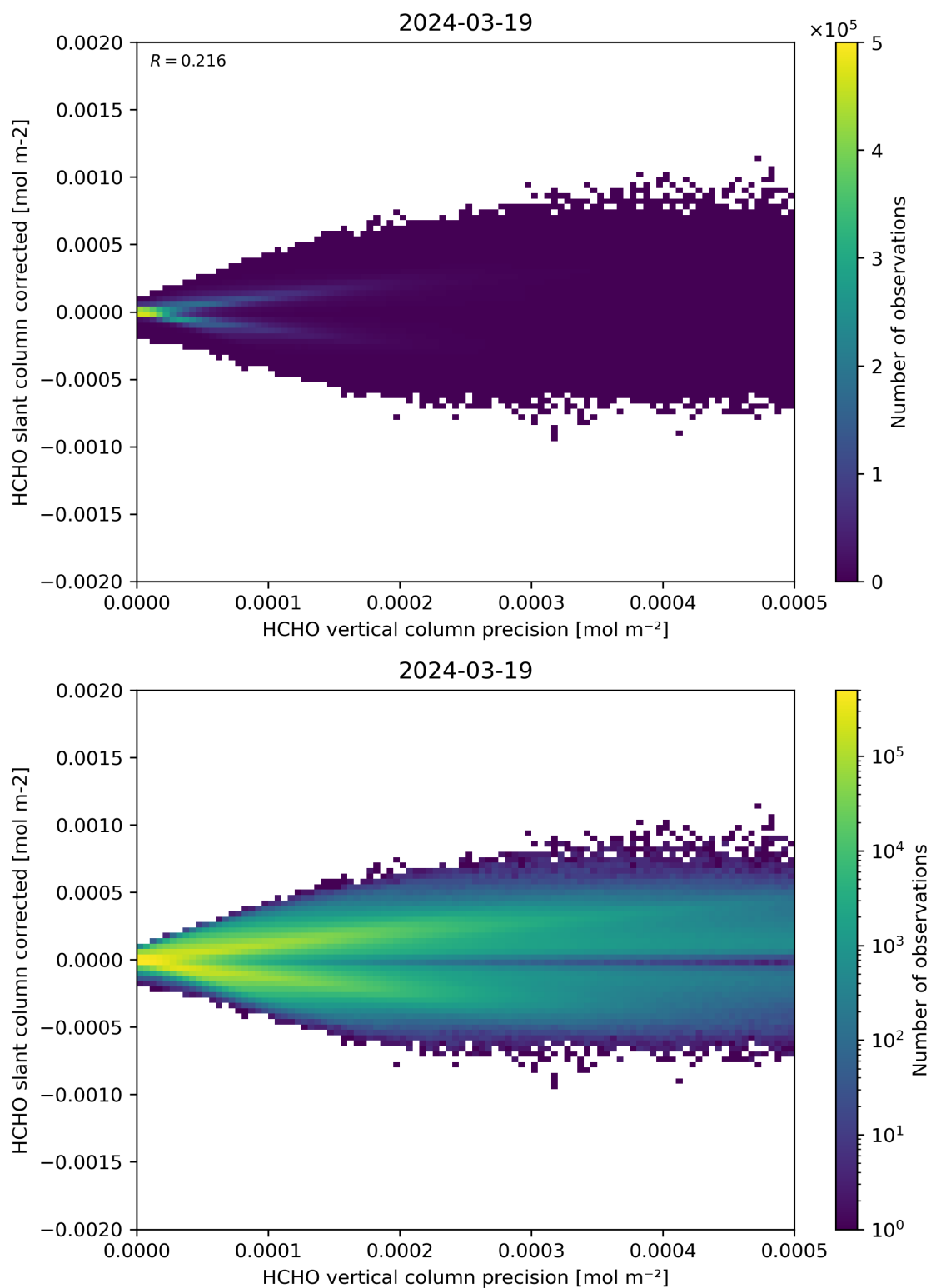
Figure 140: Scatter density plot of “HCHO vertical column precision” against “HCHO slant column corrected” for 2024-03-18 to 2024-03-20.
