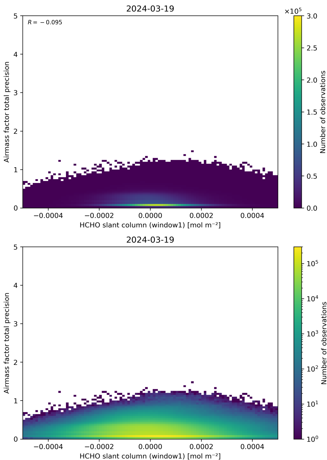
Figure 86: Scatter density plot of “HCHO slant column (window1)” against “Airmass factor total precision” for 2024-03-18 to 2024-03-20.
