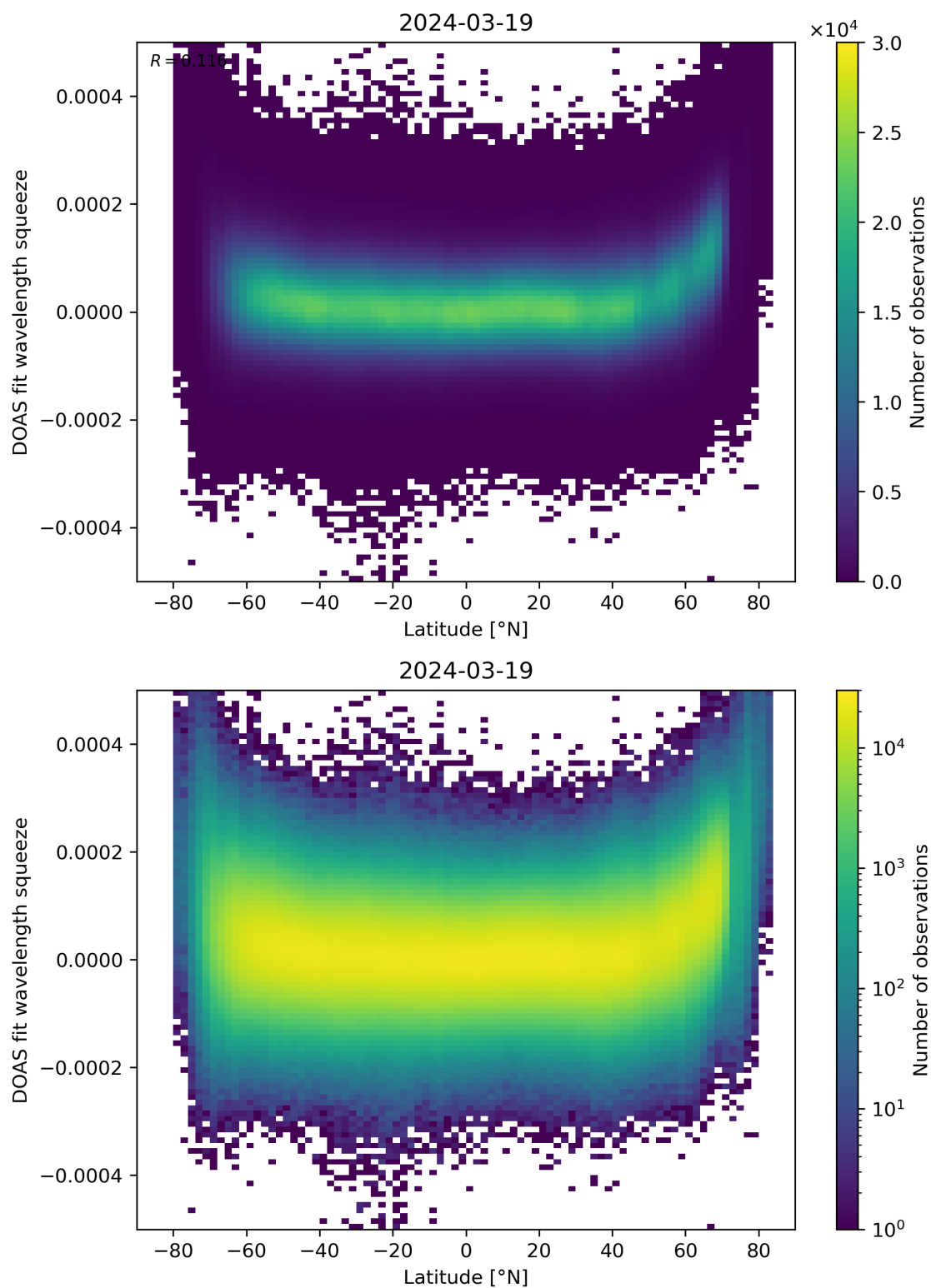
Figure 155: Scatter density plot of “Latitude” against “DOAS fit wavelength squeeze” for 2024-03-18 to 2024-03-20.
