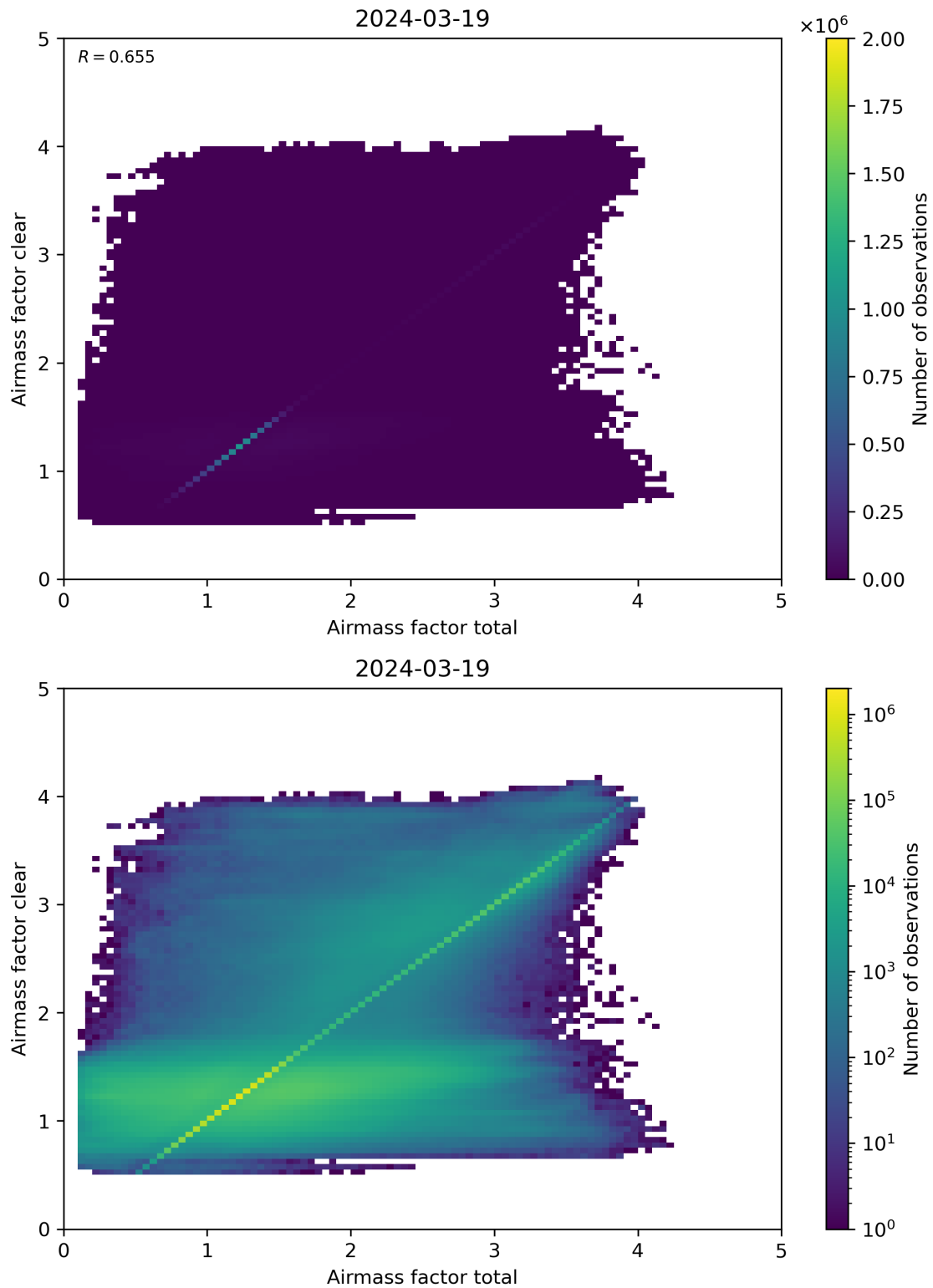
Figure 100: Scatter density plot of “Airmass factor total” against “Airmass factor clear” for 2024-03-18 to 2024-03-20.
