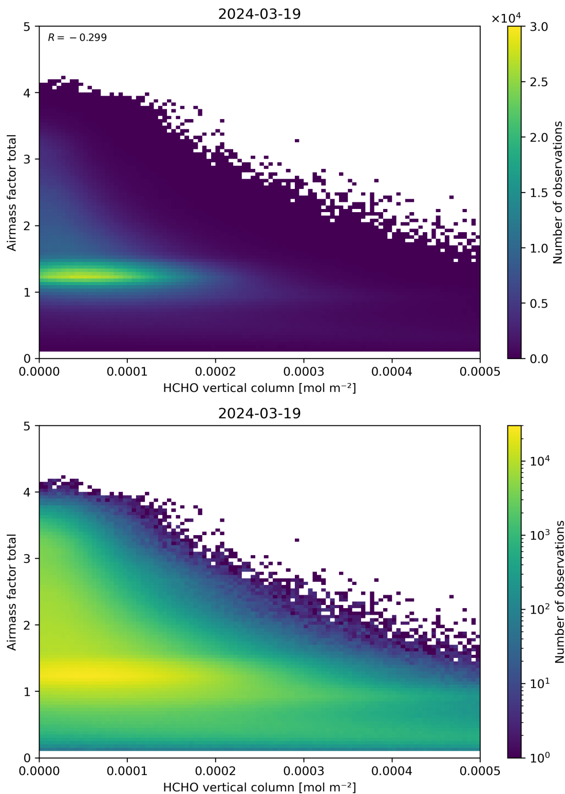
Figure 131: Scatter density plot of “HCHO vertical column” against “Airmass factor total” for 2024-03-18 to 2024-03-20.
