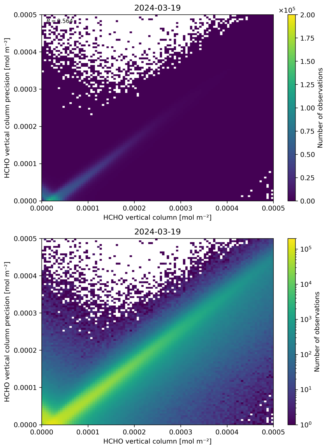
Figure 134: Scatter density plot of “HCHO vertical column” against “HCHO vertical column precision” for 2024-03-18 to 2024-03-20.
