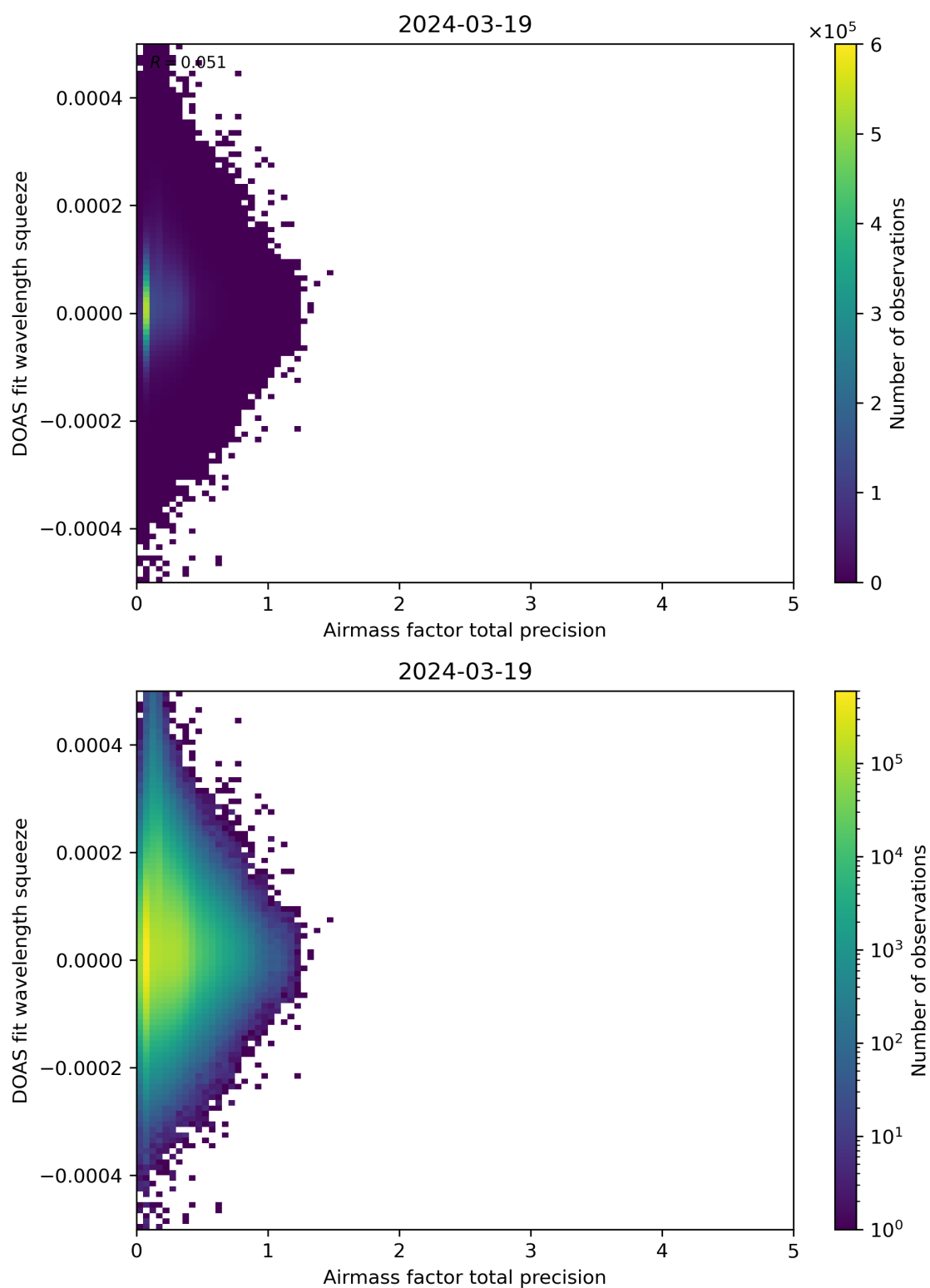
Figure 107: Scatter density plot of “Airmass factor total precision” against “DOAS fit wavelength squeeze” for 2024-03-18 to 2024-03-20.
