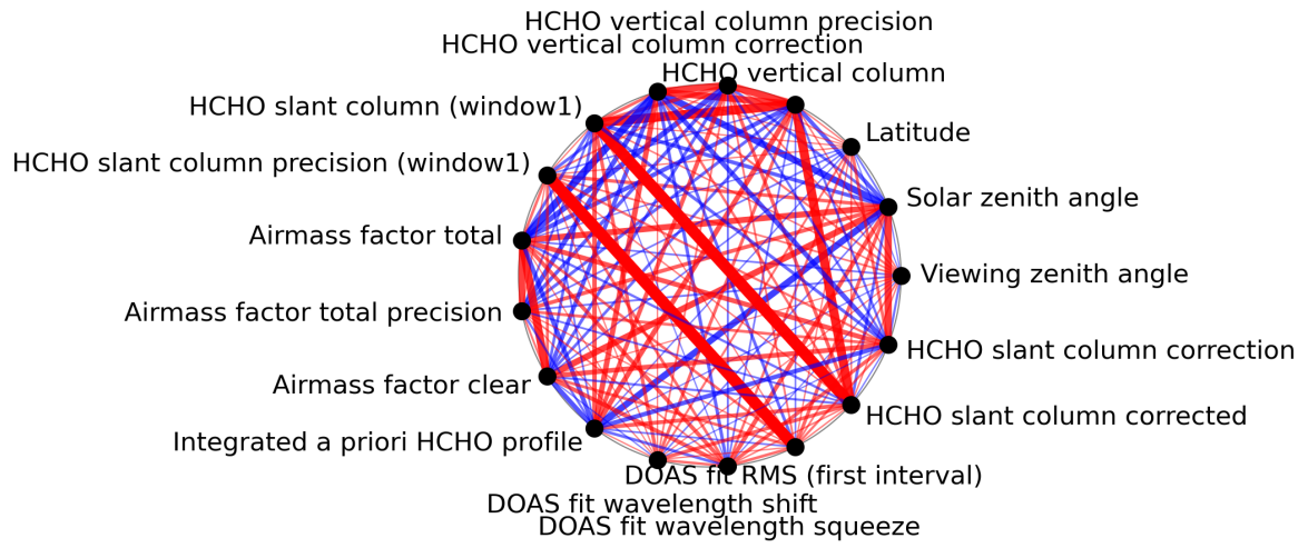
Figure 1: Map of correlation graph for 2024-03-18 to 2024-03-20.
