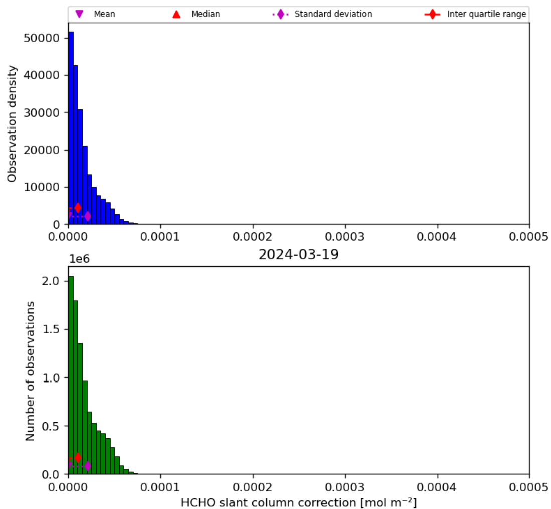
Figure 47: Histogram of “HCHO slant column correction” for 2024-03-18 to 2024-03-20
