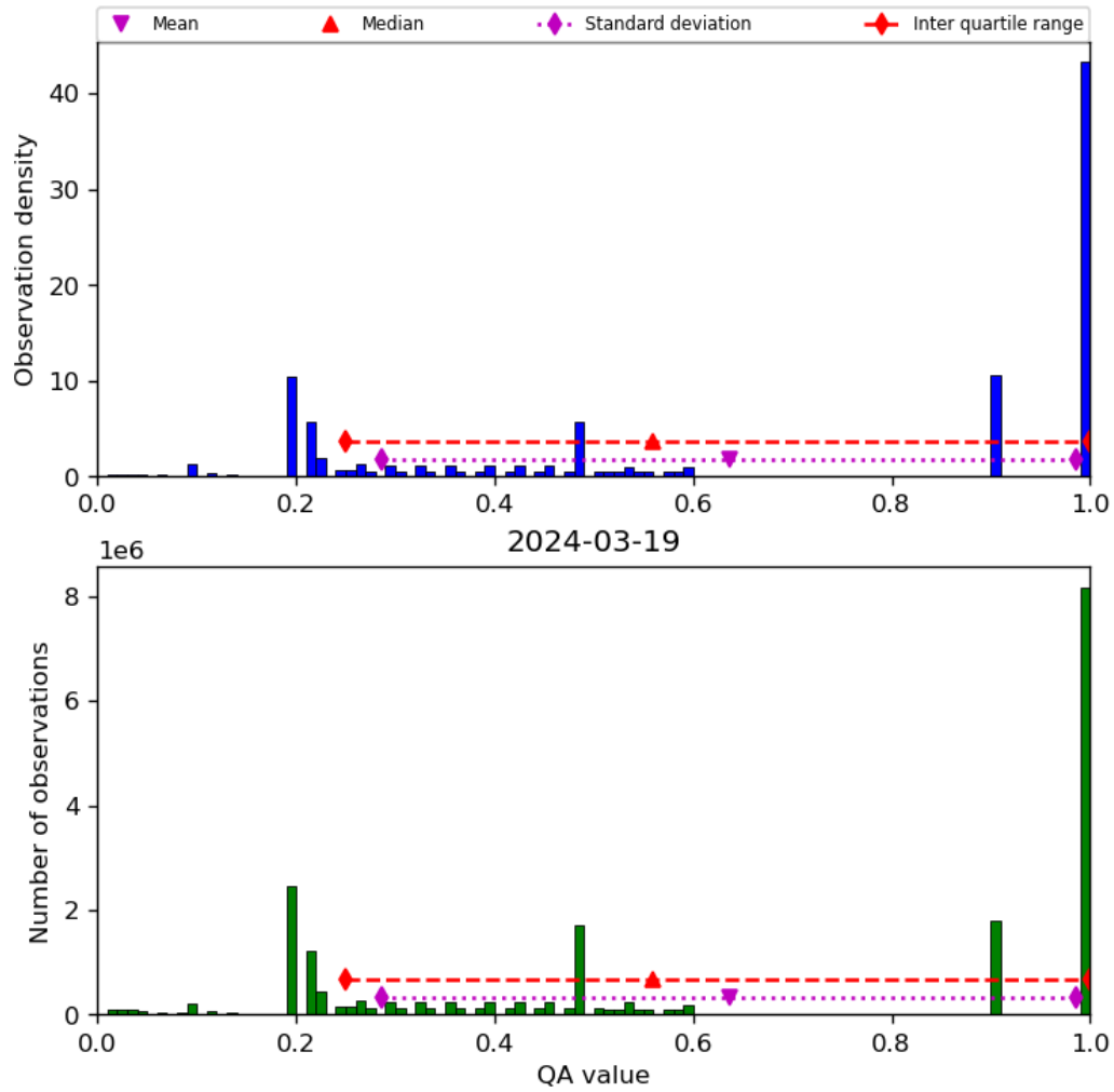
Figure 34: Histogram of “QA value” for 2024-03-18 to 2024-03-20
