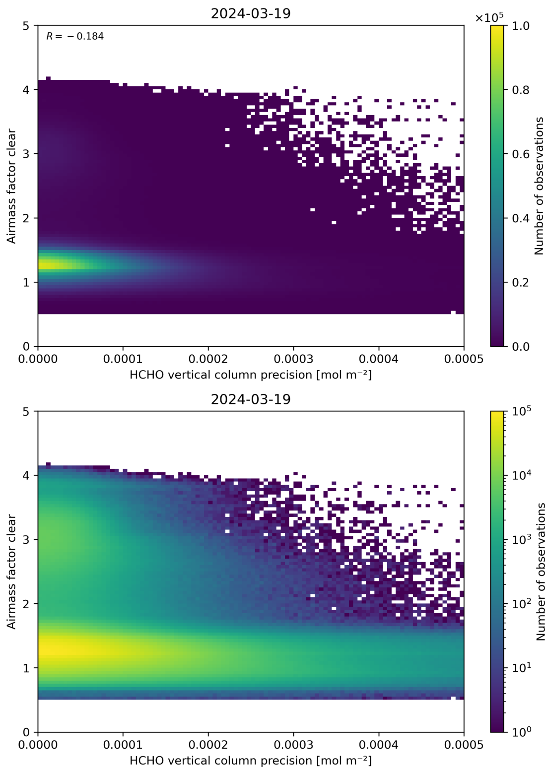
Figure 139: Scatter density plot of “HCHO vertical column precision” against “Airmass factor clear” for 2024-03-18 to 2024-03-20.
