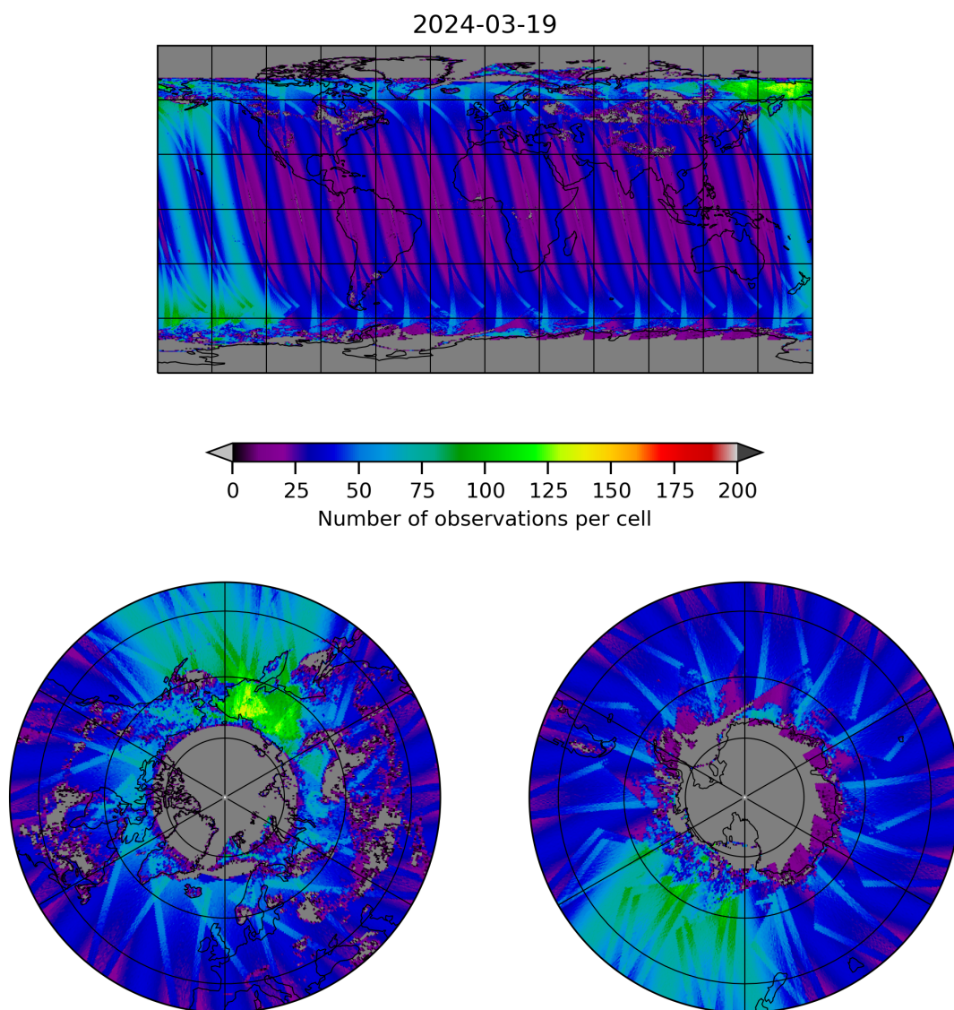
Figure 19: Map of the number of observations for 2024-03-18 to 2024-03-20
