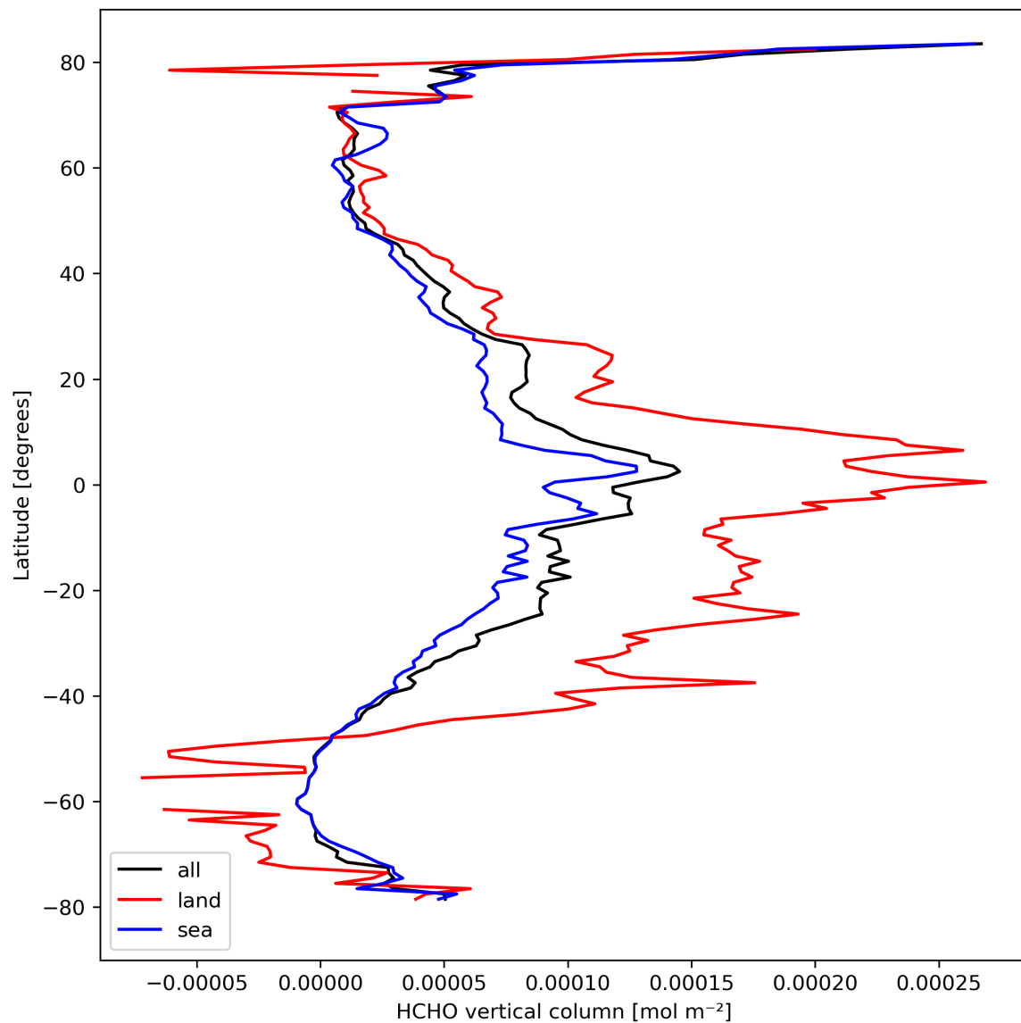
Figure 21: Zonal average of “HCHO vertical column” for 2024-03-18 to 2024-03-20.
