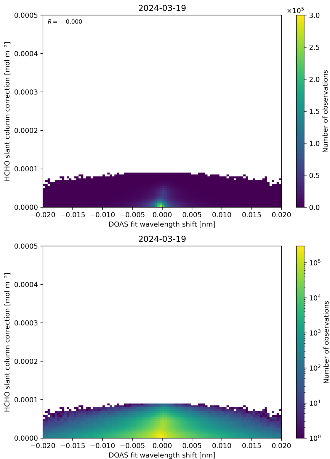
Figure 67: Scatter density plot of “DOAS fit wavelength shift” against “HCHO slant column correction” for 2024-03-18 to 2024-03-20.
