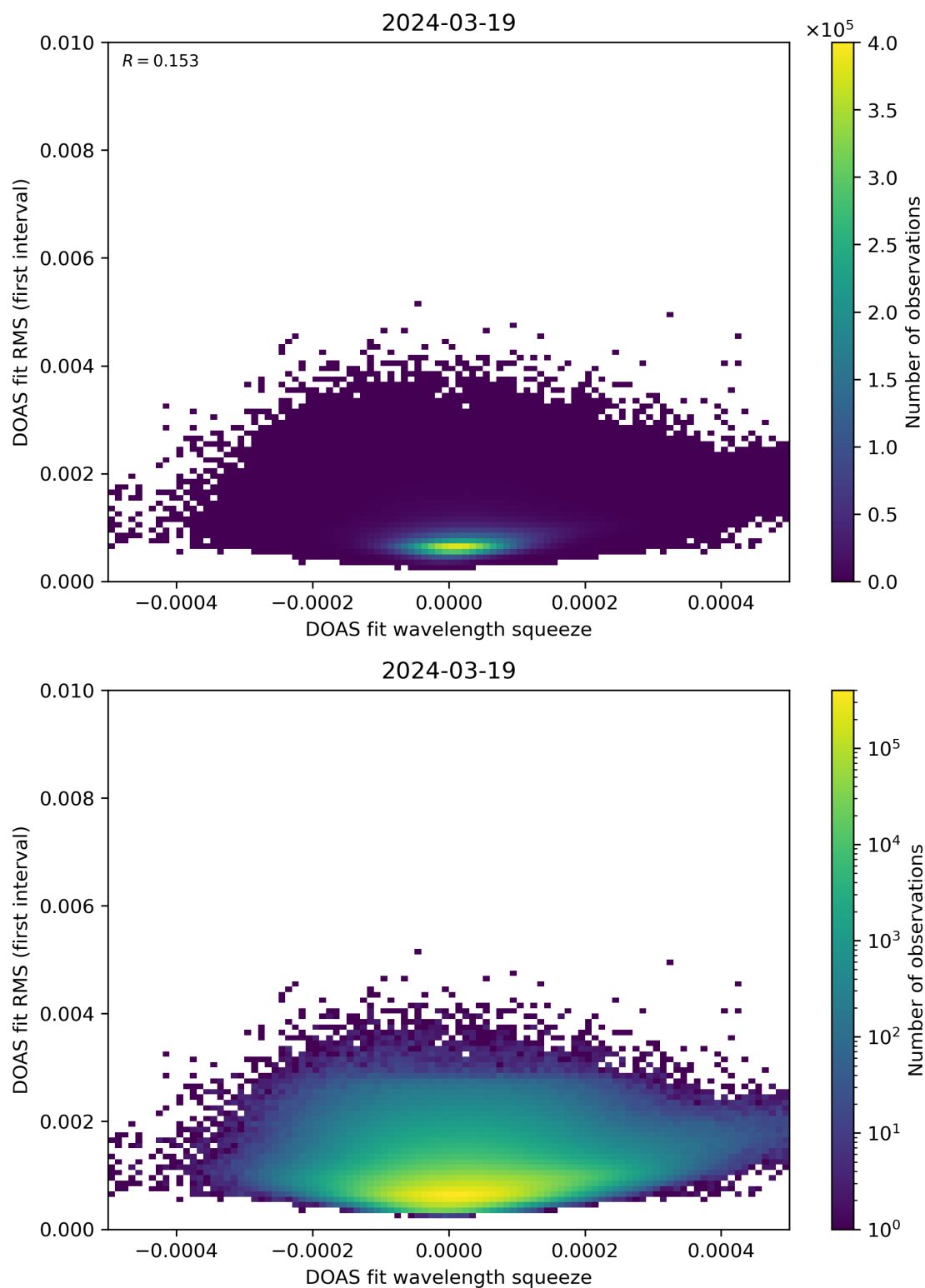
Figure 68: Scatter density plot of “DOAS fit wavelength squeeze” against “DOAS fit RMS (first interval)” for 2024-03-18 to 2024-03-20.
