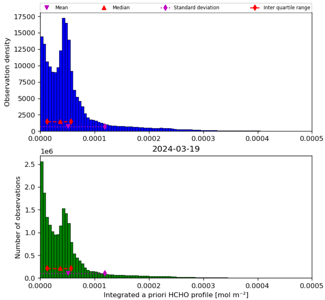
Figure 43: Histogram of “Integrated a priori HCHO profile” for 2024-03-18 to 2024-03-20
