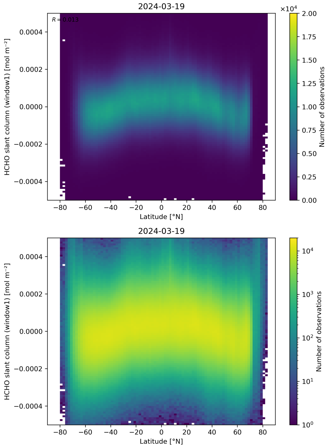
Figure 159: Scatter density plot of “Latitude” against “HCHO slant column (window1)” for 2024-03-18 to 2024-03-20.
