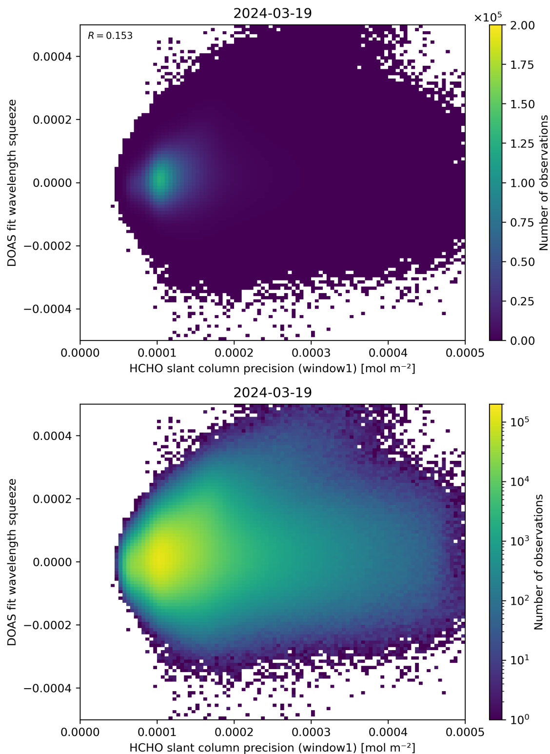
Figure 90: Scatter density plot of “HCHO slant column precision (window1)” against “DOAS fit wavelength squeeze” for 2024-03-18 to 2024-03-20.
