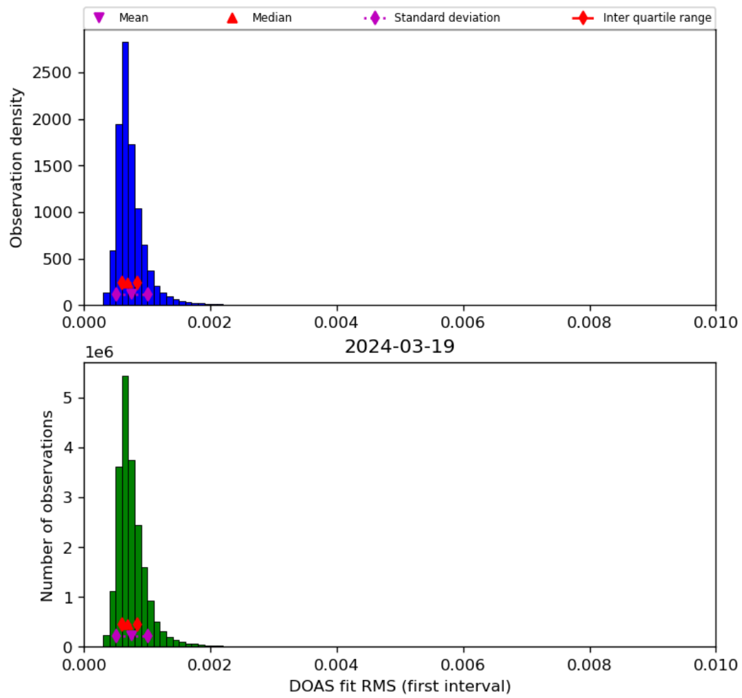
Figure 46: Histogram of “DOAS fit RMS (first interval)” for 2024-03-18 to 2024-03-20
