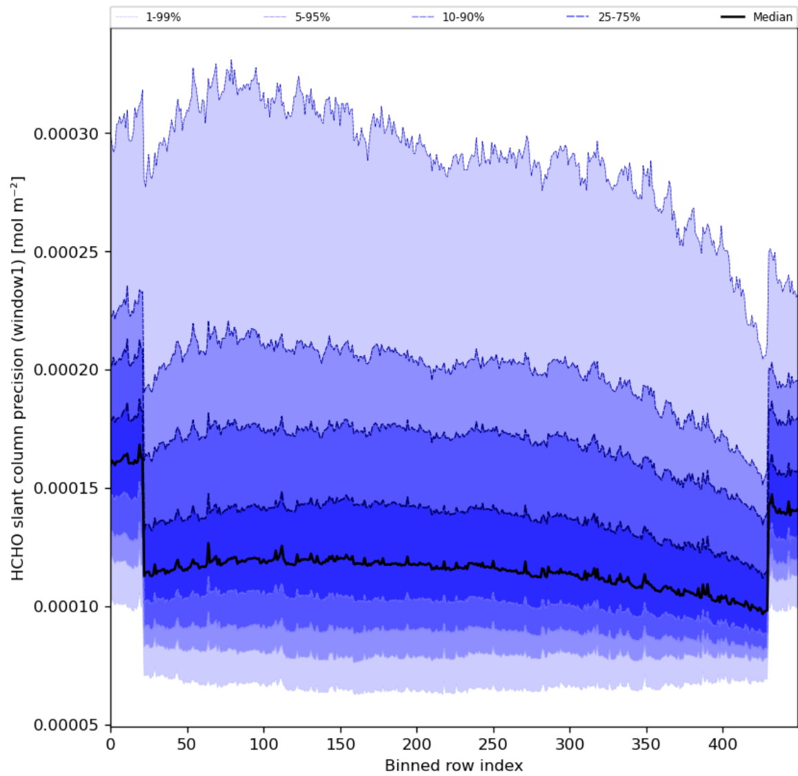
Figure 53: Along track statistics of “HCHO slant column precision (window1)” for 2024-03-18 to 2024-03-20
