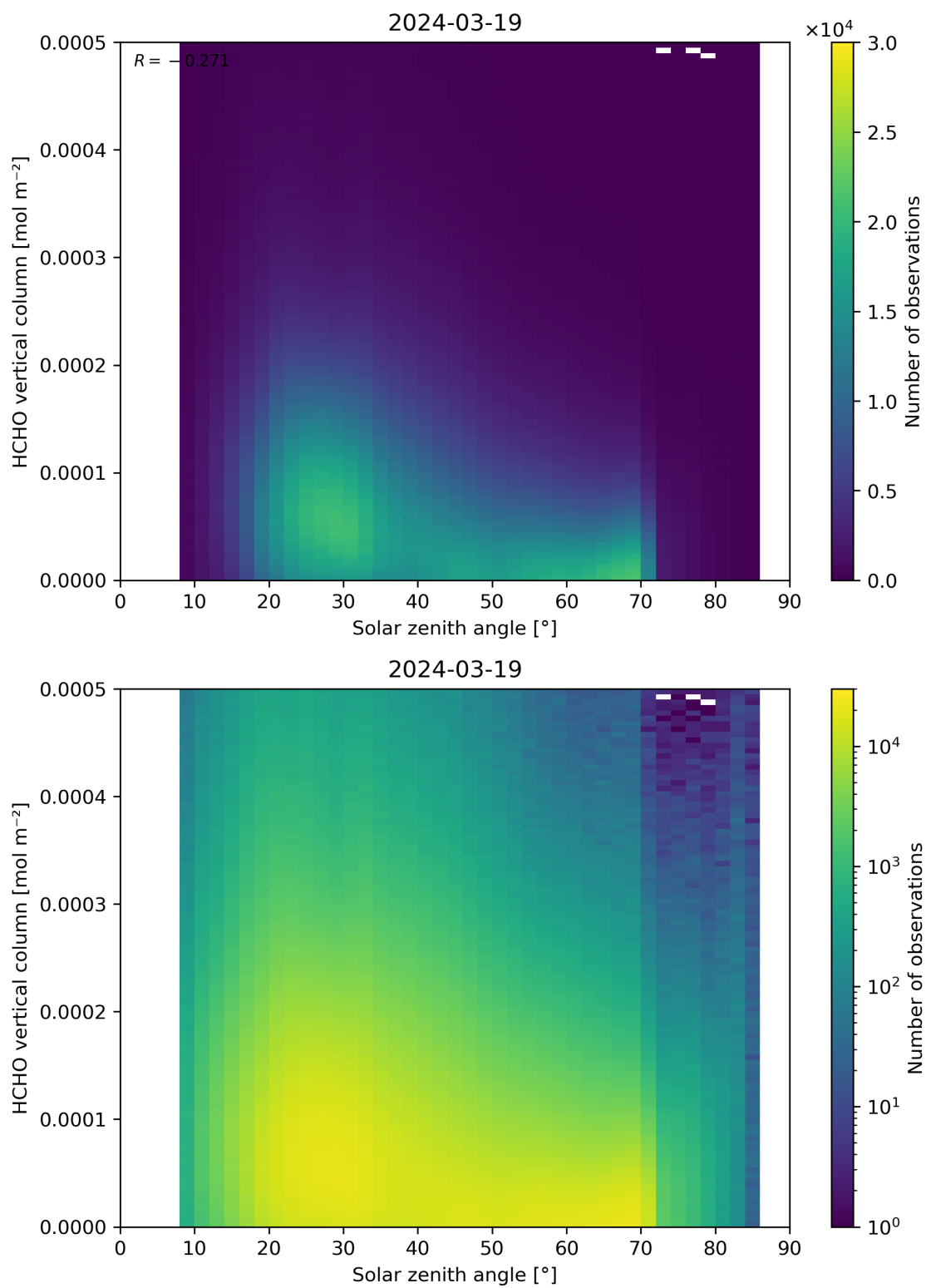
Figure 177: Scatter density plot of “Solar zenith angle” against “HCHO vertical column” for 2024-03-18 to 2024-03-20.
