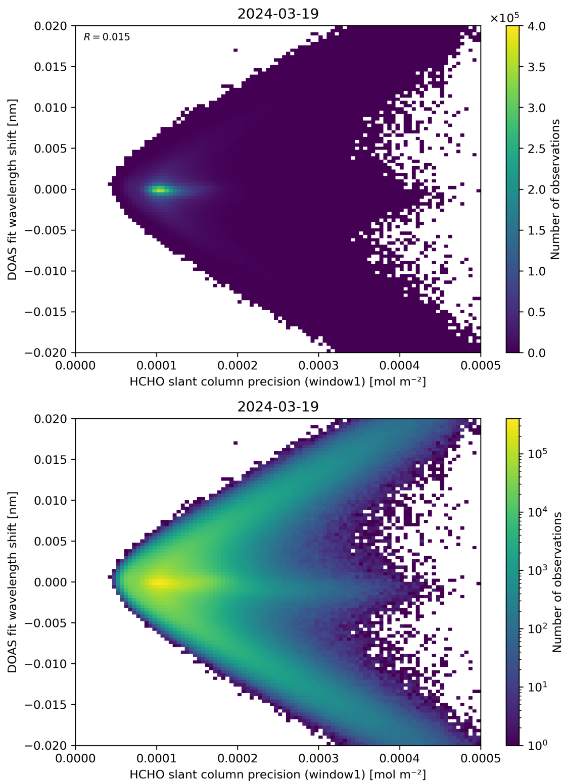
Figure 89: Scatter density plot of “HCHO slant column precision (window1)” against “DOAS fit wavelength shift” for 2024-03-18 to 2024-03-20.
