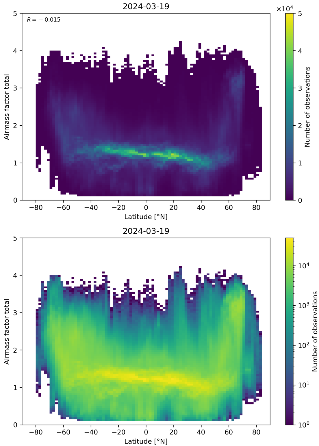
Figure 161: Scatter density plot of “Latitude” against “Airmass factor total” for 2024-03-18 to 2024-03-20.
