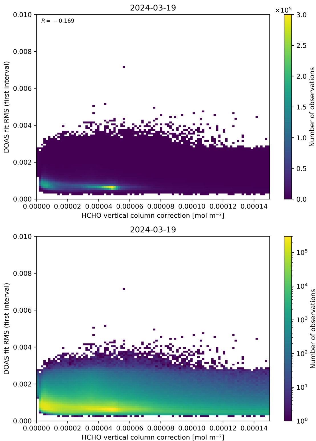
Figure 112: Scatter density plot of “HCHO vertical column correction” against “DOAS fit RMS (first interval)” for 2024-03-18 to 2024-03-20.
