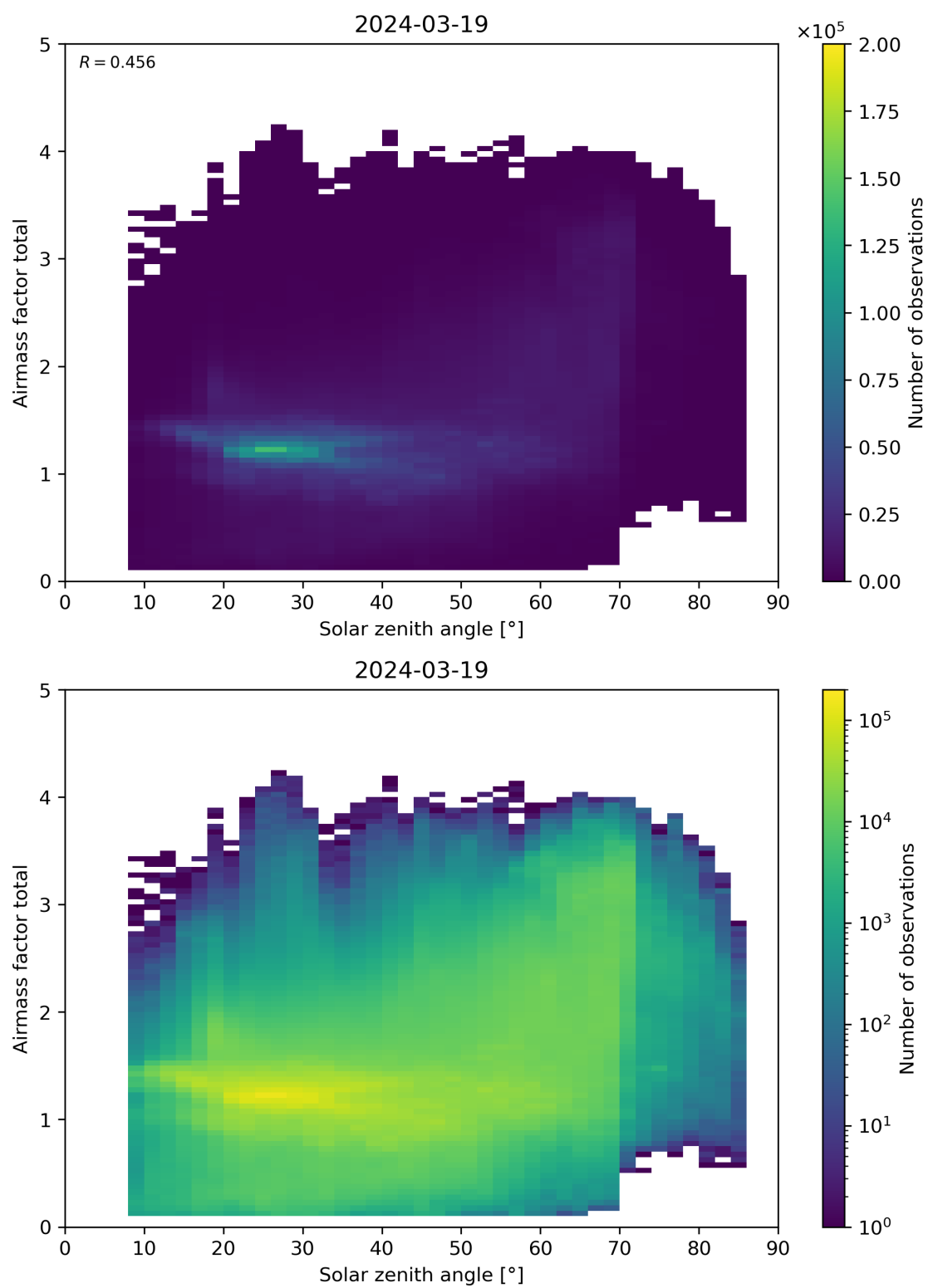
Figure 175: Scatter density plot of “Solar zenith angle” against “Airmass factor total” for 2024-03-18 to 2024-03-20.
