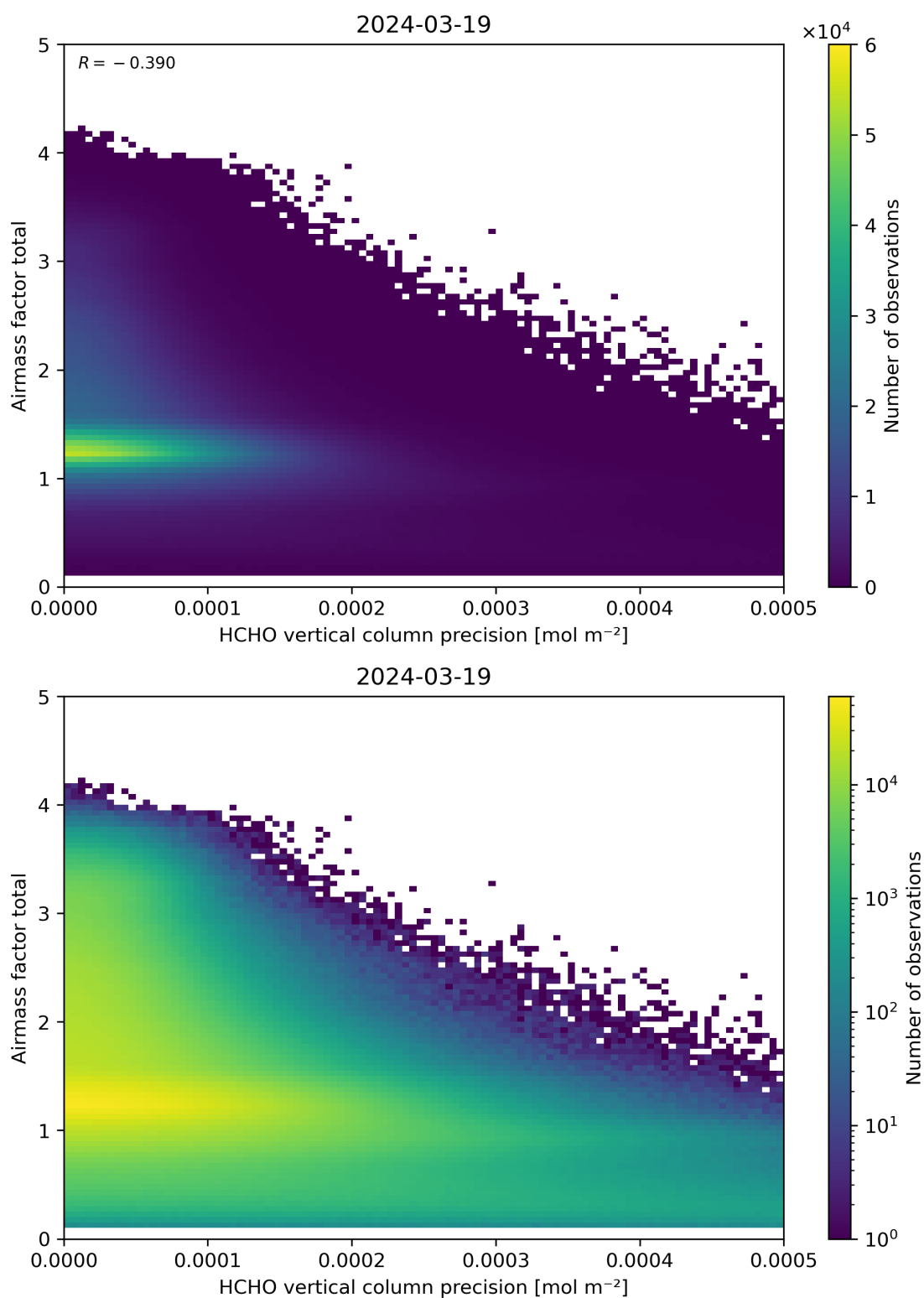
Figure 144: Scatter density plot of “HCHO vertical column precision” against “Airmass factor total” for 2024-03-18 to 2024-03-20.
