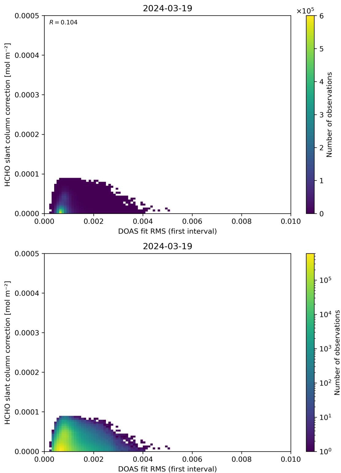
Figure 63: Scatter density plot of “DOAS fit RMS (first interval)” against “HCHO slant column correction” for 2024-03-18 to 2024-03-20.
