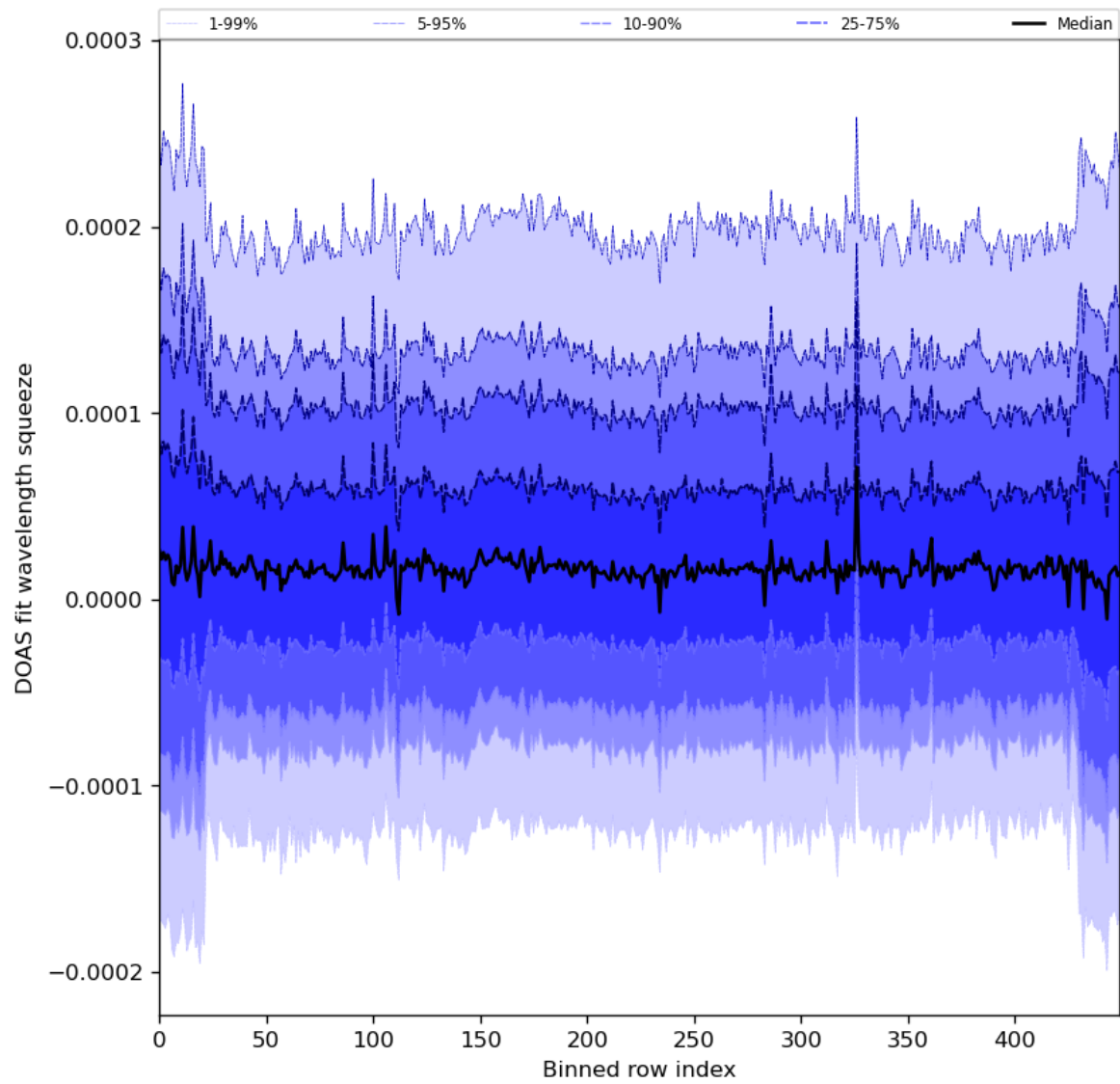
Figure 59: Along track statistics of “DOAS fit wavelength squeeze” for 2024-03-18 to 2024-03-20
