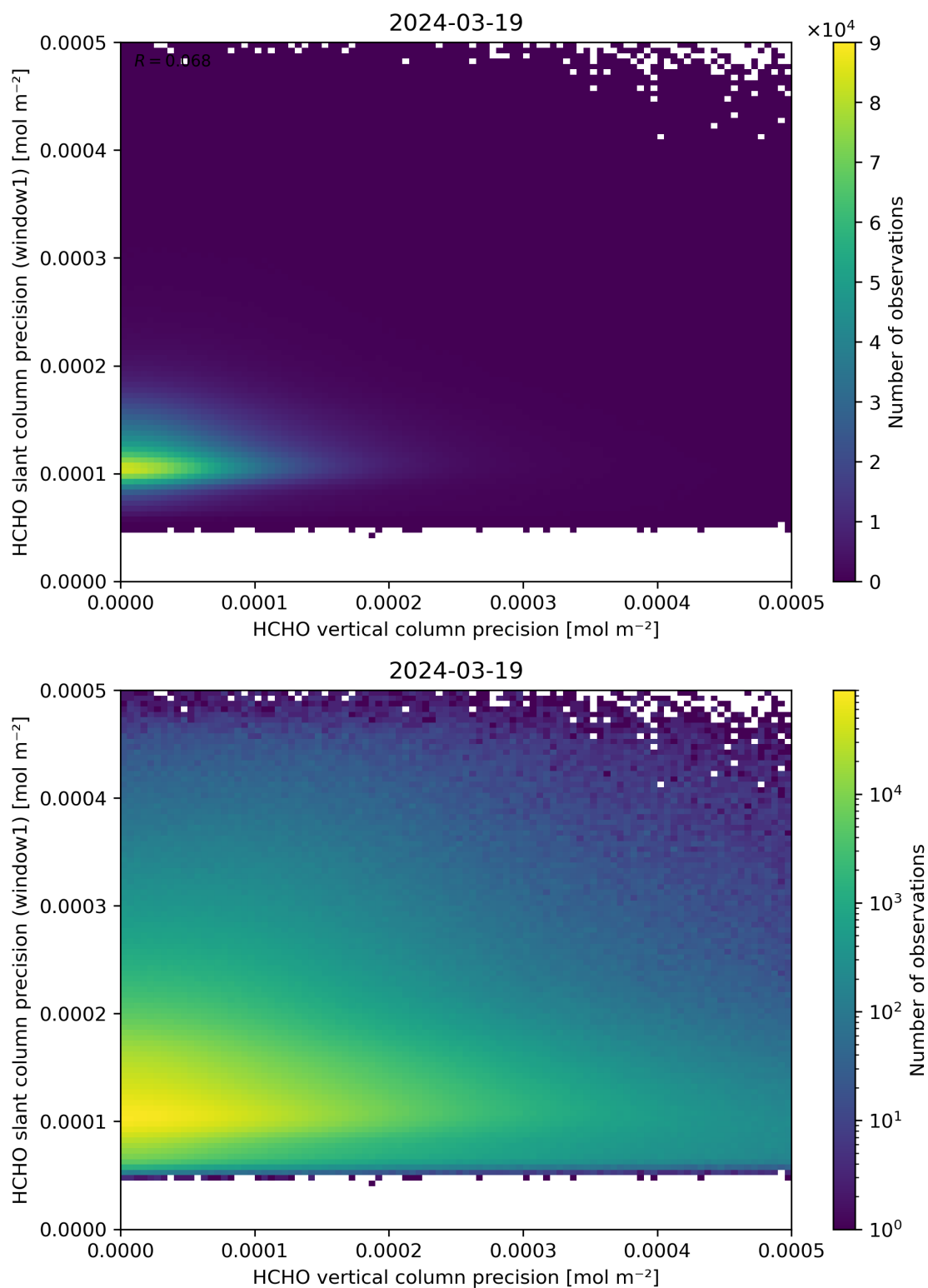
Figure 143: Scatter density plot of “HCHO vertical column precision” against “HCHO slant column precision (window1)” for 2024-03-18 to 2024-03-20.
