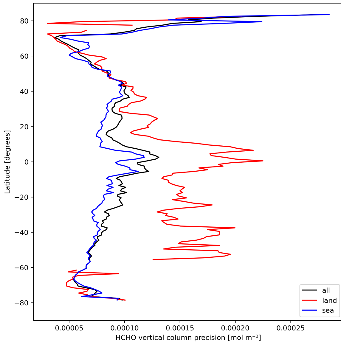
Figure 22: Zonal average of “HCHO vertical column precision” for 2024-03-18 to 2024-03-20.
