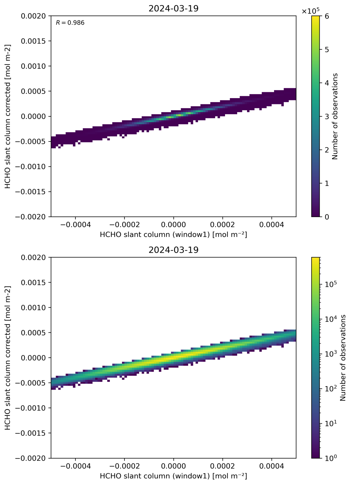
Figure 82: Scatter density plot of “HCHO slant column (window1)” against “HCHO slant column corrected” for 2024-03-18 to 2024-03-20.
