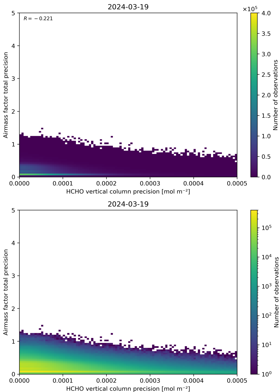
Figure 145: Scatter density plot of “HCHO vertical column precision” against “Airmass factor total precision” for 2024-03-18 to 2024-03-20.
