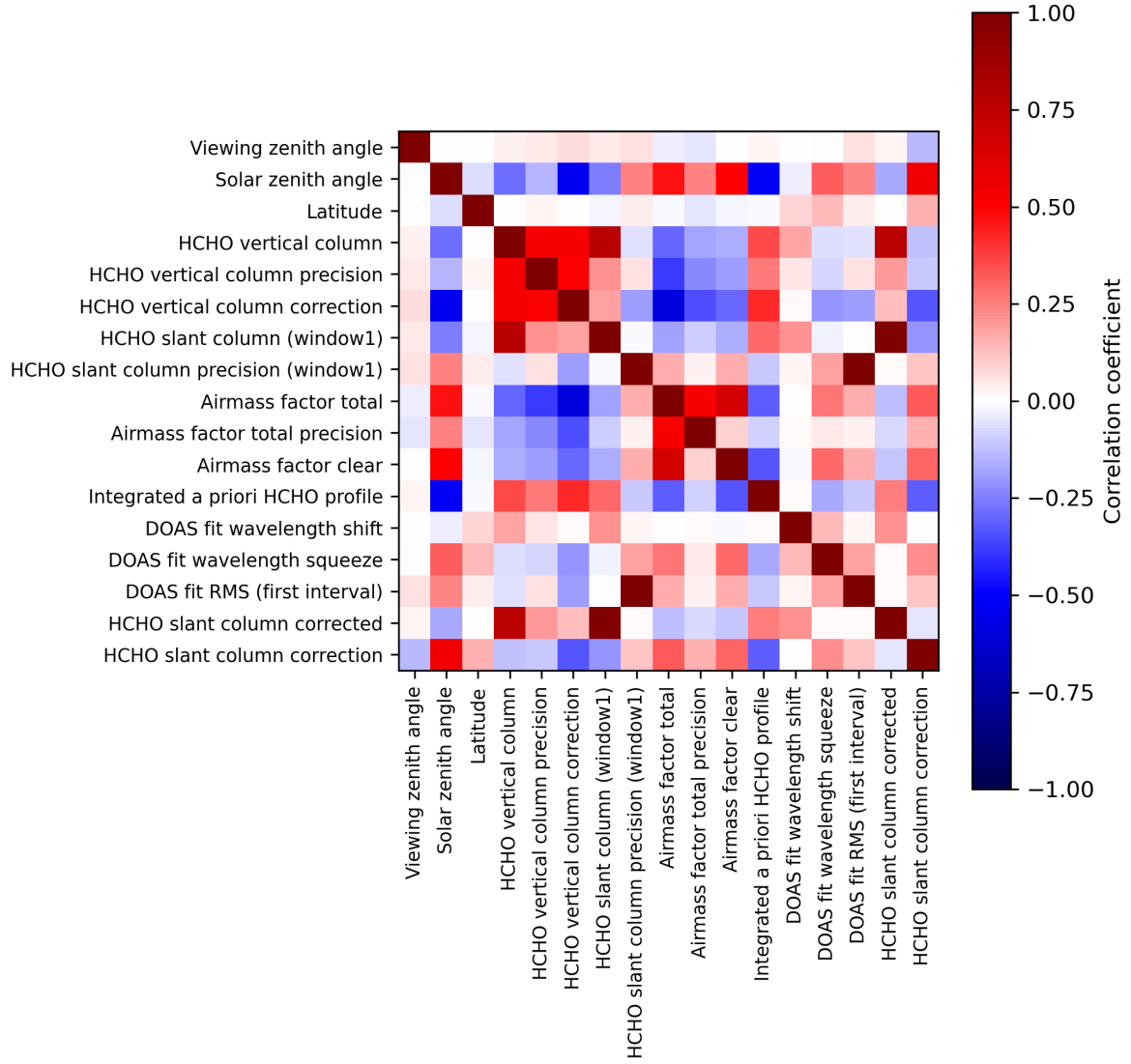
Figure 2: Map of correlation matrix for 2024-03-20 to 2024-03-22.
