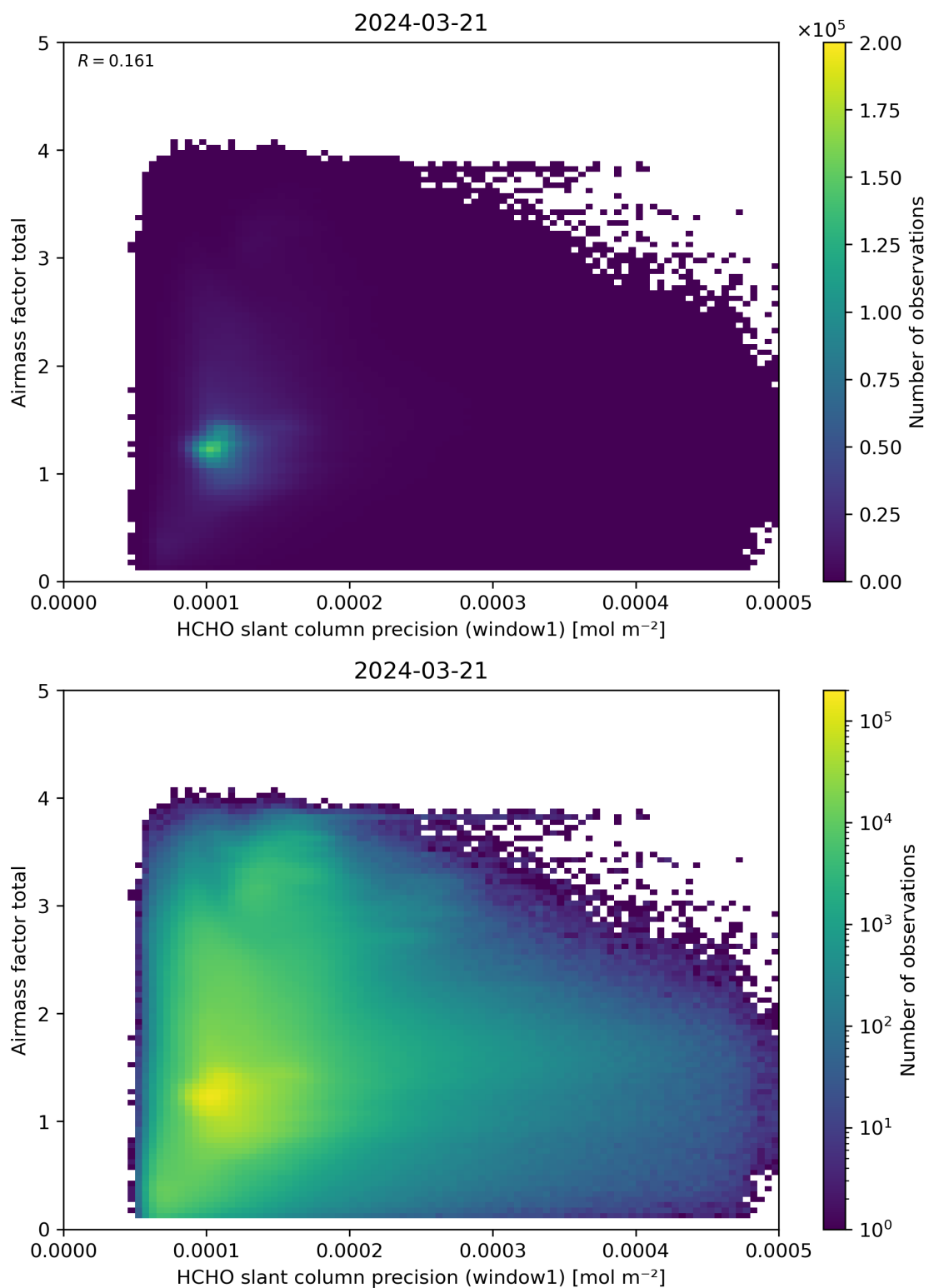
Figure 94: Scatter density plot of “HCHO slant column precision (window1)” against “Airmass factor total” for 2024-03-20 to 2024-03-22.
