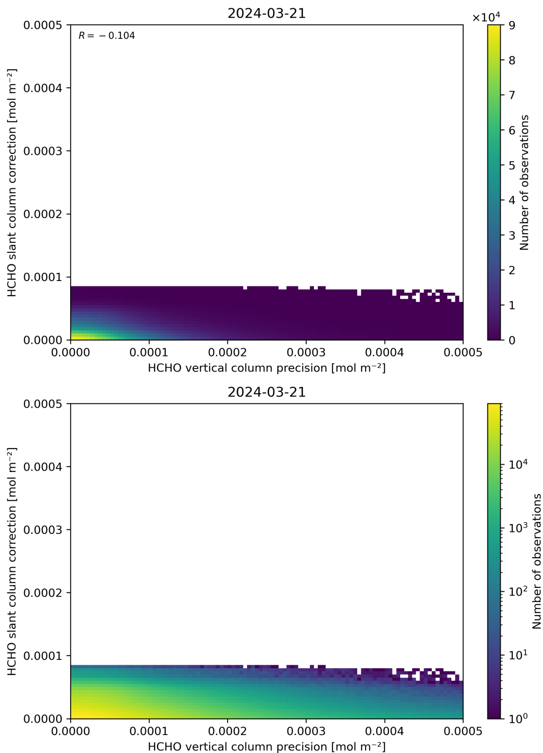
Figure 141: Scatter density plot of “HCHO vertical column precision” against “HCHO slant column correction” for 2024-03-20 to 2024-03-22.
