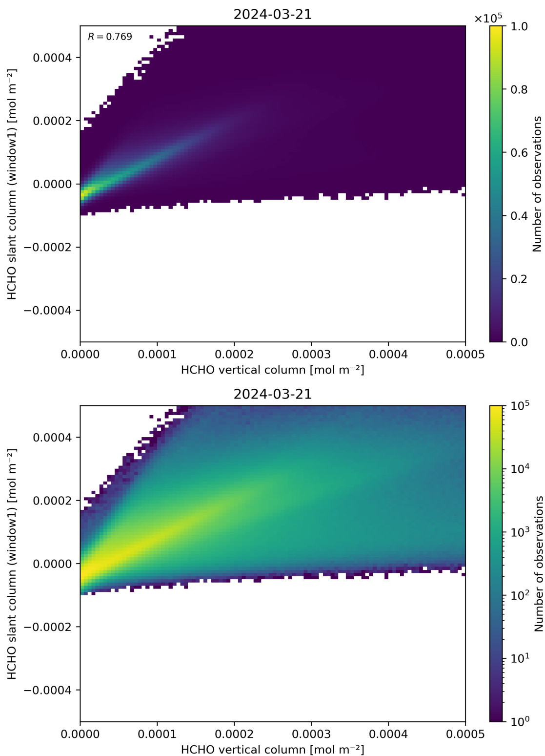
Figure 129: Scatter density plot of “HCHO vertical column” against “HCHO slant column (window1)” for 2024-03-20 to 2024-03-22.
