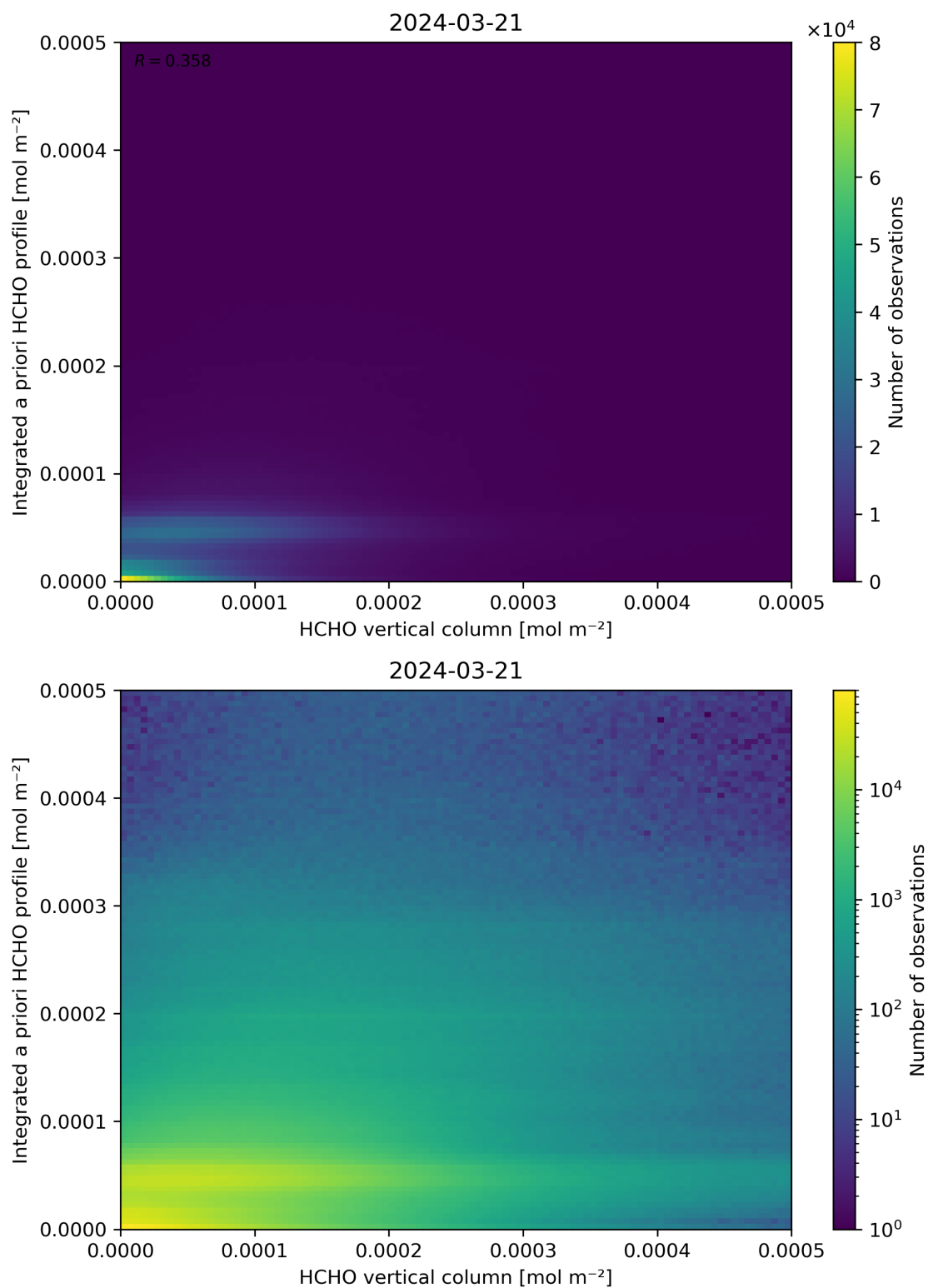
Figure 135: Scatter density plot of “HCHO vertical column” against “Integrated a priori HCHO profile” for 2024-03-20 to 2024-03-22.
