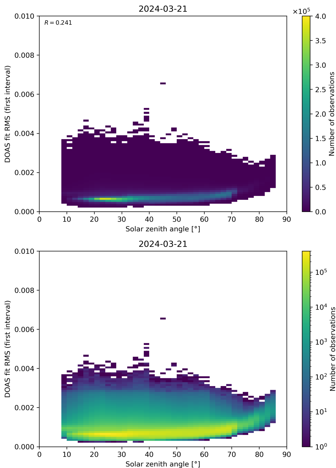
Figure 167: Scatter density plot of “Solar zenith angle” against “DOAS fit RMS (first interval)” for 2024-03-20 to 2024-03-22.
