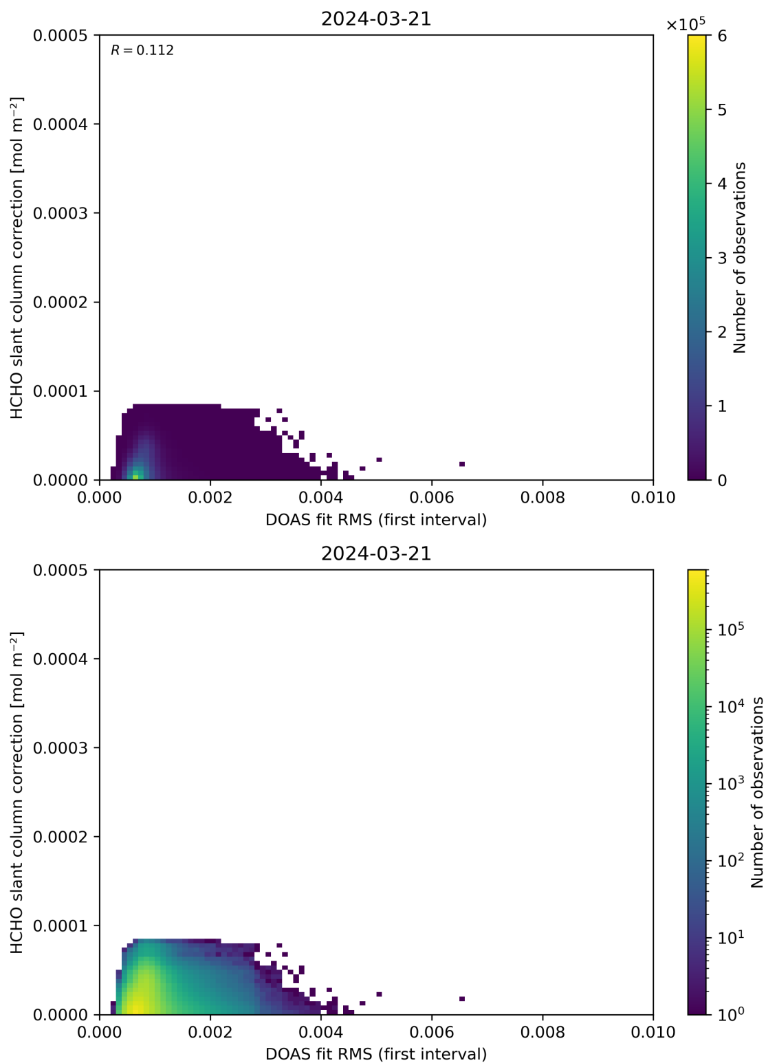
Figure 63: Scatter density plot of “DOAS fit RMS (first interval)” against “HCHO slant column correction” for 2024-03-20 to 2024-03-22.
