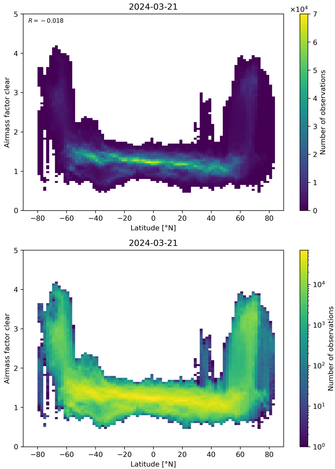
Figure 156: Scatter density plot of “Latitude” against “Airmass factor clear” for 2024-03-20 to 2024-03-22.
