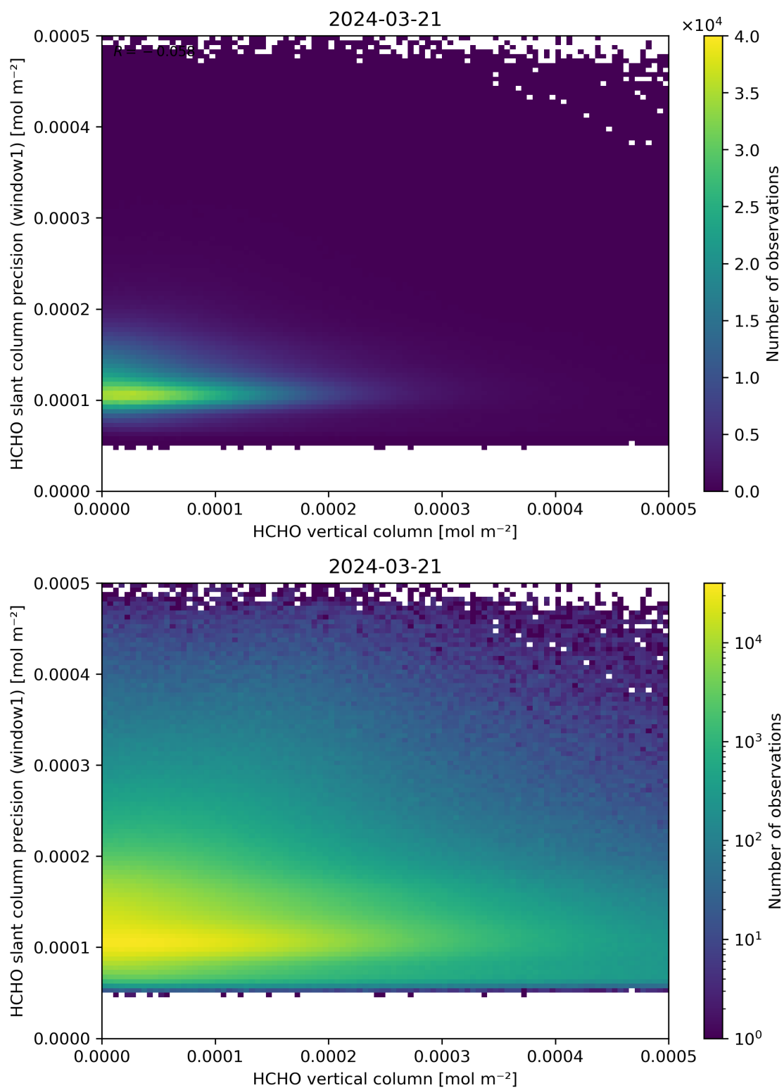
Figure 130: Scatter density plot of “HCHO vertical column” against “HCHO slant column precision (window1)” for 2024-03-20 to 2024-03-22.
