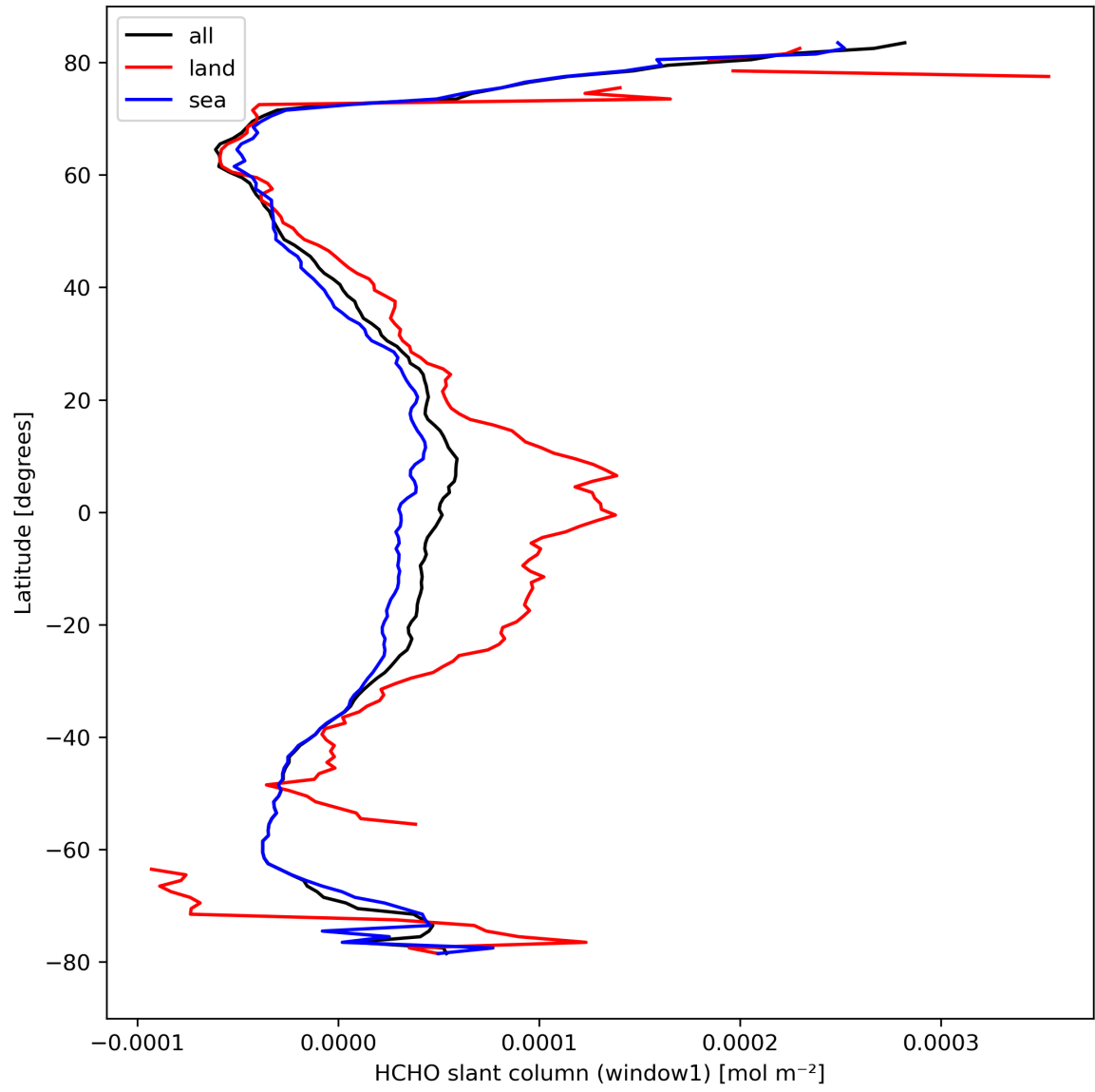
Figure 24: Zonal average of “HCHO slant column (window1)” for 2024-03-20 to 2024-03-22.
