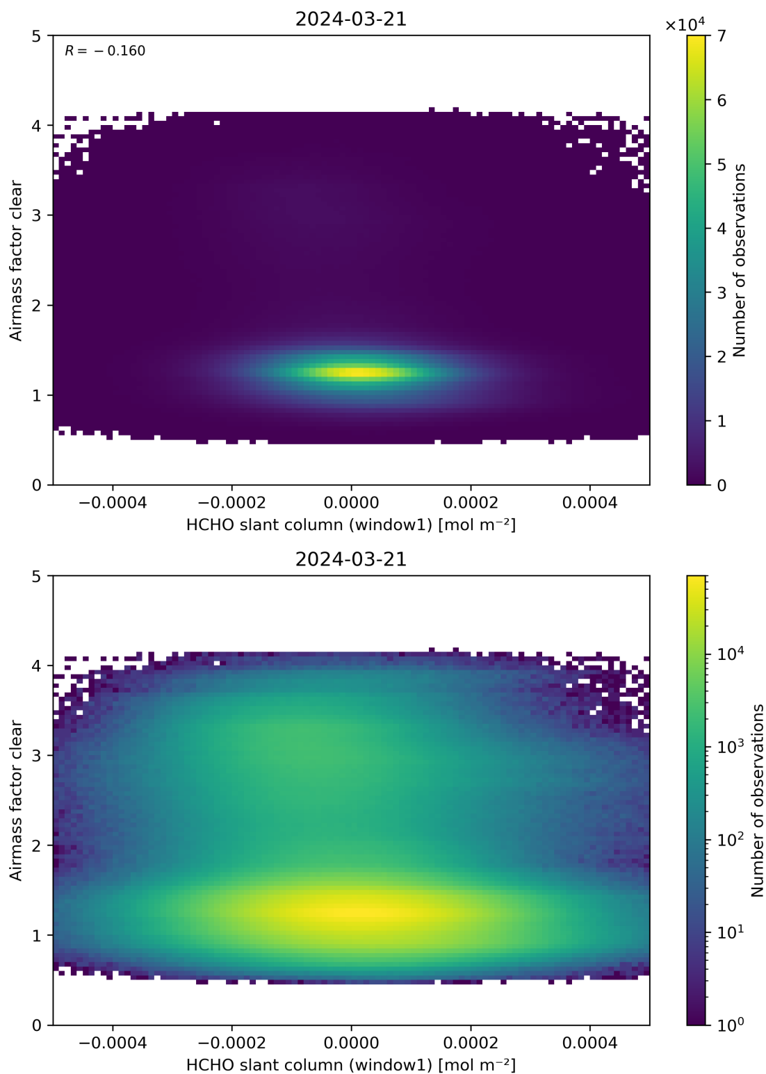
Figure 81: Scatter density plot of “HCHO slant column (window1)” against “Airmass factor clear” for 2024-03-20 to 2024-03-22.
