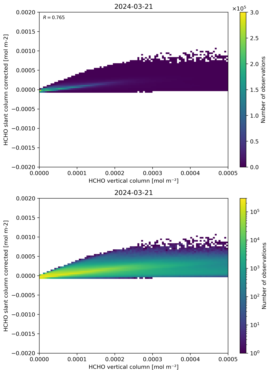
Figure 127: Scatter density plot of “HCHO vertical column” against “HCHO slant column corrected” for 2024-03-20 to 2024-03-22.
