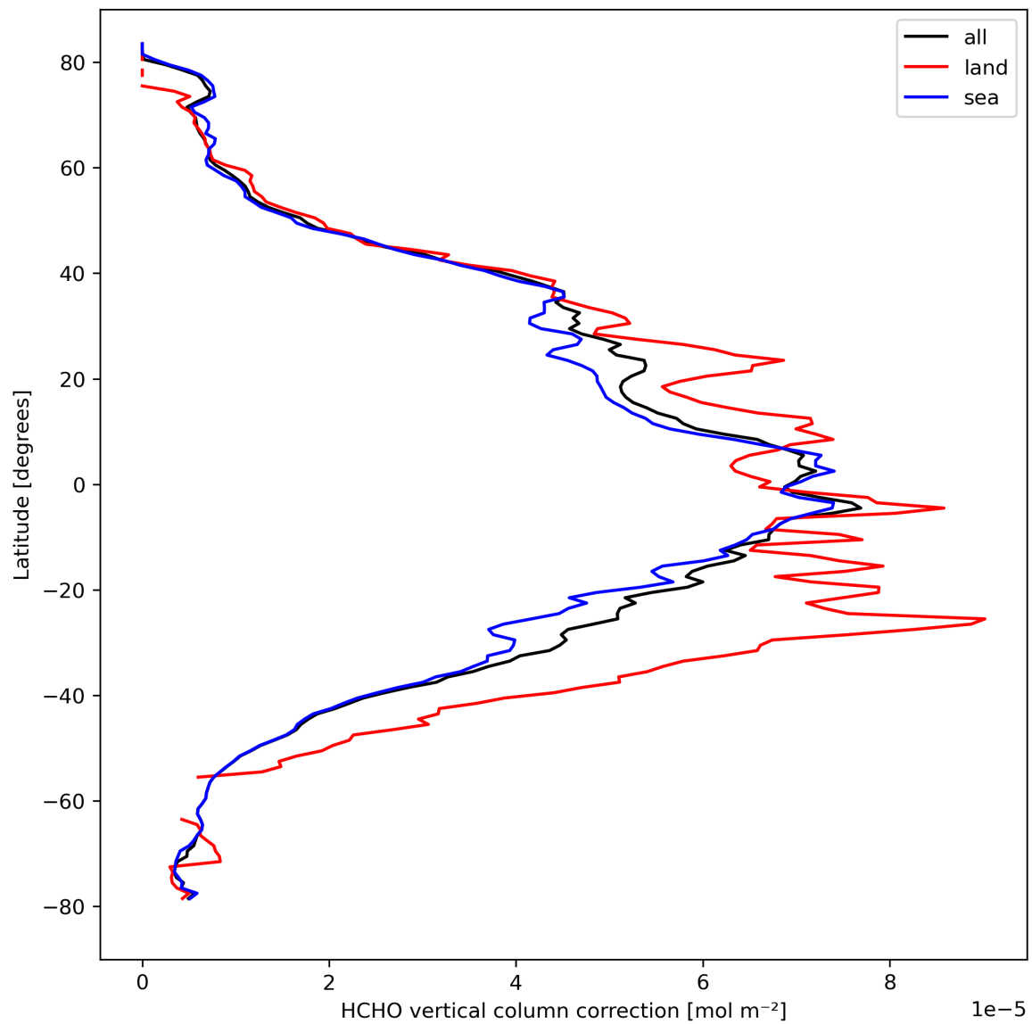
Figure 23: Zonal average of “HCHO vertical column correction” for 2024-03-20 to 2024-03-22.
