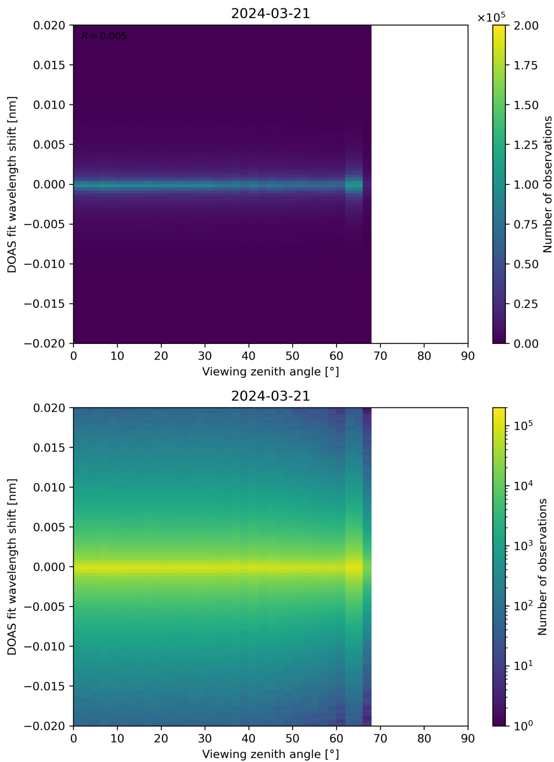
Figure 183: Scatter density plot of “Viewing zenith angle” against “DOAS fit wavelength shift” for 2024-03-20 to 2024-03-22.
