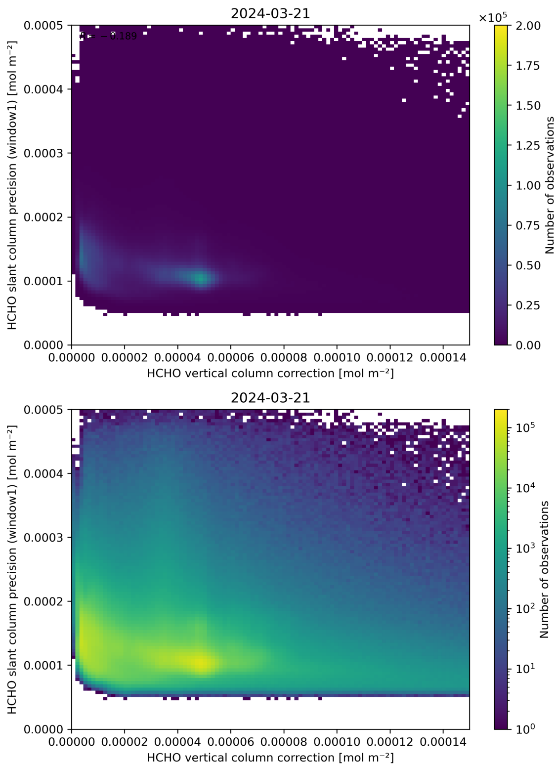
Figure 119: Scatter density plot of “HCHO vertical column correction” against “HCHO slant column precision (window1)” for 2024-03-20 to 2024-03-22.
