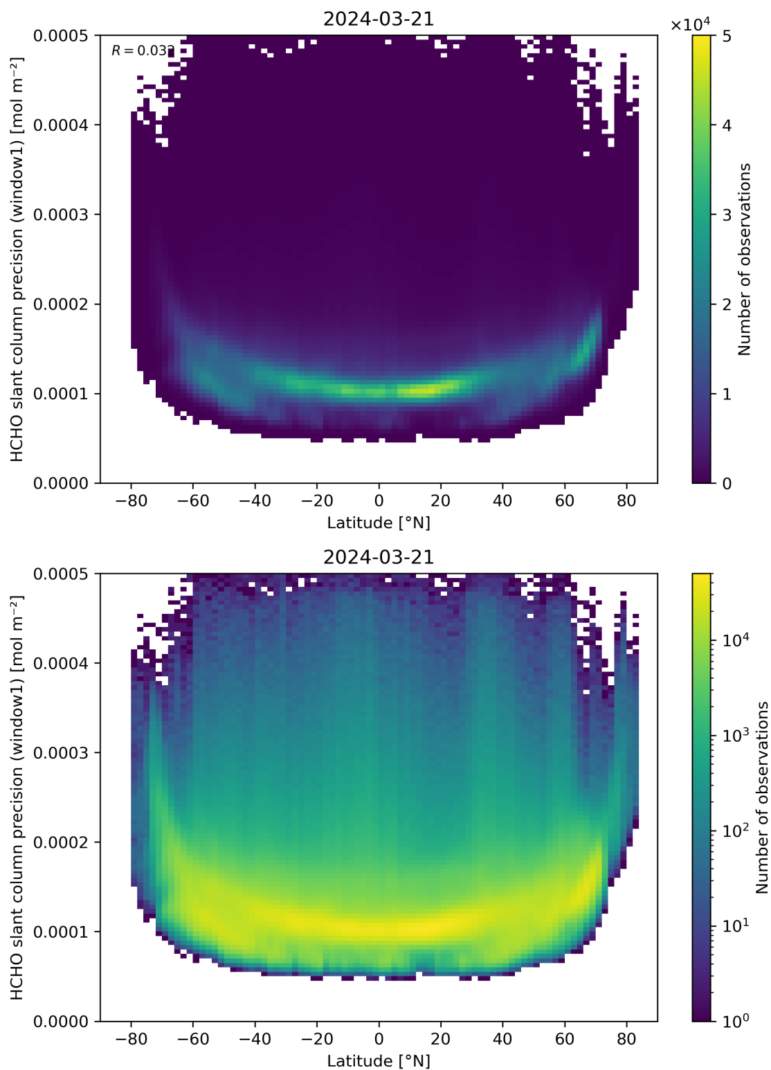
Figure 160: Scatter density plot of “Latitude” against “HCHO slant column precision (window1)” for 2024-03-20 to 2024-03-22.
