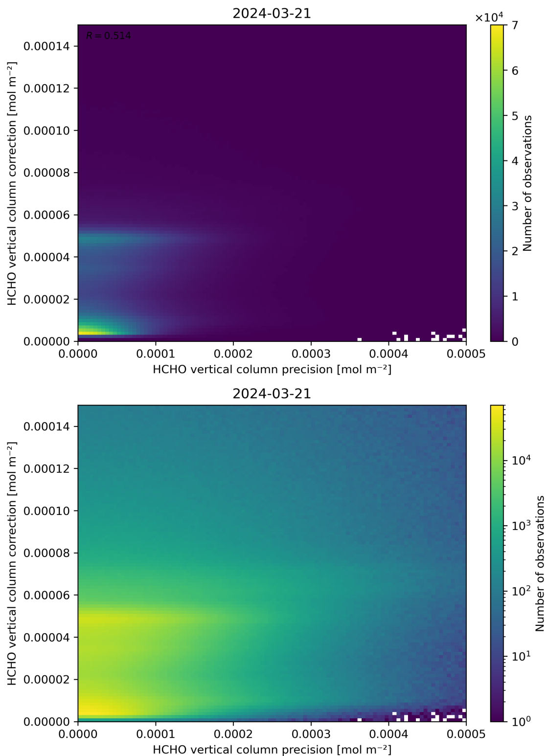
Figure 146: Scatter density plot of “HCHO vertical column precision” against “HCHO vertical column correction” for 2024-03-20 to 2024-03-22.
