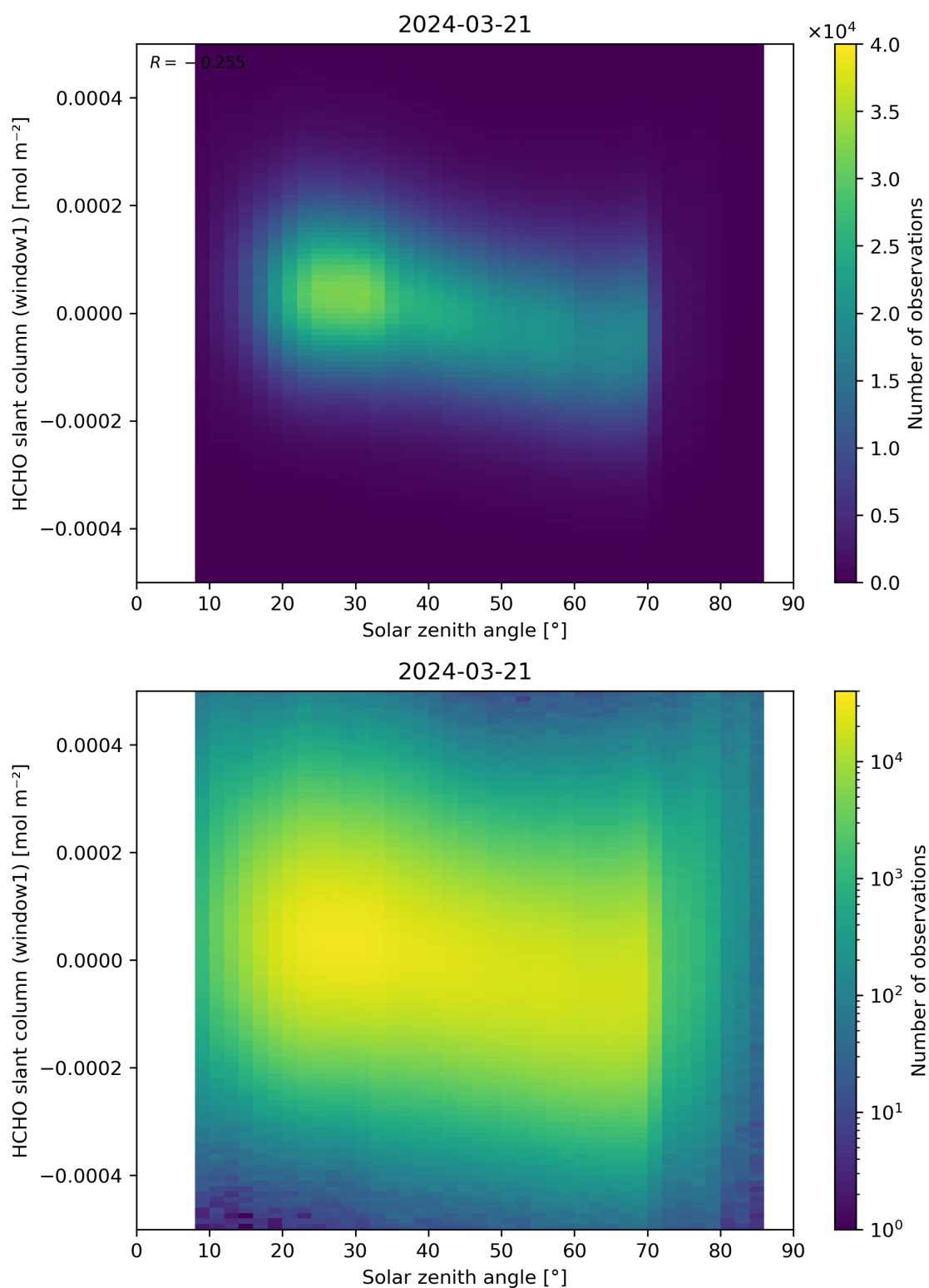
Figure 173: Scatter density plot of “Solar zenith angle” against “HCHO slant column (window1)” for 2024-03-20 to 2024-03-22.
