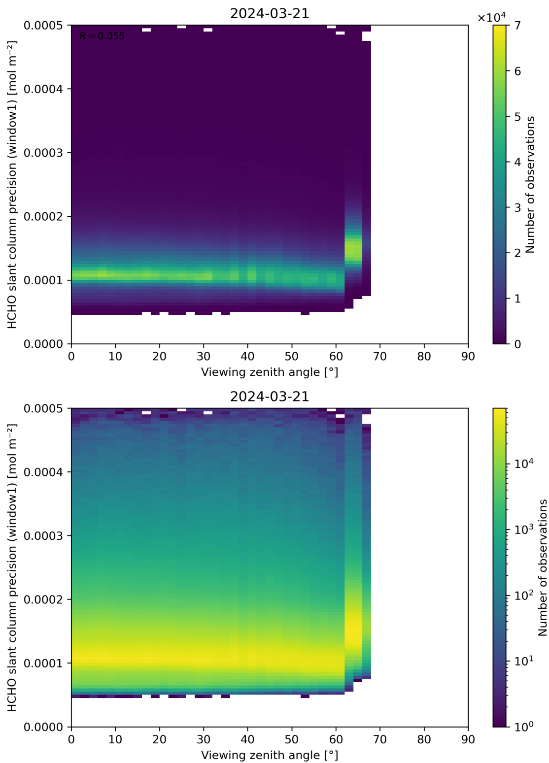
Figure 189: Scatter density plot of “Viewing zenith angle” against “HCHO slant column precision (window1)” for 2024-03-20 to 2024-03-22.
