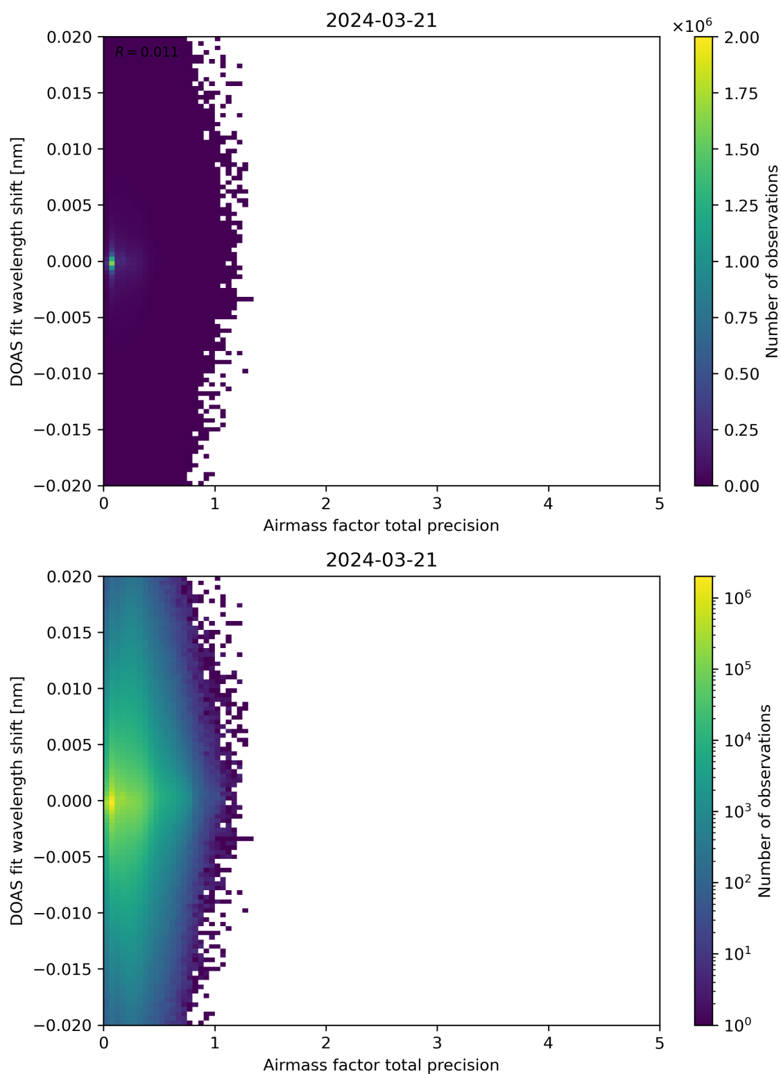
Figure 106: Scatter density plot of “Airmass factor total precision” against “DOAS fit wavelength shift” for 2024-03-20 to 2024-03-22.
