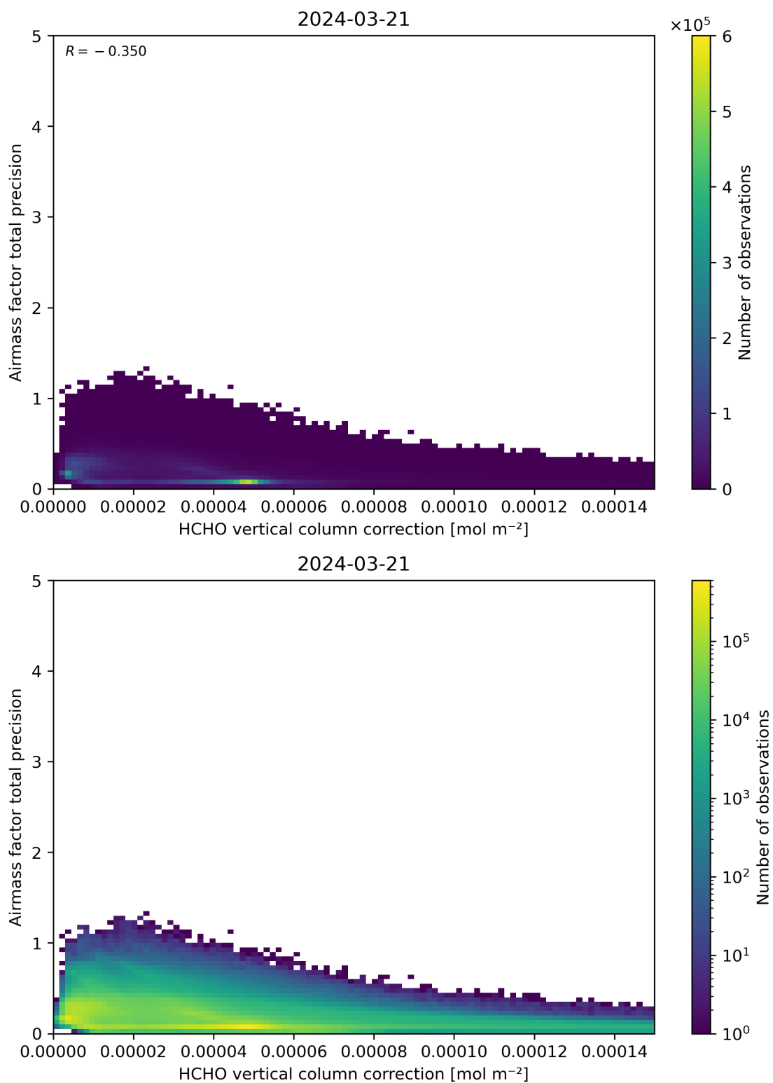
Figure 121: Scatter density plot of “HCHO vertical column correction” against “Airmass factor total precision” for 2024-03-20 to 2024-03-22.
