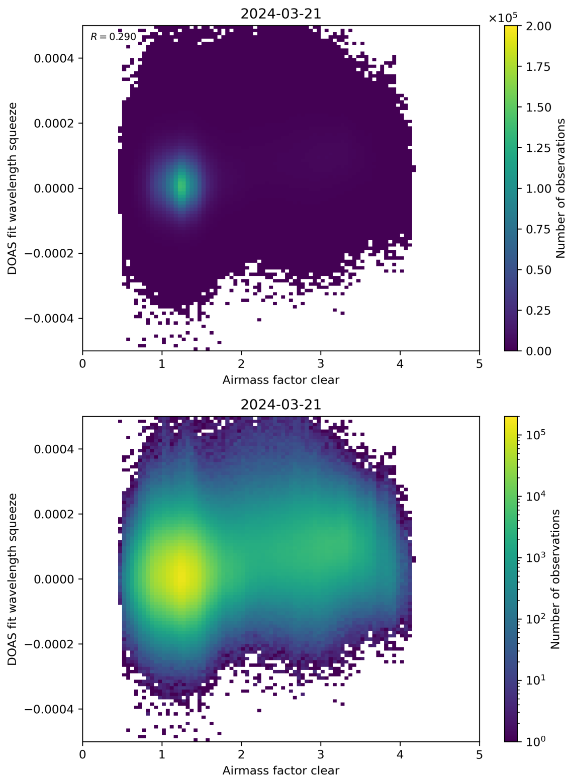
Figure 73: Scatter density plot of “Airmass factor clear” against “DOAS fit wavelength squeeze” for 2024-03-20 to 2024-03-22.
