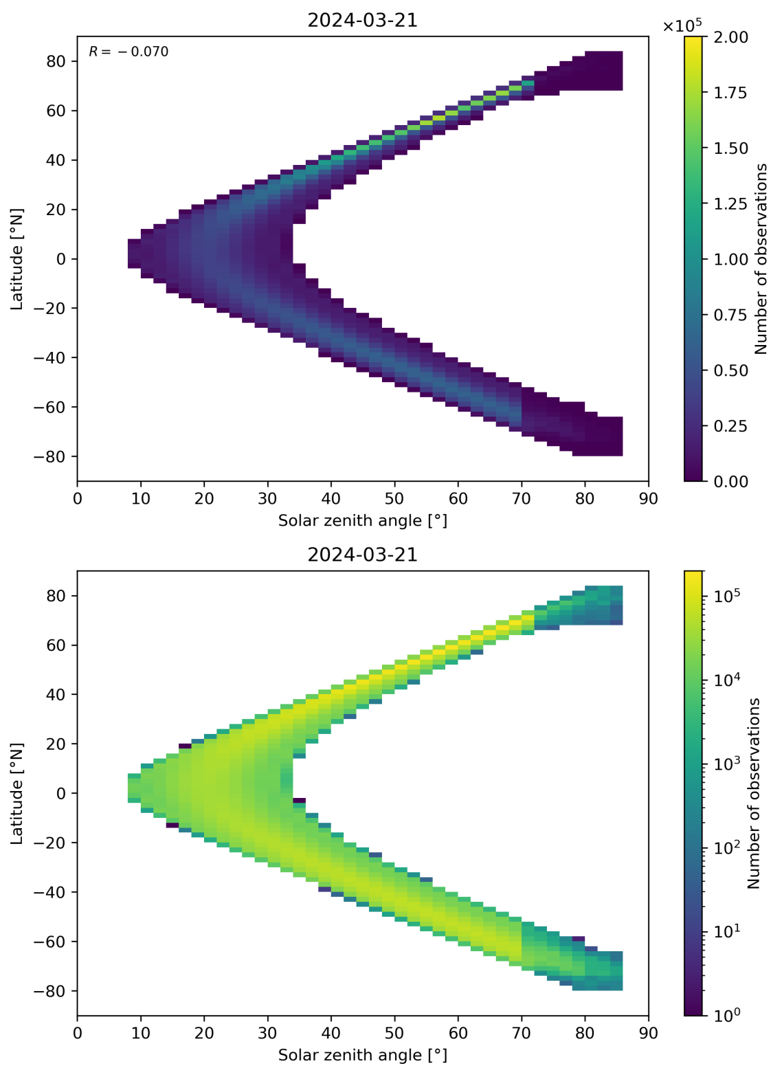
Figure 181: Scatter density plot of “Solar zenith angle” against “Latitude” for 2024-03-20 to 2024-03-22.
