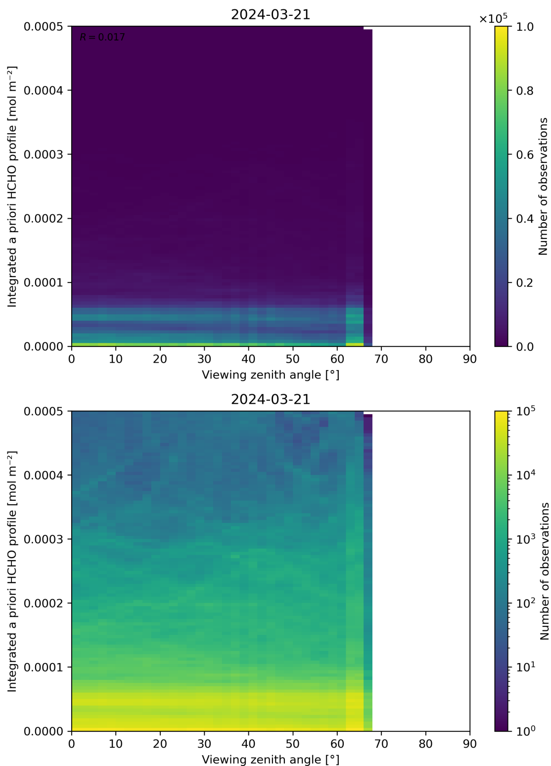
Figure 195: Scatter density plot of “Viewing zenith angle” against “Integrated a priori HCHO profile” for 2024-03-20 to 2024-03-22.
