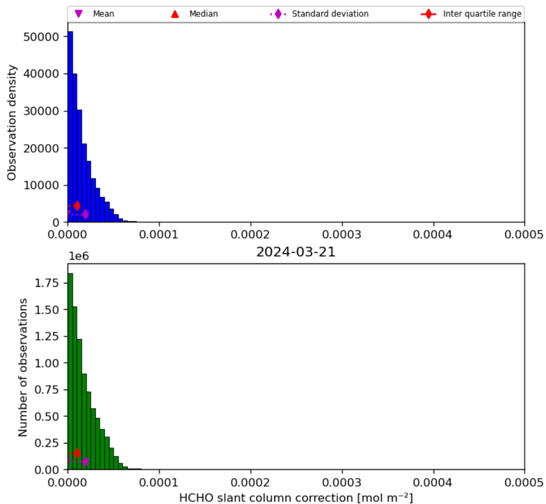
Figure 47: Histogram of “HCHO slant column correction” for 2024-03-20 to 2024-03-22
