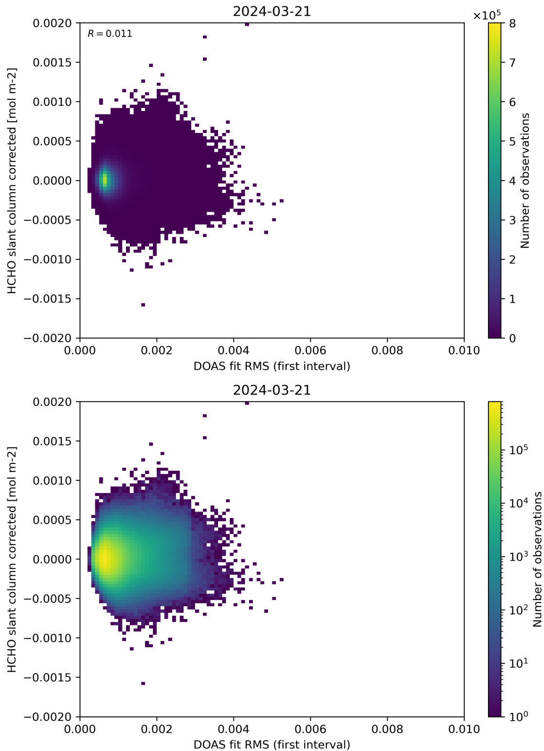
Figure 62: Scatter density plot of “DOAS fit RMS (first interval)” against “HCHO slant column corrected” for 2024-03-20 to 2024-03-22.
