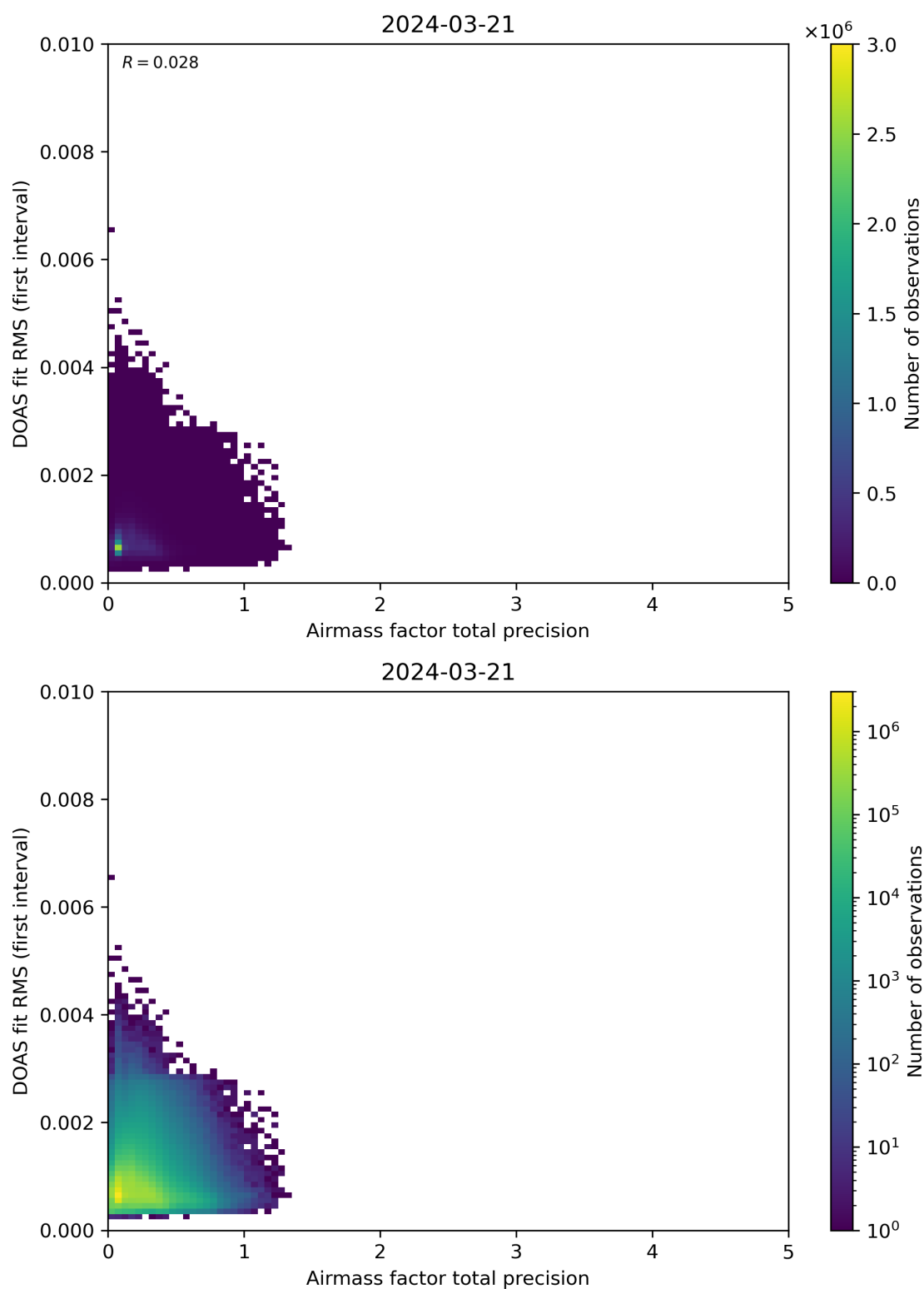
Figure 105: Scatter density plot of “Airmass factor total precision” against “DOAS fit RMS (first interval)” for 2024-03-20 to 2024-03-22.
