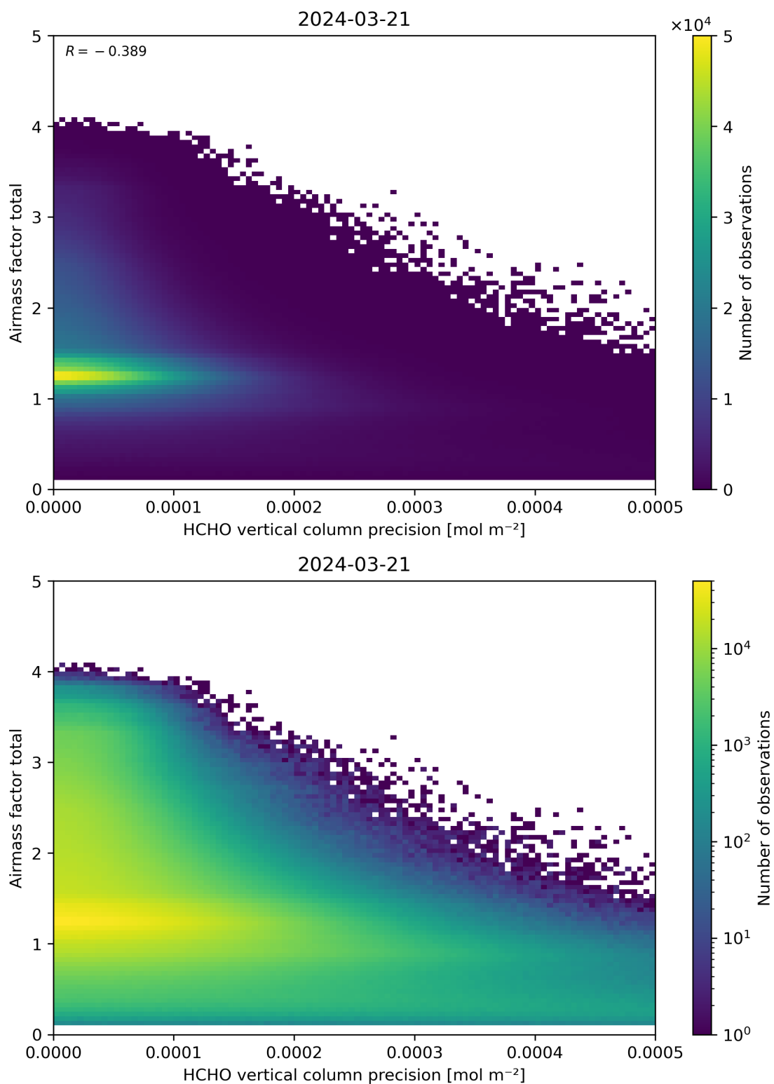
Figure 144: Scatter density plot of “HCHO vertical column precision” against “Airmass factor total” for 2024-03-20 to 2024-03-22.
