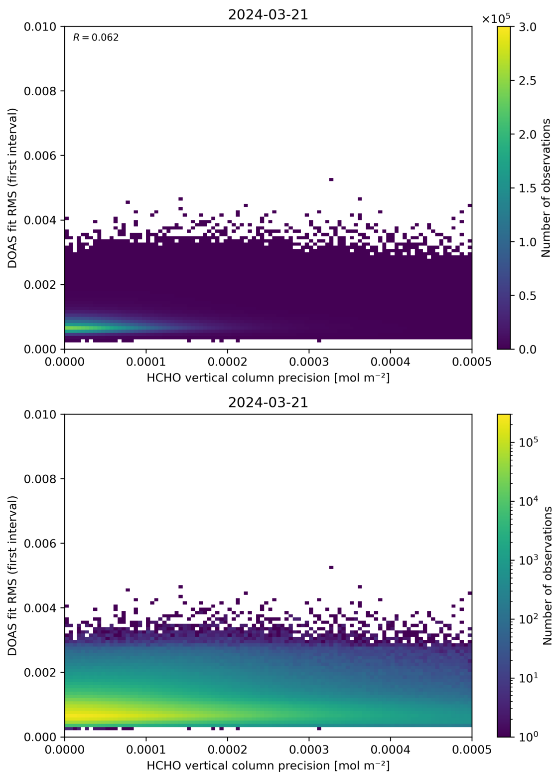
Figure 136: Scatter density plot of “HCHO vertical column precision” against “DOAS fit RMS (first interval)” for 2024-03-20 to 2024-03-22.
