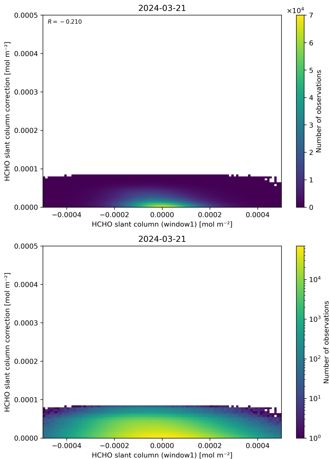
Figure 83: Scatter density plot of “HCHO slant column (window1)” against “HCHO slant column correction” for 2024-03-20 to 2024-03-22.
