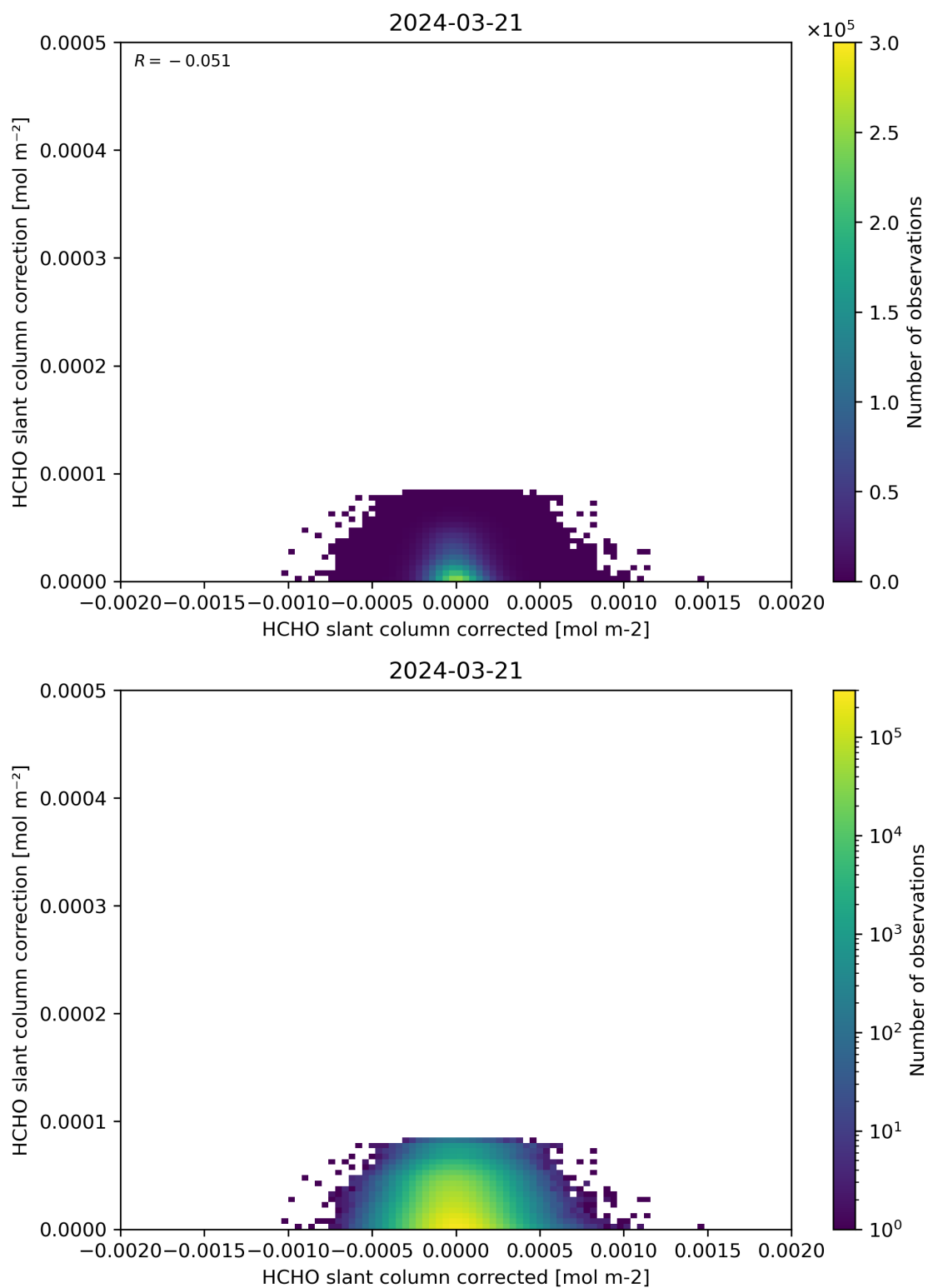
Figure 77: Scatter density plot of “HCHO slant column corrected” against “HCHO slant column correction” for 2024-03-20 to 2024-03-22.
