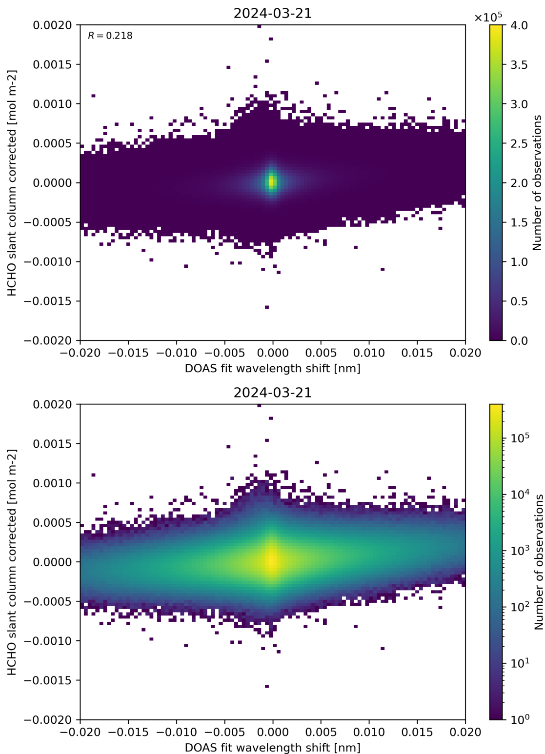
Figure 66: Scatter density plot of “DOAS fit wavelength shift” against “HCHO slant column corrected” for 2024-03-20 to 2024-03-22.
