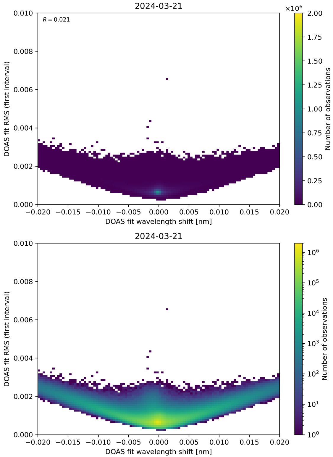
Figure 64: Scatter density plot of “DOAS fit wavelength shift” against “DOAS fit RMS (first interval)” for 2024-03-20 to 2024-03-22.
