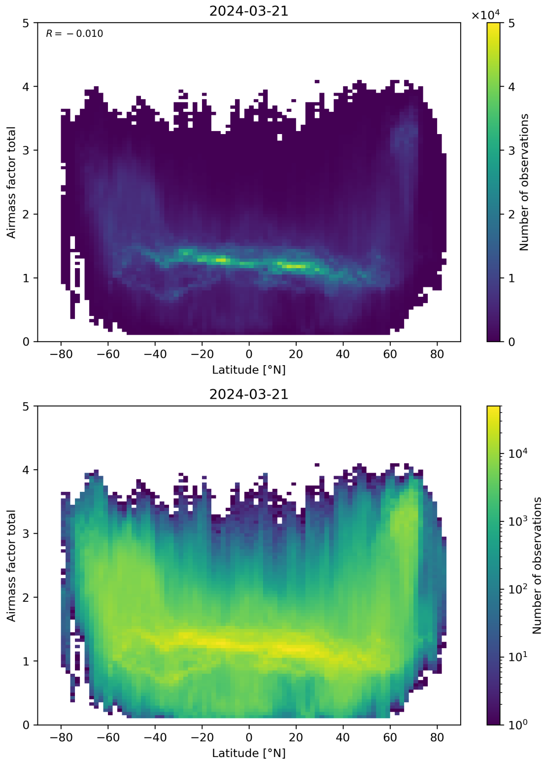
Figure 161: Scatter density plot of “Latitude” against “Airmass factor total” for 2024-03-20 to 2024-03-22.
