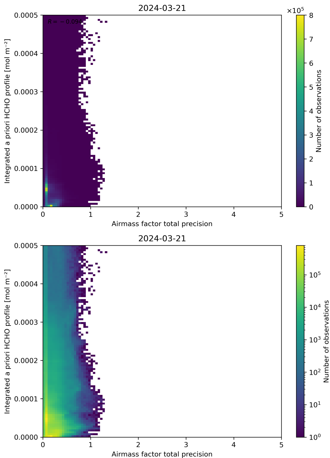
Figure 111: Scatter density plot of “Airmass factor total precision” against “Integrated a priori HCHO profile” for 2024-03-20 to 2024-03-22.
