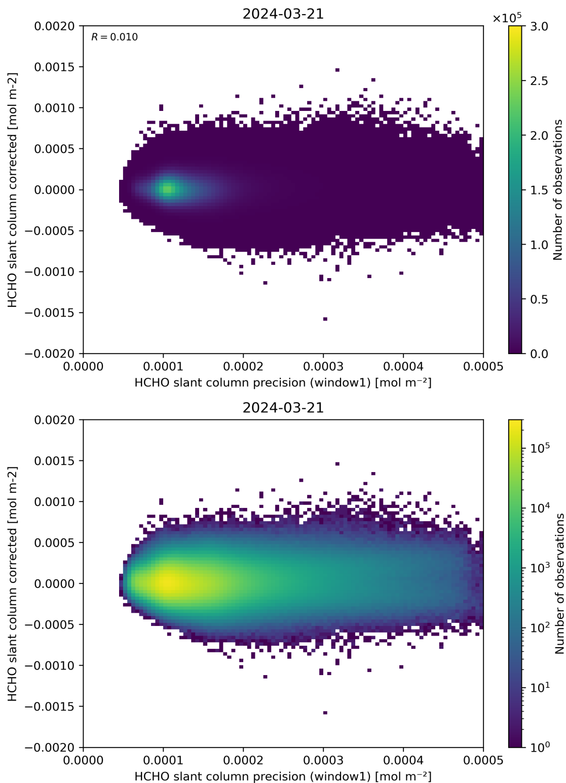
Figure 92: Scatter density plot of “HCHO slant column precision (window1)” against “HCHO slant column corrected” for 2024-03-20 to 2024-03-22.
