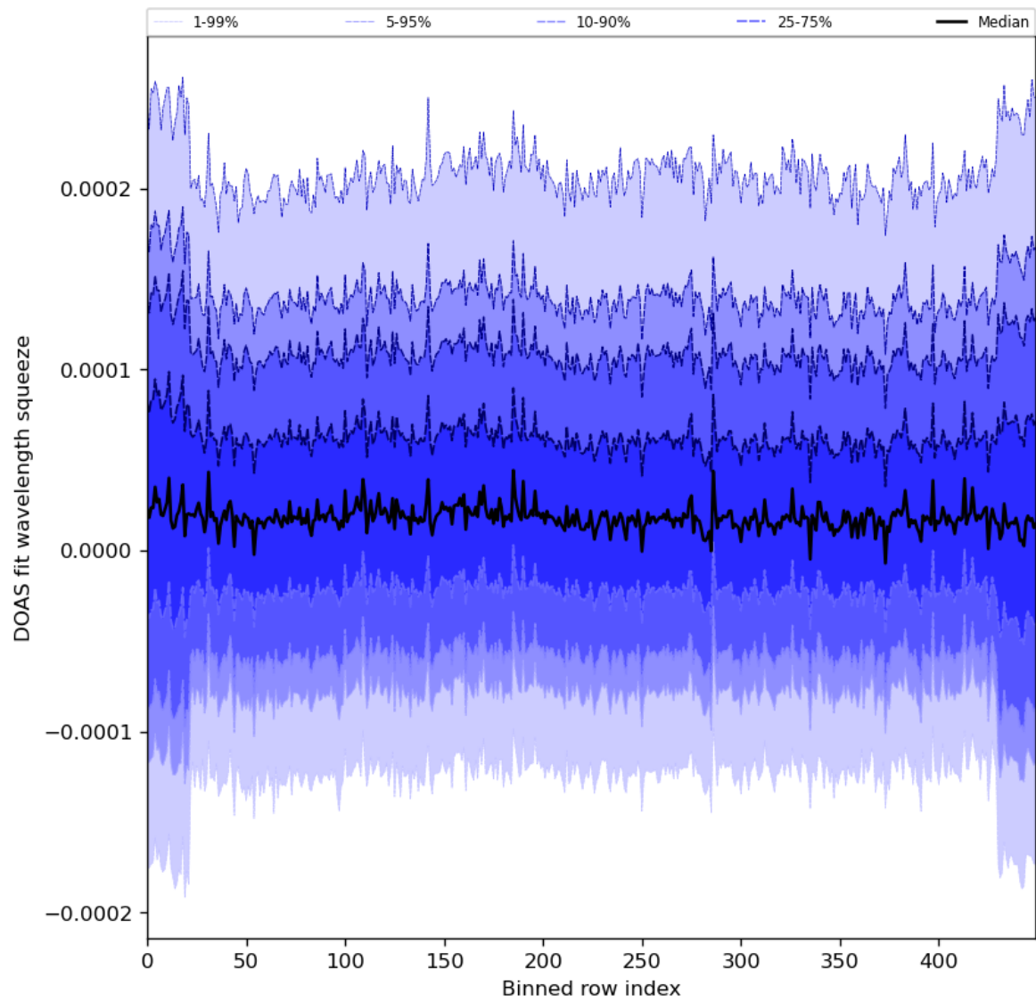
Figure 59: Along track statistics of “DOAS fit wavelength squeeze” for 2024-03-20 to 2024-03-22
