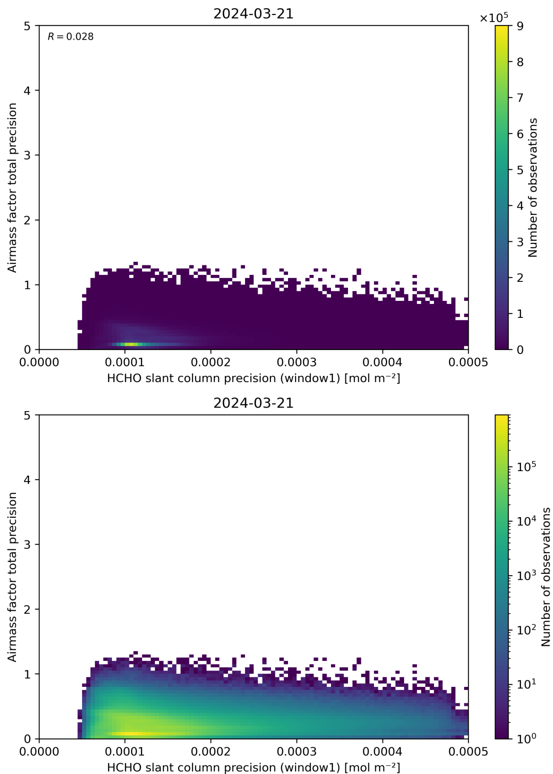
Figure 95: Scatter density plot of “HCHO slant column precision (window1)” against “Airmass factor total precision” for 2024-03-20 to 2024-03-22.
