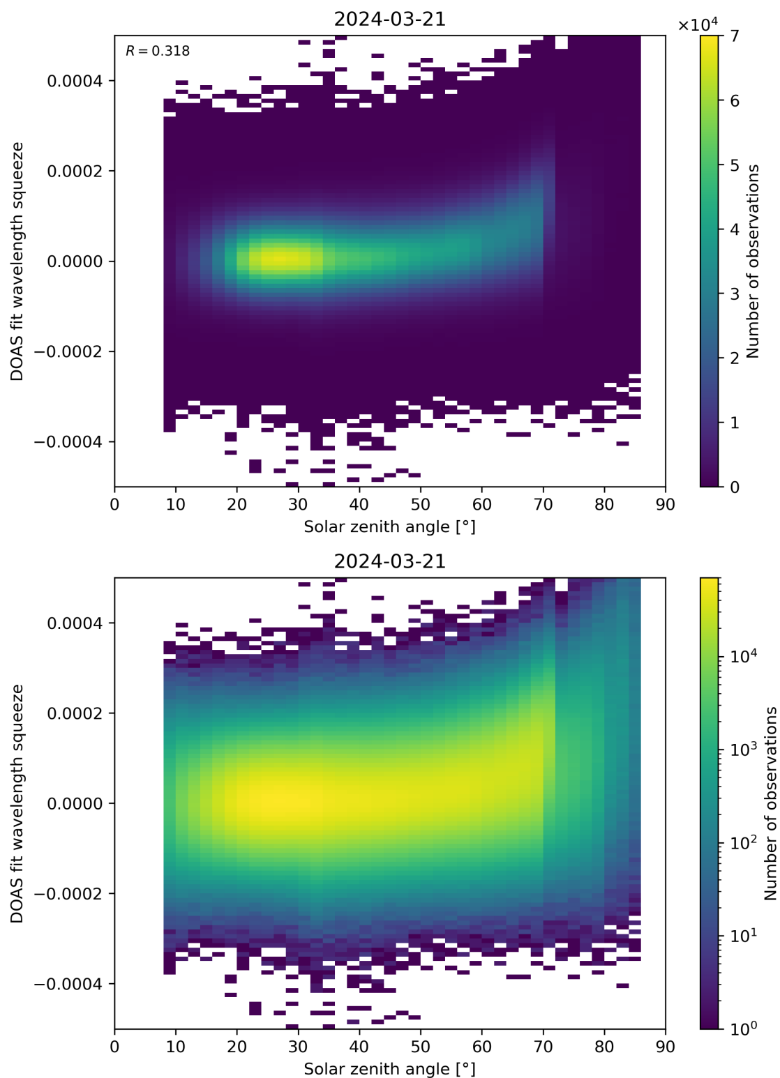
Figure 169: Scatter density plot of “Solar zenith angle” against “DOAS fit wavelength squeeze” for 2024-03-20 to 2024-03-22.
