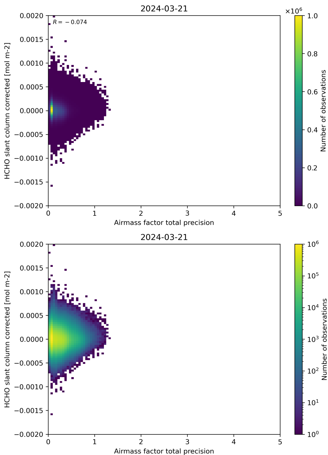
Figure 109: Scatter density plot of “Airmass factor total precision” against “HCHO slant column corrected” for 2024-03-20 to 2024-03-22.
