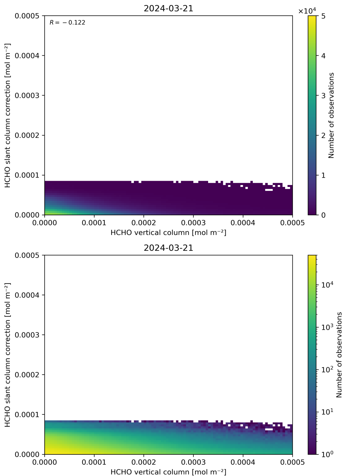
Figure 128: Scatter density plot of “HCHO vertical column” against “HCHO slant column correction” for 2024-03-20 to 2024-03-22.
