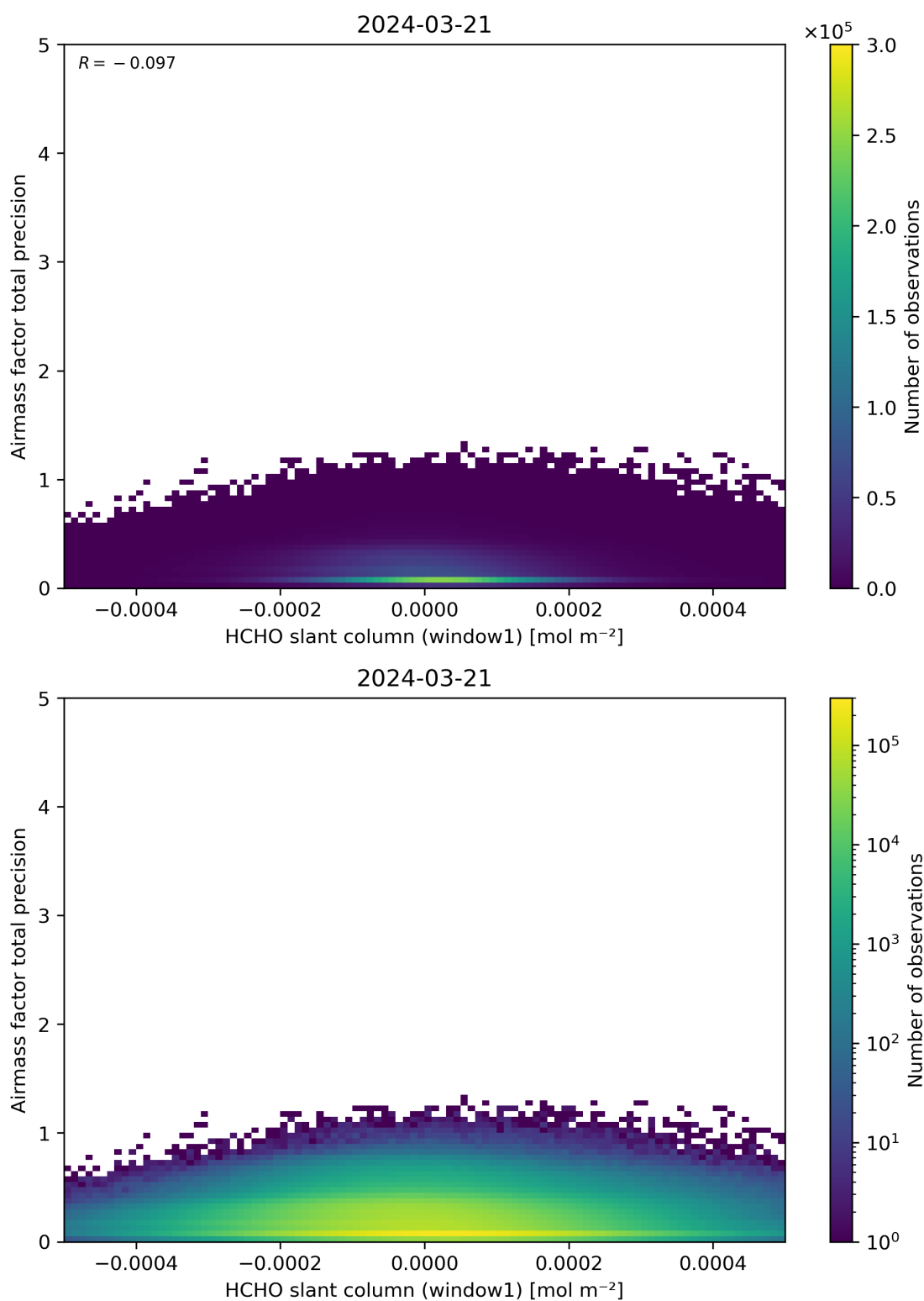
Figure 86: Scatter density plot of “HCHO slant column (window1)” against “Airmass factor total precision” for 2024-03-20 to 2024-03-22.
