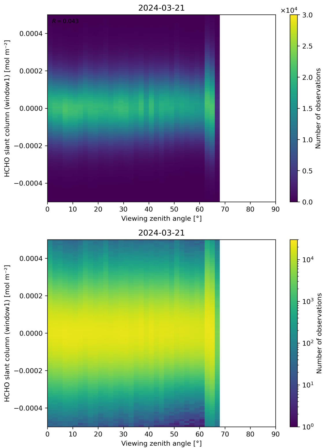
Figure 188: Scatter density plot of “Viewing zenith angle” against “HCHO slant column (window1)” for 2024-03-20 to 2024-03-22.
