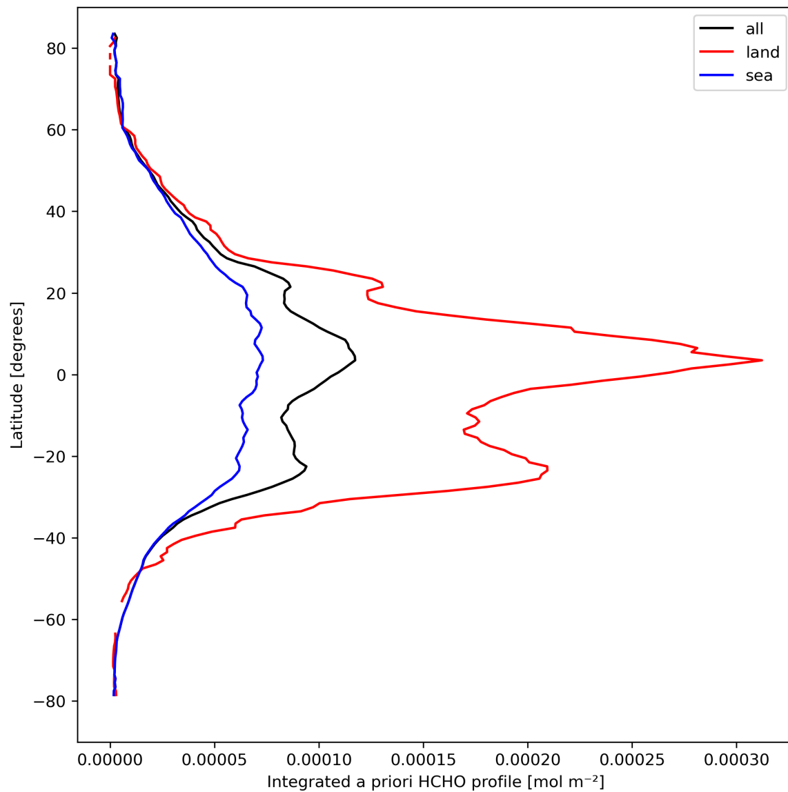
Figure 29: Zonal average of “Integrated a priori HCHO profile” for 2024-03-20 to 2024-03-22.
