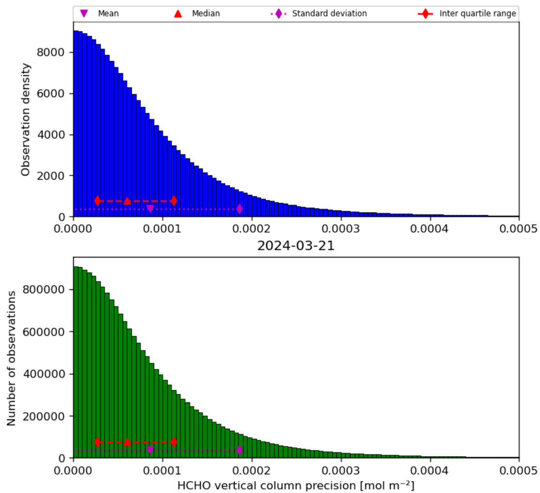
Figure 36: Histogram of "HCHO vertical column precision" for 2024-03-20 to 2024-03-22
