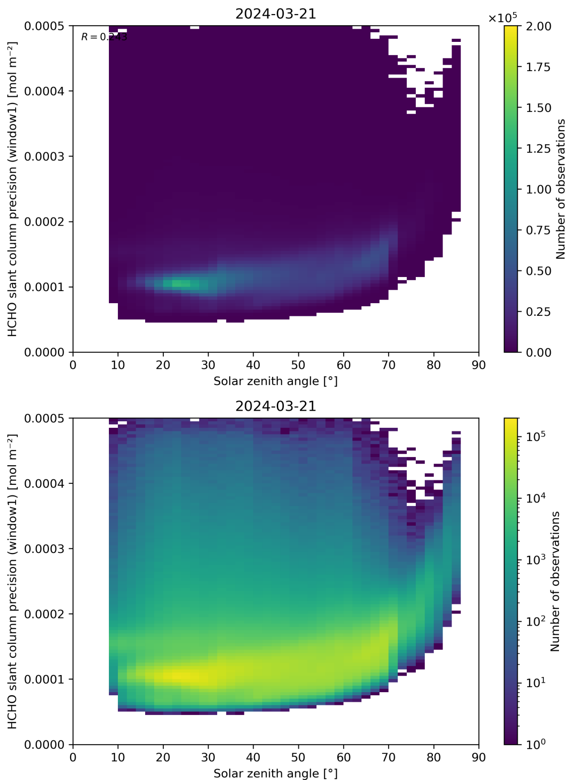
Figure 174: Scatter density plot of “Solar zenith angle” against “HCHO slant column precision (window1)” for 2024-03-20 to 2024-03-22.
