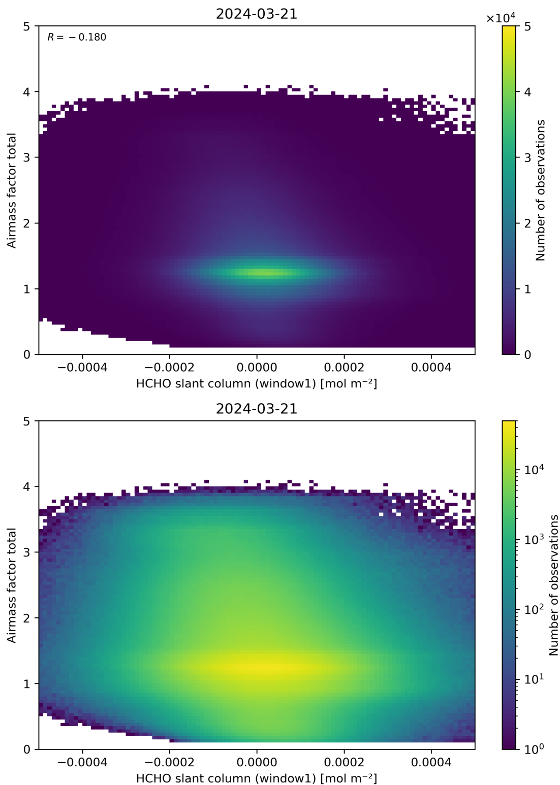
Figure 85: Scatter density plot of “HCHO slant column (window1)” against “Airmass factor total” for 2024-03-20 to 2024-03-22.
