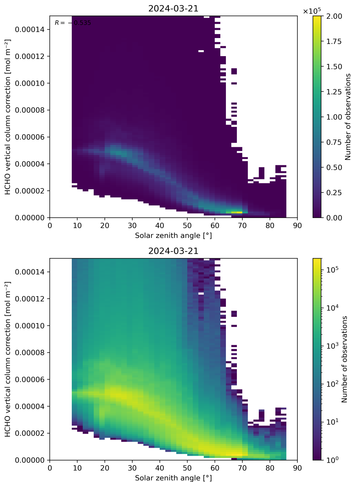
Figure 178: Scatter density plot of “Solar zenith angle” against “HCHO vertical column correction” for 2024-03-20 to 2024-03-22.
