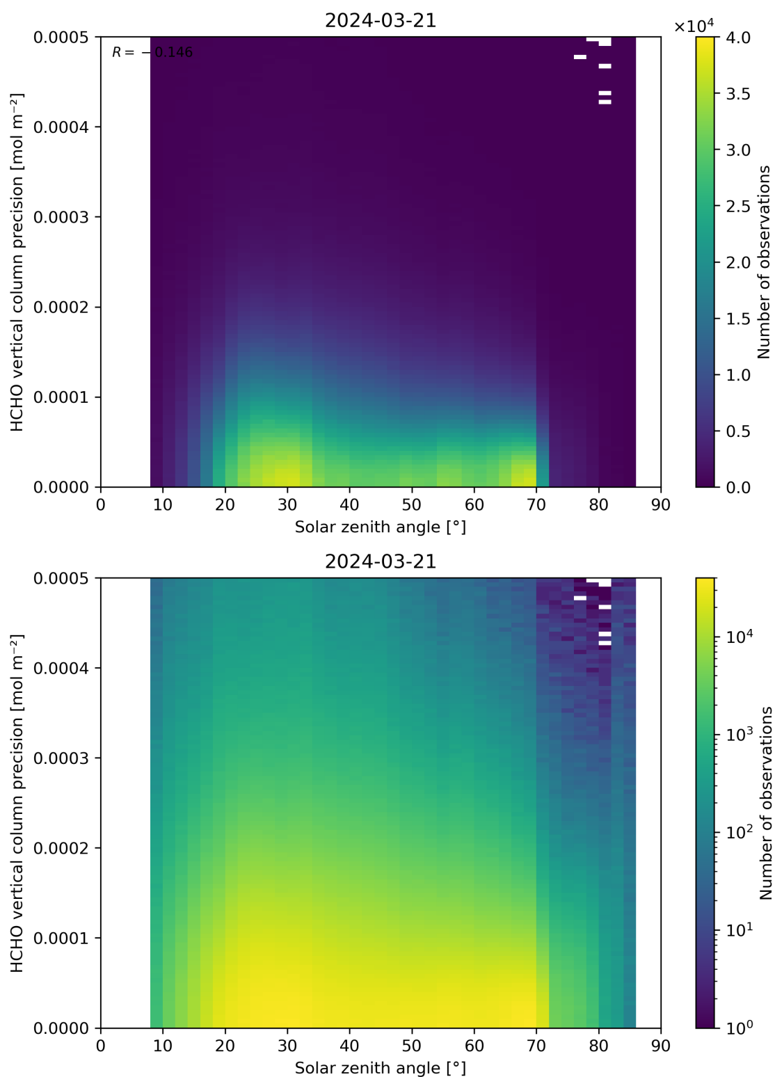
Figure 179: Scatter density plot of “Solar zenith angle” against “HCHO vertical column precision” for 2024-03-20 to 2024-03-22.
