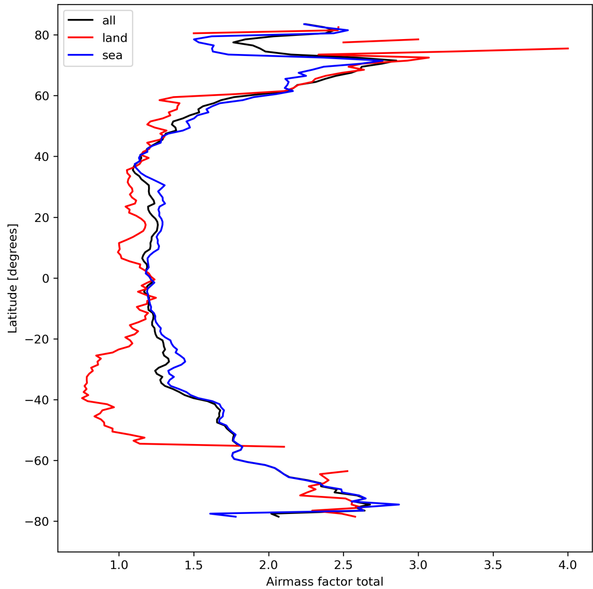
Figure 26: Zonal average of “Airmass factor total” for 2024-03-20 to 2024-03-22.
