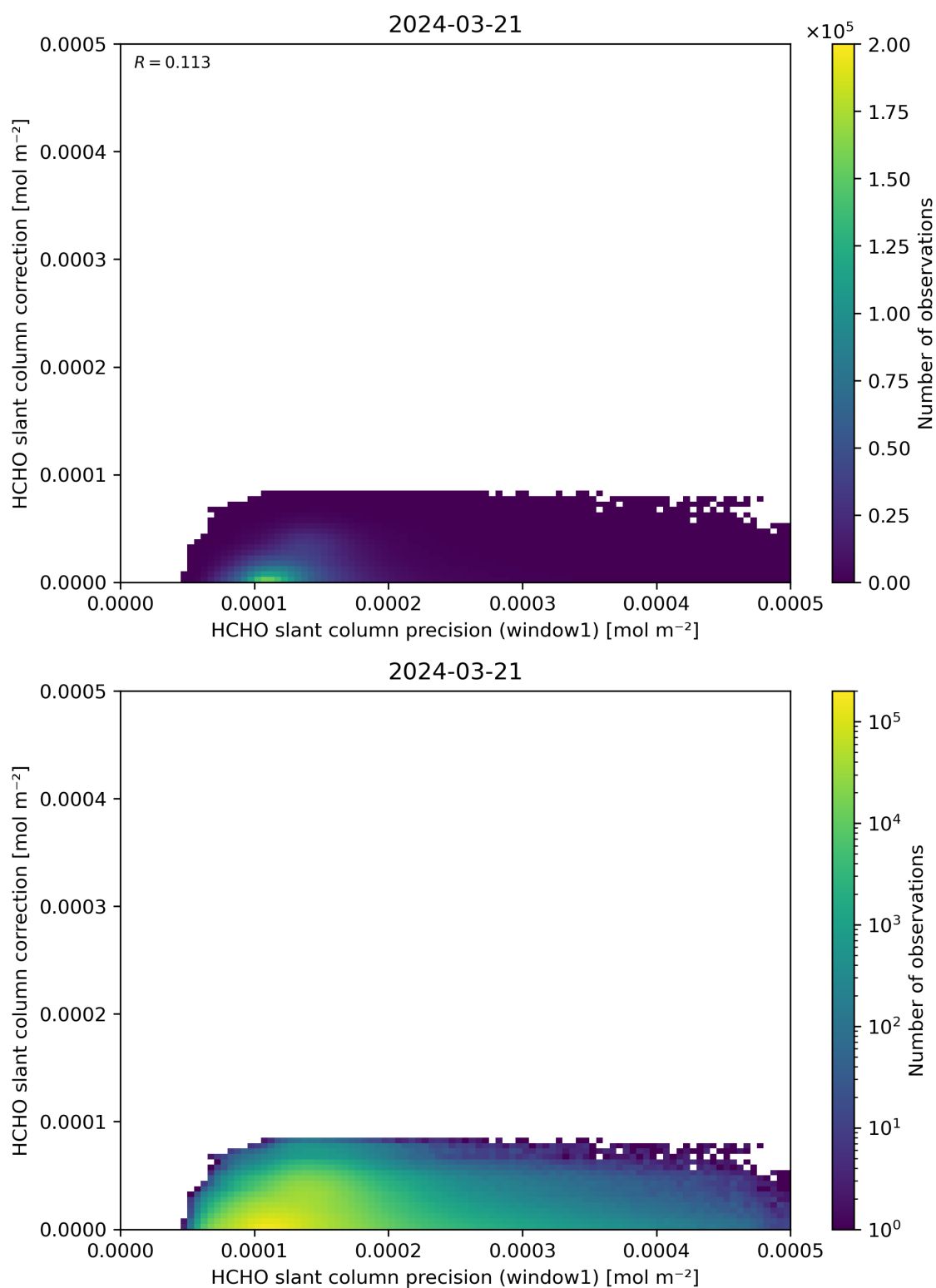
Figure 93: Scatter density plot of “HCHO slant column precision (window1)” against “HCHO slant column correction” for 2024-03-20 to 2024-03-22.
