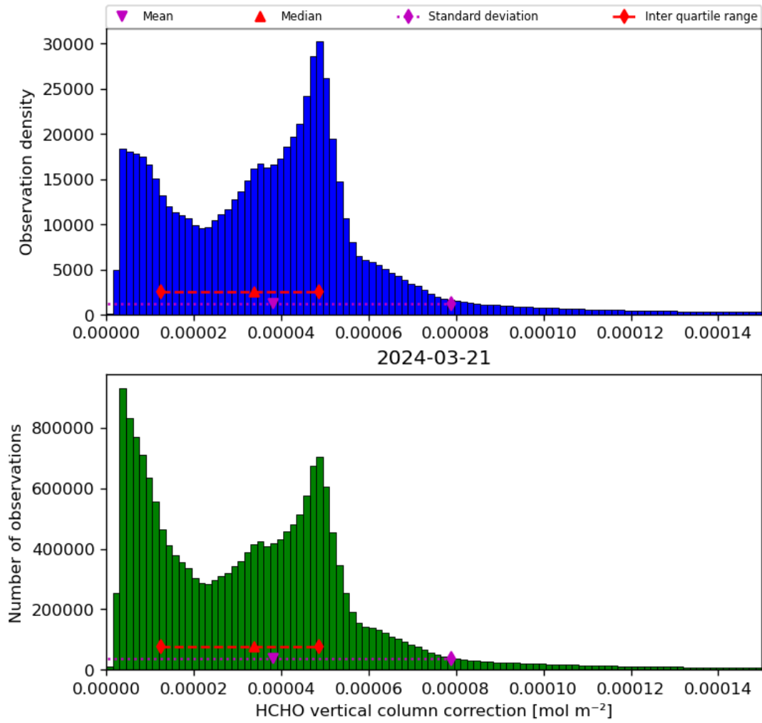
Figure 37: Histogram of “HCHO vertical column correction” for 2024-03-20 to 2024-03-22
