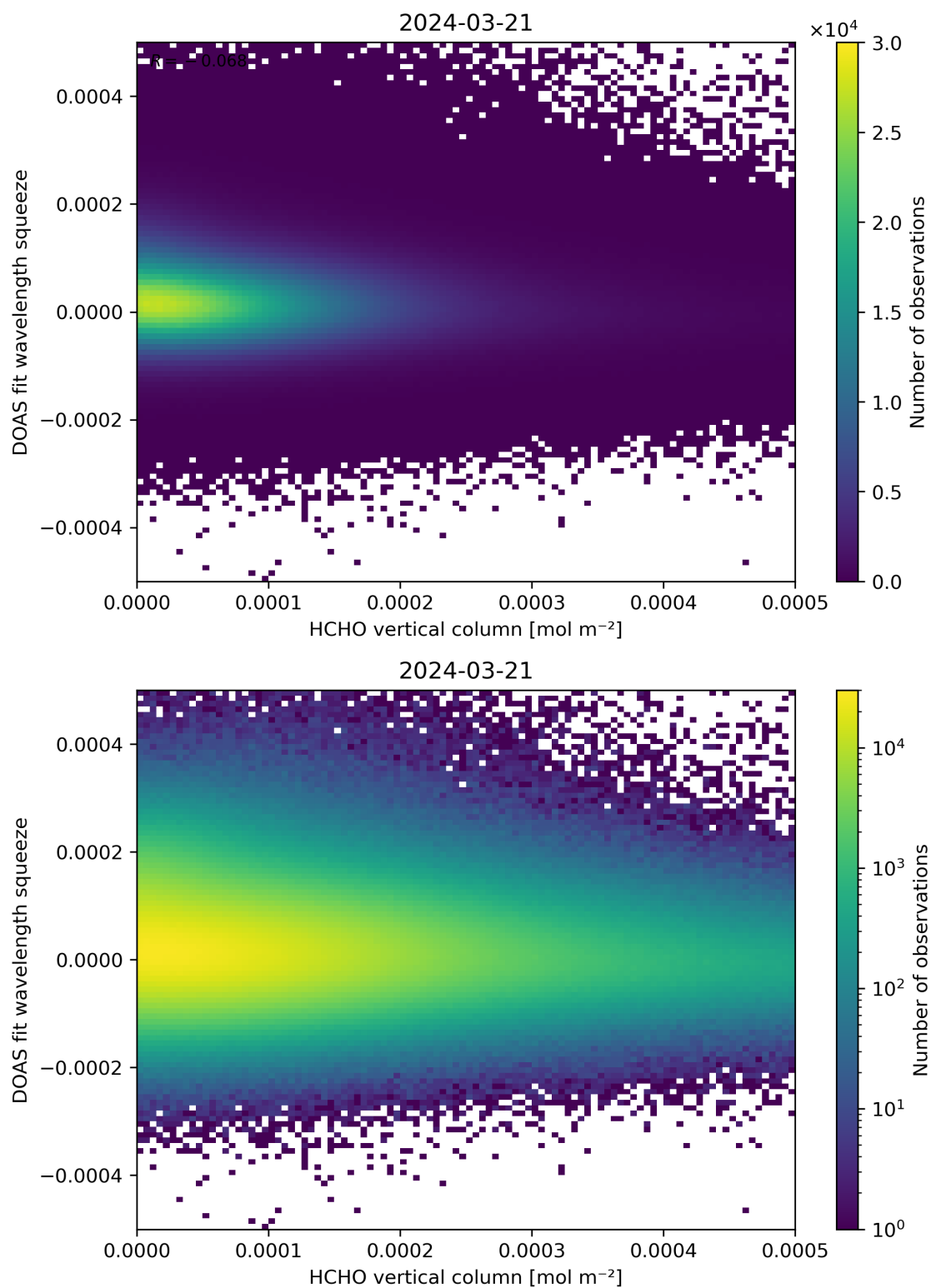
Figure 125: Scatter density plot of “HCHO vertical column” against “DOAS fit wavelength squeeze” for 2024-03-20 to 2024-03-22.
