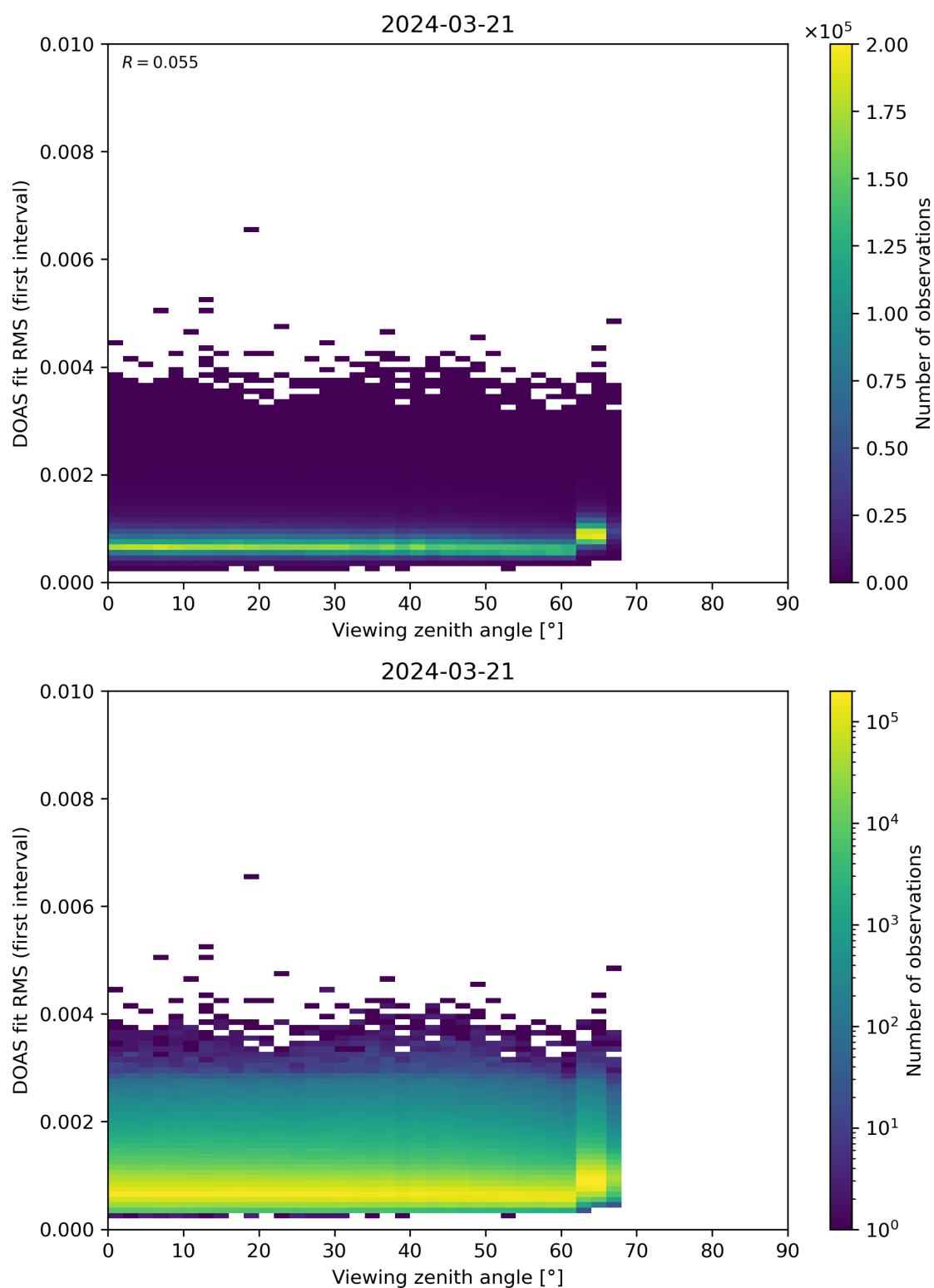
Figure 182: Scatter density plot of “Viewing zenith angle” against “DOAS fit RMS (first interval)” for 2024-03-20 to 2024-03-22.
