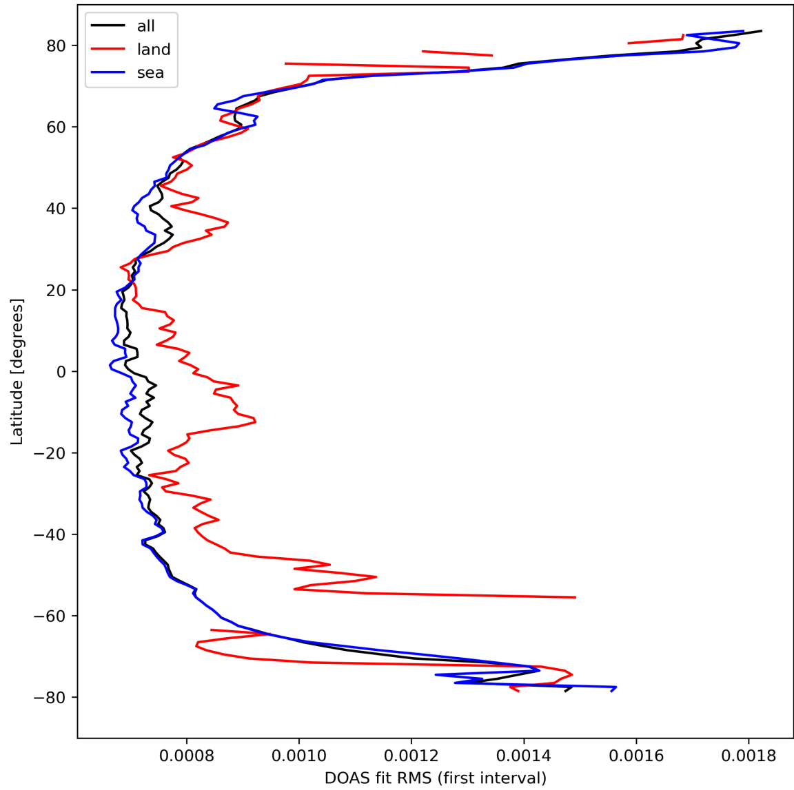
Figure 32: Zonal average of “DOAS fit RMS (first interval)” for 2024-03-20 to 2024-03-22.
