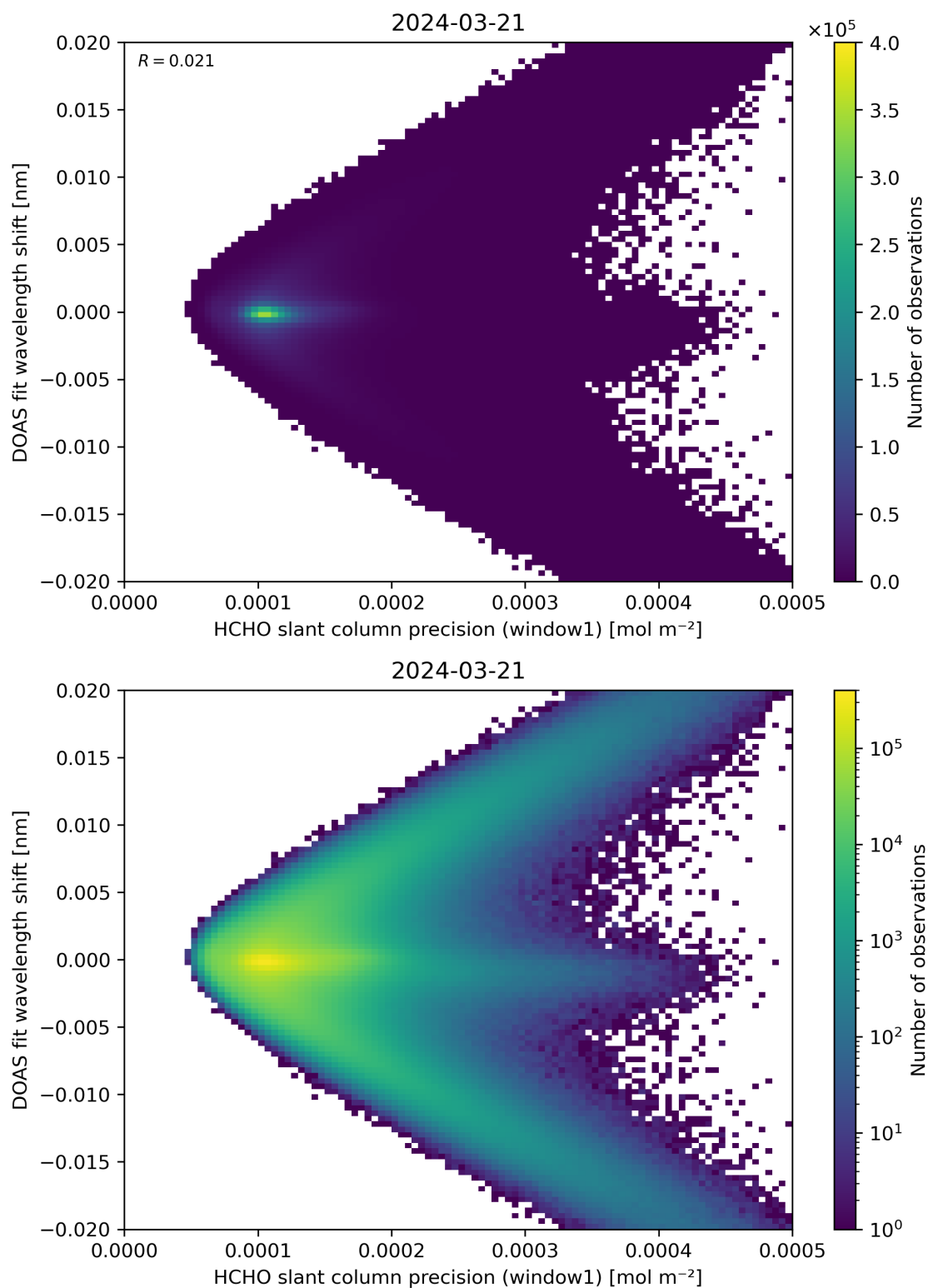
Figure 89: Scatter density plot of “HCHO slant column precision (window1)” against “DOAS fit wavelength shift” for 2024-03-20 to 2024-03-22.
