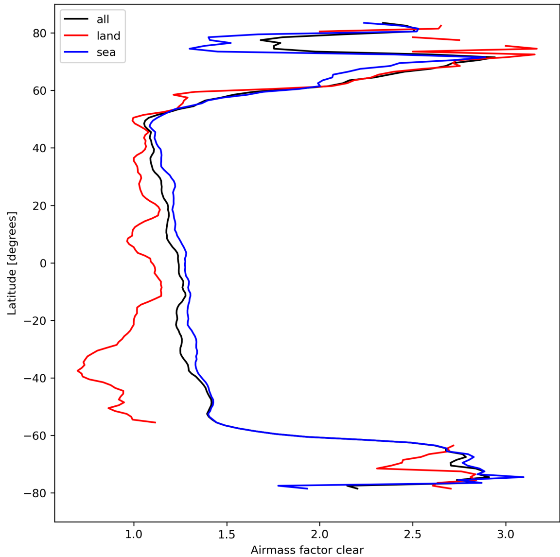
Figure 28: Zonal average of “Airmass factor clear” for 2024-03-20 to 2024-03-22.
