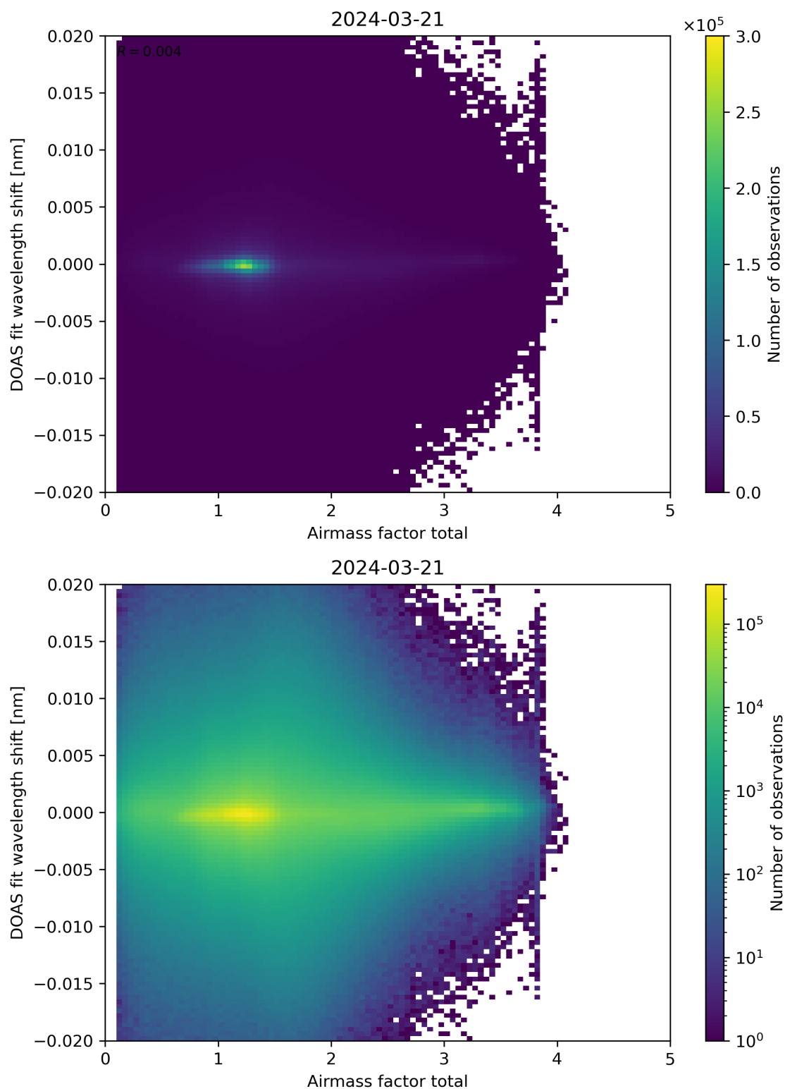
Figure 98: Scatter density plot of “Airmass factor total” against “DOAS fit wavelength shift” for 2024-03-20 to 2024-03-22.
