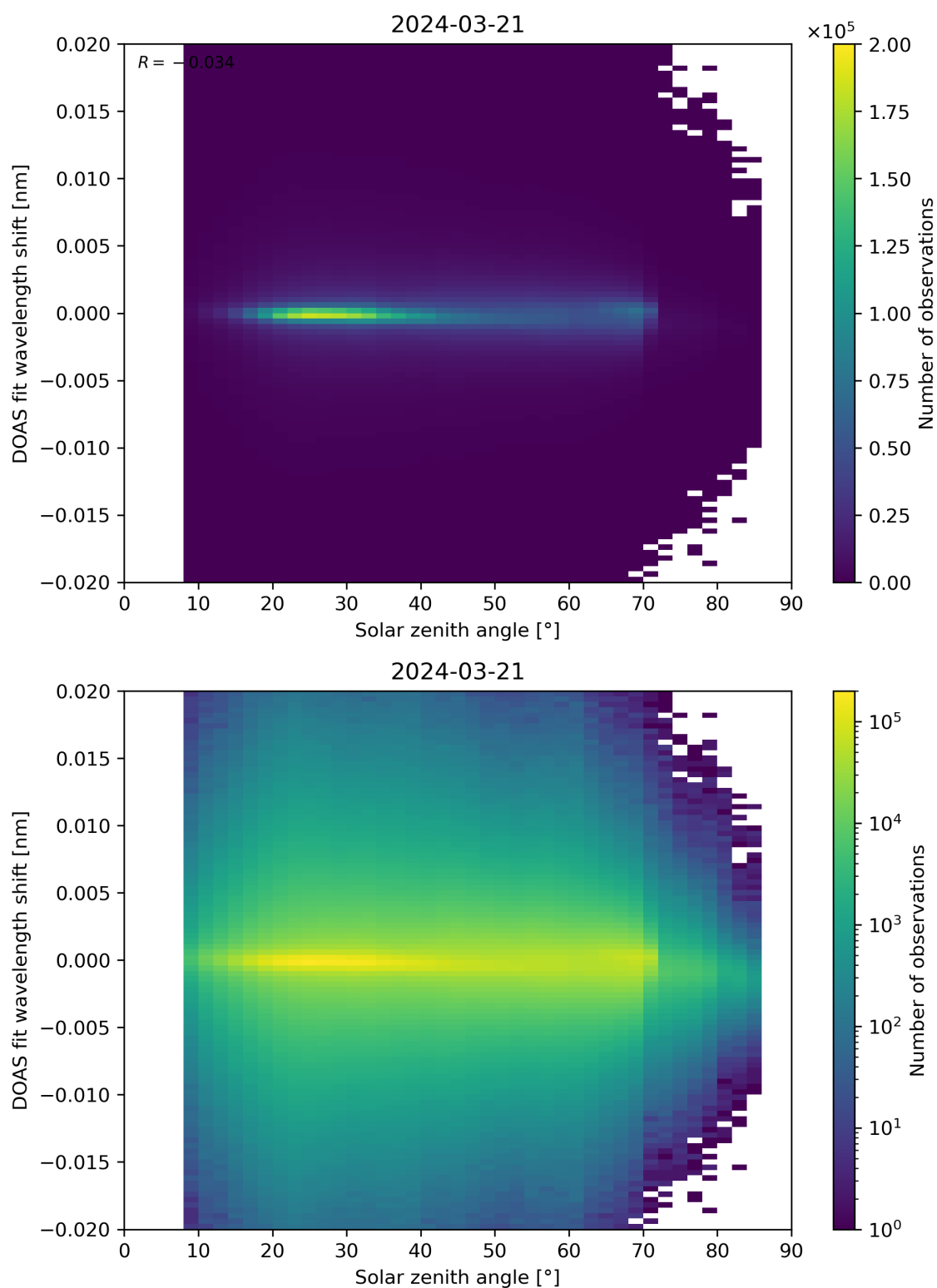
Figure 168: Scatter density plot of “Solar zenith angle” against “DOAS fit wavelength shift” for 2024-03-20 to 2024-03-22.
