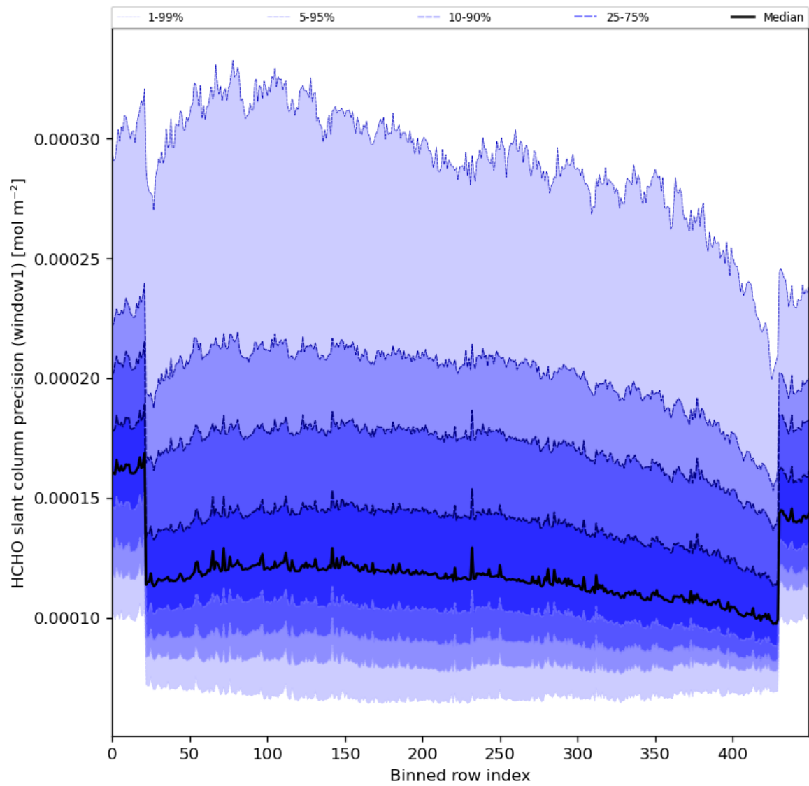
Figure 53: Along track statistics of “HCHO slant column precision (window1)” for 2024-03-20 to 2024-03-22
