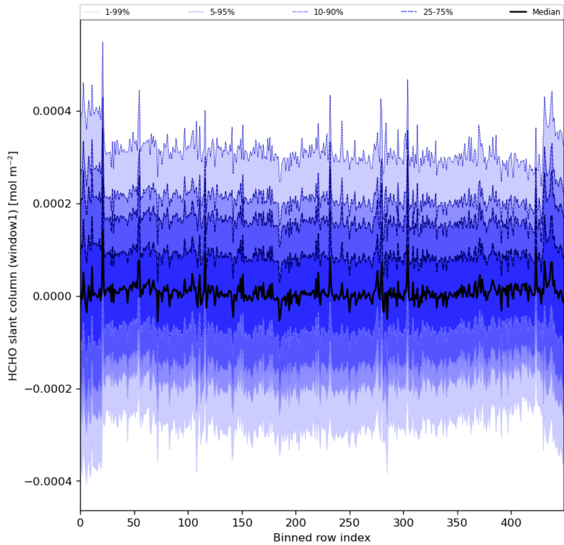
Figure 52: Along track statistics of “HCHO slant column (window1)” for 2024-03-20 to 2024-03-22
