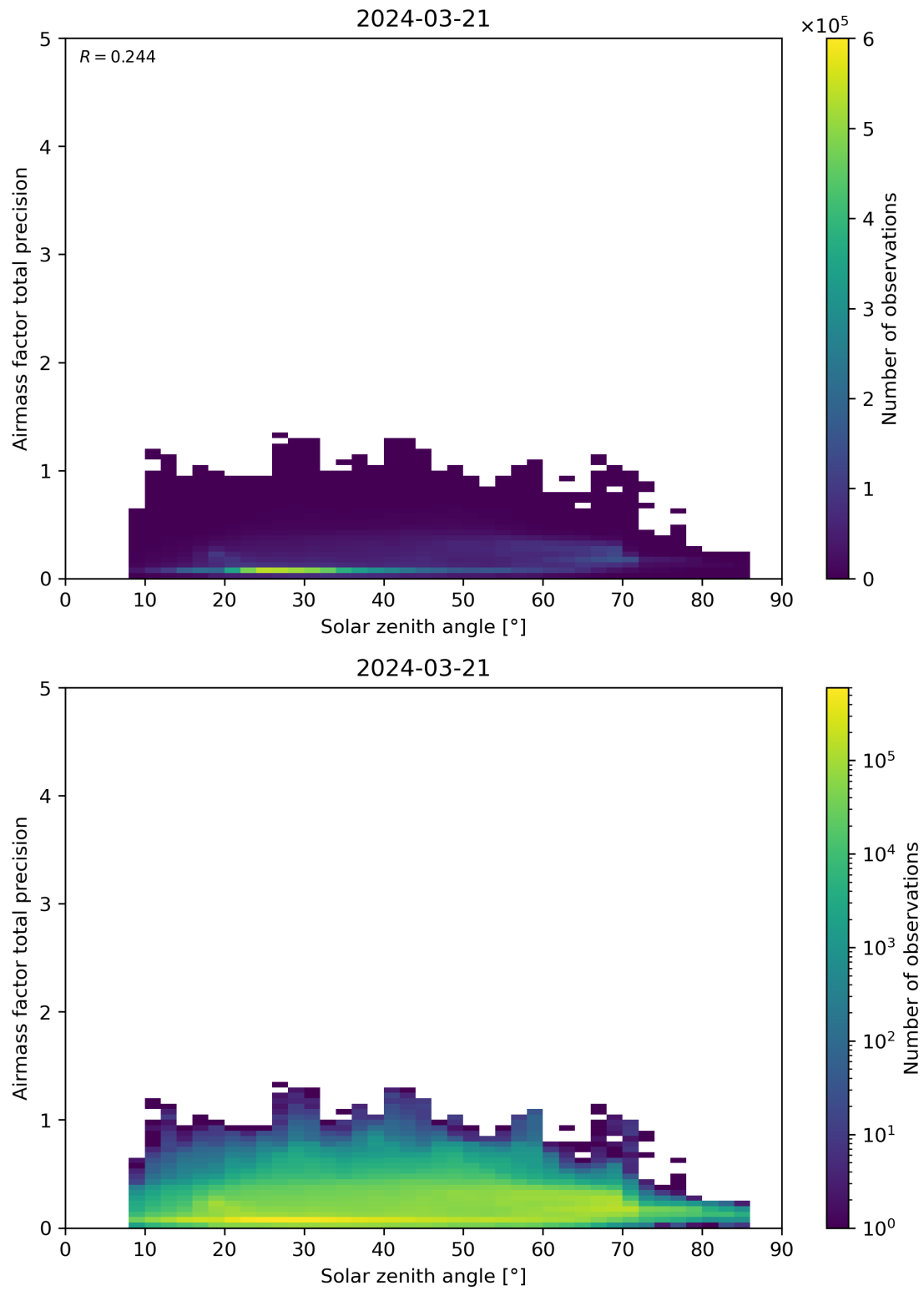
Figure 176: Scatter density plot of “Solar zenith angle” against “Airmass factor total precision” for 2024-03-20 to 2024-03-22.
