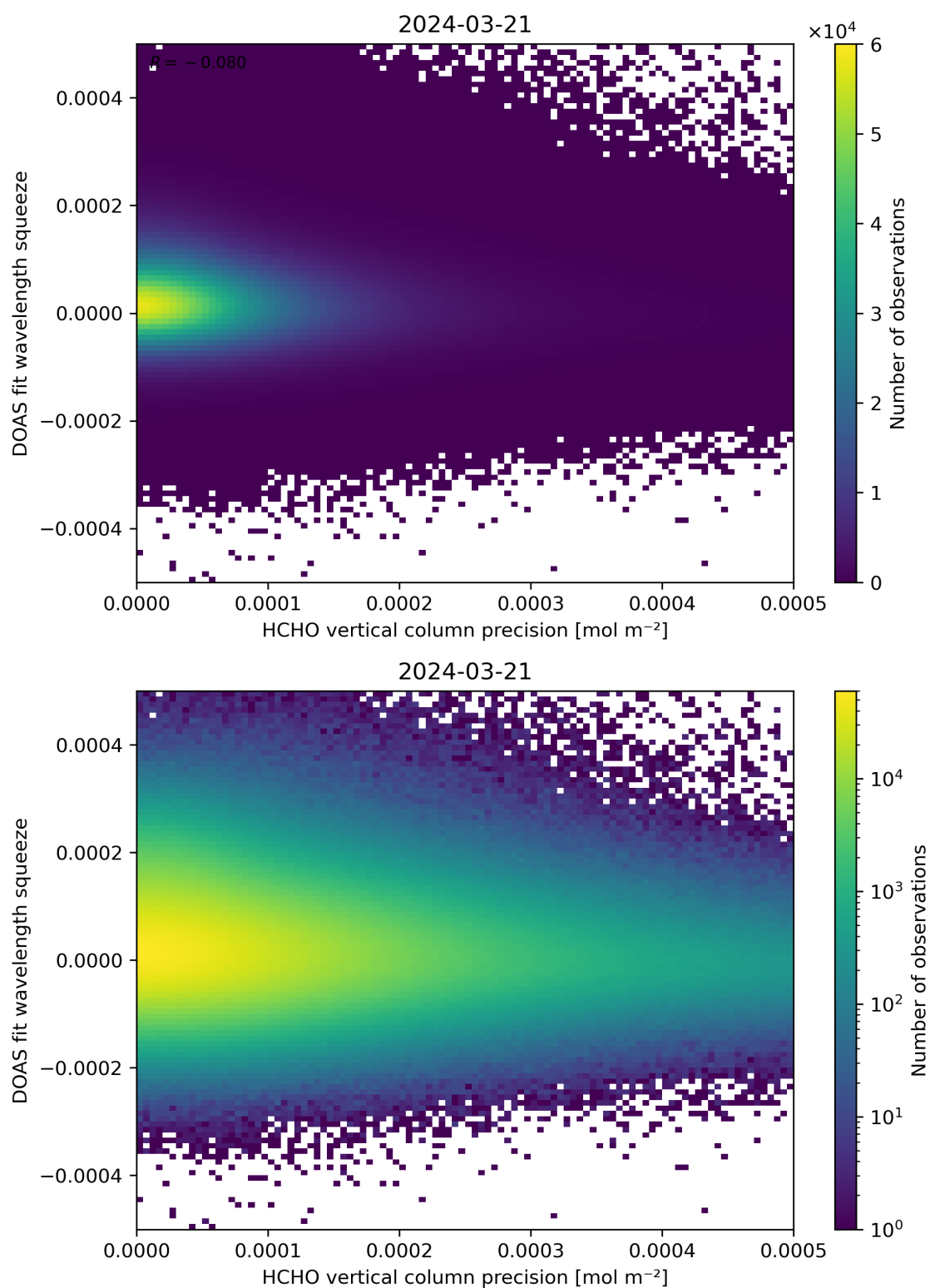
Figure 138: Scatter density plot of “HCHO vertical column precision” against “DOAS fit wavelength squeeze” for 2024-03-20 to 2024-03-22.
