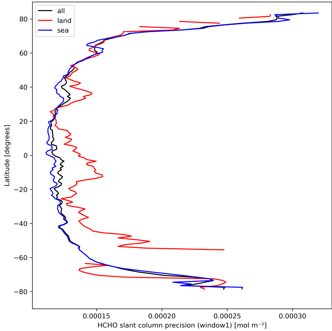
Figure 25: Zonal average of “HCHO slant column precision (window1)” for 2024-03-20 to 2024-03-22.
