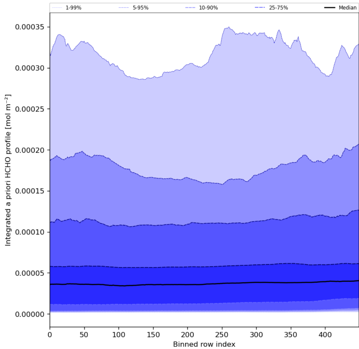
Figure 57: Along track statistics of “Integrated a priori HCHO profile” for 2024-03-20 to 2024-03-22
