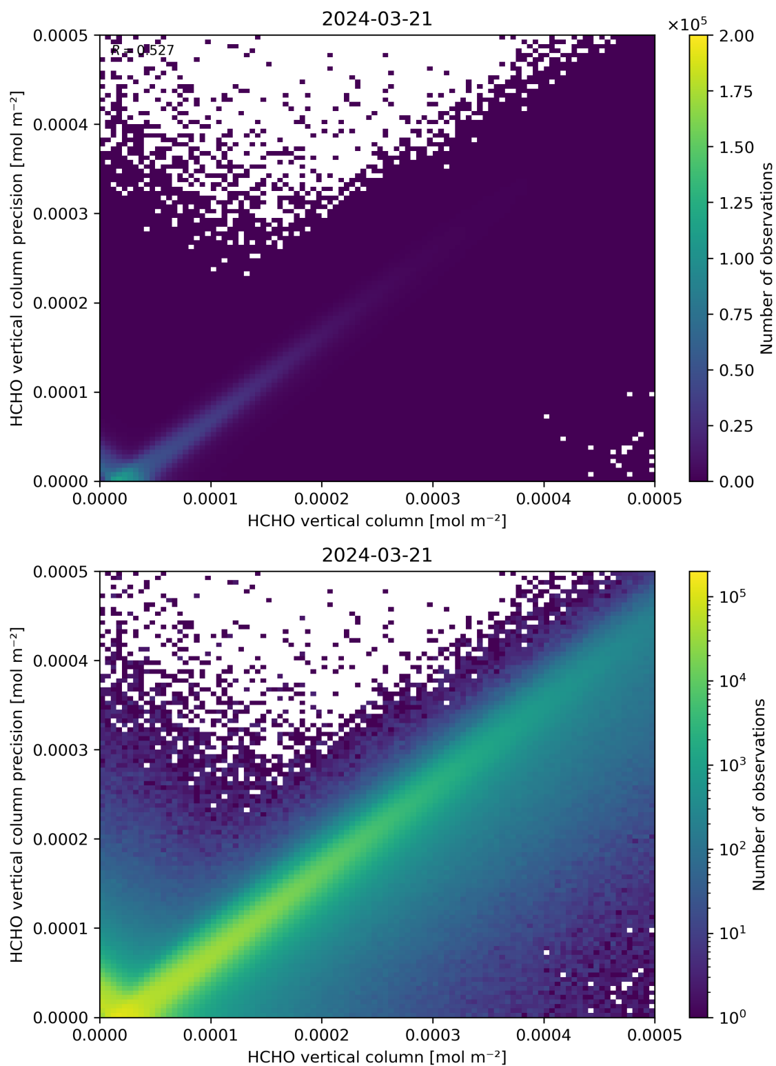
Figure 134: Scatter density plot of “HCHO vertical column” against “HCHO vertical column precision” for 2024-03-20 to 2024-03-22.
