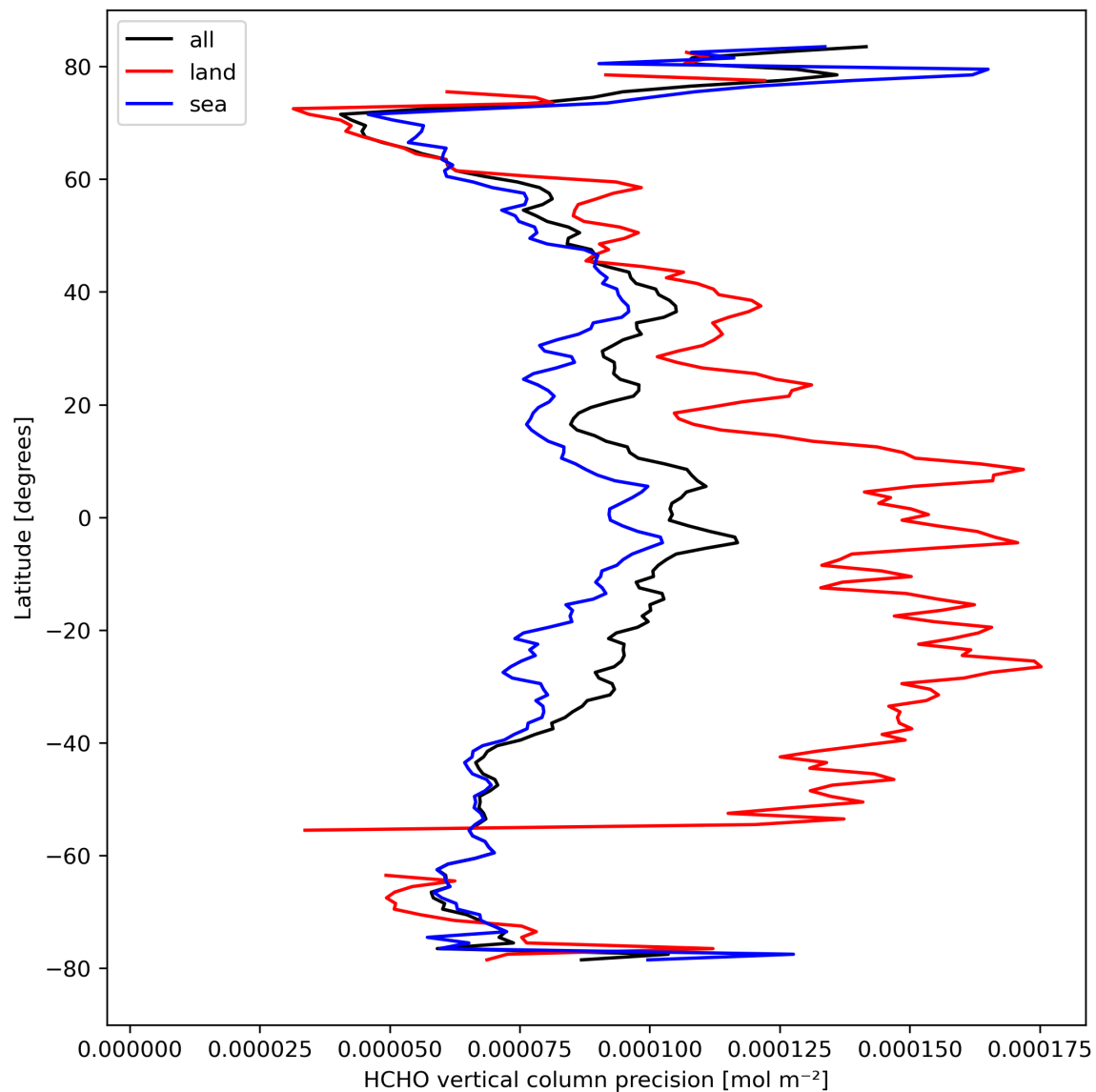
Figure 22: Zonal average of “HCHO vertical column precision” for 2024-03-20 to 2024-03-22.
