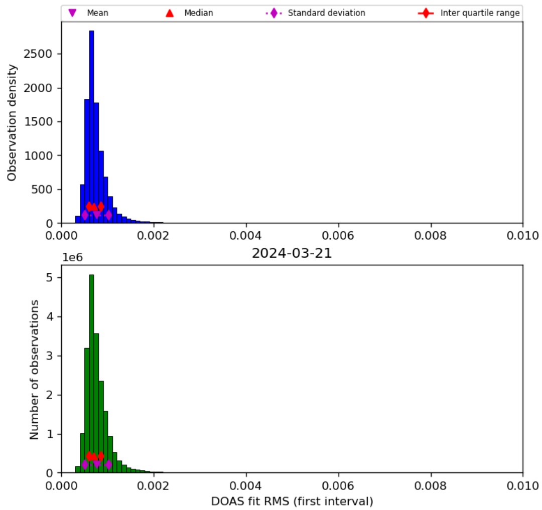
Figure 46: Histogram of “DOAS fit RMS (first interval)” for 2024-03-20 to 2024-03-22
