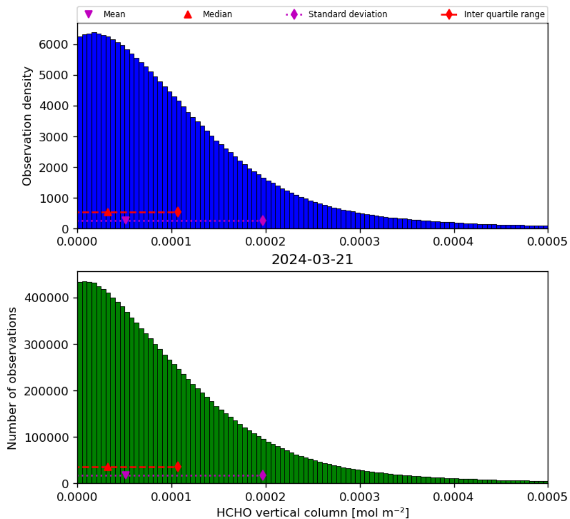
Figure 35: Histogram of “HCHO vertical column” for 2024-03-20 to 2024-03-22
