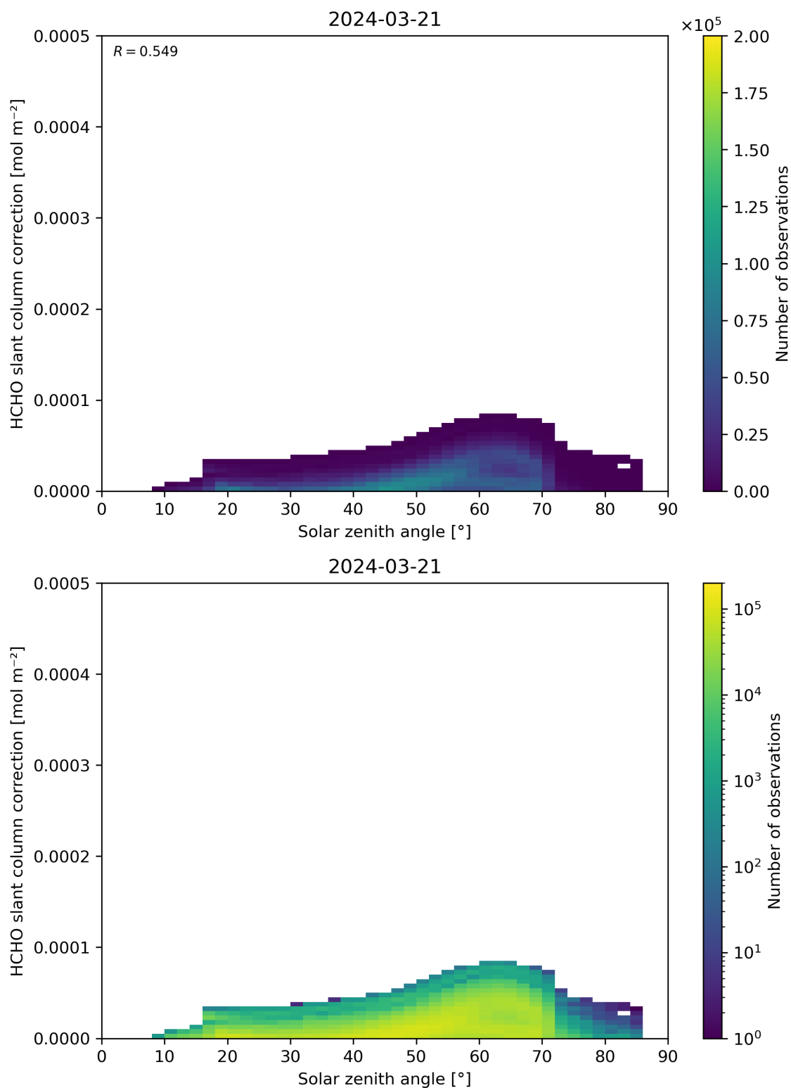
Figure 172: Scatter density plot of “Solar zenith angle” against “HCHO slant column correction” for 2024-03-20 to 2024-03-22.
