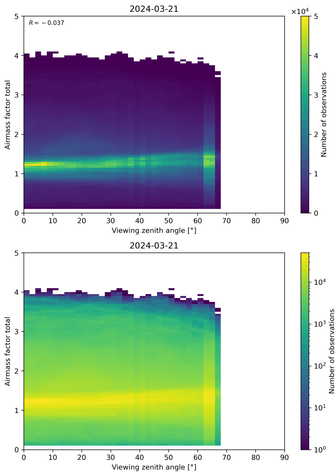
Figure 190: Scatter density plot of “Viewing zenith angle” against “Airmass factor total” for 2024-03-20 to 2024-03-22.
