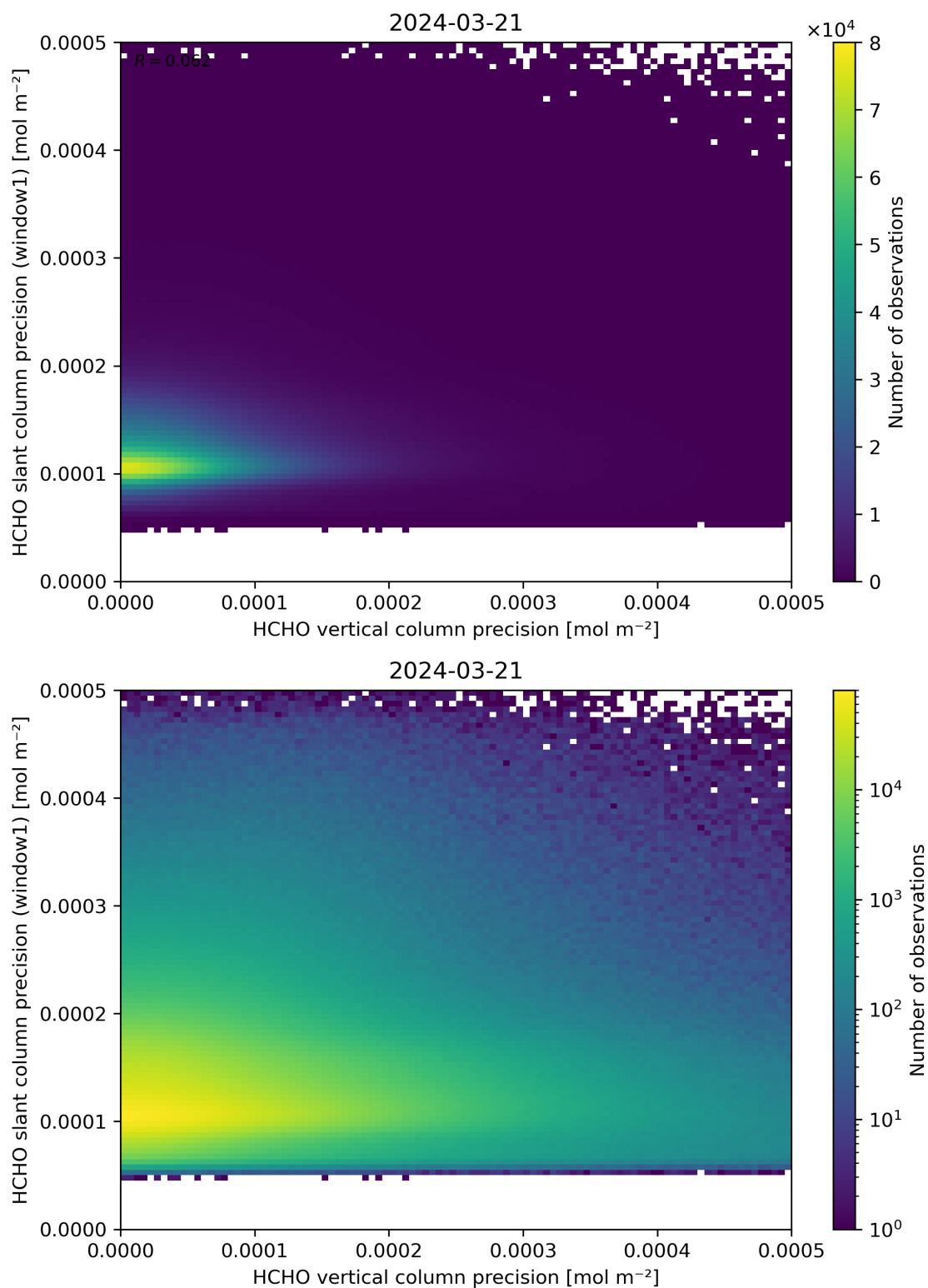
Figure 143: Scatter density plot of “HCHO vertical column precision” against “HCHO slant column precision (window1)” for 2024-03-20 to 2024-03-22.
