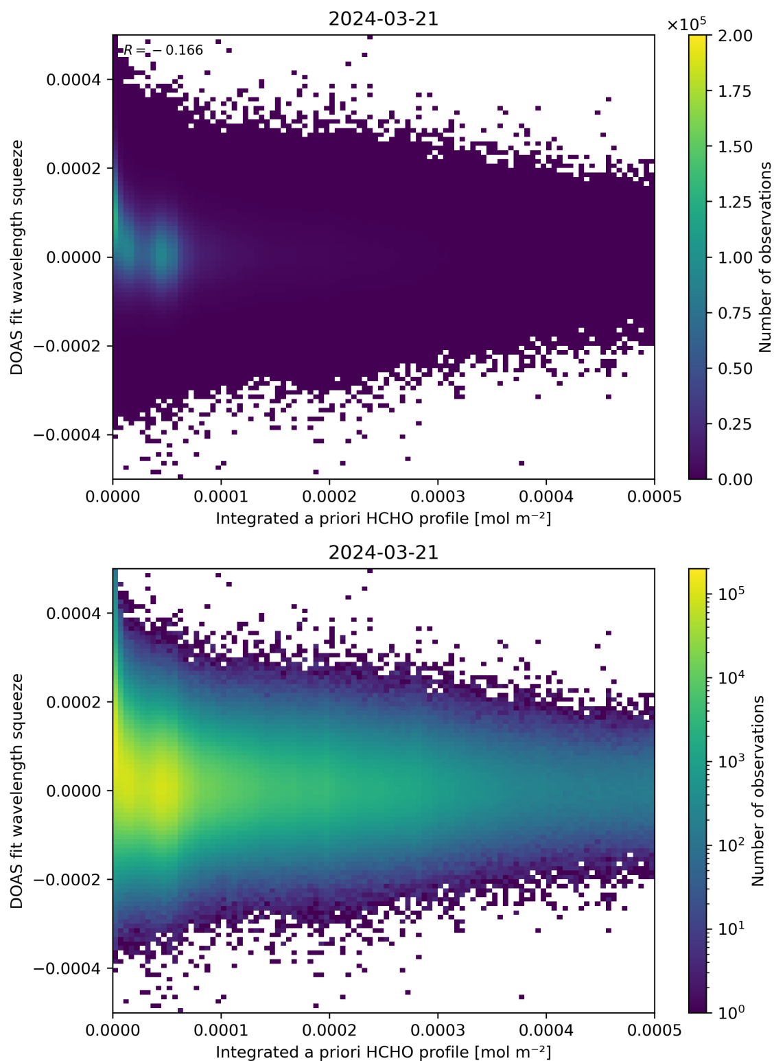
Figure 150: Scatter density plot of “Integrated a priori HCHO profile” against “DOAS fit wavelength squeeze” for 2024-03-20 to 2024-03-22.
