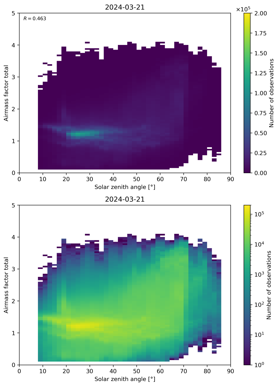
Figure 175: Scatter density plot of “Solar zenith angle” against “Airmass factor total” for 2024-03-20 to 2024-03-22.
