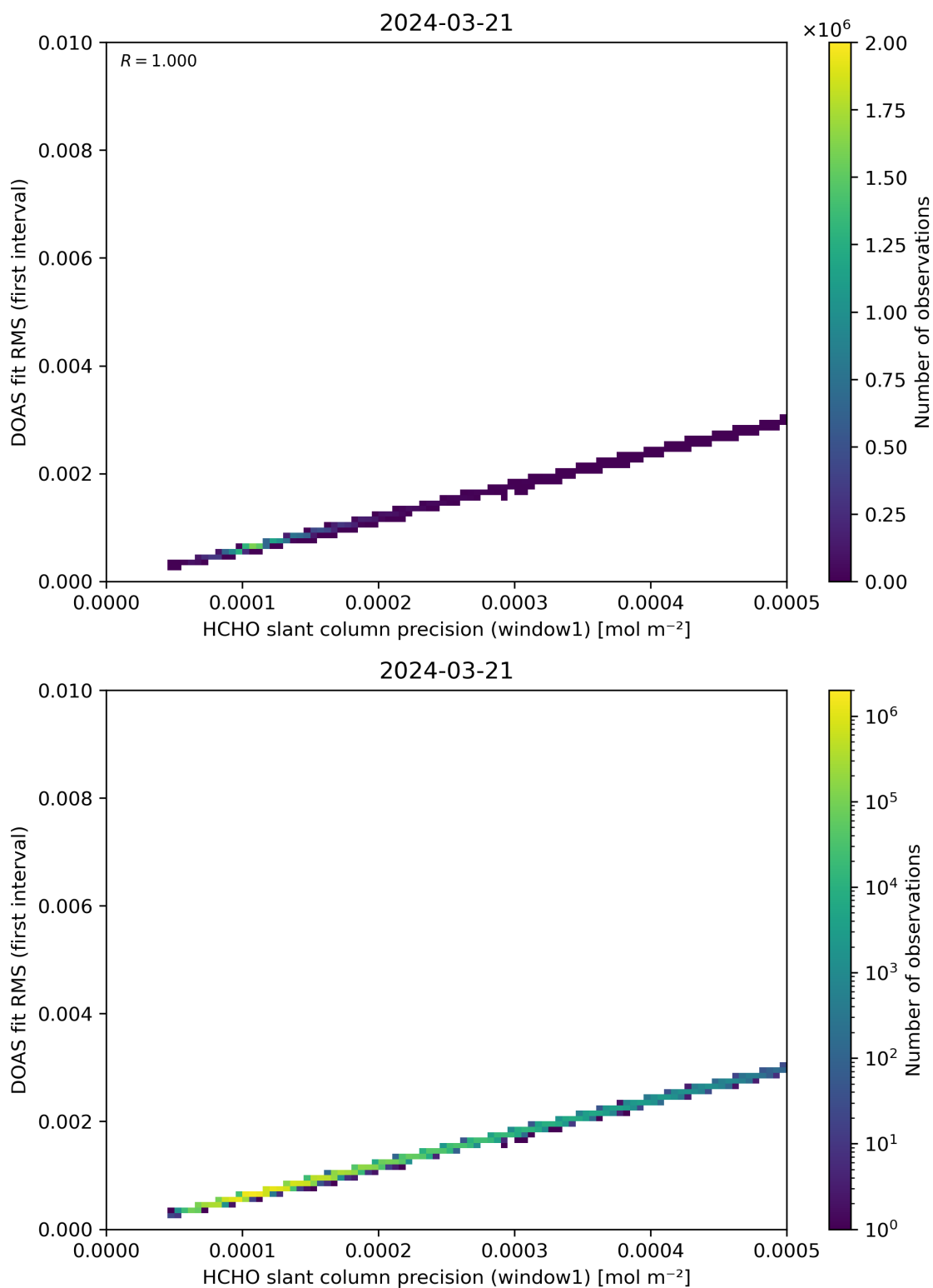
Figure 88: Scatter density plot of “HCHO slant column precision (window1)” against “DOAS fit RMS (first interval)” for 2024-03-20 to 2024-03-22.
