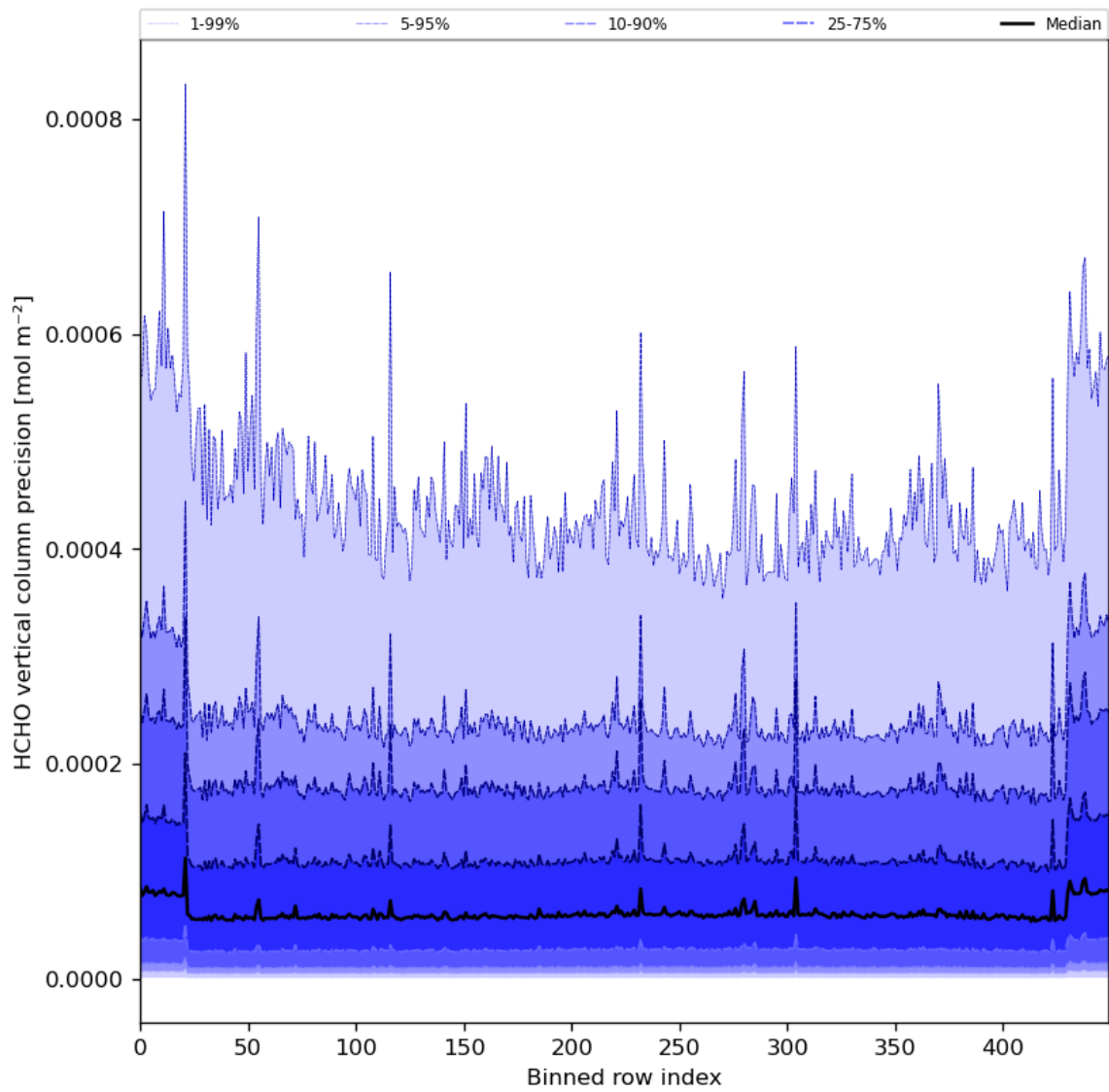
Figure 50: Along track statistics of “HCHO vertical column precision” for 2024-03-20 to 2024-03-22
