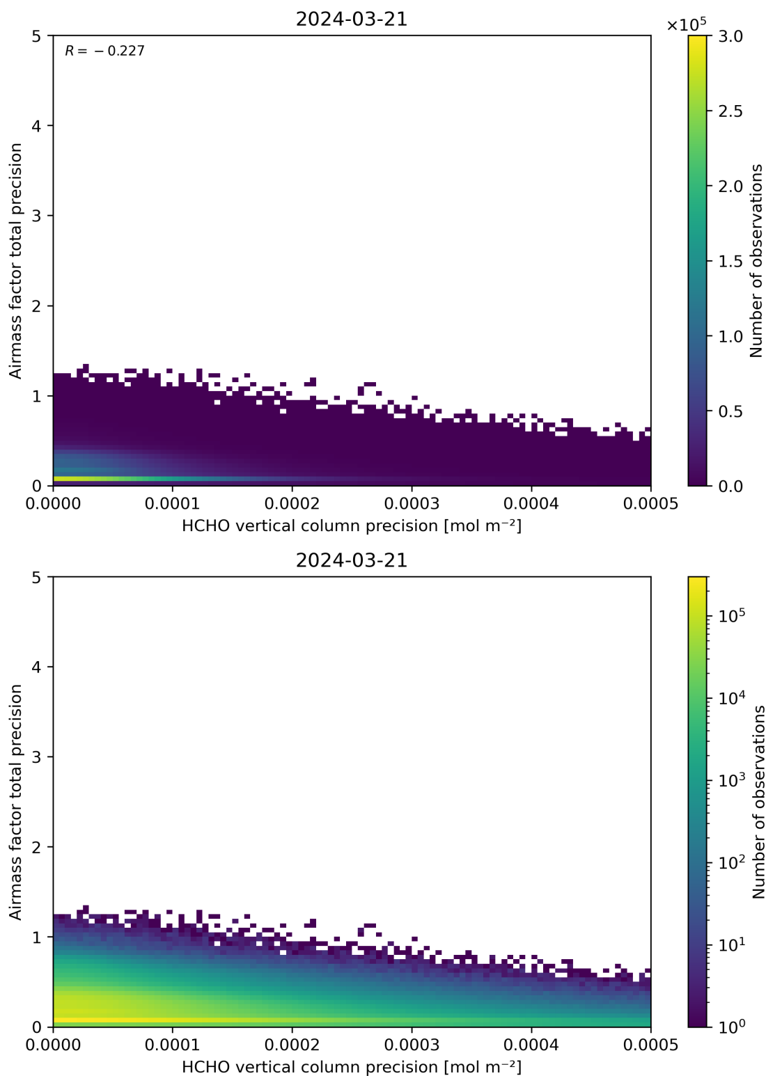
Figure 145: Scatter density plot of “HCHO vertical column precision” against “Airmass factor total precision” for 2024-03-20 to 2024-03-22.
