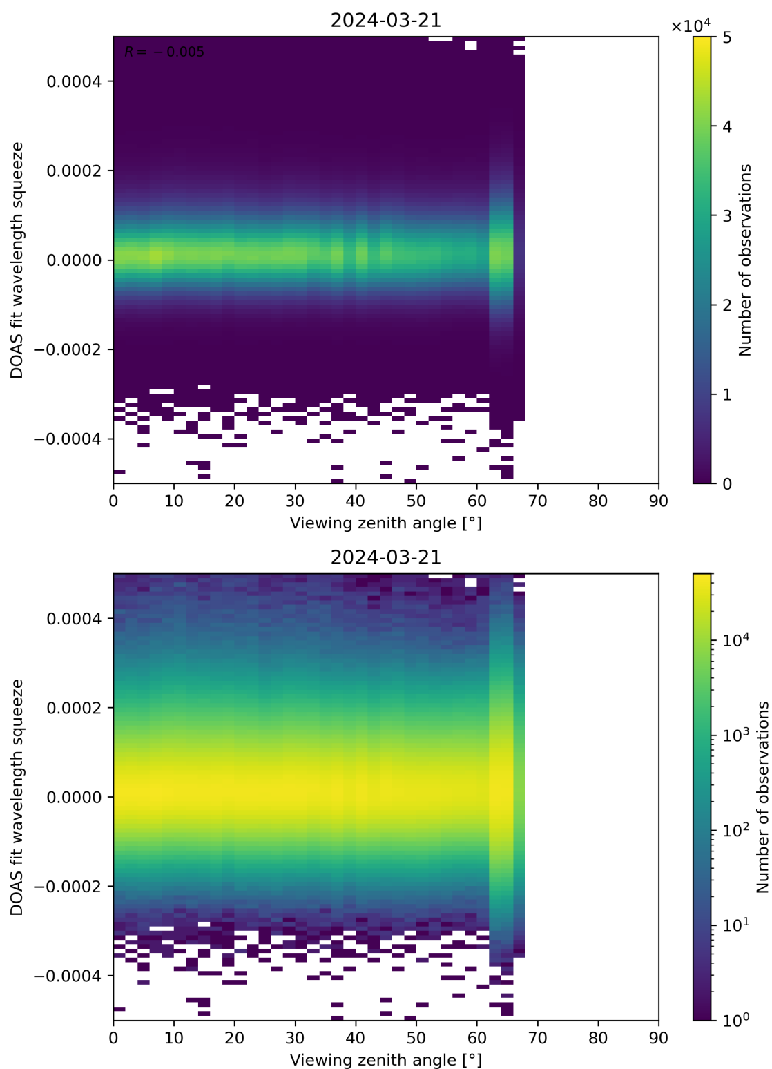
Figure 184: Scatter density plot of “Viewing zenith angle” against “DOAS fit wavelength squeeze” for 2024-03-20 to 2024-03-22.
