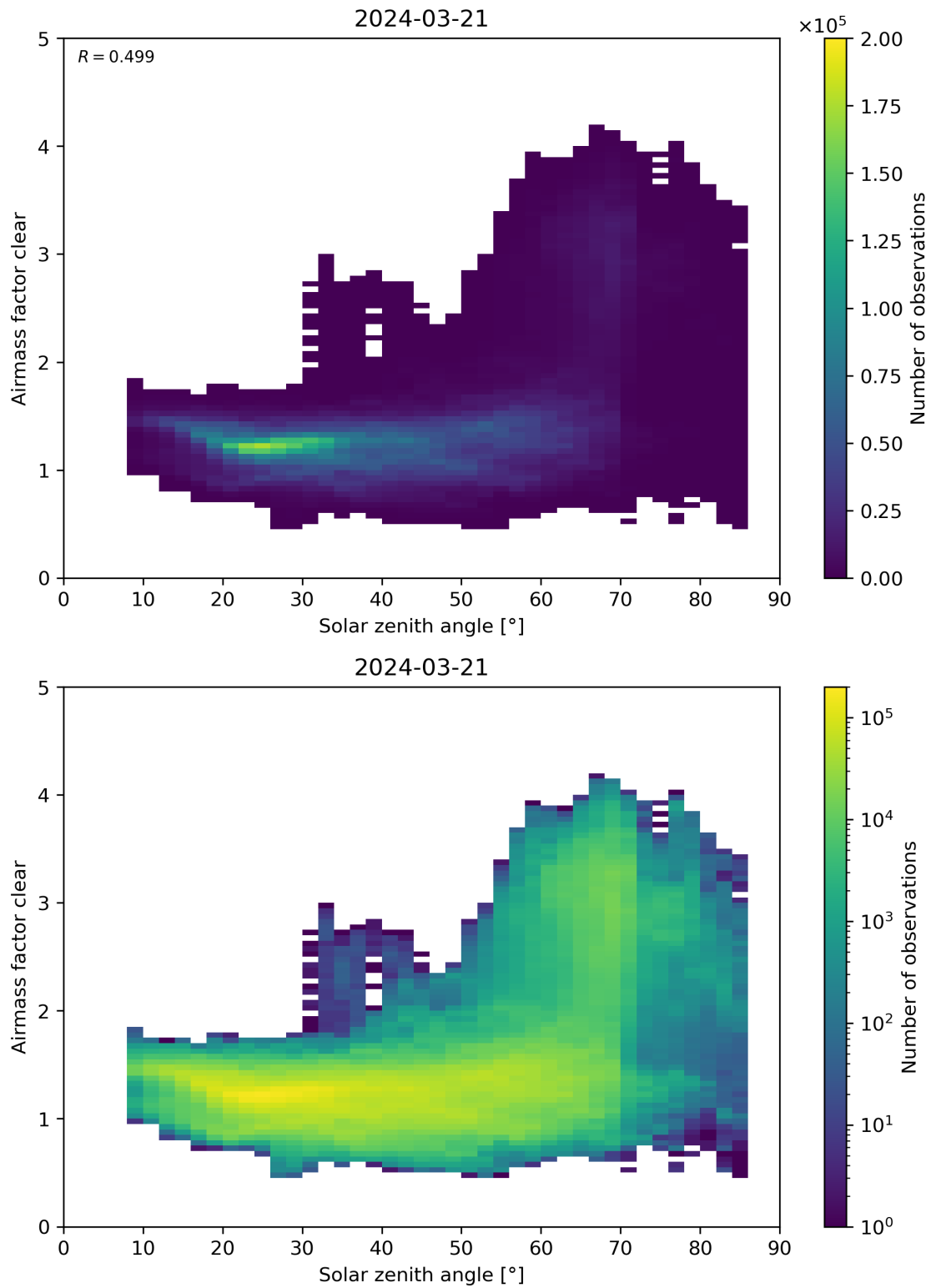
Figure 170: Scatter density plot of “Solar zenith angle” against “Airmass factor clear” for 2024-03-20 to 2024-03-22.
