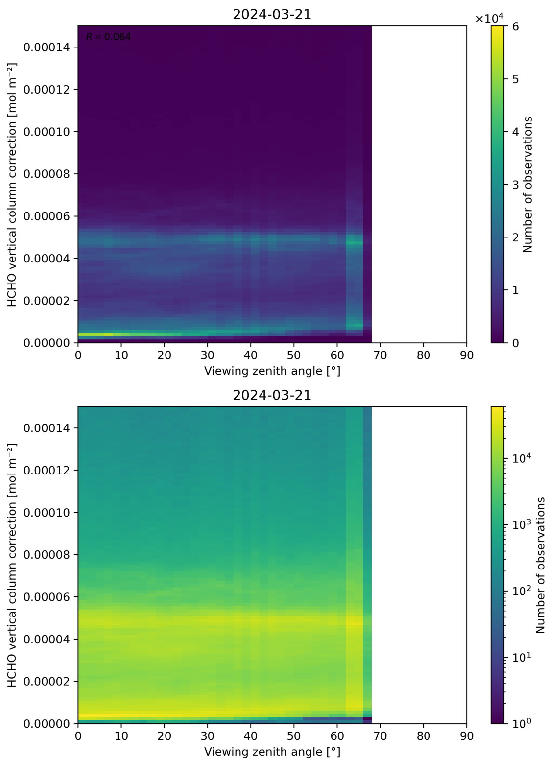
Figure 193: Scatter density plot of “Viewing zenith angle” against “HCHO vertical column correction” for 2024-03-20 to 2024-03-22.
