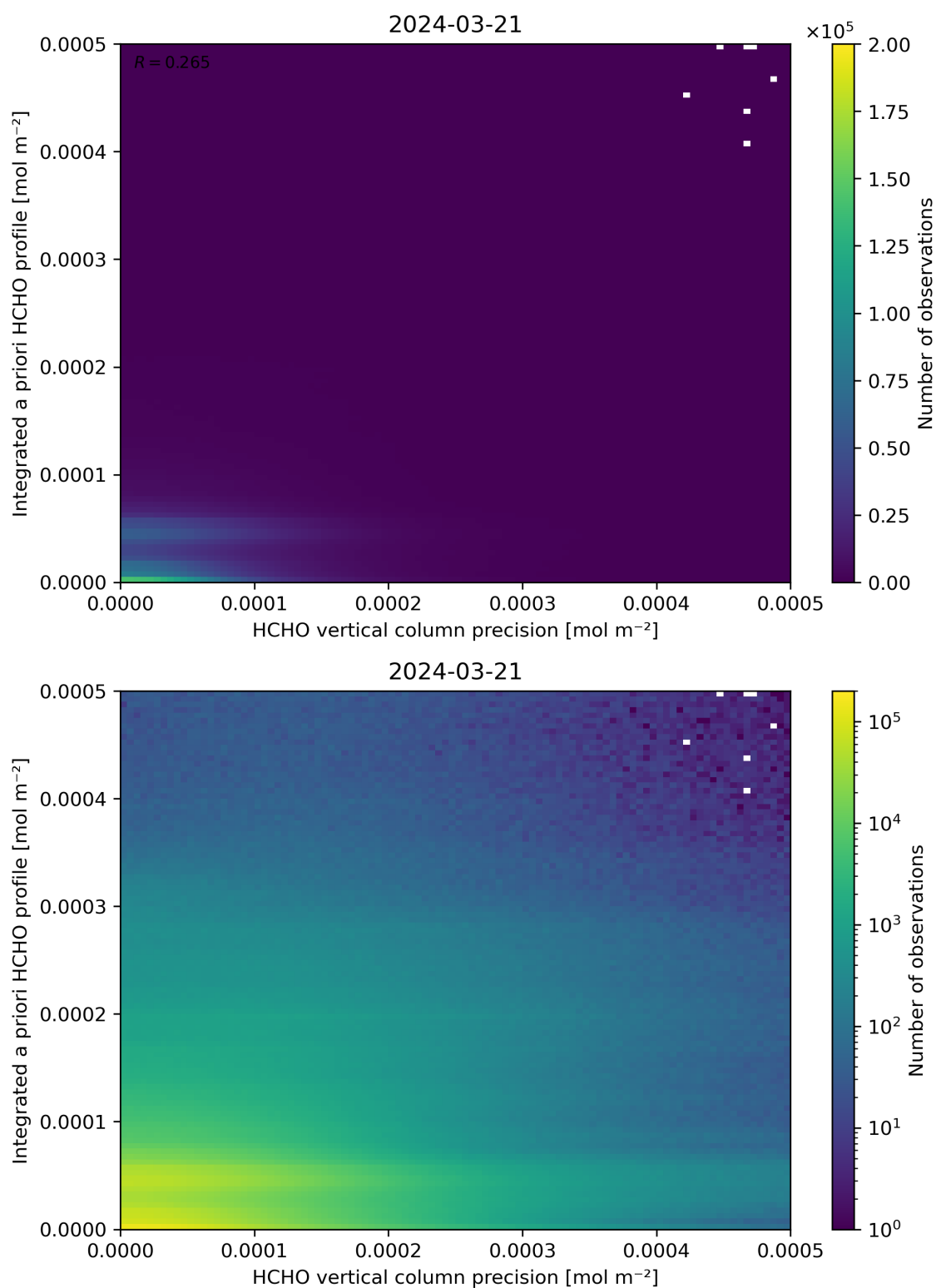
Figure 147: Scatter density plot of “HCHO vertical column precision” against “Integrated a priori HCHO profile” for 2024-03-20 to 2024-03-22.
