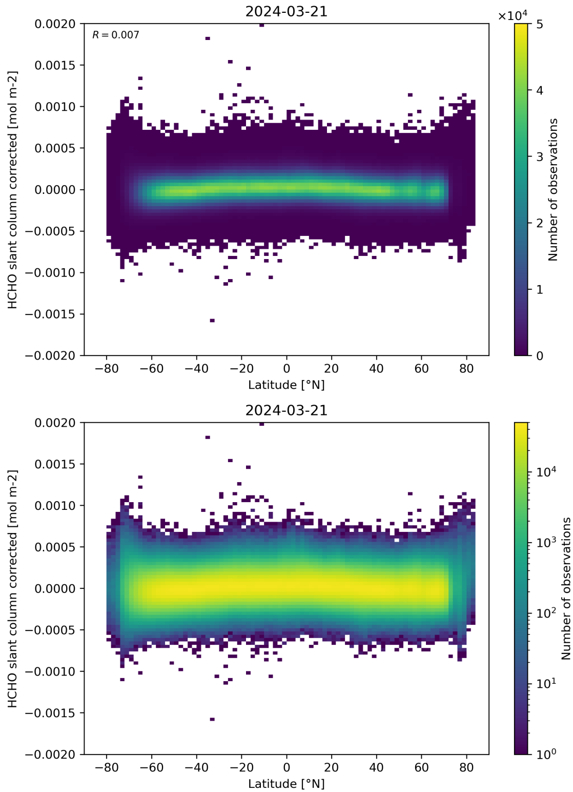
Figure 157: Scatter density plot of “Latitude” against “HCHO slant column corrected” for 2024-03-20 to 2024-03-22.
