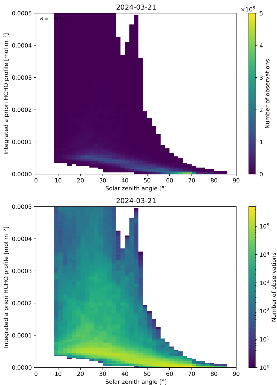
Figure 180: Scatter density plot of “Solar zenith angle” against “Integrated a priori HCHO profile” for 2024-03-20 to 2024-03-22.
