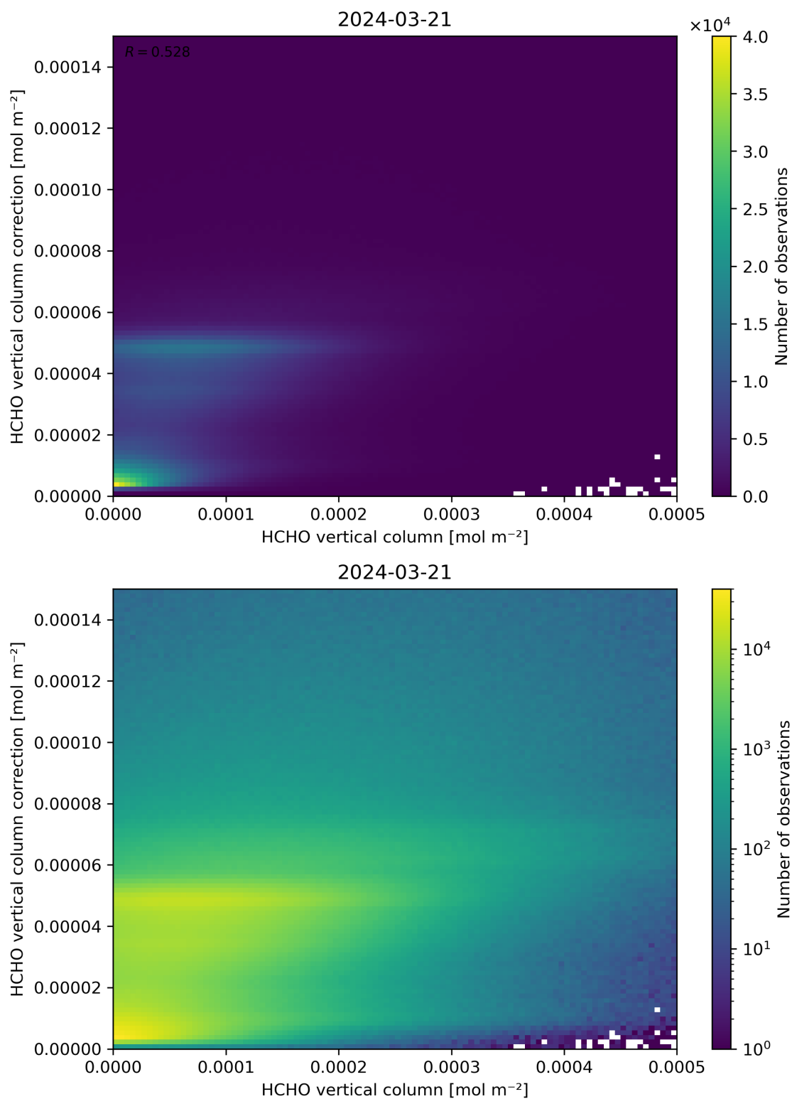
Figure 133: Scatter density plot of “HCHO vertical column” against “HCHO vertical column correction” for 2024-03-20 to 2024-03-22.
