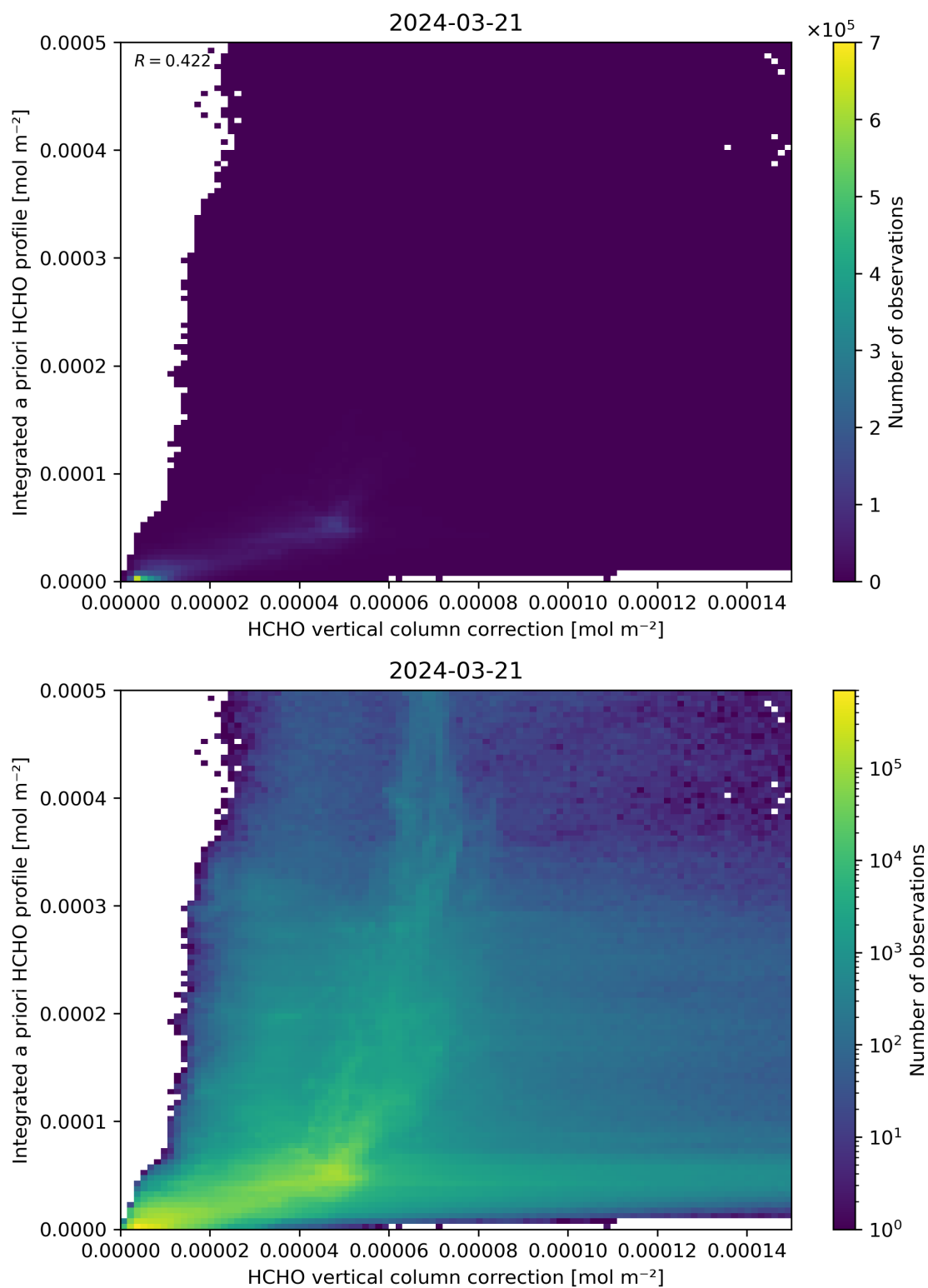
Figure 122: Scatter density plot of “HCHO vertical column correction” against “Integrated a priori HCHO profile” for 2024-03-20 to 2024-03-22.
