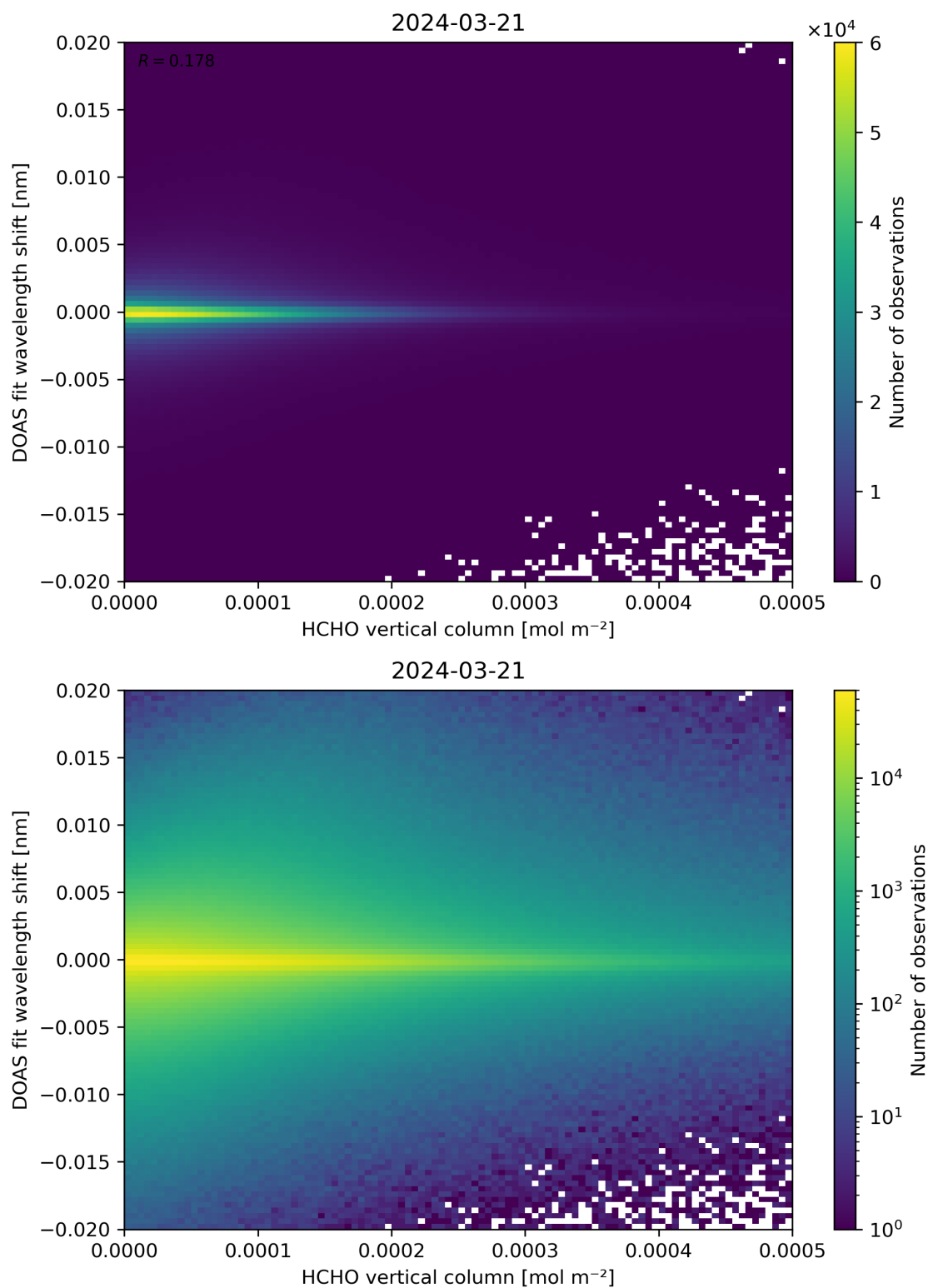
Figure 124: Scatter density plot of “HCHO vertical column” against “DOAS fit wavelength shift” for 2024-03-20 to 2024-03-22.
