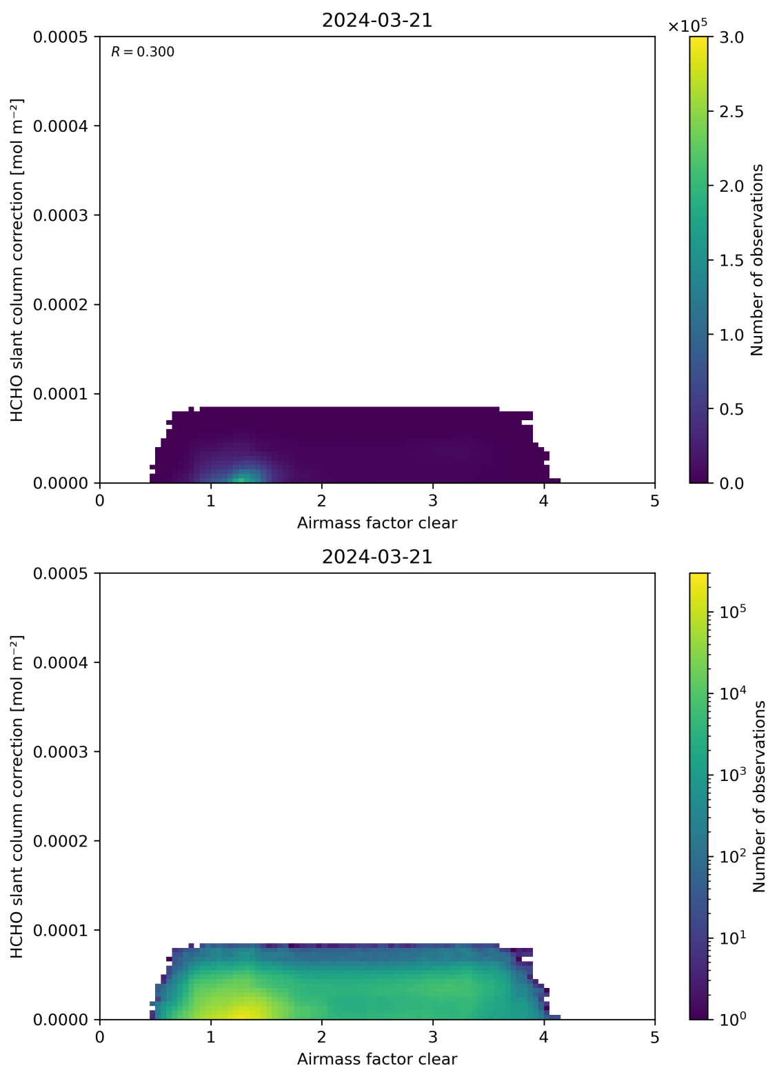
Figure 75: Scatter density plot of “Airmass factor clear” against “HCHO slant column correction” for 2024-03-20 to 2024-03-22.
