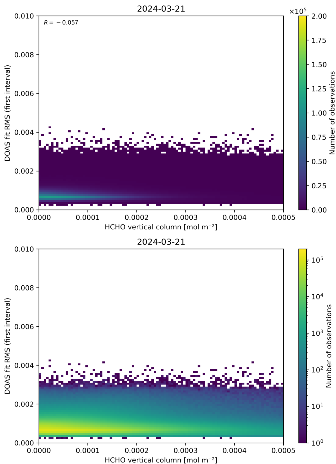
Figure 123: Scatter density plot of “HCHO vertical column” against “DOAS fit RMS (first interval)” for 2024-03-20 to 2024-03-22.
