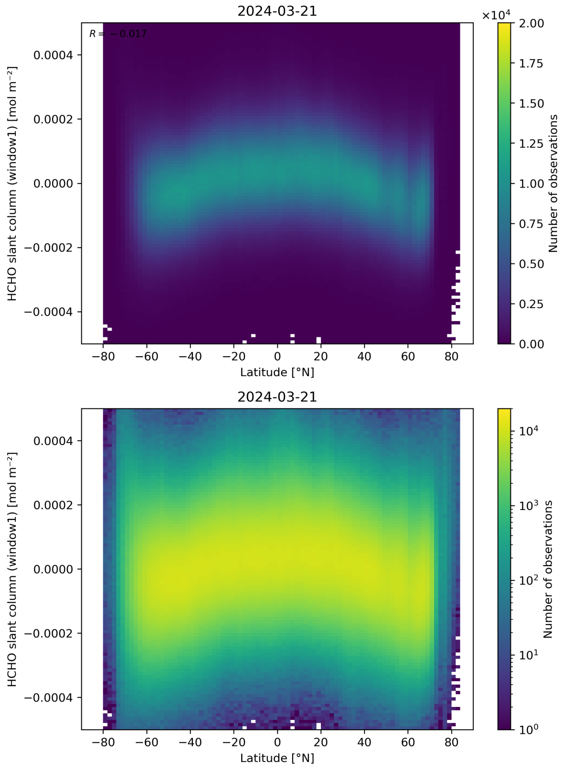
Figure 159: Scatter density plot of “Latitude” against “HCHO slant column (window1)” for 2024-03-20 to 2024-03-22.
