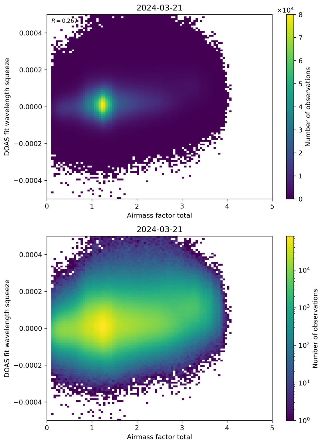
Figure 99: Scatter density plot of “Airmass factor total” against “DOAS fit wavelength squeeze” for 2024-03-20 to 2024-03-22.
