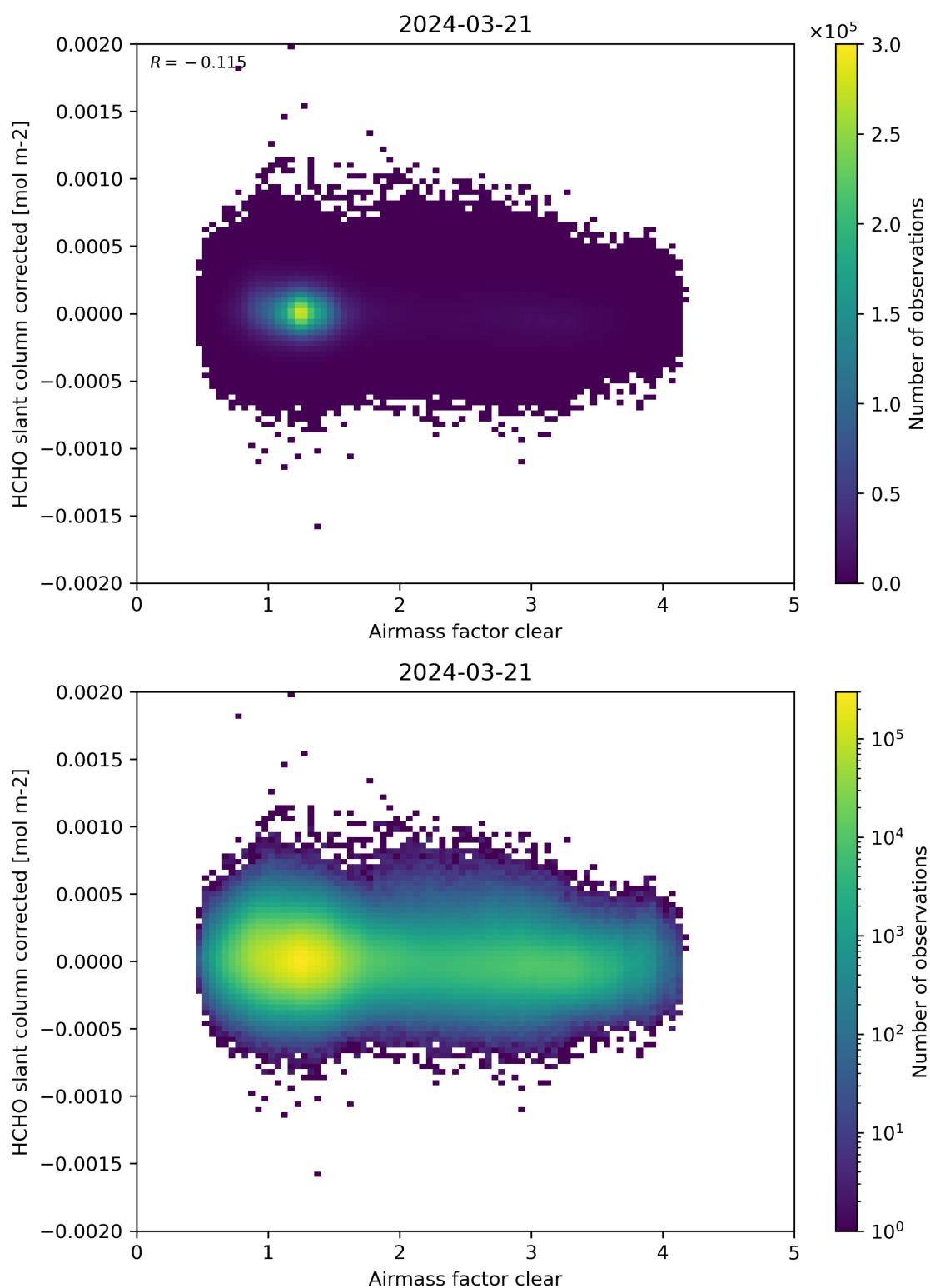
Figure 74: Scatter density plot of “Airmass factor clear” against “HCHO slant column corrected” for 2024-03-20 to 2024-03-22.
