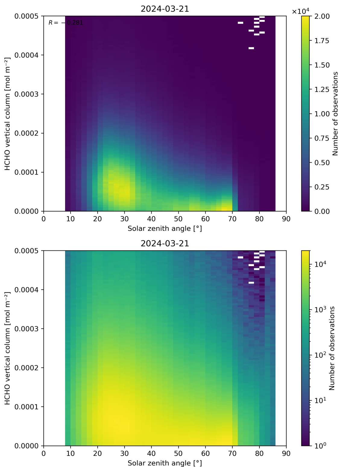
Figure 177: Scatter density plot of “Solar zenith angle” against “HCHO vertical column” for 2024-03-20 to 2024-03-22.
