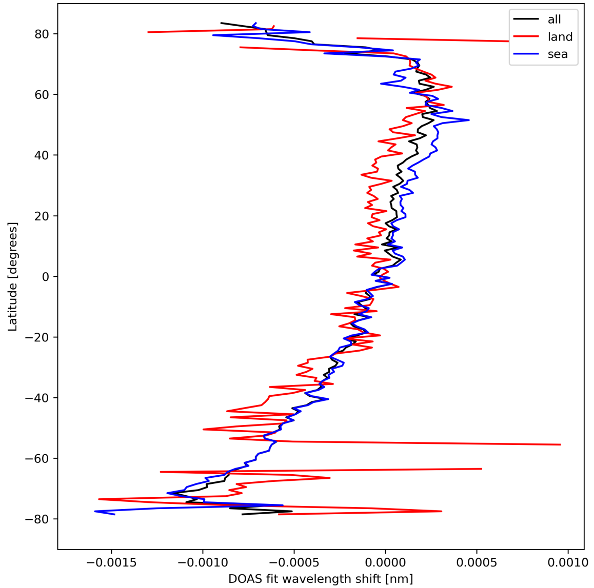
Figure 30: Zonal average of “DOAS fit wavelength shift” for 2024-03-20 to 2024-03-22.
