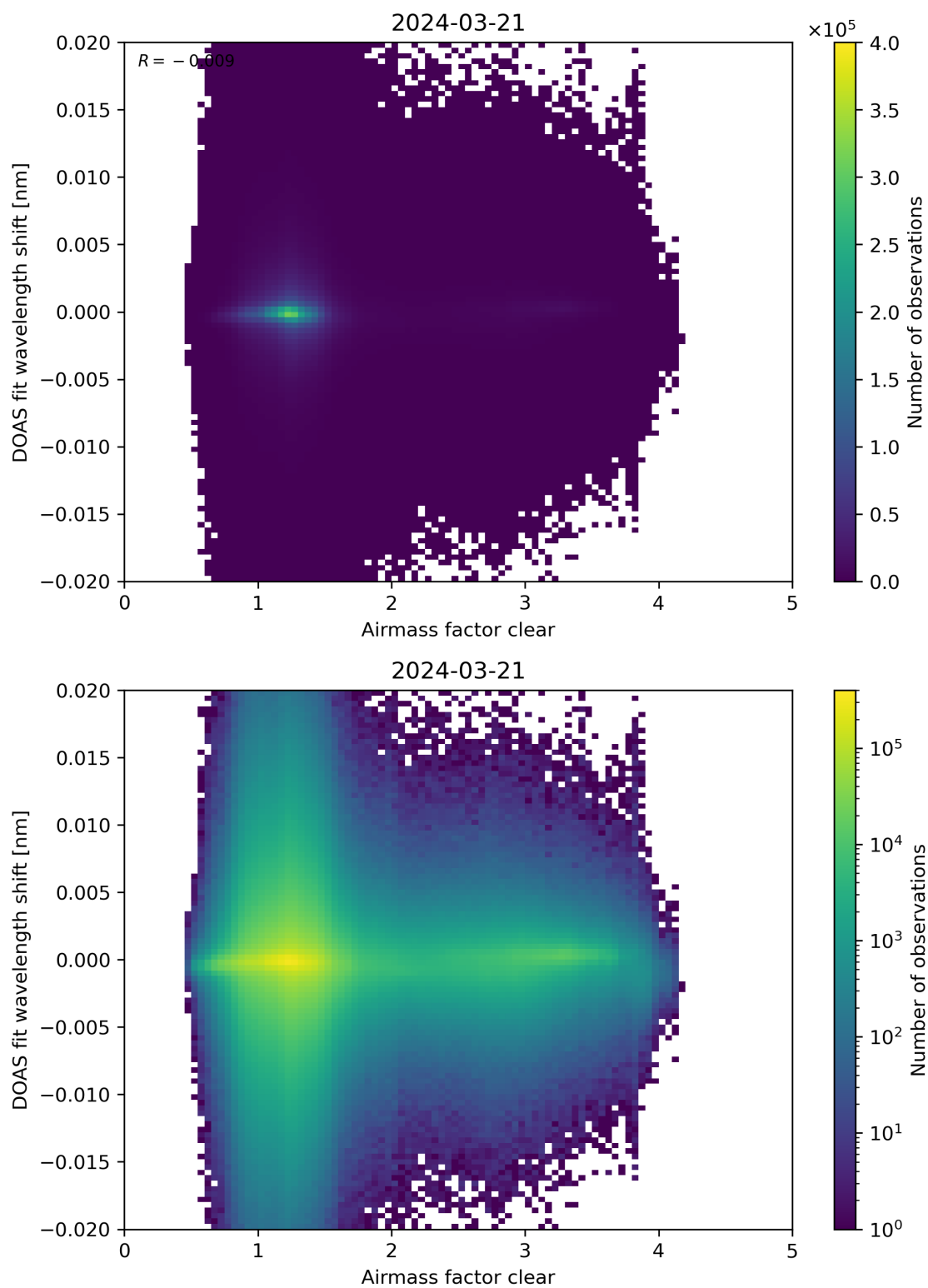
Figure 72: Scatter density plot of “Airmass factor clear” against “DOAS fit wavelength shift” for 2024-03-20 to 2024-03-22.
