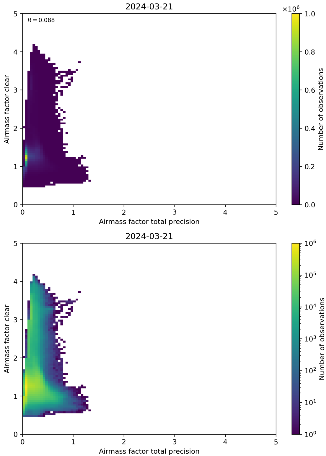
Figure 108: Scatter density plot of “Airmass factor total precision” against “Airmass factor clear” for 2024-03-20 to 2024-03-22.
