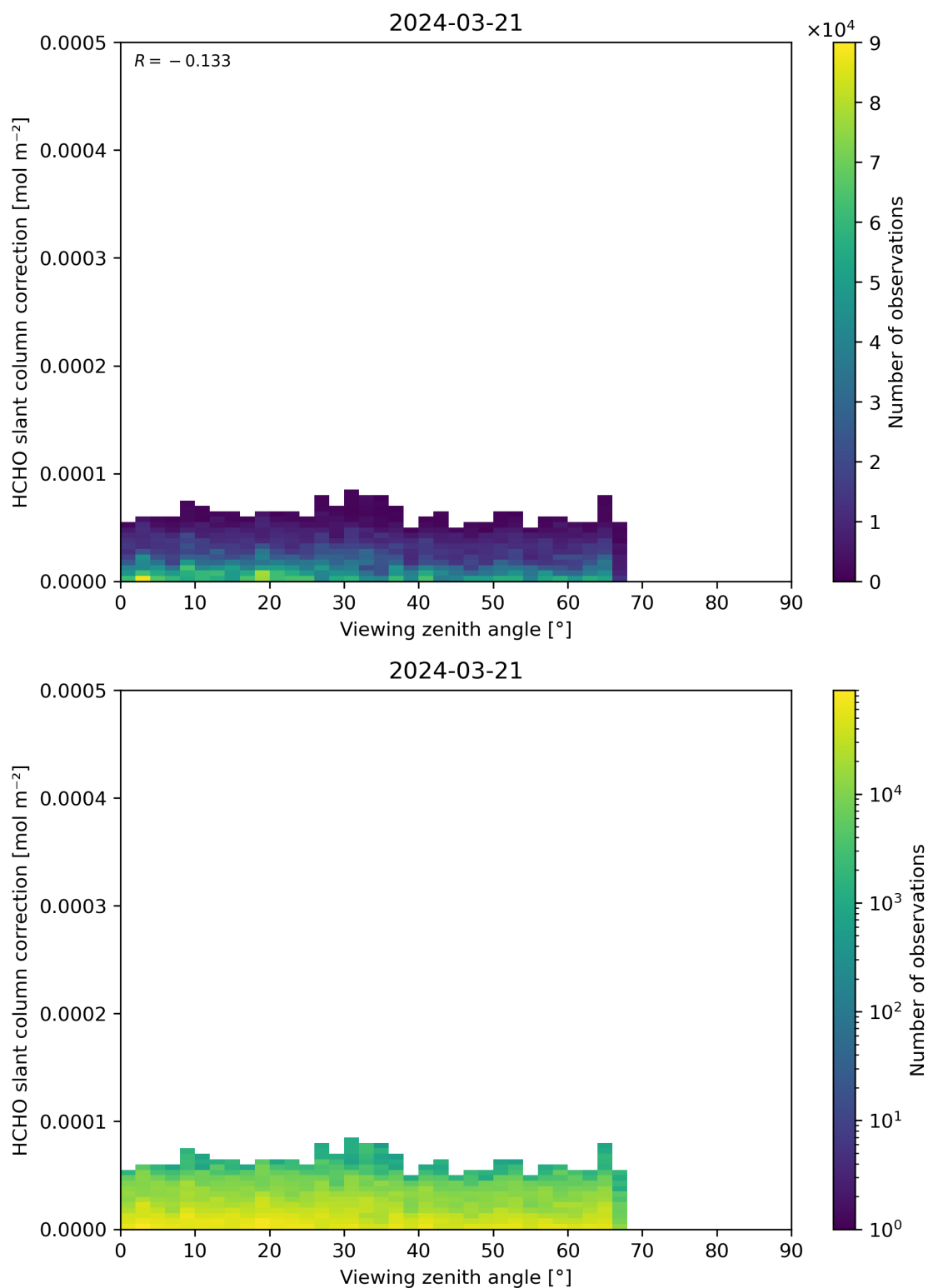
Figure 187: Scatter density plot of “Viewing zenith angle” against “HCHO slant column correction” for 2024-03-20 to 2024-03-22.
