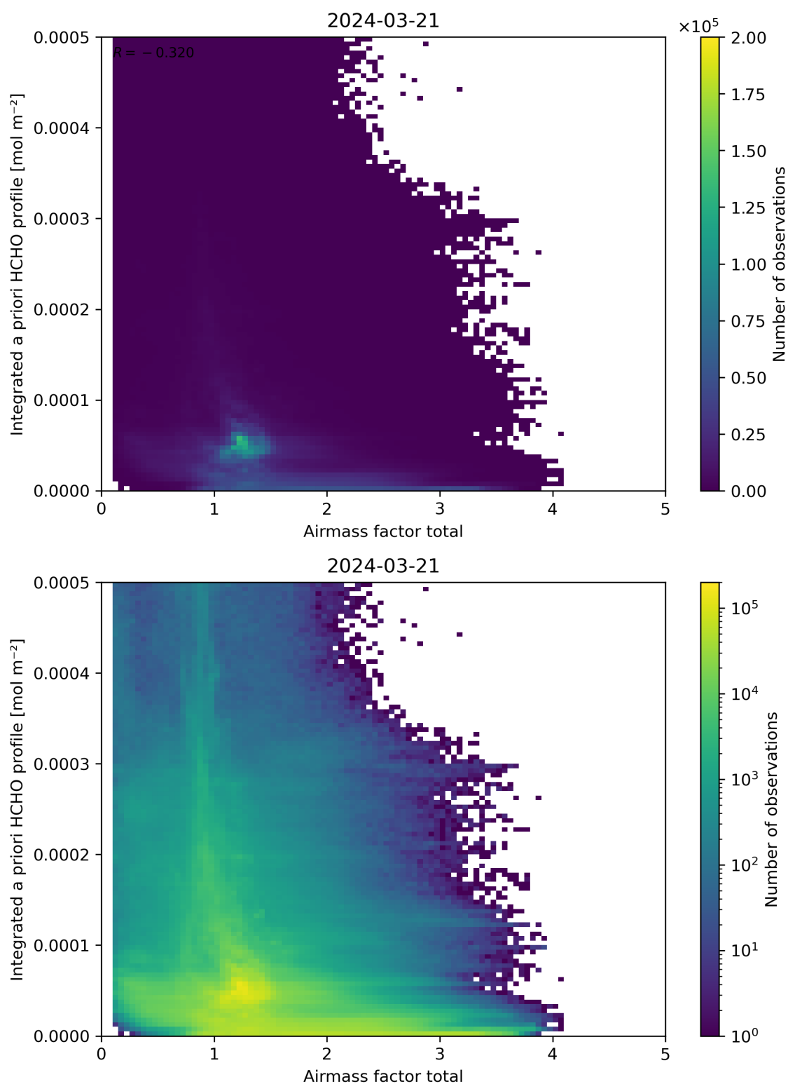
Figure 104: Scatter density plot of “Air mass factor total” against “Integrated a priori HCHO profile” for 2024-03-20 to 2024-03-22.
