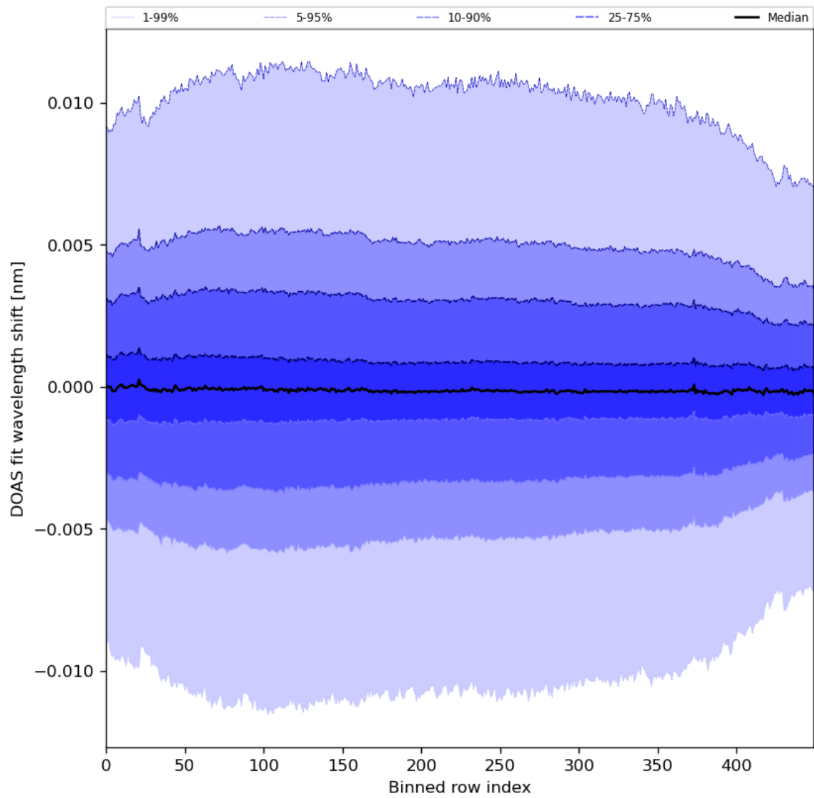
Figure 58: Along track statistics of “DOAS fit wavelength shift” for 2024-03-20 to 2024-03-22
