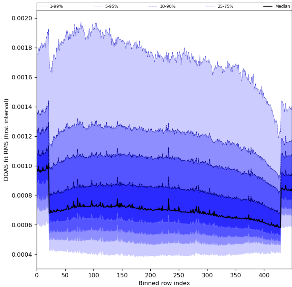
Figure 60: Along track statistics of “DOAS fit RMS (first interval)” for 2024-03-20 to 2024-03-22
