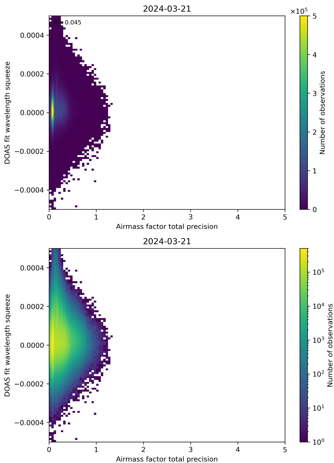
Figure 107: Scatter density plot of “Airmass factor total precision” against “DOAS fit wavelength squeeze” for 2024-03-20 to 2024-03-22.
