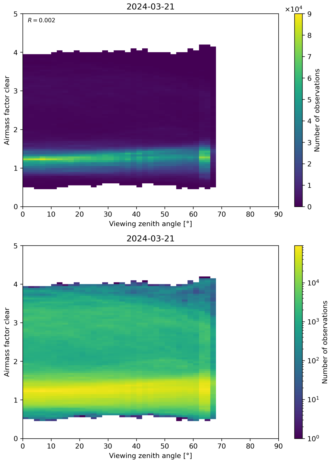
Figure 185: Scatter density plot of “Viewing zenith angle” against “Airmass factor clear” for 2024-03-20 to 2024-03-22.
