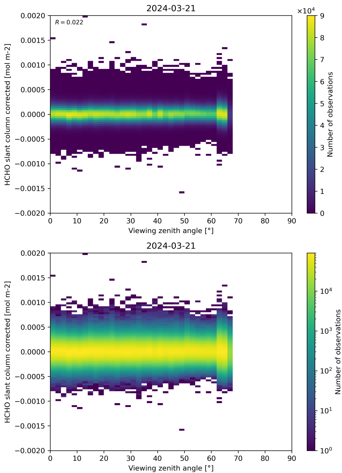
Figure 186: Scatter density plot of “Viewing zenith angle” against “HCHO slant column corrected” for 2024-03-20 to 2024-03-22.
