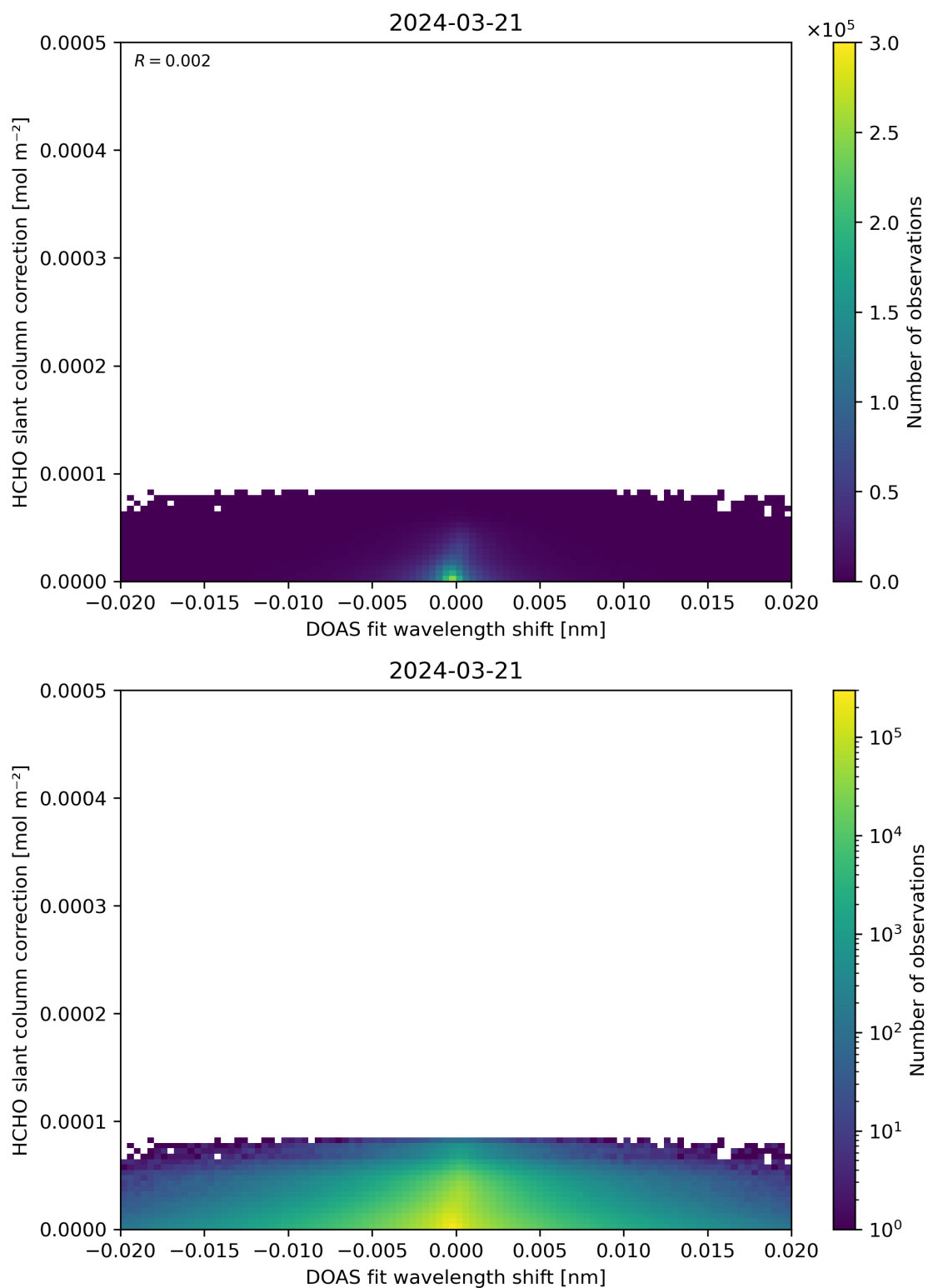
Figure 67: Scatter density plot of “DOAS fit wavelength shift” against “HCHO slant column correction” for 2024-03-20 to 2024-03-22.
