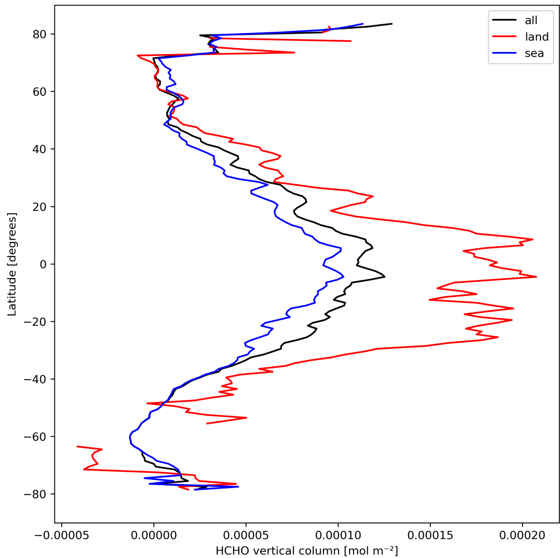
Figure 21: Zonal average of “HCHO vertical column” for 2024-03-20 to 2024-03-22.
