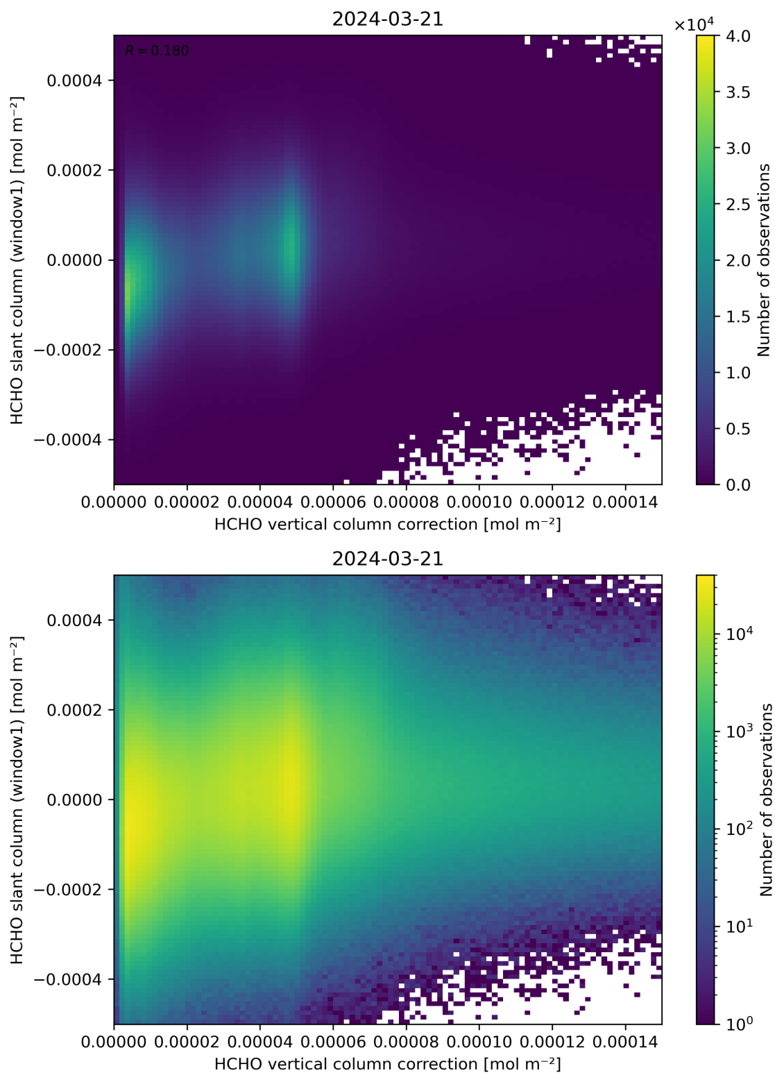
Figure 118: Scatter density plot of “HCHO vertical column correction” against “HCHO slant column (window1)” for 2024-03-20 to 2024-03-22.
