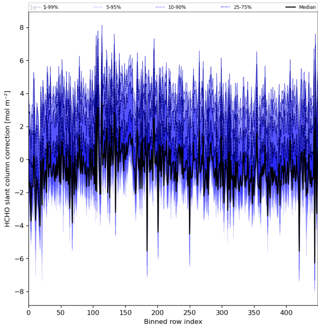
Figure 61: Along track statistics of “HCHO slant column correction” for 2024-03-20 to 2024-03-22
