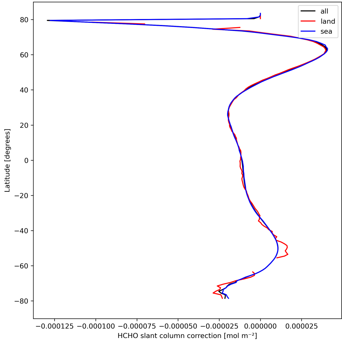
Figure 33: Zonal average of “HCHO slant column correction” for 2024-03-20 to 2024-03-22.
