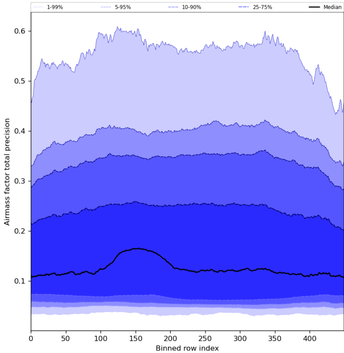
Figure 55: Along track statistics of “Airmass factor total precision” for 2024-03-20 to 2024-03-22
