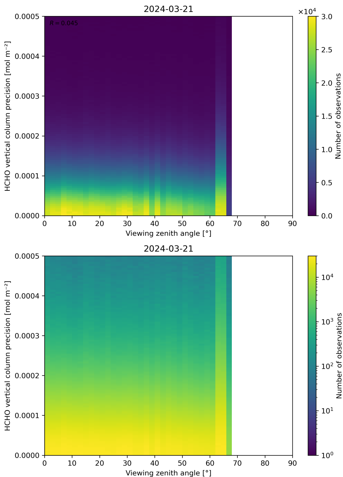
Figure 194: Scatter density plot of “Viewing zenith angle” against “HCHO vertical column precision” for 2024-03-20 to 2024-03-22.
