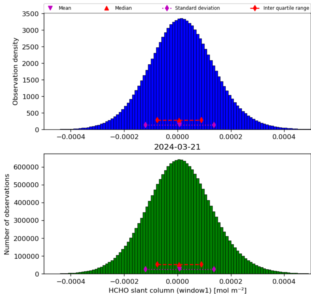
Figure 38: Histogram of “HCHO slant column (window1)” for 2024-03-20 to 2024-03-22
