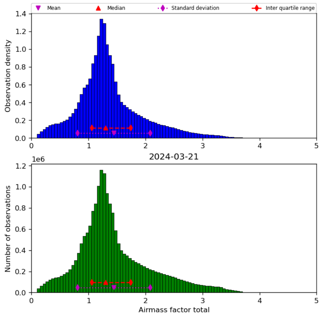
Figure 40: Histogram of “Airmass factor total” for 2024-03-20 to 2024-03-22
