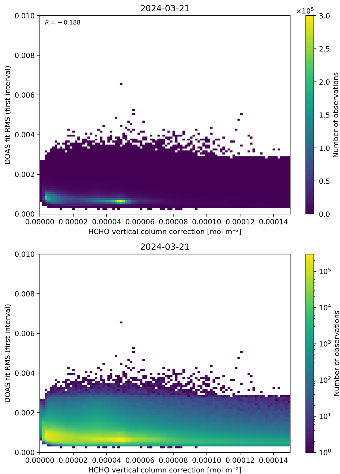
Figure 112: Scatter density plot of “HCHO vertical column correction” against “DOAS fit RMS (first interval)” for 2024-03-20 to 2024-03-22.
