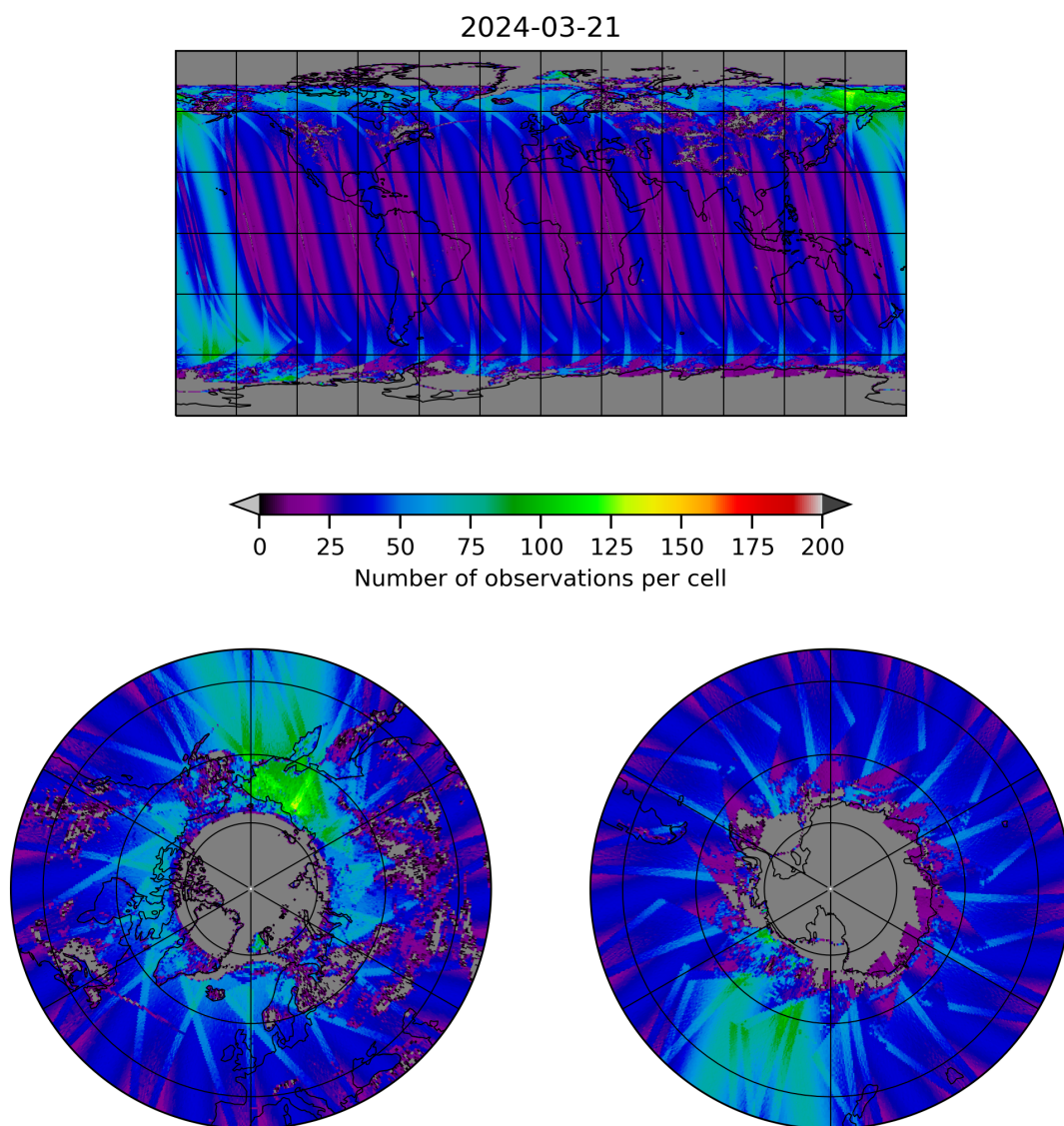
Figure 19: Map of the number of observations for 2024-03-20 to 2024-03-22
