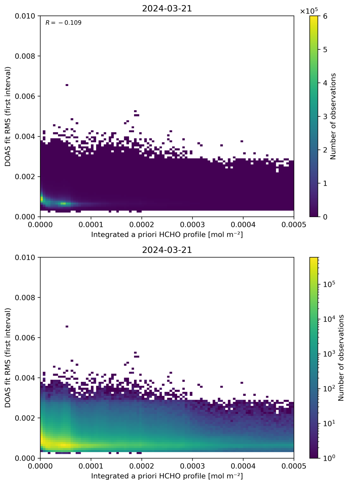
Figure 148: Scatter density plot of “Integrated a priori HCHO profile” against “DOAS fit RMS (first interval)” for 2024-03-20 to 2024-03-22.
