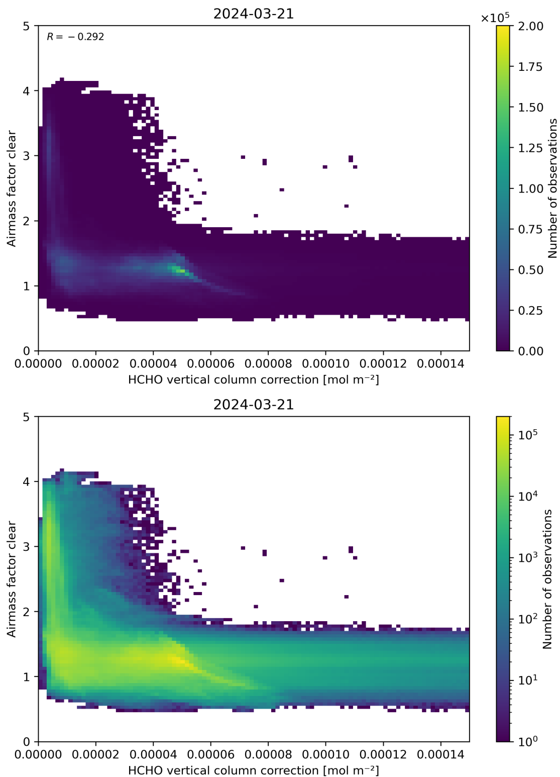
Figure 115: Scatter density plot of “HCHO vertical column correction” against “Airmass factor clear” for 2024-03-20 to 2024-03-22.
