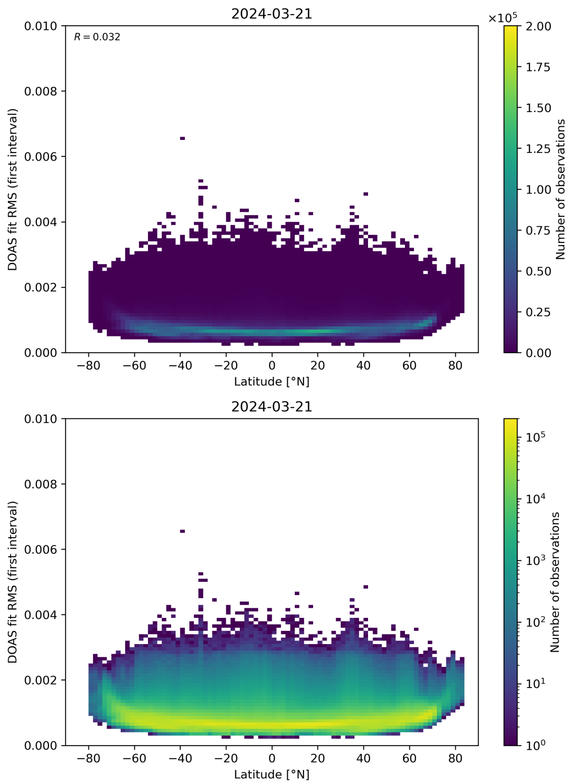
Figure 153: Scatter density plot of “Latitude” against “DOAS fit RMS (first interval)” for 2024-03-20 to 2024-03-22.
