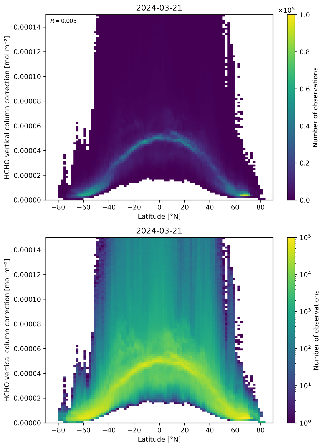
Figure 164: Scatter density plot of “Latitude” against “HCHO vertical column correction” for 2024-03-20 to 2024-03-22.
