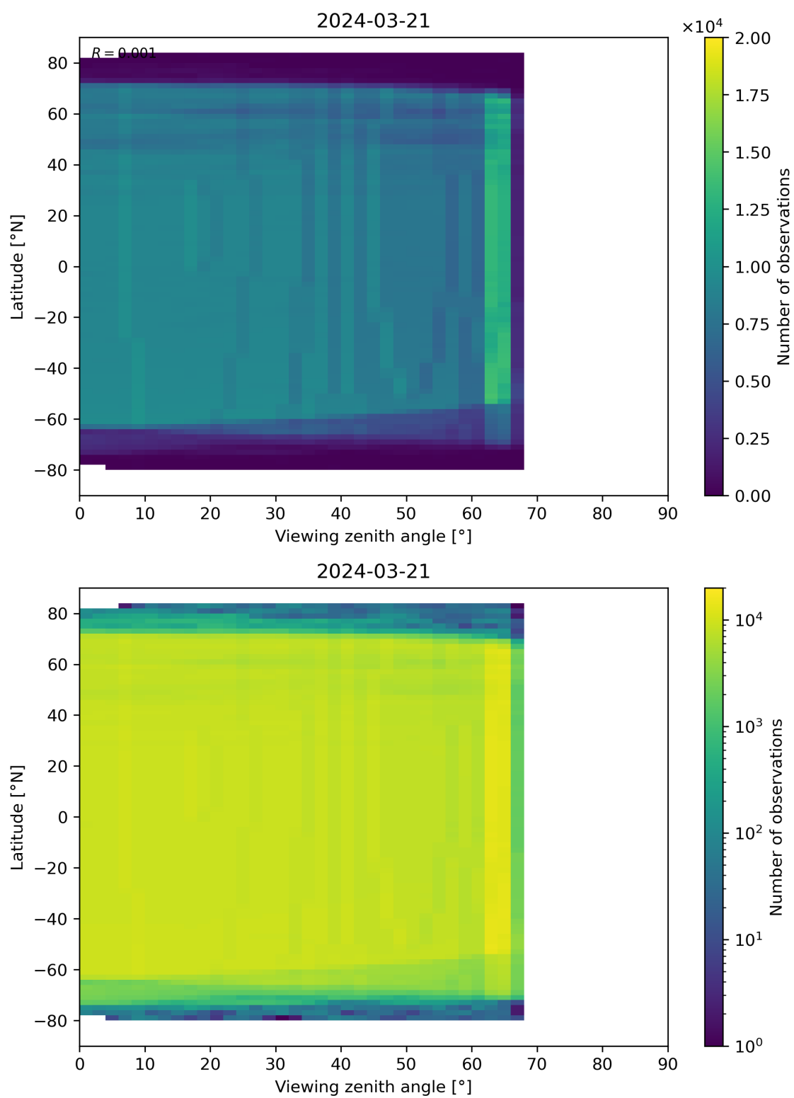
Figure 196: Scatter density plot of “Viewing zenith angle” against “Latitude” for 2024-03-20 to 2024-03-22.
