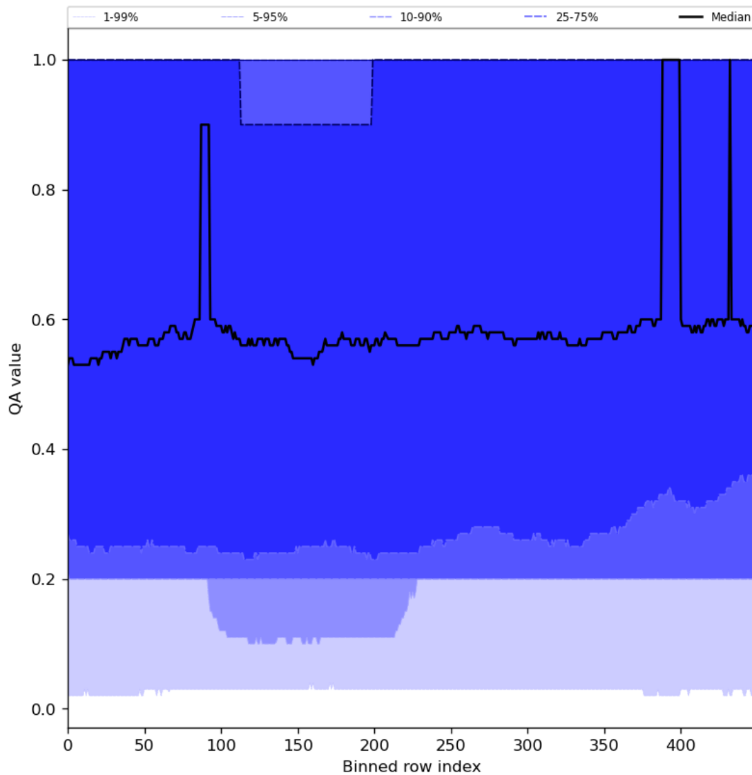
Figure 48: Along track statistics of “QA value” for 2024-03-20 to 2024-03-22
