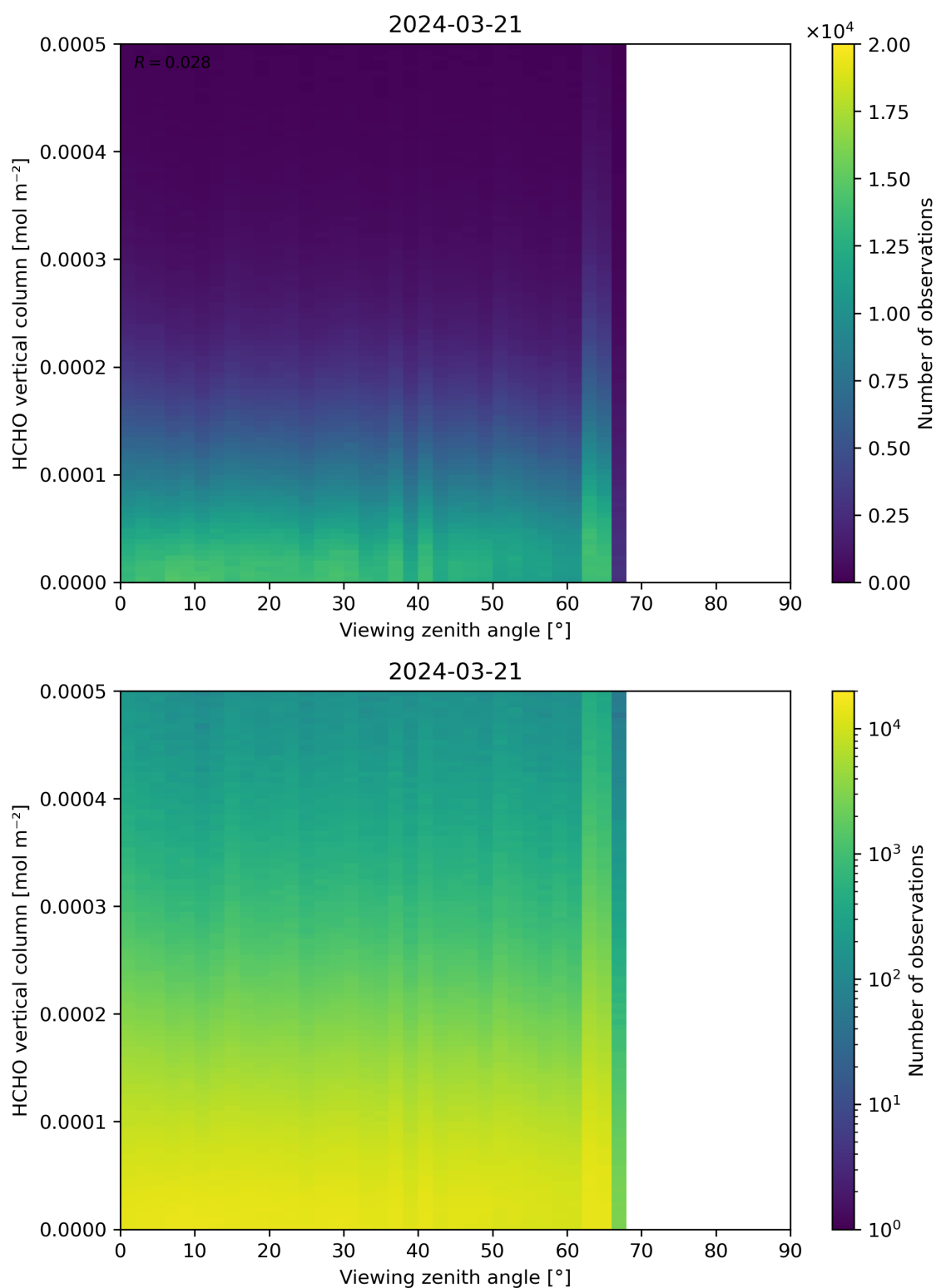
Figure 192: Scatter density plot of “Viewing zenith angle” against “HCHO vertical column” for 2024-03-20 to 2024-03-22.
