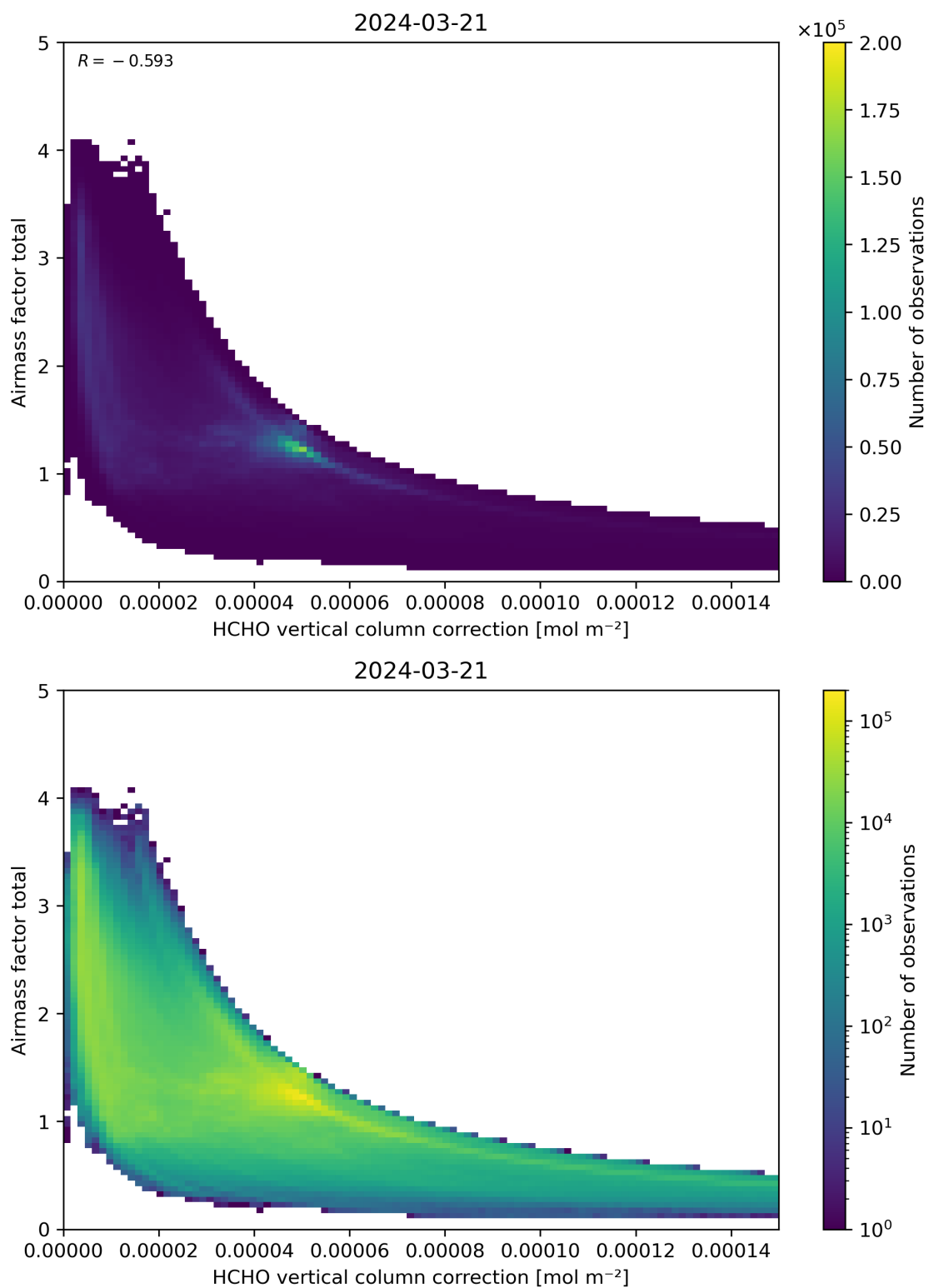
Figure 120: Scatter density plot of “HCHO vertical column correction” against “Airmass factor total” for 2024-03-20 to 2024-03-22.
