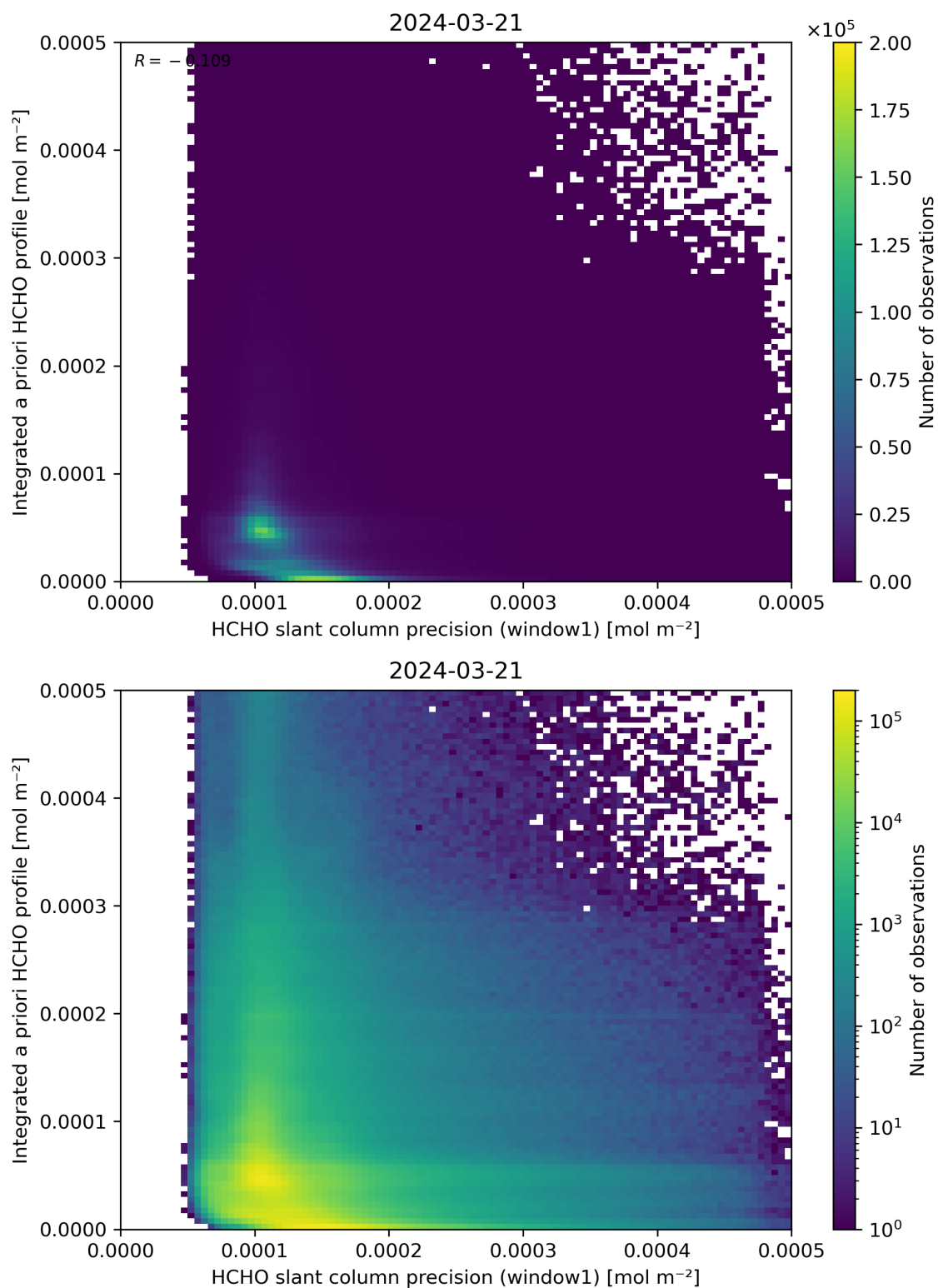
Figure 96: Scatter density plot of “HCHO slant column precision (window1)” against “Integrated a priori HCHO profile” for 2024-03-20 to 2024-03-22.
