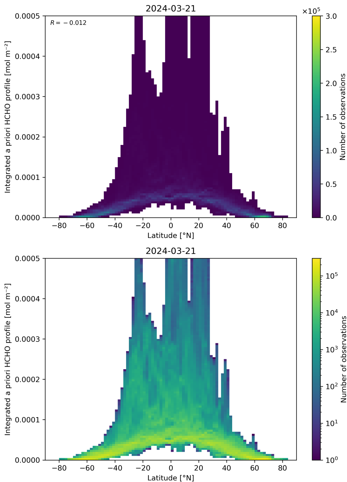
Figure 166: Scatter density plot of “Latitude” against “Integrated a priori HCHO profile” for 2024-03-20 to 2024-03-22.
