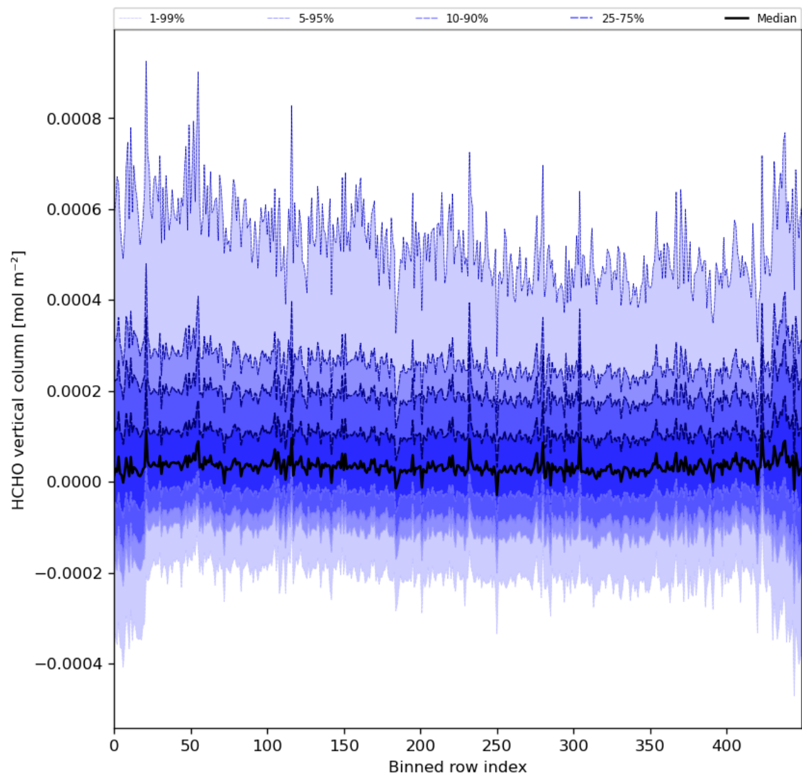
Figure 49: Along track statistics of “HCHO vertical column” for 2024-03-20 to 2024-03-22
