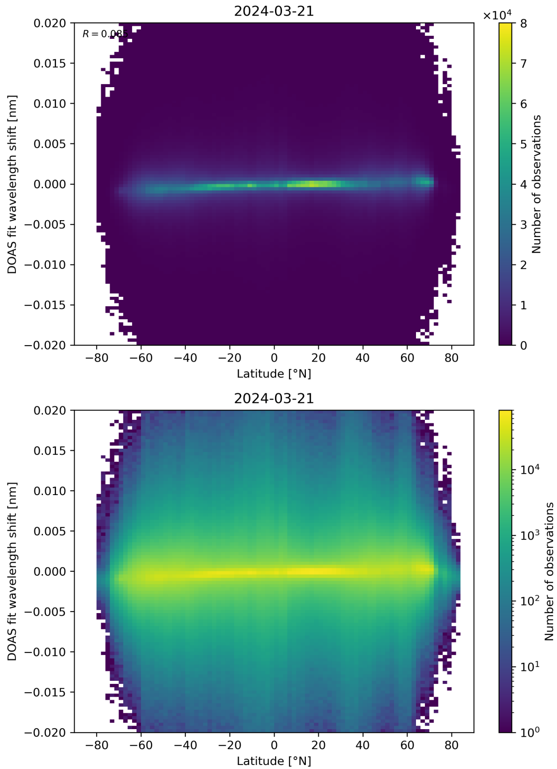
Figure 154: Scatter density plot of “Latitude” against “DOAS fit wavelength shift” for 2024-03-20 to 2024-03-22.
