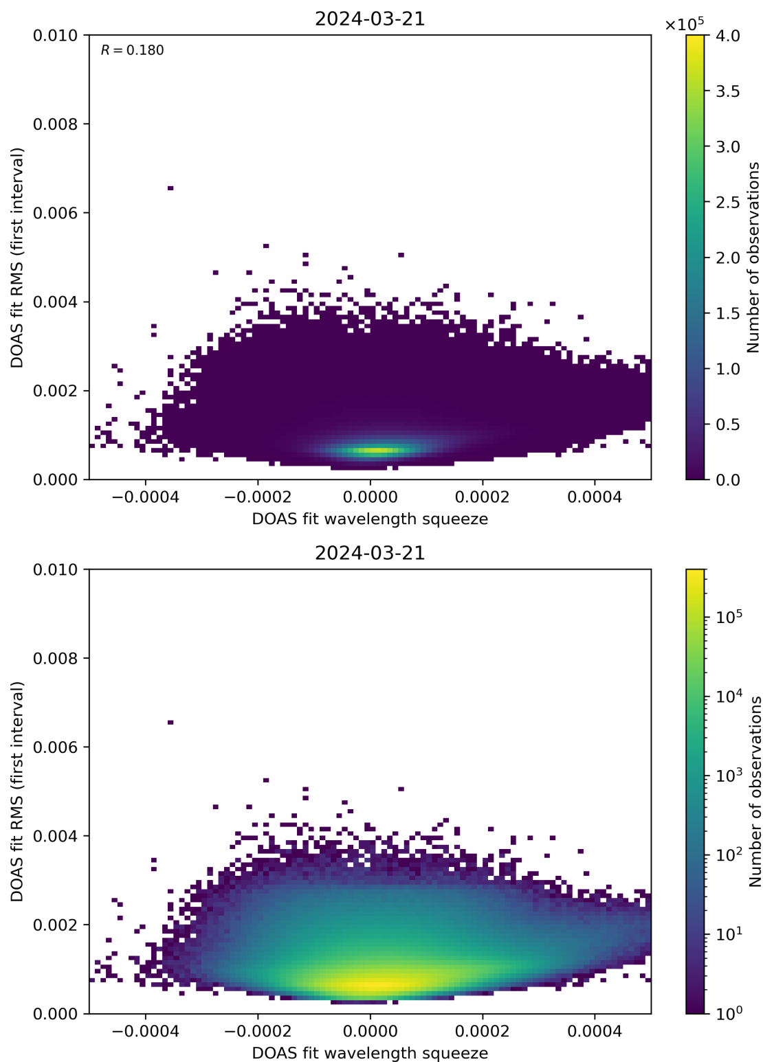
Figure 68: Scatter density plot of “DOAS fit wavelength squeeze” against “DOAS fit RMS (first interval)” for 2024-03-20 to 2024-03-22.
