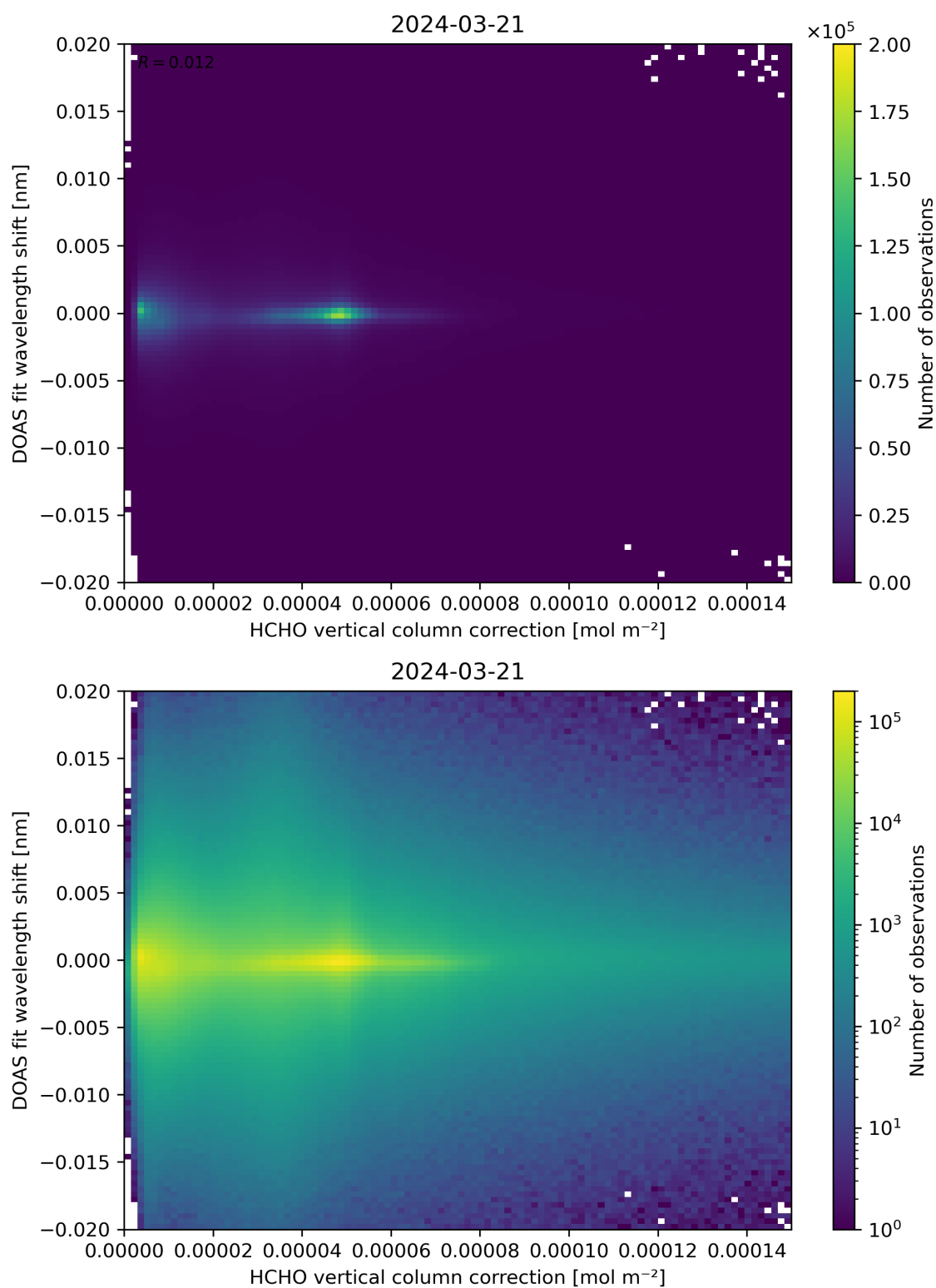
Figure 113: Scatter density plot of “HCHO vertical column correction” against “DOAS fit wavelength shift” for 2024-03-20 to 2024-03-22.
