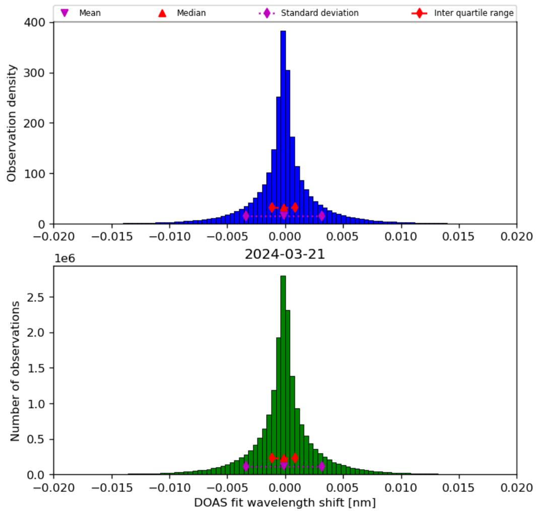
Figure 44: Histogram of “DOAS fit wavelength shift” for 2024-03-20 to 2024-03-22
