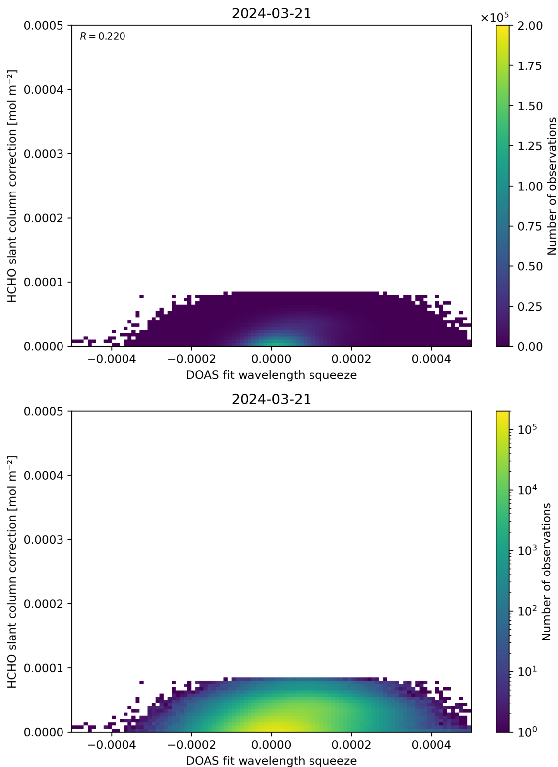
Figure 70: Scatter density plot of “DOAS fit wavelength squeeze” against “HCHO slant column correction” for 2024-03-20 to 2024-03-22.
