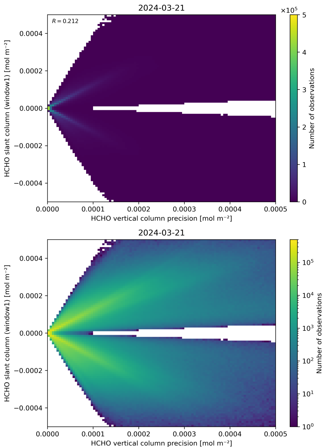
Figure 142: Scatter density plot of “HCHO vertical column precision” against “HCHO slant column (window1)” for 2024-03-20 to 2024-03-22.
