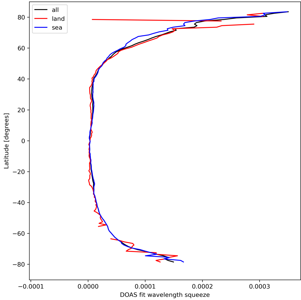
Figure 31: Zonal average of “DOAS fit wavelength squeeze” for 2024-03-20 to 2024-03-22.
