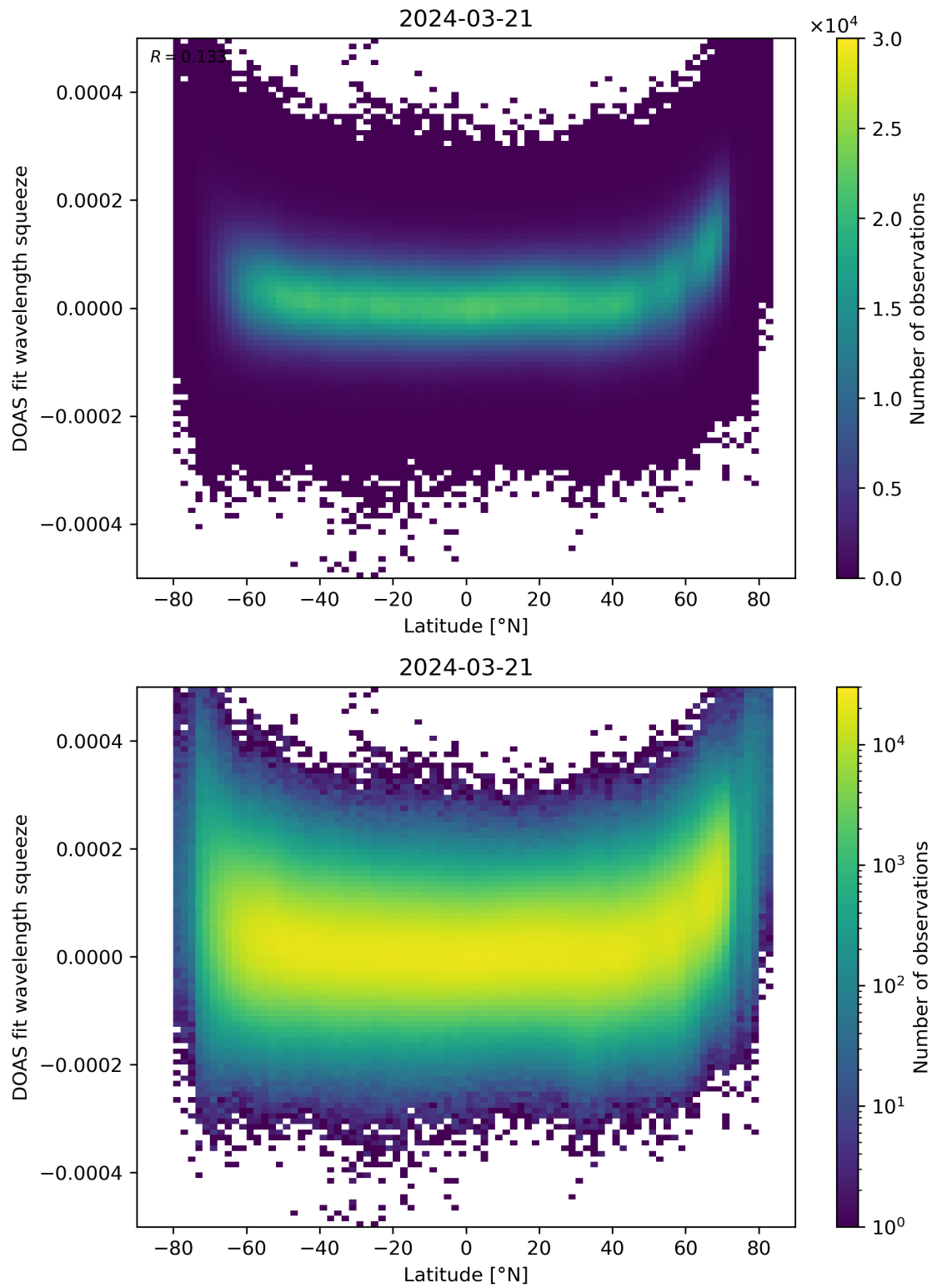
Figure 155: Scatter density plot of “Latitude” against “DOAS fit wavelength squeeze” for 2024-03-20 to 2024-03-22.
