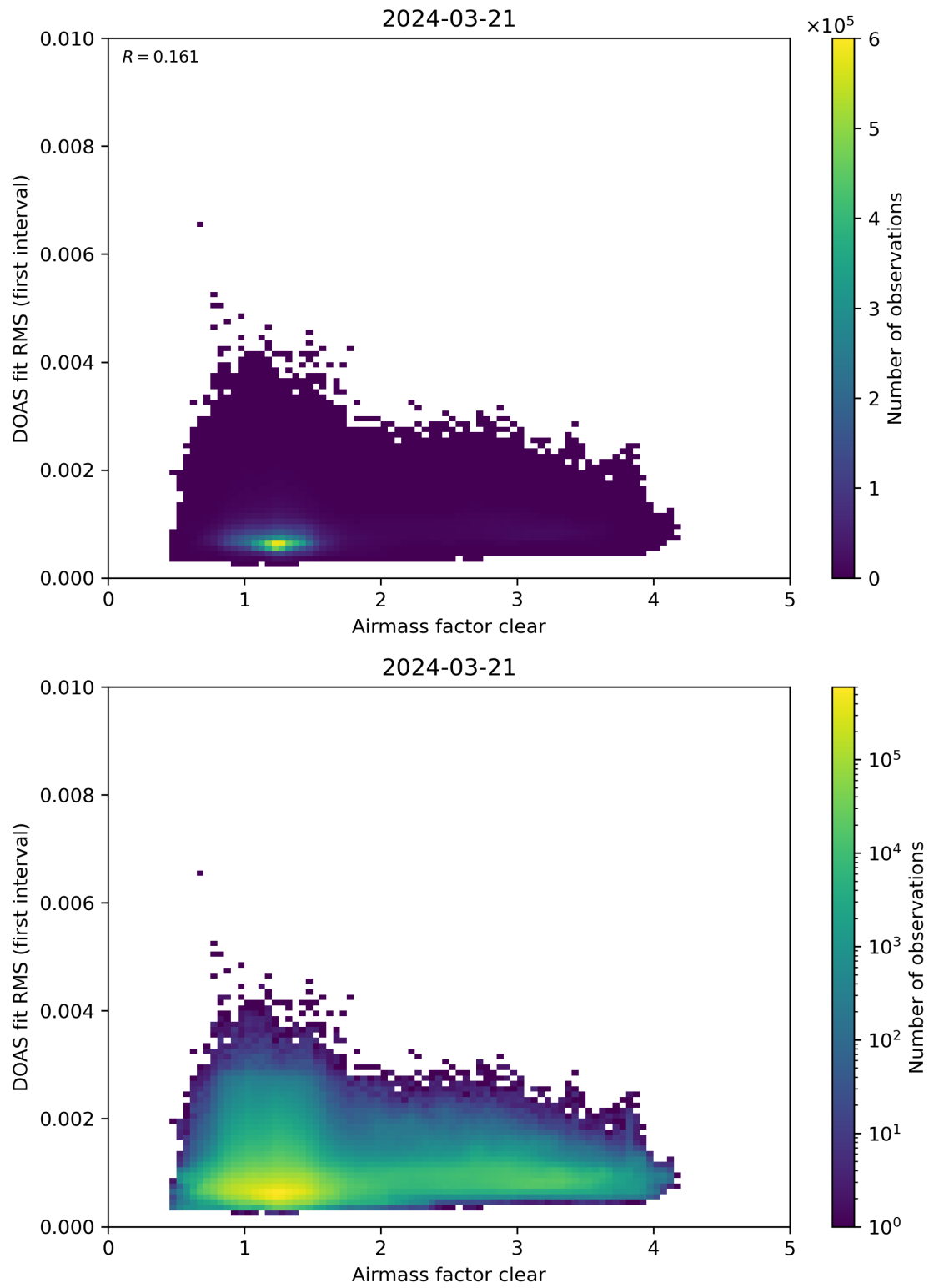
Figure 71: Scatter density plot of “Airmass factor clear” against “DOAS fit RMS (first interval)” for 2024-03-20 to 2024-03-22.
