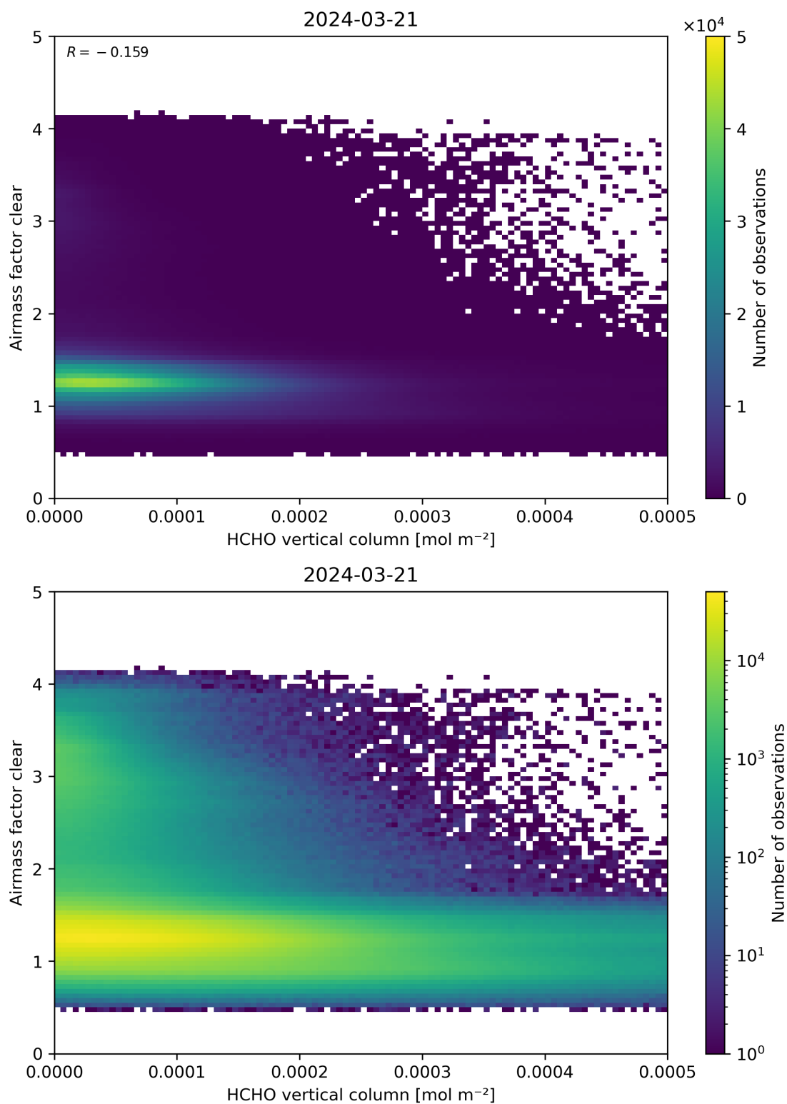
Figure 126: Scatter density plot of “HCHO vertical column” against “Airmass factor clear” for 2024-03-20 to 2024-03-22.
