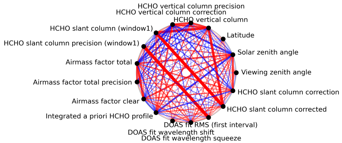
Figure 1: Map of correlation graph for 2024-03-20 to 2024-03-22.
