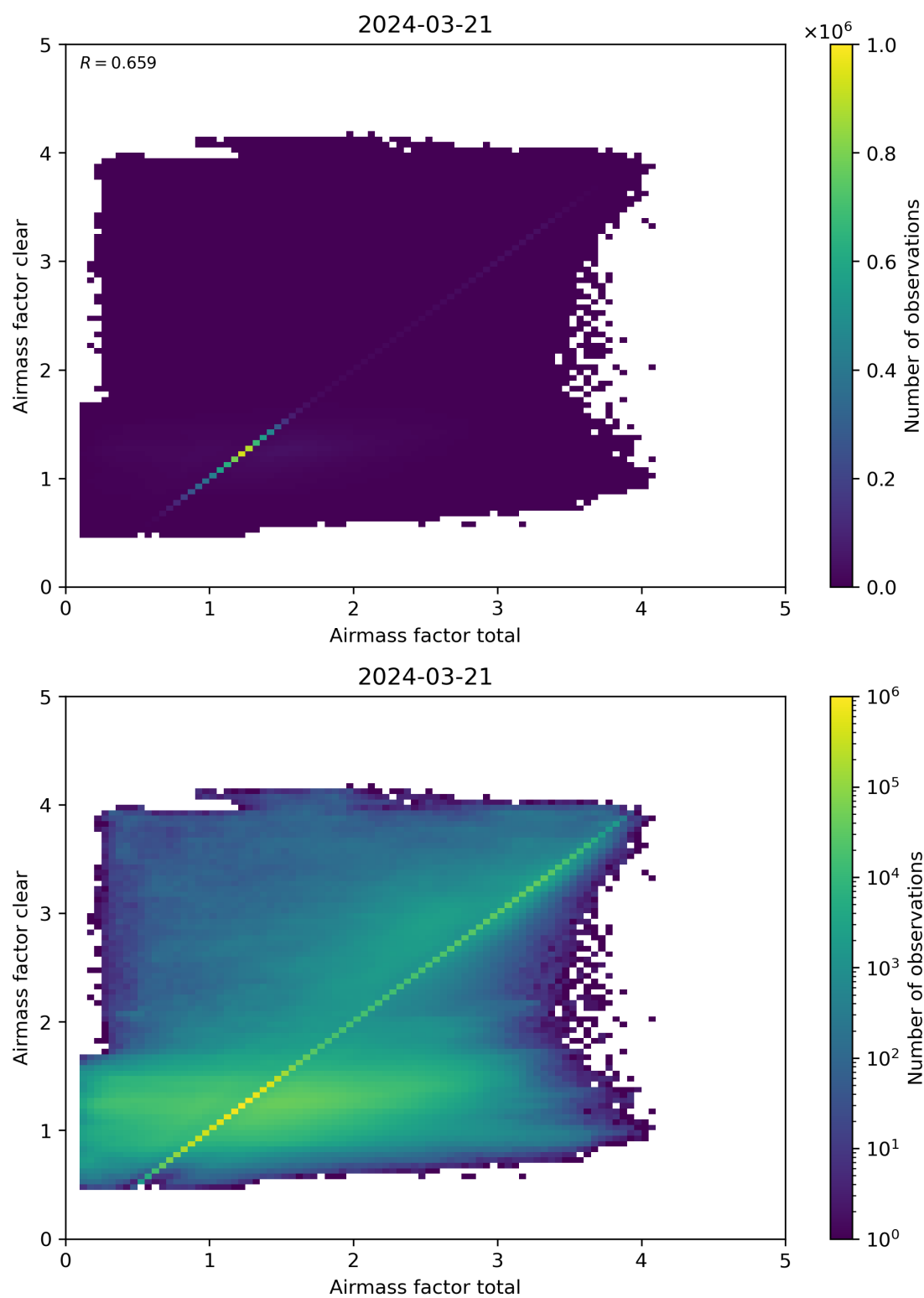
Figure 100: Scatter density plot of “Airmass factor total” against “Airmass factor clear” for 2024-03-20 to 2024-03-22.
