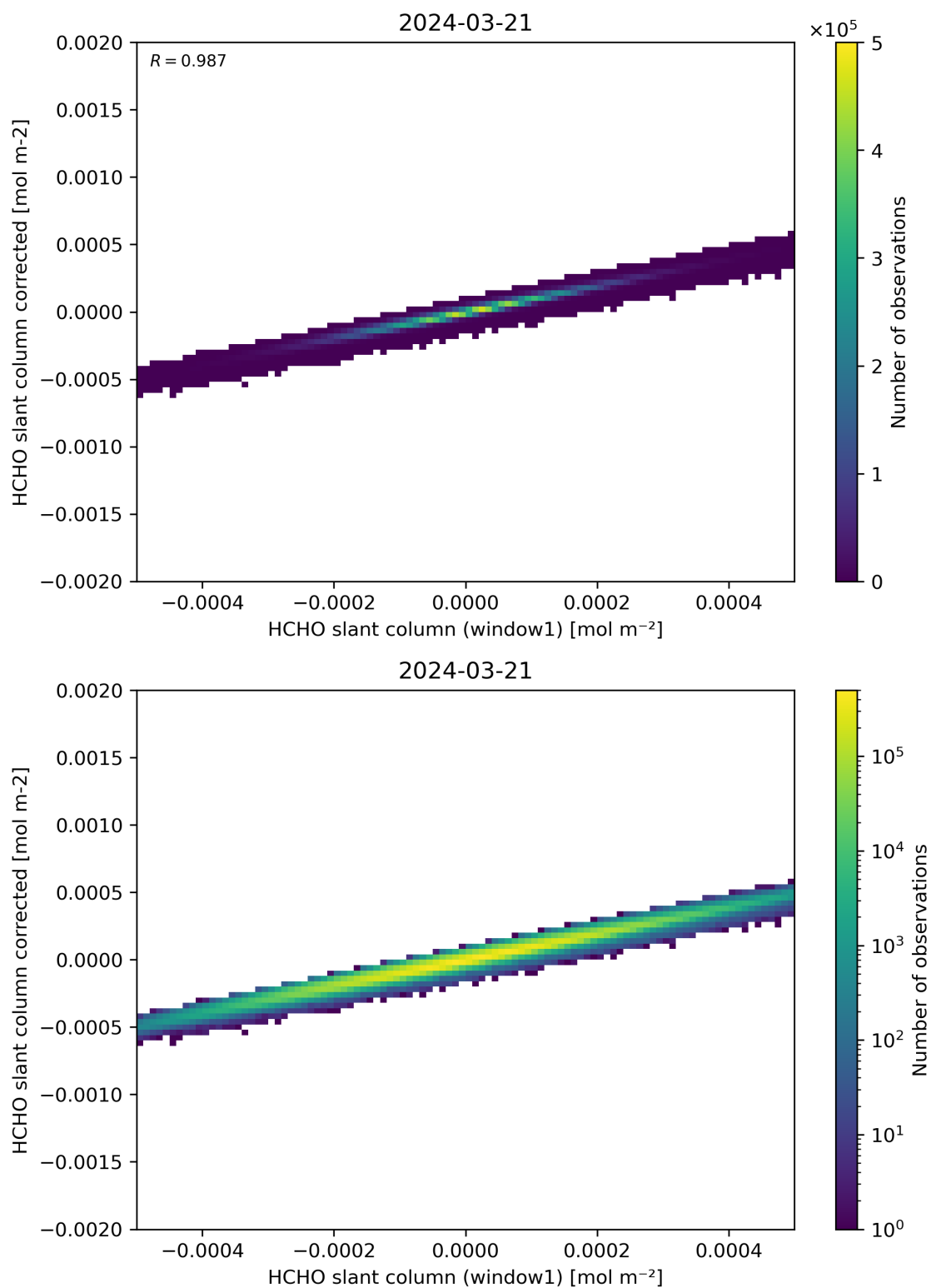
Figure 82: Scatter density plot of “HCHO slant column (window1)” against “HCHO slant column corrected” for 2024-03-20 to 2024-03-22.
