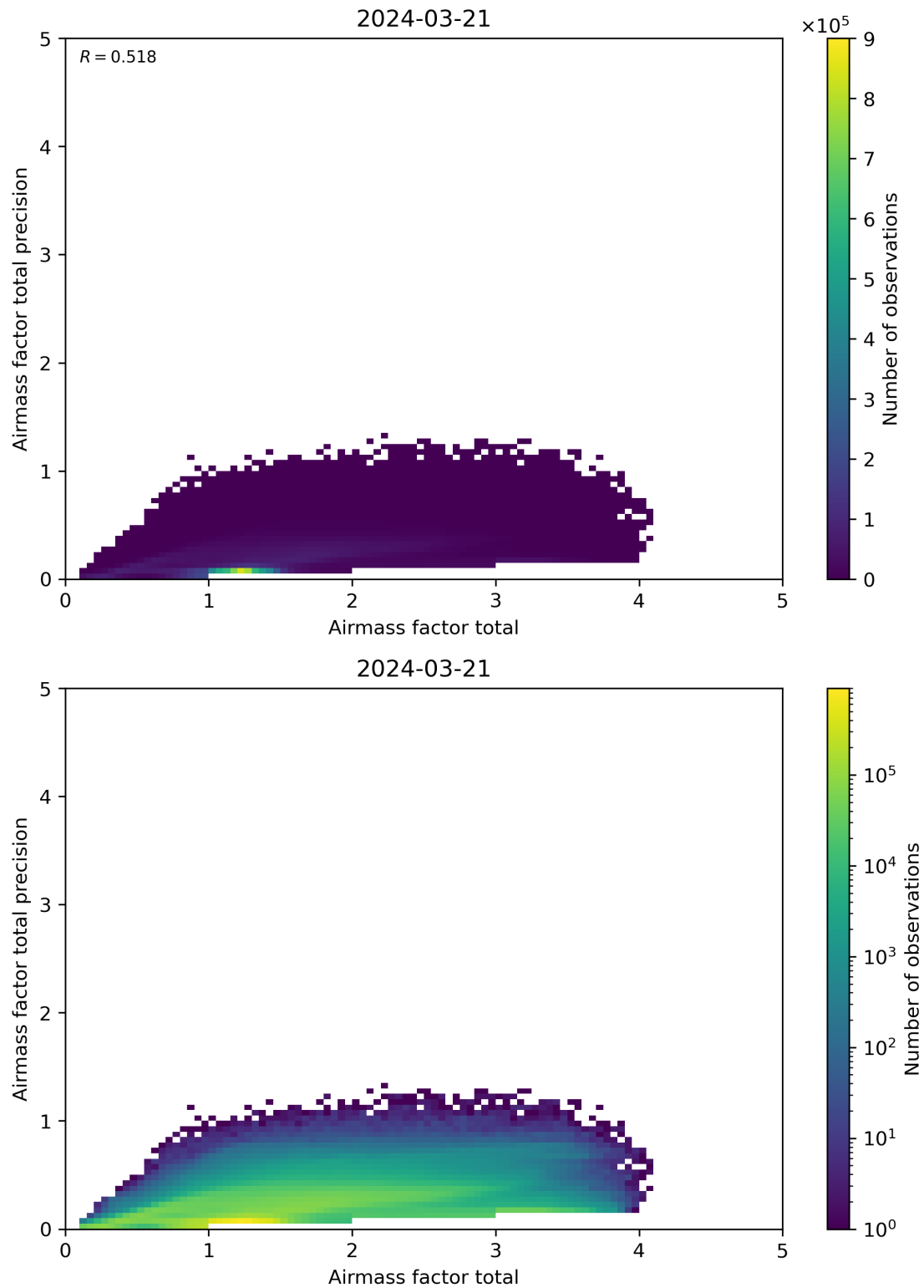
Figure 103: Scatter density plot of “Airmass factor total” against “Airmass factor total precision” for 2024-03-20 to 2024-03-22.
