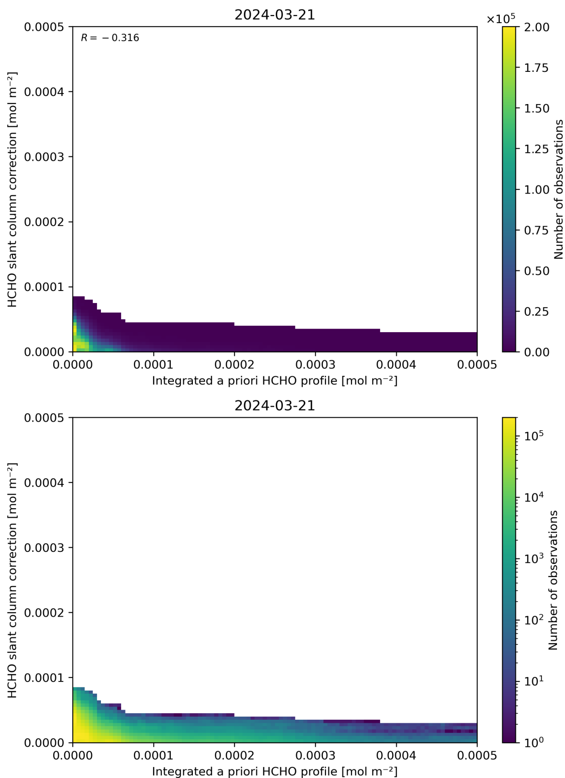
Figure 152: Scatter density plot of “Integrated a priori HCHO profile” against “HCHO slant column correction” for 2024-03-20 to 2024-03-22.
