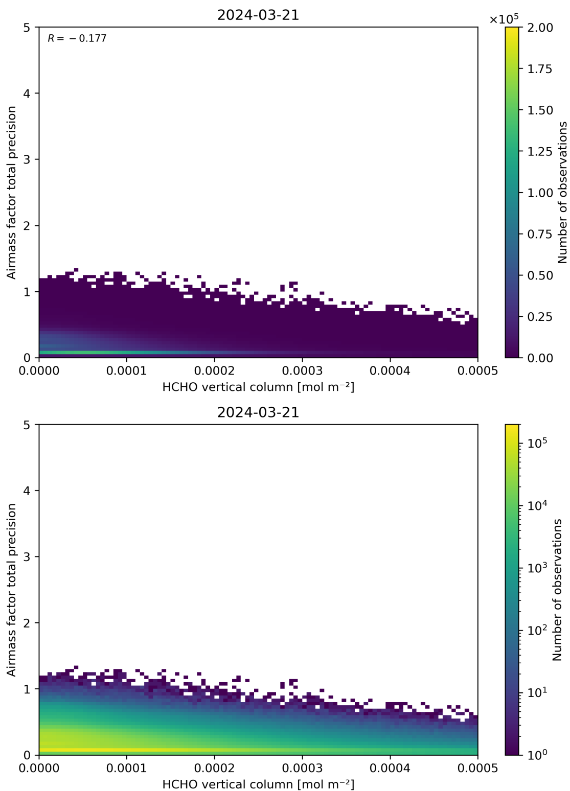
Figure 132: Scatter density plot of “HCHO vertical column” against “Airmass factor total precision” for 2024-03-20 to 2024-03-22.
