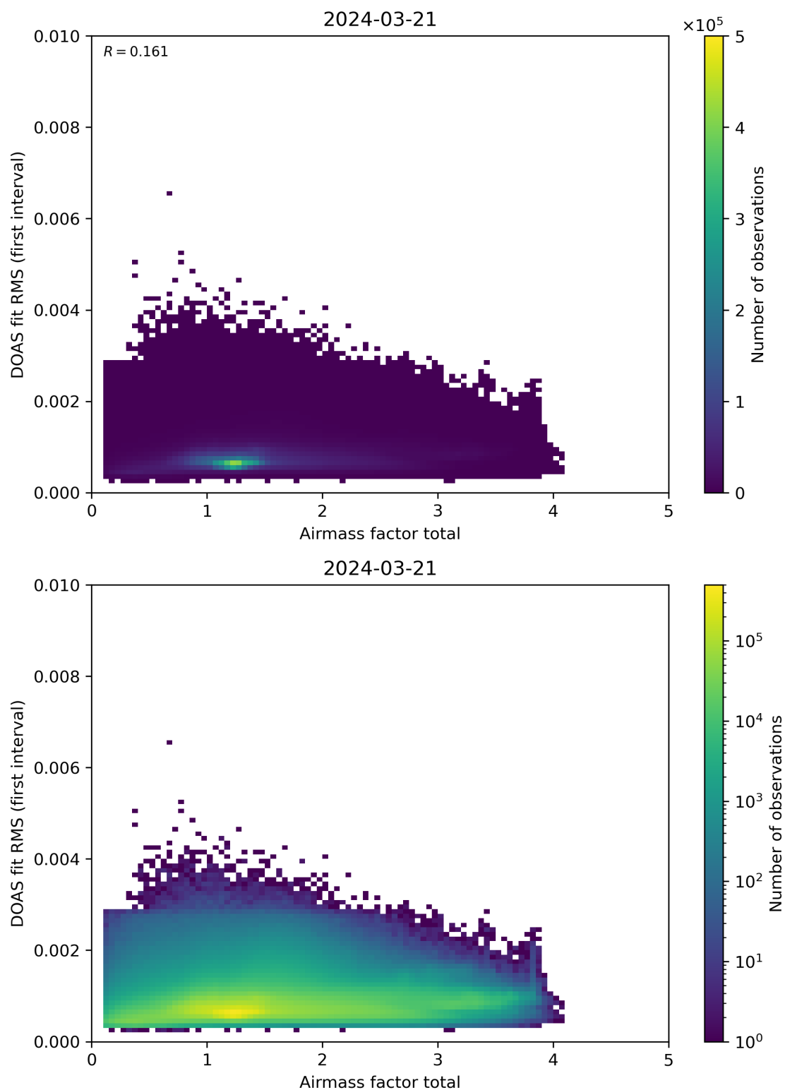
Figure 97: Scatter density plot of “Airmass factor total” against “DOAS fit RMS (first interval)” for 2024-03-20 to 2024-03-22.
