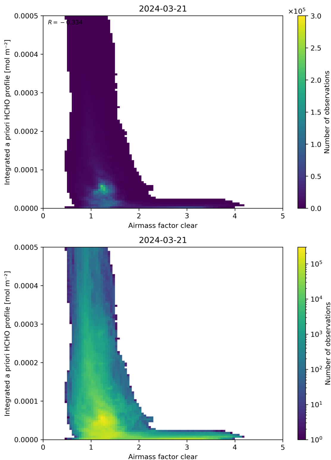
Figure 76: Scatter density plot of “Airmass factor clear” against “Integrated a priori HCHO profile” for 2024-03-20 to 2024-03-22.
