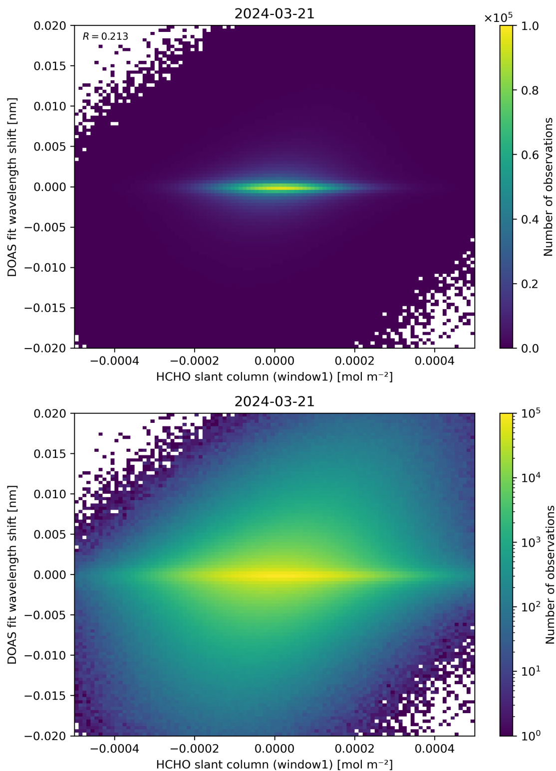
Figure 79: Scatter density plot of “HCHO slant column (window1)” against “DOAS fit wavelength shift” for 2024-03-20 to 2024-03-22.
