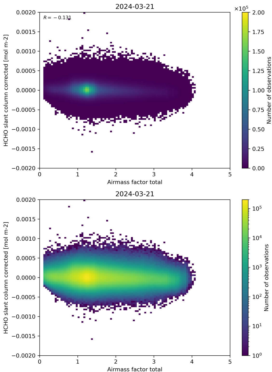
Figure 101: Scatter density plot of “Airmass factor total” against “HCHO slant column corrected” for 2024-03-20 to 2024-03-22.
