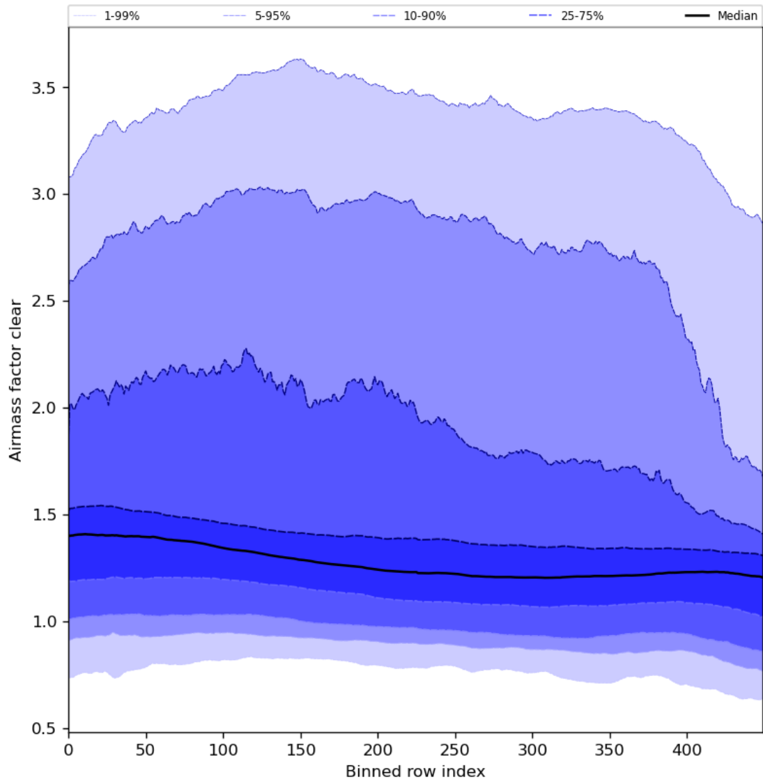
Figure 56: Along track statistics of “Airmass factor clear” for 2024-03-20 to 2024-03-22
