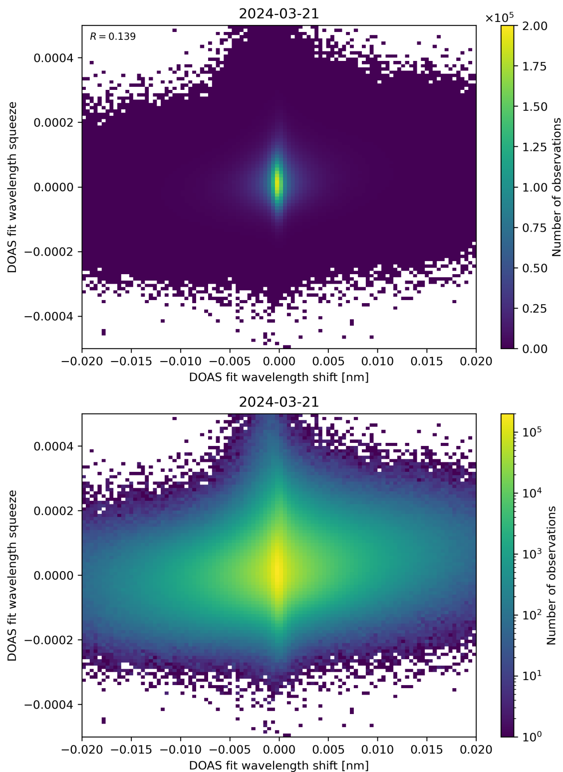
Figure 65: Scatter density plot of “DOAS fit wavelength shift” against “DOAS fit wavelength squeeze” for 2024-03-20 to 2024-03-22.
