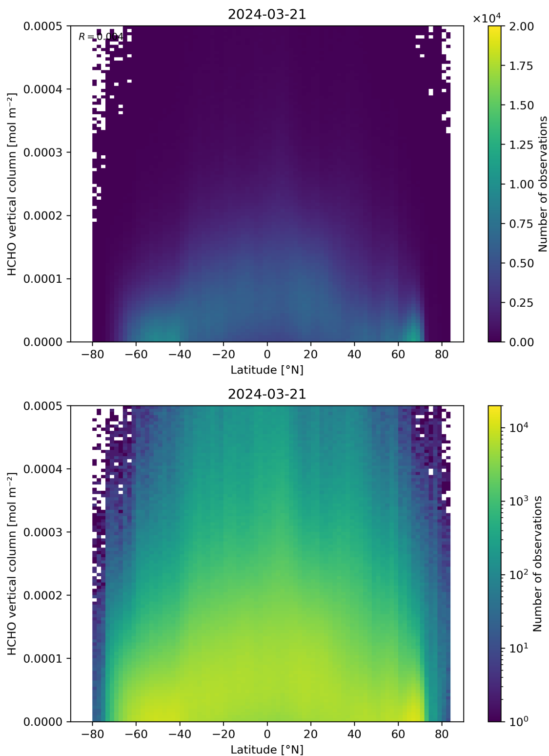
Figure 163: Scatter density plot of “Latitude” against “HCHO vertical column” for 2024-03-20 to 2024-03-22.
