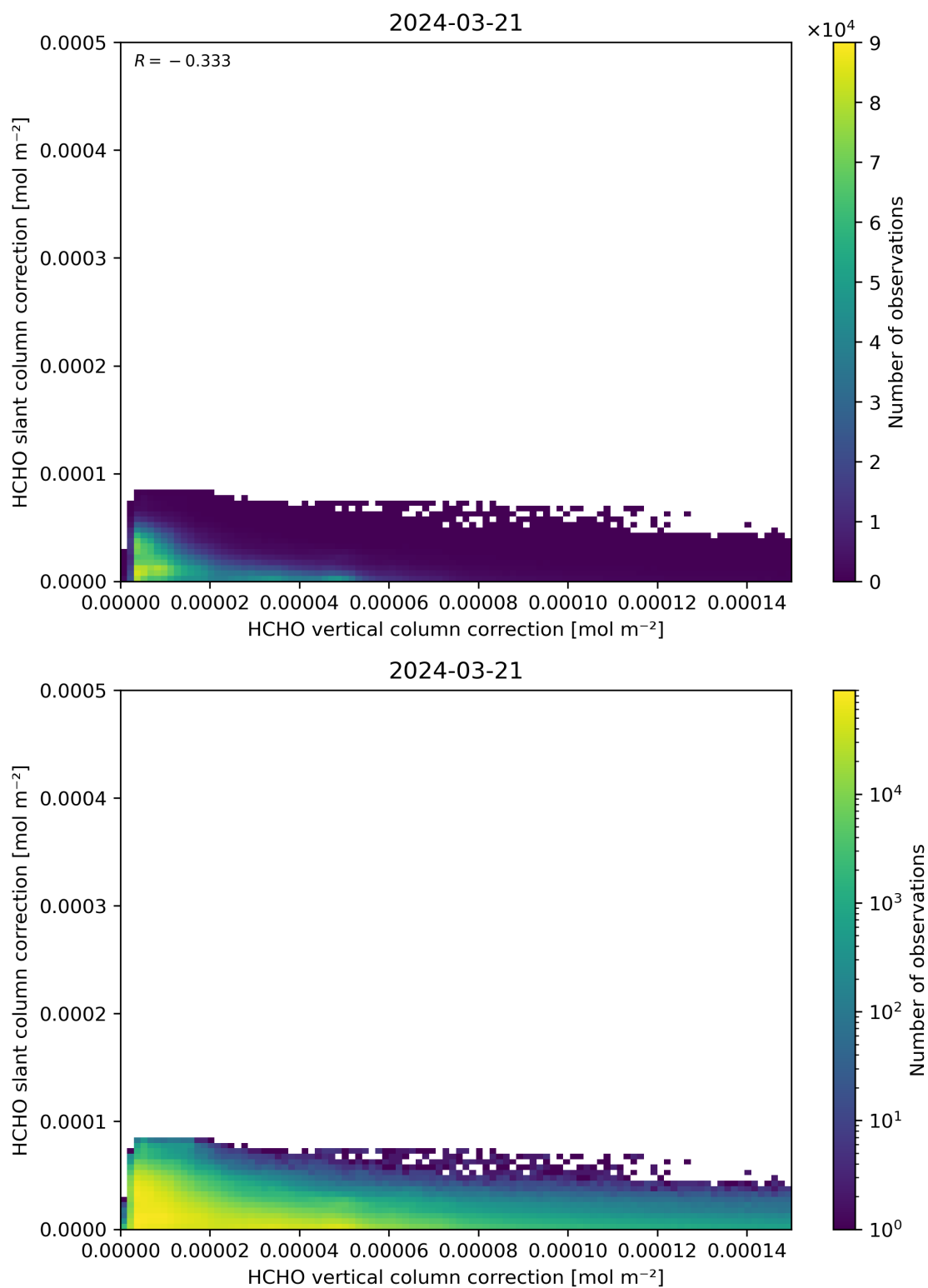
Figure 117: Scatter density plot of “HCHO vertical column correction” against “HCHO slant column correction” for 2024-03-20 to 2024-03-22.
