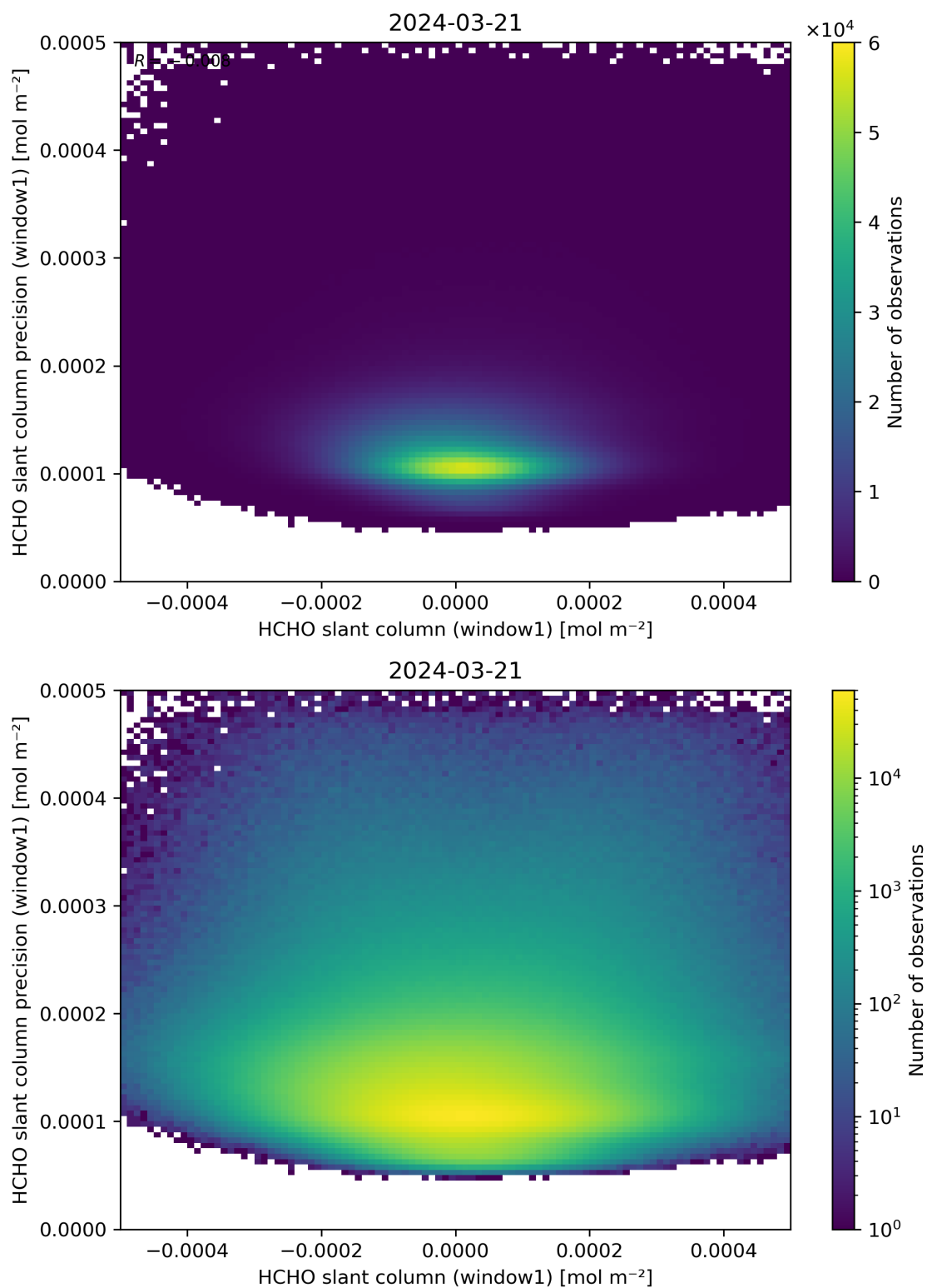
Figure 84: Scatter density plot of “HCHO slant column (window1)” against “HCHO slant column precision (window1)” for 2024-03-20 to 2024-03-22.
