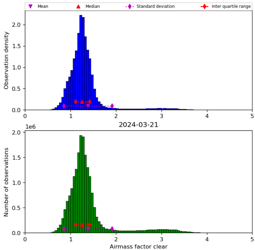
Figure 42: Histogram of “Airmass factor clear” for 2024-03-20 to 2024-03-22
