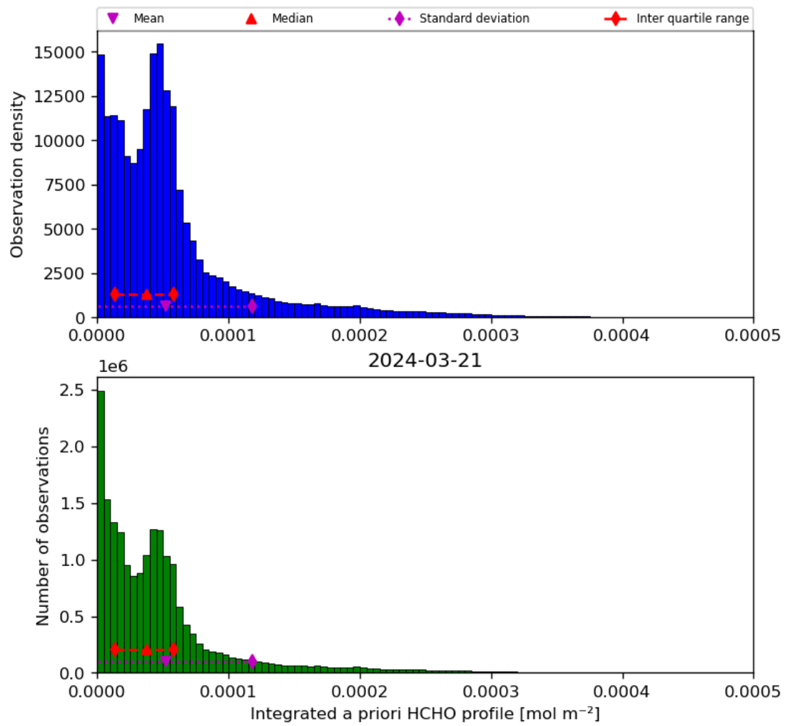
Figure 43: Histogram of “Integrated a priori HCHO profile” for 2024-03-20 to 2024-03-22
