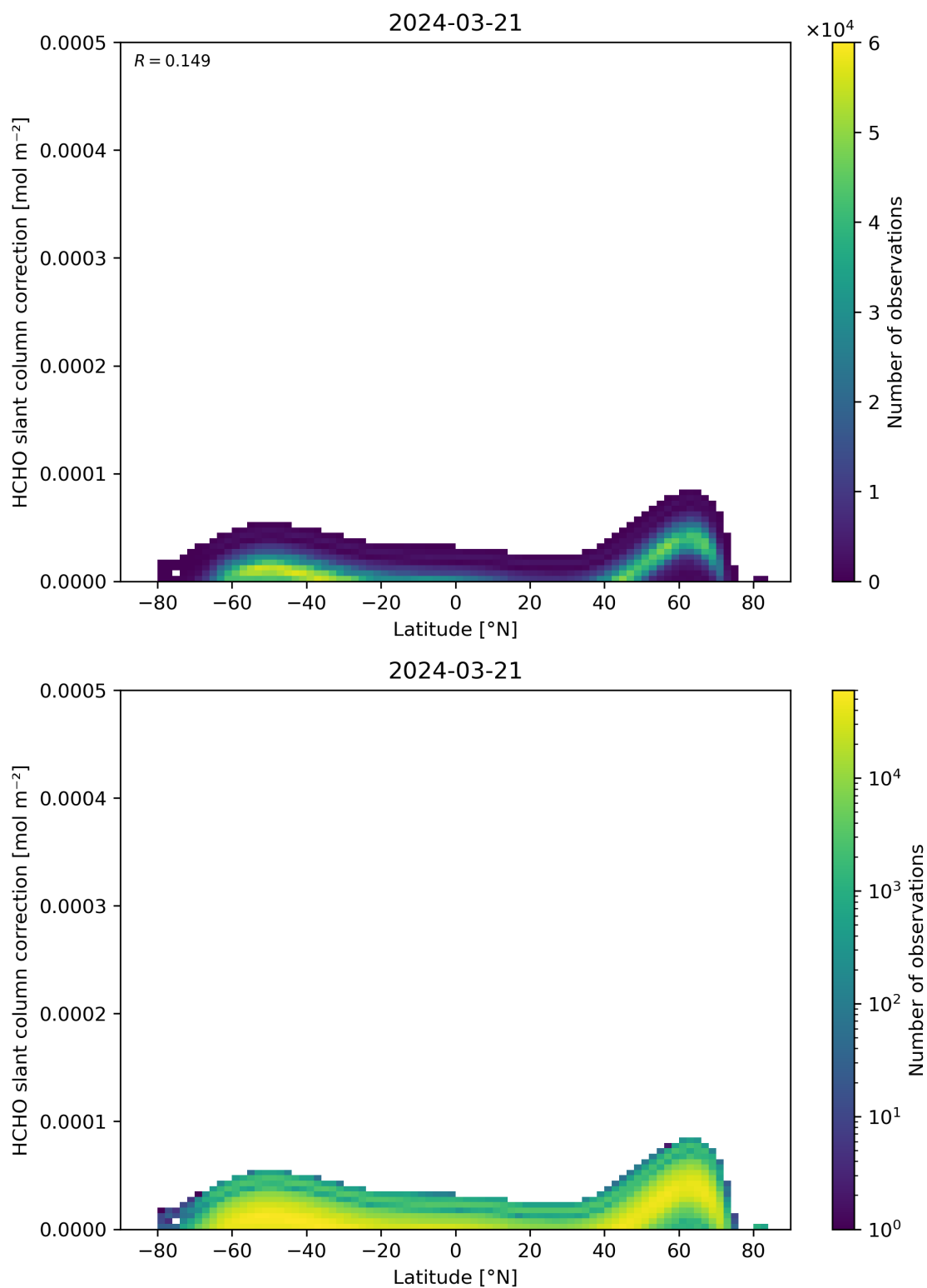
Figure 158: Scatter density plot of “Latitude” against “HCHO slant column correction” for 2024-03-20 to 2024-03-22.
