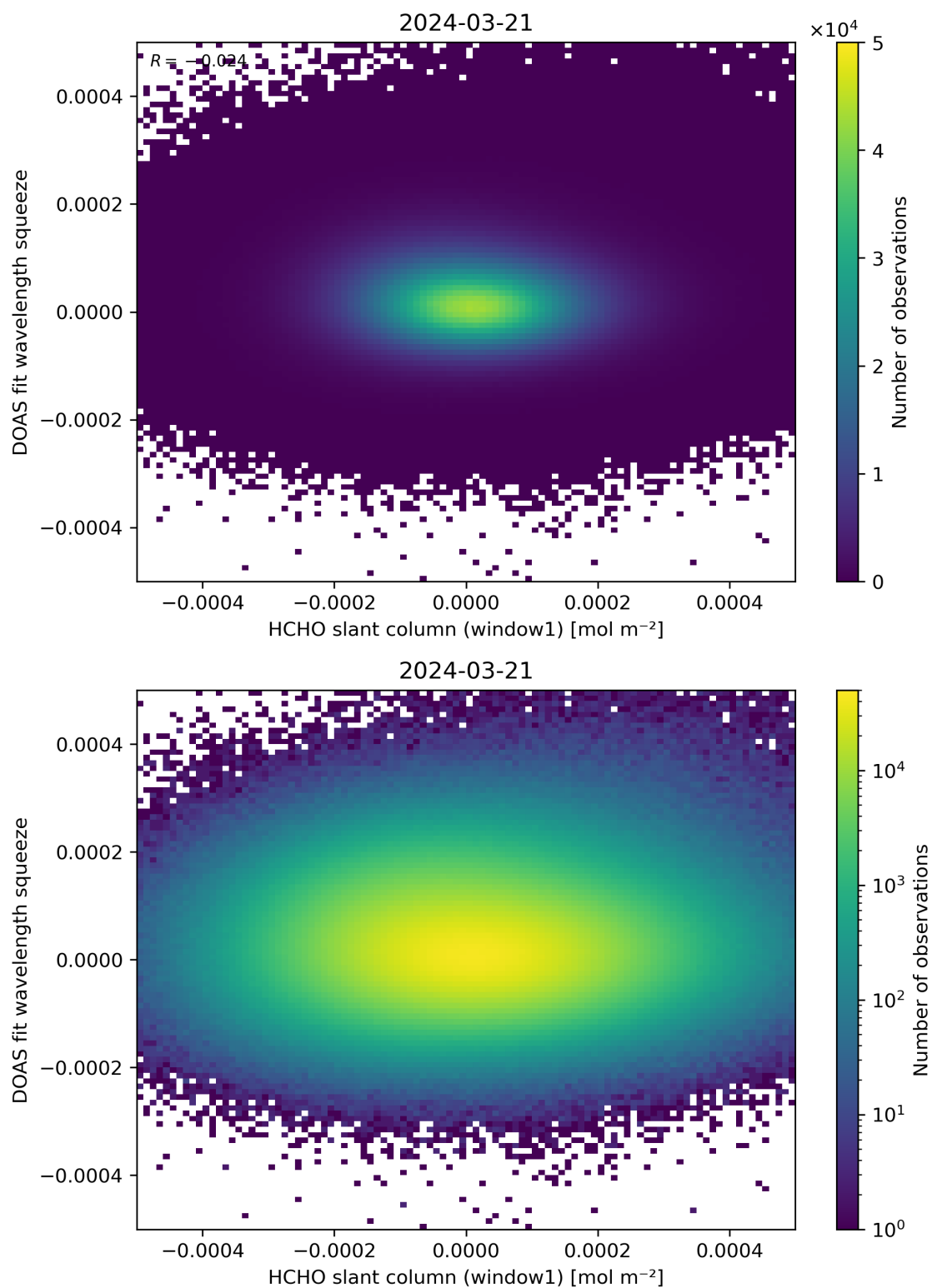
Figure 80: Scatter density plot of “HCHO slant column (window1)” against “DOAS fit wavelength squeeze” for 2024-03-20 to 2024-03-22.
