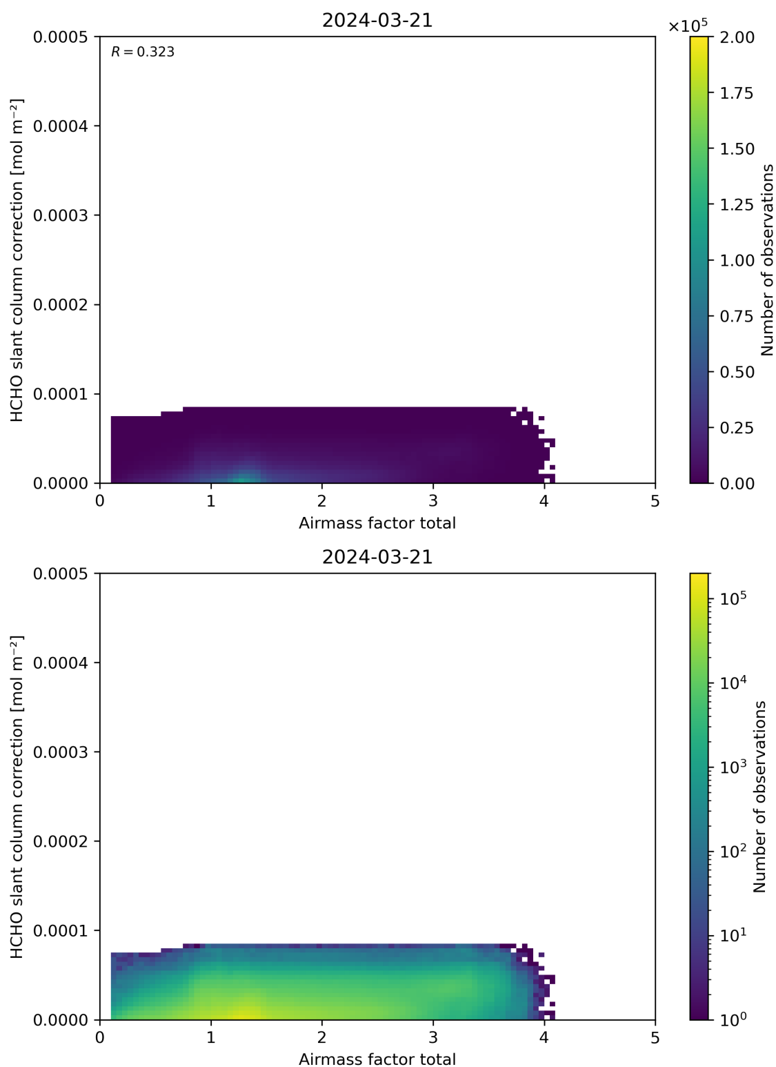
Figure 102: Scatter density plot of “Airmass factor total” against “HCHO slant column correction” for 2024-03-20 to 2024-03-22.
