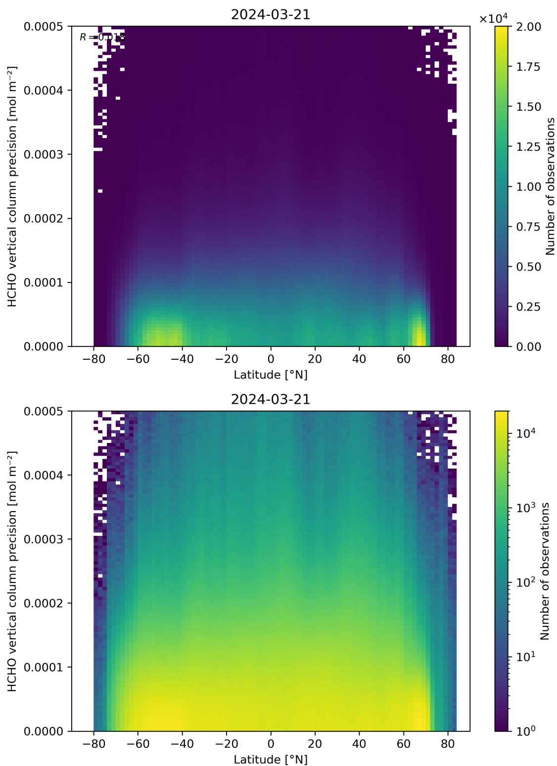
Figure 165: Scatter density plot of “Latitude” against “HCHO vertical column precision” for 2024-03-20 to 2024-03-22.
