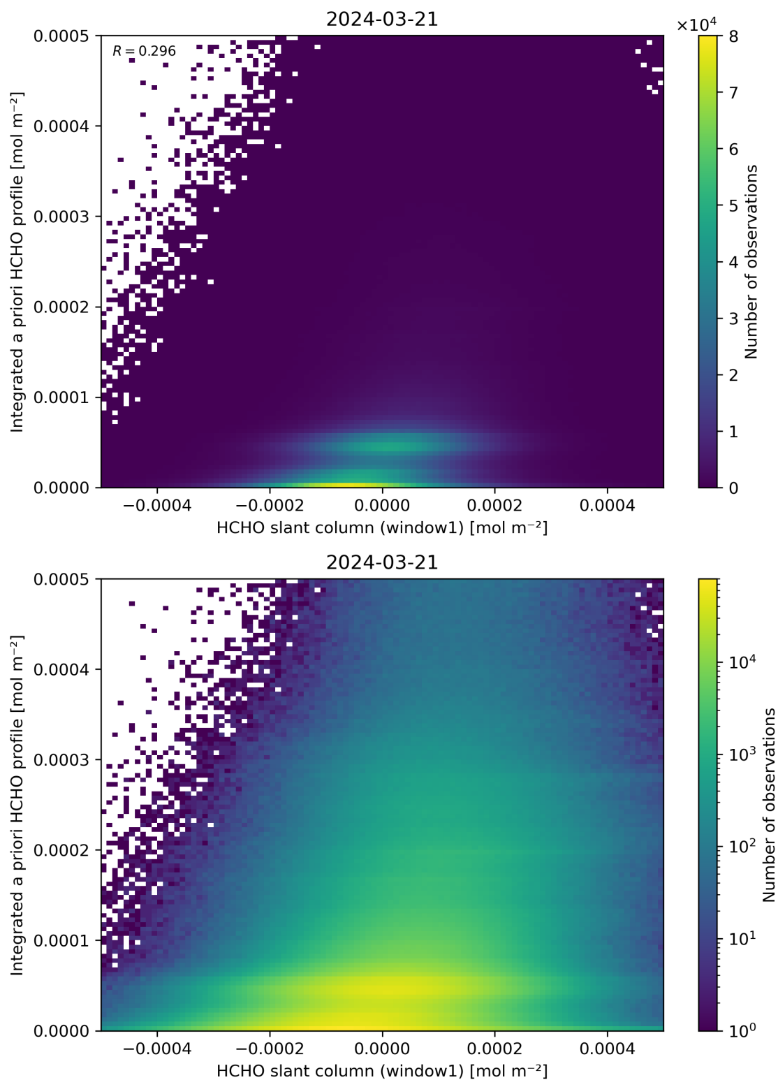
Figure 87: Scatter density plot of “HCHO slant column (window1)” against “Integrated a priori HCHO profile” for 2024-03-20 to 2024-03-22.
