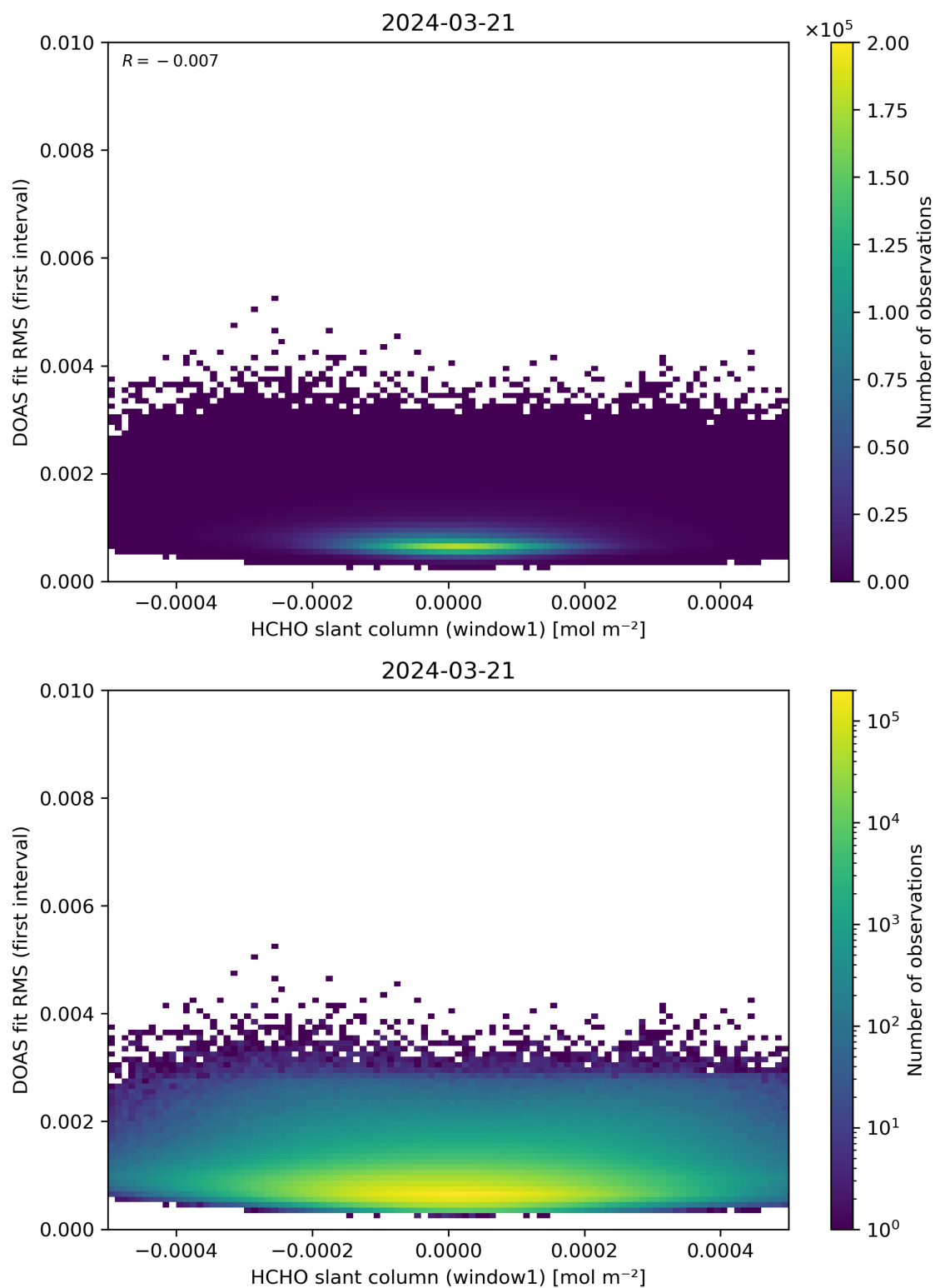
Figure 78: Scatter density plot of “HCHO slant column (window1)” against “DOAS fit RMS (first interval)” for 2024-03-20 to 2024-03-22.
