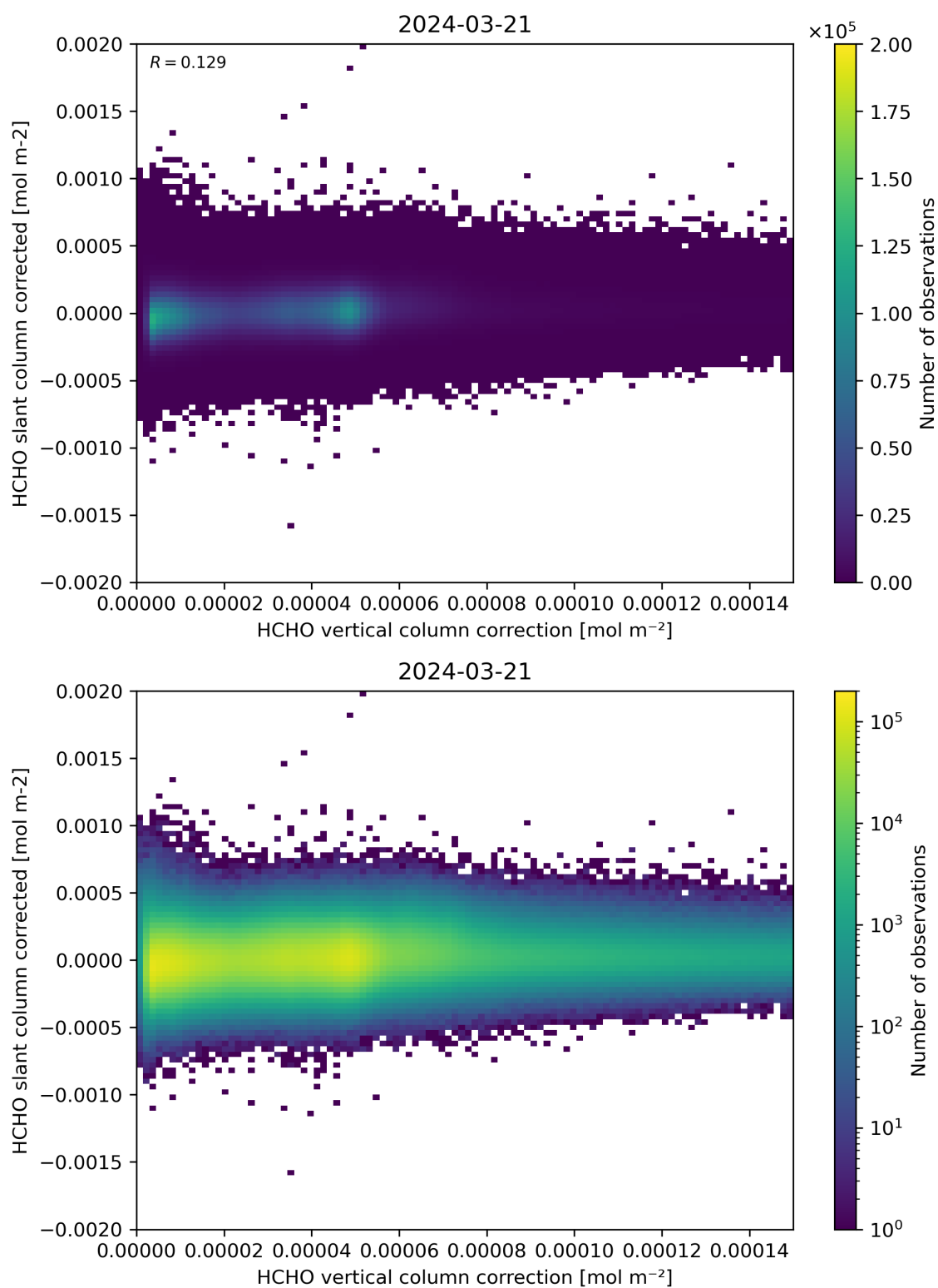
Figure 116: Scatter density plot of “HCHO vertical column correction” against “HCHO slant column corrected” for 2024-03-20 to 2024-03-22.
