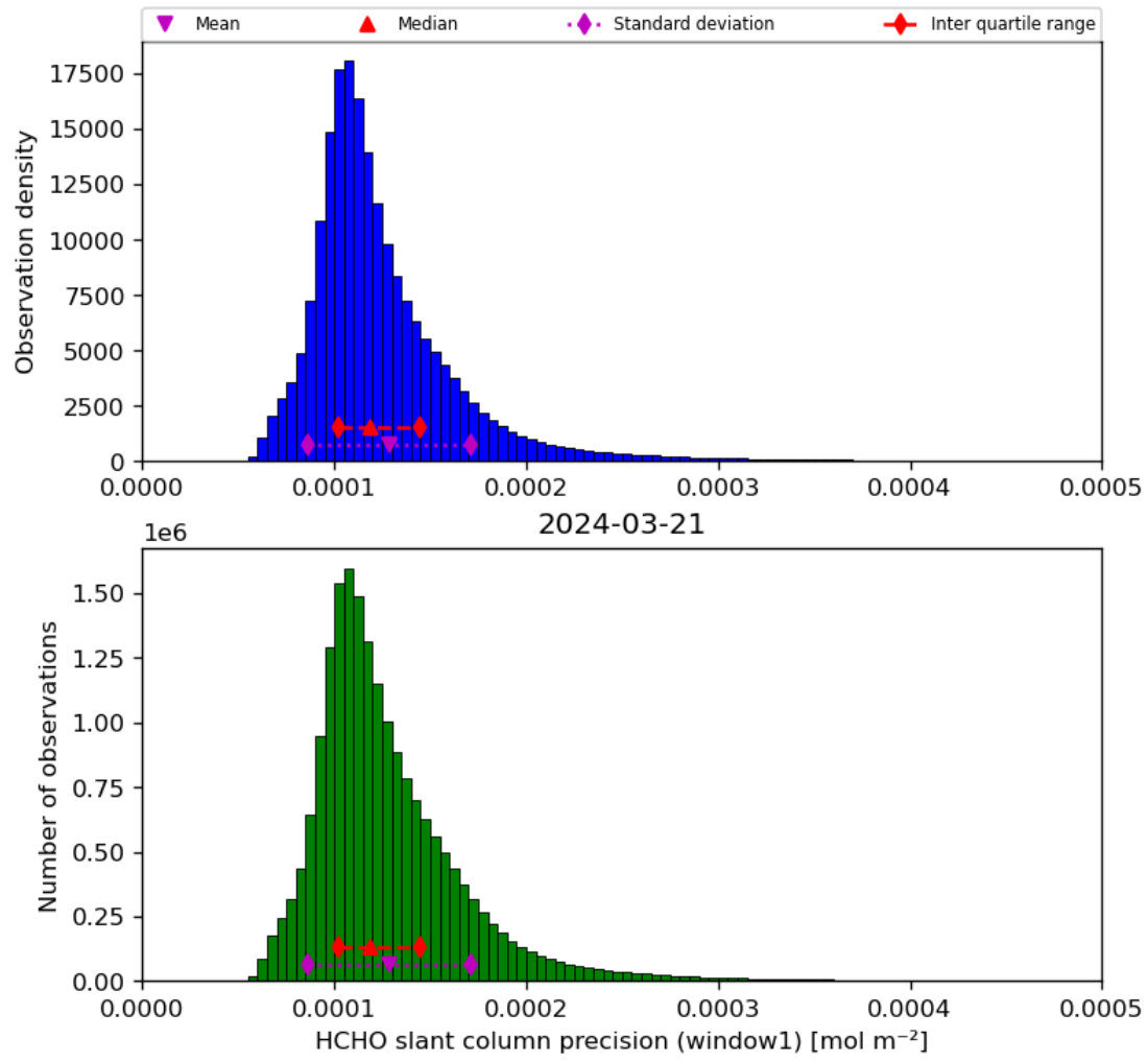
Figure 39: Histogram of “HCHO slant column precision (window1)” for 2024-03-20 to 2024-03-22
