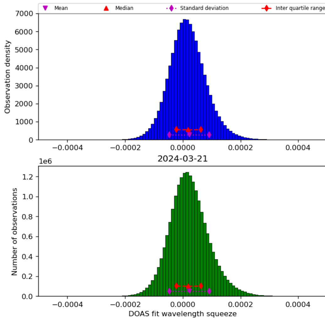
Figure 45: Histogram of “DOAS fit wavelength squeeze” for 2024-03-20 to 2024-03-22
