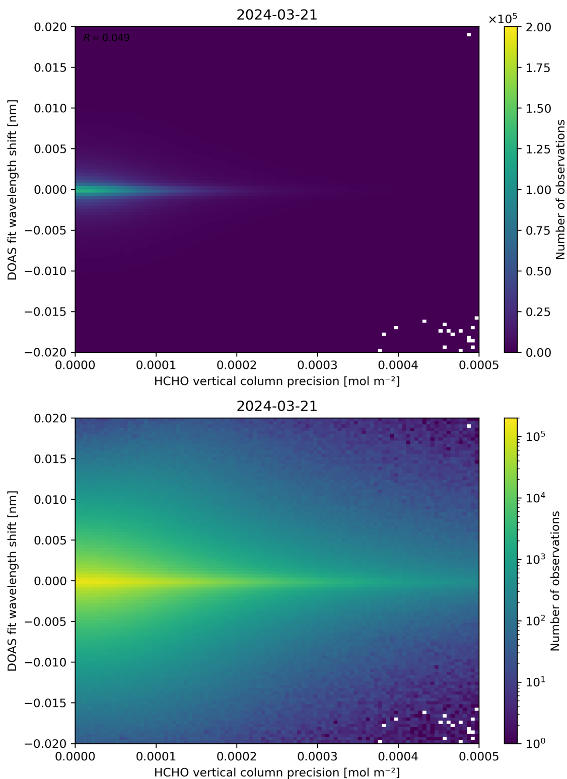
Figure 137: Scatter density plot of “HCHO vertical column precision” against “DOAS fit wavelength shift” for 2024-03-20 to 2024-03-22.
