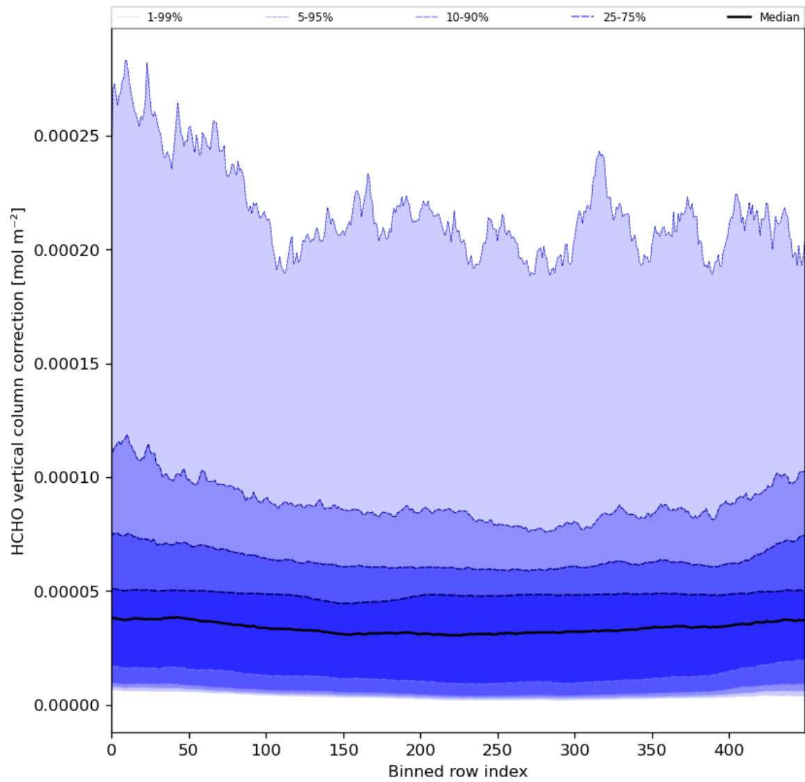
Figure 51: Along track statistics of “HCHO vertical column correction” for 2024-03-20 to 2024-03-22
