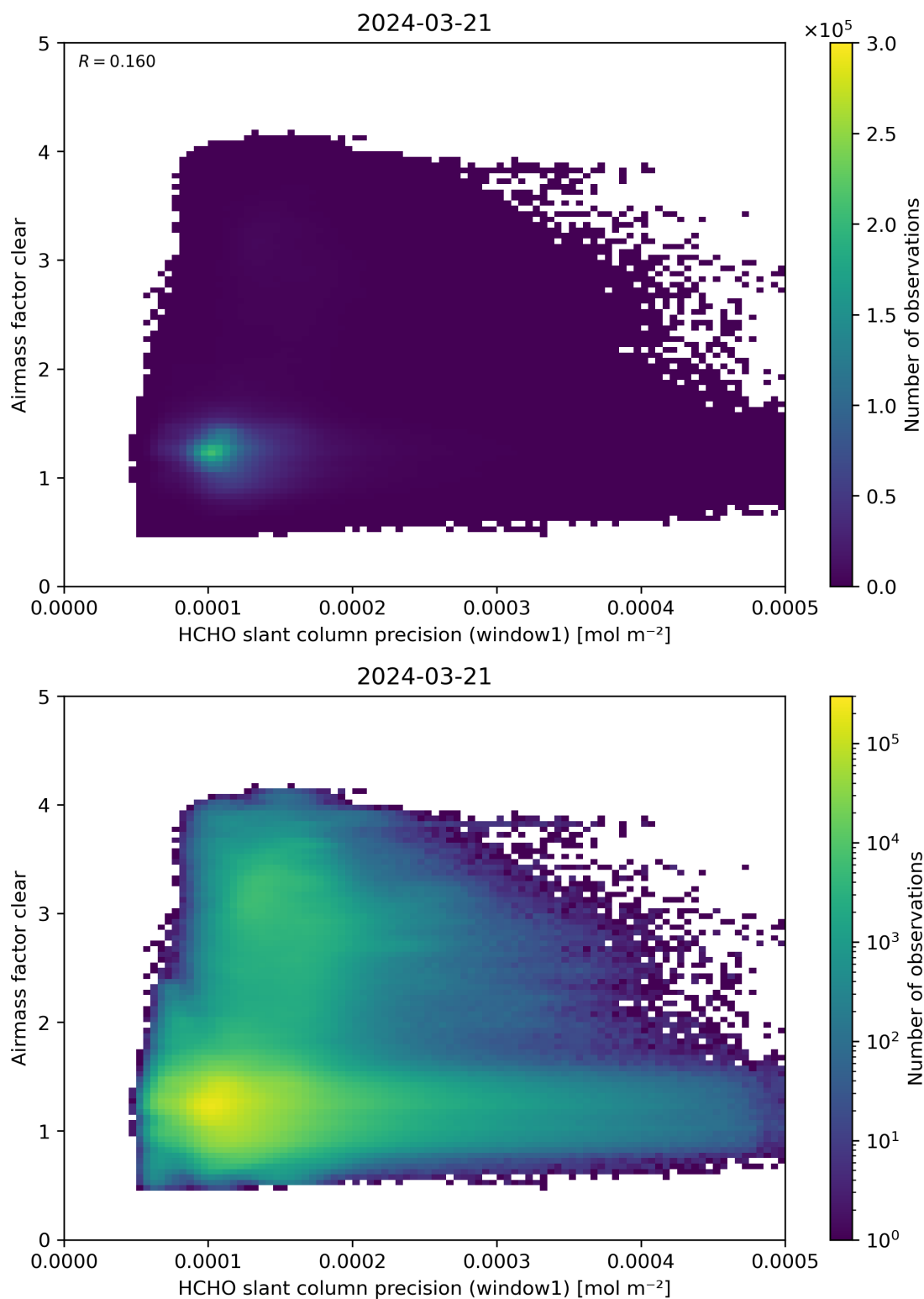
Figure 91: Scatter density plot of “HCHO slant column precision (window1)” against “Airmass factor clear” for 2024-03-20 to 2024-03-22.
