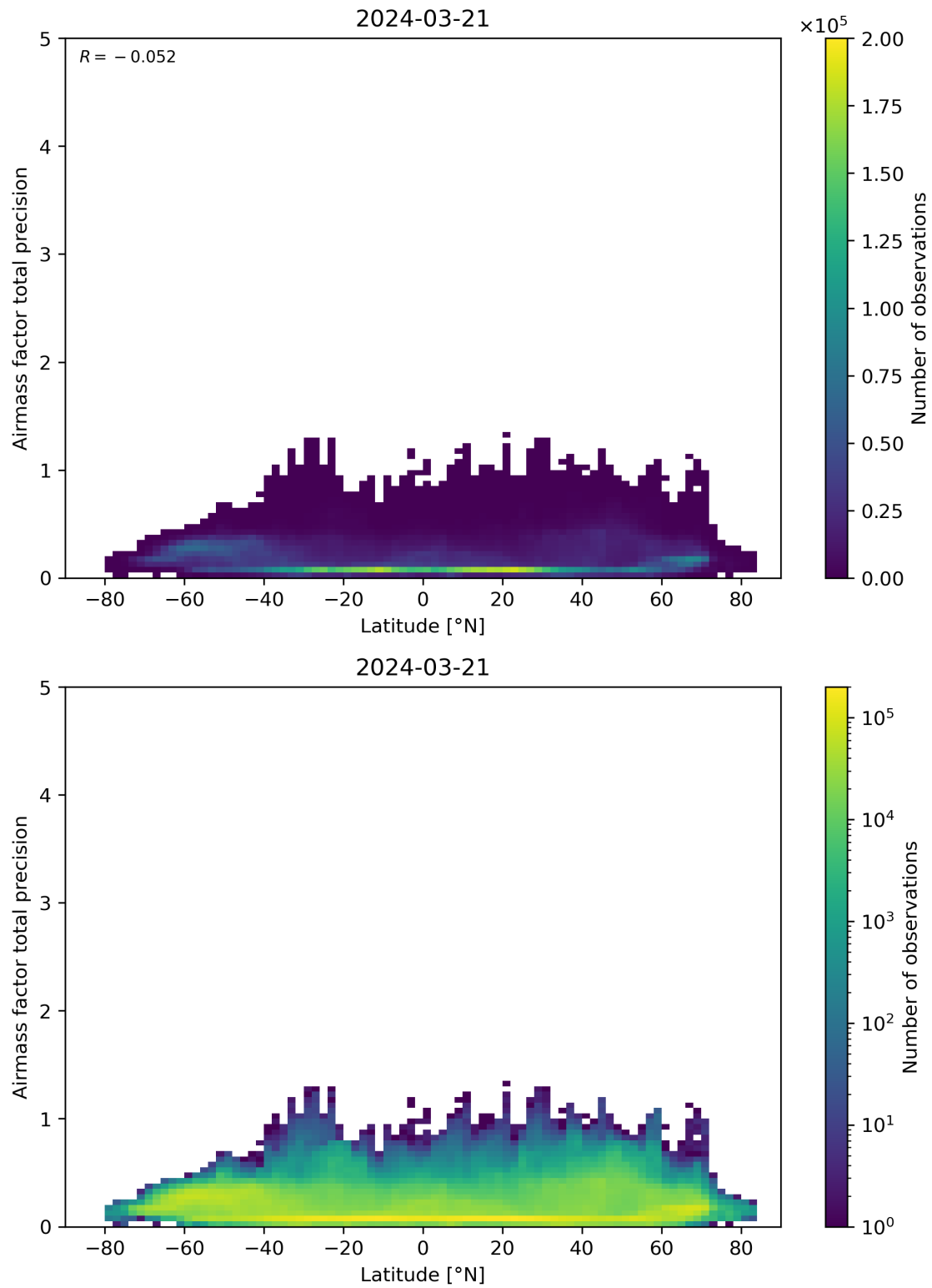
Figure 162: Scatter density plot of “Latitude” against “Airmass factor total precision” for 2024-03-20 to 2024-03-22.
