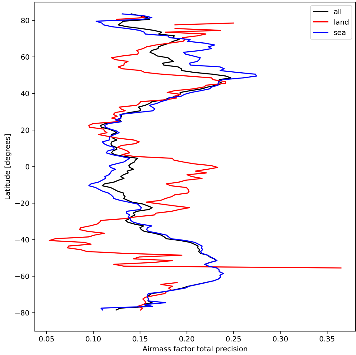
Figure 27: Zonal average of “Airmass factor total precision” for 2024-03-20 to 2024-03-22.
