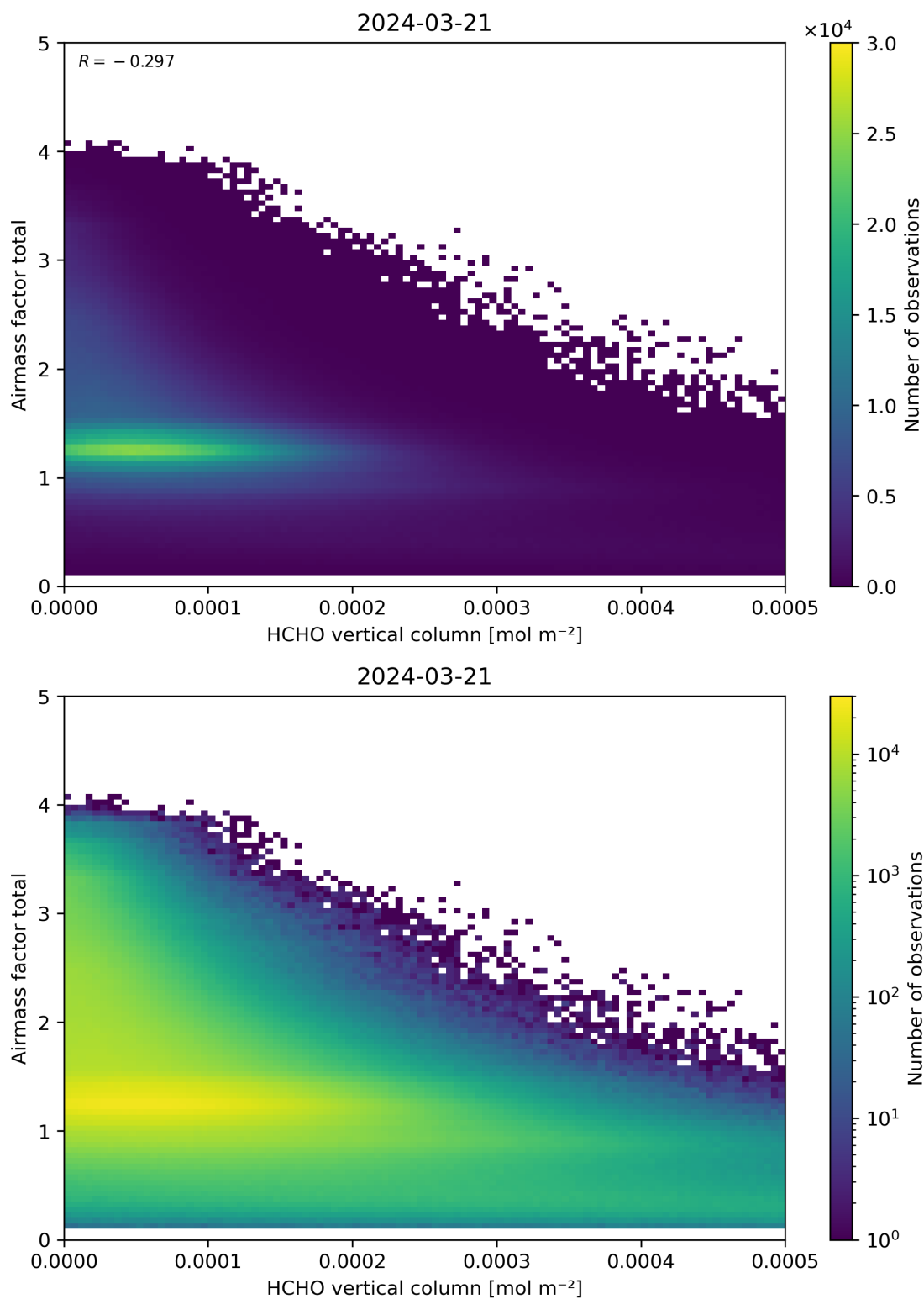
Figure 131: Scatter density plot of “HCHO vertical column” against “Airmass factor total” for 2024-03-20 to 2024-03-22.
