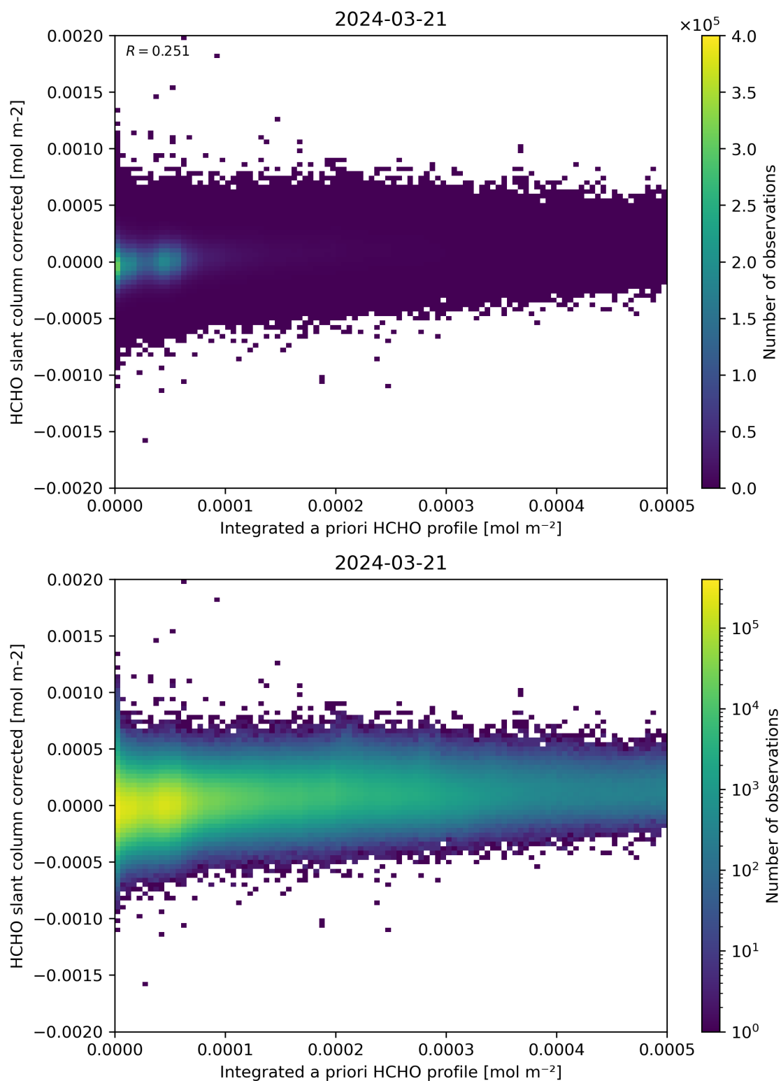
Figure 151: Scatter density plot of “Integrated a priori HCHO profile” against “HCHO slant column corrected” for 2024-03-20 to 2024-03-22.
