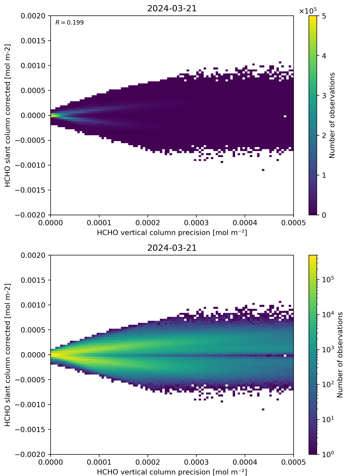
Figure 140: Scatter density plot of “HCHO vertical column precision” against “HCHO slant column corrected” for 2024-03-20 to 2024-03-22.
