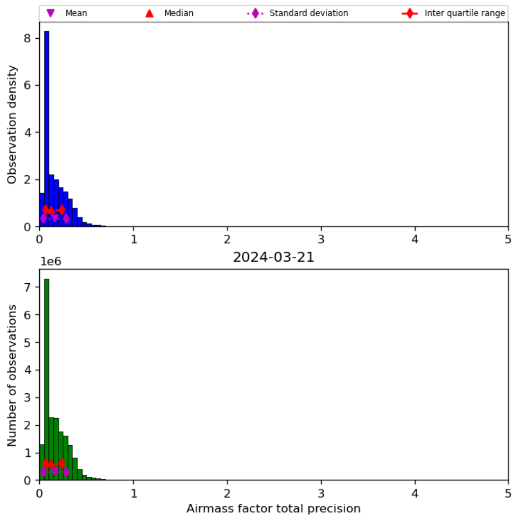
Figure 41: Histogram of “Airmass factor total precision” for 2024-03-20 to 2024-03-22
