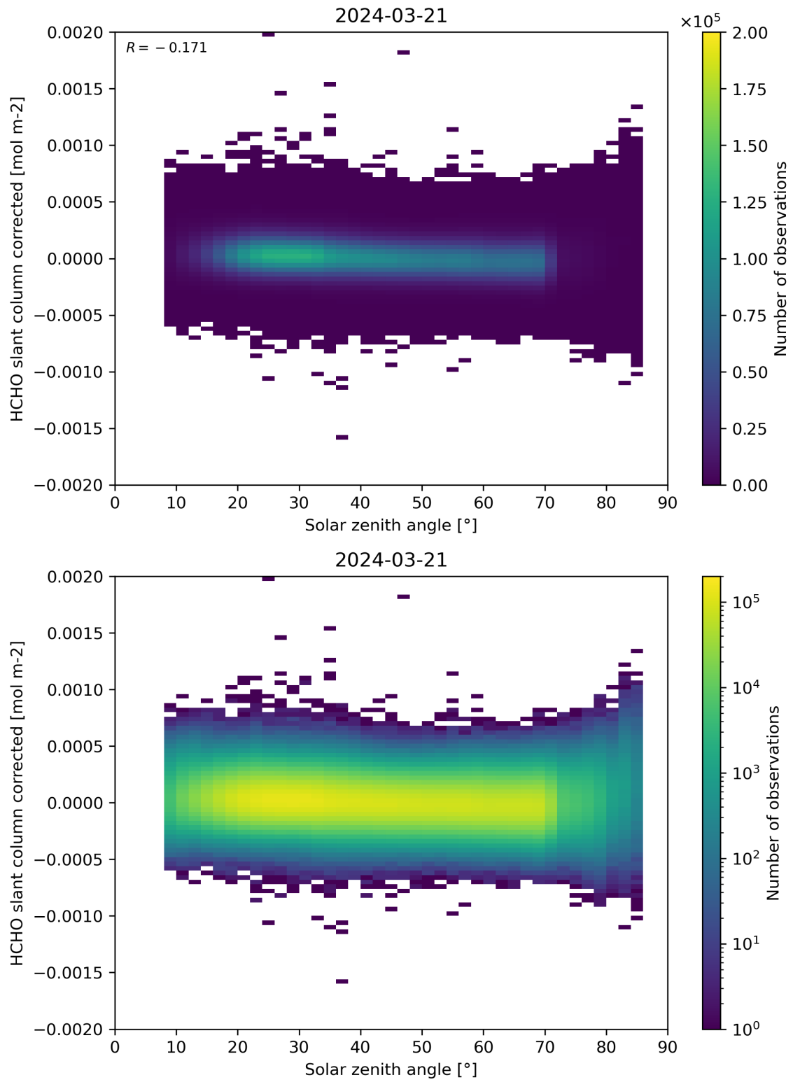
Figure 171: Scatter density plot of “Solar zenith angle” against “HCHO slant column corrected” for 2024-03-20 to 2024-03-22.
