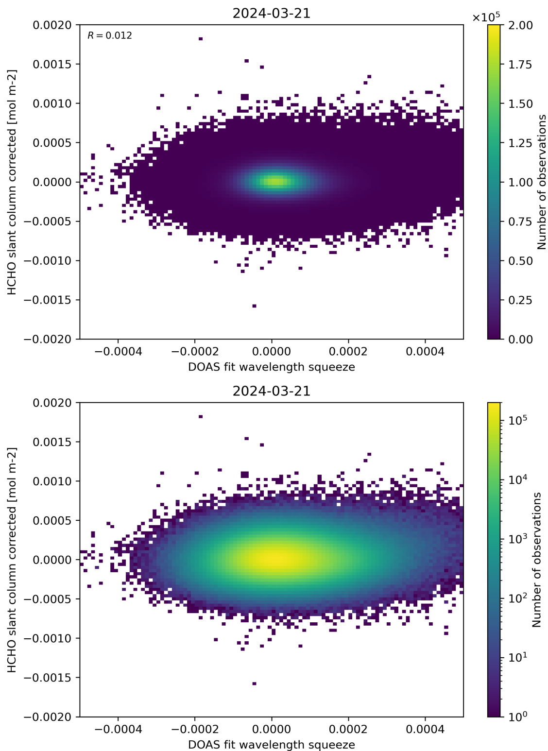
Figure 69: Scatter density plot of “DOAS fit wavelength squeeze” against “HCHO slant column corrected” for 2024-03-20 to 2024-03-22.
