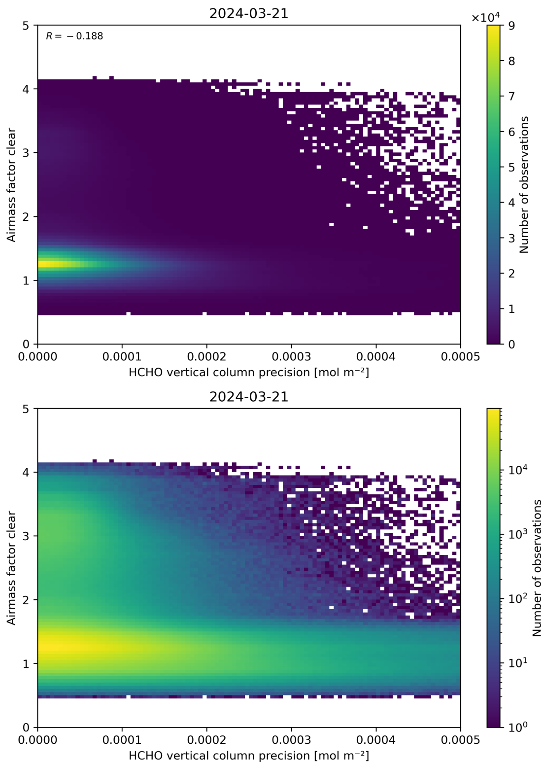
Figure 139: Scatter density plot of “HCHO vertical column precision” against “Airmass factor clear” for 2024-03-20 to 2024-03-22.
