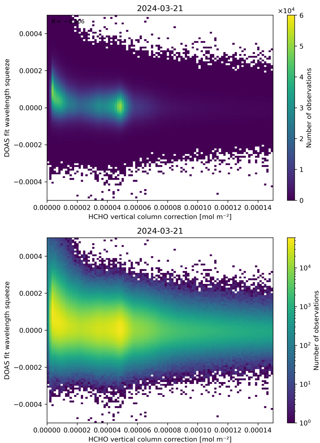
Figure 114: Scatter density plot of “HCHO vertical column correction” against “DOAS fit wavelength squeeze” for 2024-03-20 to 2024-03-22.
