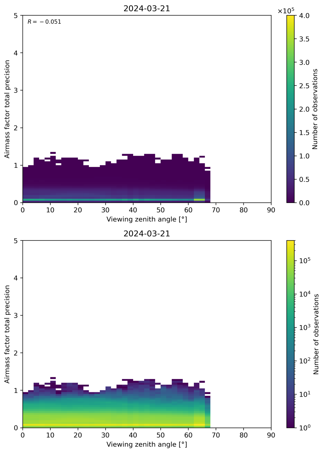
Figure 191: Scatter density plot of “Viewing zenith angle” against “Airmass factor total precision” for 2024-03-20 to 2024-03-22.
