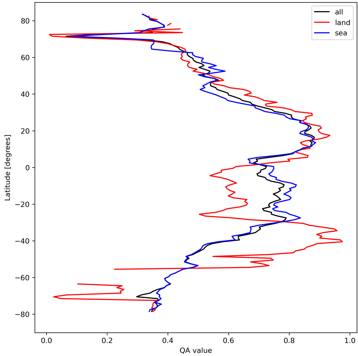
Figure 20: Zonal average of “QA value” for 2024-03-20 to 2024-03-22.
