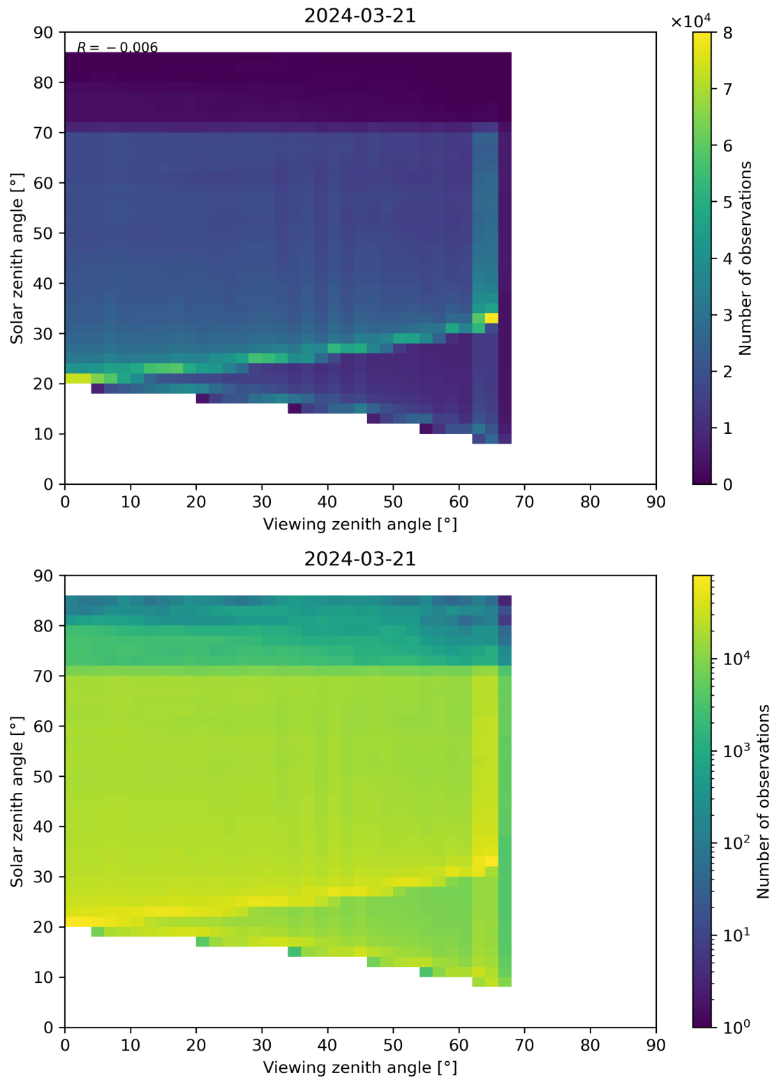
Figure 197: Scatter density plot of “Viewing zenith angle” against “Solar zenith angle” for 2024-03-20 to 2024-03-22.
