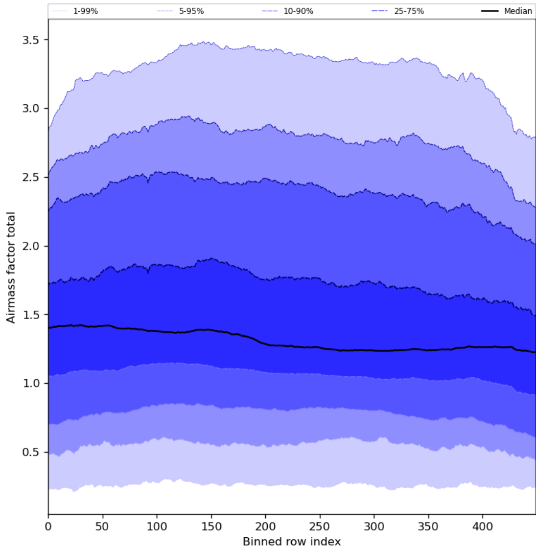
Figure 54: Along track statistics of “Airmass factor total” for 2024-03-20 to 2024-03-22
