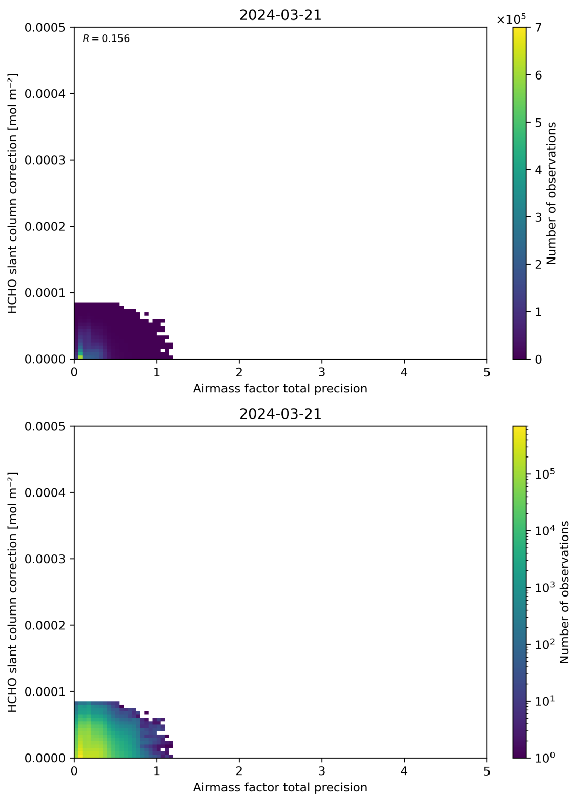
Figure 110: Scatter density plot of “Airmass factor total precision” against “HCHO slant column correction” for 2024-03-20 to 2024-03-22.
