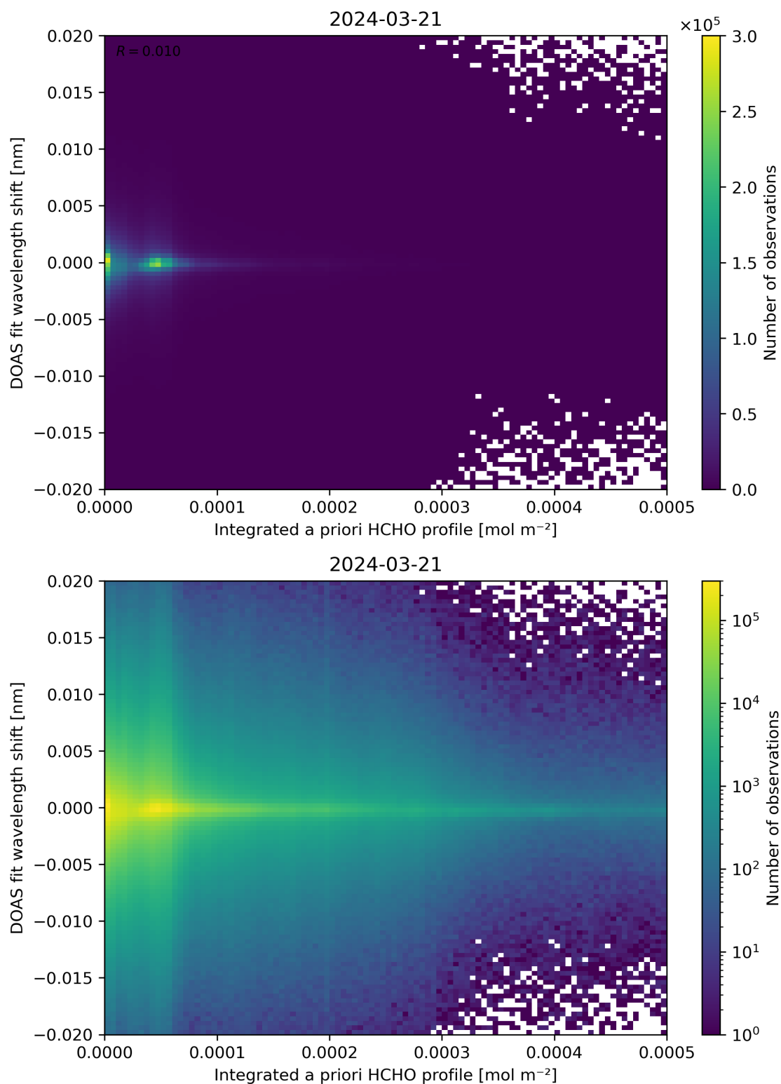
Figure 149: Scatter density plot of “Integrated a priori HCHO profile” against “DOAS fit wavelength shift” for 2024-03-20 to 2024-03-22.
