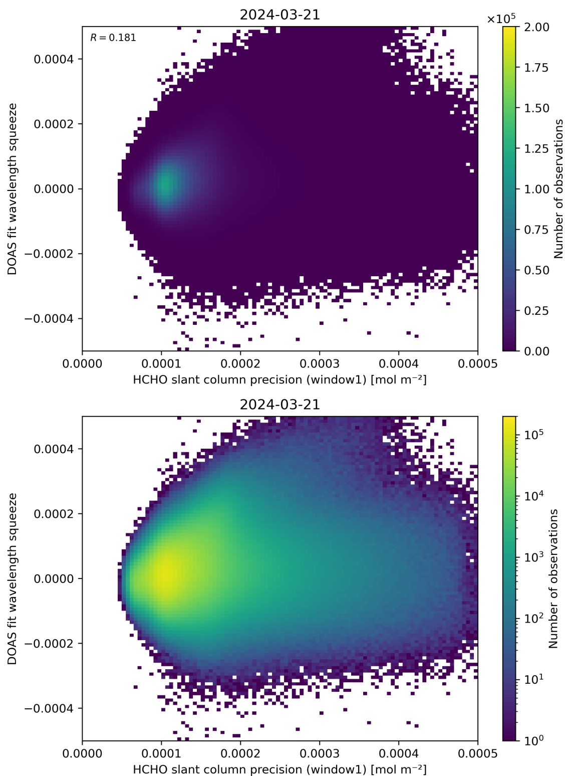
Figure 90: Scatter density plot of “HCHO slant column precision (window1)” against “DOAS fit wavelength squeeze” for 2024-03-20 to 2024-03-22.
