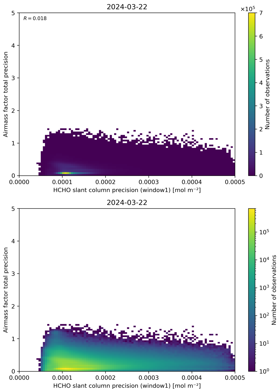
Figure 95: Scatter density plot of “HCHO slant column precision (window1)” against “Airmass factor total precision” for 2024-03-21 to 2024-03-22.
