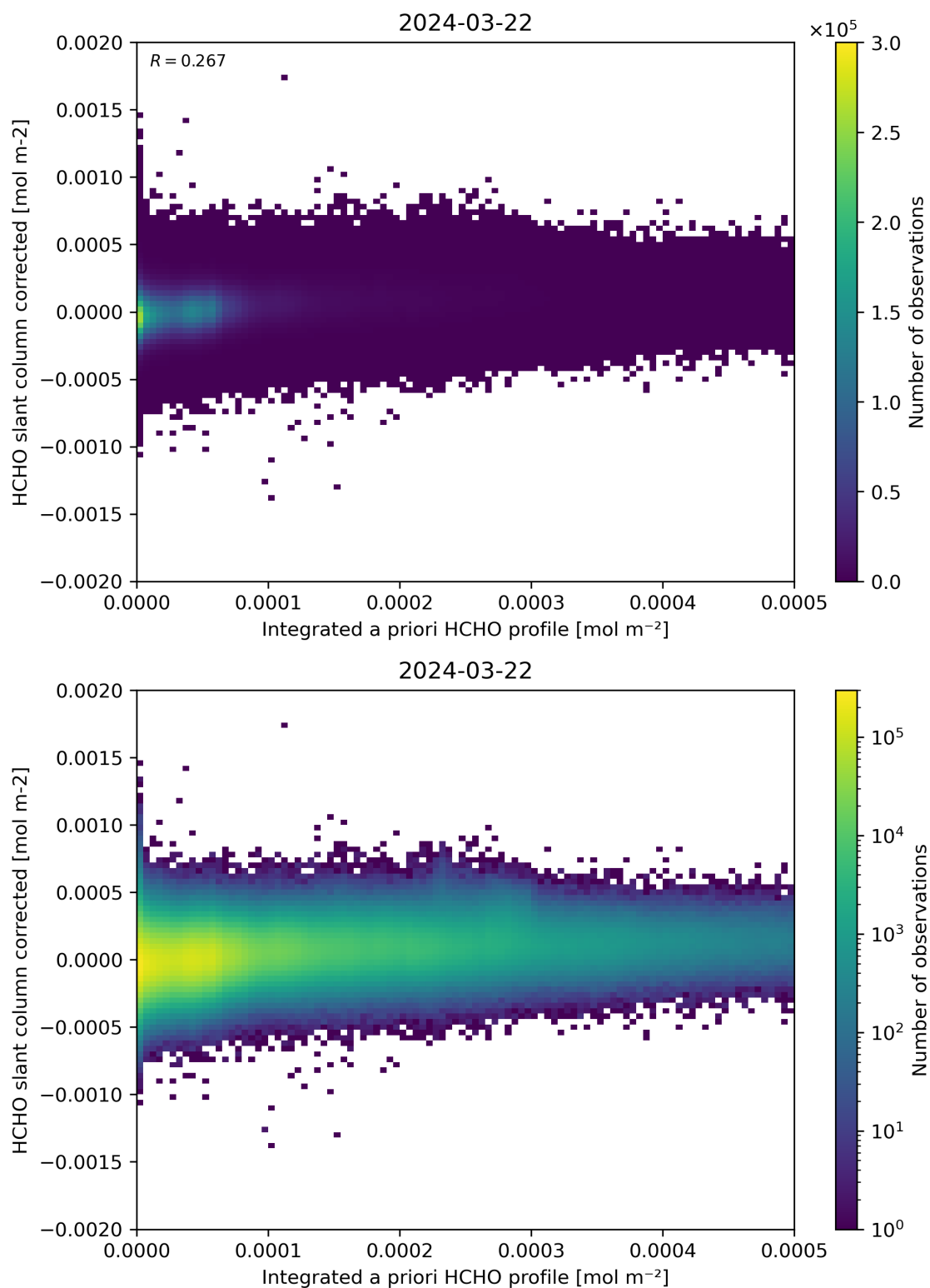
Figure 151: Scatter density plot of “Integrated a priori HCHO profile” against “HCHO slant column corrected” for 2024-03-21 to 2024-03-22.
