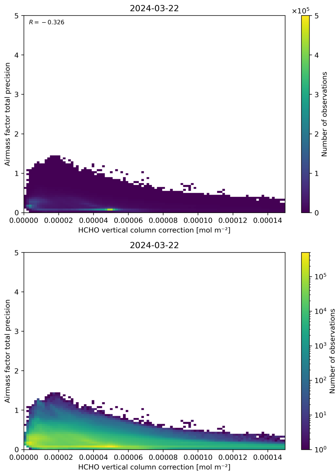
Figure 121: Scatter density plot of “HCHO vertical column correction” against “Airmass factor total precision” for 2024-03-21 to 2024-03-22.
