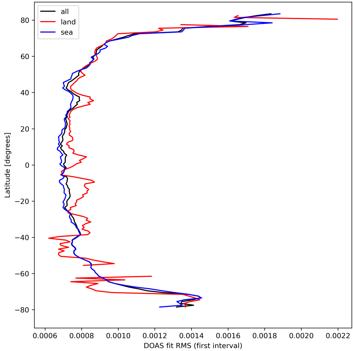
Figure 32: Zonal average of “DOAS fit RMS (first interval)” for 2024-03-21 to 2024-03-22.
