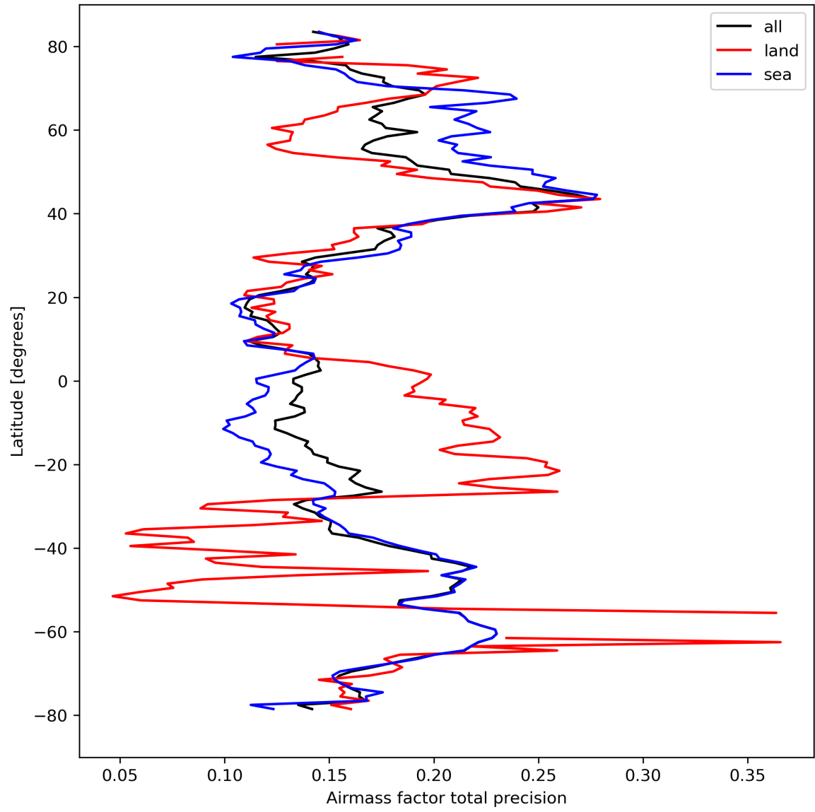
Figure 27: Zonal average of “Airmass factor total precision” for 2024-03-21 to 2024-03-22.
