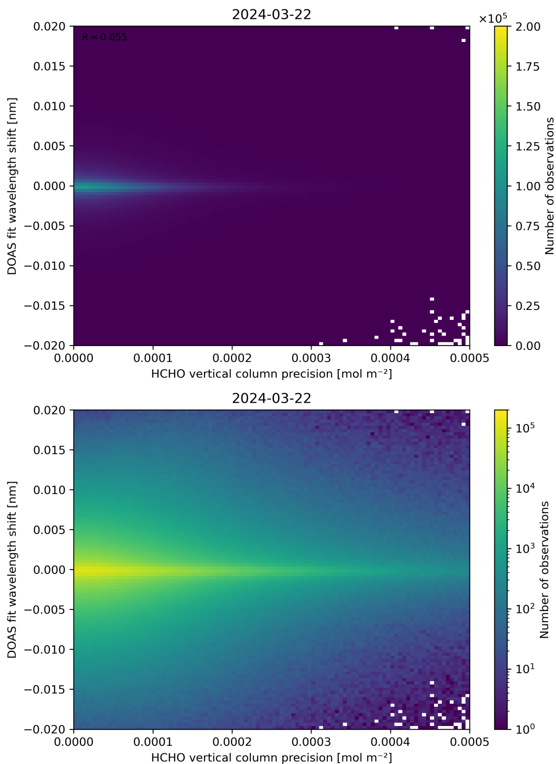
Figure 137: Scatter density plot of “HCHO vertical column precision” against “DOAS fit wavelength shift” for 2024-03-21 to 2024-03-22.
