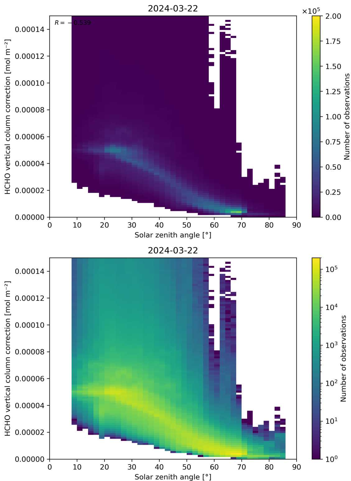
Figure 178: Scatter density plot of “Solar zenith angle” against “HCHO vertical column correction” for 2024-03-21 to 2024-03-22.
