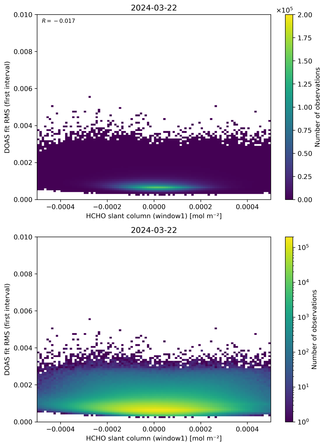
Figure 78: Scatter density plot of “HCHO slant column (window1)” against “DOAS fit RMS (first interval)” for 2024-03-21 to 2024-03-22.
