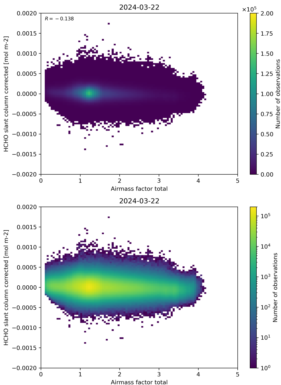
Figure 101: Scatter density plot of “Airmass factor total” against “HCHO slant column corrected” for 2024-03-21 to 2024-03-22.
