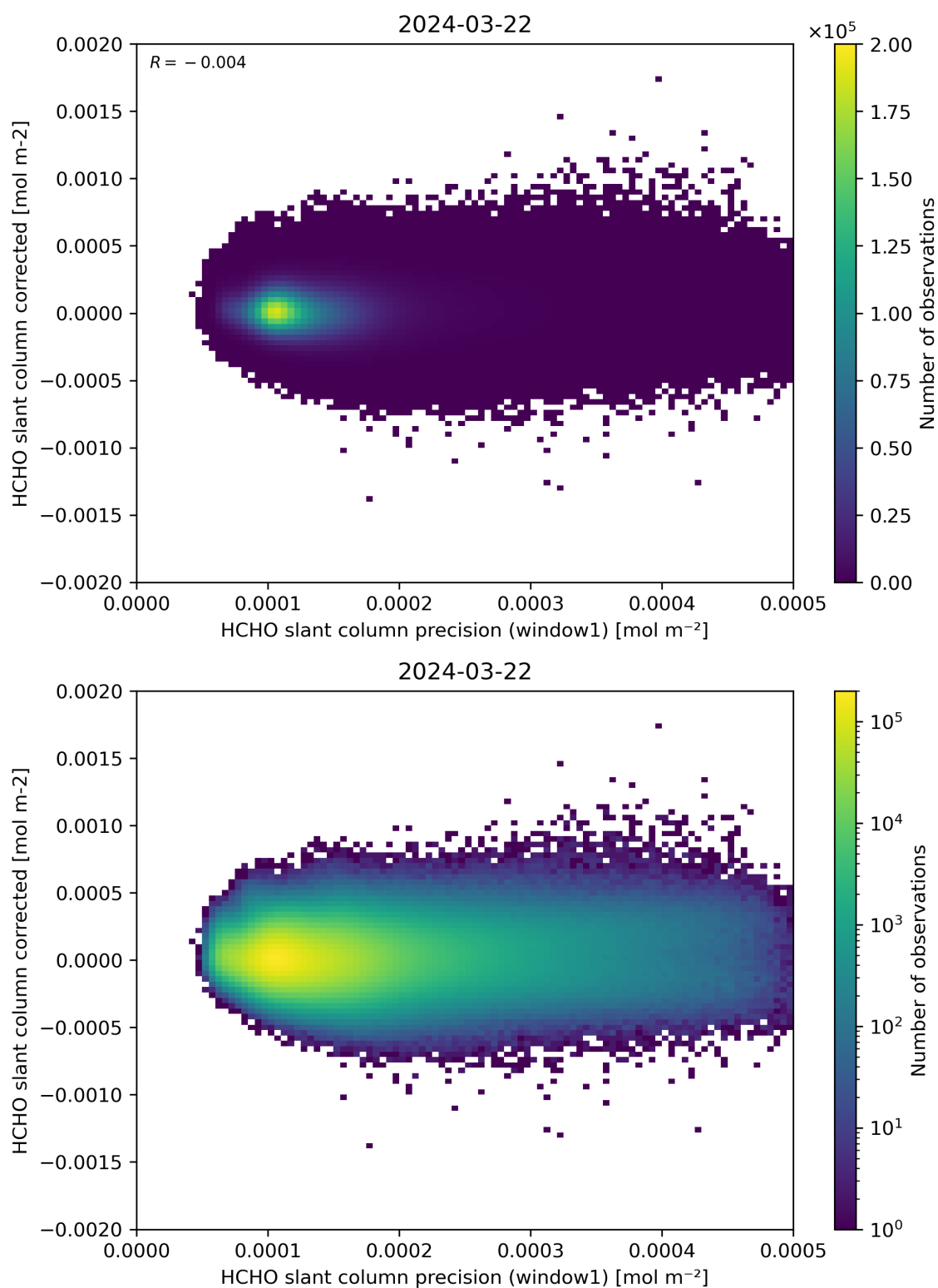
Figure 92: Scatter density plot of “HCHO slant column precision (window1)” against “HCHO slant column corrected” for 2024-03-21 to 2024-03-22.
