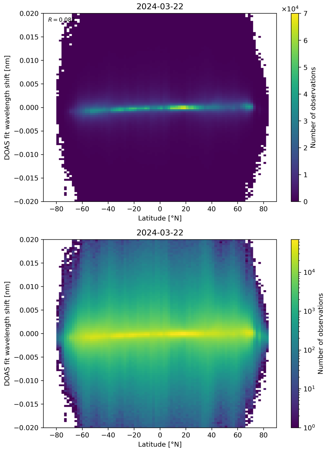
Figure 154: Scatter density plot of “Latitude” against “DOAS fit wavelength shift” for 2024-03-21 to 2024-03-22.
