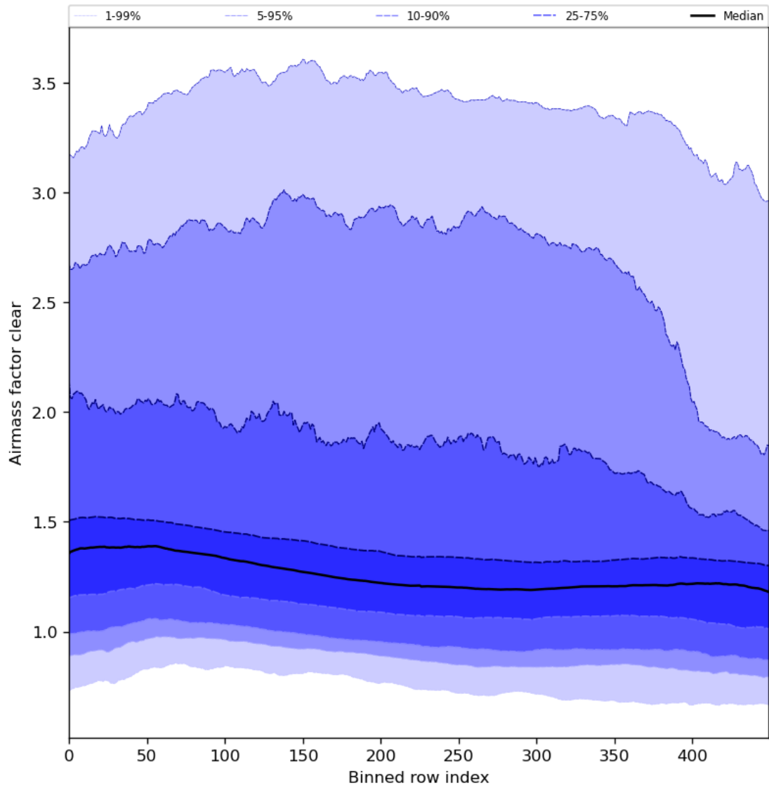
Figure 56: Along track statistics of “Airmass factor clear” for 2024-03-21 to 2024-03-22
