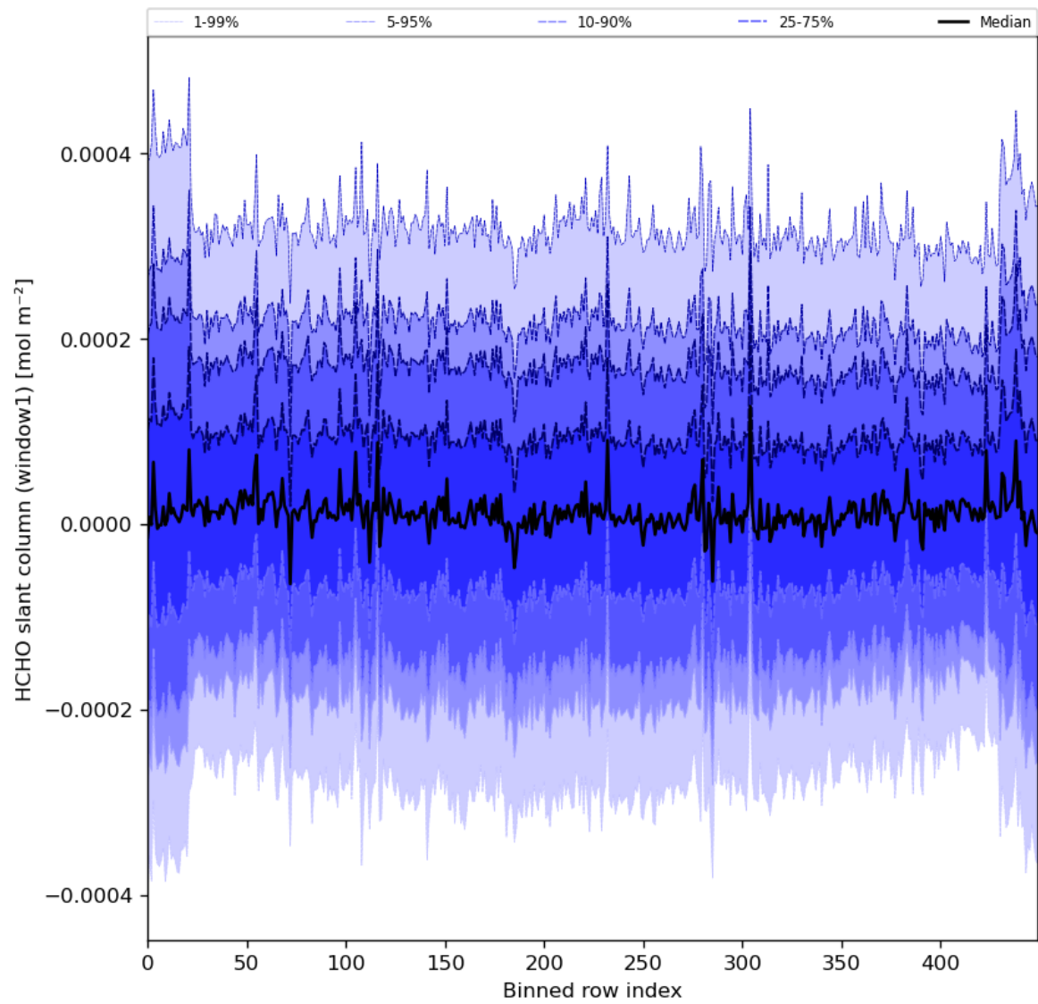
Figure 52: Along track statistics of “HCHO slant column (window1)” for 2024-03-21 to 2024-03-22
