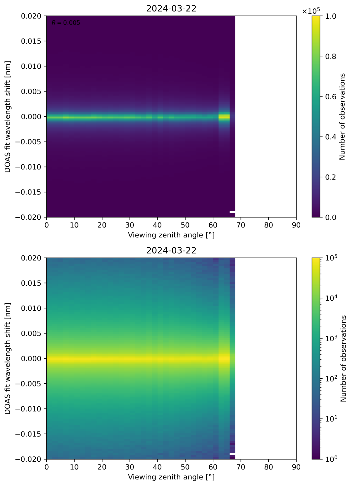
Figure 183: Scatter density plot of “Viewing zenith angle” against “DOAS fit wavelength shift” for 2024-03-21 to 2024-03-22.
