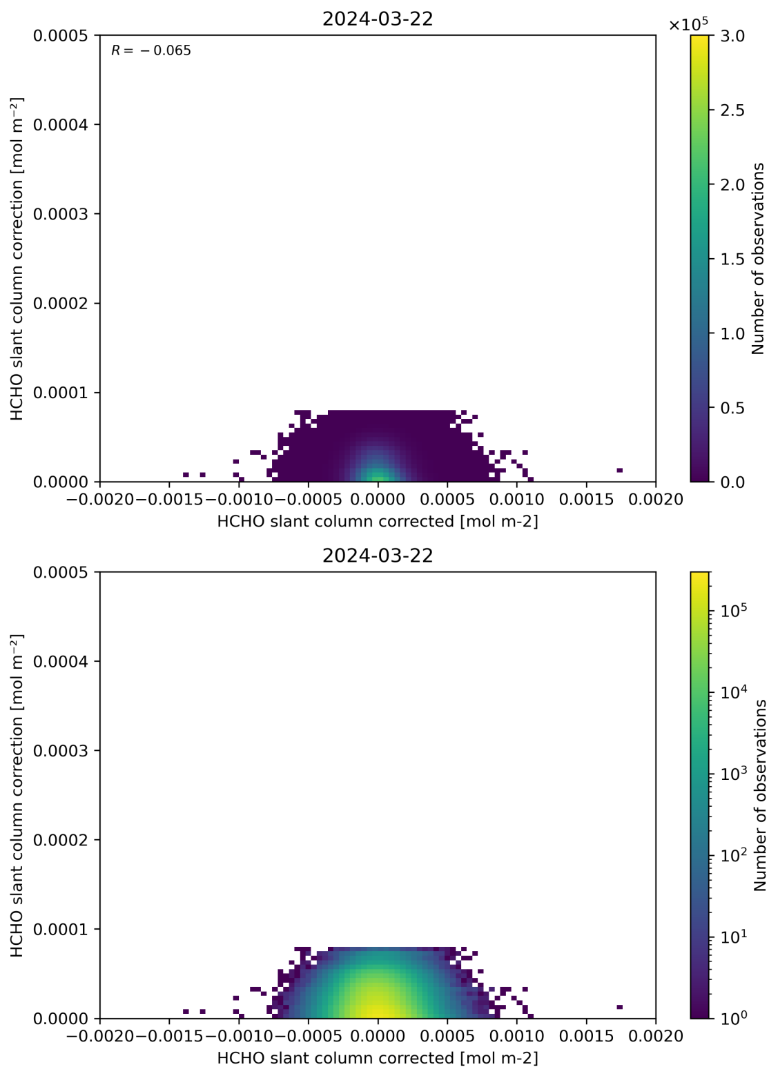
Figure 77: Scatter density plot of “HCHO slant column corrected” against “HCHO slant column correction” for 2024-03-21 to 2024-03-22.
