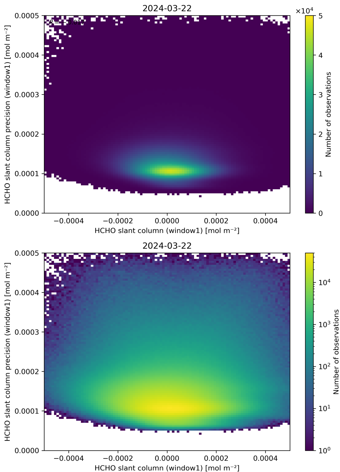
Figure 84: Scatter density plot of “HCHO slant column (window1)” against “HCHO slant column precision (window1)” for 2024-03-21 to 2024-03-22.
