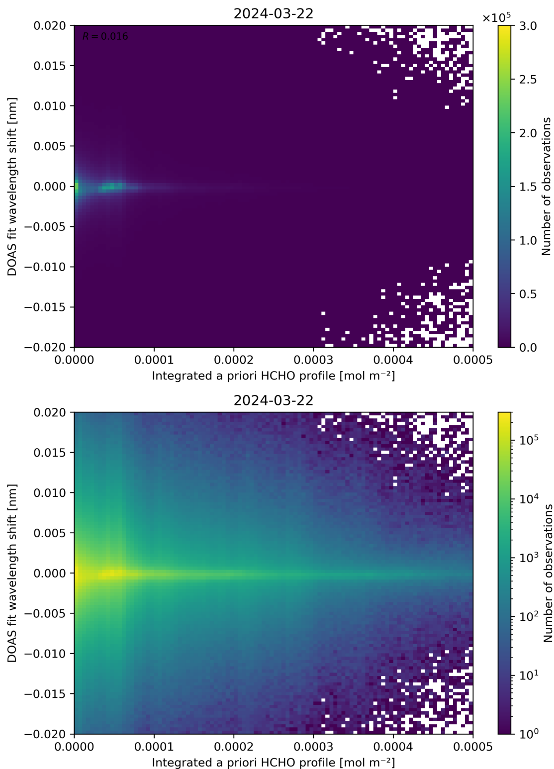
Figure 149: Scatter density plot of “Integrated a priori HCHO profile” against “DOAS fit wavelength shift” for 2024-03-21 to 2024-03-22.
