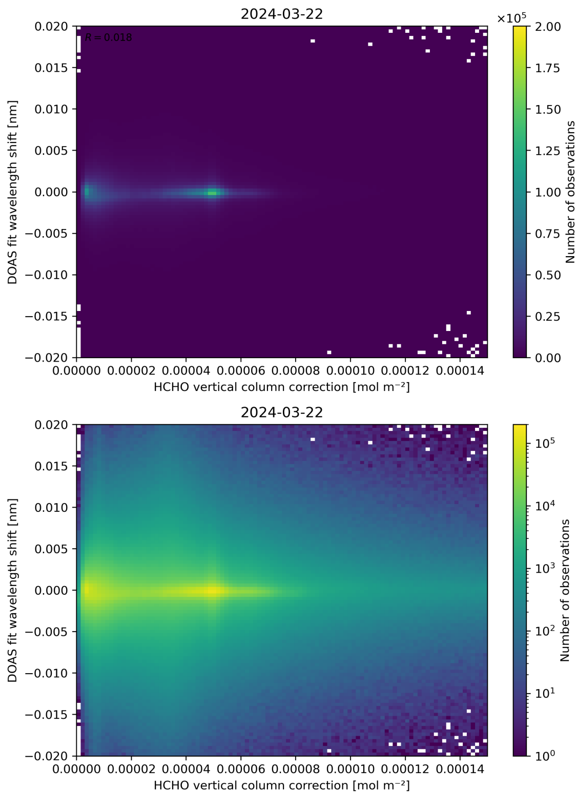
Figure 113: Scatter density plot of “HCHO vertical column correction” against “DOAS fit wavelength shift” for 2024-03-21 to 2024-03-22.
