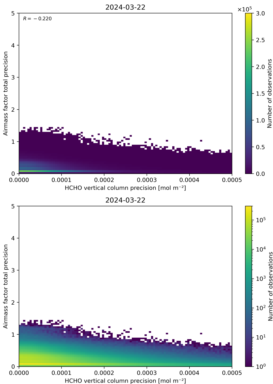
Figure 145: Scatter density plot of “HCHO vertical column precision” against “Airmass factor total precision” for 2024-03-21 to 2024-03-22.
