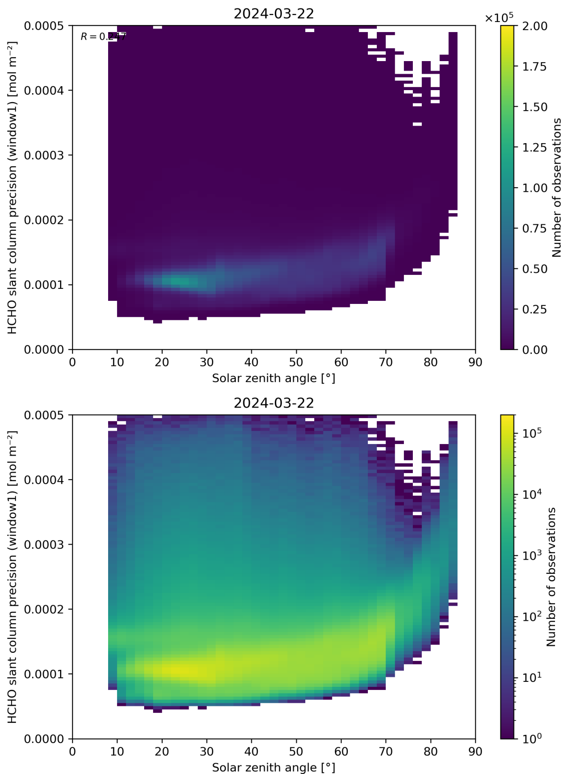
Figure 174: Scatter density plot of “Solar zenith angle” against “HCHO slant column precision (window1)” for 2024-03-21 to 2024-03-22.
