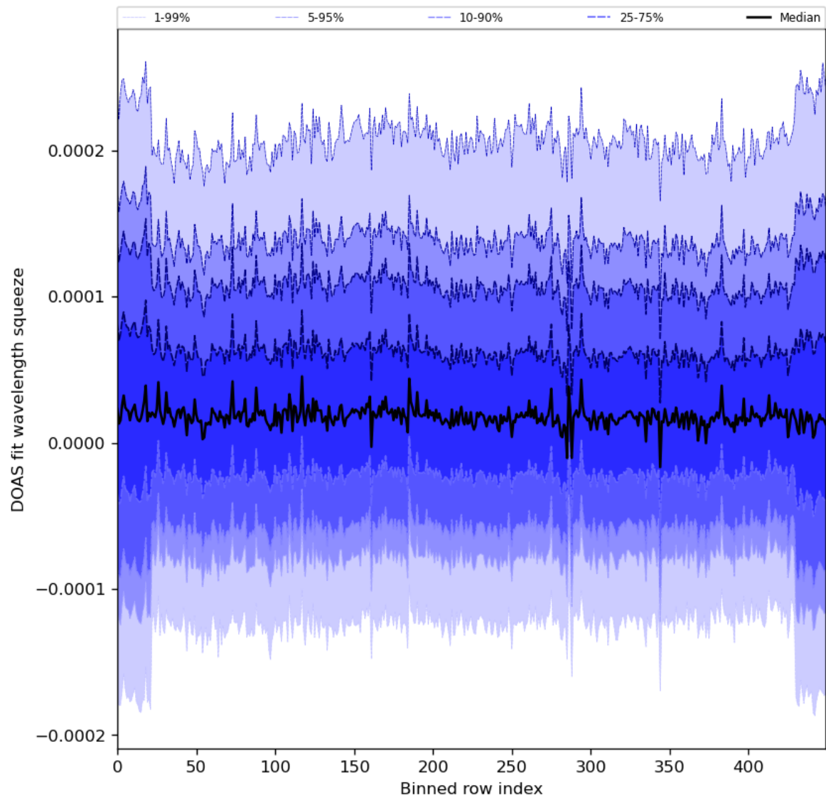
Figure 59: Along track statistics of “DOAS fit wavelength squeeze” for 2024-03-21 to 2024-03-22
