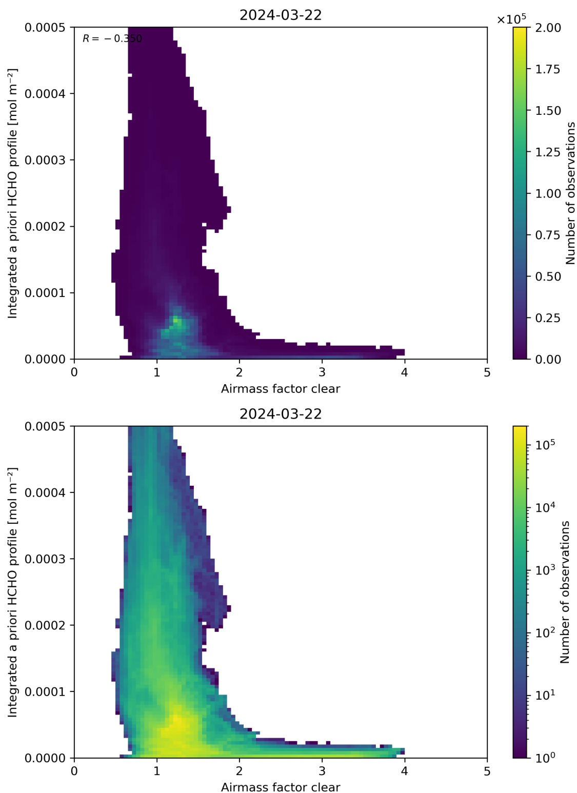
Figure 76: Scatter density plot of “Airmass factor clear” against “Integrated a priori HCHO profile” for 2024-03-21 to 2024-03-22.
