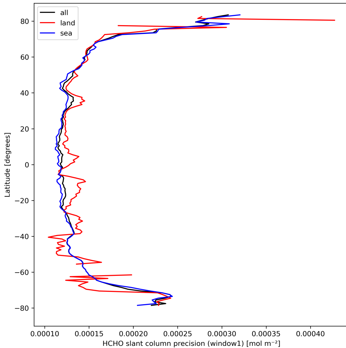
Figure 25: Zonal average of “HCHO slant column precision (window1)” for 2024-03-21 to 2024-03-22.
