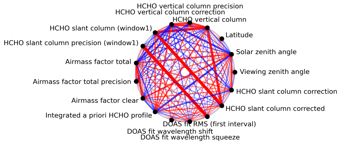
Figure 1: Map of correlation graph for 2024-03-21 to 2024-03-22.
