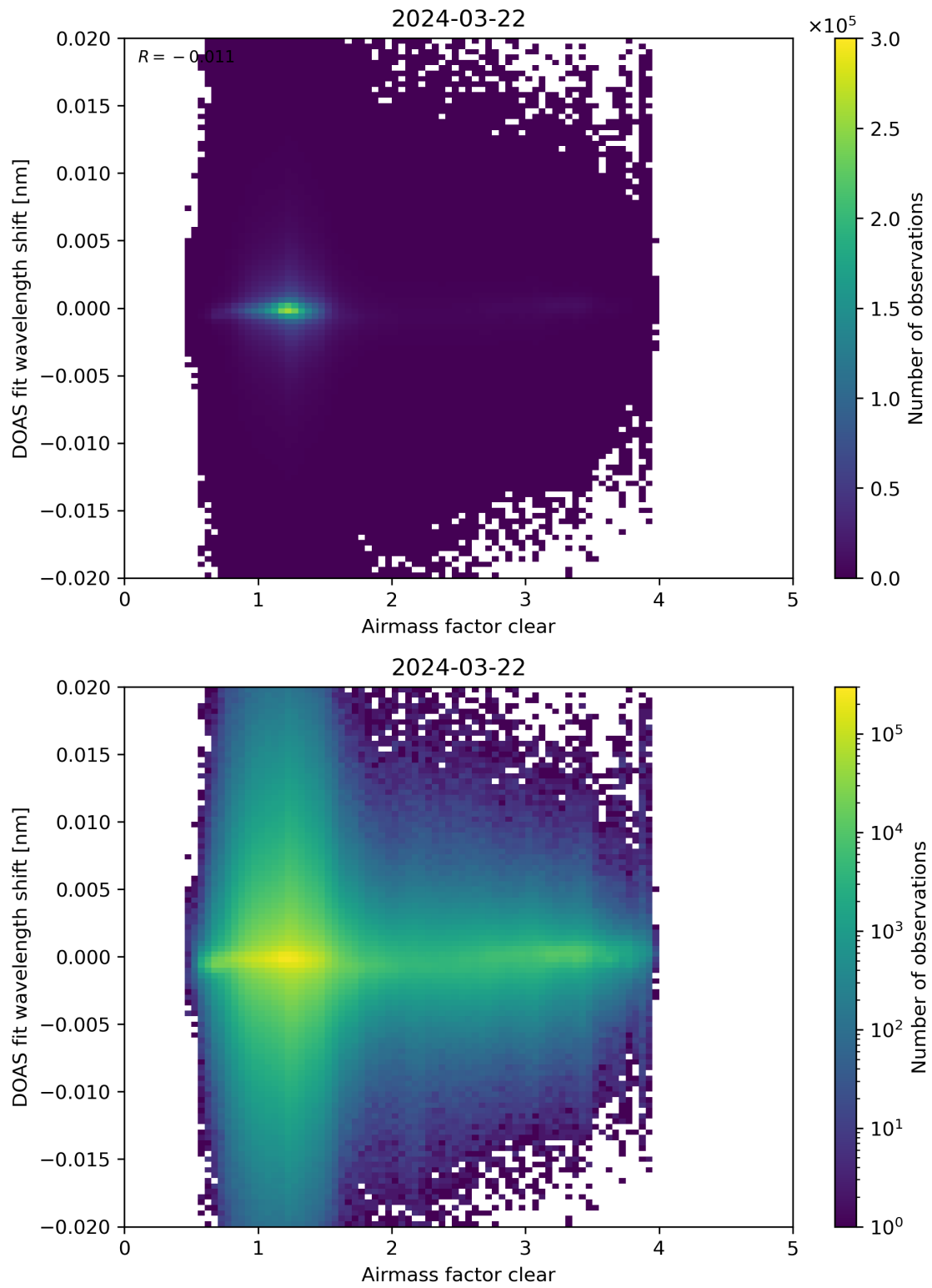
Figure 72: Scatter density plot of “Airmass factor clear” against “DOAS fit wavelength shift” for 2024-03-21 to 2024-03-22.
