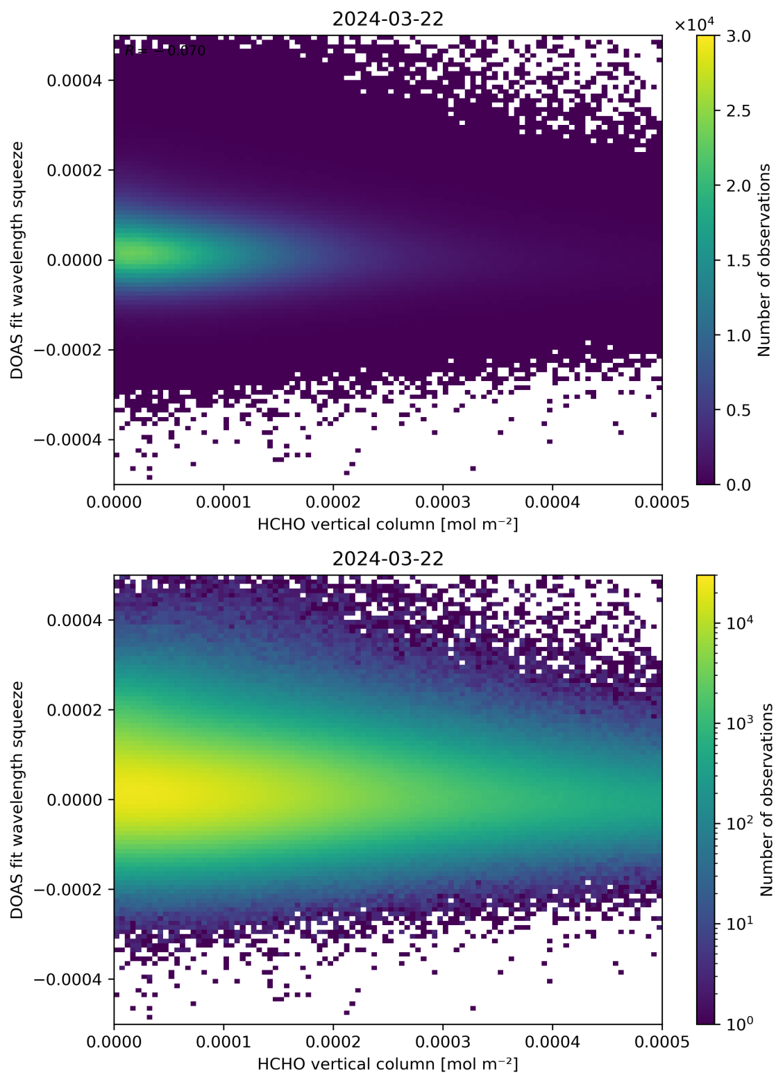
Figure 125: Scatter density plot of “HCHO vertical column” against “DOAS fit wavelength squeeze” for 2024-03-21 to 2024-03-22.
