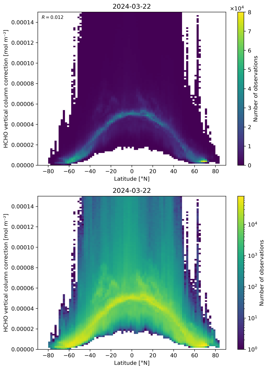
Figure 164: Scatter density plot of “Latitude” against “HCHO vertical column correction” for 2024-03-21 to 2024-03-22.
