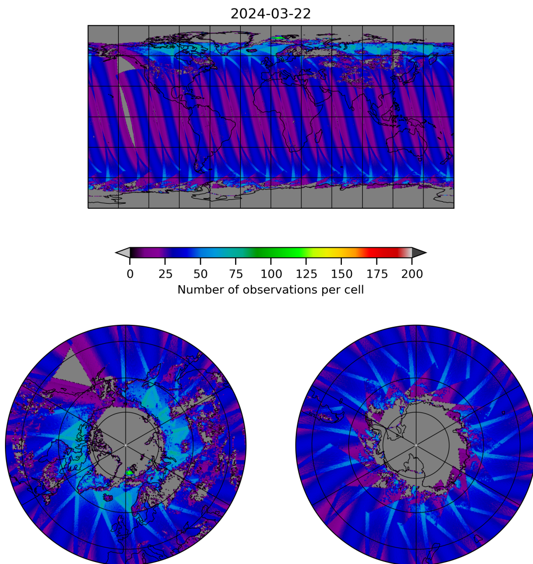
Figure 19: Map of the number of observations for 2024-03-21 to 2024-03-22
