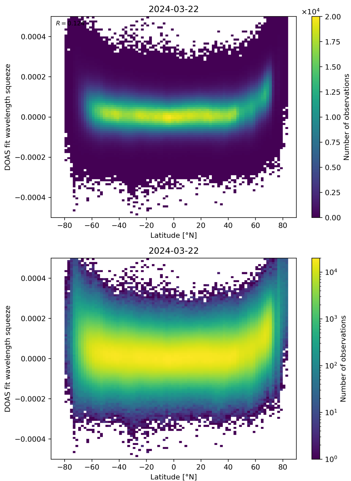
Figure 155: Scatter density plot of “Latitude” against “DOAS fit wavelength squeeze” for 2024-03-21 to 2024-03-22.
