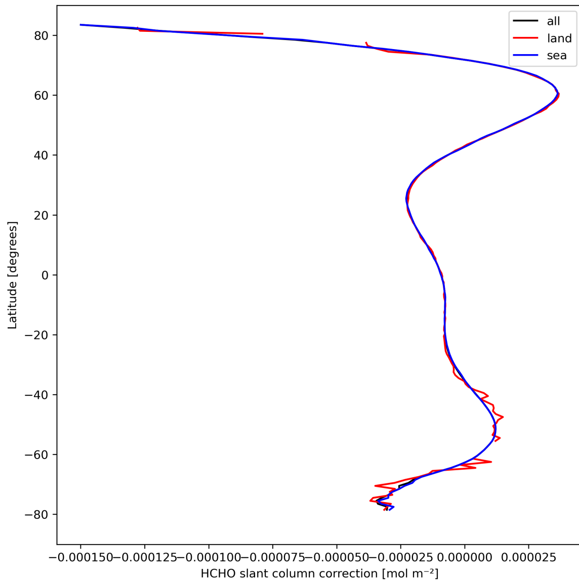
Figure 33: Zonal average of “HCHO slant column correction” for 2024-03-21 to 2024-03-22.
