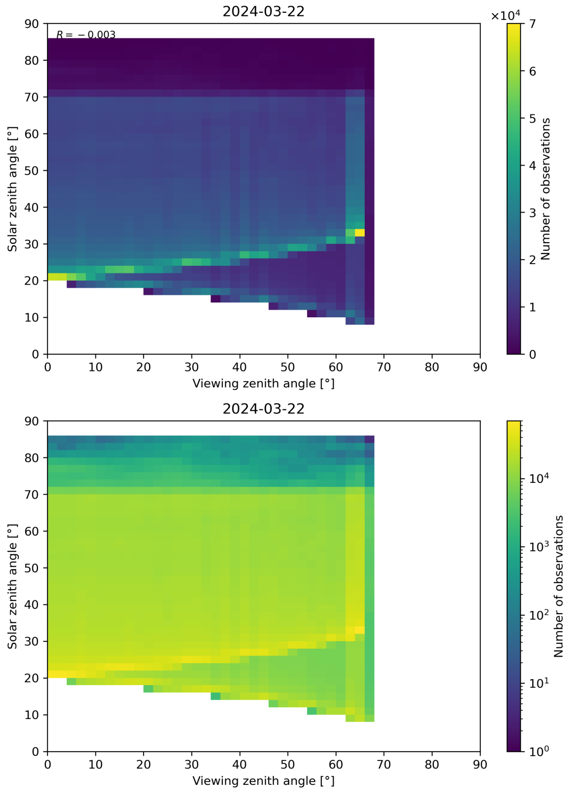
Figure 197: Scatter density plot of “Viewing zenith angle” against “Solar zenith angle” for 2024-03-21 to 2024-03-22.
