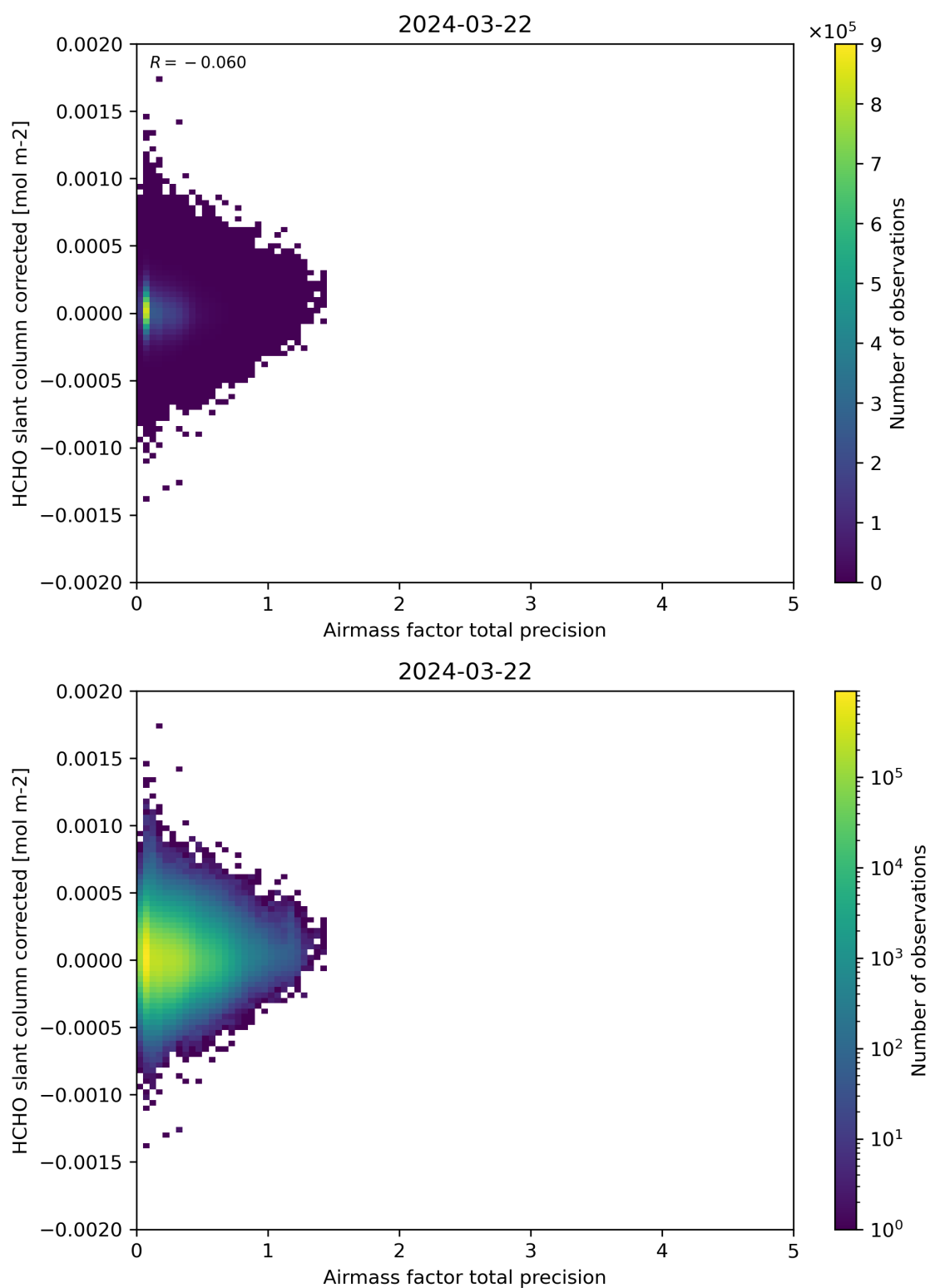
Figure 109: Scatter density plot of “Airmass factor total precision” against “HCHO slant column corrected” for 2024-03-21 to 2024-03-22.
