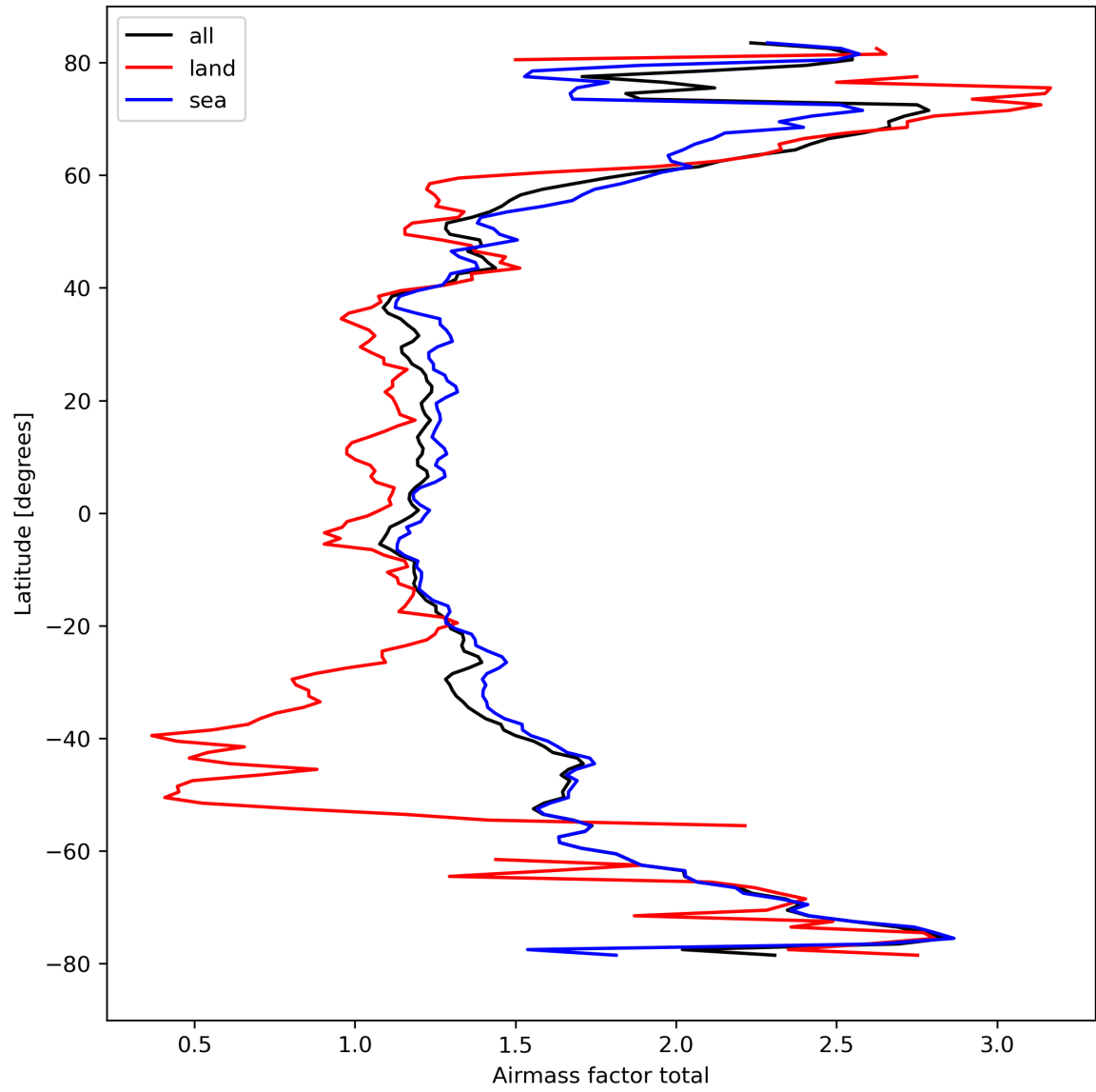
Figure 26: Zonal average of “Airmass factor total” for 2024-03-21 to 2024-03-22.
