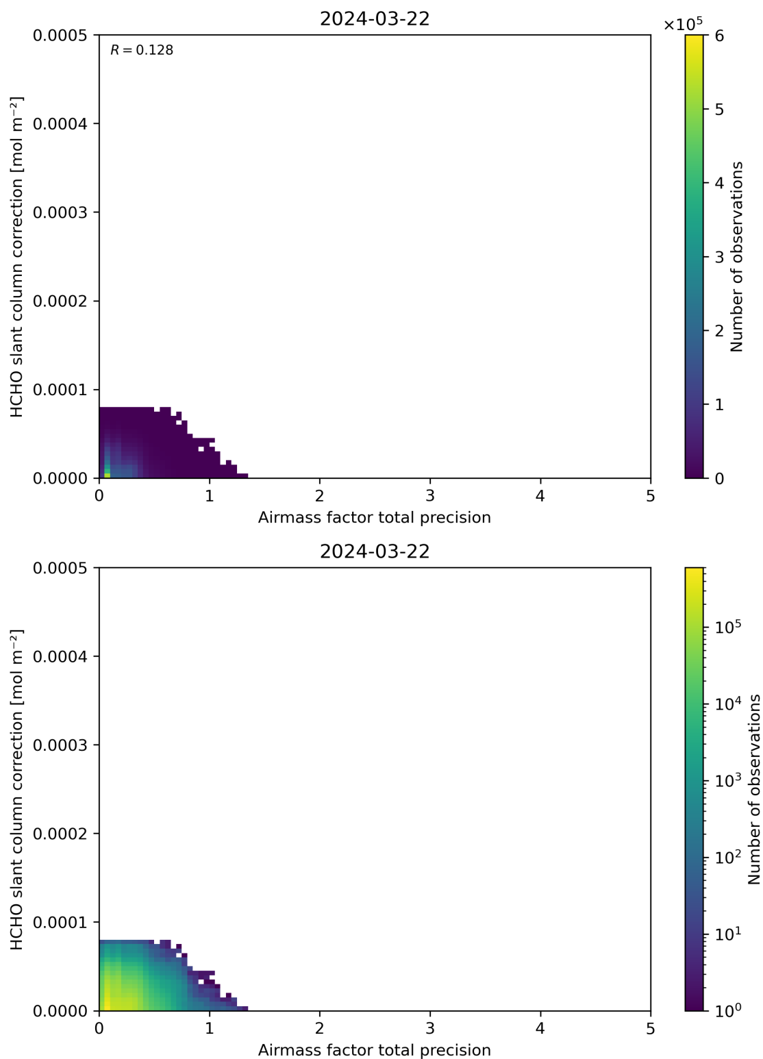
Figure 110: Scatter density plot of “Airmass factor total precision” against “HCHO slant column correction” for 2024-03-21 to 2024-03-22.
