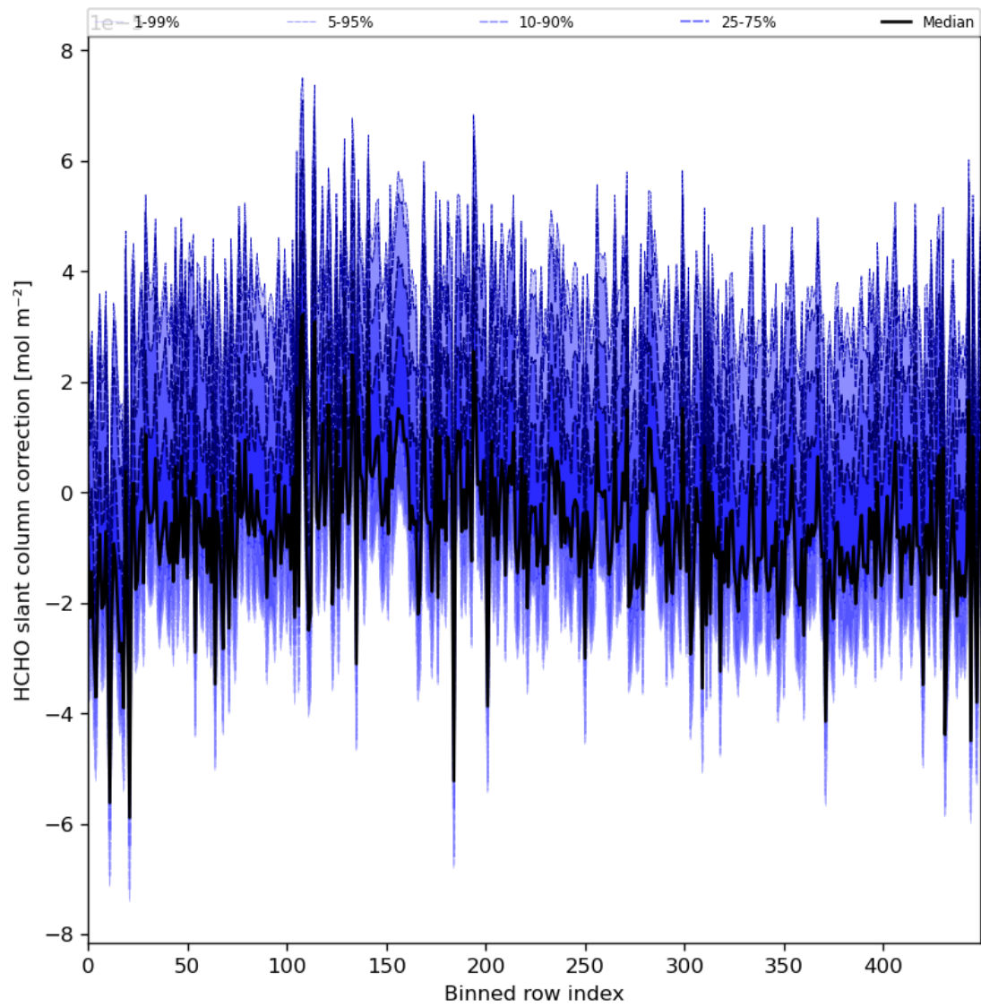
Figure 61: Along track statistics of “HCHO slant column correction” for 2024-03-21 to 2024-03-22
