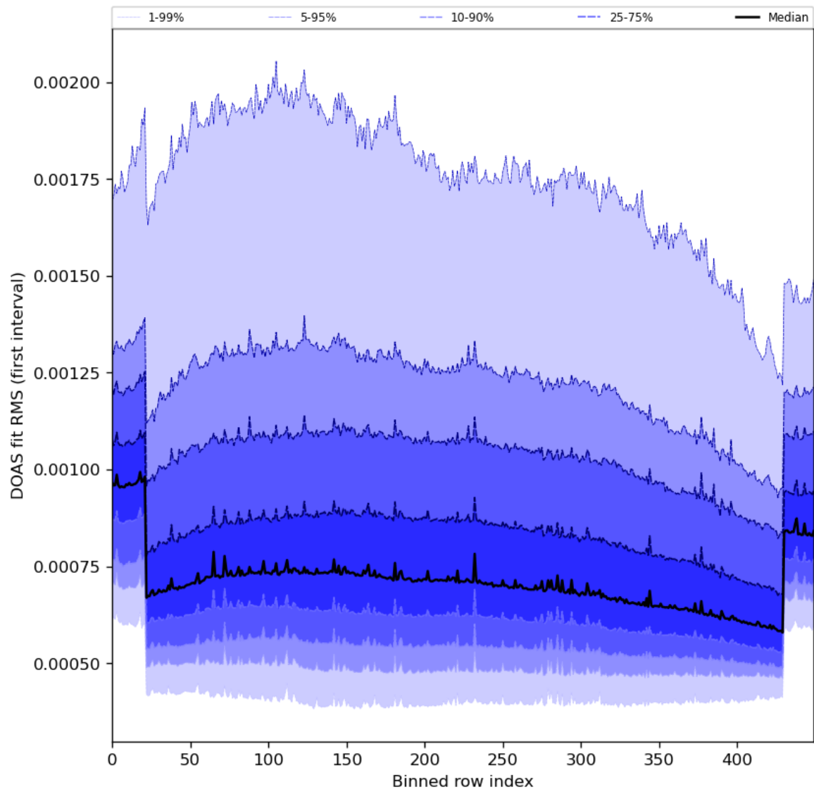
Figure 60: Along track statistics of “DOAS fit RMS (first interval)” for 2024-03-21 to 2024-03-22
