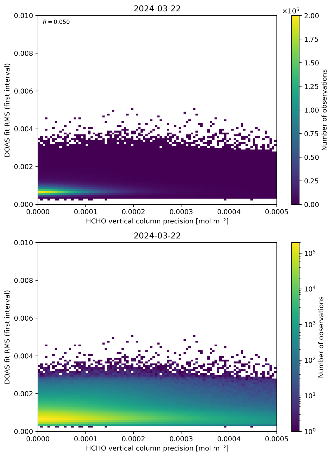
Figure 136: Scatter density plot of “HCHO vertical column precision” against “DOAS fit RMS (first interval)” for 2024-03-21 to 2024-03-22.
