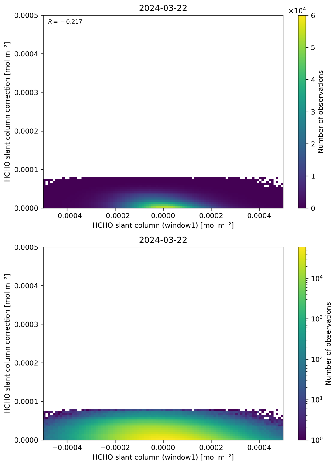
Figure 83: Scatter density plot of “HCHO slant column (window1)” against “HCHO slant column correction” for 2024-03-21 to 2024-03-22.
