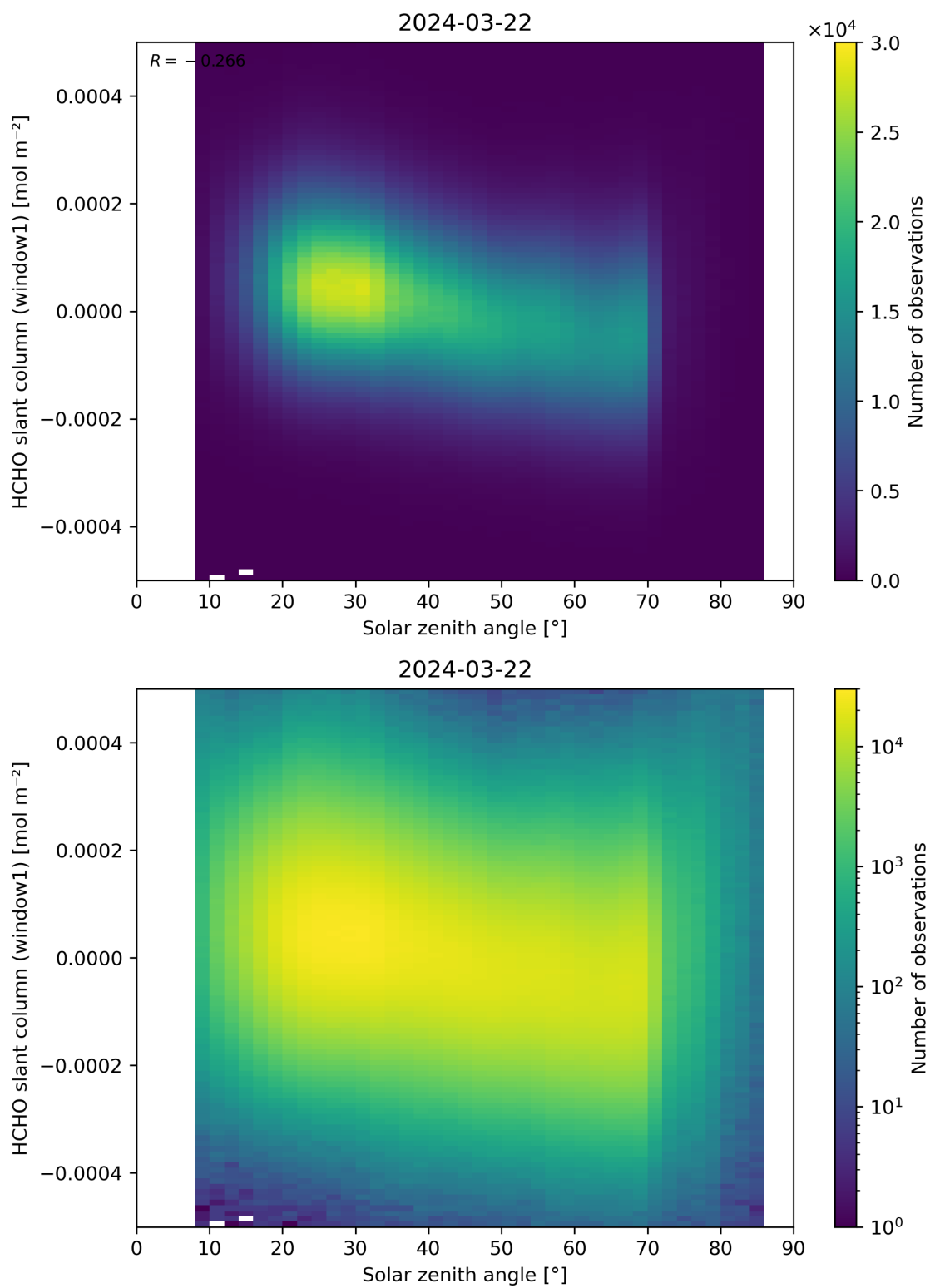
Figure 173: Scatter density plot of “Solar zenith angle” against “HCHO slant column (window1)” for 2024-03-21 to 2024-03-22.
