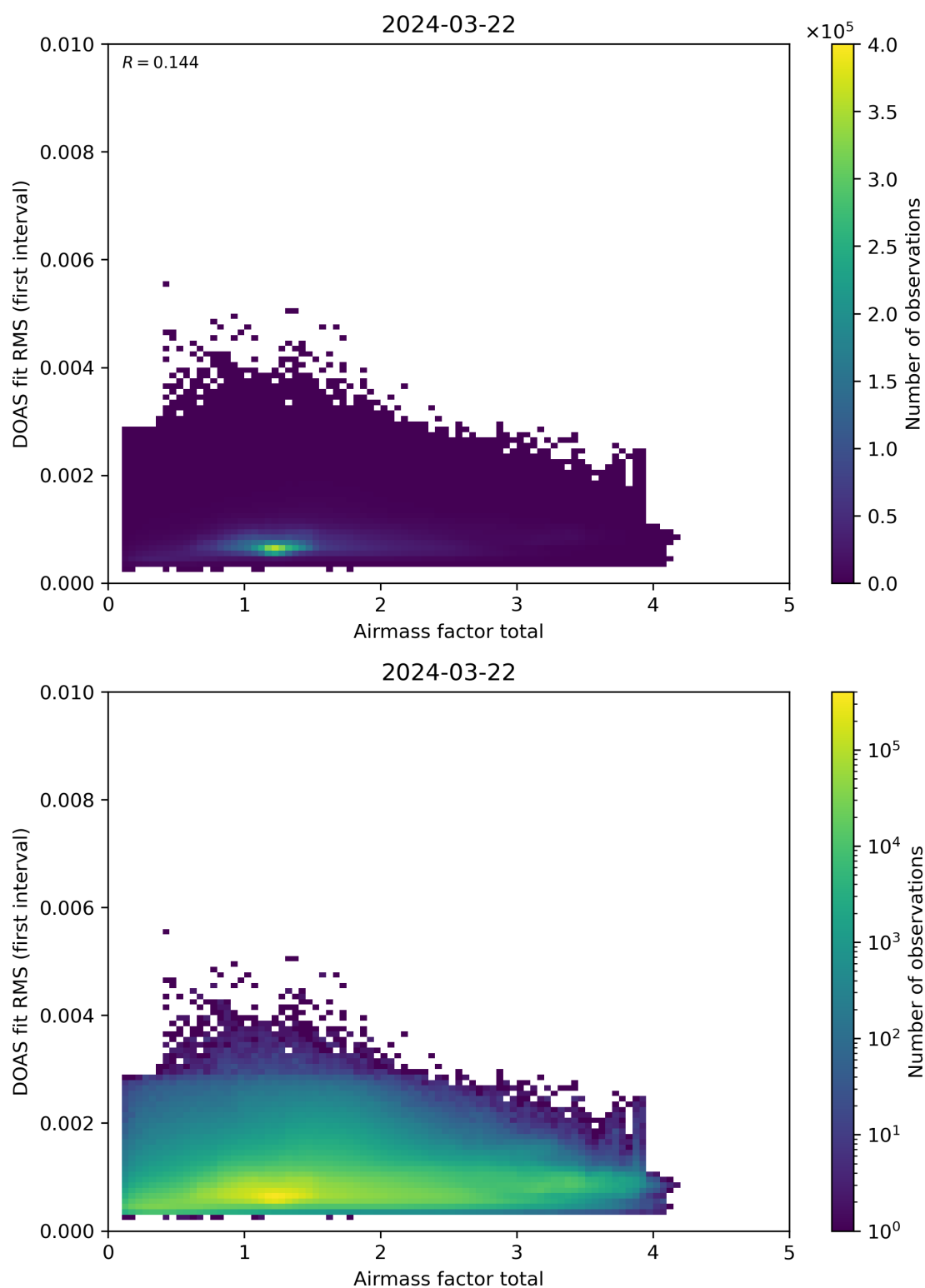
Figure 97: Scatter density plot of “Airmass factor total” against “DOAS fit RMS (first interval)” for 2024-03-21 to 2024-03-22.
