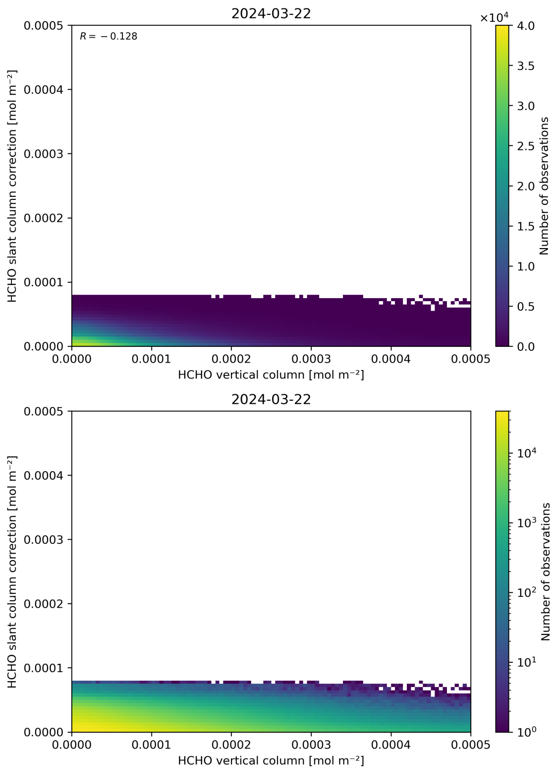
Figure 128: Scatter density plot of “HCHO vertical column” against “HCHO slant column correction” for 2024-03-21 to 2024-03-22.
