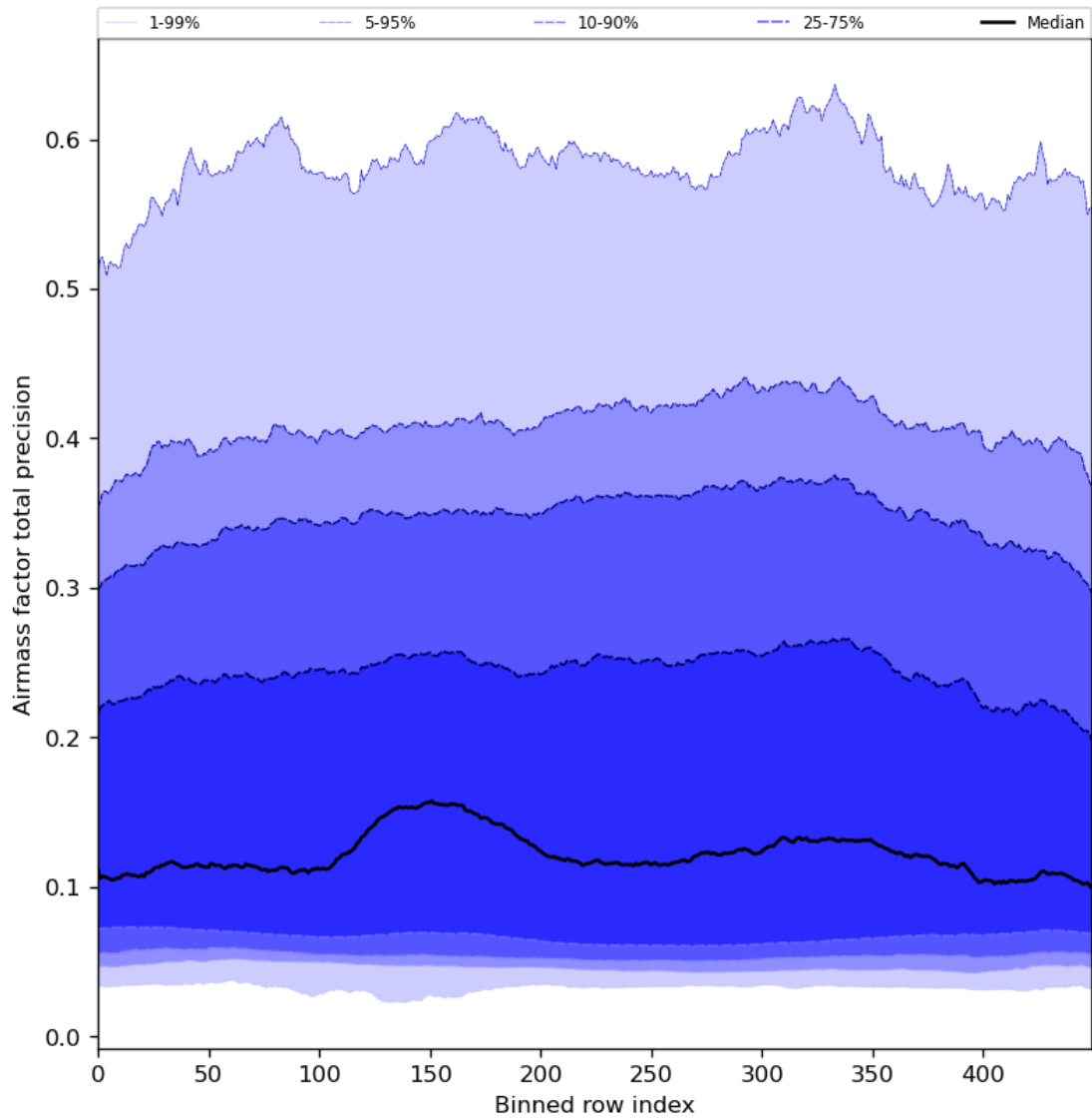
Figure 55: Along track statistics of “Airmass factor total precision” for 2024-03-21 to 2024-03-22
