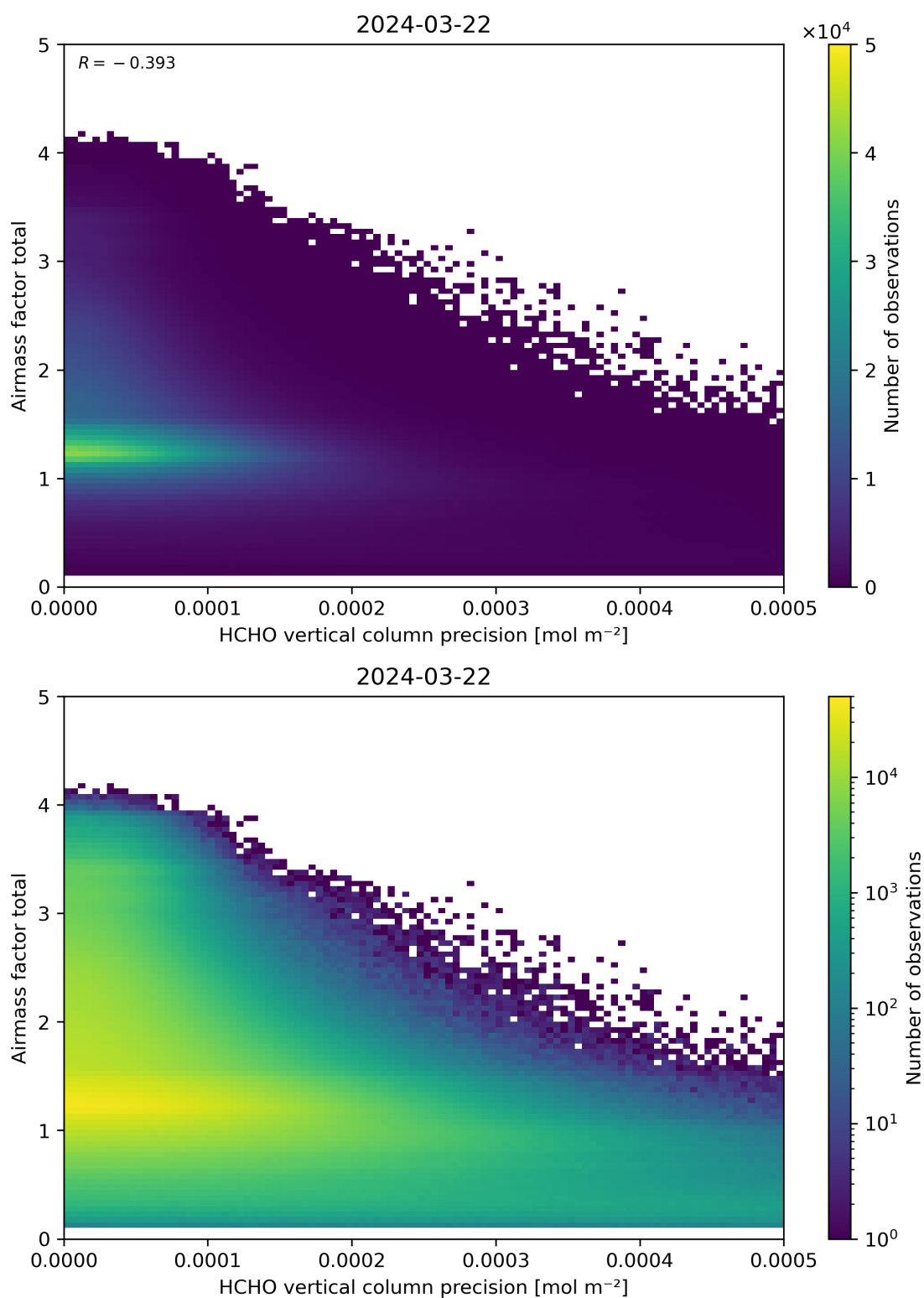
Figure 144: Scatter density plot of “HCHO vertical column precision” against “Airmass factor total” for 2024-03-21 to 2024-03-22.
