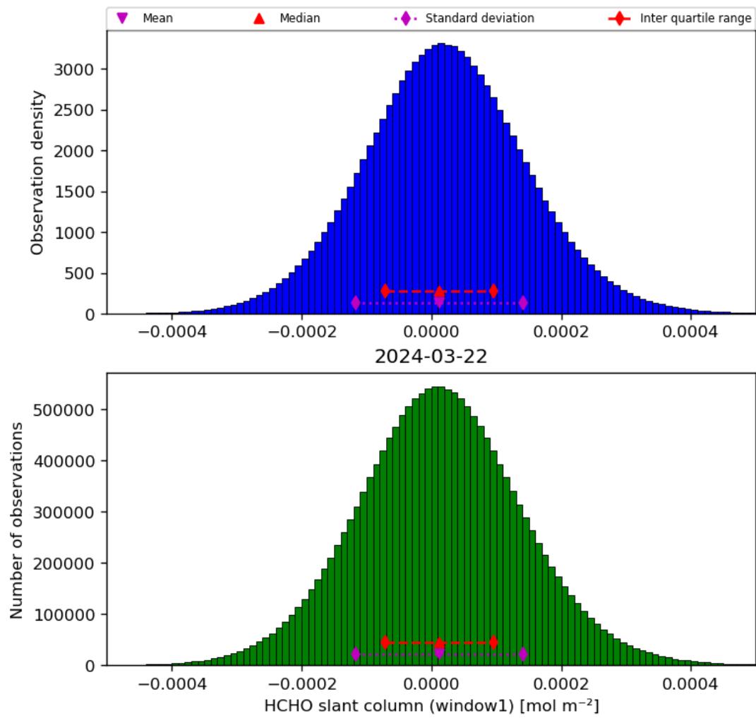
Figure 38: Histogram of “HCHO slant column (window1)” for 2024-03-21 to 2024-03-22
