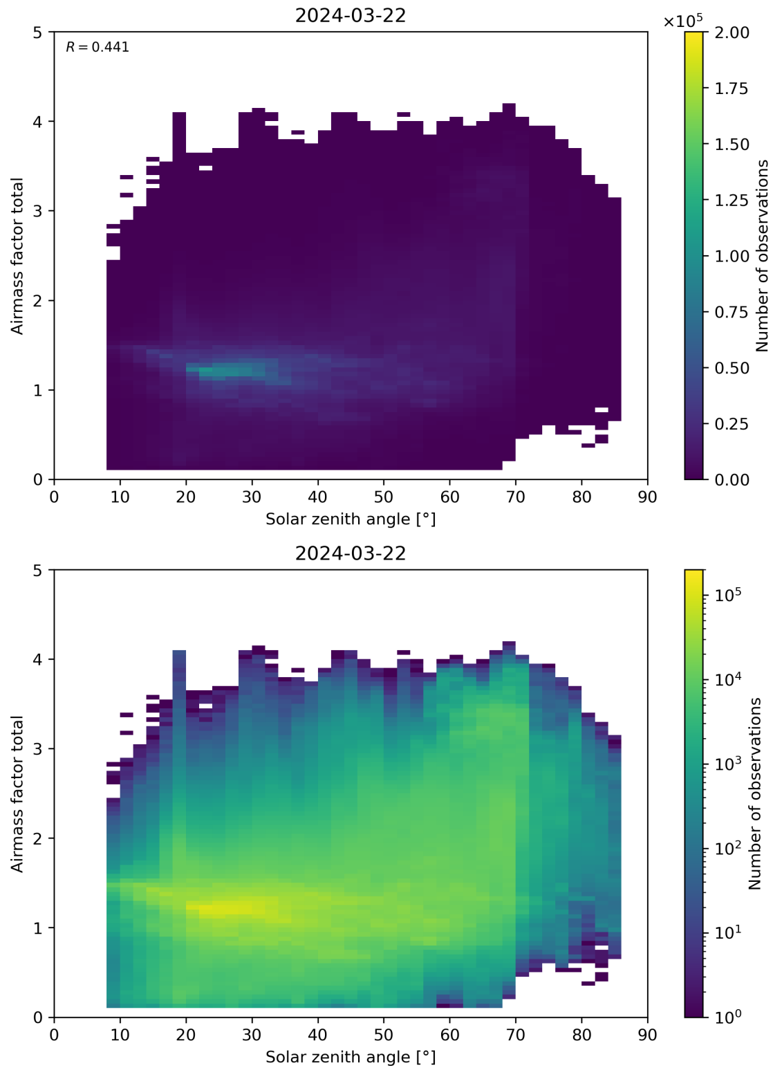
Figure 175: Scatter density plot of “Solar zenith angle” against “Airmass factor total” for 2024-03-21 to 2024-03-22.
