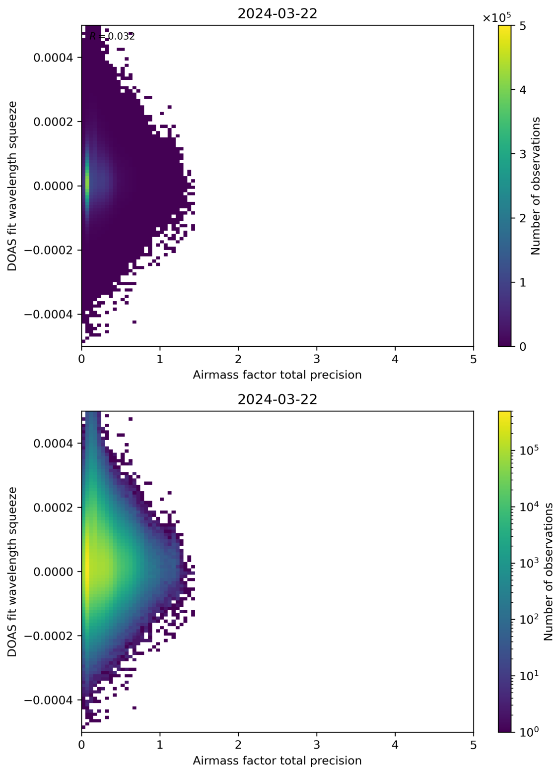
Figure 107: Scatter density plot of “Airmass factor total precision” against “DOAS fit wavelength squeeze” for 2024-03-21 to 2024-03-22.
