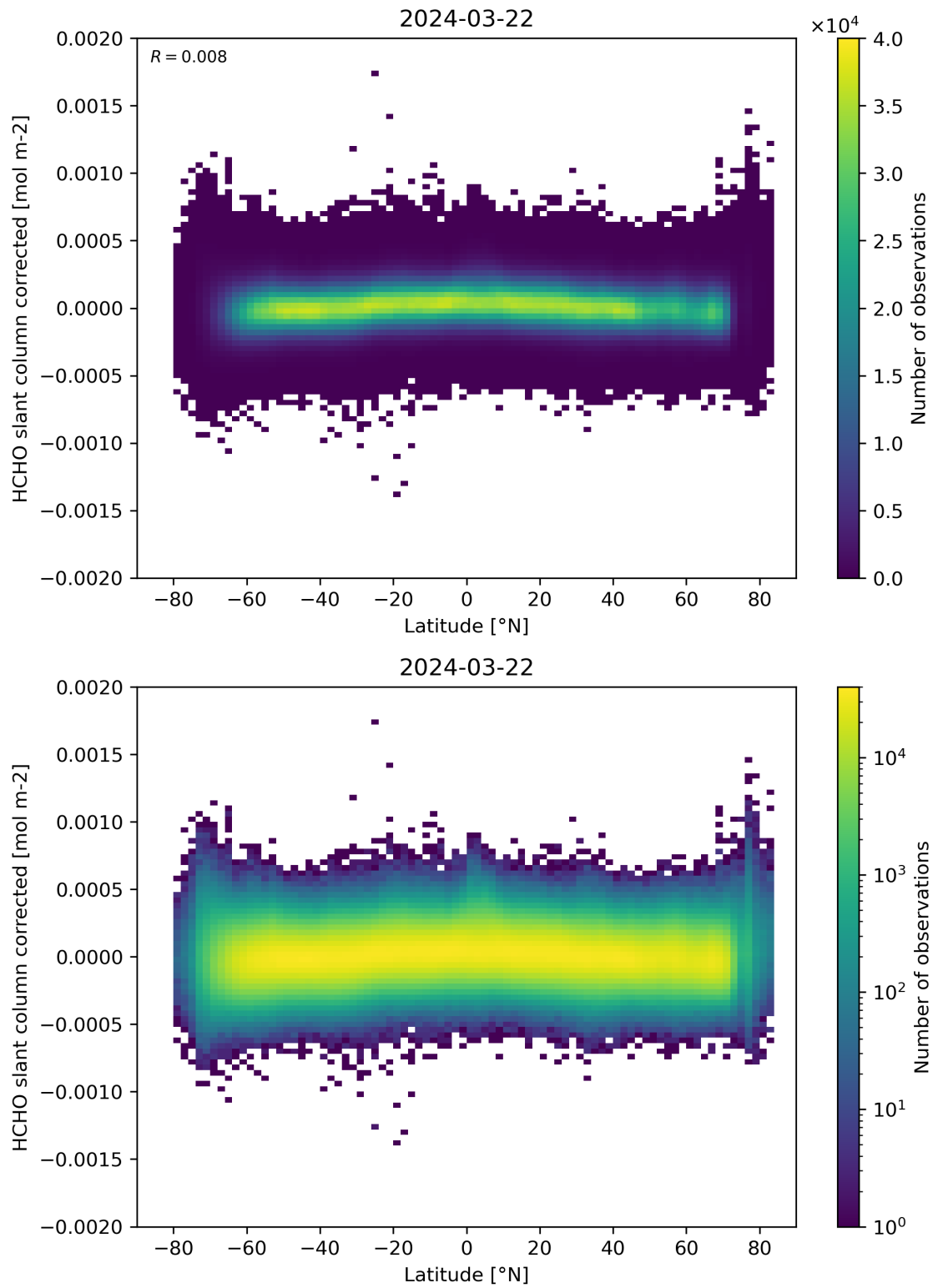
Figure 157: Scatter density plot of “Latitude” against “HCHO slant column corrected” for 2024-03-21 to 2024-03-22.
