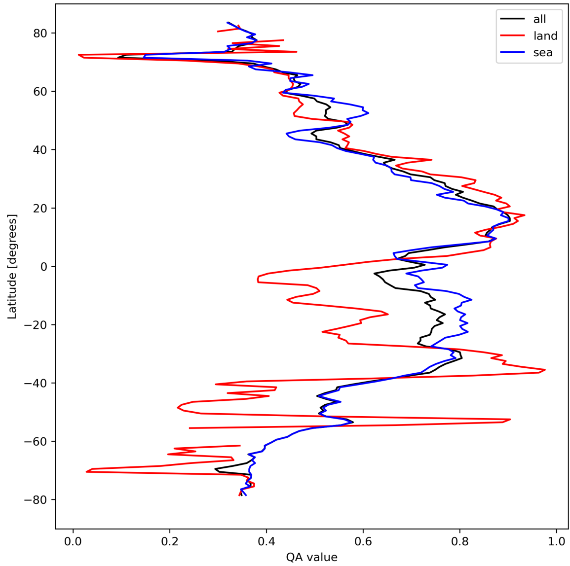
Figure 20: Zonal average of “QA value” for 2024-03-21 to 2024-03-22.
