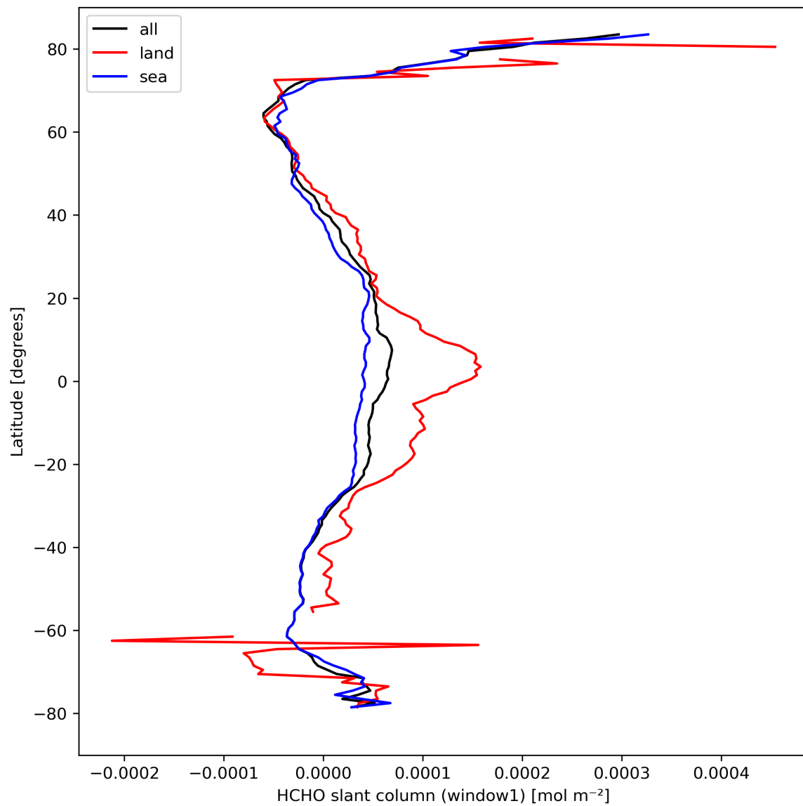
Figure 24: Zonal average of “HCHO slant column (window1)” for 2024-03-21 to 2024-03-22.
