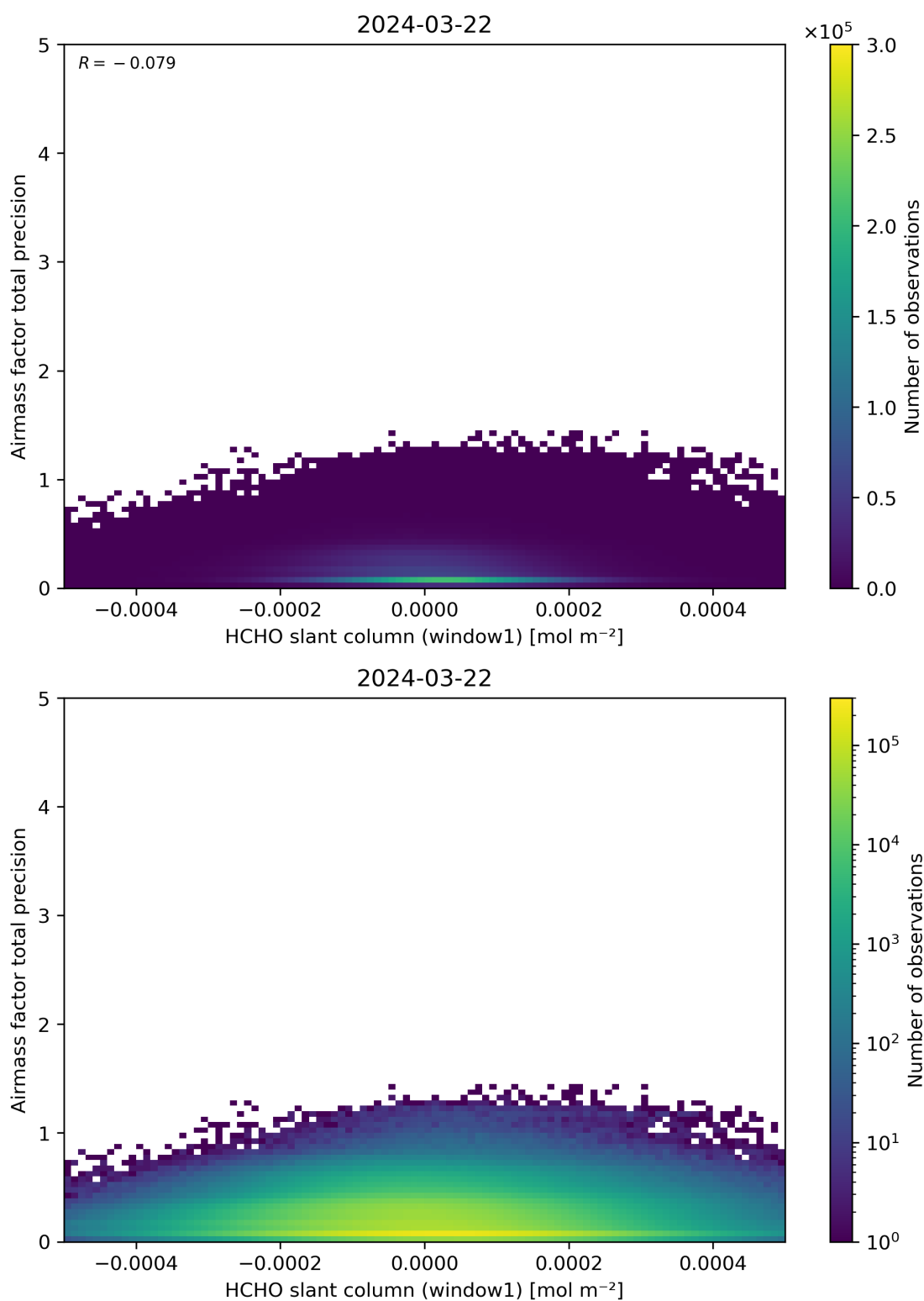
Figure 86: Scatter density plot of “HCHO slant column (window1)” against “Airmass factor total precision” for 2024-03-21 to 2024-03-22.
