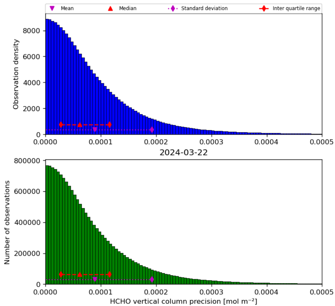
Figure 36: Histogram of “HCHO vertical column precision” for 2024-03-21 to 2024-03-22
