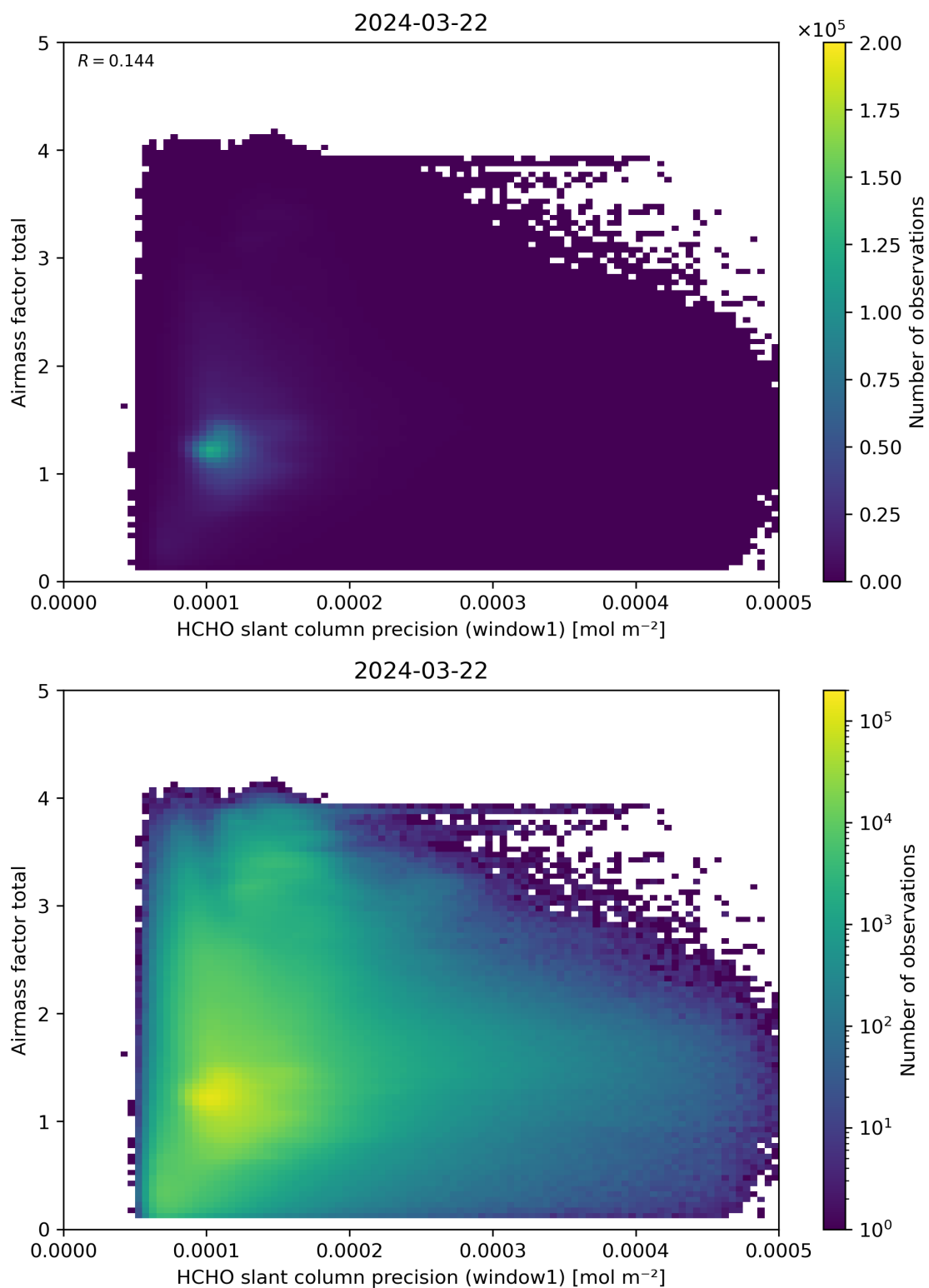
Figure 94: Scatter density plot of “HCHO slant column precision (window1)” against “Airmass factor total” for 2024-03-21 to 2024-03-22.
