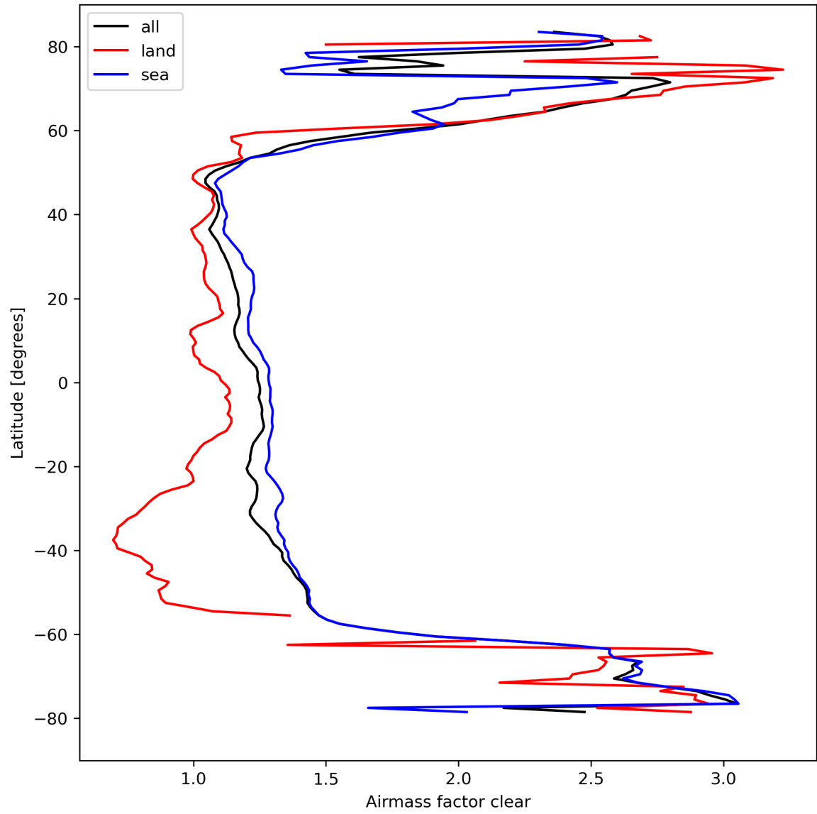
Figure 28: Zonal average of “Airmass factor clear” for 2024-03-21 to 2024-03-22.
