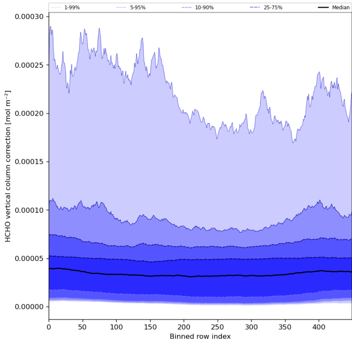
Figure 51: Along track statistics of “HCHO vertical column correction” for 2024-03-21 to 2024-03-22
