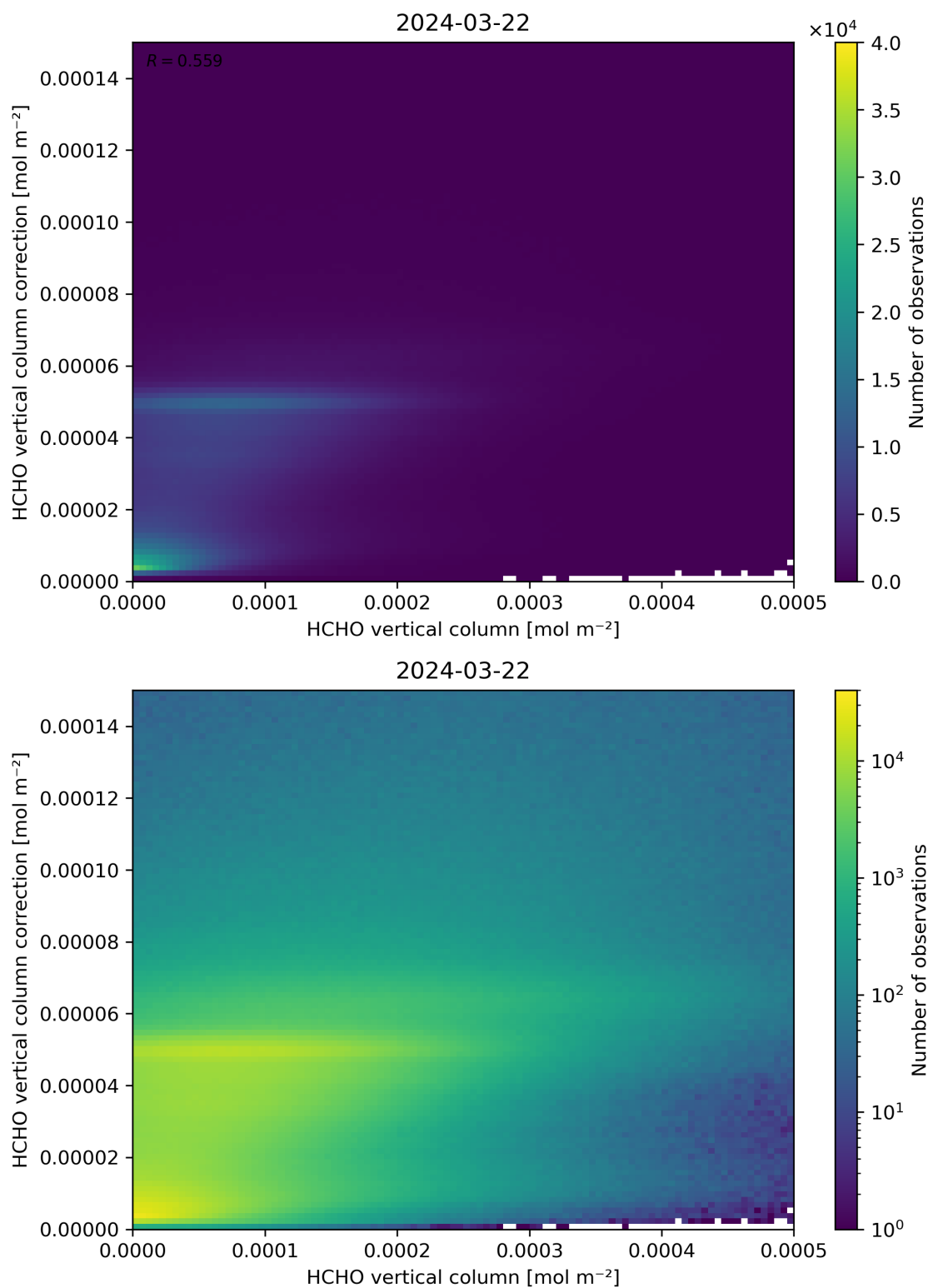
Figure 133: Scatter density plot of “HCHO vertical column” against “HCHO vertical column correction” for 2024-03-21 to 2024-03-22.
