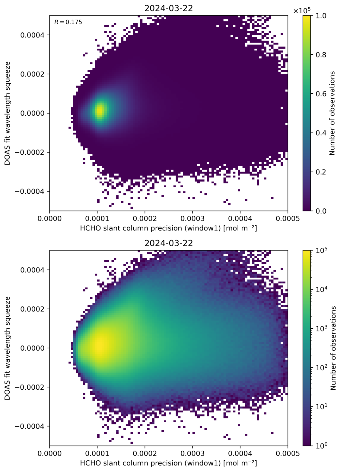
Figure 90: Scatter density plot of “HCHO slant column precision (window1)” against “DOAS fit wavelength squeeze” for 2024-03-21 to 2024-03-22.
