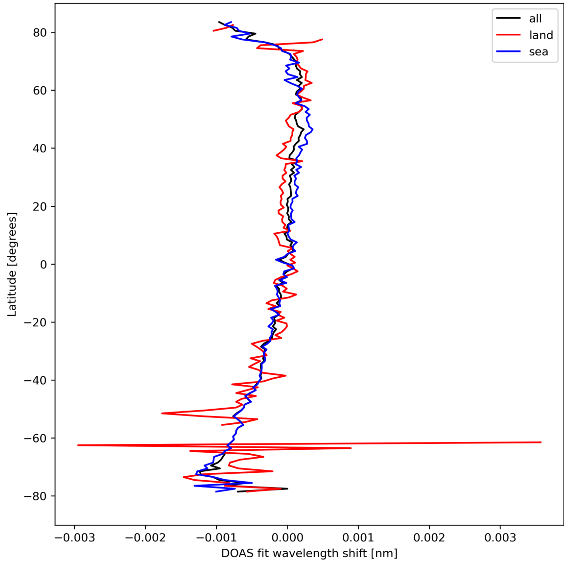
Figure 30: Zonal average of “DOAS fit wavelength shift” for 2024-03-21 to 2024-03-22.
