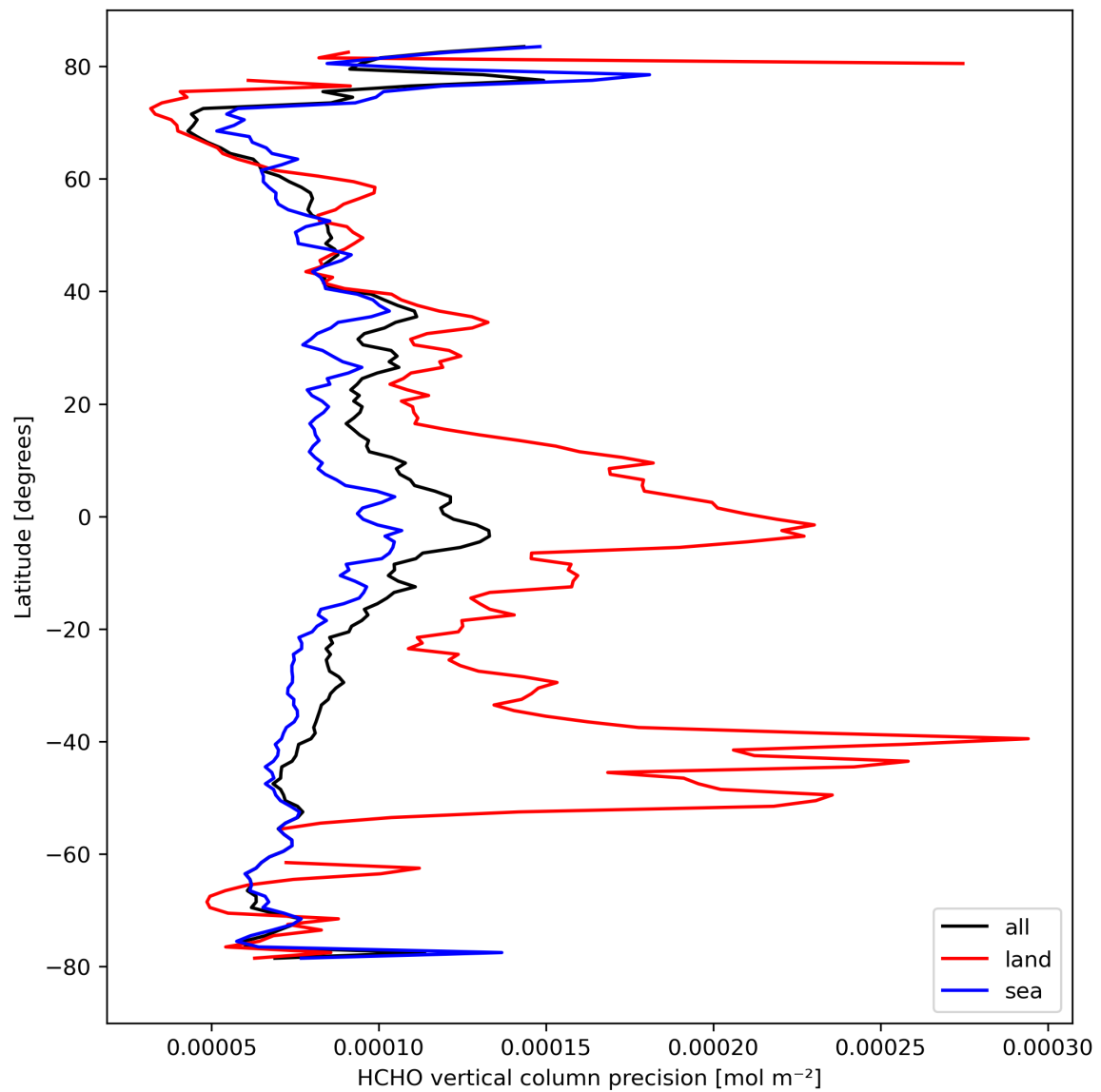
Figure 22: Zonal average of “HCHO vertical column precision” for 2024-03-21 to 2024-03-22.
