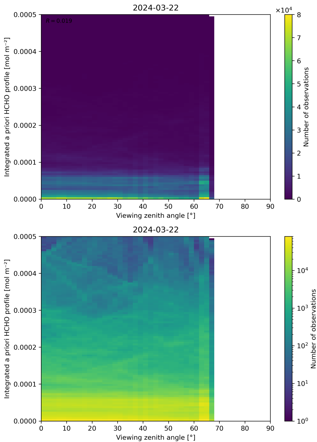
Figure 195: Scatter density plot of “Viewing zenith angle” against “Integrated a priori HCHO profile” for 2024-03-21 to 2024-03-22.
