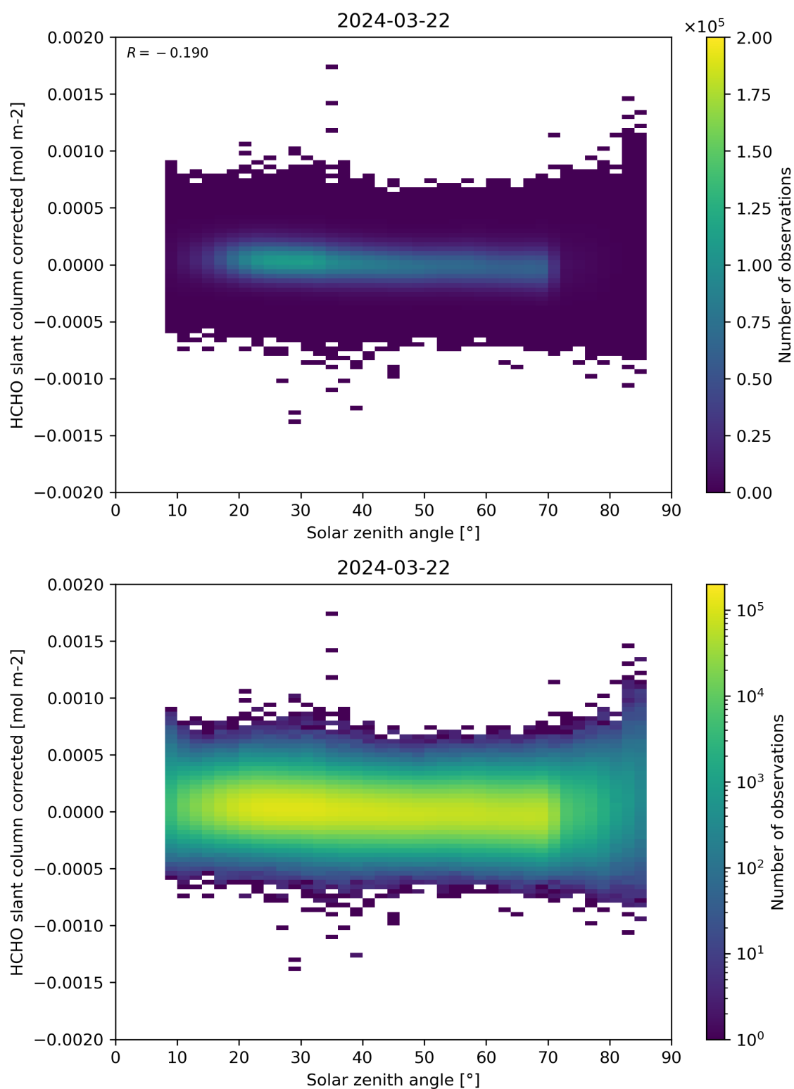
Figure 171: Scatter density plot of “Solar zenith angle” against “HCHO slant column corrected” for 2024-03-21 to 2024-03-22.
