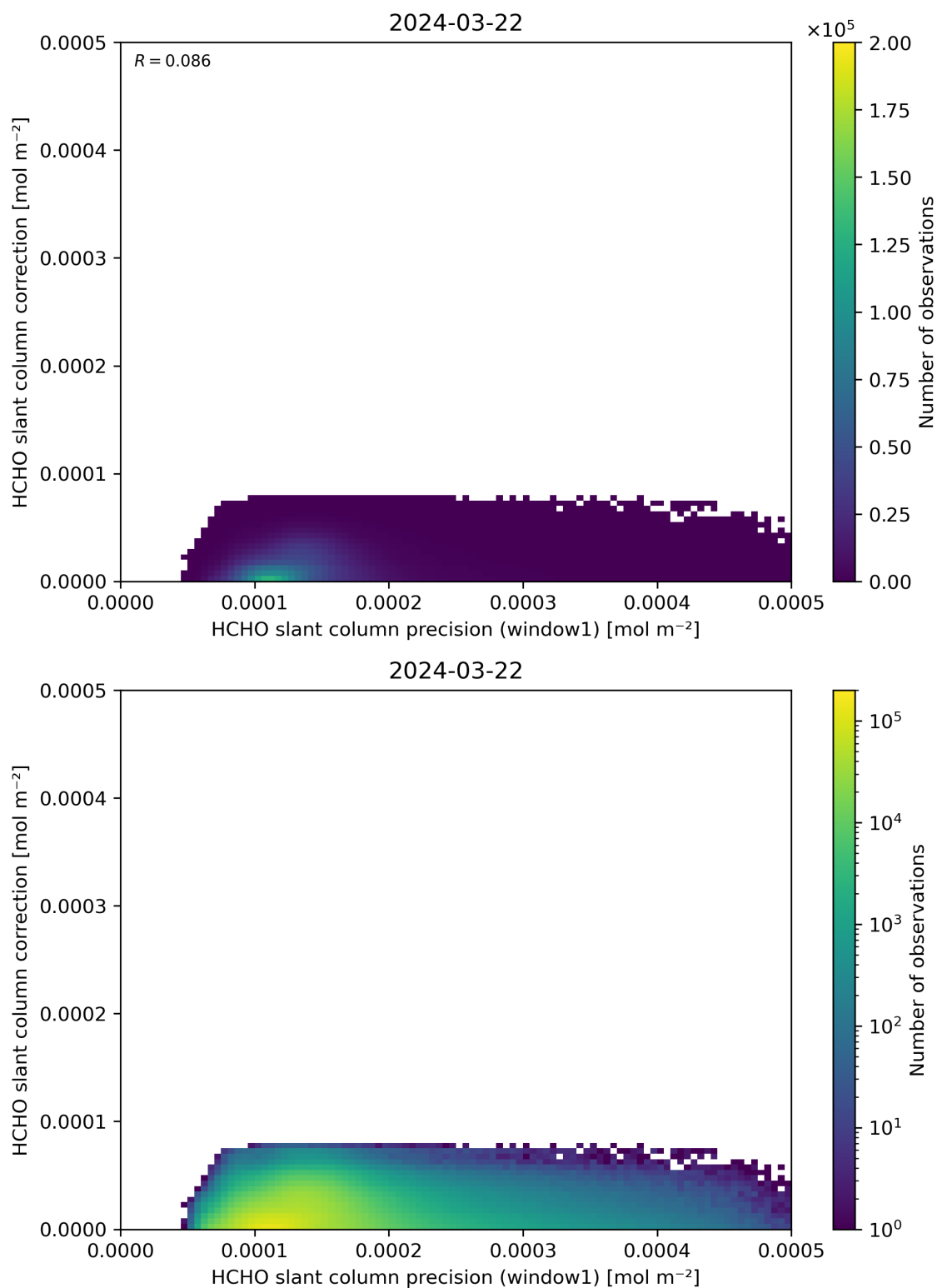
Figure 93: Scatter density plot of “HCHO slant column precision (window1)” against “HCHO slant column correction” for 2024-03-21 to 2024-03-22.
