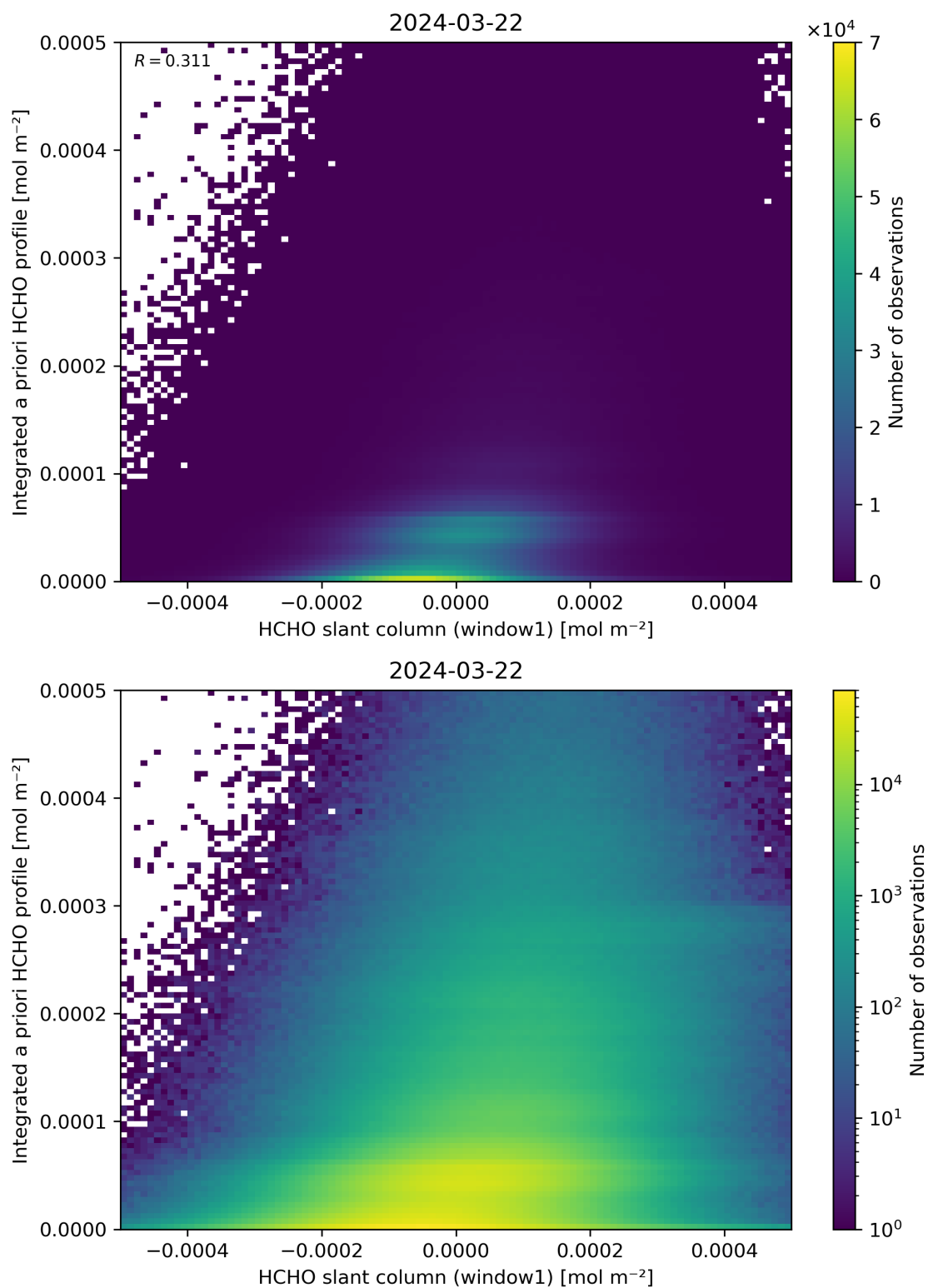
Figure 87: Scatter density plot of “HCHO slant column (window1)” against “Integrated a priori HCHO profile” for 2024-03-21 to 2024-03-22.
