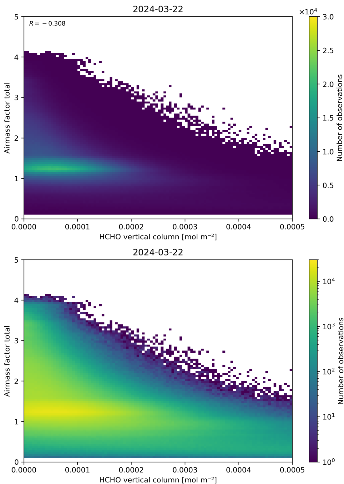
Figure 131: Scatter density plot of “HCHO vertical column” against “Airmass factor total” for 2024-03-21 to 2024-03-22.
