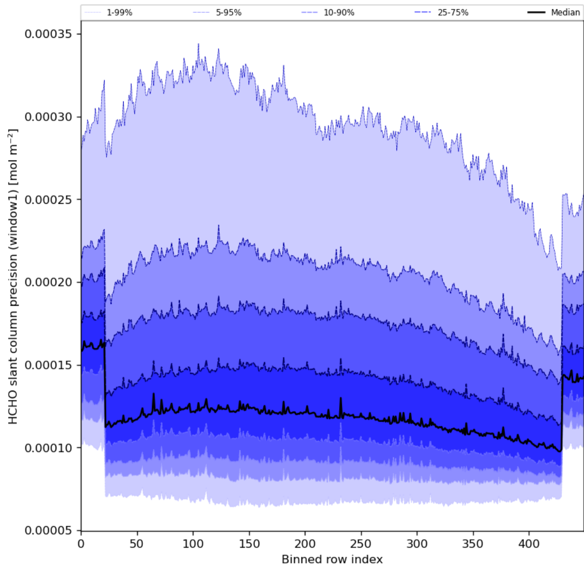
Figure 53: Along track statistics of “HCHO slant column precision (window1)” for 2024-03-21 to 2024-03-22
