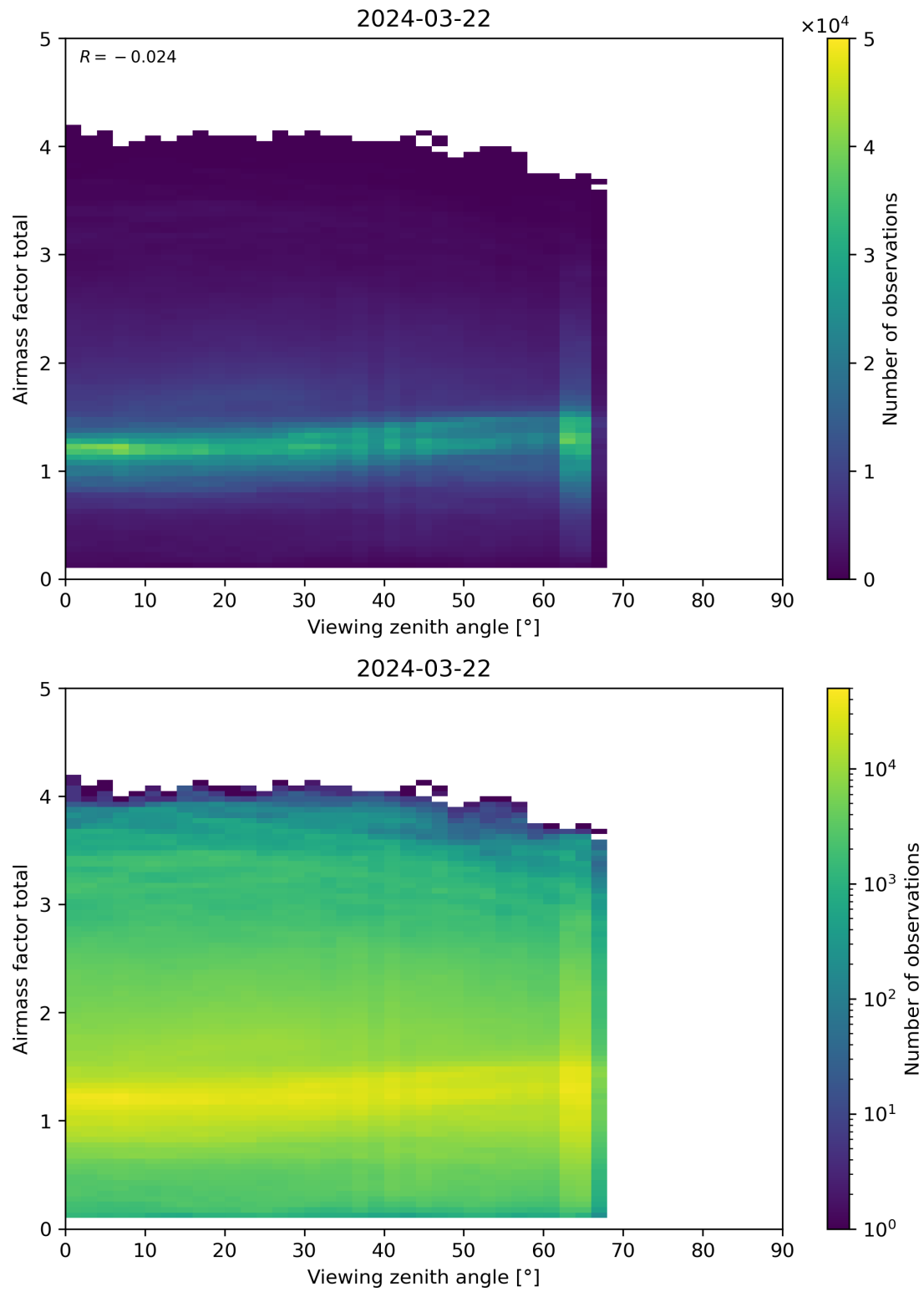
Figure 190: Scatter density plot of “Viewing zenith angle” against “Airmass factor total” for 2024-03-21 to 2024-03-22.
