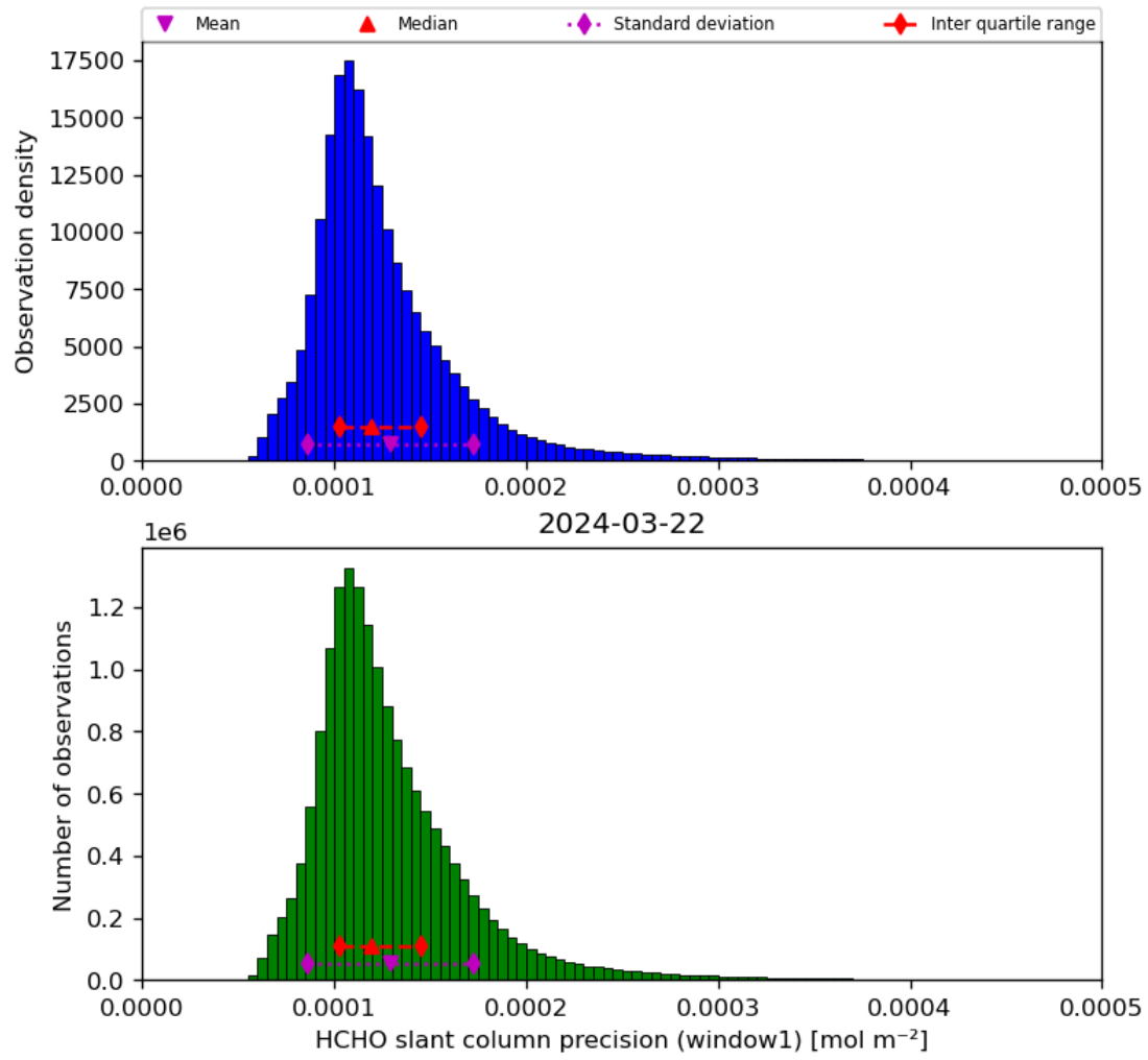
Figure 39: Histogram of “HCHO slant column precision (window1)” for 2024-03-21 to 2024-03-22
