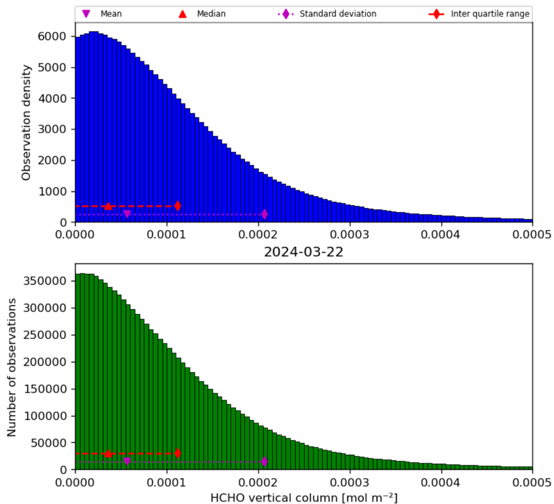
Figure 35: Histogram of “HCHO vertical column” for 2024-03-21 to 2024-03-22
