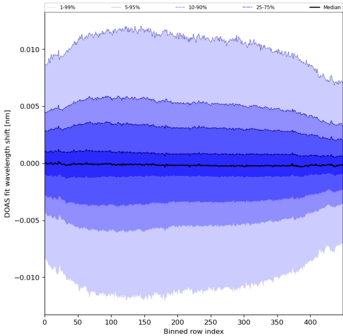
Figure 58: Along track statistics of “DOAS fit wavelength shift” for 2024-03-21 to 2024-03-22
