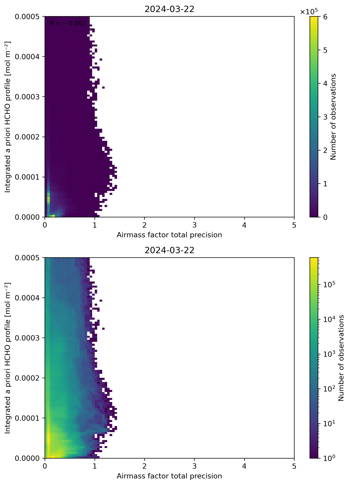
Figure 111: Scatter density plot of “Airmass factor total precision” against “Integrated a priori HCHO profile” for 2024-03-21 to 2024-03-22.
