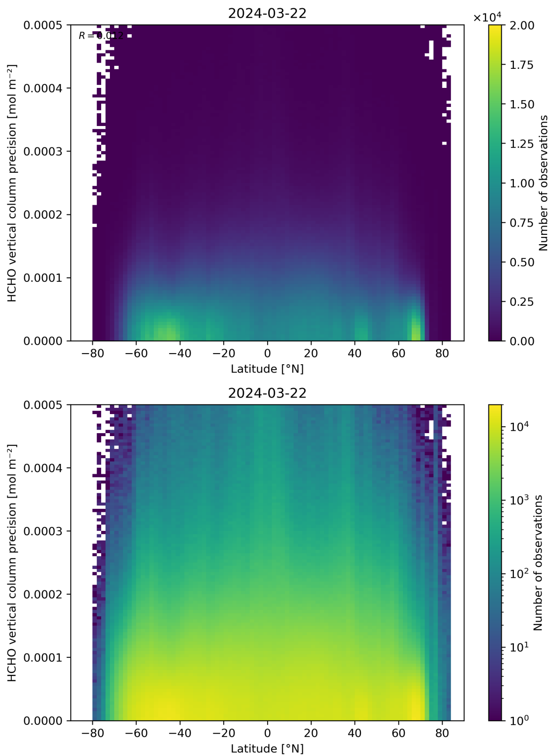
Figure 165: Scatter density plot of “Latitude” against “HCHO vertical column precision” for 2024-03-21 to 2024-03-22.
