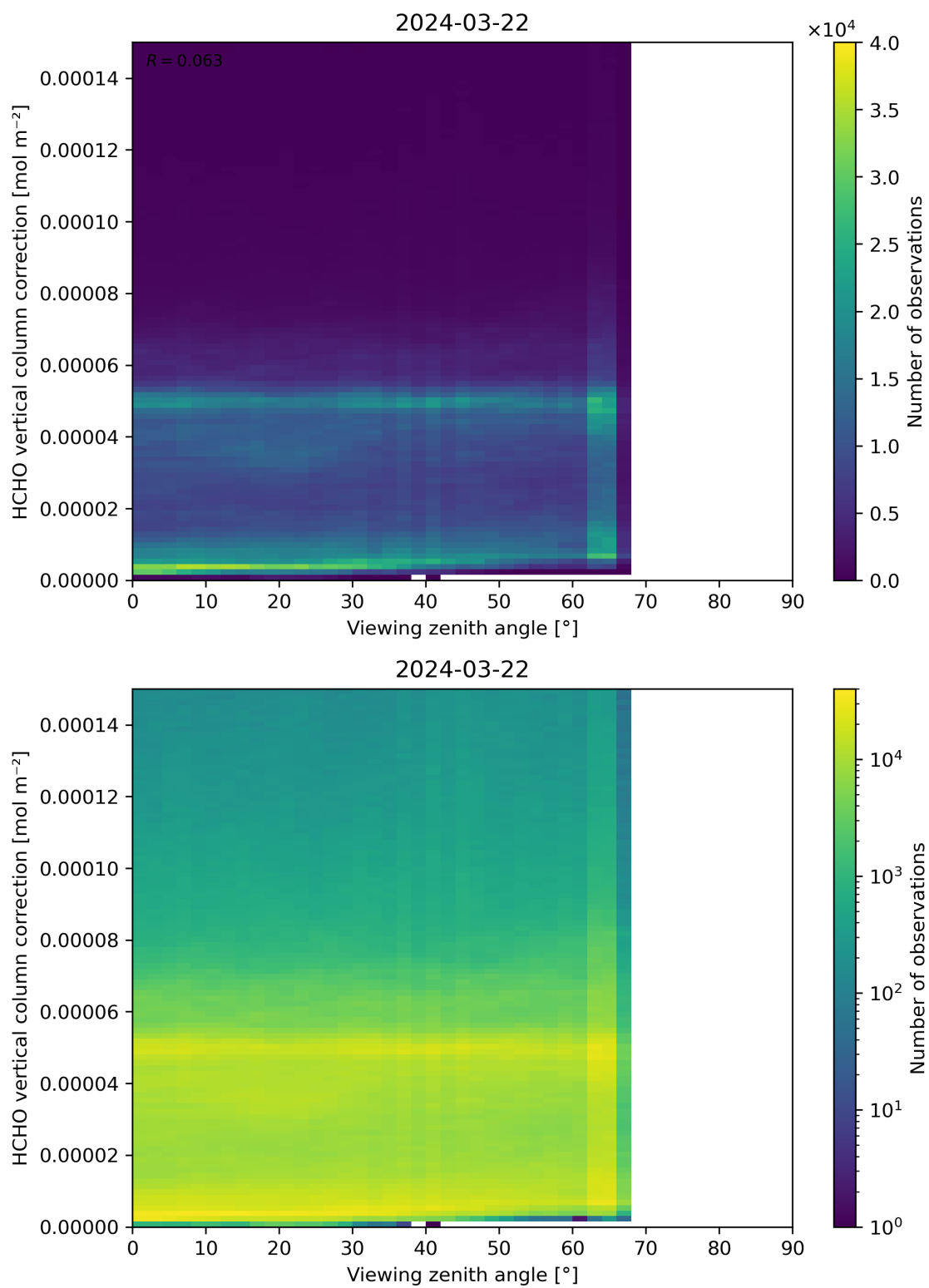
Figure 193: Scatter density plot of “Viewing zenith angle” against “HCHO vertical column correction” for 2024-03-21 to 2024-03-22.
