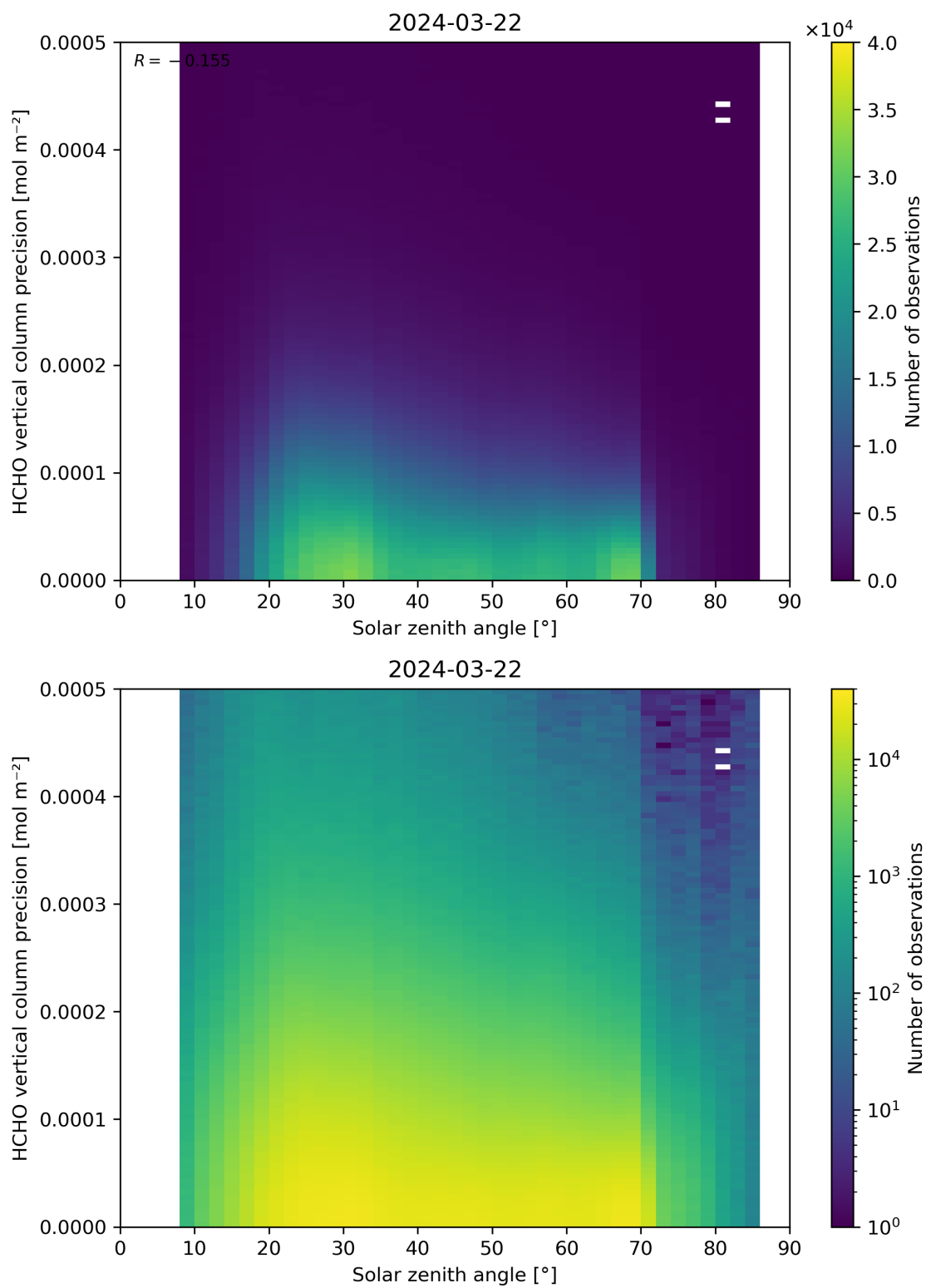
Figure 179: Scatter density plot of “Solar zenith angle” against “HCHO vertical column precision” for 2024-03-21 to 2024-03-22.
