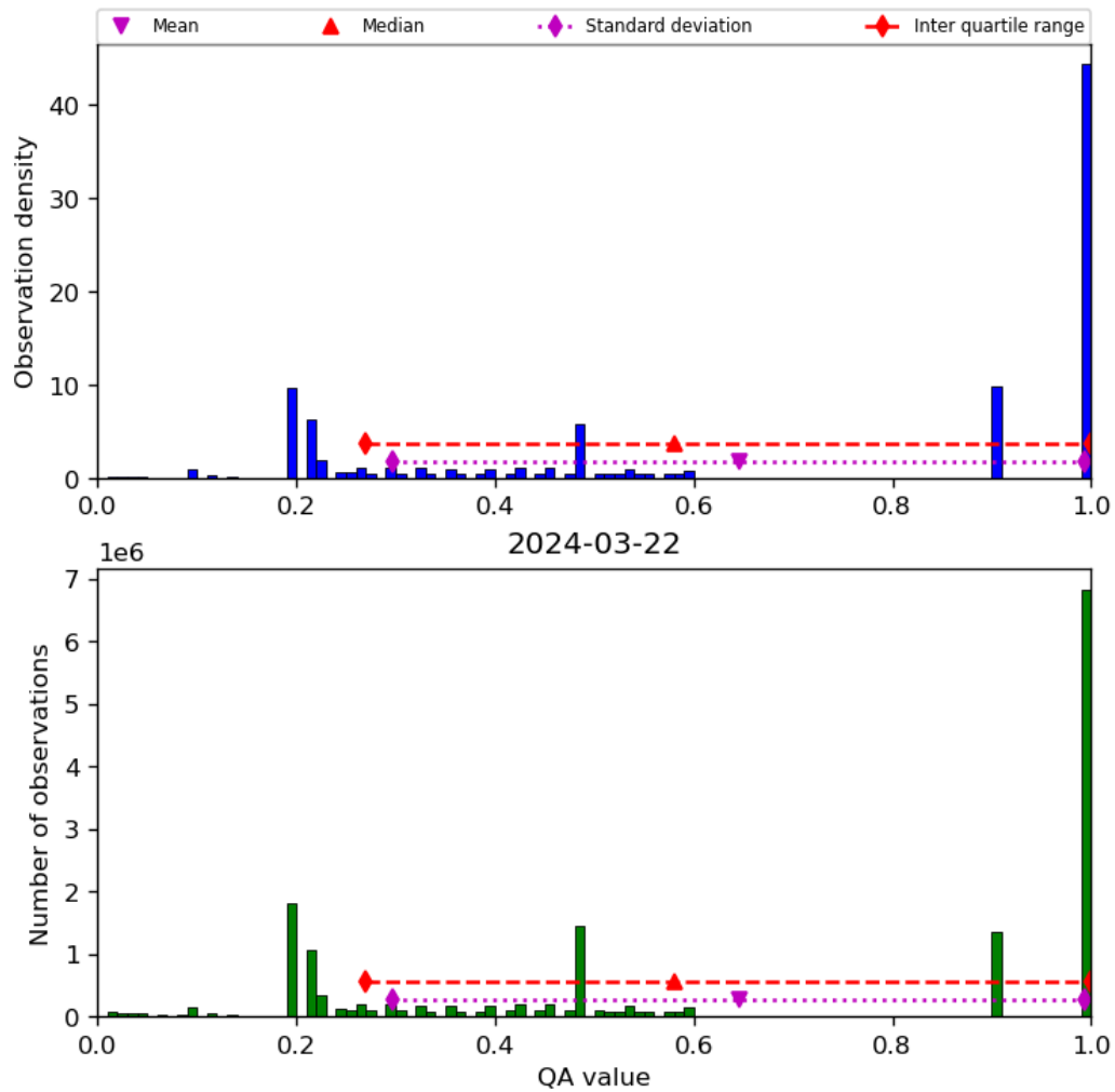
Figure 34: Histogram of “QA value” for 2024-03-21 to 2024-03-22
