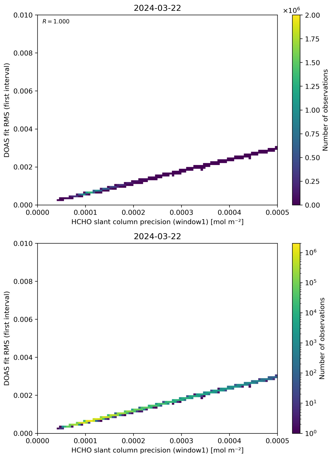
Figure 88: Scatter density plot of “HCHO slant column precision (window1)” against “DOAS fit RMS (first interval)” for 2024-03-21 to 2024-03-22.
