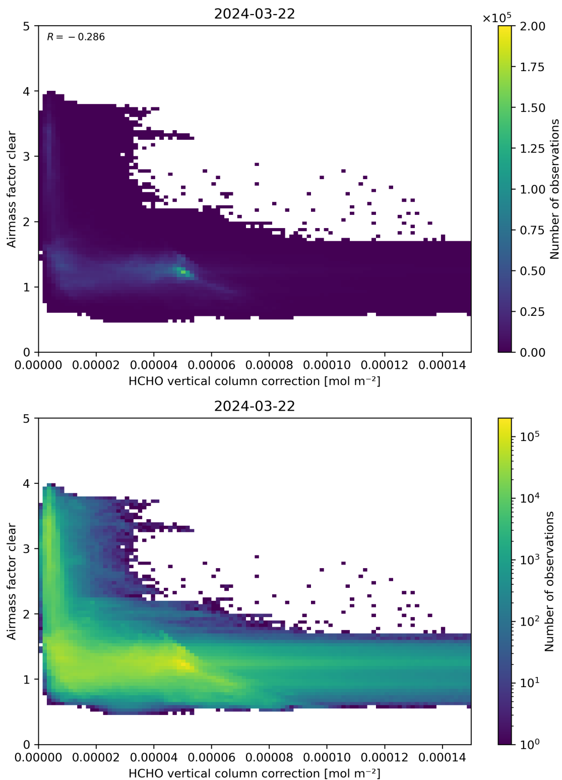
Figure 115: Scatter density plot of “HCHO vertical column correction” against “Airmass factor clear” for 2024-03-21 to 2024-03-22.
