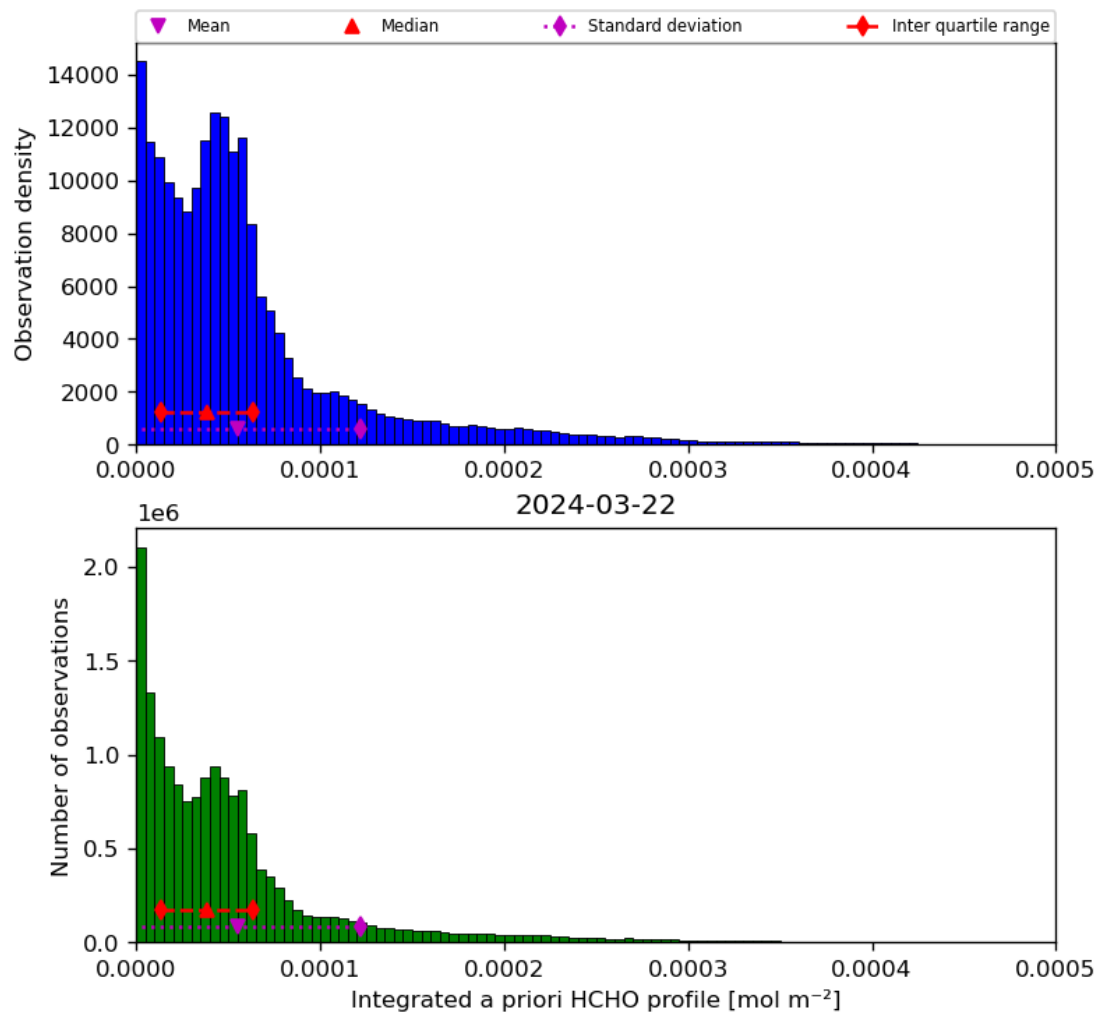
Figure 43: Histogram of “Integrated a priori HCHO profile” for 2024-03-21 to 2024-03-22
