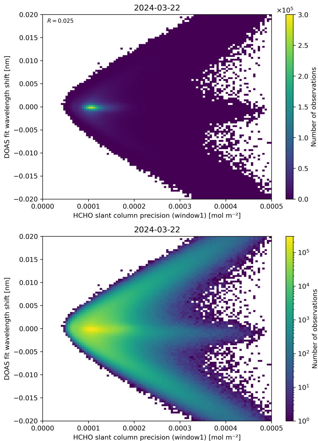
Figure 89: Scatter density plot of “HCHO slant column precision (window1)” against “DOAS fit wavelength shift” for 2024-03-21 to 2024-03-22.
