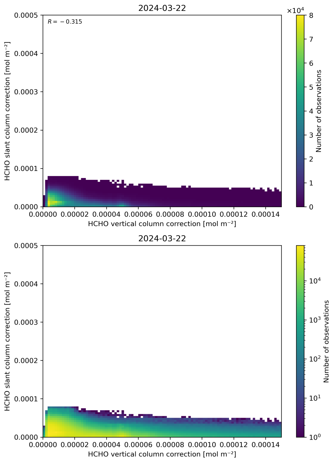
Figure 117: Scatter density plot of “HCHO vertical column correction” against “HCHO slant column correction” for 2024-03-21 to 2024-03-22.
