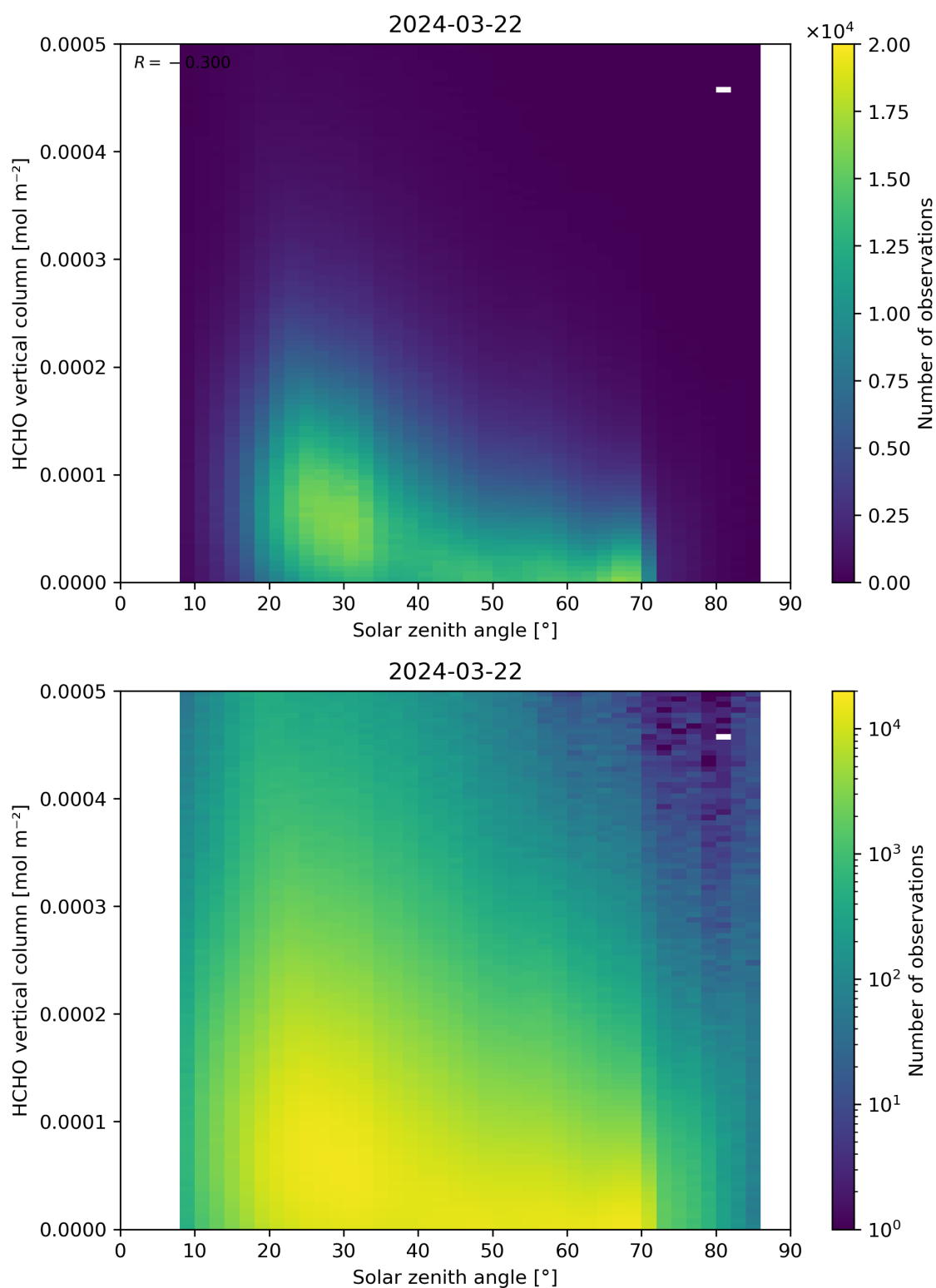
Figure 177: Scatter density plot of “Solar zenith angle” against “HCHO vertical column” for 2024-03-21 to 2024-03-22.
