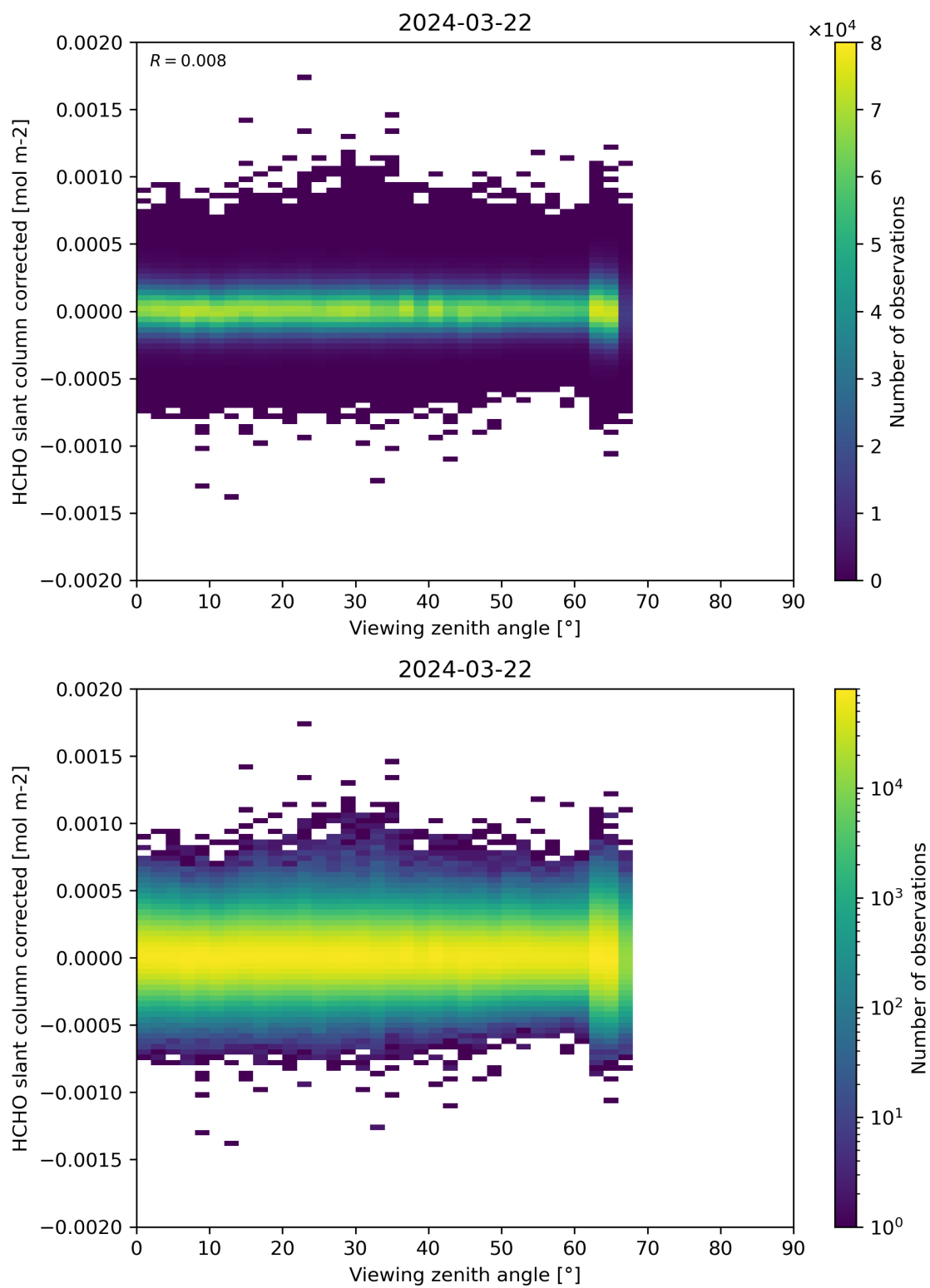
Figure 186: Scatter density plot of “Viewing zenith angle” against “HCHO slant column corrected” for 2024-03-21 to 2024-03-22.
