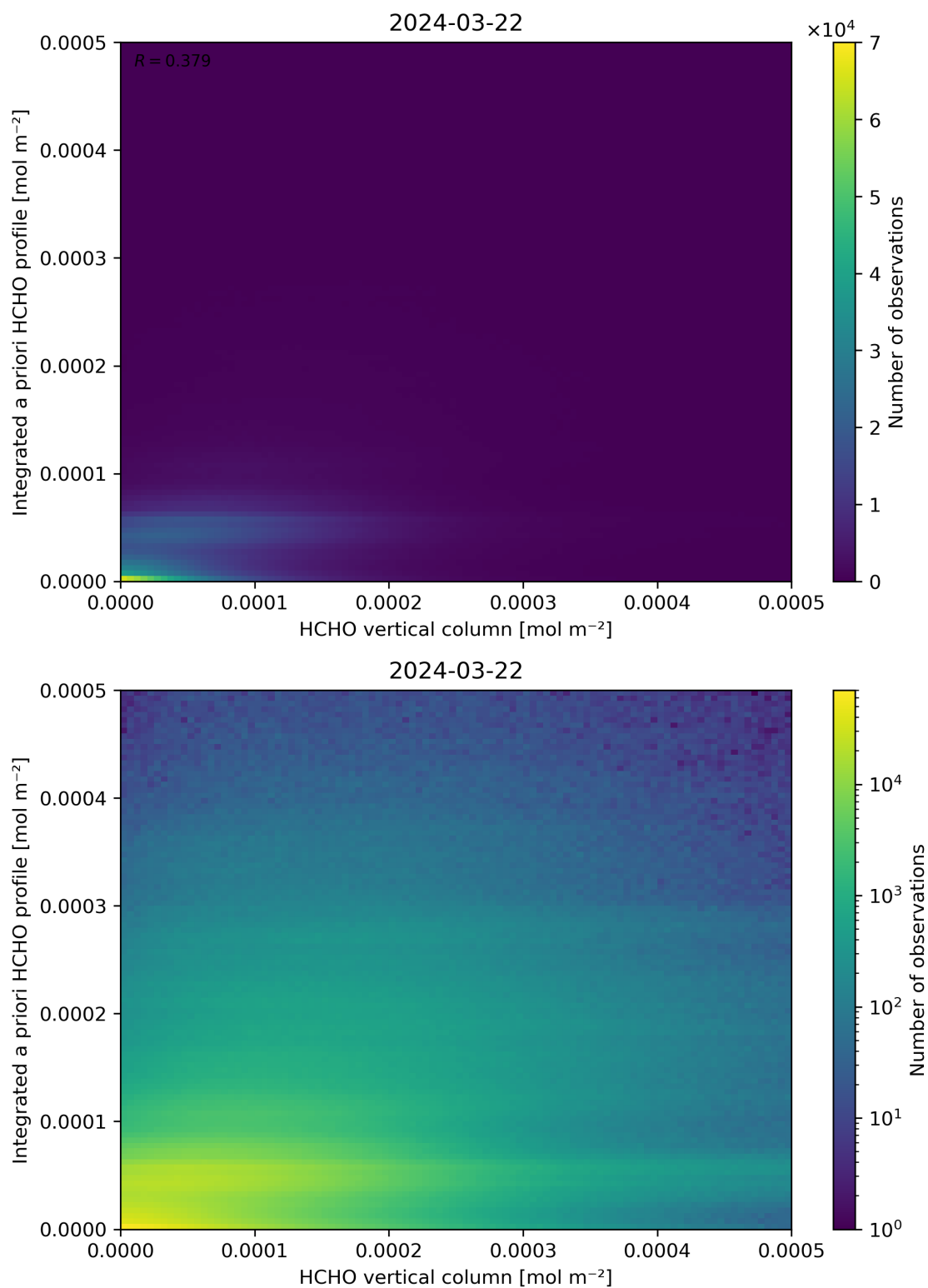
Figure 135: Scatter density plot of “HCHO vertical column” against “Integrated a priori HCHO profile” for 2024-03-21 to 2024-03-22.
