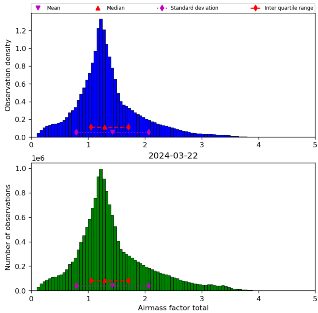
Figure 40: Histogram of “Airmass factor total” for 2024-03-21 to 2024-03-22
