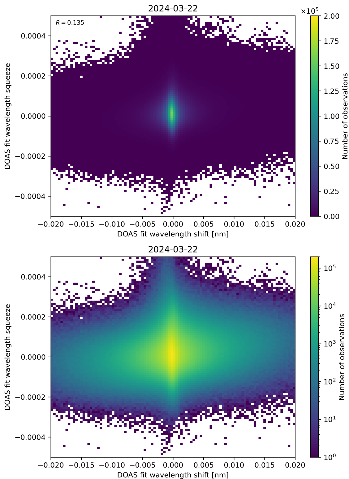
Figure 65: Scatter density plot of “DOAS fit wavelength shift” against “DOAS fit wavelength squeeze” for 2024-03-21 to 2024-03-22.
