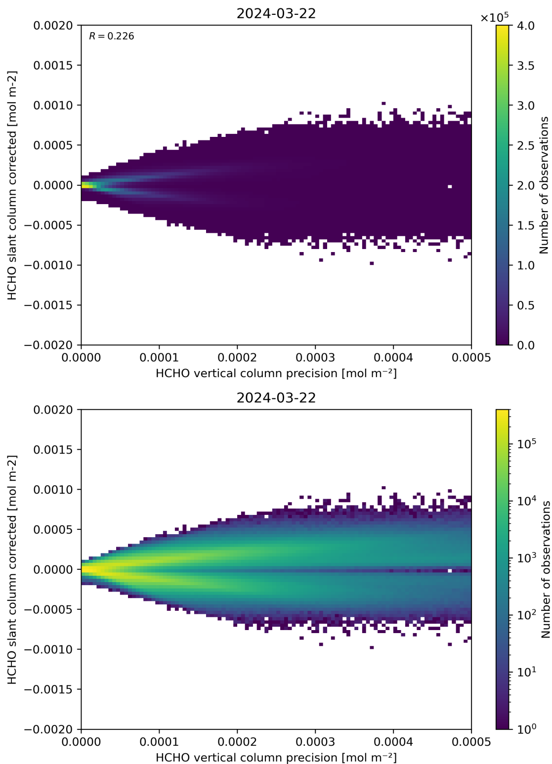
Figure 140: Scatter density plot of “HCHO vertical column precision” against “HCHO slant column corrected” for 2024-03-21 to 2024-03-22.
