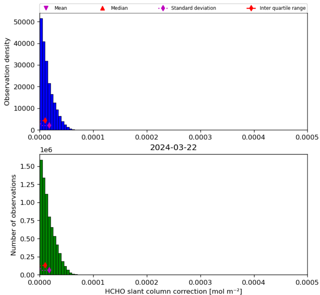
Figure 47: Histogram of “HCHO slant column correction” for 2024-03-21 to 2024-03-22
