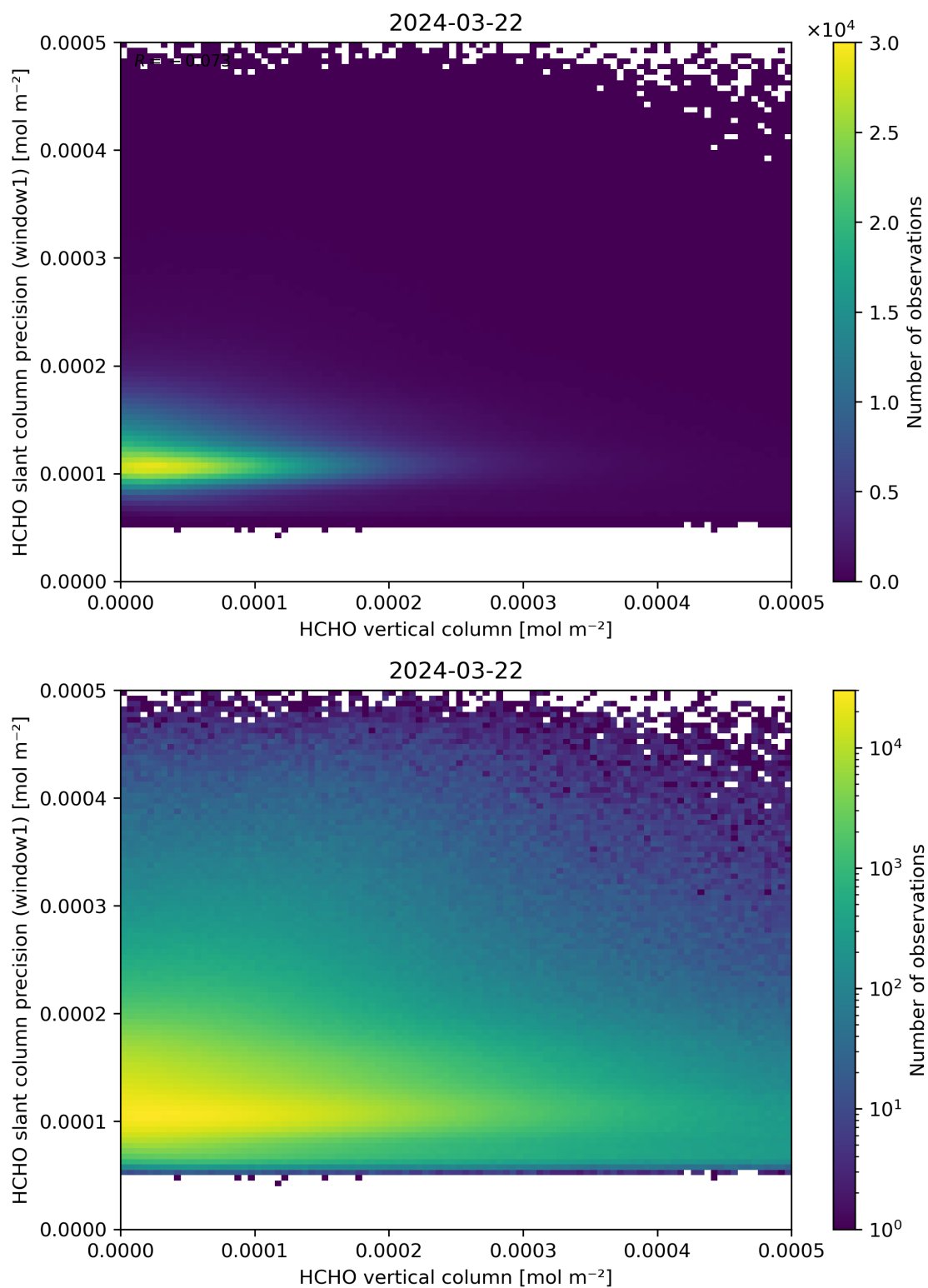
Figure 130: Scatter density plot of “HCHO vertical column” against “HCHO slant column precision (window1)” for 2024-03-21 to 2024-03-22.
