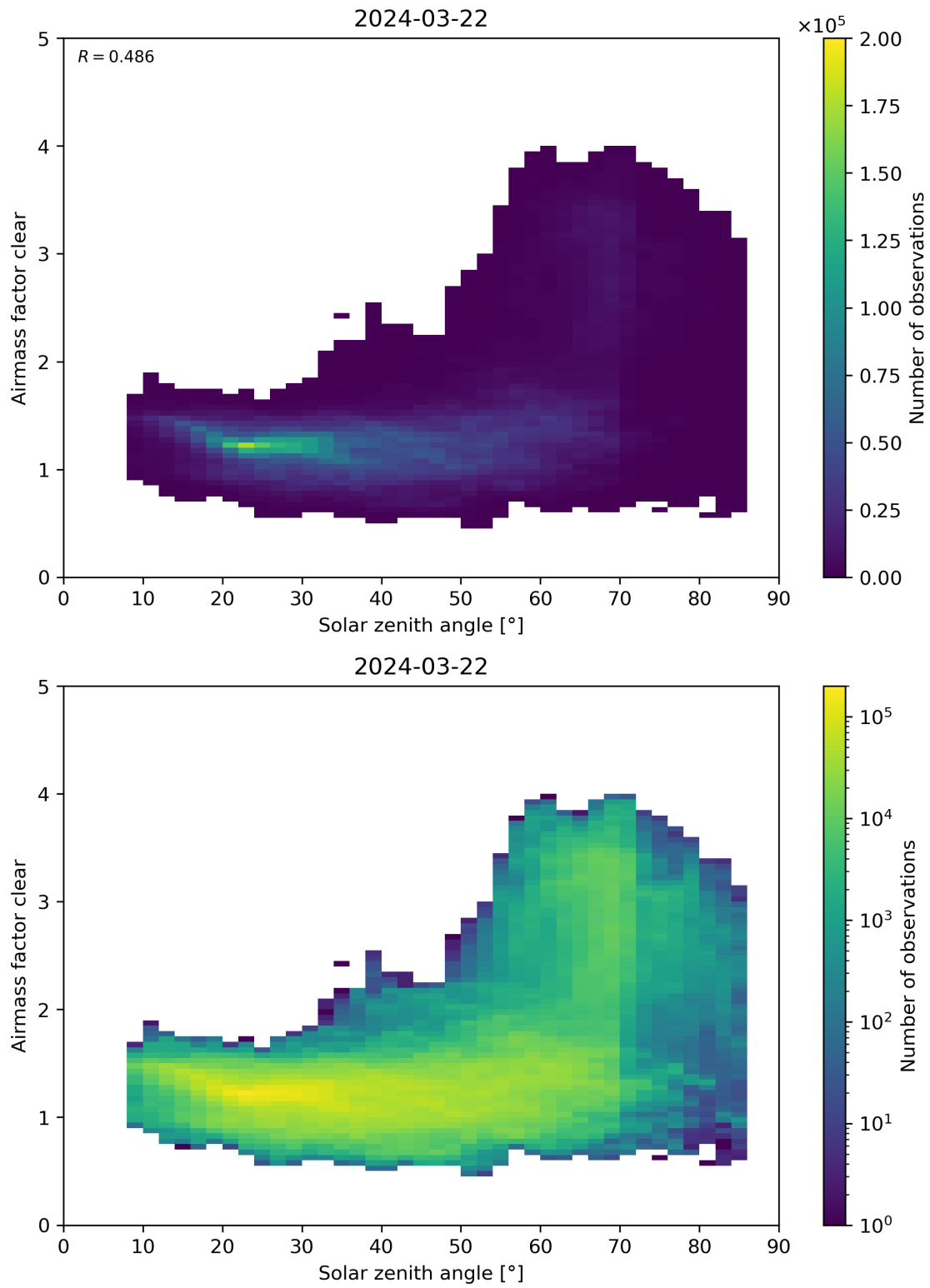
Figure 170: Scatter density plot of “Solar zenith angle” against “Airmass factor clear” for 2024-03-21 to 2024-03-22.
