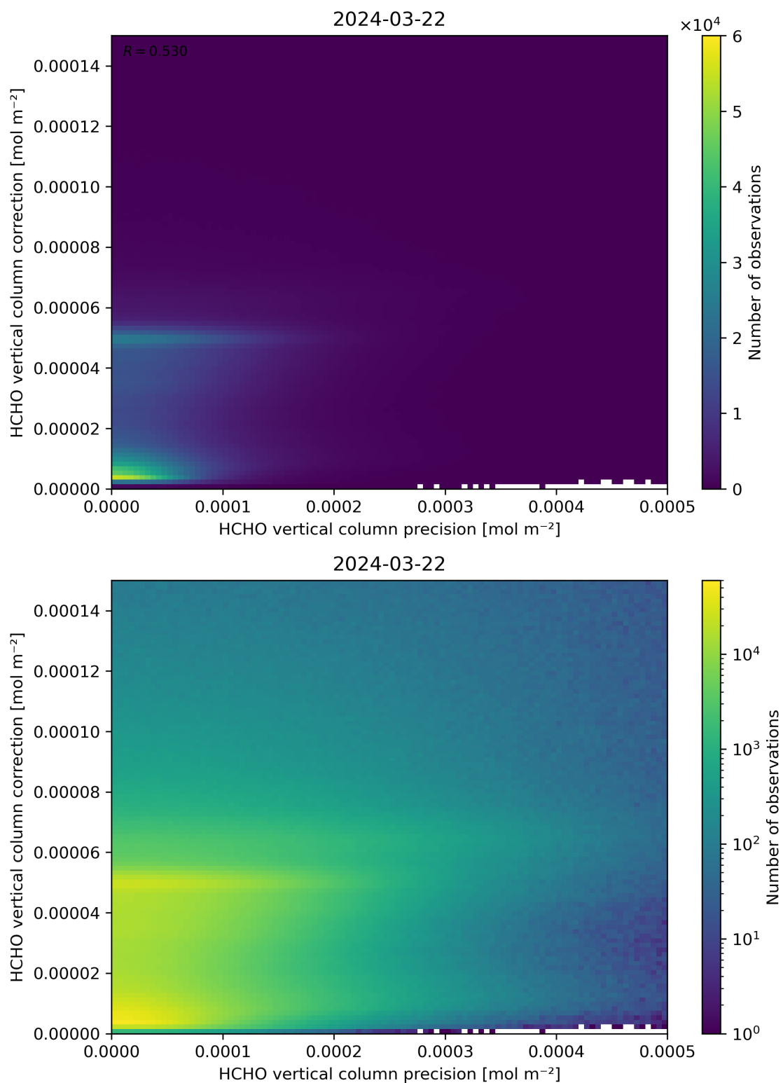
Figure 146: Scatter density plot of “HCHO vertical column precision” against “HCHO vertical column correction” for 2024-03-21 to 2024-03-22.
