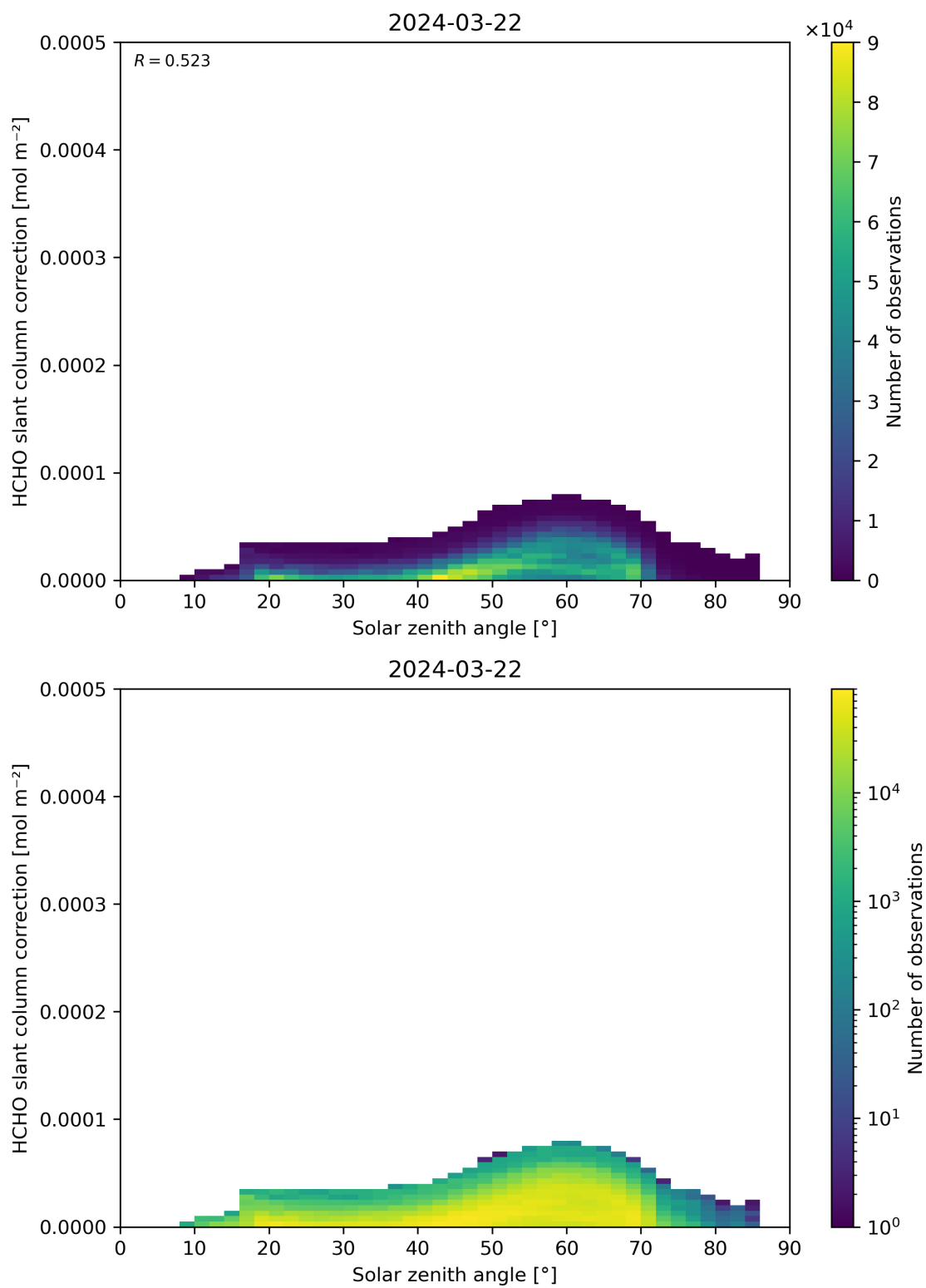
Figure 172: Scatter density plot of “Solar zenith angle” against “HCHO slant column correction” for 2024-03-21 to 2024-03-22.
