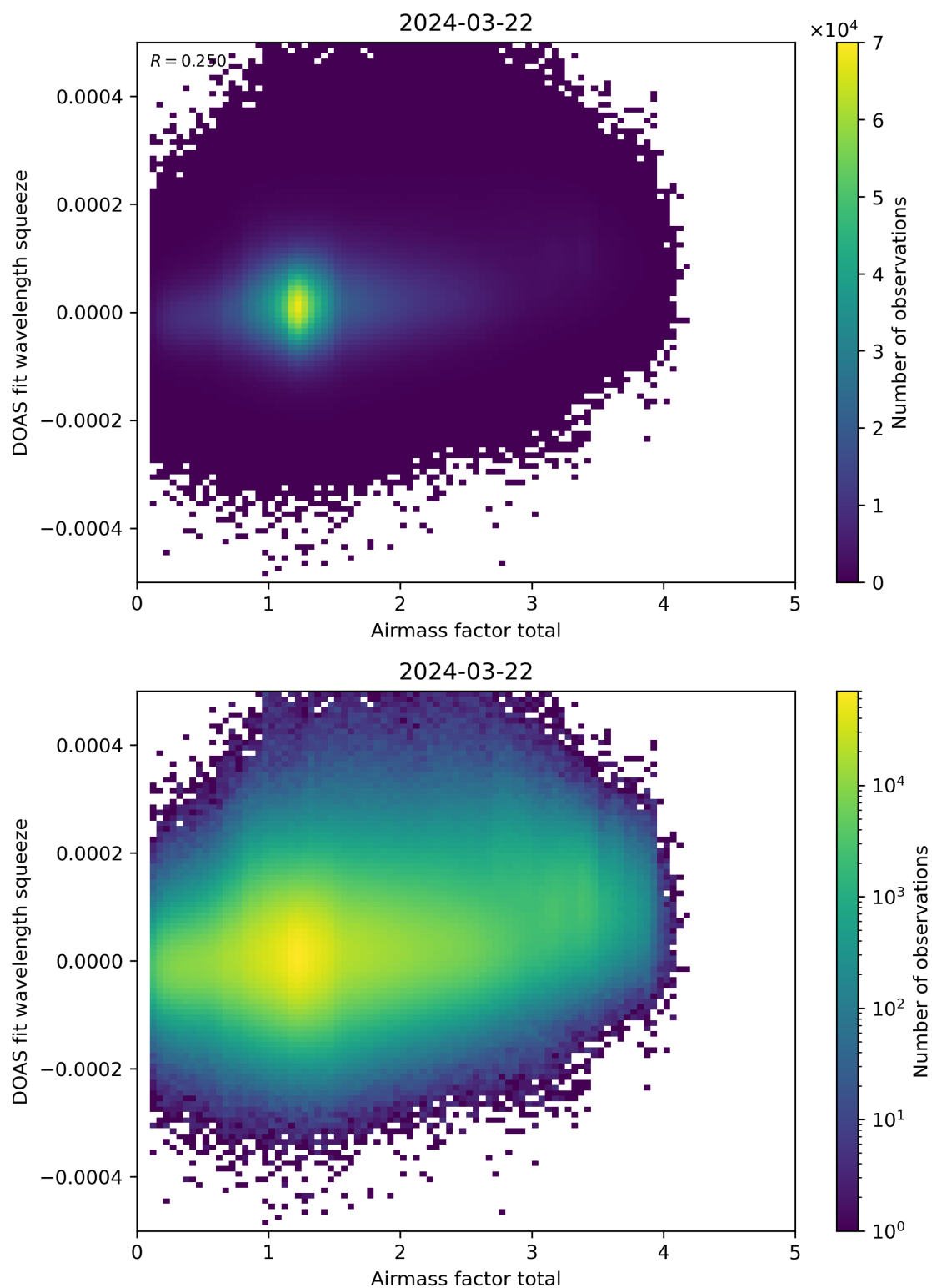
Figure 99: Scatter density plot of “Airmass factor total” against “DOAS fit wavelength squeeze” for 2024-03-21 to 2024-03-22.
