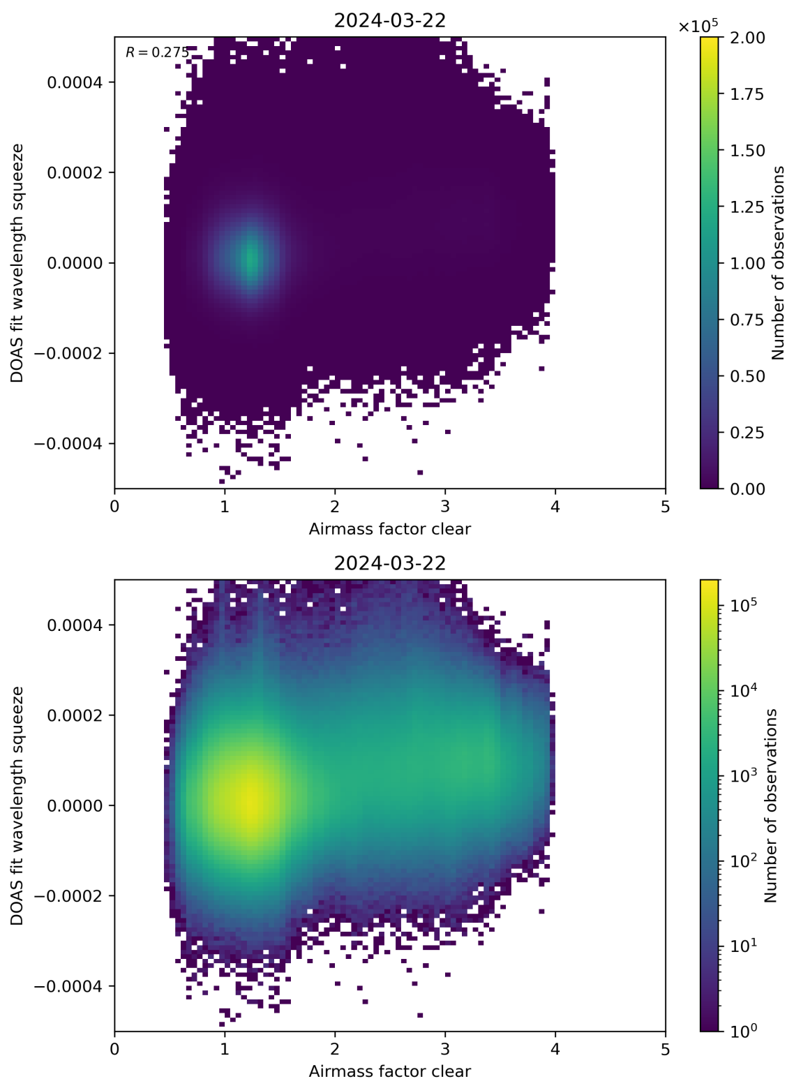
Figure 73: Scatter density plot of “Airmass factor clear” against “DOAS fit wavelength squeeze” for 2024-03-21 to 2024-03-22.
