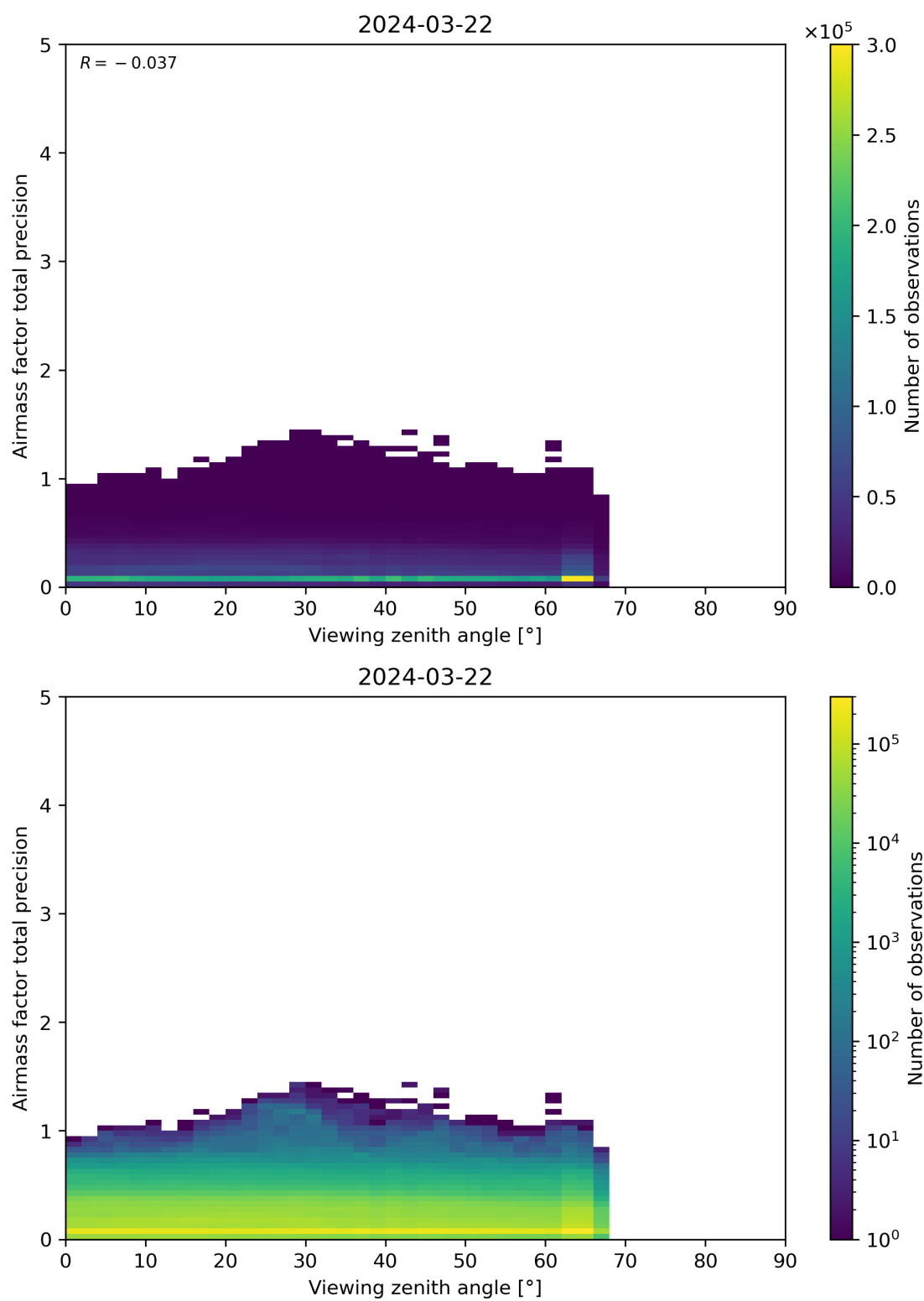
Figure 191: Scatter density plot of “Viewing zenith angle” against “Airmass factor total precision” for 2024-03-21 to 2024-03-22.
