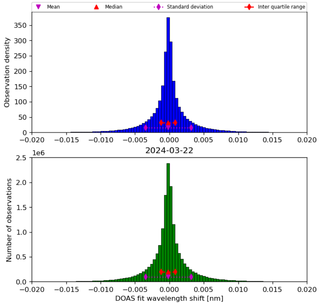
Figure 44: Histogram of “DOAS fit wavelength shift” for 2024-03-21 to 2024-03-22
