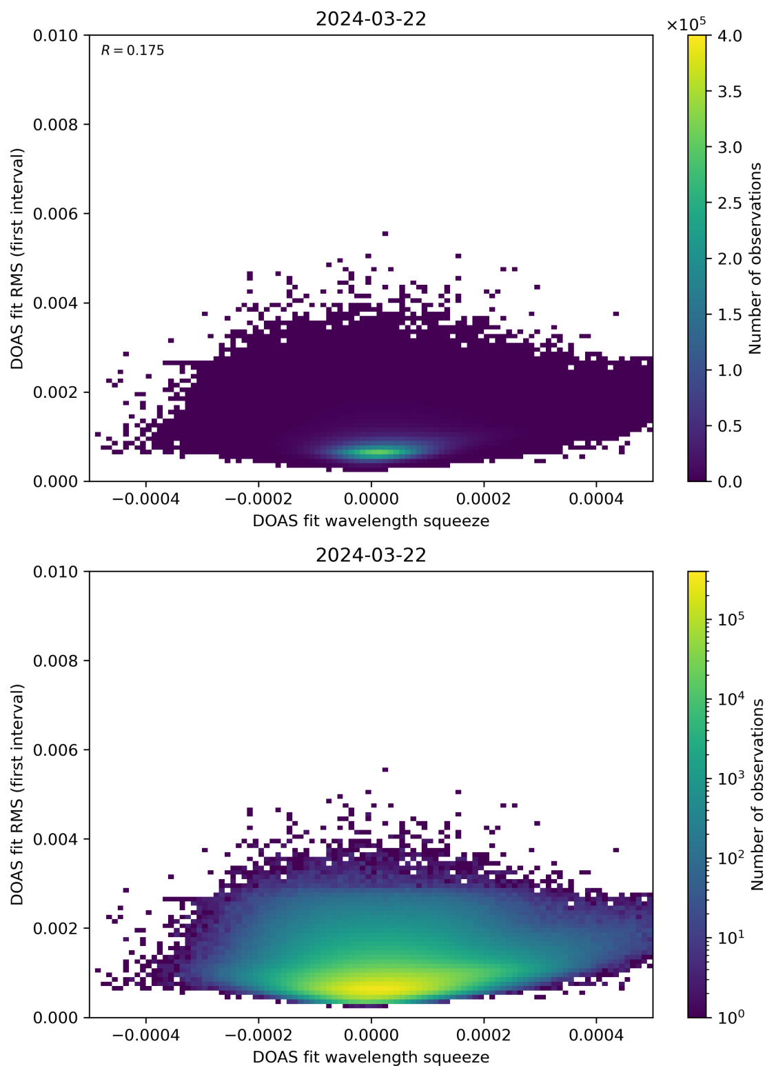
Figure 68: Scatter density plot of “DOAS fit wavelength squeeze” against “DOAS fit RMS (first interval)” for 2024-03-21 to 2024-03-22.
