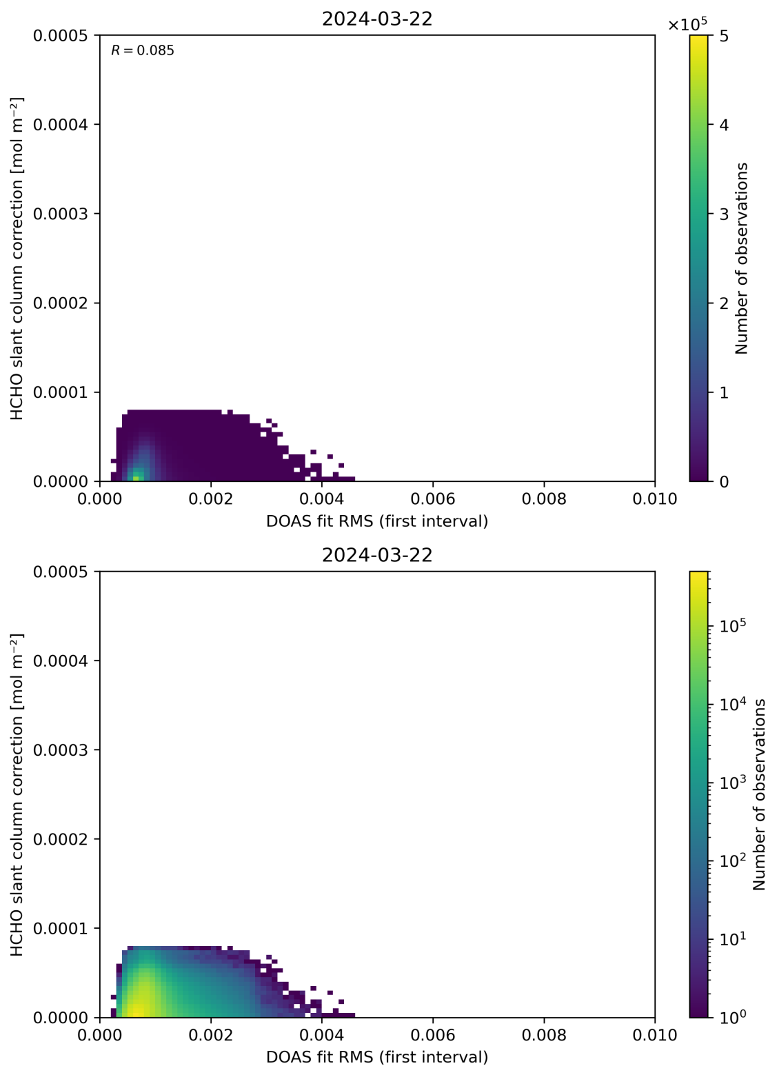
Figure 63: Scatter density plot of “DOAS fit RMS (first interval)” against “HCHO slant column correction” for 2024-03-21 to 2024-03-22.
