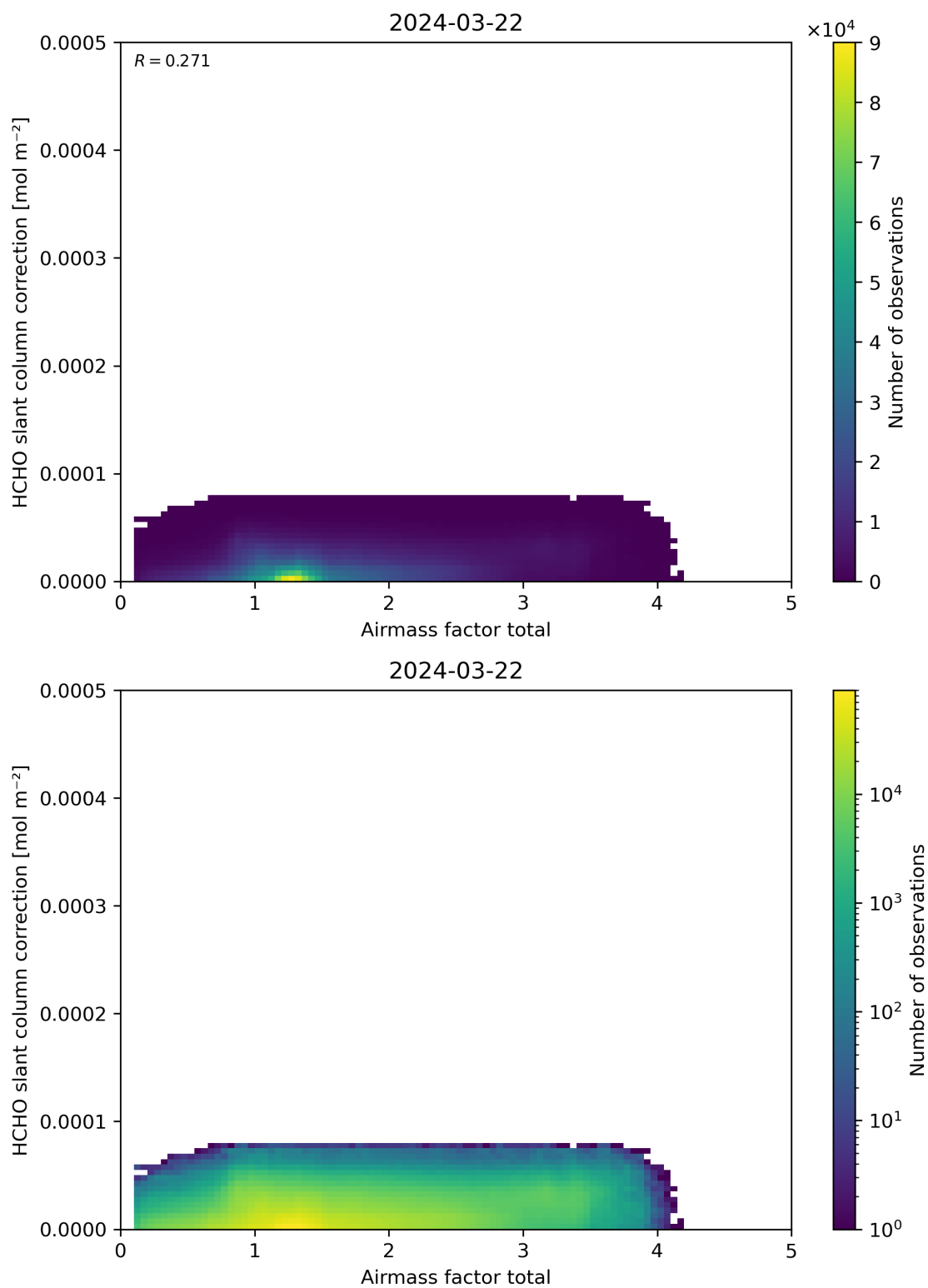
Figure 102: Scatter density plot of “Airmass factor total” against “HCHO slant column correction” for 2024-03-21 to 2024-03-22.
