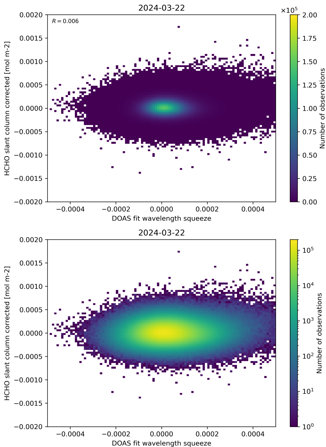
Figure 69: Scatter density plot of “DOAS fit wavelength squeeze” against “HCHO slant column corrected” for 2024-03-21 to 2024-03-22.
