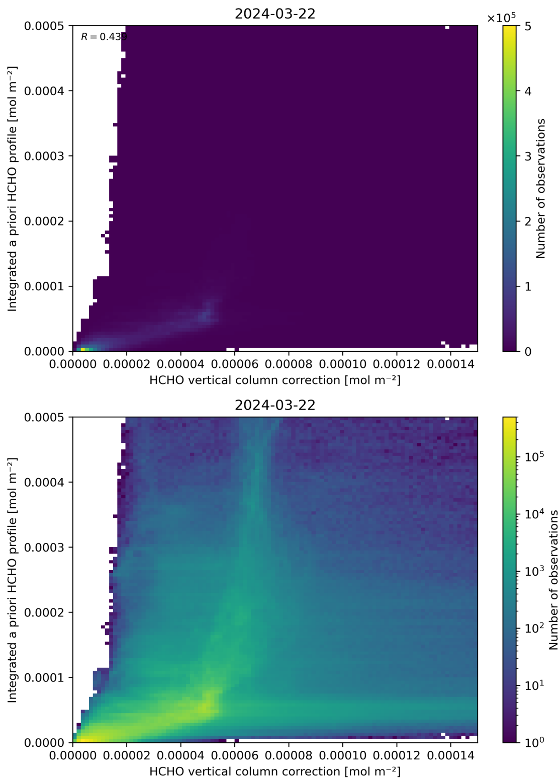
Figure 122: Scatter density plot of “HCHO vertical column correction” against “Integrated a priori HCHO profile” for 2024-03-21 to 2024-03-22.
