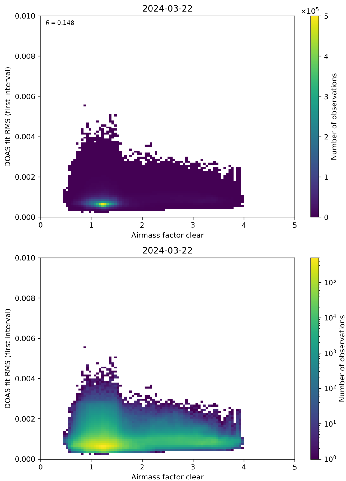
Figure 71: Scatter density plot of “Airmass factor clear” against “DOAS fit RMS (first interval)” for 2024-03-21 to 2024-03-22.
