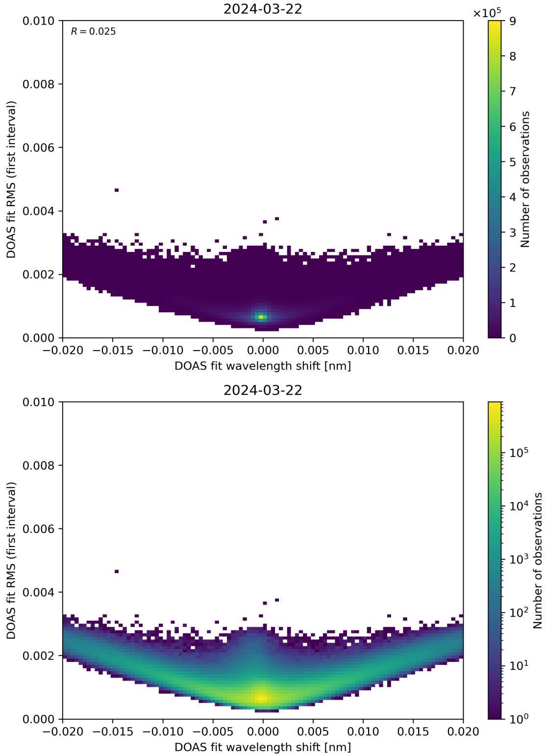
Figure 64: Scatter density plot of “DOAS fit wavelength shift” against “DOAS fit RMS (first interval)” for 2024-03-21 to 2024-03-22.
