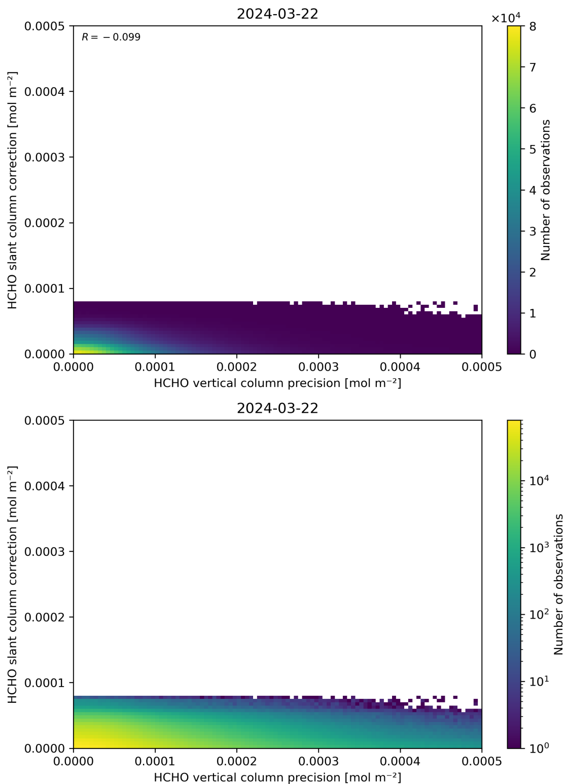
Figure 141: Scatter density plot of “HCHO vertical column precision” against “HCHO slant column correction” for 2024-03-21 to 2024-03-22.
