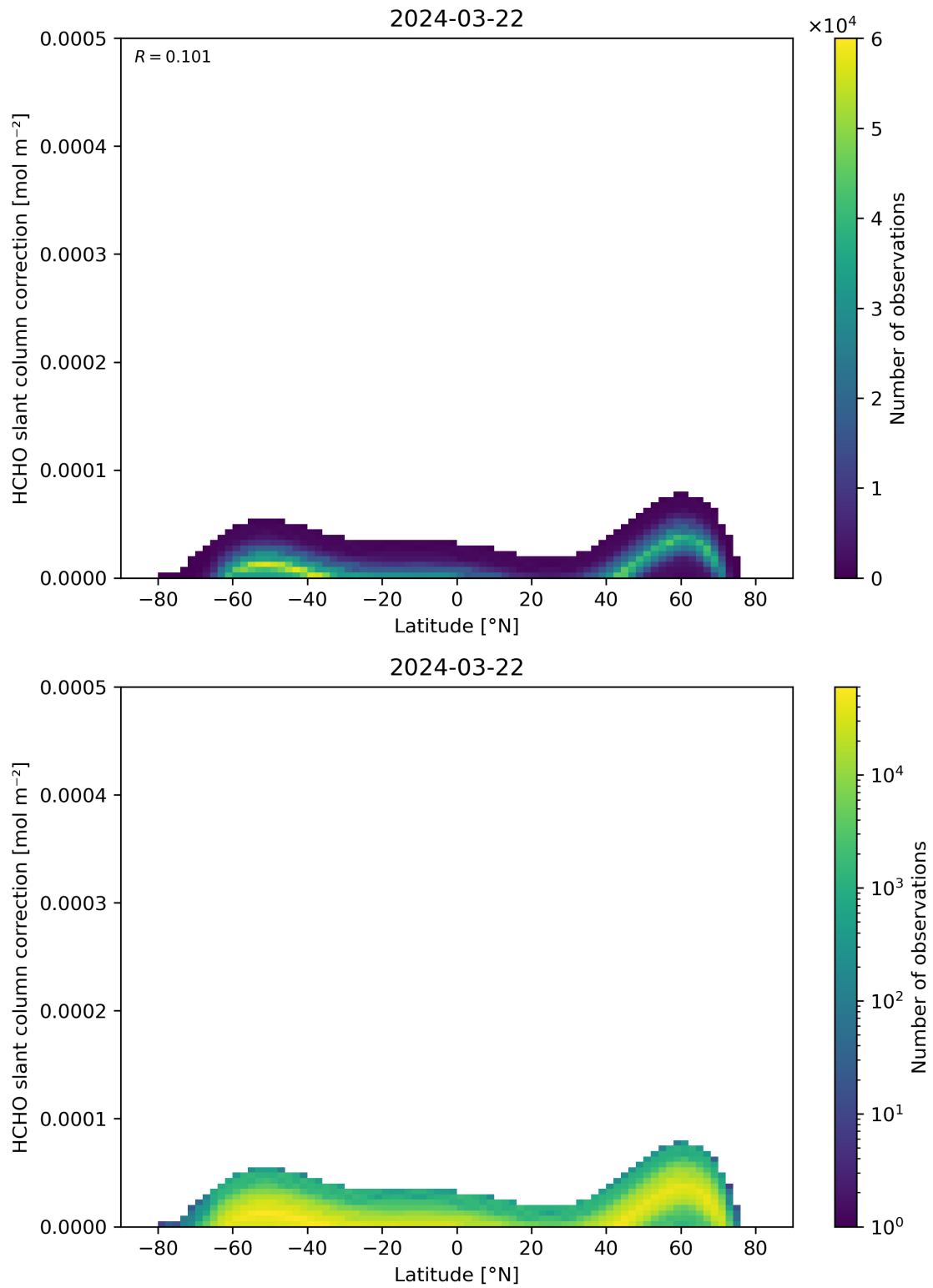
Figure 158: Scatter density plot of “Latitude” against “HCHO slant column correction” for 2024-03-21 to 2024-03-22.
