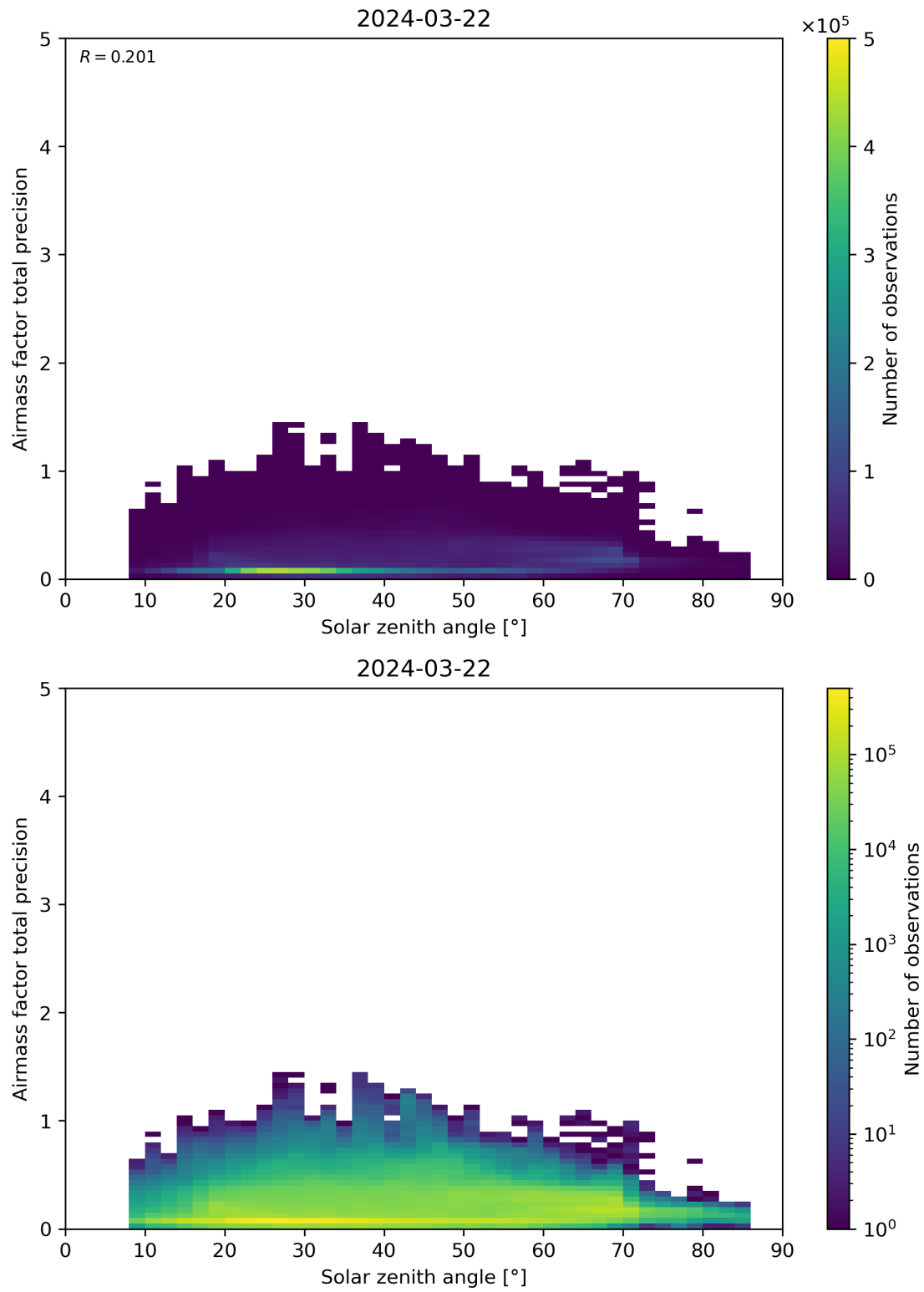
Figure 176: Scatter density plot of “Solar zenith angle” against “Airmass factor total precision” for 2024-03-21 to 2024-03-22.
