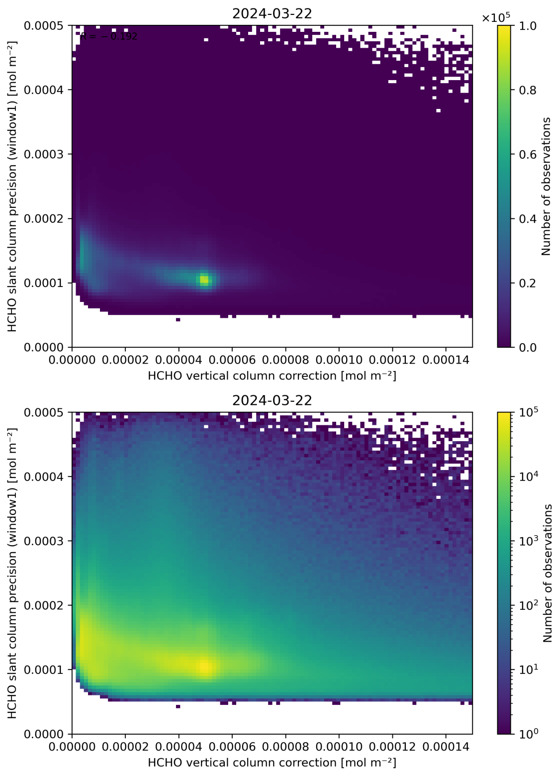
Figure 119: Scatter density plot of “HCHO vertical column correction” against “HCHO slant column precision (window1)” for 2024-03-21 to 2024-03-22.
