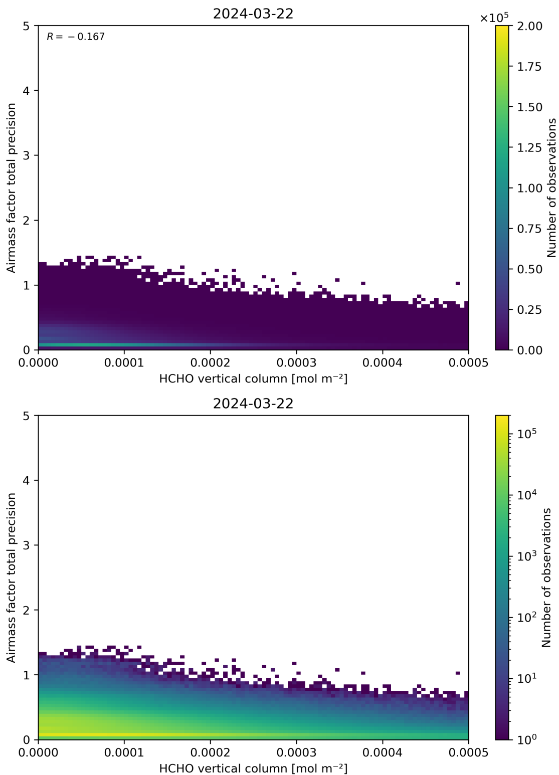
Figure 132: Scatter density plot of “HCHO vertical column” against “Airmass factor total precision” for 2024-03-21 to 2024-03-22.
