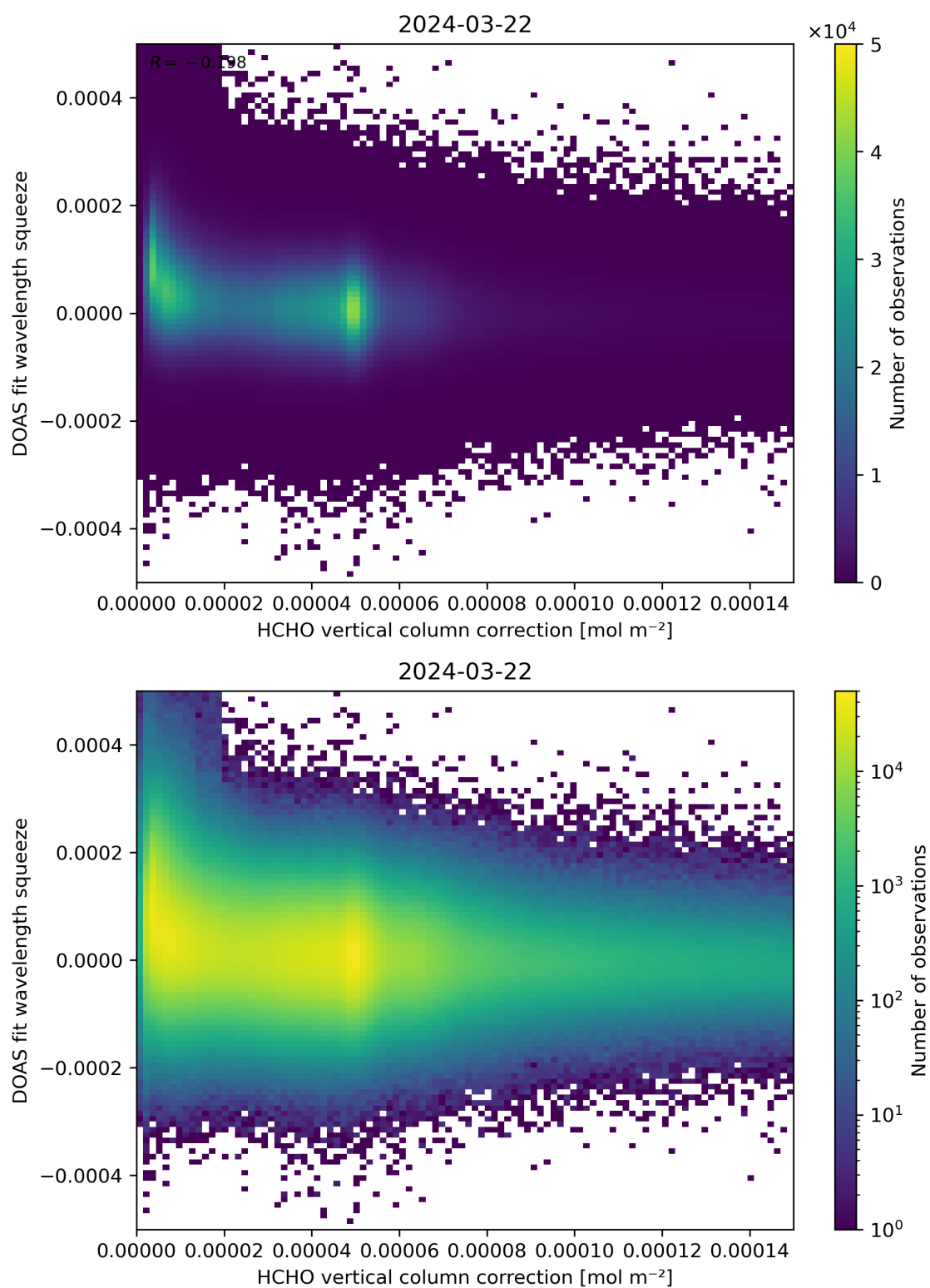
Figure 114: Scatter density plot of “HCHO vertical column correction” against “DOAS fit wavelength squeeze” for 2024-03-21 to 2024-03-22.
