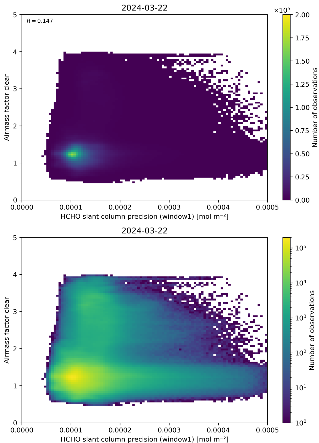
Figure 91: Scatter density plot of “HCHO slant column precision (window1)” against “Airmass factor clear” for 2024-03-21 to 2024-03-22.
