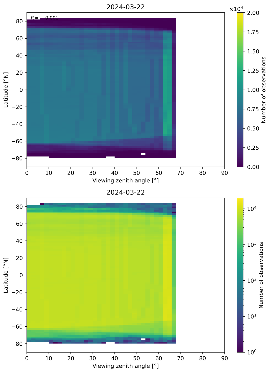
Figure 196: Scatter density plot of “Viewing zenith angle” against “Latitude” for 2024-03-21 to 2024-03-22.
