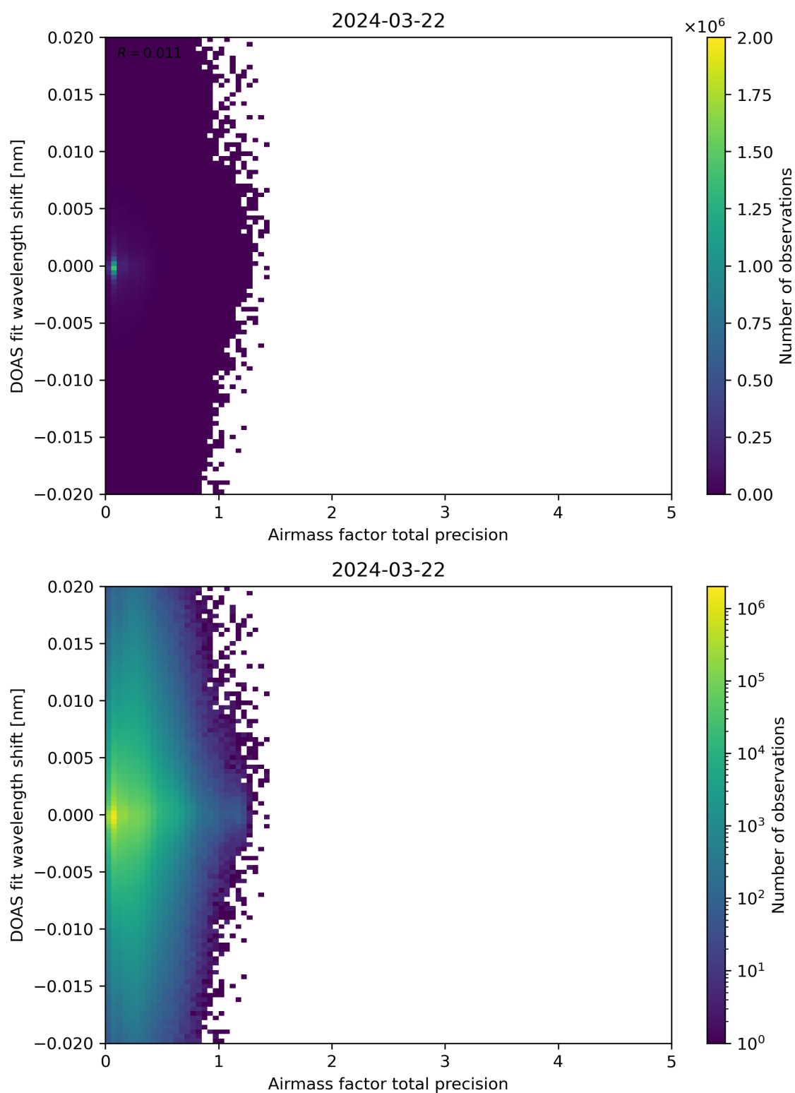
Figure 106: Scatter density plot of “Airmass factor total precision” against “DOAS fit wavelength shift” for 2024-03-21 to 2024-03-22.
