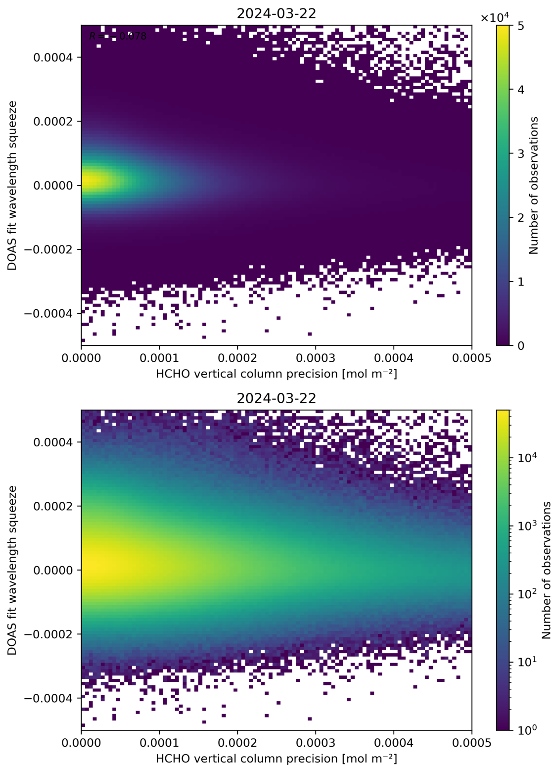
Figure 138: Scatter density plot of “HCHO vertical column precision” against “DOAS fit wavelength squeeze” for 2024-03-21 to 2024-03-22.
