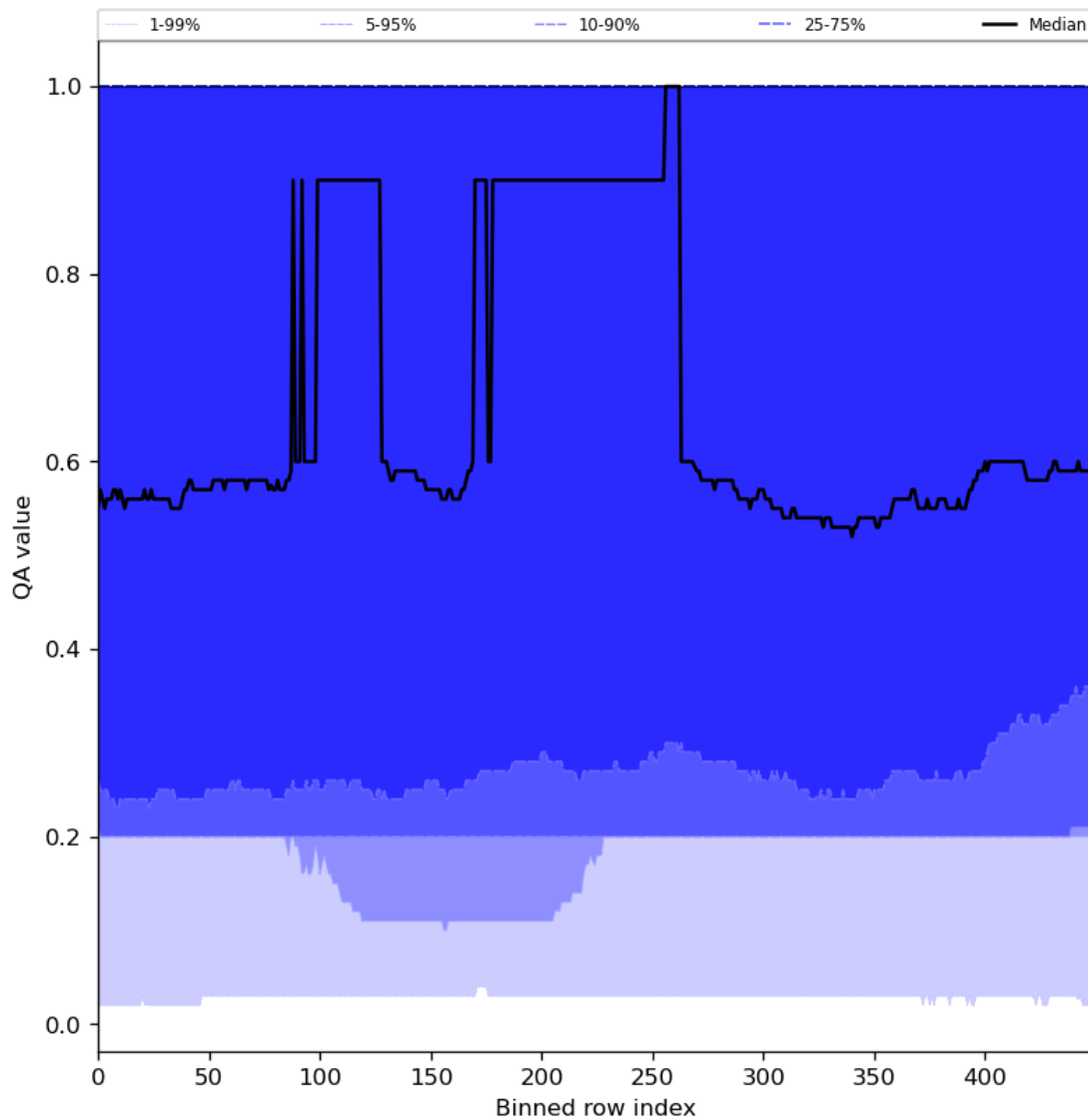
Figure 48: Along track statistics of “QA value” for 2024-03-21 to 2024-03-22
