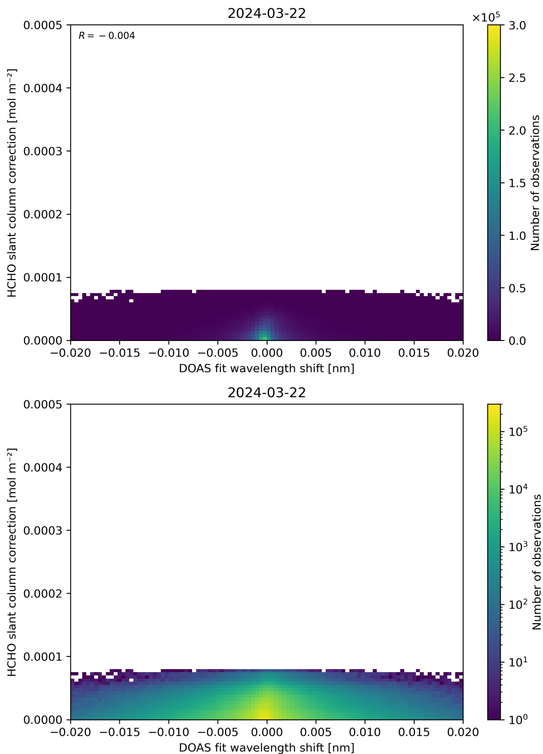
Figure 67: Scatter density plot of “DOAS fit wavelength shift” against “HCHO slant column correction” for 2024-03-21 to 2024-03-22.
