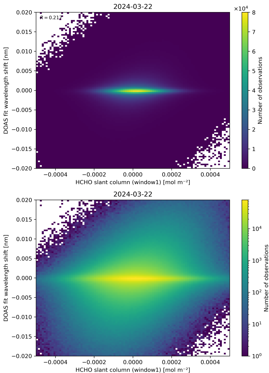
Figure 79: Scatter density plot of “HCHO slant column (window1)” against “DOAS fit wavelength shift” for 2024-03-21 to 2024-03-22.
