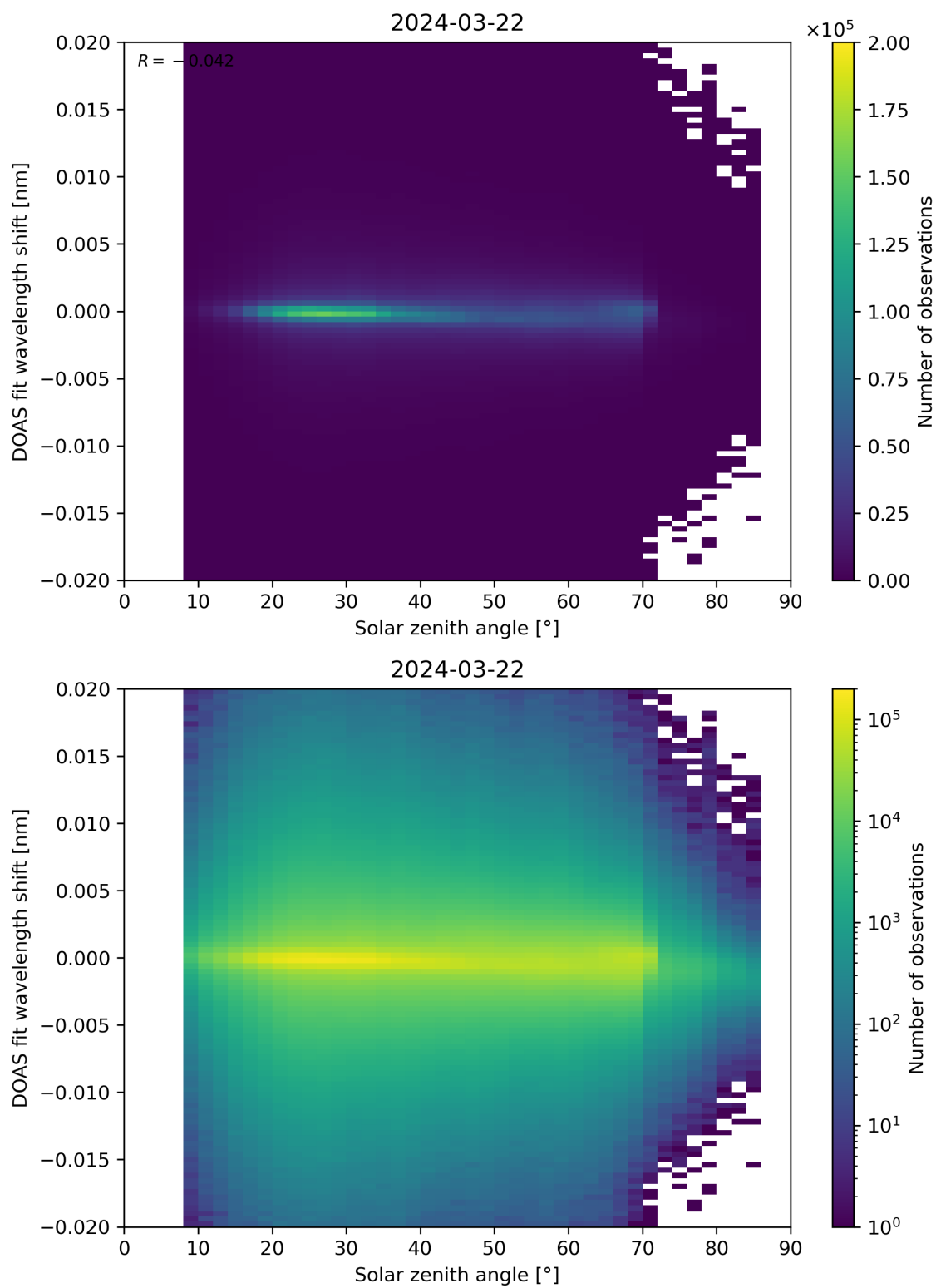
Figure 168: Scatter density plot of “Solar zenith angle” against “DOAS fit wavelength shift” for 2024-03-21 to 2024-03-22.
