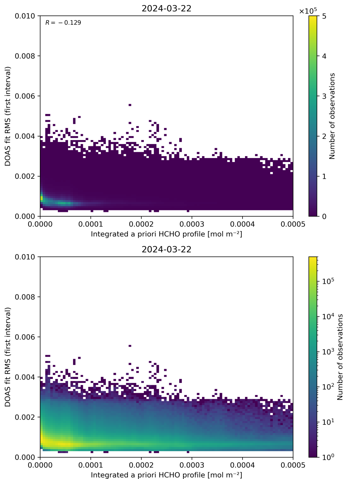
Figure 148: Scatter density plot of “Integrated a priori HCHO profile” against “DOAS fit RMS (first interval)” for 2024-03-21 to 2024-03-22.
