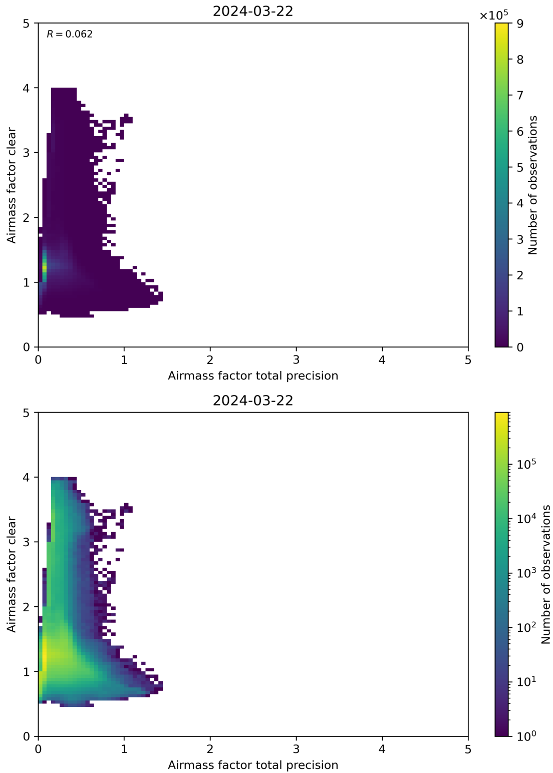
Figure 108: Scatter density plot of “Airmass factor total precision” against “Airmass factor clear” for 2024-03-21 to 2024-03-22.
