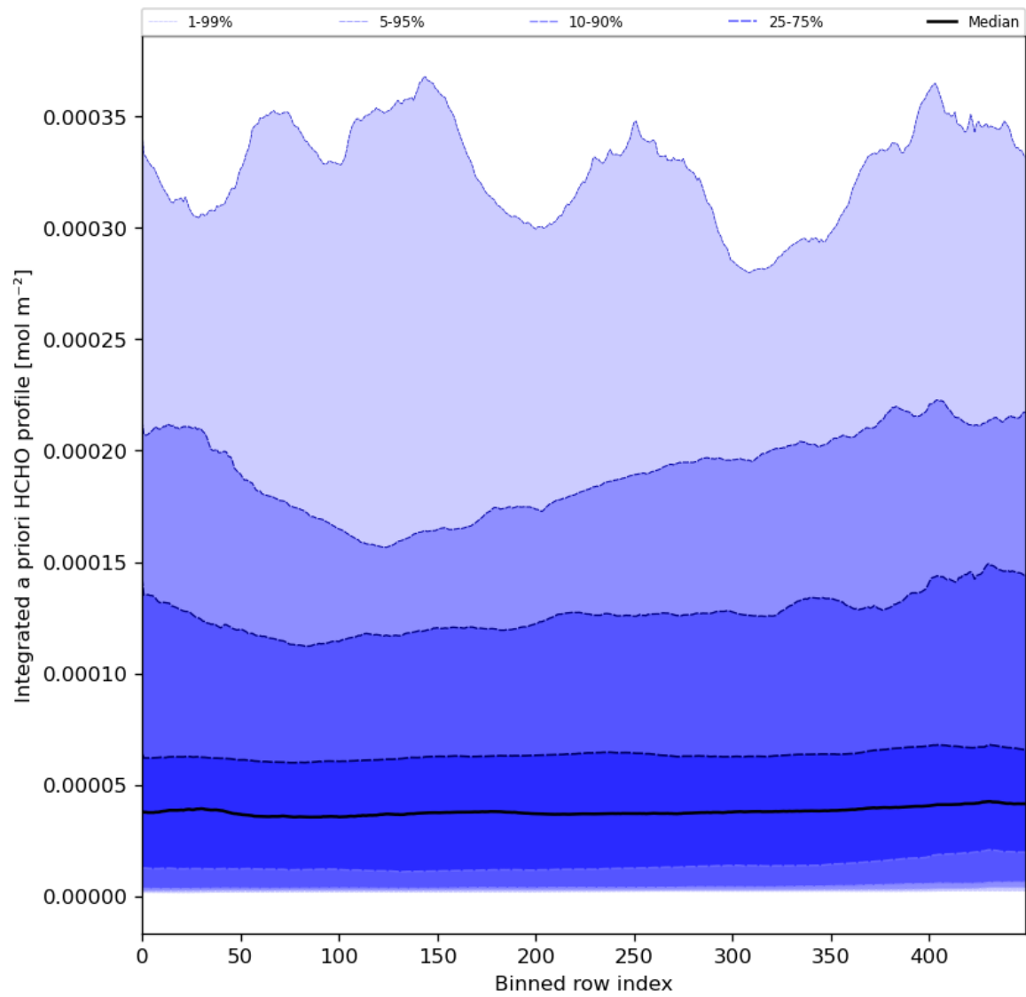
Figure 57: Along track statistics of “Integrated a priori HCHO profile” for 2024-03-21 to 2024-03-22
