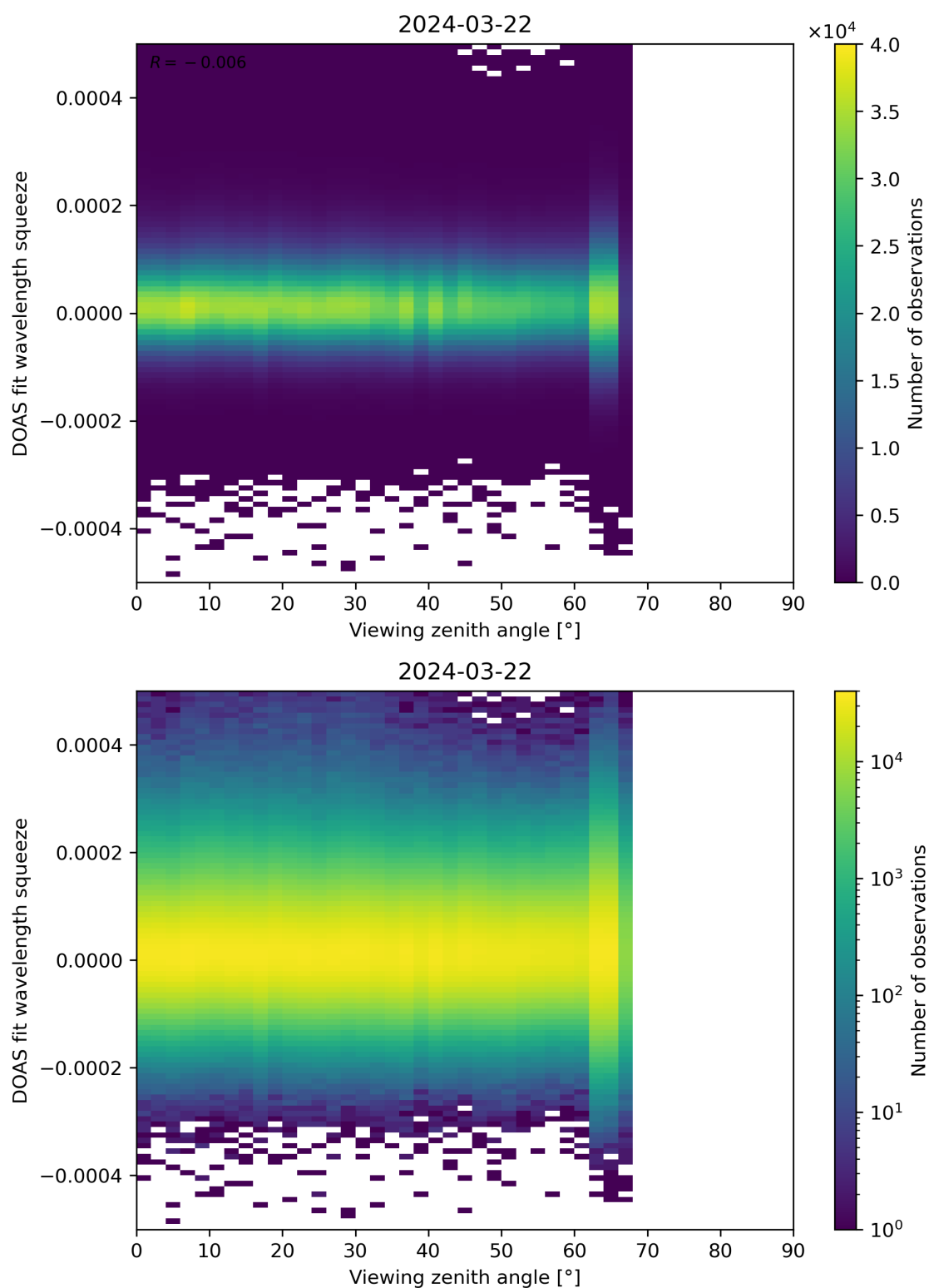
Figure 184: Scatter density plot of “Viewing zenith angle” against “DOAS fit wavelength squeeze” for 2024-03-21 to 2024-03-22.
