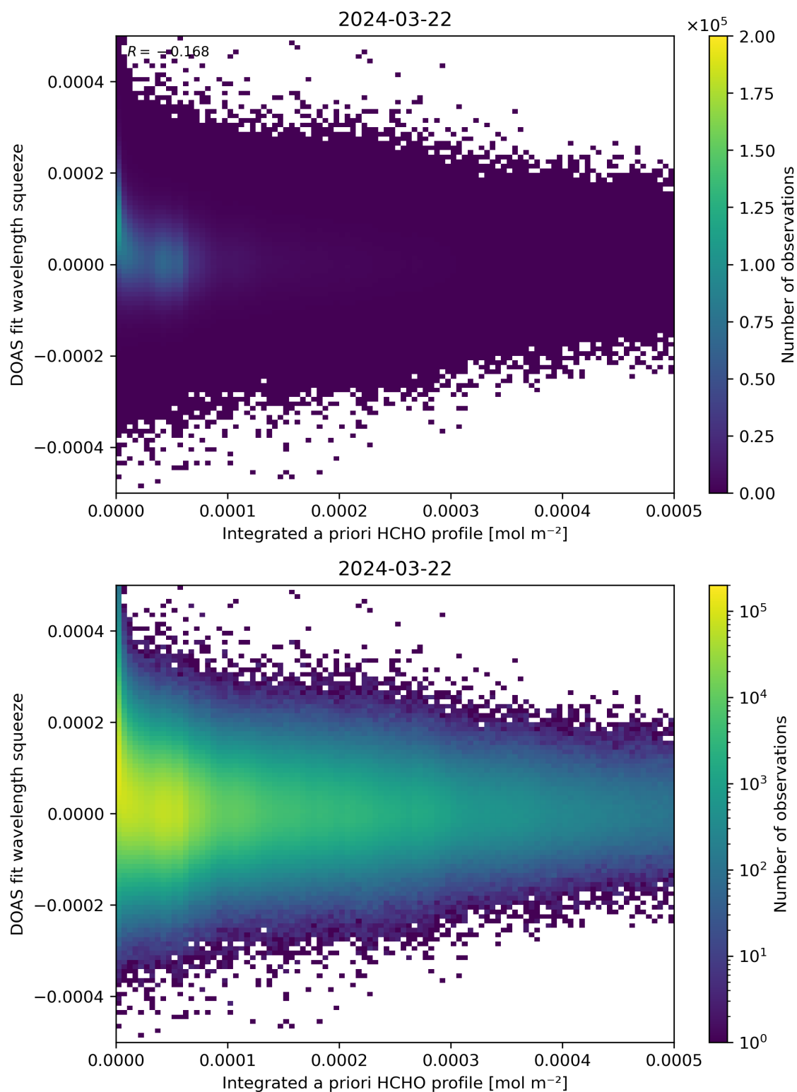
Figure 150: Scatter density plot of “Integrated a priori HCHO profile” against “DOAS fit wavelength squeeze” for 2024-03-21 to 2024-03-22.
