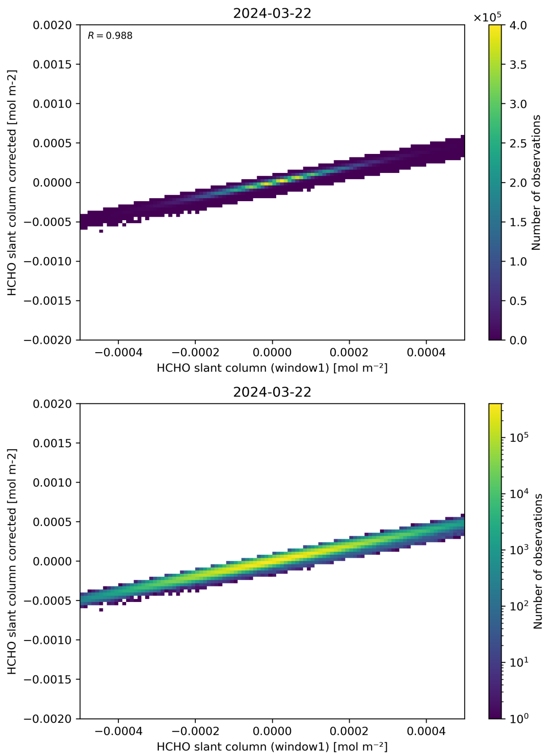
Figure 82: Scatter density plot of “HCHO slant column (window1)” against “HCHO slant column corrected” for 2024-03-21 to 2024-03-22.
