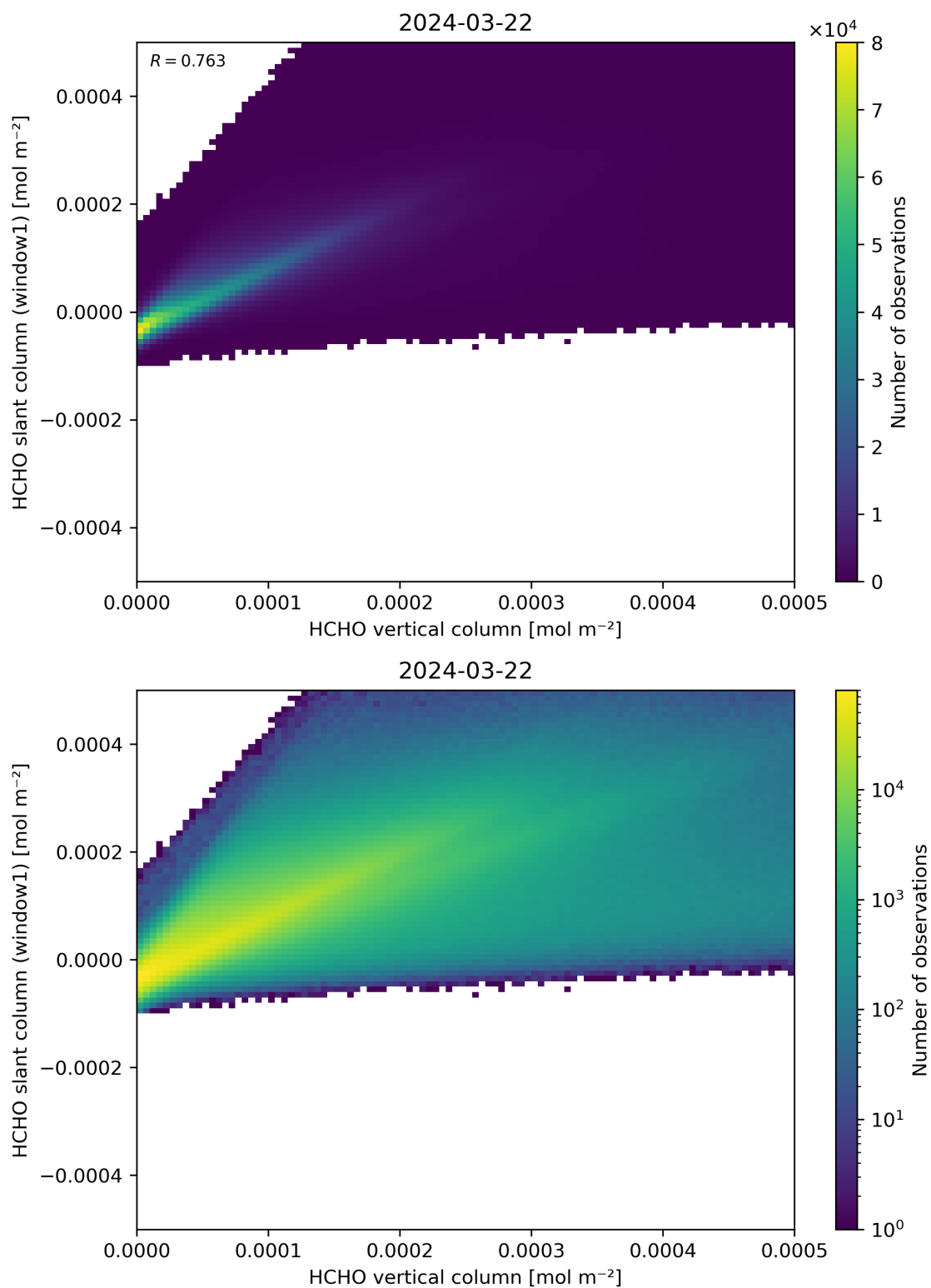
Figure 129: Scatter density plot of “HCHO vertical column” against “HCHO slant column (window1)” for 2024-03-21 to 2024-03-22.
