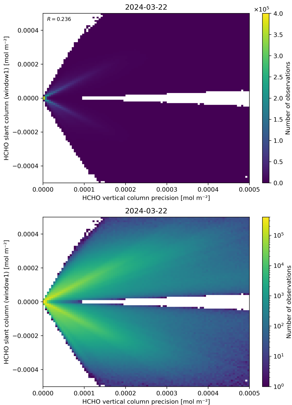
Figure 142: Scatter density plot of “HCHO vertical column precision” against “HCHO slant column (window1)” for 2024-03-21 to 2024-03-22.
