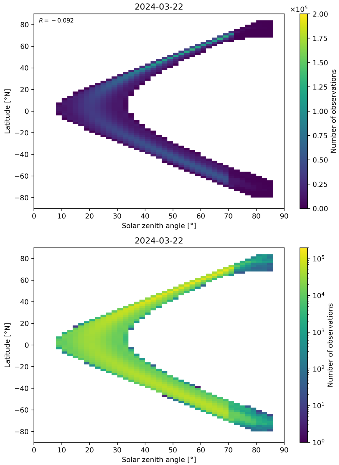
Figure 181: Scatter density plot of “Solar zenith angle” against “Latitude” for 2024-03-21 to 2024-03-22.
