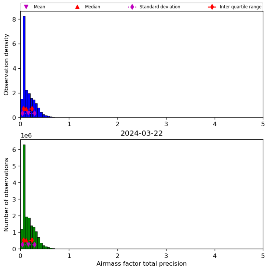
Figure 41: Histogram of “Airmass factor total precision” for 2024-03-21 to 2024-03-22
