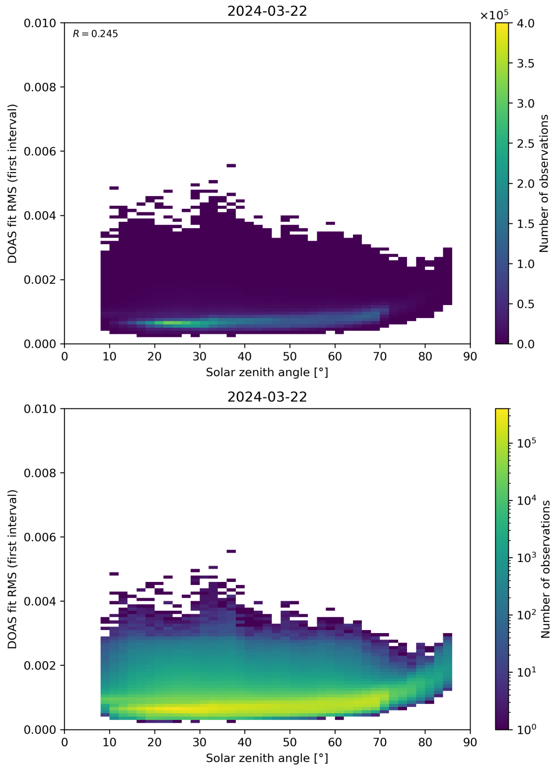
Figure 167: Scatter density plot of “Solar zenith angle” against “DOAS fit RMS (first interval)” for 2024-03-21 to 2024-03-22.
