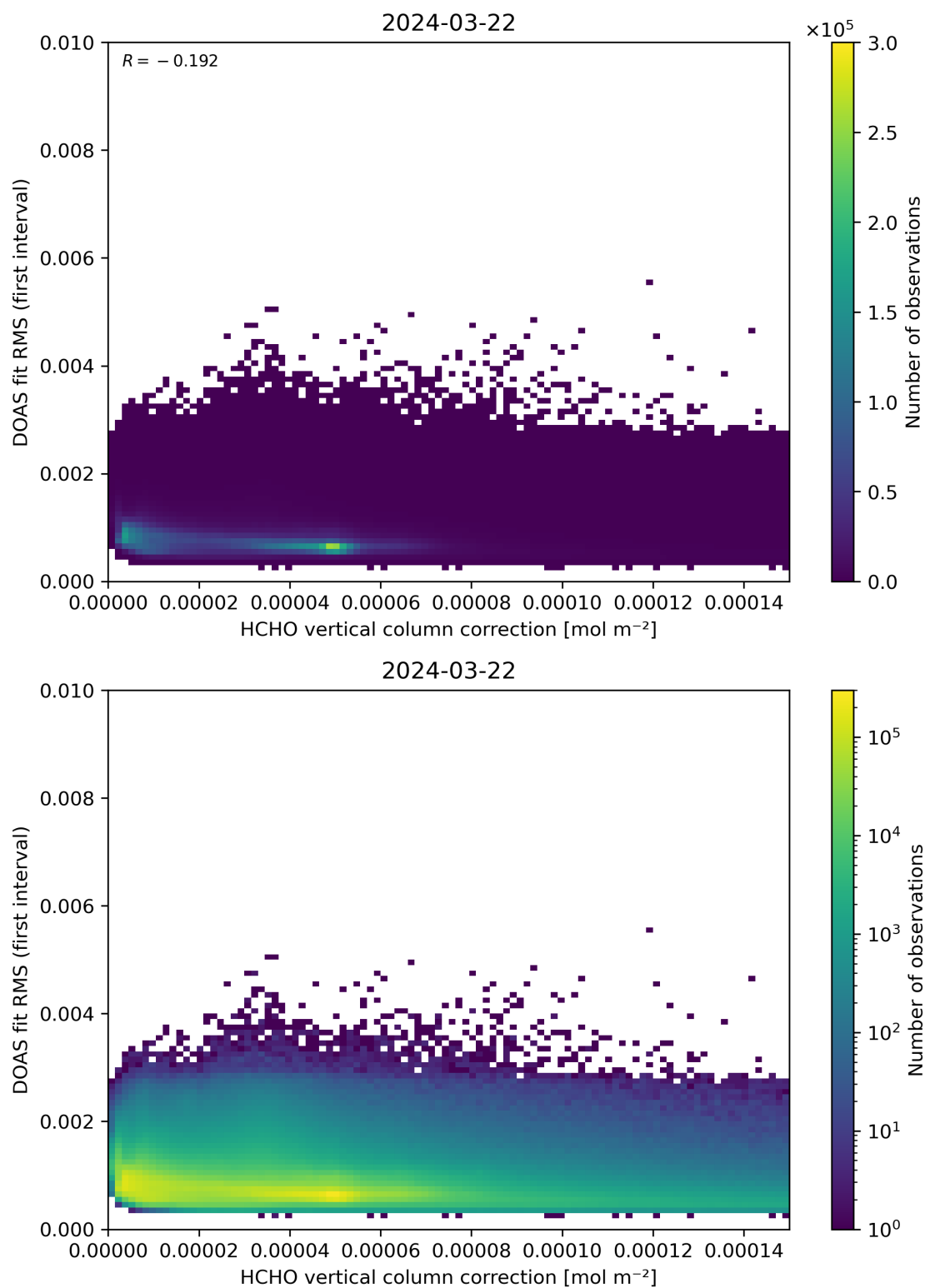
Figure 112: Scatter density plot of “HCHO vertical column correction” against “DOAS fit RMS (first interval)” for 2024-03-21 to 2024-03-22.
