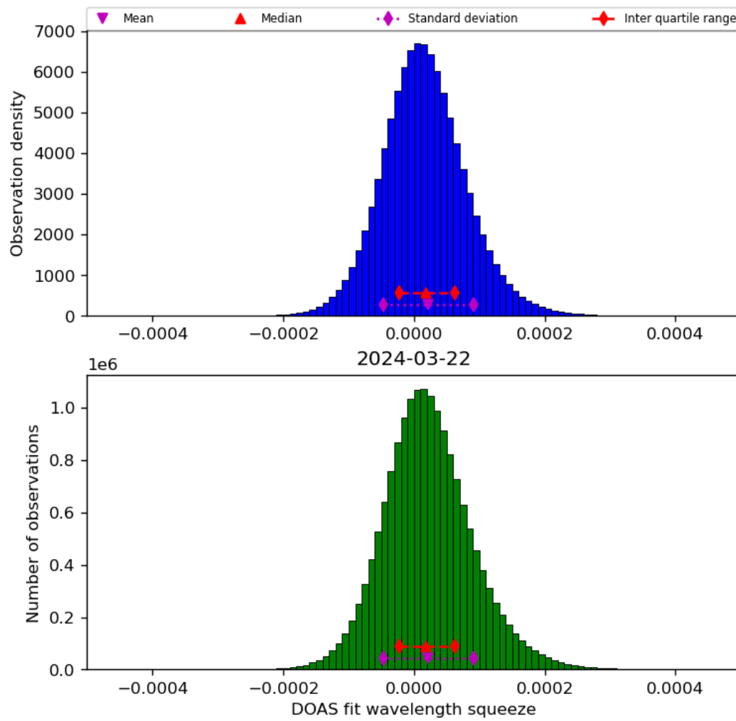
Figure 45: Histogram of “DOAS fit wavelength squeeze” for 2024-03-21 to 2024-03-22
