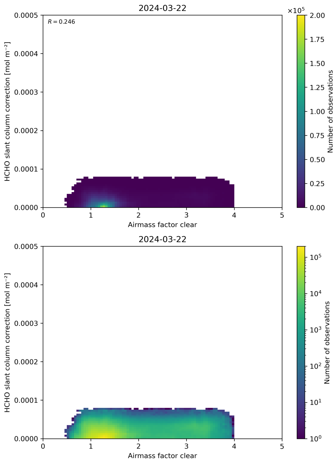
Figure 75: Scatter density plot of “Airmass factor clear” against “HCHO slant column correction” for 2024-03-21 to 2024-03-22.
