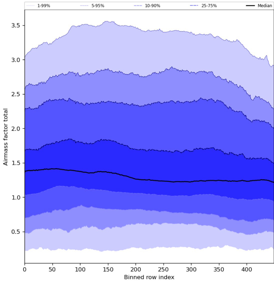
Figure 54: Along track statistics of “Airmass factor total” for 2024-03-21 to 2024-03-22
