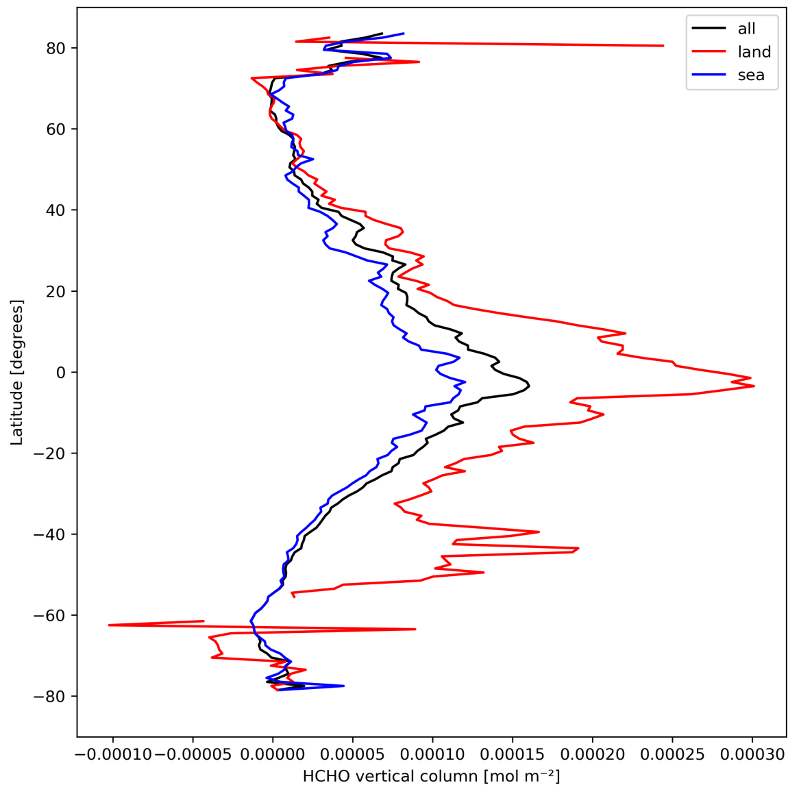
Figure 21: Zonal average of “HCHO vertical column” for 2024-03-21 to 2024-03-22.
