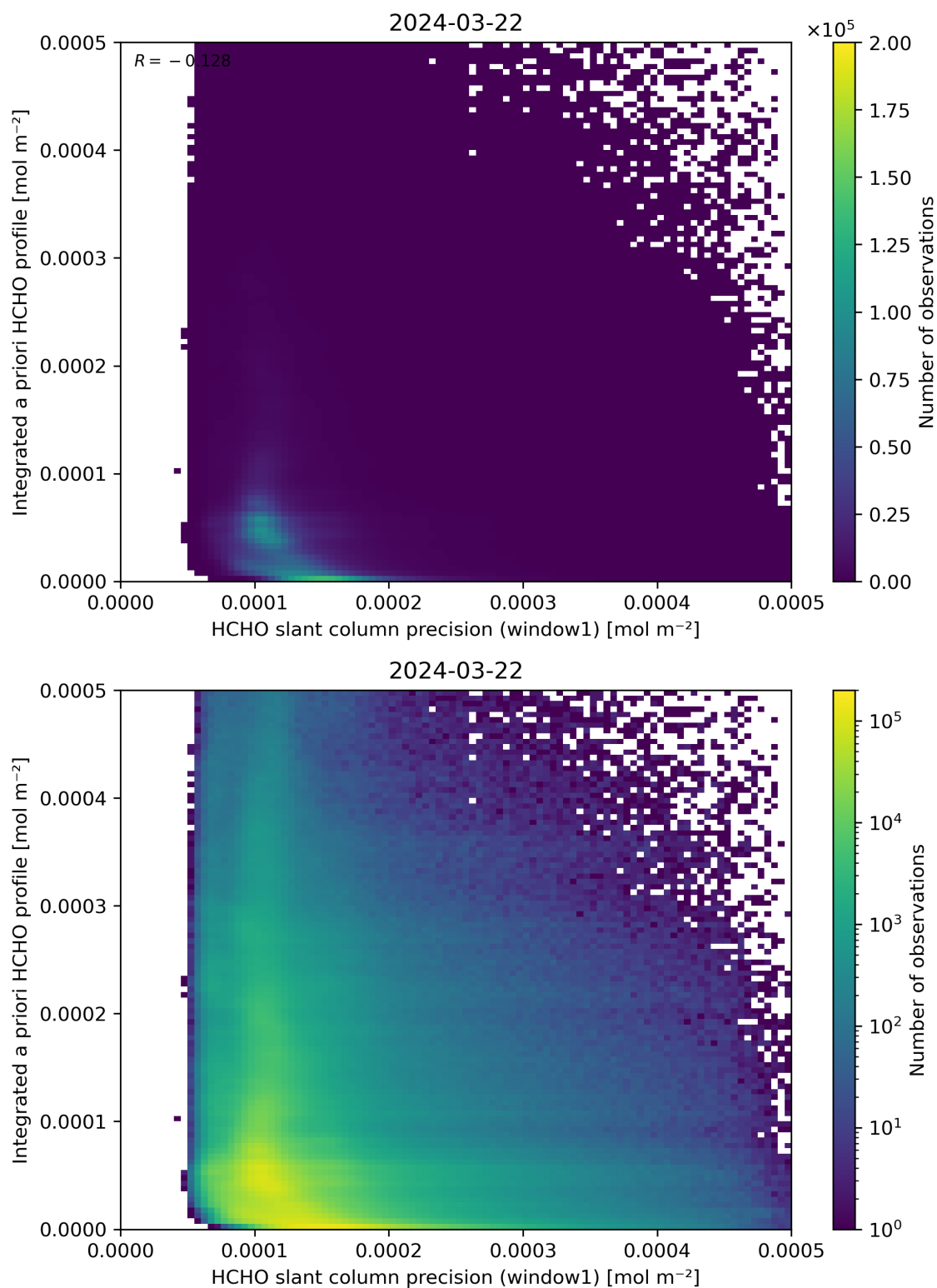
Figure 96: Scatter density plot of “HCHO slant column precision (window1)” against “Integrated a priori HCHO profile” for 2024-03-21 to 2024-03-22.
