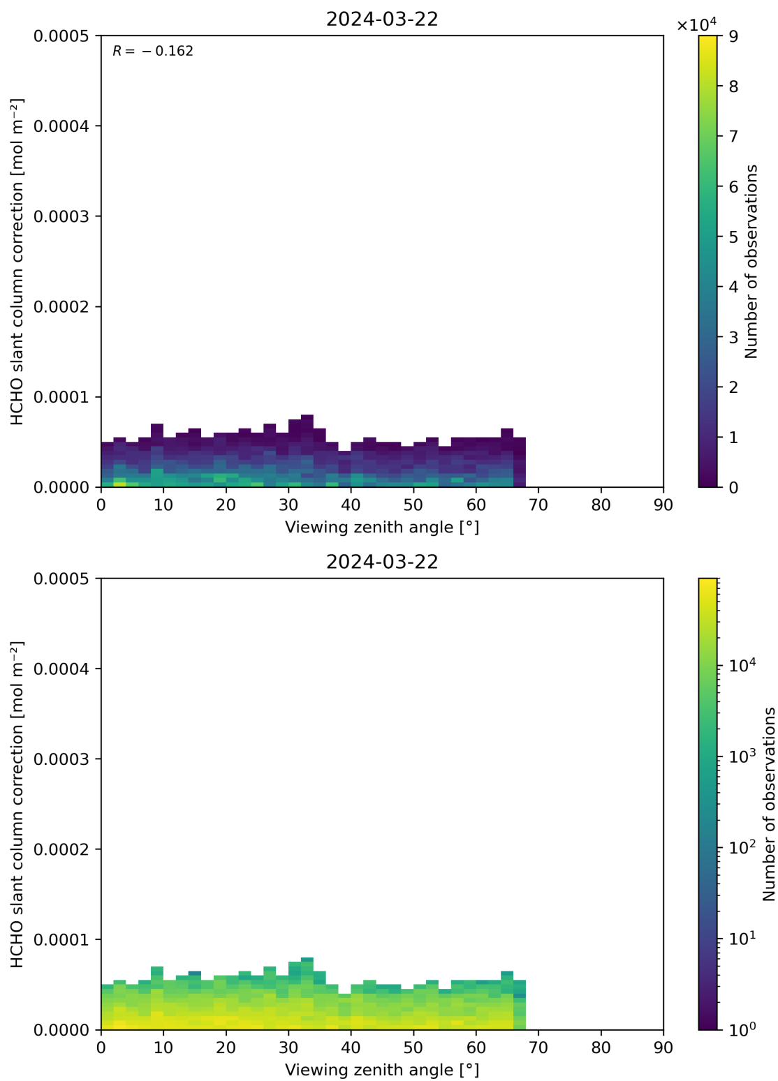
Figure 187: Scatter density plot of “Viewing zenith angle” against “HCHO slant column correction” for 2024-03-21 to 2024-03-22.
