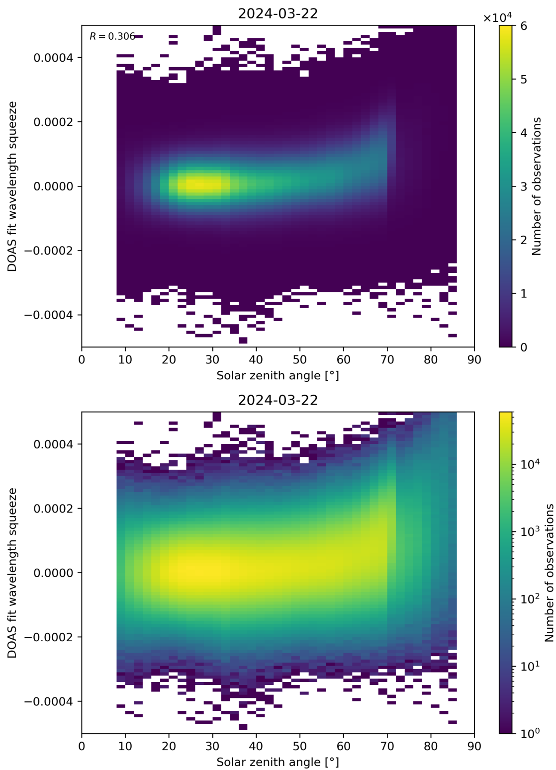
Figure 169: Scatter density plot of “Solar zenith angle” against “DOAS fit wavelength squeeze” for 2024-03-21 to 2024-03-22.
