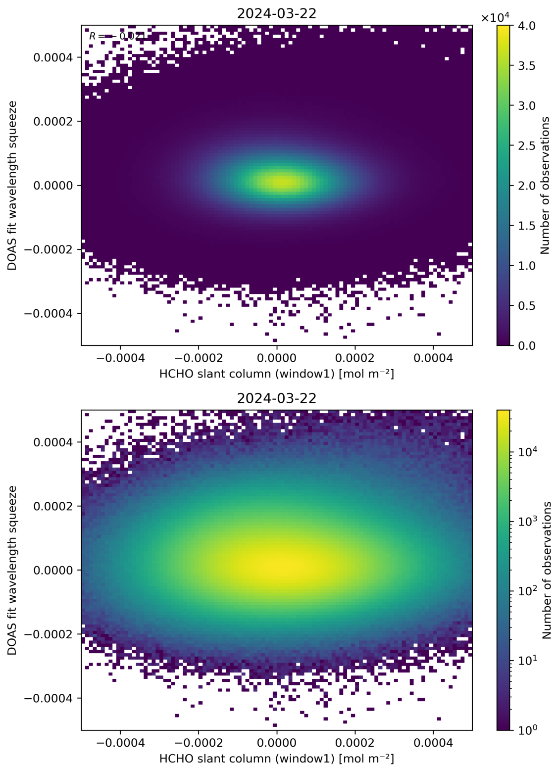
Figure 80: Scatter density plot of “HCHO slant column (window1)” against “DOAS fit wavelength squeeze” for 2024-03-21 to 2024-03-22.
