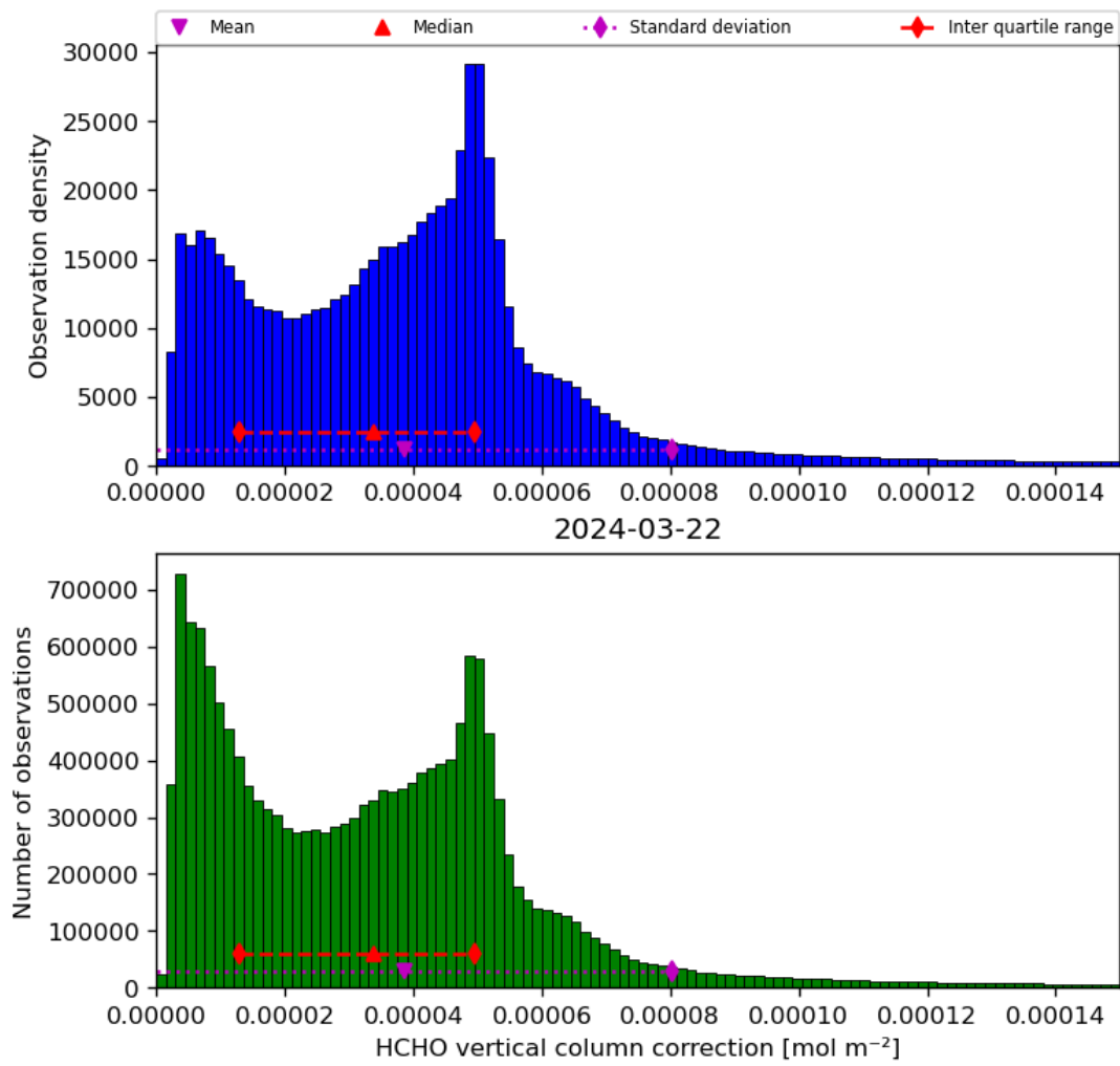
Figure 37: Histogram of “HCHO vertical column correction” for 2024-03-21 to 2024-03-22
