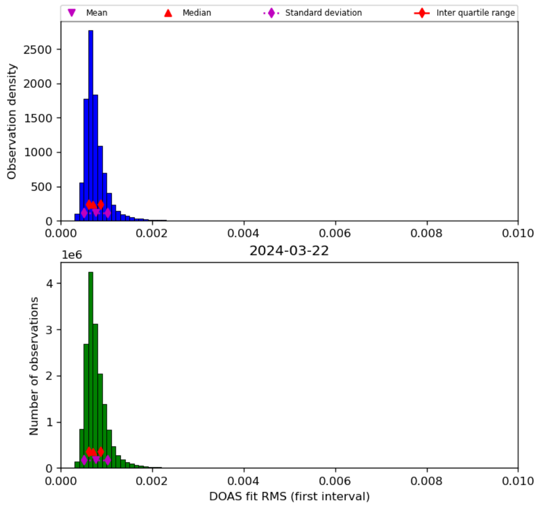
Figure 46: Histogram of “DOAS fit RMS (first interval)” for 2024-03-21 to 2024-03-22
