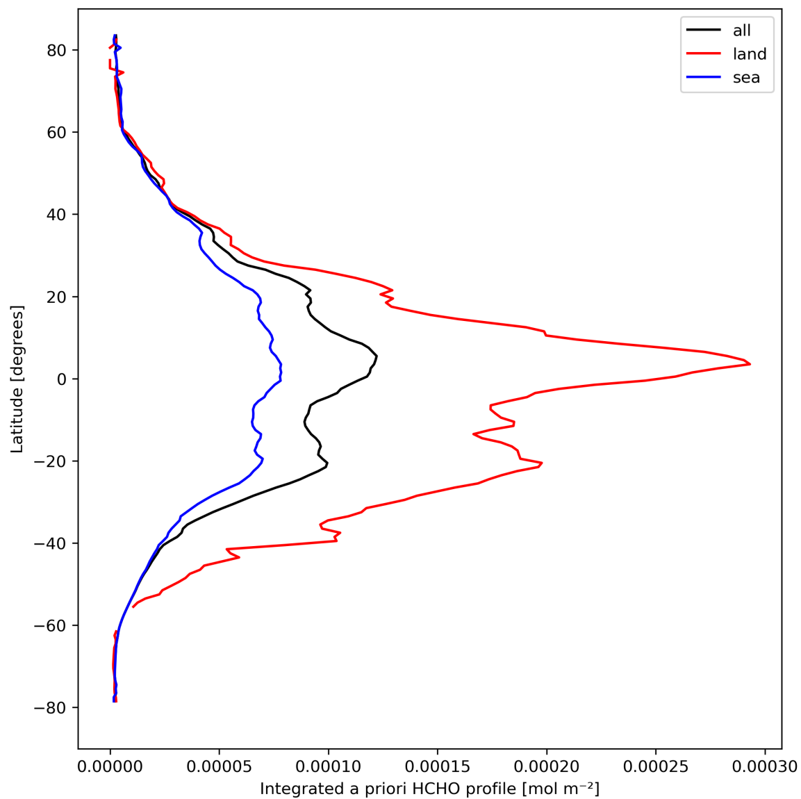
Figure 29: Zonal average of “Integrated a priori HCHO profile” for 2024-03-21 to 2024-03-22.
