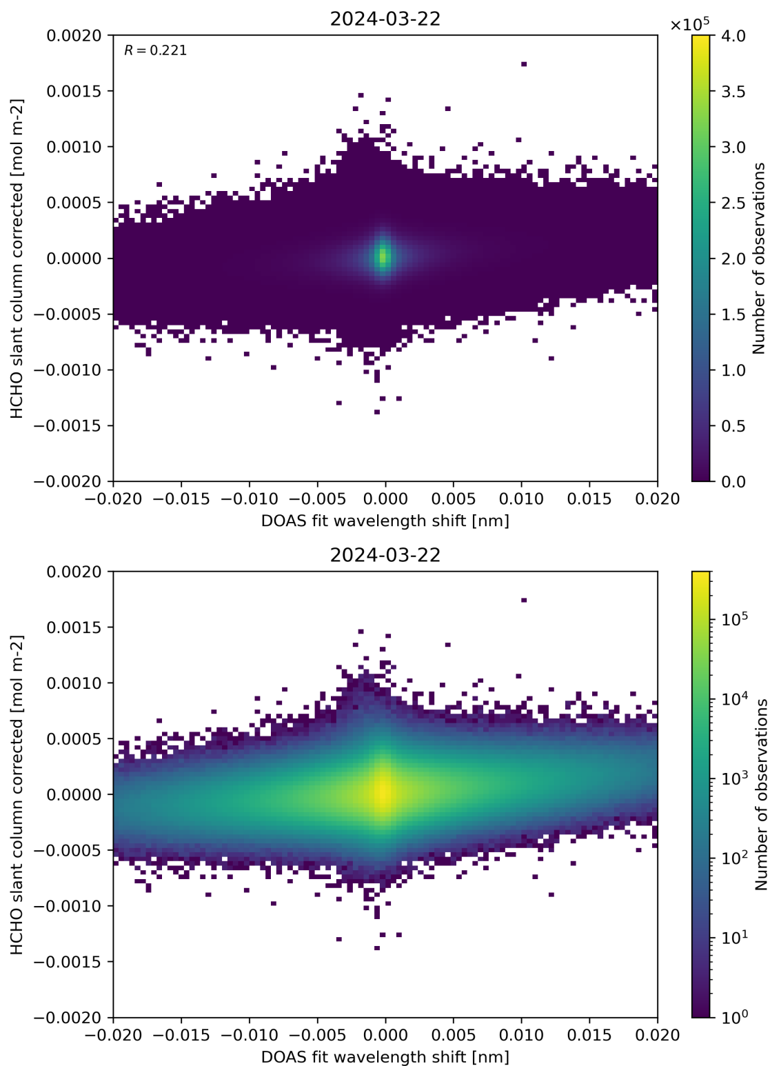
Figure 66: Scatter density plot of “DOAS fit wavelength shift” against “HCHO slant column corrected” for 2024-03-21 to 2024-03-22.
