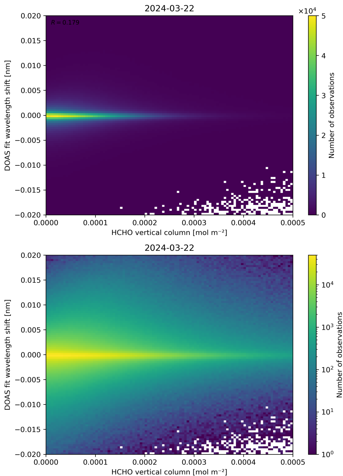
Figure 124: Scatter density plot of “HCHO vertical column” against “DOAS fit wavelength shift” for 2024-03-21 to 2024-03-22.
