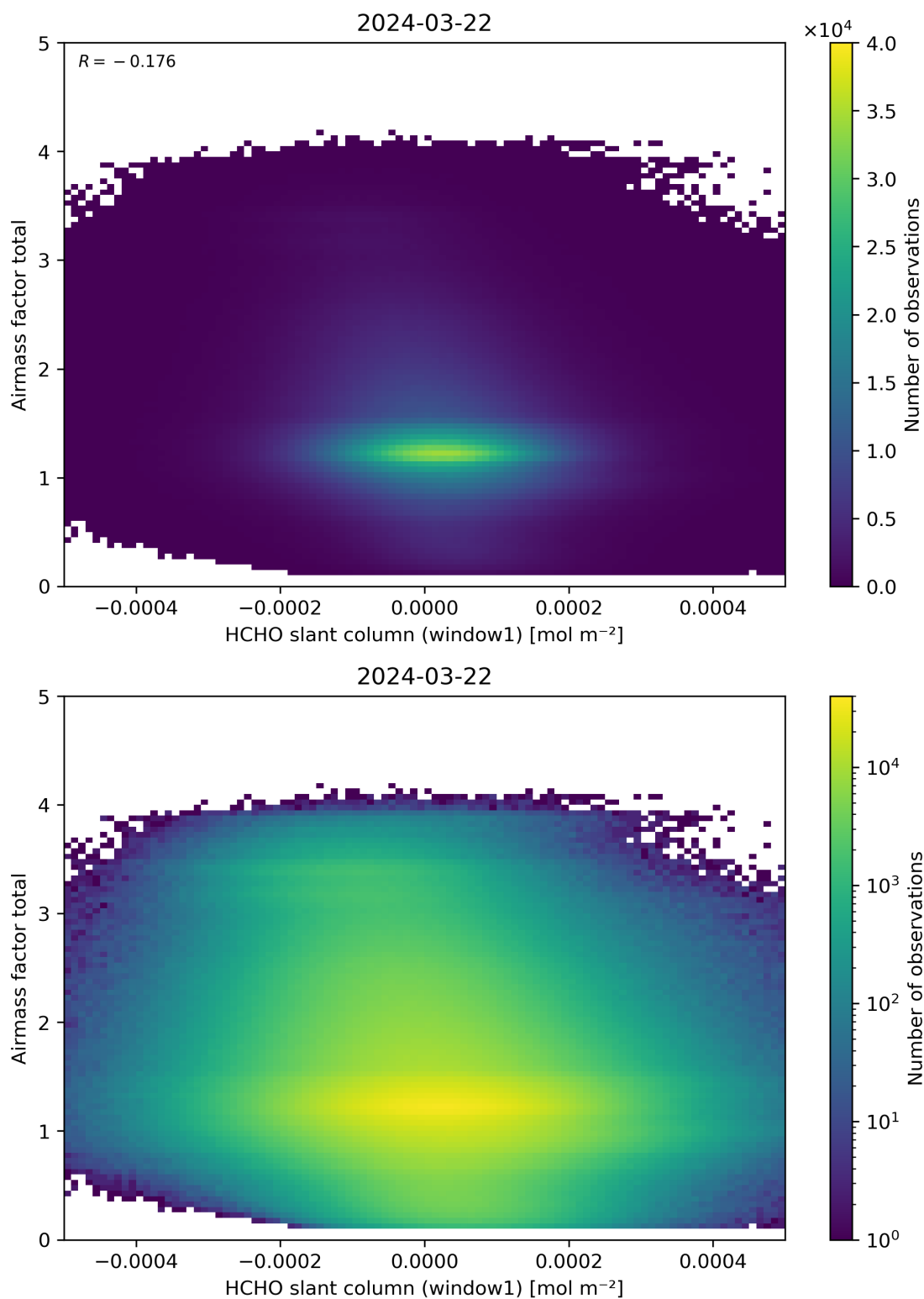
Figure 85: Scatter density plot of “HCHO slant column (window1)” against “Airmass factor total” for 2024-03-21 to 2024-03-22.
