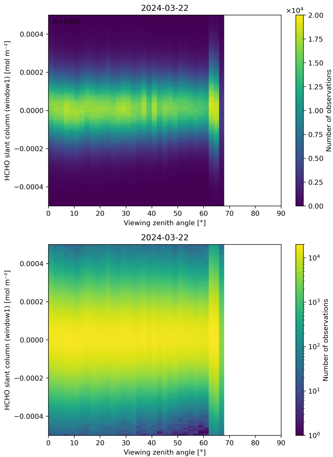
Figure 188: Scatter density plot of “Viewing zenith angle” against “HCHO slant column (window1)” for 2024-03-21 to 2024-03-22.
