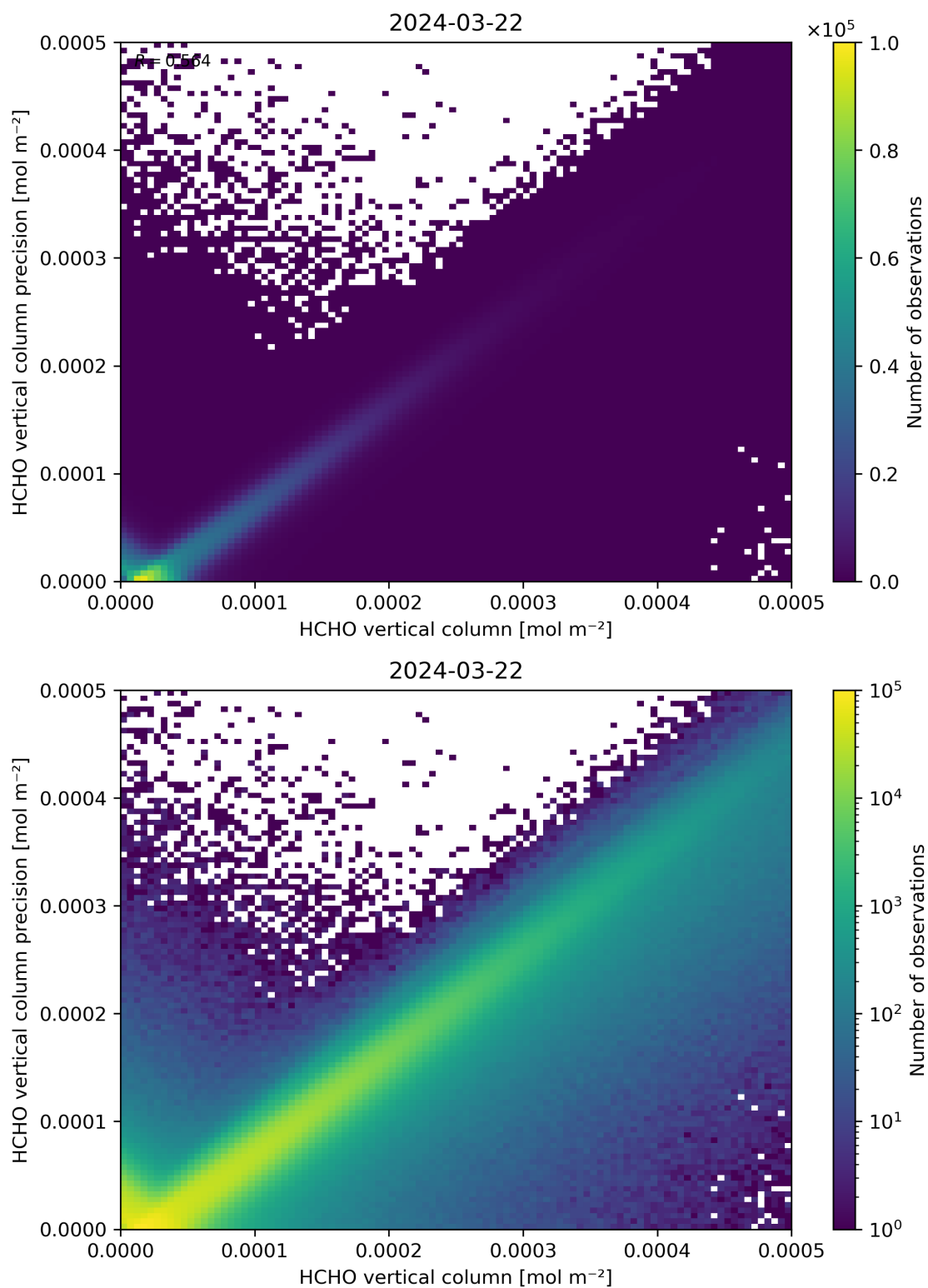
Figure 134: Scatter density plot of “HCHO vertical column” against “HCHO vertical column precision” for 2024-03-21 to 2024-03-22.
