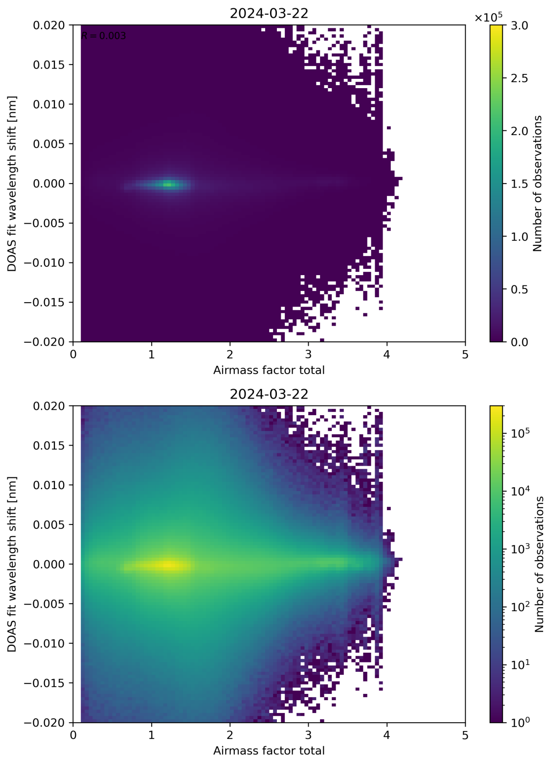
Figure 98: Scatter density plot of “Airmass factor total” against “DOAS fit wavelength shift” for 2024-03-21 to 2024-03-22.
