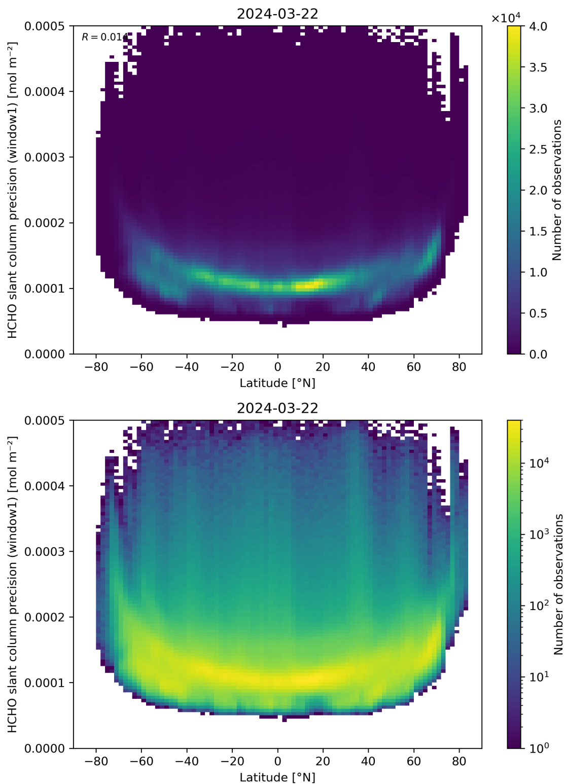
Figure 160: Scatter density plot of “Latitude” against “HCHO slant column precision (window1)” for 2024-03-21 to 2024-03-22.
