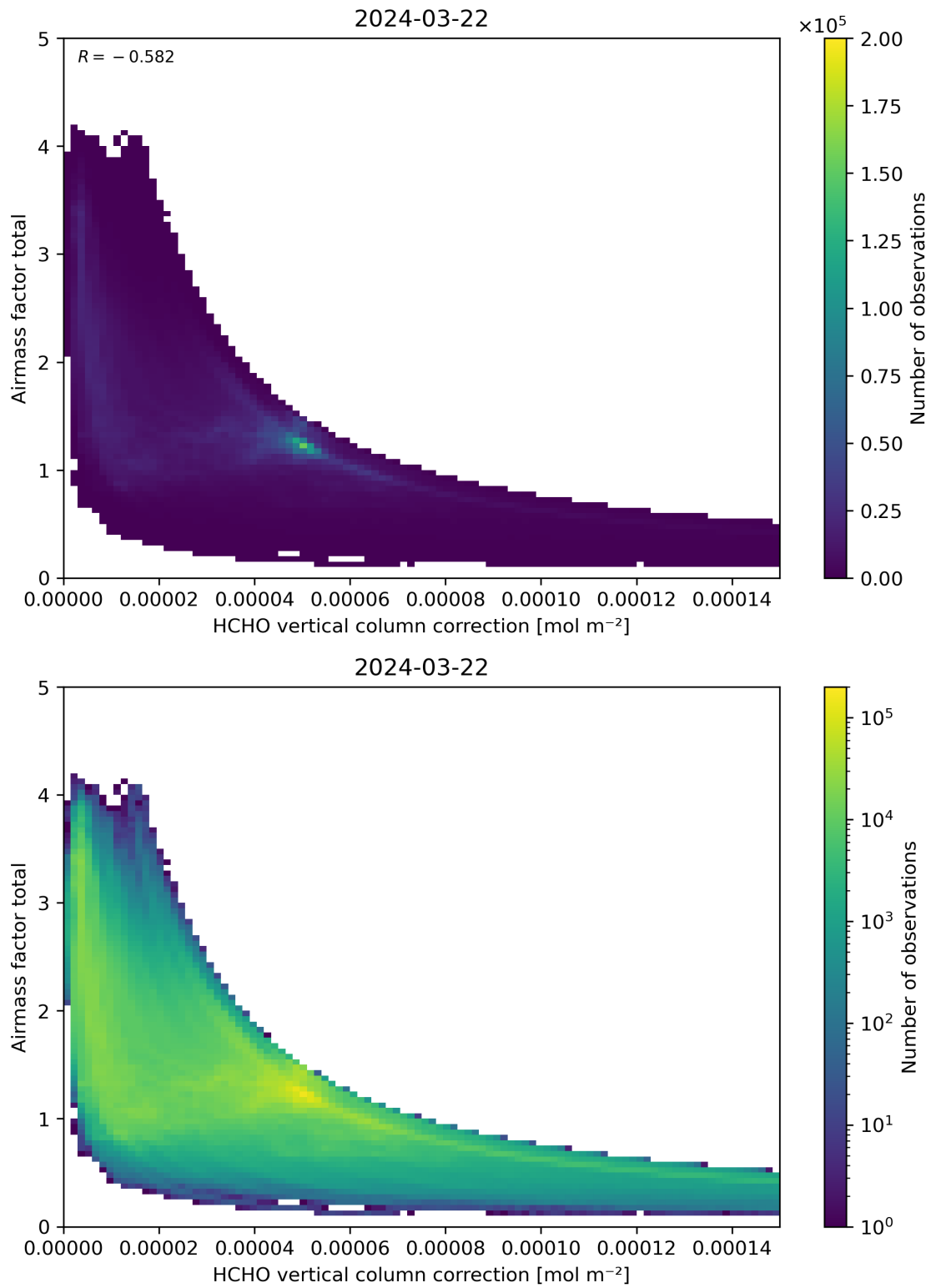
Figure 120: Scatter density plot of “HCHO vertical column correction” against “Airmass factor total” for 2024-03-21 to 2024-03-22.
