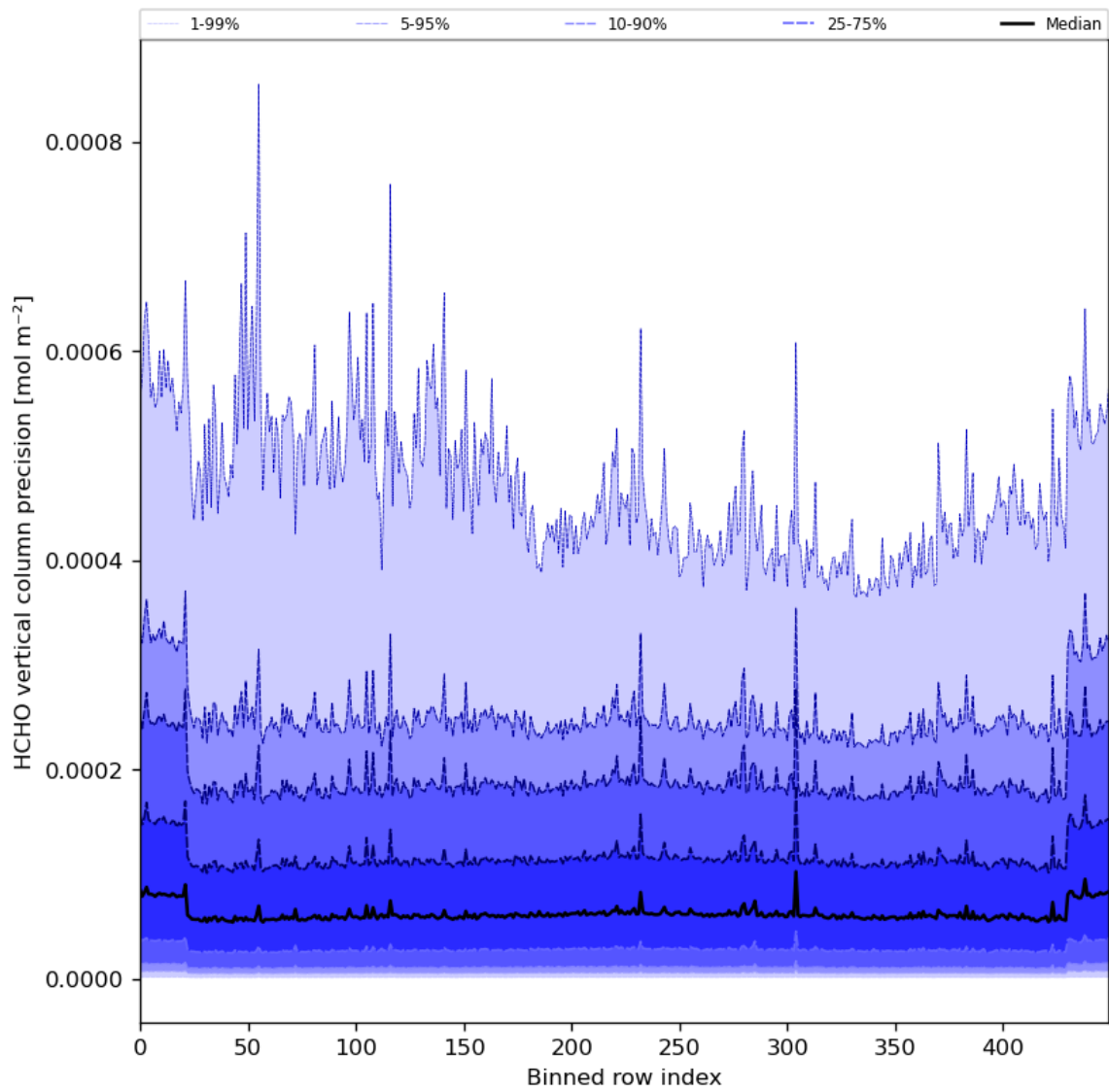
Figure 50: Along track statistics of "HCHO vertical column precision" for 2024-03-21 to 2024-03-22
