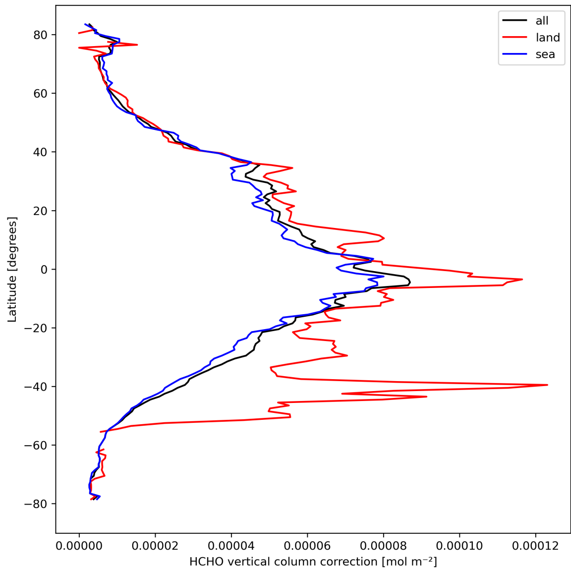
Figure 23: Zonal average of “HCHO vertical column correction” for 2024-03-21 to 2024-03-22.
