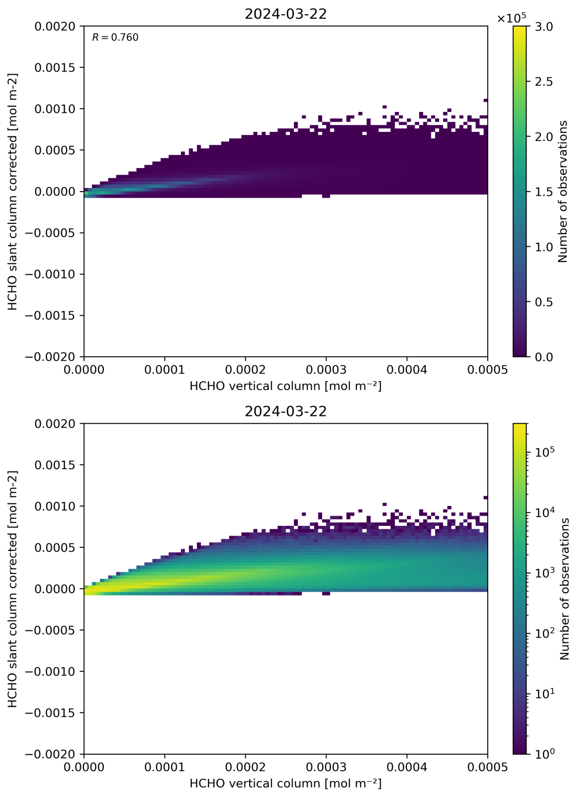
Figure 127: Scatter density plot of “HCHO vertical column” against “HCHO slant column corrected” for 2024-03-21 to 2024-03-22.
