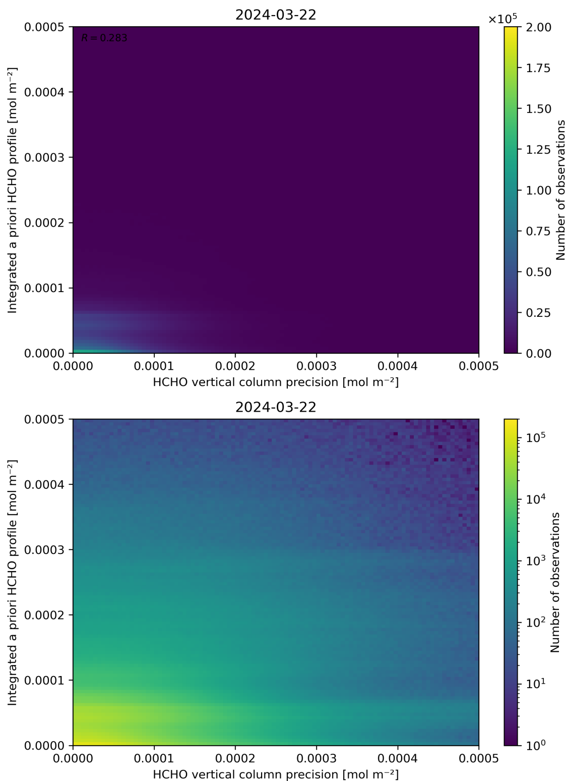
Figure 147: Scatter density plot of “HCHO vertical column precision” against “Integrated a priori HCHO profile” for 2024-03-21 to 2024-03-22.
