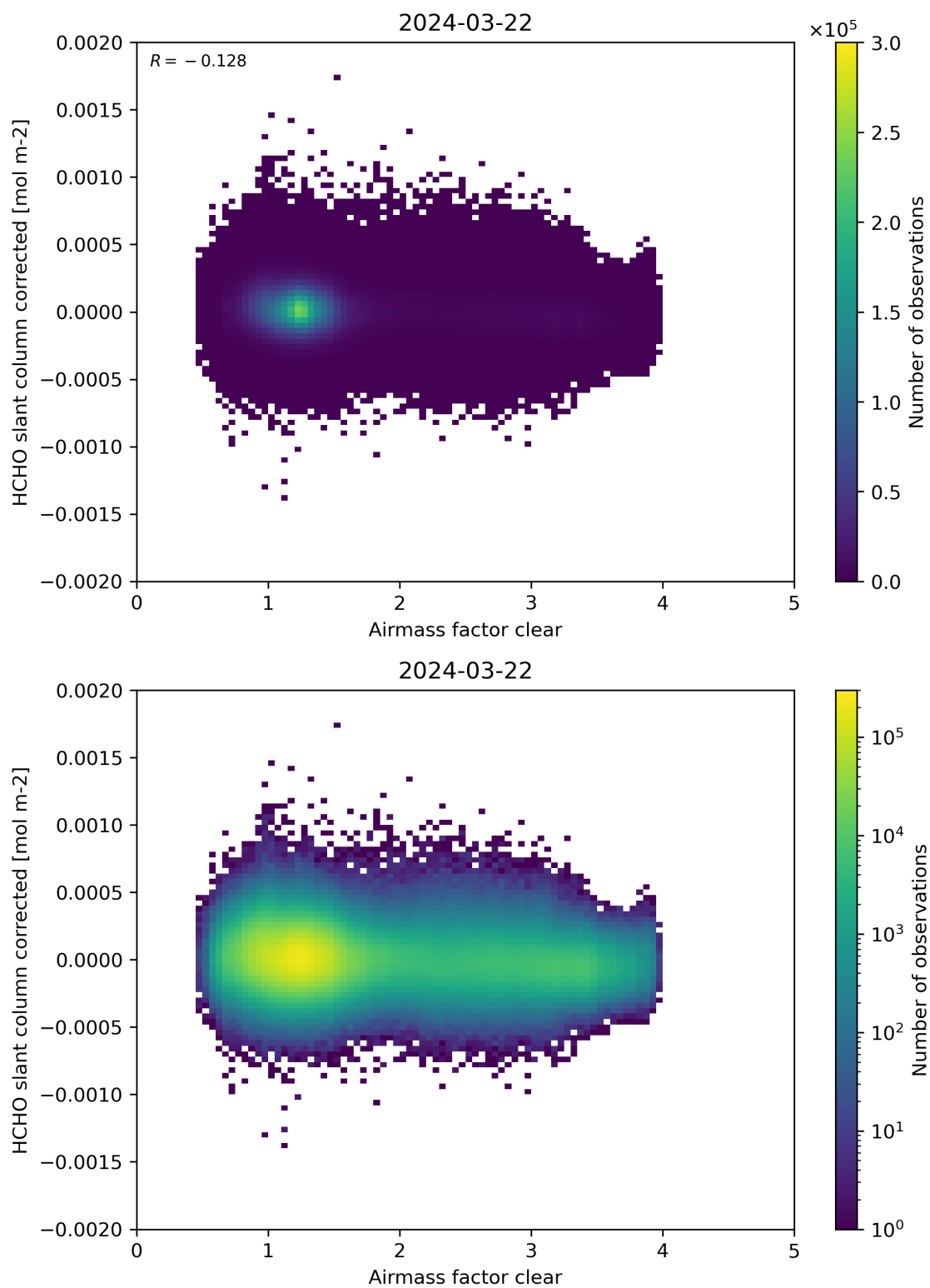
Figure 74: Scatter density plot of “Airmass factor clear” against “HCHO slant column corrected” for 2024-03-21 to 2024-03-22.
