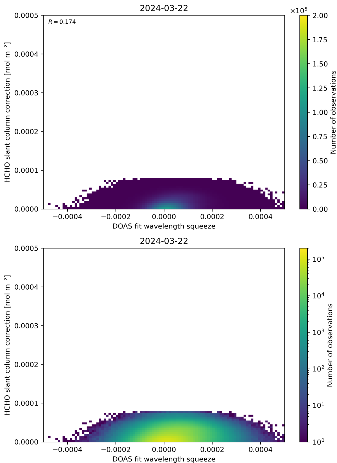
Figure 70: Scatter density plot of “DOAS fit wavelength squeeze” against “HCHO slant column correction” for 2024-03-21 to 2024-03-22.
