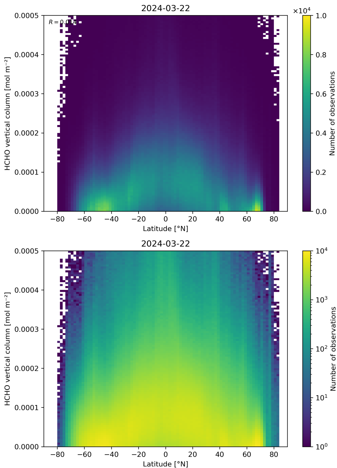
Figure 163: Scatter density plot of “Latitude” against “HCHO vertical column” for 2024-03-21 to 2024-03-22.
