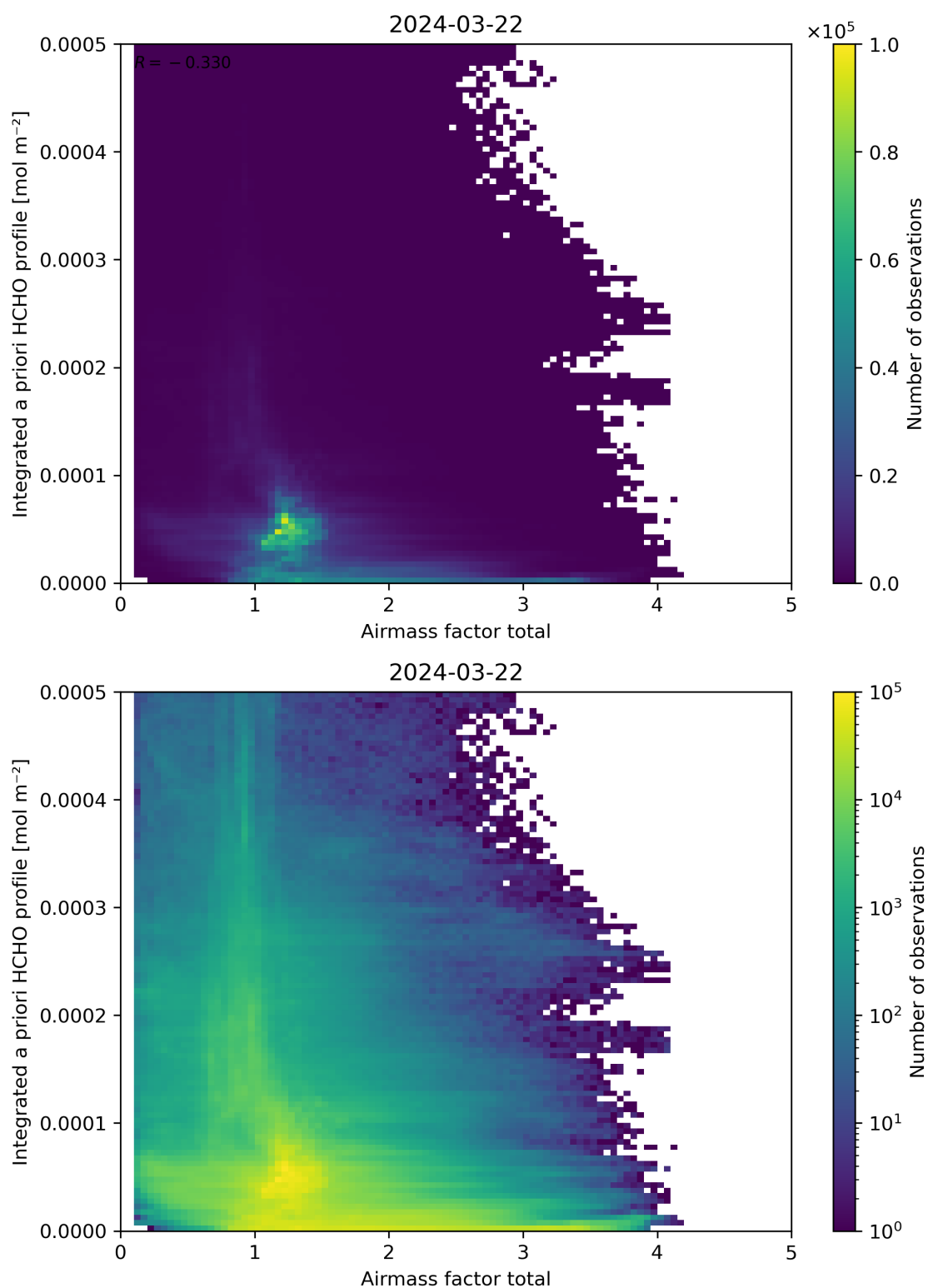
Figure 104: Scatter density plot of “Air mass factor total” against “Integrated a priori HCHO profile” for 2024-03-21 to 2024-03-22.
