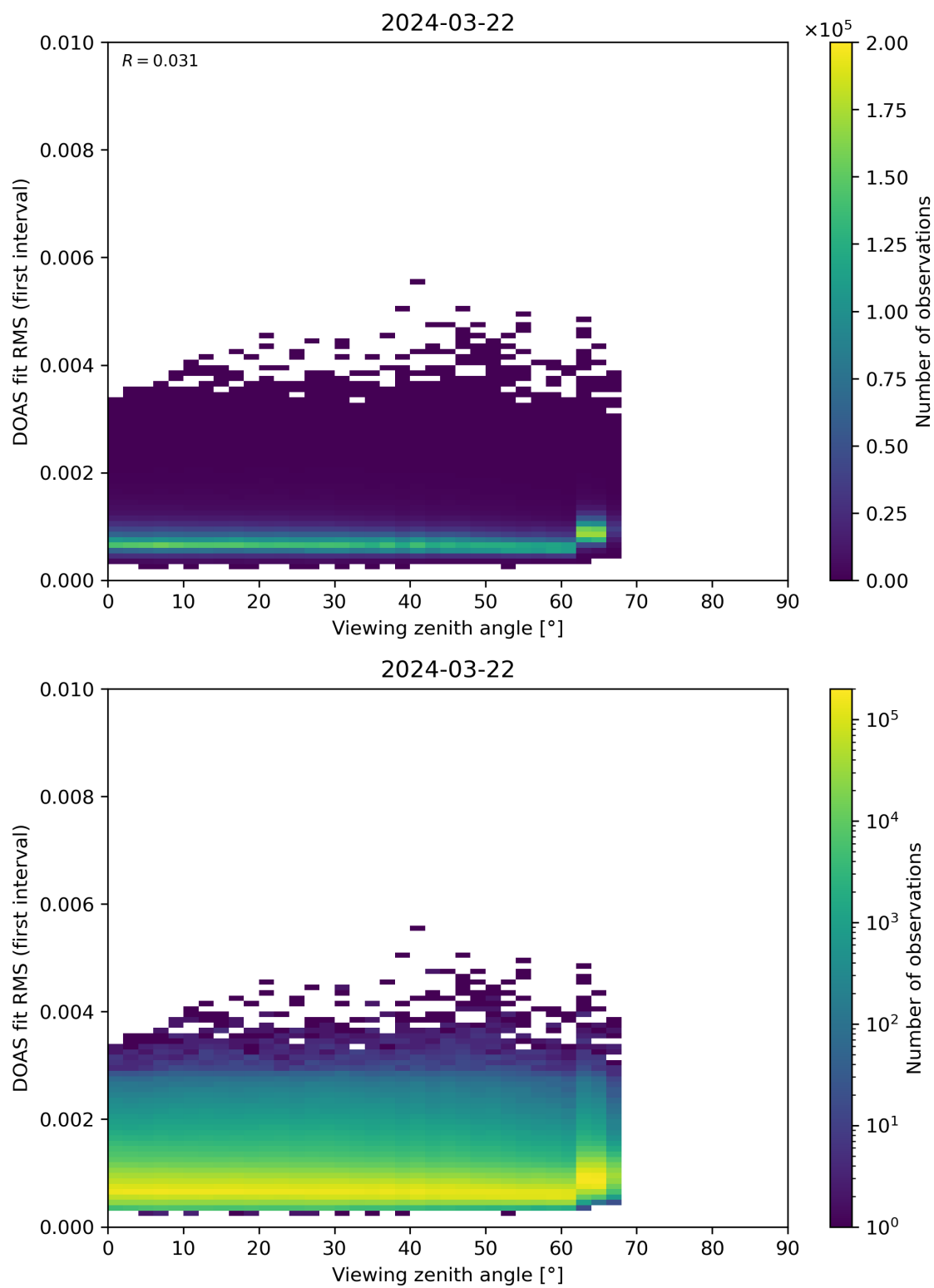
Figure 182: Scatter density plot of “Viewing zenith angle” against “DOAS fit RMS (first interval)” for 2024-03-21 to 2024-03-22.
