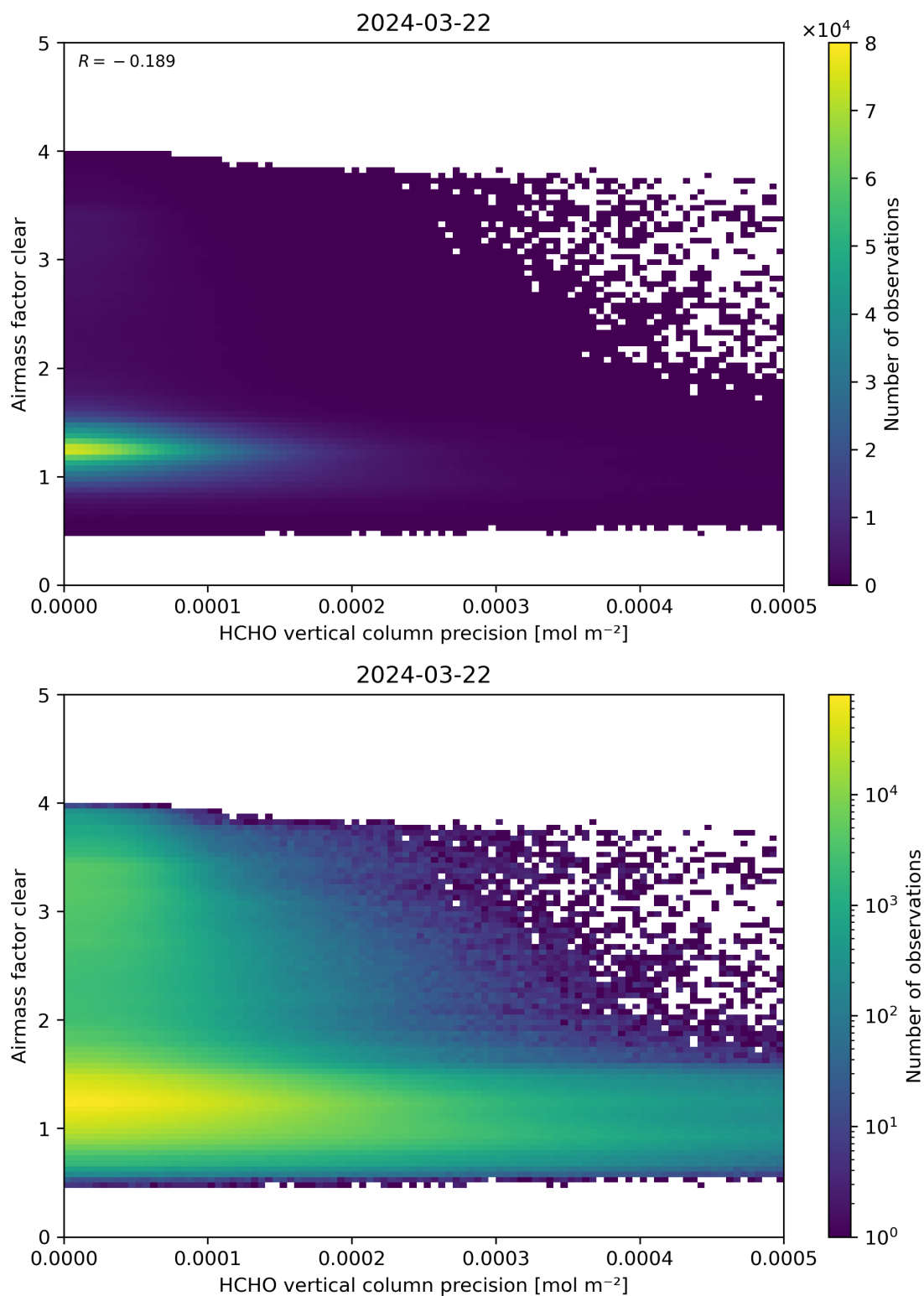
Figure 139: Scatter density plot of “HCHO vertical column precision” against “Airmass factor clear” for 2024-03-21 to 2024-03-22.
