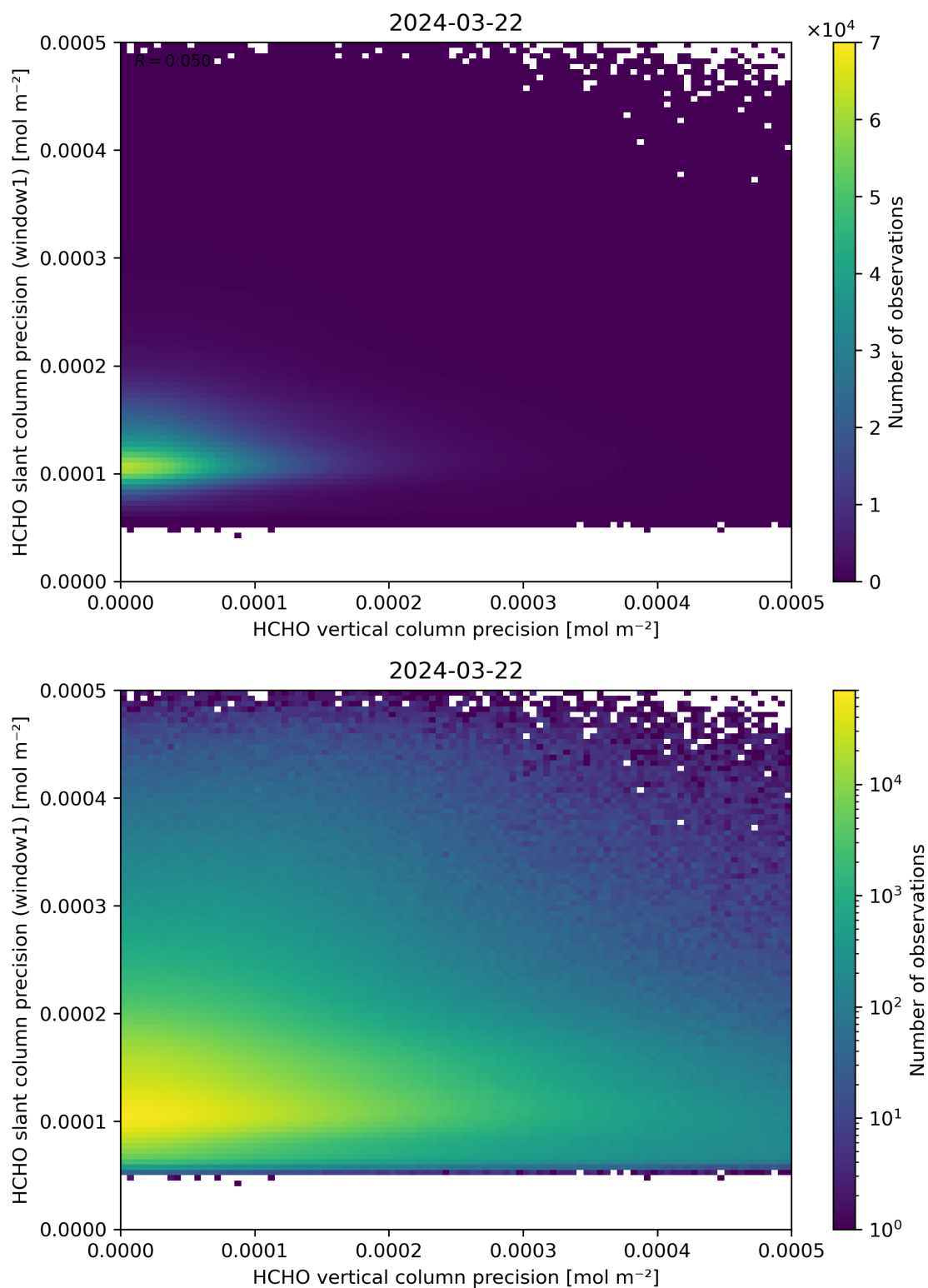
Figure 143: Scatter density plot of “HCHO vertical column precision” against “HCHO slant column precision (window1)” for 2024-03-21 to 2024-03-22.
