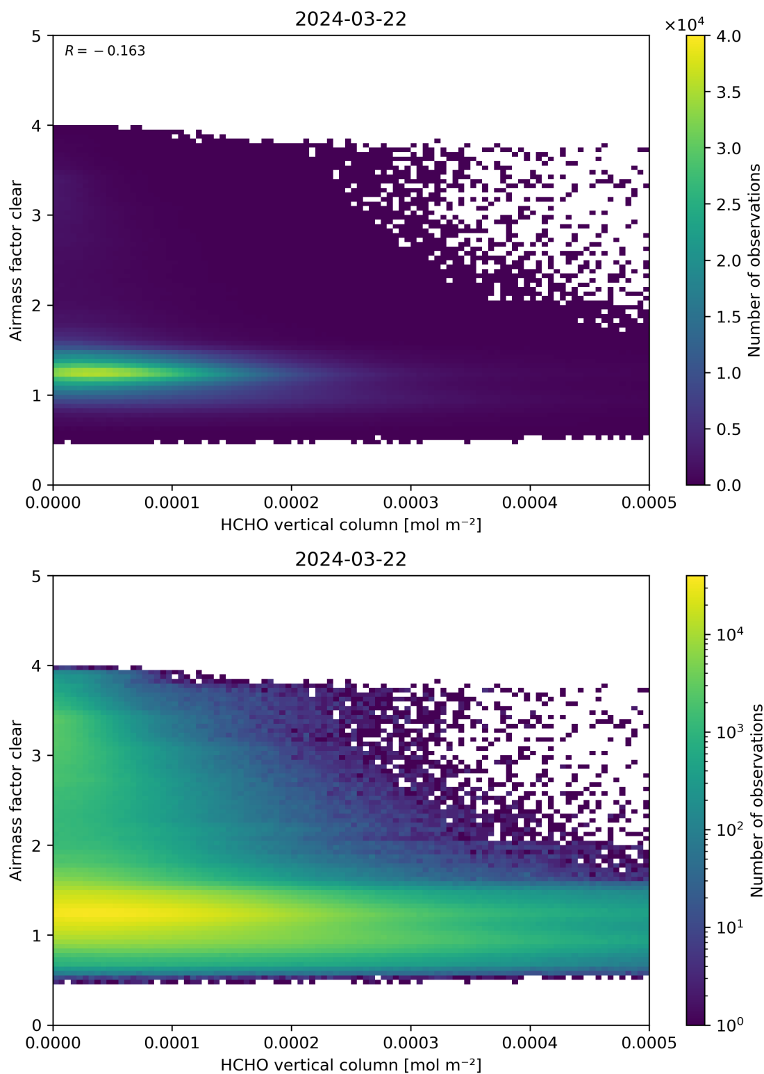
Figure 126: Scatter density plot of “HCHO vertical column” against “Airmass factor clear” for 2024-03-21 to 2024-03-22.
