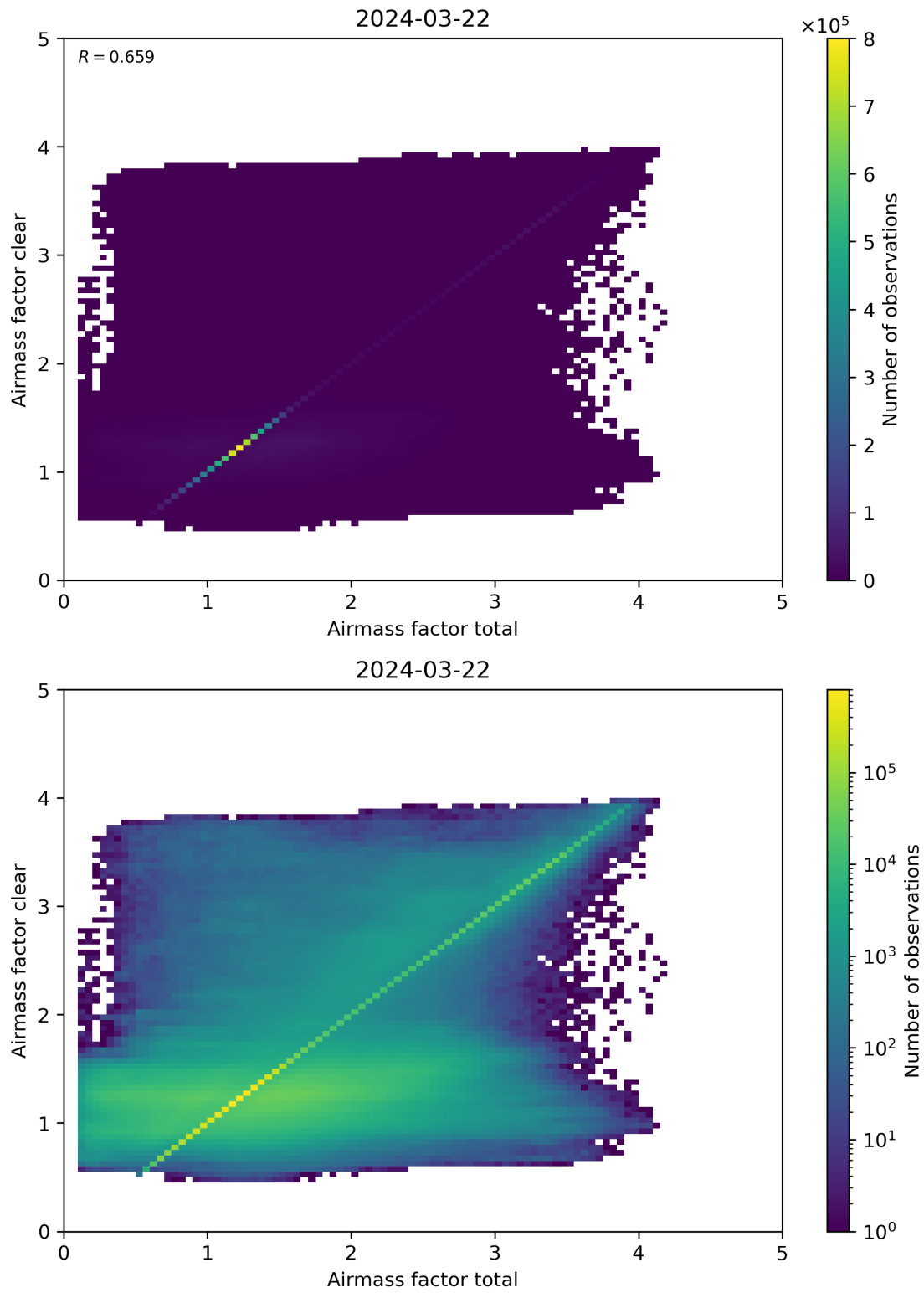
Figure 100: Scatter density plot of “Airmass factor total” against “Airmass factor clear” for 2024-03-21 to 2024-03-22.
