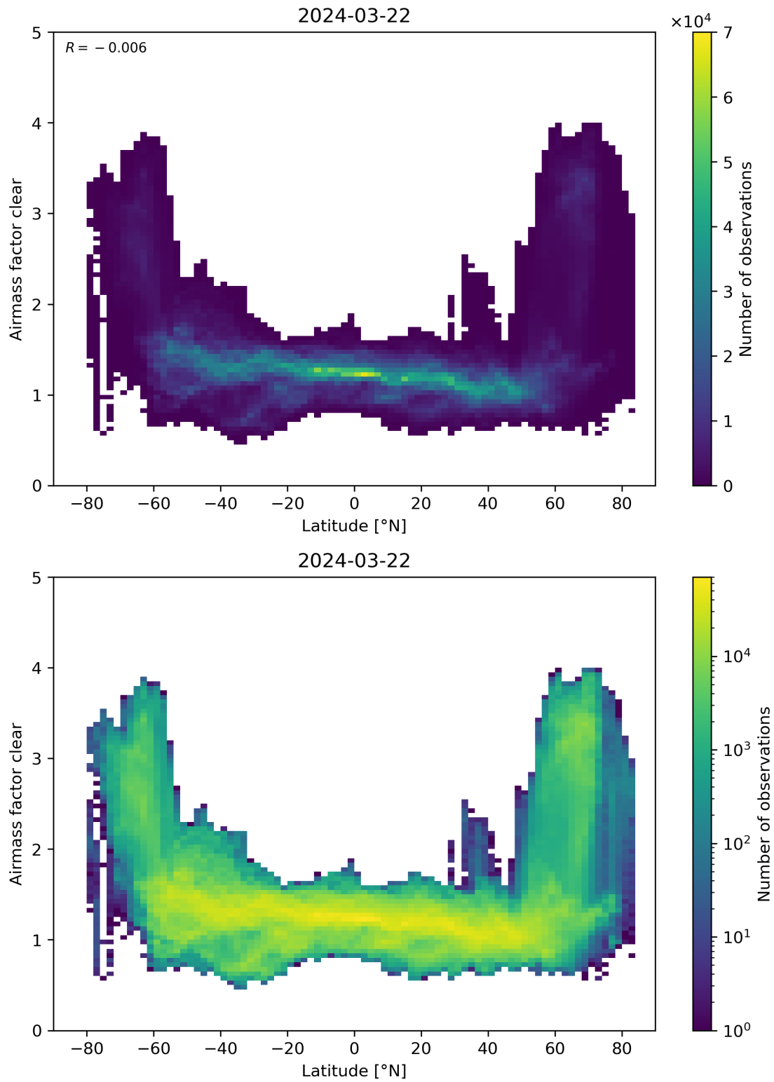
Figure 156: Scatter density plot of “Latitude” against “Airmass factor clear” for 2024-03-21 to 2024-03-22.
