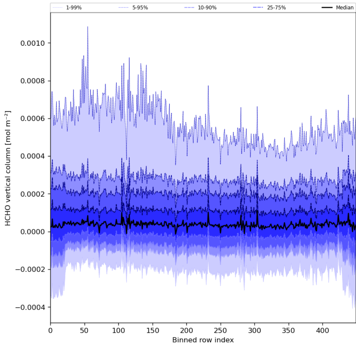
Figure 49: Along track statistics of “HCHO vertical column” for 2024-03-21 to 2024-03-22
