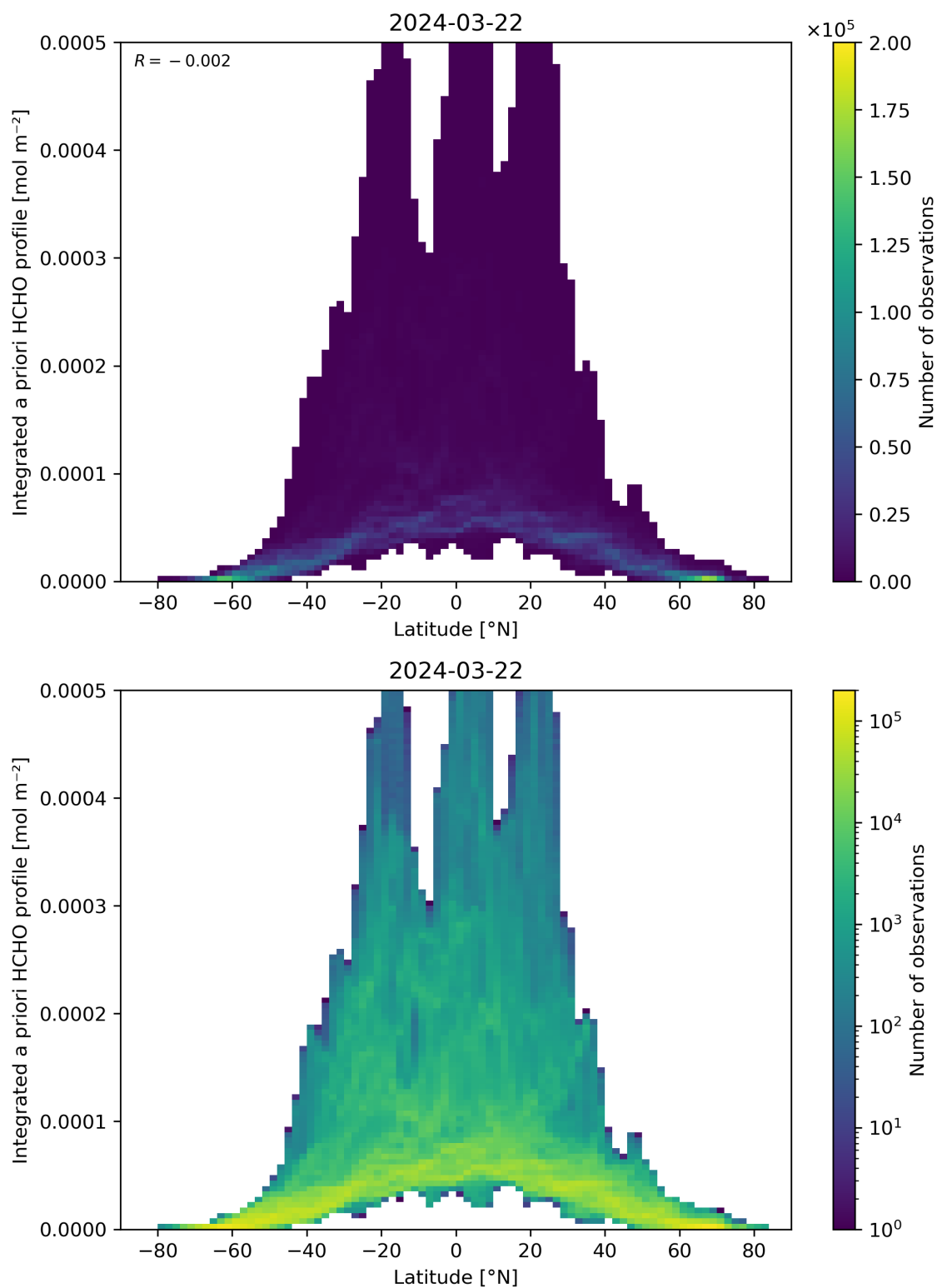
Figure 166: Scatter density plot of “Latitude” against “Integrated a priori HCHO profile” for 2024-03-21 to 2024-03-22.
