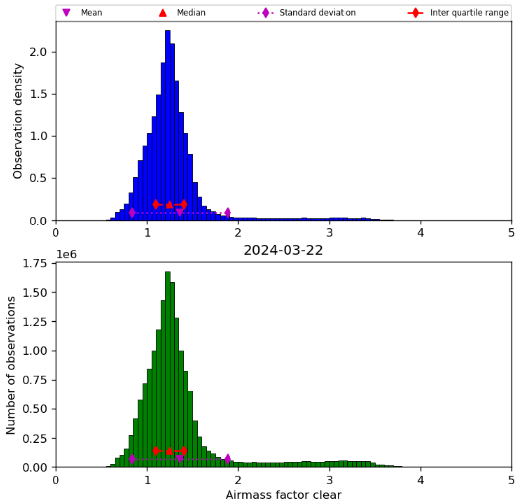
Figure 42: Histogram of “Airmass factor clear” for 2024-03-21 to 2024-03-22
