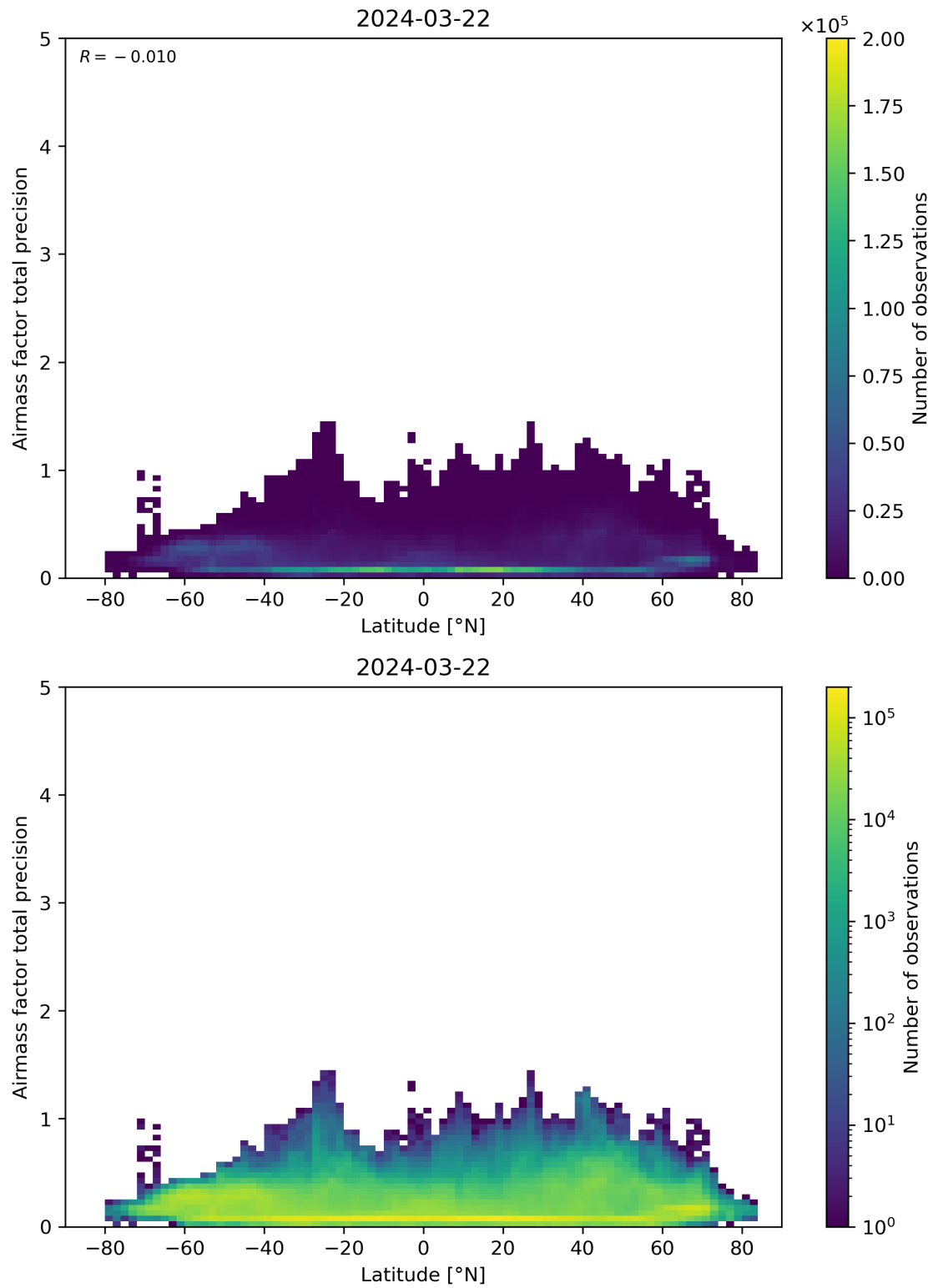
Figure 162: Scatter density plot of “Latitude” against “Airmass factor total precision” for 2024-03-21 to 2024-03-22.
