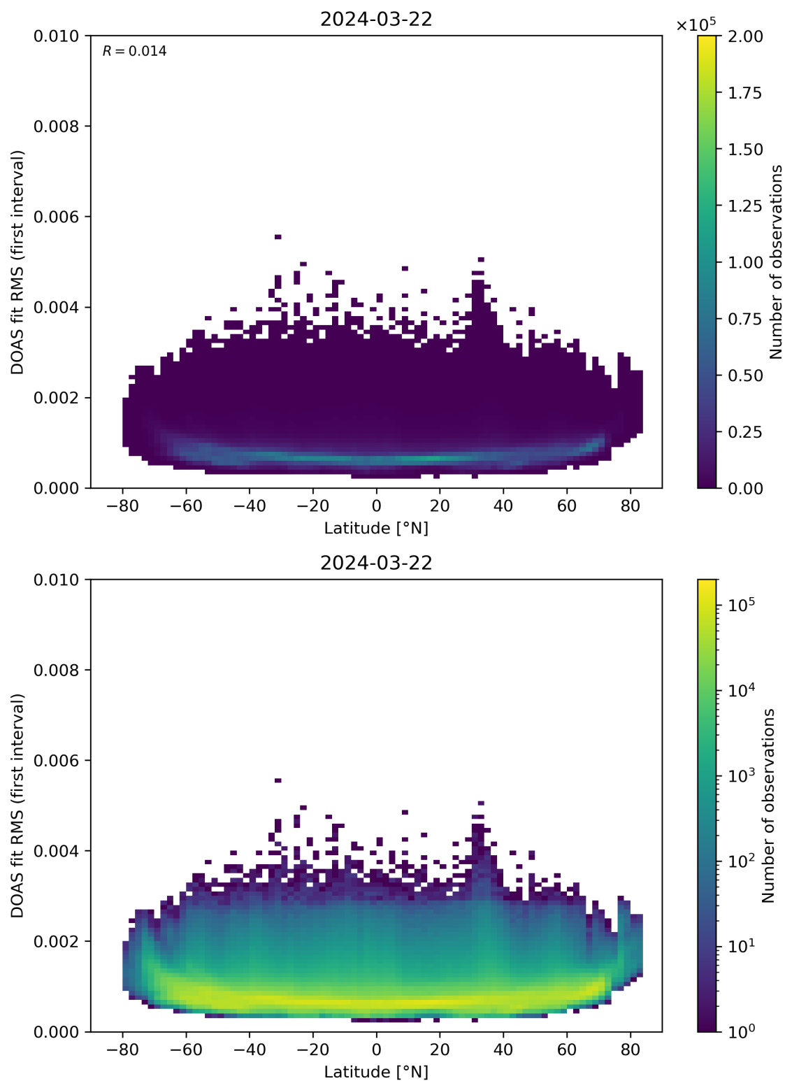
Figure 153: Scatter density plot of “Latitude” against “DOAS fit RMS (first interval)” for 2024-03-21 to 2024-03-22.
