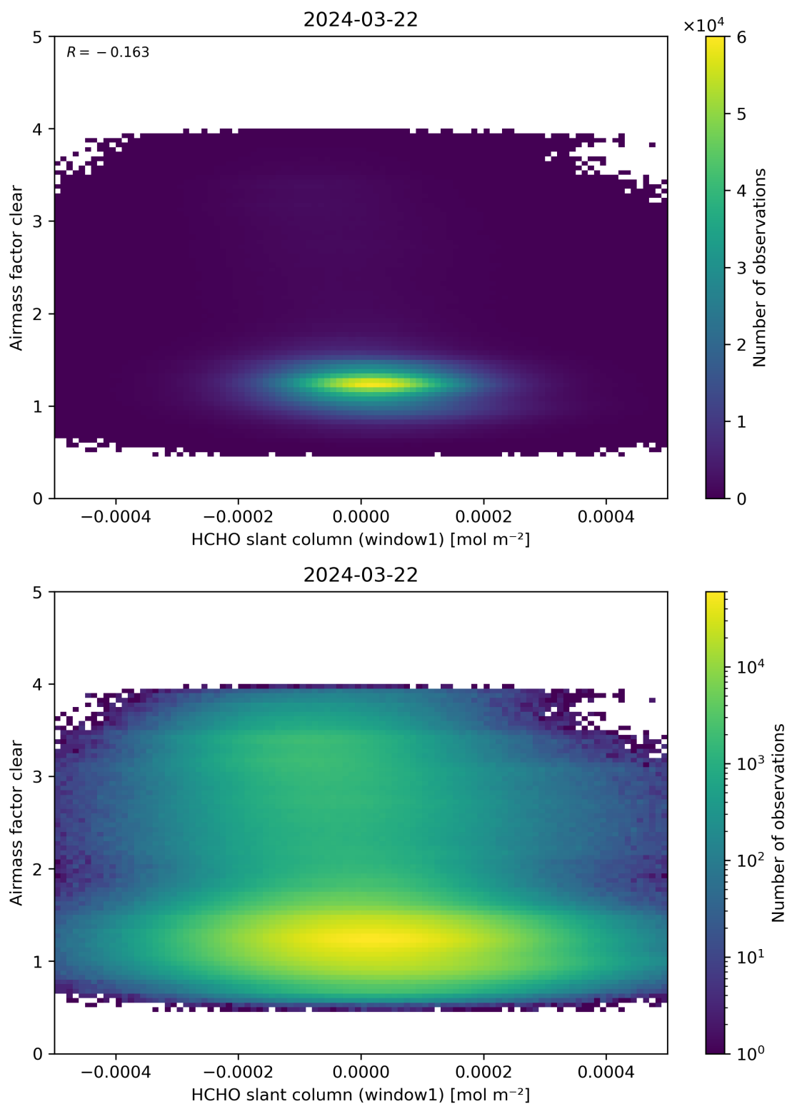
Figure 81: Scatter density plot of “HCHO slant column (window1)” against “Airmass factor clear” for 2024-03-21 to 2024-03-22.
