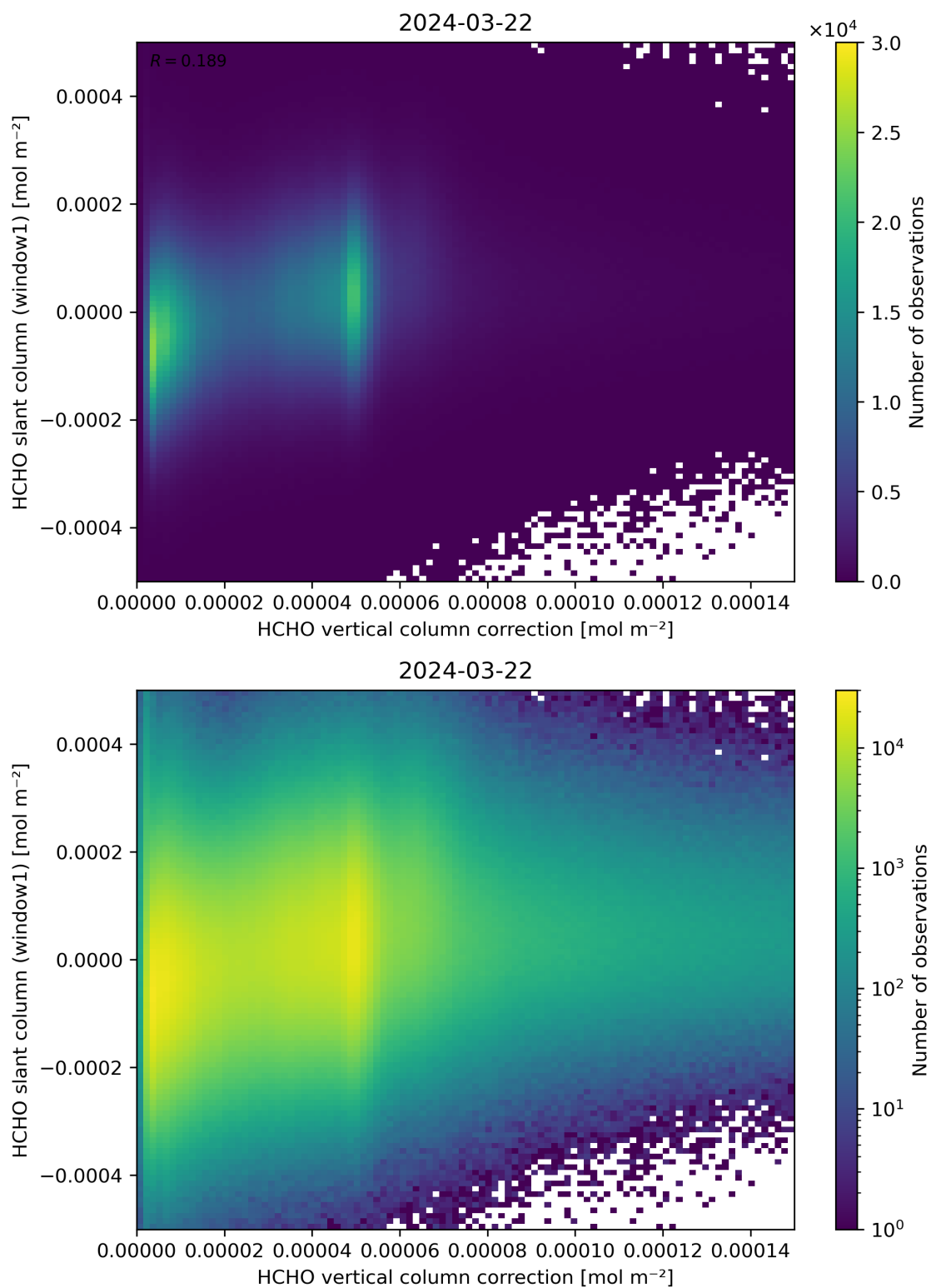
Figure 118: Scatter density plot of “HCHO vertical column correction” against “HCHO slant column (window1)” for 2024-03-21 to 2024-03-22.
