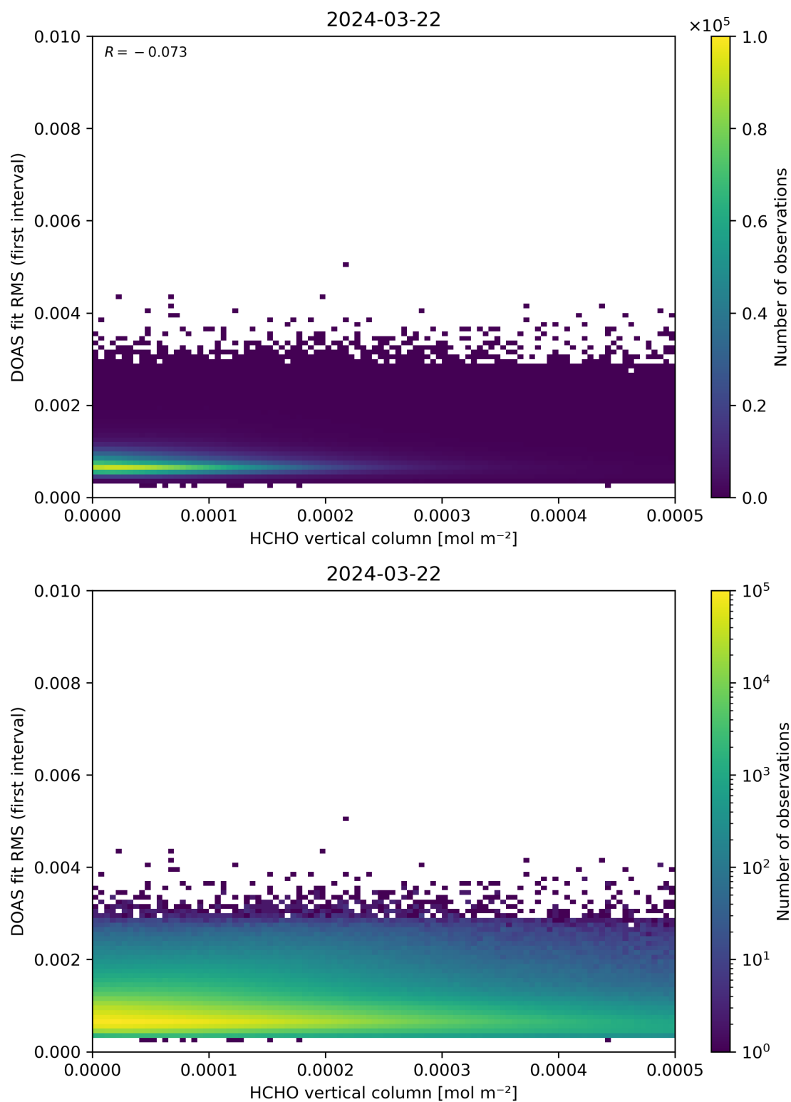
Figure 123: Scatter density plot of “HCHO vertical column” against “DOAS fit RMS (first interval)” for 2024-03-21 to 2024-03-22.
