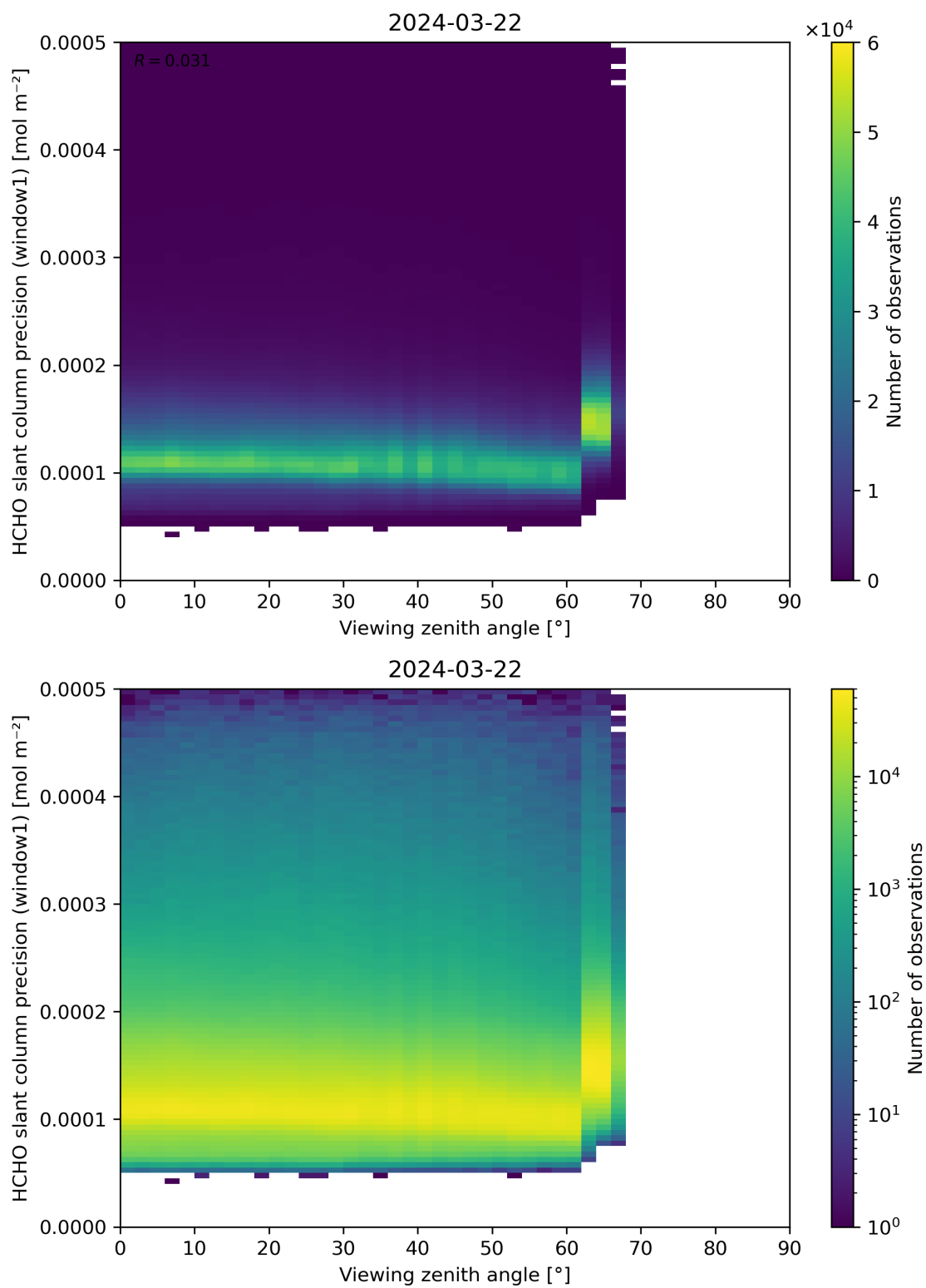
Figure 189: Scatter density plot of “Viewing zenith angle” against “HCHO slant column precision (window1)” for 2024-03-21 to 2024-03-22.
