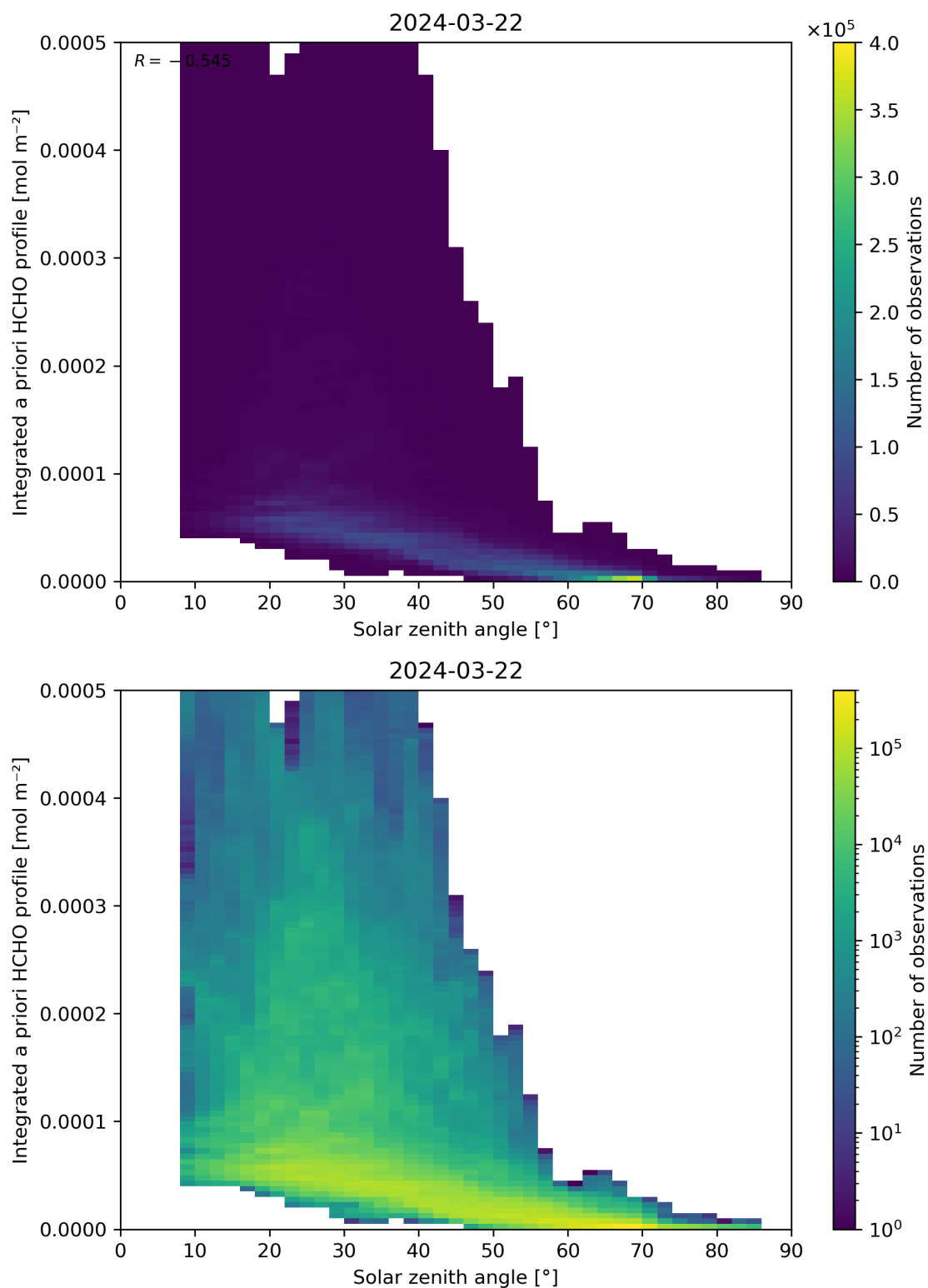
Figure 180: Scatter density plot of “Solar zenith angle” against “Integrated a priori HCHO profile” for 2024-03-21 to 2024-03-22.
