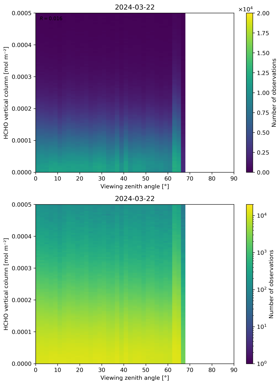
Figure 192: Scatter density plot of “Viewing zenith angle” against “HCHO vertical column” for 2024-03-21 to 2024-03-22.
