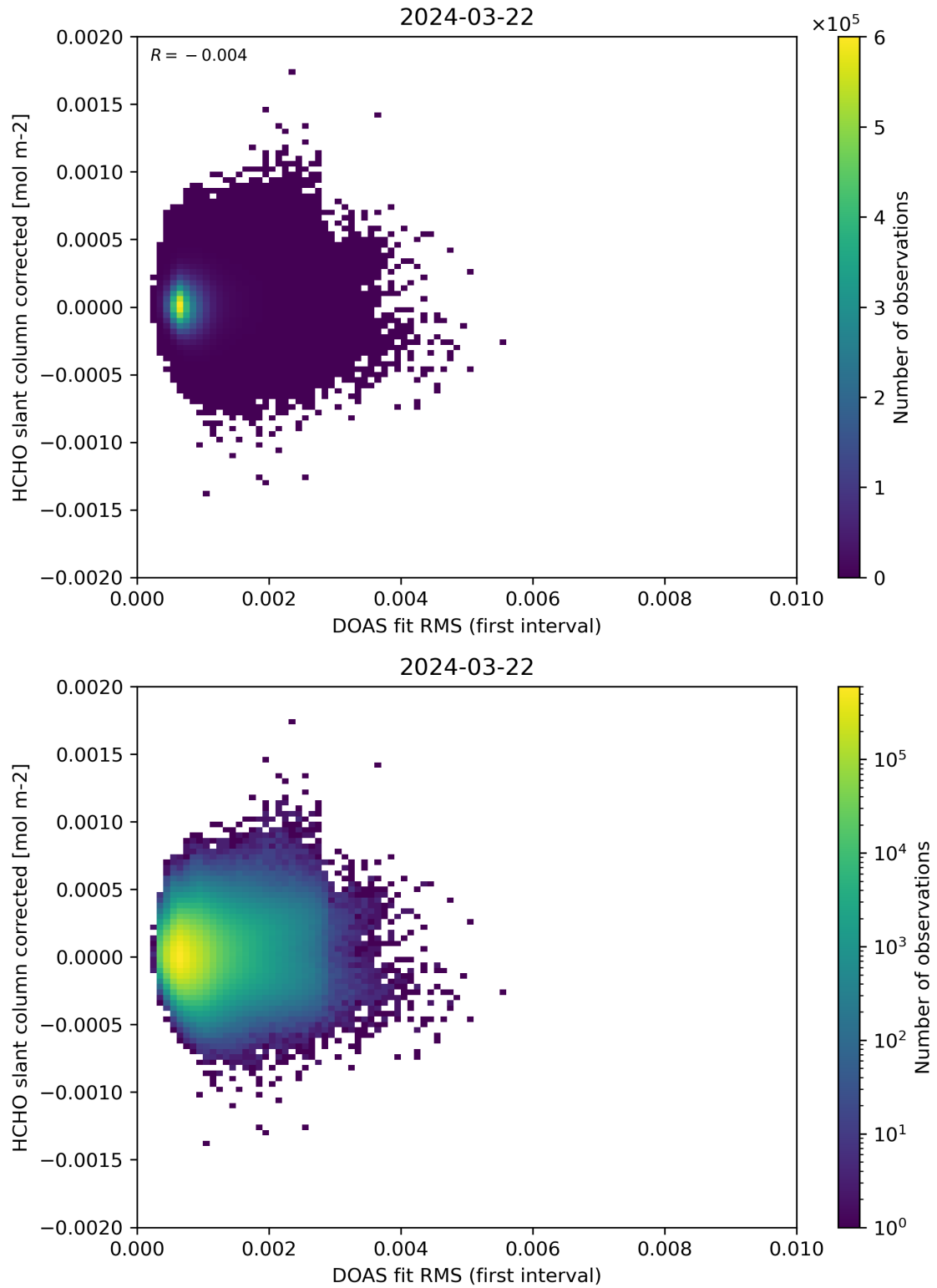
Figure 62: Scatter density plot of “DOAS fit RMS (first interval)” against “HCHO slant column corrected” for 2024-03-21 to 2024-03-22.
