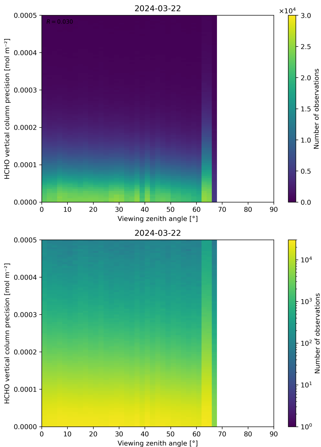
Figure 194: Scatter density plot of “Viewing zenith angle” against “HCHO vertical column precision” for 2024-03-21 to 2024-03-22.
