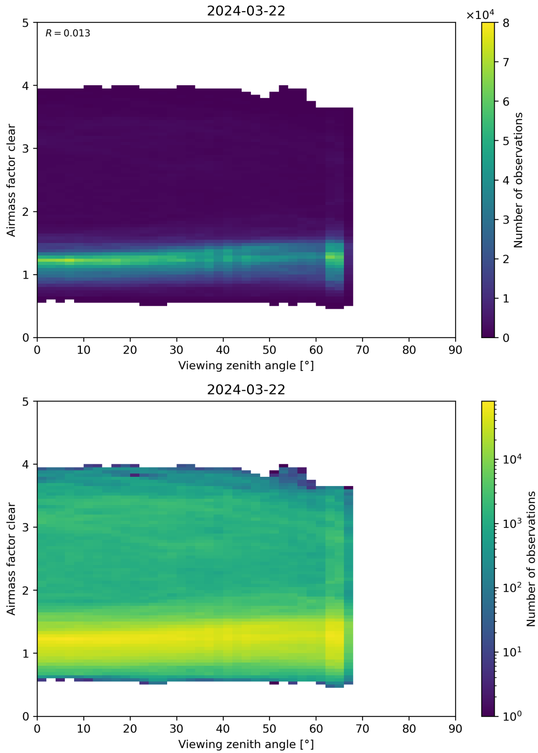
Figure 185: Scatter density plot of “Viewing zenith angle” against “Airmass factor clear” for 2024-03-21 to 2024-03-22.
