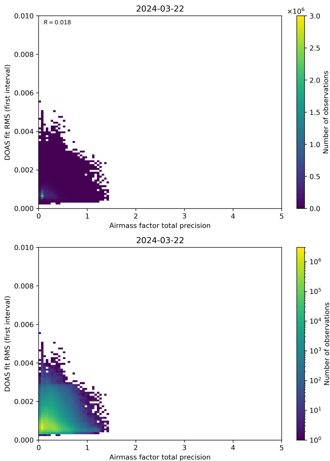
Figure 105: Scatter density plot of “Airmass factor total precision” against “DOAS fit RMS (first interval)” for 2024-03-21 to 2024-03-22.
