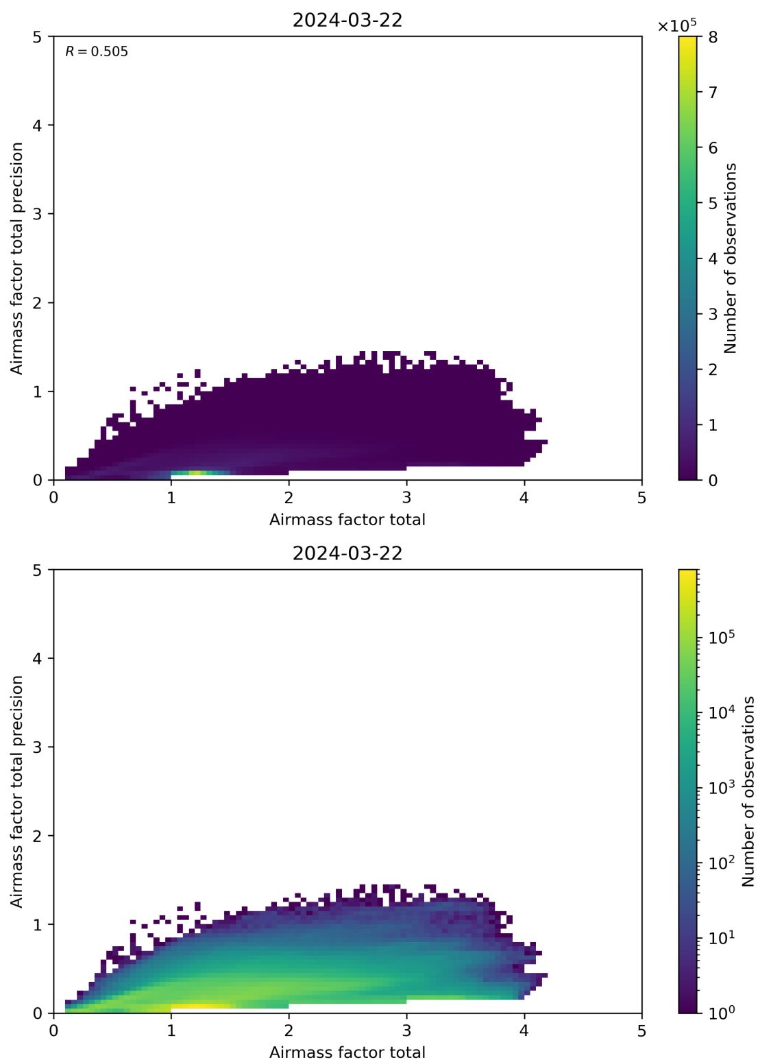
Figure 103: Scatter density plot of “Airmass factor total” against “Airmass factor total precision” for 2024-03-21 to 2024-03-22.
