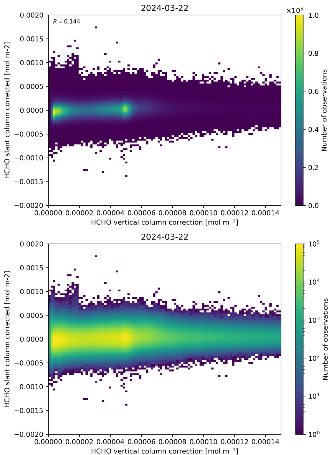
Figure 116: Scatter density plot of “HCHO vertical column correction” against “HCHO slant column corrected” for 2024-03-21 to 2024-03-22.
