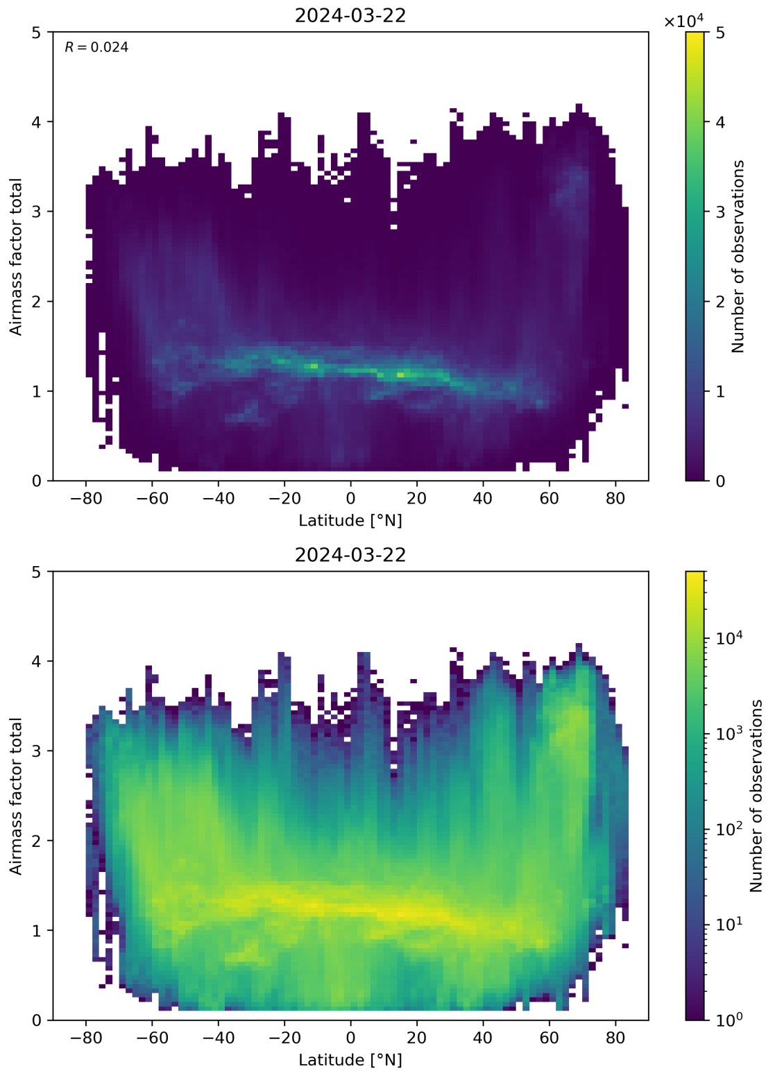
Figure 161: Scatter density plot of “Latitude” against “Airmass factor total” for 2024-03-21 to 2024-03-22.
