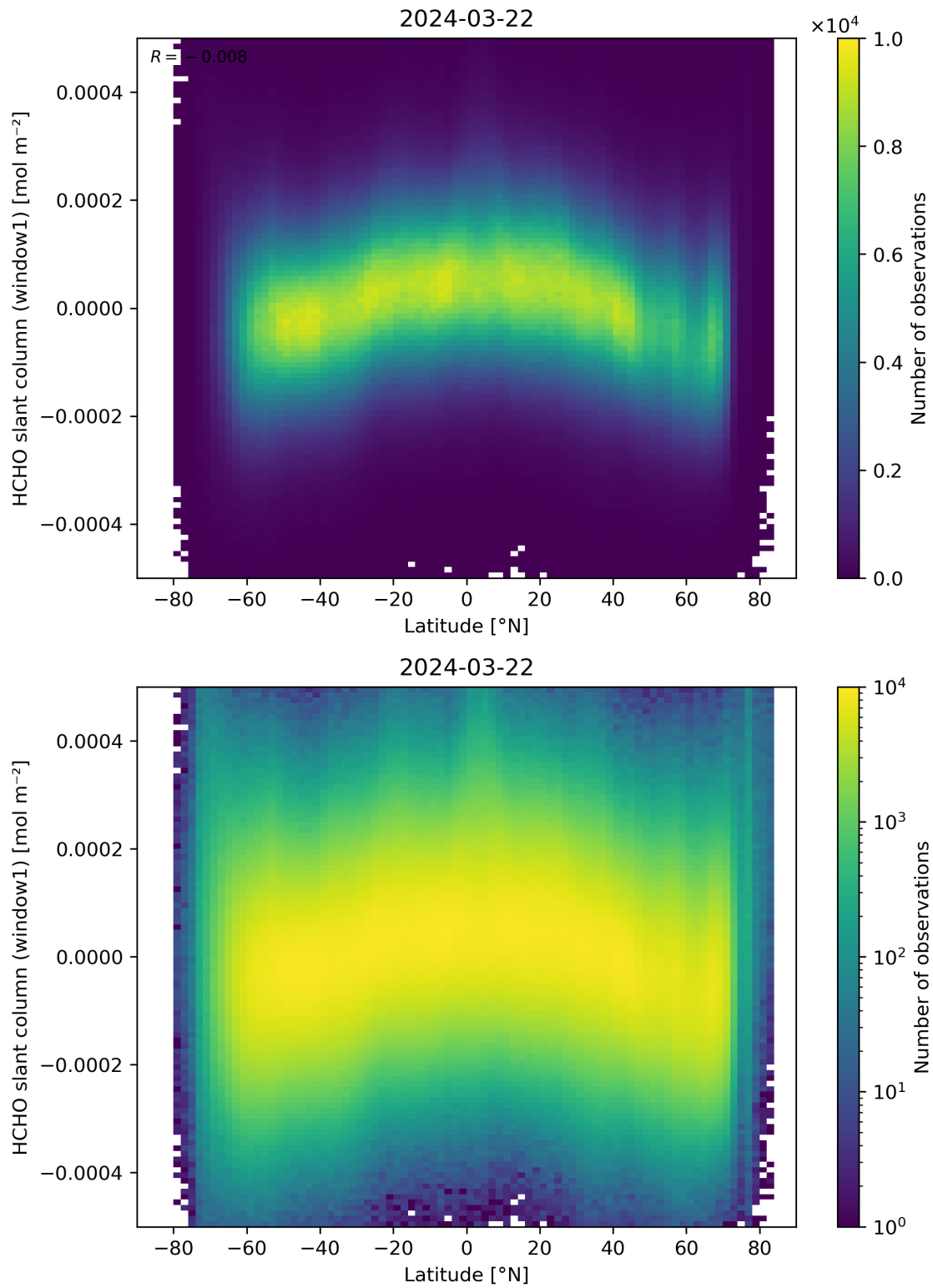
Figure 159: Scatter density plot of “Latitude” against “HCHO slant column (window1)” for 2024-03-21 to 2024-03-22.
