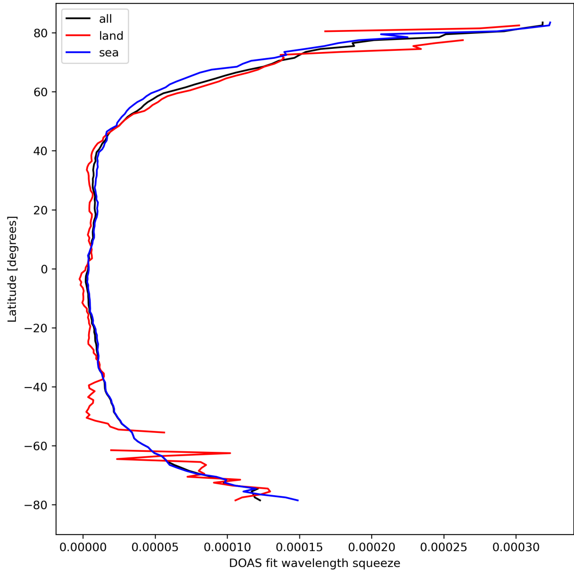
Figure 31: Zonal average of “DOAS fit wavelength squeeze” for 2024-03-21 to 2024-03-22.
