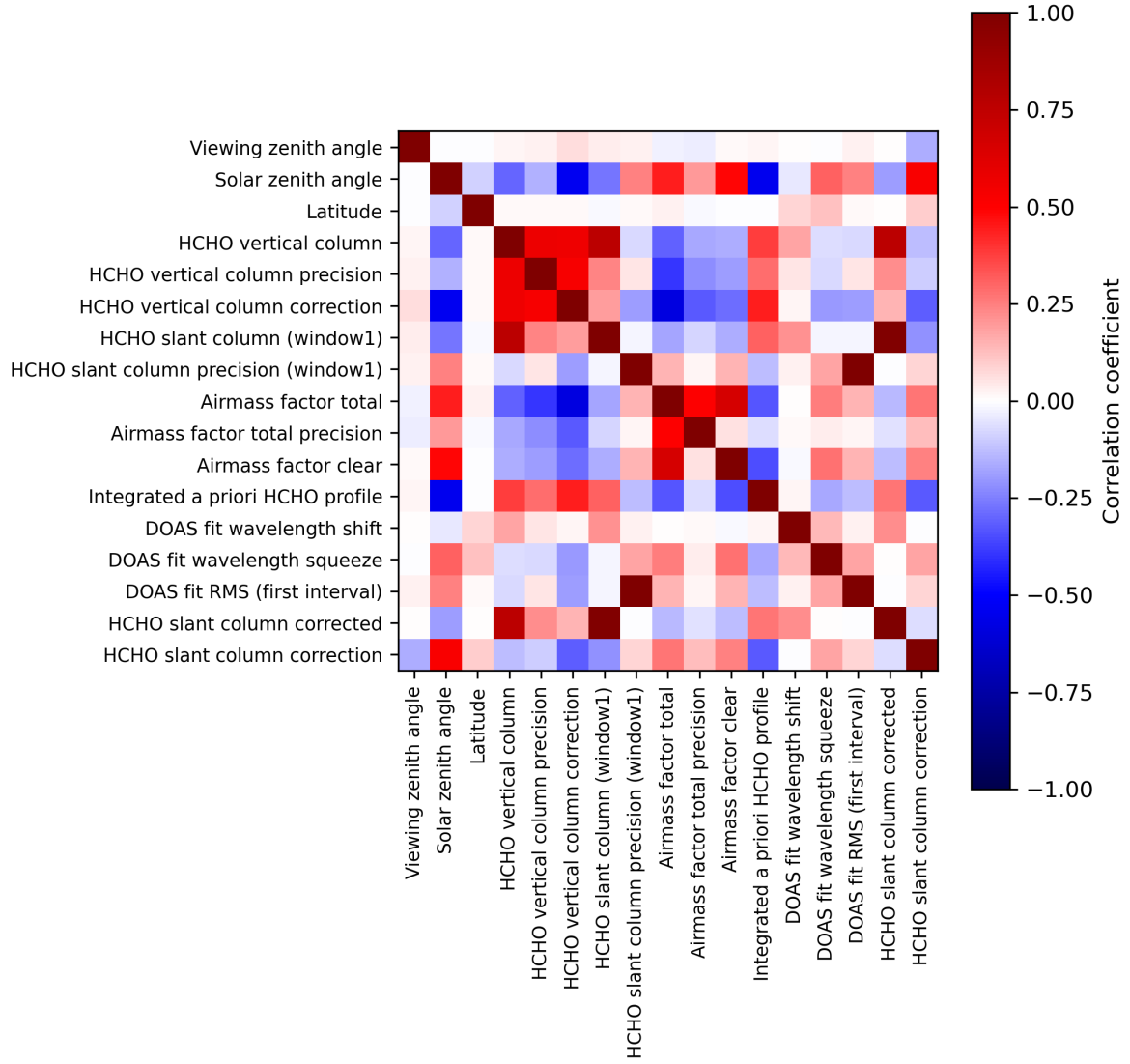
Figure 2: Map of correlation matrix for 2024-03-21 to 2024-03-22.
