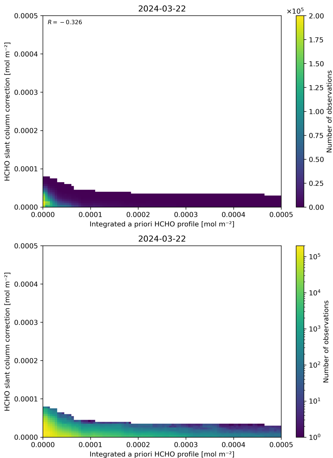
Figure 152: Scatter density plot of “Integrated a priori HCHO profile” against “HCHO slant column correction” for 2024-03-21 to 2024-03-22.
