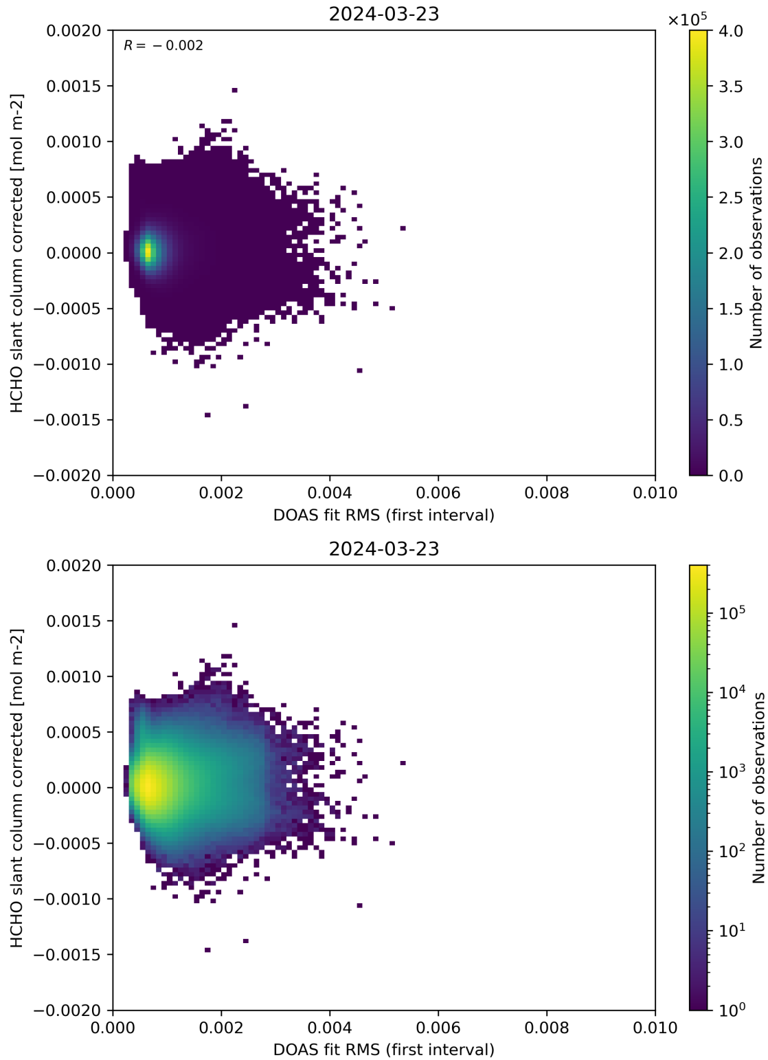
Figure 62: Scatter density plot of “DOAS fit RMS (first interval)” against “HCHO slant column corrected” for 2024-03-23 to 2024-03-24.
