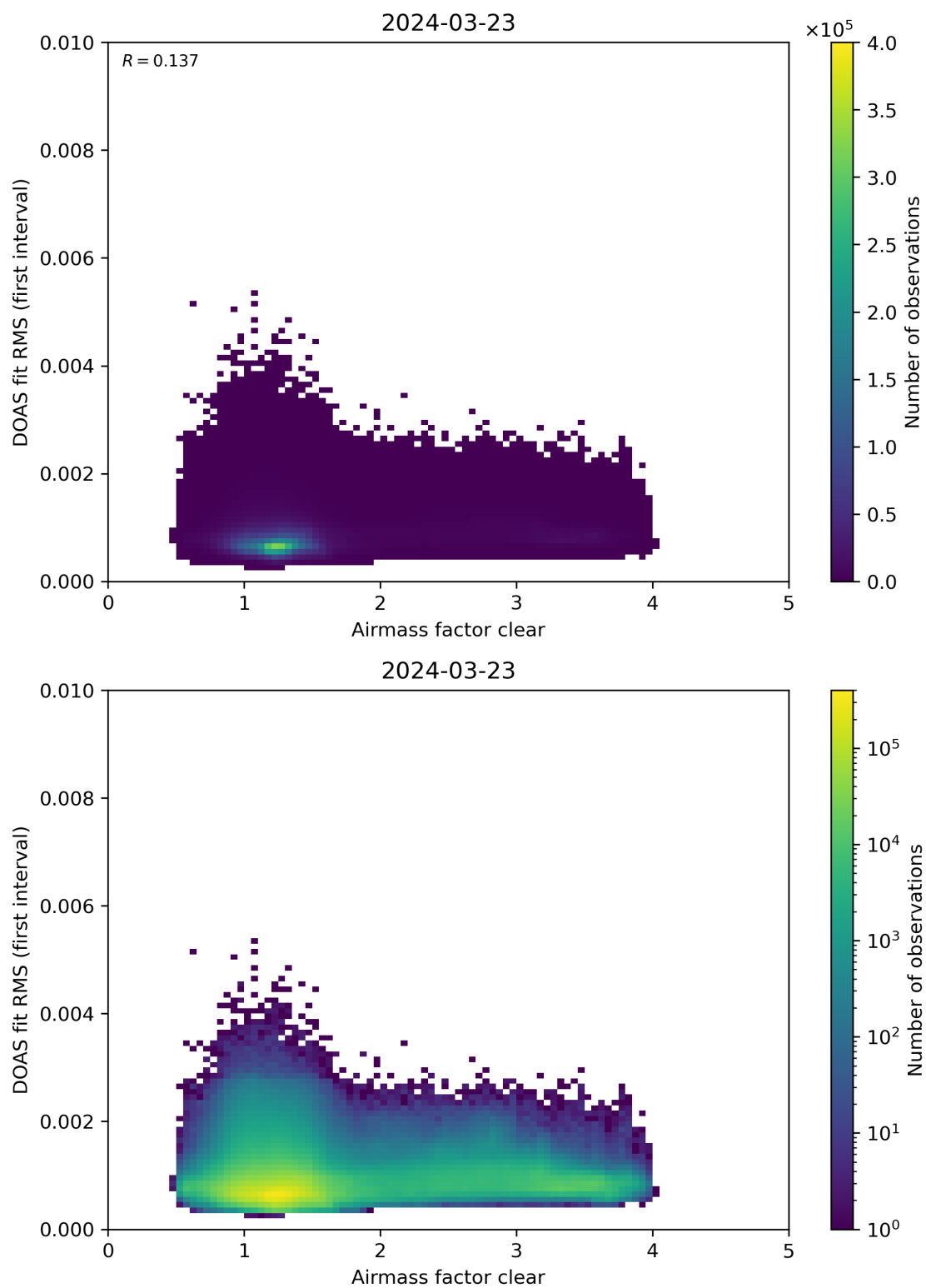
Figure 71: Scatter density plot of “Airmass factor clear” against “DOAS fit RMS (first interval)” for 2024-03-23 to 2024-03-24.
