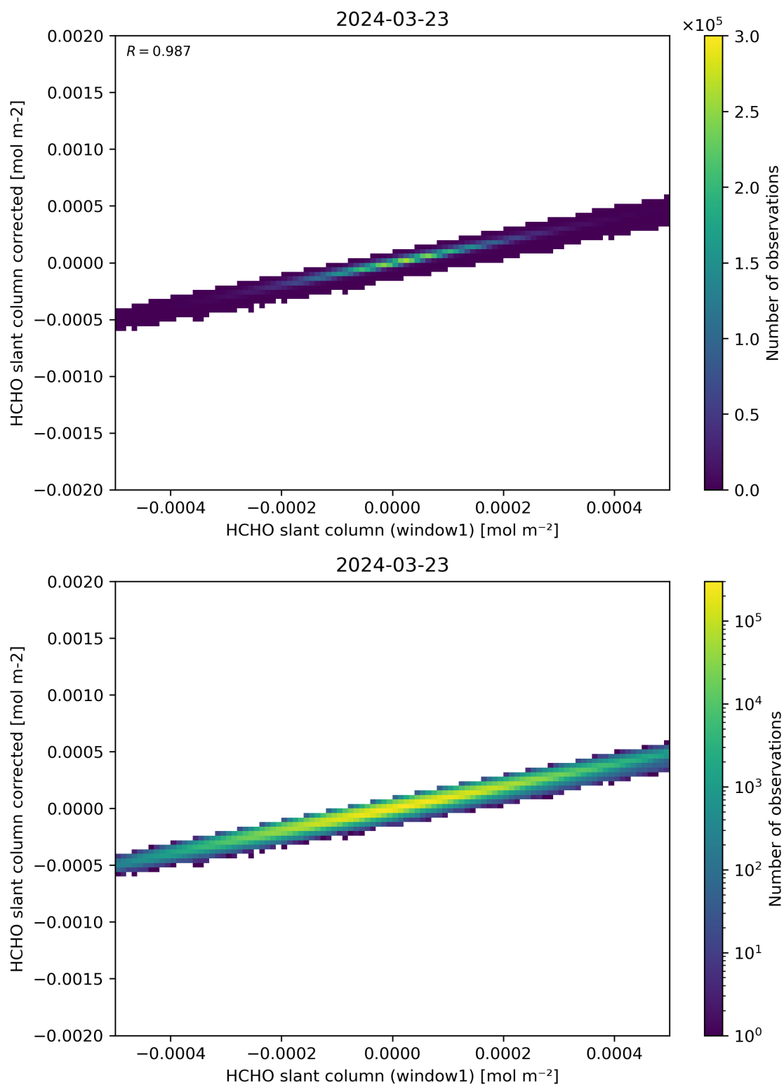
Figure 82: Scatter density plot of “HCHO slant column (window1)” against “HCHO slant column corrected” for 2024-03-23 to 2024-03-24.
