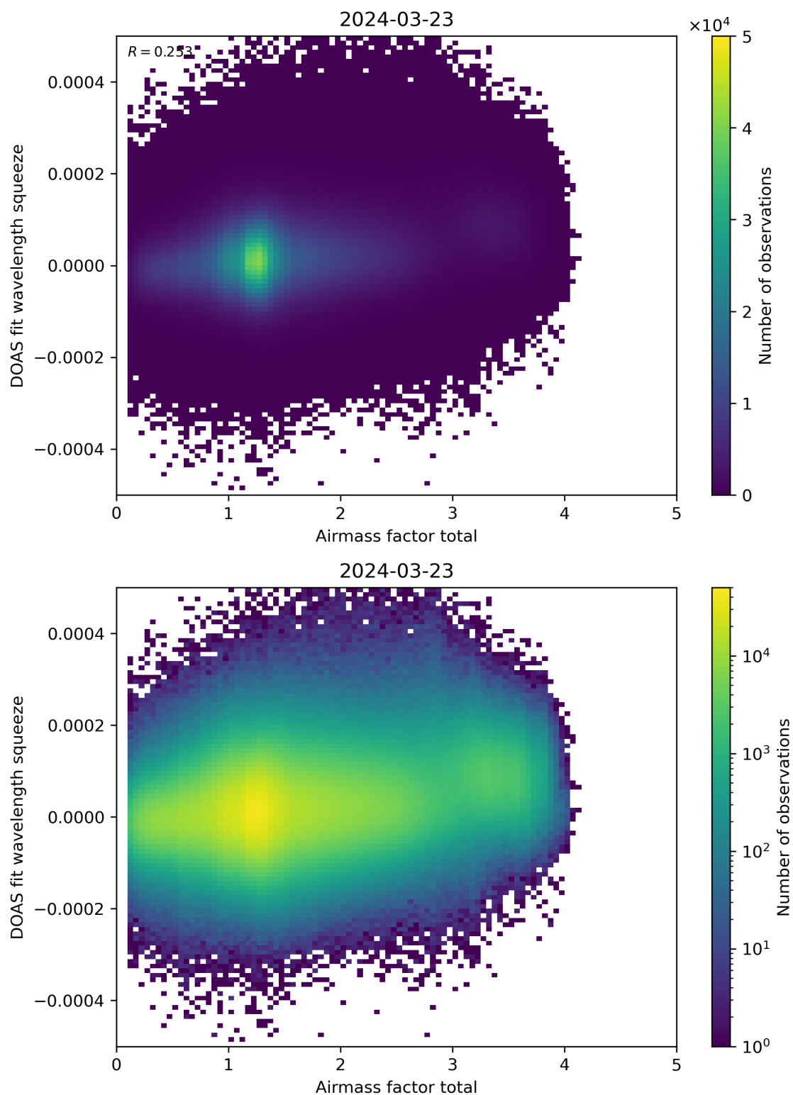
Figure 99: Scatter density plot of “Airmass factor total” against “DOAS fit wavelength squeeze” for 2024-03-23 to 2024-03-24.
