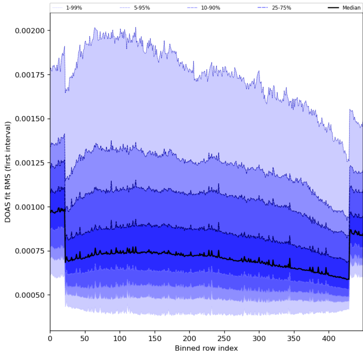
Figure 60: Along track statistics of “DOAS fit RMS (first interval)” for 2024-03-23 to 2024-03-24
