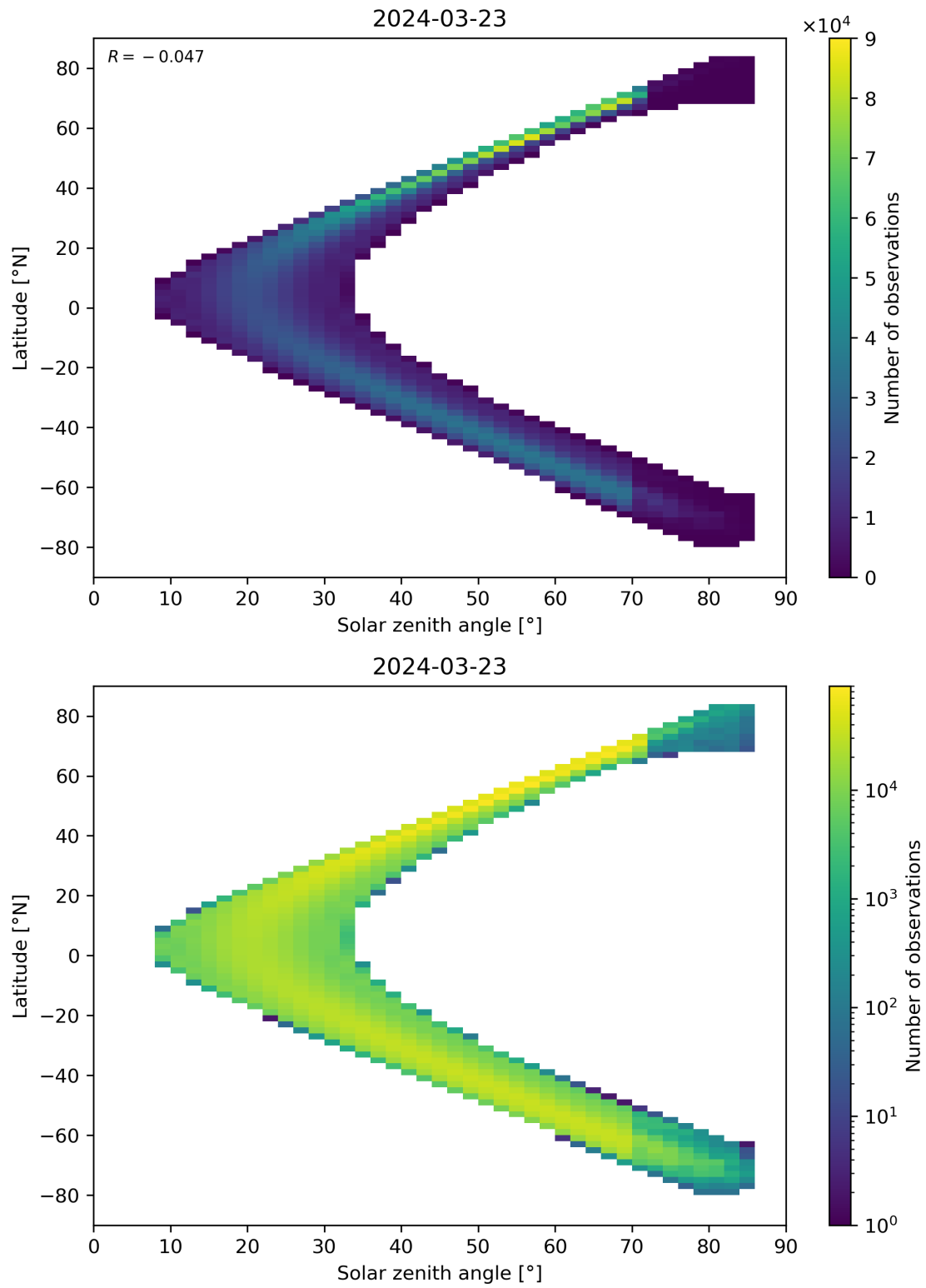
Figure 181: Scatter density plot of “Solar zenith angle” against “Latitude” for 2024-03-23 to 2024-03-24.
