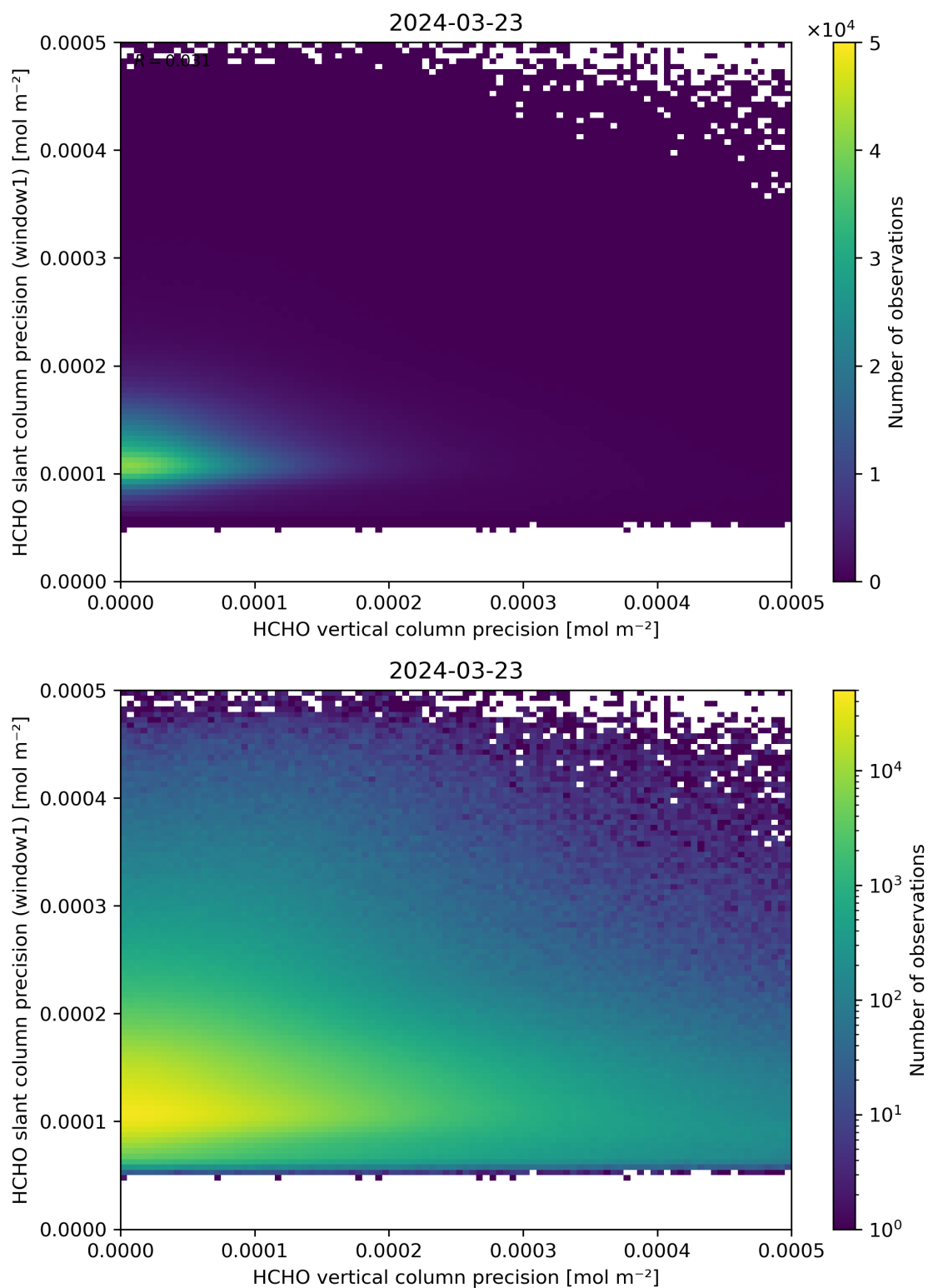
Figure 143: Scatter density plot of “HCHO vertical column precision” against “HCHO slant column precision (window1)” for 2024-03-23 to 2024-03-24.
