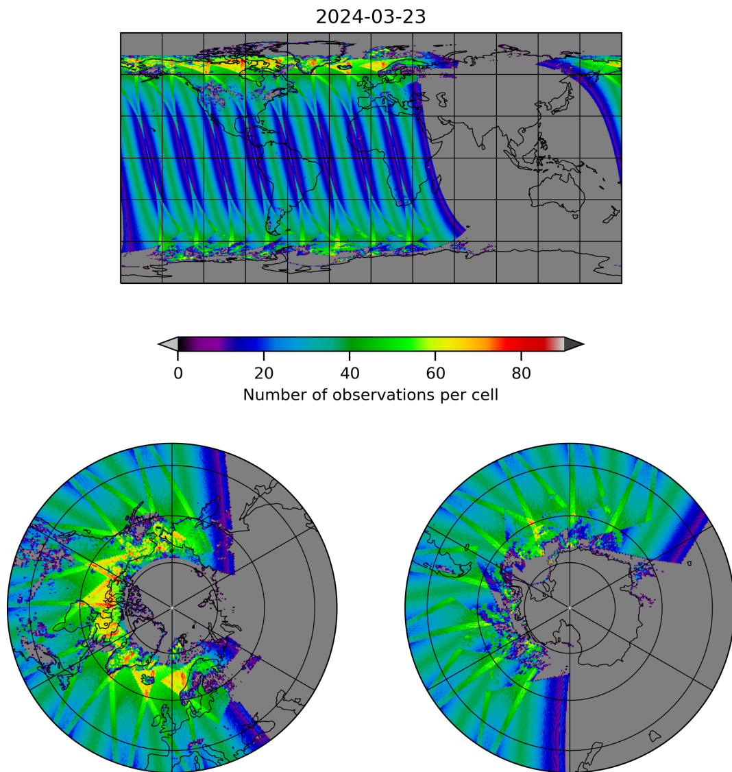
Figure 19: Map of the number of observations for 2024-03-23 to 2024-03-24
