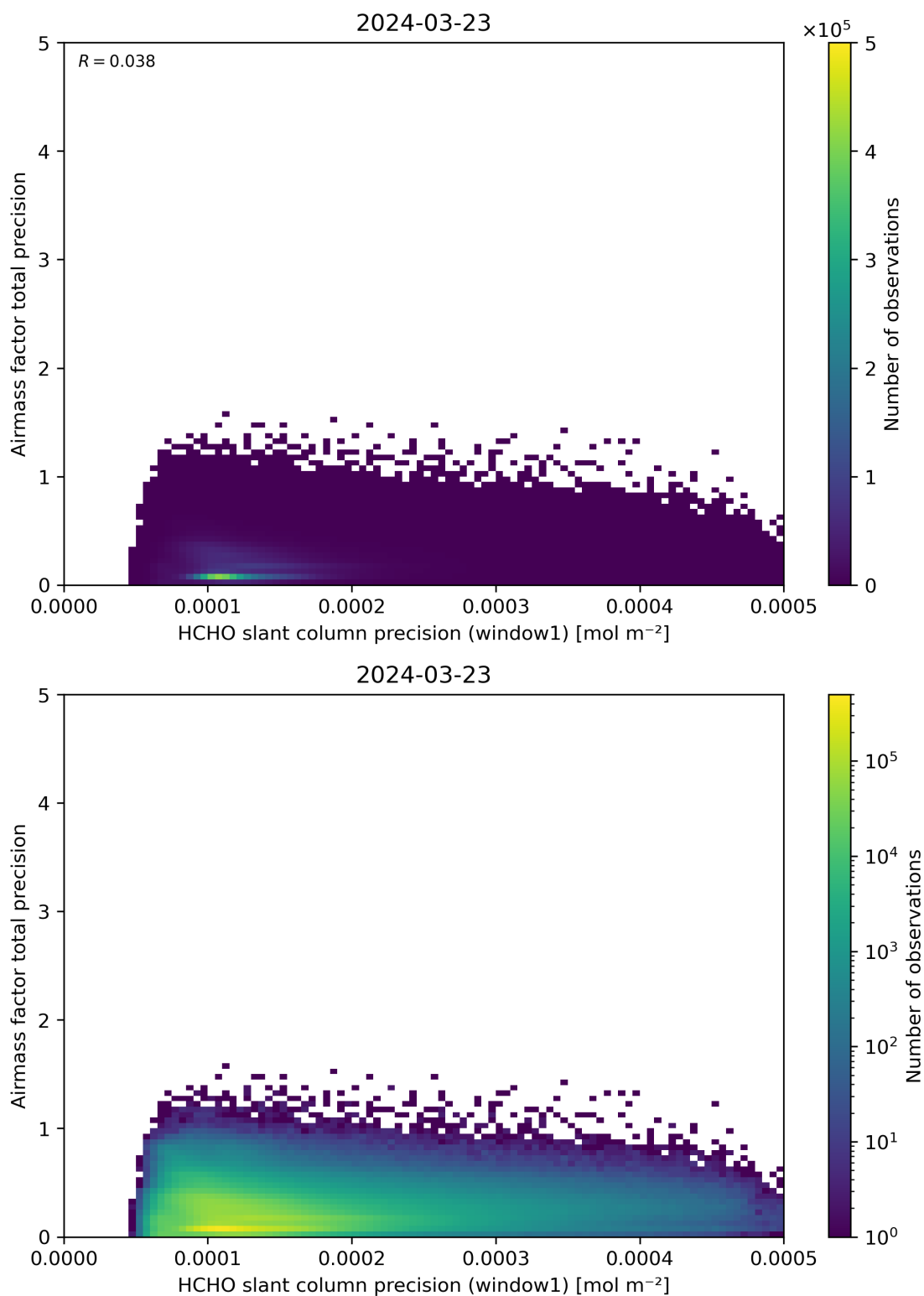
Figure 95: Scatter density plot of “HCHO slant column precision (window1)” against “Airmass factor total precision” for 2024-03-23 to 2024-03-24.
