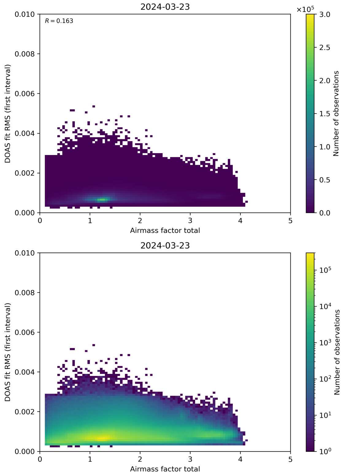
Figure 97: Scatter density plot of “Airmass factor total” against “DOAS fit RMS (first interval)” for 2024-03-23 to 2024-03-24.
