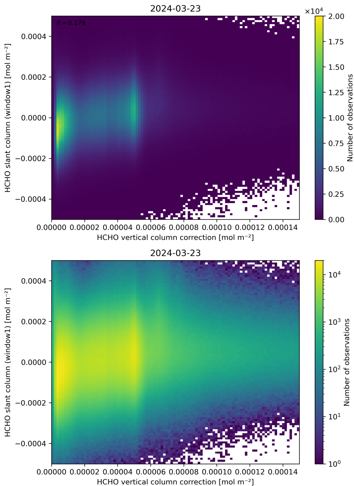
Figure 118: Scatter density plot of “HCHO vertical column correction” against “HCHO slant column (window1)” for 2024-03-23 to 2024-03-24.
