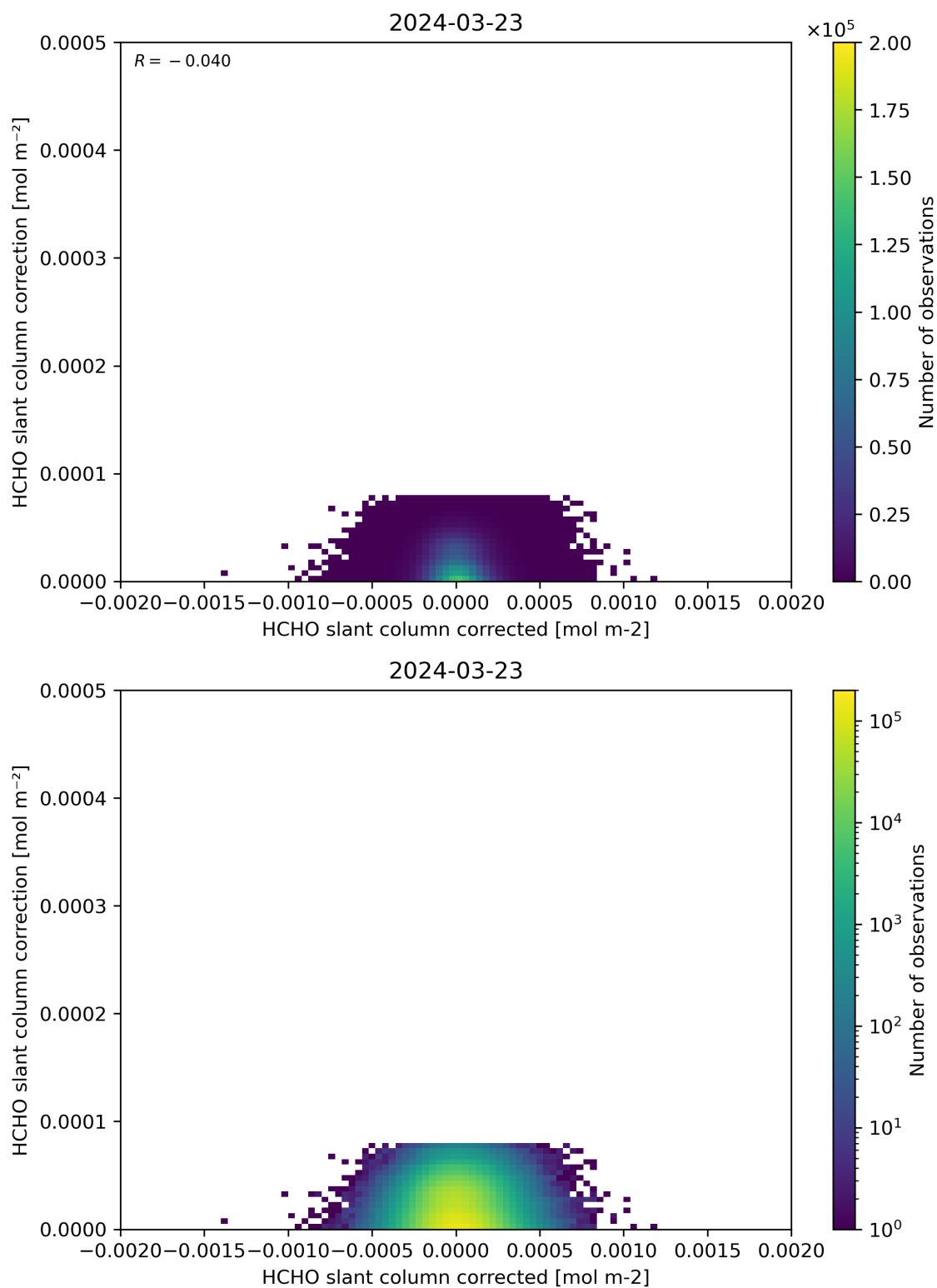
Figure 77: Scatter density plot of “HCHO slant column corrected” against “HCHO slant column correction” for 2024-03-23 to 2024-03-24.
