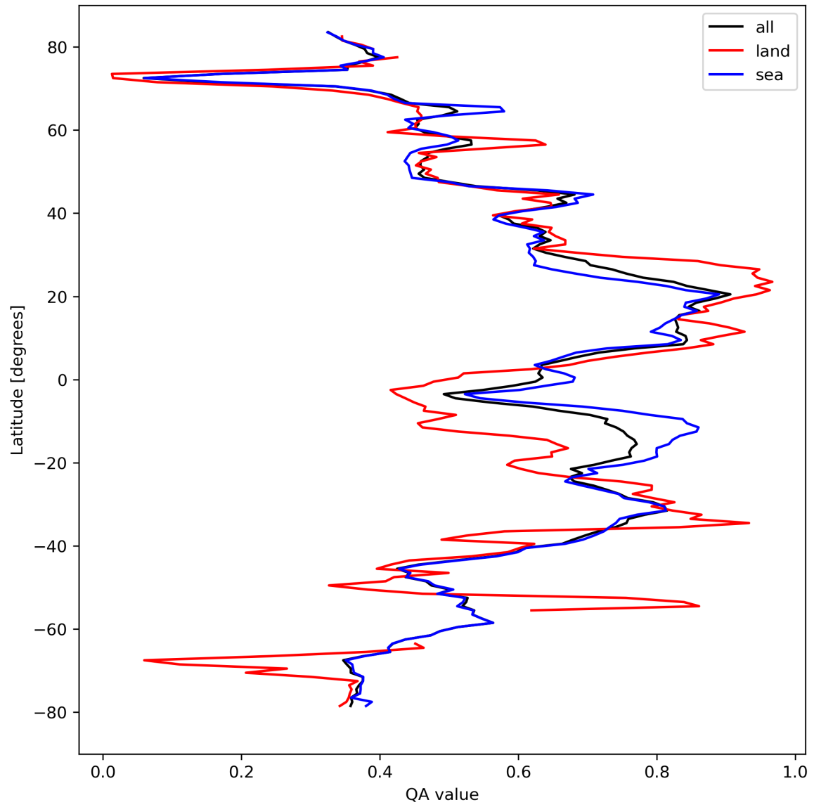
Figure 20: Zonal average of “QA value” for 2024-03-23 to 2024-03-24.
