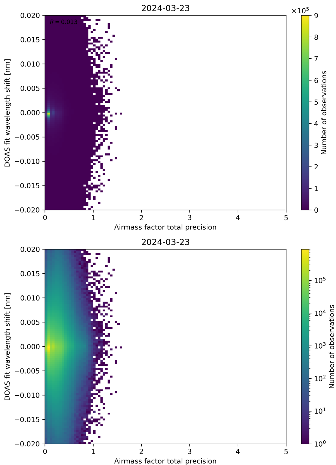
Figure 106: Scatter density plot of “Airmass factor total precision” against “DOAS fit wavelength shift” for 2024-03-23 to 2024-03-24.
