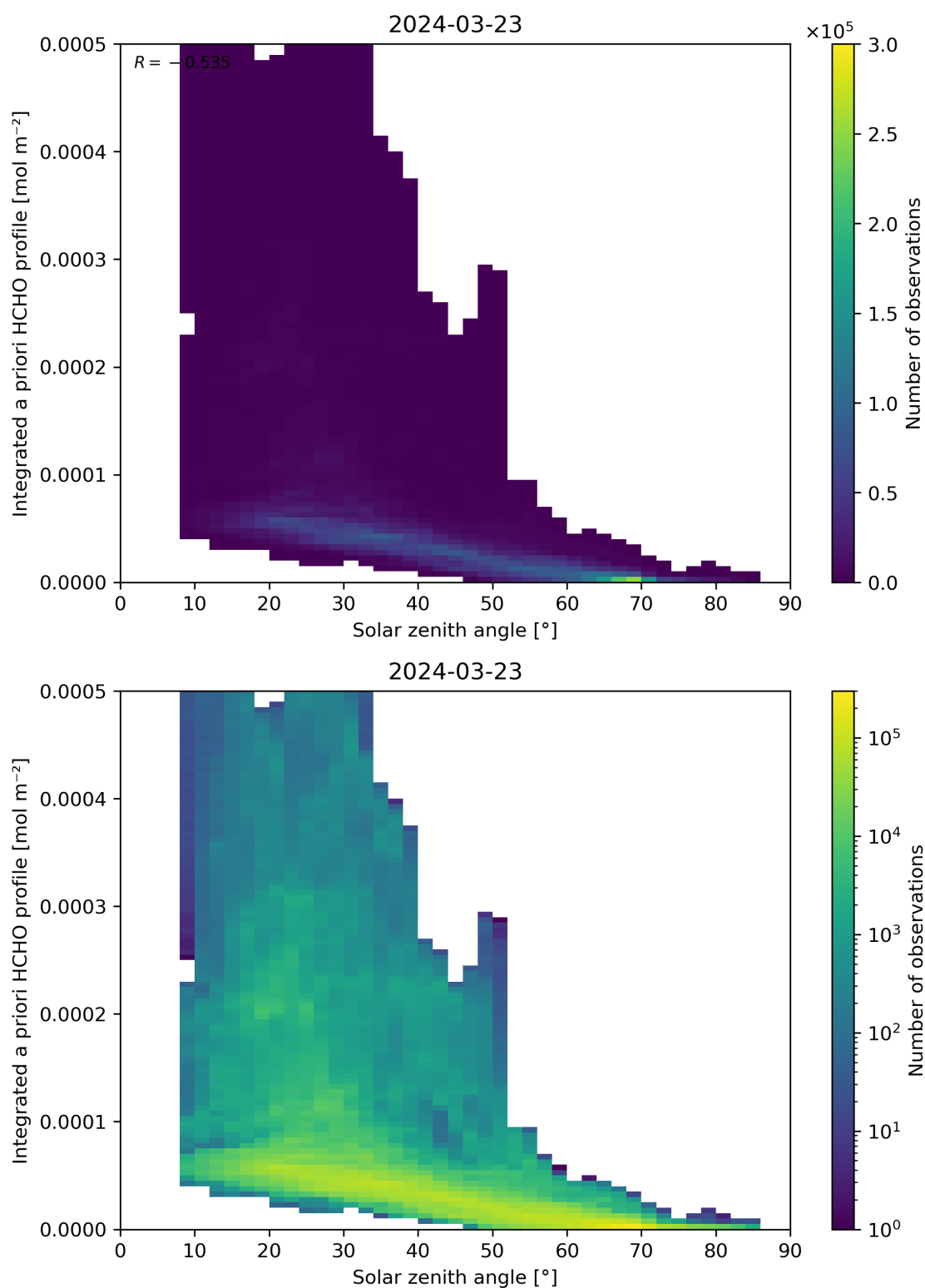
Figure 180: Scatter density plot of “Solar zenith angle” against “Integrated a priori HCHO profile” for 2024-03-23 to 2024-03-24.
