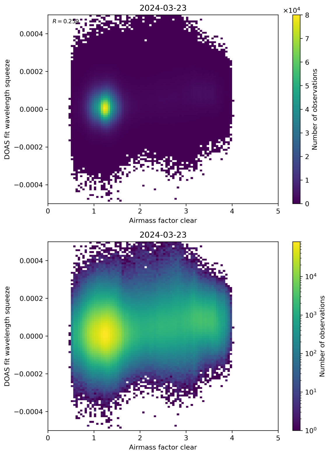
Figure 73: Scatter density plot of “Airmass factor clear” against “DOAS fit wavelength squeeze” for 2024-03-23 to 2024-03-24.
