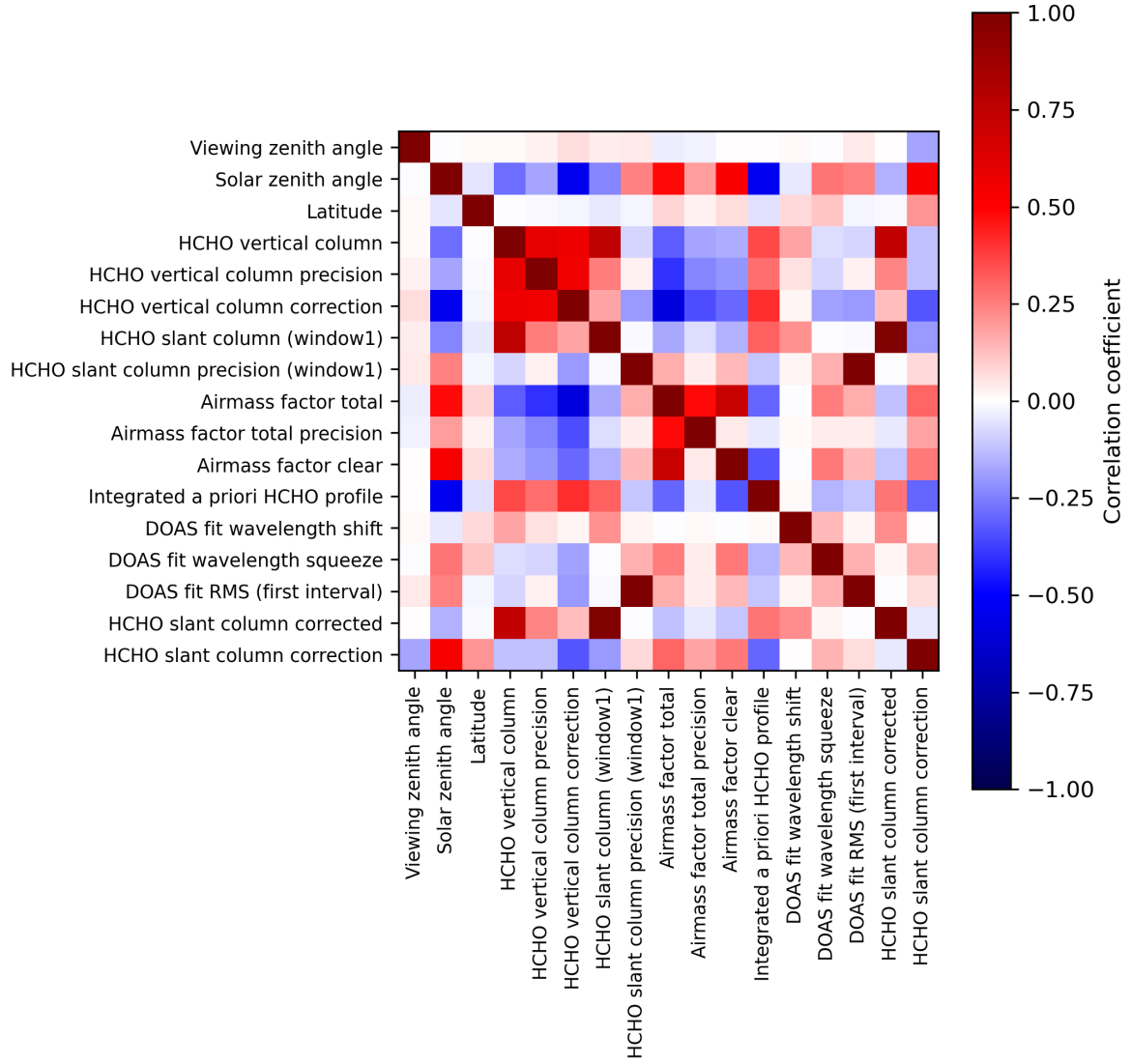
Figure 2: Map of correlation matrix for 2024-03-23 to 2024-03-24.
