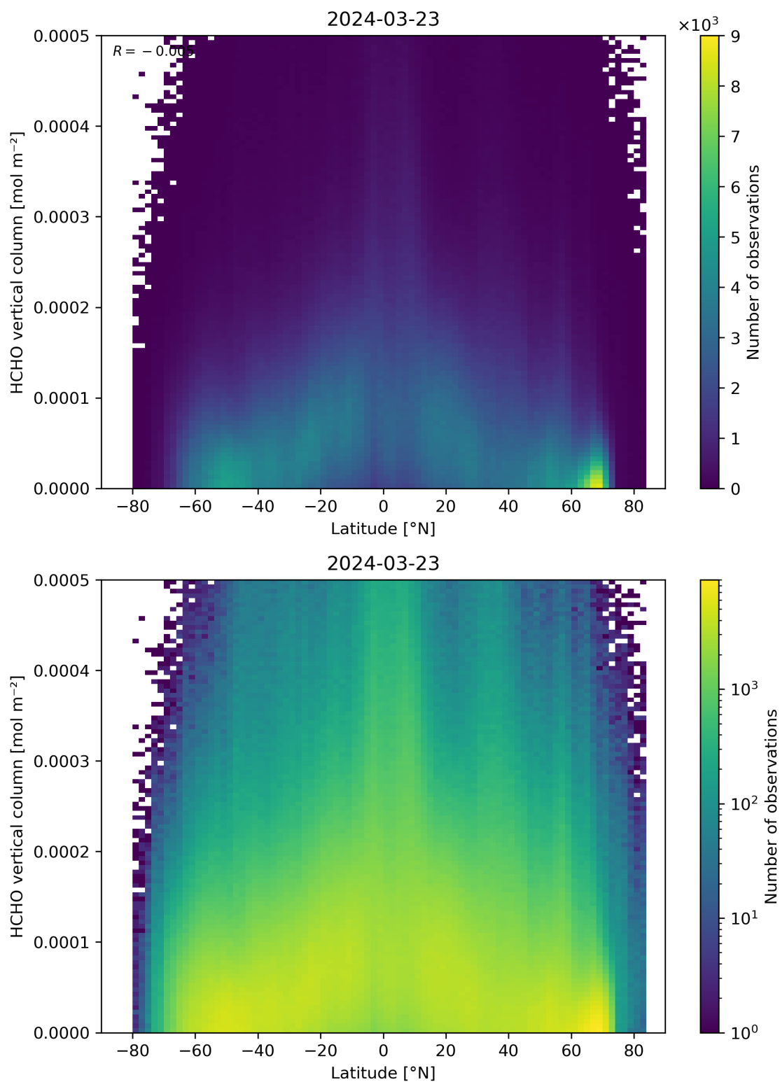
Figure 163: Scatter density plot of “Latitude” against “HCHO vertical column” for 2024-03-23 to 2024-03-24.
