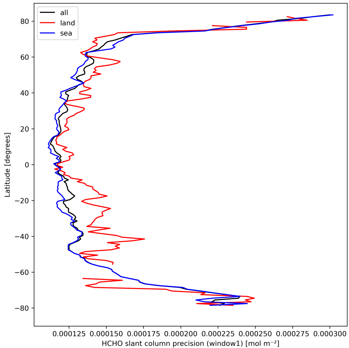
Figure 25: Zonal average of “HCHO slant column precision (window1)” for 2024-03-23 to 2024-03-24.
