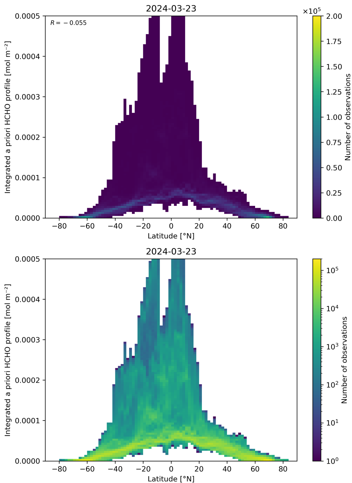
Figure 166: Scatter density plot of “Latitude” against “Integrated a priori HCHO profile” for 2024-03-23 to 2024-03-24.
