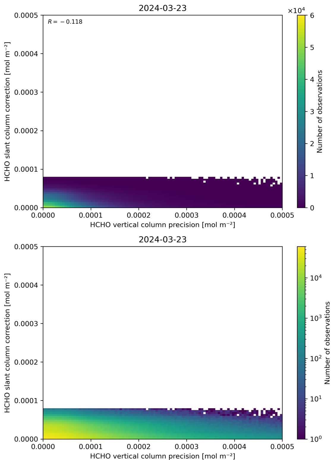
Figure 141: Scatter density plot of “HCHO vertical column precision” against “HCHO slant column correction” for 2024-03-23 to 2024-03-24.
