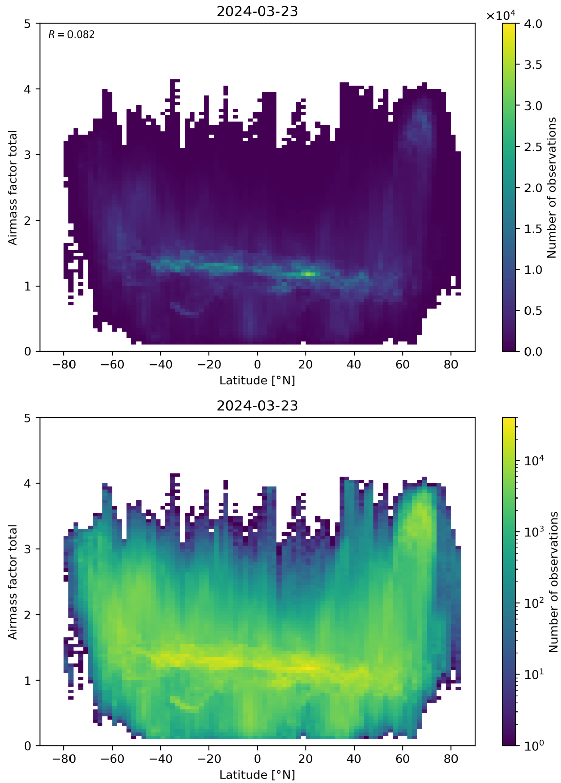
Figure 161: Scatter density plot of “Latitude” against “Airmass factor total” for 2024-03-23 to 2024-03-24.
