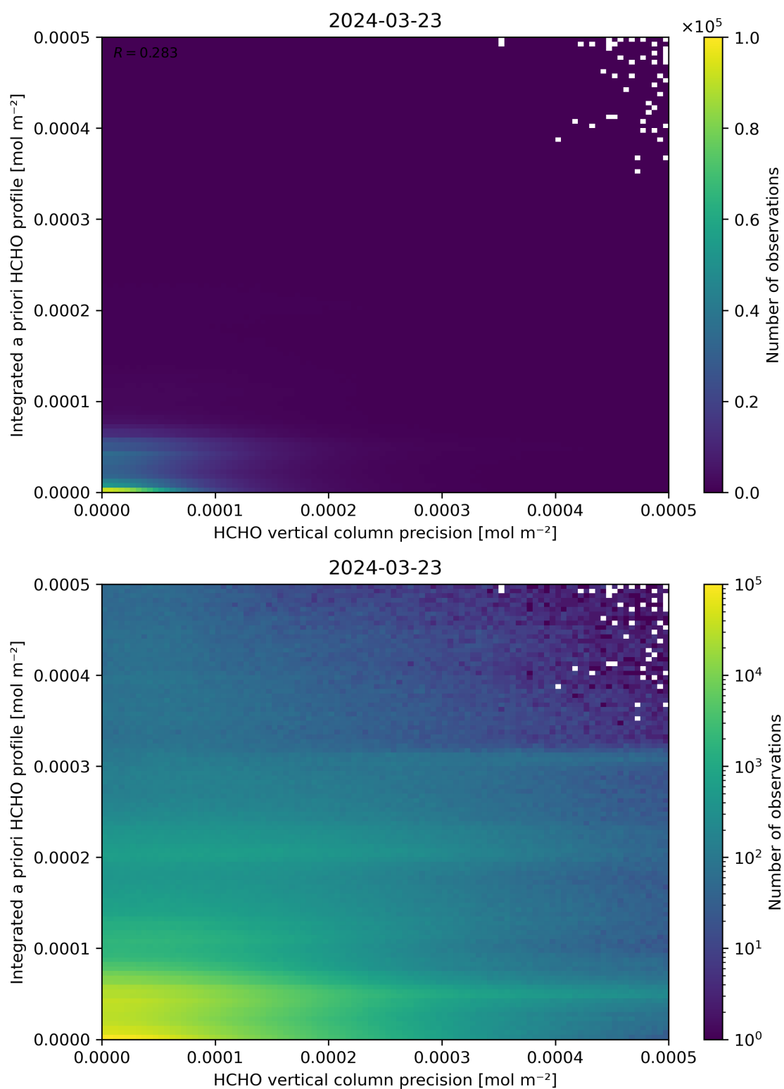
Figure 147: Scatter density plot of “HCHO vertical column precision” against “Integrated a priori HCHO profile” for 2024-03-23 to 2024-03-24.
