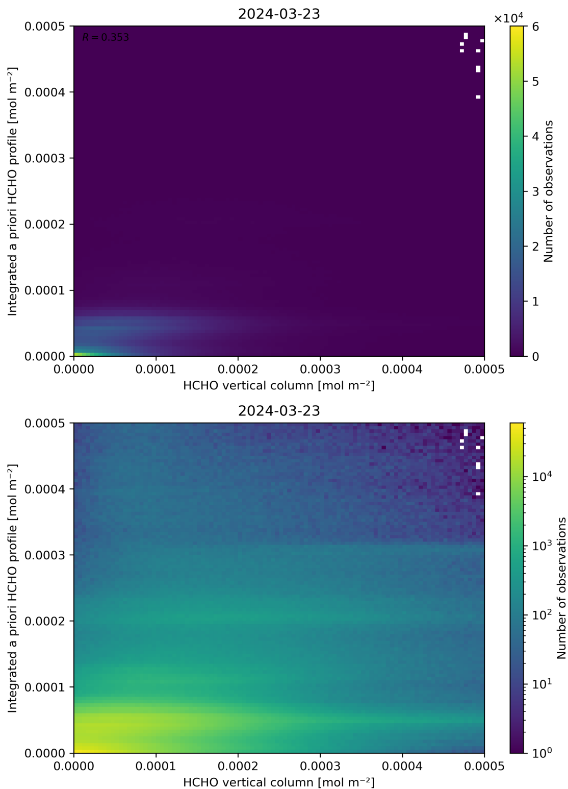
Figure 135: Scatter density plot of “HCHO vertical column” against “Integrated a priori HCHO profile” for 2024-03-23 to 2024-03-24.
