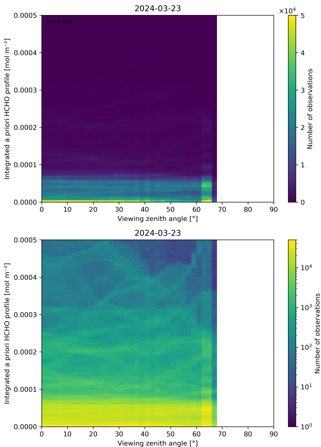
Figure 195: Scatter density plot of “Viewing zenith angle” against “Integrated a priori HCHO profile” for 2024-03-23 to 2024-03-24.
