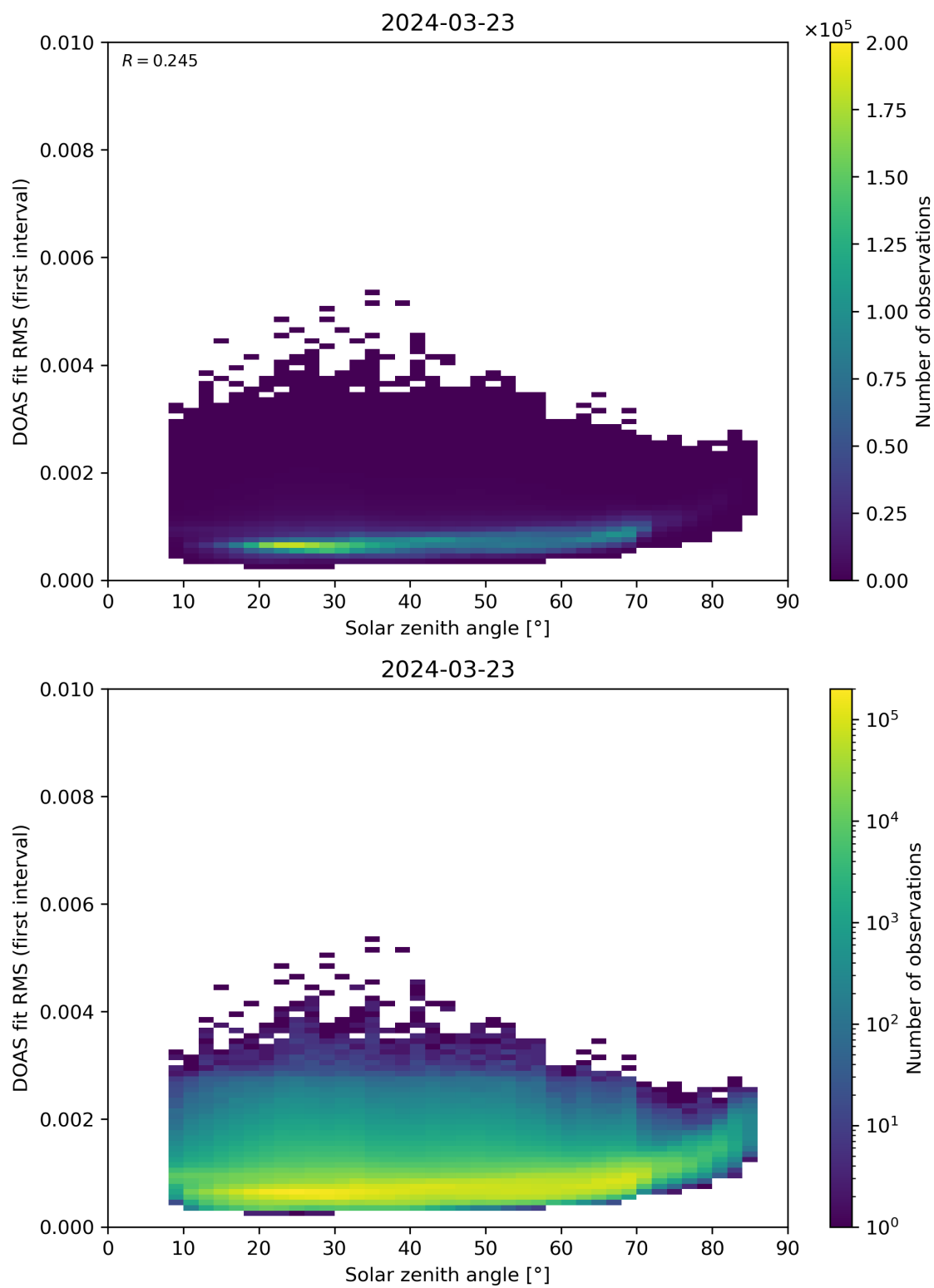
Figure 167: Scatter density plot of “Solar zenith angle” against “DOAS fit RMS (first interval)” for 2024-03-23 to 2024-03-24.
