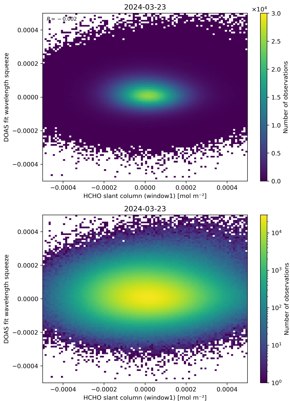
Figure 80: Scatter density plot of “HCHO slant column (window1)” against “DOAS fit wavelength squeeze” for 2024-03-23 to 2024-03-24.
