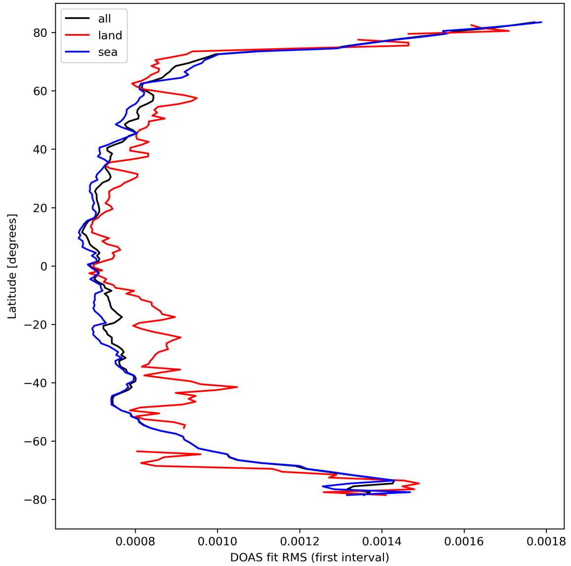
Figure 32: Zonal average of "DOAS fit RMS (first interval)" for 2024-03-23 to 2024-03-24.
