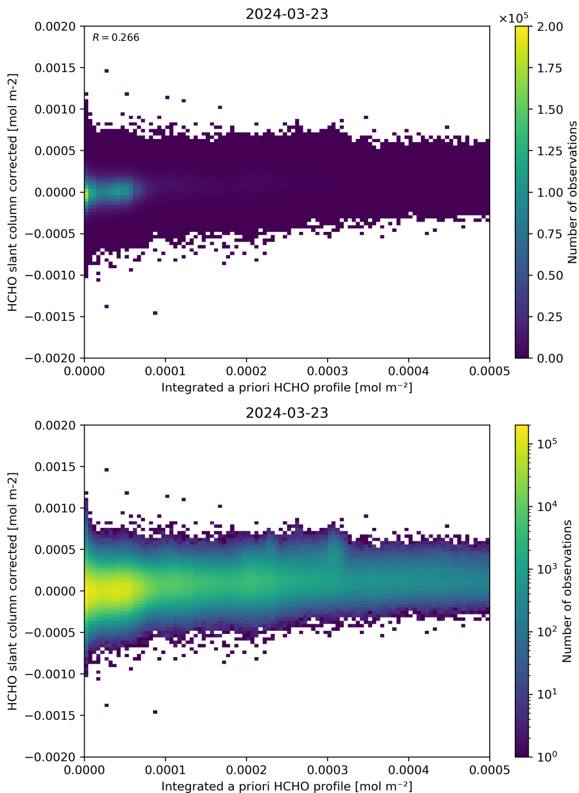
Figure 151: Scatter density plot of “Integrated a priori HCHO profile” against “HCHO slant column corrected” for 2024-03-23 to 2024-03-24.
