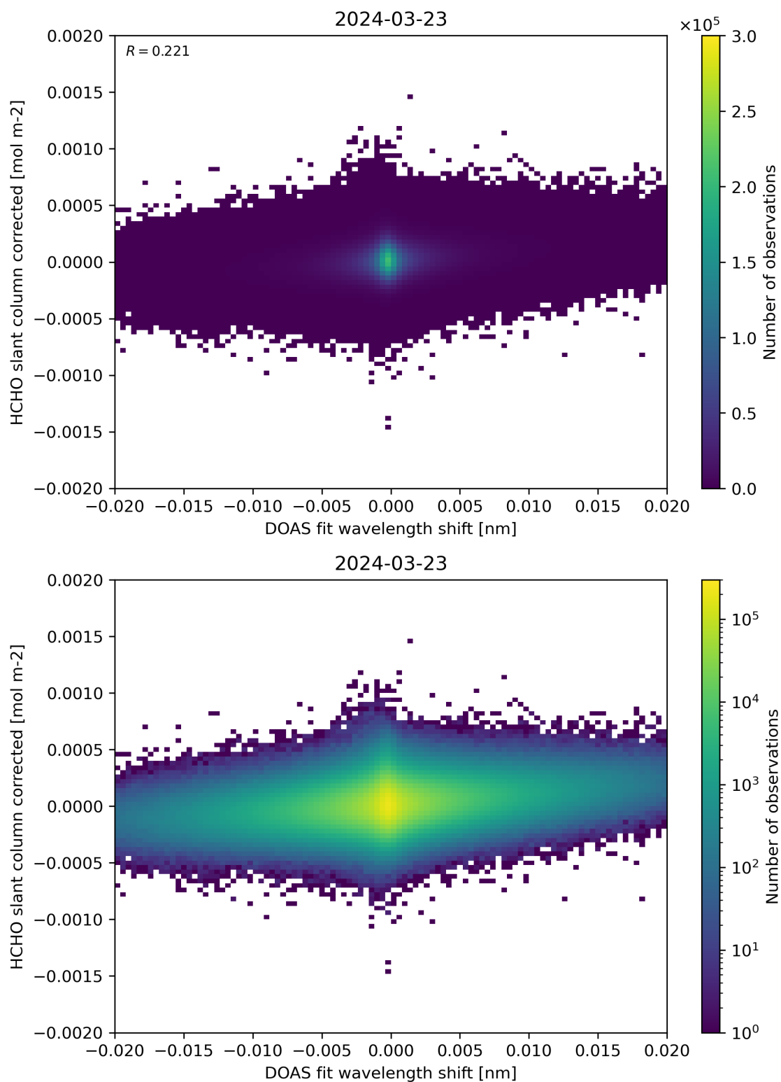
Figure 66: Scatter density plot of “DOAS fit wavelength shift” against “HCHO slant column corrected” for 2024-03-23 to 2024-03-24.
