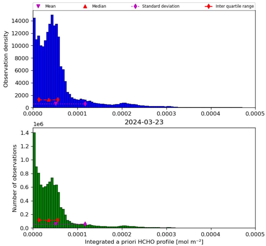
Figure 43: Histogram of “Integrated a priori HCHO profile” for 2024-03-23 to 2024-03-24
