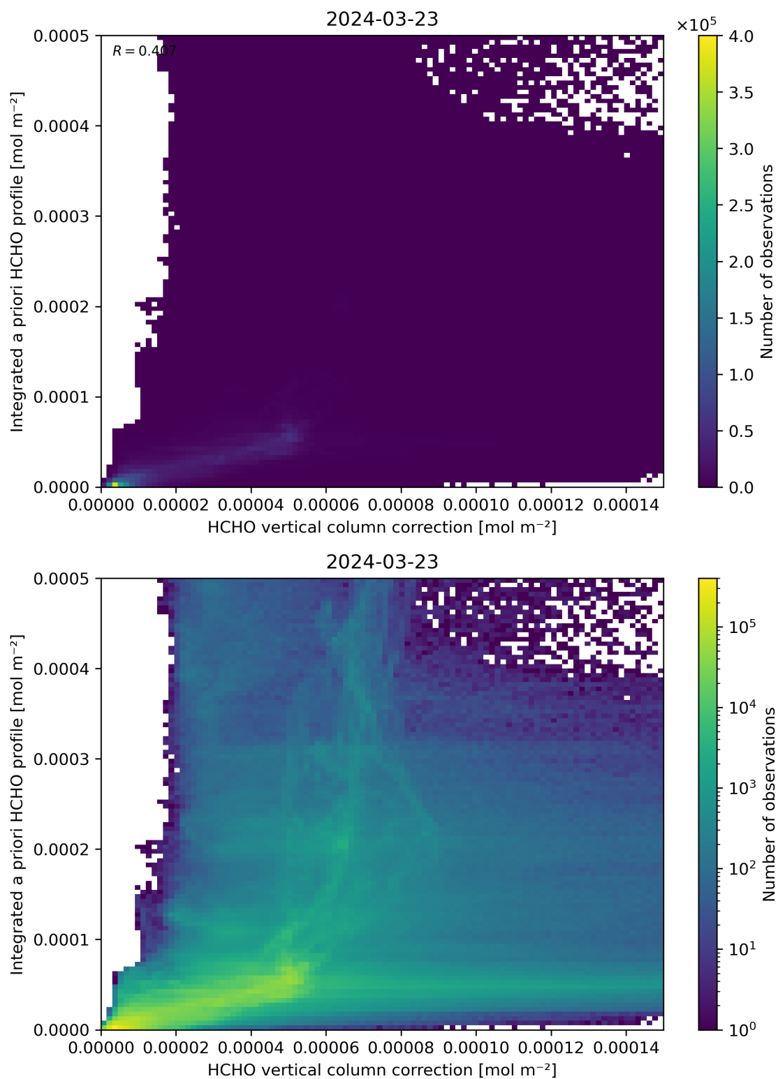
Figure 122: Scatter density plot of “HCHO vertical column correction” against “Integrated a priori HCHO profile” for 2024-03-23 to 2024-03-24.
