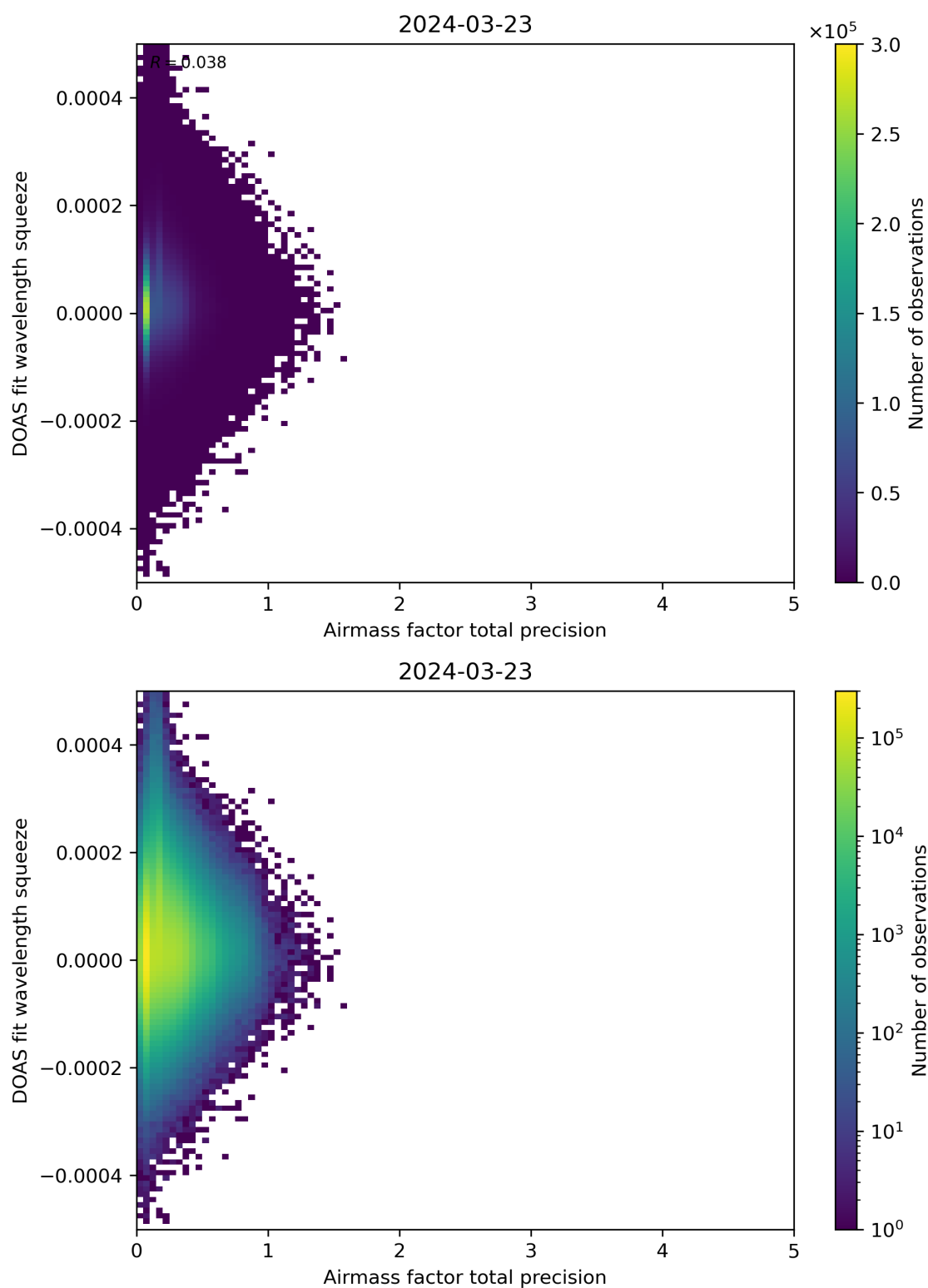
Figure 107: Scatter density plot of “Airmass factor total precision” against “DOAS fit wavelength squeeze” for 2024-03-23 to 2024-03-24.
