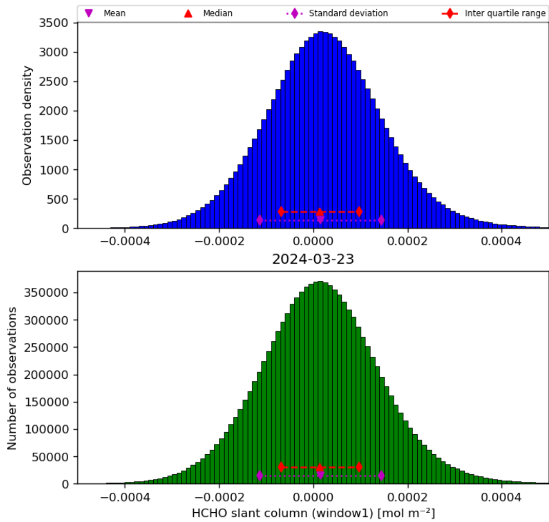
Figure 38: Histogram of “HCHO slant column (window1)” for 2024-03-23 to 2024-03-24
