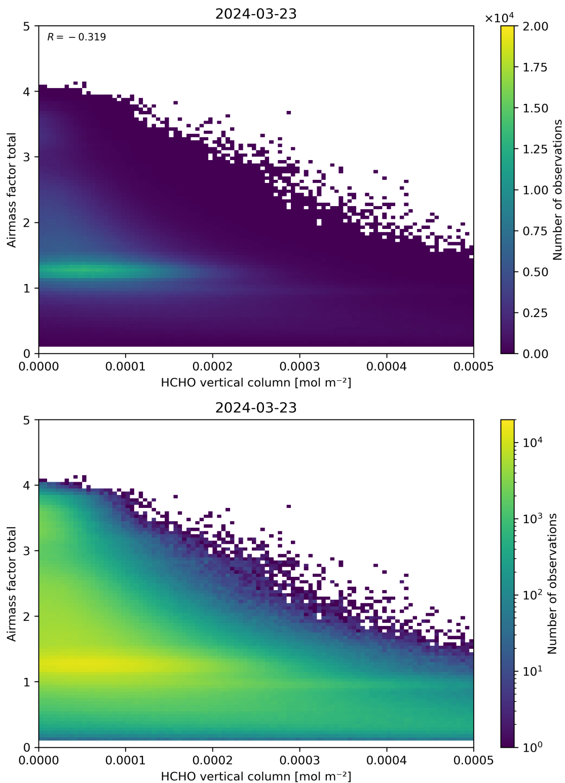
Figure 131: Scatter density plot of “HCHO vertical column” against “Airmass factor total” for 2024-03-23 to 2024-03-24.
