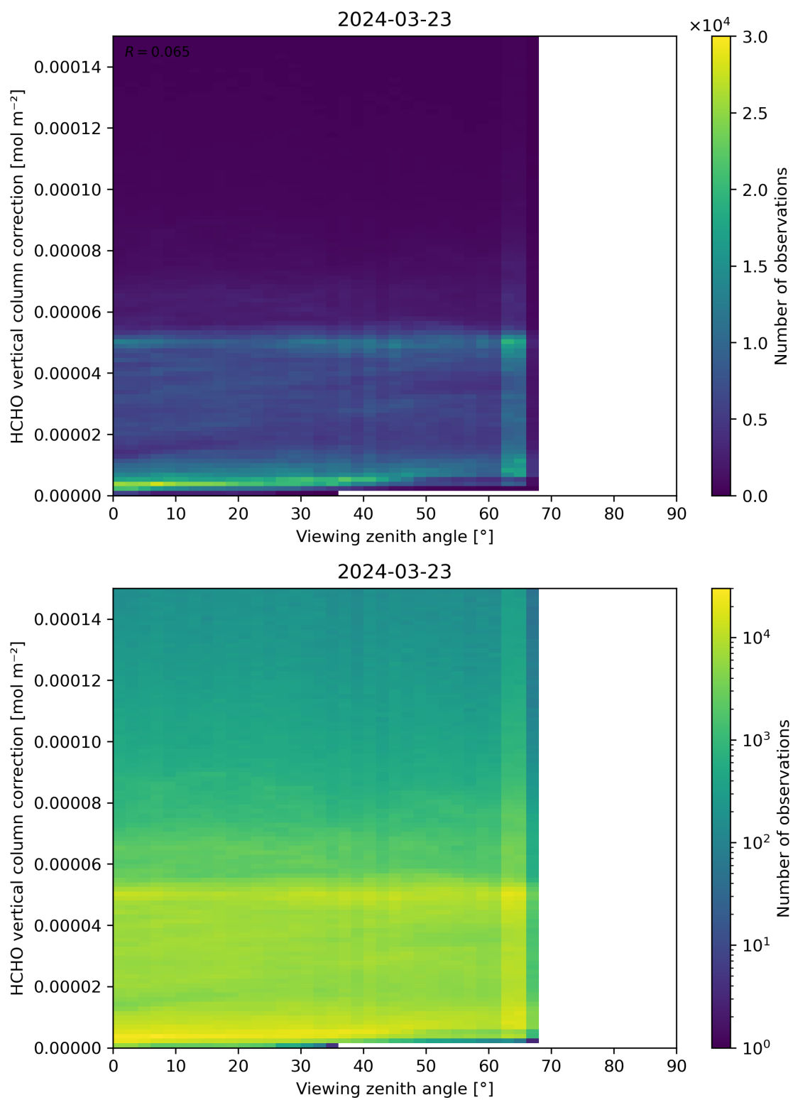
Figure 193: Scatter density plot of “Viewing zenith angle” against “HCHO vertical column correction” for 2024-03-23 to 2024-03-24.
