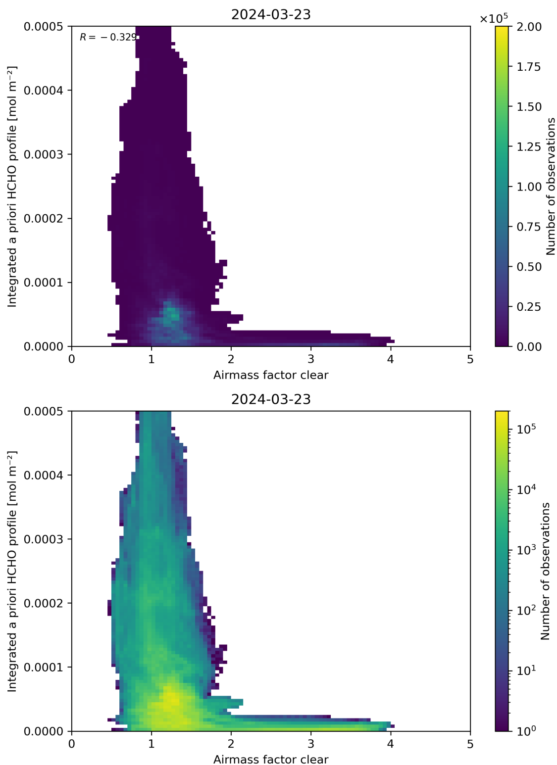
Figure 76: Scatter density plot of “Airmass factor clear” against “Integrated a priori HCHO profile” for 2024-03-23 to 2024-03-24.
