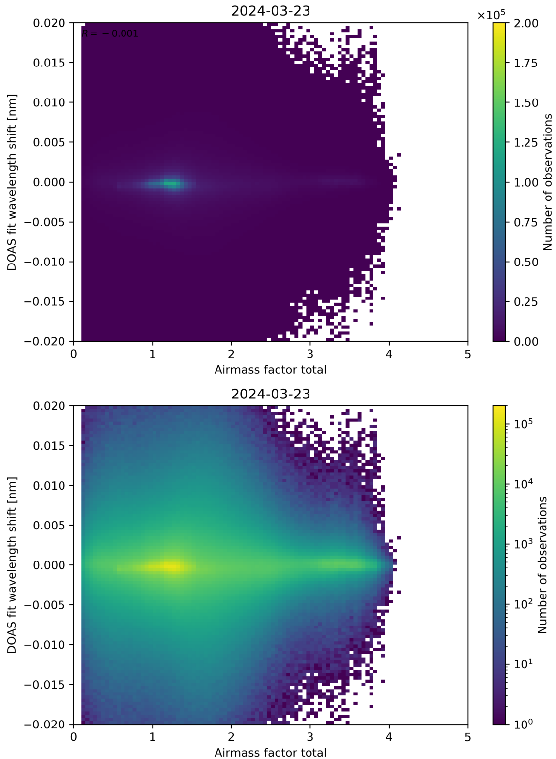
Figure 98: Scatter density plot of “Airmass factor total” against “DOAS fit wavelength shift” for 2024-03-23 to 2024-03-24.
