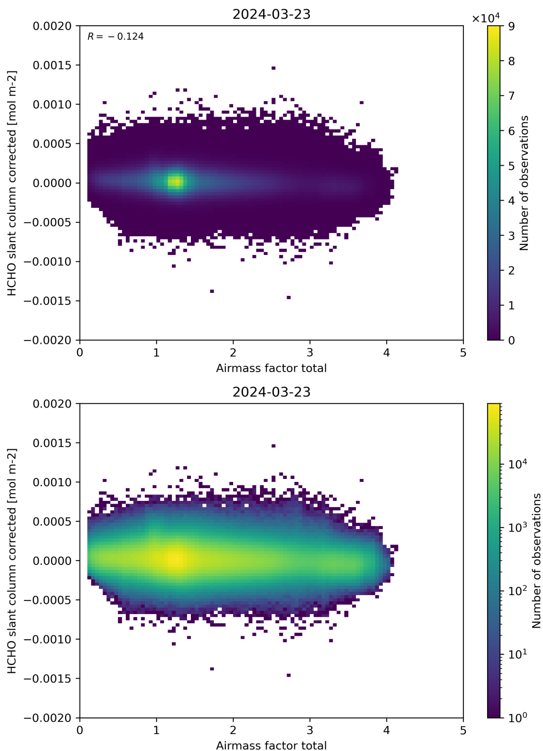
Figure 101: Scatter density plot of “Airmass factor total” against “HCHO slant column corrected” for 2024-03-23 to 2024-03-24.
