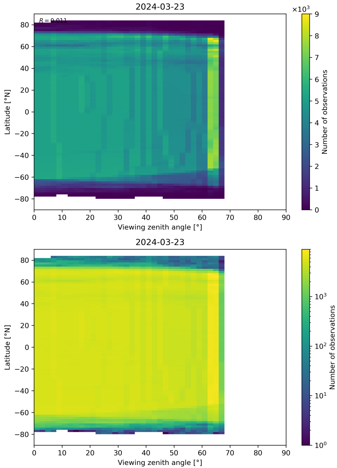
Figure 196: Scatter density plot of “Viewing zenith angle” against “Latitude” for 2024-03-23 to 2024-03-24.
