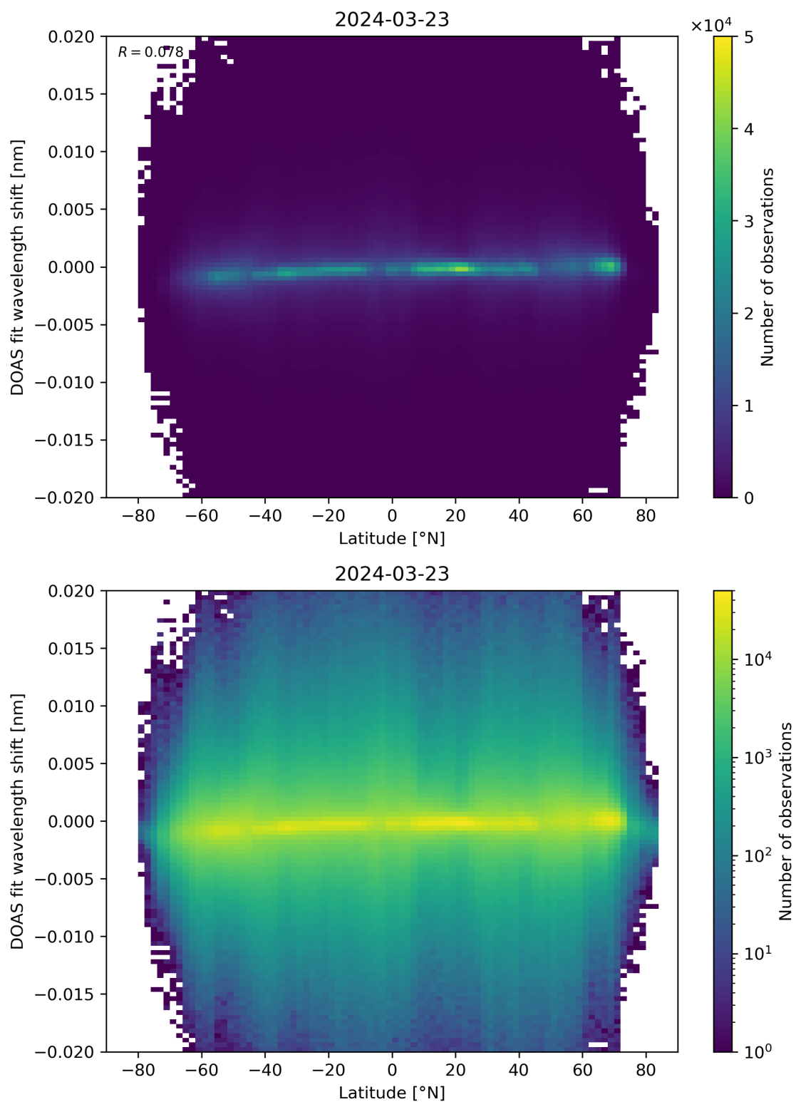
Figure 154: Scatter density plot of “Latitude” against “DOAS fit wavelength shift” for 2024-03-23 to 2024-03-24.
