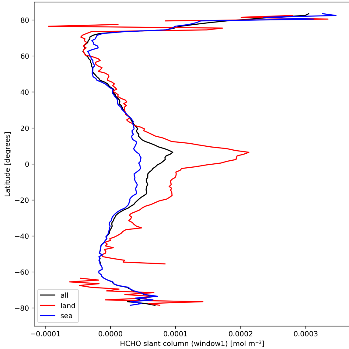
Figure 24: Zonal average of “HCHO slant column (window1)” for 2024-03-23 to 2024-03-24.
