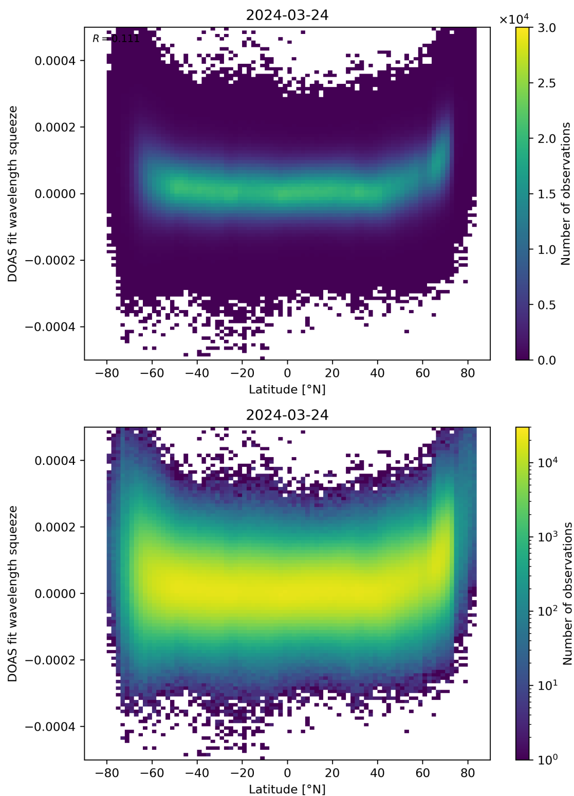
Figure 155: Scatter density plot of “Latitude” against “DOAS fit wavelength squeeze” for 2024-03-23 to 2024-03-25.
