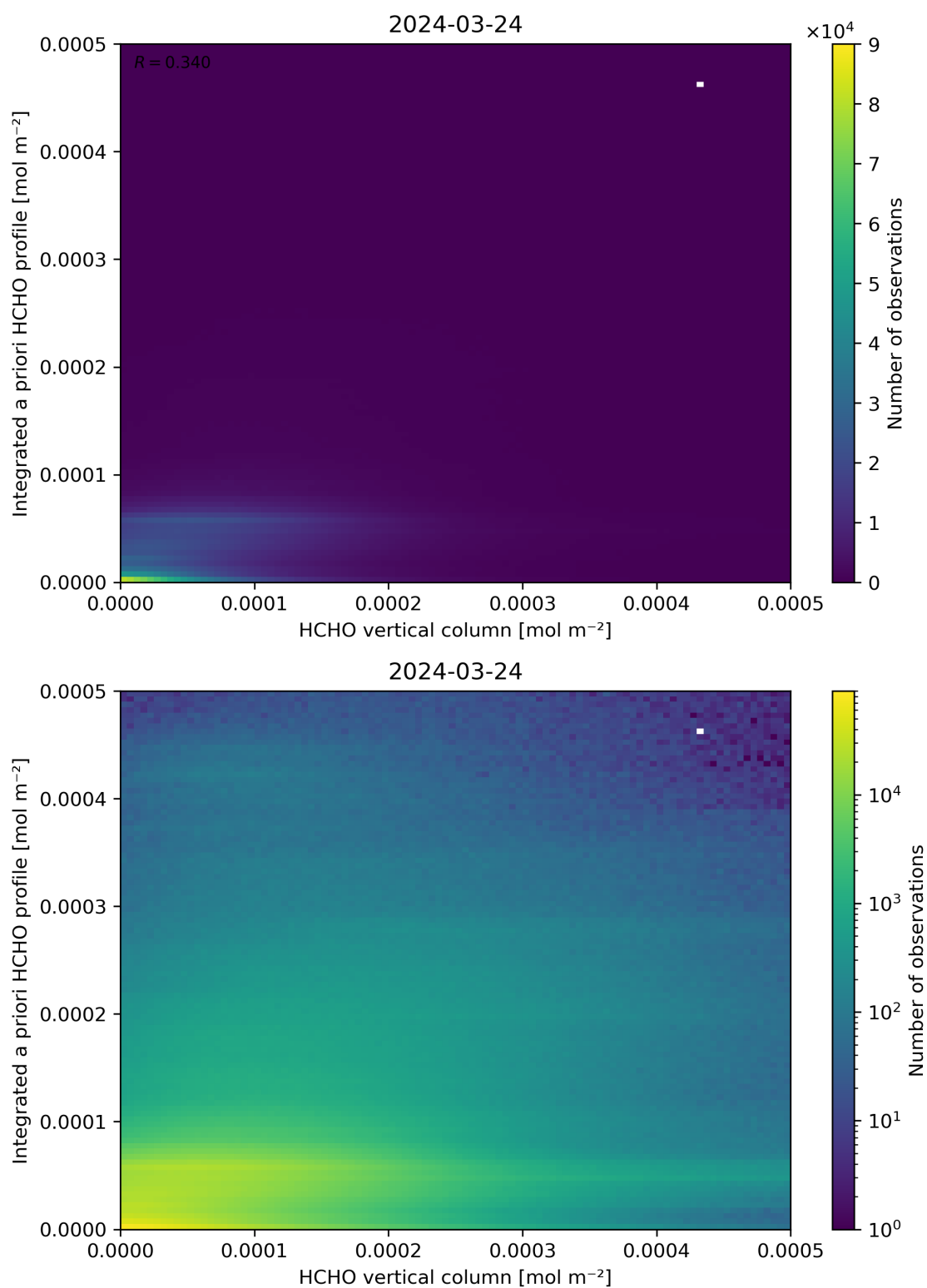
Figure 135: Scatter density plot of “HCHO vertical column” against “Integrated a priori HCHO profile” for 2024-03-23 to 2024-03-25.
