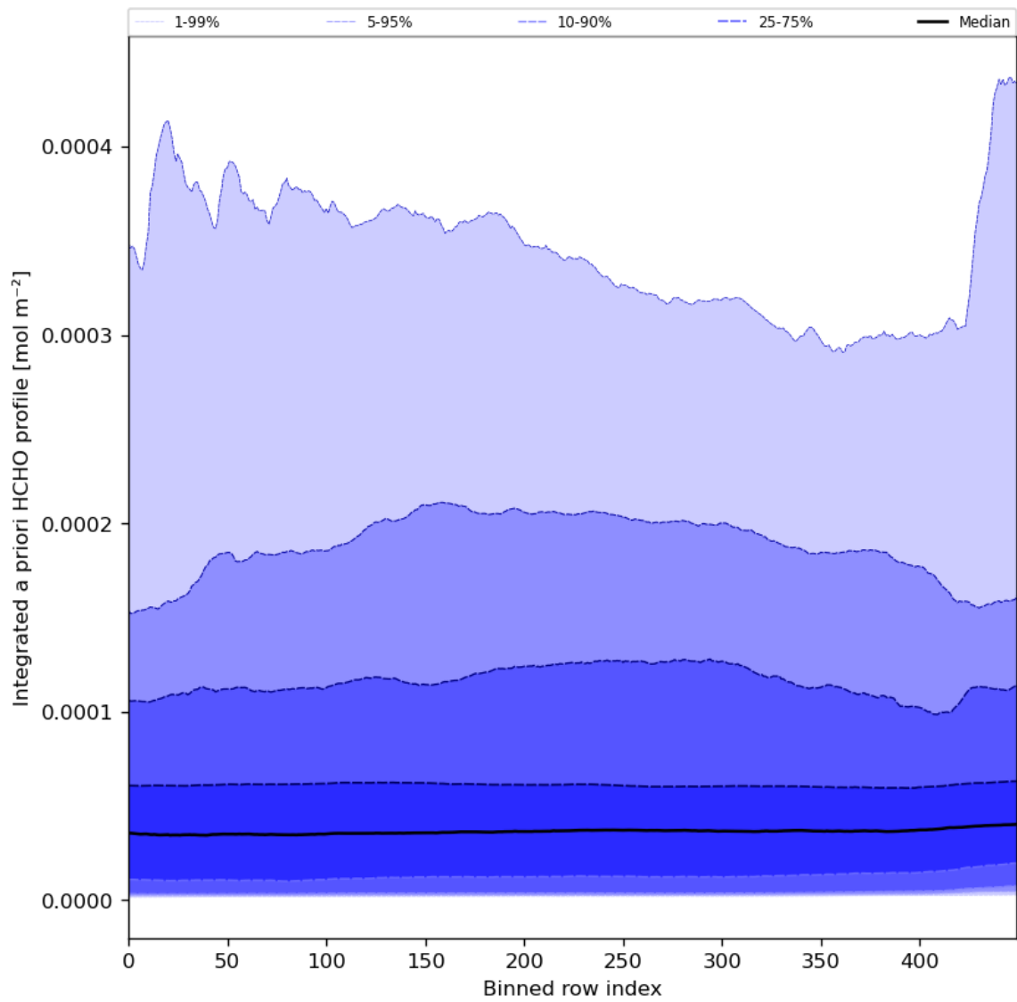
Figure 57: Along track statistics of “Integrated a priori HCHO profile” for 2024-03-23 to 2024-03-25
