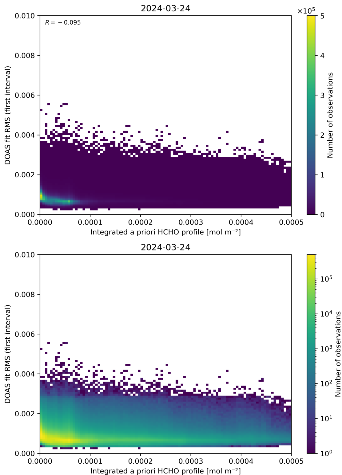
Figure 148: Scatter density plot of “Integrated a priori HCHO profile” against “DOAS fit RMS (first interval)” for 2024-03-23 to 2024-03-25.
