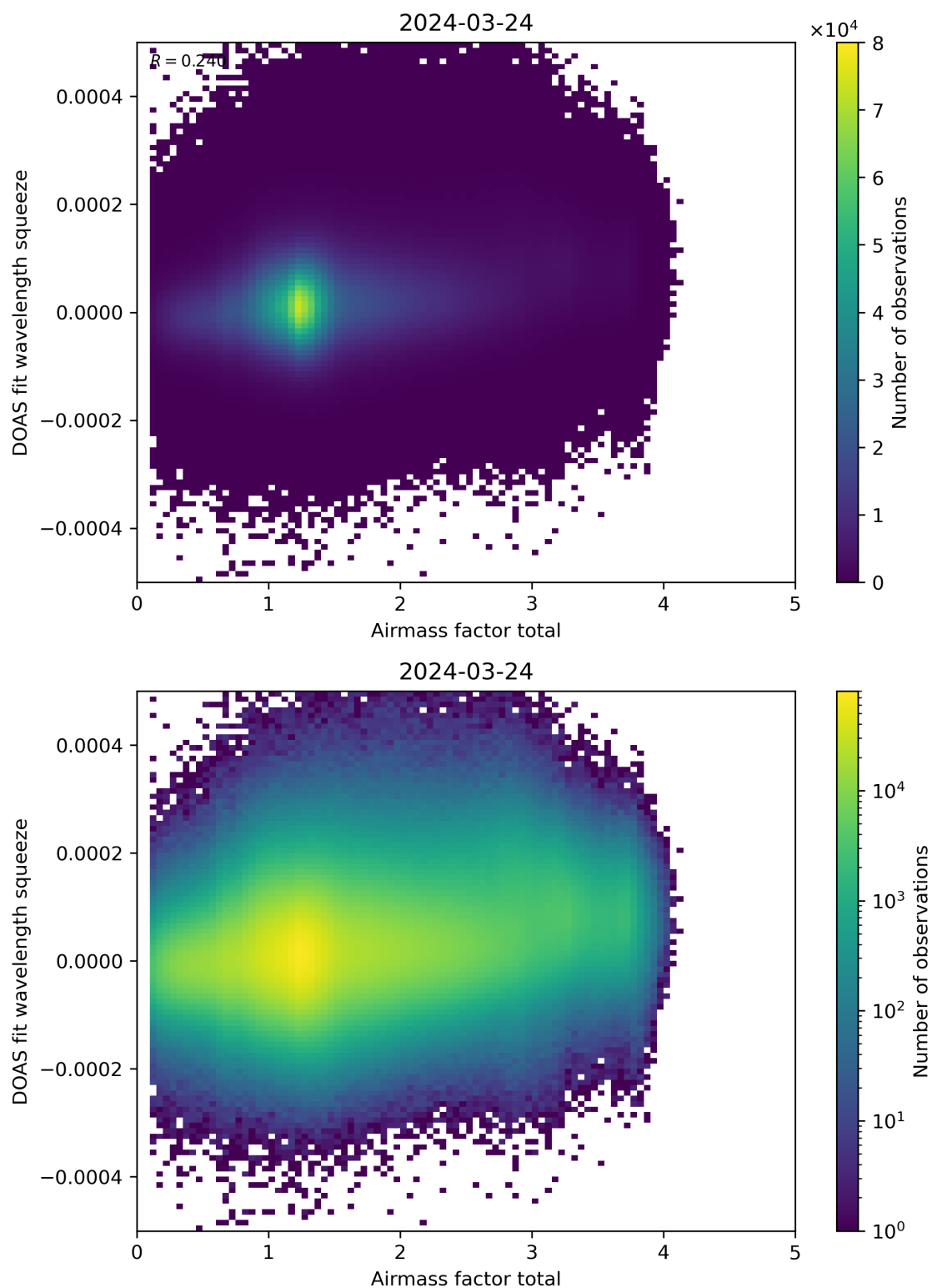
Figure 99: Scatter density plot of “Airmass factor total” against “DOAS fit wavelength squeeze” for 2024-03-23 to 2024-03-25.
