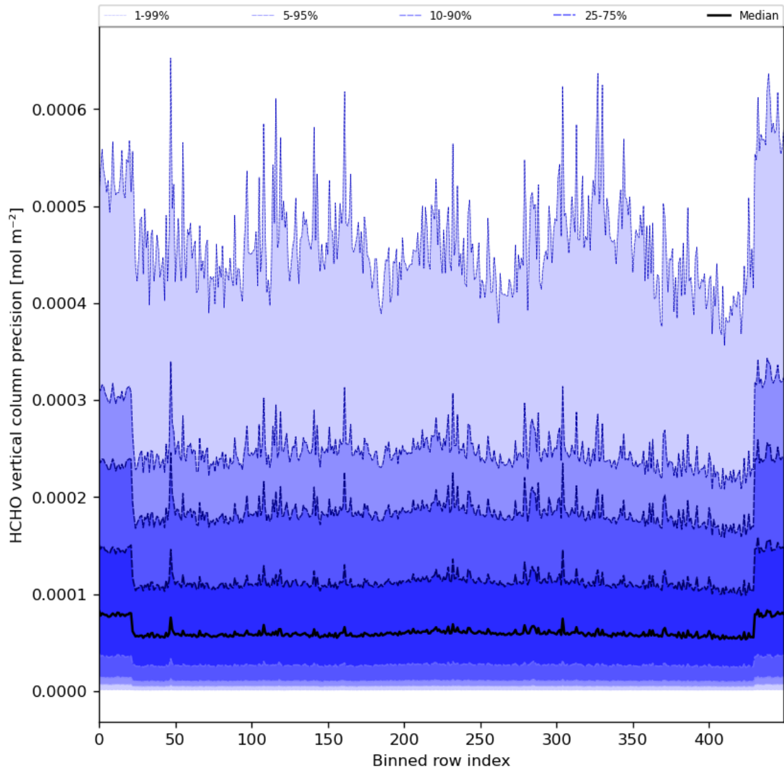
Figure 50: Along track statistics of “HCHO vertical column precision” for 2024-03-23 to 2024-03-25
