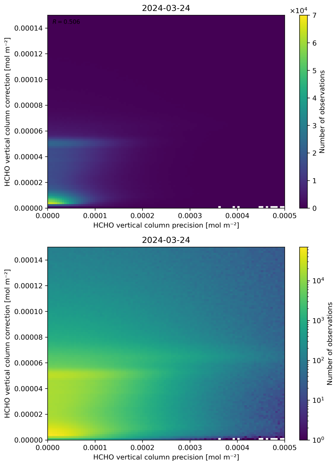
Figure 146: Scatter density plot of “HCHO vertical column precision” against “HCHO vertical column correction” for 2024-03-23 to 2024-03-25.
