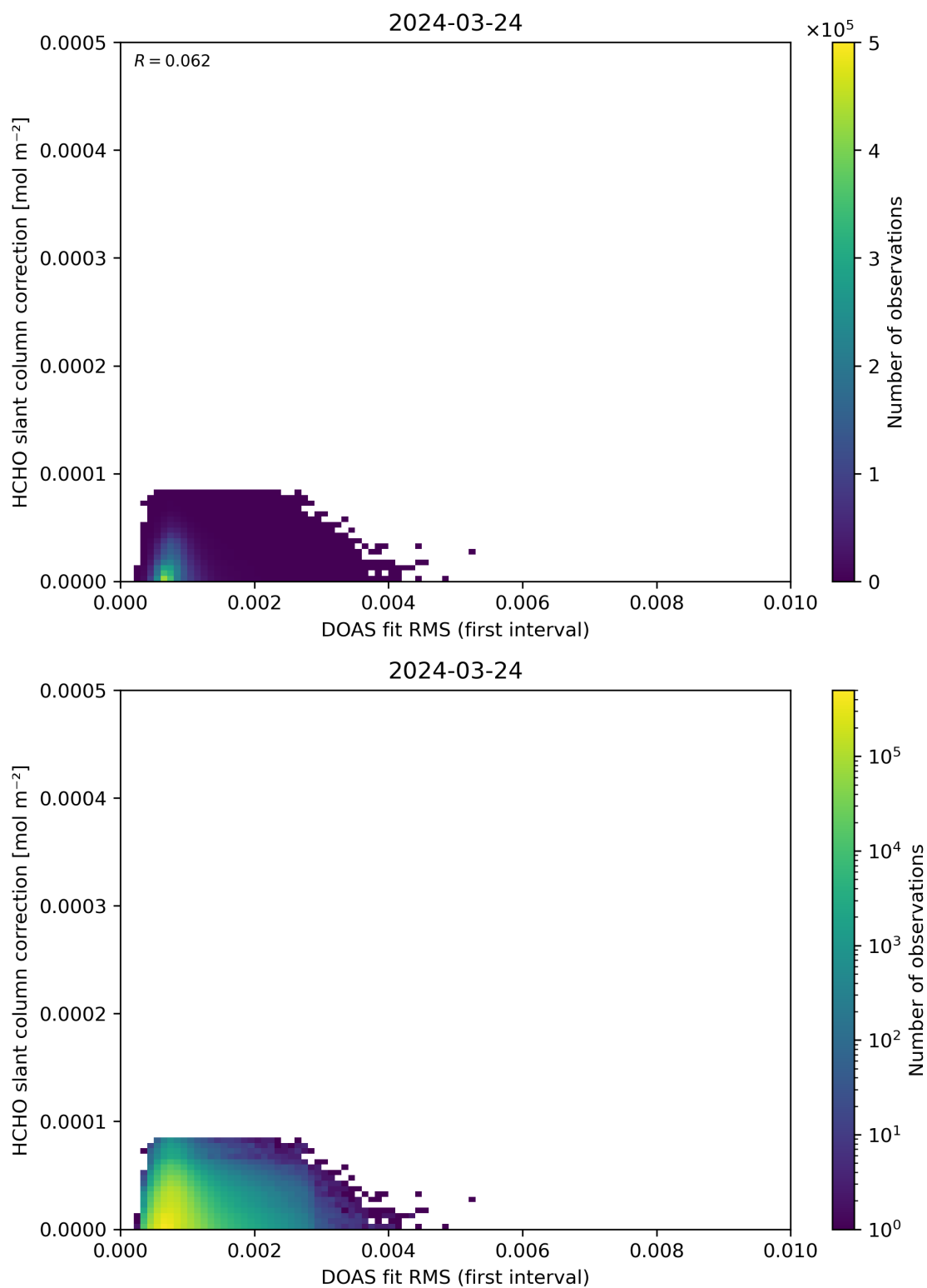
Figure 63: Scatter density plot of “DOAS fit RMS (first interval)” against “HCHO slant column correction” for 2024-03-23 to 2024-03-25.
