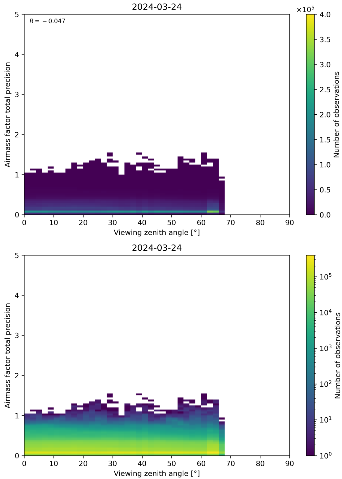
Figure 191: Scatter density plot of “Viewing zenith angle” against “Airmass factor total precision” for 2024-03-23 to 2024-03-25.
