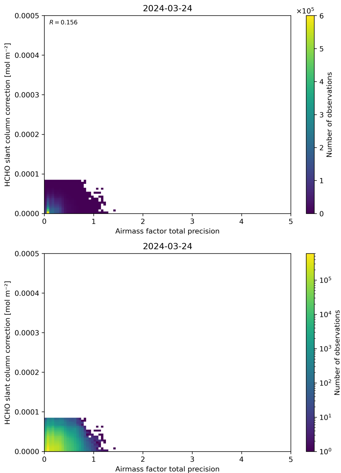
Figure 110: Scatter density plot of “Airmass factor total precision” against “HCHO slant column correction” for 2024-03-23 to 2024-03-25.
