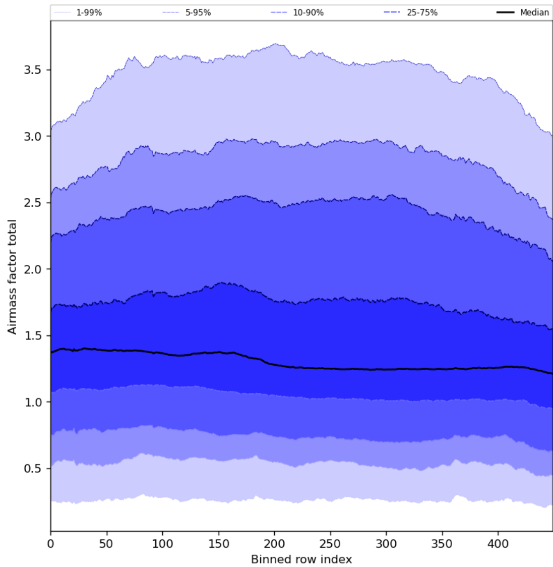
Figure 54: Along track statistics of “Airmass factor total” for 2024-03-23 to 2024-03-25
