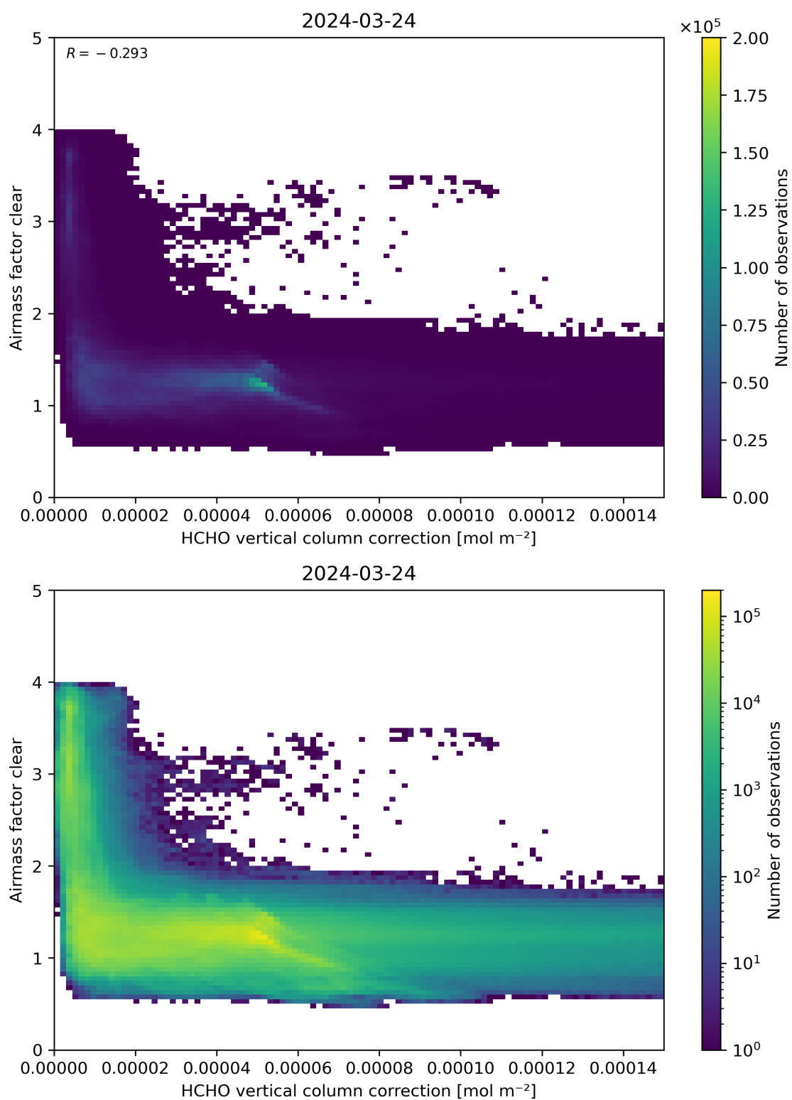
Figure 115: Scatter density plot of “HCHO vertical column correction” against “Airmass factor clear” for 2024-03-23 to 2024-03-25.
