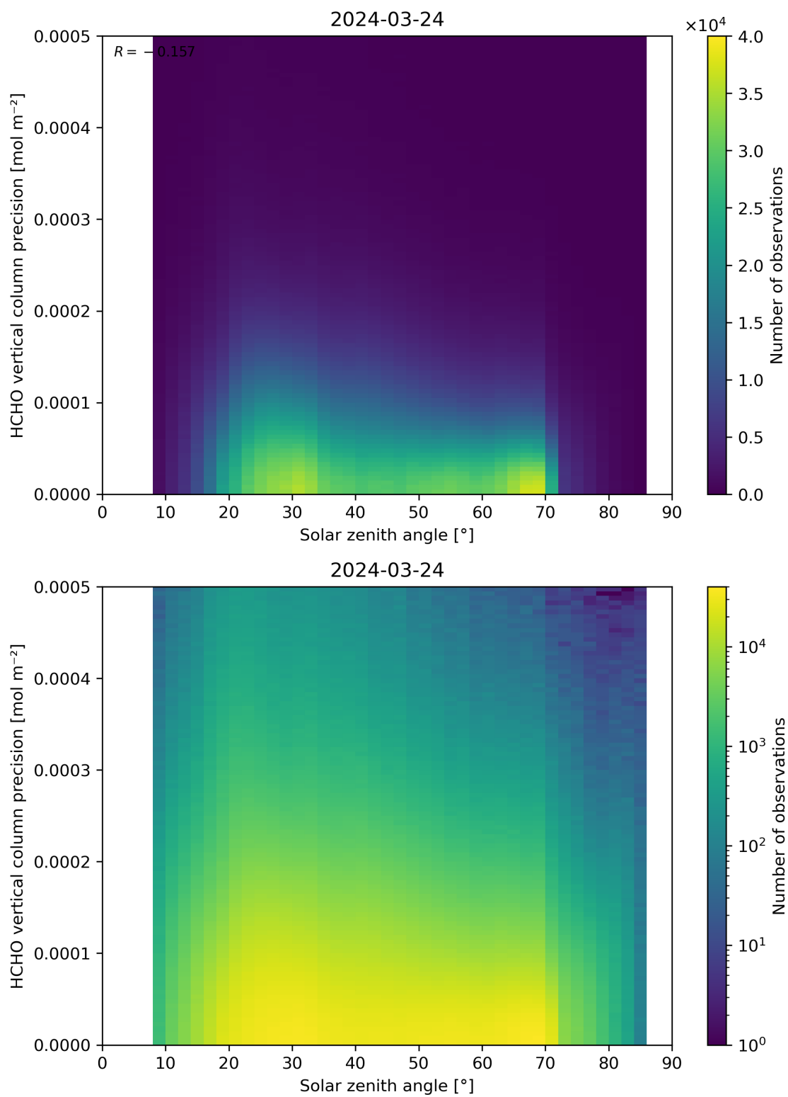
Figure 179: Scatter density plot of “Solar zenith angle” against “HCHO vertical column precision” for 2024-03-23 to 2024-03-25.
