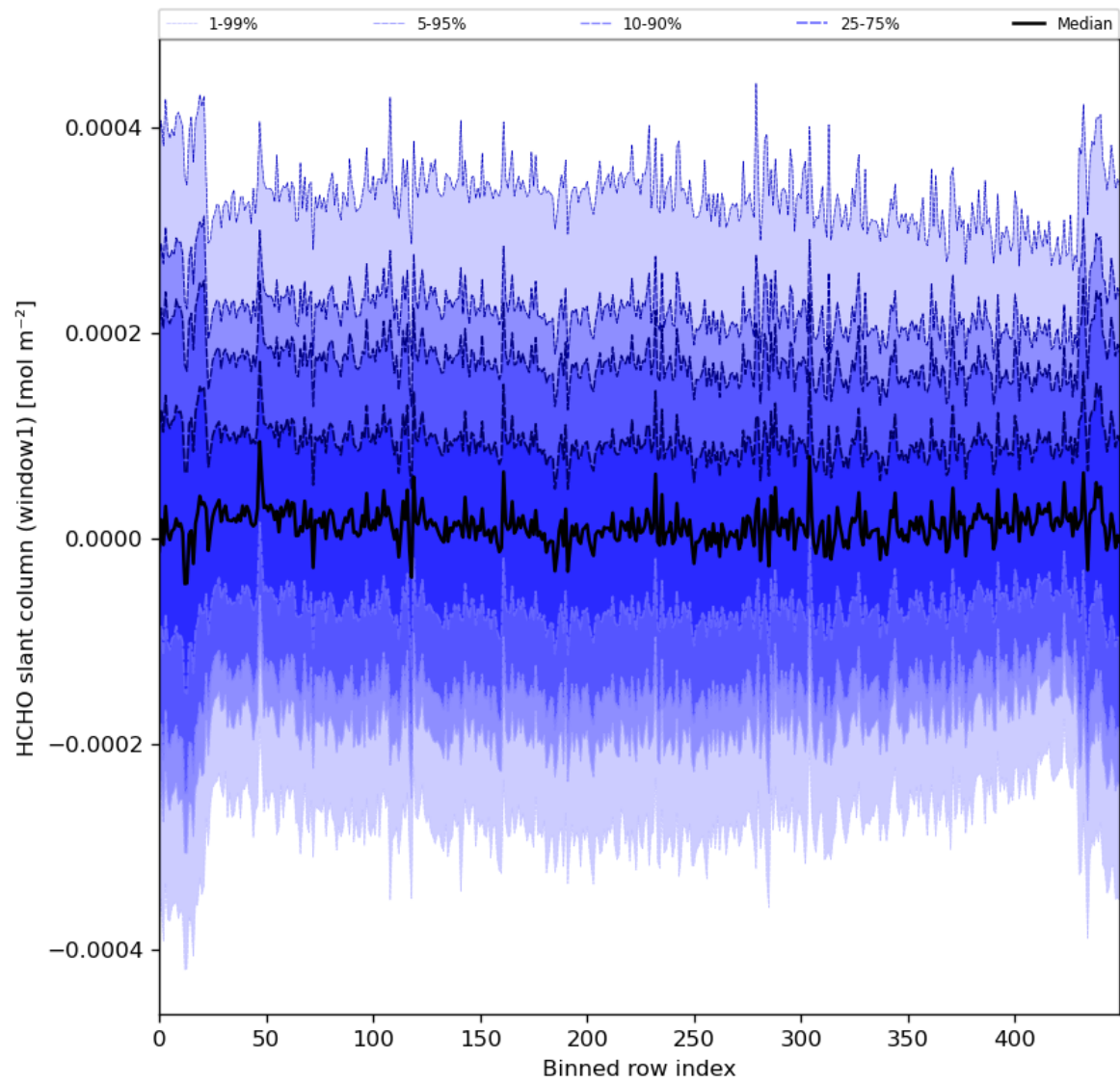
Figure 52: Along track statistics of “HCHO slant column (window1)” for 2024-03-23 to 2024-03-25
