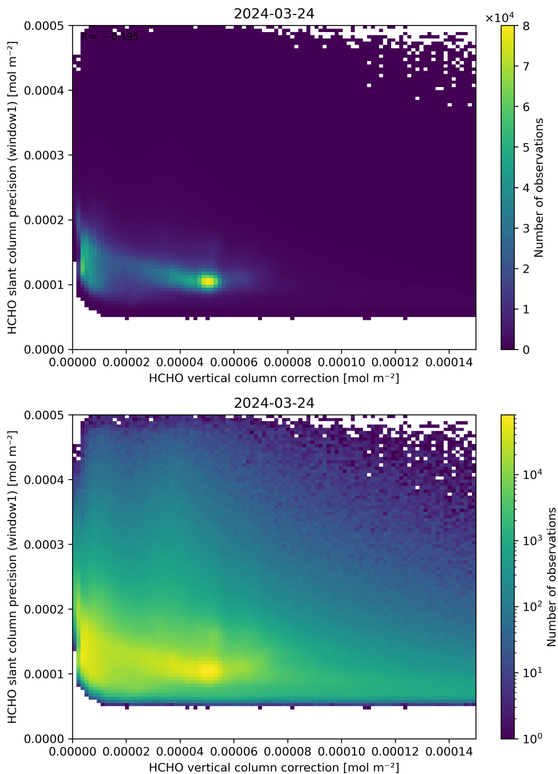
Figure 119: Scatter density plot of “HCHO vertical column correction” against “HCHO slant column precision (window1)” for 2024-03-23 to 2024-03-25.
