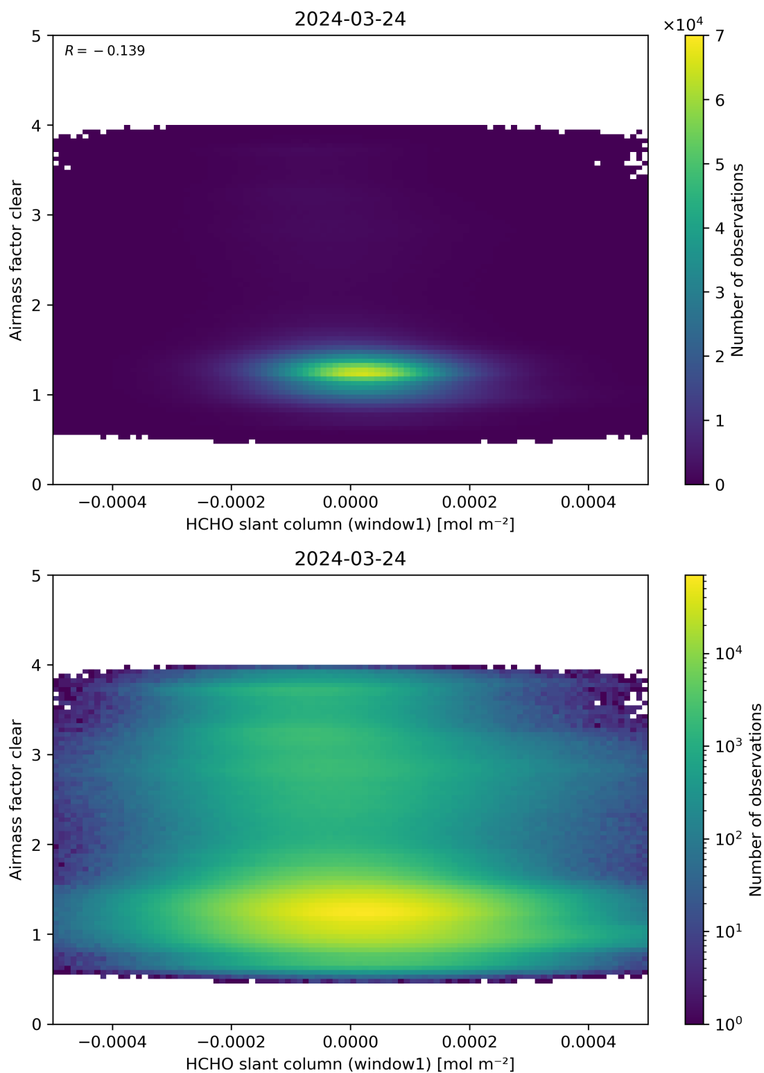
Figure 81: Scatter density plot of “HCHO slant column (window1)” against “Airmass factor clear” for 2024-03-23 to 2024-03-25.
