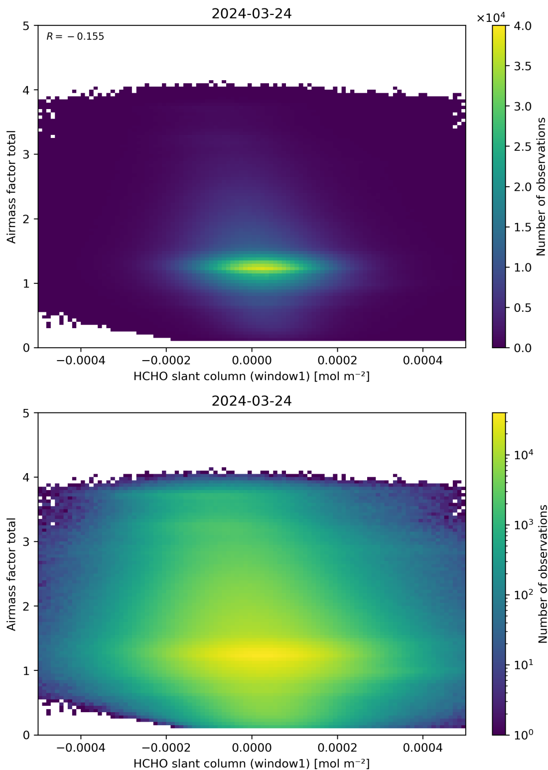
Figure 85: Scatter density plot of “HCHO slant column (window1)” against “Airmass factor total” for 2024-03-23 to 2024-03-25.
