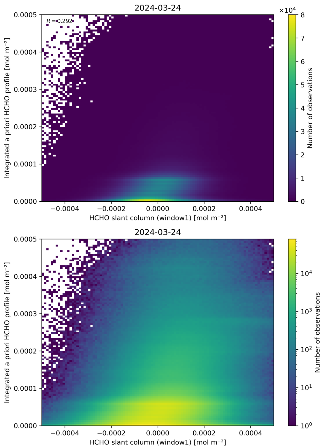
Figure 87: Scatter density plot of “HCHO slant column (window1)” against “Integrated a priori HCHO profile” for 2024-03-23 to 2024-03-25.
