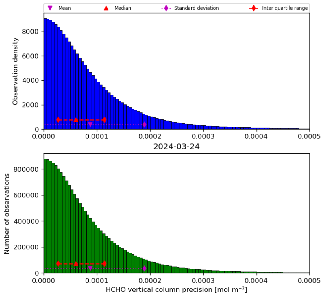
Figure 36: Histogram of “HCHO vertical column precision” for 2024-03-23 to 2024-03-25
