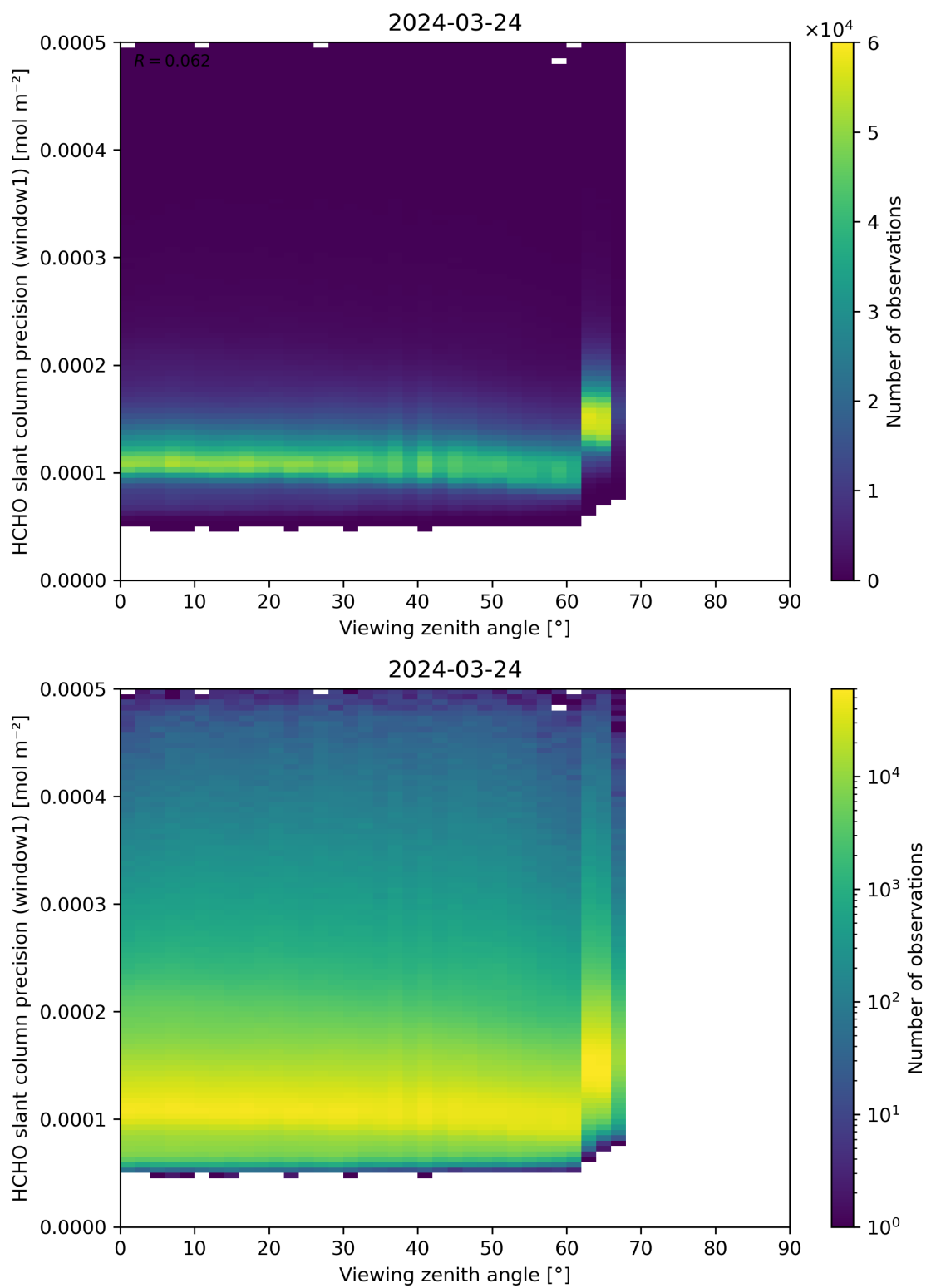
Figure 189: Scatter density plot of “Viewing zenith angle” against “HCHO slant column precision (window1)” for 2024-03-23 to 2024-03-25.
