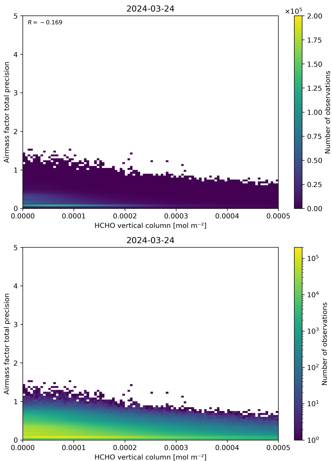
Figure 132: Scatter density plot of “HCHO vertical column” against “Airmass factor total precision” for 2024-03-23 to 2024-03-25.
