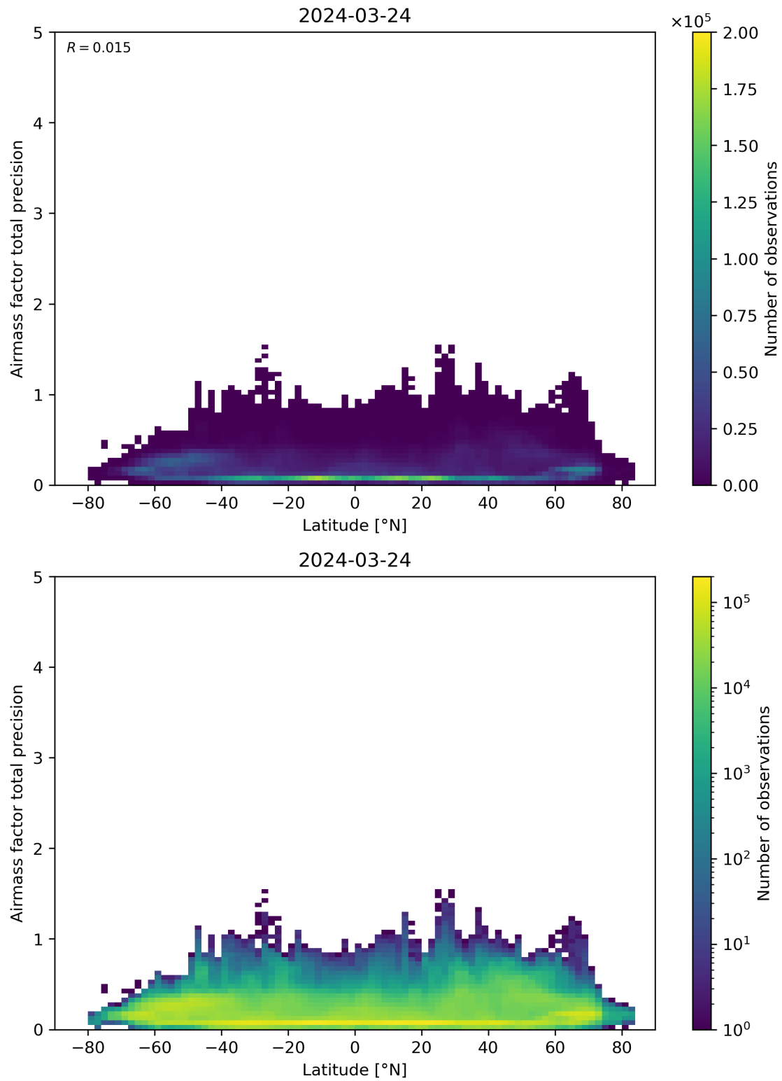
Figure 162: Scatter density plot of “Latitude” against “Airmass factor total precision” for 2024-03-23 to 2024-03-25.
