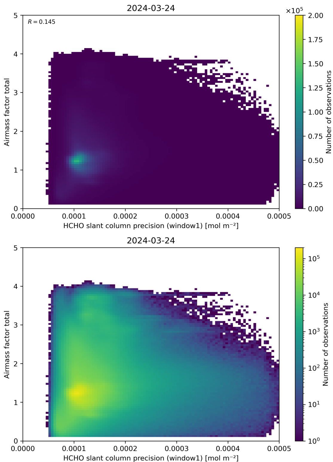
Figure 94: Scatter density plot of “HCHO slant column precision (window1)” against “Airmass factor total” for 2024-03-23 to 2024-03-25.
