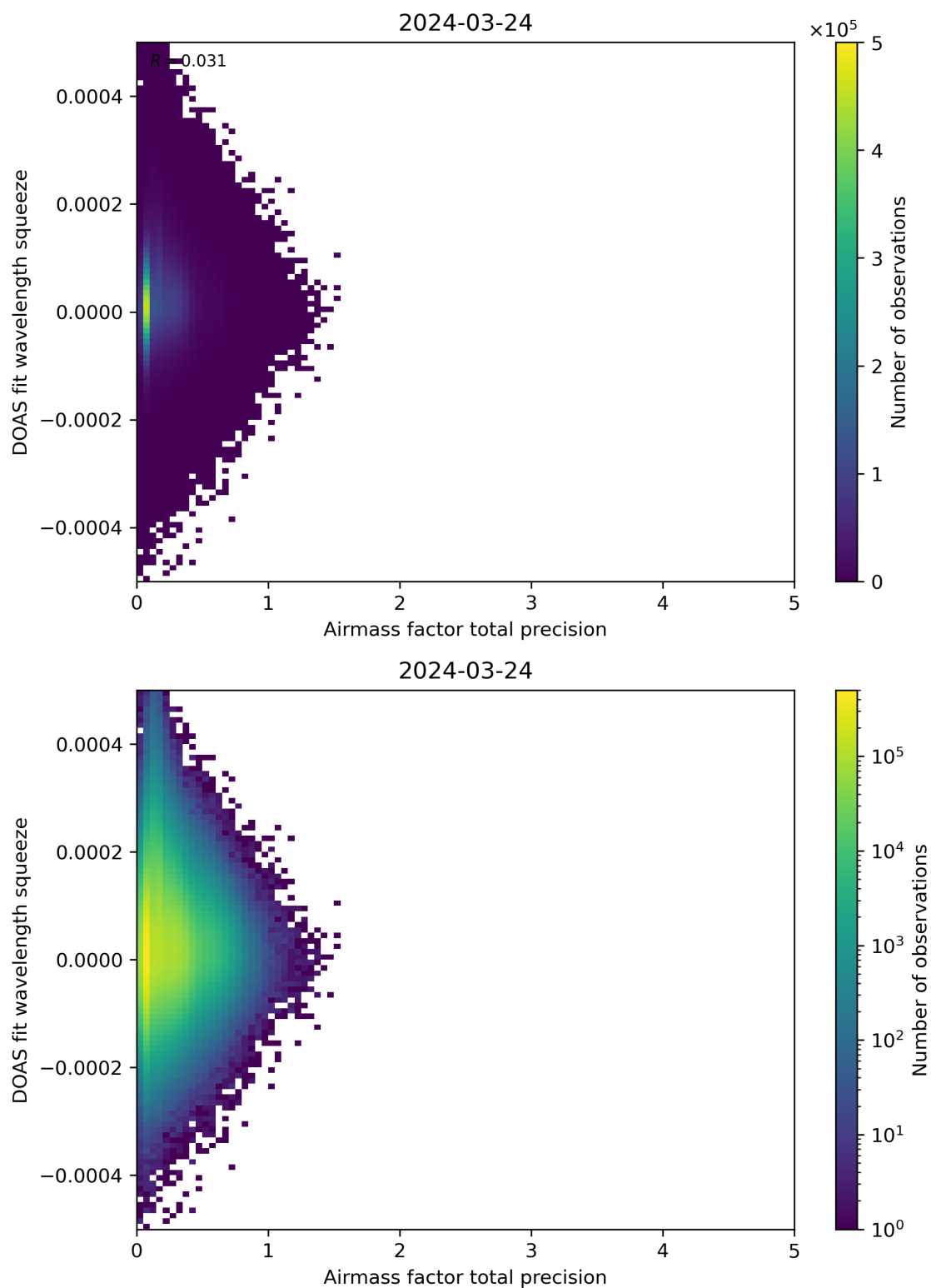
Figure 107: Scatter density plot of “Airmass factor total precision” against “DOAS fit wavelength squeeze” for 2024-03-23 to 2024-03-25.
