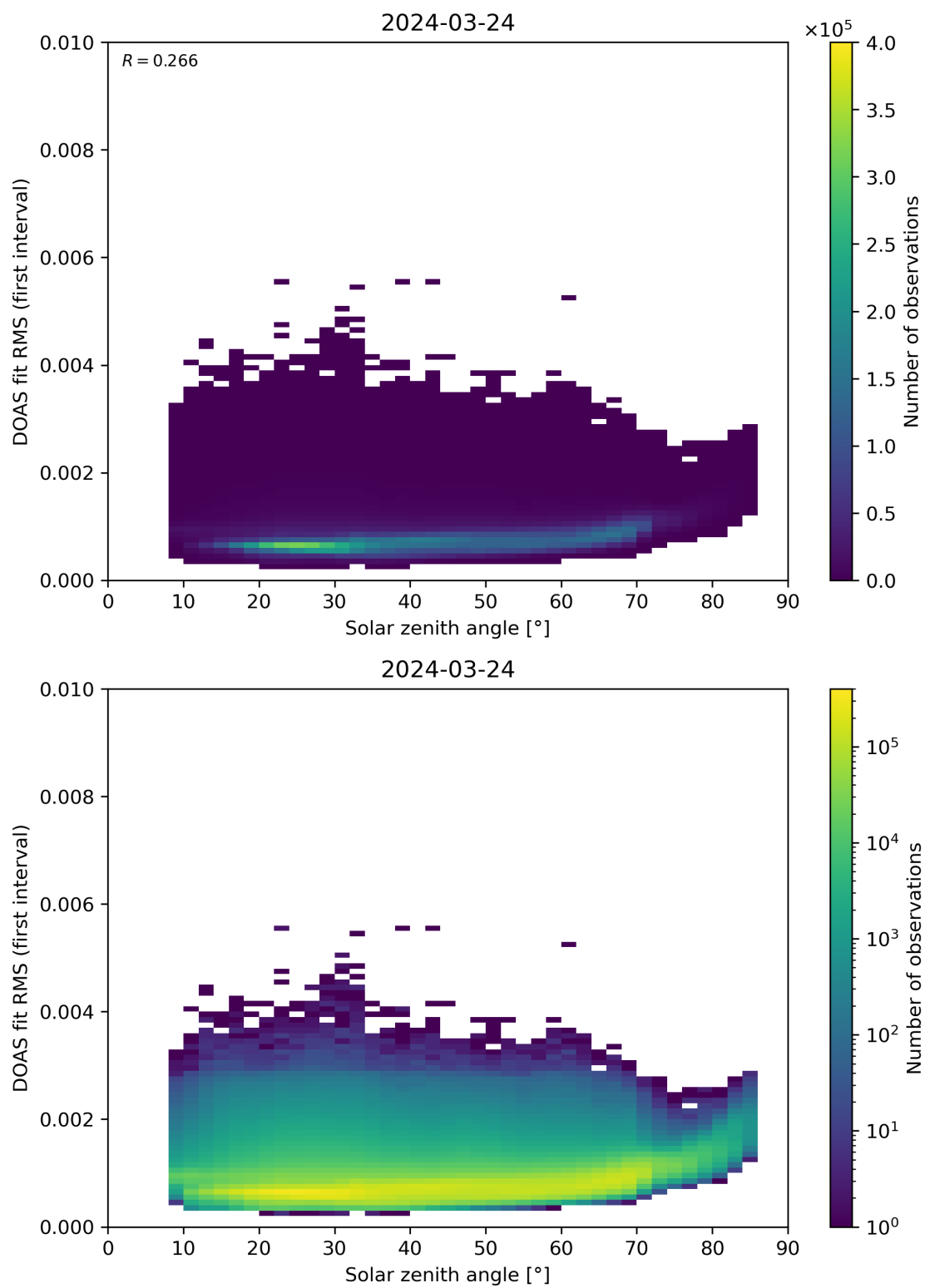
Figure 167: Scatter density plot of “Solar zenith angle” against “DOAS fit RMS (first interval)” for 2024-03-23 to 2024-03-25.
