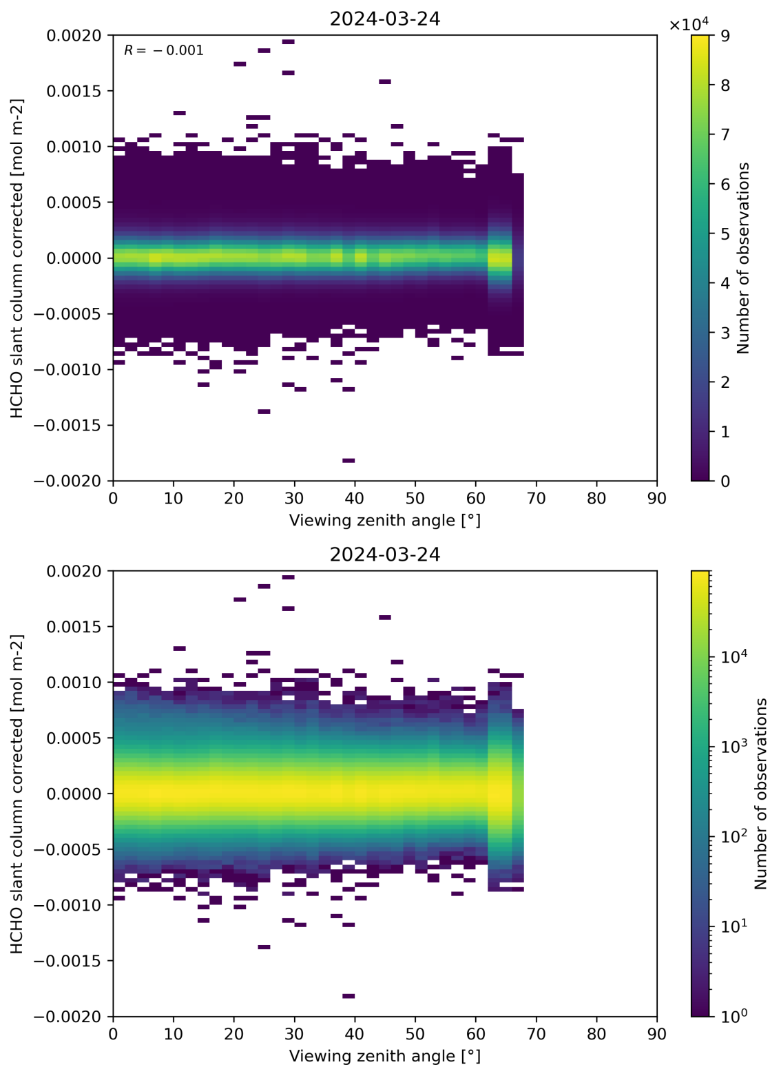
Figure 186: Scatter density plot of “Viewing zenith angle” against “HCHO slant column corrected” for 2024-03-23 to 2024-03-25.
