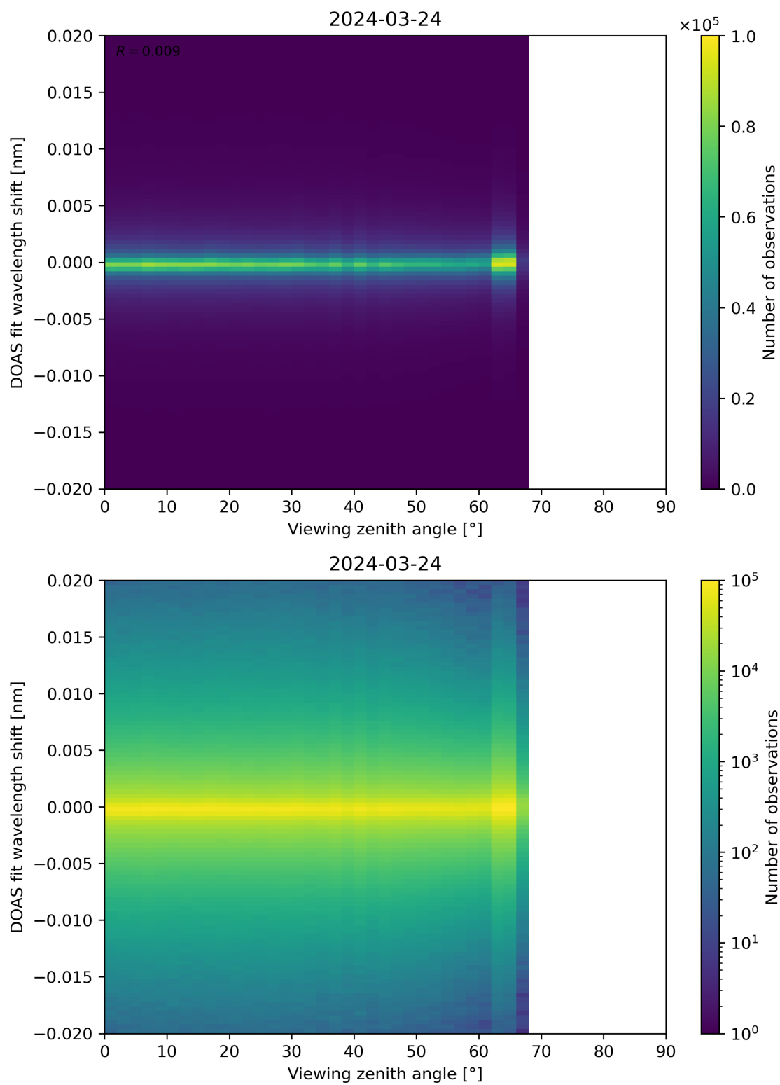
Figure 183: Scatter density plot of “Viewing zenith angle” against “DOAS fit wavelength shift” for 2024-03-23 to 2024-03-25.
