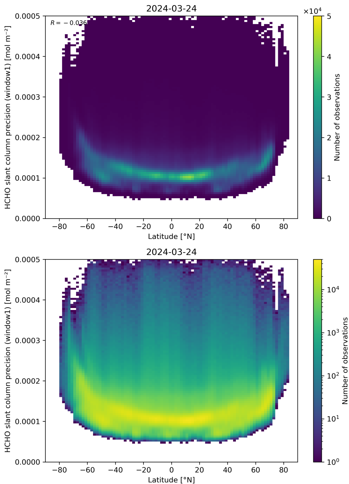
Figure 160: Scatter density plot of “Latitude” against “HCHO slant column precision (window1)” for 2024-03-23 to 2024-03-25.
