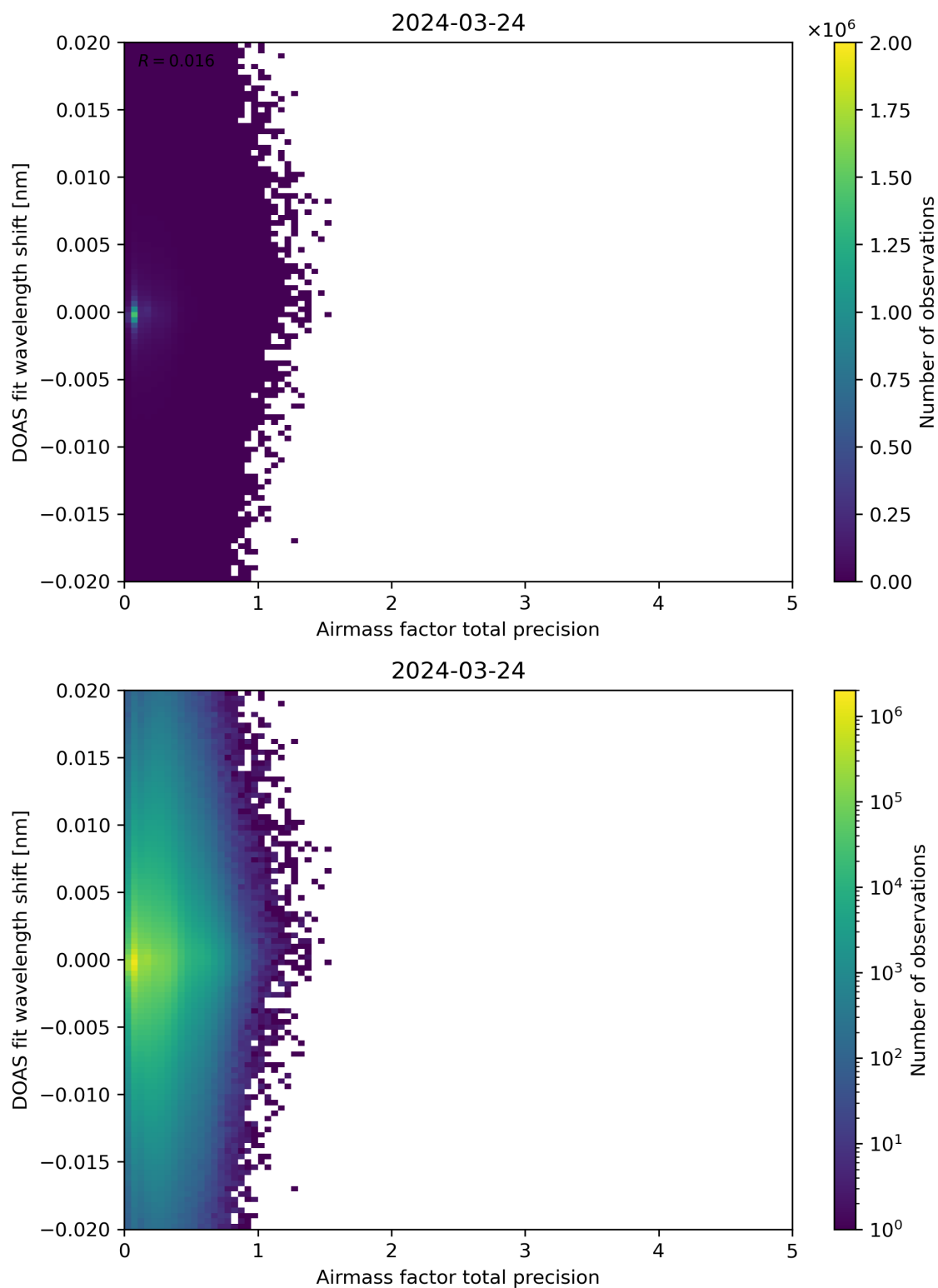
Figure 106: Scatter density plot of “Airmass factor total precision” against “DOAS fit wavelength shift” for 2024-03-23 to 2024-03-25.
