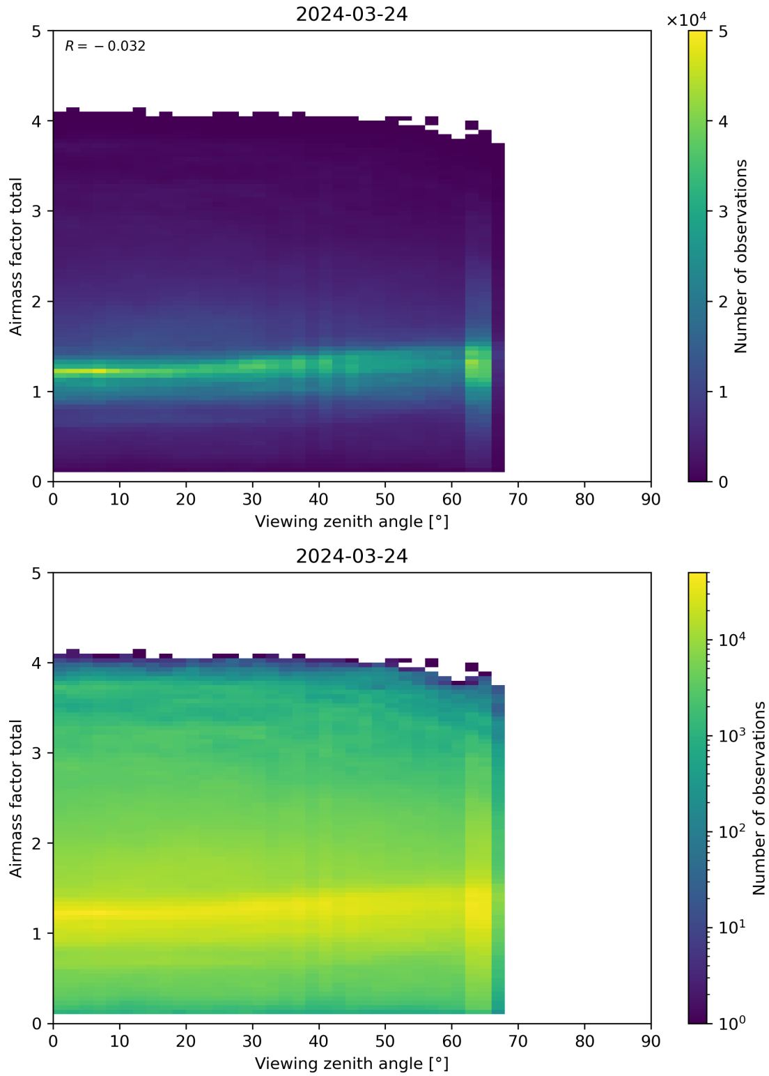
Figure 190: Scatter density plot of “Viewing zenith angle” against “Airmass factor total” for 2024-03-23 to 2024-03-25.
