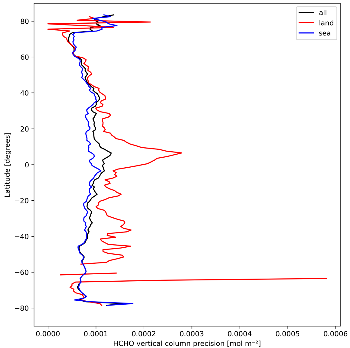
Figure 22: Zonal average of “HCHO vertical column precision” for 2024-03-23 to 2024-03-25.
