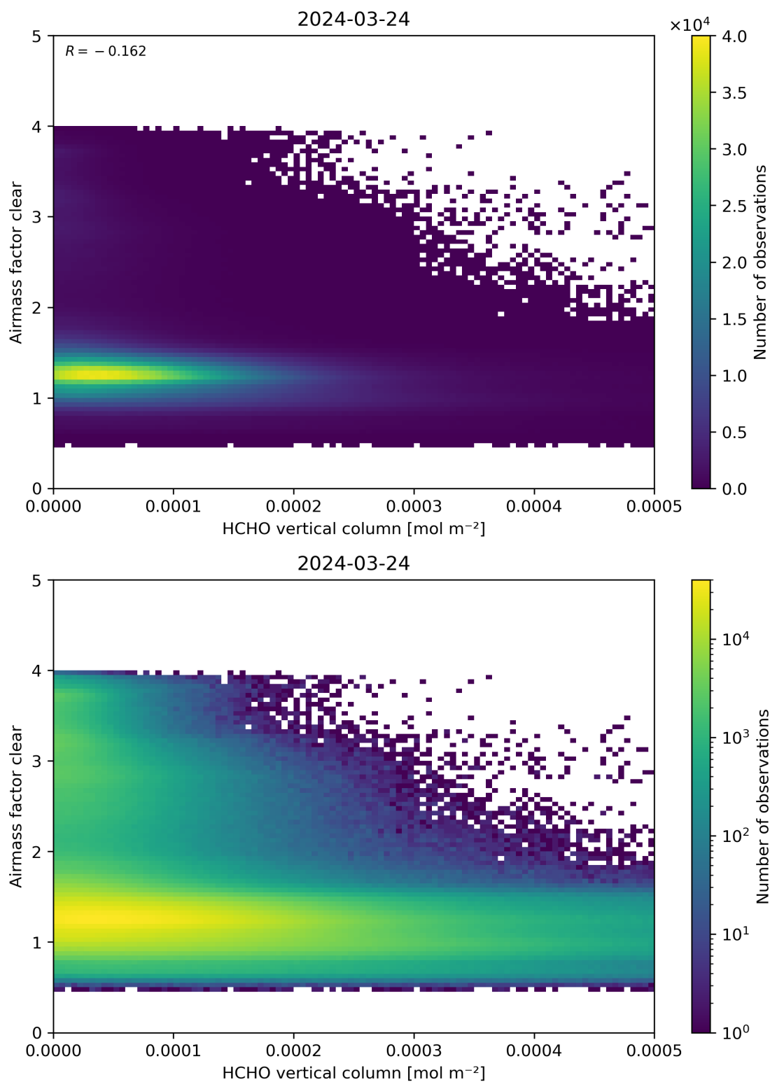
Figure 126: Scatter density plot of “HCHO vertical column” against “Airmass factor clear” for 2024-03-23 to 2024-03-25.
