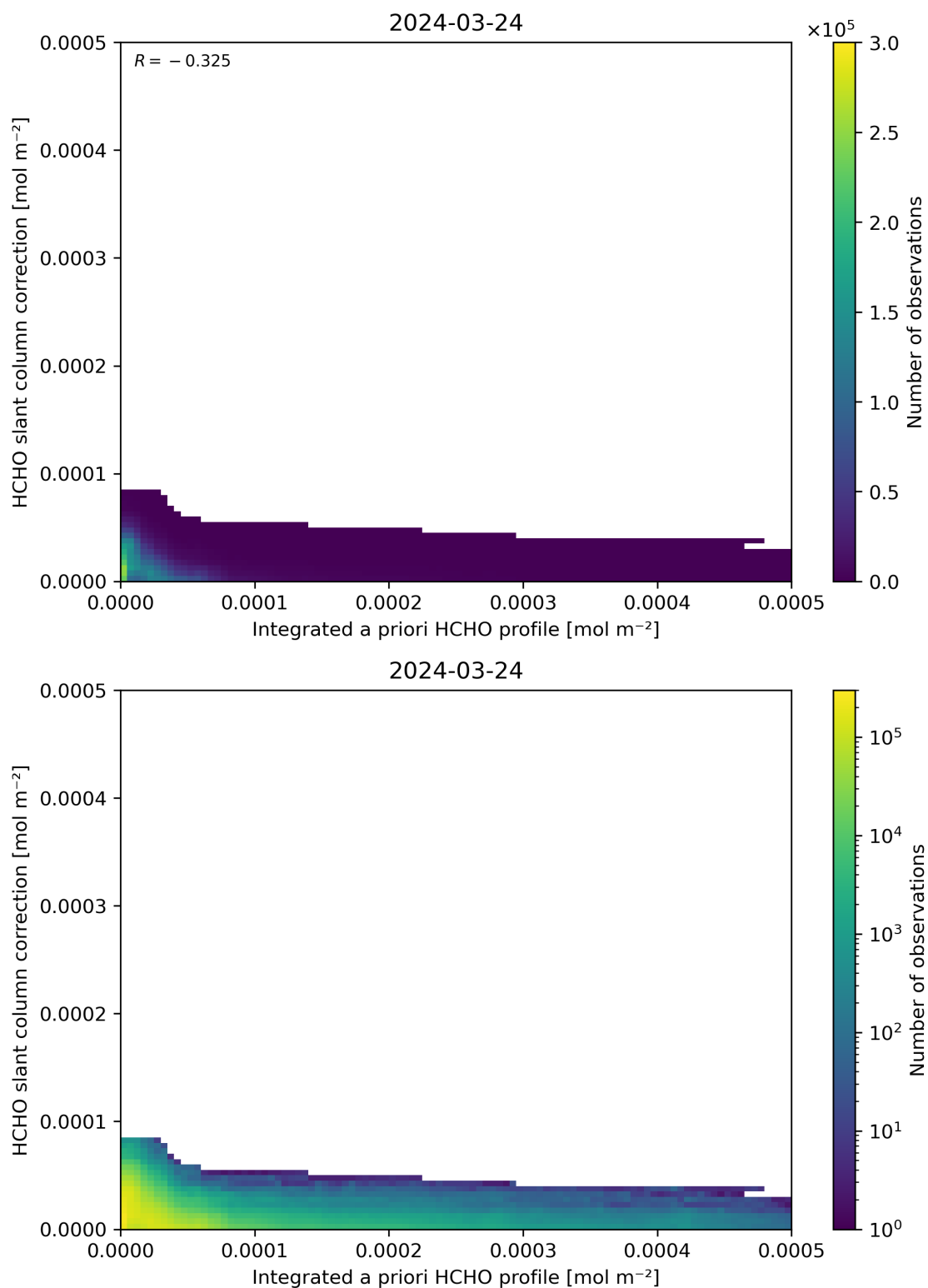
Figure 152: Scatter density plot of “Integrated a priori HCHO profile” against “HCHO slant column correction” for 2024-03-23 to 2024-03-25.
