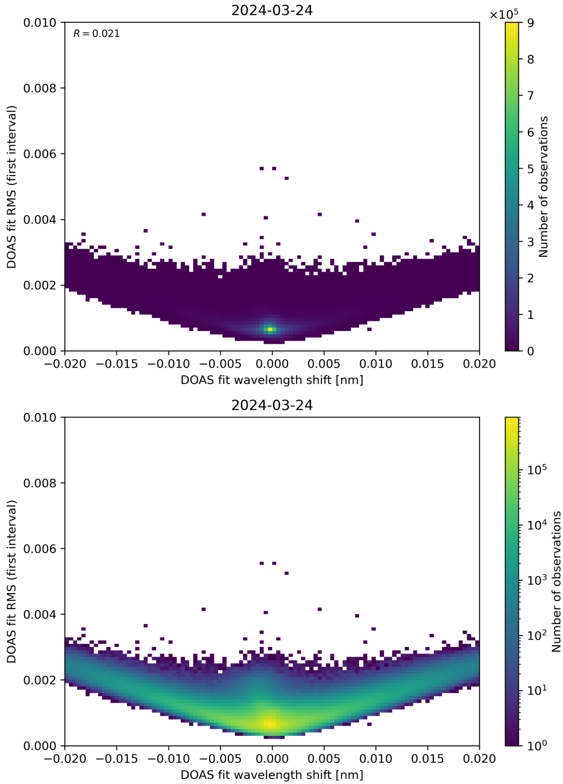
Figure 64: Scatter density plot of “DOAS fit wavelength shift” against “DOAS fit RMS (first interval)” for 2024-03-23 to 2024-03-25.
