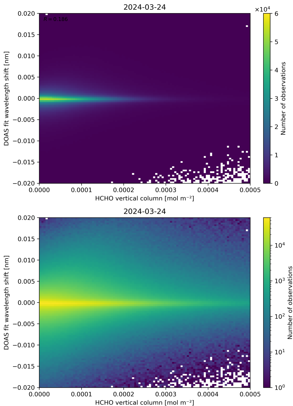
Figure 124: Scatter density plot of “HCHO vertical column” against “DOAS fit wavelength shift” for 2024-03-23 to 2024-03-25.
