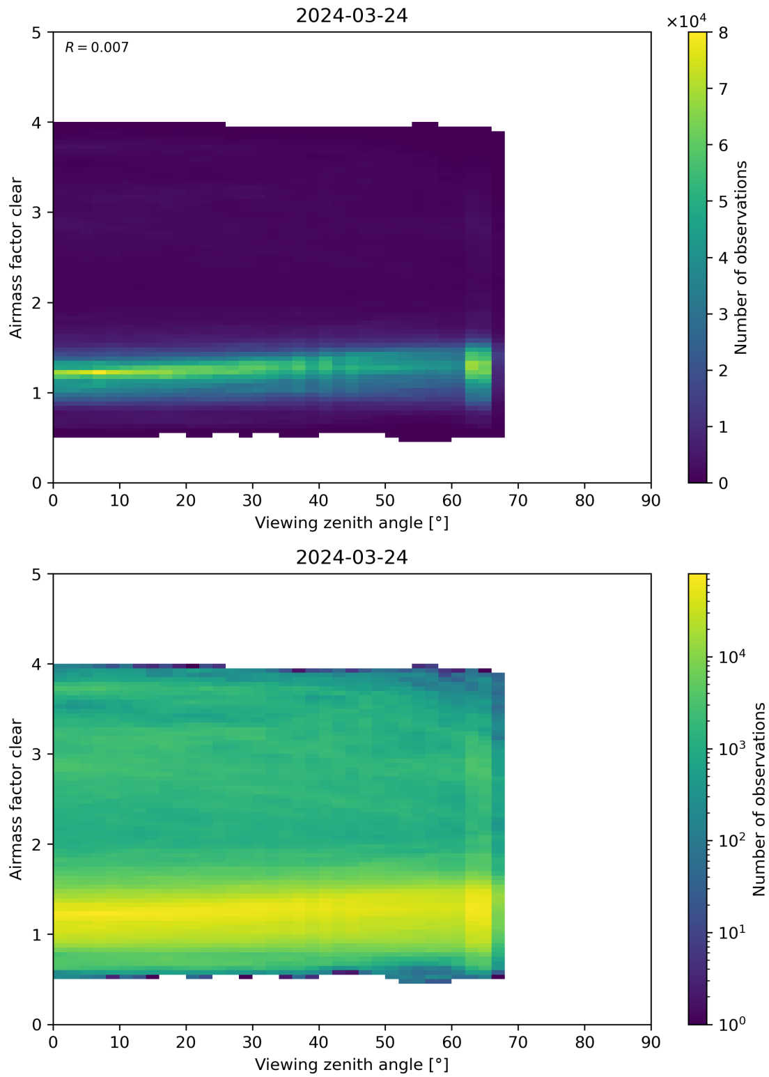
Figure 185: Scatter density plot of “Viewing zenith angle” against “Airmass factor clear” for 2024-03-23 to 2024-03-25.
