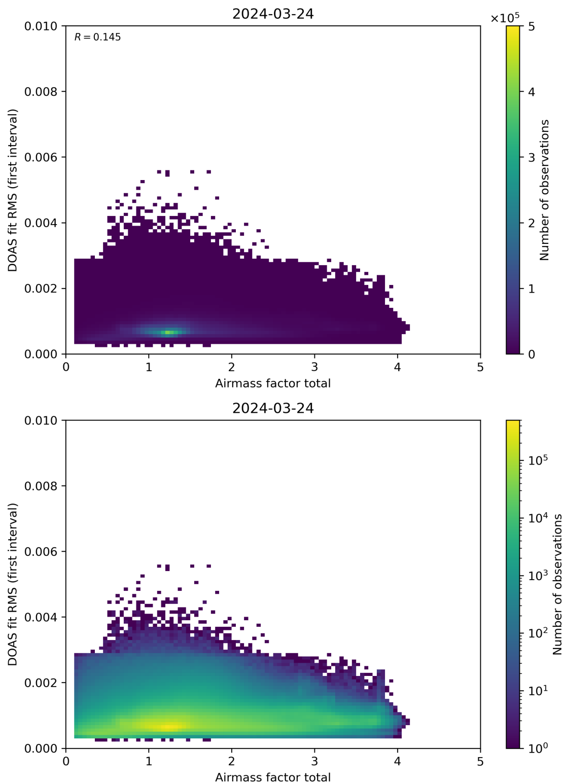
Figure 97: Scatter density plot of “Airmass factor total” against “DOAS fit RMS (first interval)” for 2024-03-23 to 2024-03-25.
