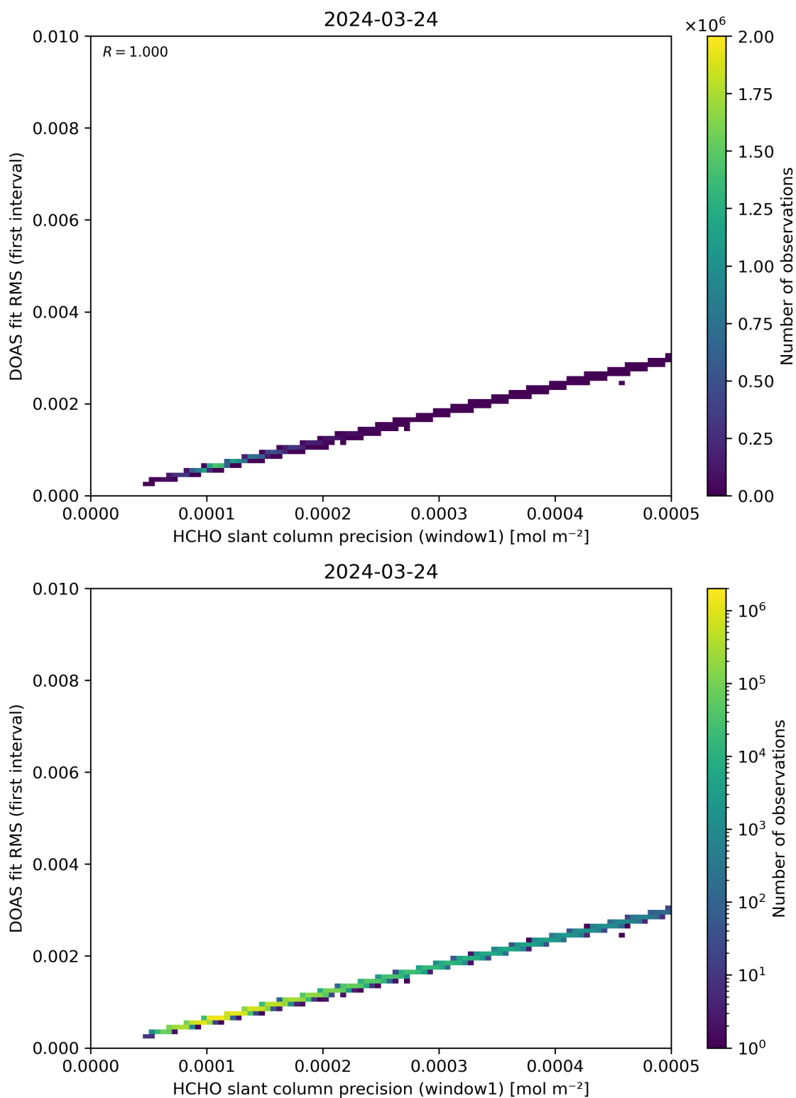
Figure 88: Scatter density plot of “HCHO slant column precision (window1)” against “DOAS fit RMS (first interval)” for 2024-03-23 to 2024-03-25.
