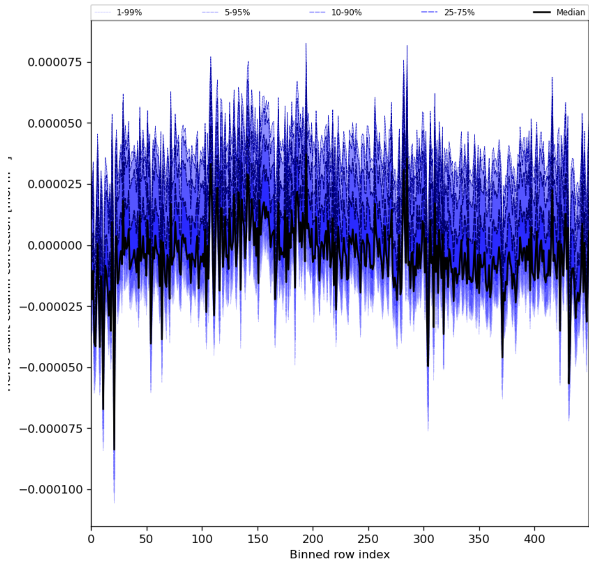
Figure 61: Along track statistics of “HCHO slant column correction” for 2024-03-23 to 2024-03-25
