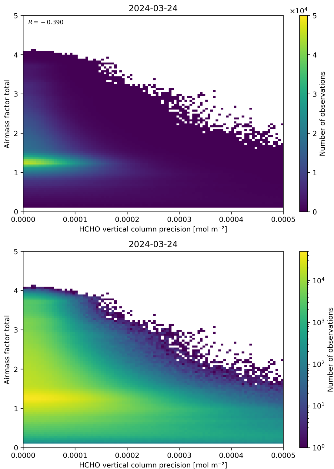
Figure 144: Scatter density plot of “HCHO vertical column precision” against “Airmass factor total” for 2024-03-23 to 2024-03-25.
