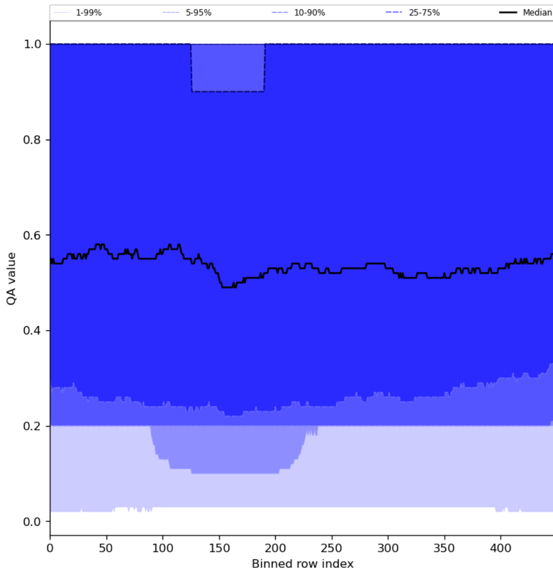
Figure 48: Along track statistics of “QA value” for 2024-03-23 to 2024-03-25
