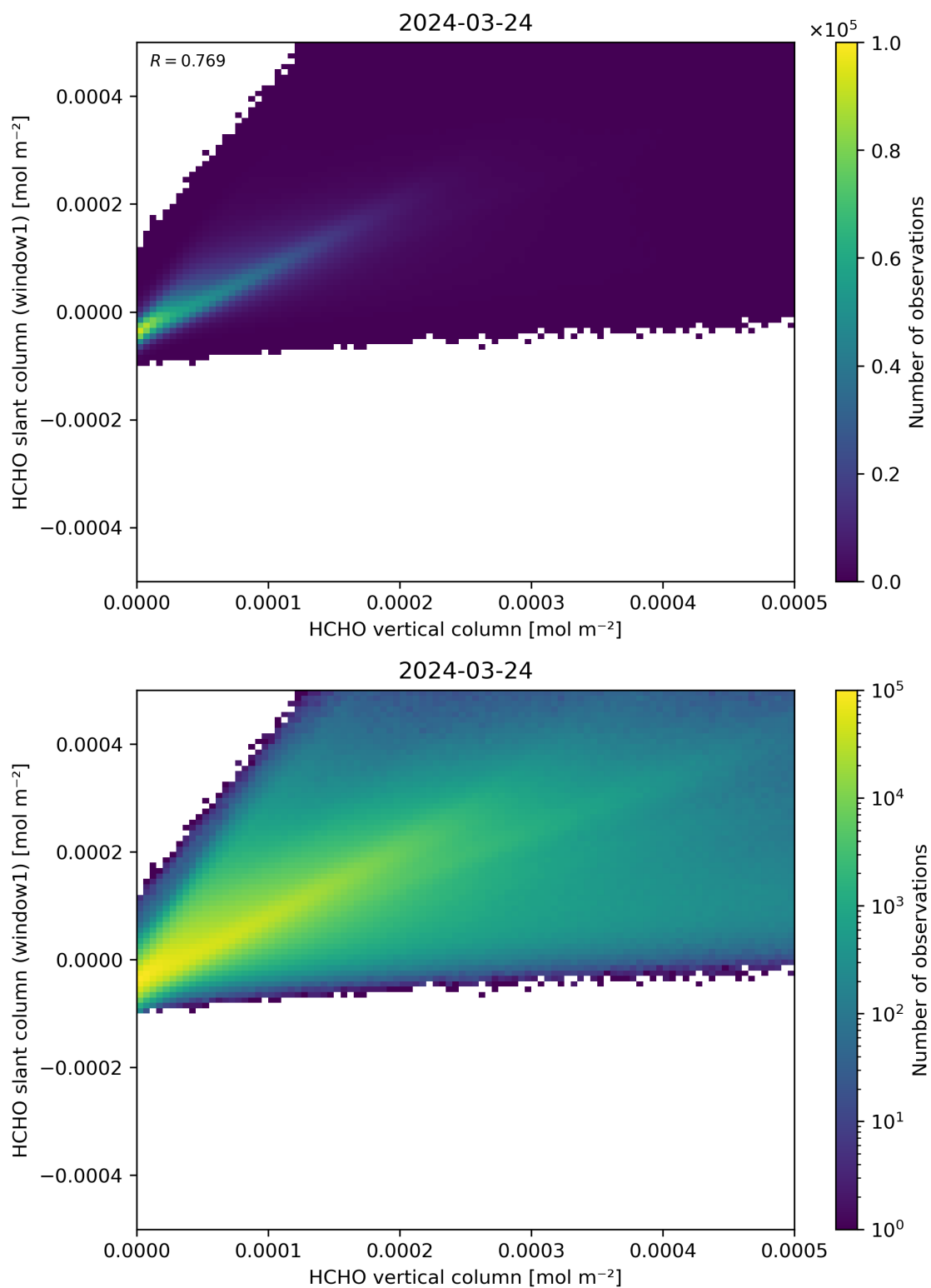
Figure 129: Scatter density plot of “HCHO vertical column” against “HCHO slant column (window1)” for 2024-03-23 to 2024-03-25.
