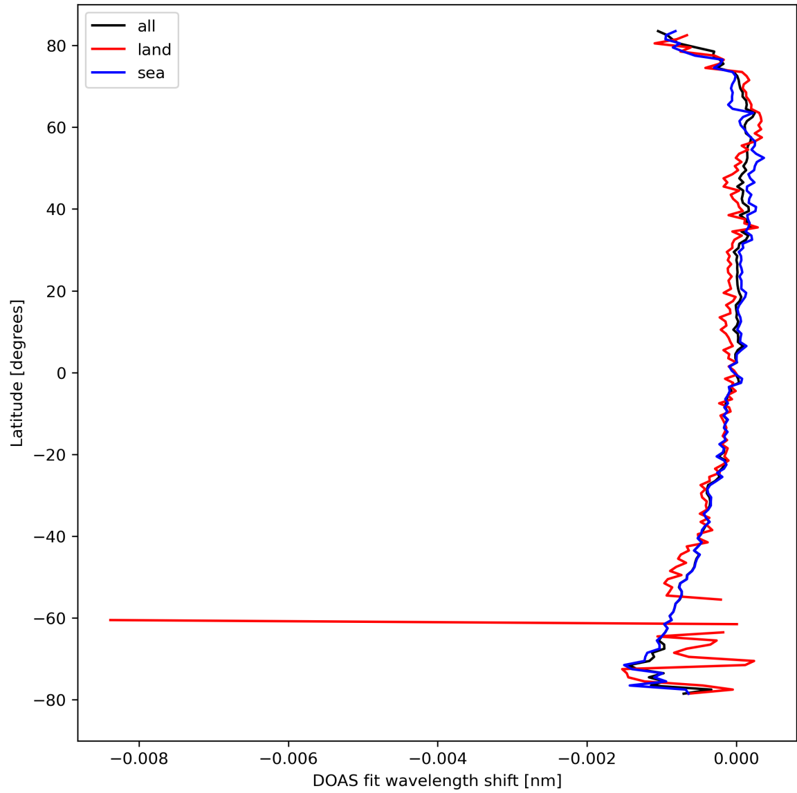
Figure 30: Zonal average of “DOAS fit wavelength shift” for 2024-03-23 to 2024-03-25.
