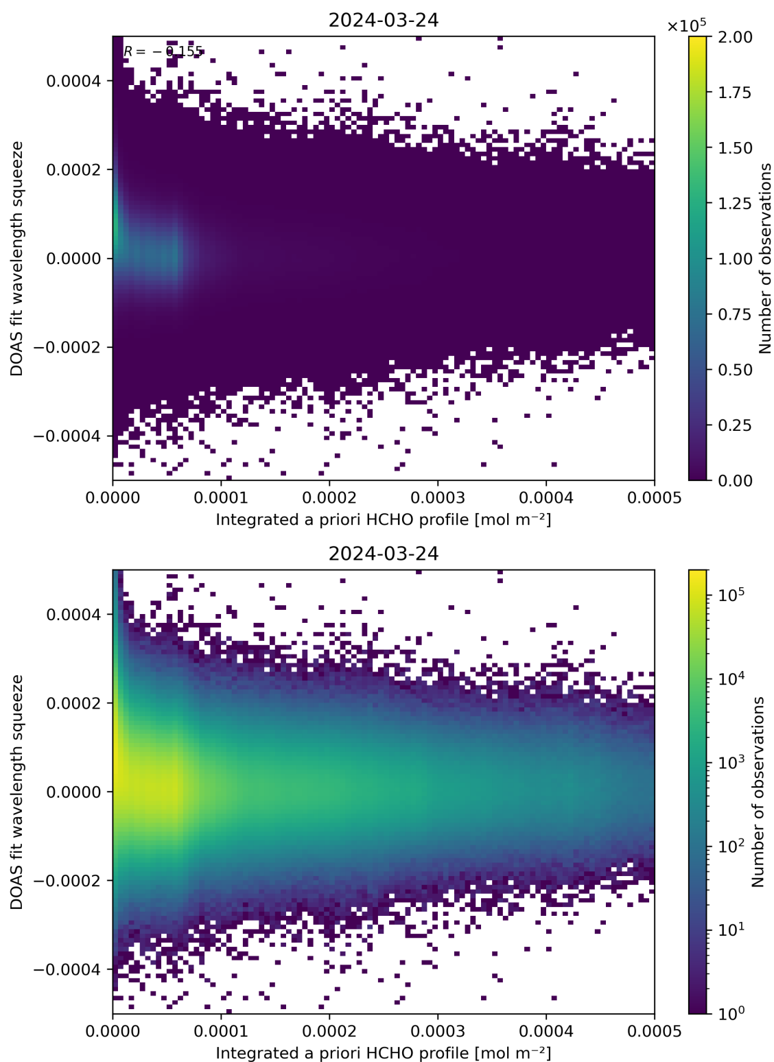
Figure 150: Scatter density plot of “Integrated a priori HCHO profile” against “DOAS fit wavelength squeeze” for 2024-03-23 to 2024-03-25.
