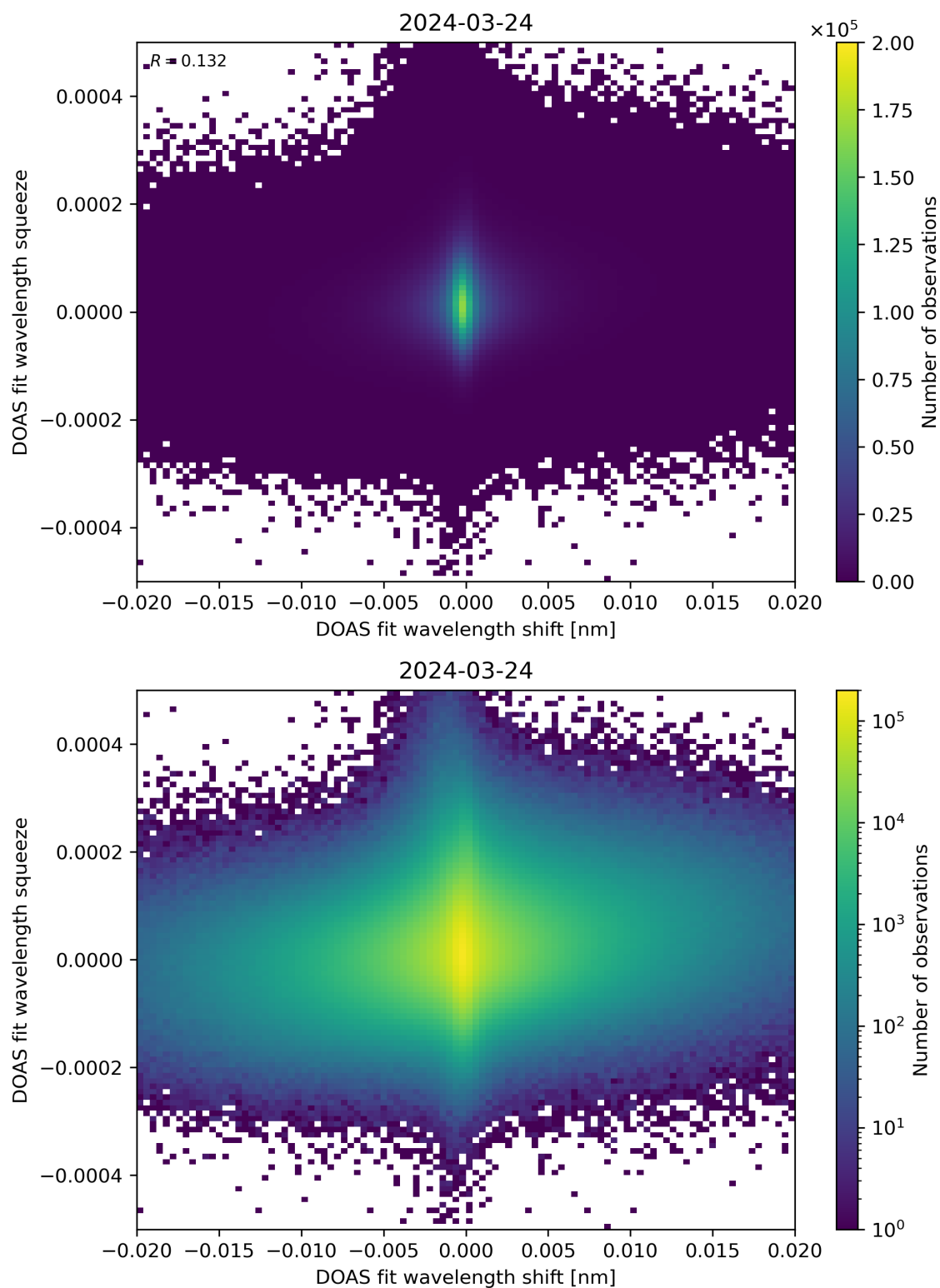
Figure 65: Scatter density plot of “DOAS fit wavelength shift” against “DOAS fit wavelength squeeze” for 2024-03-23 to 2024-03-25.
