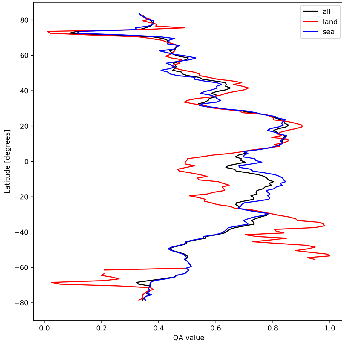
Figure 20: Zonal average of “QA value” for 2024-03-23 to 2024-03-25.
