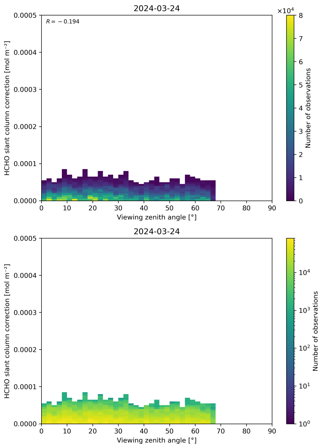
Figure 187: Scatter density plot of “Viewing zenith angle” against “HCHO slant column correction” for 2024-03-23 to 2024-03-25.
