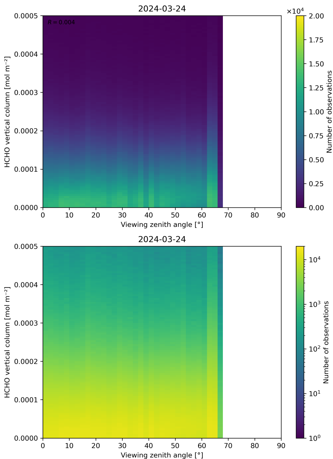
Figure 192: Scatter density plot of “Viewing zenith angle” against “HCHO vertical column” for 2024-03-23 to 2024-03-25.
