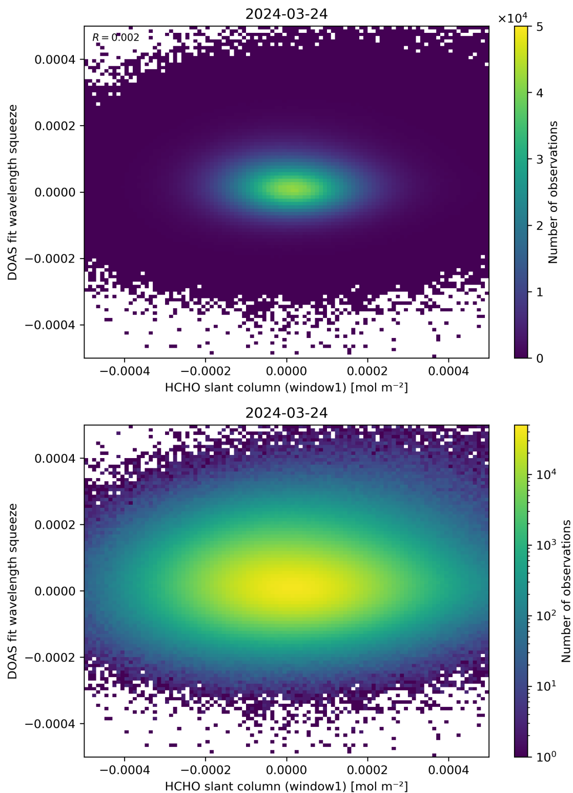
Figure 80: Scatter density plot of “HCHO slant column (window1)” against “DOAS fit wavelength squeeze” for 2024-03-23 to 2024-03-25.
