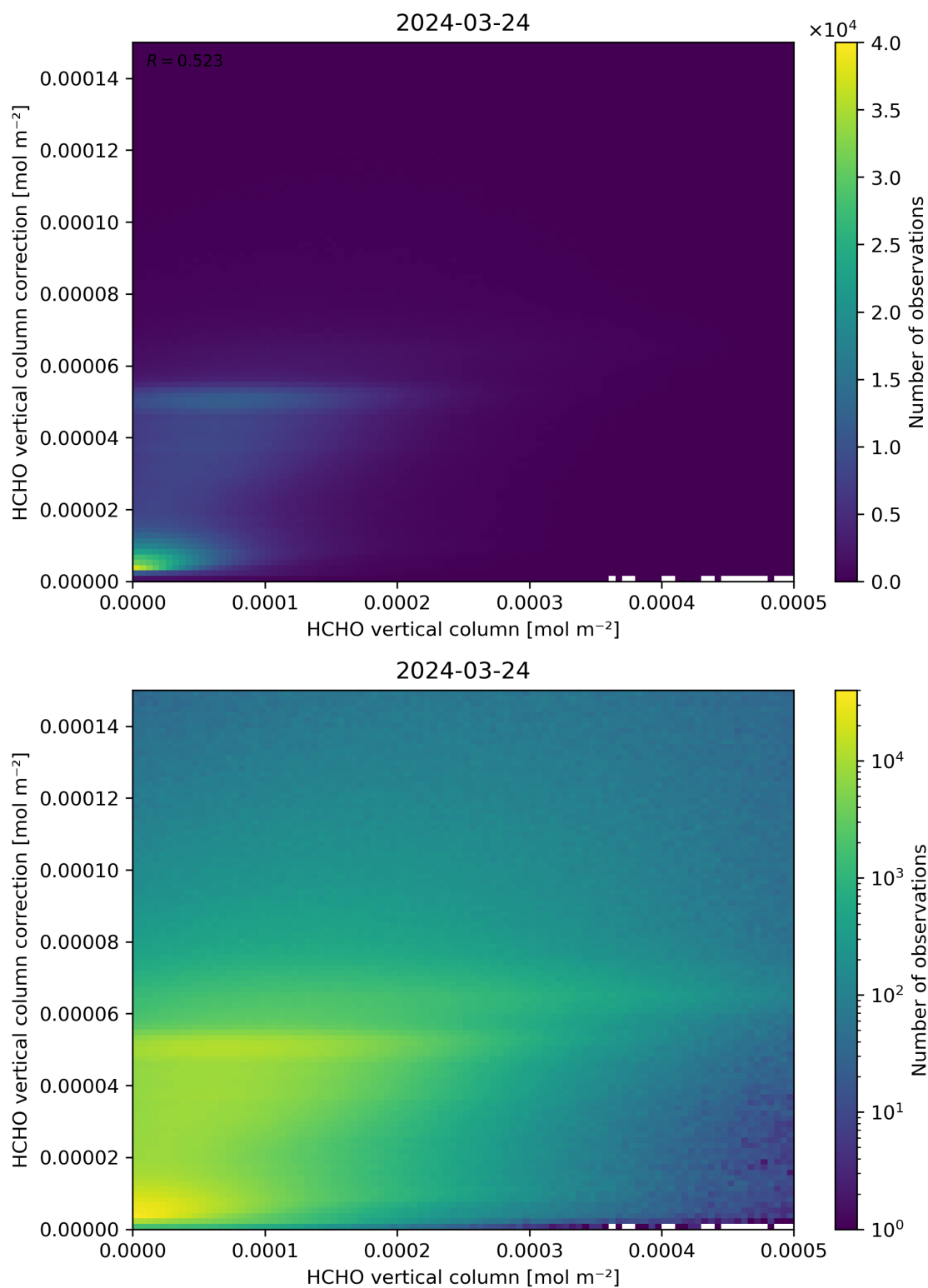
Figure 133: Scatter density plot of “HCHO vertical column” against “HCHO vertical column correction” for 2024-03-23 to 2024-03-25.
