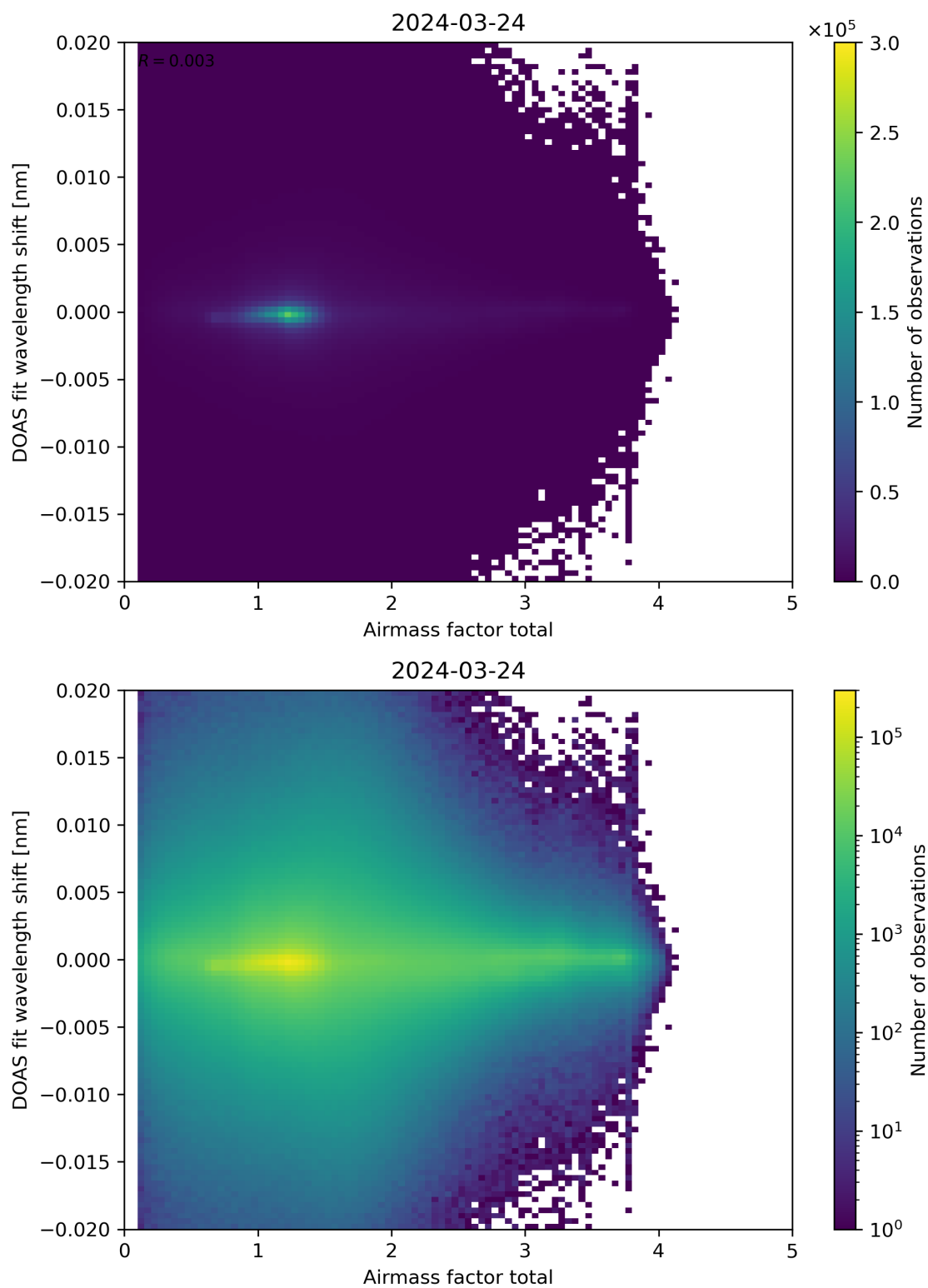
Figure 98: Scatter density plot of “Airmass factor total” against “DOAS fit wavelength shift” for 2024-03-23 to 2024-03-25.
