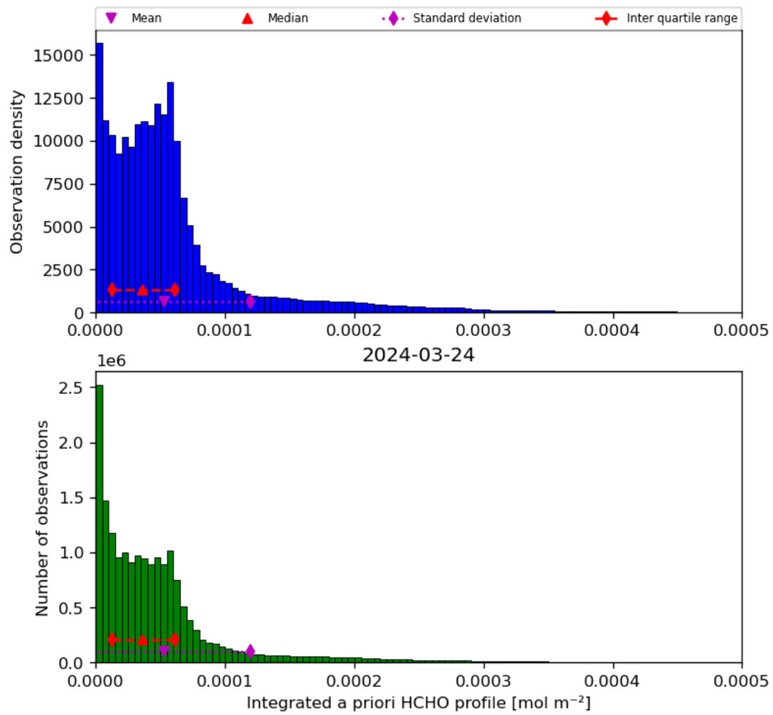
Figure 43: Histogram of “Integrated a priori HCHO profile” for 2024-03-23 to 2024-03-25
