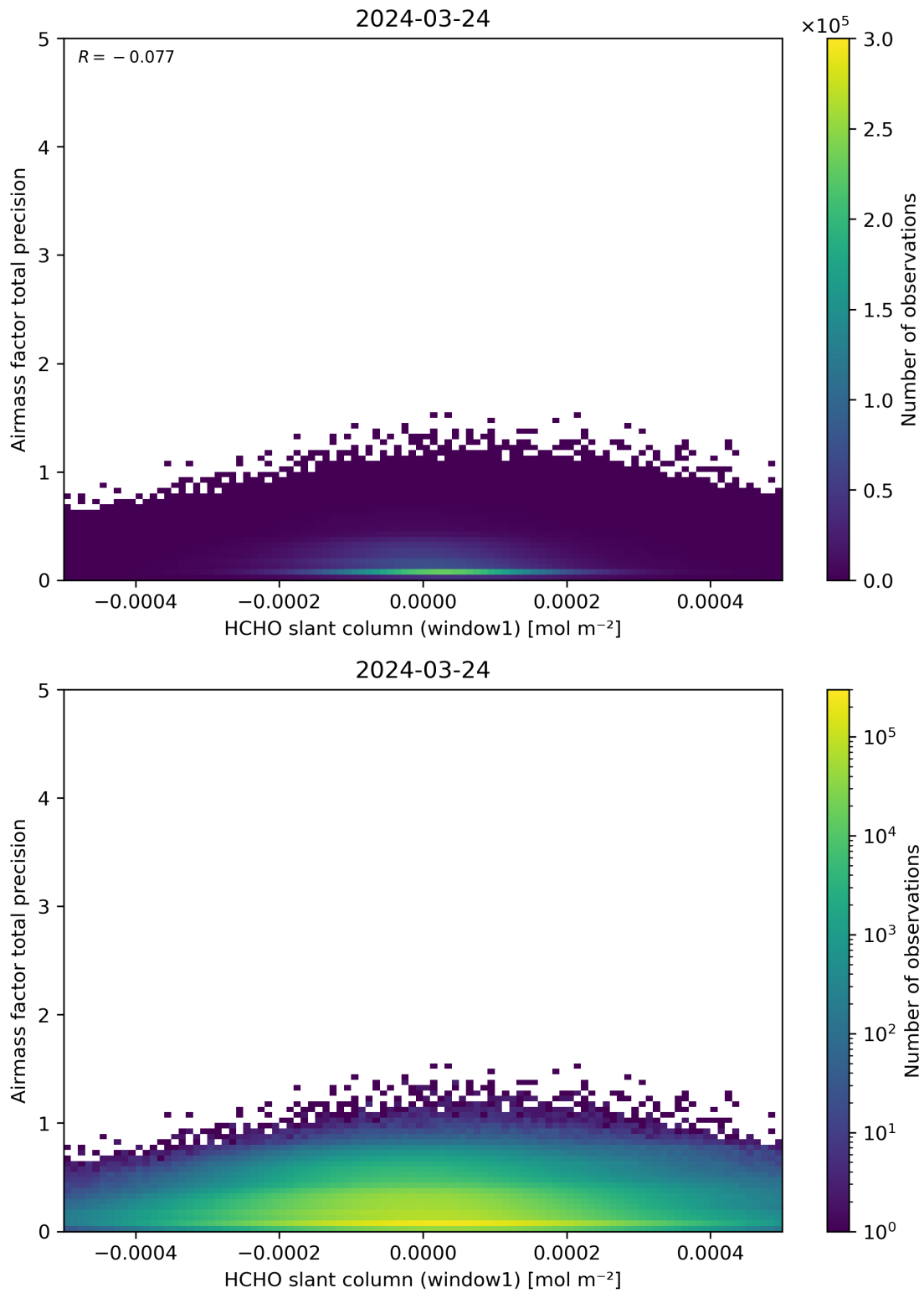
Figure 86: Scatter density plot of “HCHO slant column (window1)” against “Airmass factor total precision” for 2024-03-23 to 2024-03-25.
