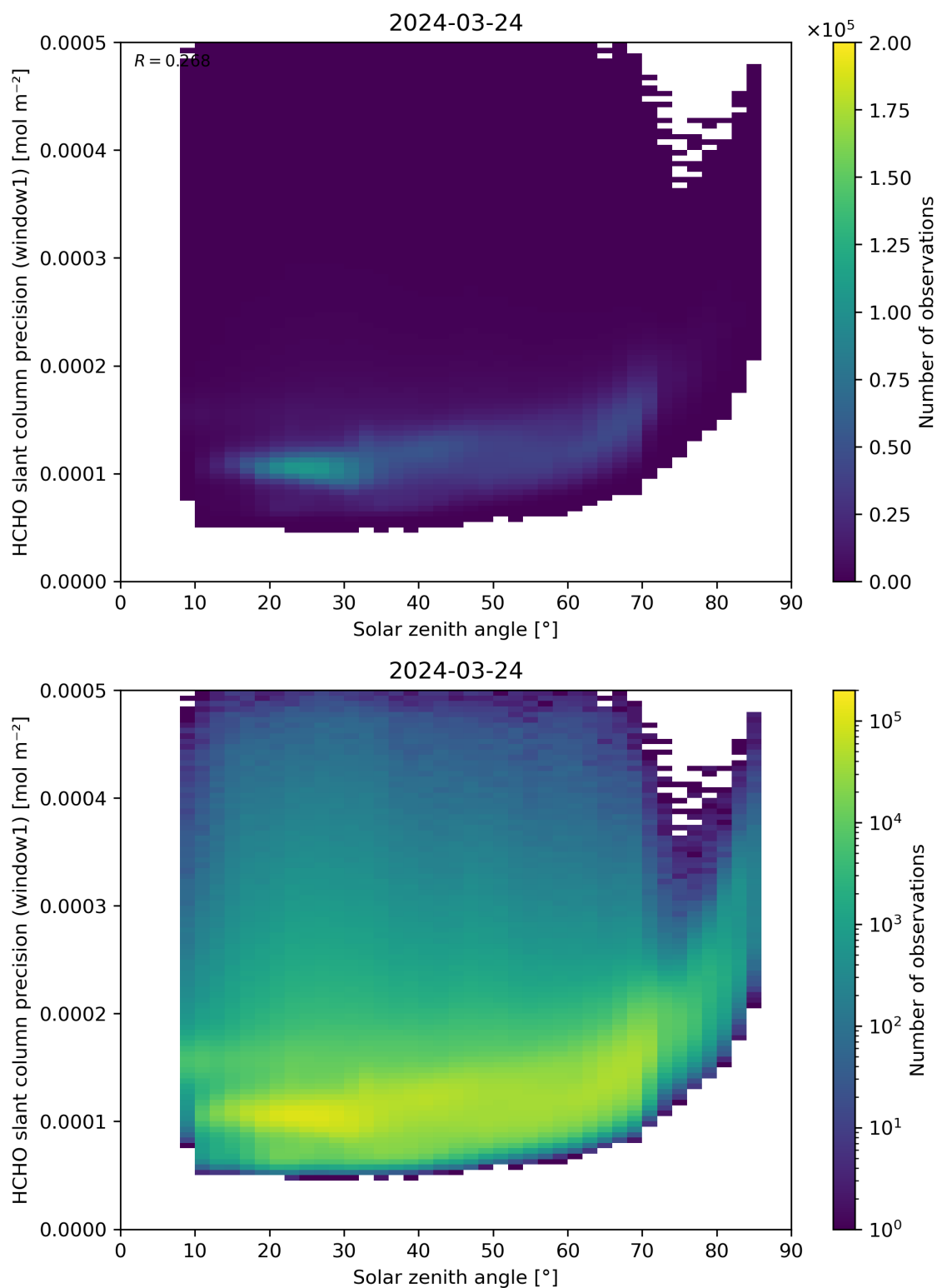
Figure 174: Scatter density plot of “Solar zenith angle” against “HCHO slant column precision (window1)” for 2024-03-23 to 2024-03-25.
