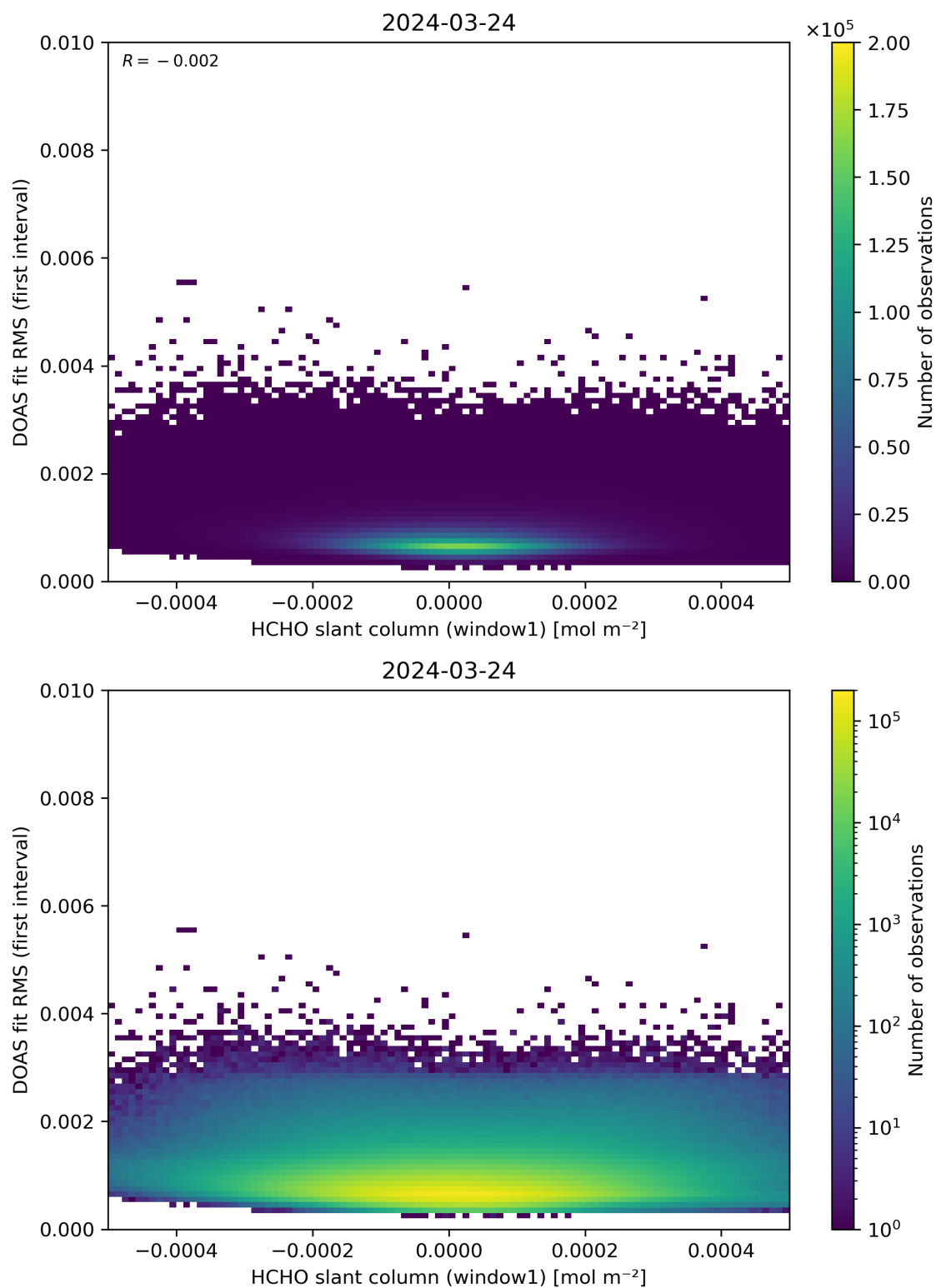
Figure 78: Scatter density plot of “HCHO slant column (window1)” against “DOAS fit RMS (first interval)” for 2024-03-23 to 2024-03-25.
