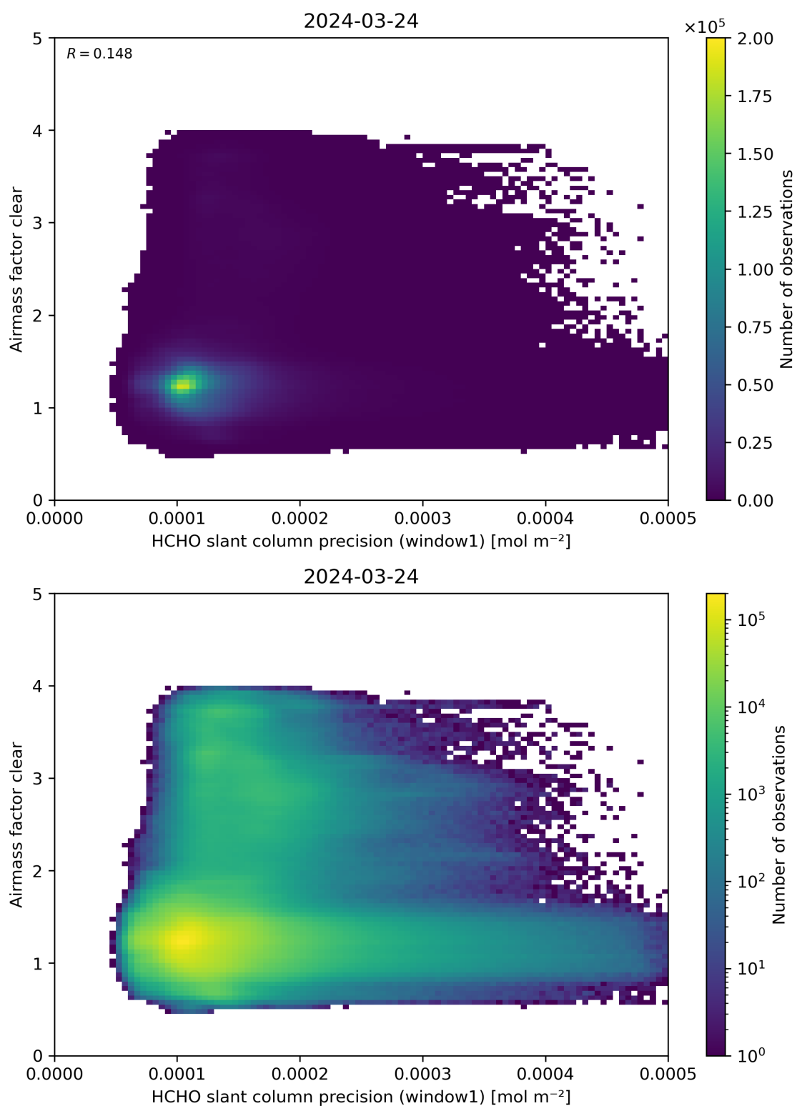
Figure 91: Scatter density plot of “HCHO slant column precision (window1)” against “Airmass factor clear” for 2024-03-23 to 2024-03-25.
