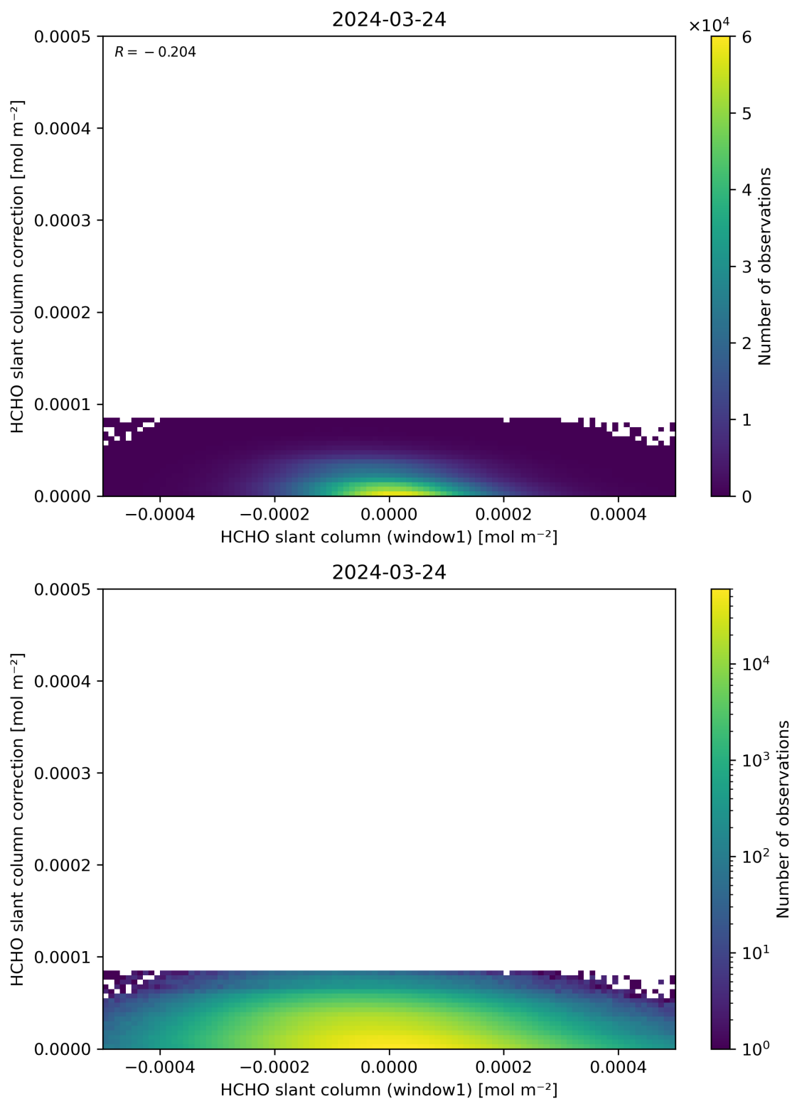
Figure 83: Scatter density plot of “HCHO slant column (window1)” against “HCHO slant column correction” for 2024-03-23 to 2024-03-25.
