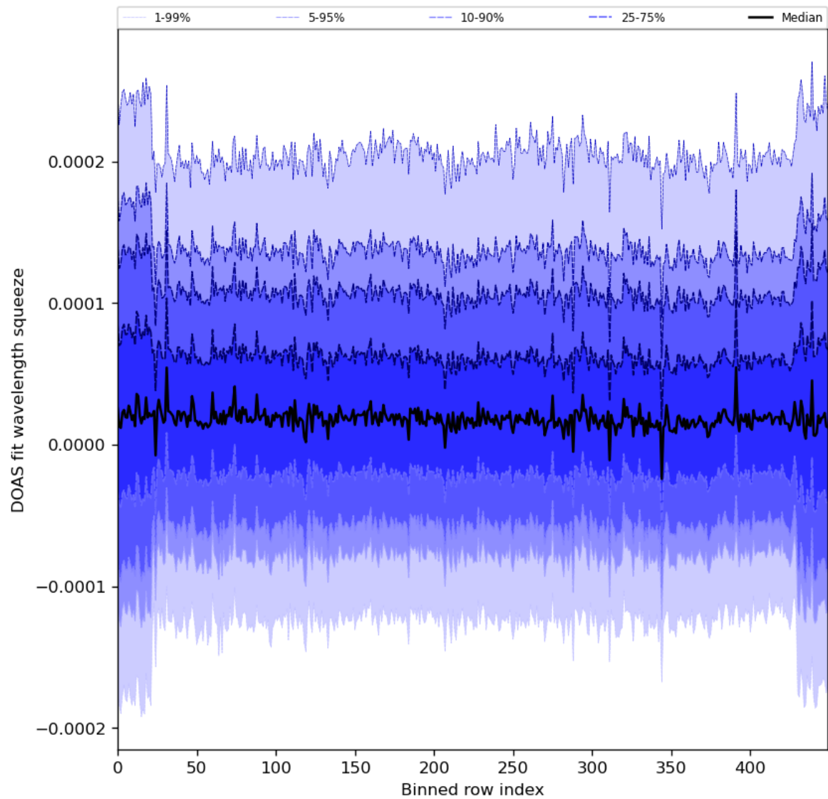
Figure 59: Along track statistics of “DOAS fit wavelength squeeze” for 2024-03-23 to 2024-03-25
