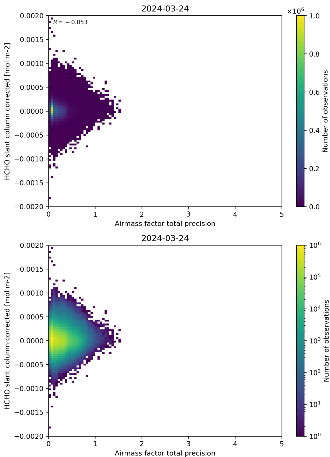
Figure 109: Scatter density plot of “Airmass factor total precision” against “HCHO slant column corrected” for 2024-03-23 to 2024-03-25.
