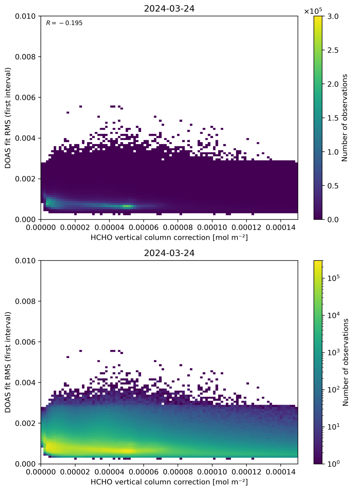
Figure 112: Scatter density plot of “HCHO vertical column correction” against “DOAS fit RMS (first interval)” for 2024-03-23 to 2024-03-25.
