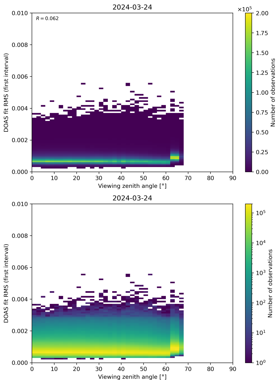
Figure 182: Scatter density plot of “Viewing zenith angle” against “DOAS fit RMS (first interval)” for 2024-03-23 to 2024-03-25.
