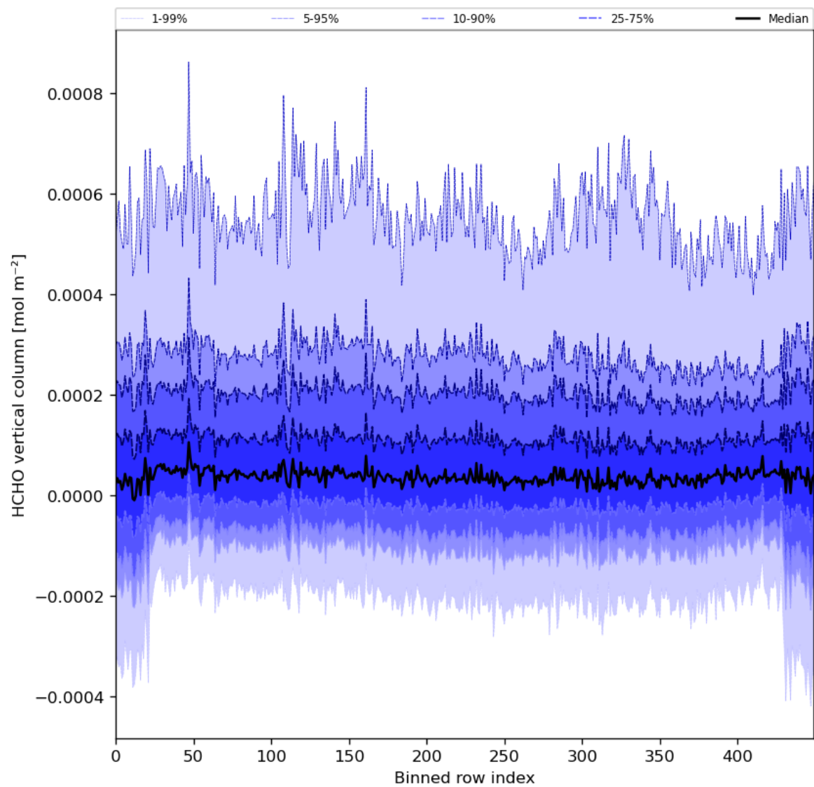
Figure 49: Along track statistics of “HCHO vertical column” for 2024-03-23 to 2024-03-25
