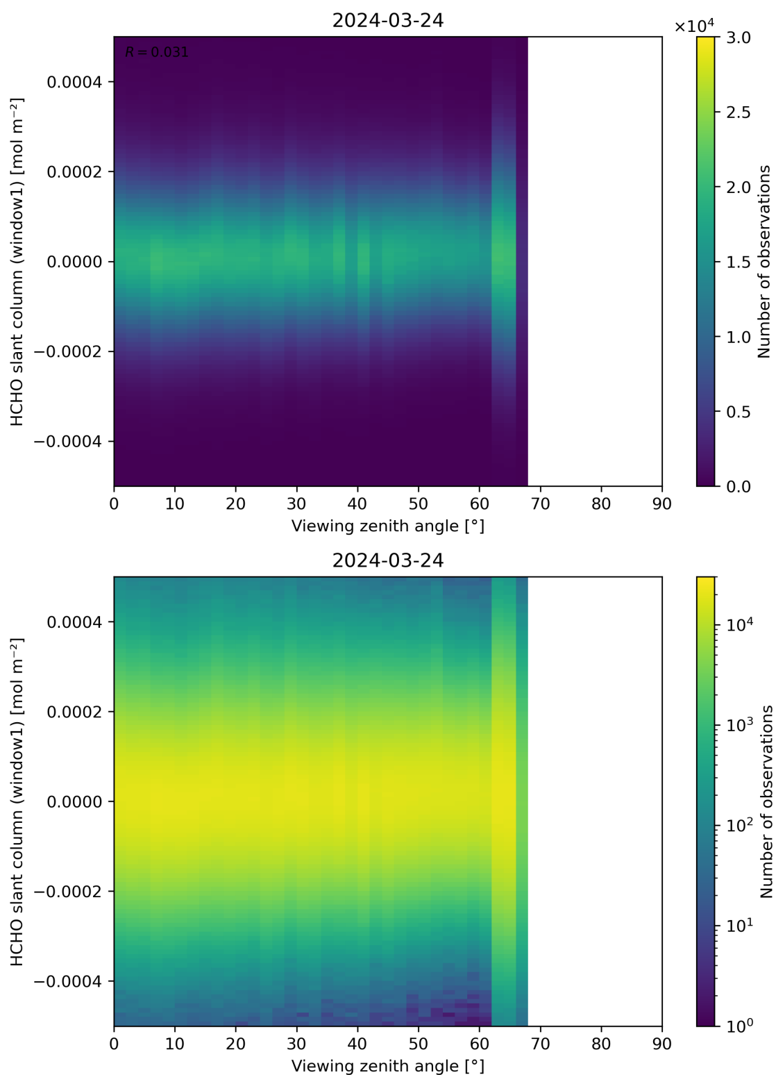
Figure 188: Scatter density plot of “Viewing zenith angle” against “HCHO slant column (window1)” for 2024-03-23 to 2024-03-25.
