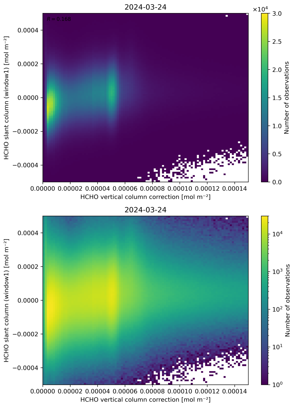
Figure 118: Scatter density plot of “HCHO vertical column correction” against “HCHO slant column (window1)” for 2024-03-23 to 2024-03-25.
