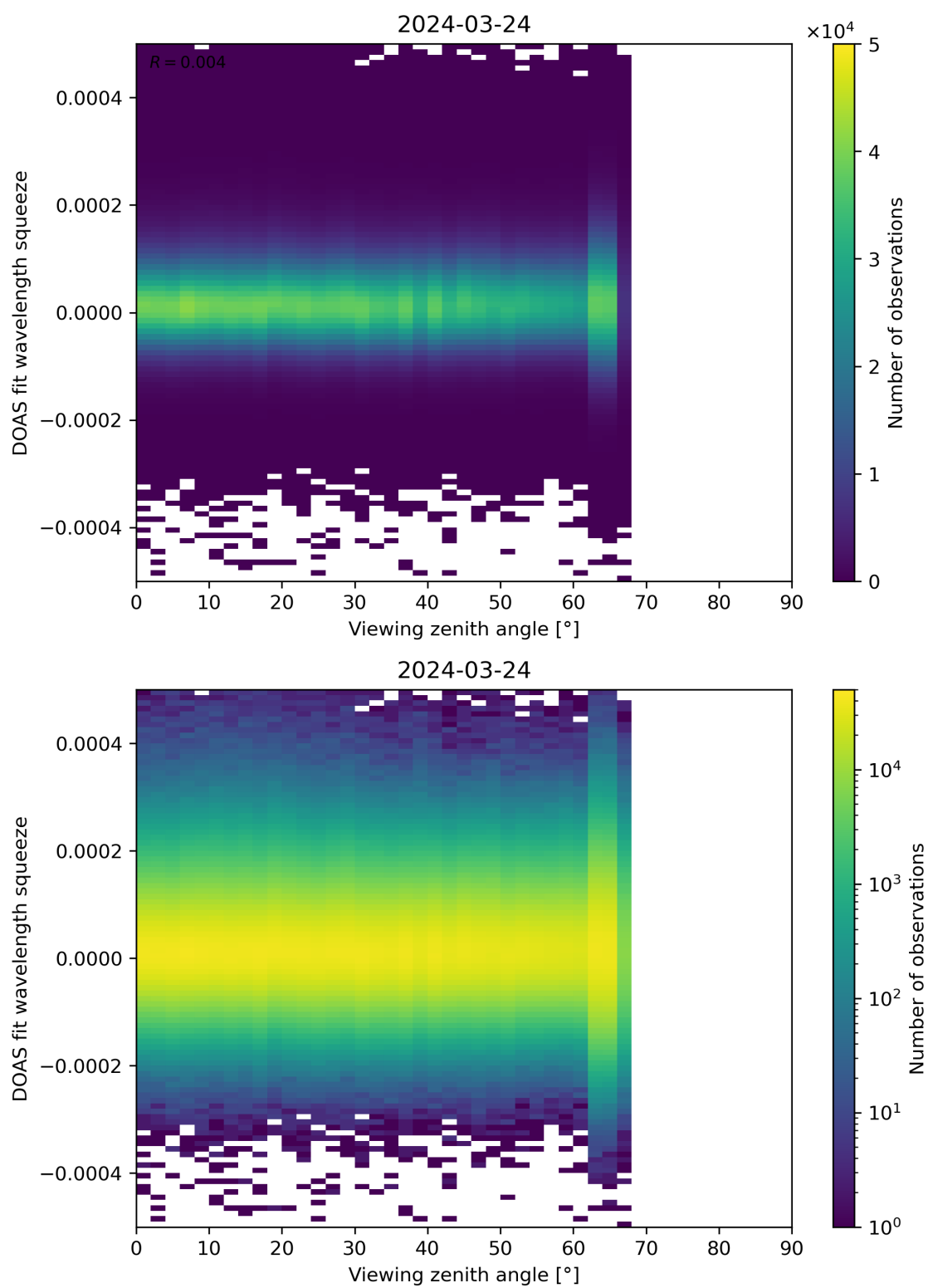
Figure 184: Scatter density plot of “Viewing zenith angle” against “DOAS fit wavelength squeeze” for 2024-03-23 to 2024-03-25.
