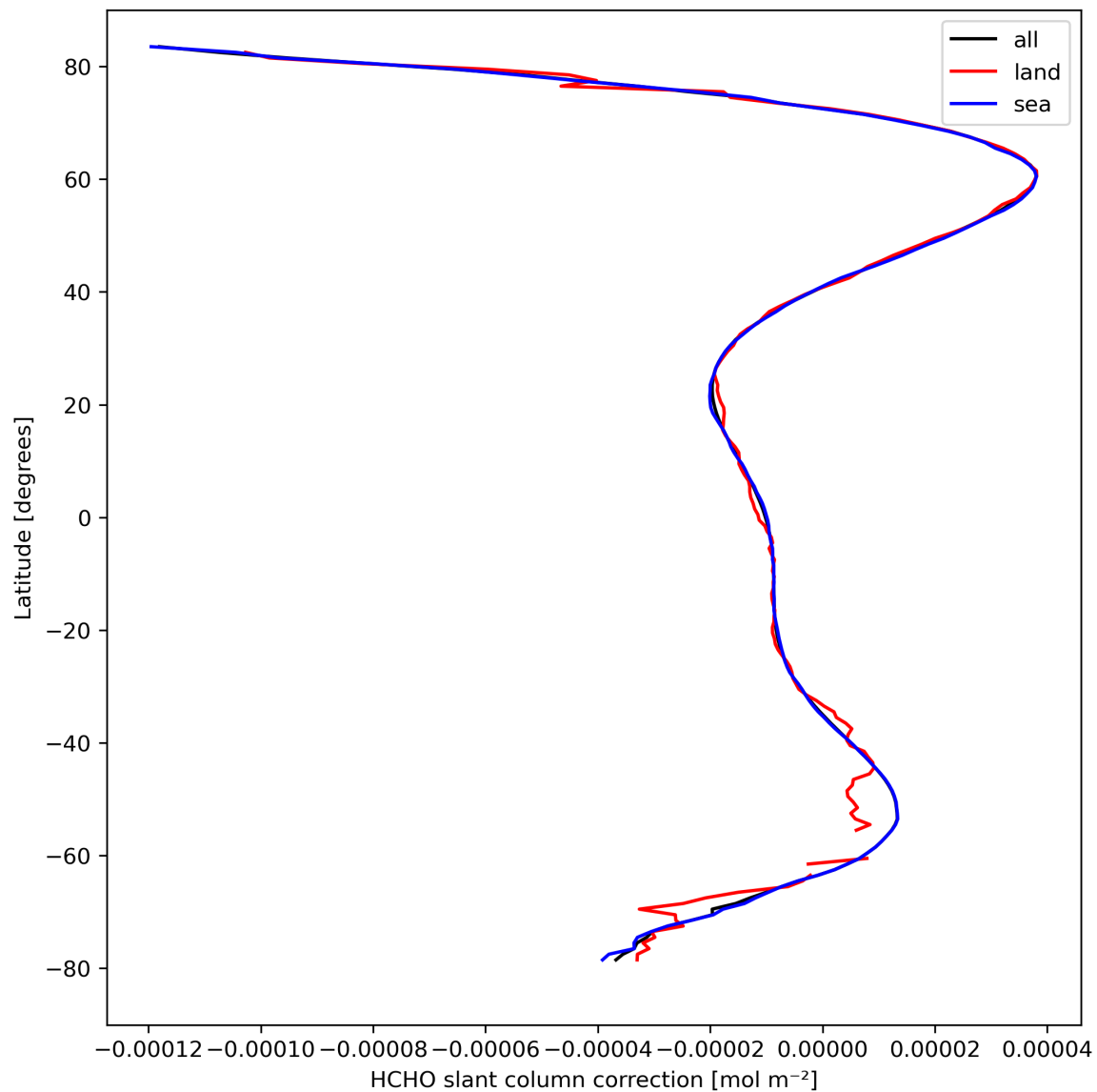
Figure 33: Zonal average of “HCHO slant column correction” for 2024-03-23 to 2024-03-25.
