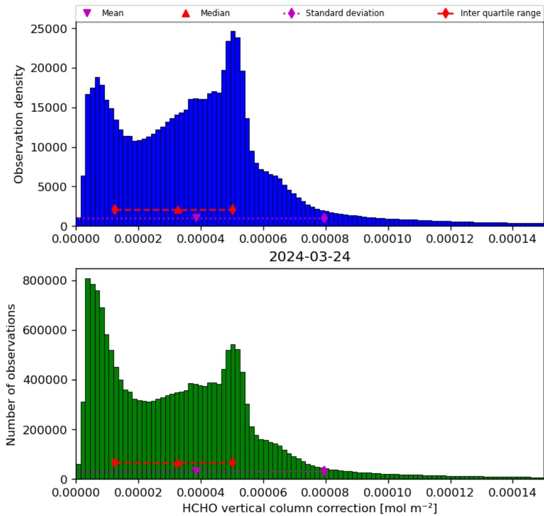
Figure 37: Histogram of “HCHO vertical column correction” for 2024-03-23 to 2024-03-25
