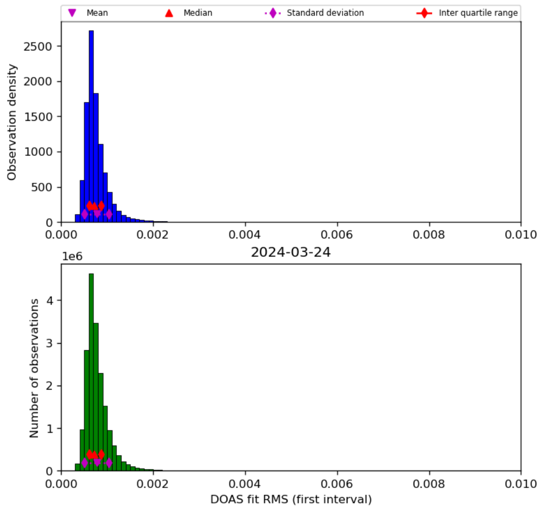
Figure 46: Histogram of “DOAS fit RMS (first interval)” for 2024-03-23 to 2024-03-25
