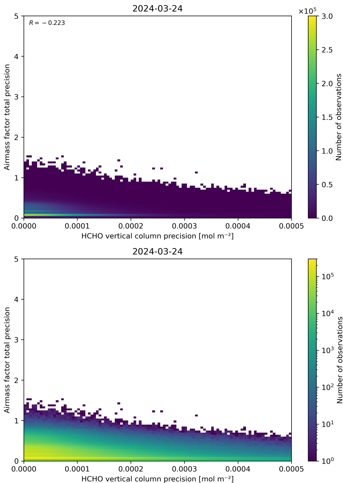
Figure 145: Scatter density plot of “HCHO vertical column precision” against “Airmass factor total precision” for 2024-03-23 to 2024-03-25.
