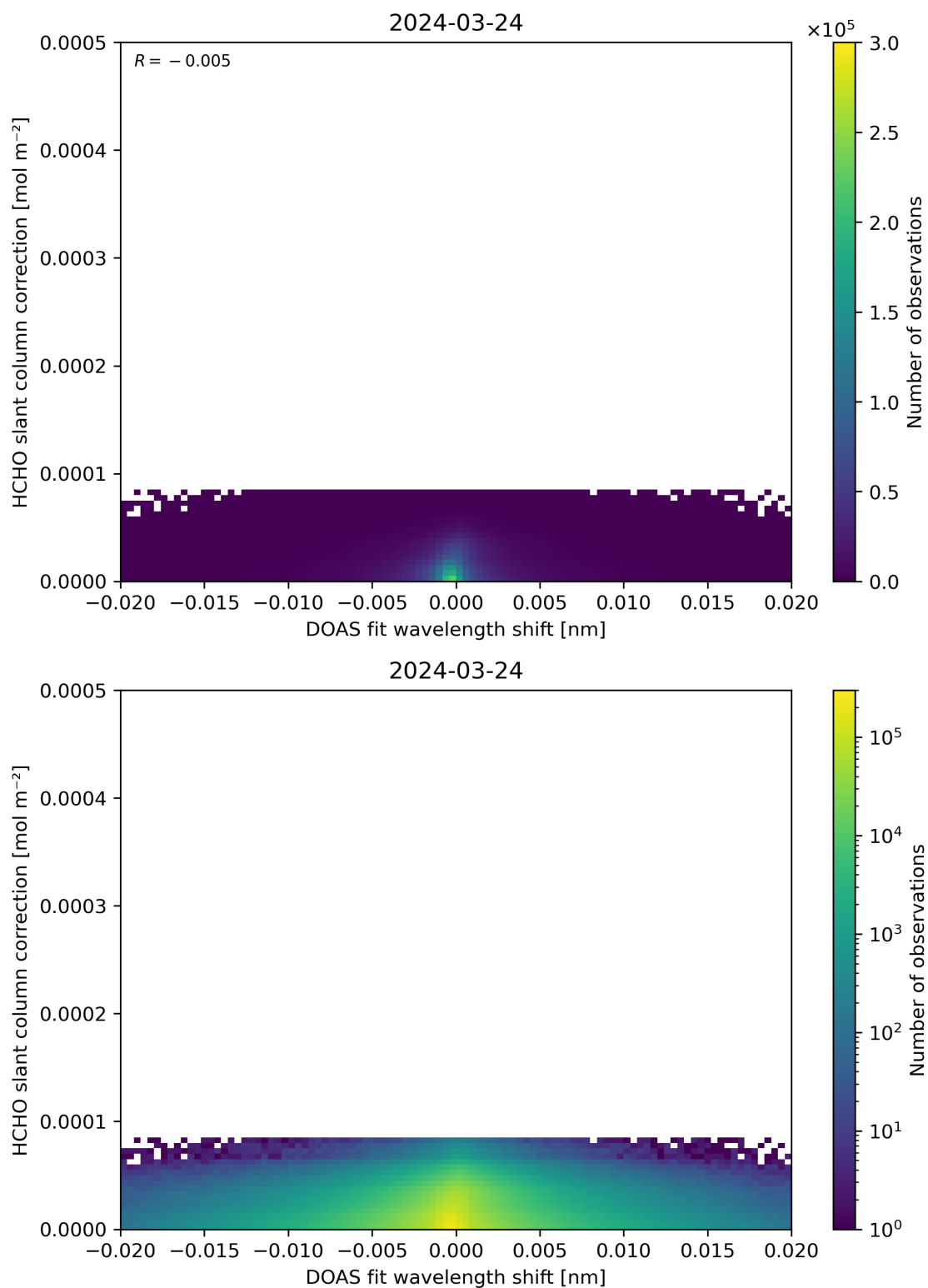
Figure 67: Scatter density plot of “DOAS fit wavelength shift” against “HCHO slant column correction” for 2024-03-23 to 2024-03-25.
