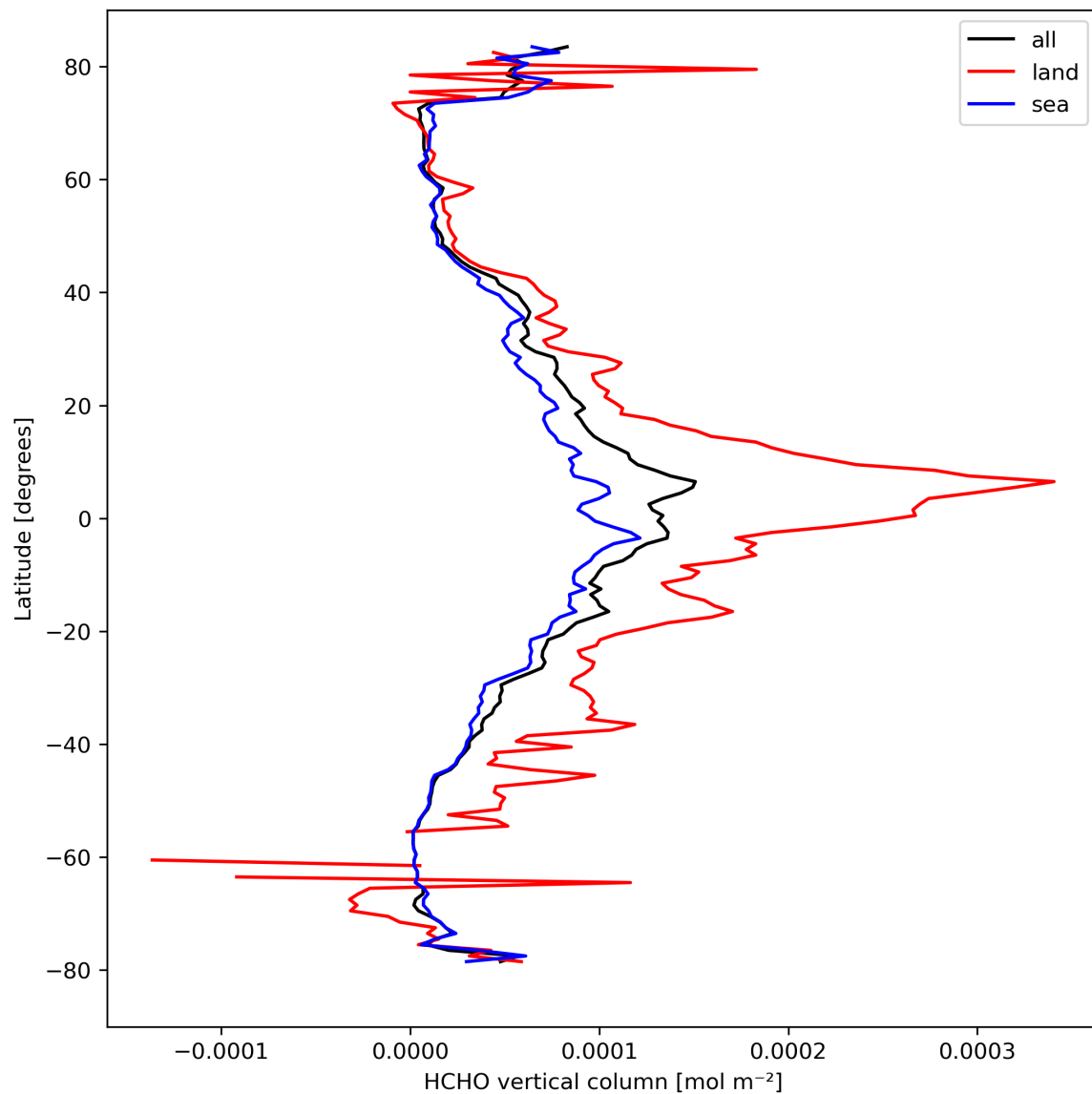
Figure 21: Zonal average of “HCHO vertical column” for 2024-03-23 to 2024-03-25.
