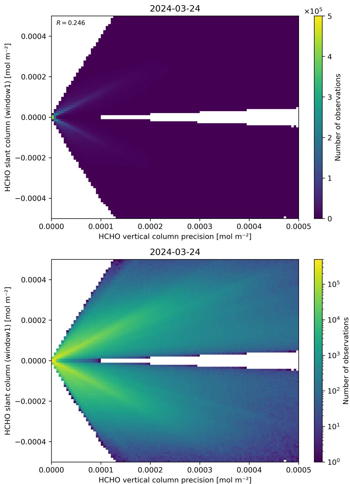
Figure 142: Scatter density plot of “HCHO vertical column precision” against “HCHO slant column (window1)” for 2024-03-23 to 2024-03-25.
