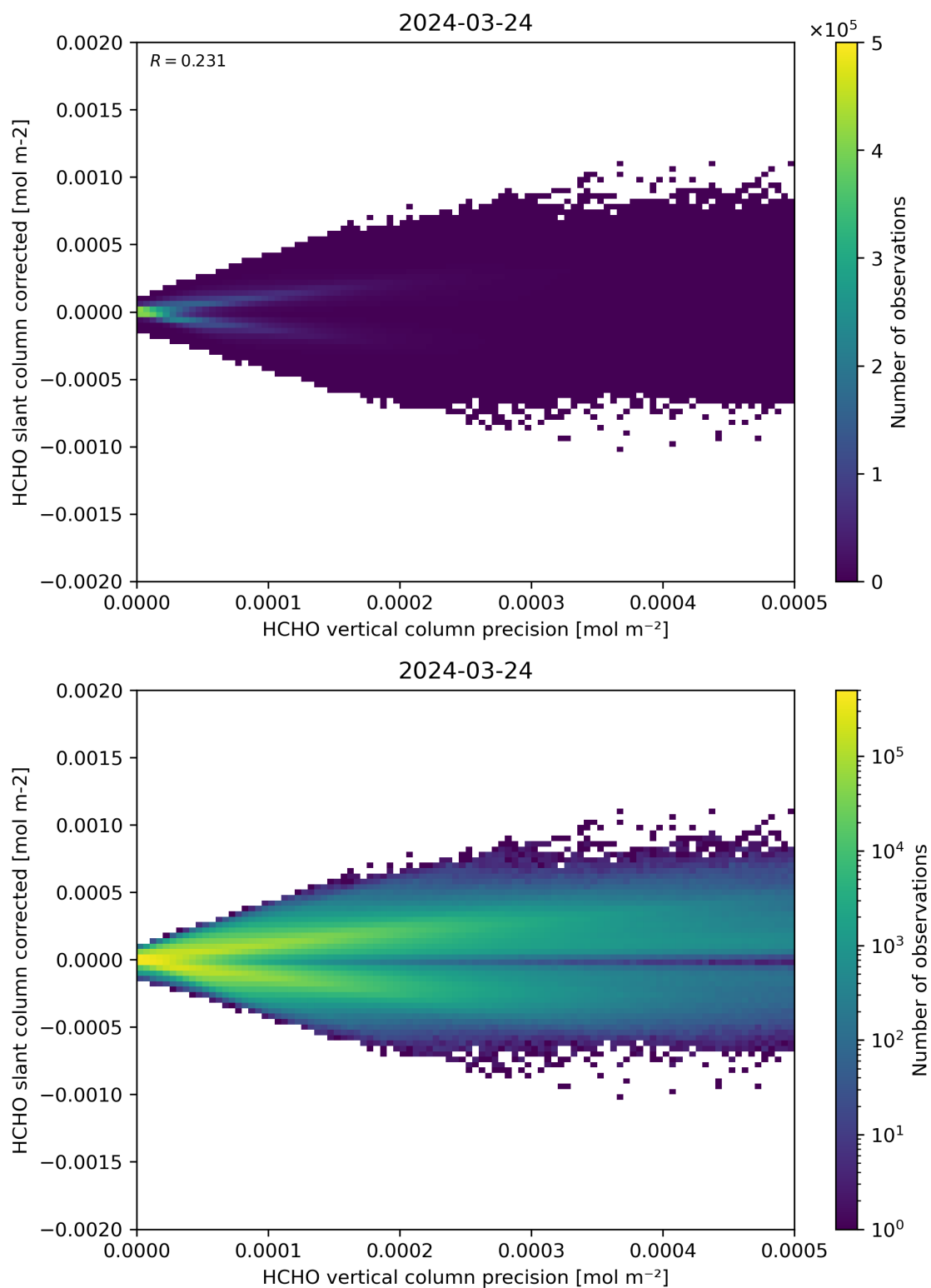
Figure 140: Scatter density plot of “HCHO vertical column precision” against “HCHO slant column corrected” for 2024-03-23 to 2024-03-25.
