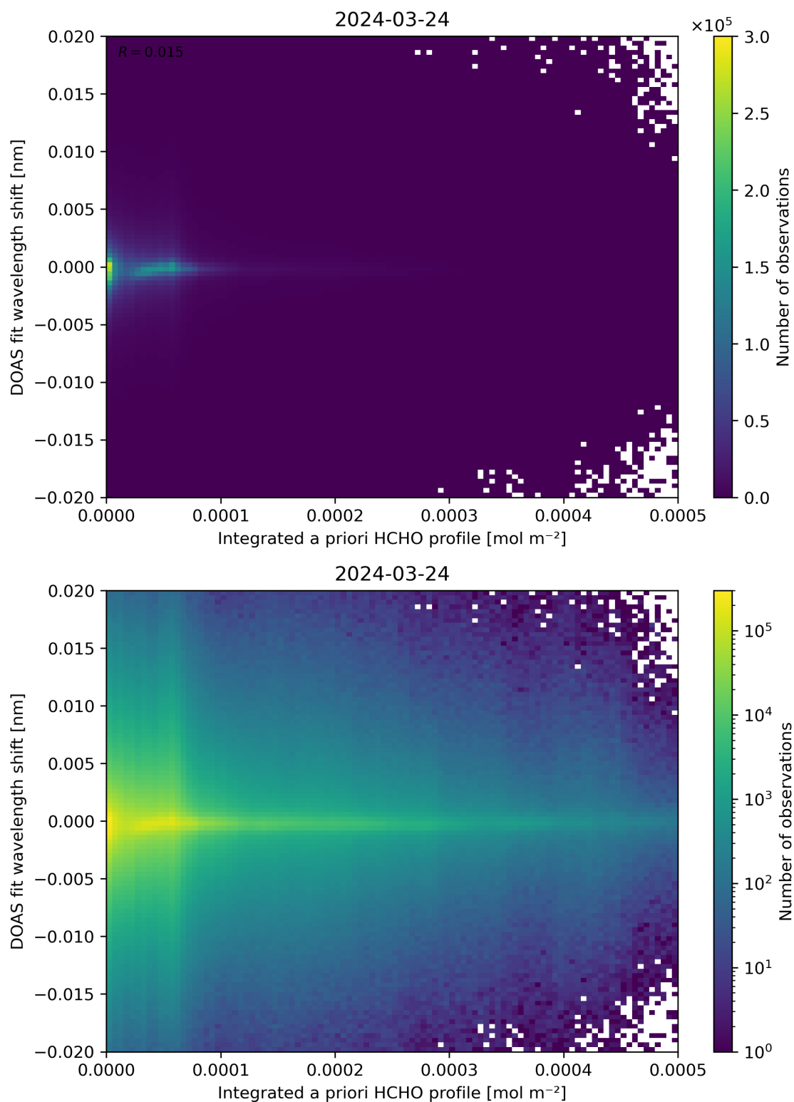
Figure 149: Scatter density plot of “Integrated a priori HCHO profile” against “DOAS fit wavelength shift” for 2024-03-23 to 2024-03-25.
