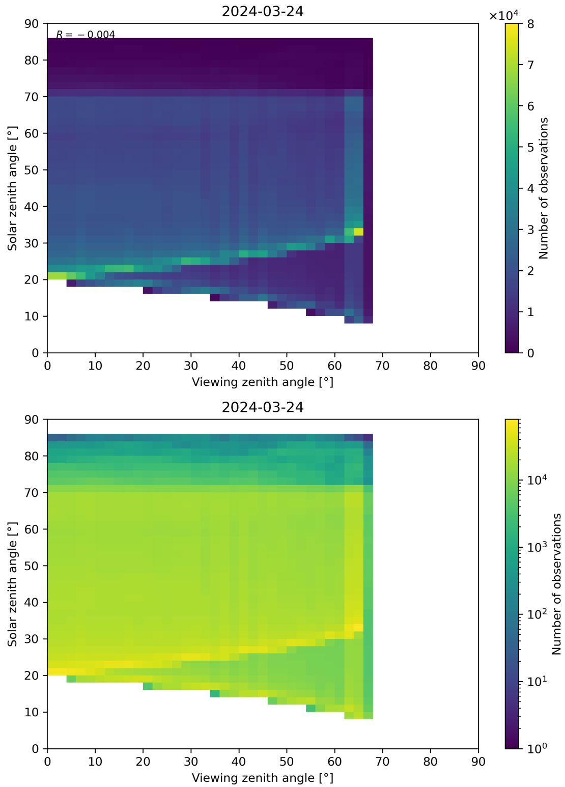
Figure 197: Scatter density plot of “Viewing zenith angle” against “Solar zenith angle” for 2024-03-23 to 2024-03-25.
