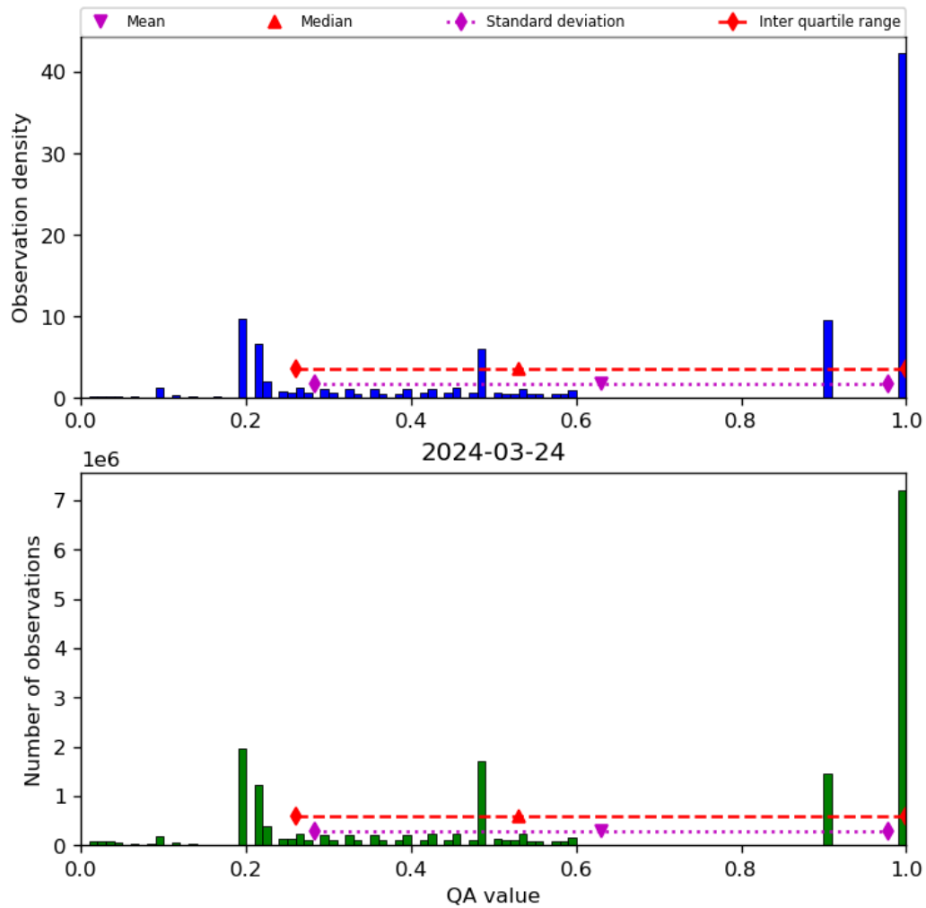
Figure 34: Histogram of “QA value” for 2024-03-23 to 2024-03-25
