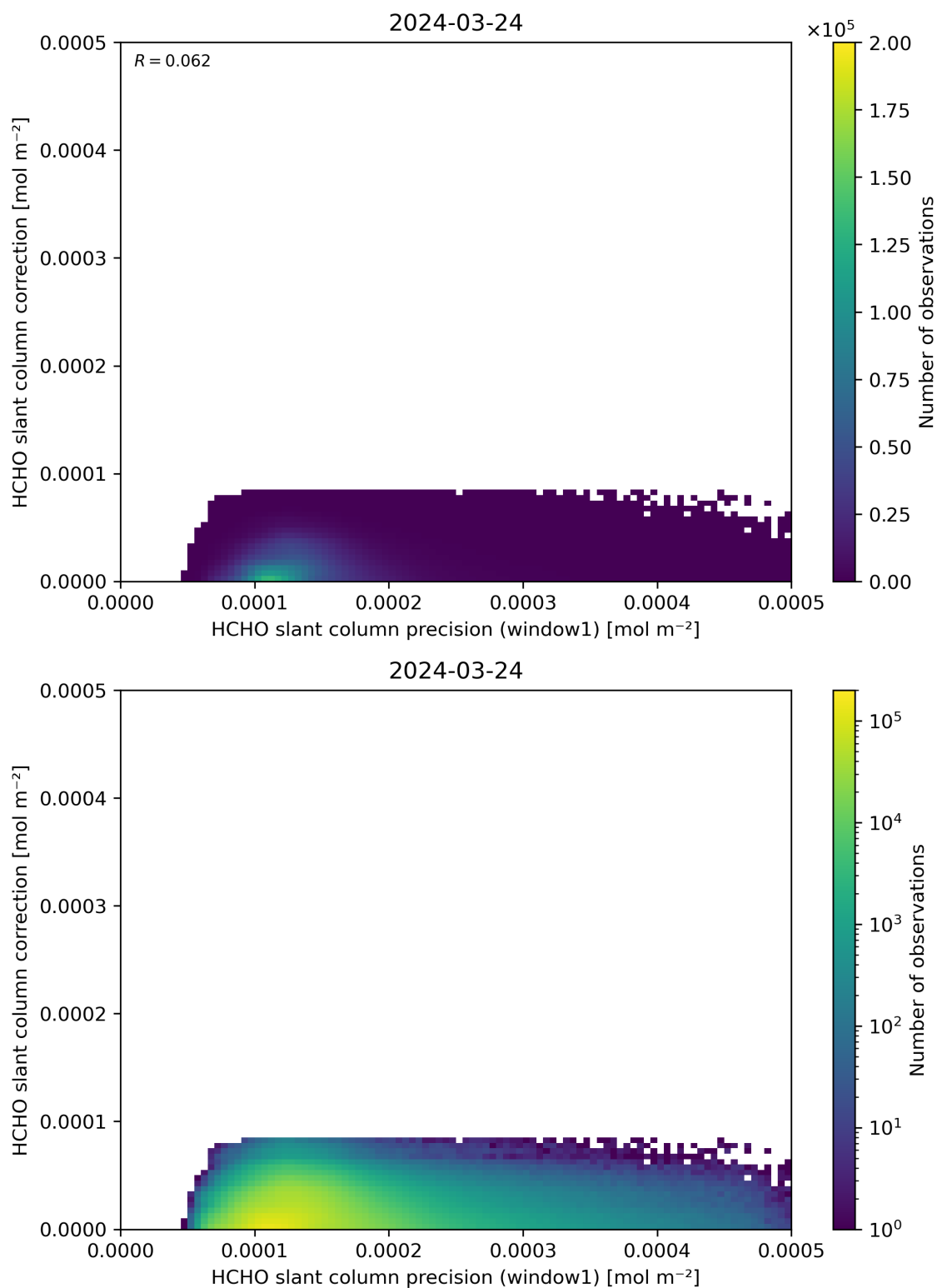
Figure 93: Scatter density plot of “HCHO slant column precision (window1)” against “HCHO slant column correction” for 2024-03-23 to 2024-03-25.
