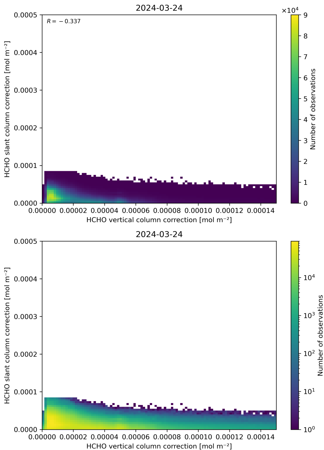
Figure 117: Scatter density plot of “HCHO vertical column correction” against “HCHO slant column correction” for 2024-03-23 to 2024-03-25.
