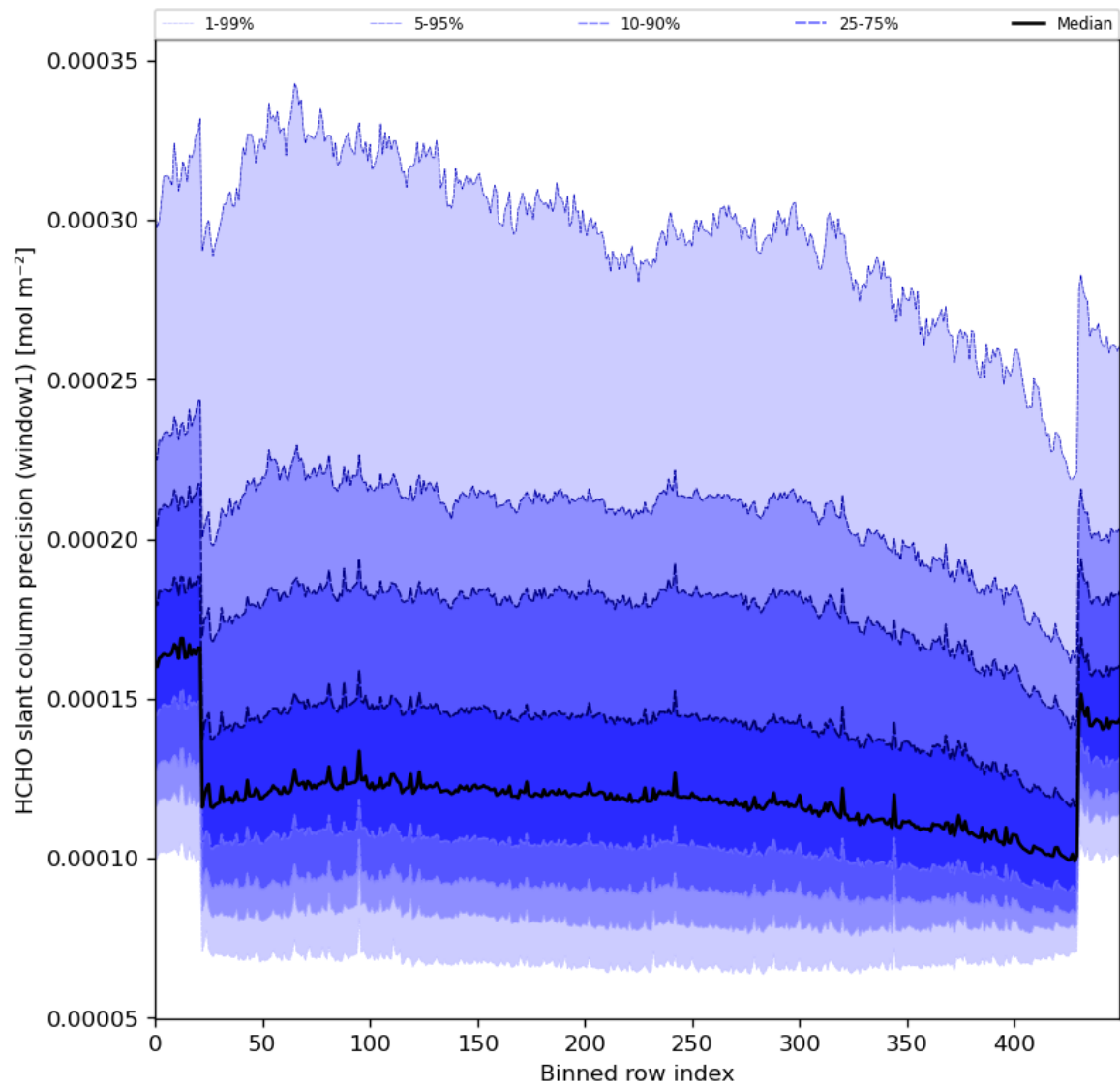
Figure 53: Along track statistics of “HCHO slant column precision (window1)” for 2024-03-23 to 2024-03-25
