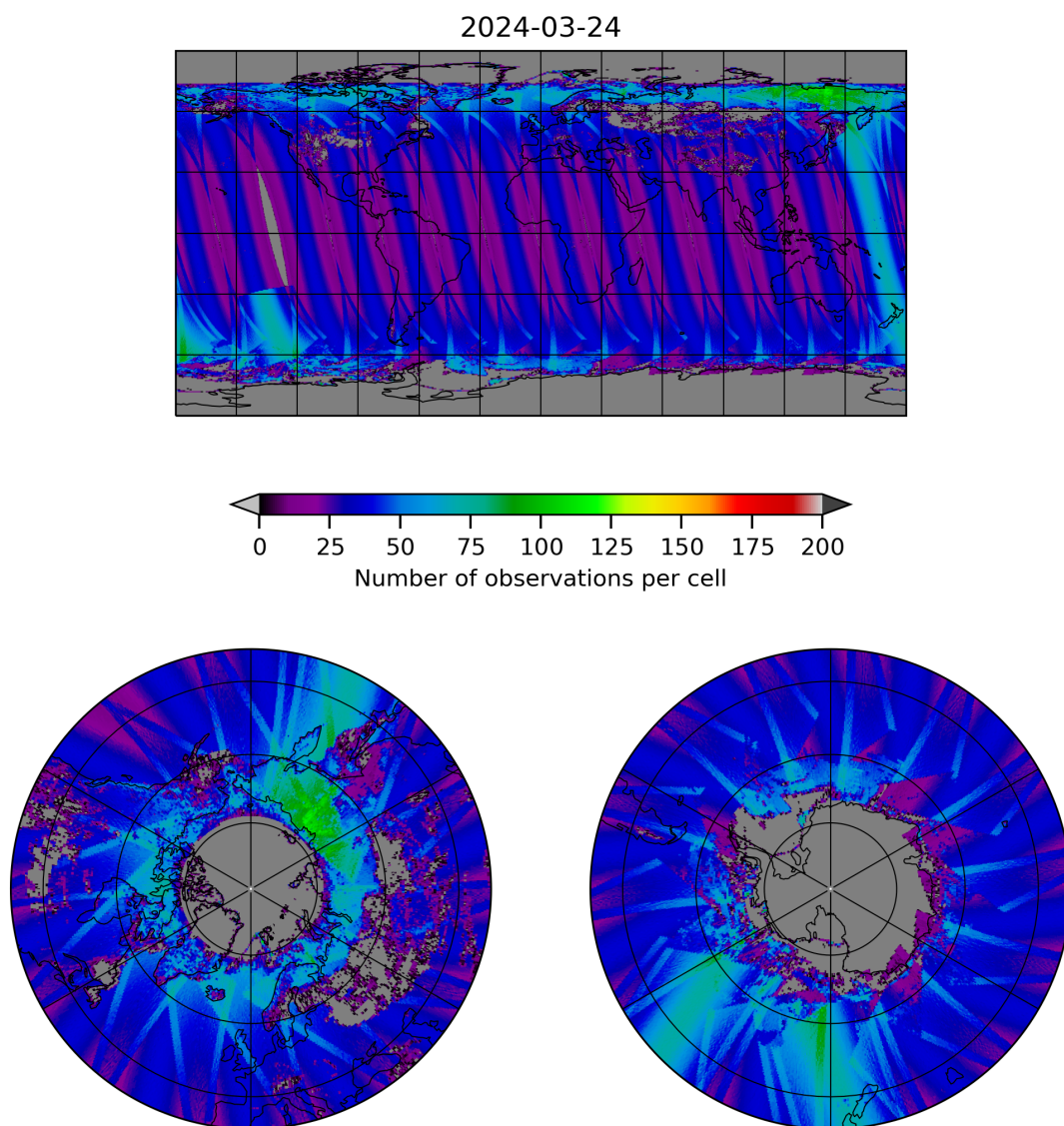
Figure 19: Map of the number of observations for 2024-03-23 to 2024-03-25
