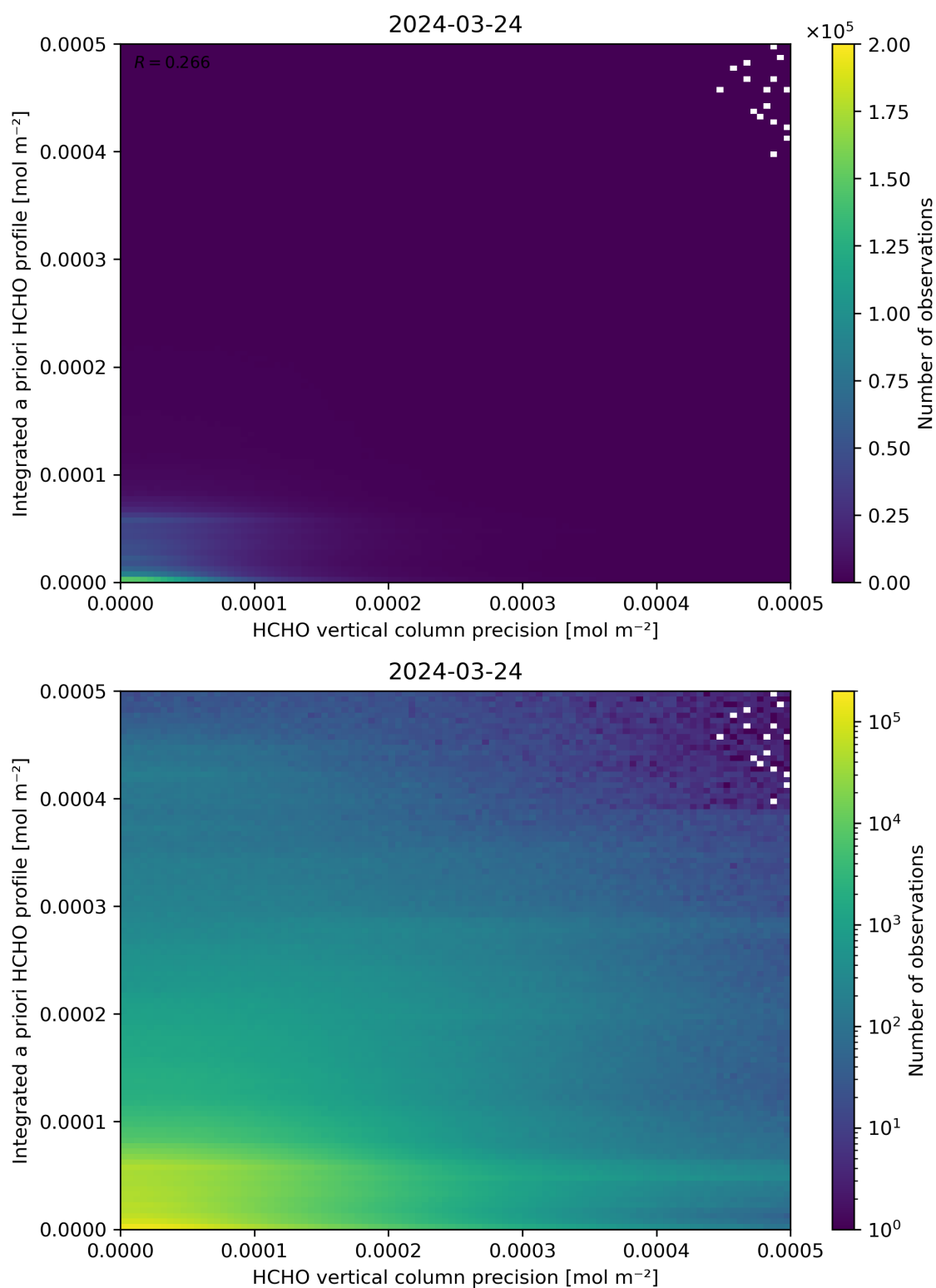
Figure 147: Scatter density plot of “HCHO vertical column precision” against “Integrated a priori HCHO profile” for 2024-03-23 to 2024-03-25.
