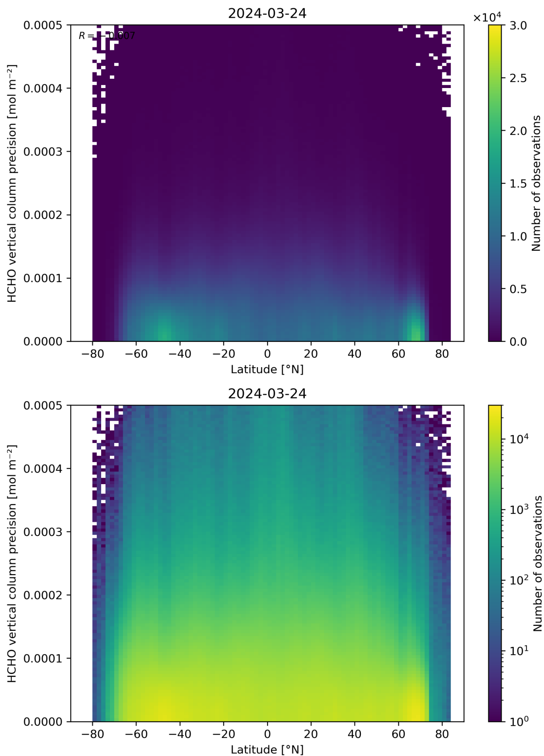
Figure 165: Scatter density plot of “Latitude” against “HCHO vertical column precision” for 2024-03-23 to 2024-03-25.
