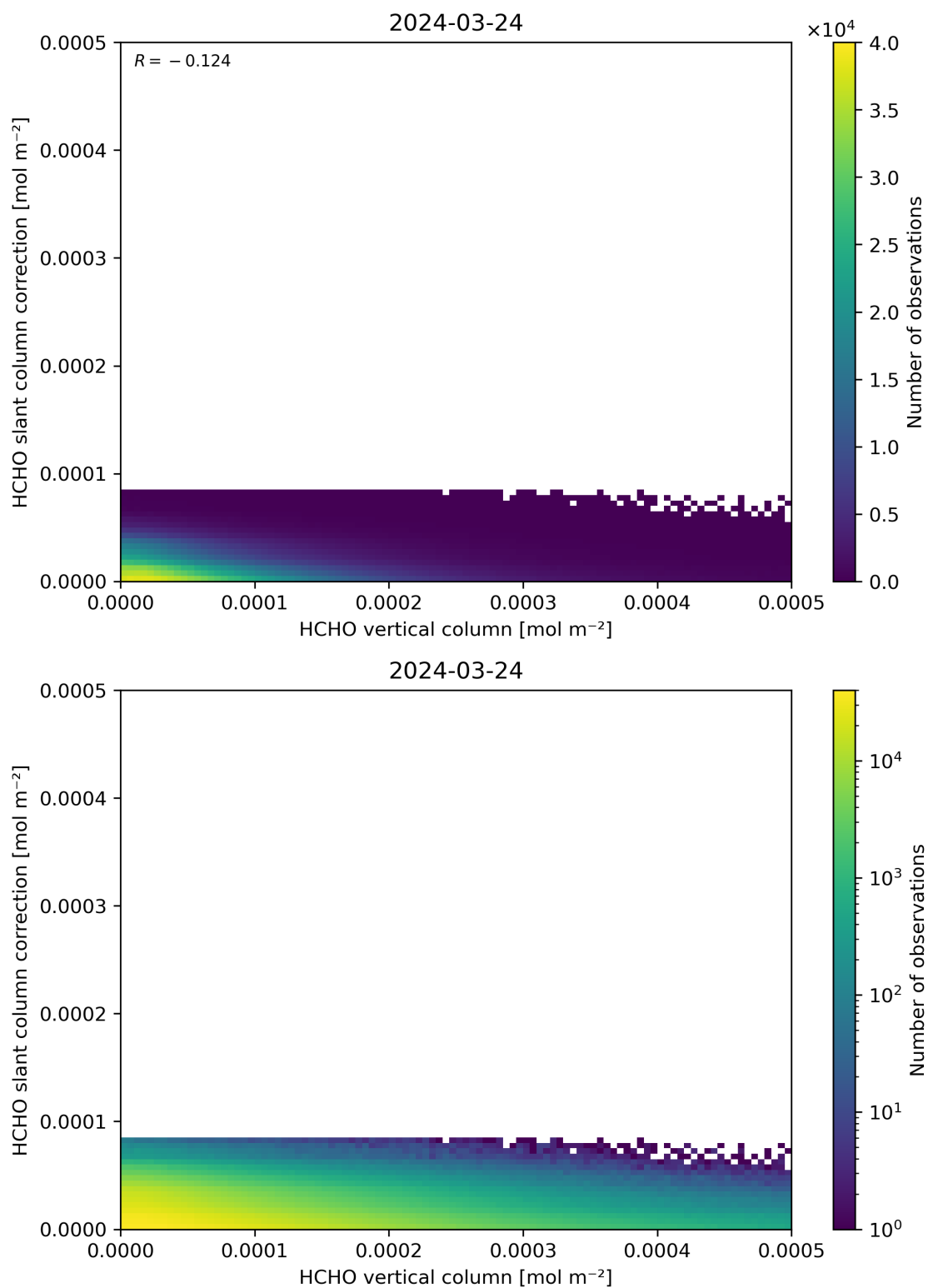
Figure 128: Scatter density plot of “HCHO vertical column” against “HCHO slant column correction” for 2024-03-23 to 2024-03-25.
