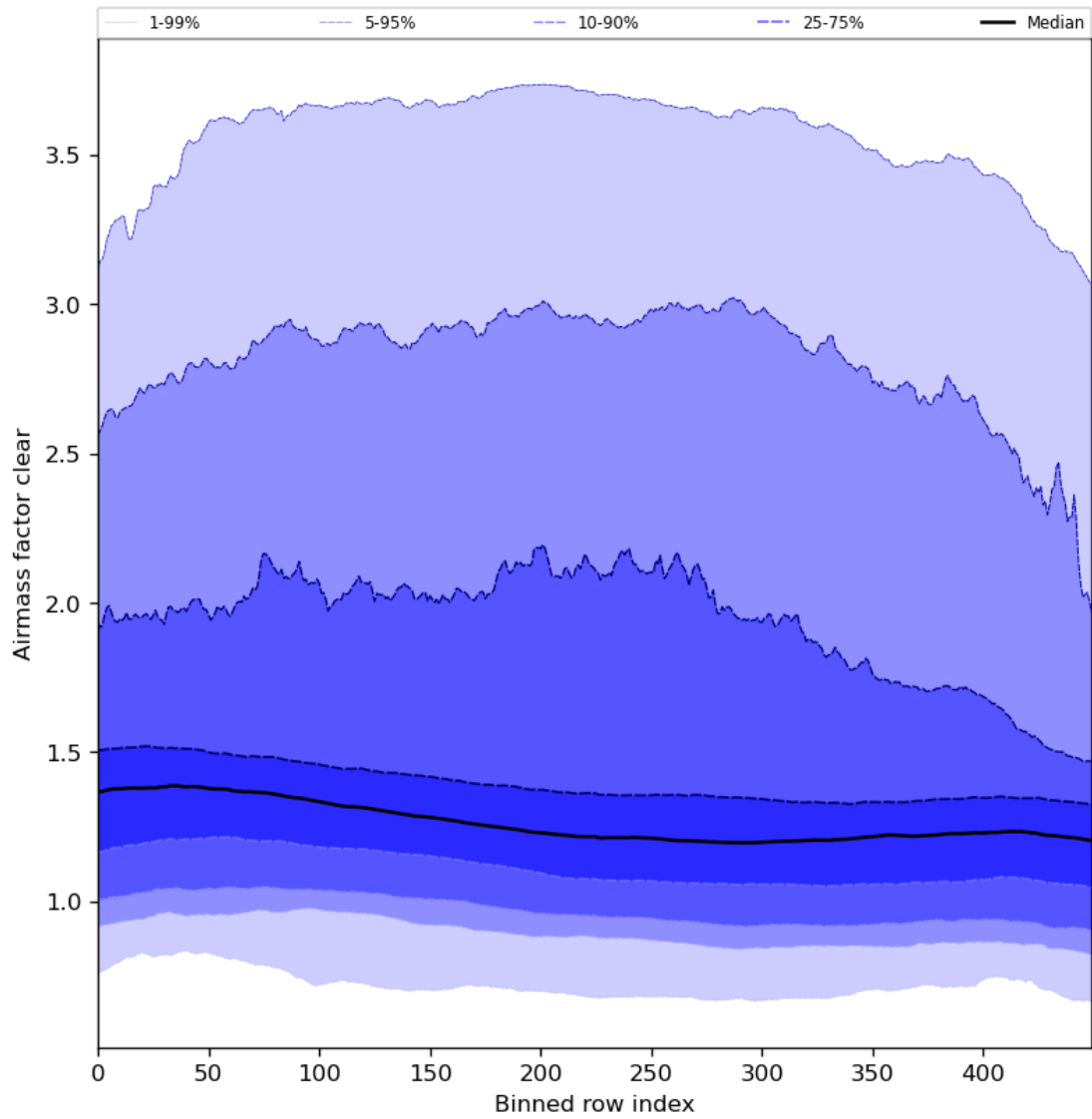
Figure 56: Along track statistics of “Airmass factor clear” for 2024-03-23 to 2024-03-25
