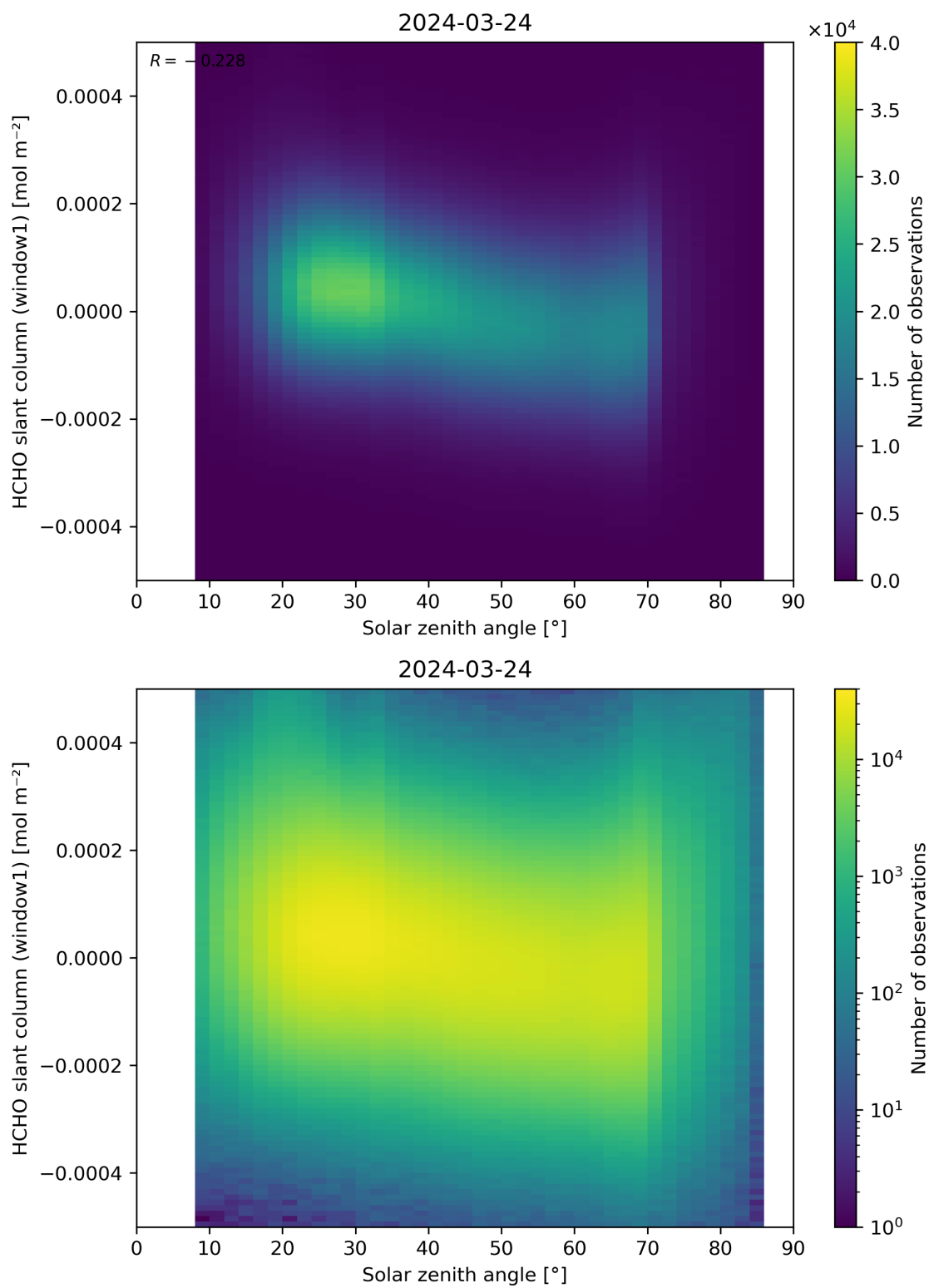
Figure 173: Scatter density plot of “Solar zenith angle” against “HCHO slant column (window1)” for 2024-03-23 to 2024-03-25.
