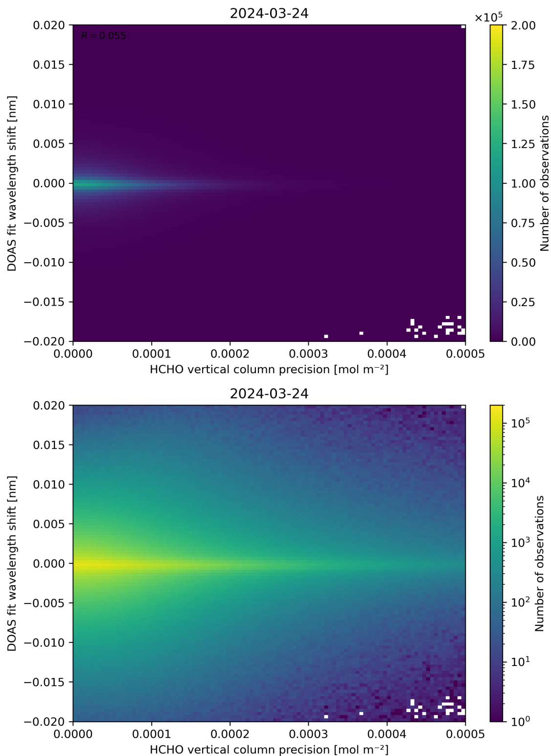
Figure 137: Scatter density plot of “HCHO vertical column precision” against “DOAS fit wavelength shift” for 2024-03-23 to 2024-03-25.
