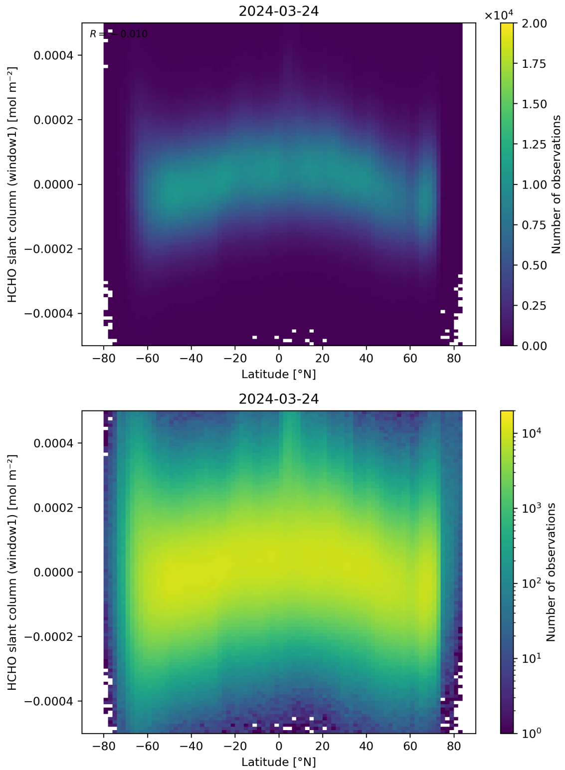
Figure 159: Scatter density plot of “Latitude” against “HCHO slant column (window1)” for 2024-03-23 to 2024-03-25.
