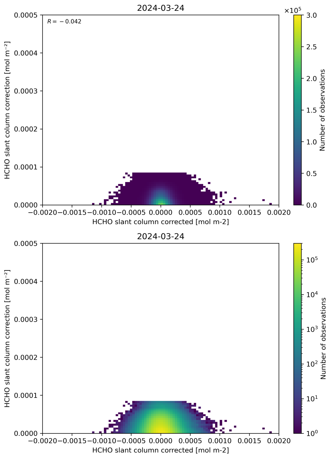
Figure 77: Scatter density plot of “HCHO slant column corrected” against “HCHO slant column correction” for 2024-03-23 to 2024-03-25.
