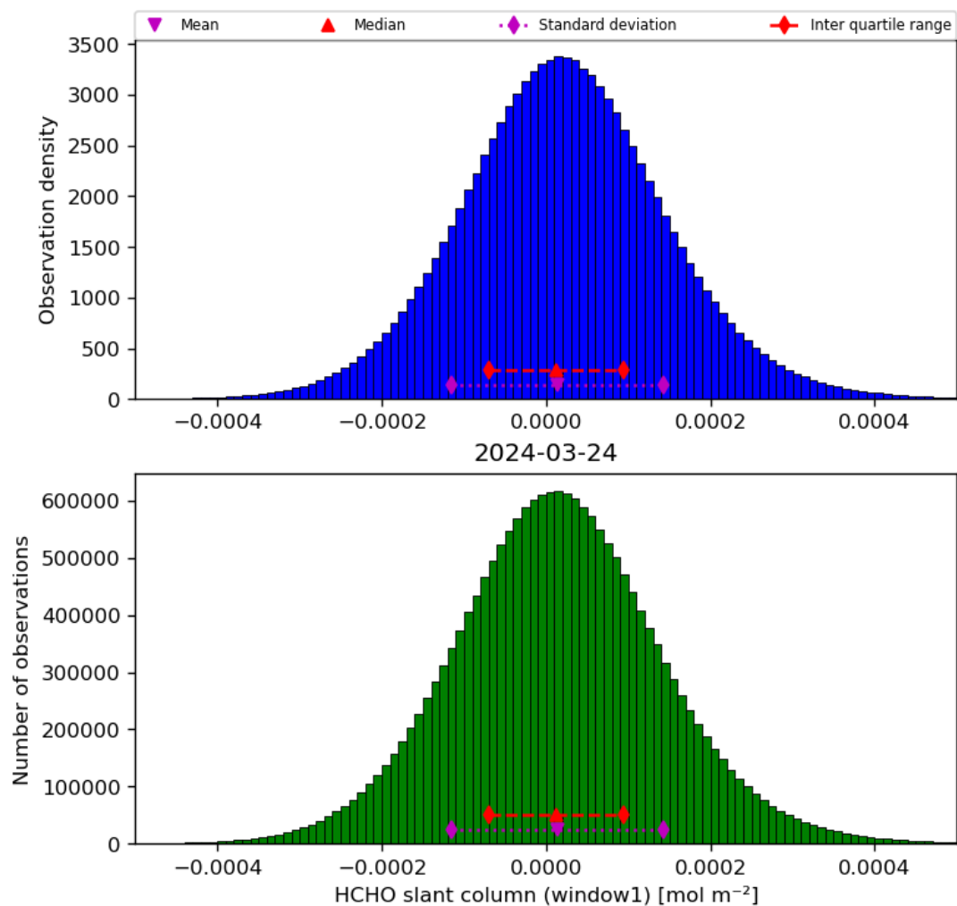
Figure 38: Histogram of “HCHO slant column (window1)” for 2024-03-23 to 2024-03-25
