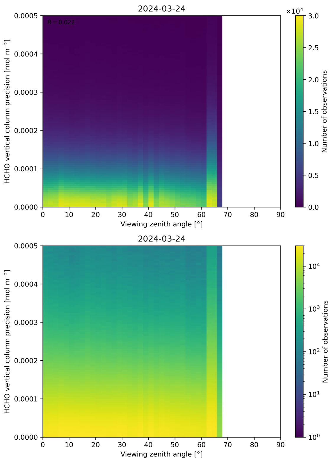
Figure 194: Scatter density plot of “Viewing zenith angle” against “HCHO vertical column precision” for 2024-03-23 to 2024-03-25.
