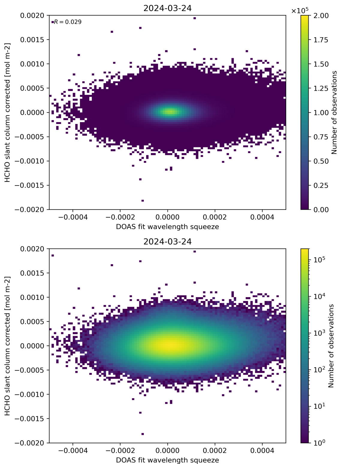
Figure 69: Scatter density plot of “DOAS fit wavelength squeeze” against “HCHO slant column corrected” for 2024-03-23 to 2024-03-25.
