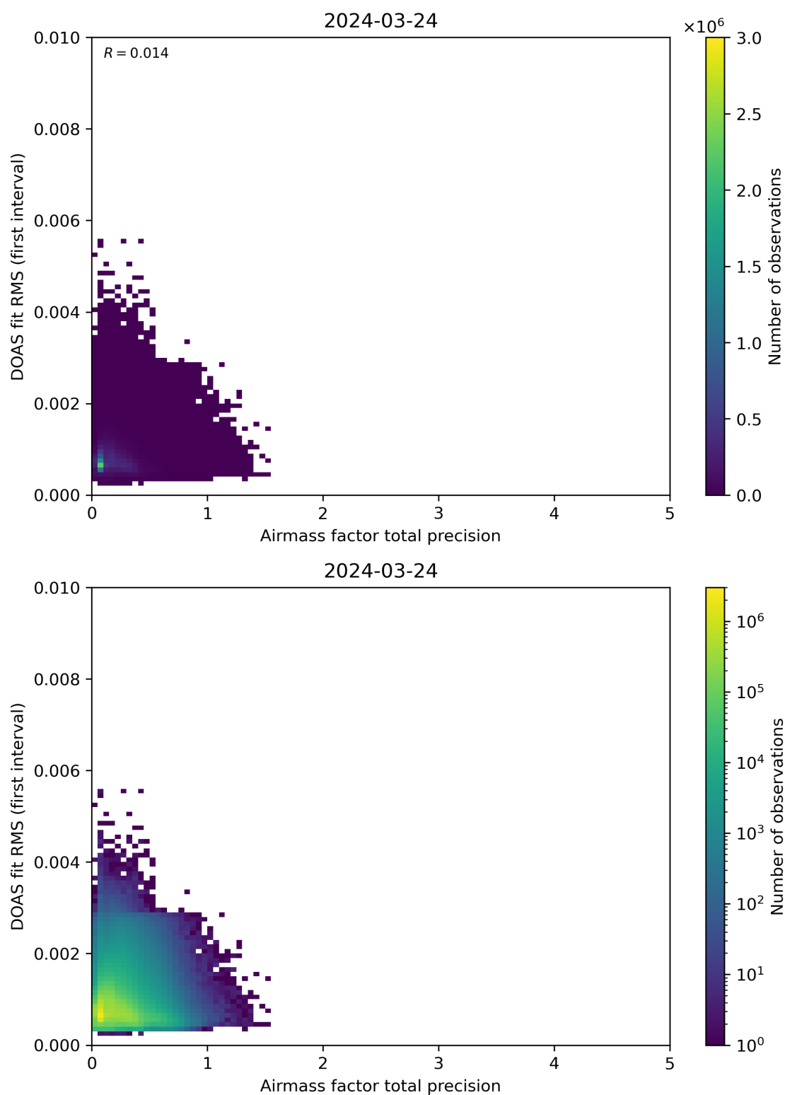
Figure 105: Scatter density plot of “Airmass factor total precision” against “DOAS fit RMS (first interval)” for 2024-03-23 to 2024-03-25.
