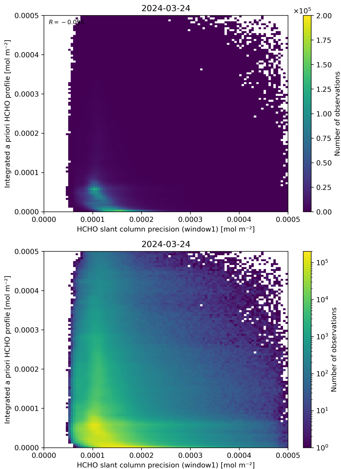
Figure 96: Scatter density plot of “HCHO slant column precision (window1)” against “Integrated a priori HCHO profile” for 2024-03-23 to 2024-03-25.
