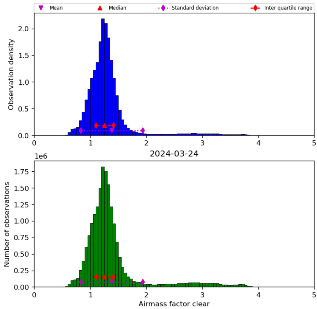
Figure 42: Histogram of “Airmass factor clear” for 2024-03-23 to 2024-03-25
