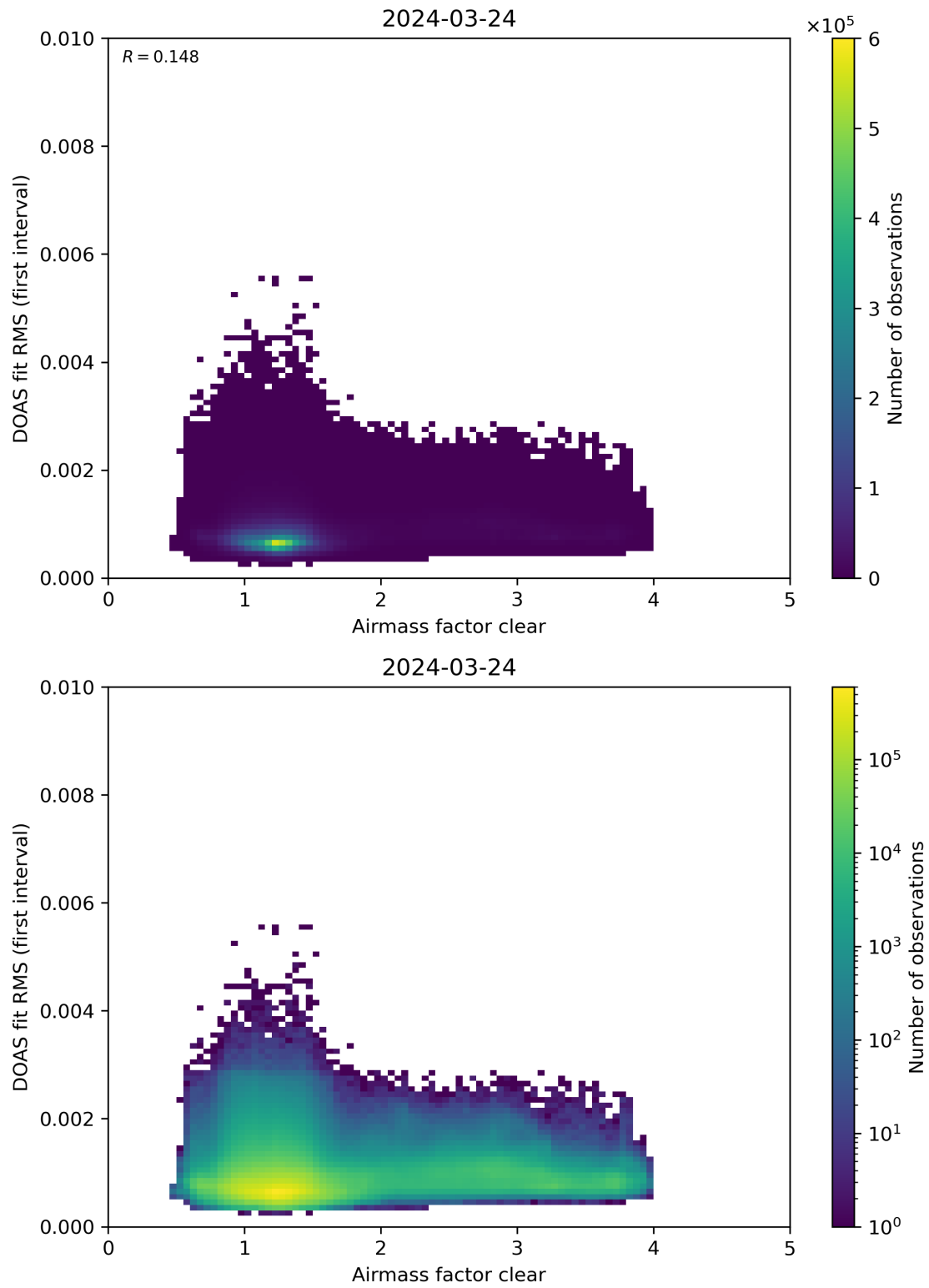
Figure 71: Scatter density plot of “Airmass factor clear” against “DOAS fit RMS (first interval)” for 2024-03-23 to 2024-03-25.
