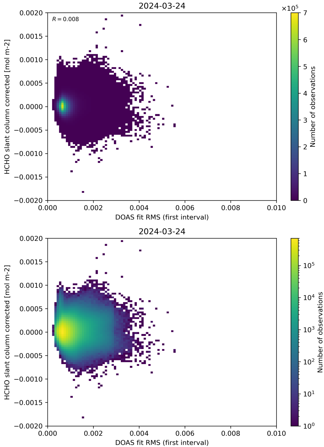
Figure 62: Scatter density plot of “DOAS fit RMS (first interval)” against “HCHO slant column corrected” for 2024-03-23 to 2024-03-25.
