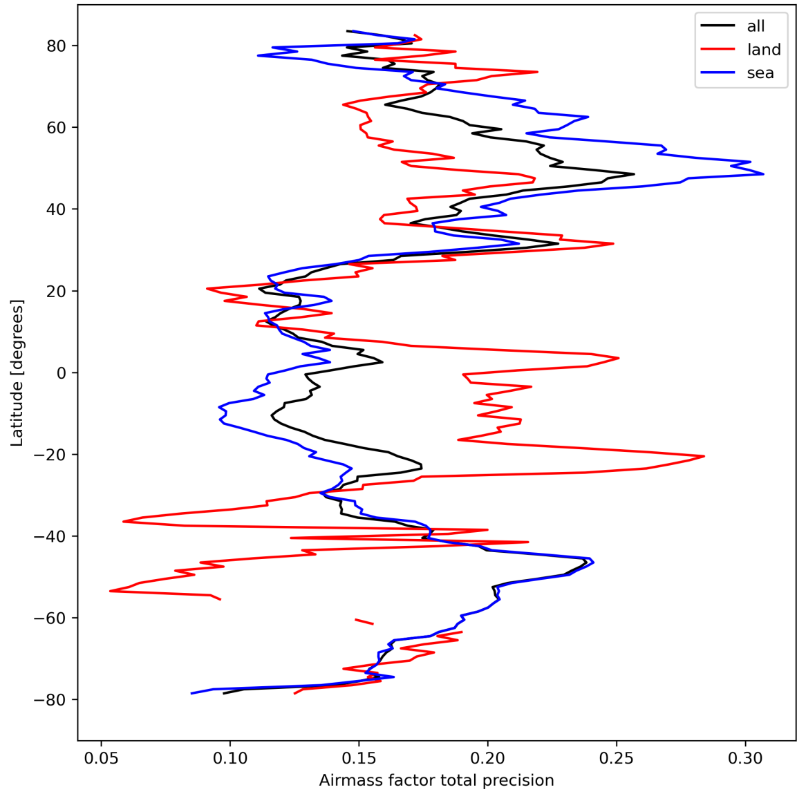
Figure 27: Zonal average of “Airmass factor total precision” for 2024-03-23 to 2024-03-25.
