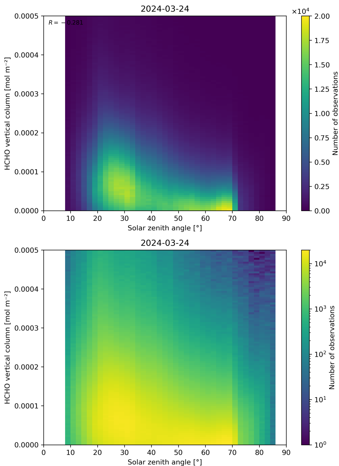
Figure 177: Scatter density plot of “Solar zenith angle” against “HCHO vertical column” for 2024-03-23 to 2024-03-25.
