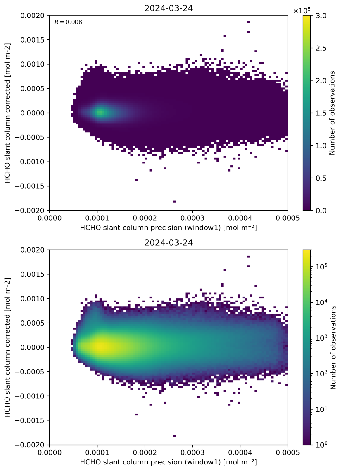
Figure 92: Scatter density plot of “HCHO slant column precision (window1)” against “HCHO slant column corrected” for 2024-03-23 to 2024-03-25.
