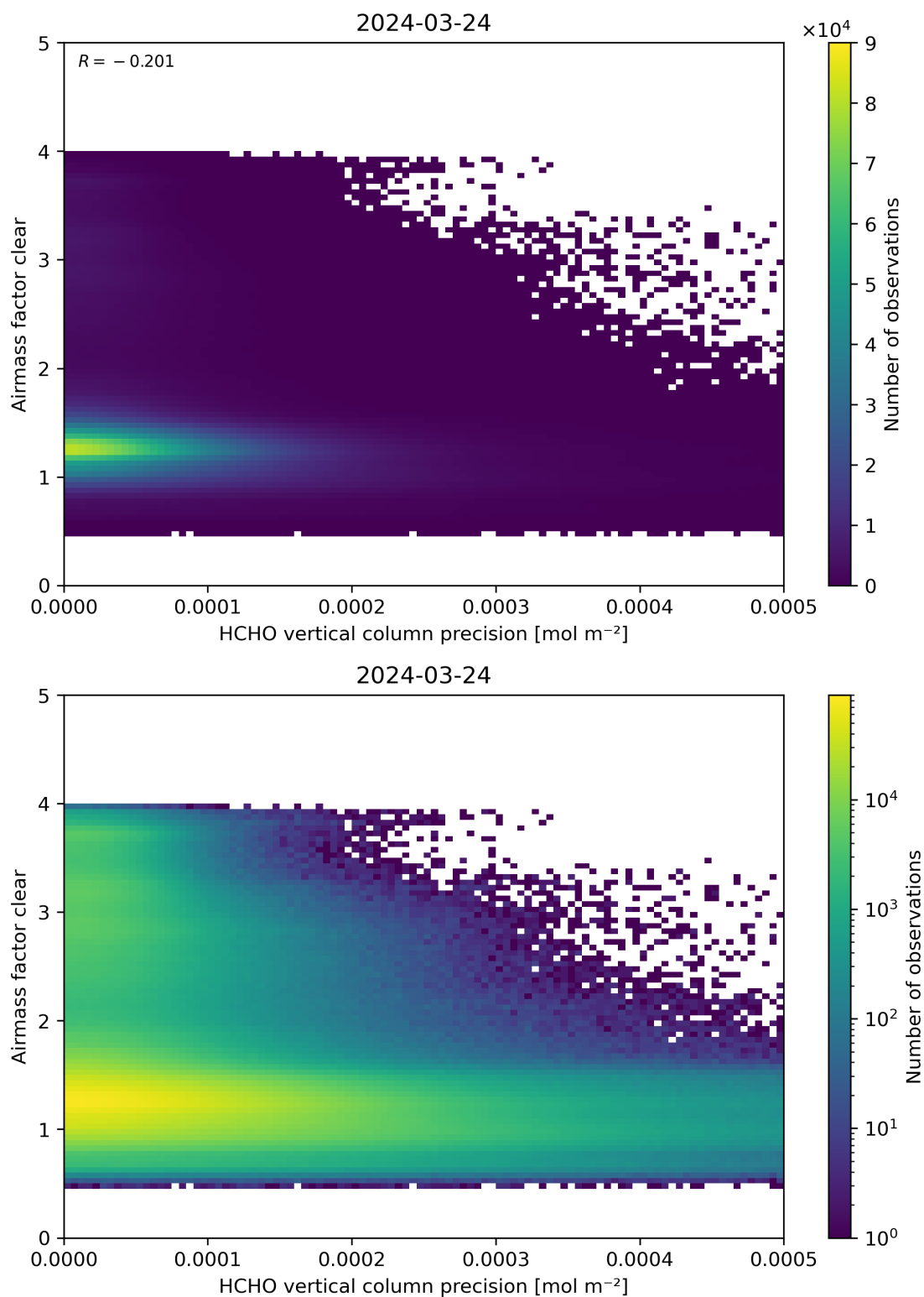
Figure 139: Scatter density plot of “HCHO vertical column precision” against “Airmass factor clear” for 2024-03-23 to 2024-03-25.
