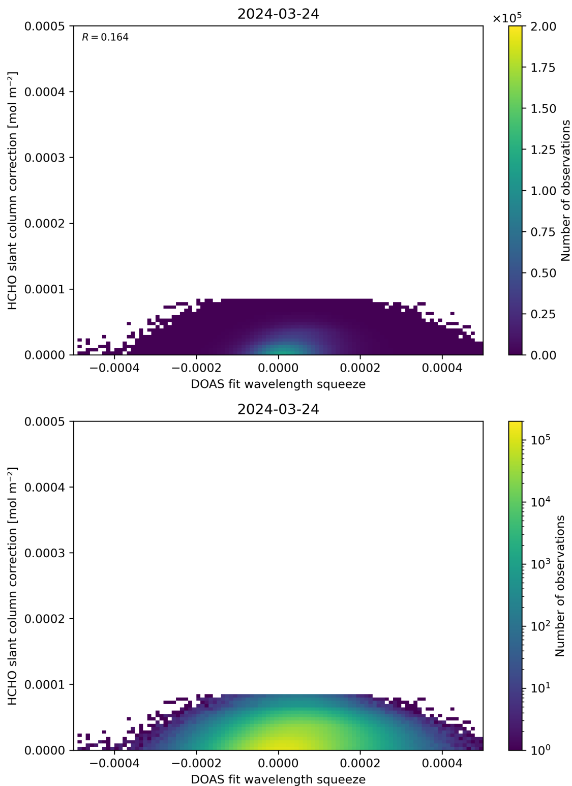
Figure 70: Scatter density plot of “DOAS fit wavelength squeeze” against “HCHO slant column correction” for 2024-03-23 to 2024-03-25.
