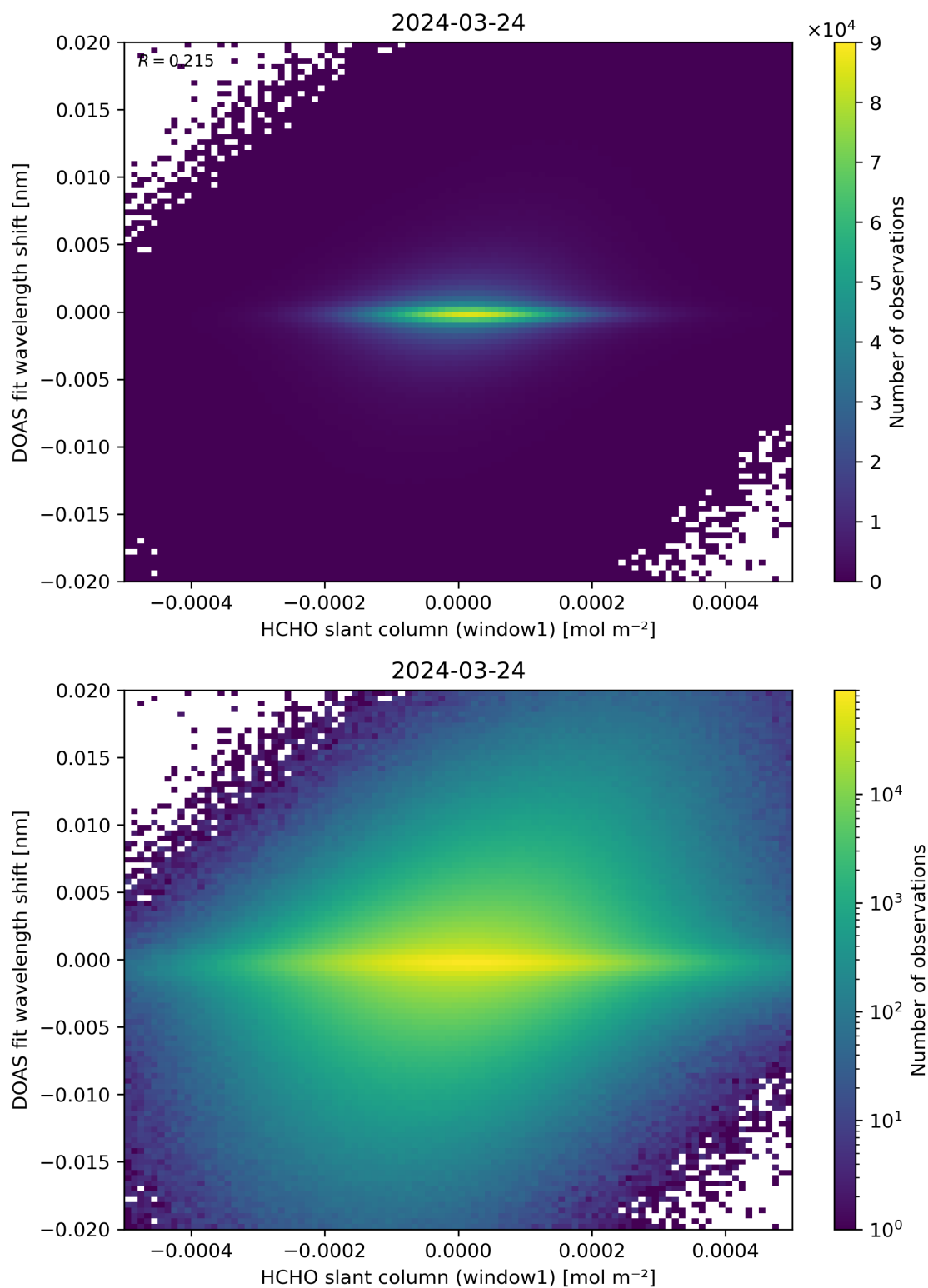
Figure 79: Scatter density plot of “HCHO slant column (window1)” against “DOAS fit wavelength shift” for 2024-03-23 to 2024-03-25.
