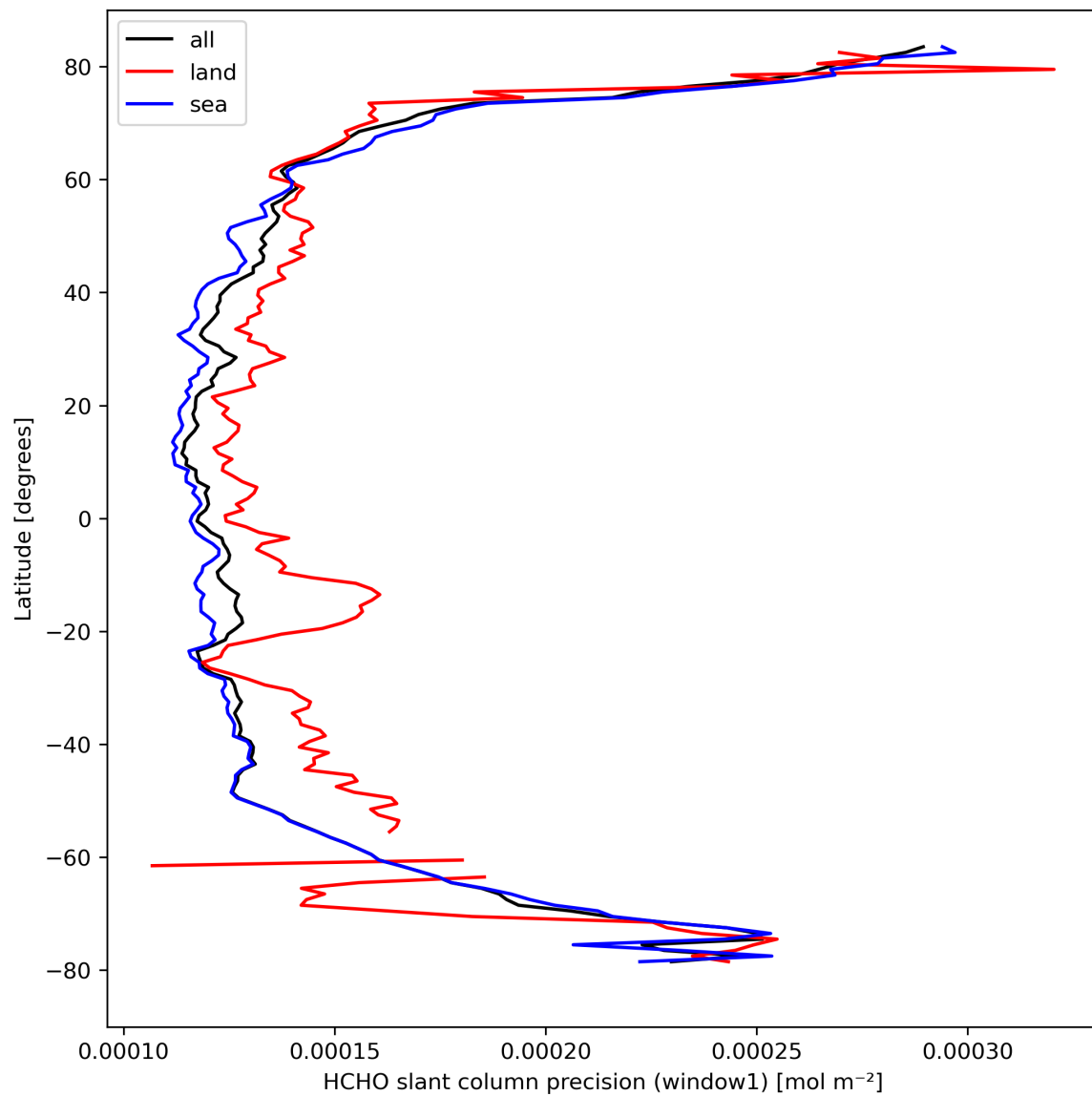
Figure 25: Zonal average of “HCHO slant column precision (window1)” for 2024-03-23 to 2024-03-25.
