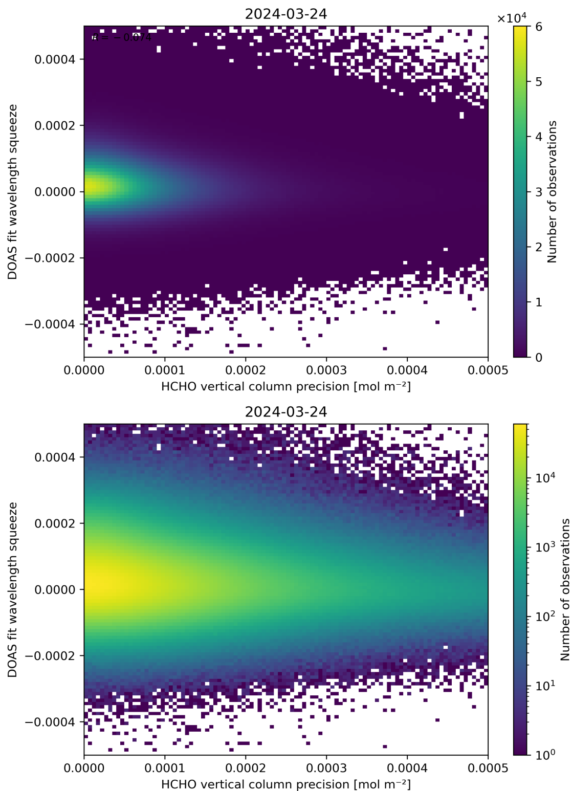
Figure 138: Scatter density plot of “HCHO vertical column precision” against “DOAS fit wavelength squeeze” for 2024-03-23 to 2024-03-25.
