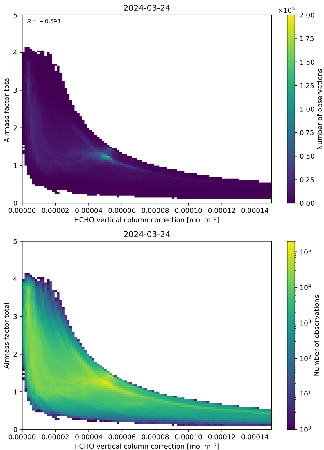
Figure 120: Scatter density plot of “HCHO vertical column correction” against “Airmass factor total” for 2024-03-23 to 2024-03-25.
