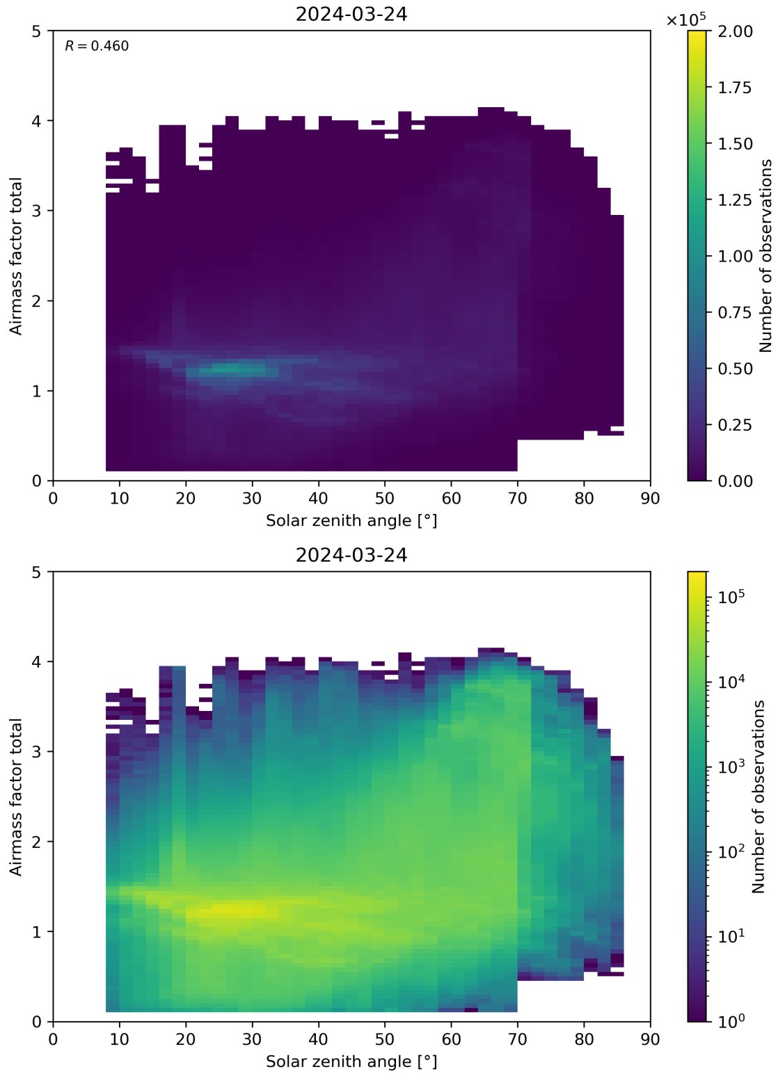
Figure 175: Scatter density plot of “Solar zenith angle” against “Airmass factor total” for 2024-03-23 to 2024-03-25.
