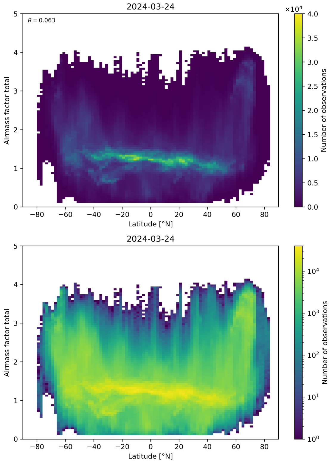
Figure 161: Scatter density plot of “Latitude” against “Airmass factor total” for 2024-03-23 to 2024-03-25.
