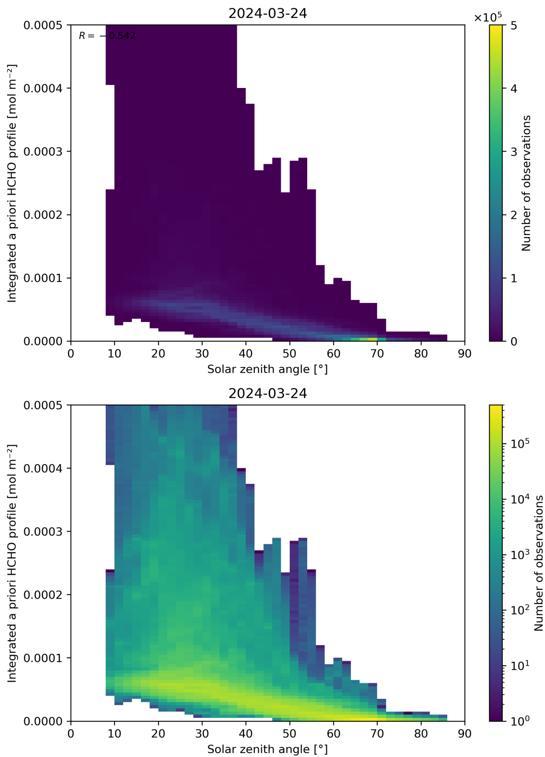
Figure 180: Scatter density plot of “Solar zenith angle” against “Integrated a priori HCHO profile” for 2024-03-23 to 2024-03-25.
