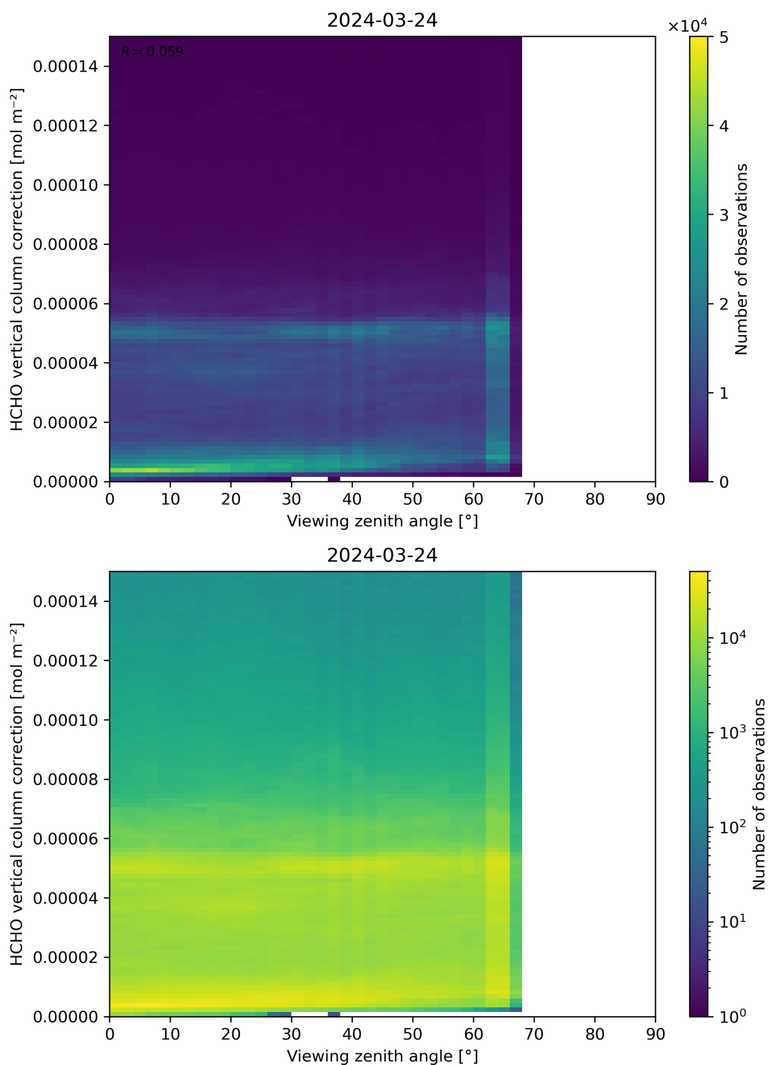
Figure 193: Scatter density plot of “Viewing zenith angle” against “HCHO vertical column correction” for 2024-03-23 to 2024-03-25.
