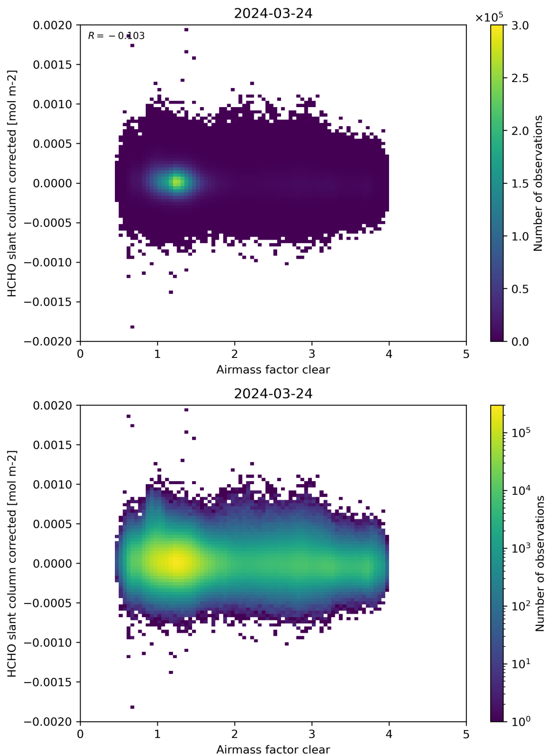
Figure 74: Scatter density plot of “Airmass factor clear” against “HCHO slant column corrected” for 2024-03-23 to 2024-03-25.
