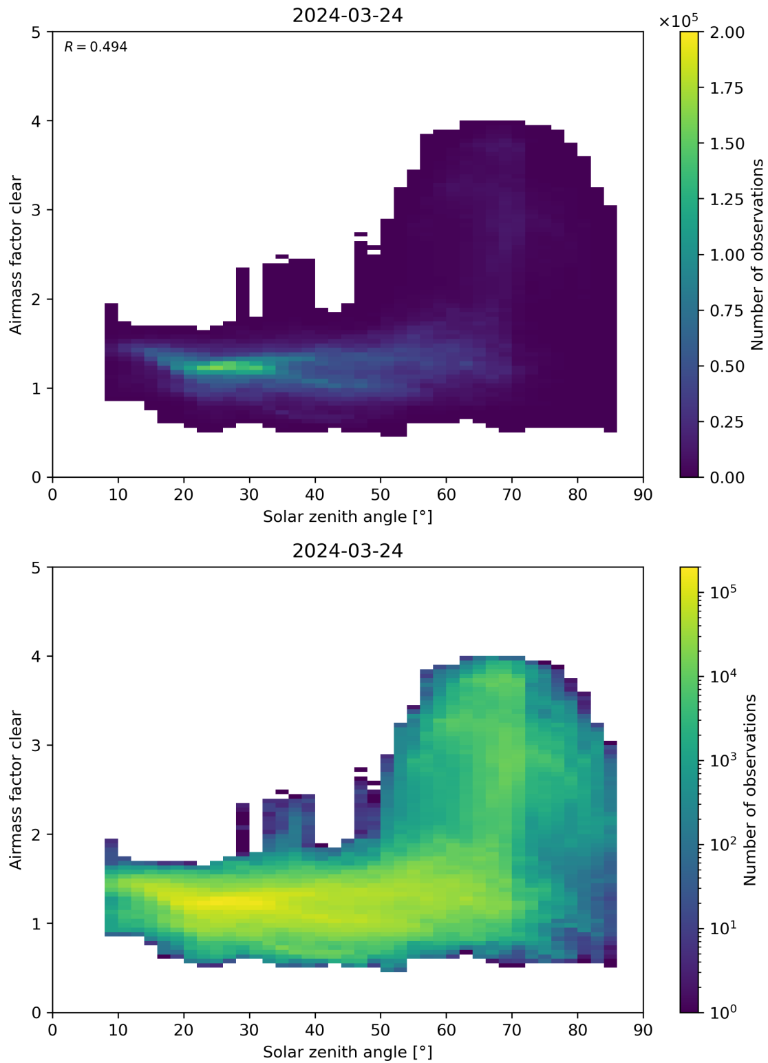
Figure 170: Scatter density plot of “Solar zenith angle” against “Airmass factor clear” for 2024-03-23 to 2024-03-25.
