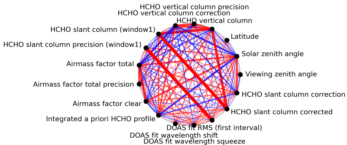
Figure 1: Map of correlation graph for 2024-03-23 to 2024-03-25.
