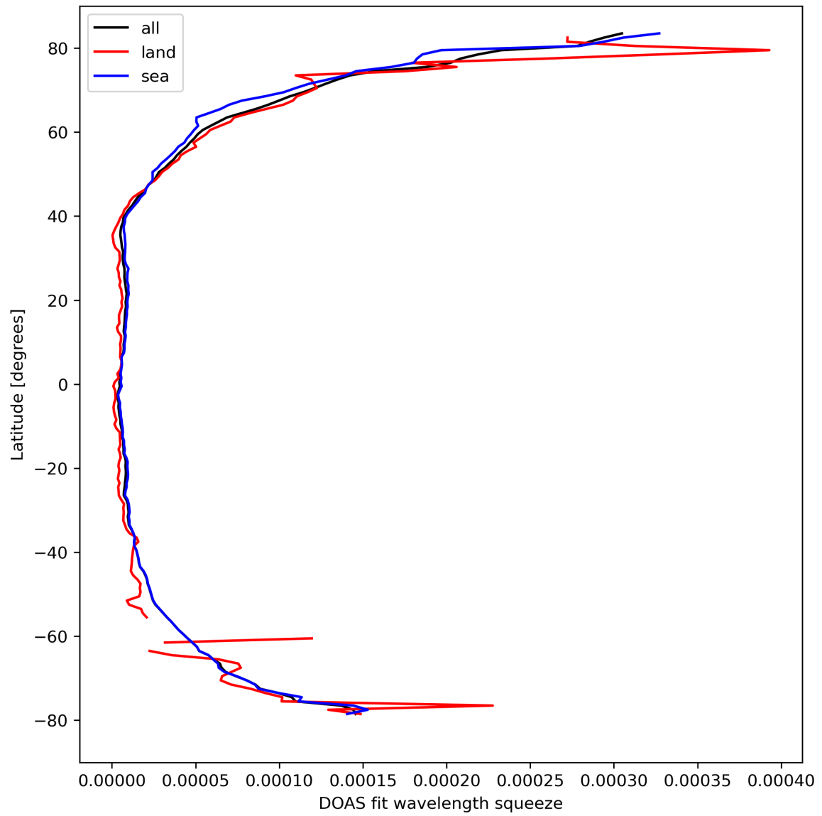
Figure 31: Zonal average of “DOAS fit wavelength squeeze” for 2024-03-23 to 2024-03-25.
