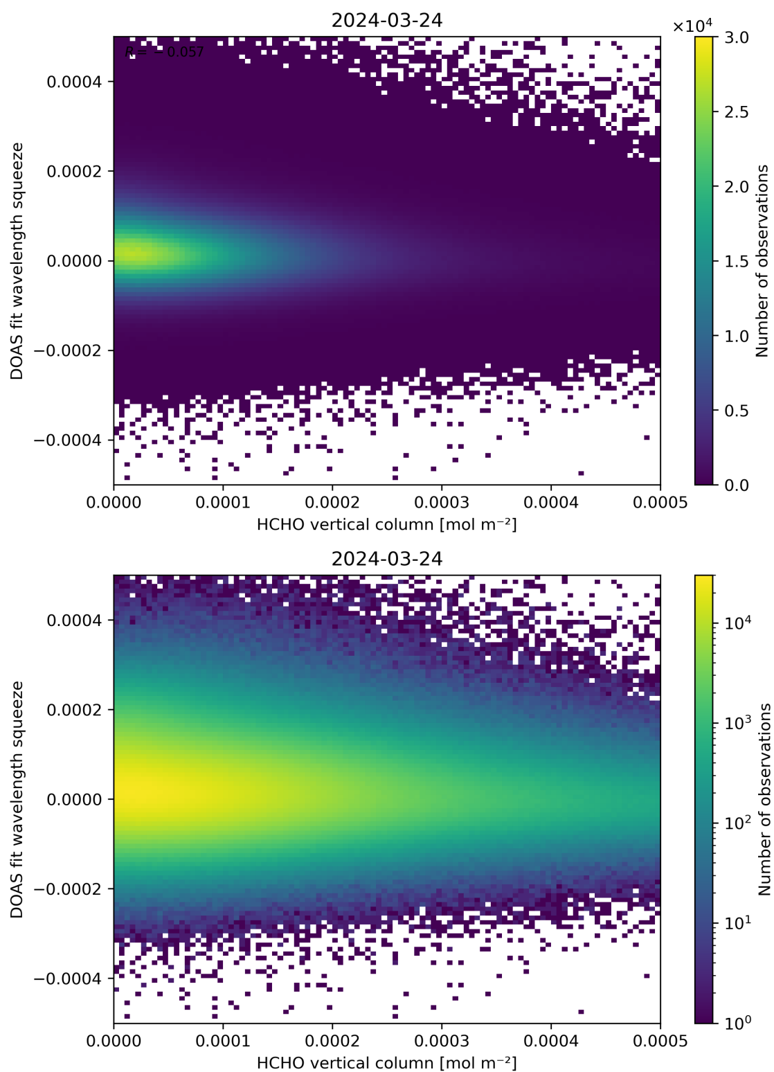
Figure 125: Scatter density plot of “HCHO vertical column” against “DOAS fit wavelength squeeze” for 2024-03-23 to 2024-03-25.
