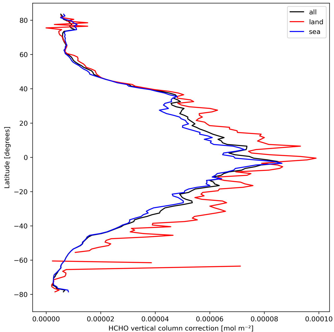
Figure 23: Zonal average of “HCHO vertical column correction” for 2024-03-23 to 2024-03-25.
