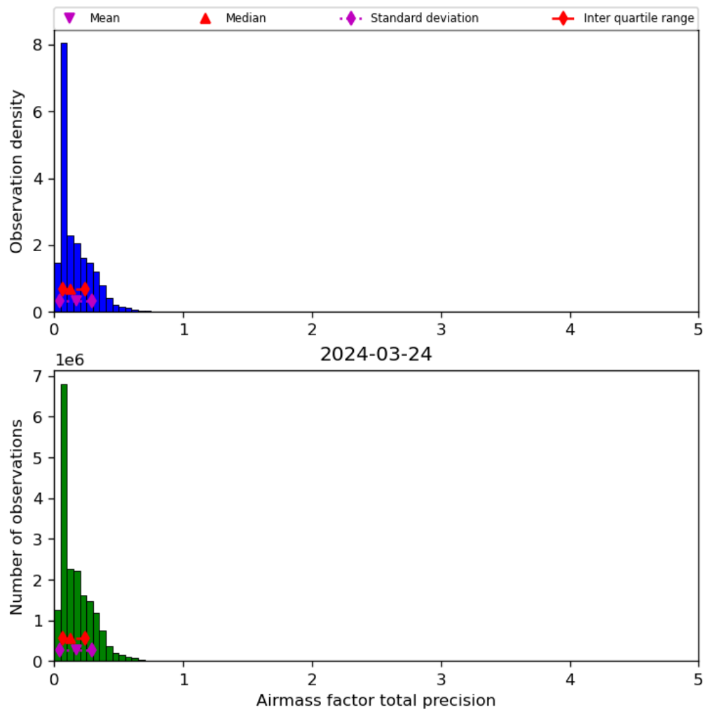
Figure 41: Histogram of “Airmass factor total precision” for 2024-03-23 to 2024-03-25
