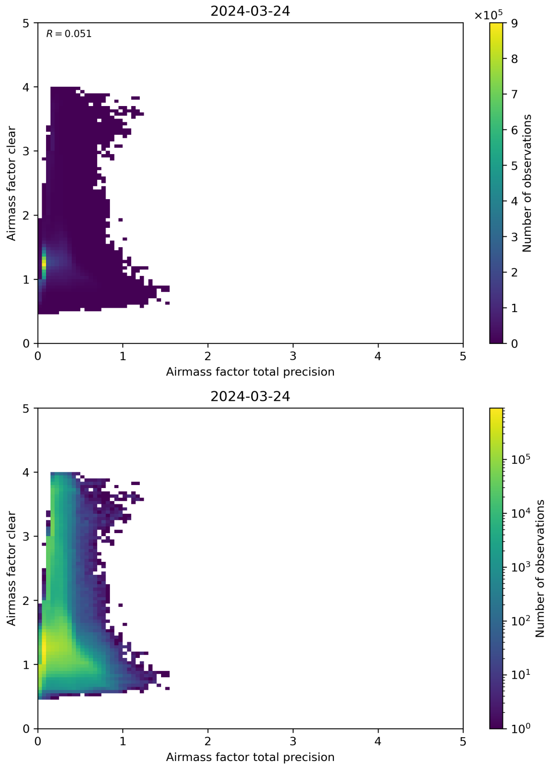
Figure 108: Scatter density plot of “Airmass factor total precision” against “Airmass factor clear” for 2024-03-23 to 2024-03-25.
