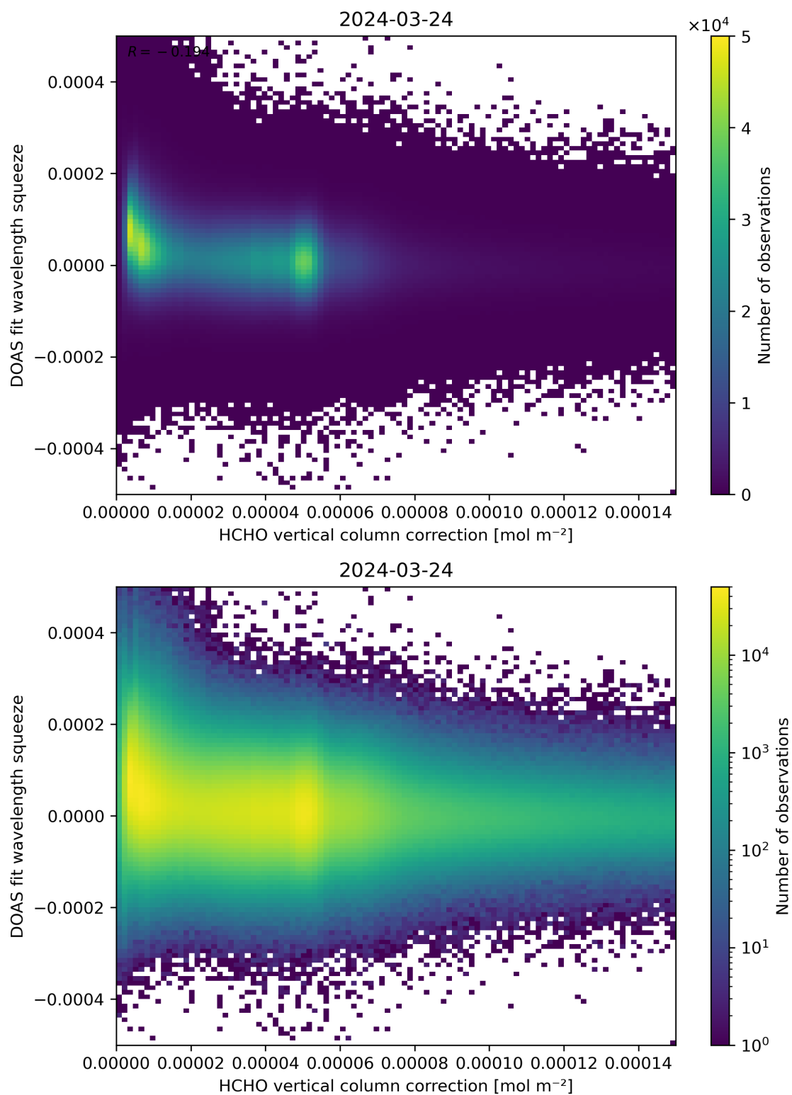
Figure 114: Scatter density plot of “HCHO vertical column correction” against “DOAS fit wavelength squeeze” for 2024-03-23 to 2024-03-25.
