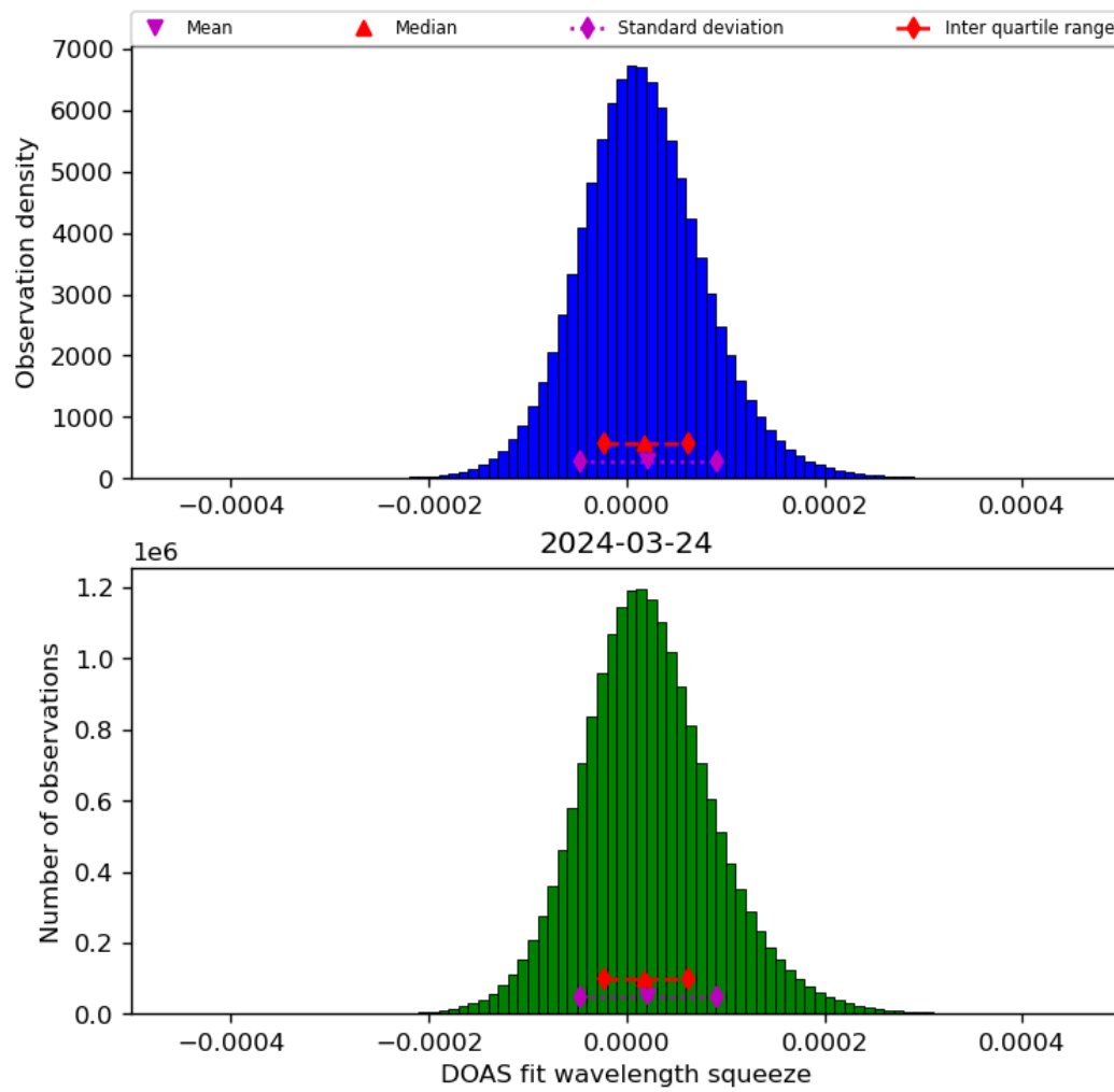
Figure 45: Histogram of “DOAS fit wavelength squeeze” for 2024-03-23 to 2024-03-25
