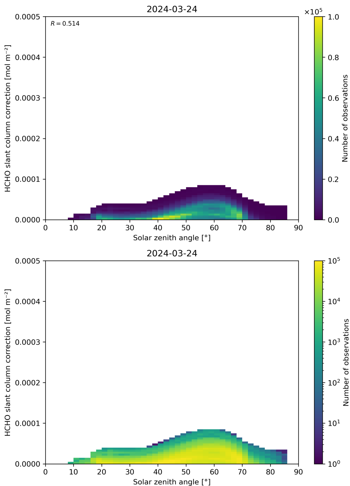
Figure 172: Scatter density plot of “Solar zenith angle” against “HCHO slant column correction” for 2024-03-23 to 2024-03-25.
