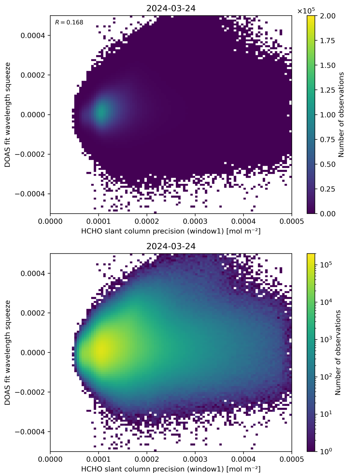
Figure 90: Scatter density plot of “HCHO slant column precision (window1)” against “DOAS fit wavelength squeeze” for 2024-03-23 to 2024-03-25.
