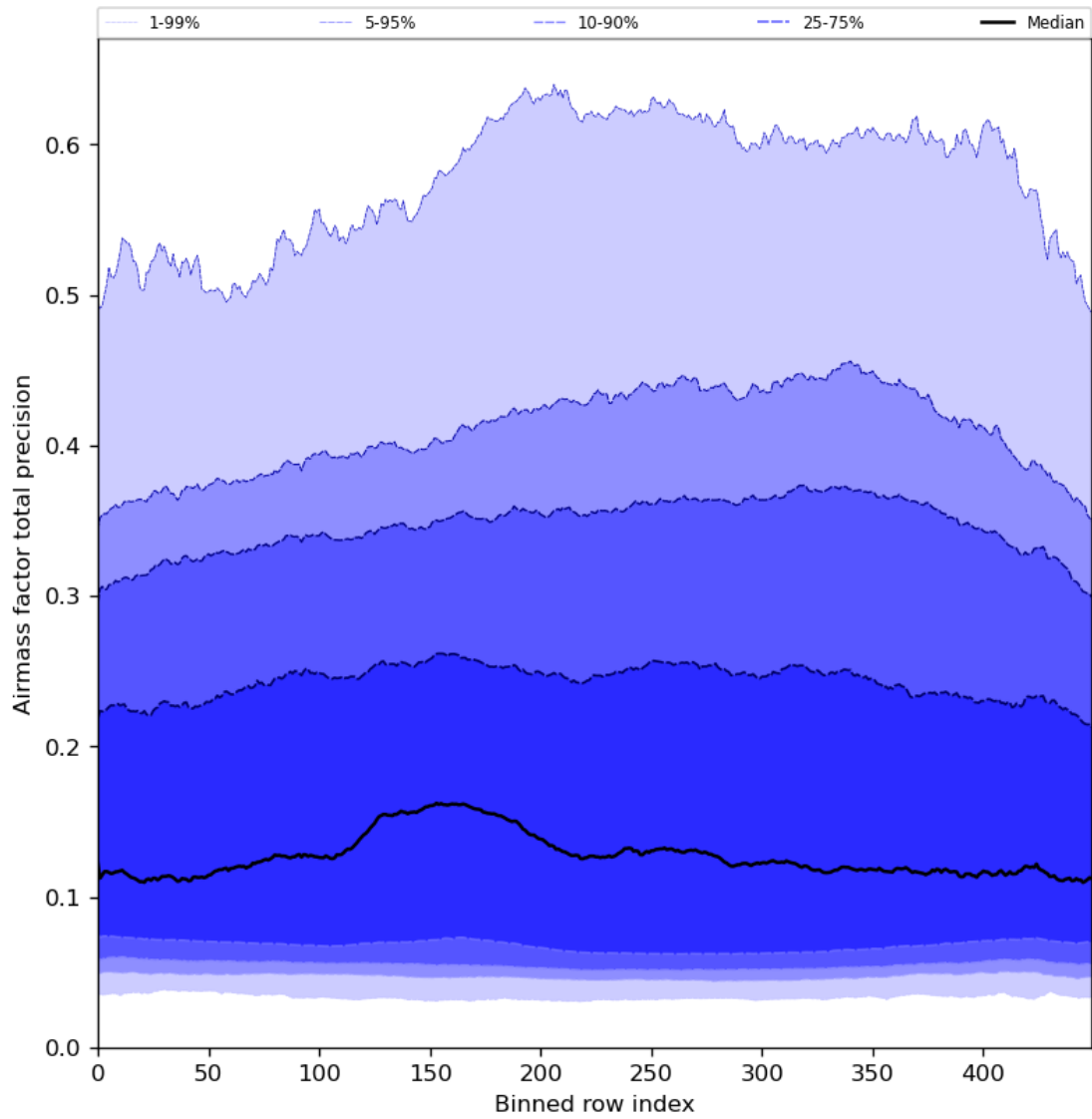
Figure 55: Along track statistics of “Airmass factor total precision” for 2024-03-23 to 2024-03-25
