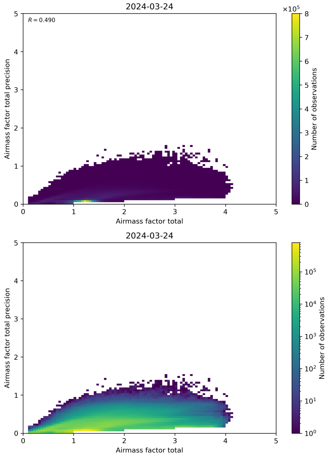
Figure 103: Scatter density plot of “Airmass factor total” against “Airmass factor total precision” for 2024-03-23 to 2024-03-25.
