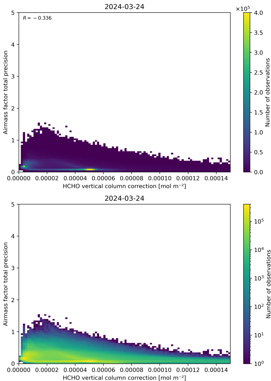
Figure 121: Scatter density plot of “HCHO vertical column correction” against “Airmass factor total precision” for 2024-03-23 to 2024-03-25.
