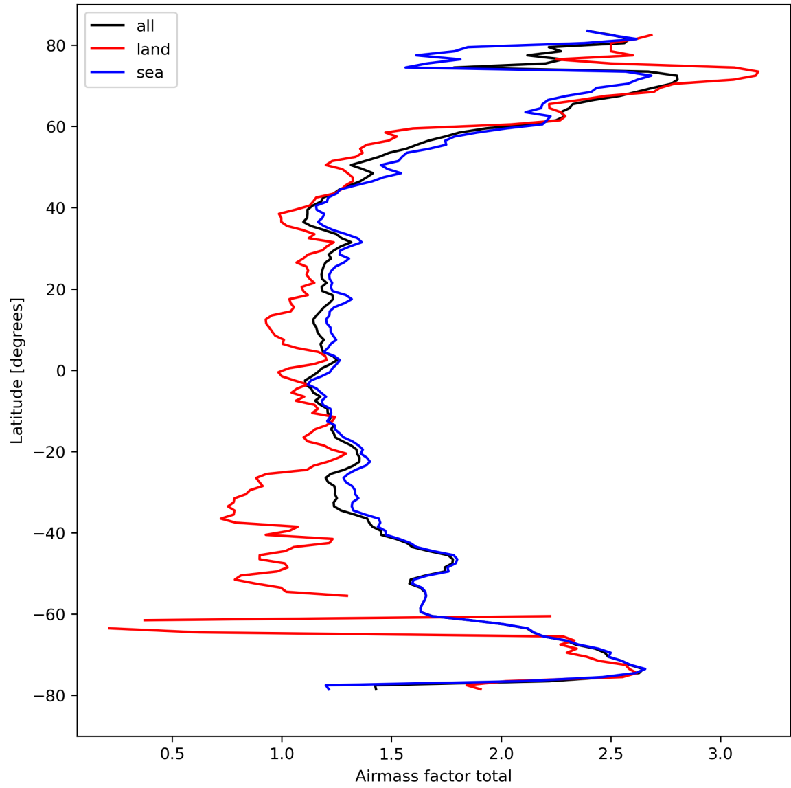
Figure 26: Zonal average of “Airmass factor total” for 2024-03-23 to 2024-03-25.
