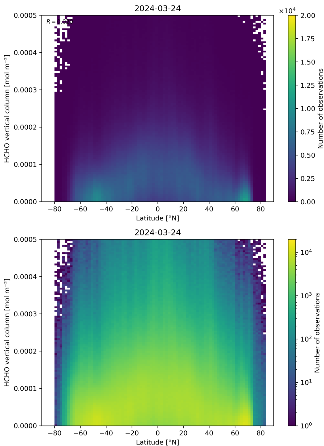
Figure 163: Scatter density plot of “Latitude” against “HCHO vertical column” for 2024-03-23 to 2024-03-25.
