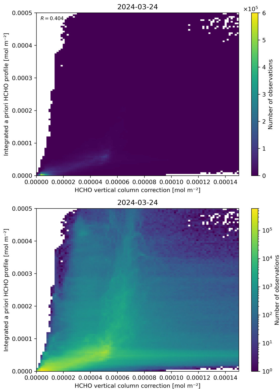
Figure 122: Scatter density plot of “HCHO vertical column correction” against “Integrated a priori HCHO profile” for 2024-03-23 to 2024-03-25.
