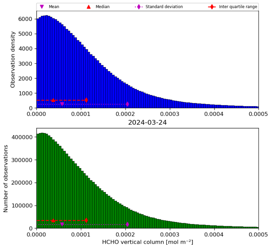
Figure 35: Histogram of “HCHO vertical column” for 2024-03-23 to 2024-03-25
