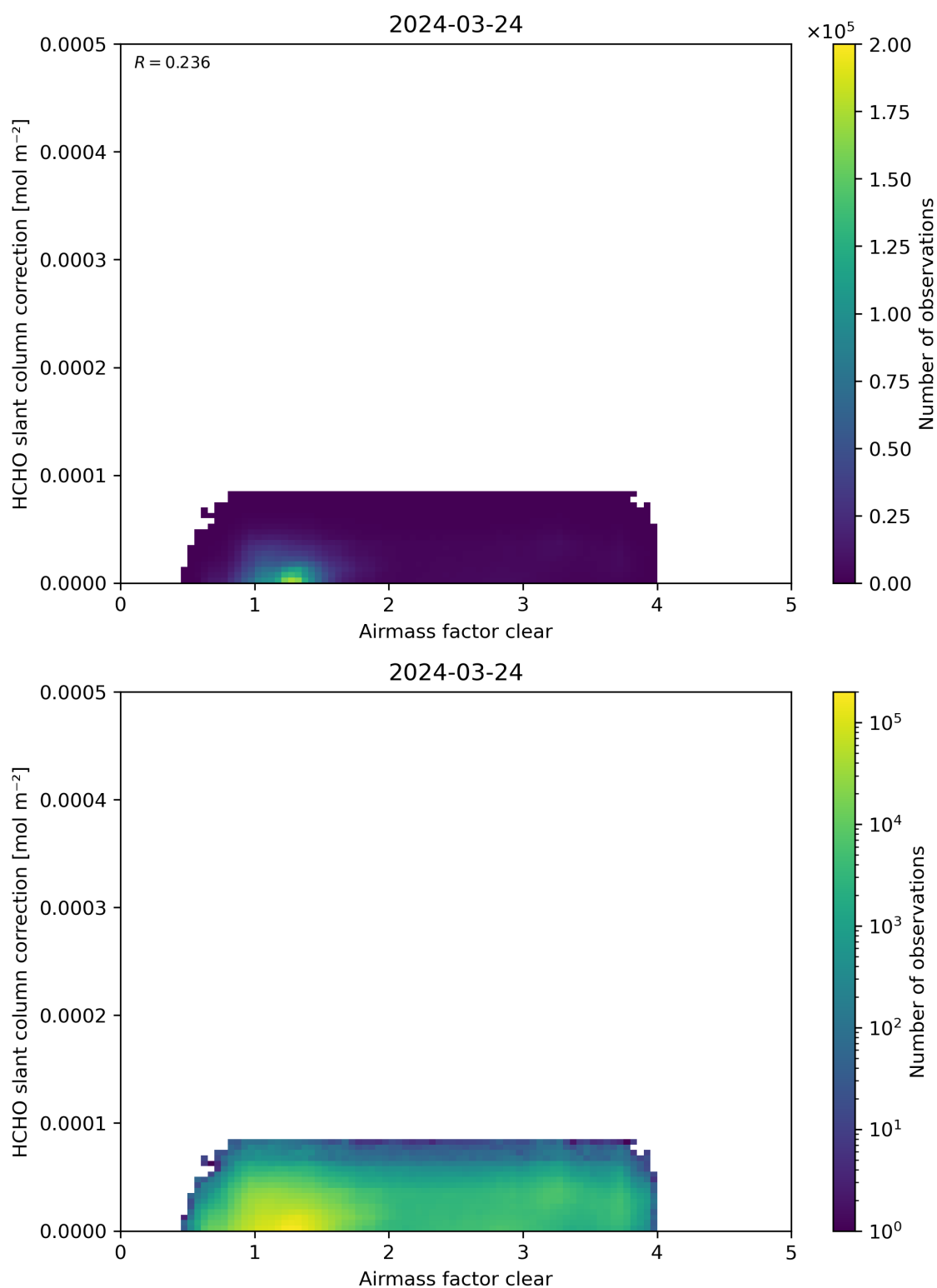
Figure 75: Scatter density plot of “Airmass factor clear” against “HCHO slant column correction” for 2024-03-23 to 2024-03-25.
