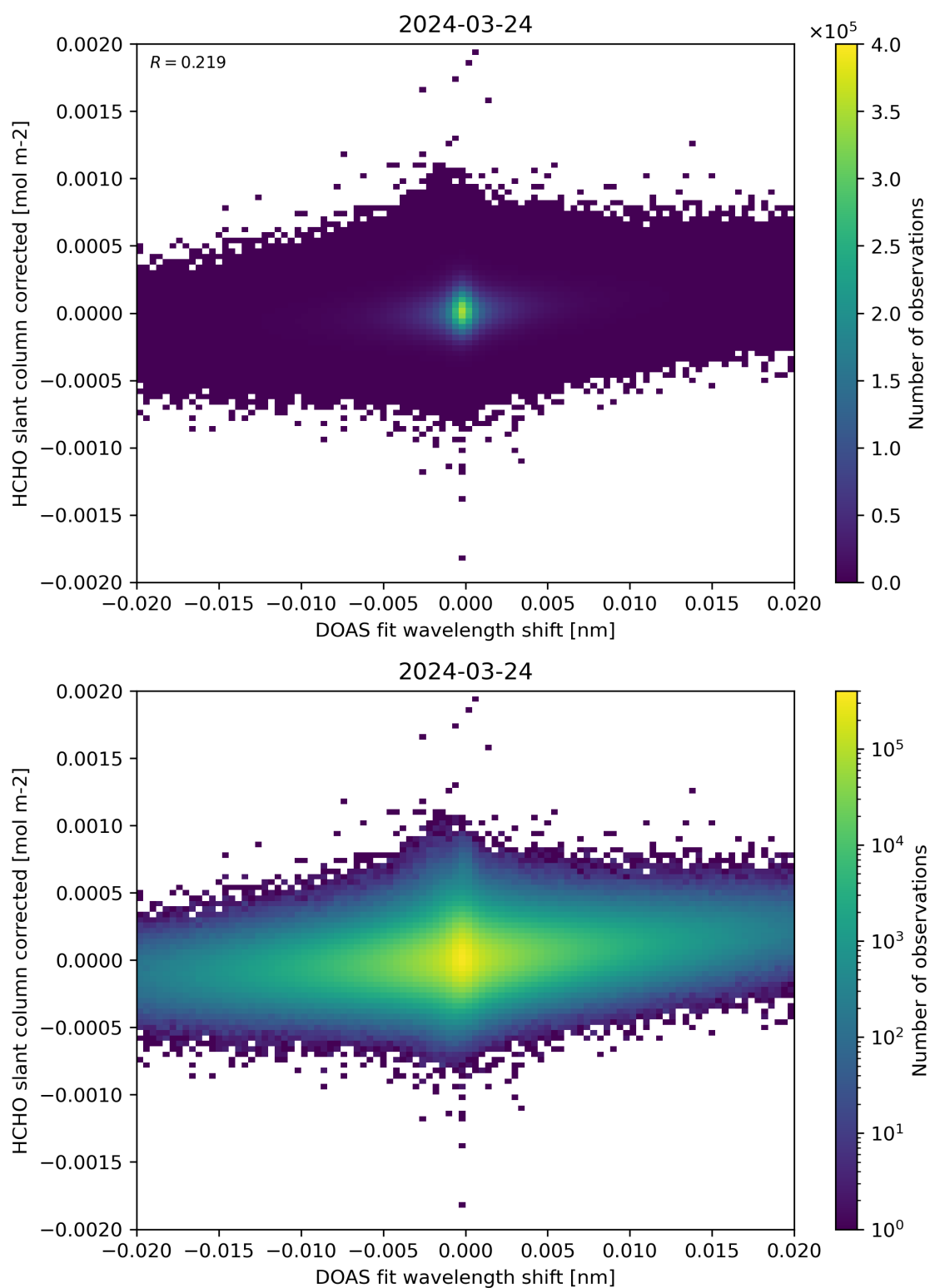
Figure 66: Scatter density plot of “DOAS fit wavelength shift” against “HCHO slant column corrected” for 2024-03-23 to 2024-03-25.
