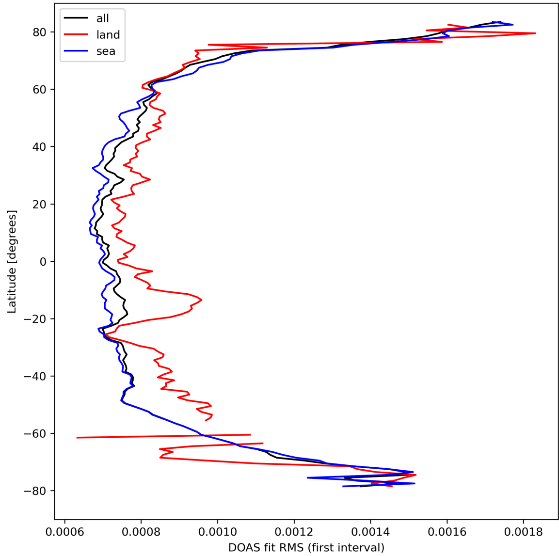
Figure 32: Zonal average of “DOAS fit RMS (first interval)” for 2024-03-23 to 2024-03-25.
