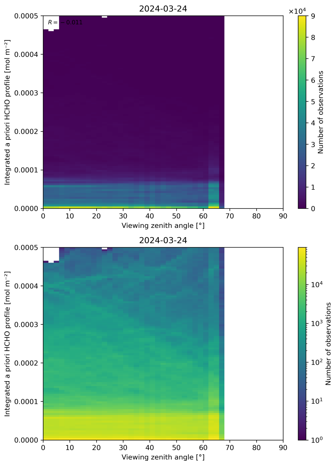
Figure 195: Scatter density plot of “Viewing zenith angle” against “Integrated a priori HCHO profile” for 2024-03-23 to 2024-03-25.
