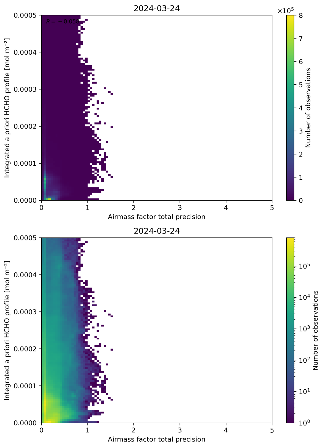
Figure 111: Scatter density plot of “Airmass factor total precision” against “Integrated a priori HCHO profile” for 2024-03-23 to 2024-03-25.
