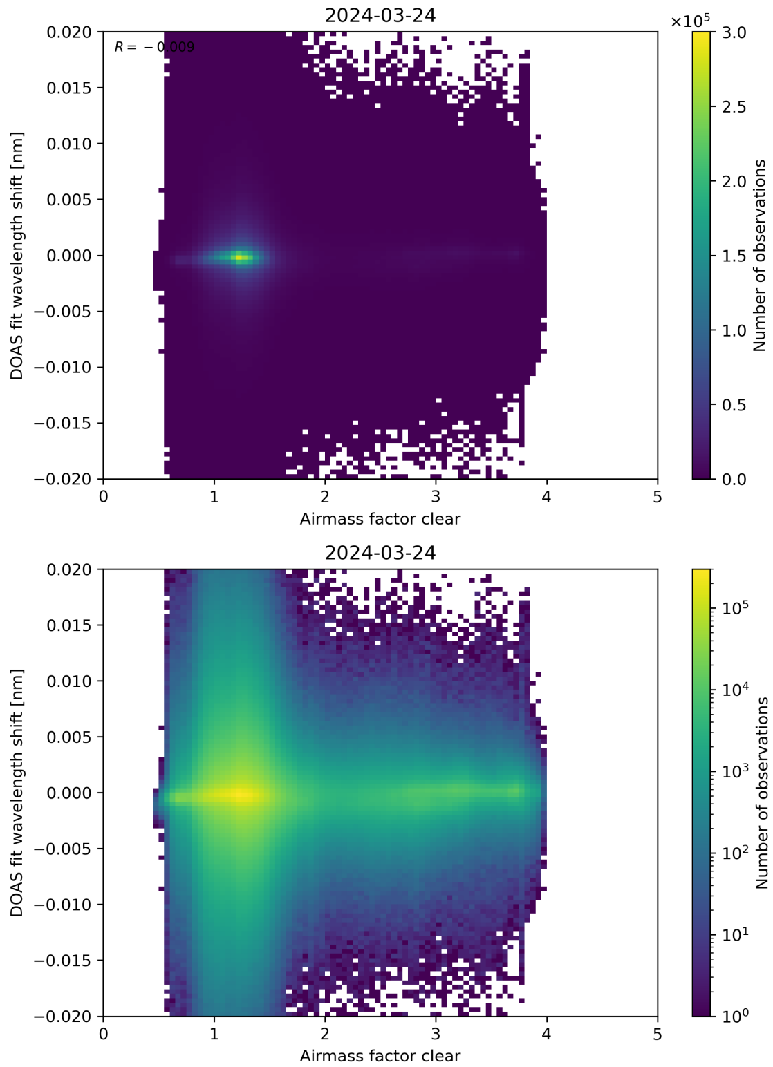
Figure 72: Scatter density plot of “Airmass factor clear” against “DOAS fit wavelength shift” for 2024-03-23 to 2024-03-25.
