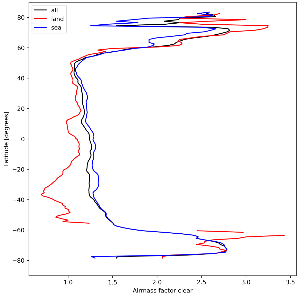
Figure 28: Zonal average of “Airmass factor clear” for 2024-03-23 to 2024-03-25.
