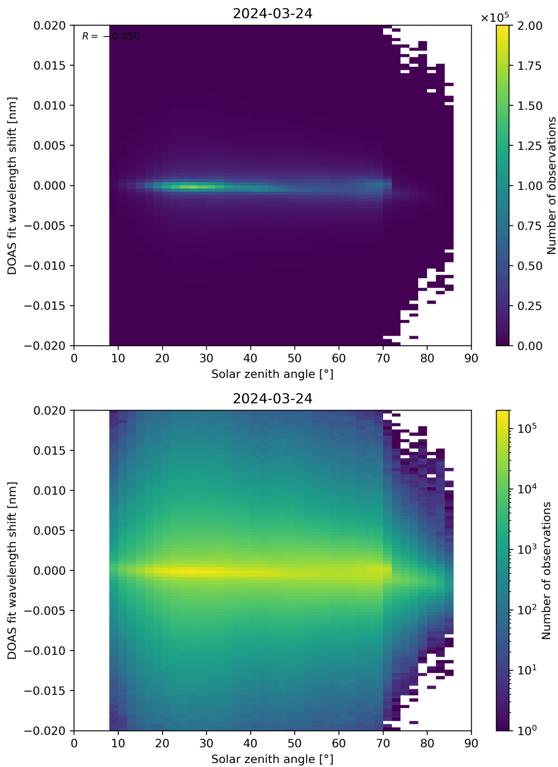
Figure 168: Scatter density plot of “Solar zenith angle” against “DOAS fit wavelength shift” for 2024-03-23 to 2024-03-25.
