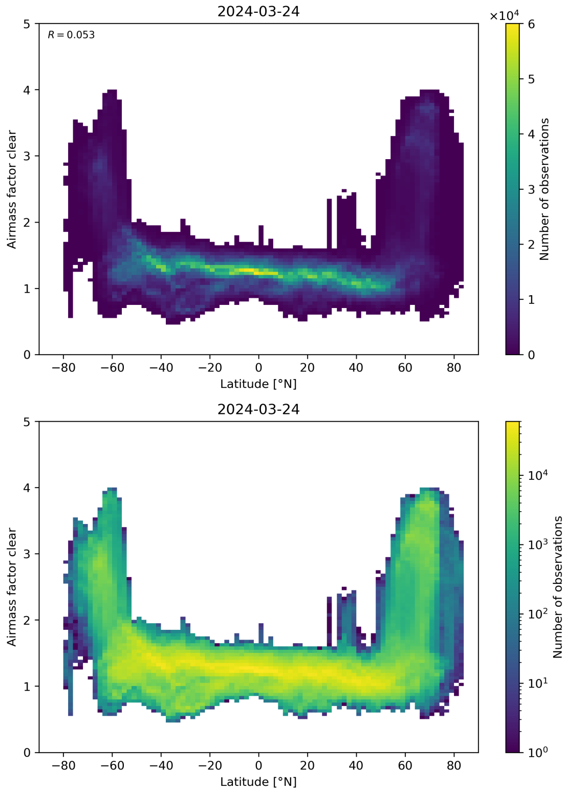
Figure 156: Scatter density plot of “Latitude” against “Airmass factor clear” for 2024-03-23 to 2024-03-25.
