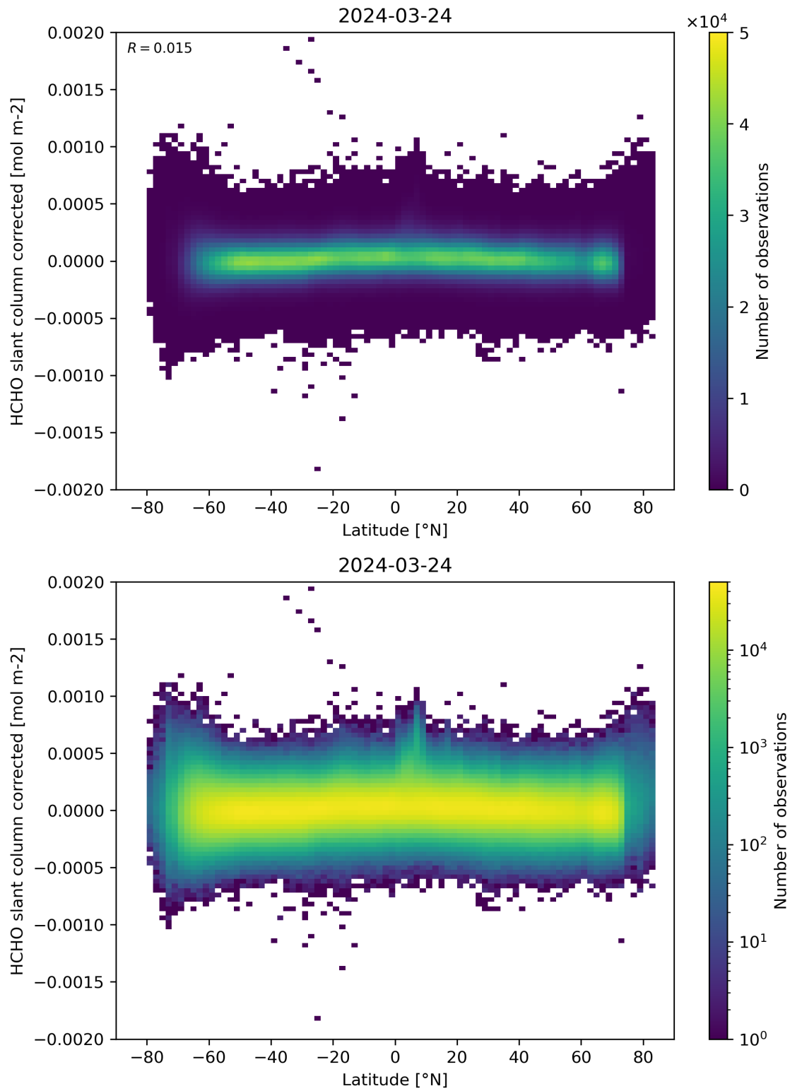
Figure 157: Scatter density plot of “Latitude” against “HCHO slant column corrected” for 2024-03-23 to 2024-03-25.
