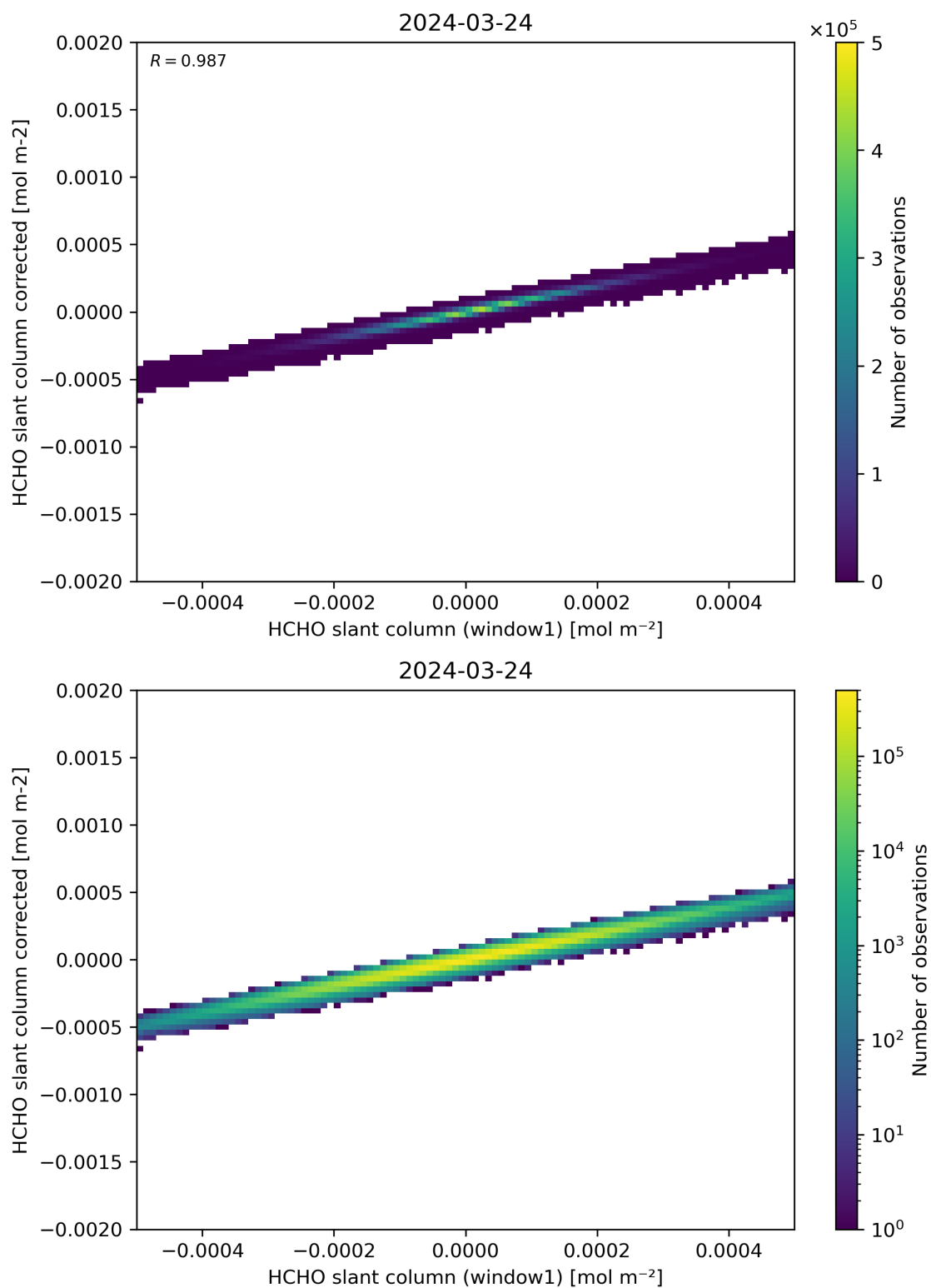
Figure 82: Scatter density plot of “HCHO slant column (window1)” against “HCHO slant column corrected” for 2024-03-23 to 2024-03-25.
