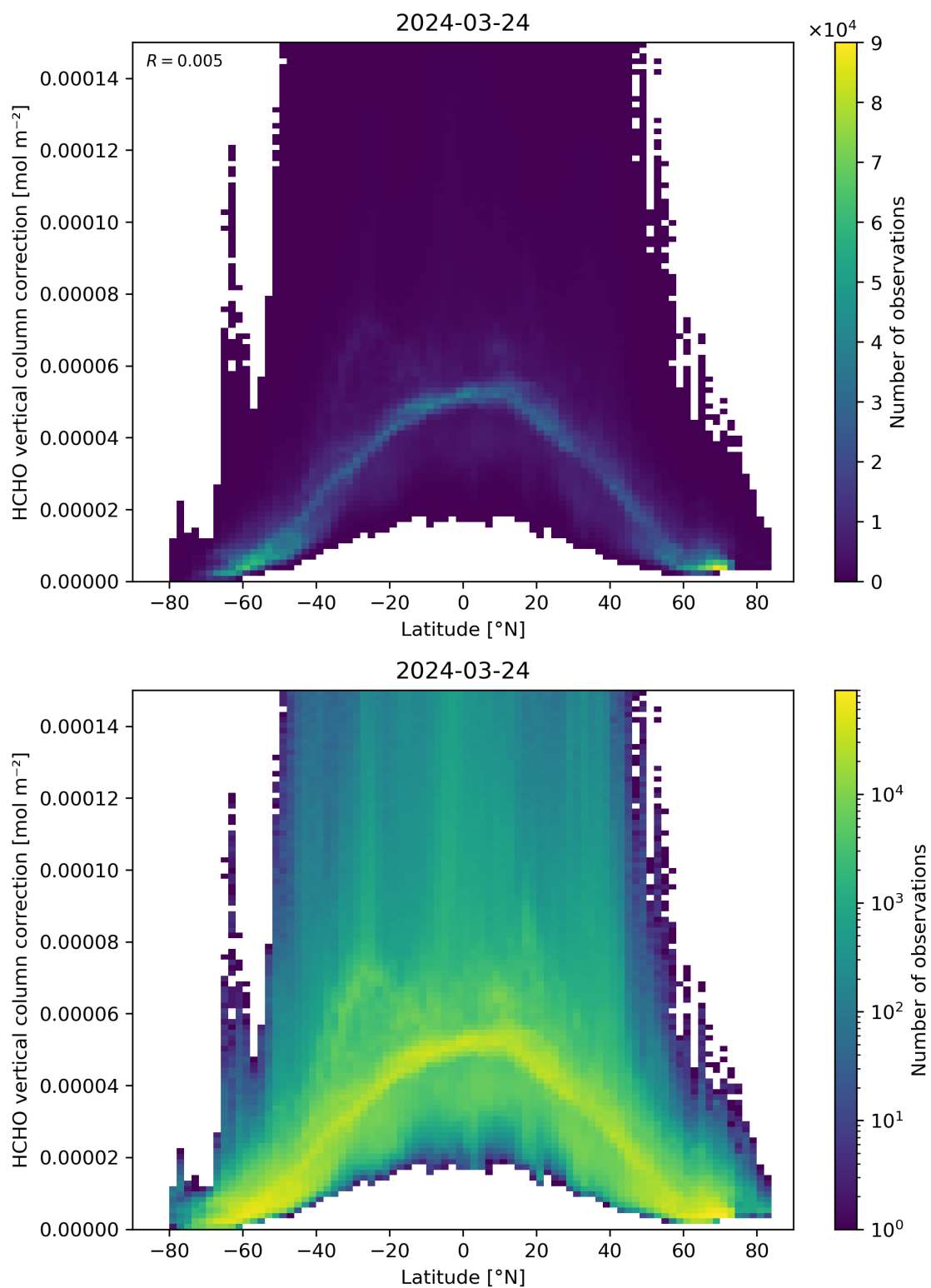
Figure 164: Scatter density plot of “Latitude” against “HCHO vertical column correction” for 2024-03-23 to 2024-03-25.
