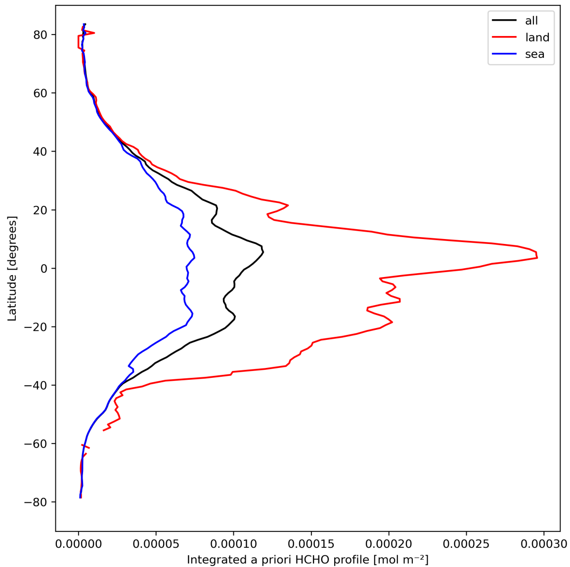
Figure 29: Zonal average of “Integrated a priori HCHO profile” for 2024-03-23 to 2024-03-25.
