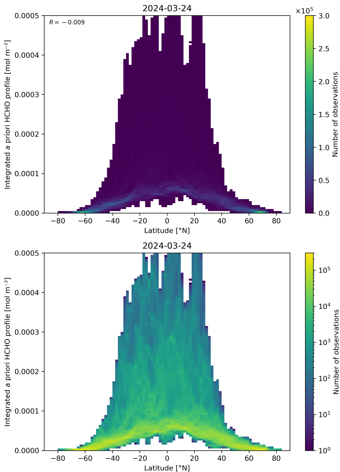
Figure 166: Scatter density plot of “Latitude” against “Integrated a priori HCHO profile” for 2024-03-23 to 2024-03-25.
