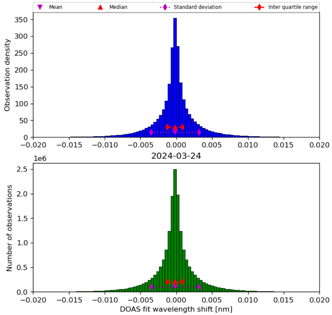
Figure 44: Histogram of “DOAS fit wavelength shift” for 2024-03-23 to 2024-03-25
