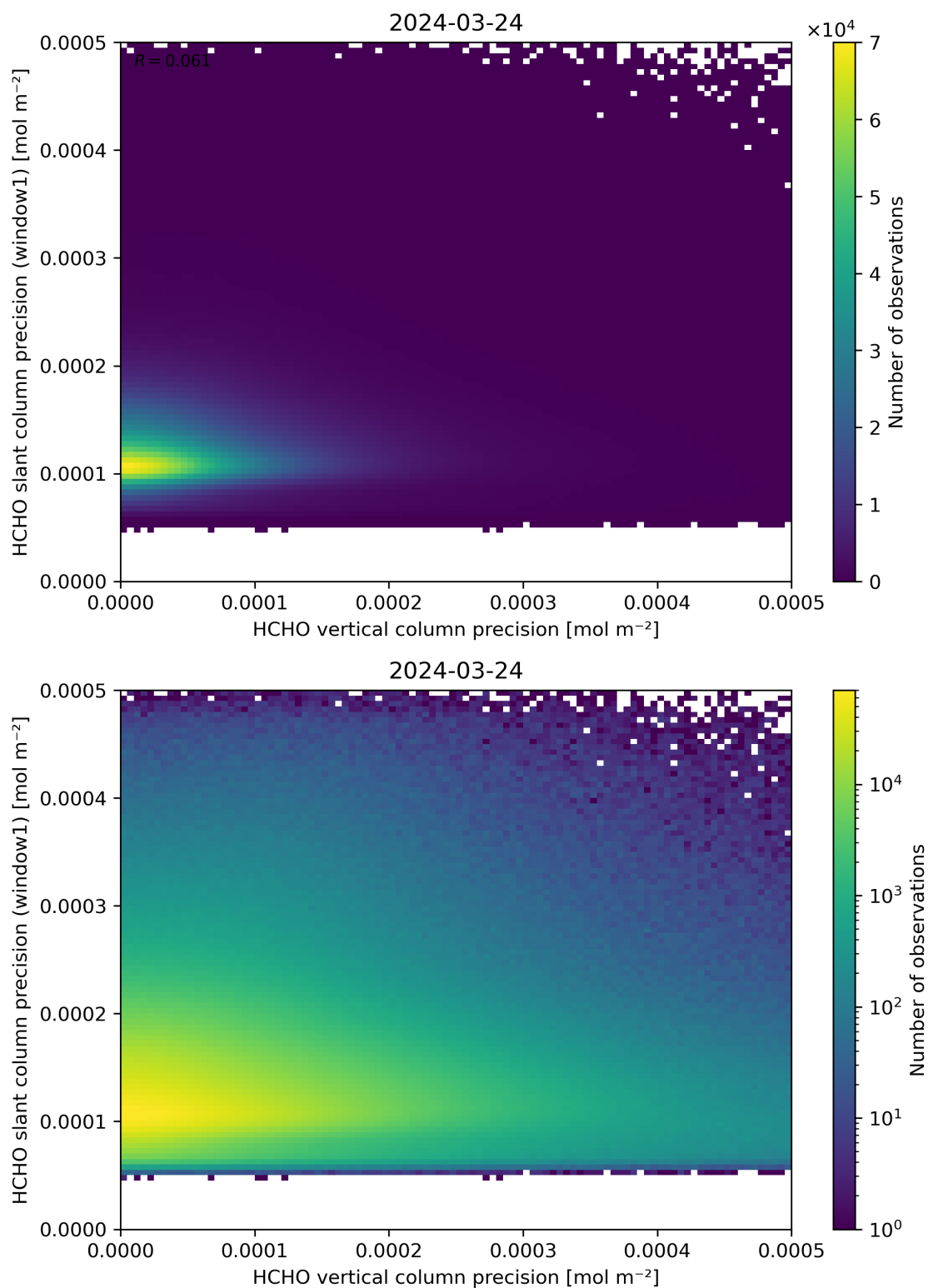
Figure 143: Scatter density plot of “HCHO vertical column precision” against “HCHO slant column precision (window1)” for 2024-03-23 to 2024-03-25.
