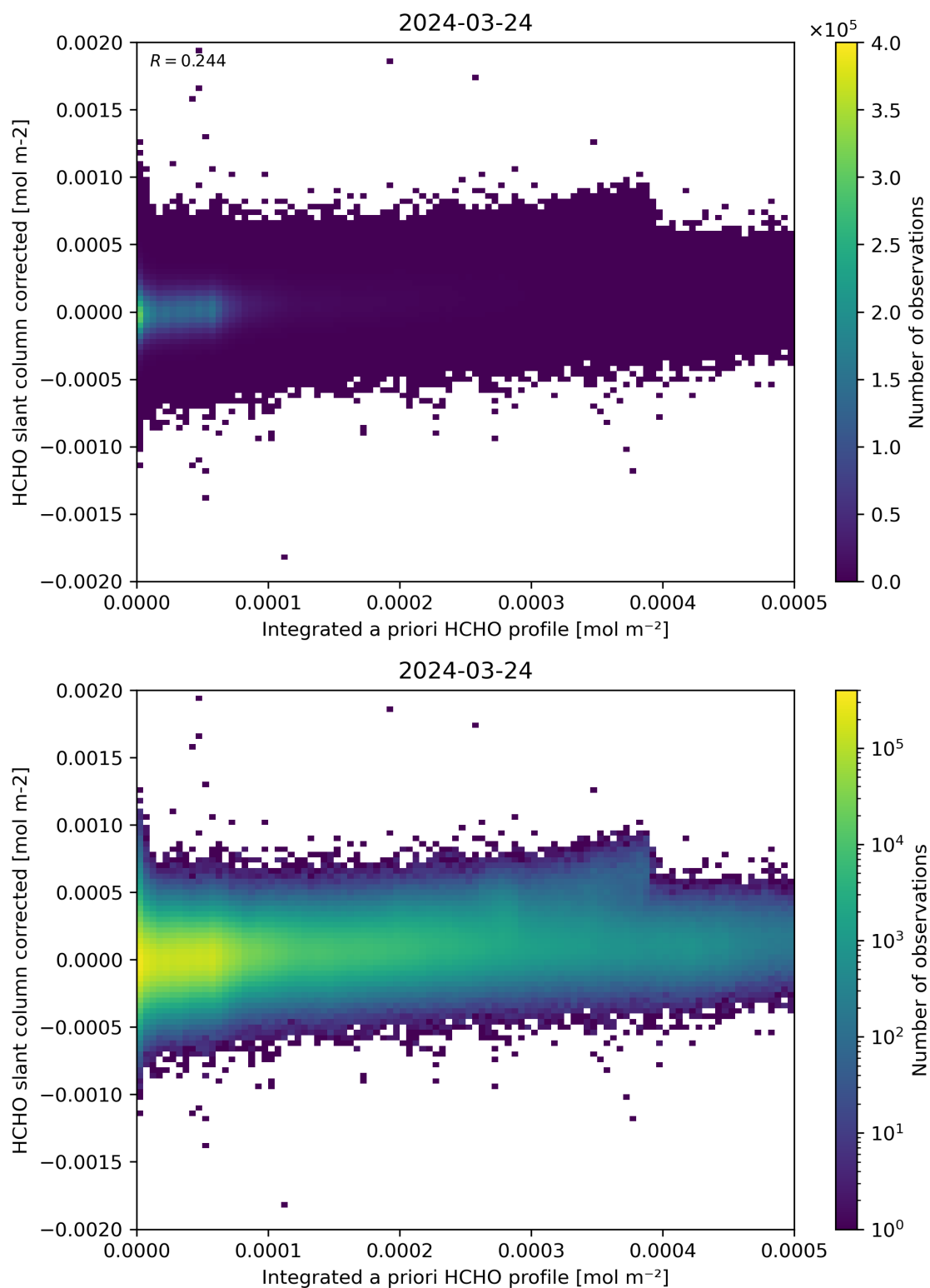
Figure 151: Scatter density plot of “Integrated a priori HCHO profile” against “HCHO slant column corrected” for 2024-03-23 to 2024-03-25.
