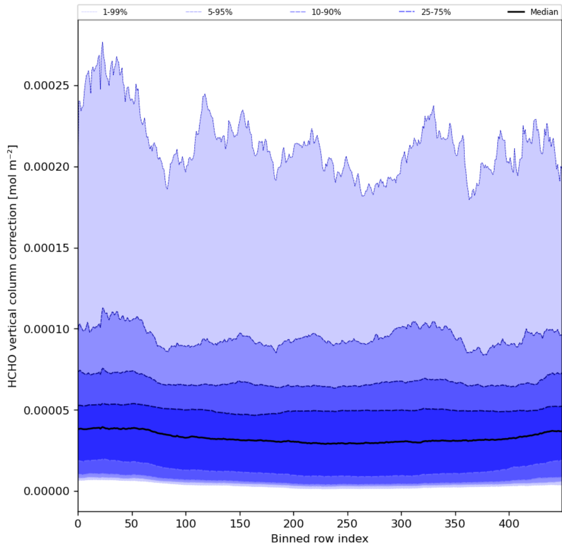
Figure 51: Along track statistics of “HCHO vertical column correction” for 2024-03-23 to 2024-03-25
