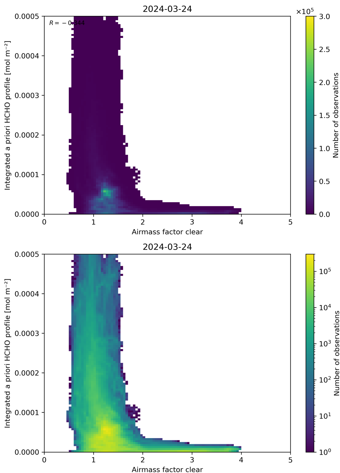
Figure 76: Scatter density plot of “Airmass factor clear” against “Integrated a priori HCHO profile” for 2024-03-23 to 2024-03-25.
