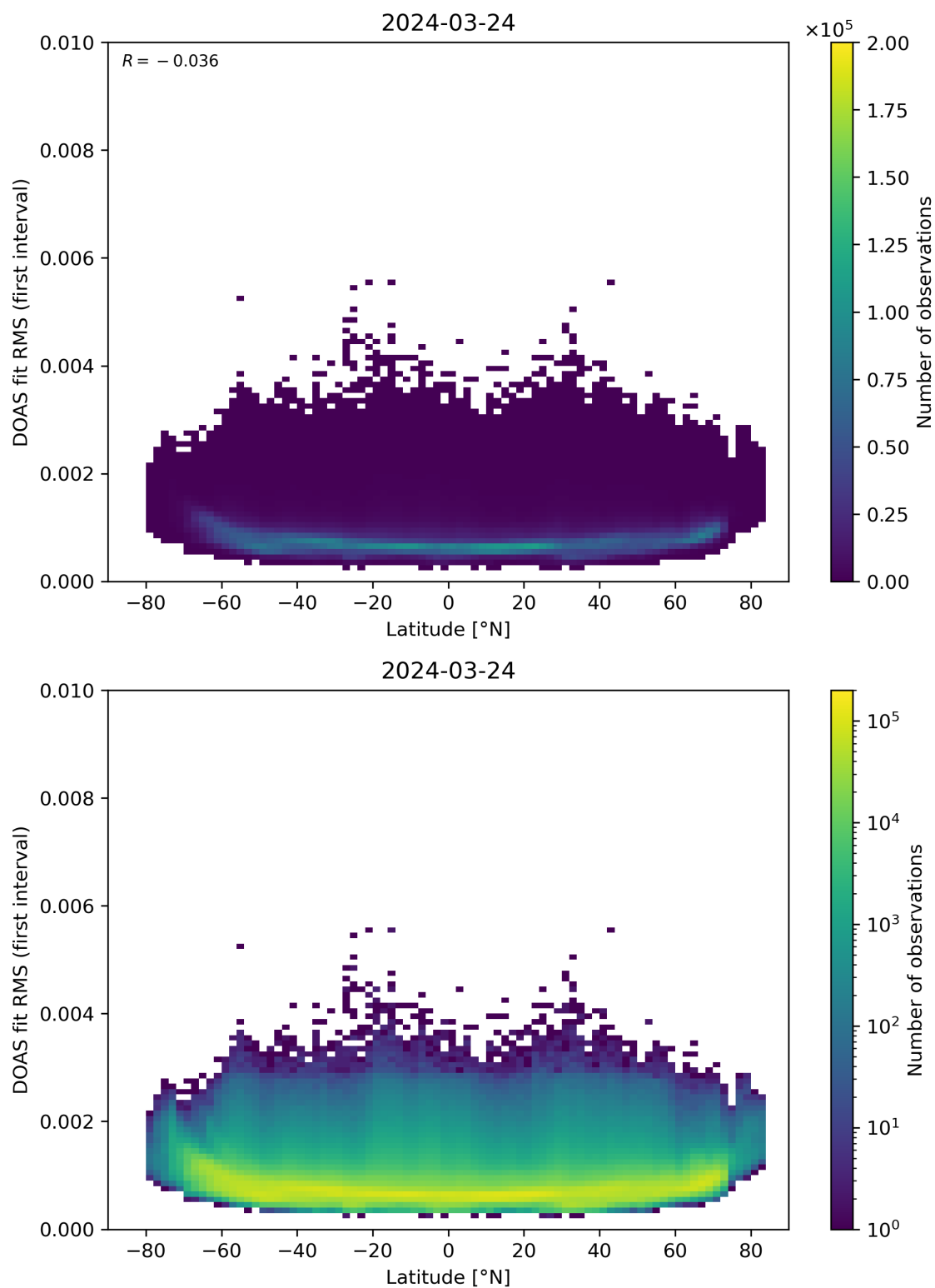
Figure 153: Scatter density plot of “Latitude” against “DOAS fit RMS (first interval)” for 2024-03-23 to 2024-03-25.
