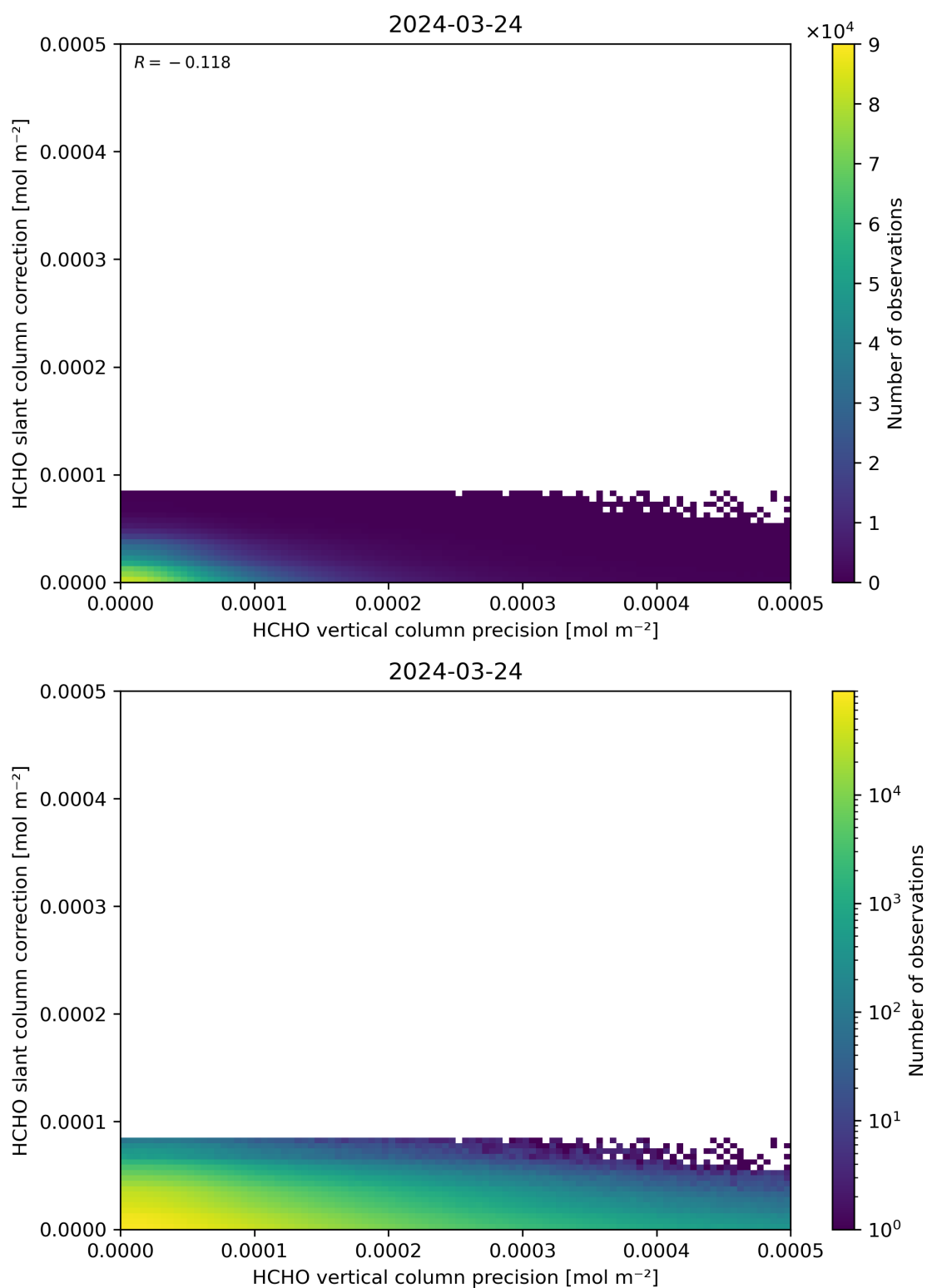
Figure 141: Scatter density plot of “HCHO vertical column precision” against “HCHO slant column correction” for 2024-03-23 to 2024-03-25.
