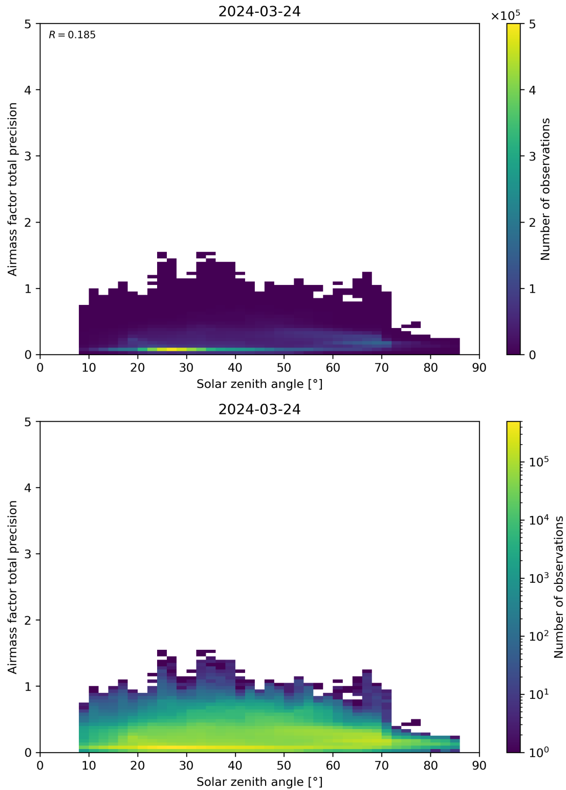
Figure 176: Scatter density plot of “Solar zenith angle” against “Airmass factor total precision” for 2024-03-23 to 2024-03-25.
