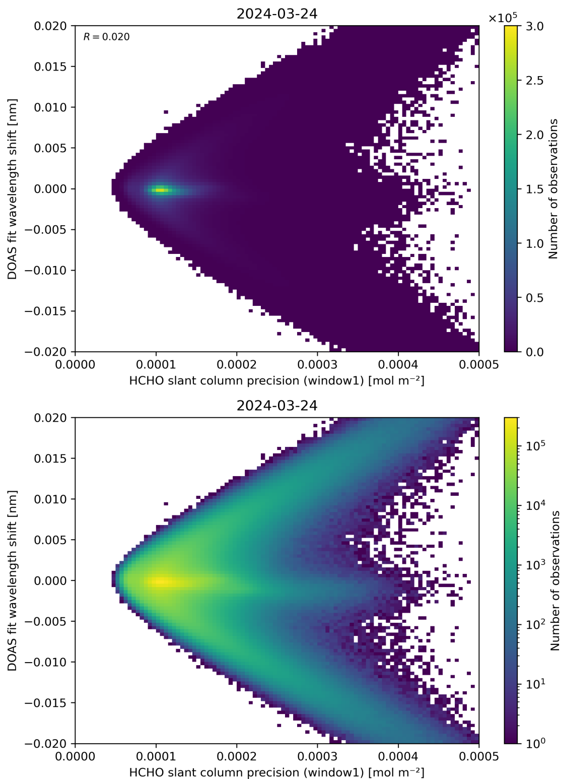
Figure 89: Scatter density plot of “HCHO slant column precision (window1)” against “DOAS fit wavelength shift” for 2024-03-23 to 2024-03-25.
