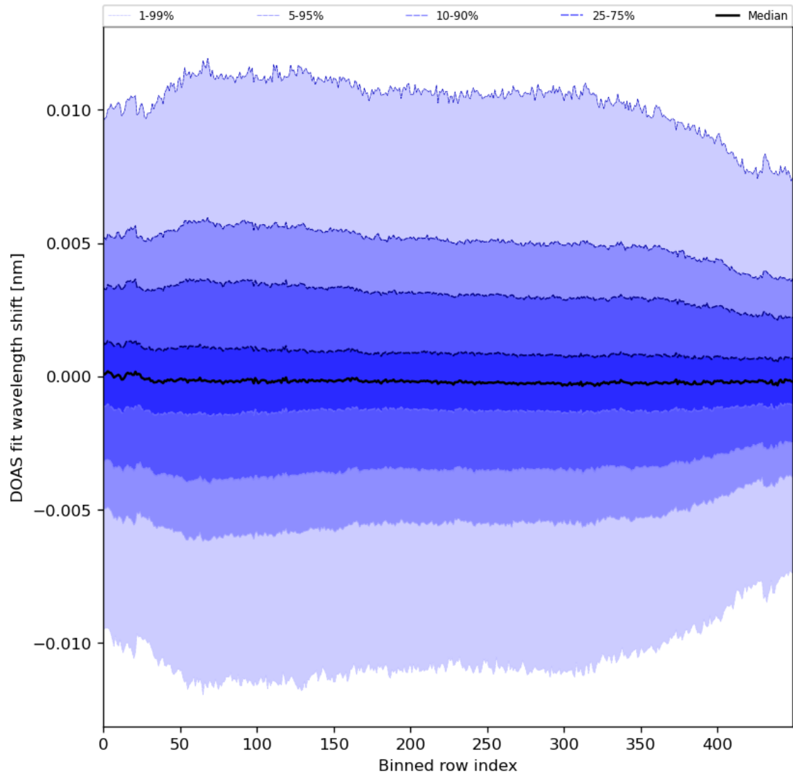
Figure 58: Along track statistics of “DOAS fit wavelength shift” for 2024-03-23 to 2024-03-25
