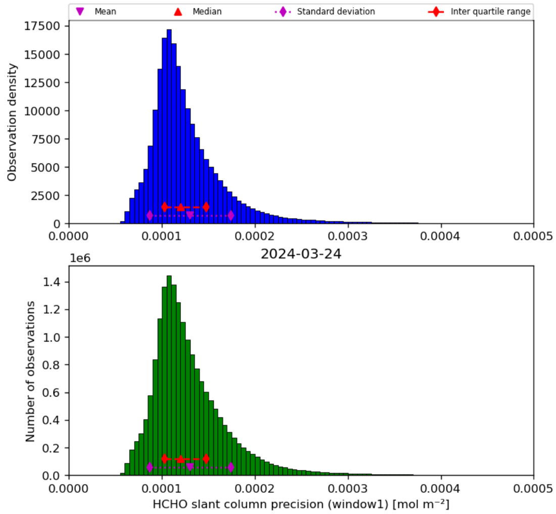
Figure 39: Histogram of “HCHO slant column precision (window1)” for 2024-03-23 to 2024-03-25
