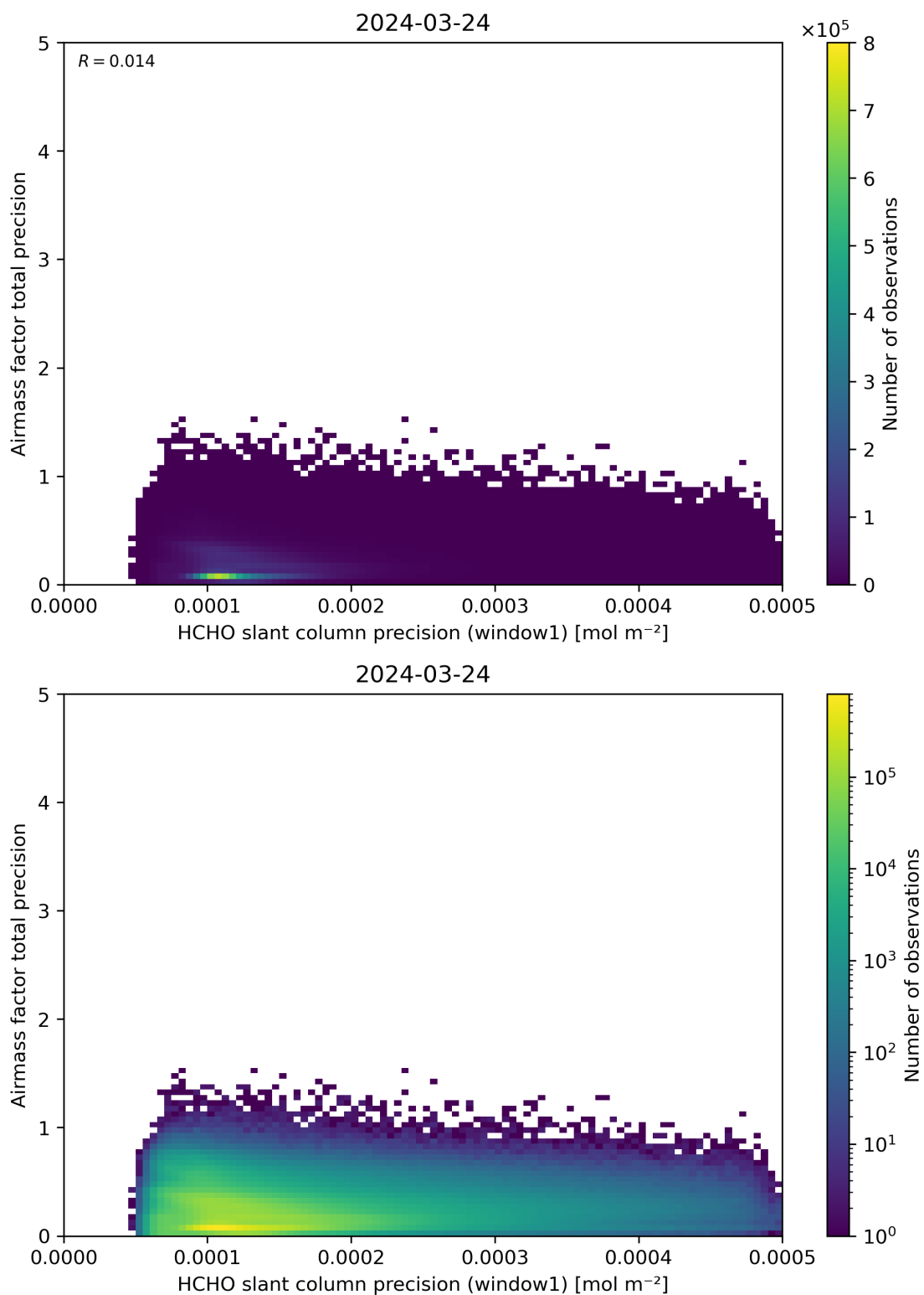
Figure 95: Scatter density plot of “HCHO slant column precision (window1)” against “Airmass factor total precision” for 2024-03-23 to 2024-03-25.
