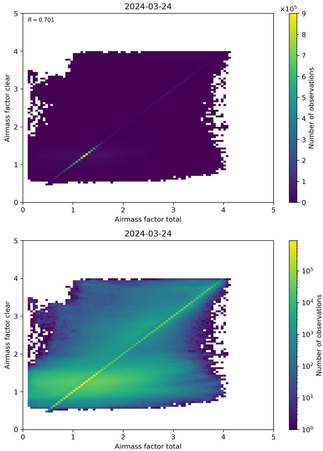
Figure 100: Scatter density plot of “Airmass factor total” against “Airmass factor clear” for 2024-03-23 to 2024-03-25.
