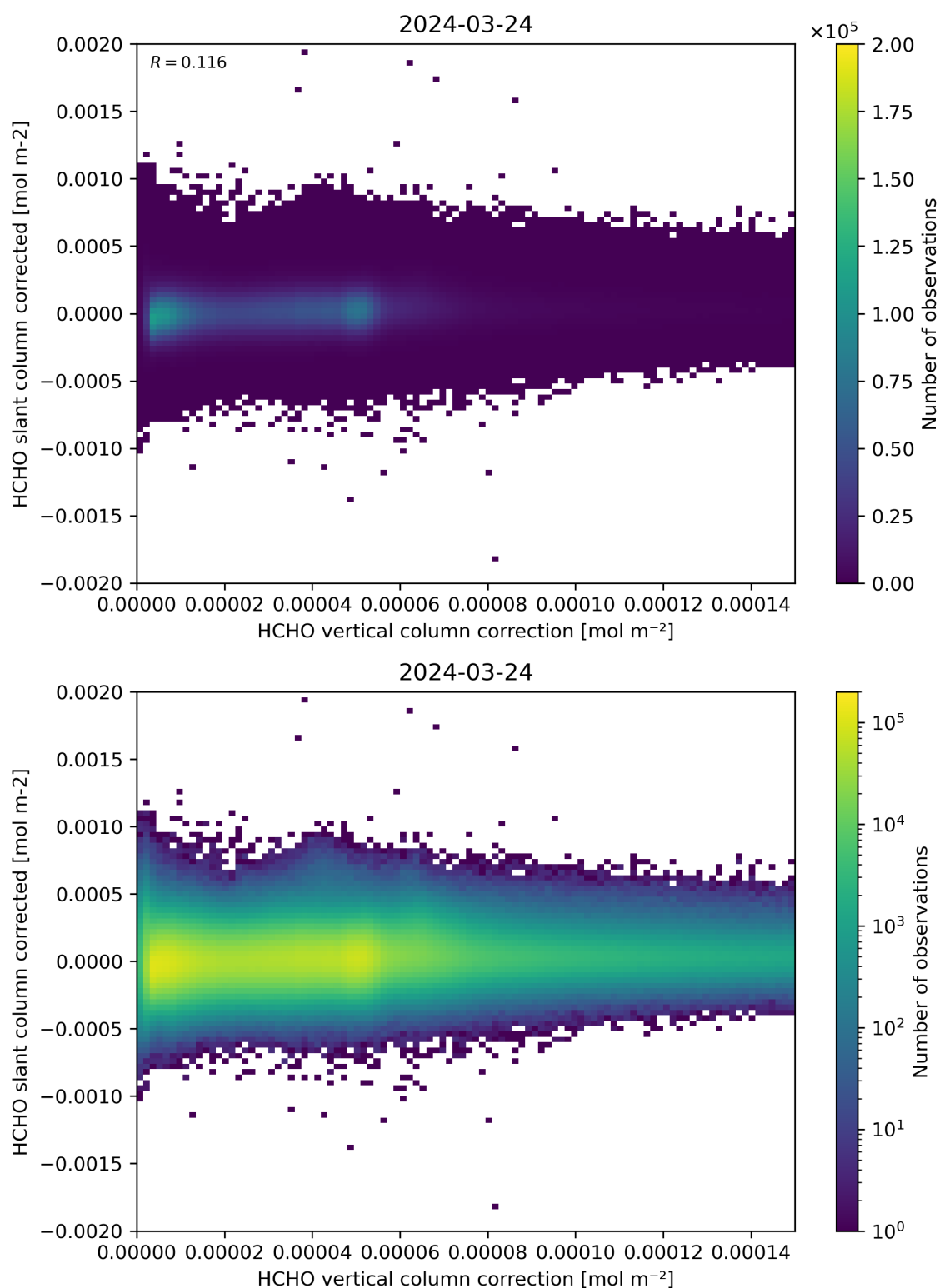
Figure 116: Scatter density plot of “HCHO vertical column correction” against “HCHO slant column corrected” for 2024-03-23 to 2024-03-25.
