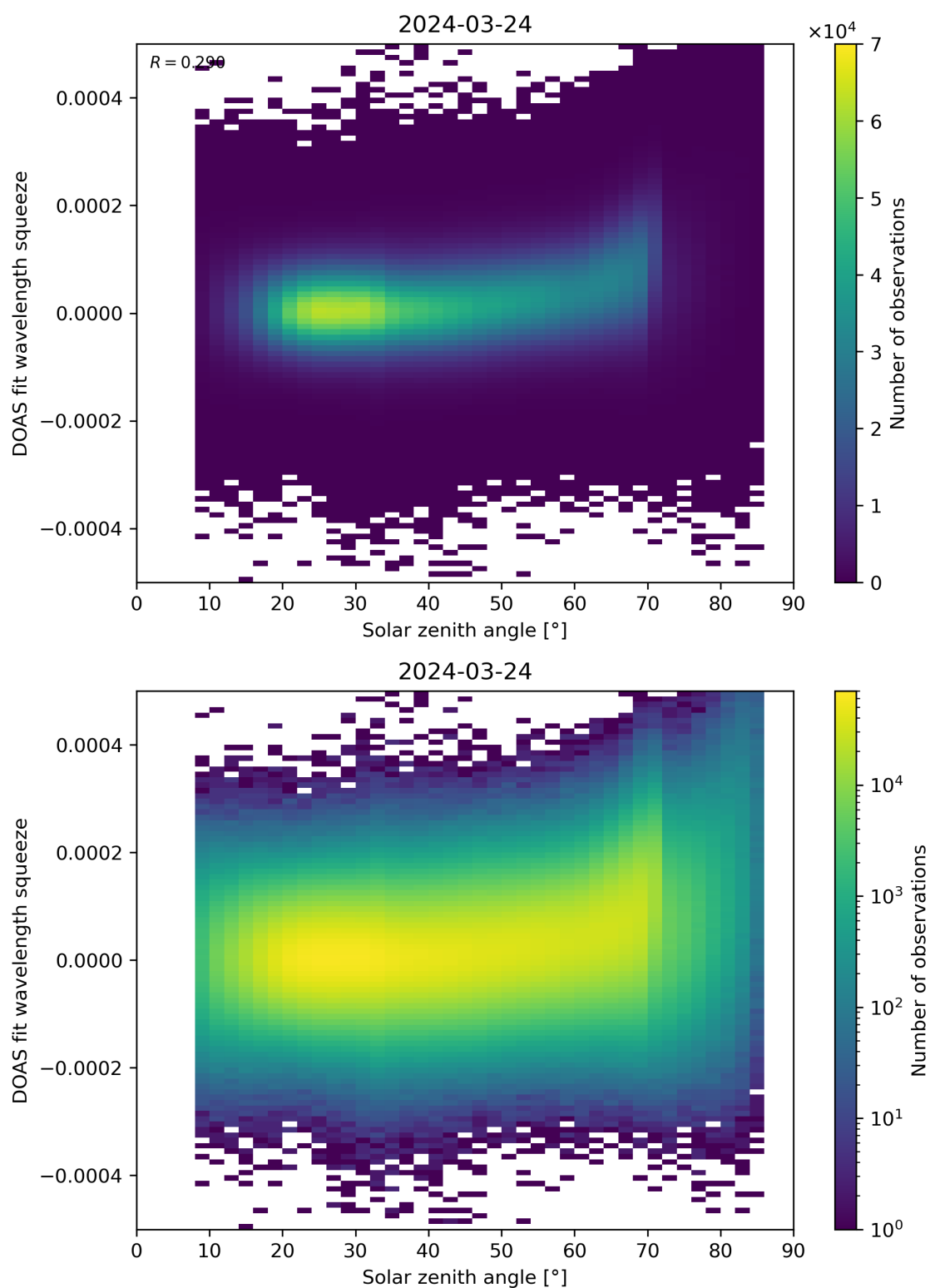
Figure 169: Scatter density plot of “Solar zenith angle” against “DOAS fit wavelength squeeze” for 2024-03-23 to 2024-03-25.
