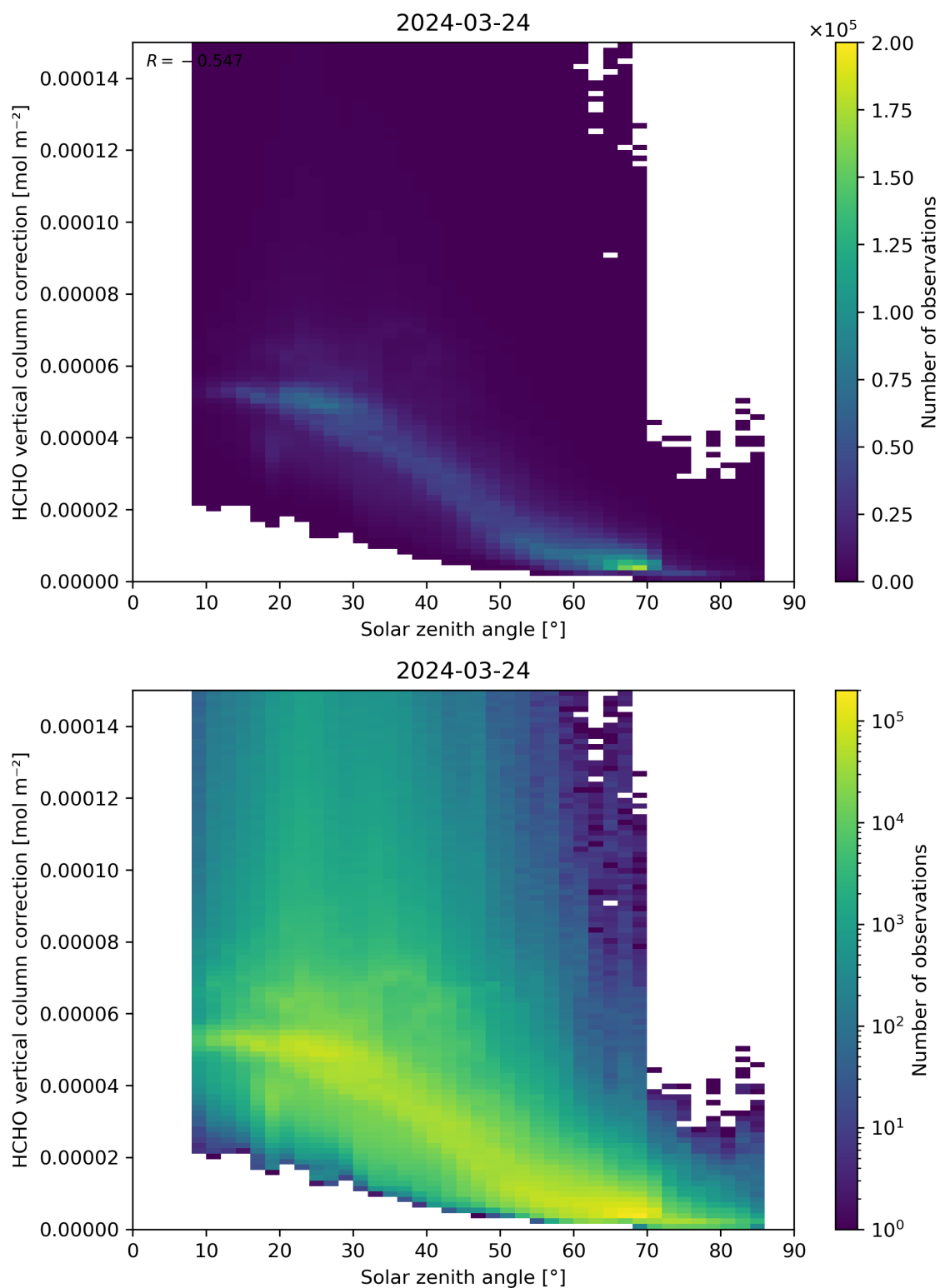
Figure 178: Scatter density plot of “Solar zenith angle” against “HCHO vertical column correction” for 2024-03-23 to 2024-03-25.
