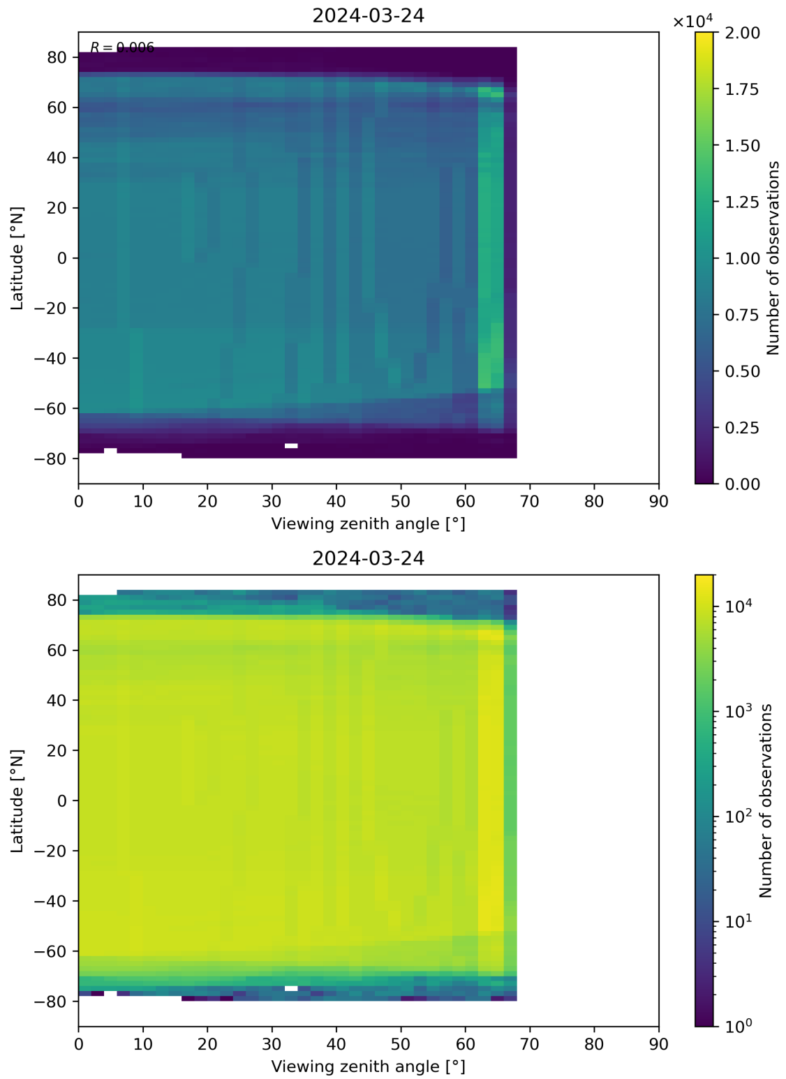
Figure 196: Scatter density plot of “Viewing zenith angle” against “Latitude” for 2024-03-23 to 2024-03-25.
