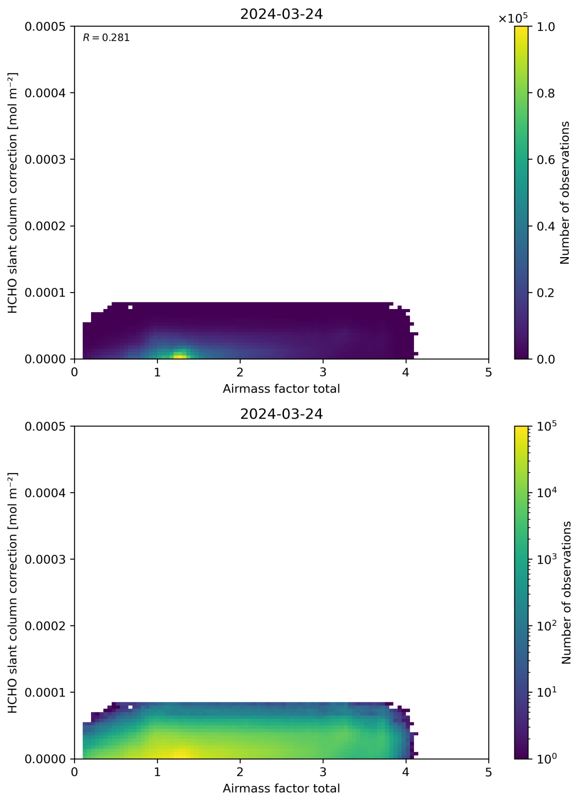
Figure 102: Scatter density plot of “Airmass factor total” against “HCHO slant column correction” for 2024-03-23 to 2024-03-25.
