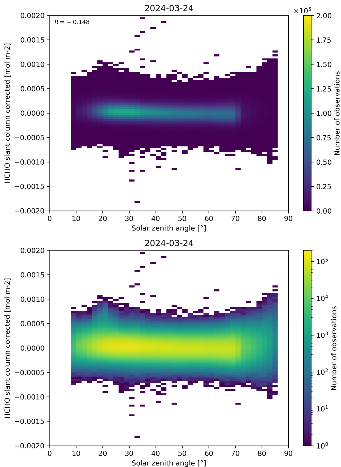
Figure 171: Scatter density plot of “Solar zenith angle” against “HCHO slant column corrected” for 2024-03-23 to 2024-03-25.
