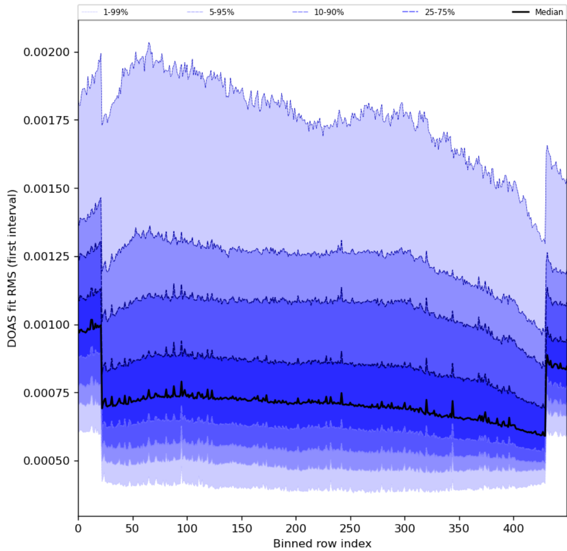
Figure 60: Along track statistics of “DOAS fit RMS (first interval)” for 2024-03-23 to 2024-03-25
