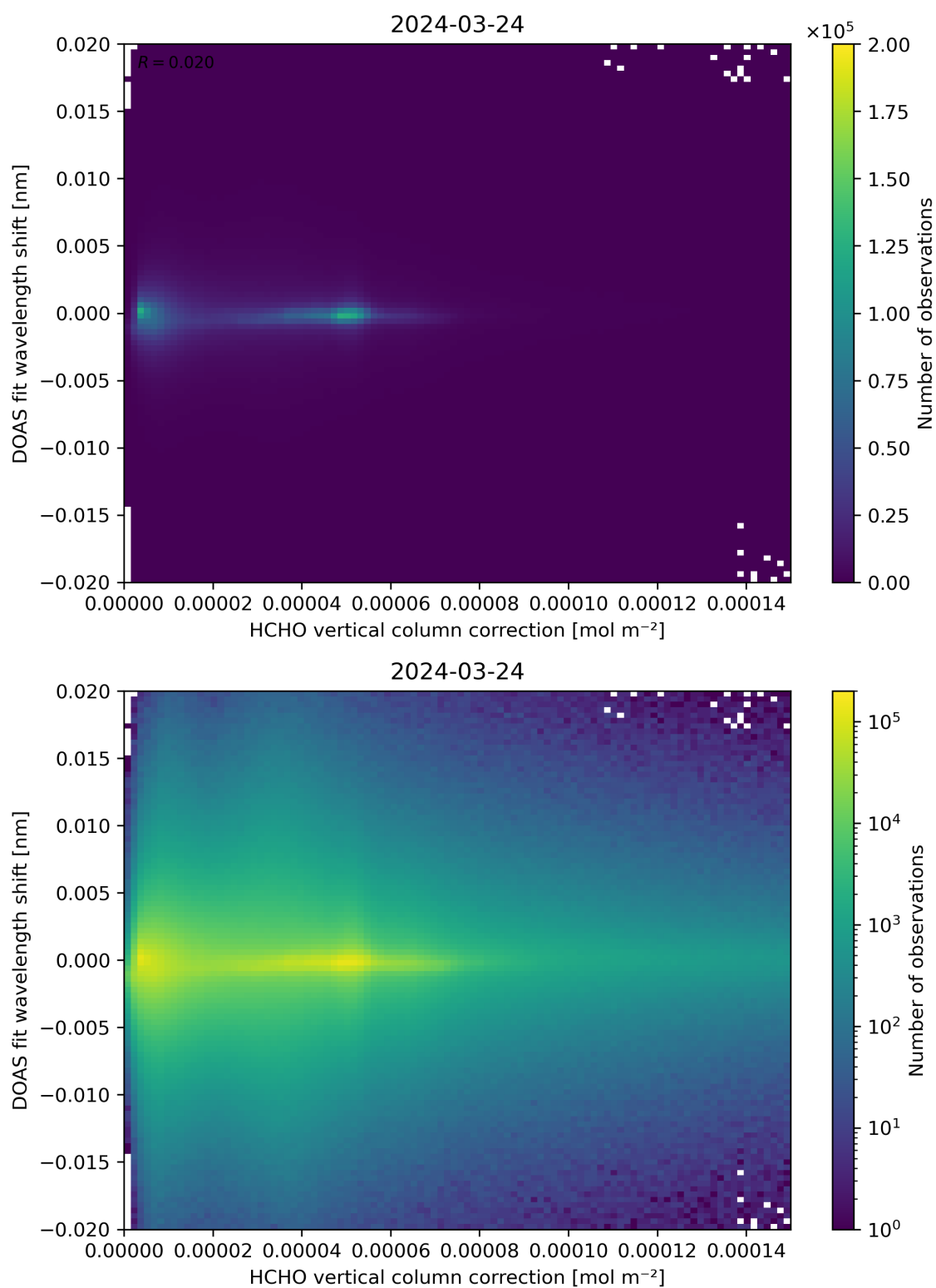
Figure 113: Scatter density plot of “HCHO vertical column correction” against “DOAS fit wavelength shift” for 2024-03-23 to 2024-03-25.
