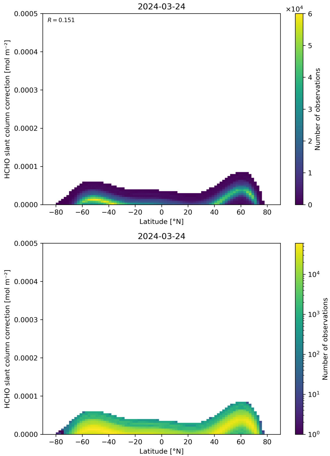
Figure 158: Scatter density plot of “Latitude” against “HCHO slant column correction” for 2024-03-23 to 2024-03-25.
