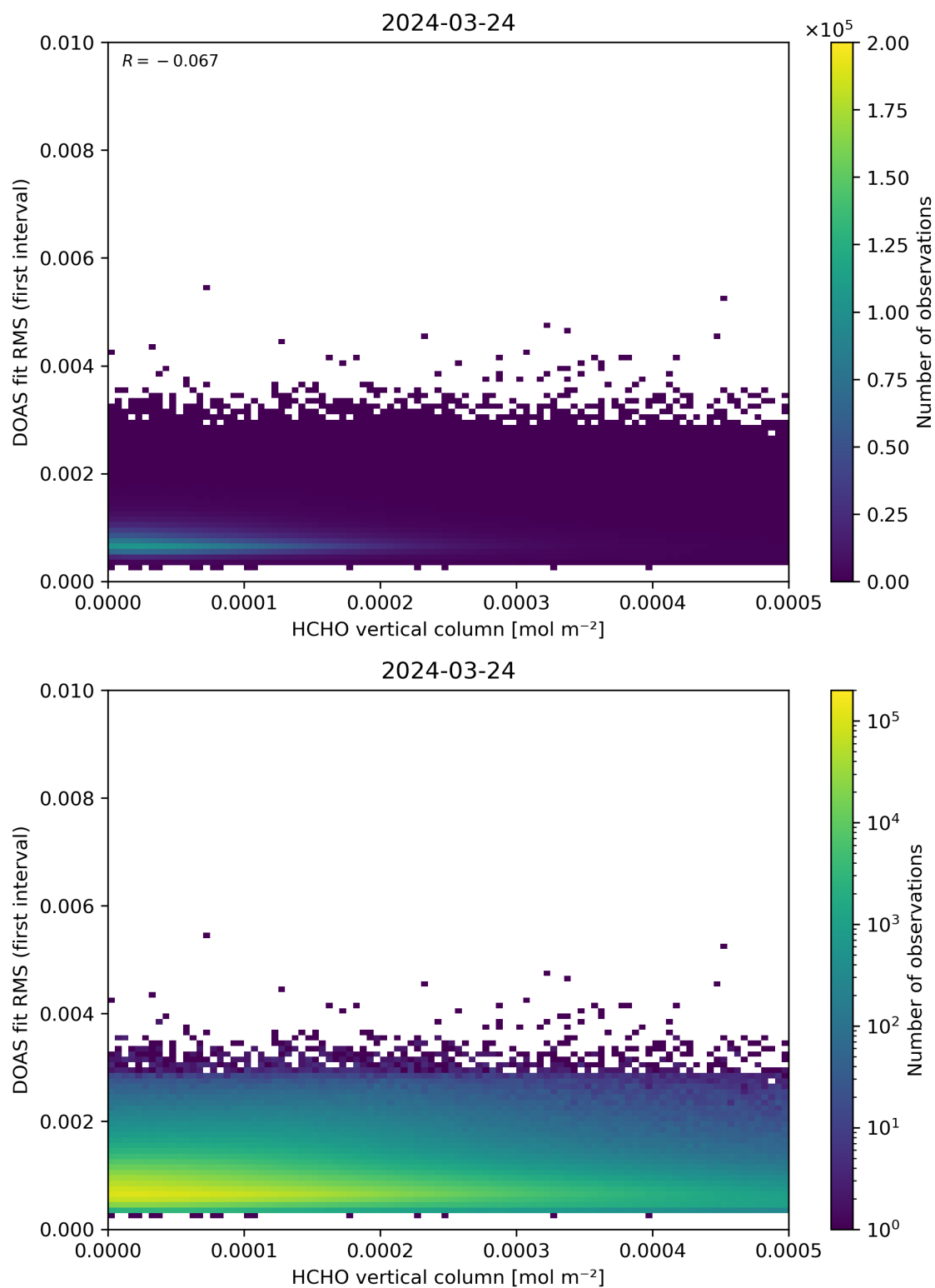
Figure 123: Scatter density plot of “HCHO vertical column” against “DOAS fit RMS (first interval)” for 2024-03-23 to 2024-03-25.
