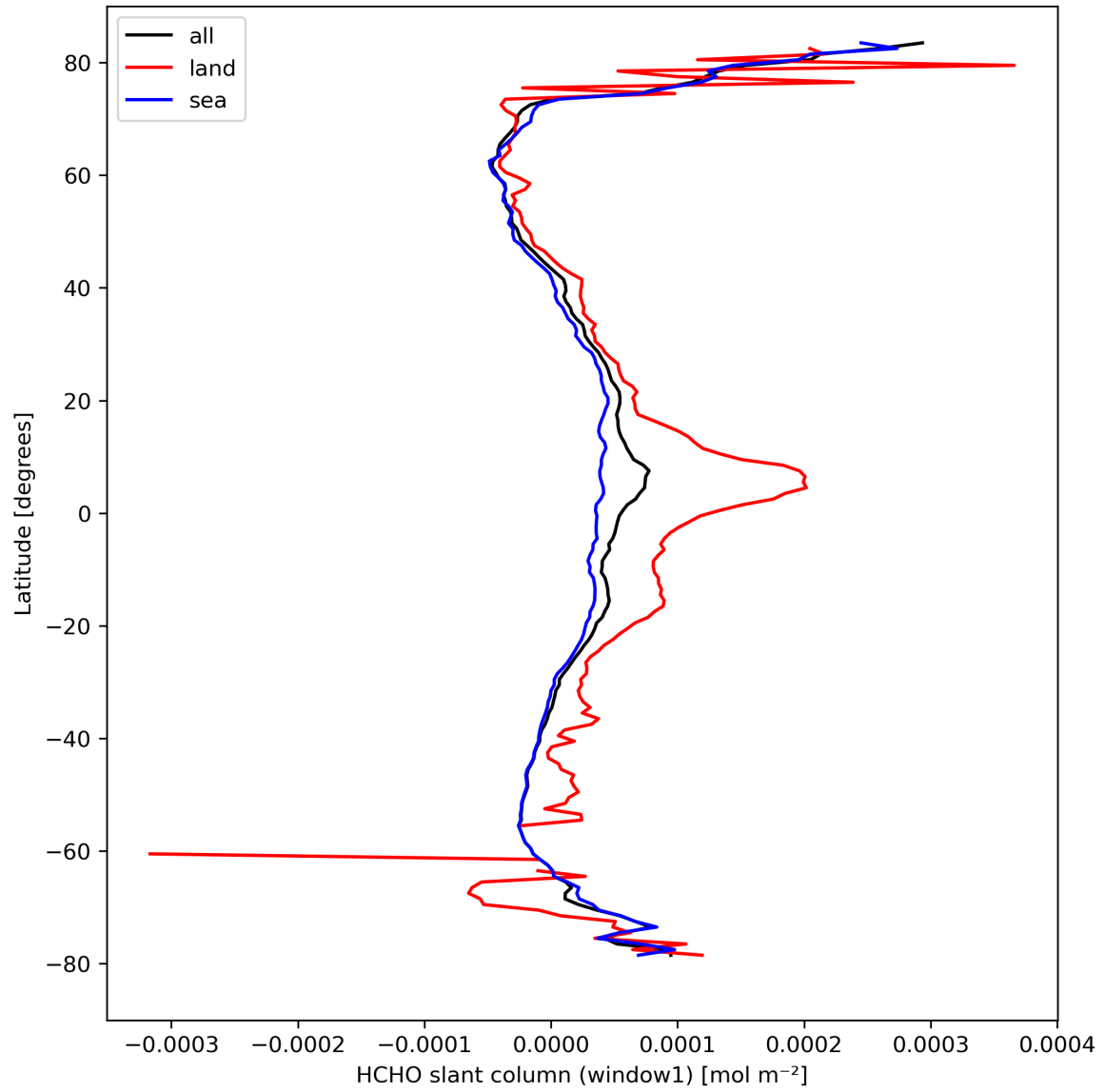
Figure 24: Zonal average of “HCHO slant column (window1)” for 2024-03-23 to 2024-03-25.
