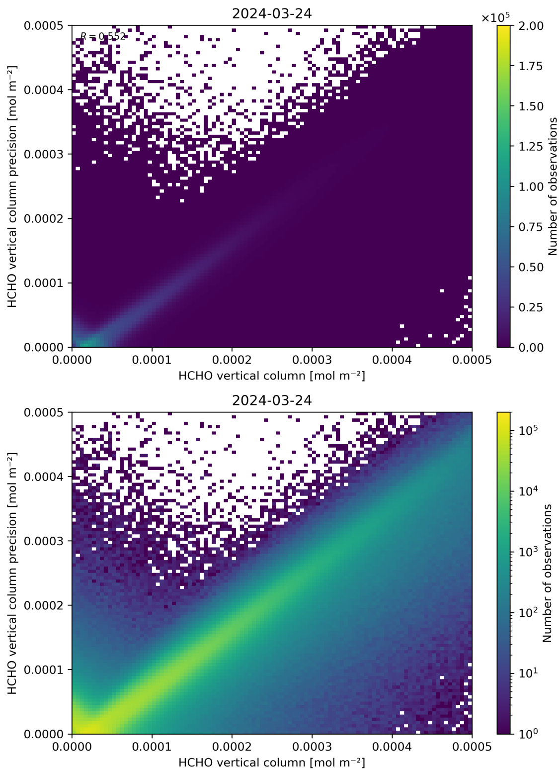
Figure 134: Scatter density plot of “HCHO vertical column” against “HCHO vertical column precision” for 2024-03-23 to 2024-03-25.
