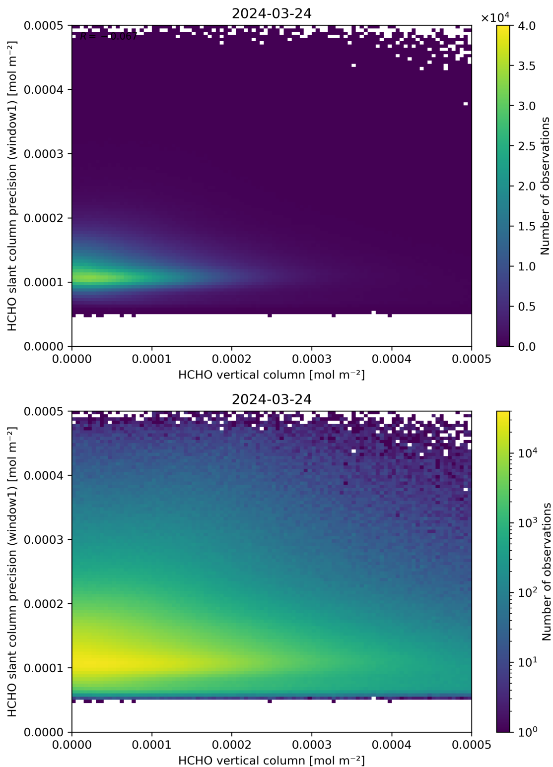
Figure 130: Scatter density plot of “HCHO vertical column” against “HCHO slant column precision (window1)” for 2024-03-23 to 2024-03-25.
