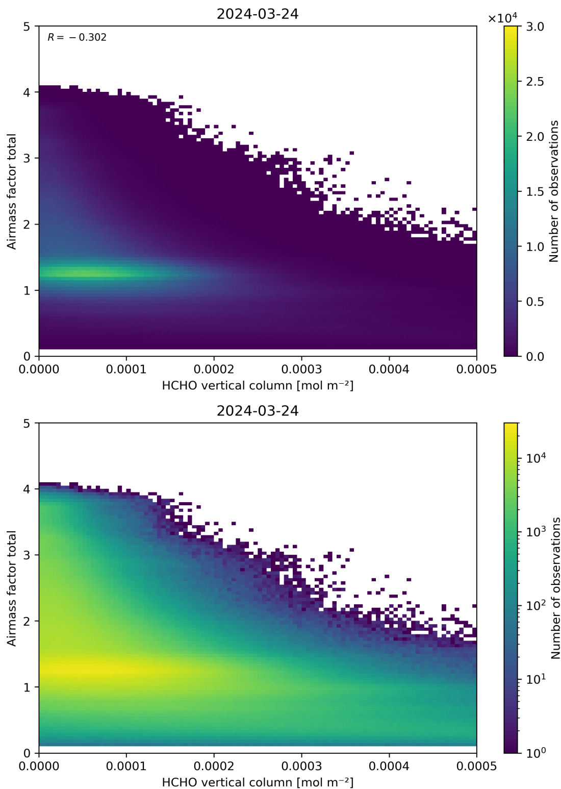
Figure 131: Scatter density plot of “HCHO vertical column” against “Airmass factor total” for 2024-03-23 to 2024-03-25.
