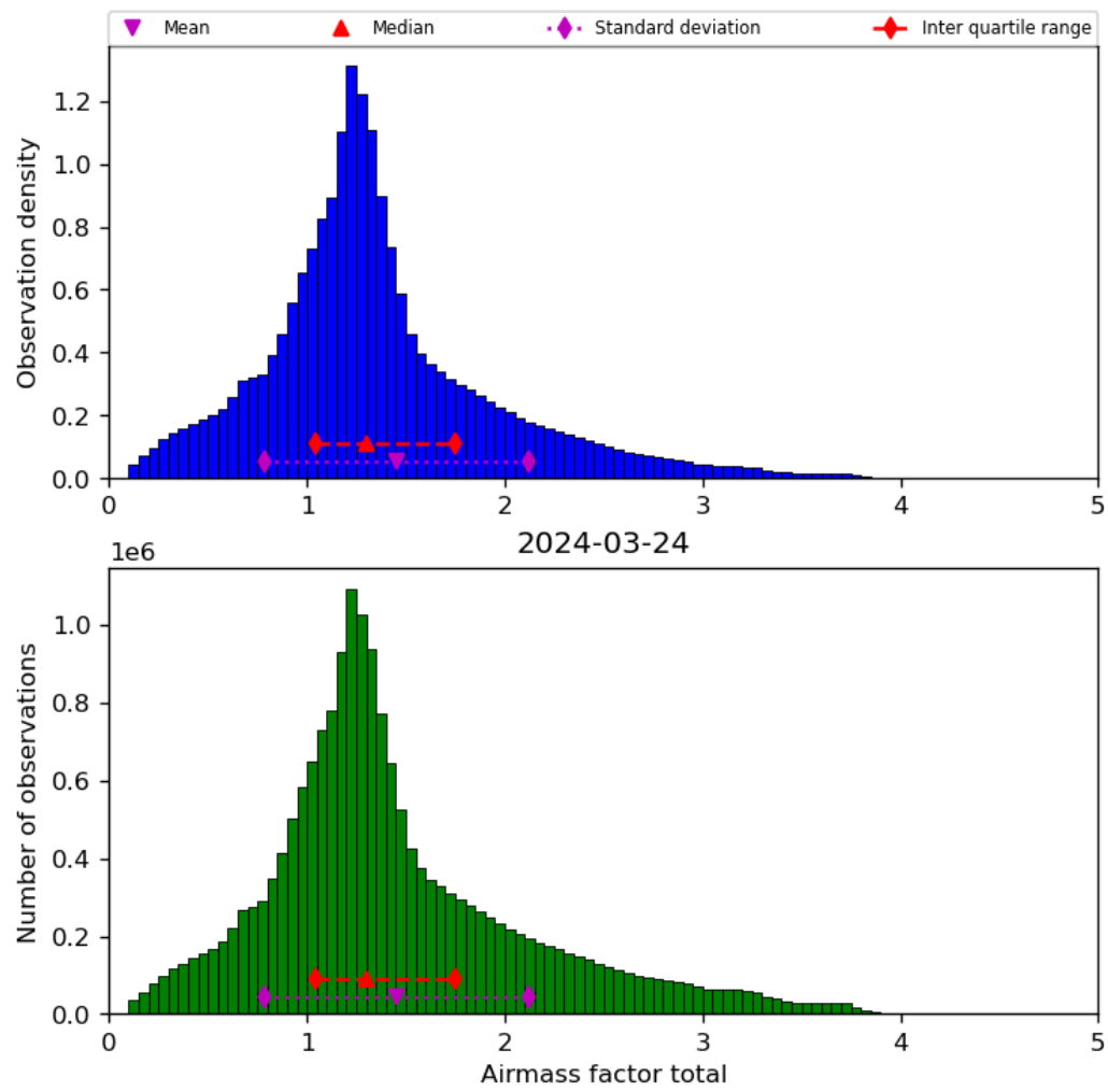
Figure 40: Histogram of “Airmass factor total” for 2024-03-23 to 2024-03-25
