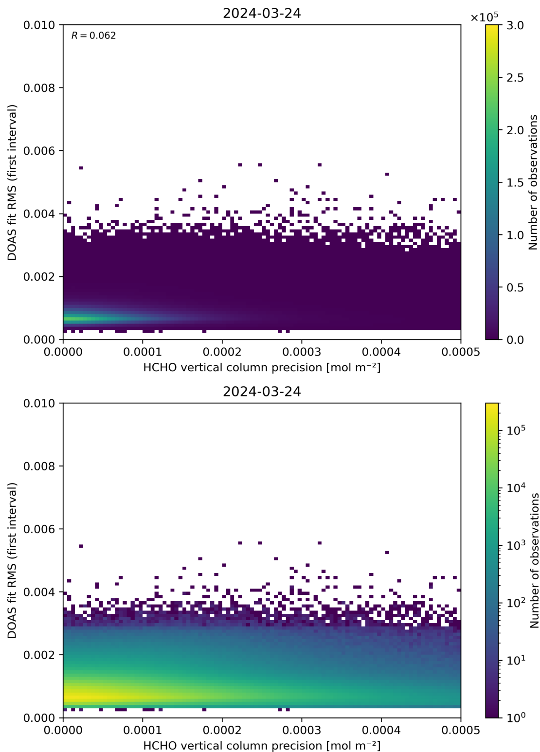
Figure 136: Scatter density plot of “HCHO vertical column precision” against “DOAS fit RMS (first interval)” for 2024-03-23 to 2024-03-25.
