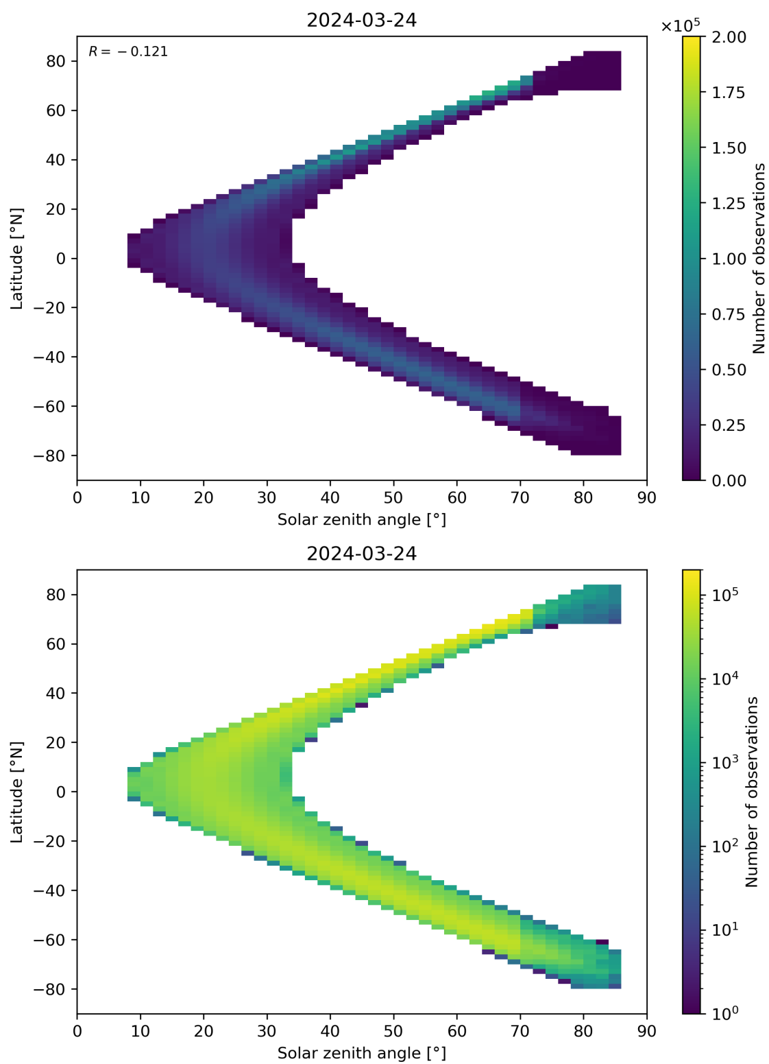
Figure 181: Scatter density plot of “Solar zenith angle” against “Latitude” for 2024-03-23 to 2024-03-25.
