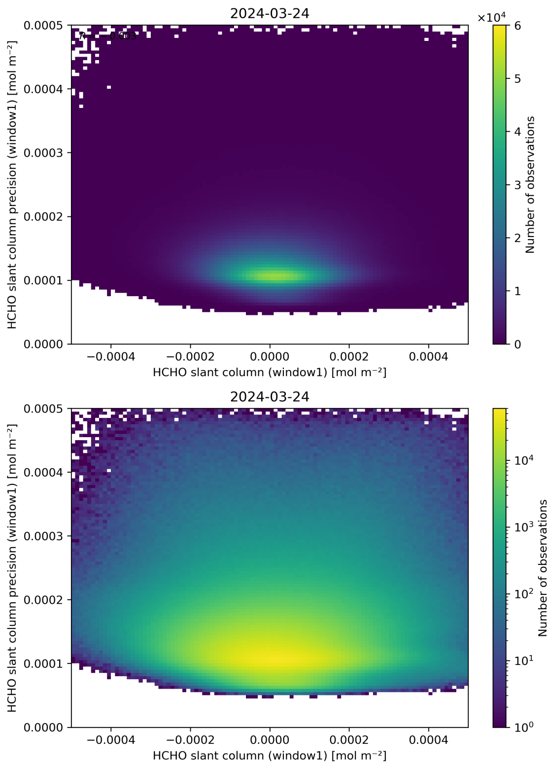
Figure 84: Scatter density plot of “HCHO slant column (window1)” against “HCHO slant column precision (window1)” for 2024-03-23 to 2024-03-25.
