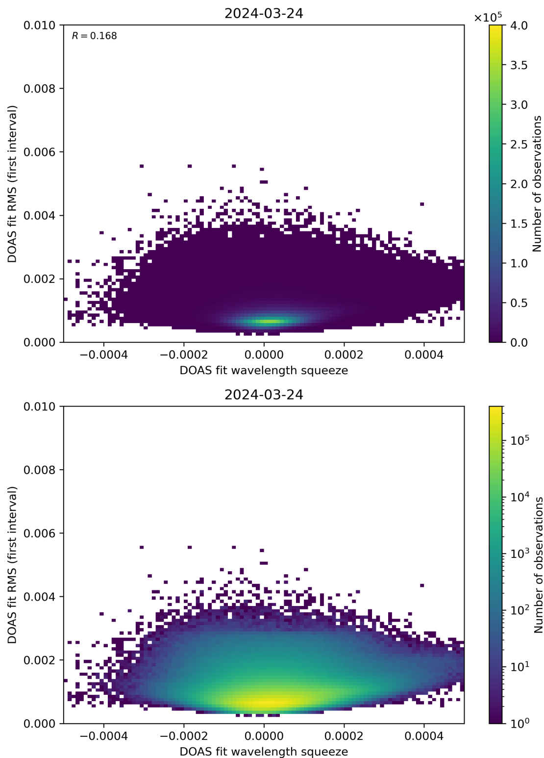
Figure 68: Scatter density plot of “DOAS fit wavelength squeeze” against “DOAS fit RMS (first interval)” for 2024-03-23 to 2024-03-25.
