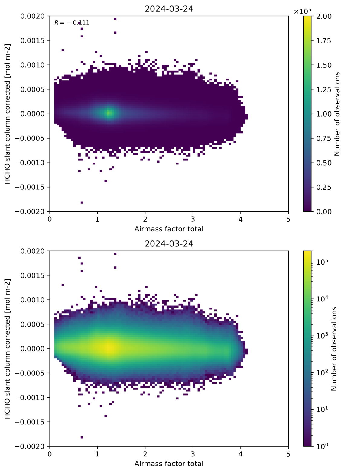
Figure 101: Scatter density plot of “Airmass factor total” against “HCHO slant column corrected” for 2024-03-23 to 2024-03-25.
