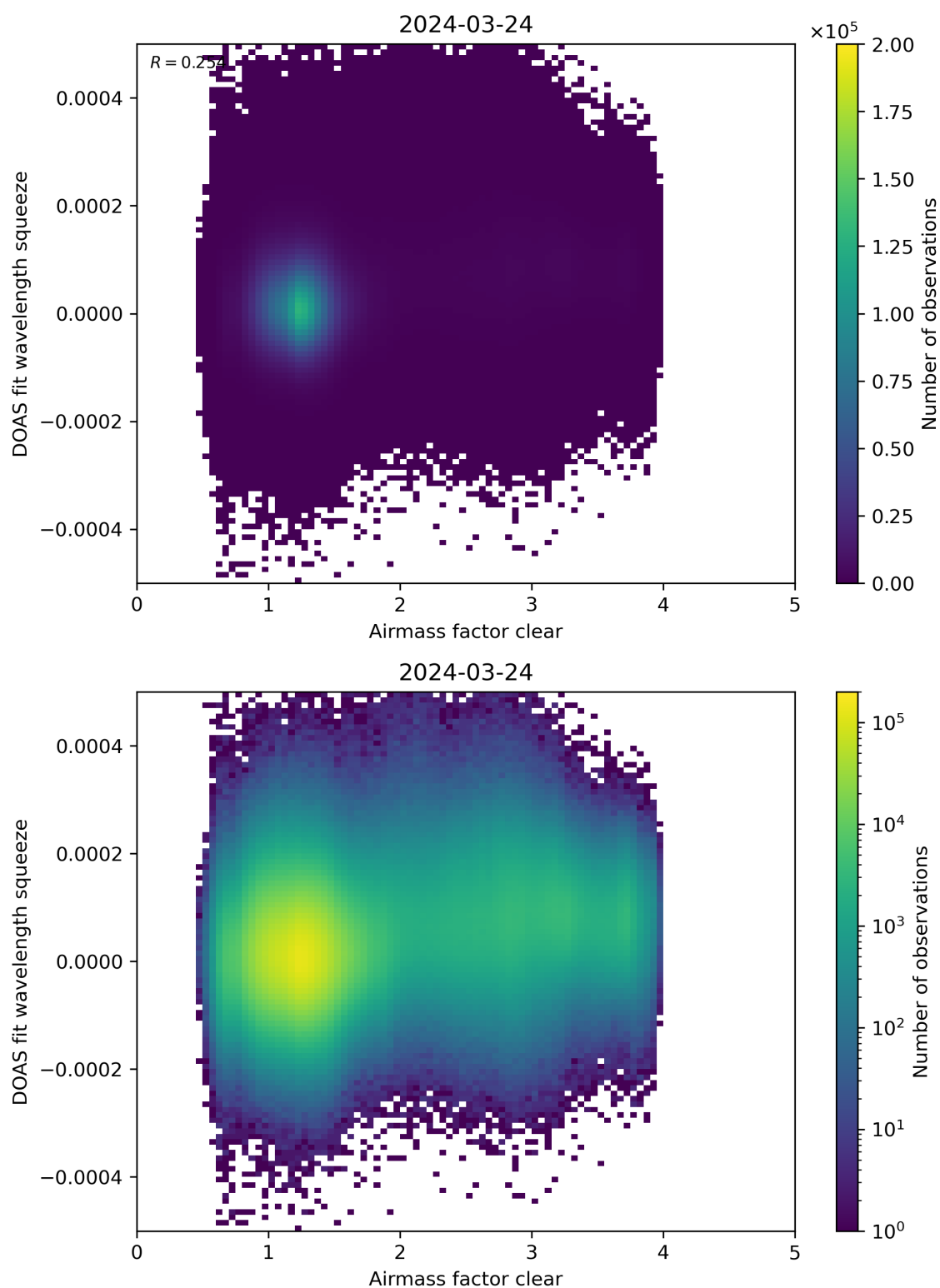
Figure 73: Scatter density plot of “Airmass factor clear” against “DOAS fit wavelength squeeze” for 2024-03-23 to 2024-03-25.
