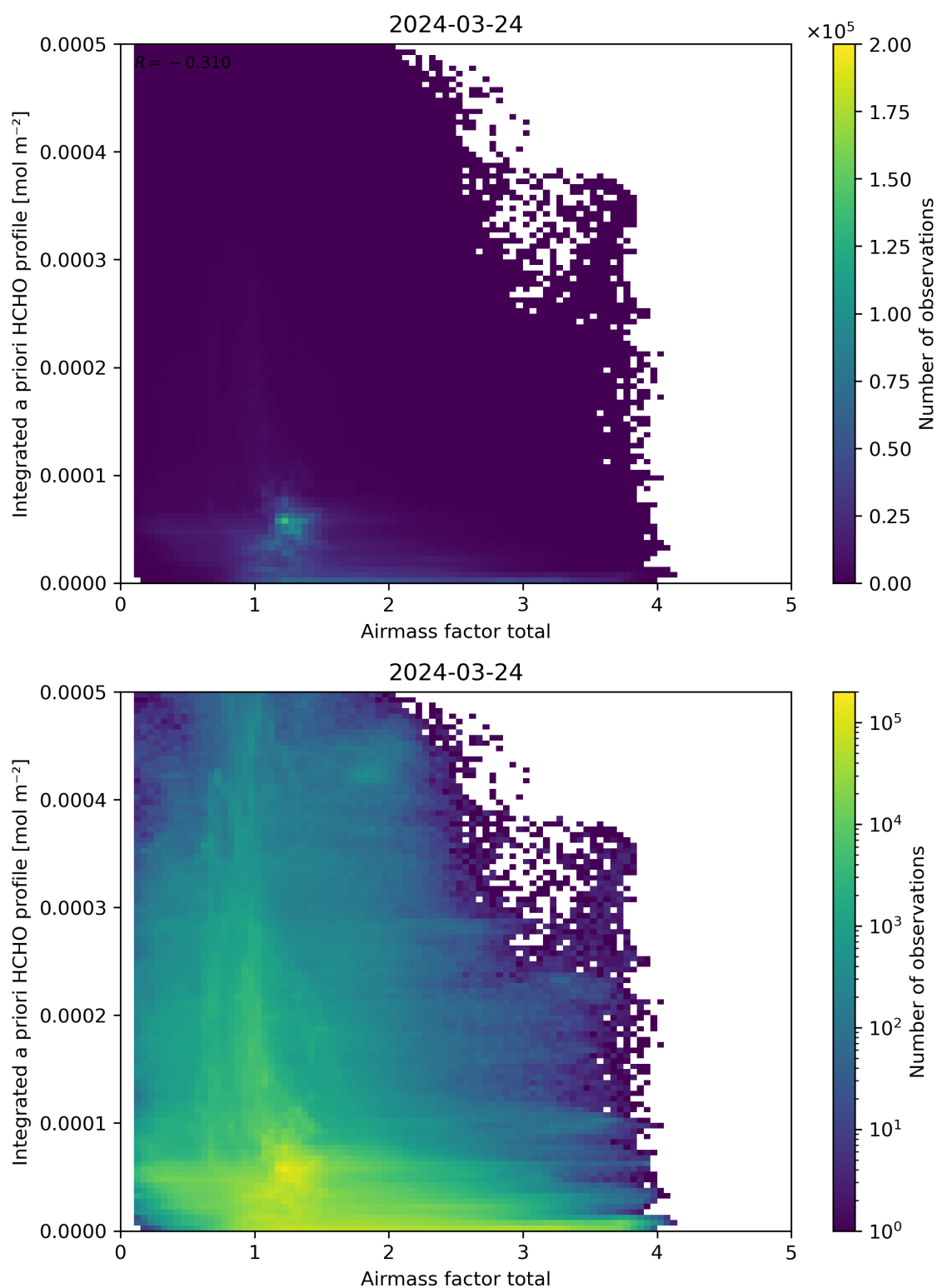
Figure 104: Scatter density plot of “Airmass factor total” against “Integrated a priori HCHO profile” for 2024-03-23 to 2024-03-25.
