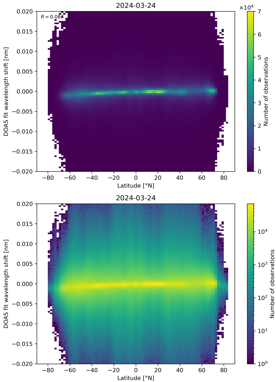
Figure 154: Scatter density plot of “Latitude” against “DOAS fit wavelength shift” for 2024-03-23 to 2024-03-25.
