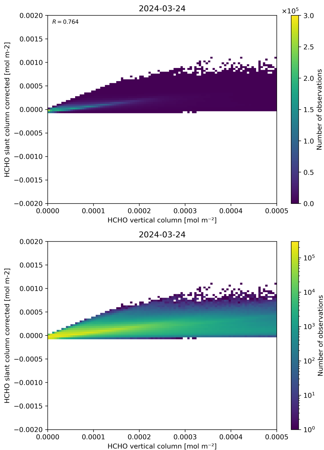
Figure 127: Scatter density plot of “HCHO vertical column” against “HCHO slant column corrected” for 2024-03-23 to 2024-03-25.
