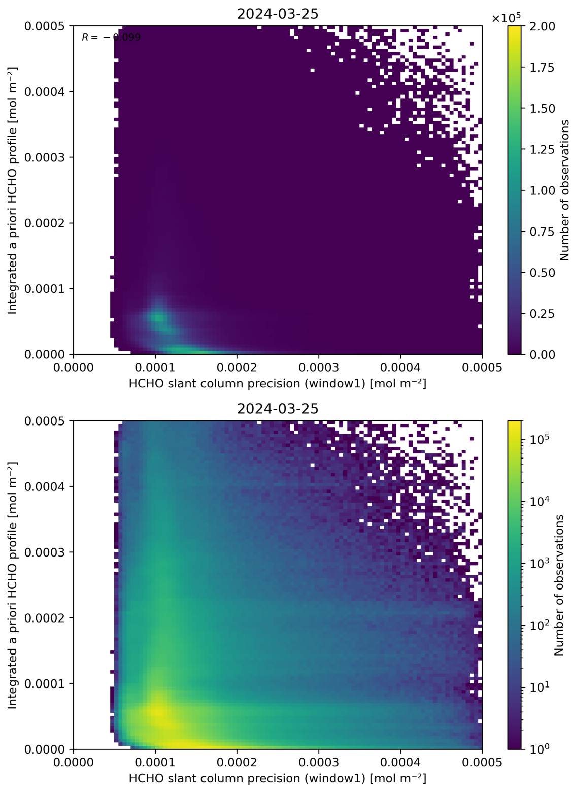
Figure 96: Scatter density plot of “HCHO slant column precision (window1)” against “Integrated a priori HCHO profile” for 2024-03-25 to 2024-03-26.
