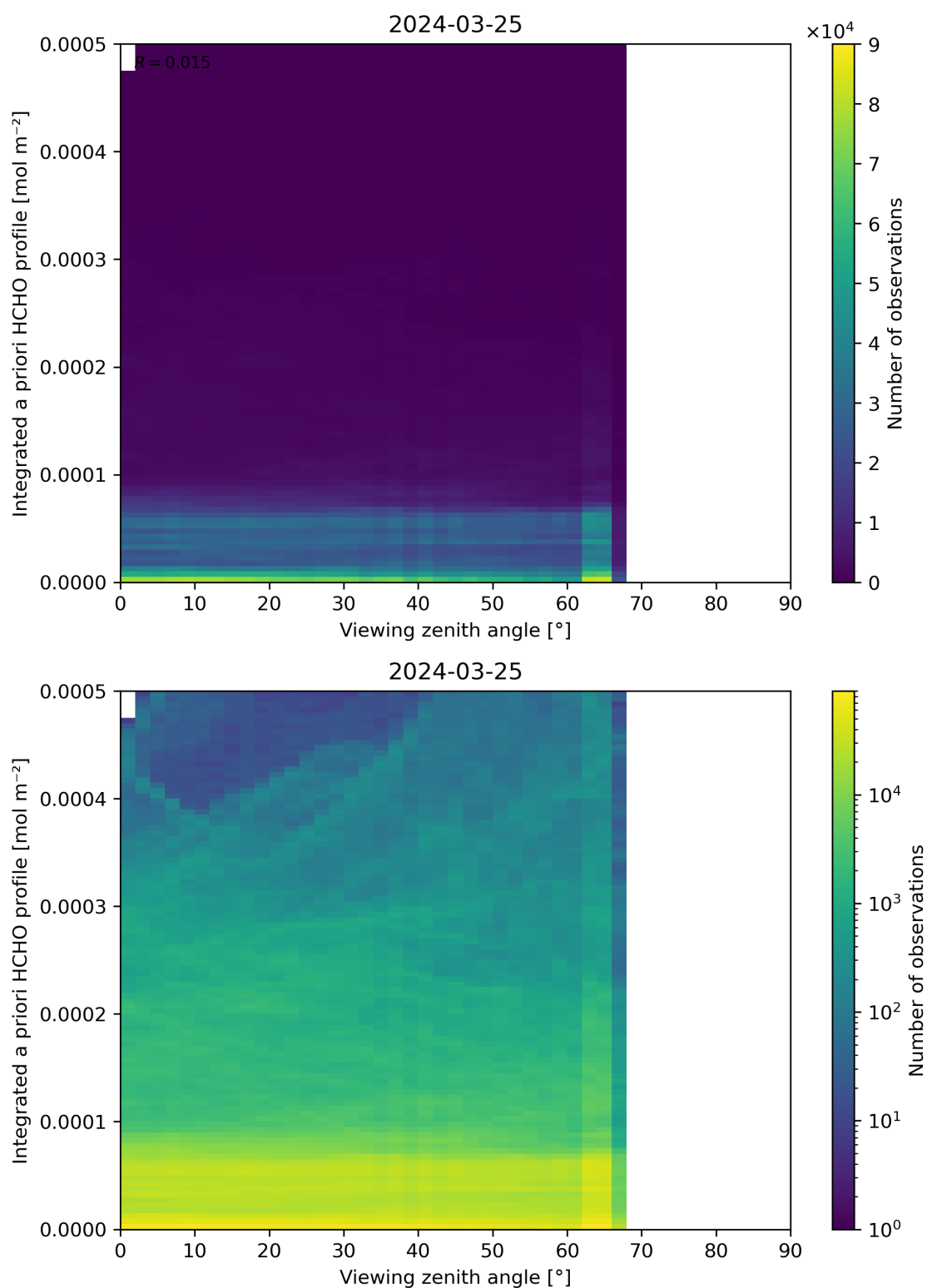
Figure 195: Scatter density plot of “Viewing zenith angle” against “Integrated a priori HCHO profile” for 2024-03-25 to 2024-03-26.
