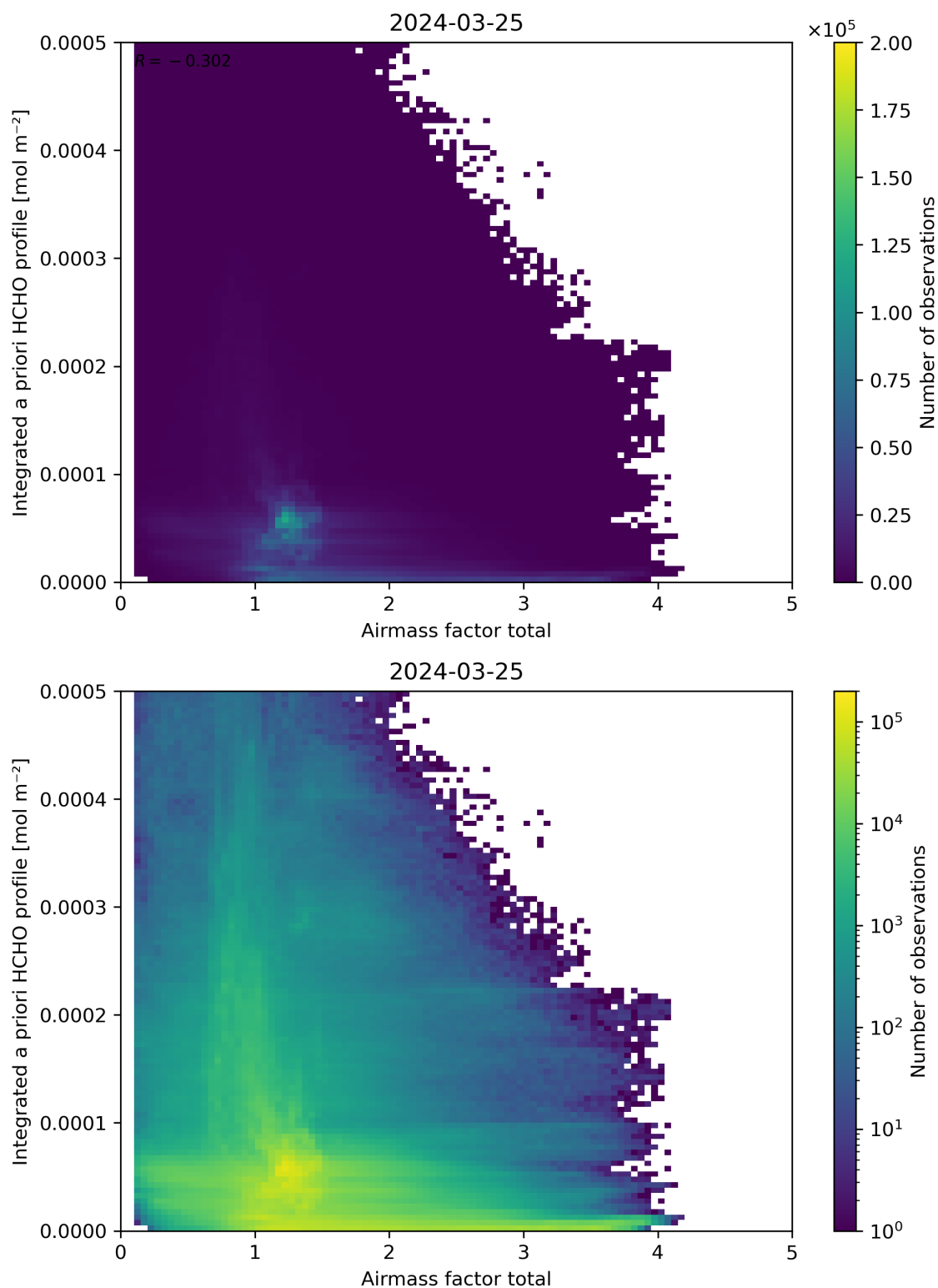
Figure 104: Scatter density plot of “Air mass factor total” against “Integrated a priori HCHO profile” for 2024-03-25 to 2024-03-26.
