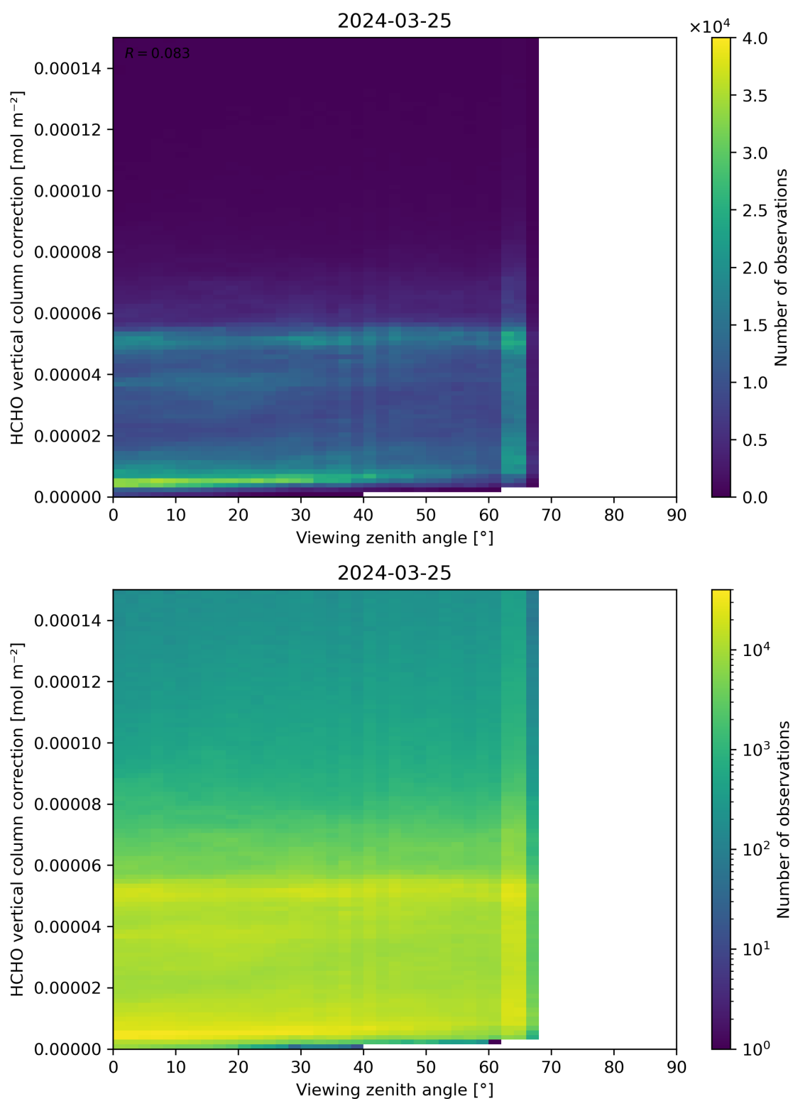
Figure 193: Scatter density plot of “Viewing zenith angle” against “HCHO vertical column correction” for 2024-03-25 to 2024-03-26.
