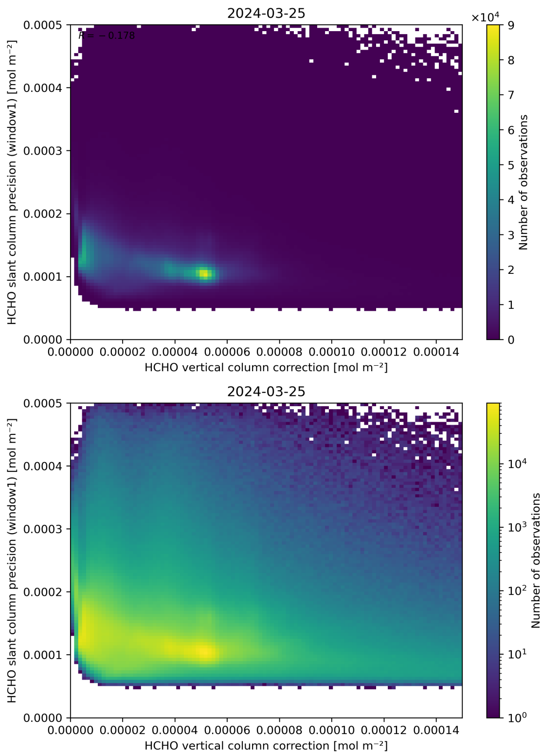
Figure 119: Scatter density plot of “HCHO vertical column correction” against “HCHO slant column precision (window1)” for 2024-03-25 to 2024-03-26.
