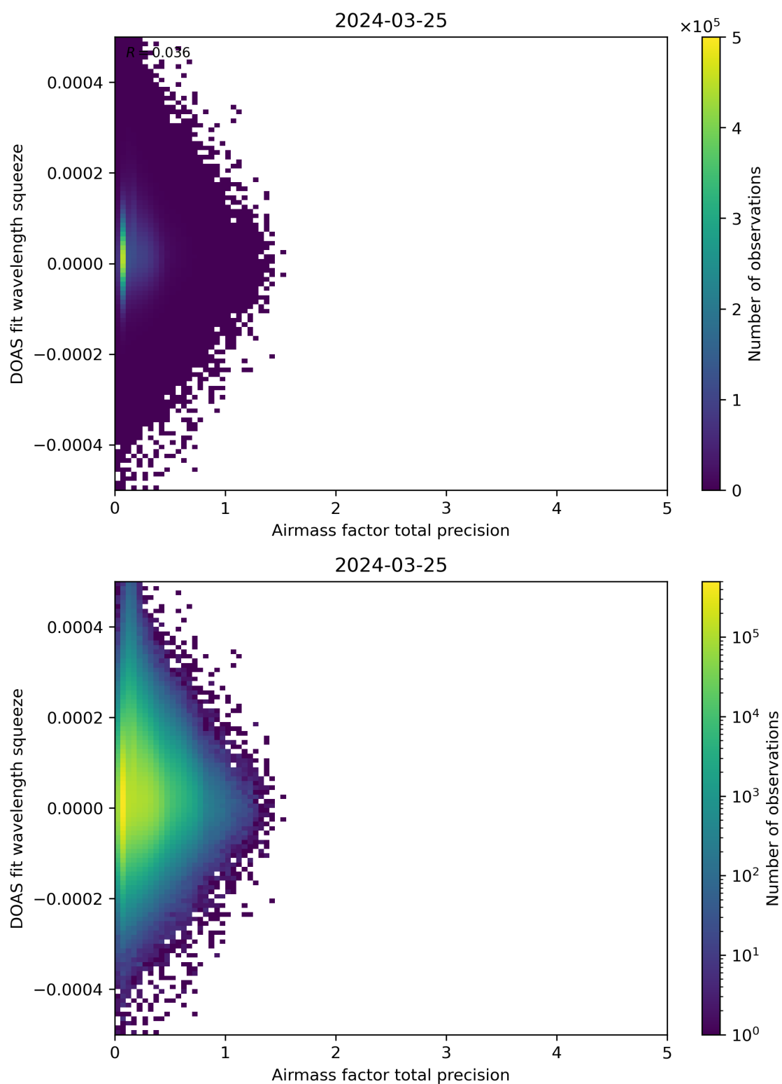
Figure 107: Scatter density plot of “Airmass factor total precision” against “DOAS fit wavelength squeeze” for 2024-03-25 to 2024-03-26.
