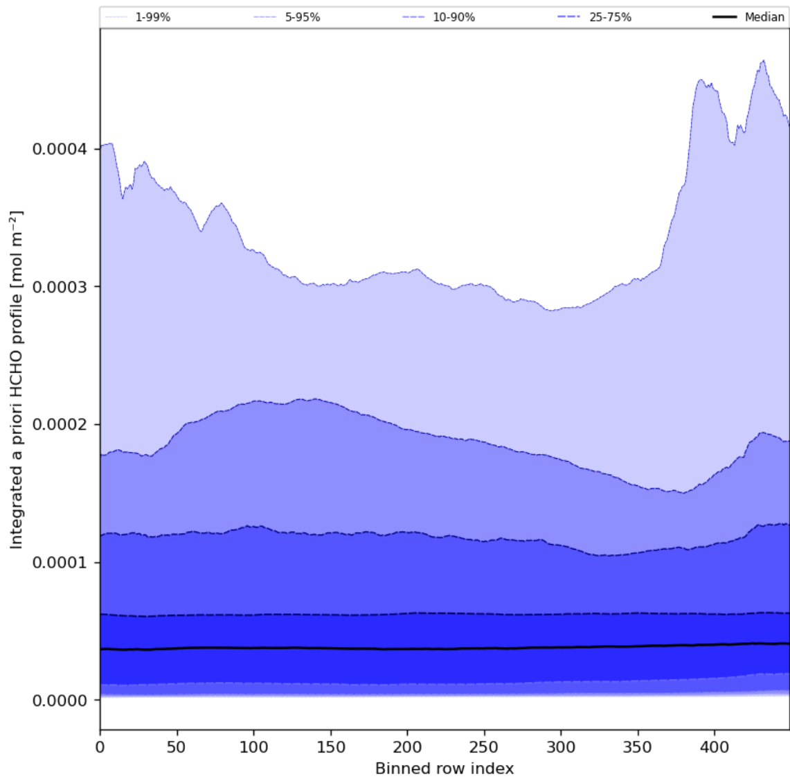
Figure 57: Along track statistics of "Integrated a priori HCHO profile" for 2024-03-25 to 2024-03-26
