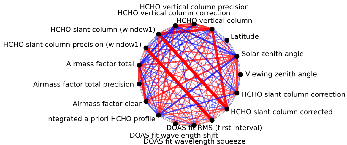
Figure 1: Map of correlation graph for 2024-03-25 to 2024-03-26.
