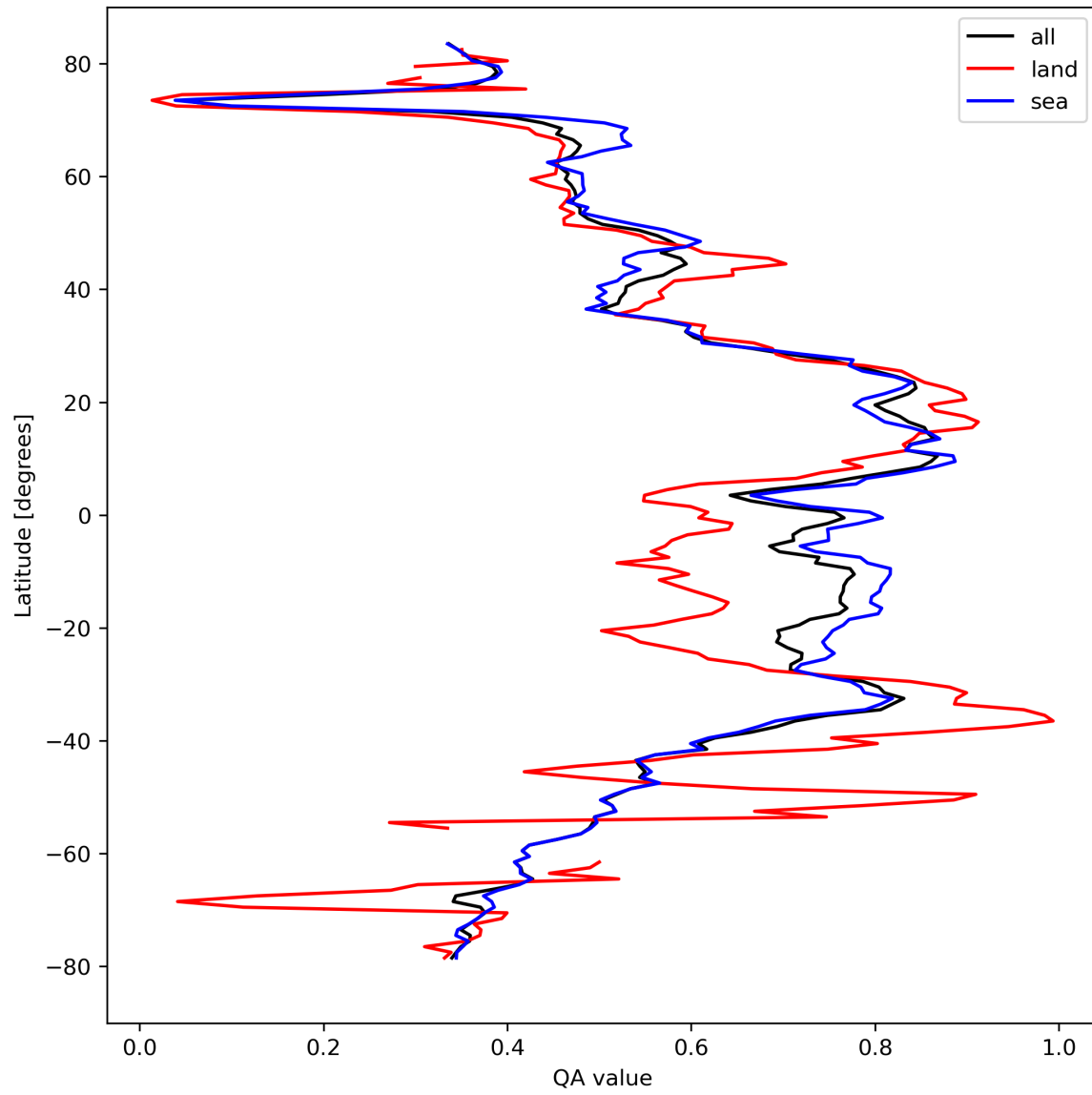
Figure 20: Zonal average of “QA value” for 2024-03-25 to 2024-03-26.
