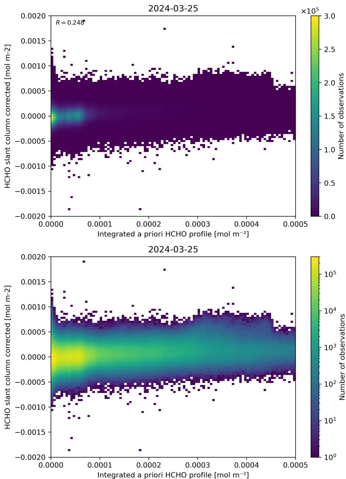
Figure 151: Scatter density plot of “Integrated a priori HCHO profile” against “HCHO slant column corrected” for 2024-03-25 to 2024-03-26.
