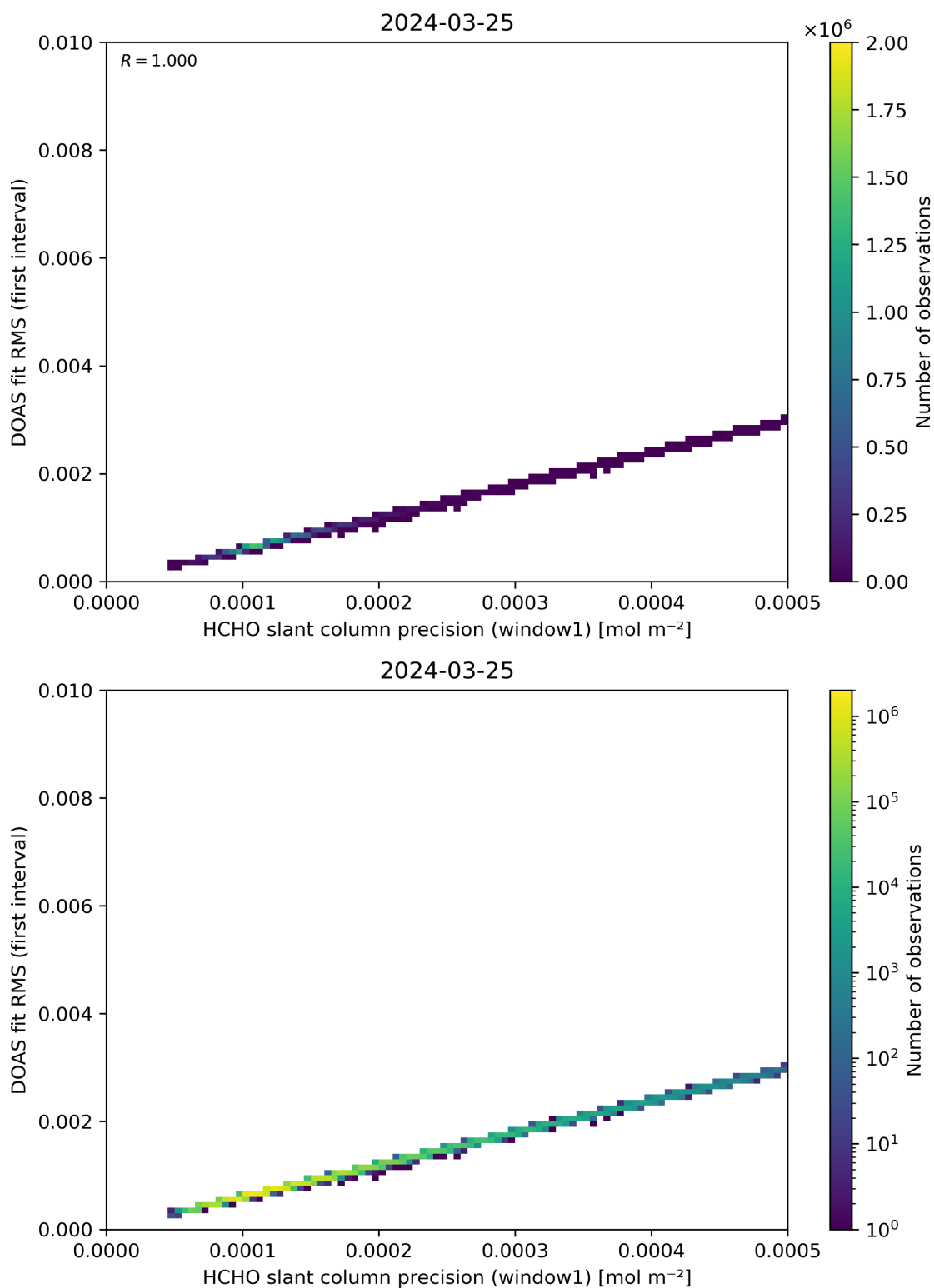
Figure 88: Scatter density plot of “HCHO slant column precision (window1)” against “DOAS fit RMS (first interval)” for 2024-03-25 to 2024-03-26.
