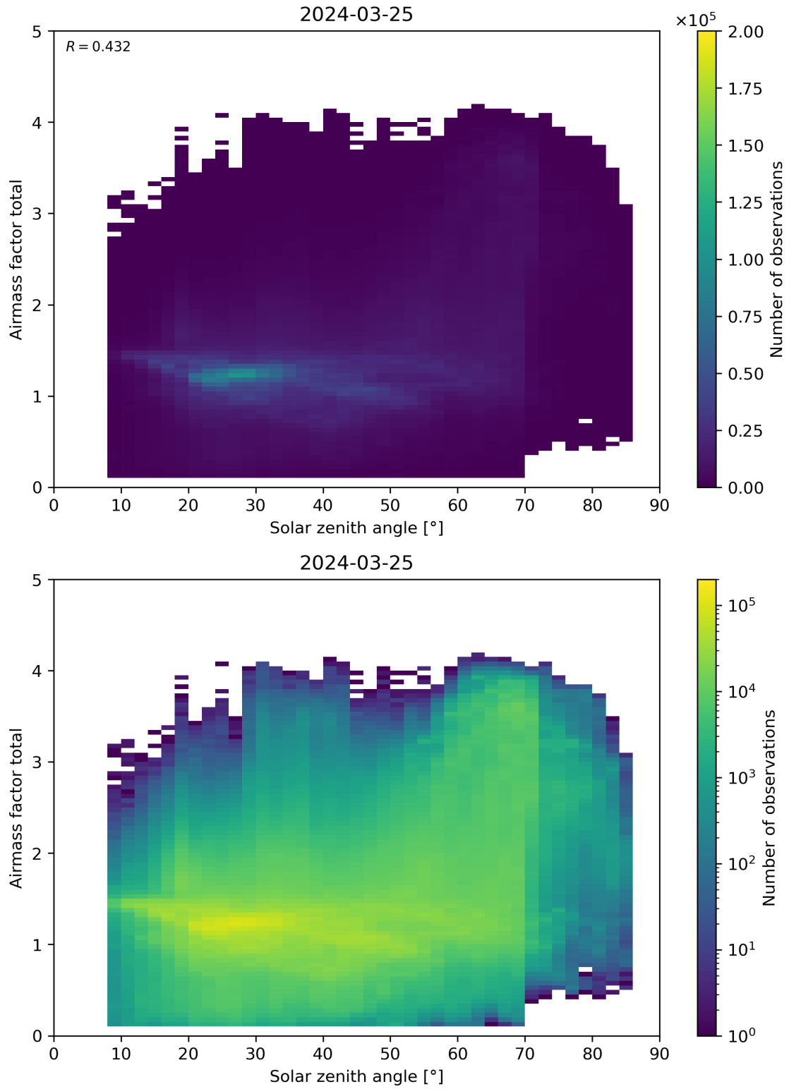
Figure 175: Scatter density plot of “Solar zenith angle” against “Airmass factor total” for 2024-03-25 to 2024-03-26.
