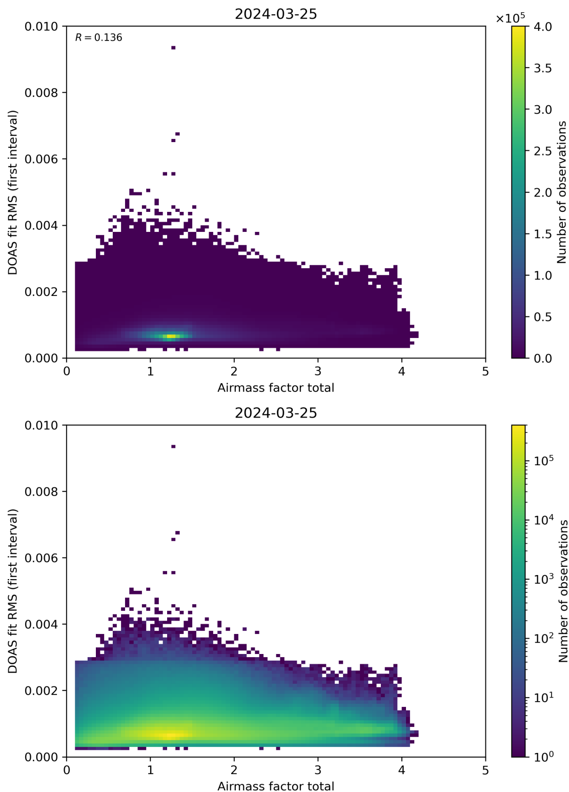
Figure 97: Scatter density plot of “Airmass factor total” against “DOAS fit RMS (first interval)” for 2024-03-25 to 2024-03-26.
