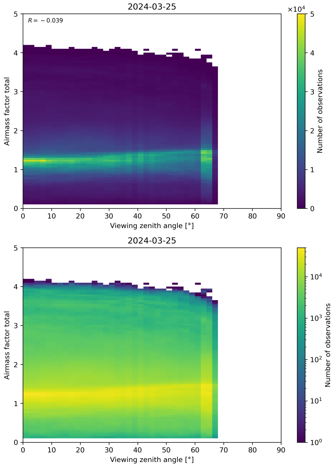
Figure 190: Scatter density plot of “Viewing zenith angle” against “Airmass factor total” for 2024-03-25 to 2024-03-26.
