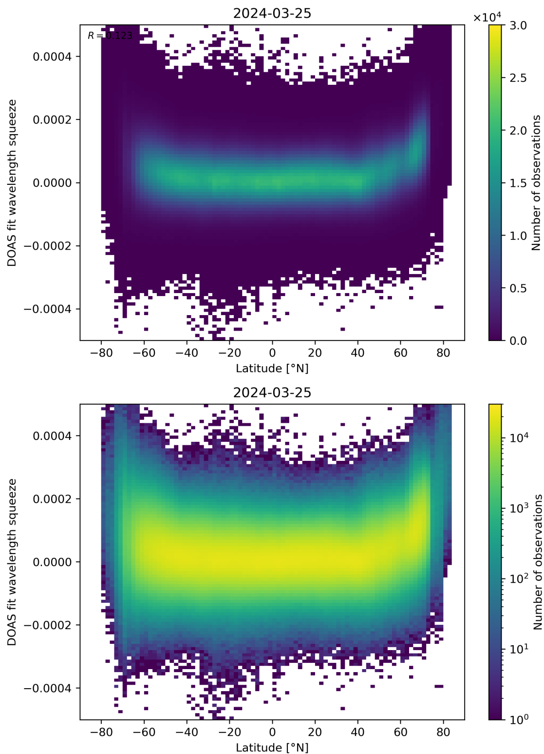
Figure 155: Scatter density plot of “Latitude” against “DOAS fit wavelength squeeze” for 2024-03-25 to 2024-03-26.
