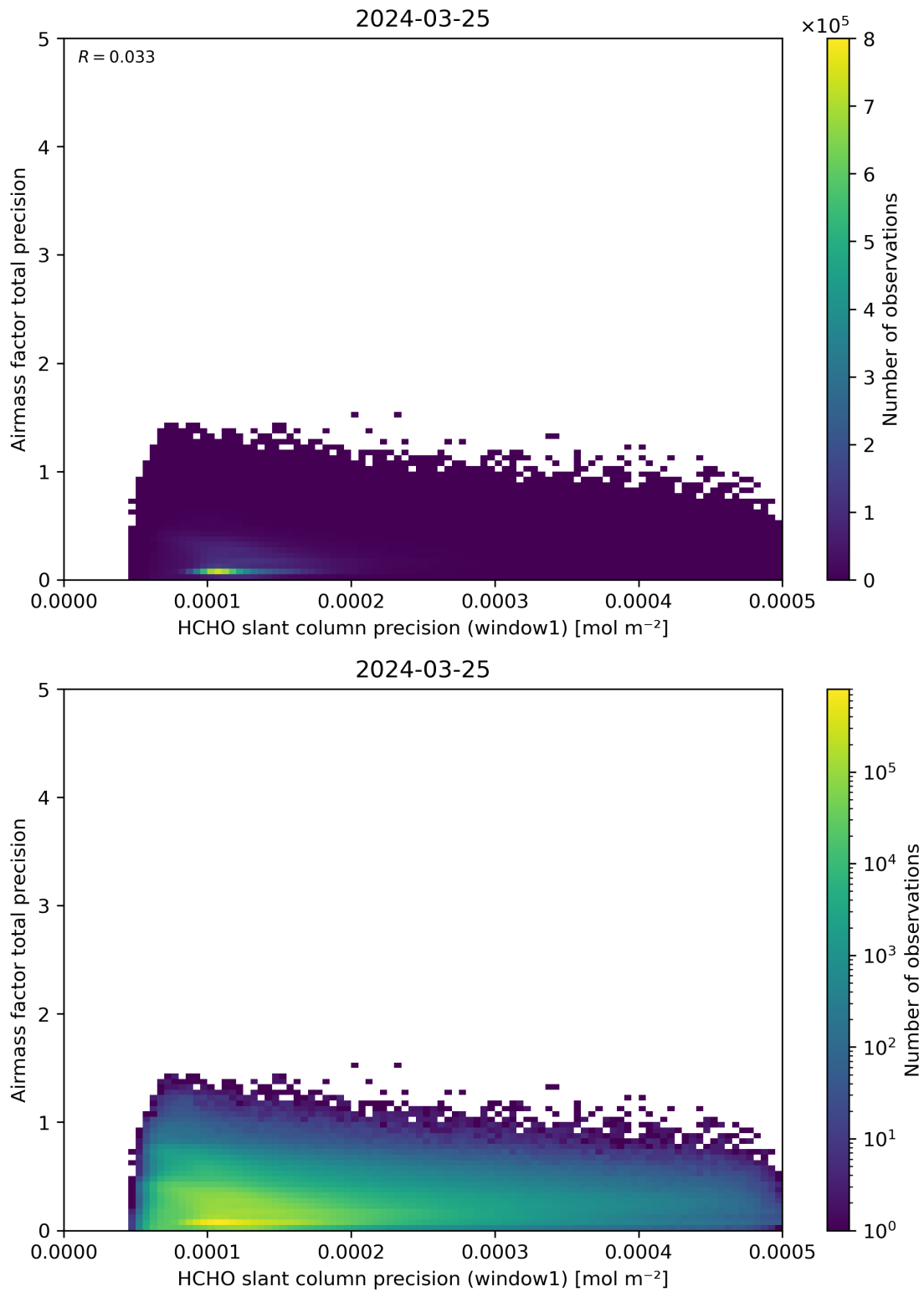
Figure 95: Scatter density plot of “HCHO slant column precision (window1)” against “Airmass factor total precision” for 2024-03-25 to 2024-03-26.
