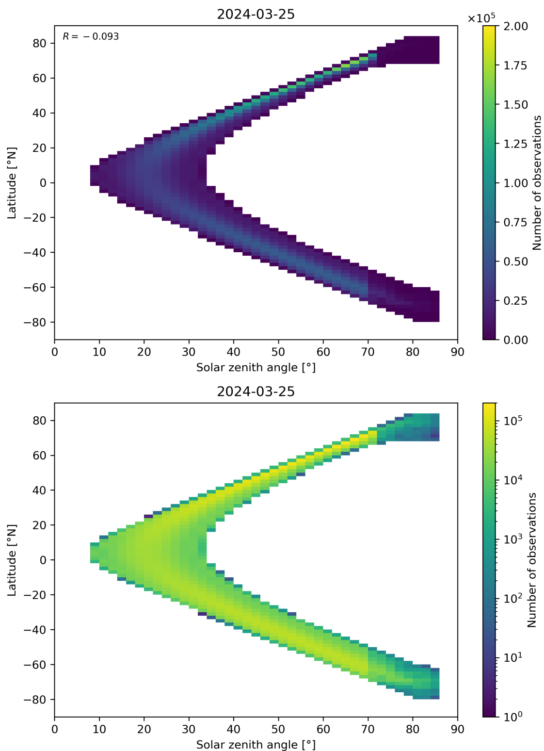
Figure 181: Scatter density plot of “Solar zenith angle” against “Latitude” for 2024-03-25 to 2024-03-26.
