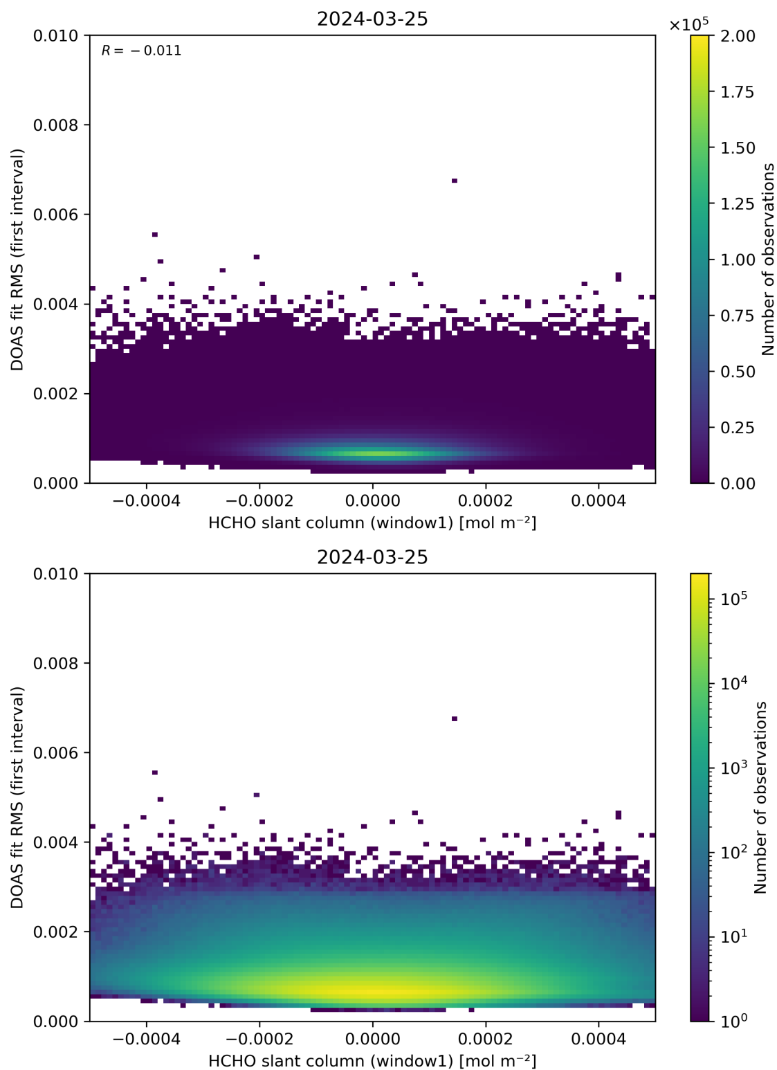
Figure 78: Scatter density plot of “HCHO slant column (window1)” against “DOAS fit RMS (first interval)” for 2024-03-25 to 2024-03-26.
