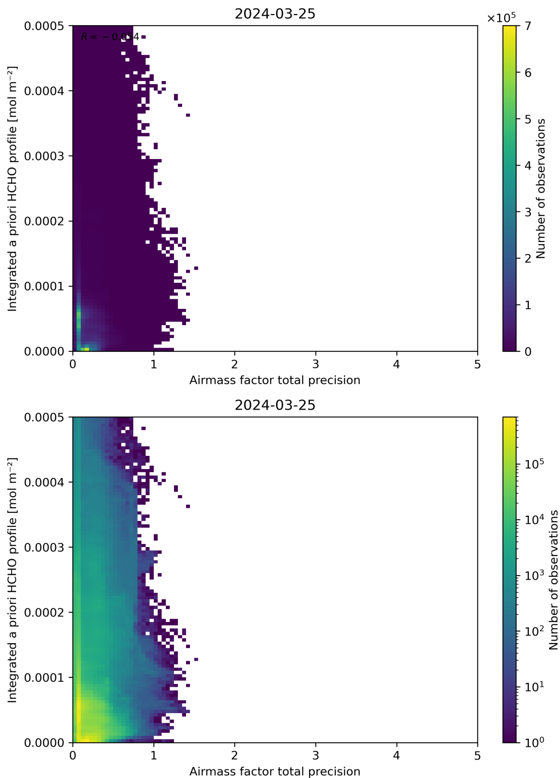
Figure 111: Scatter density plot of “Airmass factor total precision” against “Integrated a priori HCHO profile” for 2024-03-25 to 2024-03-26.
