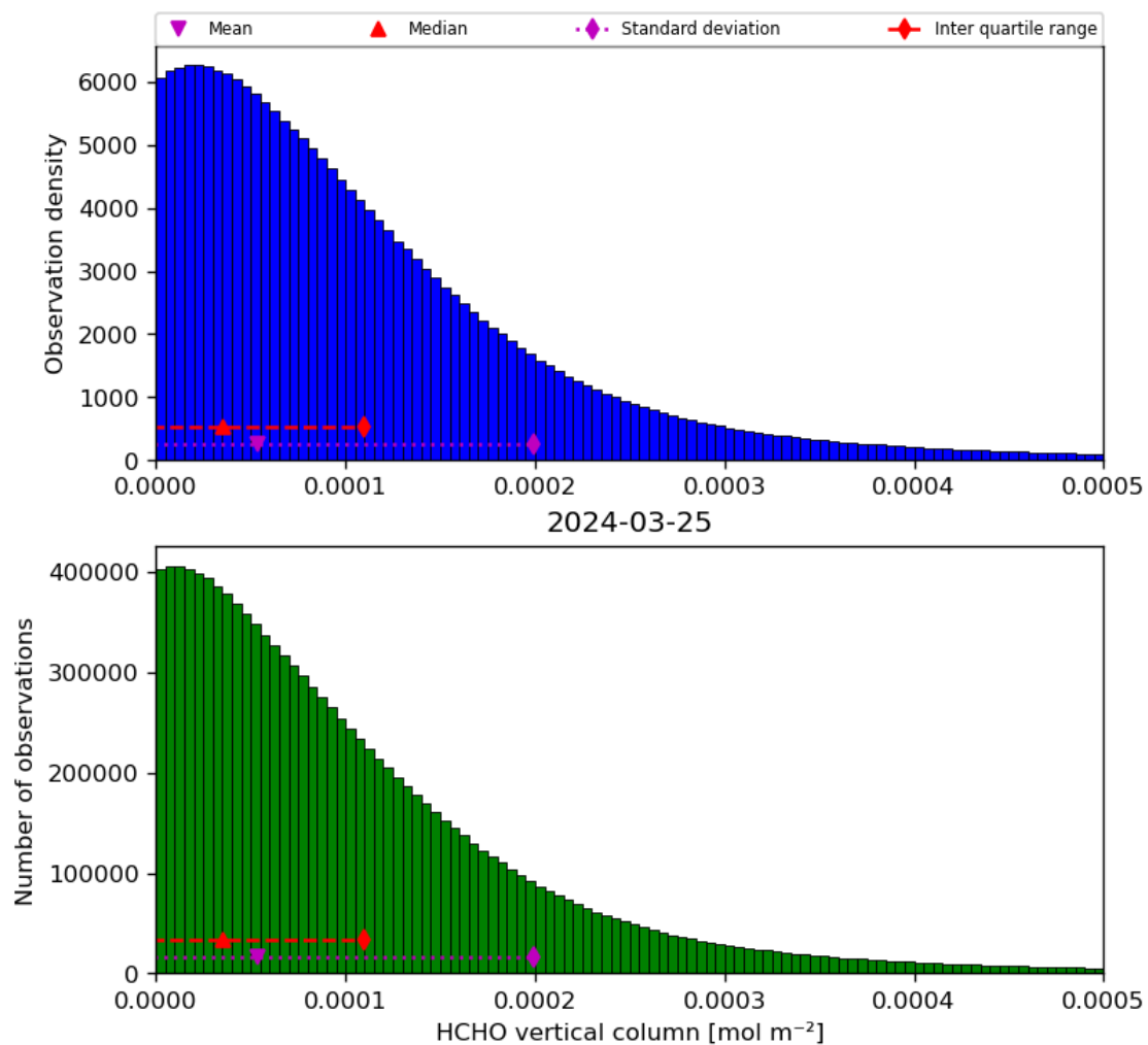
Figure 35: Histogram of “HCHO vertical column” for 2024-03-25 to 2024-03-26
