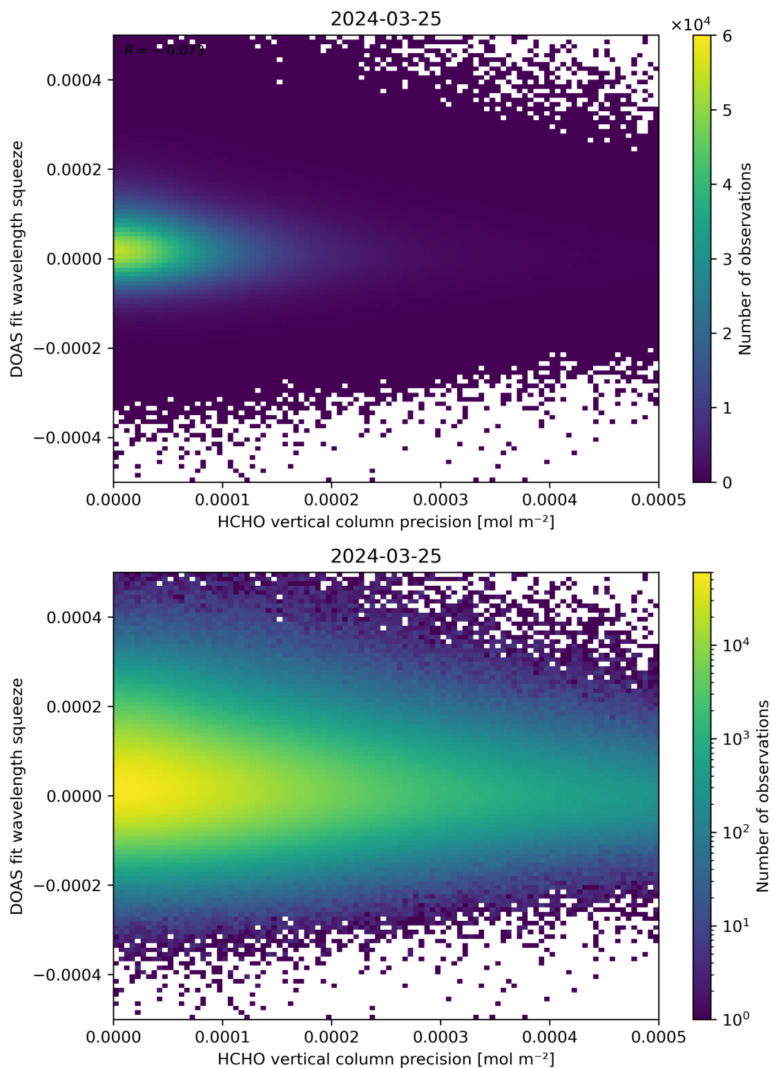
Figure 138: Scatter density plot of “HCHO vertical column precision” against “DOAS fit wavelength squeeze” for 2024-03-25 to 2024-03-26.
