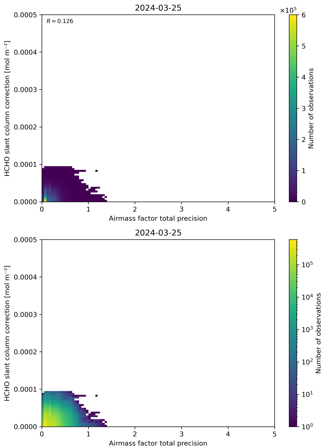
Figure 110: Scatter density plot of “Airmass factor total precision” against “HCHO slant column correction” for 2024-03-25 to 2024-03-26.
