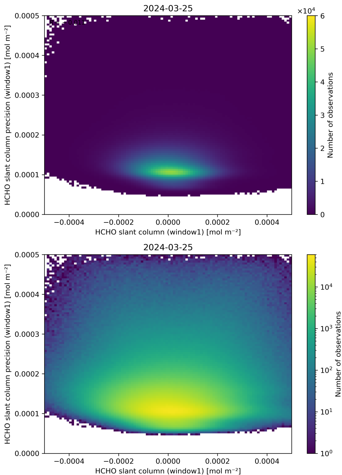
Figure 84: Scatter density plot of “HCHO slant column (window1)” against “HCHO slant column precision (window1)” for 2024-03-25 to 2024-03-26.
