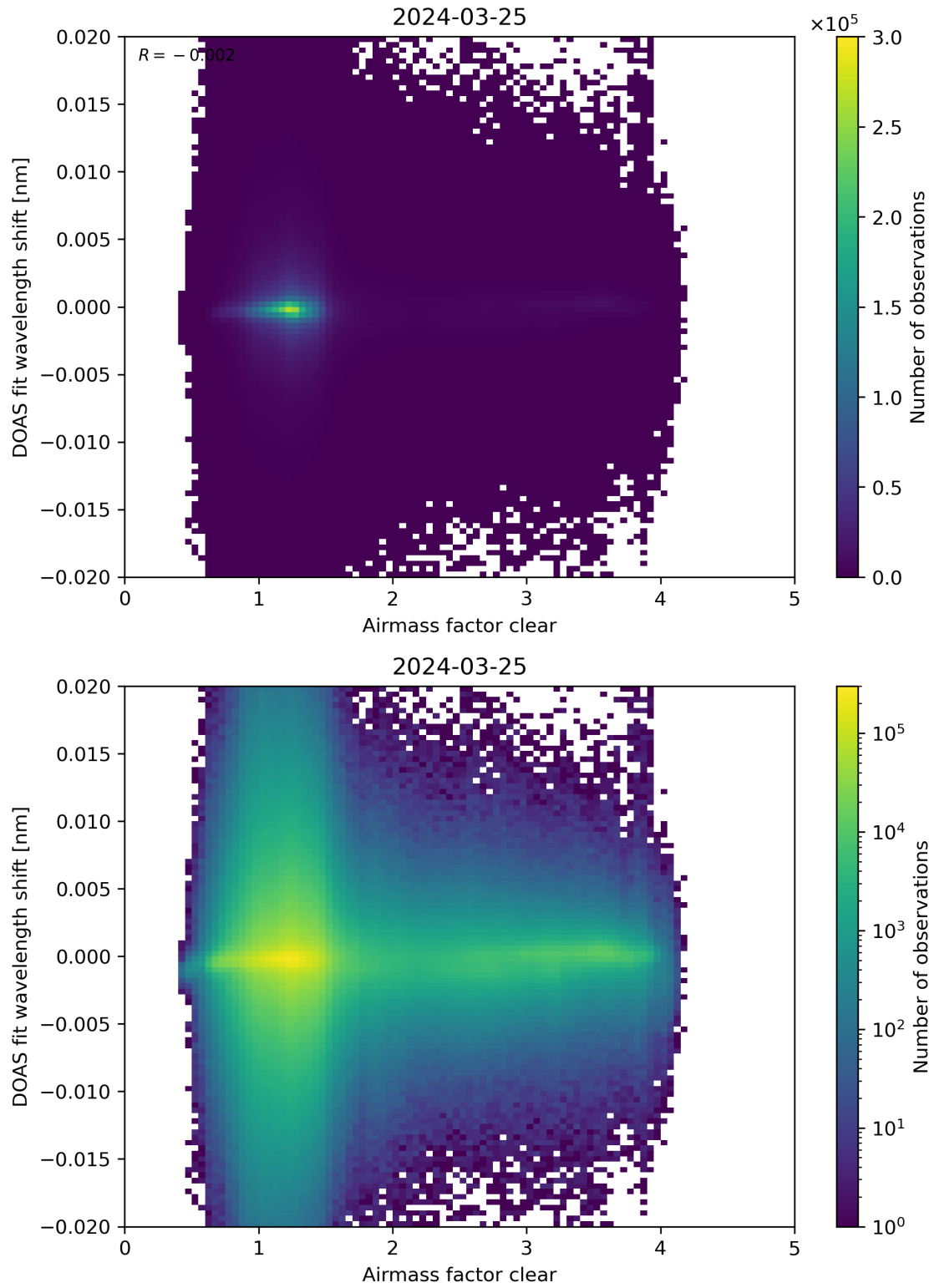
Figure 72: Scatter density plot of “Airmass factor clear” against “DOAS fit wavelength shift” for 2024-03-25 to 2024-03-26.
