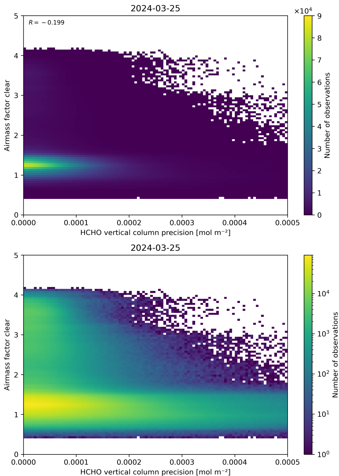
Figure 139: Scatter density plot of “HCHO vertical column precision” against “Airmass factor clear” for 2024-03-25 to 2024-03-26.
