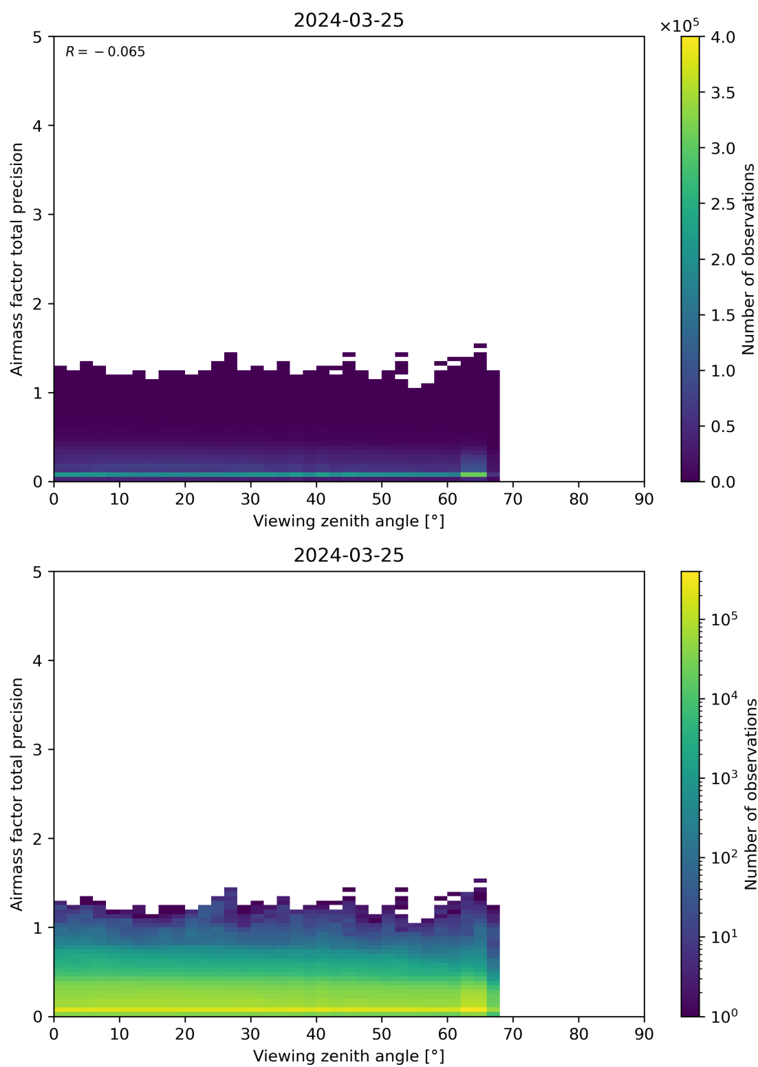
Figure 191: Scatter density plot of “Viewing zenith angle” against “Airmass factor total precision” for 2024-03-25 to 2024-03-26.
