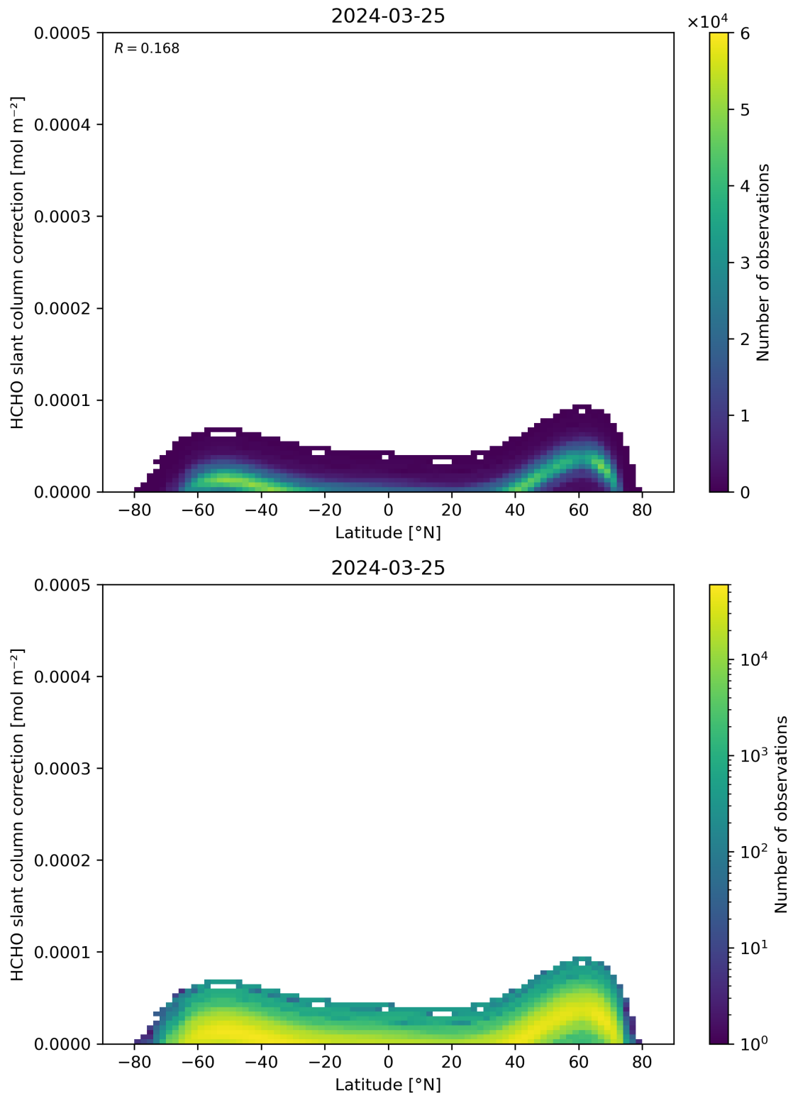
Figure 158: Scatter density plot of “Latitude” against “HCHO slant column correction” for 2024-03-25 to 2024-03-26.
