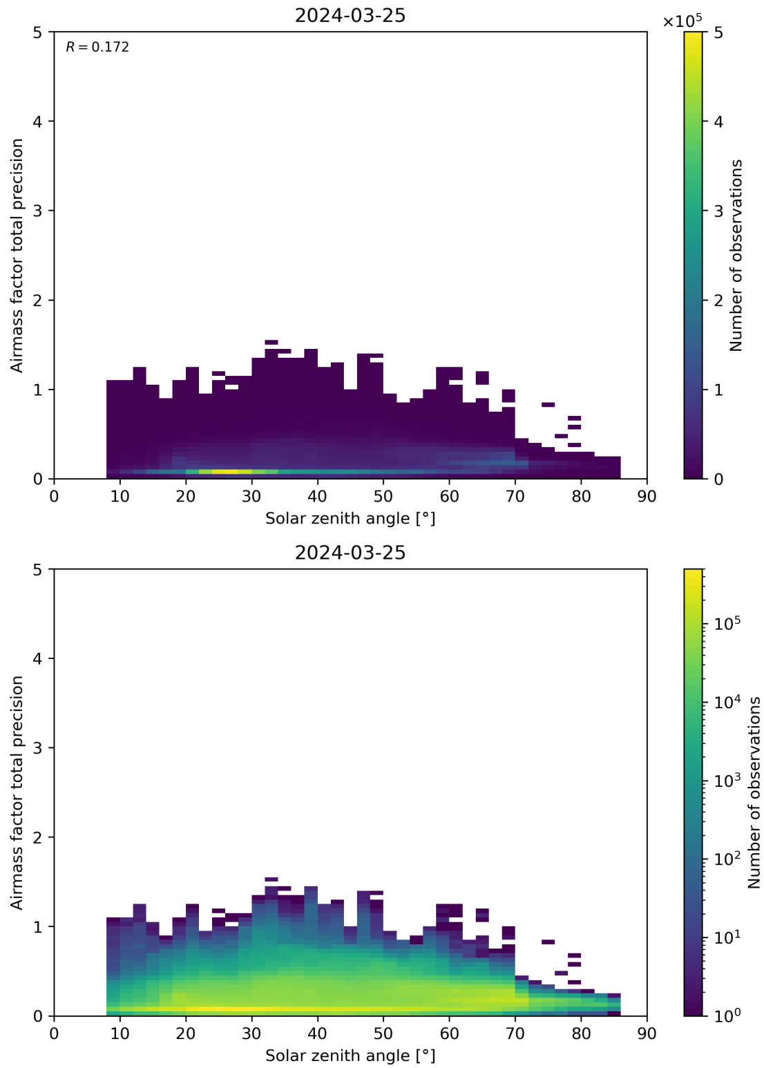
Figure 176: Scatter density plot of “Solar zenith angle” against “Airmass factor total precision” for 2024-03-25 to 2024-03-26.
