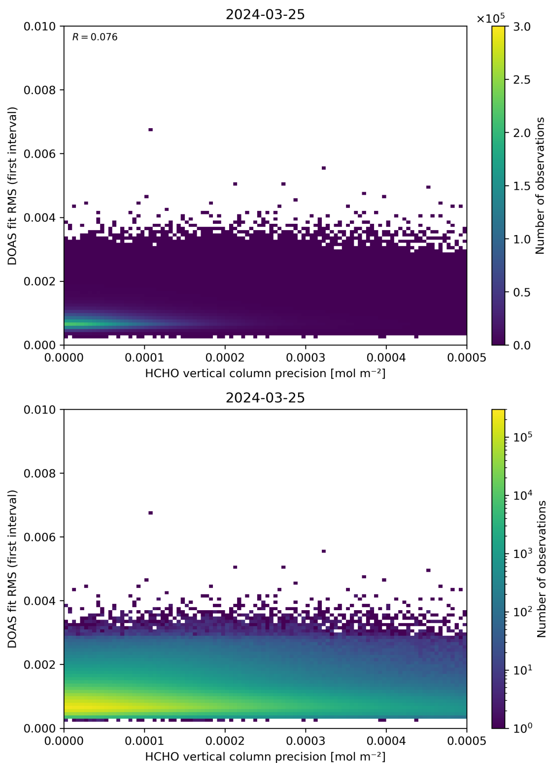
Figure 136: Scatter density plot of “HCHO vertical column precision” against “DOAS fit RMS (first interval)” for 2024-03-25 to 2024-03-26.
