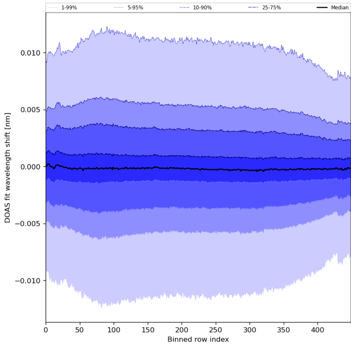
Figure 58: Along track statistics of “DOAS fit wavelength shift” for 2024-03-25 to 2024-03-26
