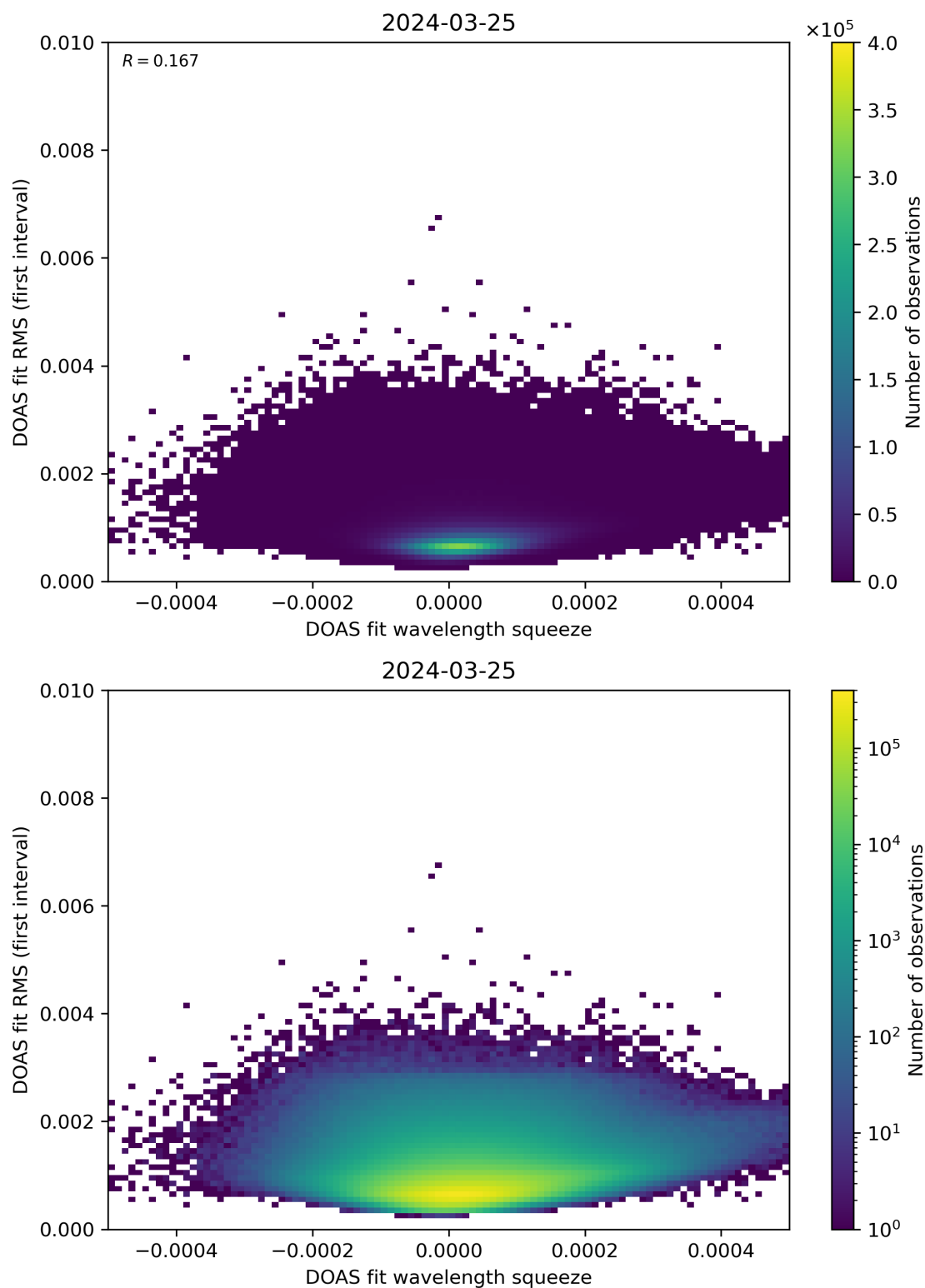
Figure 68: Scatter density plot of “DOAS fit wavelength squeeze” against “DOAS fit RMS (first interval)” for 2024-03-25 to 2024-03-26.
