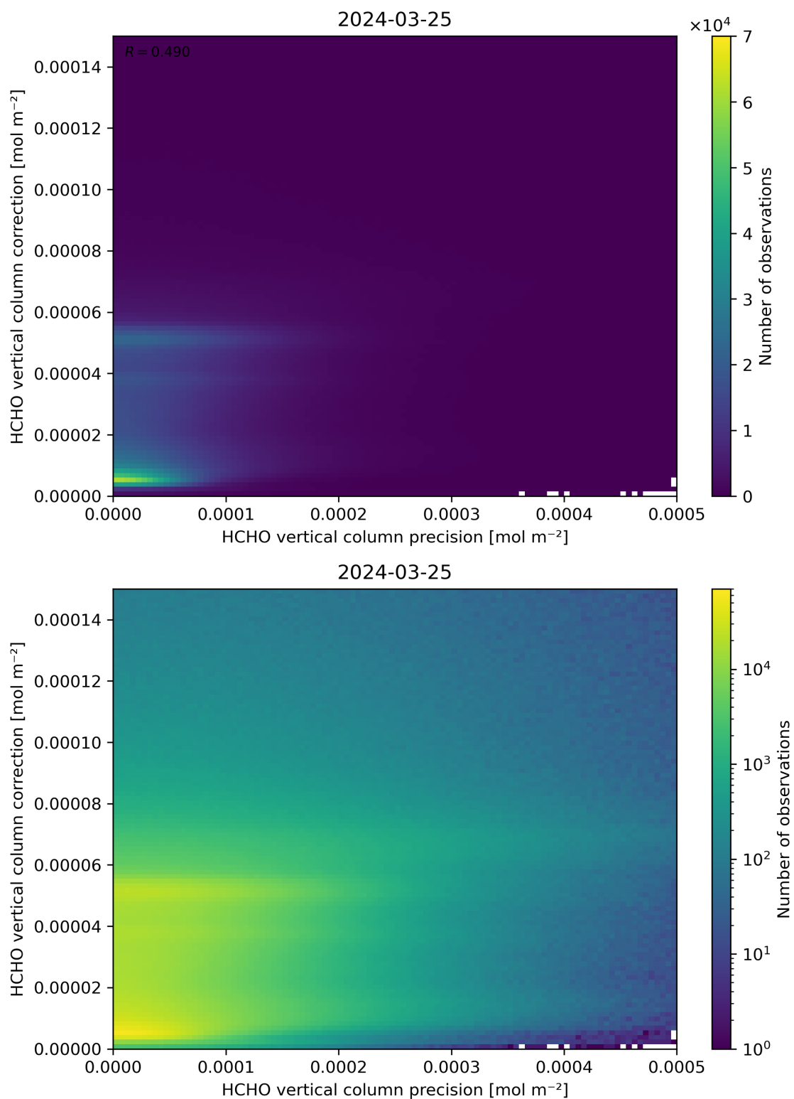
Figure 146: Scatter density plot of “HCHO vertical column precision” against “HCHO vertical column correction” for 2024-03-25 to 2024-03-26.
