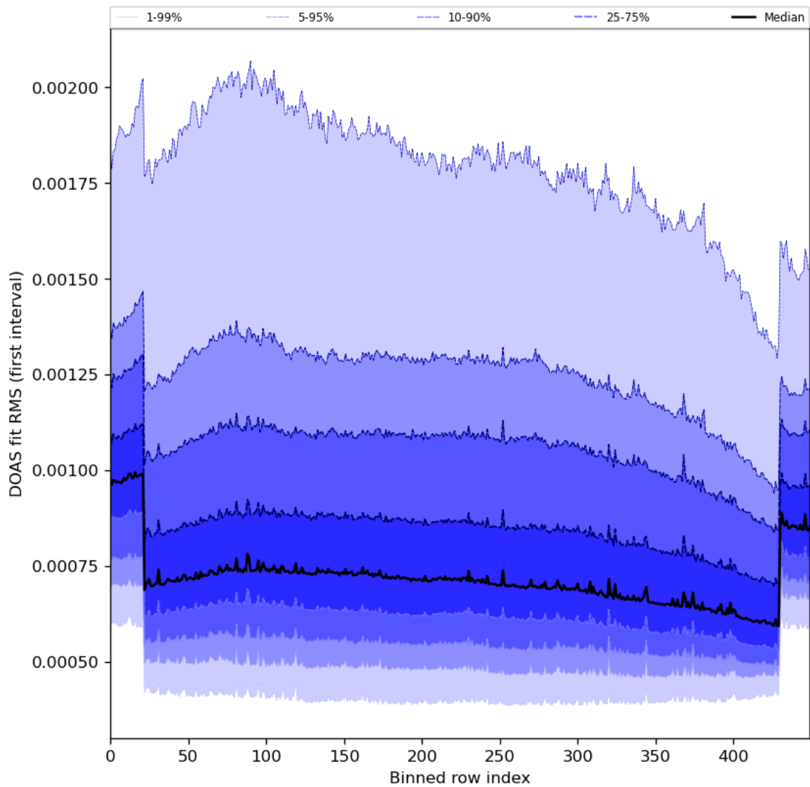
Figure 60: Along track statistics of “DOAS fit RMS (first interval)” for 2024-03-25 to 2024-03-26
