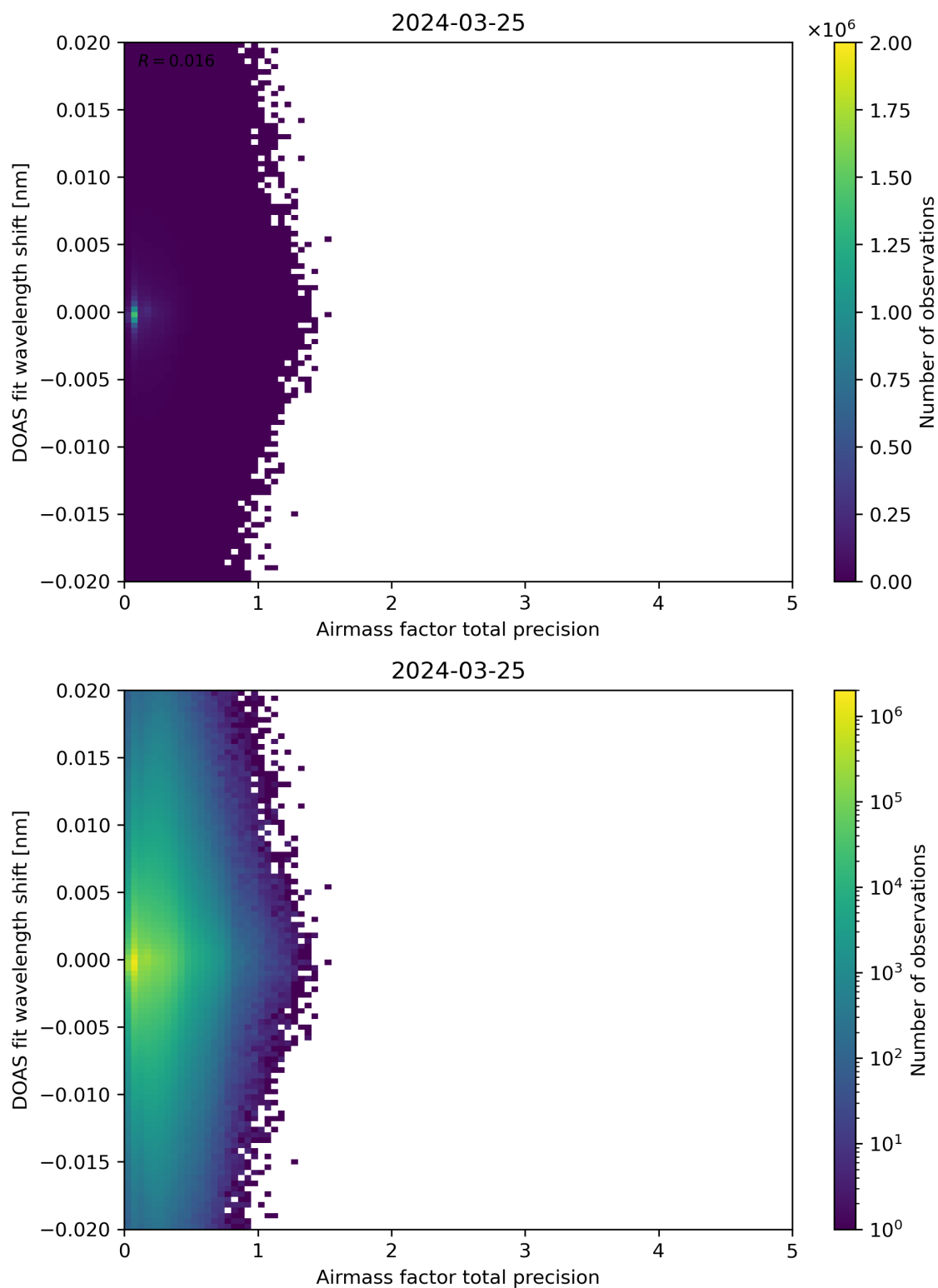
Figure 106: Scatter density plot of “Airmass factor total precision” against “DOAS fit wavelength shift” for 2024-03-25 to 2024-03-26.
