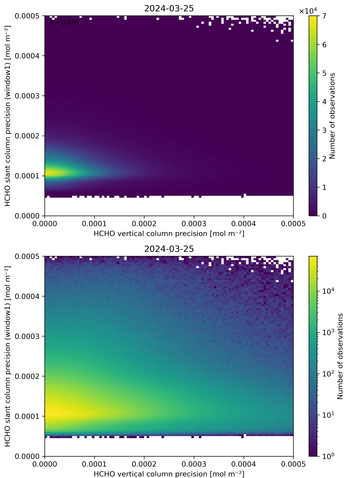
Figure 143: Scatter density plot of “HCHO vertical column precision” against “HCHO slant column precision (window1)” for 2024-03-25 to 2024-03-26.
