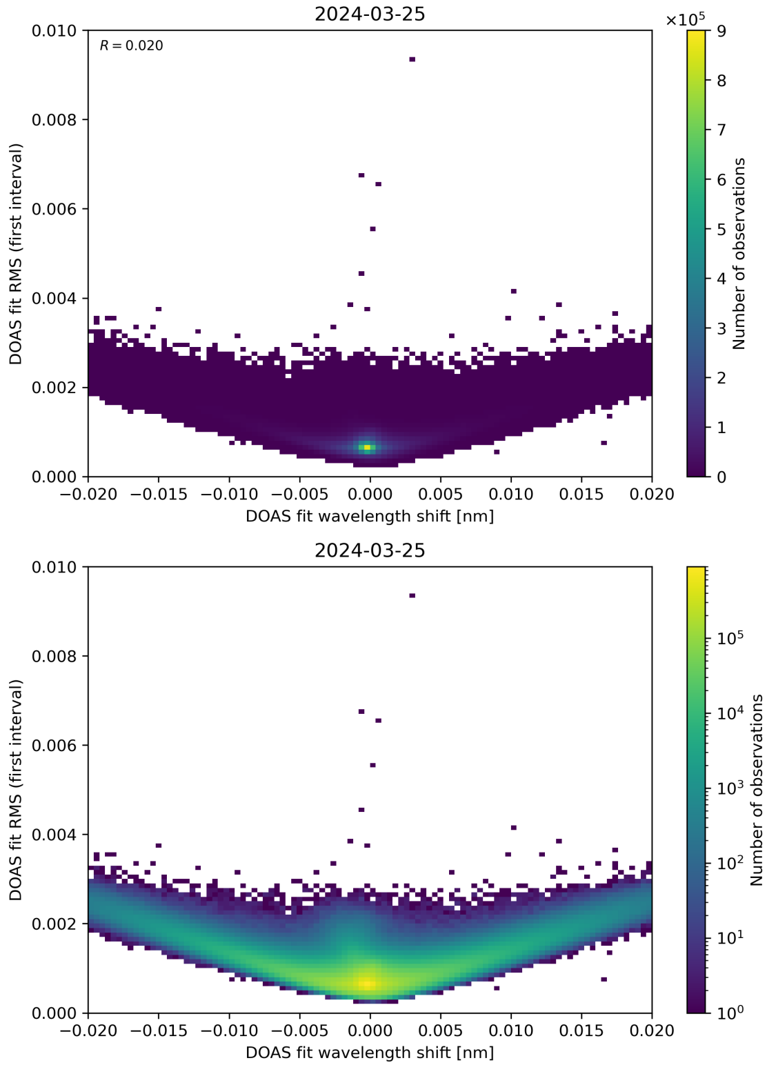
Figure 64: Scatter density plot of “DOAS fit wavelength shift” against “DOAS fit RMS (first interval)” for 2024-03-25 to 2024-03-26.
