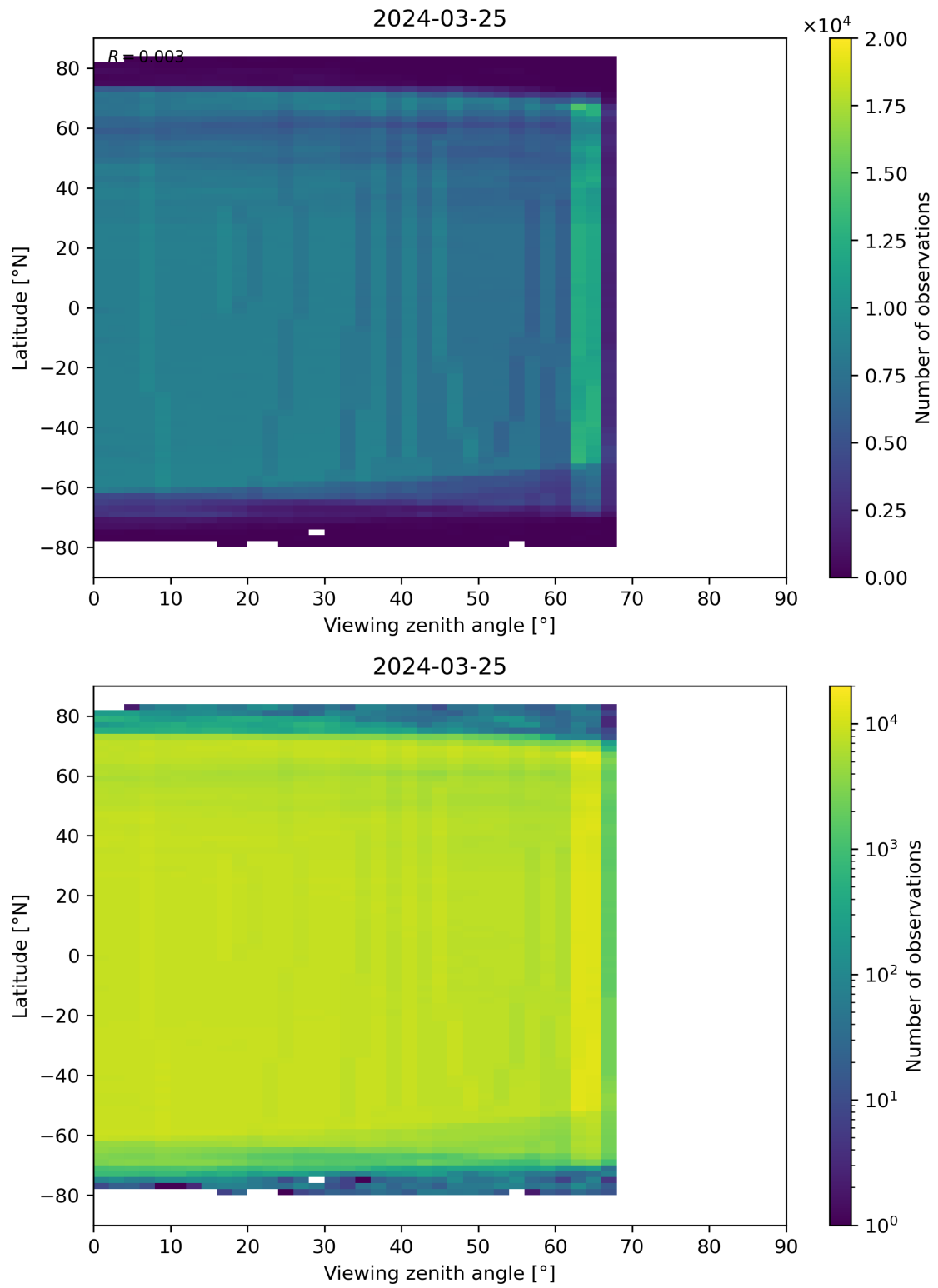
Figure 196: Scatter density plot of “Viewing zenith angle” against “Latitude” for 2024-03-25 to 2024-03-26.
