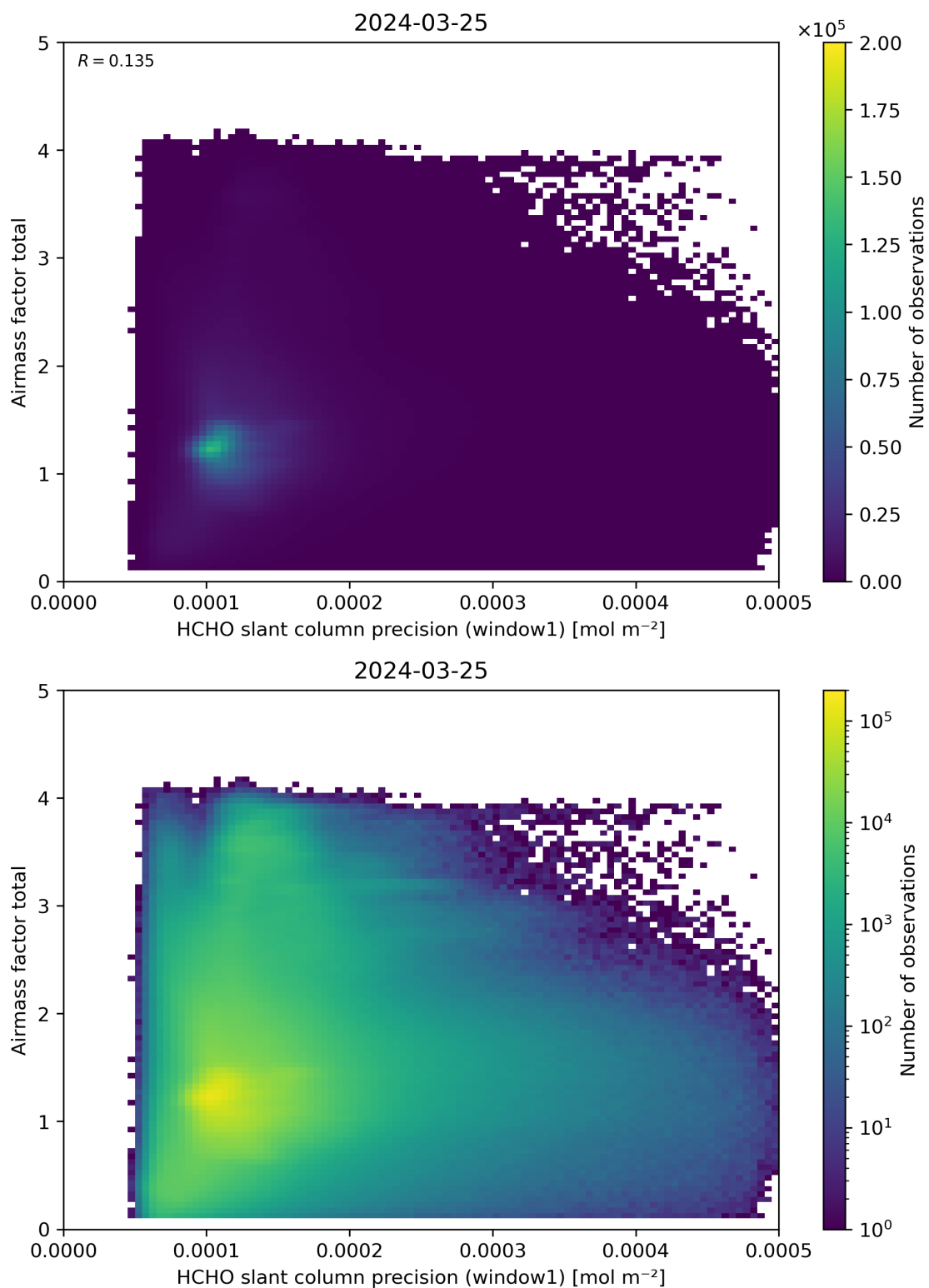
Figure 94: Scatter density plot of “HCHO slant column precision (window1)” against “Airmass factor total” for 2024-03-25 to 2024-03-26.
