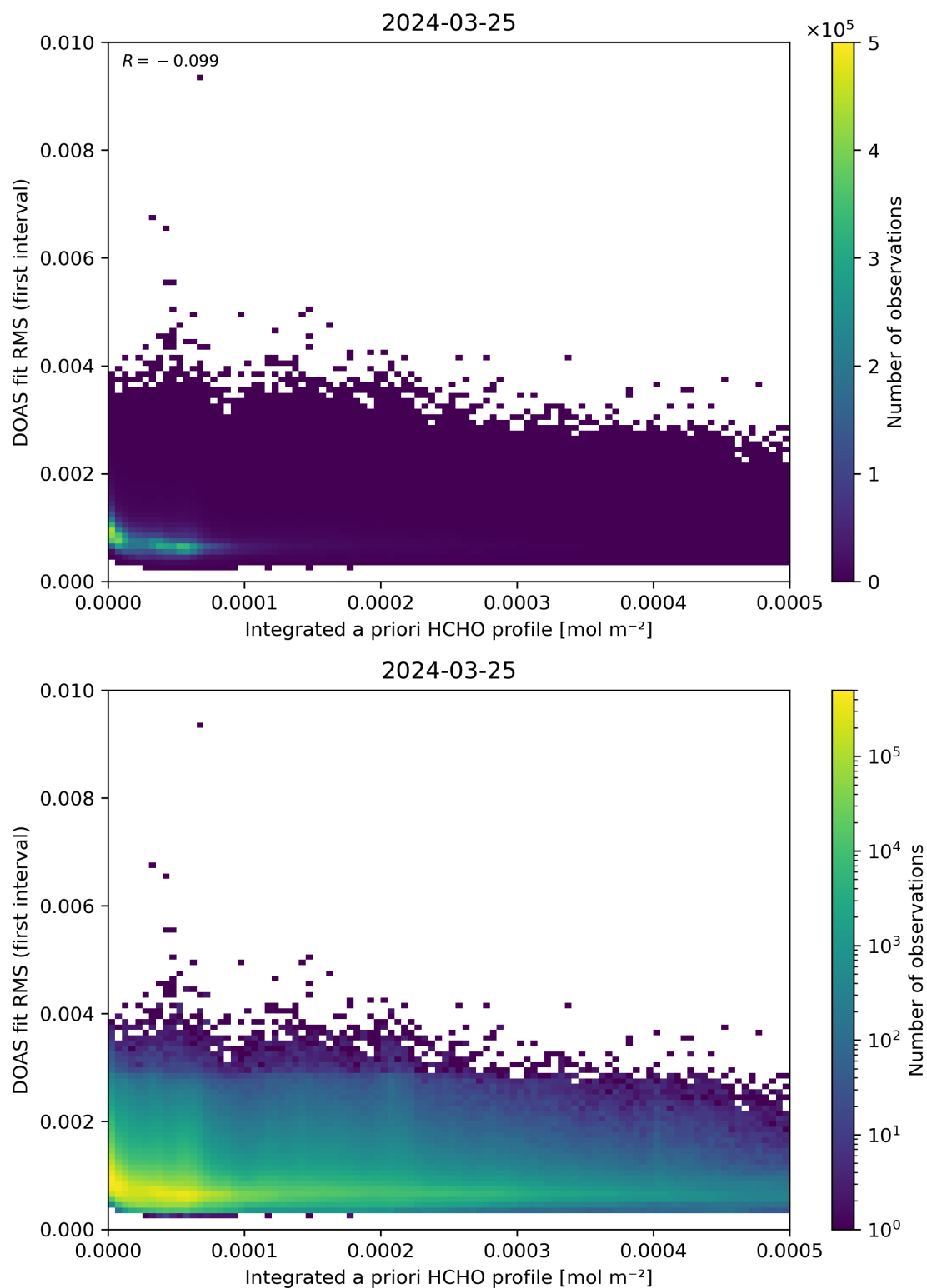
Figure 148: Scatter density plot of “Integrated a priori HCHO profile” against “DOAS fit RMS (first interval)” for 2024-03-25 to 2024-03-26.
