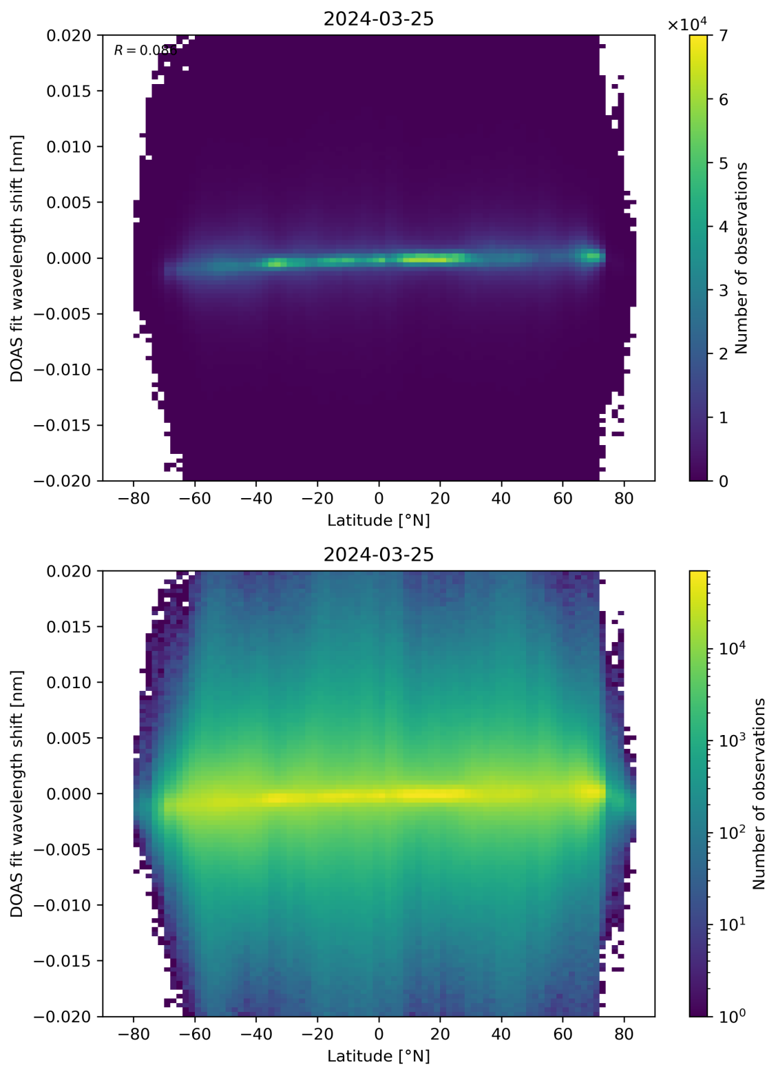
Figure 154: Scatter density plot of “Latitude” against “DOAS fit wavelength shift” for 2024-03-25 to 2024-03-26.
