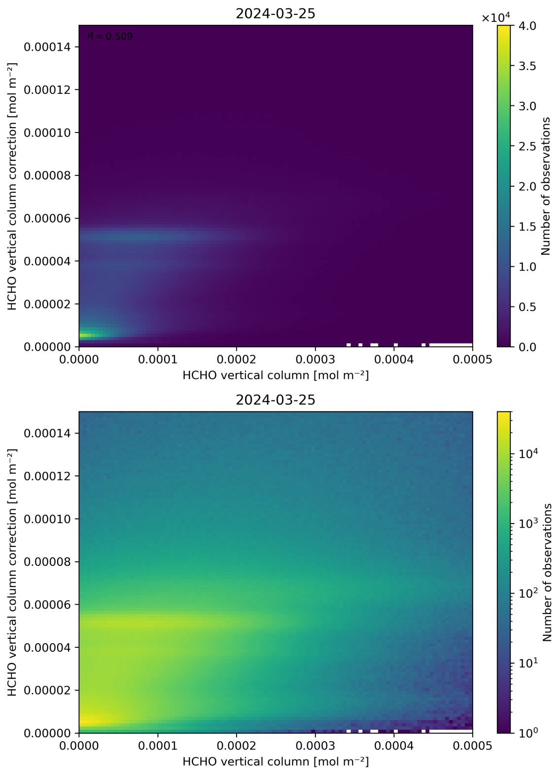
Figure 133: Scatter density plot of “HCHO vertical column” against “HCHO vertical column correction” for 2024-03-25 to 2024-03-26.
