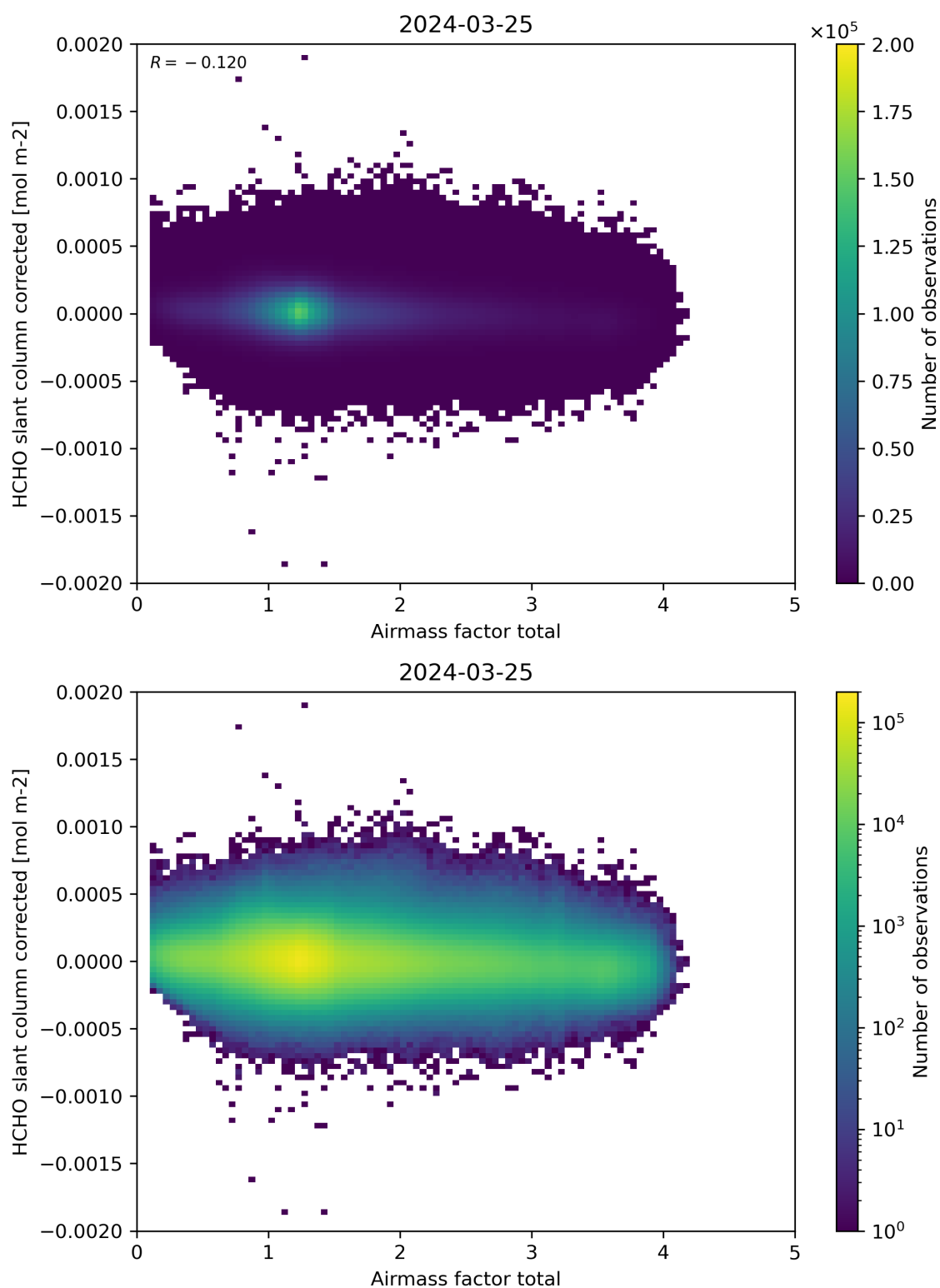
Figure 101: Scatter density plot of “Airmass factor total” against “HCHO slant column corrected” for 2024-03-25 to 2024-03-26.
