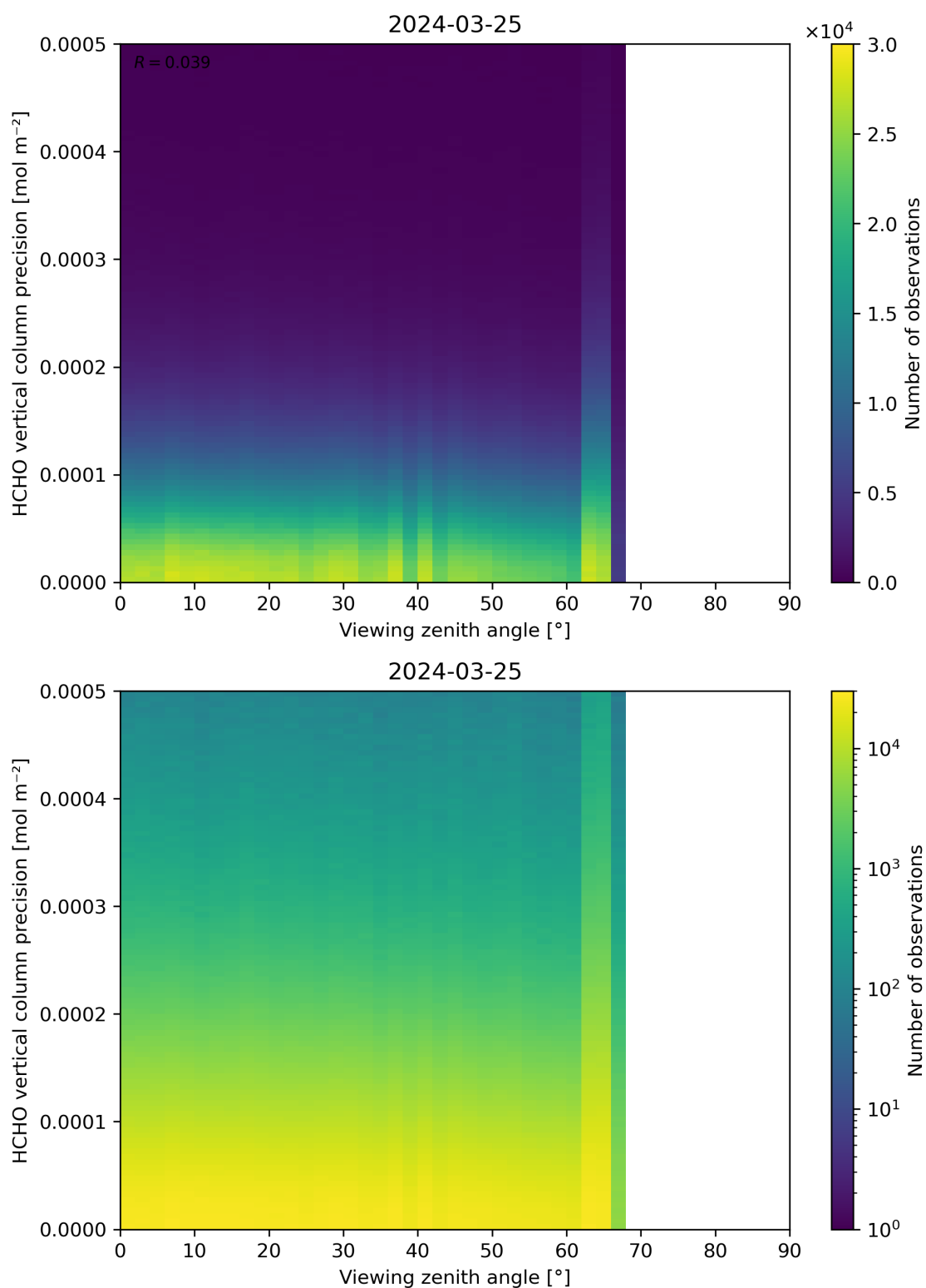
Figure 194: Scatter density plot of “Viewing zenith angle” against “HCHO vertical column precision” for 2024-03-25 to 2024-03-26.
