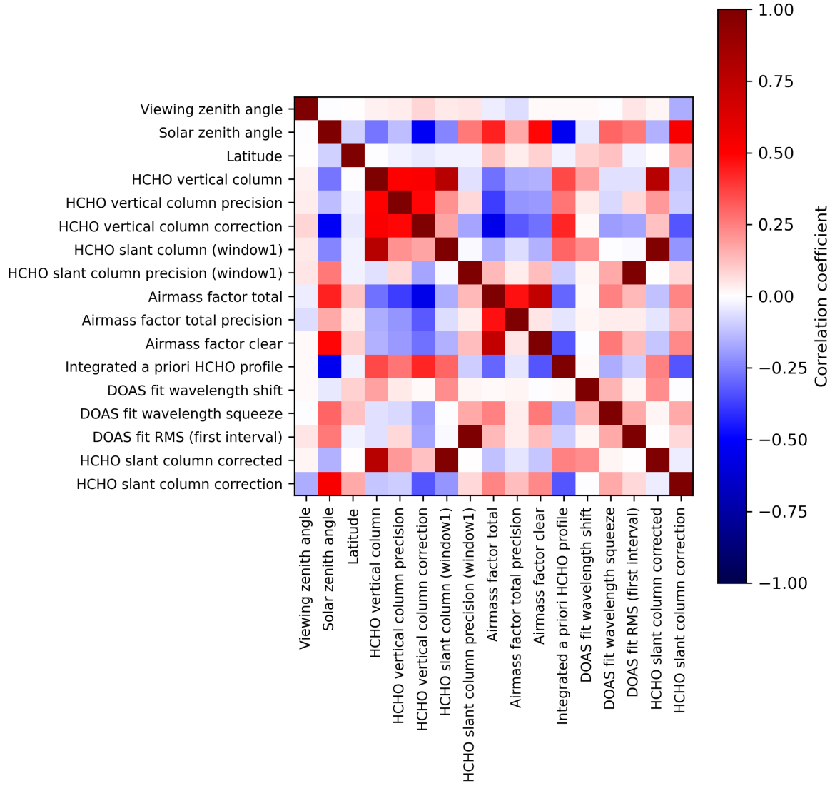
Figure 2: Map of correlation matrix for 2024-03-25 to 2024-03-26.
