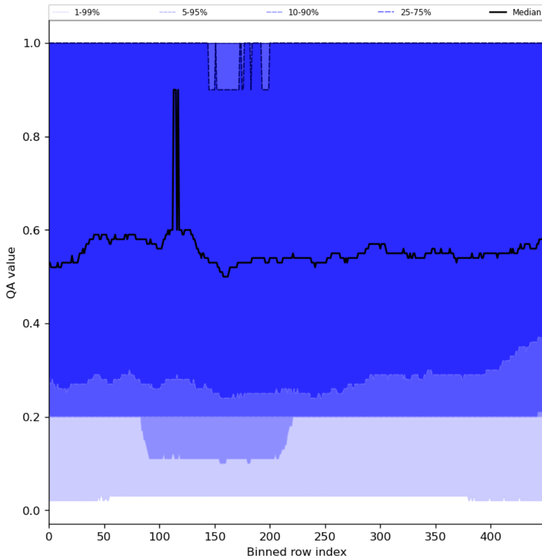
Figure 48: Along track statistics of “QA value” for 2024-03-25 to 2024-03-26
