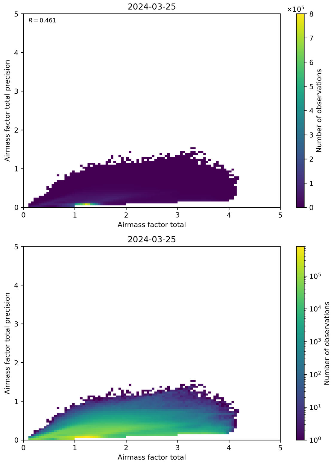
Figure 103: Scatter density plot of “Airmass factor total” against “Airmass factor total precision” for 2024-03-25 to 2024-03-26.
