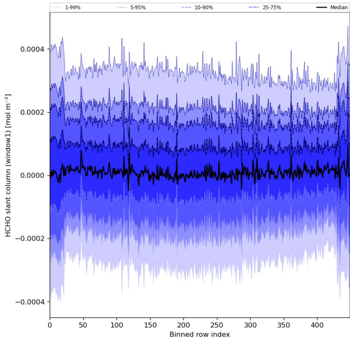
Figure 52: Along track statistics of “HCHO slant column (window1)” for 2024-03-25 to 2024-03-26
