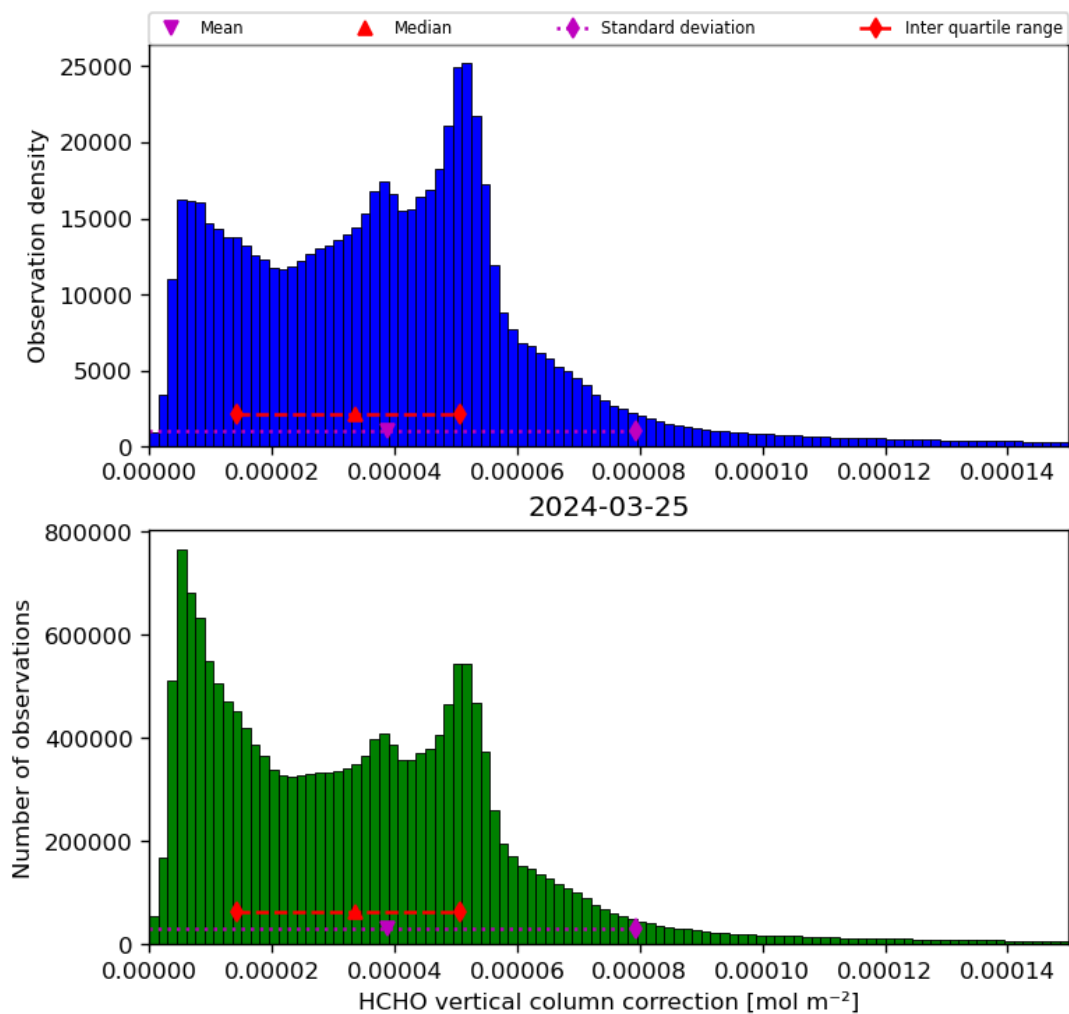
Figure 37: Histogram of “HCHO vertical column correction” for 2024-03-25 to 2024-03-26
