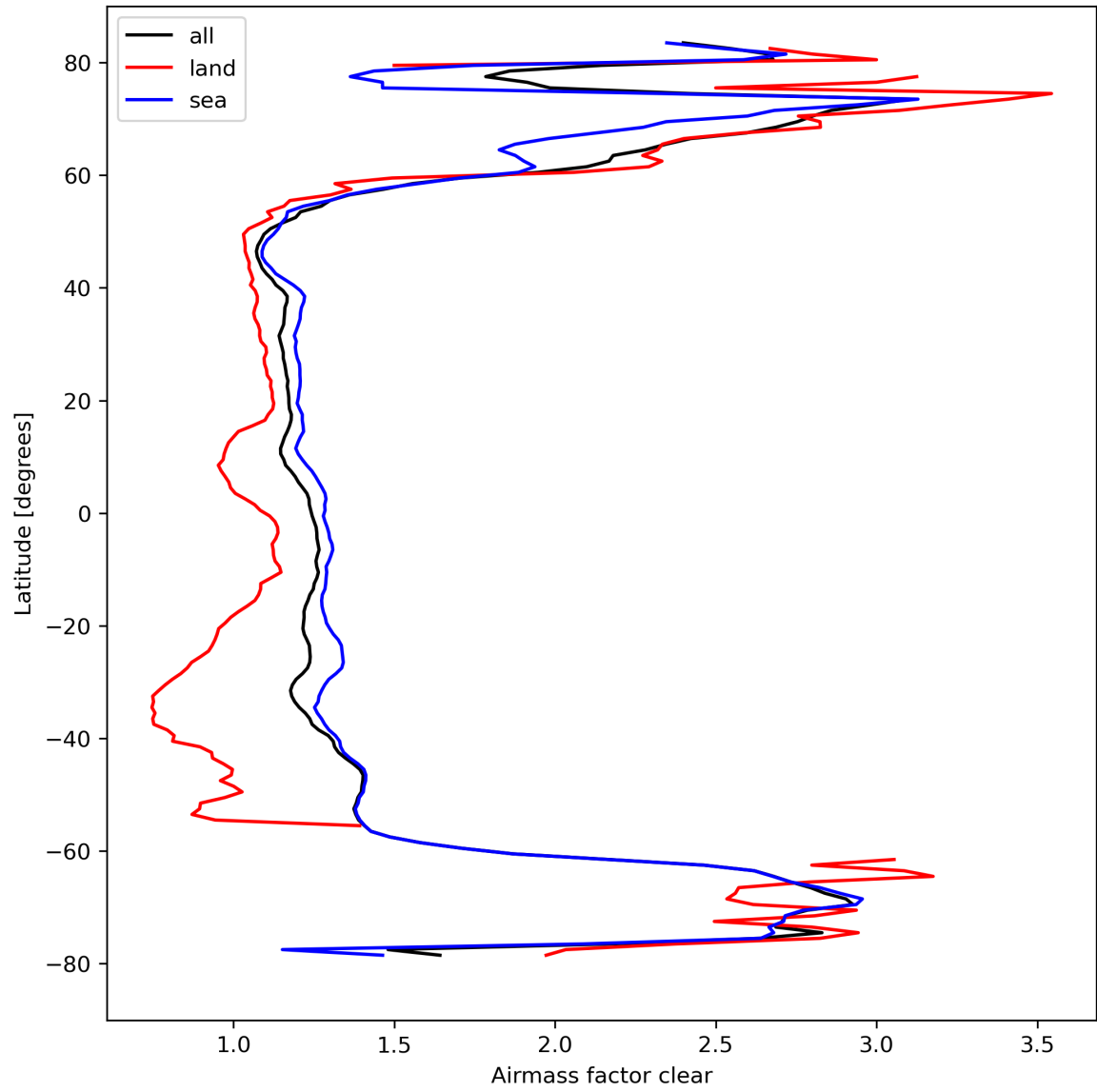
Figure 28: Zonal average of “Airmass factor clear” for 2024-03-25 to 2024-03-26.
