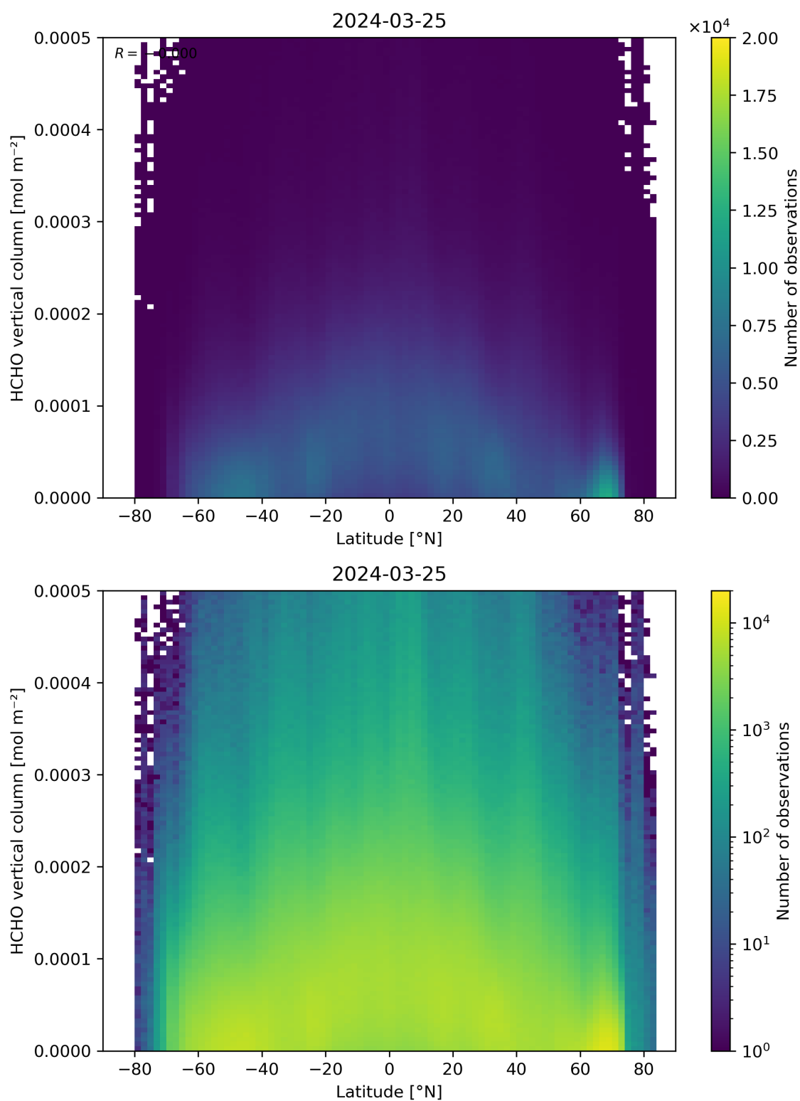
Figure 163: Scatter density plot of “Latitude” against “HCHO vertical column” for 2024-03-25 to 2024-03-26.
