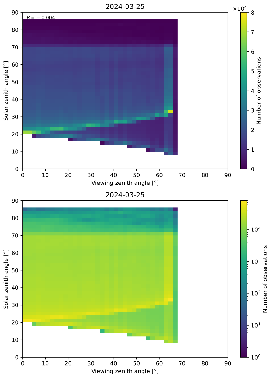
Figure 197: Scatter density plot of “Viewing zenith angle” against “Solar zenith angle” for 2024-03-25 to 2024-03-26.
