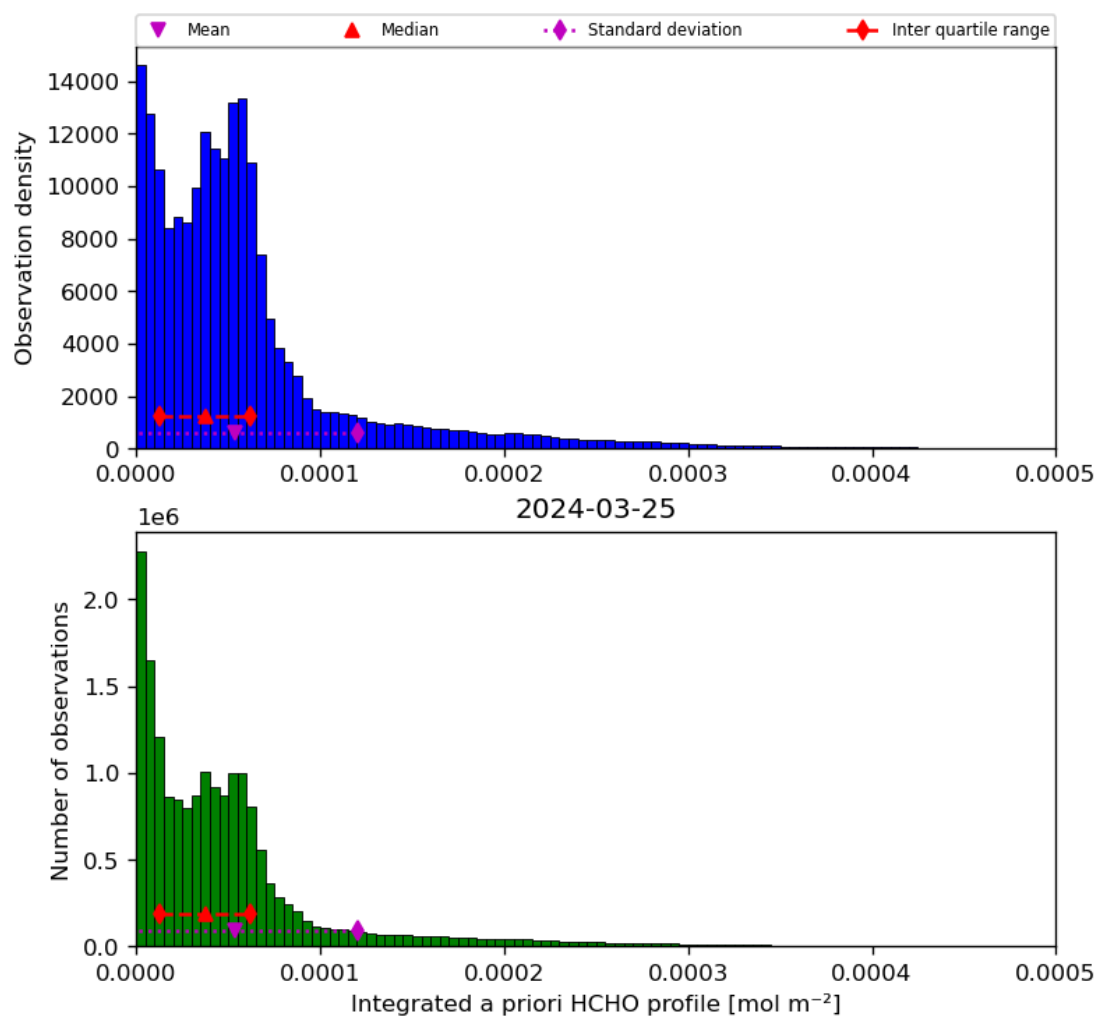
Figure 43: Histogram of “Integrated a priori HCHO profile” for 2024-03-25 to 2024-03-26
