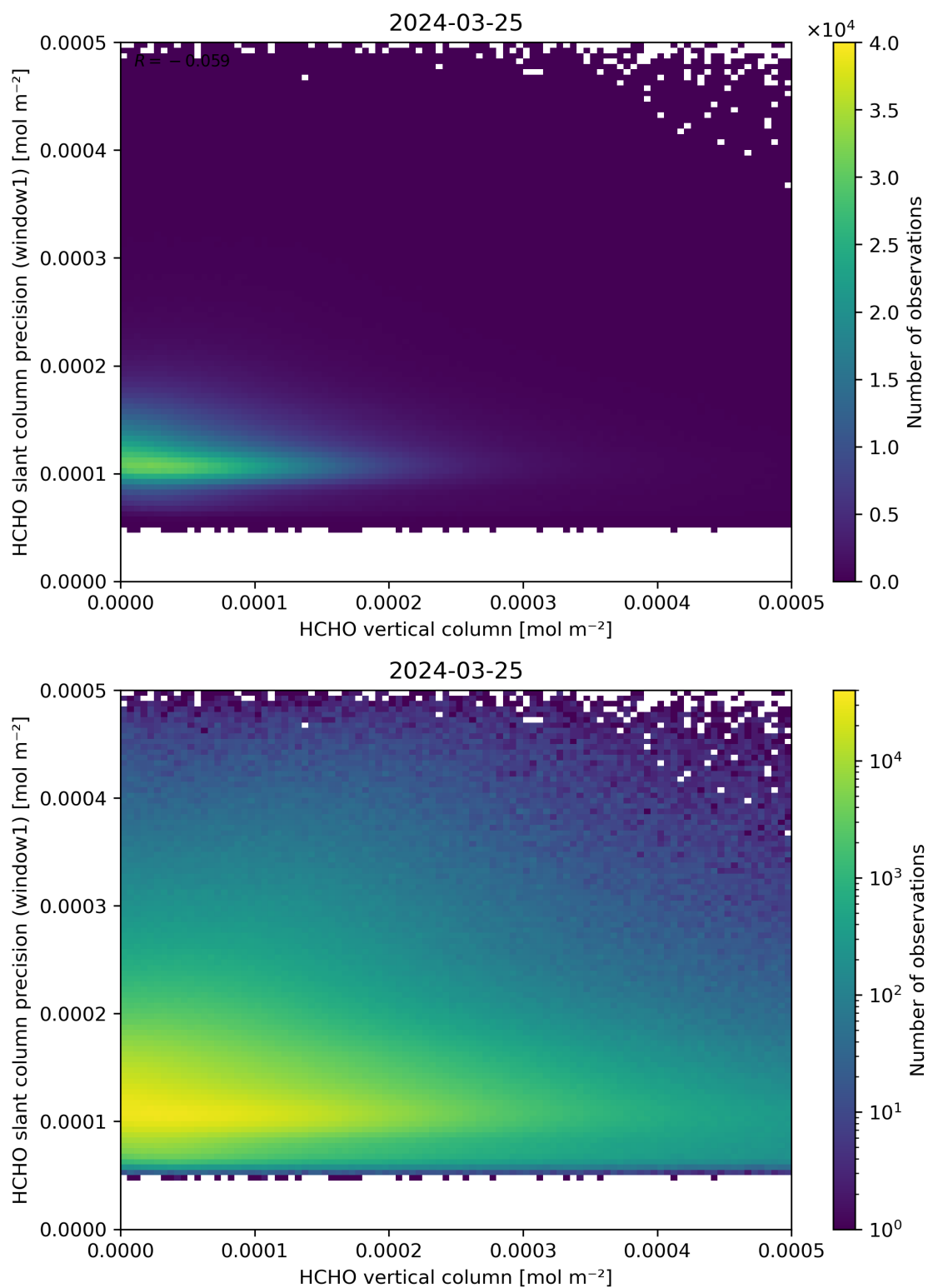
Figure 130: Scatter density plot of “HCHO vertical column” against “HCHO slant column precision (window1)” for 2024-03-25 to 2024-03-26.
