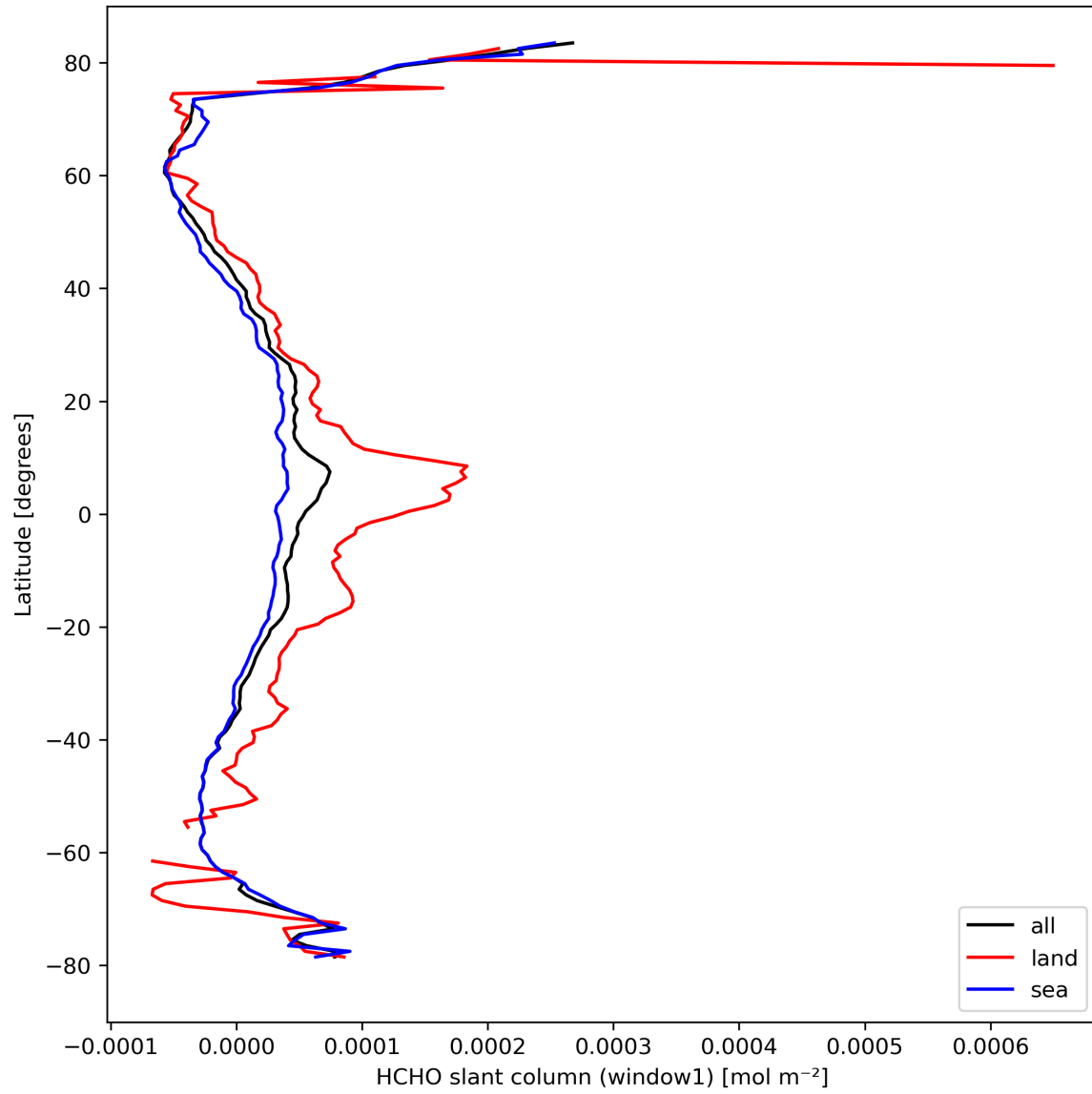
Figure 24: Zonal average of “HCHO slant column (window1)” for 2024-03-25 to 2024-03-26.
