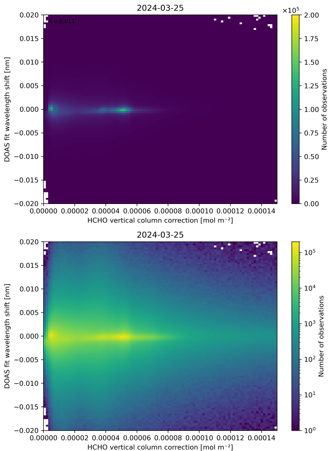
Figure 113: Scatter density plot of “HCHO vertical column correction” against “DOAS fit wavelength shift” for 2024-03-25 to 2024-03-26.
