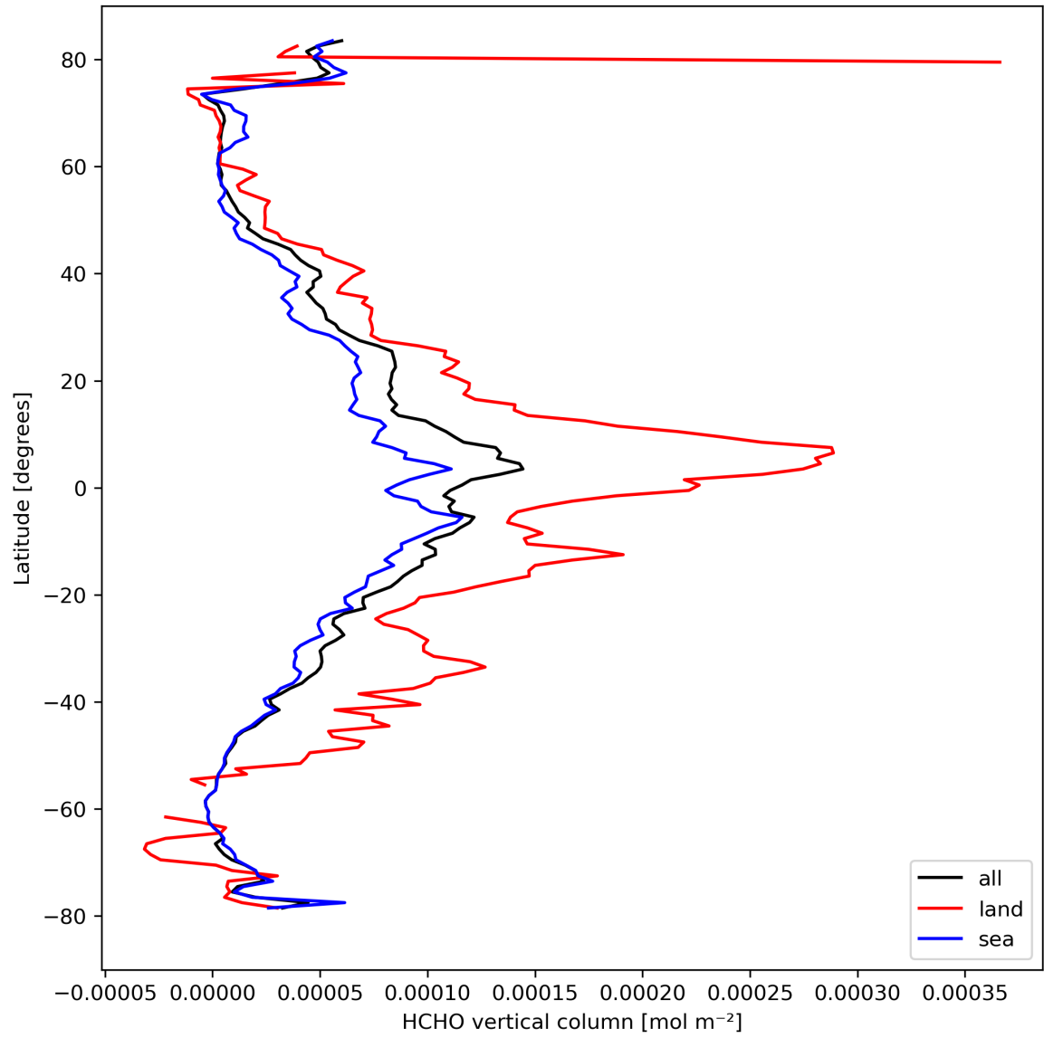
Figure 21: Zonal average of “HCHO vertical column” for 2024-03-25 to 2024-03-26.
