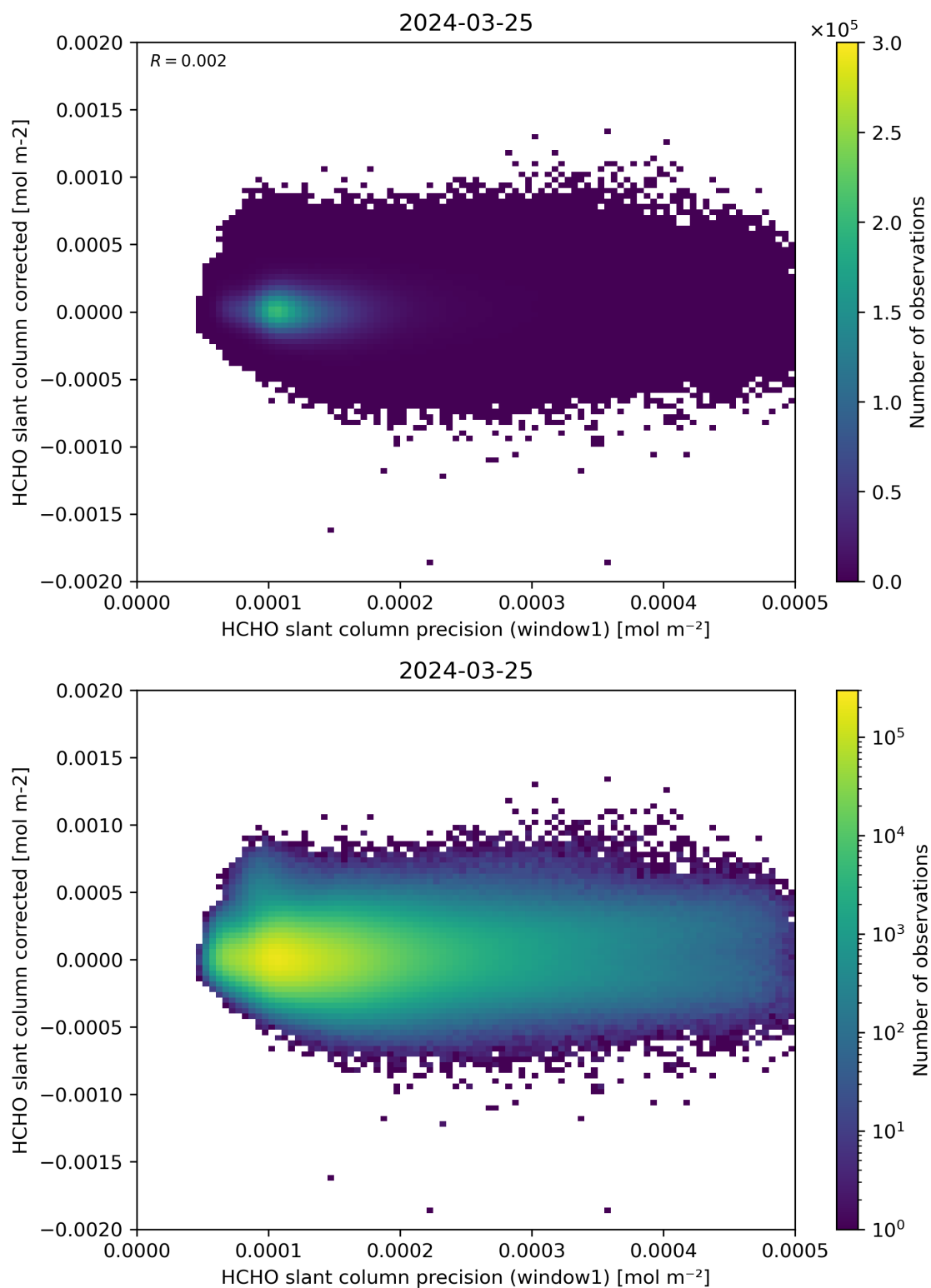
Figure 92: Scatter density plot of “HCHO slant column precision (window1)” against “HCHO slant column corrected” for 2024-03-25 to 2024-03-26.
