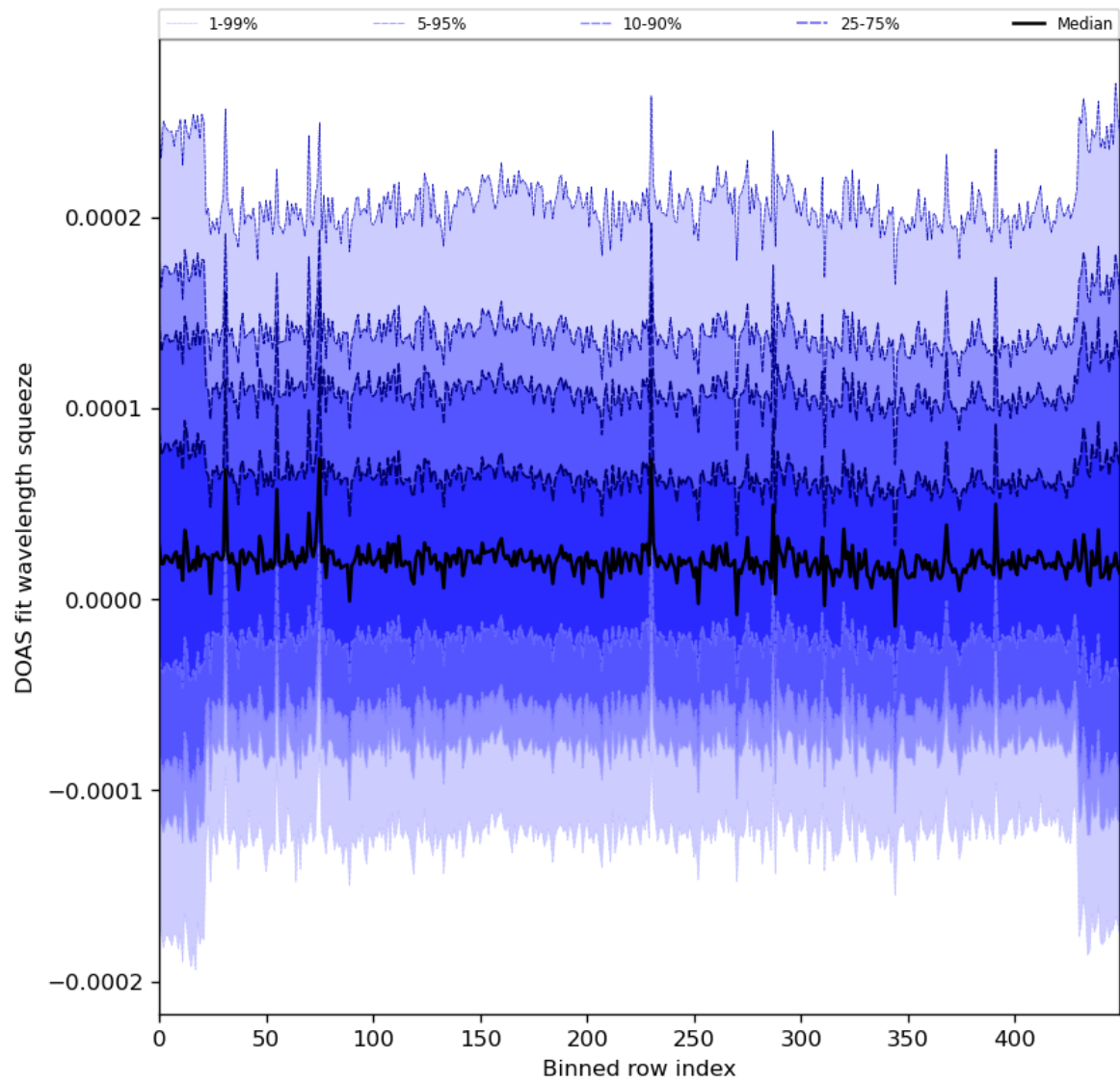
Figure 59: Along track statistics of “DOAS fit wavelength squeeze” for 2024-03-25 to 2024-03-26
