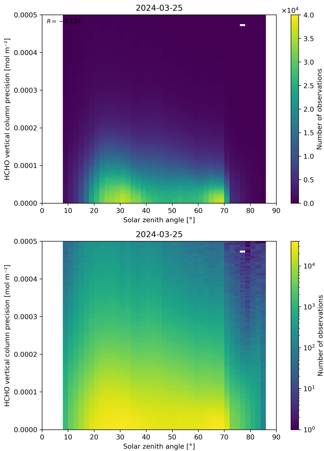
Figure 179: Scatter density plot of “Solar zenith angle” against “HCHO vertical column precision” for 2024-03-25 to 2024-03-26.
