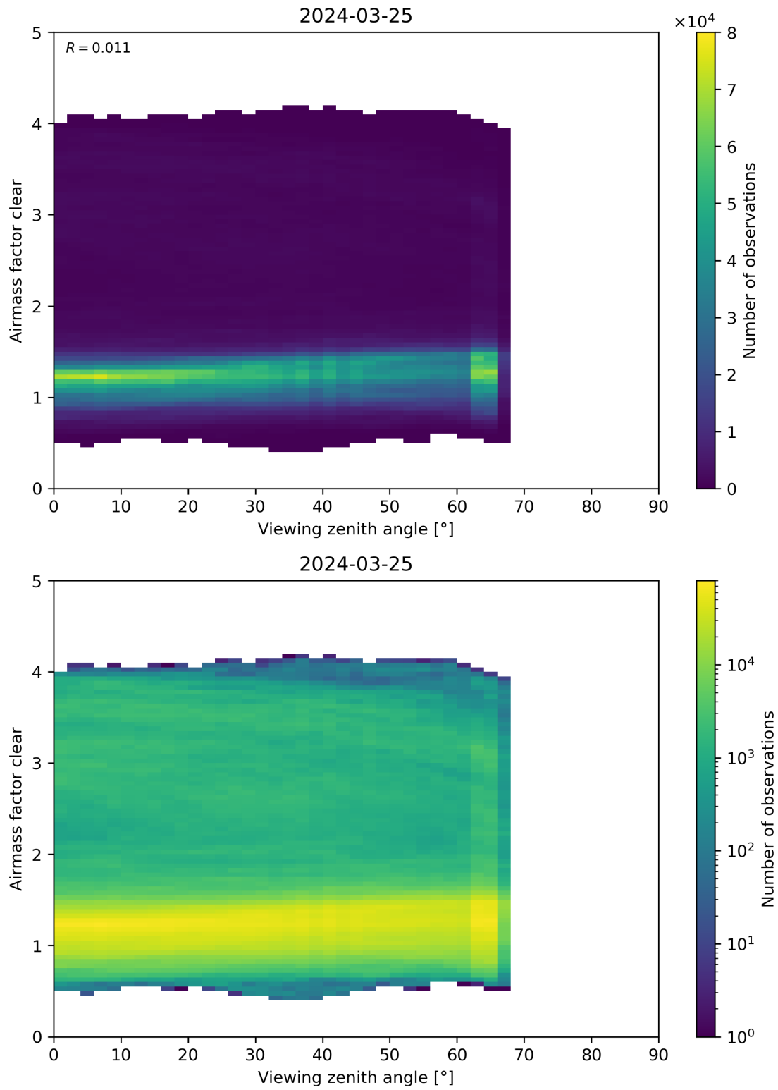
Figure 185: Scatter density plot of “Viewing zenith angle” against “Airmass factor clear” for 2024-03-25 to 2024-03-26.
