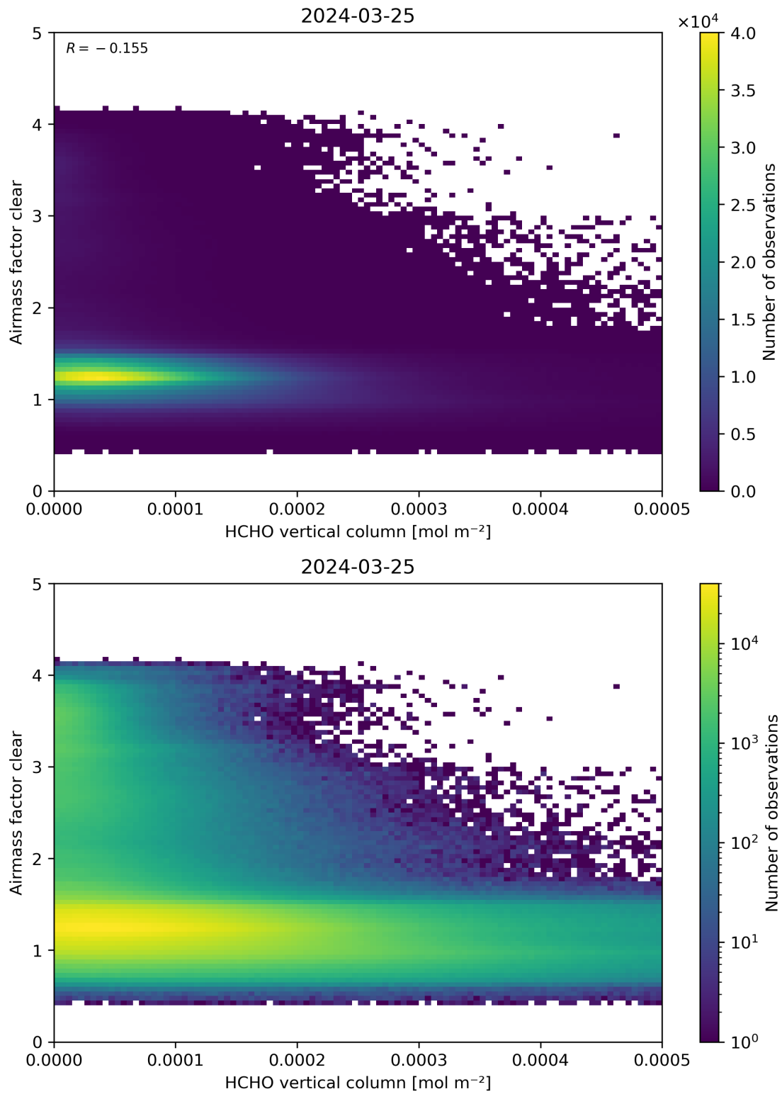
Figure 126: Scatter density plot of “HCHO vertical column” against “Airmass factor clear” for 2024-03-25 to 2024-03-26.
