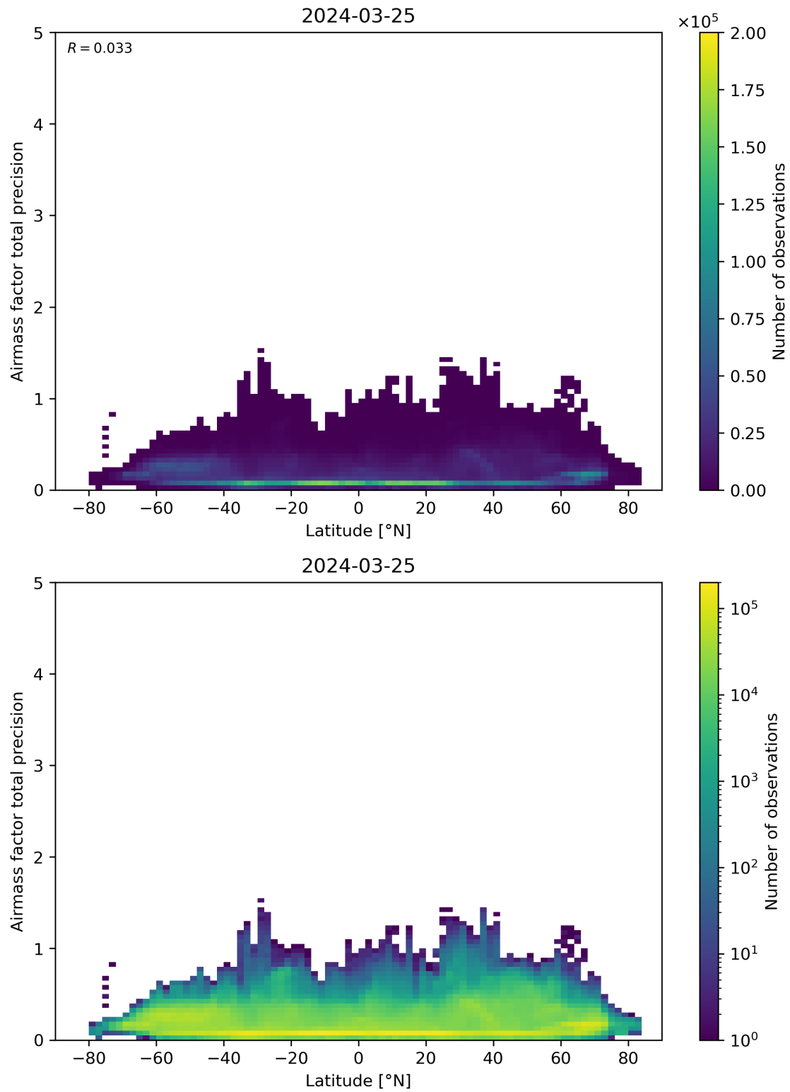
Figure 162: Scatter density plot of “Latitude” against “Airmass factor total precision” for 2024-03-25 to 2024-03-26.
