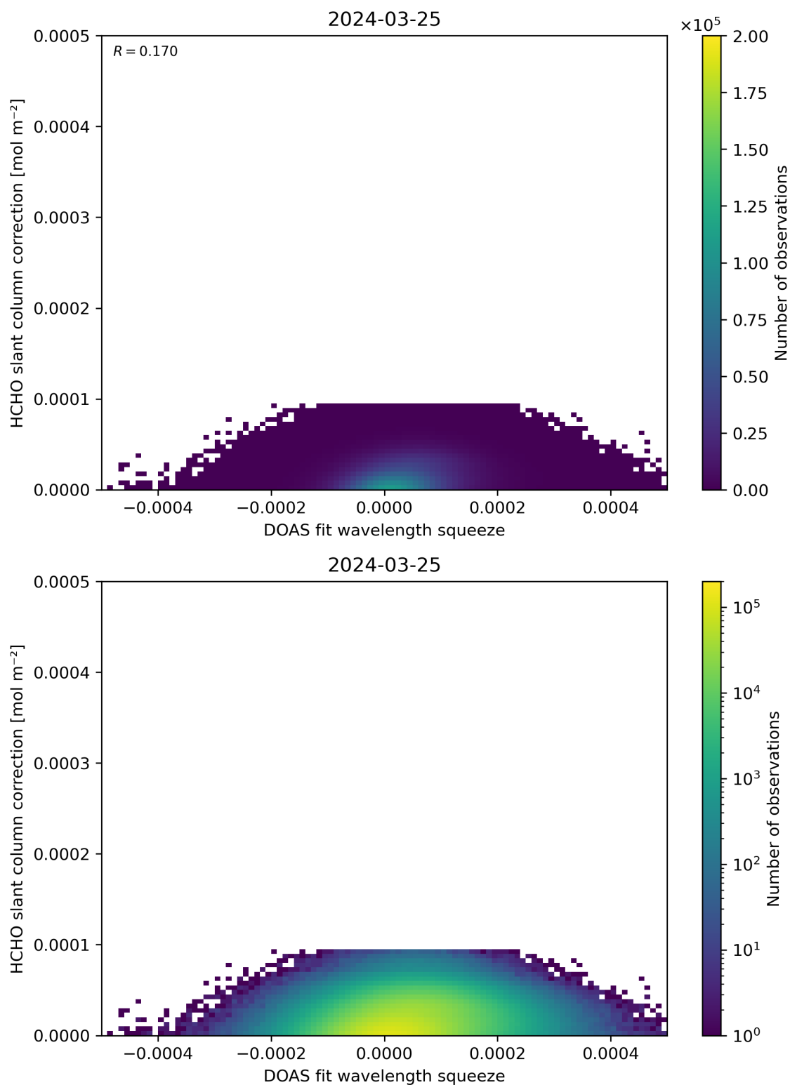
Figure 70: Scatter density plot of “DOAS fit wavelength squeeze” against “HCHO slant column correction” for 2024-03-25 to 2024-03-26.
