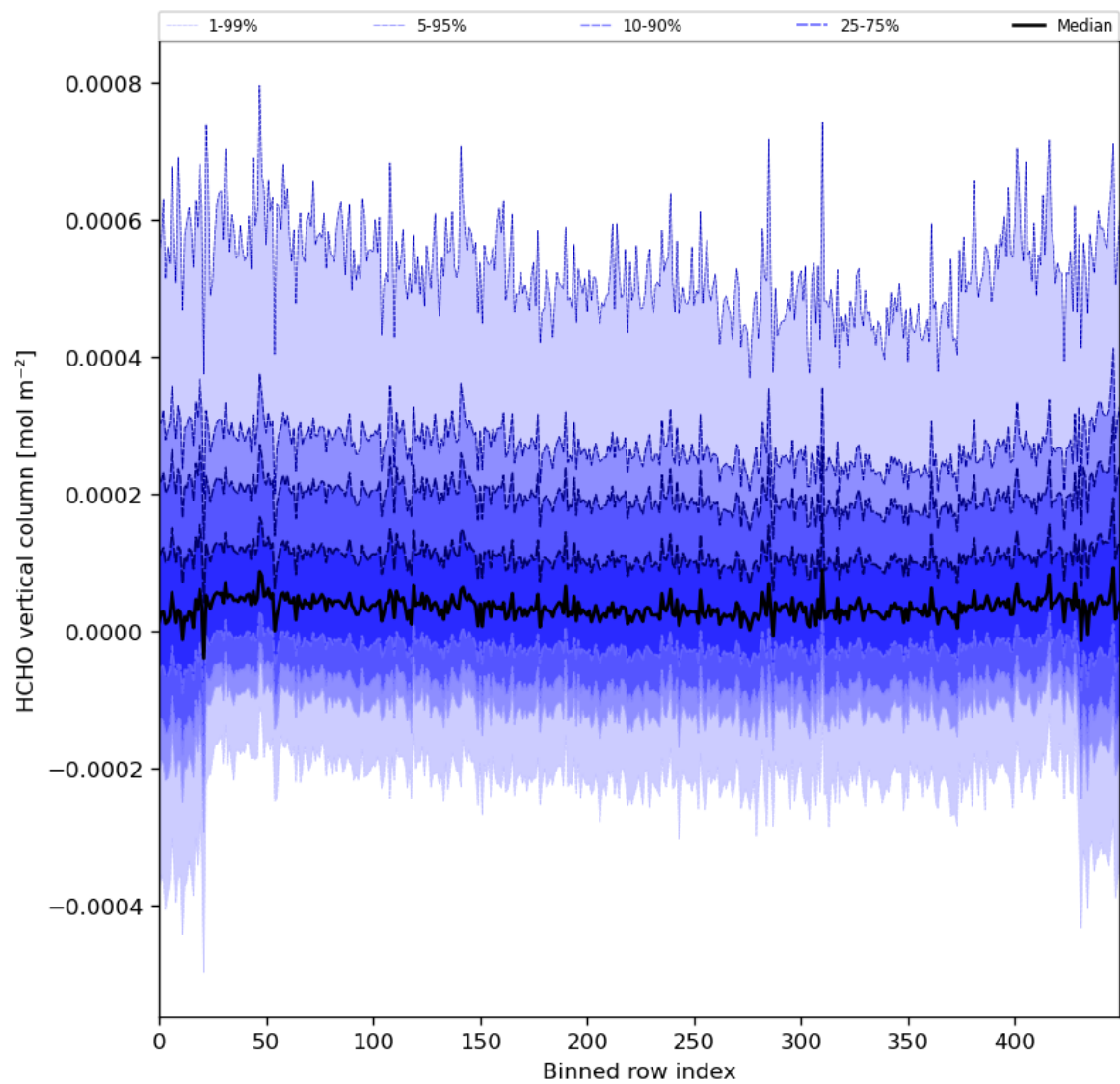
Figure 49: Along track statistics of “HCHO vertical column” for 2024-03-25 to 2024-03-26
