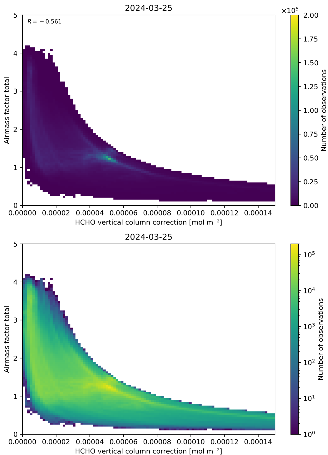
Figure 120: Scatter density plot of “HCHO vertical column correction” against “Airmass factor total” for 2024-03-25 to 2024-03-26.
