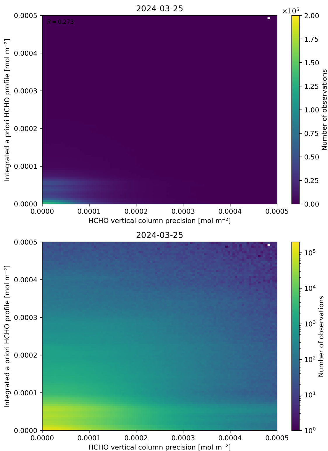
Figure 147: Scatter density plot of “HCHO vertical column precision” against “Integrated a priori HCHO profile” for 2024-03-25 to 2024-03-26.
