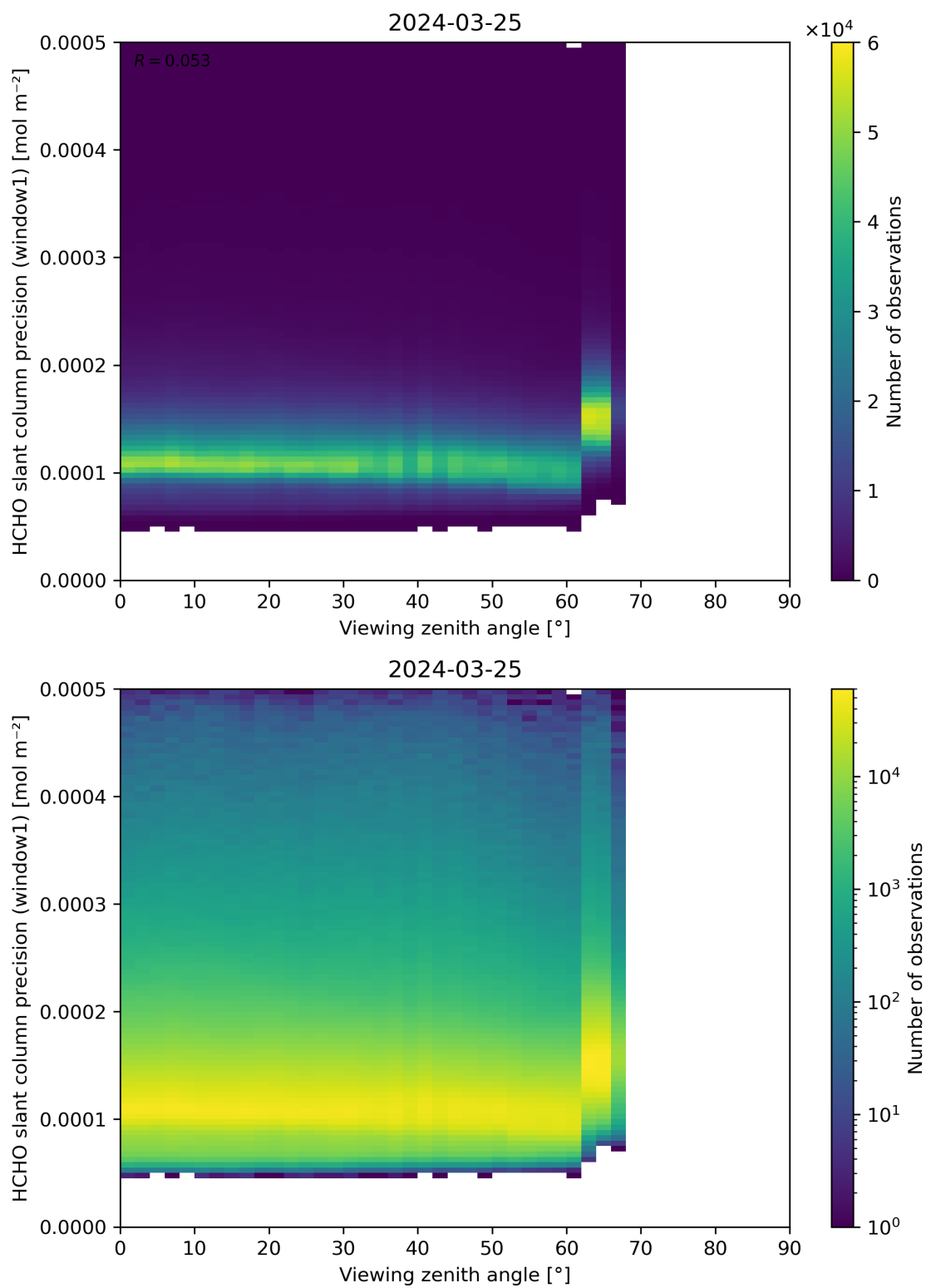
Figure 189: Scatter density plot of “Viewing zenith angle” against “HCHO slant column precision (window1)” for 2024-03-25 to 2024-03-26.
