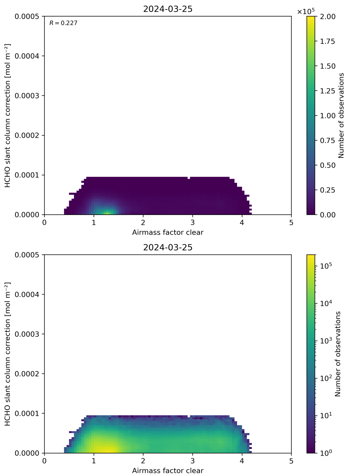
Figure 75: Scatter density plot of “Airmass factor clear” against “HCHO slant column correction” for 2024-03-25 to 2024-03-26.
