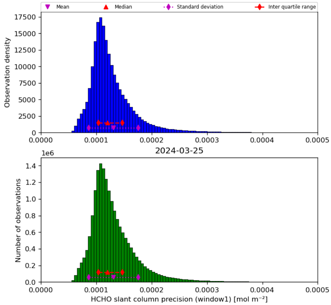
Figure 39: Histogram of “HCHO slant column precision (window1)” for 2024-03-25 to 2024-03-26
