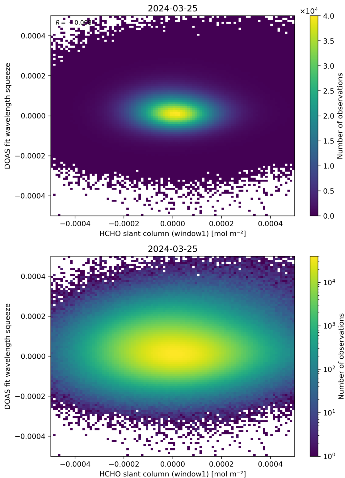
Figure 80: Scatter density plot of “HCHO slant column (window1)” against “DOAS fit wavelength squeeze” for 2024-03-25 to 2024-03-26.
