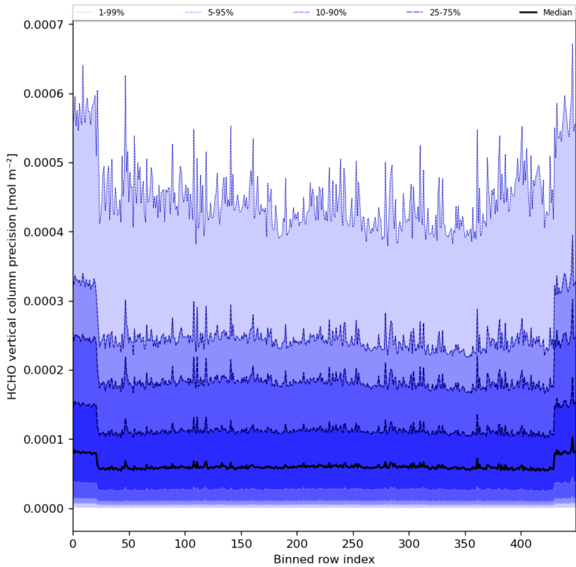
Figure 50: Along track statistics of “HCHO vertical column precision” for 2024-03-25 to 2024-03-26
