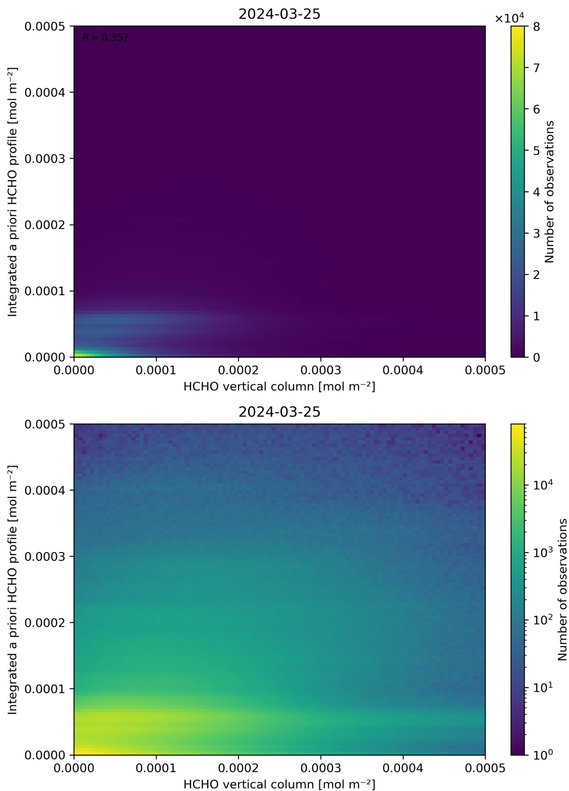
Figure 135: Scatter density plot of “HCHO vertical column” against “Integrated a priori HCHO profile” for 2024-03-25 to 2024-03-26.
