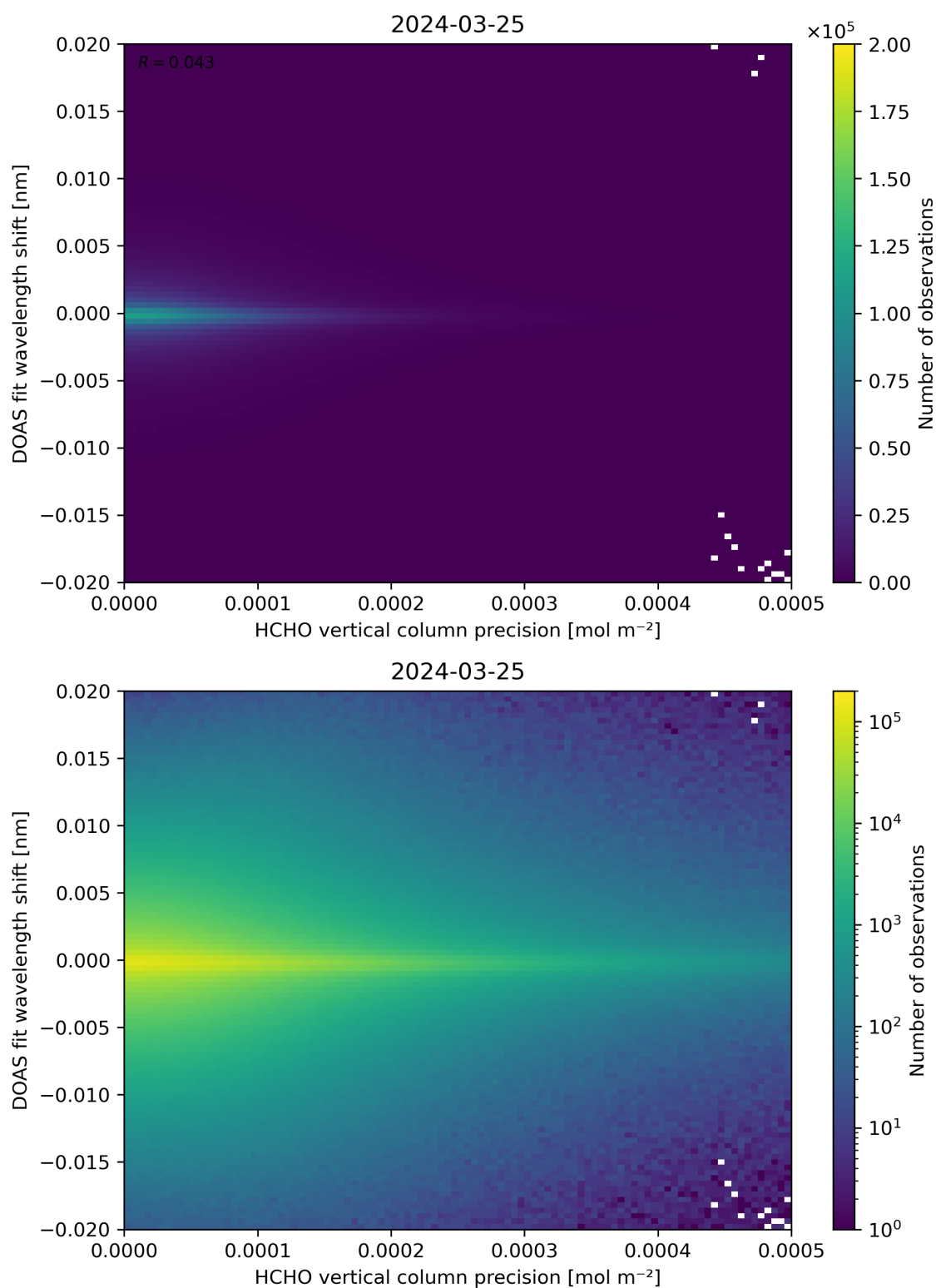
Figure 137: Scatter density plot of “HCHO vertical column precision” against “DOAS fit wavelength shift” for 2024-03-25 to 2024-03-26.
