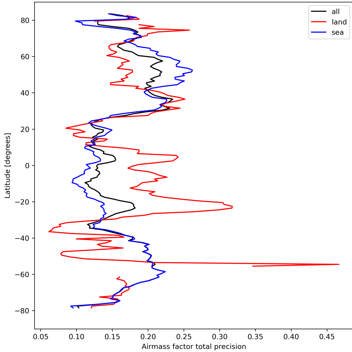
Figure 27: Zonal average of “Airmass factor total precision” for 2024-03-25 to 2024-03-26.
