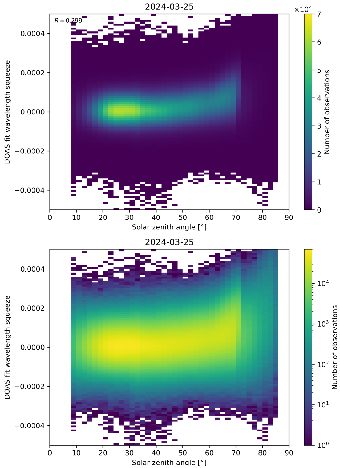
Figure 169: Scatter density plot of “Solar zenith angle” against “DOAS fit wavelength squeeze” for 2024-03-25 to 2024-03-26.
