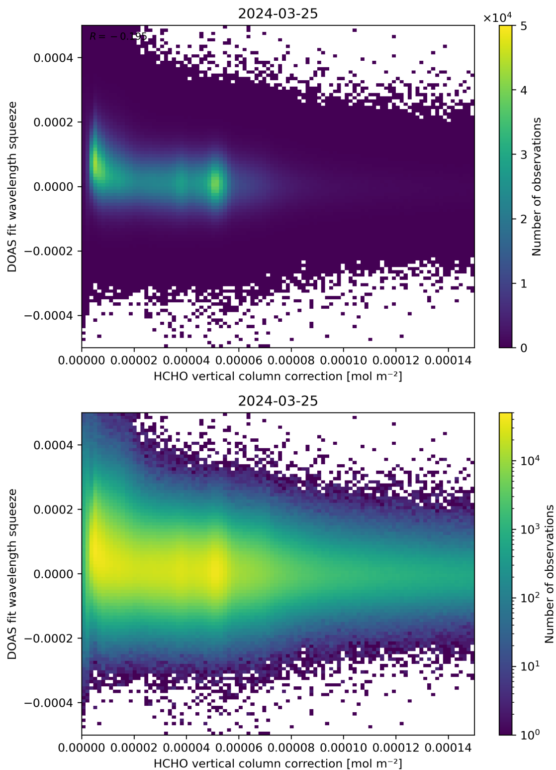
Figure 114: Scatter density plot of “HCHO vertical column correction” against “DOAS fit wavelength squeeze” for 2024-03-25 to 2024-03-26.
