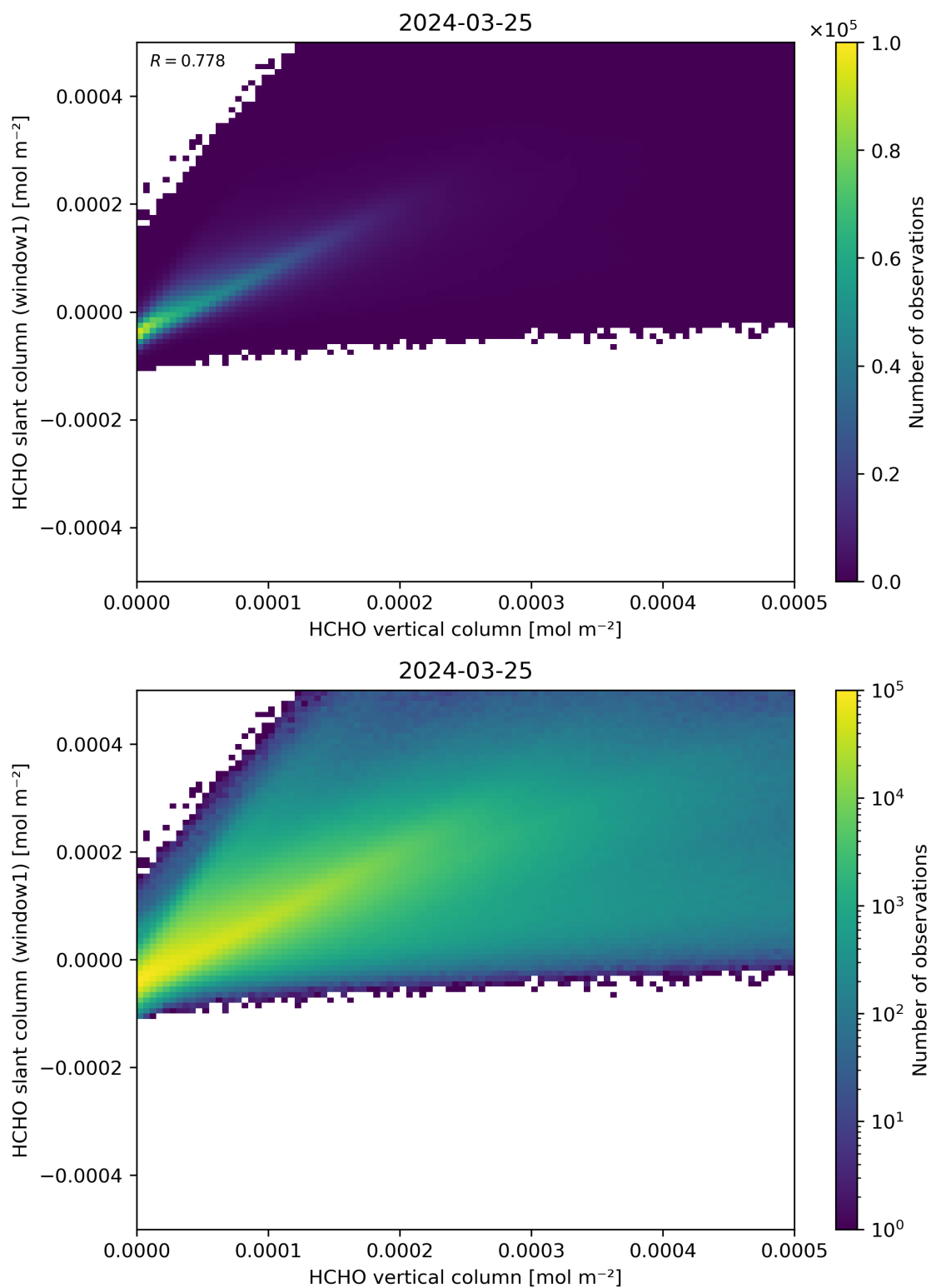
Figure 129: Scatter density plot of “HCHO vertical column” against “HCHO slant column (window1)” for 2024-03-25 to 2024-03-26.
