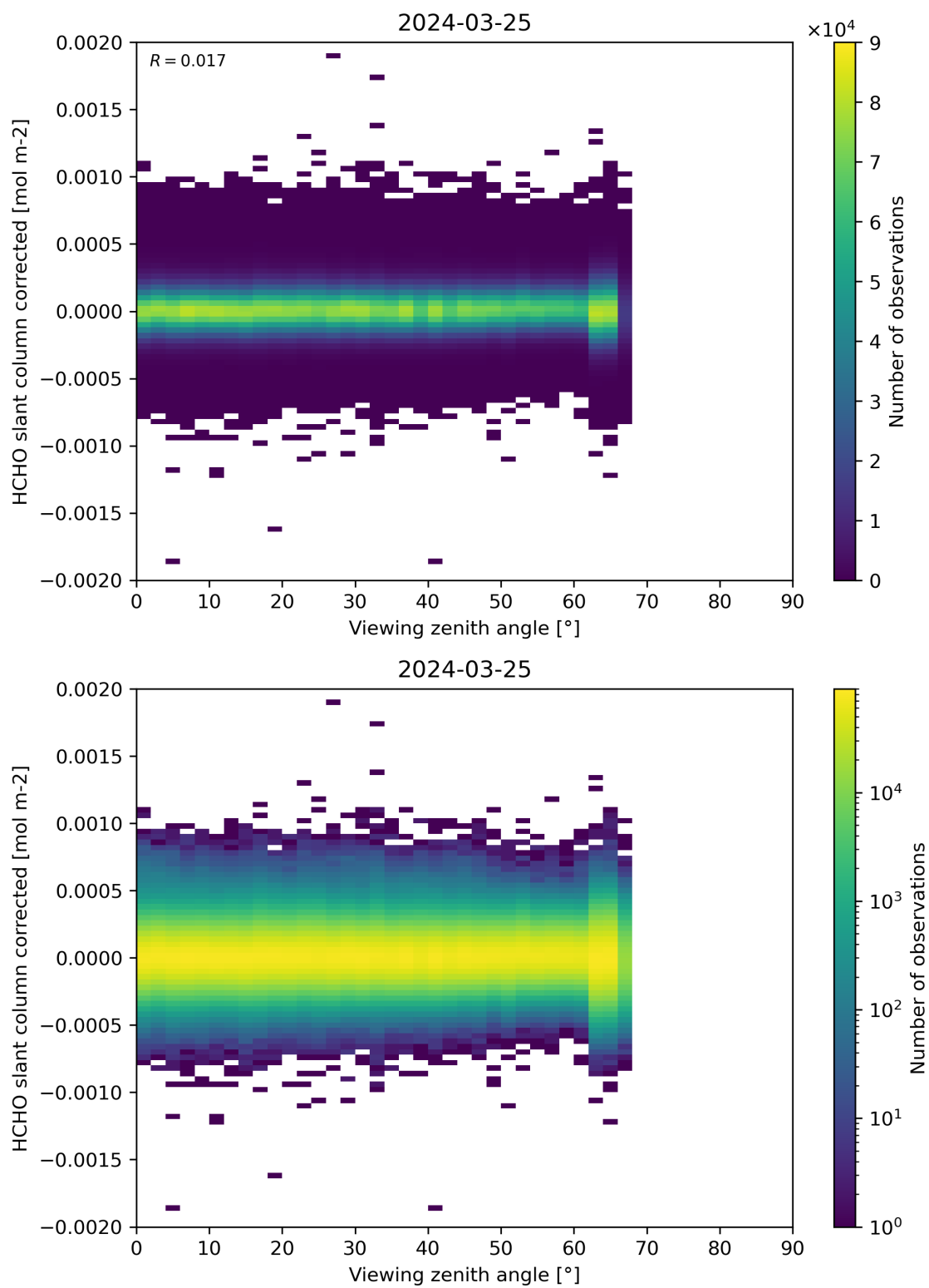
Figure 186: Scatter density plot of “Viewing zenith angle” against “HCHO slant column corrected” for 2024-03-25 to 2024-03-26.
