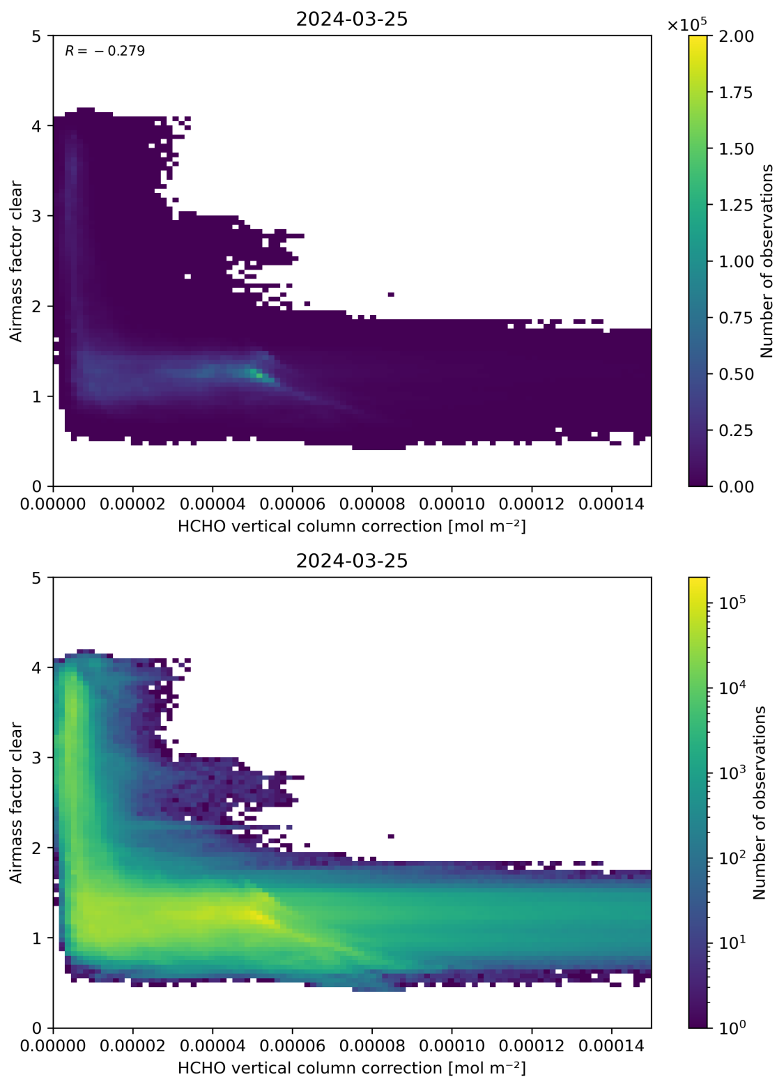
Figure 115: Scatter density plot of “HCHO vertical column correction” against “Airmass factor clear” for 2024-03-25 to 2024-03-26.
