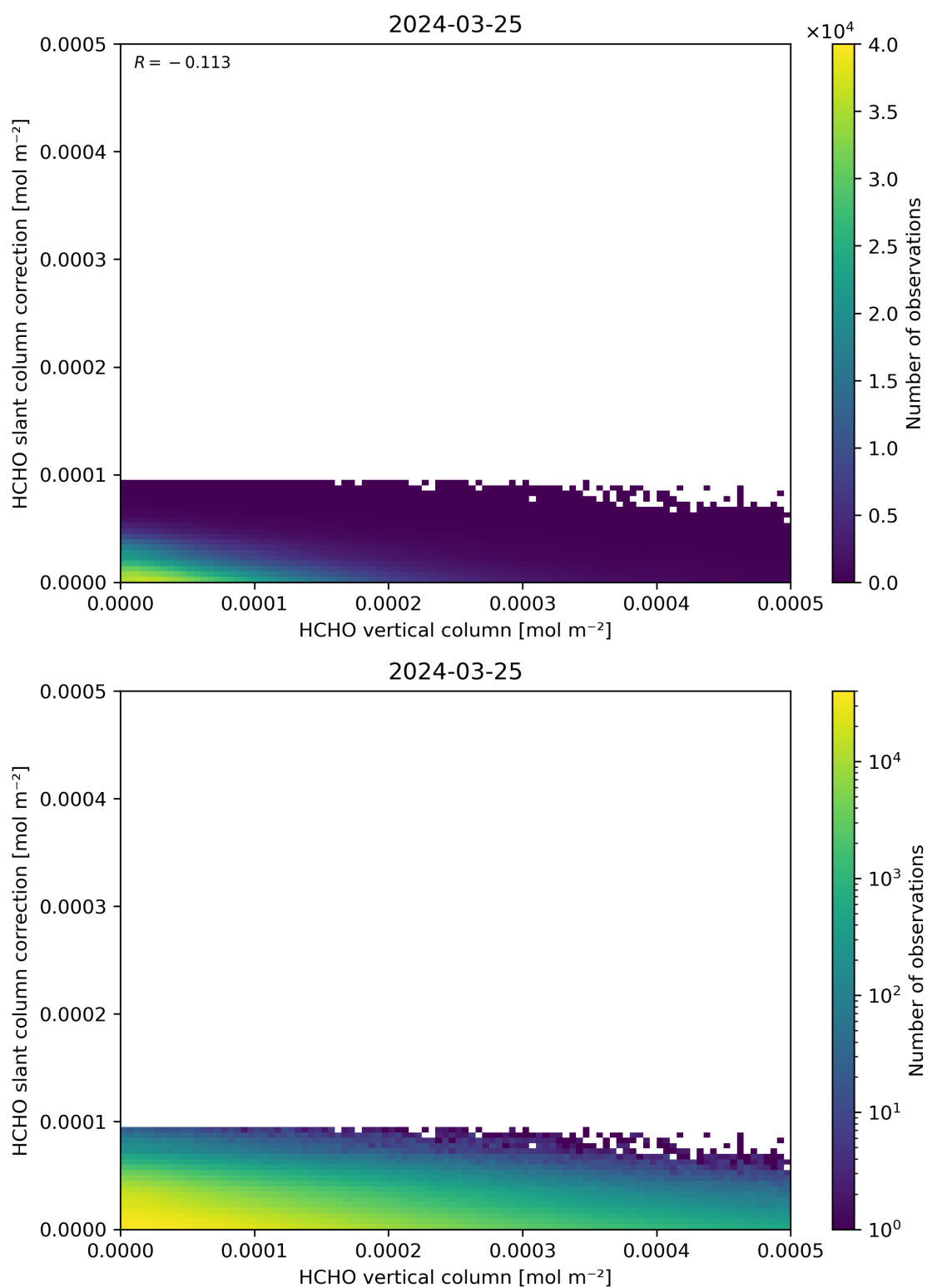
Figure 128: Scatter density plot of “HCHO vertical column” against “HCHO slant column correction” for 2024-03-25 to 2024-03-26.
