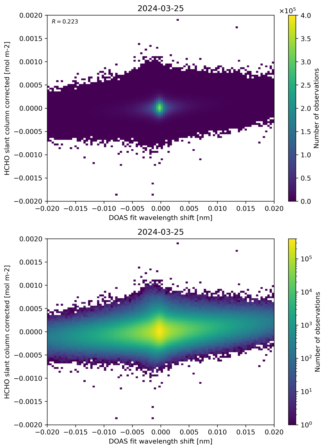
Figure 66: Scatter density plot of “DOAS fit wavelength shift” against “HCHO slant column corrected” for 2024-03-25 to 2024-03-26.
