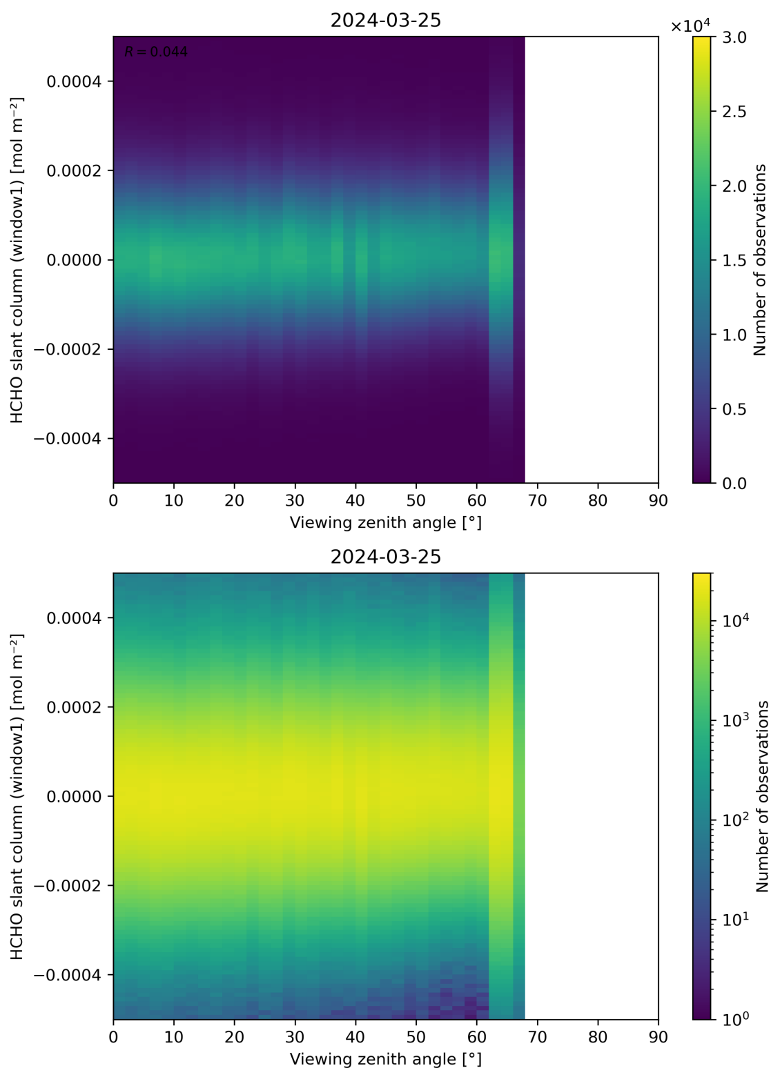
Figure 188: Scatter density plot of “Viewing zenith angle” against “HCHO slant column (window1)” for 2024-03-25 to 2024-03-26.
