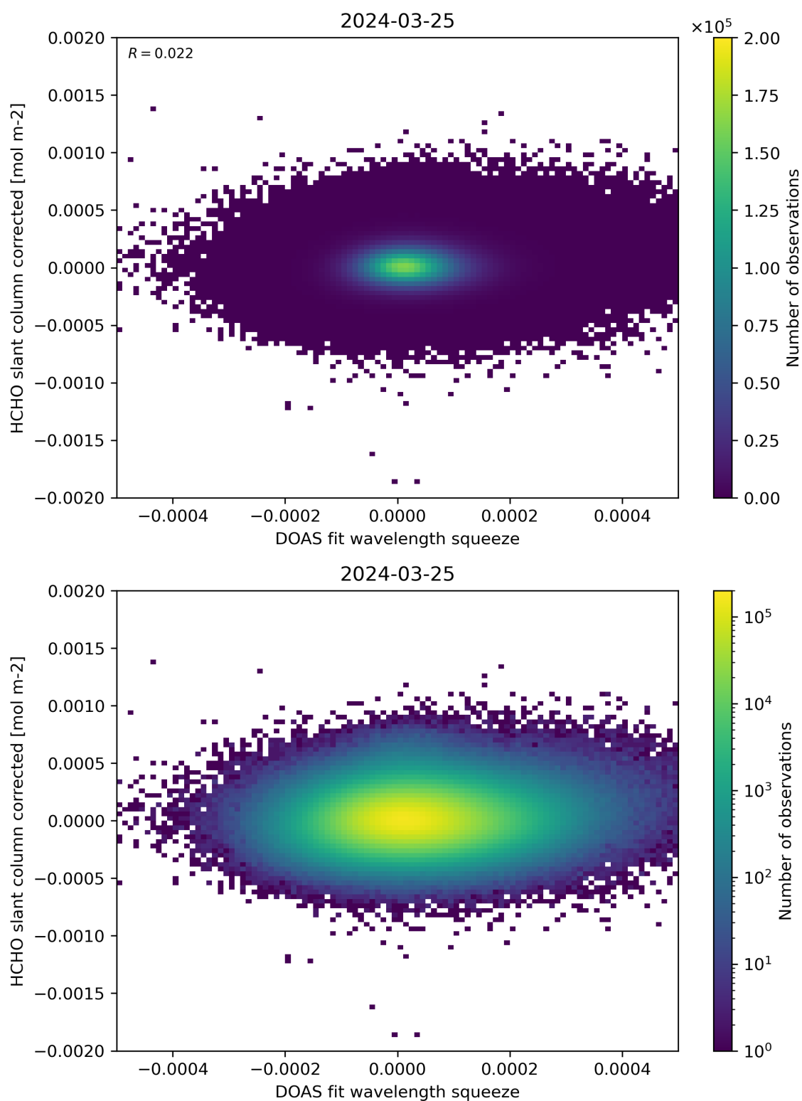
Figure 69: Scatter density plot of “DOAS fit wavelength squeeze” against “HCHO slant column corrected” for 2024-03-25 to 2024-03-26.
