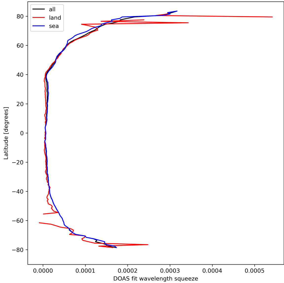
Figure 31: Zonal average of “DOAS fit wavelength squeeze” for 2024-03-25 to 2024-03-26.
