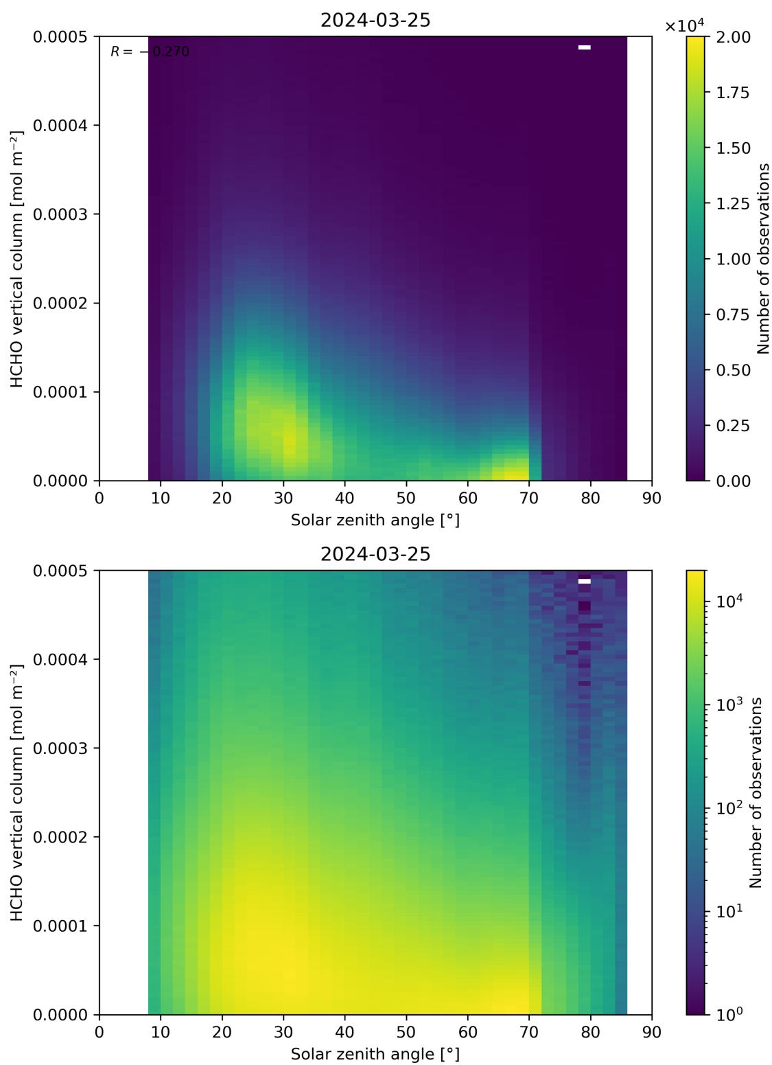
Figure 177: Scatter density plot of “Solar zenith angle” against “HCHO vertical column” for 2024-03-25 to 2024-03-26.
