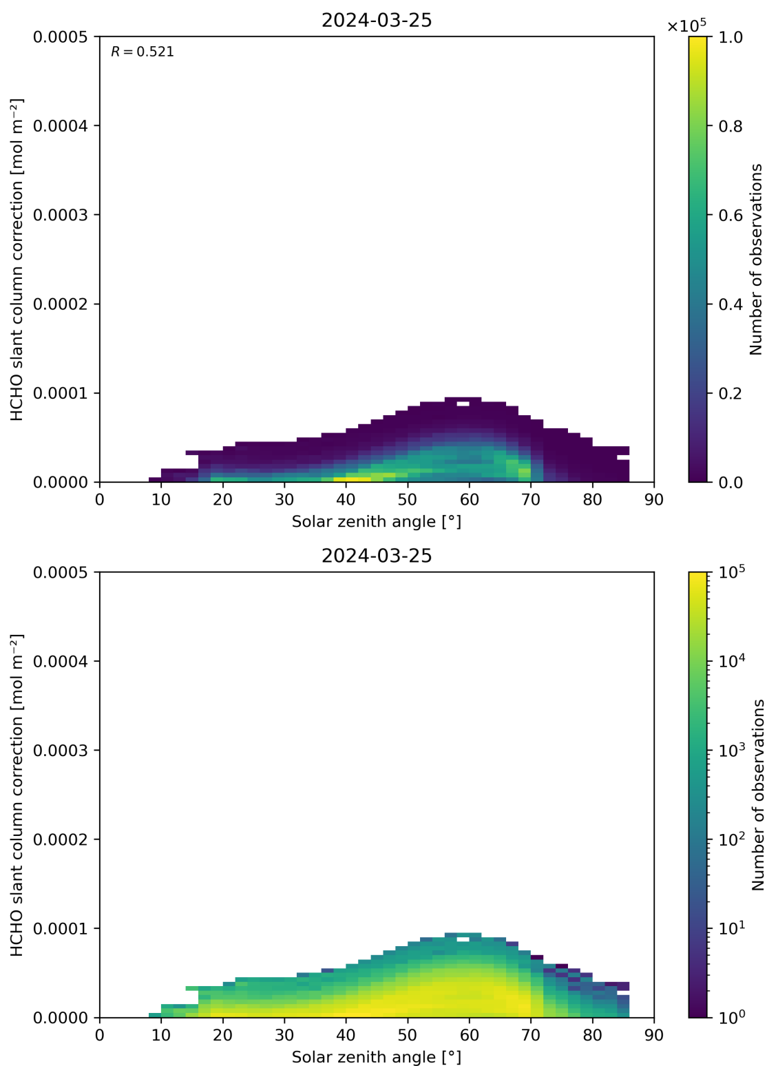
Figure 172: Scatter density plot of “Solar zenith angle” against “HCHO slant column correction” for 2024-03-25 to 2024-03-26.
