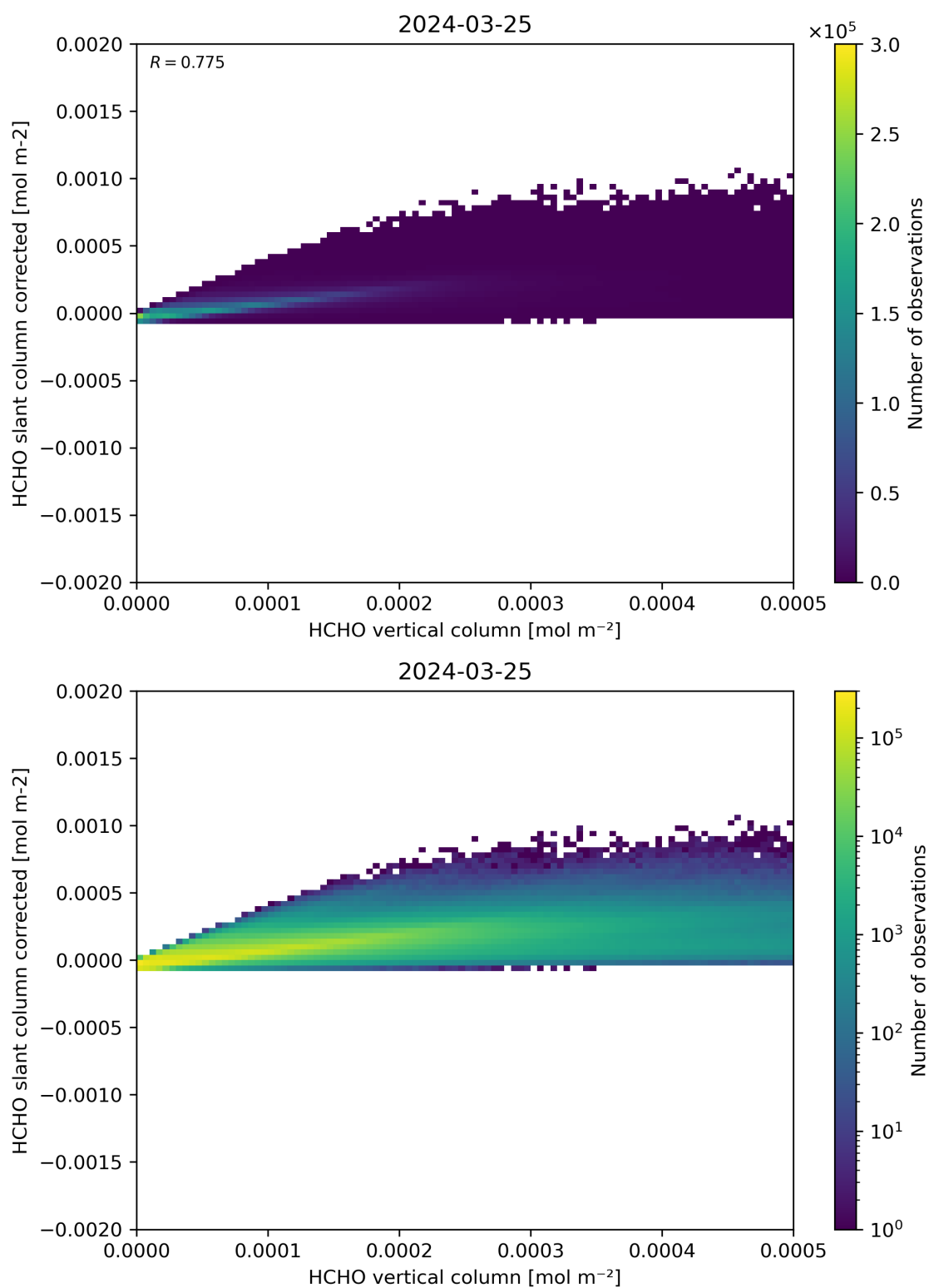
Figure 127: Scatter density plot of “HCHO vertical column” against “HCHO slant column corrected” for 2024-03-25 to 2024-03-26.
