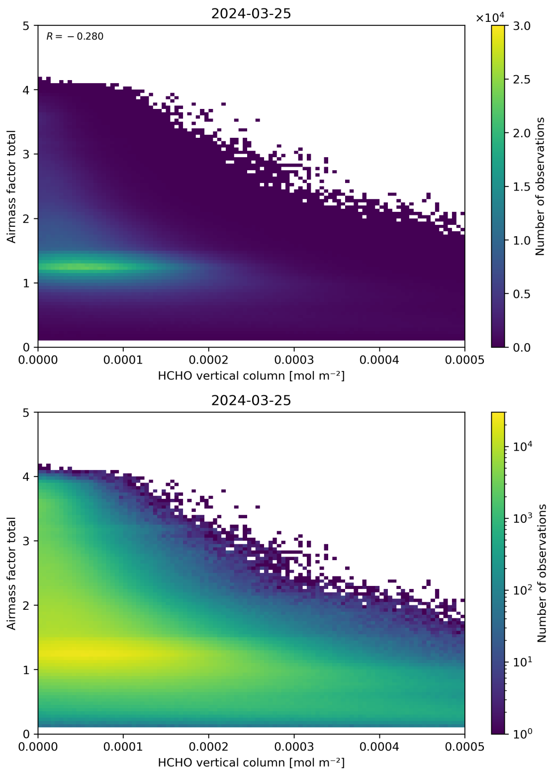
Figure 131: Scatter density plot of “HCHO vertical column” against “Airmass factor total” for 2024-03-25 to 2024-03-26.
