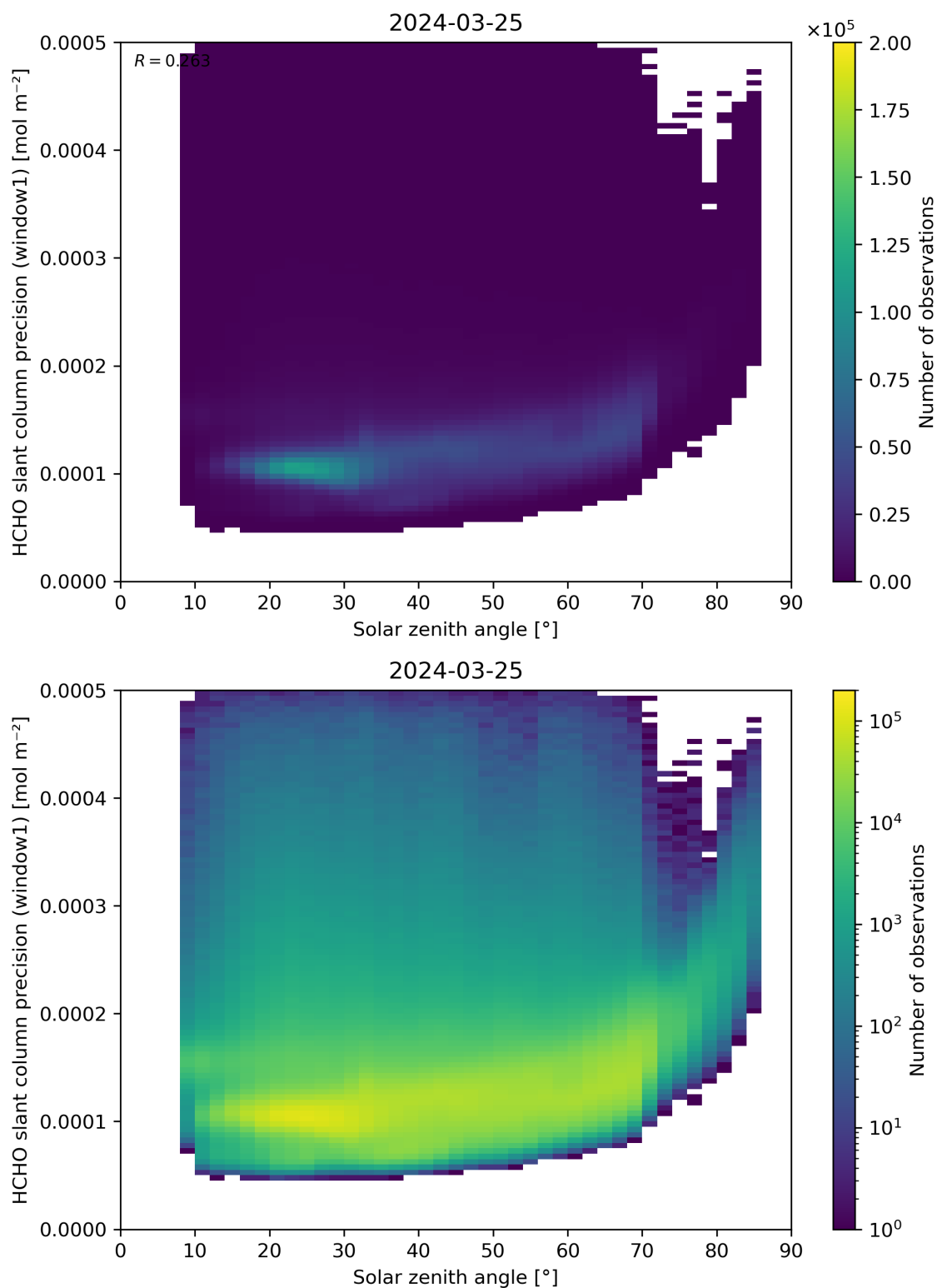
Figure 174: Scatter density plot of “Solar zenith angle” against “HCHO slant column precision (window1)” for 2024-03-25 to 2024-03-26.
