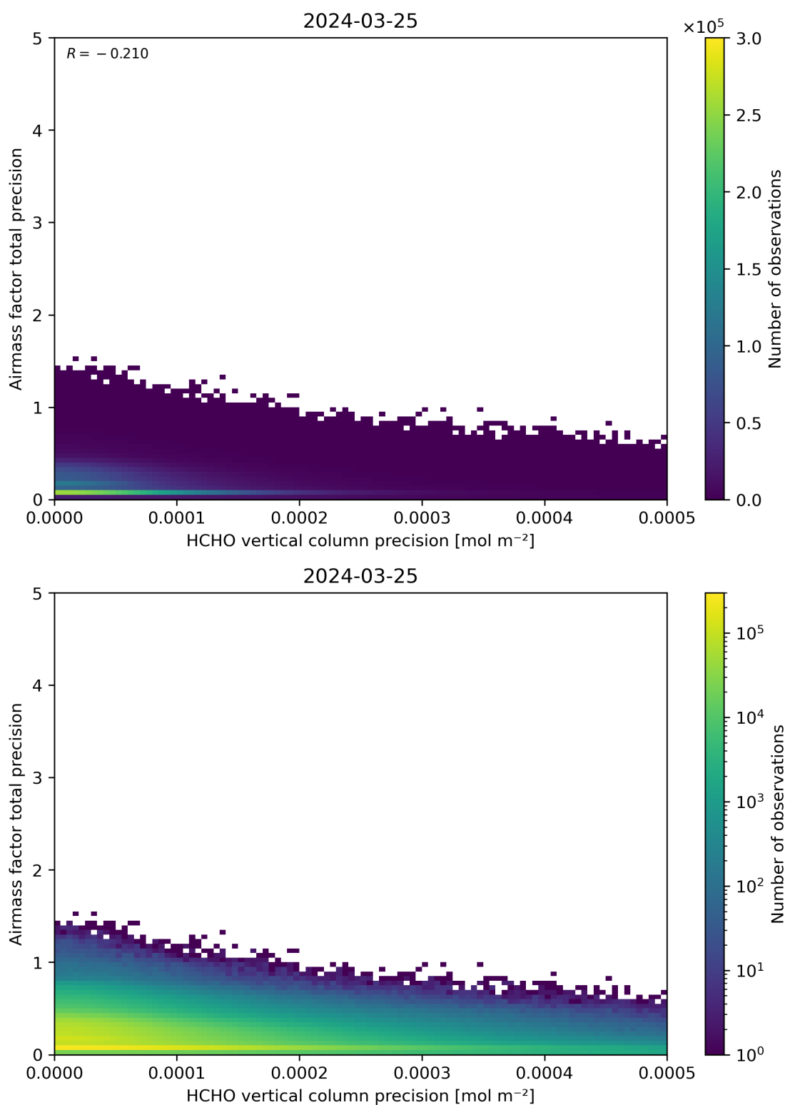
Figure 145: Scatter density plot of “HCHO vertical column precision” against “Airmass factor total precision” for 2024-03-25 to 2024-03-26.
