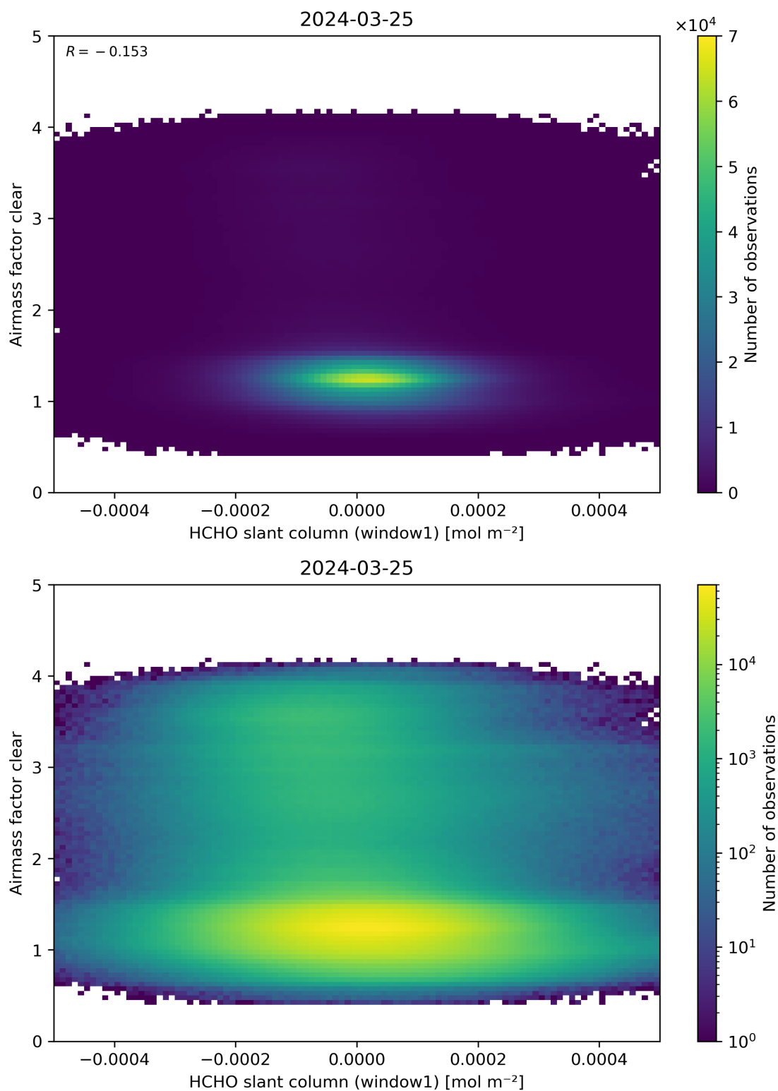
Figure 81: Scatter density plot of “HCHO slant column (window1)” against “Airmass factor clear” for 2024-03-25 to 2024-03-26.
