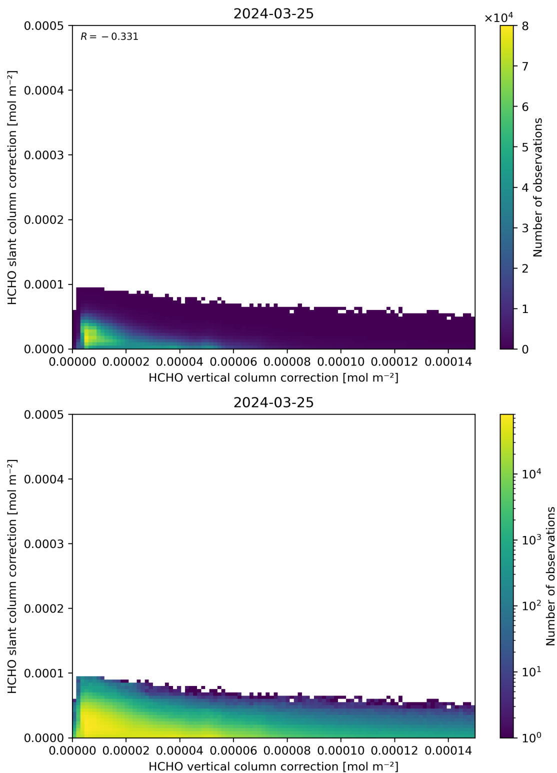
Figure 117: Scatter density plot of “HCHO vertical column correction” against “HCHO slant column correction” for 2024-03-25 to 2024-03-26.
