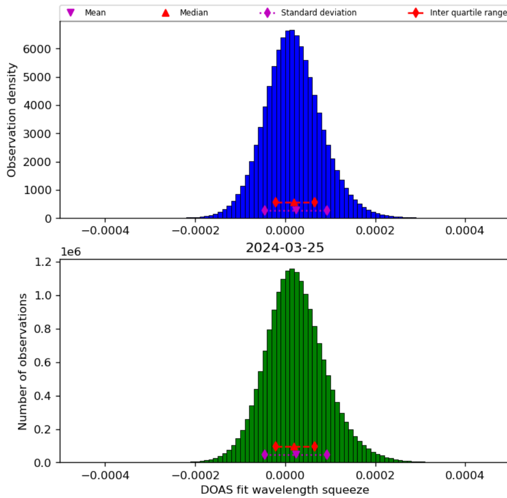
Figure 45: Histogram of “DOAS fit wavelength squeeze” for 2024-03-25 to 2024-03-26
