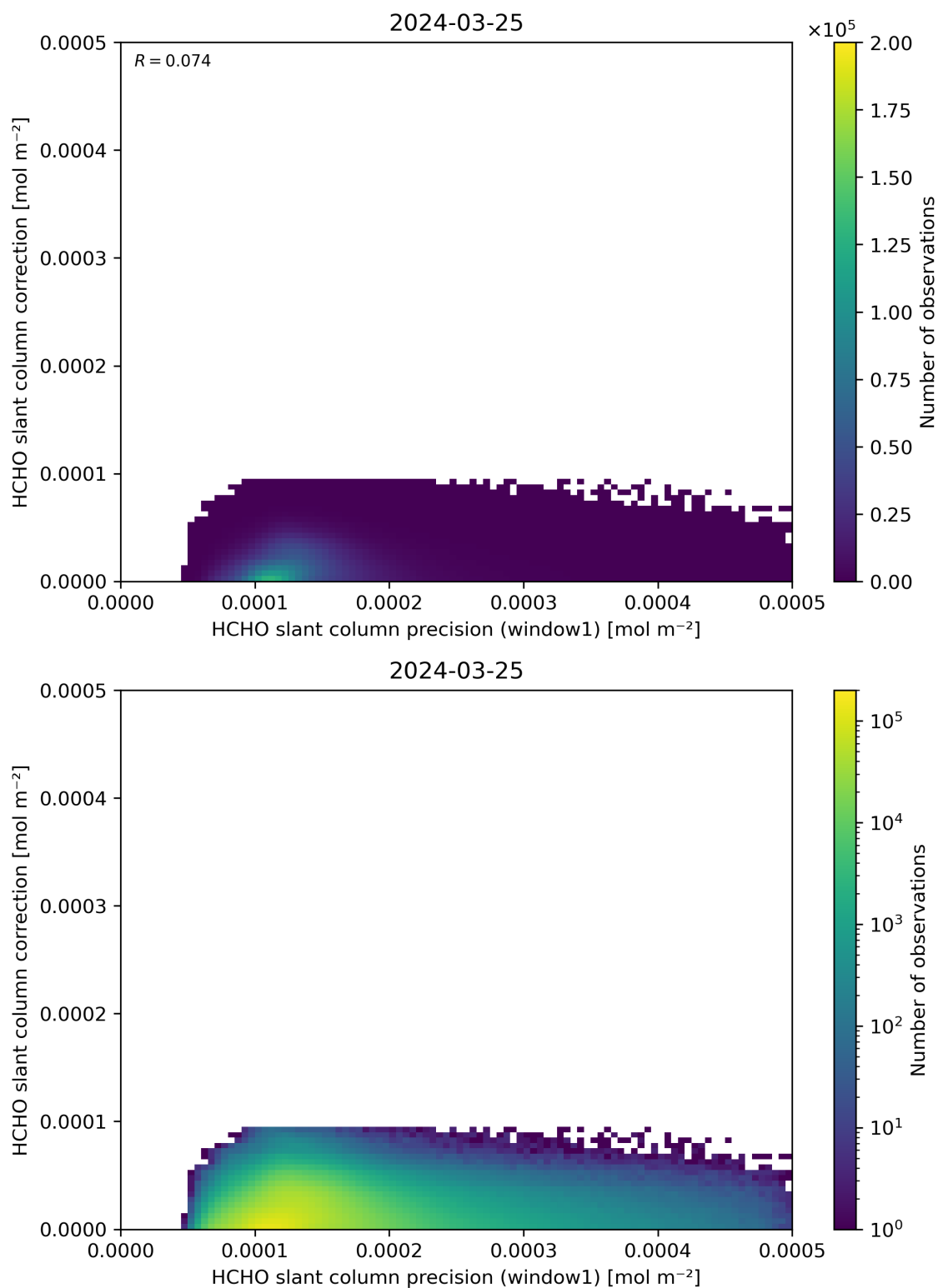
Figure 93: Scatter density plot of “HCHO slant column precision (window1)” against “HCHO slant column correction” for 2024-03-25 to 2024-03-26.
