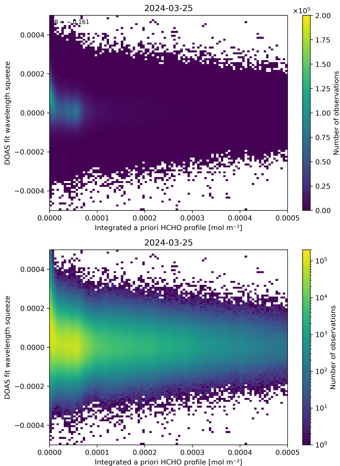
Figure 150: Scatter density plot of “Integrated a priori HCHO profile” against “DOAS fit wavelength squeeze” for 2024-03-25 to 2024-03-26.
