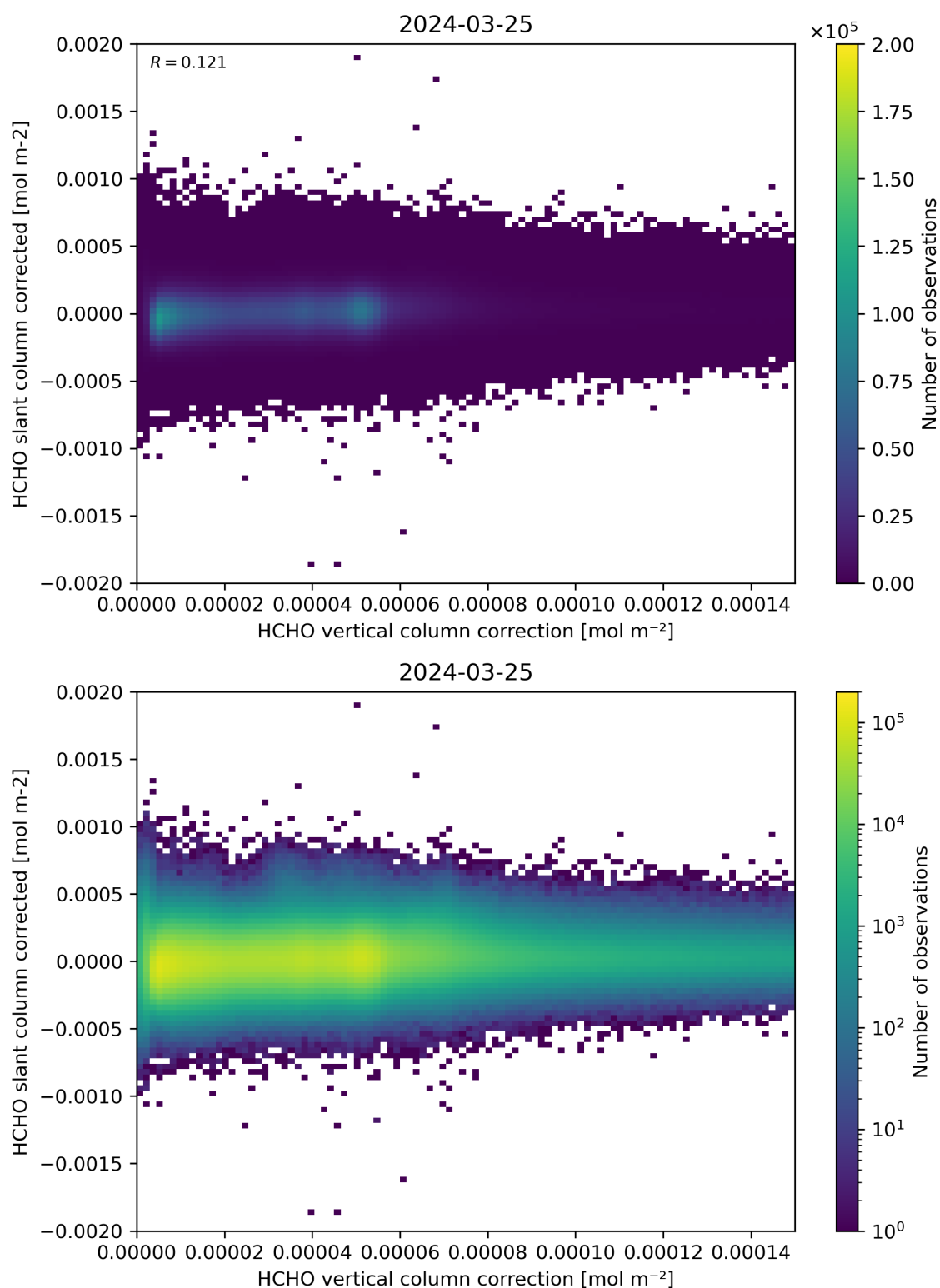
Figure 116: Scatter density plot of “HCHO vertical column correction” against “HCHO slant column corrected” for 2024-03-25 to 2024-03-26.
