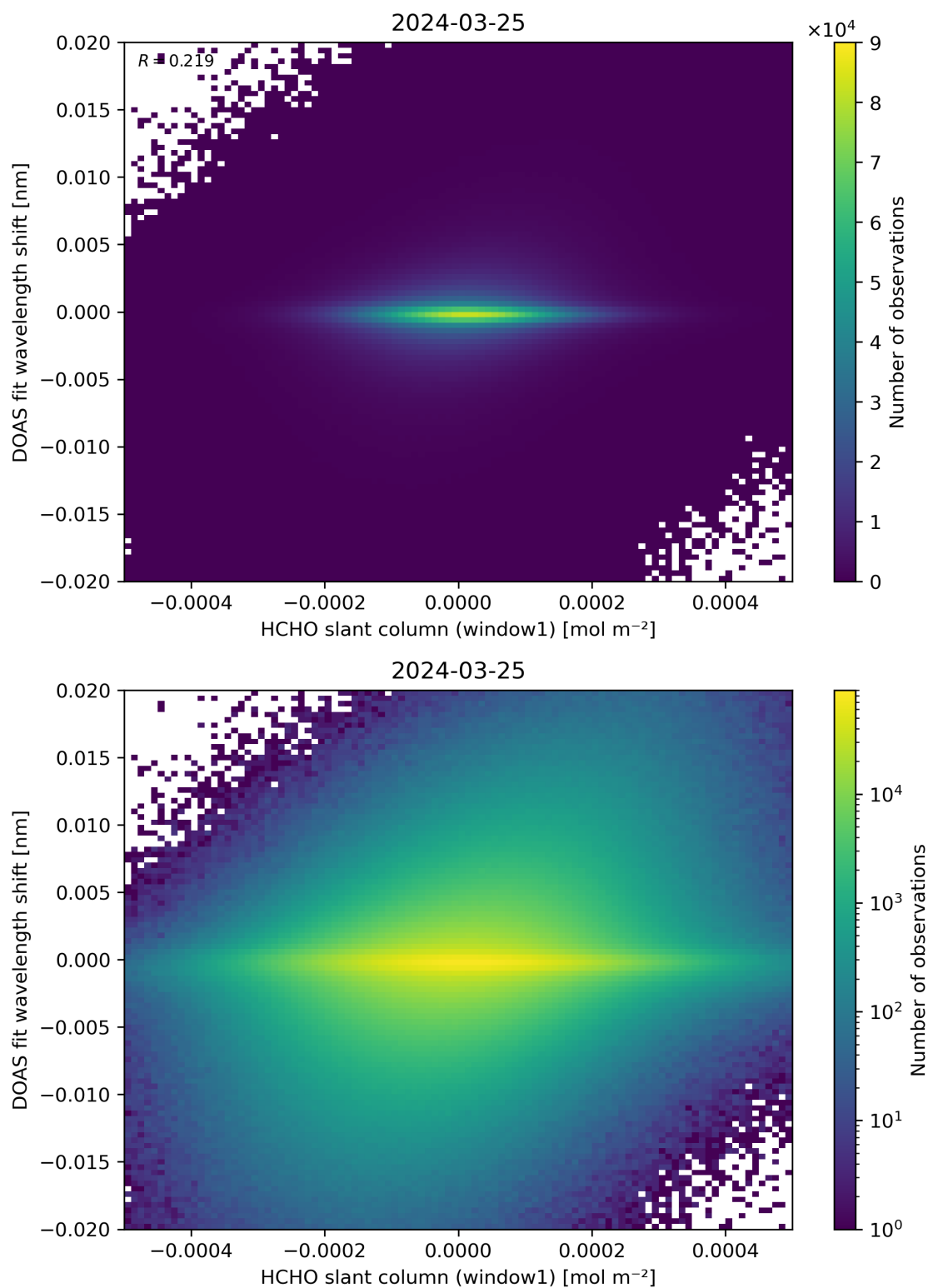
Figure 79: Scatter density plot of “HCHO slant column (window1)” against “DOAS fit wavelength shift” for 2024-03-25 to 2024-03-26.
