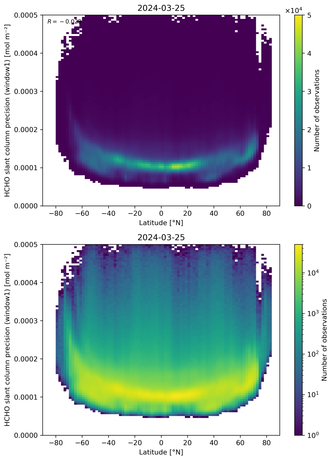
Figure 160: Scatter density plot of “Latitude” against “HCHO slant column precision (window1)” for 2024-03-25 to 2024-03-26.
