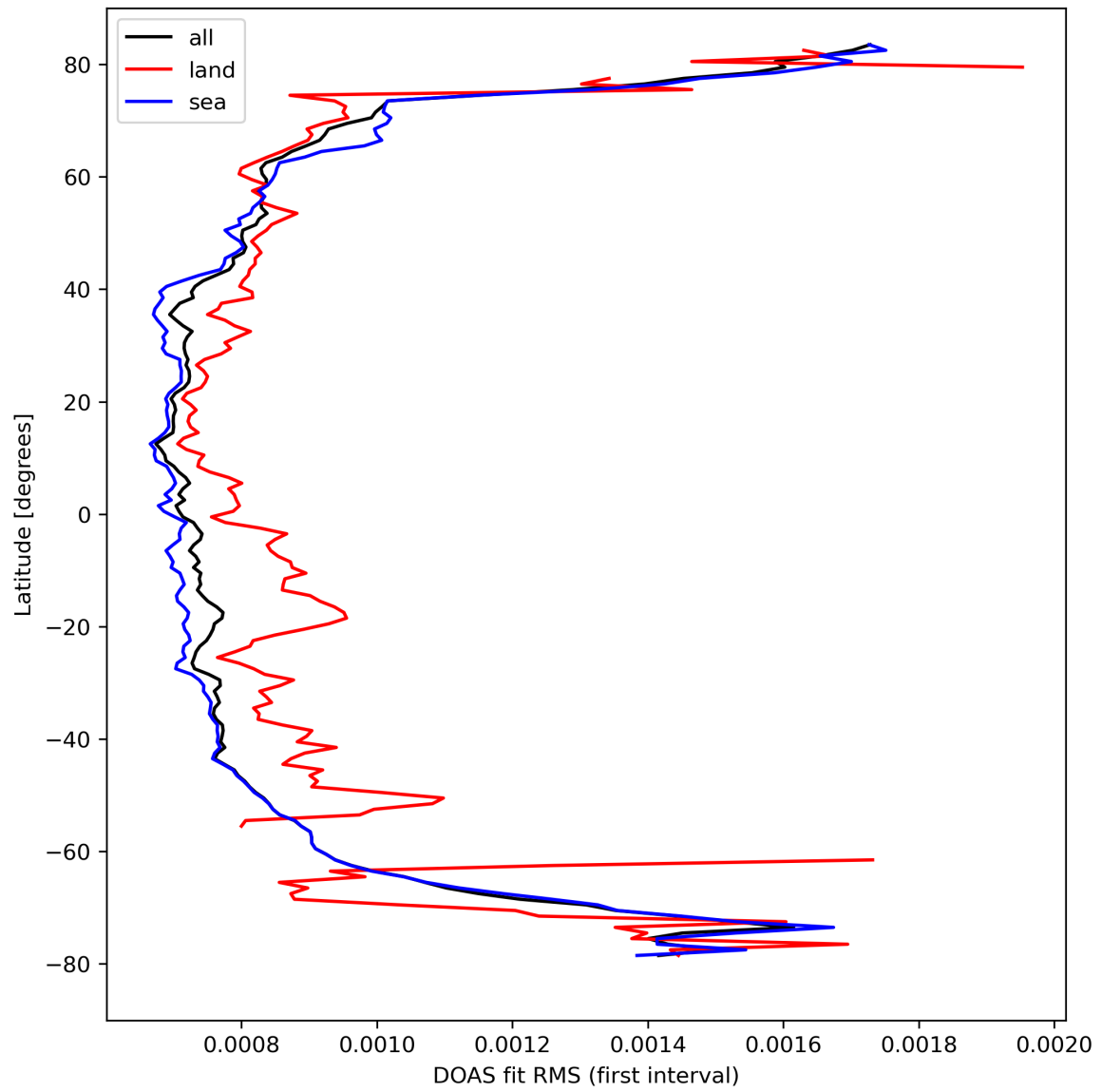
Figure 32: Zonal average of “DOAS fit RMS (first interval)” for 2024-03-25 to 2024-03-26.
