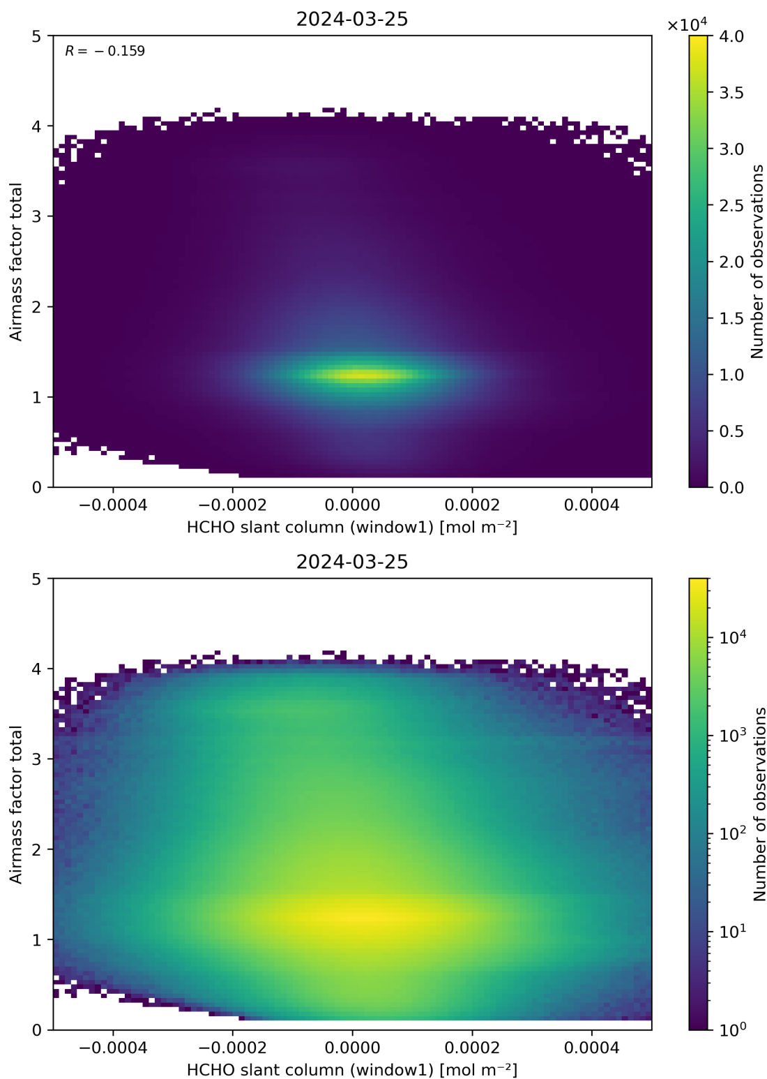
Figure 85: Scatter density plot of “HCHO slant column (window1)” against “Airmass factor total” for 2024-03-25 to 2024-03-26.
