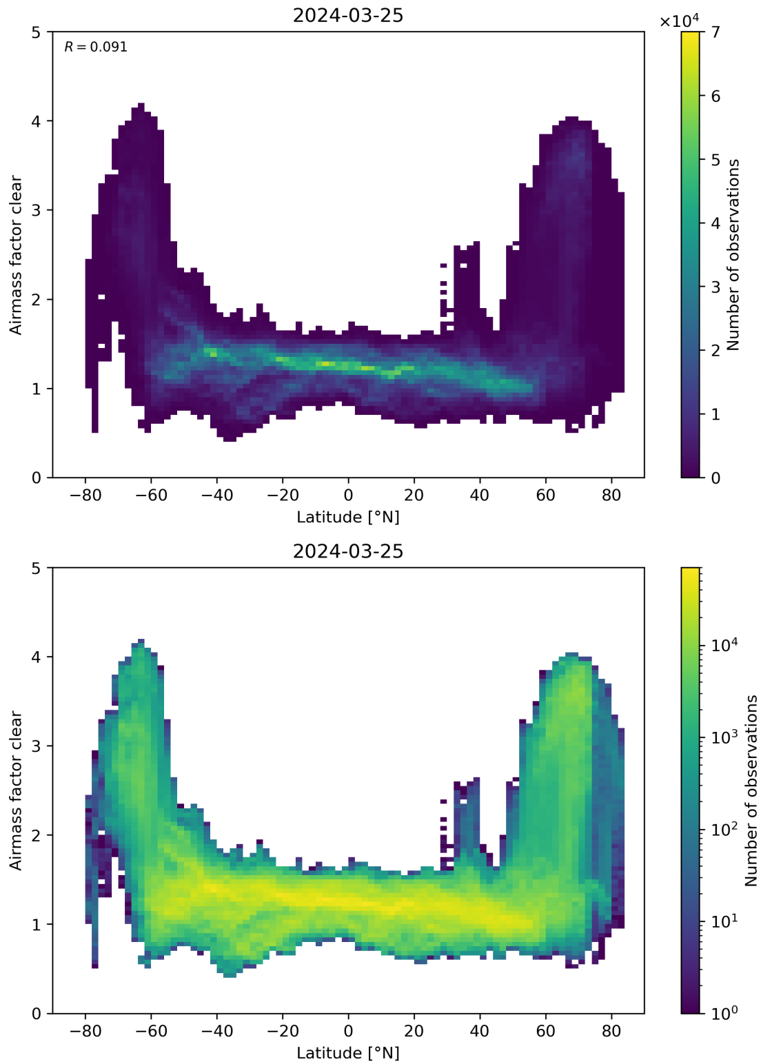
Figure 156: Scatter density plot of “Latitude” against “Airmass factor clear” for 2024-03-25 to 2024-03-26.
