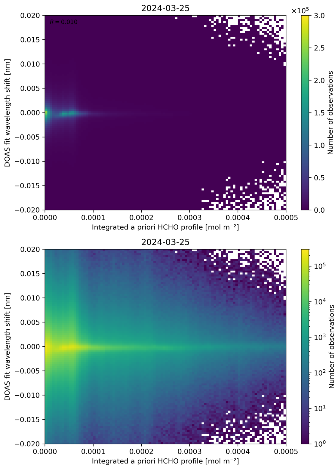
Figure 149: Scatter density plot of “Integrated a priori HCHO profile” against “DOAS fit wavelength shift” for 2024-03-25 to 2024-03-26.
