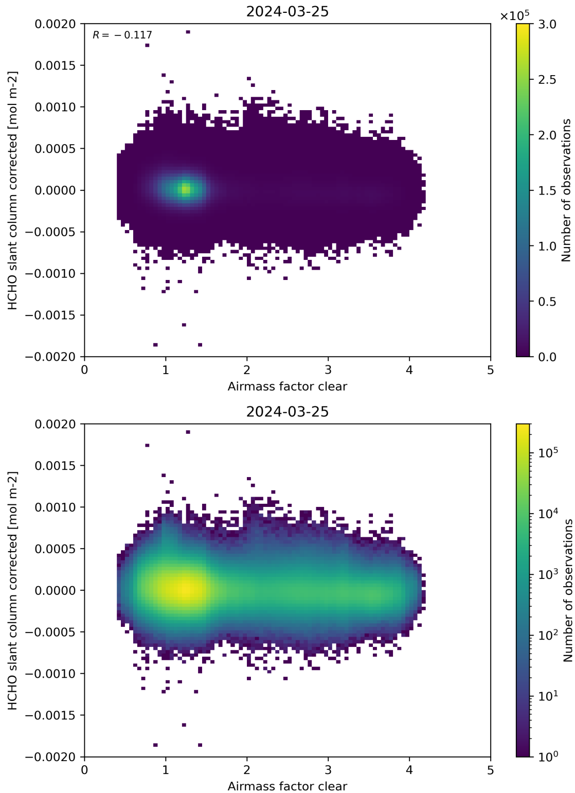
Figure 74: Scatter density plot of “Airmass factor clear” against “HCHO slant column corrected” for 2024-03-25 to 2024-03-26.
