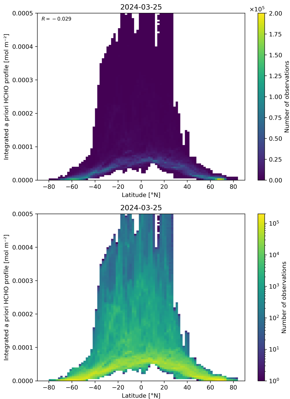
Figure 166: Scatter density plot of “Latitude” against “Integrated a priori HCHO profile” for 2024-03-25 to 2024-03-26.
