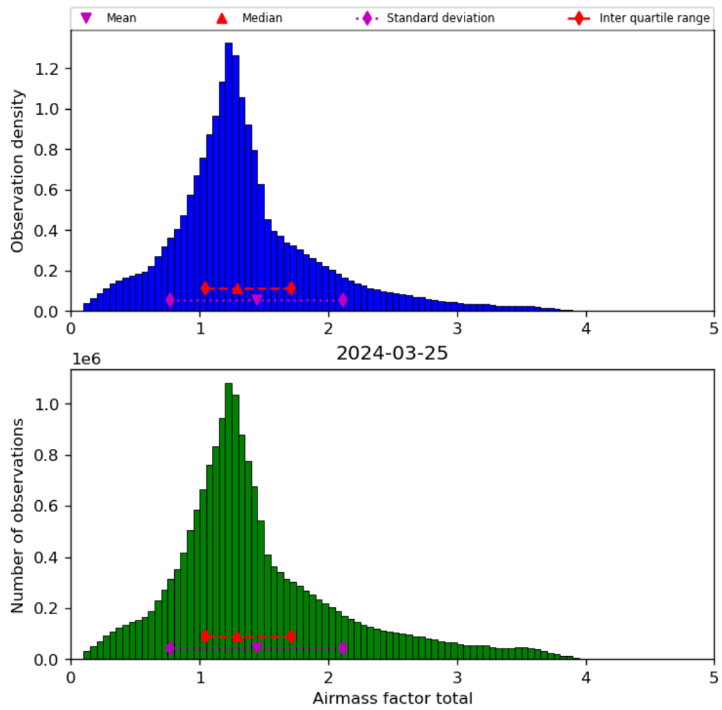
Figure 40: Histogram of “Airmass factor total” for 2024-03-25 to 2024-03-26
