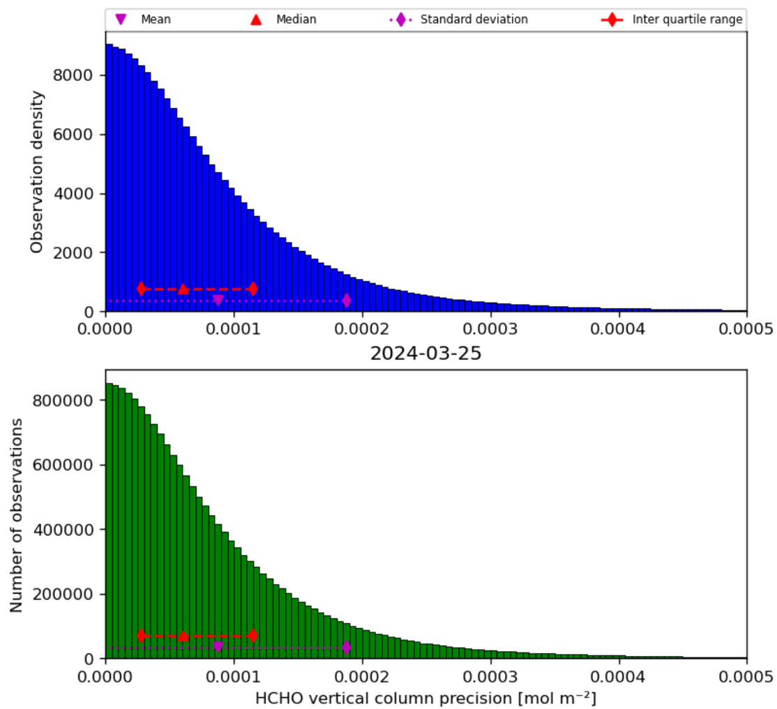
Figure 36: Histogram of “HCHO vertical column precision” for 2024-03-25 to 2024-03-26
