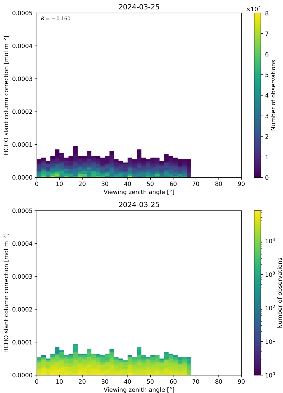
Figure 187: Scatter density plot of “Viewing zenith angle” against “HCHO slant column correction” for 2024-03-25 to 2024-03-26.
