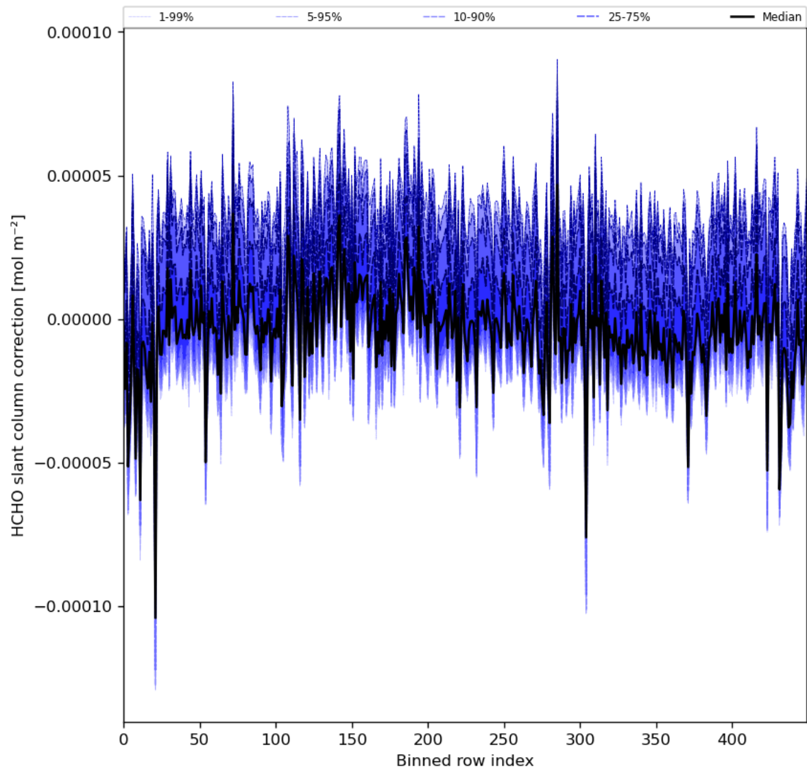
Figure 61: Along track statistics of “HCHO slant column correction” for 2024-03-25 to 2024-03-26
