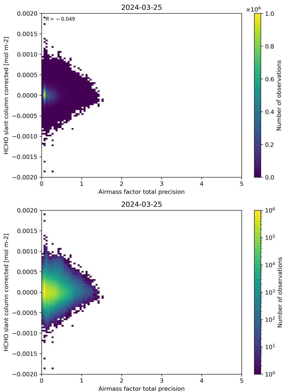
Figure 109: Scatter density plot of “Airmass factor total precision” against “HCHO slant column corrected” for 2024-03-25 to 2024-03-26.
