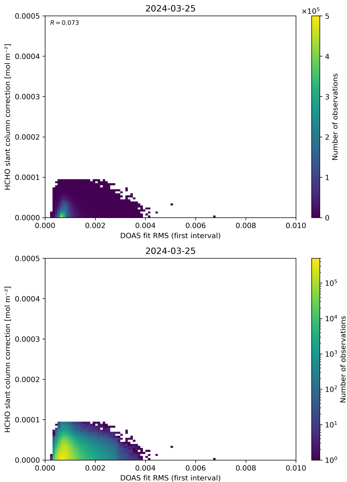
Figure 63: Scatter density plot of “DOAS fit RMS (first interval)” against “HCHO slant column correction” for 2024-03-25 to 2024-03-26.
