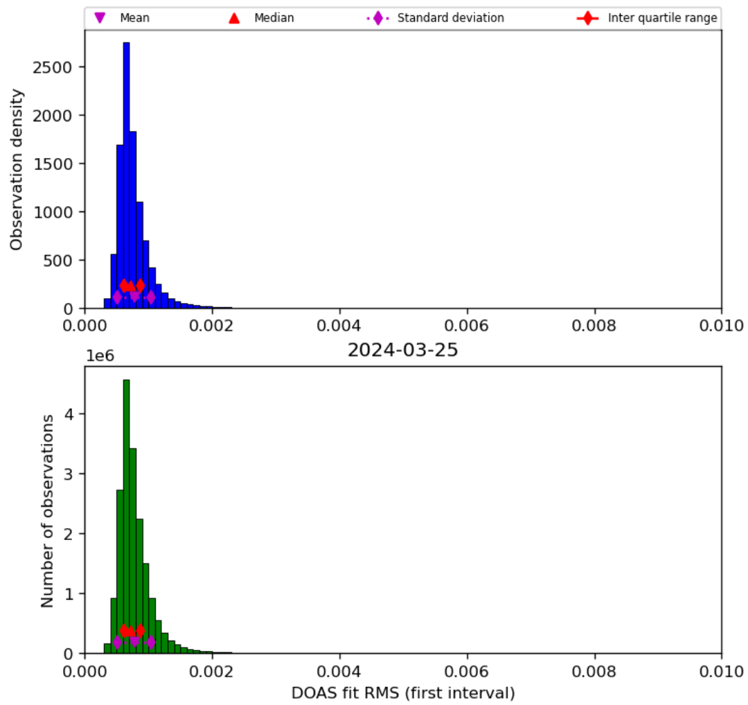
Figure 46: Histogram of “DOAS fit RMS (first interval)” for 2024-03-25 to 2024-03-26
