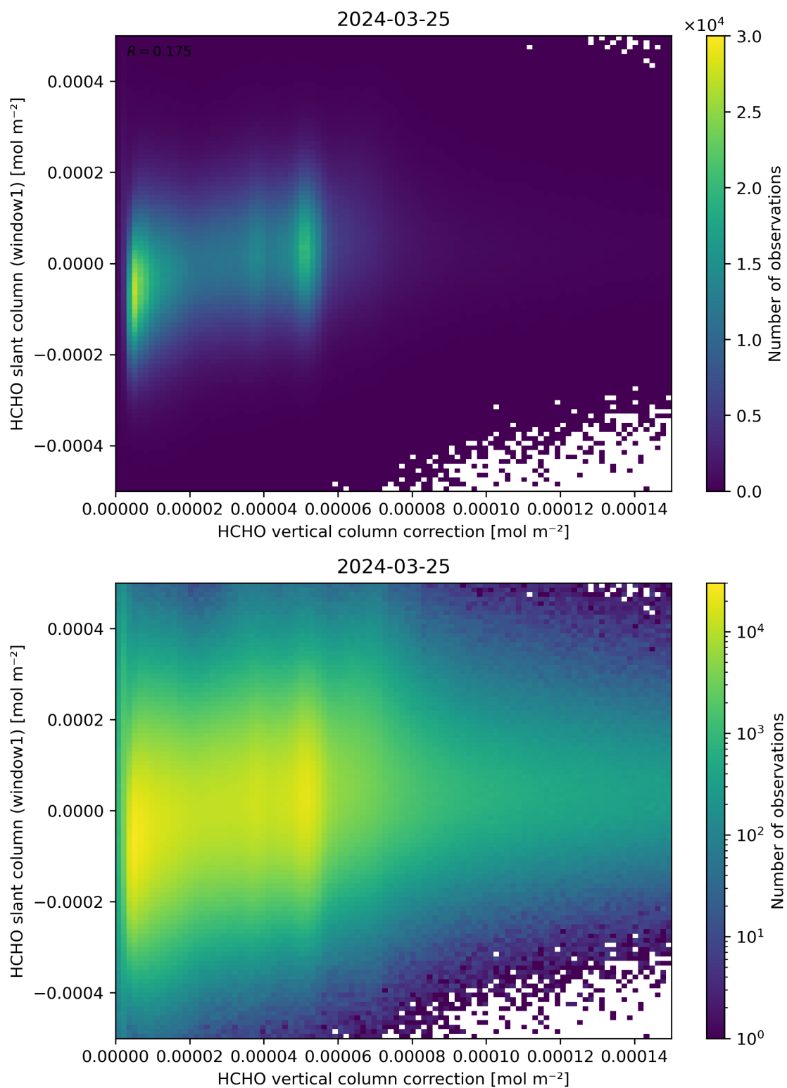
Figure 118: Scatter density plot of “HCHO vertical column correction” against “HCHO slant column (window1)” for 2024-03-25 to 2024-03-26.
