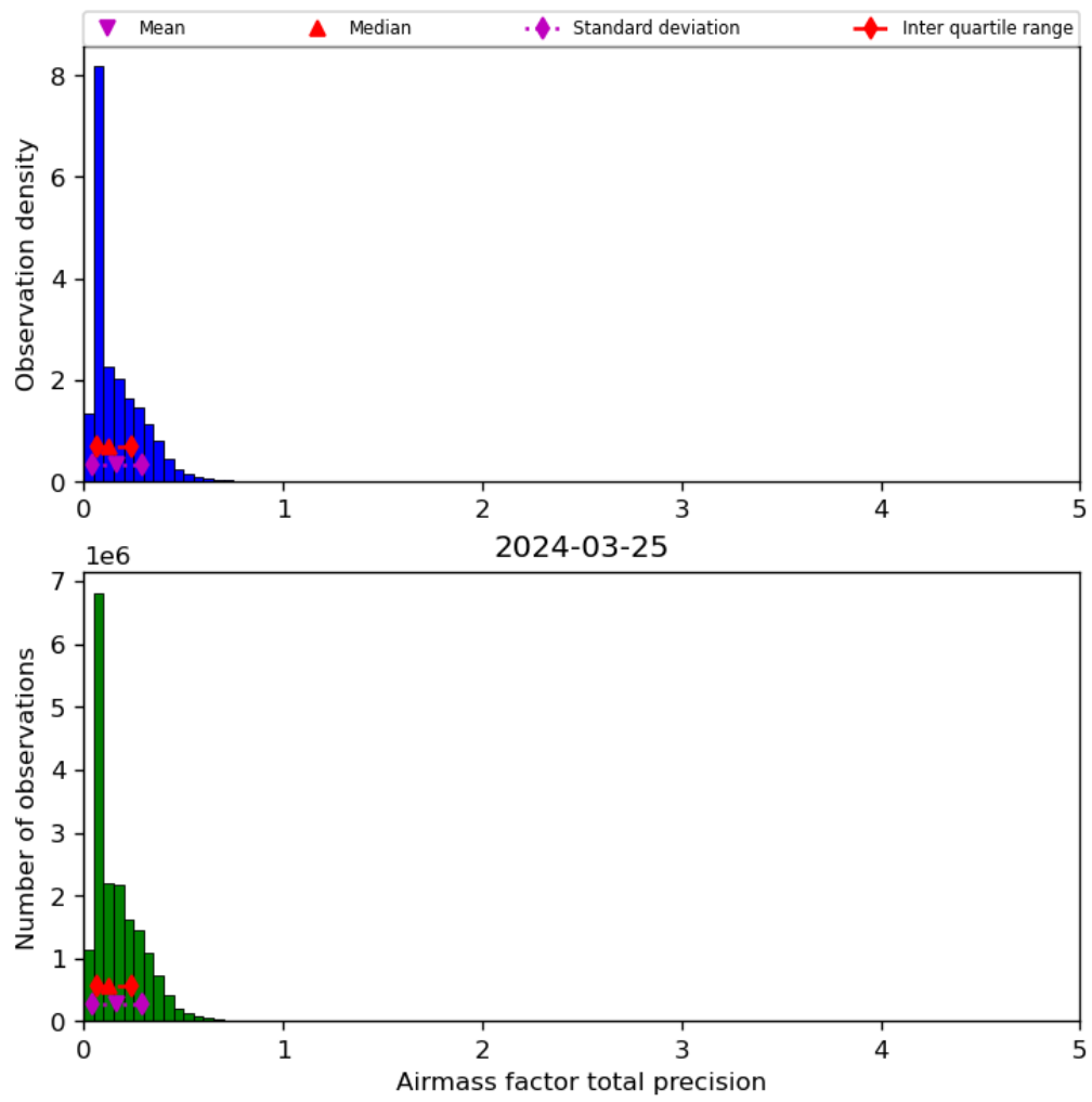
Figure 41: Histogram of “Airmass factor total precision” for 2024-03-25 to 2024-03-26
