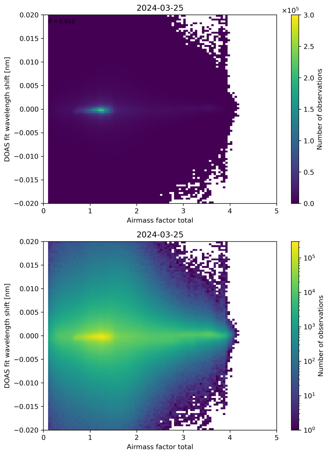
Figure 98: Scatter density plot of “Airmass factor total” against “DOAS fit wavelength shift” for 2024-03-25 to 2024-03-26.
