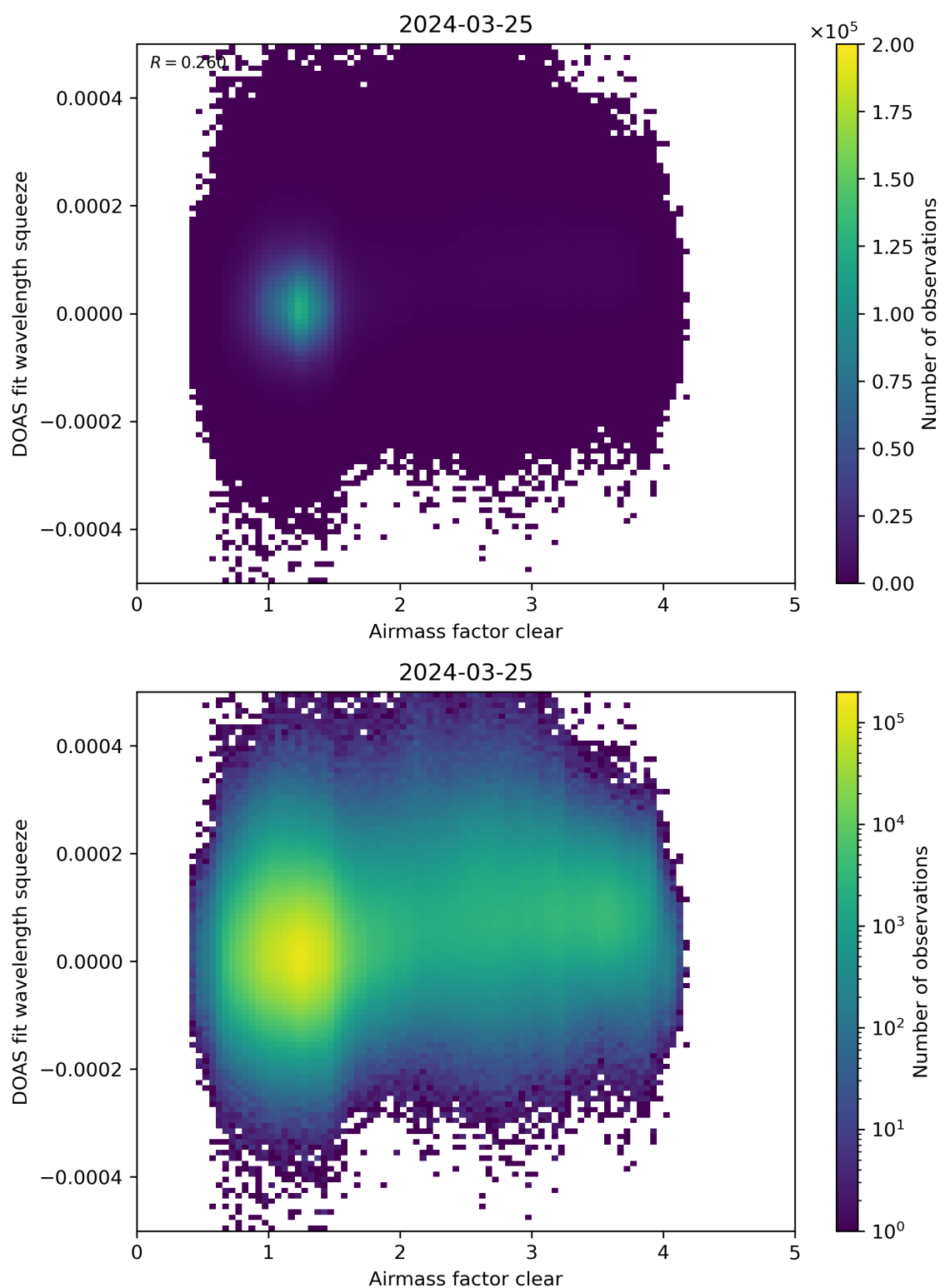
Figure 73: Scatter density plot of “Airmass factor clear” against “DOAS fit wavelength squeeze” for 2024-03-25 to 2024-03-26.
