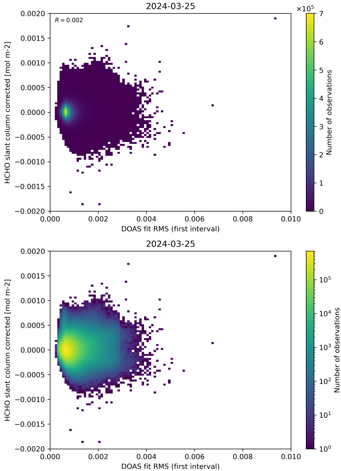
Figure 62: Scatter density plot of “DOAS fit RMS (first interval)” against “HCHO slant column corrected” for 2024-03-25 to 2024-03-26.
