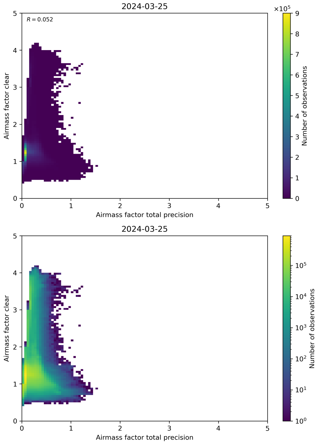
Figure 108: Scatter density plot of “Airmass factor total precision” against “Airmass factor clear” for 2024-03-25 to 2024-03-26.
