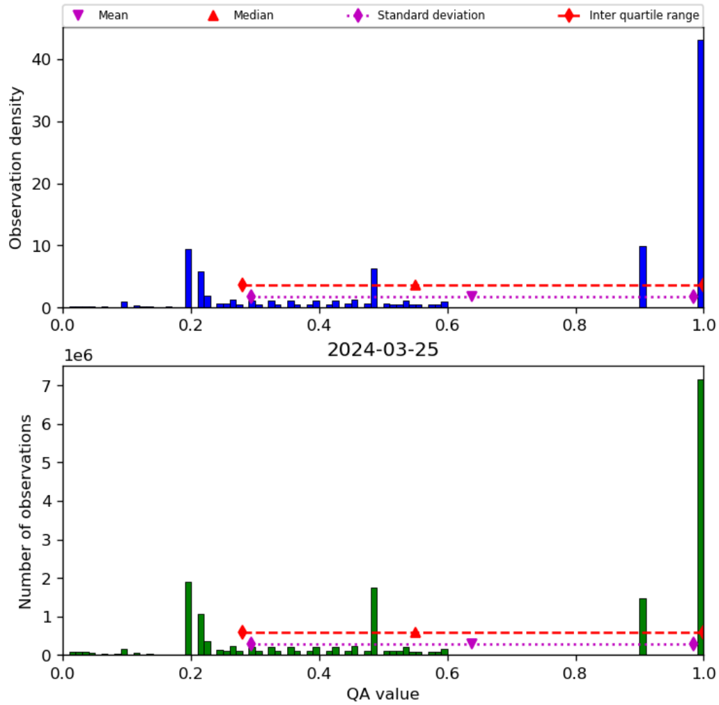
Figure 34: Histogram of “QA value” for 2024-03-25 to 2024-03-26
