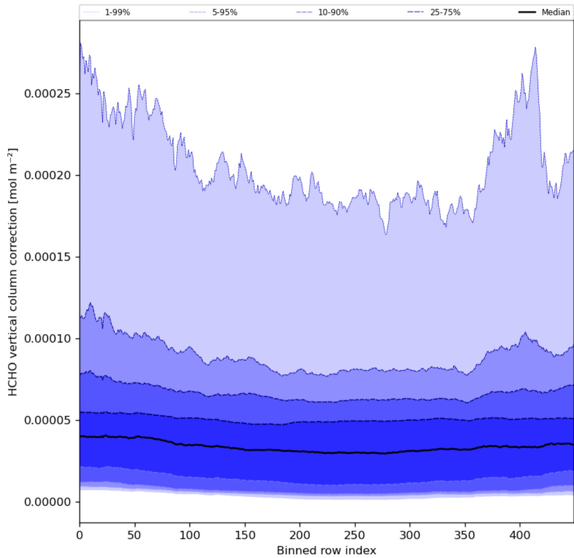
Figure 51: Along track statistics of “HCHO vertical column correction” for 2024-03-25 to 2024-03-26
