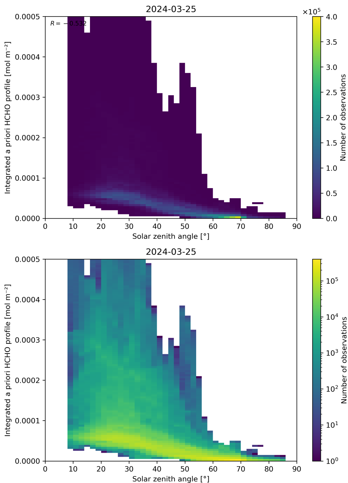
Figure 180: Scatter density plot of “Solar zenith angle” against “Integrated a priori HCHO profile” for 2024-03-25 to 2024-03-26.
