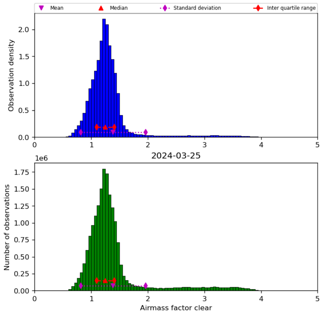
Figure 42: Histogram of “Airmass factor clear” for 2024-03-25 to 2024-03-26
