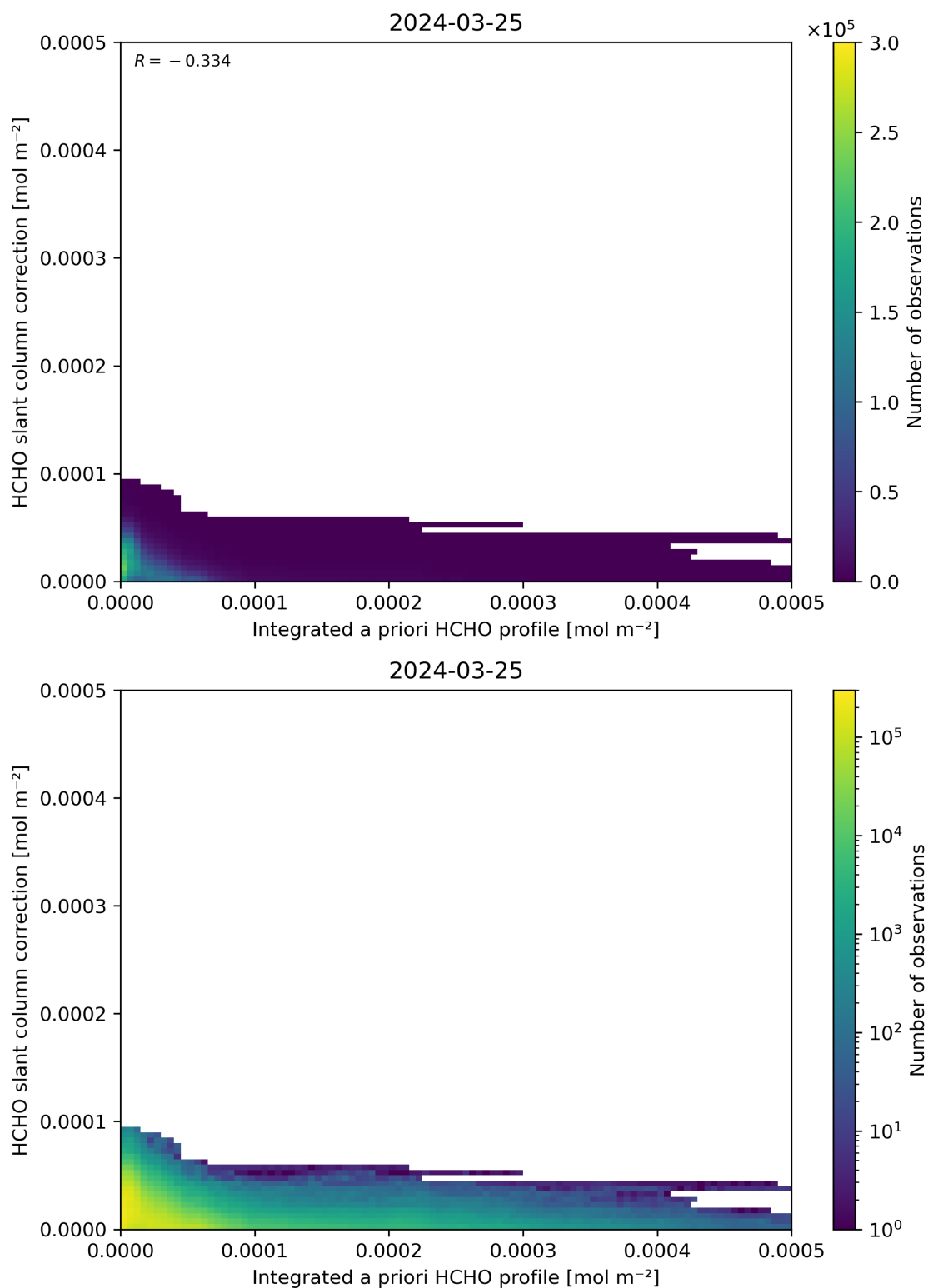
Figure 152: Scatter density plot of “Integrated a priori HCHO profile” against “HCHO slant column correction” for 2024-03-25 to 2024-03-26.
