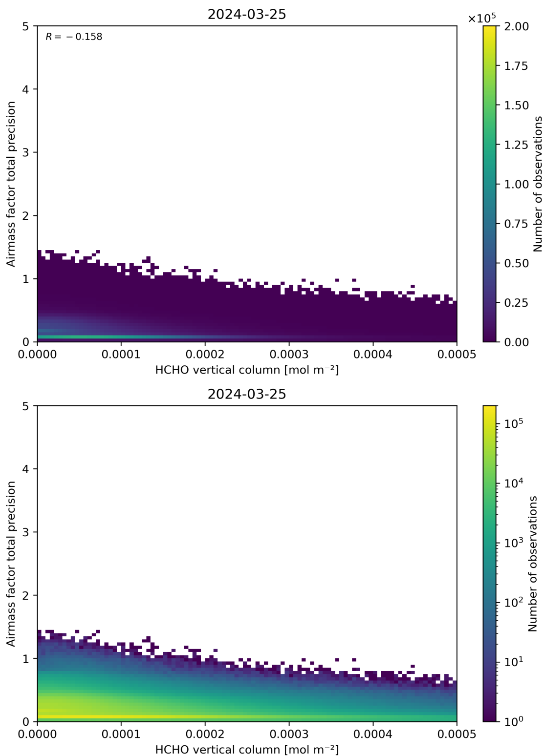
Figure 132: Scatter density plot of “HCHO vertical column” against “Airmass factor total precision” for 2024-03-25 to 2024-03-26.
