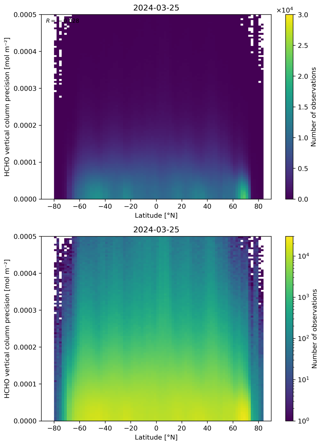
Figure 165: Scatter density plot of “Latitude” against “HCHO vertical column precision” for 2024-03-25 to 2024-03-26.
