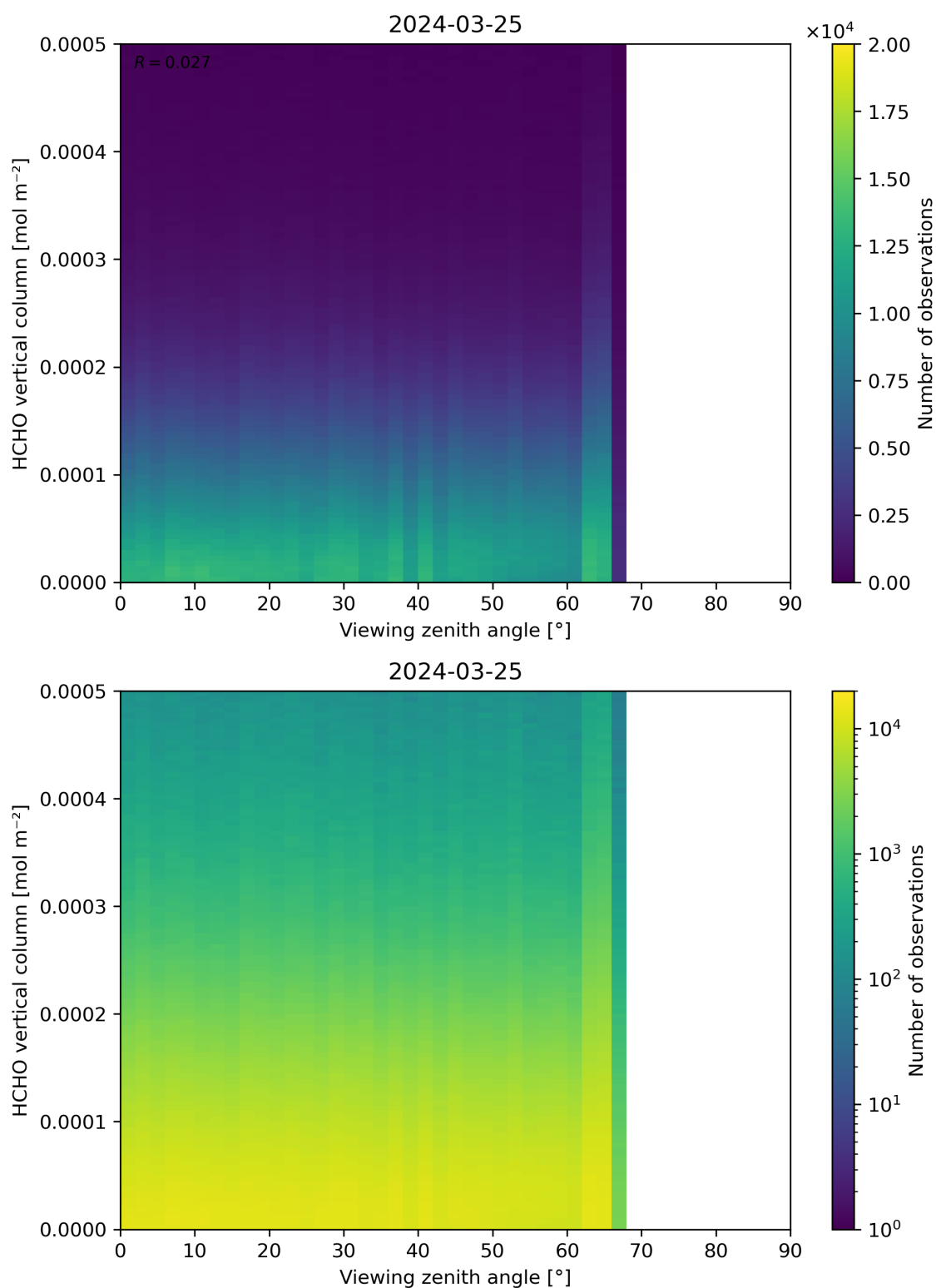
Figure 192: Scatter density plot of “Viewing zenith angle” against “HCHO vertical column” for 2024-03-25 to 2024-03-26.
