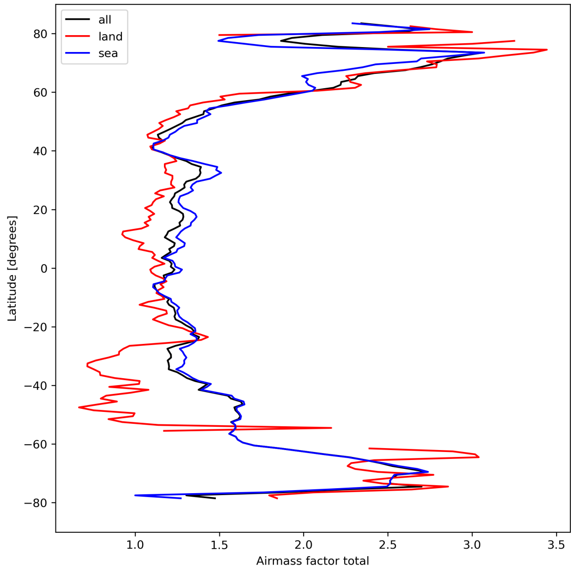
Figure 26: Zonal average of “Airmass factor total” for 2024-03-25 to 2024-03-26.
