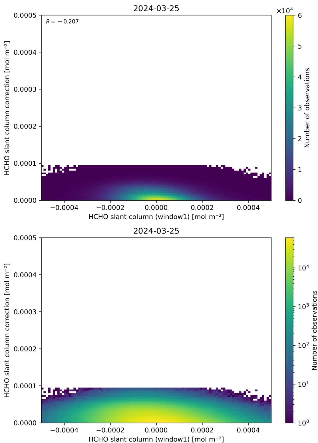
Figure 83: Scatter density plot of “HCHO slant column (window1)” against “HCHO slant column correction” for 2024-03-25 to 2024-03-26.
