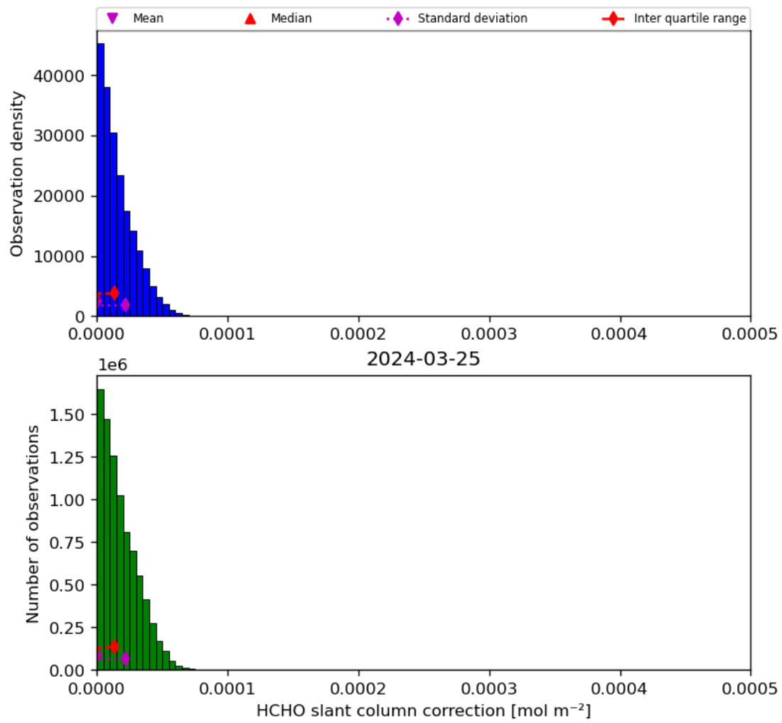
Figure 47: Histogram of “HCHO slant column correction” for 2024-03-25 to 2024-03-26
