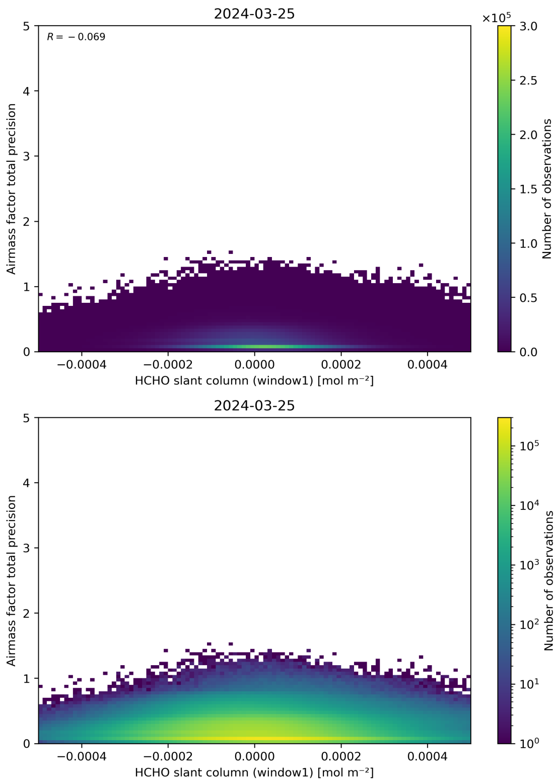
Figure 86: Scatter density plot of “HCHO slant column (window1)” against “Airmass factor total precision” for 2024-03-25 to 2024-03-26.
