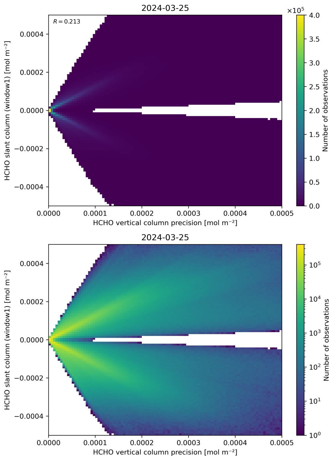
Figure 142: Scatter density plot of “HCHO vertical column precision” against “HCHO slant column (window1)” for 2024-03-25 to 2024-03-26.
