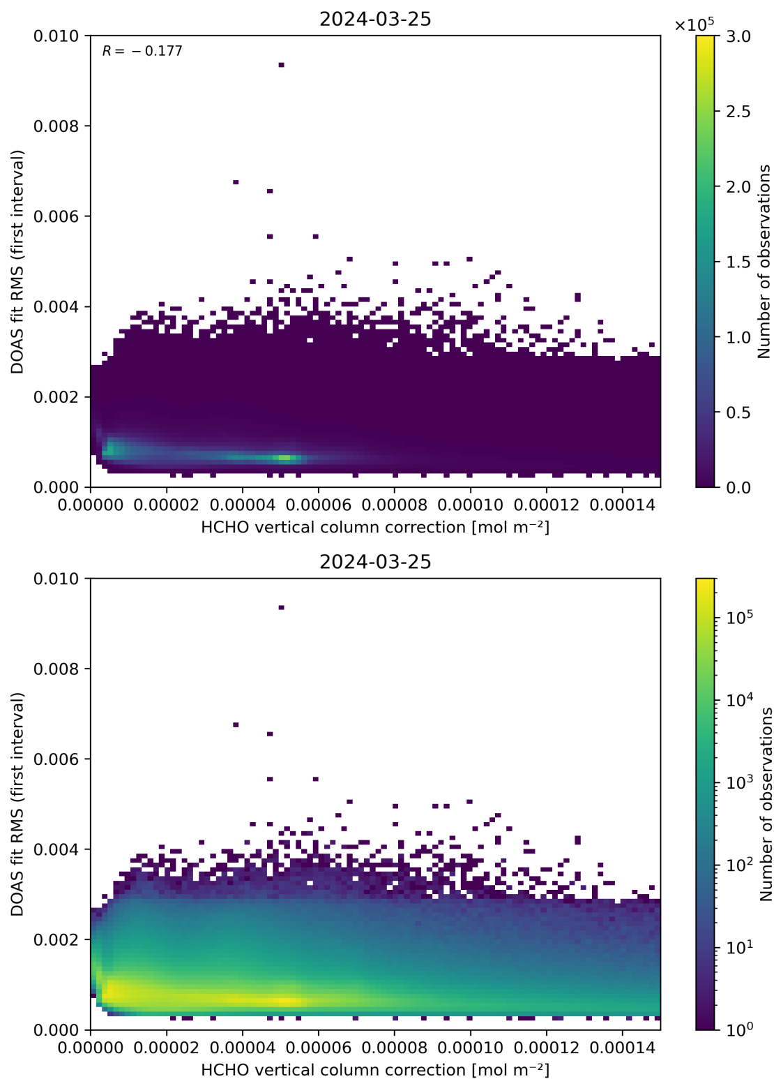
Figure 112: Scatter density plot of “HCHO vertical column correction” against “DOAS fit RMS (first interval)” for 2024-03-25 to 2024-03-26.
