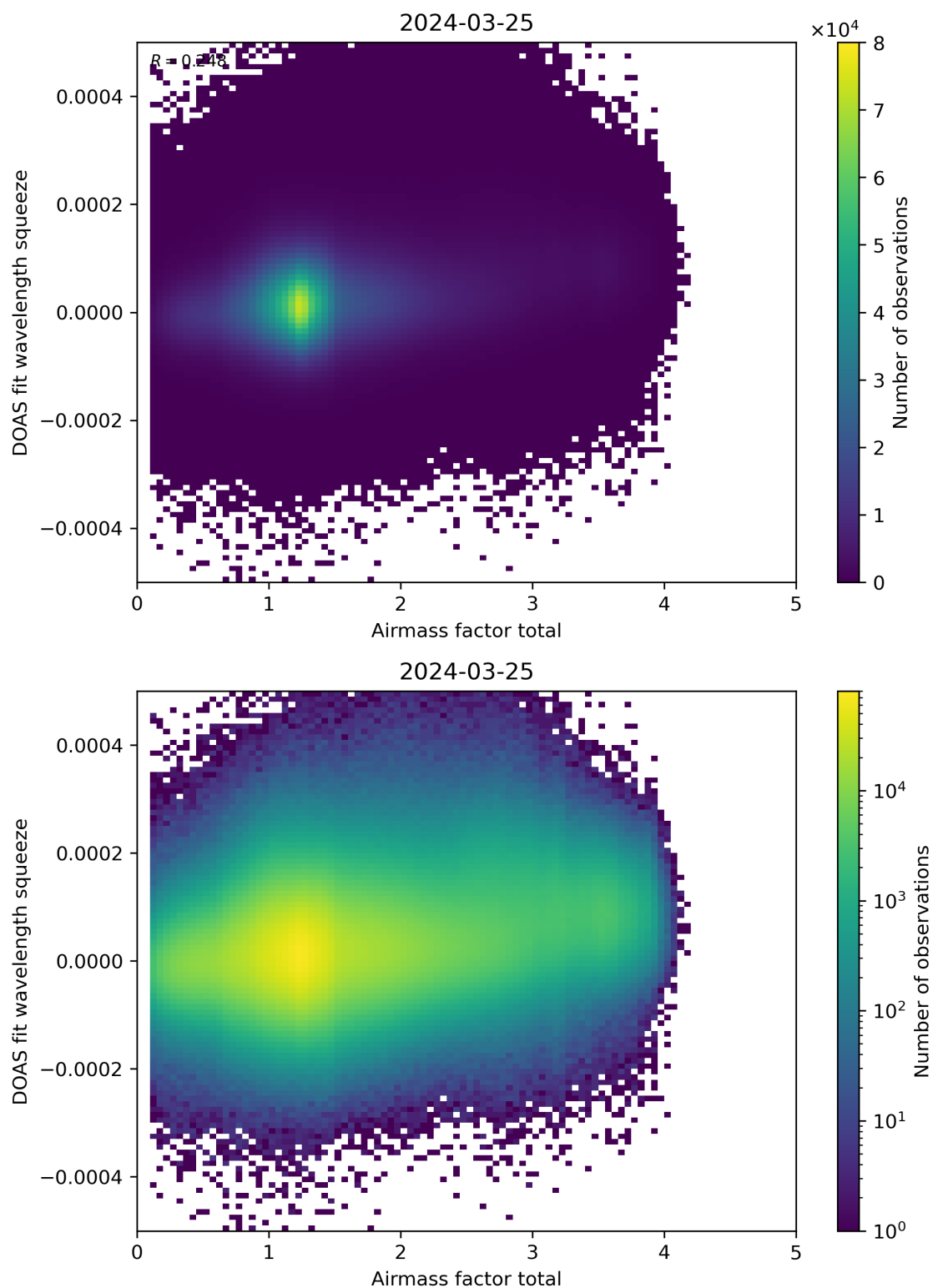
Figure 99: Scatter density plot of “Airmass factor total” against “DOAS fit wavelength squeeze” for 2024-03-25 to 2024-03-26.
