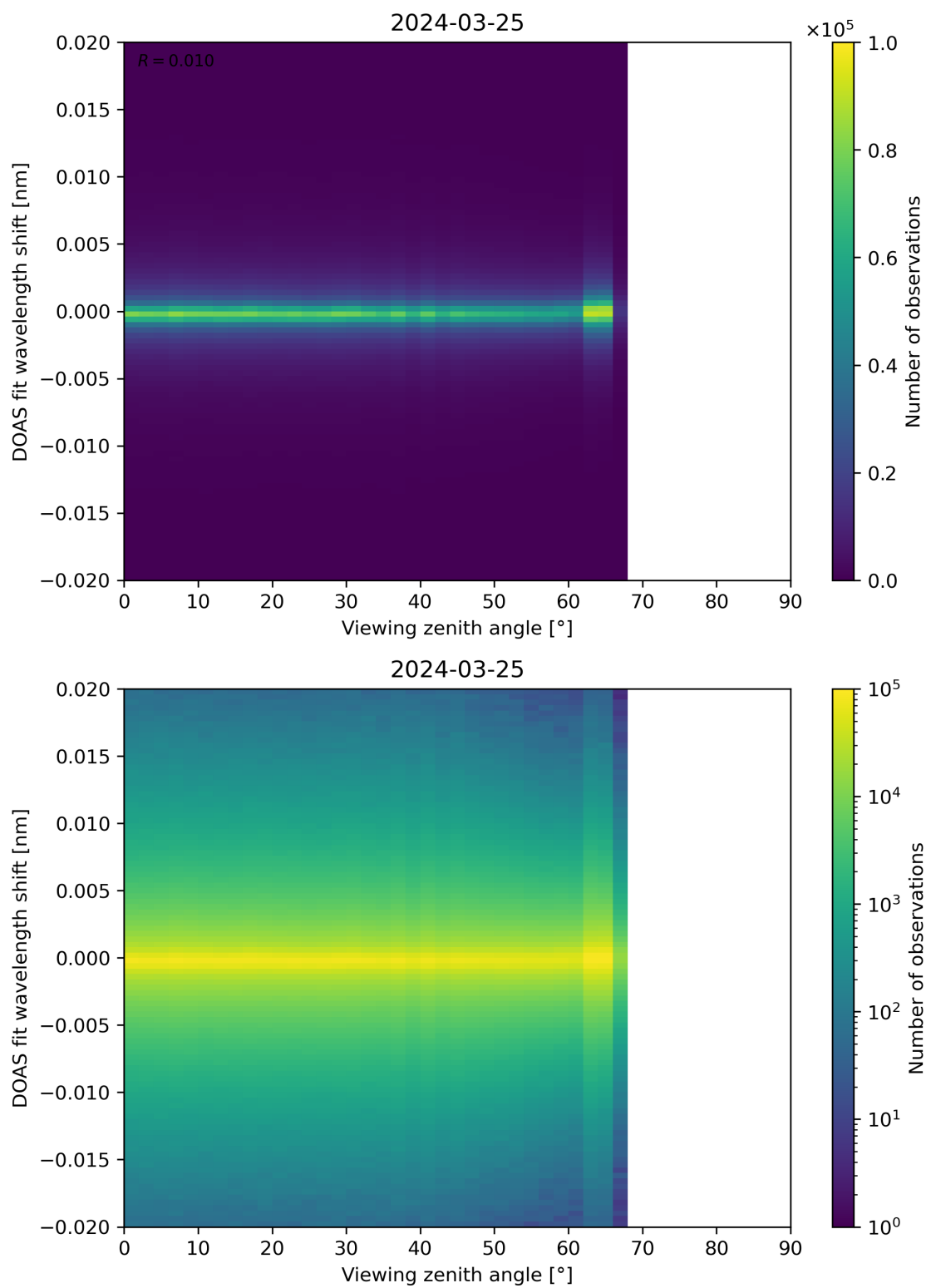
Figure 183: Scatter density plot of “Viewing zenith angle” against “DOAS fit wavelength shift” for 2024-03-25 to 2024-03-26.
