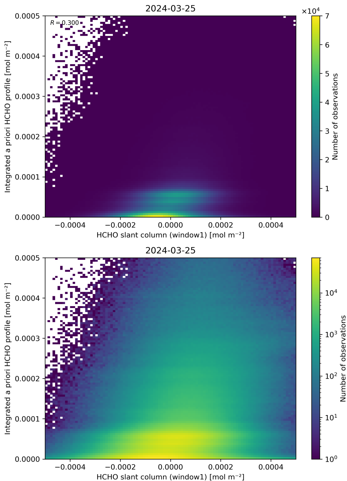
Figure 87: Scatter density plot of “HCHO slant column (window1)” against “Integrated a priori HCHO profile” for 2024-03-25 to 2024-03-26.
