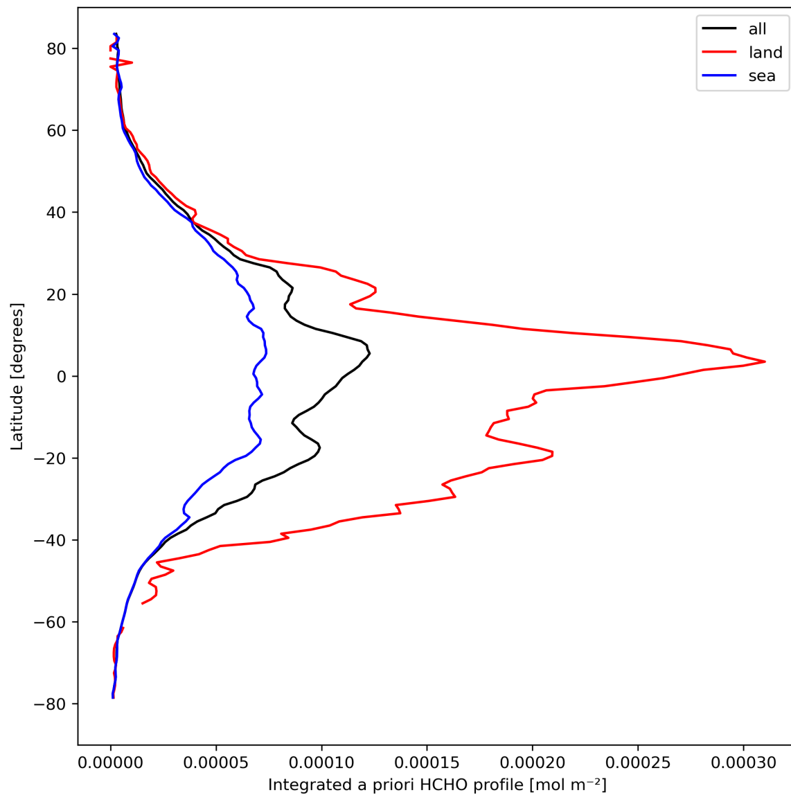
Figure 29: Zonal average of “Integrated a priori HCHO profile” for 2024-03-25 to 2024-03-26.
