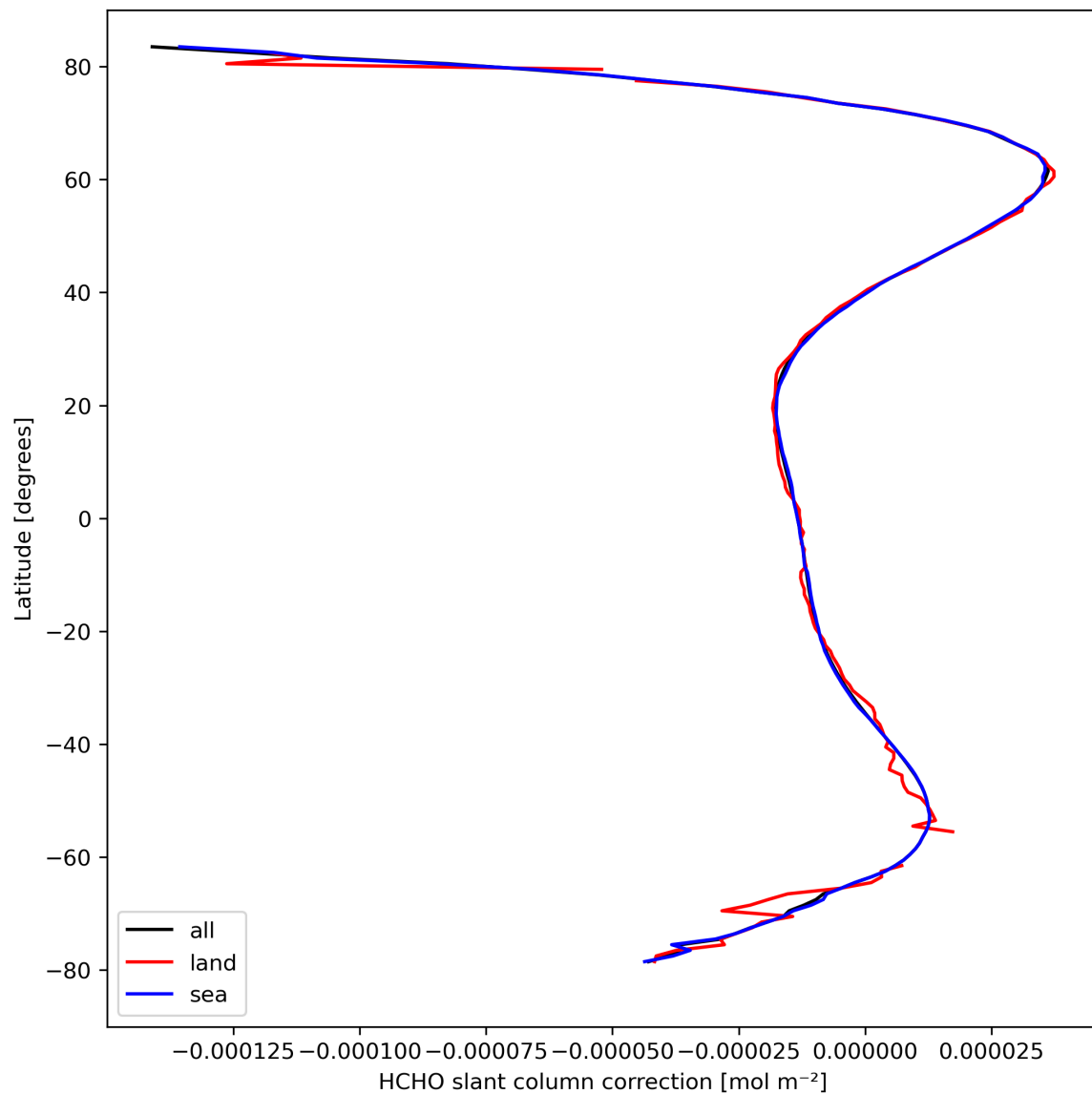
Figure 33: Zonal average of “HCHO slant column correction” for 2024-03-25 to 2024-03-26.
