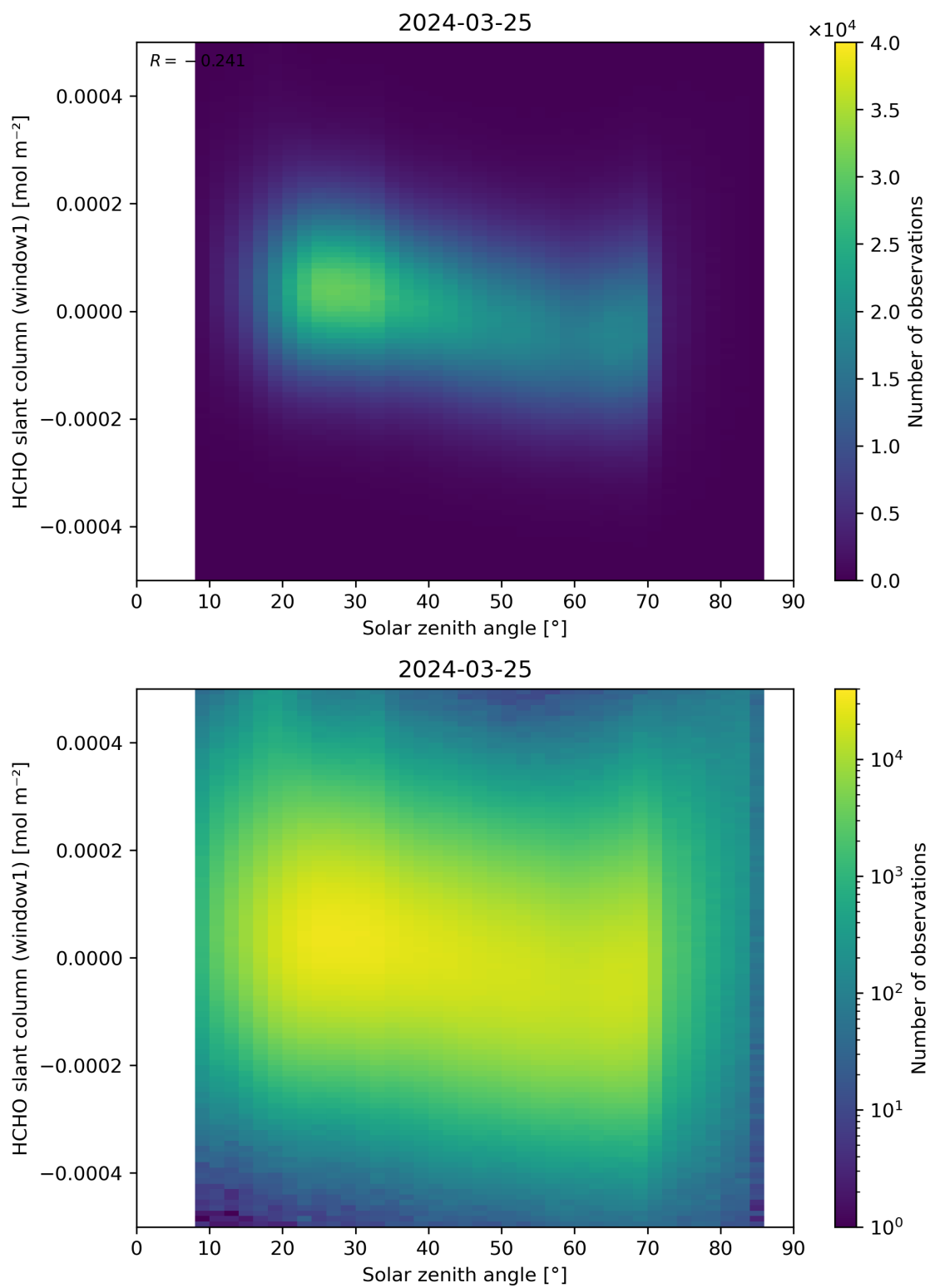
Figure 173: Scatter density plot of “Solar zenith angle” against “HCHO slant column (window1)” for 2024-03-25 to 2024-03-26.
