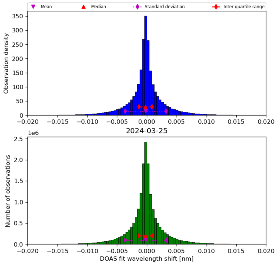
Figure 44: Histogram of “DOAS fit wavelength shift” for 2024-03-25 to 2024-03-26
