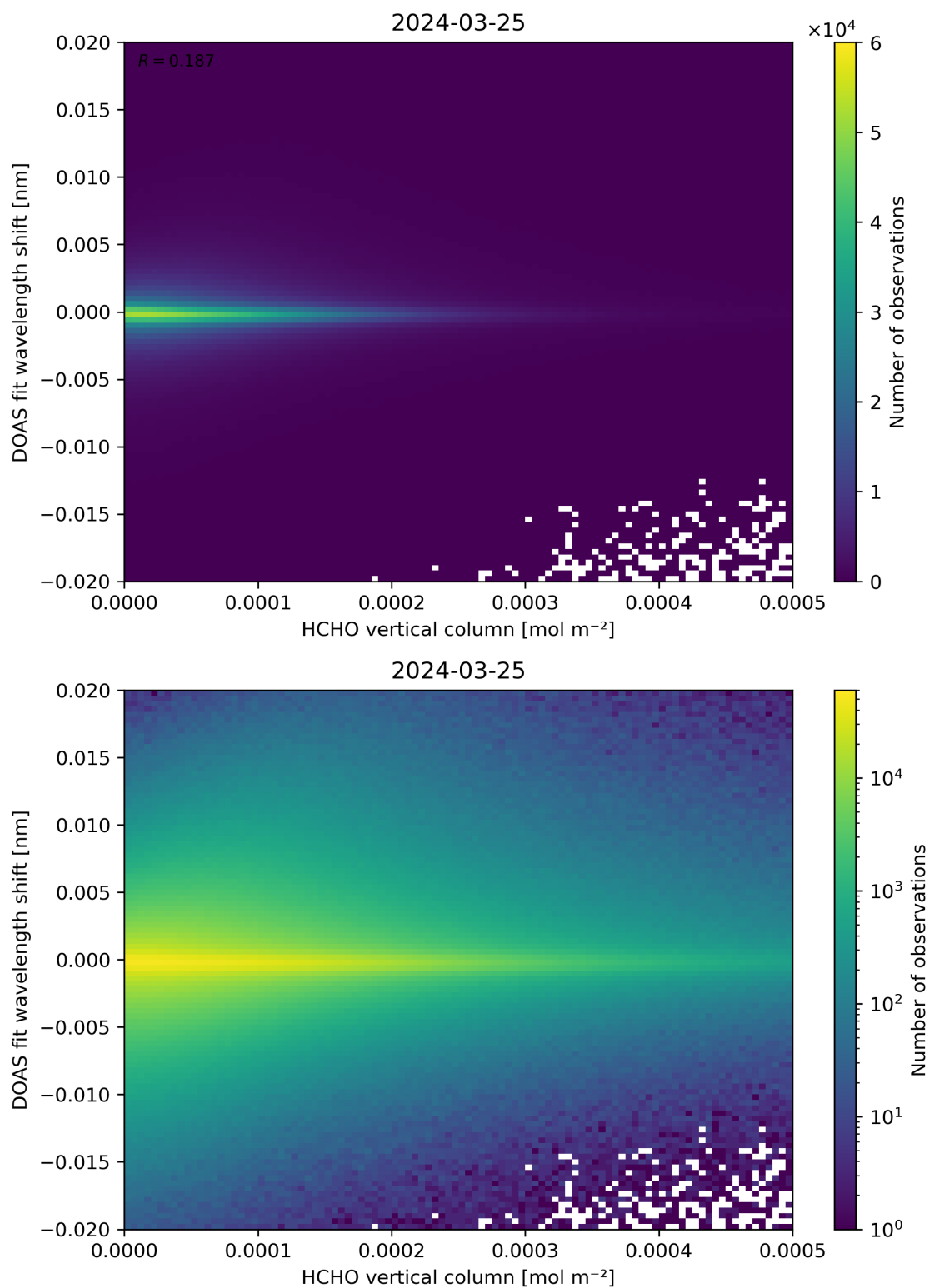
Figure 124: Scatter density plot of “HCHO vertical column” against “DOAS fit wavelength shift” for 2024-03-25 to 2024-03-26.
