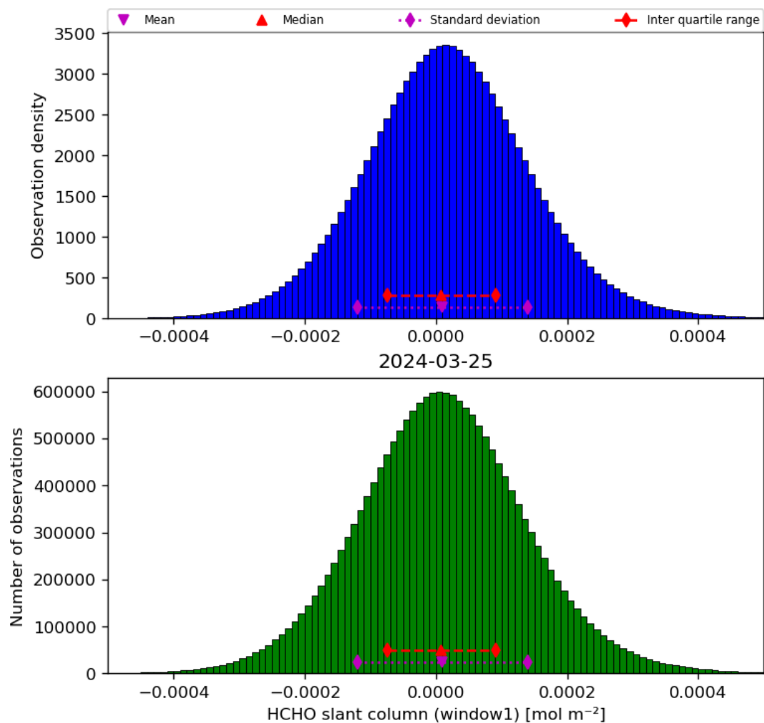
Figure 38: Histogram of “HCHO slant column (window1)” for 2024-03-25 to 2024-03-26
