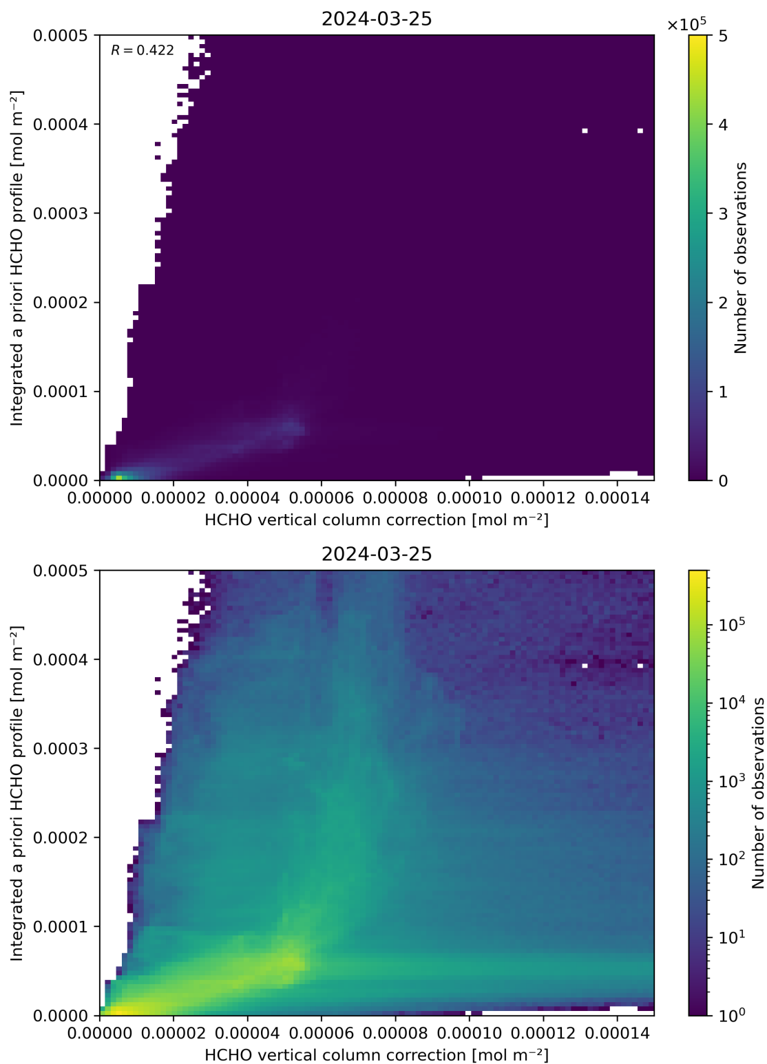
Figure 122: Scatter density plot of “HCHO vertical column correction” against “Integrated a priori HCHO profile” for 2024-03-25 to 2024-03-26.
