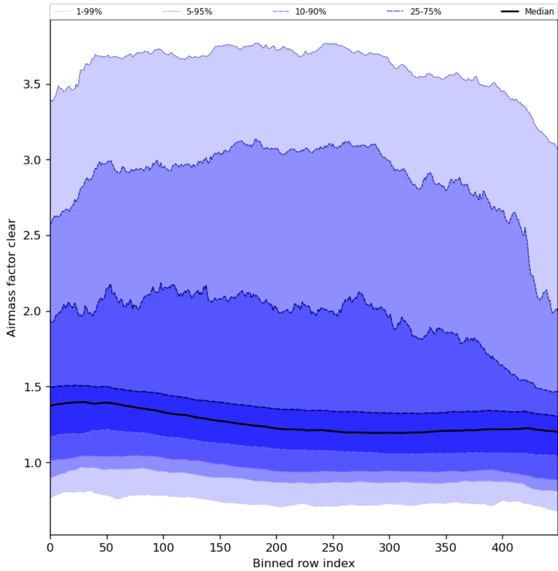
Figure 56: Along track statistics of “Airmass factor clear” for 2024-03-25 to 2024-03-26
