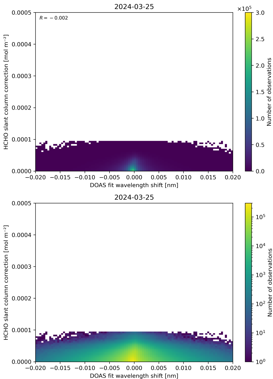
Figure 67: Scatter density plot of “DOAS fit wavelength shift” against “HCHO slant column correction” for 2024-03-25 to 2024-03-26.
