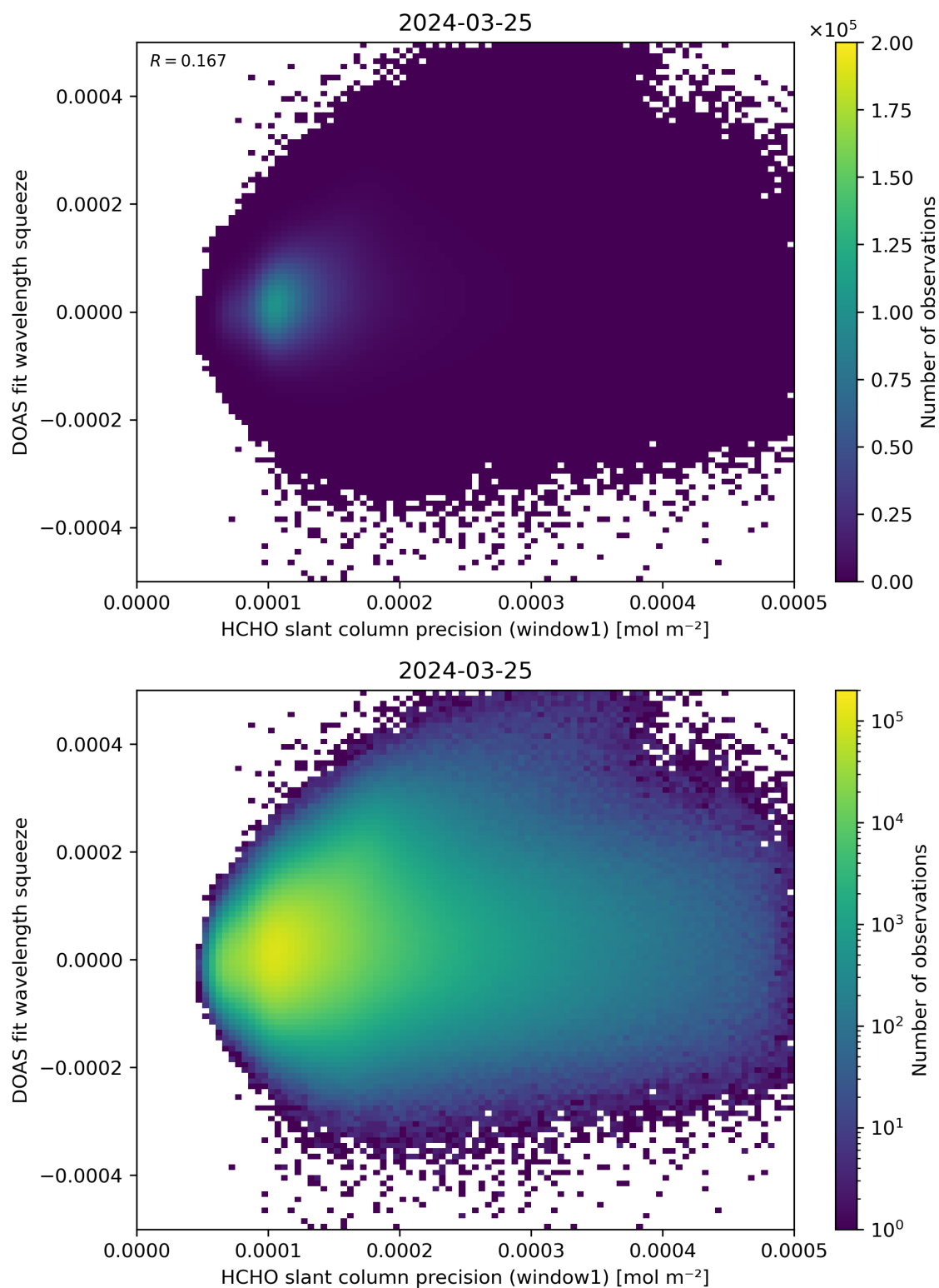
Figure 90: Scatter density plot of “HCHO slant column precision (window1)” against “DOAS fit wavelength squeeze” for 2024-03-25 to 2024-03-26.
