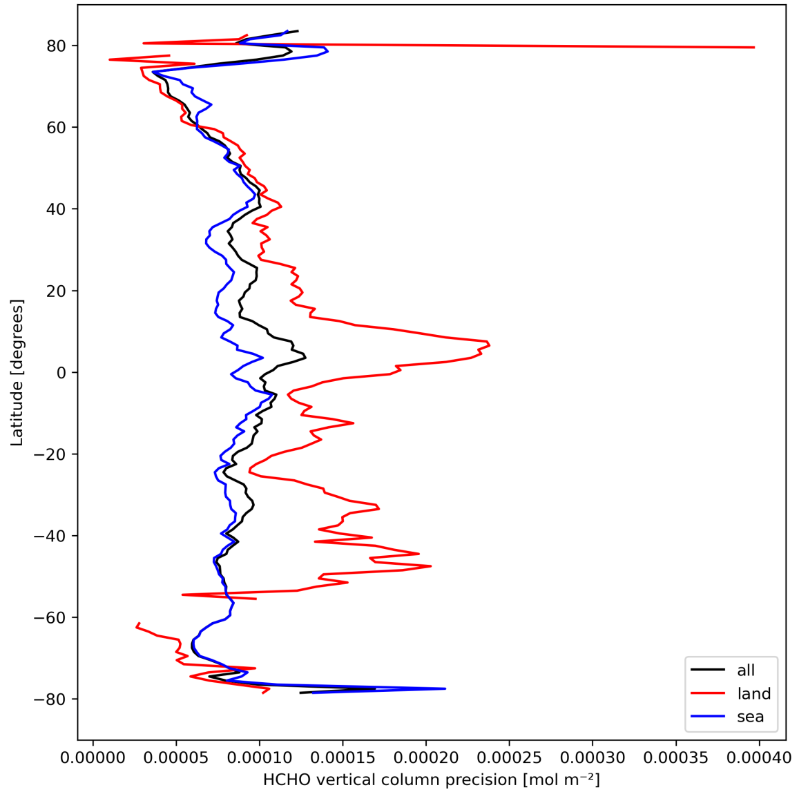
Figure 22: Zonal average of “HCHO vertical column precision” for 2024-03-25 to 2024-03-26.
