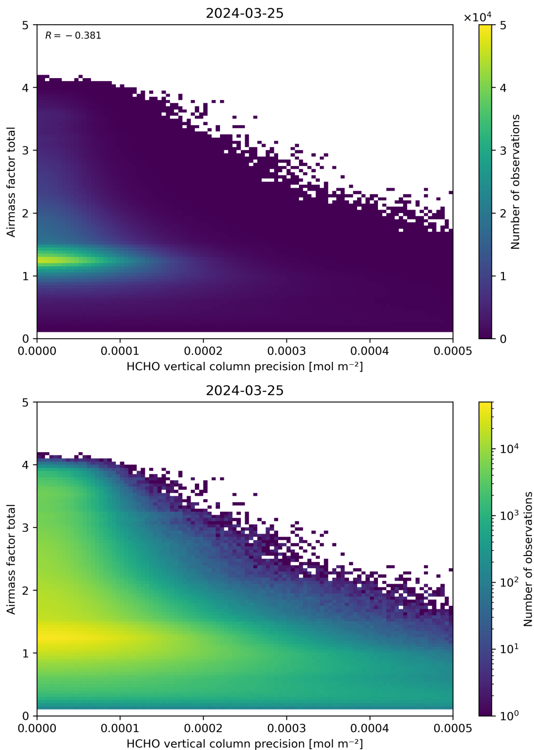
Figure 144: Scatter density plot of “HCHO vertical column precision” against “Airmass factor total” for 2024-03-25 to 2024-03-26.
