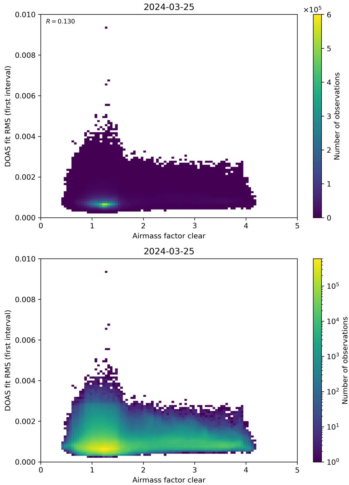
Figure 71: Scatter density plot of “Airmass factor clear” against “DOAS fit RMS (first interval)” for 2024-03-25 to 2024-03-26.
