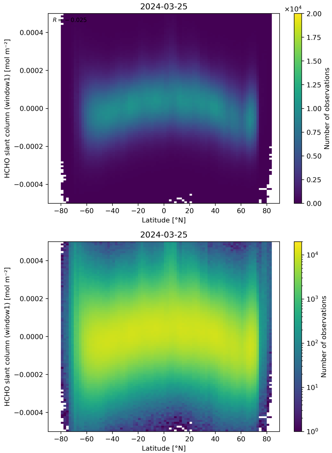
Figure 159: Scatter density plot of “Latitude” against “HCHO slant column (window1)” for 2024-03-25 to 2024-03-26.
