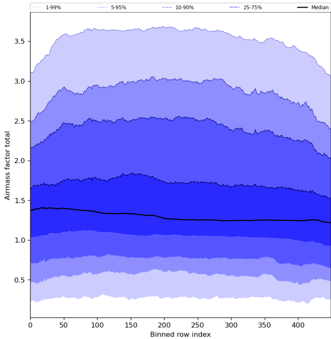
Figure 54: Along track statistics of “Airmass factor total” for 2024-03-25 to 2024-03-26
