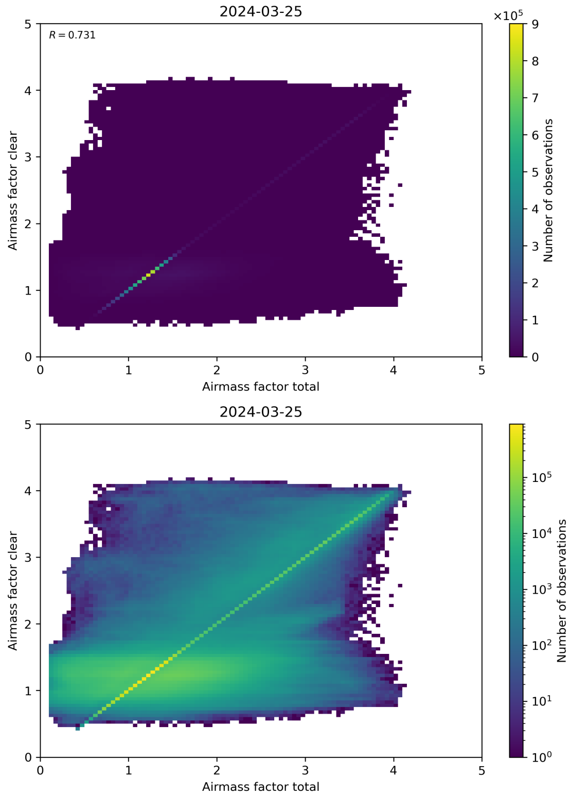
Figure 100: Scatter density plot of “Airmass factor total” against “Airmass factor clear” for 2024-03-25 to 2024-03-26.
