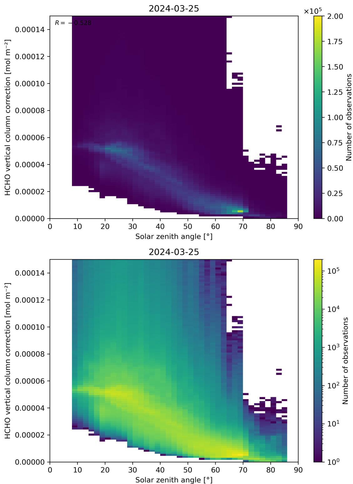
Figure 178: Scatter density plot of “Solar zenith angle” against “HCHO vertical column correction” for 2024-03-25 to 2024-03-26.
