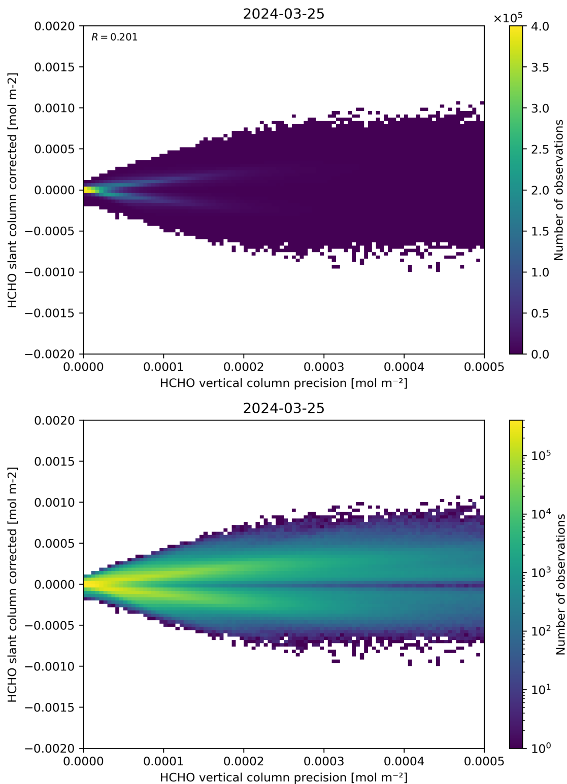
Figure 140: Scatter density plot of “HCHO vertical column precision” against “HCHO slant column corrected” for 2024-03-25 to 2024-03-26.
