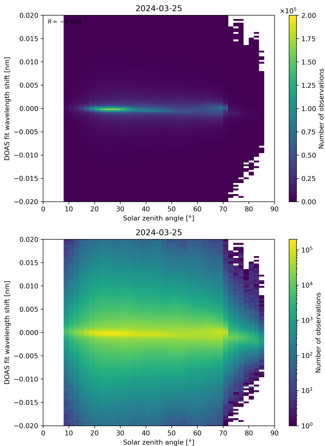
Figure 168: Scatter density plot of “Solar zenith angle” against “DOAS fit wavelength shift” for 2024-03-25 to 2024-03-26.
