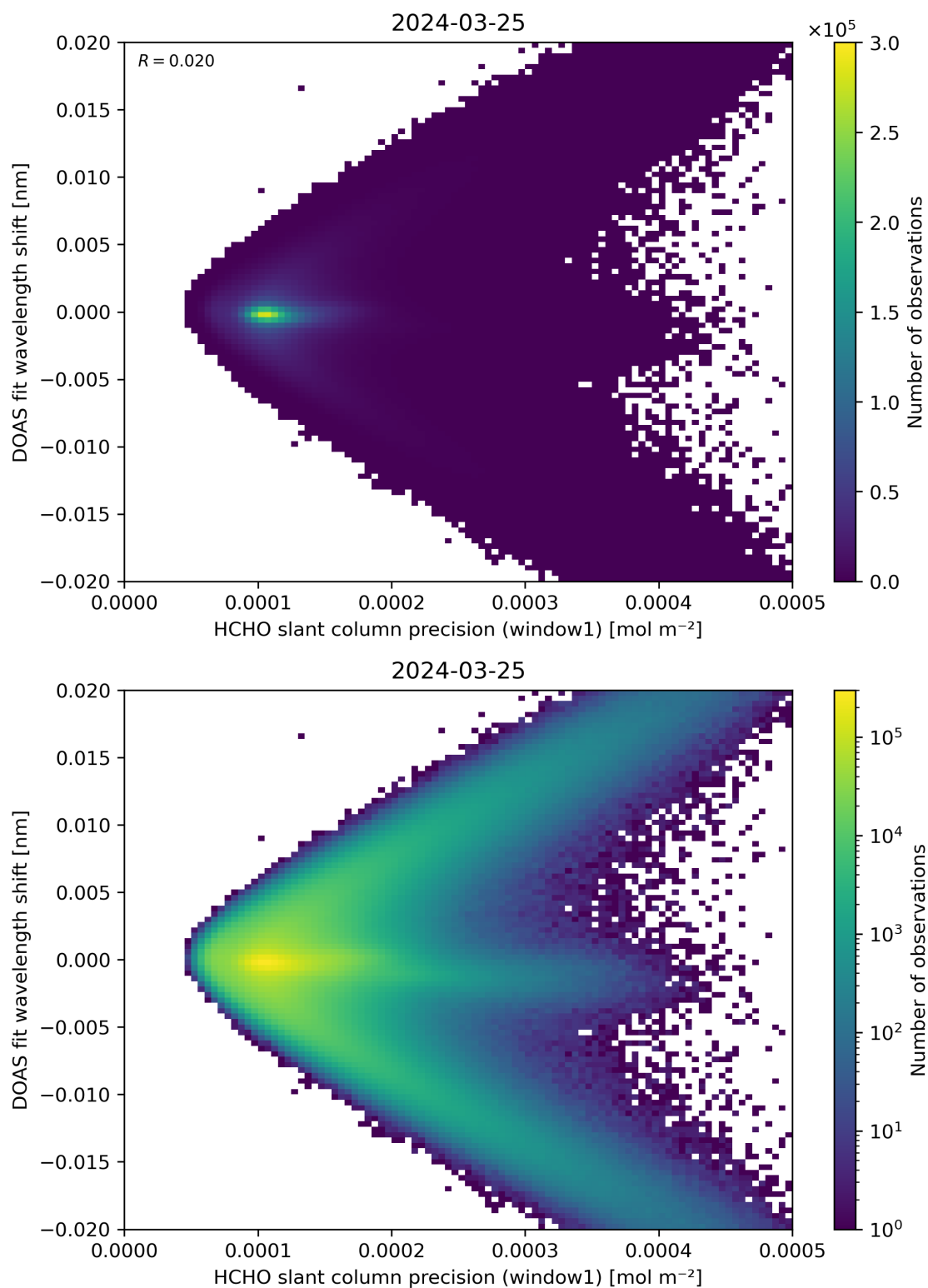
Figure 89: Scatter density plot of “HCHO slant column precision (window1)” against “DOAS fit wavelength shift” for 2024-03-25 to 2024-03-26.
