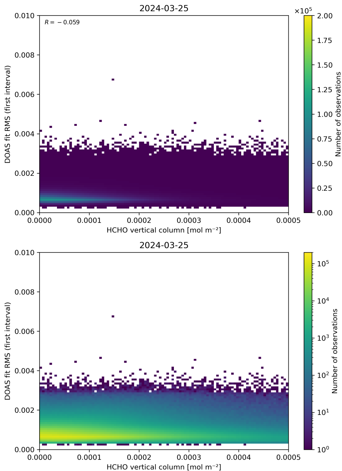
Figure 123: Scatter density plot of “HCHO vertical column” against “DOAS fit RMS (first interval)” for 2024-03-25 to 2024-03-26.
