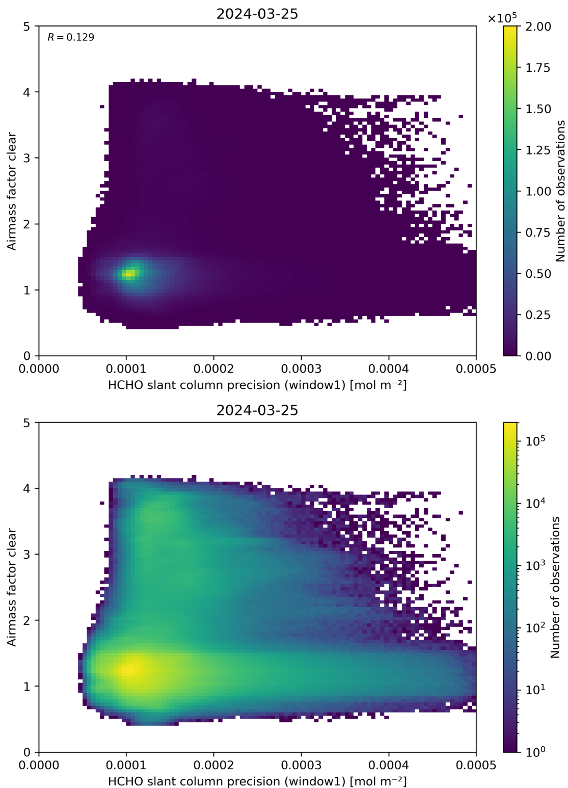
Figure 91: Scatter density plot of “HCHO slant column precision (window1)” against “Airmass factor clear” for 2024-03-25 to 2024-03-26.
