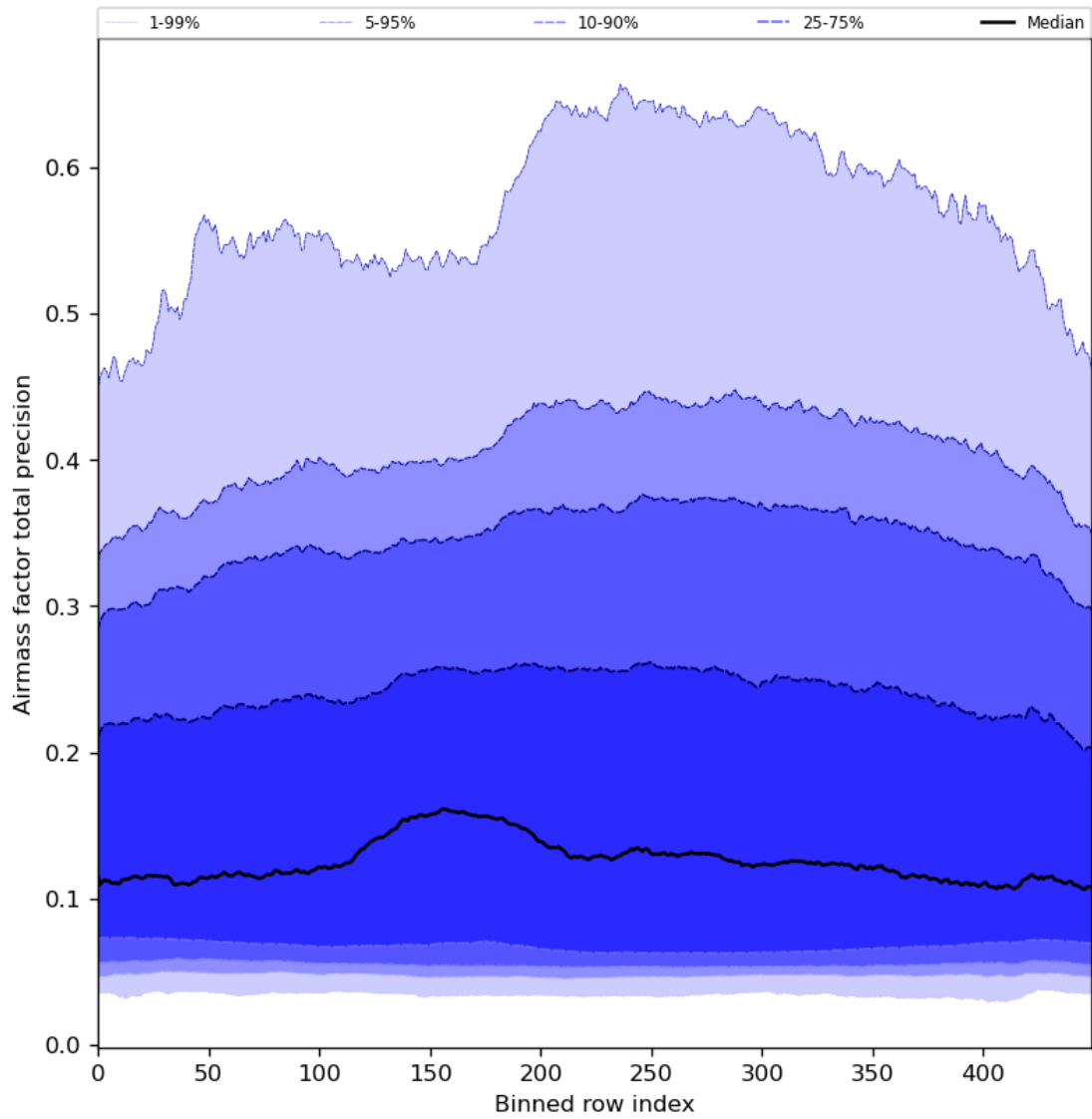
Figure 55: Along track statistics of “Airmass factor total precision” for 2024-03-25 to 2024-03-26
