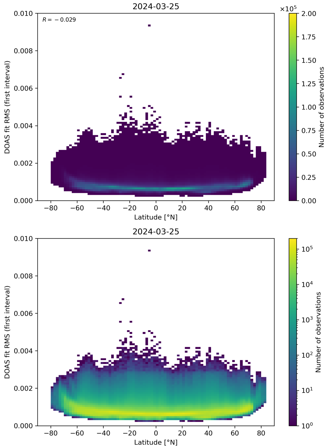
Figure 153: Scatter density plot of “Latitude” against “DOAS fit RMS (first interval)” for 2024-03-25 to 2024-03-26.
