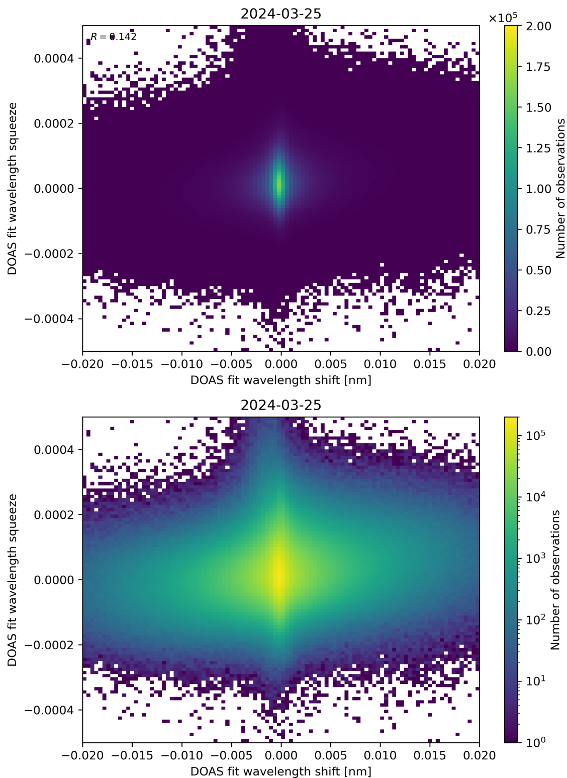
Figure 65: Scatter density plot of “DOAS fit wavelength shift” against “DOAS fit wavelength squeeze” for 2024-03-25 to 2024-03-26.
