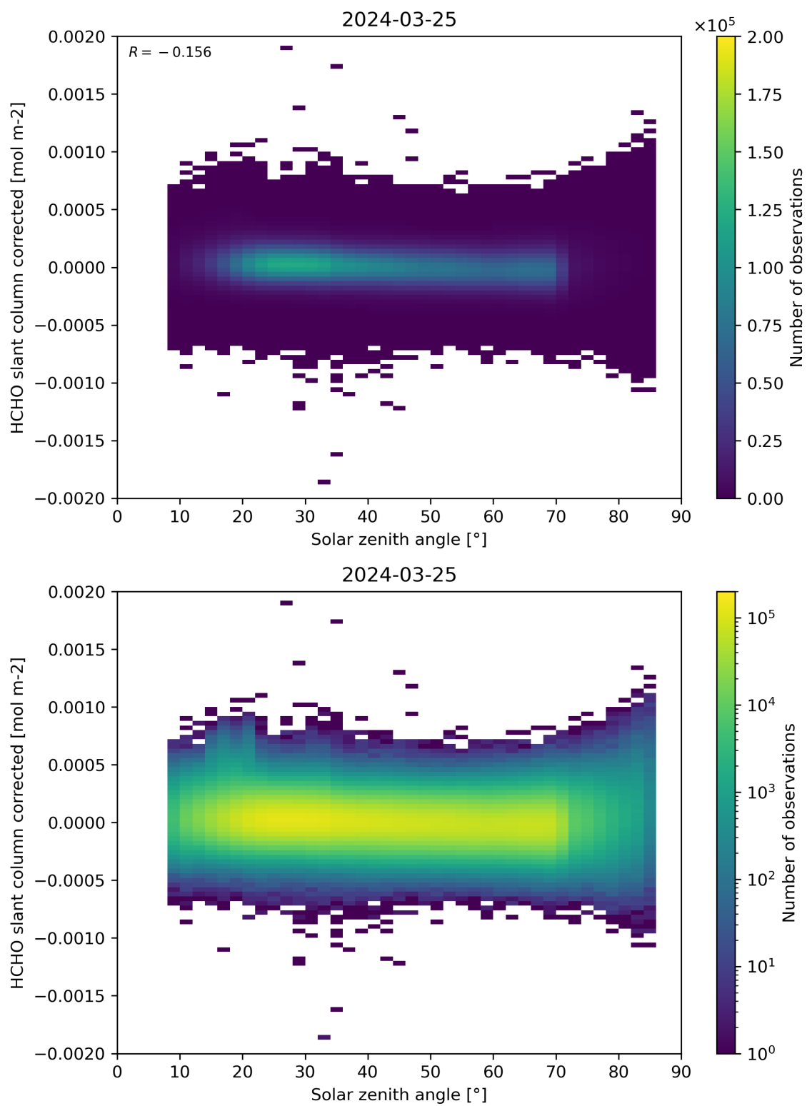
Figure 171: Scatter density plot of “Solar zenith angle” against “HCHO slant column corrected” for 2024-03-25 to 2024-03-26.
