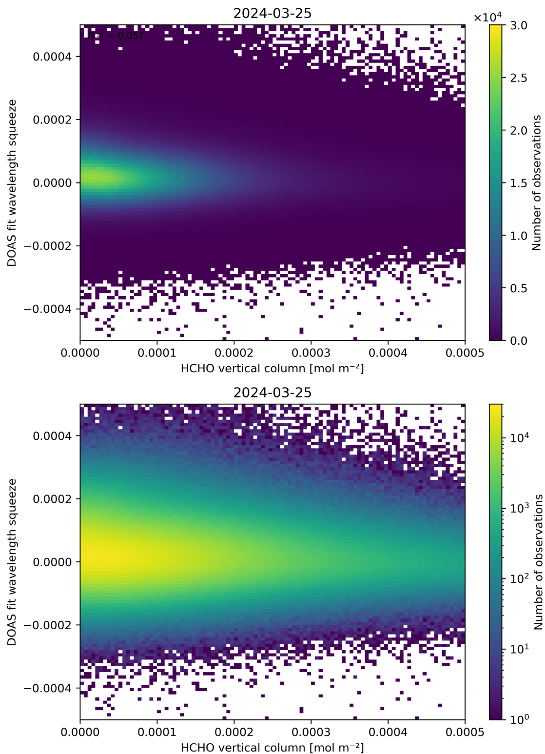
Figure 125: Scatter density plot of “HCHO vertical column” against “DOAS fit wavelength squeeze” for 2024-03-25 to 2024-03-26.
