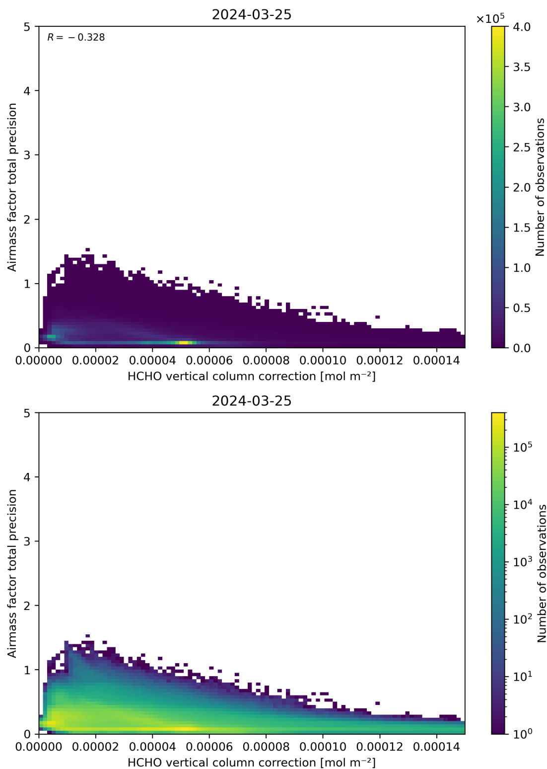
Figure 121: Scatter density plot of “HCHO vertical column correction” against “Airmass factor total precision” for 2024-03-25 to 2024-03-26.
