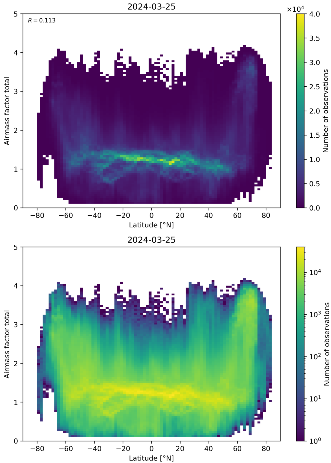
Figure 161: Scatter density plot of “Latitude” against “Airmass factor total” for 2024-03-25 to 2024-03-26.
