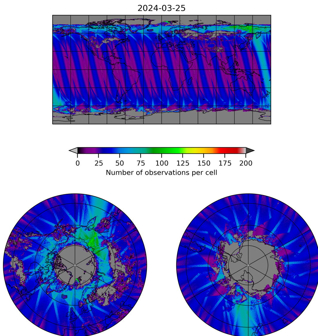
Figure 19: Map of the number of observations for 2024-03-25 to 2024-03-26
