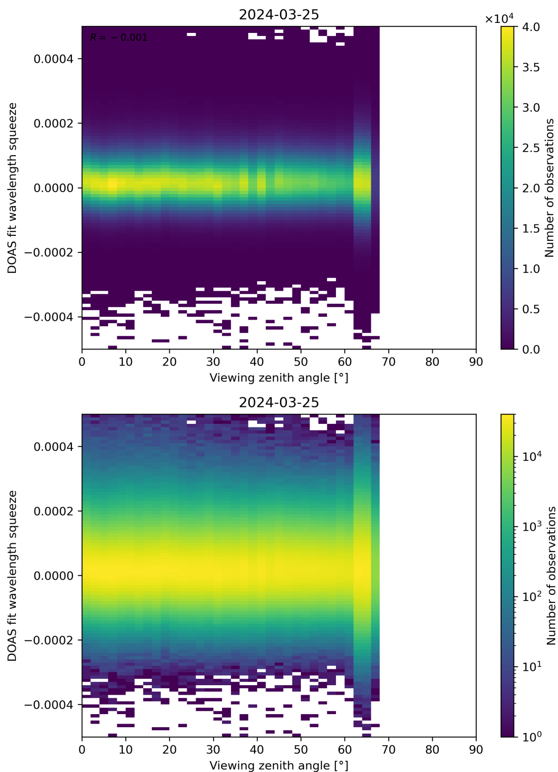
Figure 184: Scatter density plot of “Viewing zenith angle” against “DOAS fit wavelength squeeze” for 2024-03-25 to 2024-03-26.
