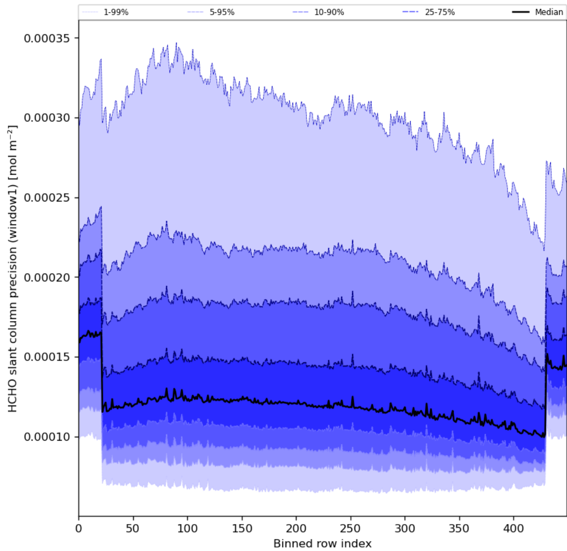
Figure 53: Along track statistics of “HCHO slant column precision (window1)” for 2024-03-25 to 2024-03-26
