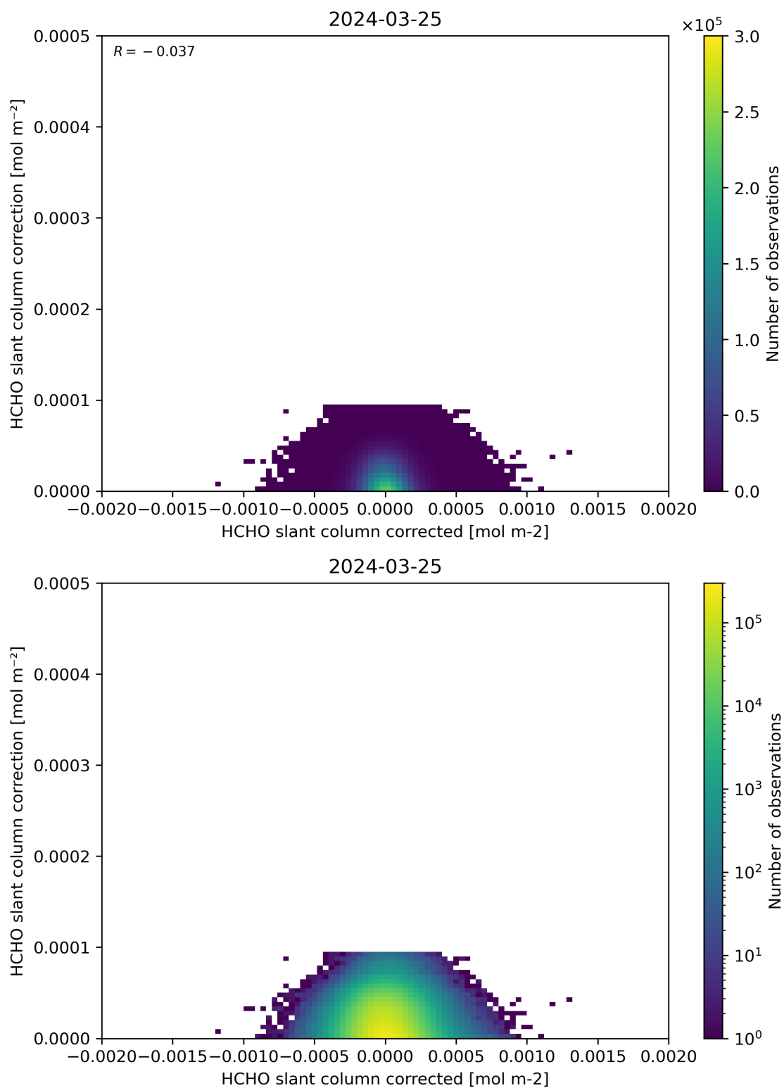
Figure 77: Scatter density plot of “HCHO slant column corrected” against “HCHO slant column correction” for 2024-03-25 to 2024-03-26.
