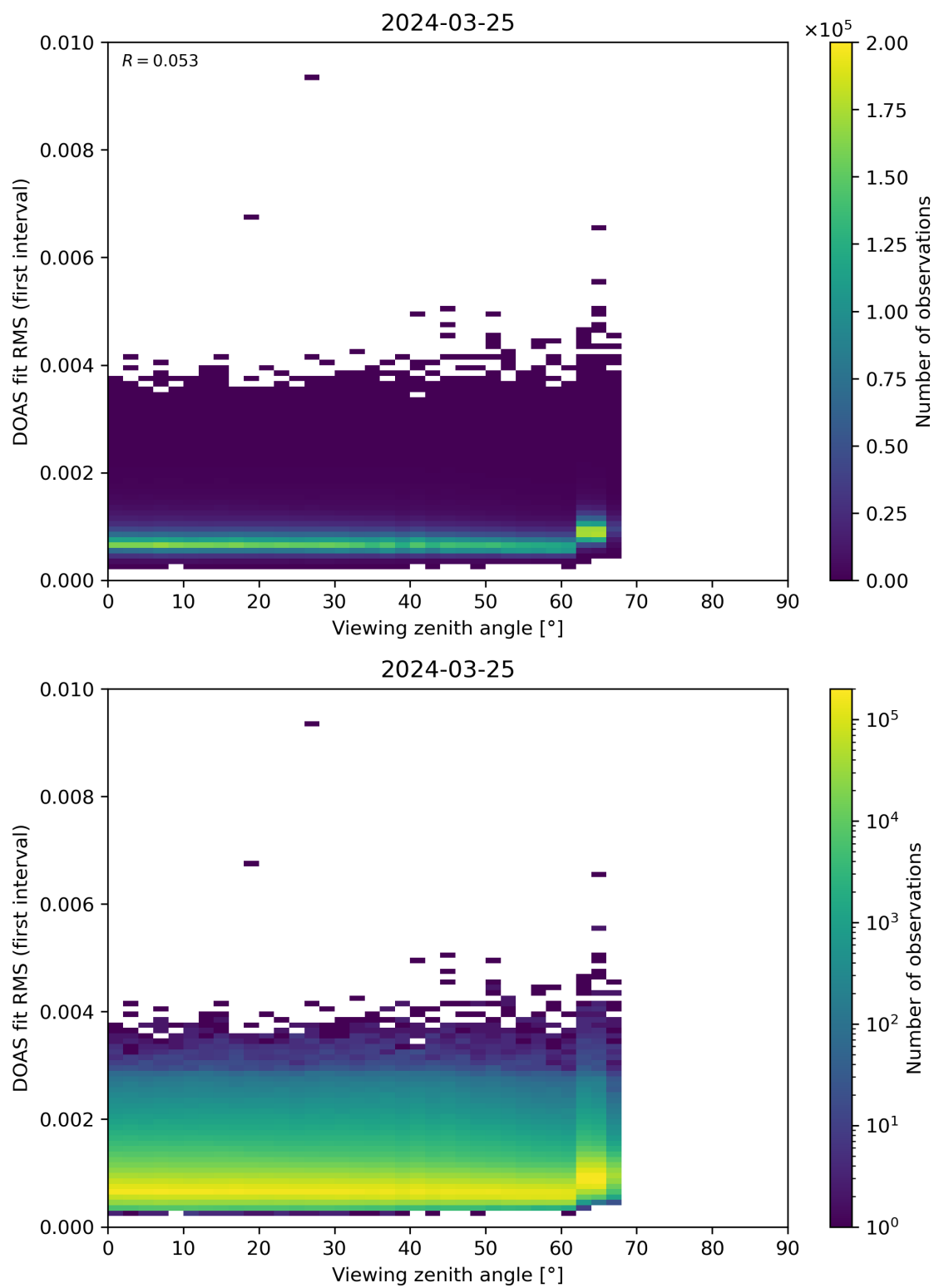
Figure 182: Scatter density plot of “Viewing zenith angle” against “DOAS fit RMS (first interval)” for 2024-03-25 to 2024-03-26.
