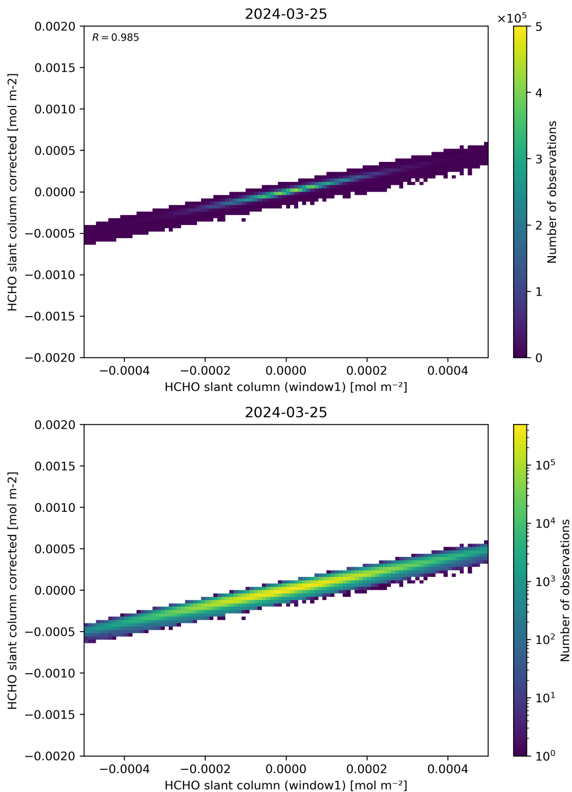
Figure 82: Scatter density plot of “HCHO slant column (window1)” against “HCHO slant column corrected” for 2024-03-25 to 2024-03-26.
