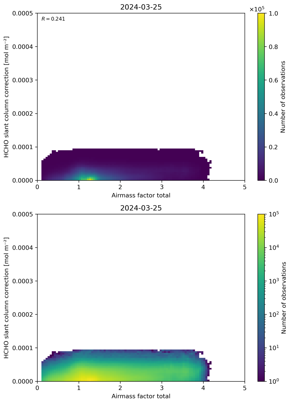
Figure 102: Scatter density plot of “Airmass factor total” against “HCHO slant column correction” for 2024-03-25 to 2024-03-26.
