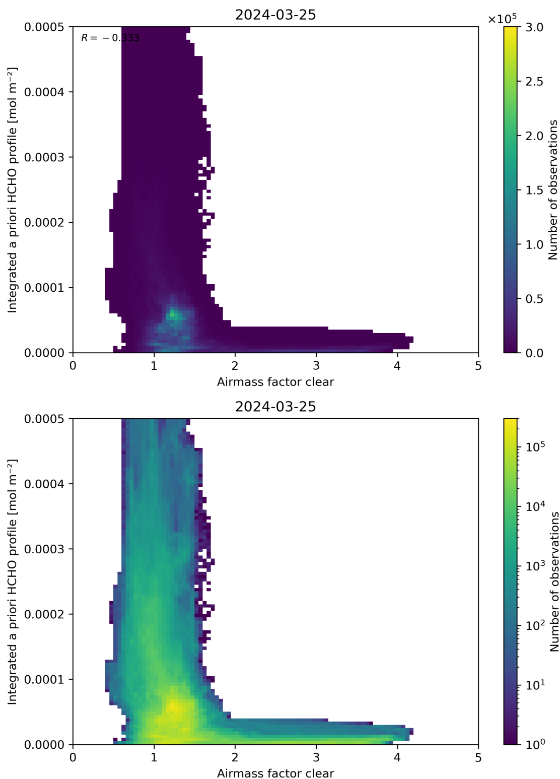
Figure 76: Scatter density plot of “Airmass factor clear” against “Integrated a priori HCHO profile” for 2024-03-25 to 2024-03-26.
