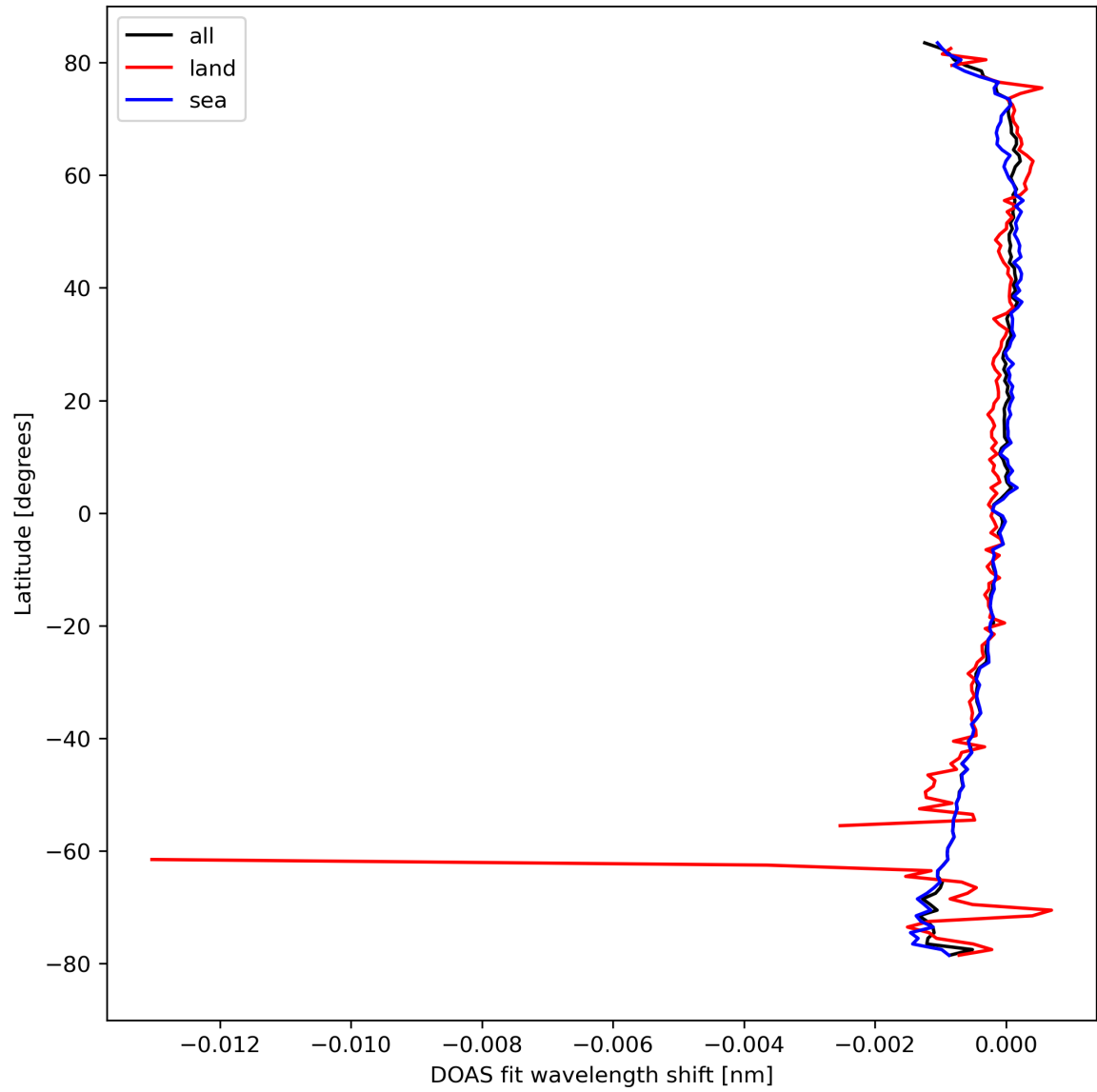
Figure 30: Zonal average of “DOAS fit wavelength shift” for 2024-03-25 to 2024-03-26.
