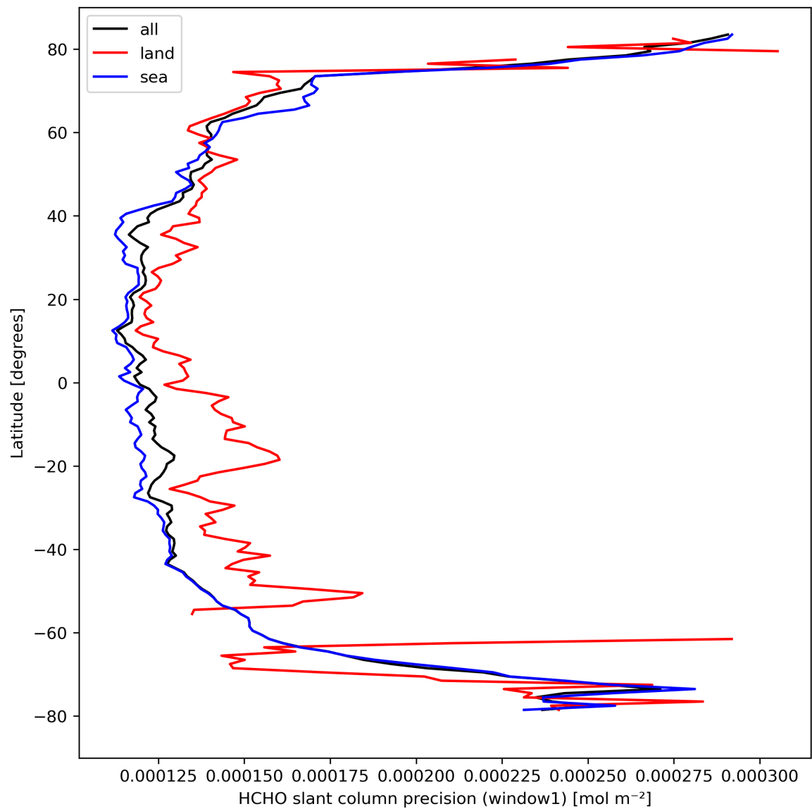
Figure 25: Zonal average of “HCHO slant column precision (window1)” for 2024-03-25 to 2024-03-26.
