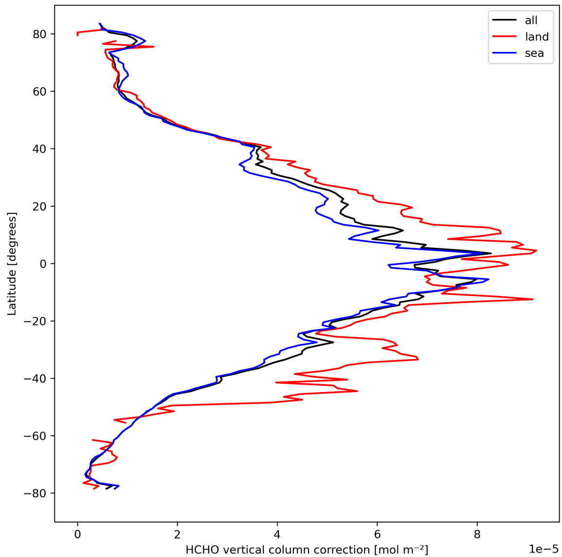
Figure 23: Zonal average of “HCHO vertical column correction” for 2024-03-25 to 2024-03-26.
