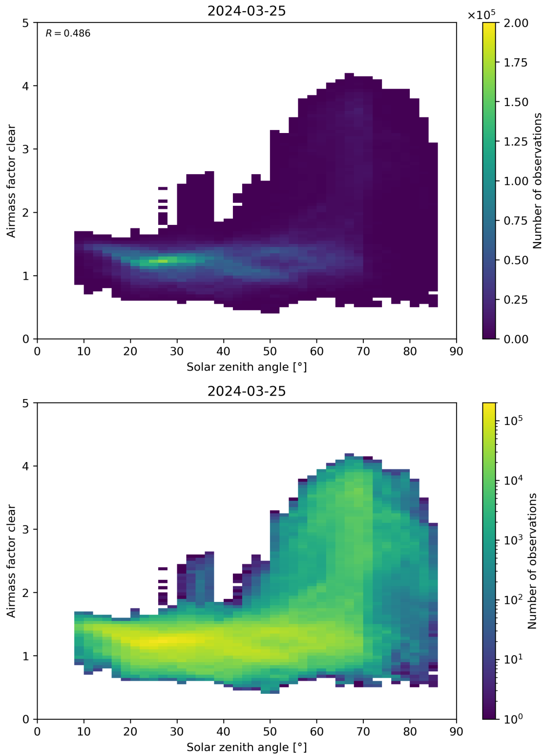
Figure 170: Scatter density plot of “Solar zenith angle” against “Airmass factor clear” for 2024-03-25 to 2024-03-26.
