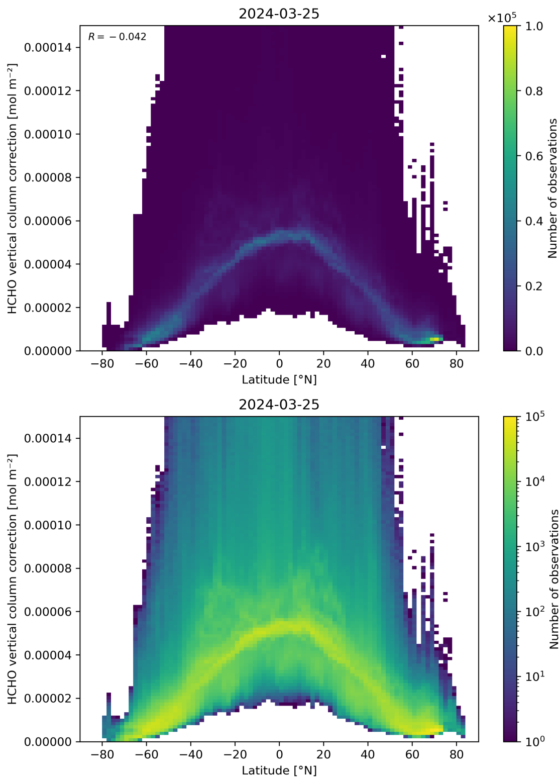
Figure 164: Scatter density plot of “Latitude” against “HCHO vertical column correction” for 2024-03-25 to 2024-03-26.
