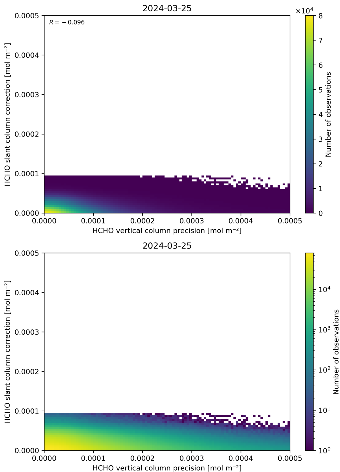
Figure 141: Scatter density plot of “HCHO vertical column precision” against “HCHO slant column correction” for 2024-03-25 to 2024-03-26.
