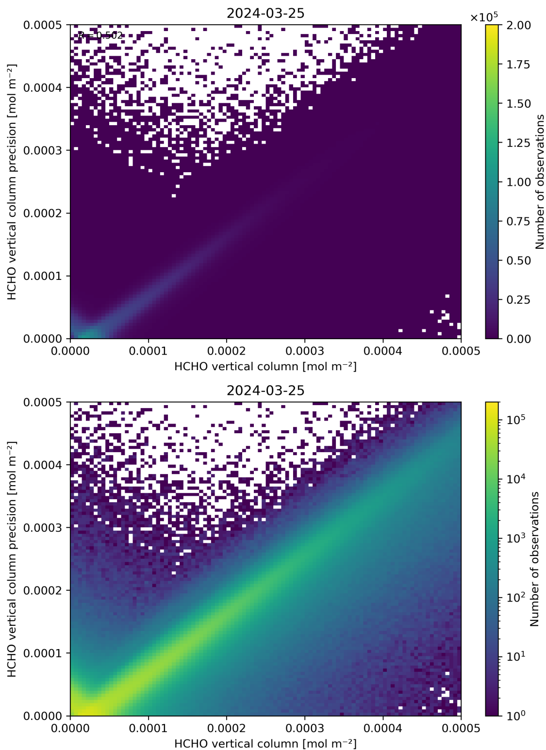
Figure 134: Scatter density plot of “HCHO vertical column” against “HCHO vertical column precision” for 2024-03-25 to 2024-03-26.
