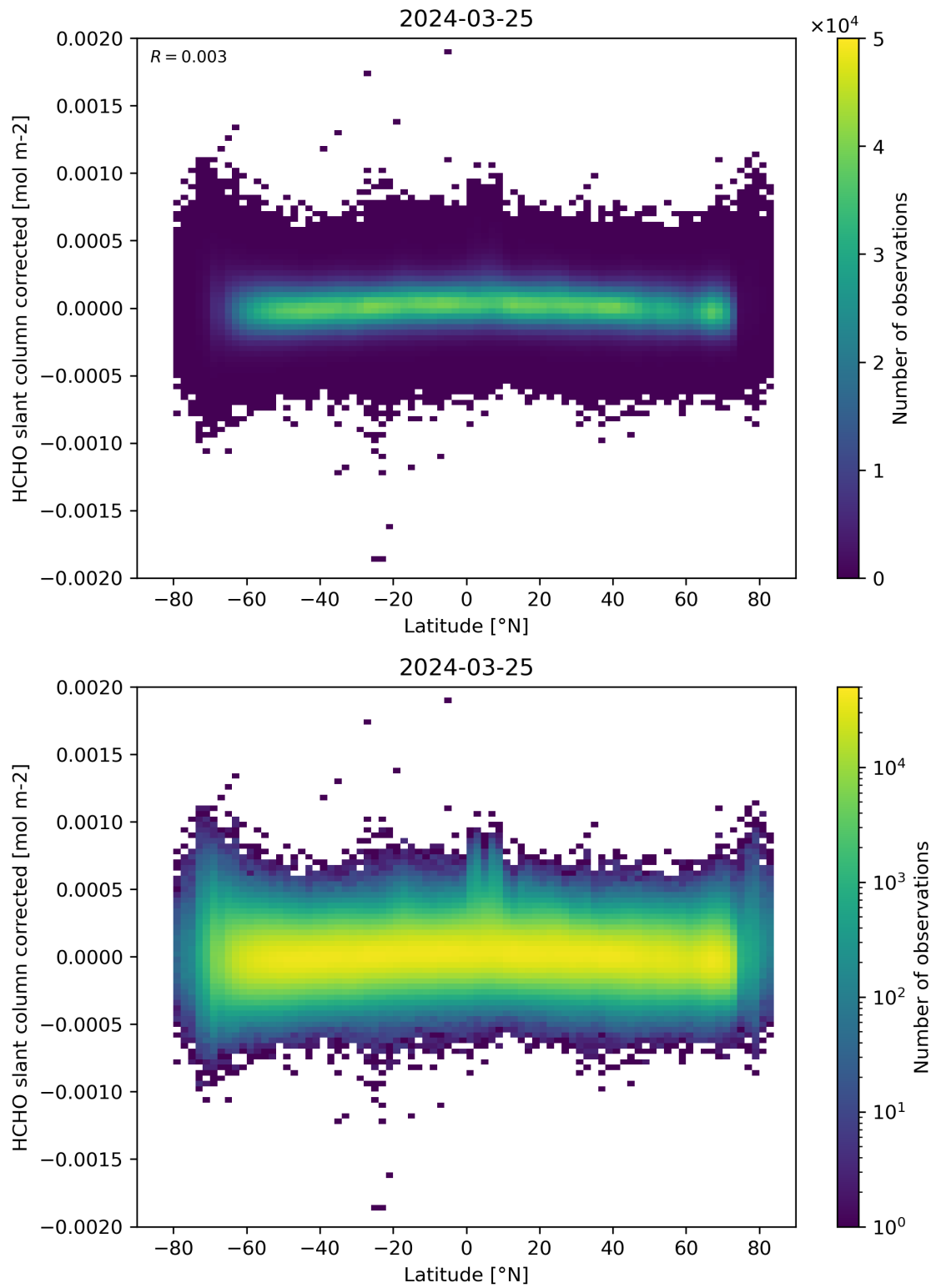
Figure 157: Scatter density plot of “Latitude” against “HCHO slant column corrected” for 2024-03-25 to 2024-03-26.
