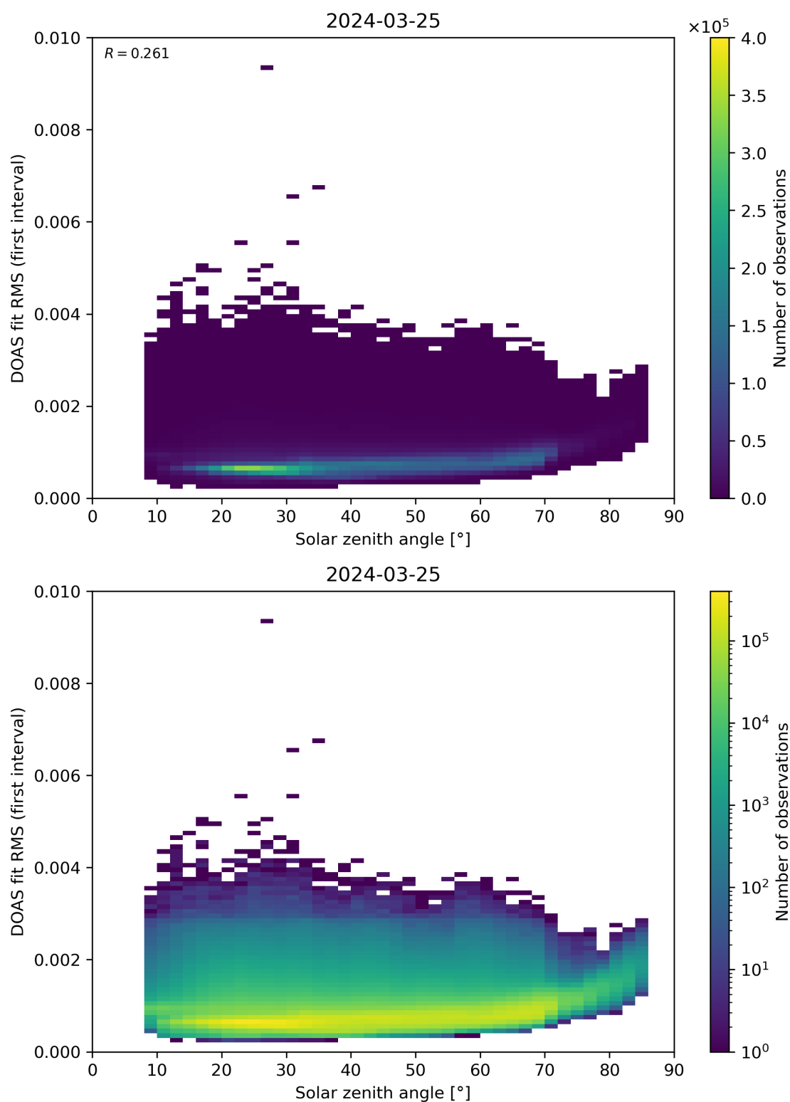
Figure 167: Scatter density plot of “Solar zenith angle” against “DOAS fit RMS (first interval)” for 2024-03-25 to 2024-03-26.
