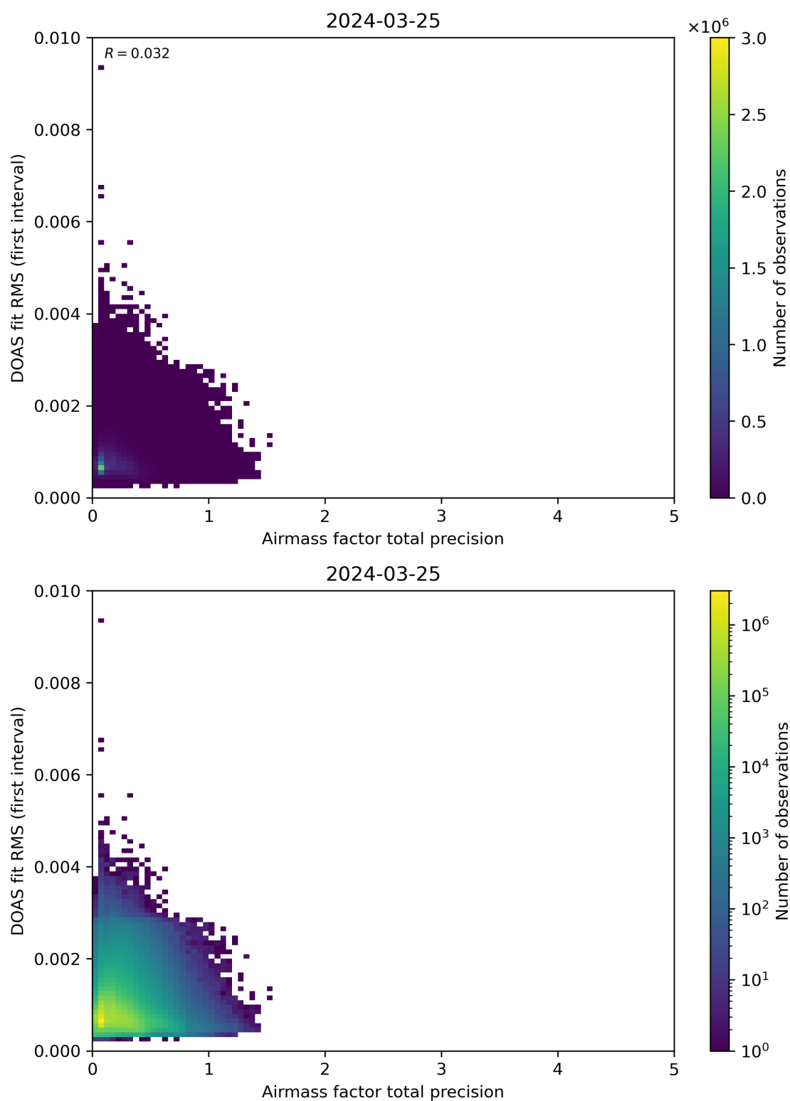
Figure 105: Scatter density plot of “Airmass factor total precision” against “DOAS fit RMS (first interval)” for 2024-03-25 to 2024-03-26.
