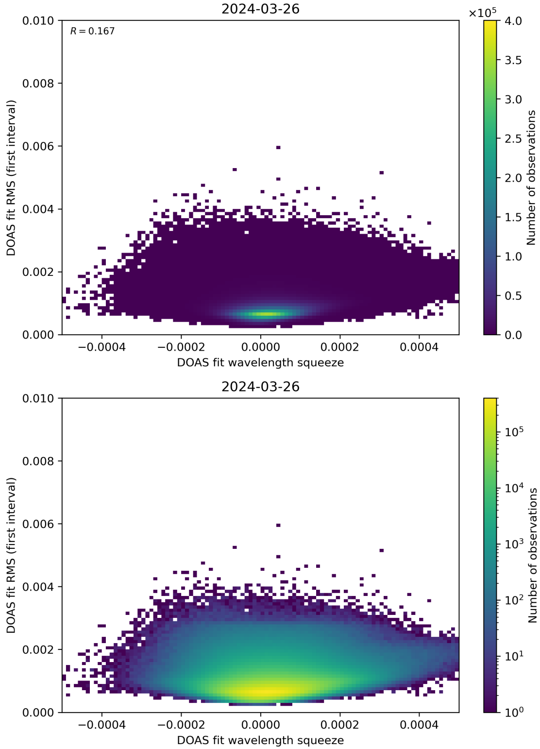
Figure 68: Scatter density plot of “DOAS fit wavelength squeeze” against “DOAS fit RMS (first interval)” for 2024-03-25 to 2024-03-27.
