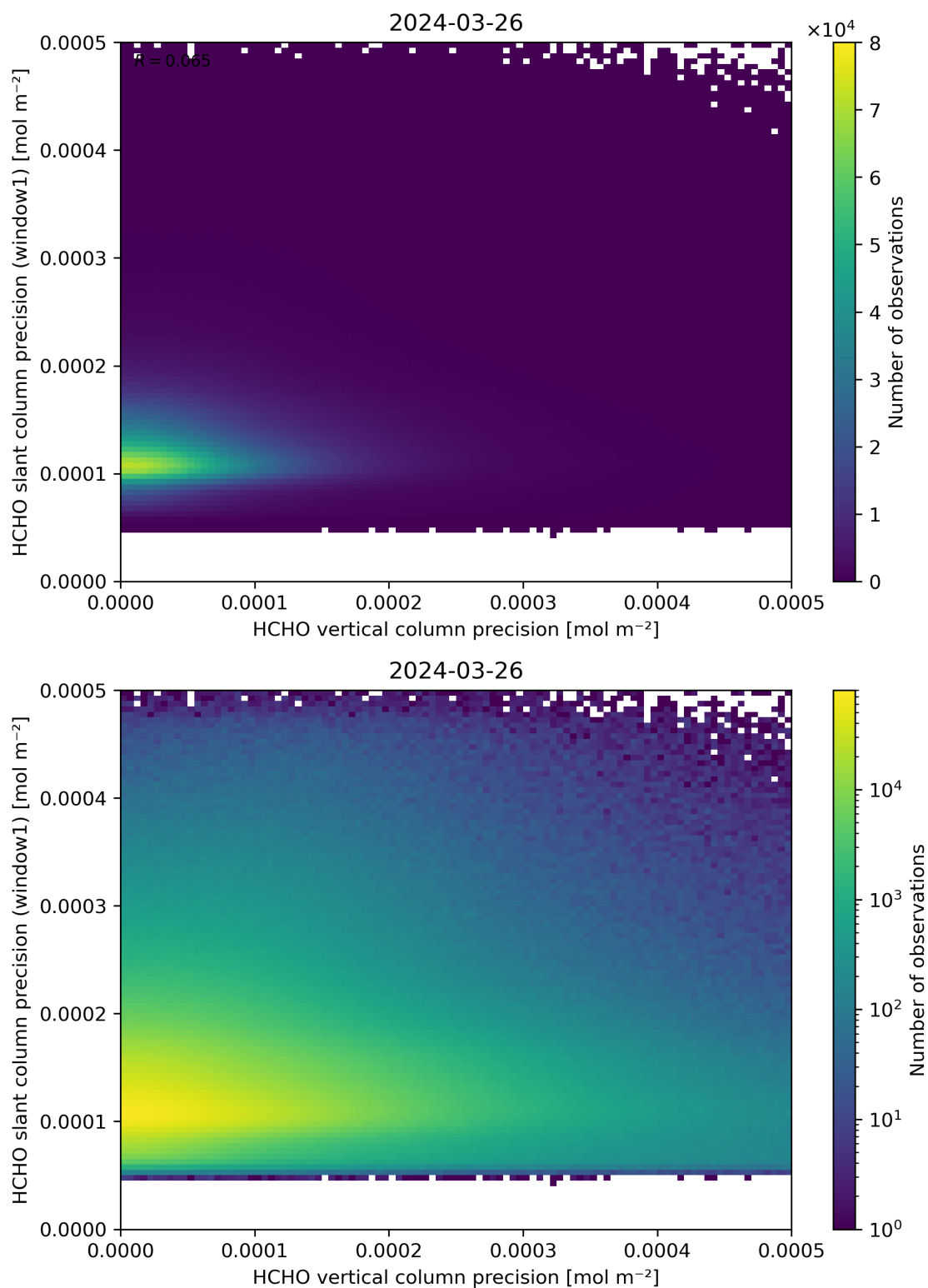
Figure 143: Scatter density plot of “HCHO vertical column precision” against “HCHO slant column precision (window1)” for 2024-03-25 to 2024-03-27.
