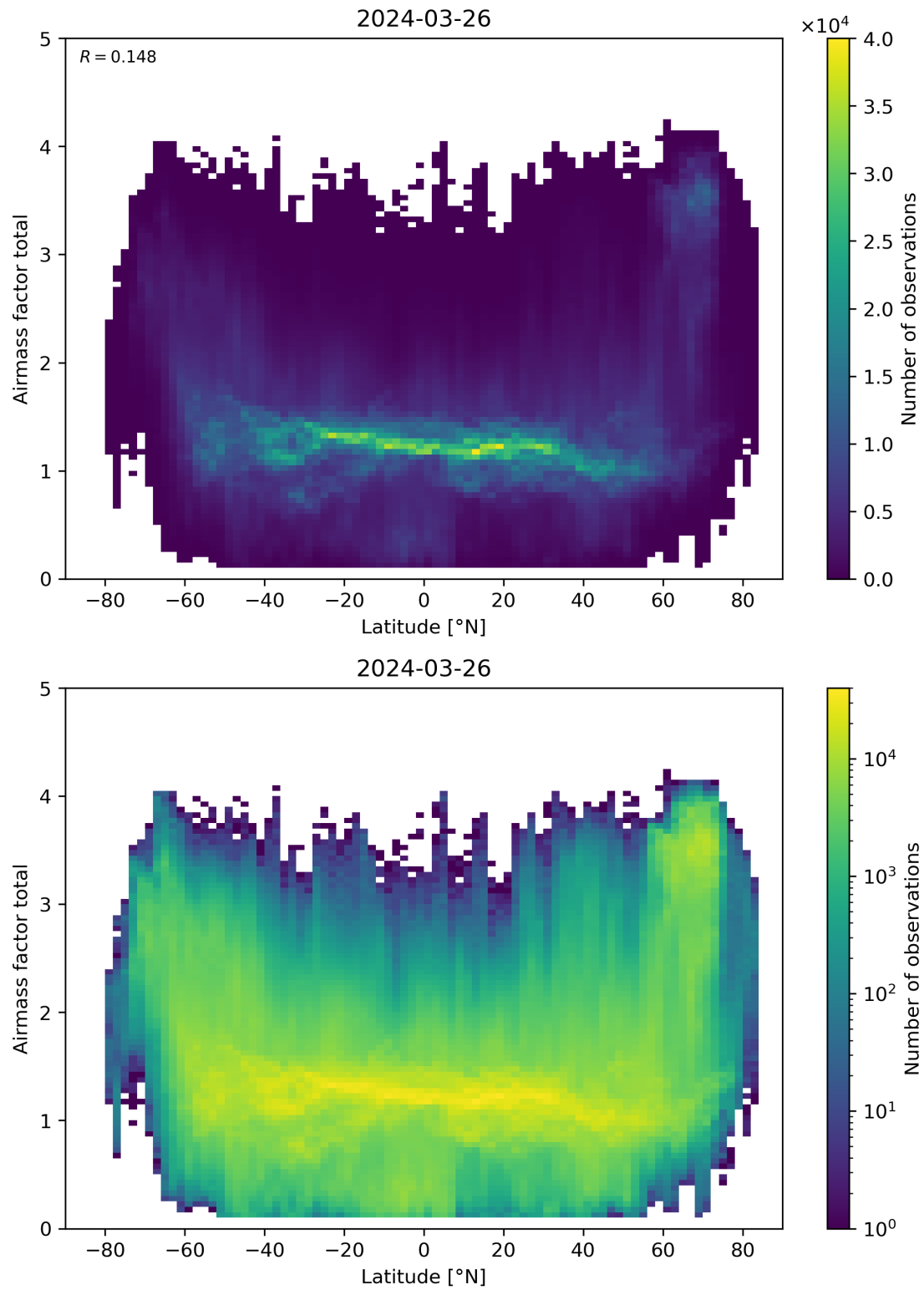
Figure 161: Scatter density plot of “Latitude” against “Airmass factor total” for 2024-03-25 to 2024-03-27.
