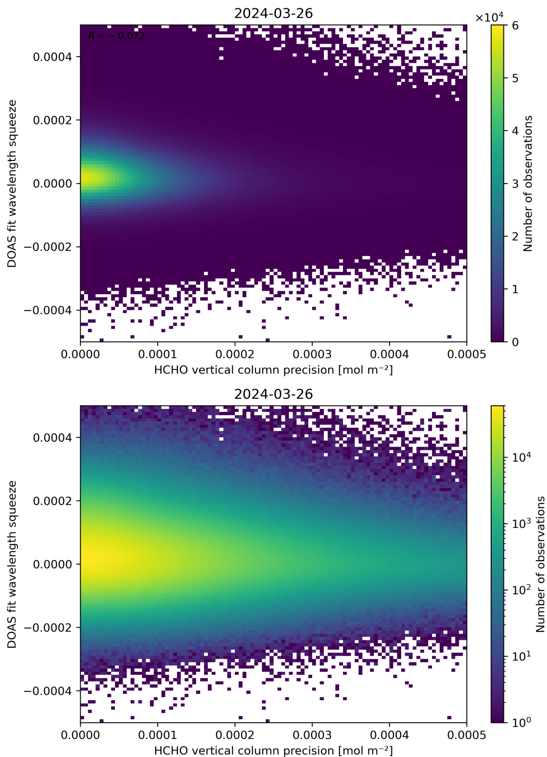
Figure 138: Scatter density plot of “HCHO vertical column precision” against “DOAS fit wavelength squeeze” for 2024-03-25 to 2024-03-27.
