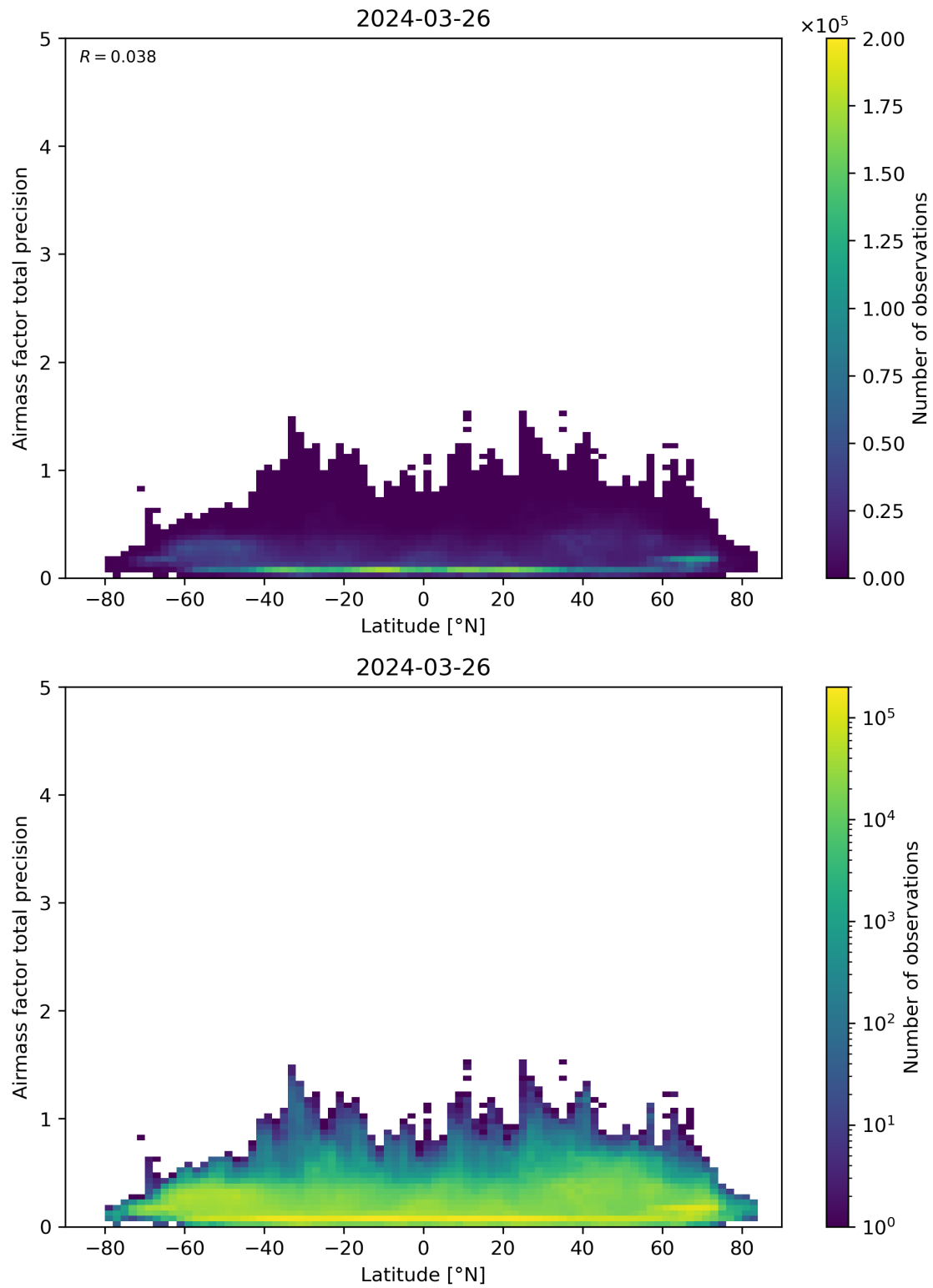
Figure 162: Scatter density plot of “Latitude” against “Airmass factor total precision” for 2024-03-25 to 2024-03-27.
