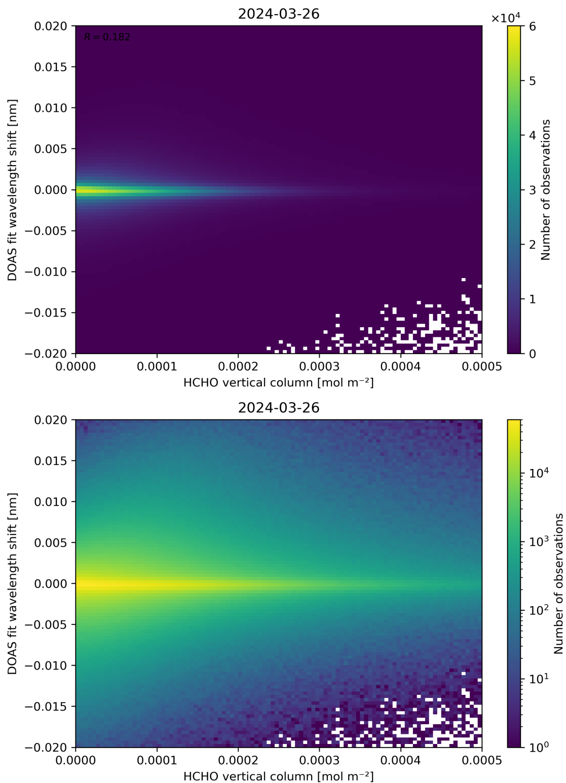
Figure 124: Scatter density plot of “HCHO vertical column” against “DOAS fit wavelength shift” for 2024-03-25 to 2024-03-27.
