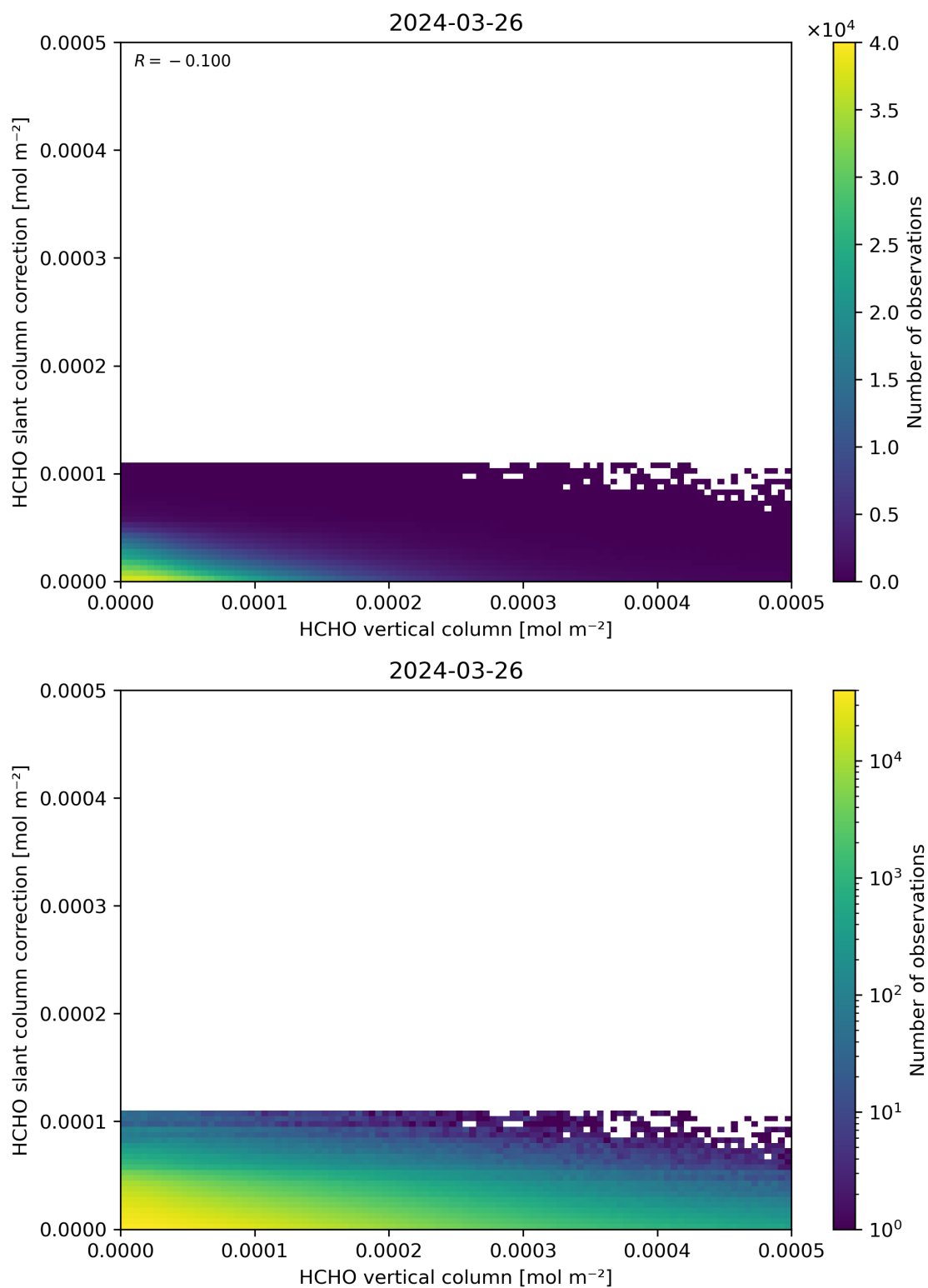
Figure 128: Scatter density plot of “HCHO vertical column” against “HCHO slant column correction” for 2024-03-25 to 2024-03-27.
