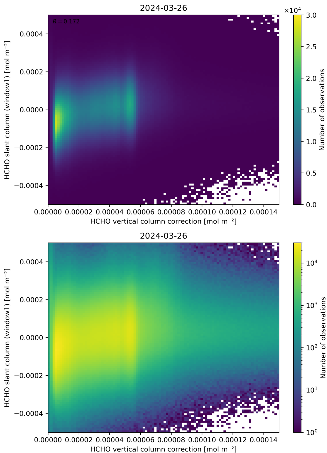
Figure 118: Scatter density plot of “HCHO vertical column correction” against “HCHO slant column (window1)” for 2024-03-25 to 2024-03-27.
