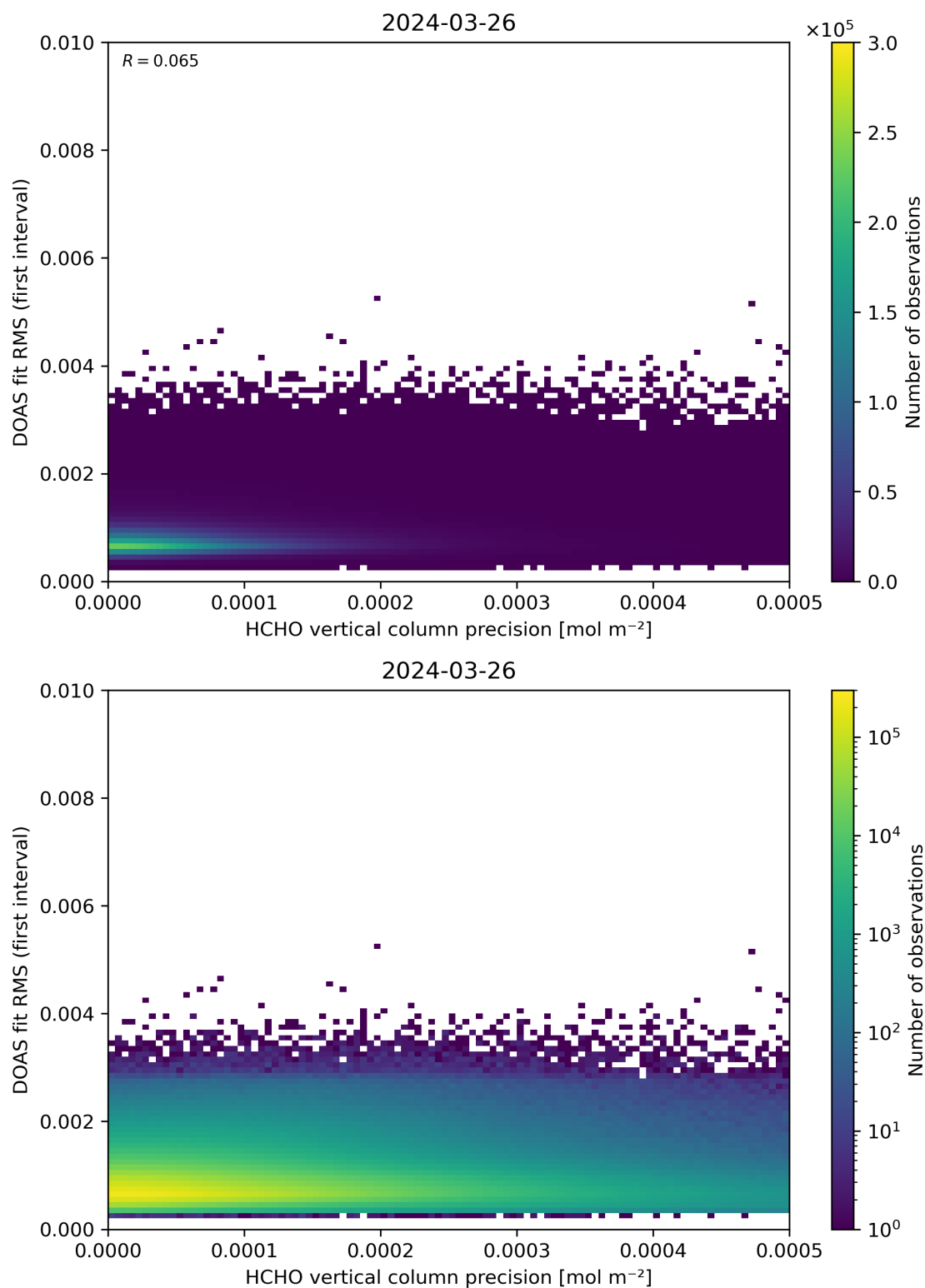
Figure 136: Scatter density plot of “HCHO vertical column precision” against “DOAS fit RMS (first interval)” for 2024-03-25 to 2024-03-27.
