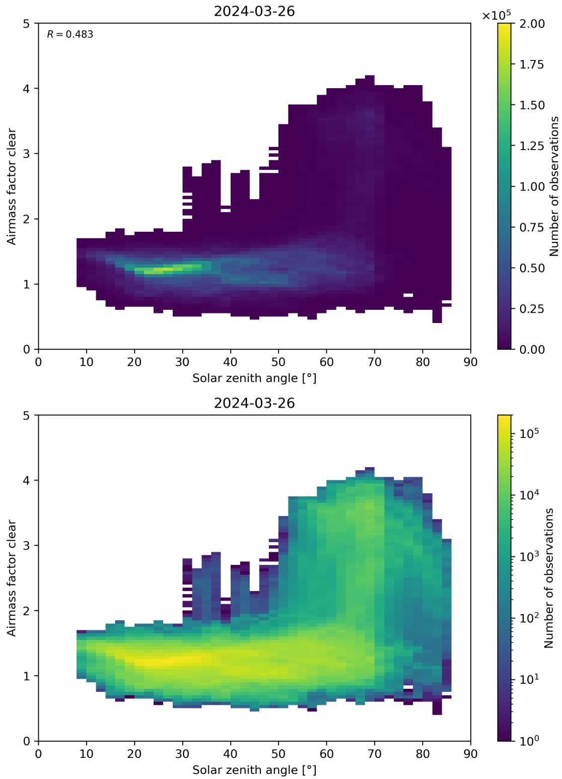
Figure 170: Scatter density plot of “Solar zenith angle” against “Airmass factor clear” for 2024-03-25 to 2024-03-27.
