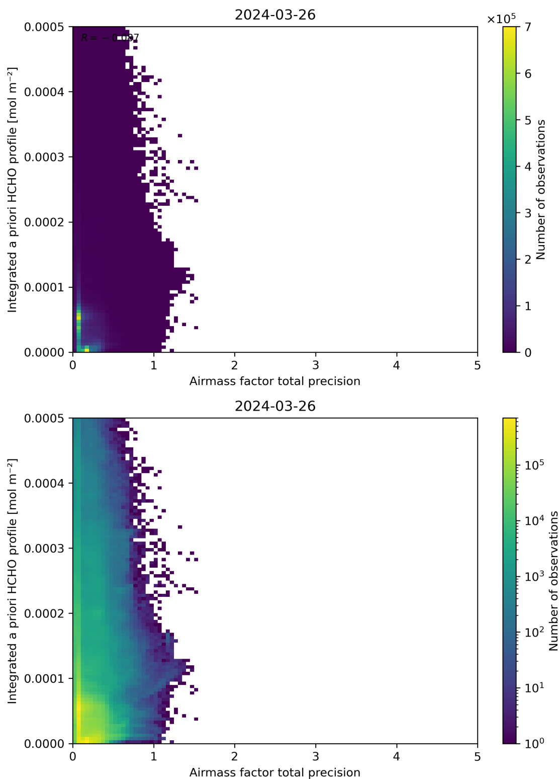
Figure 111: Scatter density plot of “Airmass factor total precision” against “Integrated a priori HCHO profile” for 2024-03-25 to 2024-03-27.
