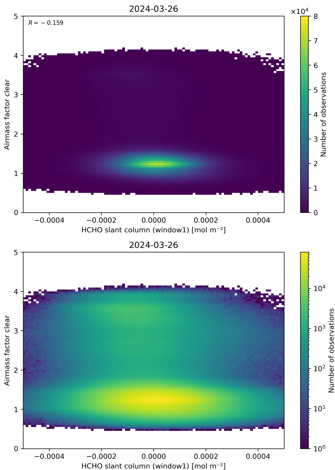
Figure 81: Scatter density plot of “HCHO slant column (window1)” against “Airmass factor clear” for 2024-03-25 to 2024-03-27.
