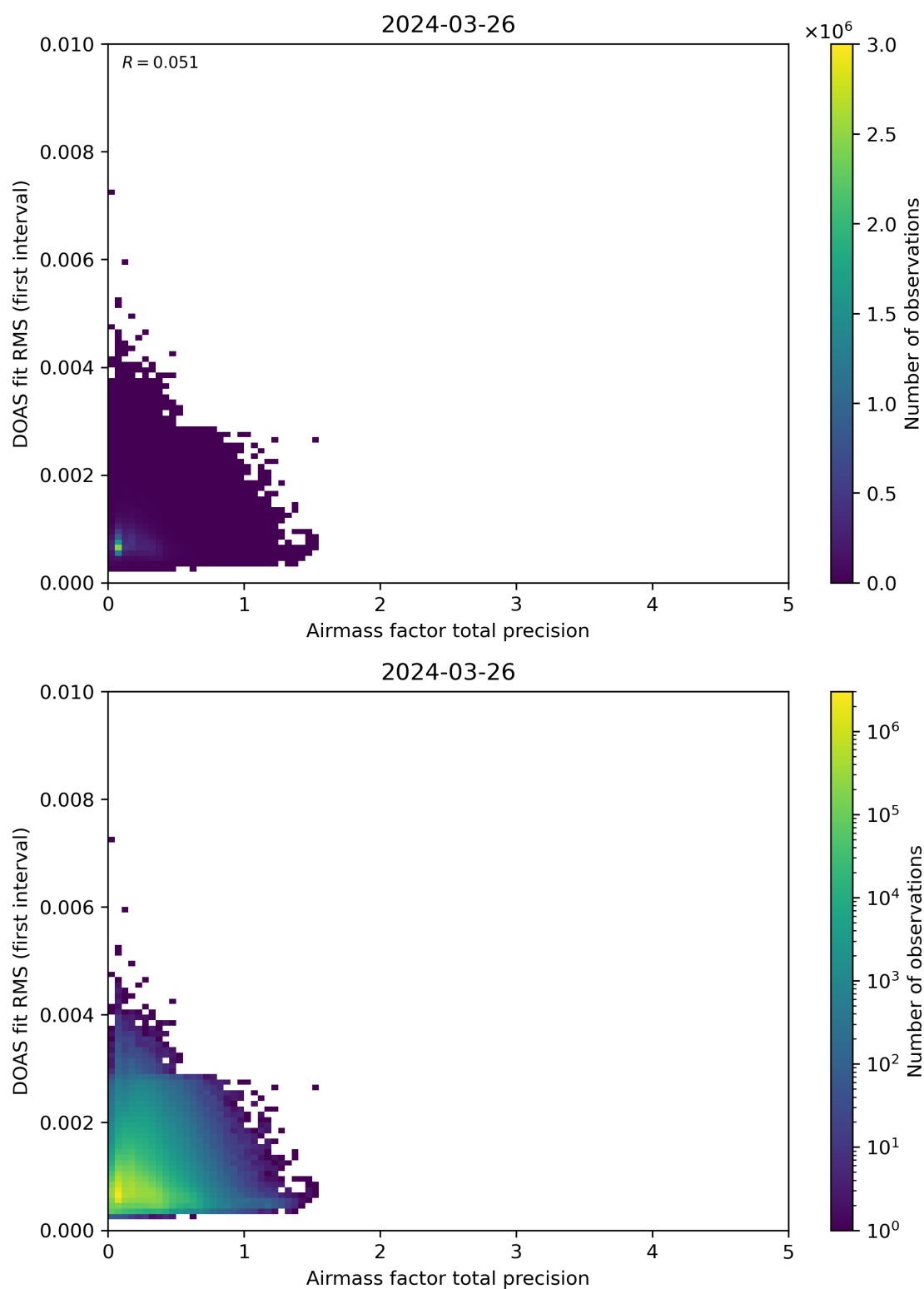
Figure 105: Scatter density plot of “Airmass factor total precision” against “DOAS fit RMS (first interval)” for 2024-03-25 to 2024-03-27.
