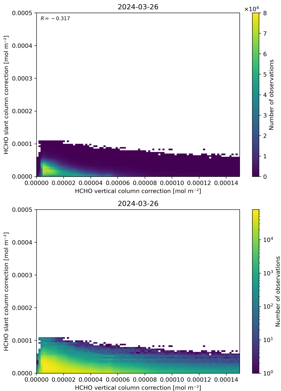
Figure 117: Scatter density plot of “HCHO vertical column correction” against “HCHO slant column correction” for 2024-03-25 to 2024-03-27.
