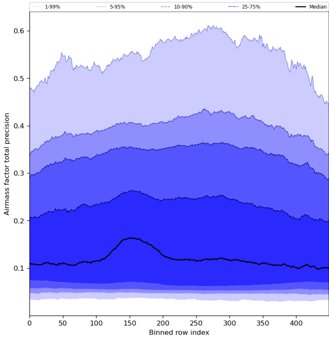
Figure 55: Along track statistics of “Airmass factor total precision” for 2024-03-25 to 2024-03-27
