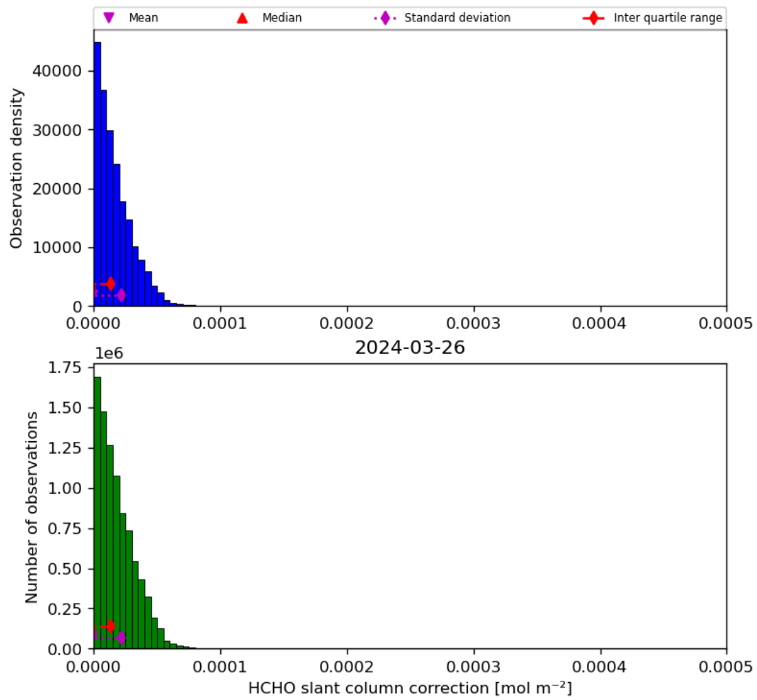
Figure 47: Histogram of “HCHO slant column correction” for 2024-03-25 to 2024-03-27
