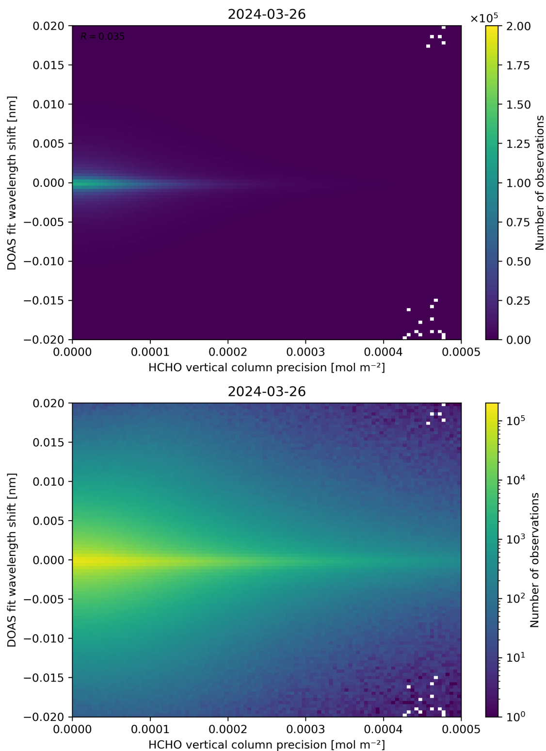
Figure 137: Scatter density plot of “HCHO vertical column precision” against “DOAS fit wavelength shift” for 2024-03-25 to 2024-03-27.
