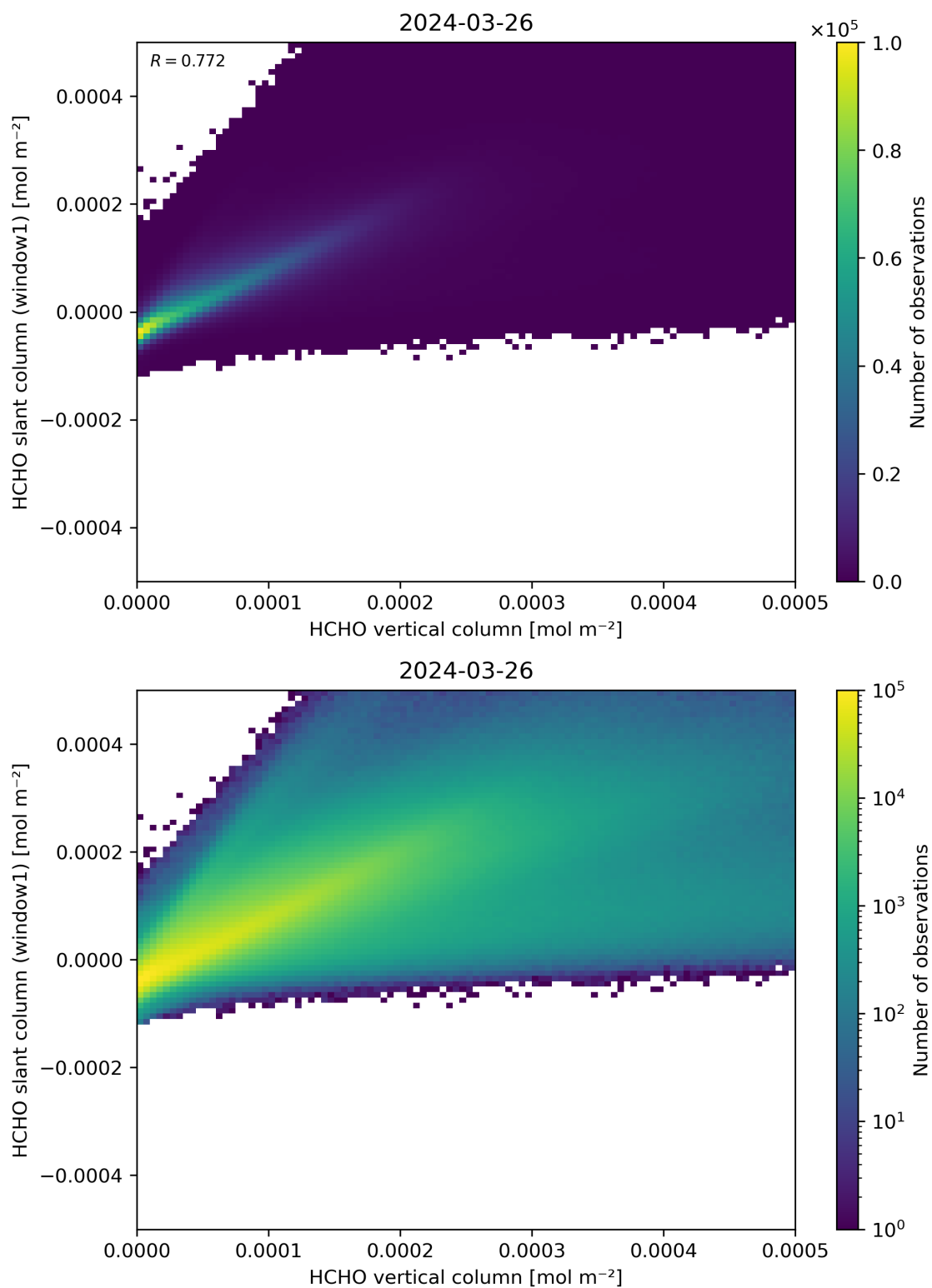
Figure 129: Scatter density plot of “HCHO vertical column” against “HCHO slant column (window1)” for 2024-03-25 to 2024-03-27.
