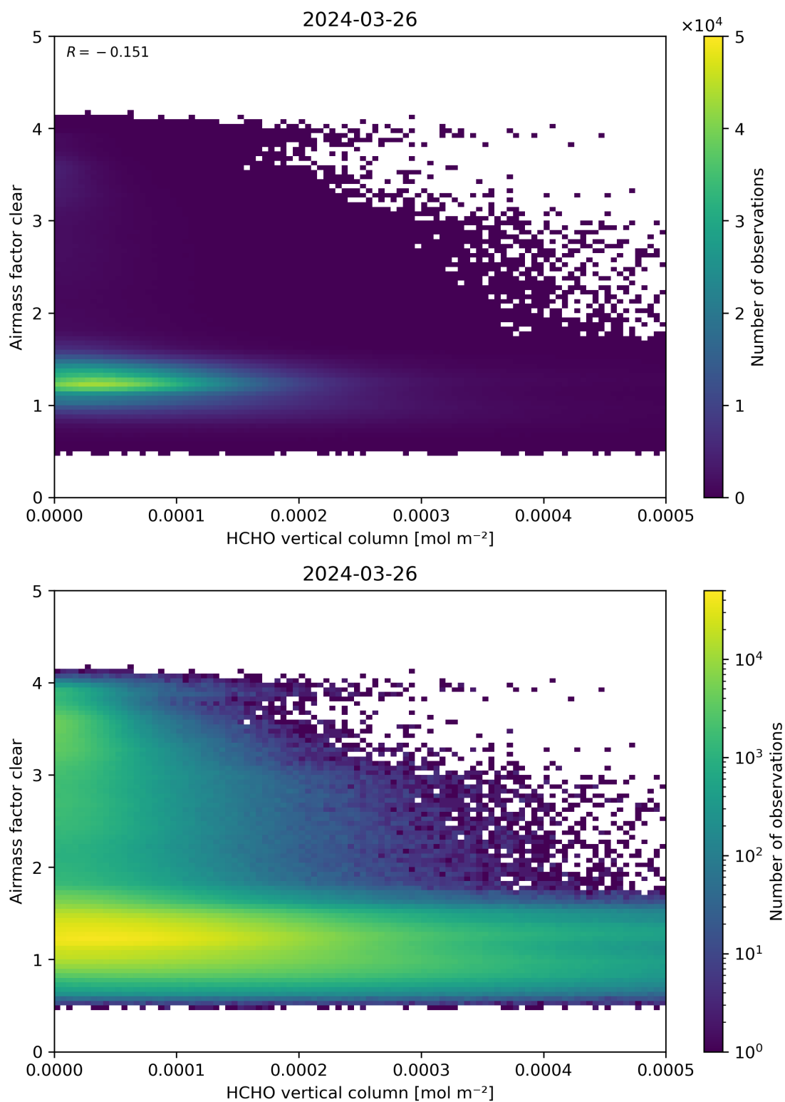
Figure 126: Scatter density plot of “HCHO vertical column” against “Airmass factor clear” for 2024-03-25 to 2024-03-27.
