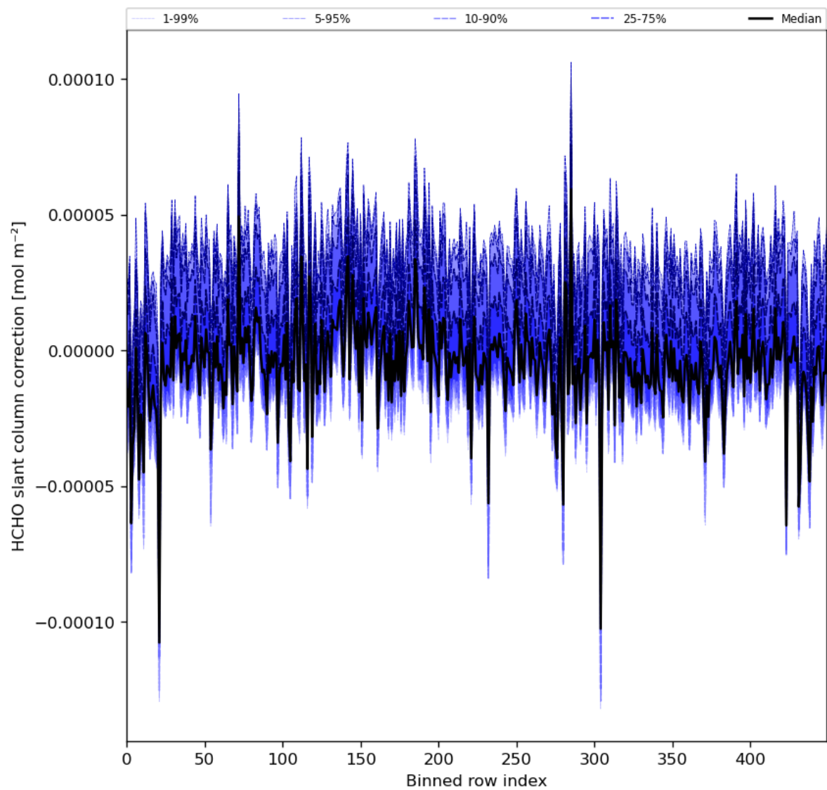
Figure 61: Along track statistics of “HCHO slant column correction” for 2024-03-25 to 2024-03-27
