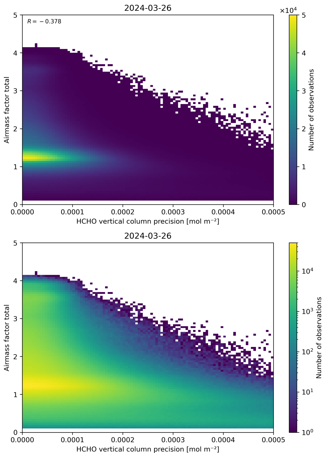
Figure 144: Scatter density plot of “HCHO vertical column precision” against “Airmass factor total” for 2024-03-25 to 2024-03-27.
