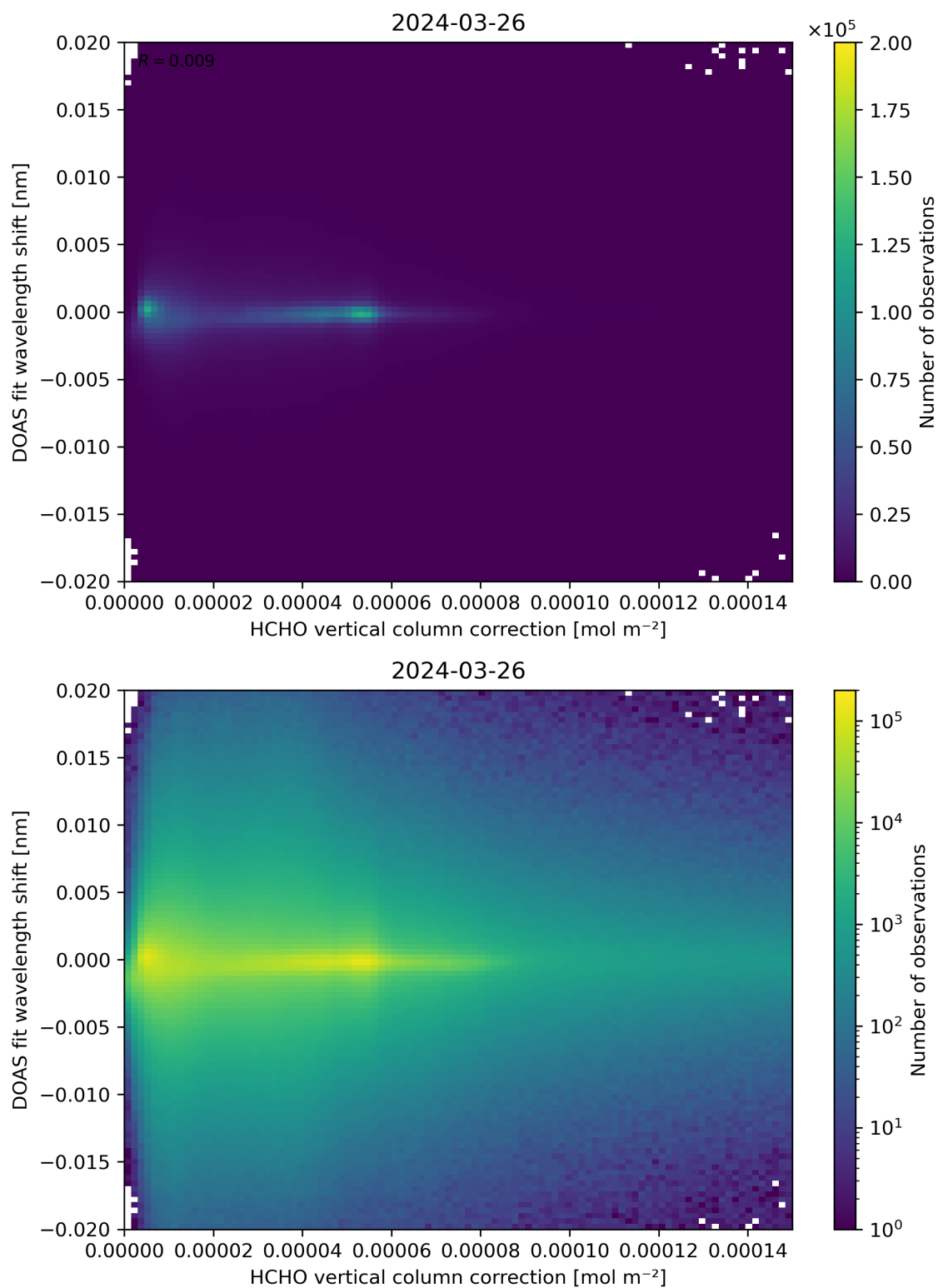
Figure 113: Scatter density plot of “HCHO vertical column correction” against “DOAS fit wavelength shift” for 2024-03-25 to 2024-03-27.
