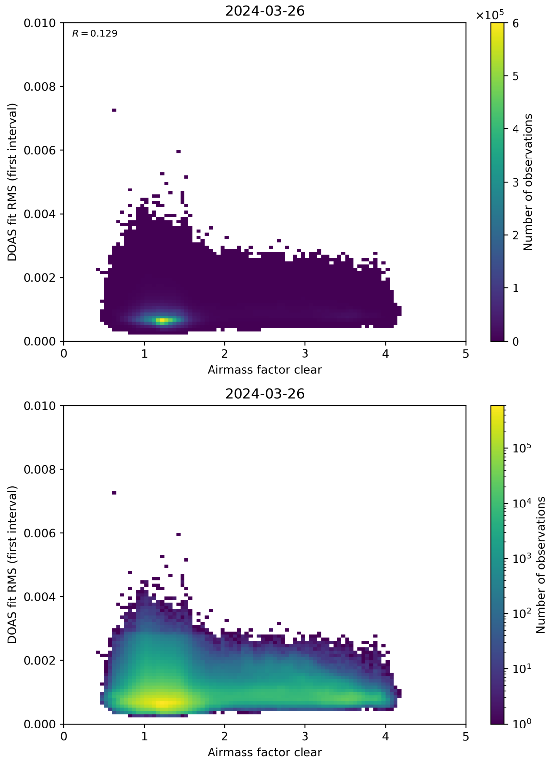
Figure 71: Scatter density plot of “Airmass factor clear” against “DOAS fit RMS (first interval)” for 2024-03-25 to 2024-03-27.
