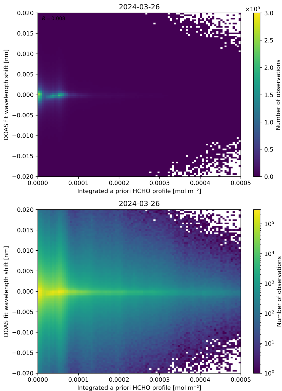
Figure 149: Scatter density plot of “Integrated a priori HCHO profile” against “DOAS fit wavelength shift” for 2024-03-25 to 2024-03-27.
