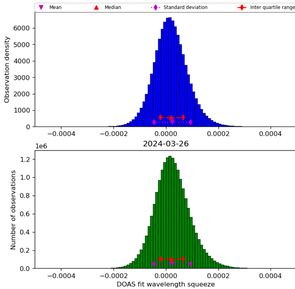
Figure 45: Histogram of “DOAS fit wavelength squeeze” for 2024-03-25 to 2024-03-27
