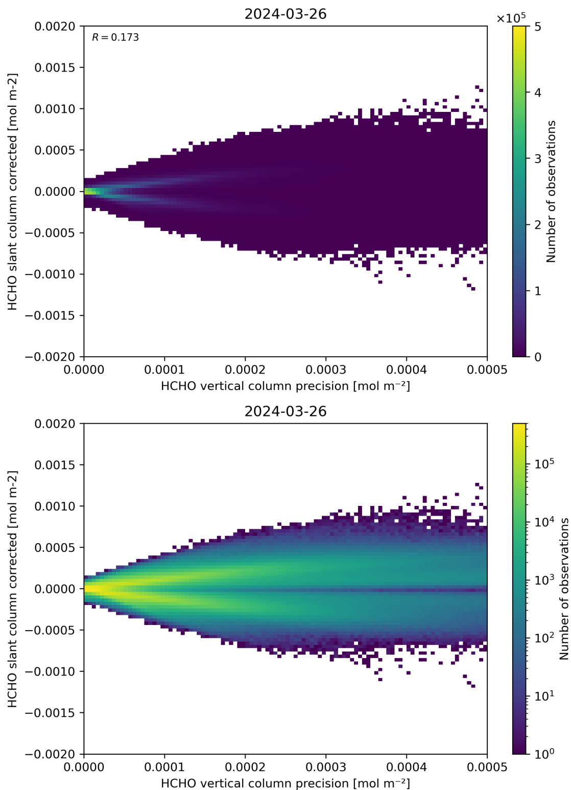
Figure 140: Scatter density plot of “HCHO vertical column precision” against “HCHO slant column corrected” for 2024-03-25 to 2024-03-27.
