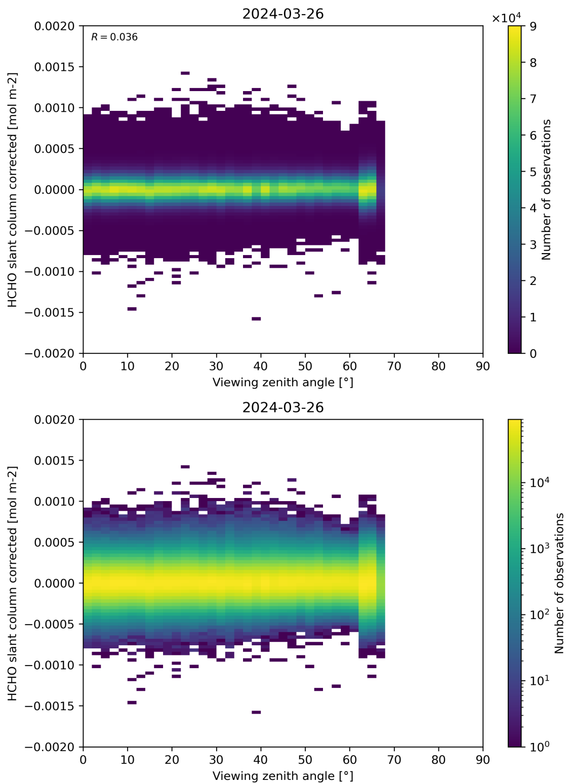
Figure 186: Scatter density plot of “Viewing zenith angle” against “HCHO slant column corrected” for 2024-03-25 to 2024-03-27.
