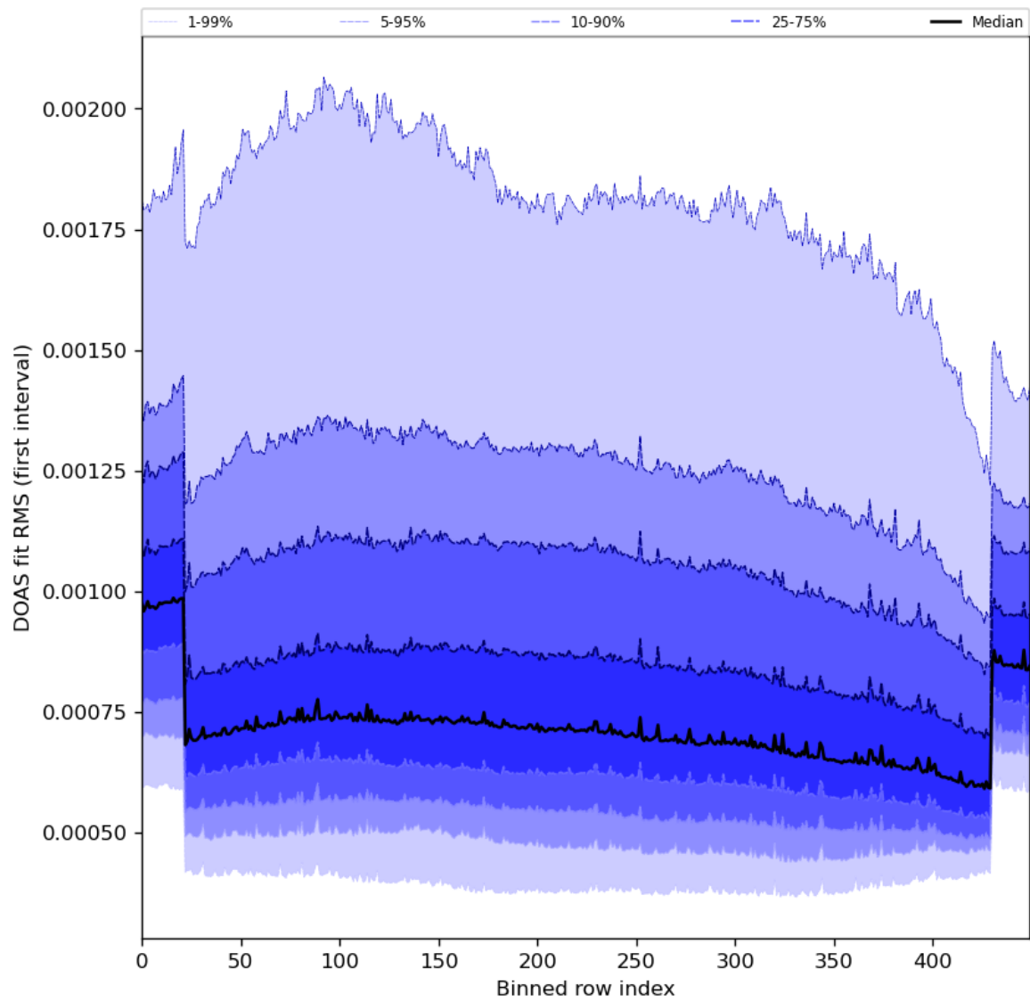
Figure 60: Along track statistics of “DOAS fit RMS (first interval)” for 2024-03-25 to 2024-03-27
