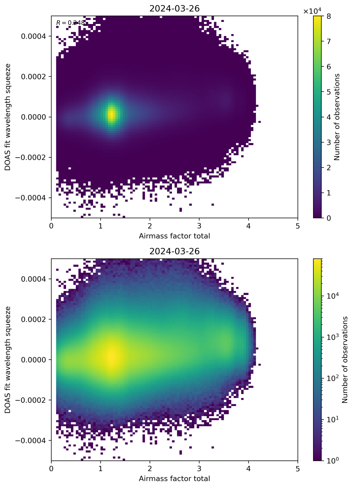
Figure 99: Scatter density plot of “Airmass factor total” against “DOAS fit wavelength squeeze” for 2024-03-25 to 2024-03-27.
