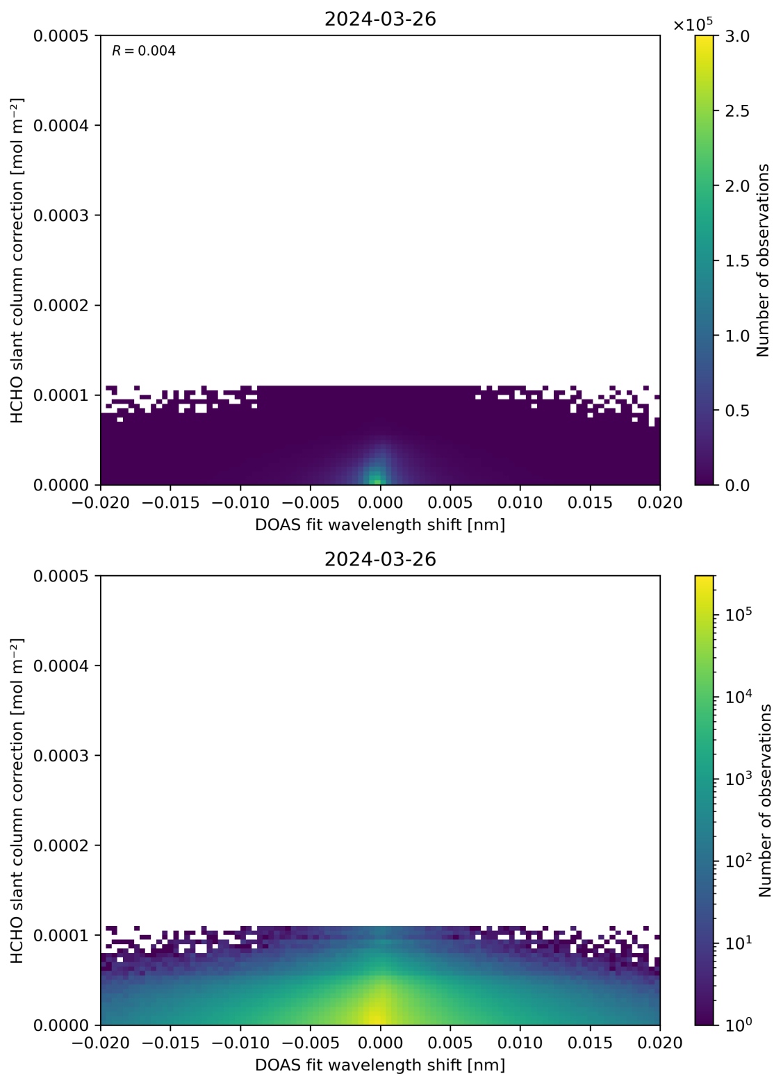
Figure 67: Scatter density plot of “DOAS fit wavelength shift” against “HCHO slant column correction” for 2024-03-25 to 2024-03-27.
