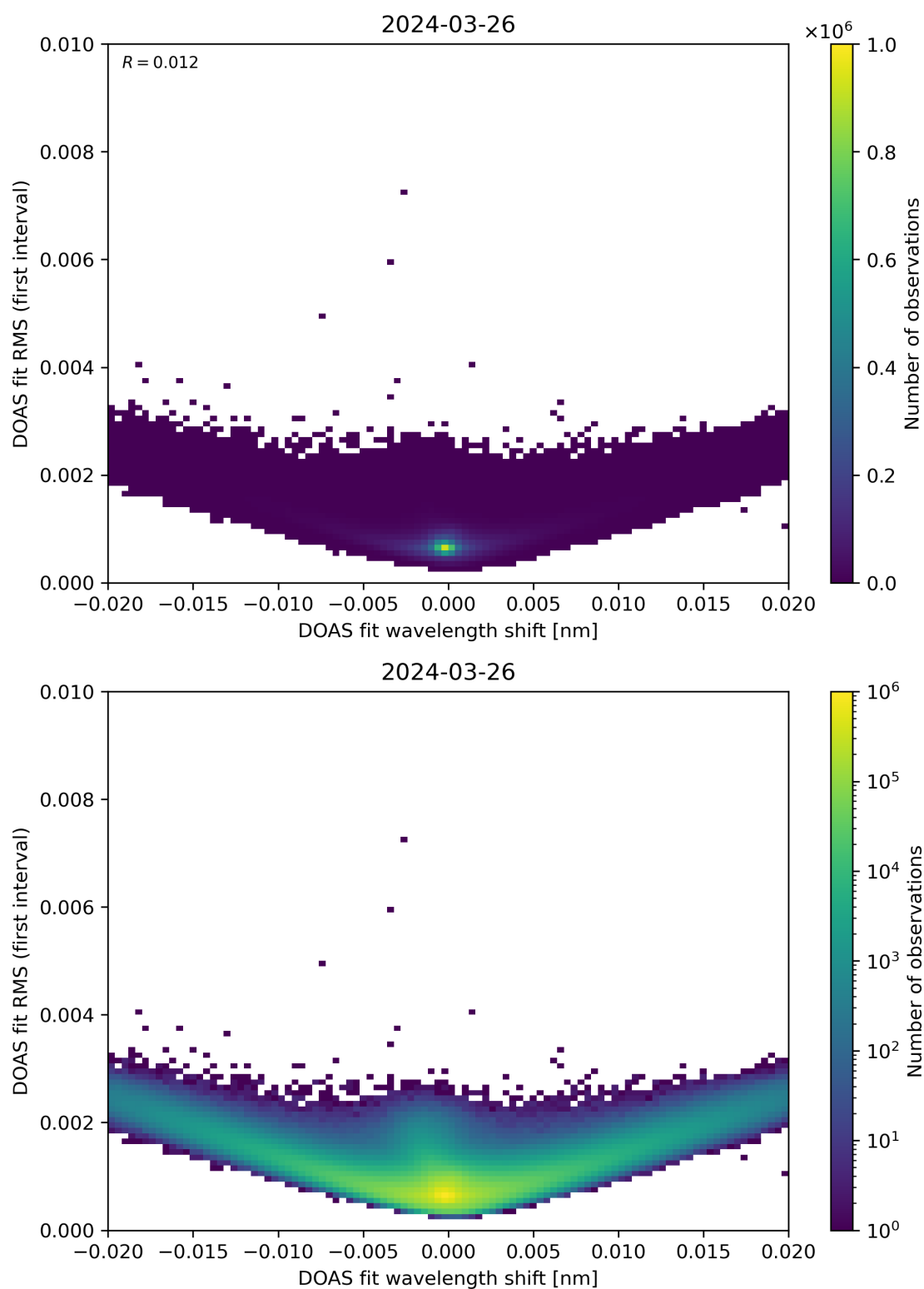
Figure 64: Scatter density plot of “DOAS fit wavelength shift” against “DOAS fit RMS (first interval)” for 2024-03-25 to 2024-03-27.
