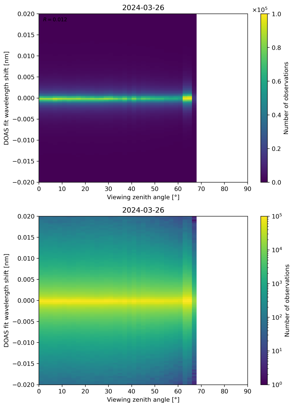
Figure 183: Scatter density plot of “Viewing zenith angle” against “DOAS fit wavelength shift” for 2024-03-25 to 2024-03-27.
