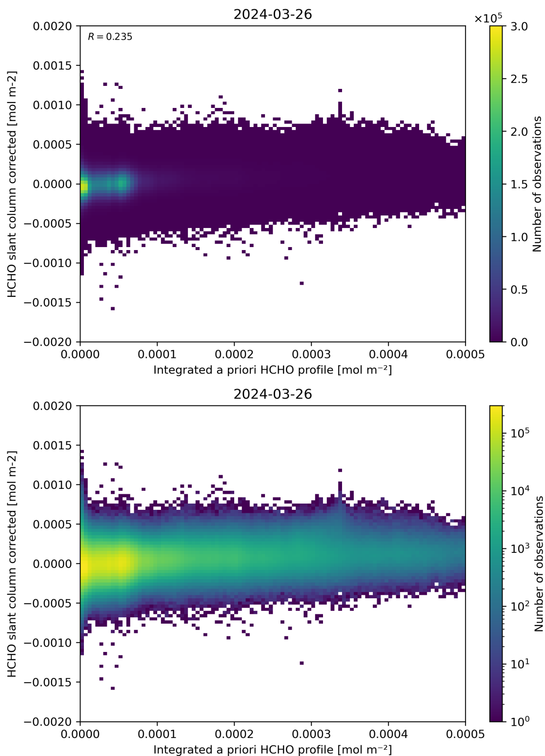
Figure 151: Scatter density plot of “Integrated a priori HCHO profile” against “HCHO slant column corrected” for 2024-03-25 to 2024-03-27.
