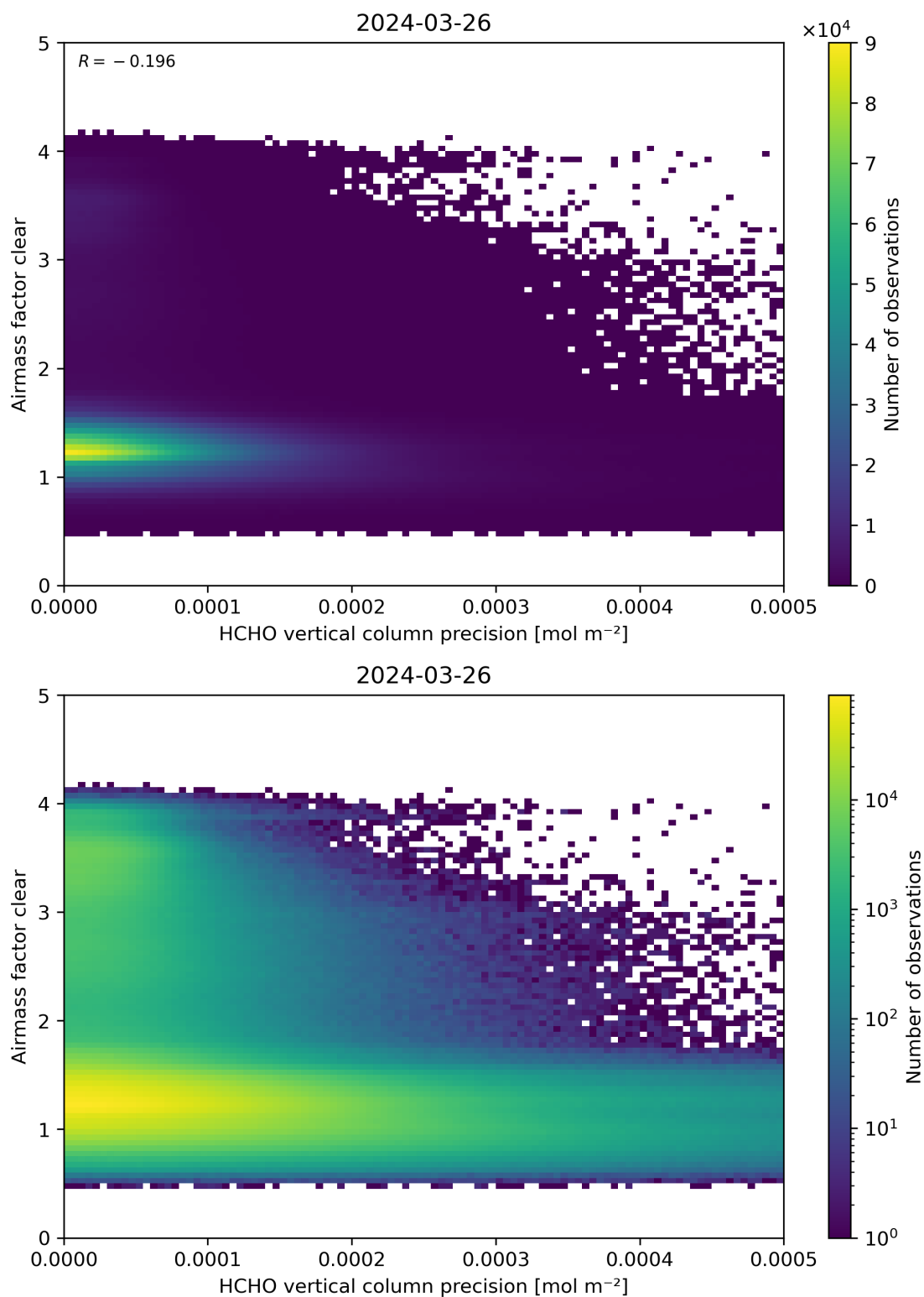
Figure 139: Scatter density plot of “HCHO vertical column precision” against “Airmass factor clear” for 2024-03-25 to 2024-03-27.
