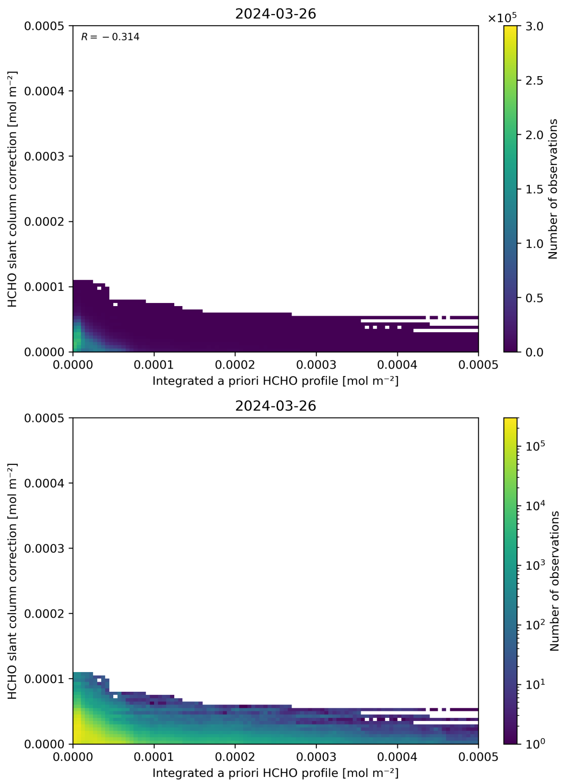
Figure 152: Scatter density plot of “Integrated a priori HCHO profile” against “HCHO slant column correction” for 2024-03-25 to 2024-03-27.
