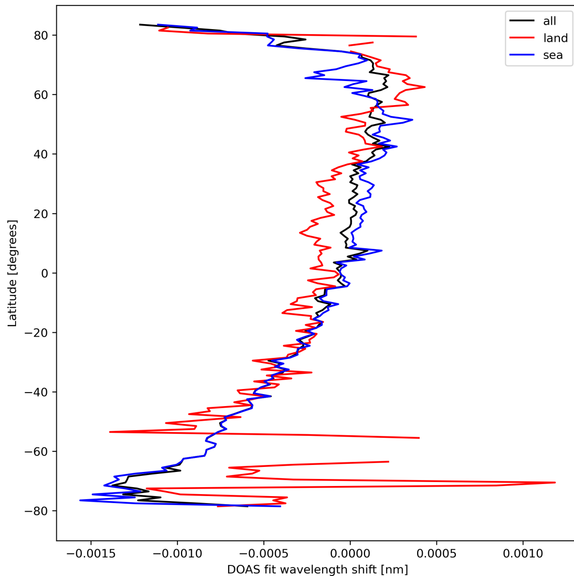
Figure 30: Zonal average of "DOAS fit wavelength shift" for 2024-03-25 to 2024-03-27.
