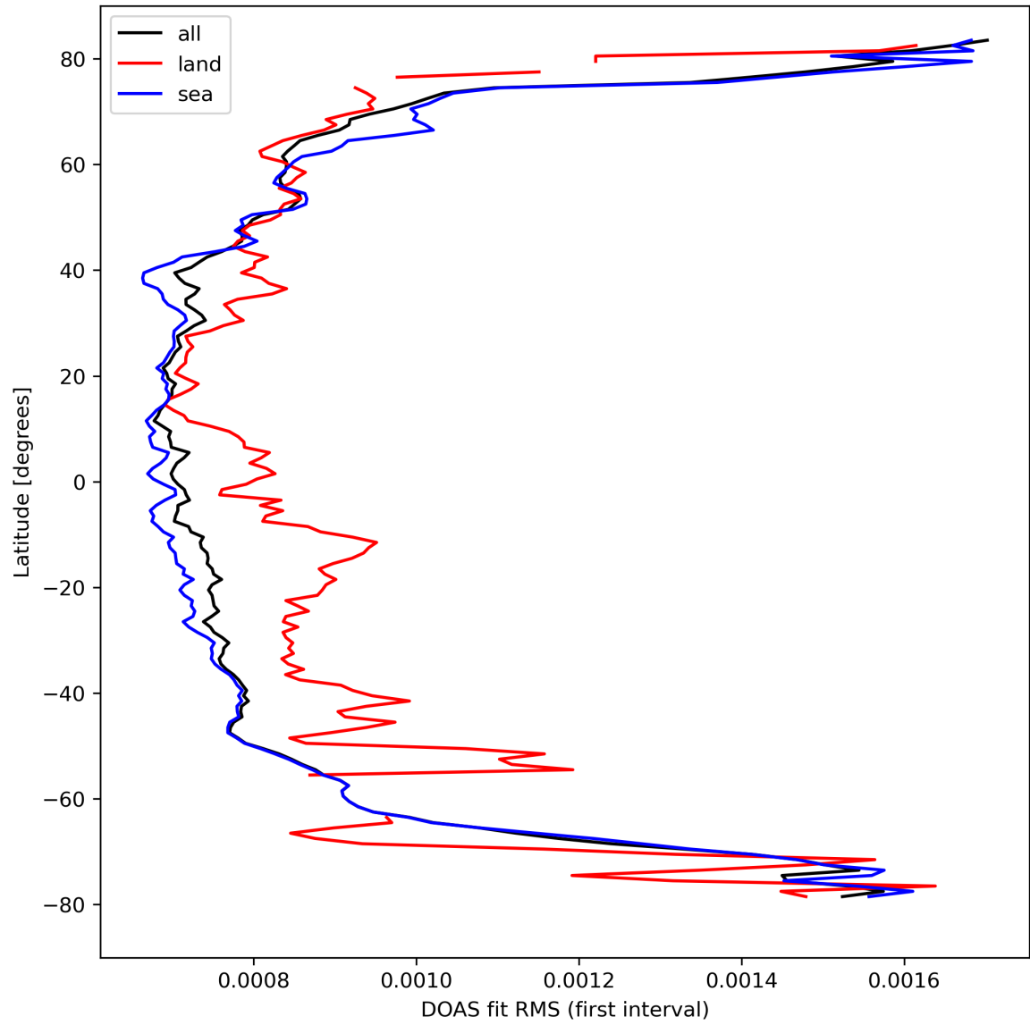
Figure 32: Zonal average of “DOAS fit RMS (first interval)” for 2024-03-25 to 2024-03-27.
