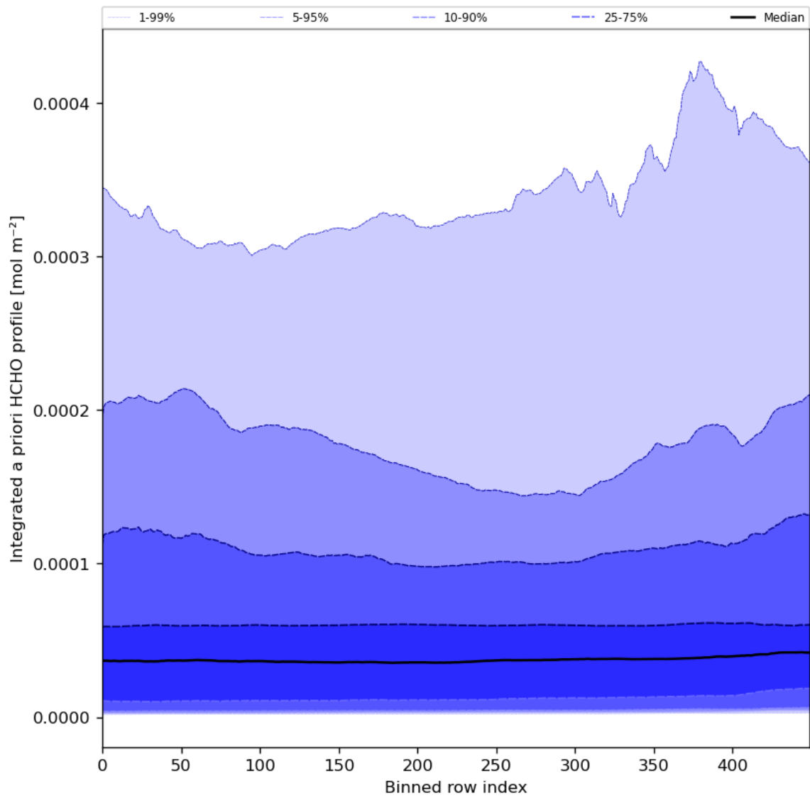
Figure 57: Along track statistics of "Integrated a priori HCHO profile" for 2024-03-25 to 2024-03-27
