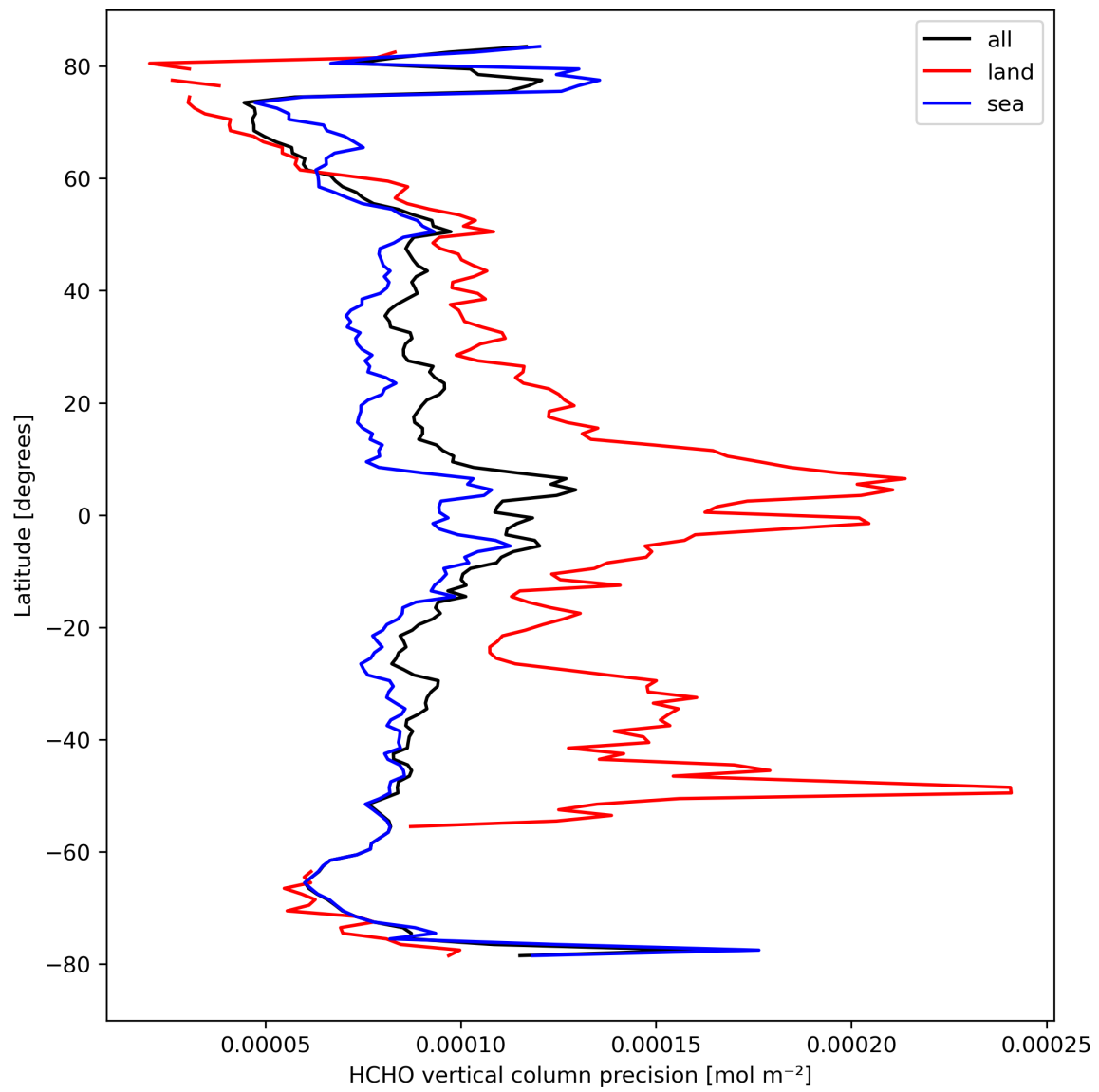
Figure 22: Zonal average of “HCHO vertical column precision” for 2024-03-25 to 2024-03-27.
