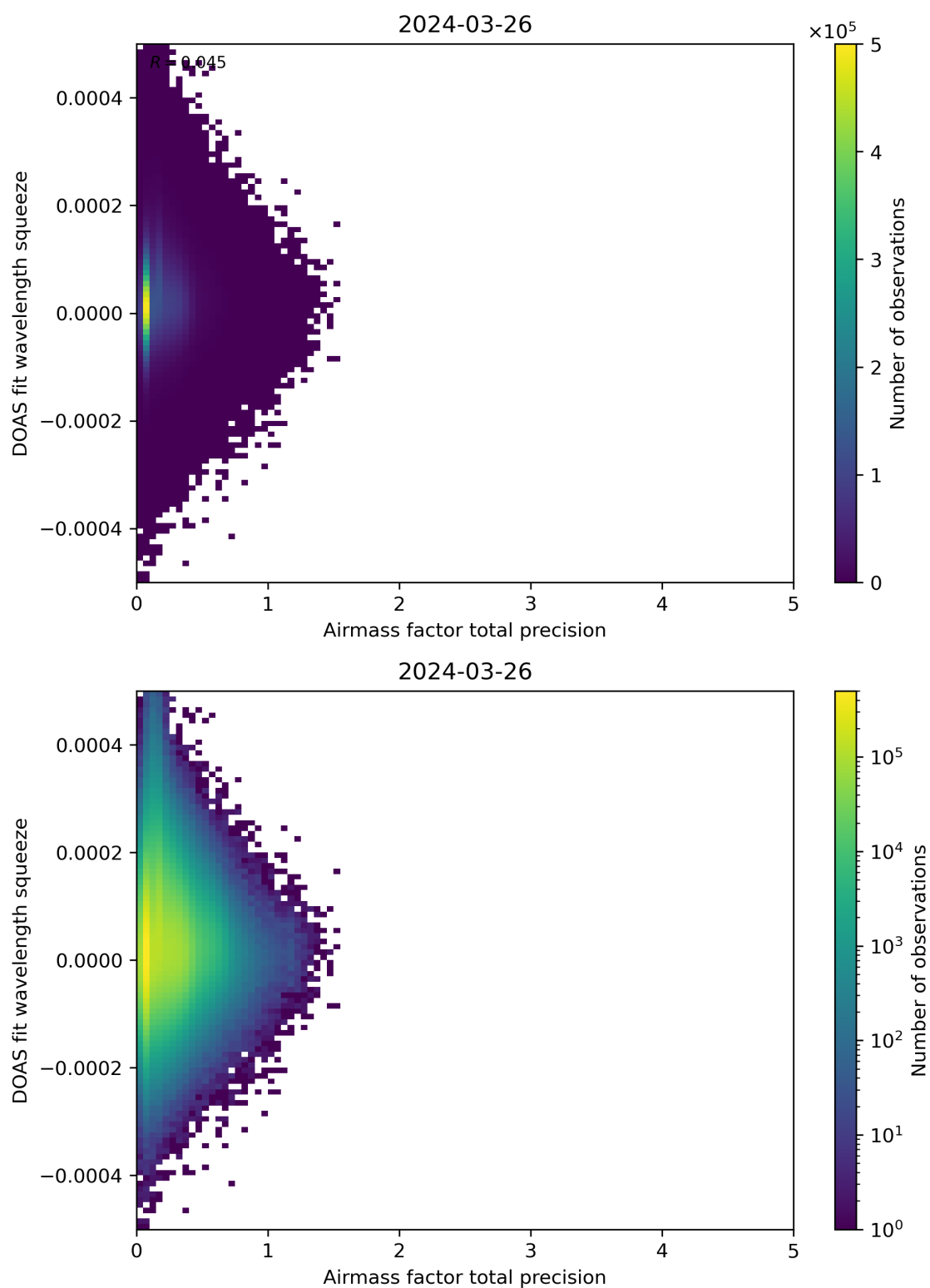
Figure 107: Scatter density plot of “Airmass factor total precision” against “DOAS fit wavelength squeeze” for 2024-03-25 to 2024-03-27.
