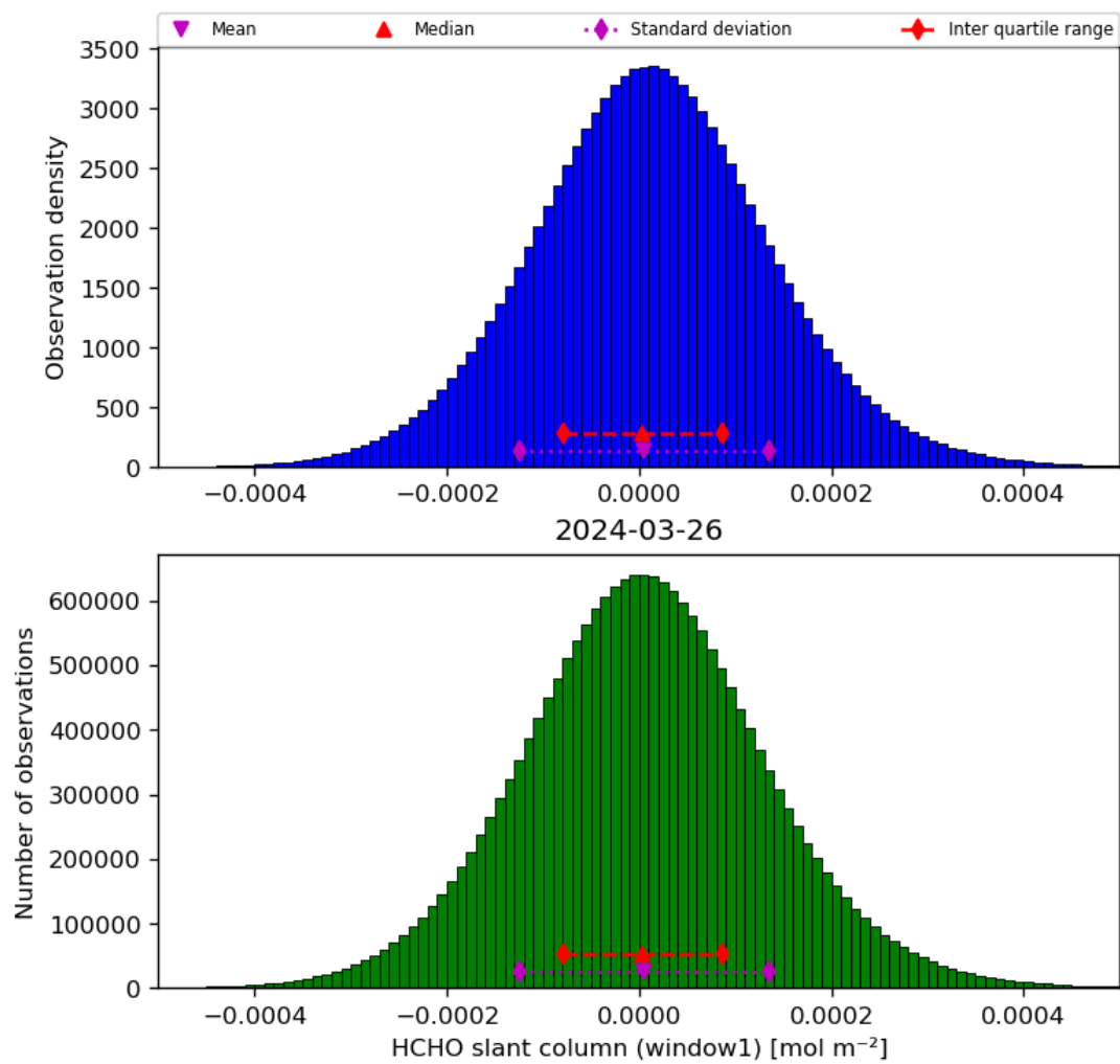
Figure 38: Histogram of “HCHO slant column (window1)” for 2024-03-25 to 2024-03-27
