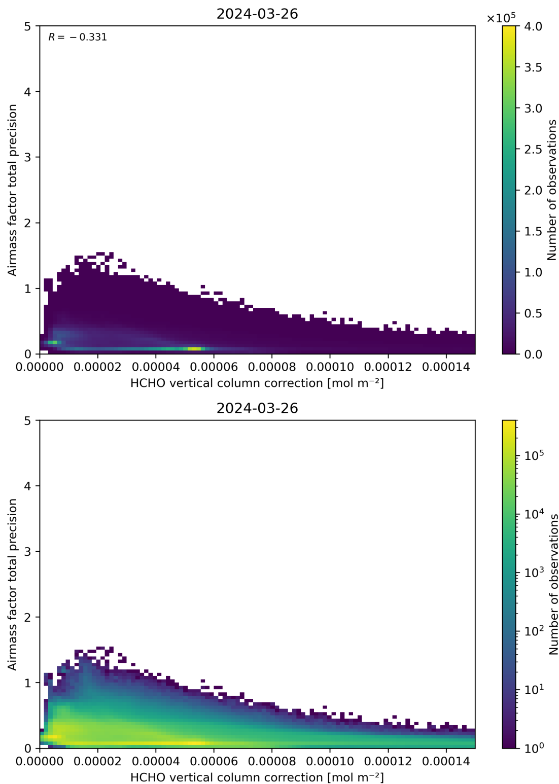
Figure 121: Scatter density plot of “HCHO vertical column correction” against “Airmass factor total precision” for 2024-03-25 to 2024-03-27.
