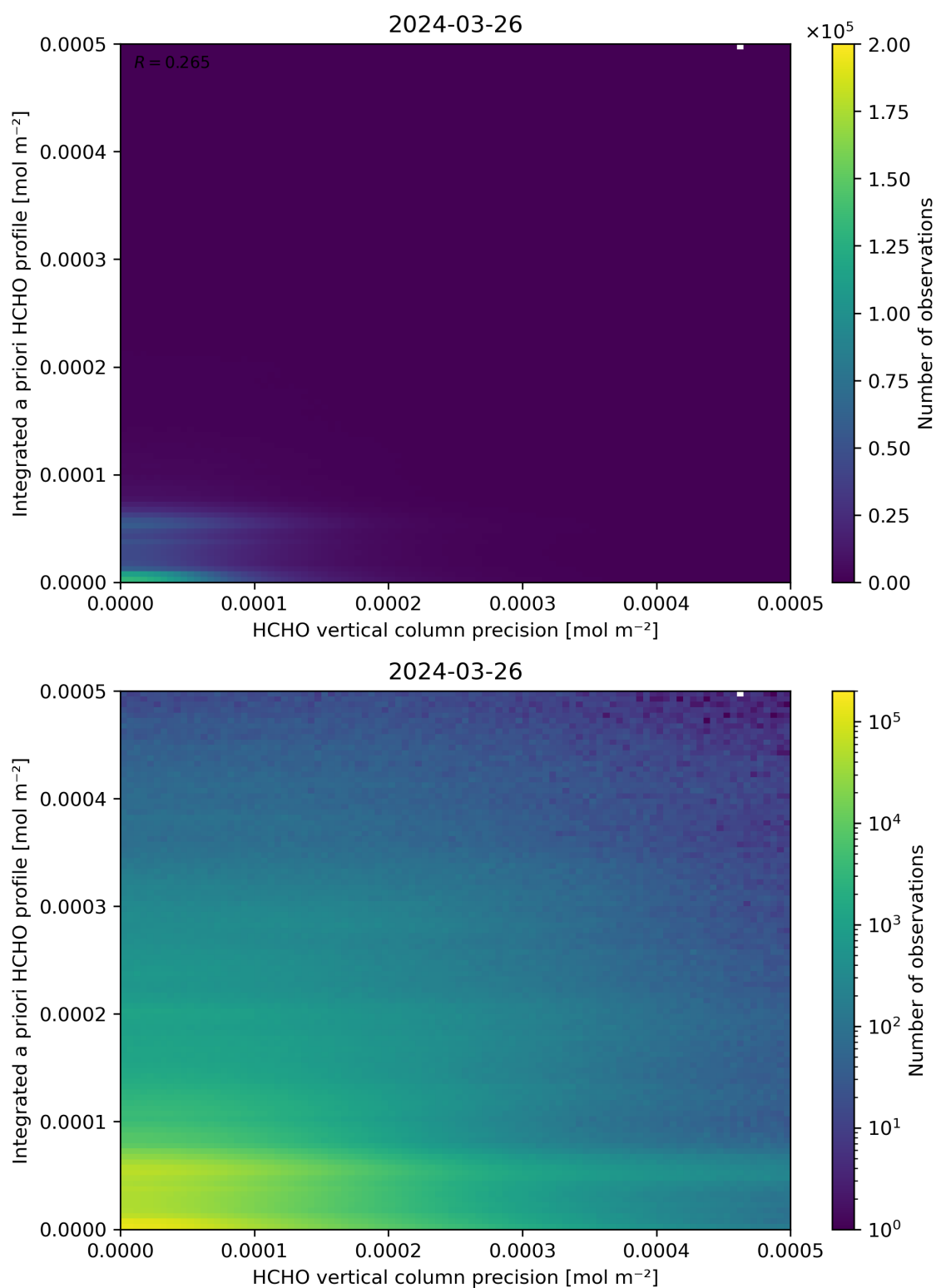
Figure 147: Scatter density plot of “HCHO vertical column precision” against “Integrated a priori HCHO profile” for 2024-03-25 to 2024-03-27.
