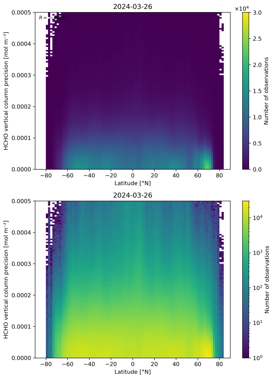
Figure 165: Scatter density plot of “Latitude” against “HCHO vertical column precision” for 2024-03-25 to 2024-03-27.
