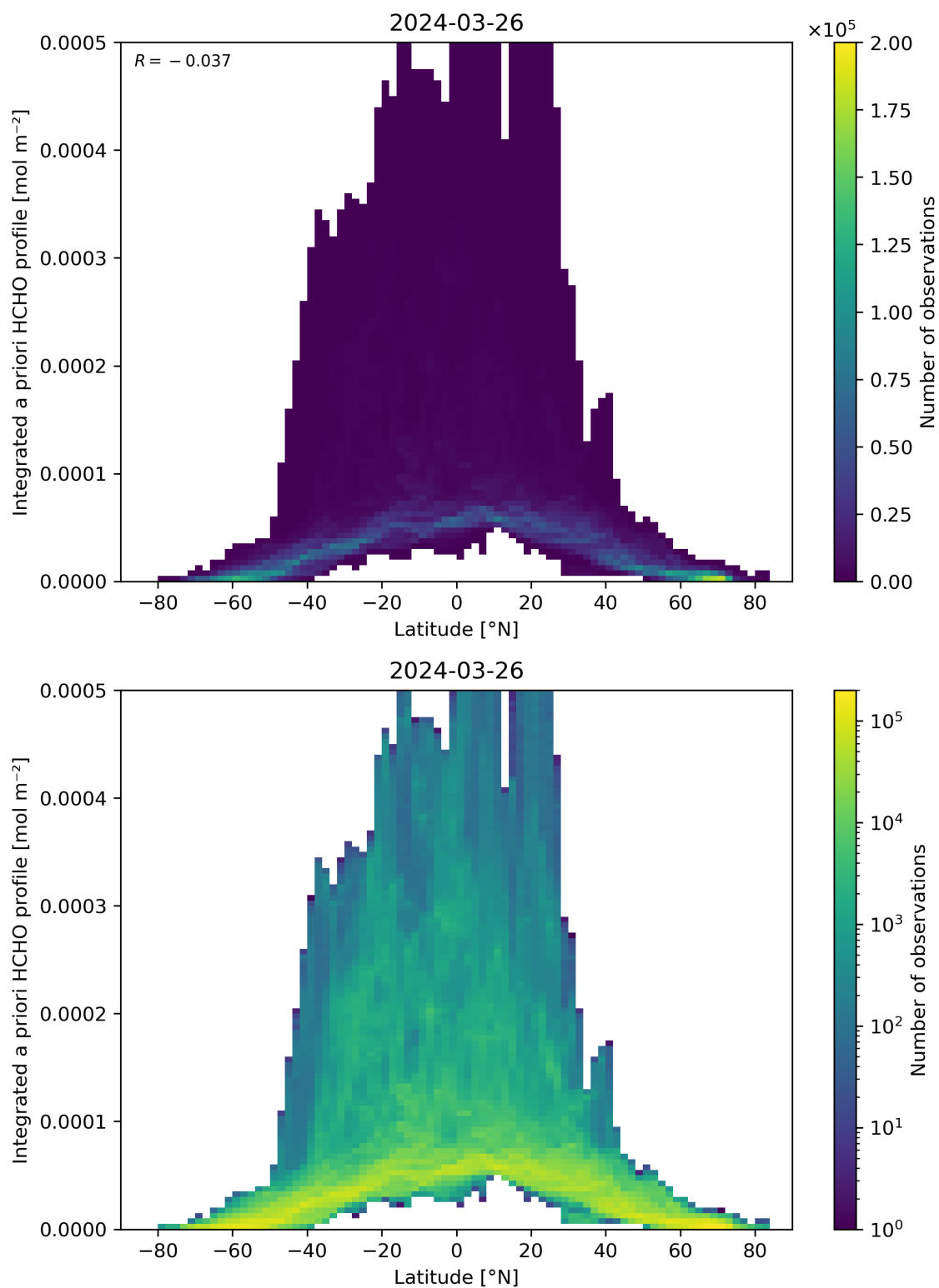
Figure 166: Scatter density plot of “Latitude” against “Integrated a priori HCHO profile” for 2024-03-25 to 2024-03-27.
