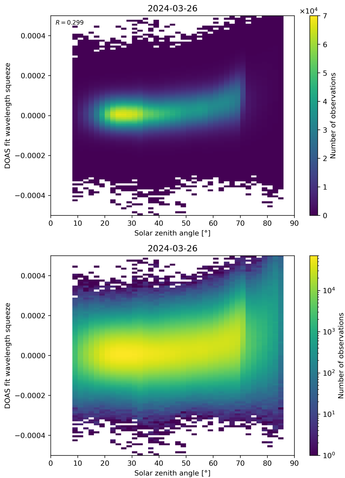
Figure 169: Scatter density plot of “Solar zenith angle” against “DOAS fit wavelength squeeze” for 2024-03-25 to 2024-03-27.
