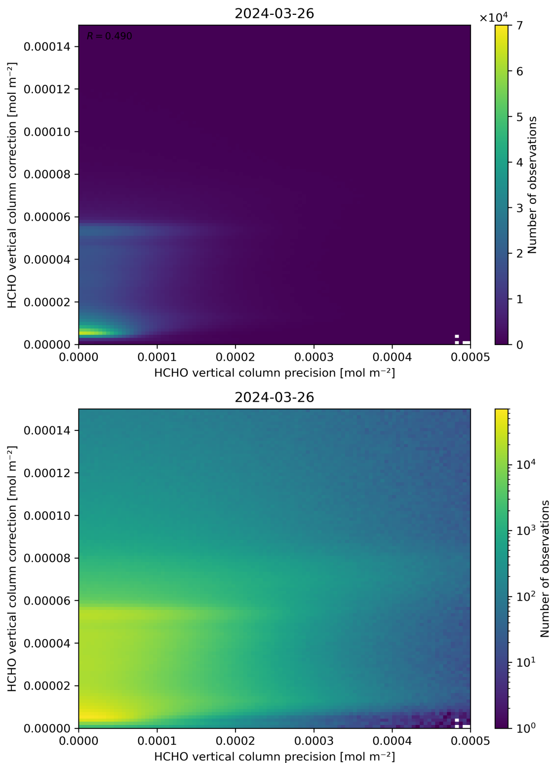
Figure 146: Scatter density plot of “HCHO vertical column precision” against “HCHO vertical column correction” for 2024-03-25 to 2024-03-27.
