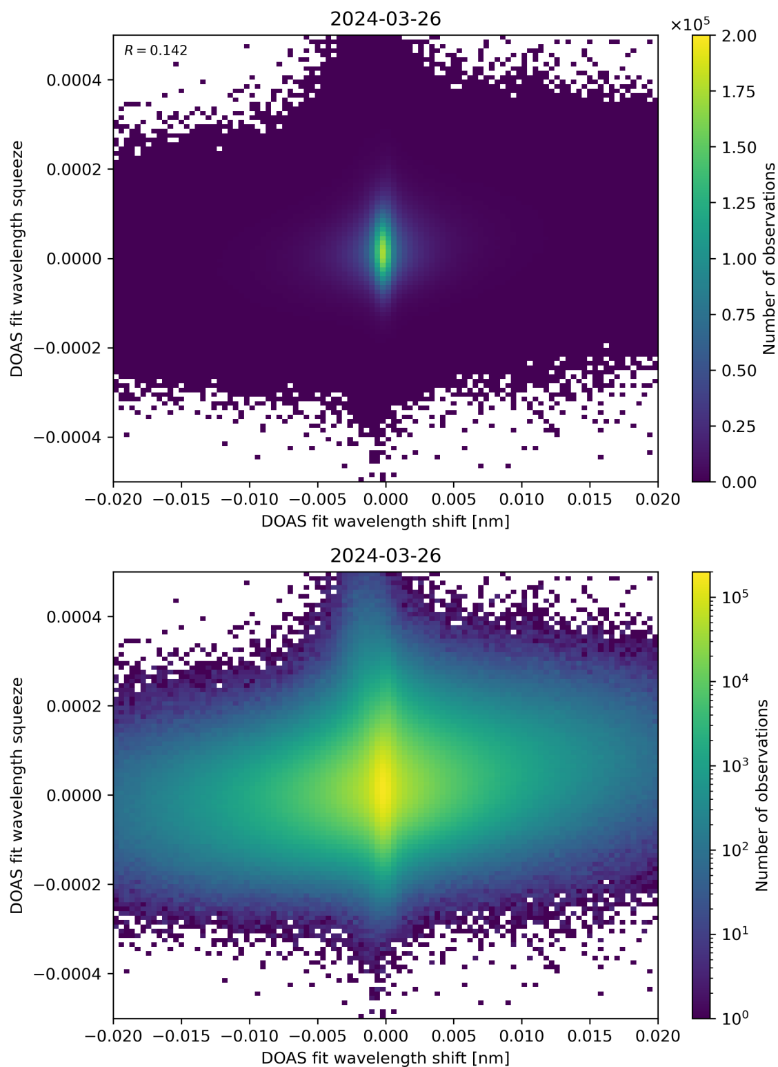
Figure 65: Scatter density plot of “DOAS fit wavelength shift” against “DOAS fit wavelength squeeze” for 2024-03-25 to 2024-03-27.
