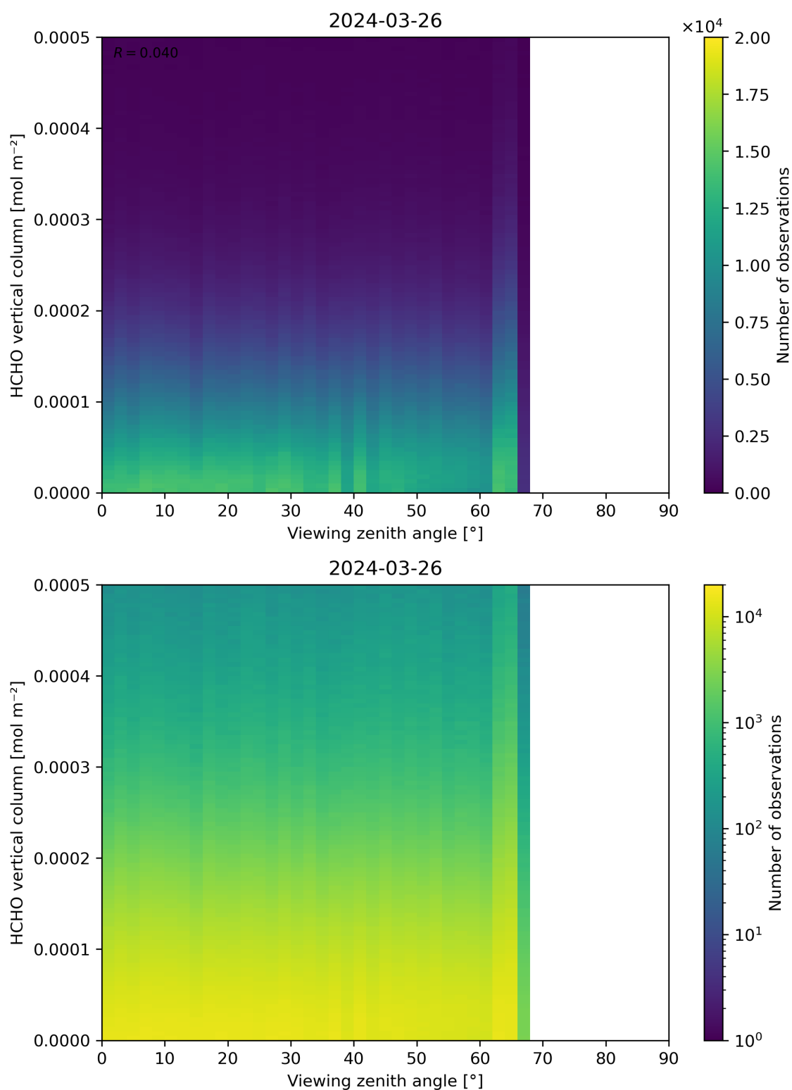
Figure 192: Scatter density plot of “Viewing zenith angle” against “HCHO vertical column” for 2024-03-25 to 2024-03-27.
