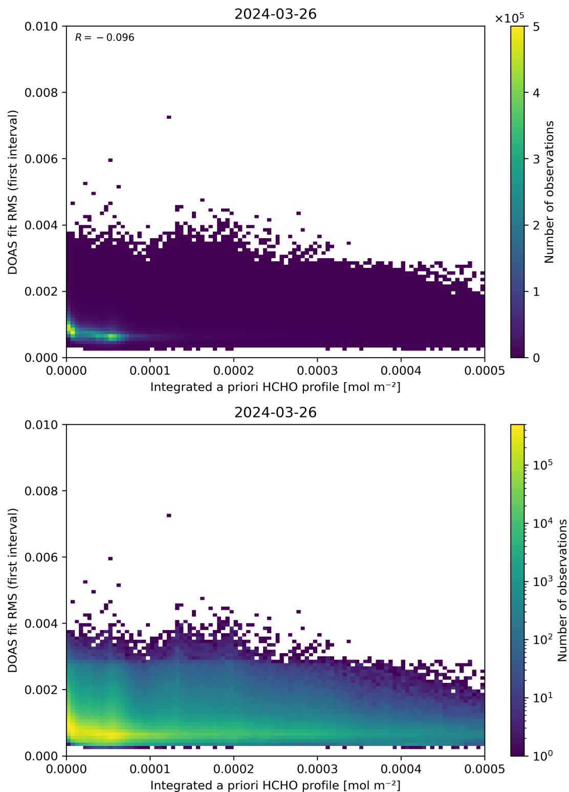
Figure 148: Scatter density plot of “Integrated a priori HCHO profile” against “DOAS fit RMS (first interval)” for 2024-03-25 to 2024-03-27.
