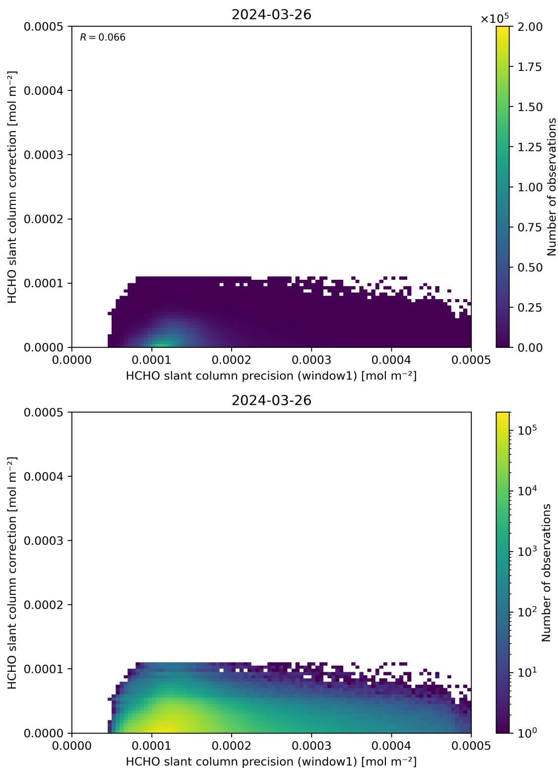
Figure 93: Scatter density plot of “HCHO slant column precision (window1)” against “HCHO slant column correction” for 2024-03-25 to 2024-03-27.
