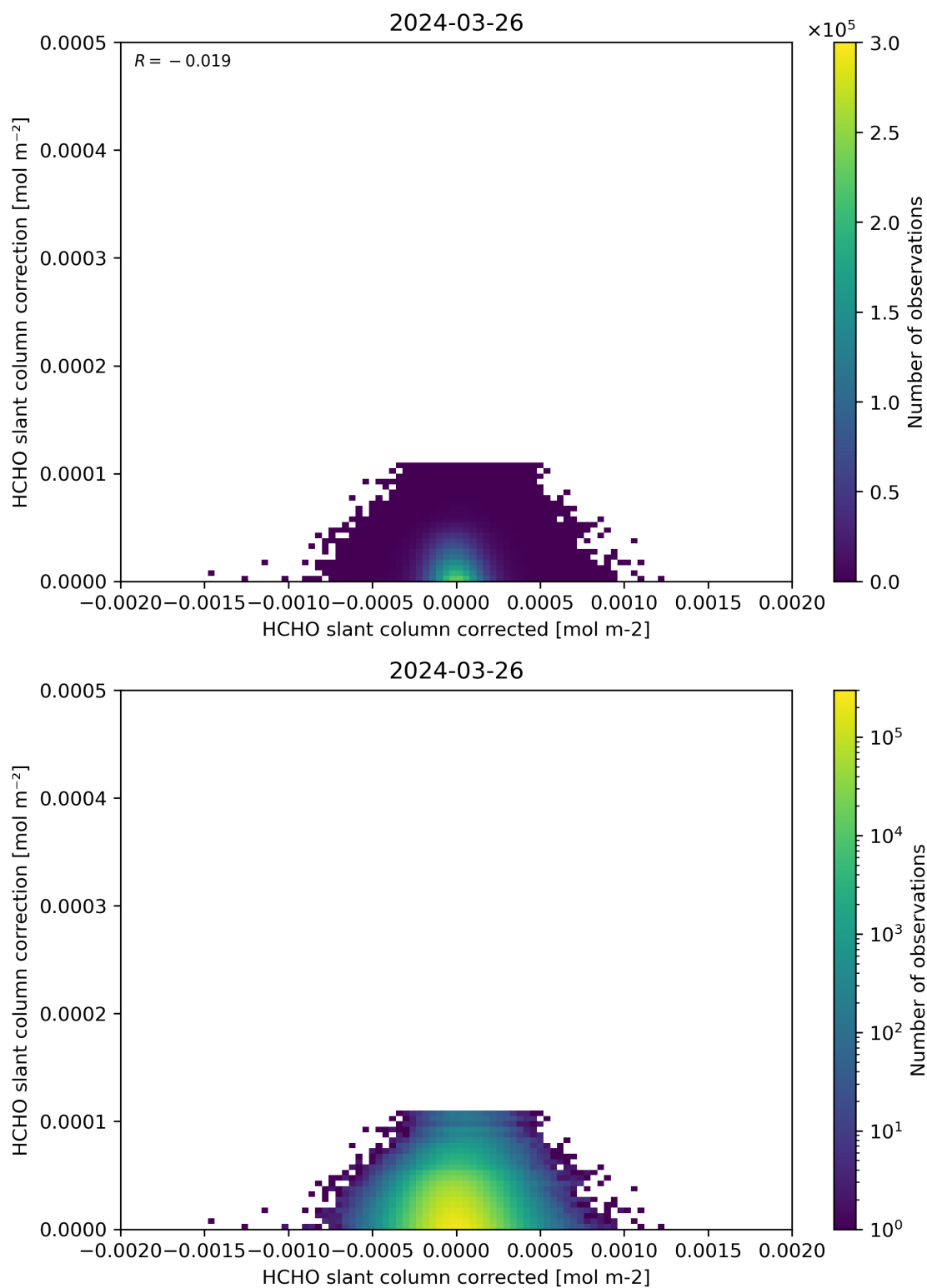
Figure 77: Scatter density plot of “HCHO slant column corrected” against “HCHO slant column correction” for 2024-03-25 to 2024-03-27.
