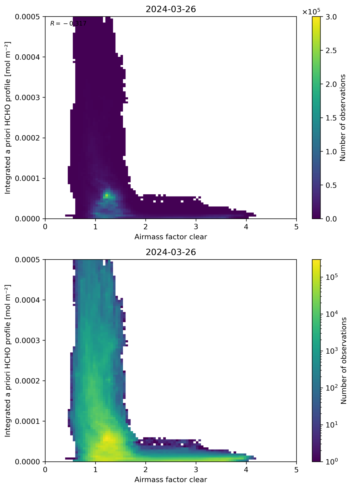
Figure 76: Scatter density plot of “Airmass factor clear” against “Integrated a priori HCHO profile” for 2024-03-25 to 2024-03-27.
