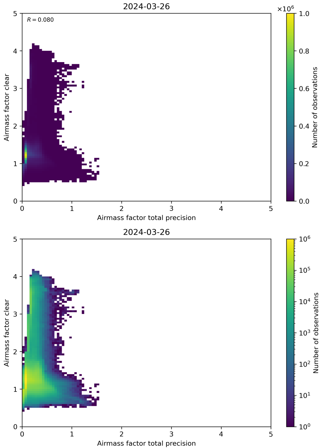
Figure 108: Scatter density plot of “Airmass factor total precision” against “Airmass factor clear” for 2024-03-25 to 2024-03-27.
