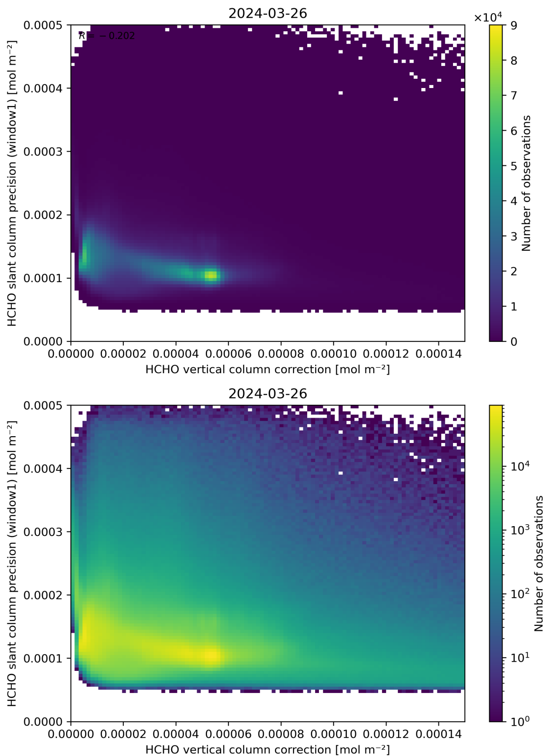
Figure 119: Scatter density plot of “HCHO vertical column correction” against “HCHO slant column precision (window1)” for 2024-03-25 to 2024-03-27.
