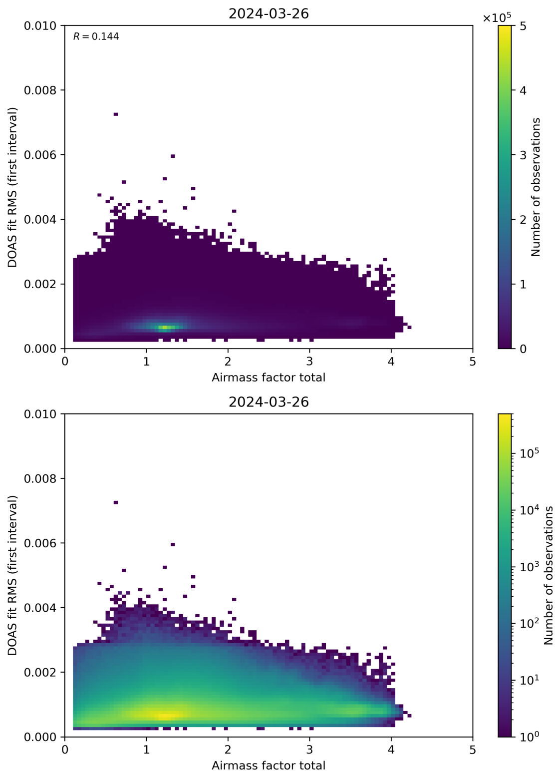
Figure 97: Scatter density plot of “Airmass factor total” against “DOAS fit RMS (first interval)” for 2024-03-25 to 2024-03-27.
