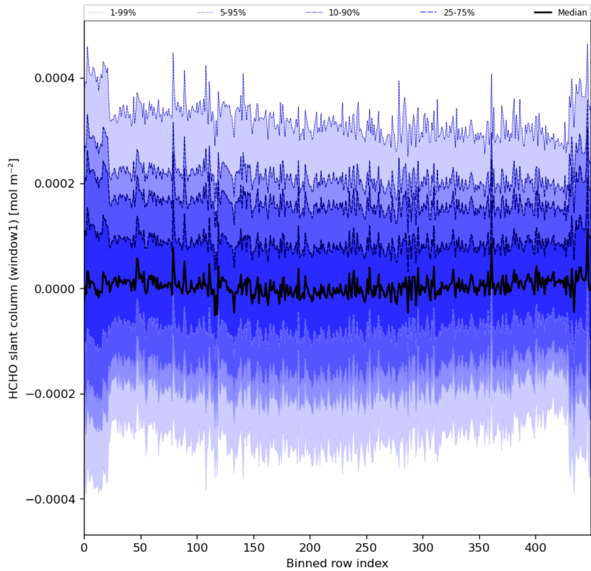
Figure 52: Along track statistics of “HCHO slant column (window1)” for 2024-03-25 to 2024-03-27
