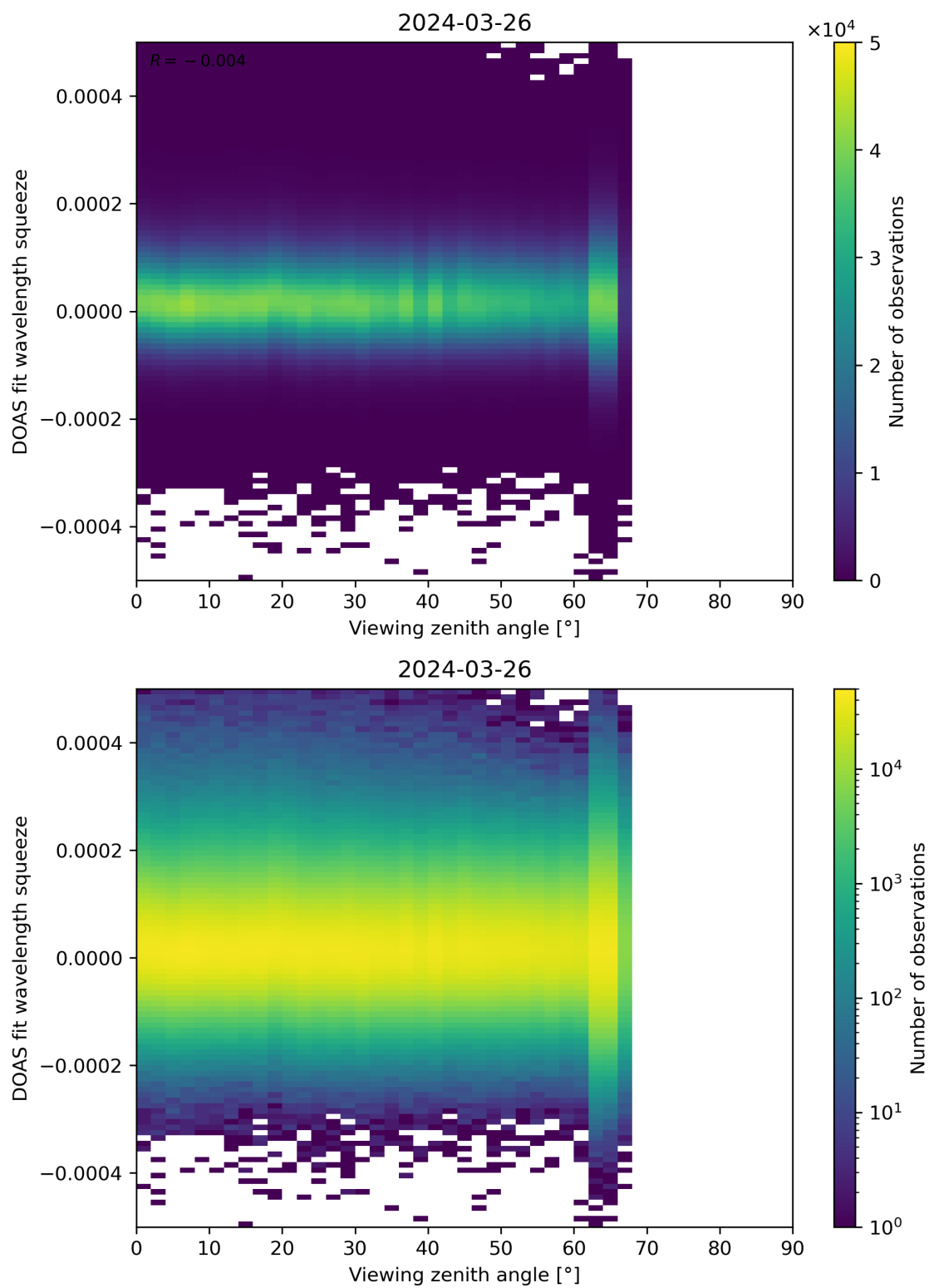
Figure 184: Scatter density plot of “Viewing zenith angle” against “DOAS fit wavelength squeeze” for 2024-03-25 to 2024-03-27.
