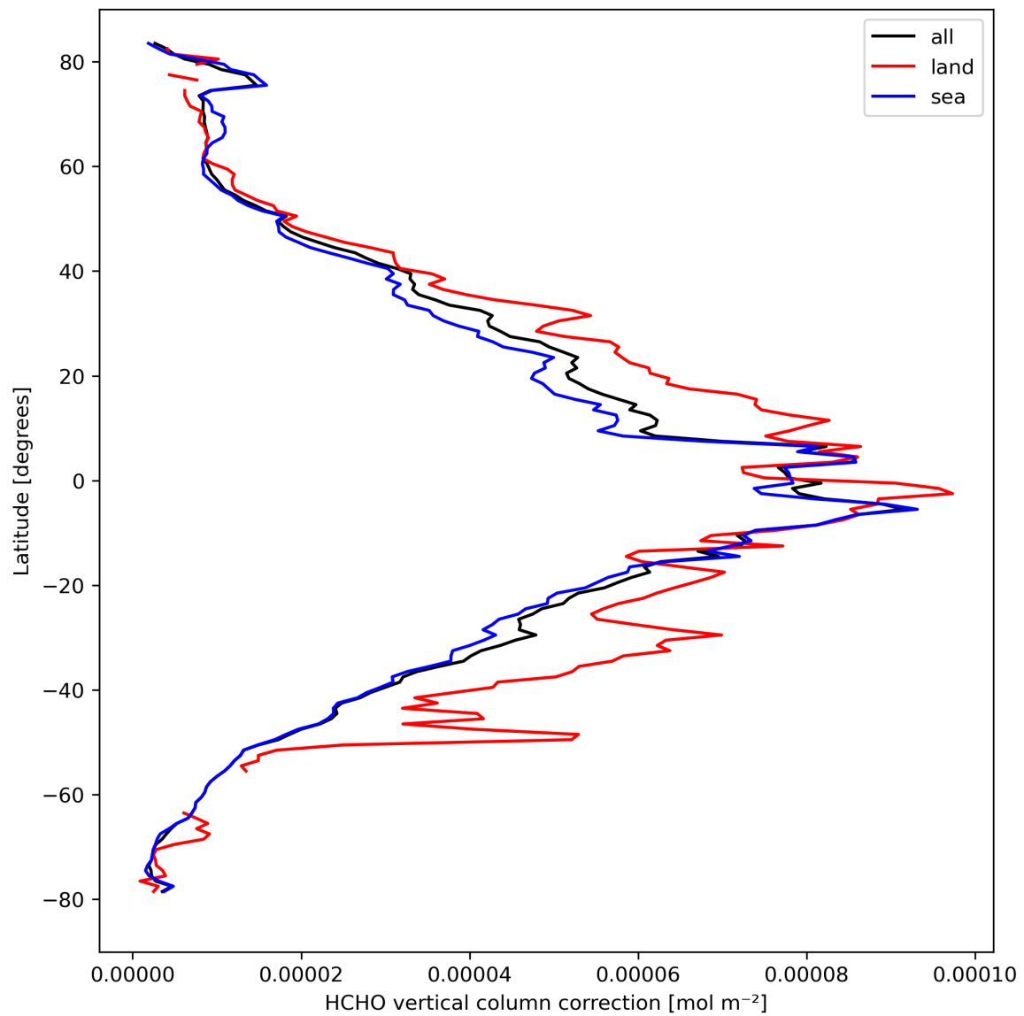
Figure 23: Zonal average of “HCHO vertical column correction” for 2024-03-25 to 2024-03-27.
