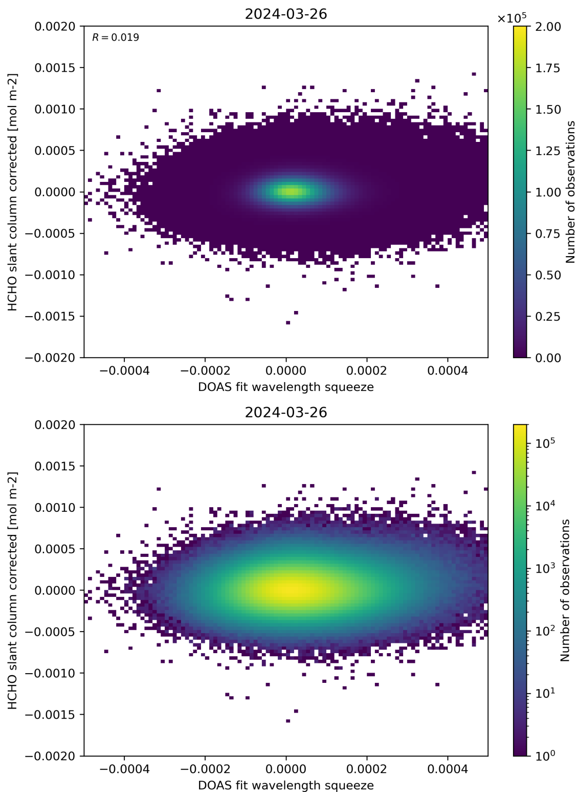
Figure 69: Scatter density plot of “DOAS fit wavelength squeeze” against “HCHO slant column corrected” for 2024-03-25 to 2024-03-27.
