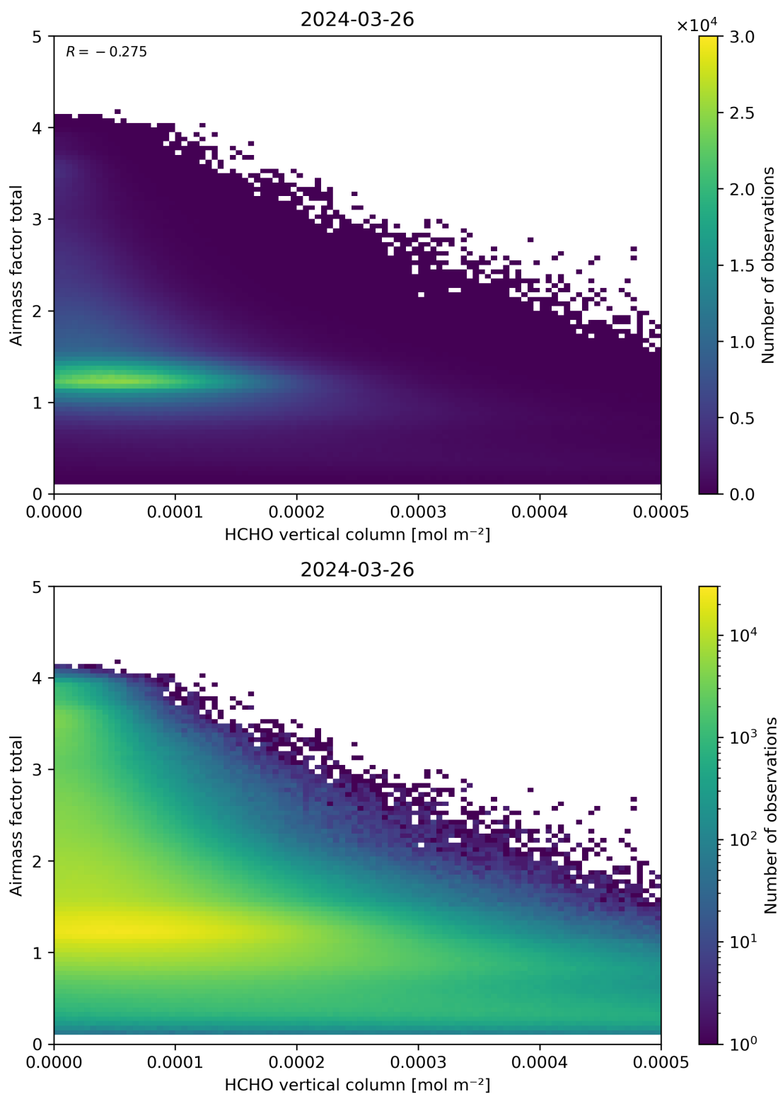
Figure 131: Scatter density plot of “HCHO vertical column” against “Airmass factor total” for 2024-03-25 to 2024-03-27.
