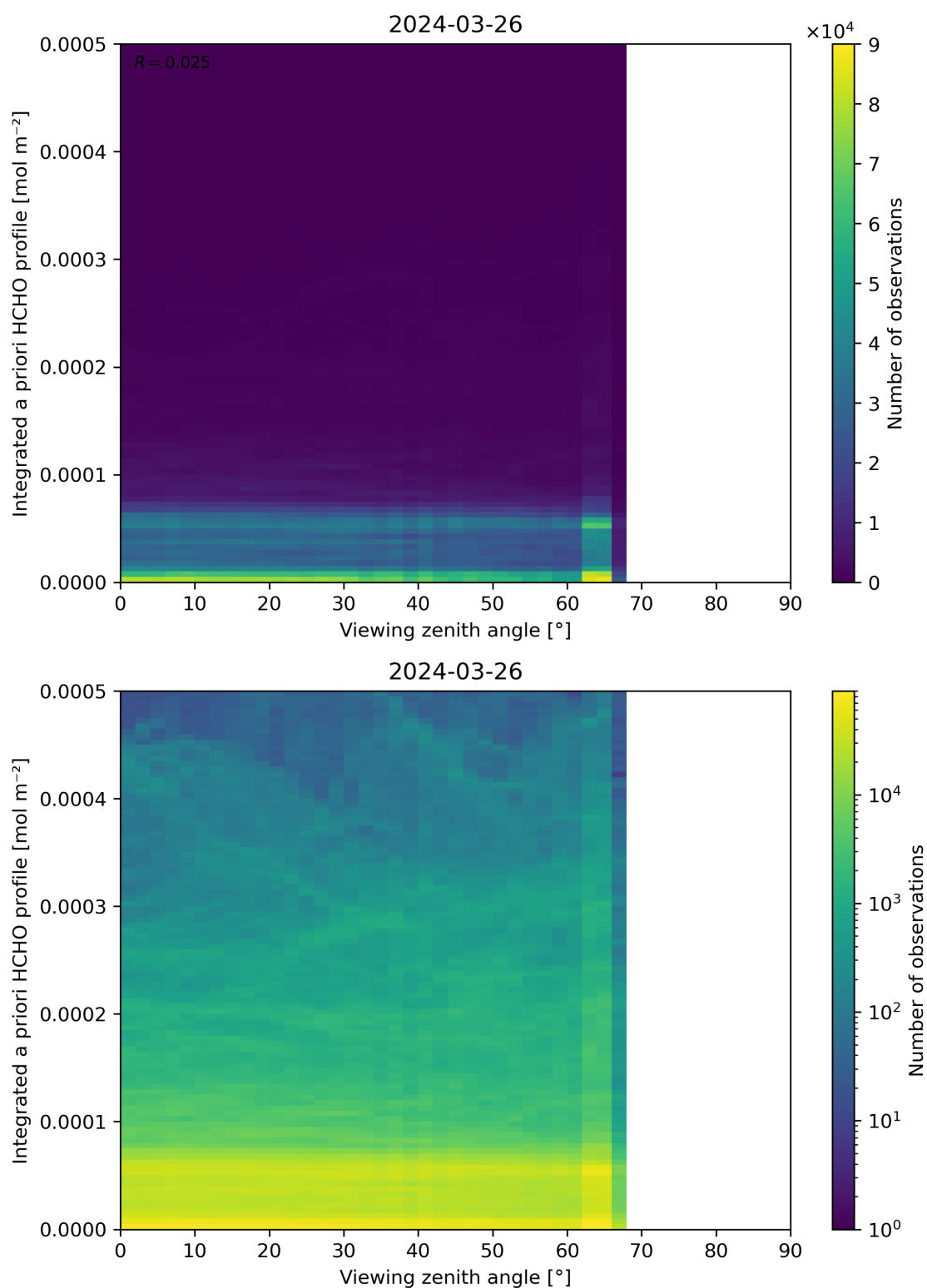
Figure 195: Scatter density plot of “Viewing zenith angle” against “Integrated a priori HCHO profile” for 2024-03-25 to 2024-03-27.
