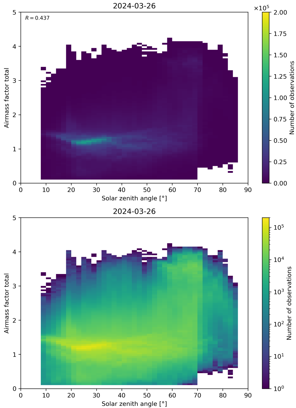
Figure 175: Scatter density plot of “Solar zenith angle” against “Airmass factor total” for 2024-03-25 to 2024-03-27.
