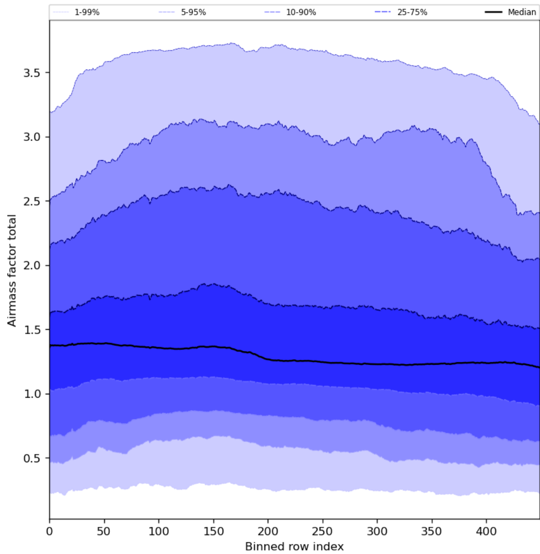
Figure 54: Along track statistics of “Airmass factor total” for 2024-03-25 to 2024-03-27
