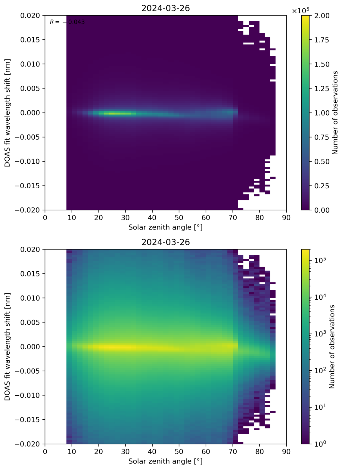
Figure 168: Scatter density plot of “Solar zenith angle” against “DOAS fit wavelength shift” for 2024-03-25 to 2024-03-27.
