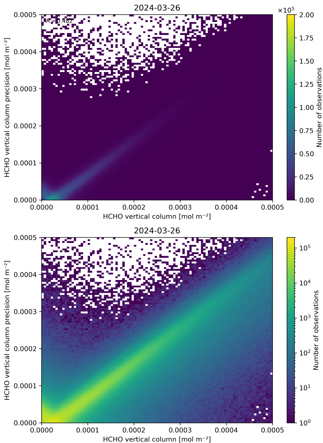
Figure 134: Scatter density plot of “HCHO vertical column” against “HCHO vertical column precision” for 2024-03-25 to 2024-03-27.
