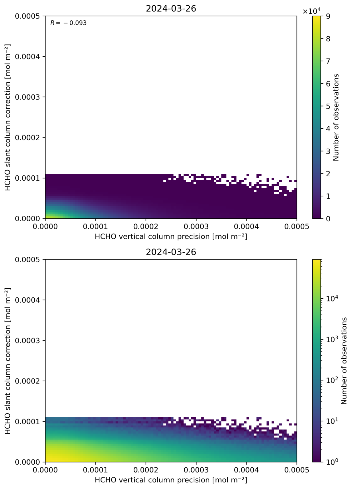
Figure 141: Scatter density plot of “HCHO vertical column precision” against “HCHO slant column correction” for 2024-03-25 to 2024-03-27.
