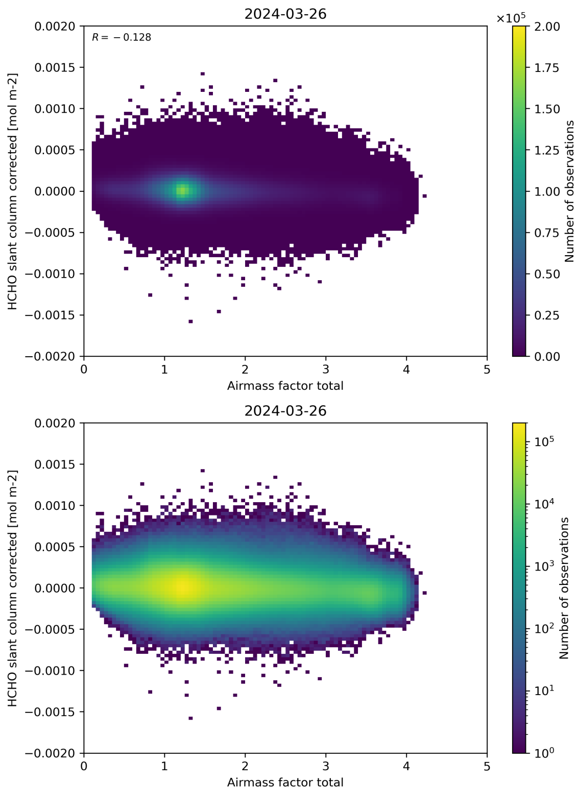
Figure 101: Scatter density plot of “Airmass factor total” against “HCHO slant column corrected” for 2024-03-25 to 2024-03-27.
