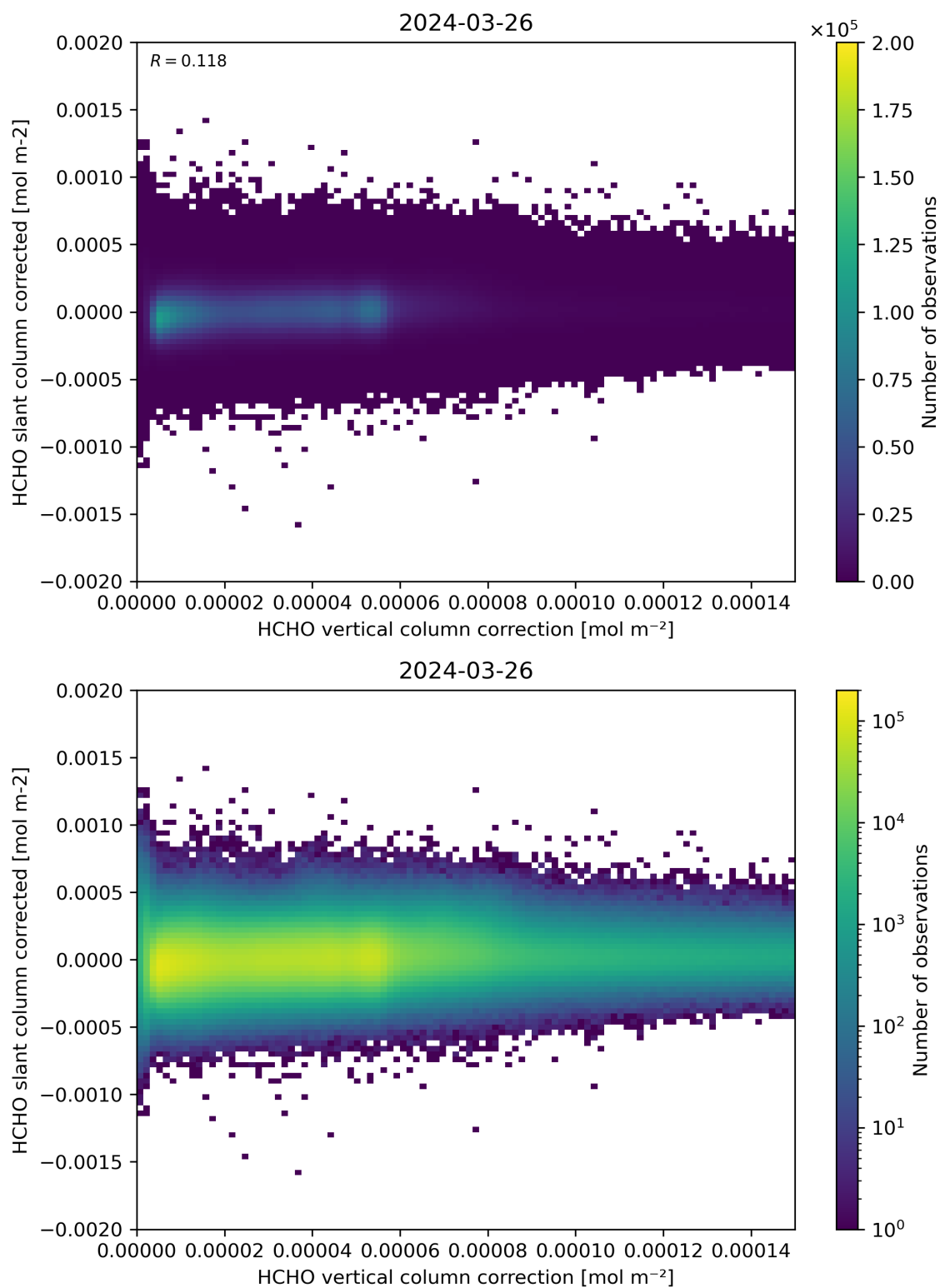
Figure 116: Scatter density plot of “HCHO vertical column correction” against “HCHO slant column corrected” for 2024-03-25 to 2024-03-27.
