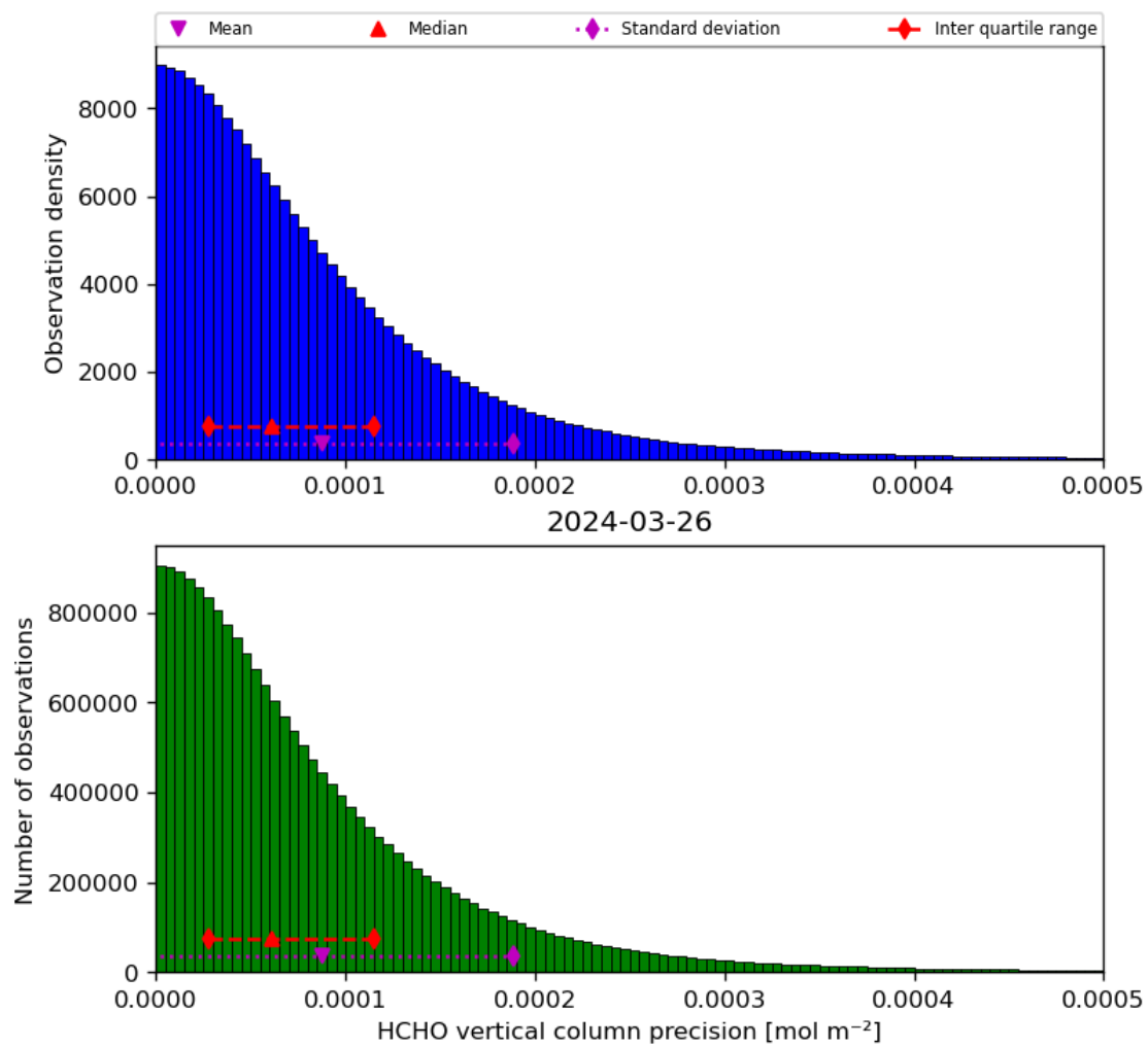
Figure 36: Histogram of “HCHO vertical column precision” for 2024-03-25 to 2024-03-27
