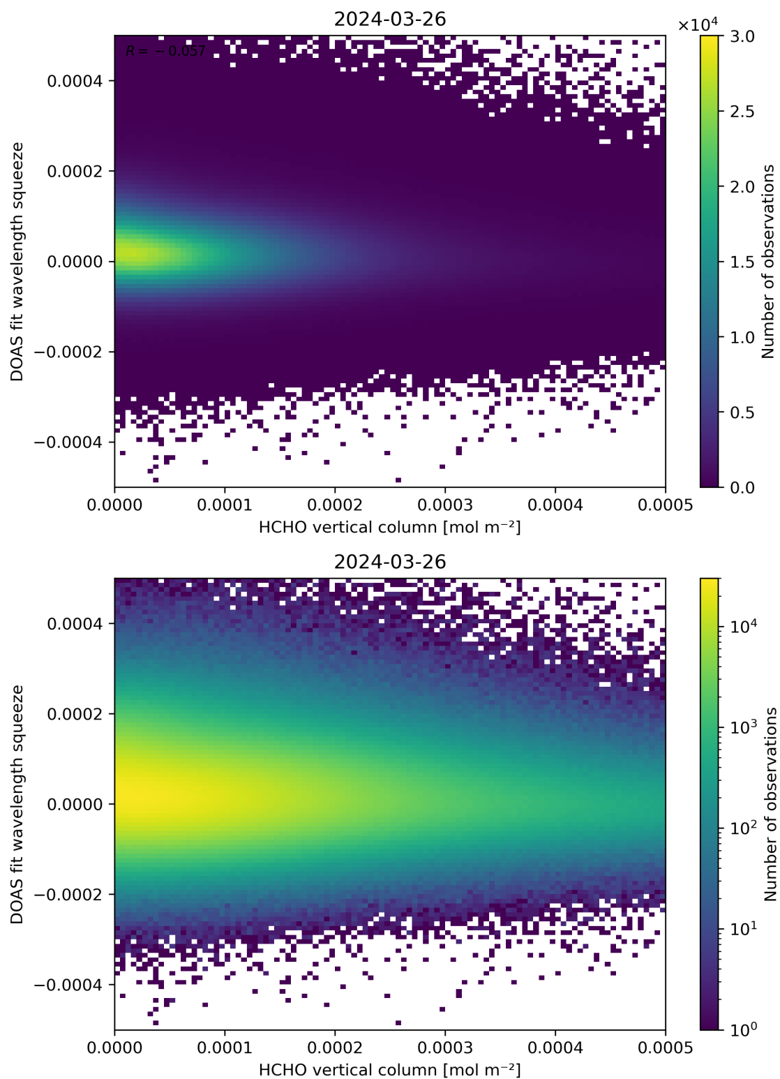
Figure 125: Scatter density plot of “HCHO vertical column” against “DOAS fit wavelength squeeze” for 2024-03-25 to 2024-03-27.
