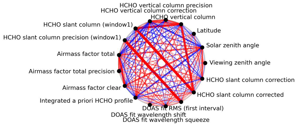
Figure 1: Map of correlation graph for 2024-03-25 to 2024-03-27.
