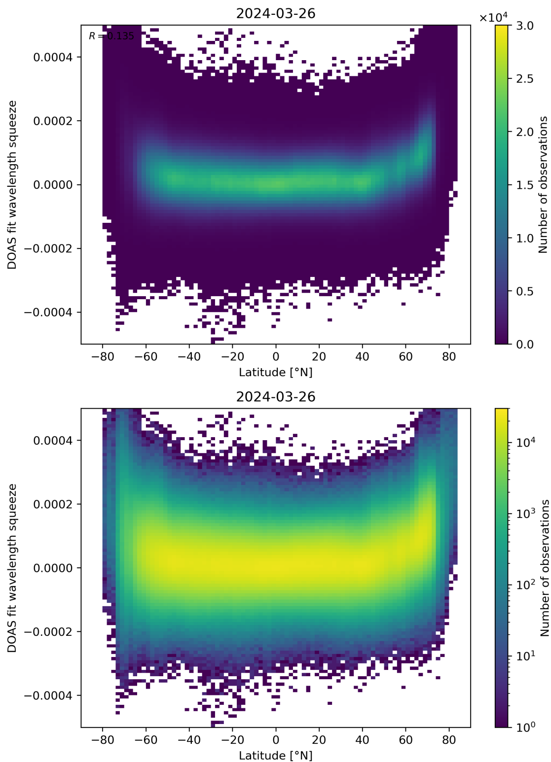
Figure 155: Scatter density plot of “Latitude” against “DOAS fit wavelength squeeze” for 2024-03-25 to 2024-03-27.
