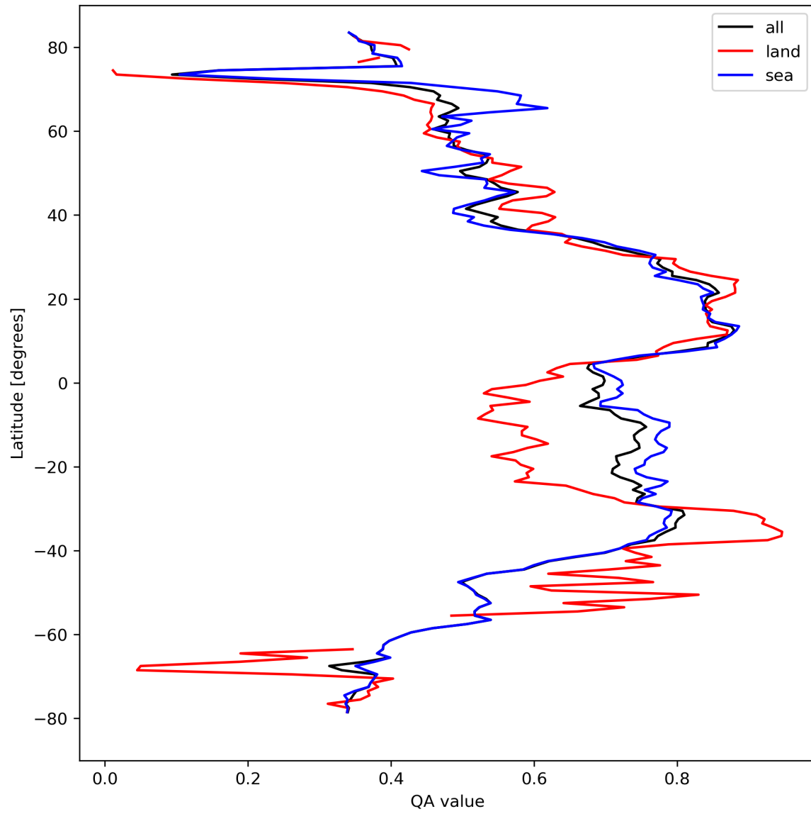
Figure 20: Zonal average of “QA value” for 2024-03-25 to 2024-03-27.
