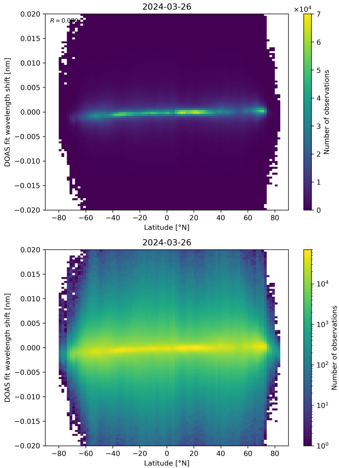
Figure 154: Scatter density plot of “Latitude” against “DOAS fit wavelength shift” for 2024-03-25 to 2024-03-27.
