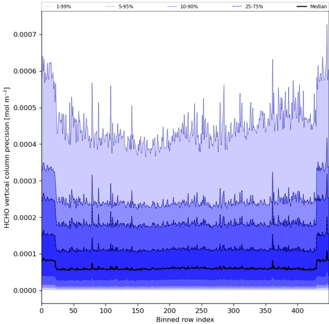
Figure 50: Along track statistics of “HCHO vertical column precision” for 2024-03-25 to 2024-03-27
