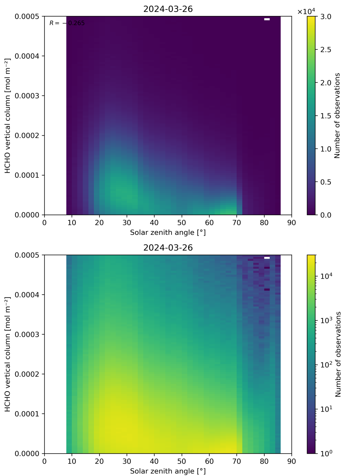
Figure 177: Scatter density plot of “Solar zenith angle” against “HCHO vertical column” for 2024-03-25 to 2024-03-27.
