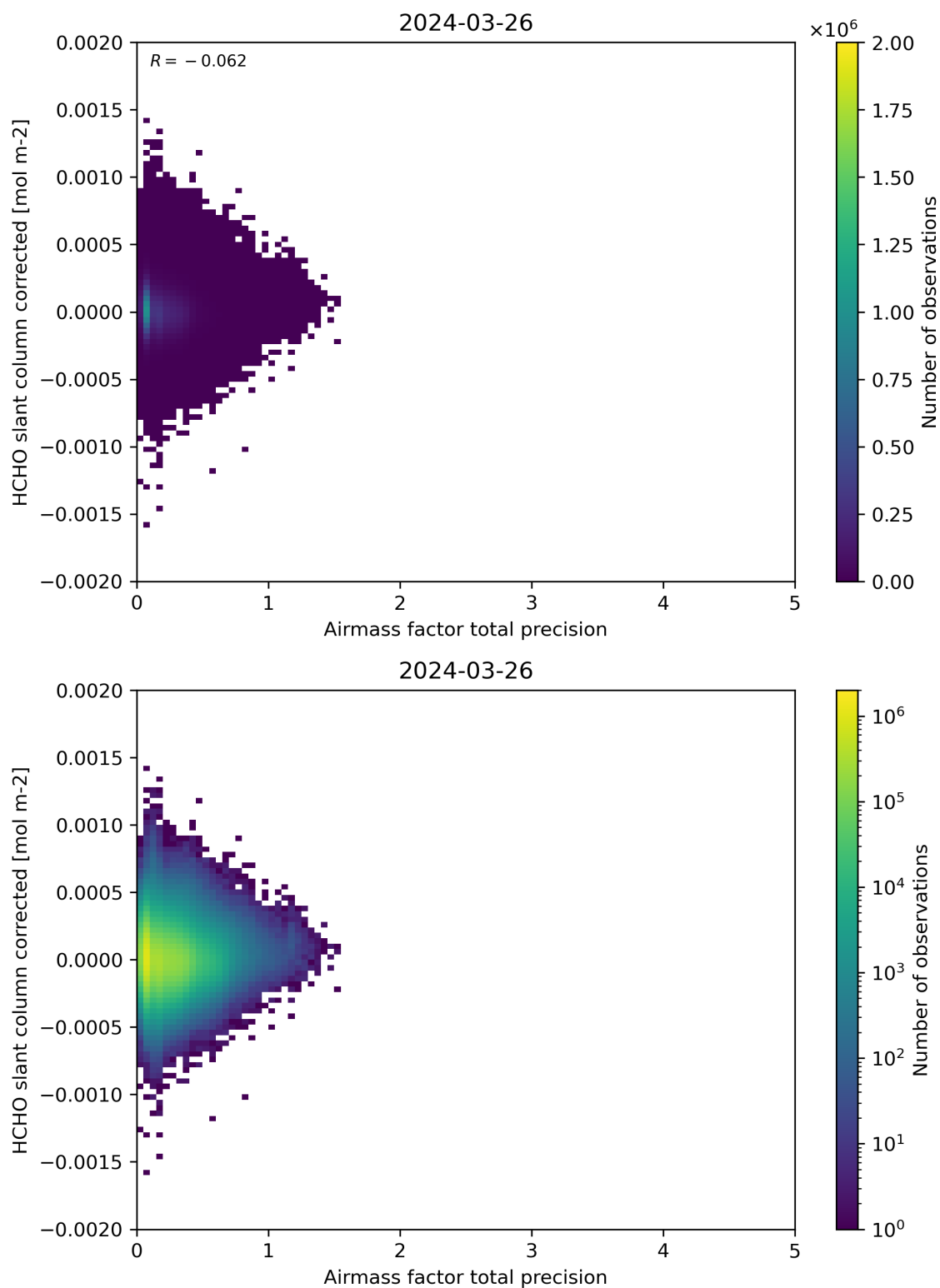
Figure 109: Scatter density plot of “Airmass factor total precision” against “HCHO slant column corrected” for 2024-03-25 to 2024-03-27.
