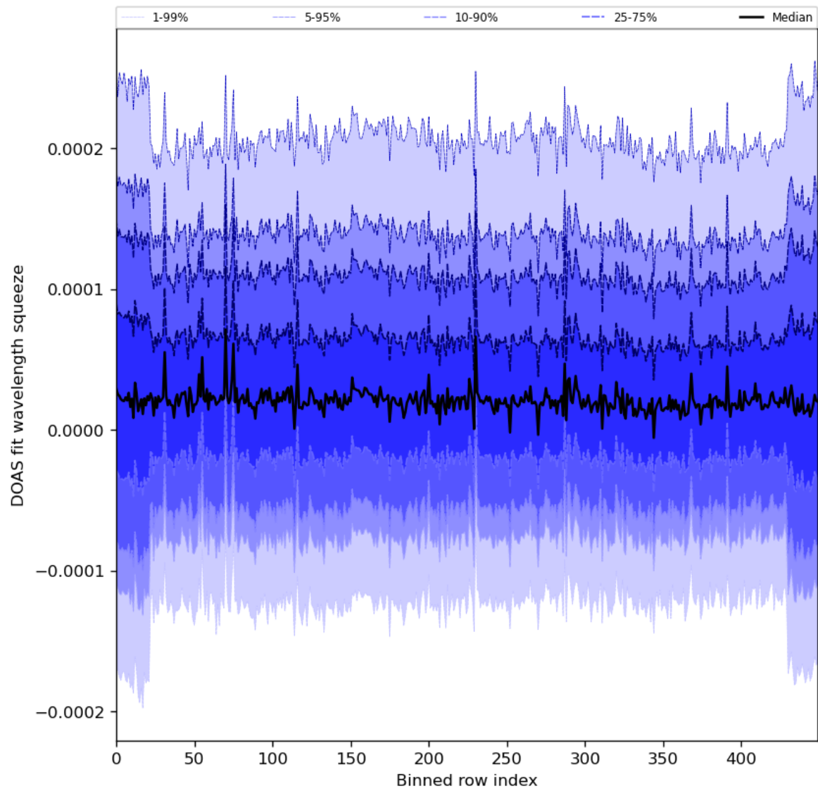
Figure 59: Along track statistics of “DOAS fit wavelength squeeze” for 2024-03-25 to 2024-03-27
