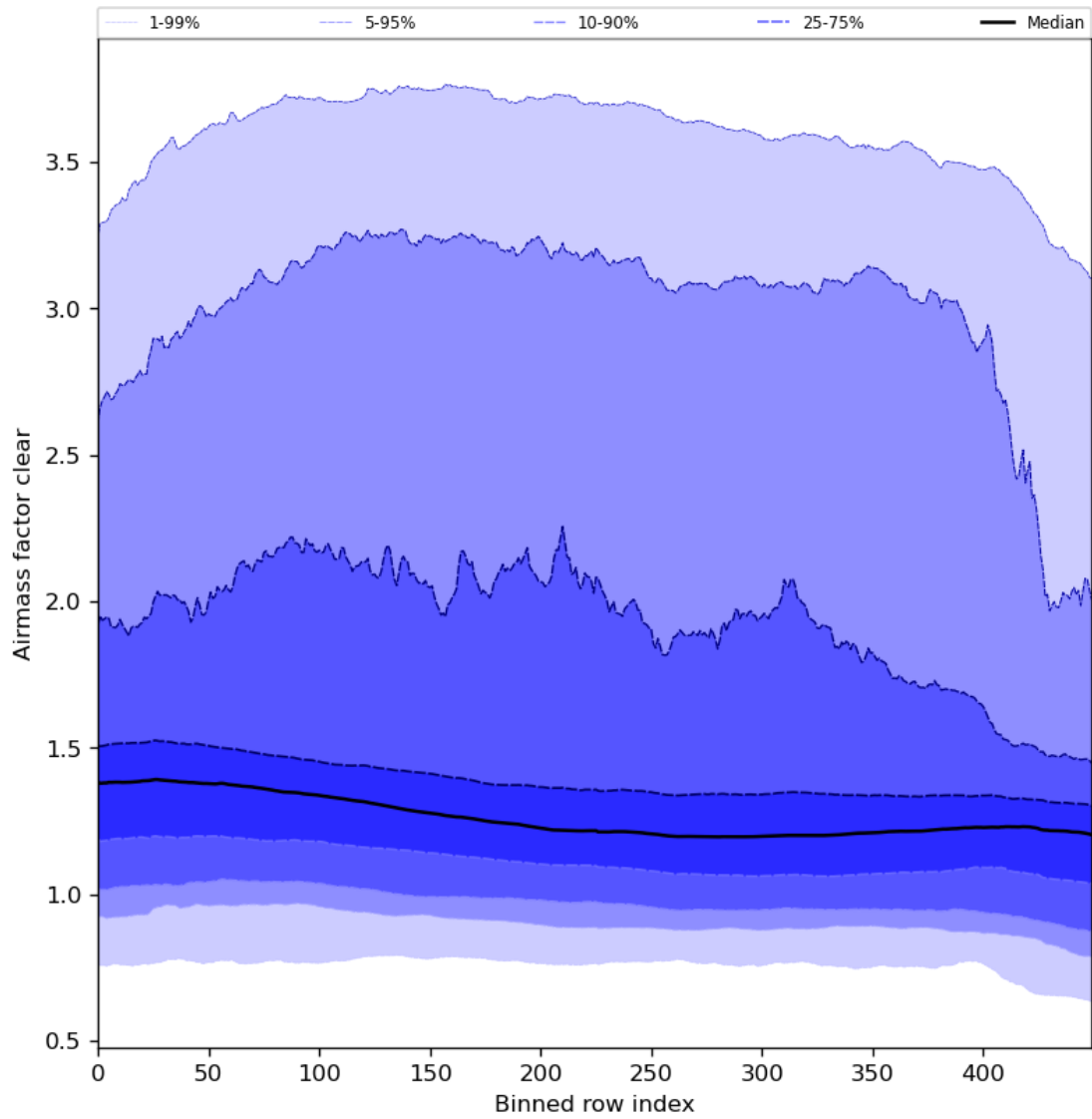
Figure 56: Along track statistics of “Airmass factor clear” for 2024-03-25 to 2024-03-27
