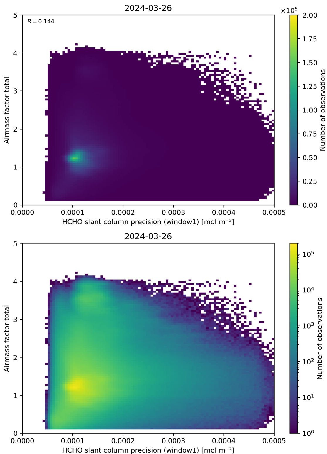
Figure 94: Scatter density plot of “HCHO slant column precision (window1)” against “Airmass factor total” for 2024-03-25 to 2024-03-27.
