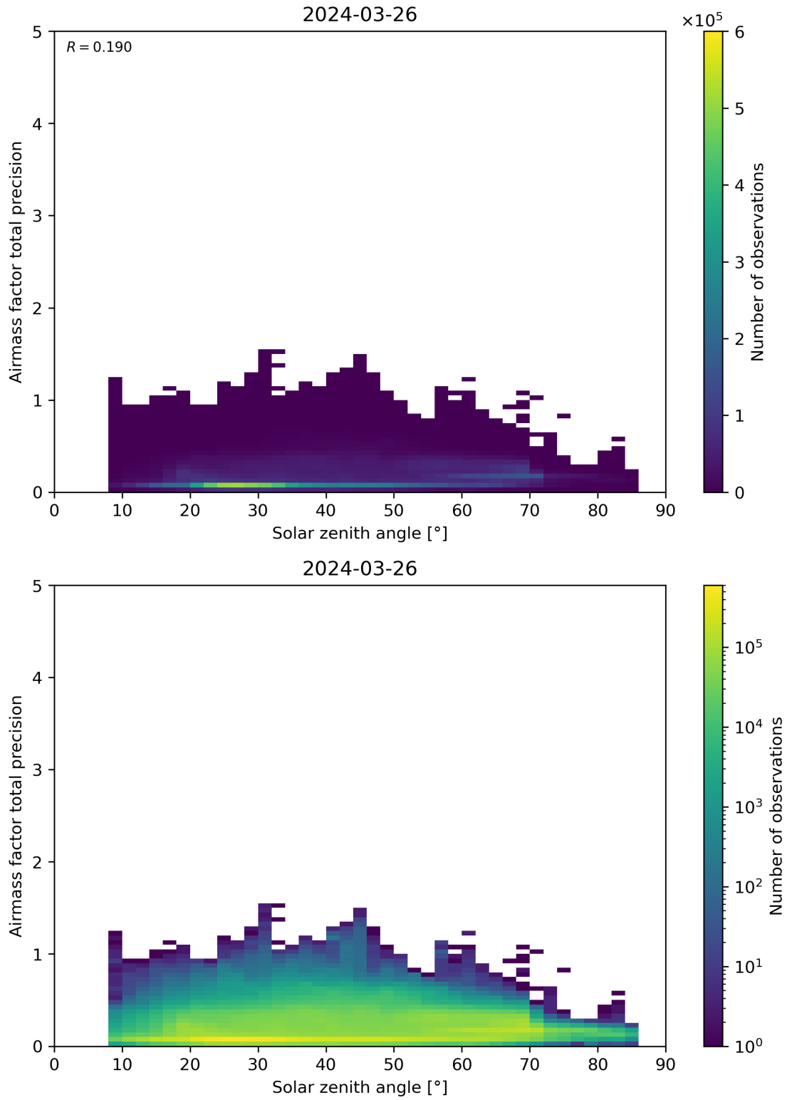
Figure 176: Scatter density plot of “Solar zenith angle” against “Airmass factor total precision” for 2024-03-25 to 2024-03-27.
