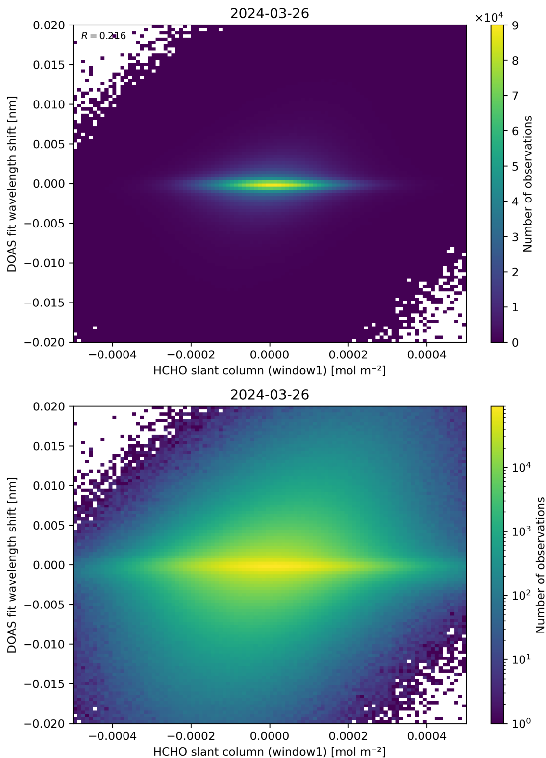
Figure 79: Scatter density plot of “HCHO slant column (window1)” against “DOAS fit wavelength shift” for 2024-03-25 to 2024-03-27.
