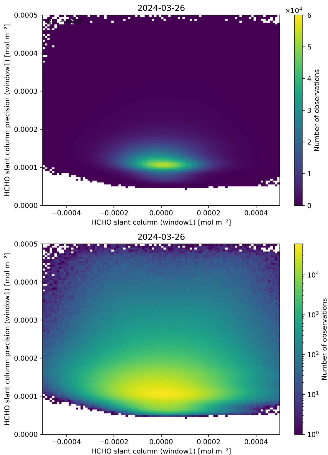
Figure 84: Scatter density plot of “HCHO slant column (window1)” against “HCHO slant column precision (window1)” for 2024-03-25 to 2024-03-27.
