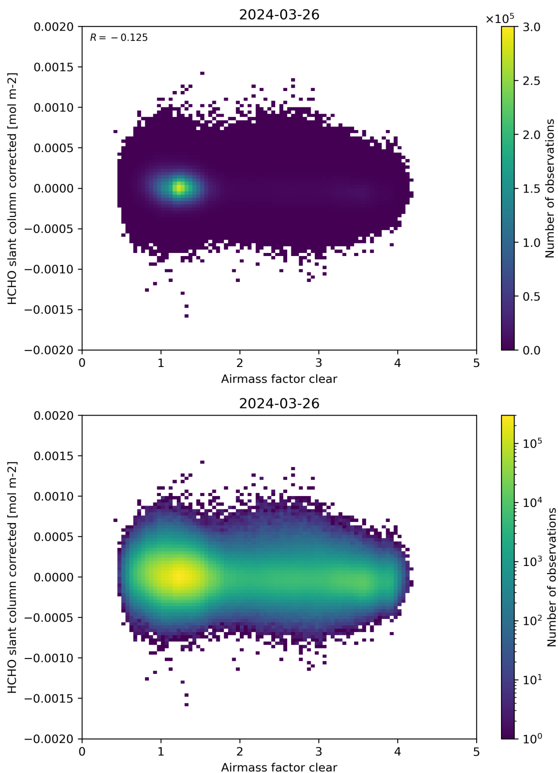
Figure 74: Scatter density plot of “Airmass factor clear” against “HCHO slant column corrected” for 2024-03-25 to 2024-03-27.
