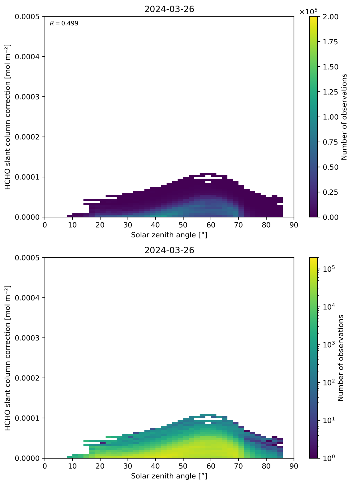
Figure 172: Scatter density plot of “Solar zenith angle” against “HCHO slant column correction” for 2024-03-25 to 2024-03-27.
