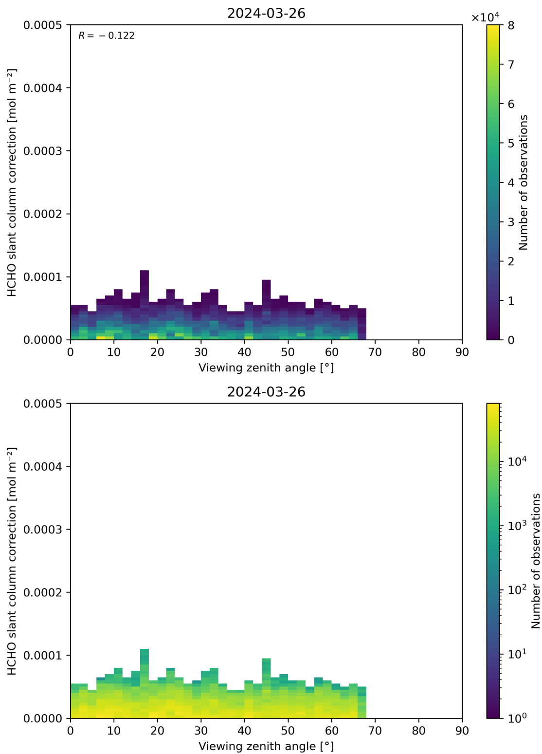
Figure 187: Scatter density plot of “Viewing zenith angle” against “HCHO slant column correction” for 2024-03-25 to 2024-03-27.
