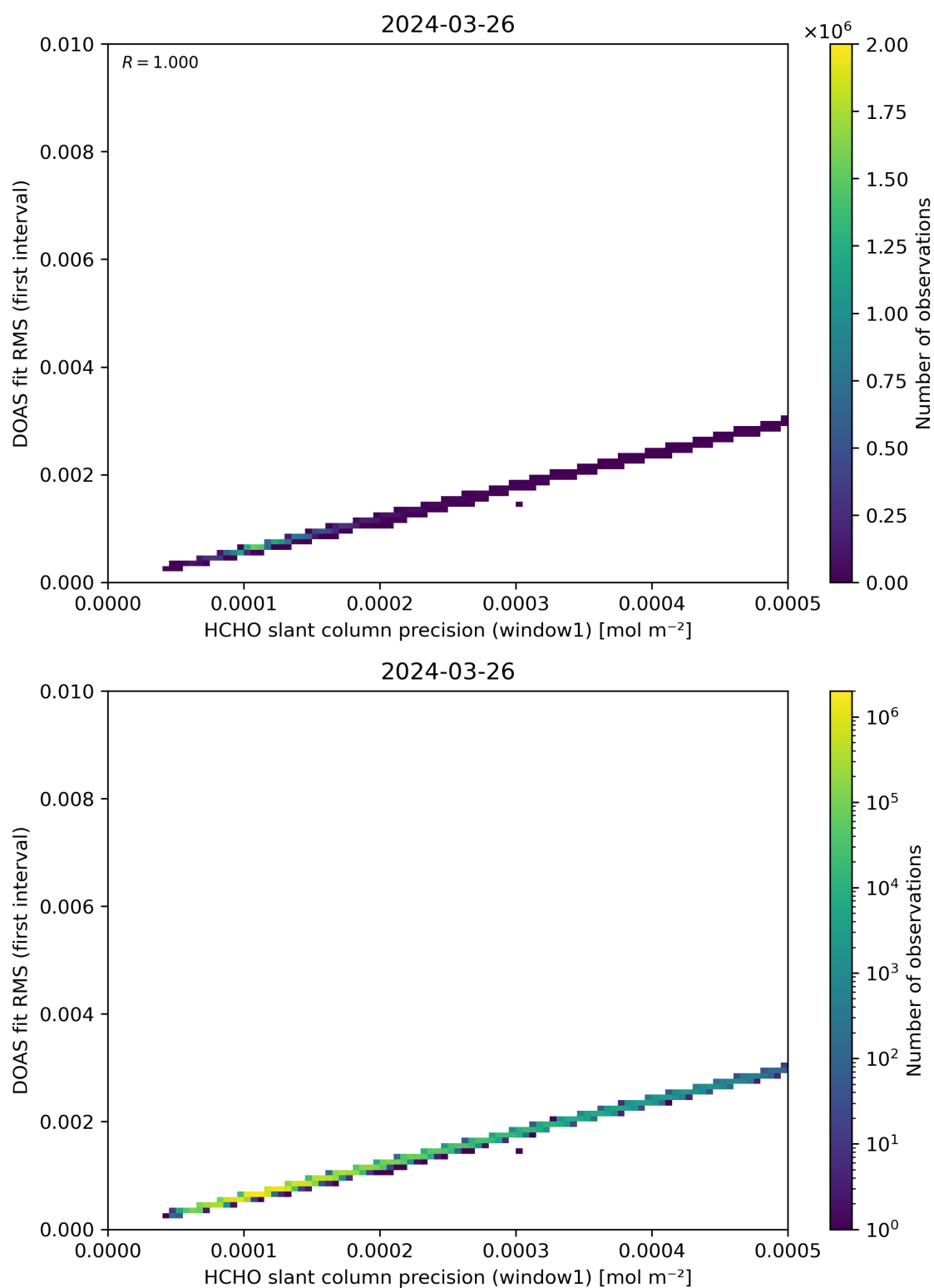
Figure 88: Scatter density plot of “HCHO slant column precision (window1)” against “DOAS fit RMS (first interval)” for 2024-03-25 to 2024-03-27.
