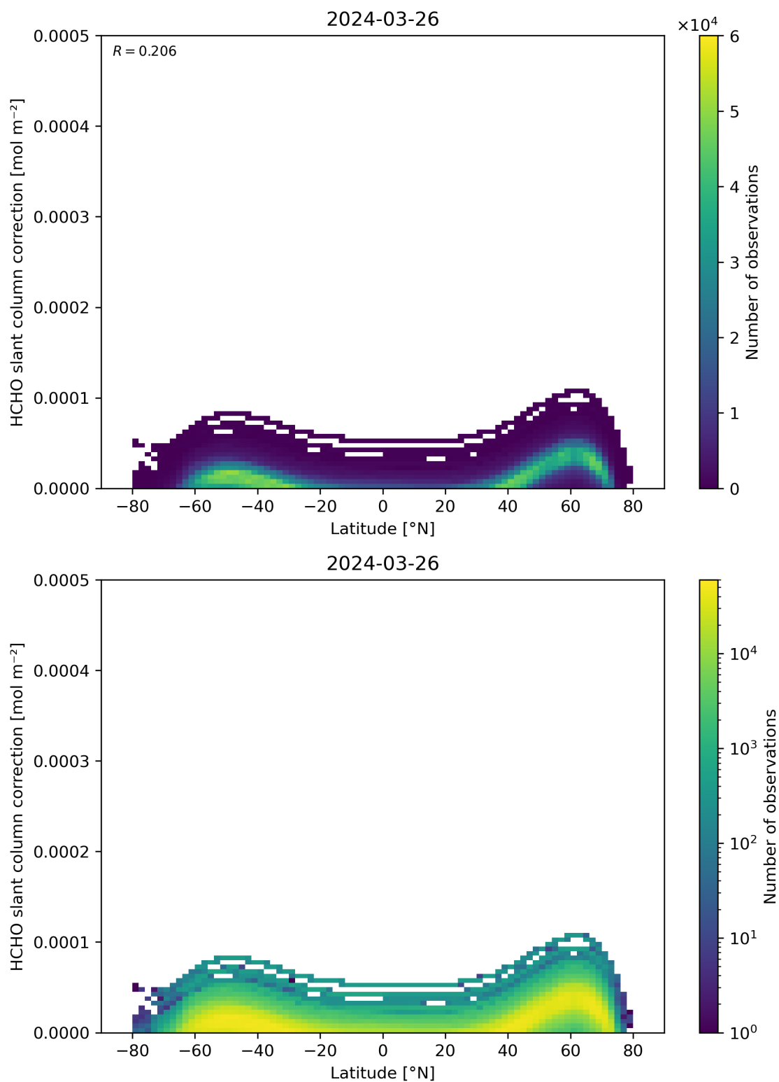
Figure 158: Scatter density plot of “Latitude” against “HCHO slant column correction” for 2024-03-25 to 2024-03-27.
