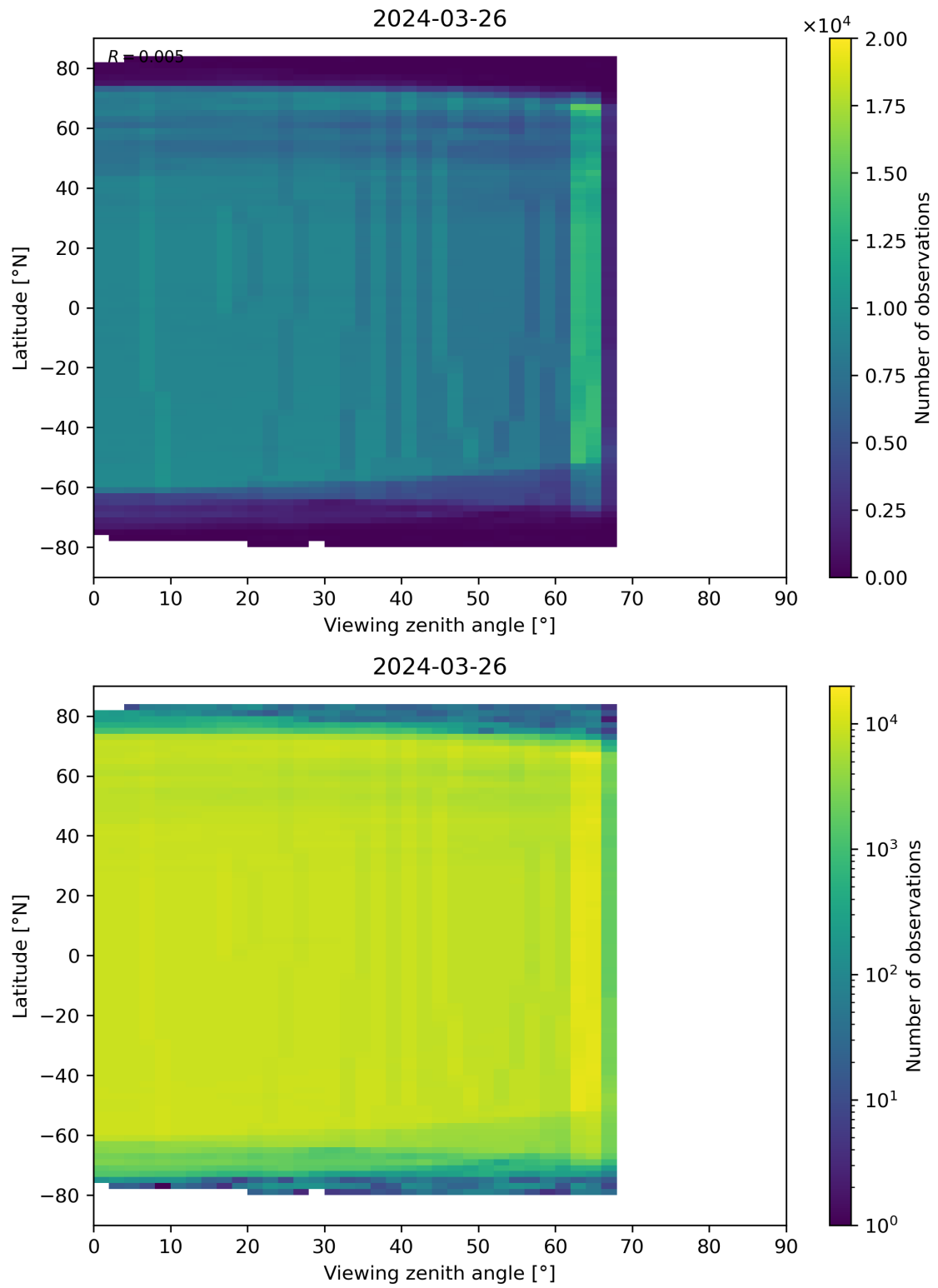
Figure 196: Scatter density plot of “Viewing zenith angle” against “Latitude” for 2024-03-25 to 2024-03-27.
