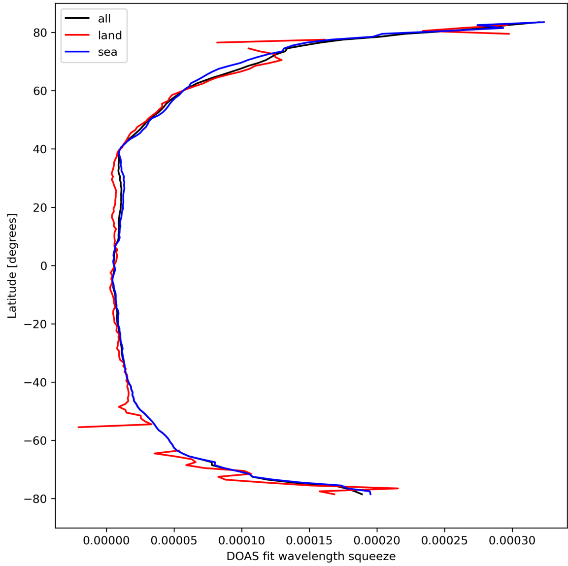
Figure 31: Zonal average of “DOAS fit wavelength squeeze” for 2024-03-25 to 2024-03-27.
