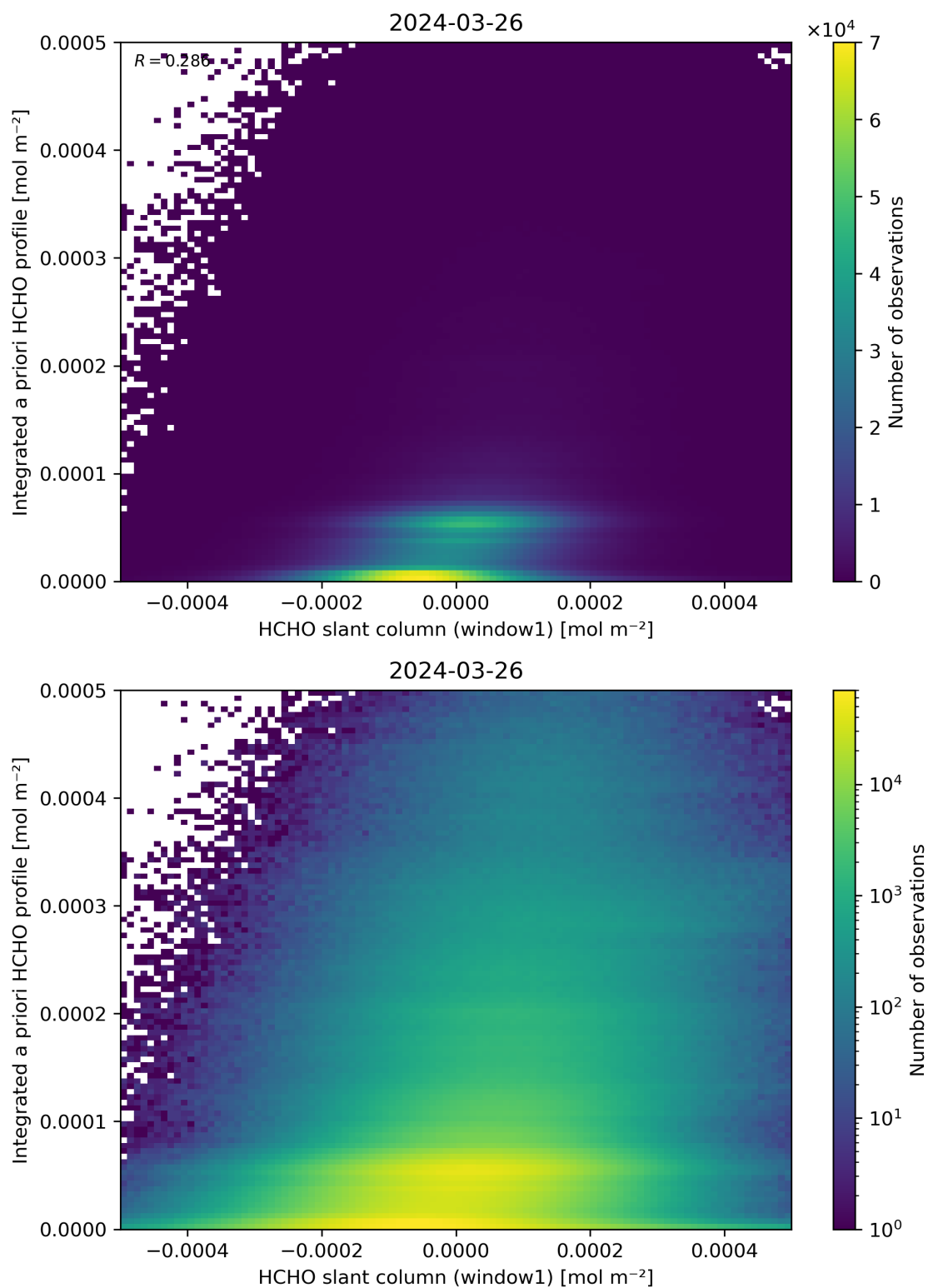
Figure 87: Scatter density plot of “HCHO slant column (window1)” against “Integrated a priori HCHO profile” for 2024-03-25 to 2024-03-27.
