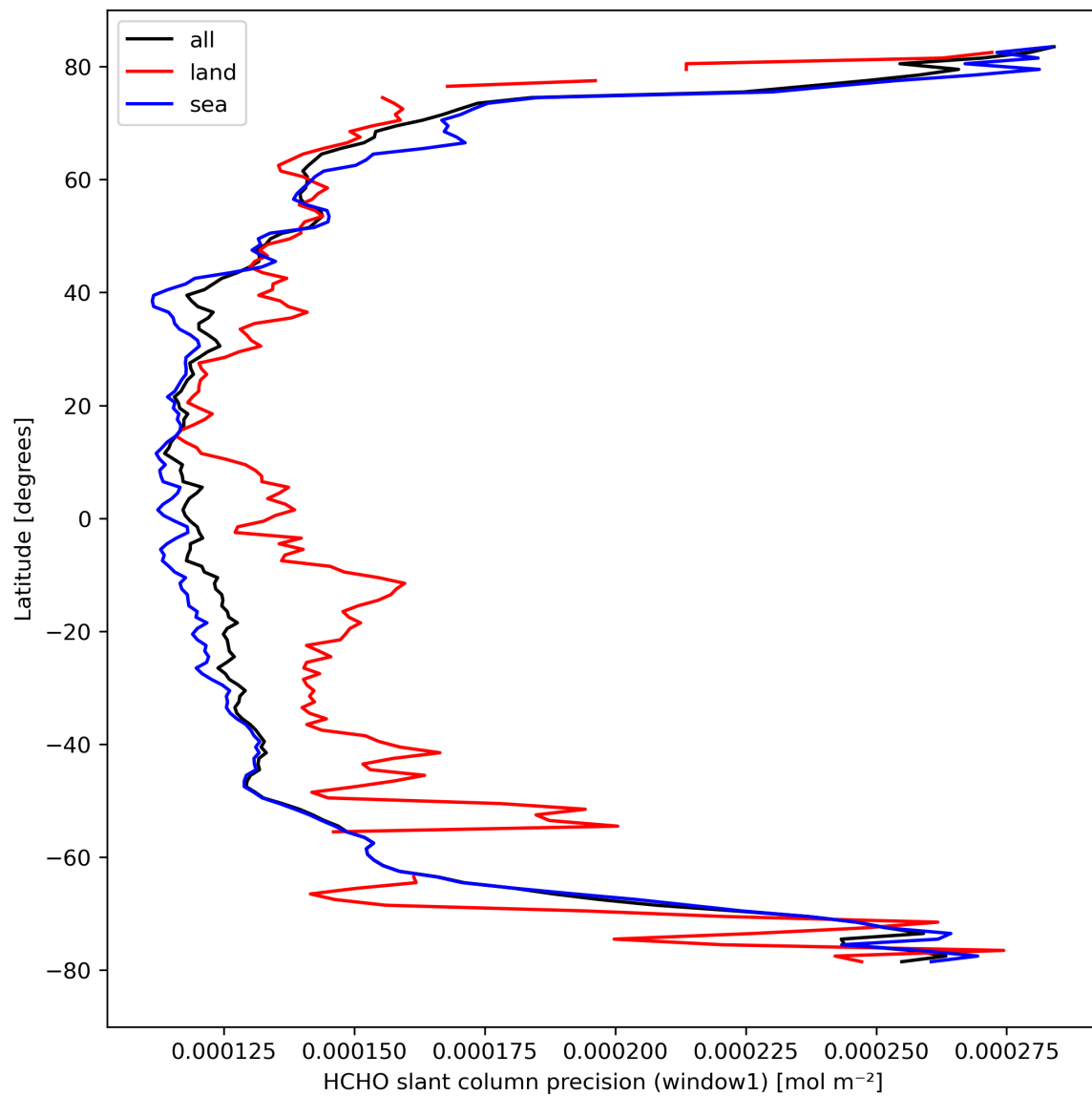
Figure 25: Zonal average of “HCHO slant column precision (window1)” for 2024-03-25 to 2024-03-27.
