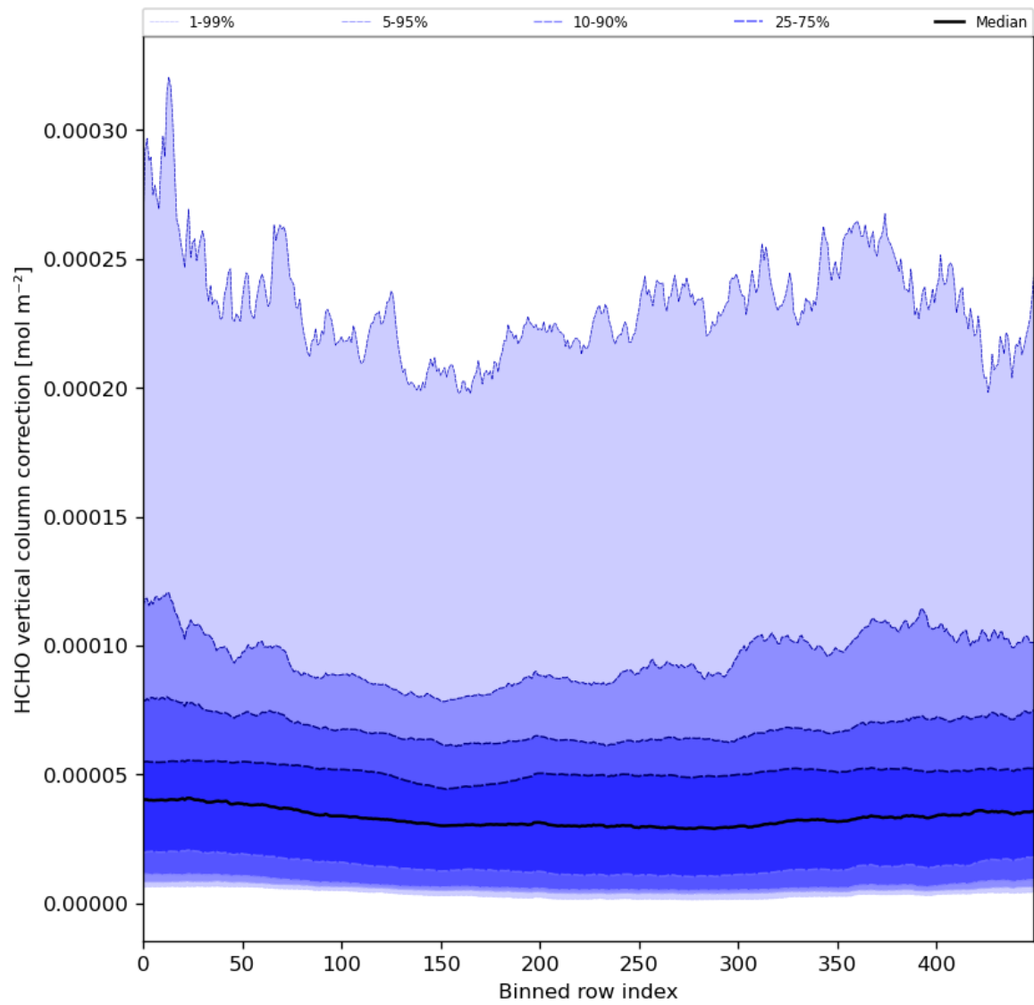
Figure 51: Along track statistics of “HCHO vertical column correction” for 2024-03-25 to 2024-03-27
