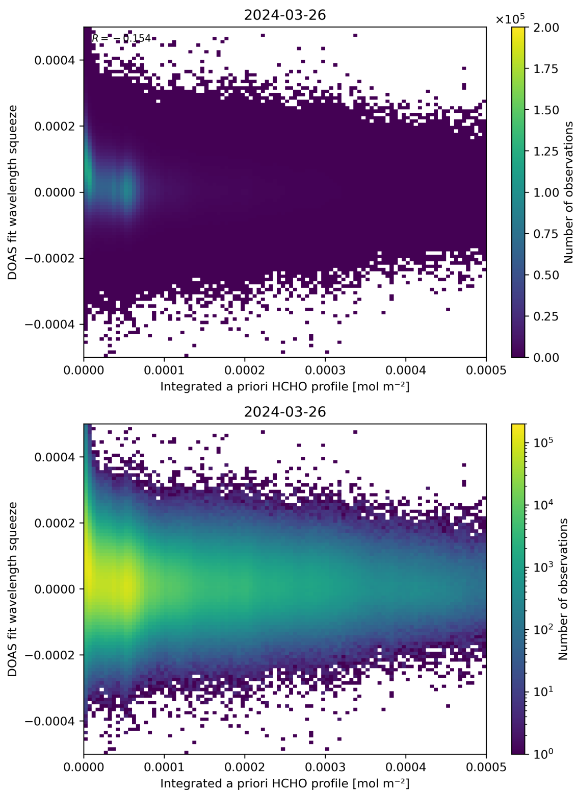
Figure 150: Scatter density plot of “Integrated a priori HCHO profile” against “DOAS fit wavelength squeeze” for 2024-03-25 to 2024-03-27.
