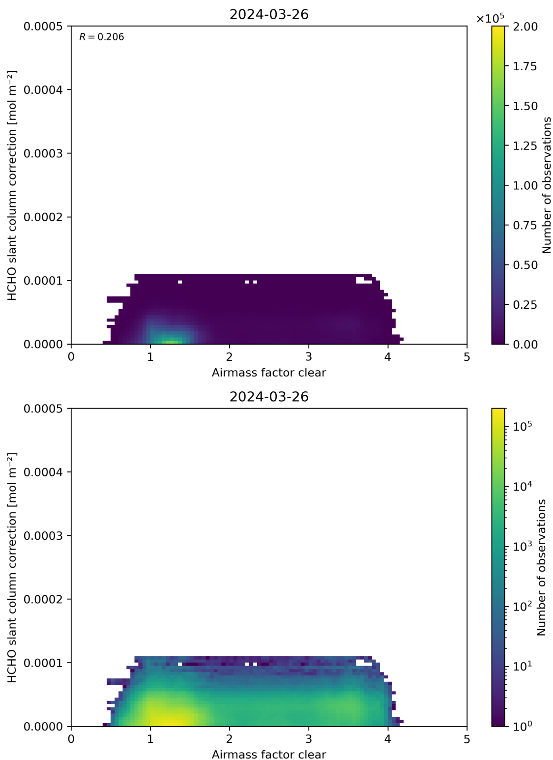
Figure 75: Scatter density plot of “Airmass factor clear” against “HCHO slant column correction” for 2024-03-25 to 2024-03-27.
