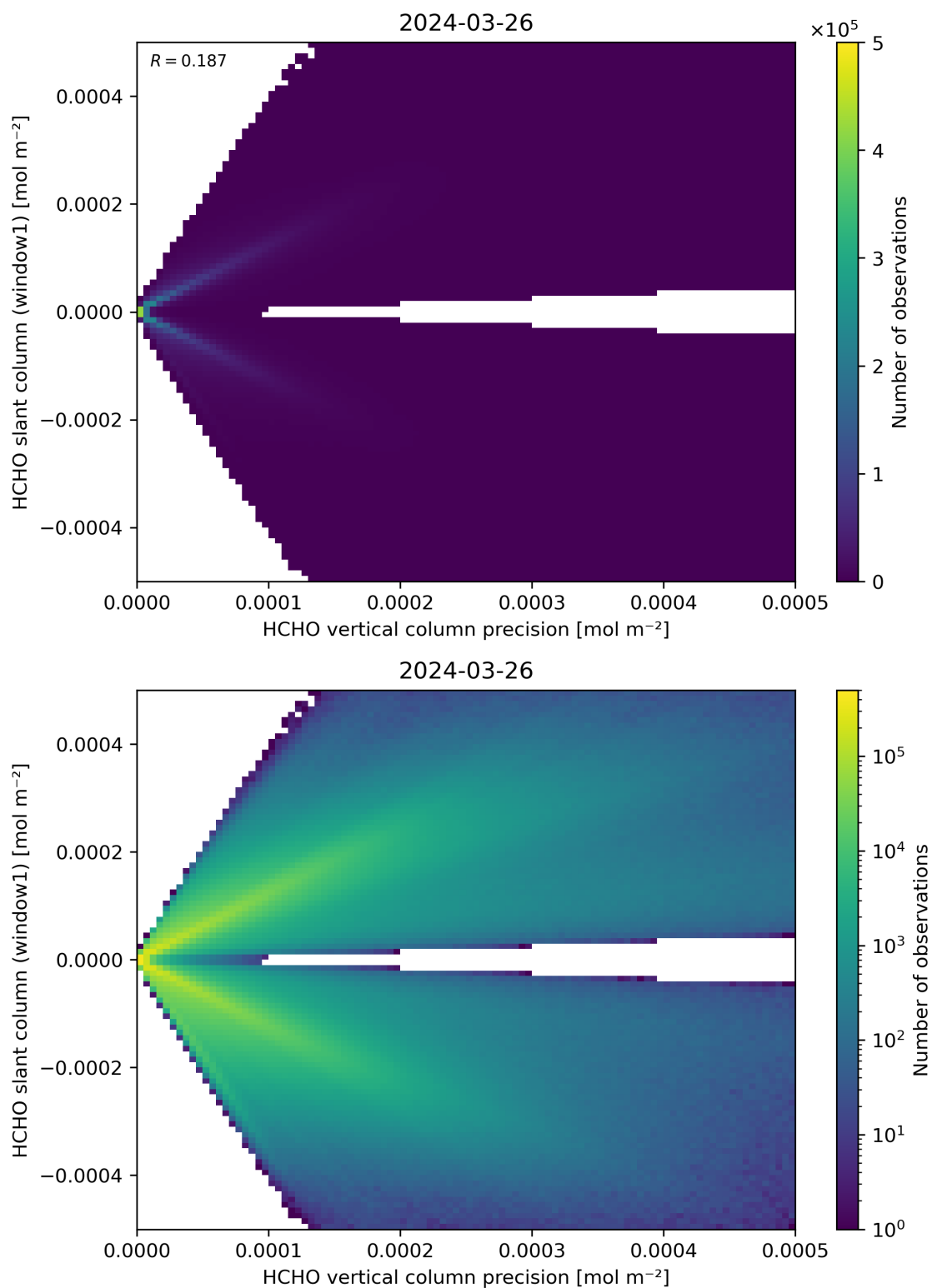
Figure 142: Scatter density plot of “HCHO vertical column precision” against “HCHO slant column (window1)” for 2024-03-25 to 2024-03-27.
