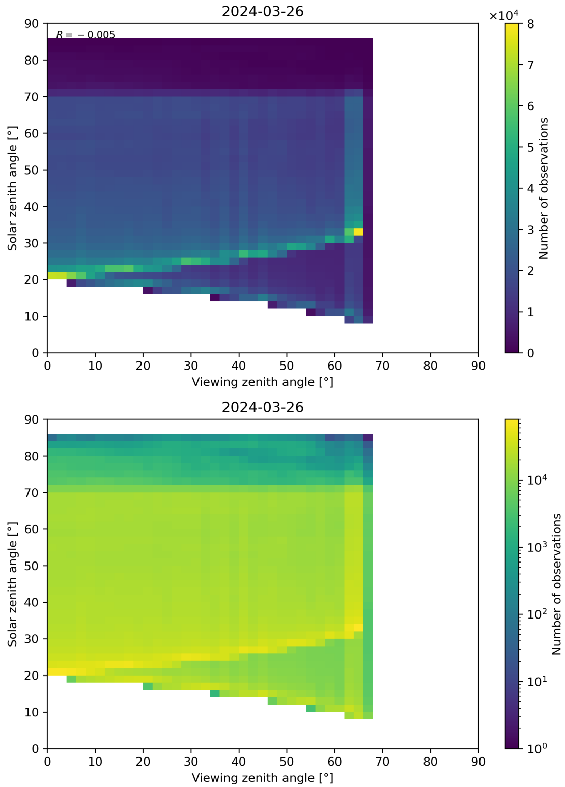
Figure 197: Scatter density plot of “Viewing zenith angle” against “Solar zenith angle” for 2024-03-25 to 2024-03-27.
