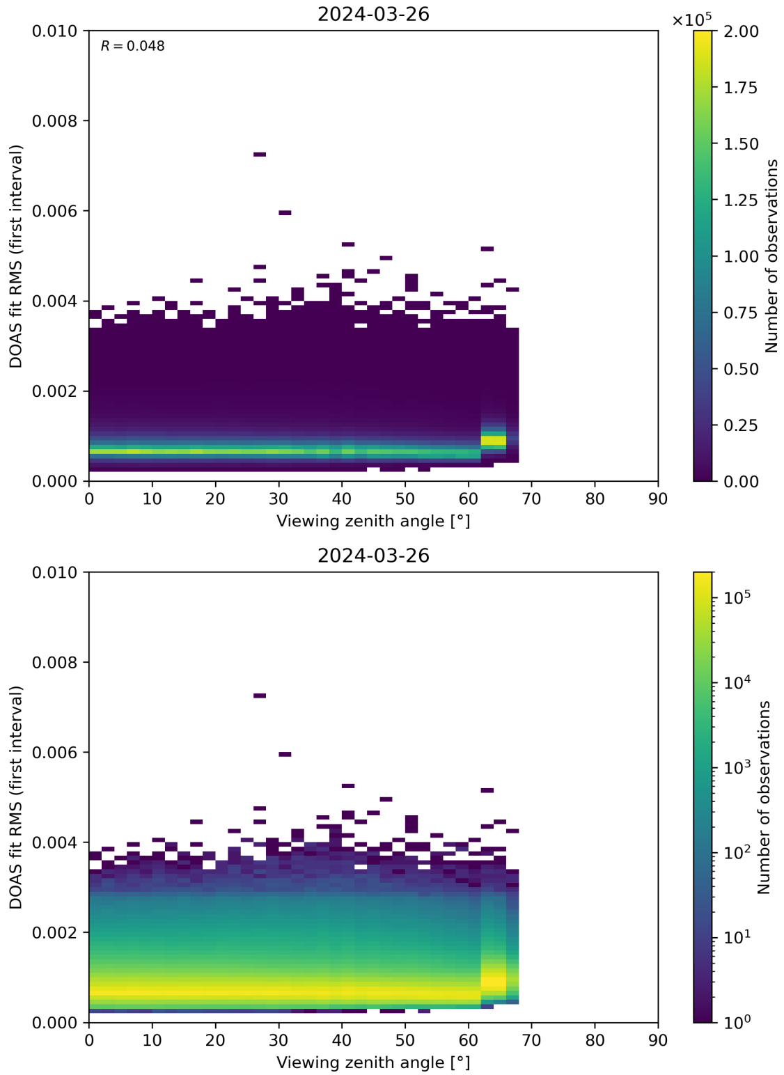
Figure 182: Scatter density plot of “Viewing zenith angle” against “DOAS fit RMS (first interval)” for 2024-03-25 to 2024-03-27.
