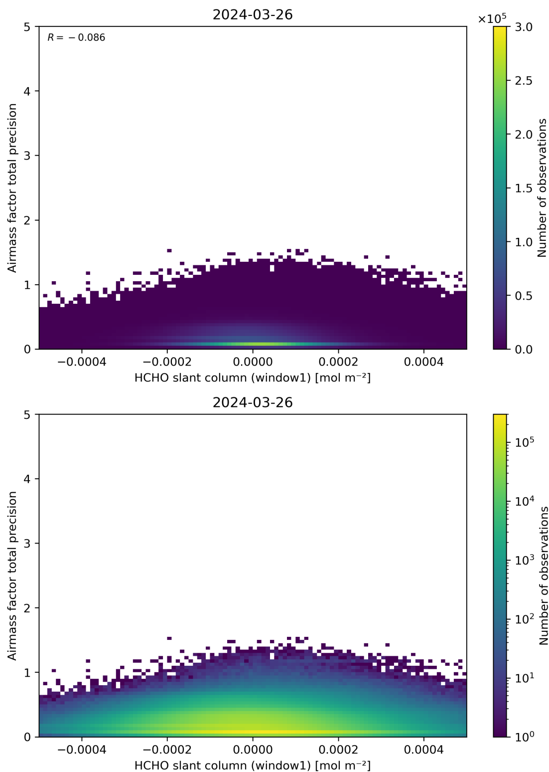
Figure 86: Scatter density plot of “HCHO slant column (window1)” against “Airmass factor total precision” for 2024-03-25 to 2024-03-27.
