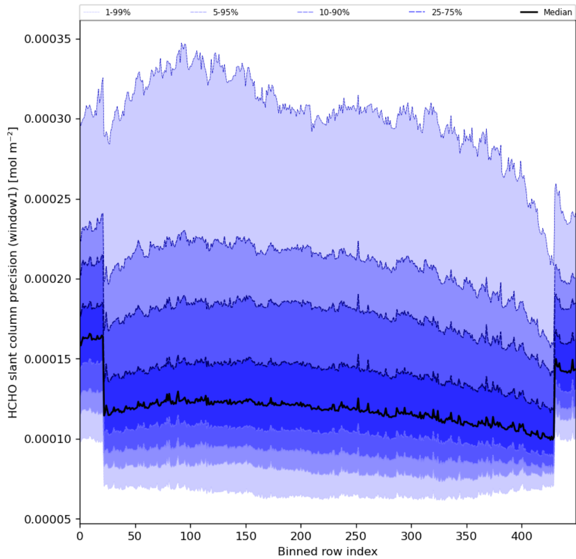
Figure 53: Along track statistics of “HCHO slant column precision (window1)” for 2024-03-25 to 2024-03-27
