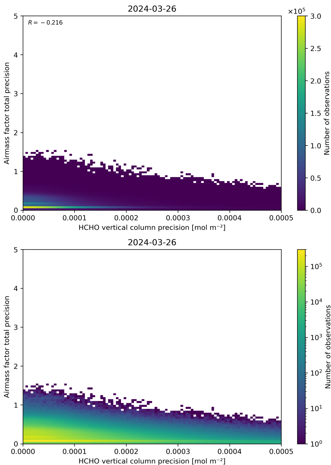
Figure 145: Scatter density plot of “HCHO vertical column precision” against “Airmass factor total precision” for 2024-03-25 to 2024-03-27.
