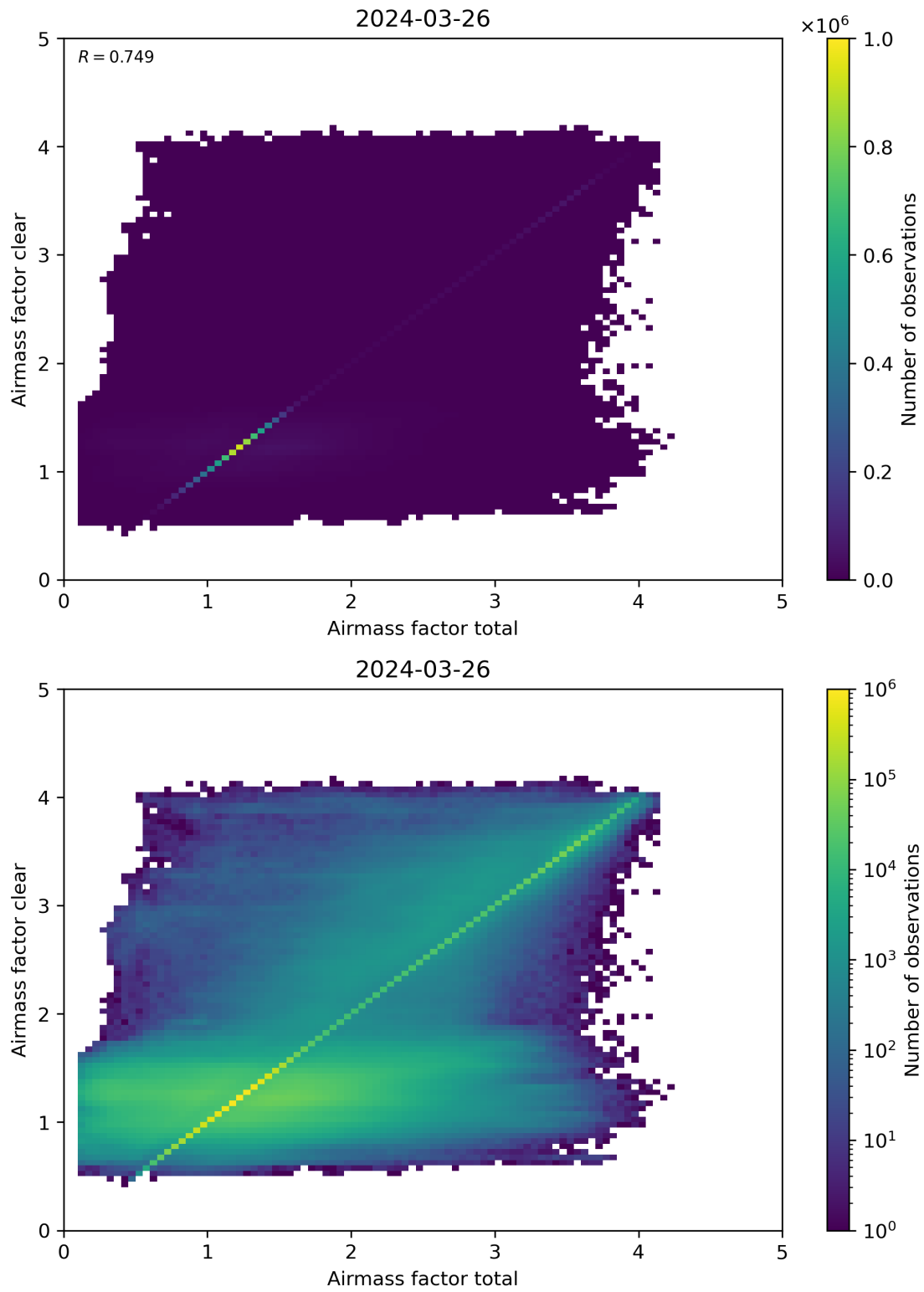
Figure 100: Scatter density plot of “Airmass factor total” against “Airmass factor clear” for 2024-03-25 to 2024-03-27.
