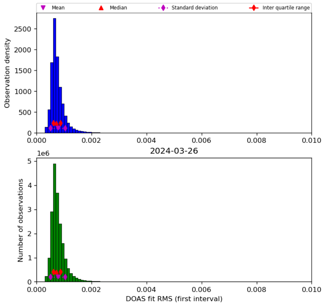
Figure 46: Histogram of “DOAS fit RMS (first interval)” for 2024-03-25 to 2024-03-27
