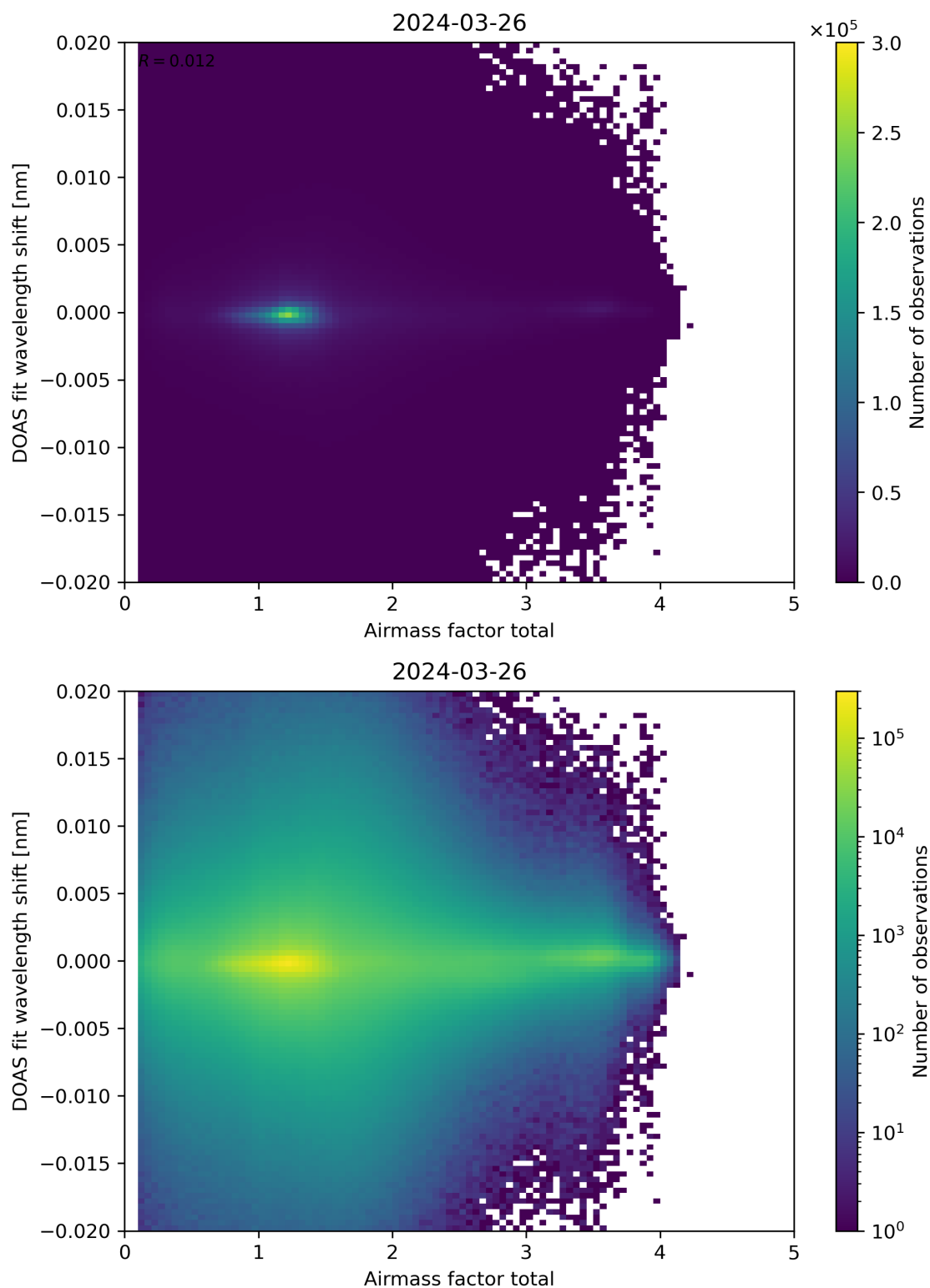
Figure 98: Scatter density plot of “Airmass factor total” against “DOAS fit wavelength shift” for 2024-03-25 to 2024-03-27.
