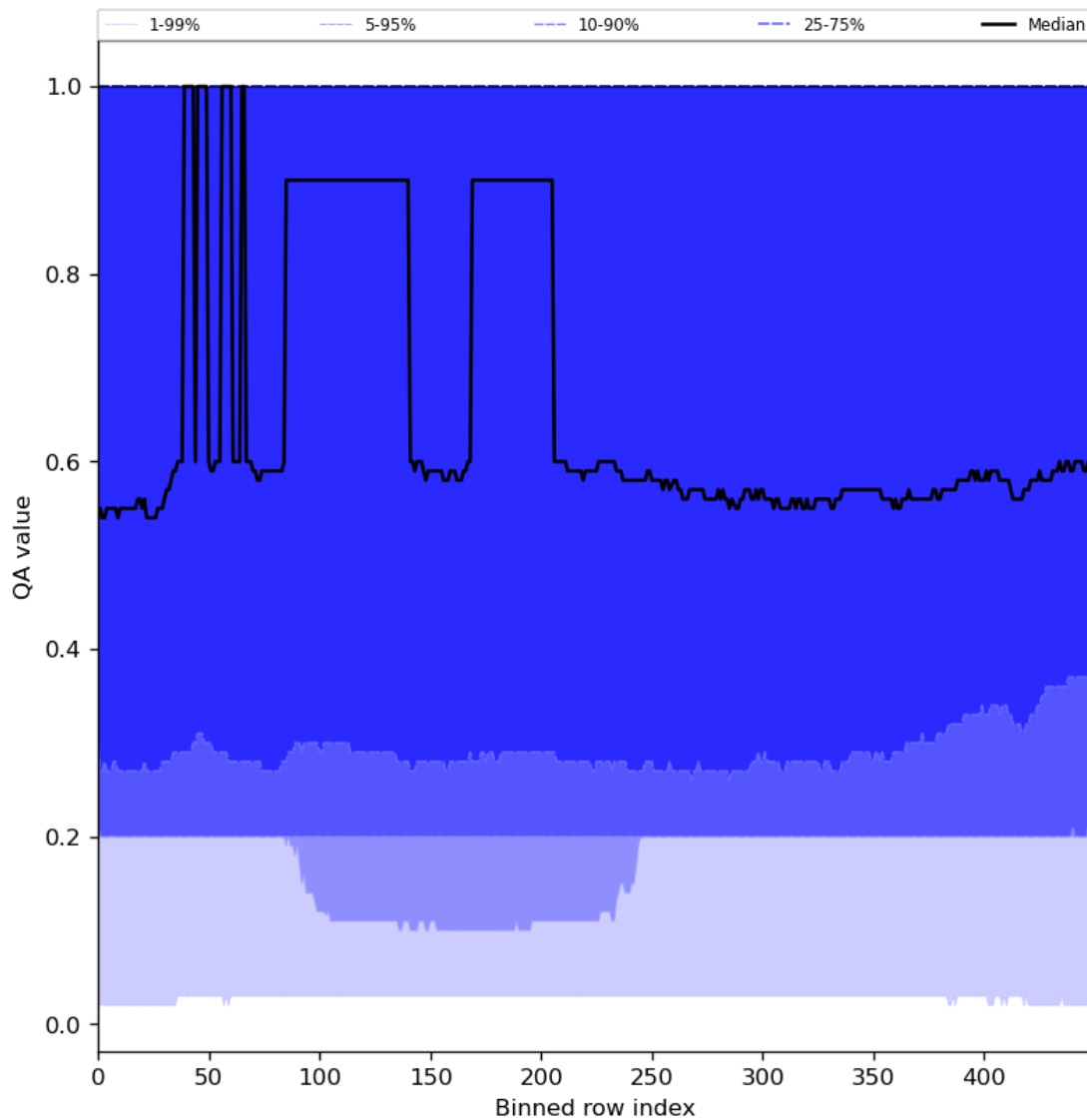
Figure 48: Along track statistics of “QA value” for 2024-03-25 to 2024-03-27
