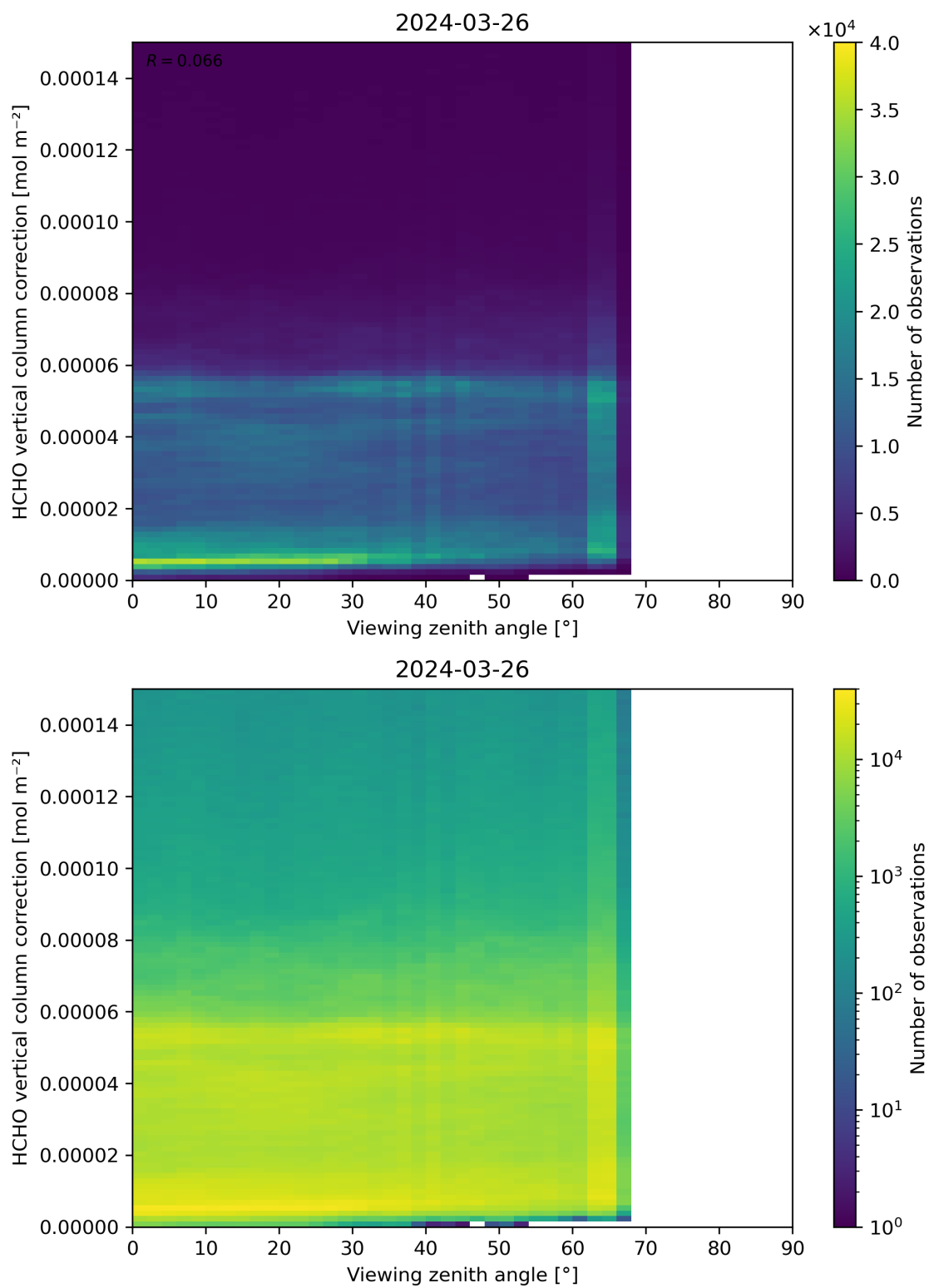
Figure 193: Scatter density plot of “Viewing zenith angle” against “HCHO vertical column correction” for 2024-03-25 to 2024-03-27.
