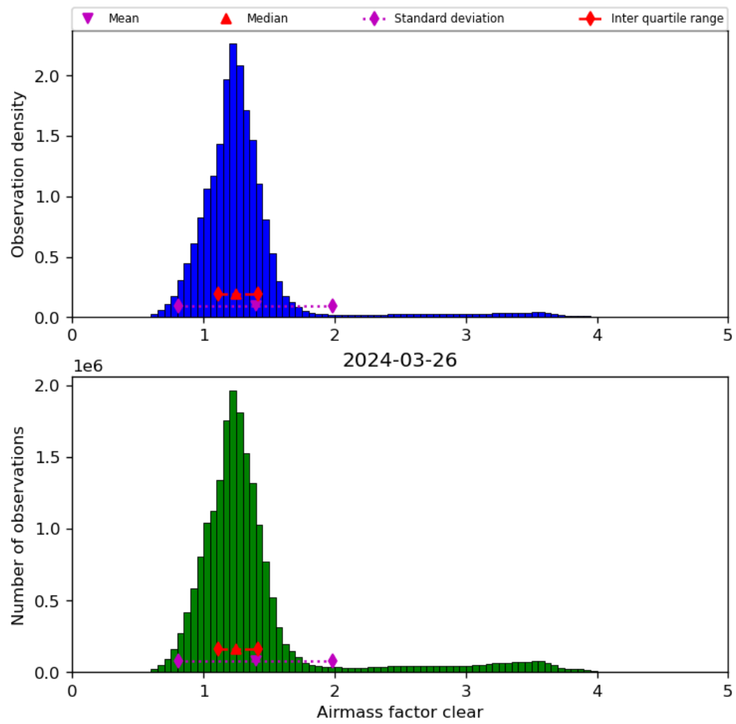
Figure 42: Histogram of “Airmass factor clear” for 2024-03-25 to 2024-03-27
