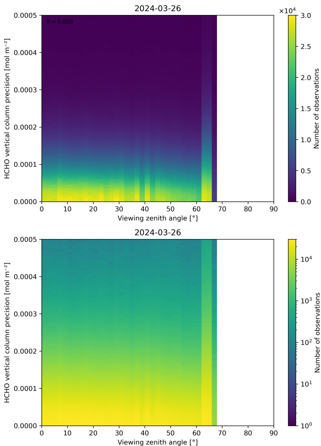
Figure 194: Scatter density plot of “Viewing zenith angle” against “HCHO vertical column precision” for 2024-03-25 to 2024-03-27.
