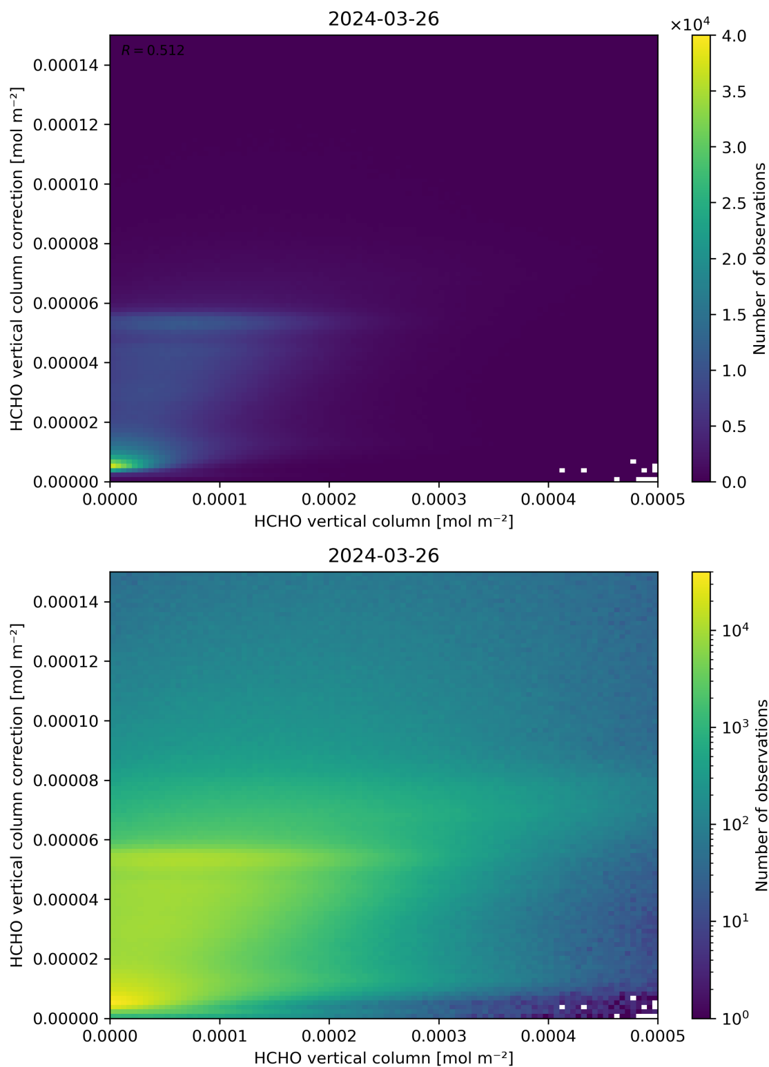
Figure 133: Scatter density plot of “HCHO vertical column” against “HCHO vertical column correction” for 2024-03-25 to 2024-03-27.
