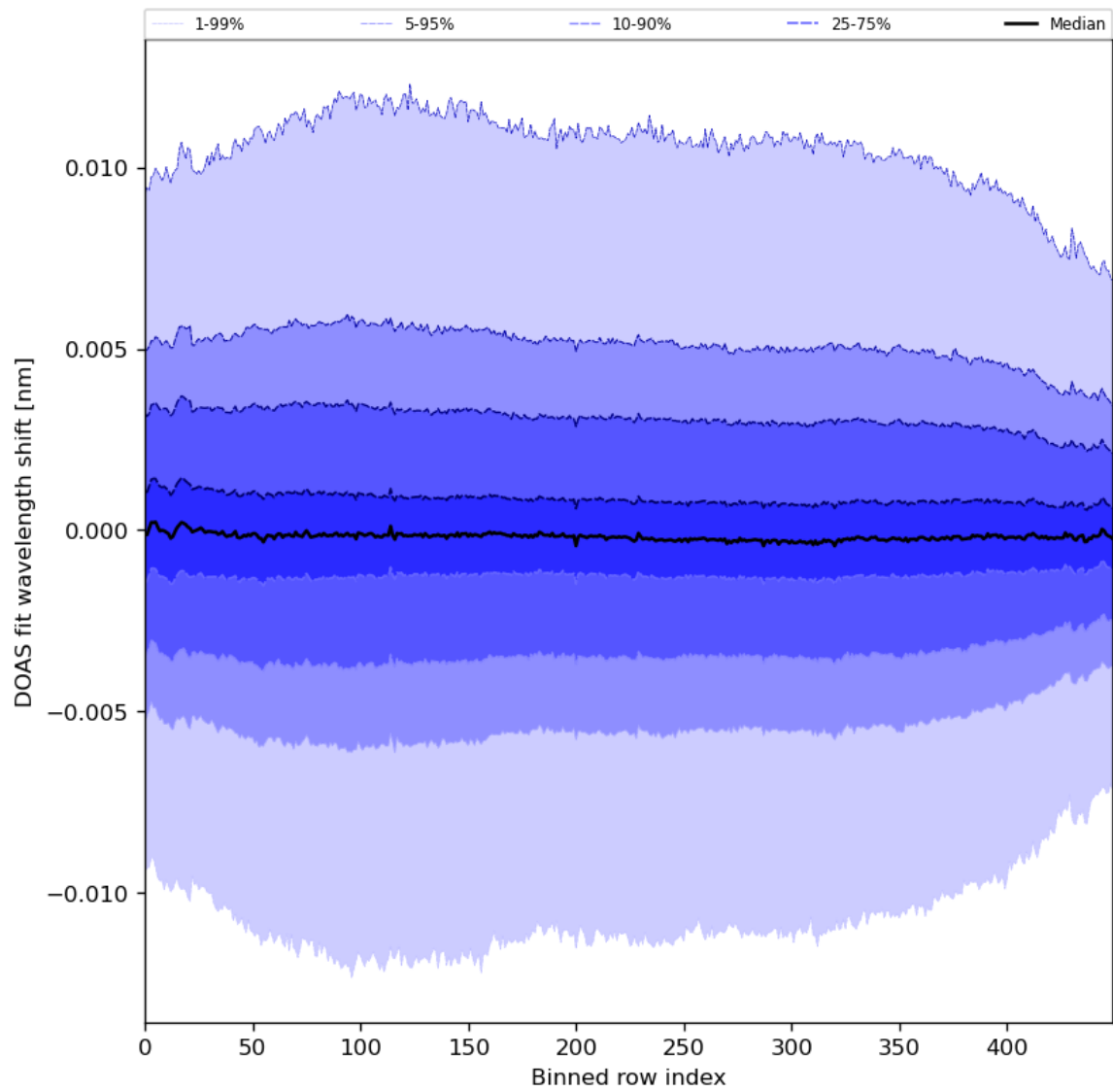
Figure 58: Along track statistics of “DOAS fit wavelength shift” for 2024-03-25 to 2024-03-27
