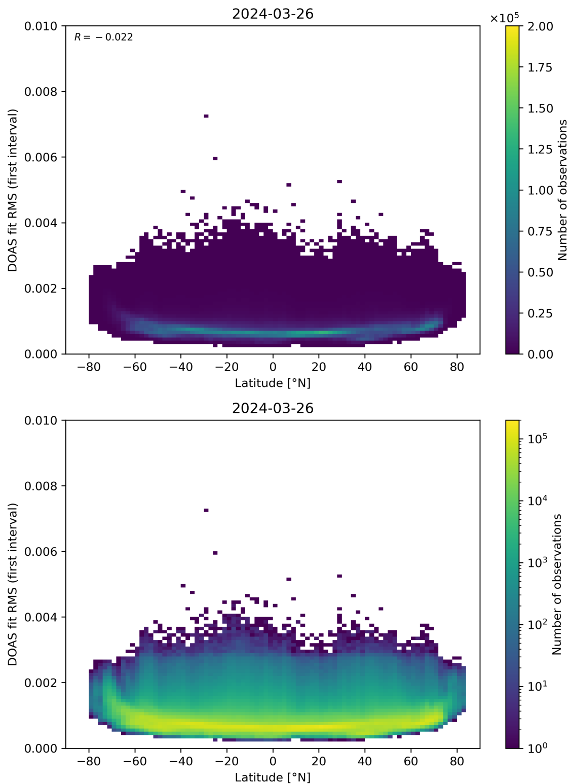
Figure 153: Scatter density plot of “Latitude” against “DOAS fit RMS (first interval)” for 2024-03-25 to 2024-03-27.
