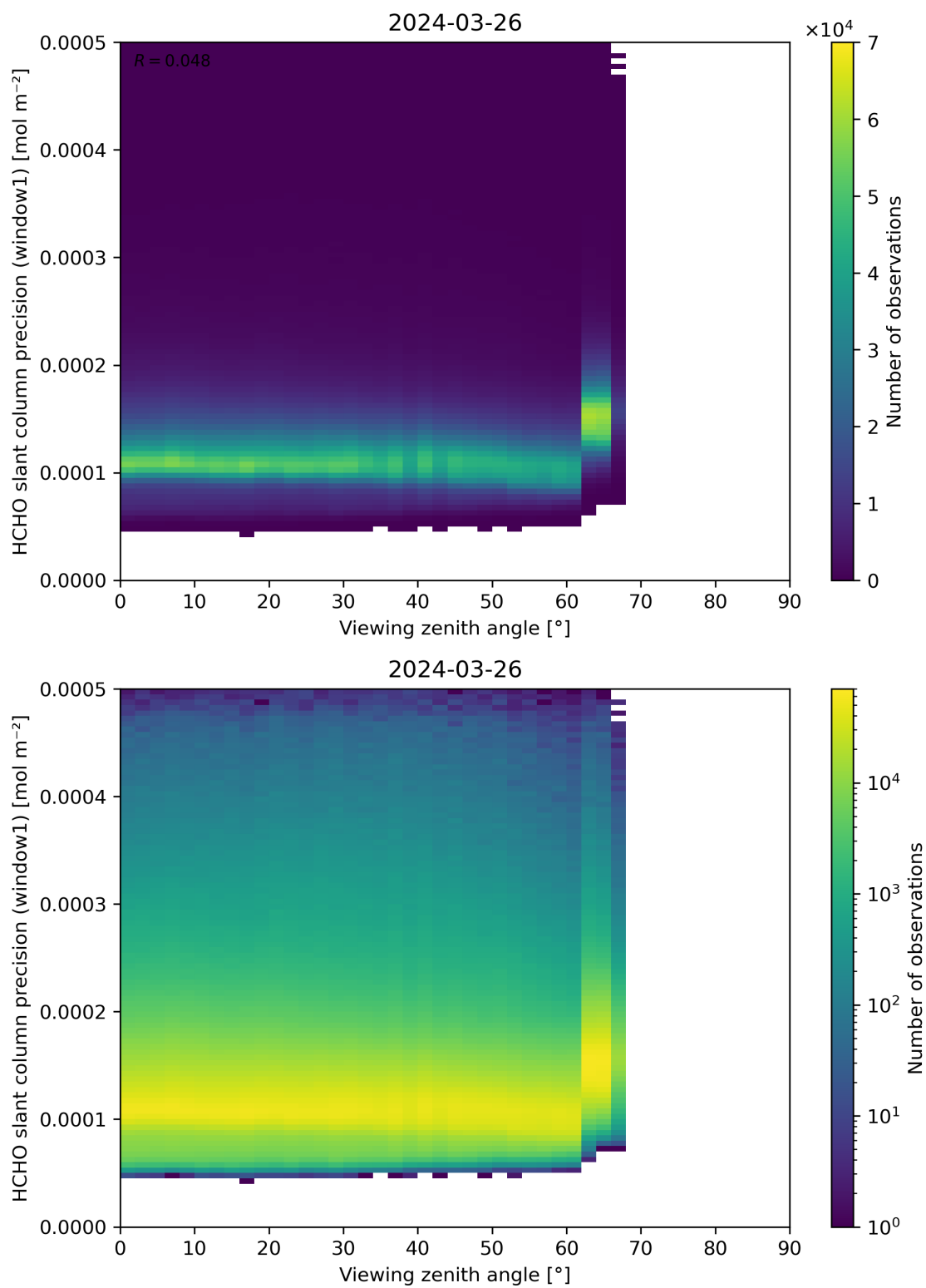
Figure 189: Scatter density plot of “Viewing zenith angle” against “HCHO slant column precision (window1)” for 2024-03-25 to 2024-03-27.
