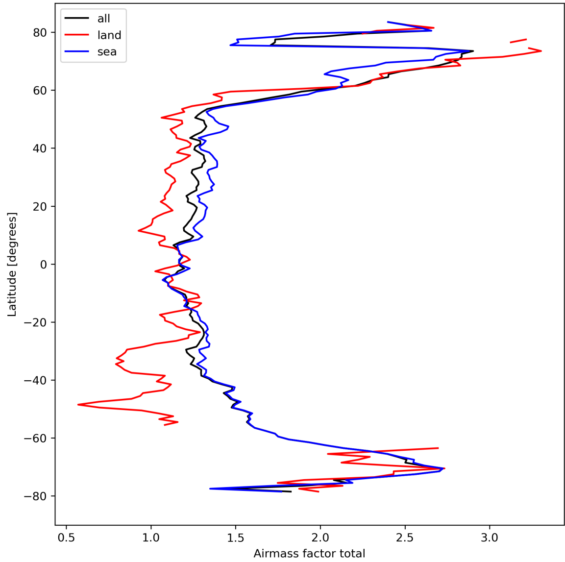
Figure 26: Zonal average of “Airmass factor total” for 2024-03-25 to 2024-03-27.
