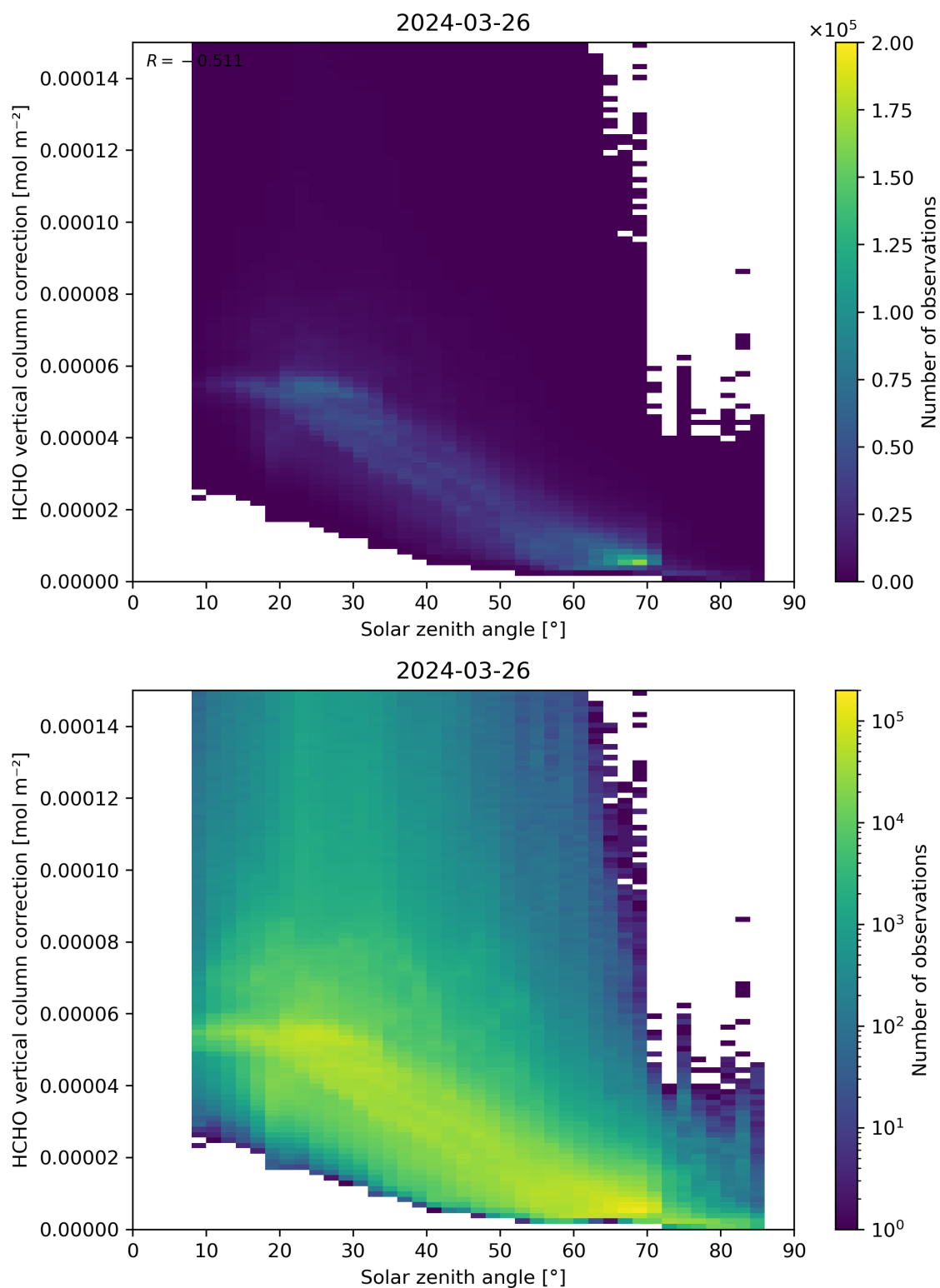
Figure 178: Scatter density plot of “Solar zenith angle” against “HCHO vertical column correction” for 2024-03-25 to 2024-03-27.
