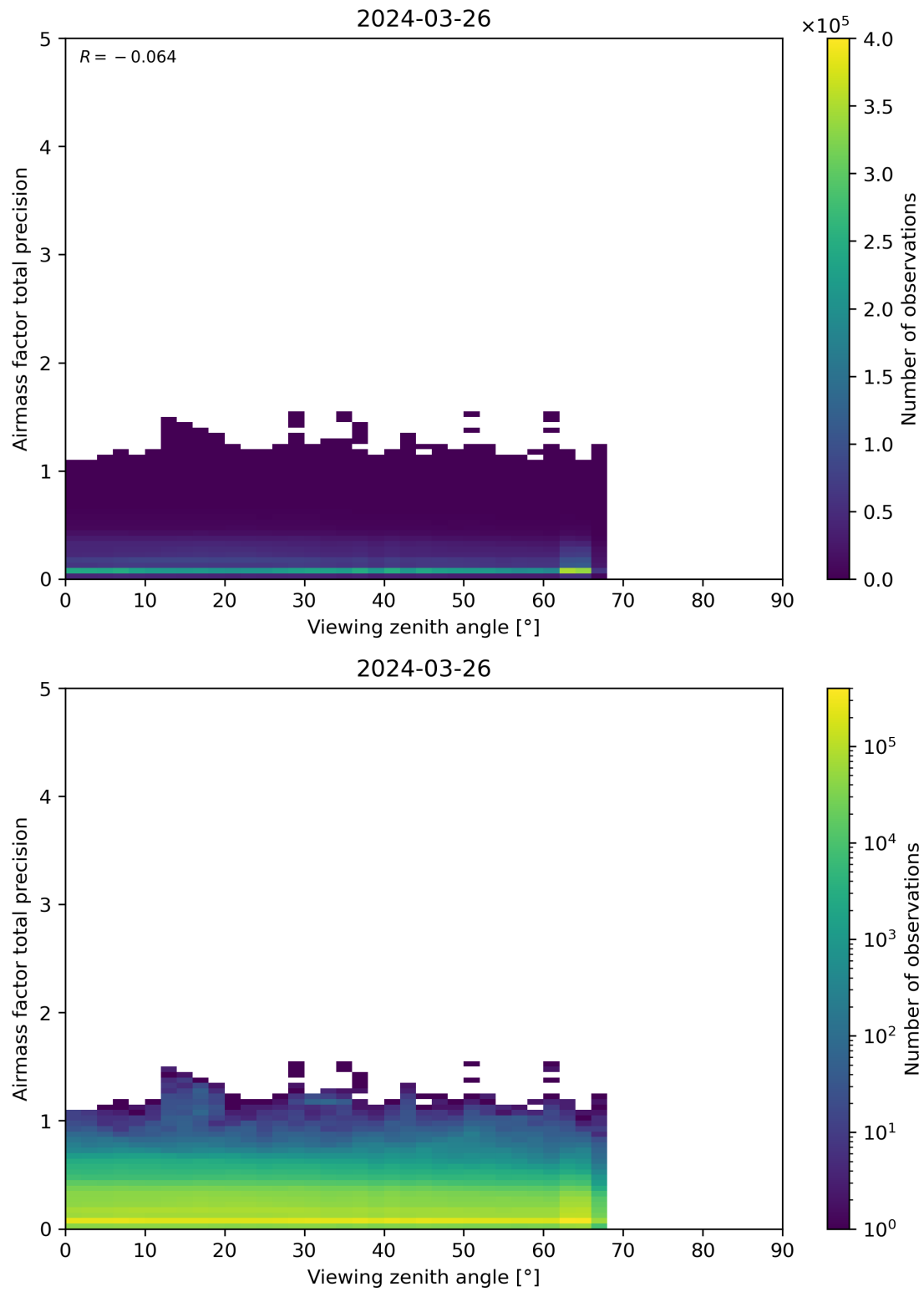
Figure 191: Scatter density plot of “Viewing zenith angle” against “Airmass factor total precision” for 2024-03-25 to 2024-03-27.
