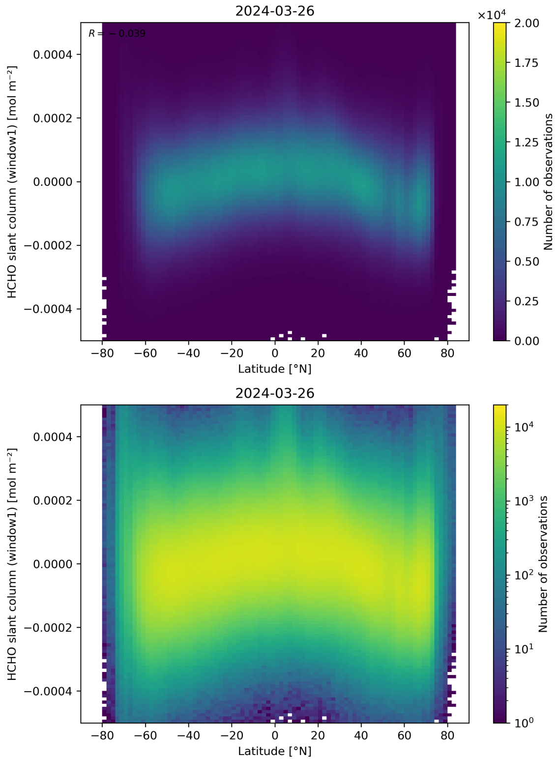
Figure 159: Scatter density plot of “Latitude” against “HCHO slant column (window1)” for 2024-03-25 to 2024-03-27.
