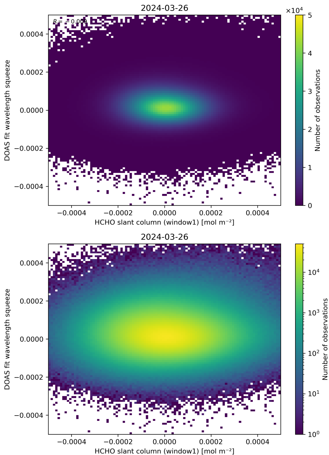
Figure 80: Scatter density plot of “HCHO slant column (window1)” against “DOAS fit wavelength squeeze” for 2024-03-25 to 2024-03-27.
