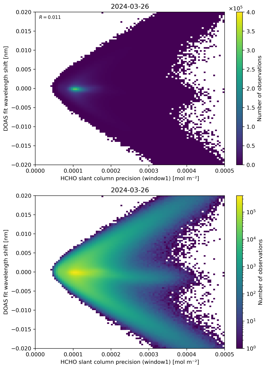
Figure 89: Scatter density plot of “HCHO slant column precision (window1)” against “DOAS fit wavelength shift” for 2024-03-25 to 2024-03-27.
