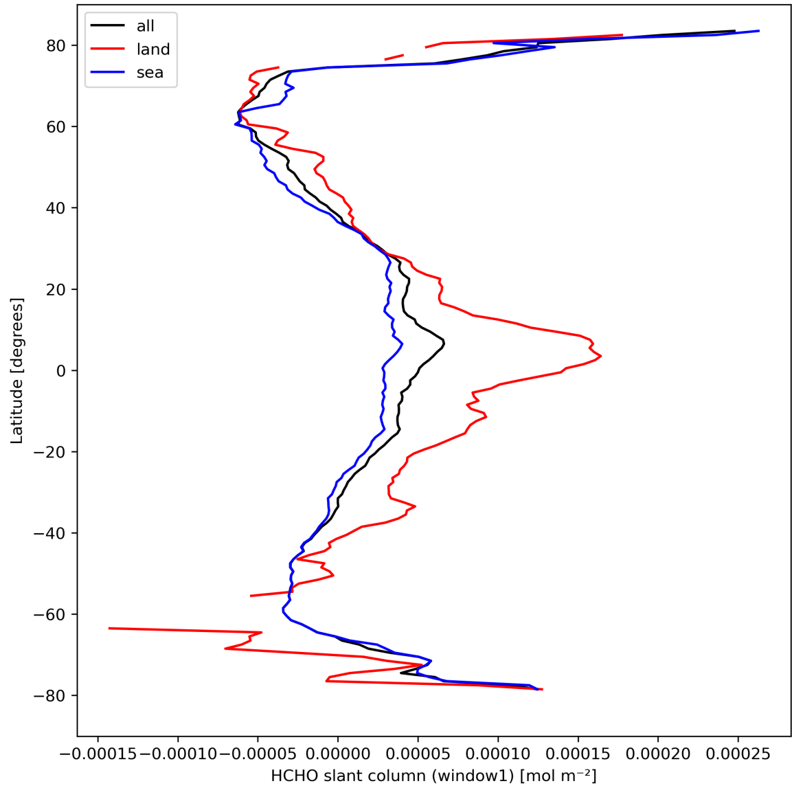
Figure 24: Zonal average of “HCHO slant column (window1)” for 2024-03-25 to 2024-03-27.
