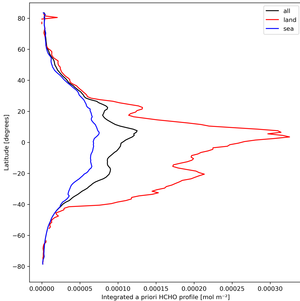
Figure 29: Zonal average of “Integrated a priori HCHO profile” for 2024-03-25 to 2024-03-27.
