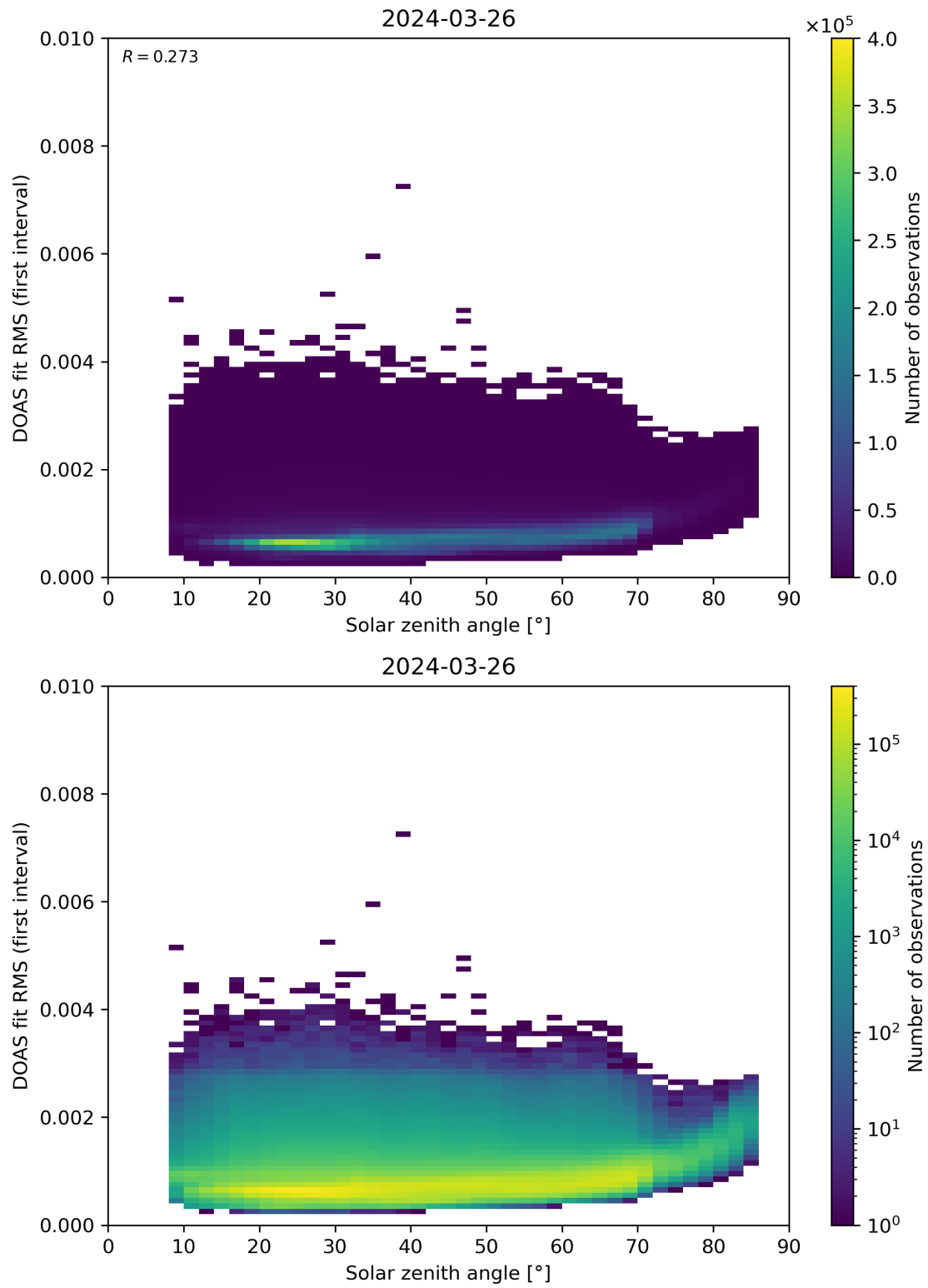
Figure 167: Scatter density plot of “Solar zenith angle” against “DOAS fit RMS (first interval)” for 2024-03-25 to 2024-03-27.
