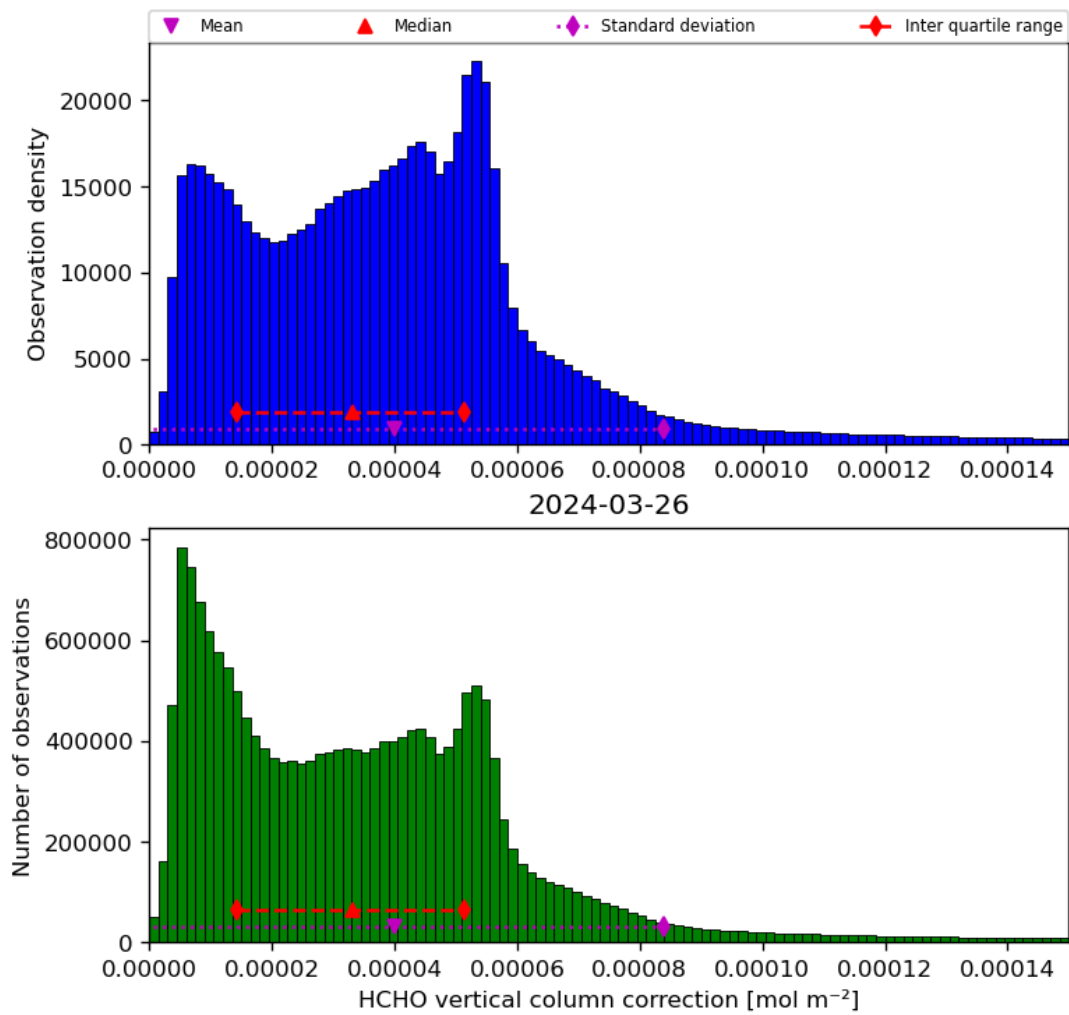
Figure 37: Histogram of “HCHO vertical column correction” for 2024-03-25 to 2024-03-27
