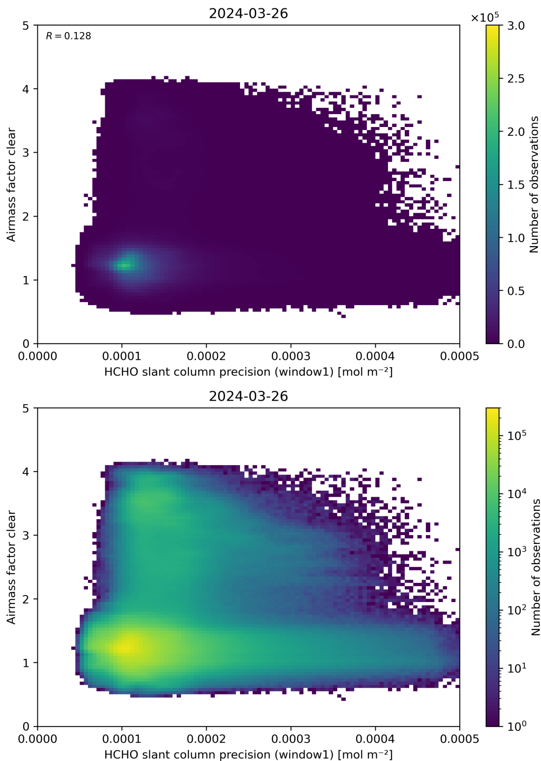
Figure 91: Scatter density plot of “HCHO slant column precision (window1)” against “Airmass factor clear” for 2024-03-25 to 2024-03-27.
