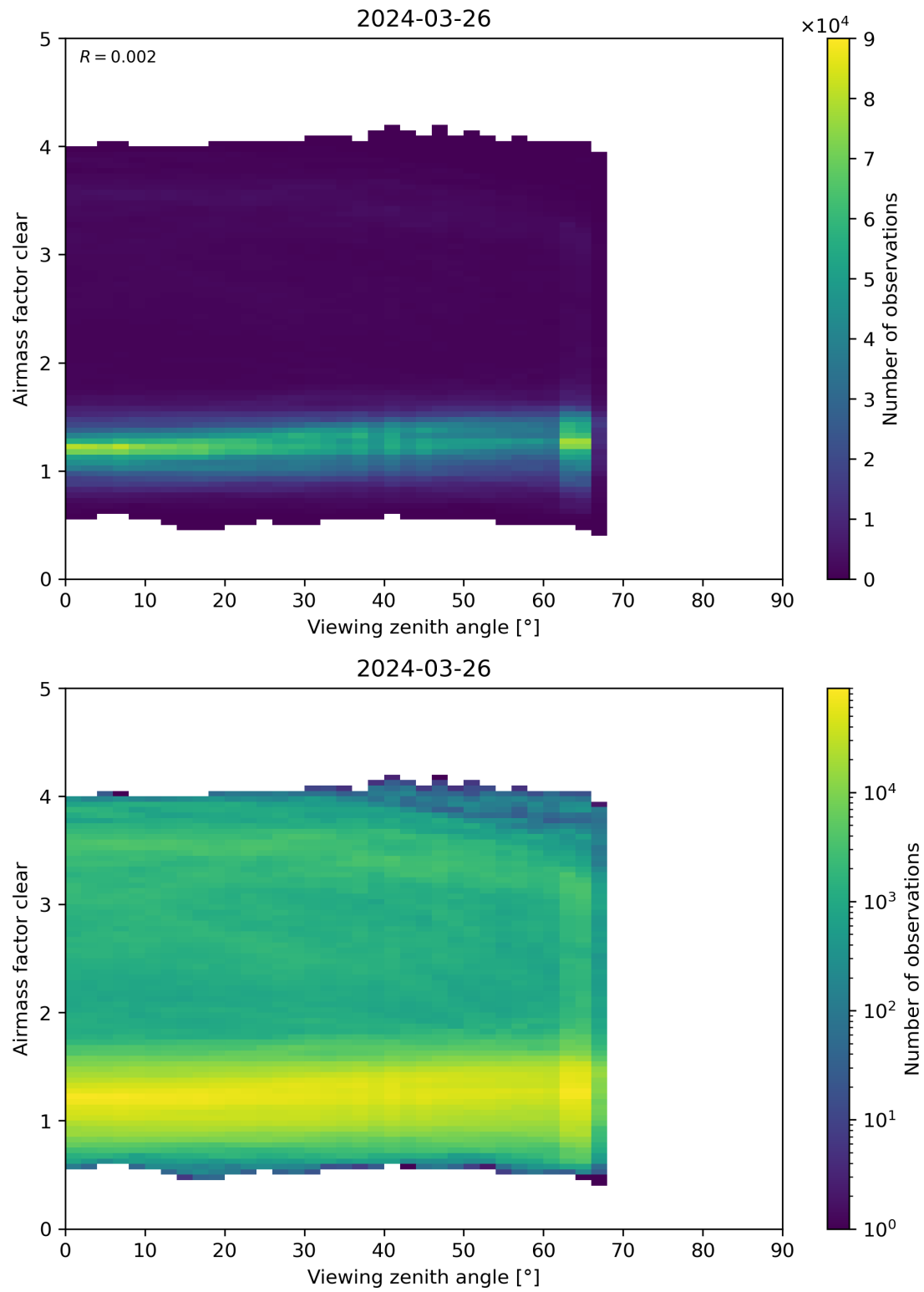
Figure 185: Scatter density plot of “Viewing zenith angle” against “Airmass factor clear” for 2024-03-25 to 2024-03-27.
