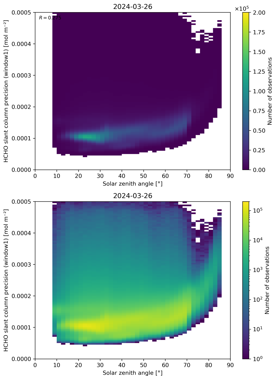
Figure 174: Scatter density plot of “Solar zenith angle” against “HCHO slant column precision (window1)” for 2024-03-25 to 2024-03-27.
