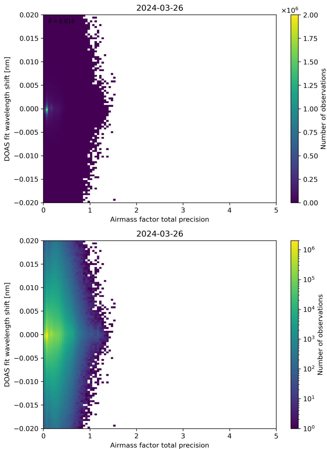
Figure 106: Scatter density plot of “Airmass factor total precision” against “DOAS fit wavelength shift” for 2024-03-25 to 2024-03-27.
