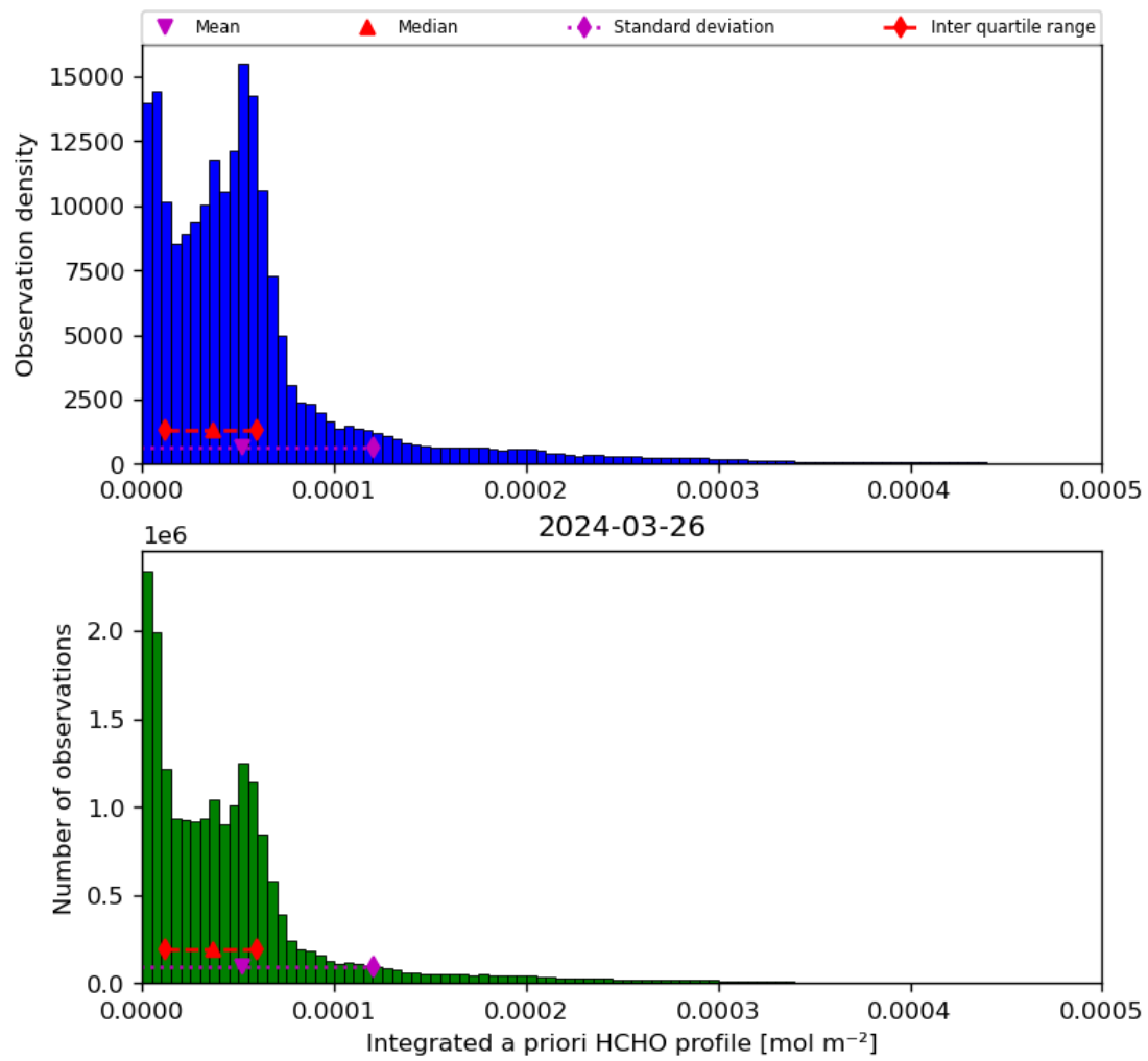
Figure 43: Histogram of “Integrated a priori HCHO profile” for 2024-03-25 to 2024-03-27
