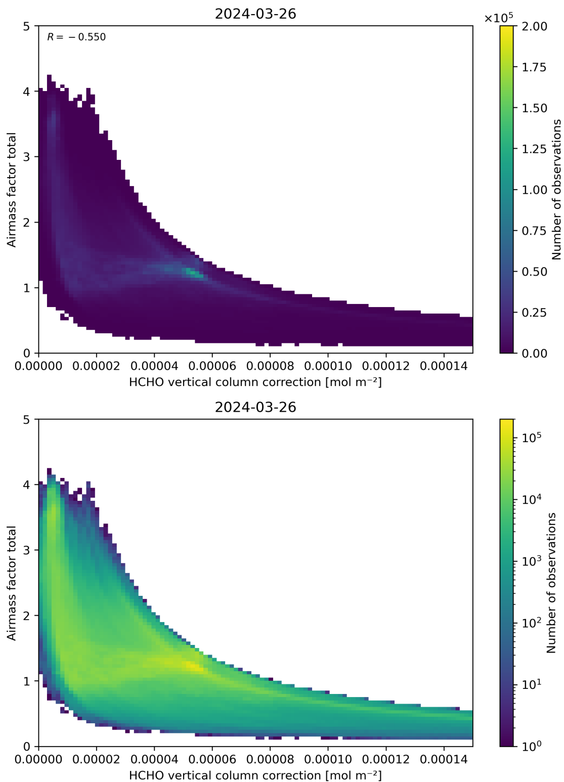
Figure 120: Scatter density plot of “HCHO vertical column correction” against “Airmass factor total” for 2024-03-25 to 2024-03-27.
