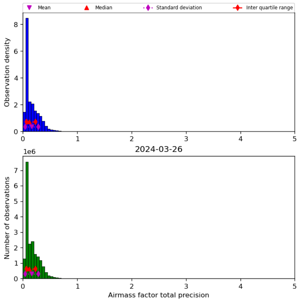
Figure 41: Histogram of “Airmass factor total precision” for 2024-03-25 to 2024-03-27
