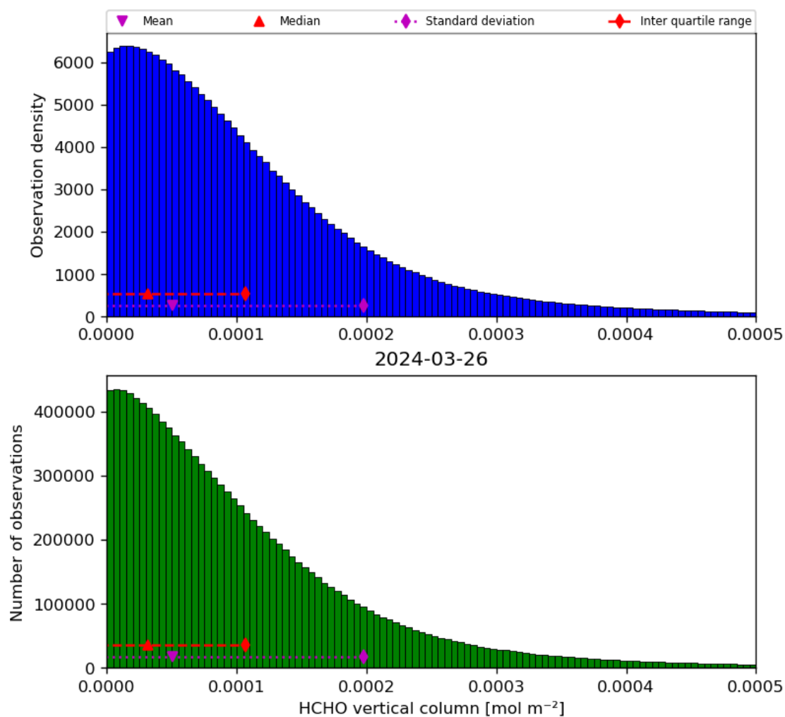
Figure 35: Histogram of “HCHO vertical column” for 2024-03-25 to 2024-03-27
