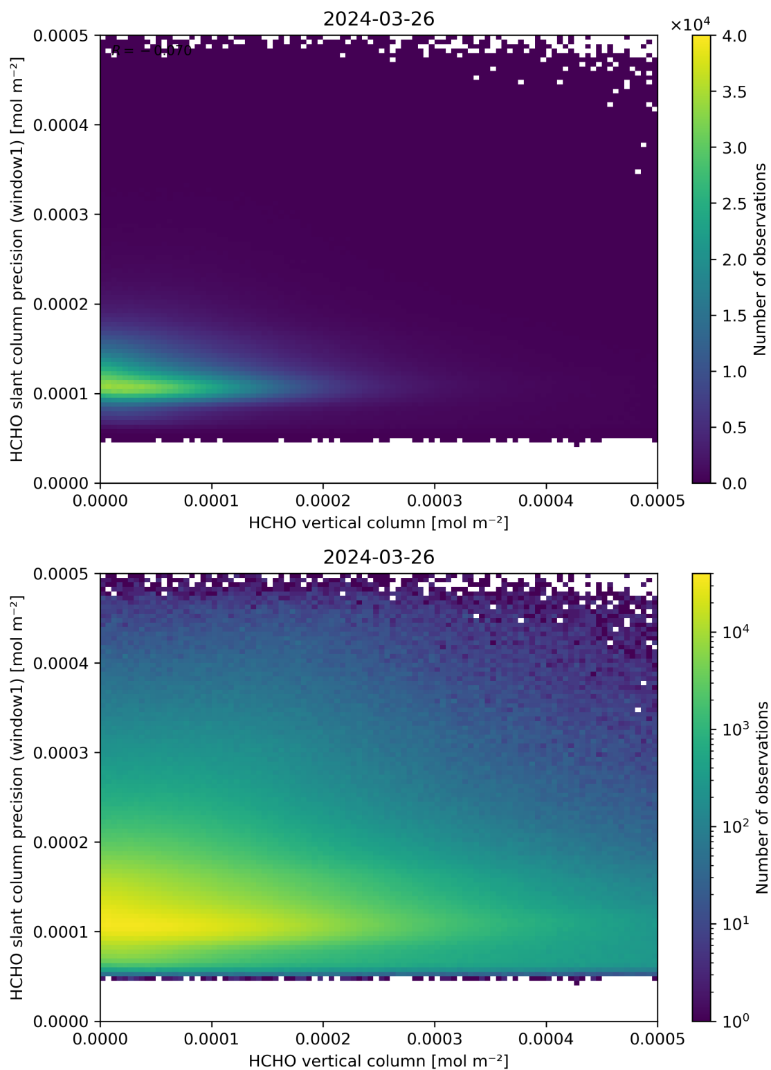
Figure 130: Scatter density plot of “HCHO vertical column” against “HCHO slant column precision (window1)” for 2024-03-25 to 2024-03-27.
