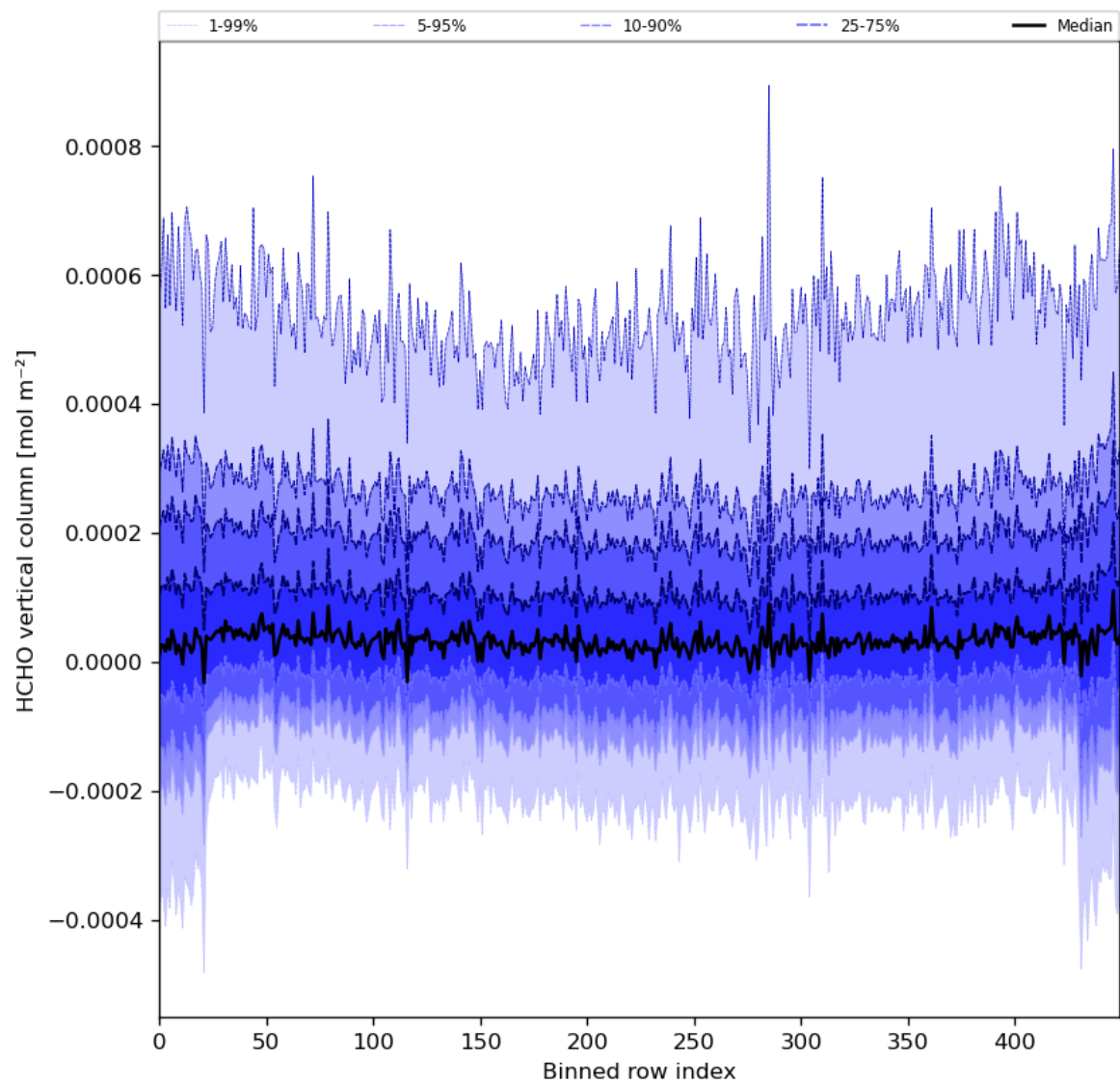
Figure 49: Along track statistics of “HCHO vertical column” for 2024-03-25 to 2024-03-27
