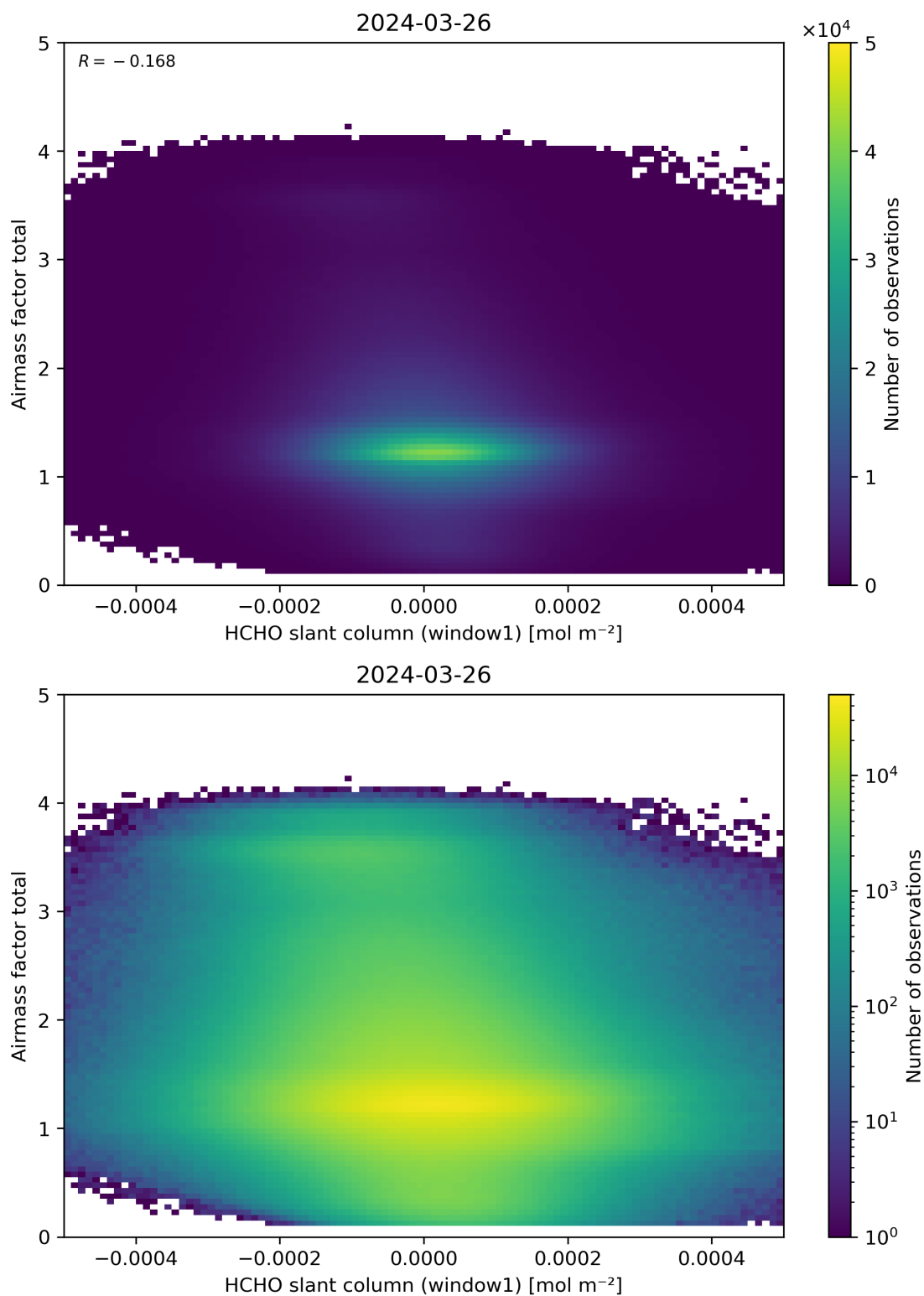
Figure 85: Scatter density plot of “HCHO slant column (window1)” against “Airmass factor total” for 2024-03-25 to 2024-03-27.
