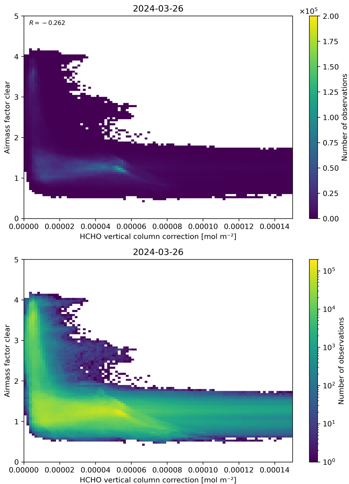
Figure 115: Scatter density plot of “HCHO vertical column correction” against “Airmass factor clear” for 2024-03-25 to 2024-03-27.
