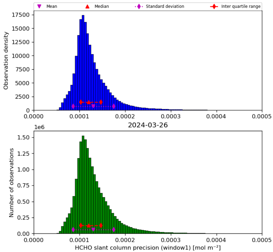
Figure 39: Histogram of “HCHO slant column precision (window1)” for 2024-03-25 to 2024-03-27
