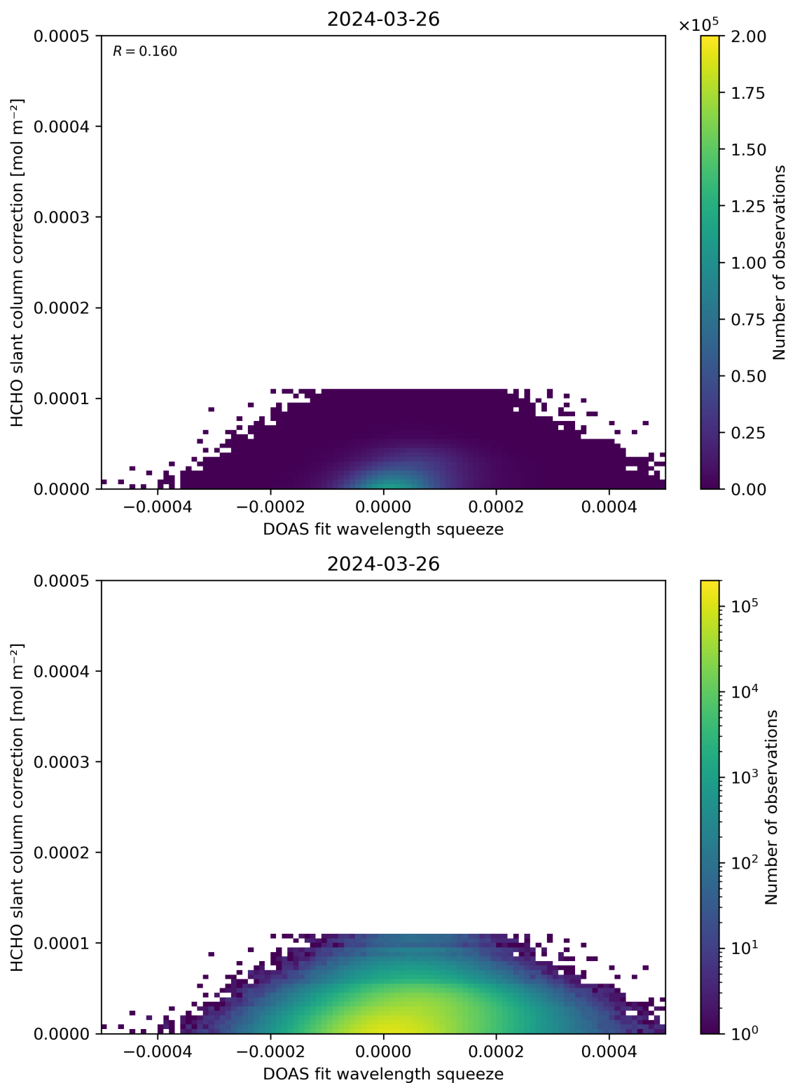
Figure 70: Scatter density plot of “DOAS fit wavelength squeeze” against “HCHO slant column correction” for 2024-03-25 to 2024-03-27.
