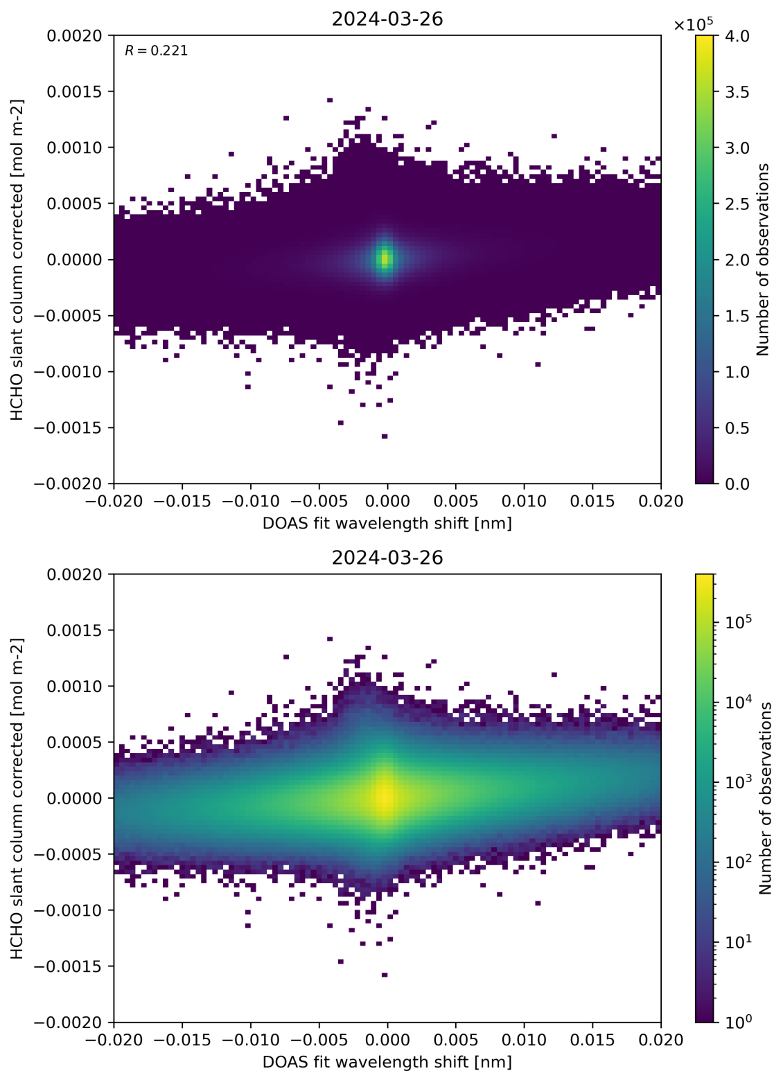
Figure 66: Scatter density plot of “DOAS fit wavelength shift” against “HCHO slant column corrected” for 2024-03-25 to 2024-03-27.
