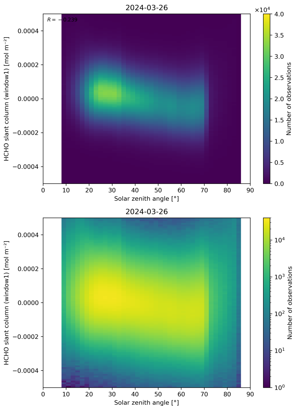
Figure 173: Scatter density plot of “Solar zenith angle” against “HCHO slant column (window1)” for 2024-03-25 to 2024-03-27.
