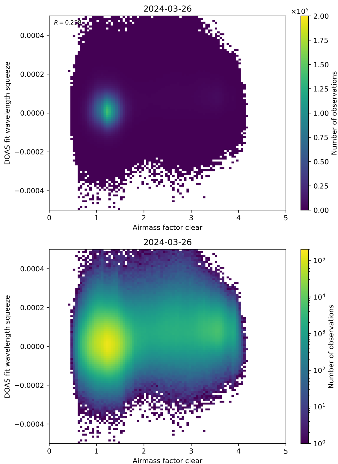
Figure 73: Scatter density plot of “Airmass factor clear” against “DOAS fit wavelength squeeze” for 2024-03-25 to 2024-03-27.
