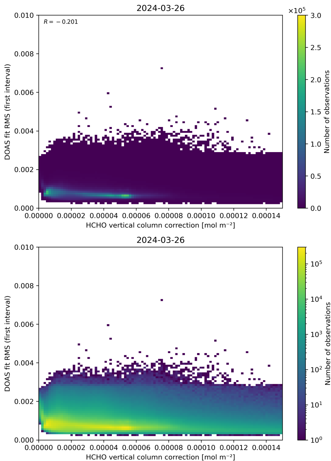
Figure 112: Scatter density plot of “HCHO vertical column correction” against “DOAS fit RMS (first interval)” for 2024-03-25 to 2024-03-27.
