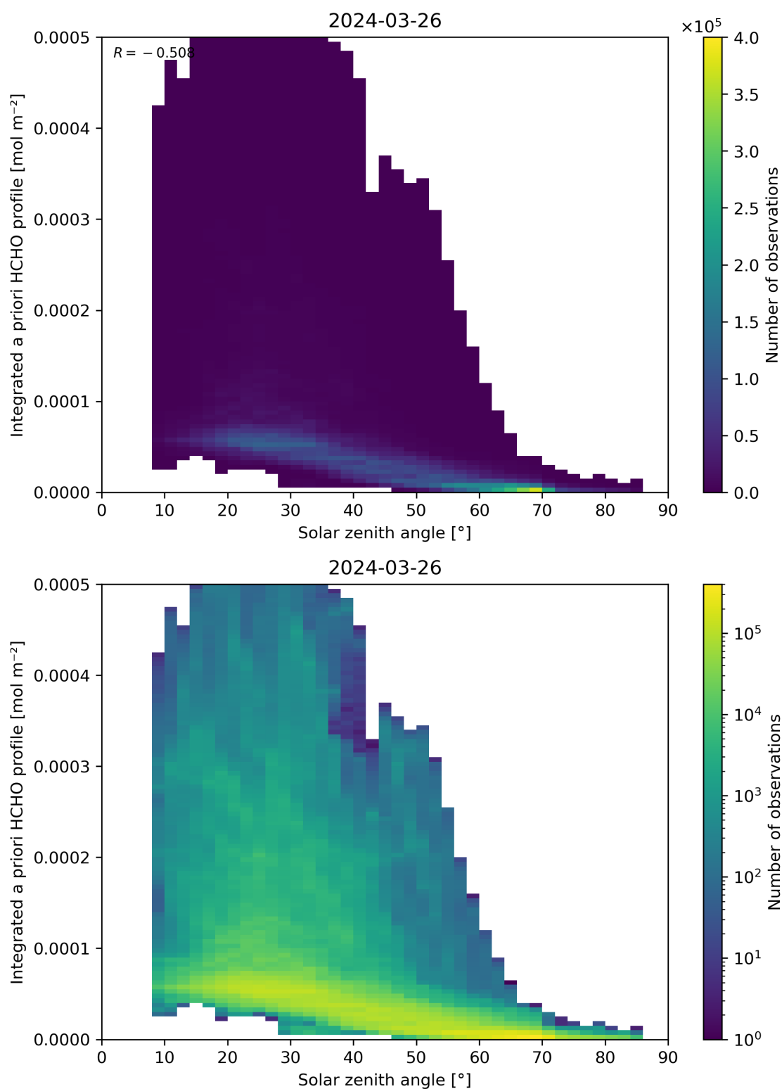
Figure 180: Scatter density plot of “Solar zenith angle” against “Integrated a priori HCHO profile” for 2024-03-25 to 2024-03-27.
