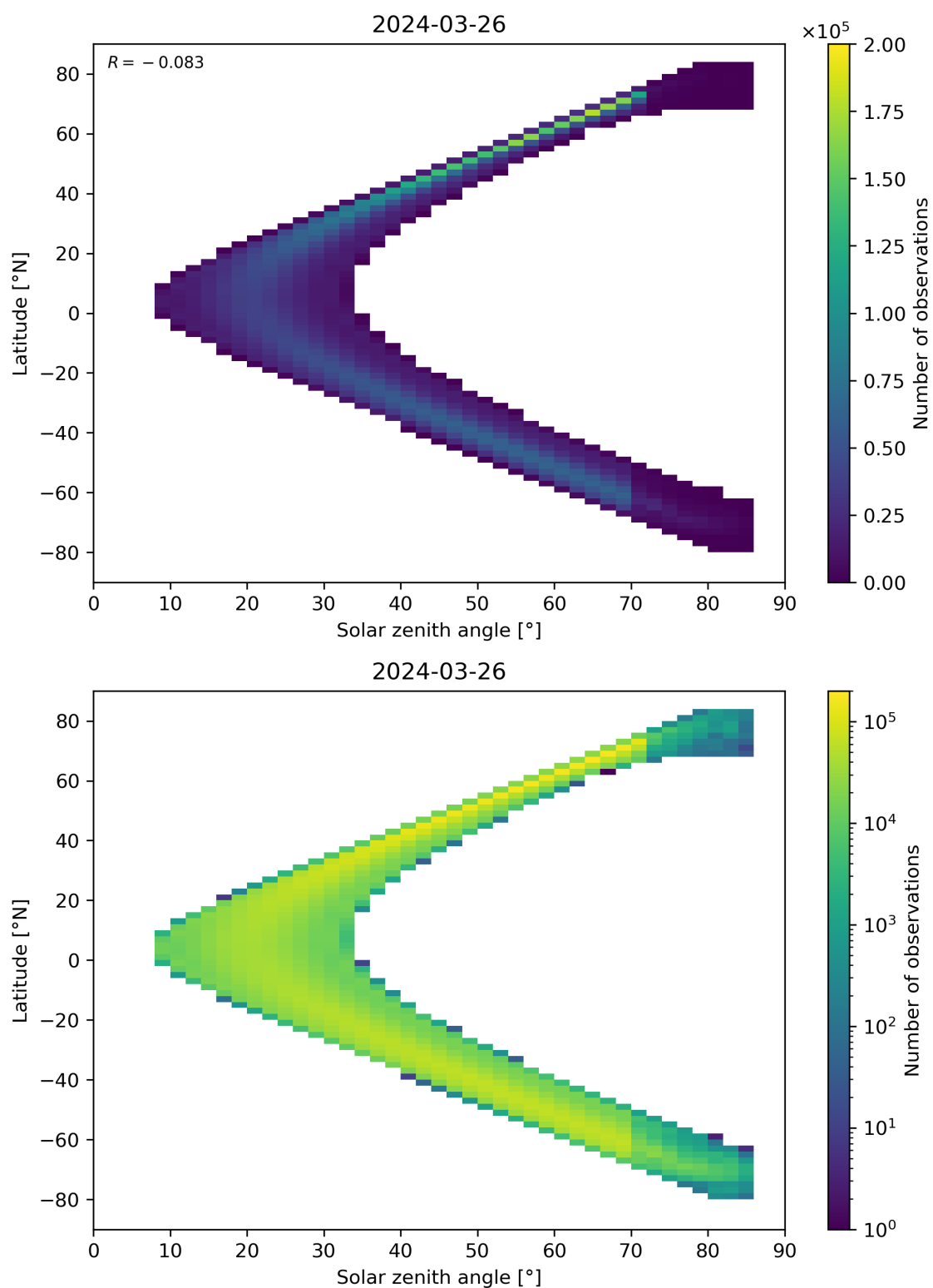
Figure 181: Scatter density plot of “Solar zenith angle” against “Latitude” for 2024-03-25 to 2024-03-27.
