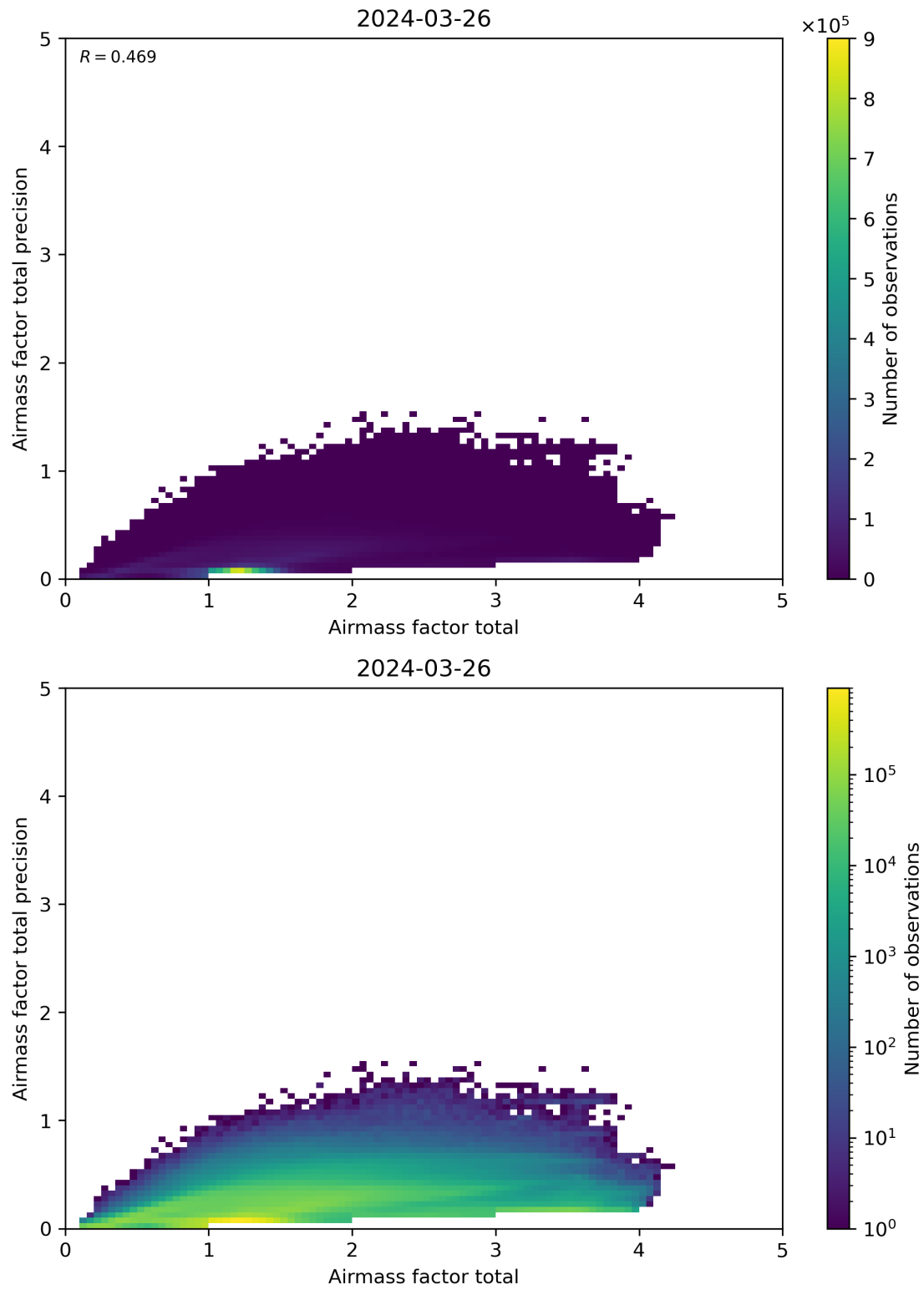
Figure 103: Scatter density plot of “Airmass factor total” against “Airmass factor total precision” for 2024-03-25 to 2024-03-27.
