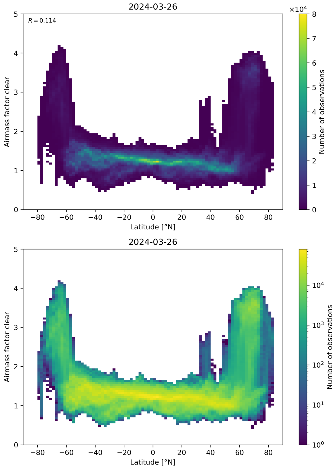
Figure 156: Scatter density plot of “Latitude” against “Airmass factor clear” for 2024-03-25 to 2024-03-27.
