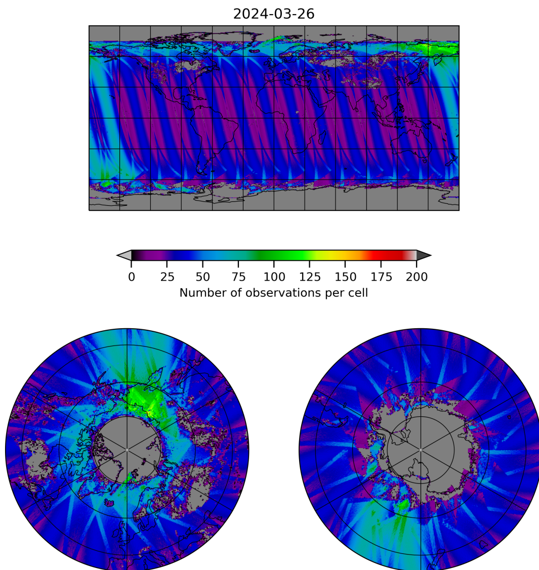
Figure 19: Map of the number of observations for 2024-03-25 to 2024-03-27
