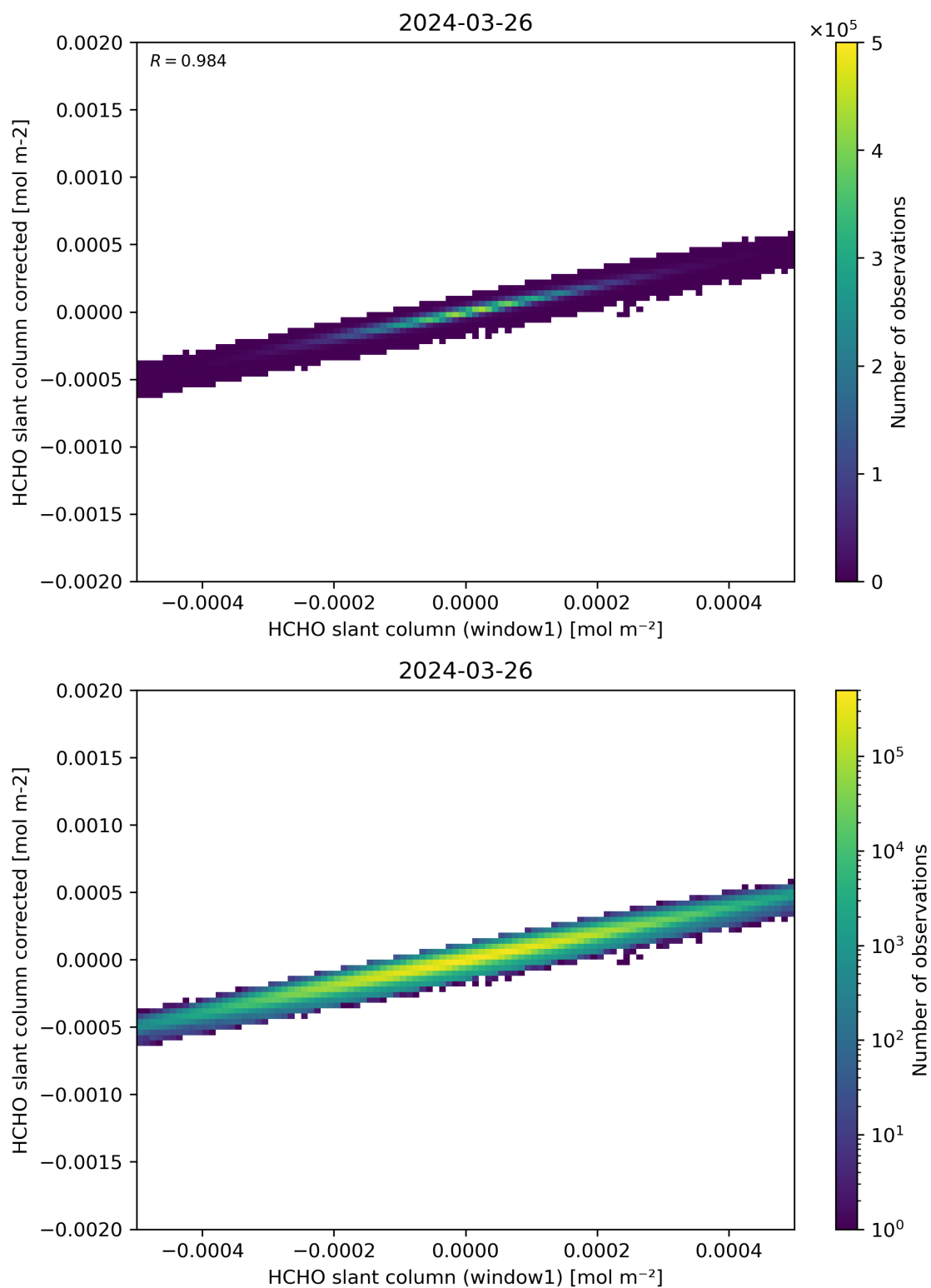
Figure 82: Scatter density plot of “HCHO slant column (window1)” against “HCHO slant column corrected” for 2024-03-25 to 2024-03-27.
