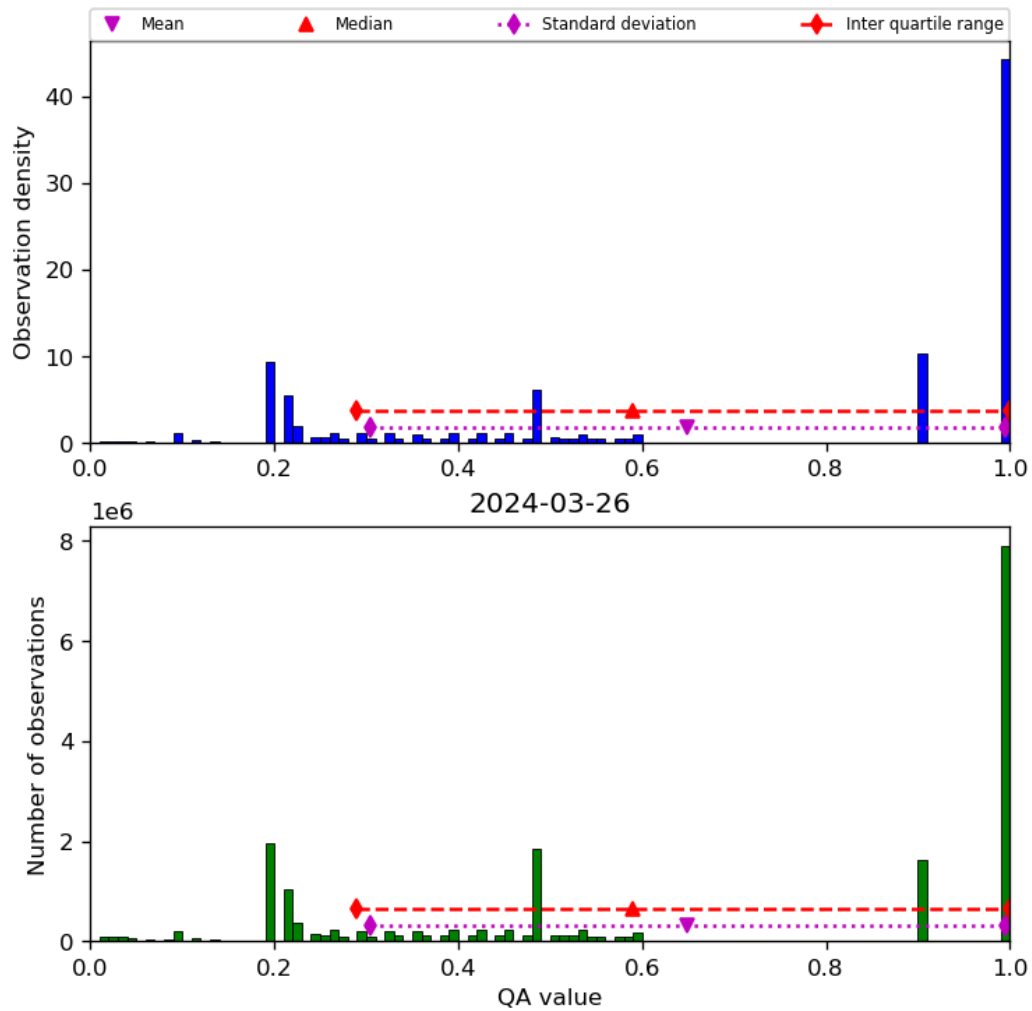
Figure 34: Histogram of “QA value” for 2024-03-25 to 2024-03-27
