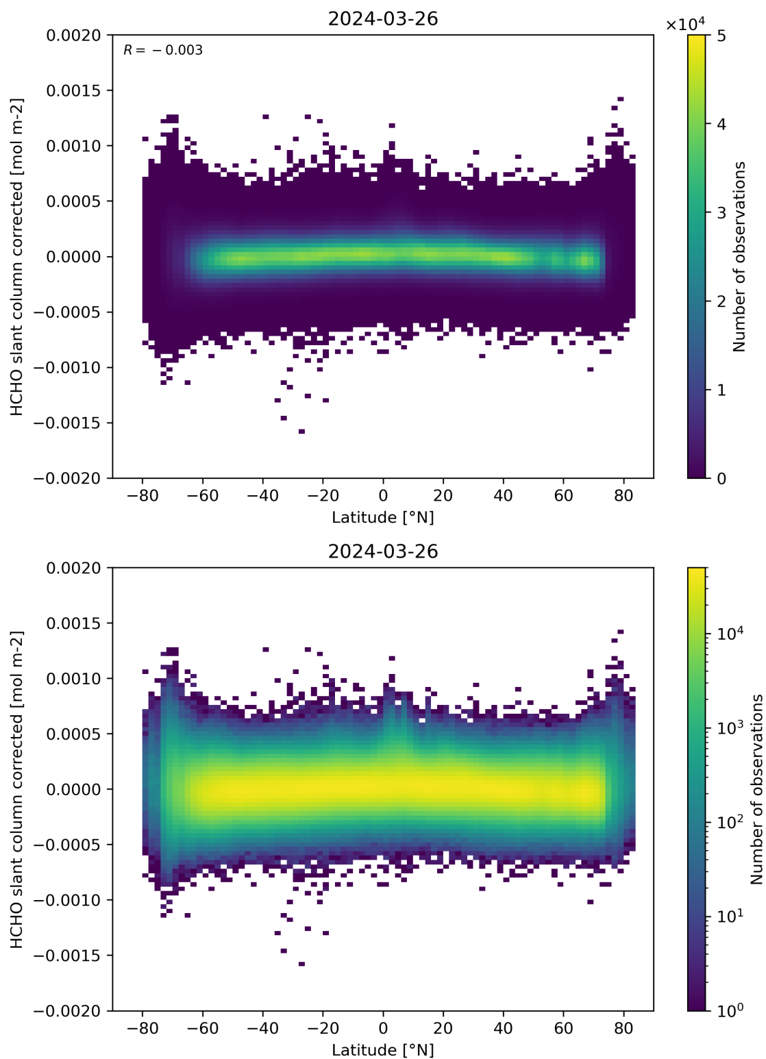
Figure 157: Scatter density plot of “Latitude” against “HCHO slant column corrected” for 2024-03-25 to 2024-03-27.
