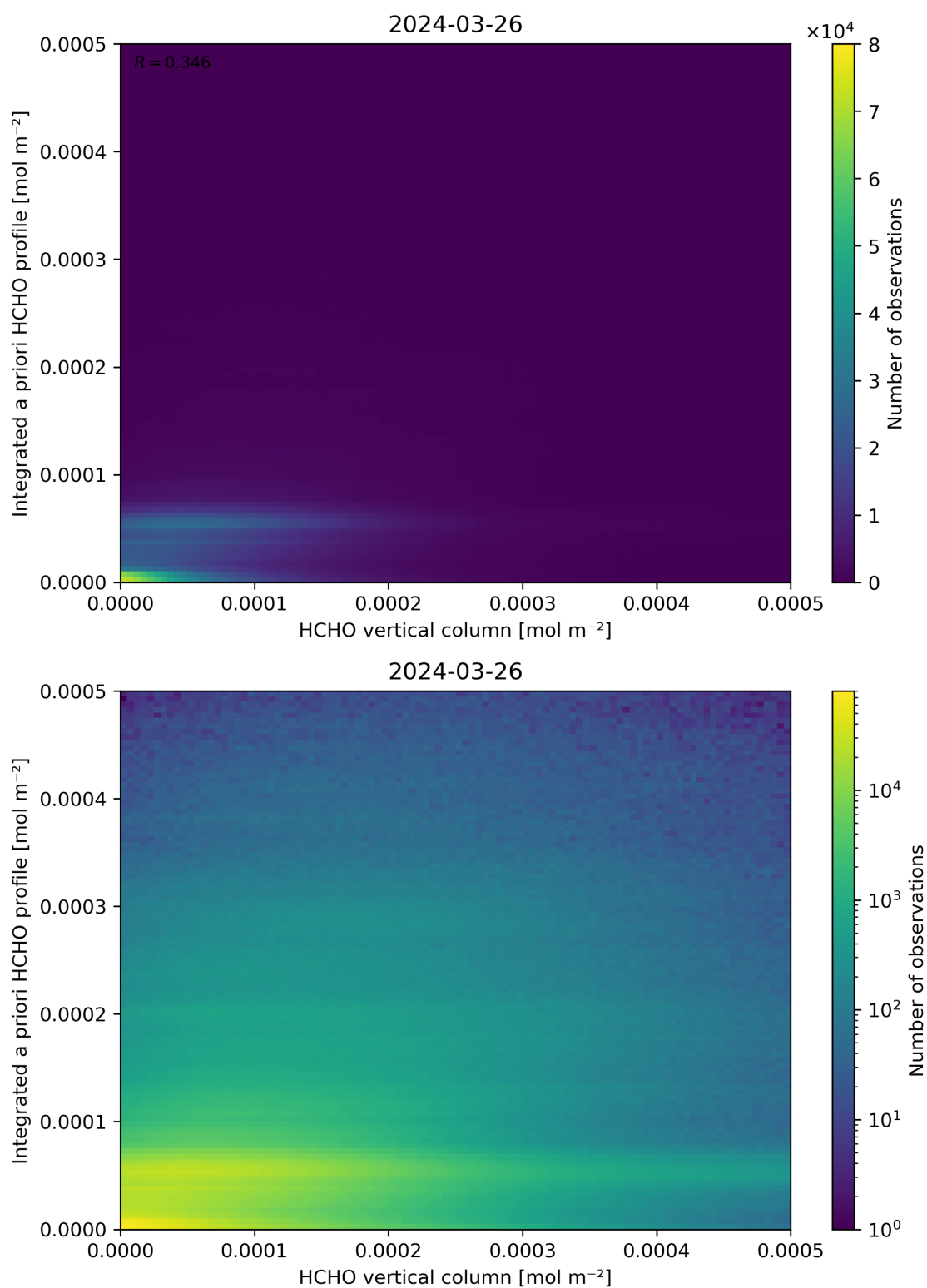
Figure 135: Scatter density plot of “HCHO vertical column” against “Integrated a priori HCHO profile” for 2024-03-25 to 2024-03-27.
