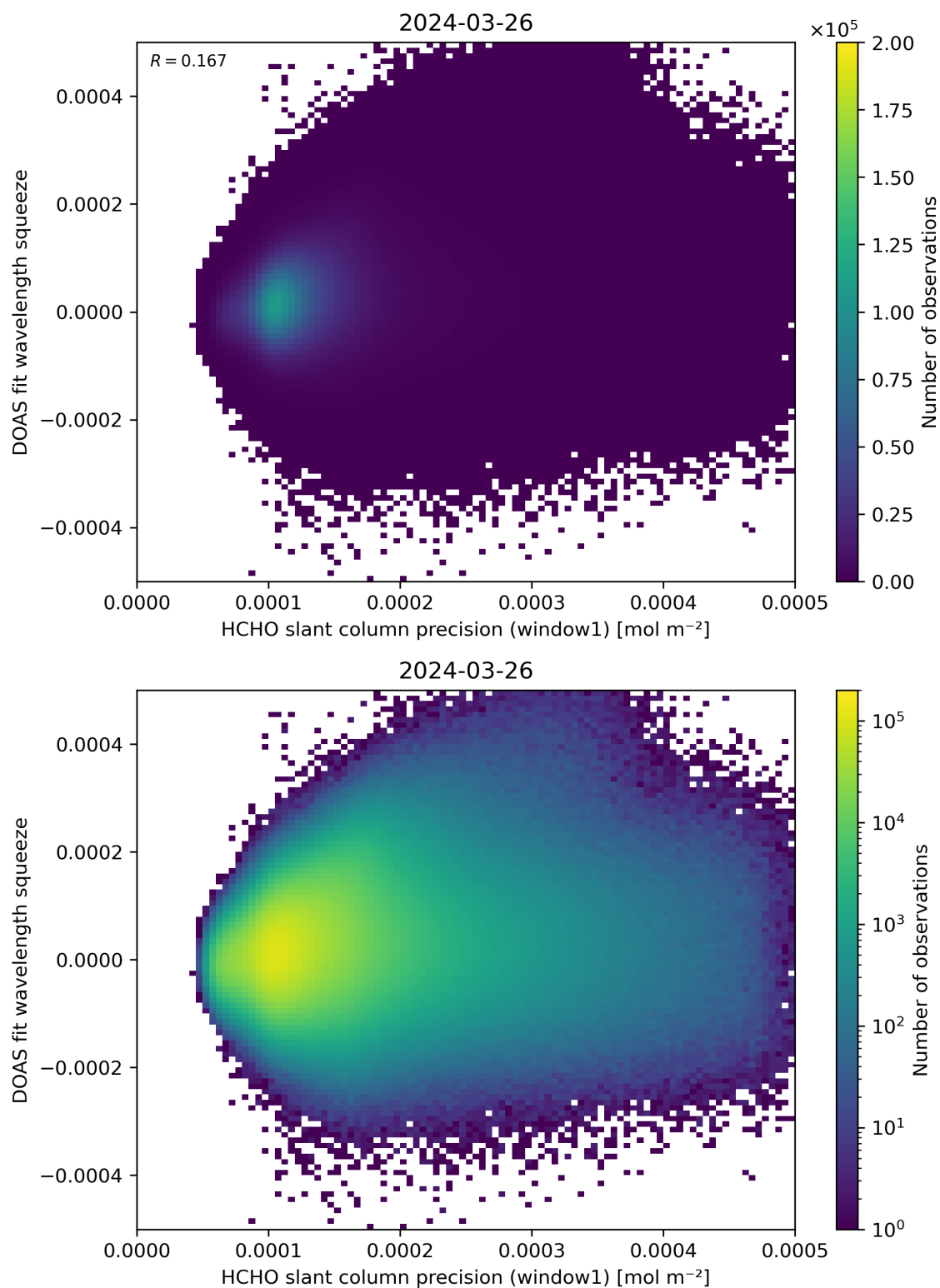
Figure 90: Scatter density plot of “HCHO slant column precision (window1)” against “DOAS fit wavelength squeeze” for 2024-03-25 to 2024-03-27.
