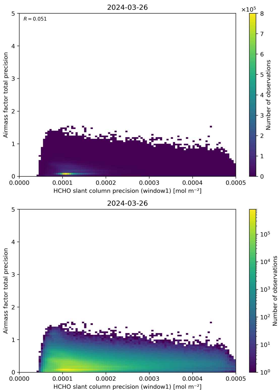
Figure 95: Scatter density plot of “HCHO slant column precision (window1)” against “Airmass factor total precision” for 2024-03-25 to 2024-03-27.
