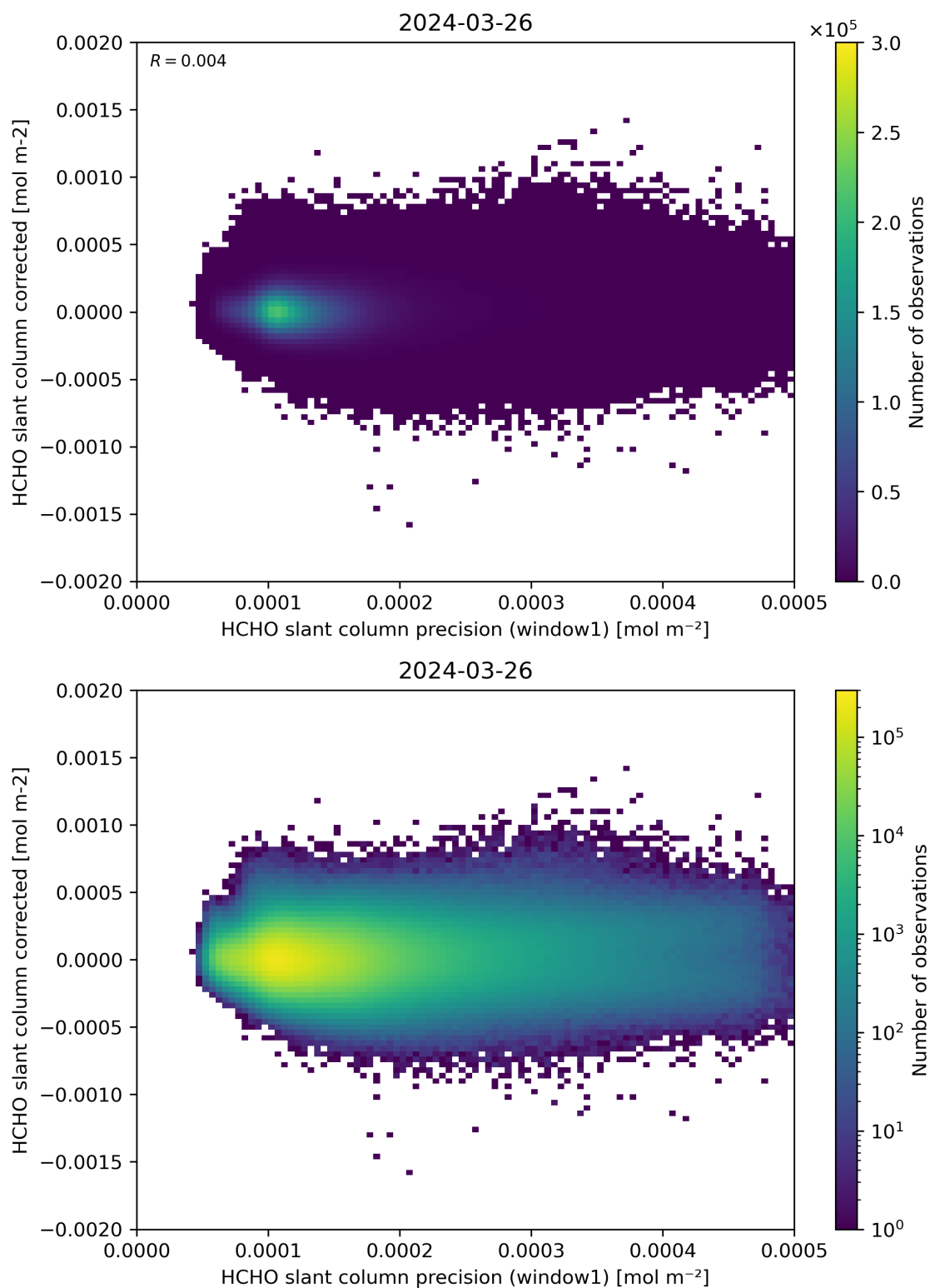
Figure 92: Scatter density plot of “HCHO slant column precision (window1)” against “HCHO slant column corrected” for 2024-03-25 to 2024-03-27.
