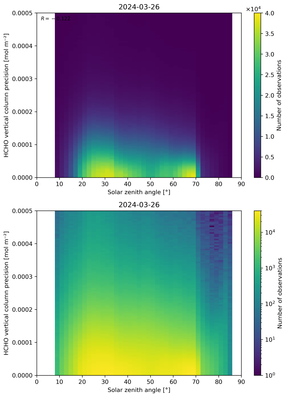
Figure 179: Scatter density plot of “Solar zenith angle” against “HCHO vertical column precision” for 2024-03-25 to 2024-03-27.
