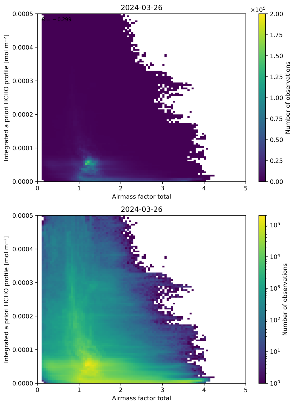
Figure 104: Scatter density plot of “Air mass factor total” against “Integrated a priori HCHO profile” for 2024-03-25 to 2024-03-27.
