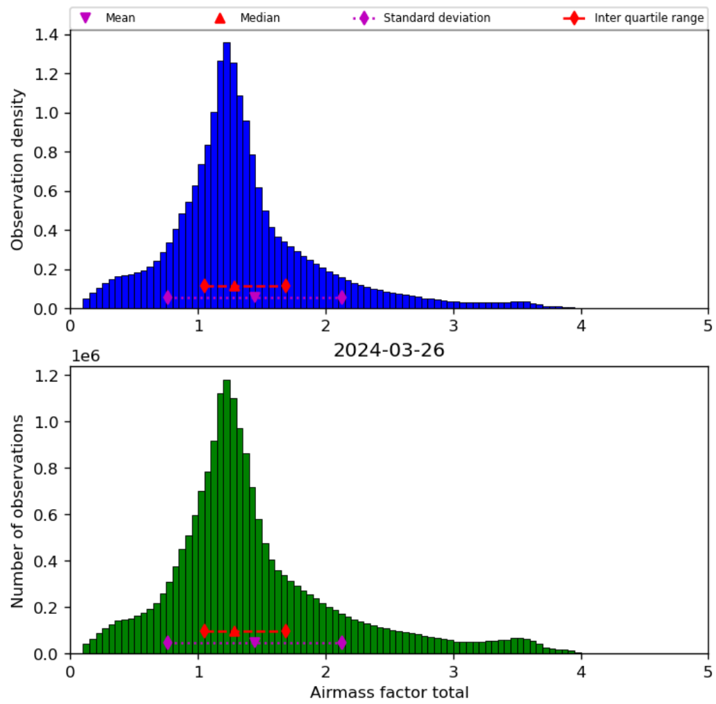
Figure 40: Histogram of “Airmass factor total” for 2024-03-25 to 2024-03-27
