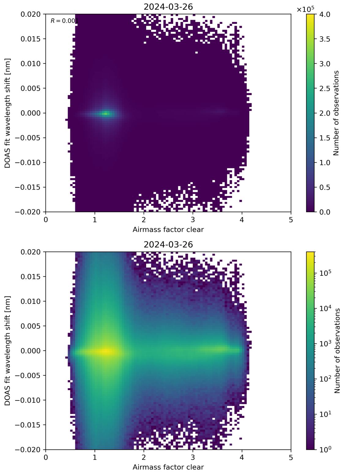
Figure 72: Scatter density plot of “Airmass factor clear” against “DOAS fit wavelength shift” for 2024-03-25 to 2024-03-27.
