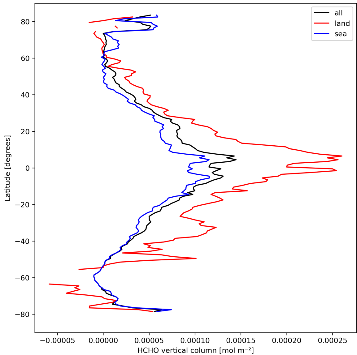
Figure 21: Zonal average of “HCHO vertical column” for 2024-03-25 to 2024-03-27.
