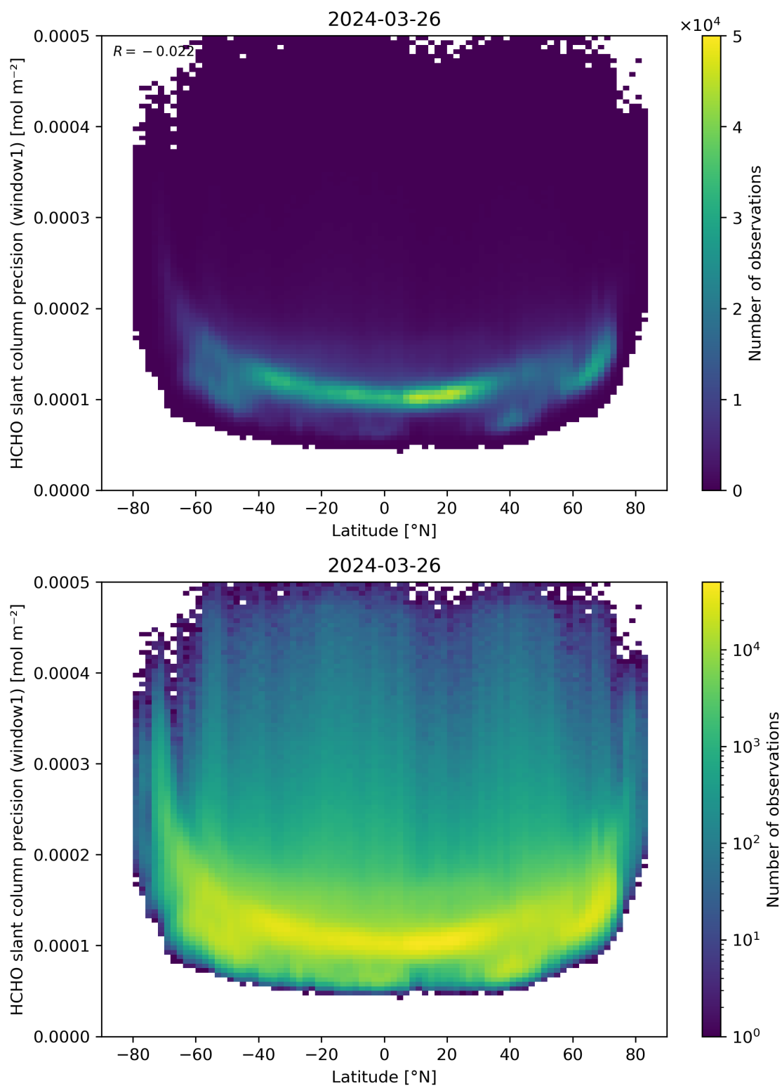
Figure 160: Scatter density plot of “Latitude” against “HCHO slant column precision (window1)” for 2024-03-25 to 2024-03-27.
