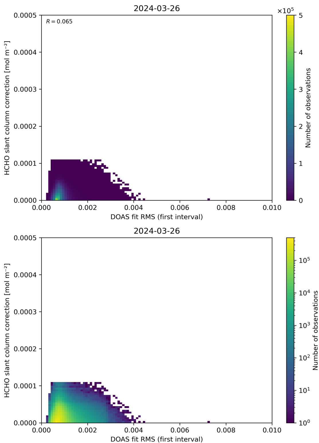
Figure 63: Scatter density plot of “DOAS fit RMS (first interval)” against “HCHO slant column correction” for 2024-03-25 to 2024-03-27.
