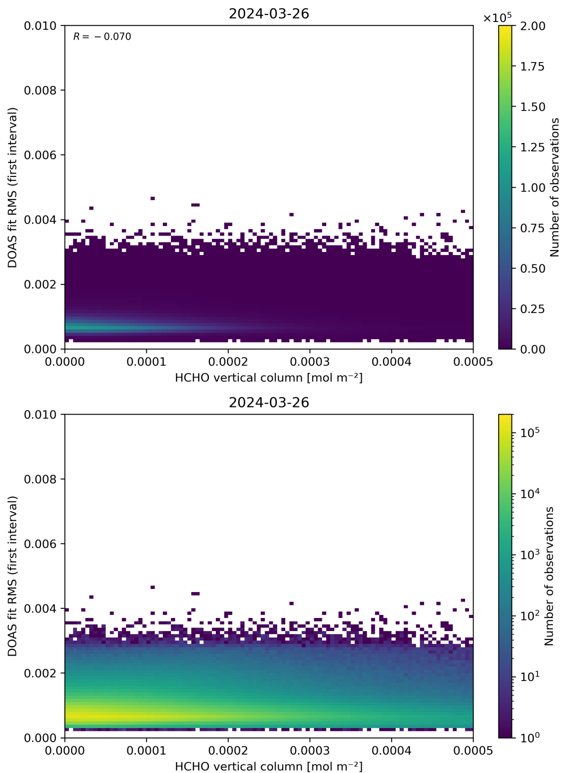
Figure 123: Scatter density plot of “HCHO vertical column” against “DOAS fit RMS (first interval)” for 2024-03-25 to 2024-03-27.
