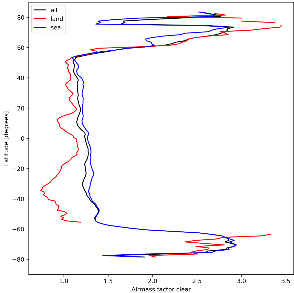
Figure 28: Zonal average of “Airmass factor clear” for 2024-03-25 to 2024-03-27.
