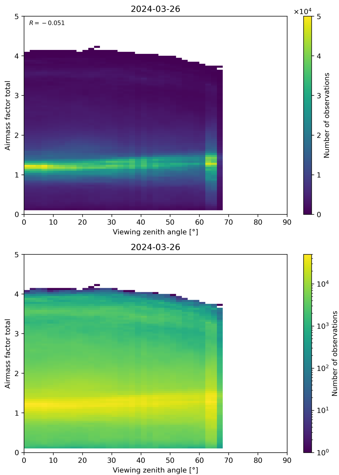
Figure 190: Scatter density plot of “Viewing zenith angle” against “Airmass factor total” for 2024-03-25 to 2024-03-27.
