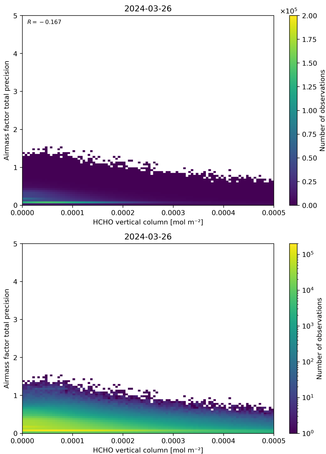
Figure 132: Scatter density plot of “HCHO vertical column” against “Airmass factor total precision” for 2024-03-25 to 2024-03-27.
