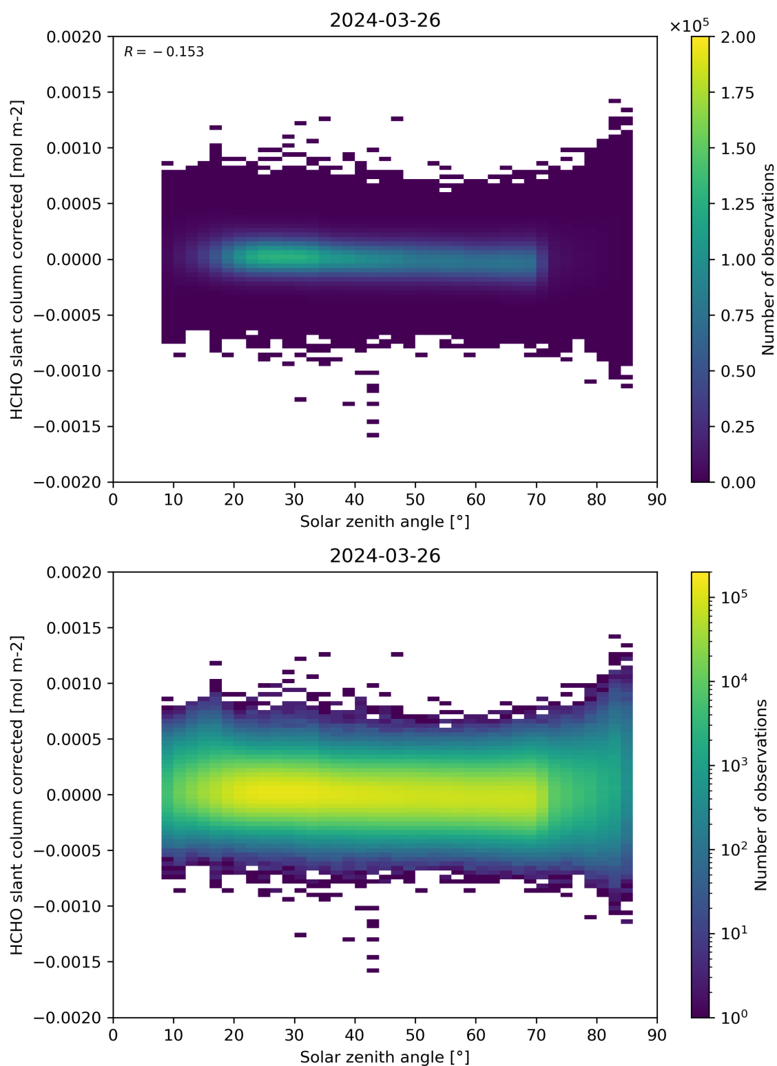
Figure 171: Scatter density plot of “Solar zenith angle” against “HCHO slant column corrected” for 2024-03-25 to 2024-03-27.
