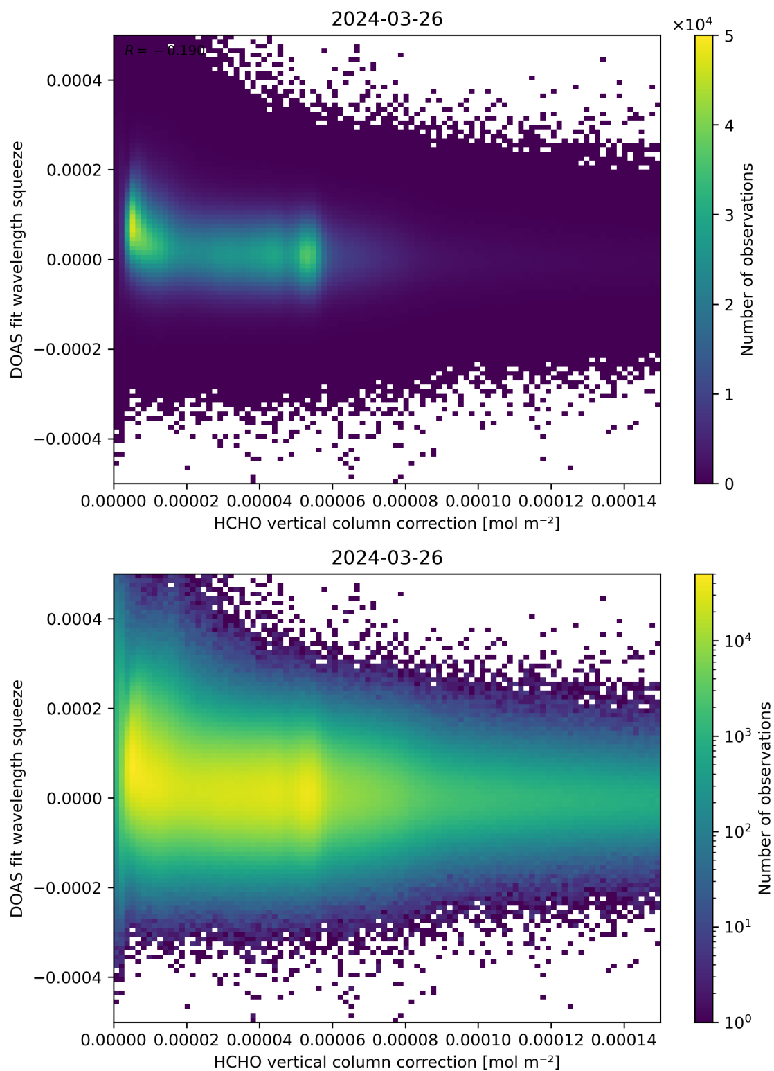
Figure 114: Scatter density plot of “HCHO vertical column correction” against “DOAS fit wavelength squeeze” for 2024-03-25 to 2024-03-27.
