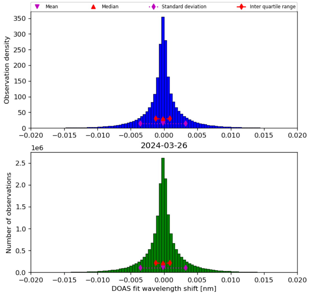
Figure 44: Histogram of “DOAS fit wavelength shift” for 2024-03-25 to 2024-03-27
