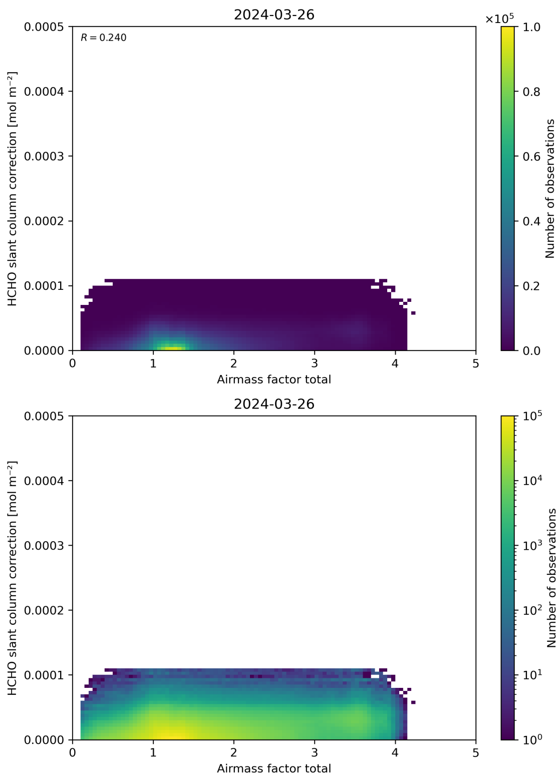
Figure 102: Scatter density plot of “Airmass factor total” against “HCHO slant column correction” for 2024-03-25 to 2024-03-27.
