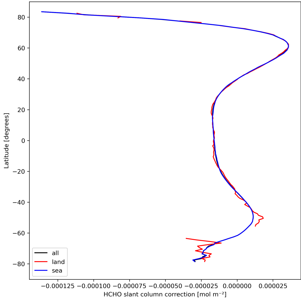
Figure 33: Zonal average of “HCHO slant column correction” for 2024-03-25 to 2024-03-27.
