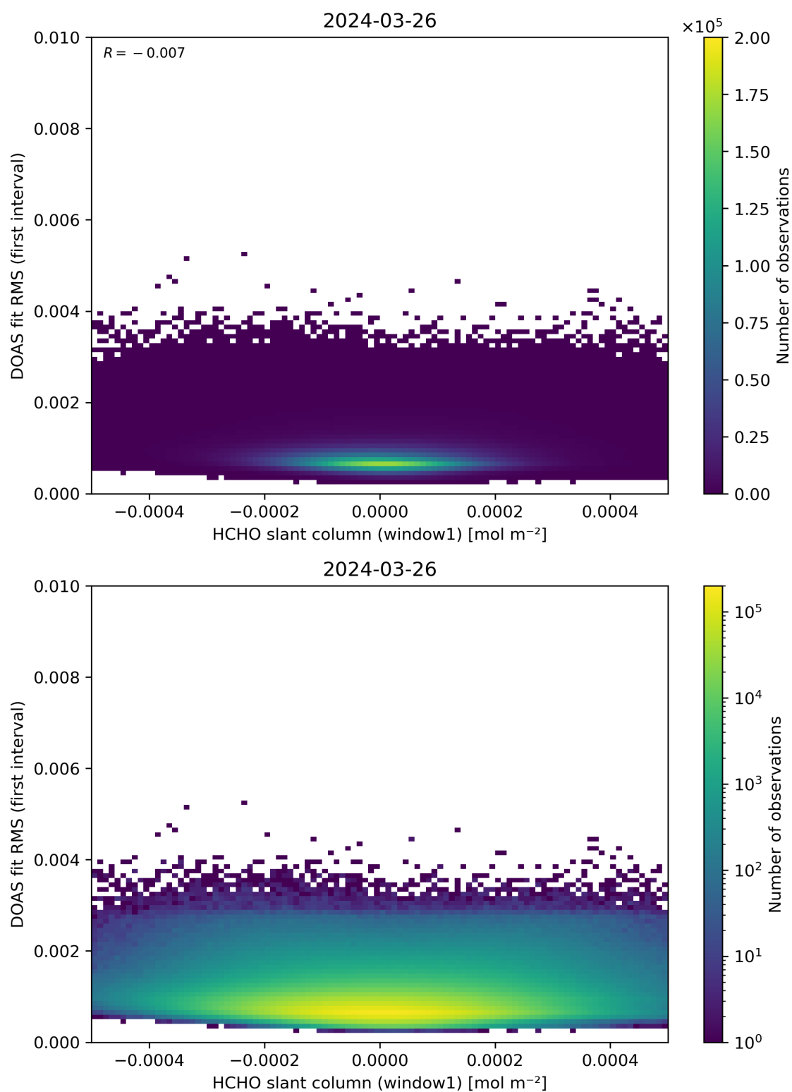
Figure 78: Scatter density plot of “HCHO slant column (window1)” against “DOAS fit RMS (first interval)” for 2024-03-25 to 2024-03-27.
