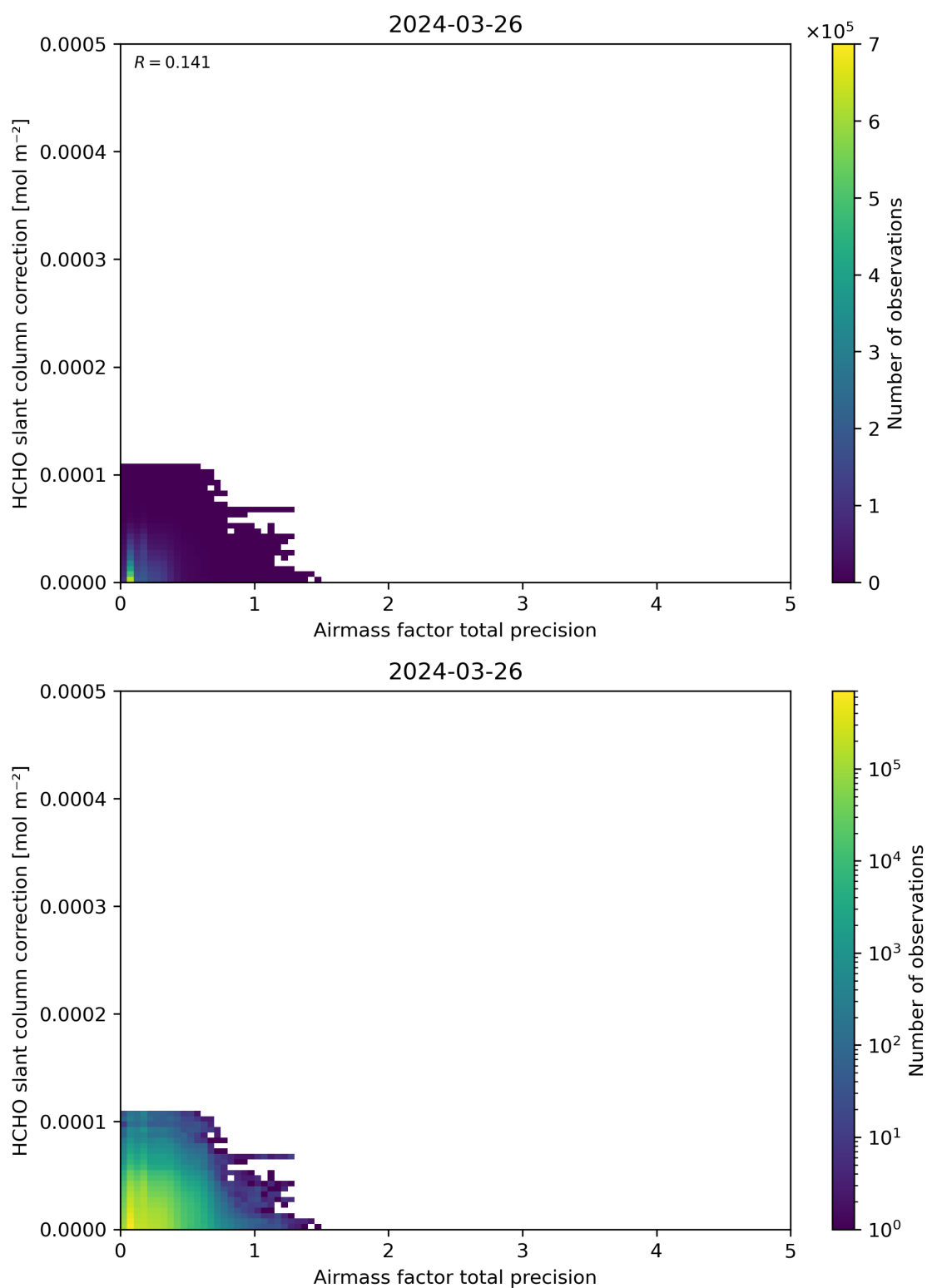
Figure 110: Scatter density plot of “Airmass factor total precision” against “HCHO slant column correction” for 2024-03-25 to 2024-03-27.
