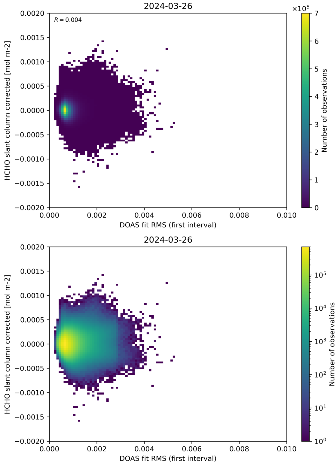
Figure 62: Scatter density plot of “DOAS fit RMS (first interval)” against “HCHO slant column corrected” for 2024-03-25 to 2024-03-27.
