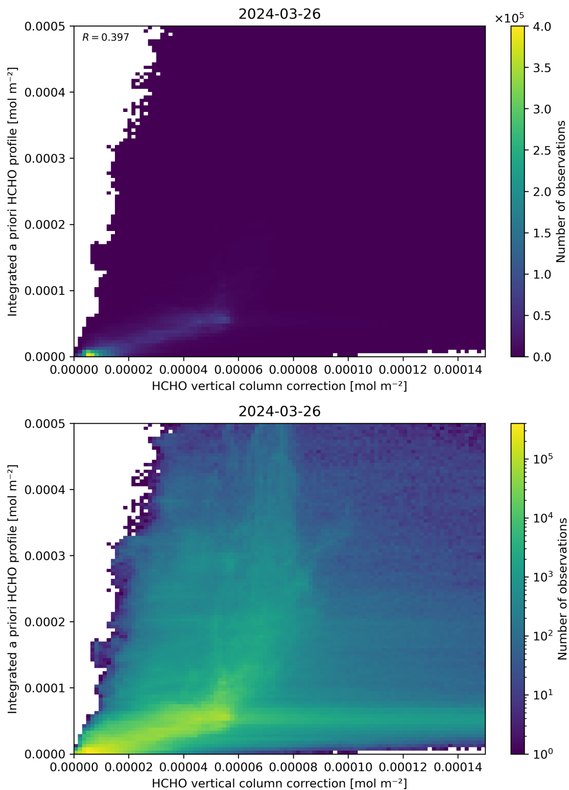
Figure 122: Scatter density plot of “HCHO vertical column correction” against “Integrated a priori HCHO profile” for 2024-03-25 to 2024-03-27.
