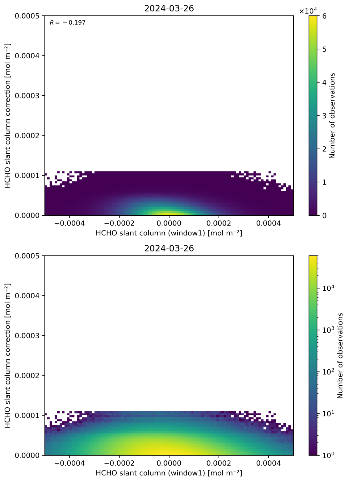
Figure 83: Scatter density plot of “HCHO slant column (window1)” against “HCHO slant column correction” for 2024-03-25 to 2024-03-27.
