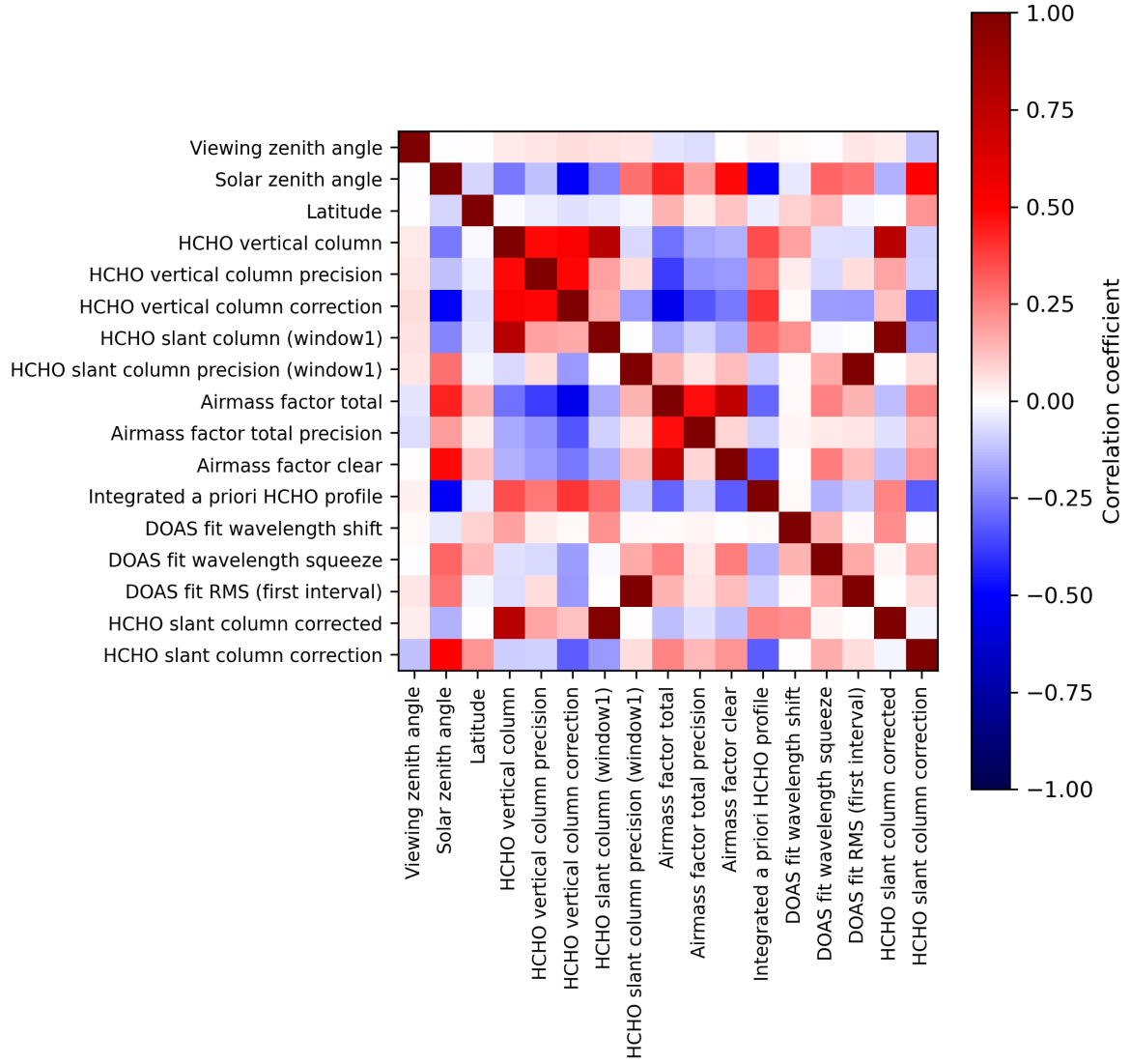
Figure 2: Map of correlation matrix for 2024-03-25 to 2024-03-27.
