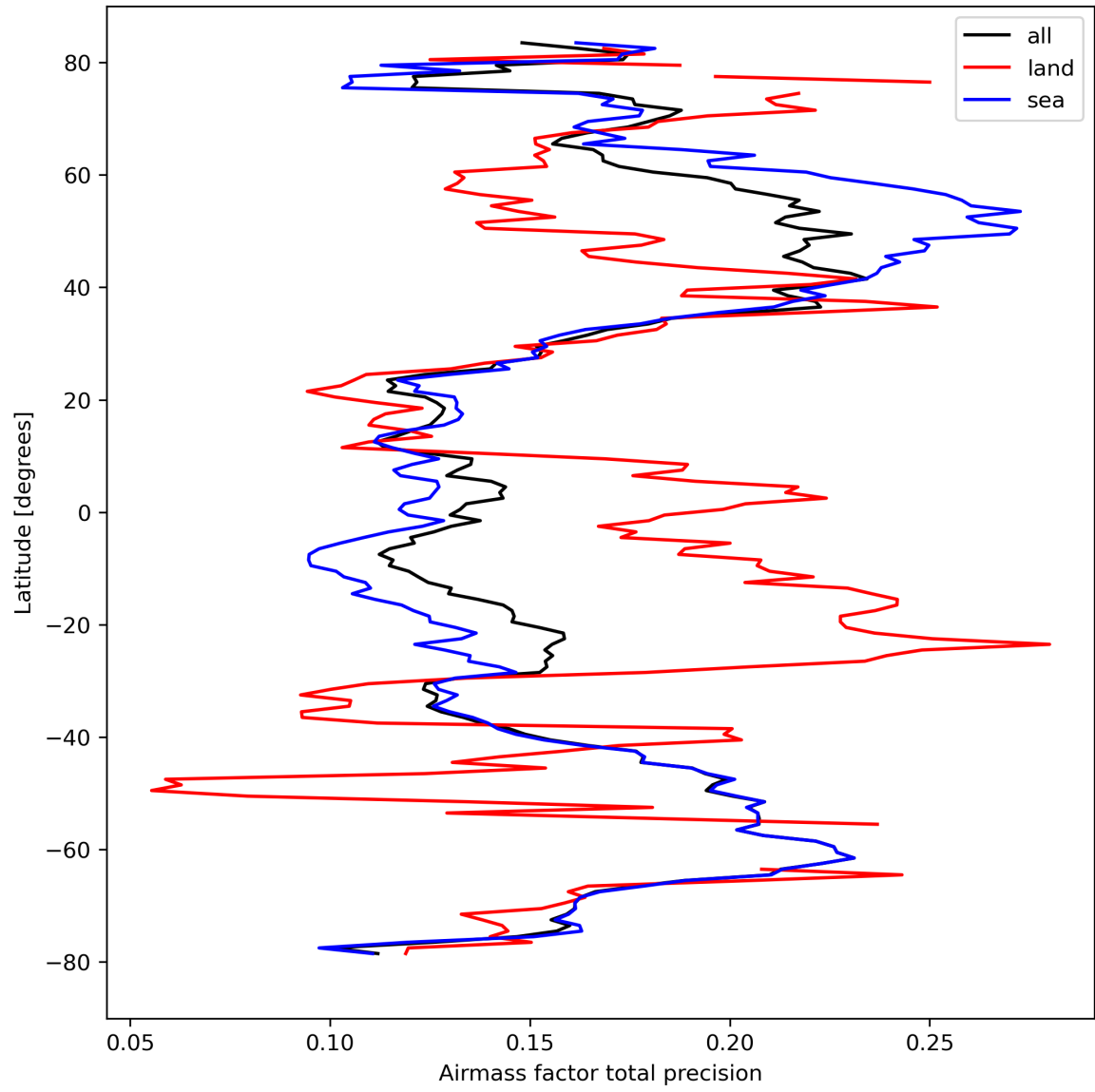
Figure 27: Zonal average of “Airmass factor total precision” for 2024-03-25 to 2024-03-27.
