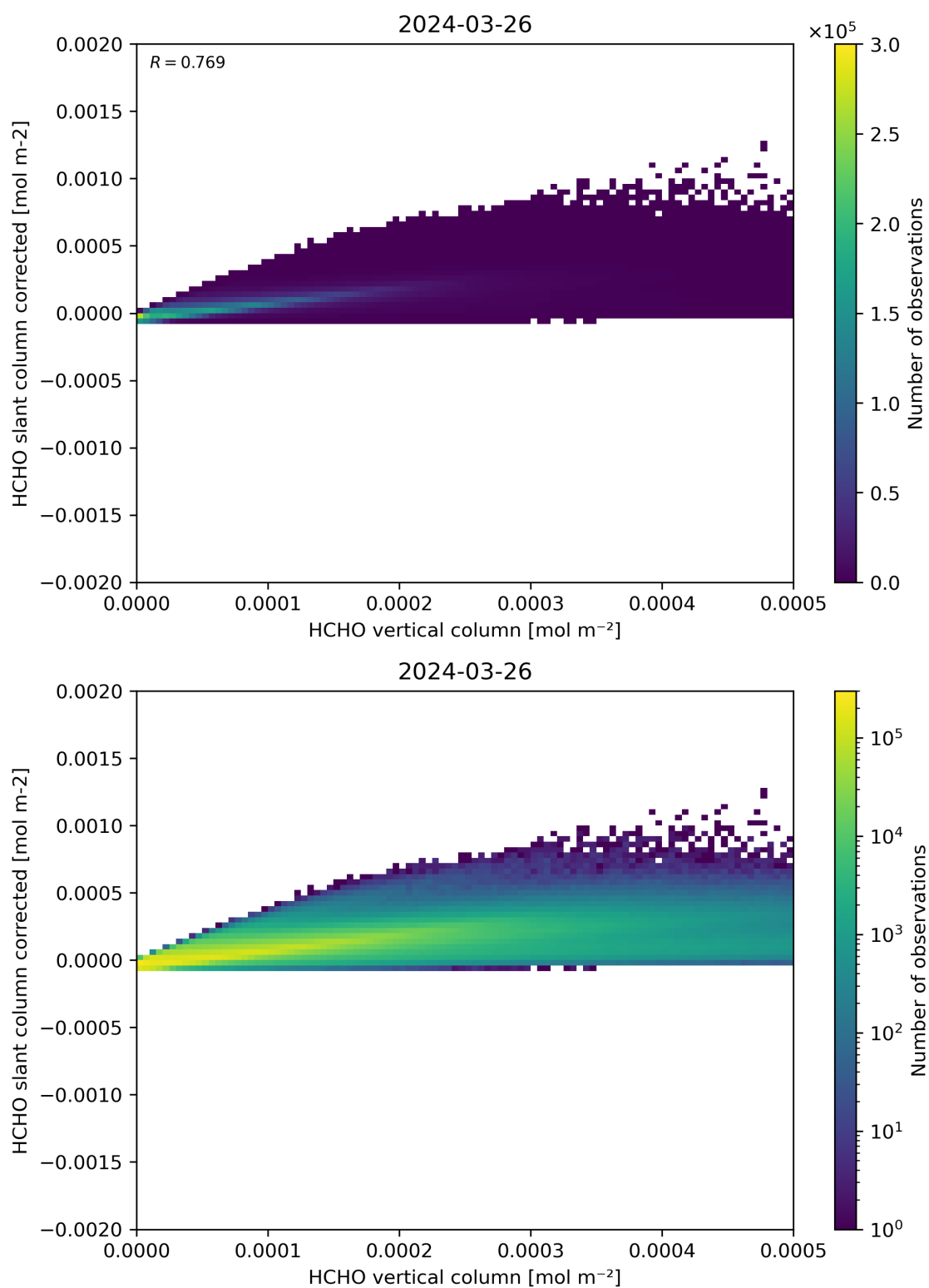
Figure 127: Scatter density plot of “HCHO vertical column” against “HCHO slant column corrected” for 2024-03-25 to 2024-03-27.
