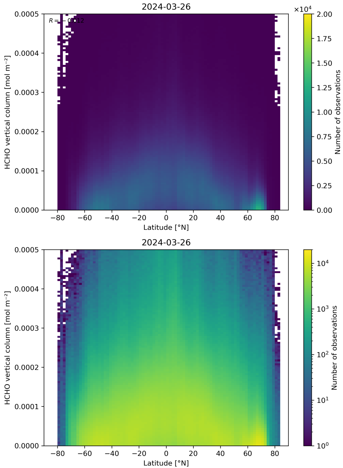
Figure 163: Scatter density plot of “Latitude” against “HCHO vertical column” for 2024-03-25 to 2024-03-27.
