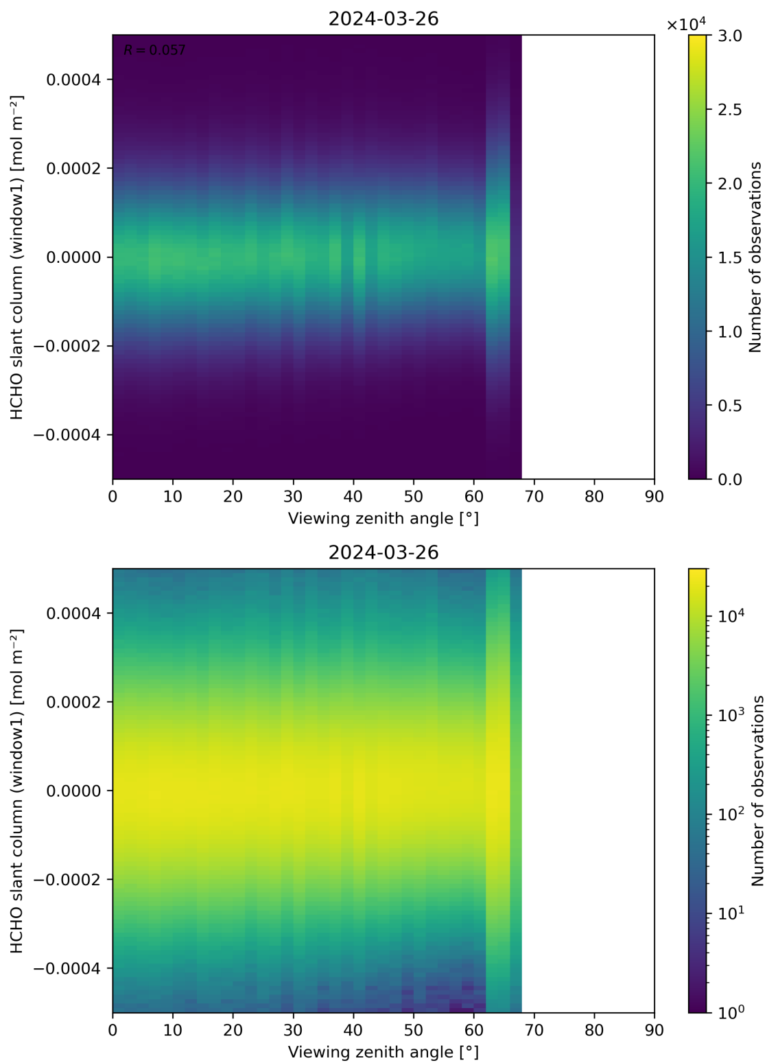
Figure 188: Scatter density plot of “Viewing zenith angle” against “HCHO slant column (window1)” for 2024-03-25 to 2024-03-27.
