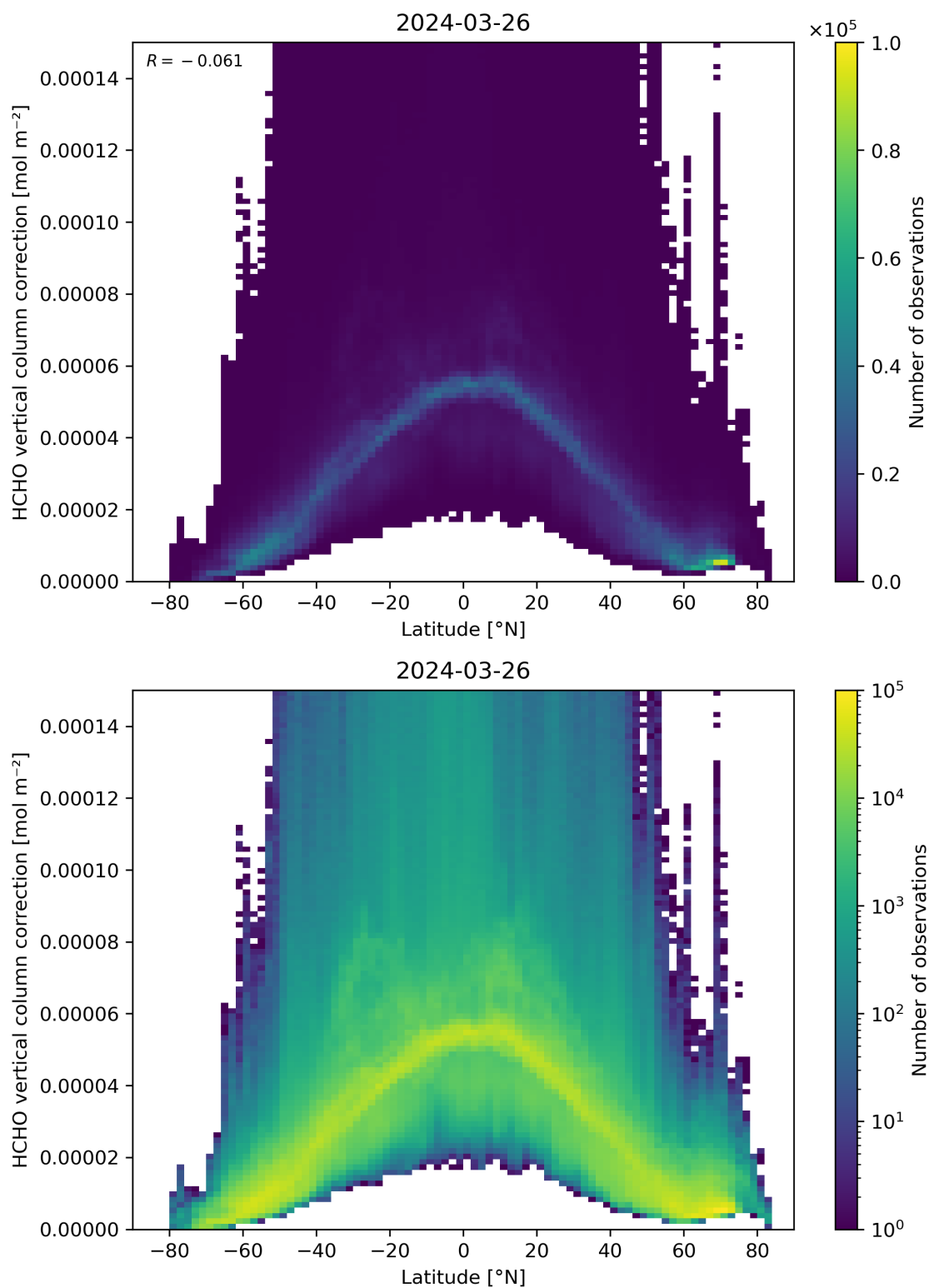
Figure 164: Scatter density plot of “Latitude” against “HCHO vertical column correction” for 2024-03-25 to 2024-03-27.
