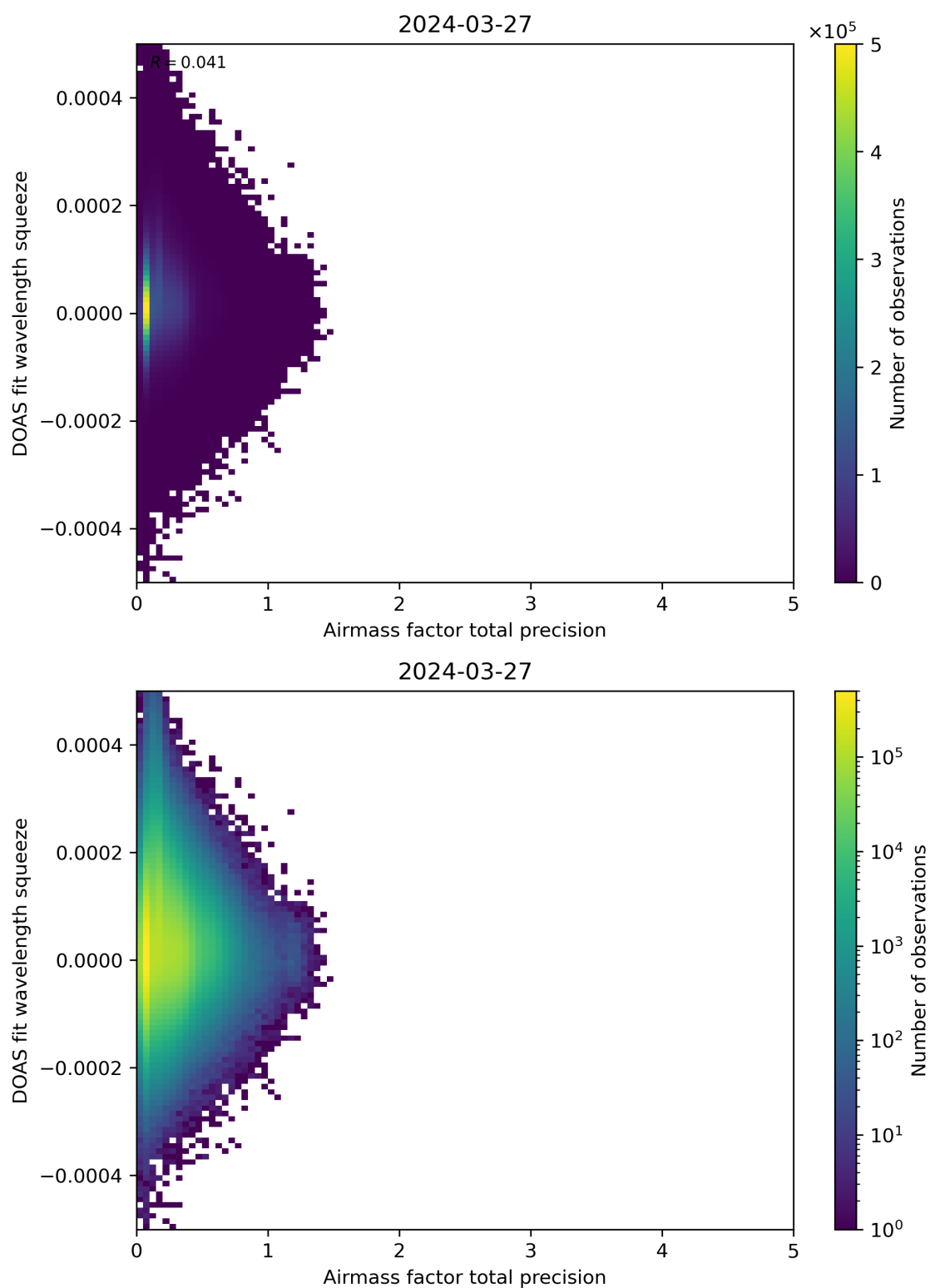
Figure 107: Scatter density plot of “Airmass factor total precision” against “DOAS fit wavelength squeeze” for 2024-03-26 to 2024-03-28.
