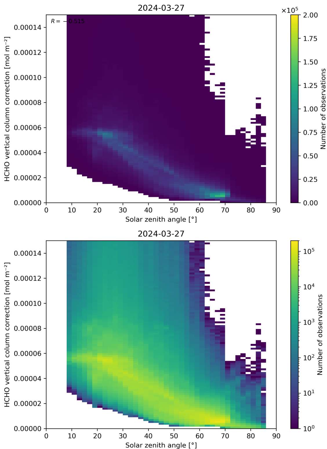
Figure 178: Scatter density plot of “Solar zenith angle” against “HCHO vertical column correction” for 2024-03-26 to 2024-03-28.
