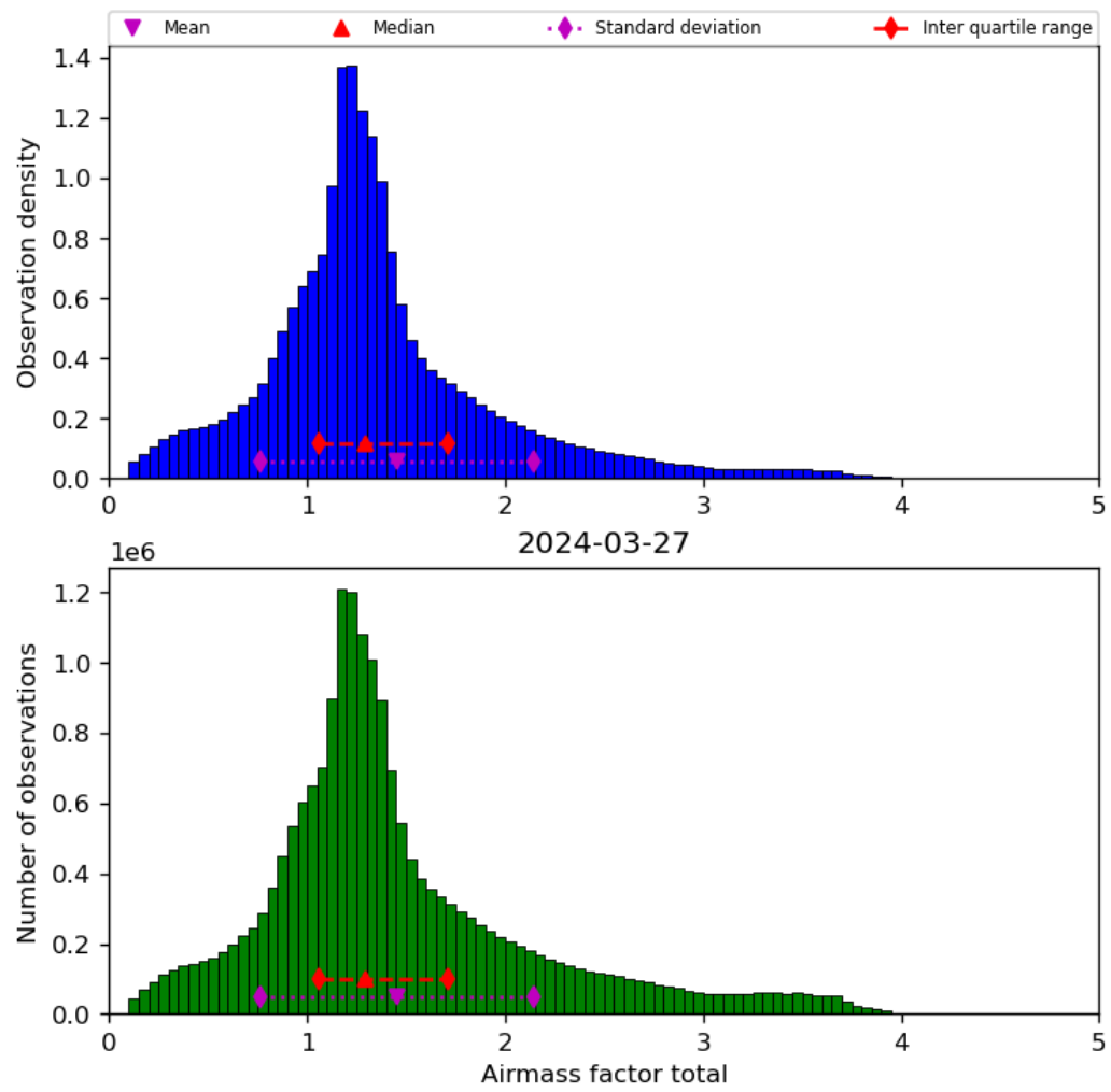
Figure 40: Histogram of “Airmass factor total” for 2024-03-26 to 2024-03-28
