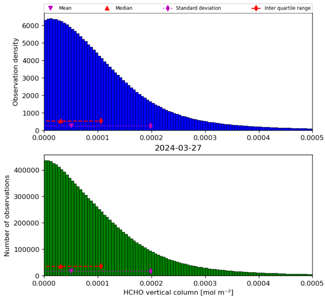
Figure 35: Histogram of “HCHO vertical column” for 2024-03-26 to 2024-03-28
