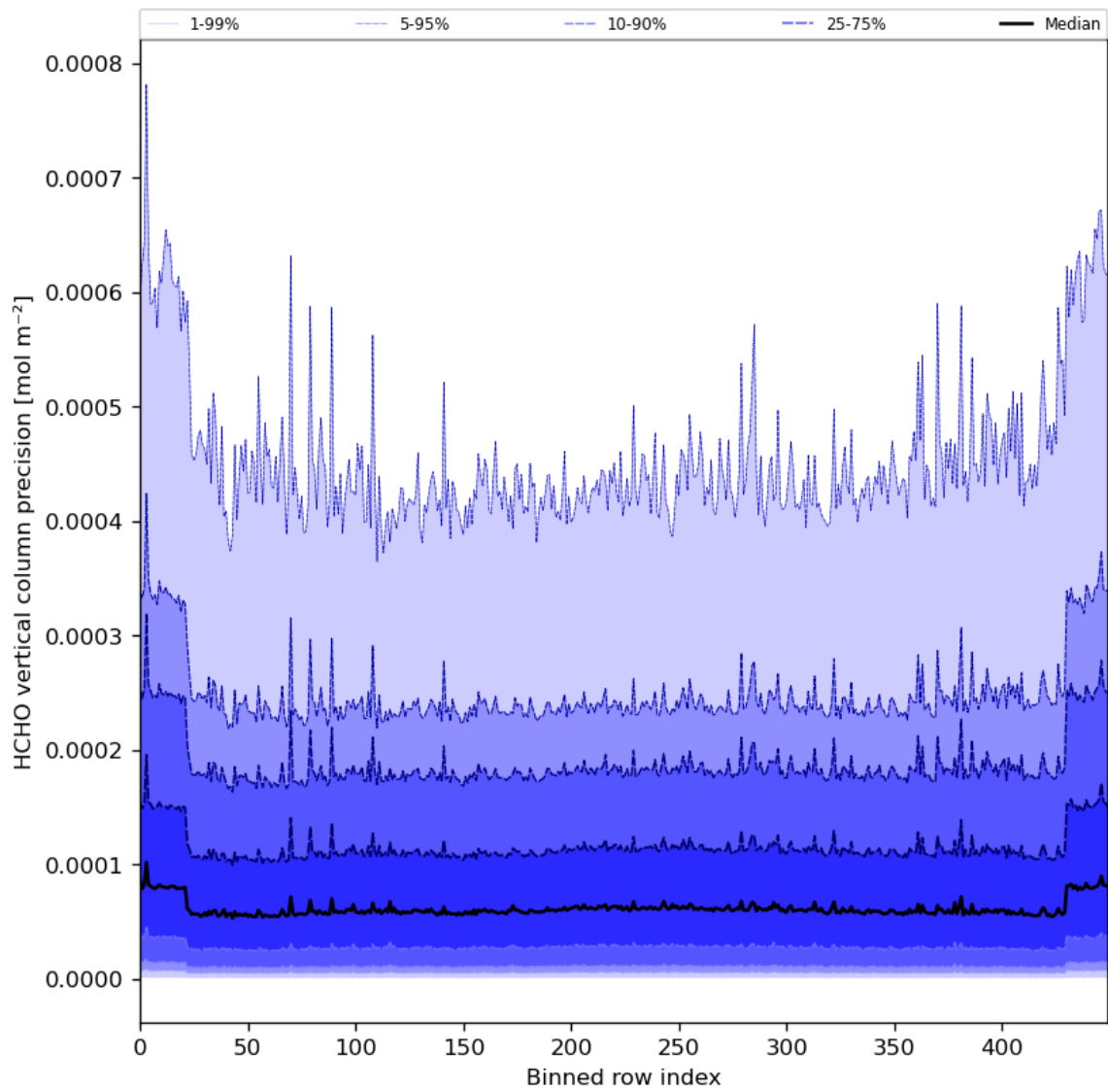
Figure 50: Along track statistics of “HCHO vertical column precision” for 2024-03-26 to 2024-03-28
