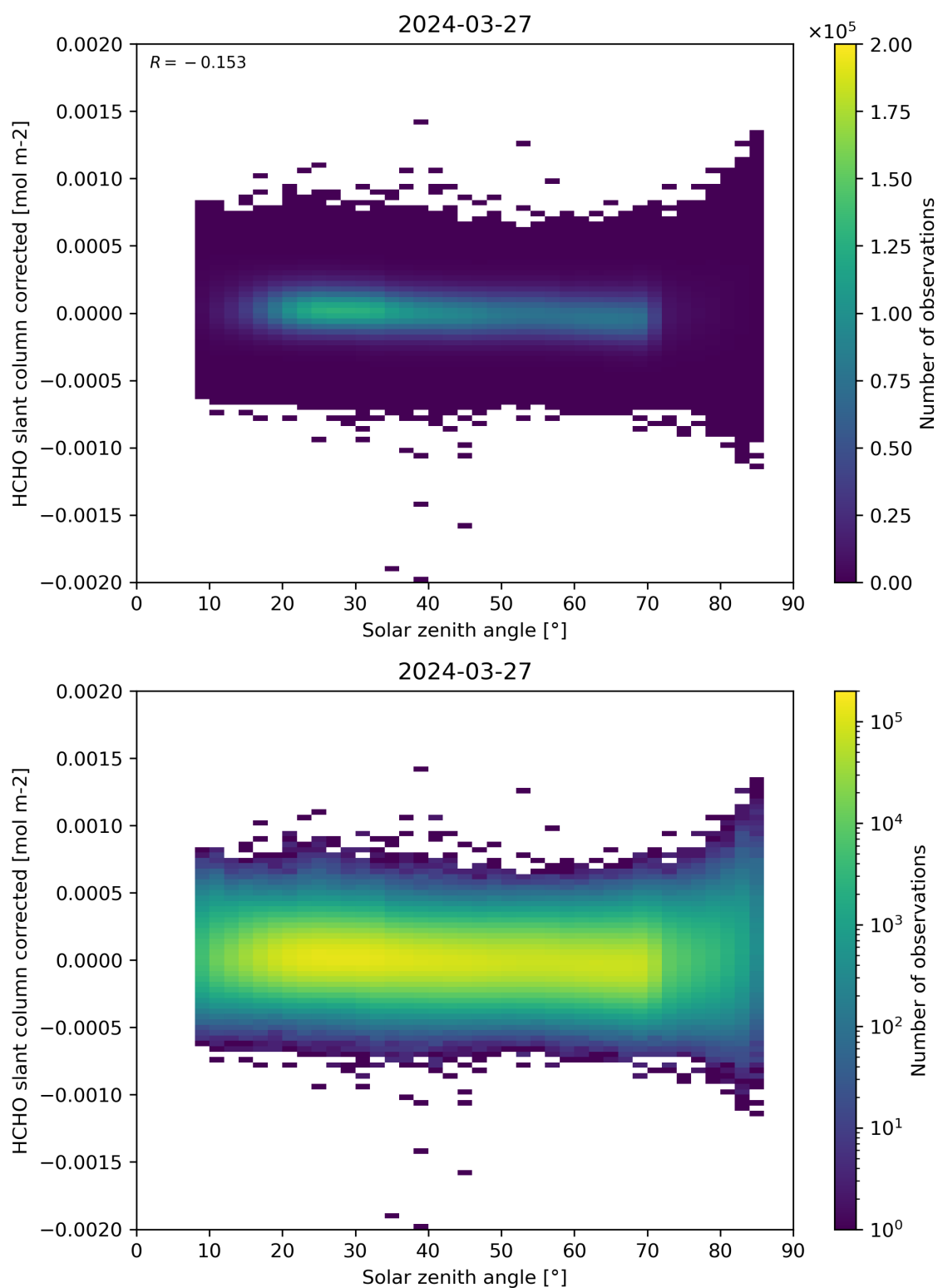
Figure 171: Scatter density plot of “Solar zenith angle” against “HCHO slant column corrected” for 2024-03-26 to 2024-03-28.
