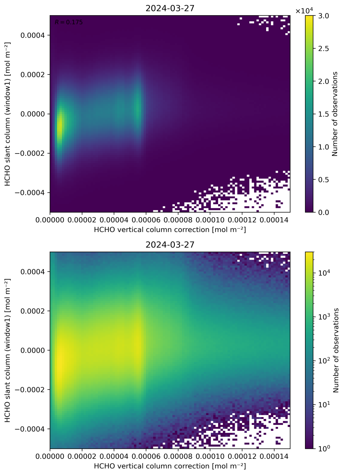
Figure 118: Scatter density plot of “HCHO vertical column correction” against “HCHO slant column (window1)” for 2024-03-26 to 2024-03-28.
