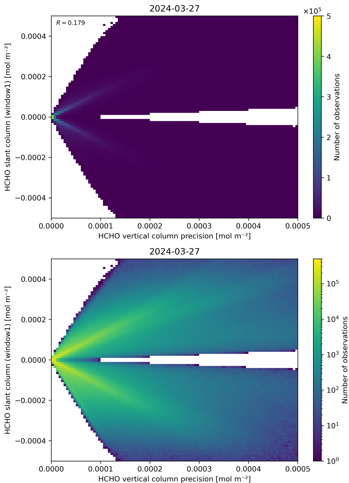
Figure 142: Scatter density plot of “HCHO vertical column precision” against “HCHO slant column (window1)” for 2024-03-26 to 2024-03-28.
