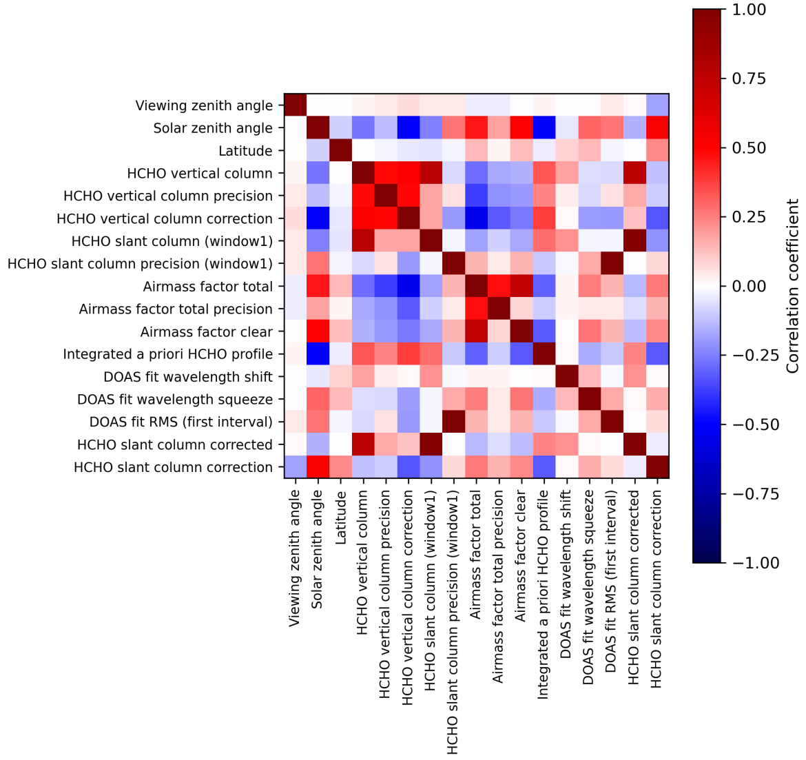
Figure 2: Map of correlation matrix for 2024-03-26 to 2024-03-28.
