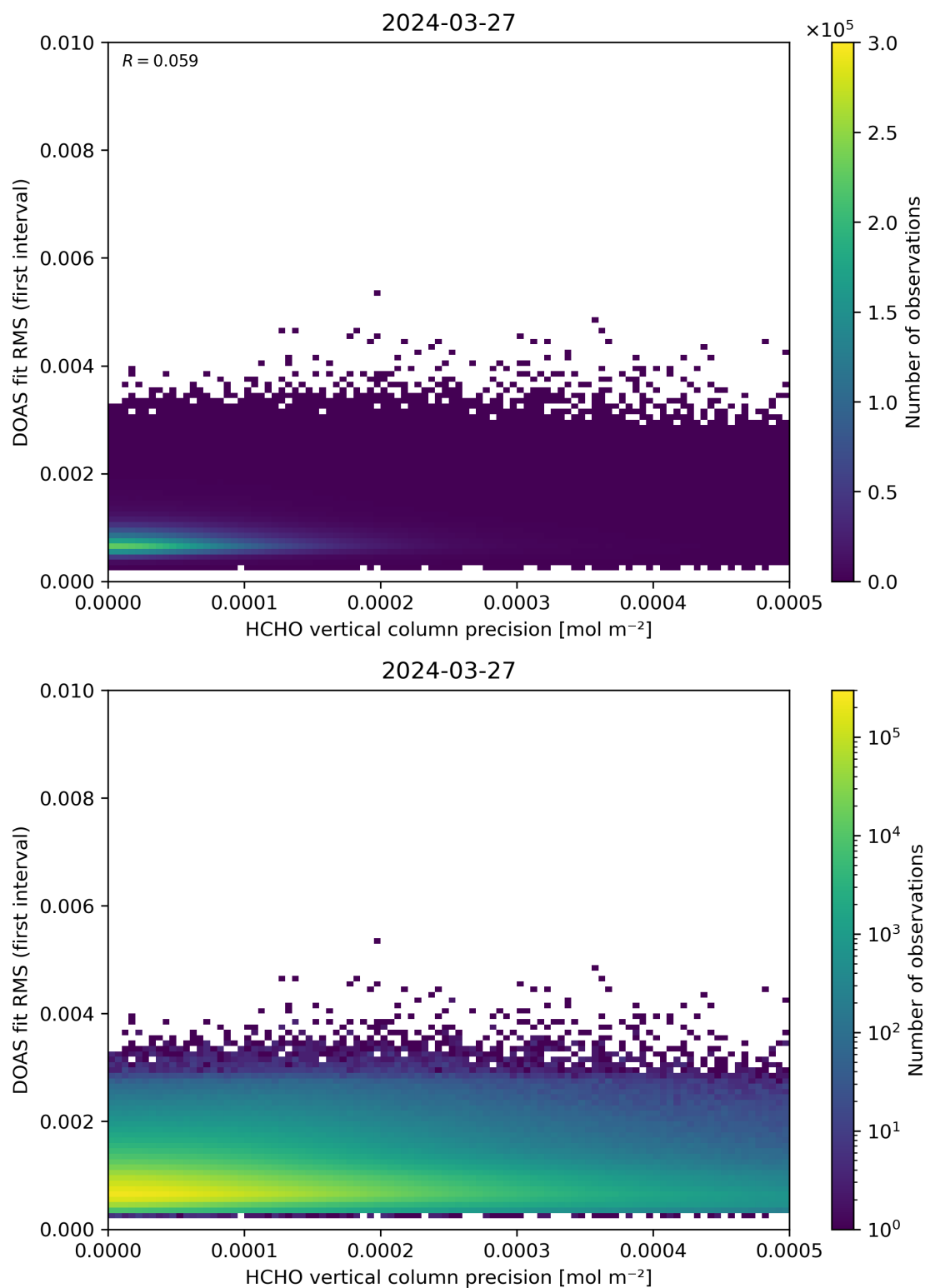
Figure 136: Scatter density plot of “HCHO vertical column precision” against “DOAS fit RMS (first interval)” for 2024-03-26 to 2024-03-28.
