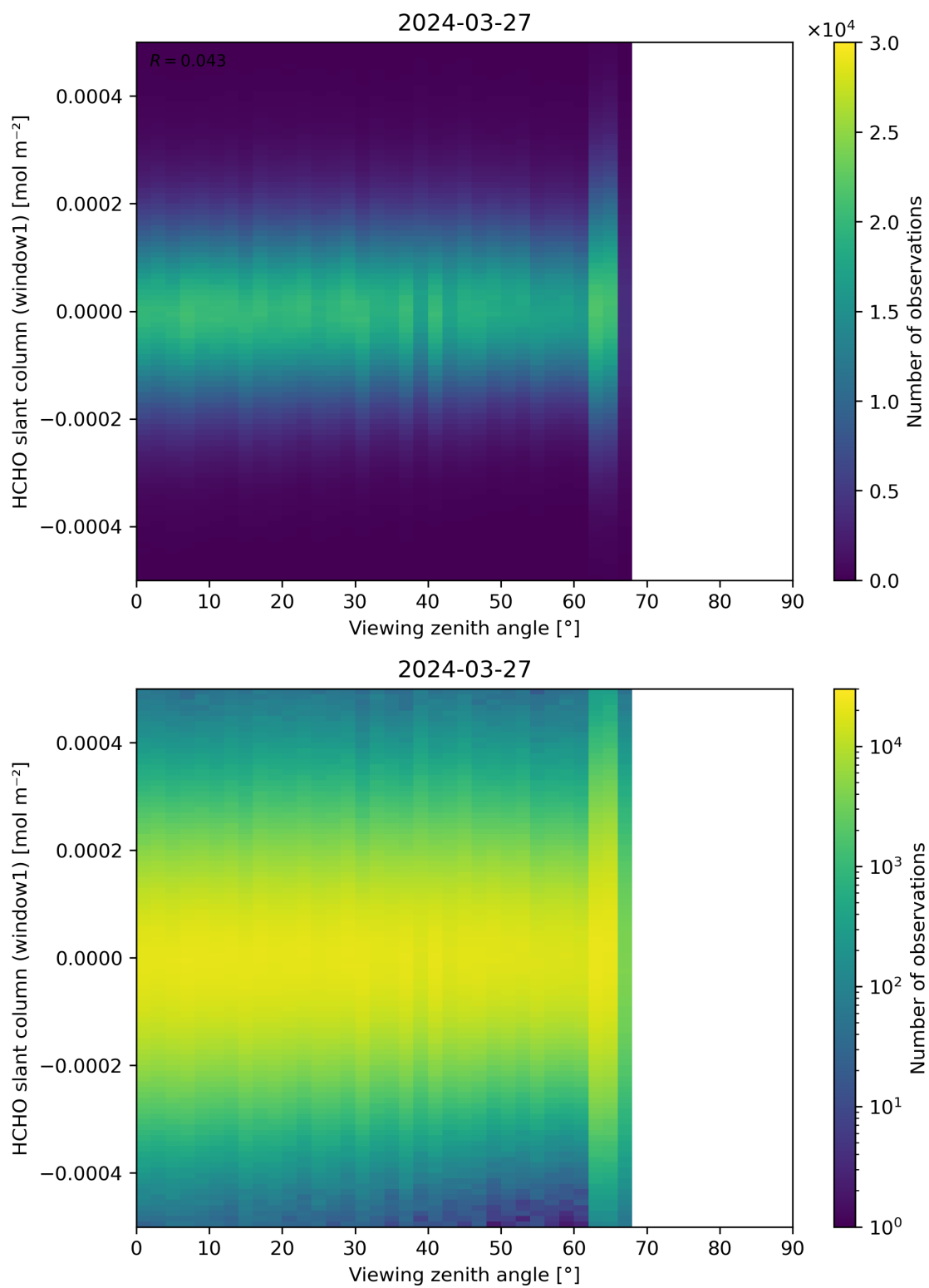
Figure 188: Scatter density plot of “Viewing zenith angle” against “HCHO slant column (window1)” for 2024-03-26 to 2024-03-28.
