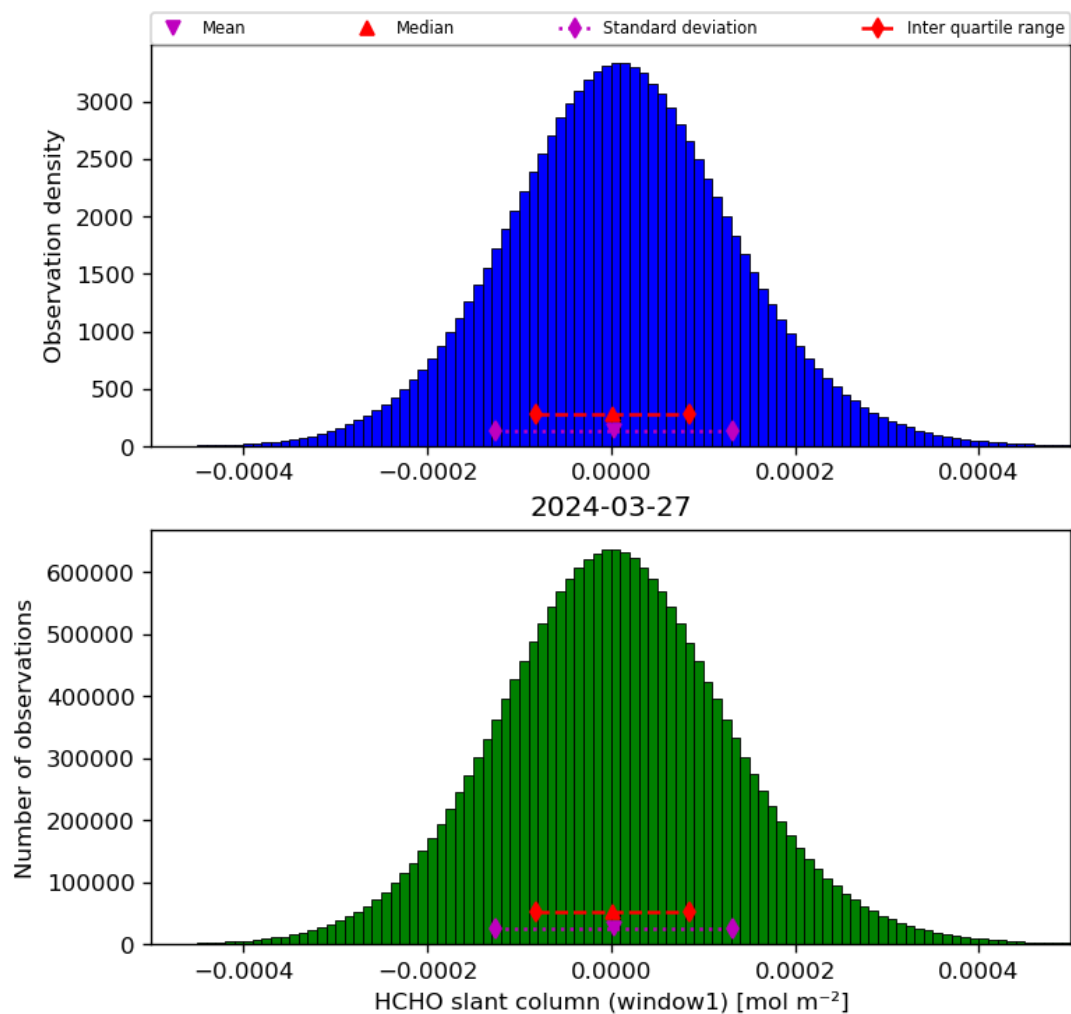
Figure 38: Histogram of “HCHO slant column (window1)” for 2024-03-26 to 2024-03-28
