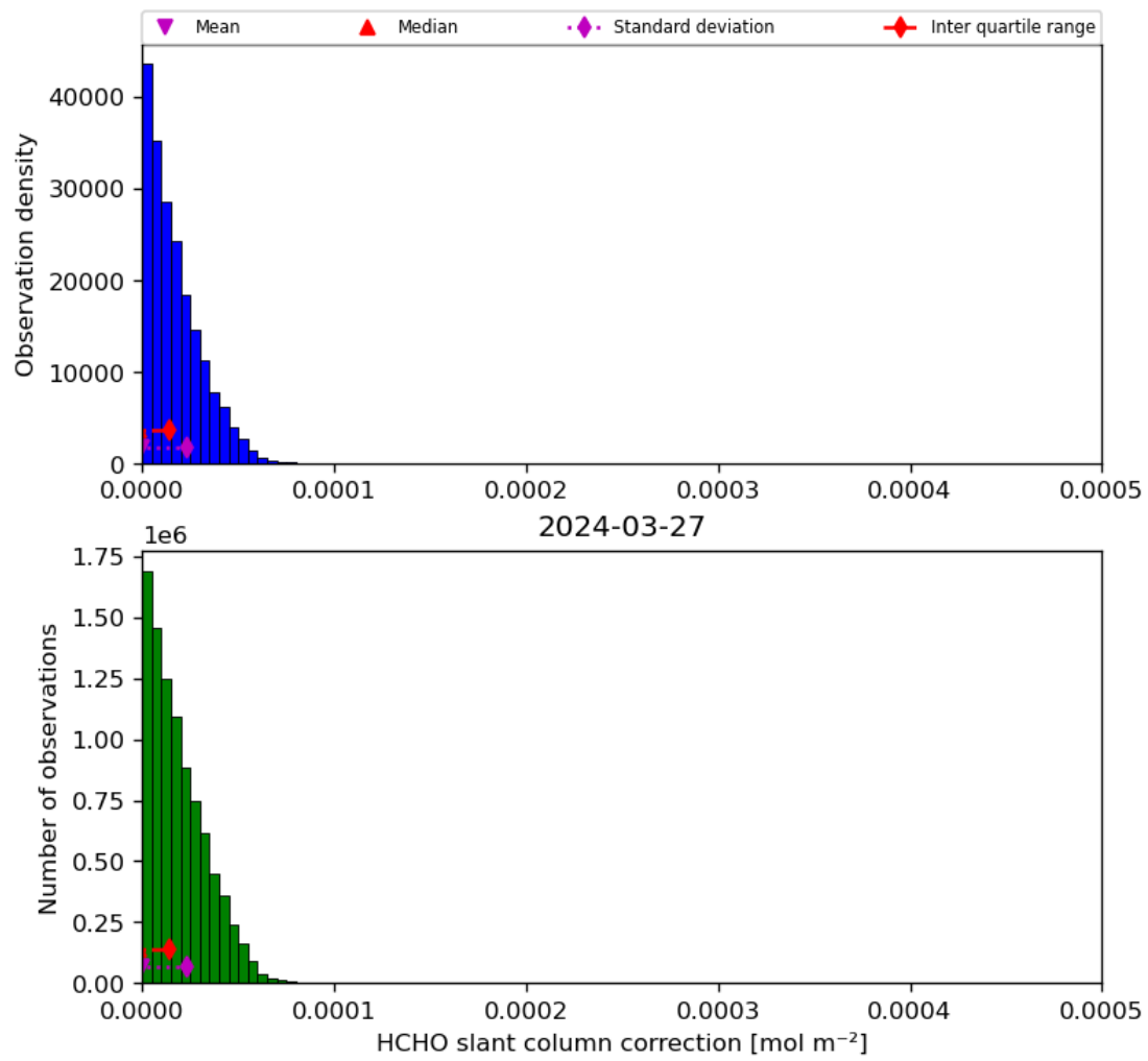
Figure 47: Histogram of “HCHO slant column correction” for 2024-03-26 to 2024-03-28
