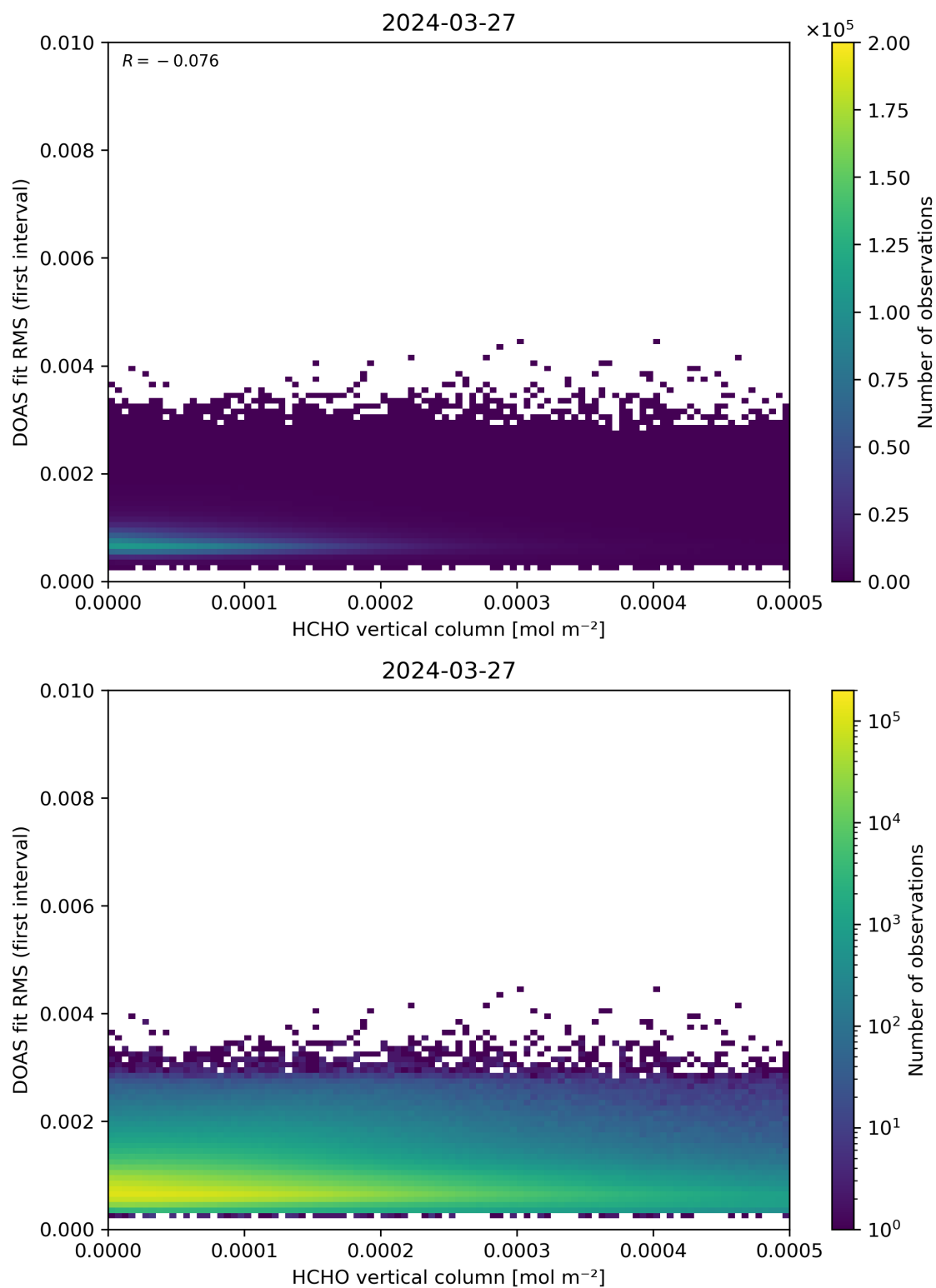
Figure 123: Scatter density plot of “HCHO vertical column” against “DOAS fit RMS (first interval)” for 2024-03-26 to 2024-03-28.
