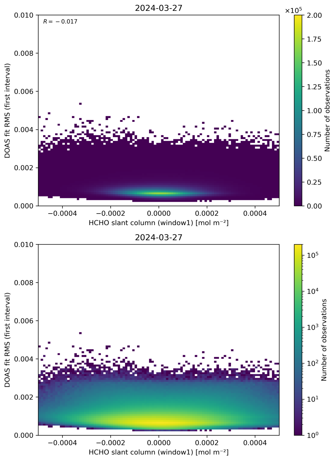
Figure 78: Scatter density plot of “HCHO slant column (window1)” against “DOAS fit RMS (first interval)” for 2024-03-26 to 2024-03-28.
