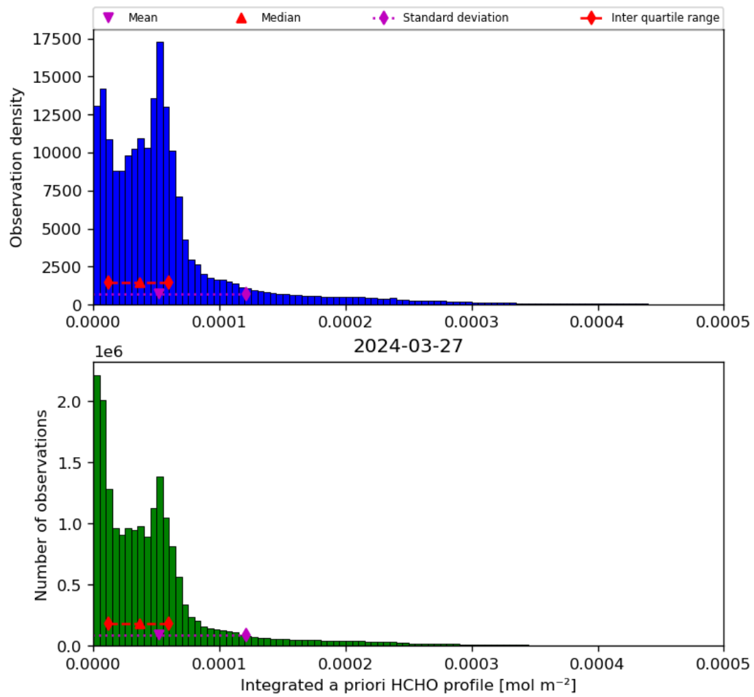
Figure 43: Histogram of “Integrated a priori HCHO profile” for 2024-03-26 to 2024-03-28
