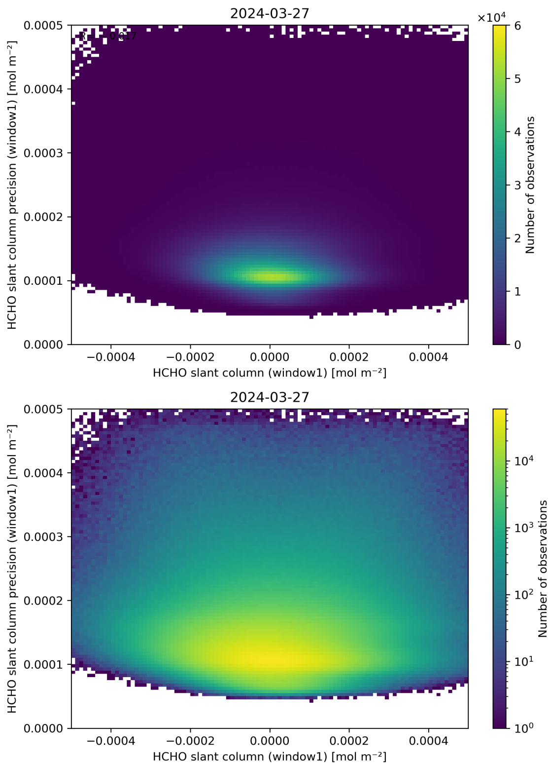
Figure 84: Scatter density plot of “HCHO slant column (window1)” against “HCHO slant column precision (window1)” for 2024-03-26 to 2024-03-28.
