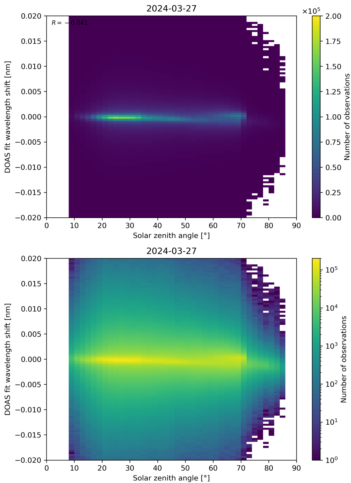
Figure 168: Scatter density plot of “Solar zenith angle” against “DOAS fit wavelength shift” for 2024-03-26 to 2024-03-28.
