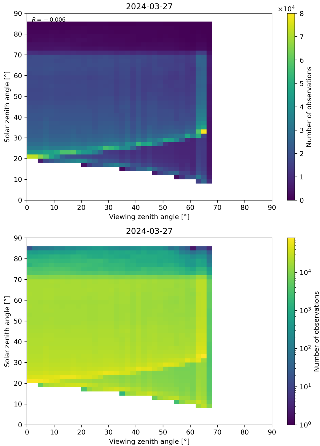
Figure 197: Scatter density plot of “Viewing zenith angle” against “Solar zenith angle” for 2024-03-26 to 2024-03-28.
