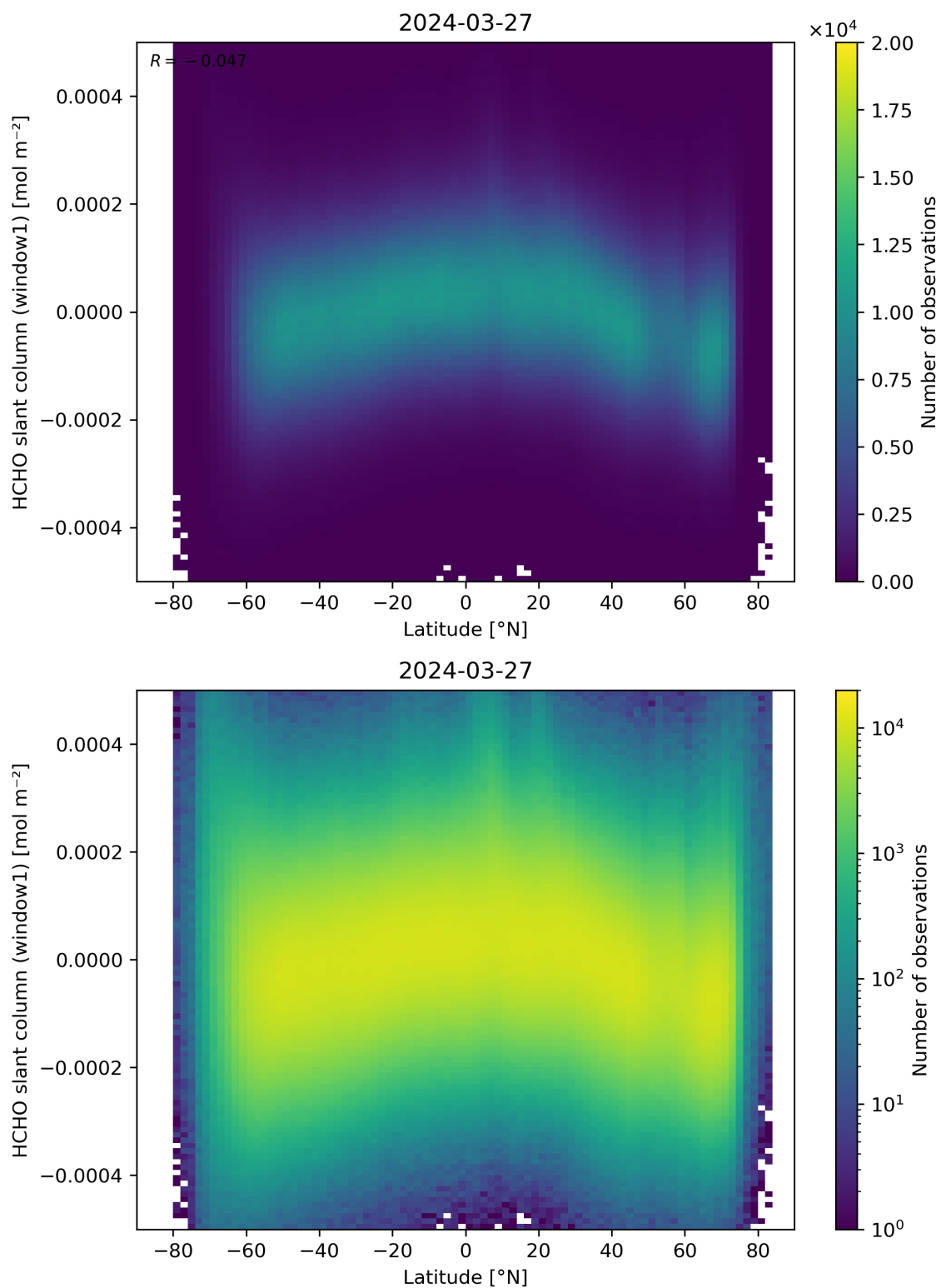
Figure 159: Scatter density plot of “Latitude” against “HCHO slant column (window1)” for 2024-03-26 to 2024-03-28.
