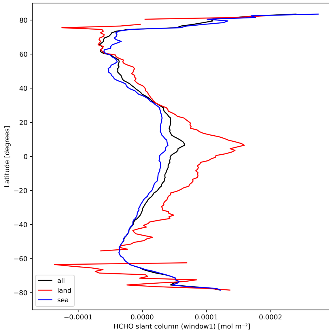
Figure 24: Zonal average of “HCHO slant column (window1)” for 2024-03-26 to 2024-03-28.
