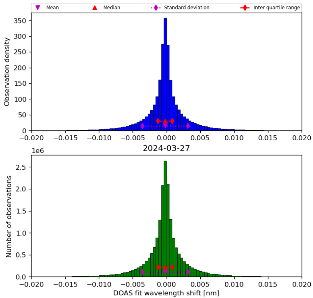
Figure 44: Histogram of “DOAS fit wavelength shift” for 2024-03-26 to 2024-03-28
