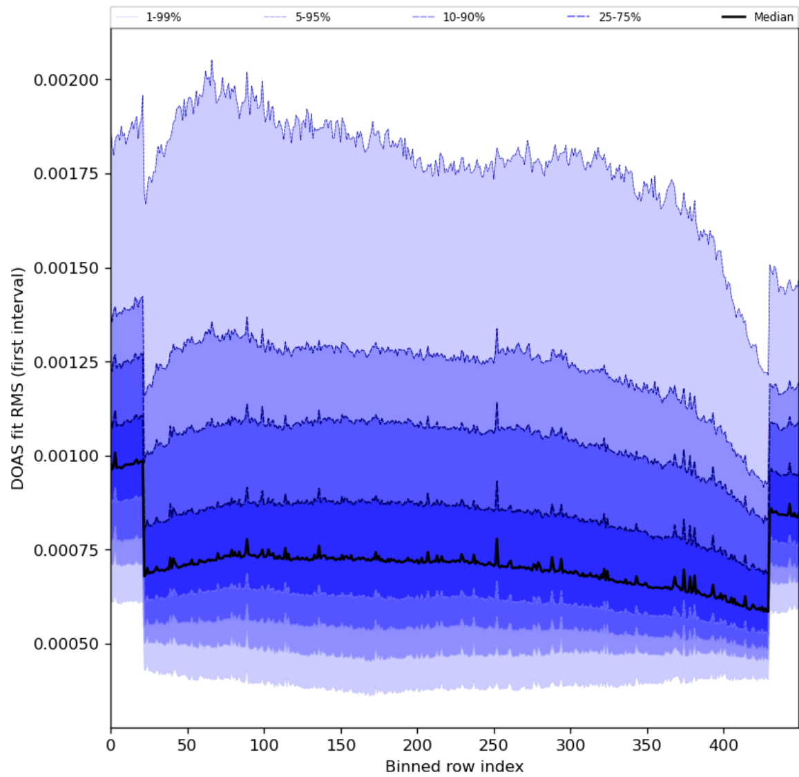
Figure 60: Along track statistics of “DOAS fit RMS (first interval)” for 2024-03-26 to 2024-03-28
