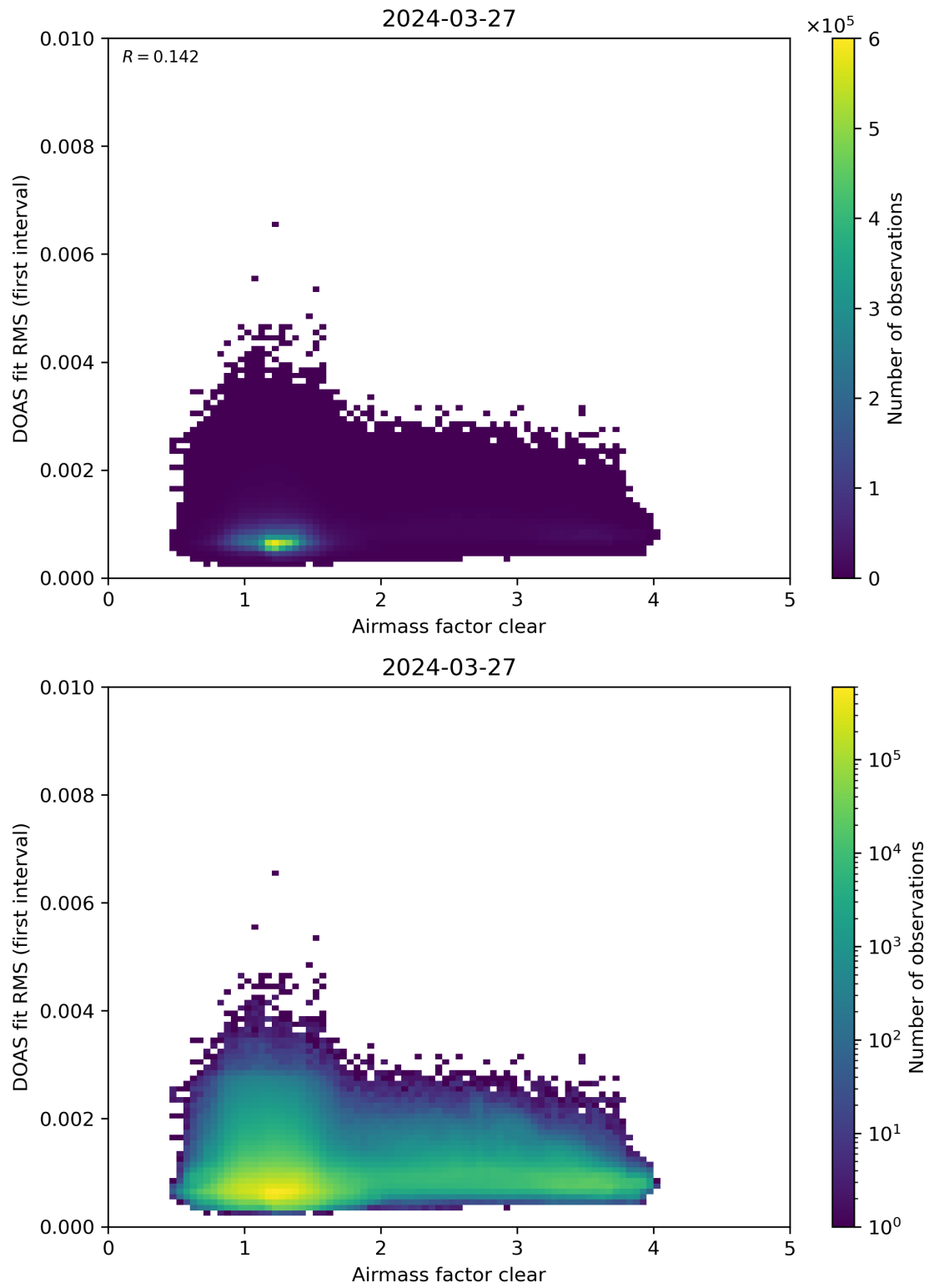
Figure 71: Scatter density plot of “Airmass factor clear” against “DOAS fit RMS (first interval)” for 2024-03-26 to 2024-03-28.
