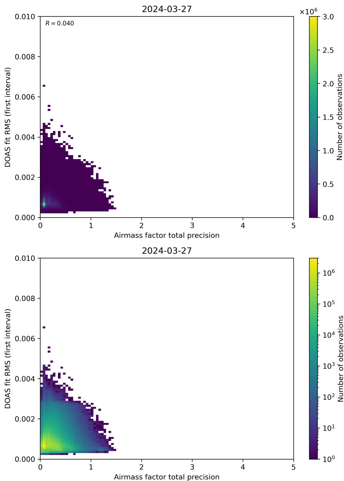
Figure 105: Scatter density plot of “Airmass factor total precision” against “DOAS fit RMS (first interval)” for 2024-03-26 to 2024-03-28.
