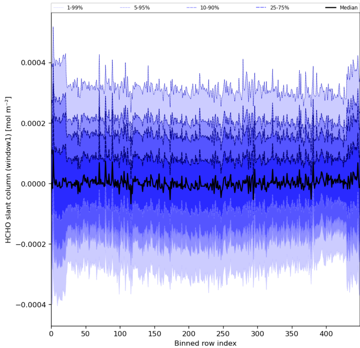
Figure 52: Along track statistics of “HCHO slant column (window1)” for 2024-03-26 to 2024-03-28
