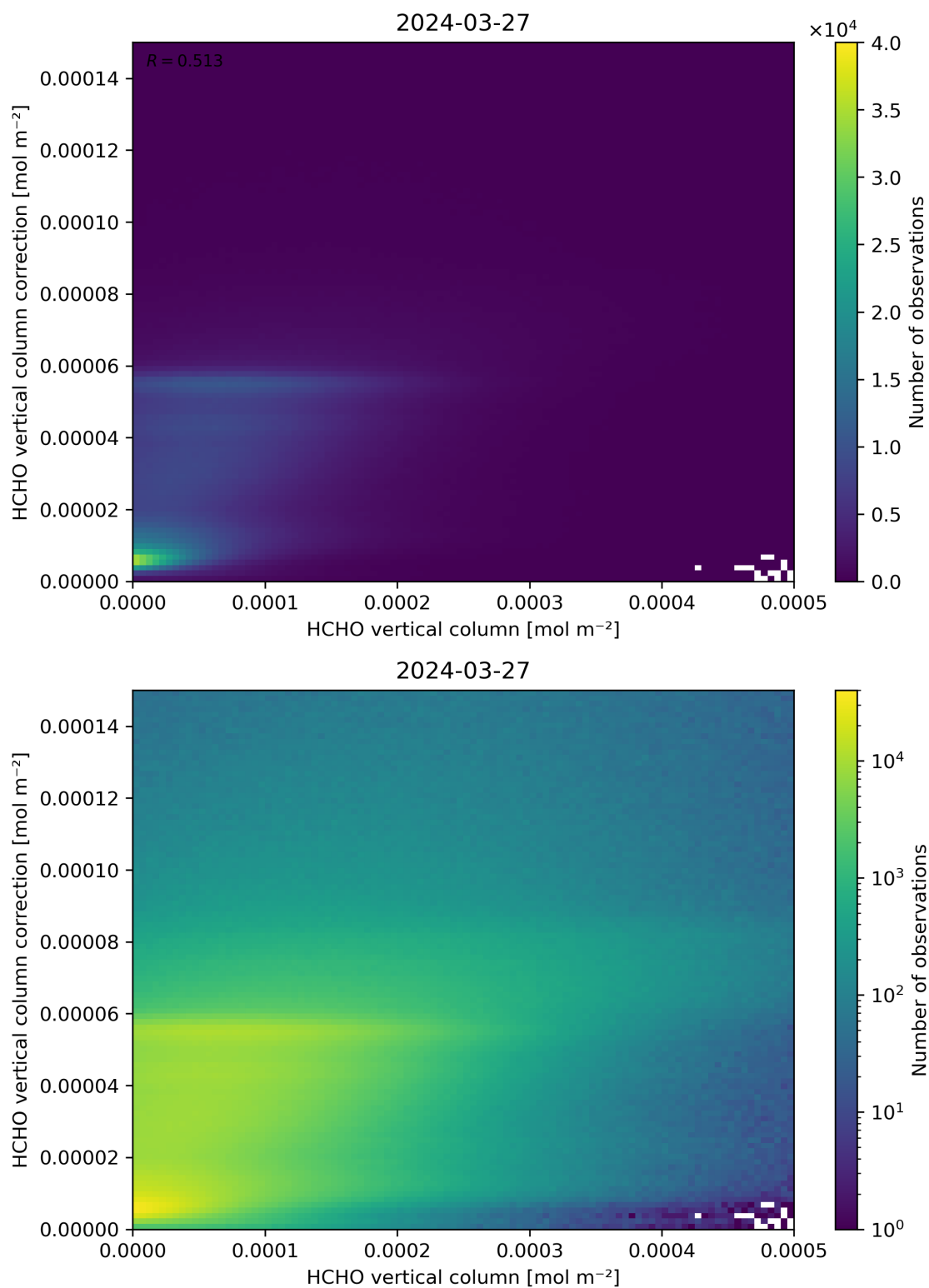
Figure 133: Scatter density plot of “HCHO vertical column” against “HCHO vertical column correction” for 2024-03-26 to 2024-03-28.
