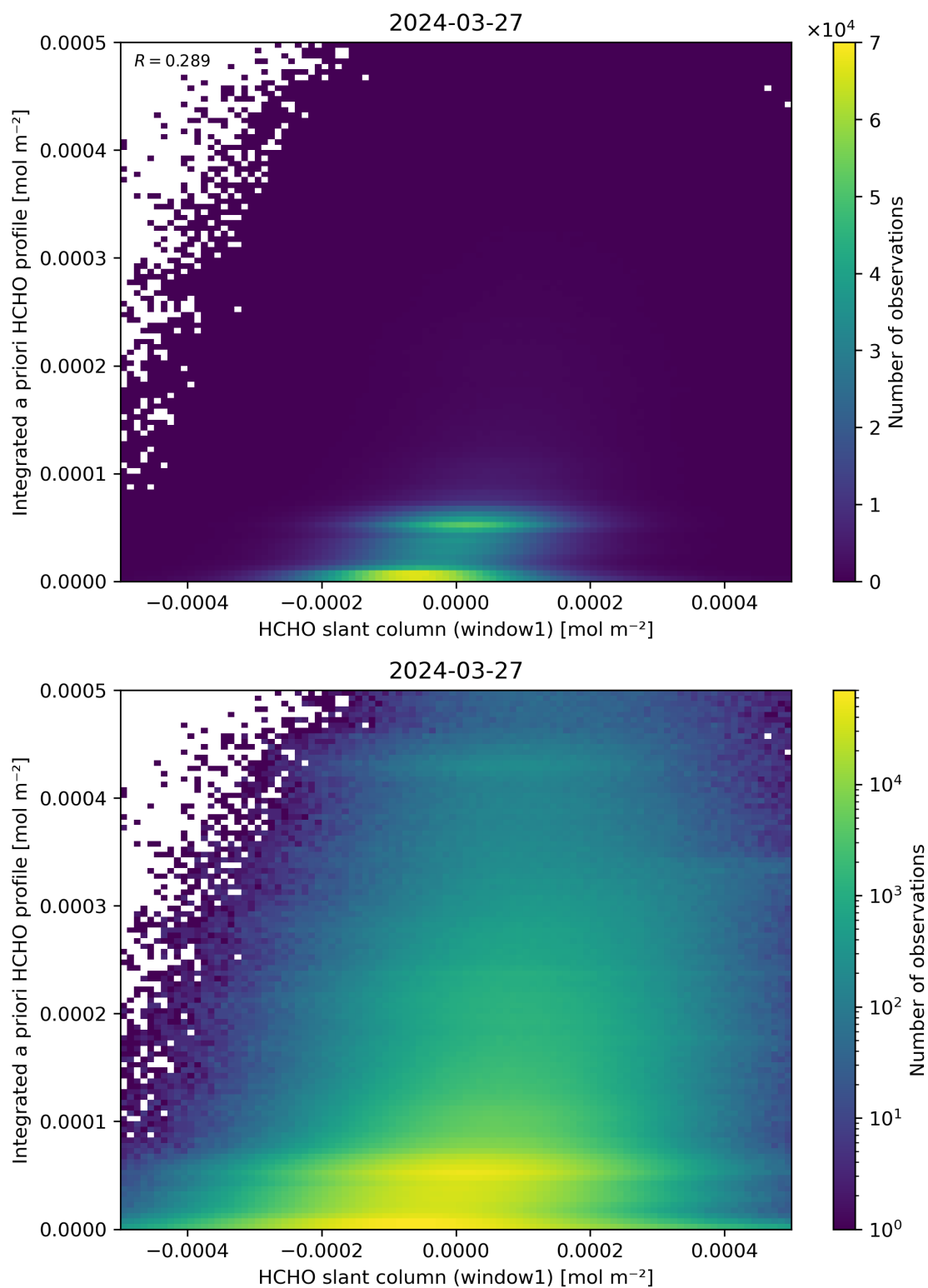
Figure 87: Scatter density plot of “HCHO slant column (window1)” against “Integrated a priori HCHO profile” for 2024-03-26 to 2024-03-28.
