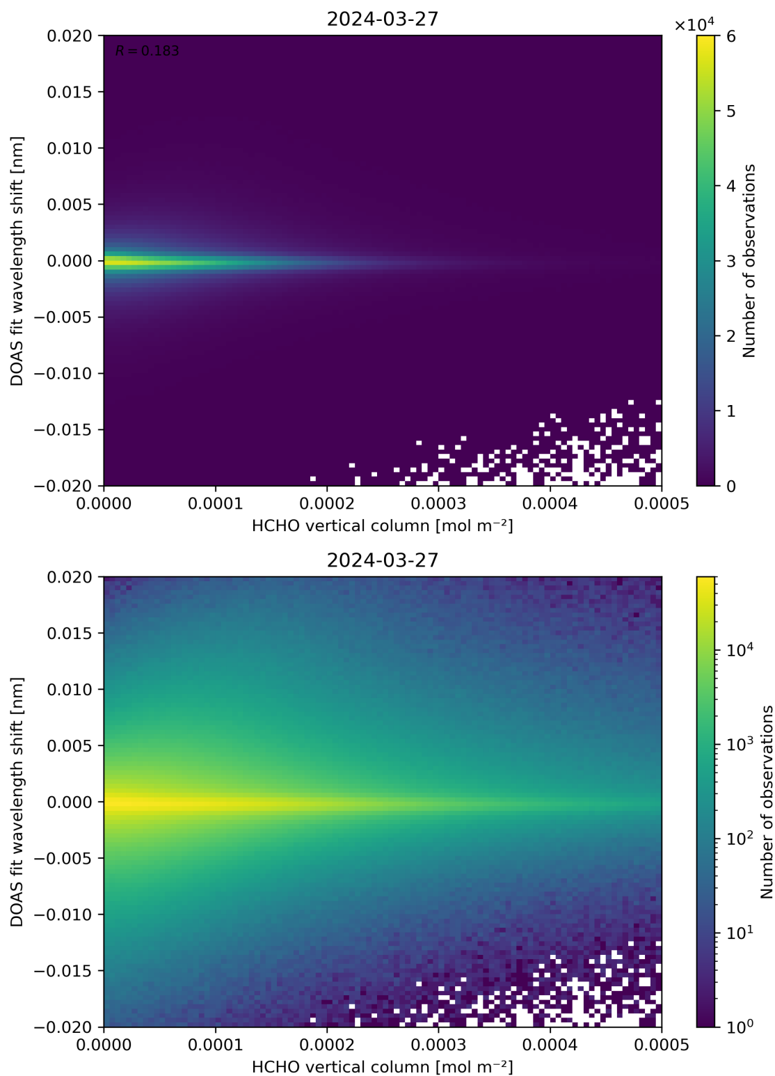
Figure 124: Scatter density plot of “HCHO vertical column” against “DOAS fit wavelength shift” for 2024-03-26 to 2024-03-28.
