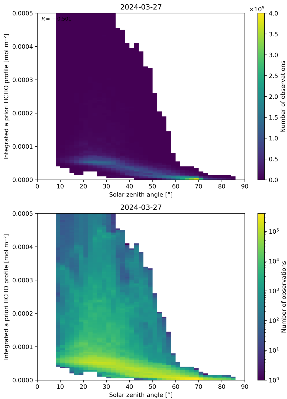
Figure 180: Scatter density plot of “Solar zenith angle” against “Integrated a priori HCHO profile” for 2024-03-26 to 2024-03-28.
