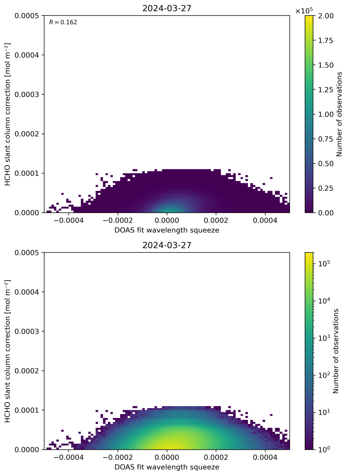
Figure 70: Scatter density plot of “DOAS fit wavelength squeeze” against “HCHO slant column correction” for 2024-03-26 to 2024-03-28.
