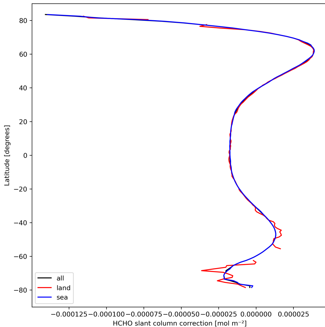
Figure 33: Zonal average of “HCHO slant column correction” for 2024-03-26 to 2024-03-28.
