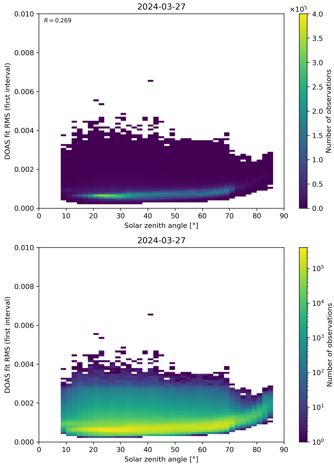
Figure 167: Scatter density plot of “Solar zenith angle” against “DOAS fit RMS (first interval)” for 2024-03-26 to 2024-03-28.
