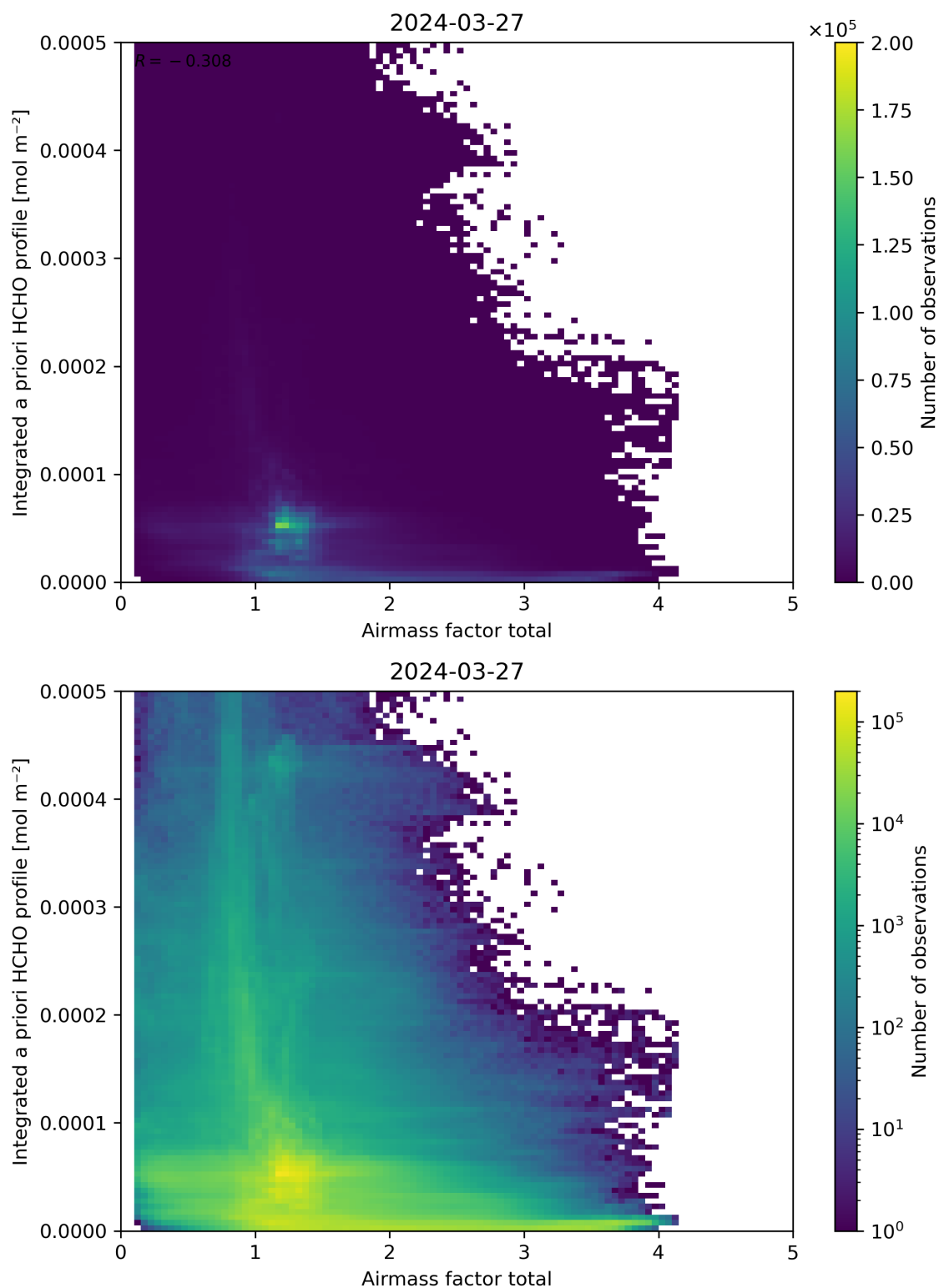
Figure 104: Scatter density plot of “Air mass factor total” against “Integrated a priori HCHO profile” for 2024-03-26 to 2024-03-28.
