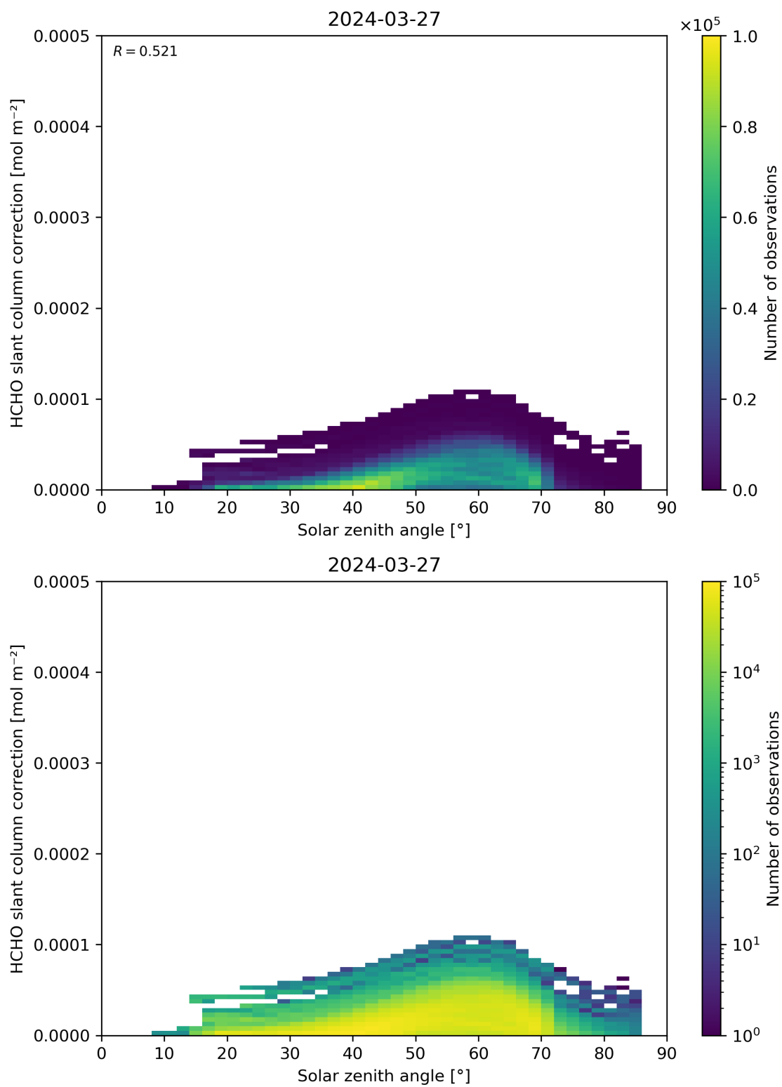
Figure 172: Scatter density plot of “Solar zenith angle” against “HCHO slant column correction” for 2024-03-26 to 2024-03-28.
