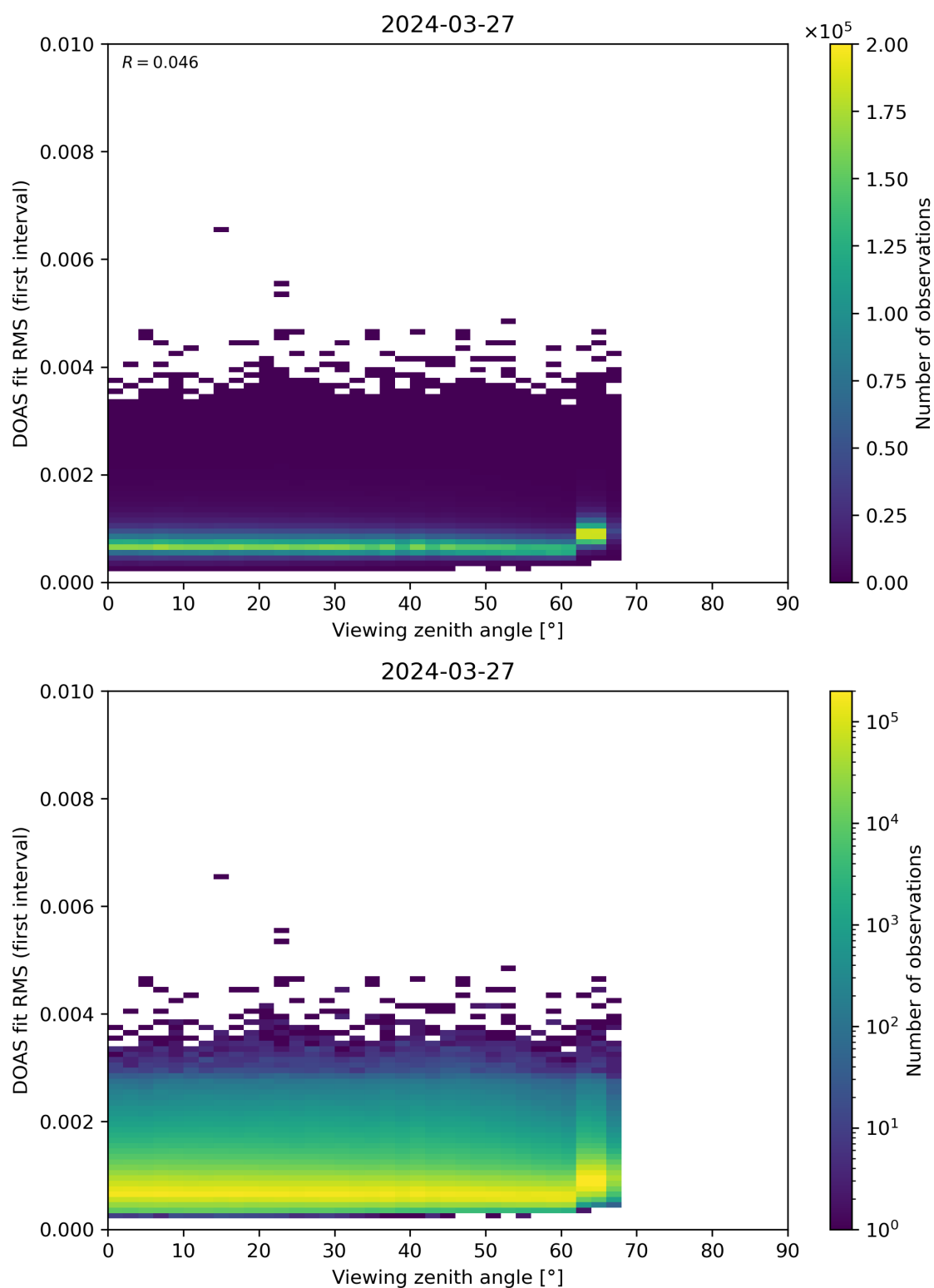
Figure 182: Scatter density plot of “Viewing zenith angle” against “DOAS fit RMS (first interval)” for 2024-03-26 to 2024-03-28.
