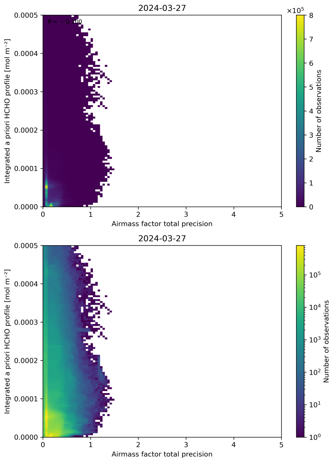
Figure 111: Scatter density plot of “Airmass factor total precision” against “Integrated a priori HCHO profile” for 2024-03-26 to 2024-03-28.
