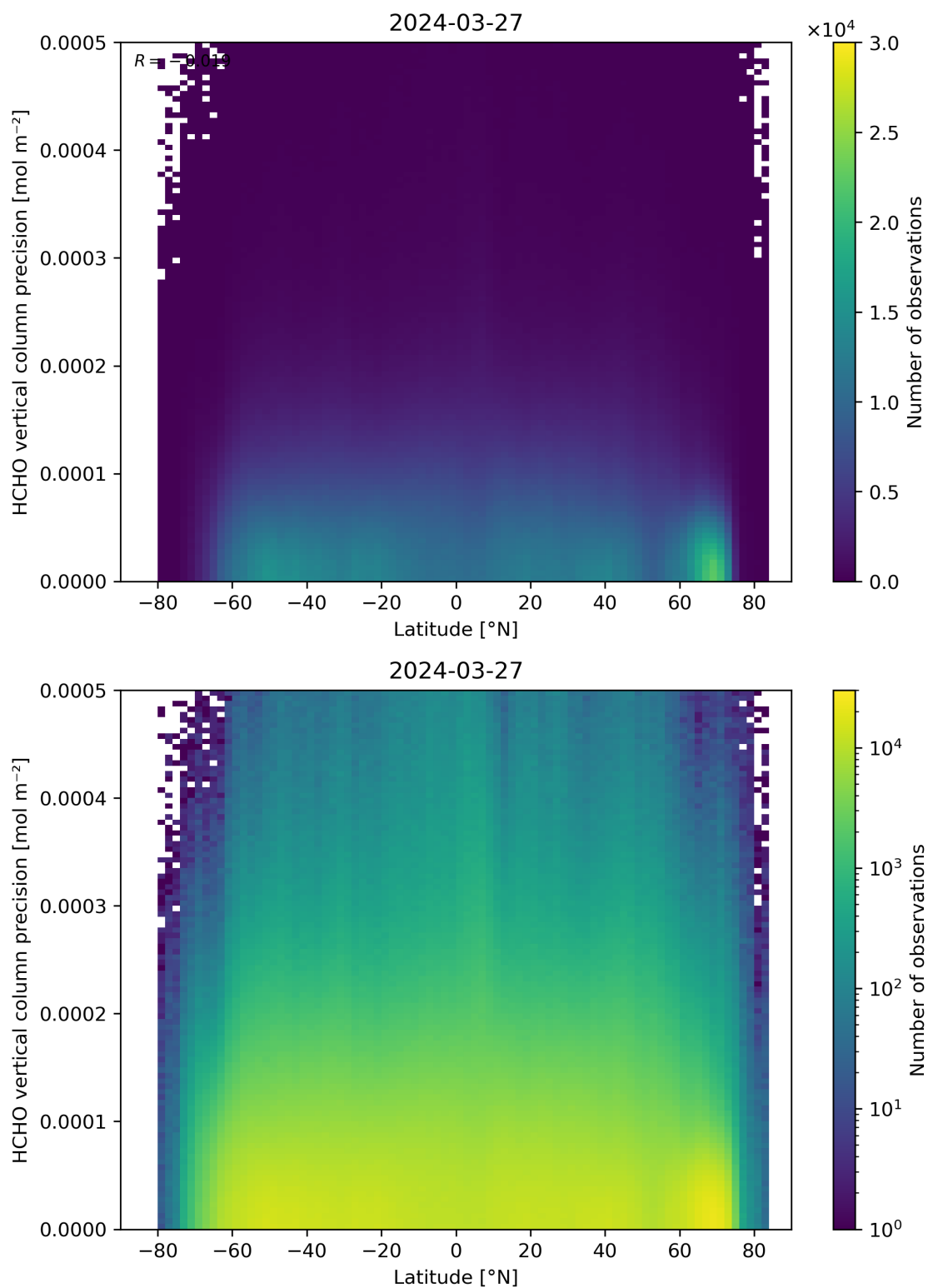
Figure 165: Scatter density plot of “Latitude” against “HCHO vertical column precision” for 2024-03-26 to 2024-03-28.
