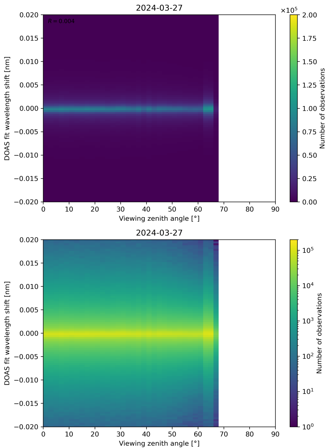
Figure 183: Scatter density plot of “Viewing zenith angle” against “DOAS fit wavelength shift” for 2024-03-26 to 2024-03-28.
