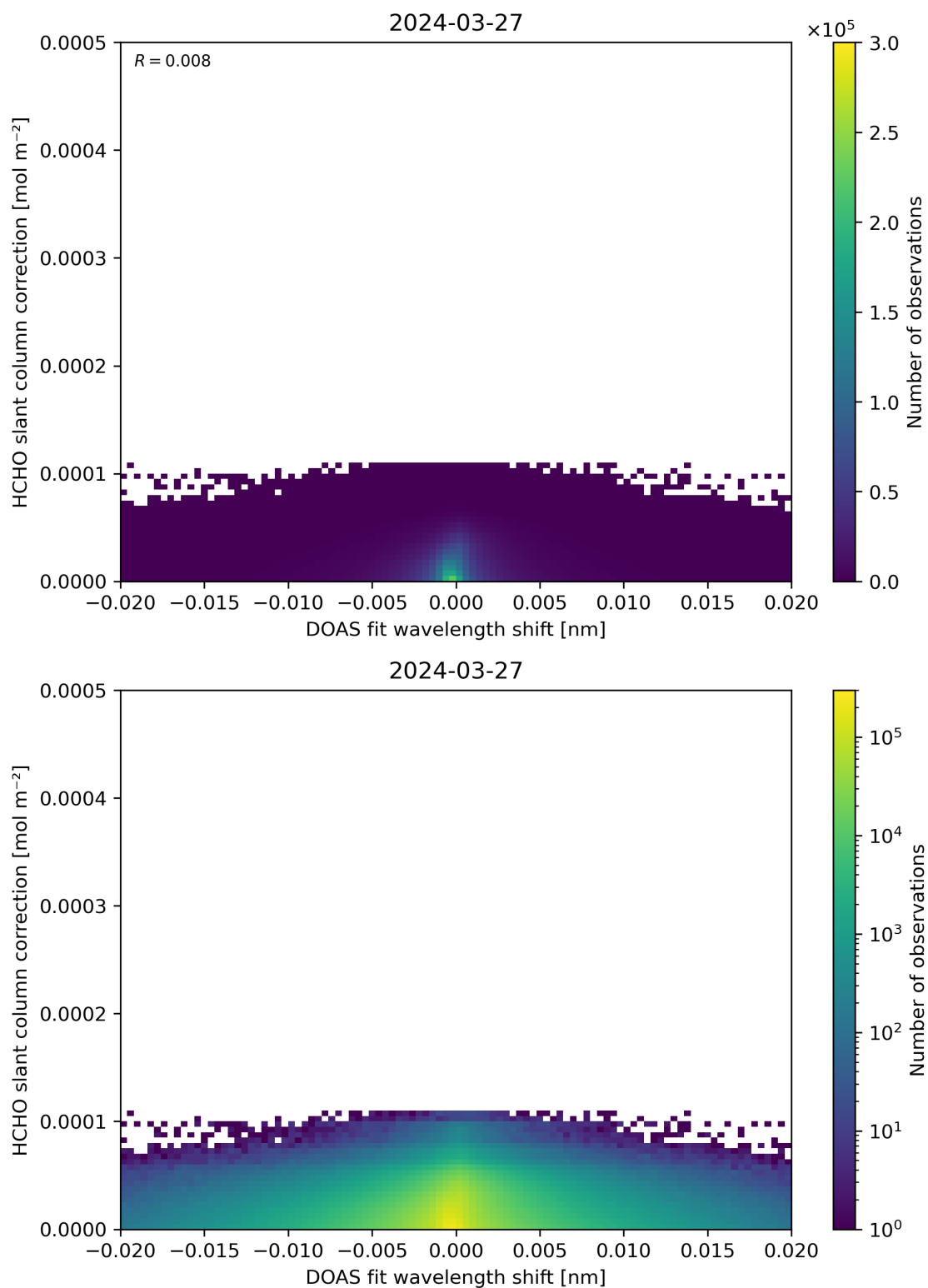
Figure 67: Scatter density plot of “DOAS fit wavelength shift” against “HCHO slant column correction” for 2024-03-26 to 2024-03-28.
