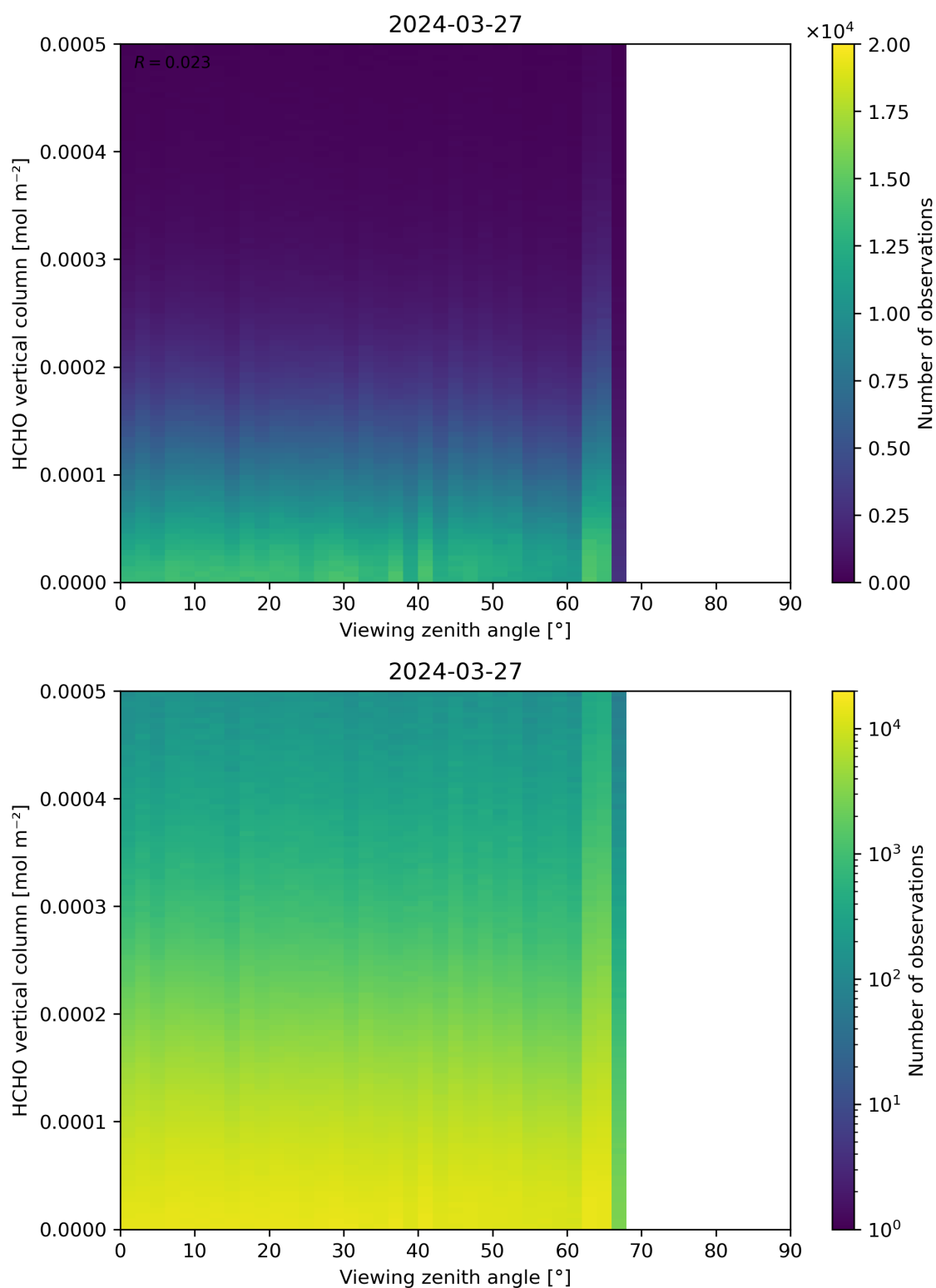
Figure 192: Scatter density plot of “Viewing zenith angle” against “HCHO vertical column” for 2024-03-26 to 2024-03-28.
