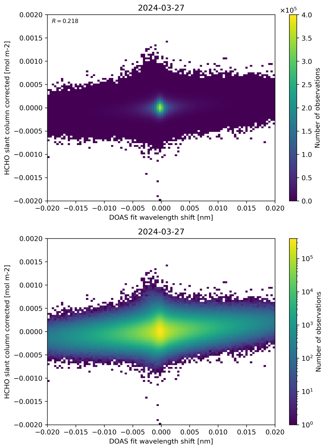
Figure 66: Scatter density plot of “DOAS fit wavelength shift” against “HCHO slant column corrected” for 2024-03-26 to 2024-03-28.
