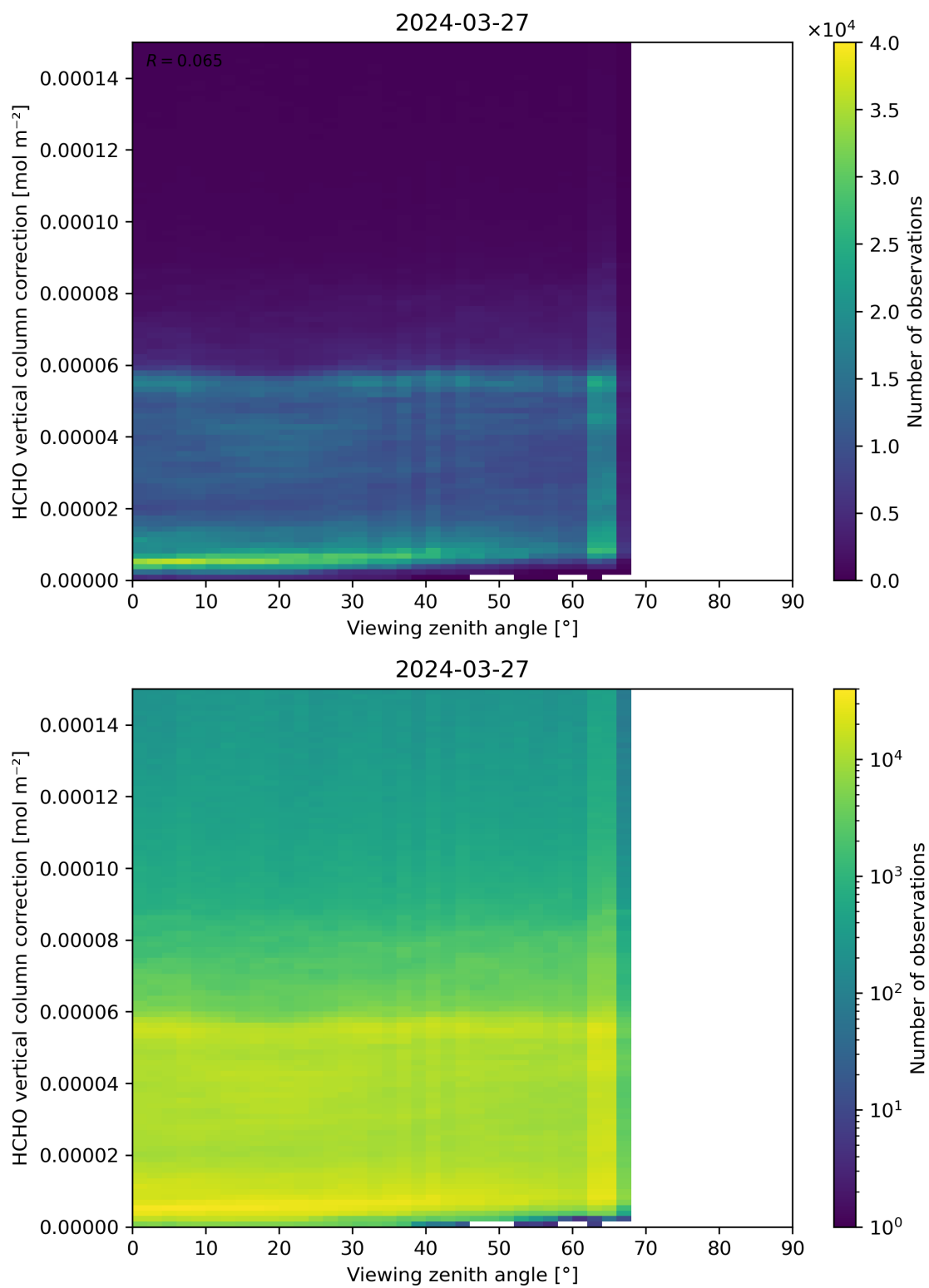
Figure 193: Scatter density plot of “Viewing zenith angle” against “HCHO vertical column correction” for 2024-03-26 to 2024-03-28.
