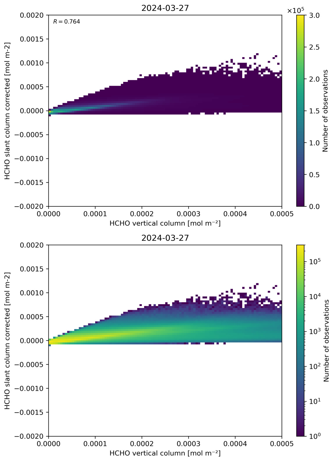
Figure 127: Scatter density plot of “HCHO vertical column” against “HCHO slant column corrected” for 2024-03-26 to 2024-03-28.
