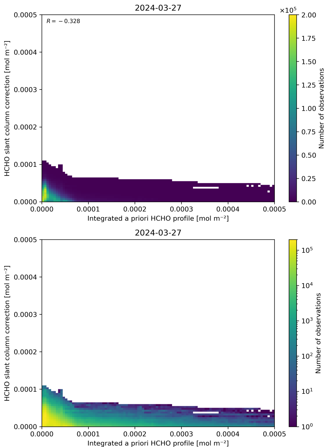
Figure 152: Scatter density plot of “Integrated a priori HCHO profile” against “HCHO slant column correction” for 2024-03-26 to 2024-03-28.
