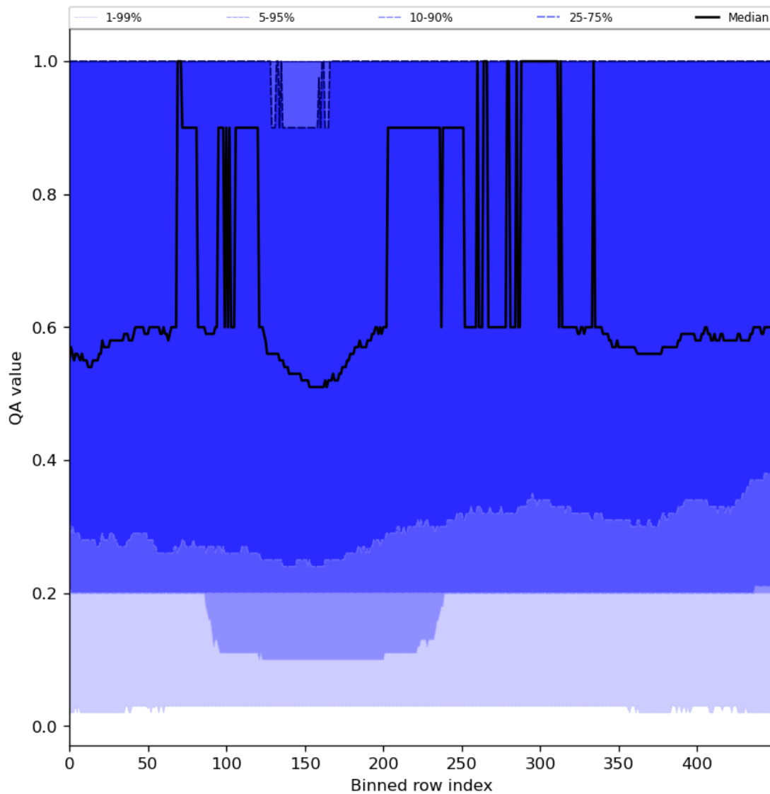
Figure 48: Along track statistics of “QA value” for 2024-03-26 to 2024-03-28
