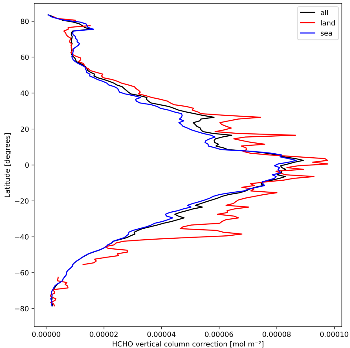
Figure 23: Zonal average of “HCHO vertical column correction” for 2024-03-26 to 2024-03-28.
