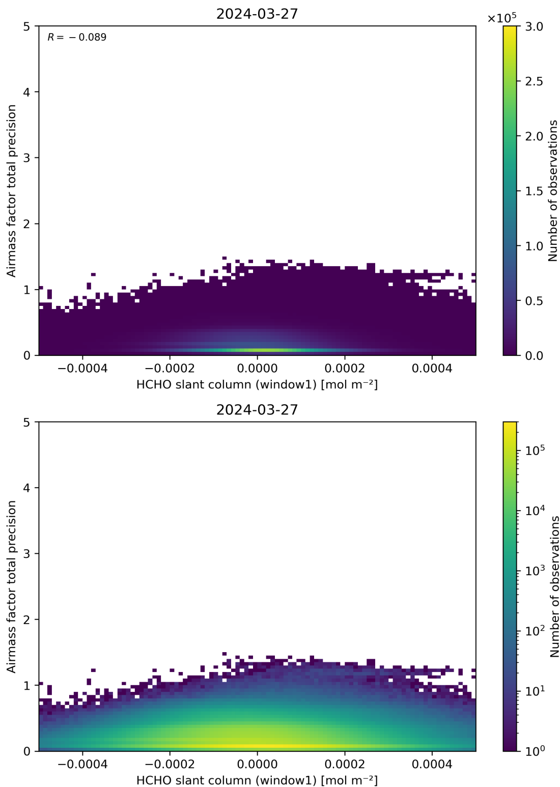
Figure 86: Scatter density plot of “HCHO slant column (window1)” against “Airmass factor total precision” for 2024-03-26 to 2024-03-28.
