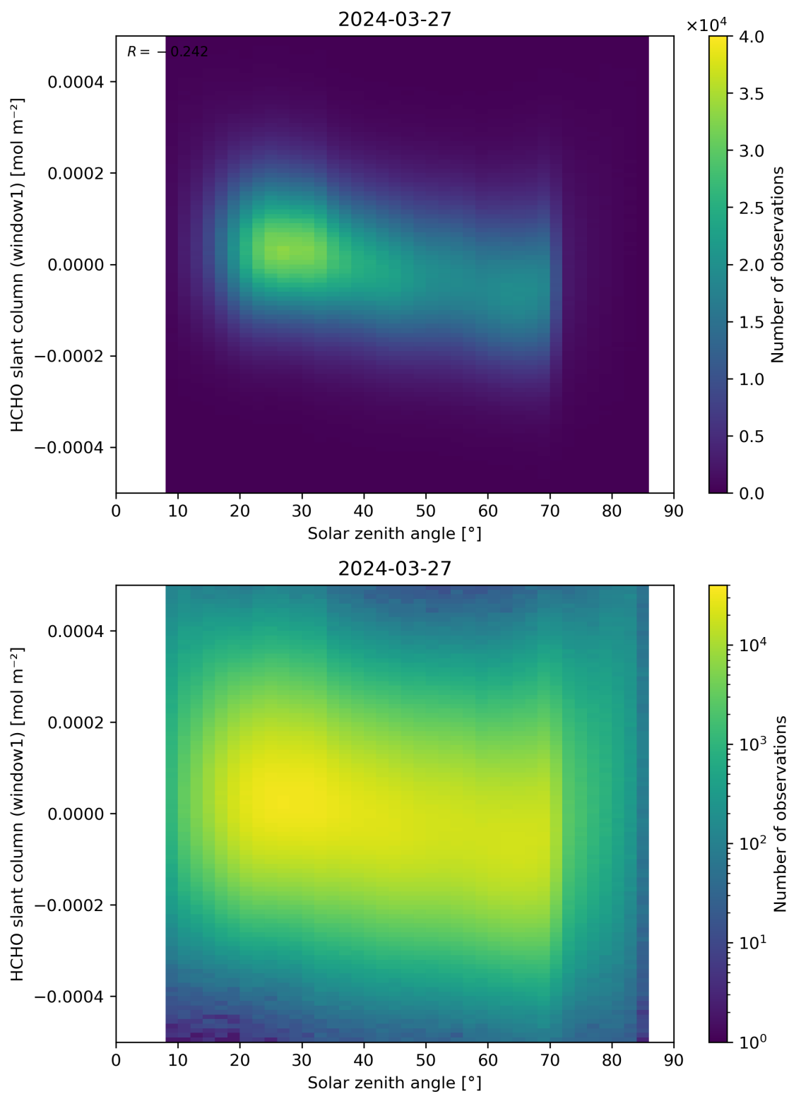
Figure 173: Scatter density plot of “Solar zenith angle” against “HCHO slant column (window1)” for 2024-03-26 to 2024-03-28.
