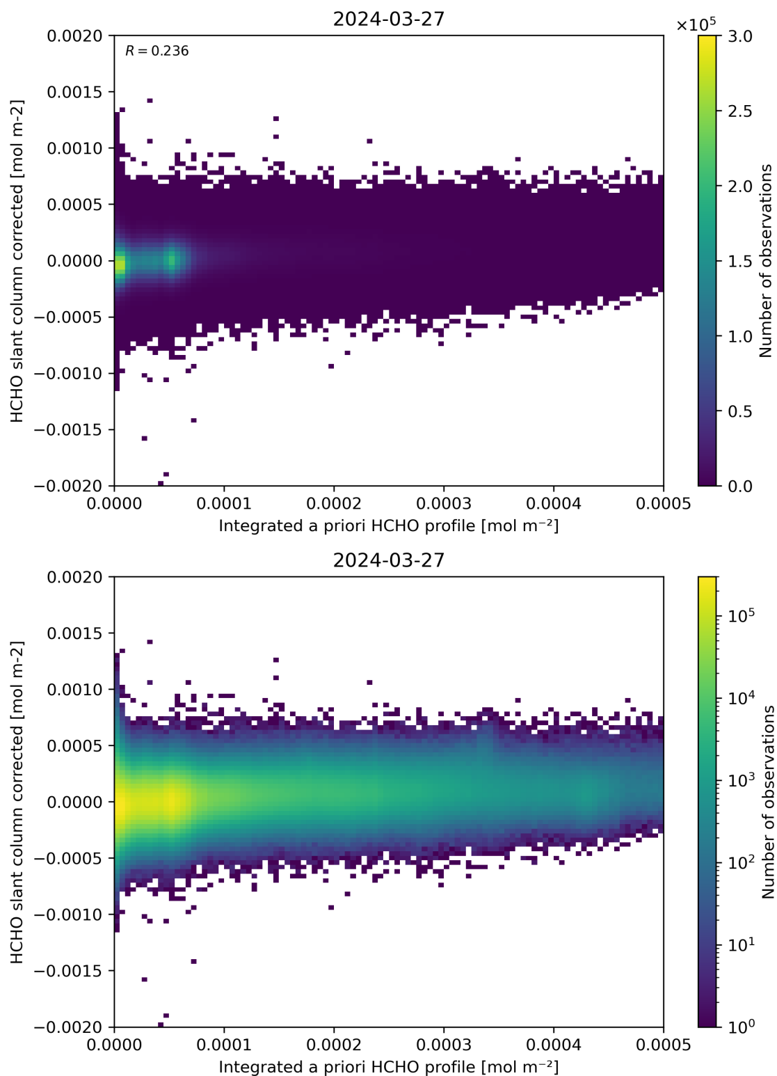
Figure 151: Scatter density plot of “Integrated a priori HCHO profile” against “HCHO slant column corrected” for 2024-03-26 to 2024-03-28.
