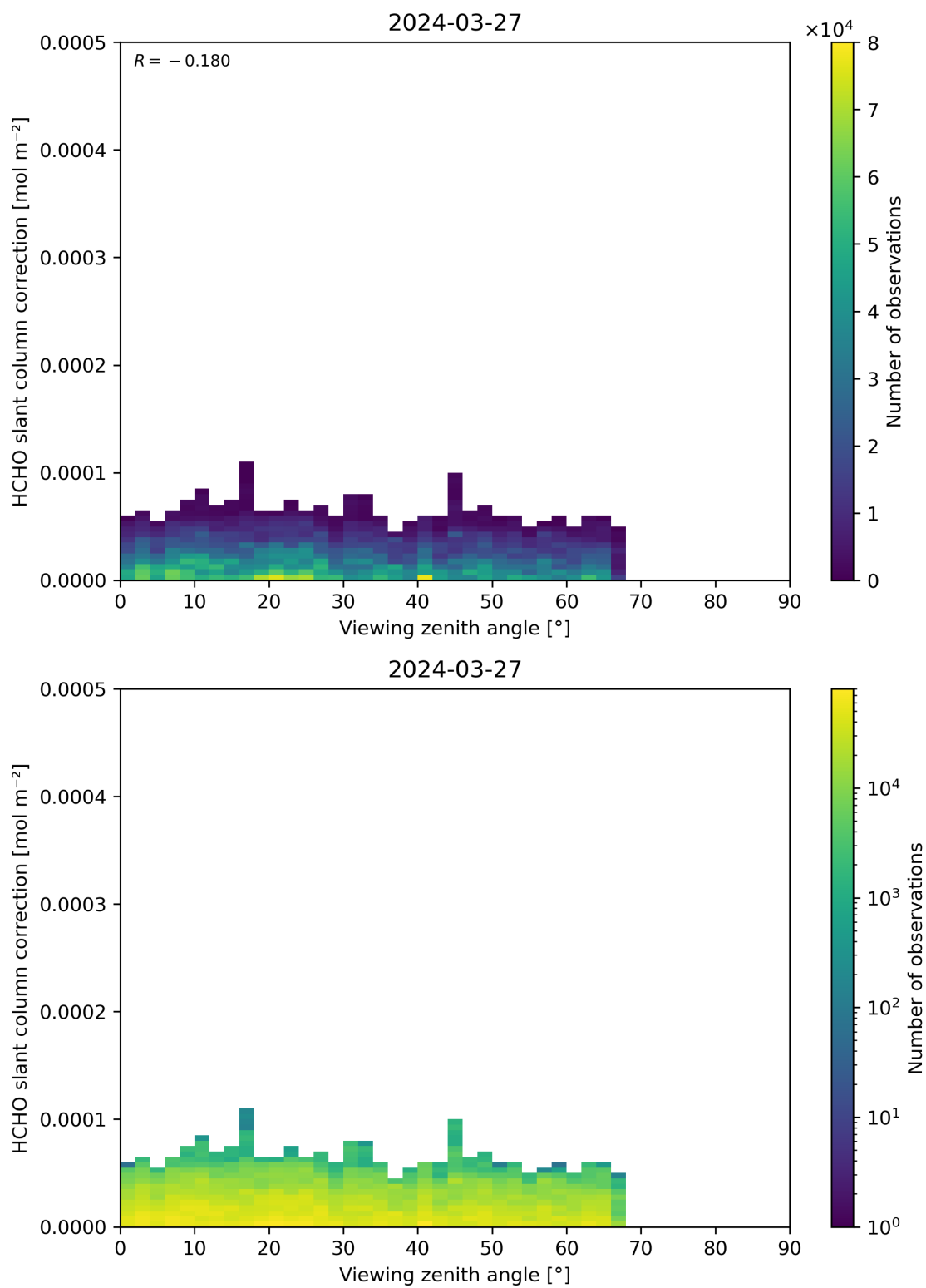
Figure 187: Scatter density plot of “Viewing zenith angle” against “HCHO slant column correction” for 2024-03-26 to 2024-03-28.
