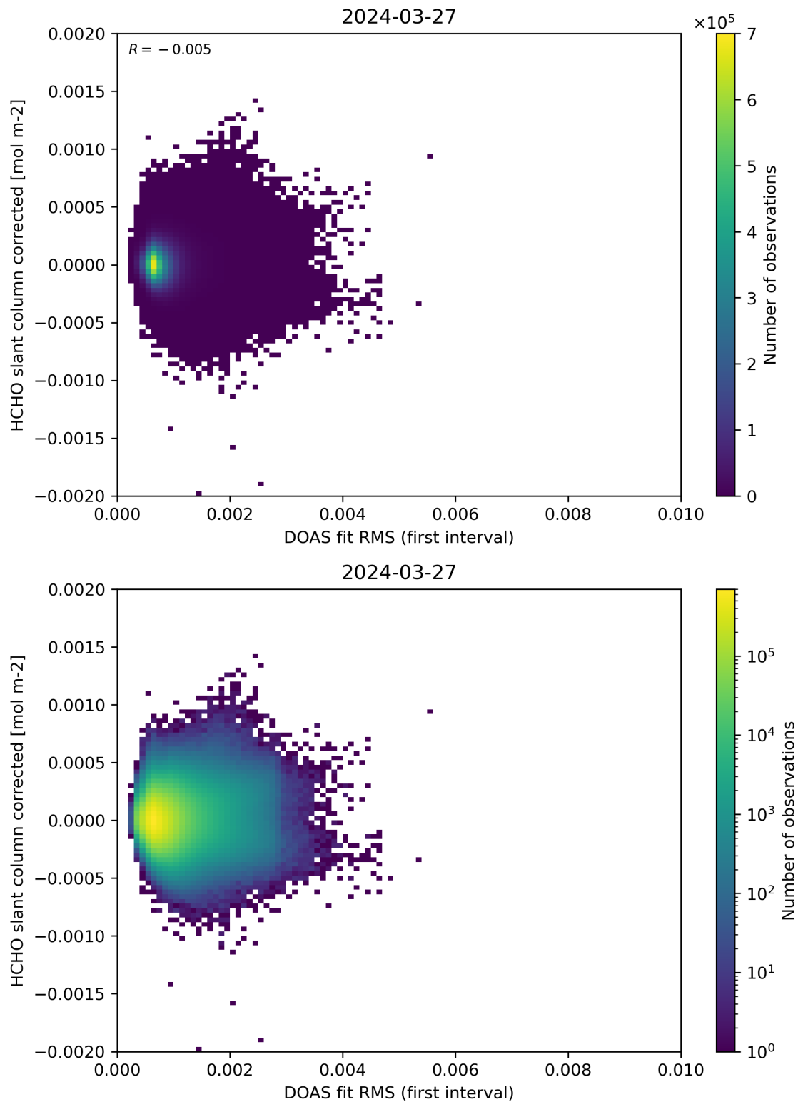
Figure 62: Scatter density plot of “DOAS fit RMS (first interval)” against “HCHO slant column corrected” for 2024-03-26 to 2024-03-28.
