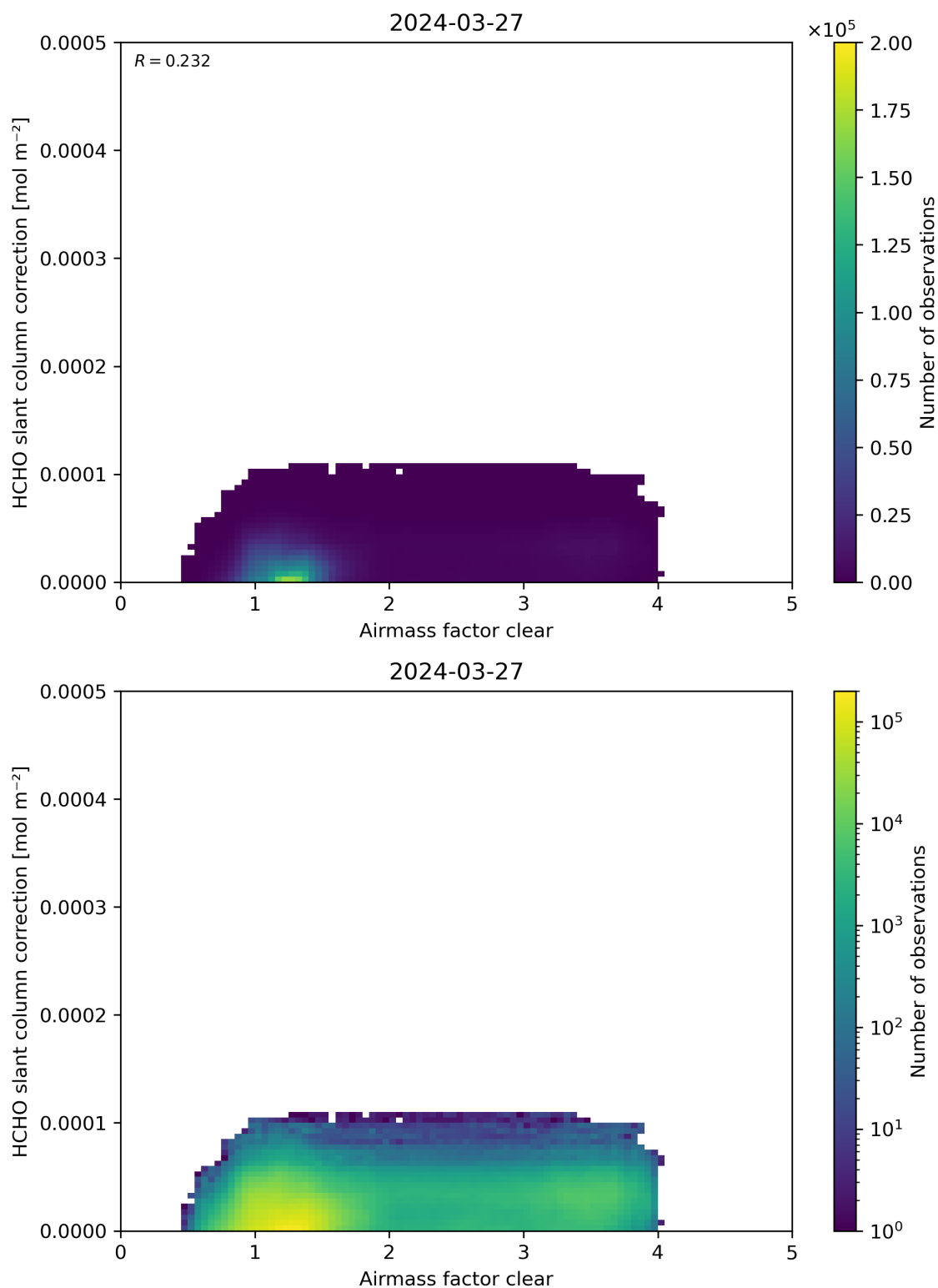
Figure 75: Scatter density plot of “Airmass factor clear” against “HCHO slant column correction” for 2024-03-26 to 2024-03-28.
