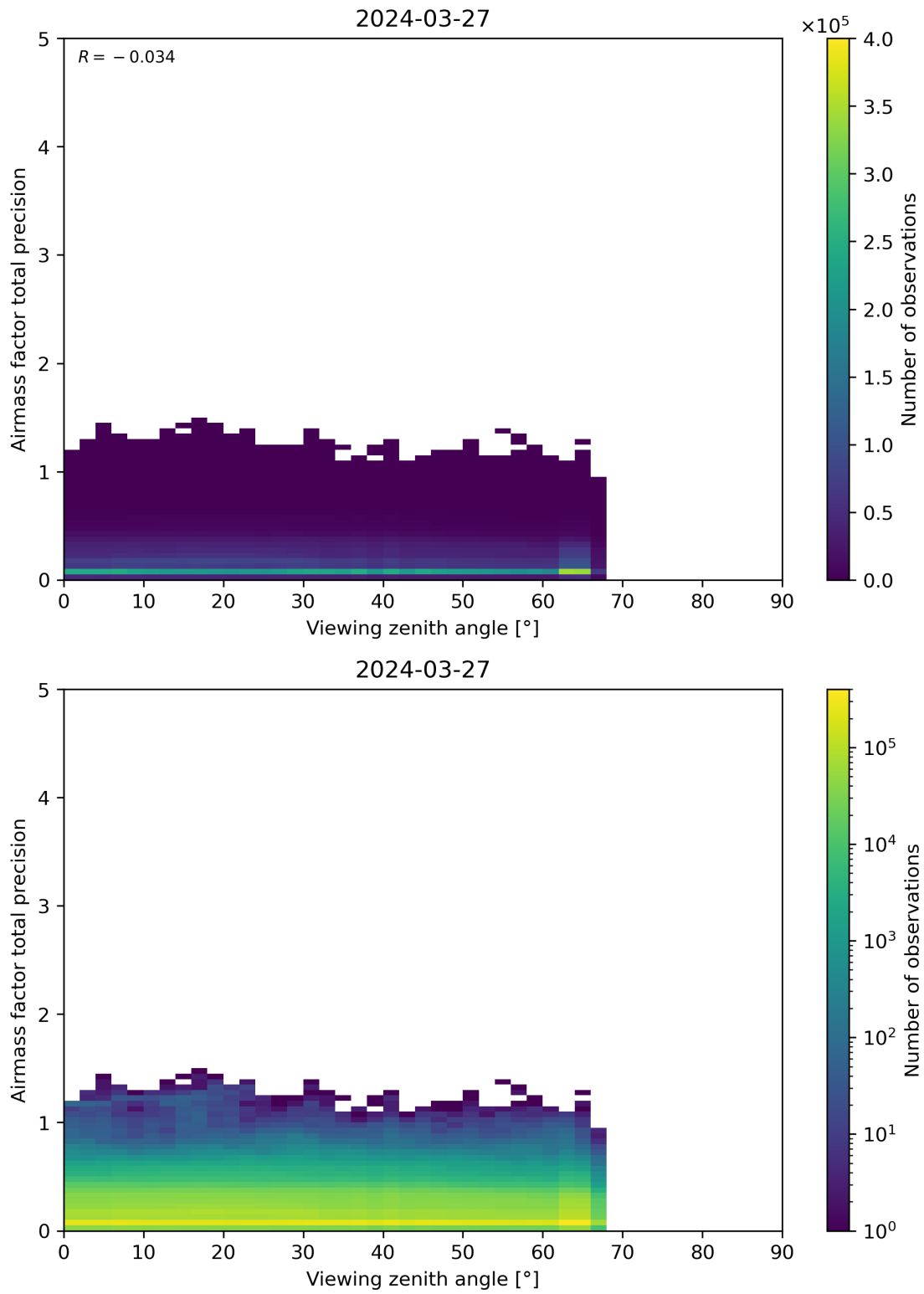
Figure 191: Scatter density plot of “Viewing zenith angle” against “Airmass factor total precision” for 2024-03-26 to 2024-03-28.
