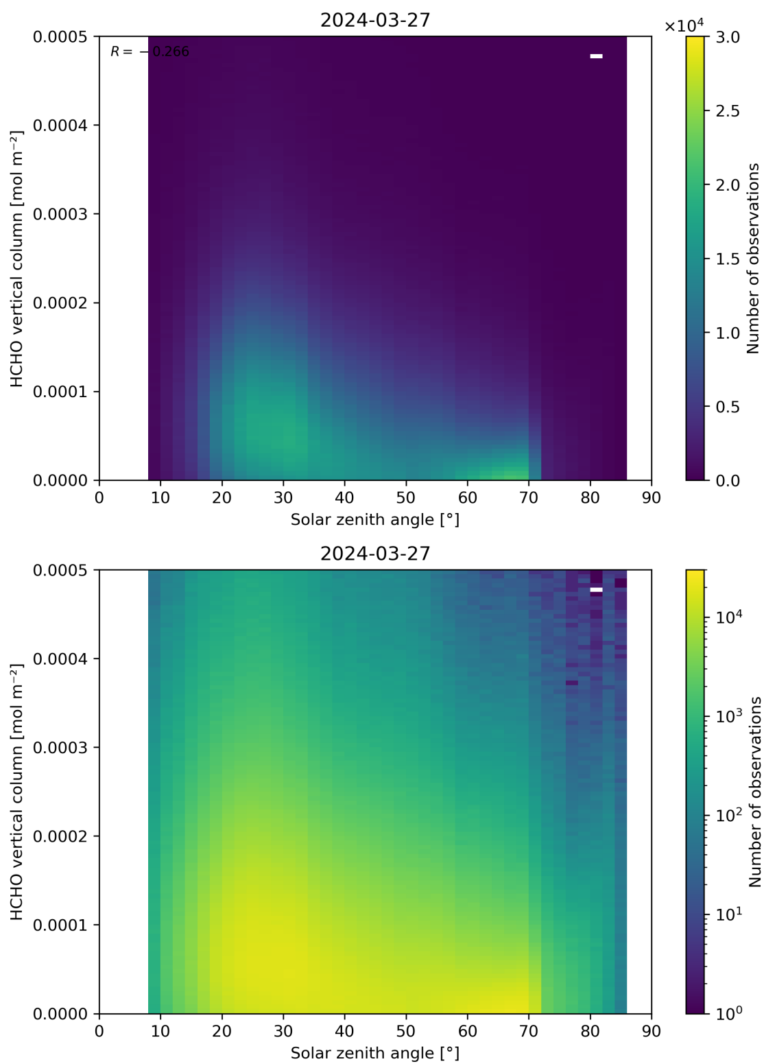
Figure 177: Scatter density plot of “Solar zenith angle” against “HCHO vertical column” for 2024-03-26 to 2024-03-28.
