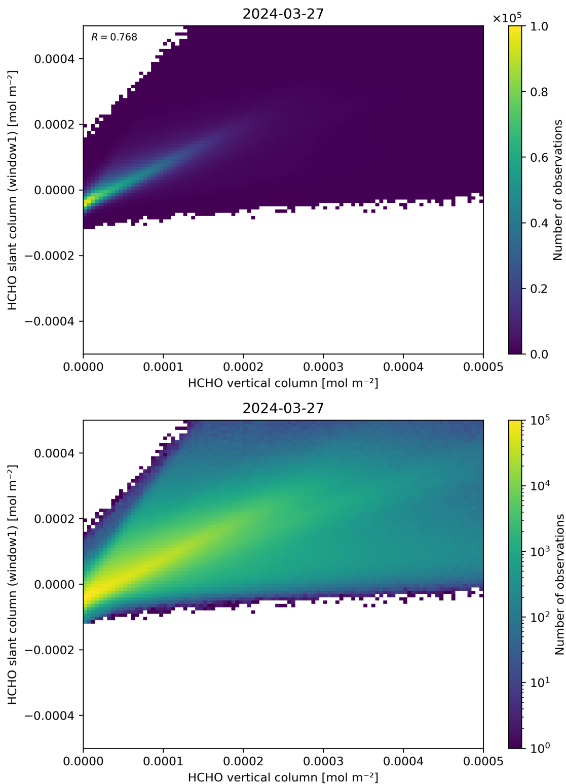
Figure 129: Scatter density plot of “HCHO vertical column” against “HCHO slant column (window1)” for 2024-03-26 to 2024-03-28.
