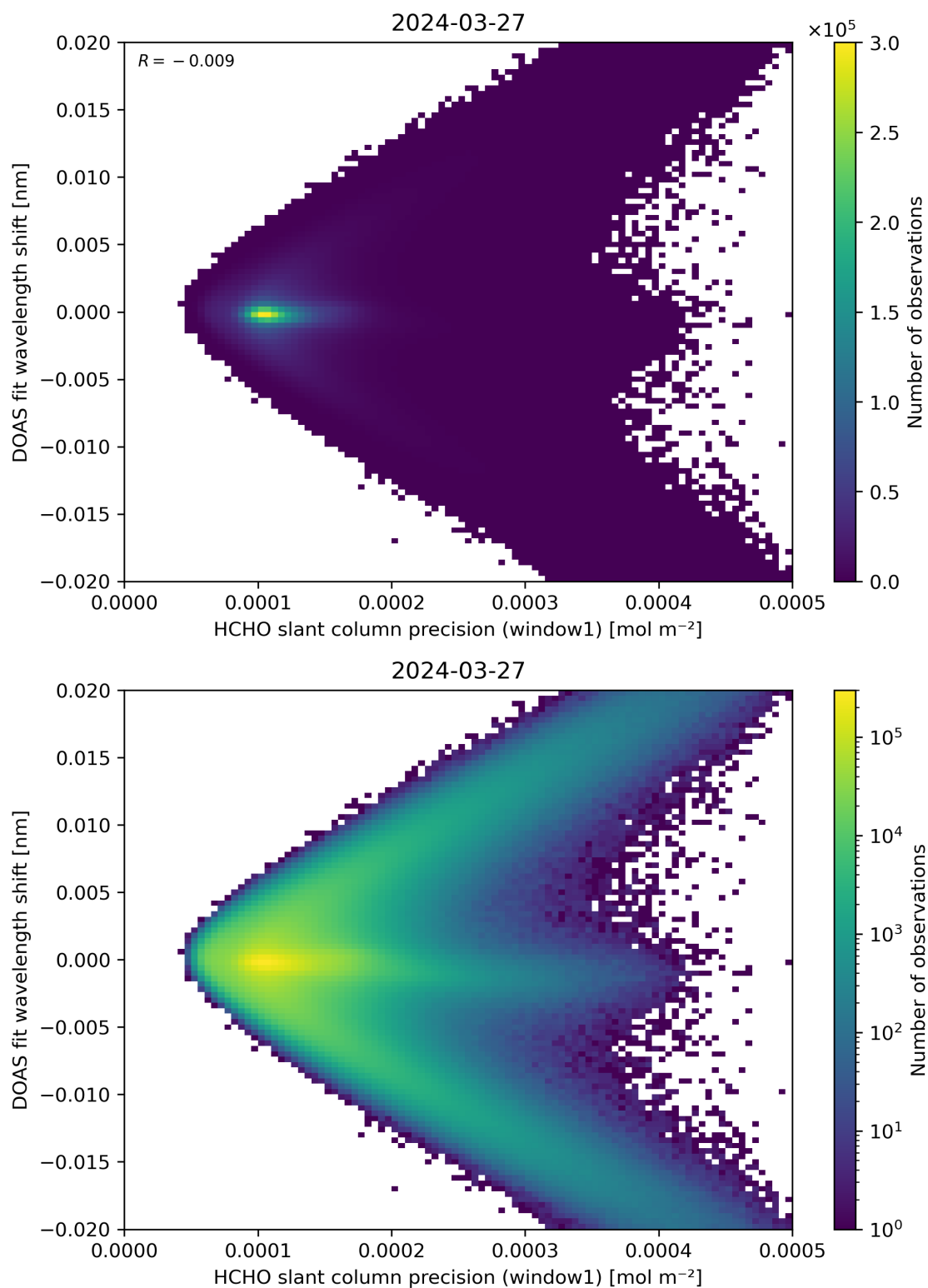
Figure 89: Scatter density plot of “HCHO slant column precision (window1)” against “DOAS fit wavelength shift” for 2024-03-26 to 2024-03-28.
