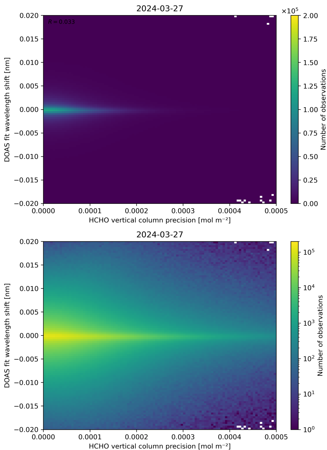
Figure 137: Scatter density plot of “HCHO vertical column precision” against “DOAS fit wavelength shift” for 2024-03-26 to 2024-03-28.
