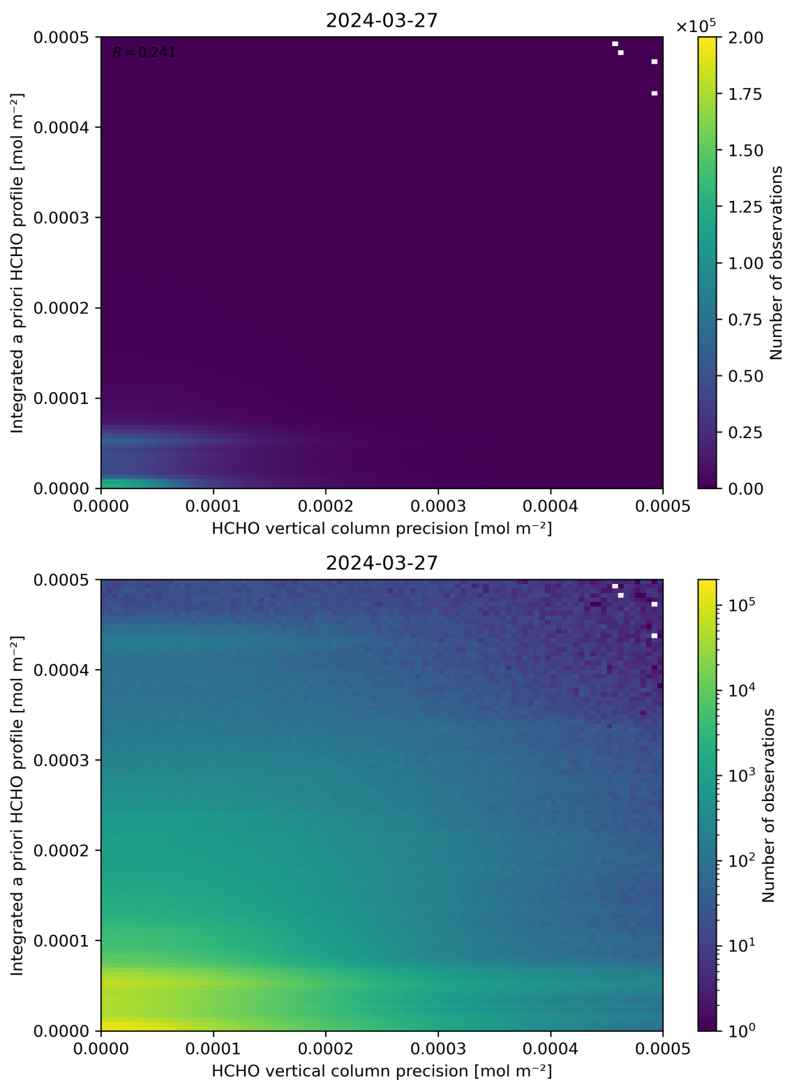
Figure 147: Scatter density plot of “HCHO vertical column precision” against “Integrated a priori HCHO profile” for 2024-03-26 to 2024-03-28.
