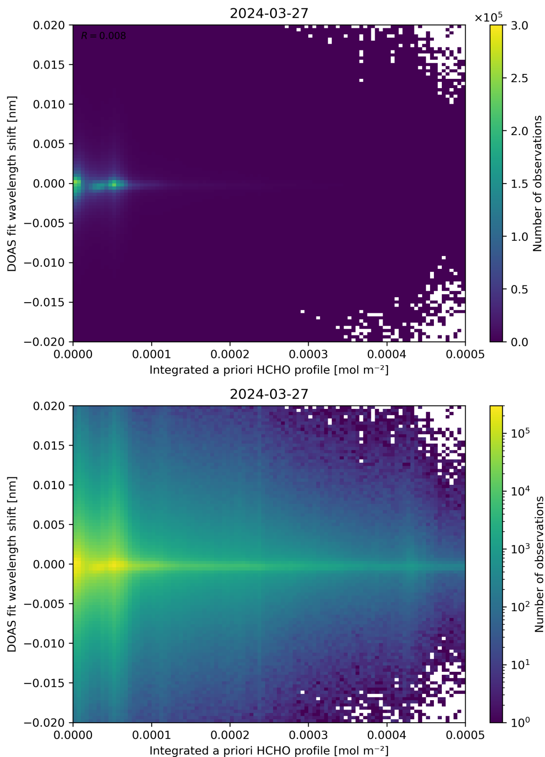
Figure 149: Scatter density plot of “Integrated a priori HCHO profile” against “DOAS fit wavelength shift” for 2024-03-26 to 2024-03-28.
