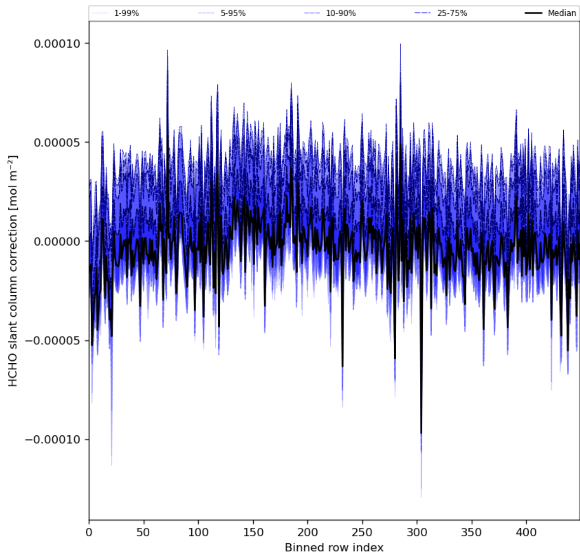
Figure 61: Along track statistics of “HCHO slant column correction” for 2024-03-26 to 2024-03-28
