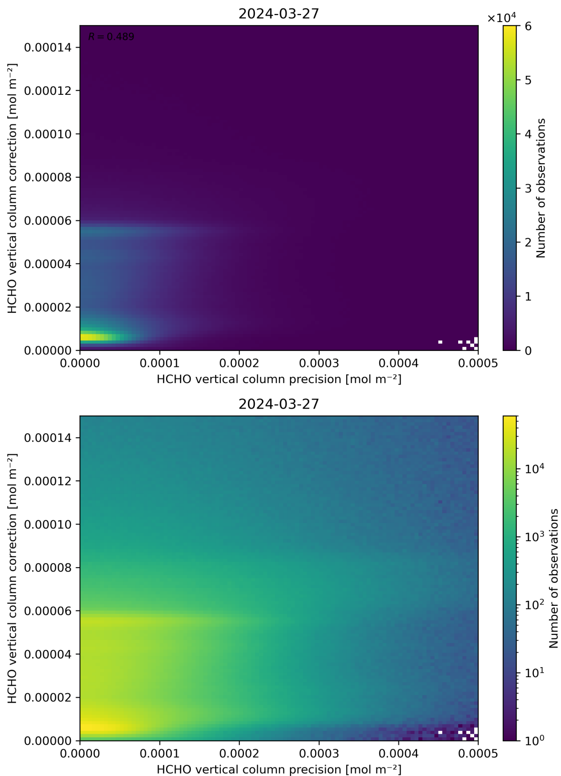
Figure 146: Scatter density plot of “HCHO vertical column precision” against “HCHO vertical column correction” for 2024-03-26 to 2024-03-28.
