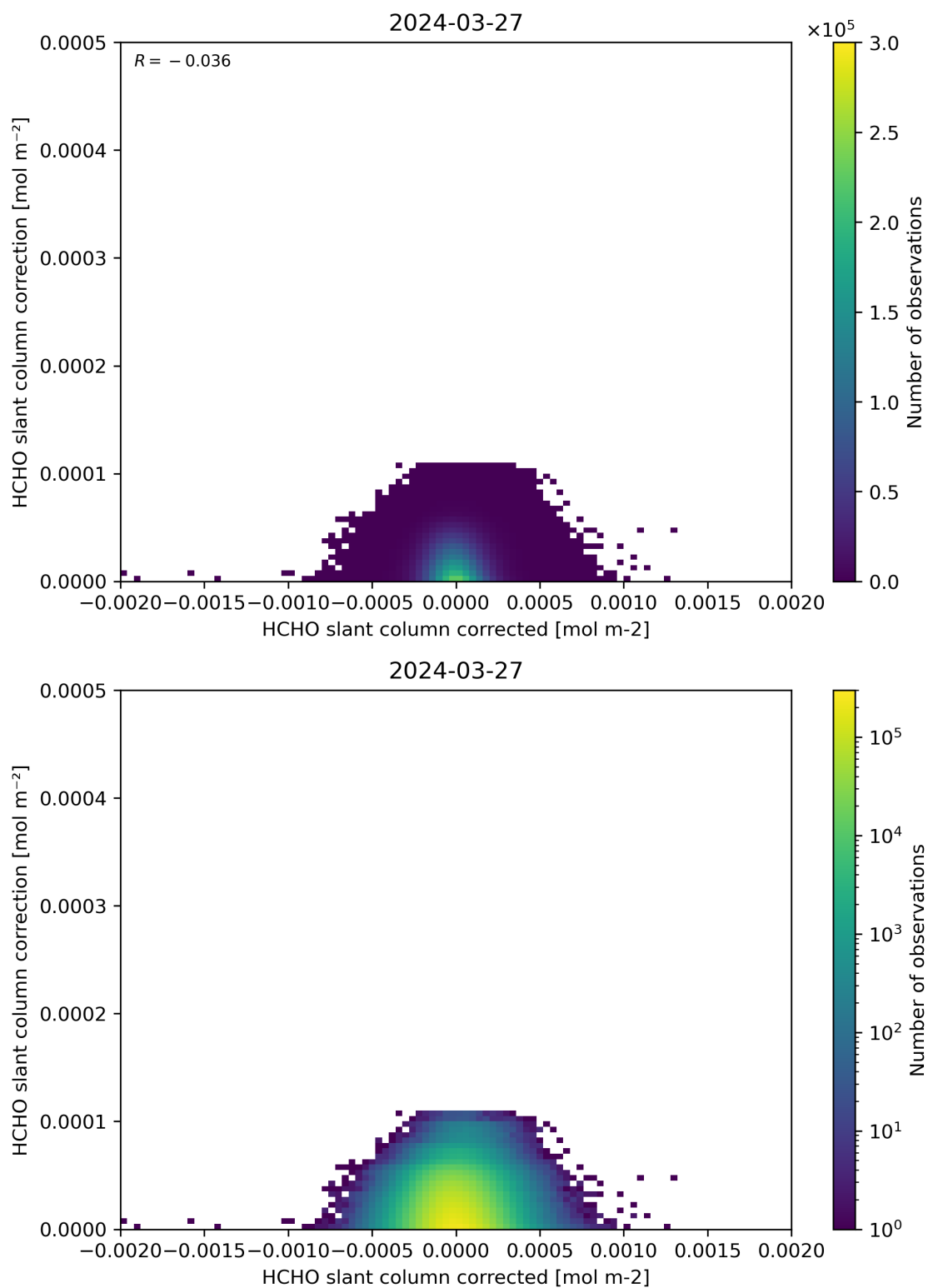
Figure 77: Scatter density plot of “HCHO slant column corrected” against “HCHO slant column correction” for 2024-03-26 to 2024-03-28.
