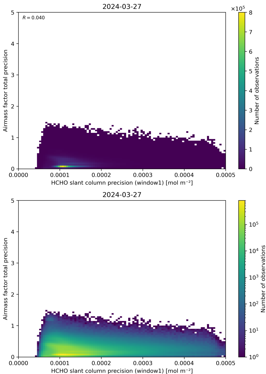
Figure 95: Scatter density plot of “HCHO slant column precision (window1)” against “Airmass factor total precision” for 2024-03-26 to 2024-03-28.
