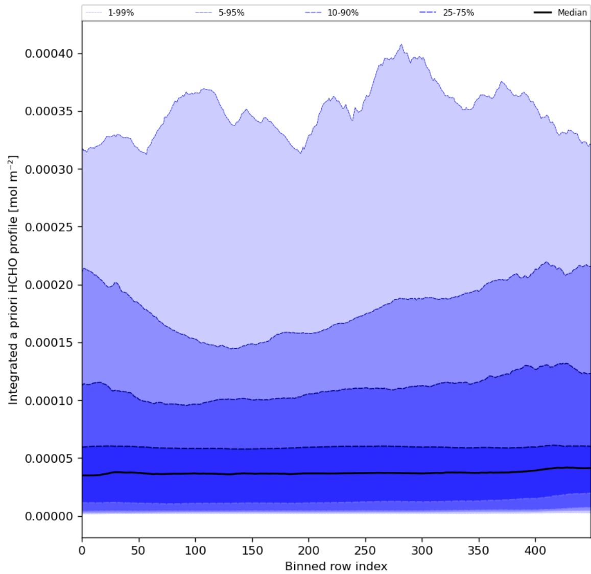
Figure 57: Along track statistics of “Integrated a priori HCHO profile” for 2024-03-26 to 2024-03-28
