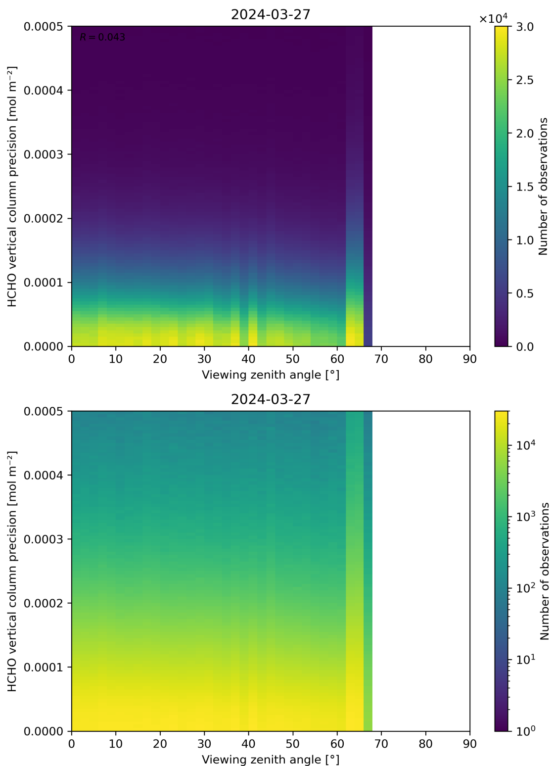
Figure 194: Scatter density plot of “Viewing zenith angle” against “HCHO vertical column precision” for 2024-03-26 to 2024-03-28.
