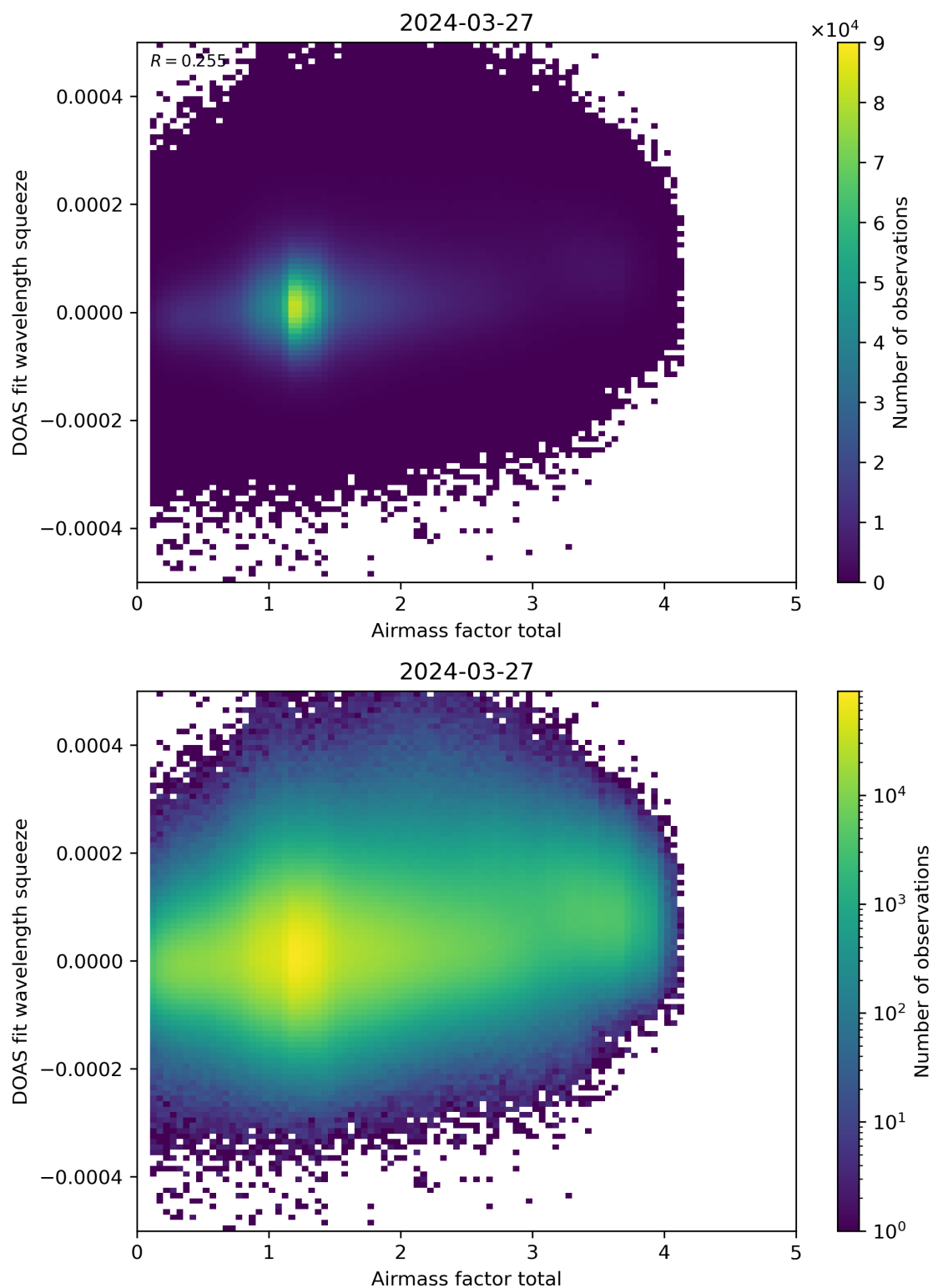
Figure 99: Scatter density plot of “Airmass factor total” against “DOAS fit wavelength squeeze” for 2024-03-26 to 2024-03-28.
