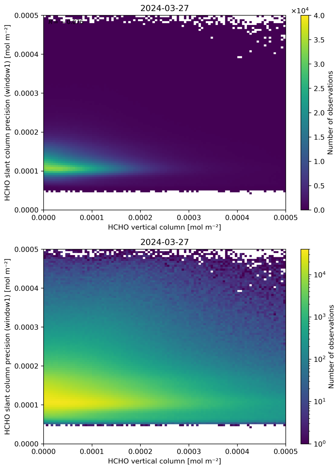
Figure 130: Scatter density plot of “HCHO vertical column” against “HCHO slant column precision (window1)” for 2024-03-26 to 2024-03-28.
