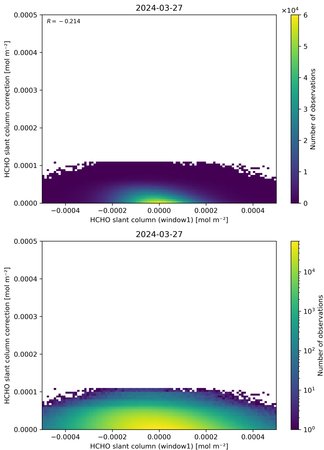
Figure 83: Scatter density plot of “HCHO slant column (window1)” against “HCHO slant column correction” for 2024-03-26 to 2024-03-28.
