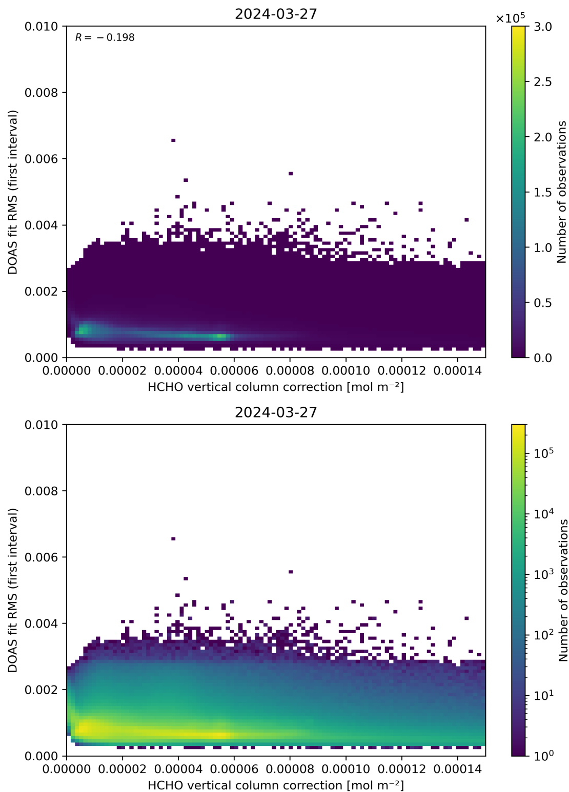
Figure 112: Scatter density plot of “HCHO vertical column correction” against “DOAS fit RMS (first interval)” for 2024-03-26 to 2024-03-28.
