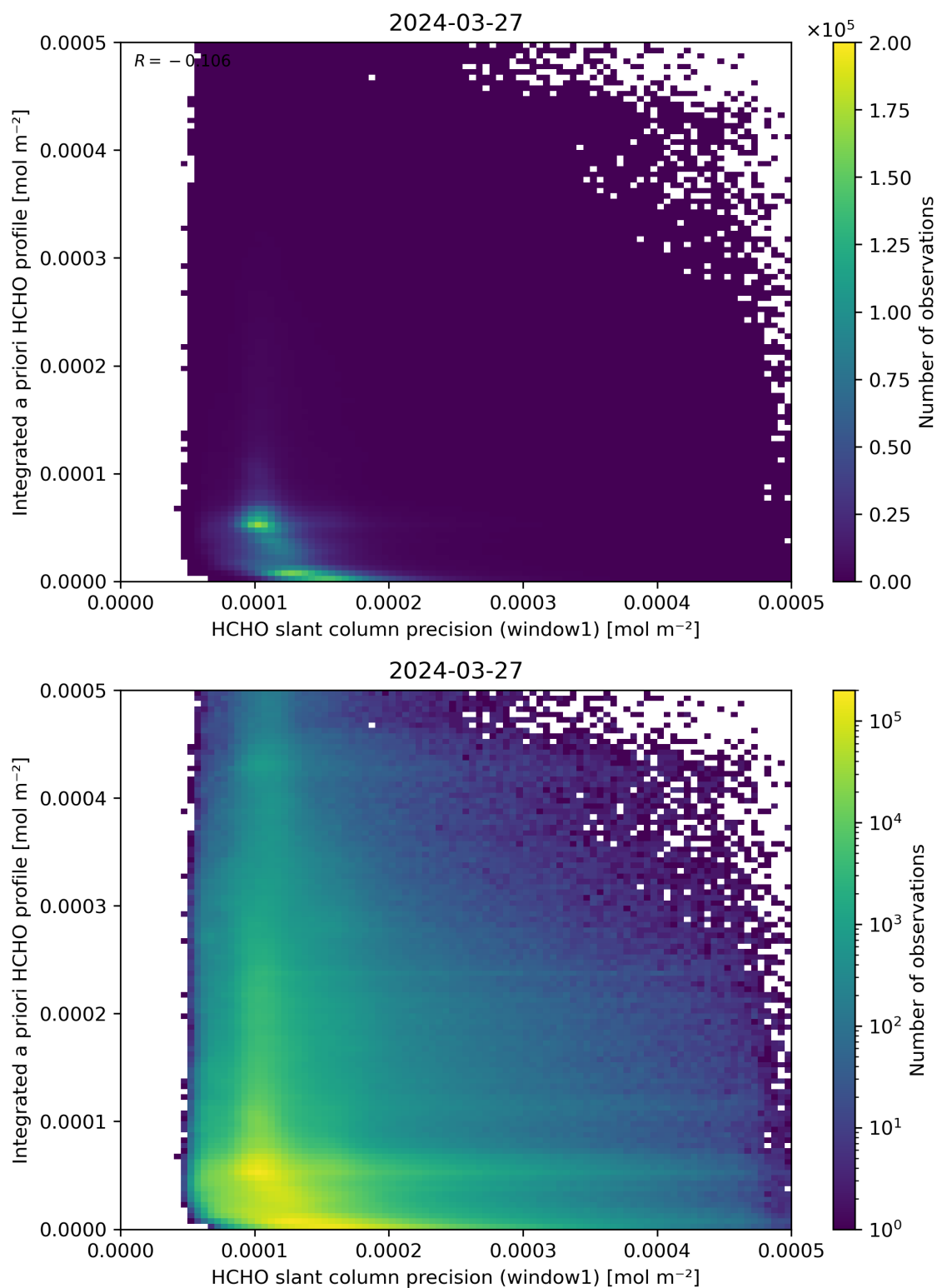
Figure 96: Scatter density plot of “HCHO slant column precision (window1)” against “Integrated a priori HCHO profile” for 2024-03-26 to 2024-03-28.
