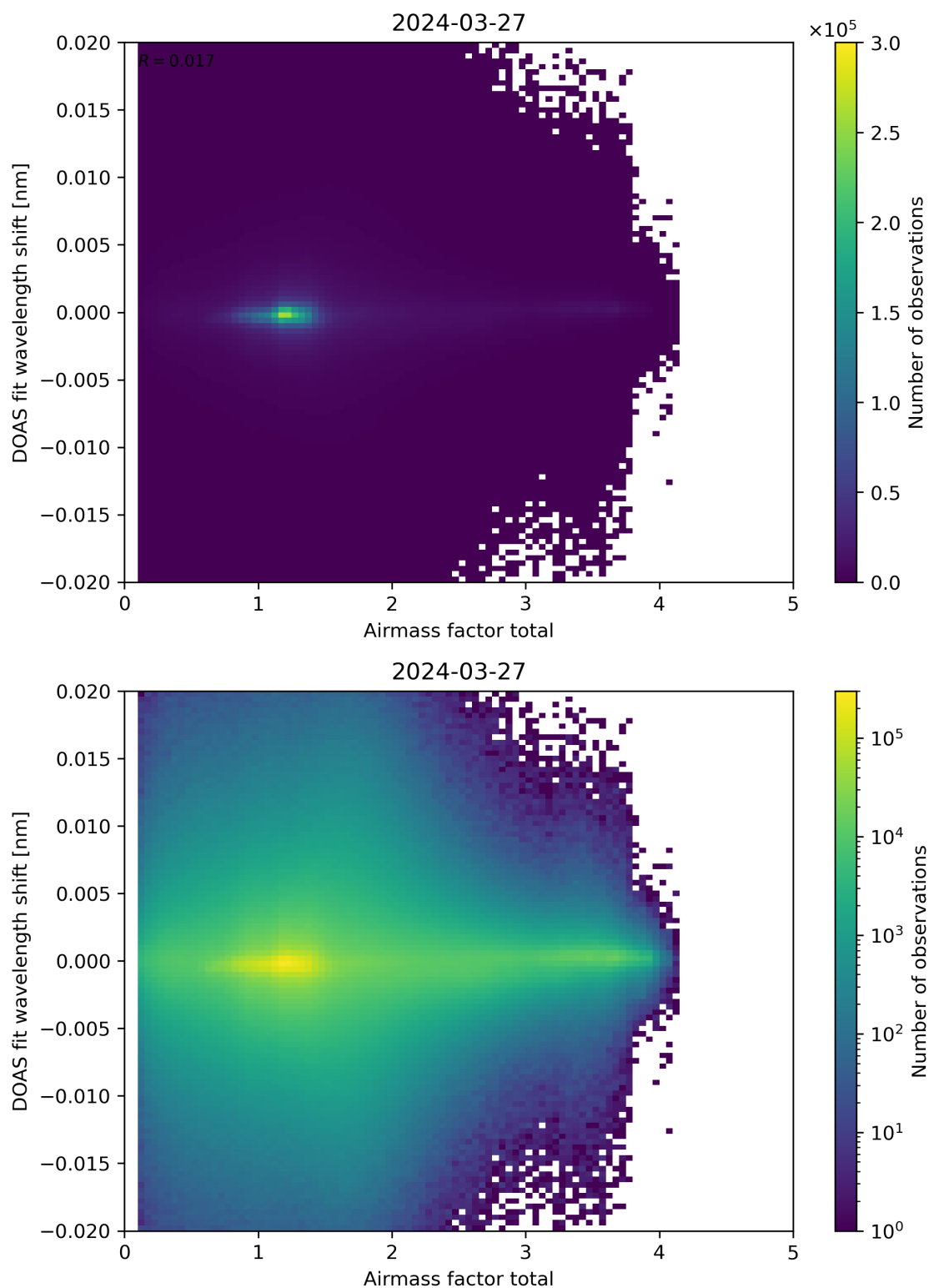
Figure 98: Scatter density plot of “Airmass factor total” against “DOAS fit wavelength shift” for 2024-03-26 to 2024-03-28.
