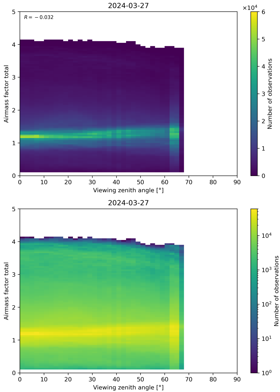
Figure 190: Scatter density plot of “Viewing zenith angle” against “Airmass factor total” for 2024-03-26 to 2024-03-28.
