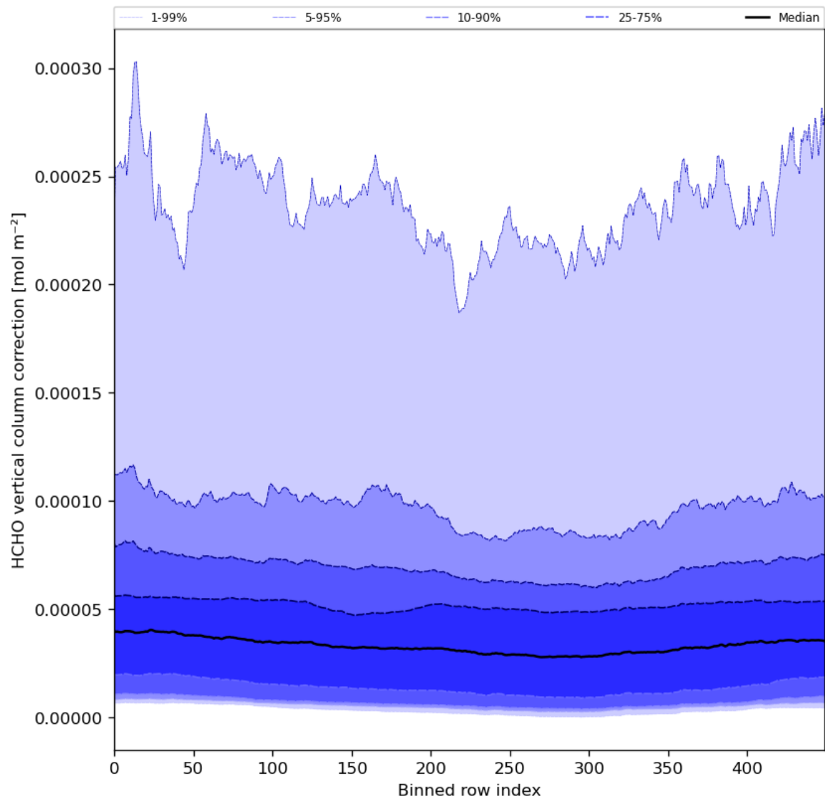
Figure 51: Along track statistics of “HCHO vertical column correction” for 2024-03-26 to 2024-03-28
