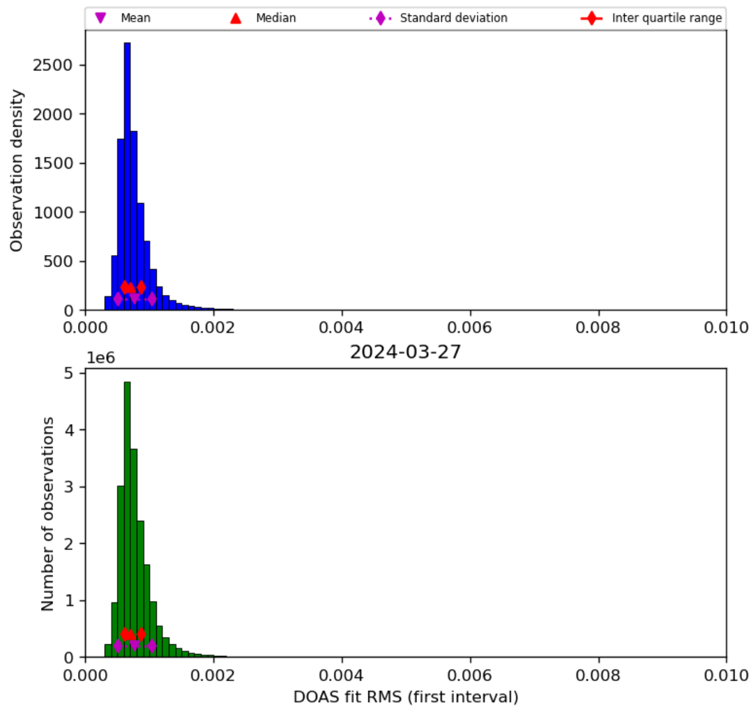
Figure 46: Histogram of “DOAS fit RMS (first interval)” for 2024-03-26 to 2024-03-28
