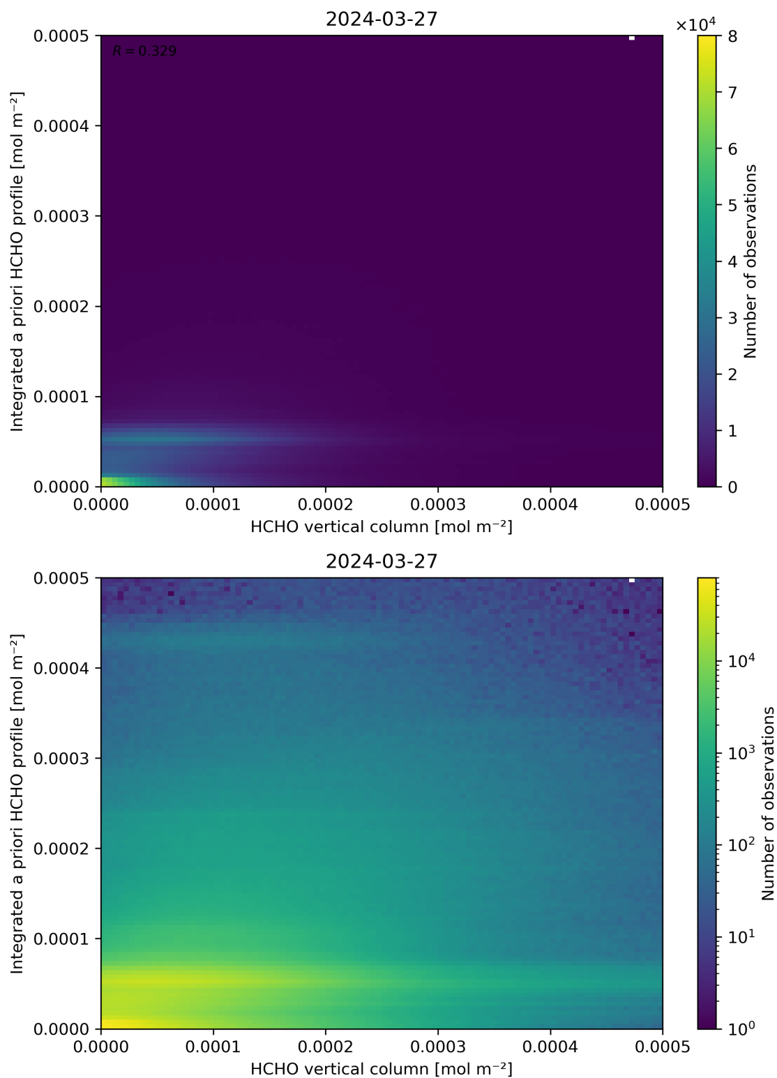
Figure 135: Scatter density plot of “HCHO vertical column” against “Integrated a priori HCHO profile” for 2024-03-26 to 2024-03-28.
