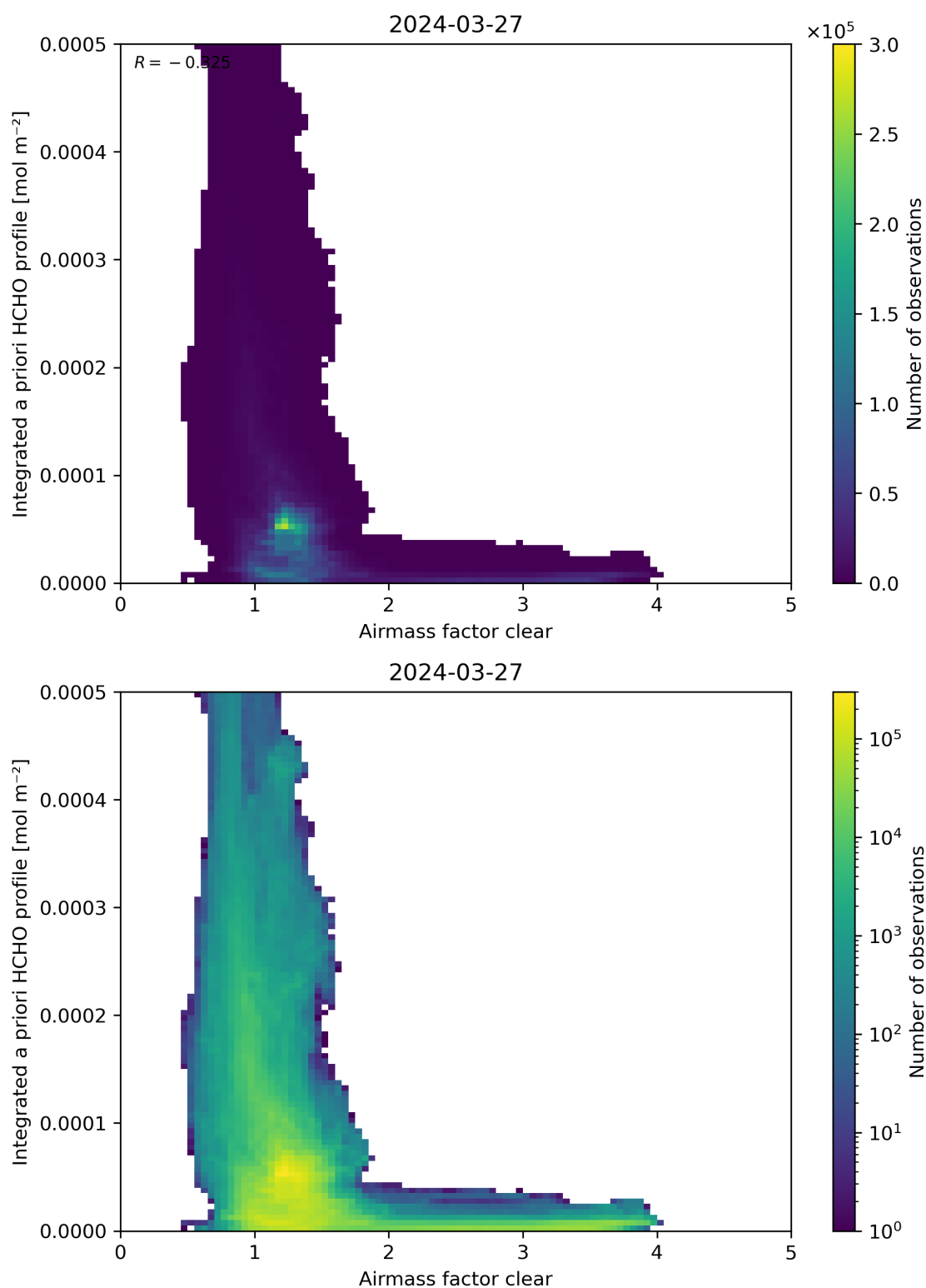
Figure 76: Scatter density plot of “Airmass factor clear” against “Integrated a priori HCHO profile” for 2024-03-26 to 2024-03-28.
