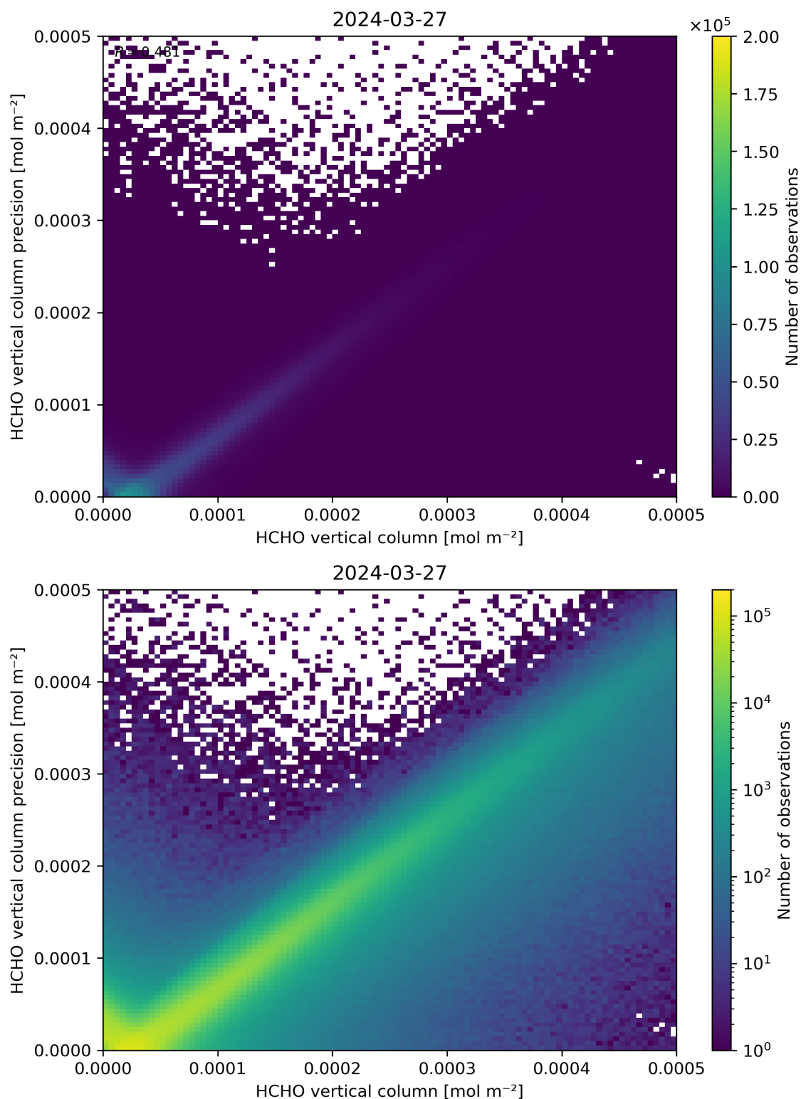
Figure 134: Scatter density plot of “HCHO vertical column” against “HCHO vertical column precision” for 2024-03-26 to 2024-03-28.
