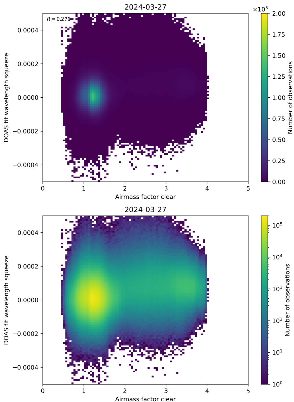
Figure 73: Scatter density plot of “Airmass factor clear” against “DOAS fit wavelength squeeze” for 2024-03-26 to 2024-03-28.
