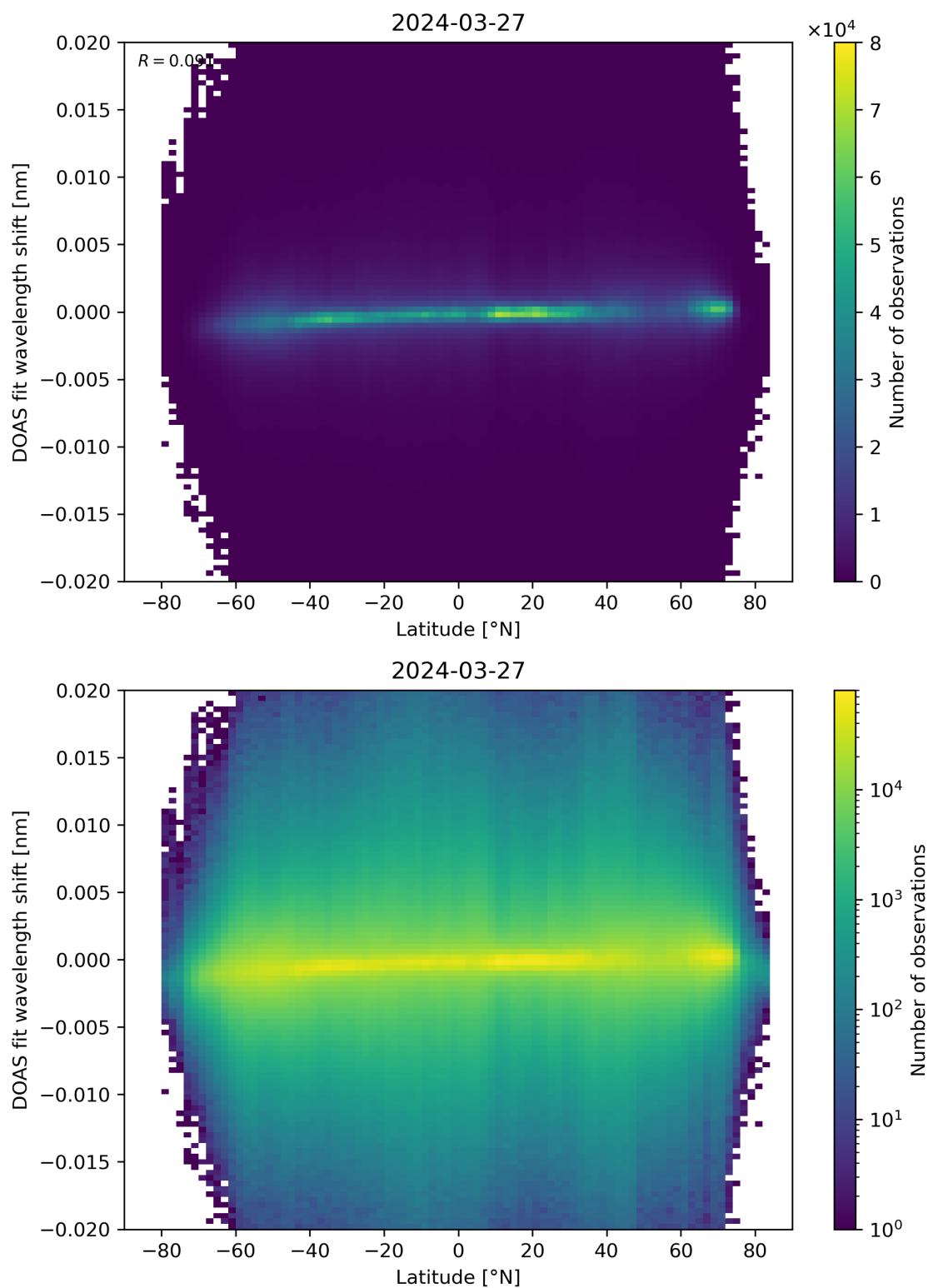
Figure 154: Scatter density plot of “Latitude” against “DOAS fit wavelength shift” for 2024-03-26 to 2024-03-28.
