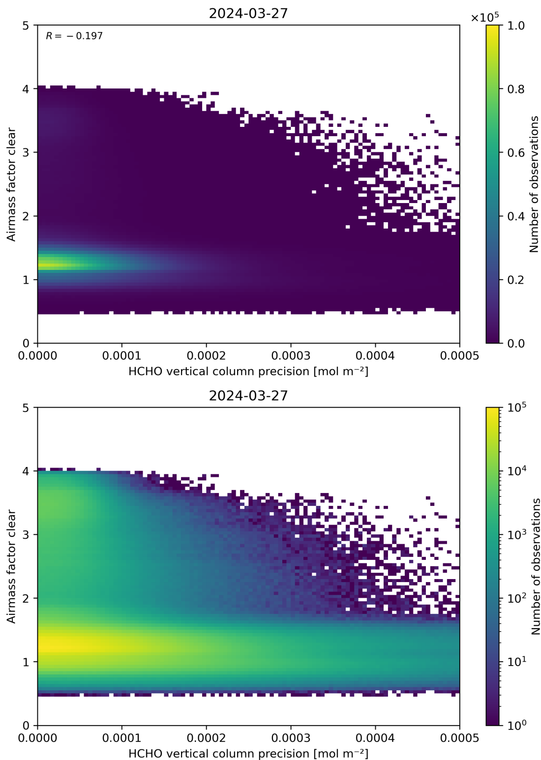
Figure 139: Scatter density plot of “HCHO vertical column precision” against “Airmass factor clear” for 2024-03-26 to 2024-03-28.
