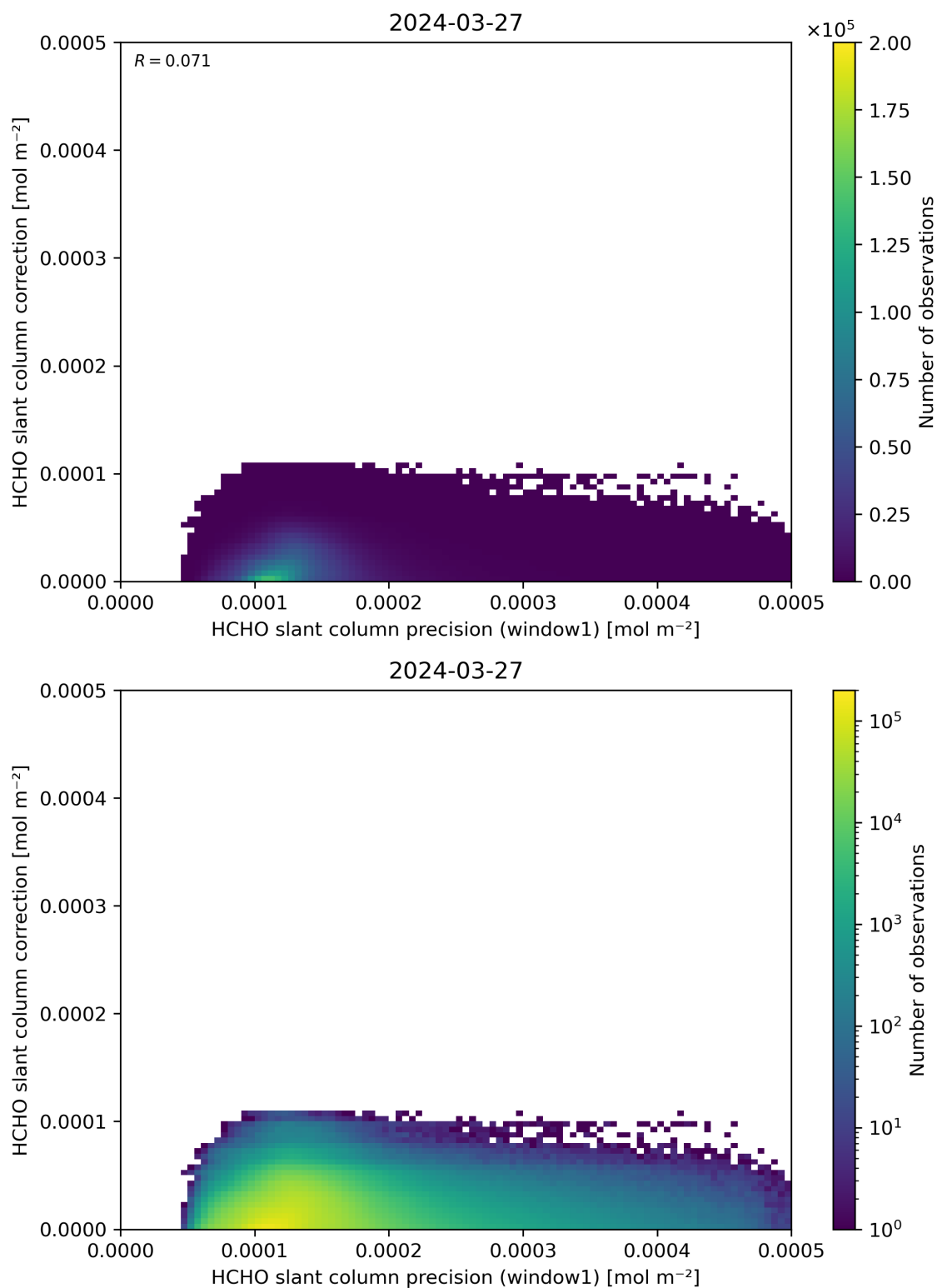
Figure 93: Scatter density plot of “HCHO slant column precision (window1)” against “HCHO slant column correction” for 2024-03-26 to 2024-03-28.
