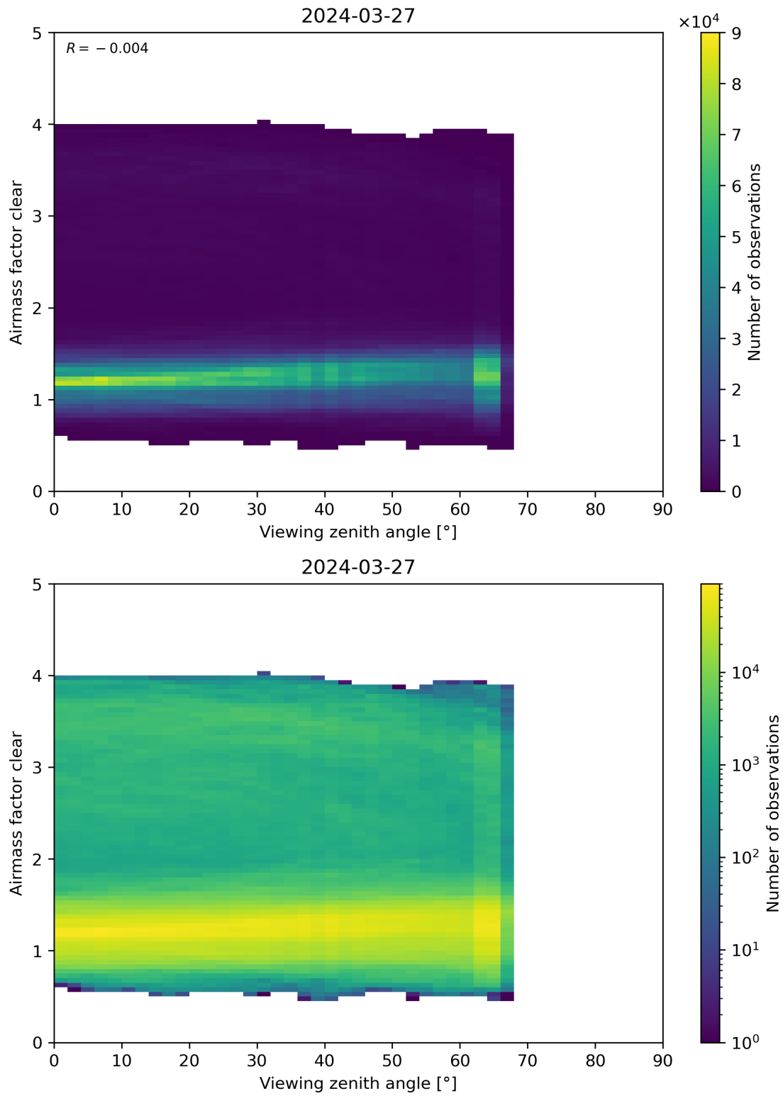
Figure 185: Scatter density plot of “Viewing zenith angle” against “Airmass factor clear” for 2024-03-26 to 2024-03-28.
