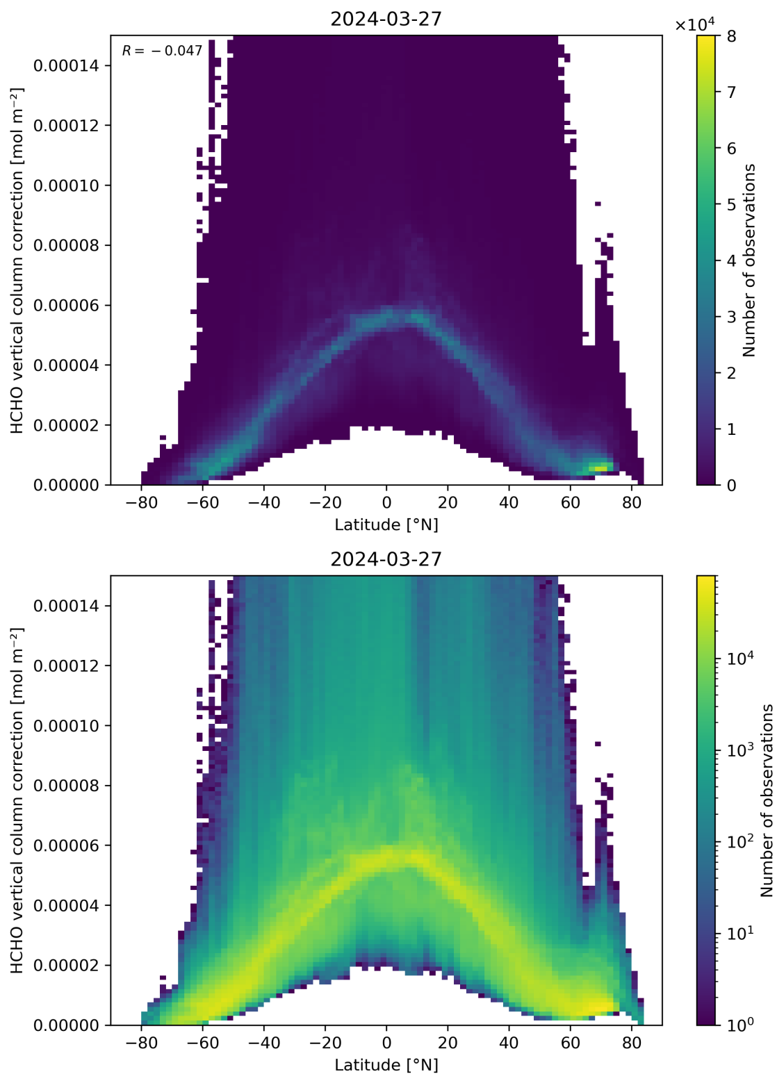
Figure 164: Scatter density plot of “Latitude” against “HCHO vertical column correction” for 2024-03-26 to 2024-03-28.
