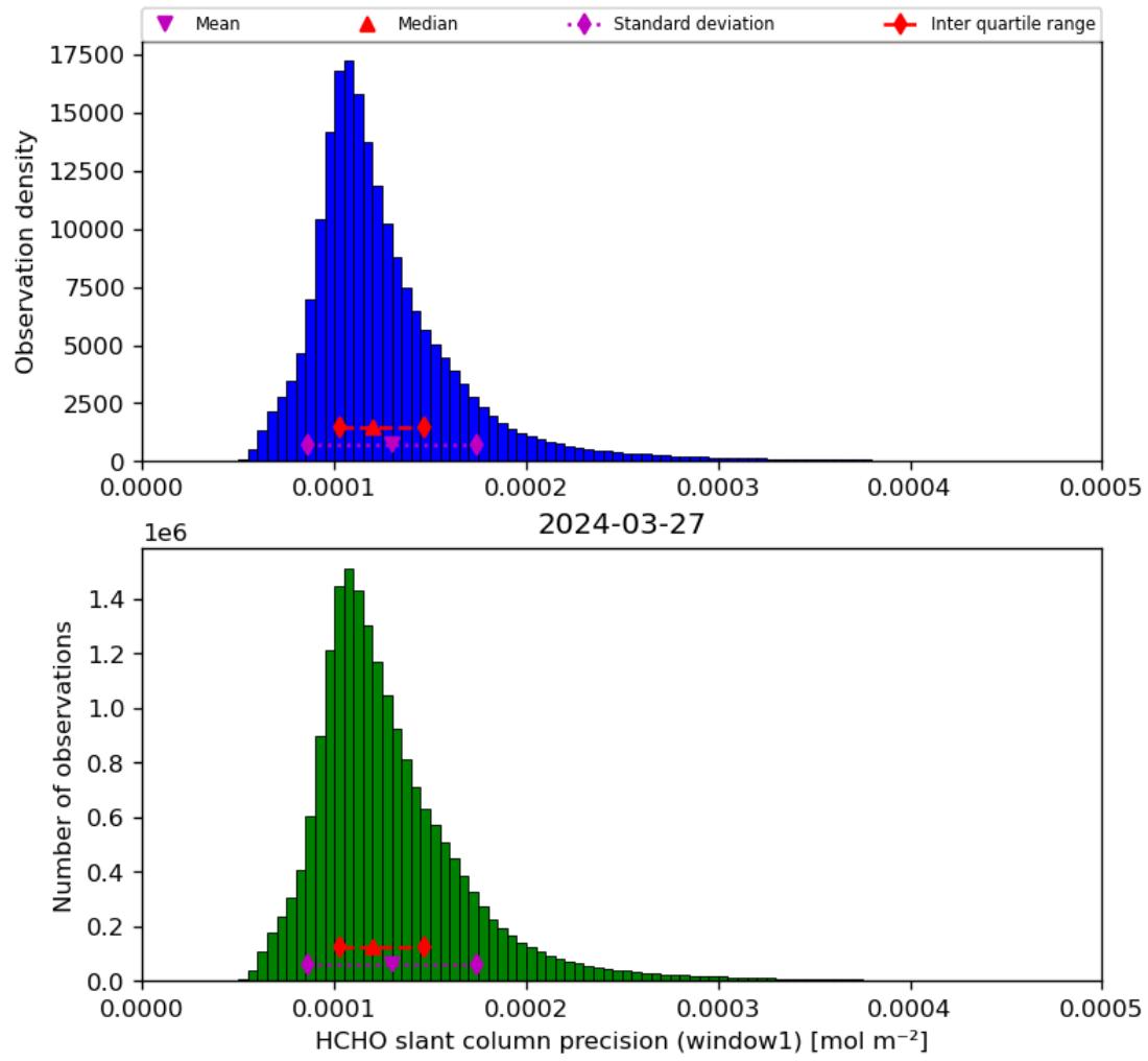
Figure 39: Histogram of “HCHO slant column precision (window1)” for 2024-03-26 to 2024-03-28
