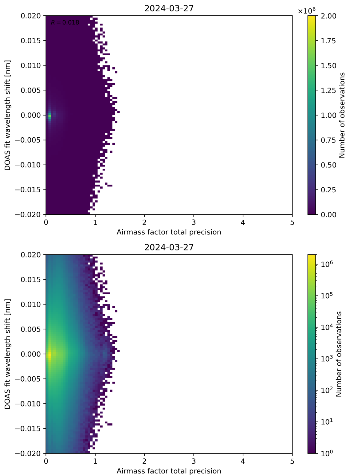
Figure 106: Scatter density plot of “Airmass factor total precision” against “DOAS fit wavelength shift” for 2024-03-26 to 2024-03-28.
