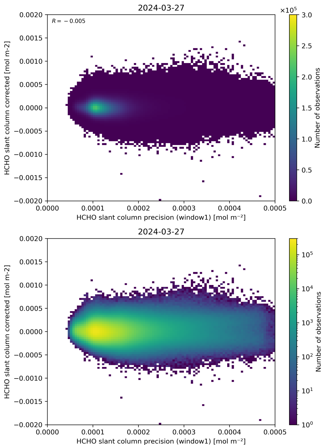
Figure 92: Scatter density plot of “HCHO slant column precision (window1)” against “HCHO slant column corrected” for 2024-03-26 to 2024-03-28.
