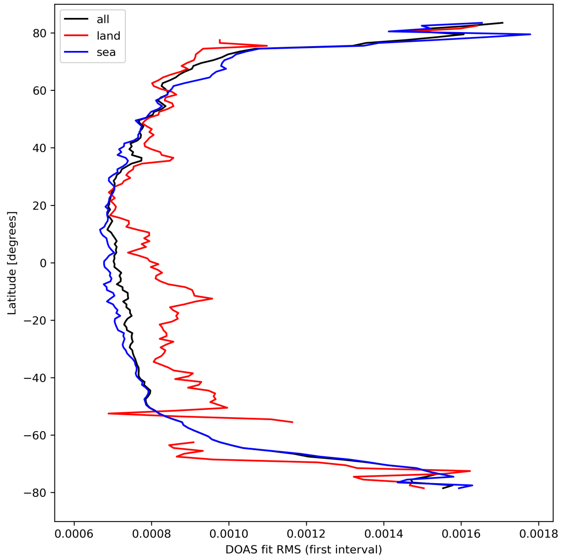
Figure 32: Zonal average of “DOAS fit RMS (first interval)” for 2024-03-26 to 2024-03-28.
