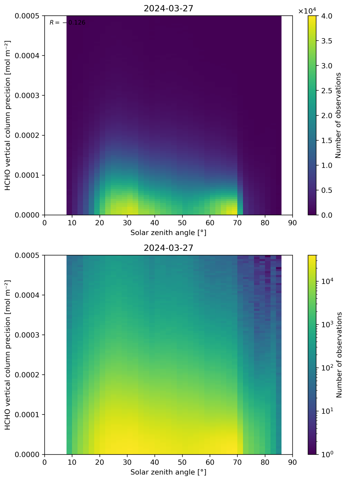
Figure 179: Scatter density plot of “Solar zenith angle” against “HCHO vertical column precision” for 2024-03-26 to 2024-03-28.
