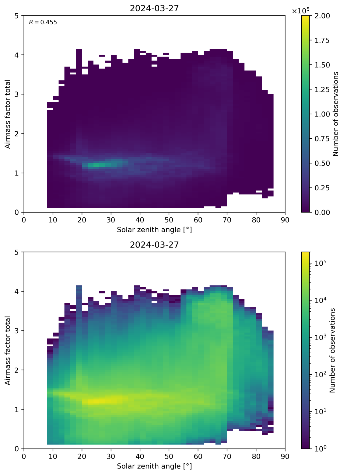
Figure 175: Scatter density plot of “Solar zenith angle” against “Airmass factor total” for 2024-03-26 to 2024-03-28.
