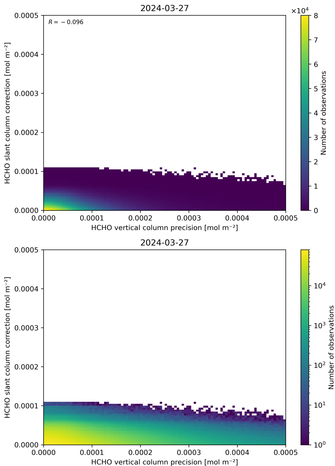
Figure 141: Scatter density plot of “HCHO vertical column precision” against “HCHO slant column correction” for 2024-03-26 to 2024-03-28.
