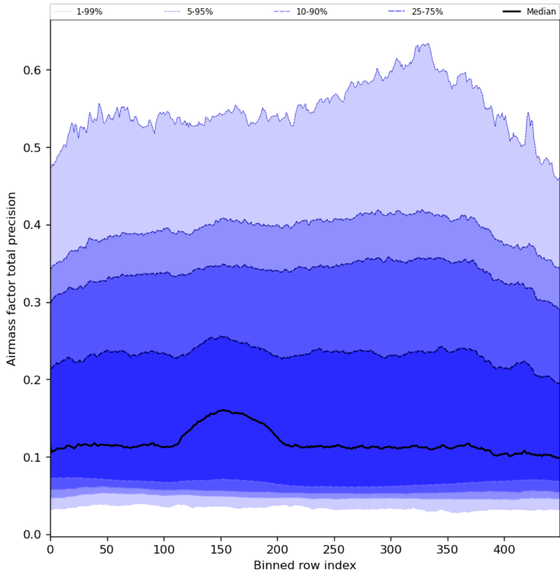
Figure 55: Along track statistics of “Airmass factor total precision” for 2024-03-26 to 2024-03-28
