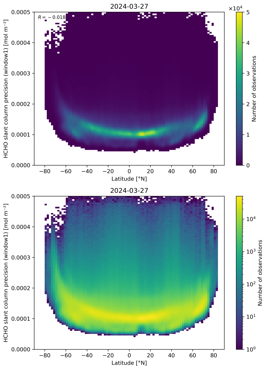
Figure 160: Scatter density plot of “Latitude” against “HCHO slant column precision (window1)” for 2024-03-26 to 2024-03-28.
