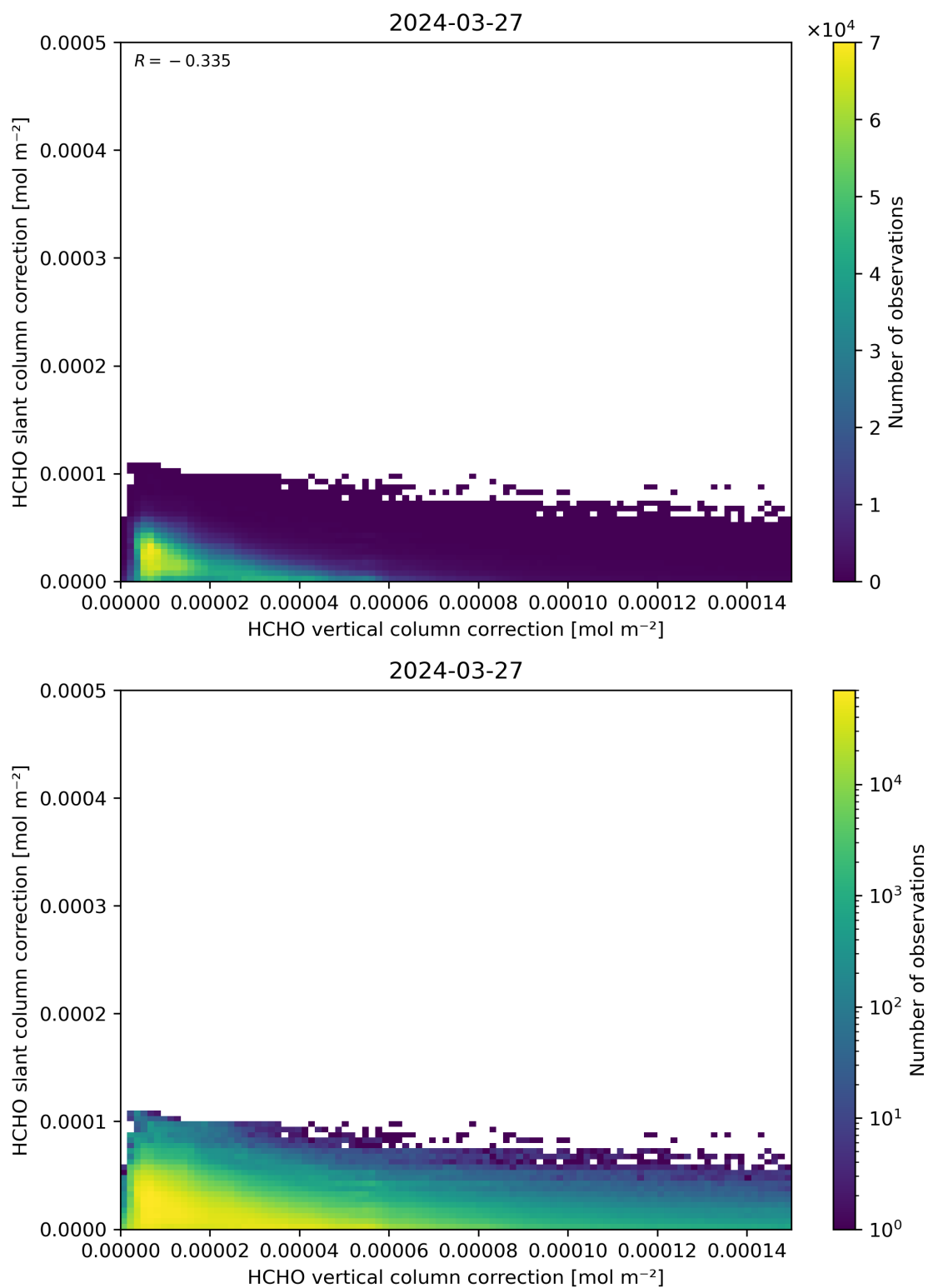
Figure 117: Scatter density plot of “HCHO vertical column correction” against “HCHO slant column correction” for 2024-03-26 to 2024-03-28.
