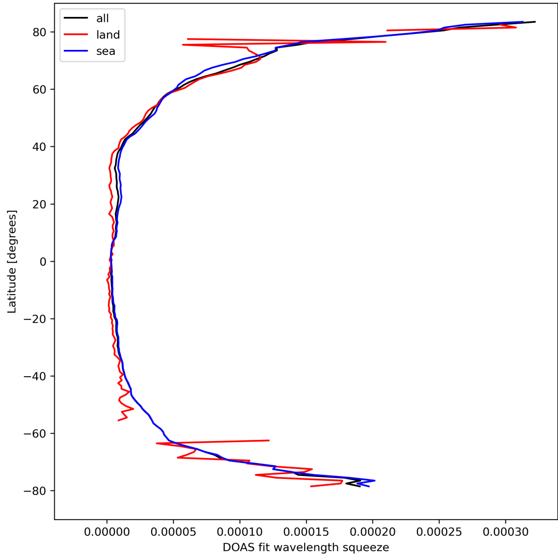
Figure 31: Zonal average of “DOAS fit wavelength squeeze” for 2024-03-26 to 2024-03-28.
