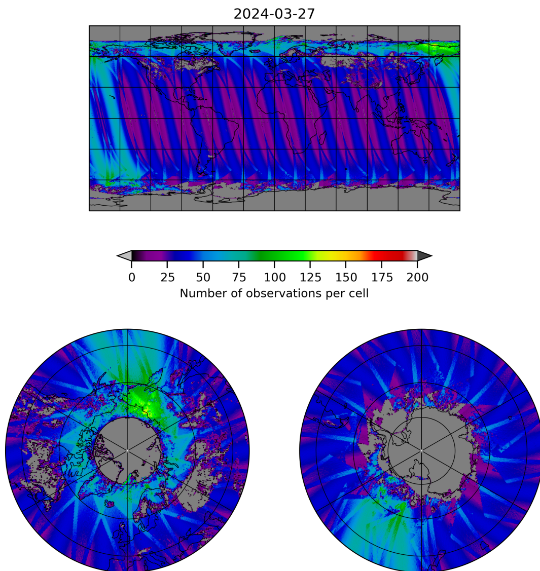
Figure 19: Map of the number of observations for 2024-03-26 to 2024-03-28
