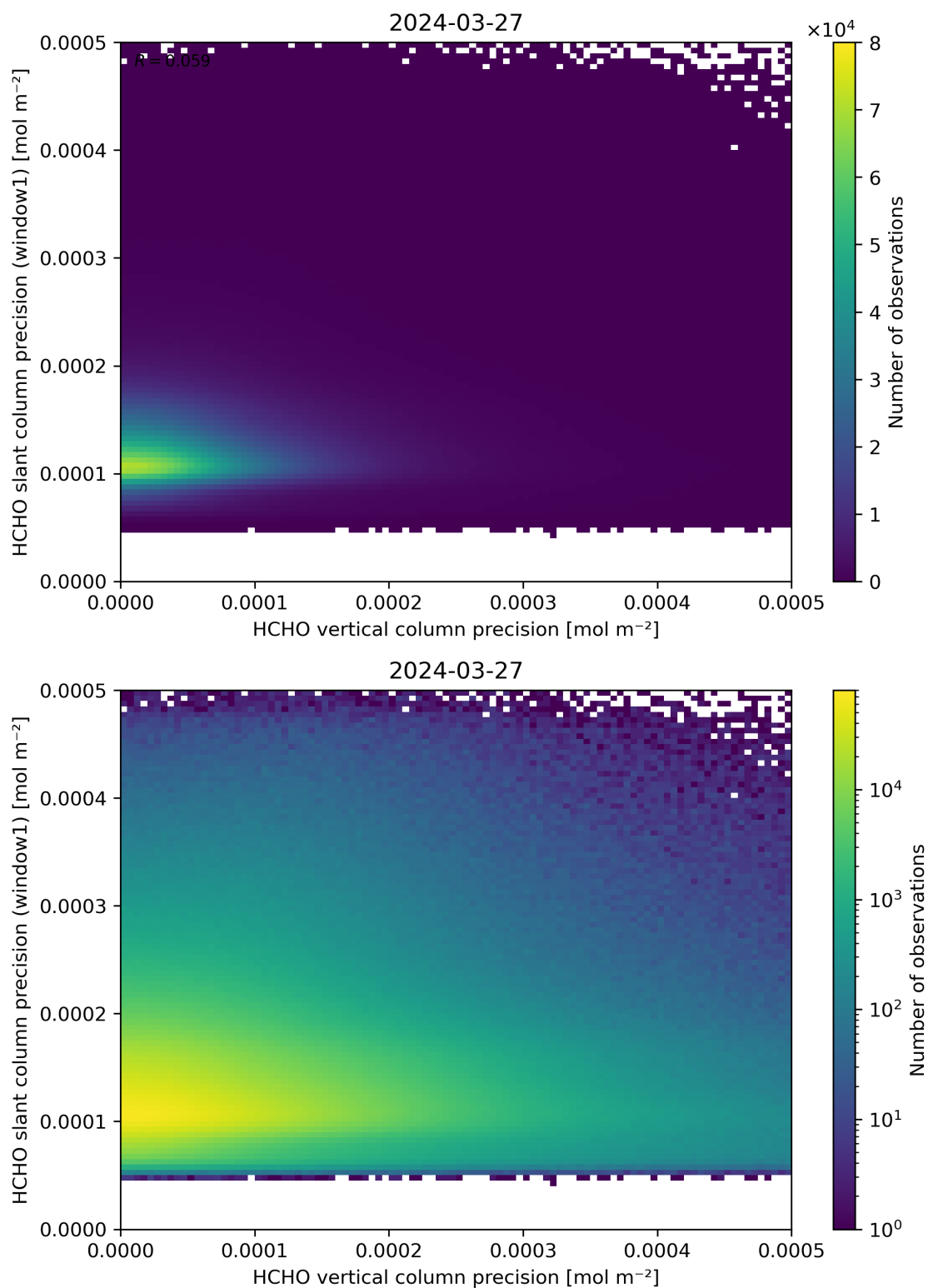
Figure 143: Scatter density plot of “HCHO vertical column precision” against “HCHO slant column precision (window1)” for 2024-03-26 to 2024-03-28.
