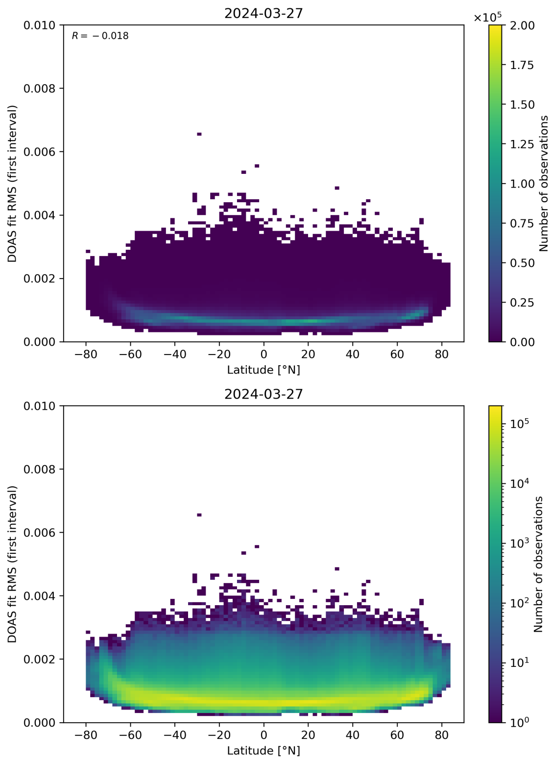
Figure 153: Scatter density plot of “Latitude” against “DOAS fit RMS (first interval)” for 2024-03-26 to 2024-03-28.
