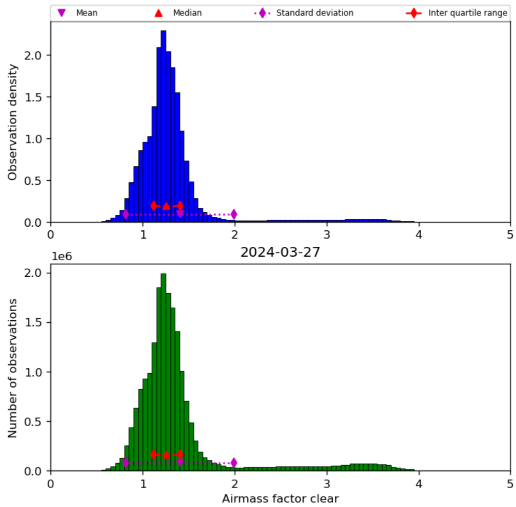
Figure 42: Histogram of "Airmass factor clear" for 2024-03-26 to 2024-03-28
