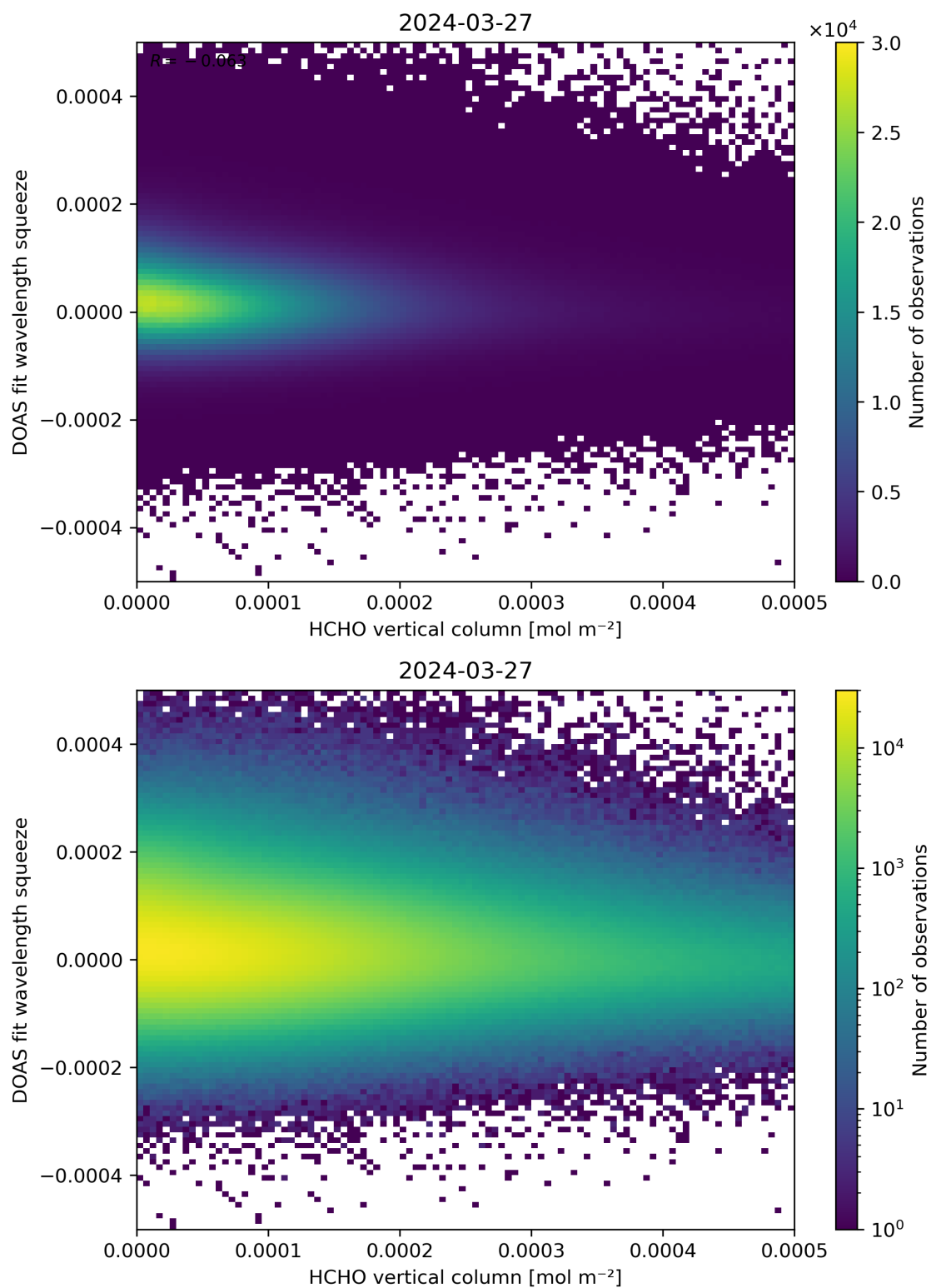
Figure 125: Scatter density plot of “HCHO vertical column” against “DOAS fit wavelength squeeze” for 2024-03-26 to 2024-03-28.
