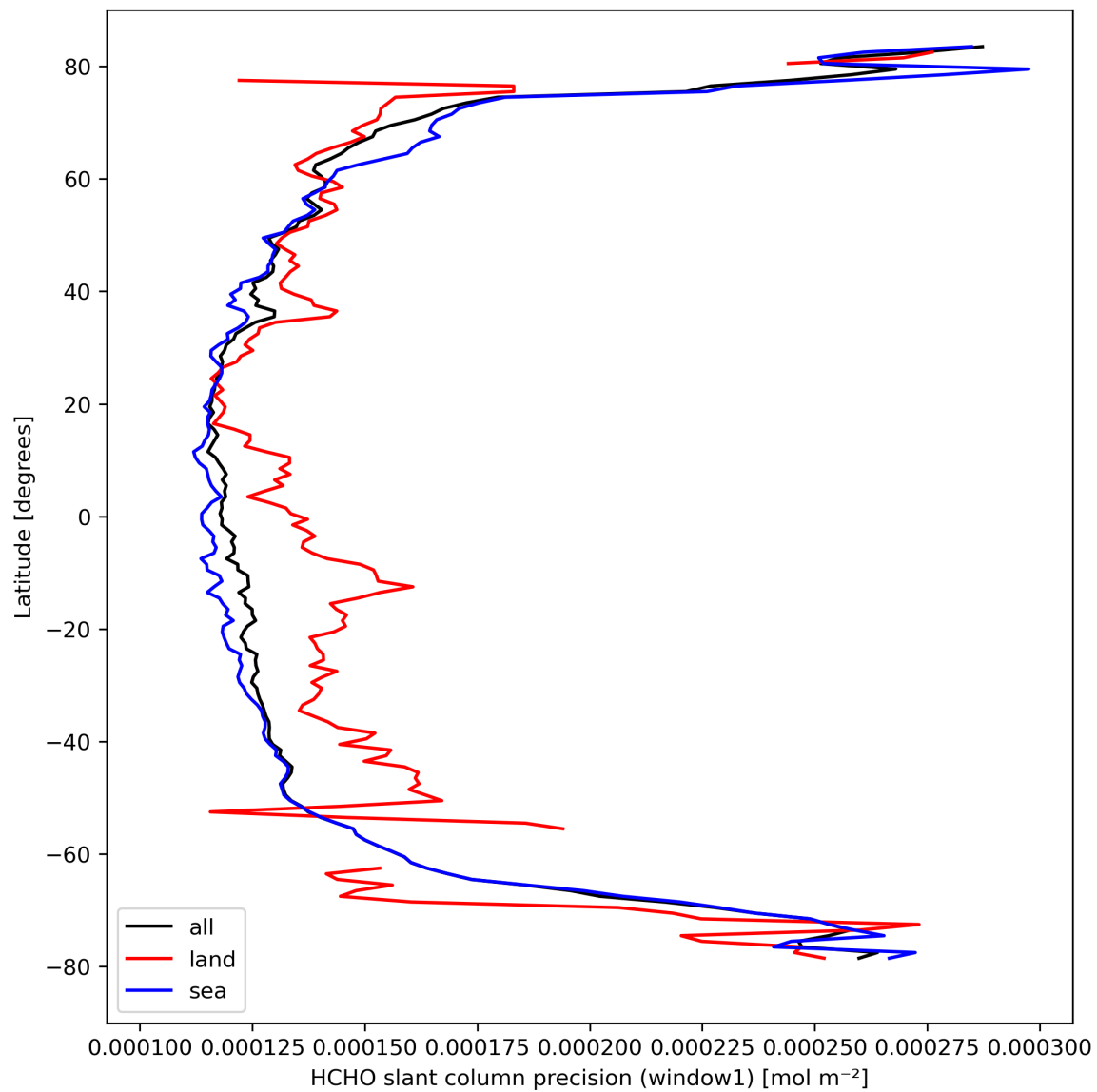
Figure 25: Zonal average of “HCHO slant column precision (window1)” for 2024-03-26 to 2024-03-28.
