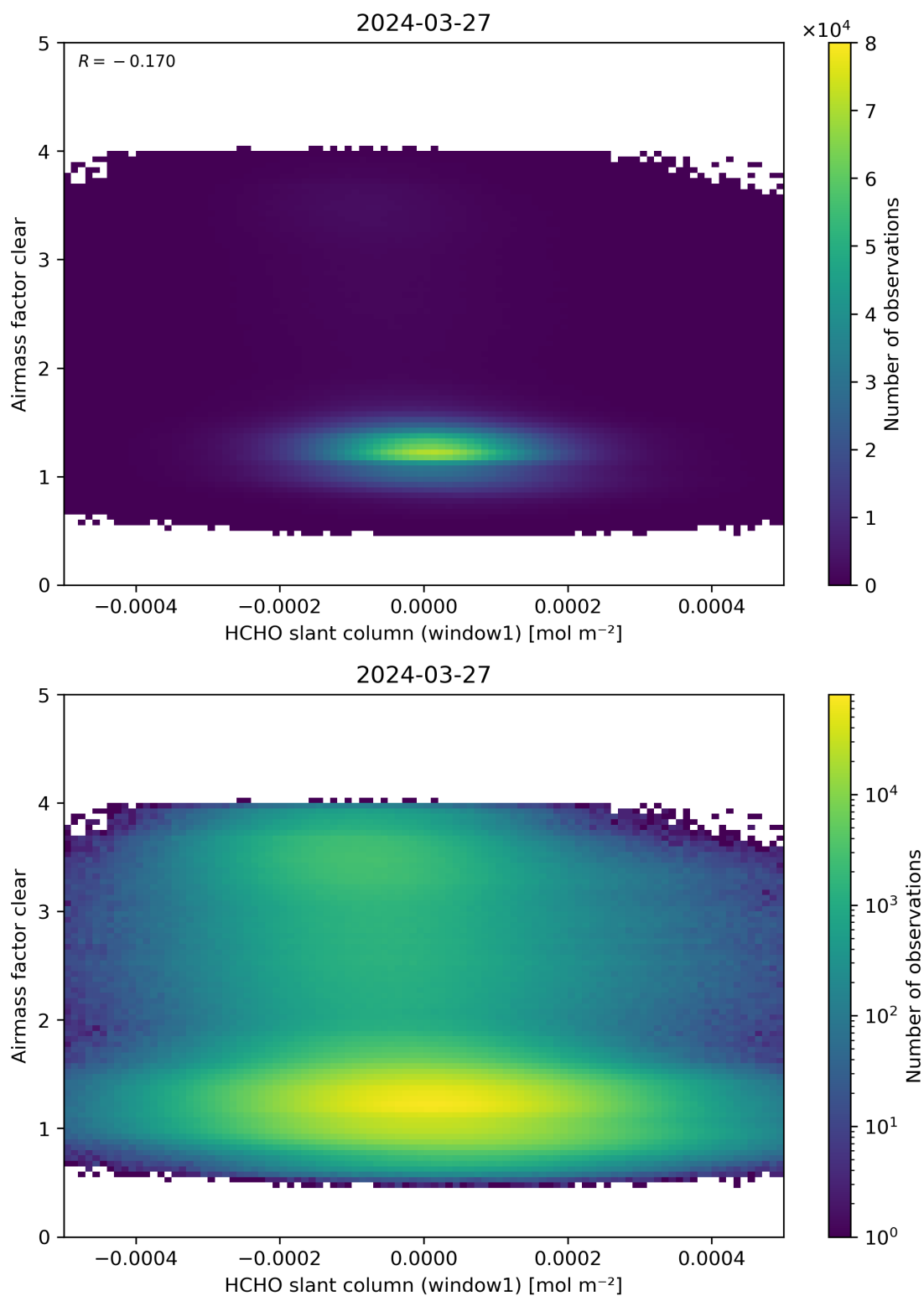
Figure 81: Scatter density plot of “HCHO slant column (window1)” against “Airmass factor clear” for 2024-03-26 to 2024-03-28.
