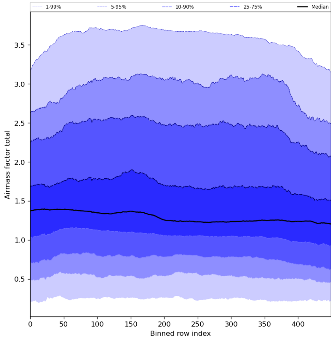
Figure 54: Along track statistics of “Airmass factor total” for 2024-03-26 to 2024-03-28
