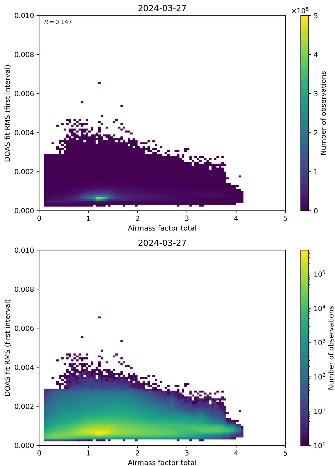
Figure 97: Scatter density plot of “Airmass factor total” against “DOAS fit RMS (first interval)” for 2024-03-26 to 2024-03-28.
