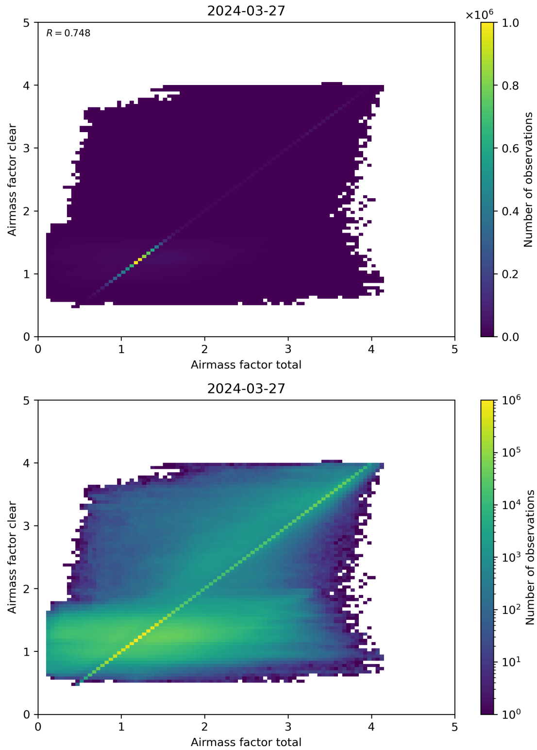
Figure 100: Scatter density plot of “Airmass factor total” against “Airmass factor clear” for 2024-03-26 to 2024-03-28.
