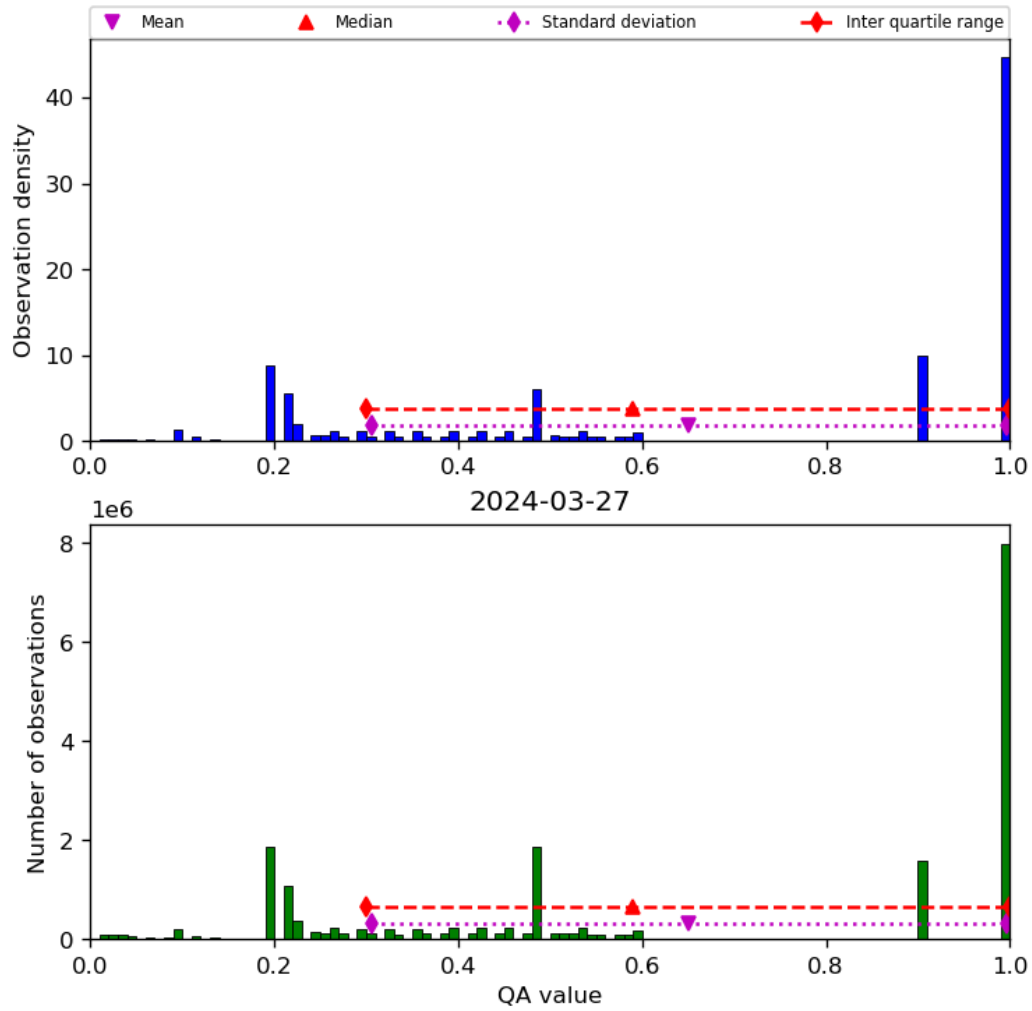
Figure 34: Histogram of “QA value” for 2024-03-26 to 2024-03-28
