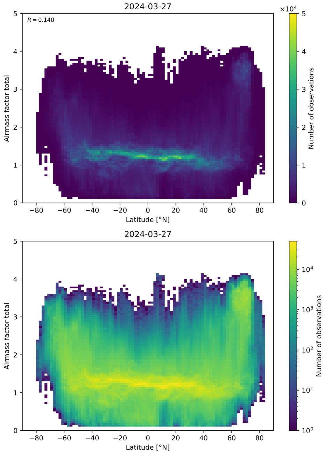
Figure 161: Scatter density plot of “Latitude” against “Airmass factor total” for 2024-03-26 to 2024-03-28.
