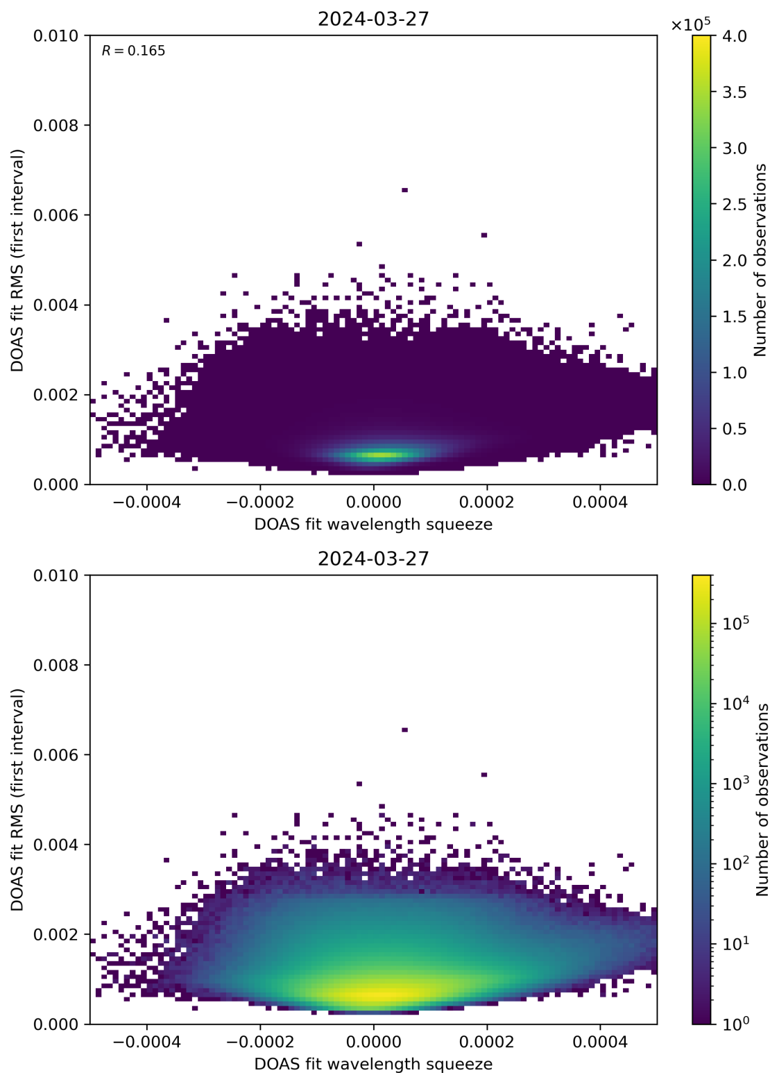
Figure 68: Scatter density plot of “DOAS fit wavelength squeeze” against “DOAS fit RMS (first interval)” for 2024-03-26 to 2024-03-28.
