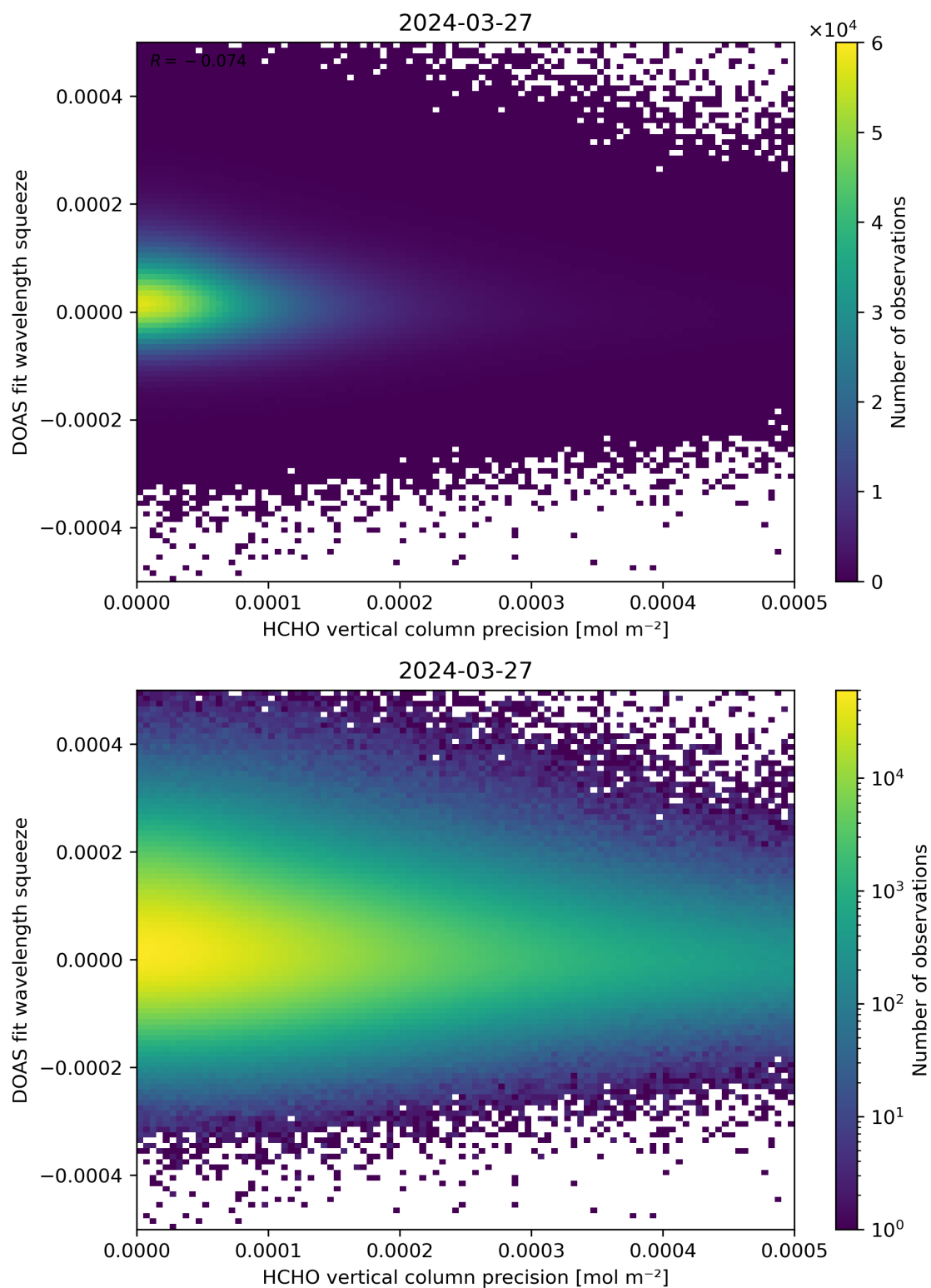
Figure 138: Scatter density plot of “HCHO vertical column precision” against “DOAS fit wavelength squeeze” for 2024-03-26 to 2024-03-28.
