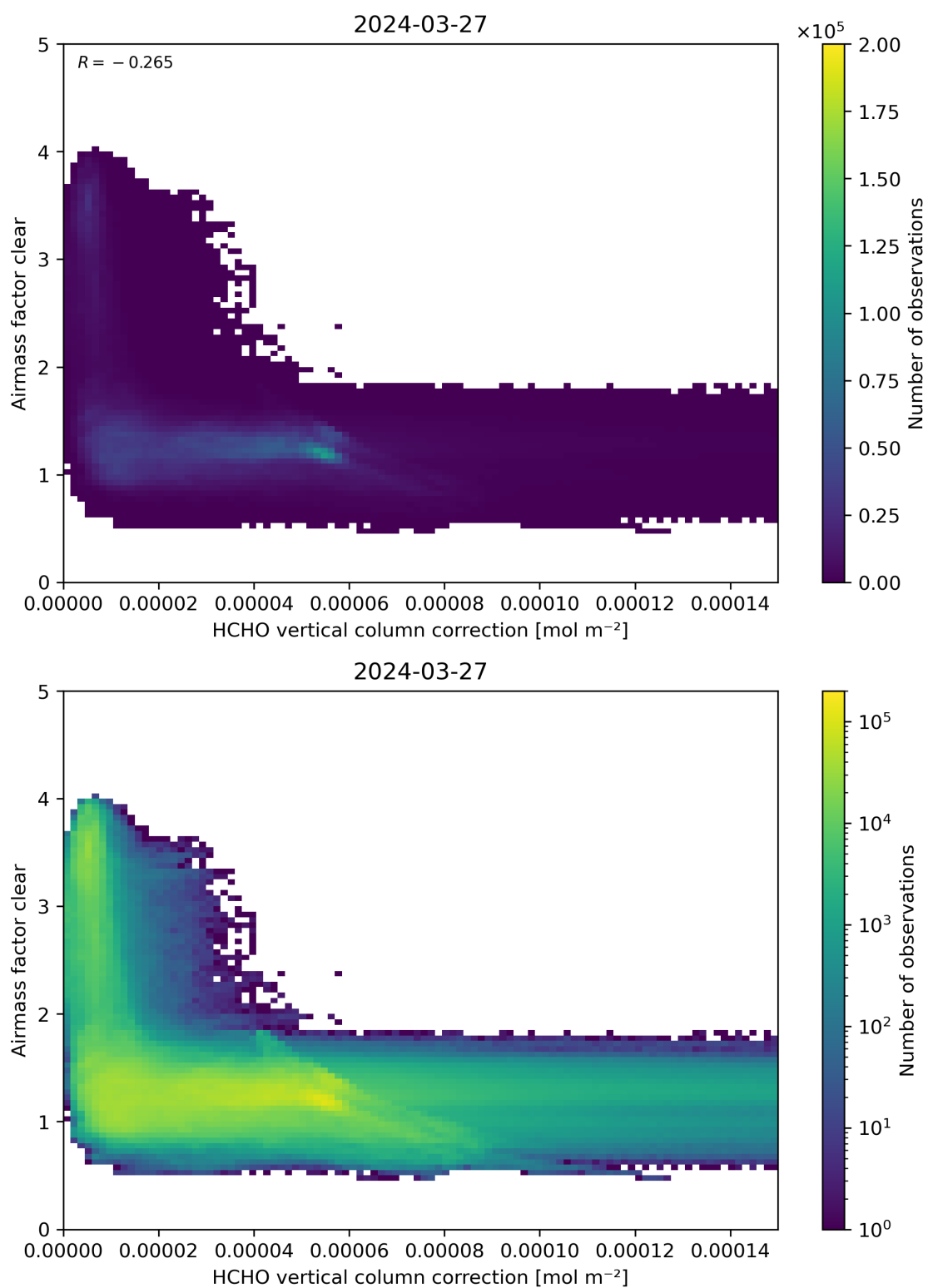
Figure 115: Scatter density plot of “HCHO vertical column correction” against “Airmass factor clear” for 2024-03-26 to 2024-03-28.
