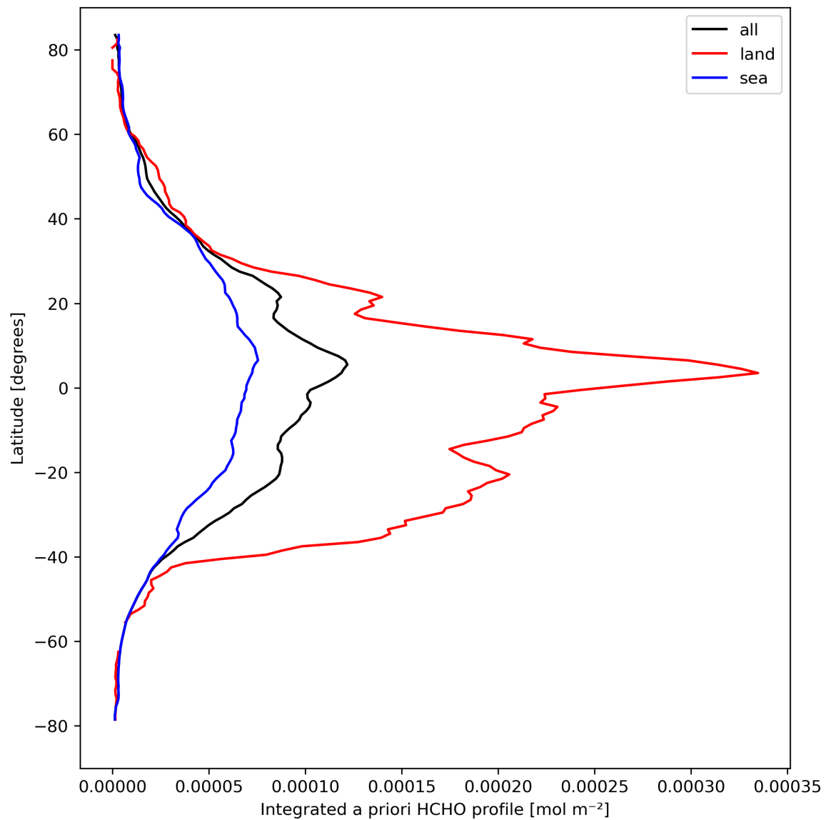
Figure 29: Zonal average of “Integrated a priori HCHO profile” for 2024-03-26 to 2024-03-28.
