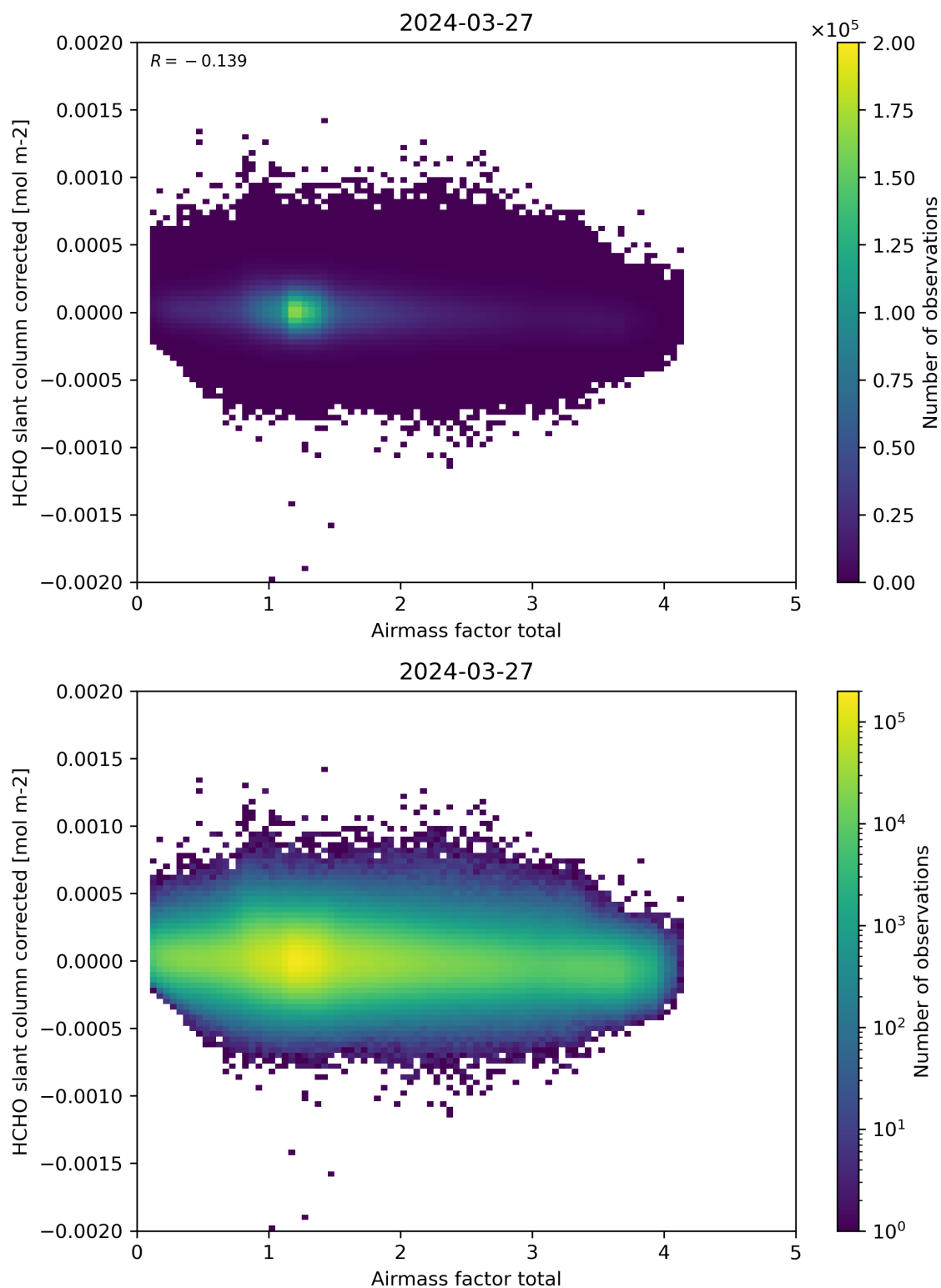
Figure 101: Scatter density plot of “Airmass factor total” against “HCHO slant column corrected” for 2024-03-26 to 2024-03-28.
