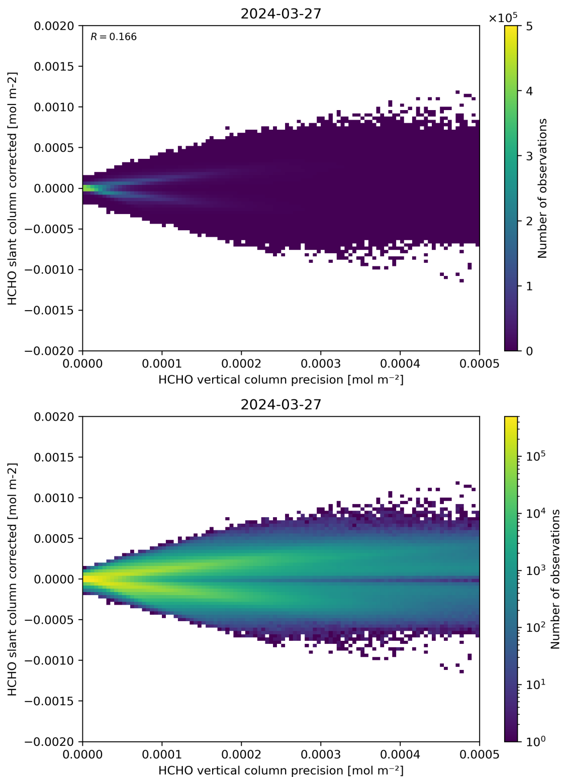
Figure 140: Scatter density plot of “HCHO vertical column precision” against “HCHO slant column corrected” for 2024-03-26 to 2024-03-28.
