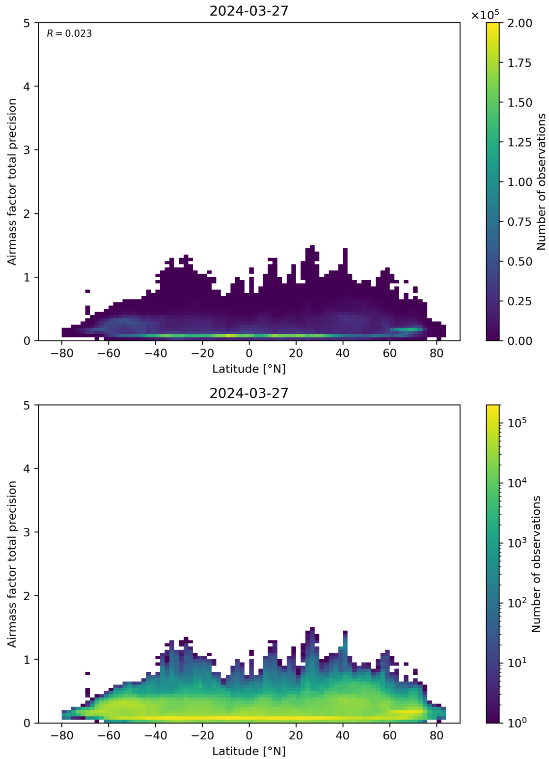
Figure 162: Scatter density plot of “Latitude” against “Airmass factor total precision” for 2024-03-26 to 2024-03-28.
