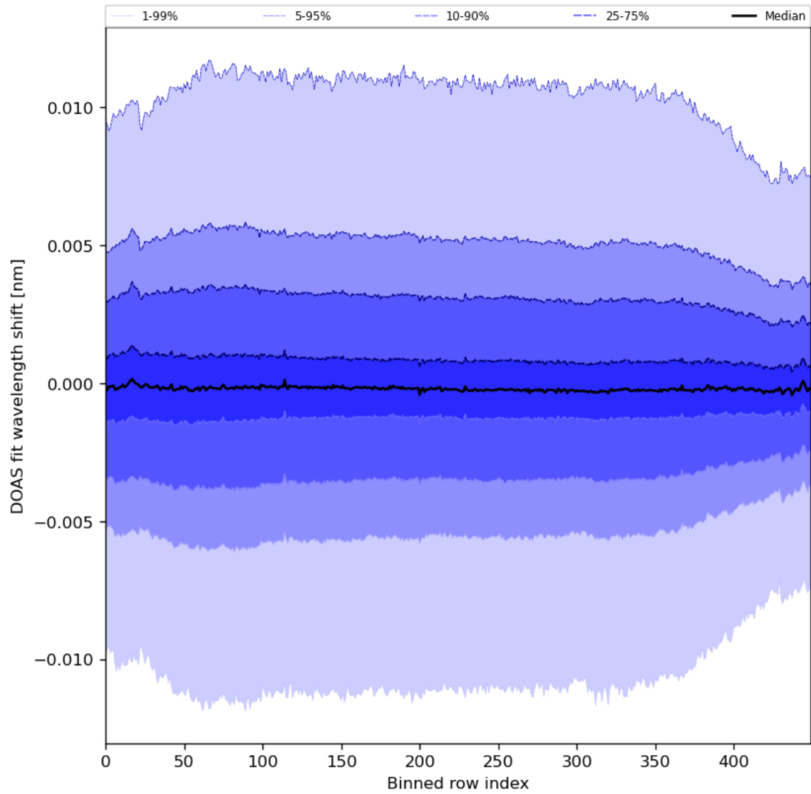
Figure 58: Along track statistics of “DOAS fit wavelength shift” for 2024-03-26 to 2024-03-28
