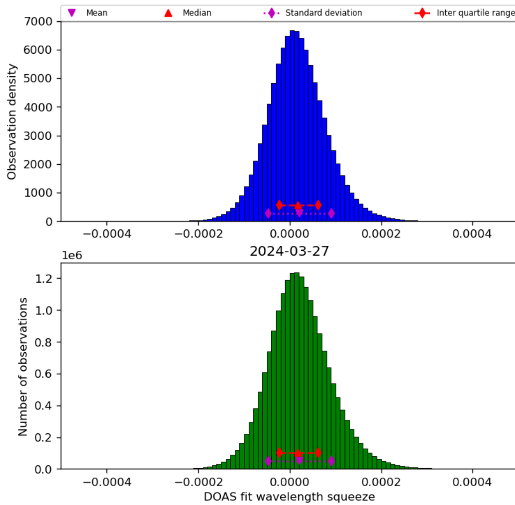
Figure 45: Histogram of “DOAS fit wavelength squeeze” for 2024-03-26 to 2024-03-28
