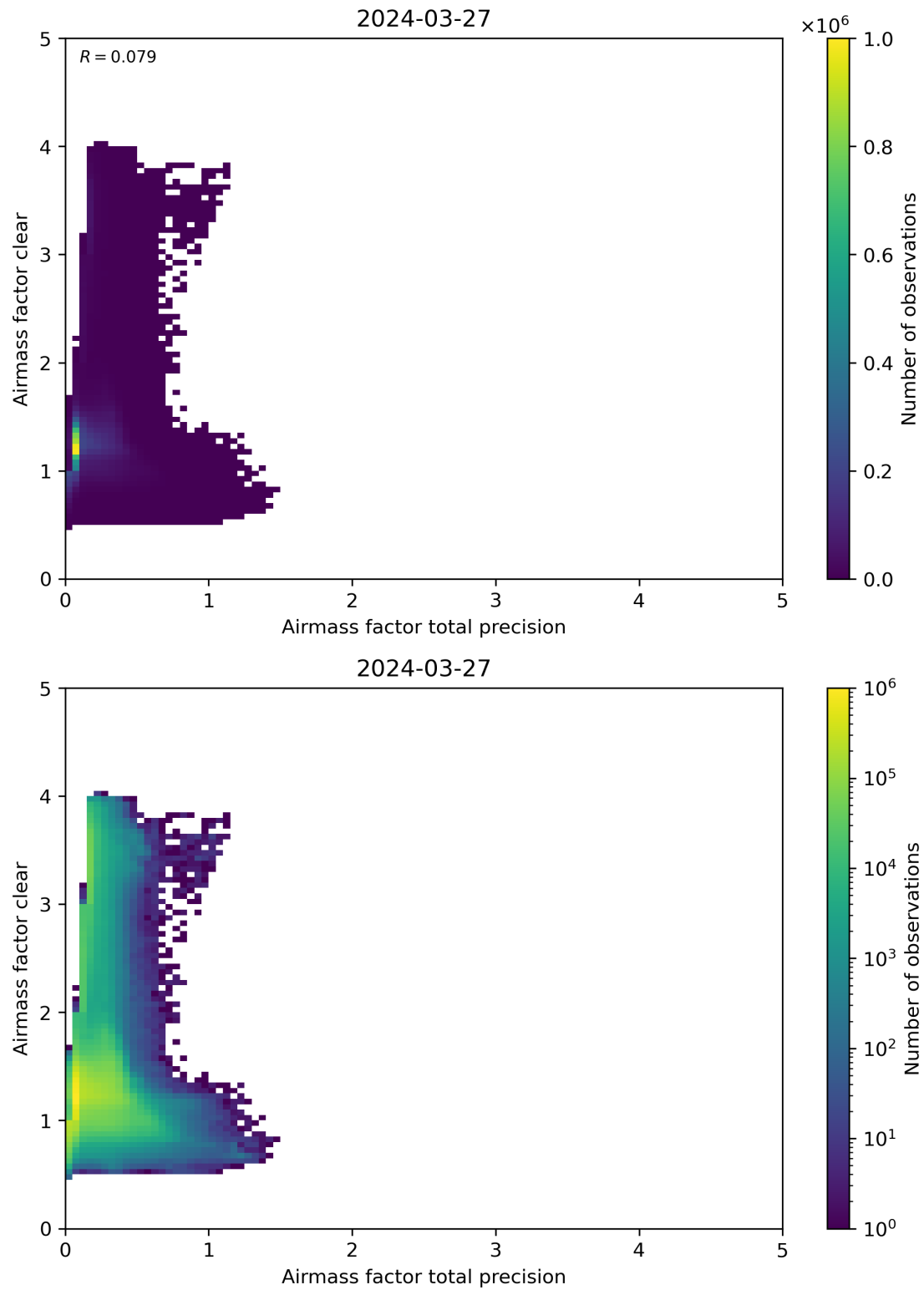
Figure 108: Scatter density plot of “Airmass factor total precision” against “Airmass factor clear” for 2024-03-26 to 2024-03-28.
