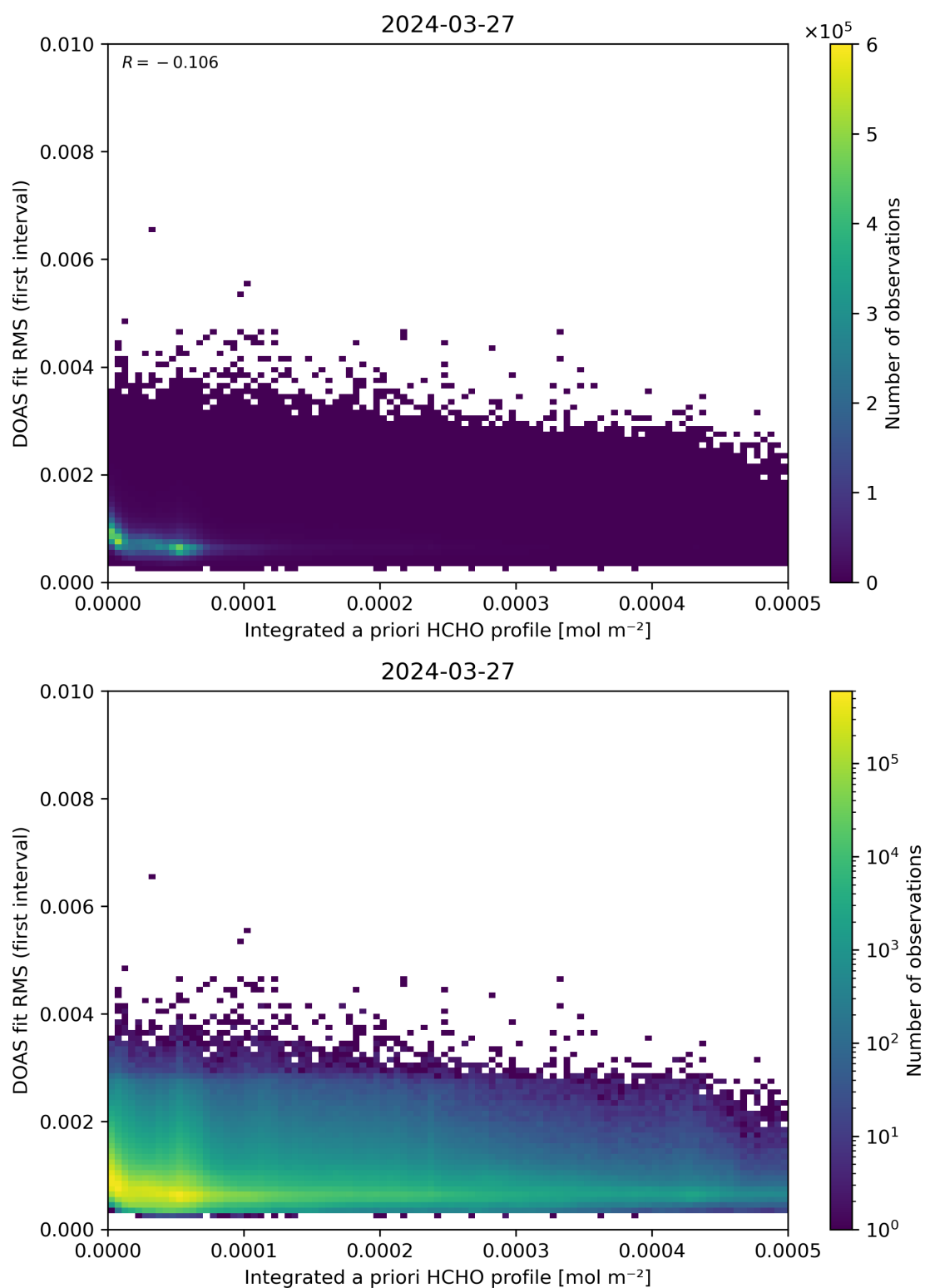
Figure 148: Scatter density plot of “Integrated a priori HCHO profile” against “DOAS fit RMS (first interval)” for 2024-03-26 to 2024-03-28.
