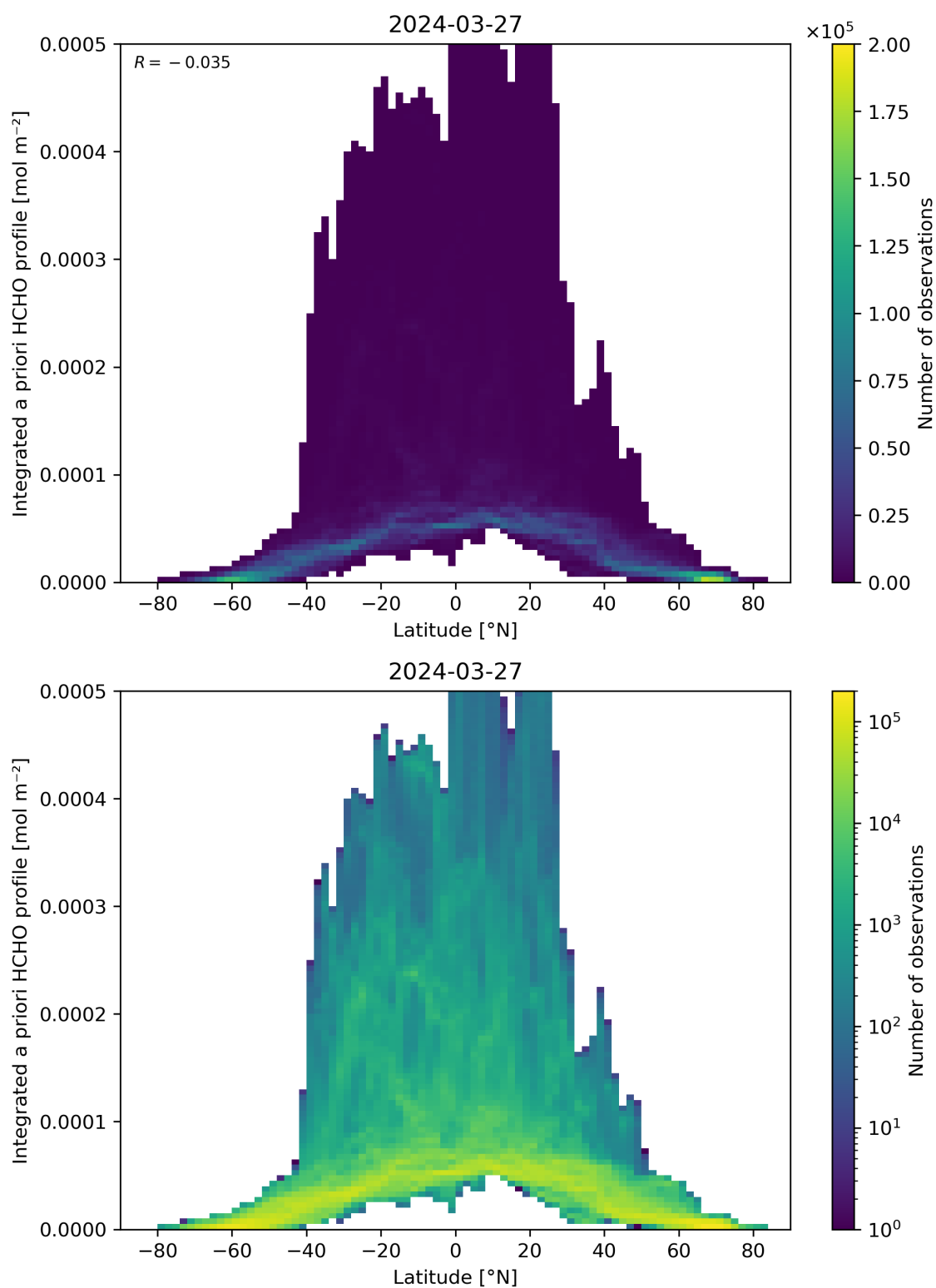
Figure 166: Scatter density plot of “Latitude” against “Integrated a priori HCHO profile” for 2024-03-26 to 2024-03-28.
