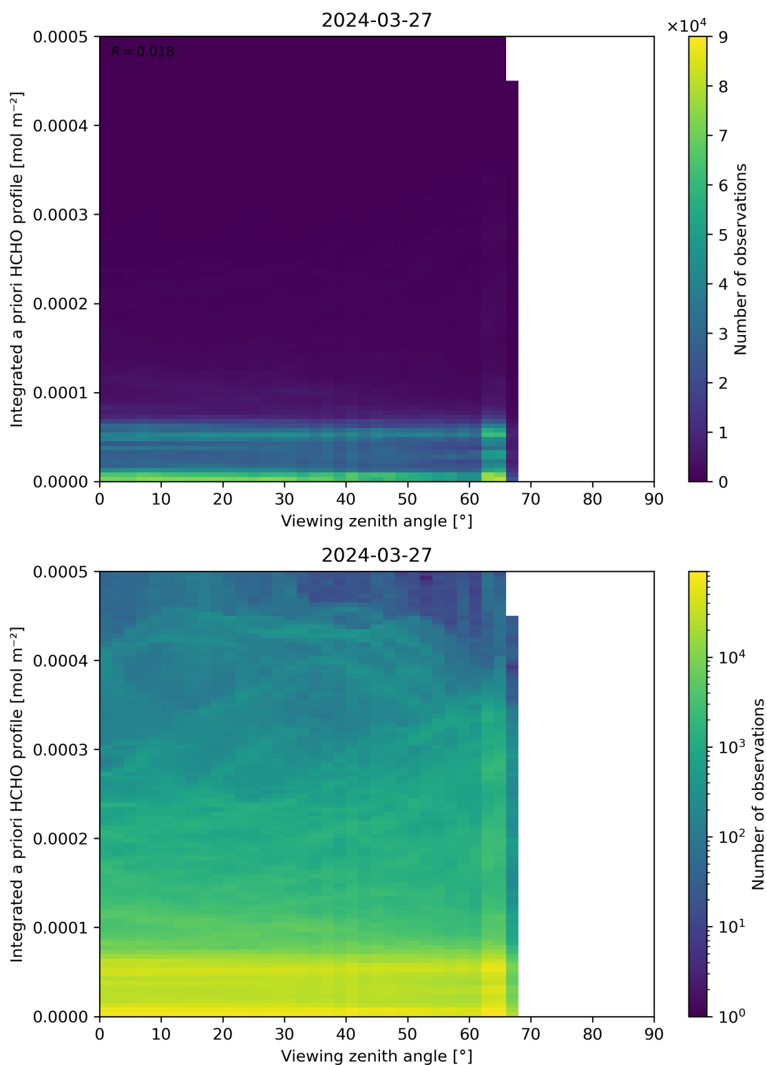
Figure 195: Scatter density plot of “Viewing zenith angle” against “Integrated a priori HCHO profile” for 2024-03-26 to 2024-03-28.
