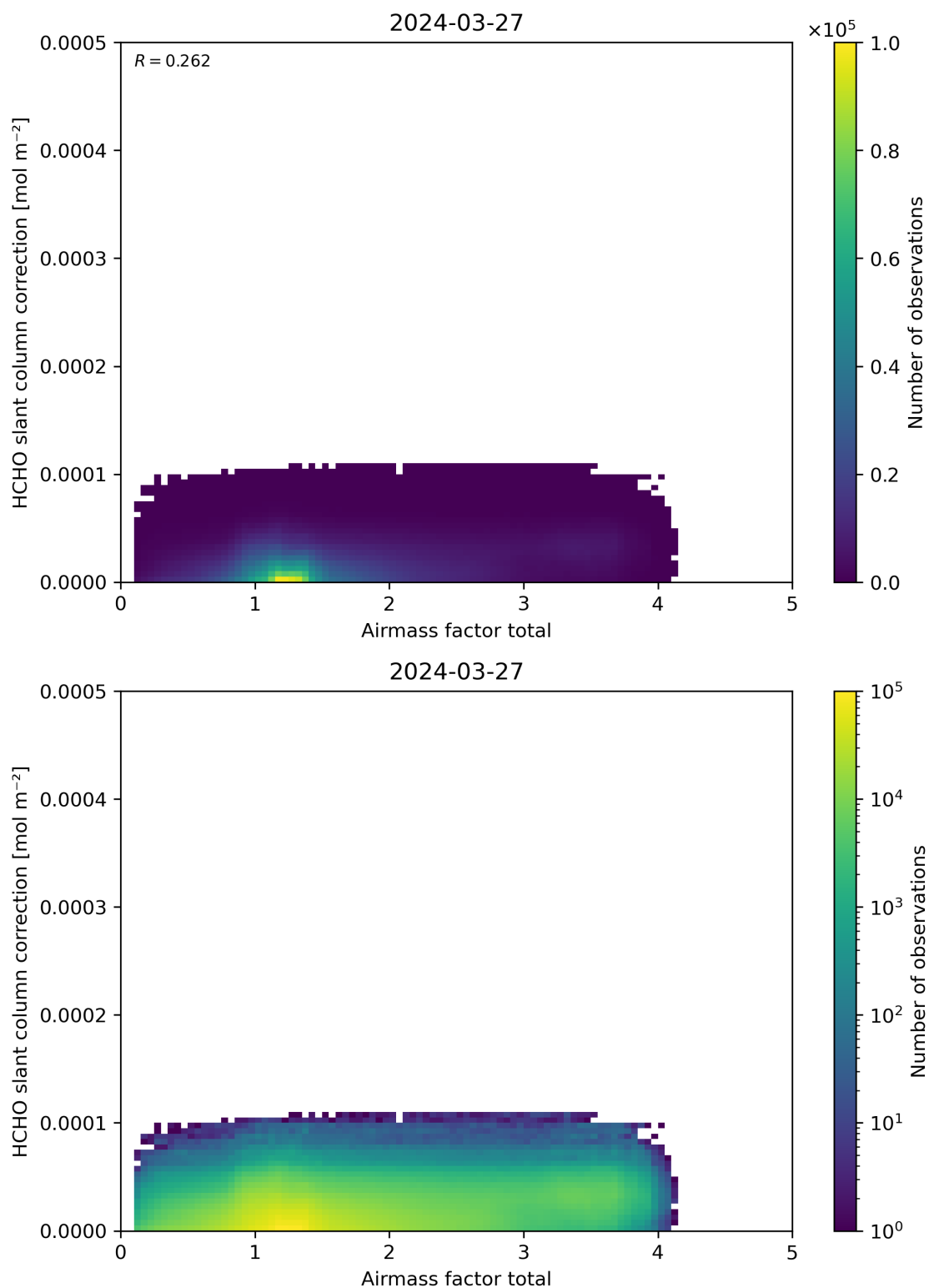
Figure 102: Scatter density plot of “Airmass factor total” against “HCHO slant column correction” for 2024-03-26 to 2024-03-28.
