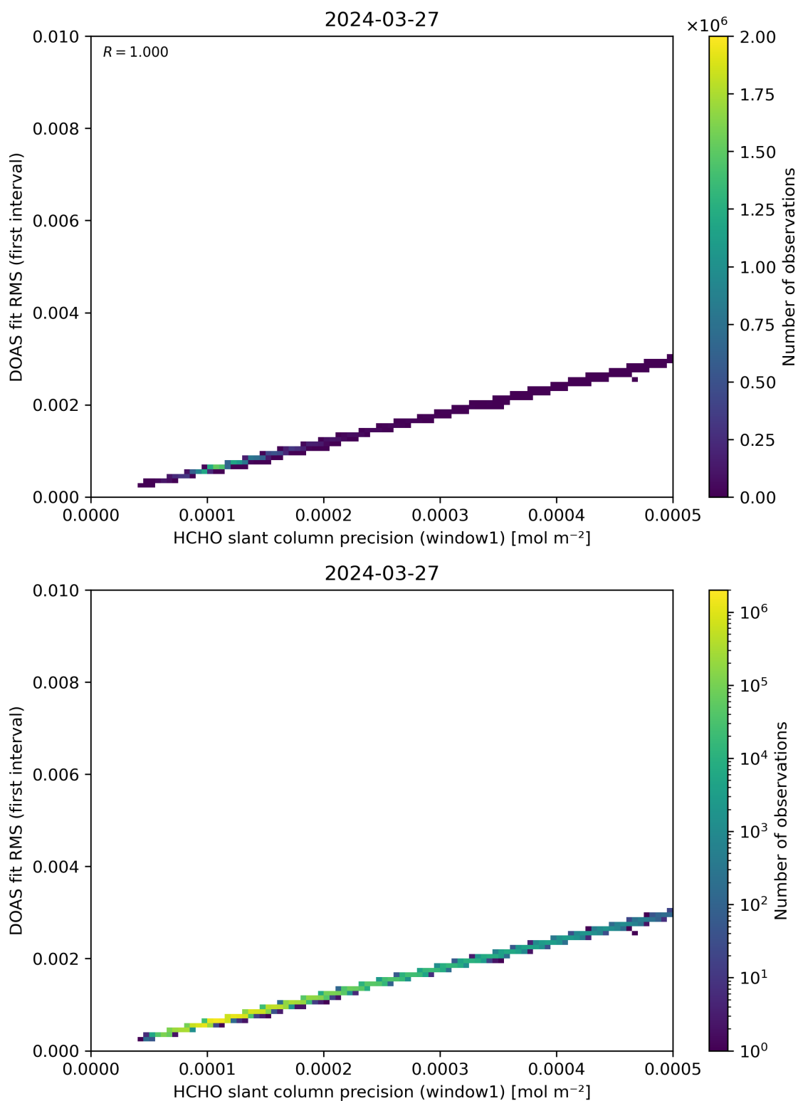
Figure 88: Scatter density plot of “HCHO slant column precision (window1)” against “DOAS fit RMS (first interval)” for 2024-03-26 to 2024-03-28.
