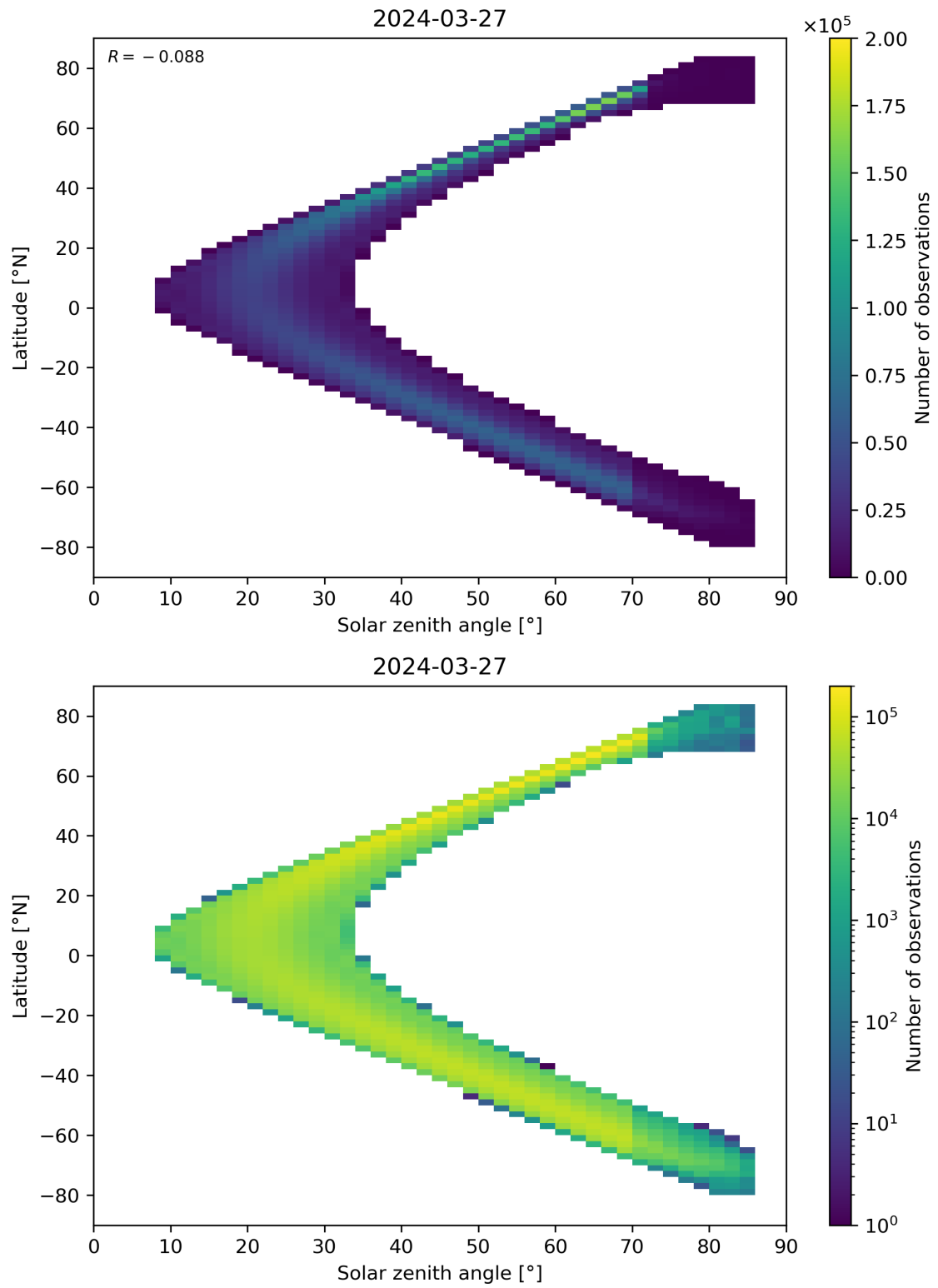
Figure 181: Scatter density plot of “Solar zenith angle” against “Latitude” for 2024-03-26 to 2024-03-28.
