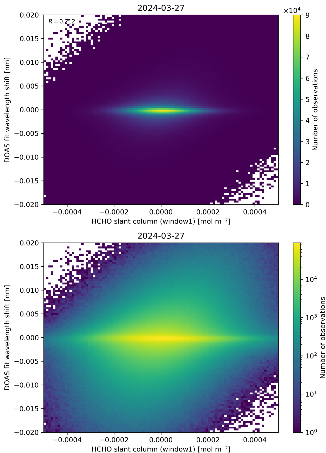
Figure 79: Scatter density plot of “HCHO slant column (window1)” against “DOAS fit wavelength shift” for 2024-03-26 to 2024-03-28.
