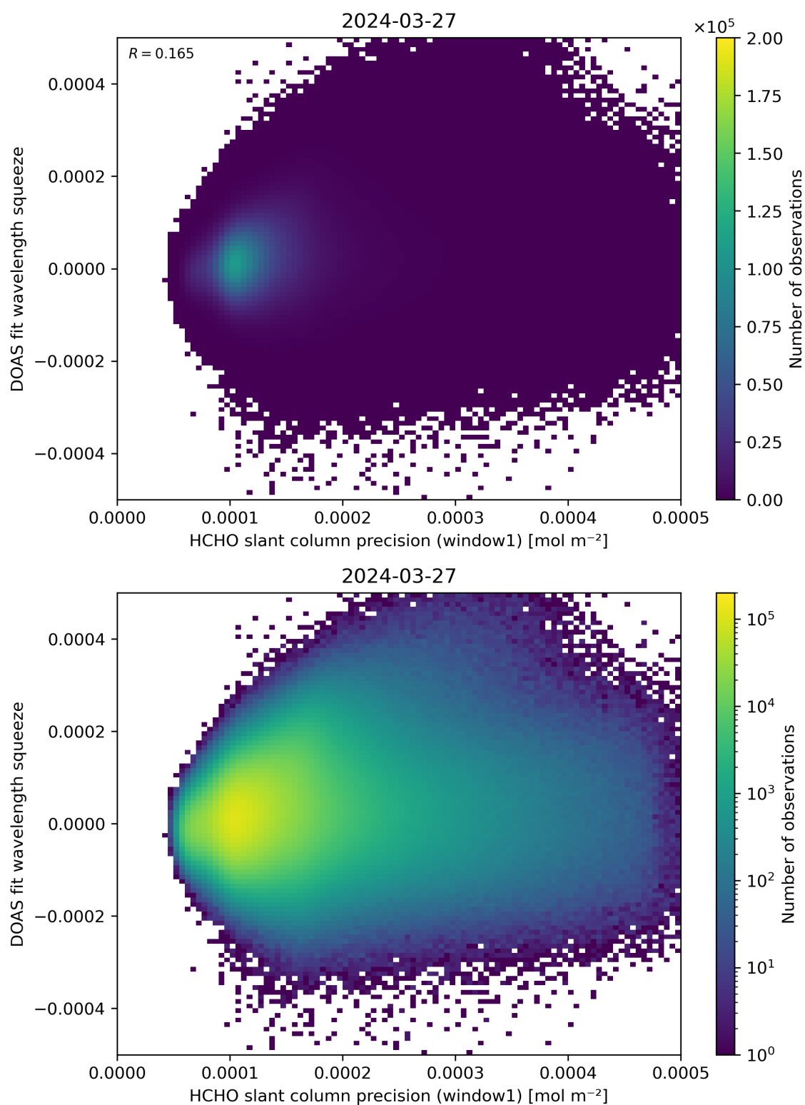
Figure 90: Scatter density plot of “HCHO slant column precision (window1)” against “DOAS fit wavelength squeeze” for 2024-03-26 to 2024-03-28.
