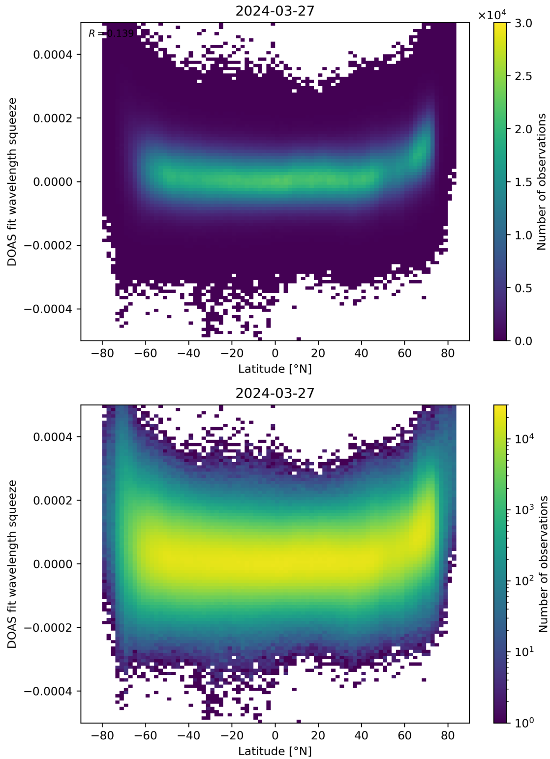
Figure 155: Scatter density plot of “Latitude” against “DOAS fit wavelength squeeze” for 2024-03-26 to 2024-03-28.
