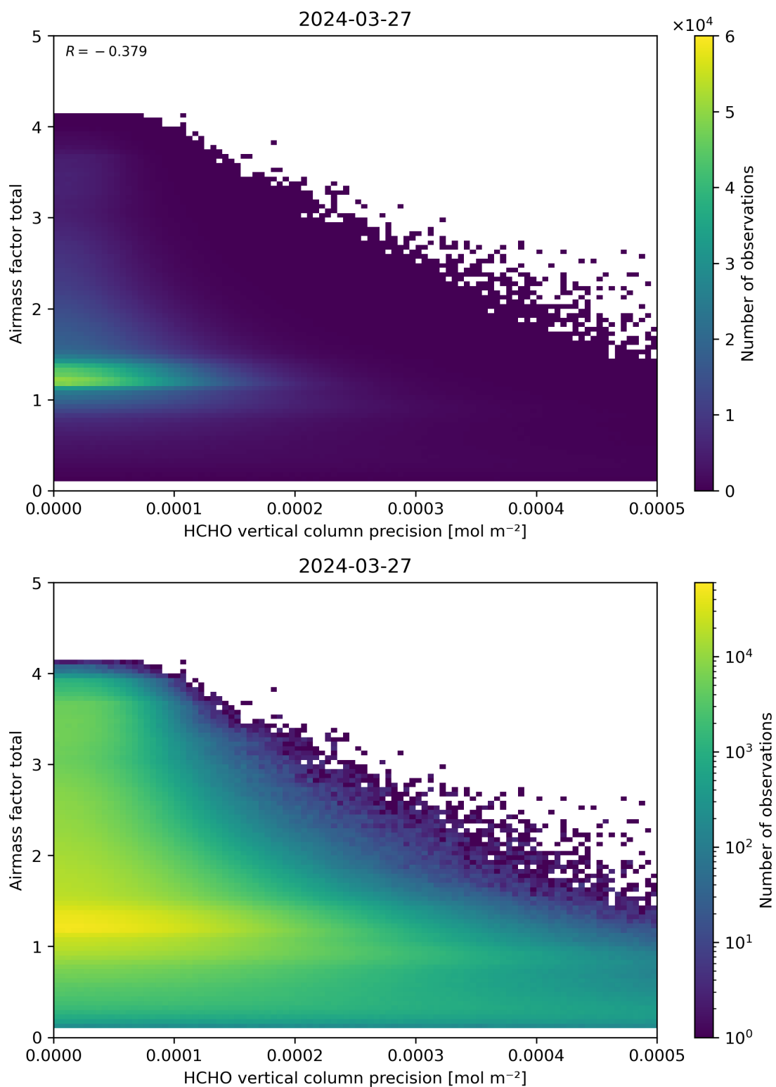
Figure 144: Scatter density plot of “HCHO vertical column precision” against “Airmass factor total” for 2024-03-26 to 2024-03-28.
