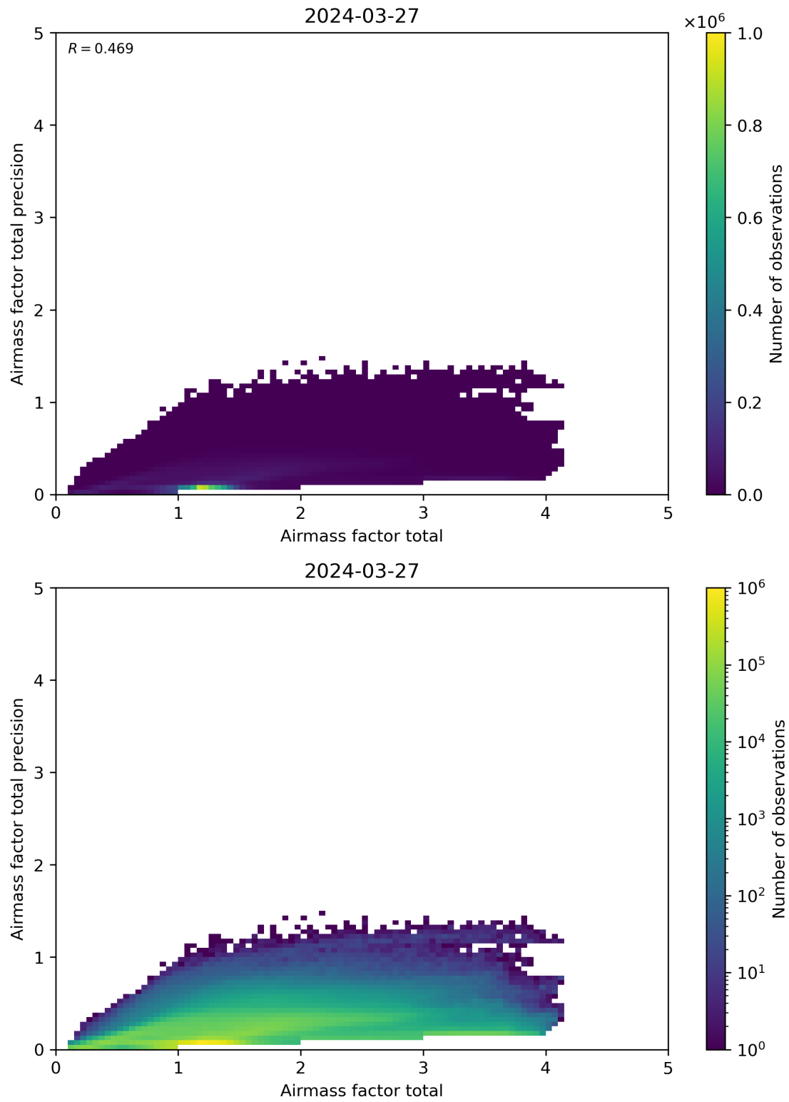
Figure 103: Scatter density plot of “Airmass factor total” against “Airmass factor total precision” for 2024-03-26 to 2024-03-28.
