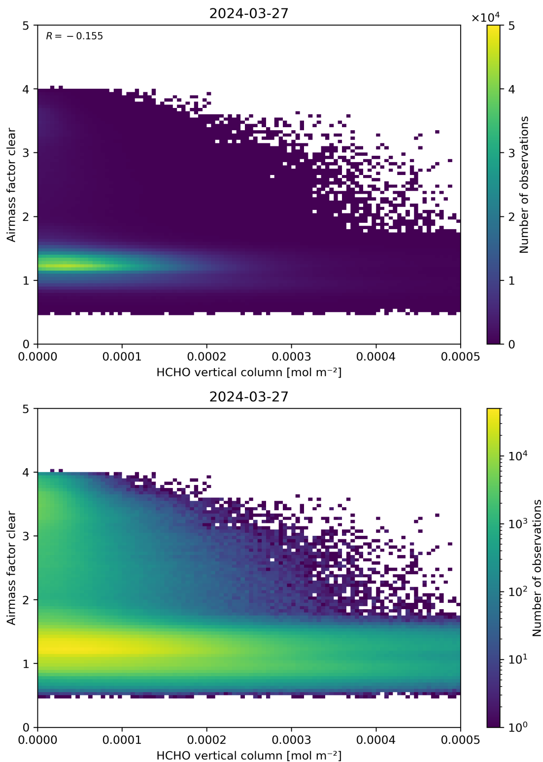
Figure 126: Scatter density plot of “HCHO vertical column” against “Airmass factor clear” for 2024-03-26 to 2024-03-28.
