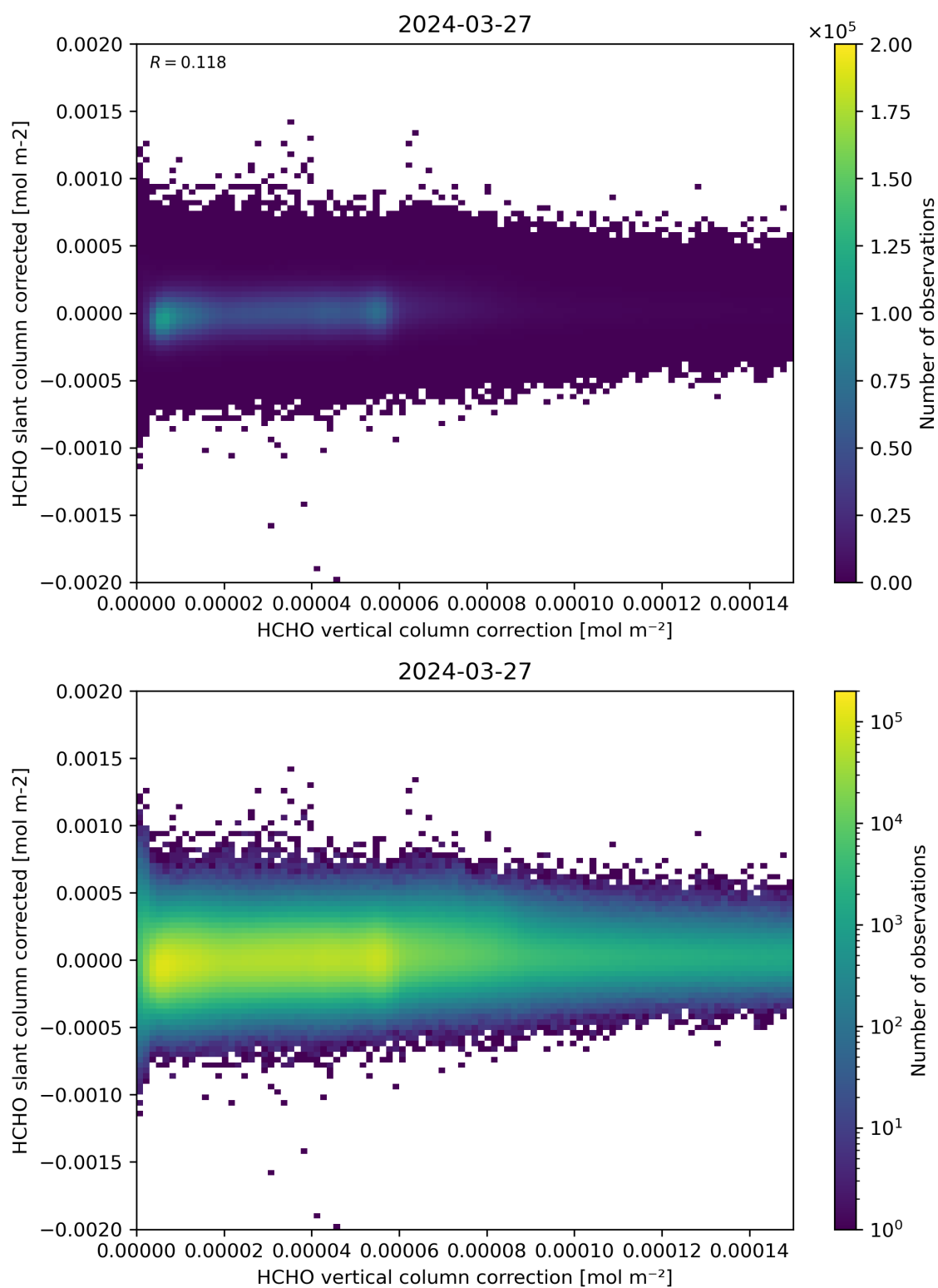
Figure 116: Scatter density plot of “HCHO vertical column correction” against “HCHO slant column corrected” for 2024-03-26 to 2024-03-28.
