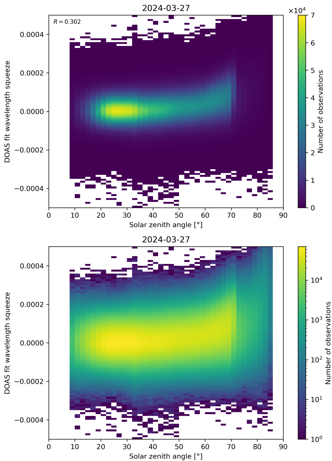
Figure 169: Scatter density plot of “Solar zenith angle” against “DOAS fit wavelength squeeze” for 2024-03-26 to 2024-03-28.
