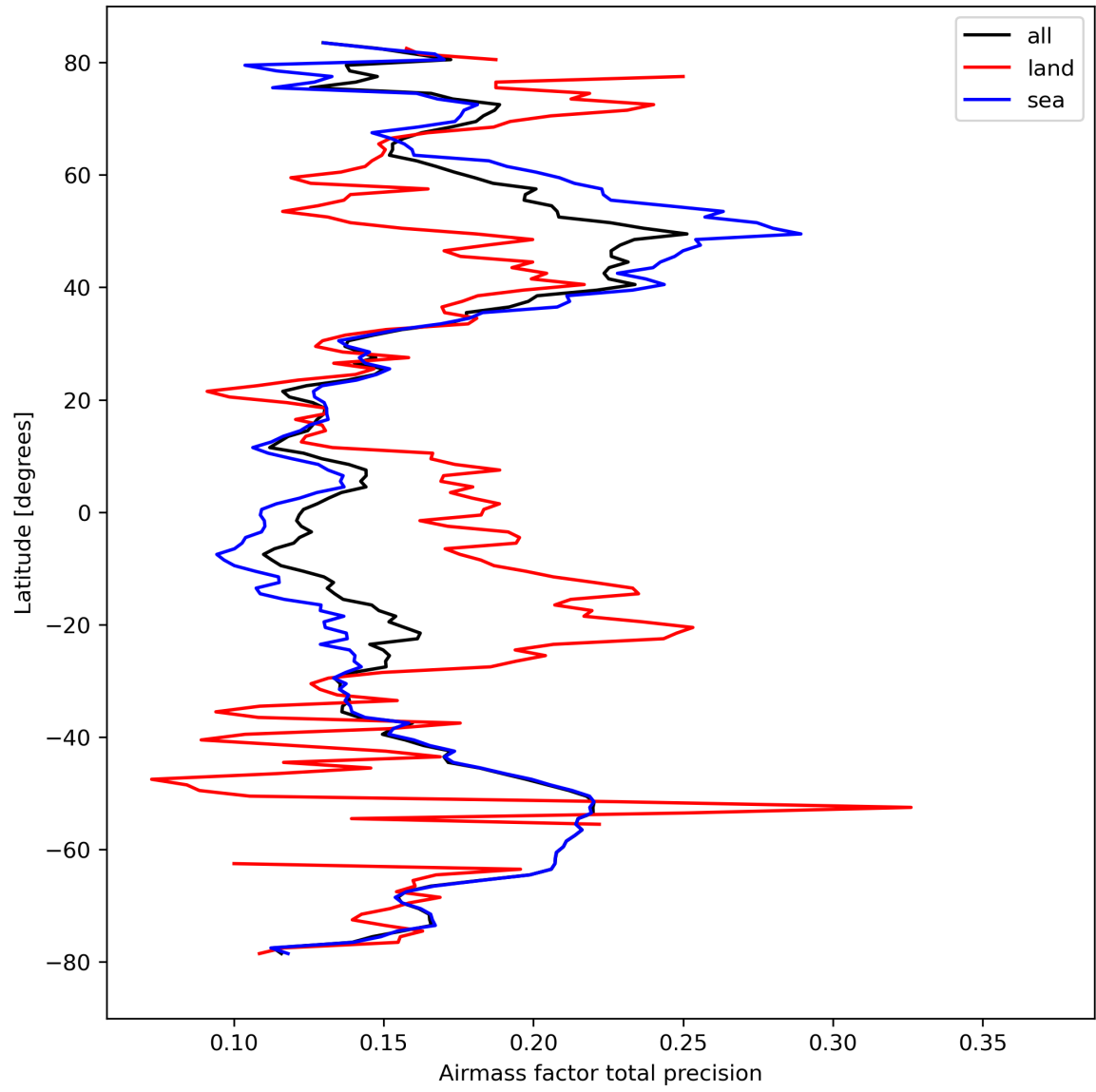
Figure 27: Zonal average of “Airmass factor total precision” for 2024-03-26 to 2024-03-28.
