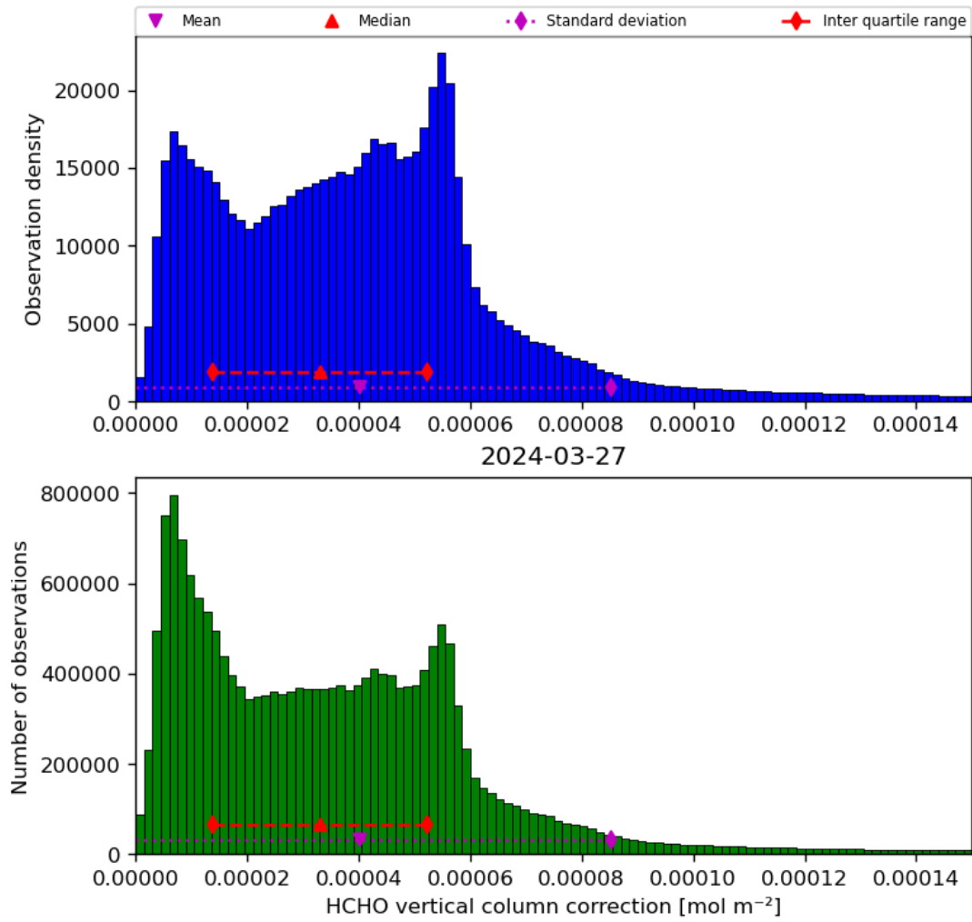
Figure 37: Histogram of “HCHO vertical column correction” for 2024-03-26 to 2024-03-28
