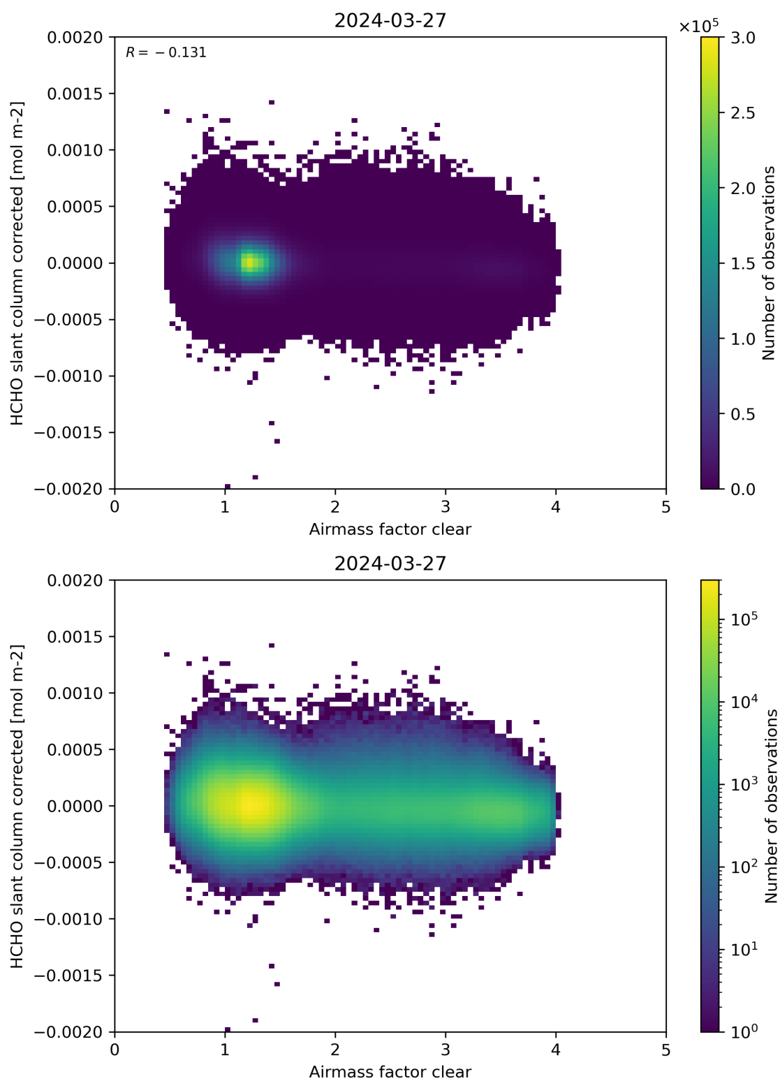
Figure 74: Scatter density plot of “Airmass factor clear” against “HCHO slant column corrected” for 2024-03-26 to 2024-03-28.
