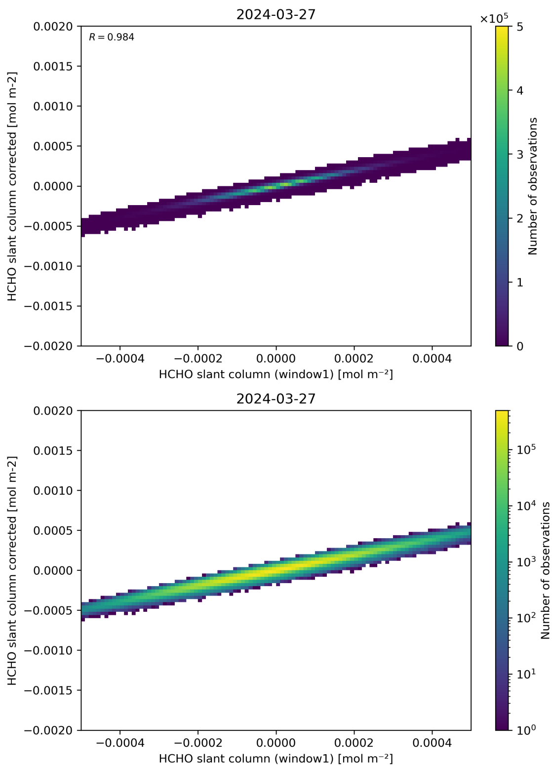
Figure 82: Scatter density plot of “HCHO slant column (window1)” against “HCHO slant column corrected” for 2024-03-26 to 2024-03-28.
