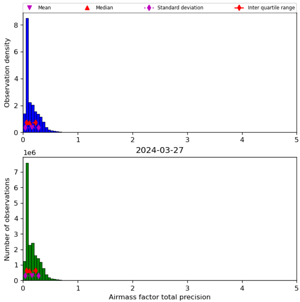
Figure 41: Histogram of “Airmass factor total precision” for 2024-03-26 to 2024-03-28
