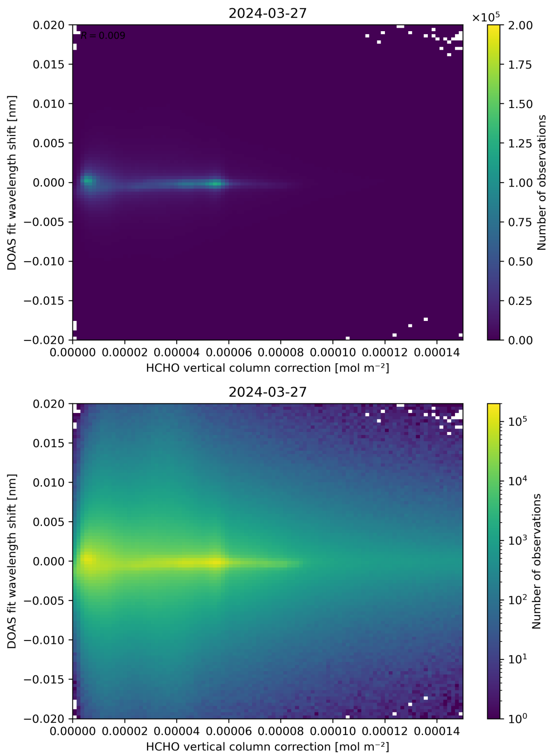
Figure 113: Scatter density plot of “HCHO vertical column correction” against “DOAS fit wavelength shift” for 2024-03-26 to 2024-03-28.
