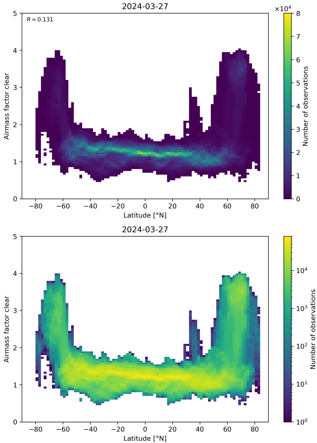
Figure 156: Scatter density plot of “Latitude” against “Airmass factor clear” for 2024-03-26 to 2024-03-28.
