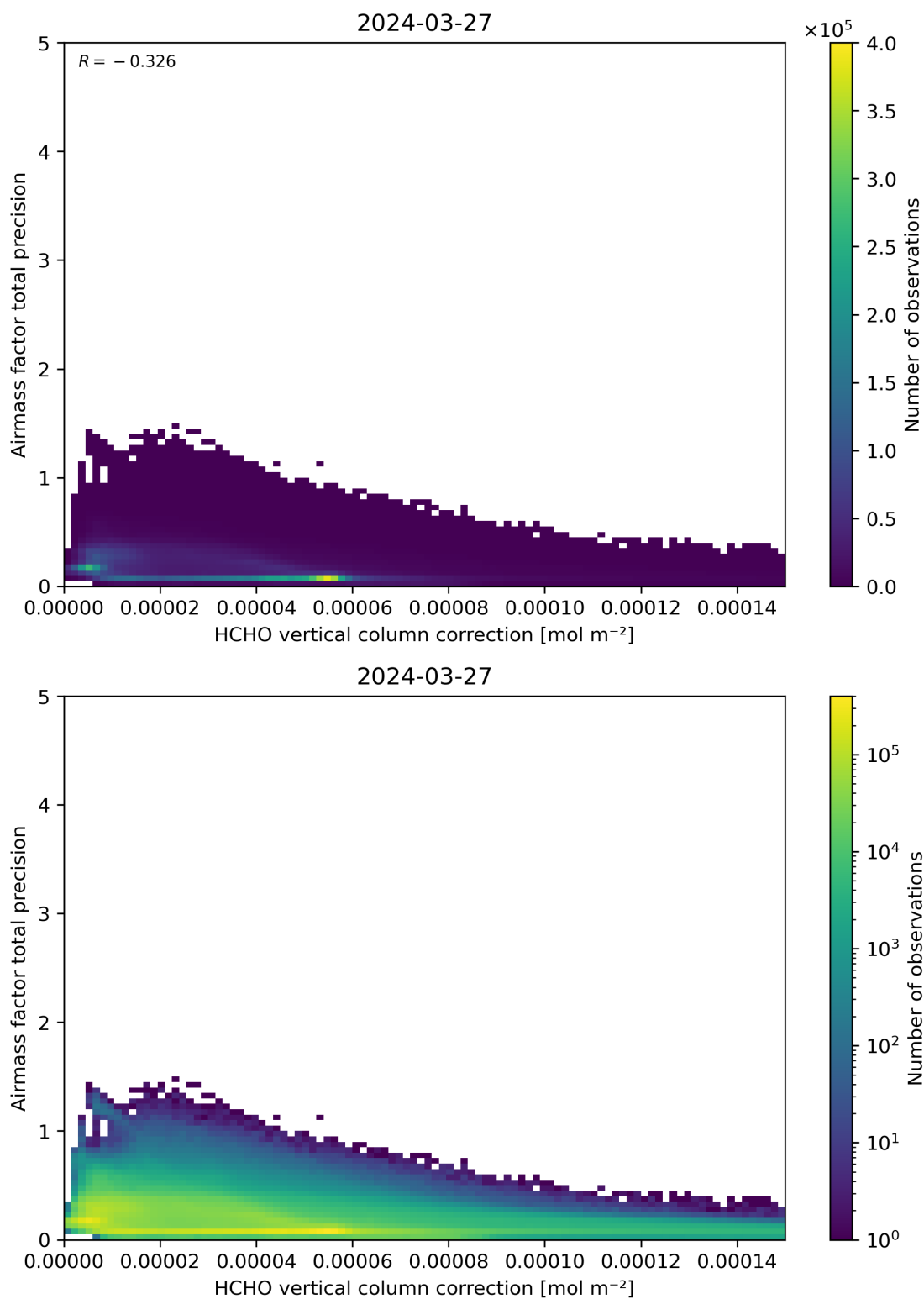
Figure 121: Scatter density plot of “HCHO vertical column correction” against “Airmass factor total precision” for 2024-03-26 to 2024-03-28.
