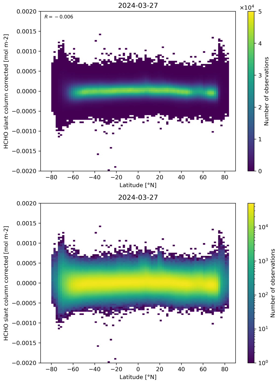
Figure 157: Scatter density plot of “Latitude” against “HCHO slant column corrected” for 2024-03-26 to 2024-03-28.
