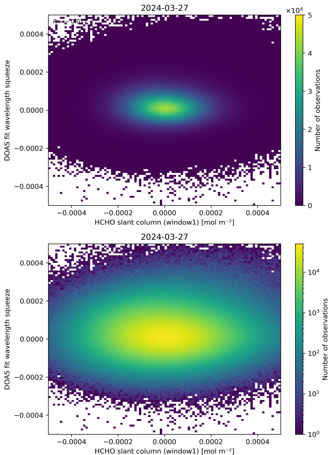
Figure 80: Scatter density plot of “HCHO slant column (window1)” against “DOAS fit wavelength squeeze” for 2024-03-26 to 2024-03-28.
