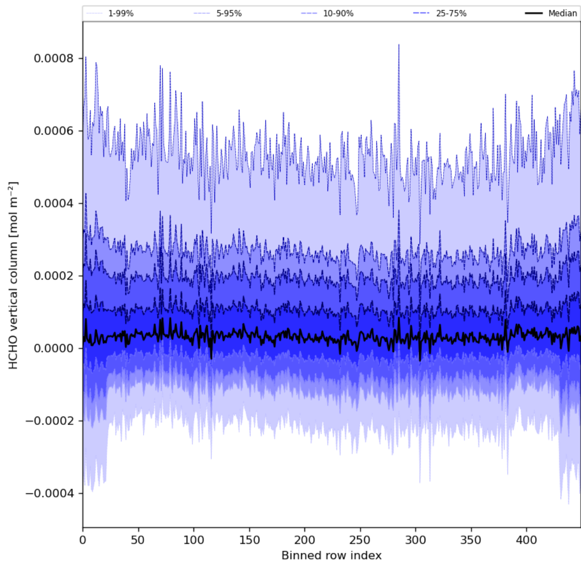
Figure 49: Along track statistics of “HCHO vertical column” for 2024-03-26 to 2024-03-28
