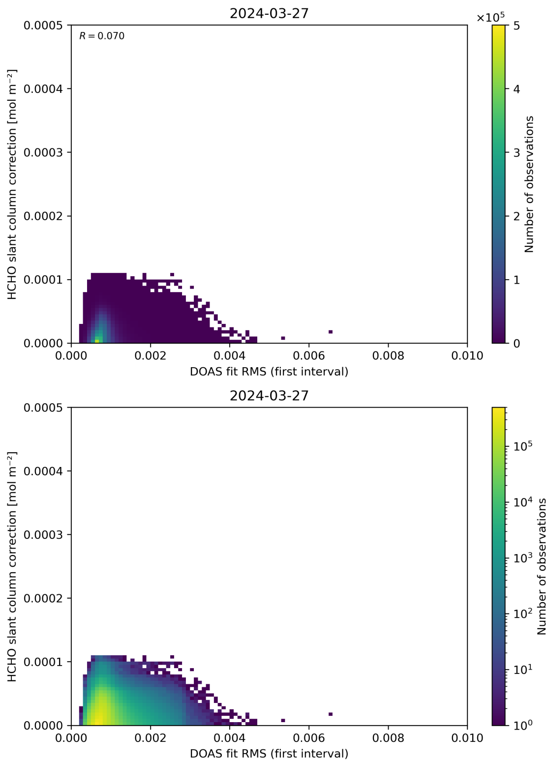
Figure 63: Scatter density plot of “DOAS fit RMS (first interval)” against “HCHO slant column correction” for 2024-03-26 to 2024-03-28.
