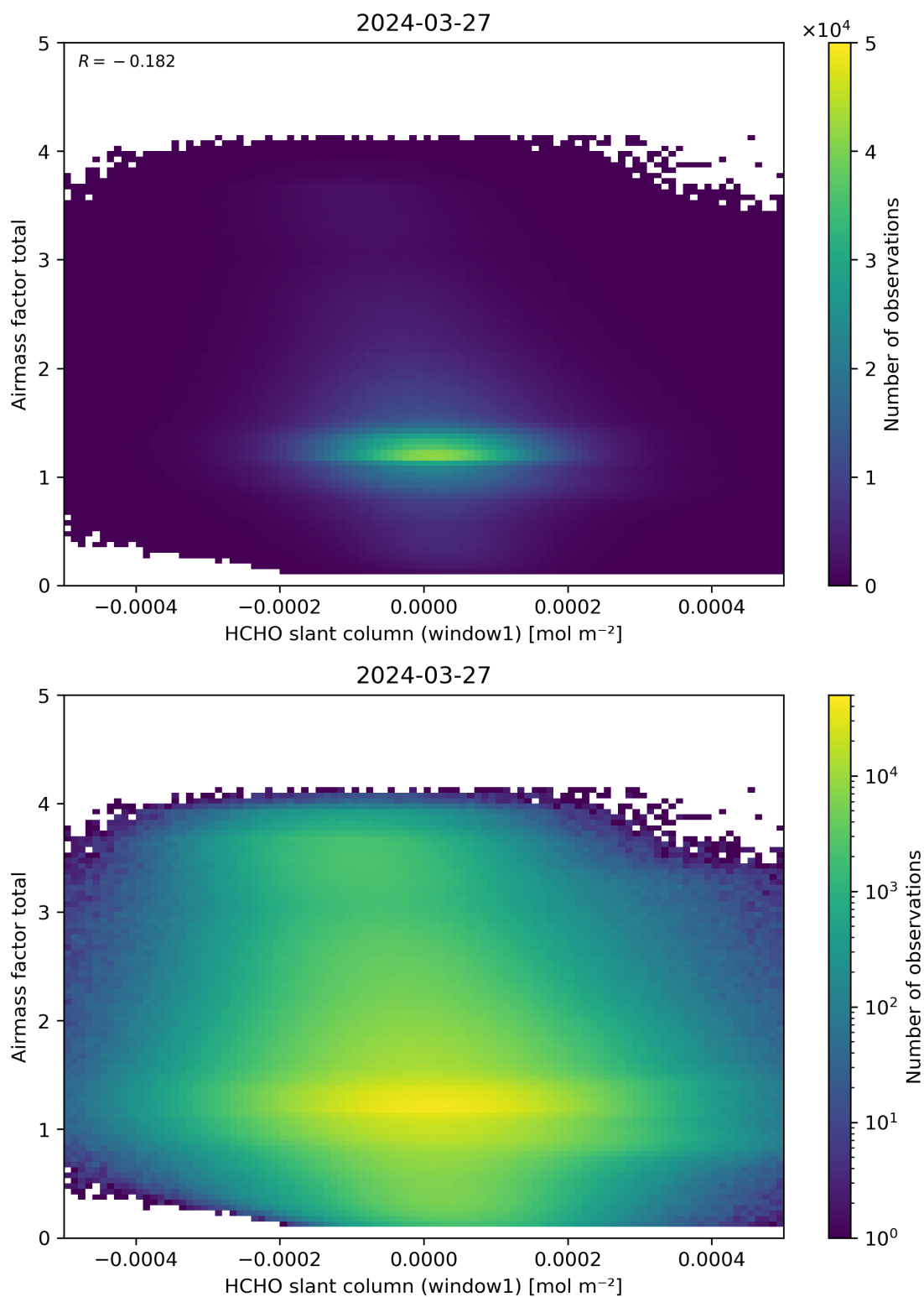
Figure 85: Scatter density plot of “HCHO slant column (window1)” against “Airmass factor total” for 2024-03-26 to 2024-03-28.
