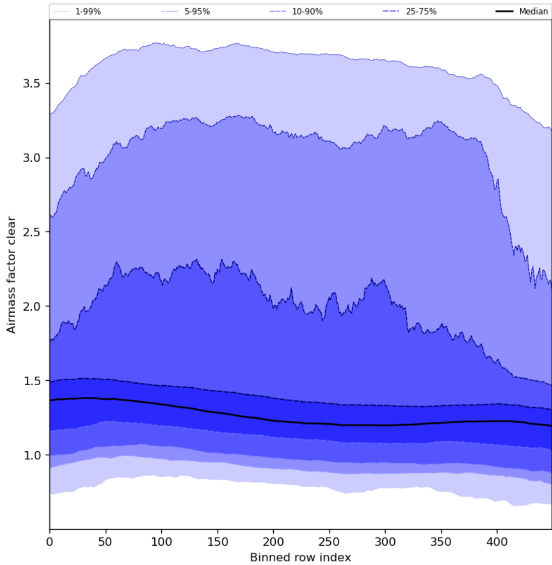
Figure 56: Along track statistics of “Airmass factor clear” for 2024-03-26 to 2024-03-28
