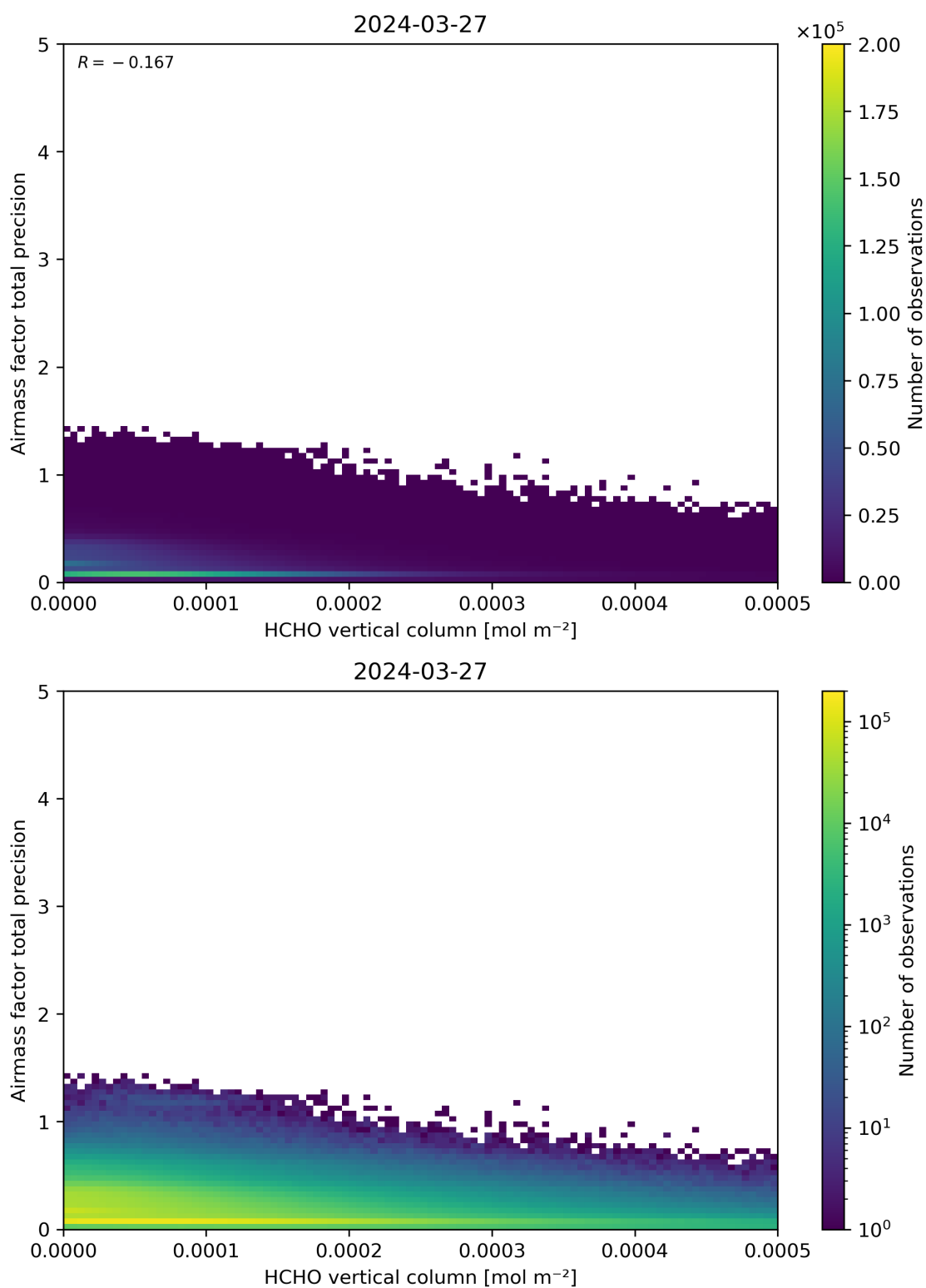
Figure 132: Scatter density plot of “HCHO vertical column” against “Airmass factor total precision” for 2024-03-26 to 2024-03-28.
