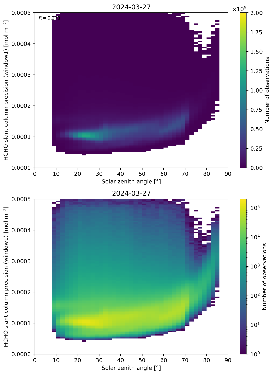
Figure 174: Scatter density plot of “Solar zenith angle” against “HCHO slant column precision (window1)” for 2024-03-26 to 2024-03-28.
