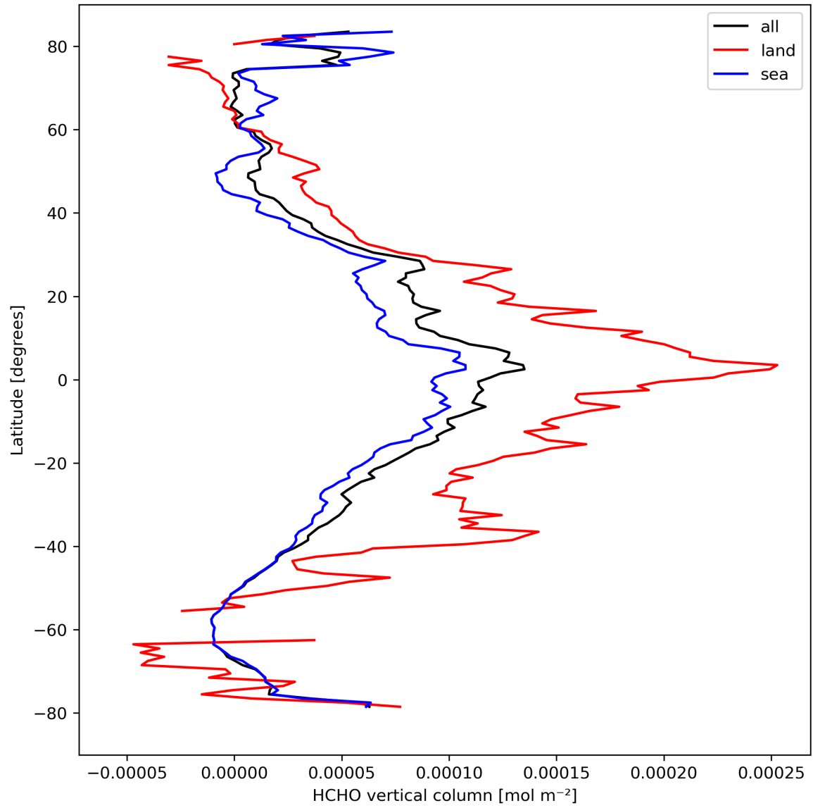
Figure 21: Zonal average of “HCHO vertical column” for 2024-03-26 to 2024-03-28.
