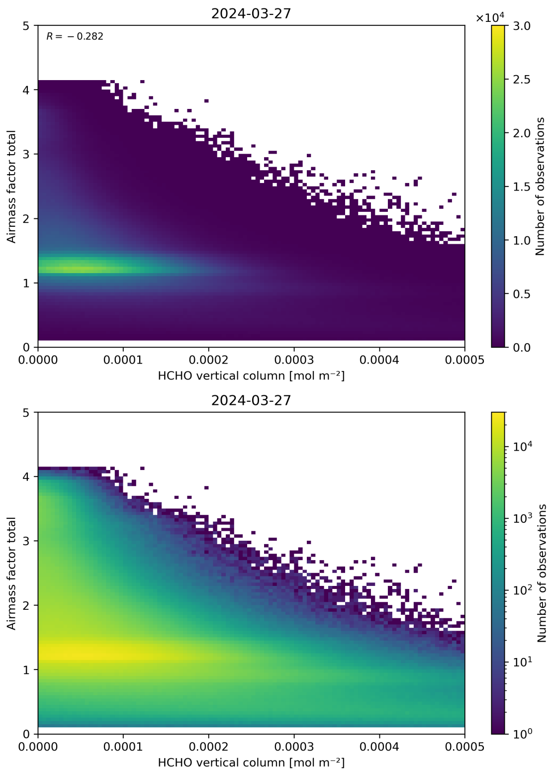
Figure 131: Scatter density plot of “HCHO vertical column” against “Airmass factor total” for 2024-03-26 to 2024-03-28.
