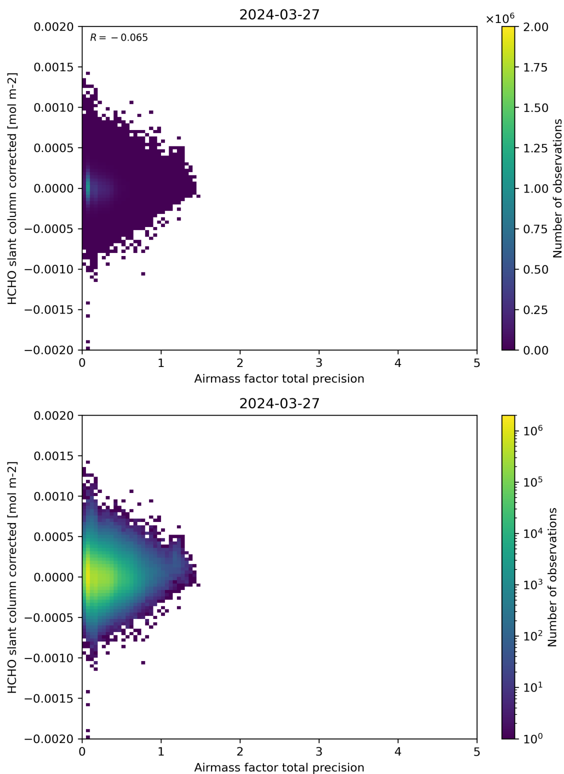
Figure 109: Scatter density plot of “Airmass factor total precision” against “HCHO slant column corrected” for 2024-03-26 to 2024-03-28.
