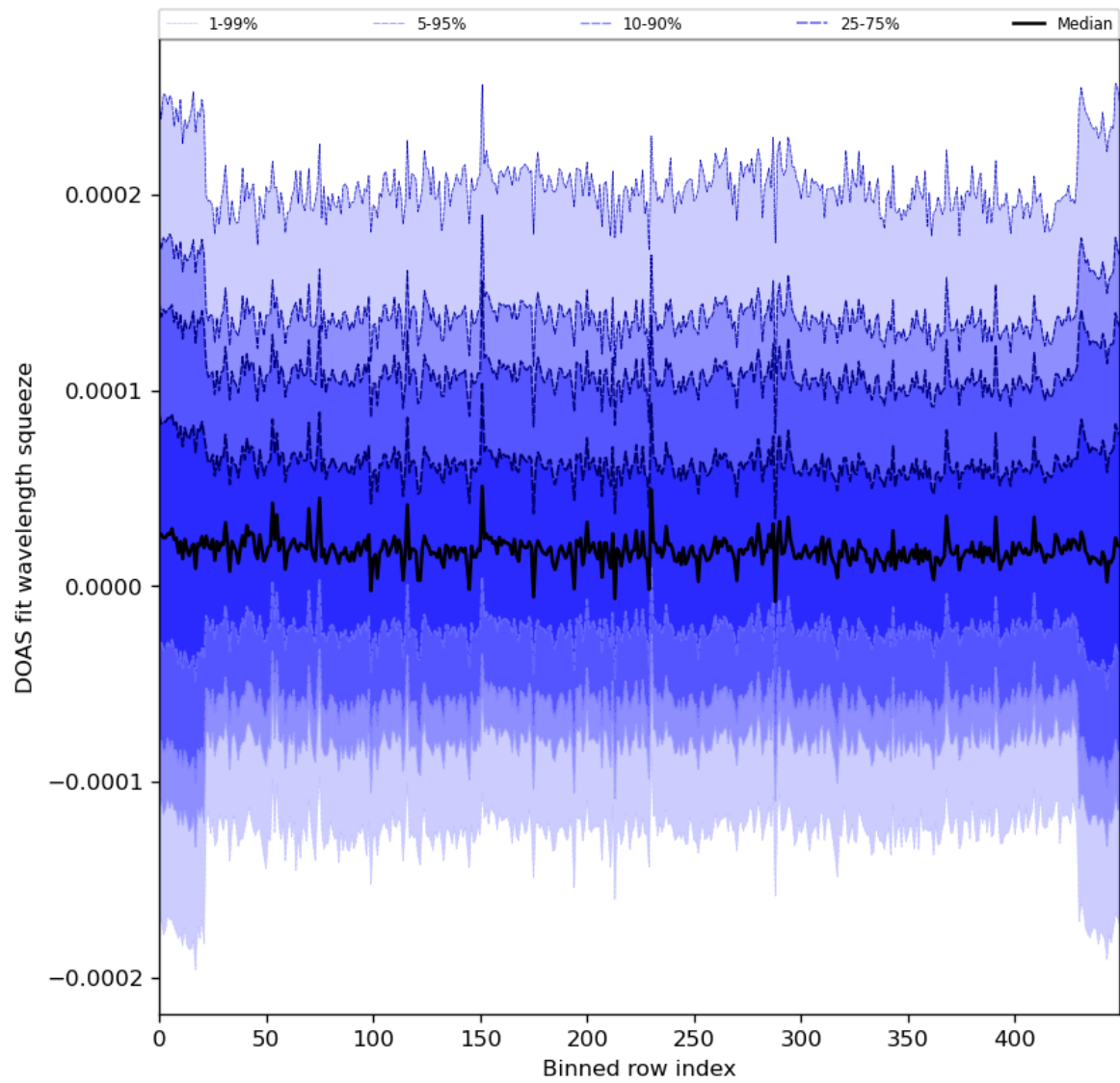
Figure 59: Along track statistics of “DOAS fit wavelength squeeze” for 2024-03-26 to 2024-03-28
