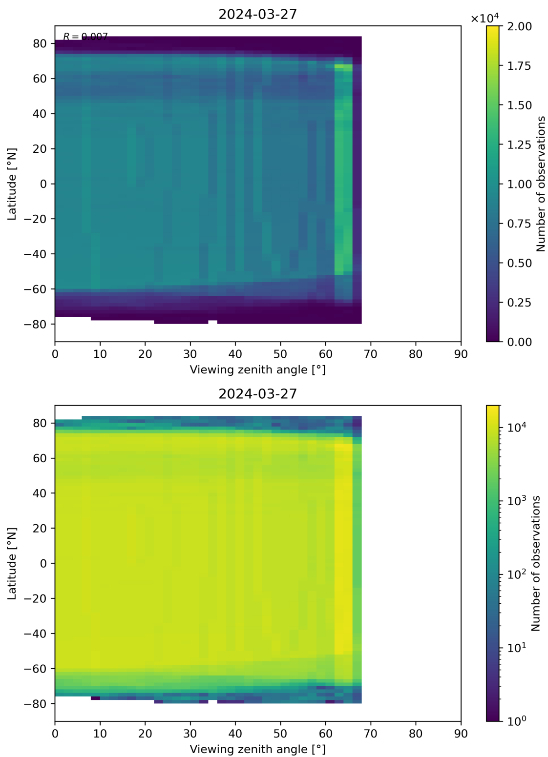
Figure 196: Scatter density plot of “Viewing zenith angle” against “Latitude” for 2024-03-26 to 2024-03-28.
