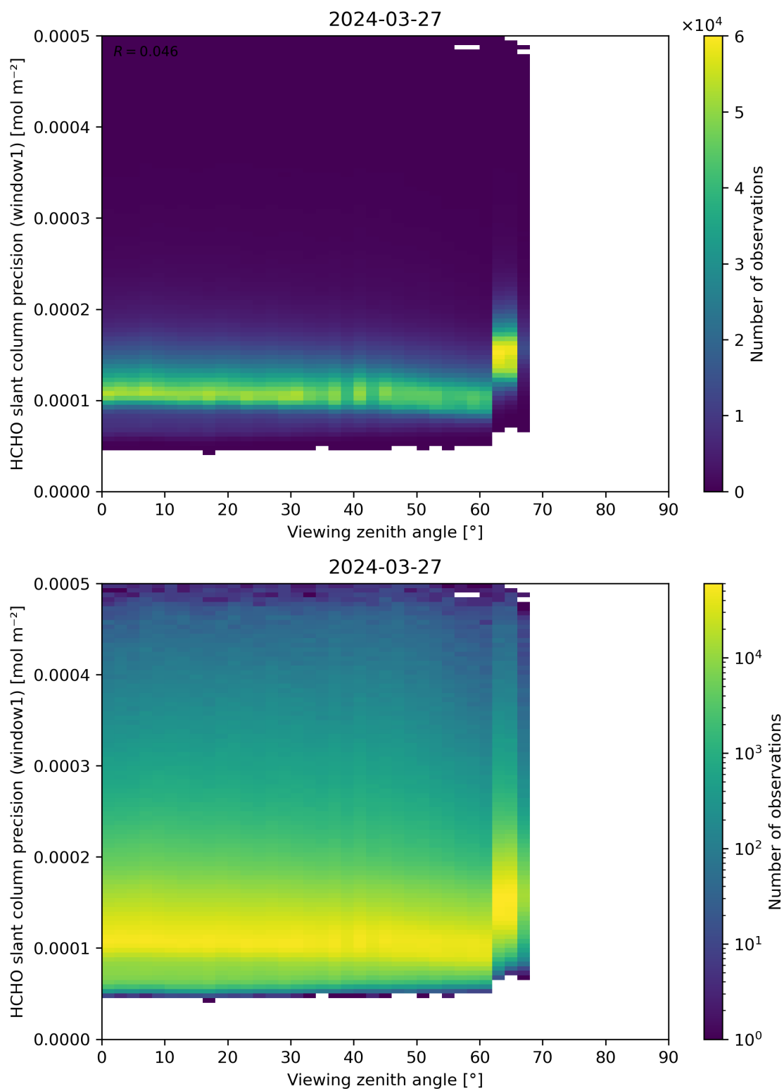
Figure 189: Scatter density plot of “Viewing zenith angle” against “HCHO slant column precision (window1)” for 2024-03-26 to 2024-03-28.
