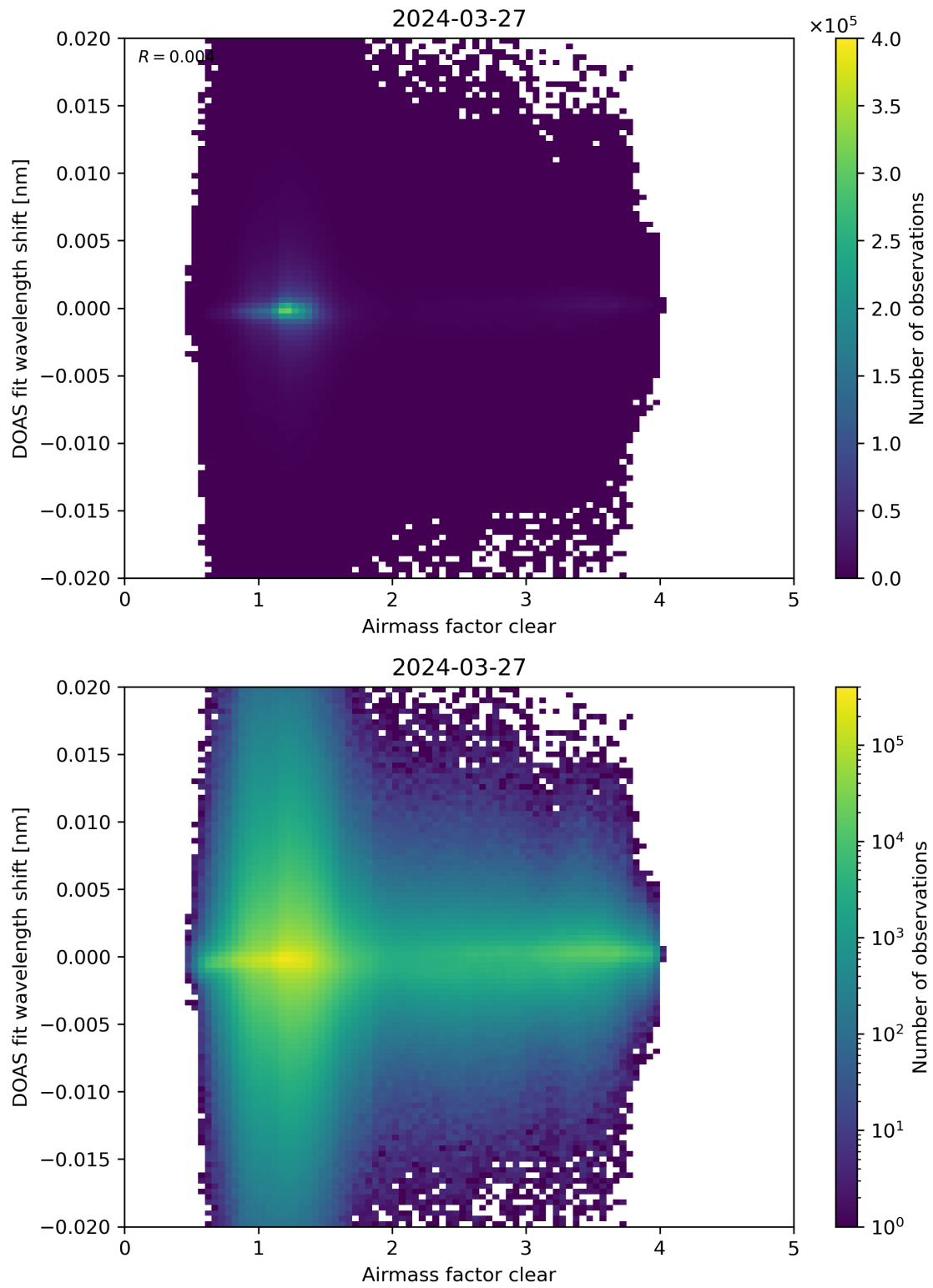
Figure 72: Scatter density plot of “Airmass factor clear” against “DOAS fit wavelength shift” for 2024-03-26 to 2024-03-28.
