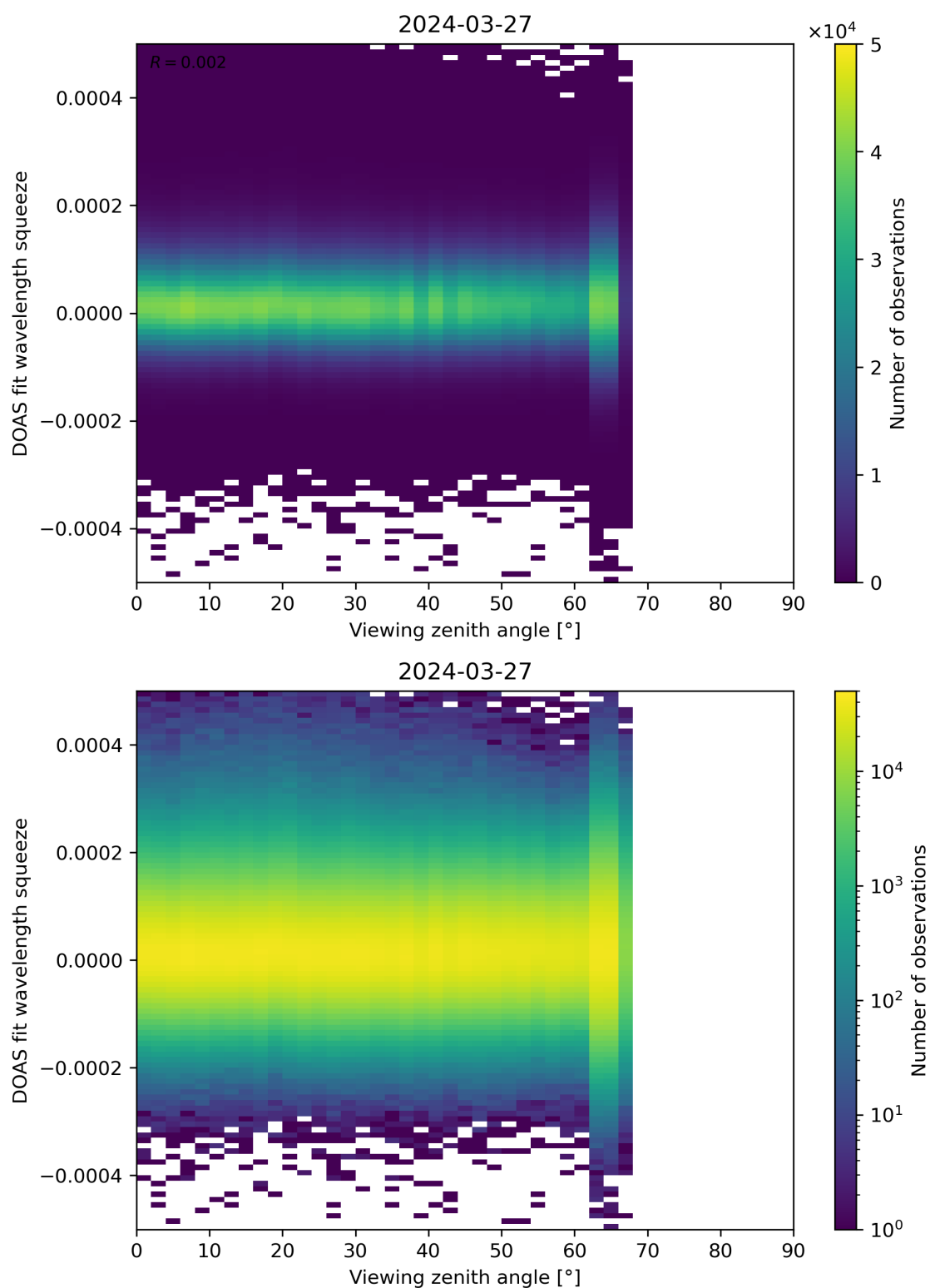
Figure 184: Scatter density plot of “Viewing zenith angle” against “DOAS fit wavelength squeeze” for 2024-03-26 to 2024-03-28.
