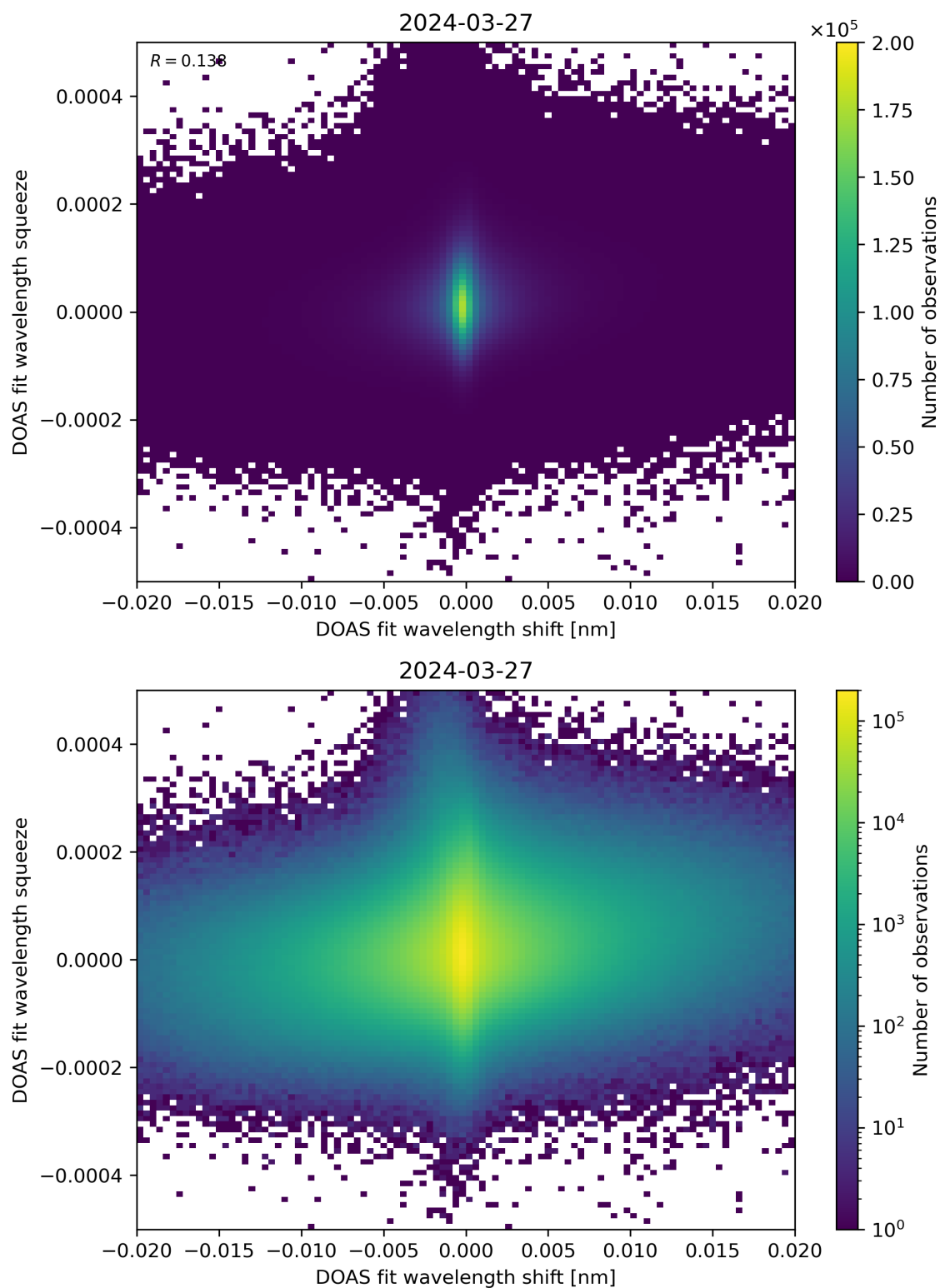
Figure 65: Scatter density plot of “DOAS fit wavelength shift” against “DOAS fit wavelength squeeze” for 2024-03-26 to 2024-03-28.
