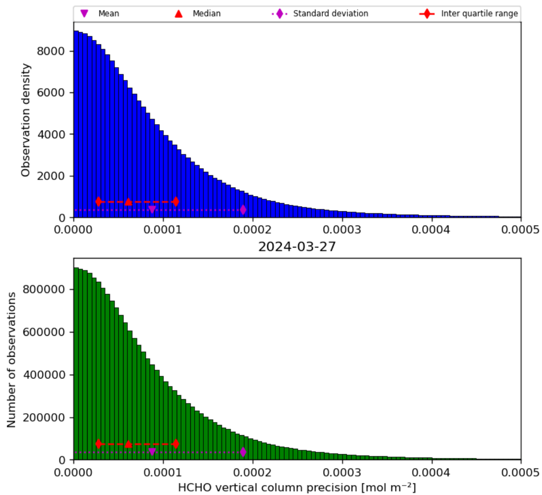
Figure 36: Histogram of “HCHO vertical column precision” for 2024-03-26 to 2024-03-28
