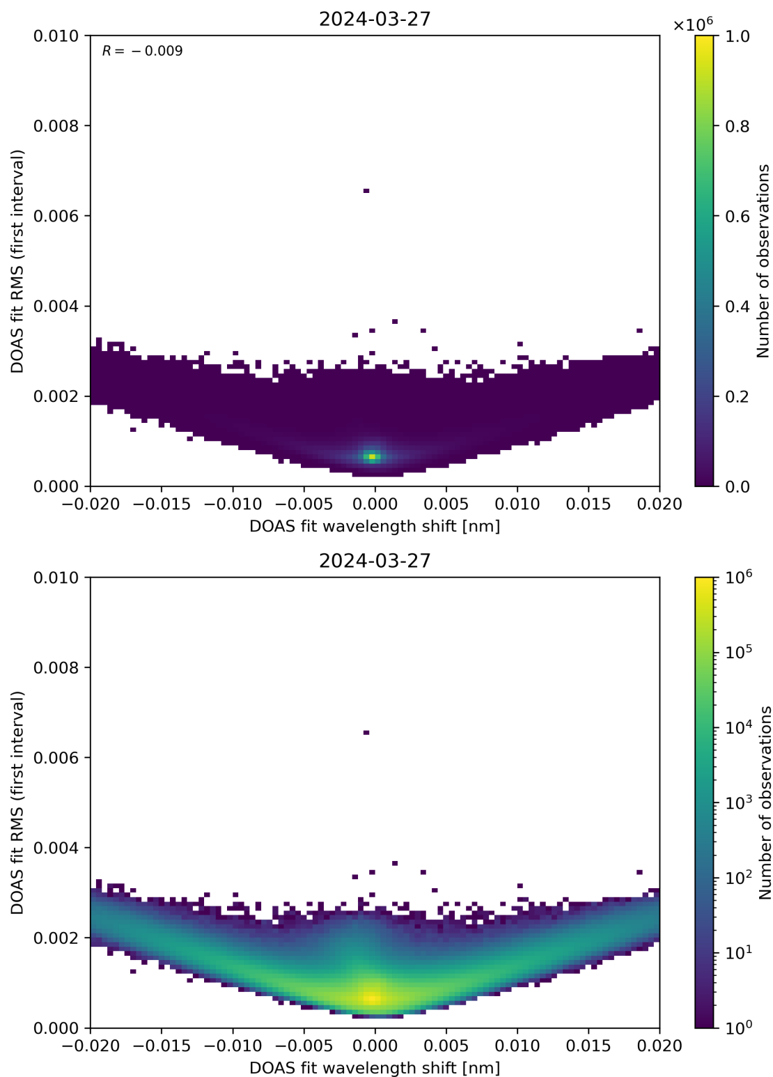
Figure 64: Scatter density plot of “DOAS fit wavelength shift” against “DOAS fit RMS (first interval)” for 2024-03-26 to 2024-03-28.
