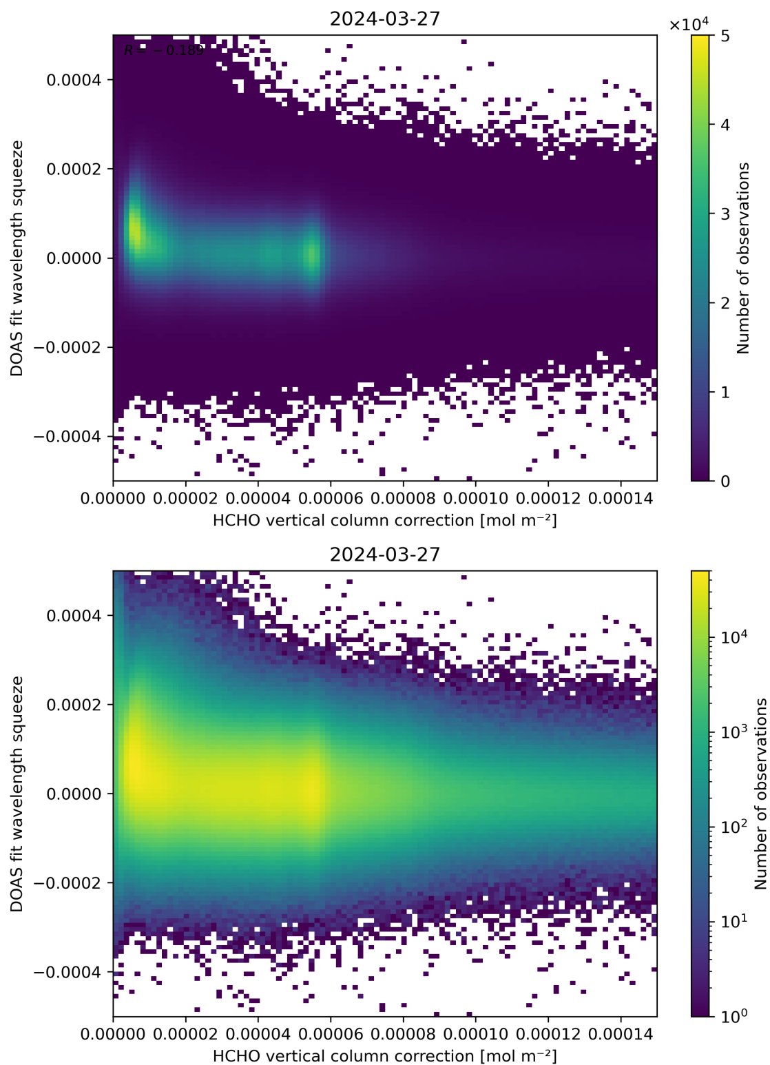
Figure 114: Scatter density plot of “HCHO vertical column correction” against “DOAS fit wavelength squeeze” for 2024-03-26 to 2024-03-28.
