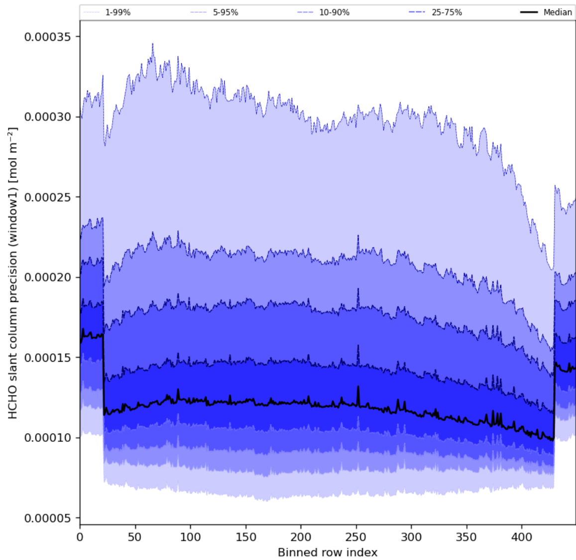
Figure 53: Along track statistics of “HCHO slant column precision (window1)” for 2024-03-26 to 2024-03-28
