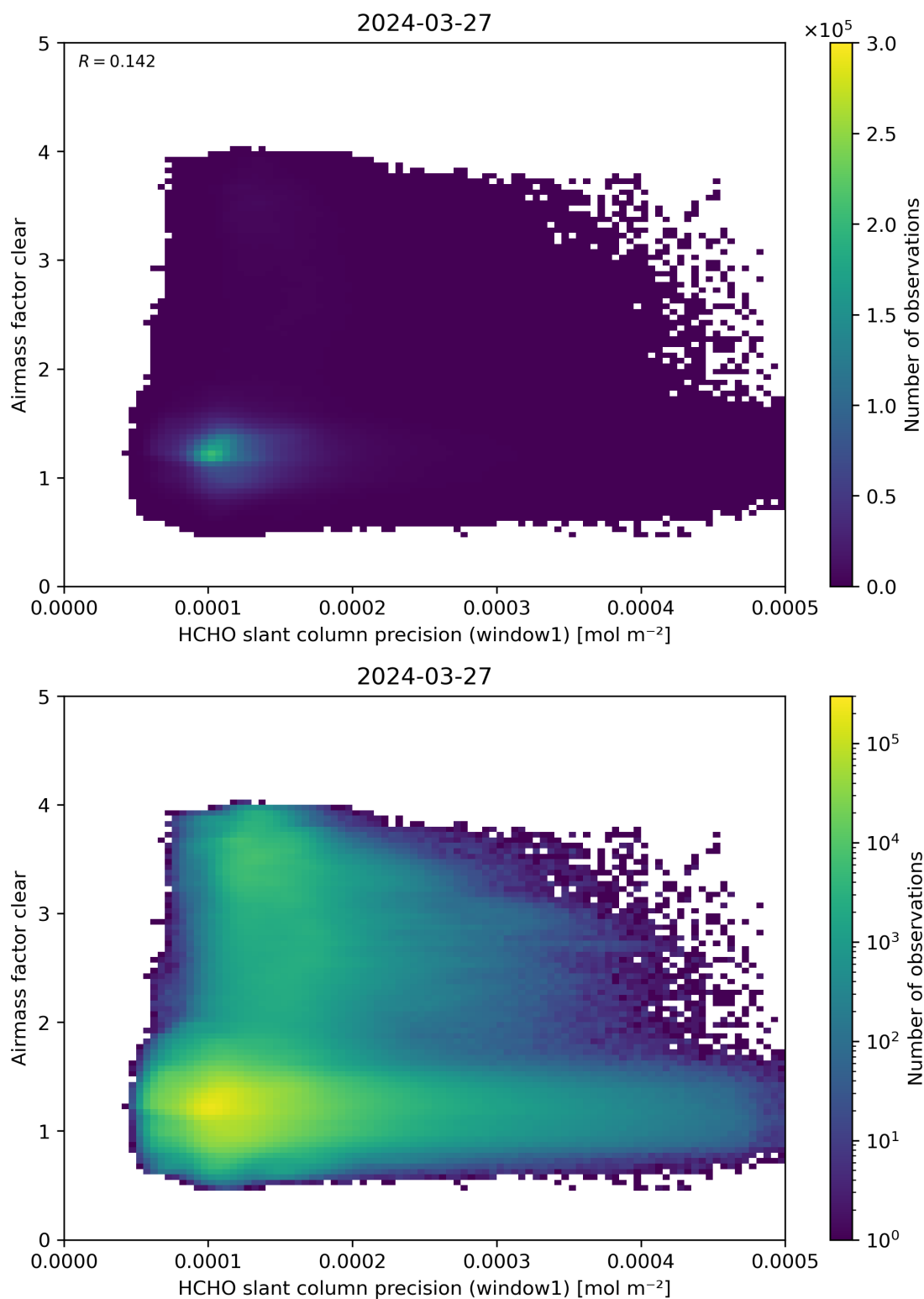
Figure 91: Scatter density plot of “HCHO slant column precision (window1)” against “Airmass factor clear” for 2024-03-26 to 2024-03-28.
