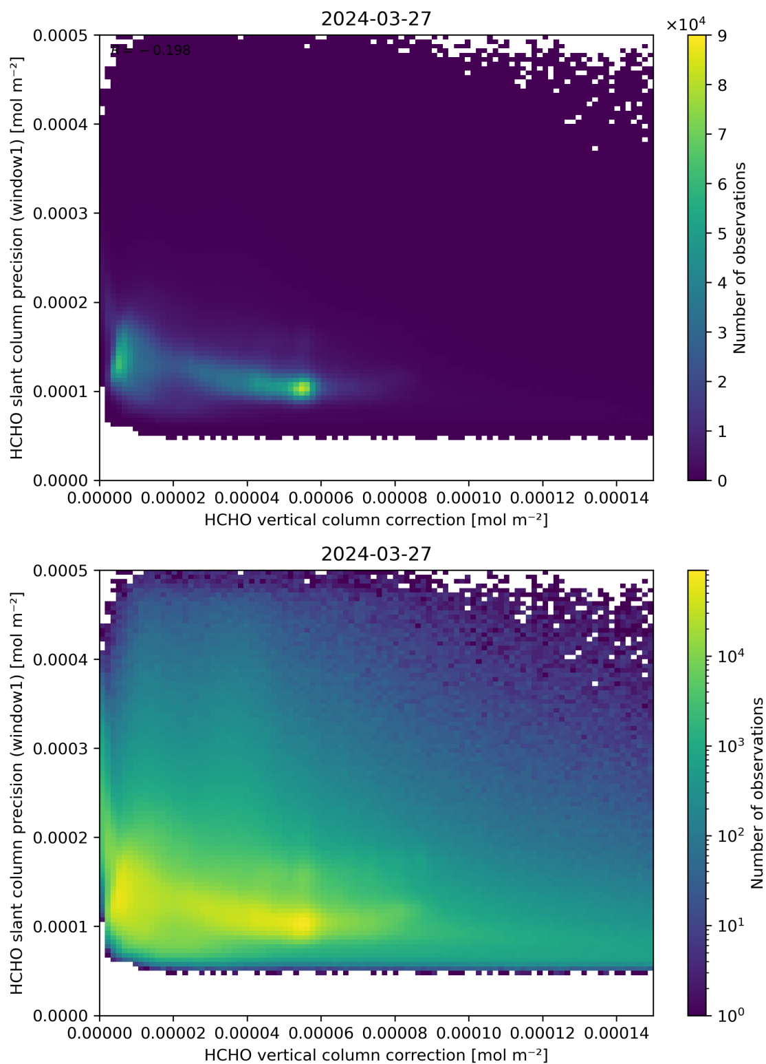
Figure 119: Scatter density plot of “HCHO vertical column correction” against “HCHO slant column precision (window1)” for 2024-03-26 to 2024-03-28.
