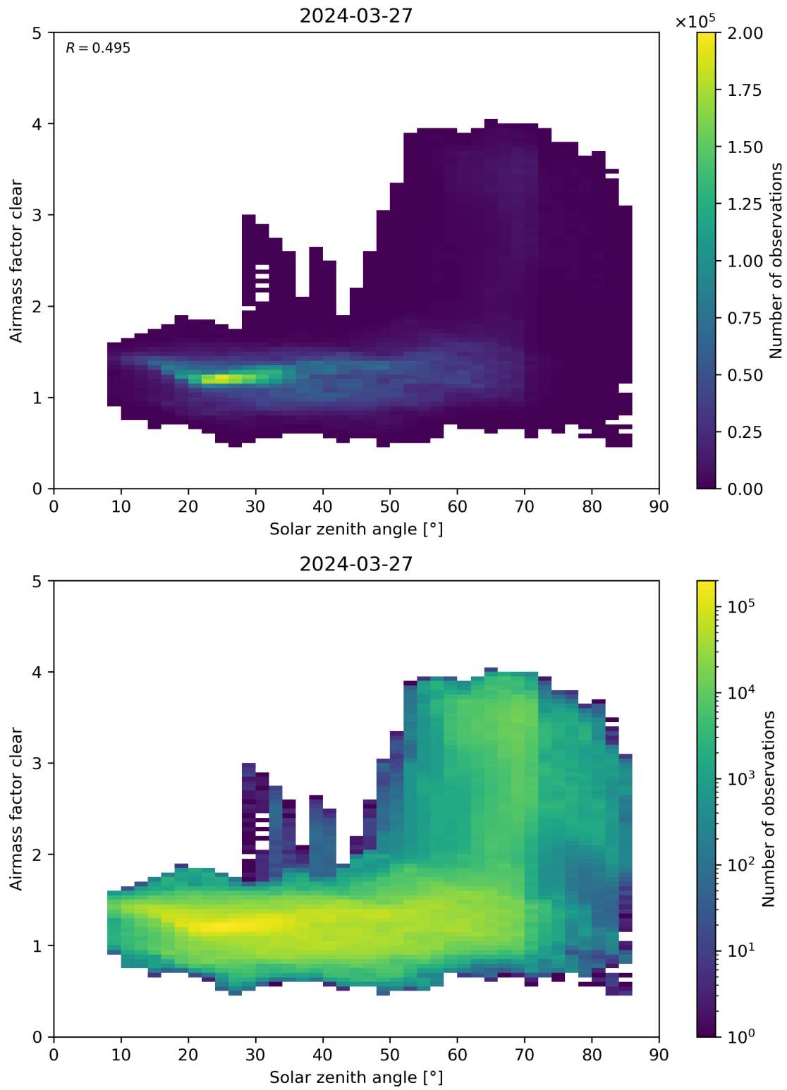
Figure 170: Scatter density plot of “Solar zenith angle” against “Airmass factor clear” for 2024-03-26 to 2024-03-28.
