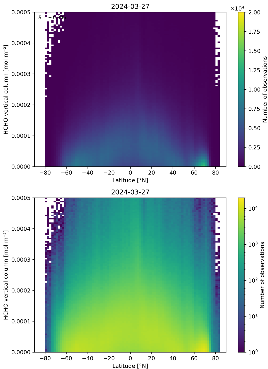
Figure 163: Scatter density plot of “Latitude” against “HCHO vertical column” for 2024-03-26 to 2024-03-28.
