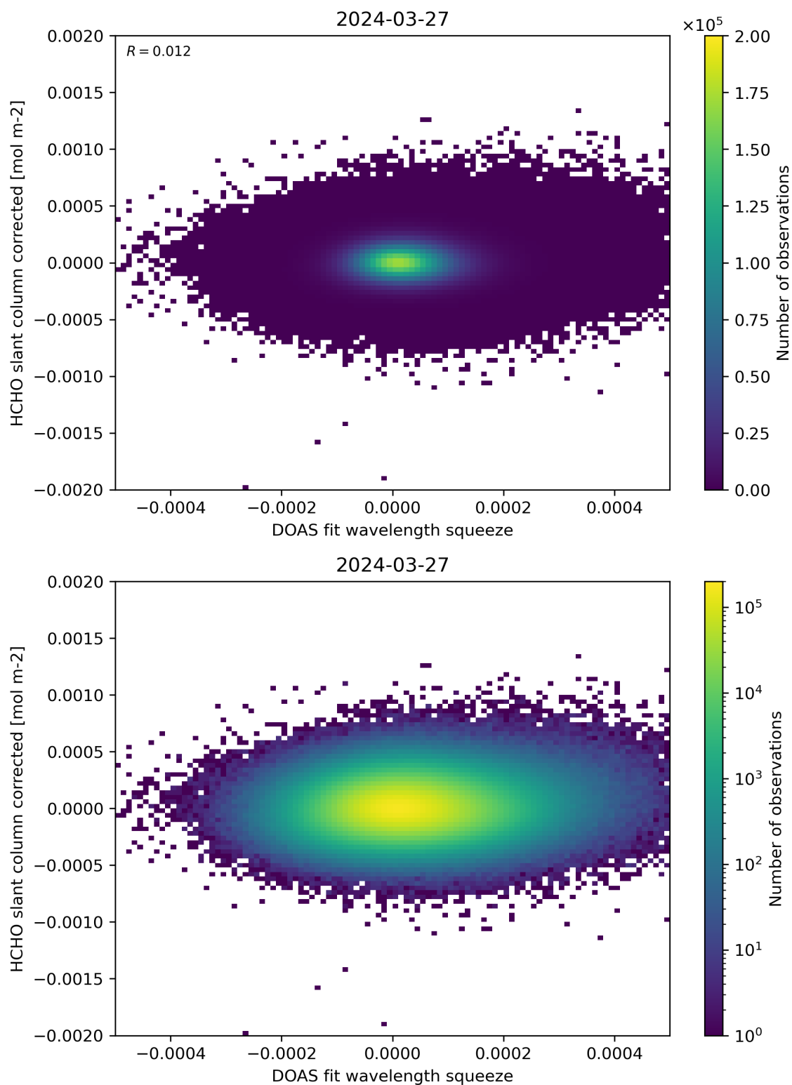
Figure 69: Scatter density plot of “DOAS fit wavelength squeeze” against “HCHO slant column corrected” for 2024-03-26 to 2024-03-28.
