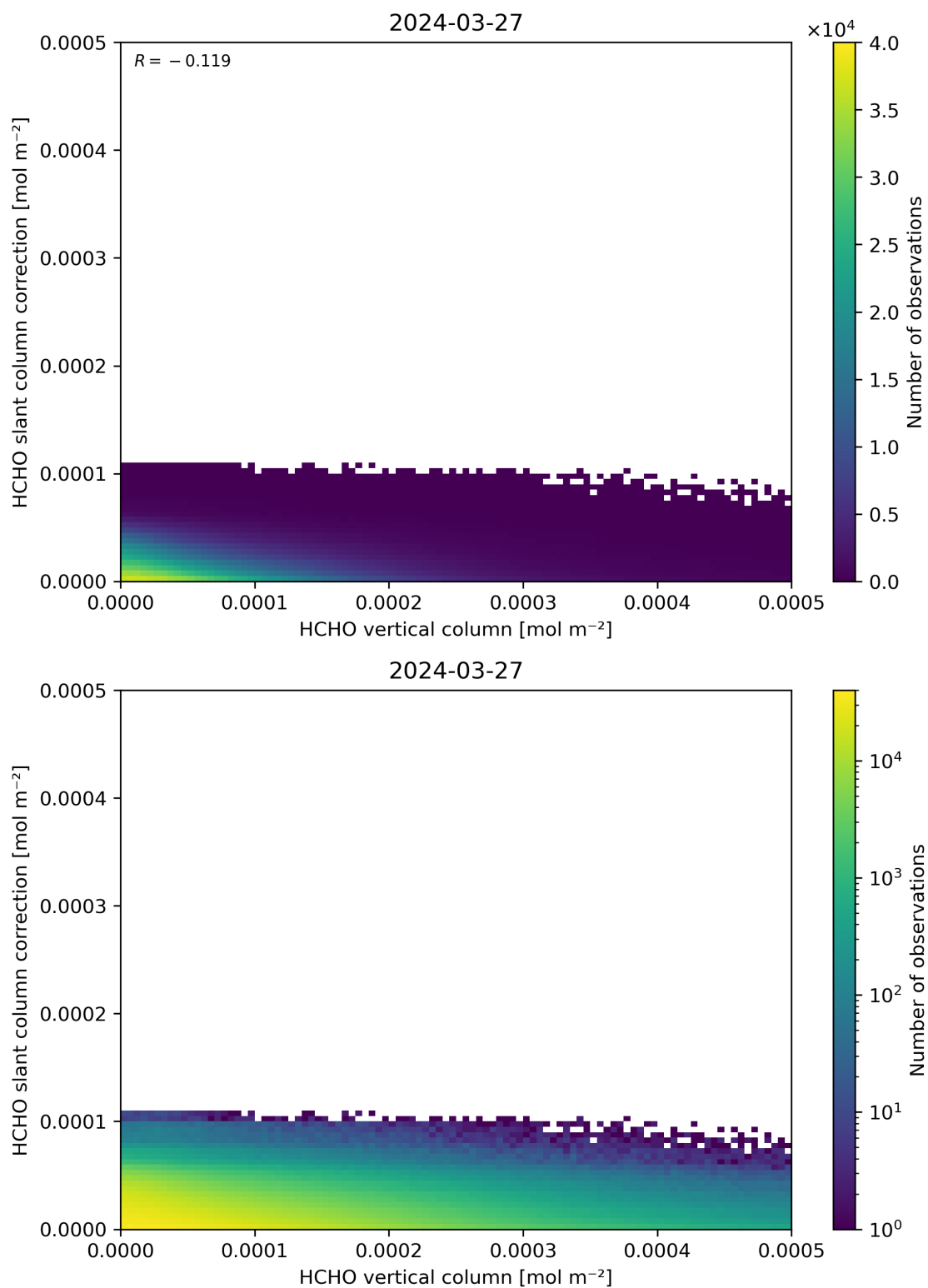
Figure 128: Scatter density plot of “HCHO vertical column” against “HCHO slant column correction” for 2024-03-26 to 2024-03-28.
