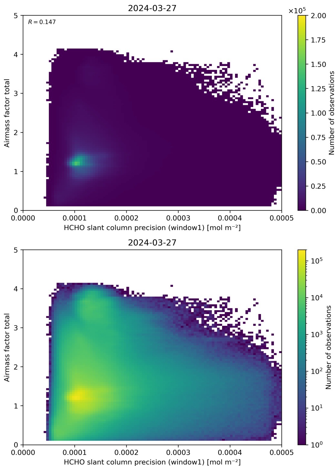
Figure 94: Scatter density plot of “HCHO slant column precision (window1)” against “Airmass factor total” for 2024-03-26 to 2024-03-28.
