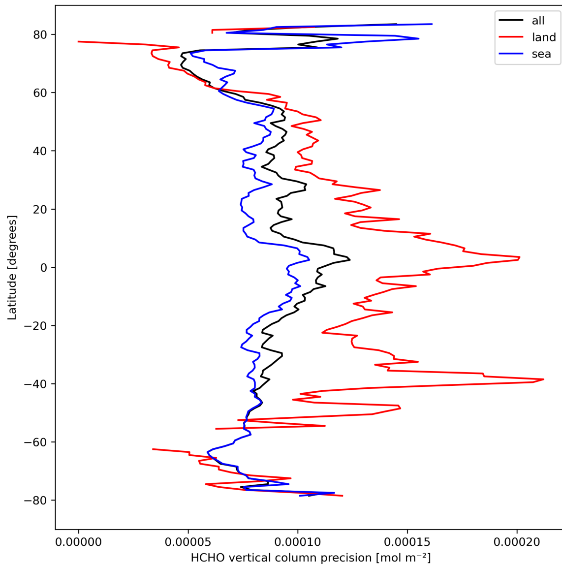
Figure 22: Zonal average of “HCHO vertical column precision” for 2024-03-26 to 2024-03-28.
