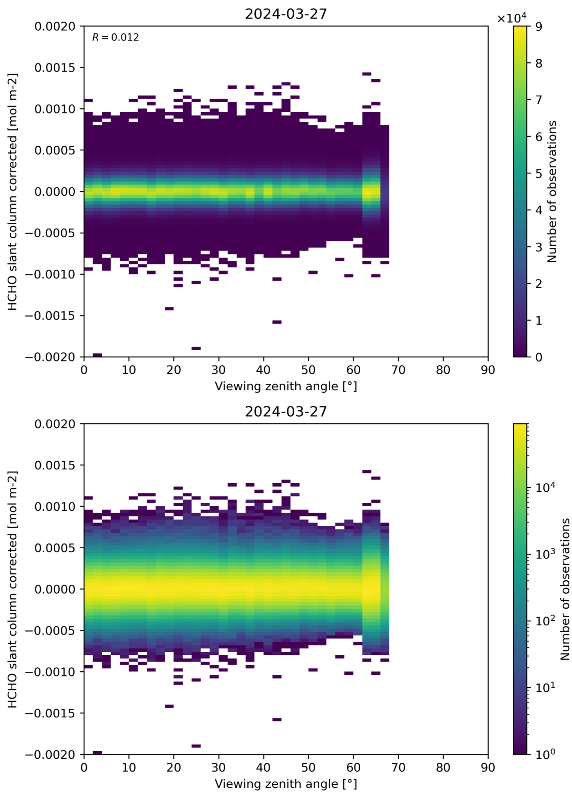
Figure 186: Scatter density plot of “Viewing zenith angle” against “HCHO slant column corrected” for 2024-03-26 to 2024-03-28.
