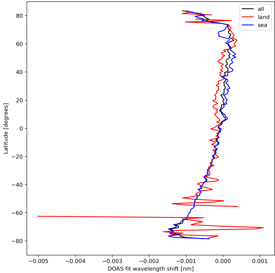
Figure 30: Zonal average of “DOAS fit wavelength shift” for 2024-03-26 to 2024-03-28.
