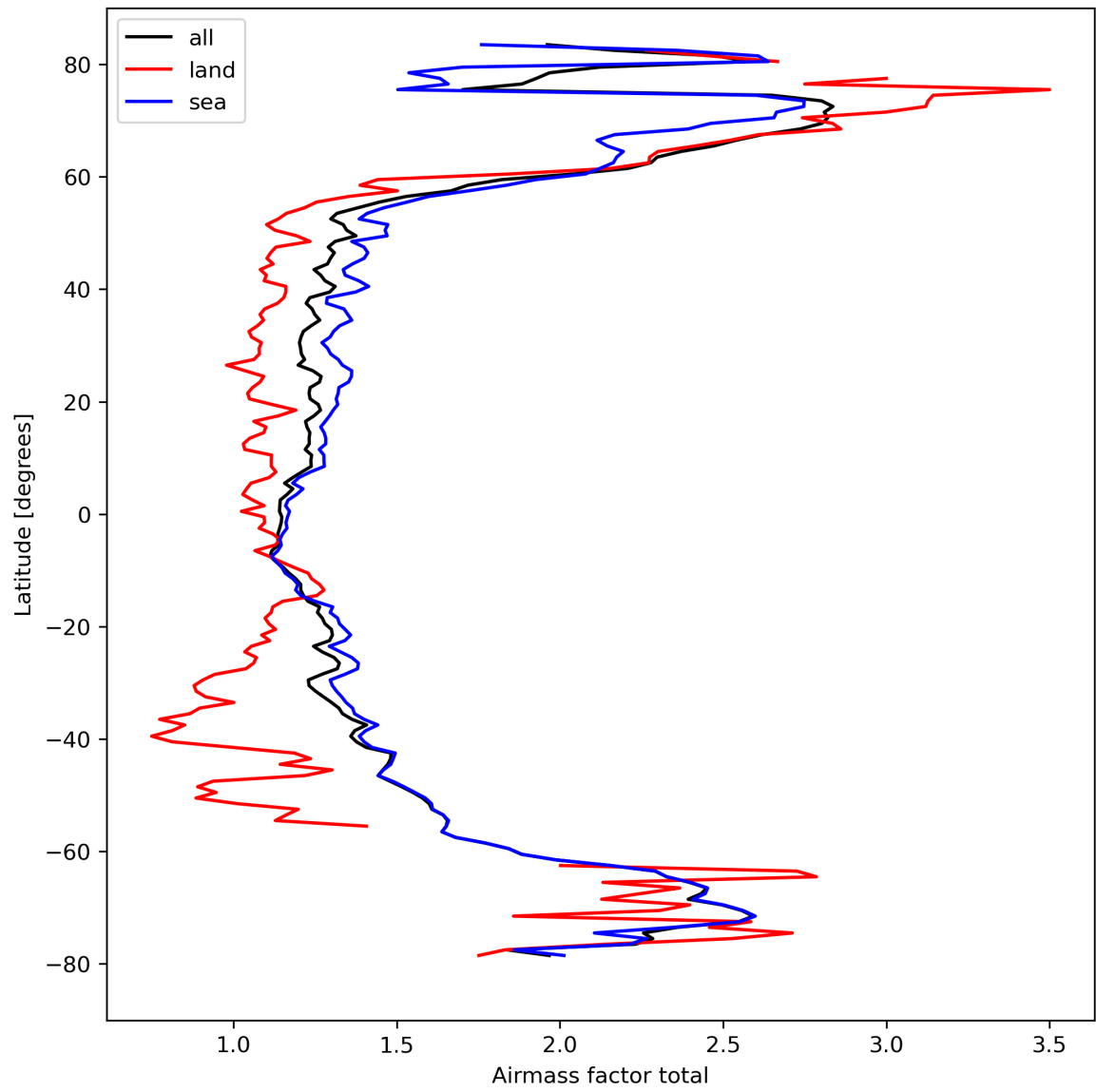
Figure 26: Zonal average of “Airmass factor total” for 2024-03-26 to 2024-03-28.
