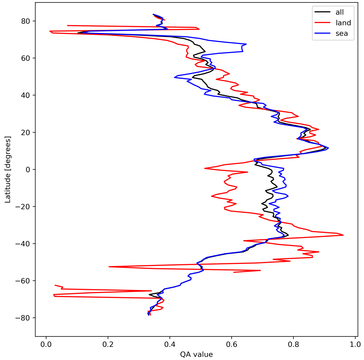
Figure 20: Zonal average of “QA value” for 2024-03-26 to 2024-03-28.
