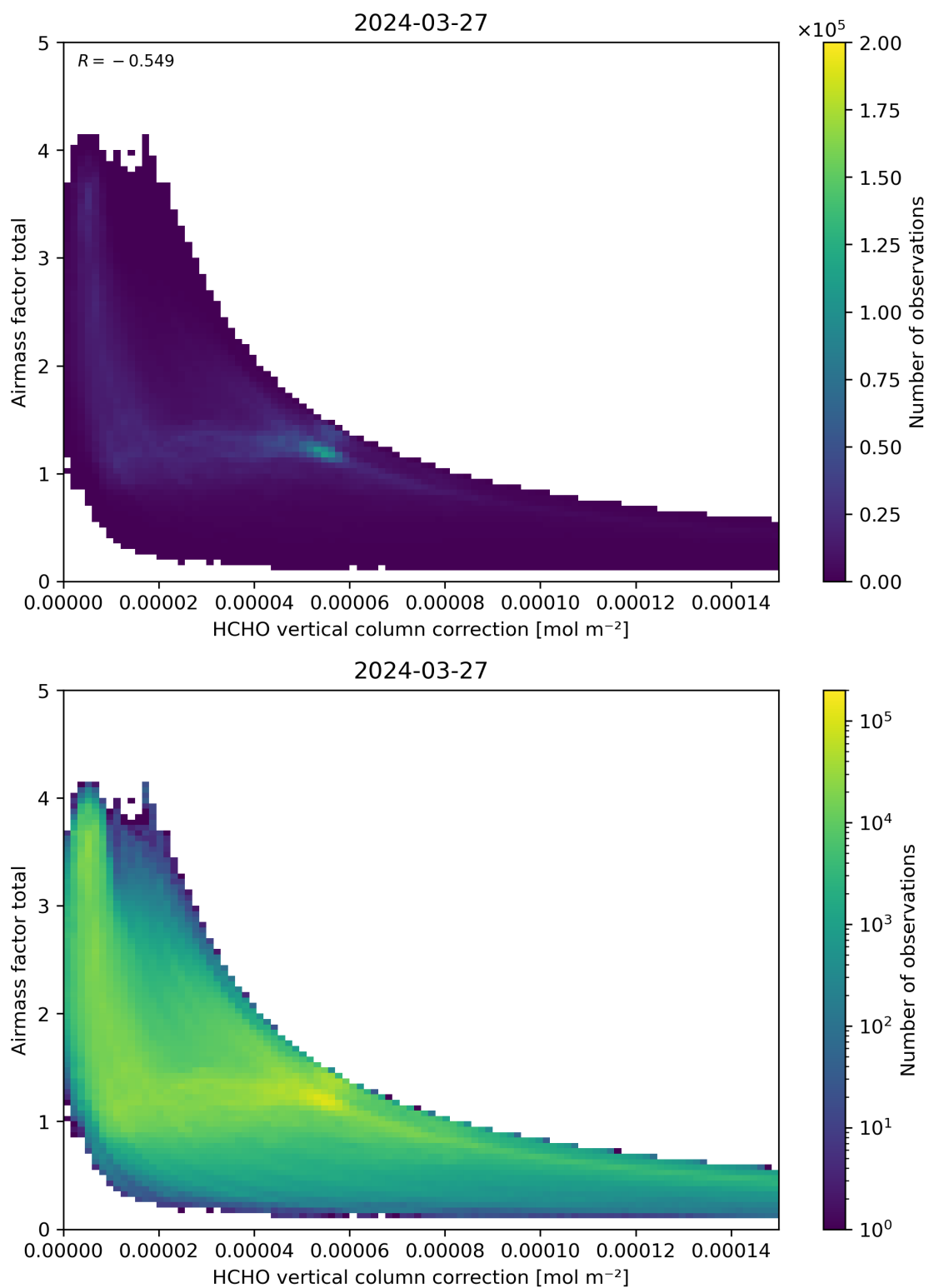
Figure 120: Scatter density plot of “HCHO vertical column correction” against “Airmass factor total” for 2024-03-26 to 2024-03-28.
