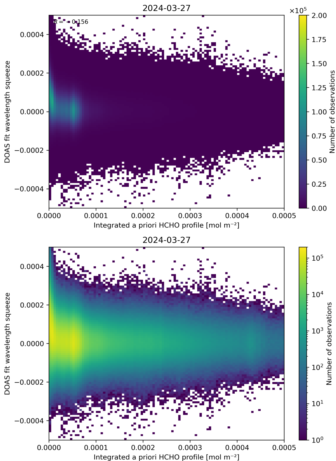
Figure 150: Scatter density plot of “Integrated a priori HCHO profile” against “DOAS fit wavelength squeeze” for 2024-03-26 to 2024-03-28.
