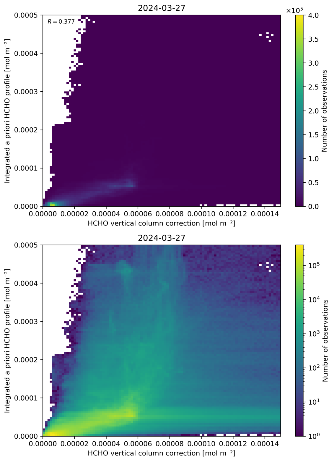
Figure 122: Scatter density plot of “HCHO vertical column correction” against “Integrated a priori HCHO profile” for 2024-03-26 to 2024-03-28.
