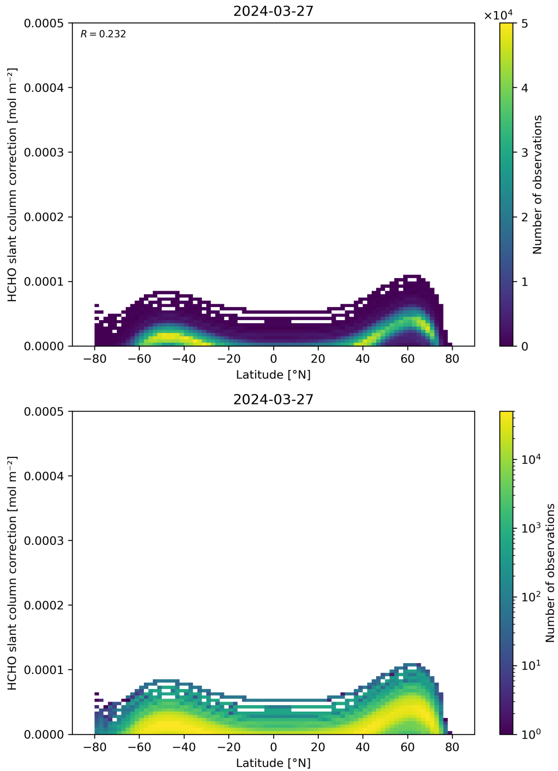
Figure 158: Scatter density plot of “Latitude” against “HCHO slant column correction” for 2024-03-26 to 2024-03-28.
