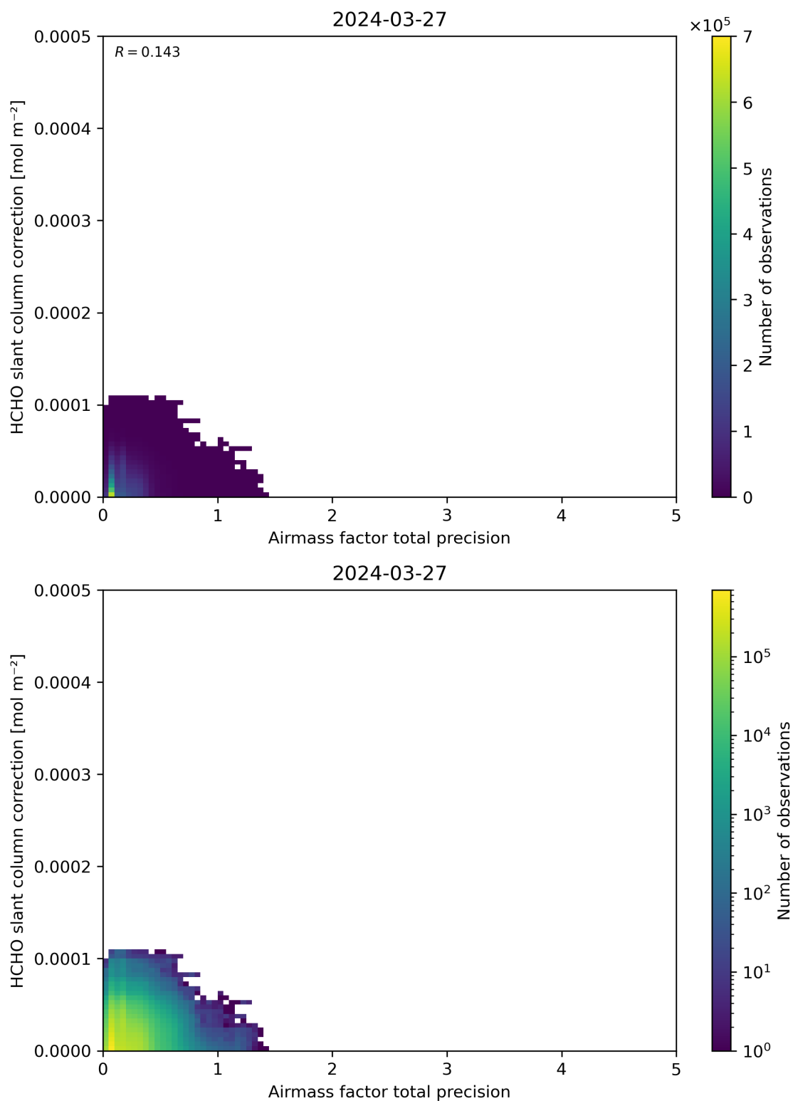
Figure 110: Scatter density plot of “Airmass factor total precision” against “HCHO slant column correction” for 2024-03-26 to 2024-03-28.
