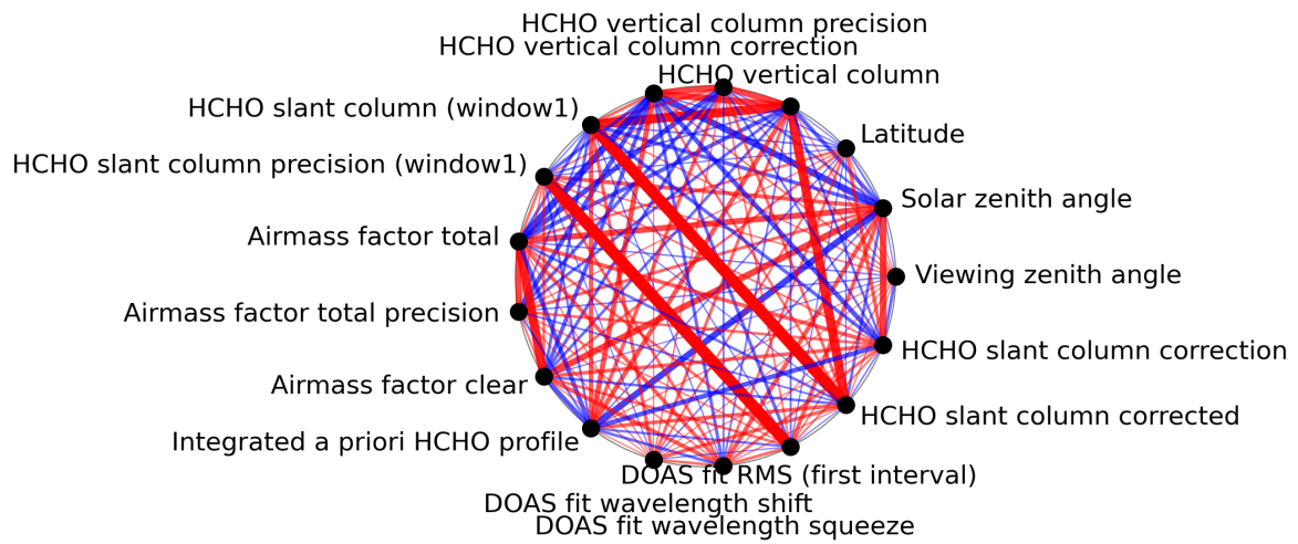
Figure 1: Map of correlation graph for 2024-03-26 to 2024-03-28.
