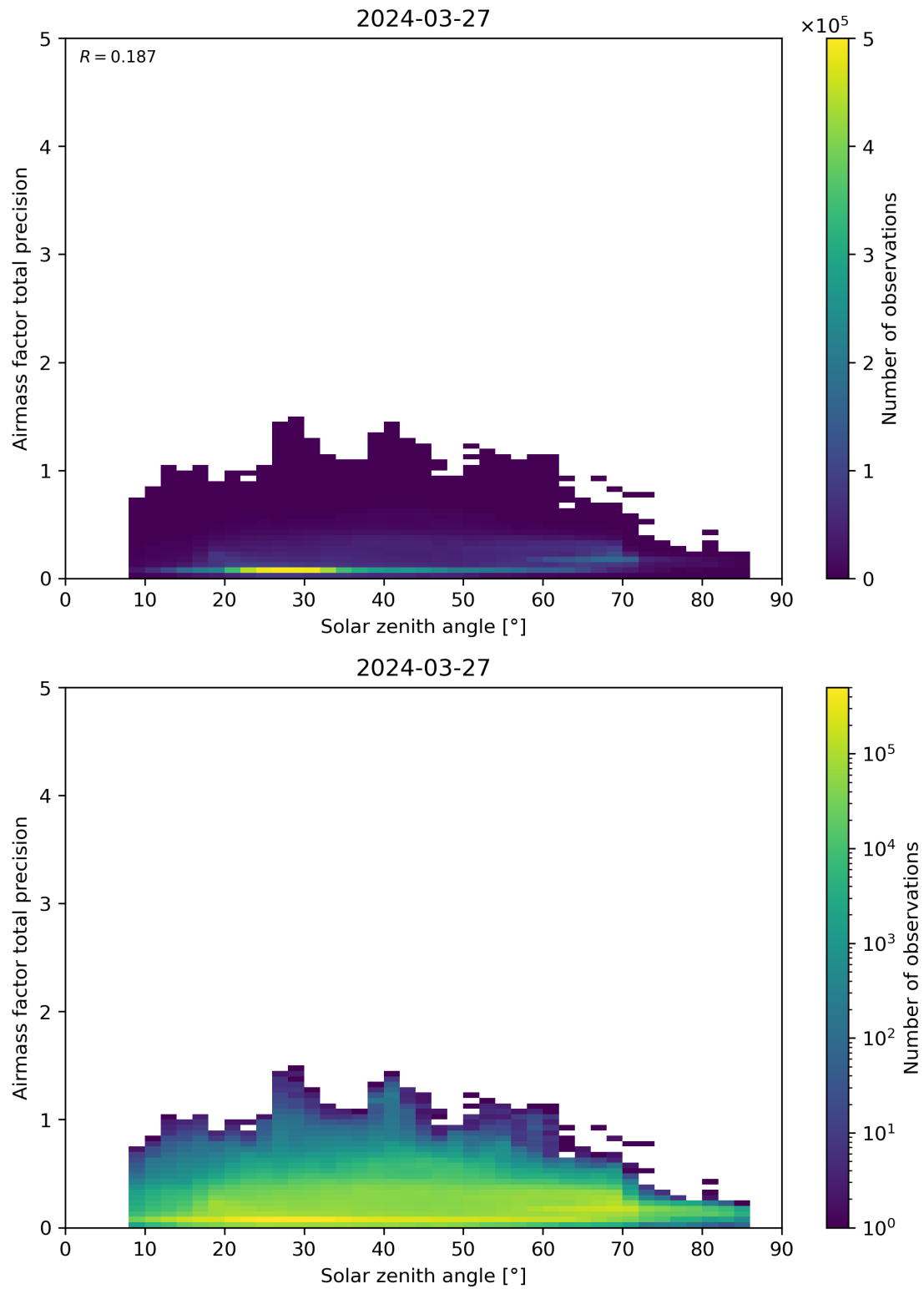
Figure 176: Scatter density plot of “Solar zenith angle” against “Airmass factor total precision” for 2024-03-26 to 2024-03-28.
