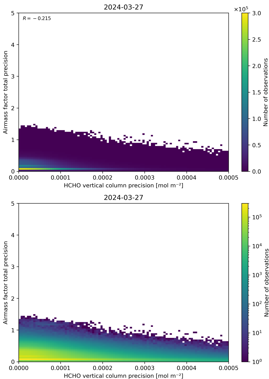
Figure 145: Scatter density plot of “HCHO vertical column precision” against “Airmass factor total precision” for 2024-03-26 to 2024-03-28.
