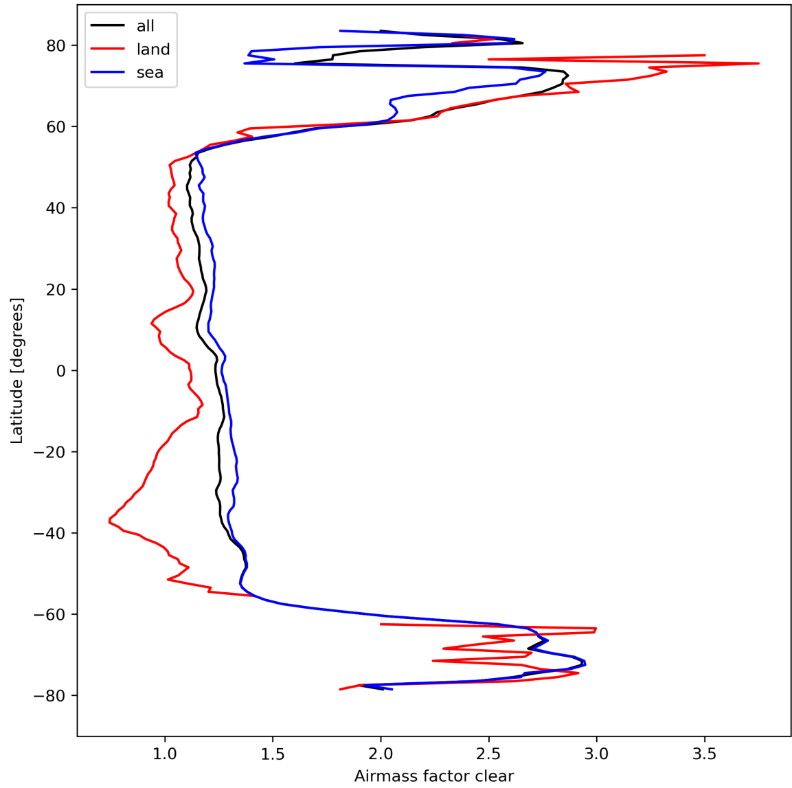
Figure 28: Zonal average of “Airmass factor clear” for 2024-03-26 to 2024-03-28.
