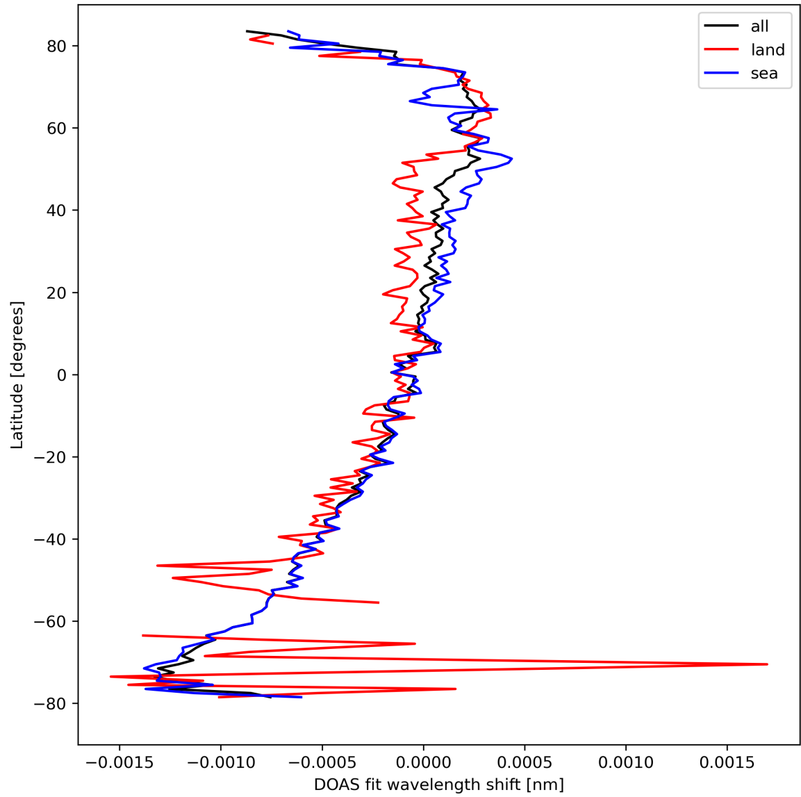
Figure 30: Zonal average of “DOAS fit wavelength shift” for 2024-03-27 to 2024-03-29.
