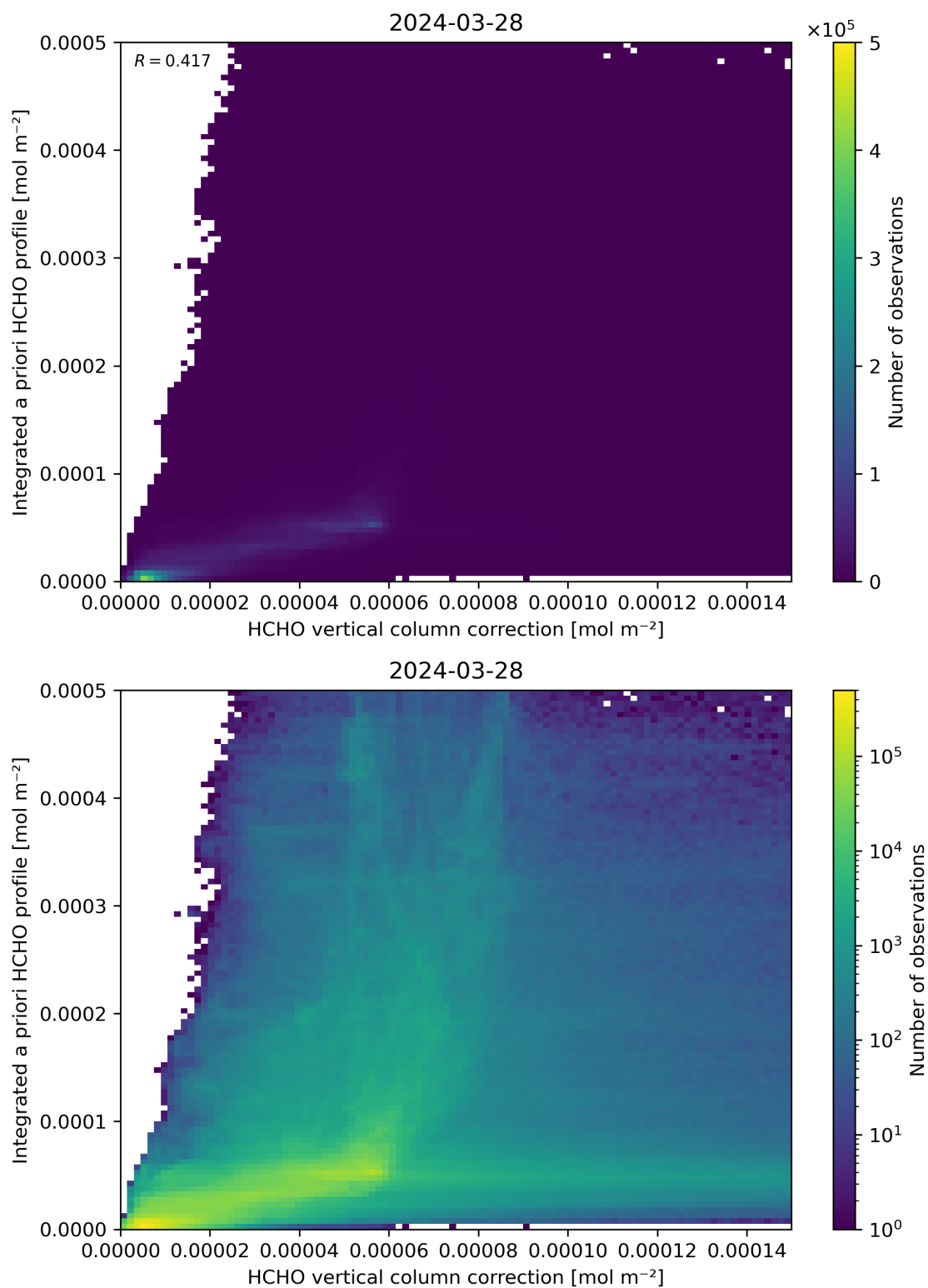
Figure 122: Scatter density plot of “HCHO vertical column correction” against “Integrated a priori HCHO profile” for 2024-03-27 to 2024-03-29.
