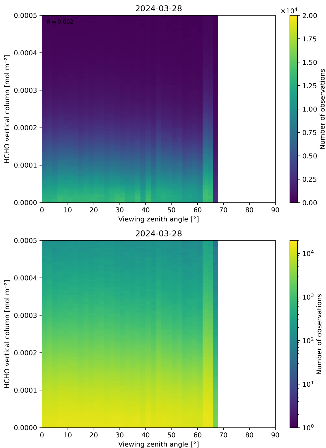
Figure 192: Scatter density plot of “Viewing zenith angle” against “HCHO vertical column” for 2024-03-27 to 2024-03-29.
