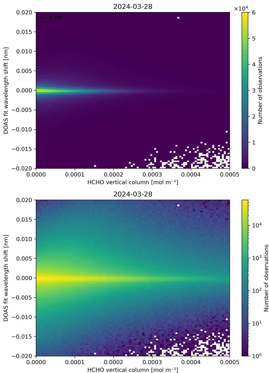
Figure 124: Scatter density plot of “HCHO vertical column” against “DOAS fit wavelength shift” for 2024-03-27 to 2024-03-29.
