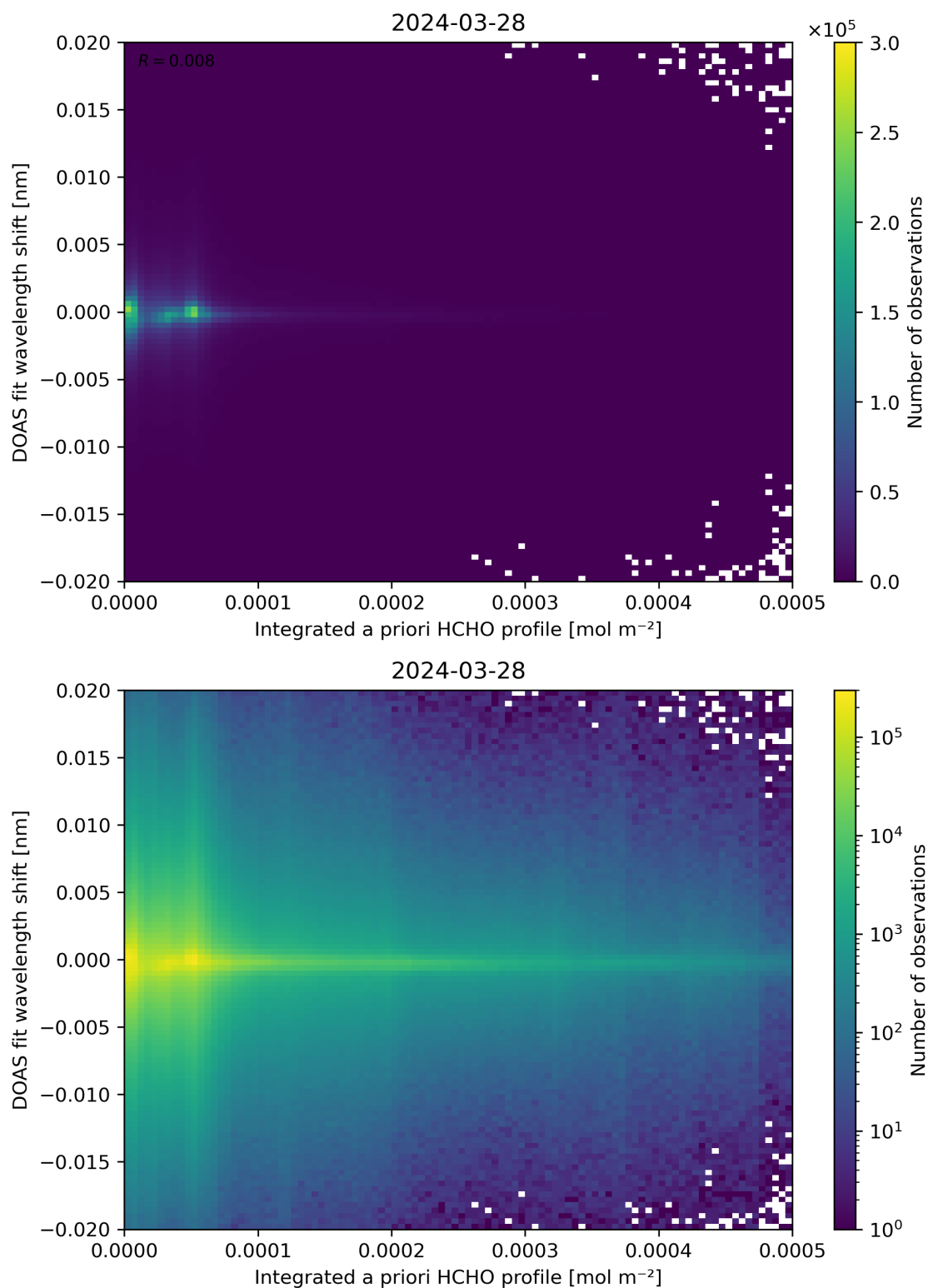
Figure 149: Scatter density plot of “Integrated a priori HCHO profile” against “DOAS fit wavelength shift” for 2024-03-27 to 2024-03-29.
