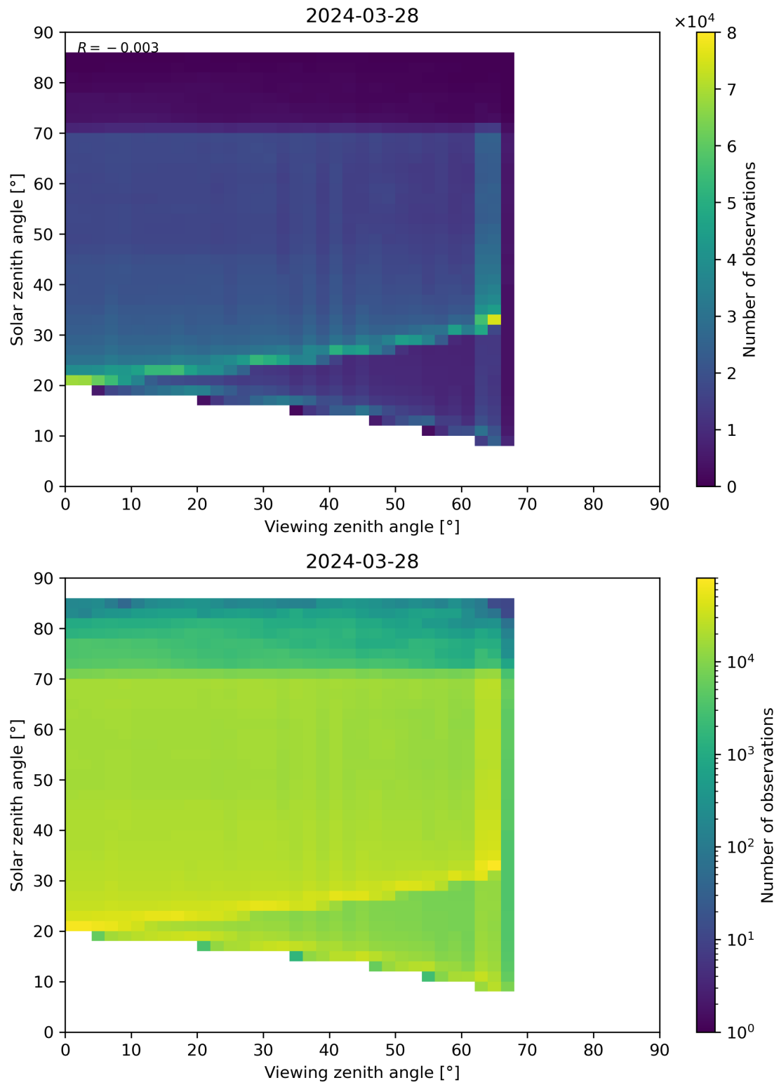
Figure 197: Scatter density plot of “Viewing zenith angle” against “Solar zenith angle” for 2024-03-27 to 2024-03-29.
