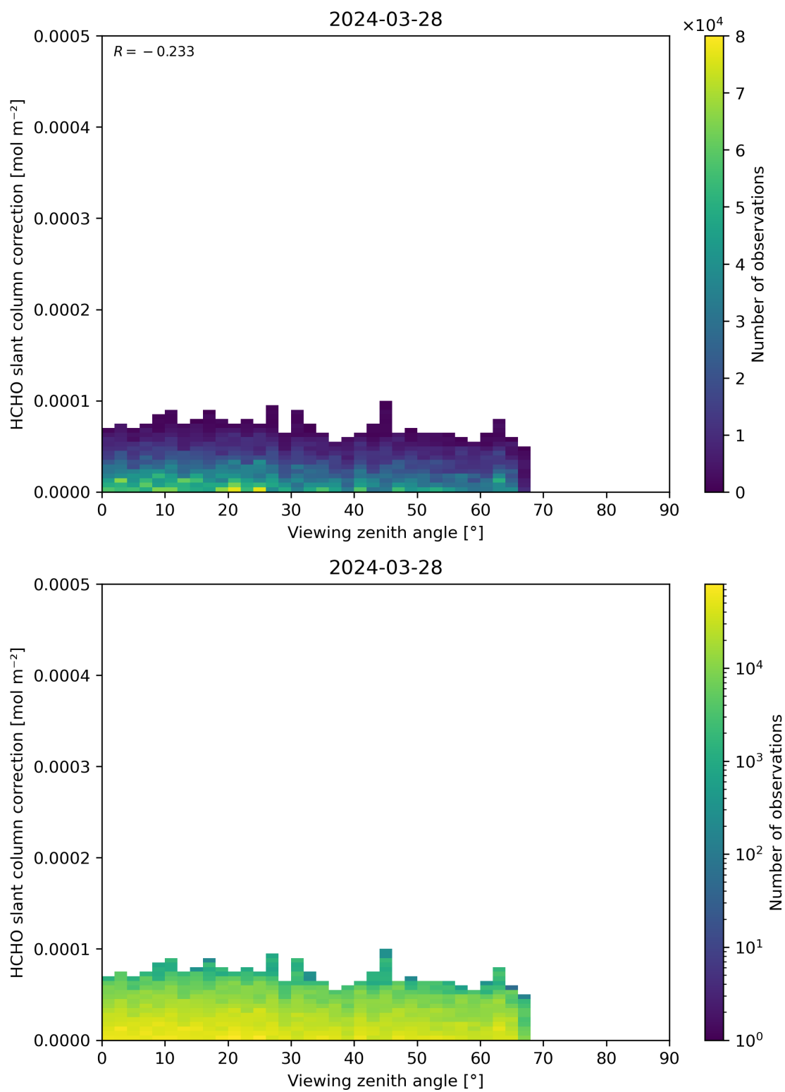
Figure 187: Scatter density plot of “Viewing zenith angle” against “HCHO slant column correction” for 2024-03-27 to 2024-03-29.
