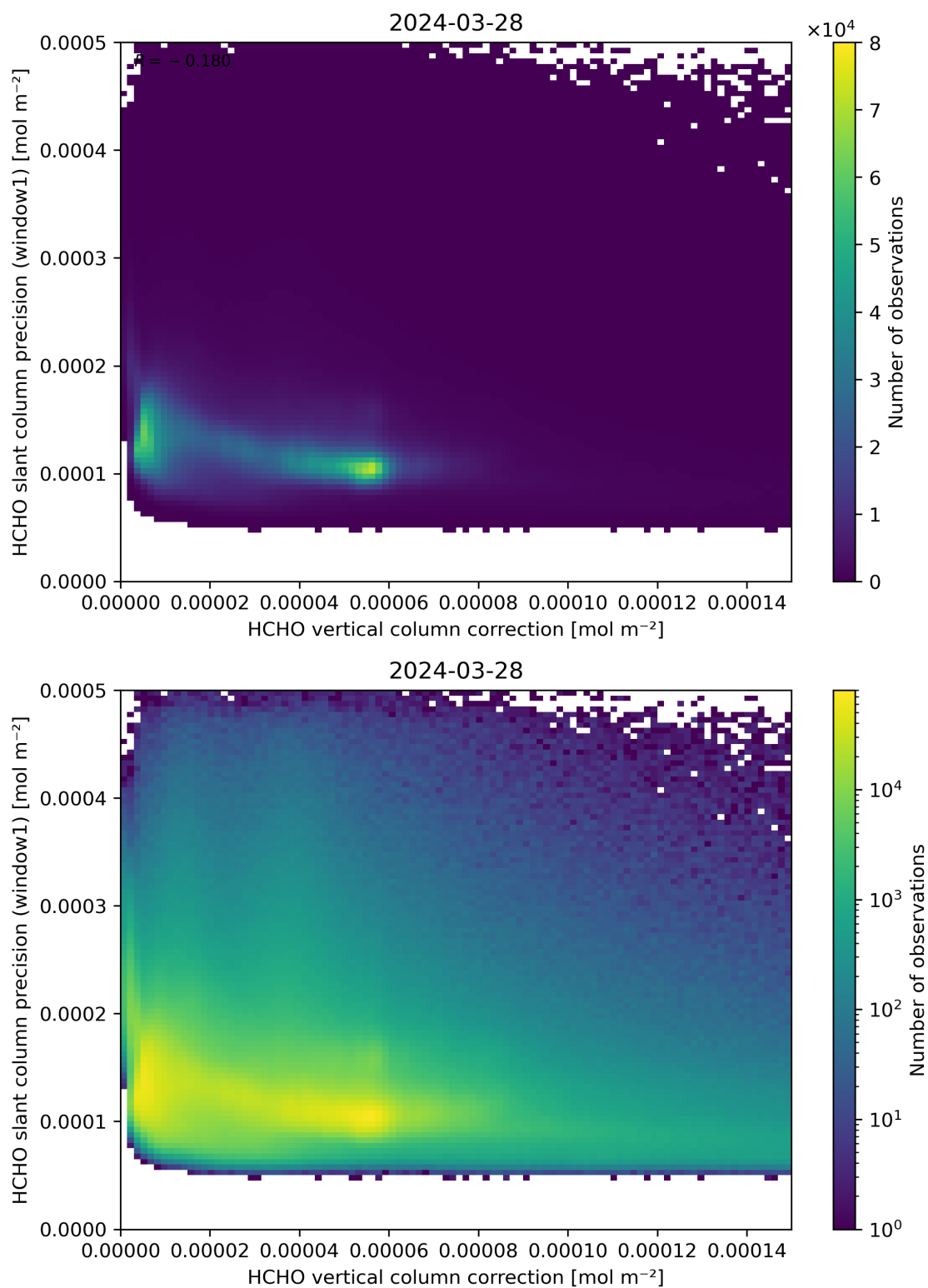
Figure 119: Scatter density plot of “HCHO vertical column correction” against “HCHO slant column precision (window1)” for 2024-03-27 to 2024-03-29.
