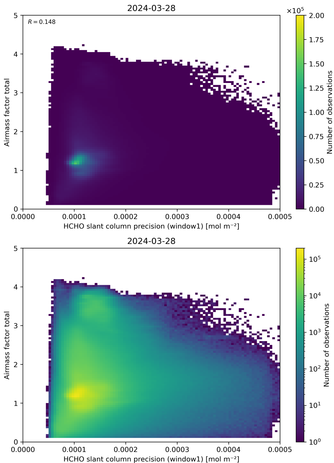
Figure 94: Scatter density plot of “HCHO slant column precision (window1)” against “Airmass factor total” for 2024-03-27 to 2024-03-29.
