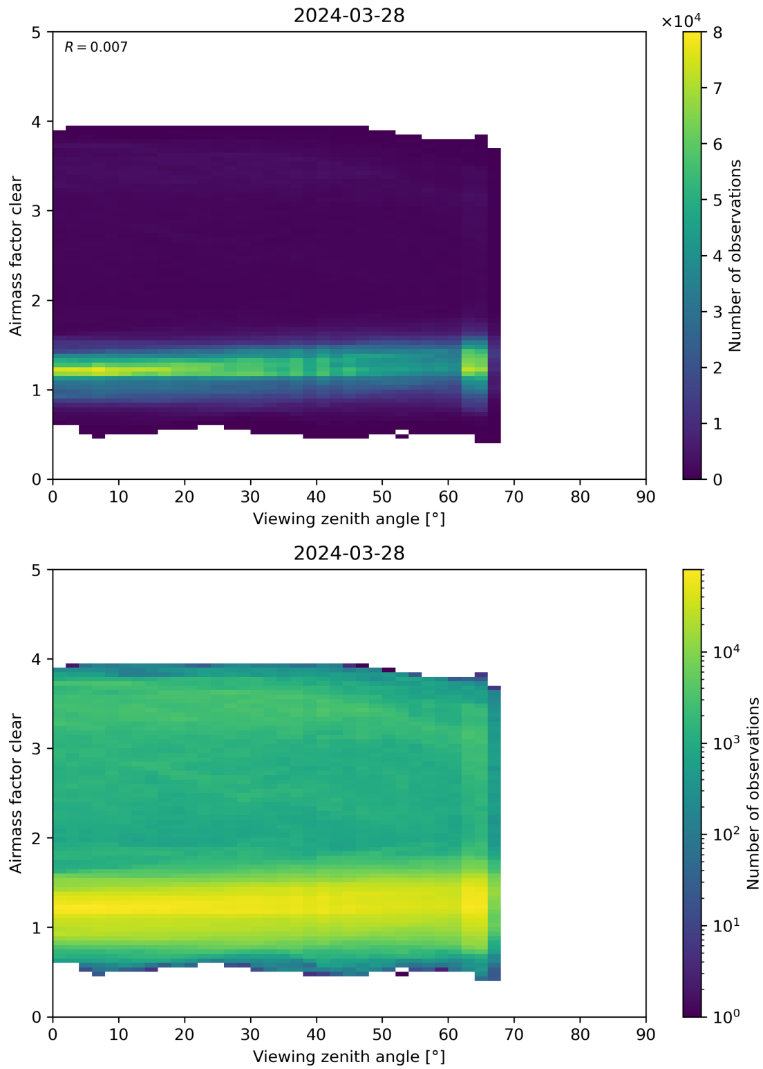
Figure 185: Scatter density plot of “Viewing zenith angle” against “Airmass factor clear” for 2024-03-27 to 2024-03-29.
