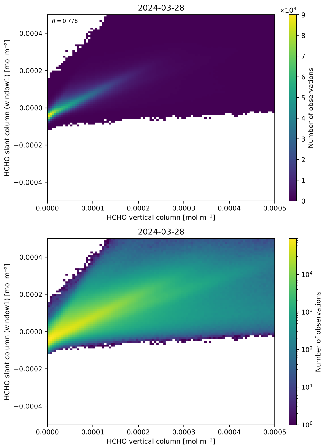
Figure 129: Scatter density plot of “HCHO vertical column” against “HCHO slant column (window1)” for 2024-03-27 to 2024-03-29.
