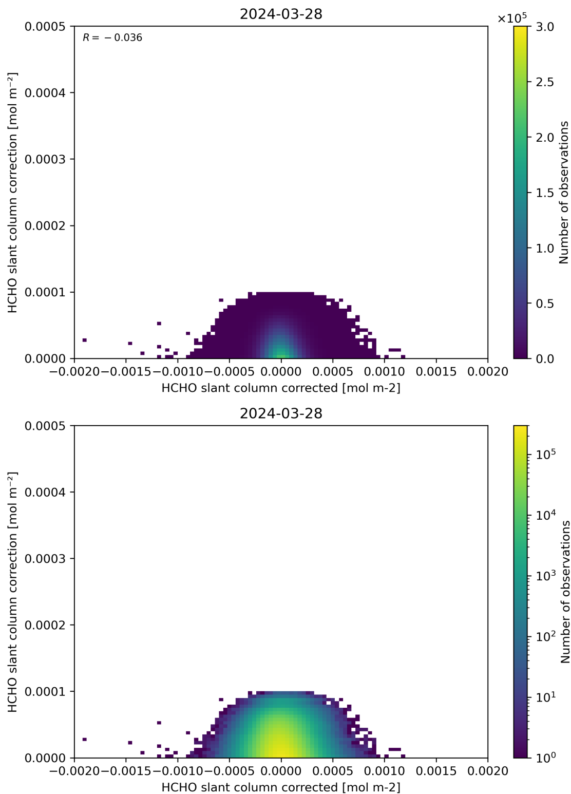
Figure 77: Scatter density plot of “HCHO slant column corrected” against “HCHO slant column correction” for 2024-03-27 to 2024-03-29.
