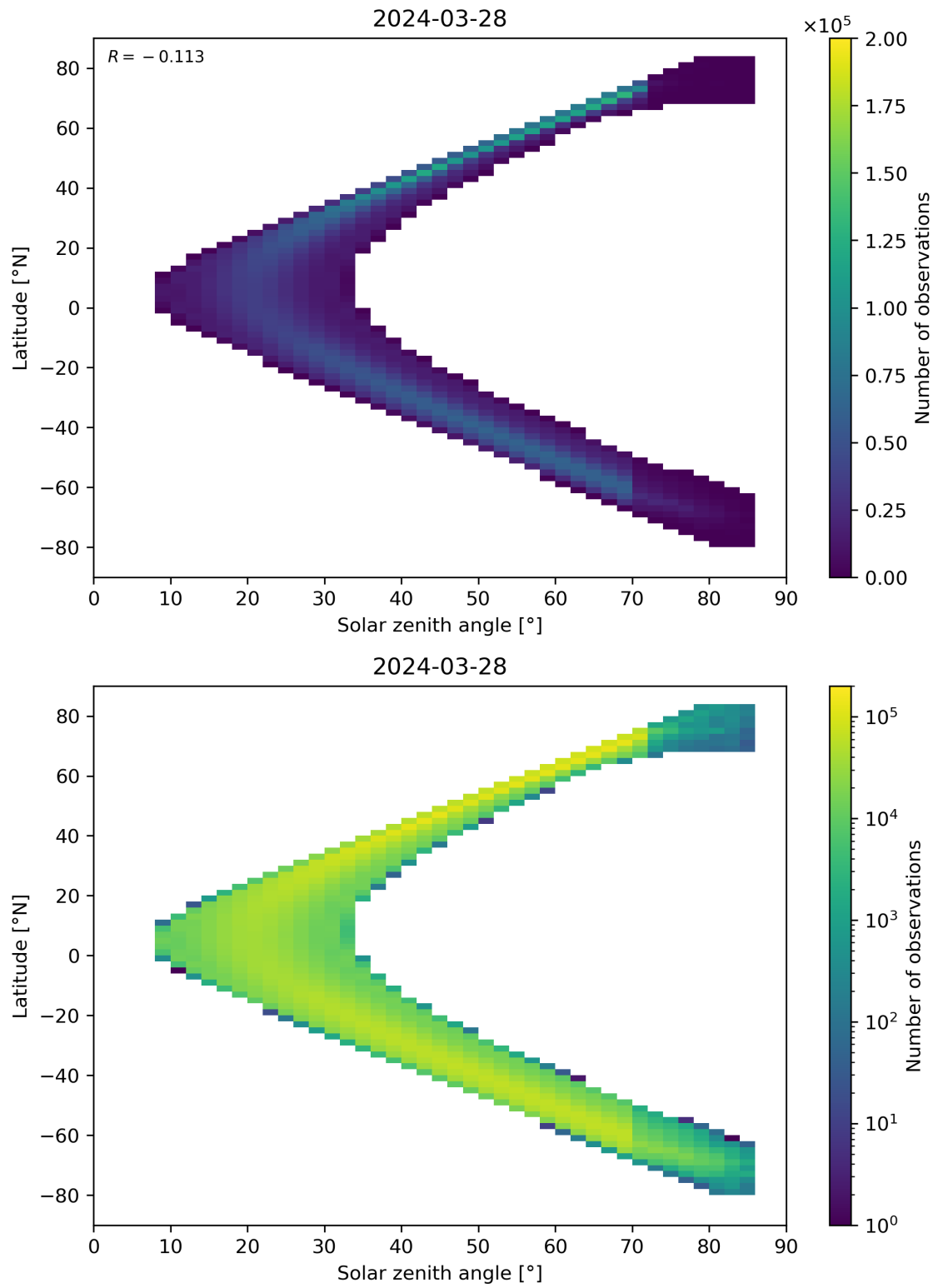
Figure 181: Scatter density plot of “Solar zenith angle” against “Latitude” for 2024-03-27 to 2024-03-29.
