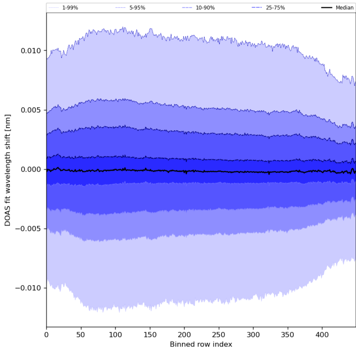
Figure 58: Along track statistics of “DOAS fit wavelength shift” for 2024-03-27 to 2024-03-29
