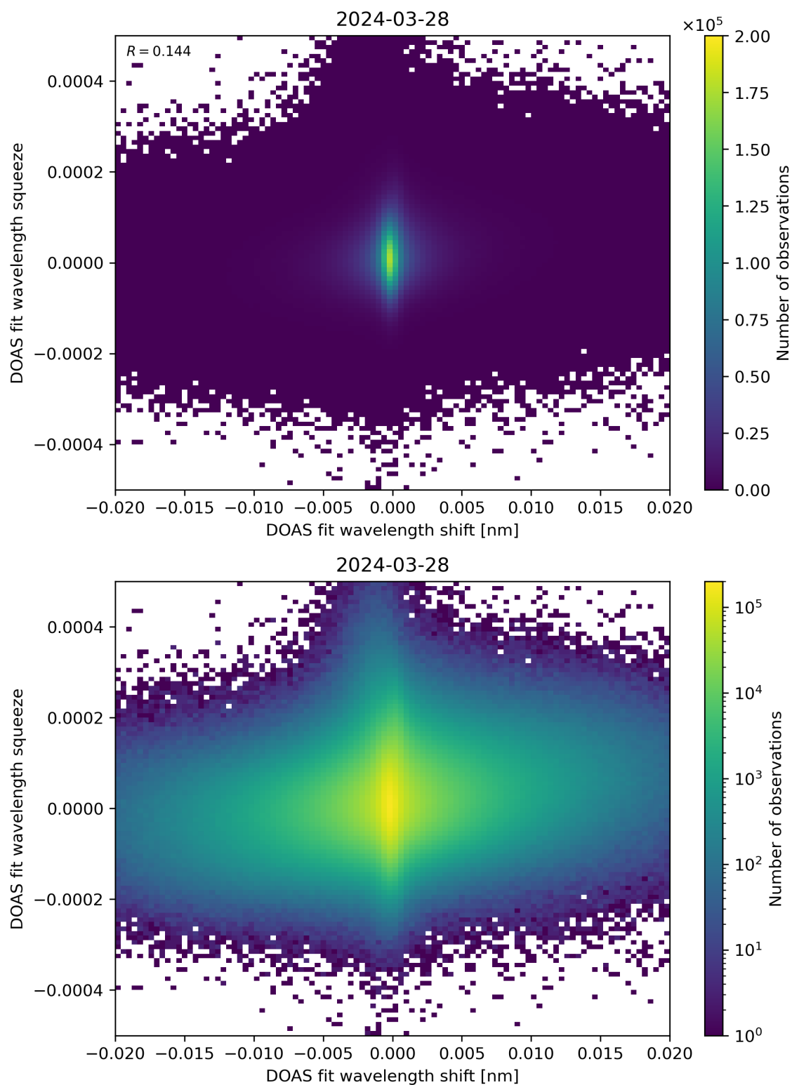
Figure 65: Scatter density plot of “DOAS fit wavelength shift” against “DOAS fit wavelength squeeze” for 2024-03-27 to 2024-03-29.
