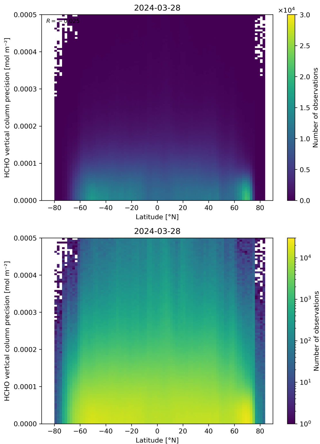
Figure 165: Scatter density plot of “Latitude” against “HCHO vertical column precision” for 2024-03-27 to 2024-03-29.
