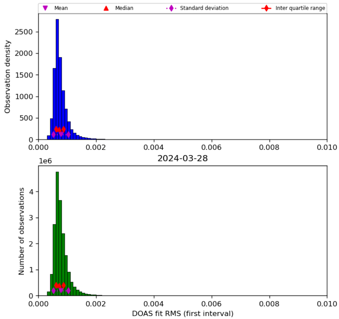
Figure 46: Histogram of “DOAS fit RMS (first interval)” for 2024-03-27 to 2024-03-29
