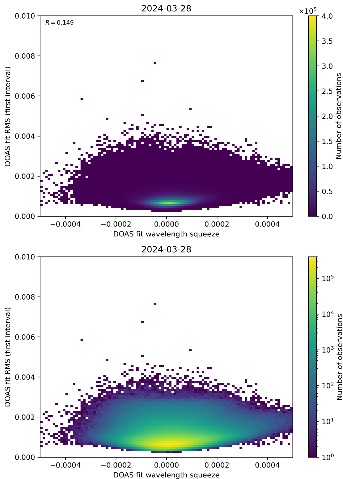
Figure 68: Scatter density plot of “DOAS fit wavelength squeeze” against “DOAS fit RMS (first interval)” for 2024-03-27 to 2024-03-29.
