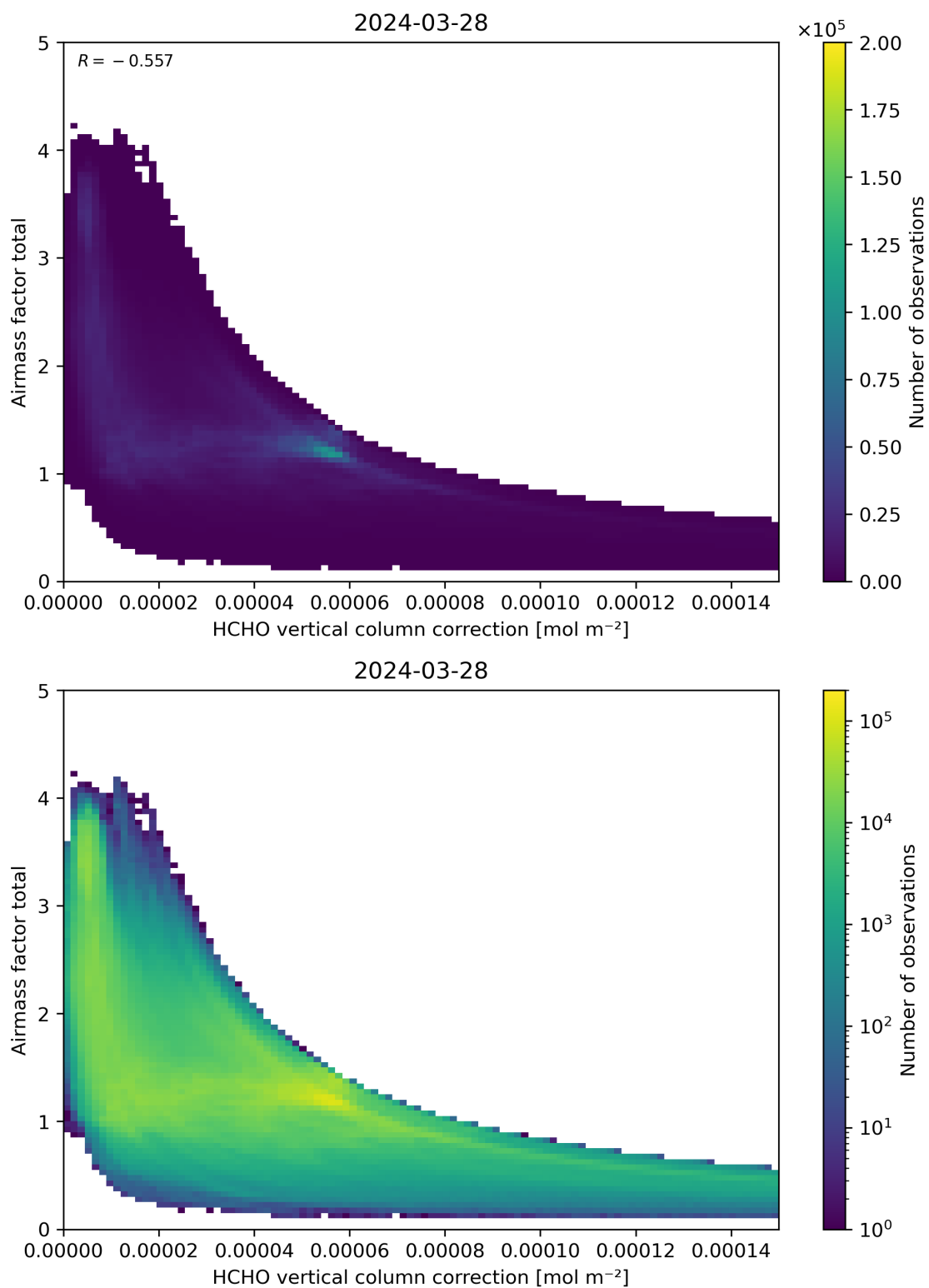
Figure 120: Scatter density plot of “HCHO vertical column correction” against “Airmass factor total” for 2024-03-27 to 2024-03-29.
