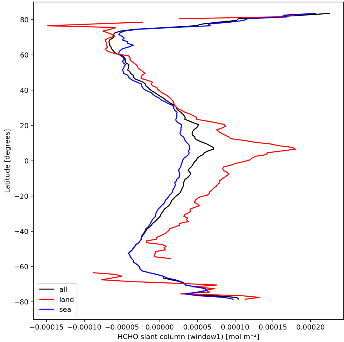
Figure 24: Zonal average of “HCHO slant column (window1)” for 2024-03-27 to 2024-03-29.
