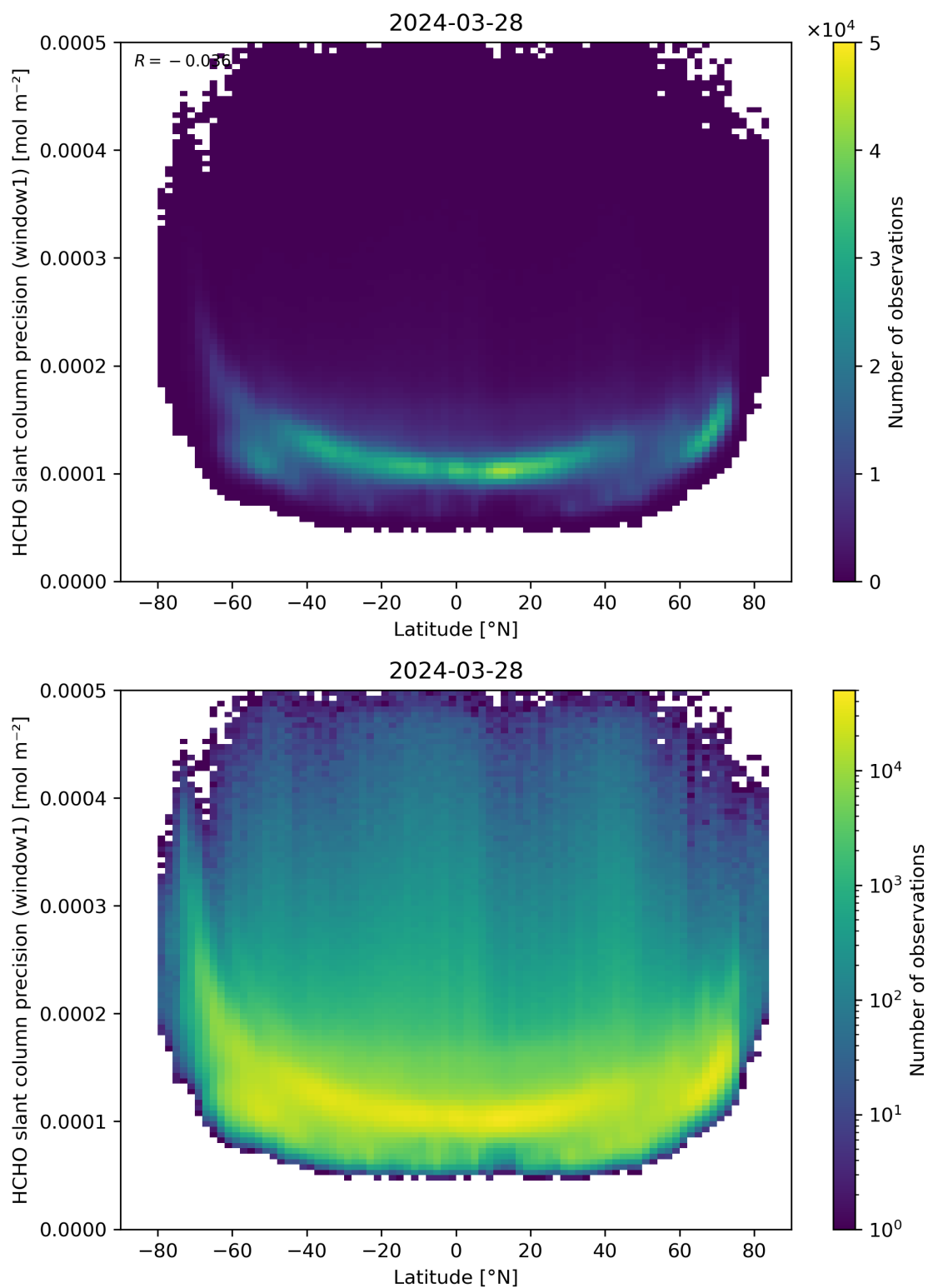
Figure 160: Scatter density plot of “Latitude” against “HCHO slant column precision (window1)” for 2024-03-27 to 2024-03-29.
