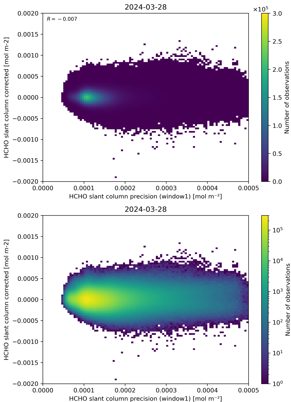
Figure 92: Scatter density plot of “HCHO slant column precision (window1)” against “HCHO slant column corrected” for 2024-03-27 to 2024-03-29.
