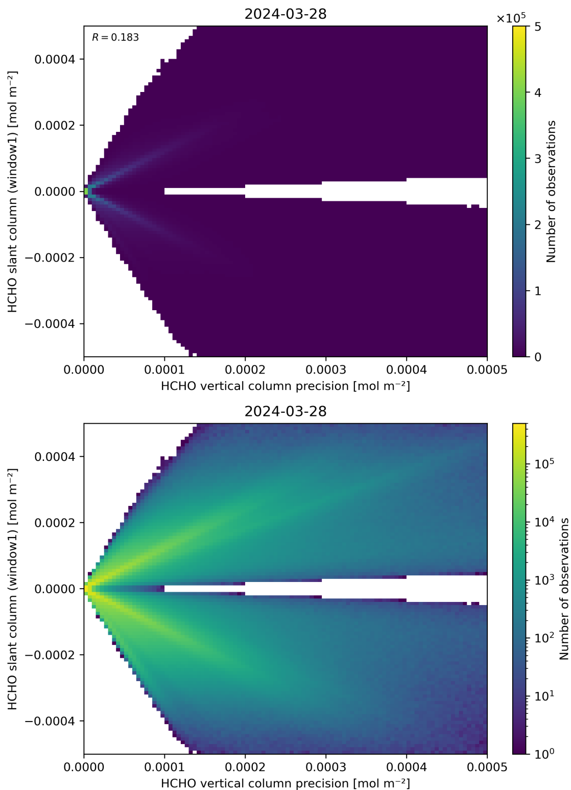
Figure 142: Scatter density plot of “HCHO vertical column precision” against “HCHO slant column (window1)” for 2024-03-27 to 2024-03-29.
