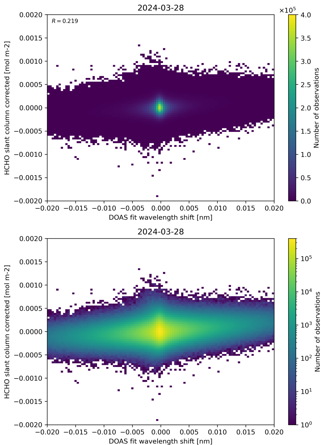
Figure 66: Scatter density plot of “DOAS fit wavelength shift” against “HCHO slant column corrected” for 2024-03-27 to 2024-03-29.
