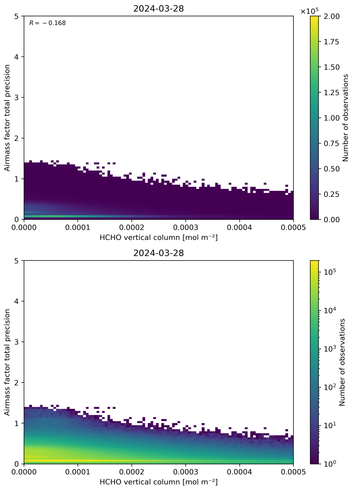
Figure 132: Scatter density plot of “HCHO vertical column” against “Airmass factor total precision” for 2024-03-27 to 2024-03-29.
