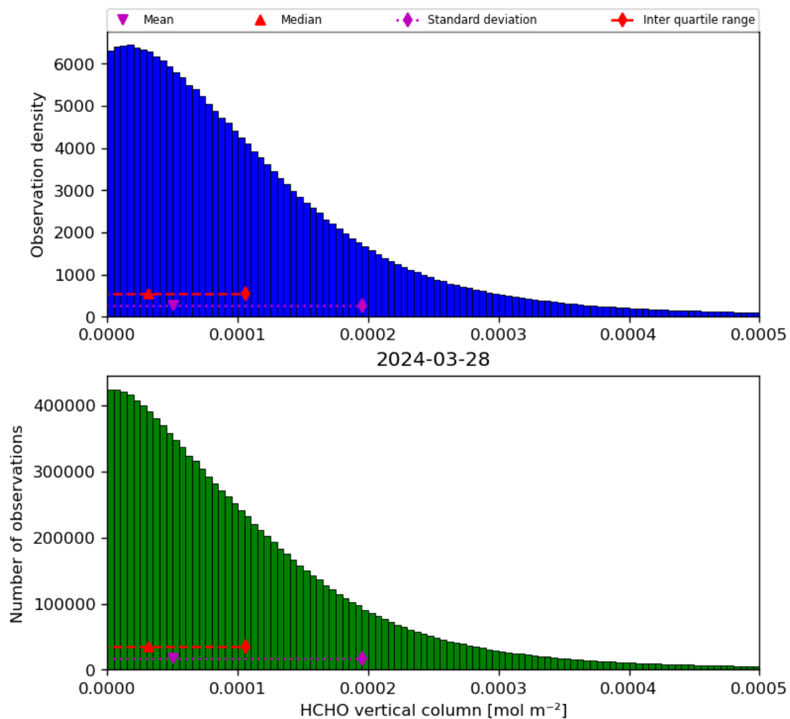
Figure 35: Histogram of “HCHO vertical column” for 2024-03-27 to 2024-03-29
