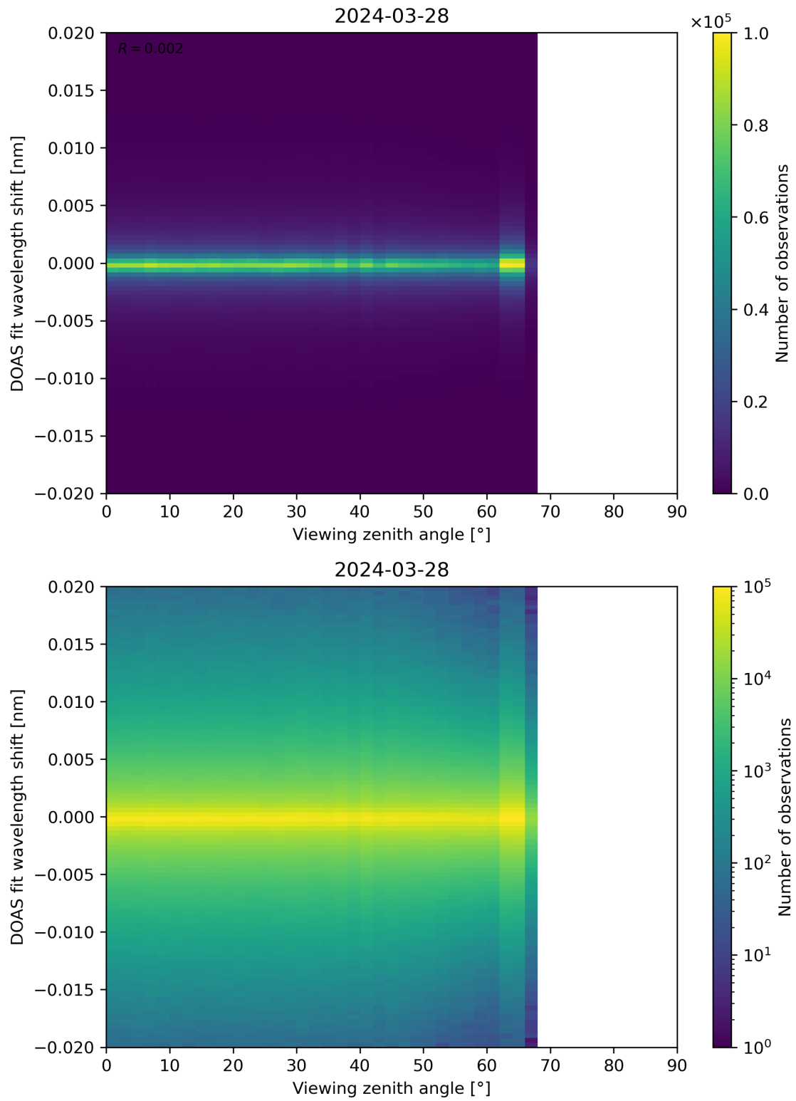
Figure 183: Scatter density plot of “Viewing zenith angle” against “DOAS fit wavelength shift” for 2024-03-27 to 2024-03-29.
