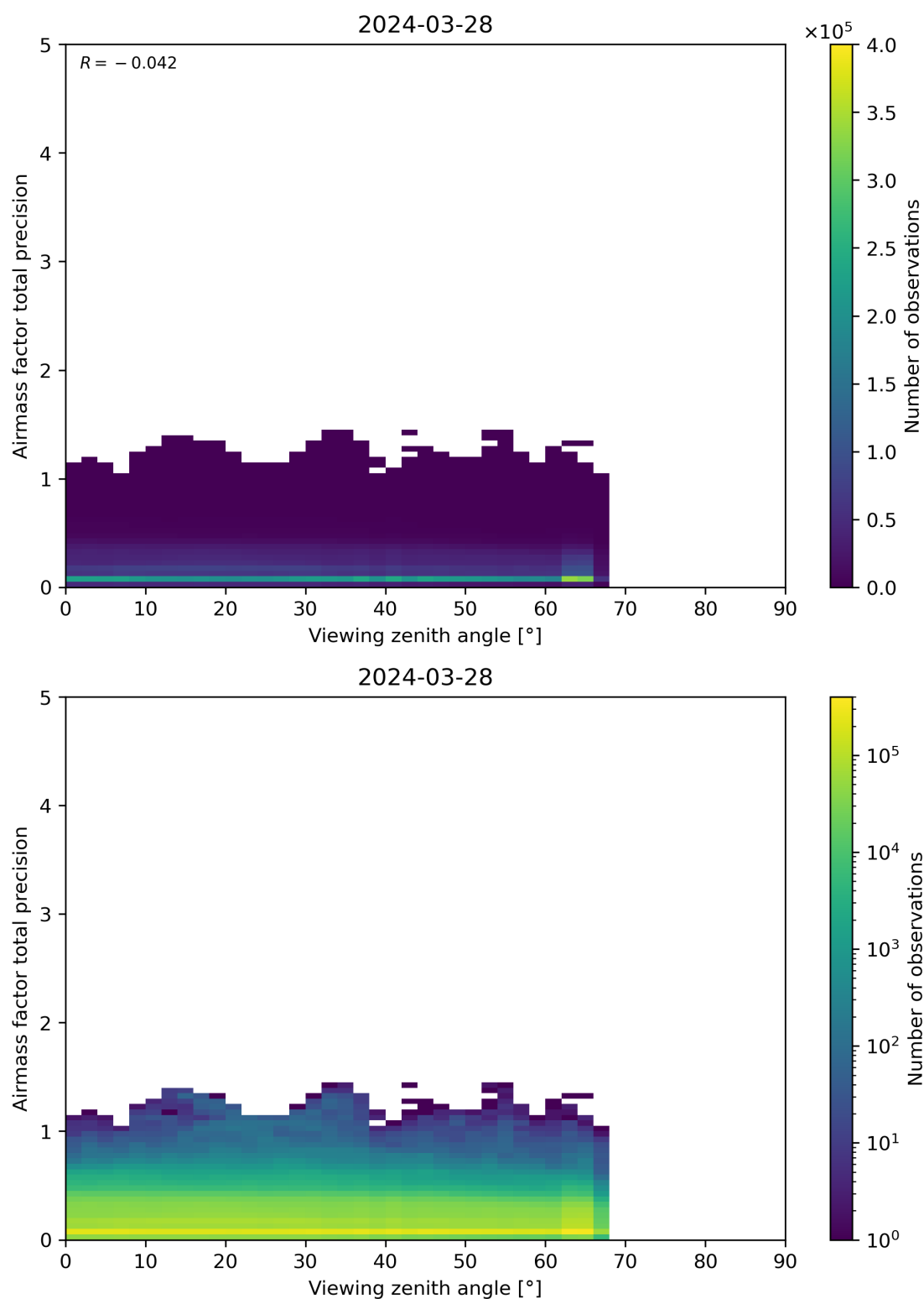
Figure 191: Scatter density plot of “Viewing zenith angle” against “Airmass factor total precision” for 2024-03-27 to 2024-03-29.
