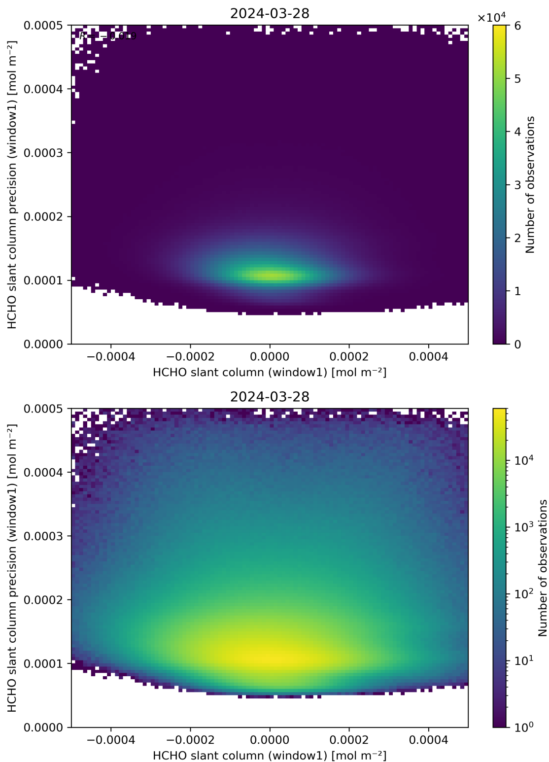
Figure 84: Scatter density plot of “HCHO slant column (window1)” against “HCHO slant column precision (window1)” for 2024-03-27 to 2024-03-29.
