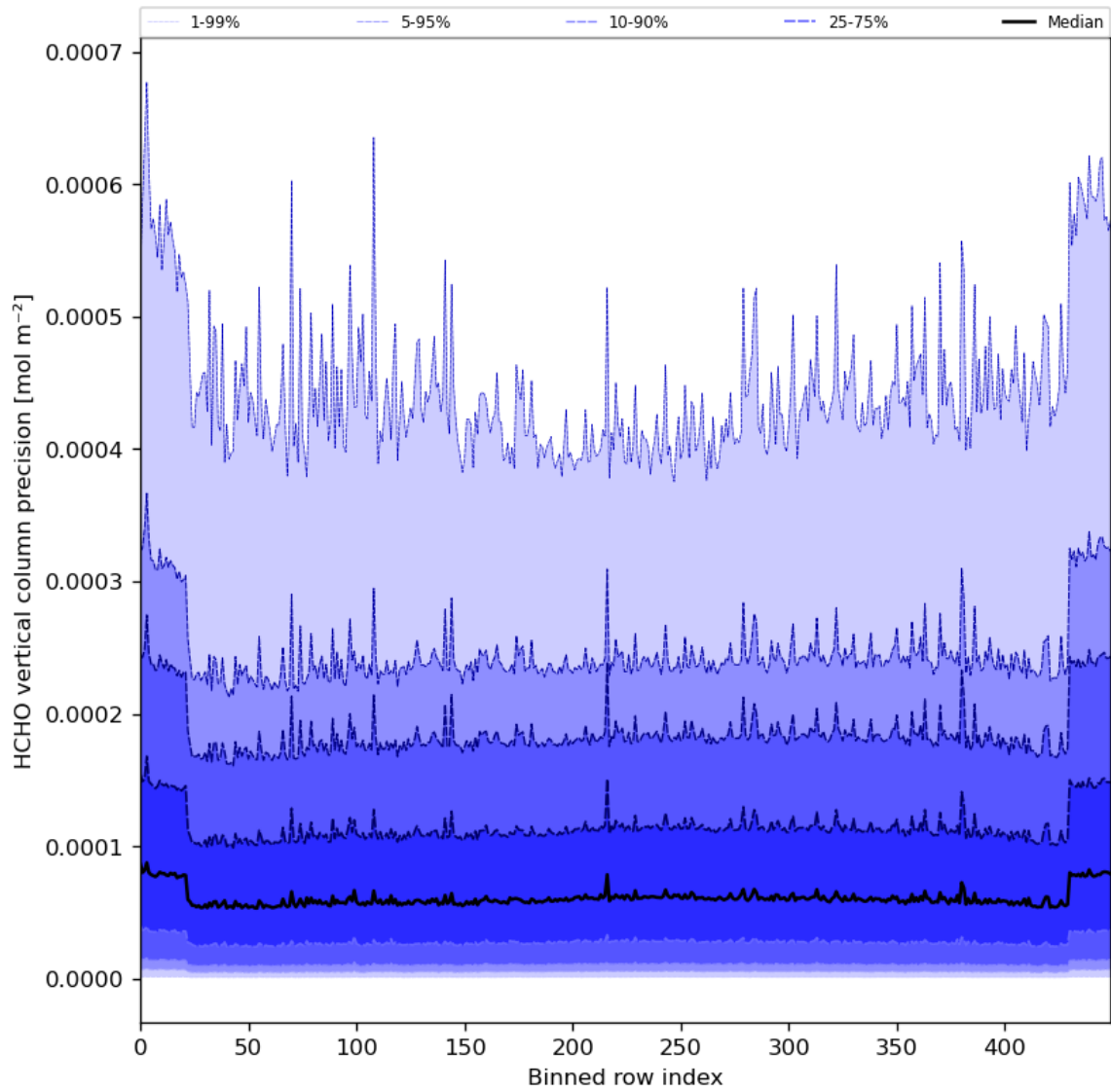
Figure 50: Along track statistics of “HCHO vertical column precision” for 2024-03-27 to 2024-03-29
