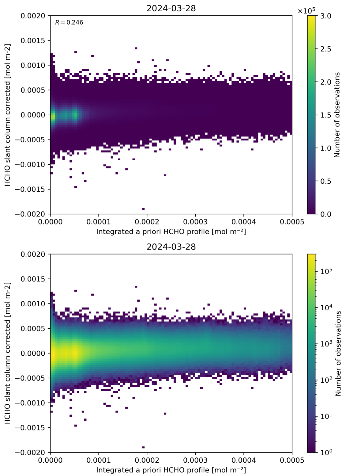
Figure 151: Scatter density plot of “Integrated a priori HCHO profile” against “HCHO slant column corrected” for 2024-03-27 to 2024-03-29.
