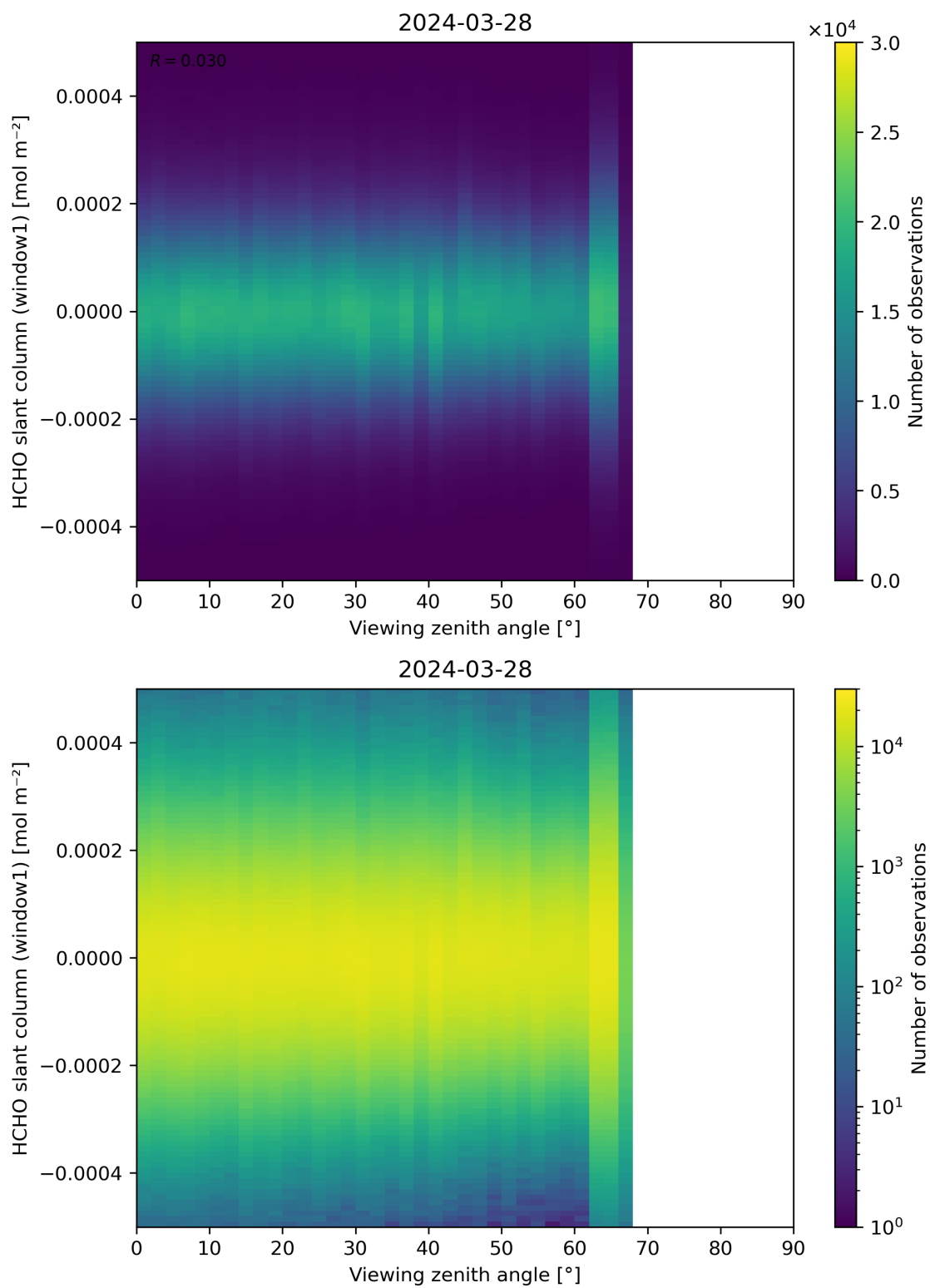
Figure 188: Scatter density plot of “Viewing zenith angle” against “HCHO slant column (window1)” for 2024-03-27 to 2024-03-29.
