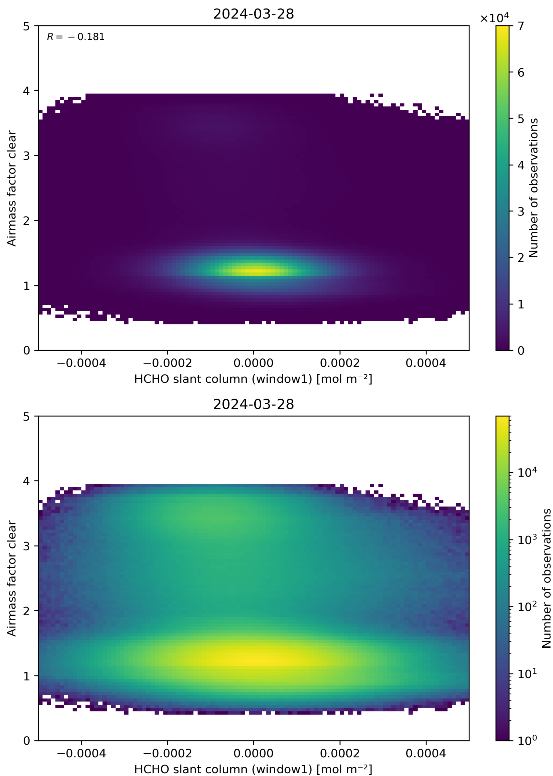
Figure 81: Scatter density plot of “HCHO slant column (window1)” against “Airmass factor clear” for 2024-03-27 to 2024-03-29.
