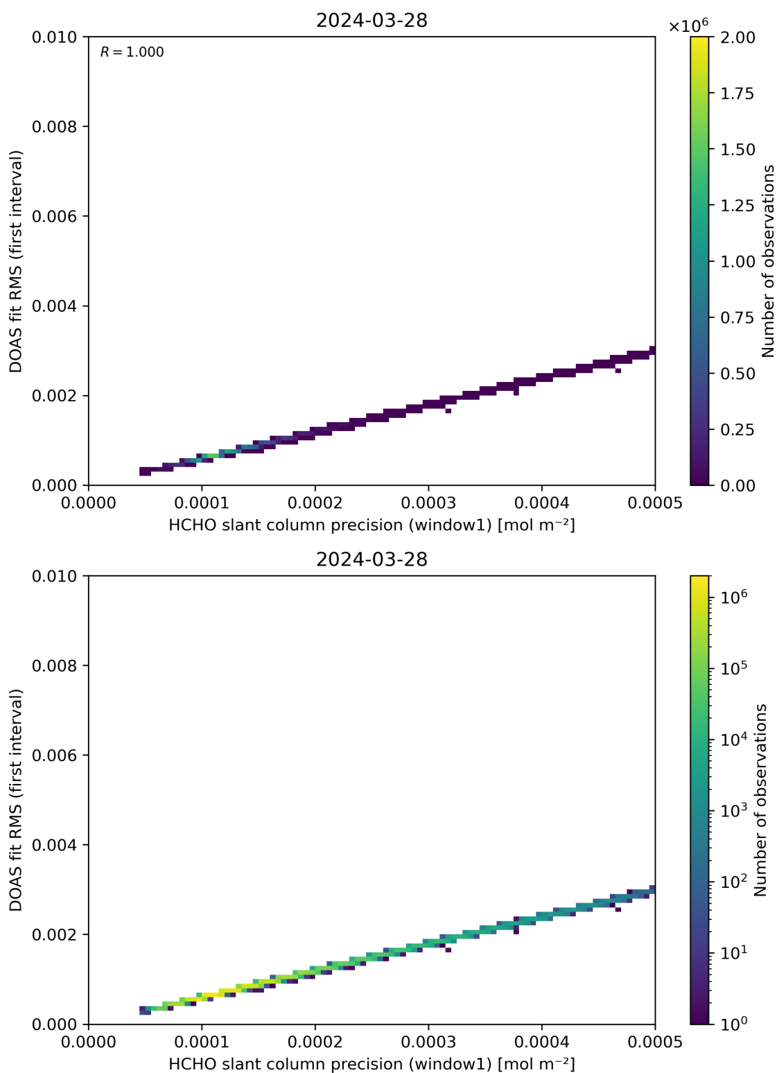
Figure 88: Scatter density plot of “HCHO slant column precision (window1)” against “DOAS fit RMS (first interval)” for 2024-03-27 to 2024-03-29.
