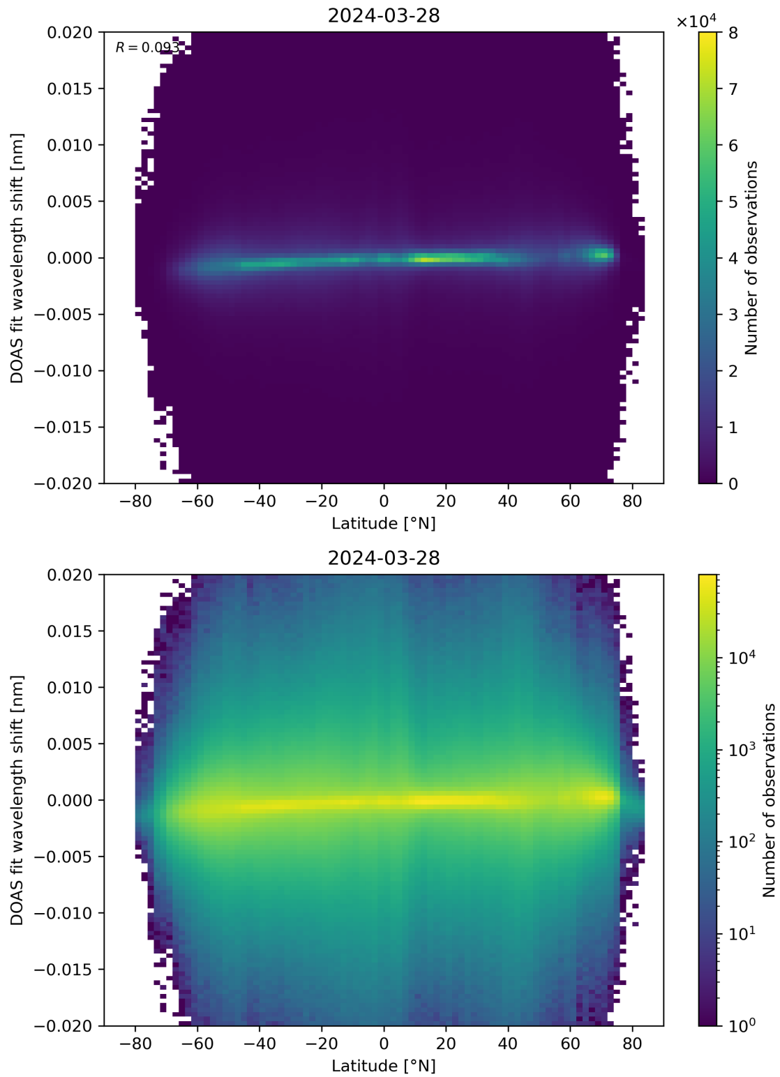
Figure 154: Scatter density plot of “Latitude” against “DOAS fit wavelength shift” for 2024-03-27 to 2024-03-29.
