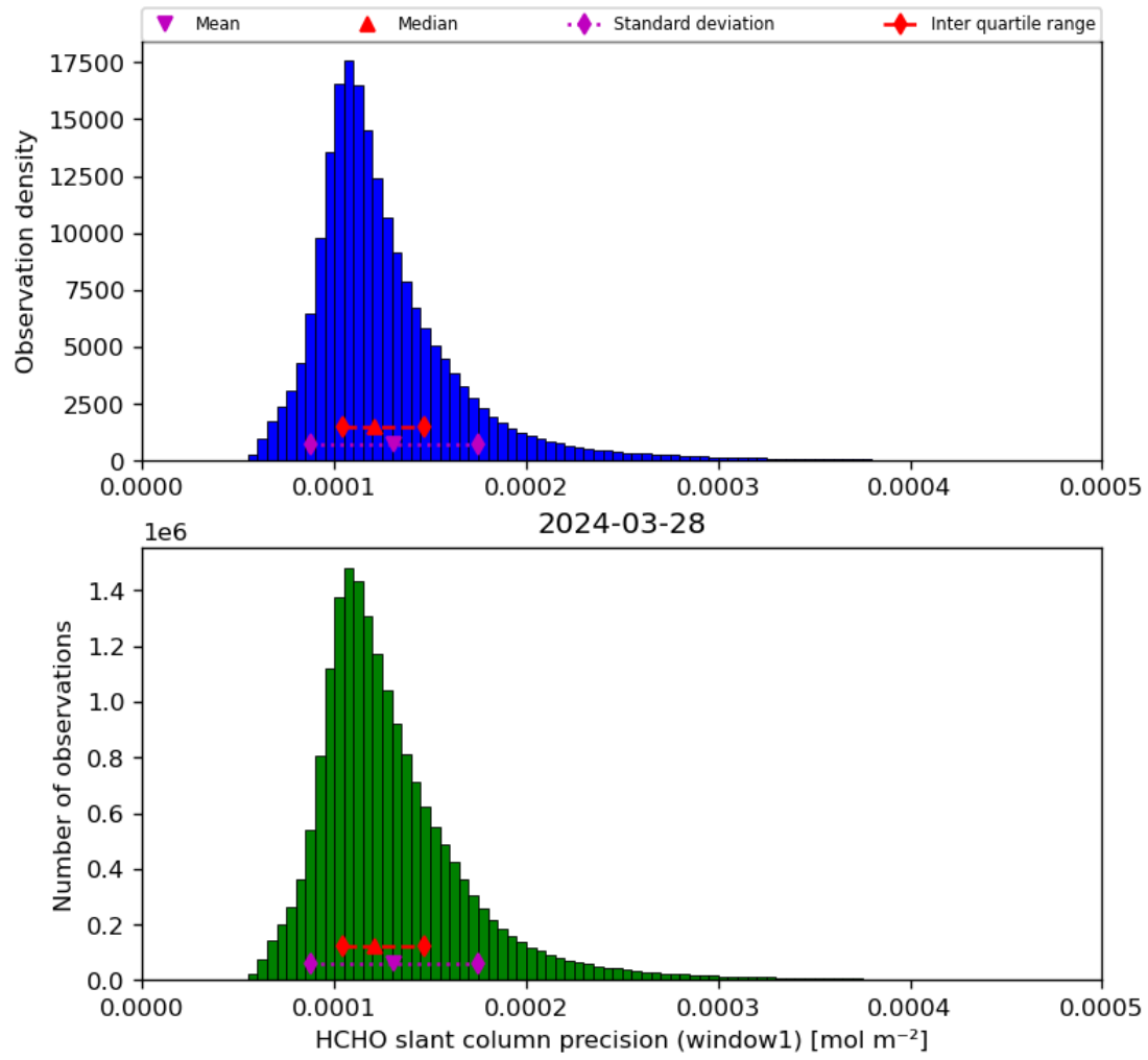
Figure 39: Histogram of “HCHO slant column precision (window1)” for 2024-03-27 to 2024-03-29
