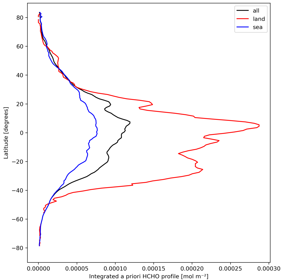
Figure 29: Zonal average of “Integrated a priori HCHO profile” for 2024-03-27 to 2024-03-29.
