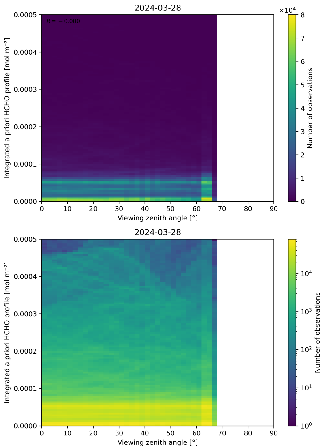
Figure 195: Scatter density plot of “Viewing zenith angle” against “Integrated a priori HCHO profile” for 2024-03-27 to 2024-03-29.
