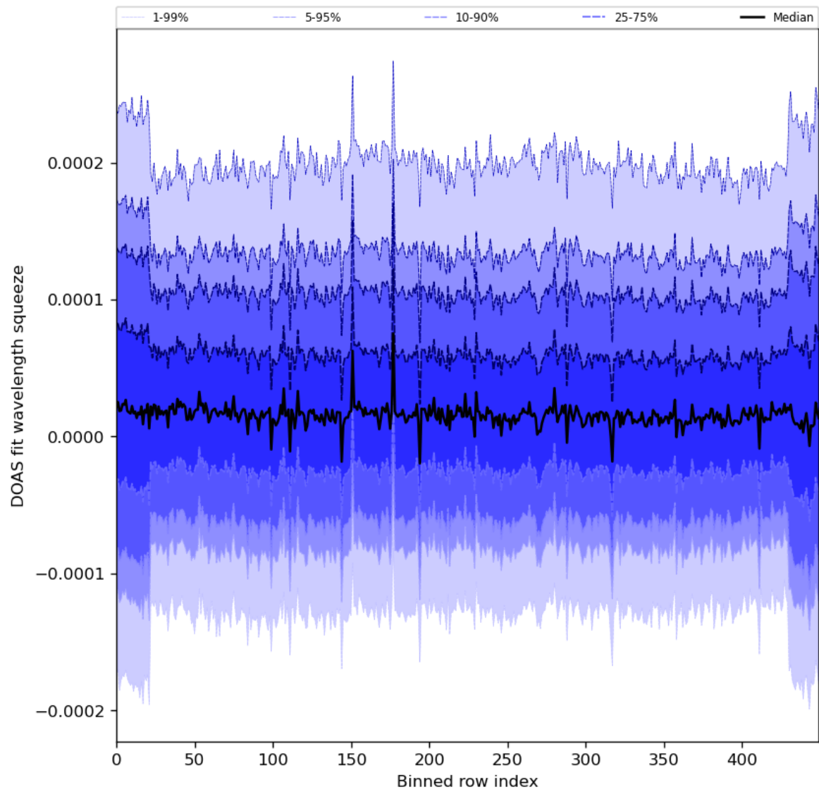
Figure 59: Along track statistics of “DOAS fit wavelength squeeze” for 2024-03-27 to 2024-03-29
