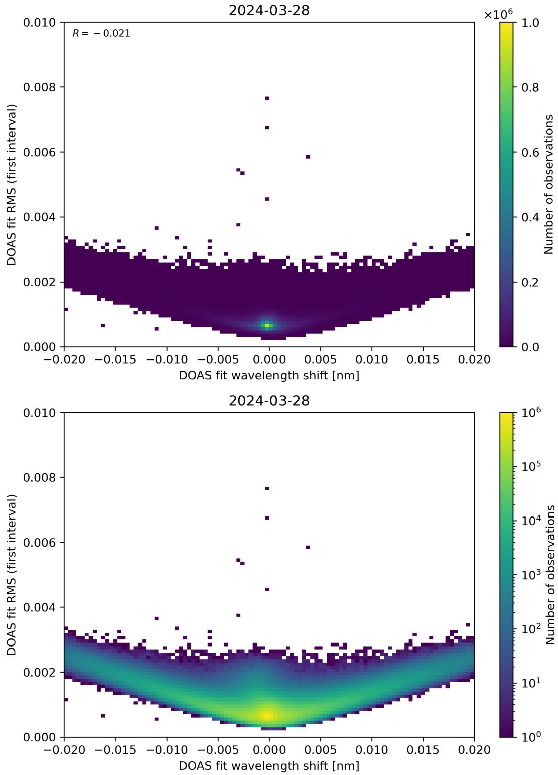
Figure 64: Scatter density plot of “DOAS fit wavelength shift” against “DOAS fit RMS (first interval)” for 2024-03-27 to 2024-03-29.
