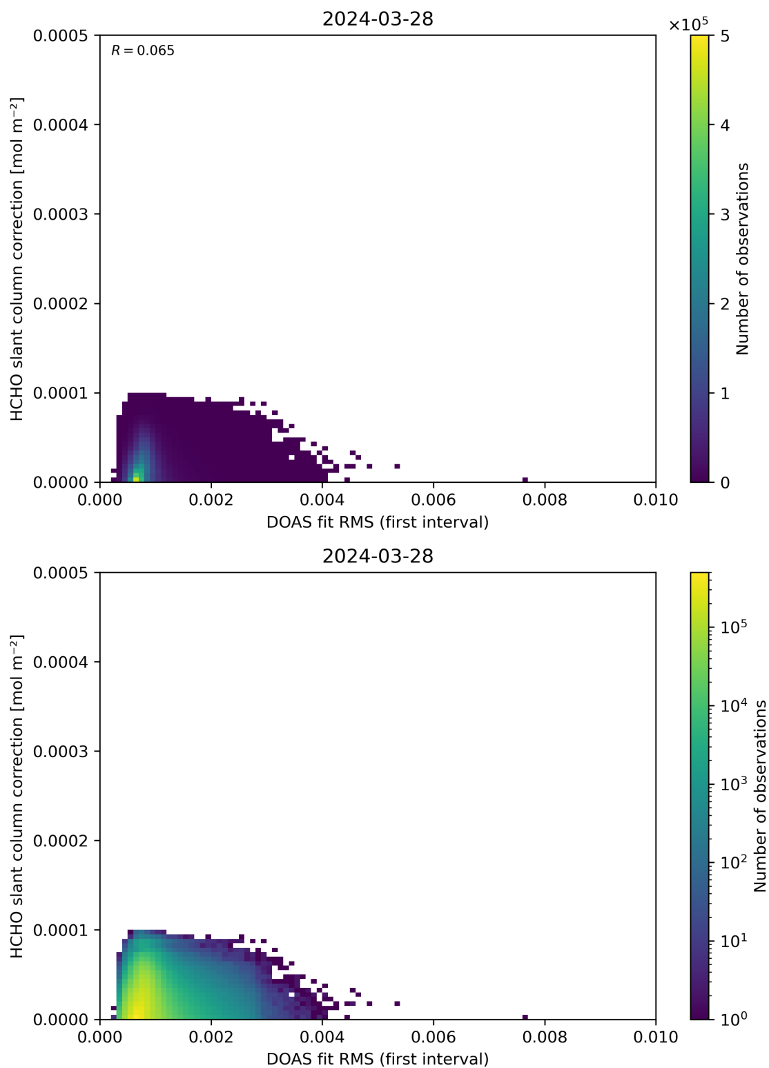
Figure 63: Scatter density plot of “DOAS fit RMS (first interval)” against “HCHO slant column correction” for 2024-03-27 to 2024-03-29.
