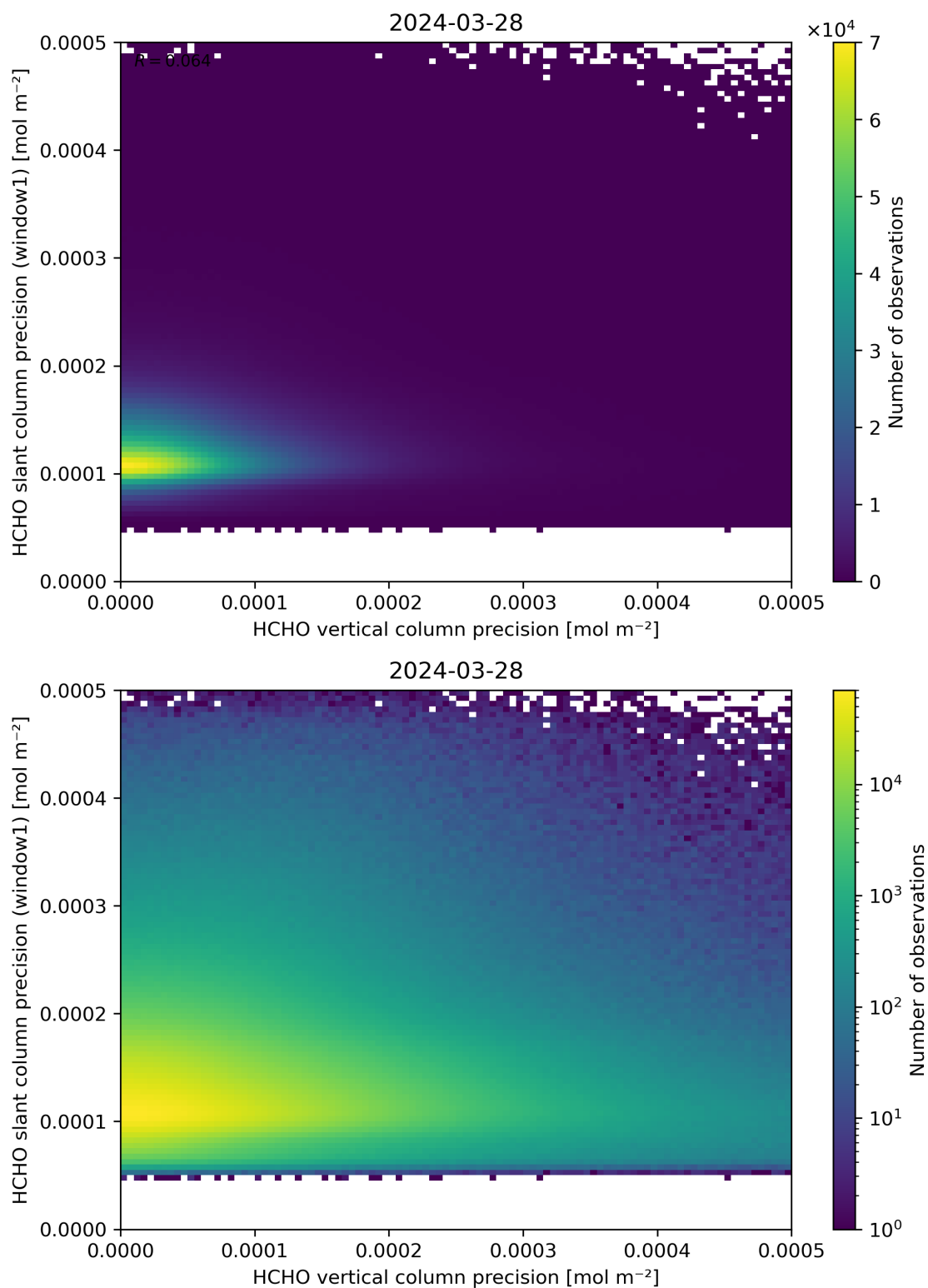
Figure 143: Scatter density plot of “HCHO vertical column precision” against “HCHO slant column precision (window1)” for 2024-03-27 to 2024-03-29.
