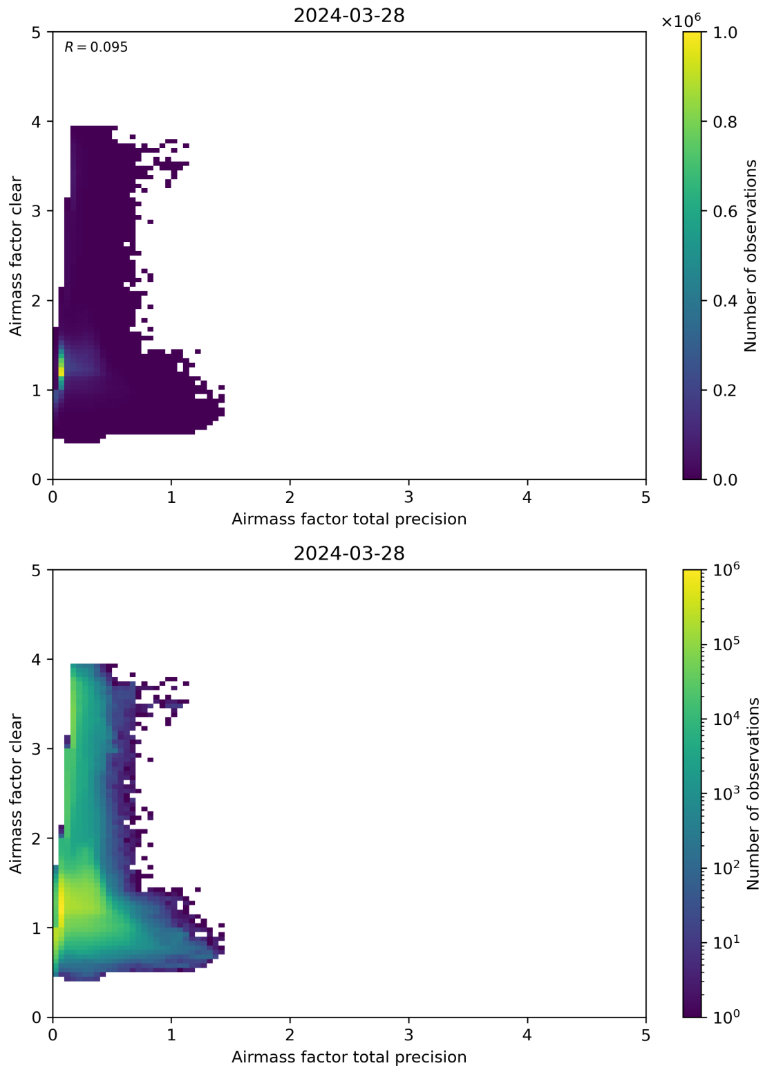
Figure 108: Scatter density plot of “Airmass factor total precision” against “Airmass factor clear” for 2024-03-27 to 2024-03-29.
