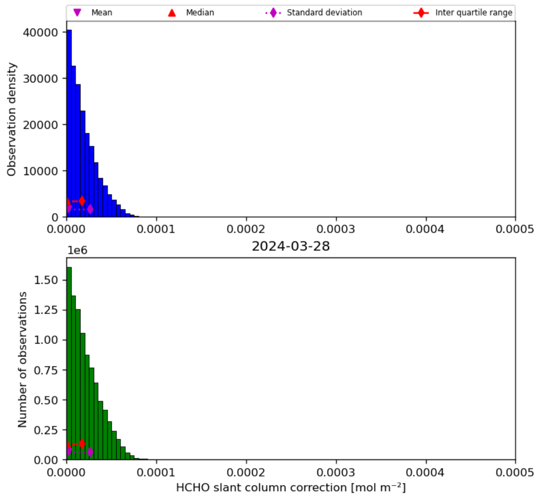
Figure 47: Histogram of “HCHO slant column correction” for 2024-03-27 to 2024-03-29
