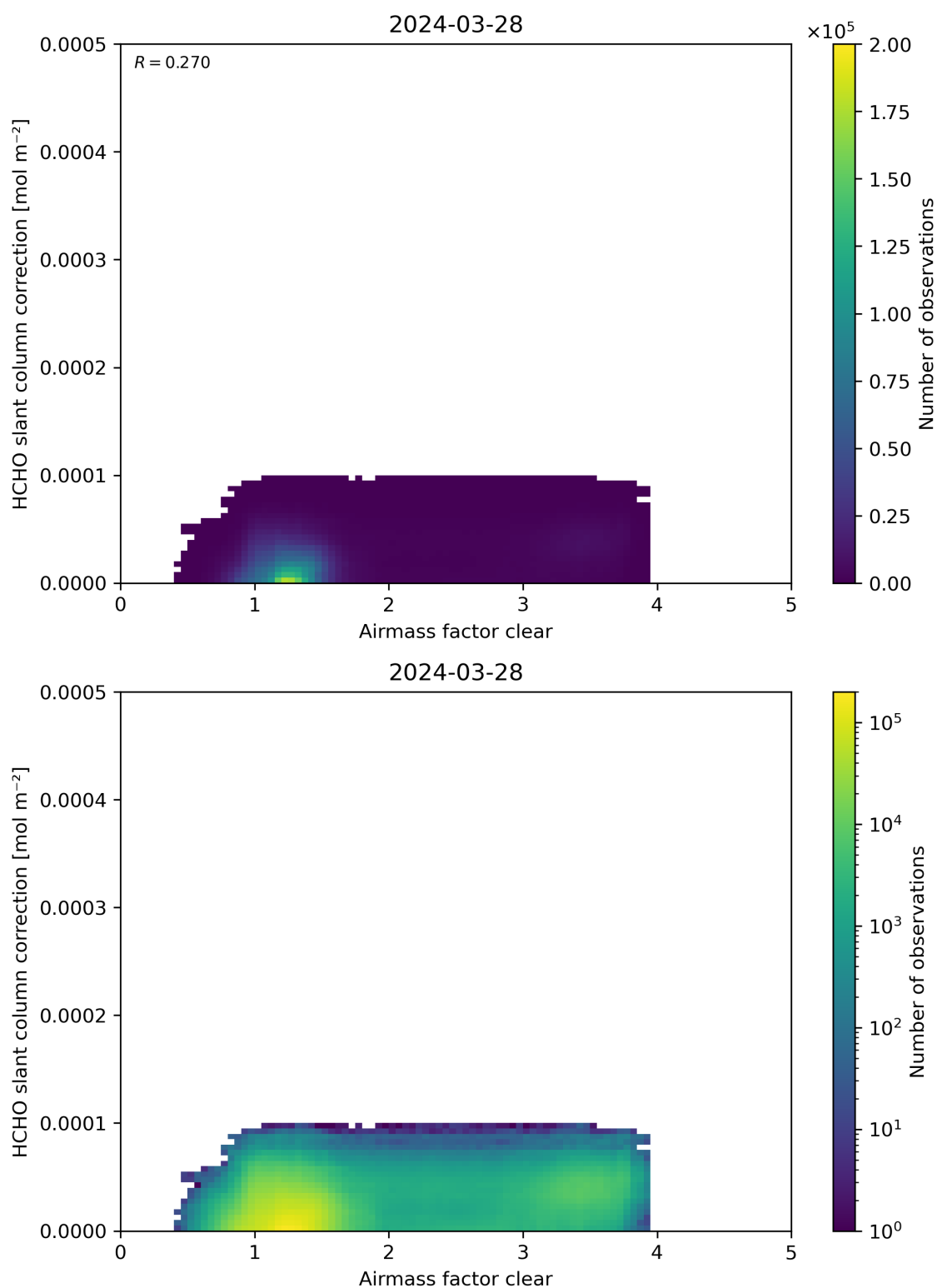
Figure 75: Scatter density plot of “Airmass factor clear” against “HCHO slant column correction” for 2024-03-27 to 2024-03-29.
