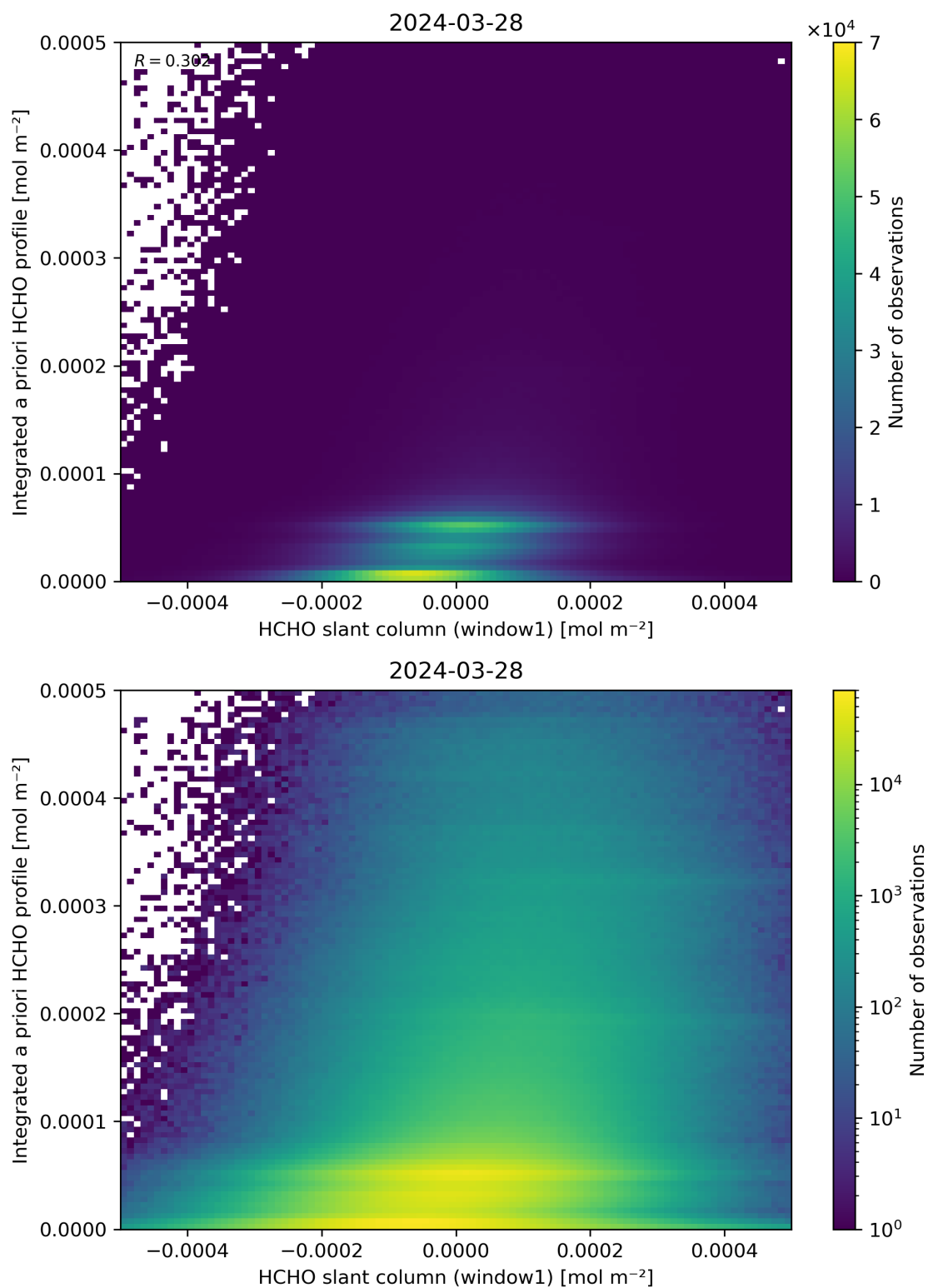
Figure 87: Scatter density plot of “HCHO slant column (window1)” against “Integrated a priori HCHO profile” for 2024-03-27 to 2024-03-29.
