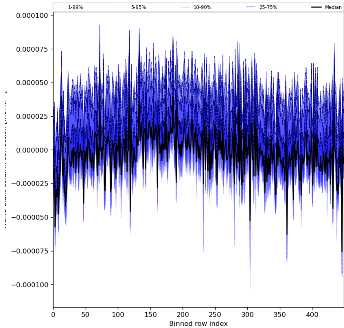
Figure 61: Along track statistics of “HCHO slant column correction” for 2024-03-27 to 2024-03-29
