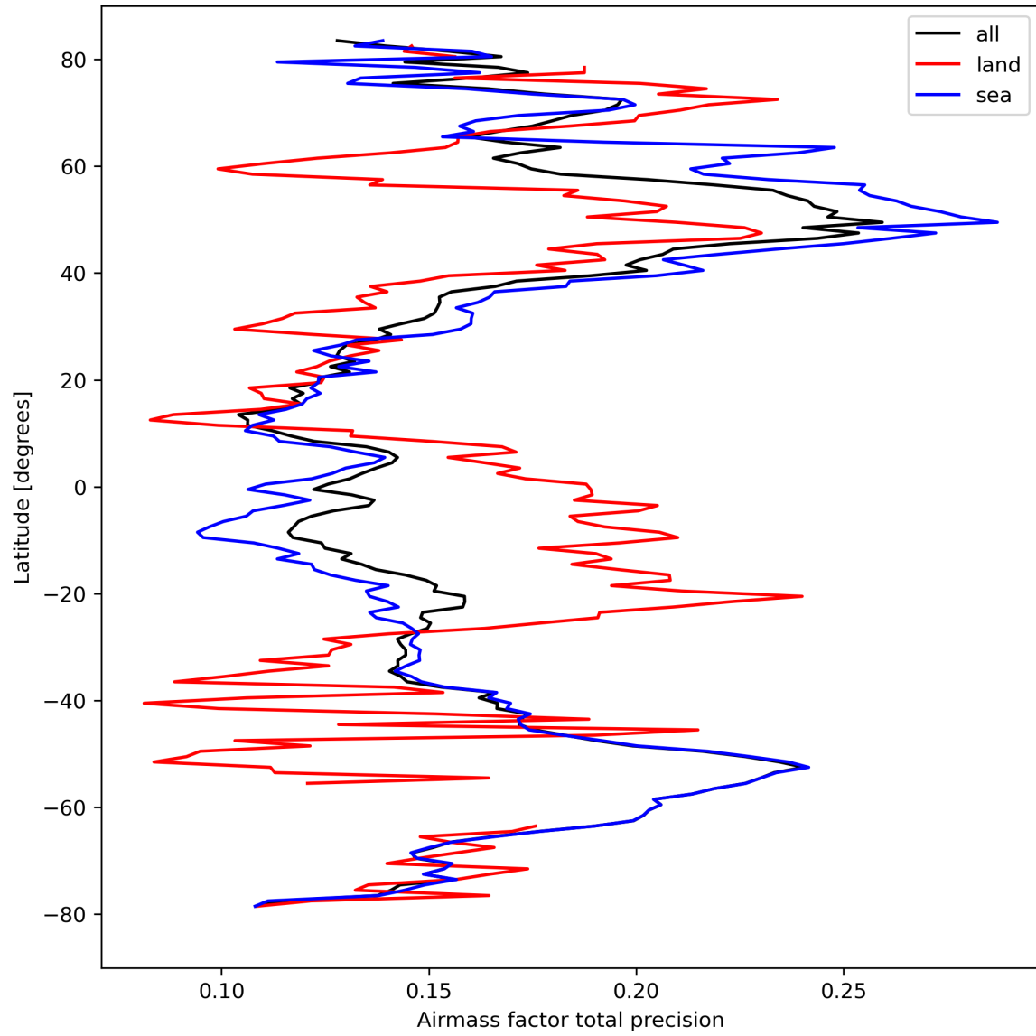
Figure 27: Zonal average of “Airmass factor total precision” for 2024-03-27 to 2024-03-29.
