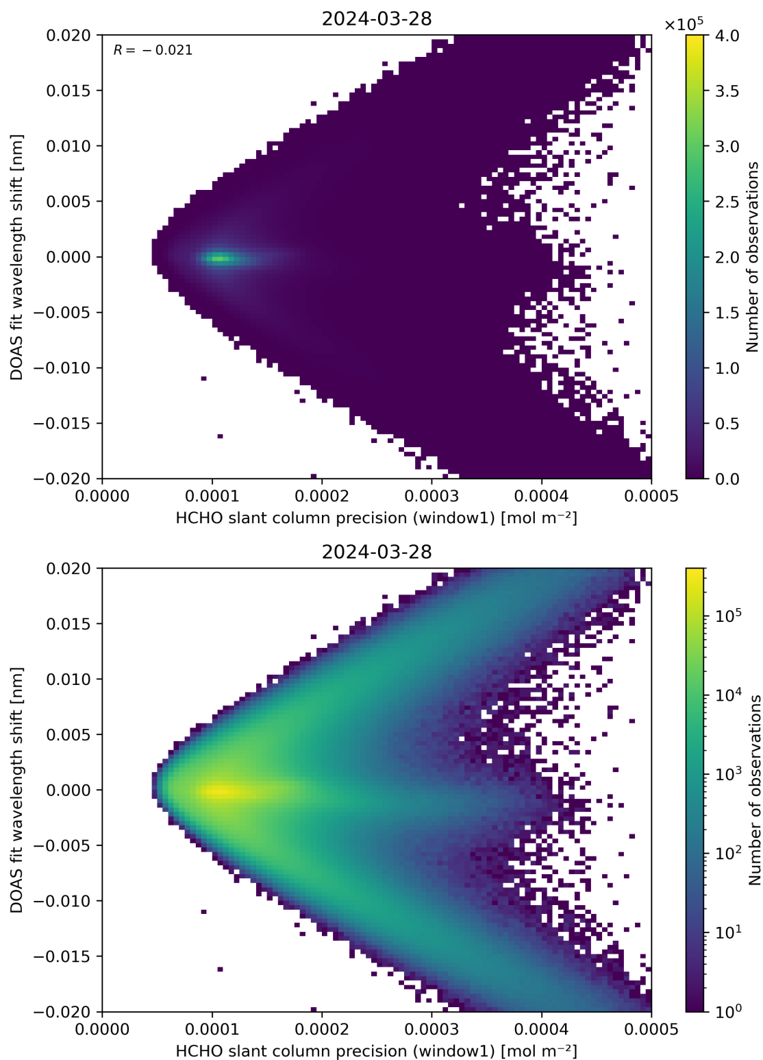
Figure 89: Scatter density plot of “HCHO slant column precision (window1)” against “DOAS fit wavelength shift” for 2024-03-27 to 2024-03-29.
