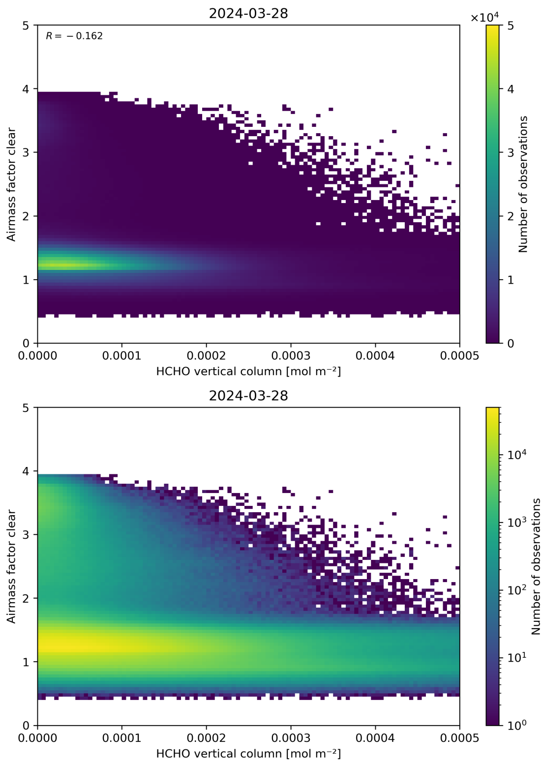
Figure 126: Scatter density plot of “HCHO vertical column” against “Airmass factor clear” for 2024-03-27 to 2024-03-29.
