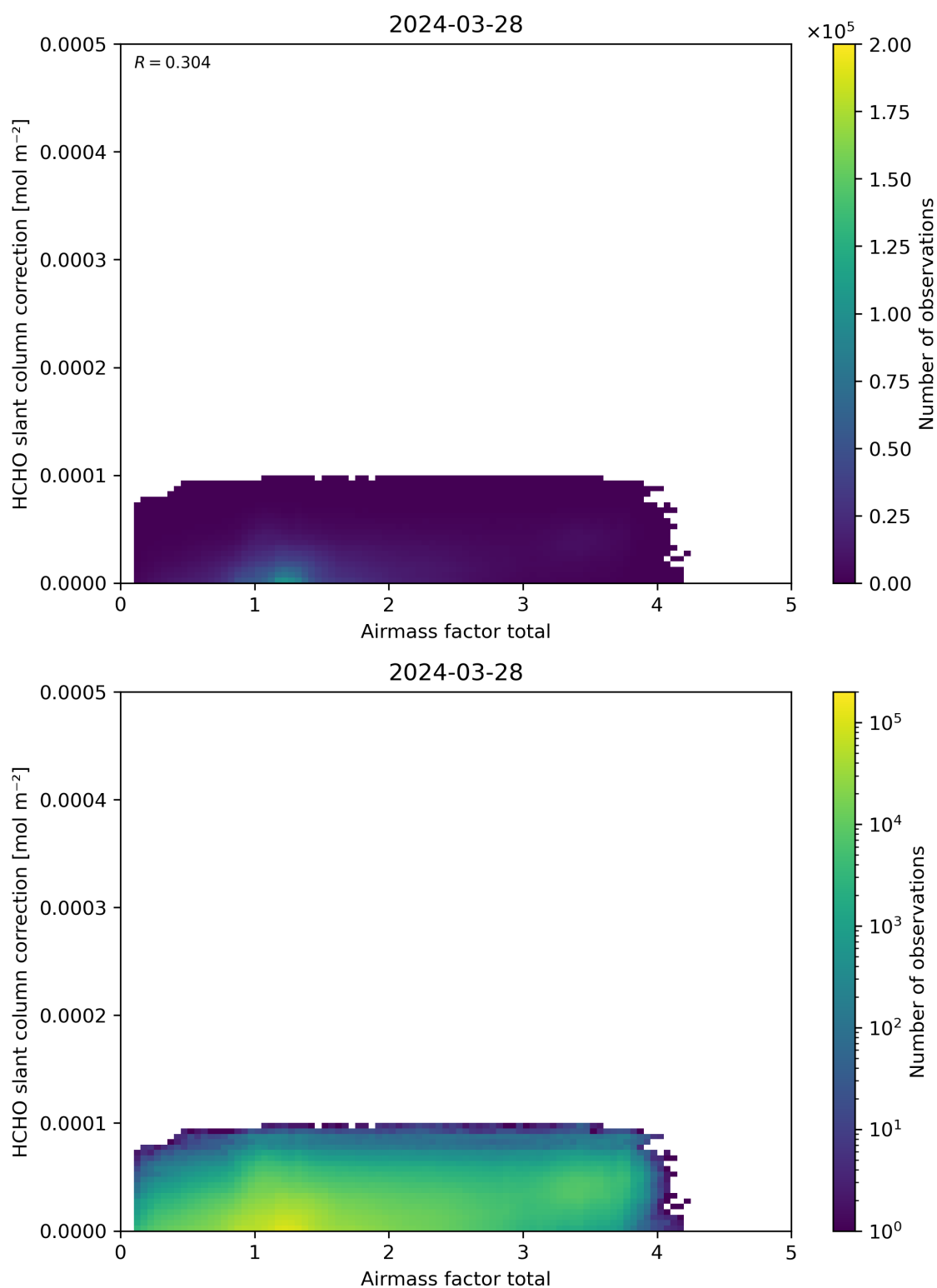
Figure 102: Scatter density plot of “Airmass factor total” against “HCHO slant column correction” for 2024-03-27 to 2024-03-29.
