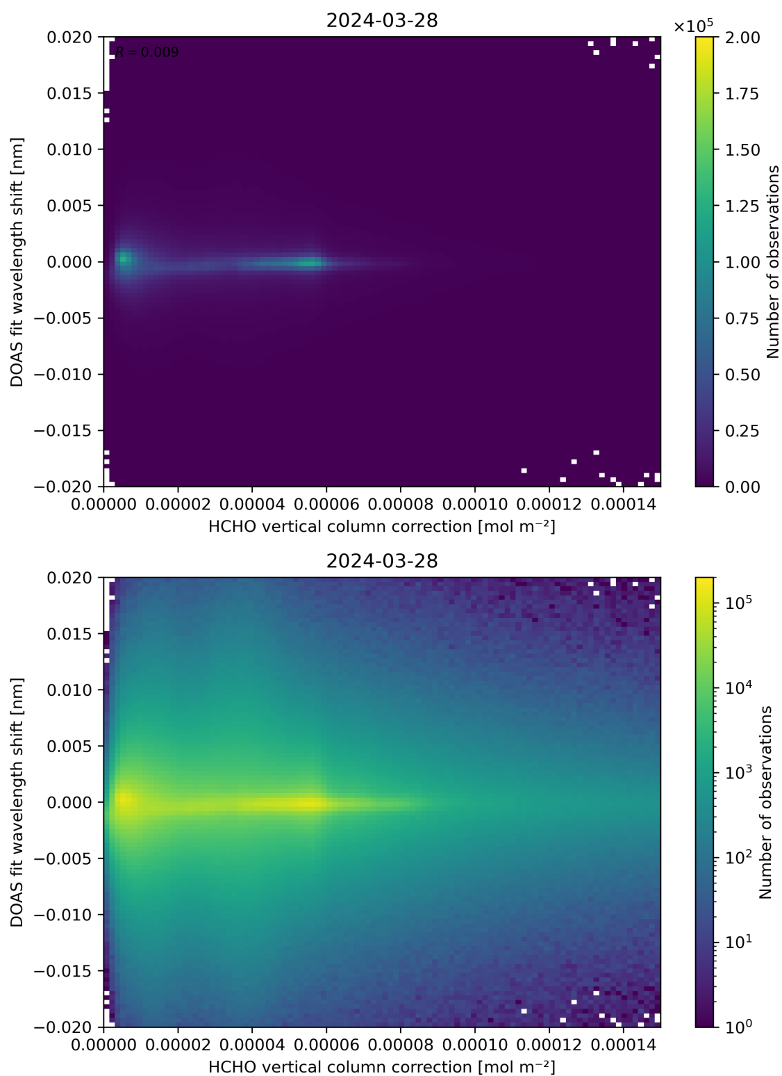
Figure 113: Scatter density plot of “HCHO vertical column correction” against “DOAS fit wavelength shift” for 2024-03-27 to 2024-03-29.
