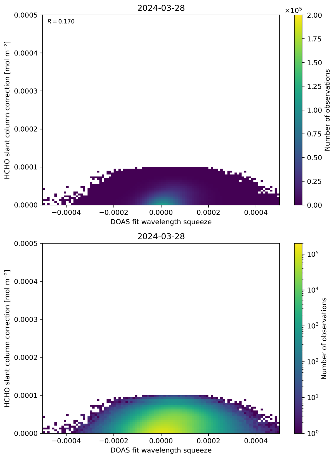
Figure 70: Scatter density plot of “DOAS fit wavelength squeeze” against “HCHO slant column correction” for 2024-03-27 to 2024-03-29.
