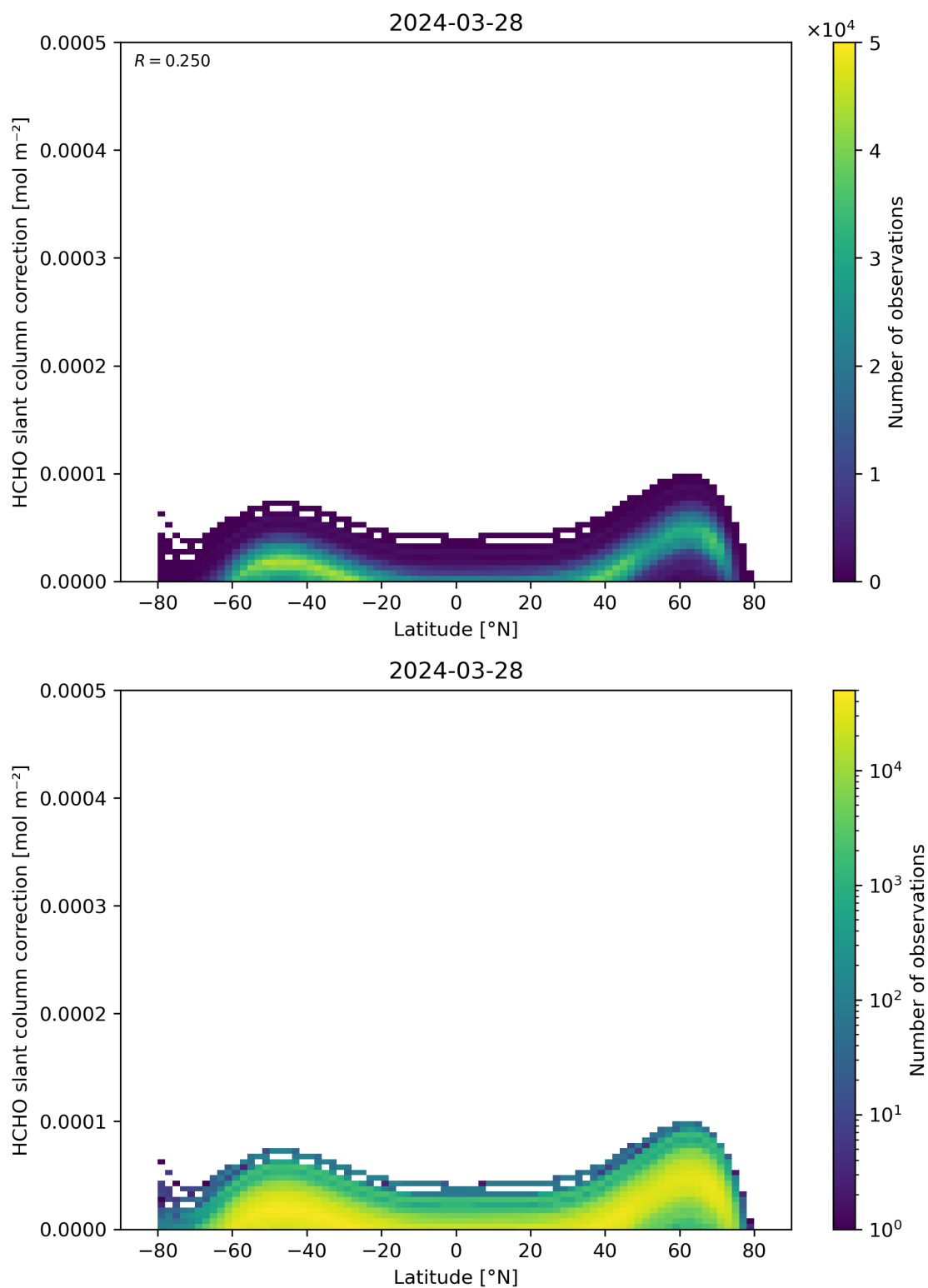
Figure 158: Scatter density plot of “Latitude” against “HCHO slant column correction” for 2024-03-27 to 2024-03-29.
