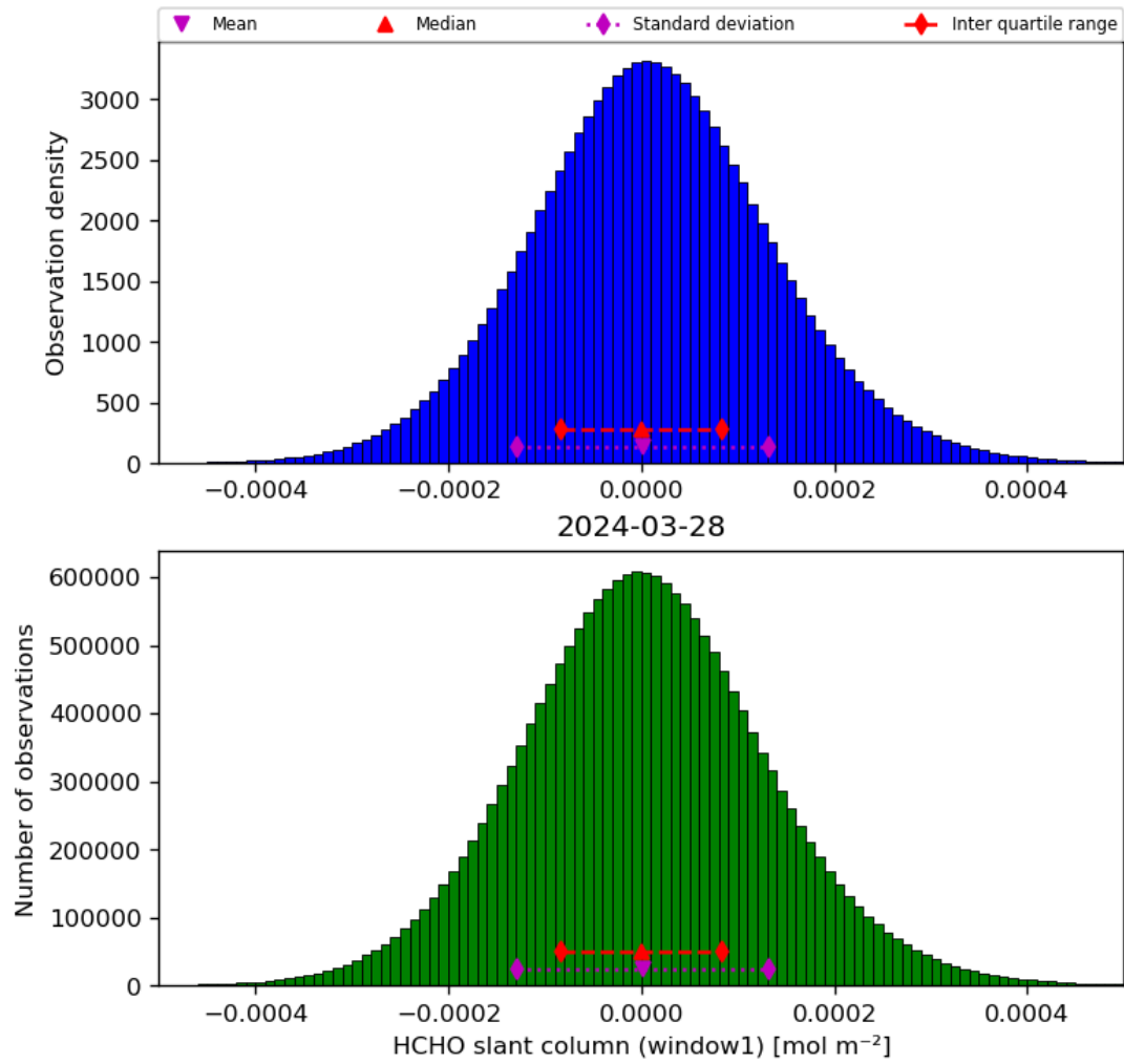
Figure 38: Histogram of “HCHO slant column (window1)” for 2024-03-27 to 2024-03-29
