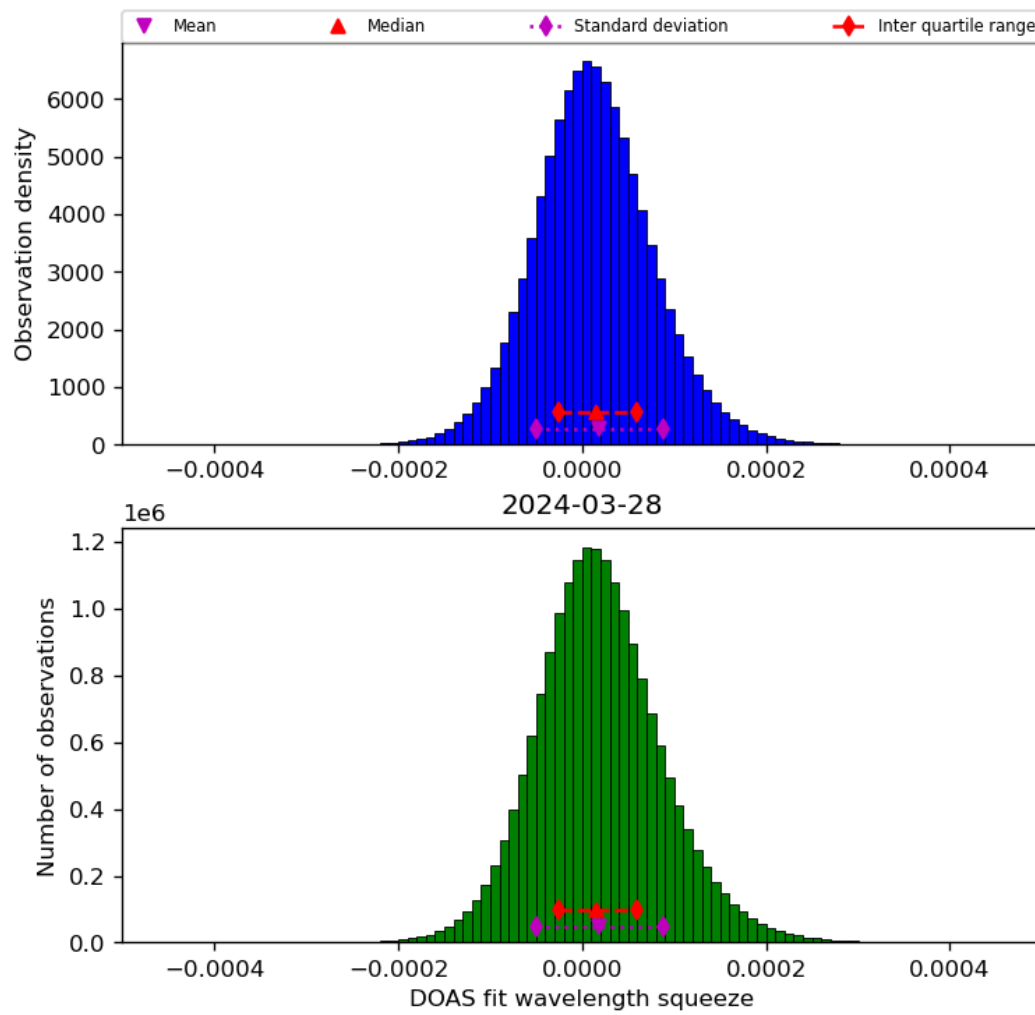
Figure 45: Histogram of “DOAS fit wavelength squeeze” for 2024-03-27 to 2024-03-29
