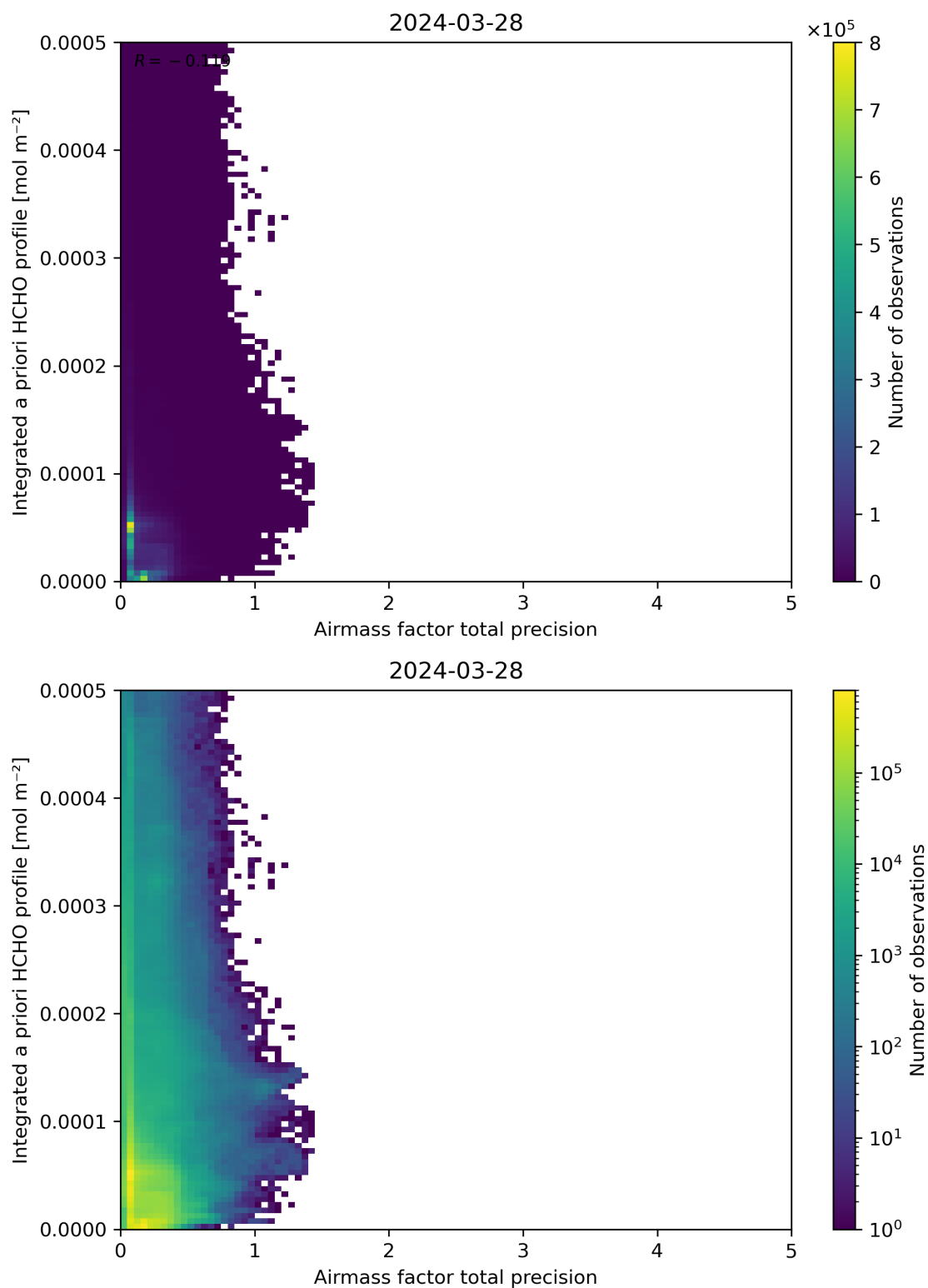
Figure 111: Scatter density plot of “Airmass factor total precision” against “Integrated a priori HCHO profile” for 2024-03-27 to 2024-03-29.
