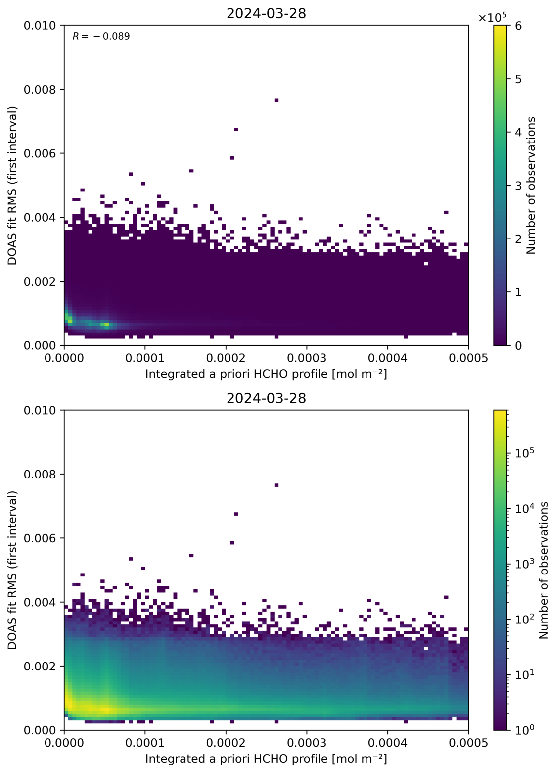
Figure 148: Scatter density plot of “Integrated a priori HCHO profile” against “DOAS fit RMS (first interval)” for 2024-03-27 to 2024-03-29.
