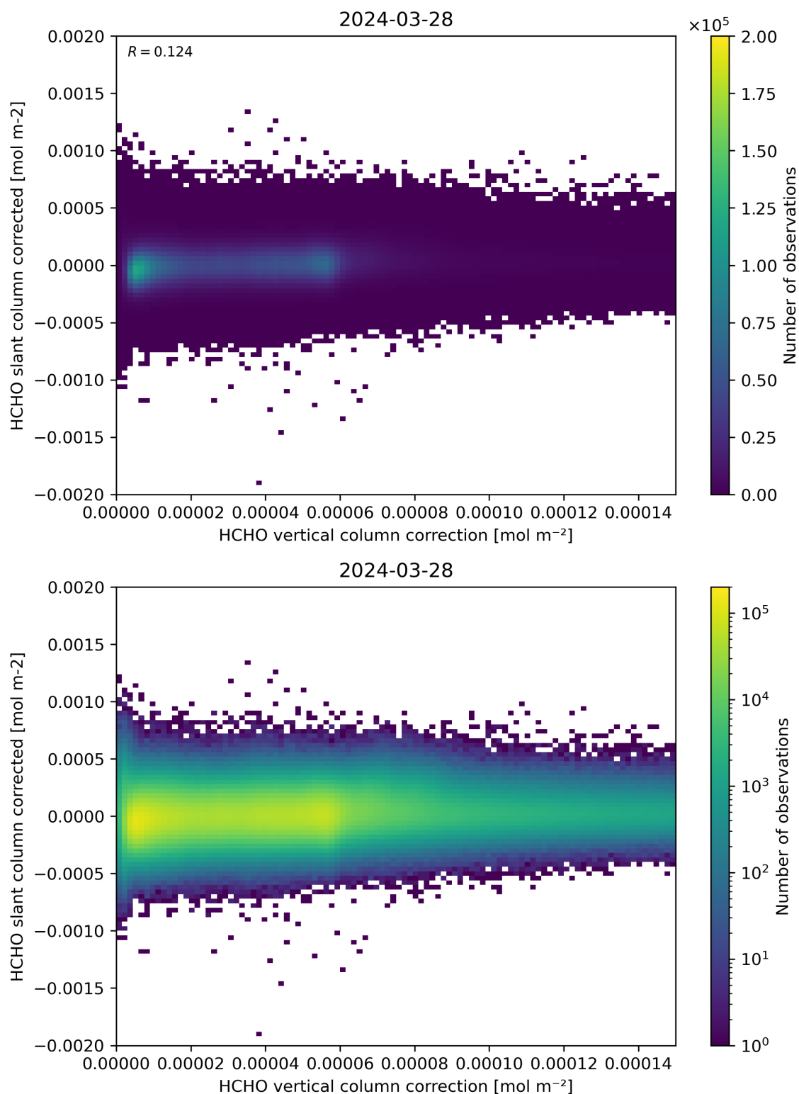
Figure 116: Scatter density plot of “HCHO vertical column correction” against “HCHO slant column corrected” for 2024-03-27 to 2024-03-29.
