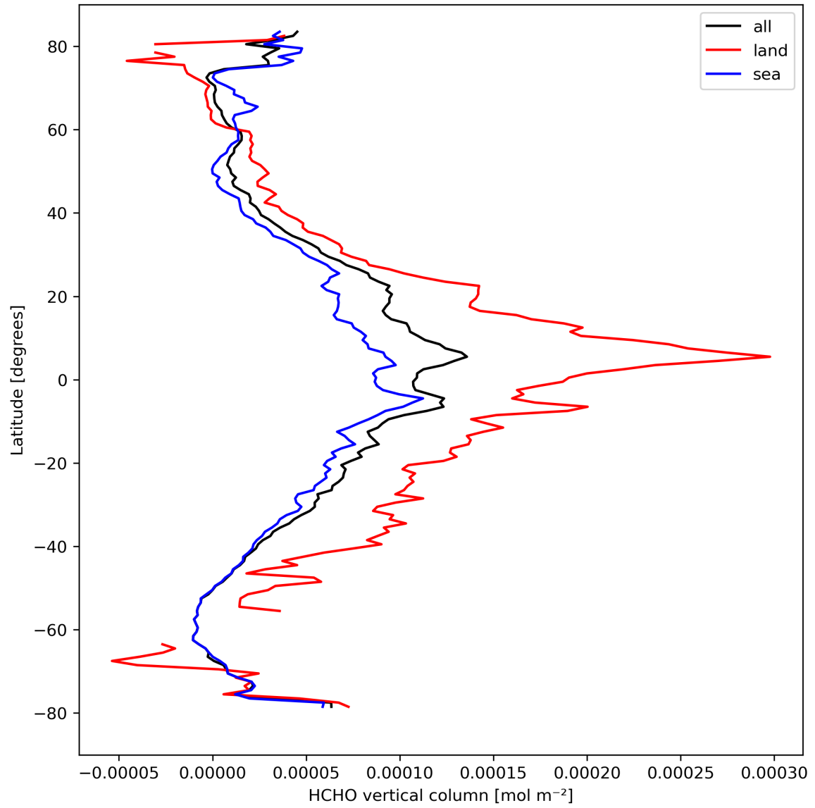
Figure 21: Zonal average of “HCHO vertical column” for 2024-03-27 to 2024-03-29.
