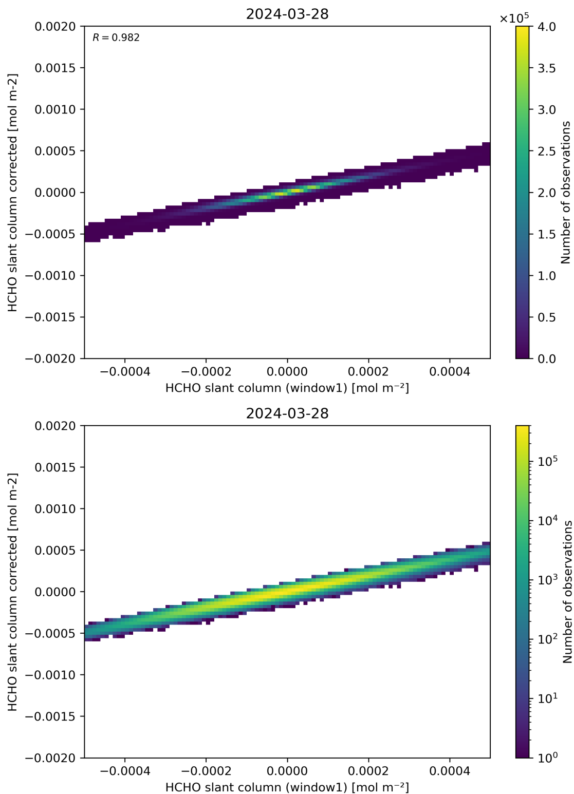
Figure 82: Scatter density plot of “HCHO slant column (window1)” against “HCHO slant column corrected” for 2024-03-27 to 2024-03-29.
