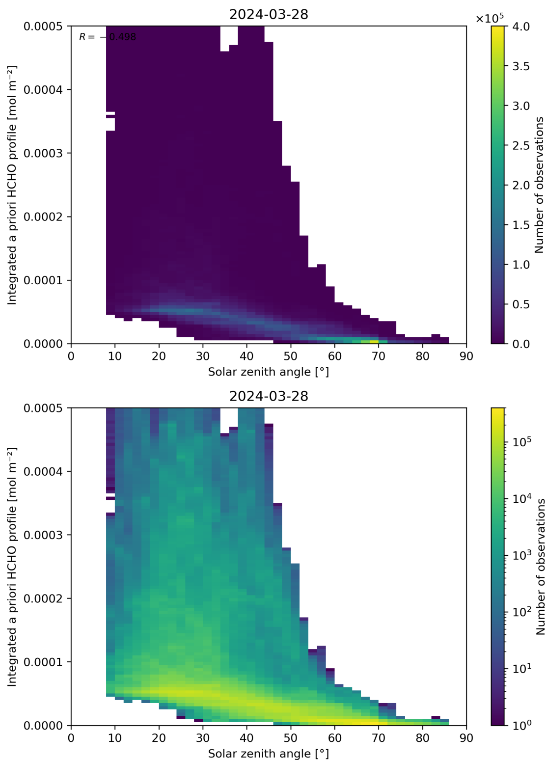
Figure 180: Scatter density plot of “Solar zenith angle” against “Integrated a priori HCHO profile” for 2024-03-27 to 2024-03-29.
