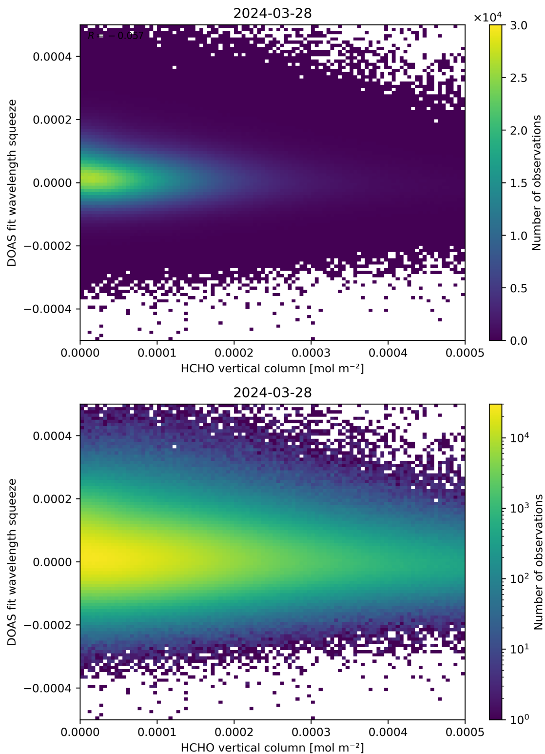
Figure 125: Scatter density plot of “HCHO vertical column” against “DOAS fit wavelength squeeze” for 2024-03-27 to 2024-03-29.
