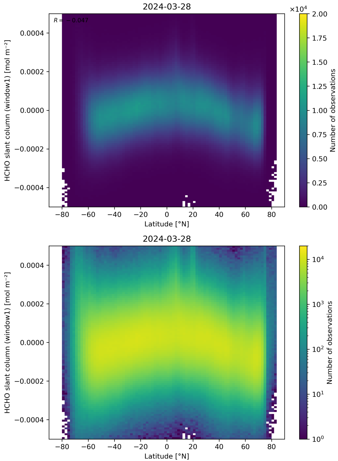
Figure 159: Scatter density plot of “Latitude” against “HCHO slant column (window1)” for 2024-03-27 to 2024-03-29.
