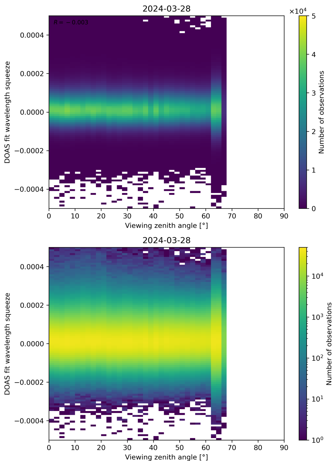
Figure 184: Scatter density plot of “Viewing zenith angle” against “DOAS fit wavelength squeeze” for 2024-03-27 to 2024-03-29.
