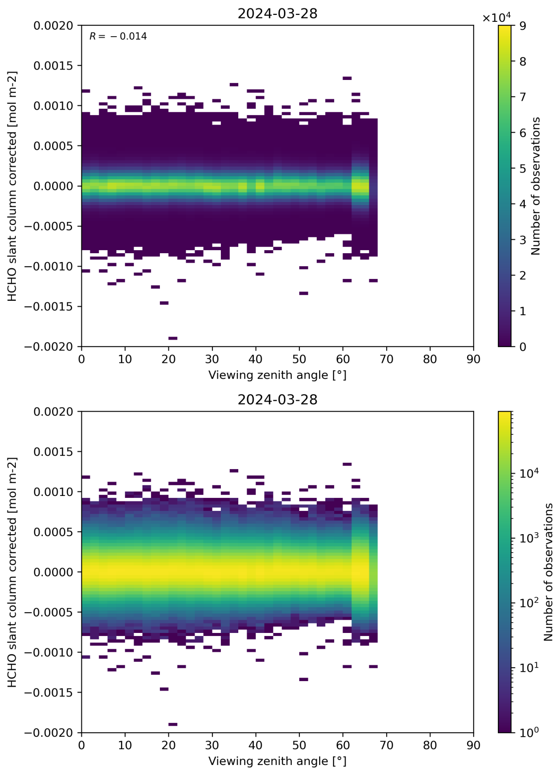
Figure 186: Scatter density plot of “Viewing zenith angle” against “HCHO slant column corrected” for 2024-03-27 to 2024-03-29.
