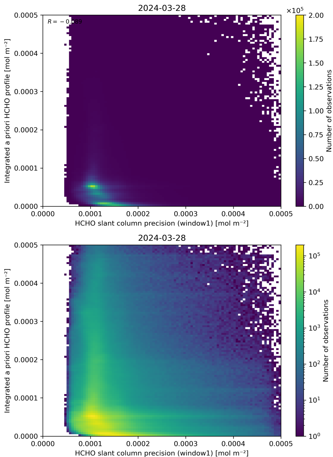
Figure 96: Scatter density plot of “HCHO slant column precision (window1)” against “Integrated a priori HCHO profile” for 2024-03-27 to 2024-03-29.
