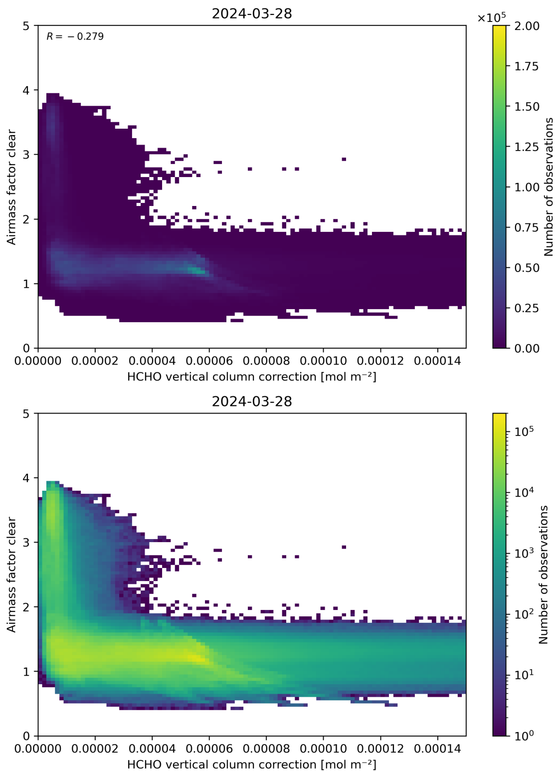
Figure 115: Scatter density plot of “HCHO vertical column correction” against “Airmass factor clear” for 2024-03-27 to 2024-03-29.
