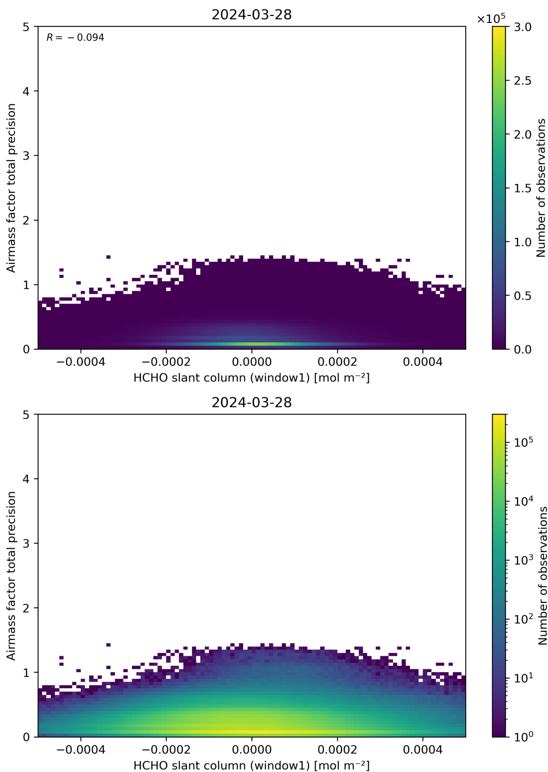
Figure 86: Scatter density plot of “HCHO slant column (window1)” against “Airmass factor total precision” for 2024-03-27 to 2024-03-29.
