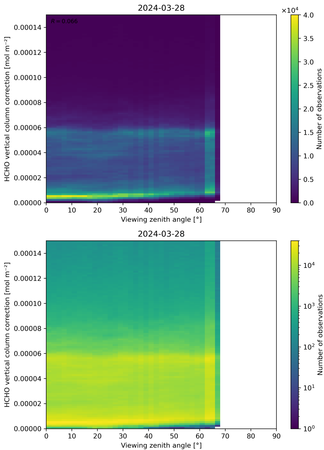
Figure 193: Scatter density plot of “Viewing zenith angle” against “HCHO vertical column correction” for 2024-03-27 to 2024-03-29.
