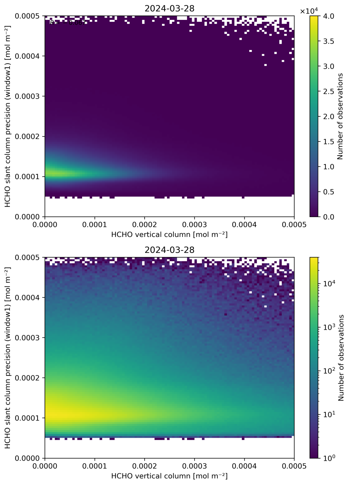
Figure 130: Scatter density plot of “HCHO vertical column” against “HCHO slant column precision (window1)” for 2024-03-27 to 2024-03-29.
