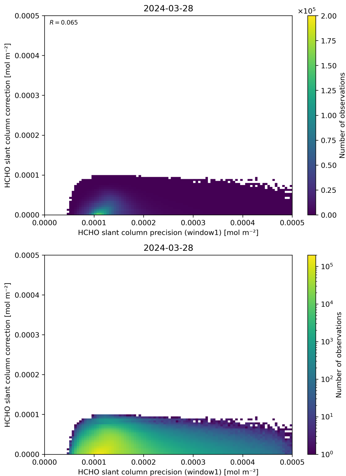
Figure 93: Scatter density plot of “HCHO slant column precision (window1)” against “HCHO slant column correction” for 2024-03-27 to 2024-03-29.
