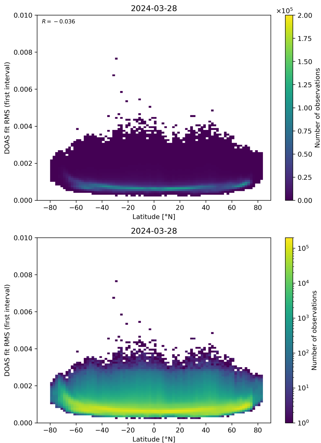
Figure 153: Scatter density plot of “Latitude” against “DOAS fit RMS (first interval)” for 2024-03-27 to 2024-03-29.
