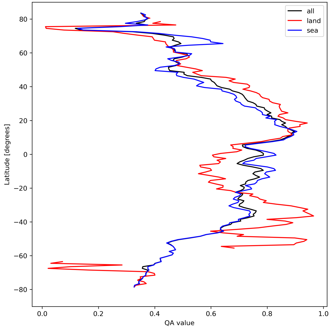
Figure 20: Zonal average of “QA value” for 2024-03-27 to 2024-03-29.
