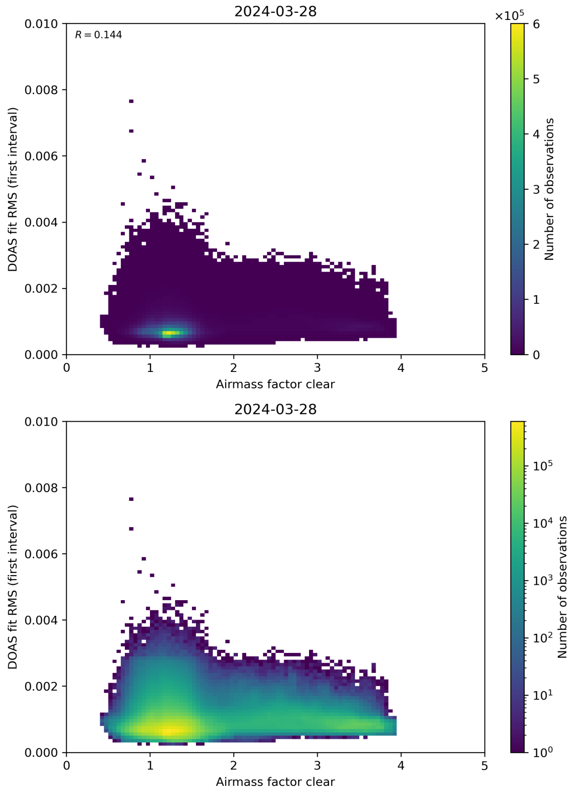
Figure 71: Scatter density plot of “Airmass factor clear” against “DOAS fit RMS (first interval)” for 2024-03-27 to 2024-03-29.
