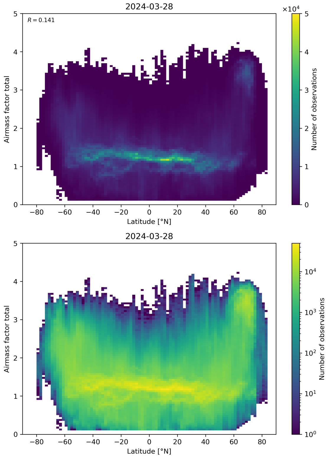
Figure 161: Scatter density plot of “Latitude” against “Airmass factor total” for 2024-03-27 to 2024-03-29.
