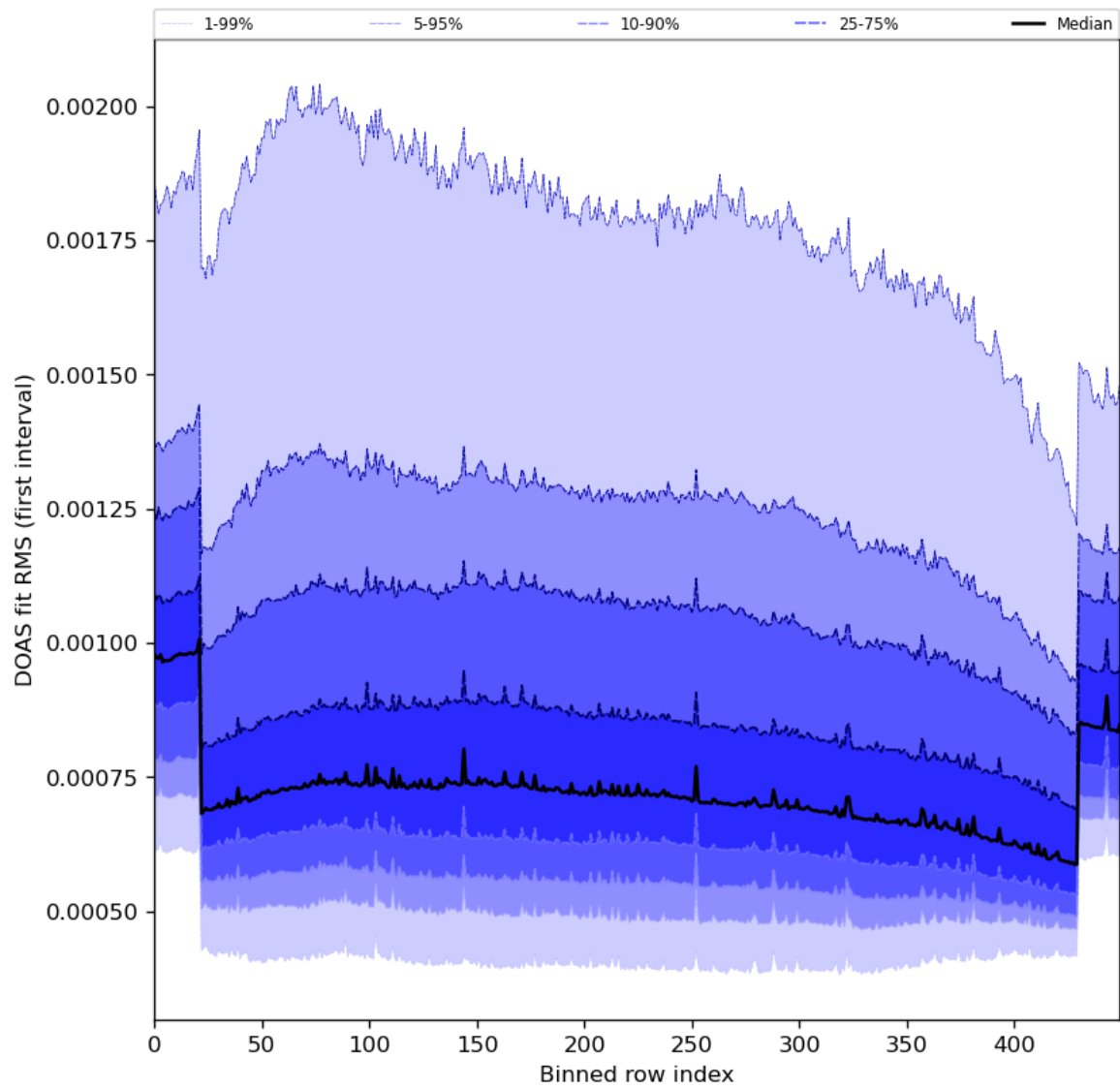
Figure 60: Along track statistics of “DOAS fit RMS (first interval)” for 2024-03-27 to 2024-03-29
