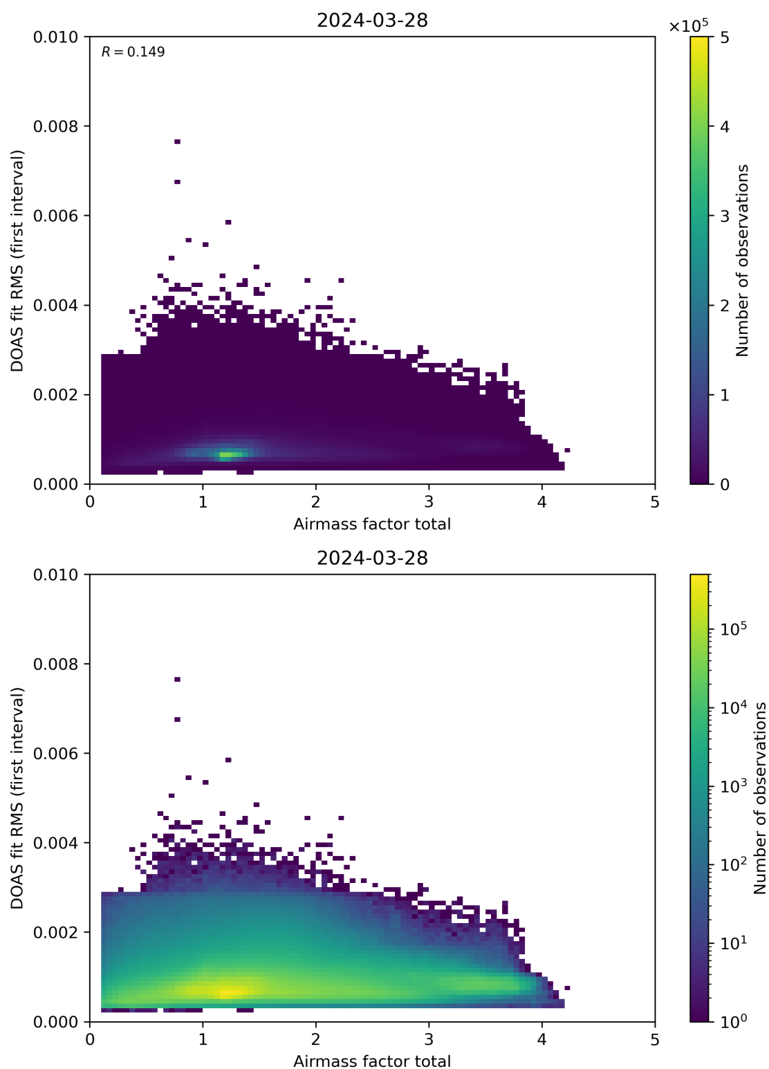
Figure 97: Scatter density plot of “Airmass factor total” against “DOAS fit RMS (first interval)” for 2024-03-27 to 2024-03-29.
