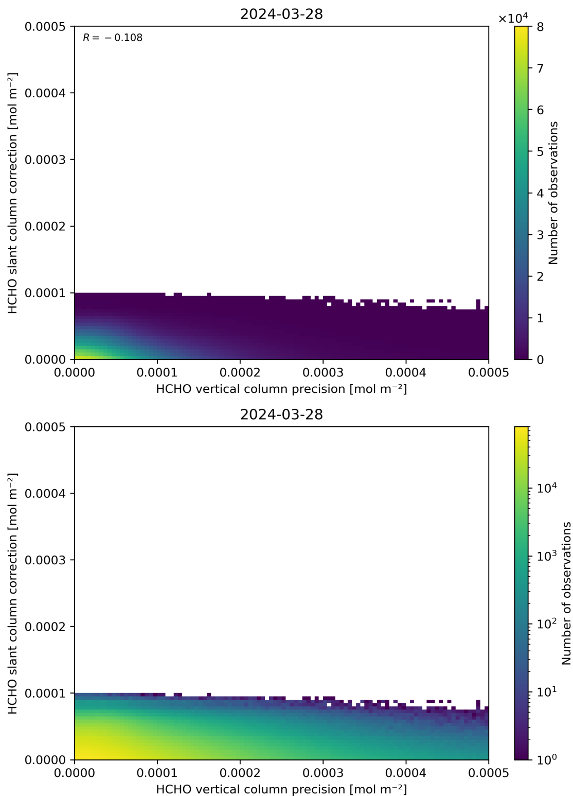
Figure 141: Scatter density plot of “HCHO vertical column precision” against “HCHO slant column correction” for 2024-03-27 to 2024-03-29.
