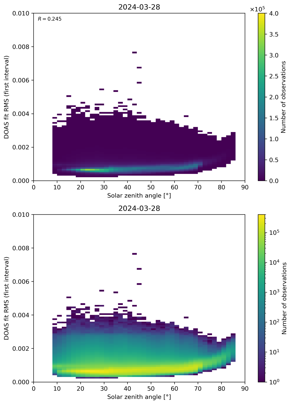
Figure 167: Scatter density plot of “Solar zenith angle” against “DOAS fit RMS (first interval)” for 2024-03-27 to 2024-03-29.
