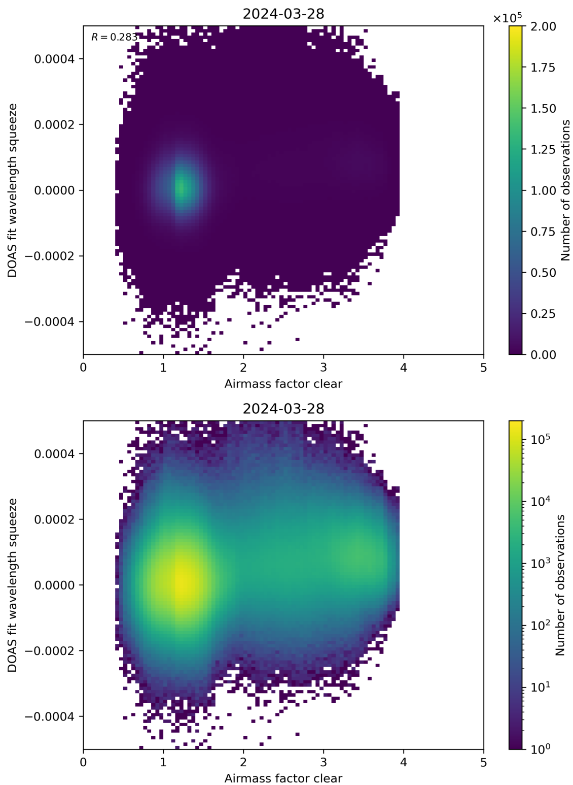
Figure 73: Scatter density plot of “Airmass factor clear” against “DOAS fit wavelength squeeze” for 2024-03-27 to 2024-03-29.
