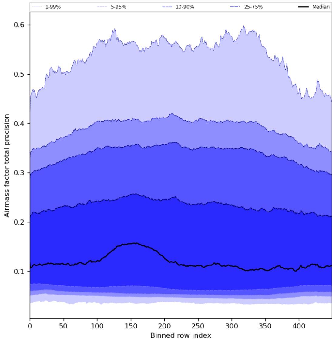
Figure 55: Along track statistics of “Airmass factor total precision” for 2024-03-27 to 2024-03-29
