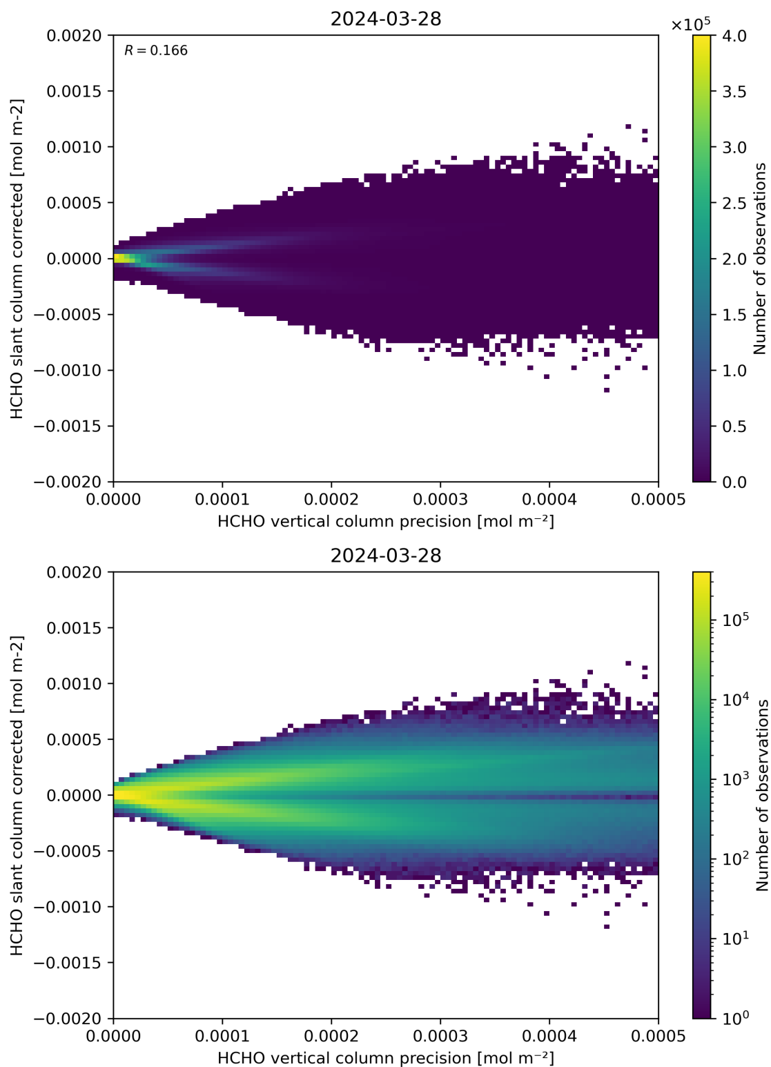
Figure 140: Scatter density plot of “HCHO vertical column precision” against “HCHO slant column corrected” for 2024-03-27 to 2024-03-29.
