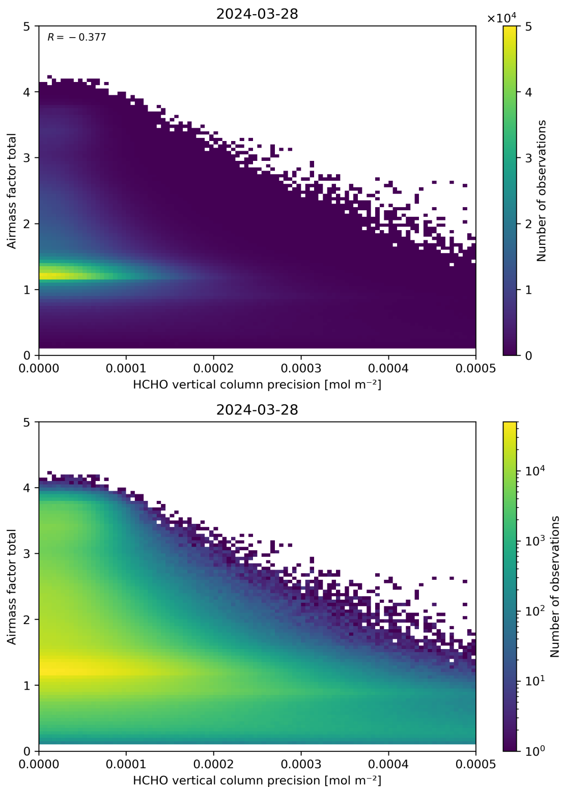
Figure 144: Scatter density plot of “HCHO vertical column precision” against “Airmass factor total” for 2024-03-27 to 2024-03-29.
