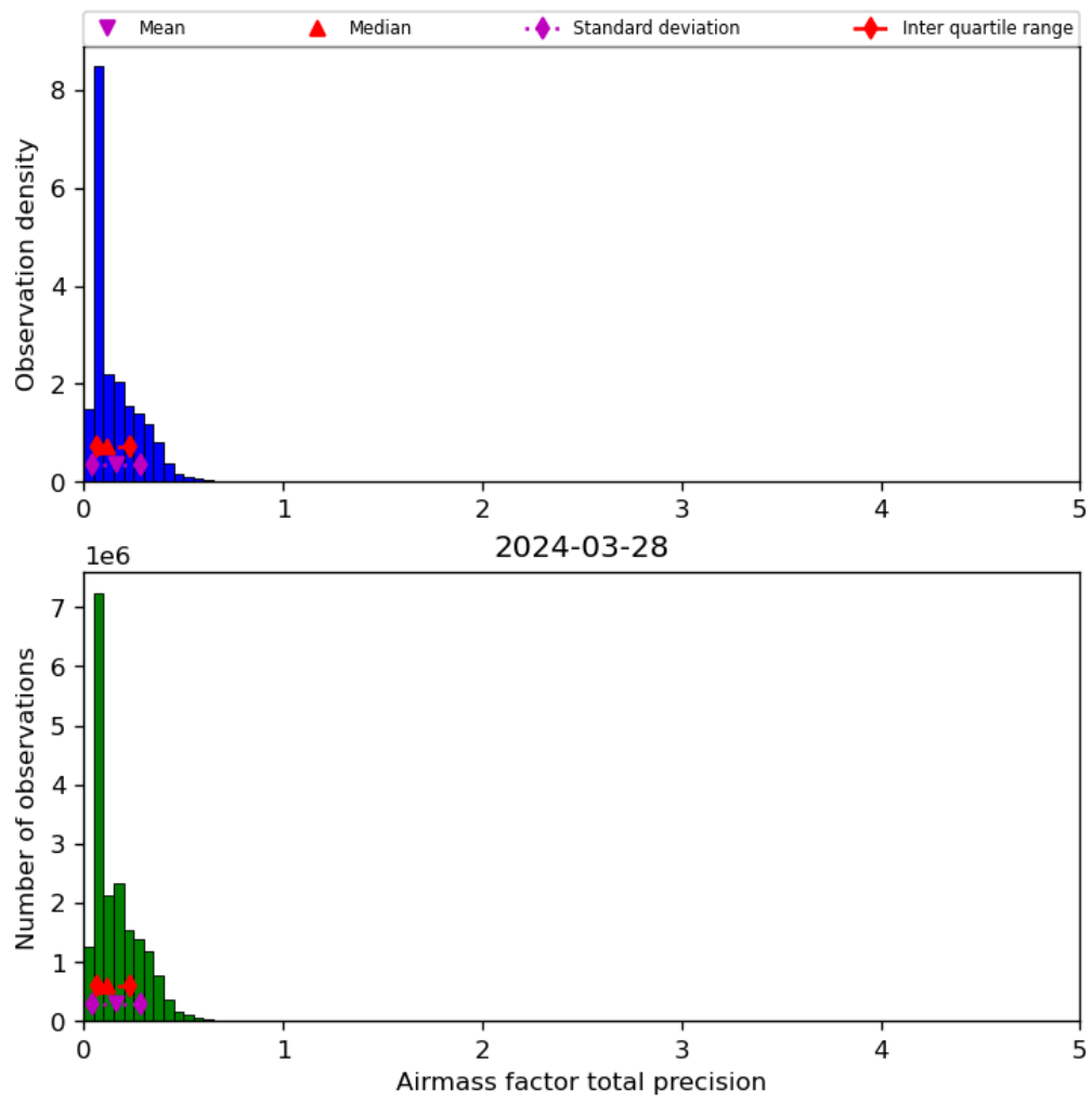
Figure 41: Histogram of "Airmass factor total precision" for 2024-03-27 to 2024-03-29
