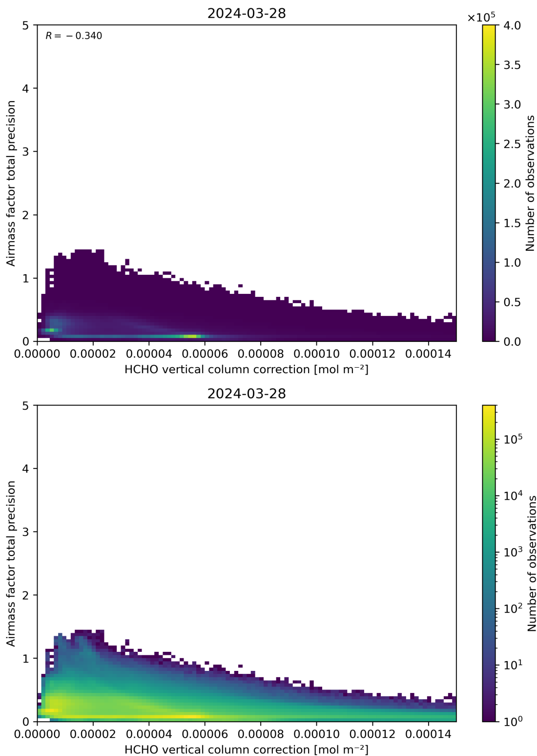
Figure 121: Scatter density plot of “HCHO vertical column correction” against “Airmass factor total precision” for 2024-03-27 to 2024-03-29.
