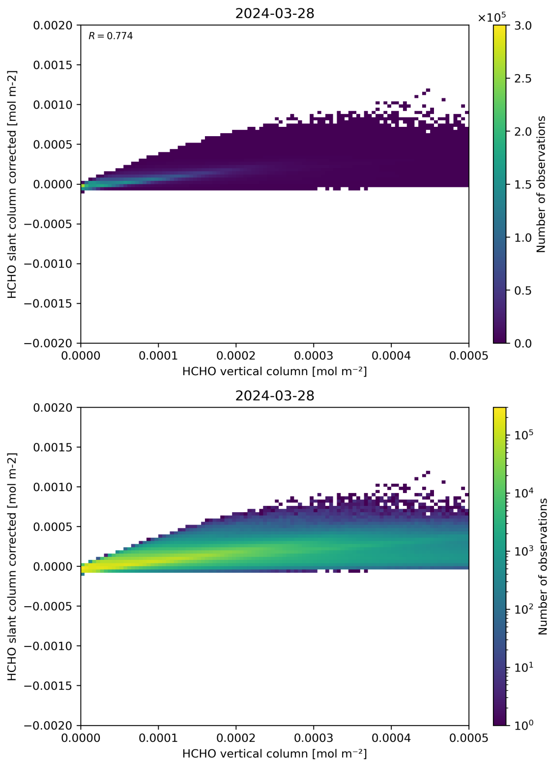
Figure 127: Scatter density plot of “HCHO vertical column” against “HCHO slant column corrected” for 2024-03-27 to 2024-03-29.
