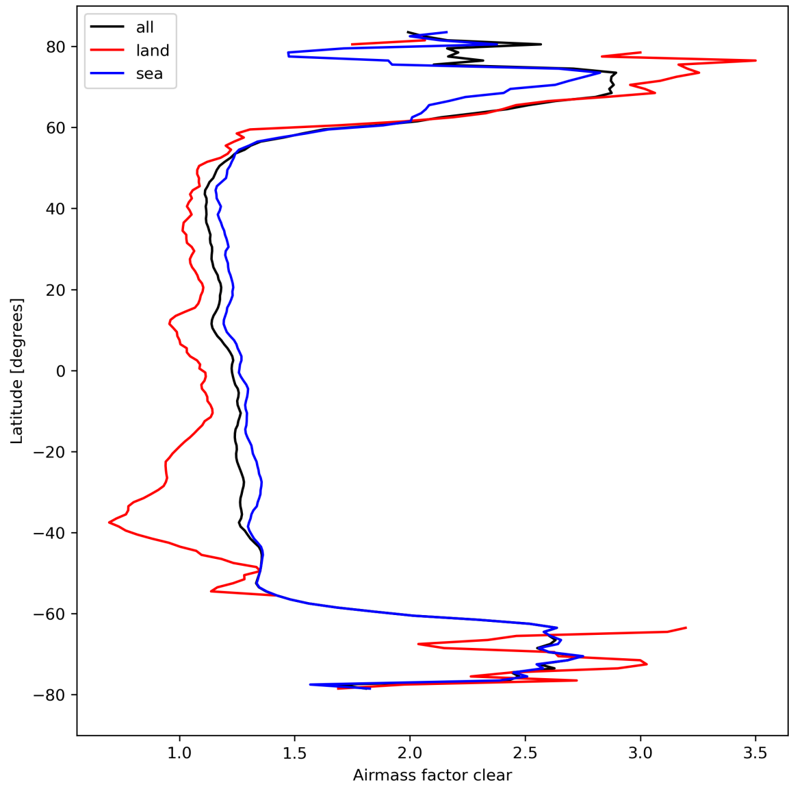
Figure 28: Zonal average of “Airmass factor clear” for 2024-03-27 to 2024-03-29.
