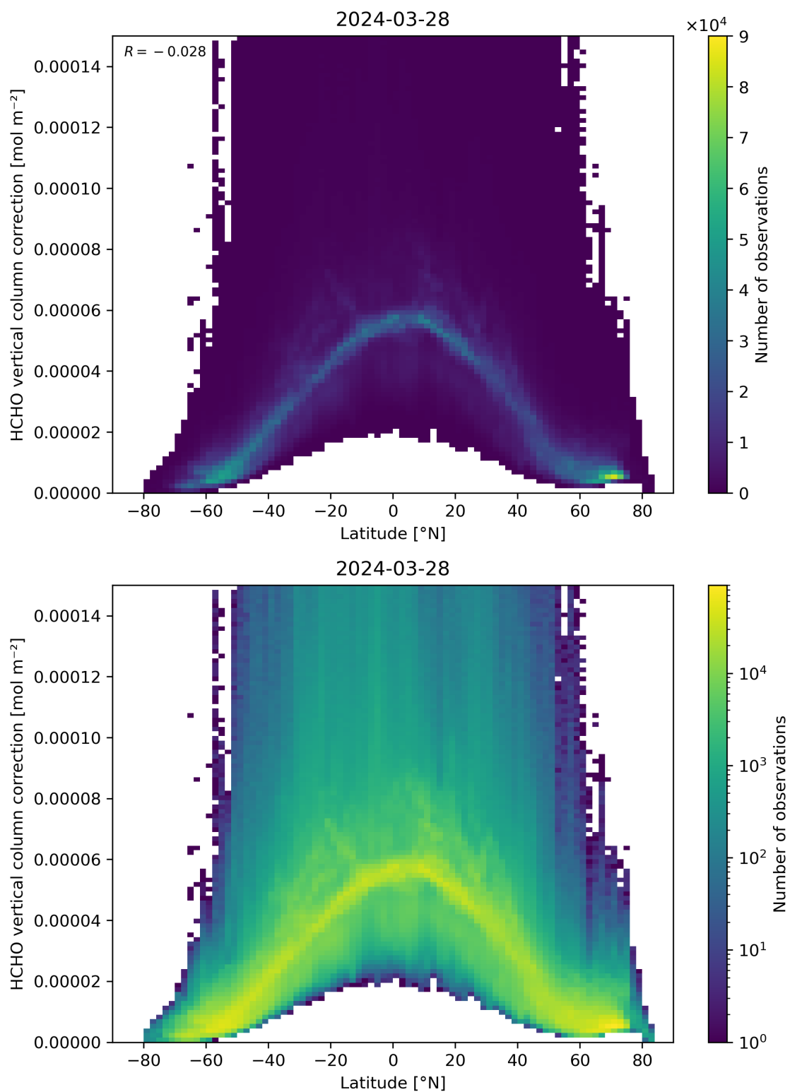
Figure 164: Scatter density plot of “Latitude” against “HCHO vertical column correction” for 2024-03-27 to 2024-03-29.
