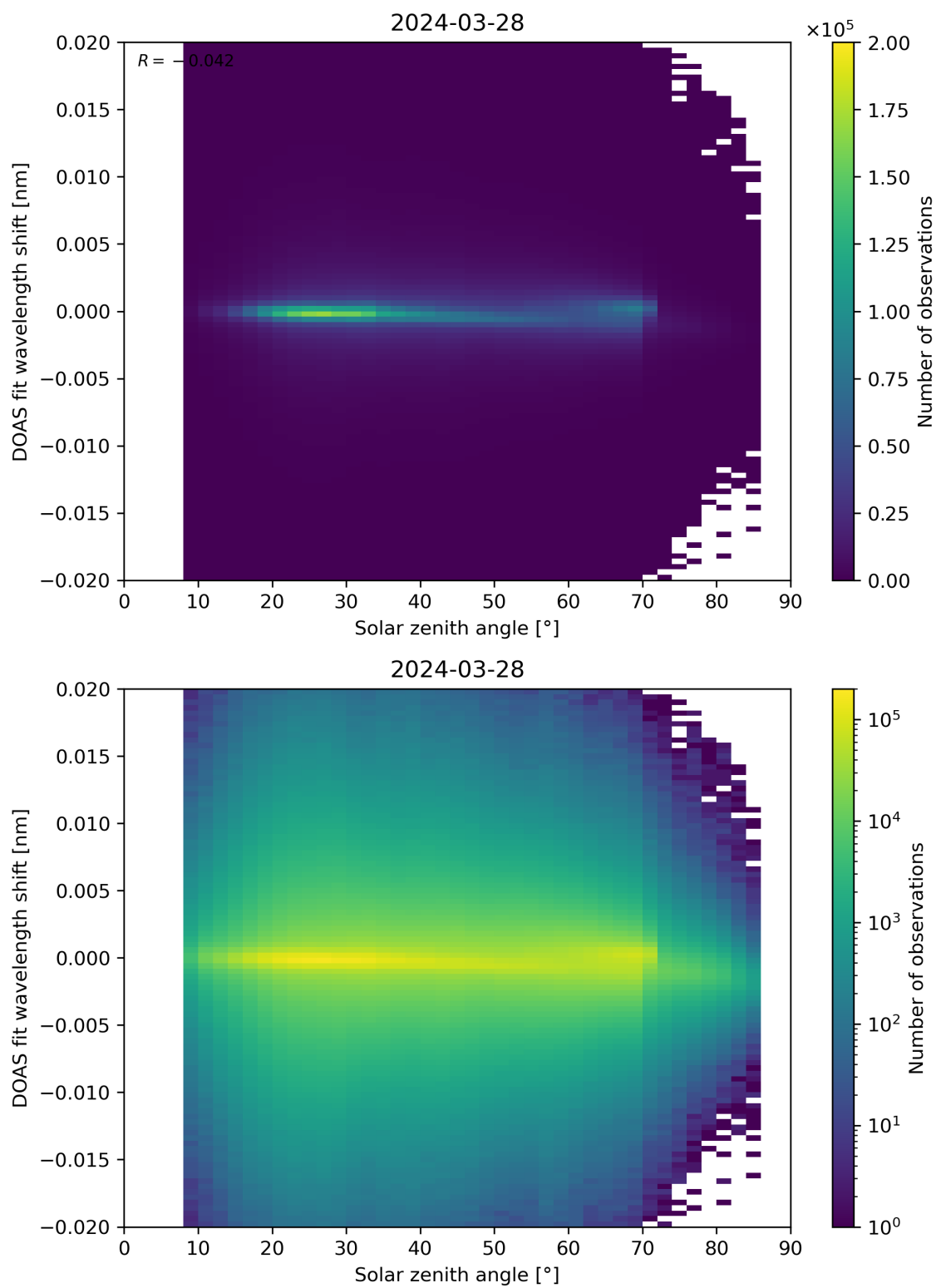
Figure 168: Scatter density plot of “Solar zenith angle” against “DOAS fit wavelength shift” for 2024-03-27 to 2024-03-29.
