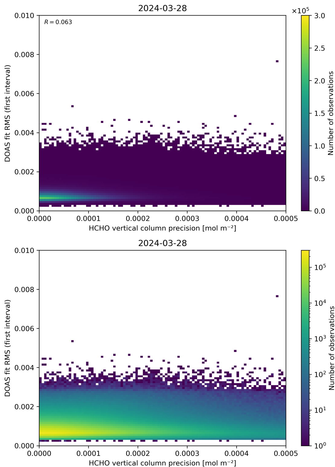
Figure 136: Scatter density plot of “HCHO vertical column precision” against “DOAS fit RMS (first interval)” for 2024-03-27 to 2024-03-29.
