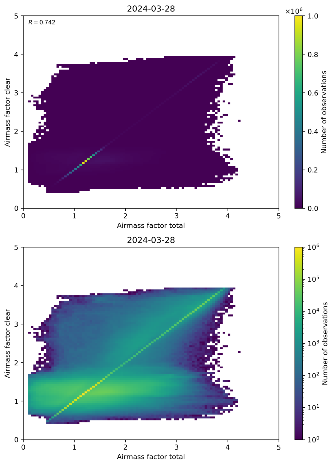
Figure 100: Scatter density plot of “Airmass factor total” against “Airmass factor clear” for 2024-03-27 to 2024-03-29.
