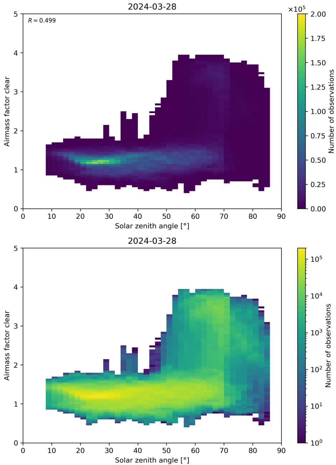
Figure 170: Scatter density plot of “Solar zenith angle” against “Airmass factor clear” for 2024-03-27 to 2024-03-29.
