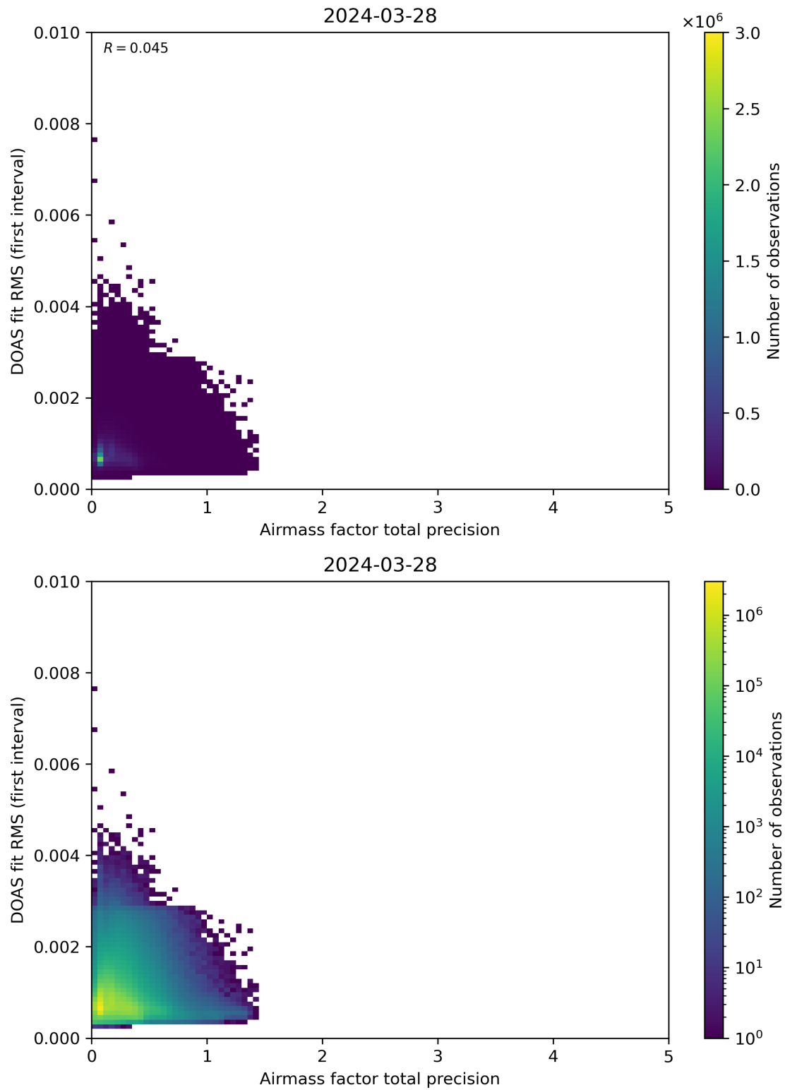
Figure 105: Scatter density plot of “Airmass factor total precision” against “DOAS fit RMS (first interval)” for 2024-03-27 to 2024-03-29.
