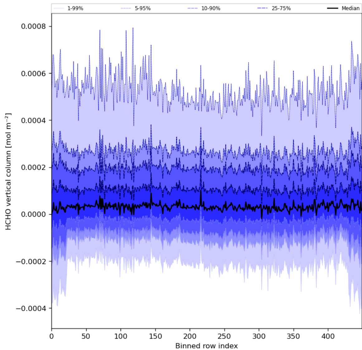
Figure 49: Along track statistics of “HCHO vertical column” for 2024-03-27 to 2024-03-29
