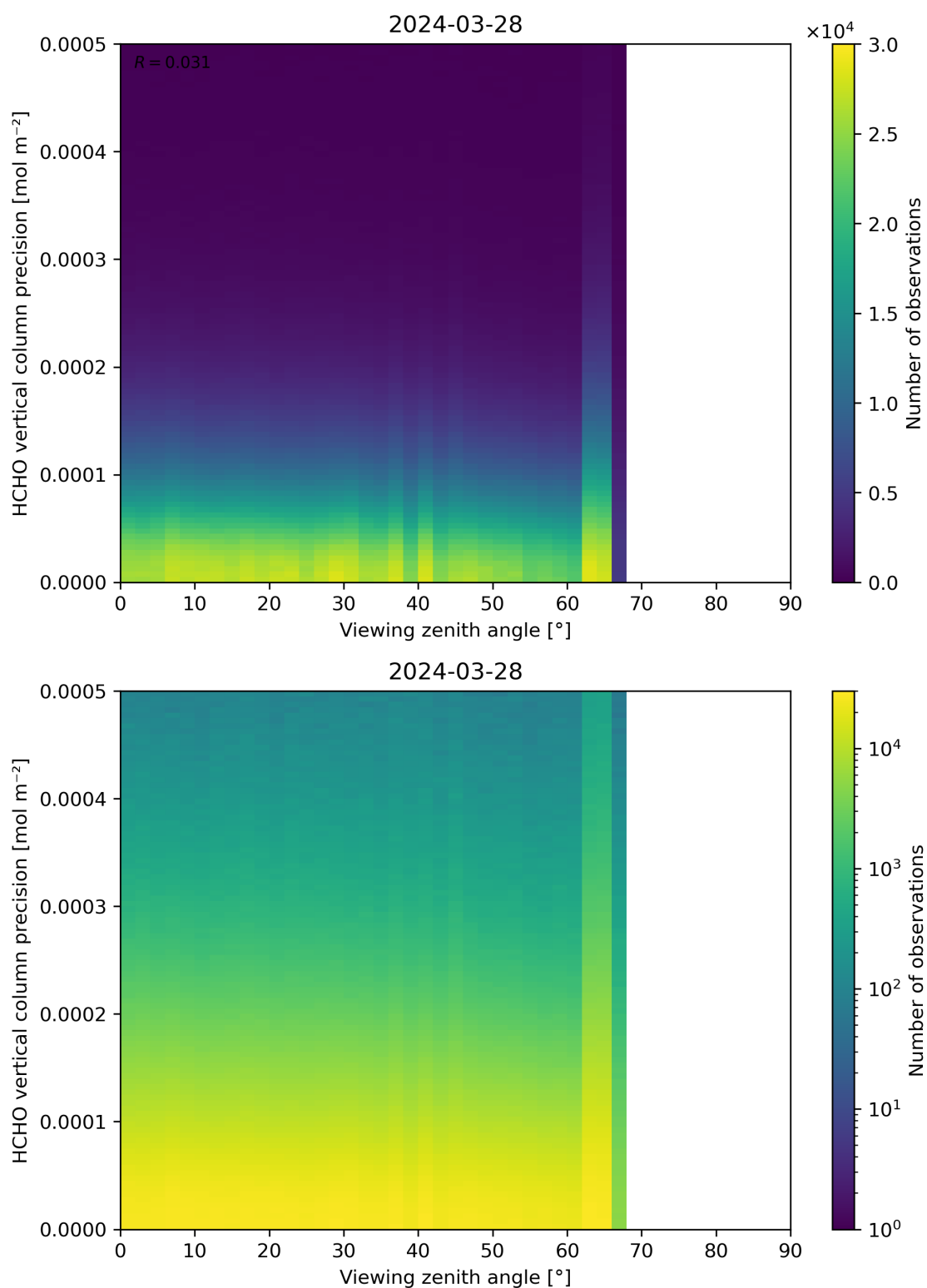
Figure 194: Scatter density plot of “Viewing zenith angle” against “HCHO vertical column precision” for 2024-03-27 to 2024-03-29.
