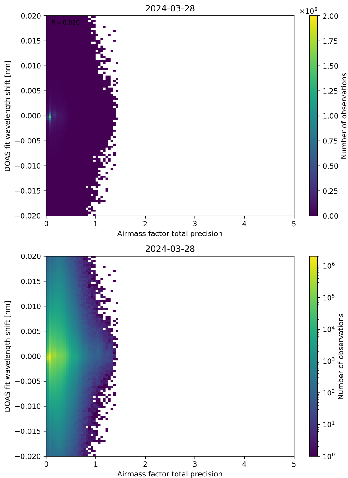
Figure 106: Scatter density plot of “Airmass factor total precision” against “DOAS fit wavelength shift” for 2024-03-27 to 2024-03-29.
