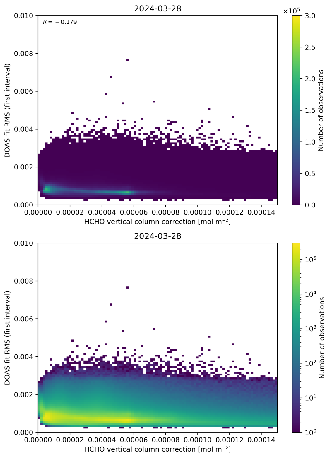
Figure 112: Scatter density plot of “HCHO vertical column correction” against “DOAS fit RMS (first interval)” for 2024-03-27 to 2024-03-29.
