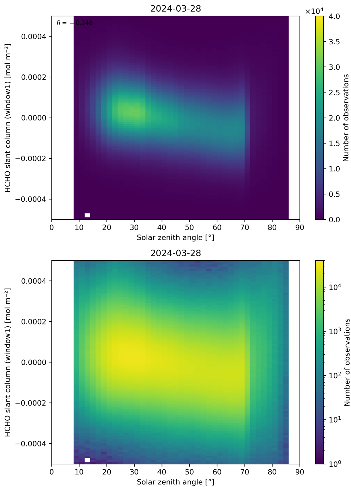
Figure 173: Scatter density plot of “Solar zenith angle” against “HCHO slant column (window1)” for 2024-03-27 to 2024-03-29.
