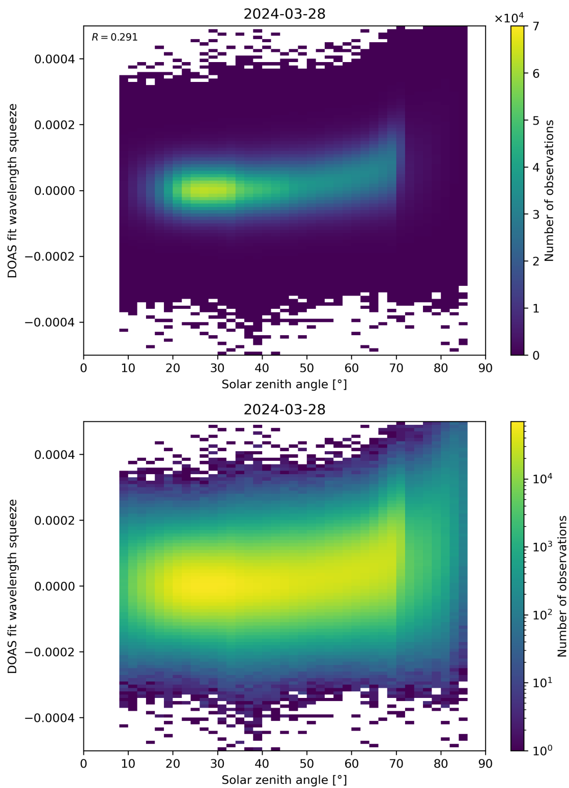
Figure 169: Scatter density plot of “Solar zenith angle” against “DOAS fit wavelength squeeze” for 2024-03-27 to 2024-03-29.
