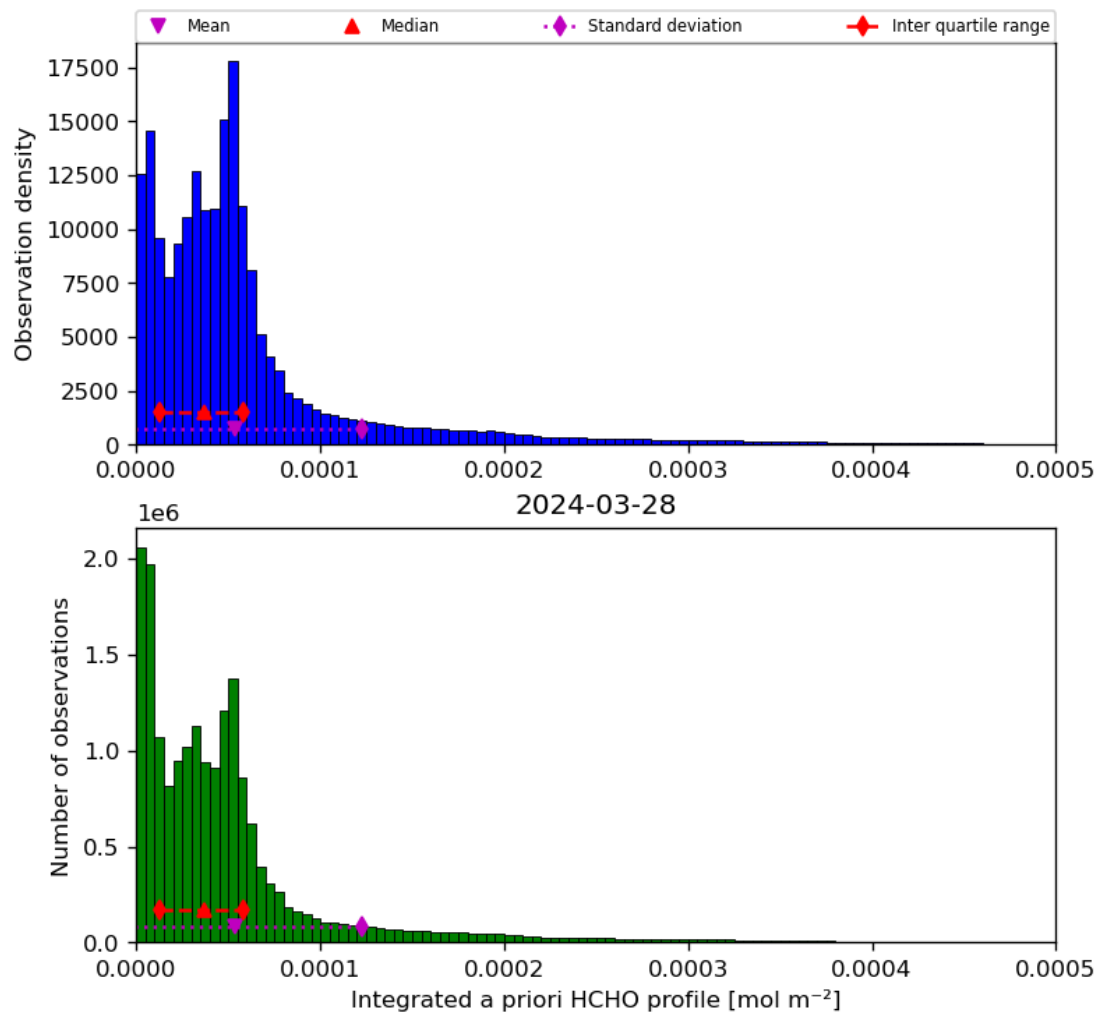
Figure 43: Histogram of “Integrated a priori HCHO profile” for 2024-03-27 to 2024-03-29
