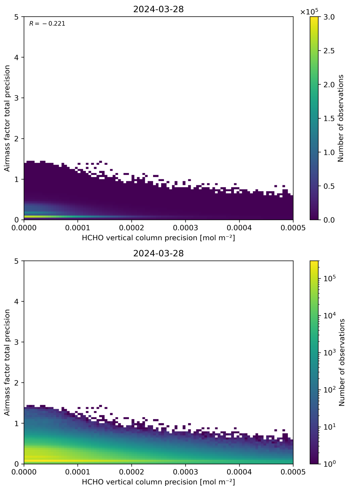
Figure 145: Scatter density plot of “HCHO vertical column precision” against “Airmass factor total precision” for 2024-03-27 to 2024-03-29.
