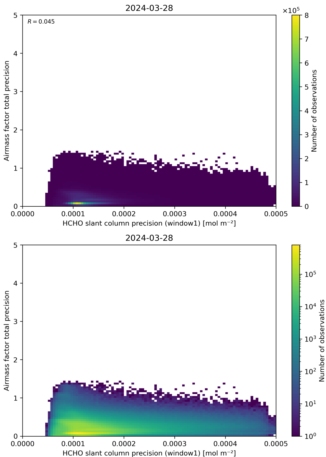
Figure 95: Scatter density plot of “HCHO slant column precision (window1)” against “Airmass factor total precision” for 2024-03-27 to 2024-03-29.
