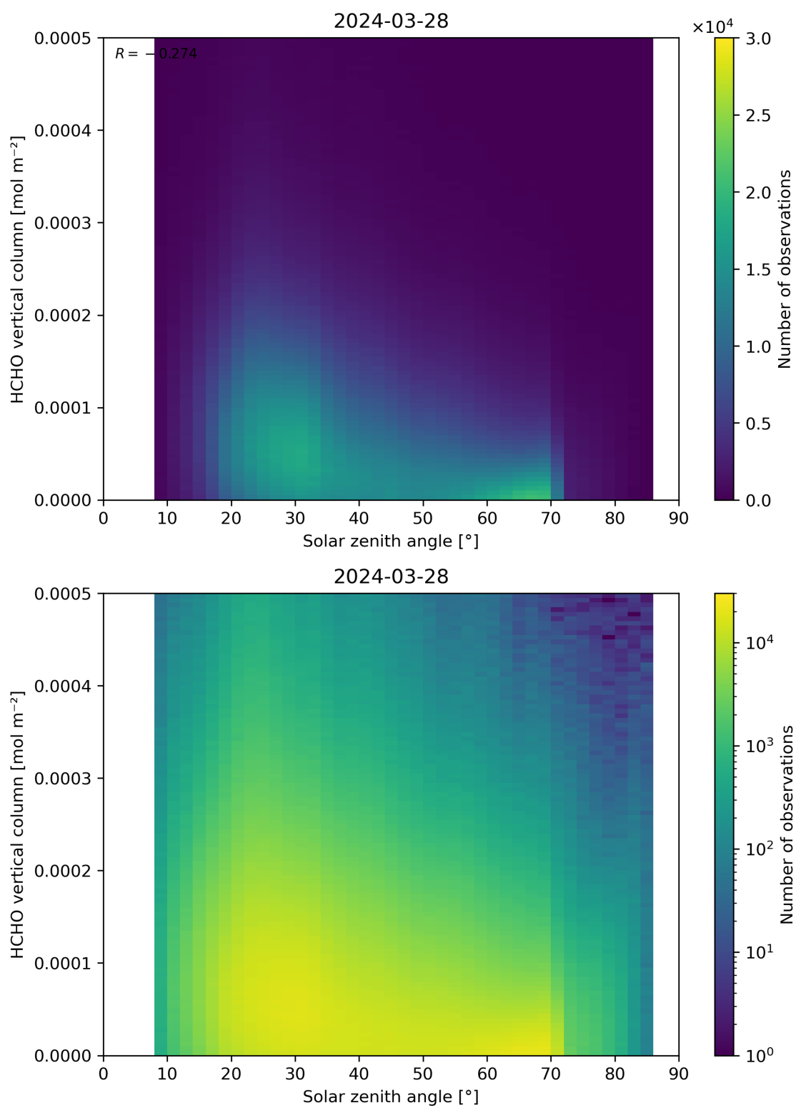
Figure 177: Scatter density plot of “Solar zenith angle” against “HCHO vertical column” for 2024-03-27 to 2024-03-29.
