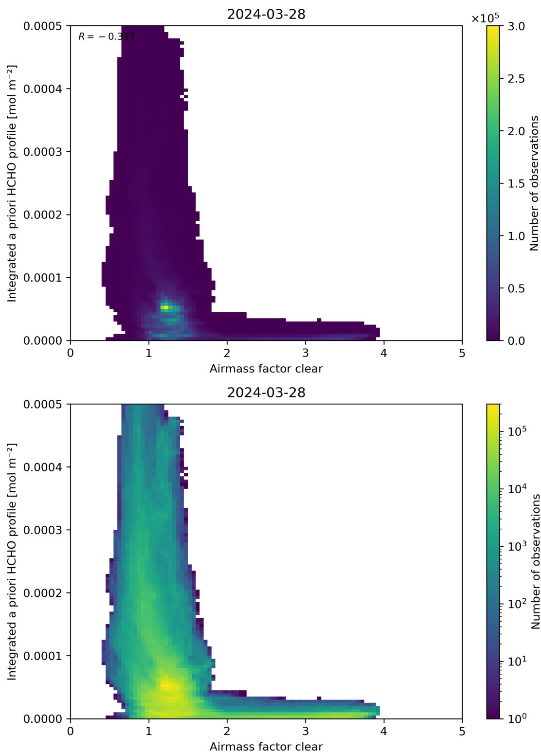
Figure 76: Scatter density plot of “Airmass factor clear” against “Integrated a priori HCHO profile” for 2024-03-27 to 2024-03-29.
