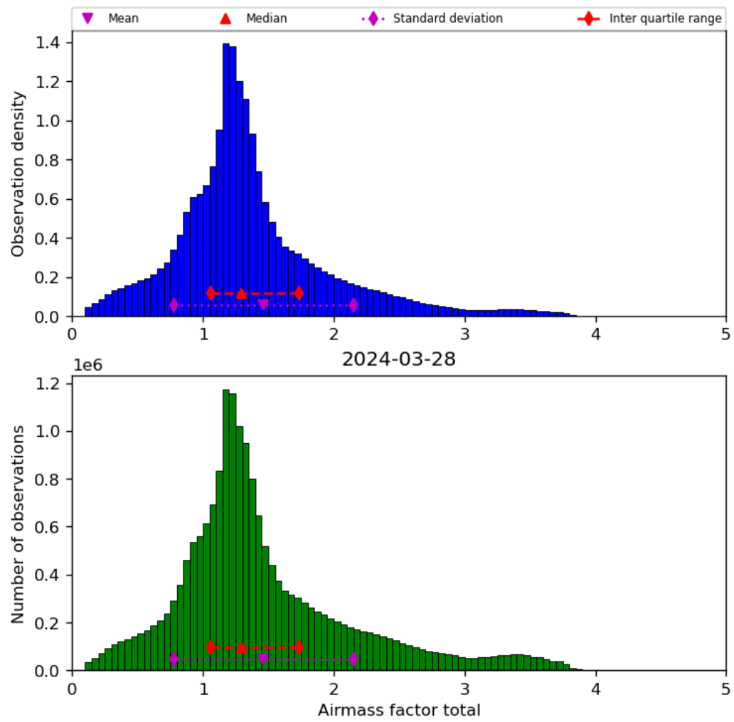
Figure 40: Histogram of “Airmass factor total” for 2024-03-27 to 2024-03-29
