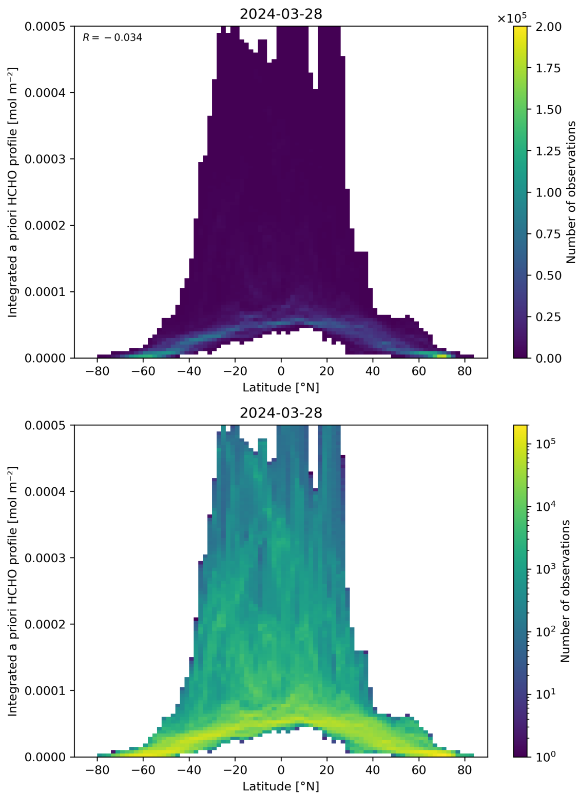
Figure 166: Scatter density plot of “Latitude” against “Integrated a priori HCHO profile” for 2024-03-27 to 2024-03-29.
