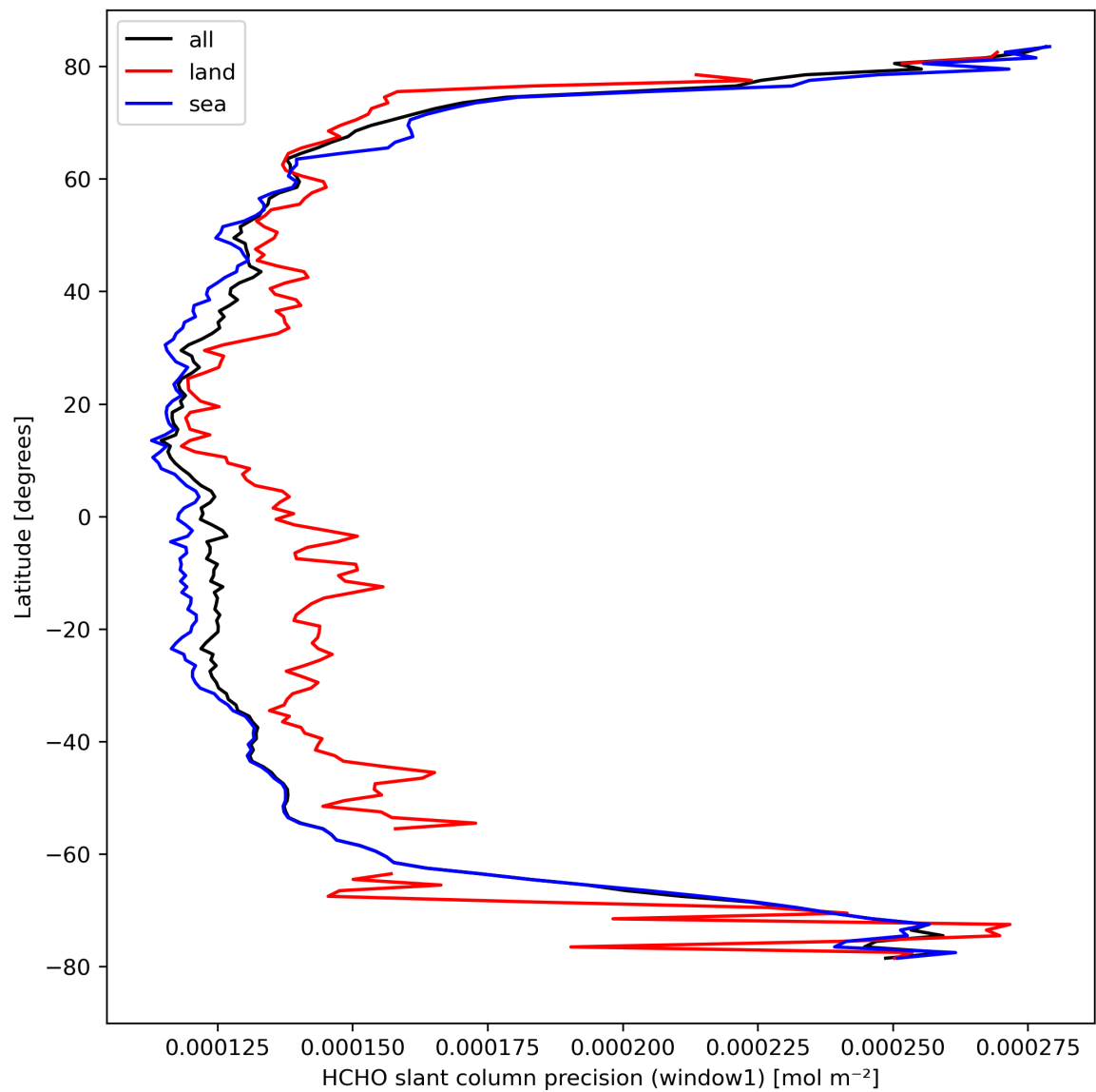
Figure 25: Zonal average of “HCHO slant column precision (window1)” for 2024-03-27 to 2024-03-29.
