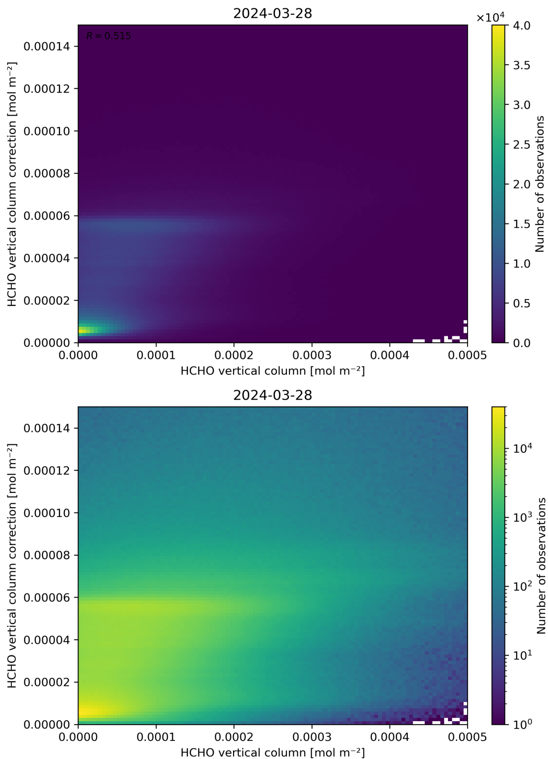
Figure 133: Scatter density plot of “HCHO vertical column” against “HCHO vertical column correction” for 2024-03-27 to 2024-03-29.
