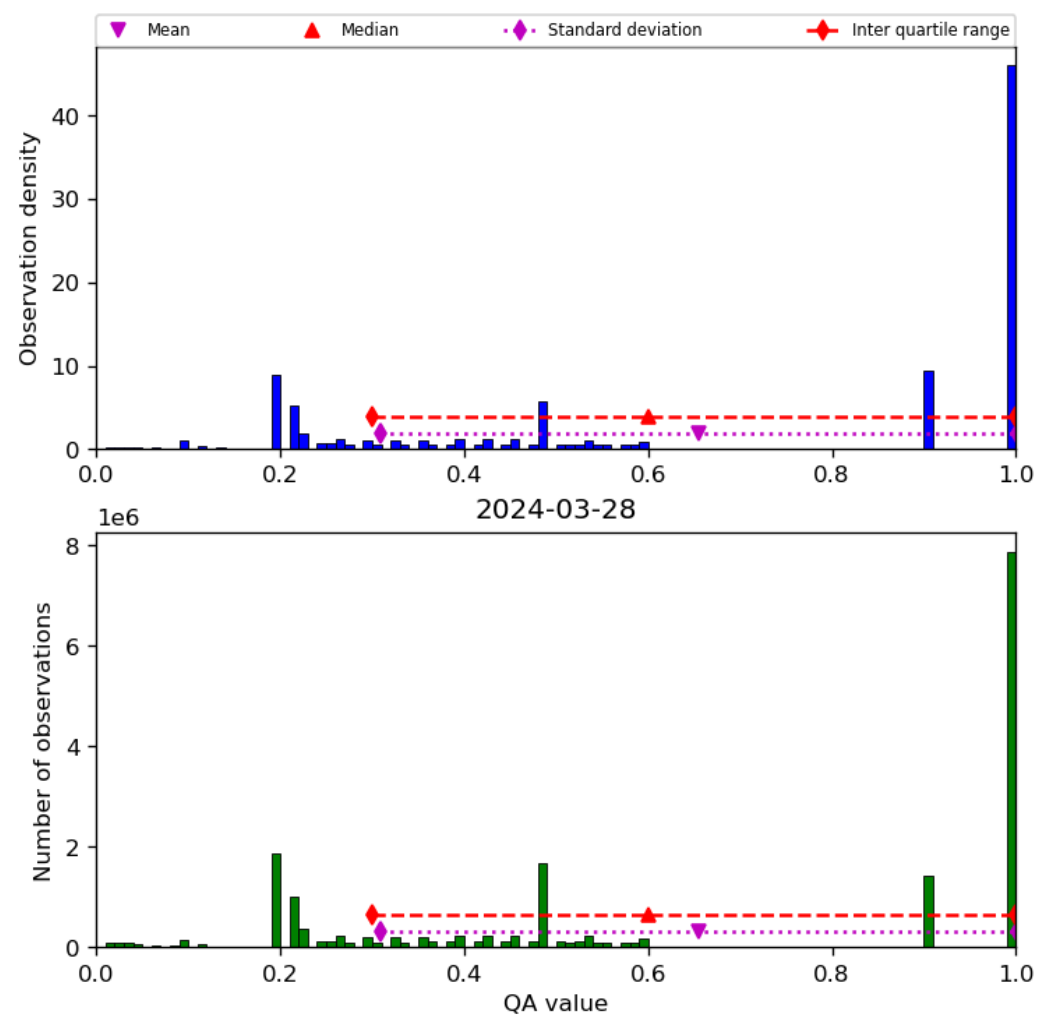
Figure 34: Histogram of “QA value” for 2024-03-27 to 2024-03-29
