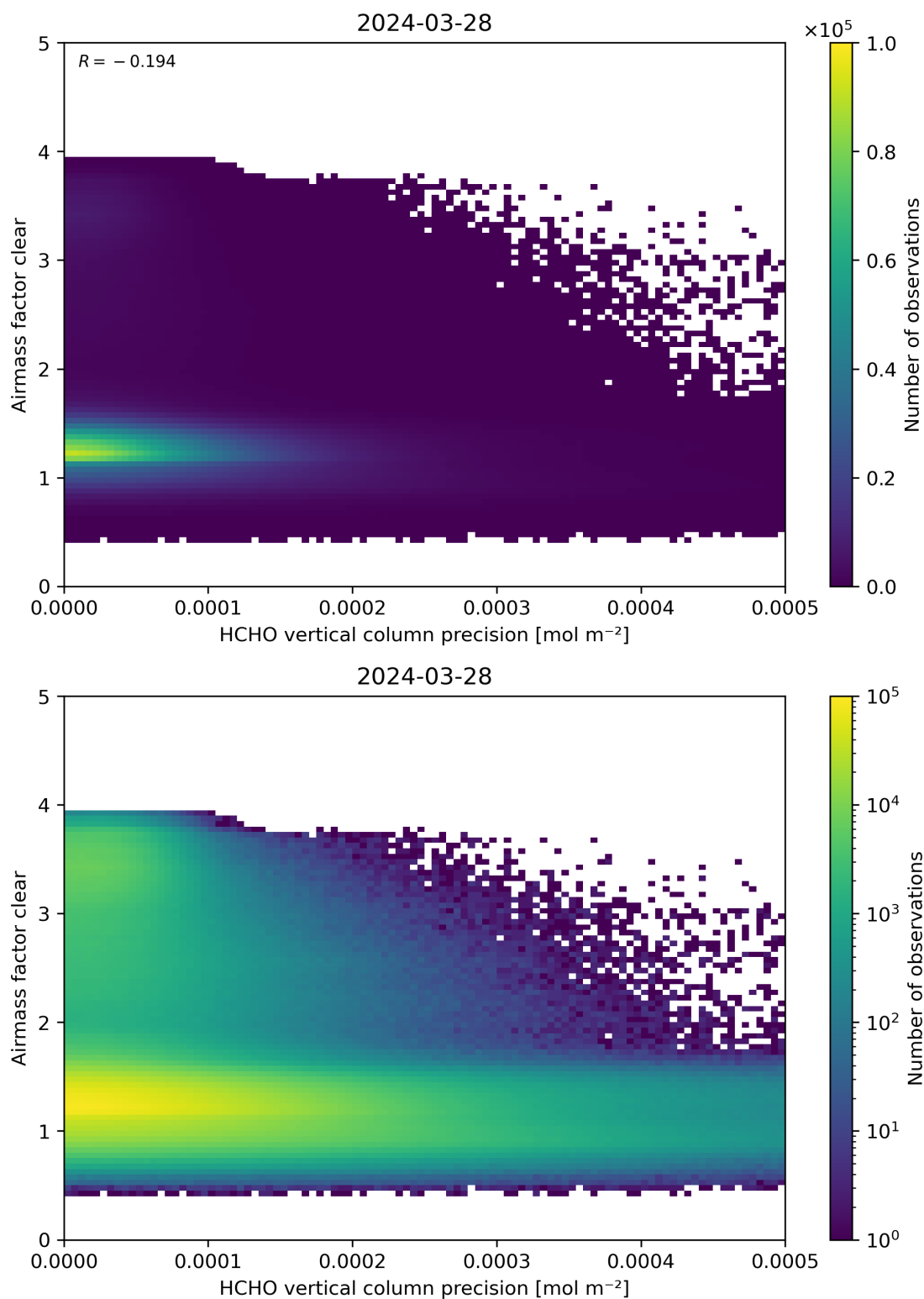
Figure 139: Scatter density plot of “HCHO vertical column precision” against “Airmass factor clear” for 2024-03-27 to 2024-03-29.
