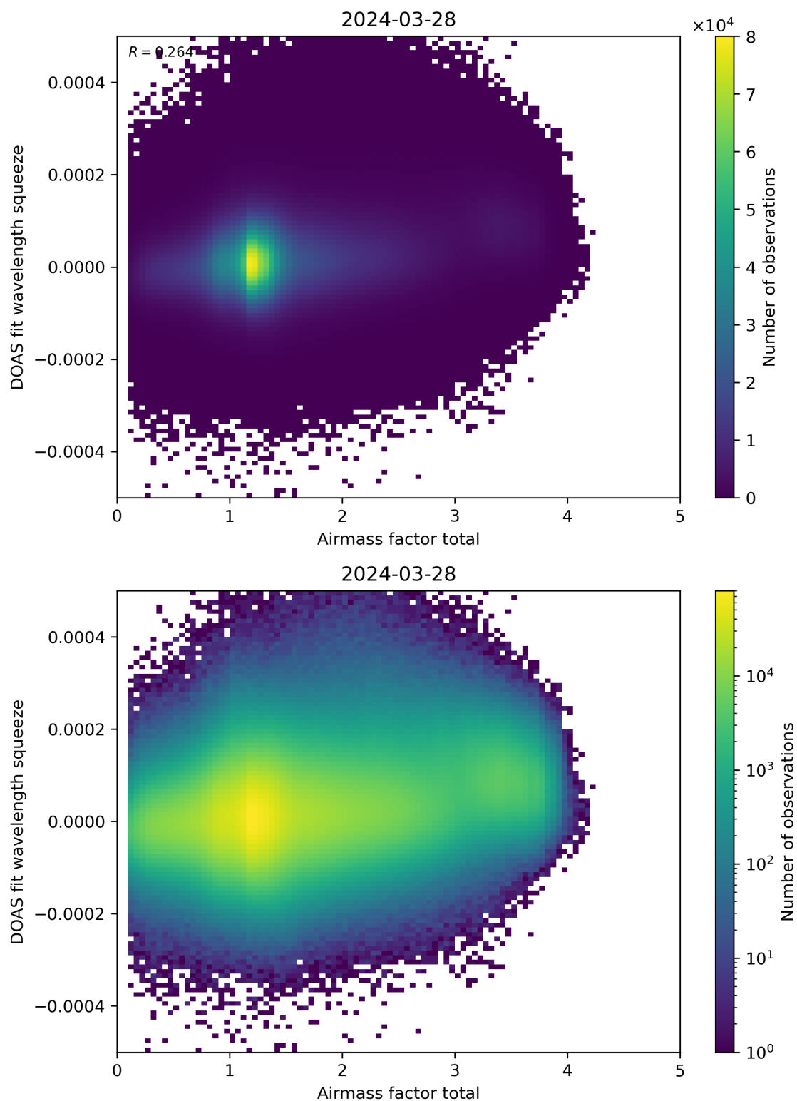
Figure 99: Scatter density plot of “Airmass factor total” against “DOAS fit wavelength squeeze” for 2024-03-27 to 2024-03-29.
