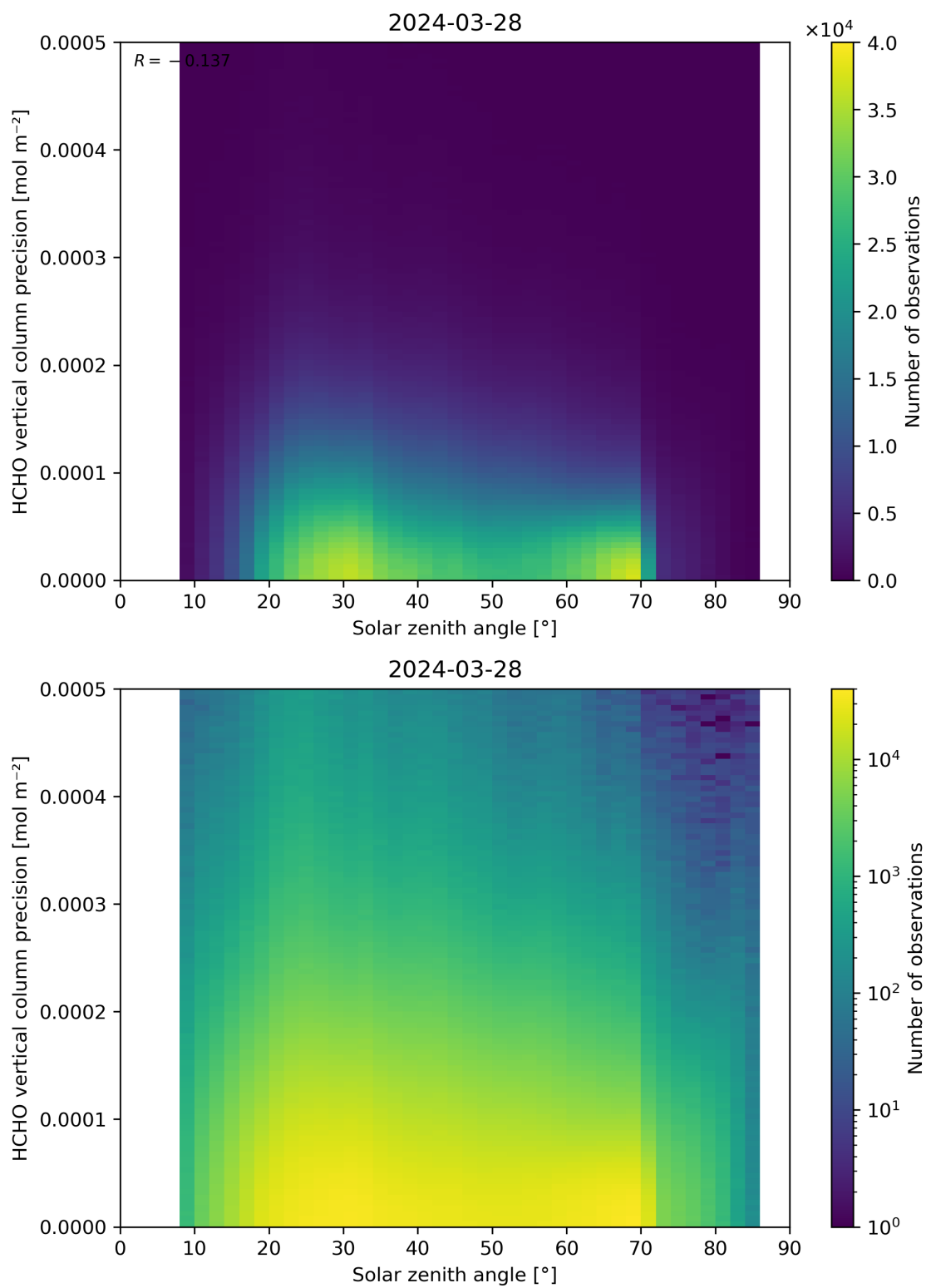
Figure 179: Scatter density plot of “Solar zenith angle” against “HCHO vertical column precision” for 2024-03-27 to 2024-03-29.
