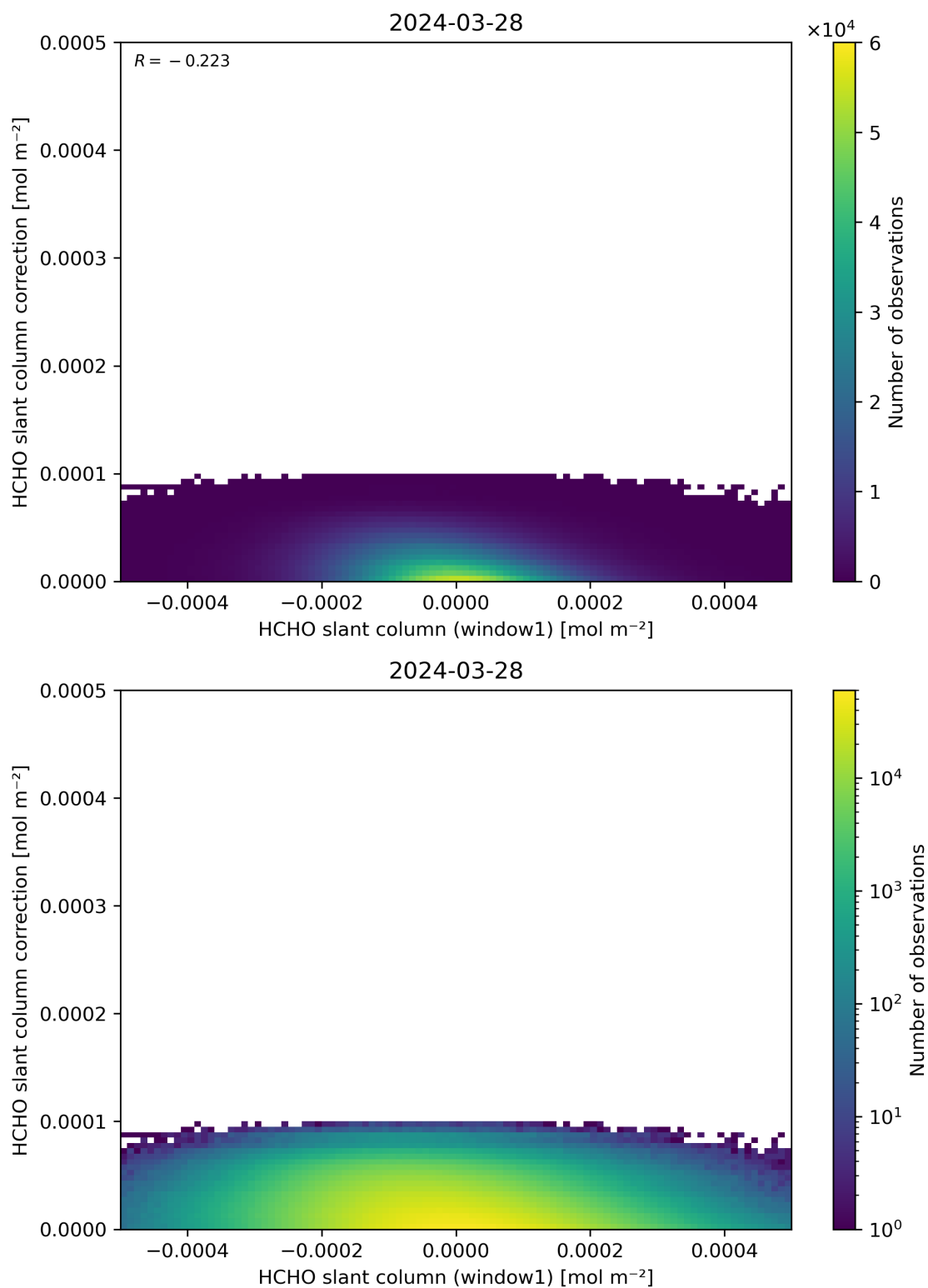
Figure 83: Scatter density plot of “HCHO slant column (window1)” against “HCHO slant column correction” for 2024-03-27 to 2024-03-29.
