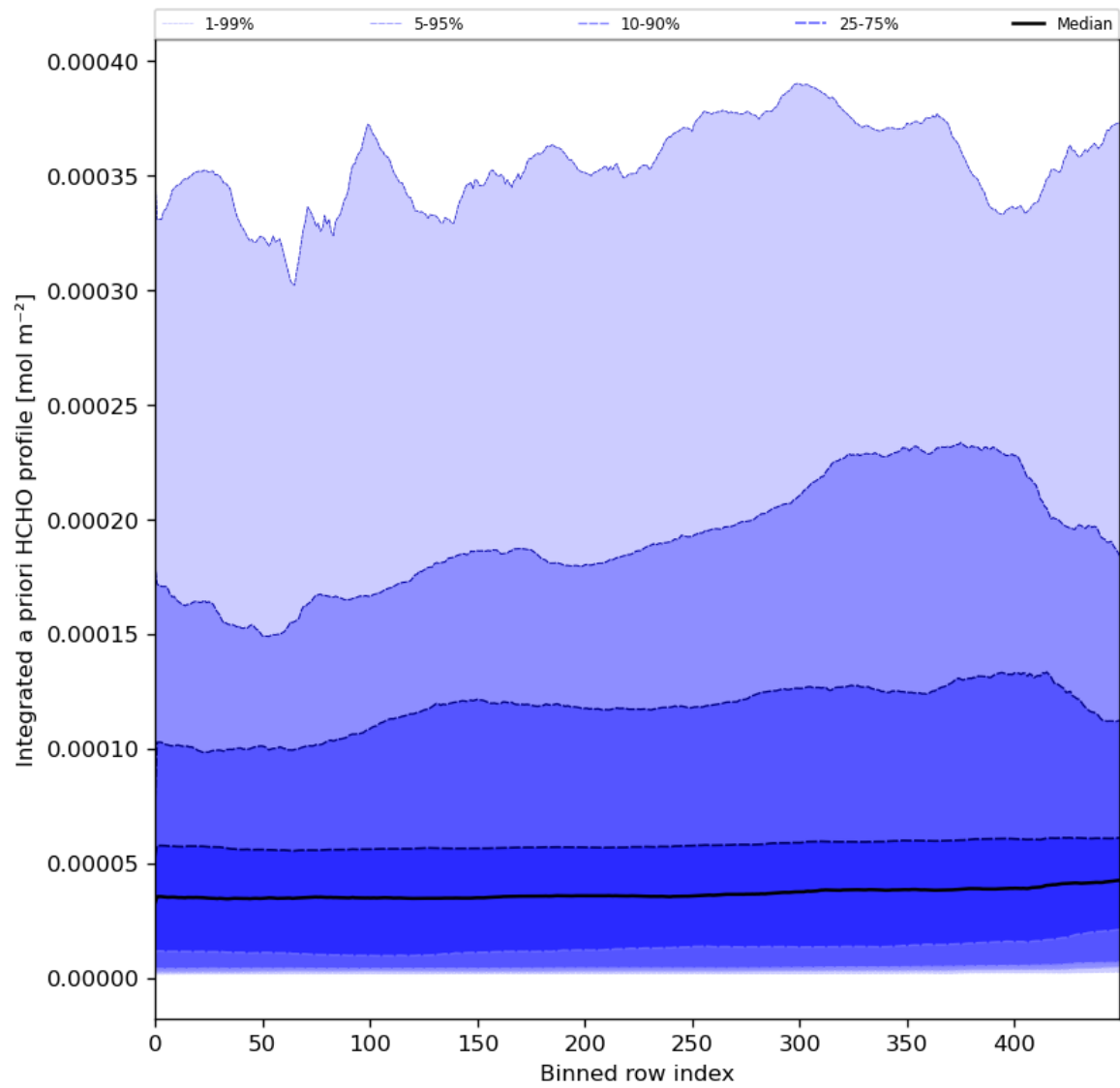
Figure 57: Along track statistics of “Integrated a priori HCHO profile” for 2024-03-27 to 2024-03-29
