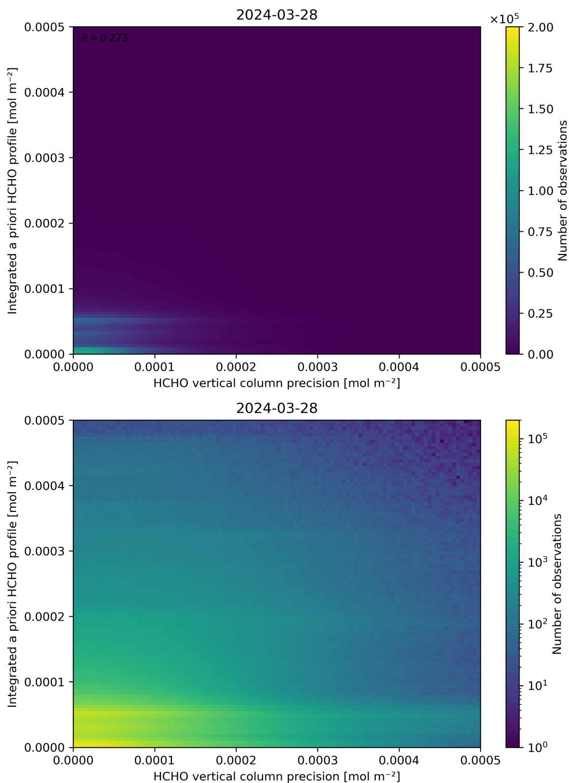
Figure 147: Scatter density plot of “HCHO vertical column precision” against “Integrated a priori HCHO profile” for 2024-03-27 to 2024-03-29.
