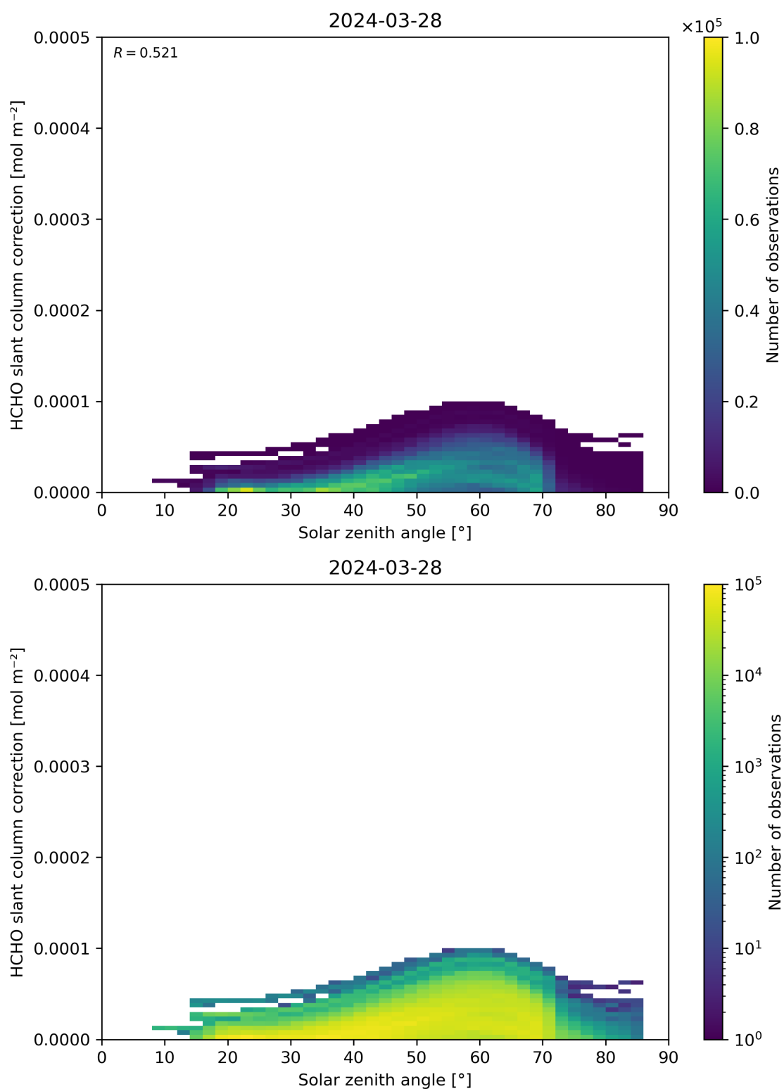
Figure 172: Scatter density plot of “Solar zenith angle” against “HCHO slant column correction” for 2024-03-27 to 2024-03-29.
