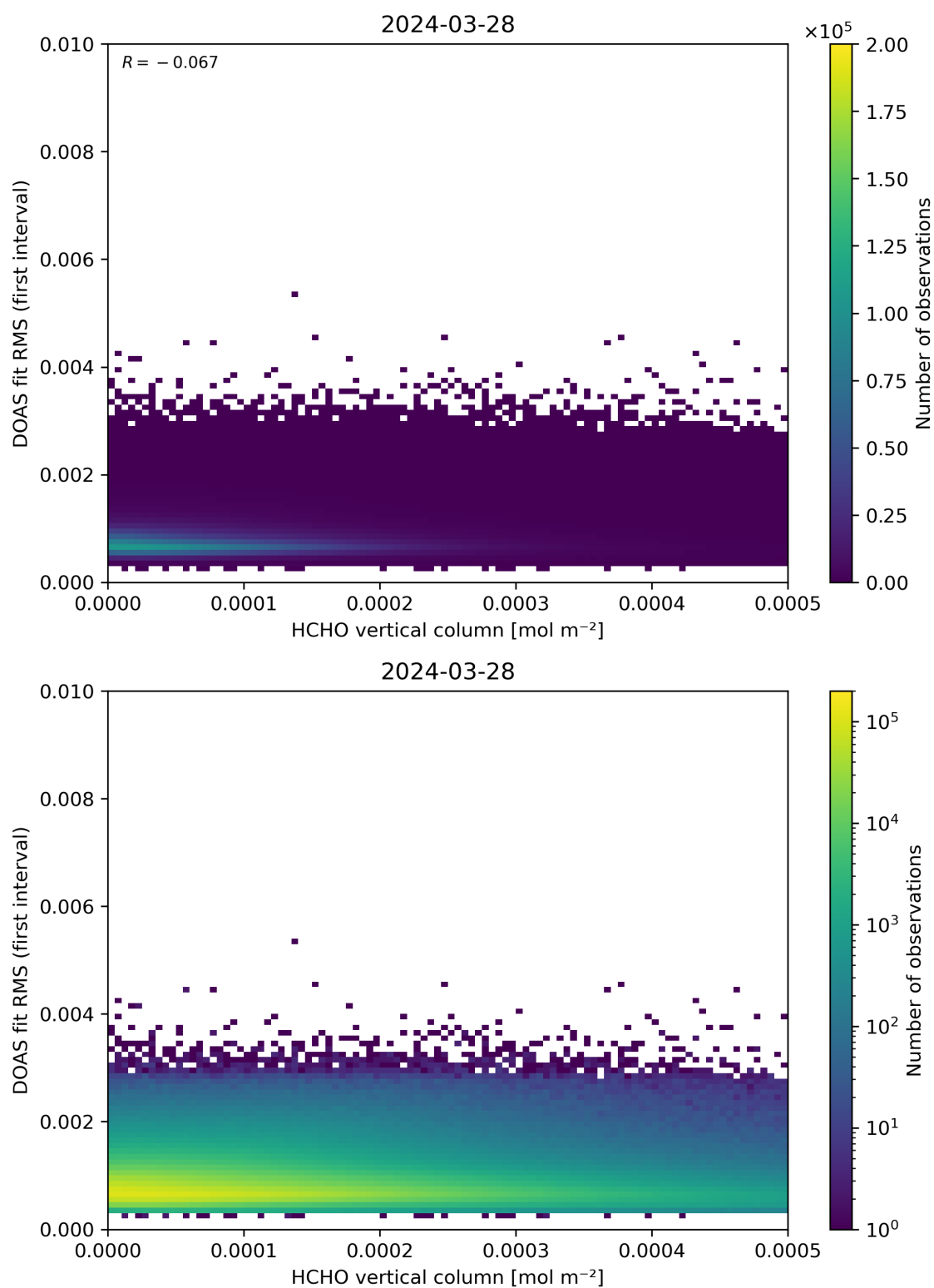
Figure 123: Scatter density plot of “HCHO vertical column” against “DOAS fit RMS (first interval)” for 2024-03-27 to 2024-03-29.
