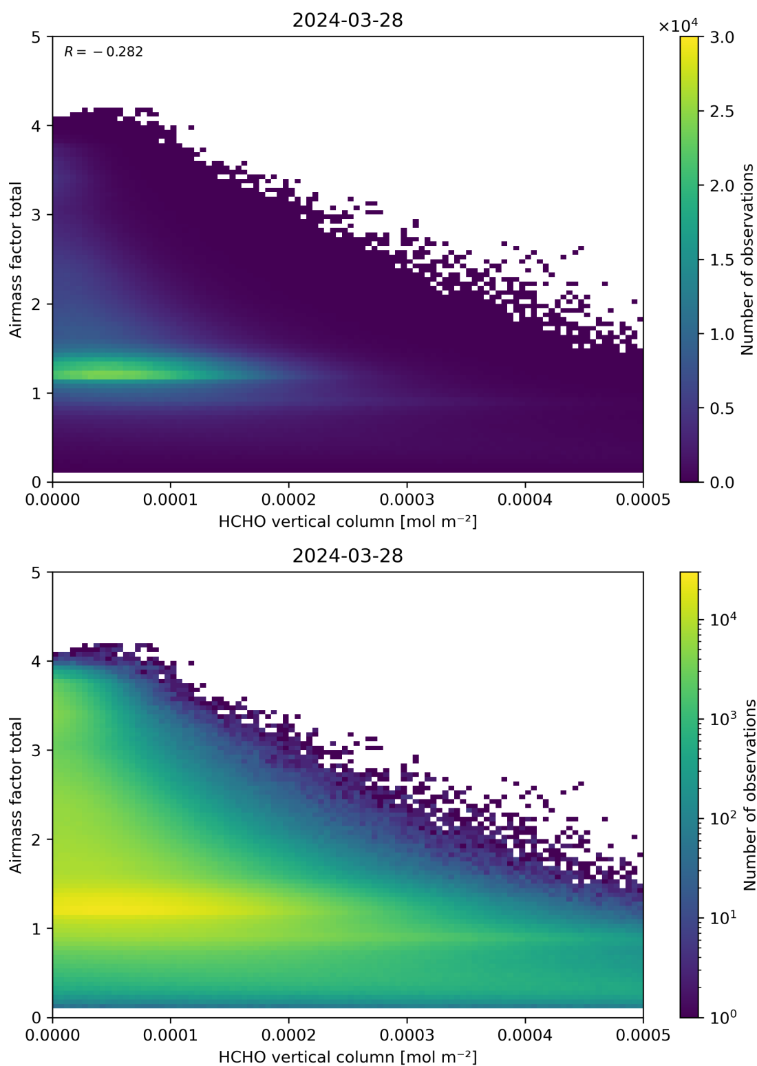
Figure 131: Scatter density plot of “HCHO vertical column” against “Airmass factor total” for 2024-03-27 to 2024-03-29.
