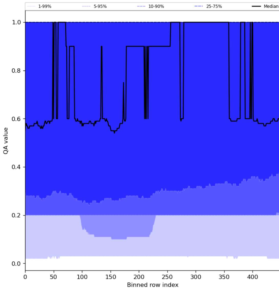
Figure 48: Along track statistics of “QA value” for 2024-03-27 to 2024-03-29
