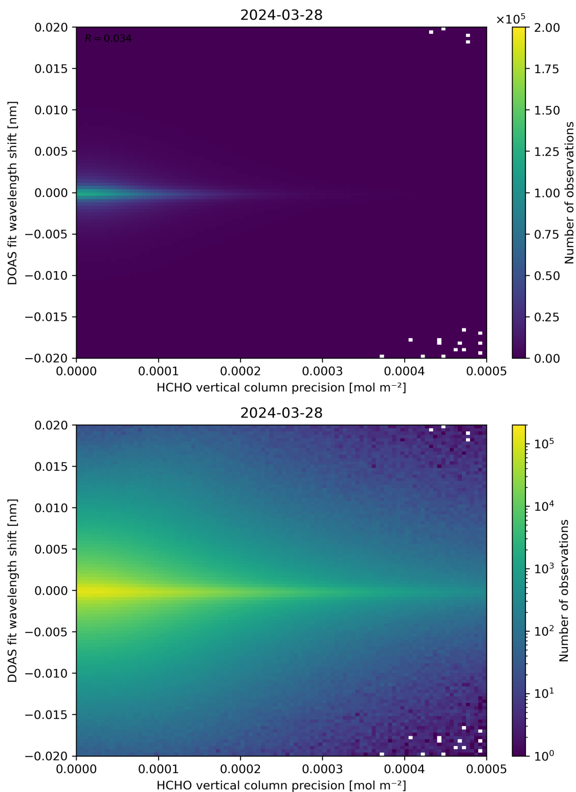
Figure 137: Scatter density plot of “HCHO vertical column precision” against “DOAS fit wavelength shift” for 2024-03-27 to 2024-03-29.
