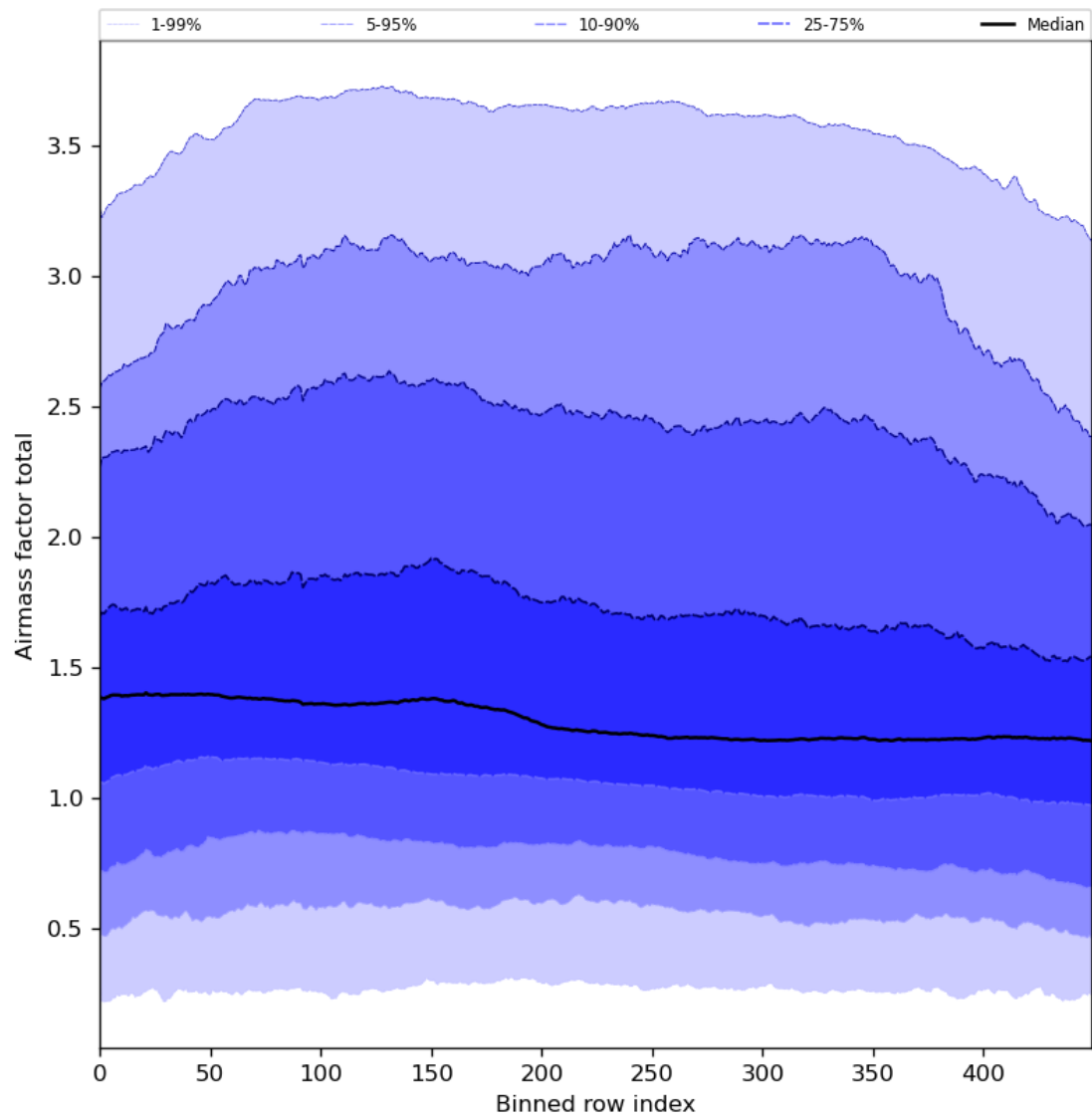
Figure 54: Along track statistics of “Airmass factor total” for 2024-03-27 to 2024-03-29
