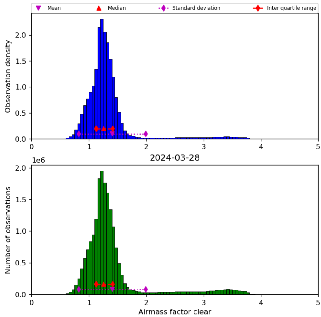
Figure 42: Histogram of “Airmass factor clear” for 2024-03-27 to 2024-03-29
