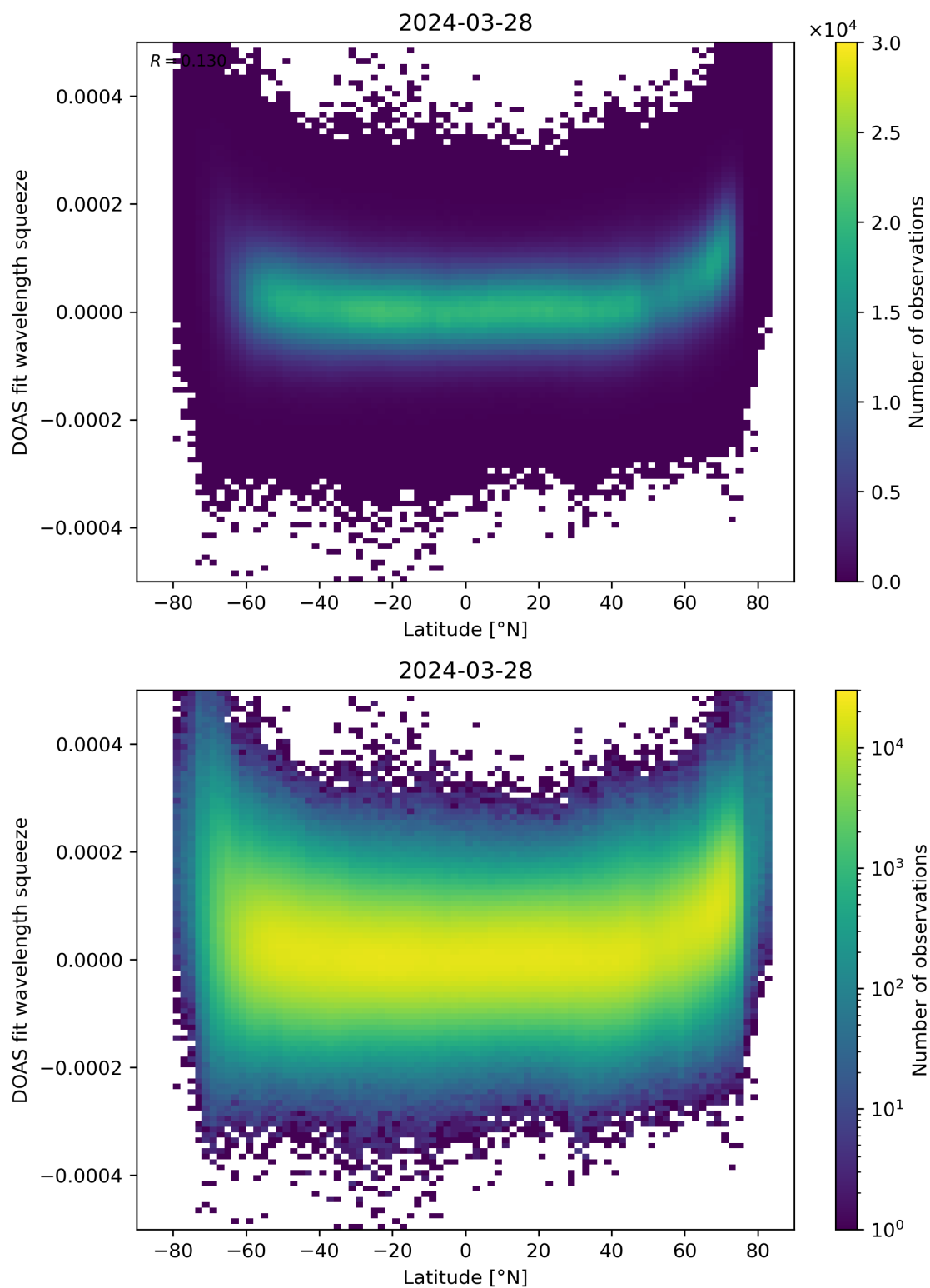
Figure 155: Scatter density plot of “Latitude” against “DOAS fit wavelength squeeze” for 2024-03-27 to 2024-03-29.
