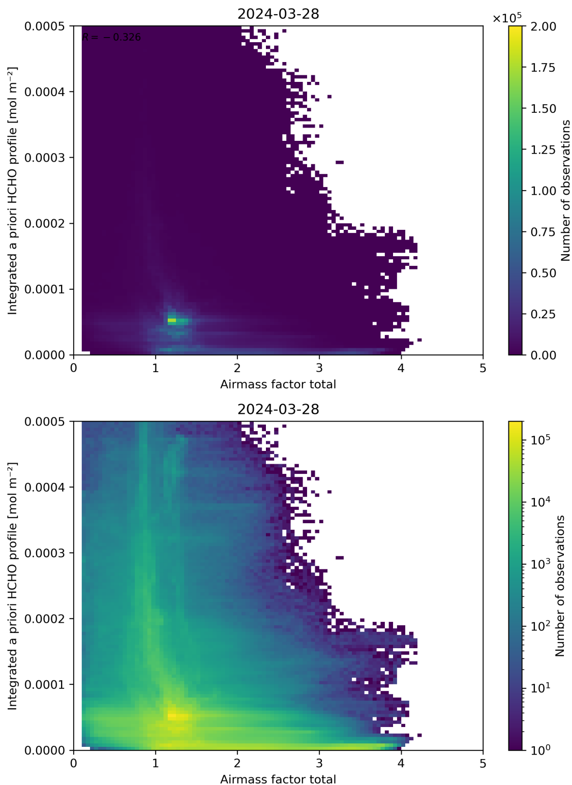
Figure 104: Scatter density plot of “Airmass factor total” against “Integrated a priori HCHO profile” for 2024-03-27 to 2024-03-29.
