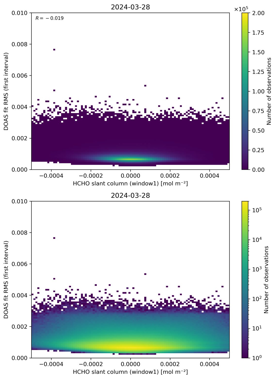
Figure 78: Scatter density plot of “HCHO slant column (window1)” against “DOAS fit RMS (first interval)” for 2024-03-27 to 2024-03-29.
