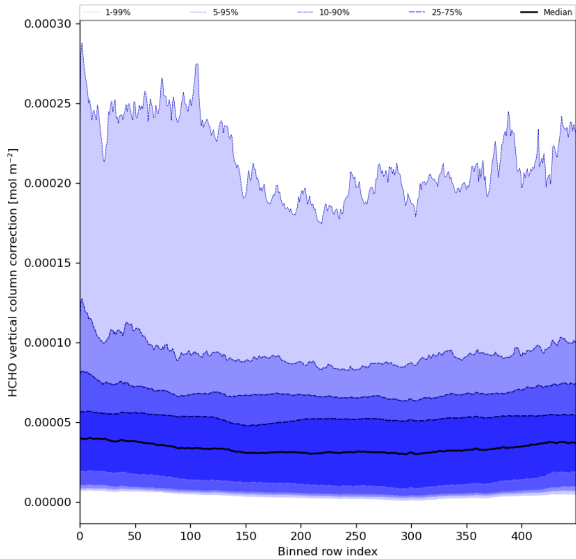
Figure 51: Along track statistics of “HCHO vertical column correction” for 2024-03-27 to 2024-03-29
