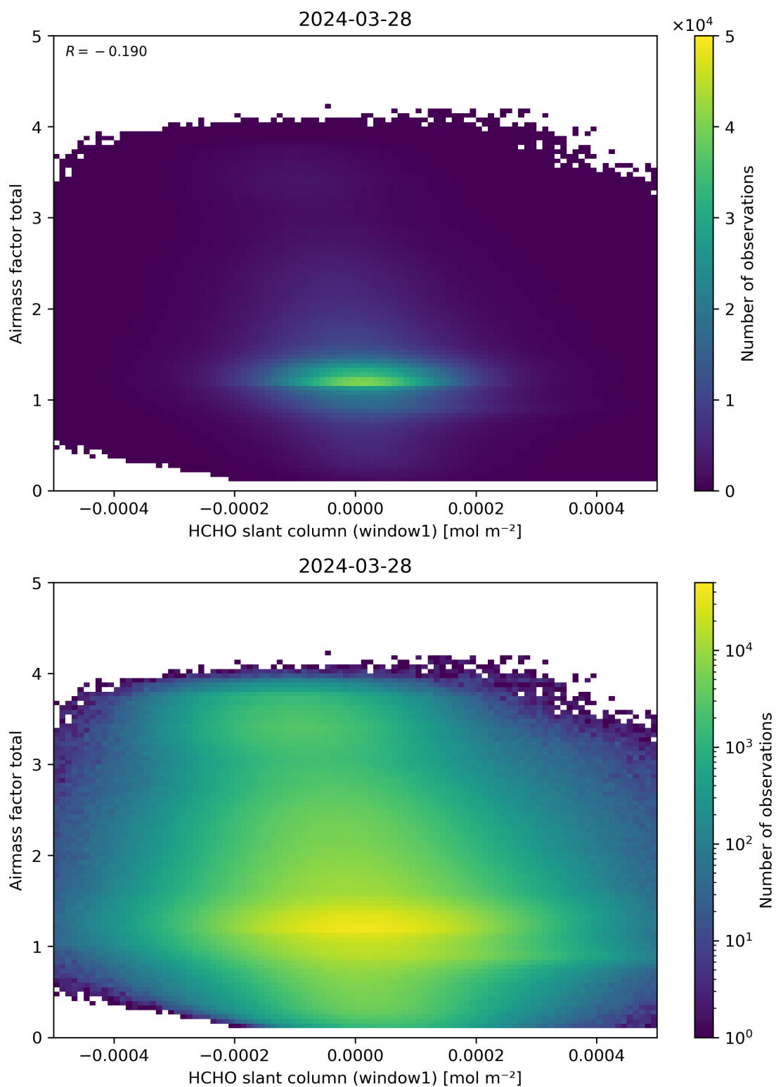
Figure 85: Scatter density plot of “HCHO slant column (window1)” against “Airmass factor total” for 2024-03-27 to 2024-03-29.
