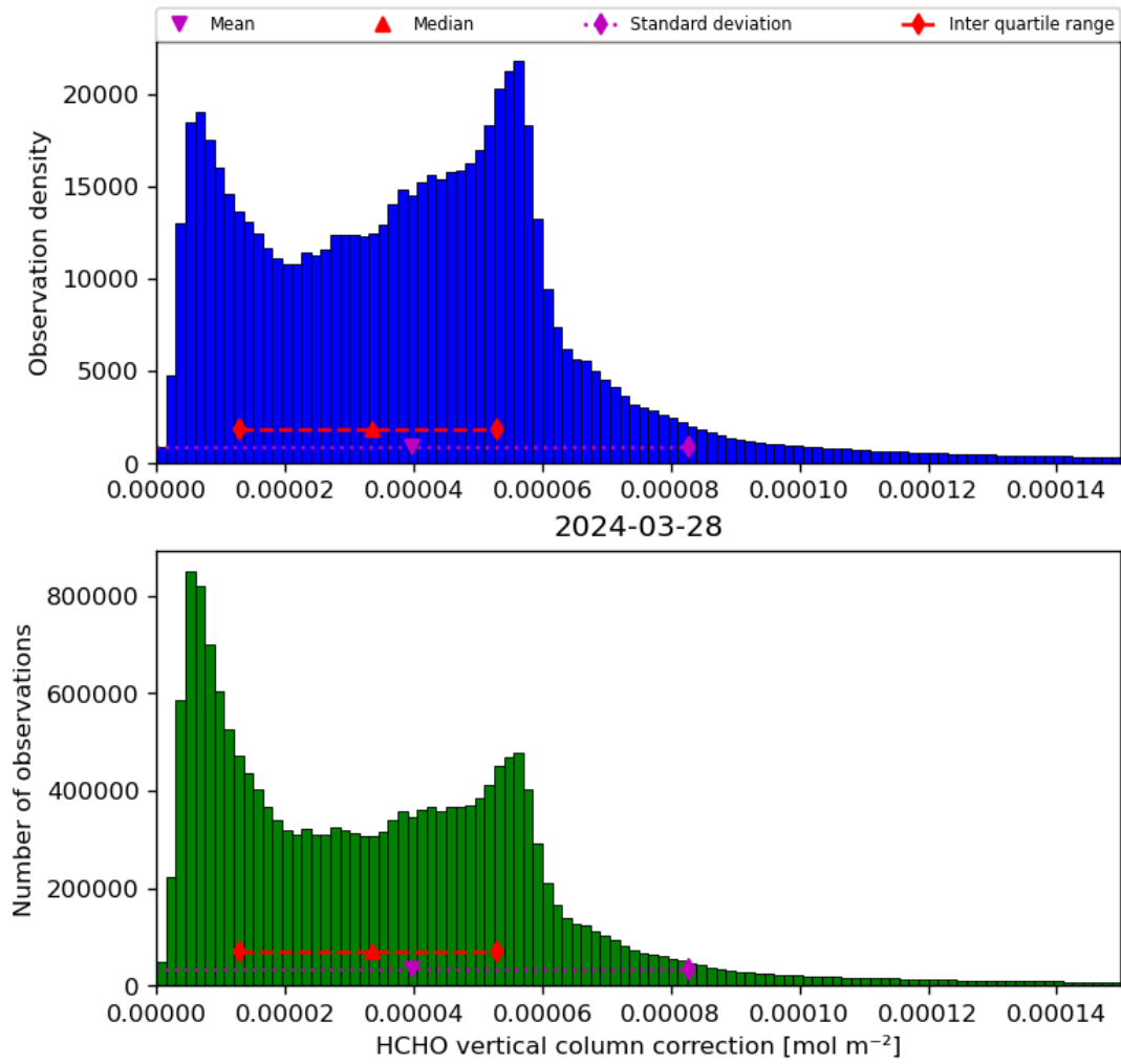
Figure 37: Histogram of “HCHO vertical column correction” for 2024-03-27 to 2024-03-29
