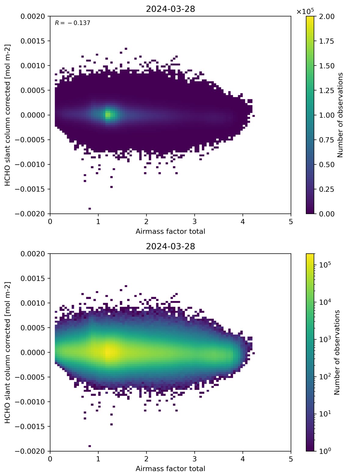
Figure 101: Scatter density plot of “Airmass factor total” against “HCHO slant column corrected” for 2024-03-27 to 2024-03-29.
