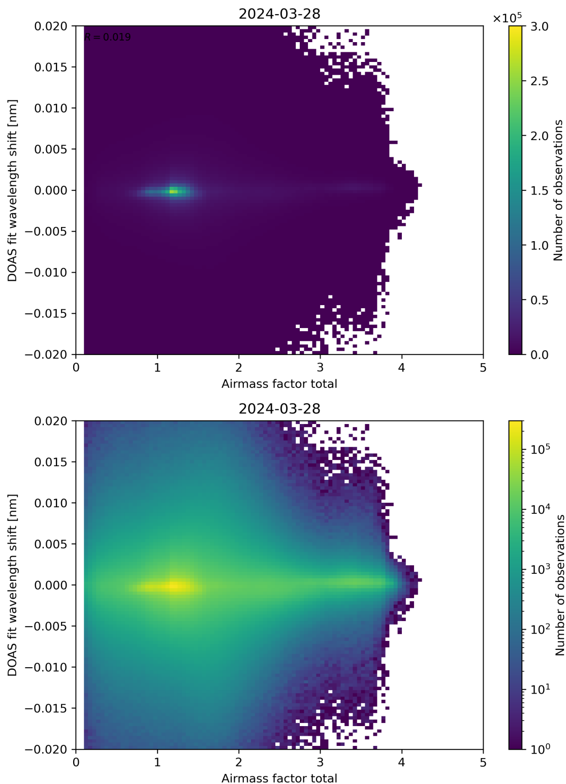
Figure 98: Scatter density plot of “Airmass factor total” against “DOAS fit wavelength shift” for 2024-03-27 to 2024-03-29.
