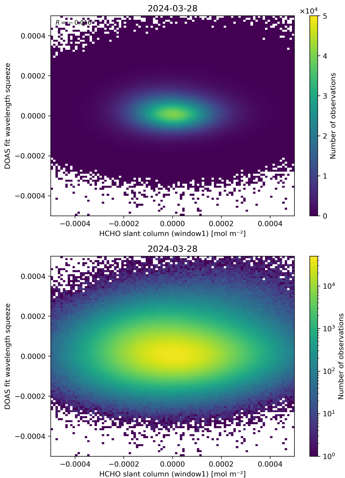
Figure 80: Scatter density plot of “HCHO slant column (window1)” against “DOAS fit wavelength squeeze” for 2024-03-27 to 2024-03-29.
