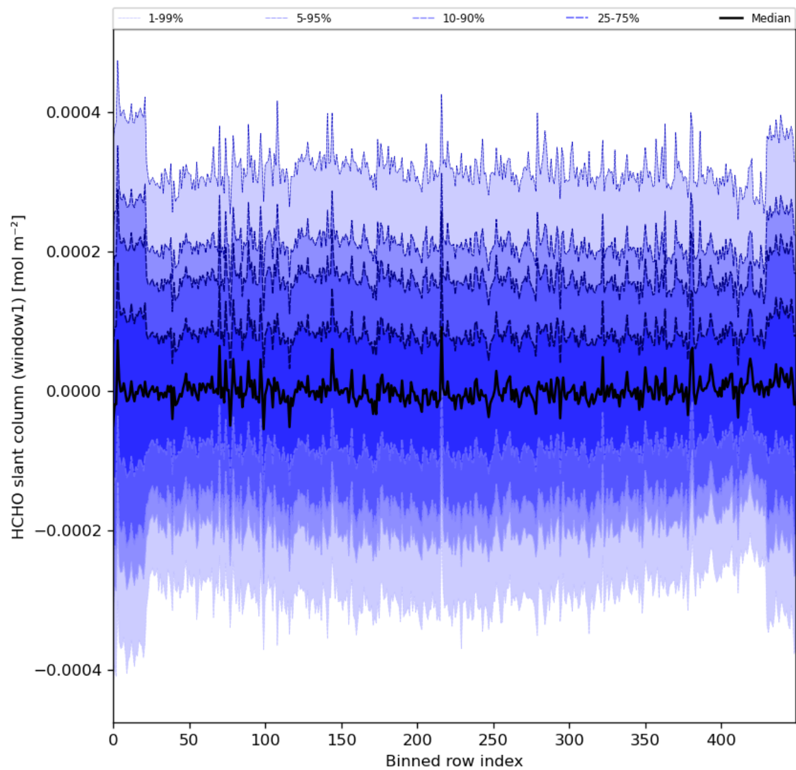
Figure 52: Along track statistics of “HCHO slant column (window1)” for 2024-03-27 to 2024-03-29
