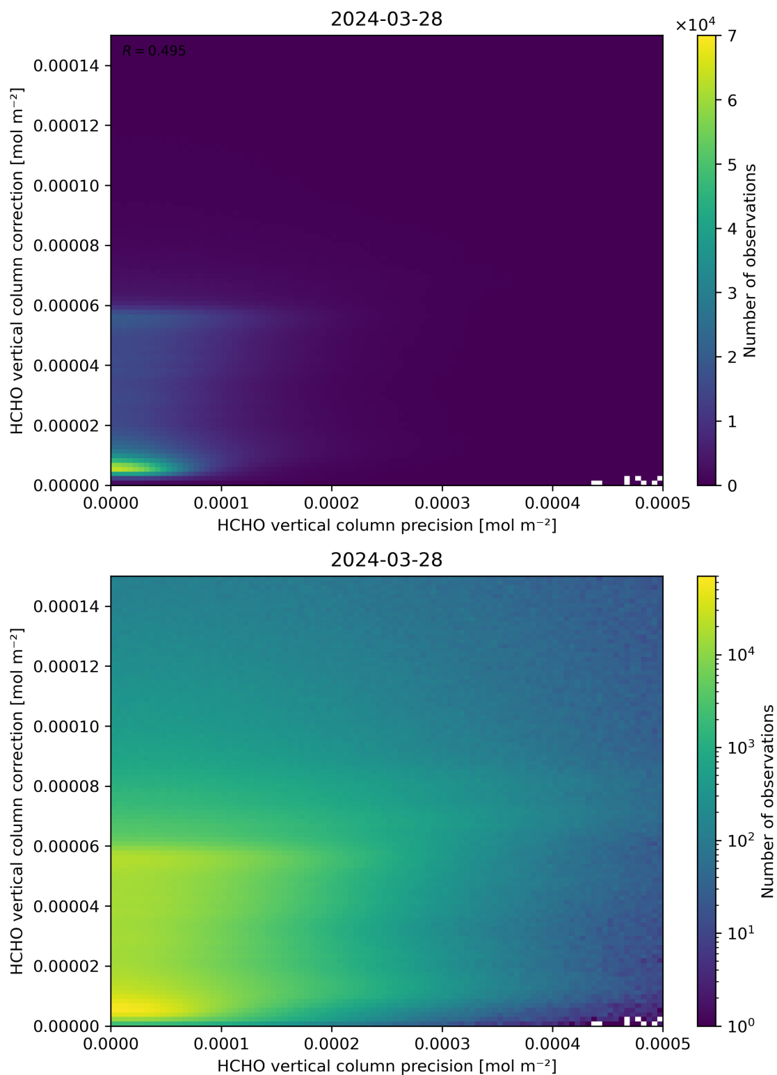
Figure 146: Scatter density plot of “HCHO vertical column precision” against “HCHO vertical column correction” for 2024-03-27 to 2024-03-29.
