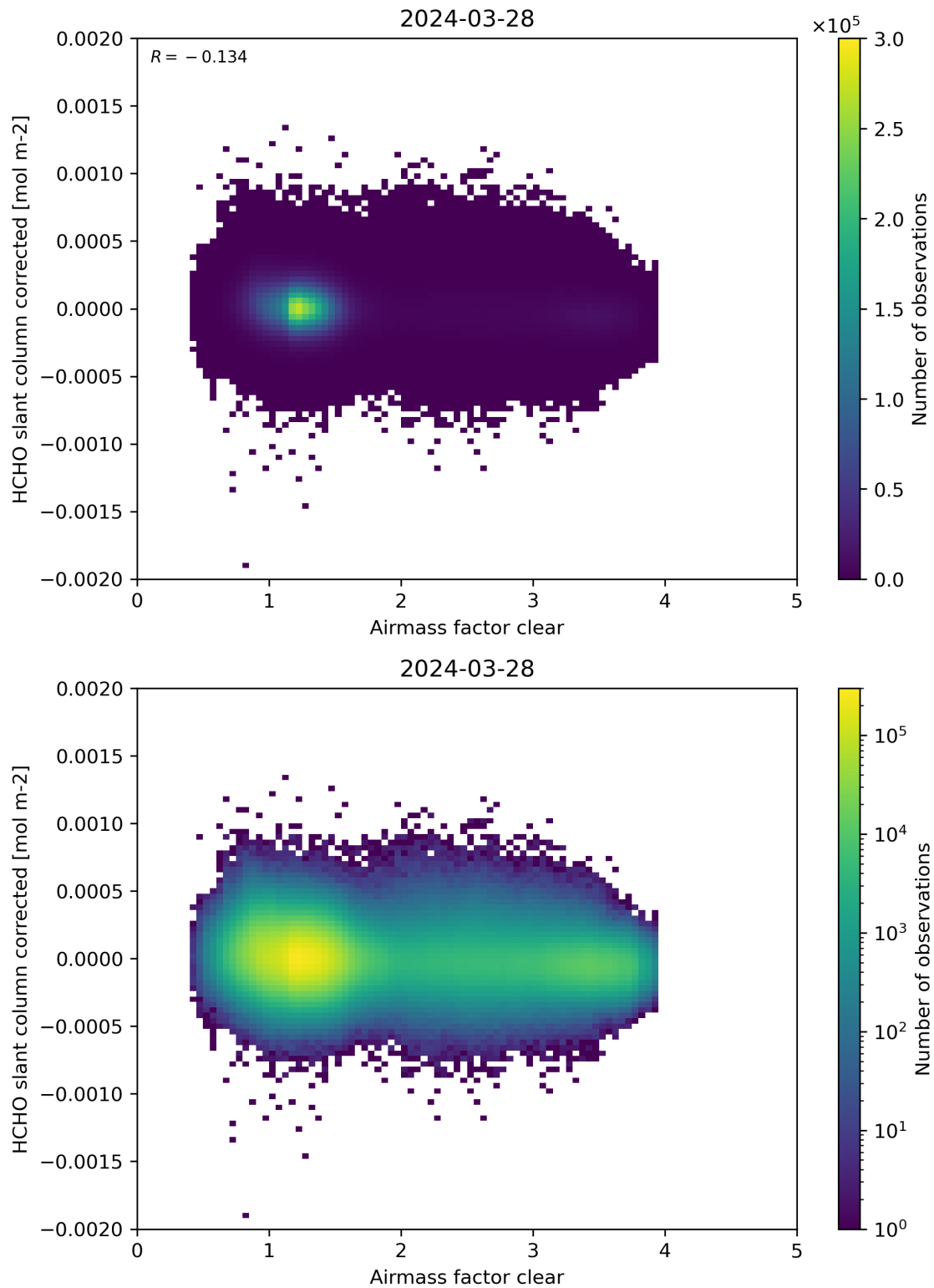
Figure 74: Scatter density plot of “Airmass factor clear” against “HCHO slant column corrected” for 2024-03-27 to 2024-03-29.
