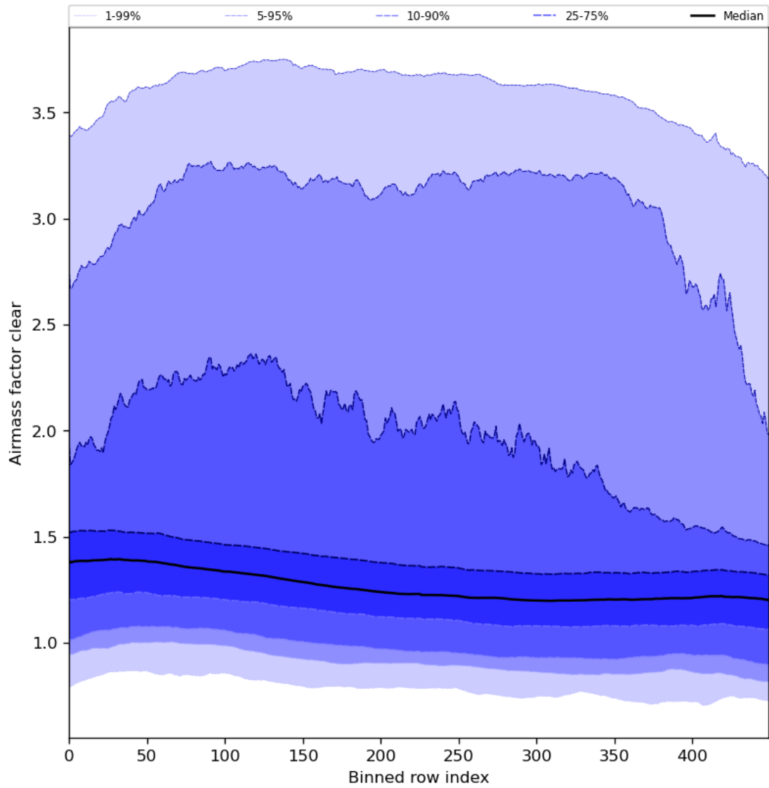
Figure 56: Along track statistics of “Airmass factor clear” for 2024-03-27 to 2024-03-29
