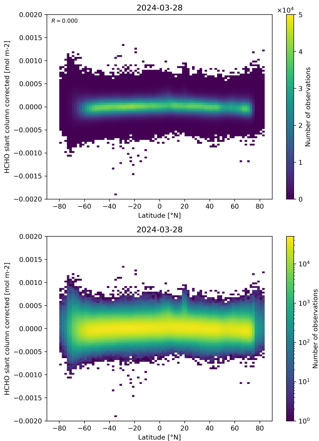
Figure 157: Scatter density plot of “Latitude” against “HCHO slant column corrected” for 2024-03-27 to 2024-03-29.
