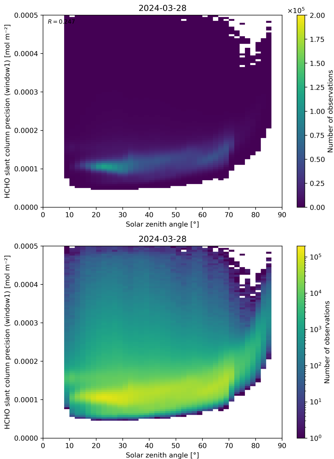
Figure 174: Scatter density plot of “Solar zenith angle” against “HCHO slant column precision (window1)” for 2024-03-27 to 2024-03-29.
