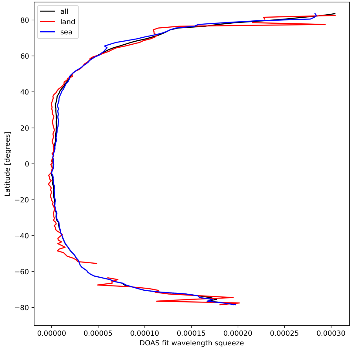
Figure 31: Zonal average of “DOAS fit wavelength squeeze” for 2024-03-27 to 2024-03-29.
