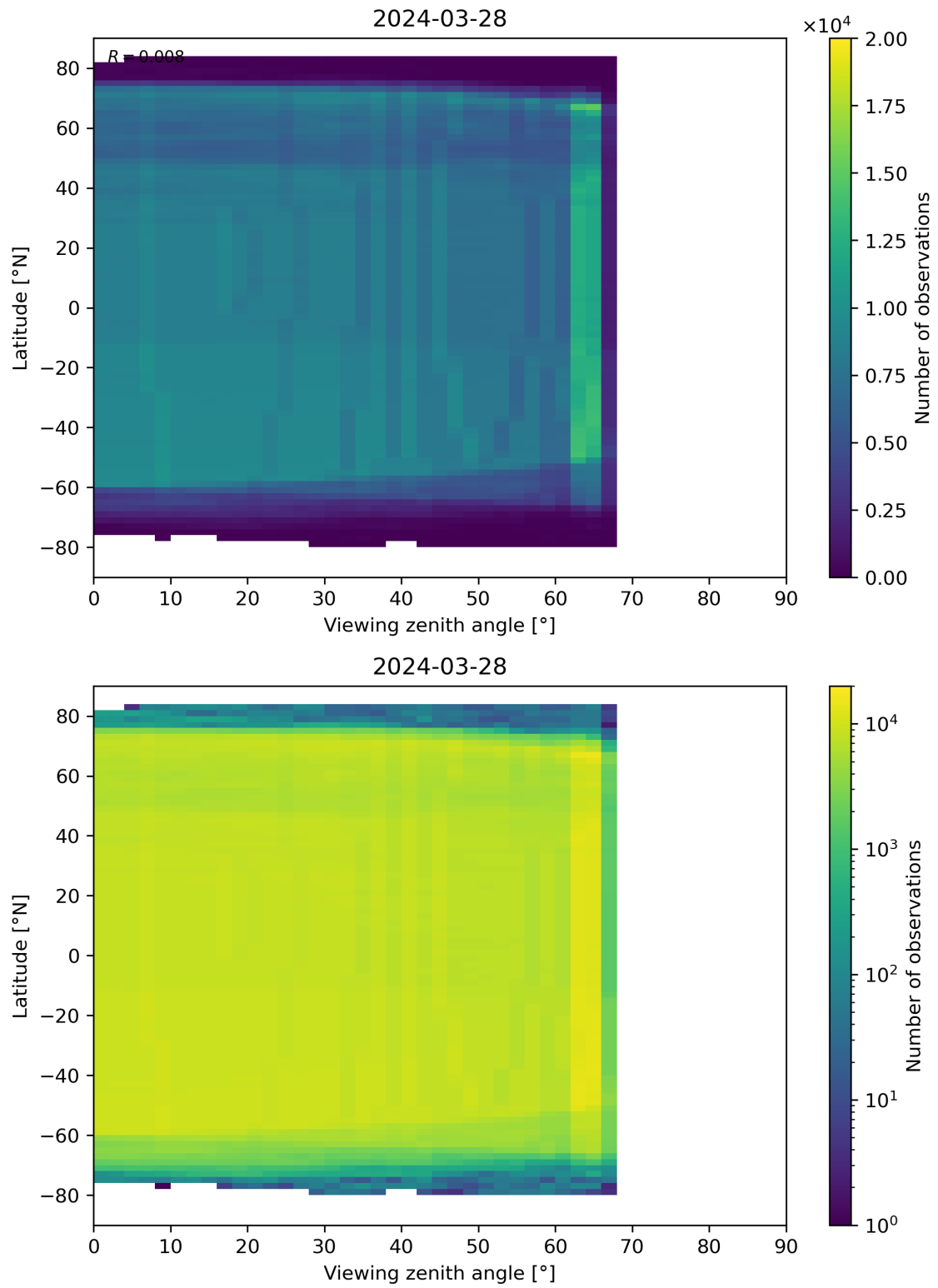
Figure 196: Scatter density plot of “Viewing zenith angle” against “Latitude” for 2024-03-27 to 2024-03-29.
