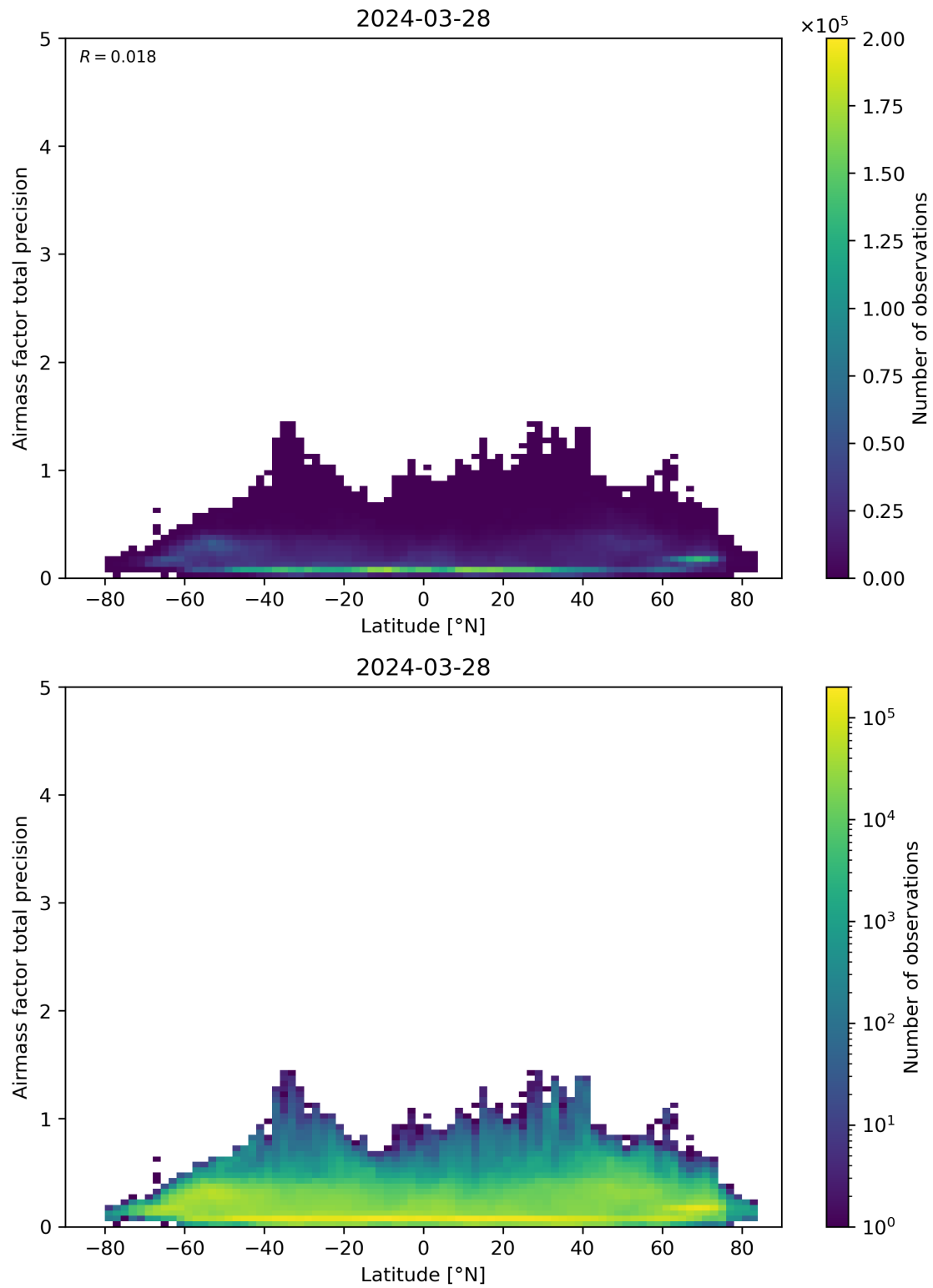
Figure 162: Scatter density plot of “Latitude” against “Airmass factor total precision” for 2024-03-27 to 2024-03-29.
