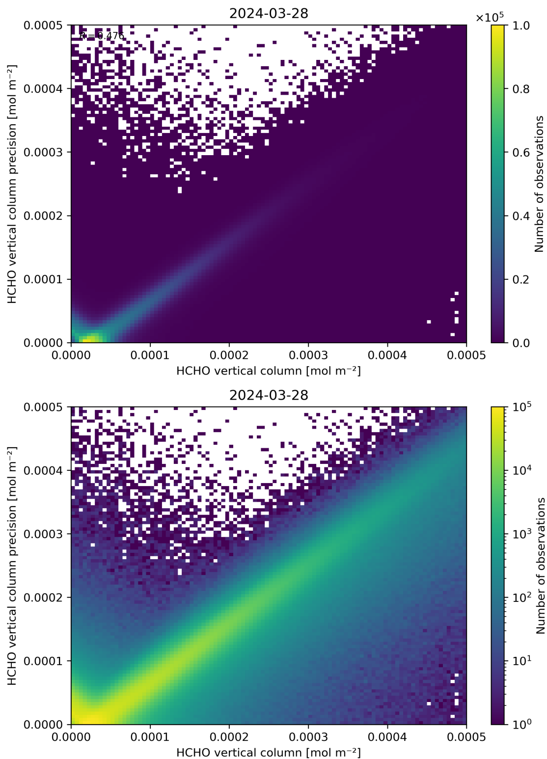
Figure 134: Scatter density plot of “HCHO vertical column” against “HCHO vertical column precision” for 2024-03-27 to 2024-03-29.
