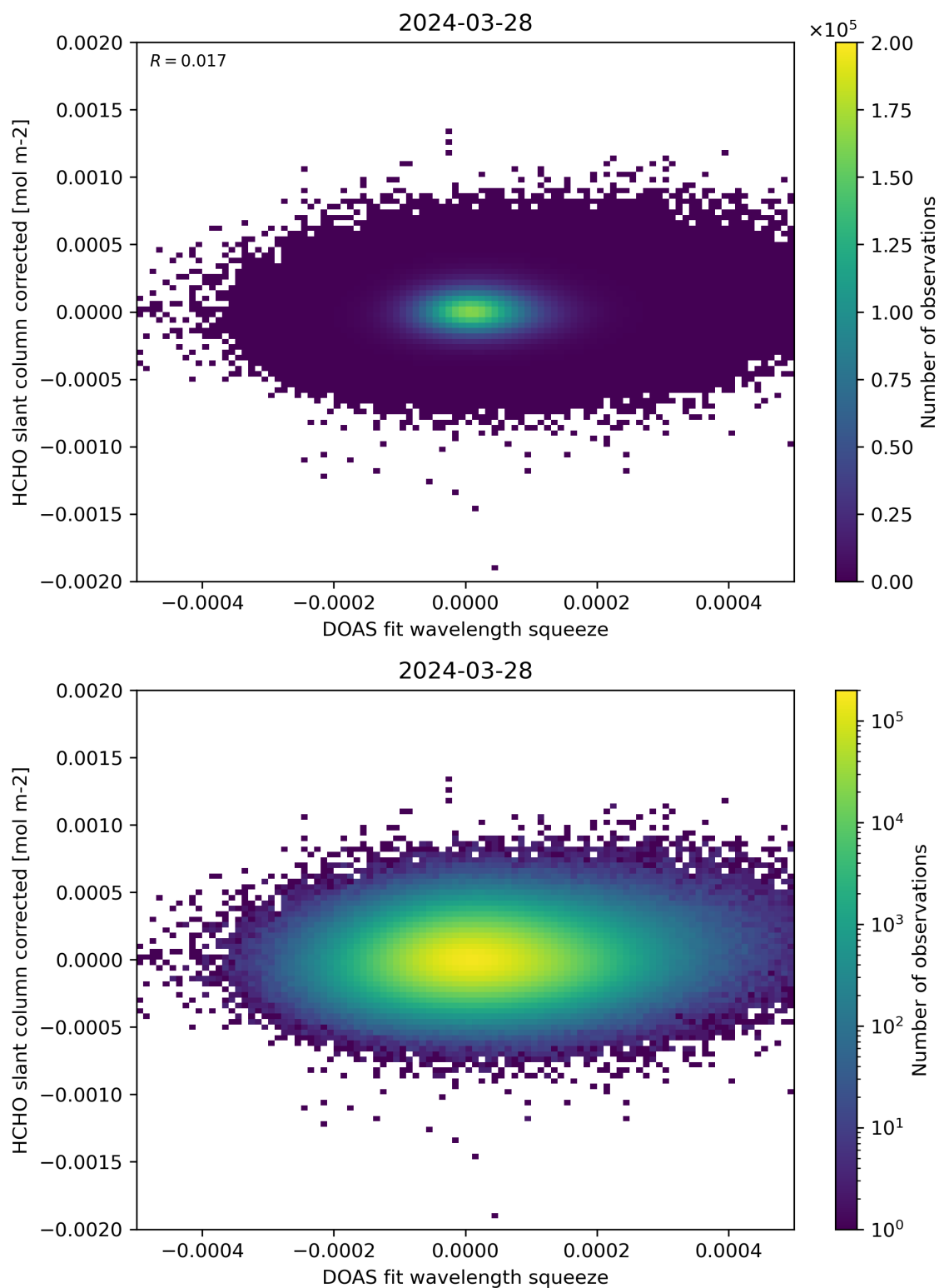
Figure 69: Scatter density plot of “DOAS fit wavelength squeeze” against “HCHO slant column corrected” for 2024-03-27 to 2024-03-29.
