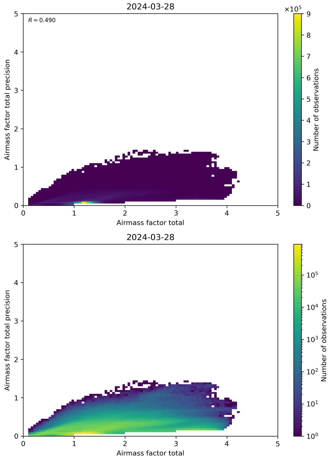
Figure 103: Scatter density plot of “Airmass factor total” against “Airmass factor total precision” for 2024-03-27 to 2024-03-29.
