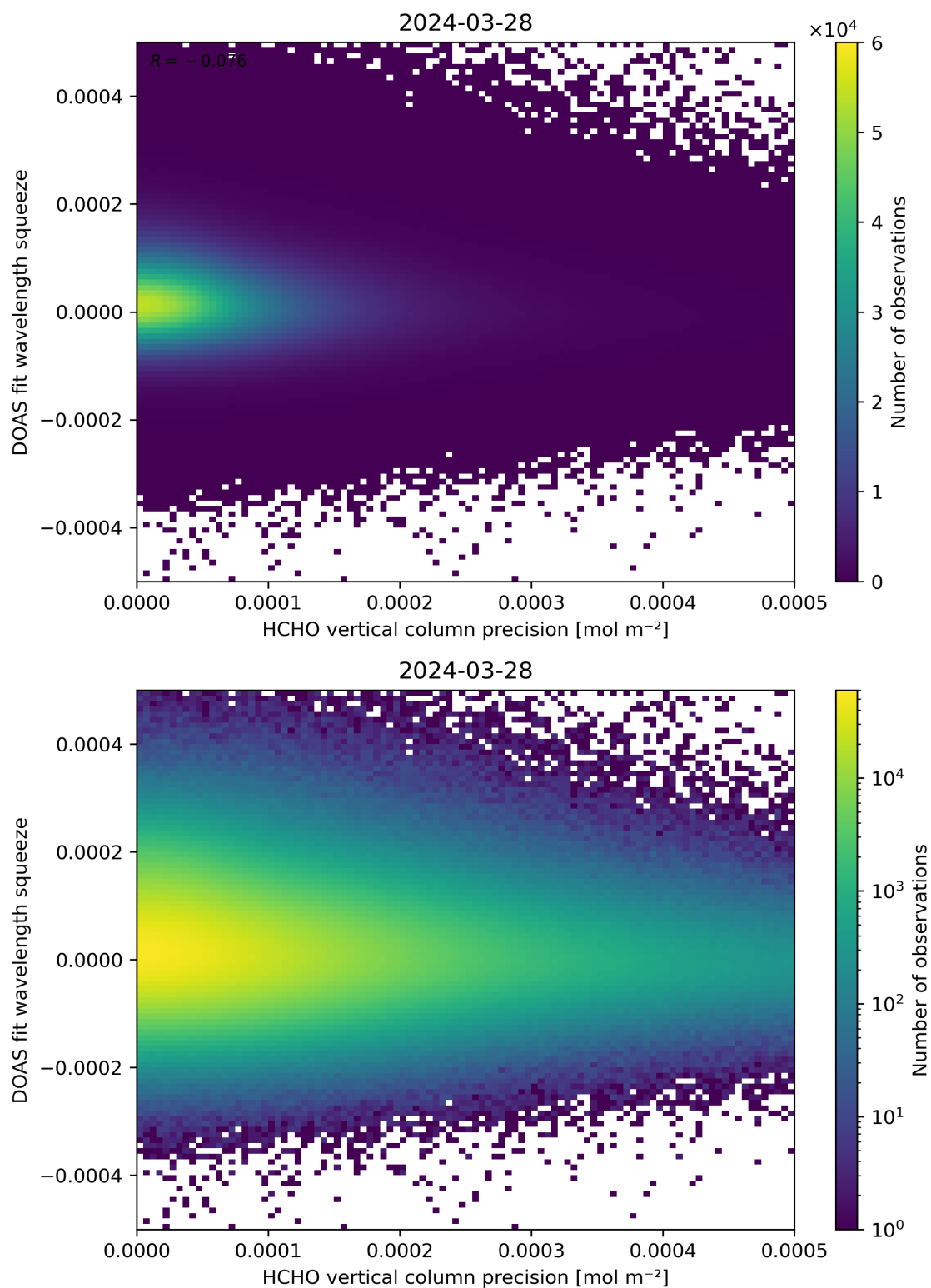
Figure 138: Scatter density plot of “HCHO vertical column precision” against “DOAS fit wavelength squeeze” for 2024-03-27 to 2024-03-29.
