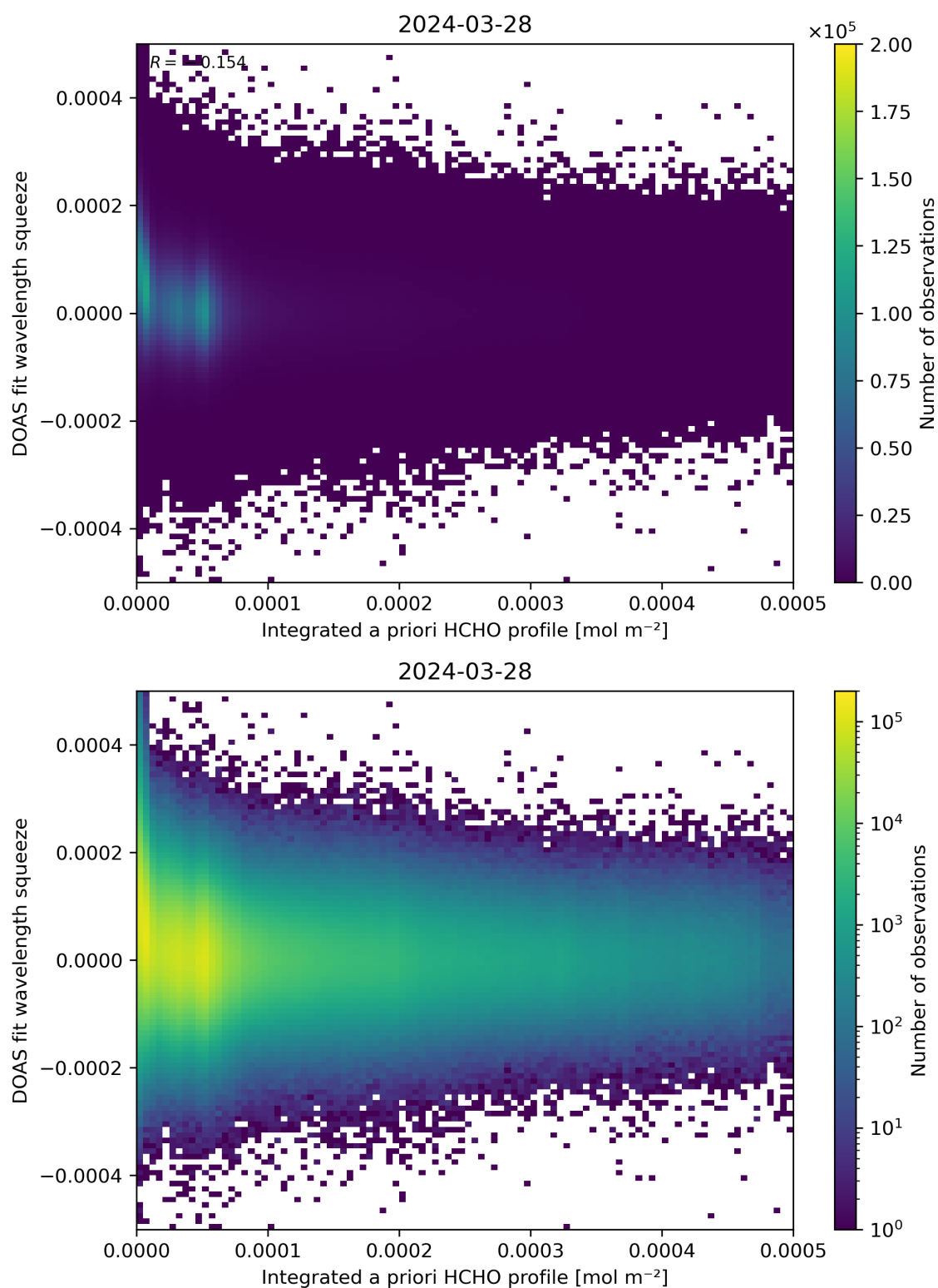
Figure 150: Scatter density plot of “Integrated a priori HCHO profile” against “DOAS fit wavelength squeeze” for 2024-03-27 to 2024-03-29.
