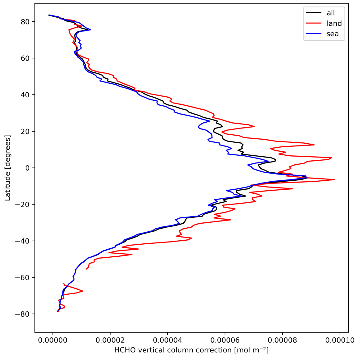
Figure 23: Zonal average of “HCHO vertical column correction” for 2024-03-27 to 2024-03-29.
