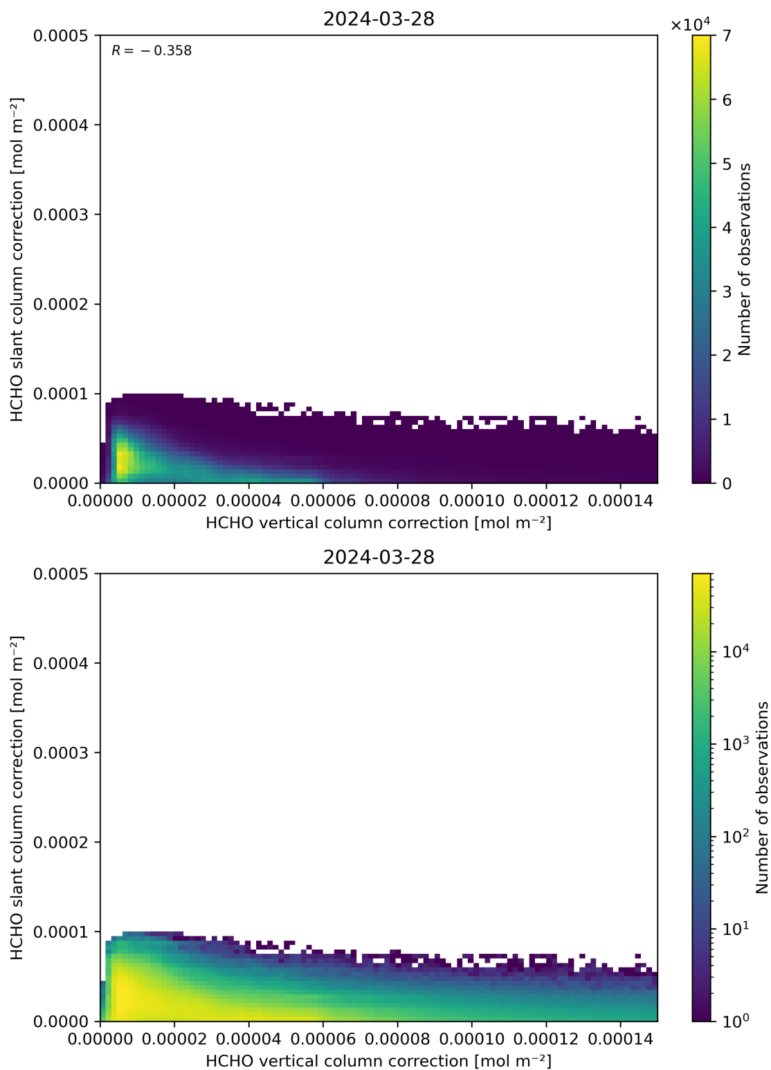
Figure 117: Scatter density plot of “HCHO vertical column correction” against “HCHO slant column correction” for 2024-03-27 to 2024-03-29.
