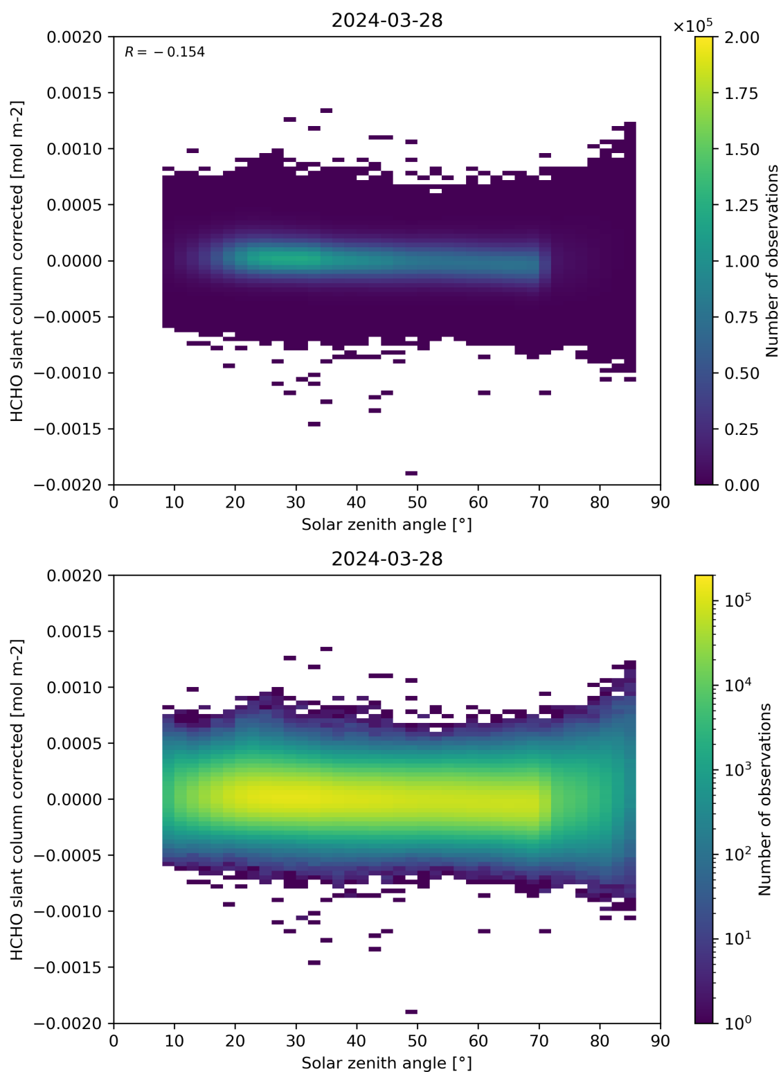
Figure 171: Scatter density plot of “Solar zenith angle” against “HCHO slant column corrected” for 2024-03-27 to 2024-03-29.
