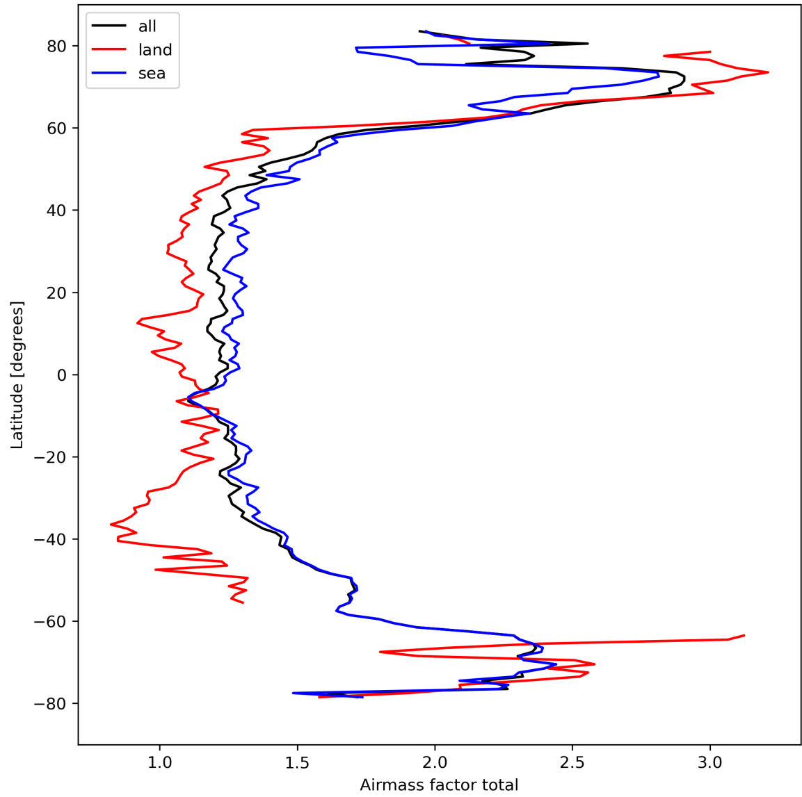
Figure 26: Zonal average of “Airmass factor total” for 2024-03-27 to 2024-03-29.
