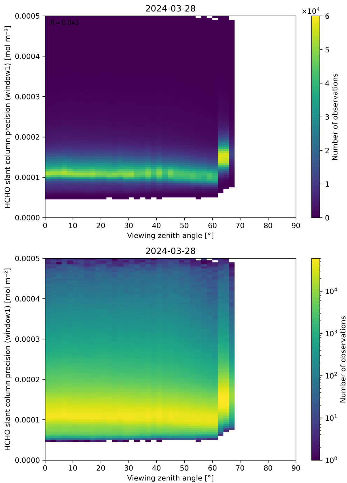
Figure 189: Scatter density plot of “Viewing zenith angle” against “HCHO slant column precision (window1)” for 2024-03-27 to 2024-03-29.
