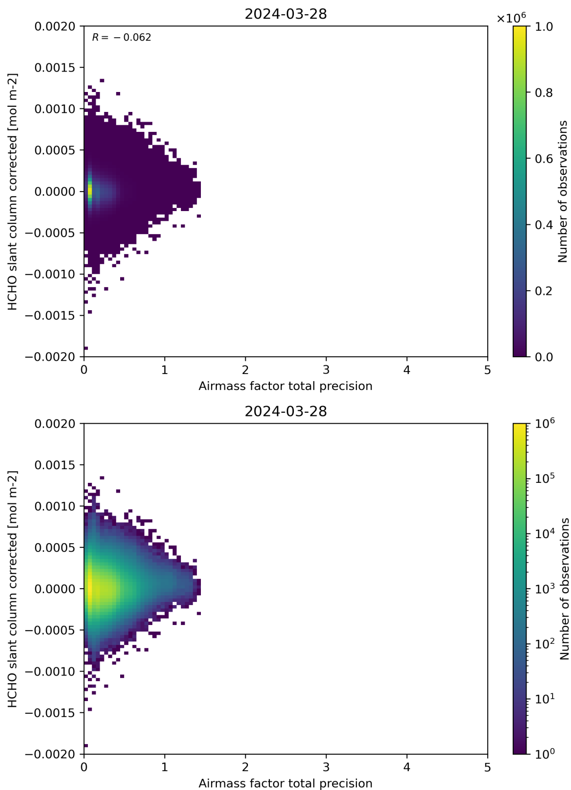
Figure 109: Scatter density plot of “Airmass factor total precision” against “HCHO slant column corrected” for 2024-03-27 to 2024-03-29.
