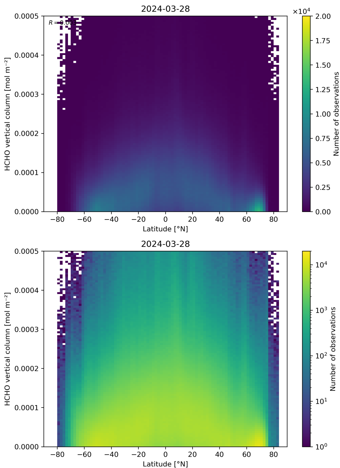
Figure 163: Scatter density plot of “Latitude” against “HCHO vertical column” for 2024-03-27 to 2024-03-29.
