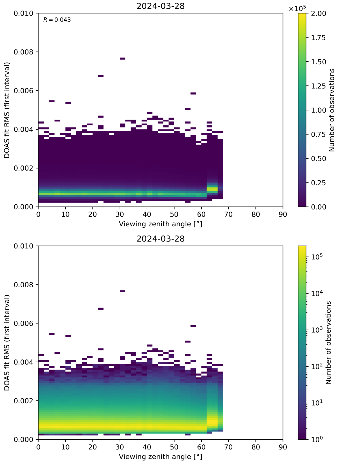
Figure 182: Scatter density plot of “Viewing zenith angle” against “DOAS fit RMS (first interval)” for 2024-03-27 to 2024-03-29.
