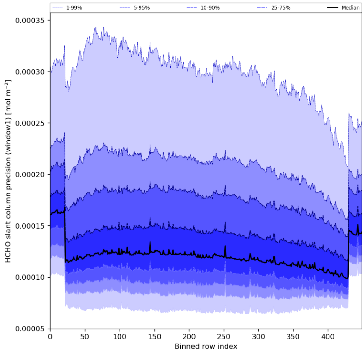
Figure 53: Along track statistics of “HCHO slant column precision (window1)” for 2024-03-27 to 2024-03-29
