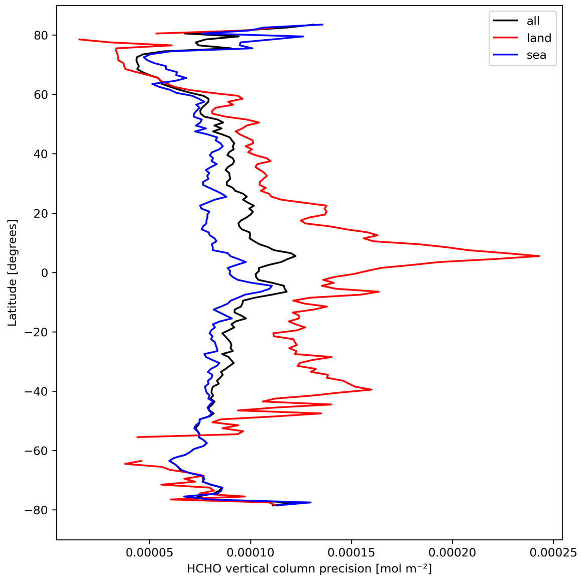
Figure 22: Zonal average of “HCHO vertical column precision” for 2024-03-27 to 2024-03-29.
