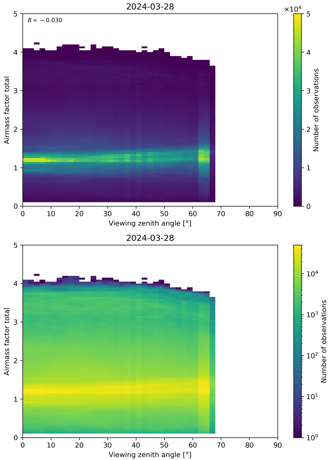
Figure 190: Scatter density plot of “Viewing zenith angle” against “Airmass factor total” for 2024-03-27 to 2024-03-29.
