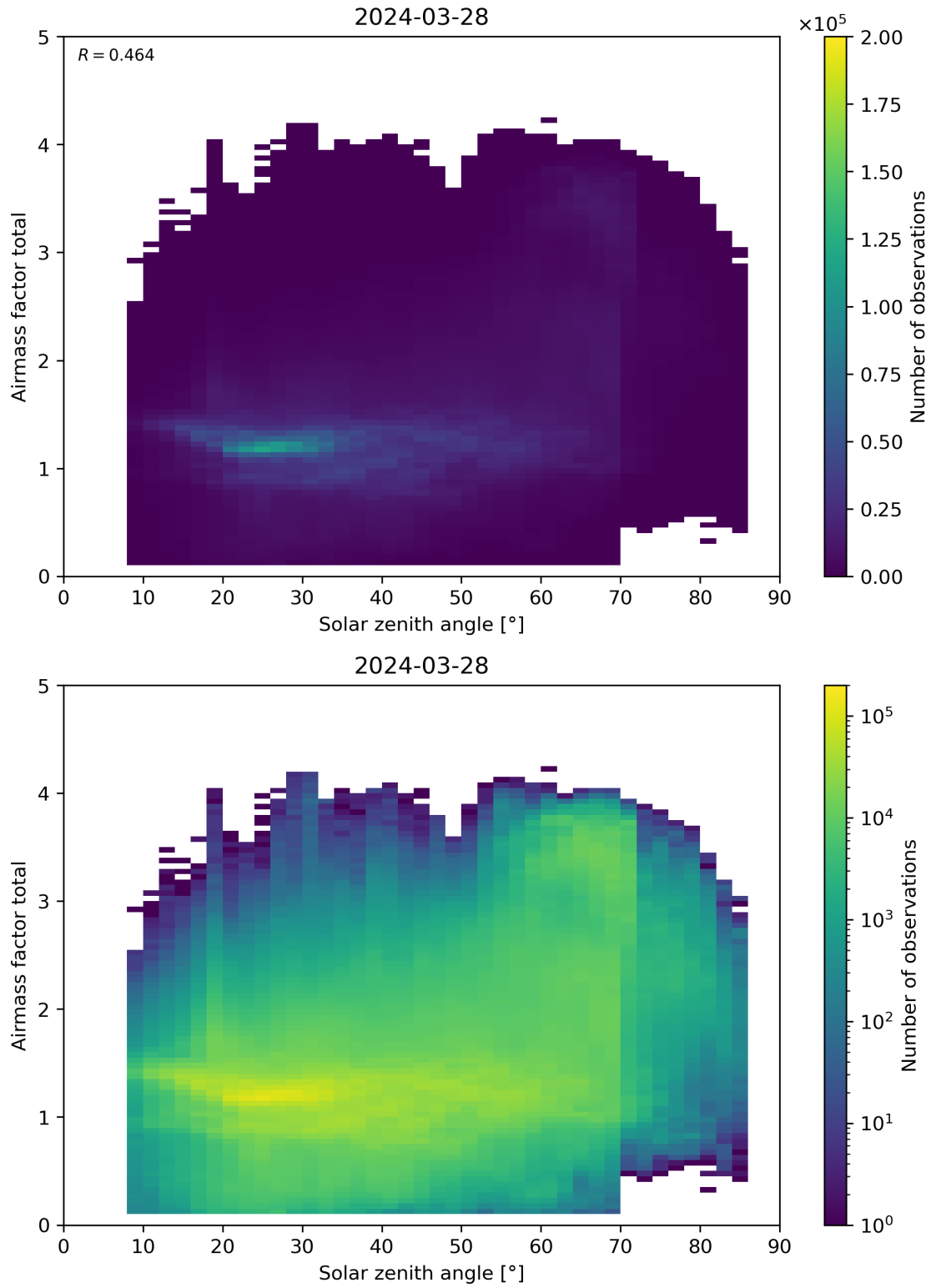
Figure 175: Scatter density plot of “Solar zenith angle” against “Airmass factor total” for 2024-03-27 to 2024-03-29.
