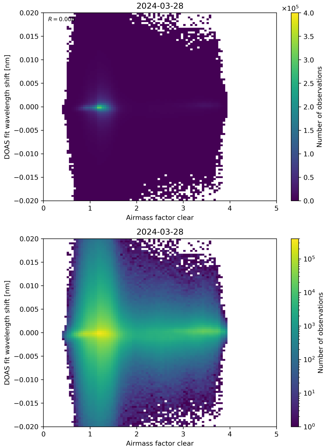
Figure 72: Scatter density plot of “Airmass factor clear” against “DOAS fit wavelength shift” for 2024-03-27 to 2024-03-29.
