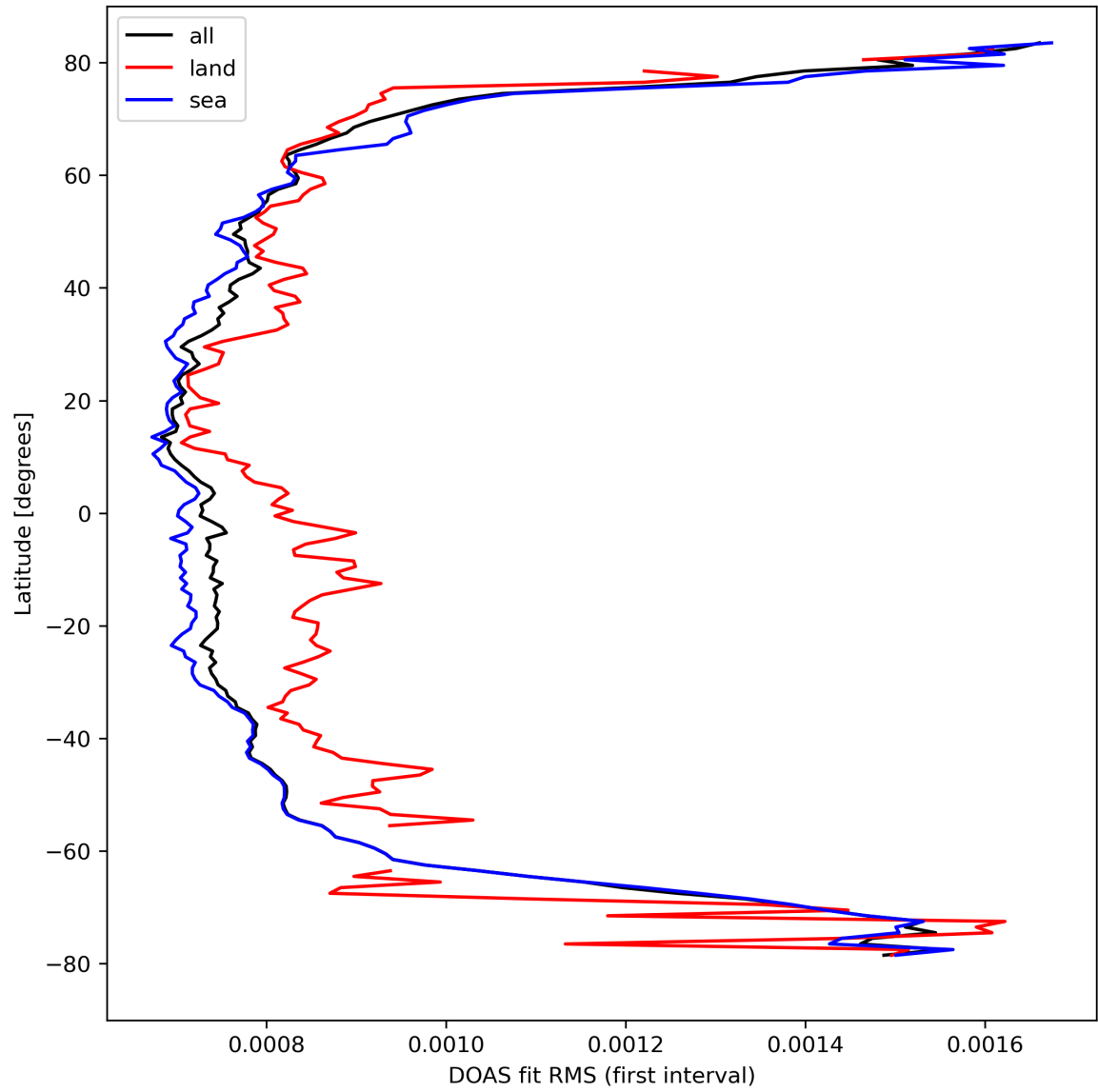
Figure 32: Zonal average of “DOAS fit RMS (first interval)” for 2024-03-27 to 2024-03-29.
