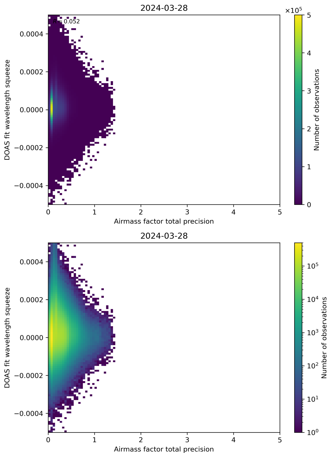
Figure 107: Scatter density plot of “Airmass factor total precision” against “DOAS fit wavelength squeeze” for 2024-03-27 to 2024-03-29.
