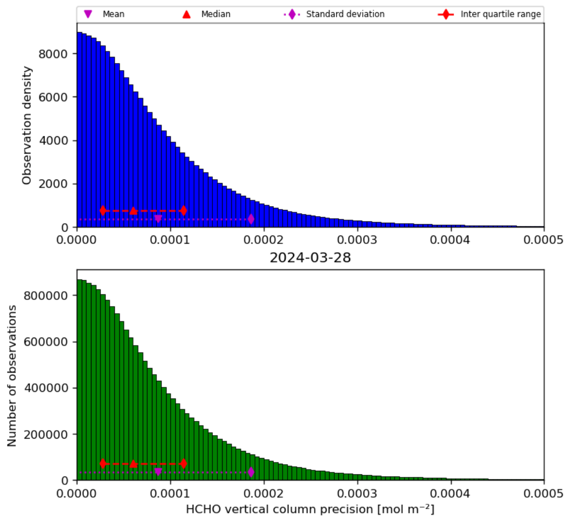
Figure 36: Histogram of “HCHO vertical column precision” for 2024-03-27 to 2024-03-29
