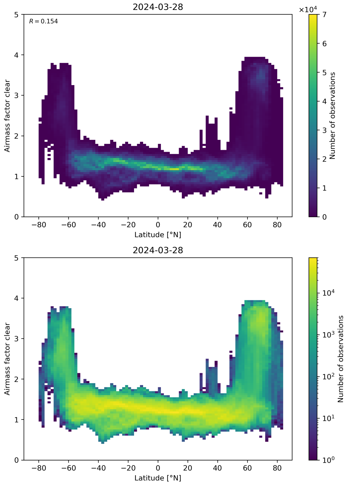
Figure 156: Scatter density plot of “Latitude” against “Airmass factor clear” for 2024-03-27 to 2024-03-29.
