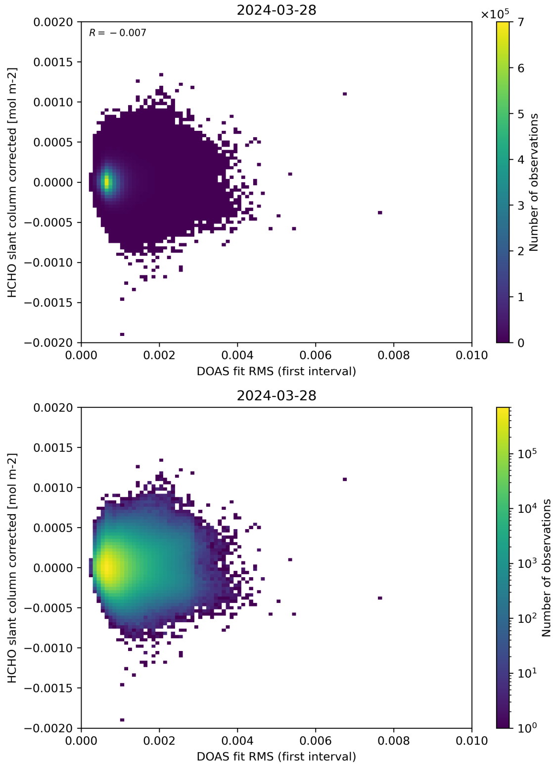
Figure 62: Scatter density plot of “DOAS fit RMS (first interval)” against “HCHO slant column corrected” for 2024-03-27 to 2024-03-29.
