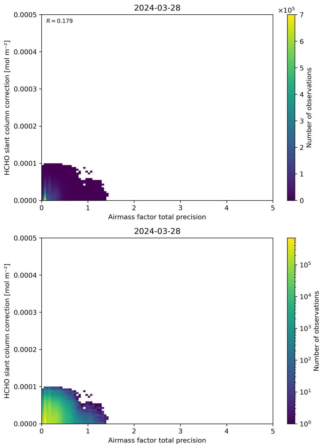
Figure 110: Scatter density plot of “Airmass factor total precision” against “HCHO slant column correction” for 2024-03-27 to 2024-03-29.
