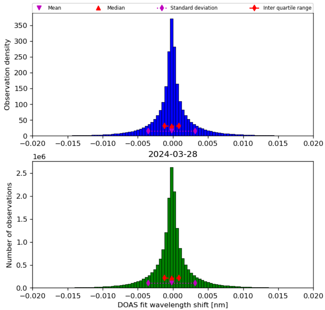
Figure 44: Histogram of “DOAS fit wavelength shift” for 2024-03-27 to 2024-03-29
