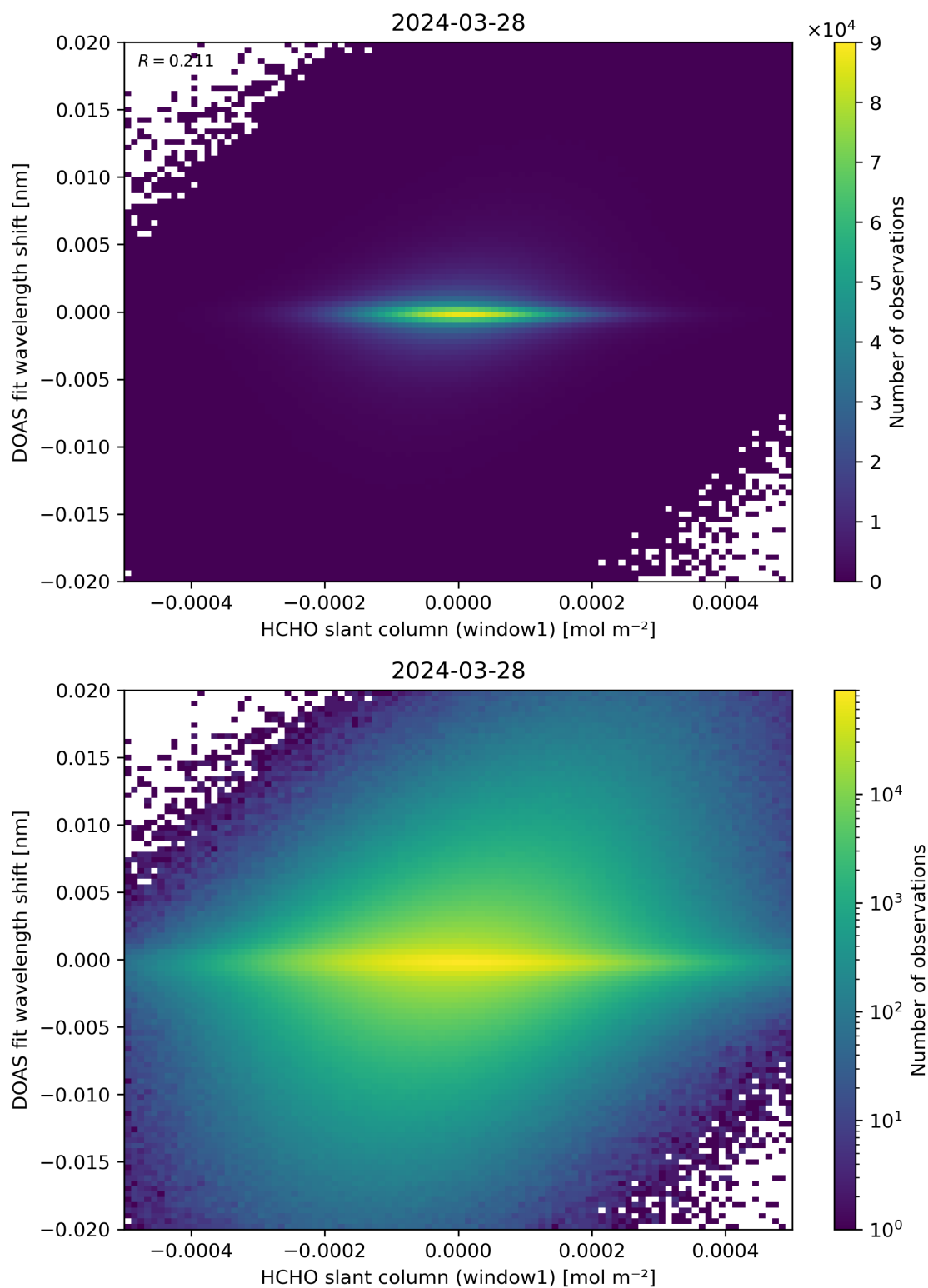
Figure 79: Scatter density plot of “HCHO slant column (window1)” against “DOAS fit wavelength shift” for 2024-03-27 to 2024-03-29.
