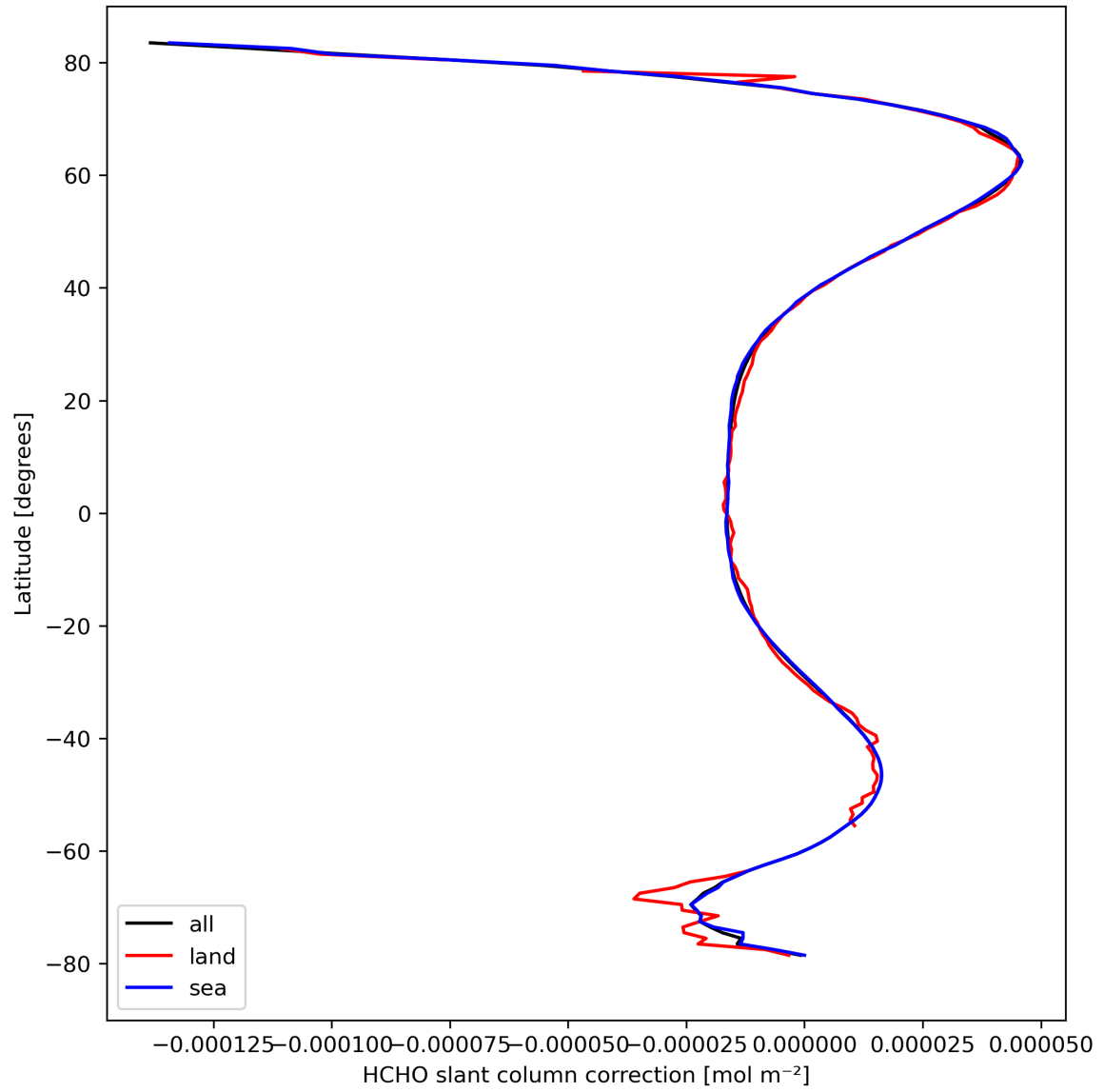
Figure 33: Zonal average of “HCHO slant column correction” for 2024-03-27 to 2024-03-29.
