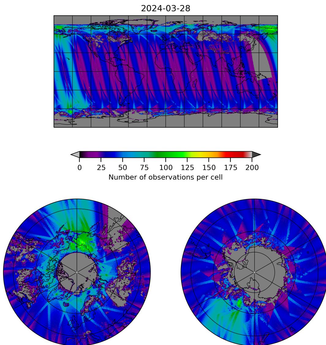
Figure 19: Map of the number of observations for 2024-03-27 to 2024-03-29
