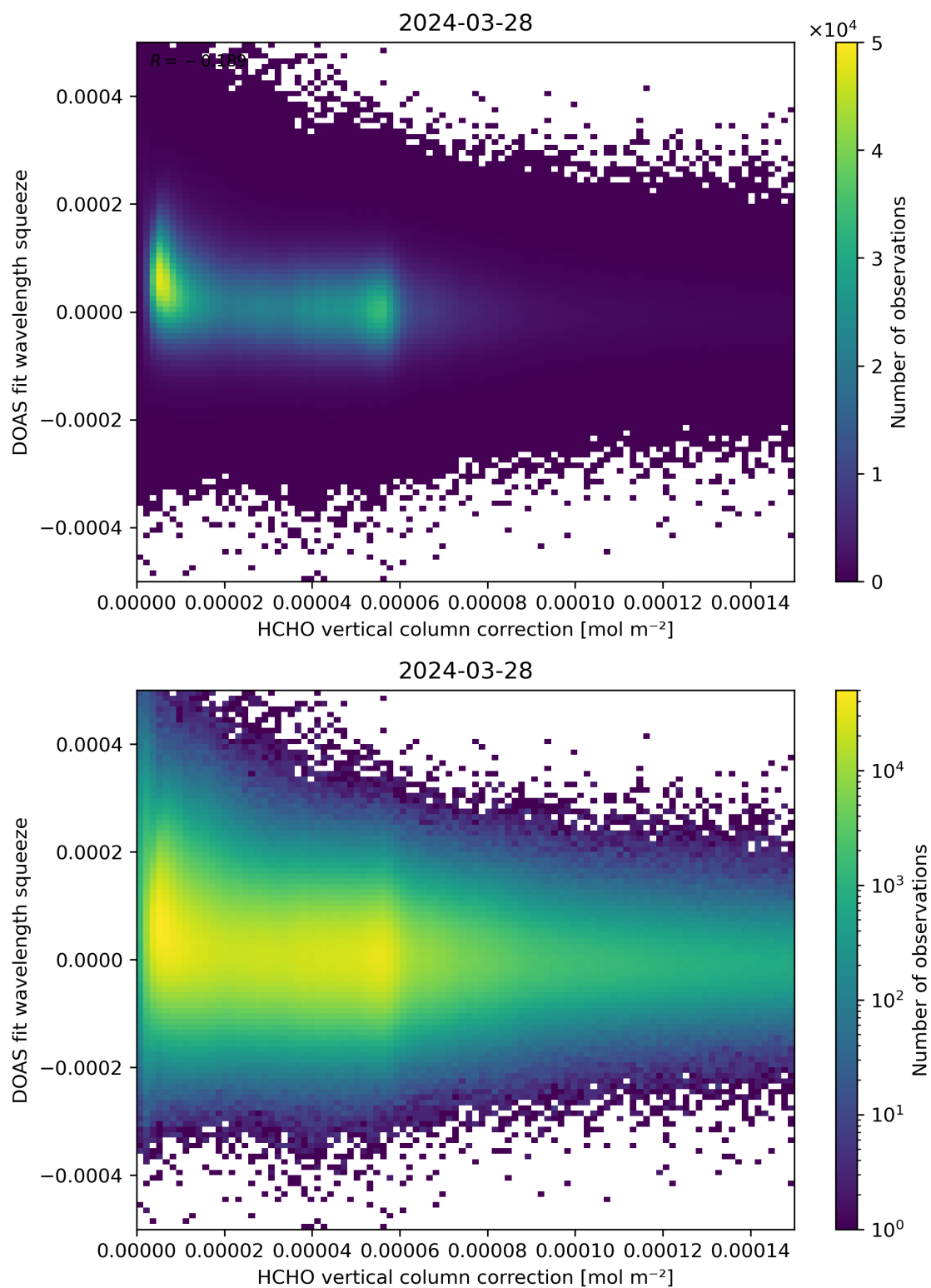
Figure 114: Scatter density plot of “HCHO vertical column correction” against “DOAS fit wavelength squeeze” for 2024-03-27 to 2024-03-29.
