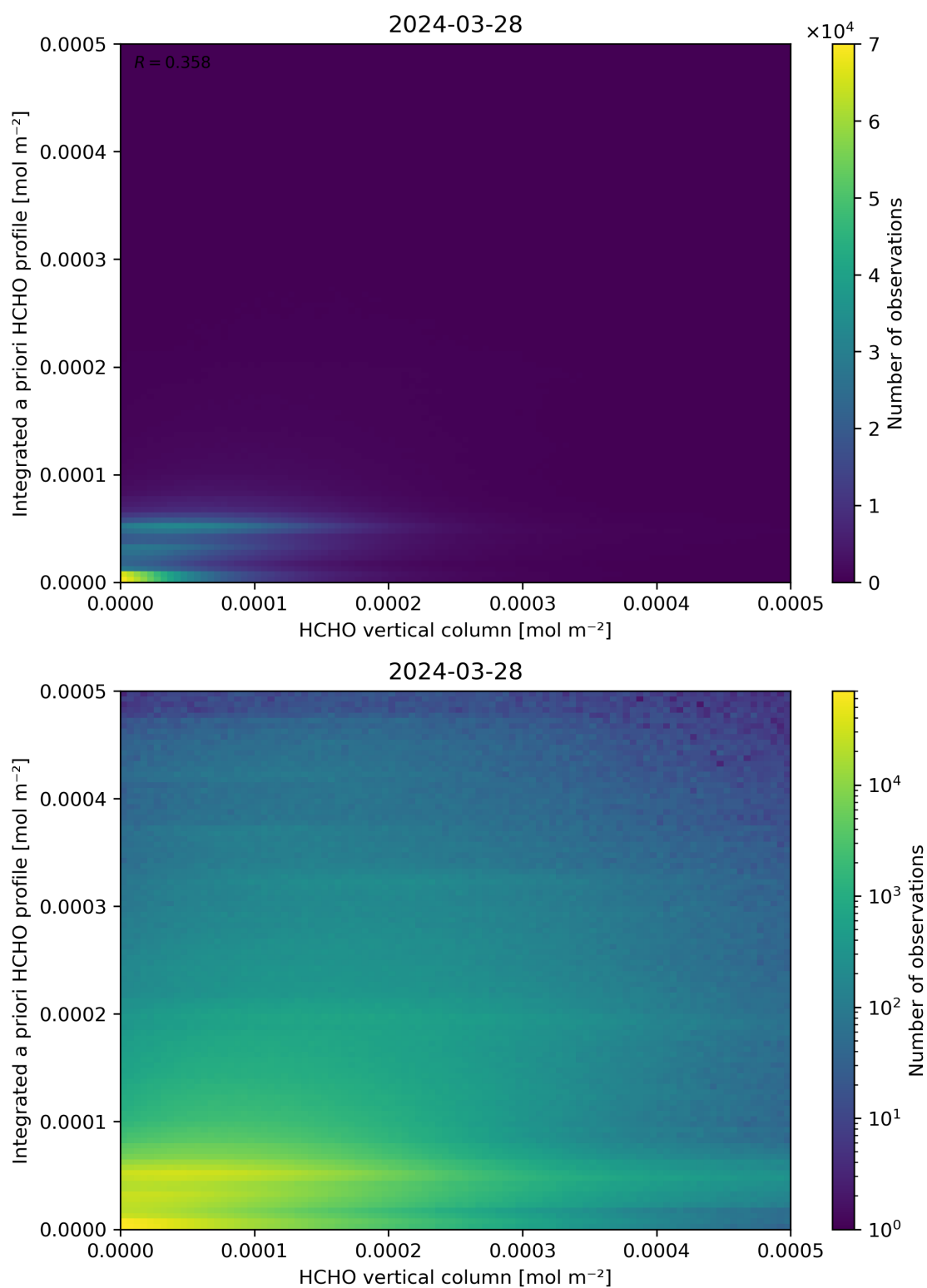
Figure 135: Scatter density plot of “HCHO vertical column” against “Integrated a priori HCHO profile” for 2024-03-27 to 2024-03-29.
