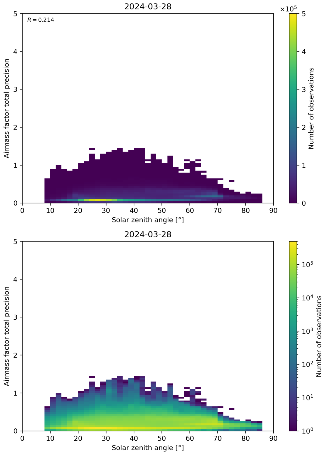
Figure 176: Scatter density plot of “Solar zenith angle” against “Airmass factor total precision” for 2024-03-27 to 2024-03-29.
