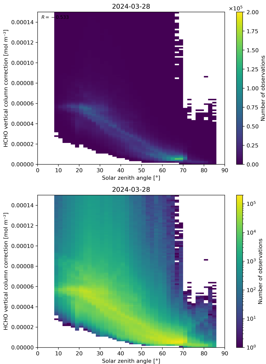
Figure 178: Scatter density plot of “Solar zenith angle” against “HCHO vertical column correction” for 2024-03-27 to 2024-03-29.
