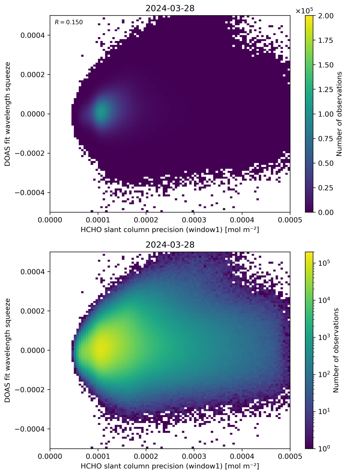
Figure 90: Scatter density plot of “HCHO slant column precision (window1)” against “DOAS fit wavelength squeeze” for 2024-03-27 to 2024-03-29.
