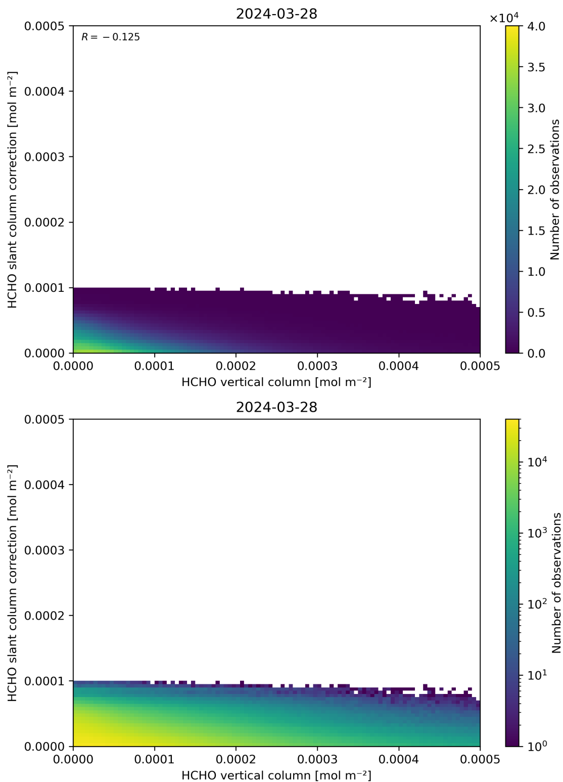
Figure 128: Scatter density plot of “HCHO vertical column” against “HCHO slant column correction” for 2024-03-27 to 2024-03-29.
