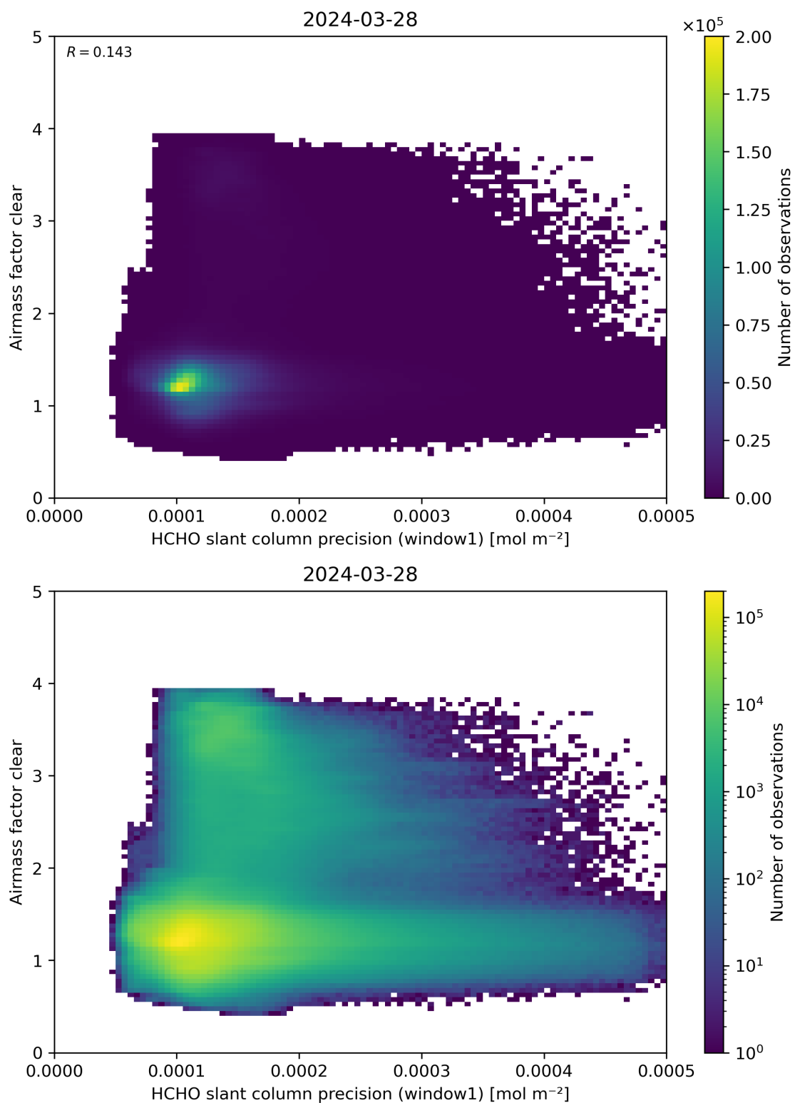
Figure 91: Scatter density plot of “HCHO slant column precision (window1)” against “Airmass factor clear” for 2024-03-27 to 2024-03-29.
