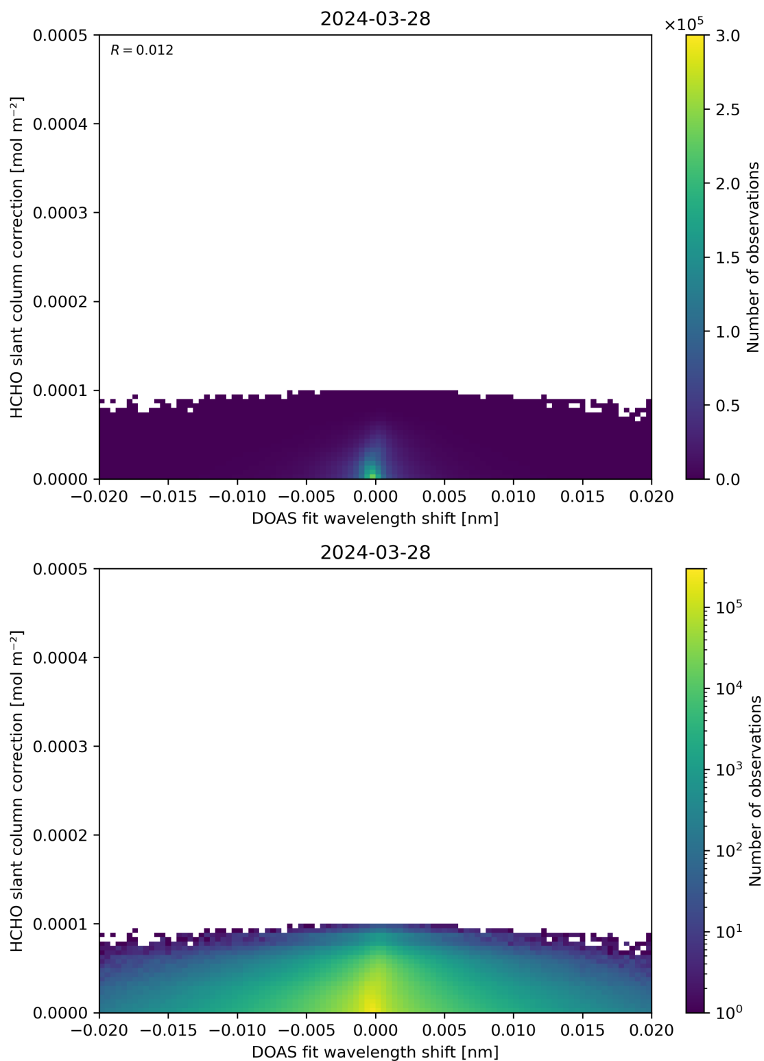
Figure 67: Scatter density plot of “DOAS fit wavelength shift” against “HCHO slant column correction” for 2024-03-27 to 2024-03-29.
