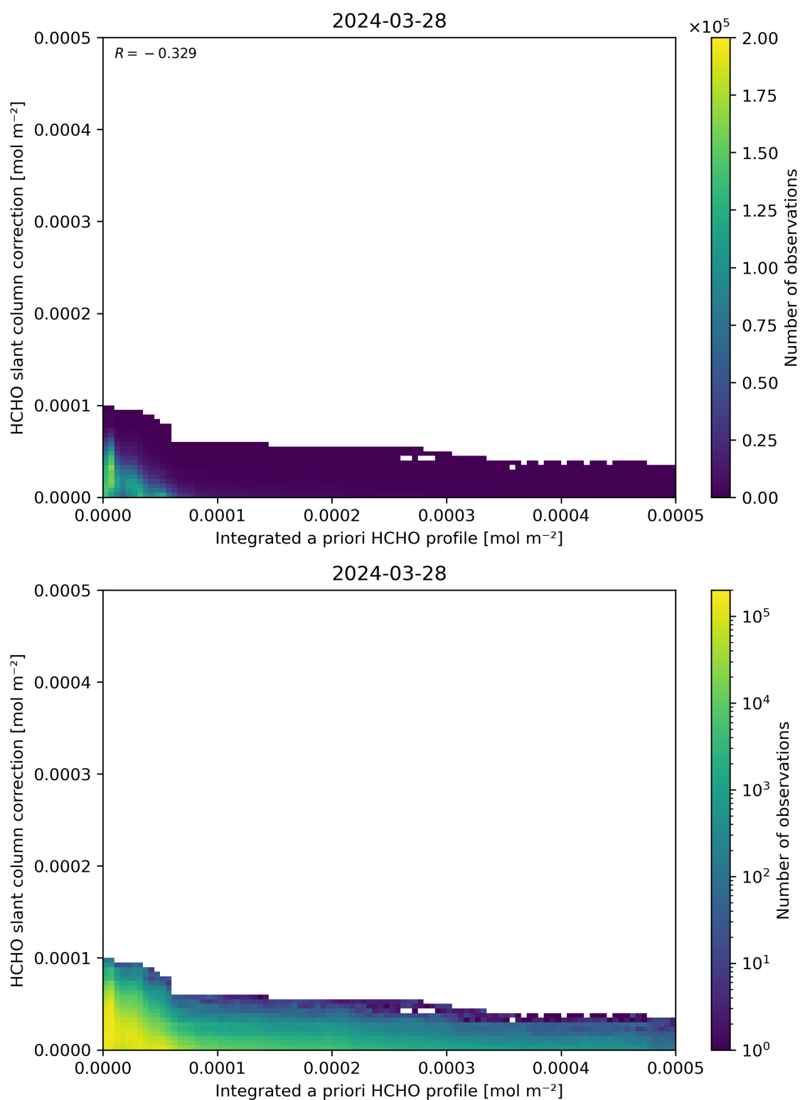
Figure 152: Scatter density plot of “Integrated a priori HCHO profile” against “HCHO slant column correction” for 2024-03-27 to 2024-03-29.
