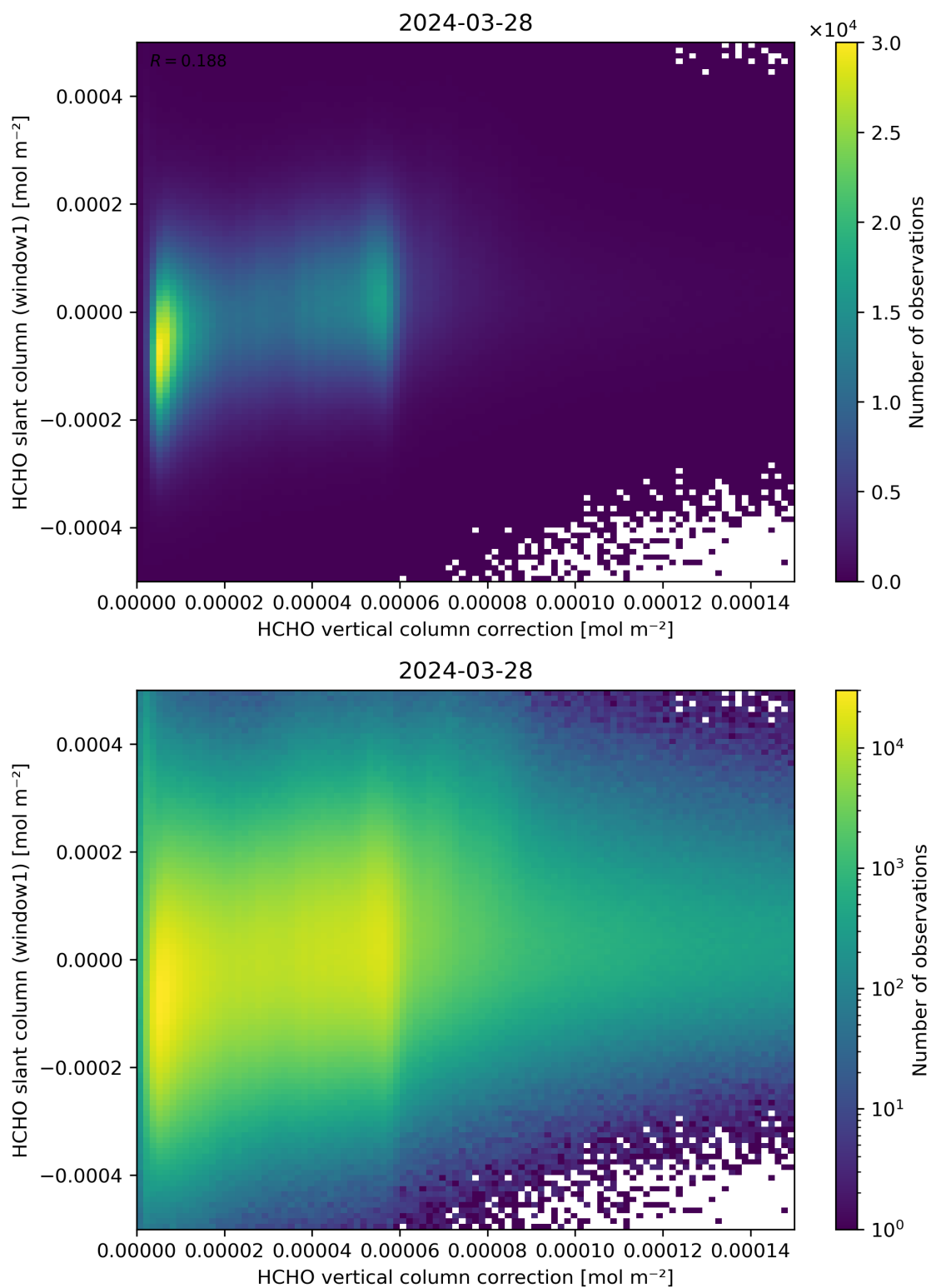
Figure 118: Scatter density plot of “HCHO vertical column correction” against “HCHO slant column (window1)” for 2024-03-27 to 2024-03-29.
