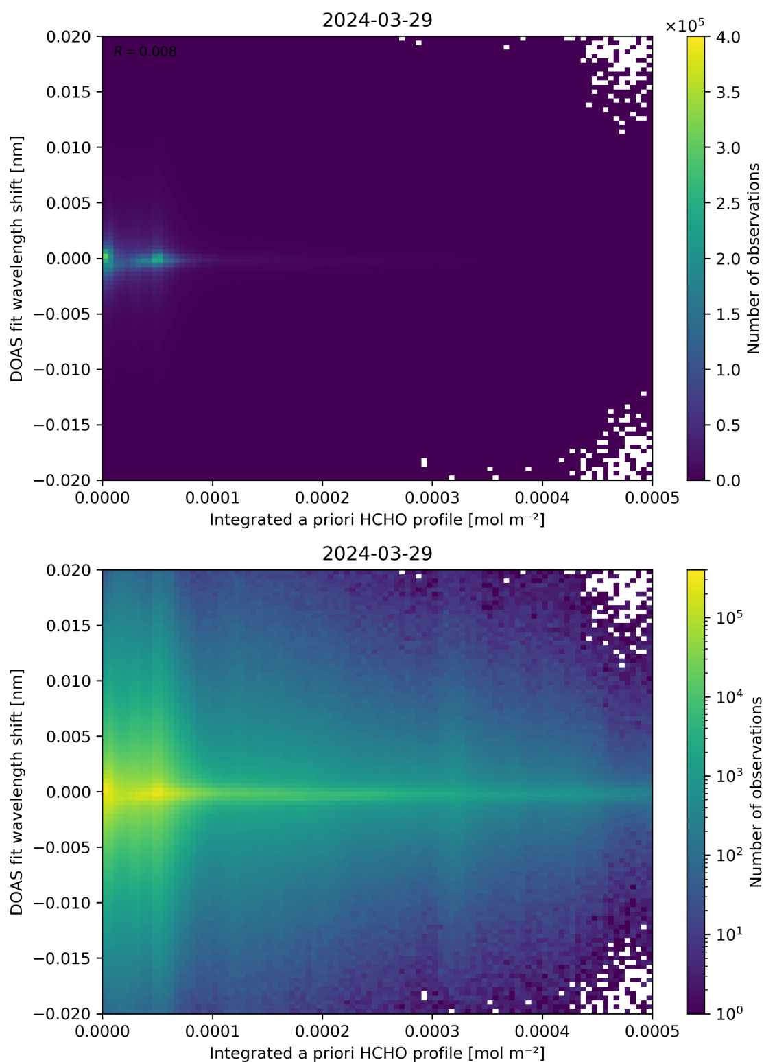
Figure 149: Scatter density plot of “Integrated a priori HCHO profile” against “DOAS fit wavelength shift” for 2024-03-28 to 2024-03-30.
