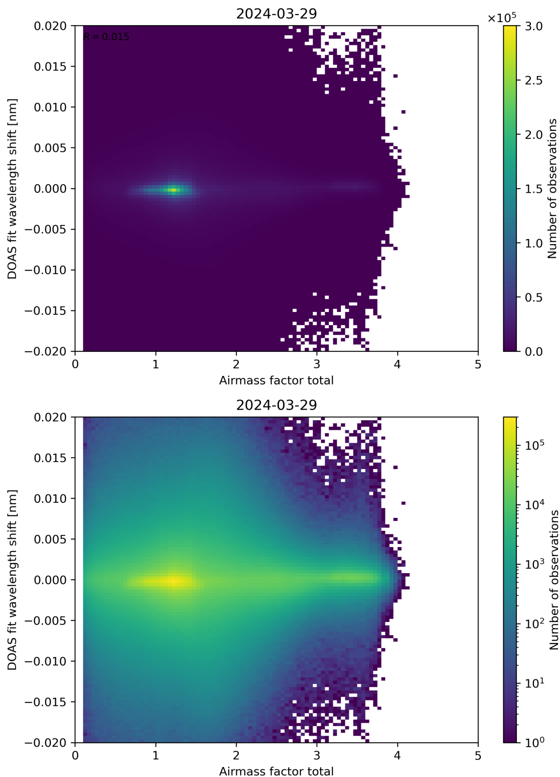
Figure 98: Scatter density plot of “Airmass factor total” against “DOAS fit wavelength shift” for 2024-03-28 to 2024-03-30.
