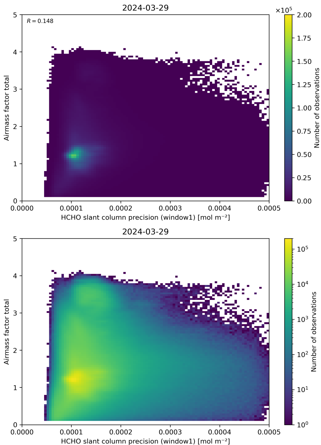
Figure 94: Scatter density plot of “HCHO slant column precision (window1)” against “Airmass factor total” for 2024-03-28 to 2024-03-30.
