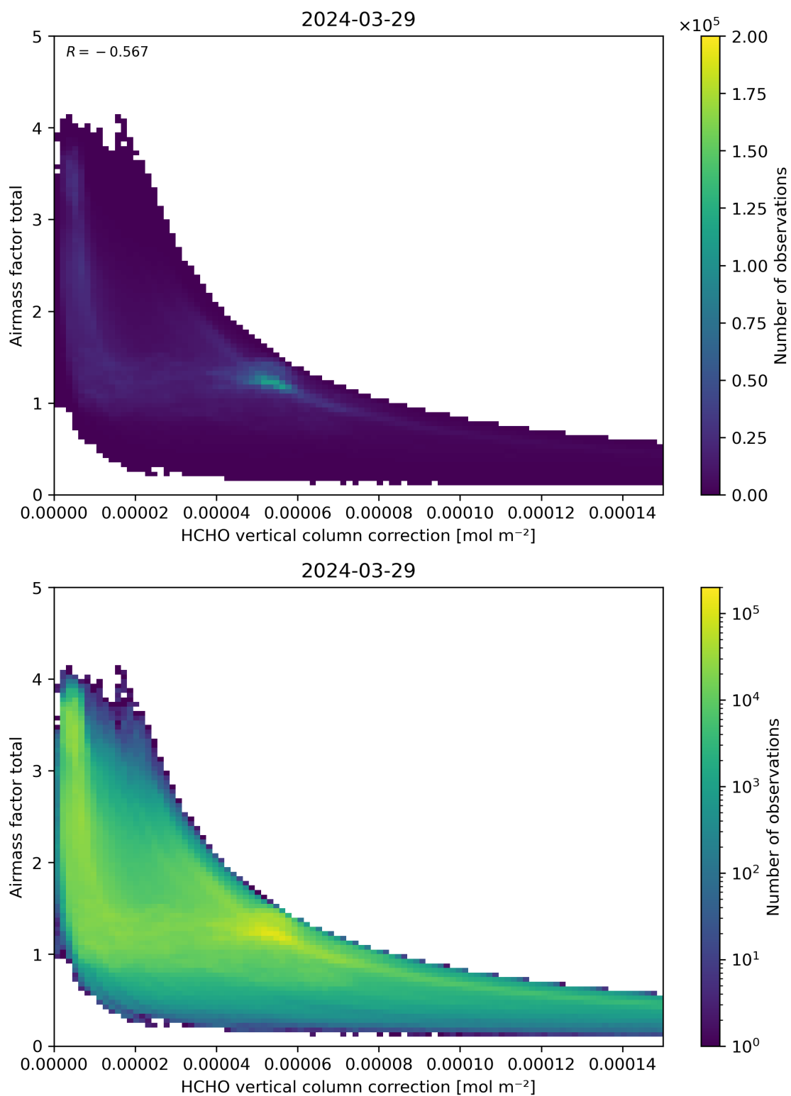
Figure 120: Scatter density plot of “HCHO vertical column correction” against “Airmass factor total” for 2024-03-28 to 2024-03-30.
