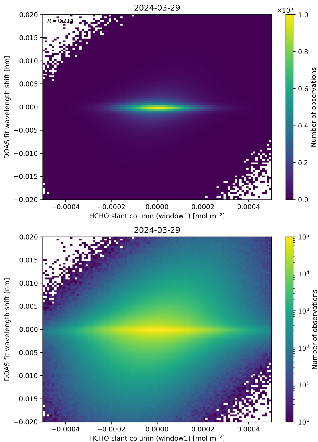
Figure 79: Scatter density plot of “HCHO slant column (window1)” against “DOAS fit wavelength shift” for 2024-03-28 to 2024-03-30.
