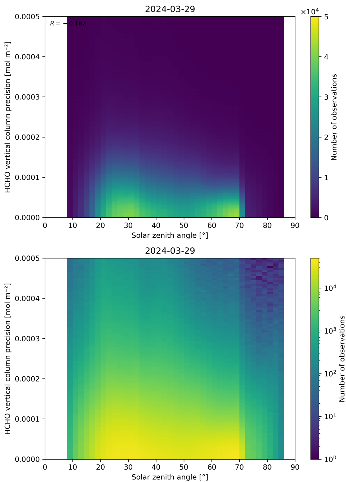
Figure 179: Scatter density plot of “Solar zenith angle” against “HCHO vertical column precision” for 2024-03-28 to 2024-03-30.
