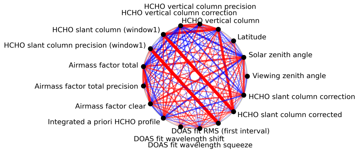
Figure 1: Map of correlation graph for 2024-03-28 to 2024-03-30.
