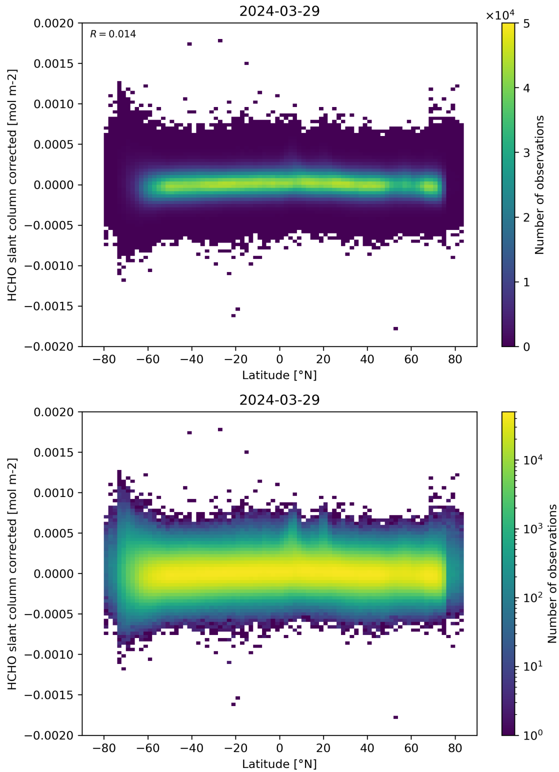
Figure 157: Scatter density plot of “Latitude” against “HCHO slant column corrected” for 2024-03-28 to 2024-03-30.
