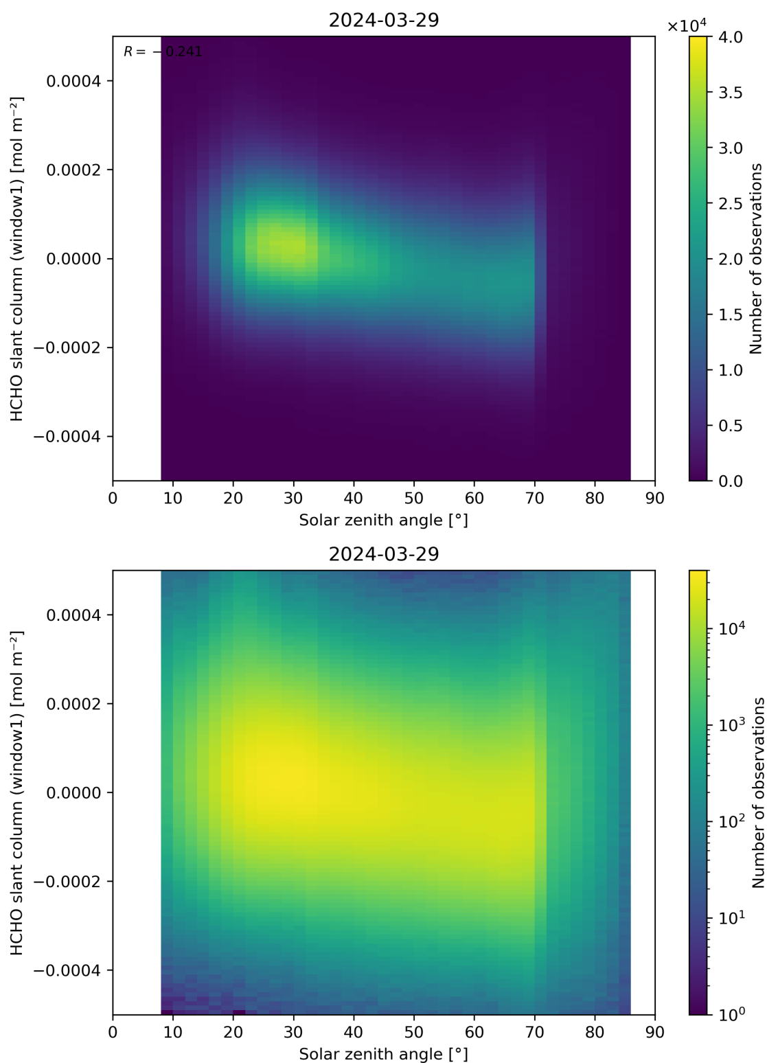
Figure 173: Scatter density plot of “Solar zenith angle” against “HCHO slant column (window1)” for 2024-03-28 to 2024-03-30.
