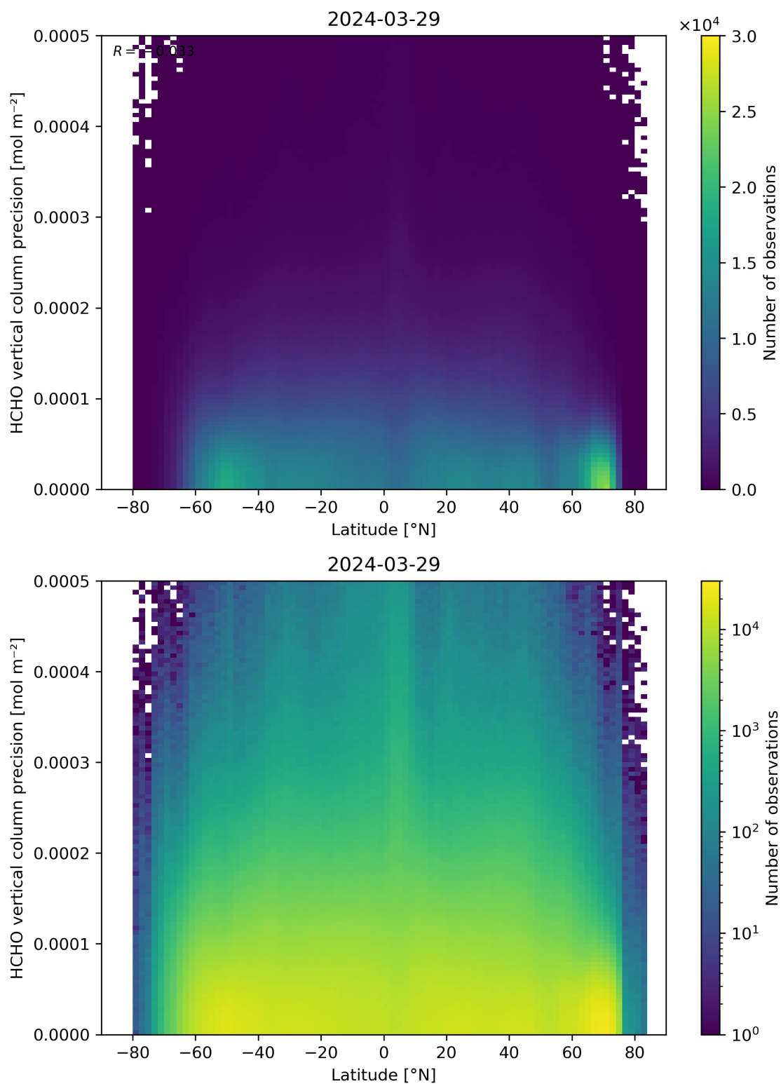
Figure 165: Scatter density plot of “Latitude” against “HCHO vertical column precision” for 2024-03-28 to 2024-03-30.
