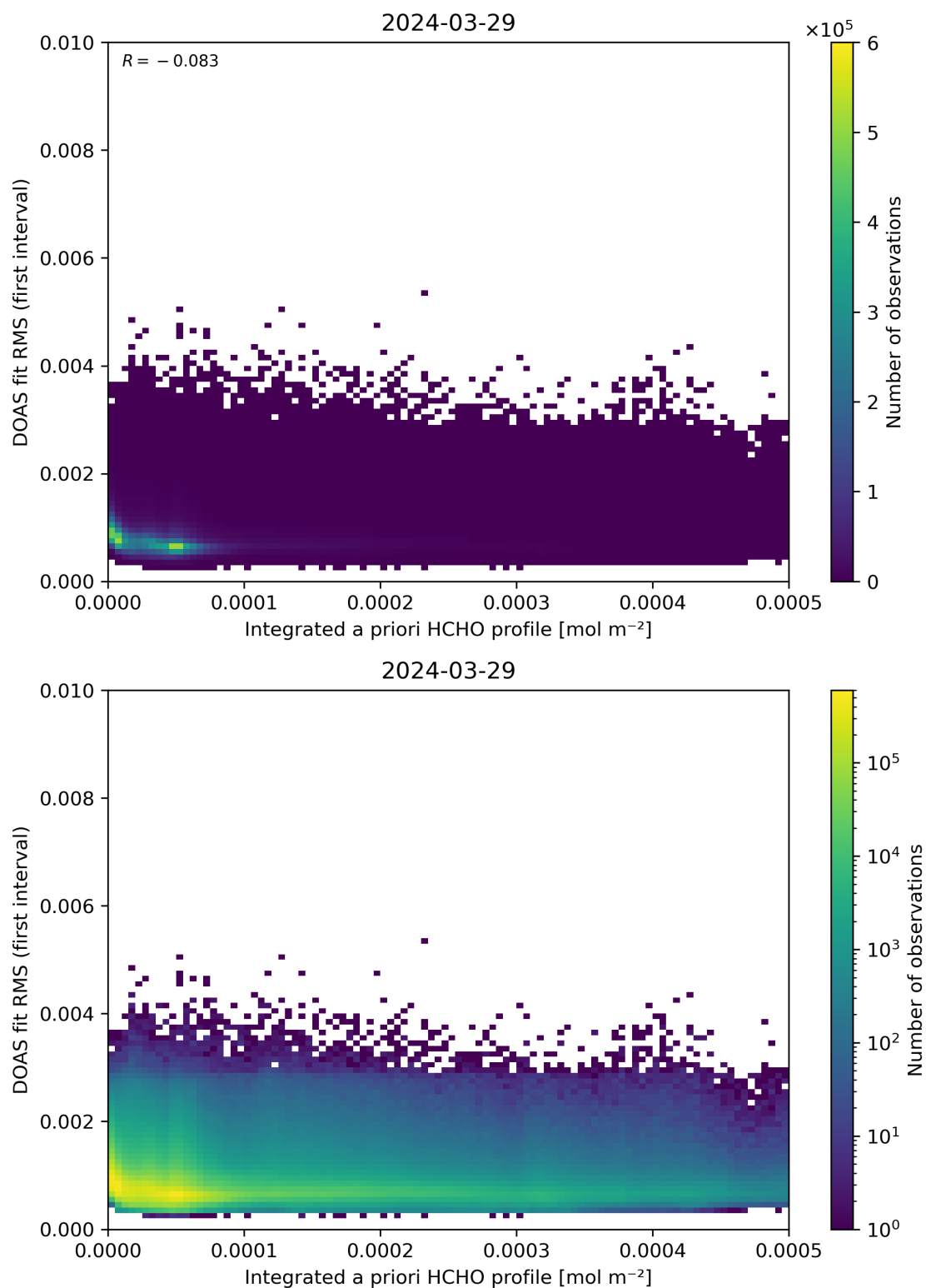
Figure 148: Scatter density plot of “Integrated a priori HCHO profile” against “DOAS fit RMS (first interval)” for 2024-03-28 to 2024-03-30.
