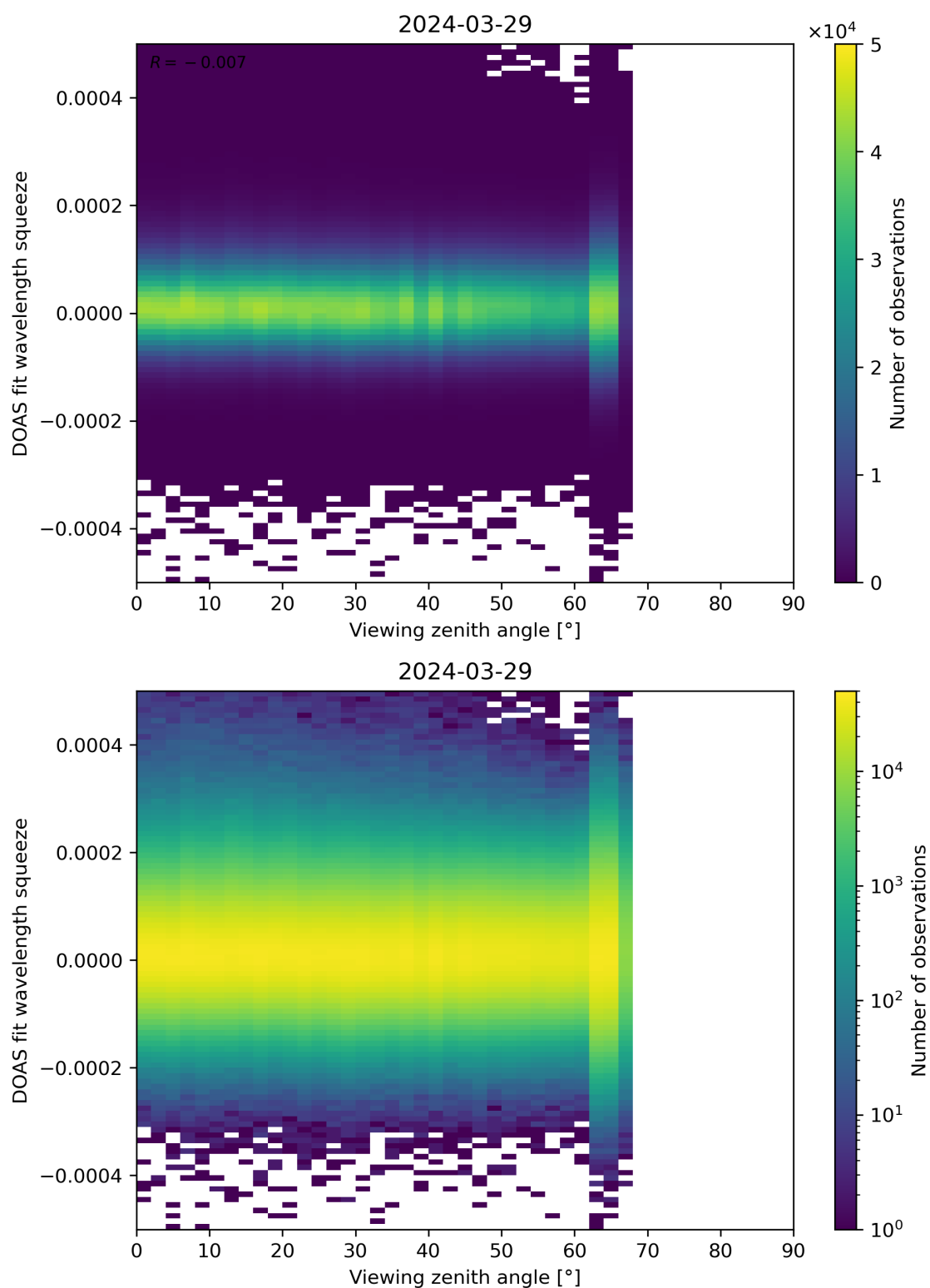
Figure 184: Scatter density plot of “Viewing zenith angle” against “DOAS fit wavelength squeeze” for 2024-03-28 to 2024-03-30.
