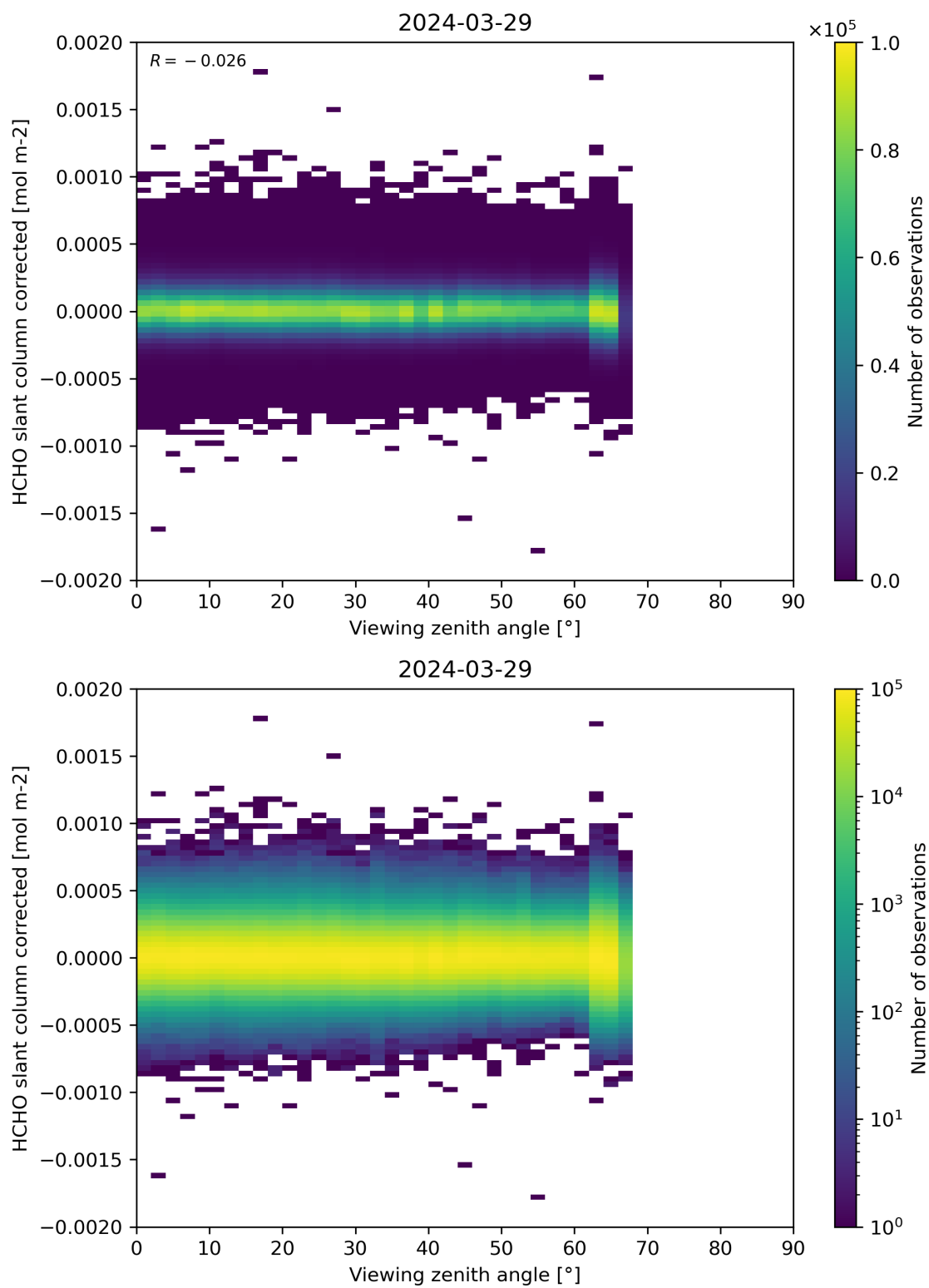
Figure 186: Scatter density plot of “Viewing zenith angle” against “HCHO slant column corrected” for 2024-03-28 to 2024-03-30.
