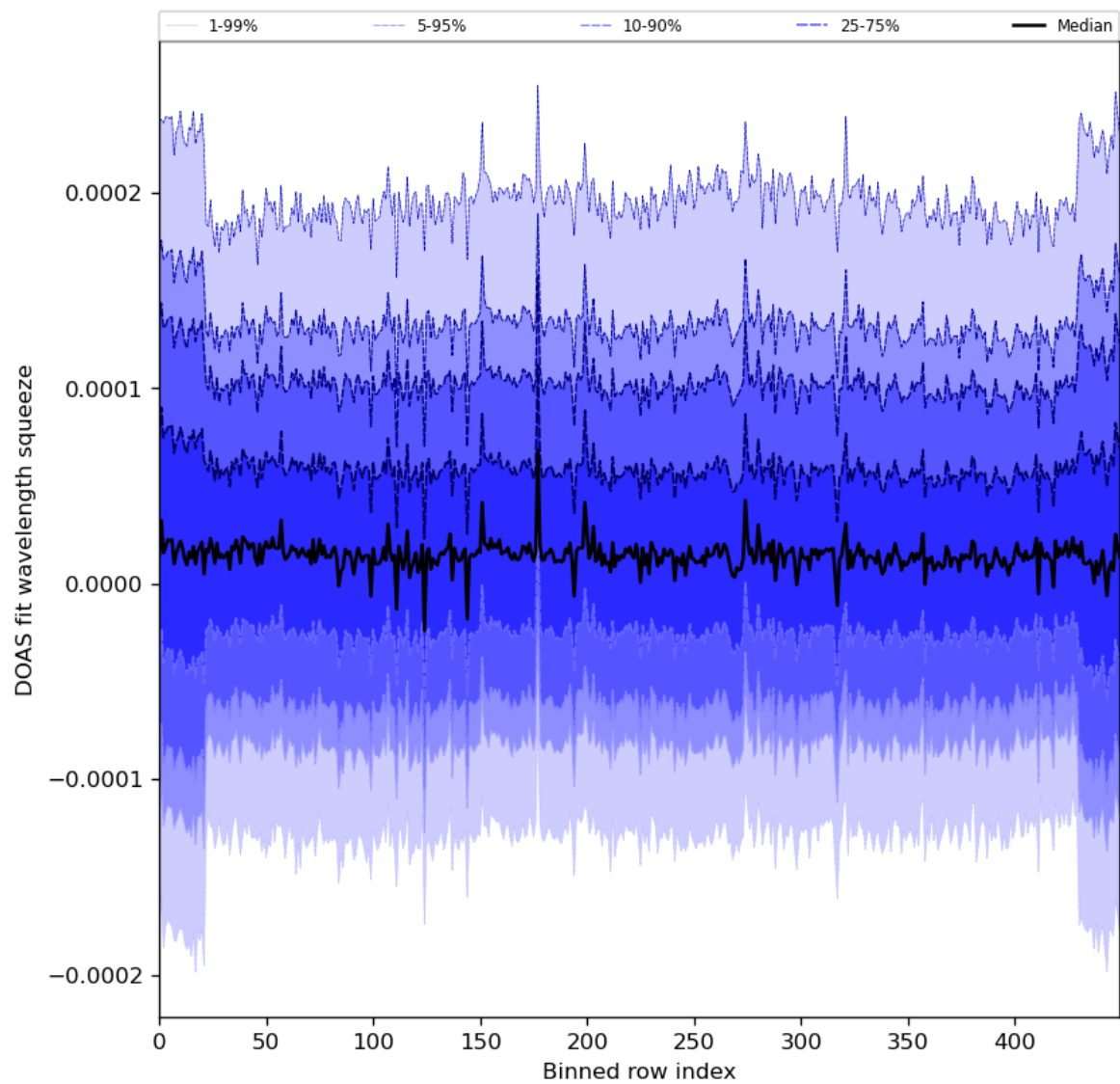
Figure 59: Along track statistics of “DOAS fit wavelength squeeze” for 2024-03-28 to 2024-03-30
