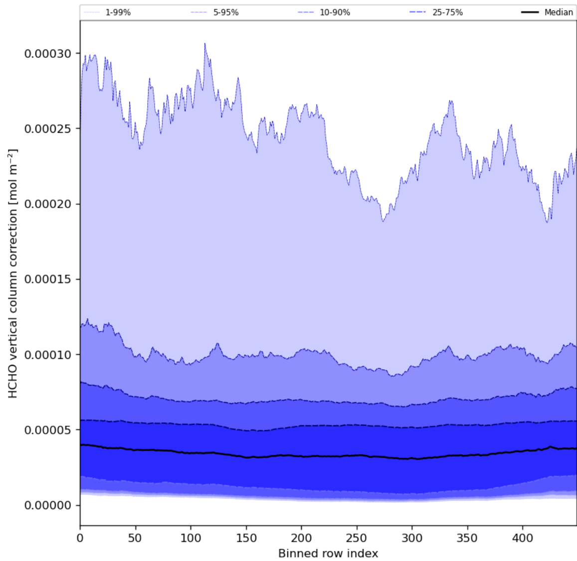
Figure 51: Along track statistics of “HCHO vertical column correction” for 2024-03-28 to 2024-03-30
