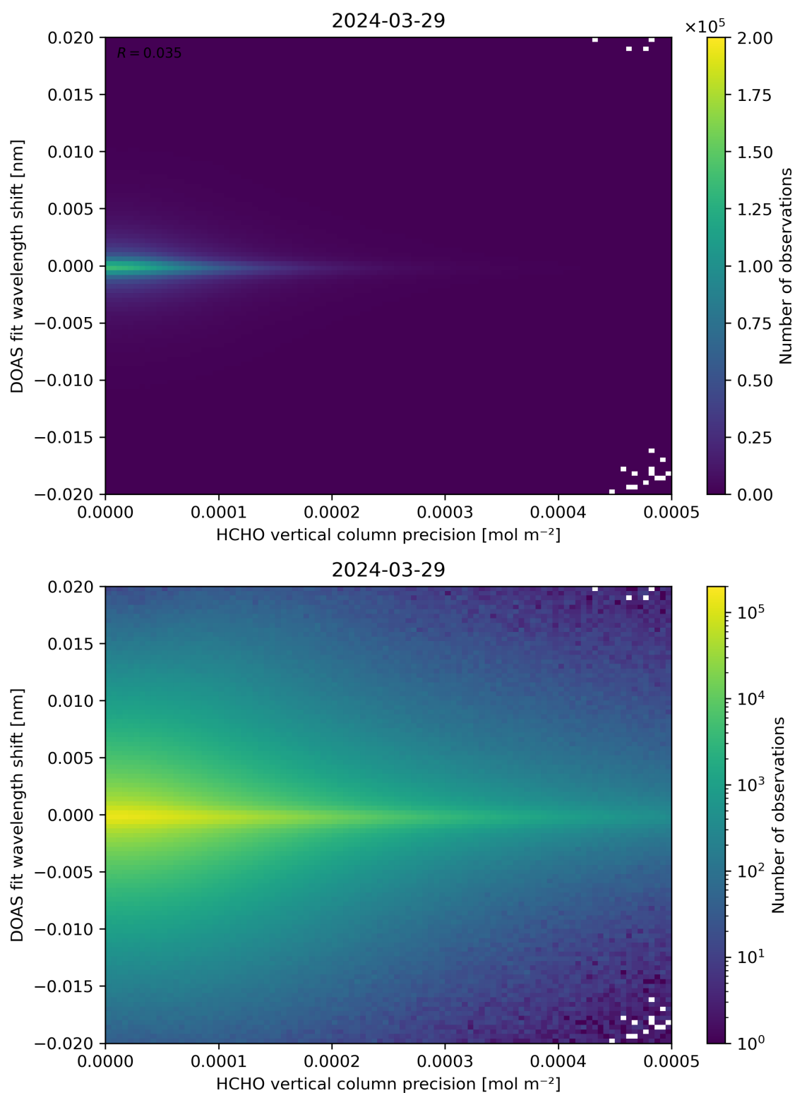
Figure 137: Scatter density plot of “HCHO vertical column precision” against “DOAS fit wavelength shift” for 2024-03-28 to 2024-03-30.
