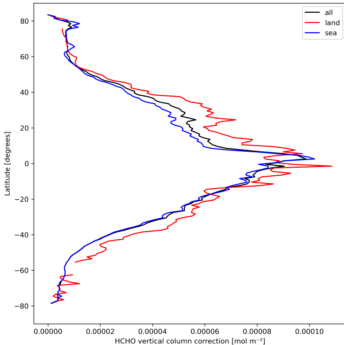
Figure 23: Zonal average of “HCHO vertical column correction” for 2024-03-28 to 2024-03-30.
