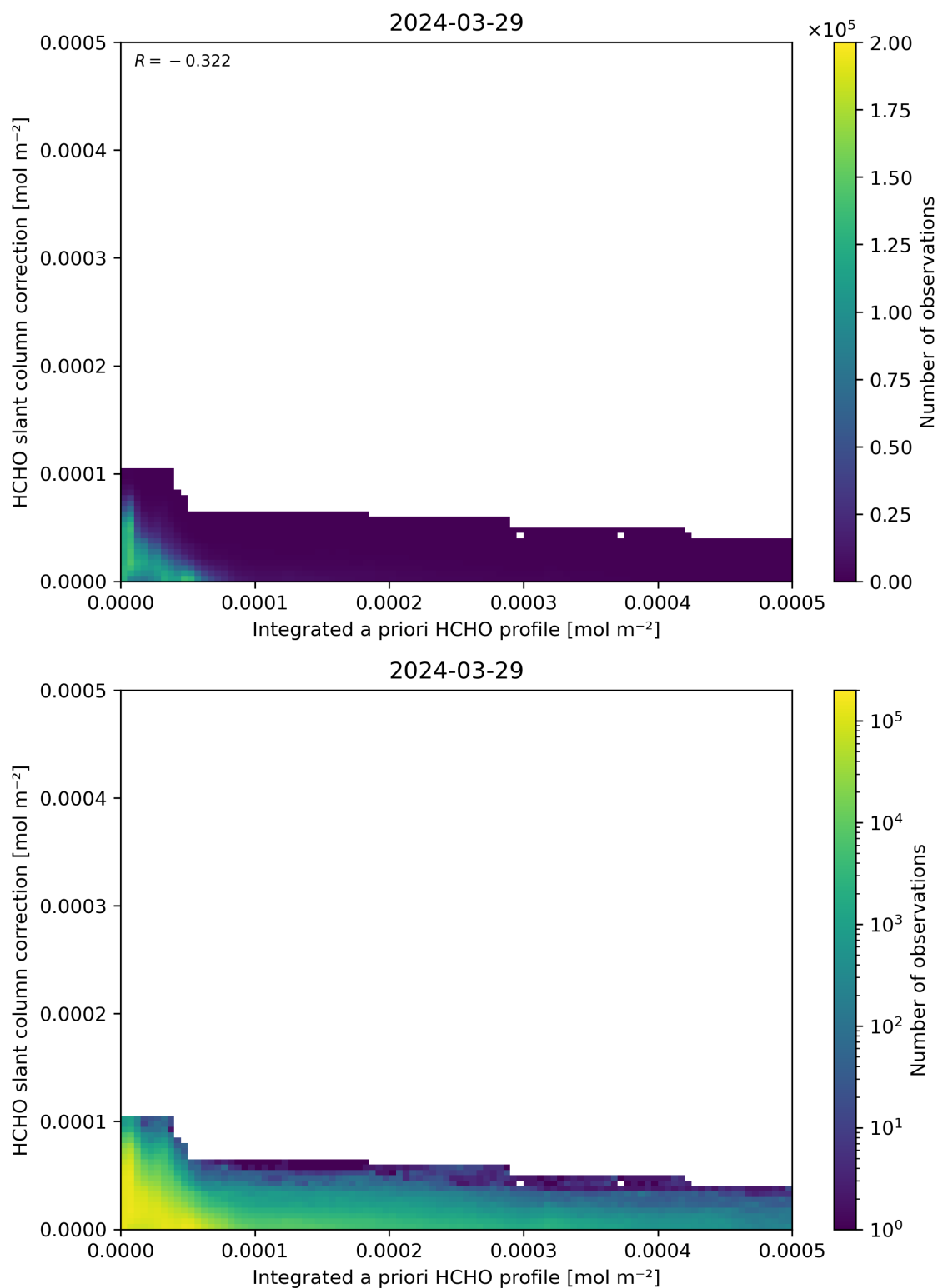
Figure 152: Scatter density plot of “Integrated a priori HCHO profile” against “HCHO slant column correction” for 2024-03-28 to 2024-03-30.
