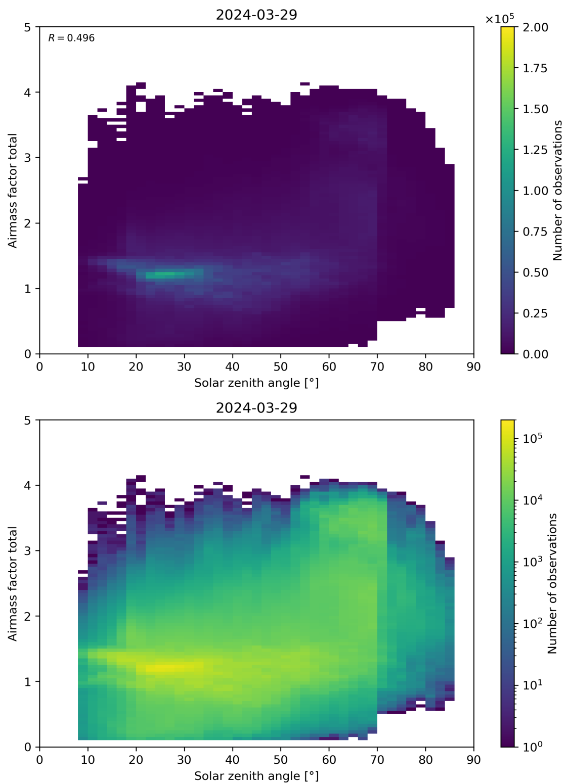
Figure 175: Scatter density plot of “Solar zenith angle” against “Airmass factor total” for 2024-03-28 to 2024-03-30.
