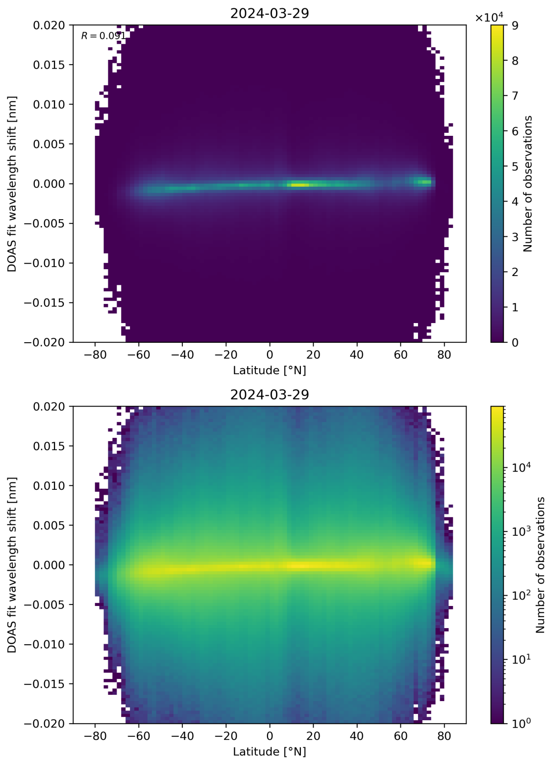
Figure 154: Scatter density plot of “Latitude” against “DOAS fit wavelength shift” for 2024-03-28 to 2024-03-30.
