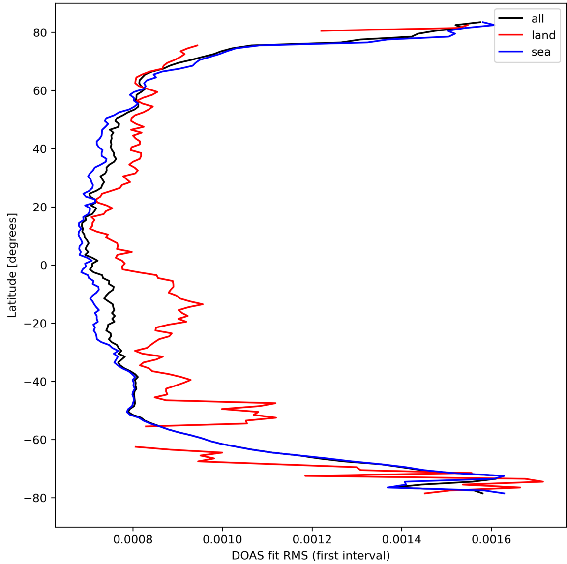
Figure 32: Zonal average of "DOAS fit RMS (first interval)" for 2024-03-28 to 2024-03-30.
