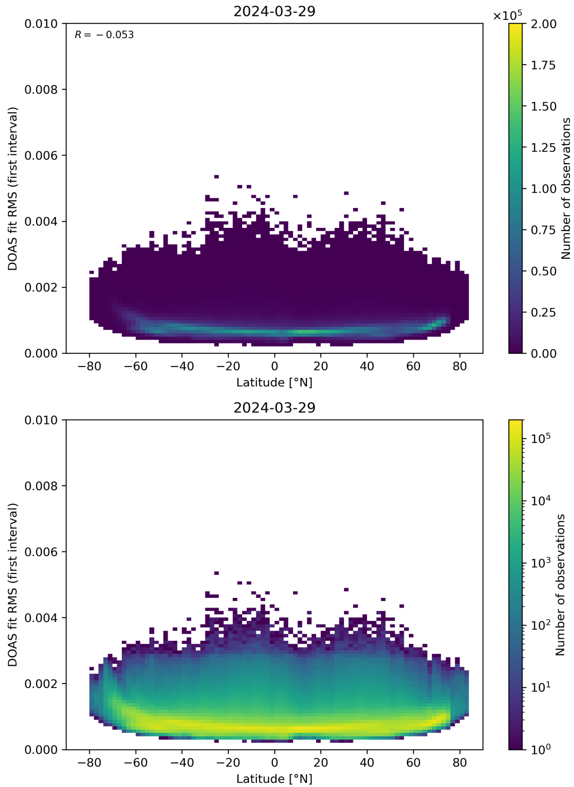
Figure 153: Scatter density plot of “Latitude” against “DOAS fit RMS (first interval)” for 2024-03-28 to 2024-03-30.
