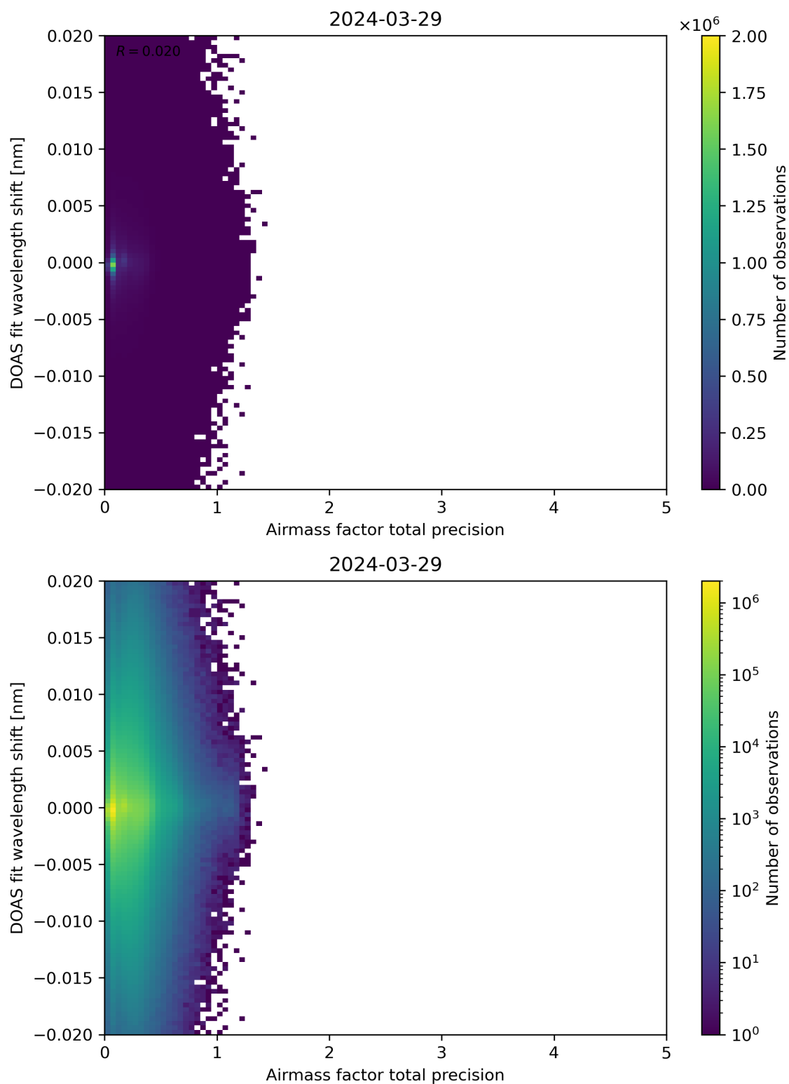
Figure 106: Scatter density plot of “Airmass factor total precision” against “DOAS fit wavelength shift” for 2024-03-28 to 2024-03-30.
