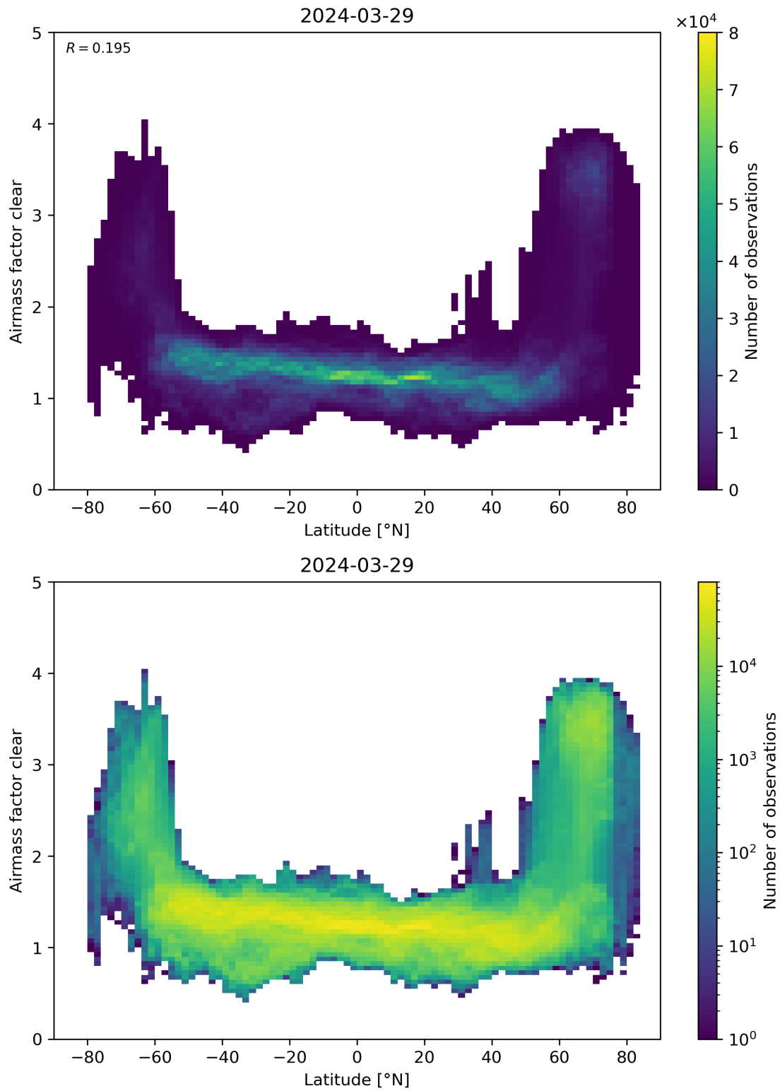
Figure 156: Scatter density plot of “Latitude” against “Airmass factor clear” for 2024-03-28 to 2024-03-30.
