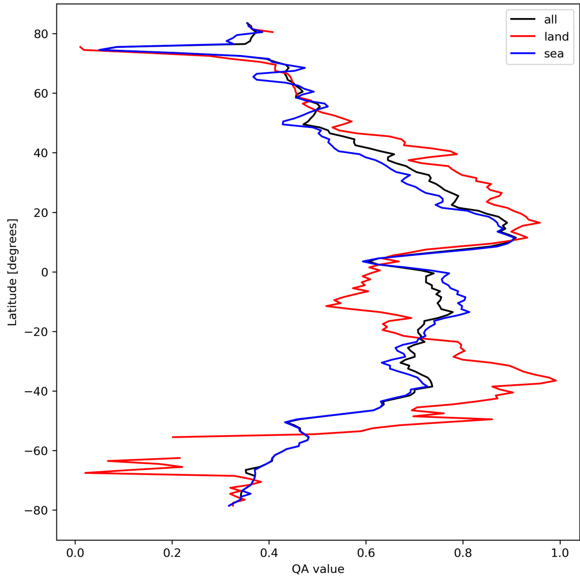
Figure 20: Zonal average of “QA value” for 2024-03-28 to 2024-03-30.
