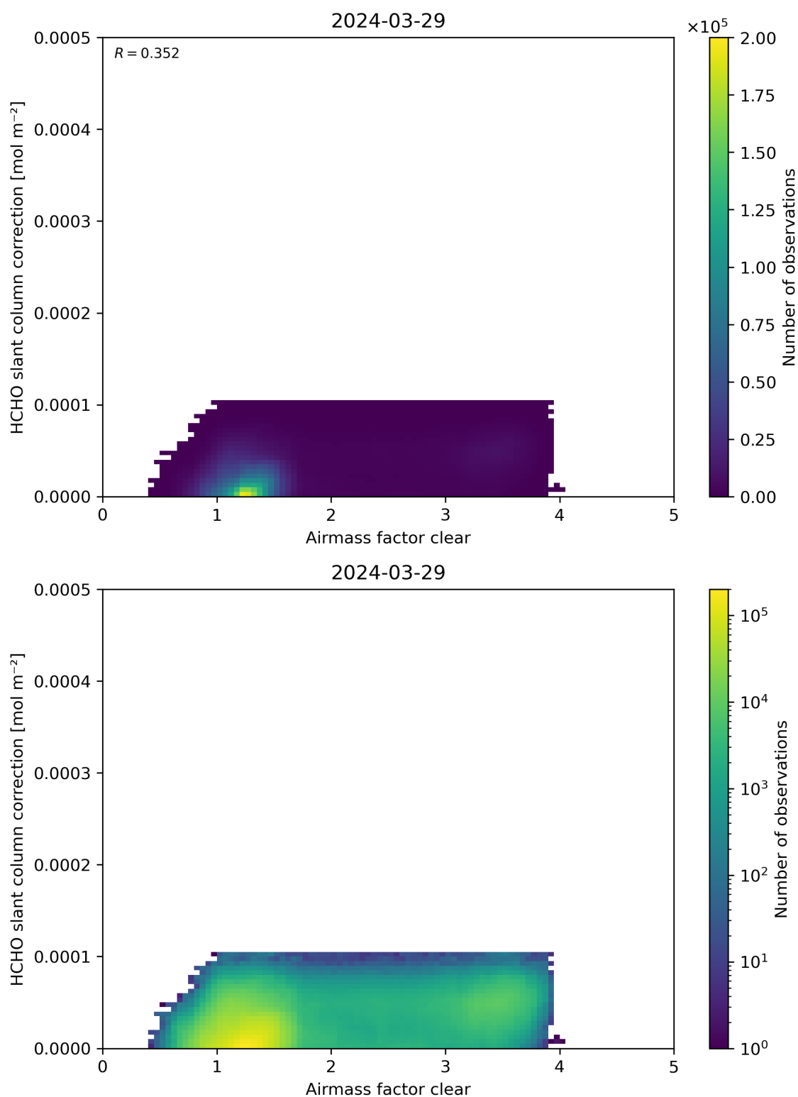
Figure 75: Scatter density plot of “Airmass factor clear” against “HCHO slant column correction” for 2024-03-28 to 2024-03-30.
