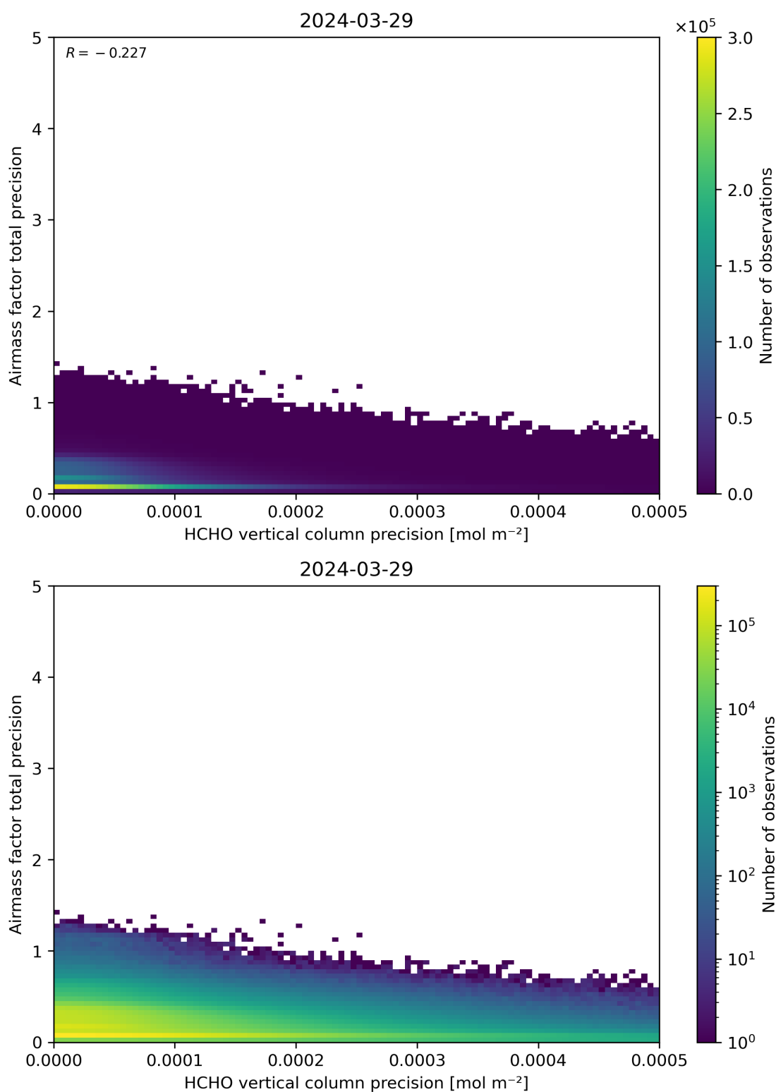
Figure 145: Scatter density plot of “HCHO vertical column precision” against “Airmass factor total precision” for 2024-03-28 to 2024-03-30.
