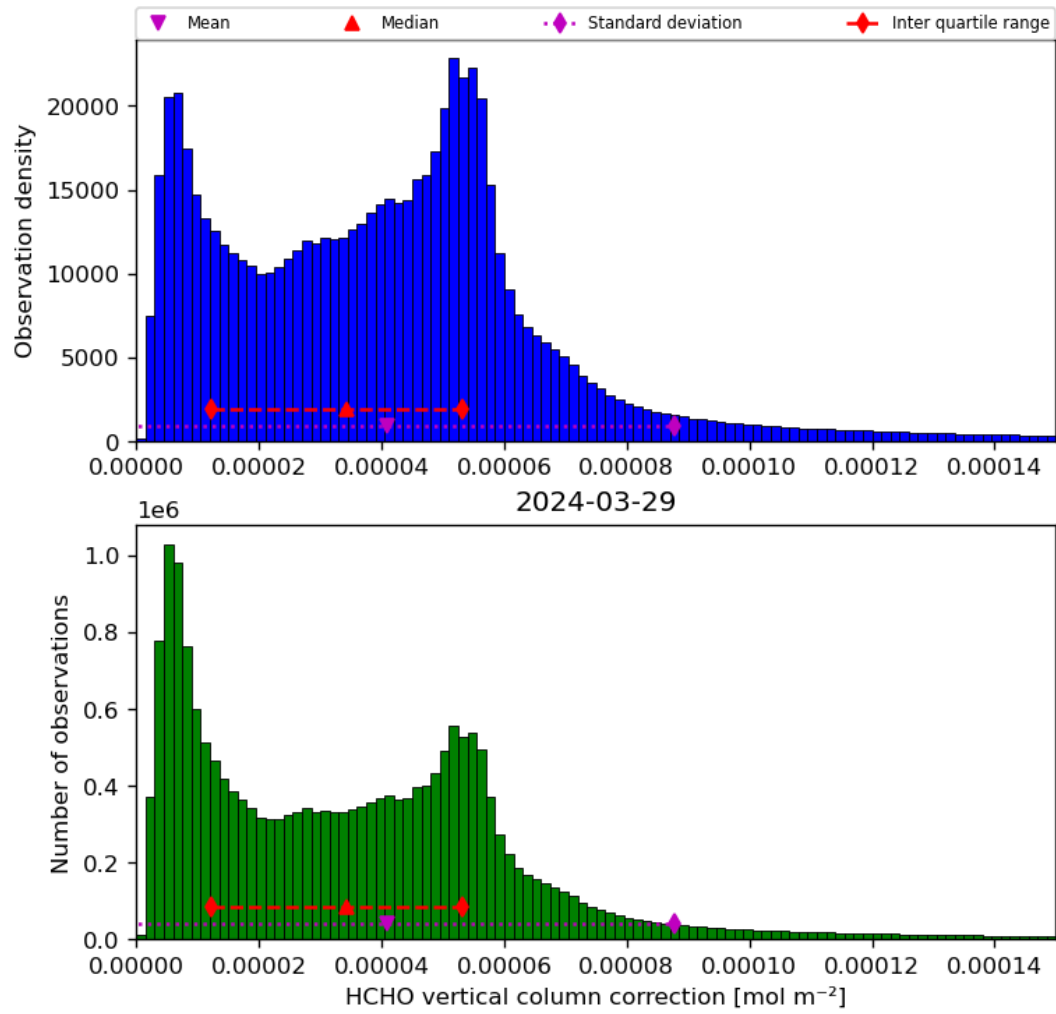
Figure 37: Histogram of “HCHO vertical column correction” for 2024-03-28 to 2024-03-30
