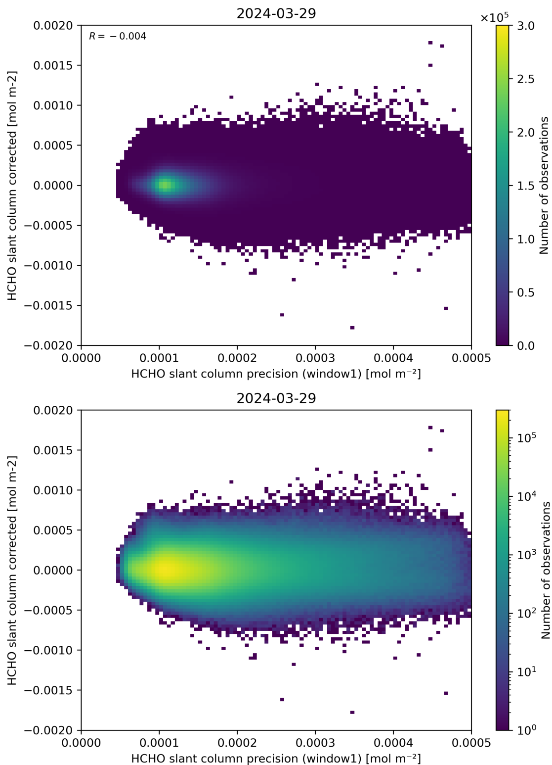
Figure 92: Scatter density plot of “HCHO slant column precision (window1)” against “HCHO slant column corrected” for 2024-03-28 to 2024-03-30.
