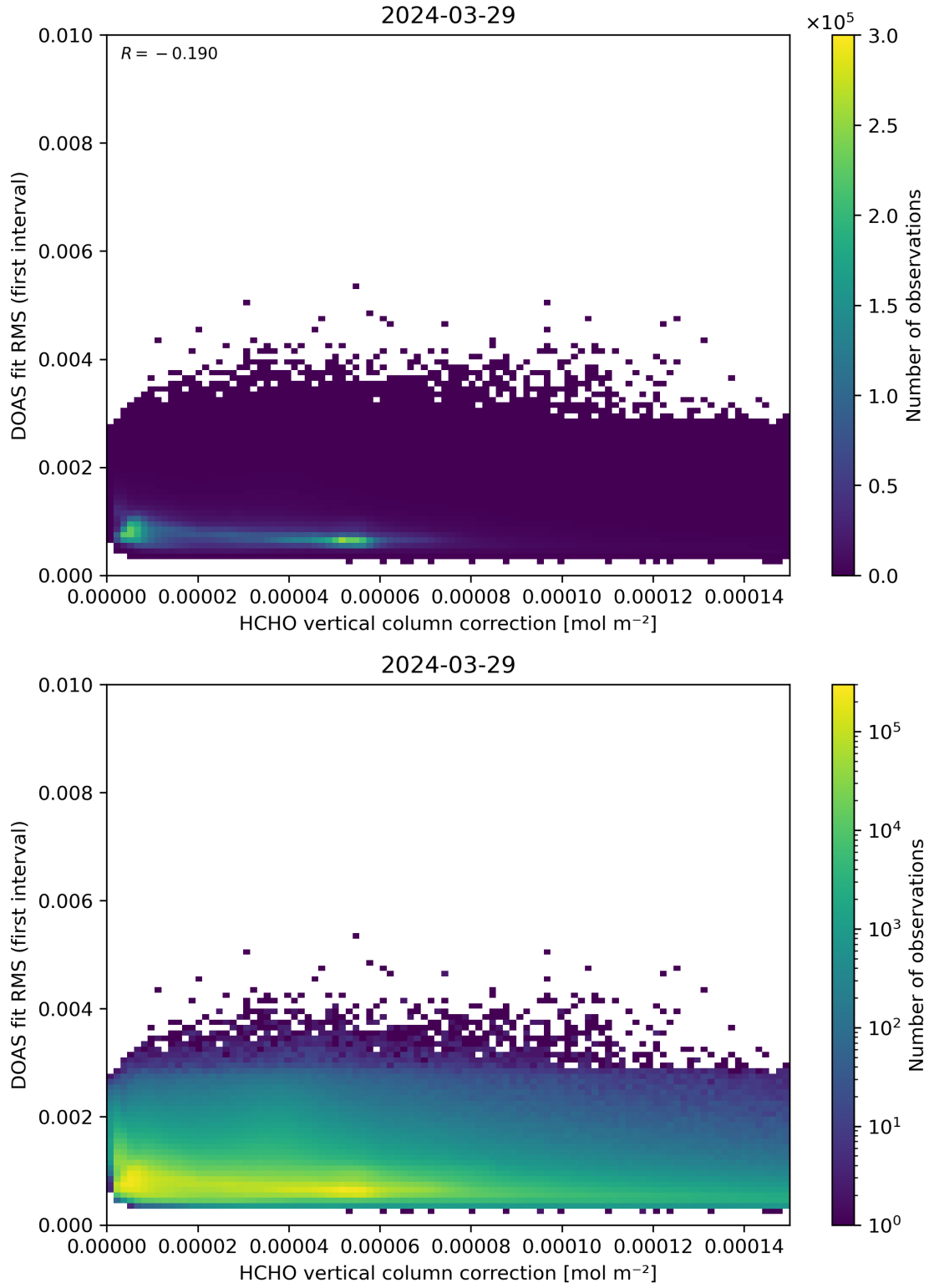
Figure 112: Scatter density plot of “HCHO vertical column correction” against “DOAS fit RMS (first interval)” for 2024-03-28 to 2024-03-30.
