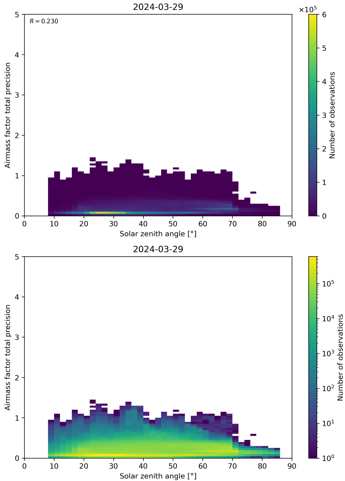
Figure 176: Scatter density plot of “Solar zenith angle” against “Airmass factor total precision” for 2024-03-28 to 2024-03-30.
