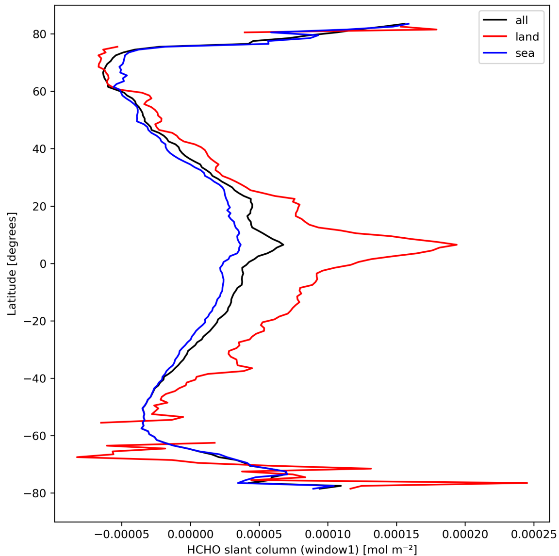
Figure 24: Zonal average of “HCHO slant column (window1)” for 2024-03-28 to 2024-03-30.
