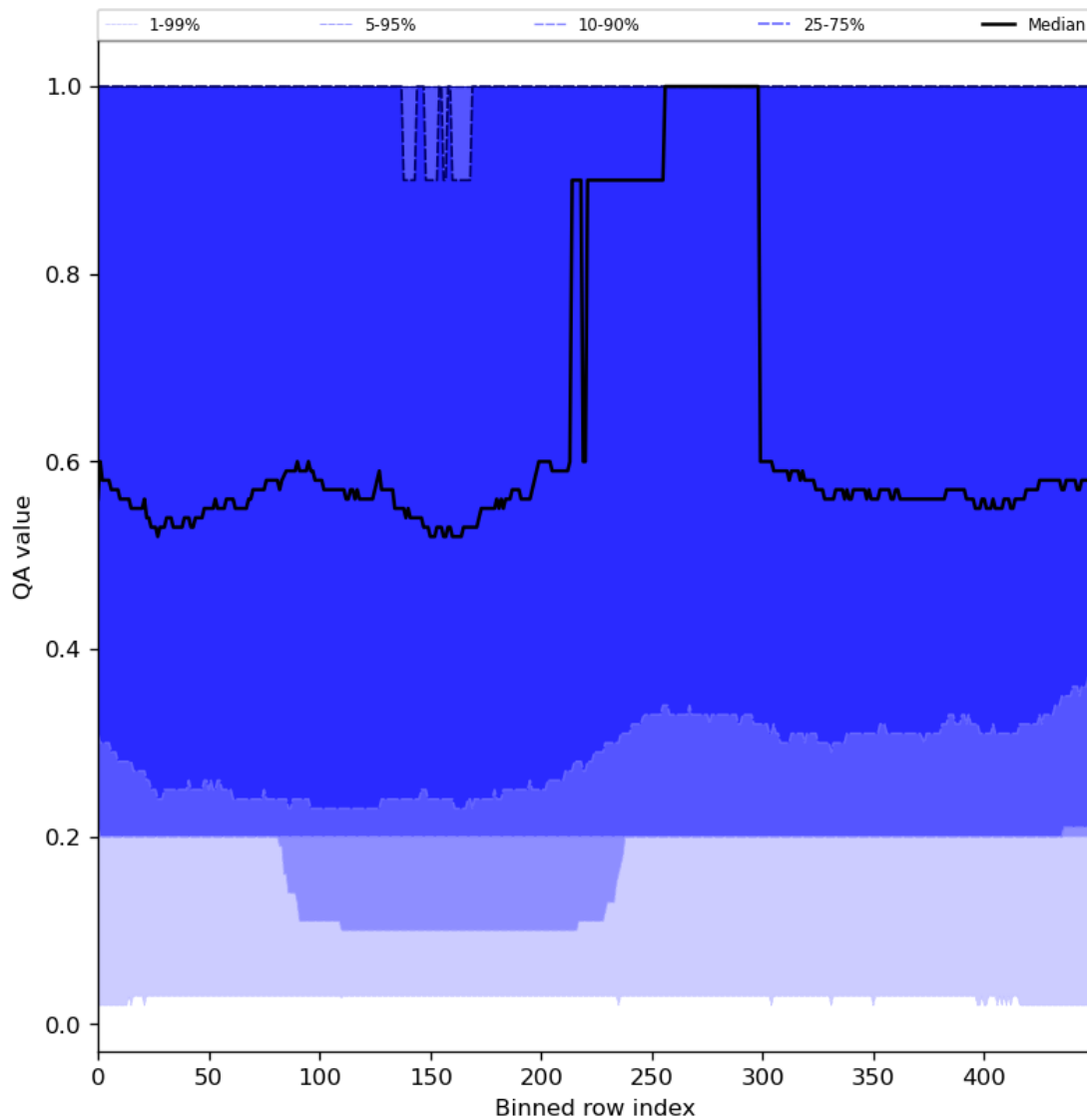
Figure 48: Along track statistics of “QA value” for 2024-03-28 to 2024-03-30
