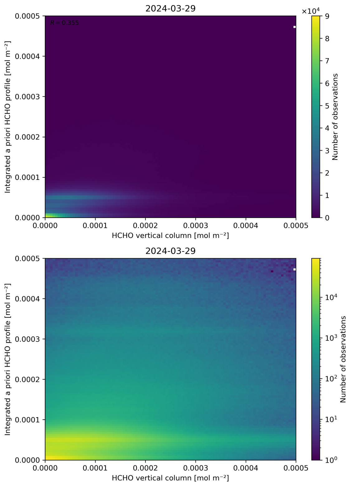
Figure 135: Scatter density plot of “HCHO vertical column” against “Integrated a priori HCHO profile” for 2024-03-28 to 2024-03-30.
