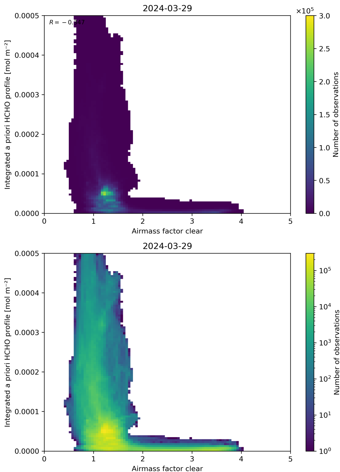
Figure 76: Scatter density plot of “Airmass factor clear” against “Integrated a priori HCHO profile” for 2024-03-28 to 2024-03-30.
