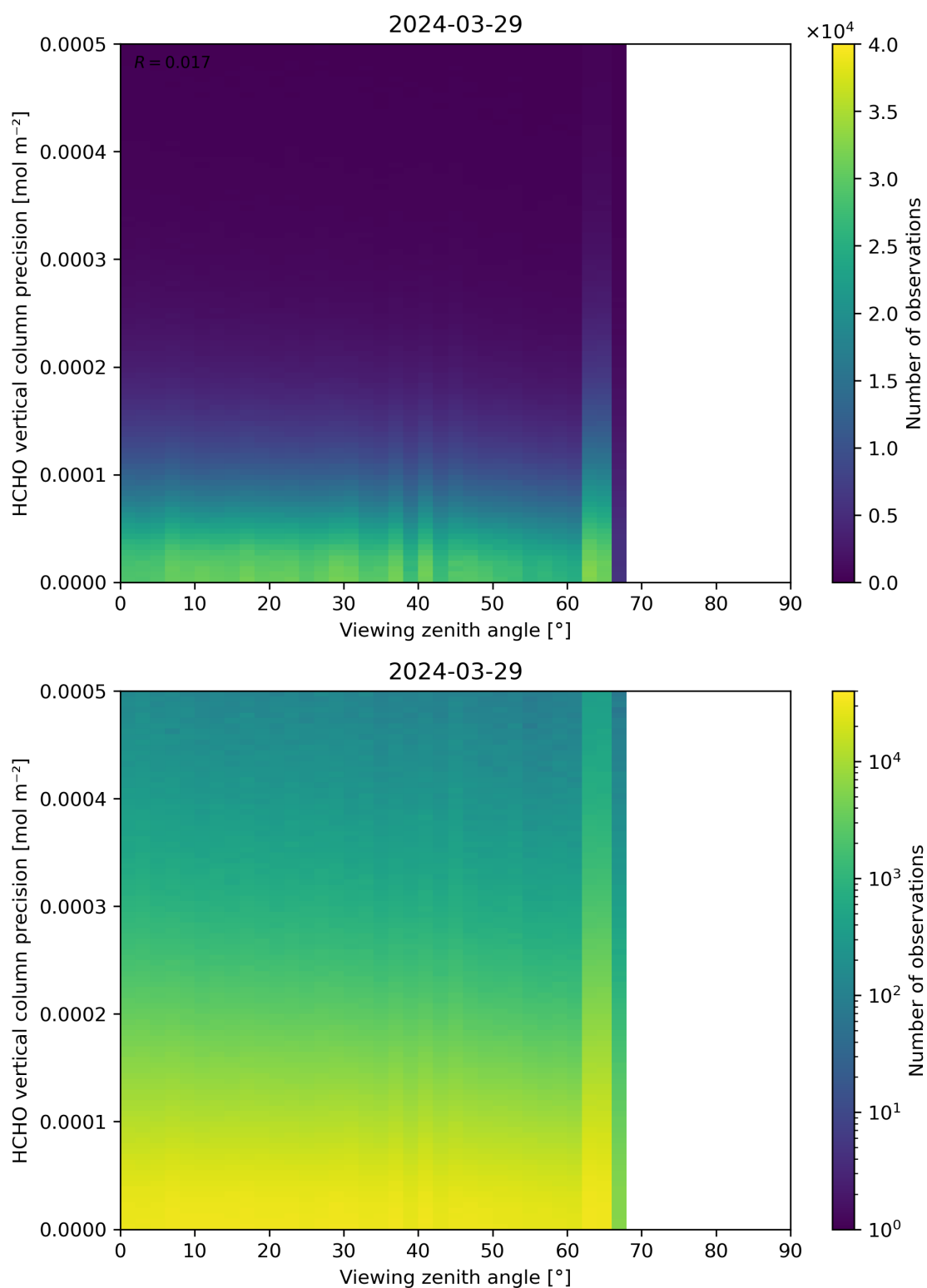
Figure 194: Scatter density plot of “Viewing zenith angle” against “HCHO vertical column precision” for 2024-03-28 to 2024-03-30.
