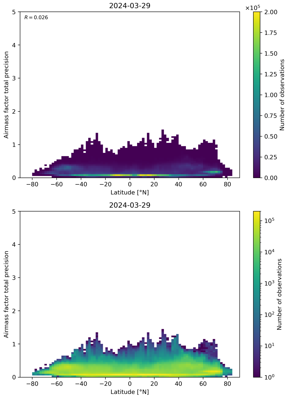
Figure 162: Scatter density plot of “Latitude” against “Airmass factor total precision” for 2024-03-28 to 2024-03-30.
