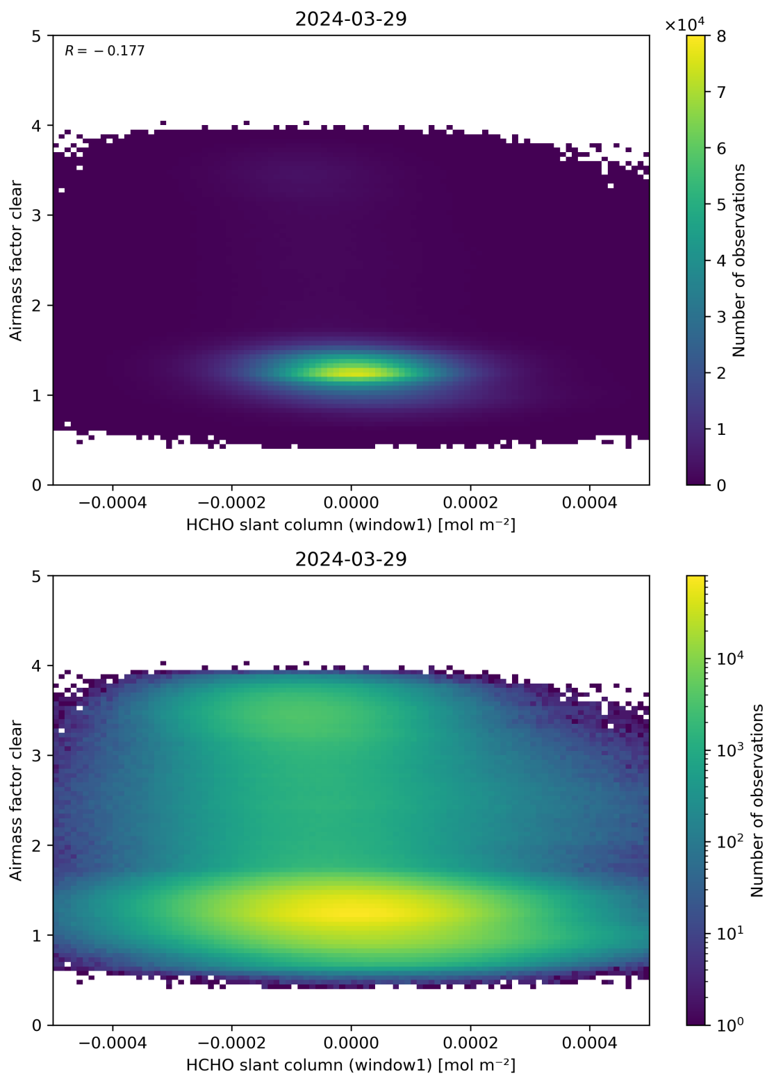
Figure 81: Scatter density plot of “HCHO slant column (window1)” against “Airmass factor clear” for 2024-03-28 to 2024-03-30.
