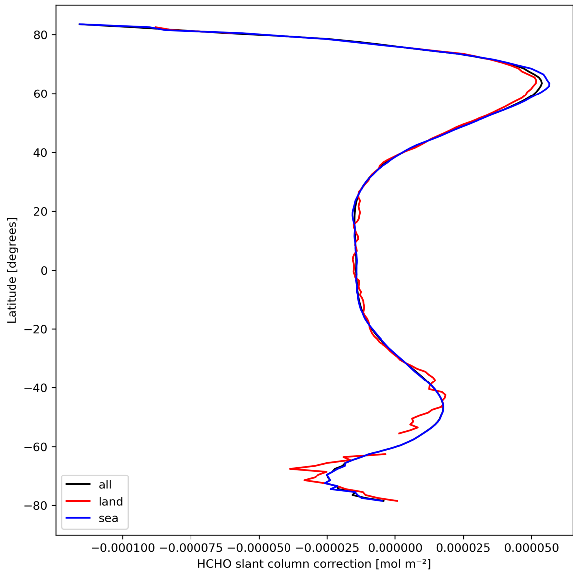
Figure 33: Zonal average of “HCHO slant column correction” for 2024-03-28 to 2024-03-30.
