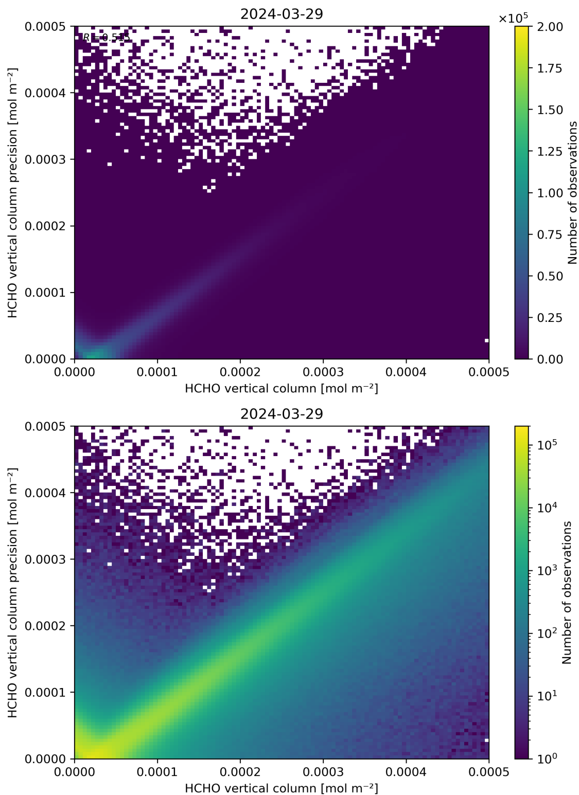
Figure 134: Scatter density plot of “HCHO vertical column” against “HCHO vertical column precision” for 2024-03-28 to 2024-03-30.
