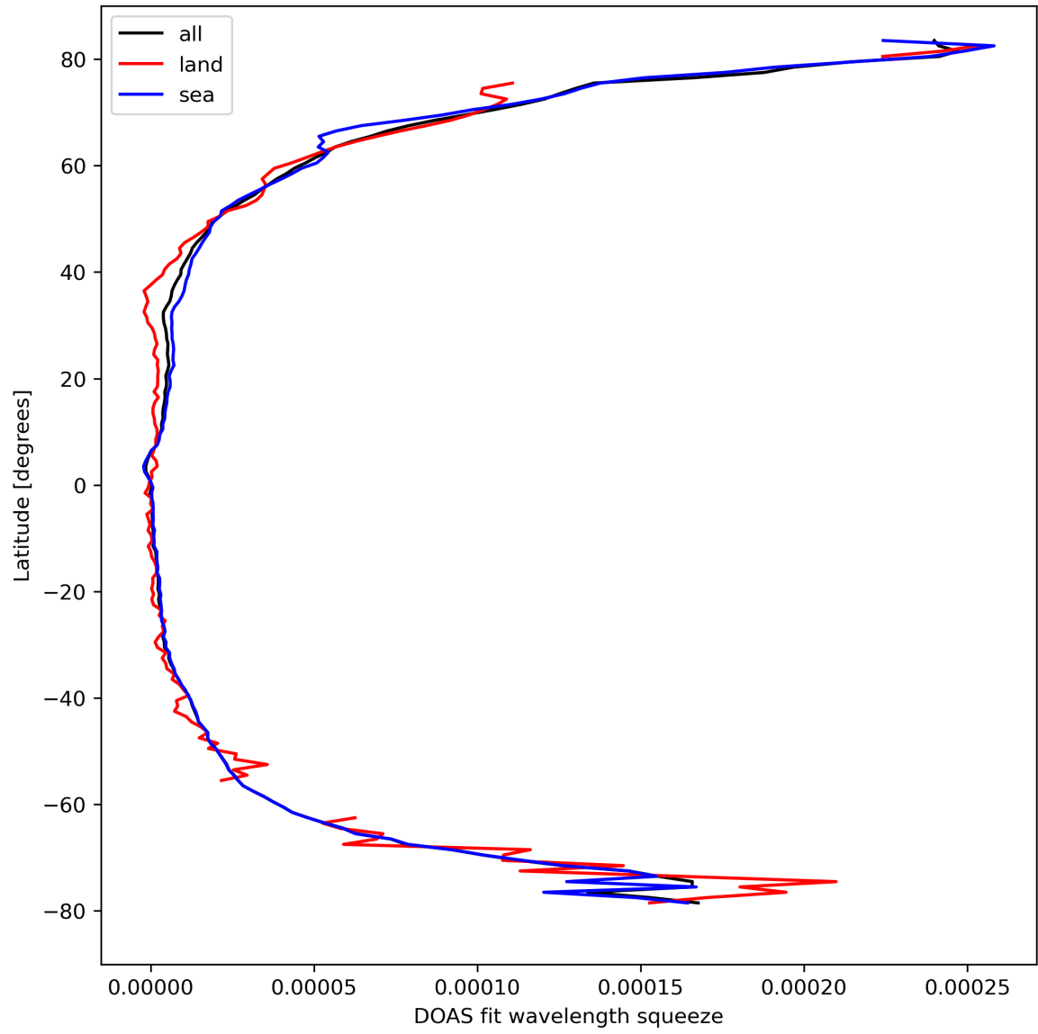
Figure 31: Zonal average of “DOAS fit wavelength squeeze” for 2024-03-28 to 2024-03-30.
