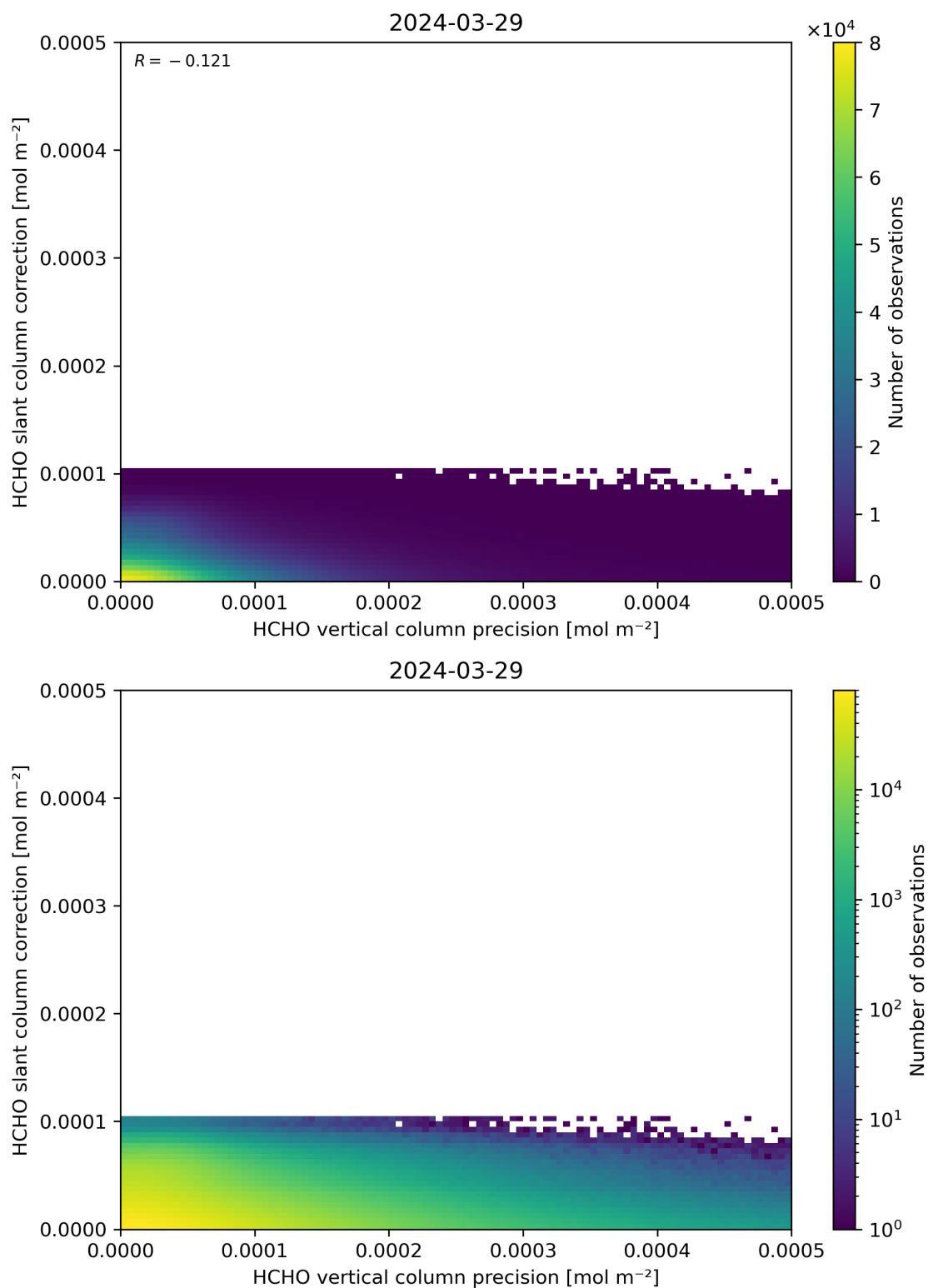
Figure 141: Scatter density plot of “HCHO vertical column precision” against “HCHO slant column correction” for 2024-03-28 to 2024-03-30.
