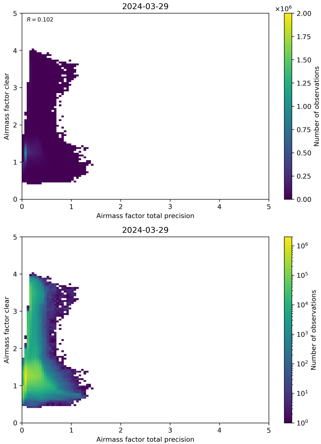
Figure 108: Scatter density plot of “Airmass factor total precision” against “Airmass factor clear” for 2024-03-28 to 2024-03-30.
