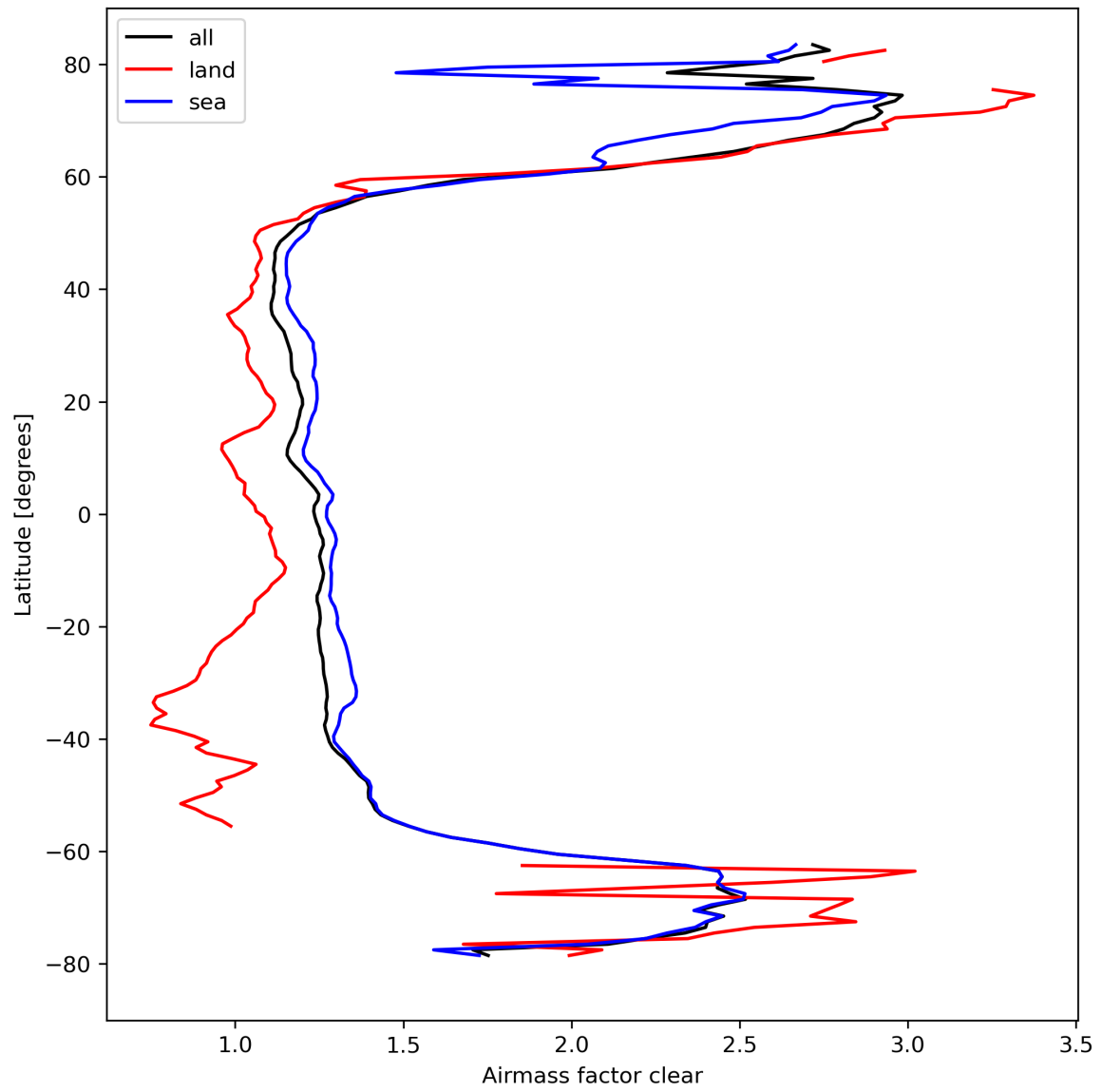
Figure 28: Zonal average of “Airmass factor clear” for 2024-03-28 to 2024-03-30.
