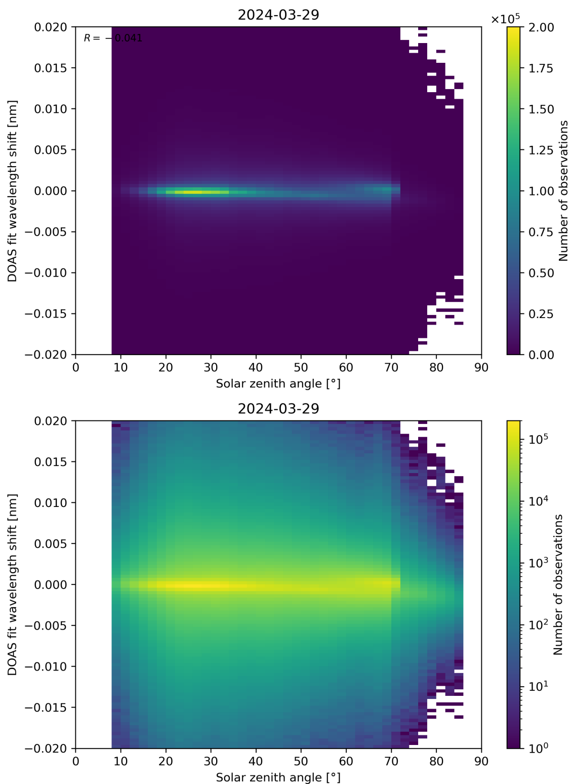
Figure 168: Scatter density plot of “Solar zenith angle” against “DOAS fit wavelength shift” for 2024-03-28 to 2024-03-30.
