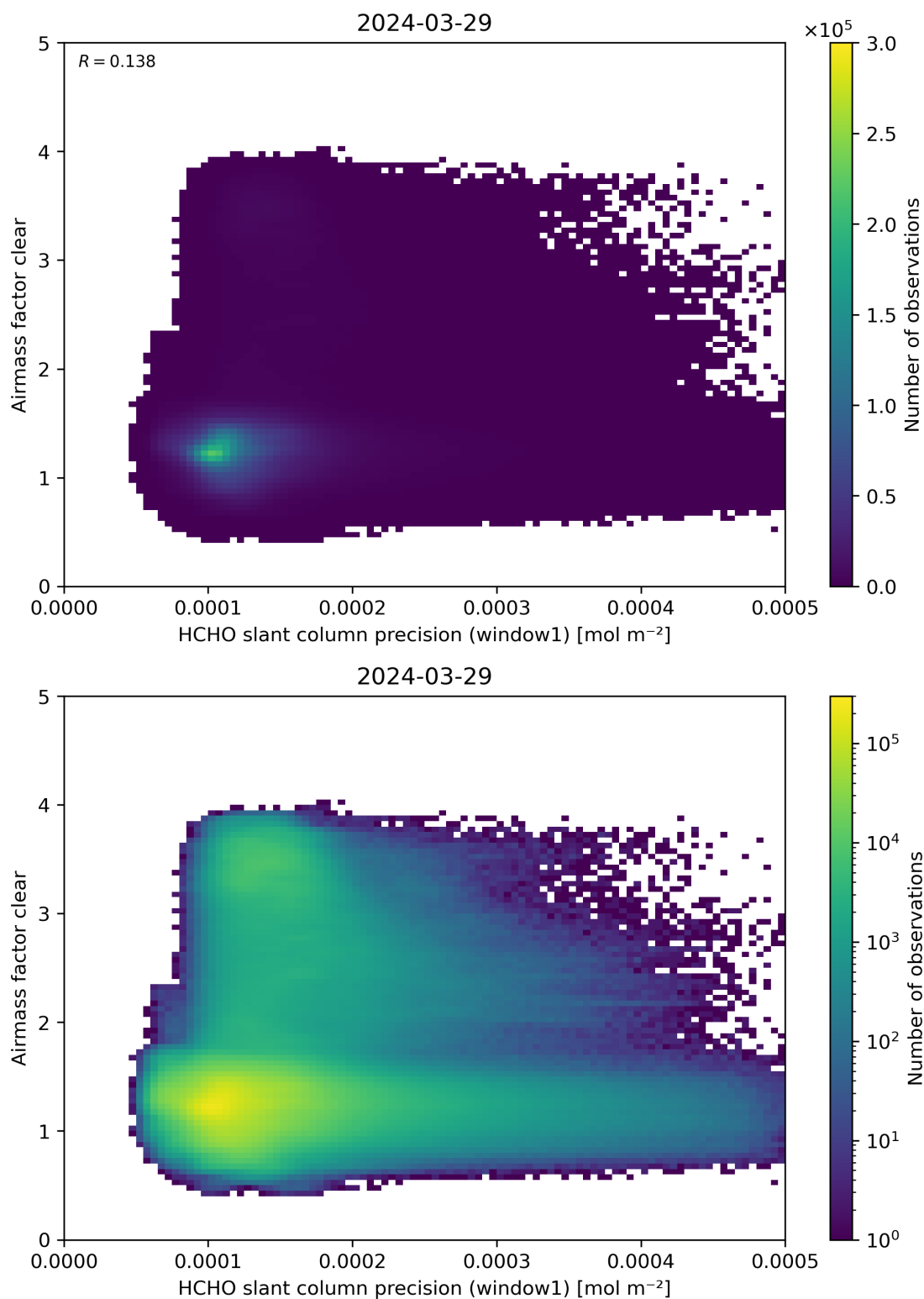
Figure 91: Scatter density plot of “HCHO slant column precision (window1)” against “Airmass factor clear” for 2024-03-28 to 2024-03-30.
