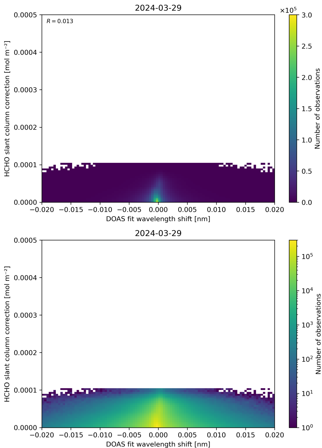
Figure 67: Scatter density plot of “DOAS fit wavelength shift” against “HCHO slant column correction” for 2024-03-28 to 2024-03-30.
