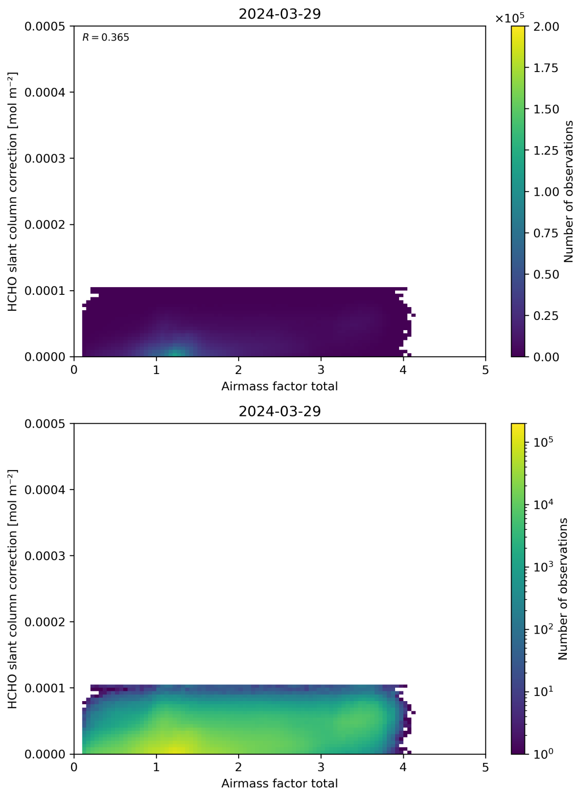
Figure 102: Scatter density plot of “Airmass factor total” against “HCHO slant column correction” for 2024-03-28 to 2024-03-30.
