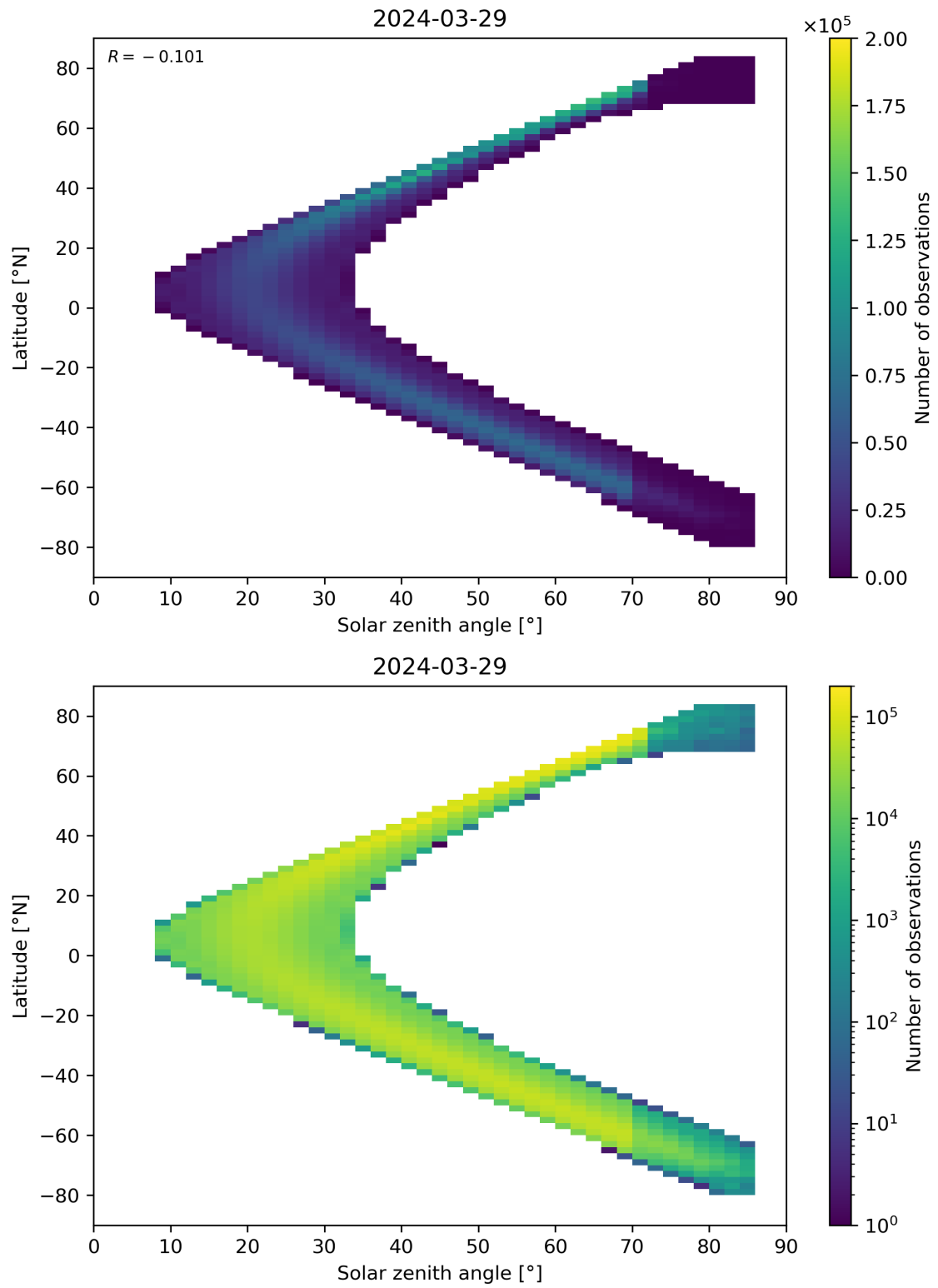
Figure 181: Scatter density plot of “Solar zenith angle” against “Latitude” for 2024-03-28 to 2024-03-30.
