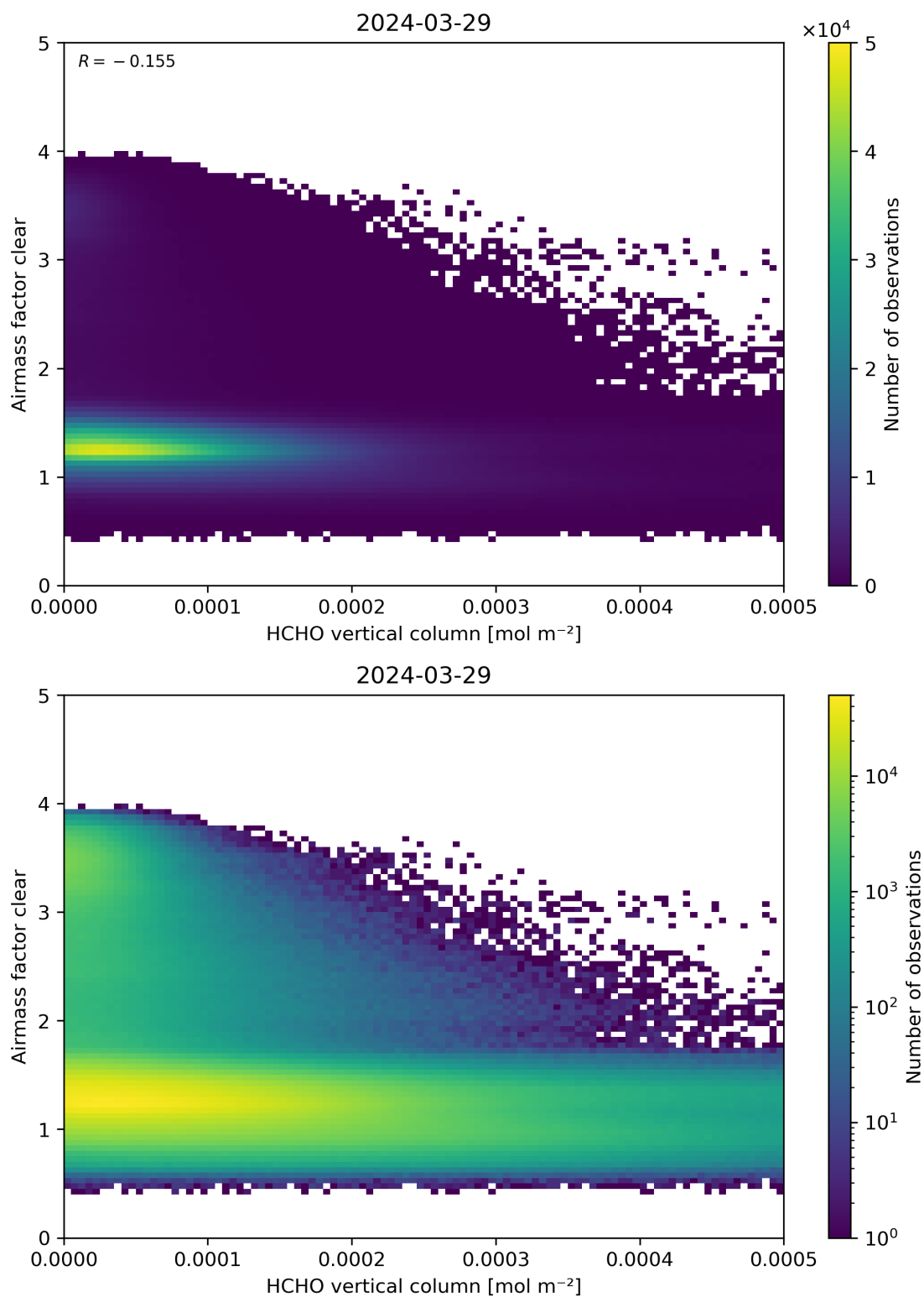
Figure 126: Scatter density plot of “HCHO vertical column” against “Airmass factor clear” for 2024-03-28 to 2024-03-30.
