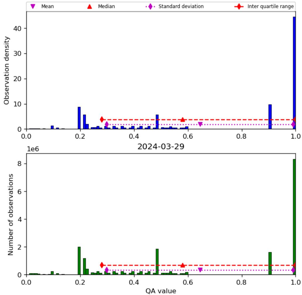
Figure 34: Histogram of “QA value” for 2024-03-28 to 2024-03-30
