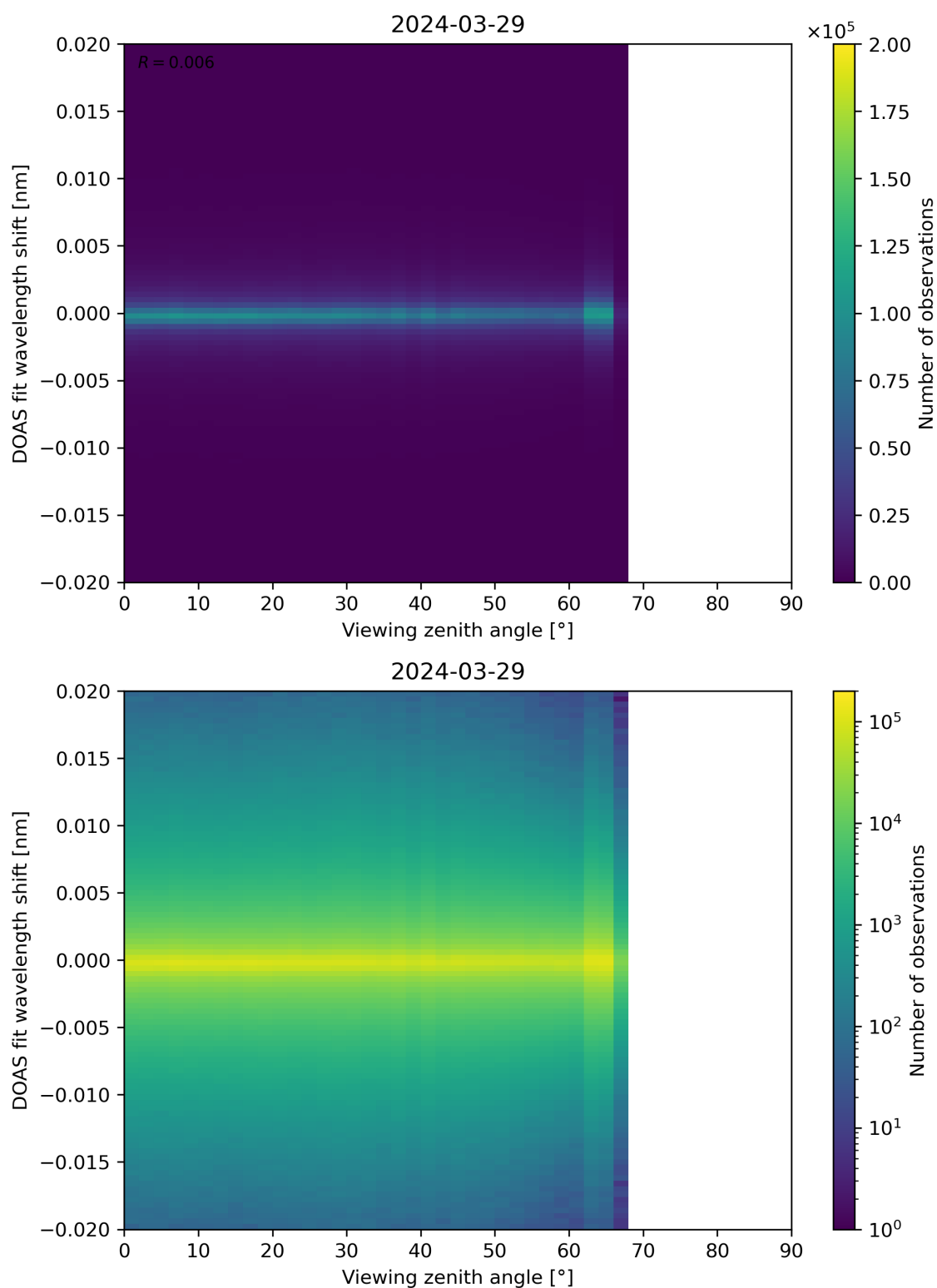
Figure 183: Scatter density plot of “Viewing zenith angle” against “DOAS fit wavelength shift” for 2024-03-28 to 2024-03-30.
