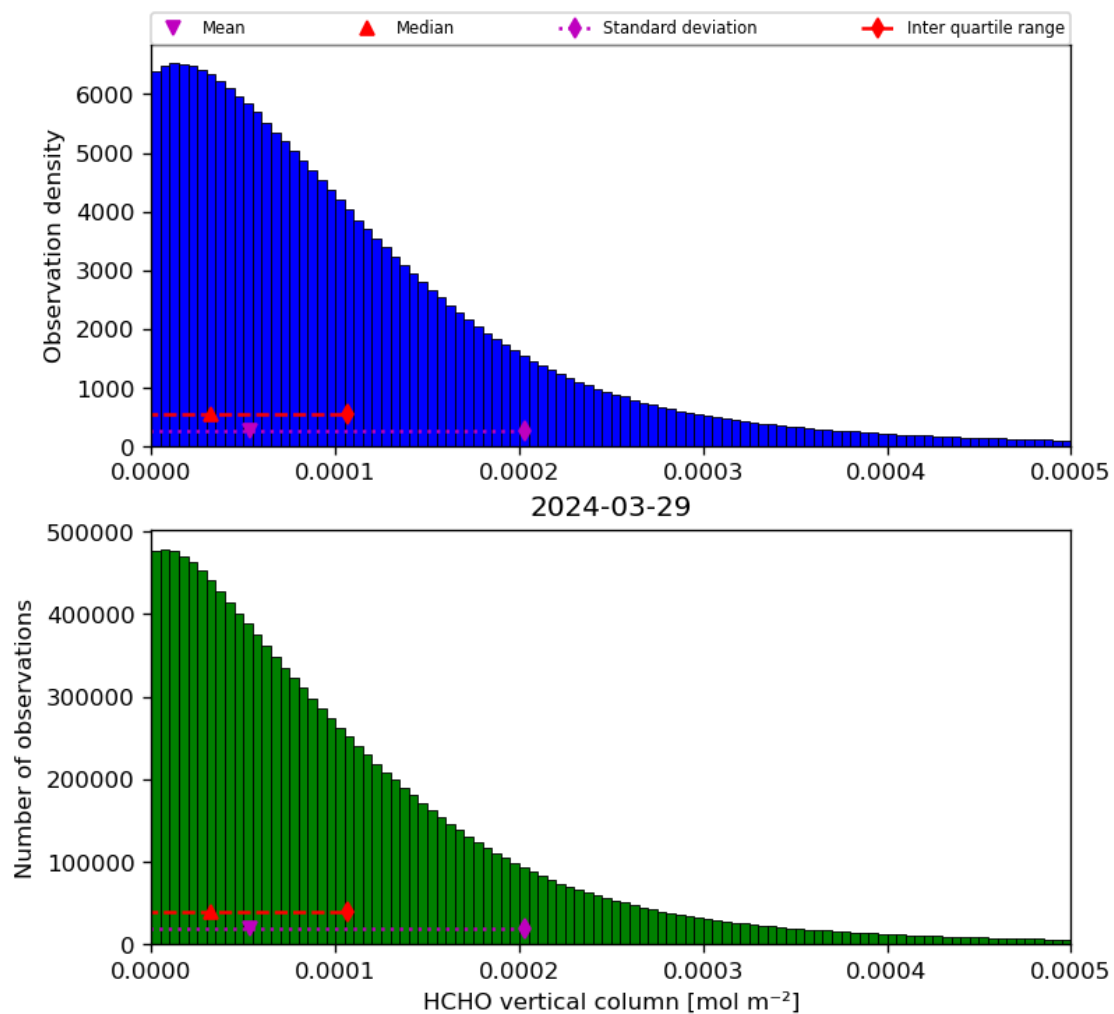
Figure 35: Histogram of “HCHO vertical column” for 2024-03-28 to 2024-03-30
