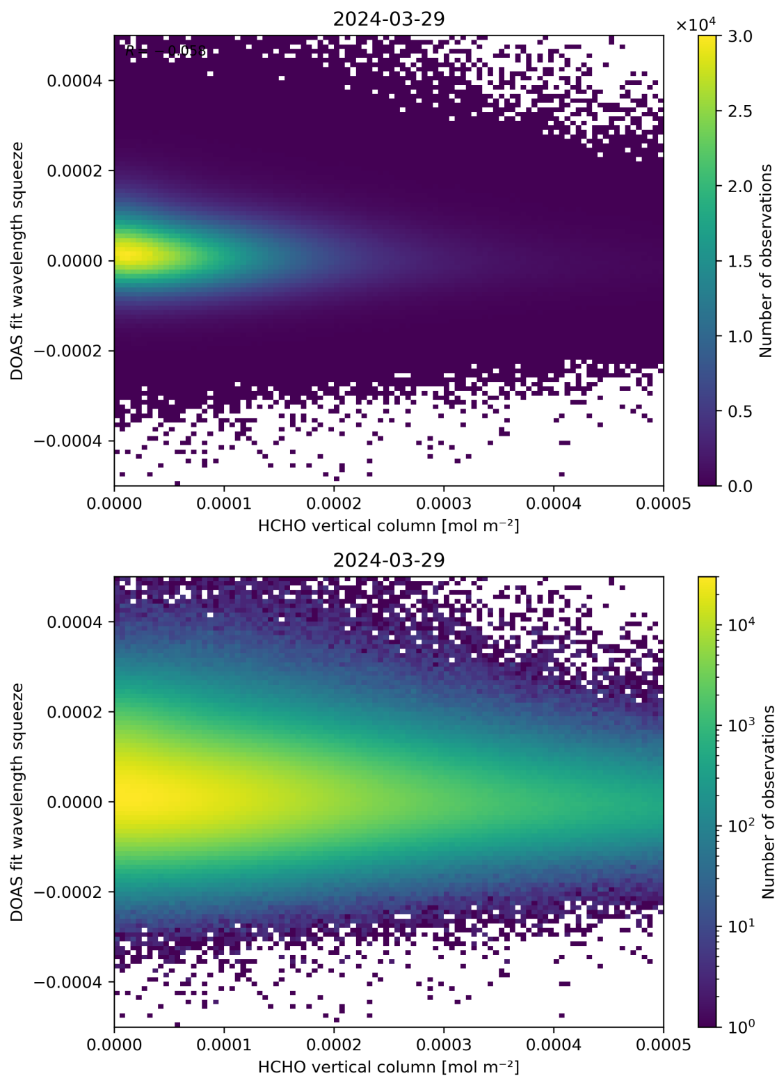
Figure 125: Scatter density plot of “HCHO vertical column” against “DOAS fit wavelength squeeze” for 2024-03-28 to 2024-03-30.
