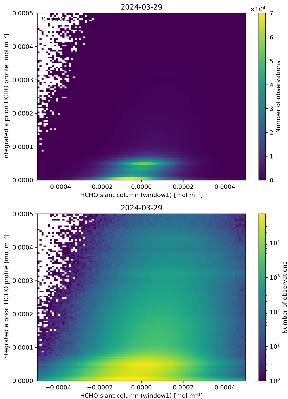
Figure 87: Scatter density plot of “HCHO slant column (window1)” against “Integrated a priori HCHO profile” for 2024-03-28 to 2024-03-30.
