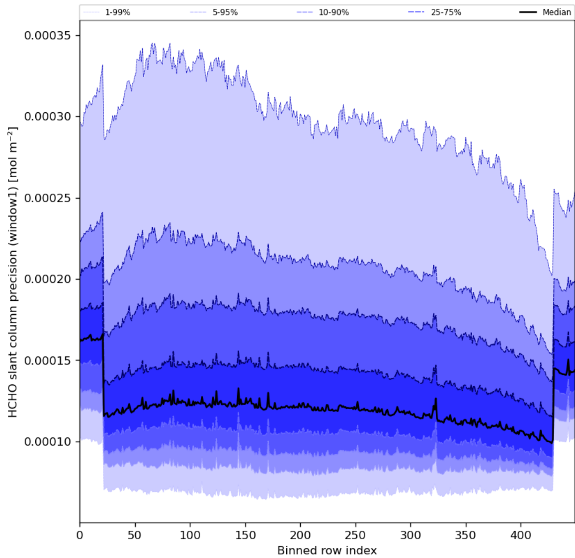
Figure 53: Along track statistics of “HCHO slant column precision (window1)” for 2024-03-28 to 2024-03-30
