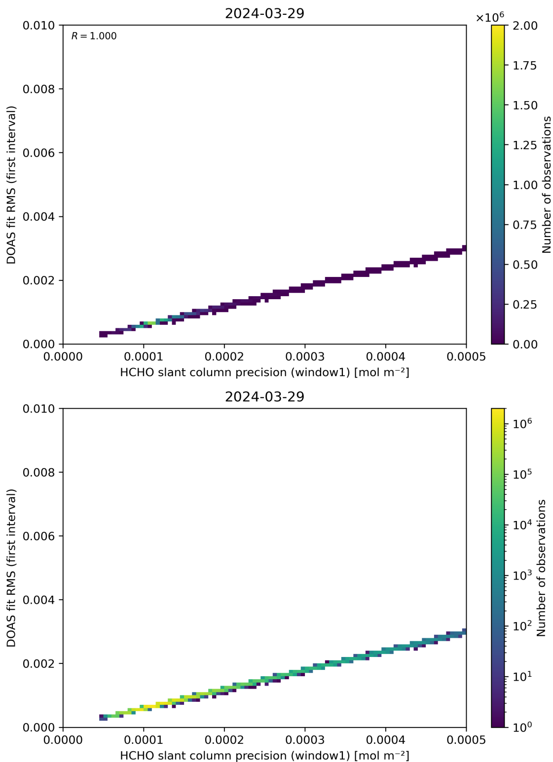
Figure 88: Scatter density plot of “HCHO slant column precision (window1)” against “DOAS fit RMS (first interval)” for 2024-03-28 to 2024-03-30.
