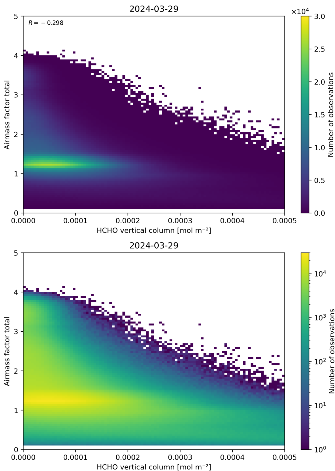
Figure 131: Scatter density plot of “HCHO vertical column” against “Airmass factor total” for 2024-03-28 to 2024-03-30.
