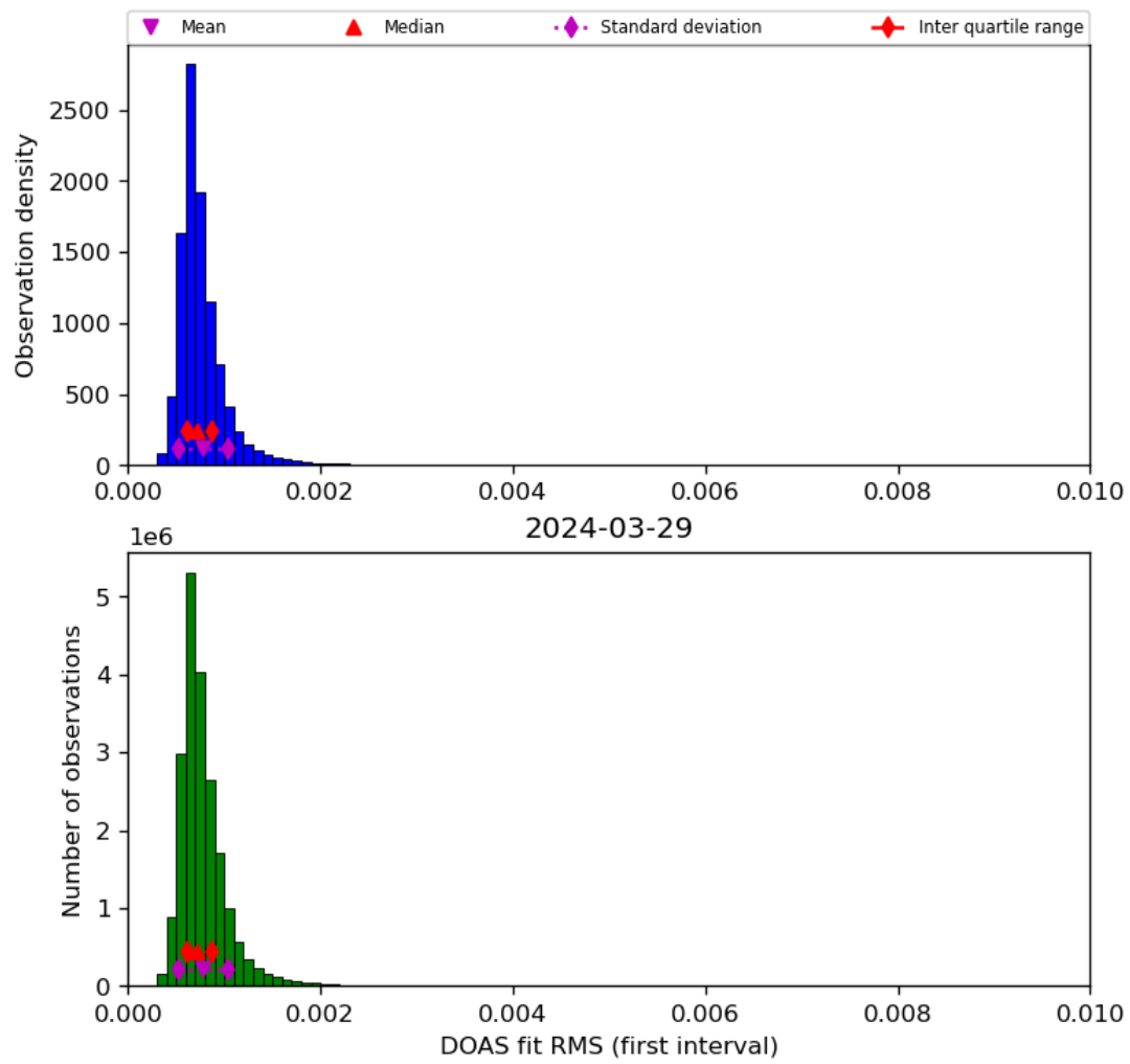
Figure 46: Histogram of “DOAS fit RMS (first interval)” for 2024-03-28 to 2024-03-30
