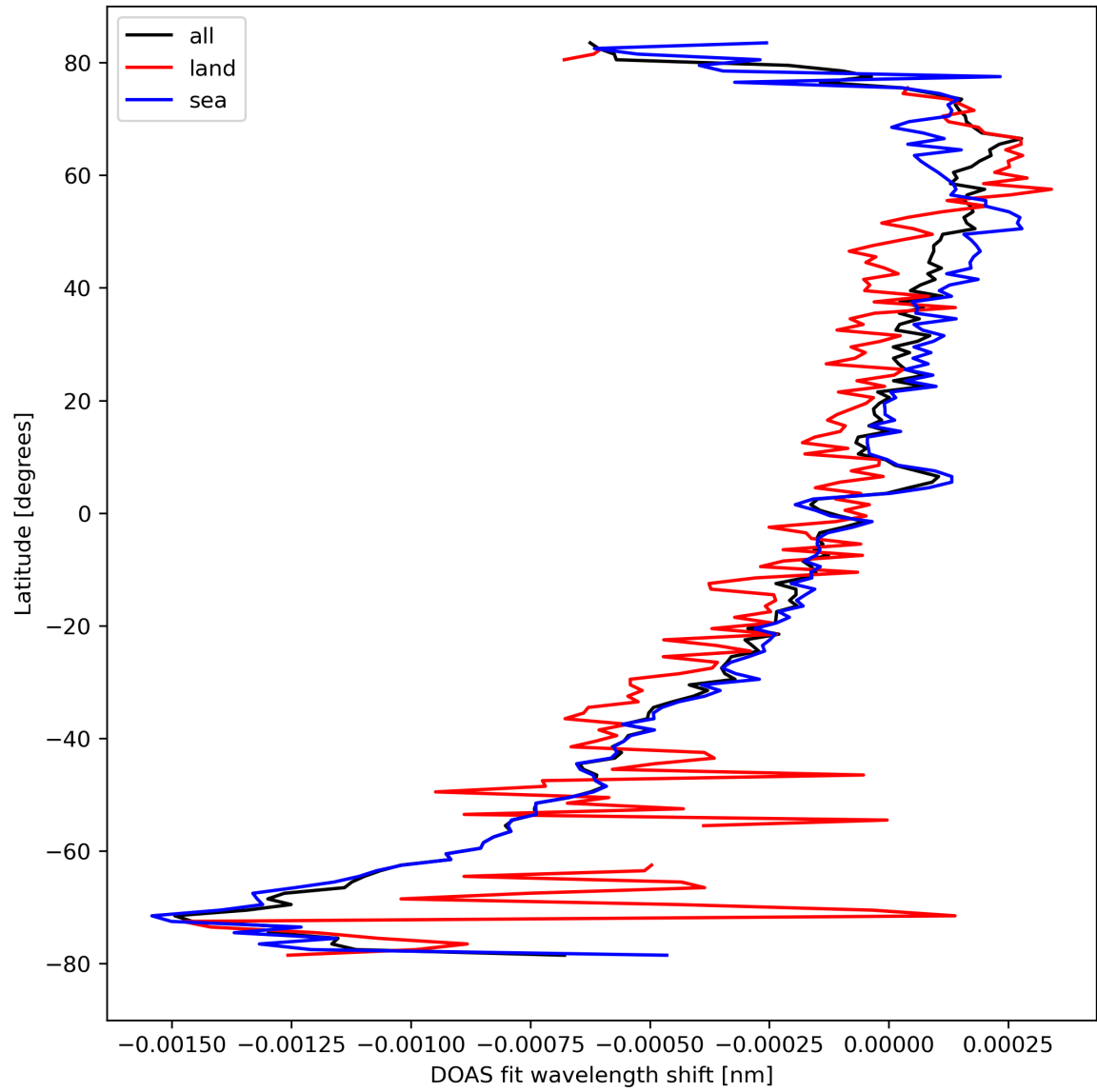
Figure 30: Zonal average of “DOAS fit wavelength shift” for 2024-03-28 to 2024-03-30.
