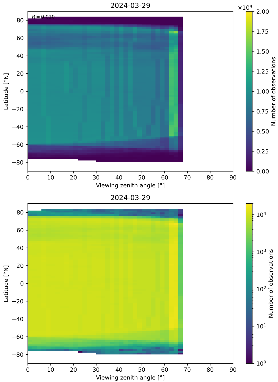
Figure 196: Scatter density plot of “Viewing zenith angle” against “Latitude” for 2024-03-28 to 2024-03-30.
