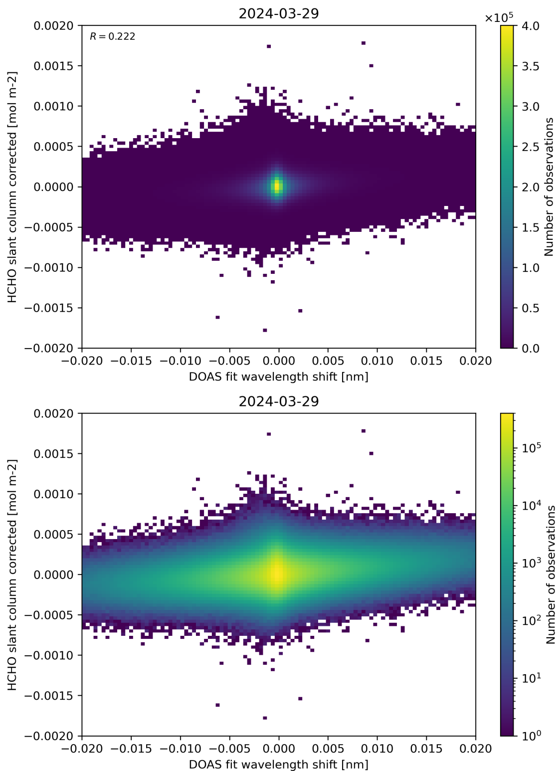
Figure 66: Scatter density plot of “DOAS fit wavelength shift” against “HCHO slant column corrected” for 2024-03-28 to 2024-03-30.
