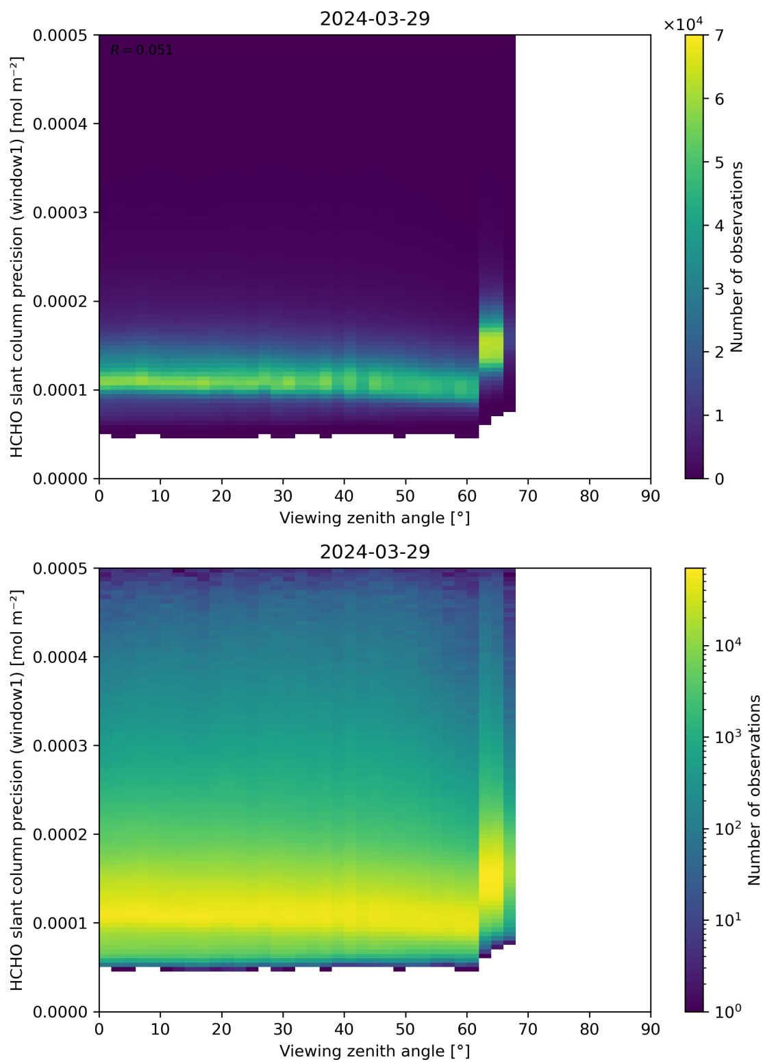
Figure 189: Scatter density plot of “Viewing zenith angle” against “HCHO slant column precision (window1)” for 2024-03-28 to 2024-03-30.
