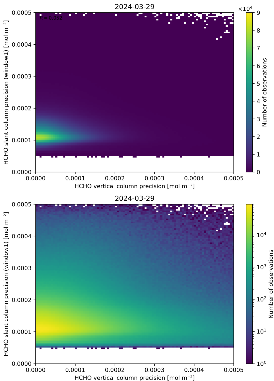
Figure 143: Scatter density plot of “HCHO vertical column precision” against “HCHO slant column precision (window1)” for 2024-03-28 to 2024-03-30.
