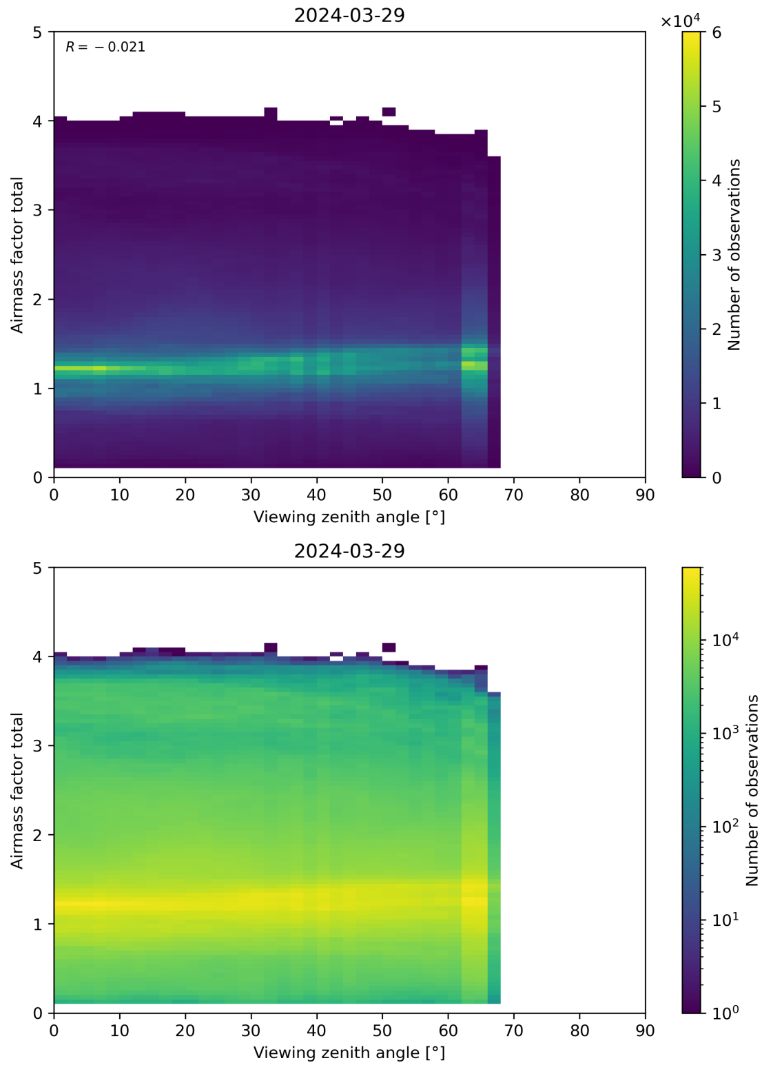
Figure 190: Scatter density plot of “Viewing zenith angle” against “Airmass factor total” for 2024-03-28 to 2024-03-30.
