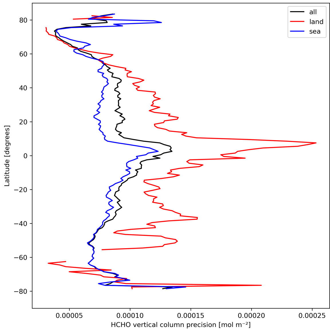
Figure 22: Zonal average of “HCHO vertical column precision” for 2024-03-28 to 2024-03-30.
