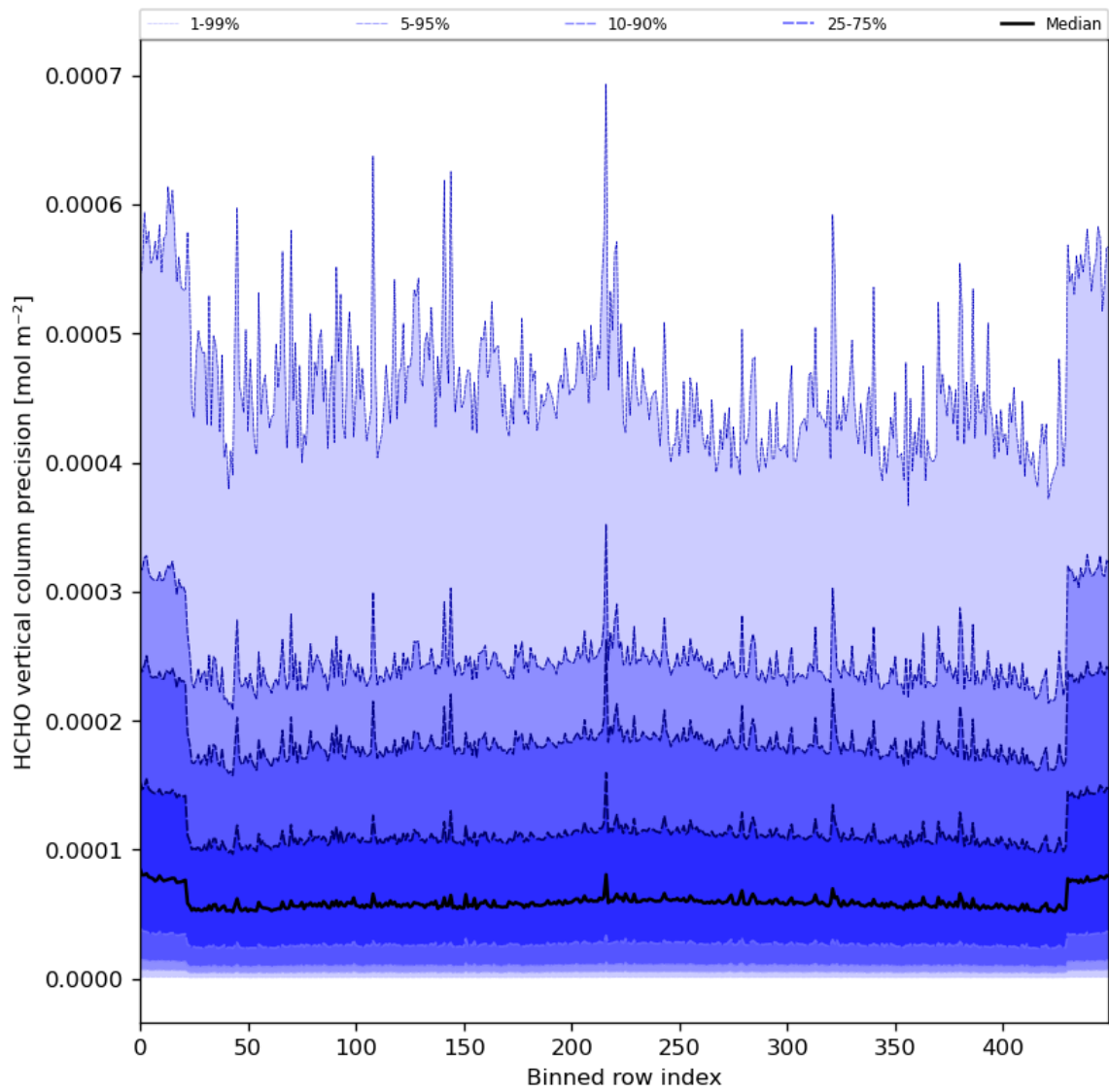
Figure 50: Along track statistics of “HCHO vertical column precision” for 2024-03-28 to 2024-03-30
