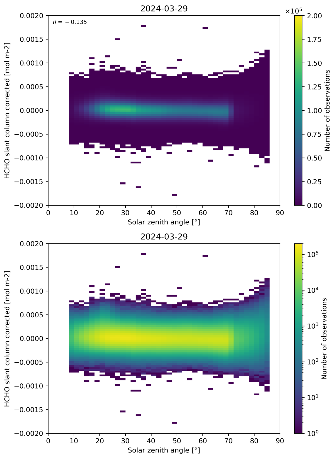
Figure 171: Scatter density plot of “Solar zenith angle” against “HCHO slant column corrected” for 2024-03-28 to 2024-03-30.
