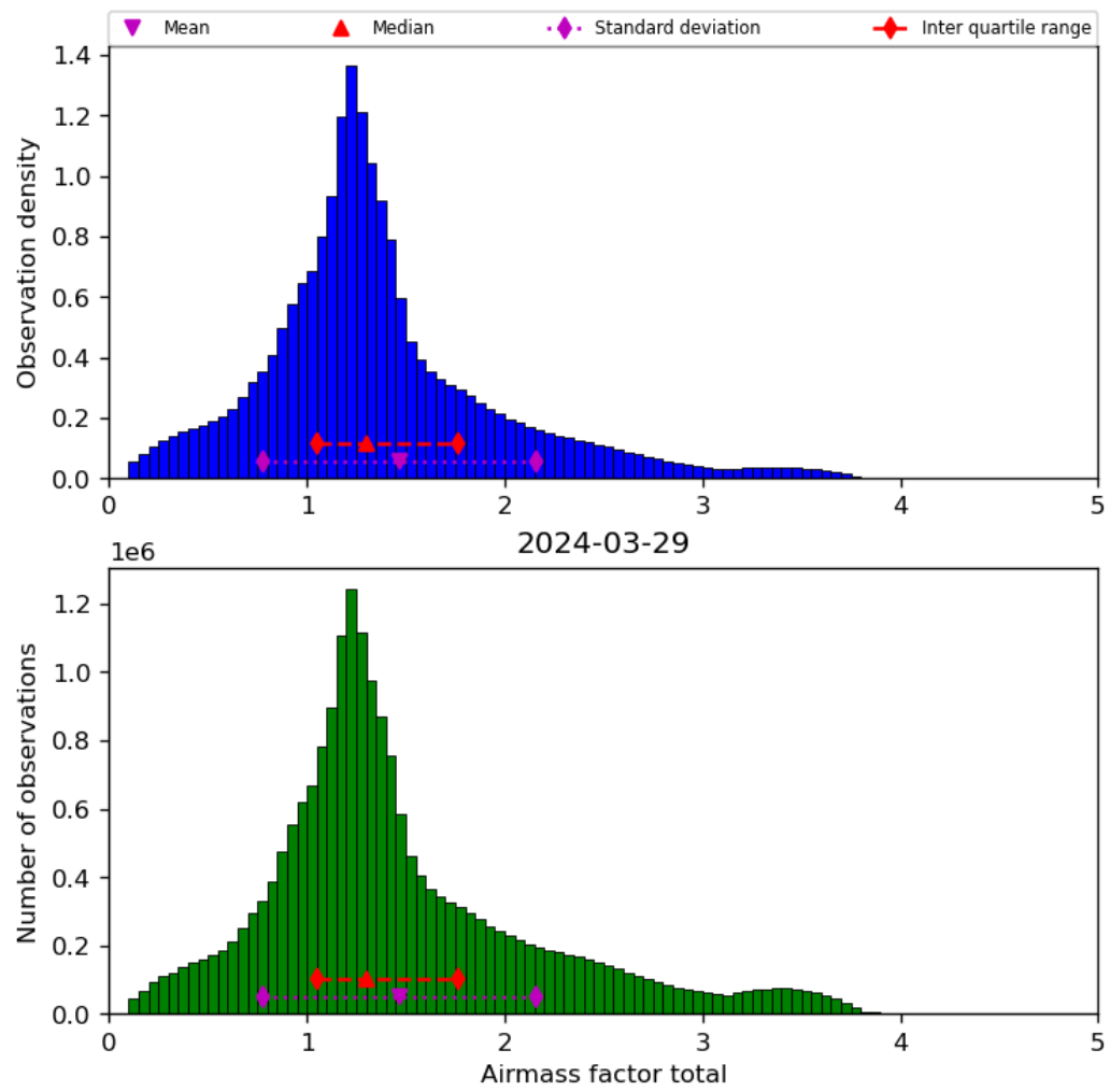
Figure 40: Histogram of “Airmass factor total” for 2024-03-28 to 2024-03-30
