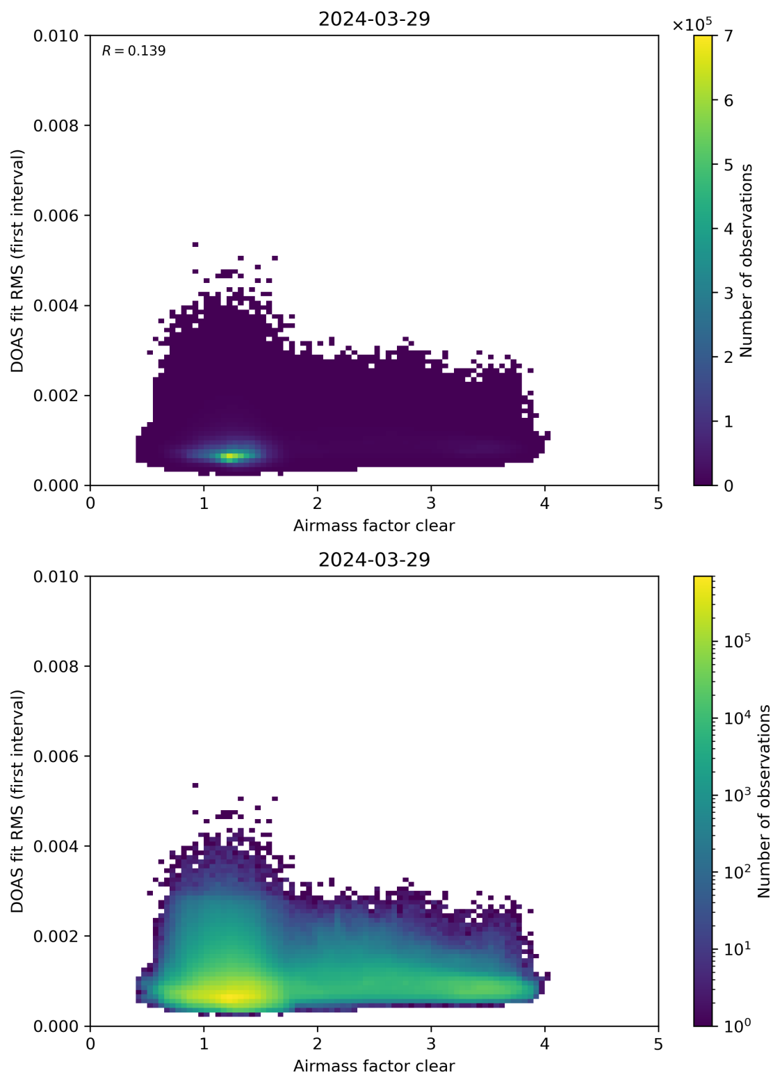
Figure 71: Scatter density plot of “Airmass factor clear” against “DOAS fit RMS (first interval)” for 2024-03-28 to 2024-03-30.
