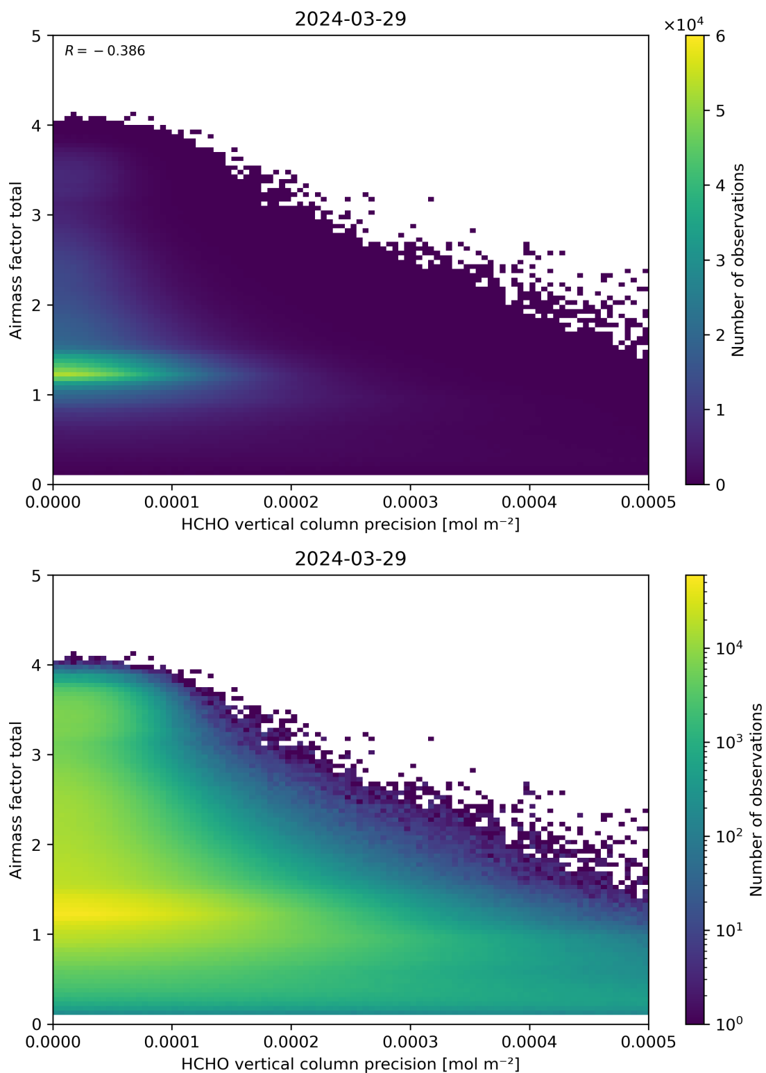
Figure 144: Scatter density plot of “HCHO vertical column precision” against “Airmass factor total” for 2024-03-28 to 2024-03-30.
