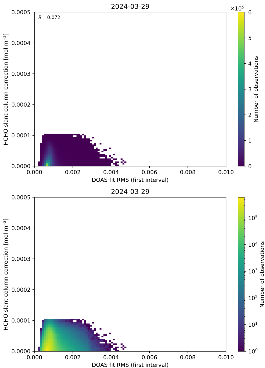
Figure 63: Scatter density plot of “DOAS fit RMS (first interval)” against “HCHO slant column correction” for 2024-03-28 to 2024-03-30.
