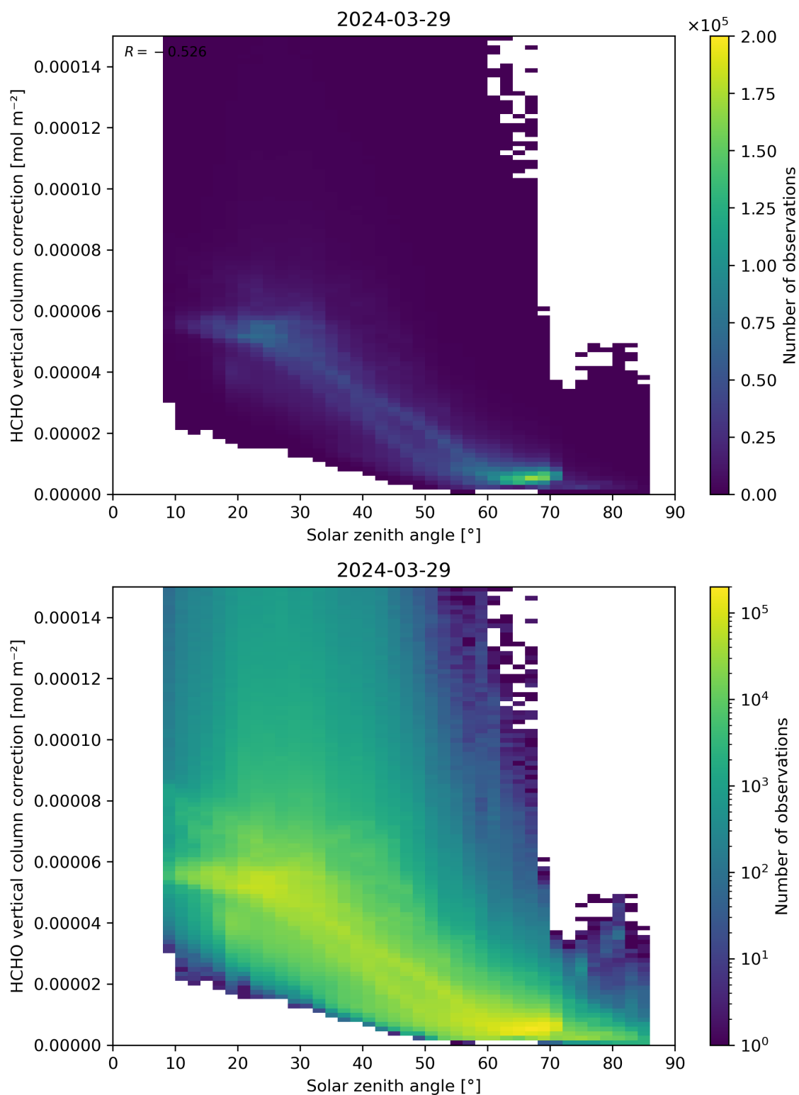
Figure 178: Scatter density plot of “Solar zenith angle” against “HCHO vertical column correction” for 2024-03-28 to 2024-03-30.
