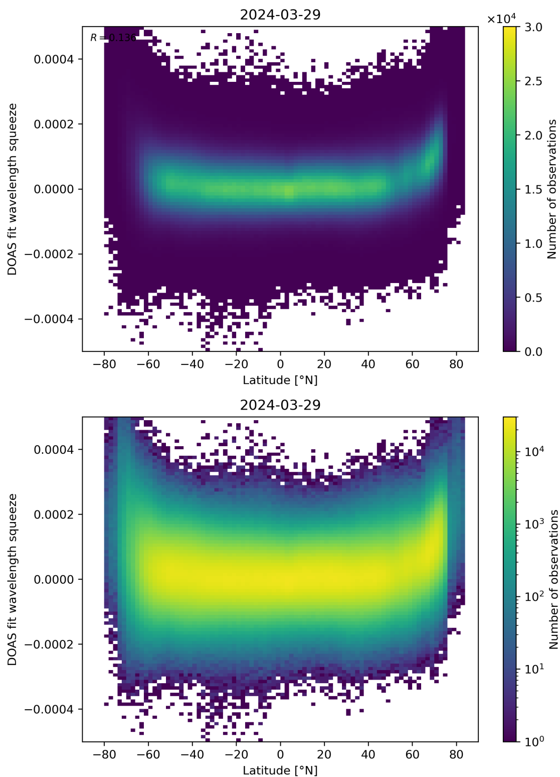
Figure 155: Scatter density plot of “Latitude” against “DOAS fit wavelength squeeze” for 2024-03-28 to 2024-03-30.
