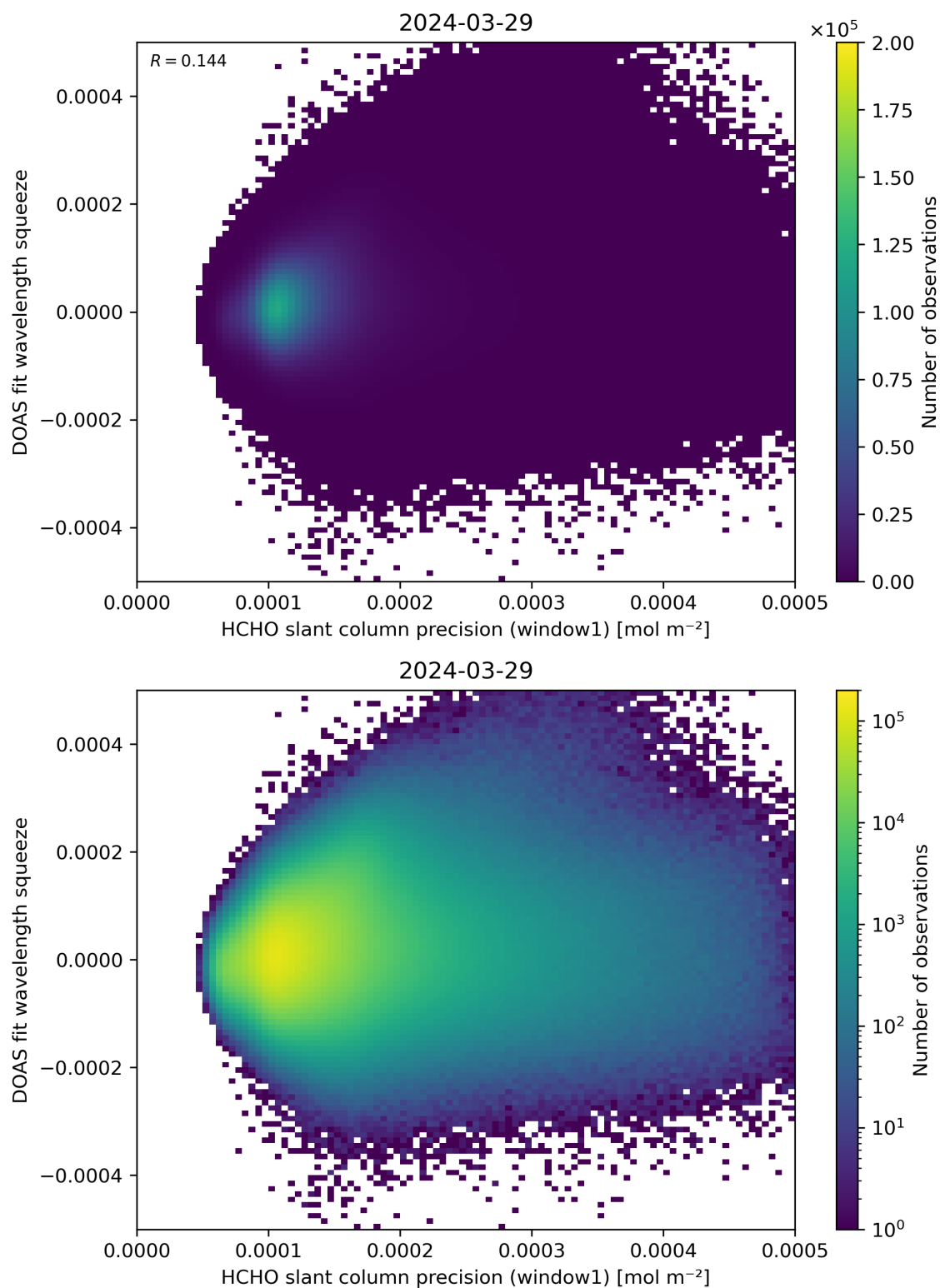
Figure 90: Scatter density plot of “HCHO slant column precision (window1)” against “DOAS fit wavelength squeeze” for 2024-03-28 to 2024-03-30.
