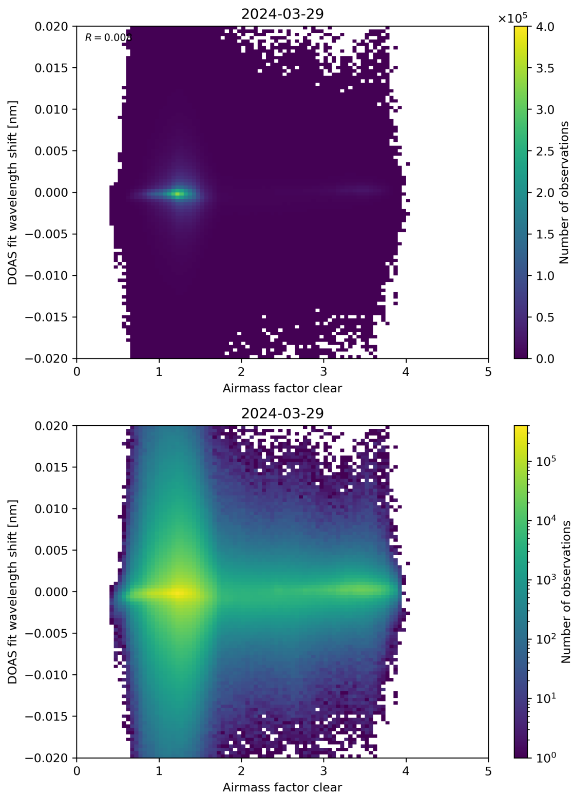
Figure 72: Scatter density plot of “Airmass factor clear” against “DOAS fit wavelength shift” for 2024-03-28 to 2024-03-30.
