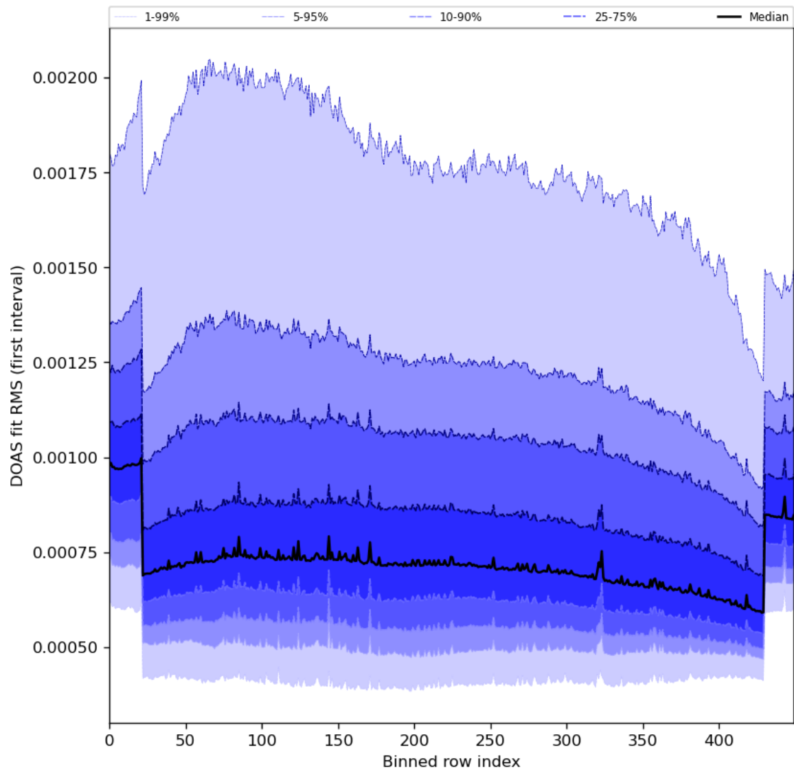
Figure 60: Along track statistics of “DOAS fit RMS (first interval)” for 2024-03-28 to 2024-03-30
