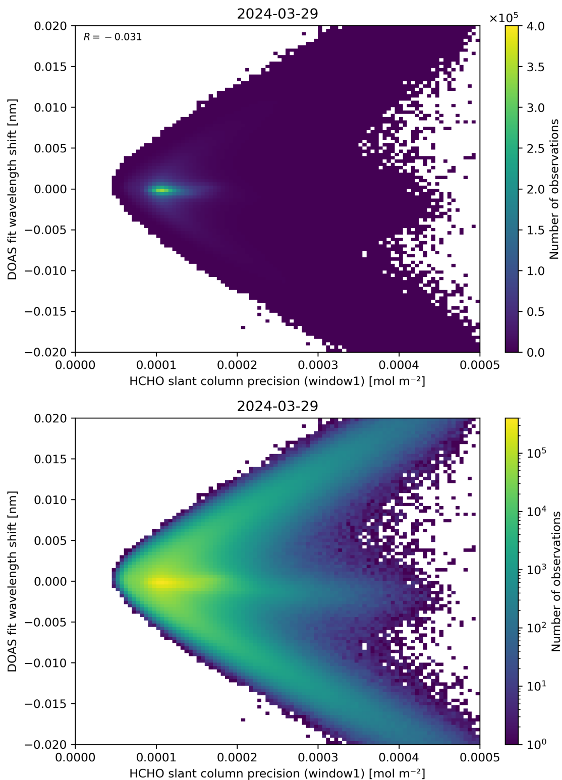
Figure 89: Scatter density plot of “HCHO slant column precision (window1)” against “DOAS fit wavelength shift” for 2024-03-28 to 2024-03-30.
