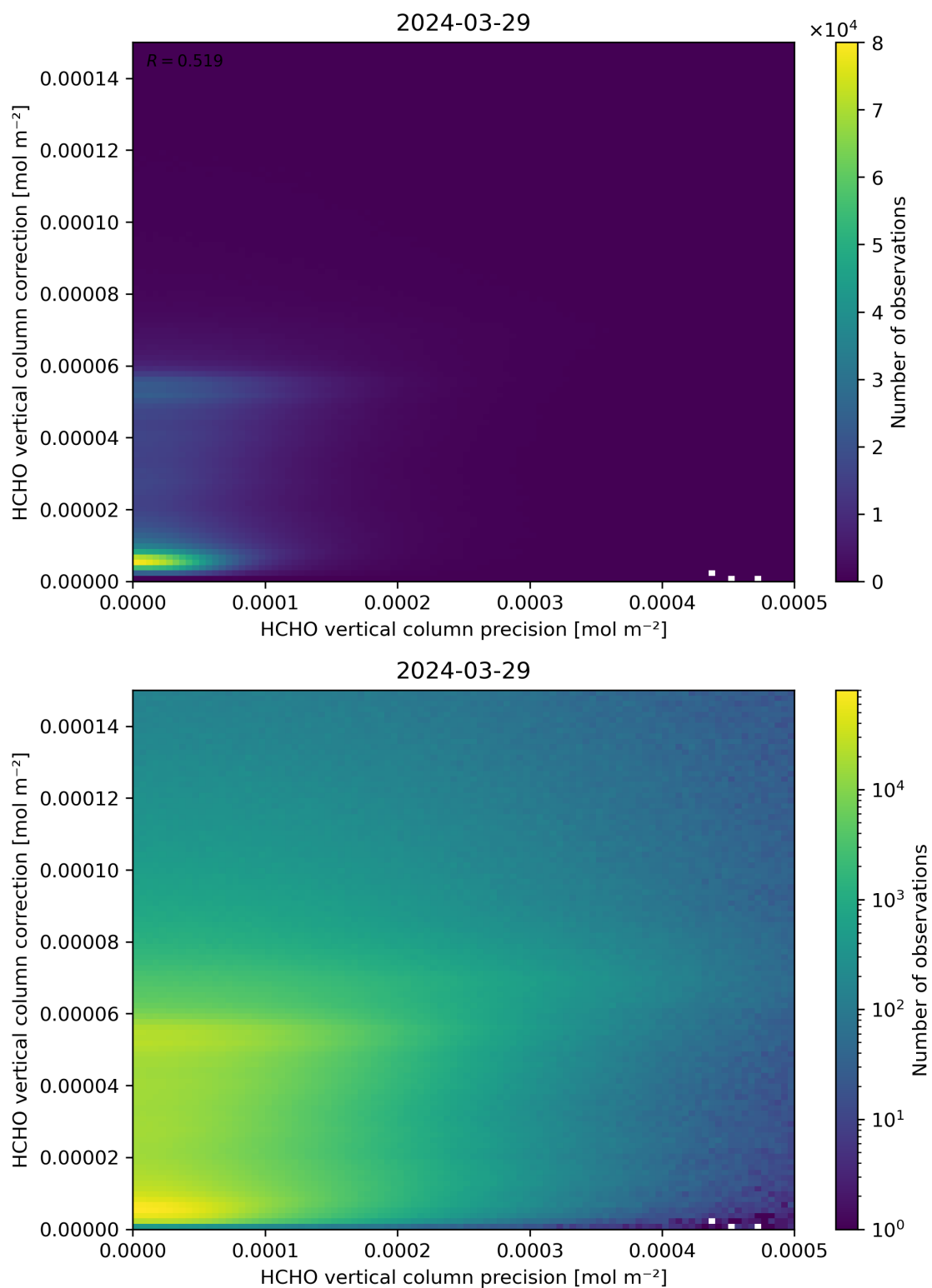
Figure 146: Scatter density plot of “HCHO vertical column precision” against “HCHO vertical column correction” for 2024-03-28 to 2024-03-30.
