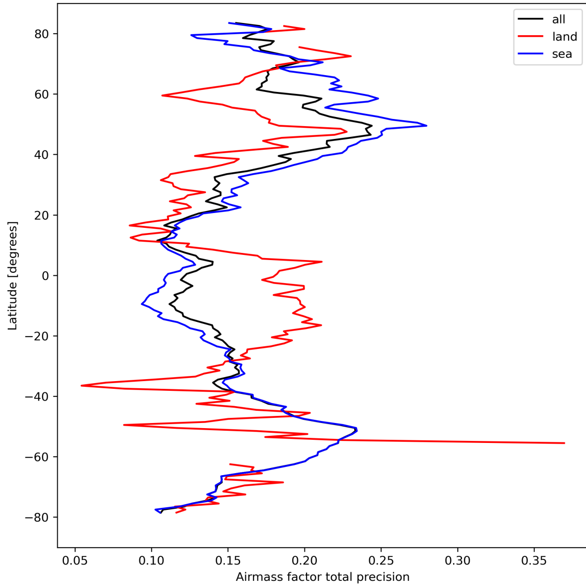
Figure 27: Zonal average of “Airmass factor total precision” for 2024-03-28 to 2024-03-30.
