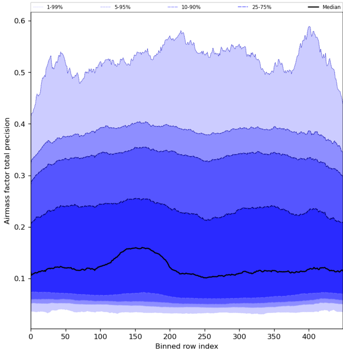
Figure 55: Along track statistics of “Airmass factor total precision” for 2024-03-28 to 2024-03-30
