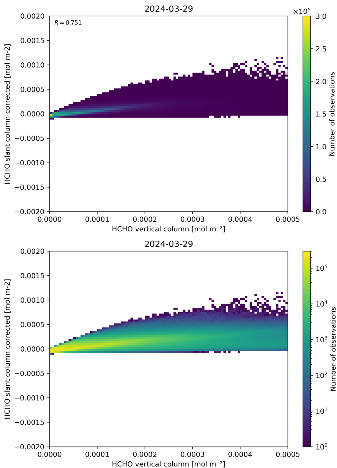
Figure 127: Scatter density plot of “HCHO vertical column” against “HCHO slant column corrected” for 2024-03-28 to 2024-03-30.
