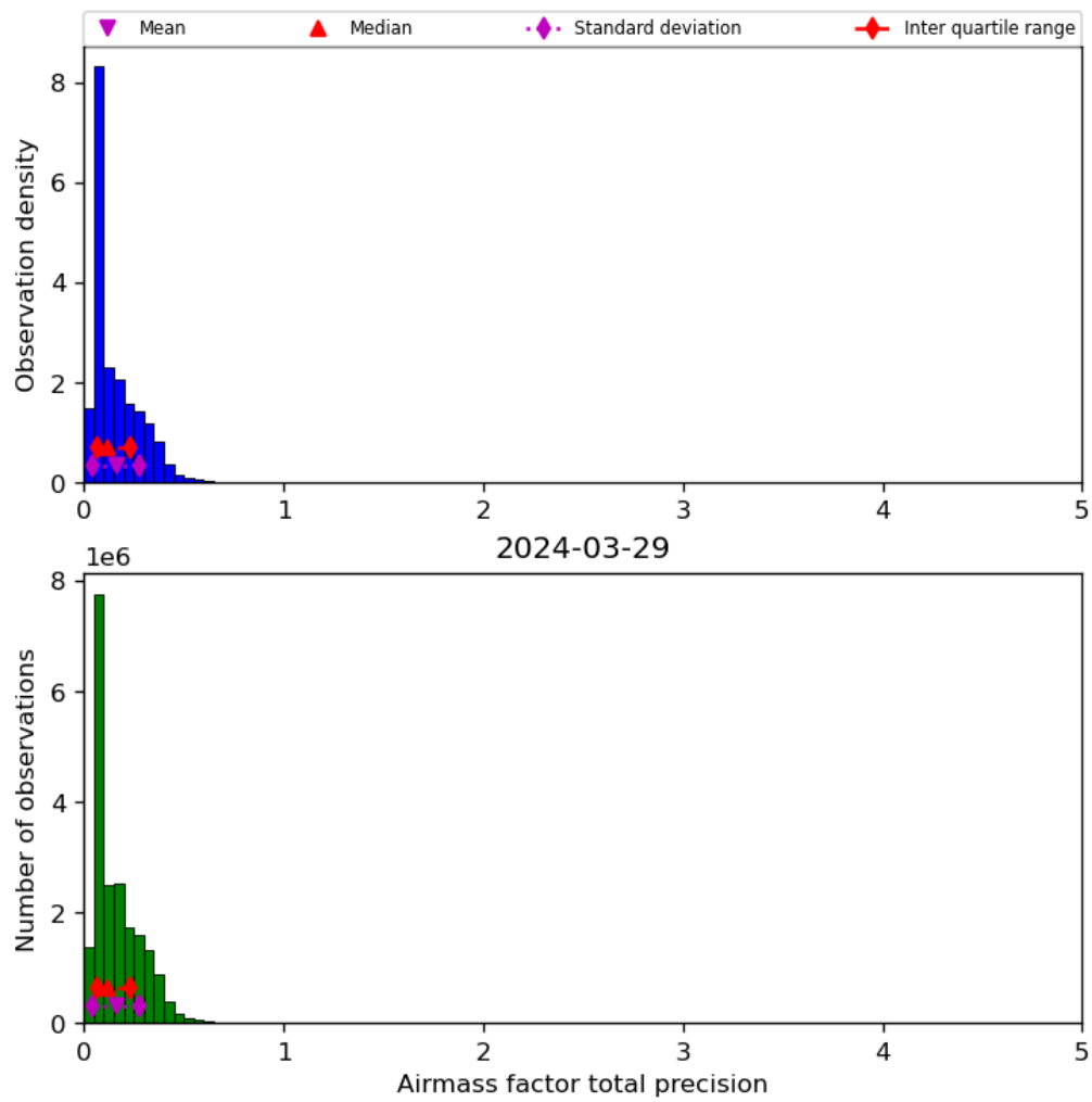
Figure 41: Histogram of "Airmass factor total precision" for 2024-03-28 to 2024-03-30
