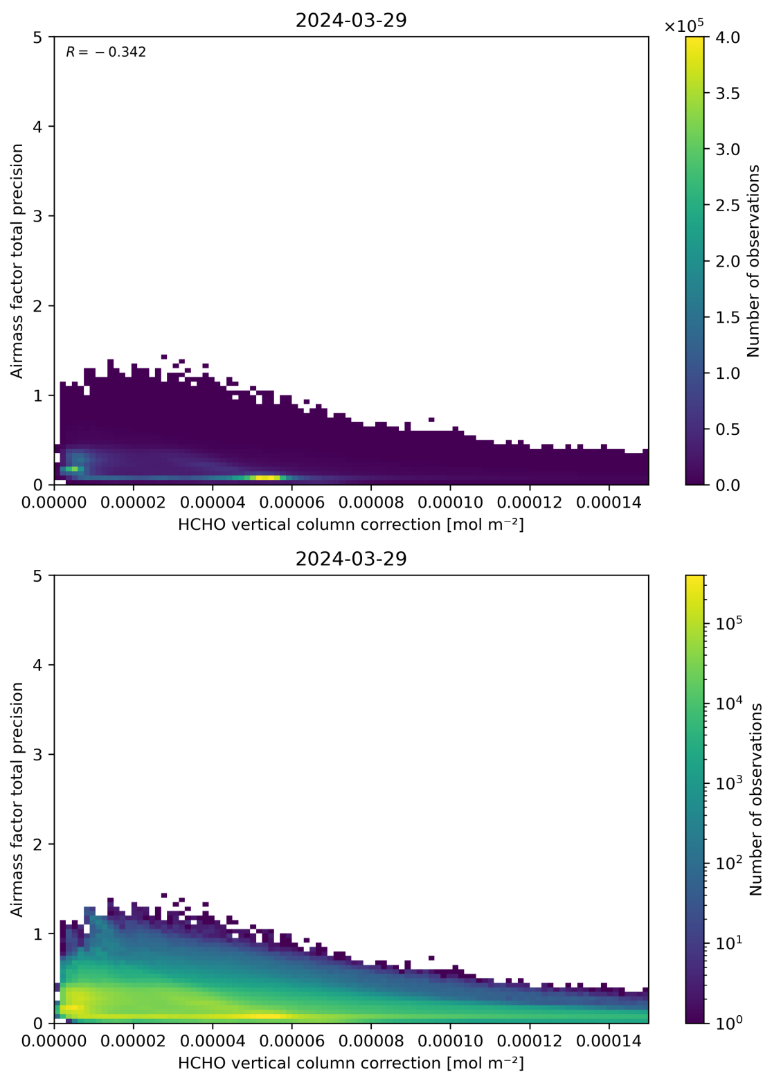
Figure 121: Scatter density plot of “HCHO vertical column correction” against “Airmass factor total precision” for 2024-03-28 to 2024-03-30.
