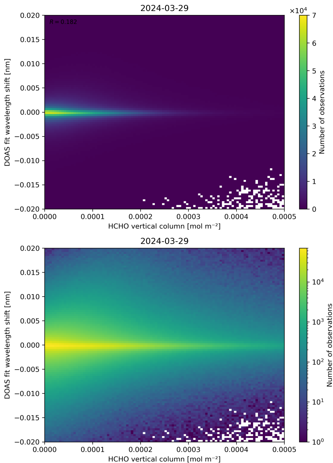
Figure 124: Scatter density plot of “HCHO vertical column” against “DOAS fit wavelength shift” for 2024-03-28 to 2024-03-30.
