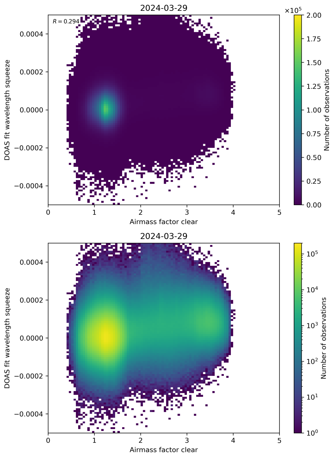
Figure 73: Scatter density plot of “Airmass factor clear” against “DOAS fit wavelength squeeze” for 2024-03-28 to 2024-03-30.
