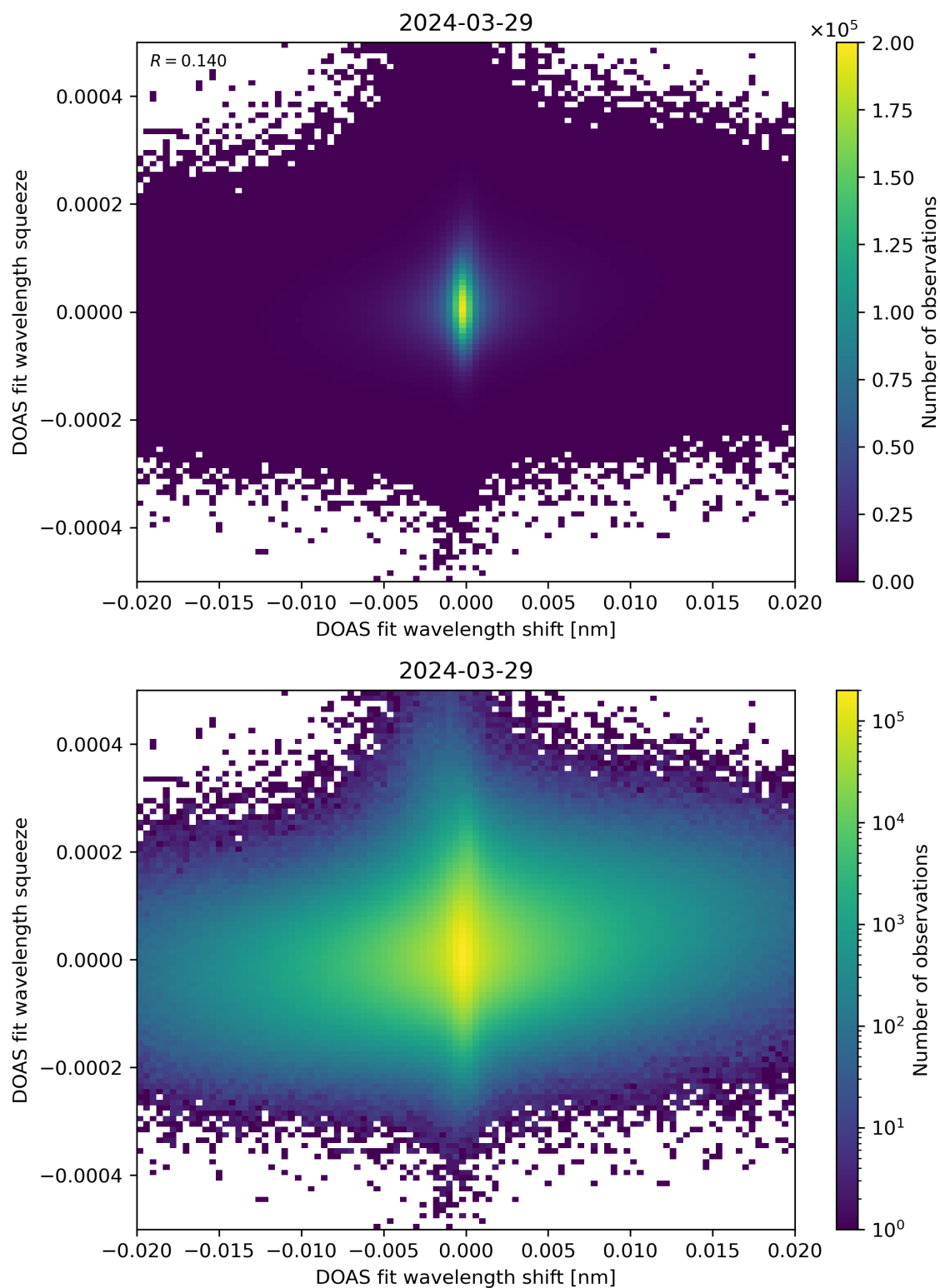
Figure 65: Scatter density plot of “DOAS fit wavelength shift” against “DOAS fit wavelength squeeze” for 2024-03-28 to 2024-03-30.
