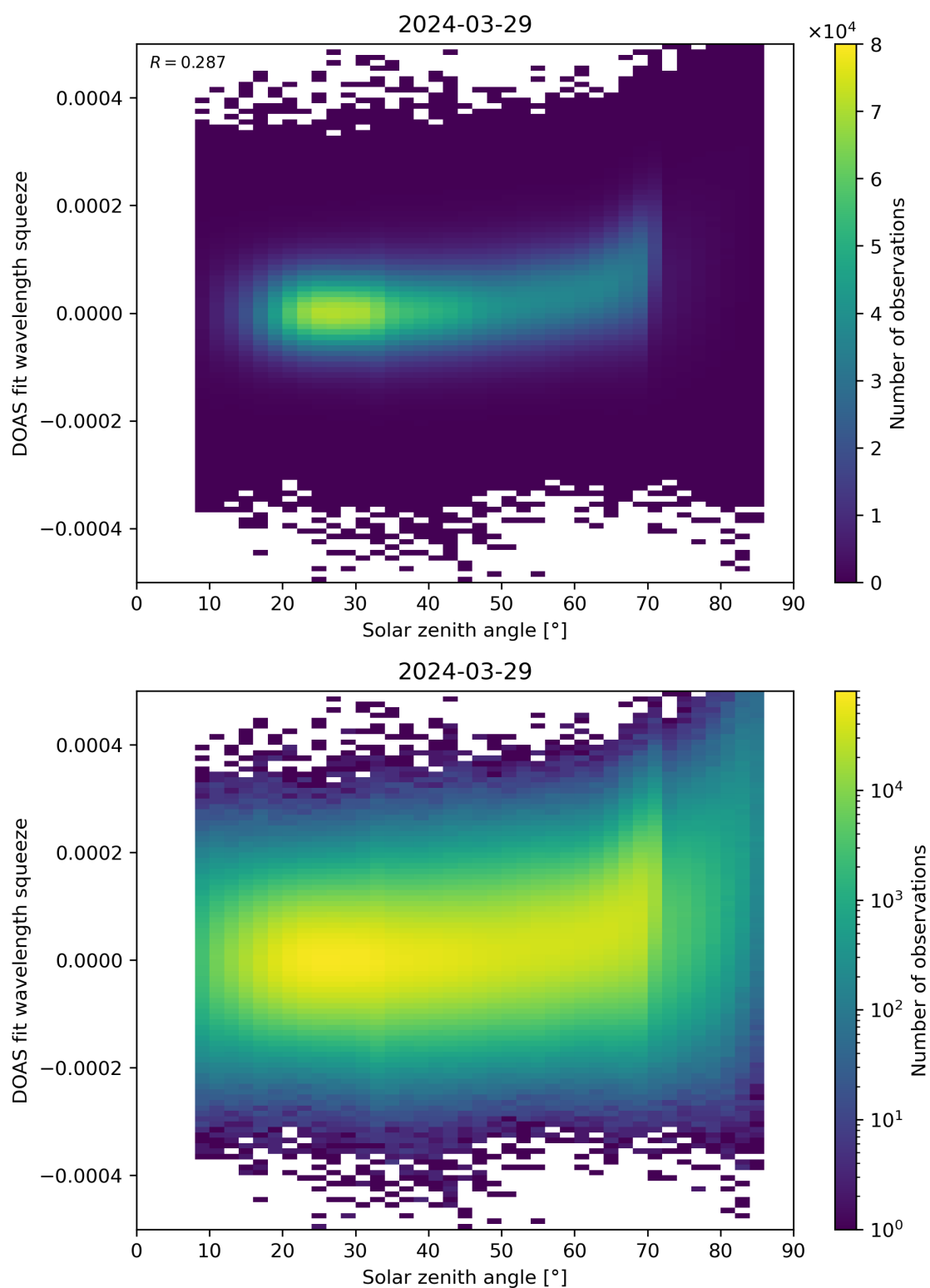
Figure 169: Scatter density plot of “Solar zenith angle” against “DOAS fit wavelength squeeze” for 2024-03-28 to 2024-03-30.
