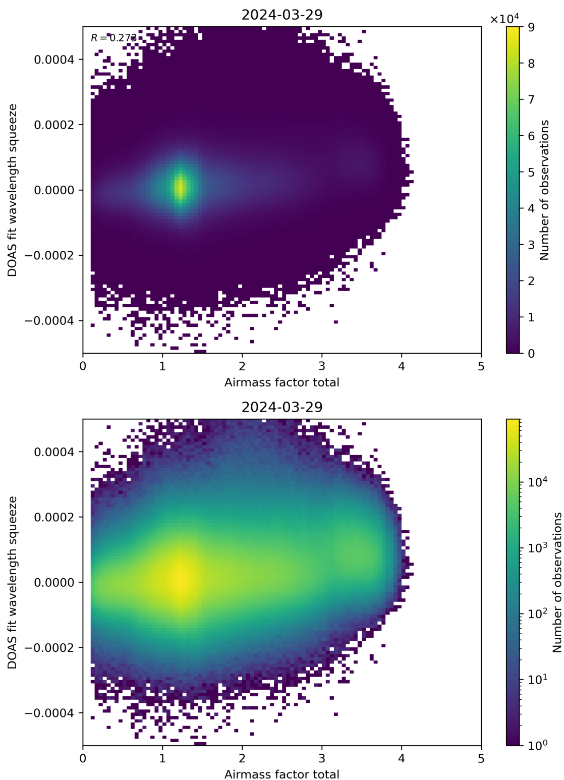
Figure 99: Scatter density plot of “Airmass factor total” against “DOAS fit wavelength squeeze” for 2024-03-28 to 2024-03-30.
