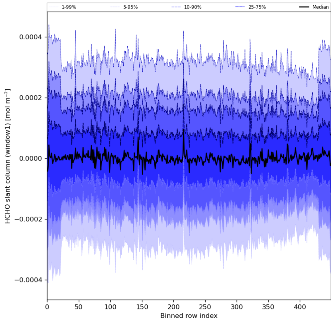
Figure 52: Along track statistics of “HCHO slant column (window1)” for 2024-03-28 to 2024-03-30
