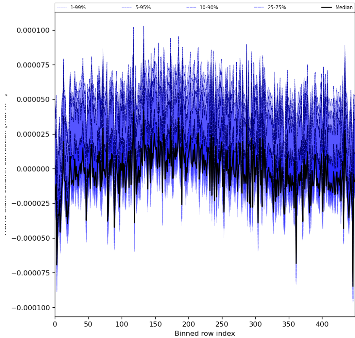
Figure 61: Along track statistics of “HCHO slant column correction” for 2024-03-28 to 2024-03-30
