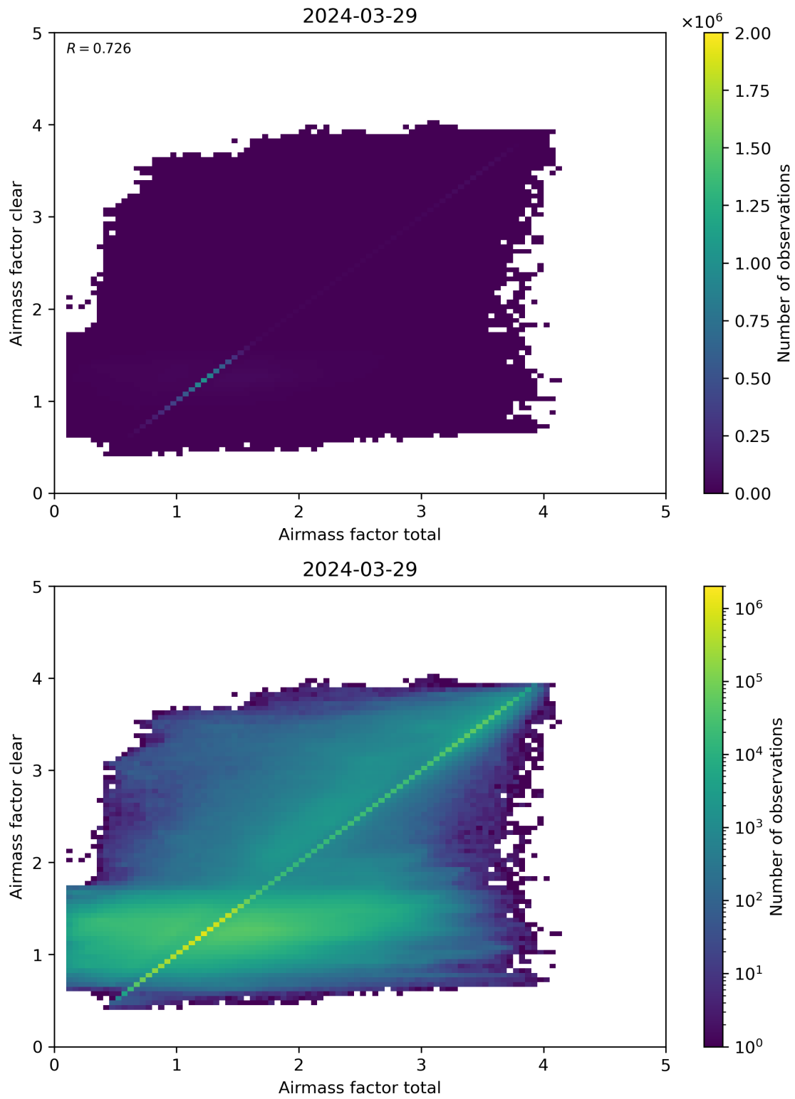
Figure 100: Scatter density plot of “Airmass factor total” against “Airmass factor clear” for 2024-03-28 to 2024-03-30.
