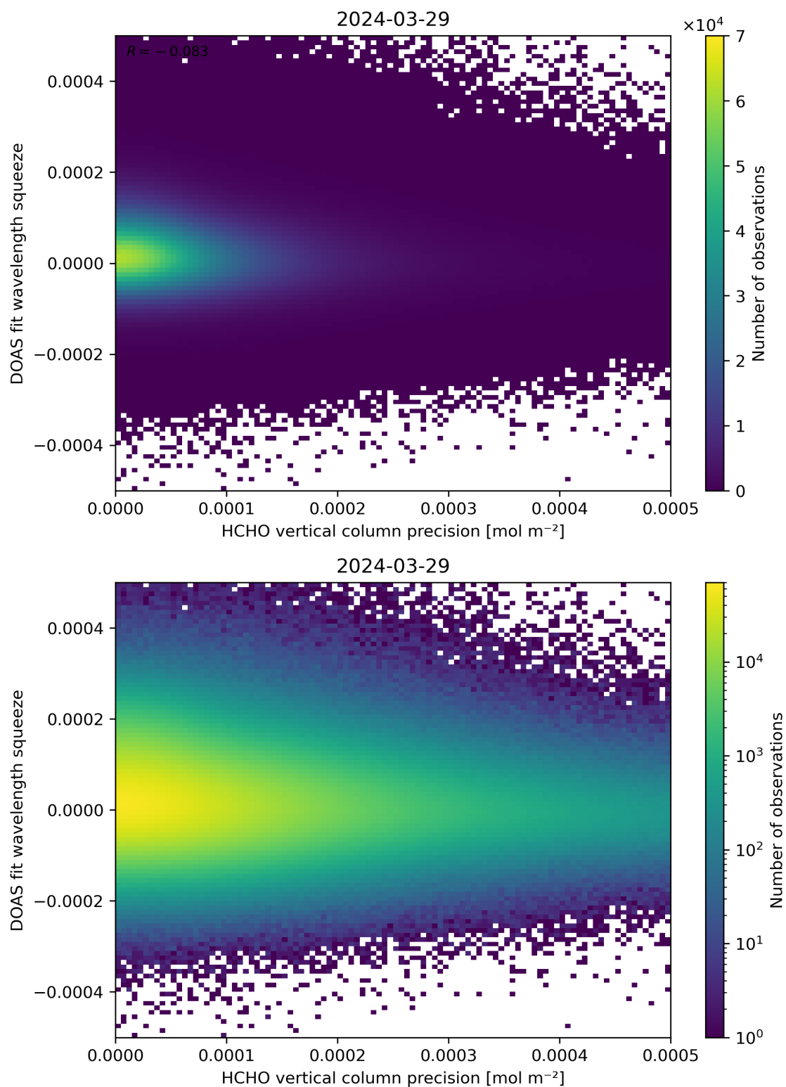
Figure 138: Scatter density plot of “HCHO vertical column precision” against “DOAS fit wavelength squeeze” for 2024-03-28 to 2024-03-30.
