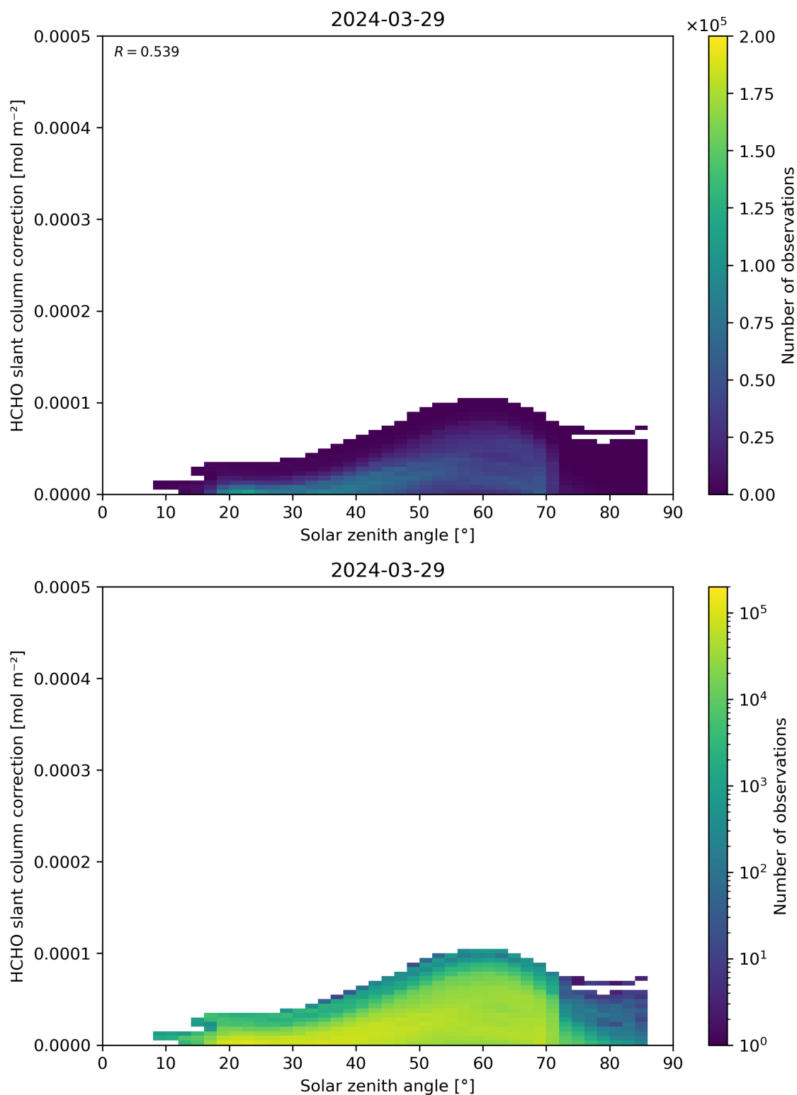
Figure 172: Scatter density plot of “Solar zenith angle” against “HCHO slant column correction” for 2024-03-28 to 2024-03-30.
