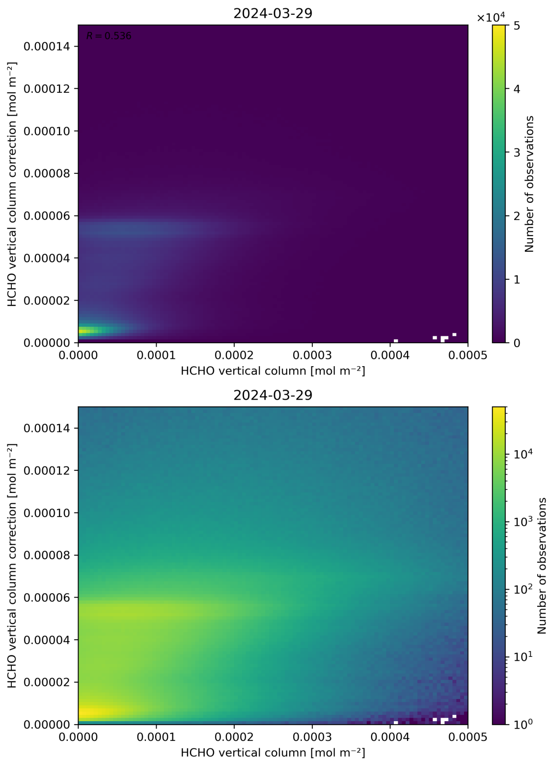
Figure 133: Scatter density plot of “HCHO vertical column” against “HCHO vertical column correction” for 2024-03-28 to 2024-03-30.
