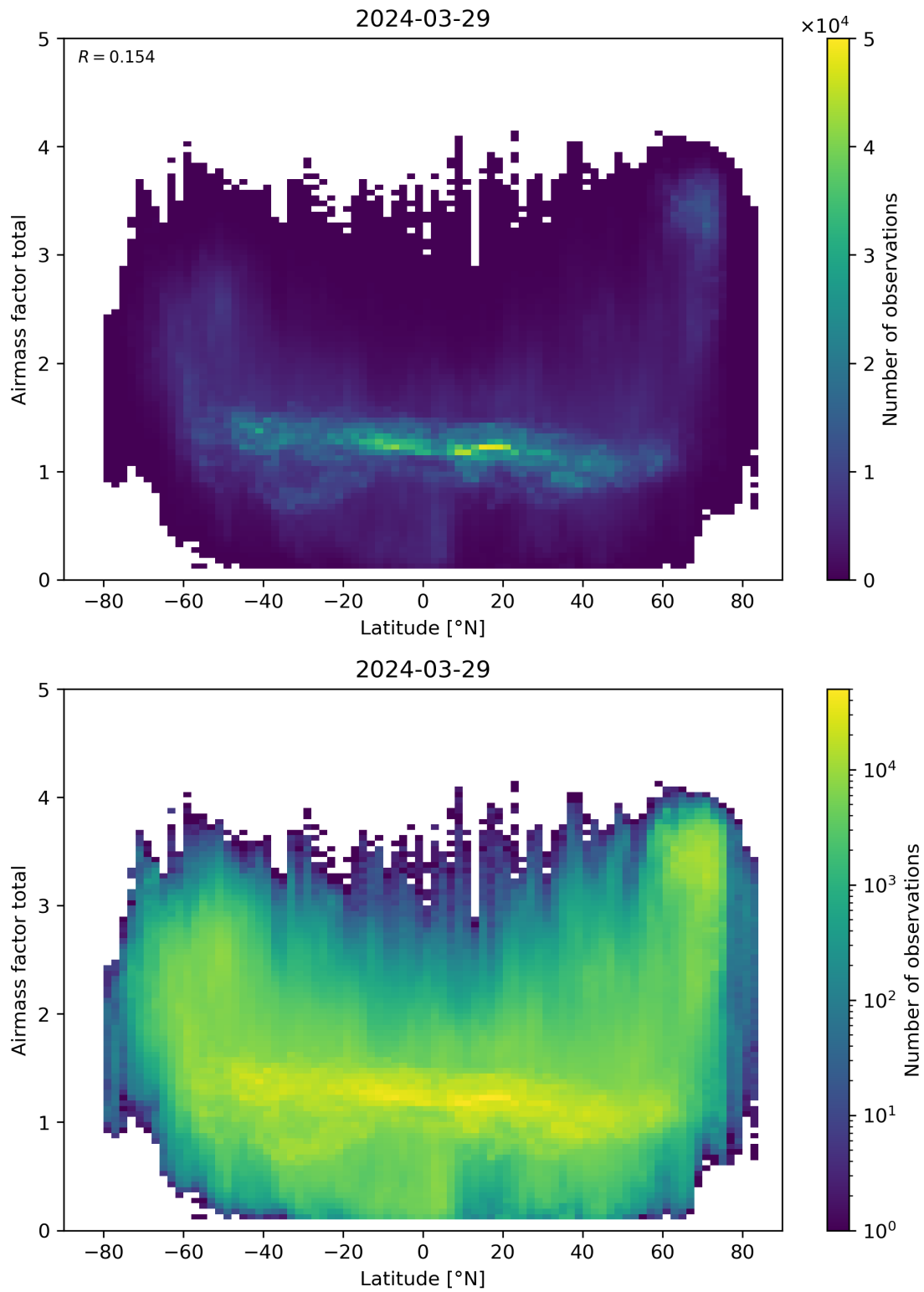
Figure 161: Scatter density plot of “Latitude” against “Airmass factor total” for 2024-03-28 to 2024-03-30.
