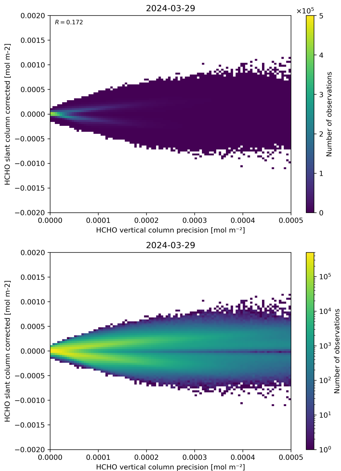
Figure 140: Scatter density plot of “HCHO vertical column precision” against “HCHO slant column corrected” for 2024-03-28 to 2024-03-30.
