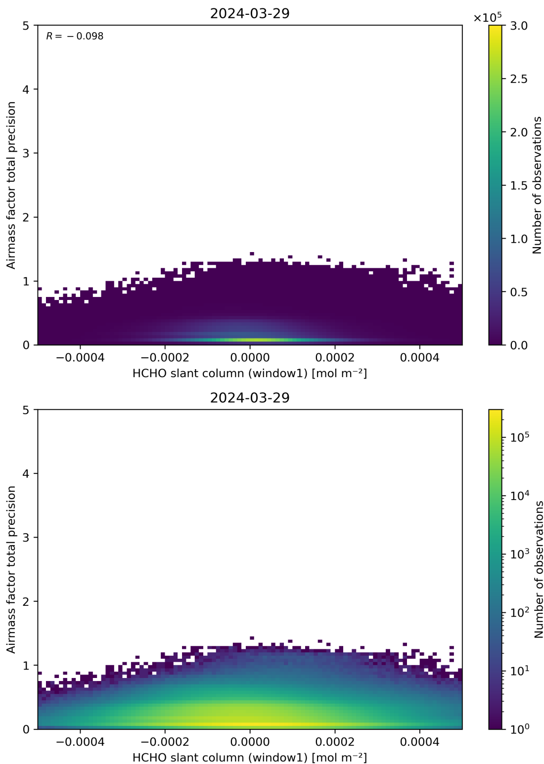
Figure 86: Scatter density plot of “HCHO slant column (window1)” against “Airmass factor total precision” for 2024-03-28 to 2024-03-30.
