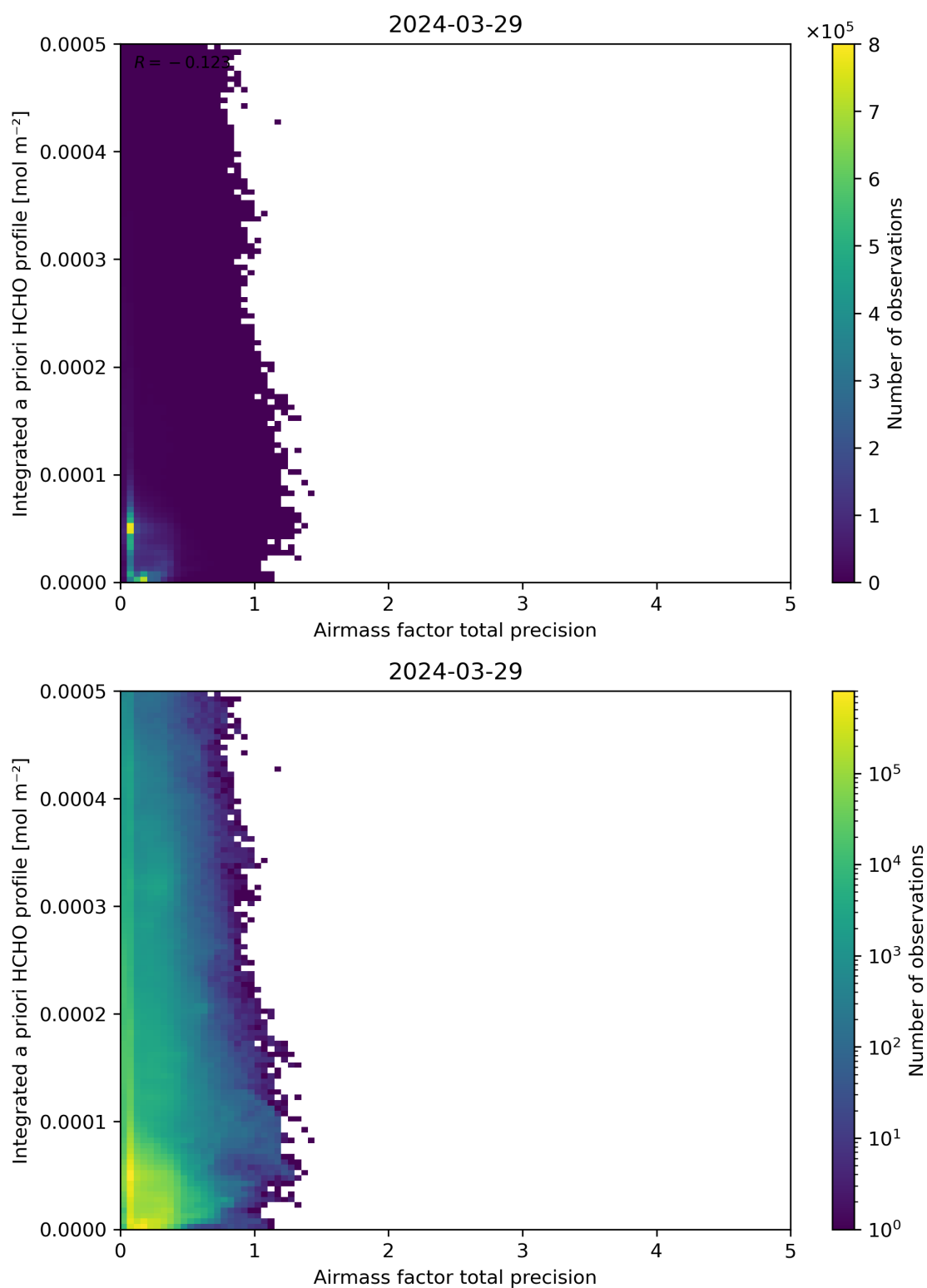
Figure 111: Scatter density plot of “Airmass factor total precision” against “Integrated a priori HCHO profile” for 2024-03-28 to 2024-03-30.
