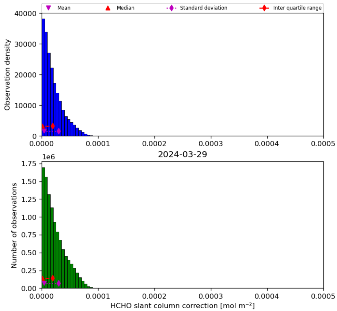
Figure 47: Histogram of “HCHO slant column correction” for 2024-03-28 to 2024-03-30
