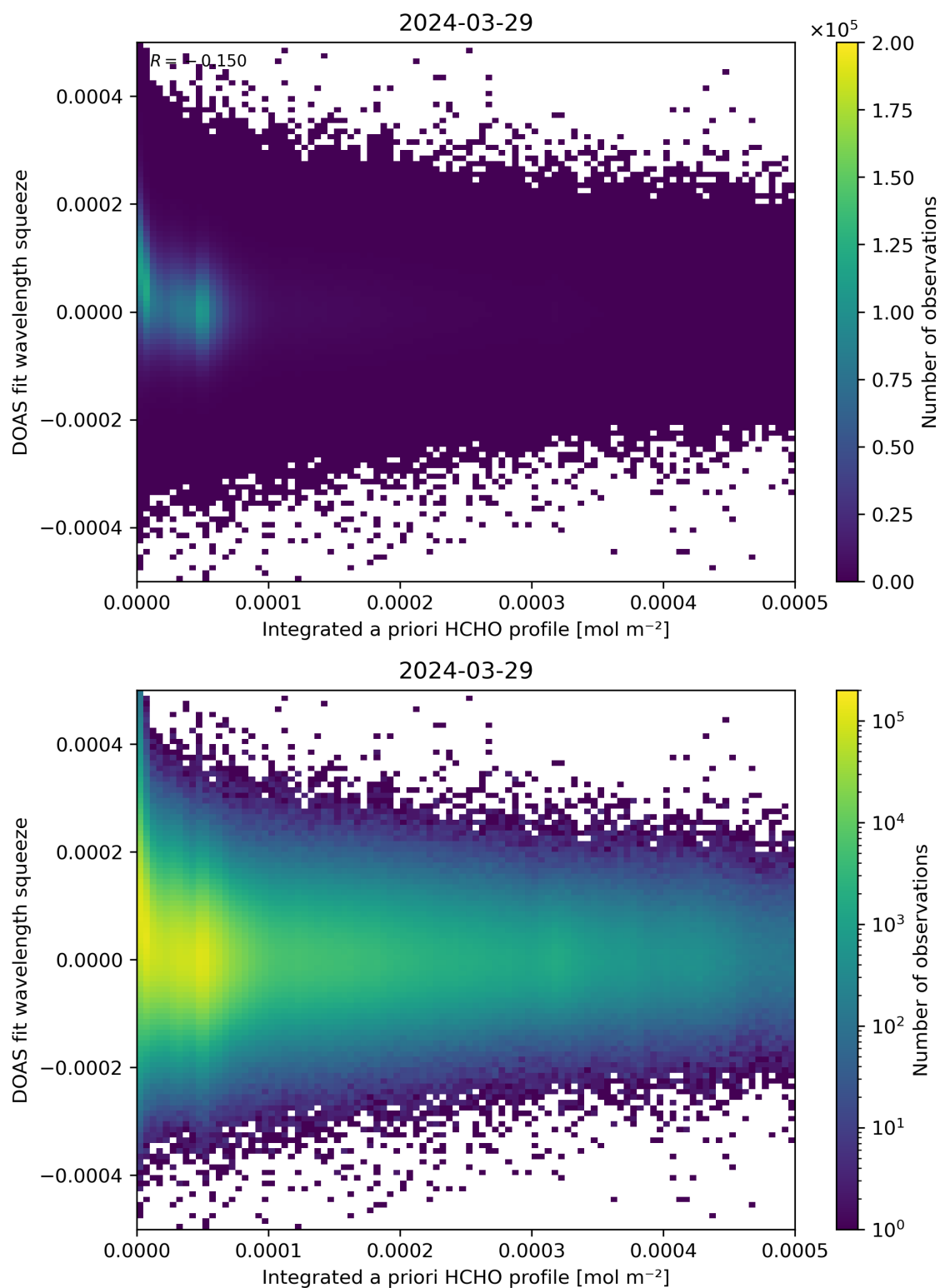
Figure 150: Scatter density plot of “Integrated a priori HCHO profile” against “DOAS fit wavelength squeeze” for 2024-03-28 to 2024-03-30.
