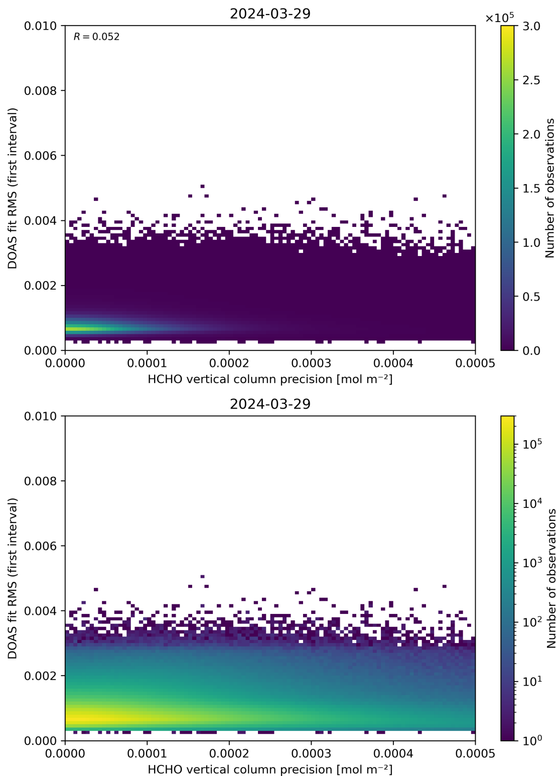
Figure 136: Scatter density plot of “HCHO vertical column precision” against “DOAS fit RMS (first interval)” for 2024-03-28 to 2024-03-30.
