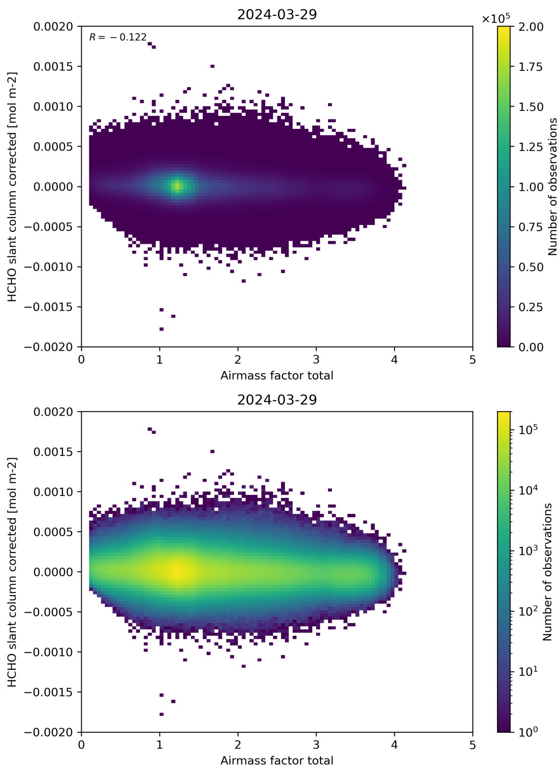
Figure 101: Scatter density plot of “Airmass factor total” against “HCHO slant column corrected” for 2024-03-28 to 2024-03-30.
