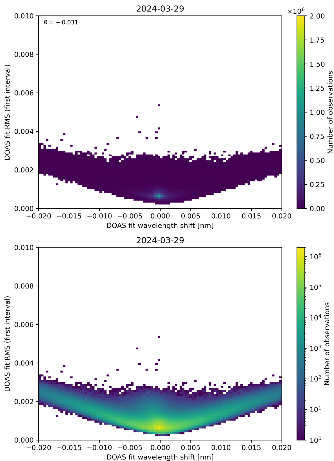
Figure 64: Scatter density plot of “DOAS fit wavelength shift” against “DOAS fit RMS (first interval)” for 2024-03-28 to 2024-03-30.
