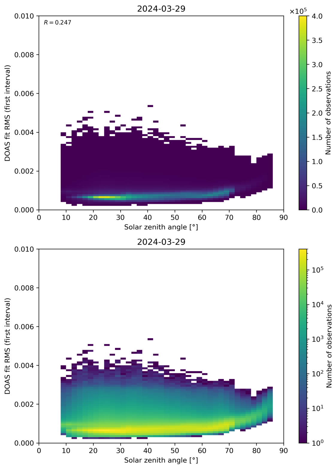
Figure 167: Scatter density plot of “Solar zenith angle” against “DOAS fit RMS (first interval)” for 2024-03-28 to 2024-03-30.
