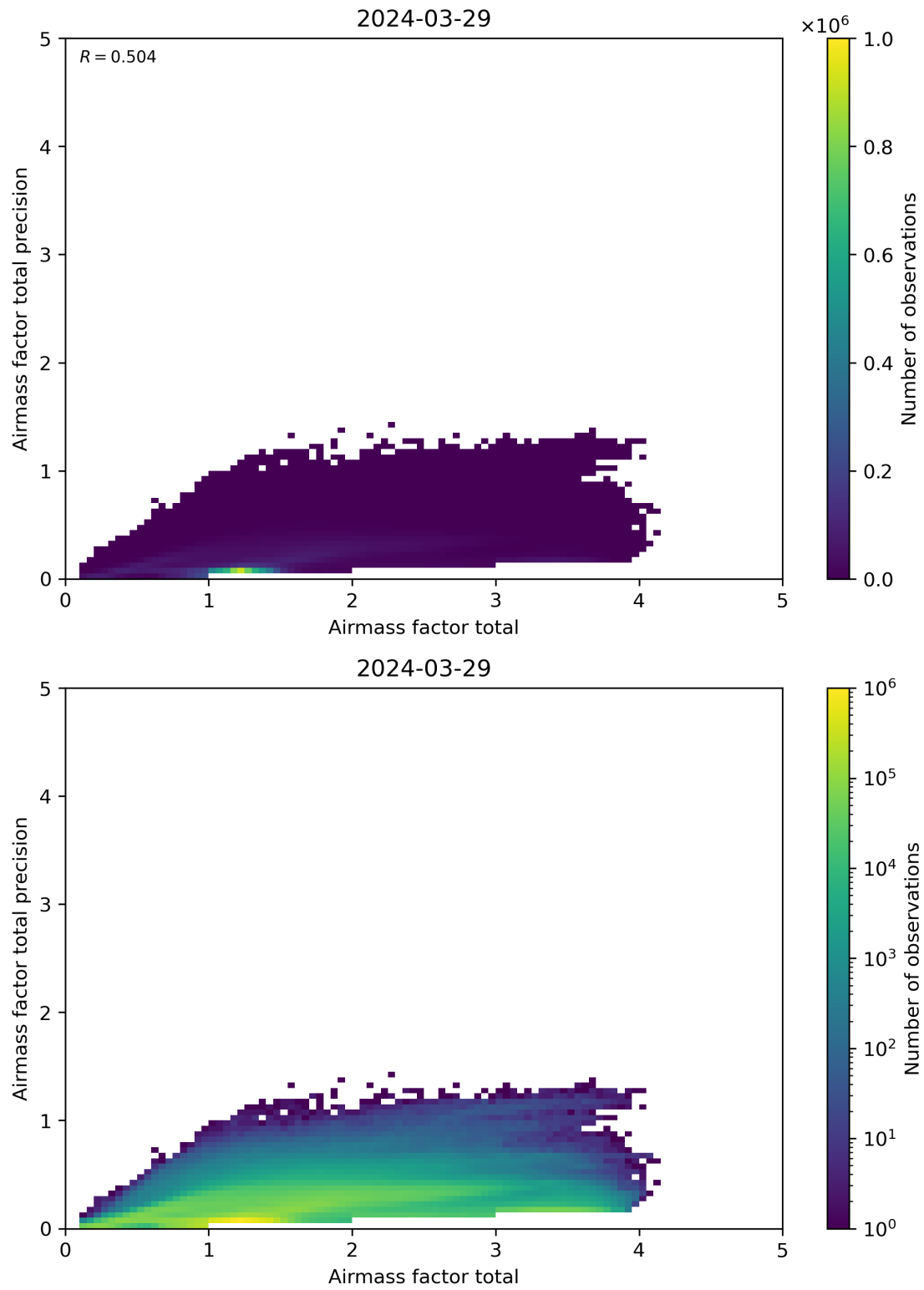
Figure 103: Scatter density plot of “Airmass factor total” against “Airmass factor total precision” for 2024-03-28 to 2024-03-30.
