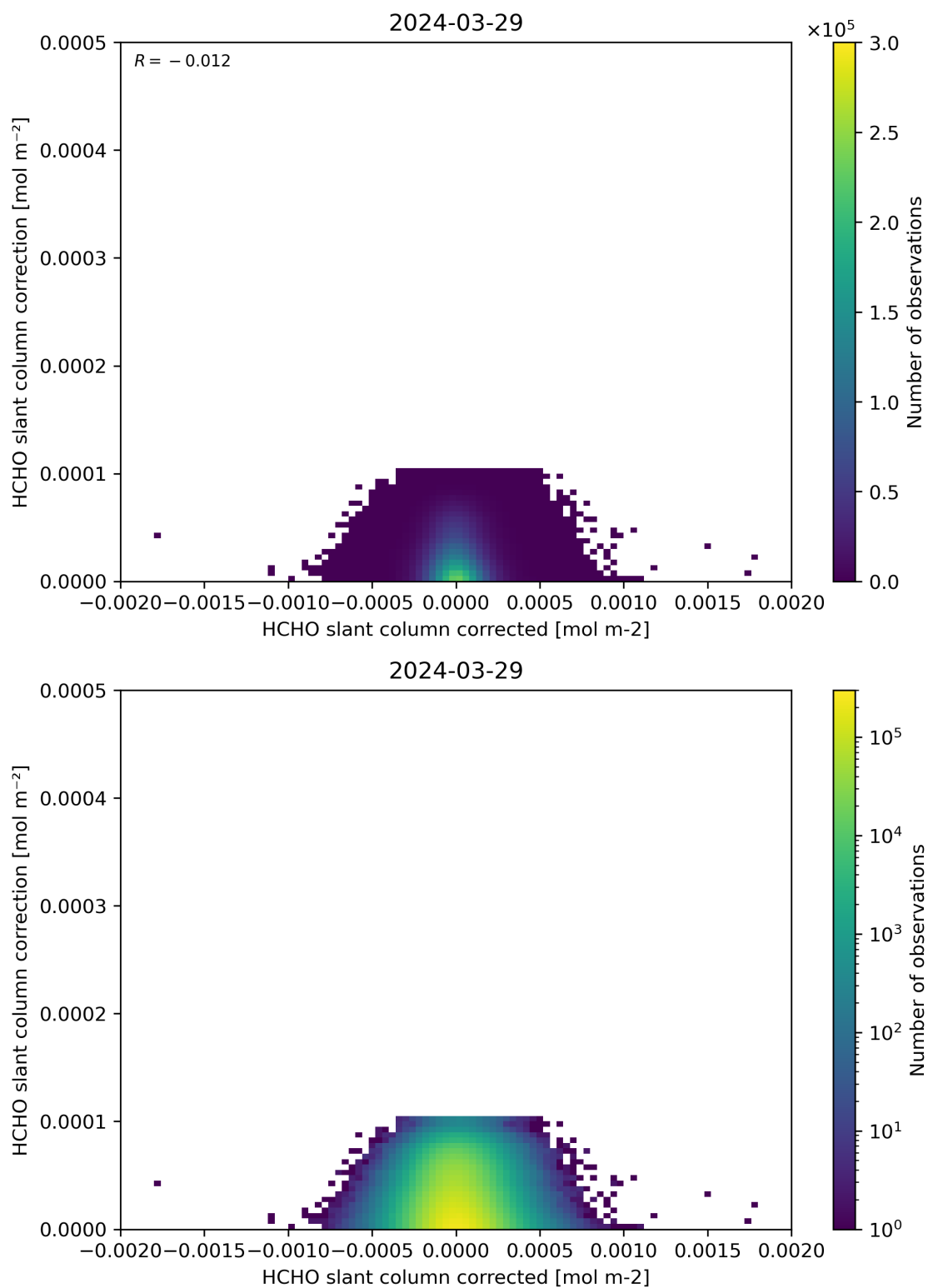
Figure 77: Scatter density plot of “HCHO slant column corrected” against “HCHO slant column correction” for 2024-03-28 to 2024-03-30.
