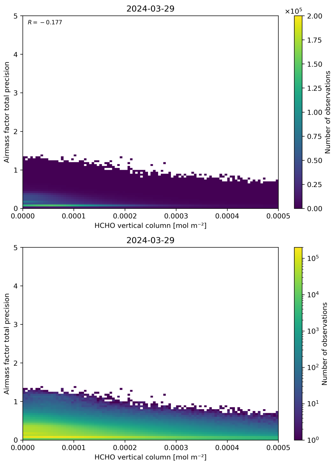
Figure 132: Scatter density plot of “HCHO vertical column” against “Airmass factor total precision” for 2024-03-28 to 2024-03-30.
