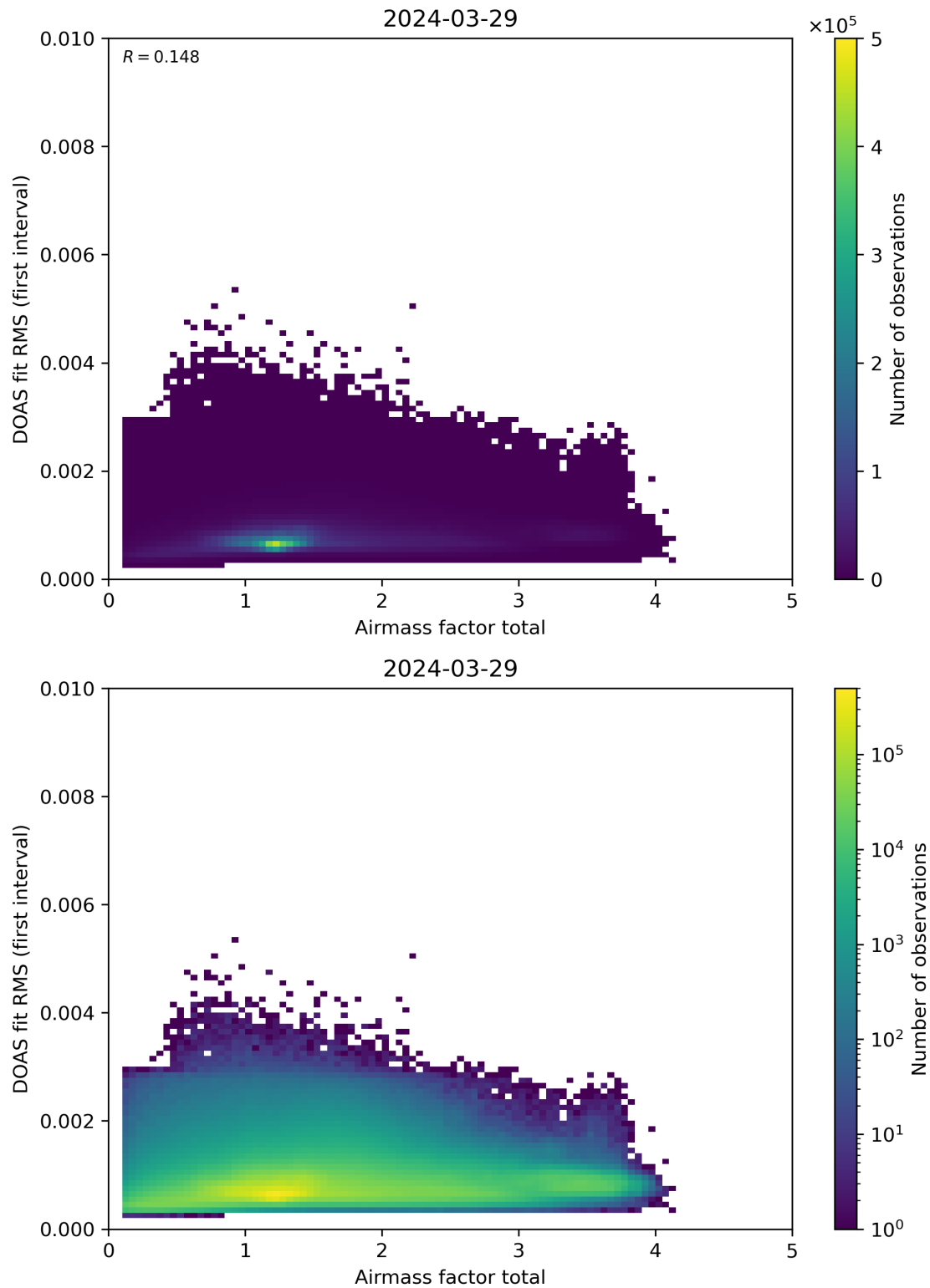
Figure 97: Scatter density plot of “Airmass factor total” against “DOAS fit RMS (first interval)” for 2024-03-28 to 2024-03-30.
