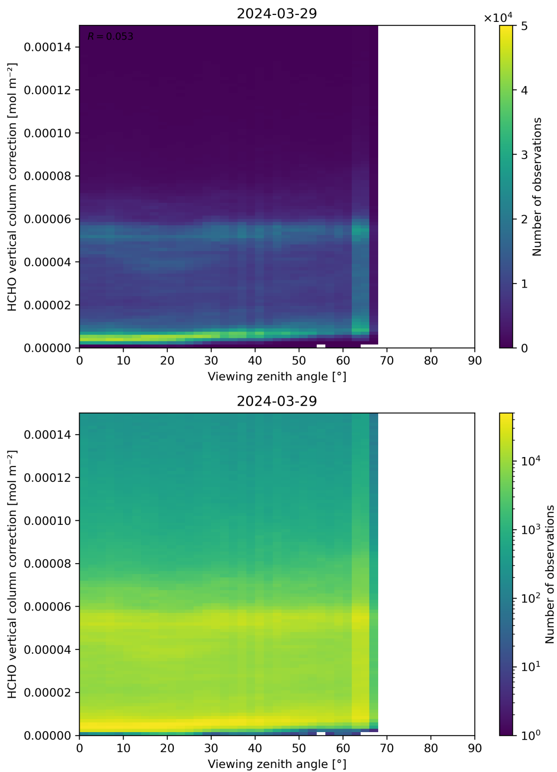
Figure 193: Scatter density plot of “Viewing zenith angle” against “HCHO vertical column correction” for 2024-03-28 to 2024-03-30.
