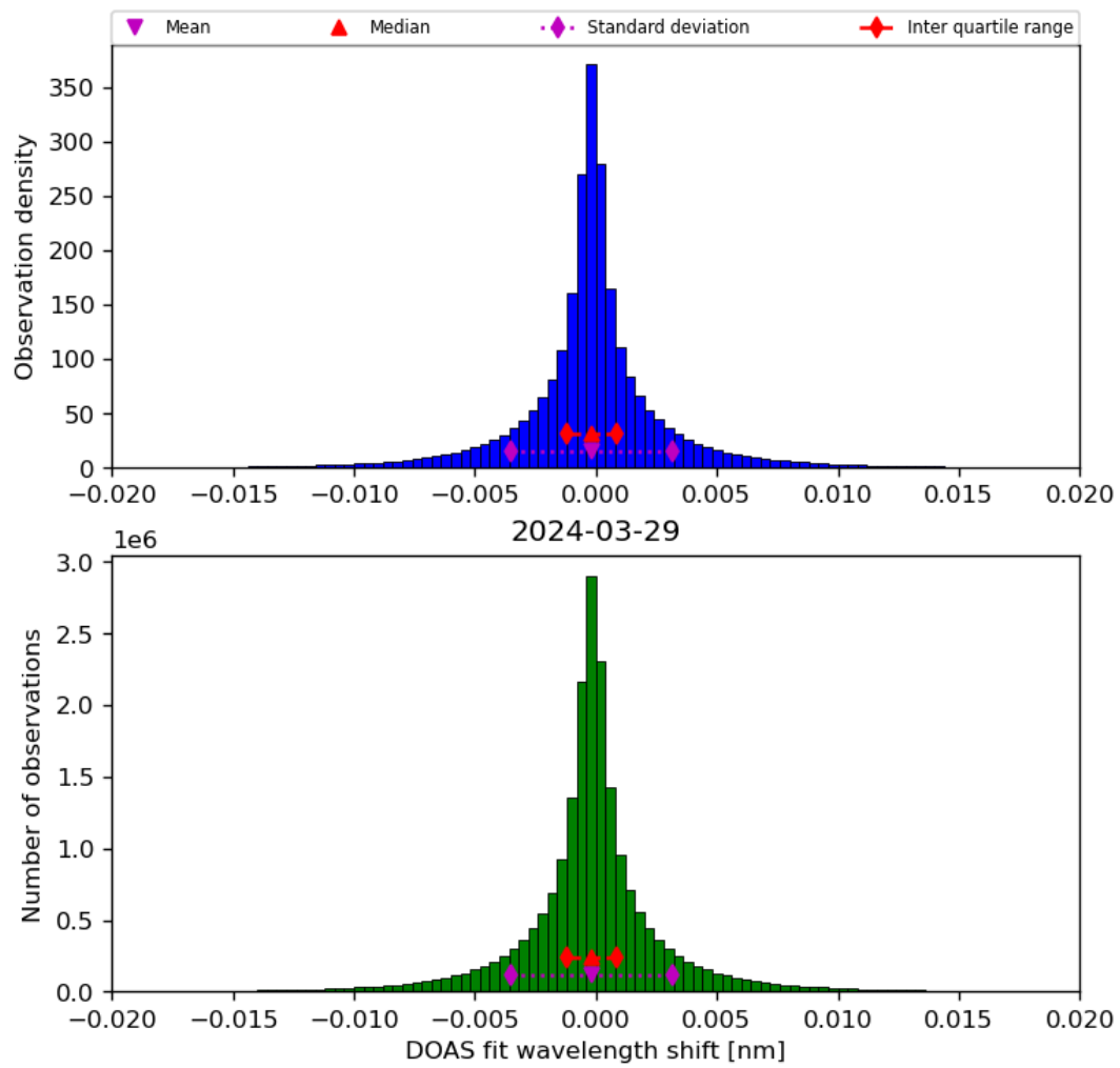
Figure 44: Histogram of “DOAS fit wavelength shift” for 2024-03-28 to 2024-03-30
