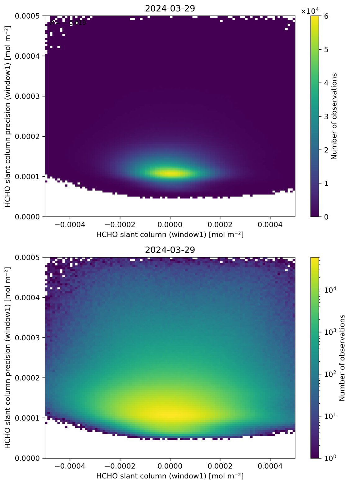
Figure 84: Scatter density plot of “HCHO slant column (window1)” against “HCHO slant column precision (window1)” for 2024-03-28 to 2024-03-30.
