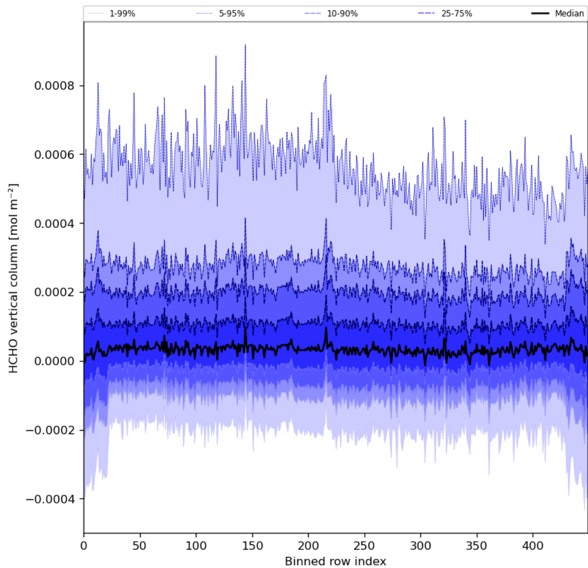
Figure 49: Along track statistics of “HCHO vertical column” for 2024-03-28 to 2024-03-30
