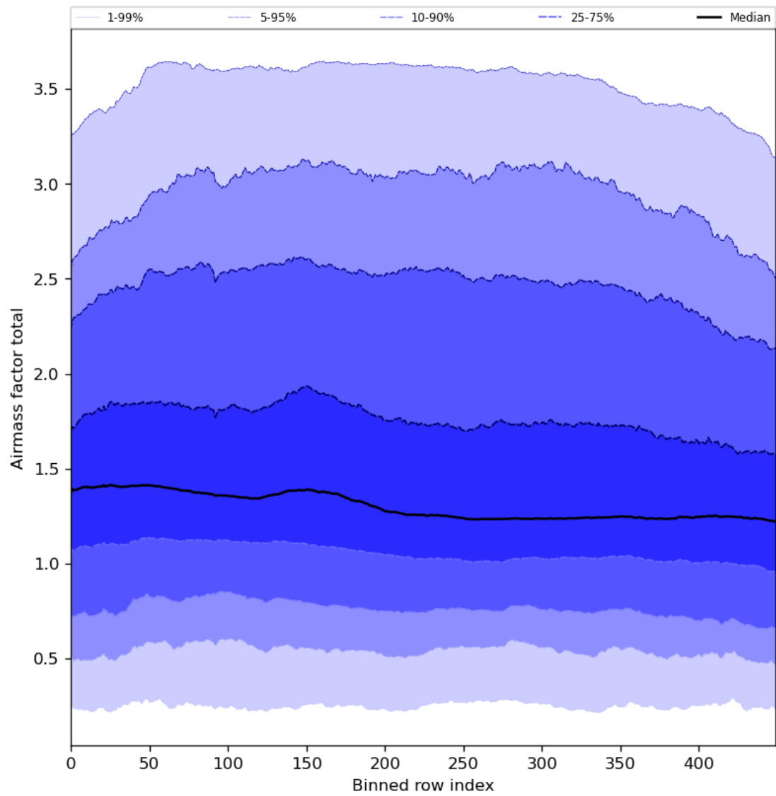
Figure 54: Along track statistics of “Airmass factor total” for 2024-03-28 to 2024-03-30
