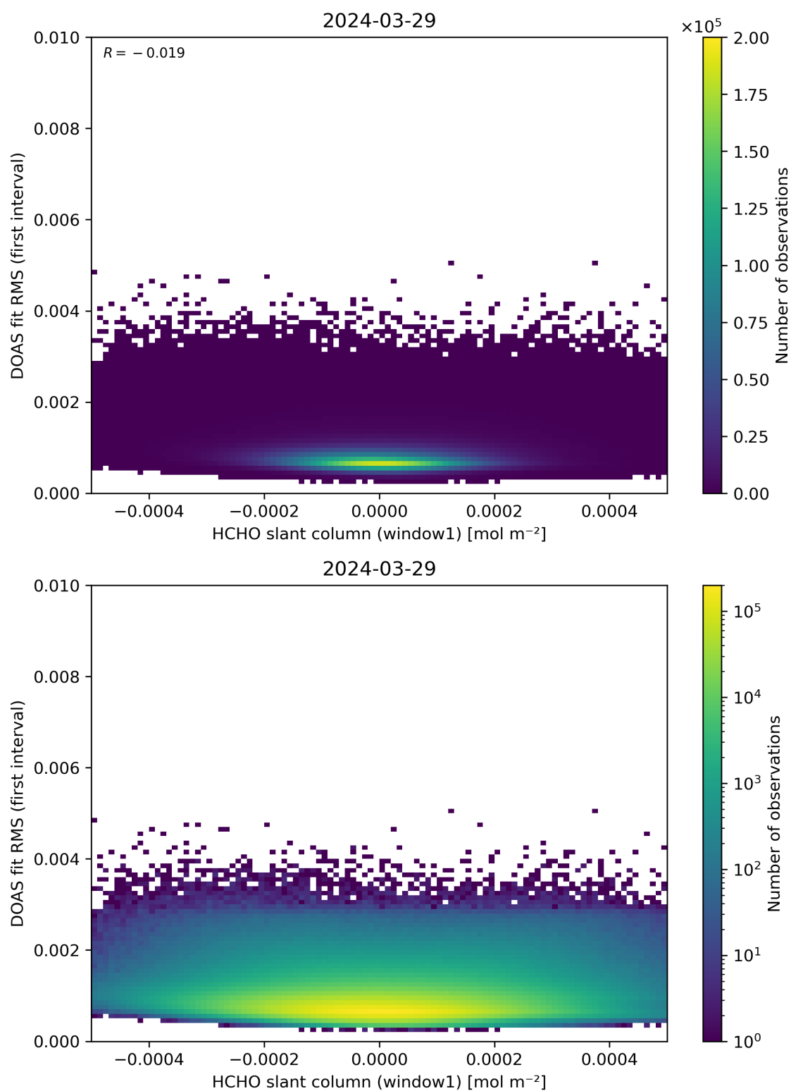
Figure 78: Scatter density plot of “HCHO slant column (window1)” against “DOAS fit RMS (first interval)” for 2024-03-28 to 2024-03-30.
