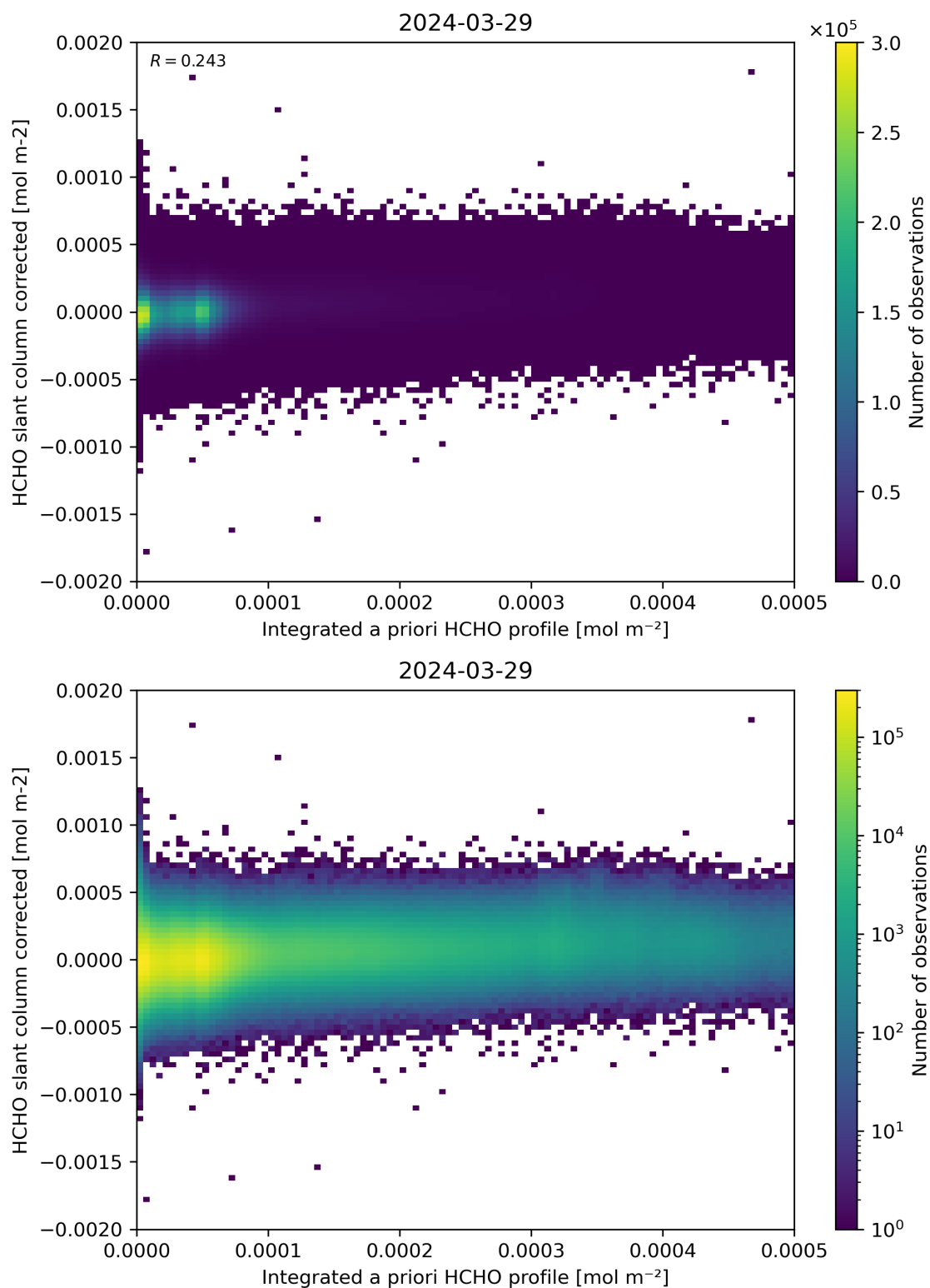
Figure 151: Scatter density plot of “Integrated a priori HCHO profile” against “HCHO slant column corrected” for 2024-03-28 to 2024-03-30.
