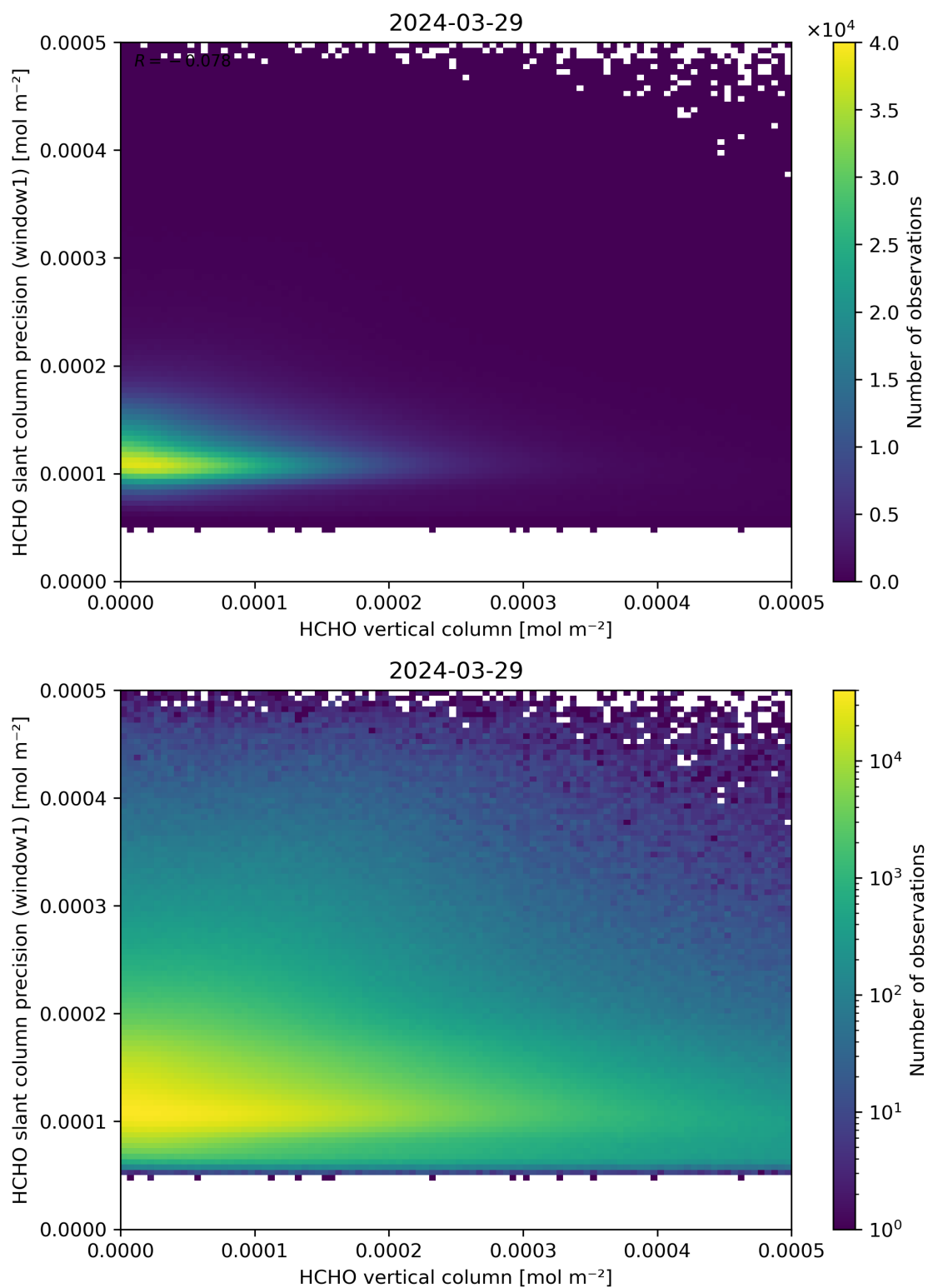
Figure 130: Scatter density plot of “HCHO vertical column” against “HCHO slant column precision (window1)” for 2024-03-28 to 2024-03-30.
