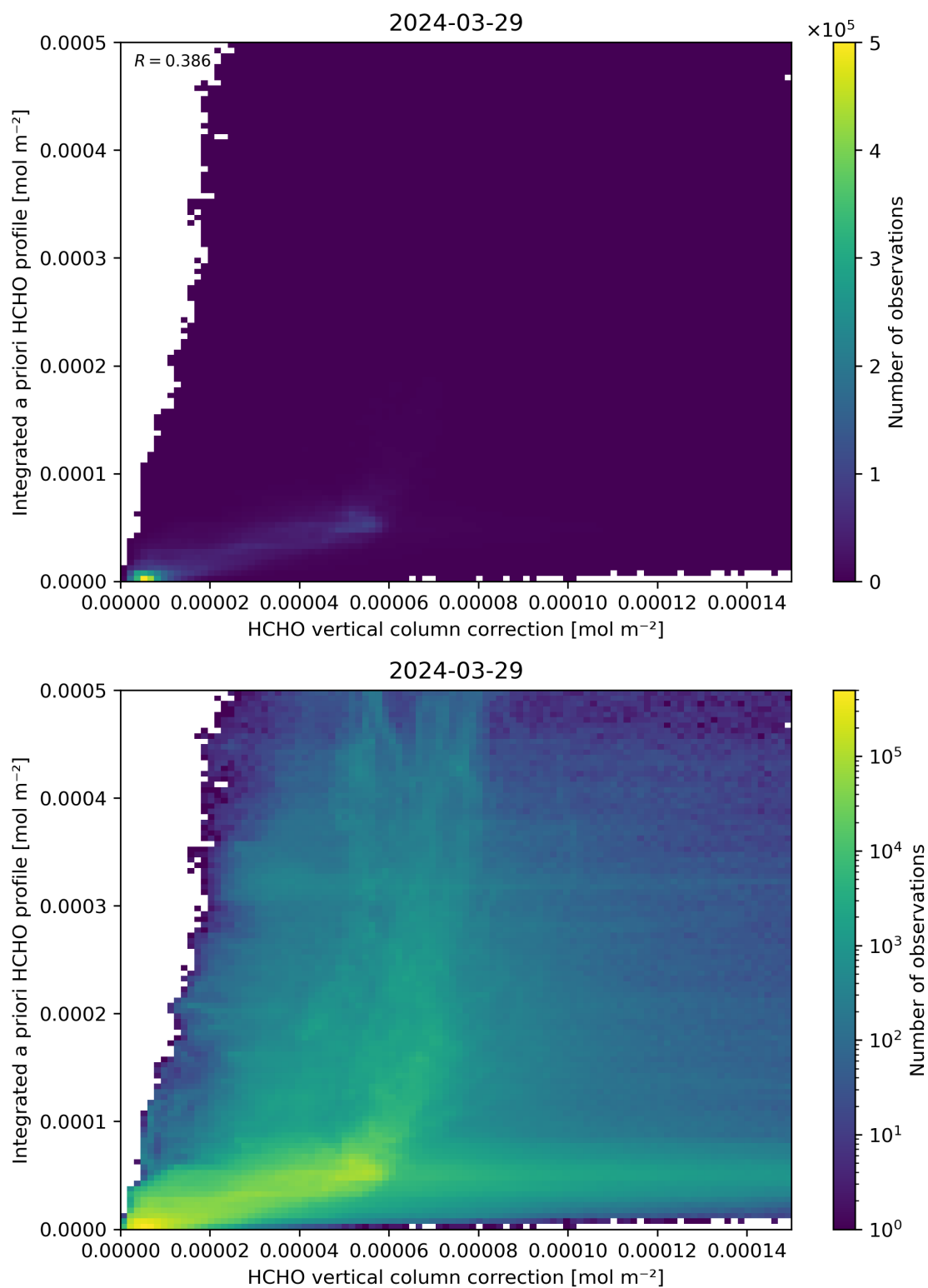
Figure 122: Scatter density plot of “HCHO vertical column correction” against “Integrated a priori HCHO profile” for 2024-03-28 to 2024-03-30.
