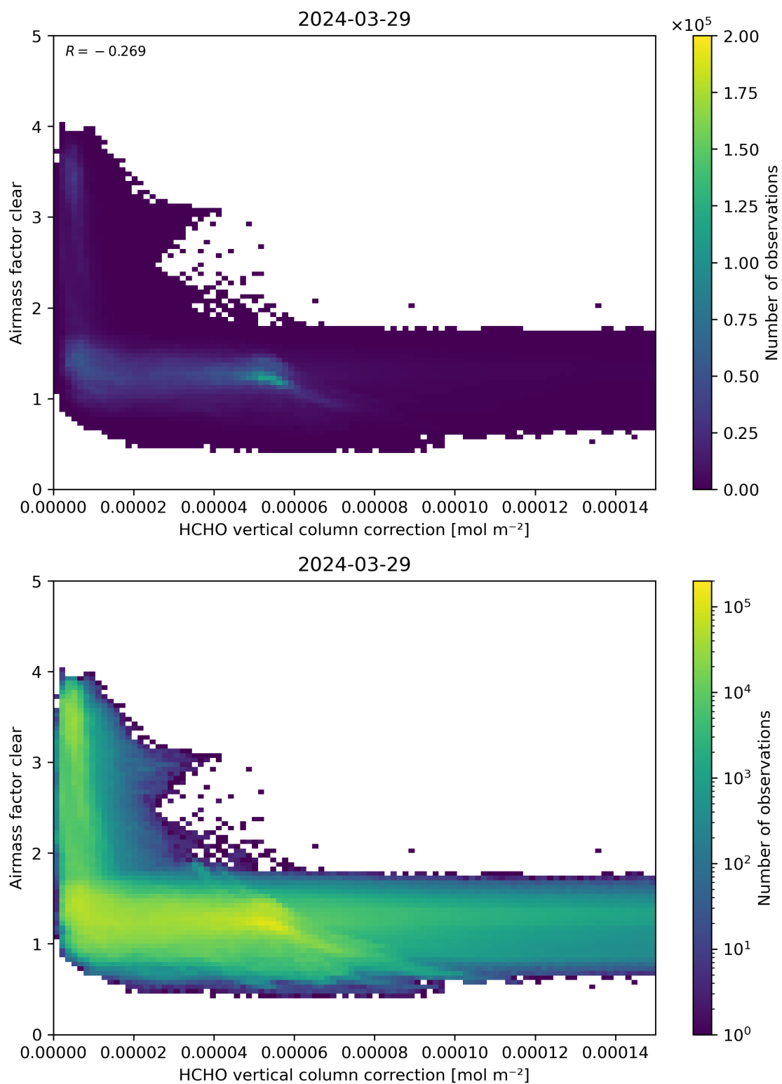
Figure 115: Scatter density plot of “HCHO vertical column correction” against “Airmass factor clear” for 2024-03-28 to 2024-03-30.
