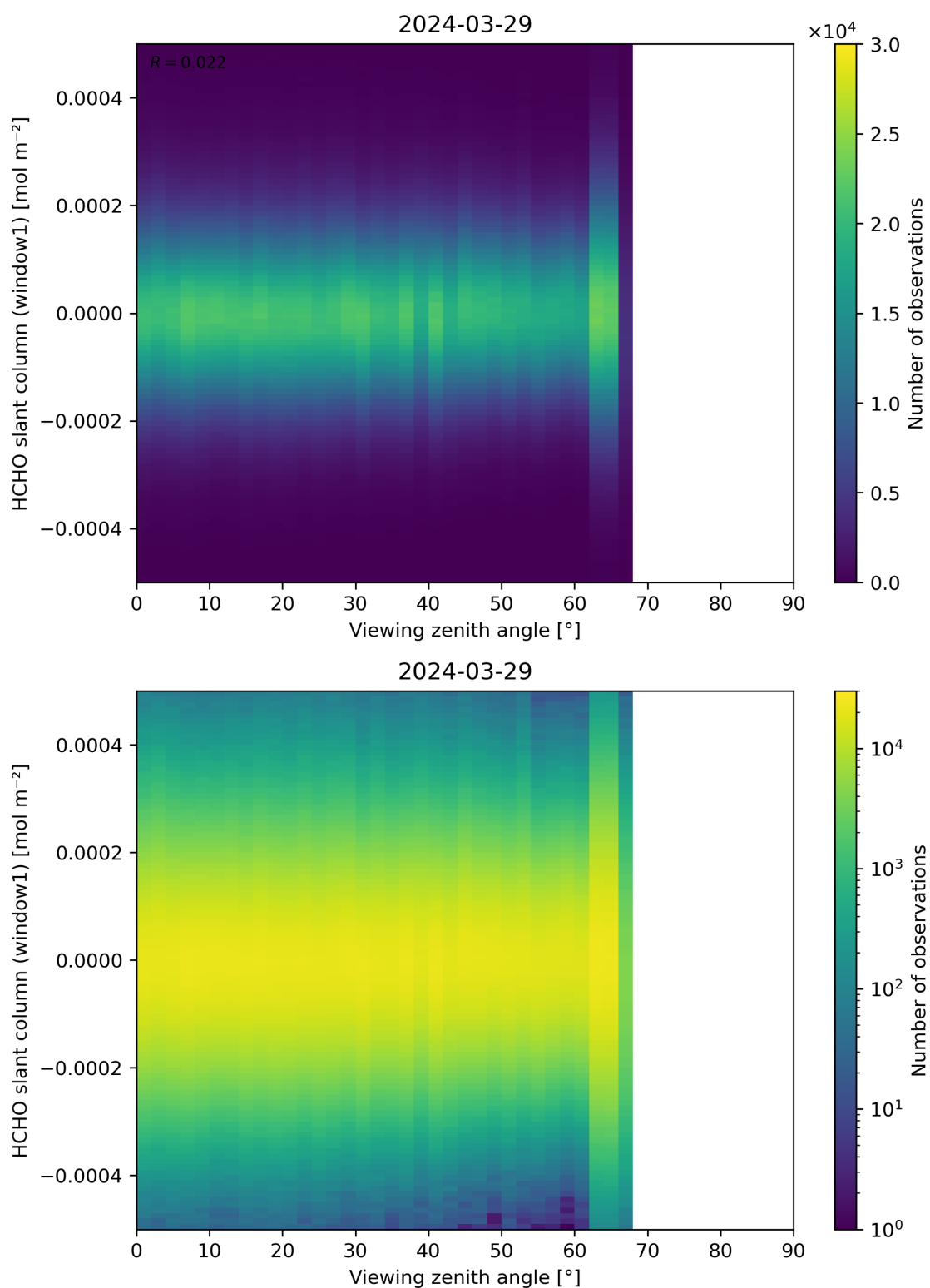
Figure 188: Scatter density plot of “Viewing zenith angle” against “HCHO slant column (window1)” for 2024-03-28 to 2024-03-30.
