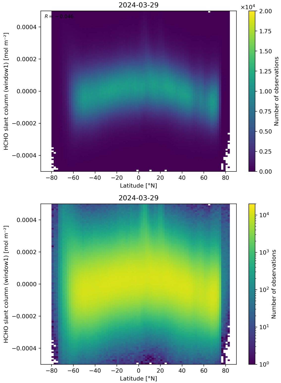
Figure 159: Scatter density plot of “Latitude” against “HCHO slant column (window1)” for 2024-03-28 to 2024-03-30.
