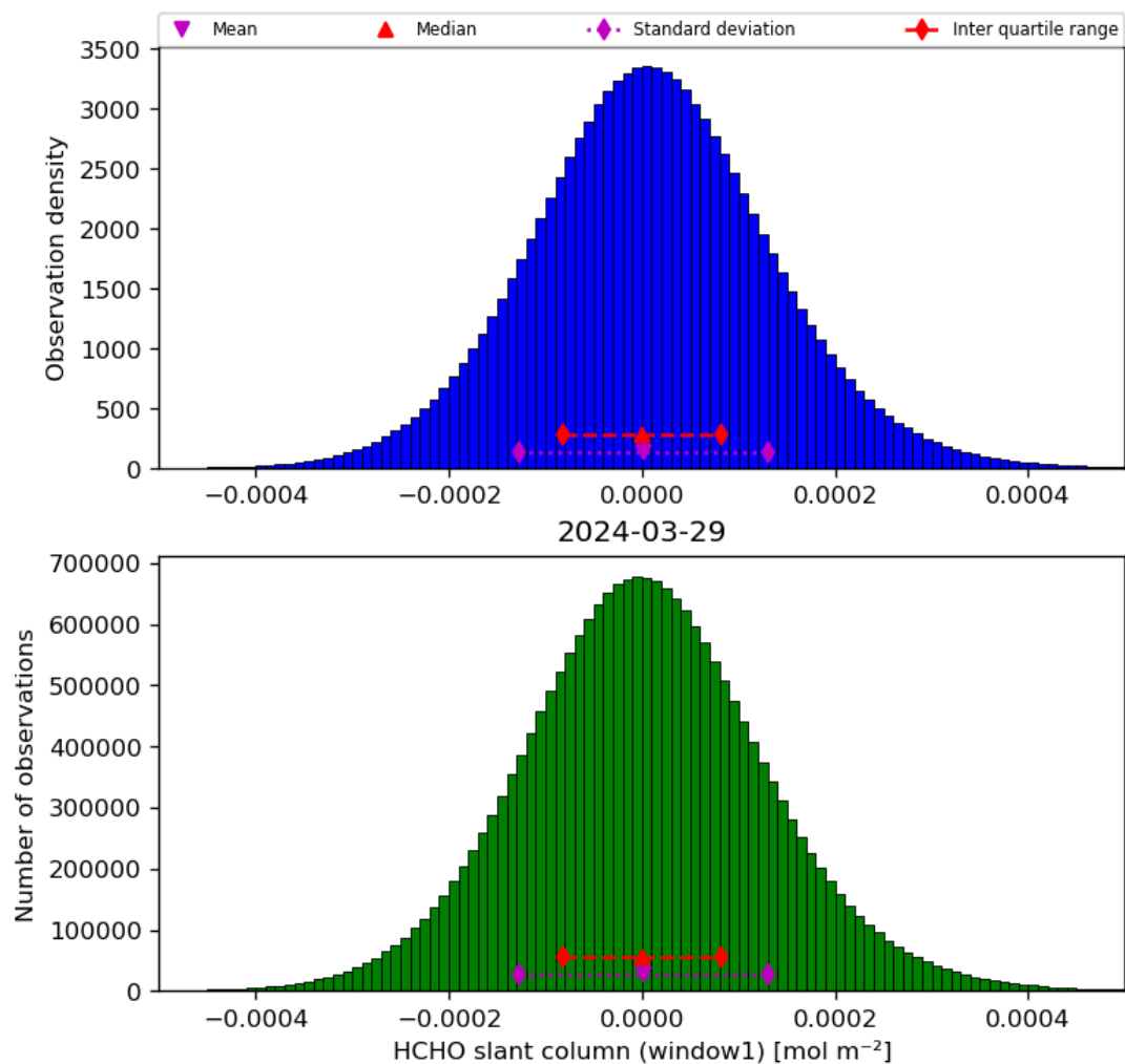
Figure 38: Histogram of “HCHO slant column (window1)” for 2024-03-28 to 2024-03-30
