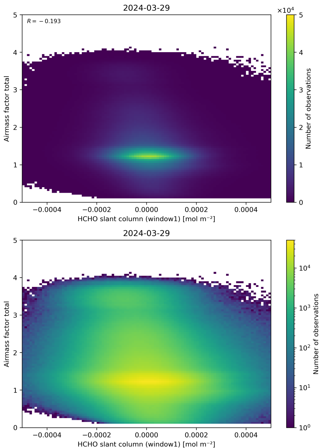
Figure 85: Scatter density plot of “HCHO slant column (window1)” against “Airmass factor total” for 2024-03-28 to 2024-03-30.
