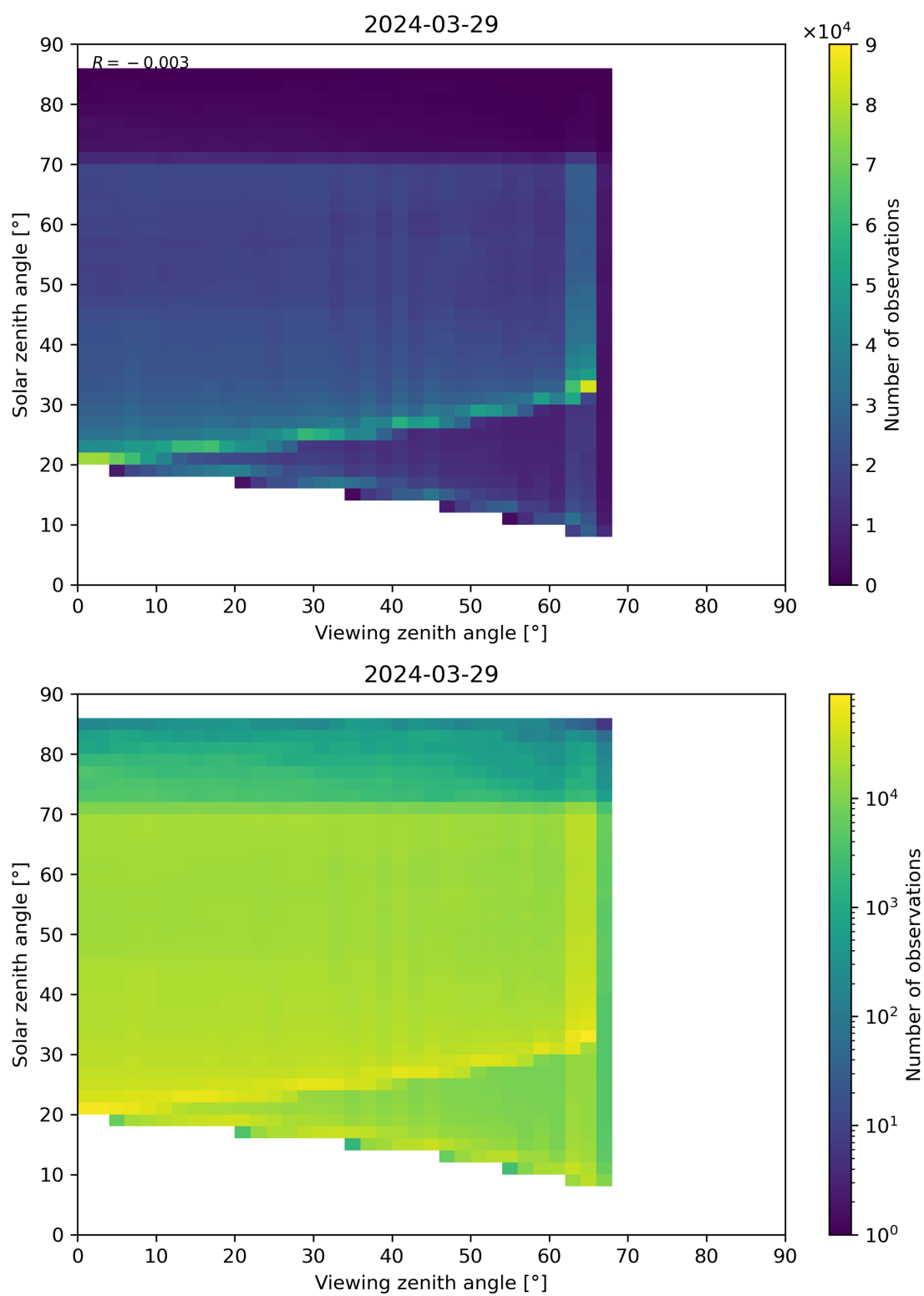
Figure 197: Scatter density plot of “Viewing zenith angle” against “Solar zenith angle” for 2024-03-28 to 2024-03-30.
