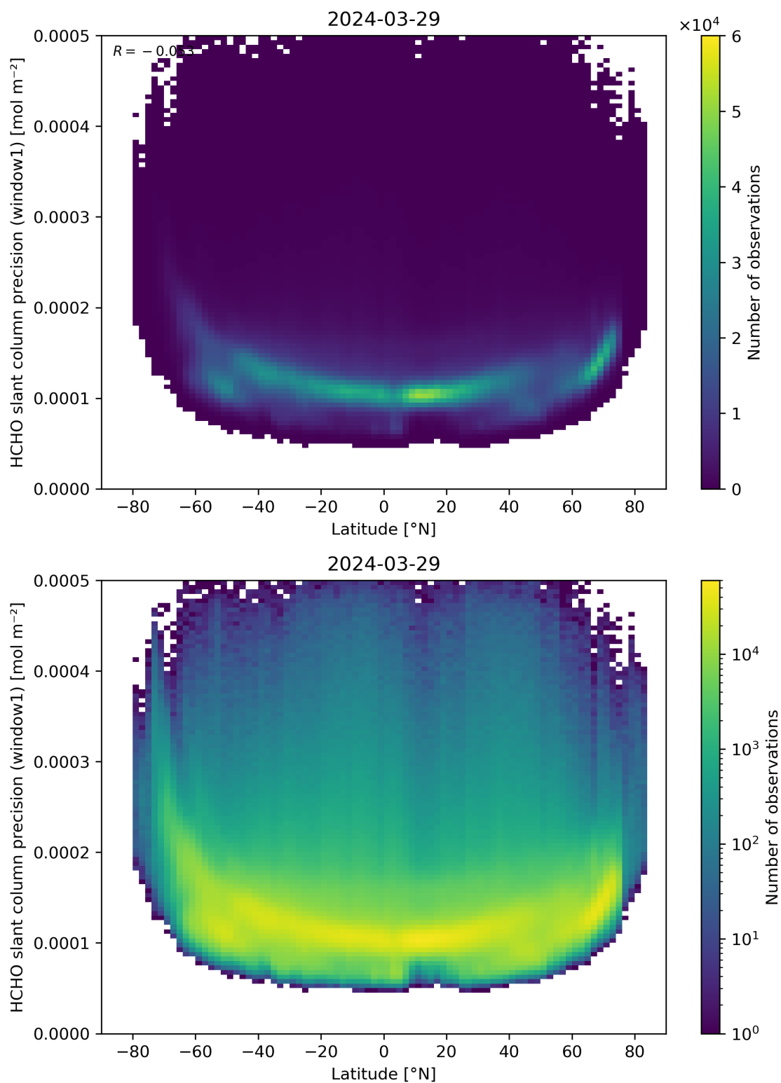
Figure 160: Scatter density plot of “Latitude” against “HCHO slant column precision (window1)” for 2024-03-28 to 2024-03-30.
