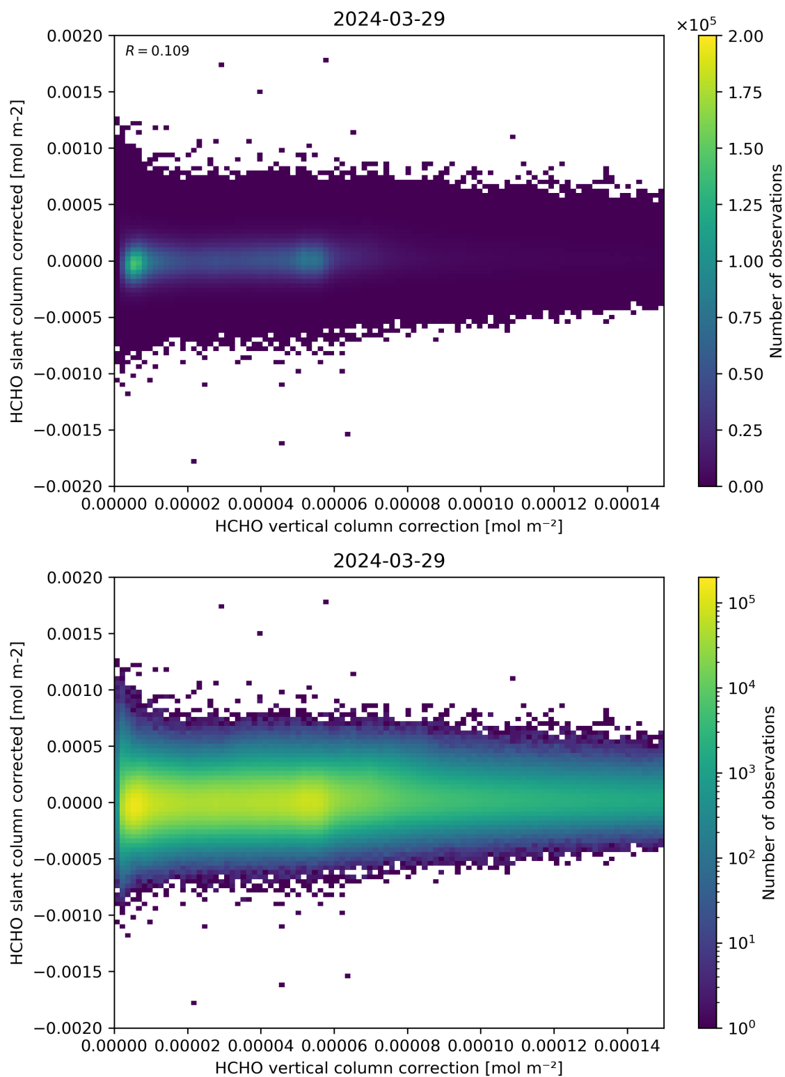
Figure 116: Scatter density plot of “HCHO vertical column correction” against “HCHO slant column corrected” for 2024-03-28 to 2024-03-30.
