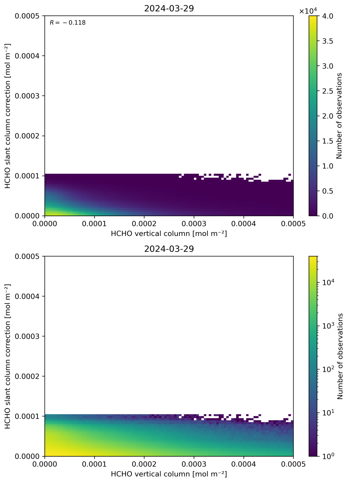
Figure 128: Scatter density plot of “HCHO vertical column” against “HCHO slant column correction” for 2024-03-28 to 2024-03-30.
