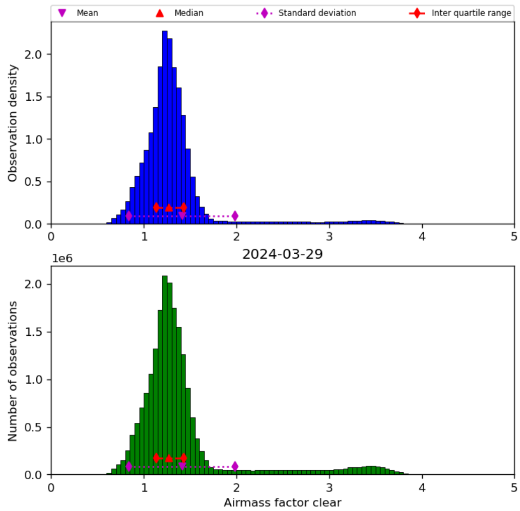
Figure 42: Histogram of “Airmass factor clear” for 2024-03-28 to 2024-03-30
