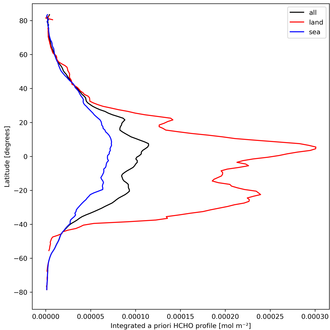
Figure 29: Zonal average of “Integrated a priori HCHO profile” for 2024-03-28 to 2024-03-30.
