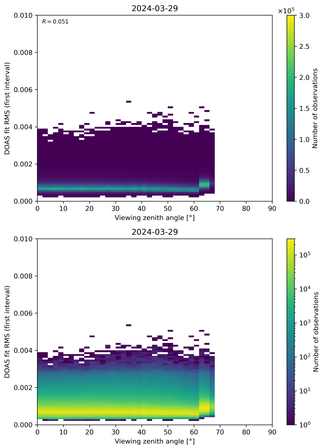
Figure 182: Scatter density plot of “Viewing zenith angle” against “DOAS fit RMS (first interval)” for 2024-03-28 to 2024-03-30.
