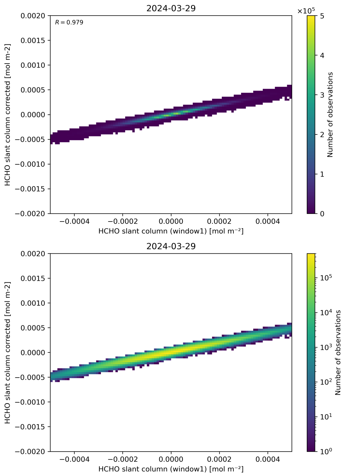
Figure 82: Scatter density plot of “HCHO slant column (window1)” against “HCHO slant column corrected” for 2024-03-28 to 2024-03-30.
