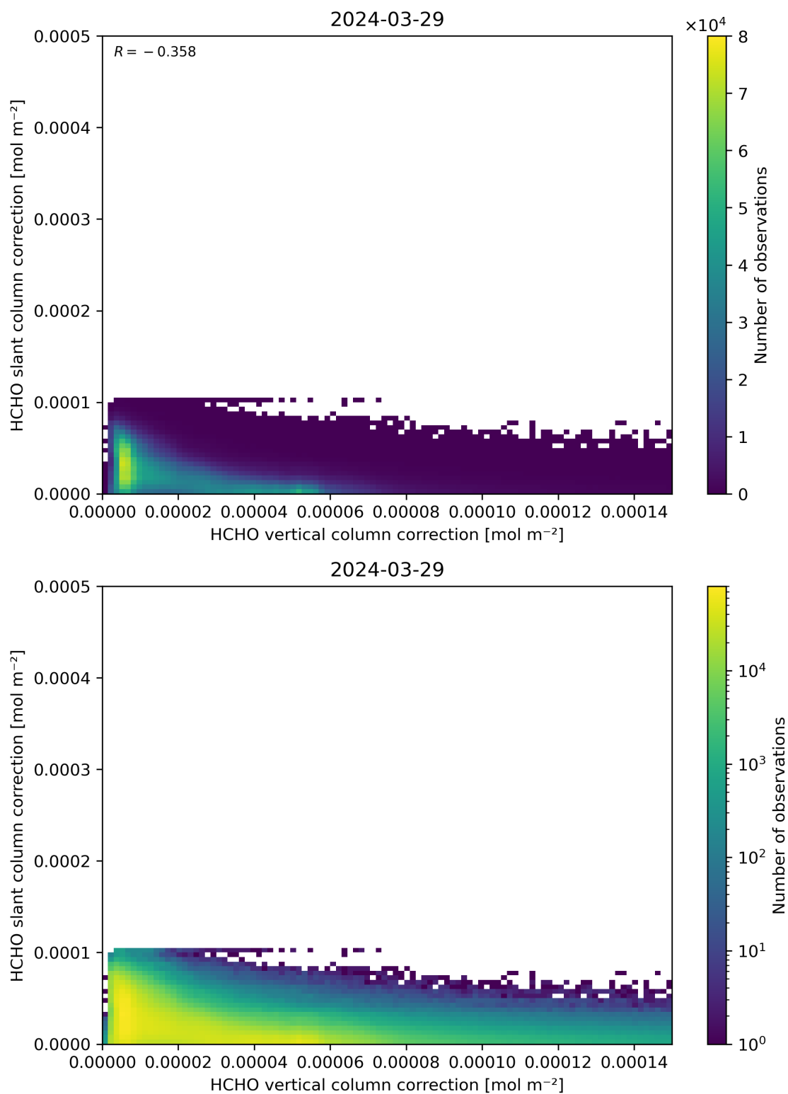
Figure 117: Scatter density plot of “HCHO vertical column correction” against “HCHO slant column correction” for 2024-03-28 to 2024-03-30.
