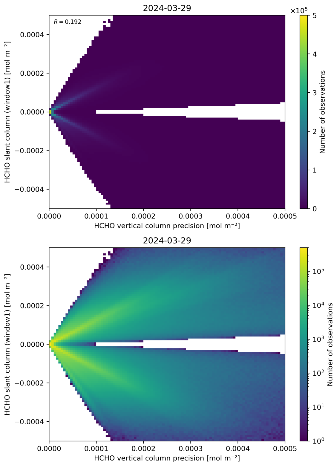
Figure 142: Scatter density plot of “HCHO vertical column precision” against “HCHO slant column (window1)” for 2024-03-28 to 2024-03-30.
