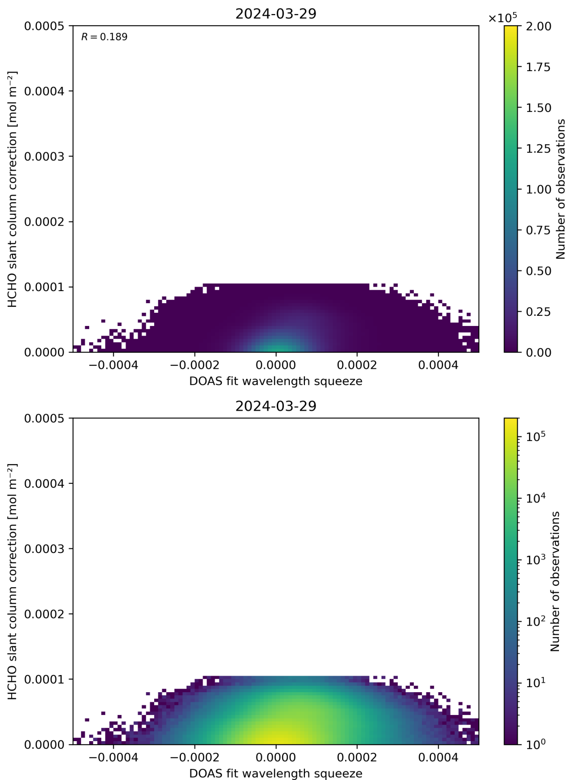
Figure 70: Scatter density plot of “DOAS fit wavelength squeeze” against “HCHO slant column correction” for 2024-03-28 to 2024-03-30.
