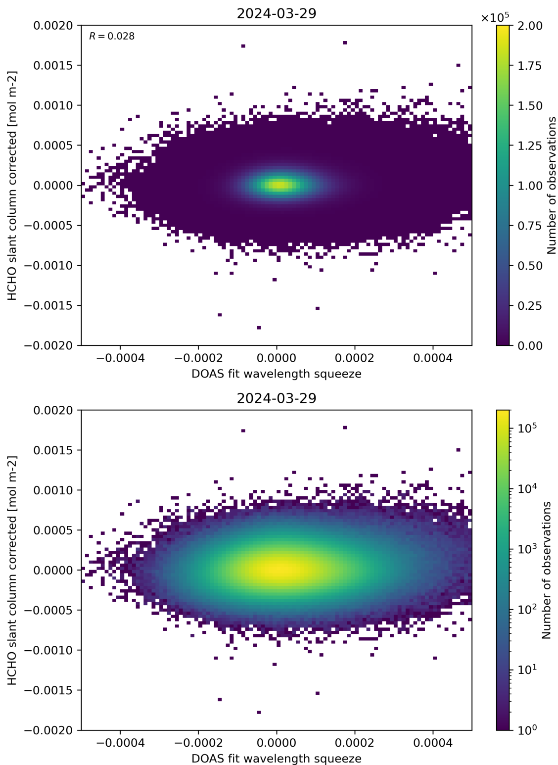
Figure 69: Scatter density plot of “DOAS fit wavelength squeeze” against “HCHO slant column corrected” for 2024-03-28 to 2024-03-30.
