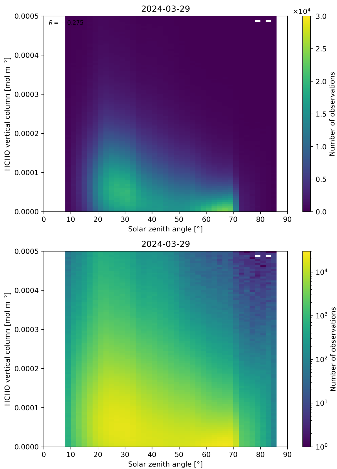
Figure 177: Scatter density plot of “Solar zenith angle” against “HCHO vertical column” for 2024-03-28 to 2024-03-30.
