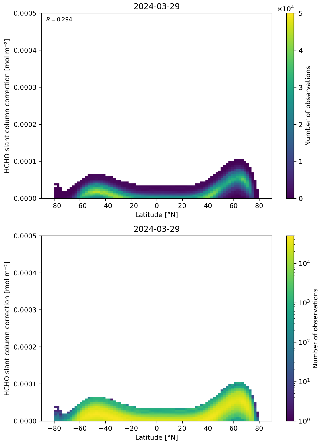
Figure 158: Scatter density plot of “Latitude” against “HCHO slant column correction” for 2024-03-28 to 2024-03-30.
