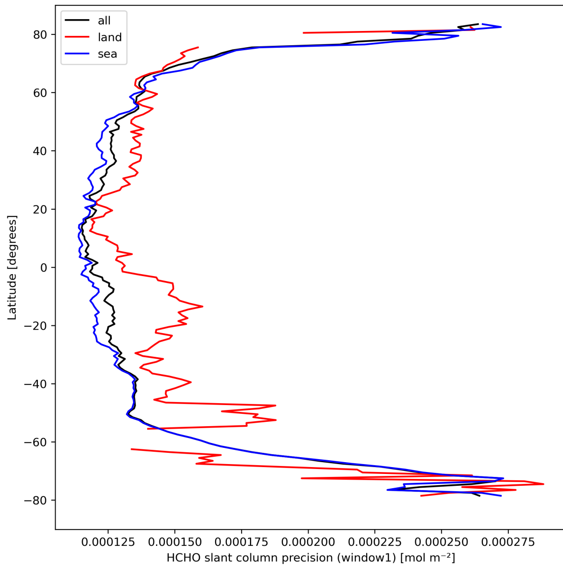
Figure 25: Zonal average of “HCHO slant column precision (window1)” for 2024-03-28 to 2024-03-30.
