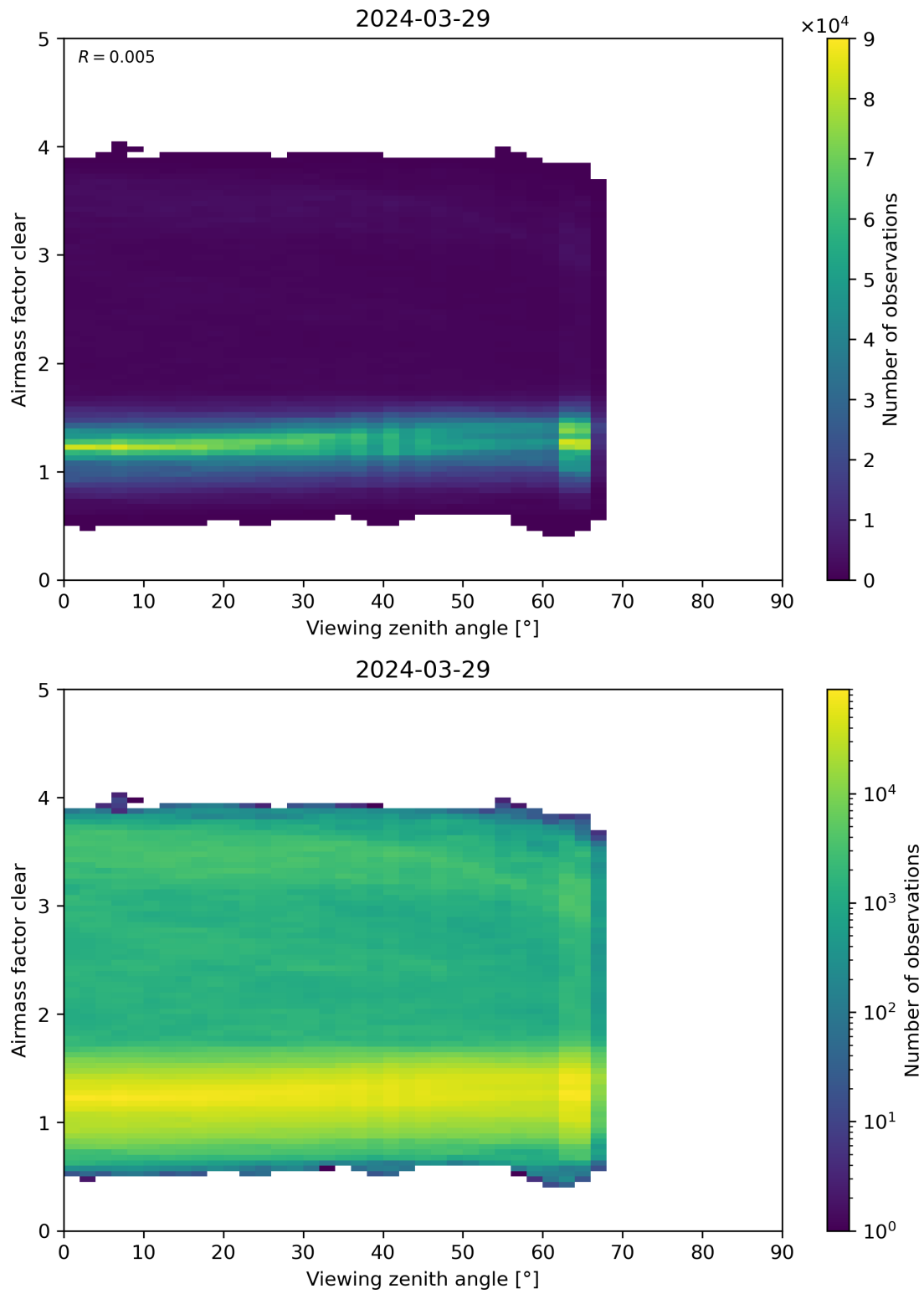
Figure 185: Scatter density plot of “Viewing zenith angle” against “Airmass factor clear” for 2024-03-28 to 2024-03-30.
