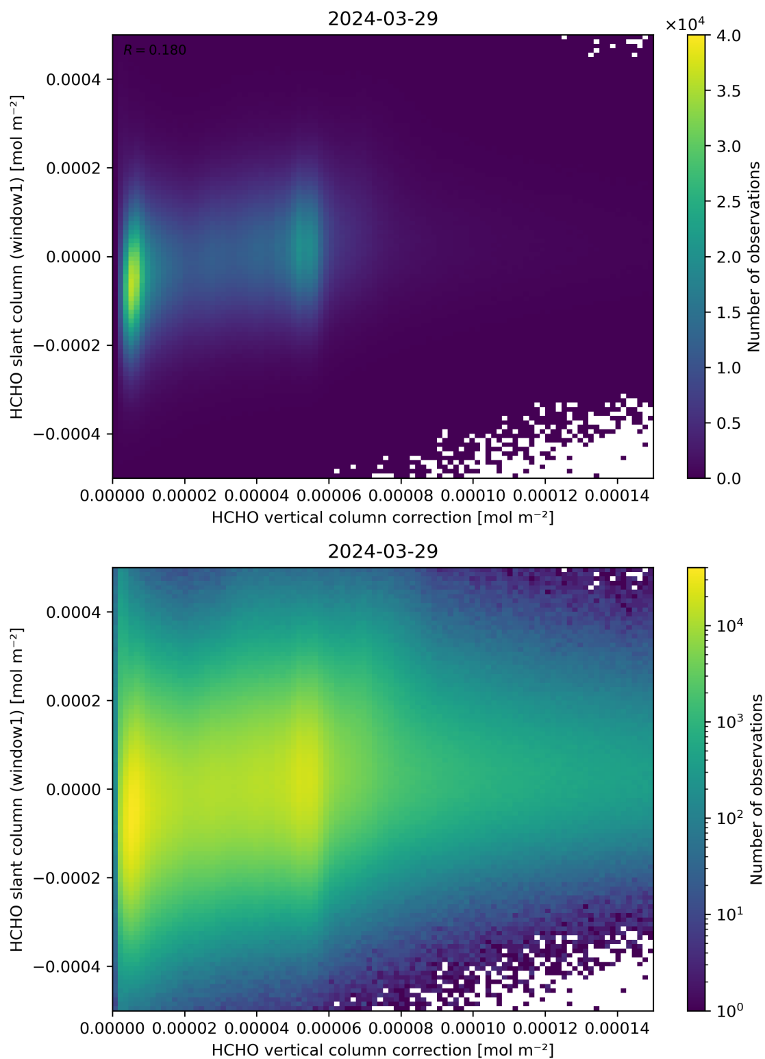
Figure 118: Scatter density plot of “HCHO vertical column correction” against “HCHO slant column (window1)” for 2024-03-28 to 2024-03-30.
