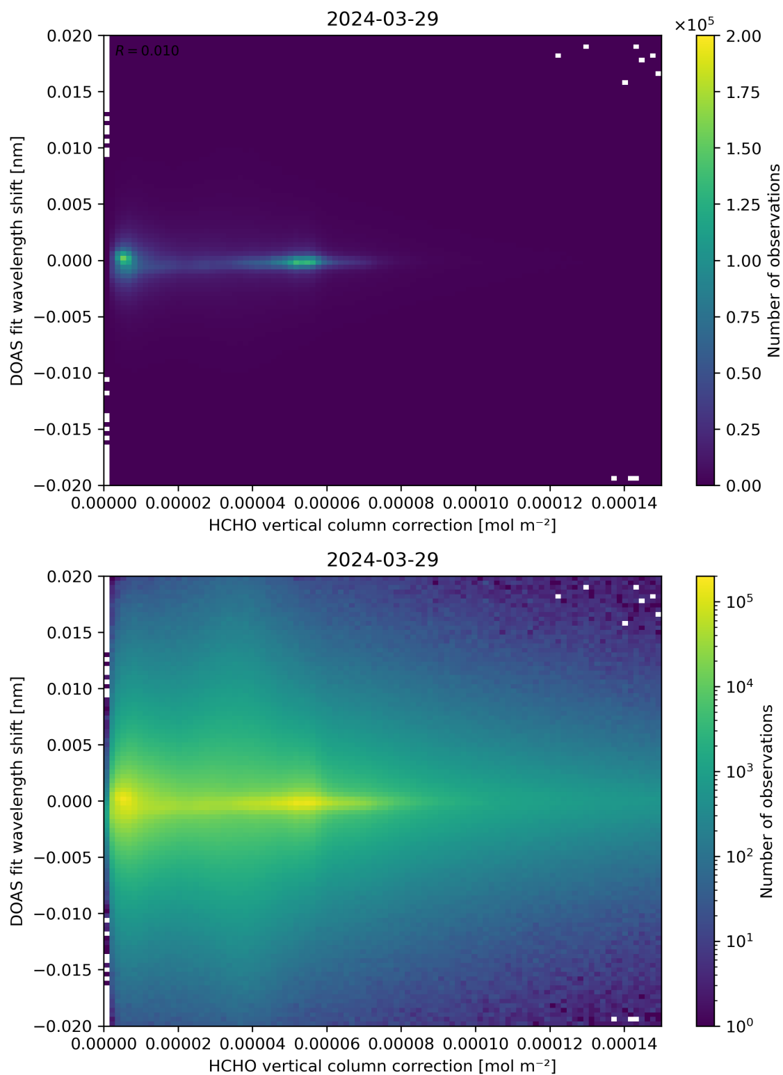
Figure 113: Scatter density plot of “HCHO vertical column correction” against “DOAS fit wavelength shift” for 2024-03-28 to 2024-03-30.
