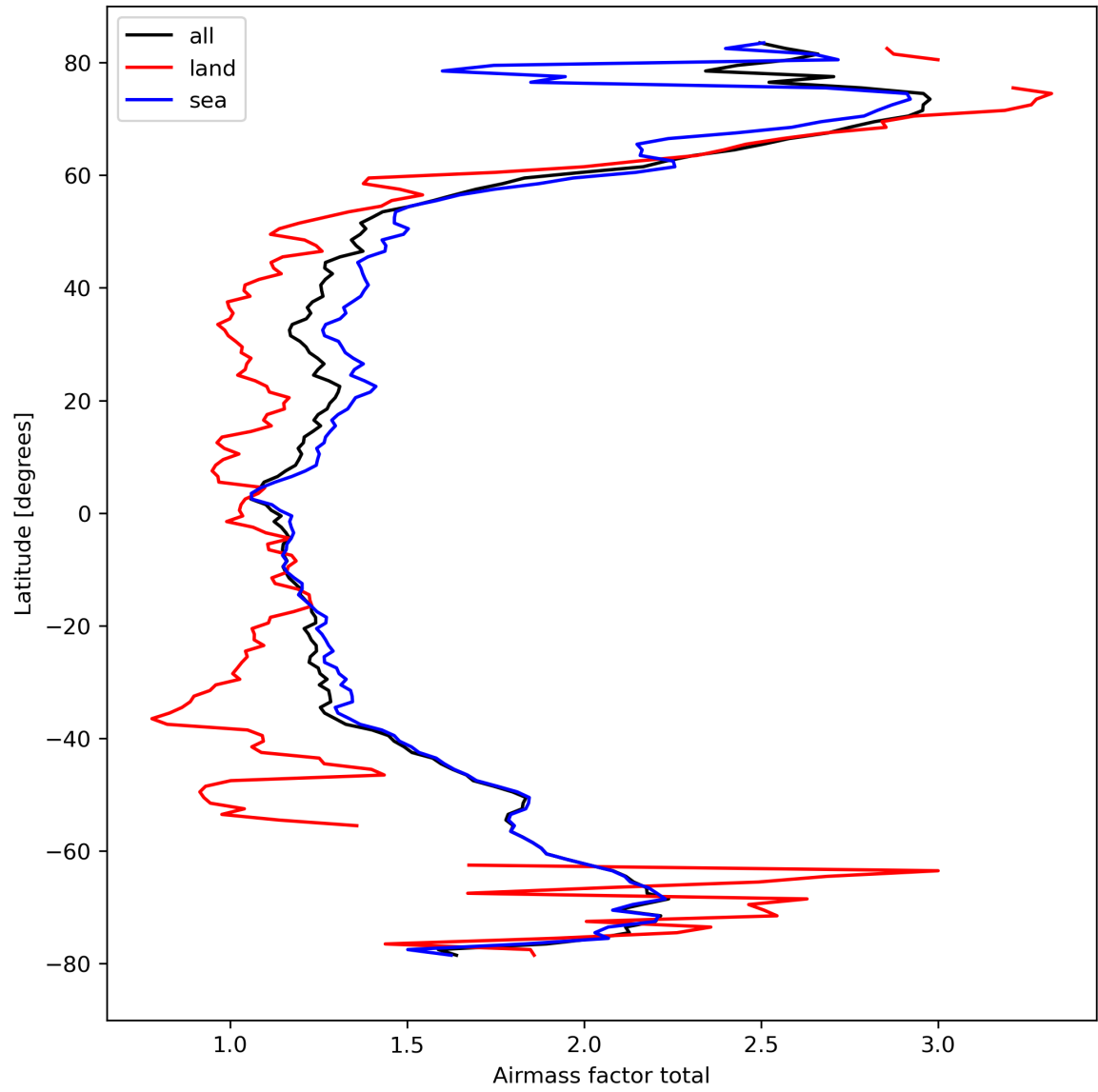
Figure 26: Zonal average of “Airmass factor total” for 2024-03-28 to 2024-03-30.
