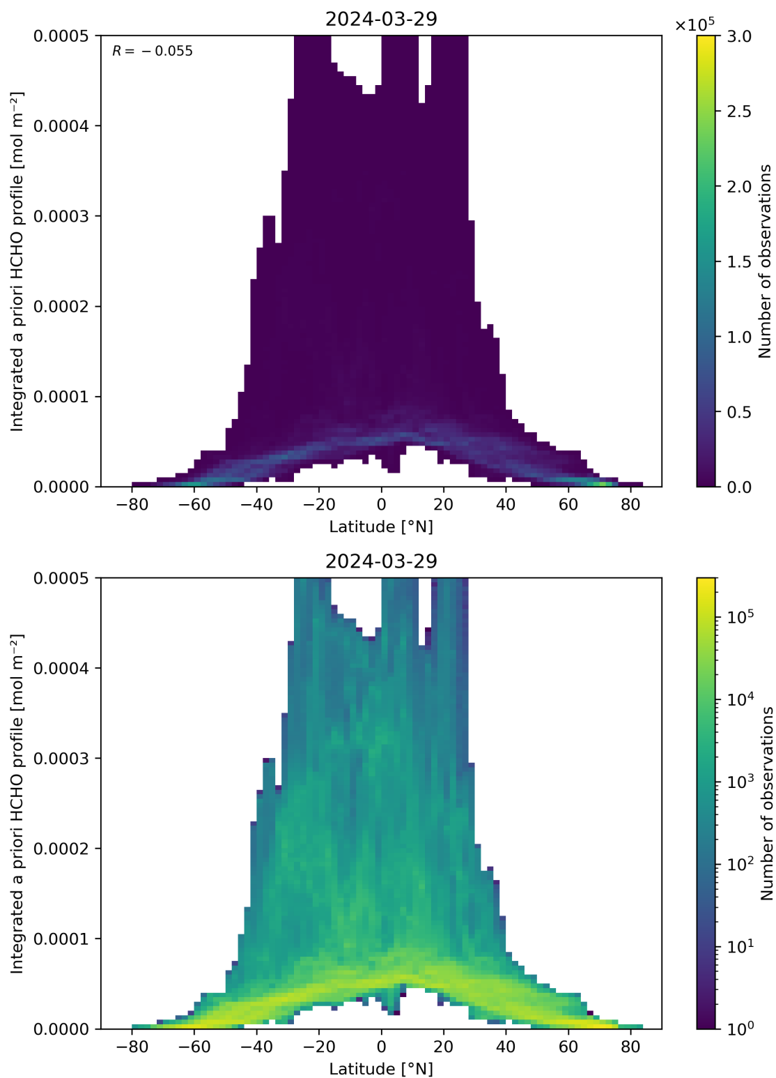
Figure 166: Scatter density plot of “Latitude” against “Integrated a priori HCHO profile” for 2024-03-28 to 2024-03-30.
