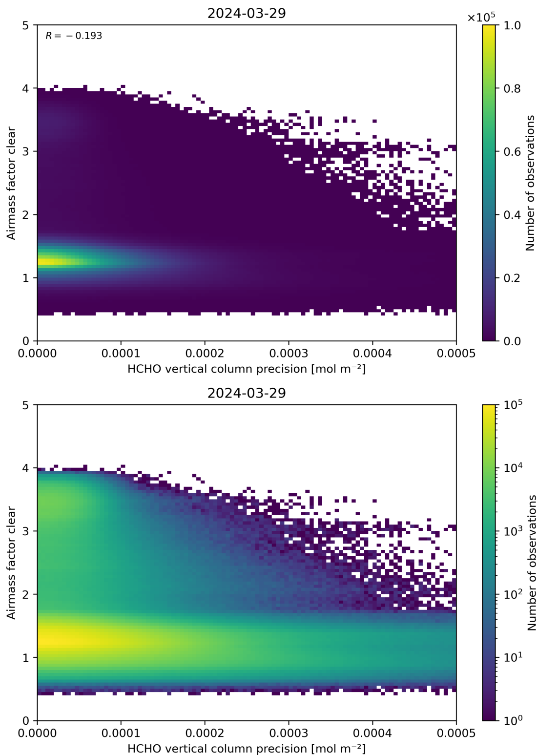
Figure 139: Scatter density plot of “HCHO vertical column precision” against “Airmass factor clear” for 2024-03-28 to 2024-03-30.
