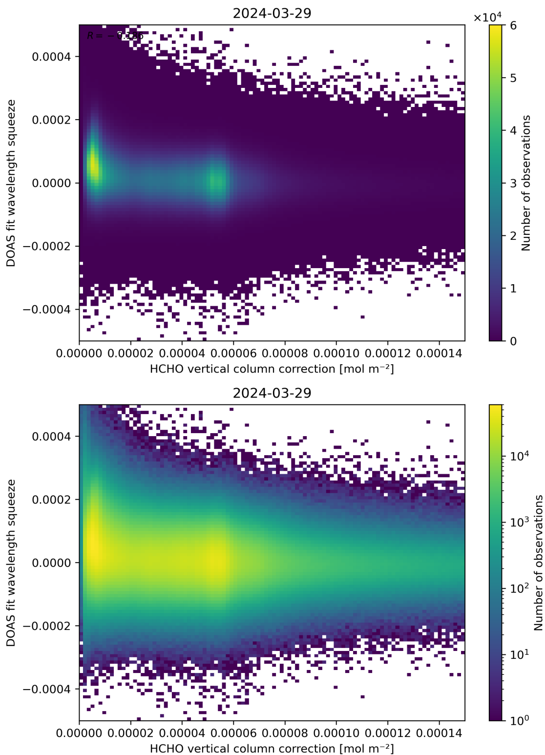
Figure 114: Scatter density plot of “HCHO vertical column correction” against “DOAS fit wavelength squeeze” for 2024-03-28 to 2024-03-30.
