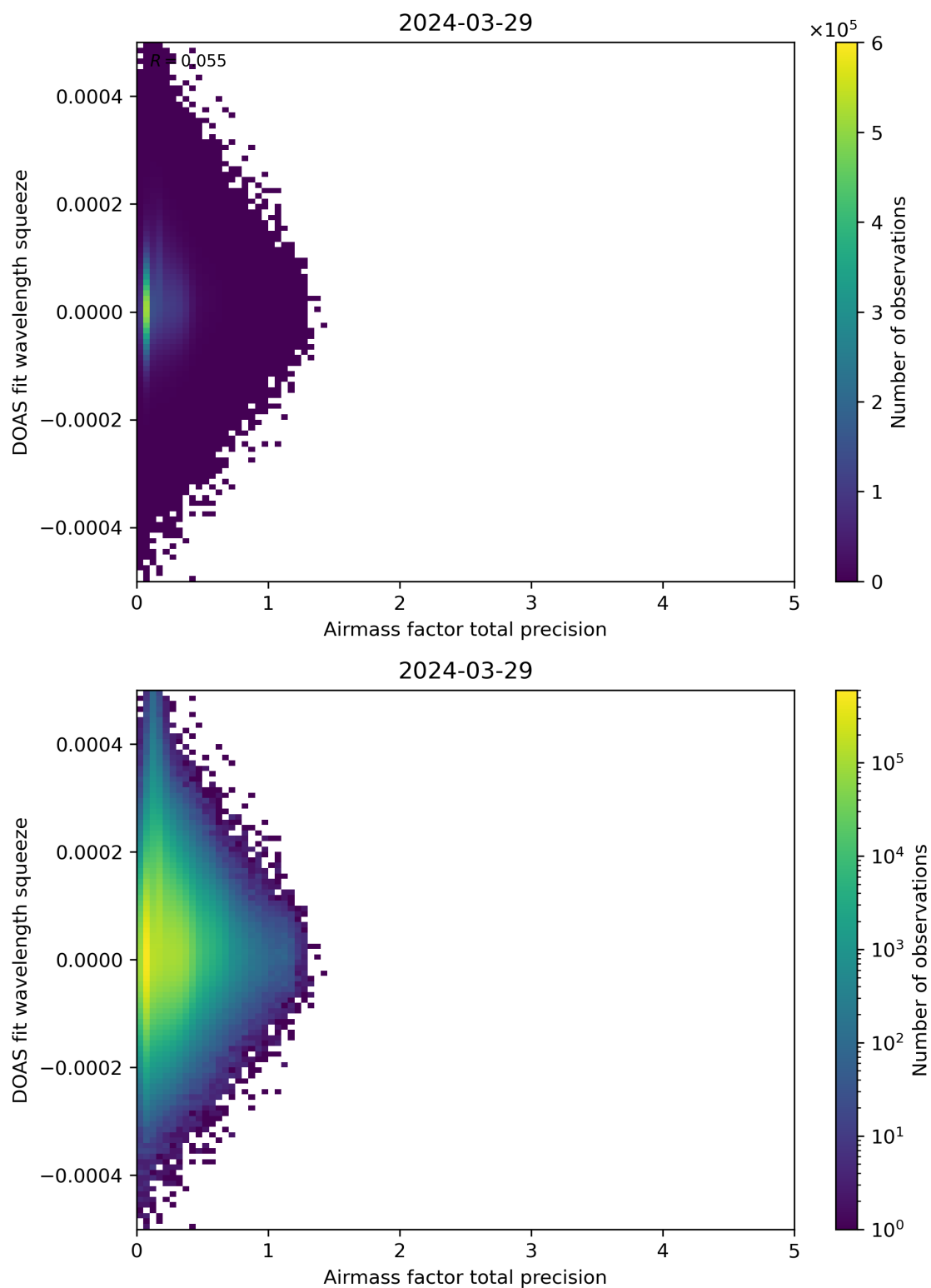
Figure 107: Scatter density plot of “Airmass factor total precision” against “DOAS fit wavelength squeeze” for 2024-03-28 to 2024-03-30.
