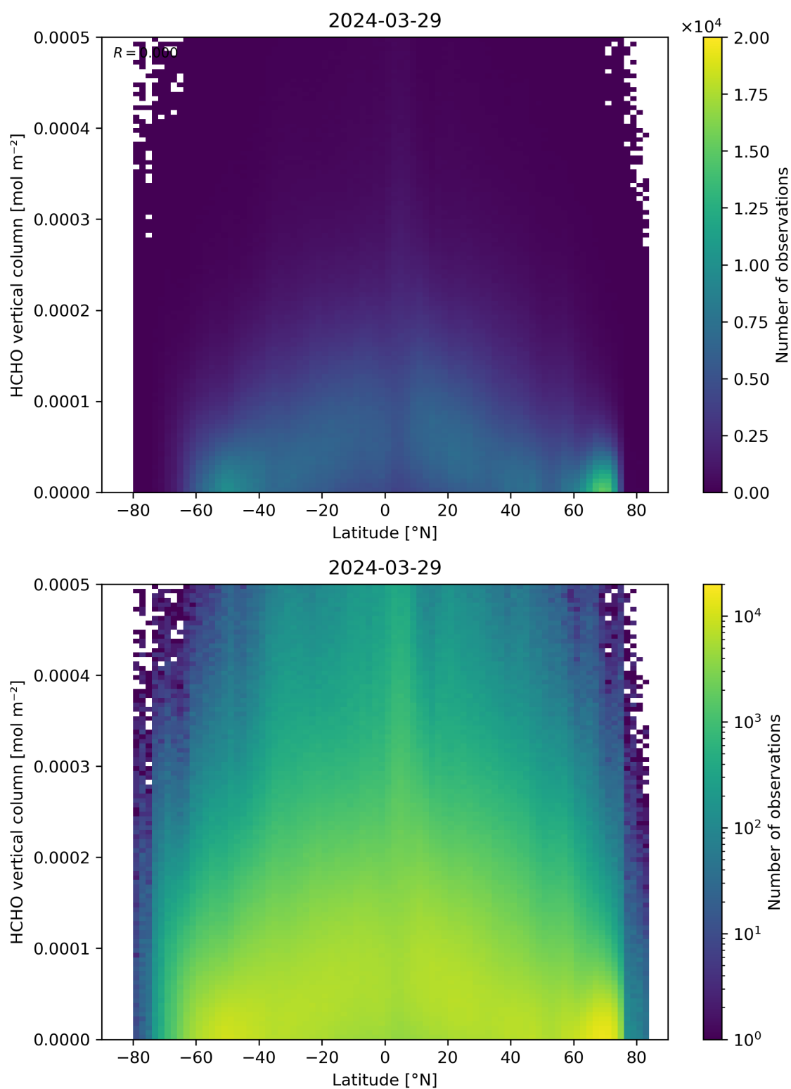
Figure 163: Scatter density plot of “Latitude” against “HCHO vertical column” for 2024-03-28 to 2024-03-30.
