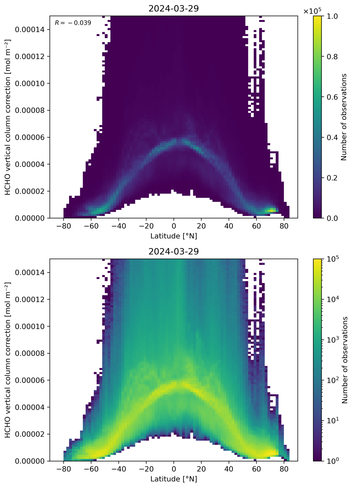
Figure 164: Scatter density plot of “Latitude” against “HCHO vertical column correction” for 2024-03-28 to 2024-03-30.
