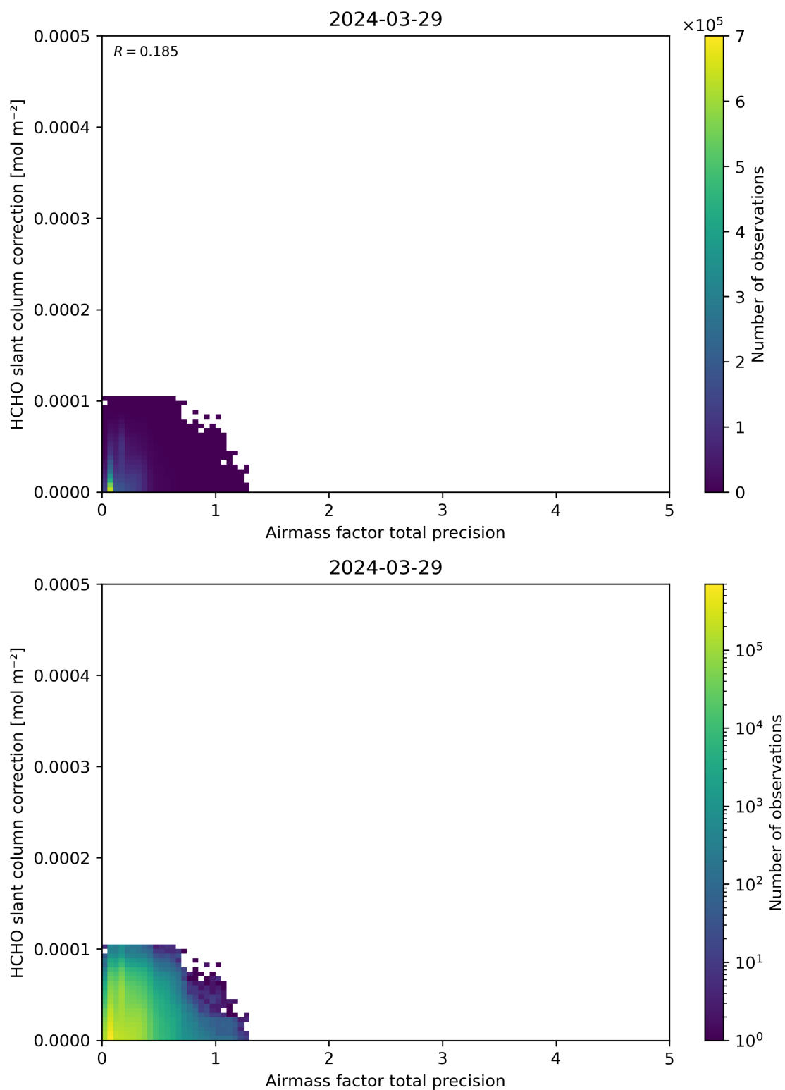
Figure 110: Scatter density plot of “Airmass factor total precision” against “HCHO slant column correction” for 2024-03-28 to 2024-03-30.
