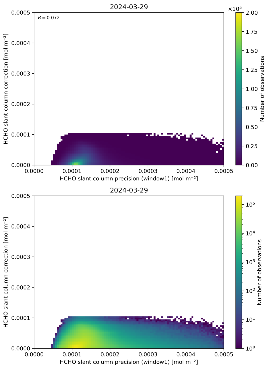
Figure 93: Scatter density plot of “HCHO slant column precision (window1)” against “HCHO slant column correction” for 2024-03-28 to 2024-03-30.
