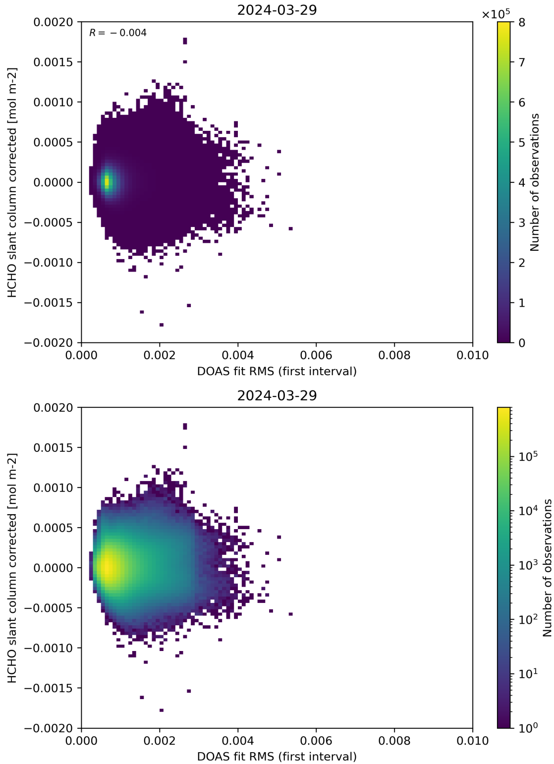
Figure 62: Scatter density plot of “DOAS fit RMS (first interval)” against “HCHO slant column corrected” for 2024-03-28 to 2024-03-30.
