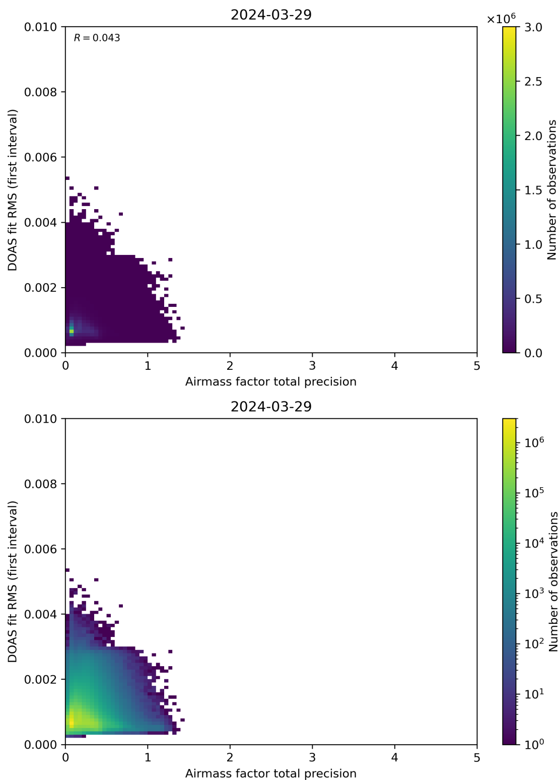
Figure 105: Scatter density plot of “Airmass factor total precision” against “DOAS fit RMS (first interval)” for 2024-03-28 to 2024-03-30.
