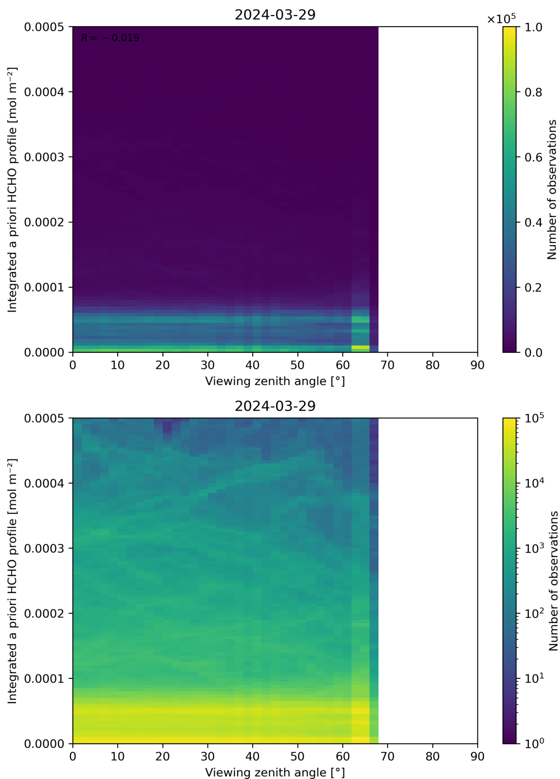
Figure 195: Scatter density plot of “Viewing zenith angle” against “Integrated a priori HCHO profile” for 2024-03-28 to 2024-03-30.
