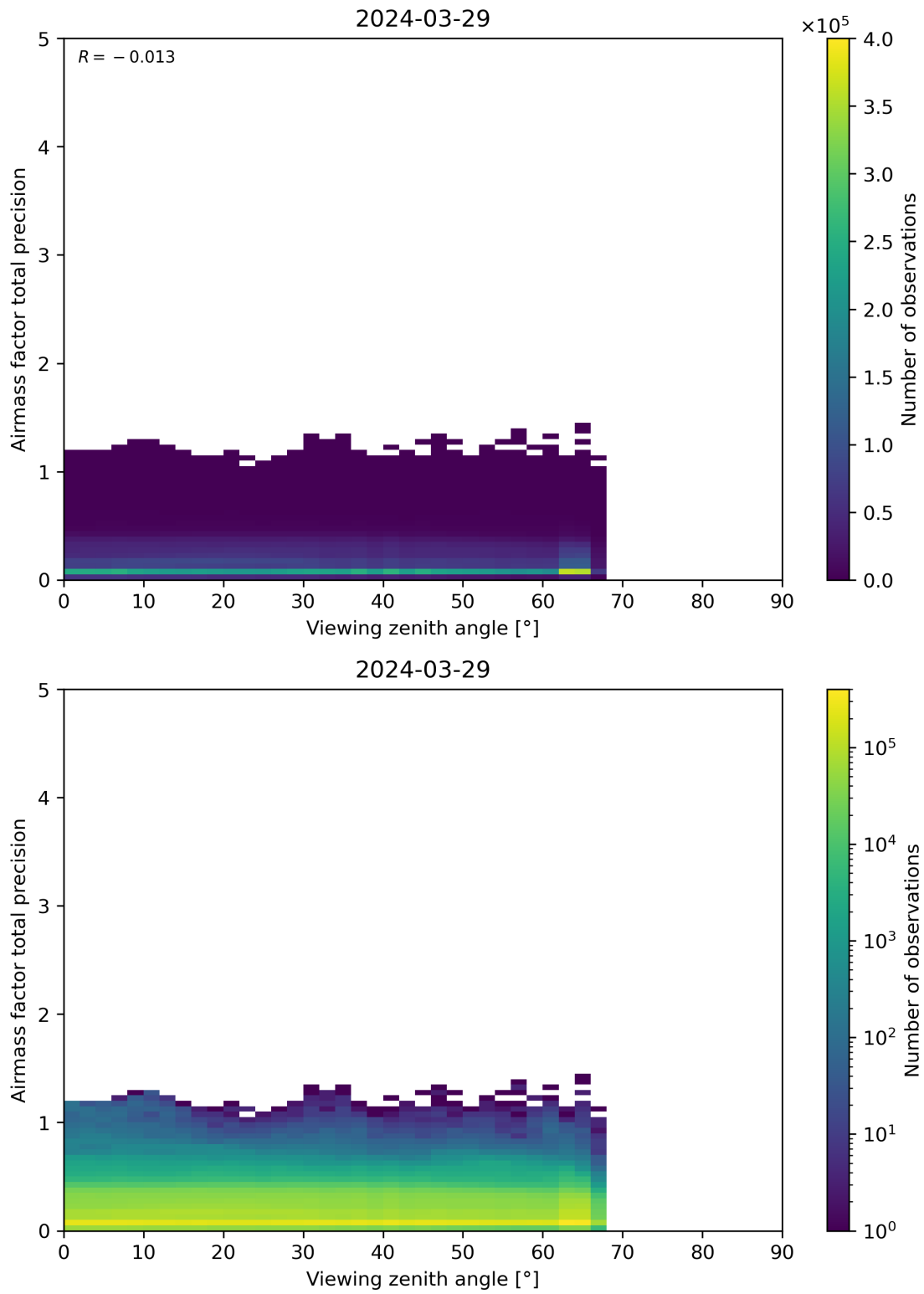
Figure 191: Scatter density plot of “Viewing zenith angle” against “Airmass factor total precision” for 2024-03-28 to 2024-03-30.
