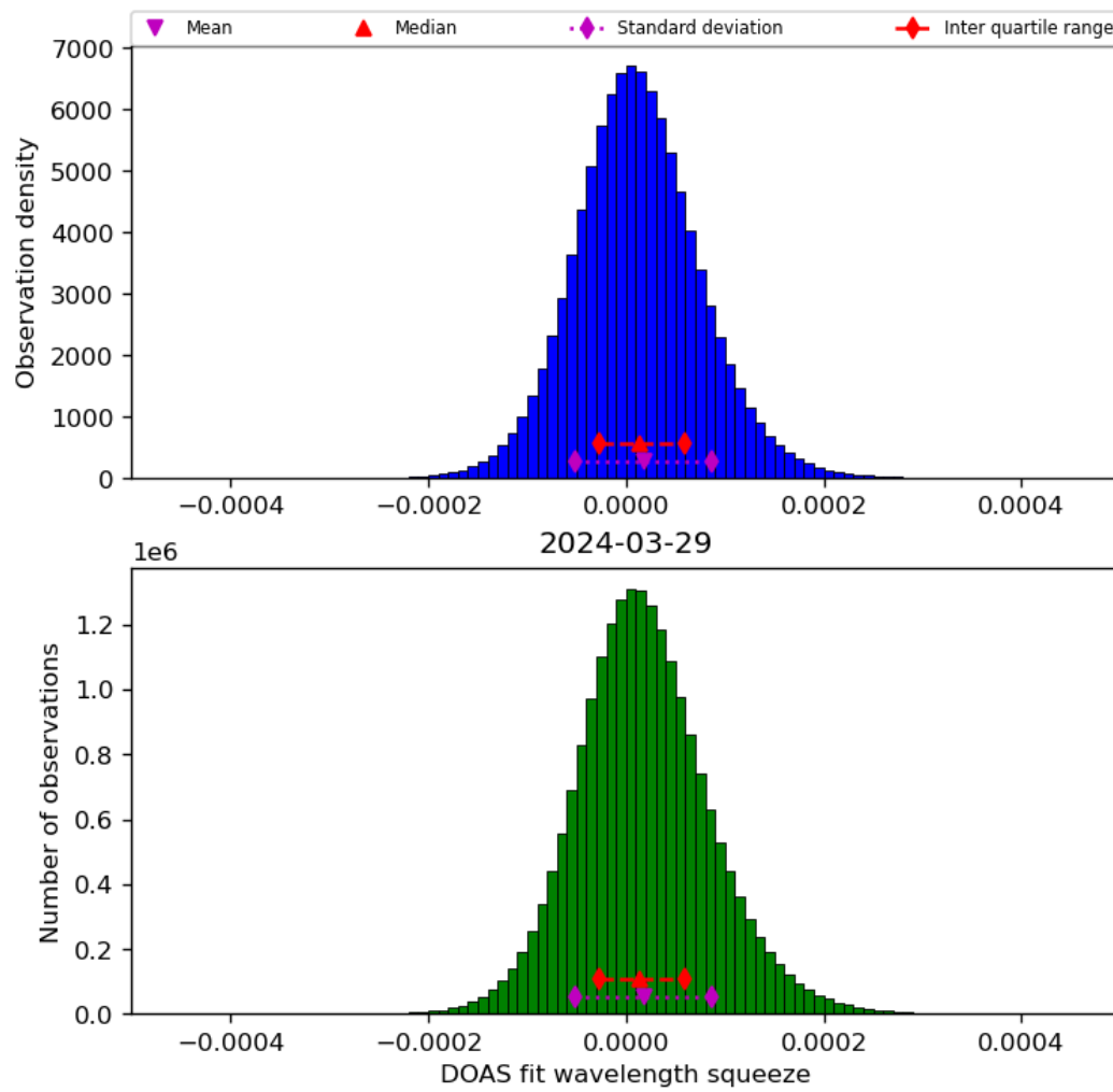
Figure 45: Histogram of “DOAS fit wavelength squeeze” for 2024-03-28 to 2024-03-30
