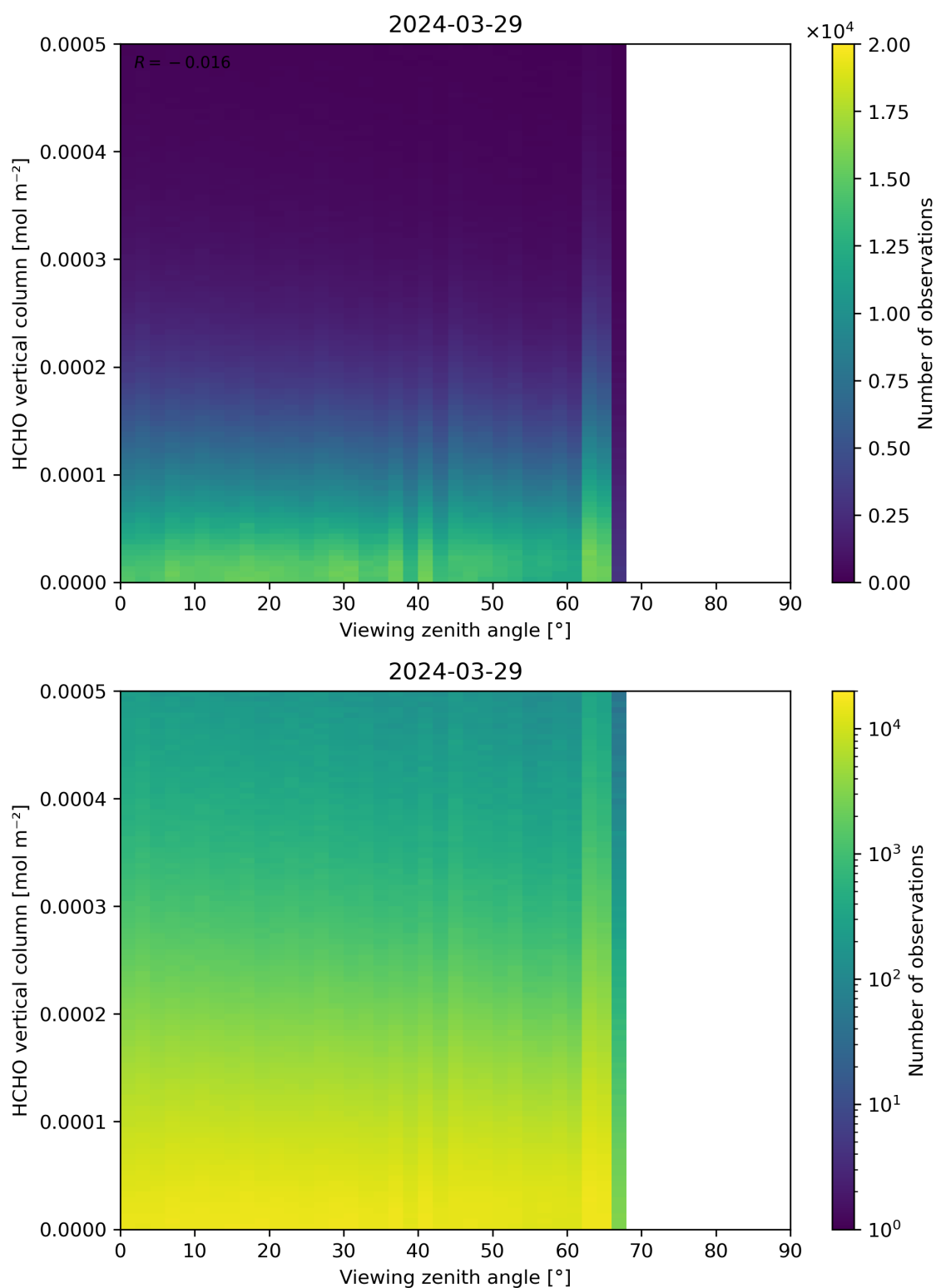
Figure 192: Scatter density plot of “Viewing zenith angle” against “HCHO vertical column” for 2024-03-28 to 2024-03-30.
