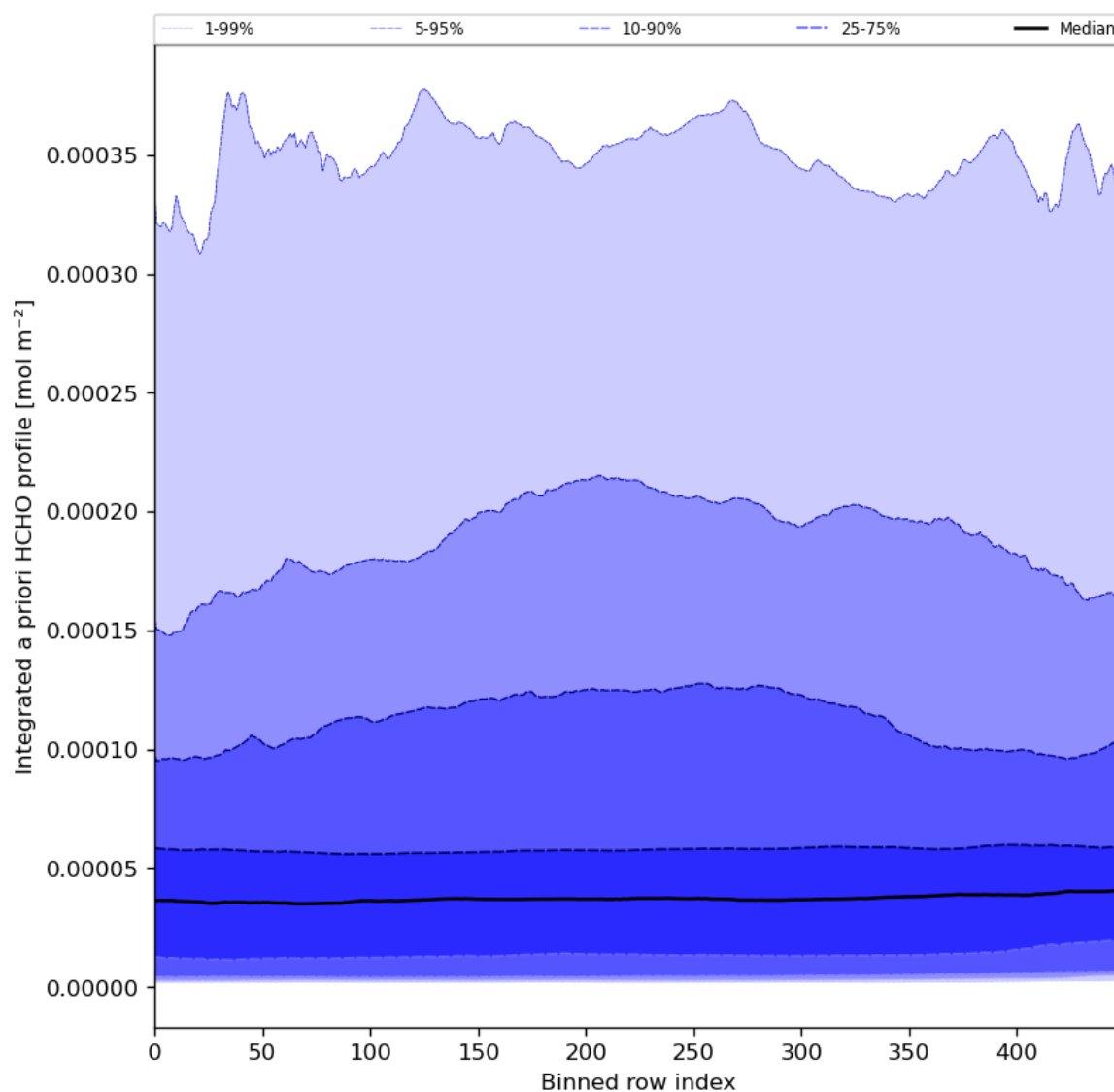
Figure 57: Along track statistics of “Integrated a priori HCHO profile” for 2024-03-28 to 2024-03-30
