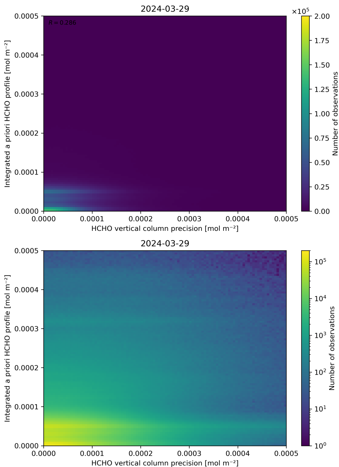
Figure 147: Scatter density plot of “HCHO vertical column precision” against “Integrated a priori HCHO profile” for 2024-03-28 to 2024-03-30.
