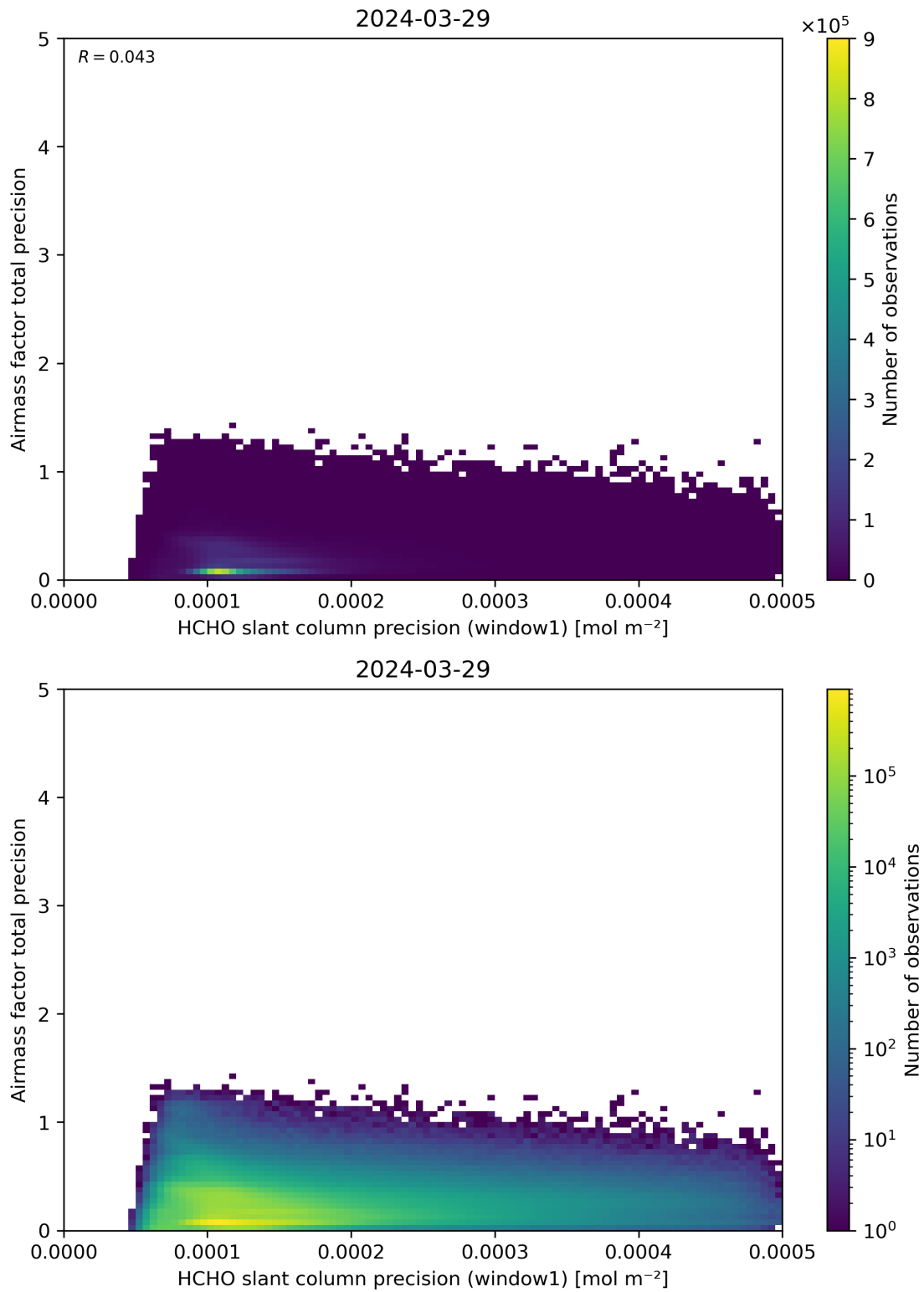
Figure 95: Scatter density plot of “HCHO slant column precision (window1)” against “Airmass factor total precision” for 2024-03-28 to 2024-03-30.
