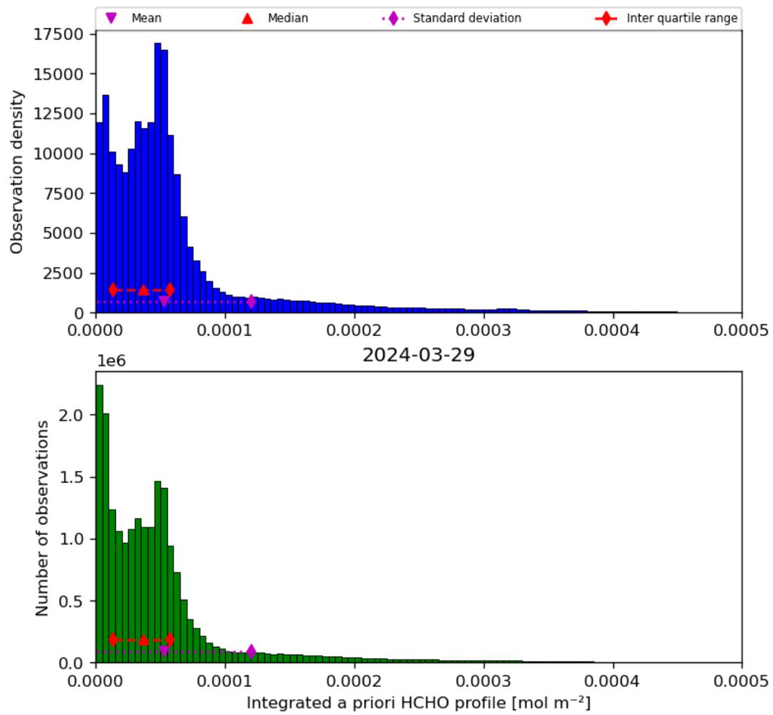
Figure 43: Histogram of “Integrated a priori HCHO profile” for 2024-03-28 to 2024-03-30
