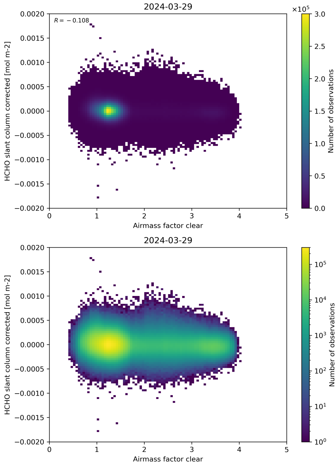
Figure 74: Scatter density plot of “Airmass factor clear” against “HCHO slant column corrected” for 2024-03-28 to 2024-03-30.
