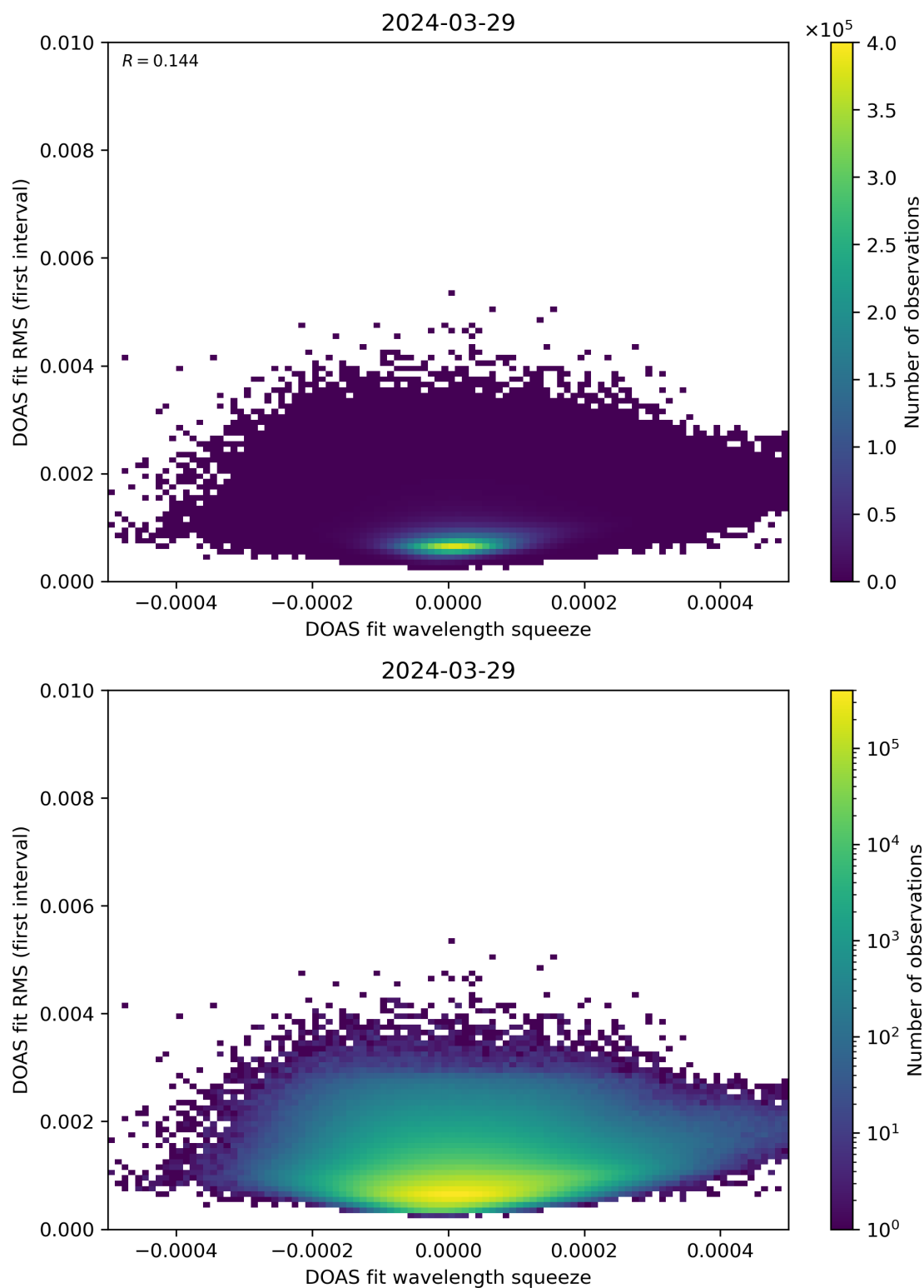
Figure 68: Scatter density plot of “DOAS fit wavelength squeeze” against “DOAS fit RMS (first interval)” for 2024-03-28 to 2024-03-30.
