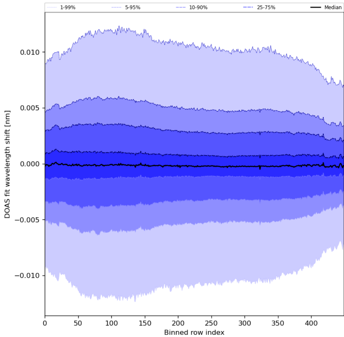
Figure 58: Along track statistics of “DOAS fit wavelength shift” for 2024-03-28 to 2024-03-30
