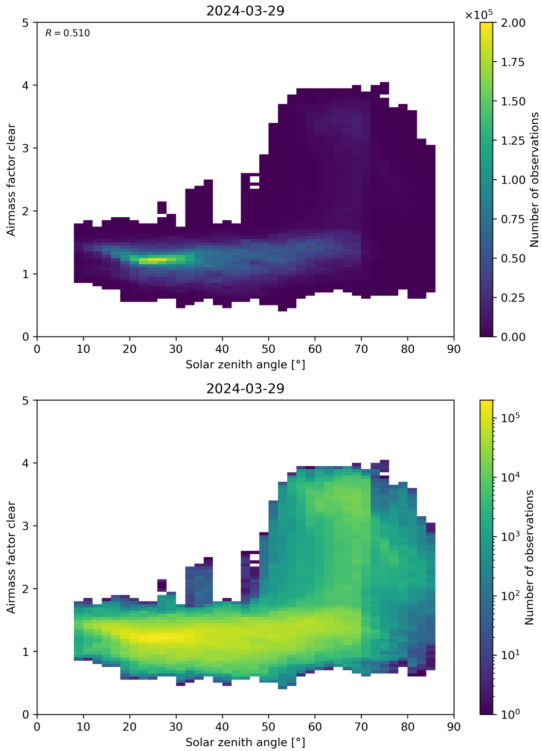
Figure 170: Scatter density plot of “Solar zenith angle” against “Airmass factor clear” for 2024-03-28 to 2024-03-30.
