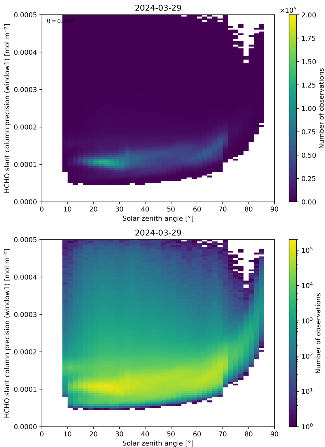
Figure 174: Scatter density plot of “Solar zenith angle” against “HCHO slant column precision (window1)” for 2024-03-28 to 2024-03-30.
