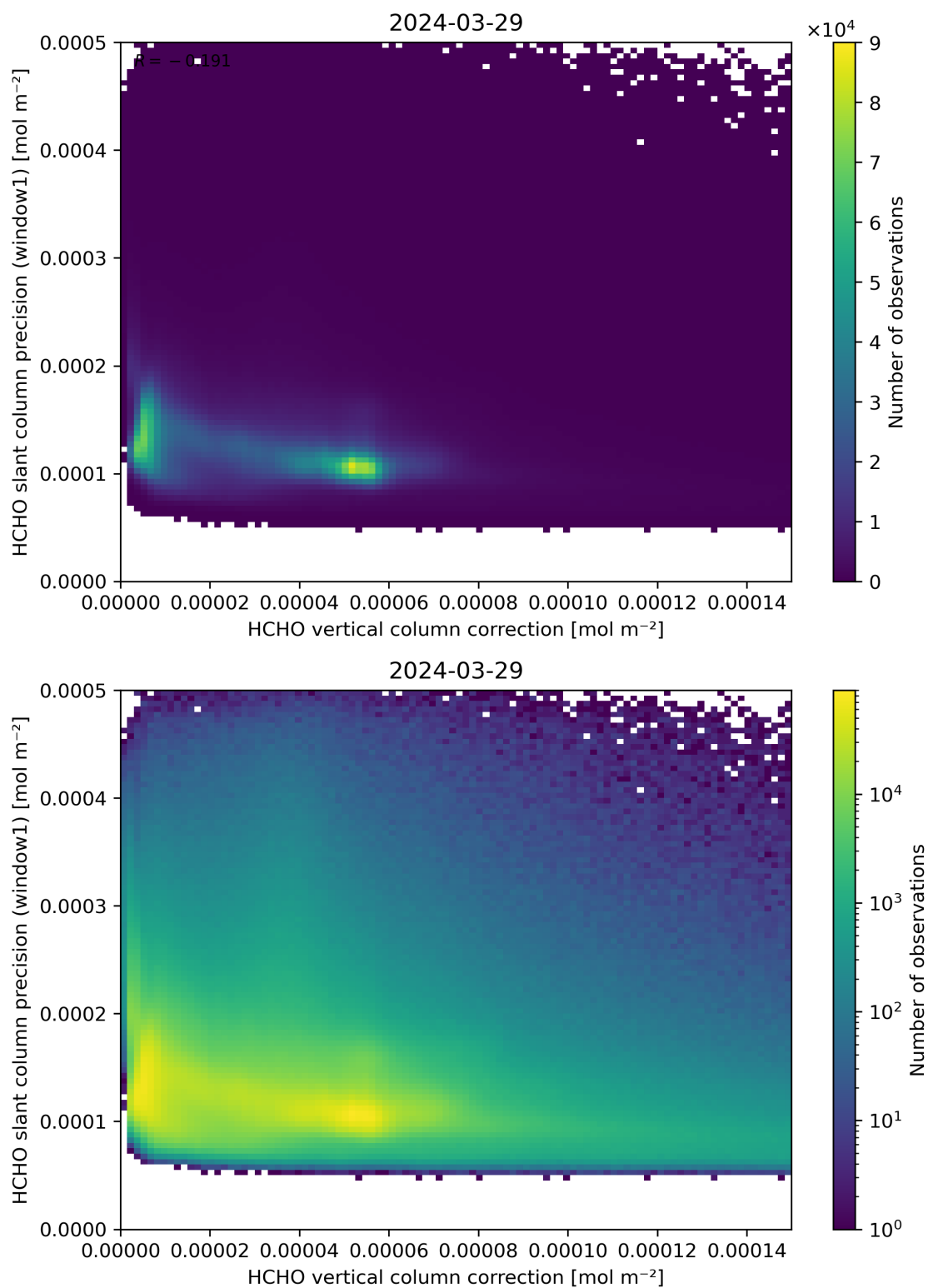
Figure 119: Scatter density plot of “HCHO vertical column correction” against “HCHO slant column precision (window1)” for 2024-03-28 to 2024-03-30.
