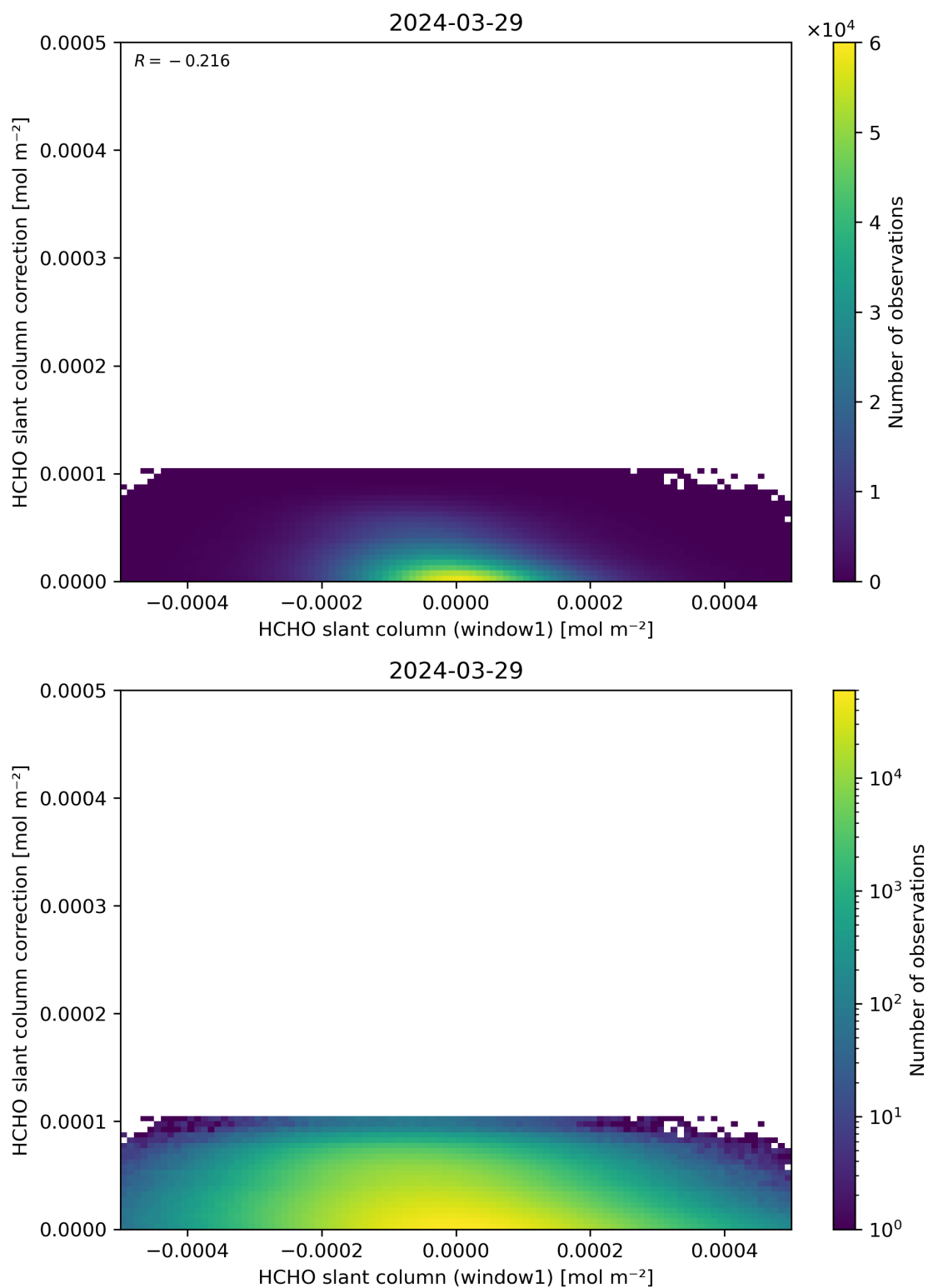
Figure 83: Scatter density plot of “HCHO slant column (window1)” against “HCHO slant column correction” for 2024-03-28 to 2024-03-30.
