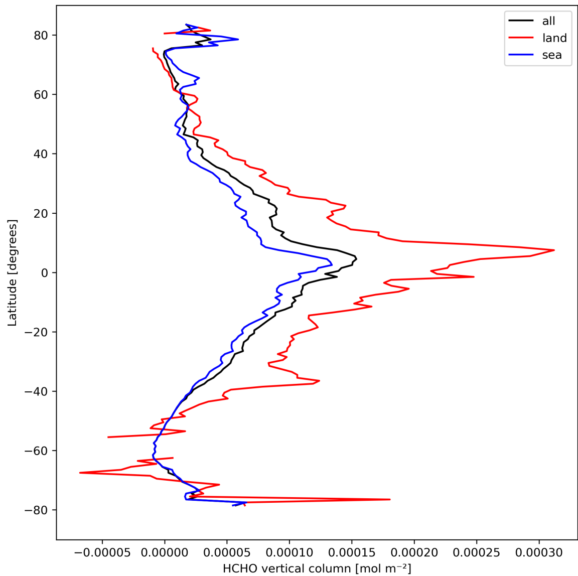
Figure 21: Zonal average of “HCHO vertical column” for 2024-03-28 to 2024-03-30.
