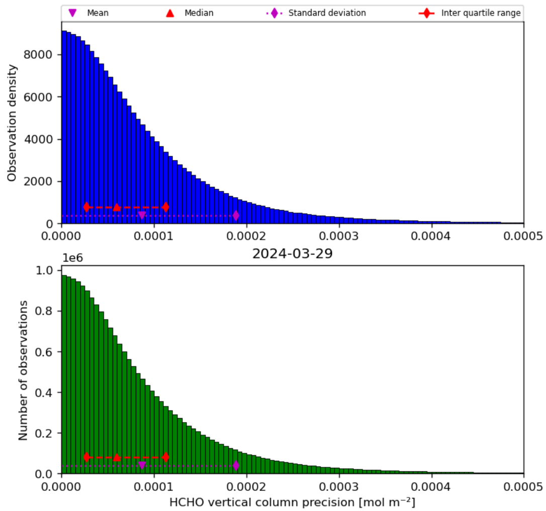
Figure 36: Histogram of “HCHO vertical column precision” for 2024-03-28 to 2024-03-30
