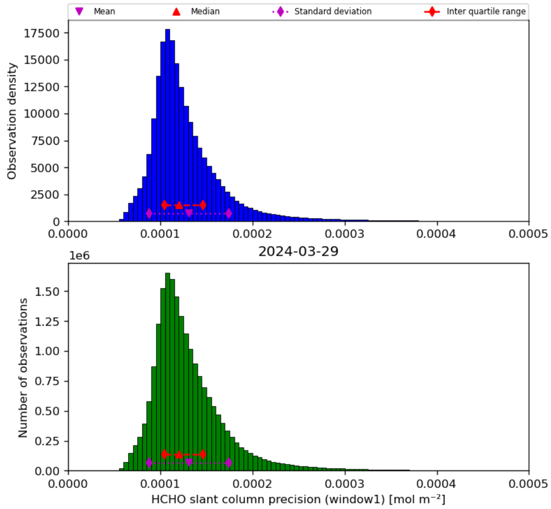
Figure 39: Histogram of “HCHO slant column precision (window1)” for 2024-03-28 to 2024-03-30
