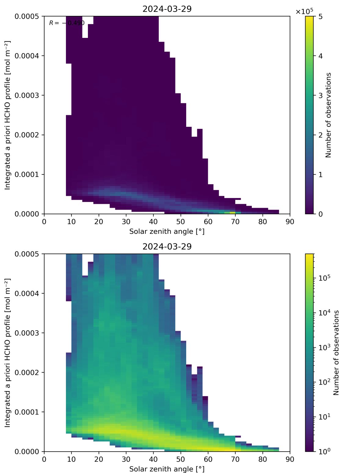
Figure 180: Scatter density plot of “Solar zenith angle” against “Integrated a priori HCHO profile” for 2024-03-28 to 2024-03-30.
