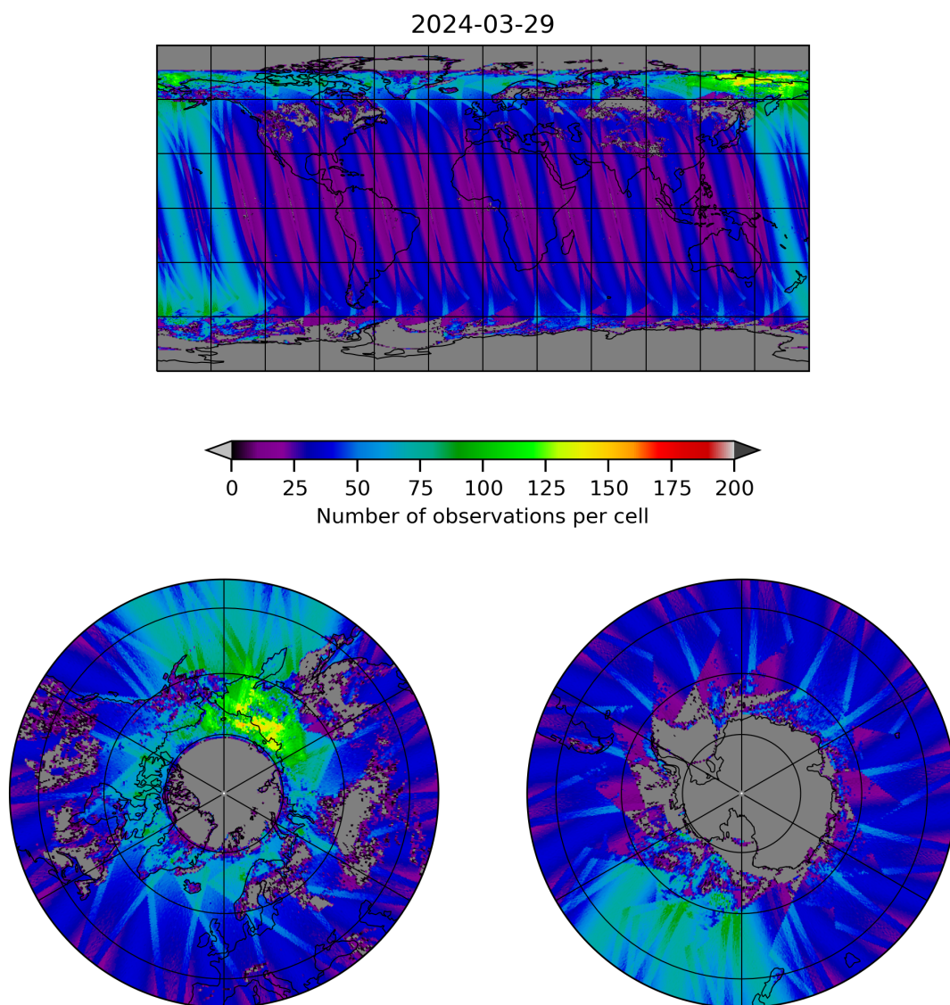
Figure 19: Map of the number of observations for 2024-03-28 to 2024-03-30
