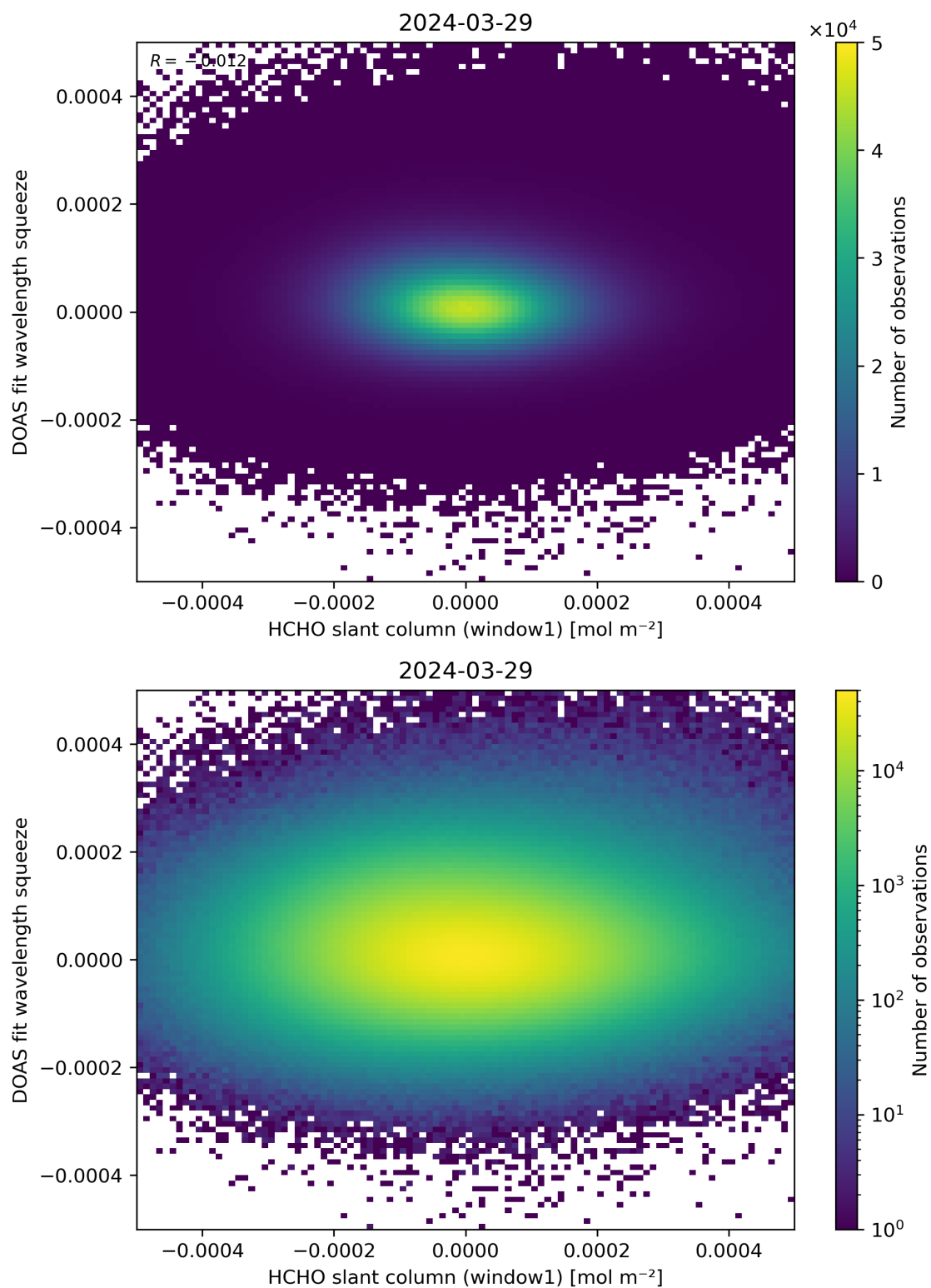
Figure 80: Scatter density plot of “HCHO slant column (window1)” against “DOAS fit wavelength squeeze” for 2024-03-28 to 2024-03-30.
