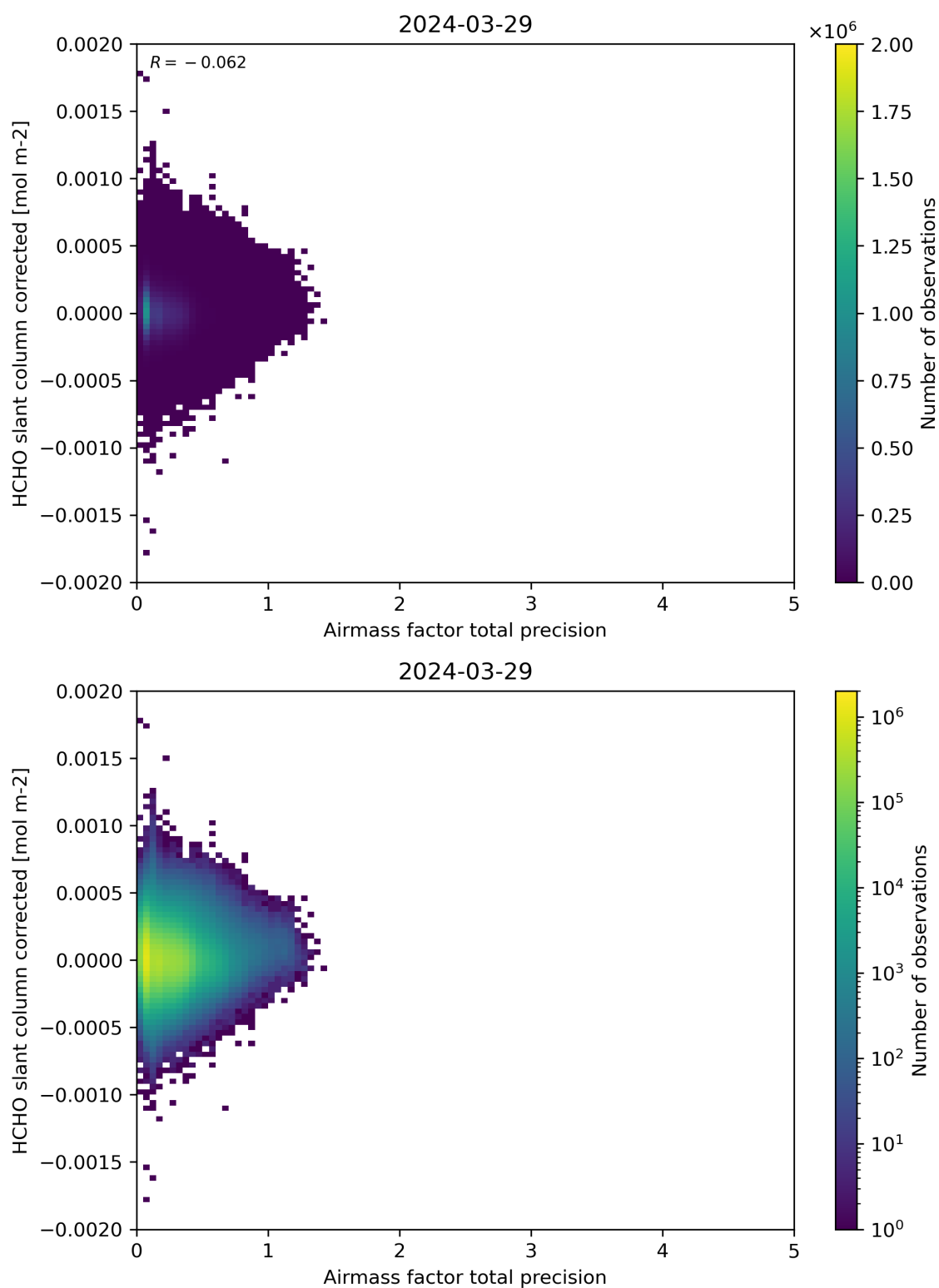
Figure 109: Scatter density plot of “Airmass factor total precision” against “HCHO slant column corrected” for 2024-03-28 to 2024-03-30.
