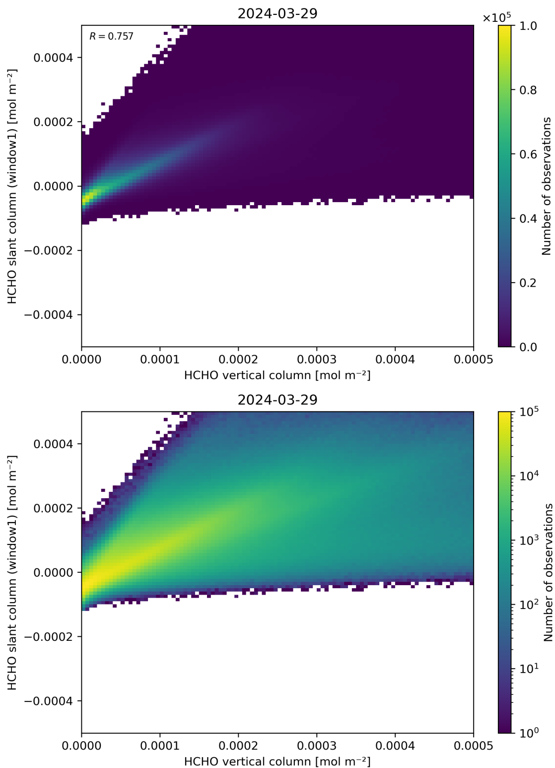
Figure 129: Scatter density plot of “HCHO vertical column” against “HCHO slant column (window1)” for 2024-03-28 to 2024-03-30.
