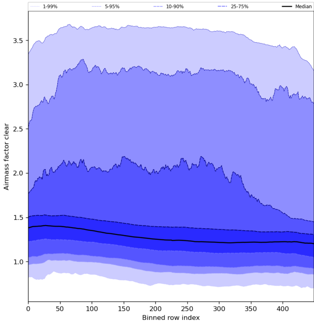
Figure 56: Along track statistics of “Airmass factor clear” for 2024-03-28 to 2024-03-30
