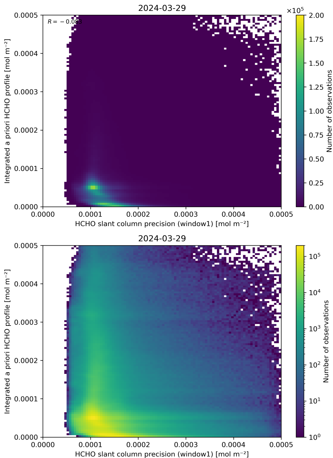
Figure 96: Scatter density plot of “HCHO slant column precision (window1)” against “Integrated a priori HCHO profile” for 2024-03-28 to 2024-03-30.
