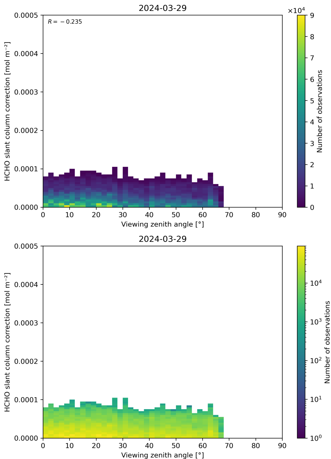
Figure 187: Scatter density plot of “Viewing zenith angle” against “HCHO slant column correction” for 2024-03-28 to 2024-03-30.
