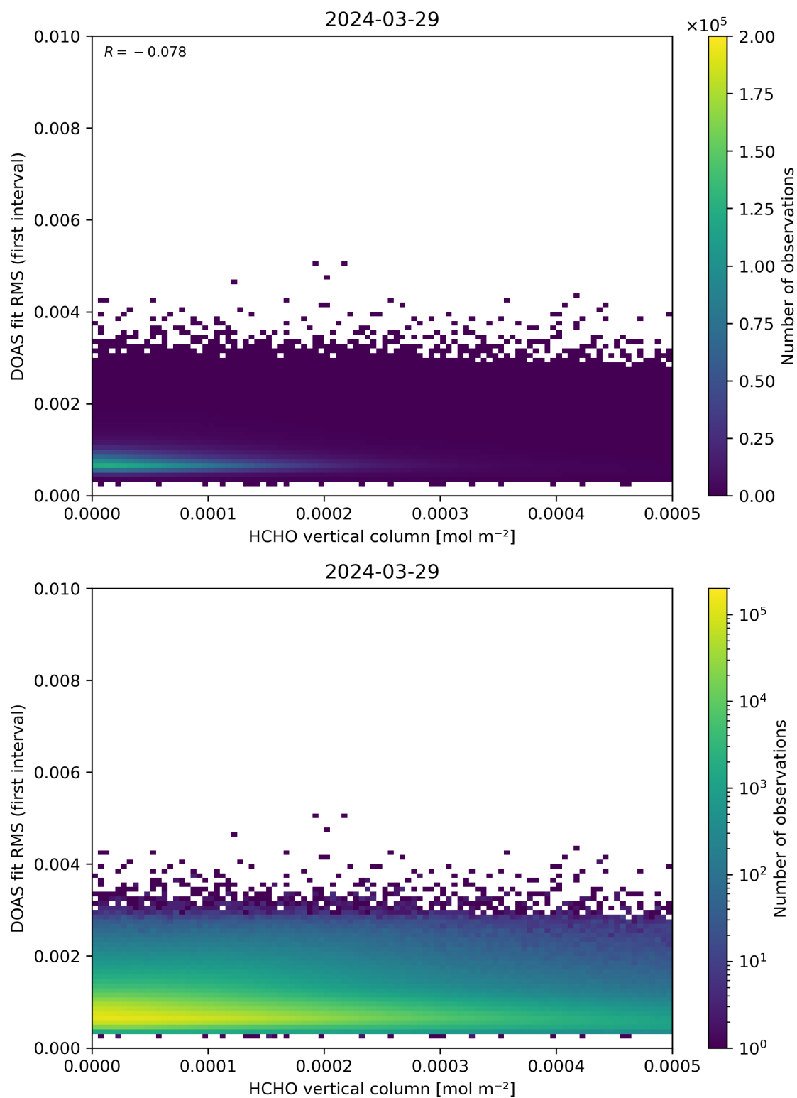
Figure 123: Scatter density plot of “HCHO vertical column” against “DOAS fit RMS (first interval)” for 2024-03-28 to 2024-03-30.
