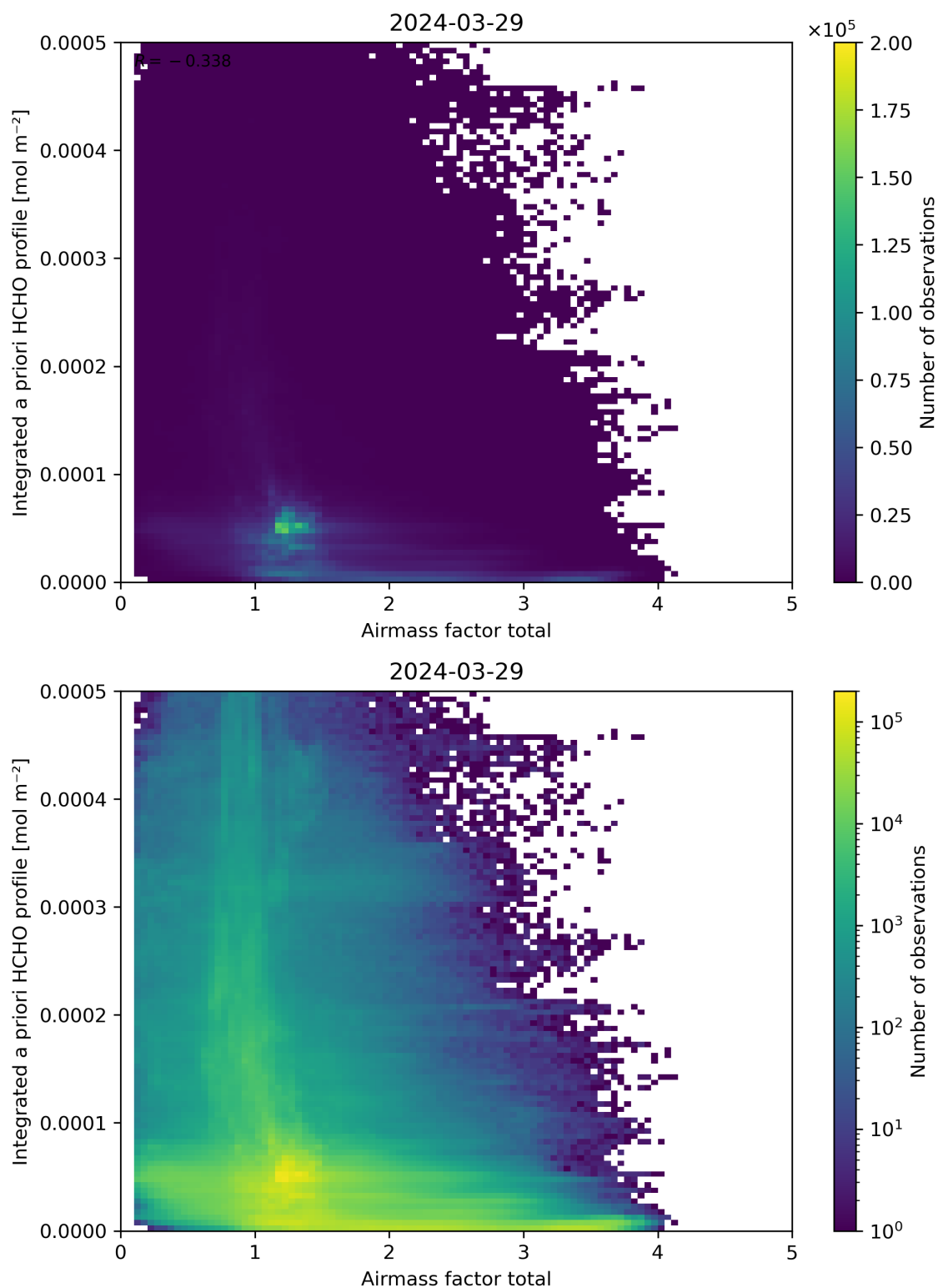
Figure 104: Scatter density plot of “Airmass factor total” against “Integrated a priori HCHO profile” for 2024-03-28 to 2024-03-30.
