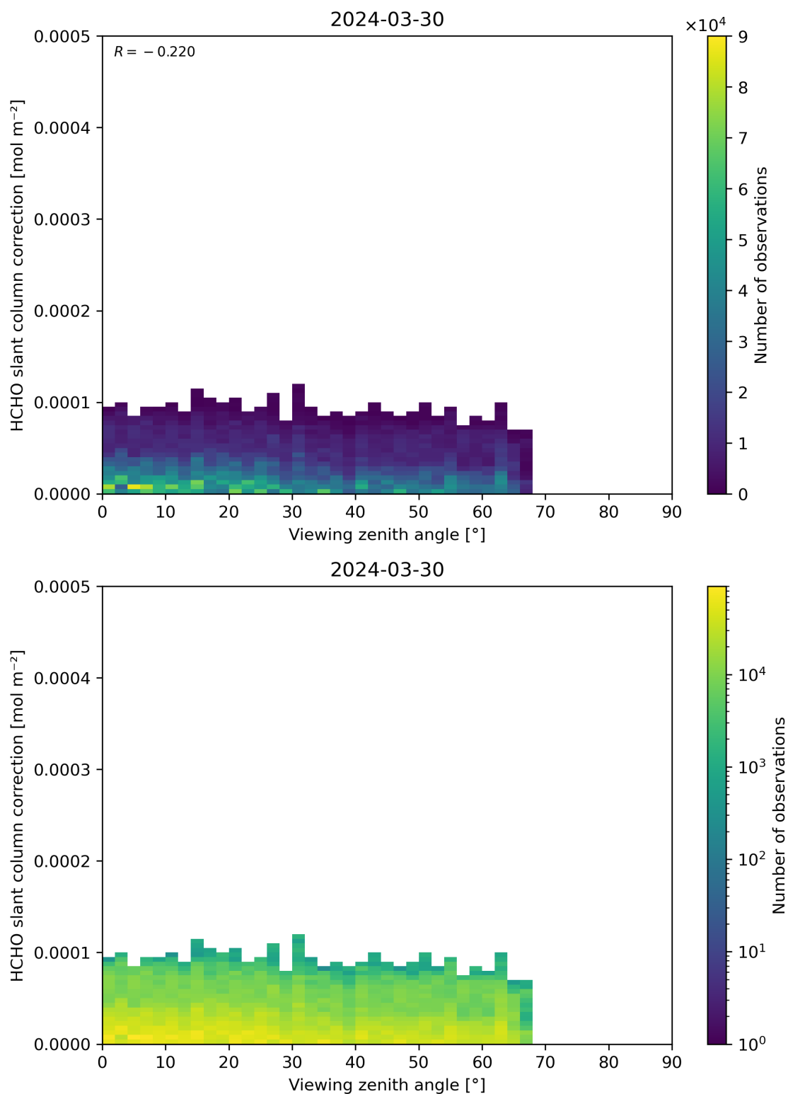
Figure 187: Scatter density plot of “Viewing zenith angle” against “HCHO slant column correction” for 2024-03-30 to 2024-03-31.
