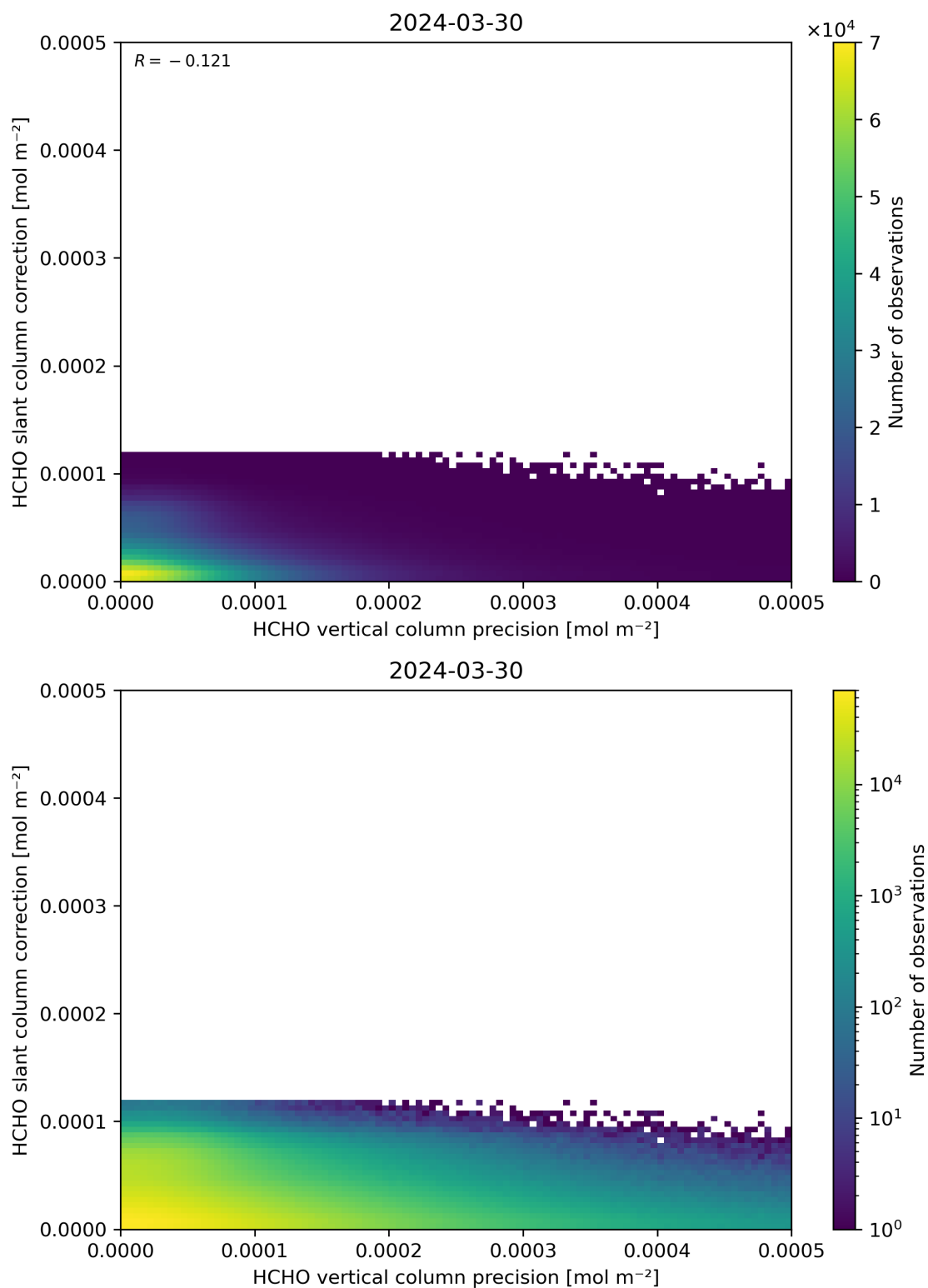
Figure 141: Scatter density plot of “HCHO vertical column precision” against “HCHO slant column correction” for 2024-03-30 to 2024-03-31.
