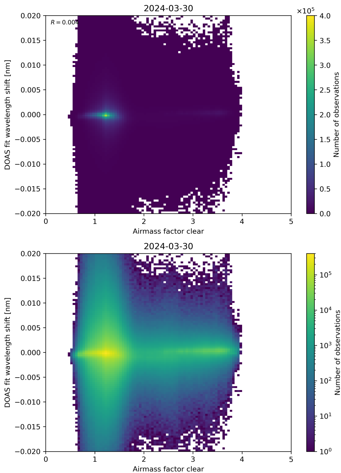
Figure 72: Scatter density plot of “Airmass factor clear” against “DOAS fit wavelength shift” for 2024-03-30 to 2024-03-31.
