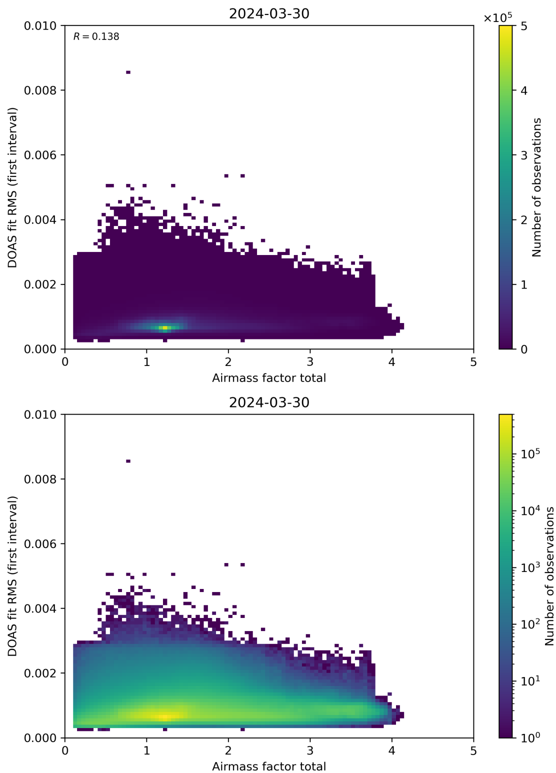
Figure 97: Scatter density plot of “Airmass factor total” against “DOAS fit RMS (first interval)” for 2024-03-30 to 2024-03-31.
