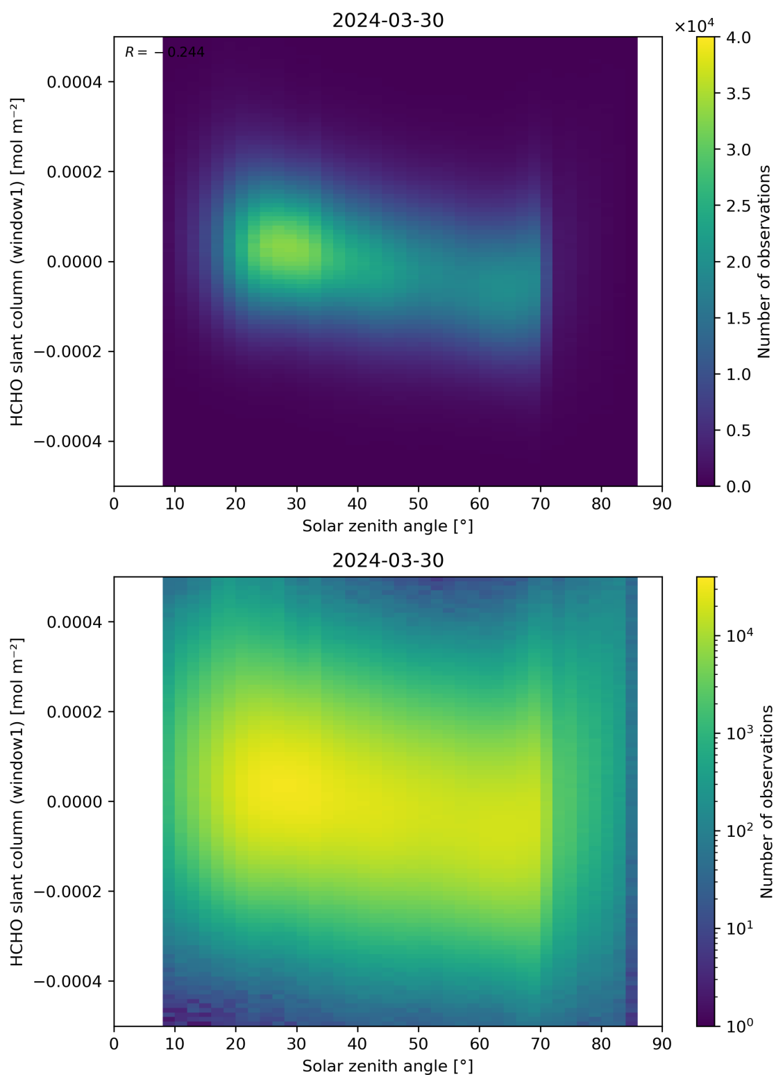
Figure 173: Scatter density plot of “Solar zenith angle” against “HCHO slant column (window1)” for 2024-03-30 to 2024-03-31.
