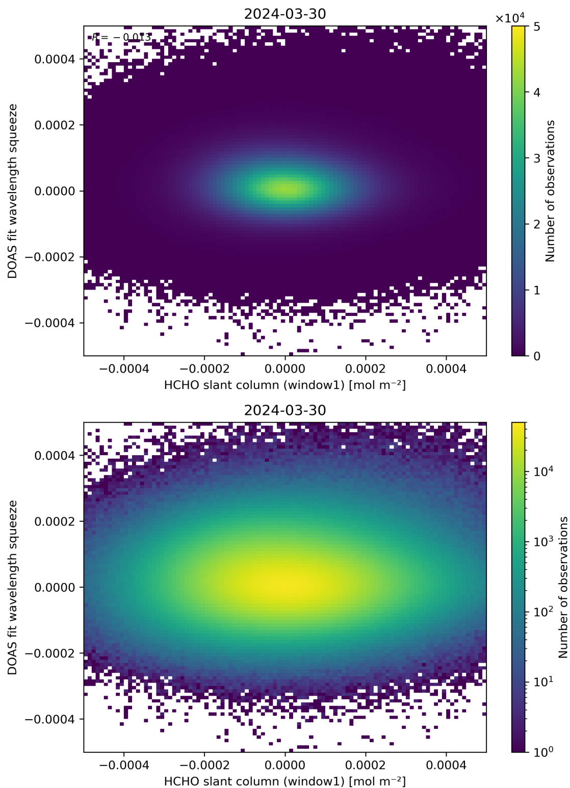
Figure 80: Scatter density plot of “HCHO slant column (window1)” against “DOAS fit wavelength squeeze” for 2024-03-30 to 2024-03-31.
