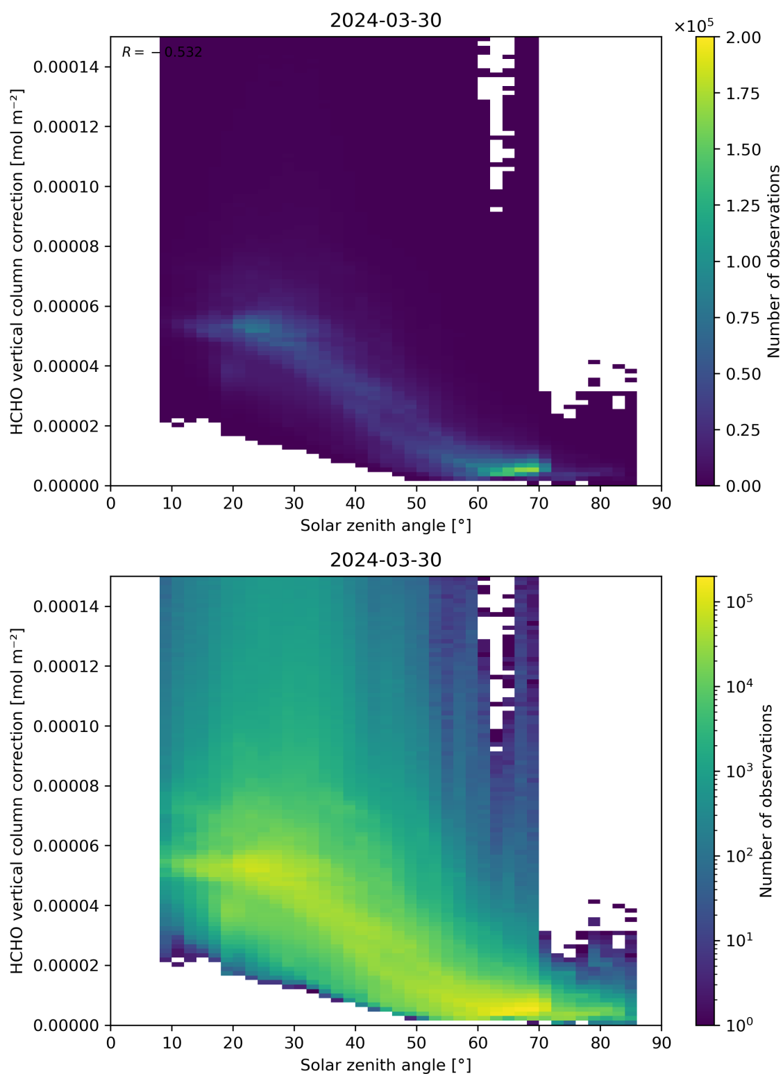
Figure 178: Scatter density plot of “Solar zenith angle” against “HCHO vertical column correction” for 2024-03-30 to 2024-03-31.
