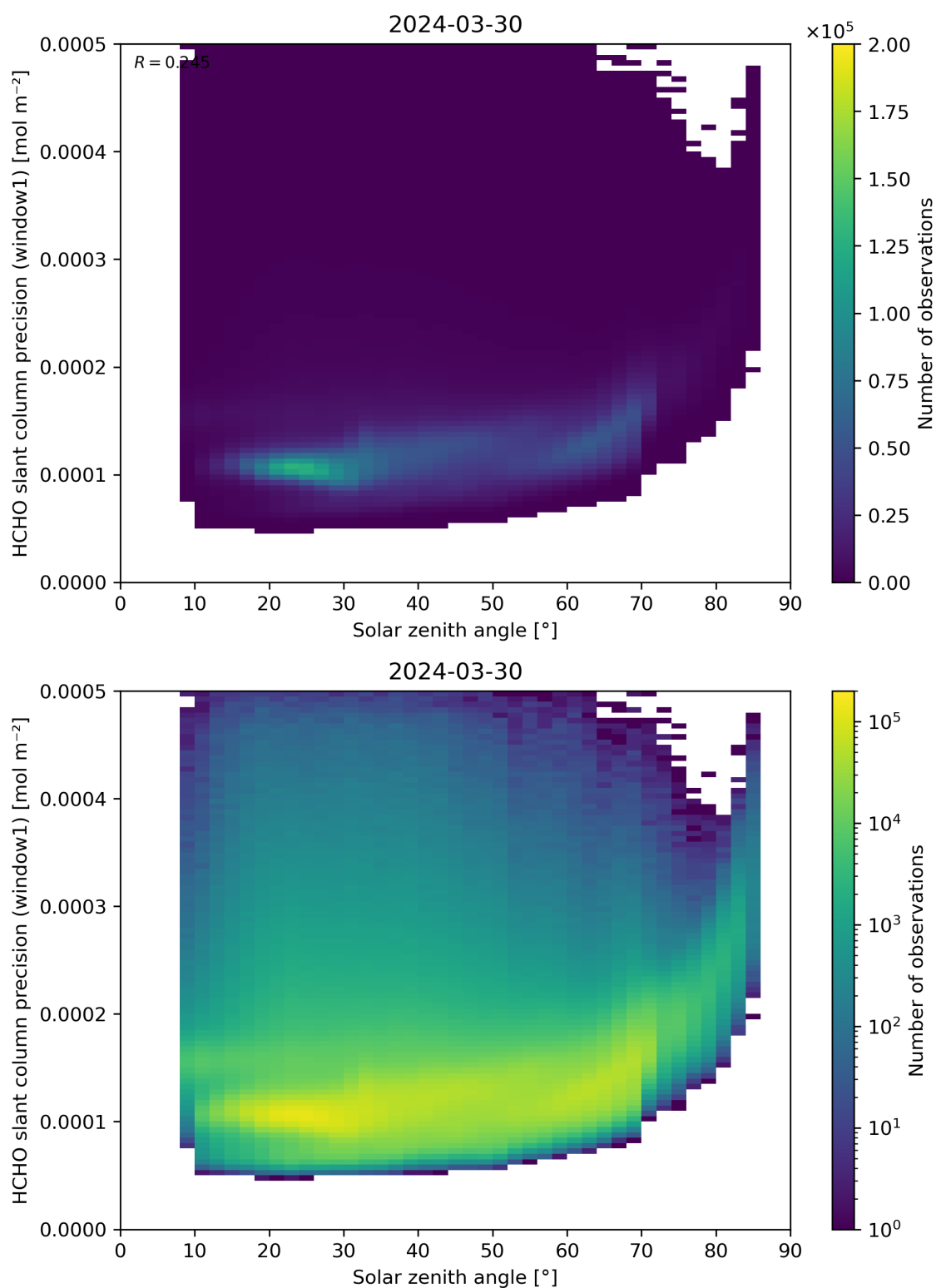
Figure 174: Scatter density plot of “Solar zenith angle” against “HCHO slant column precision (window1)” for 2024-03-30 to 2024-03-31.
