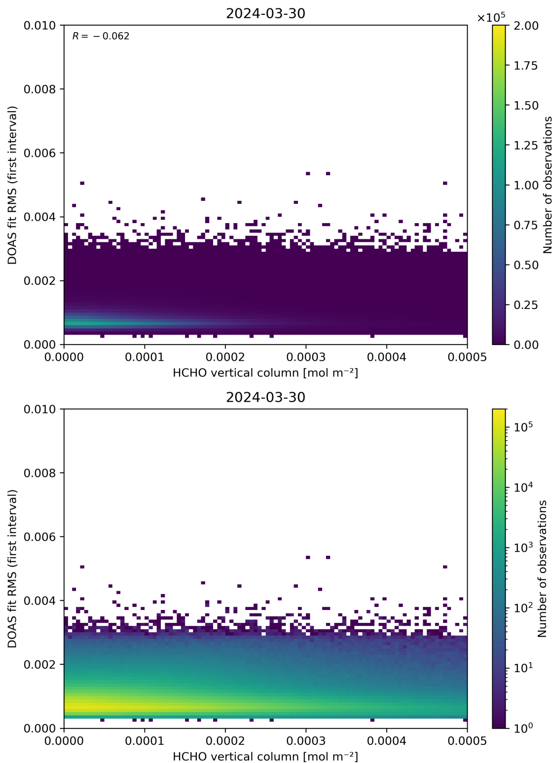
Figure 123: Scatter density plot of “HCHO vertical column” against “DOAS fit RMS (first interval)” for 2024-03-30 to 2024-03-31.
