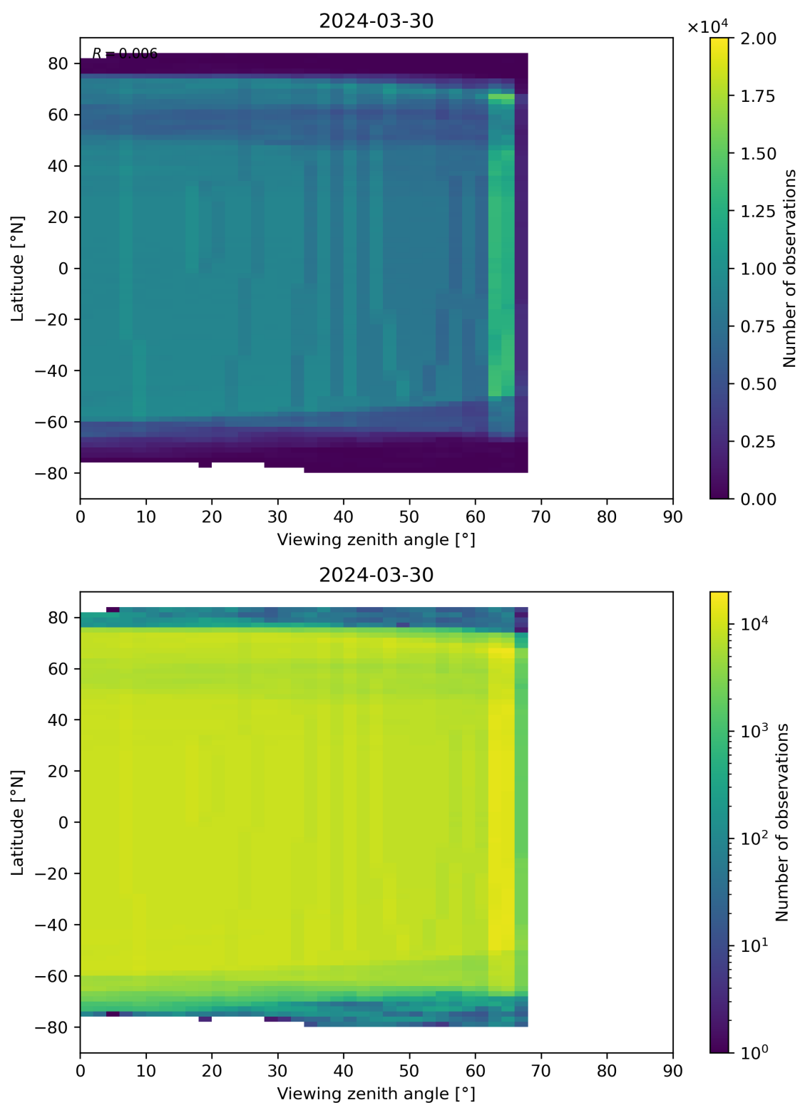
Figure 196: Scatter density plot of “Viewing zenith angle” against “Latitude” for 2024-03-30 to 2024-03-31.
