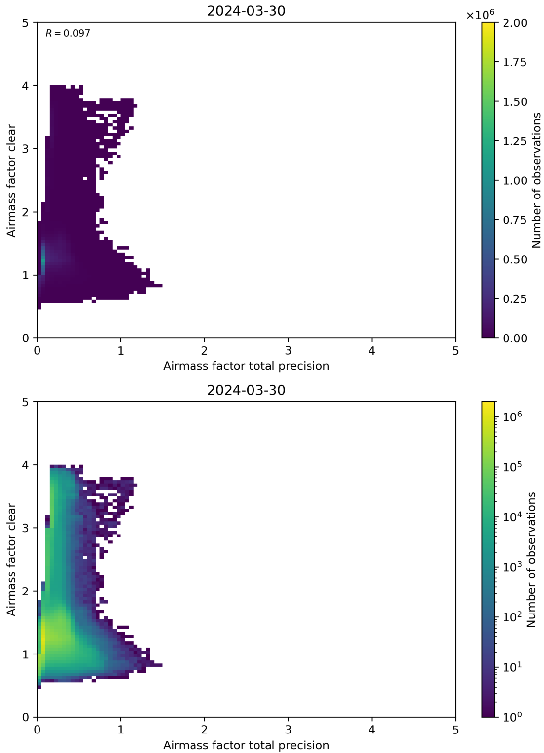
Figure 108: Scatter density plot of “Airmass factor total precision” against “Airmass factor clear” for 2024-03-30 to 2024-03-31.
