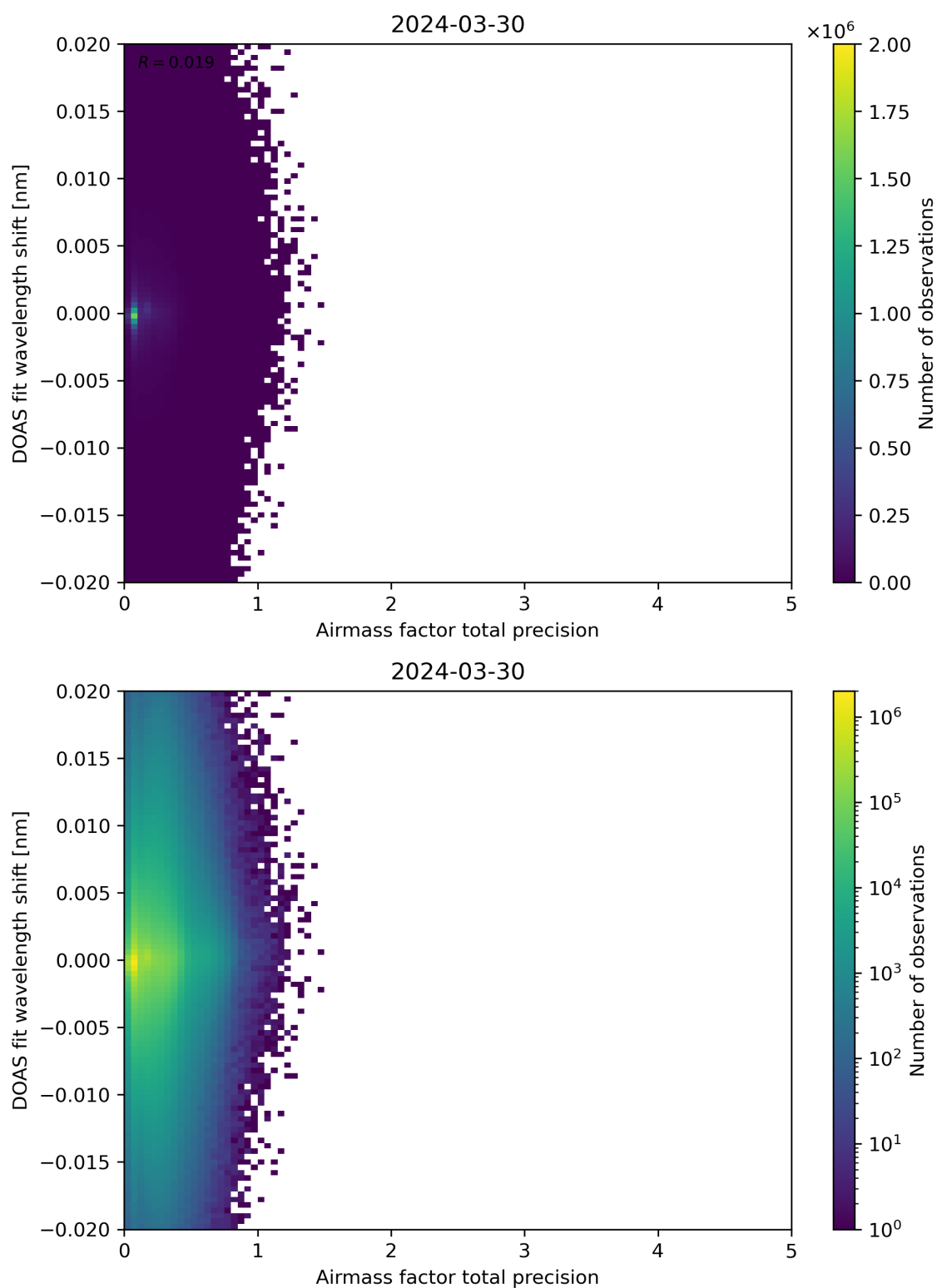
Figure 106: Scatter density plot of “Airmass factor total precision” against “DOAS fit wavelength shift” for 2024-03-30 to 2024-03-31.
