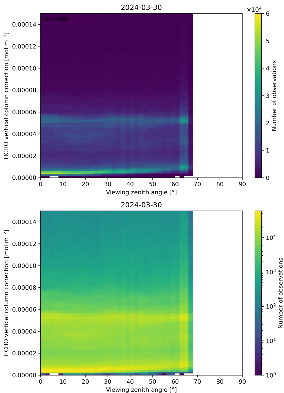
Figure 193: Scatter density plot of “Viewing zenith angle” against “HCHO vertical column correction” for 2024-03-30 to 2024-03-31.
