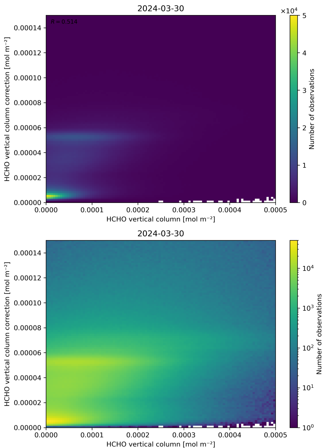
Figure 133: Scatter density plot of “HCHO vertical column” against “HCHO vertical column correction” for 2024-03-30 to 2024-03-31.
