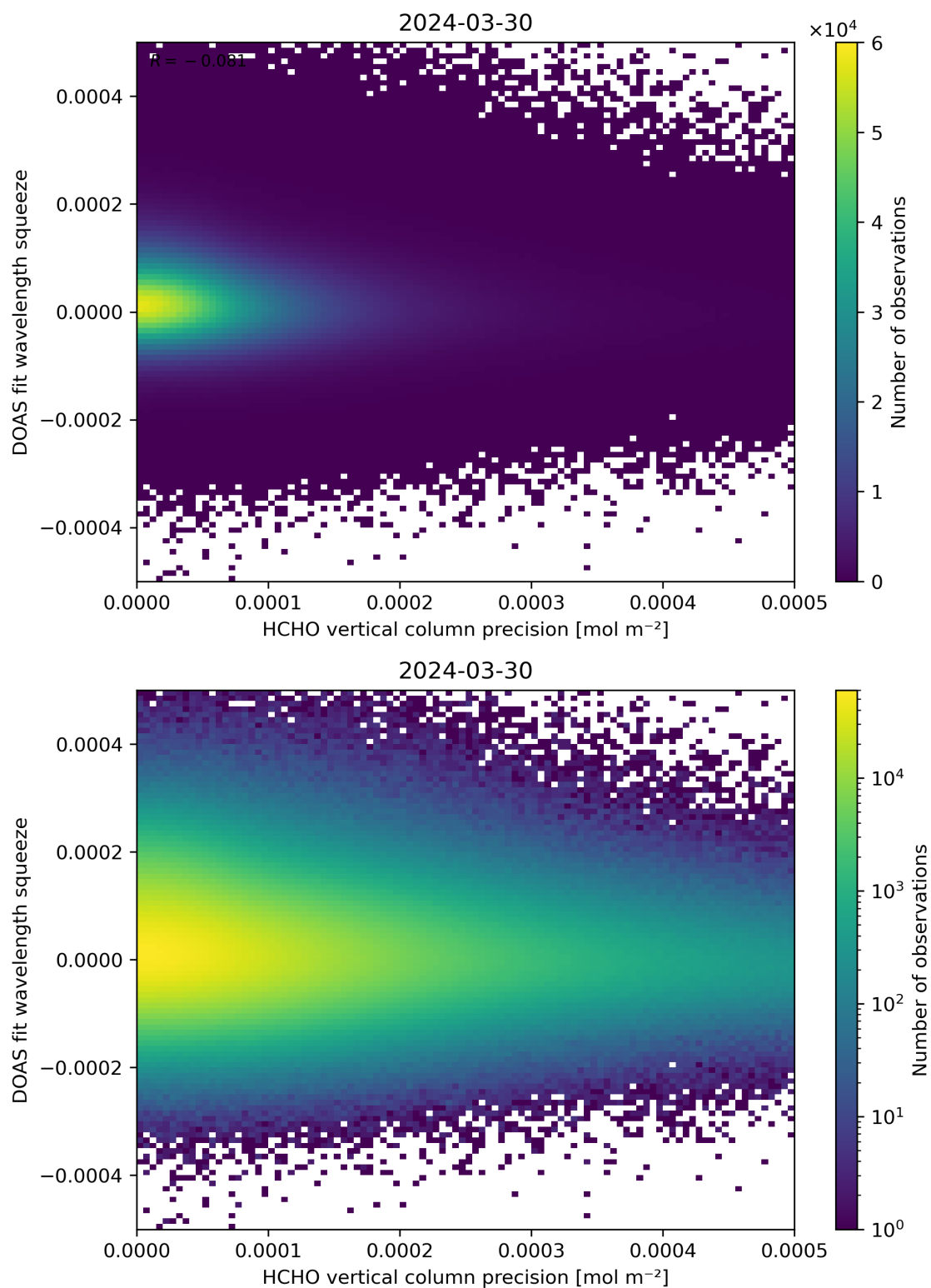
Figure 138: Scatter density plot of “HCHO vertical column precision” against “DOAS fit wavelength squeeze” for 2024-03-30 to 2024-03-31.
