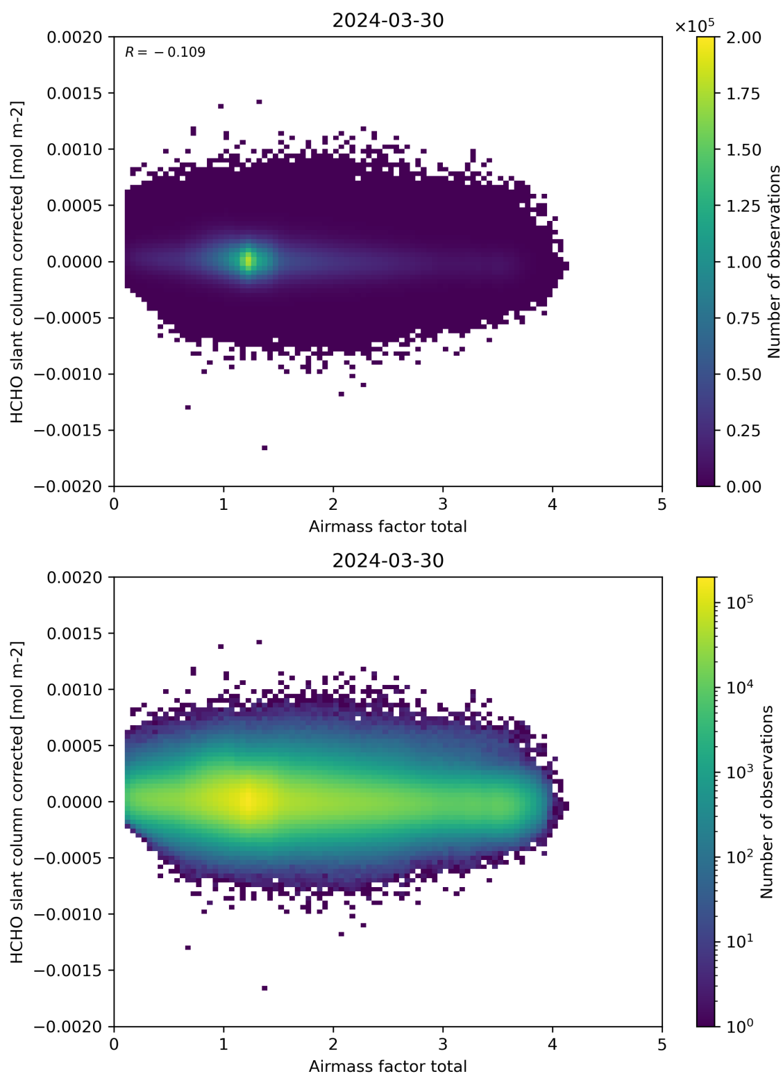
Figure 101: Scatter density plot of “Airmass factor total” against “HCHO slant column corrected” for 2024-03-30 to 2024-03-31.
