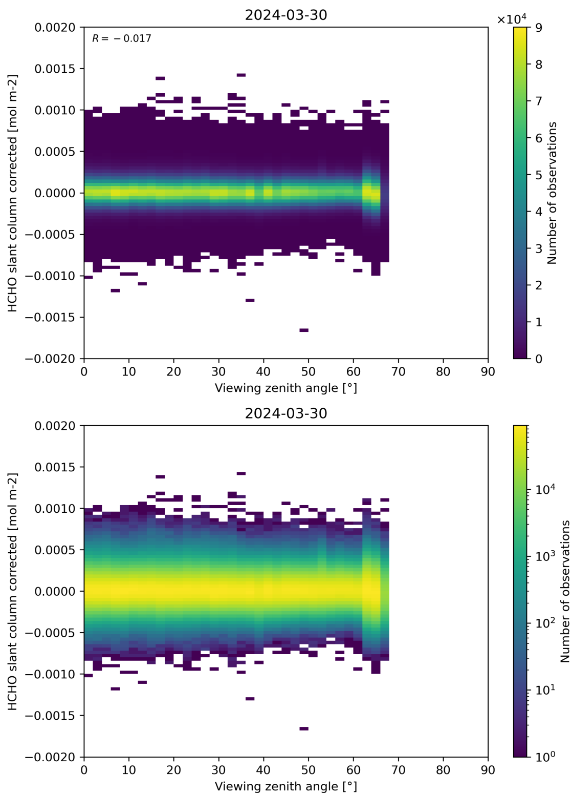
Figure 186: Scatter density plot of “Viewing zenith angle” against “HCHO slant column corrected” for 2024-03-30 to 2024-03-31.
