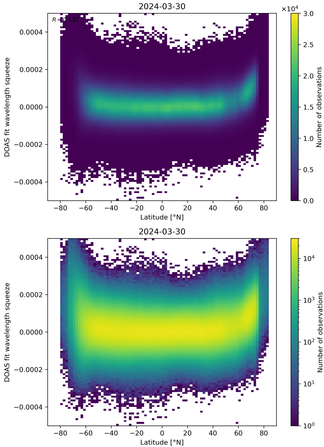
Figure 155: Scatter density plot of “Latitude” against “DOAS fit wavelength squeeze” for 2024-03-30 to 2024-03-31.
