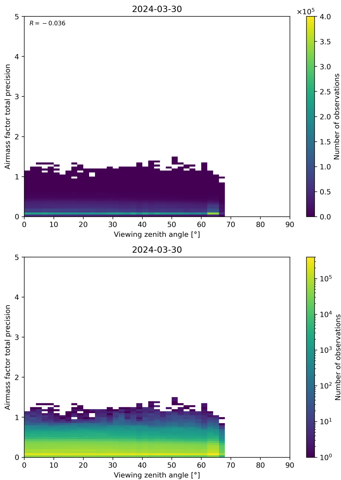
Figure 191: Scatter density plot of “Viewing zenith angle” against “Airmass factor total precision” for 2024-03-30 to 2024-03-31.
