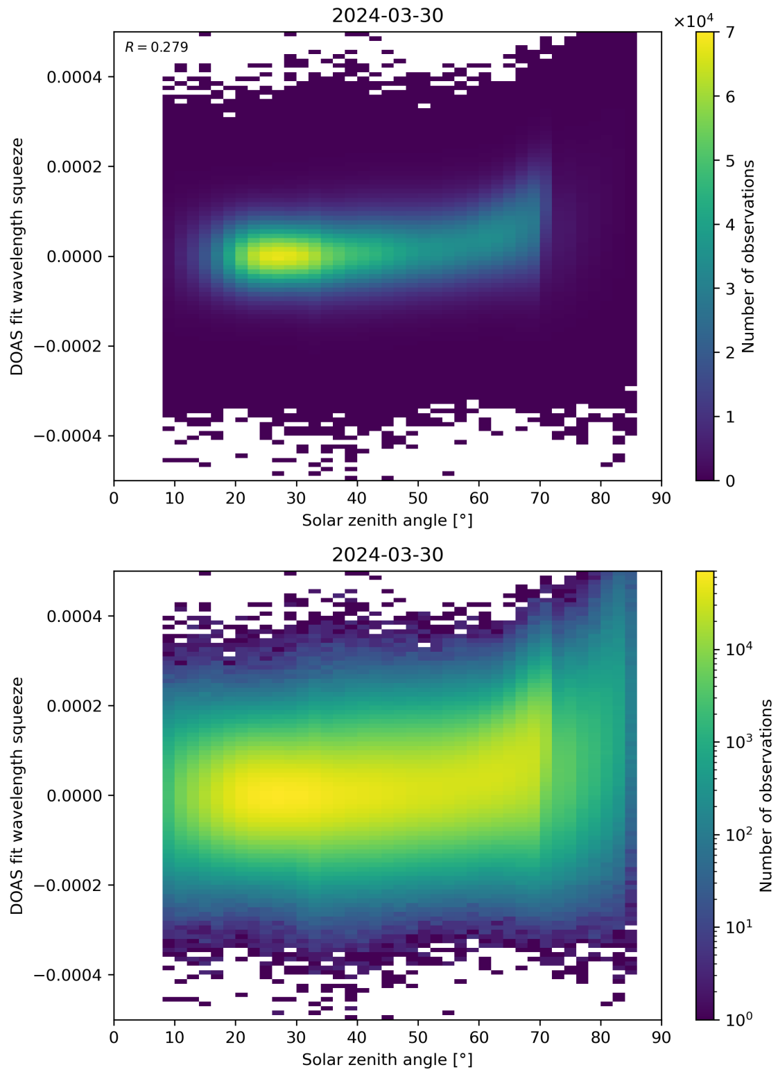
Figure 169: Scatter density plot of “Solar zenith angle” against “DOAS fit wavelength squeeze” for 2024-03-30 to 2024-03-31.
