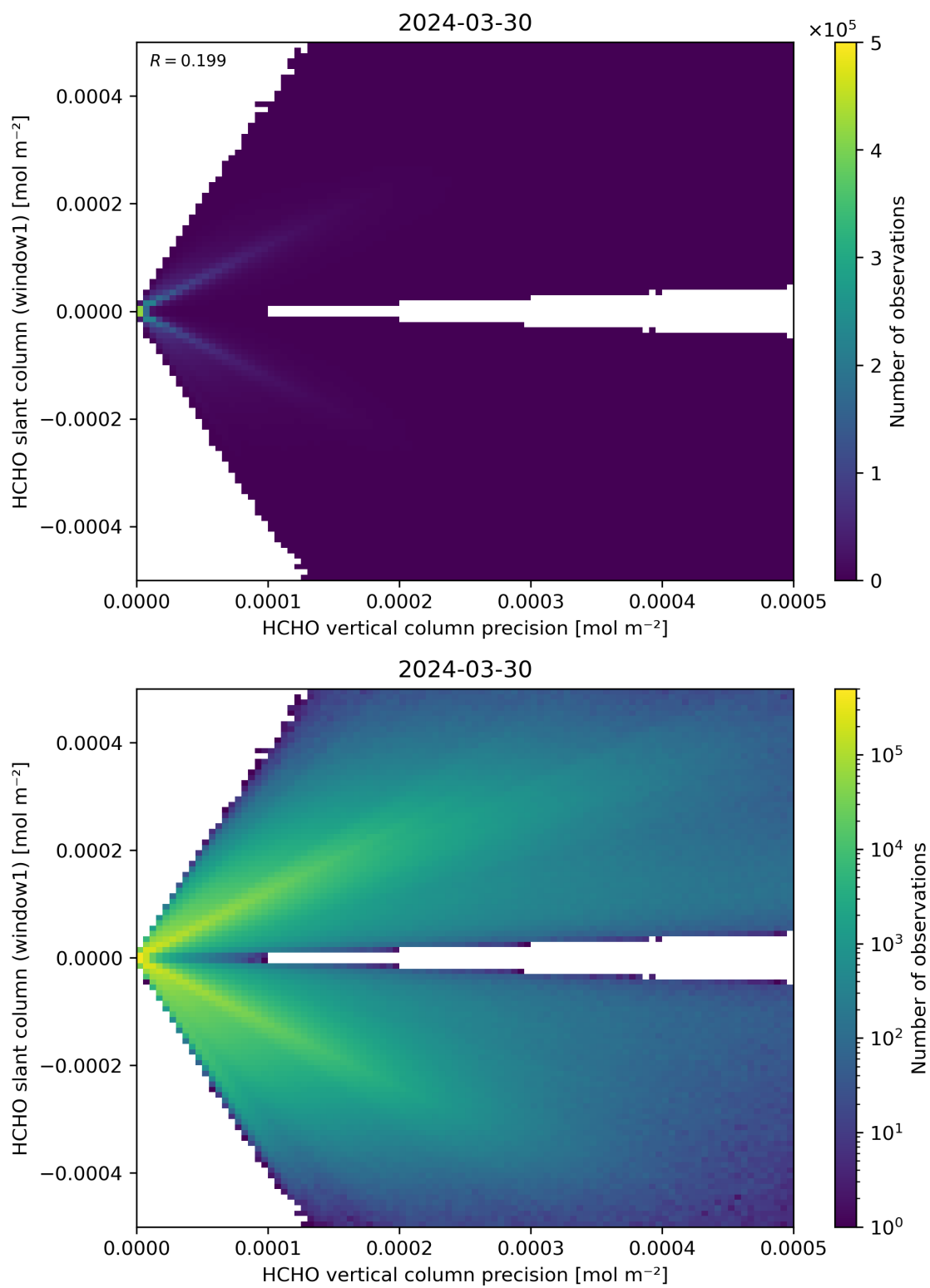
Figure 142: Scatter density plot of “HCHO vertical column precision” against “HCHO slant column (window1)” for 2024-03-30 to 2024-03-31.
