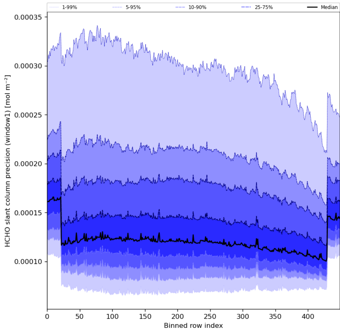
Figure 53: Along track statistics of “HCHO slant column precision (window1)” for 2024-03-30 to 2024-03-31
