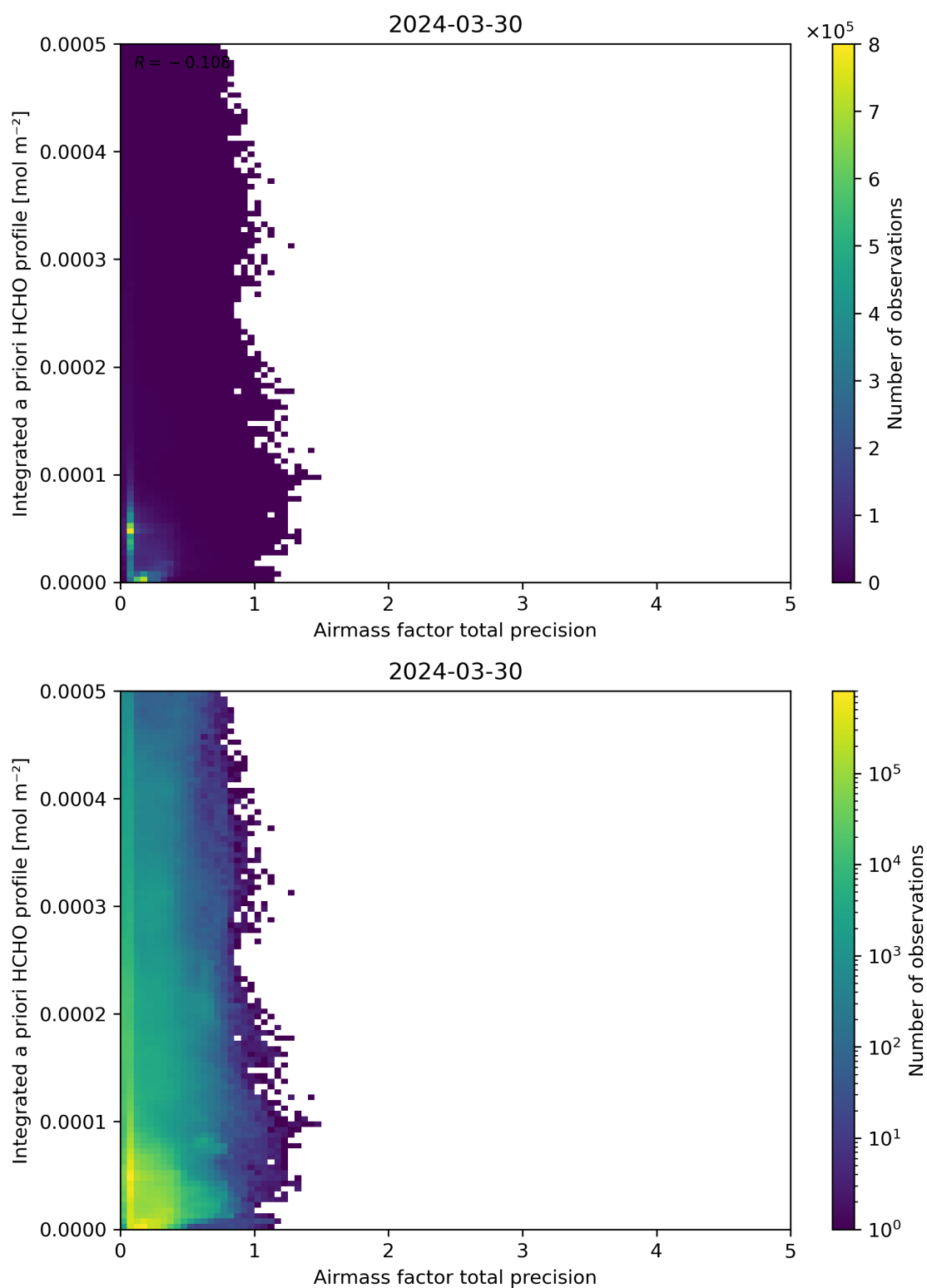
Figure 111: Scatter density plot of “Airmass factor total precision” against “Integrated a priori HCHO profile” for 2024-03-30 to 2024-03-31.
