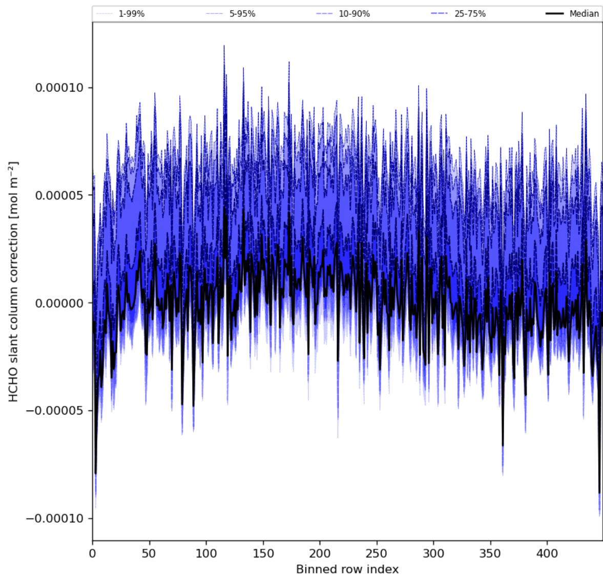
Figure 61: Along track statistics of “HCHO slant column correction” for 2024-03-30 to 2024-03-31
