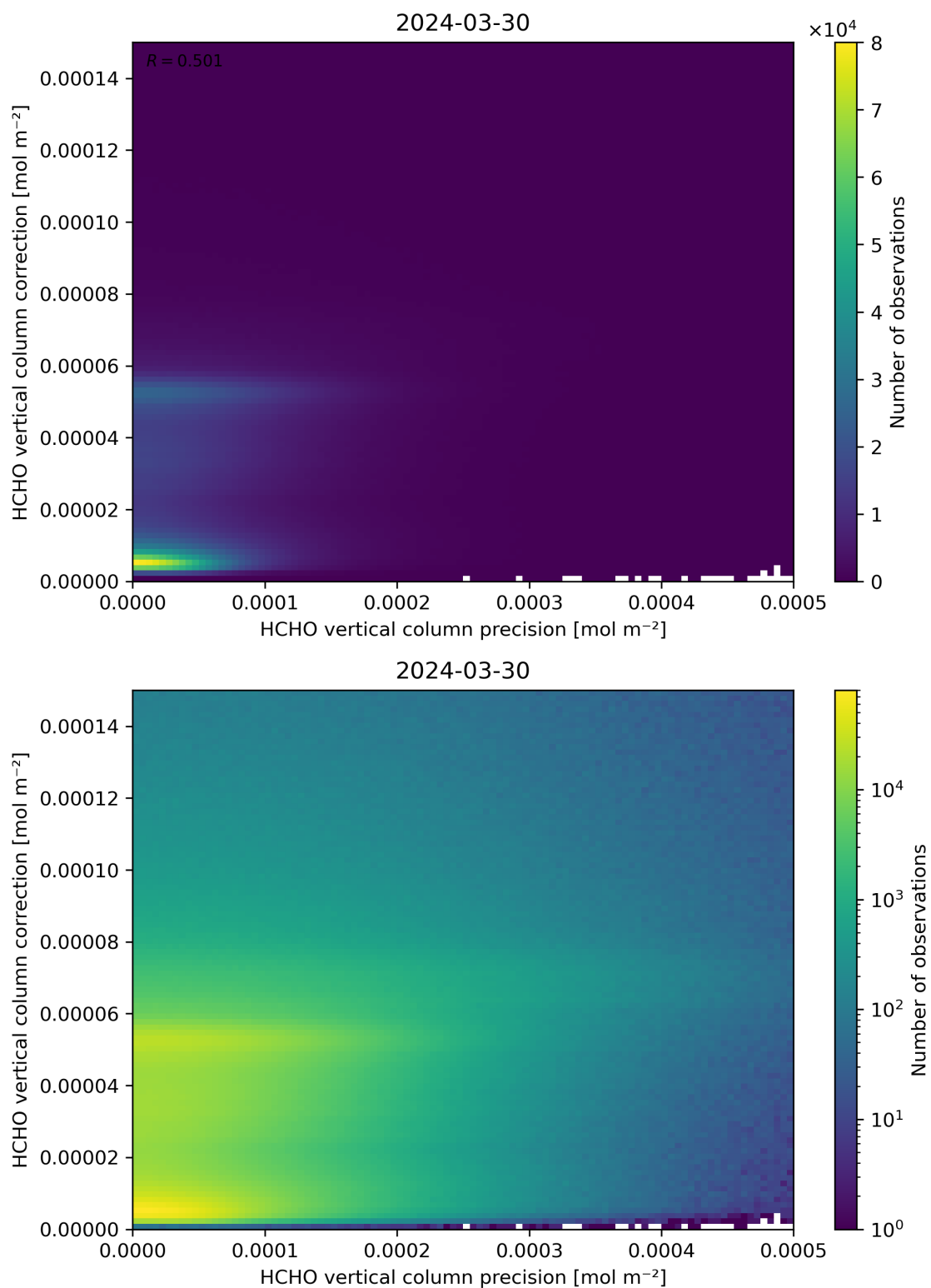
Figure 146: Scatter density plot of “HCHO vertical column precision” against “HCHO vertical column correction” for 2024-03-30 to 2024-03-31.
