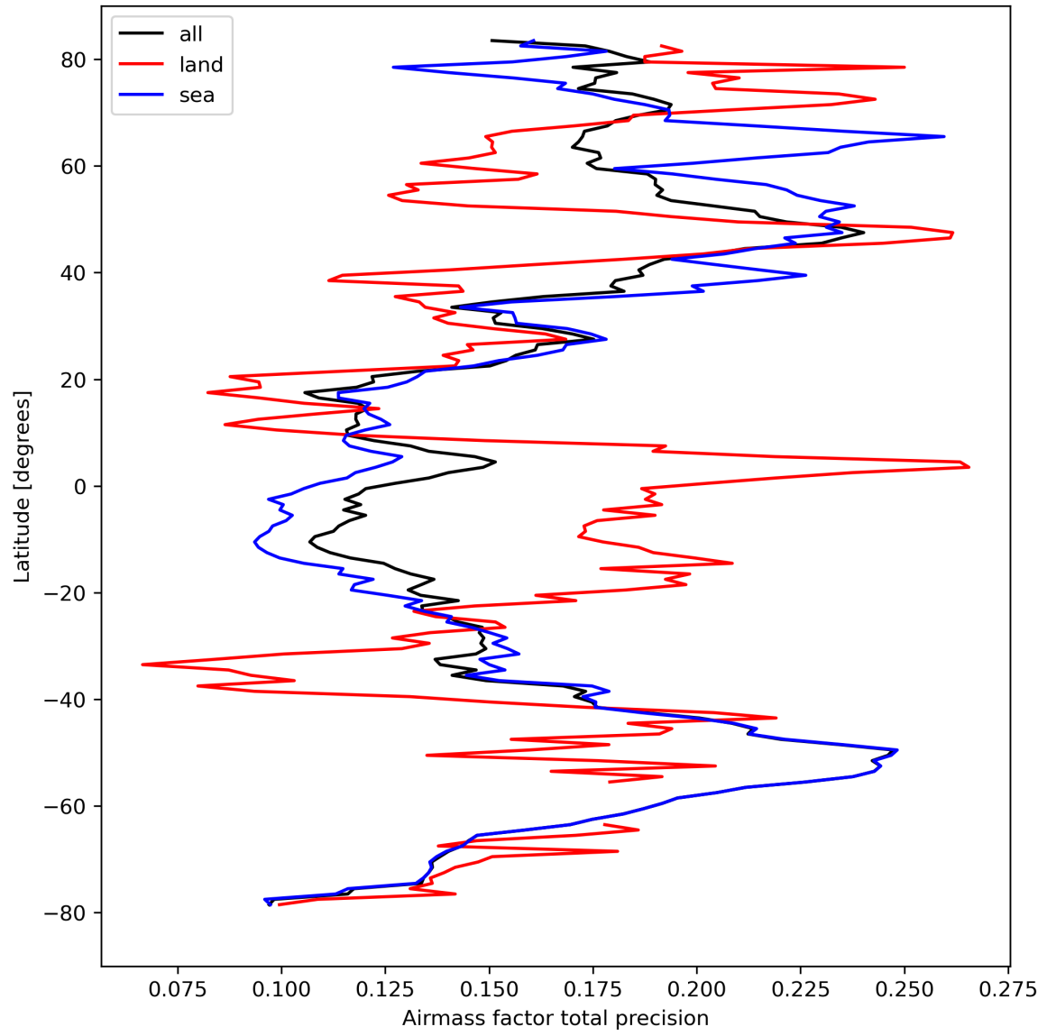
Figure 27: Zonal average of “Airmass factor total precision” for 2024-03-30 to 2024-03-31.
