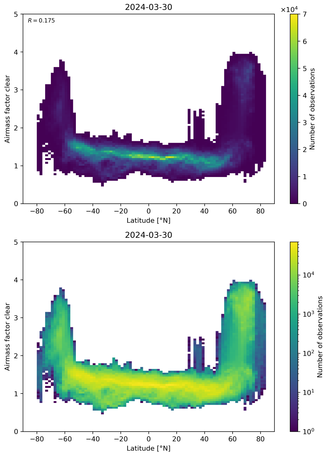
Figure 156: Scatter density plot of “Latitude” against “Airmass factor clear” for 2024-03-30 to 2024-03-31.
