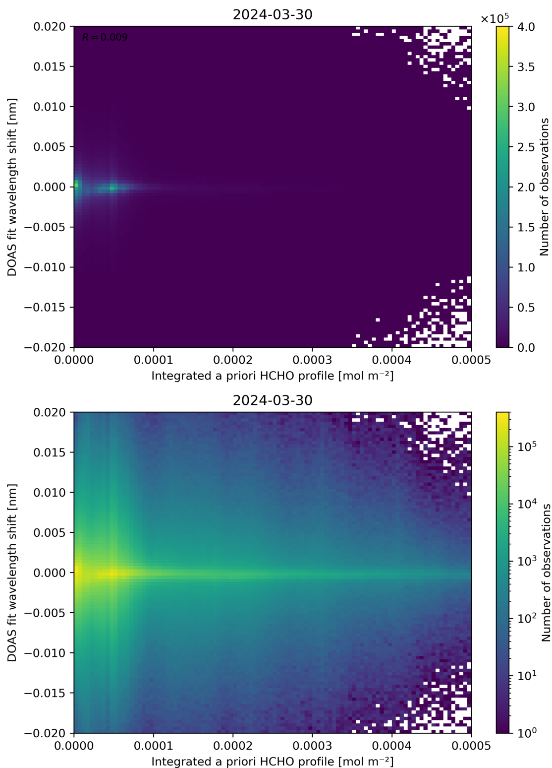
Figure 149: Scatter density plot of “Integrated a priori HCHO profile” against “DOAS fit wavelength shift” for 2024-03-30 to 2024-03-31.
