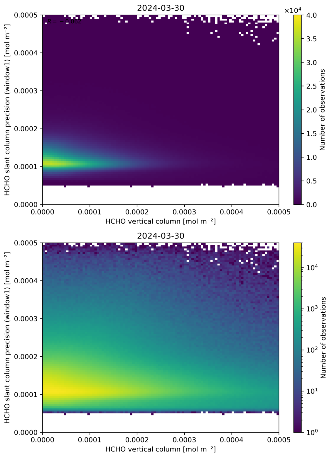
Figure 130: Scatter density plot of “HCHO vertical column” against “HCHO slant column precision (window1)” for 2024-03-30 to 2024-03-31.
