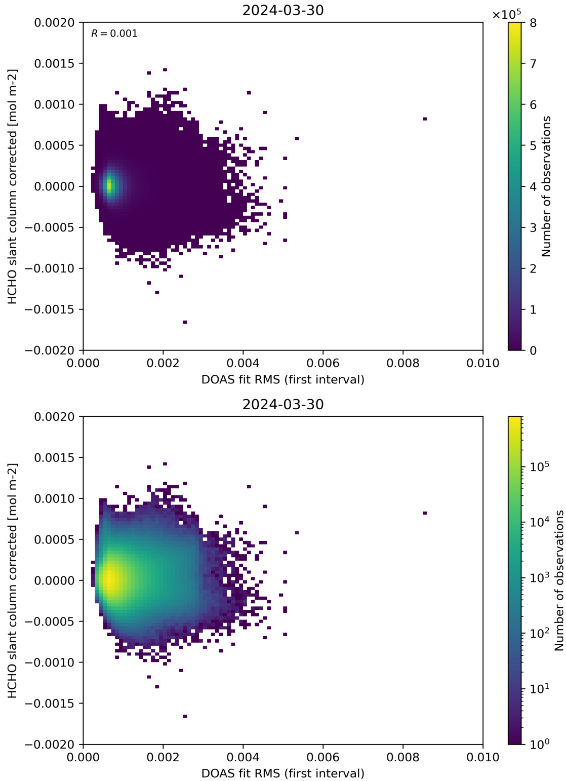
Figure 62: Scatter density plot of “DOAS fit RMS (first interval)” against “HCHO slant column corrected” for 2024-03-30 to 2024-03-31.
