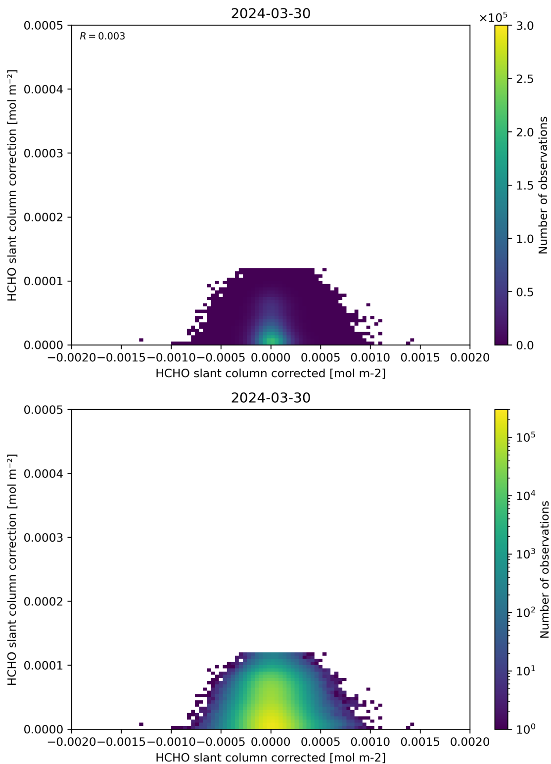
Figure 77: Scatter density plot of “HCHO slant column corrected” against “HCHO slant column correction” for 2024-03-30 to 2024-03-31.
