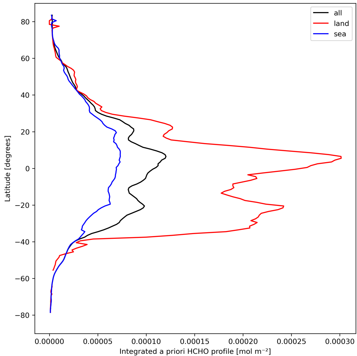
Figure 29: Zonal average of “Integrated a priori HCHO profile” for 2024-03-30 to 2024-03-31.
