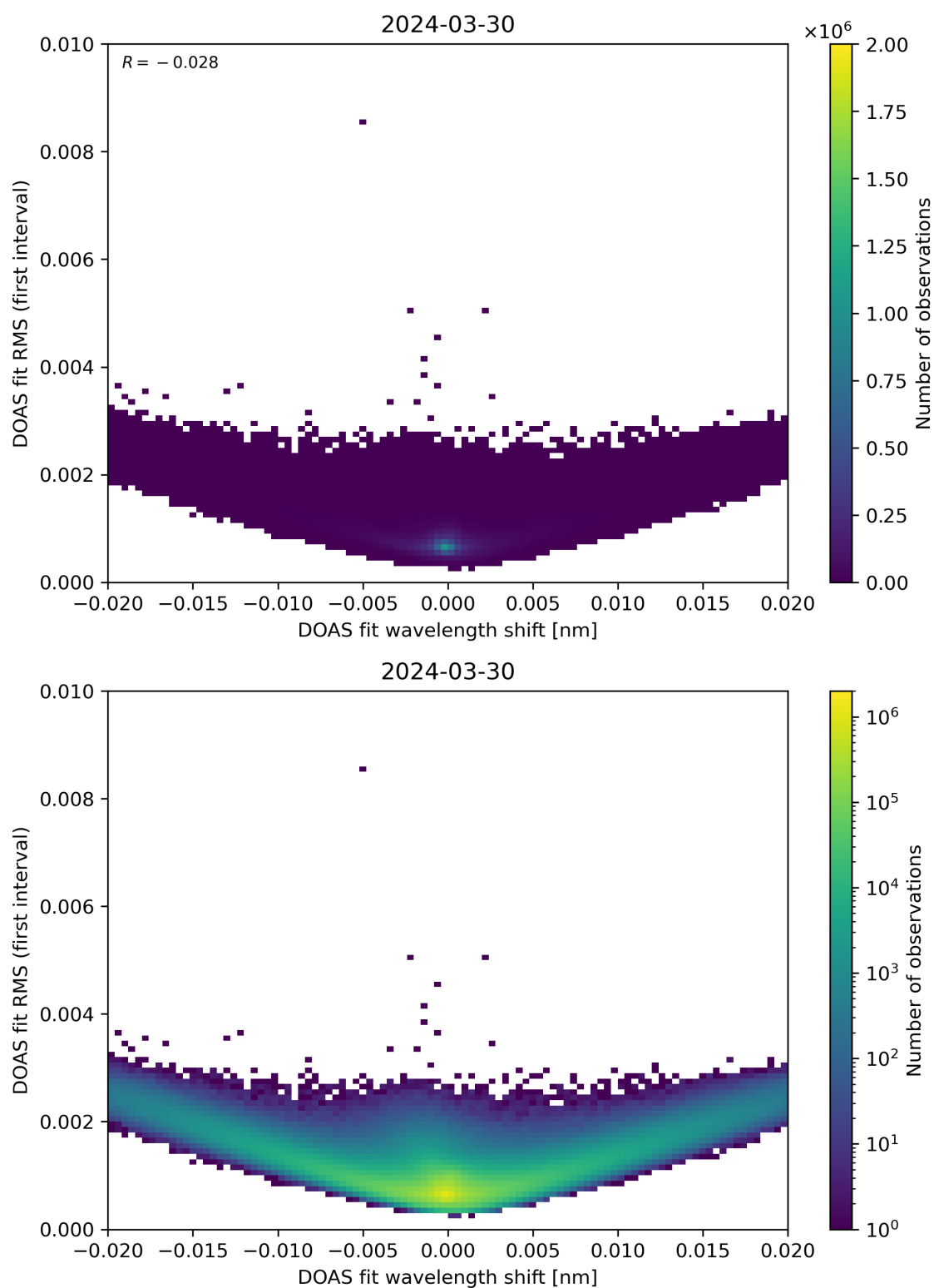
Figure 64: Scatter density plot of “DOAS fit wavelength shift” against “DOAS fit RMS (first interval)” for 2024-03-30 to 2024-03-31.
