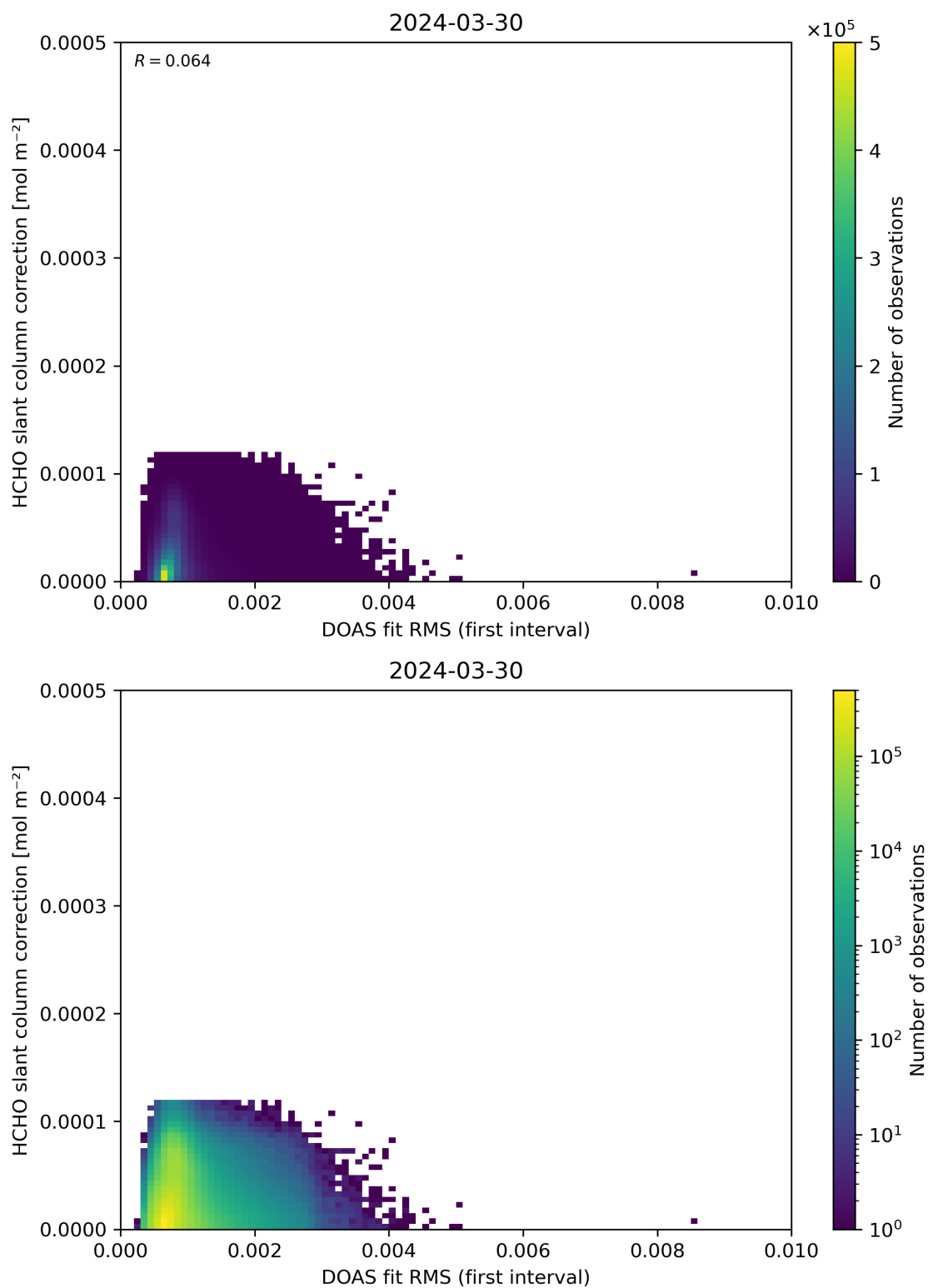
Figure 63: Scatter density plot of “DOAS fit RMS (first interval)” against “HCHO slant column correction” for 2024-03-30 to 2024-03-31.
