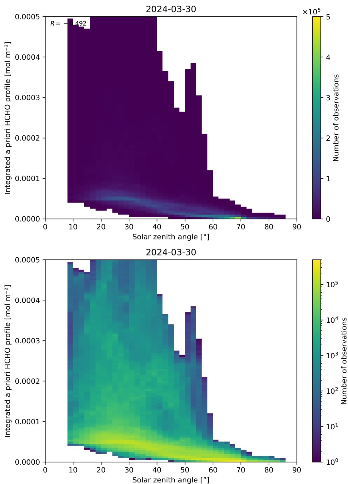
Figure 180: Scatter density plot of “Solar zenith angle” against “Integrated a priori HCHO profile” for 2024-03-30 to 2024-03-31.
