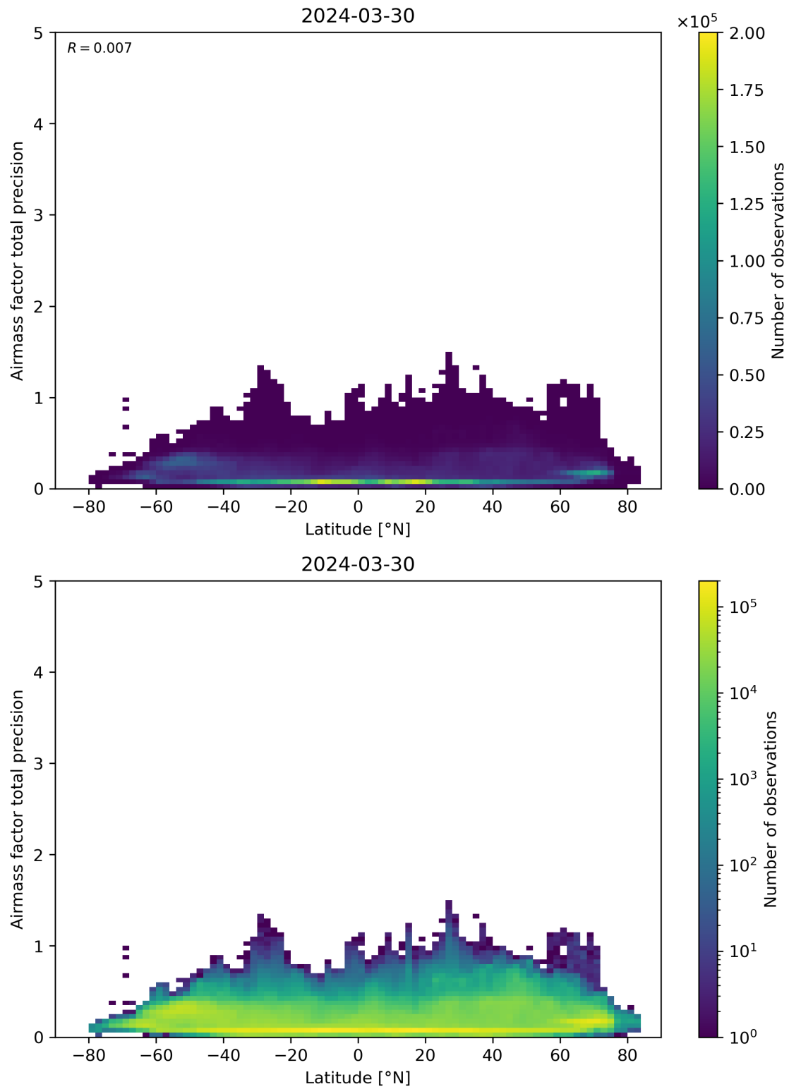
Figure 162: Scatter density plot of “Latitude” against “Airmass factor total precision” for 2024-03-30 to 2024-03-31.
