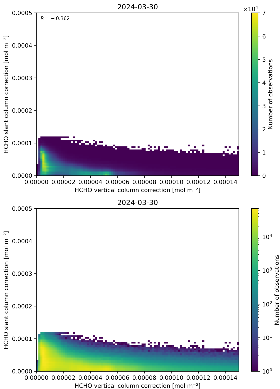
Figure 117: Scatter density plot of “HCHO vertical column correction” against “HCHO slant column correction” for 2024-03-30 to 2024-03-31.
