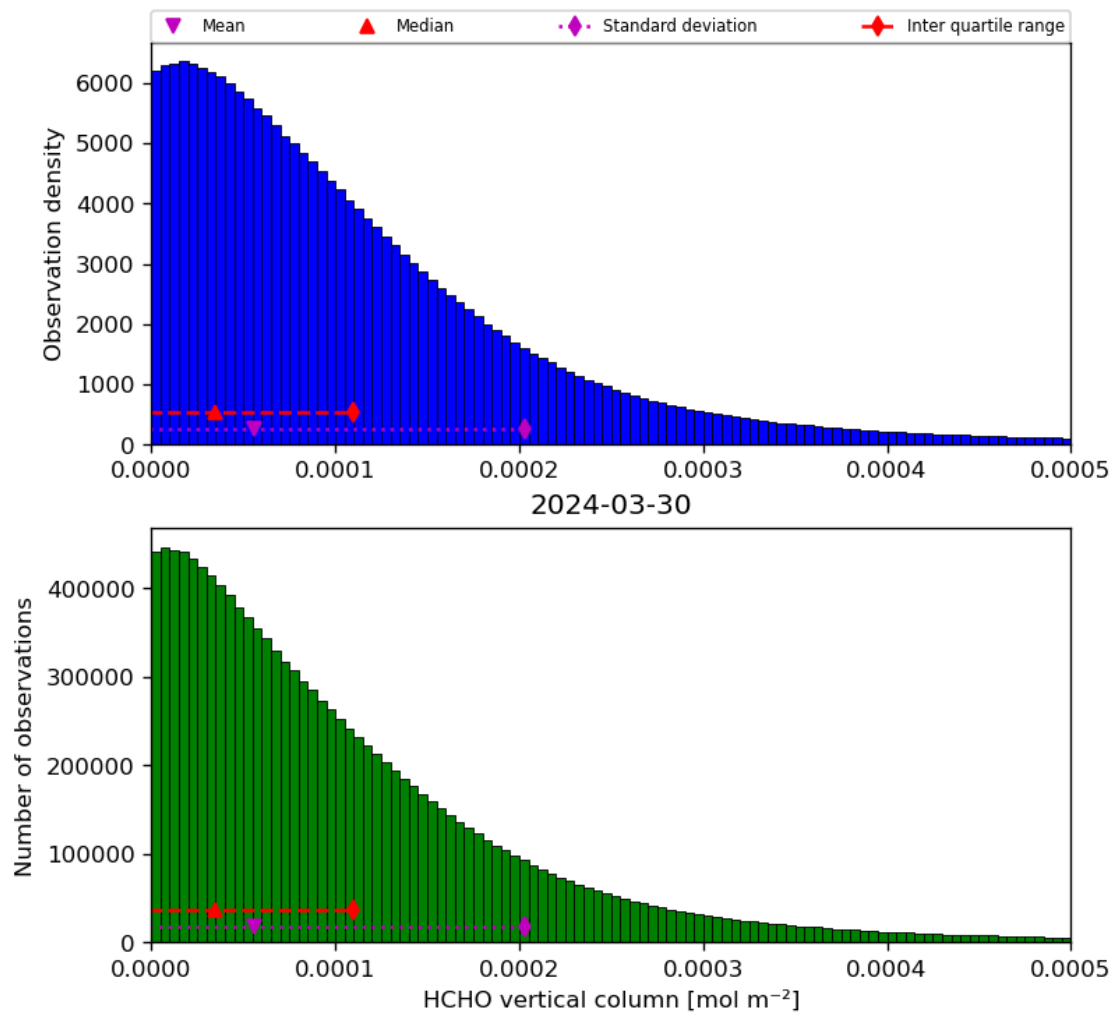
Figure 35: Histogram of “HCHO vertical column” for 2024-03-30 to 2024-03-31
