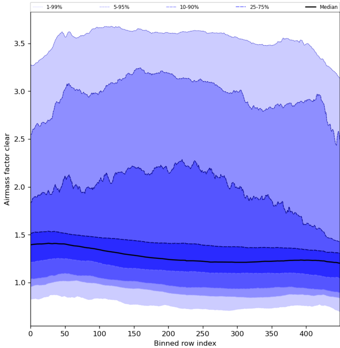
Figure 56: Along track statistics of “Airmass factor clear” for 2024-03-30 to 2024-03-31
