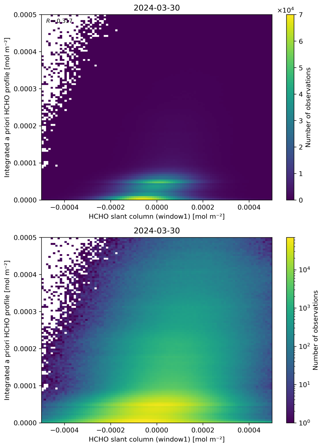
Figure 87: Scatter density plot of “HCHO slant column (window1)” against “Integrated a priori HCHO profile” for 2024-03-30 to 2024-03-31.
