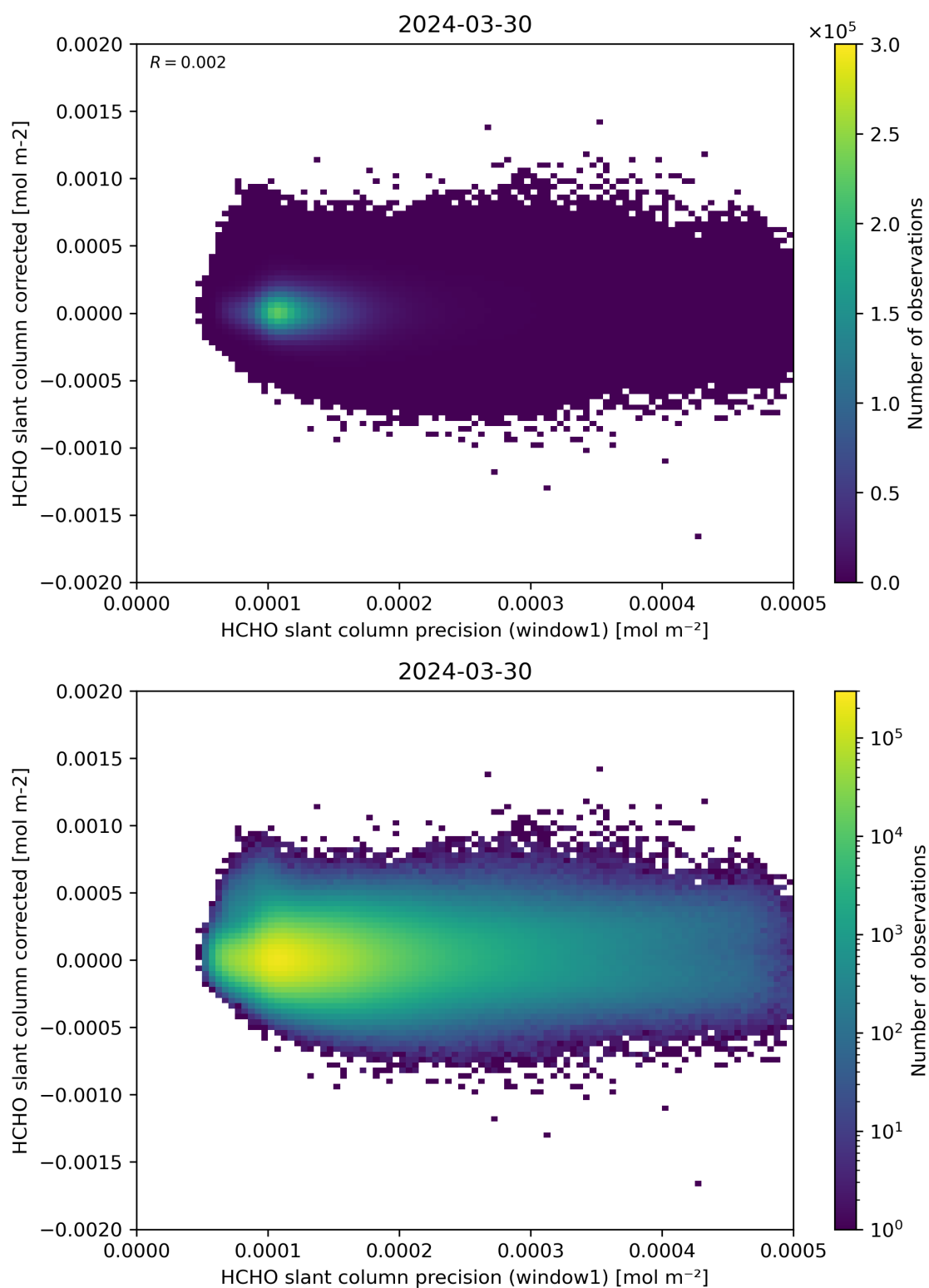
Figure 92: Scatter density plot of “HCHO slant column precision (window1)” against “HCHO slant column corrected” for 2024-03-30 to 2024-03-31.
