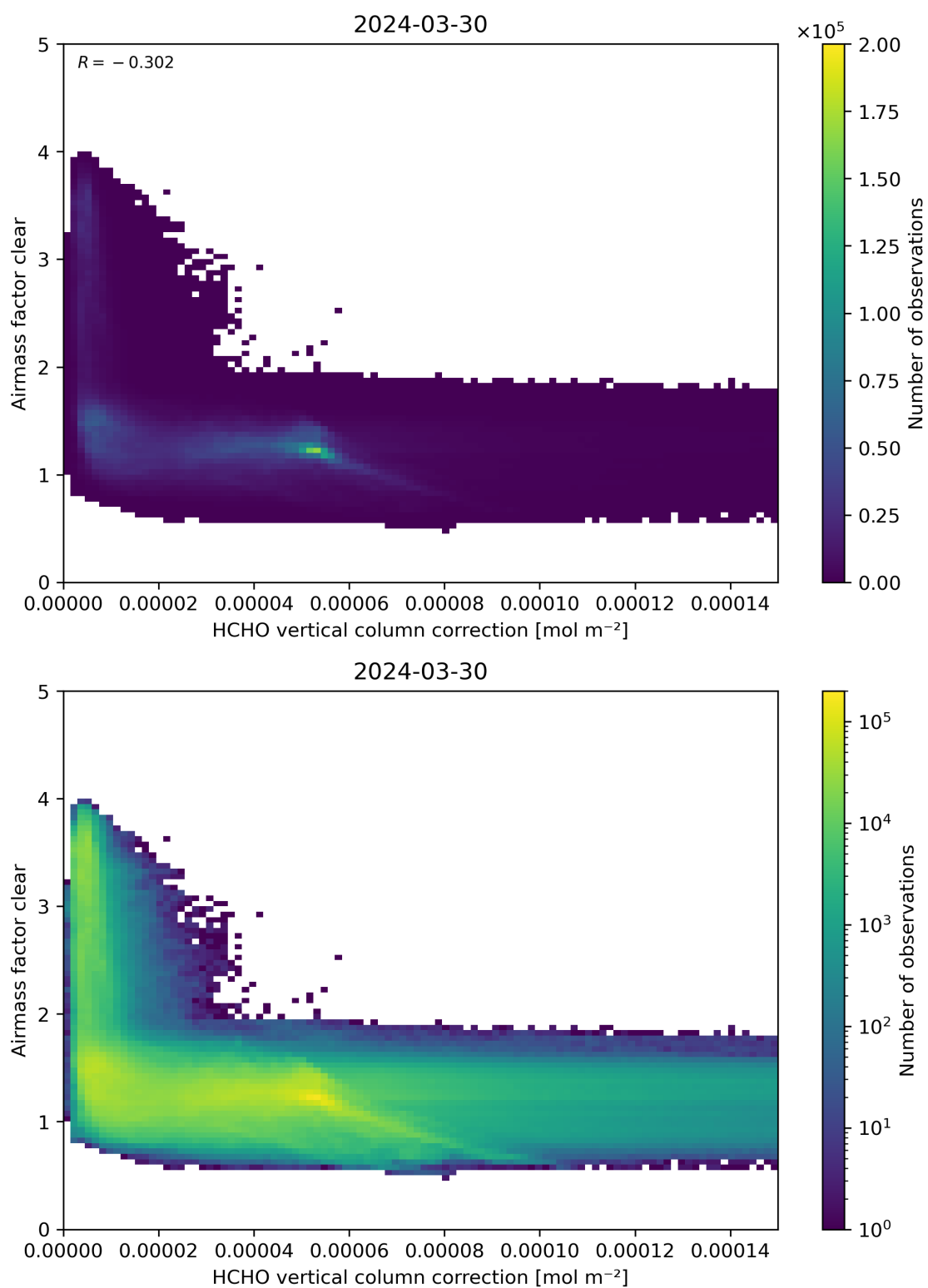
Figure 115: Scatter density plot of “HCHO vertical column correction” against “Airmass factor clear” for 2024-03-30 to 2024-03-31.
