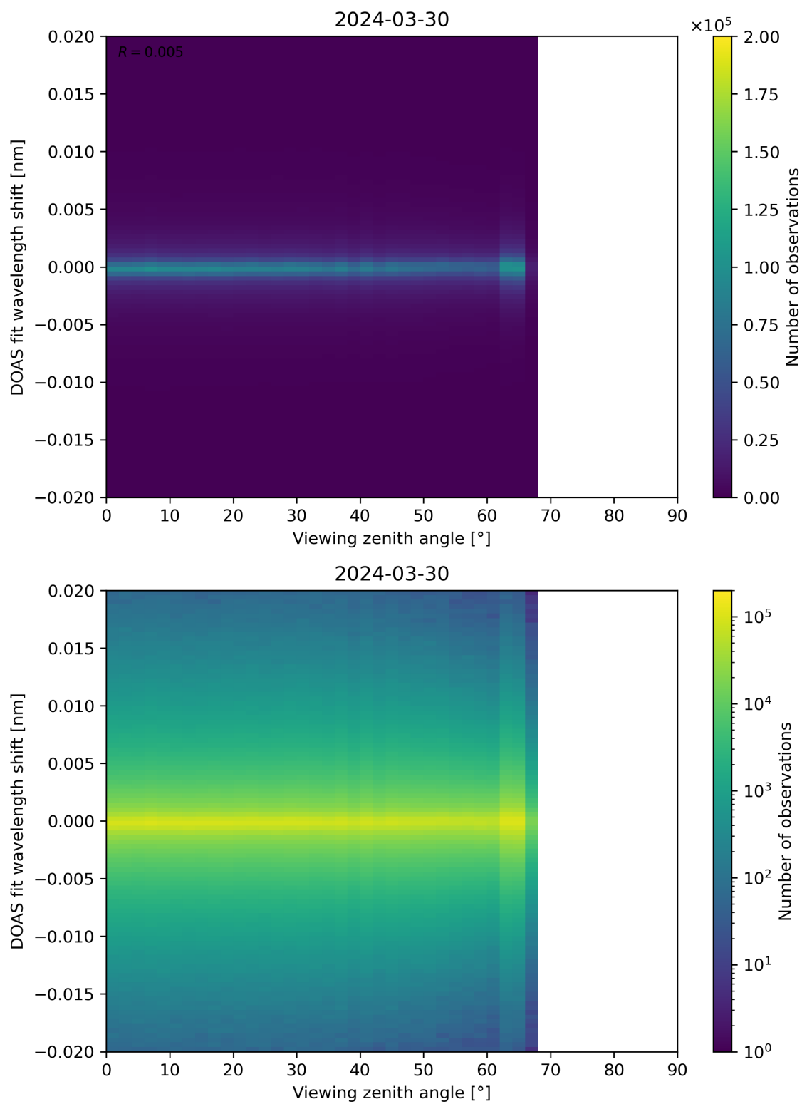
Figure 183: Scatter density plot of “Viewing zenith angle” against “DOAS fit wavelength shift” for 2024-03-30 to 2024-03-31.
