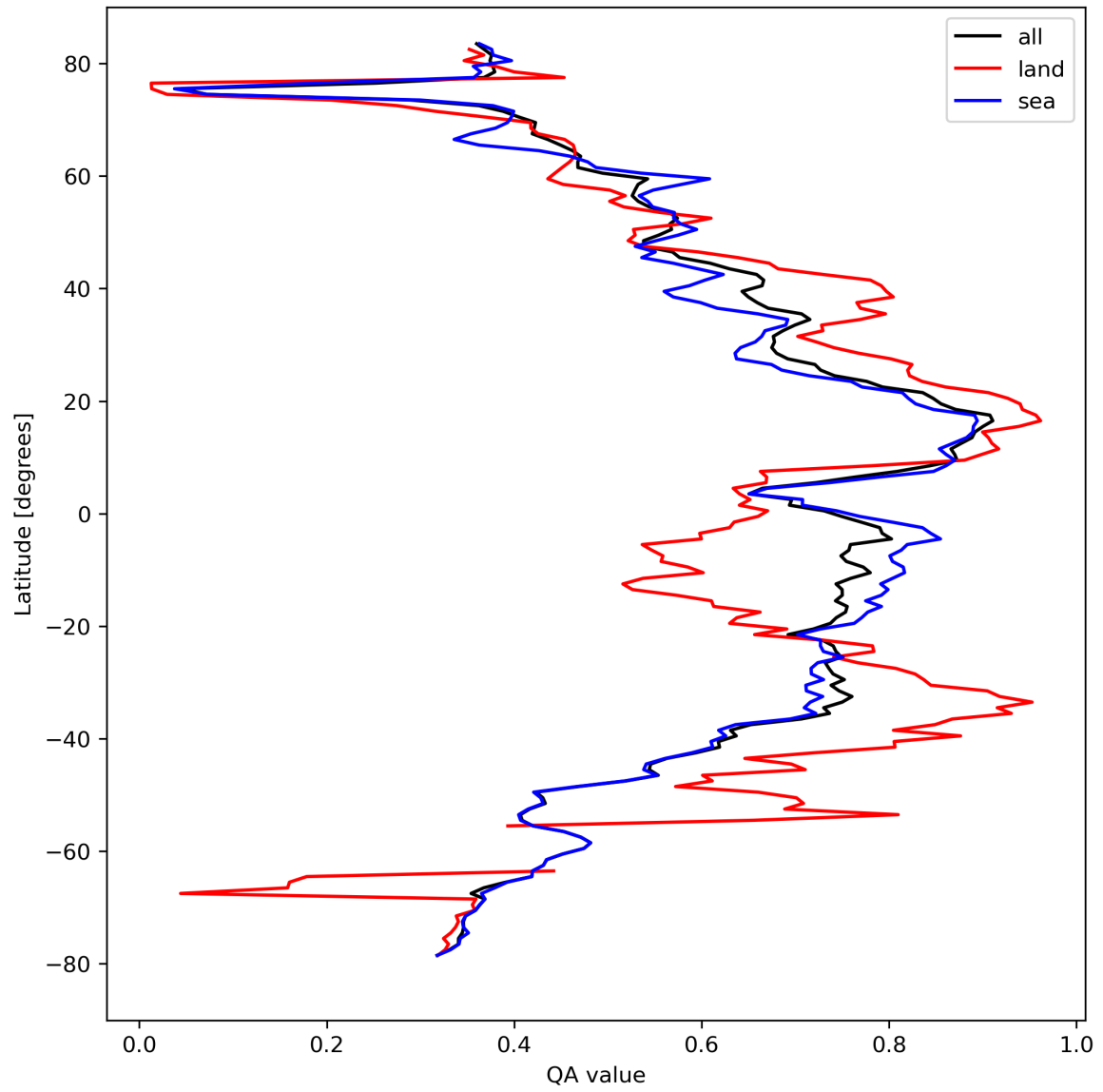
Figure 20: Zonal average of “QA value” for 2024-03-30 to 2024-03-31.
