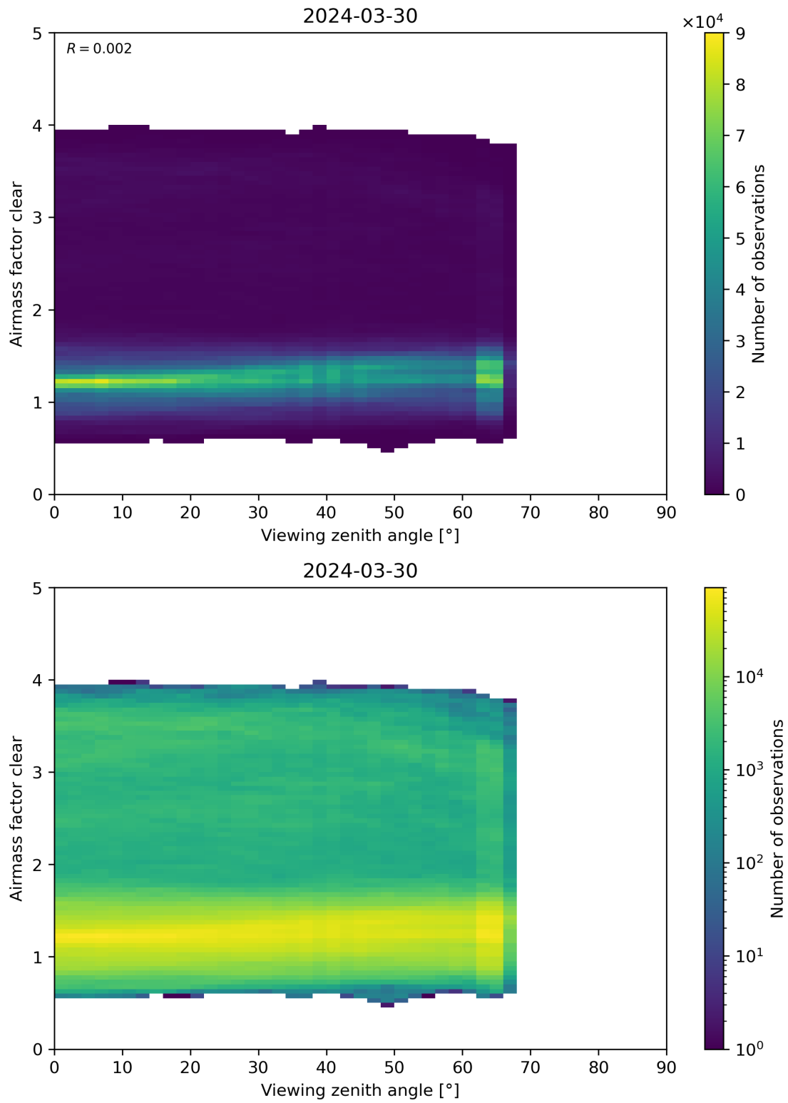
Figure 185: Scatter density plot of “Viewing zenith angle” against “Airmass factor clear” for 2024-03-30 to 2024-03-31.
