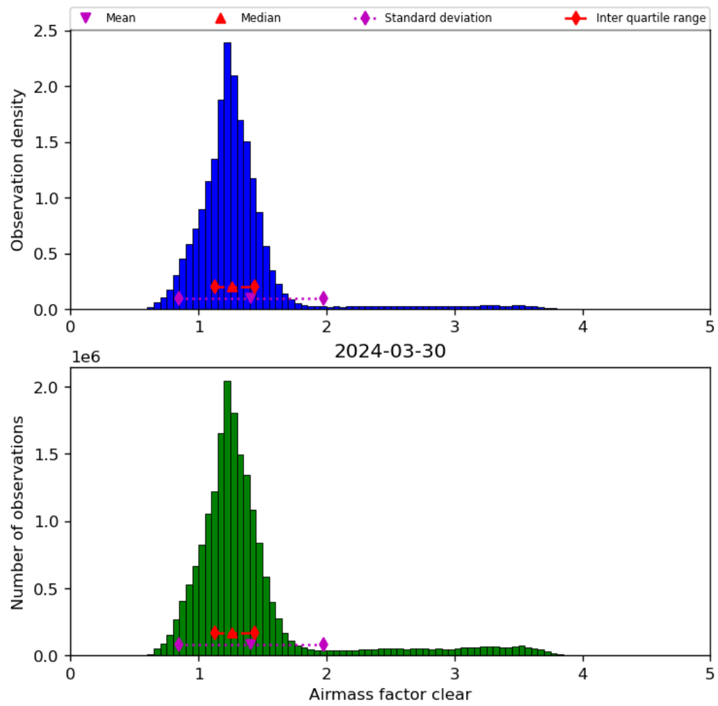
Figure 42: Histogram of “Airmass factor clear” for 2024-03-30 to 2024-03-31
