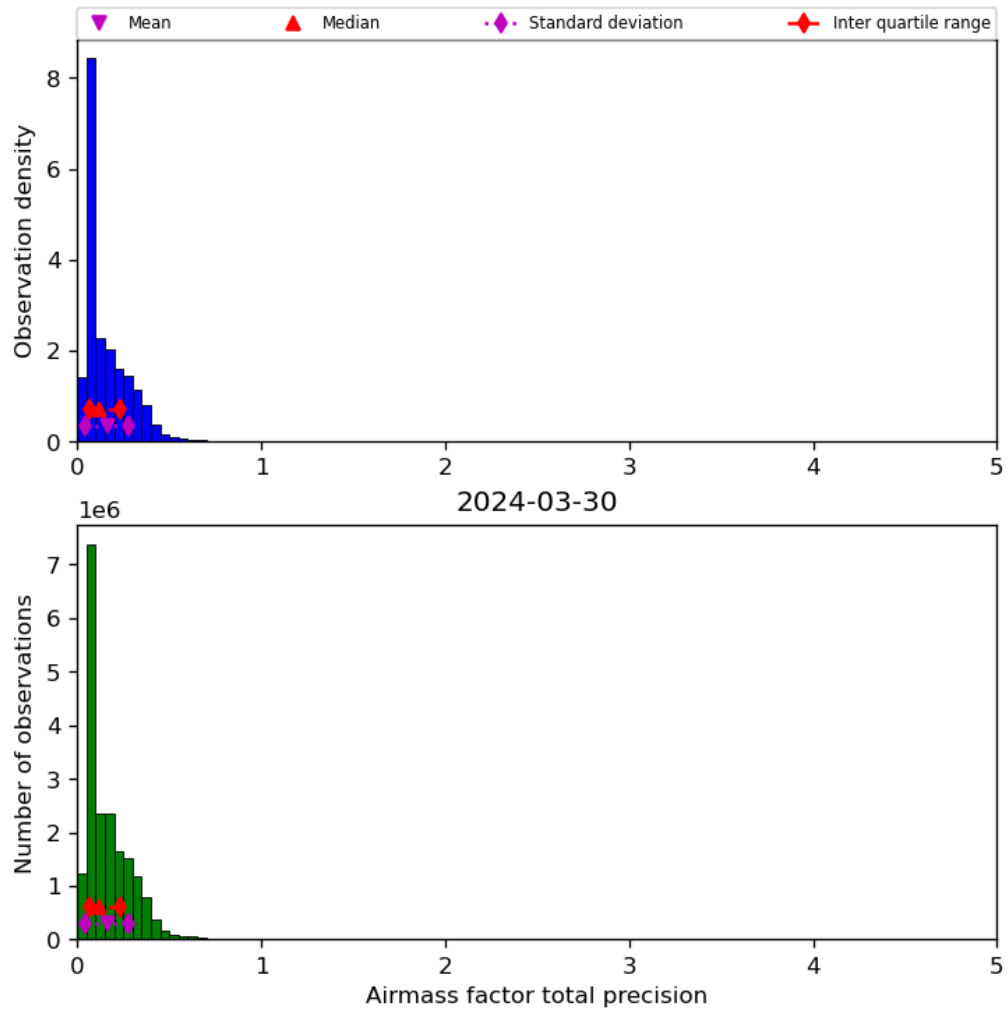
Figure 41: Histogram of “Airmass factor total precision” for 2024-03-30 to 2024-03-31
