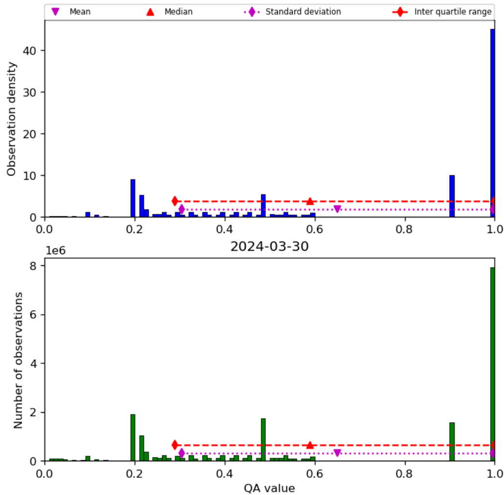
Figure 34: Histogram of “QA value” for 2024-03-30 to 2024-03-31
