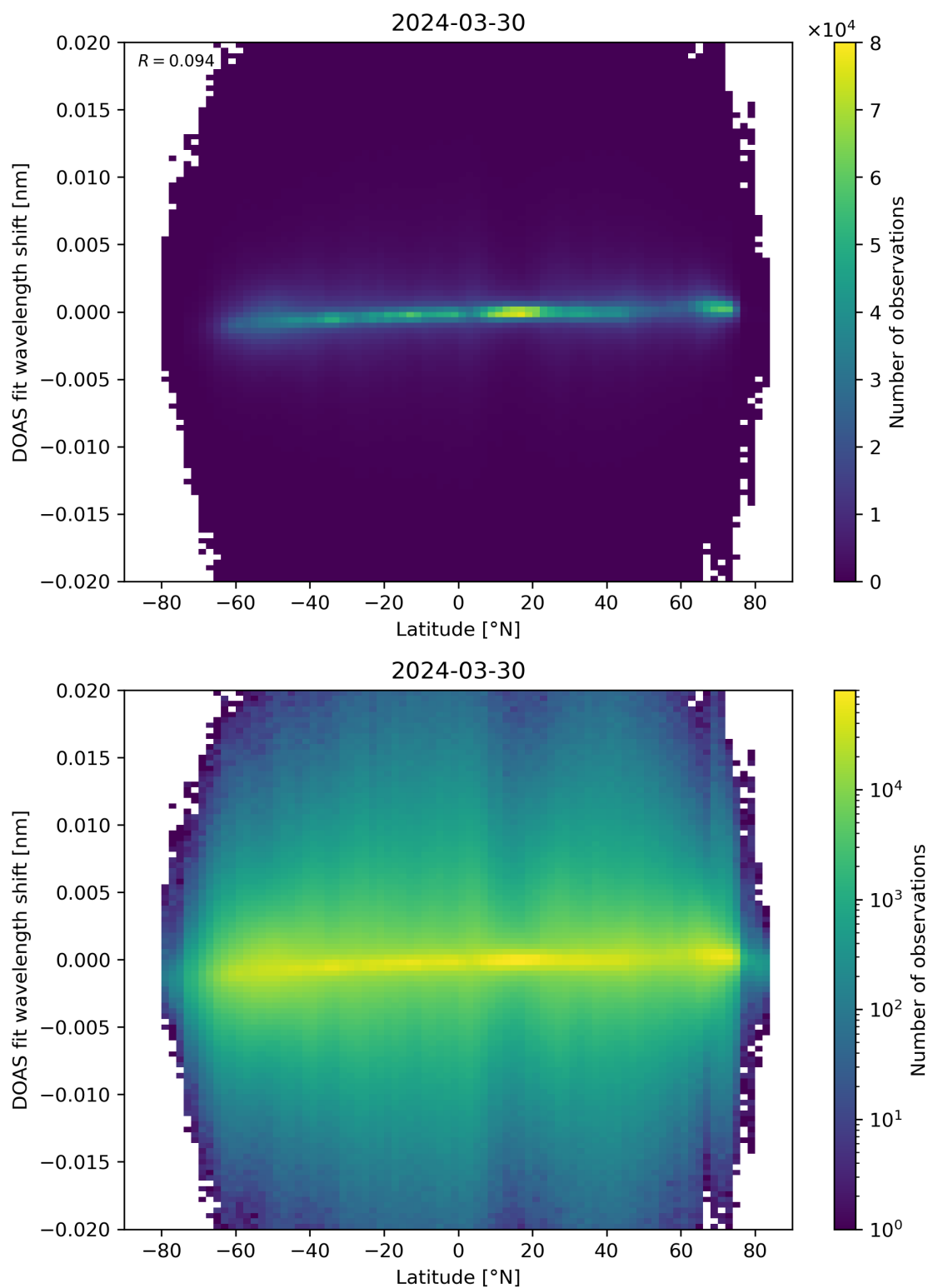
Figure 154: Scatter density plot of “Latitude” against “DOAS fit wavelength shift” for 2024-03-30 to 2024-03-31.
