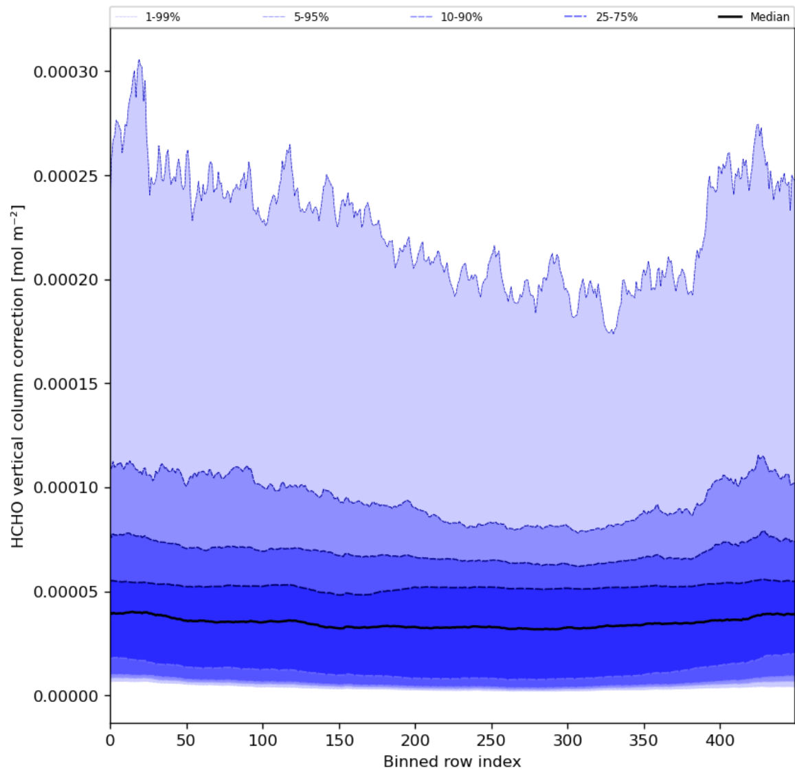
Figure 51: Along track statistics of “HCHO vertical column correction” for 2024-03-30 to 2024-03-31
