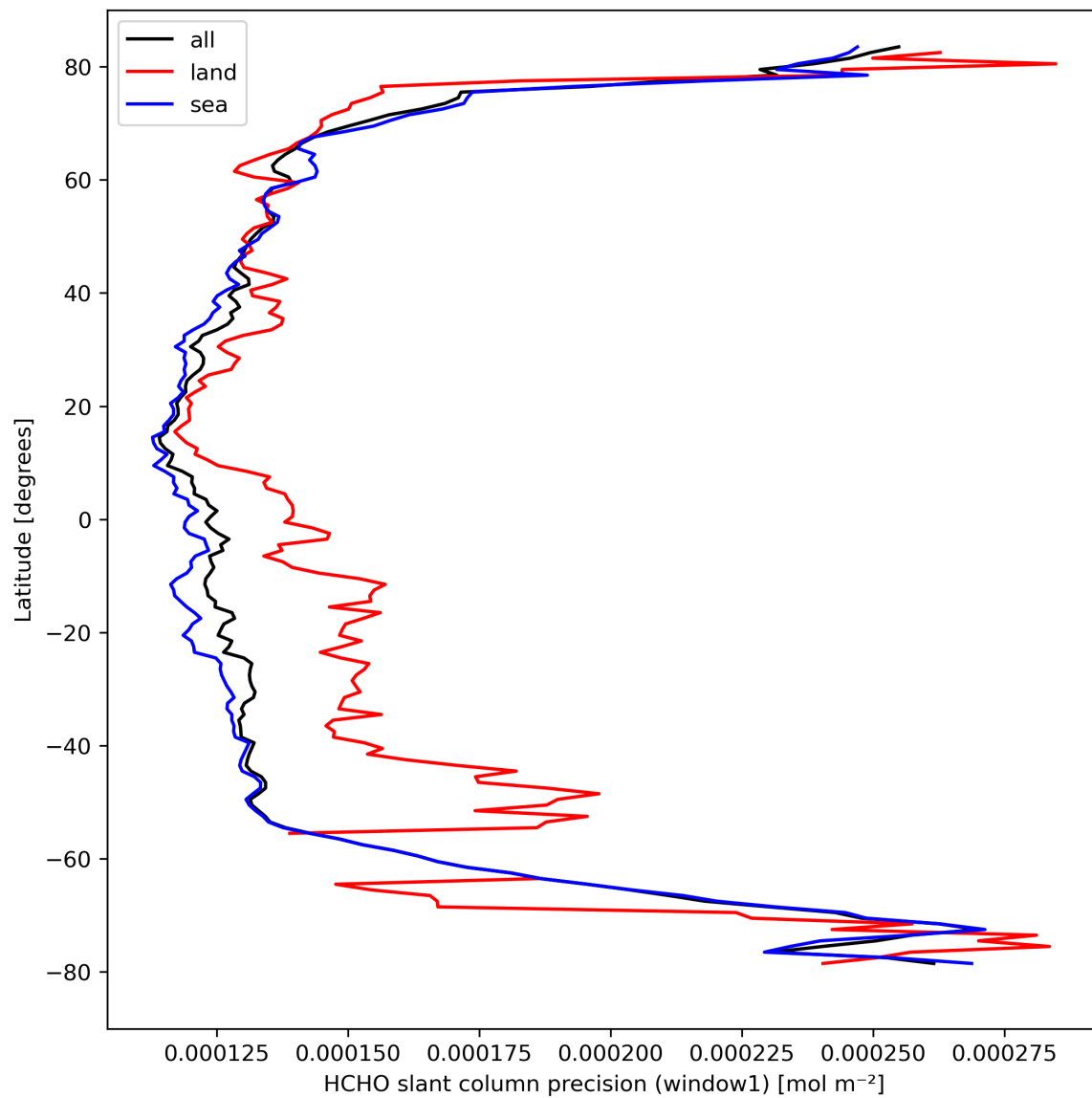
Figure 25: Zonal average of “HCHO slant column precision (window1)” for 2024-03-30 to 2024-03-31.
