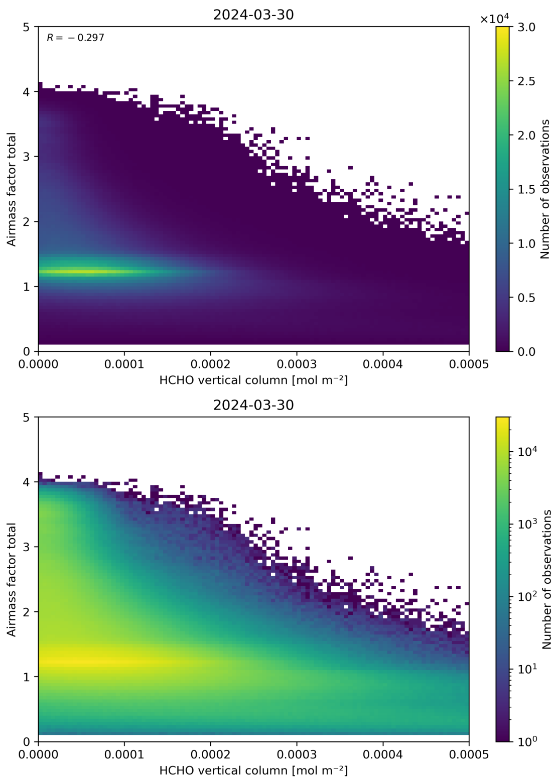
Figure 131: Scatter density plot of “HCHO vertical column” against “Airmass factor total” for 2024-03-30 to 2024-03-31.
