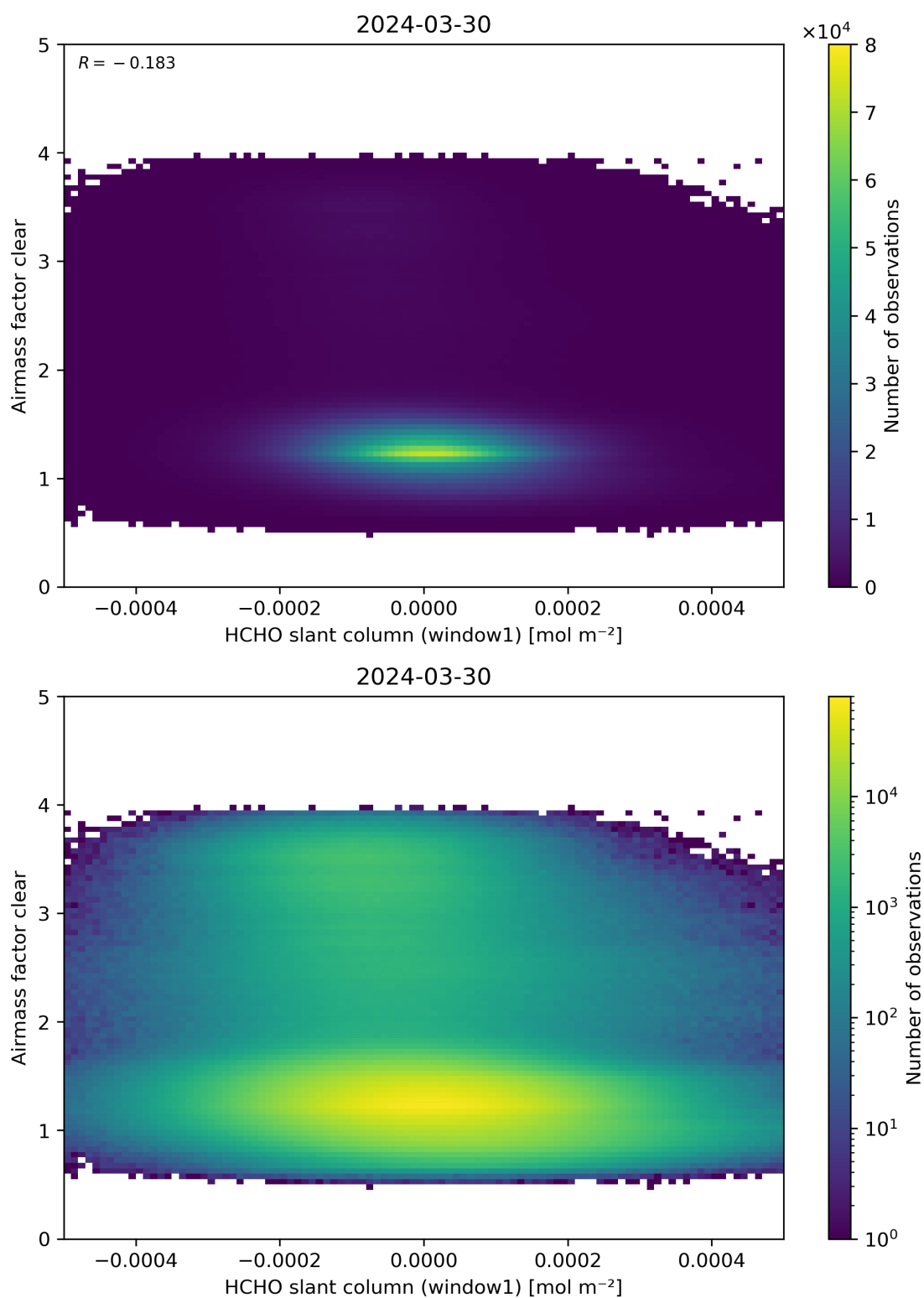
Figure 81: Scatter density plot of “HCHO slant column (window1)” against “Airmass factor clear” for 2024-03-30 to 2024-03-31.
