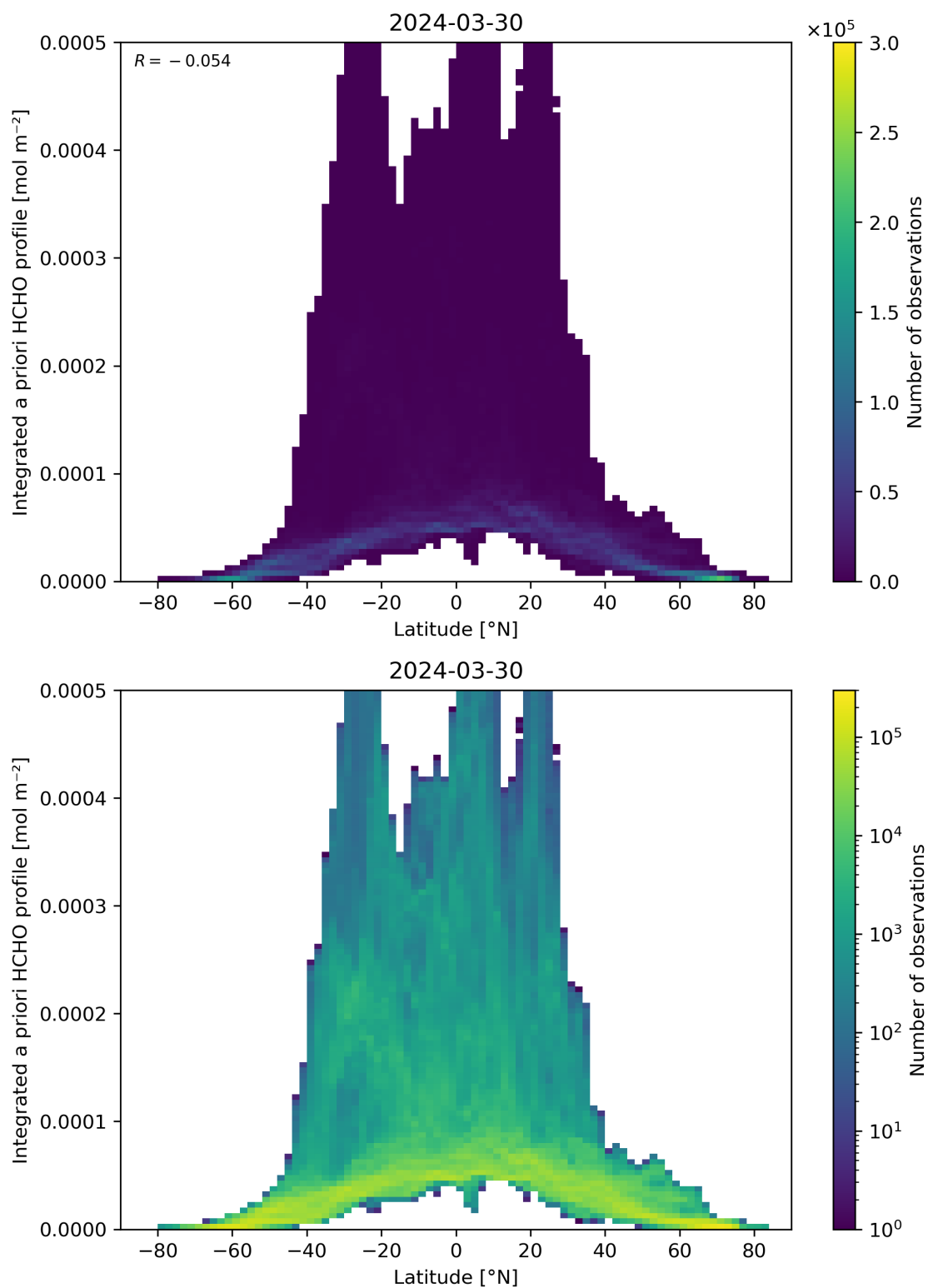
Figure 166: Scatter density plot of “Latitude” against “Integrated a priori HCHO profile” for 2024-03-30 to 2024-03-31.
