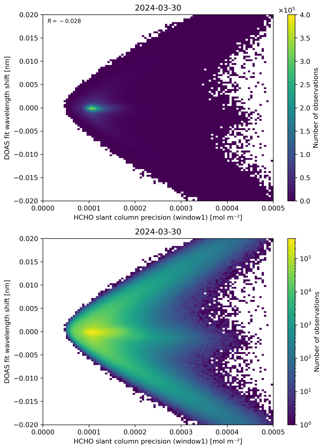
Figure 89: Scatter density plot of “HCHO slant column precision (window1)” against “DOAS fit wavelength shift” for 2024-03-30 to 2024-03-31.
