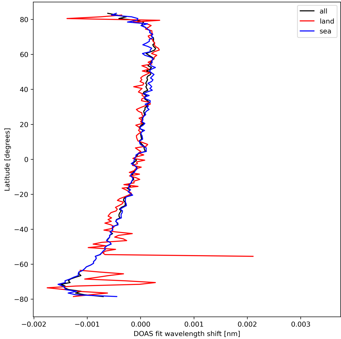
Figure 30: Zonal average of "DOAS fit wavelength shift" for 2024-03-30 to 2024-03-31.
