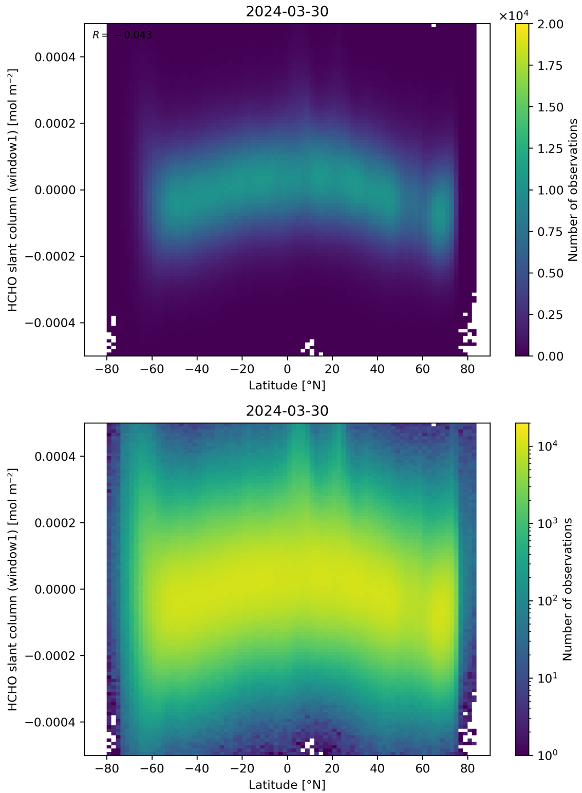
Figure 159: Scatter density plot of “Latitude” against “HCHO slant column (window1)” for 2024-03-30 to 2024-03-31.
