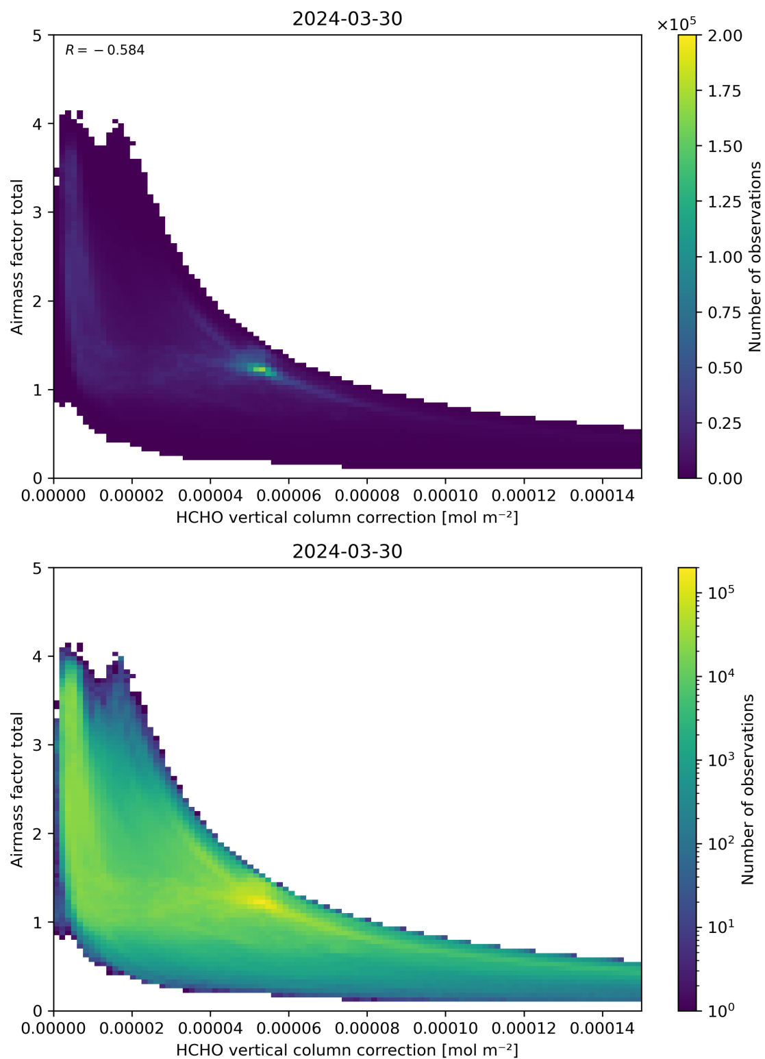
Figure 120: Scatter density plot of “HCHO vertical column correction” against “Airmass factor total” for 2024-03-30 to 2024-03-31.
