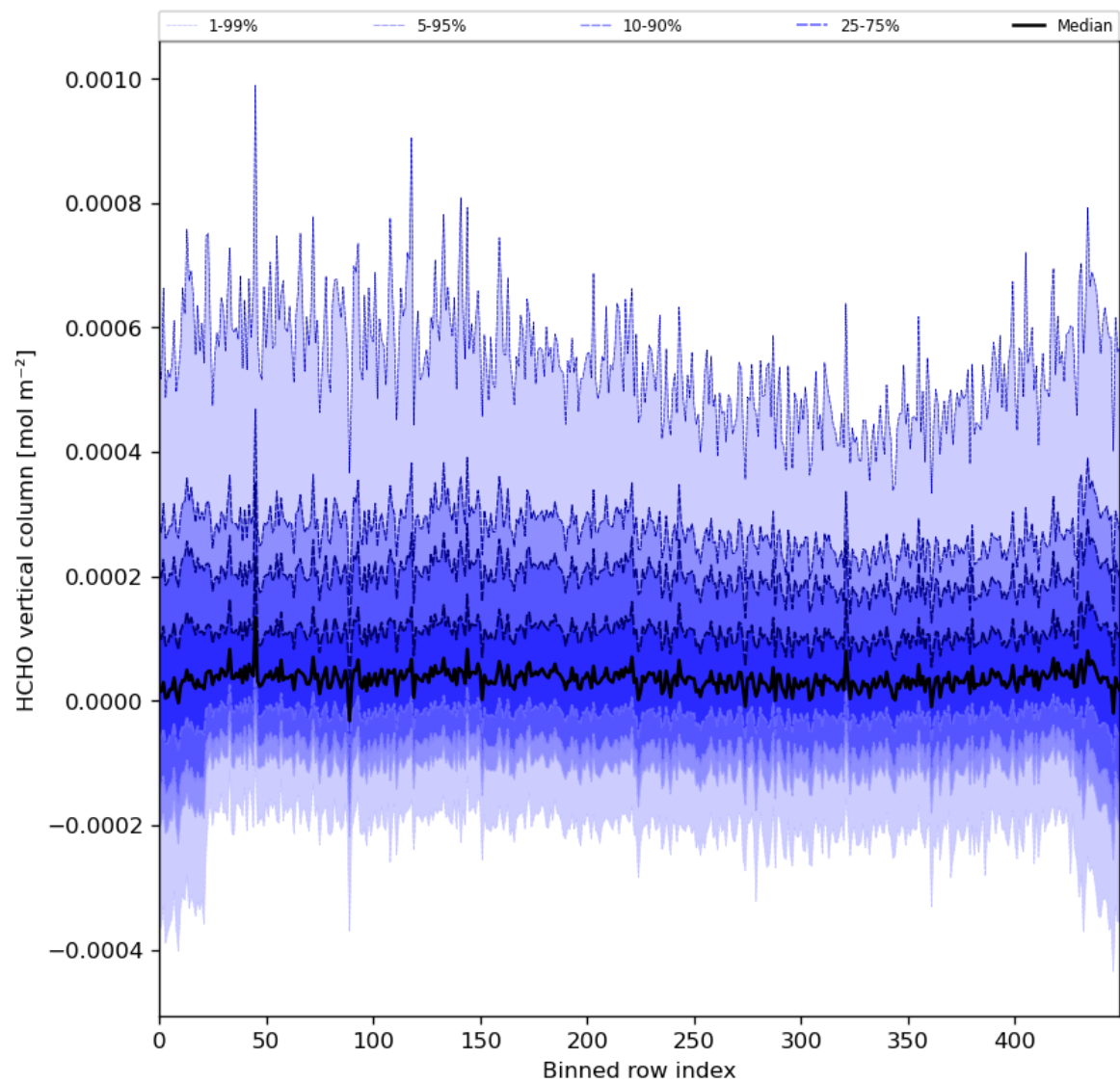
Figure 49: Along track statistics of “HCHO vertical column” for 2024-03-30 to 2024-03-31
