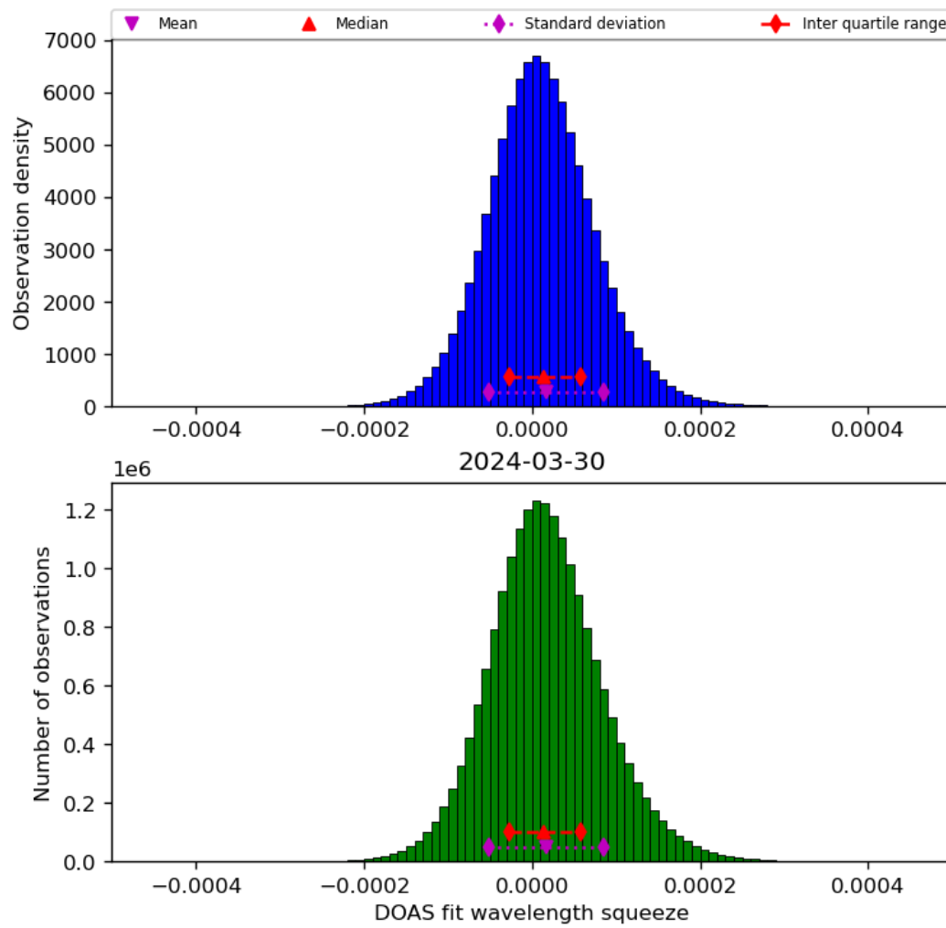
Figure 45: Histogram of “DOAS fit wavelength squeeze” for 2024-03-30 to 2024-03-31
