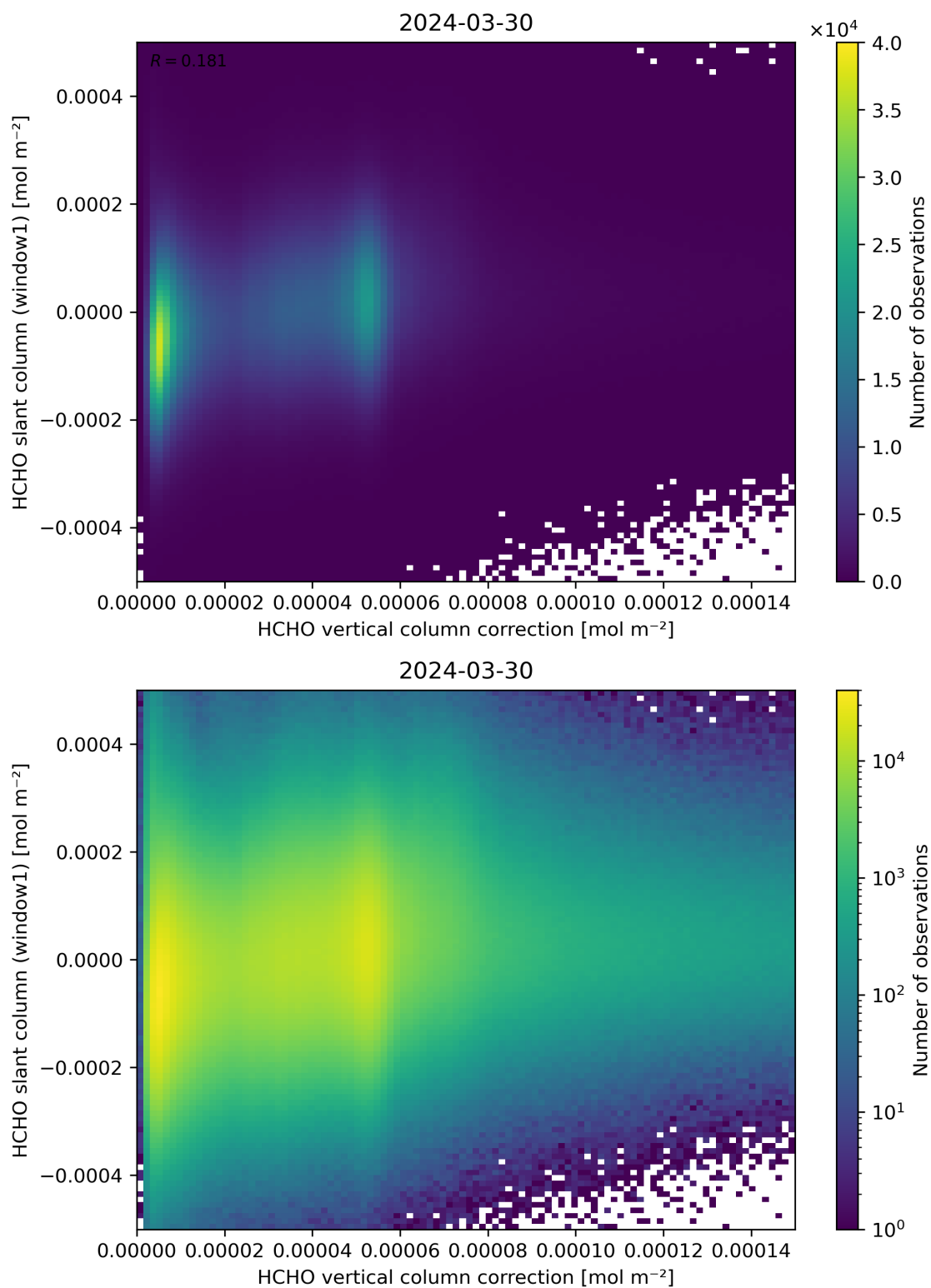
Figure 118: Scatter density plot of “HCHO vertical column correction” against “HCHO slant column (window1)” for 2024-03-30 to 2024-03-31.
