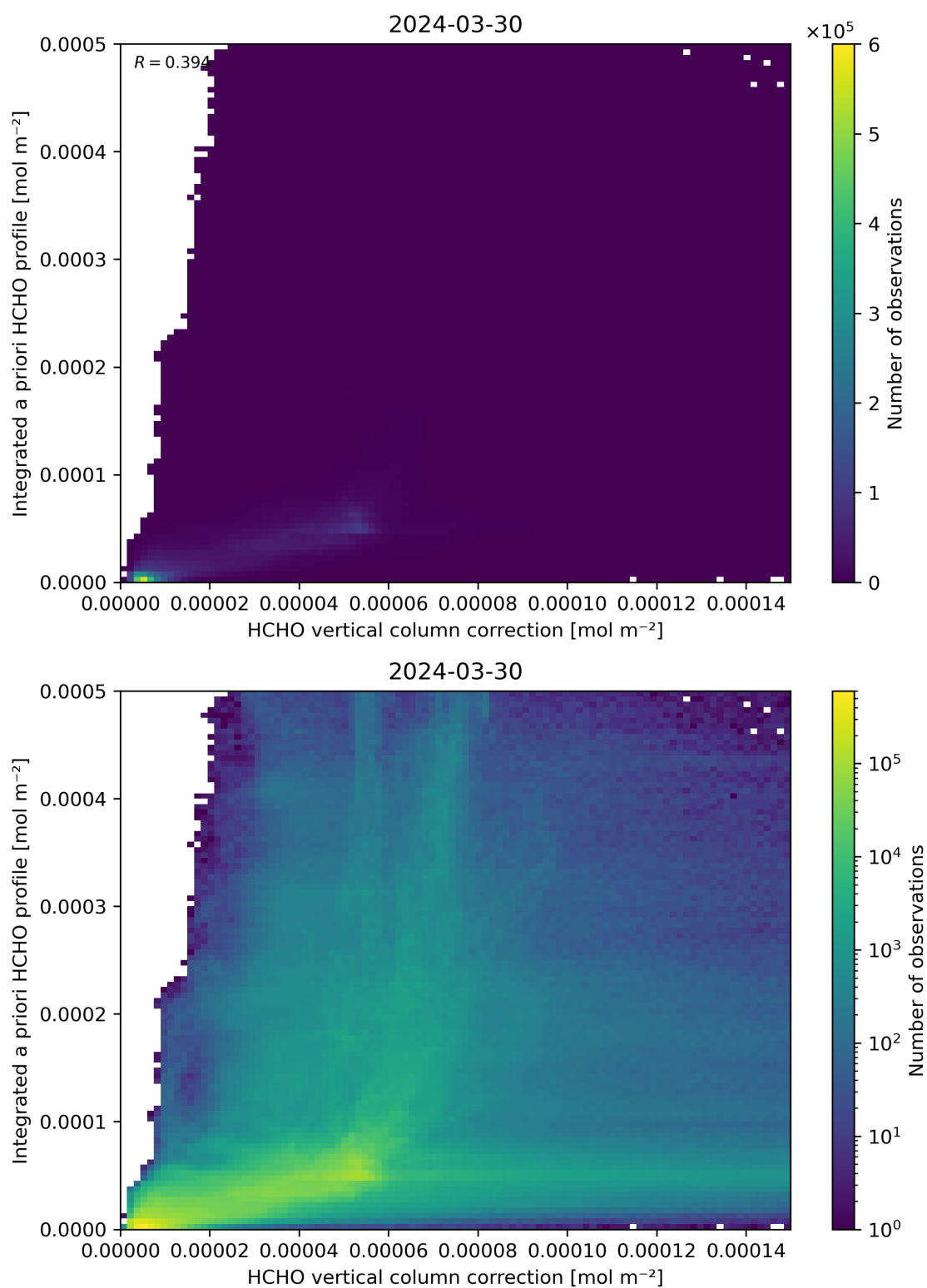
Figure 122: Scatter density plot of “HCHO vertical column correction” against “Integrated a priori HCHO profile” for 2024-03-30 to 2024-03-31.
