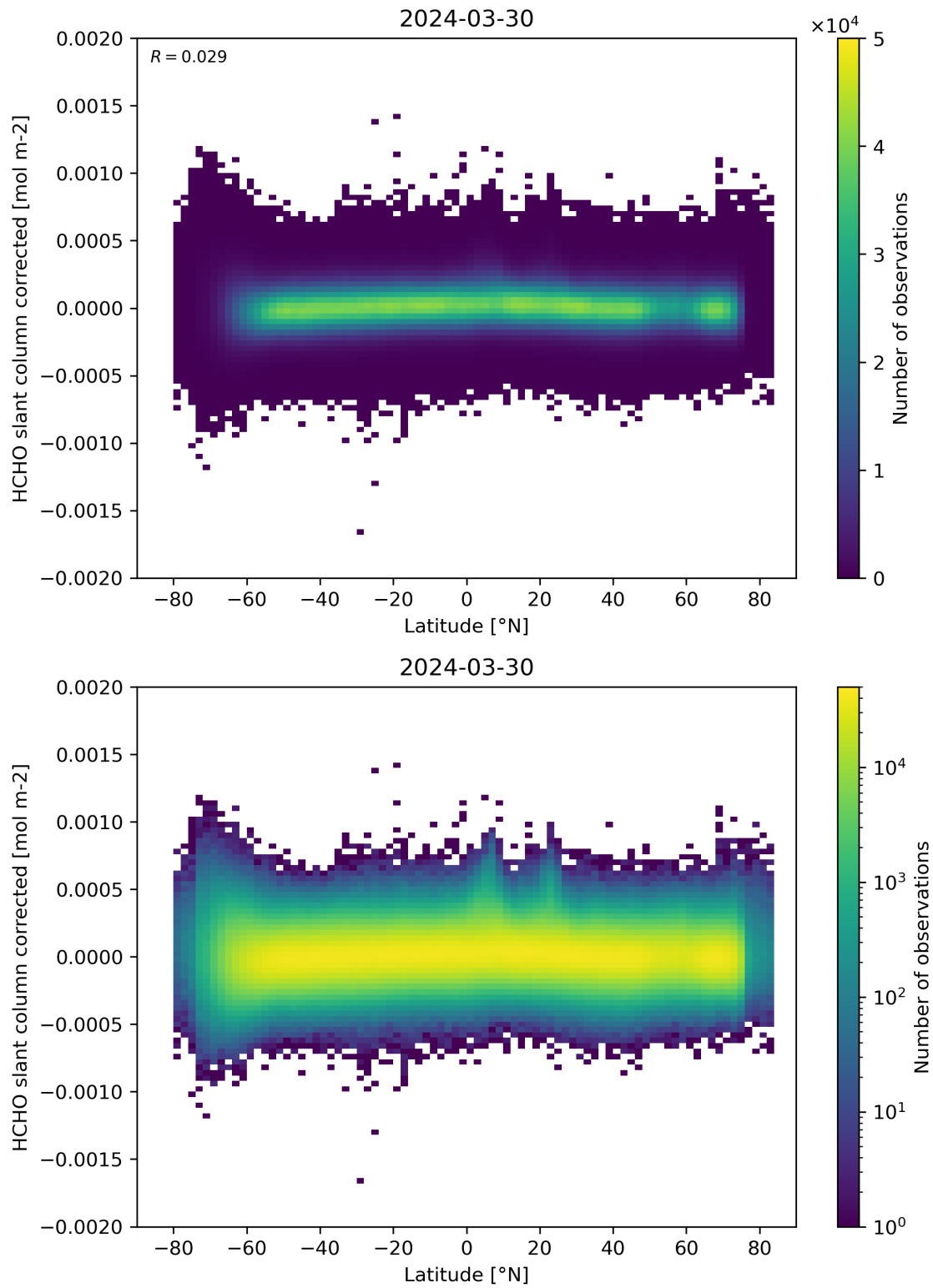
Figure 157: Scatter density plot of “Latitude” against “HCHO slant column corrected” for 2024-03-30 to 2024-03-31.
