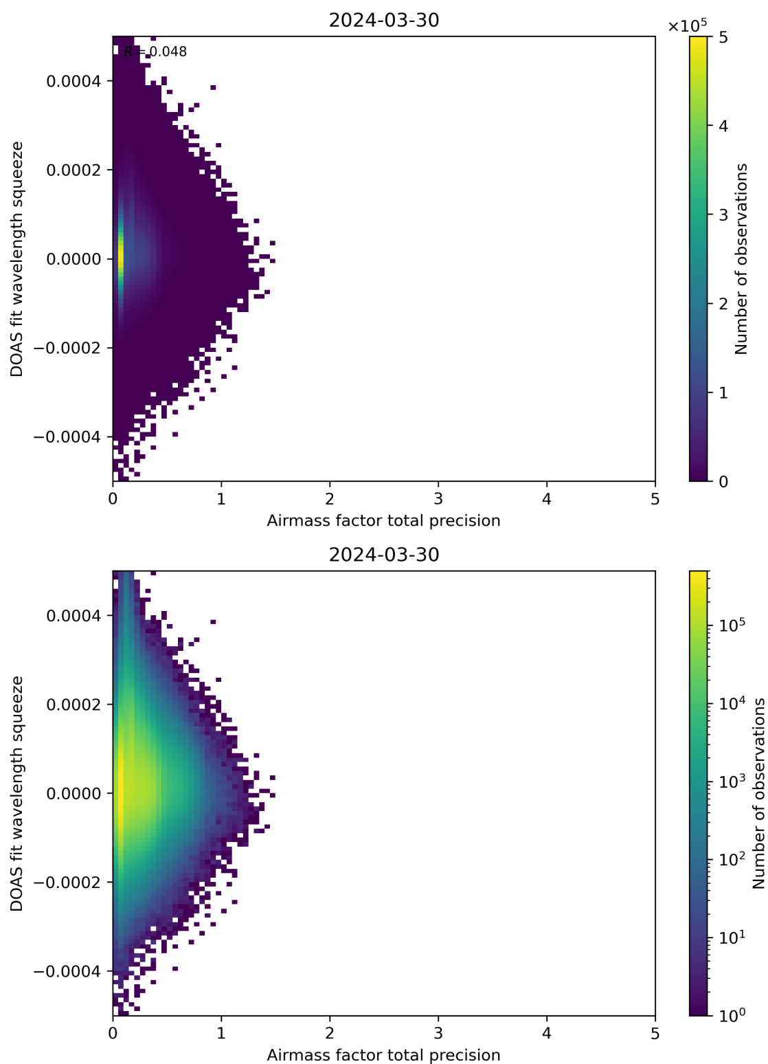
Figure 107: Scatter density plot of “Airmass factor total precision” against “DOAS fit wavelength squeeze” for 2024-03-30 to 2024-03-31.
