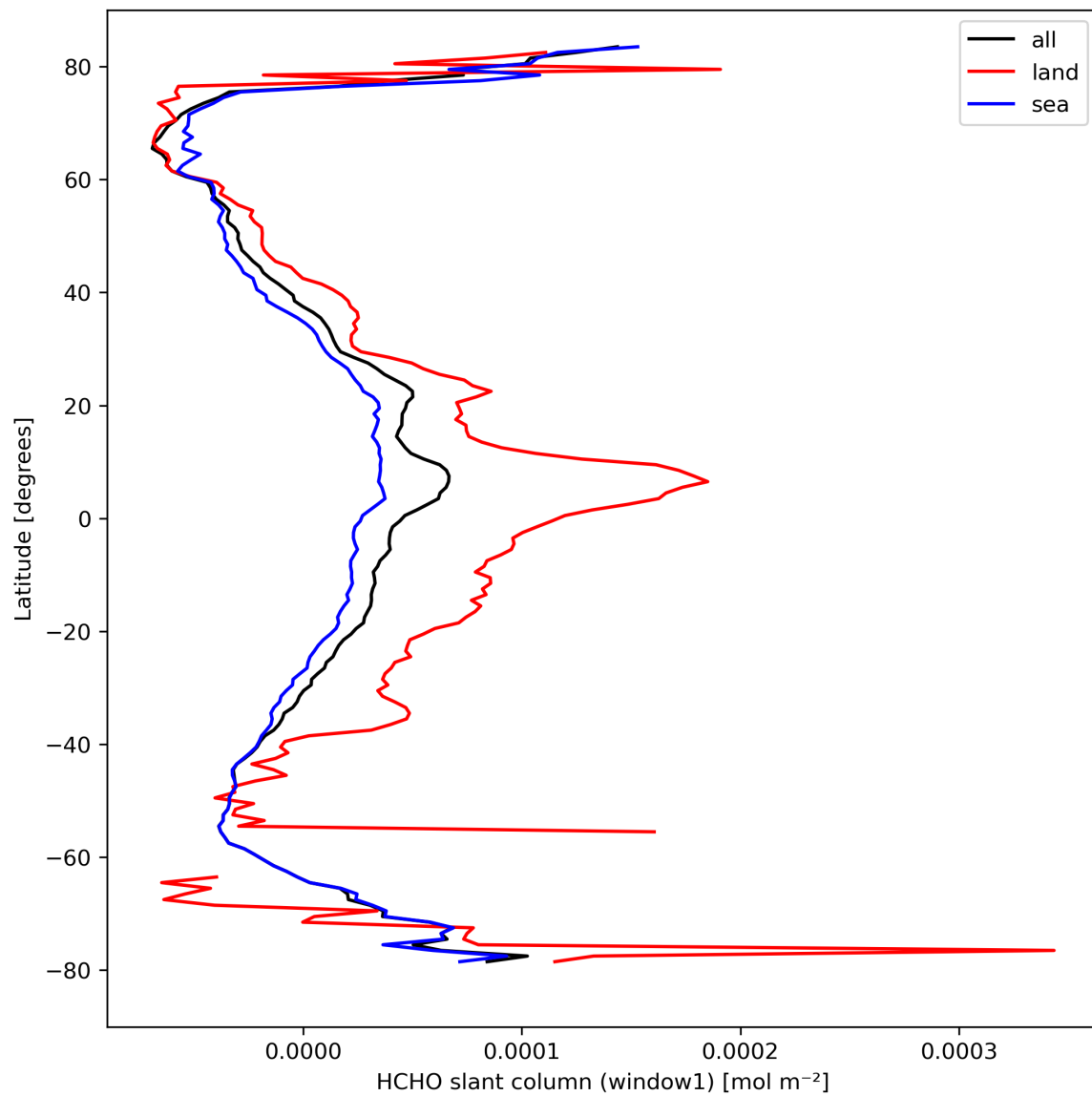
Figure 24: Zonal average of “HCHO slant column (window1)” for 2024-03-30 to 2024-03-31.
