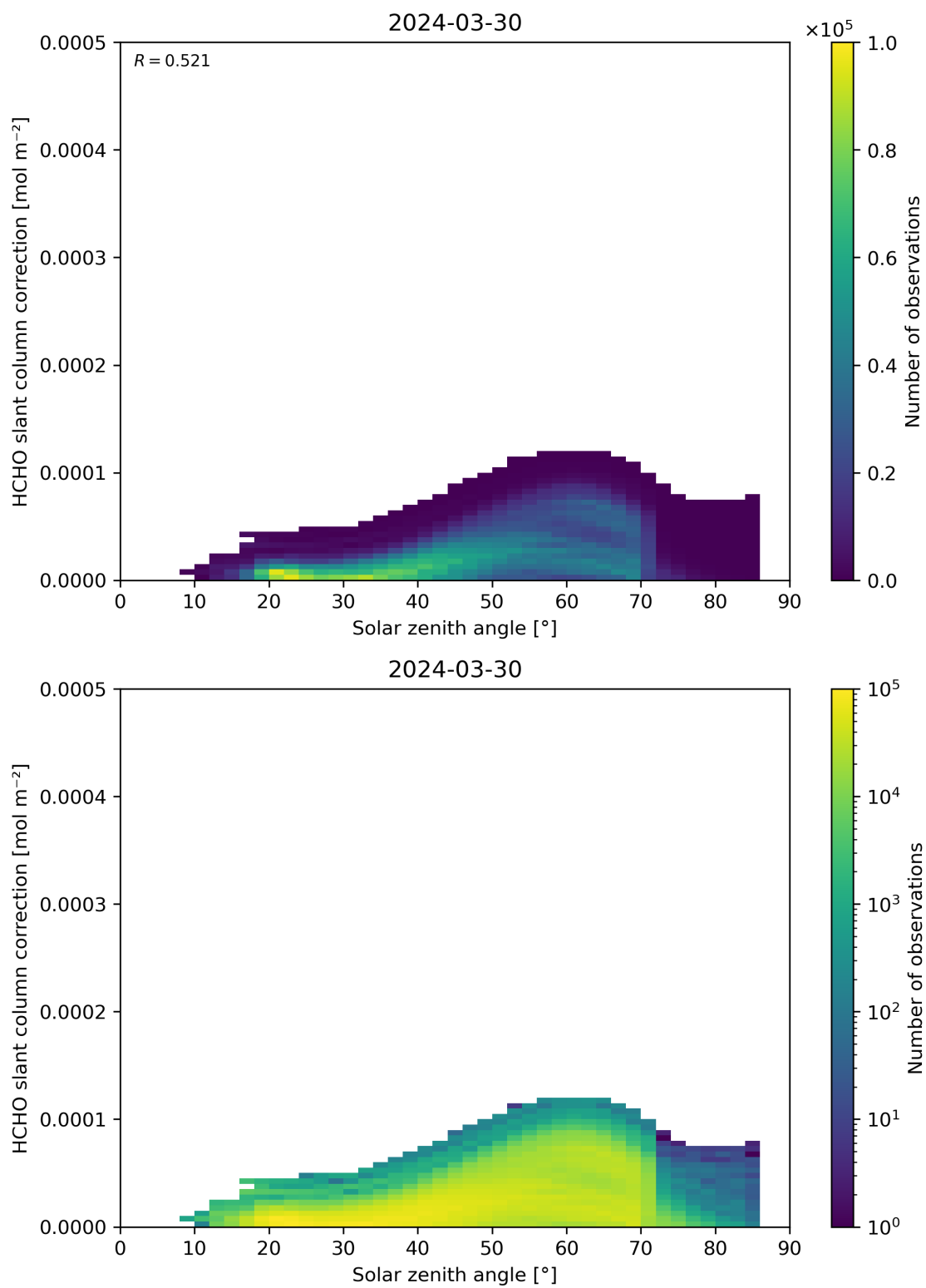
Figure 172: Scatter density plot of “Solar zenith angle” against “HCHO slant column correction” for 2024-03-30 to 2024-03-31.
