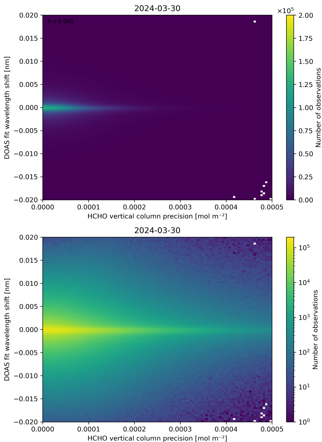
Figure 137: Scatter density plot of “HCHO vertical column precision” against “DOAS fit wavelength shift” for 2024-03-30 to 2024-03-31.
