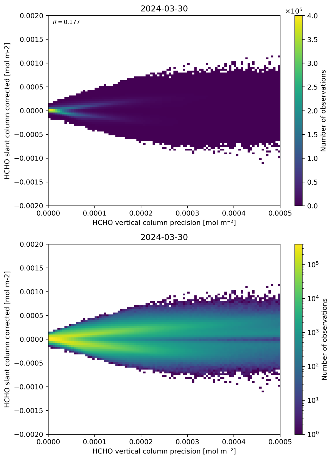
Figure 140: Scatter density plot of “HCHO vertical column precision” against “HCHO slant column corrected” for 2024-03-30 to 2024-03-31.
