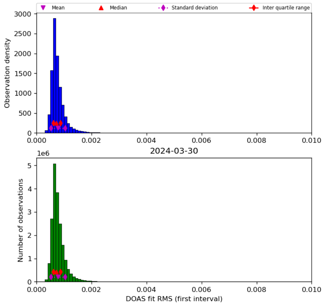
Figure 46: Histogram of “DOAS fit RMS (first interval)” for 2024-03-30 to 2024-03-31
