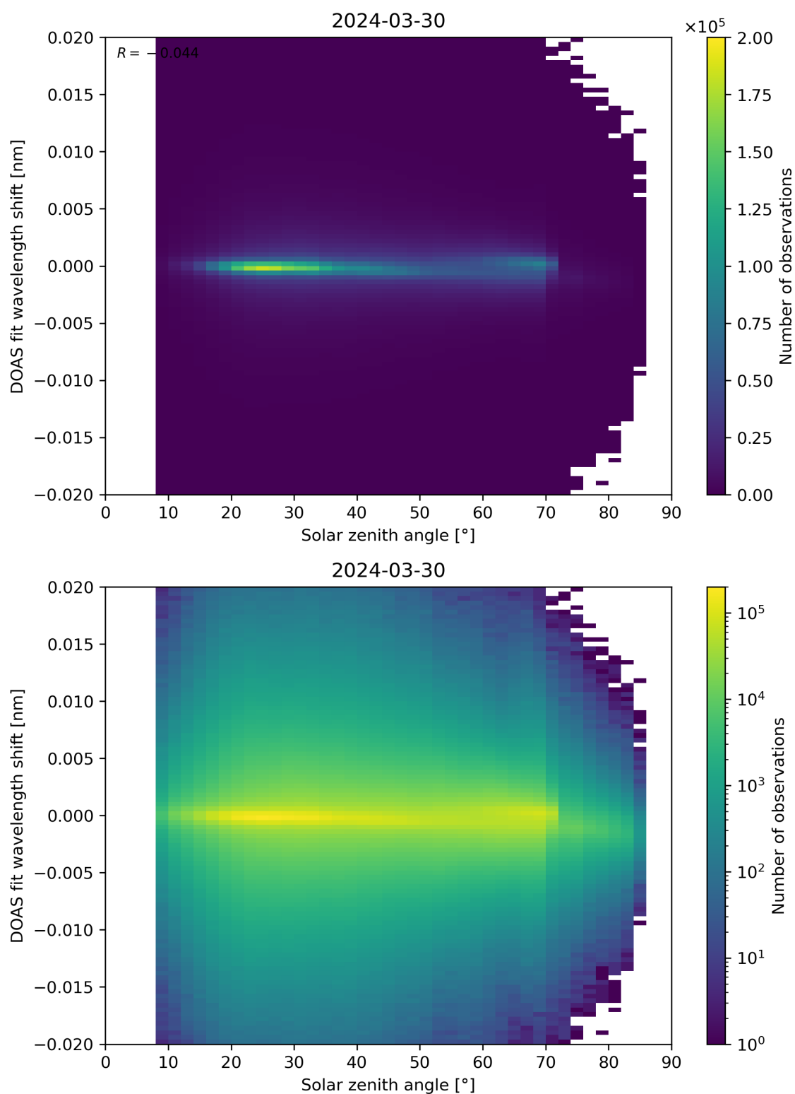
Figure 168: Scatter density plot of “Solar zenith angle” against “DOAS fit wavelength shift” for 2024-03-30 to 2024-03-31.
