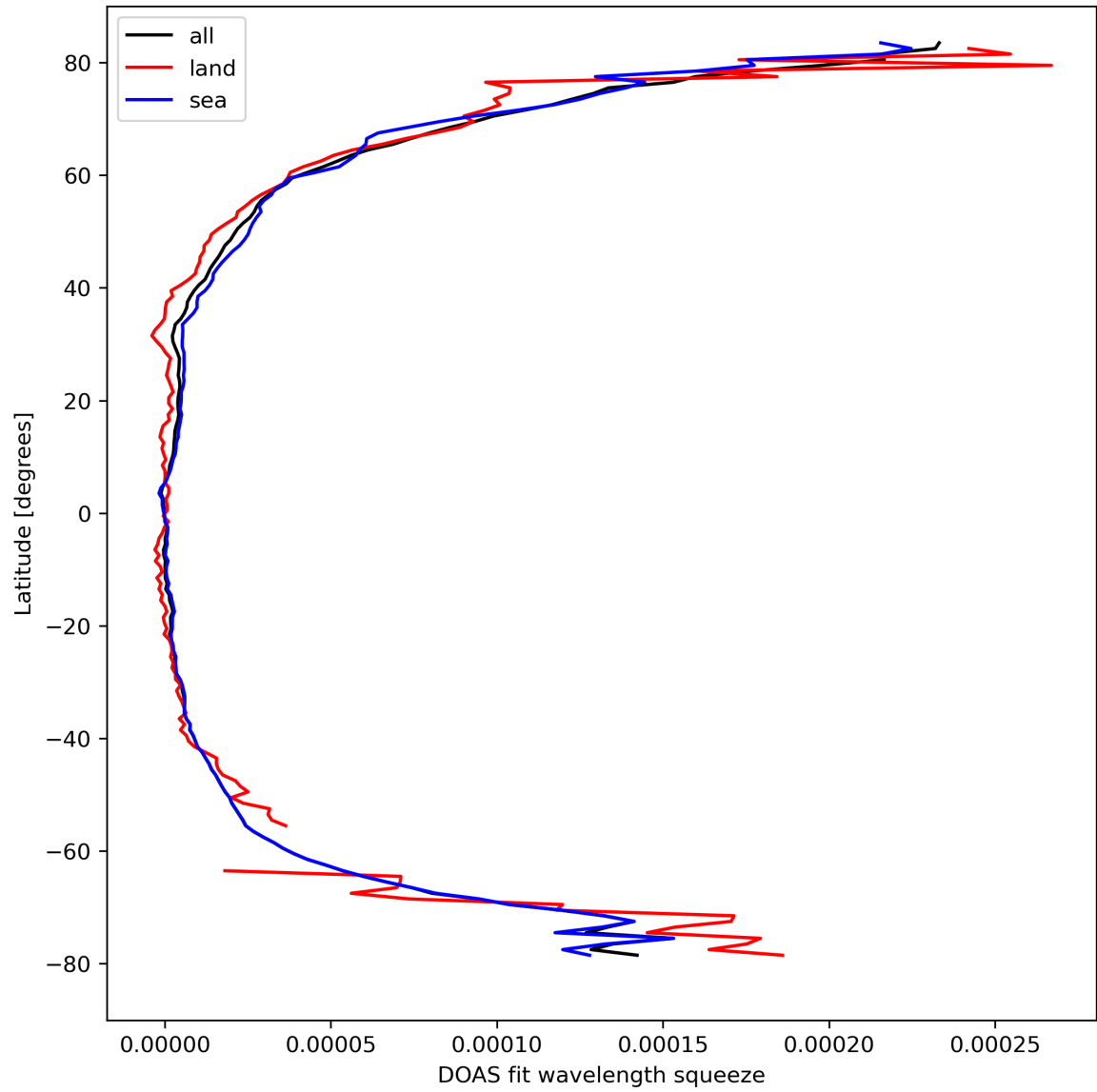
Figure 31: Zonal average of “DOAS fit wavelength squeeze” for 2024-03-30 to 2024-03-31.
