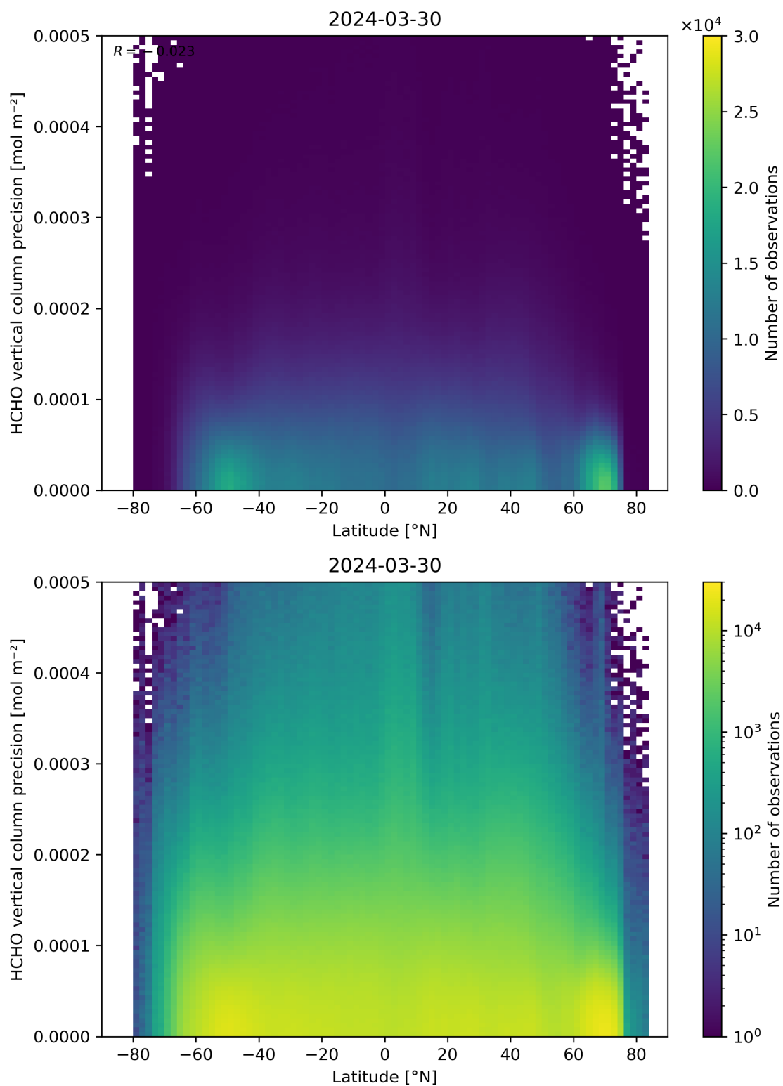
Figure 165: Scatter density plot of “Latitude” against “HCHO vertical column precision” for 2024-03-30 to 2024-03-31.
