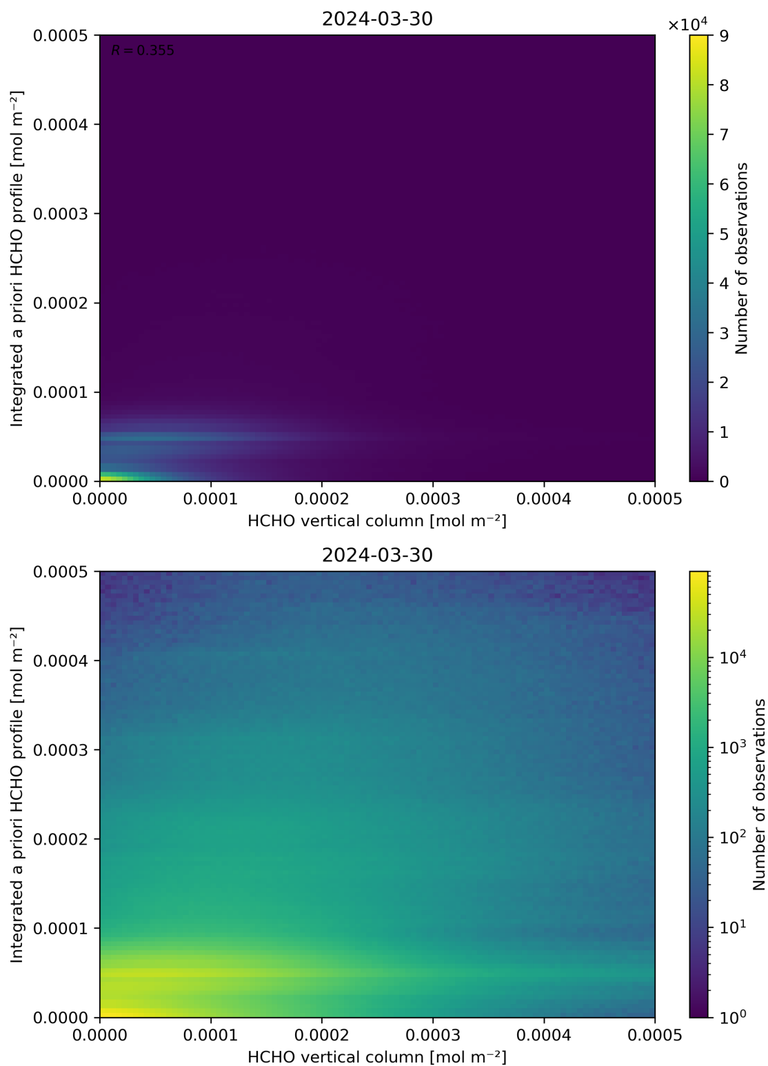
Figure 135: Scatter density plot of “HCHO vertical column” against “Integrated a priori HCHO profile” for 2024-03-30 to 2024-03-31.
