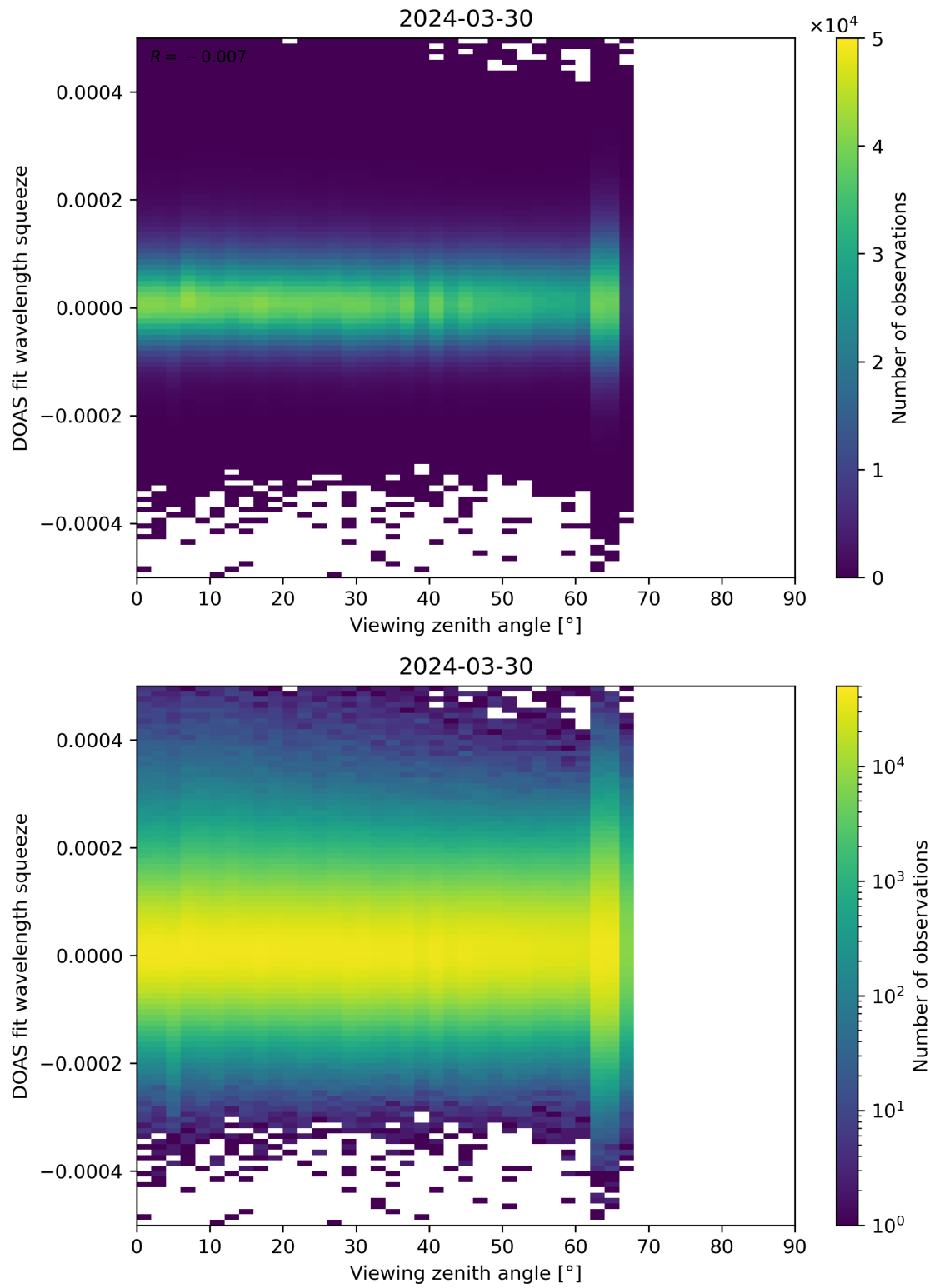
Figure 184: Scatter density plot of “Viewing zenith angle” against “DOAS fit wavelength squeeze” for 2024-03-30 to 2024-03-31.
