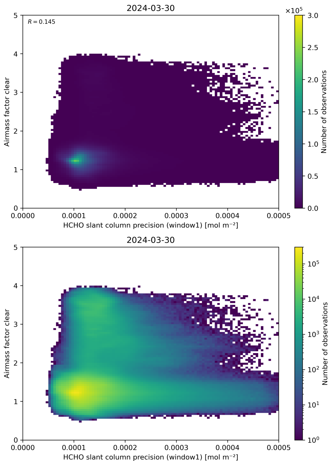
Figure 91: Scatter density plot of “HCHO slant column precision (window1)” against “Airmass factor clear” for 2024-03-30 to 2024-03-31.
