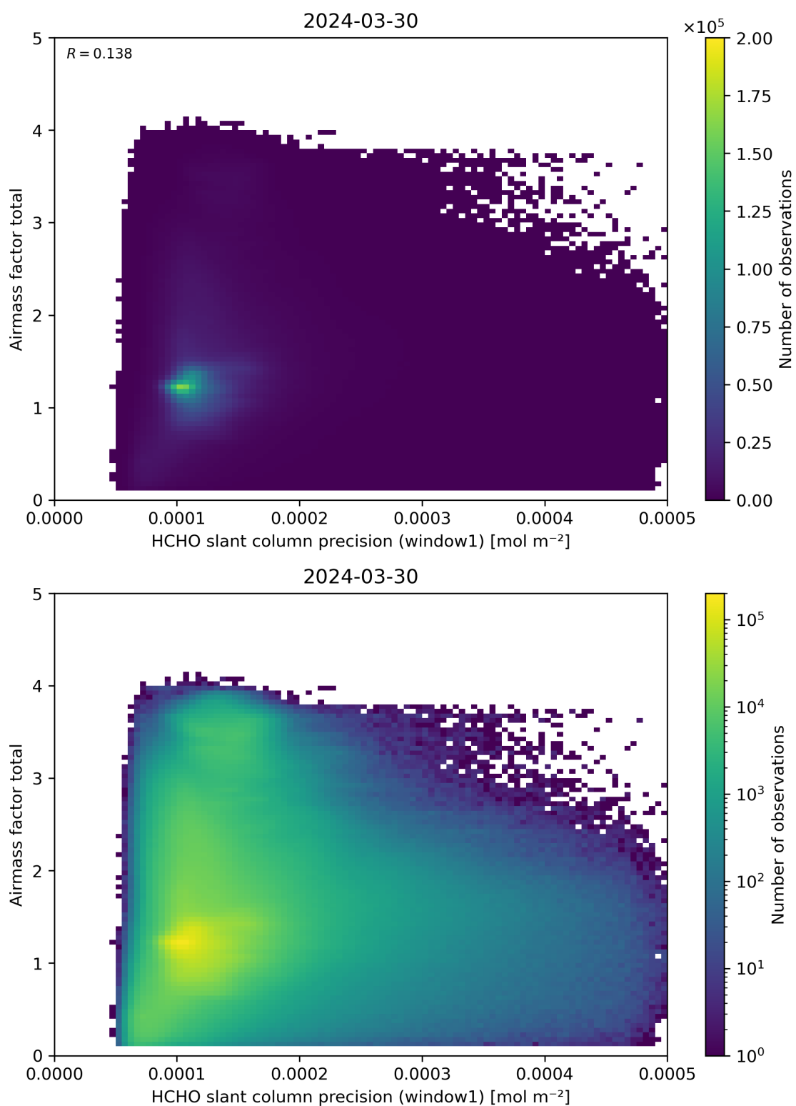
Figure 94: Scatter density plot of “HCHO slant column precision (window1)” against “Airmass factor total” for 2024-03-30 to 2024-03-31.
