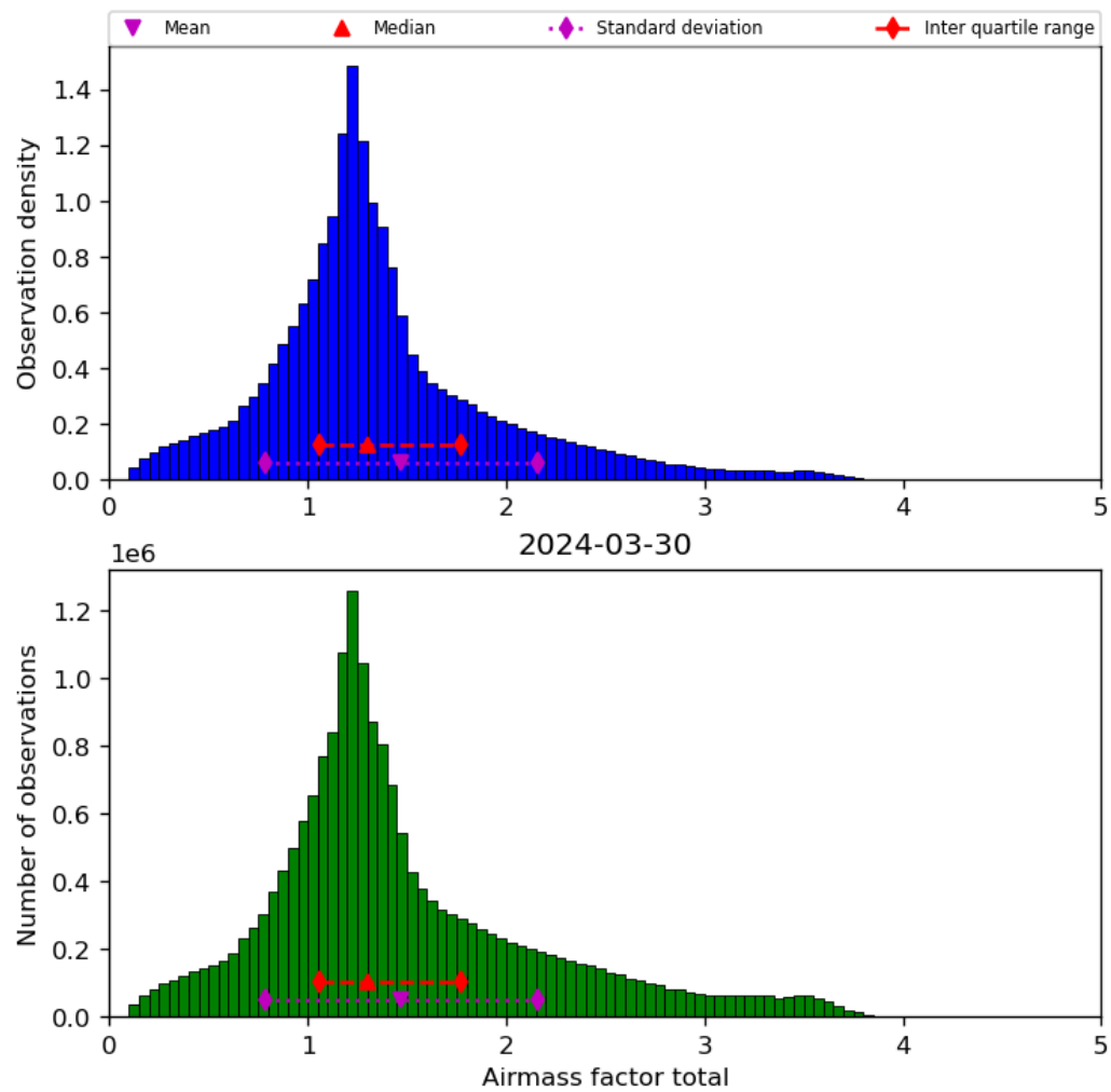
Figure 40: Histogram of “Airmass factor total” for 2024-03-30 to 2024-03-31
