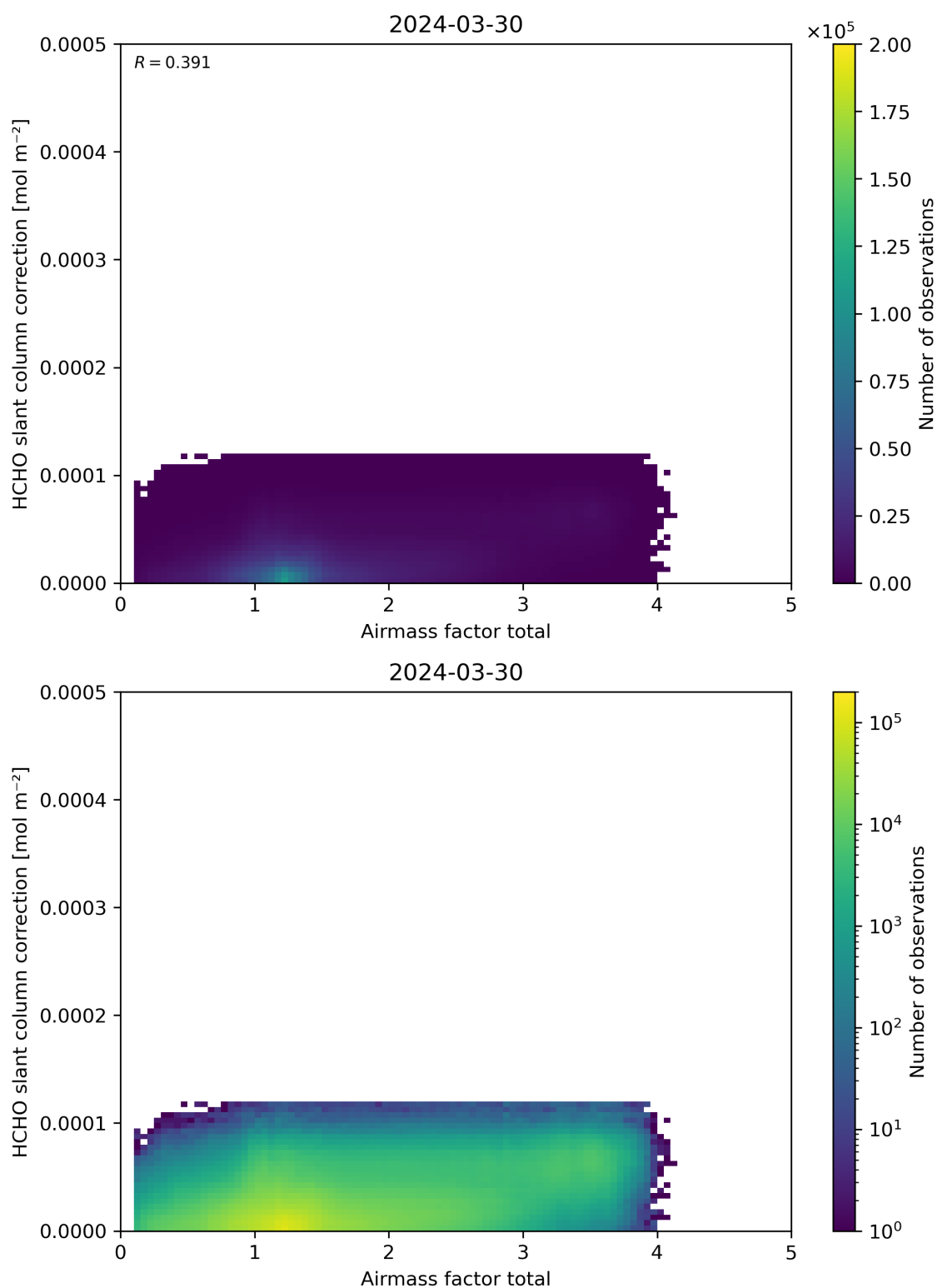
Figure 102: Scatter density plot of “Airmass factor total” against “HCHO slant column correction” for 2024-03-30 to 2024-03-31.
