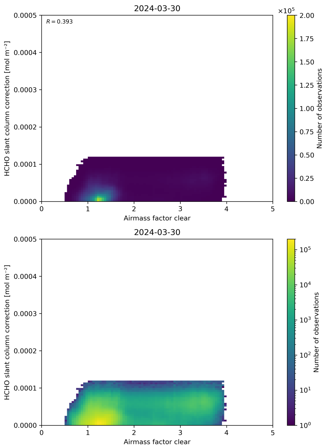
Figure 75: Scatter density plot of “Airmass factor clear” against “HCHO slant column correction” for 2024-03-30 to 2024-03-31.
