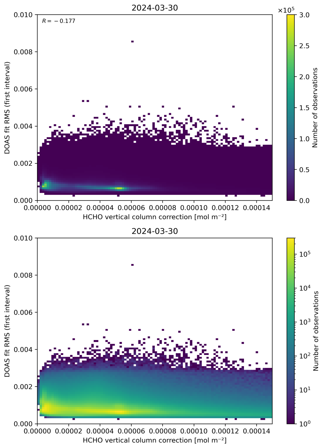
Figure 112: Scatter density plot of “HCHO vertical column correction” against “DOAS fit RMS (first interval)” for 2024-03-30 to 2024-03-31.
