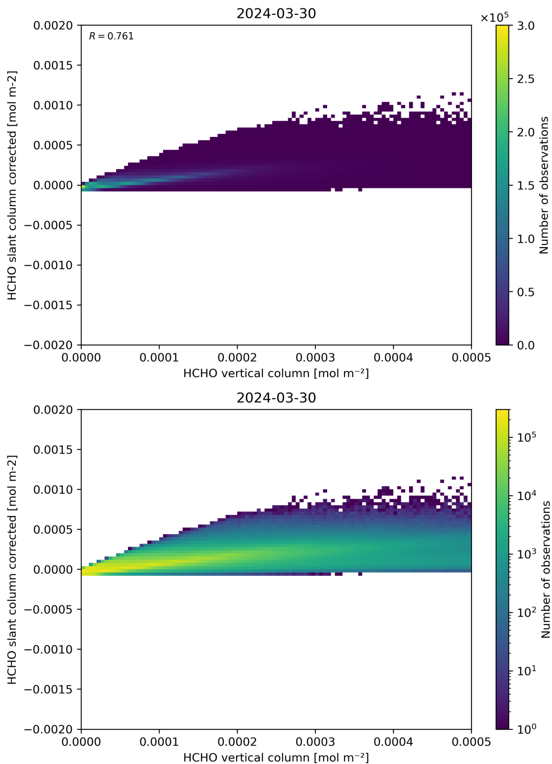
Figure 127: Scatter density plot of “HCHO vertical column” against “HCHO slant column corrected” for 2024-03-30 to 2024-03-31.
