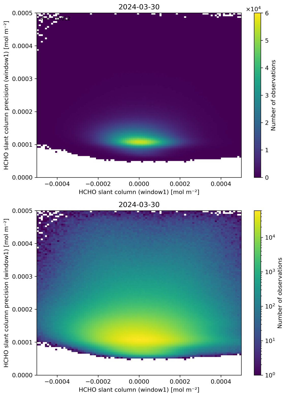
Figure 84: Scatter density plot of “HCHO slant column (window1)” against “HCHO slant column precision (window1)” for 2024-03-30 to 2024-03-31.
