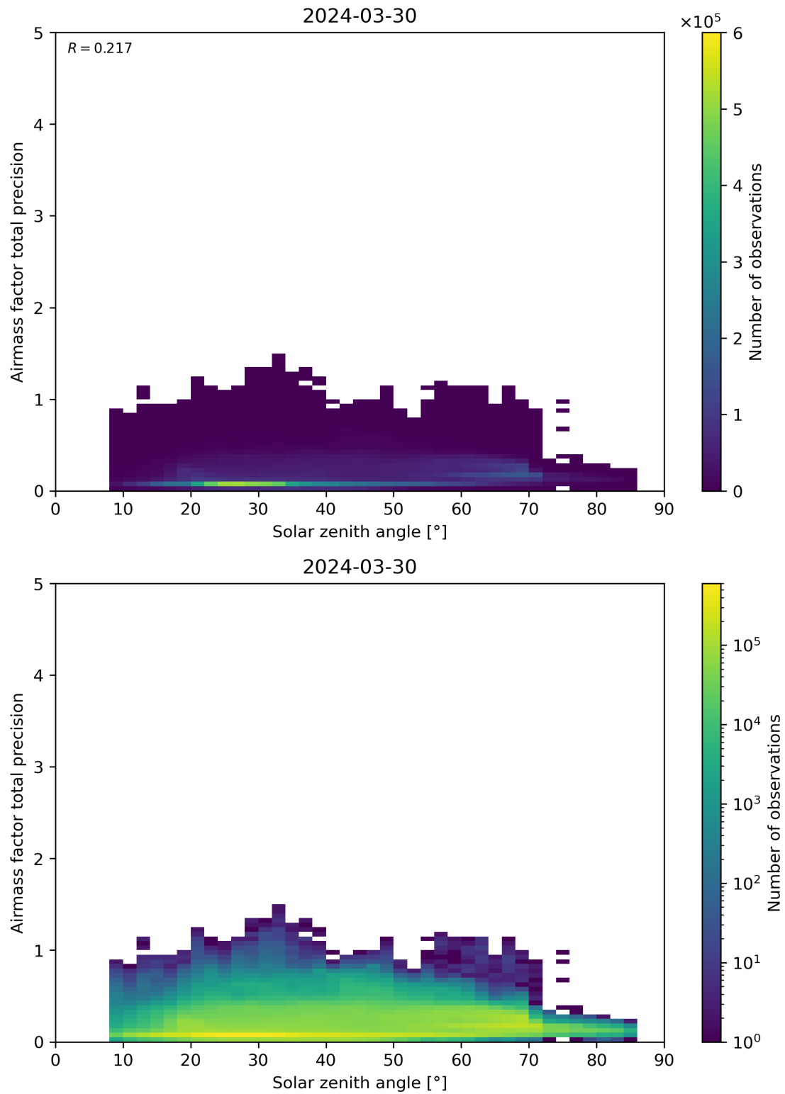
Figure 176: Scatter density plot of “Solar zenith angle” against “Airmass factor total precision” for 2024-03-30 to 2024-03-31.
