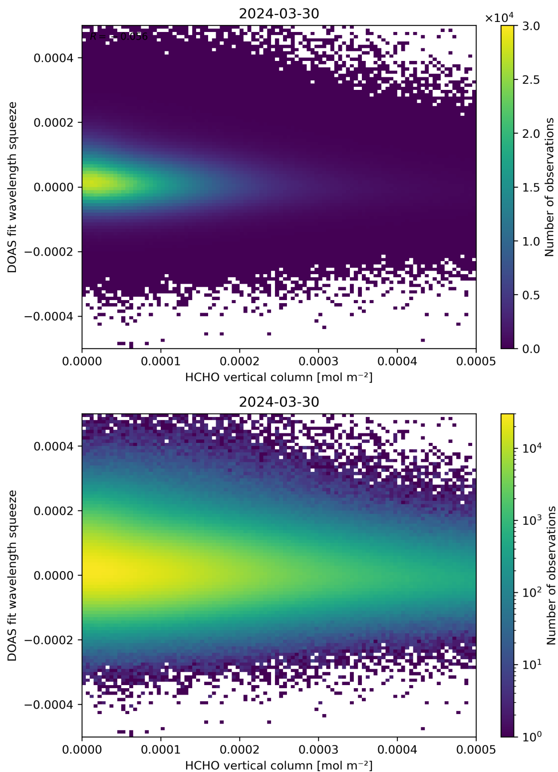
Figure 125: Scatter density plot of “HCHO vertical column” against “DOAS fit wavelength squeeze” for 2024-03-30 to 2024-03-31.
