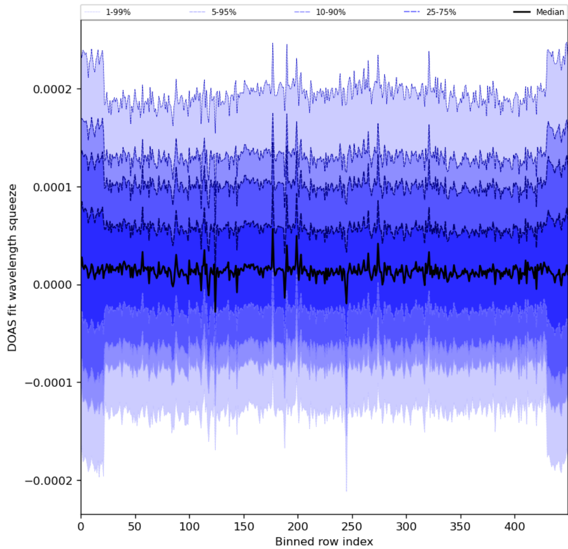
Figure 59: Along track statistics of “DOAS fit wavelength squeeze” for 2024-03-30 to 2024-03-31
