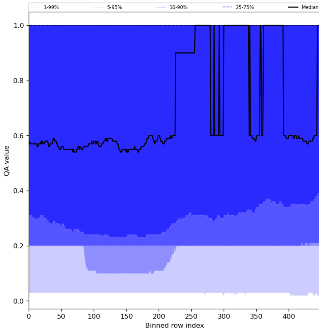
Figure 48: Along track statistics of “QA value” for 2024-03-30 to 2024-03-31
