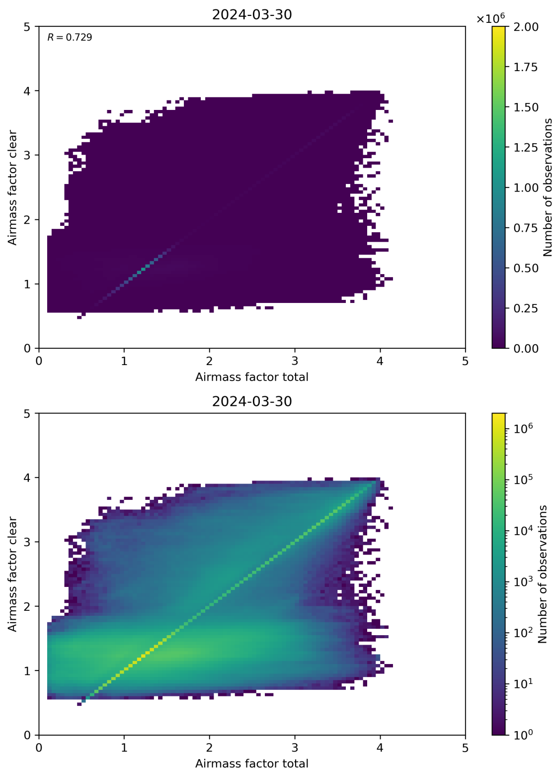
Figure 100: Scatter density plot of “Airmass factor total” against “Airmass factor clear” for 2024-03-30 to 2024-03-31.
