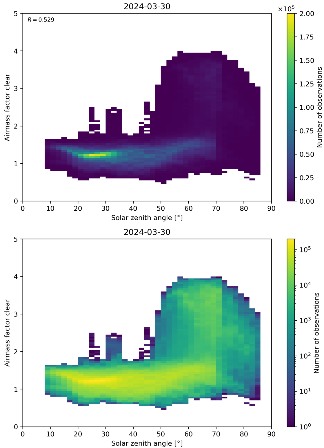
Figure 170: Scatter density plot of “Solar zenith angle” against “Airmass factor clear” for 2024-03-30 to 2024-03-31.
