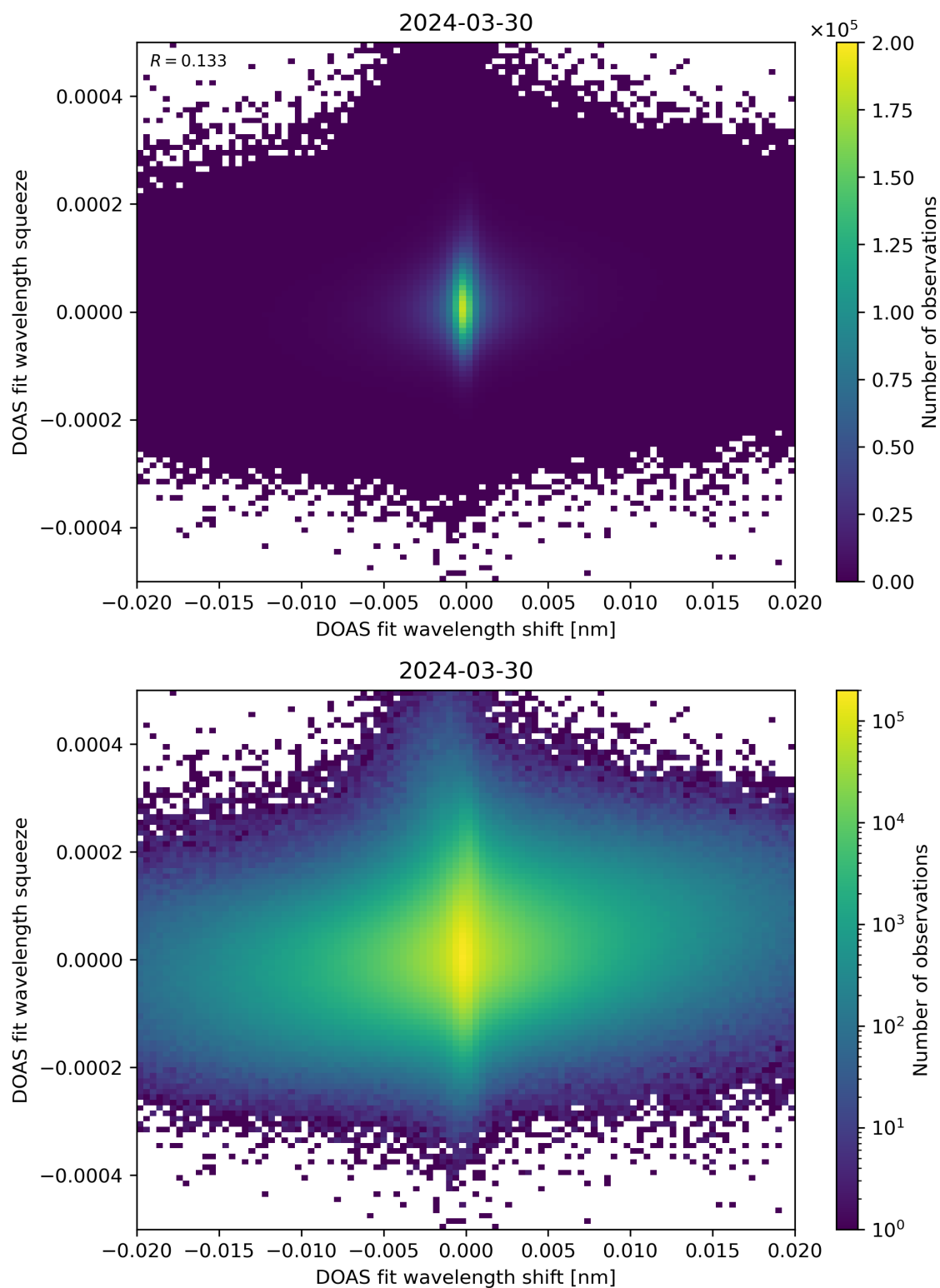
Figure 65: Scatter density plot of “DOAS fit wavelength shift” against “DOAS fit wavelength squeeze” for 2024-03-30 to 2024-03-31.
