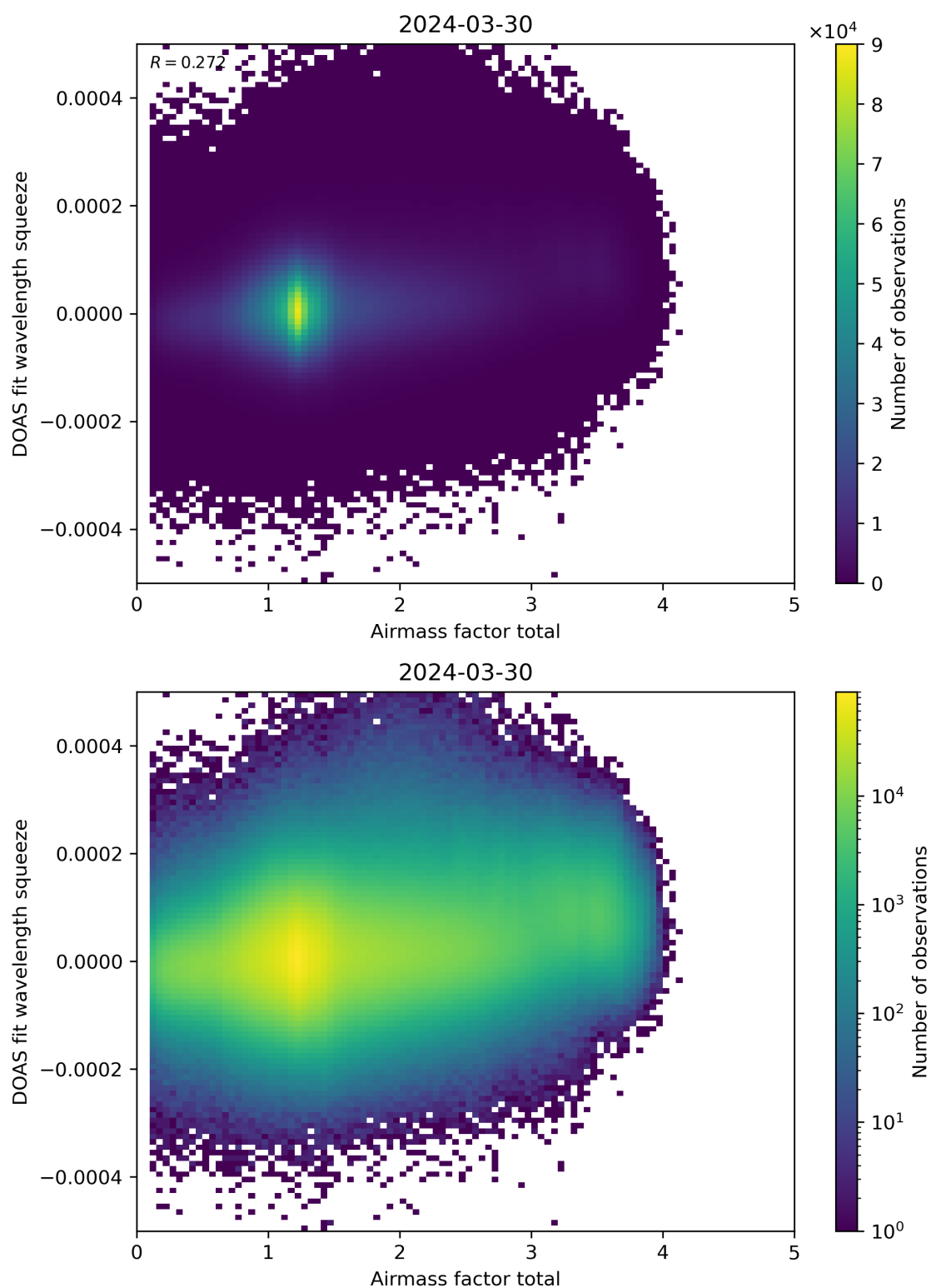
Figure 99: Scatter density plot of “Airmass factor total” against “DOAS fit wavelength squeeze” for 2024-03-30 to 2024-03-31.
