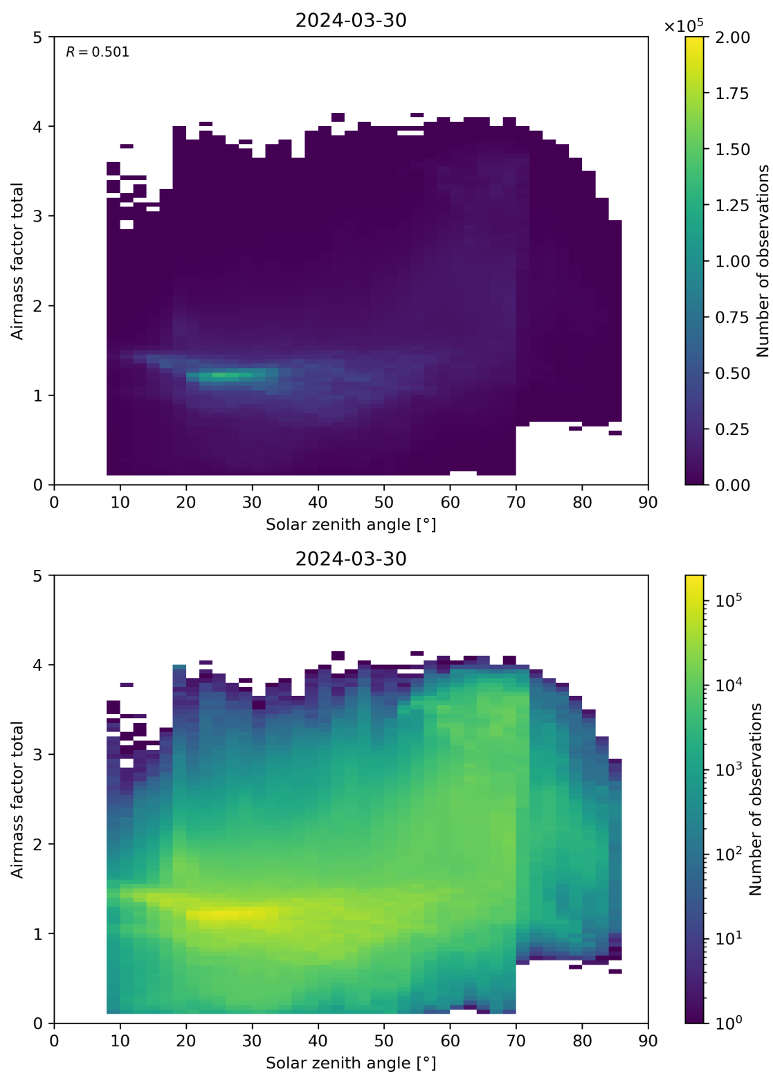
Figure 175: Scatter density plot of “Solar zenith angle” against “Airmass factor total” for 2024-03-30 to 2024-03-31.
