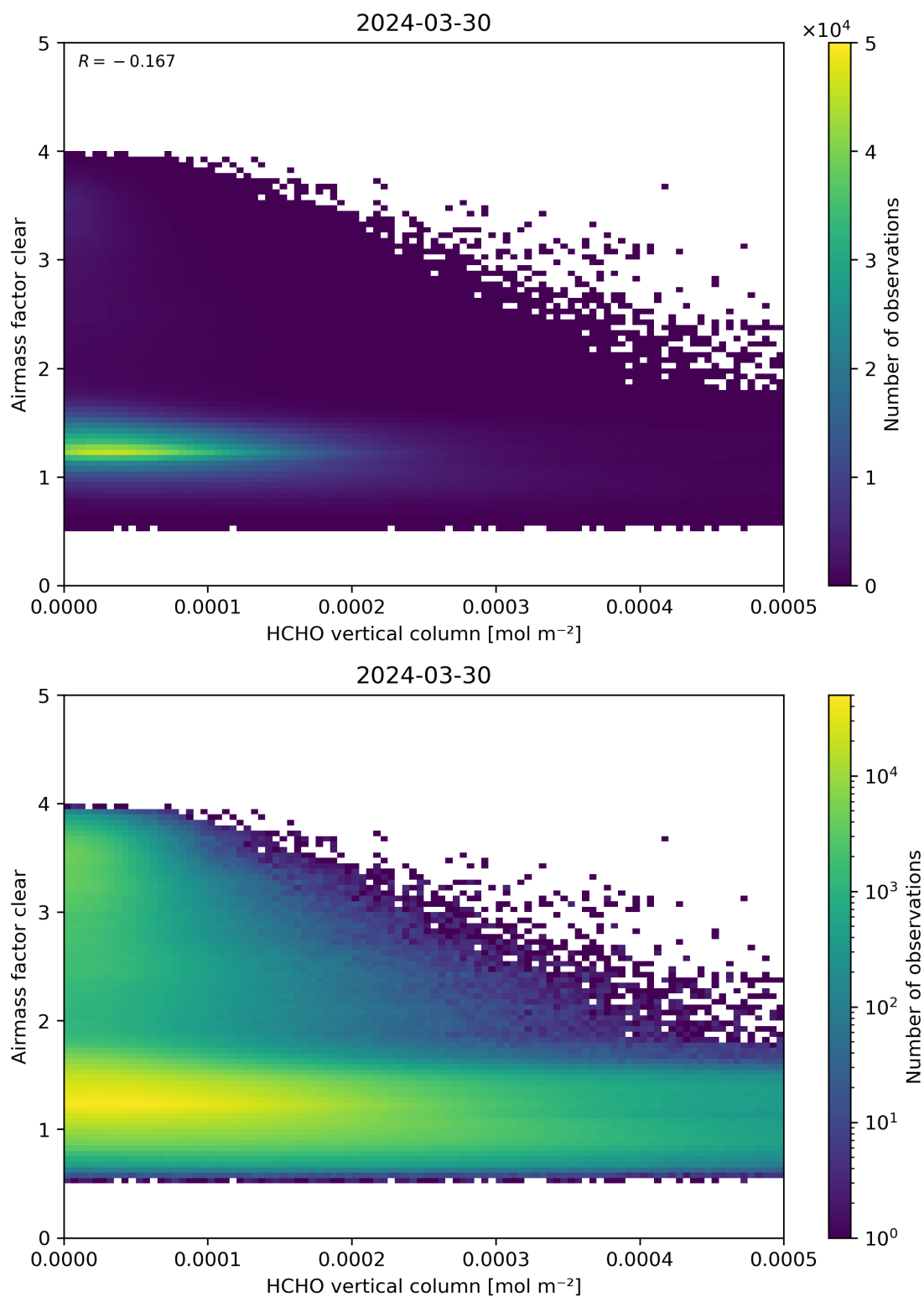
Figure 126: Scatter density plot of “HCHO vertical column” against “Airmass factor clear” for 2024-03-30 to 2024-03-31.
