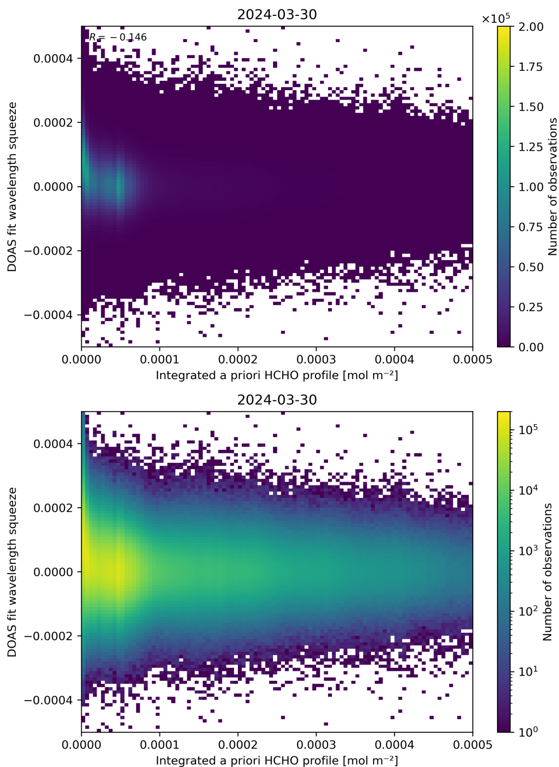
Figure 150: Scatter density plot of “Integrated a priori HCHO profile” against “DOAS fit wavelength squeeze” for 2024-03-30 to 2024-03-31.
