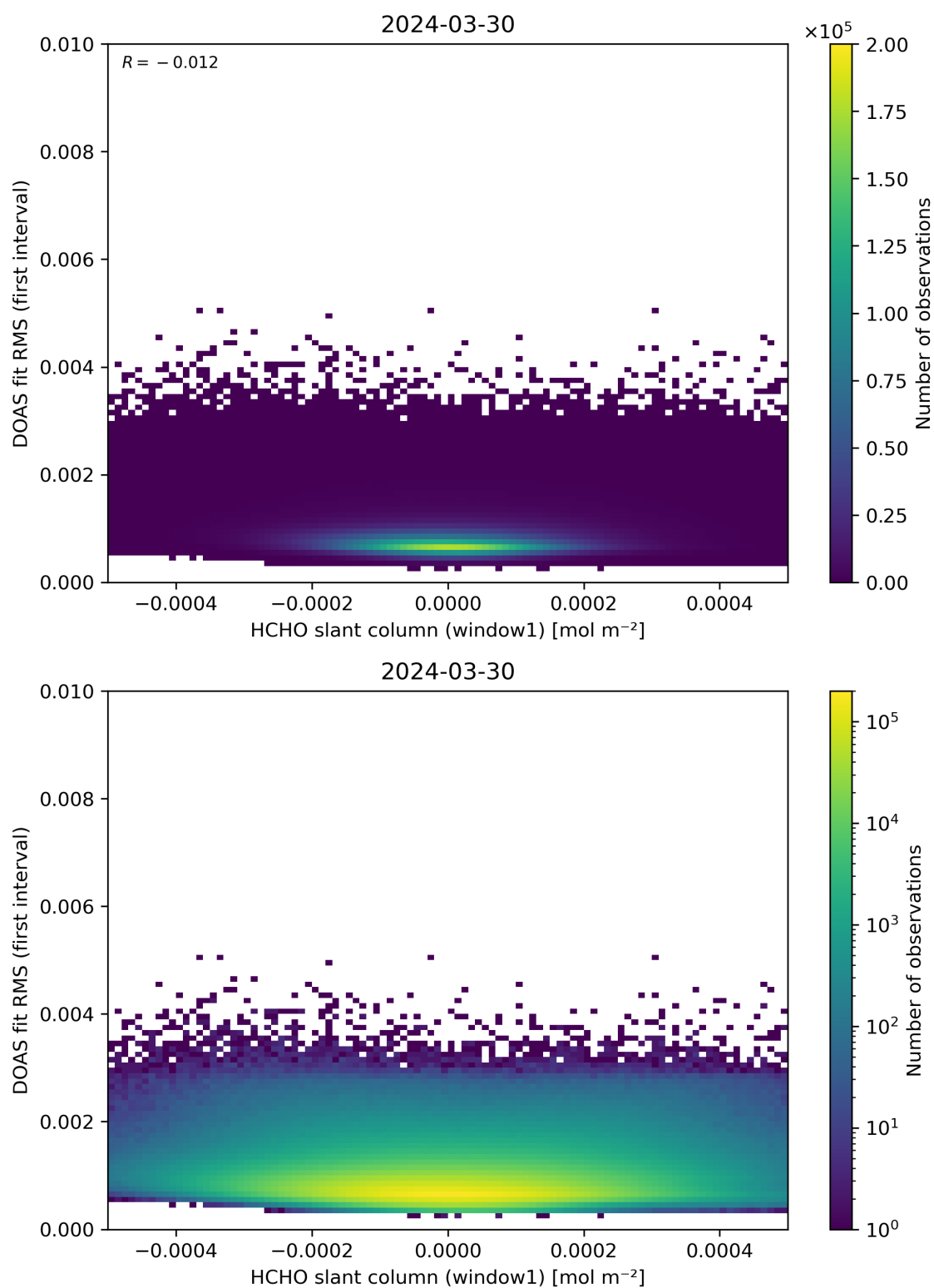
Figure 78: Scatter density plot of “HCHO slant column (window1)” against “DOAS fit RMS (first interval)” for 2024-03-30 to 2024-03-31.
