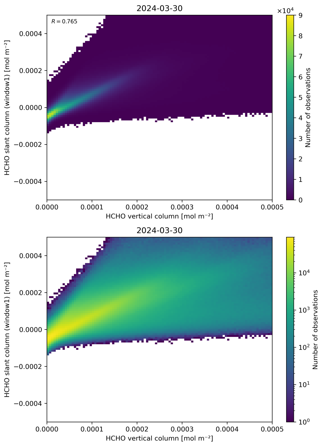
Figure 129: Scatter density plot of “HCHO vertical column” against “HCHO slant column (window1)” for 2024-03-30 to 2024-03-31.
