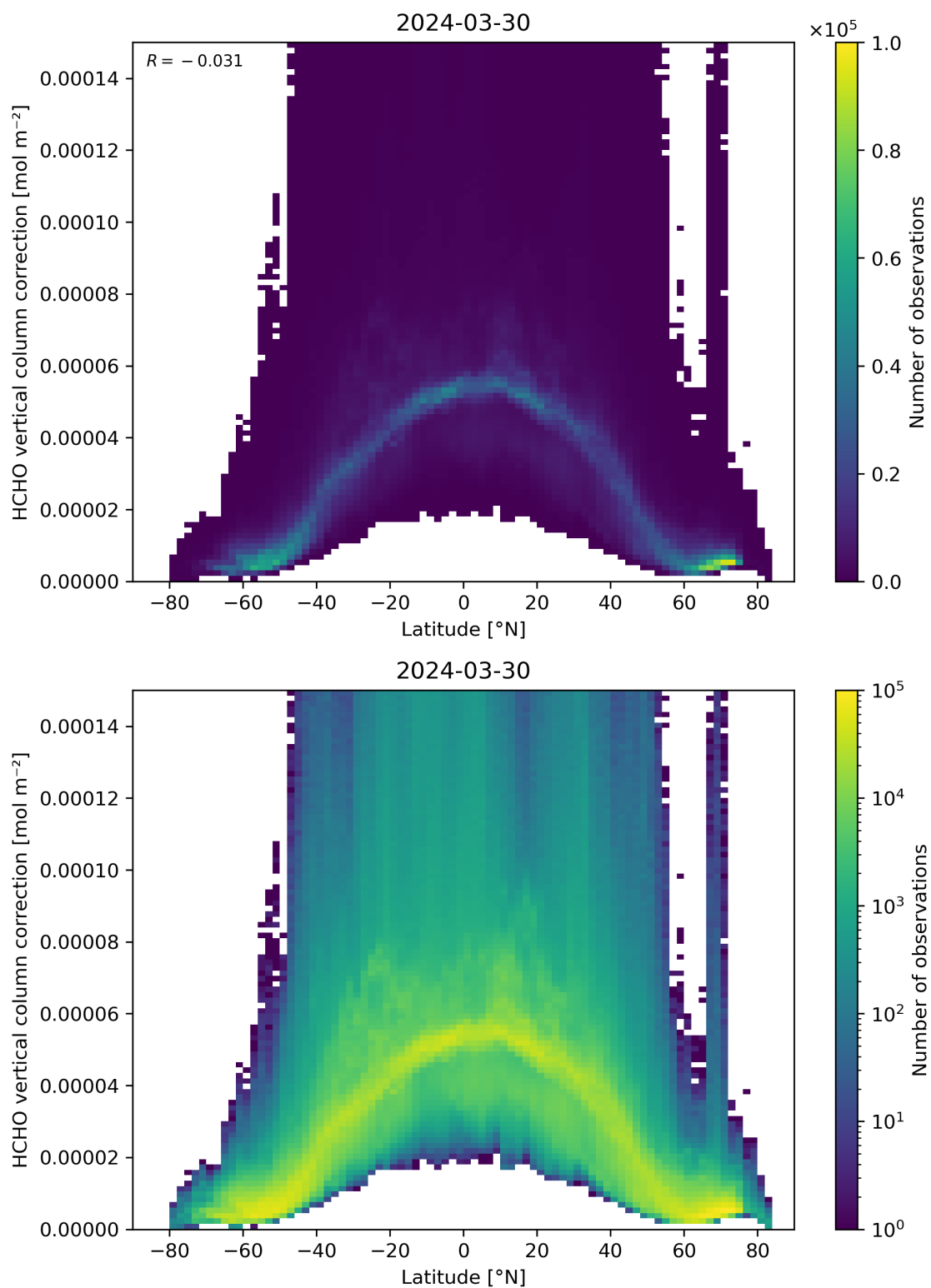
Figure 164: Scatter density plot of “Latitude” against “HCHO vertical column correction” for 2024-03-30 to 2024-03-31.
