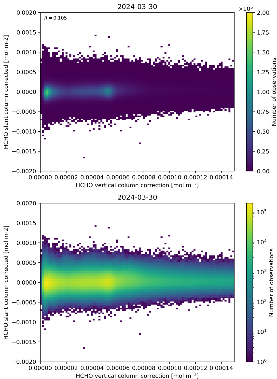
Figure 116: Scatter density plot of “HCHO vertical column correction” against “HCHO slant column corrected” for 2024-03-30 to 2024-03-31.
