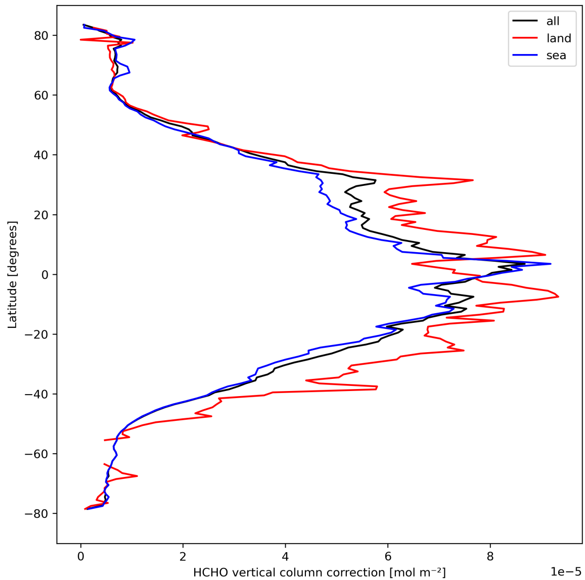
Figure 23: Zonal average of “HCHO vertical column correction” for 2024-03-30 to 2024-03-31.
