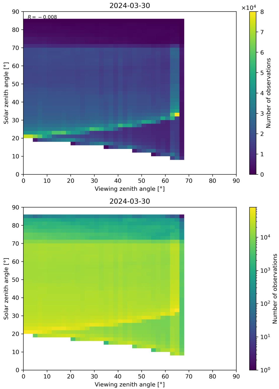
Figure 197: Scatter density plot of “Viewing zenith angle” against “Solar zenith angle” for 2024-03-30 to 2024-03-31.
