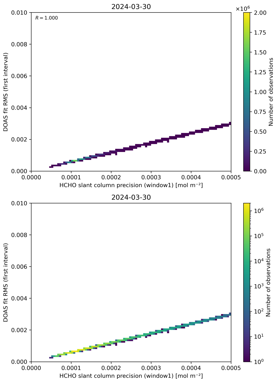
Figure 88: Scatter density plot of “HCHO slant column precision (window1)” against “DOAS fit RMS (first interval)” for 2024-03-30 to 2024-03-31.
