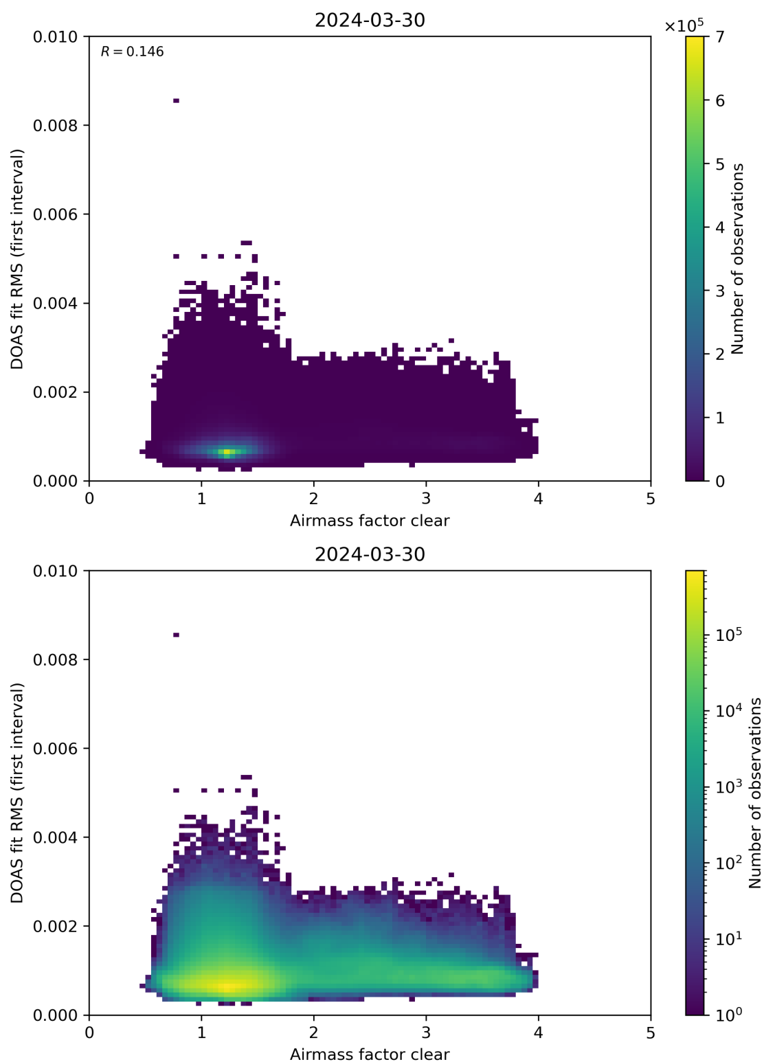
Figure 71: Scatter density plot of “Airmass factor clear” against “DOAS fit RMS (first interval)” for 2024-03-30 to 2024-03-31.
