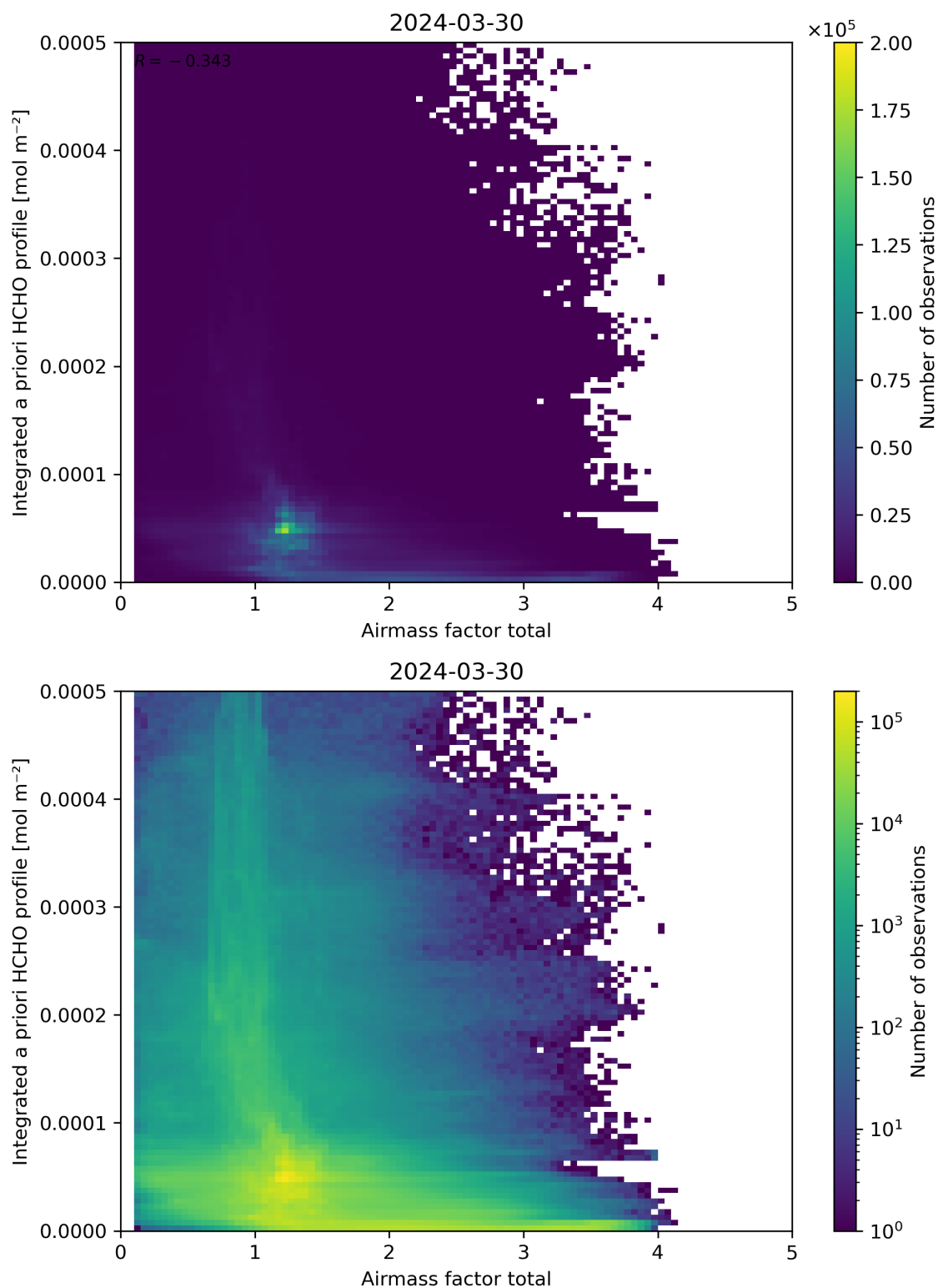
Figure 104: Scatter density plot of “Airmass factor total” against “Integrated a priori HCHO profile” for 2024-03-30 to 2024-03-31.
