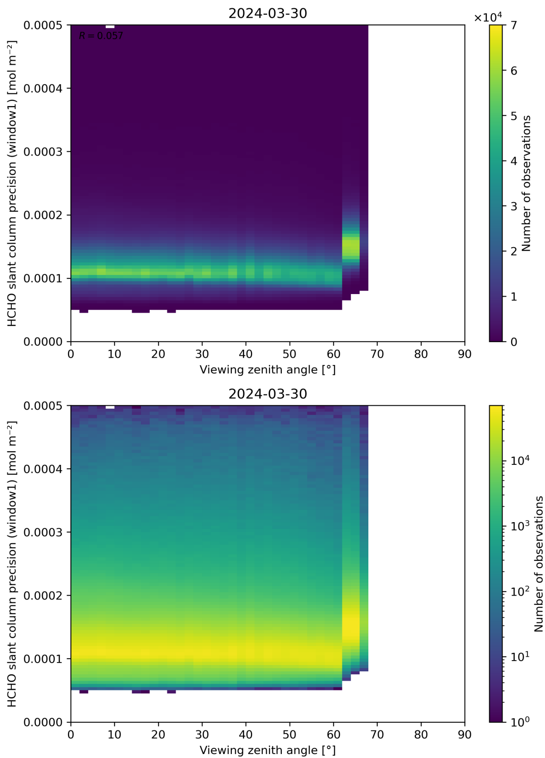
Figure 189: Scatter density plot of “Viewing zenith angle” against “HCHO slant column precision (window1)” for 2024-03-30 to 2024-03-31.
