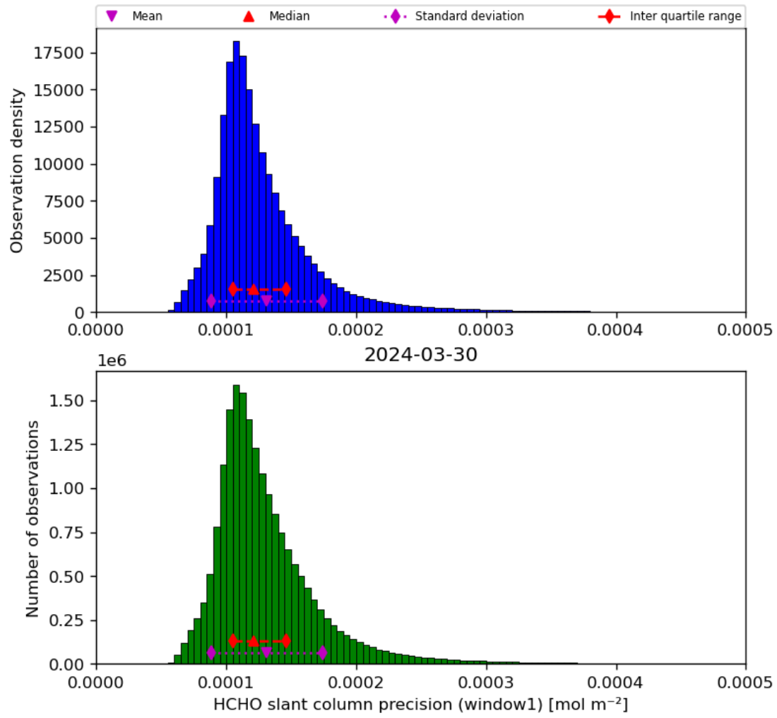
Figure 39: Histogram of “HCHO slant column precision (window1)” for 2024-03-30 to 2024-03-31
