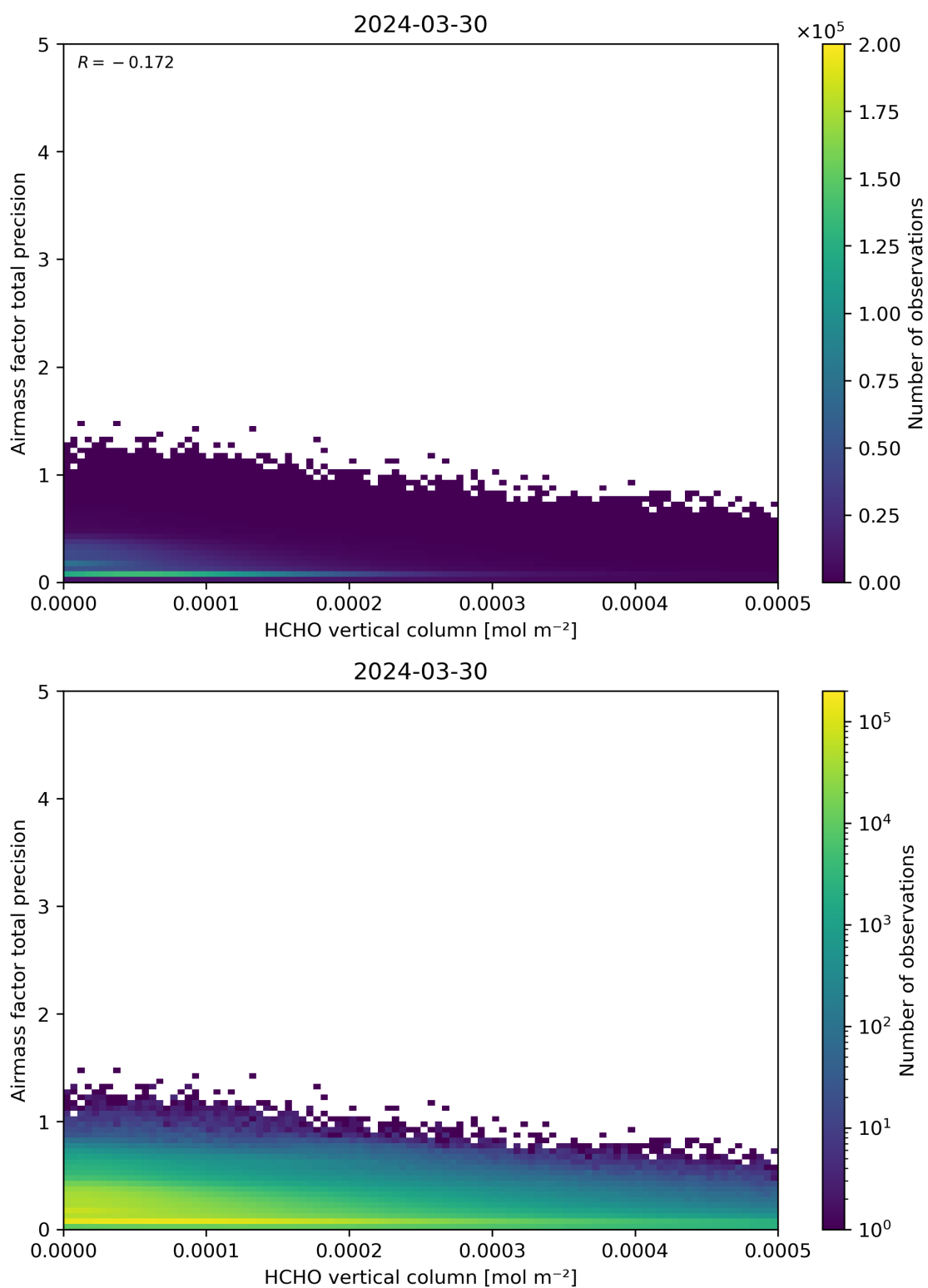
Figure 132: Scatter density plot of “HCHO vertical column” against “Airmass factor total precision” for 2024-03-30 to 2024-03-31.
