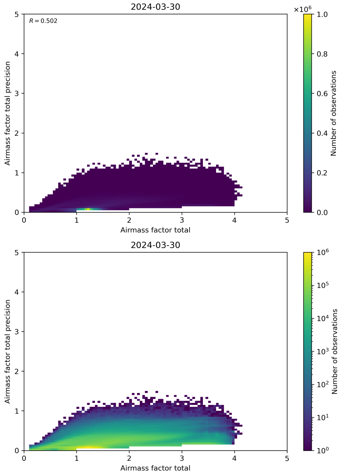
Figure 103: Scatter density plot of “Airmass factor total” against “Airmass factor total precision” for 2024-03-30 to 2024-03-31.
