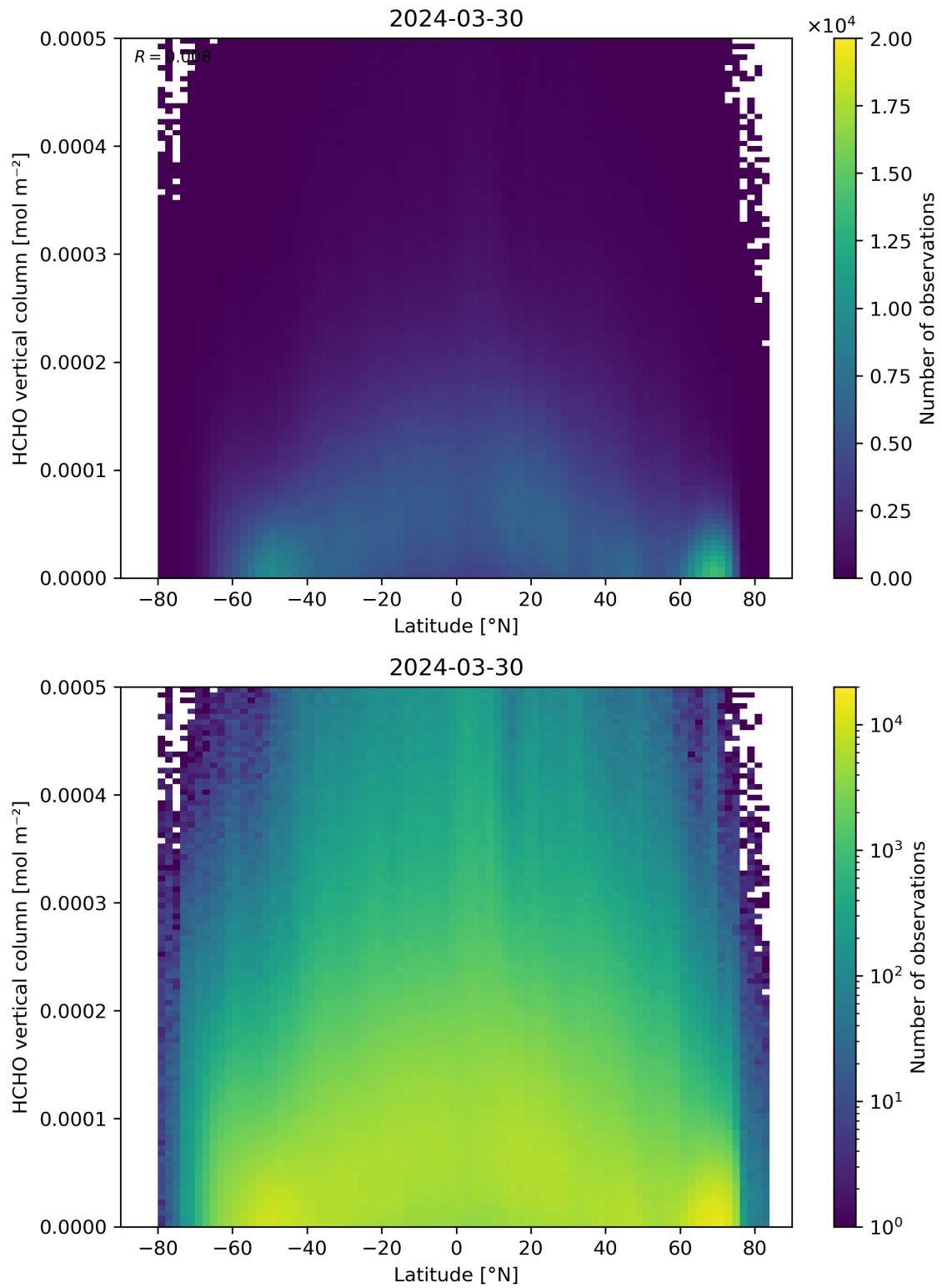
Figure 163: Scatter density plot of “Latitude” against “HCHO vertical column” for 2024-03-30 to 2024-03-31.
