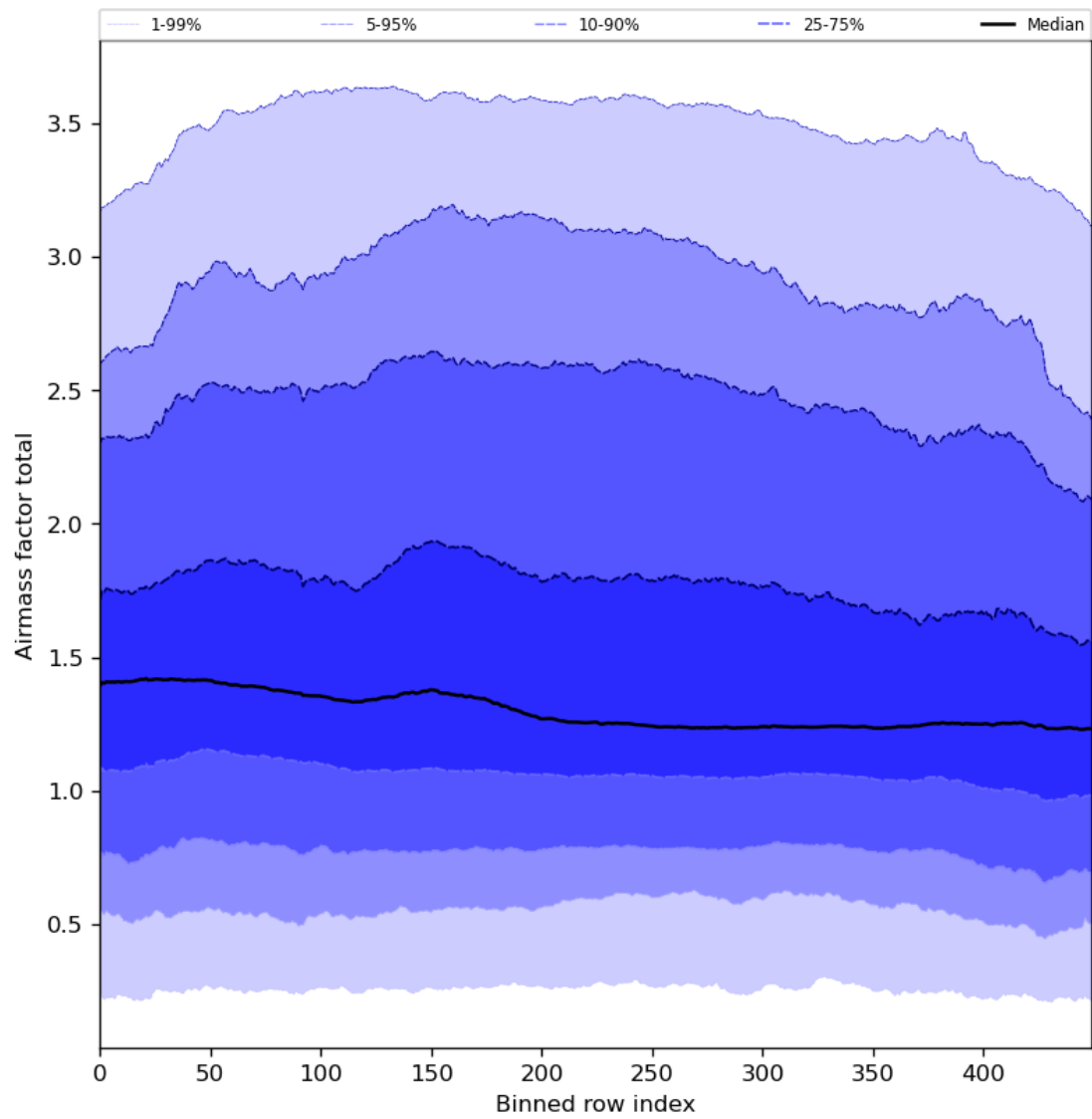
Figure 54: Along track statistics of “Airmass factor total” for 2024-03-30 to 2024-03-31
