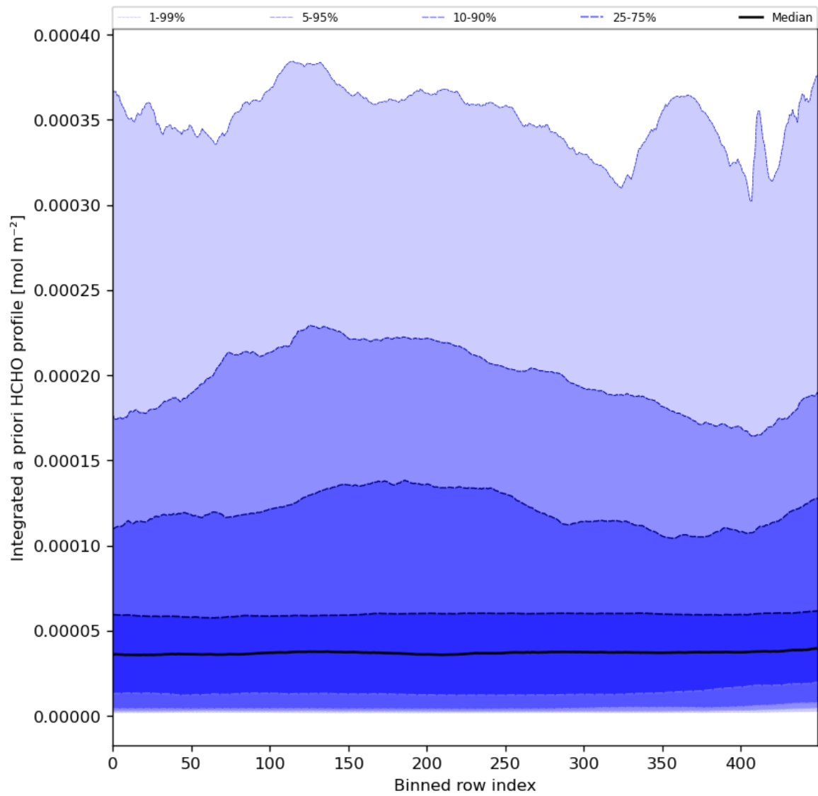
Figure 57: Along track statistics of “Integrated a priori HCHO profile” for 2024-03-30 to 2024-03-31
