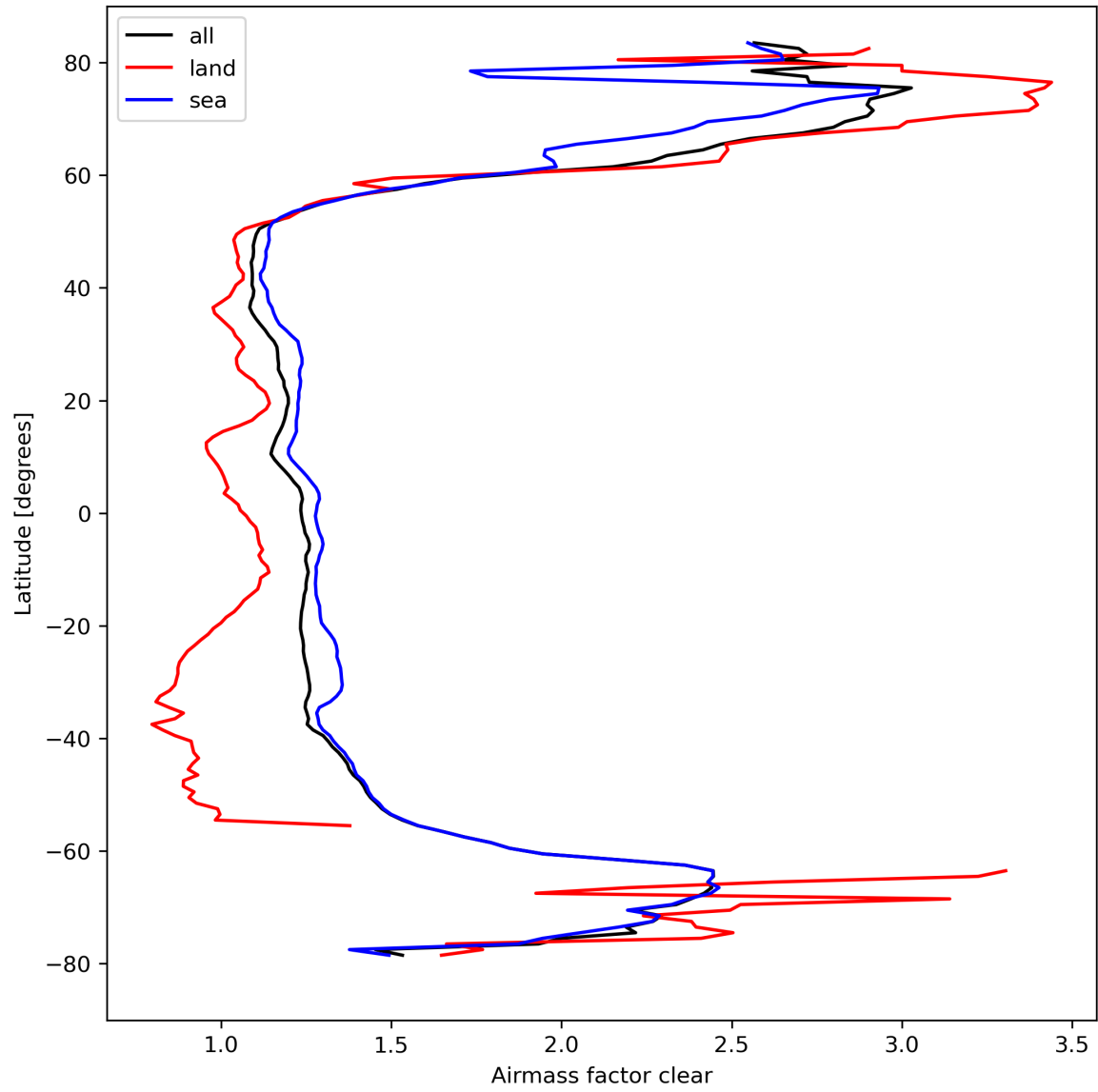
Figure 28: Zonal average of “Airmass factor clear” for 2024-03-30 to 2024-03-31.
