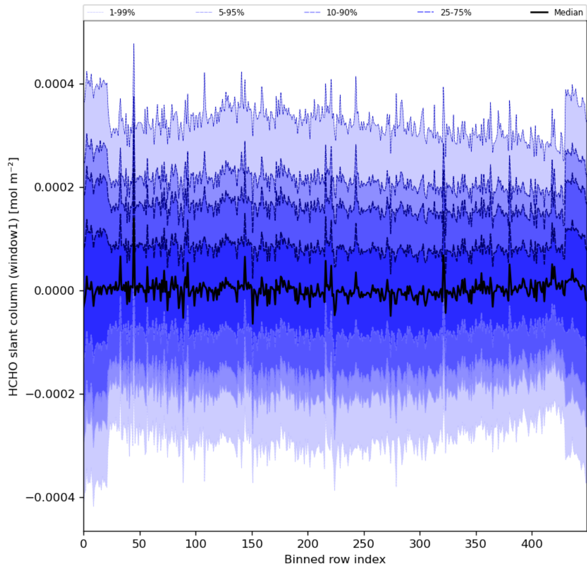
Figure 52: Along track statistics of “HCHO slant column (window1)” for 2024-03-30 to 2024-03-31
