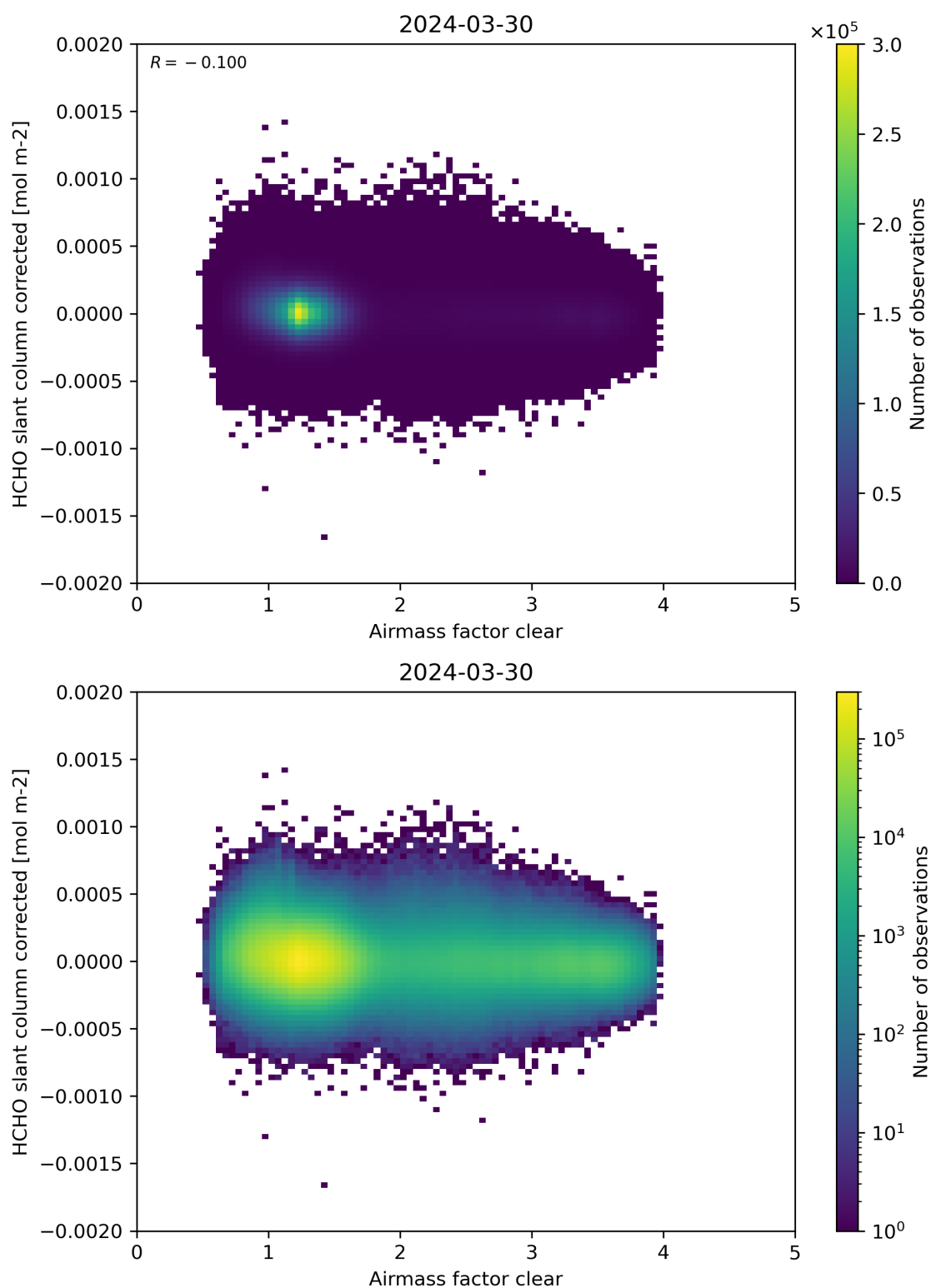
Figure 74: Scatter density plot of “Airmass factor clear” against “HCHO slant column corrected” for 2024-03-30 to 2024-03-31.
