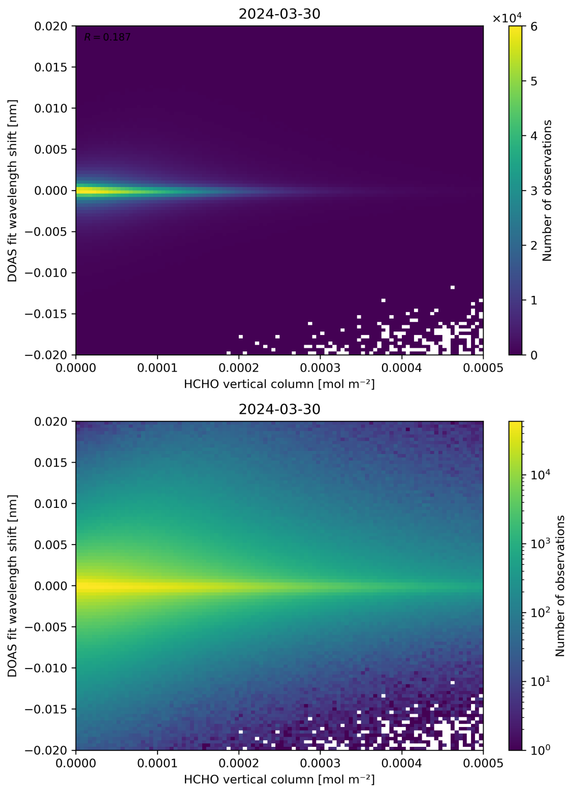
Figure 124: Scatter density plot of “HCHO vertical column” against “DOAS fit wavelength shift” for 2024-03-30 to 2024-03-31.
