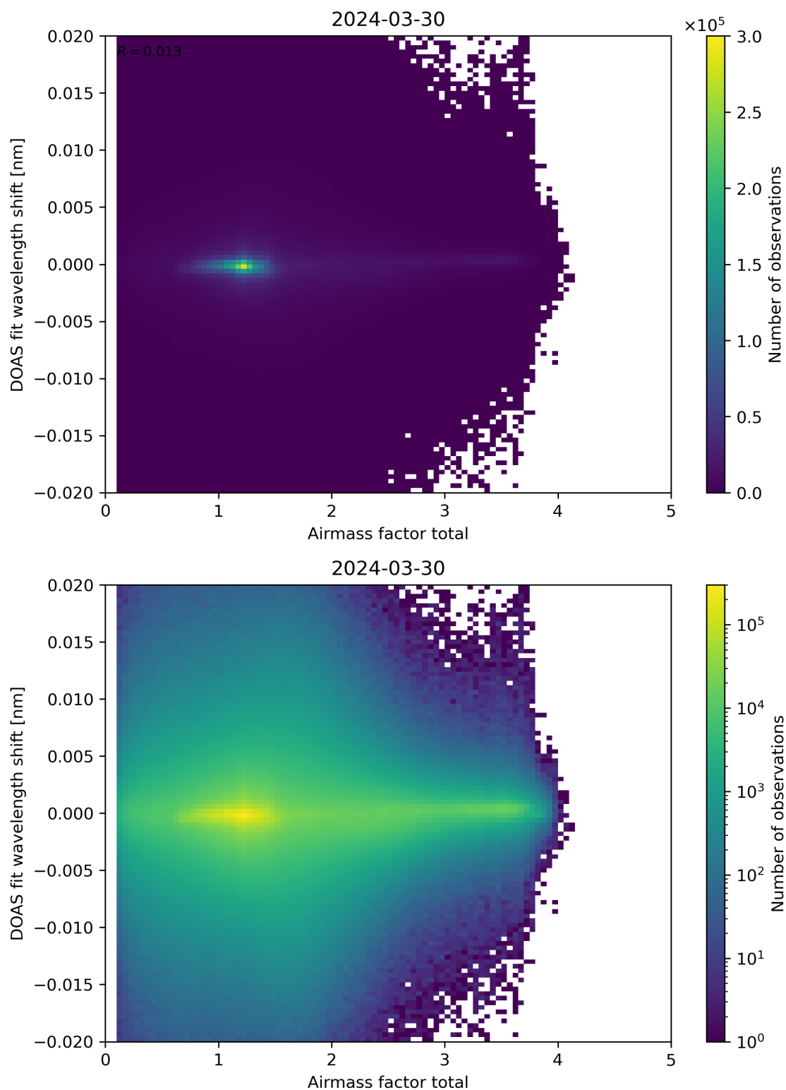
Figure 98: Scatter density plot of “Airmass factor total” against “DOAS fit wavelength shift” for 2024-03-30 to 2024-03-31.
