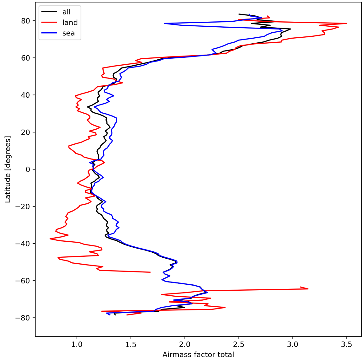
Figure 26: Zonal average of “Airmass factor total” for 2024-03-30 to 2024-03-31.
