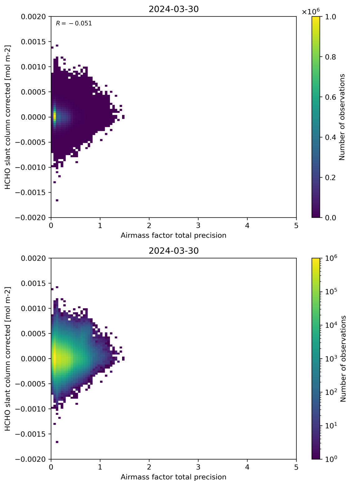
Figure 109: Scatter density plot of “Airmass factor total precision” against “HCHO slant column corrected” for 2024-03-30 to 2024-03-31.
