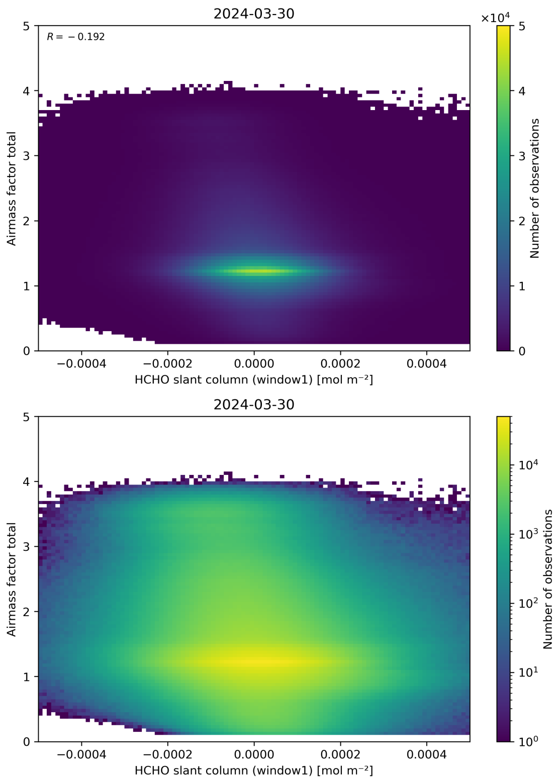
Figure 85: Scatter density plot of “HCHO slant column (window1)” against “Airmass factor total” for 2024-03-30 to 2024-03-31.
