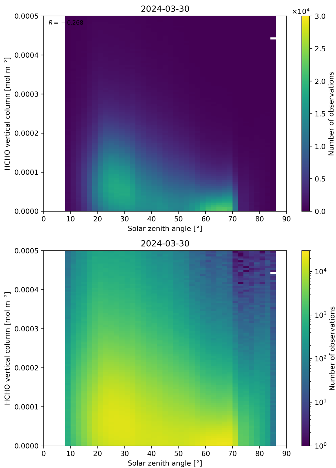
Figure 177: Scatter density plot of “Solar zenith angle” against “HCHO vertical column” for 2024-03-30 to 2024-03-31.
