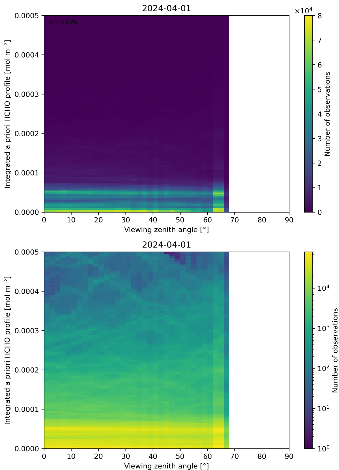
Figure 195: Scatter density plot of “Viewing zenith angle” against “Integrated a priori HCHO profile” for 2024-03-31 to 2024-04-02.
