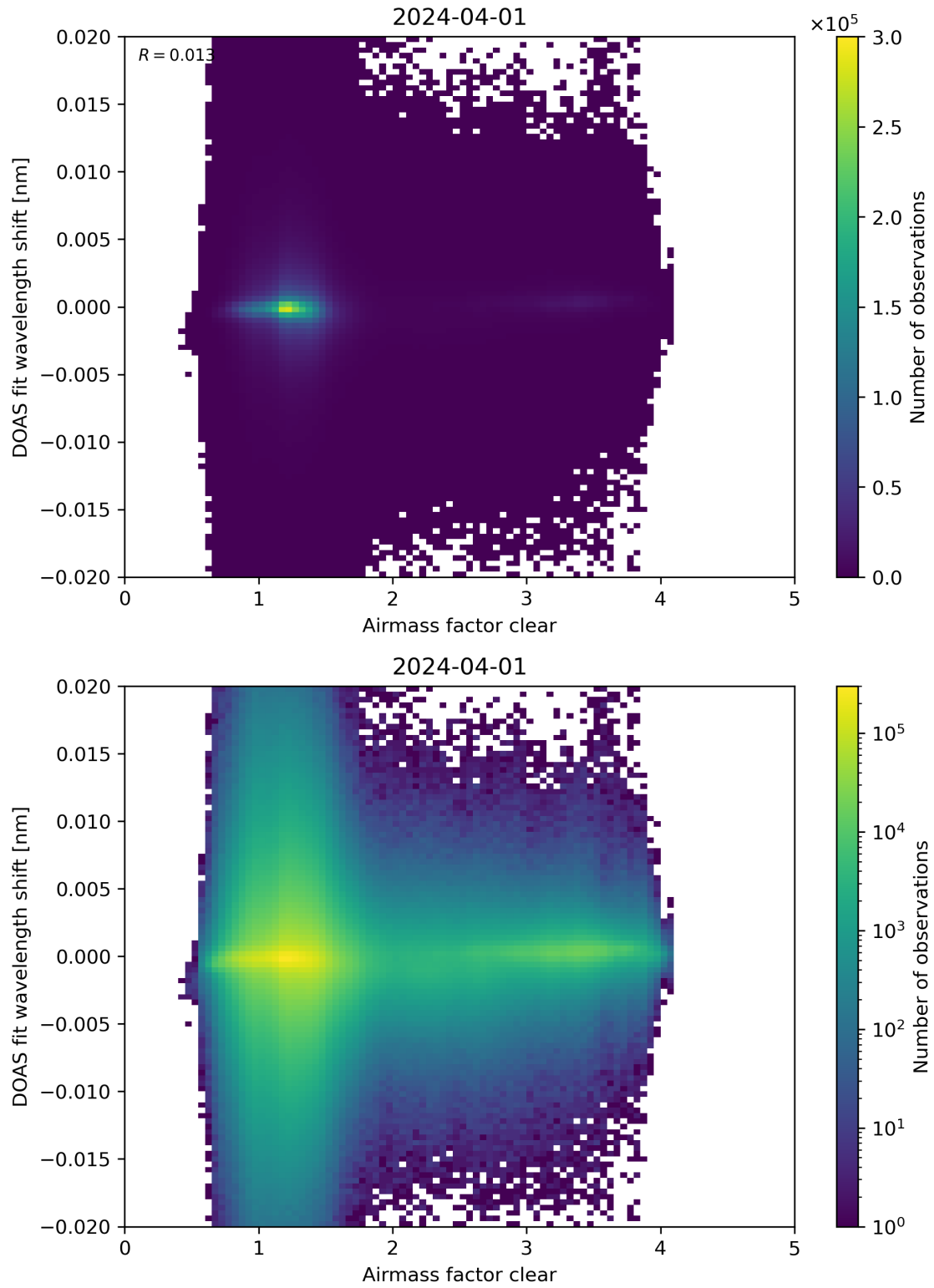
Figure 72: Scatter density plot of “Airmass factor clear” against “DOAS fit wavelength shift” for 2024-03-31 to 2024-04-02.
