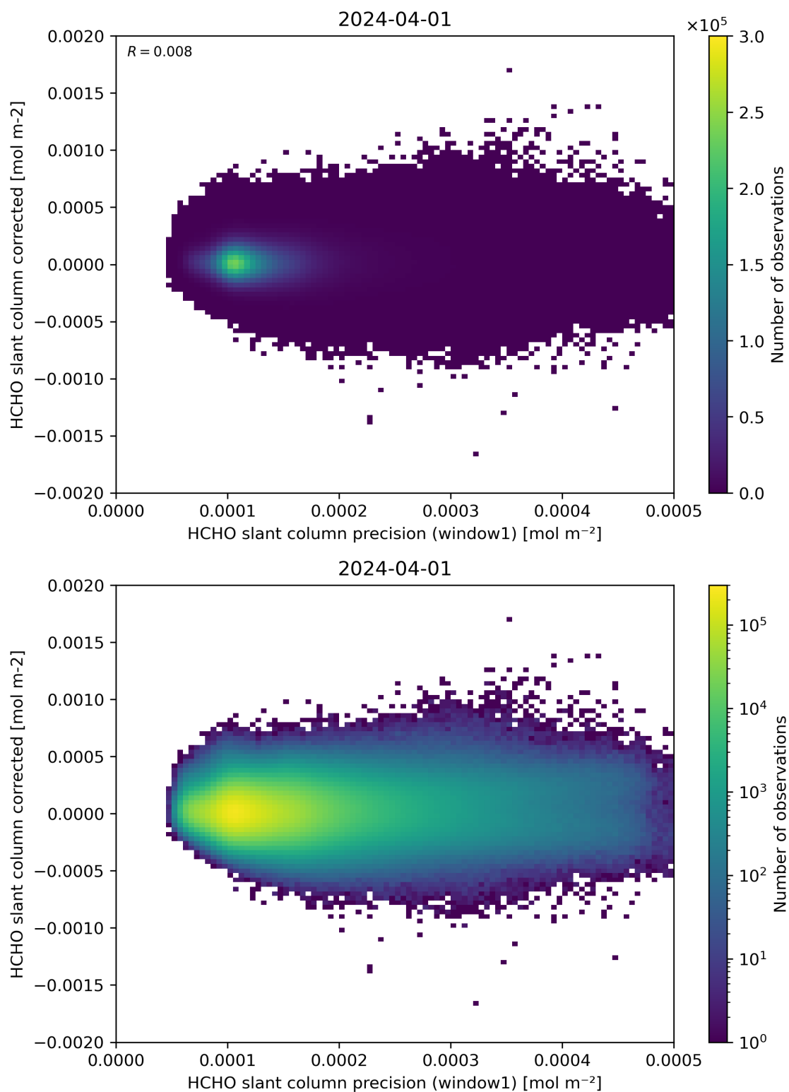
Figure 92: Scatter density plot of “HCHO slant column precision (window1)” against “HCHO slant column corrected” for 2024-03-31 to 2024-04-02.
