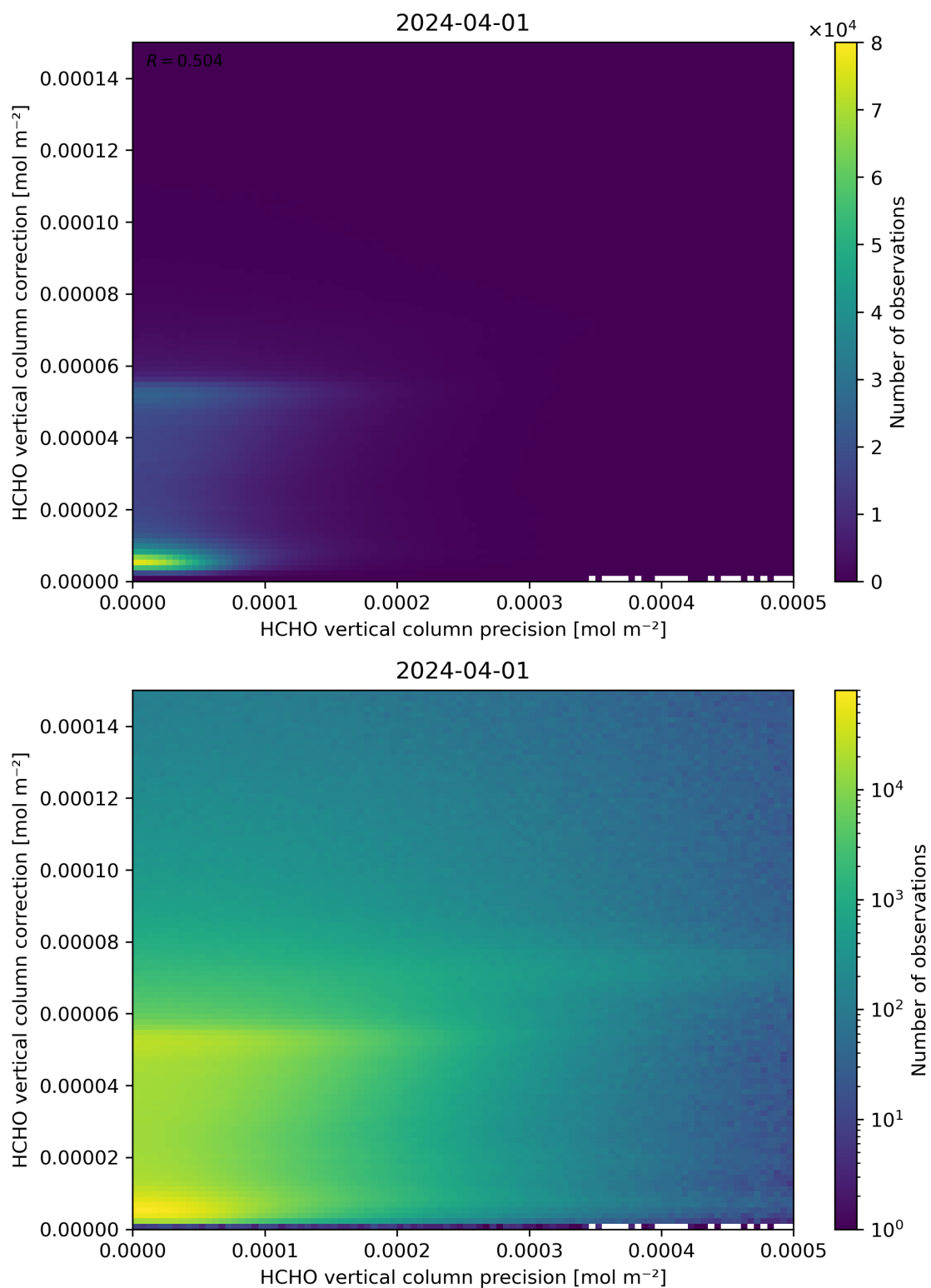
Figure 146: Scatter density plot of “HCHO vertical column precision” against “HCHO vertical column correction” for 2024-03-31 to 2024-04-02.
