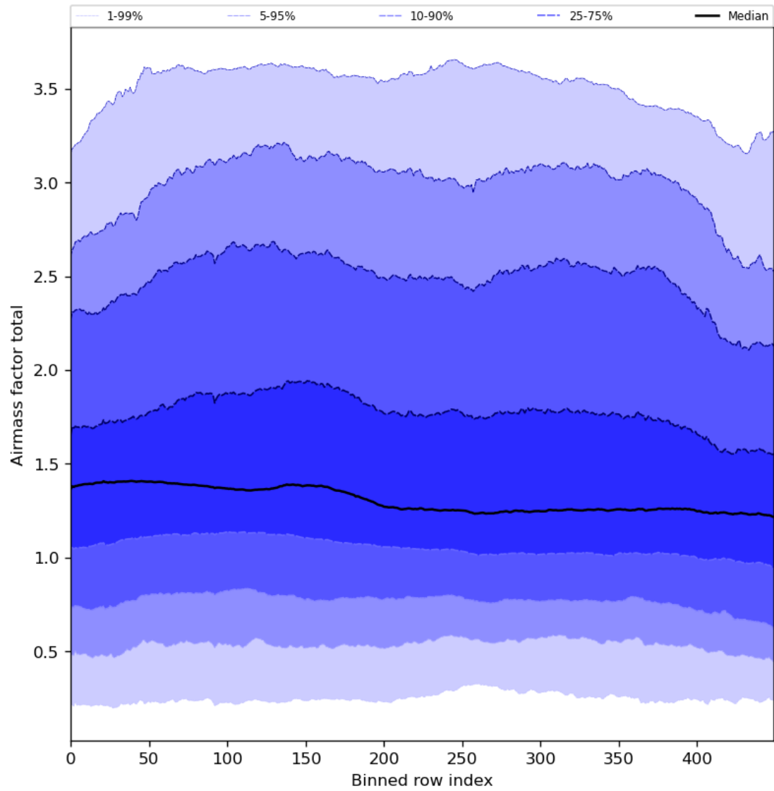
Figure 54: Along track statistics of “Airmass factor total” for 2024-03-31 to 2024-04-02
