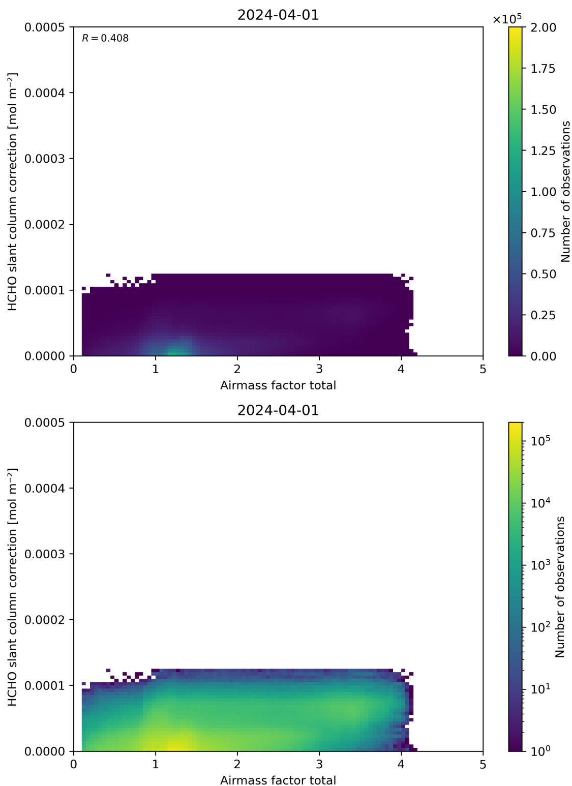
Figure 102: Scatter density plot of “Airmass factor total” against “HCHO slant column correction” for 2024-03-31 to 2024-04-02.
