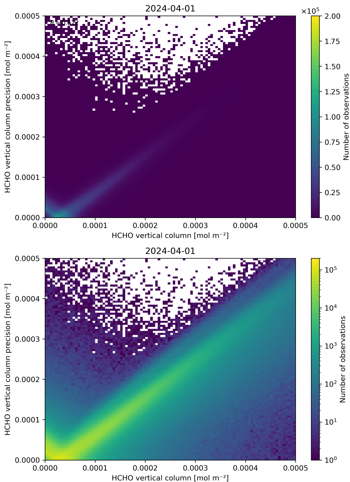
Figure 134: Scatter density plot of “HCHO vertical column” against “HCHO vertical column precision” for 2024-03-31 to 2024-04-02.
