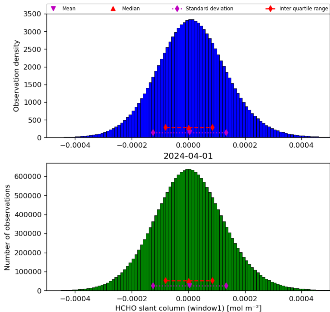
Figure 38: Histogram of “HCHO slant column (window1)” for 2024-03-31 to 2024-04-02
