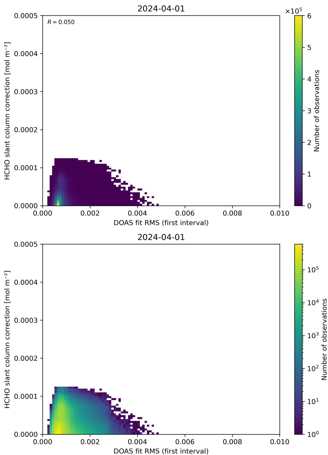
Figure 63: Scatter density plot of “DOAS fit RMS (first interval)” against “HCHO slant column correction” for 2024-03-31 to 2024-04-02.
