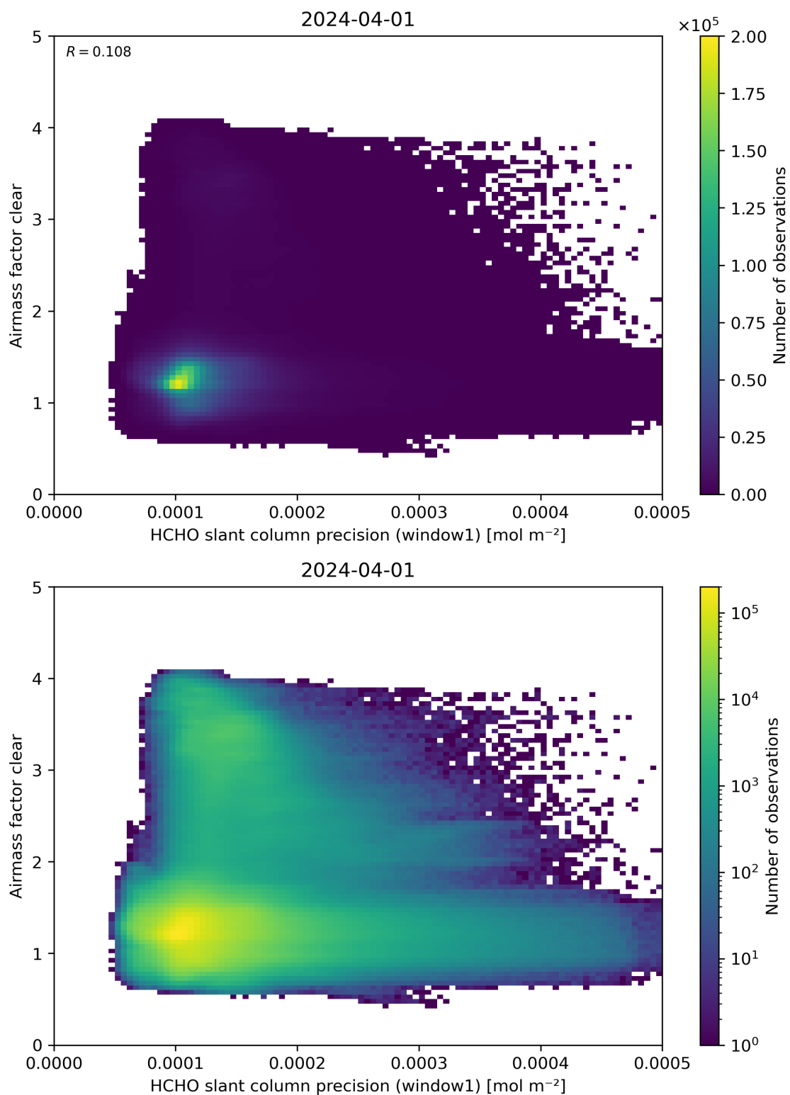
Figure 91: Scatter density plot of “HCHO slant column precision (window1)” against “Airmass factor clear” for 2024-03-31 to 2024-04-02.
