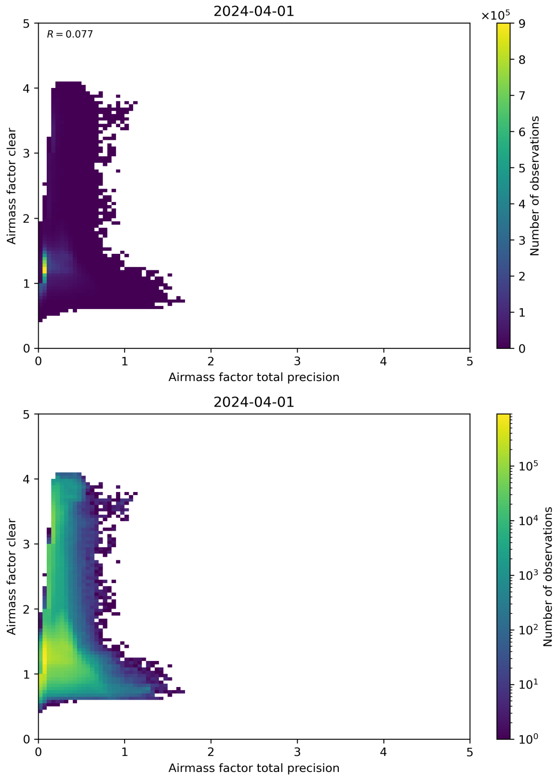
Figure 108: Scatter density plot of “Airmass factor total precision” against “Airmass factor clear” for 2024-03-31 to 2024-04-02.
