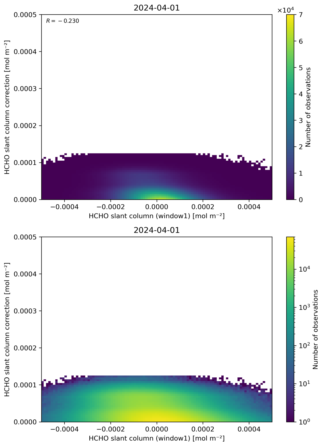
Figure 83: Scatter density plot of “HCHO slant column (window1)” against “HCHO slant column correction” for 2024-03-31 to 2024-04-02.
