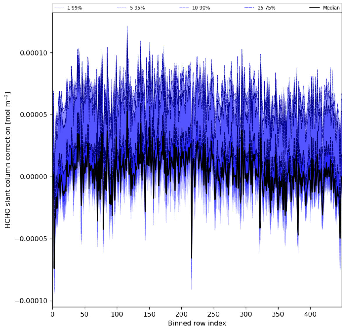
Figure 61: Along track statistics of “HCHO slant column correction” for 2024-03-31 to 2024-04-02
