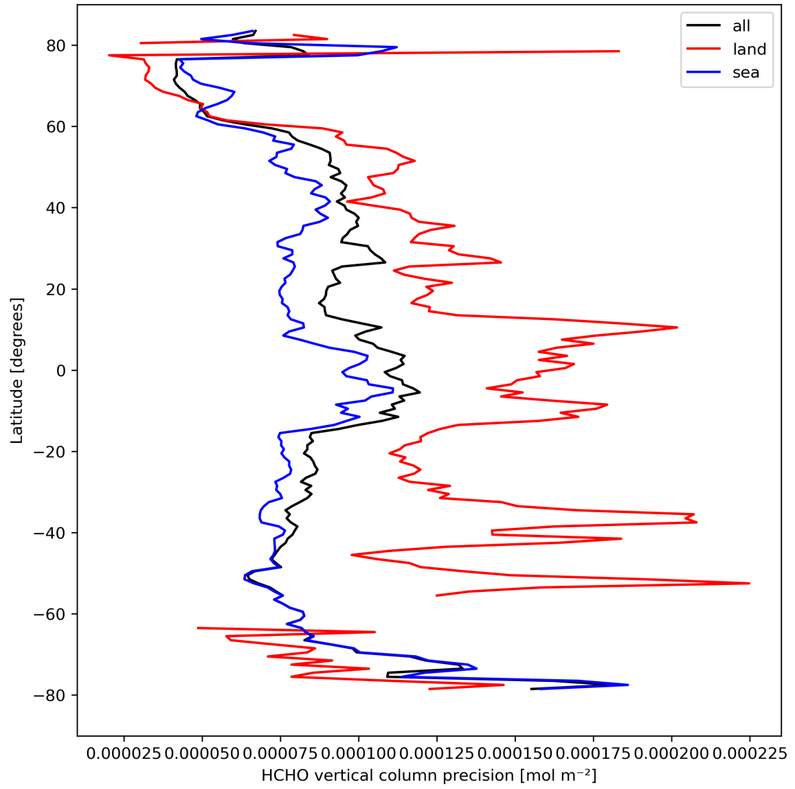
Figure 22: Zonal average of “HCHO vertical column precision” for 2024-03-31 to 2024-04-02.
