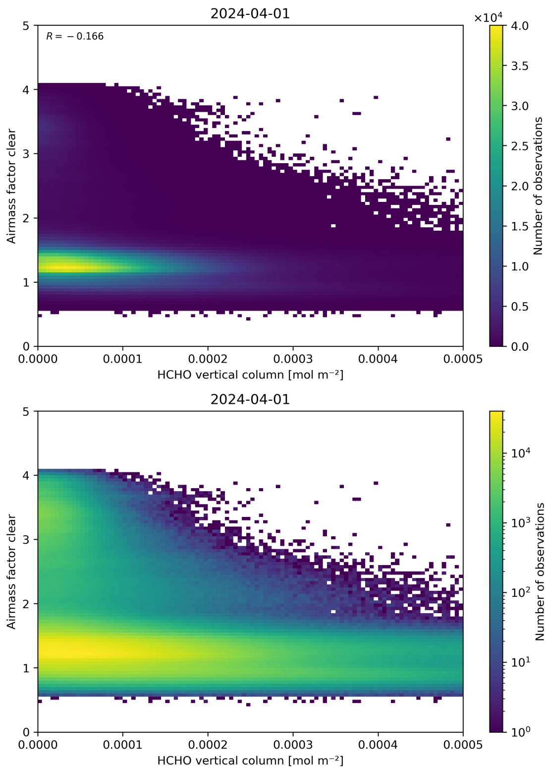
Figure 126: Scatter density plot of “HCHO vertical column” against “Airmass factor clear” for 2024-03-31 to 2024-04-02.
