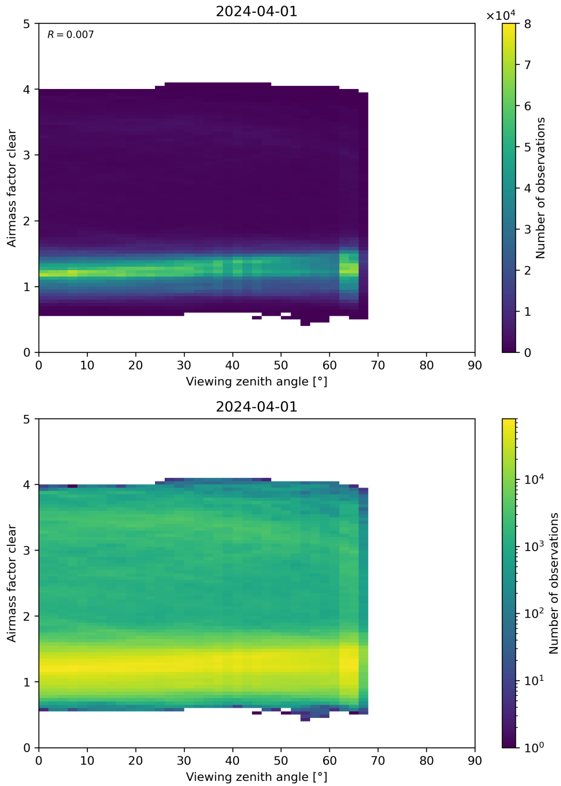
Figure 185: Scatter density plot of “Viewing zenith angle” against “Airmass factor clear” for 2024-03-31 to 2024-04-02.
