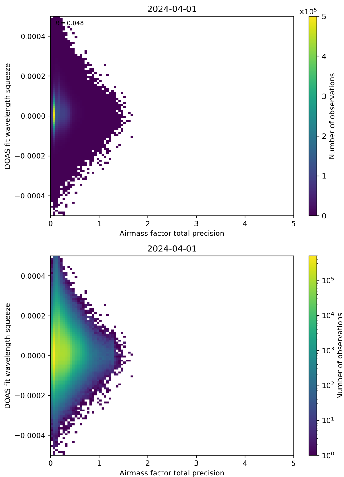
Figure 107: Scatter density plot of “Airmass factor total precision” against “DOAS fit wavelength squeeze” for 2024-03-31 to 2024-04-02.
