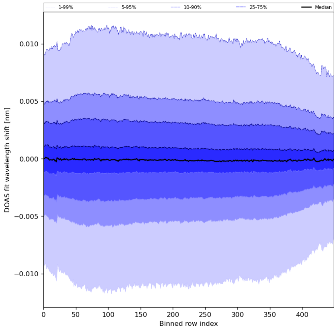
Figure 58: Along track statistics of “DOAS fit wavelength shift” for 2024-03-31 to 2024-04-02
