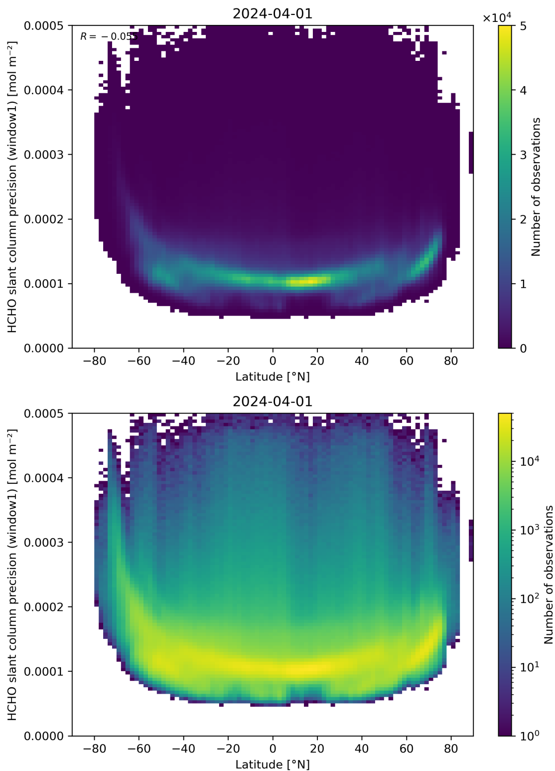
Figure 160: Scatter density plot of “Latitude” against “HCHO slant column precision (window1)” for 2024-03-31 to 2024-04-02.
