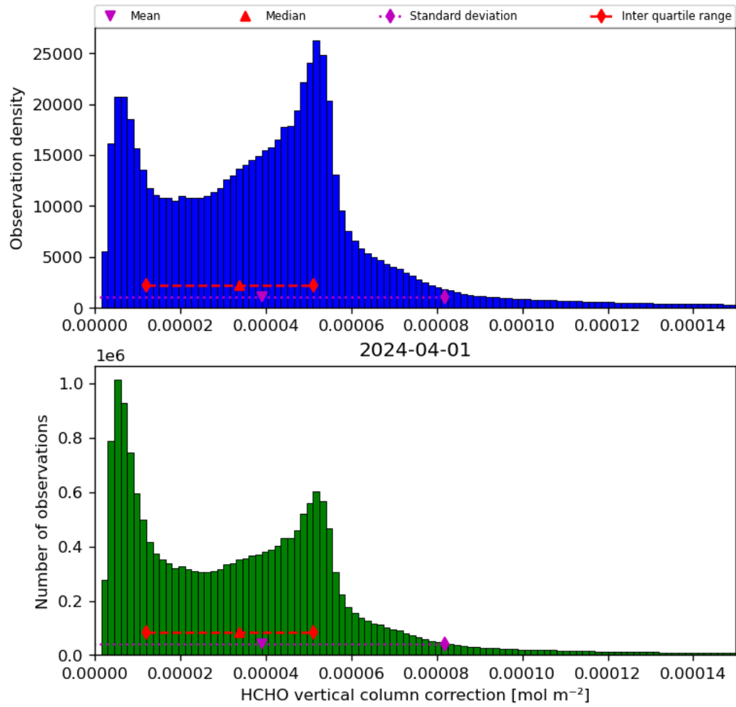
Figure 37: Histogram of “HCHO vertical column correction” for 2024-03-31 to 2024-04-02
