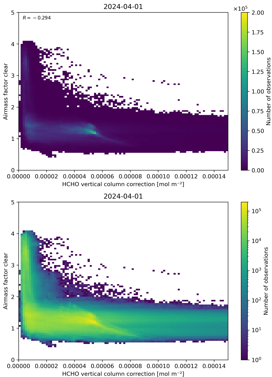
Figure 115: Scatter density plot of “HCHO vertical column correction” against “Airmass factor clear” for 2024-03-31 to 2024-04-02.
