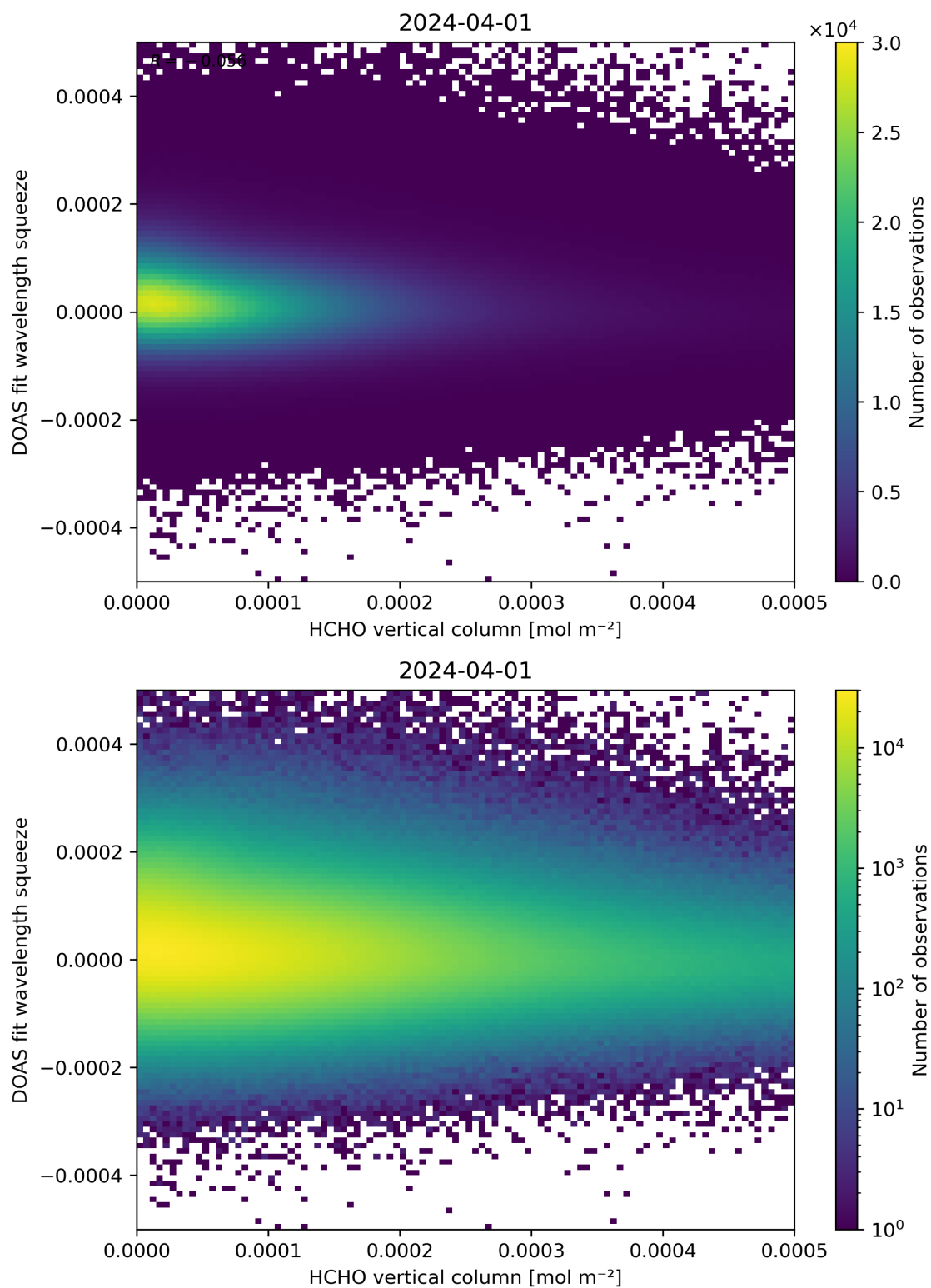
Figure 125: Scatter density plot of “HCHO vertical column” against “DOAS fit wavelength squeeze” for 2024-03-31 to 2024-04-02.
