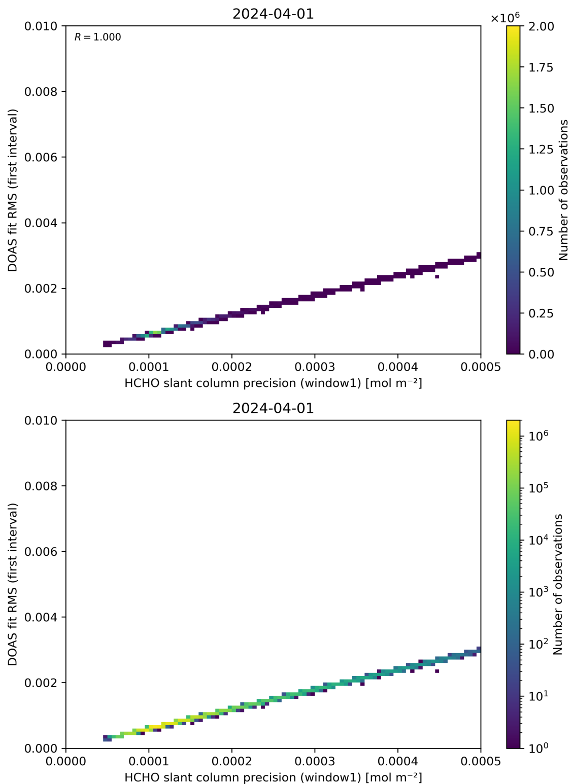
Figure 88: Scatter density plot of “HCHO slant column precision (window1)” against “DOAS fit RMS (first interval)” for 2024-03-31 to 2024-04-02.
