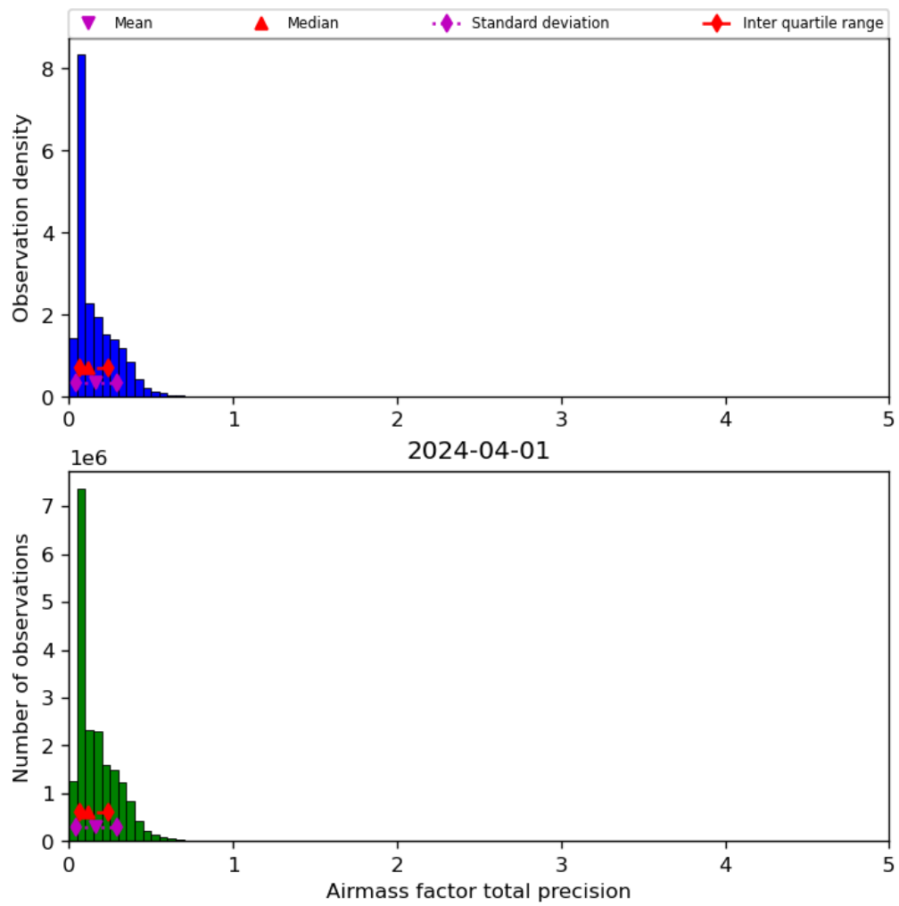
Figure 41: Histogram of “Airmass factor total precision” for 2024-03-31 to 2024-04-02
