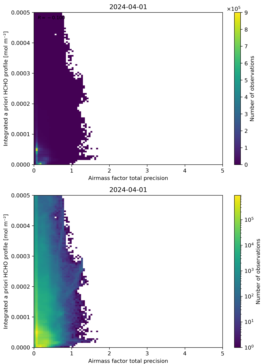
Figure 111: Scatter density plot of “Airmass factor total precision” against “Integrated a priori HCHO profile” for 2024-03-31 to 2024-04-02.
