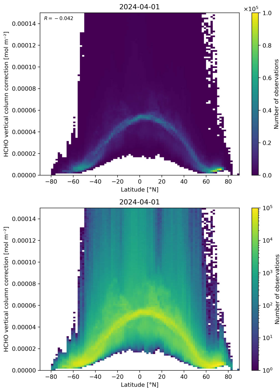
Figure 164: Scatter density plot of “Latitude” against “HCHO vertical column correction” for 2024-03-31 to 2024-04-02.
