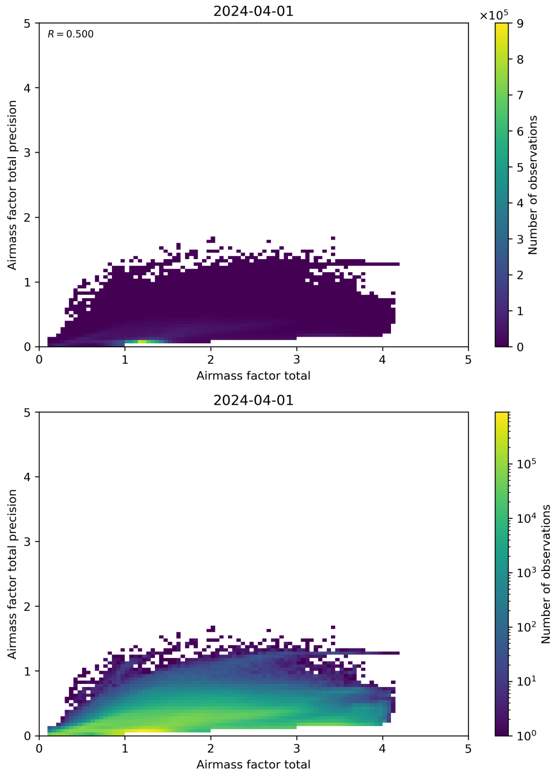
Figure 103: Scatter density plot of “Airmass factor total” against “Airmass factor total precision” for 2024-03-31 to 2024-04-02.
