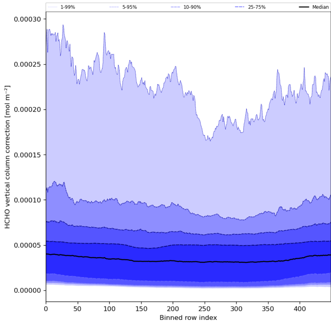
Figure 51: Along track statistics of “HCHO vertical column correction” for 2024-03-31 to 2024-04-02
