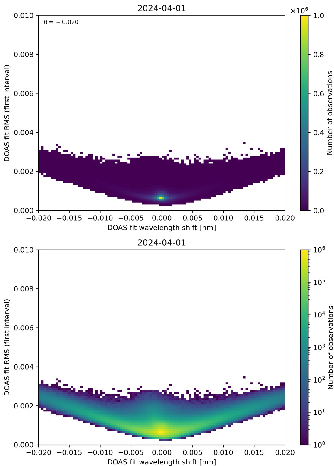
Figure 64: Scatter density plot of “DOAS fit wavelength shift” against “DOAS fit RMS (first interval)” for 2024-03-31 to 2024-04-02.
