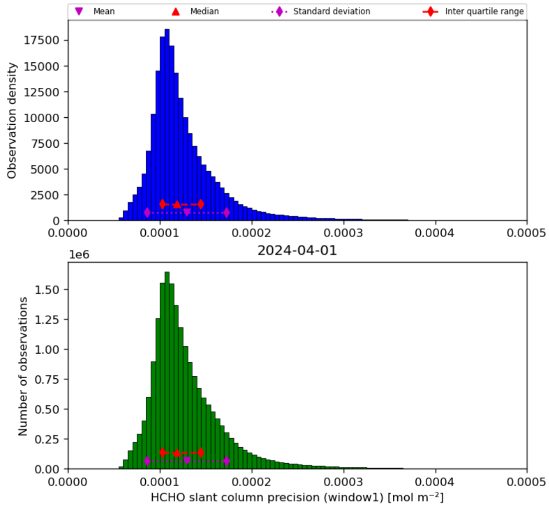
Figure 39: Histogram of “HCHO slant column precision (window1)” for 2024-03-31 to 2024-04-02
