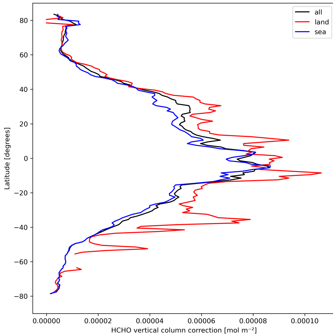
Figure 23: Zonal average of “HCHO vertical column correction” for 2024-03-31 to 2024-04-02.
