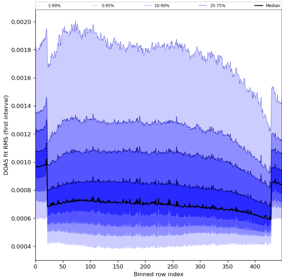
Figure 60: Along track statistics of “DOAS fit RMS (first interval)” for 2024-03-31 to 2024-04-02
