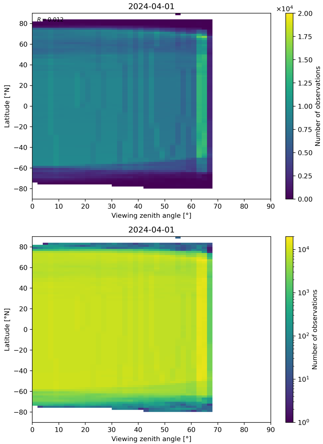
Figure 196: Scatter density plot of “Viewing zenith angle” against “Latitude” for 2024-03-31 to 2024-04-02.
