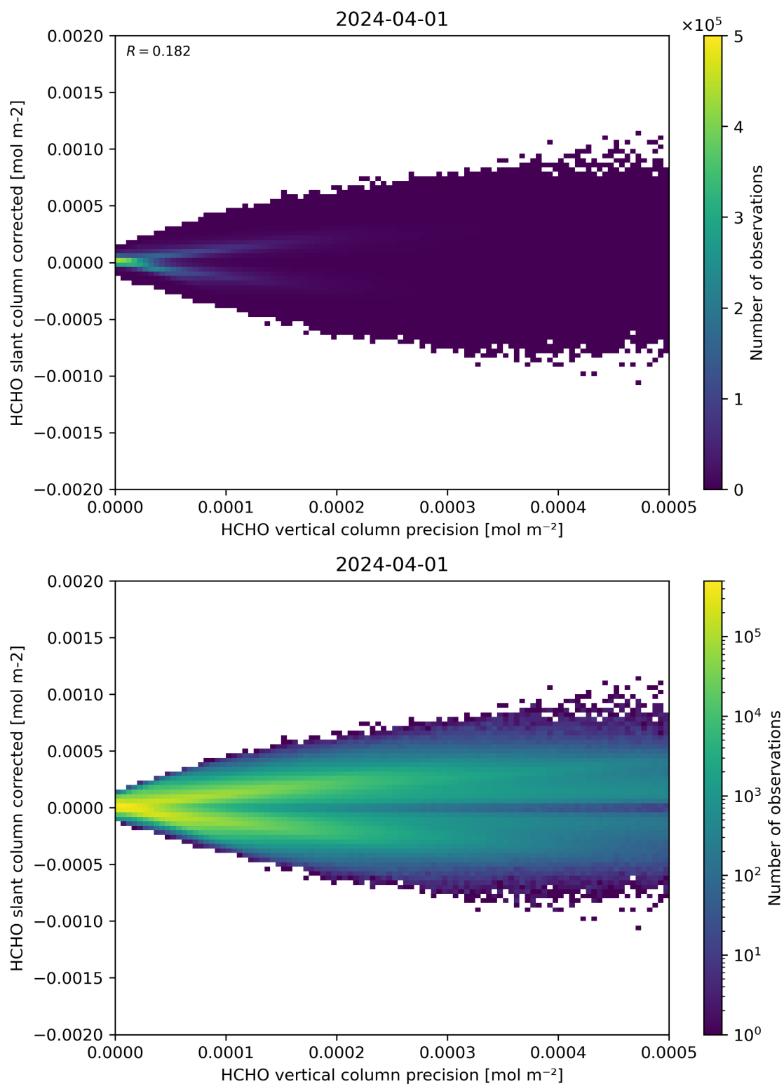
Figure 140: Scatter density plot of “HCHO vertical column precision” against “HCHO slant column corrected” for 2024-03-31 to 2024-04-02.
