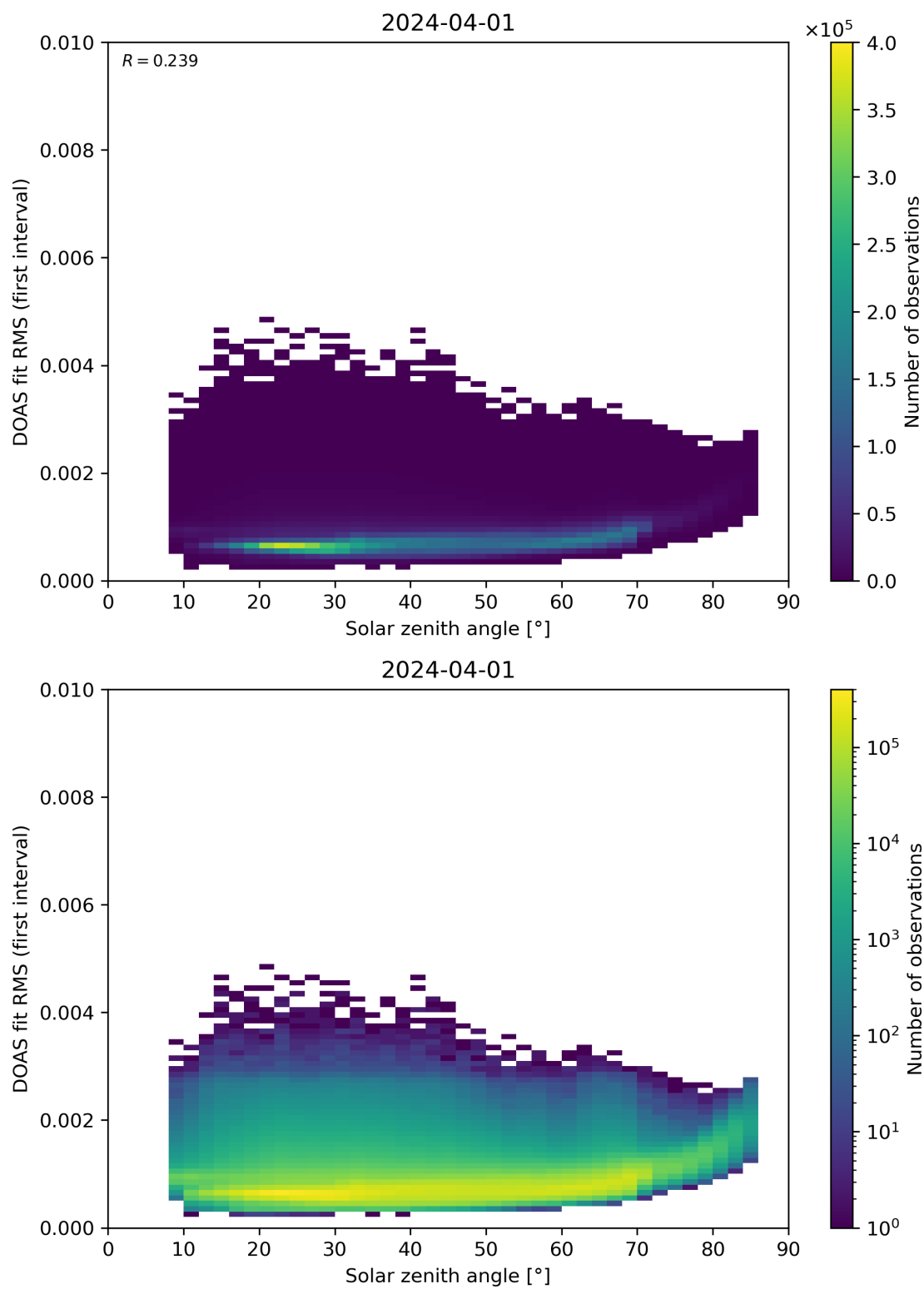
Figure 167: Scatter density plot of “Solar zenith angle” against “DOAS fit RMS (first interval)” for 2024-03-31 to 2024-04-02.
