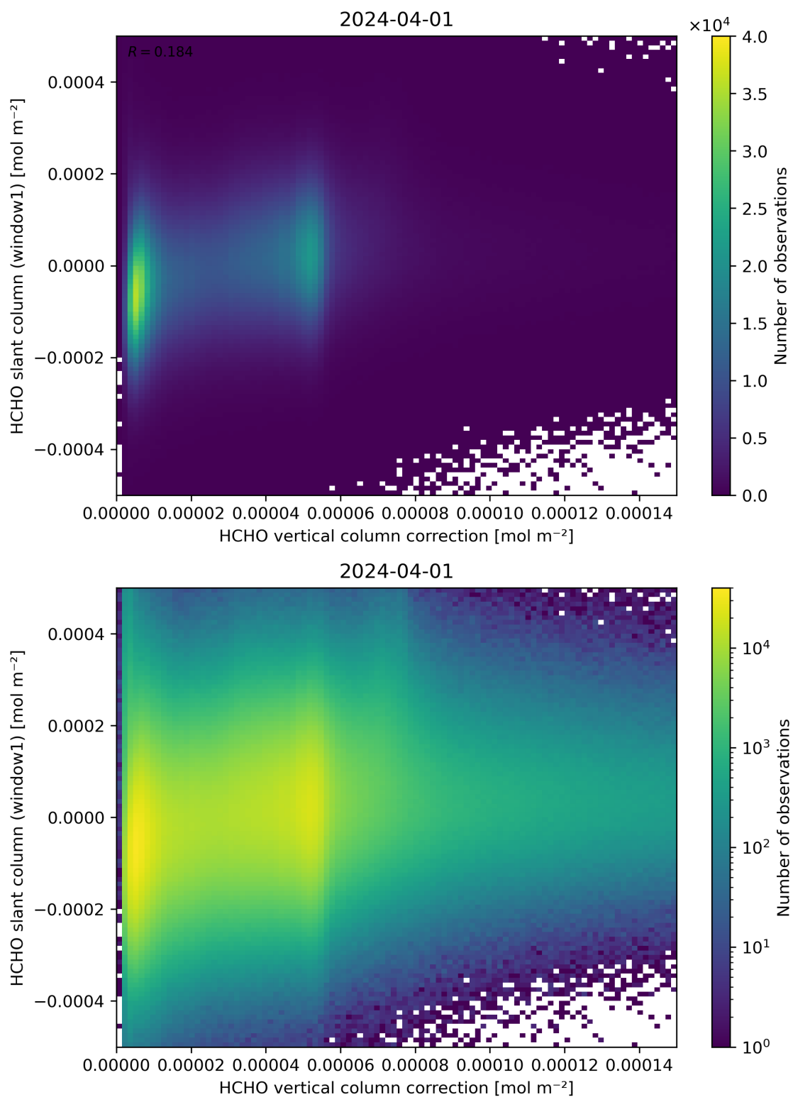
Figure 118: Scatter density plot of “HCHO vertical column correction” against “HCHO slant column (window1)” for 2024-03-31 to 2024-04-02.
