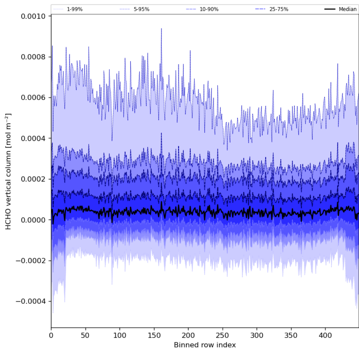
Figure 49: Along track statistics of “HCHO vertical column” for 2024-03-31 to 2024-04-02
