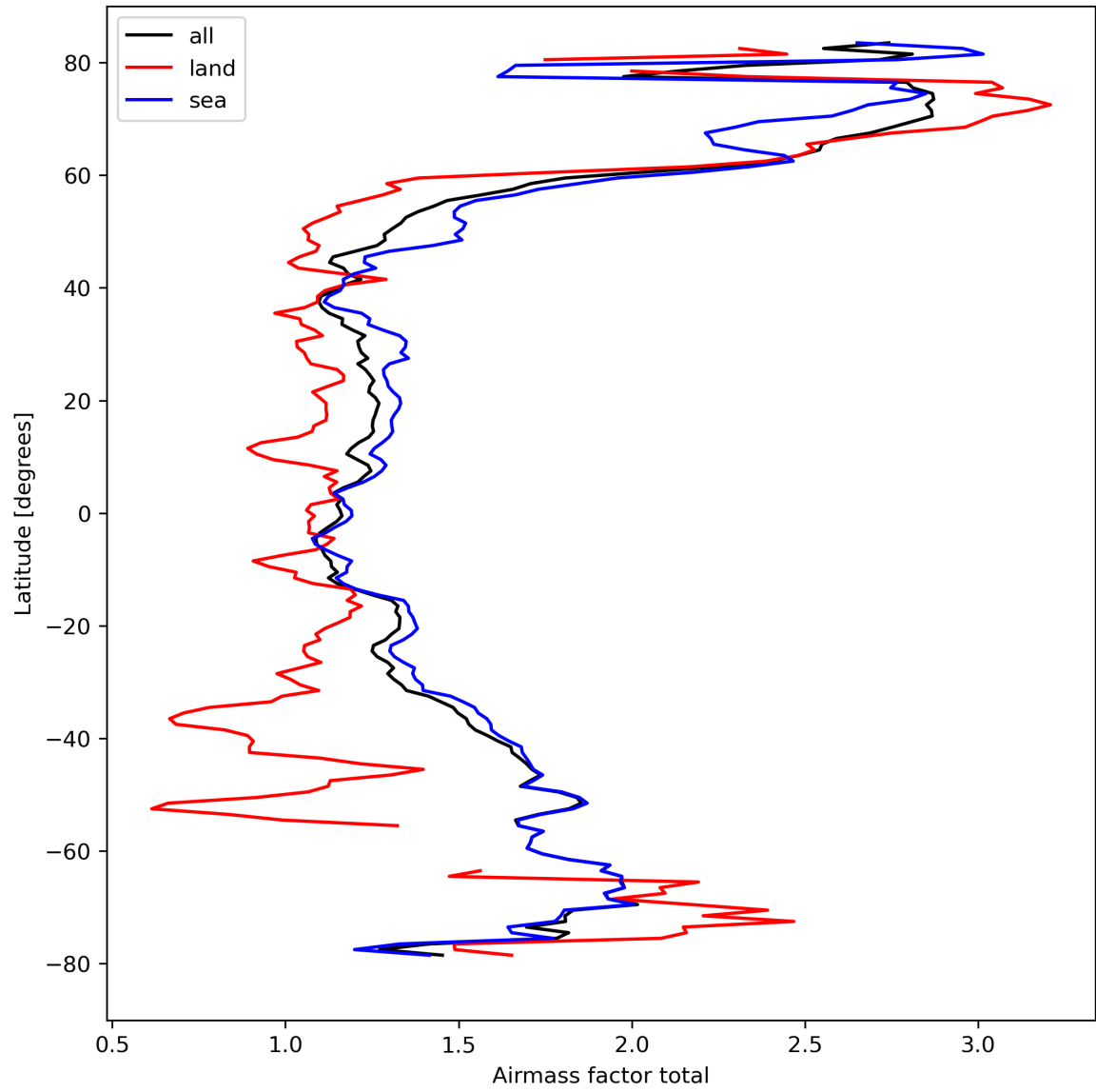
Figure 26: Zonal average of “Airmass factor total” for 2024-03-31 to 2024-04-02.
