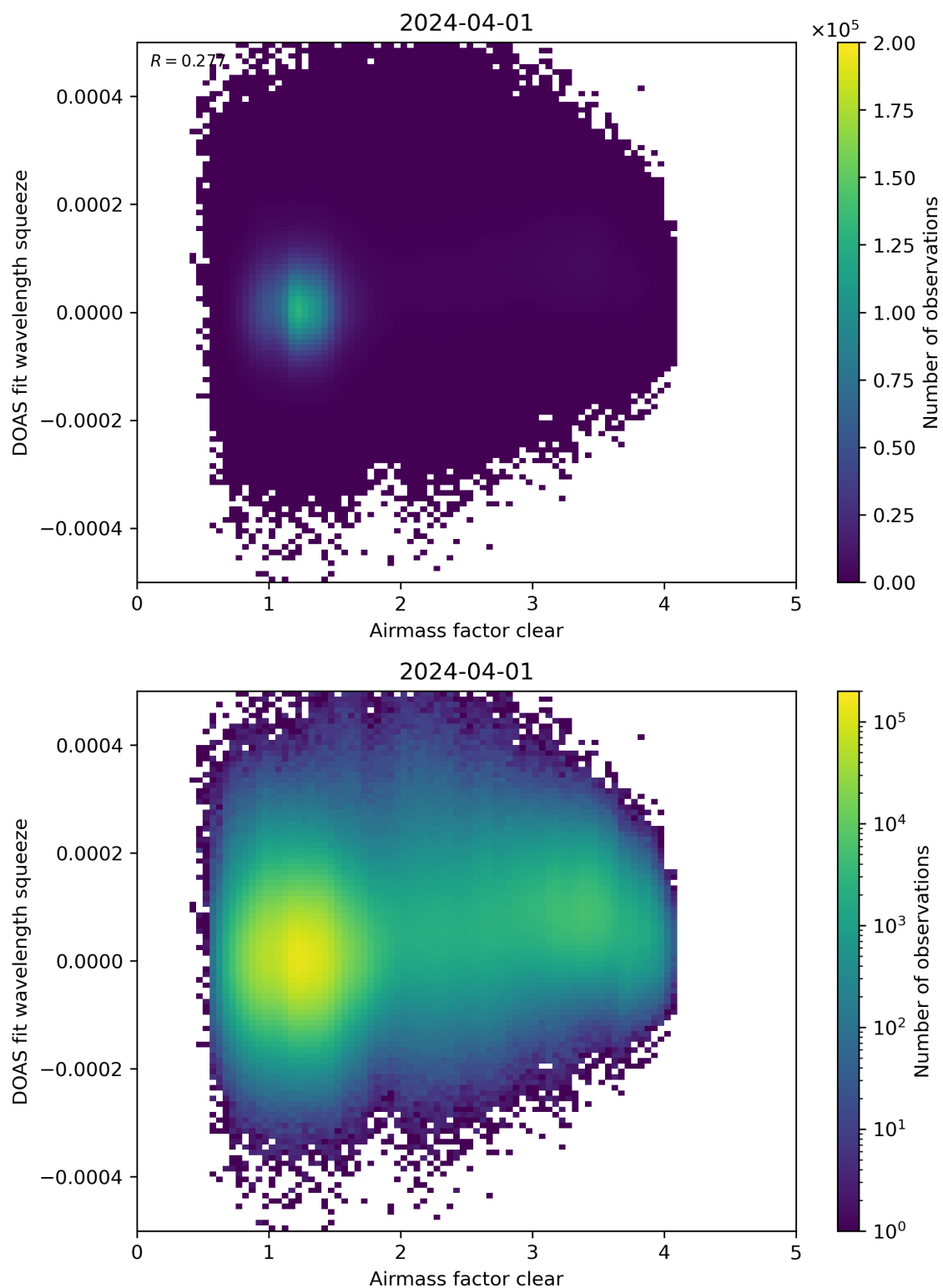
Figure 73: Scatter density plot of “Airmass factor clear” against “DOAS fit wavelength squeeze” for 2024-03-31 to 2024-04-02.
