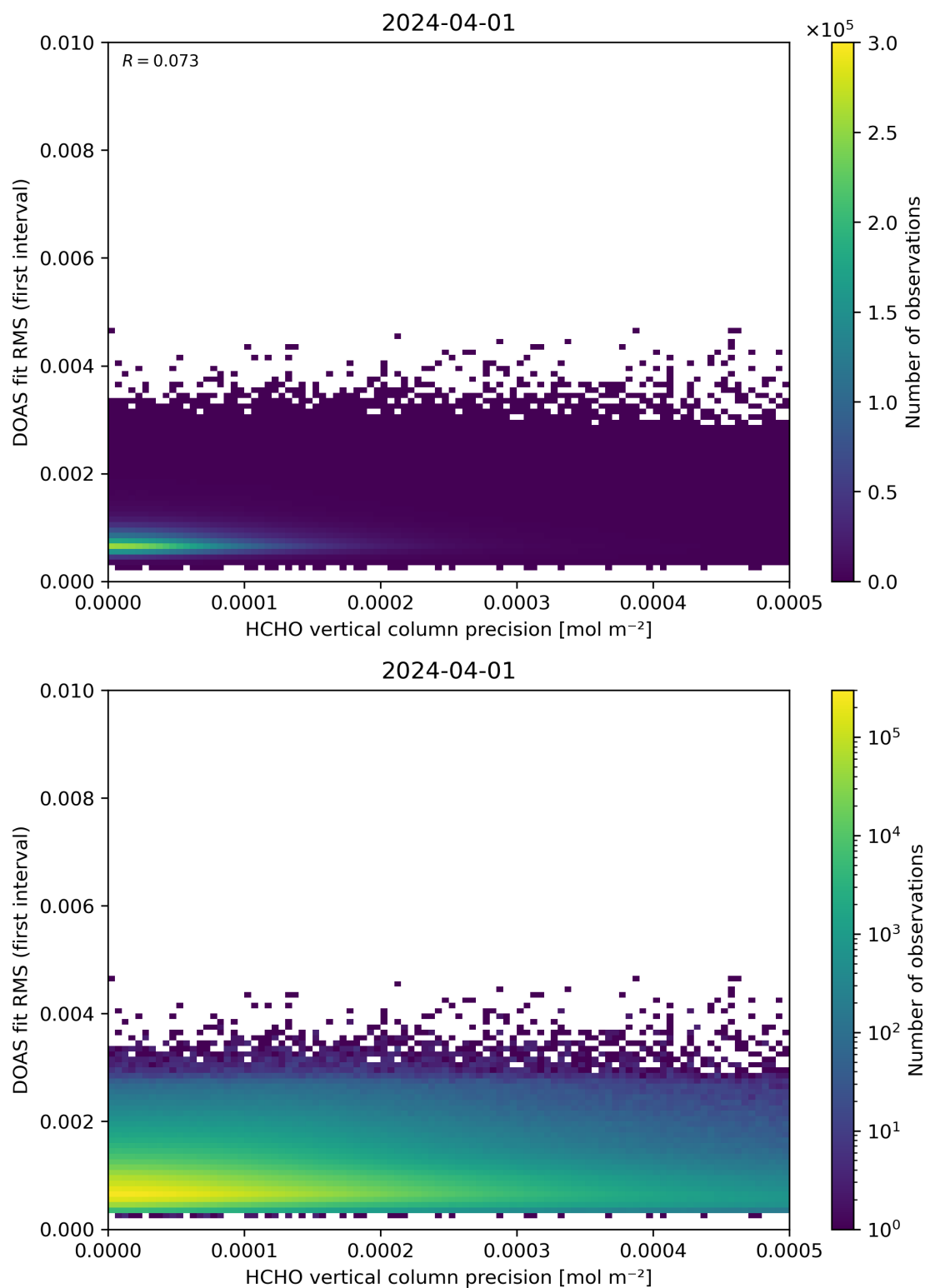
Figure 136: Scatter density plot of “HCHO vertical column precision” against “DOAS fit RMS (first interval)” for 2024-03-31 to 2024-04-02.
