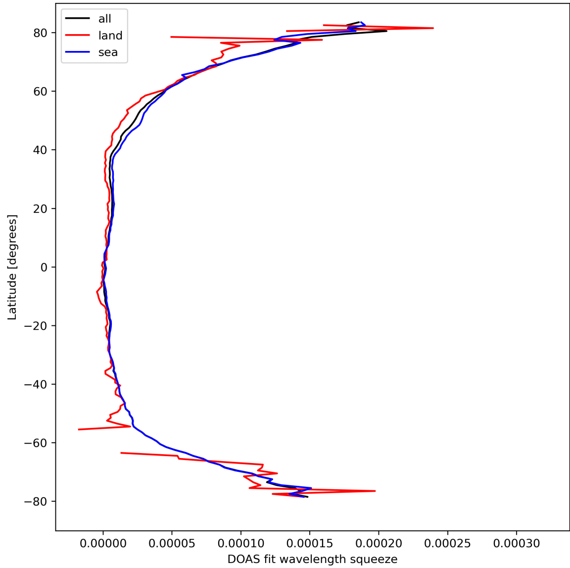
Figure 31: Zonal average of “DOAS fit wavelength squeeze” for 2024-03-31 to 2024-04-02.
