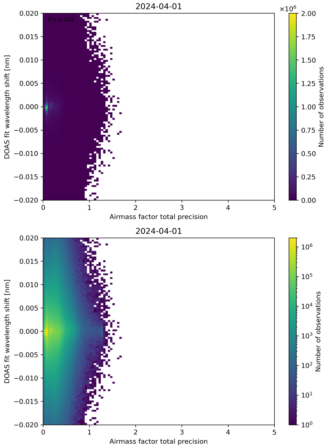
Figure 106: Scatter density plot of “Airmass factor total precision” against “DOAS fit wavelength shift” for 2024-03-31 to 2024-04-02.
