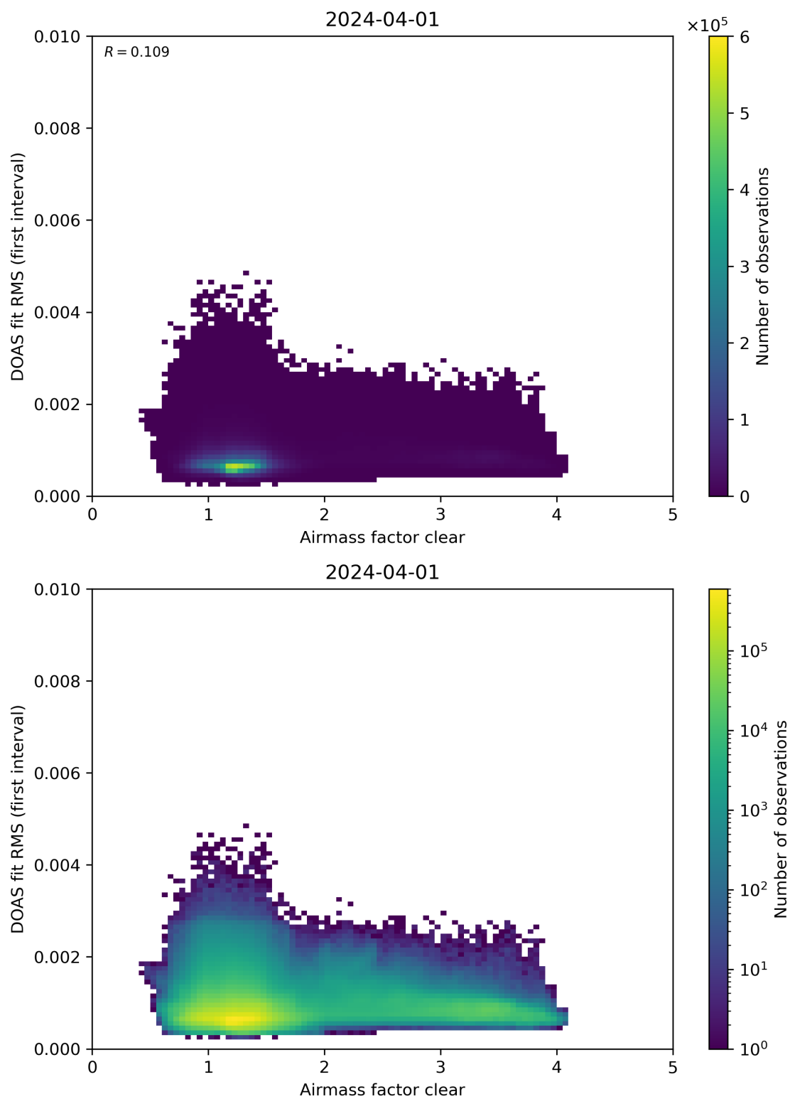
Figure 71: Scatter density plot of “Airmass factor clear” against “DOAS fit RMS (first interval)” for 2024-03-31 to 2024-04-02.
