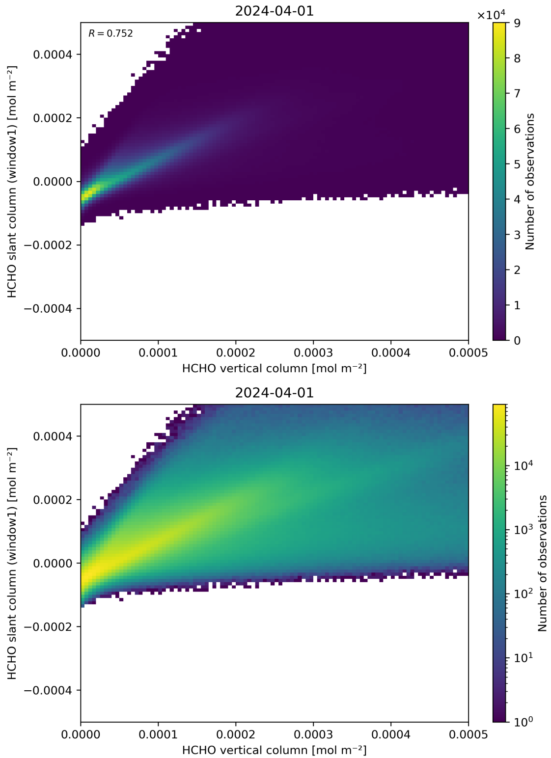
Figure 129: Scatter density plot of “HCHO vertical column” against “HCHO slant column (window1)” for 2024-03-31 to 2024-04-02.
