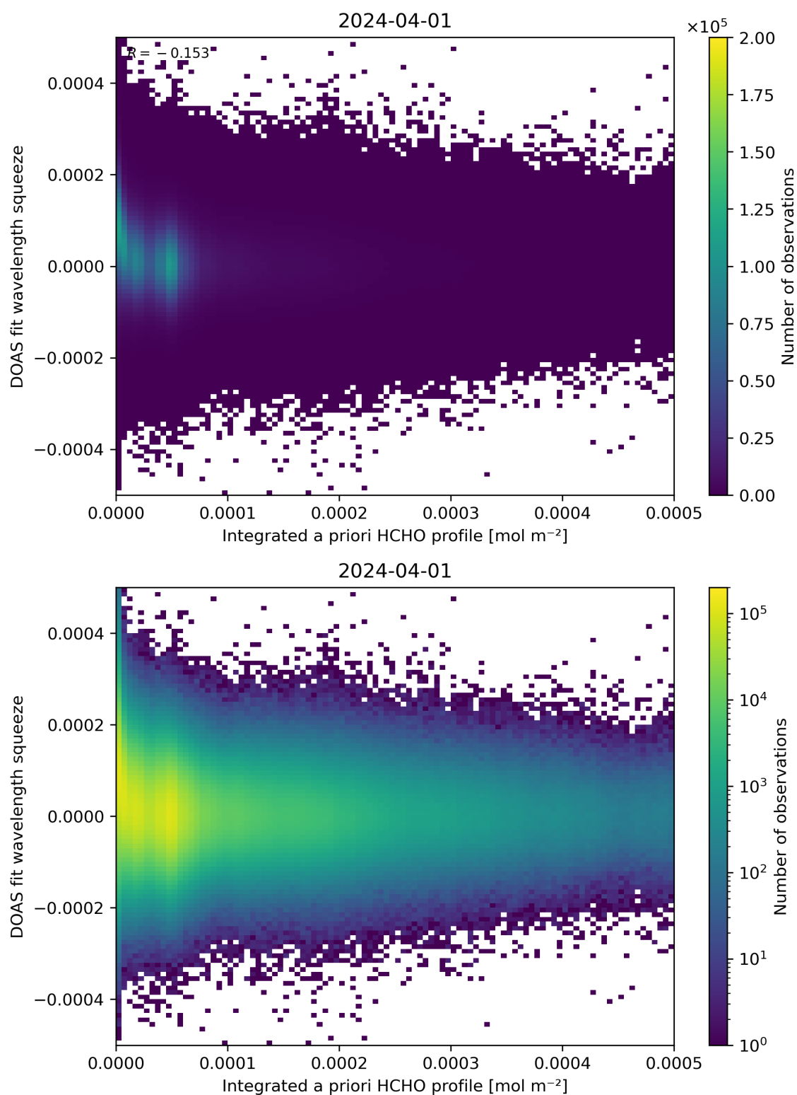
Figure 150: Scatter density plot of “Integrated a priori HCHO profile” against “DOAS fit wavelength squeeze” for 2024-03-31 to 2024-04-02.
