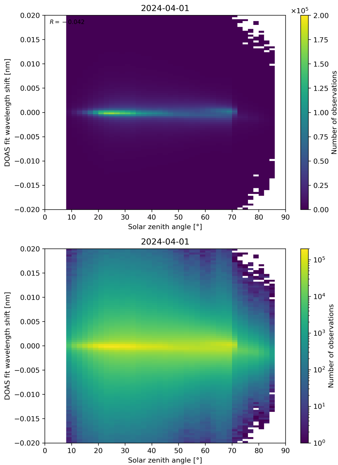
Figure 168: Scatter density plot of “Solar zenith angle” against “DOAS fit wavelength shift” for 2024-03-31 to 2024-04-02.
