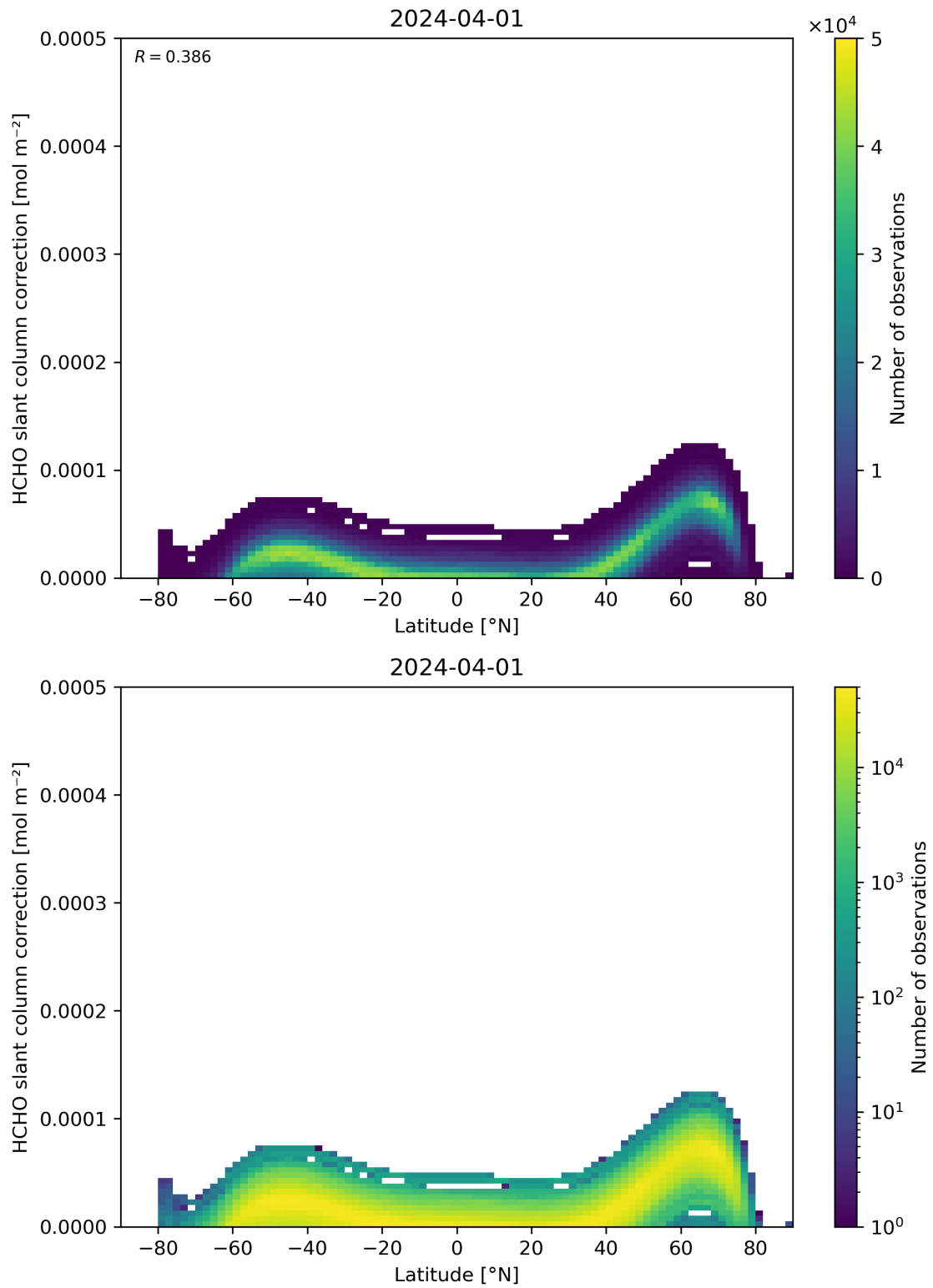
Figure 158: Scatter density plot of “Latitude” against “HCHO slant column correction” for 2024-03-31 to 2024-04-02.
