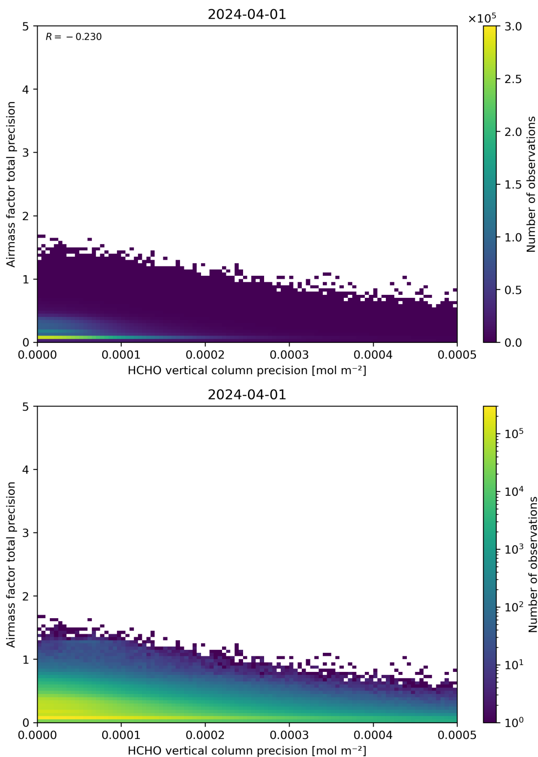
Figure 145: Scatter density plot of “HCHO vertical column precision” against “Airmass factor total precision” for 2024-03-31 to 2024-04-02.
