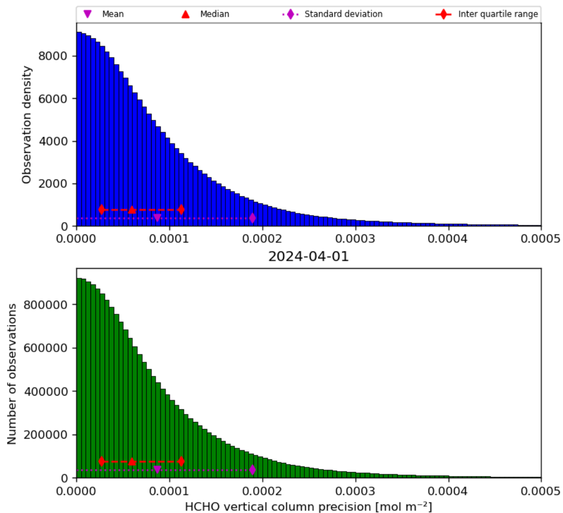
Figure 36: Histogram of “HCHO vertical column precision” for 2024-03-31 to 2024-04-02
