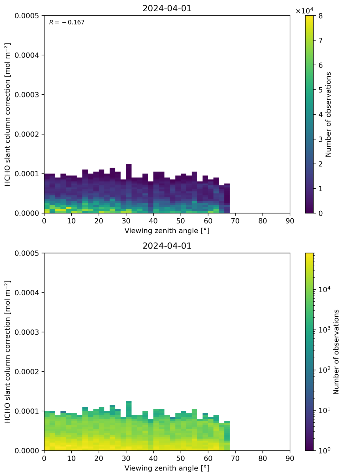
Figure 187: Scatter density plot of “Viewing zenith angle” against “HCHO slant column correction” for 2024-03-31 to 2024-04-02.
