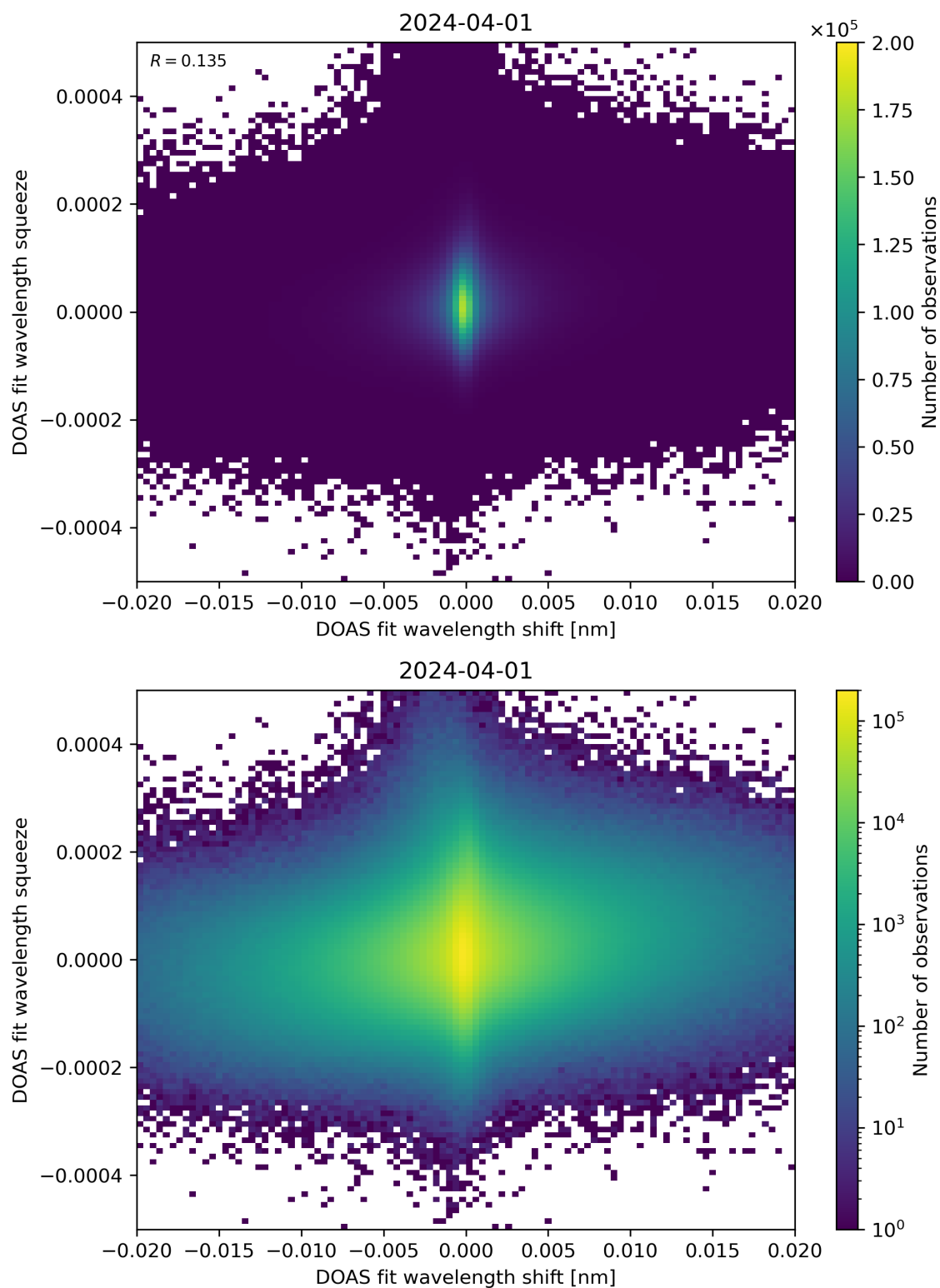
Figure 65: Scatter density plot of “DOAS fit wavelength shift” against “DOAS fit wavelength squeeze” for 2024-03-31 to 2024-04-02.
