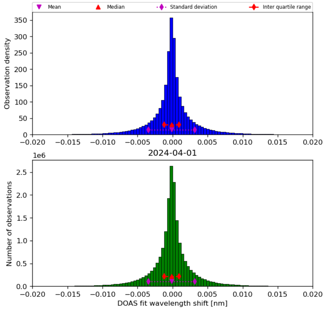
Figure 44: Histogram of “DOAS fit wavelength shift” for 2024-03-31 to 2024-04-02
