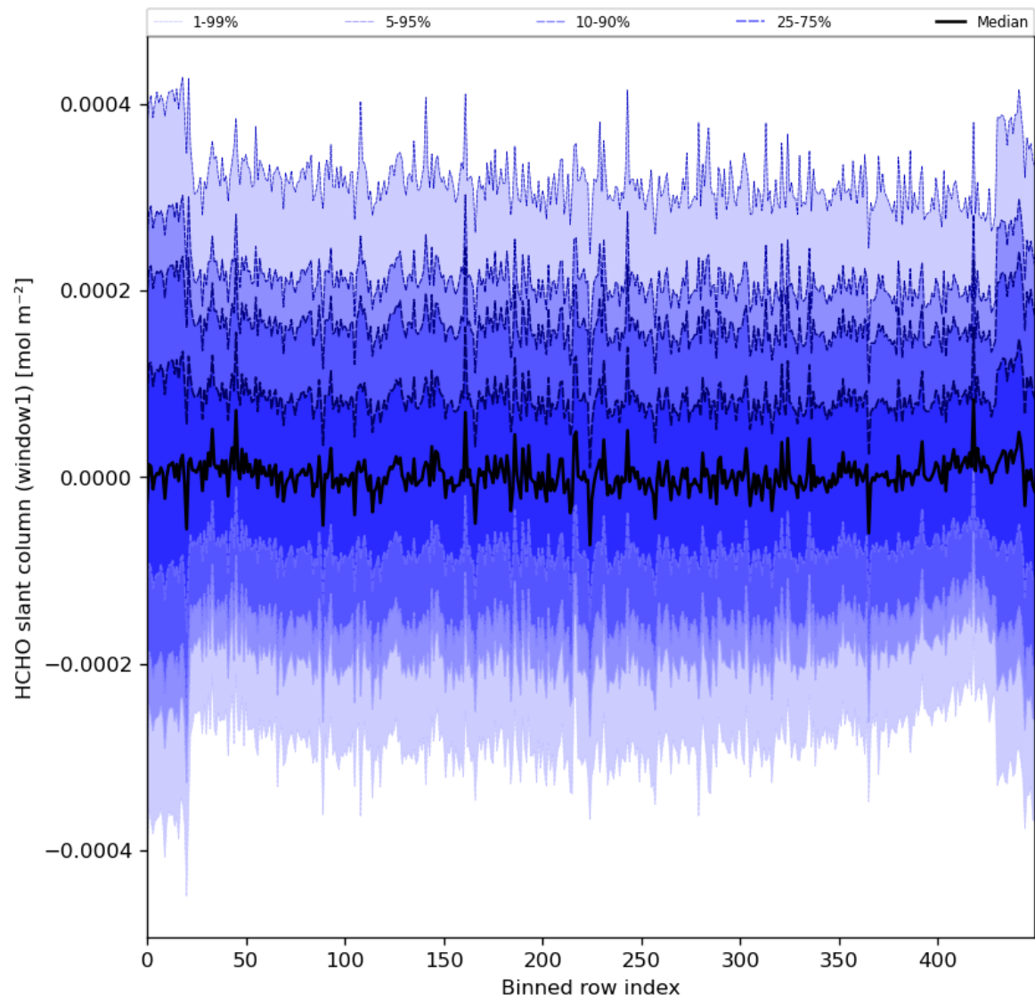
Figure 52: Along track statistics of “HCHO slant column (window1)” for 2024-03-31 to 2024-04-02
