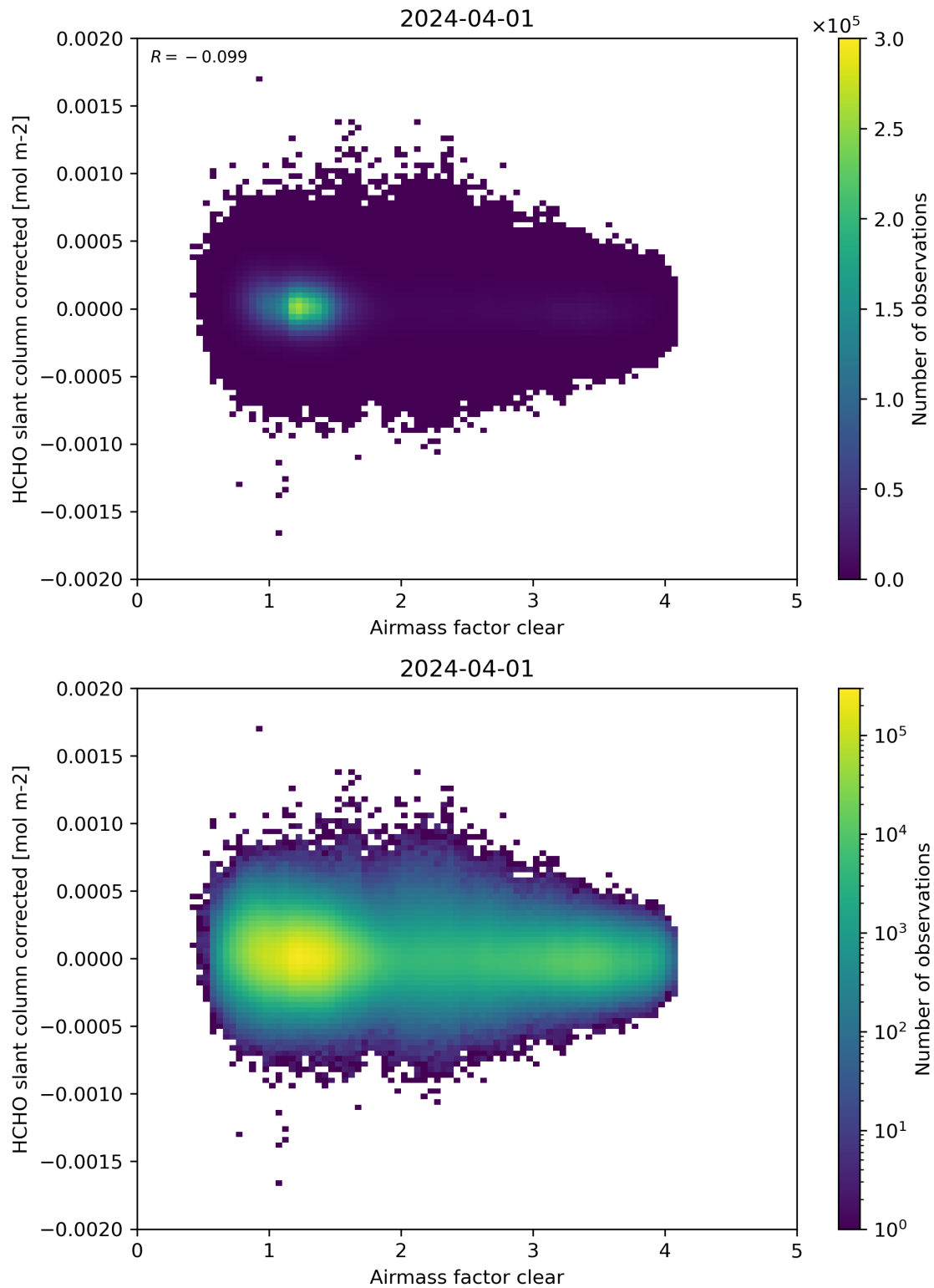
Figure 74: Scatter density plot of “Airmass factor clear” against “HCHO slant column corrected” for 2024-03-31 to 2024-04-02.
