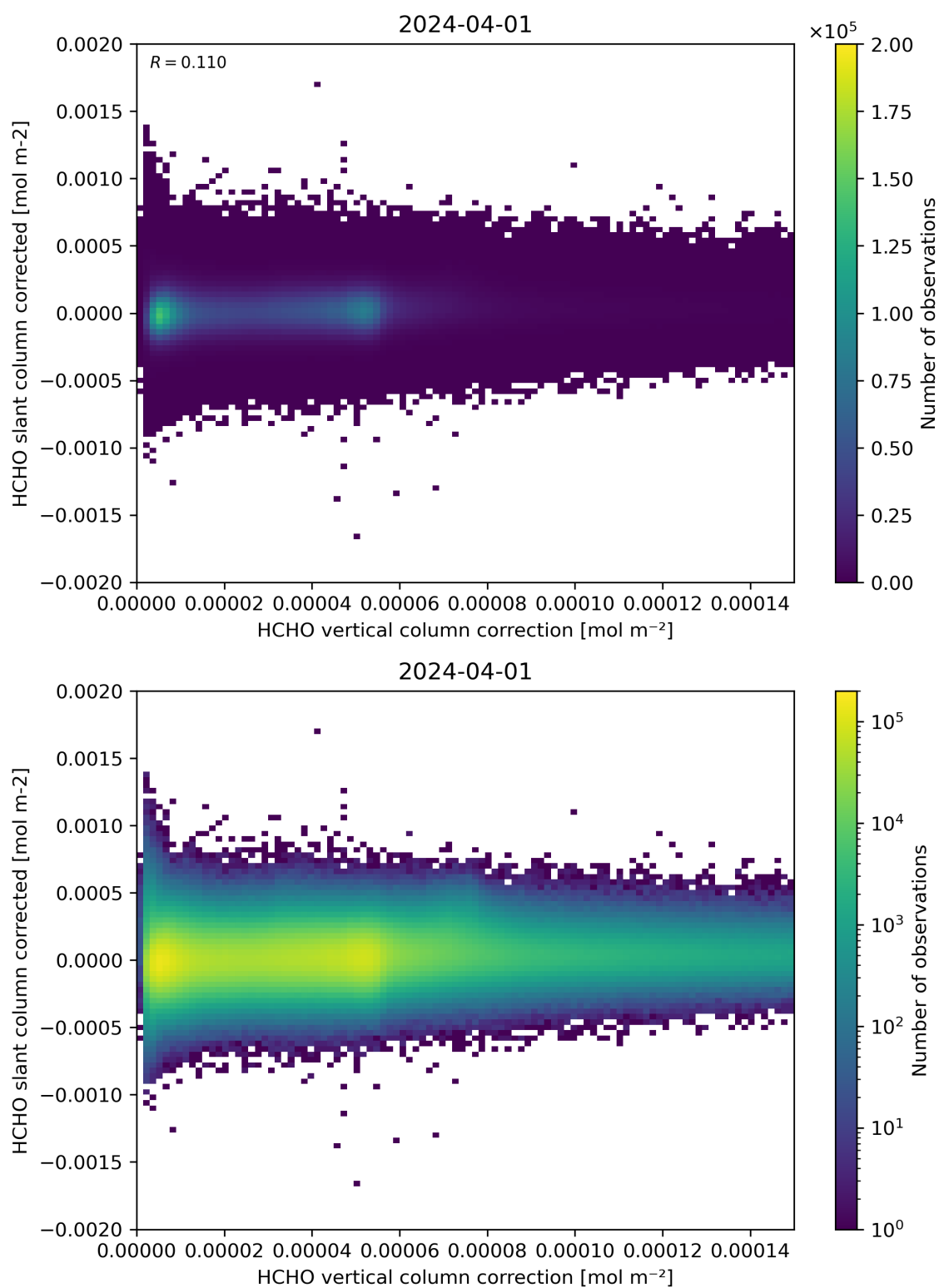
Figure 116: Scatter density plot of “HCHO vertical column correction” against “HCHO slant column corrected” for 2024-03-31 to 2024-04-02.
