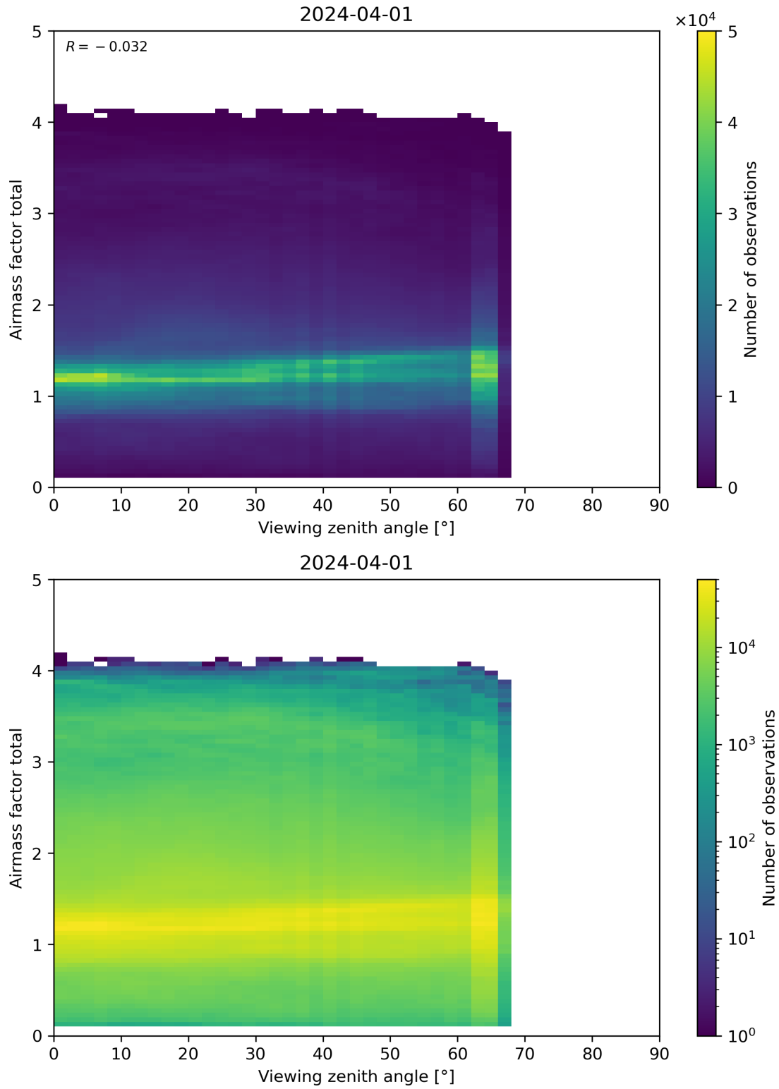
Figure 190: Scatter density plot of “Viewing zenith angle” against “Airmass factor total” for 2024-03-31 to 2024-04-02.
