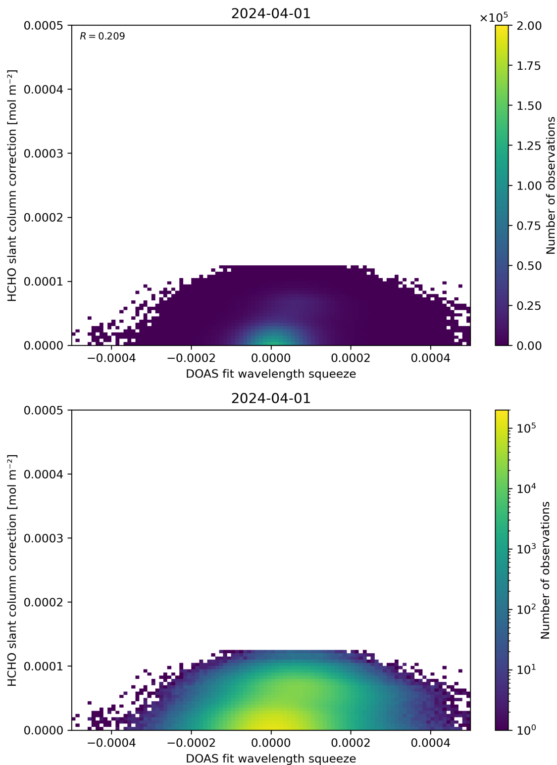
Figure 70: Scatter density plot of “DOAS fit wavelength squeeze” against “HCHO slant column correction” for 2024-03-31 to 2024-04-02.
