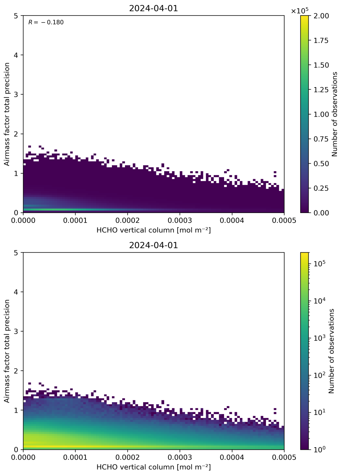
Figure 132: Scatter density plot of “HCHO vertical column” against “Airmass factor total precision” for 2024-03-31 to 2024-04-02.
