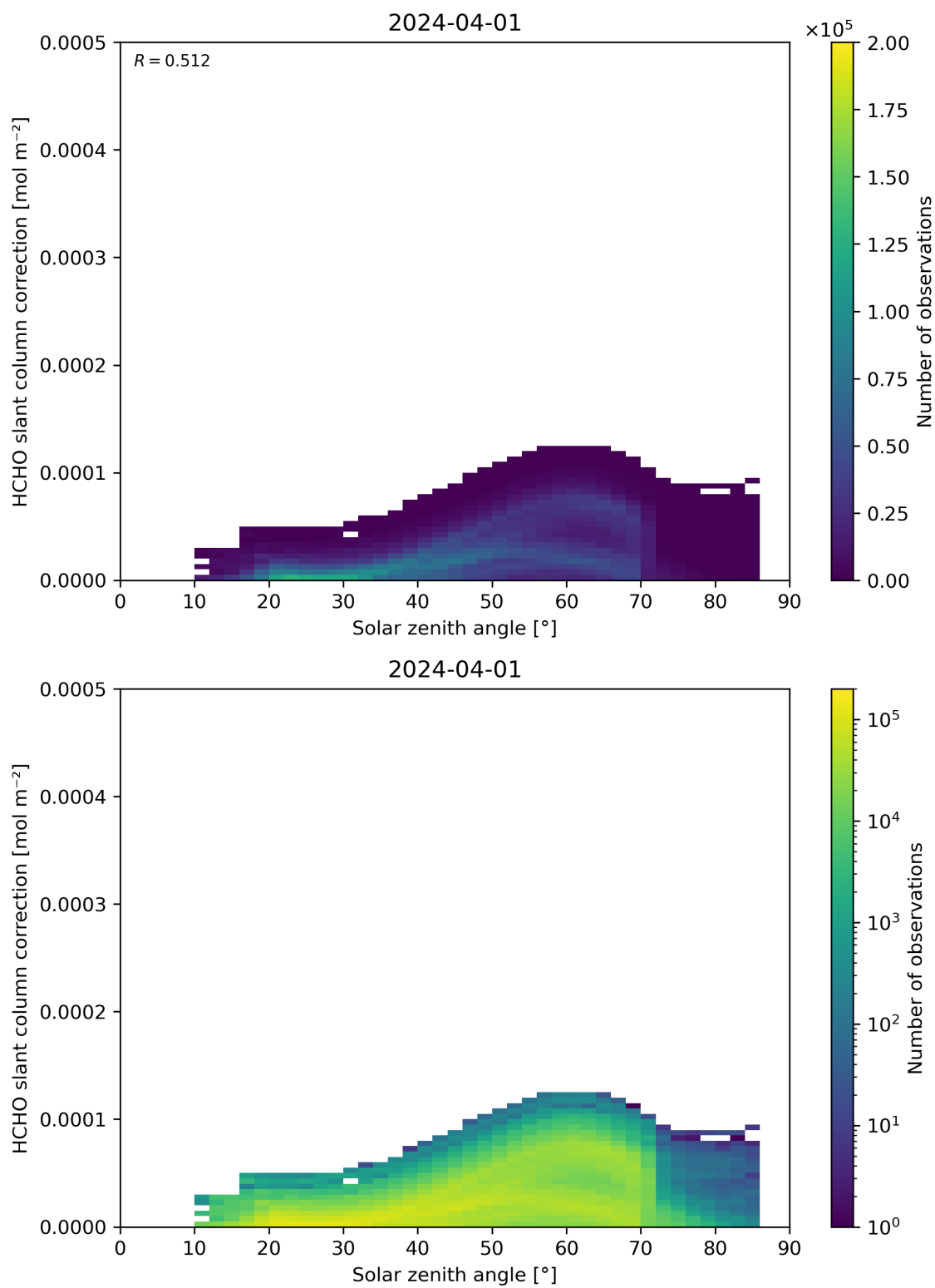
Figure 172: Scatter density plot of “Solar zenith angle” against “HCHO slant column correction” for 2024-03-31 to 2024-04-02.
