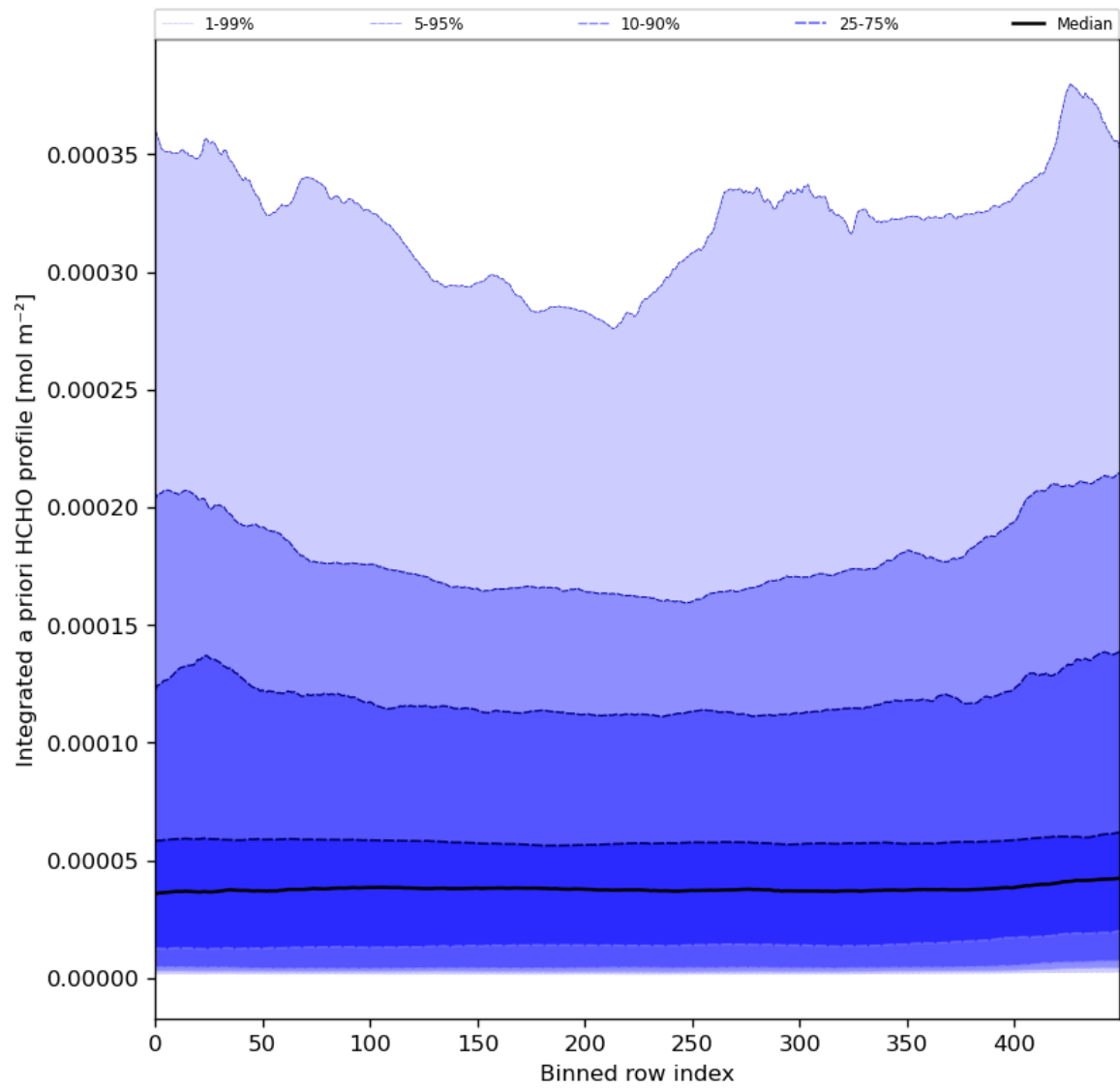
Figure 57: Along track statistics of “Integrated a priori HCHO profile” for 2024-03-31 to 2024-04-02
