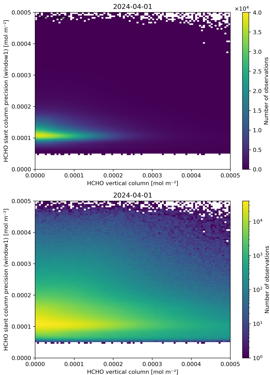
Figure 130: Scatter density plot of “HCHO vertical column” against “HCHO slant column precision (window1)” for 2024-03-31 to 2024-04-02.
