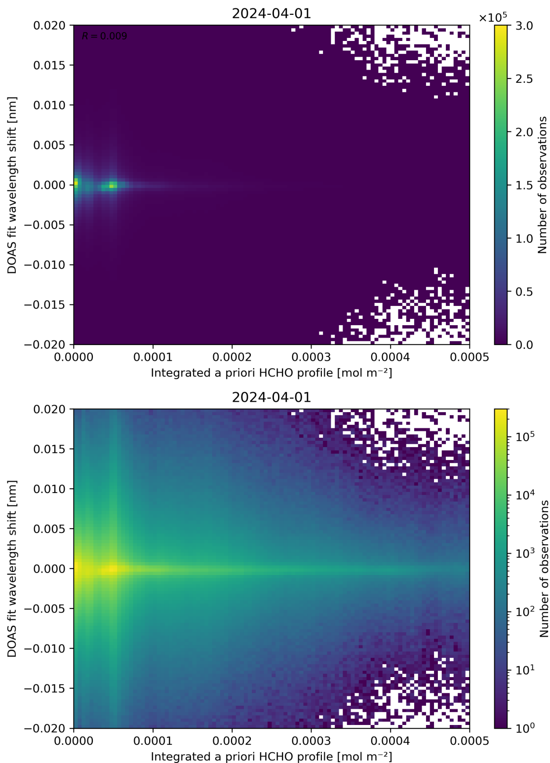
Figure 149: Scatter density plot of “Integrated a priori HCHO profile” against “DOAS fit wavelength shift” for 2024-03-31 to 2024-04-02.
