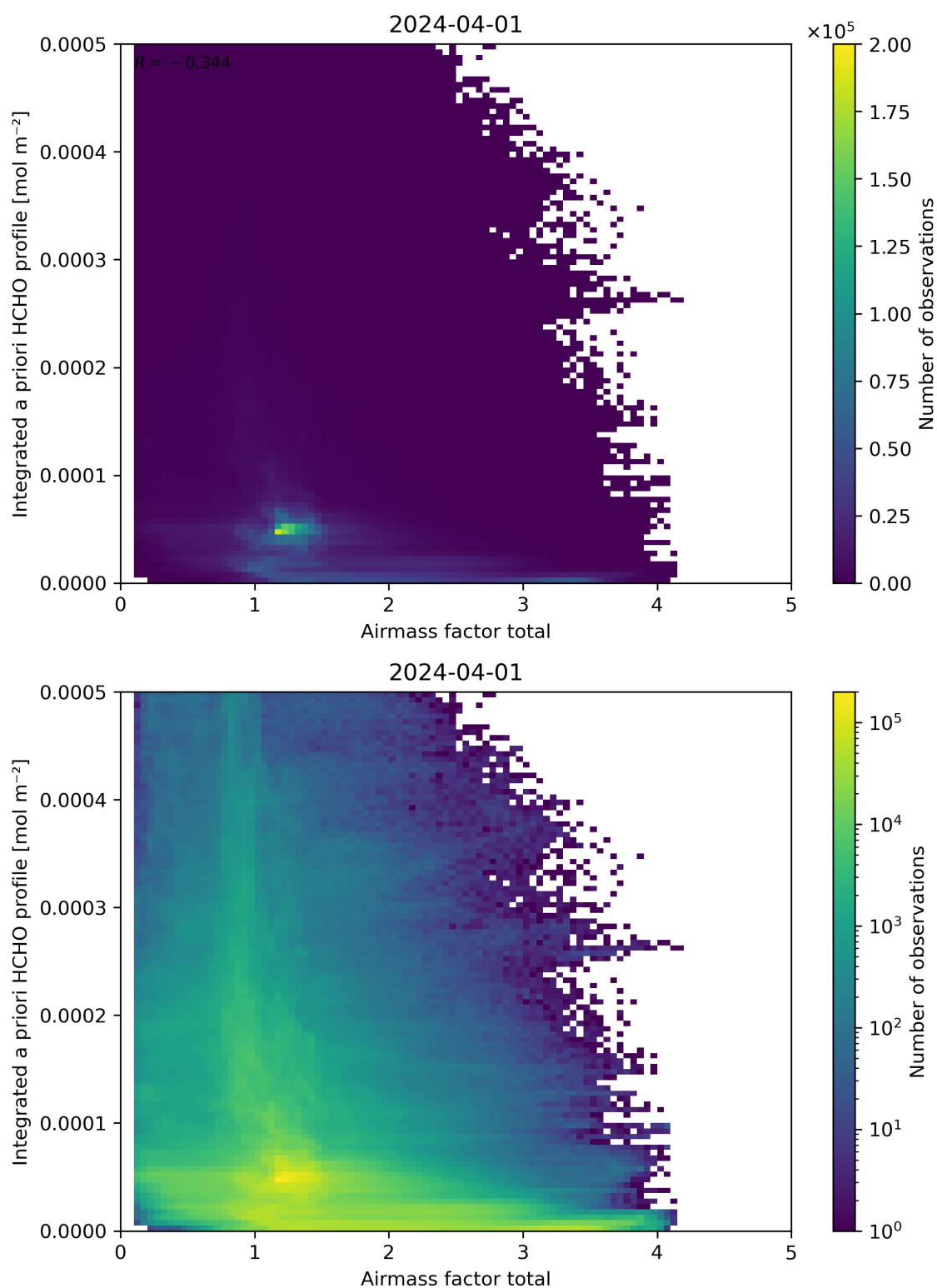
Figure 104: Scatter density plot of “Airmass factor total” against “Integrated a priori HCHO profile” for 2024-03-31 to 2024-04-02.
