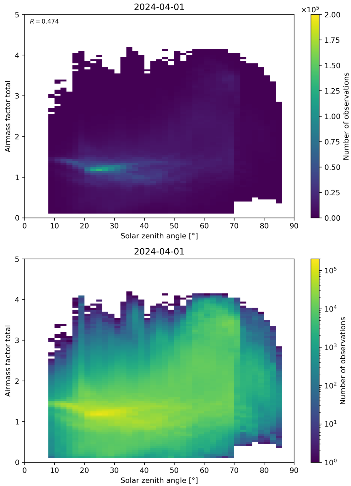
Figure 175: Scatter density plot of “Solar zenith angle” against “Airmass factor total” for 2024-03-31 to 2024-04-02.
