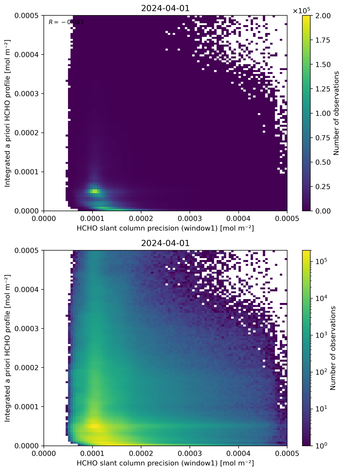
Figure 96: Scatter density plot of “HCHO slant column precision (window1)” against “Integrated a priori HCHO profile” for 2024-03-31 to 2024-04-02.
