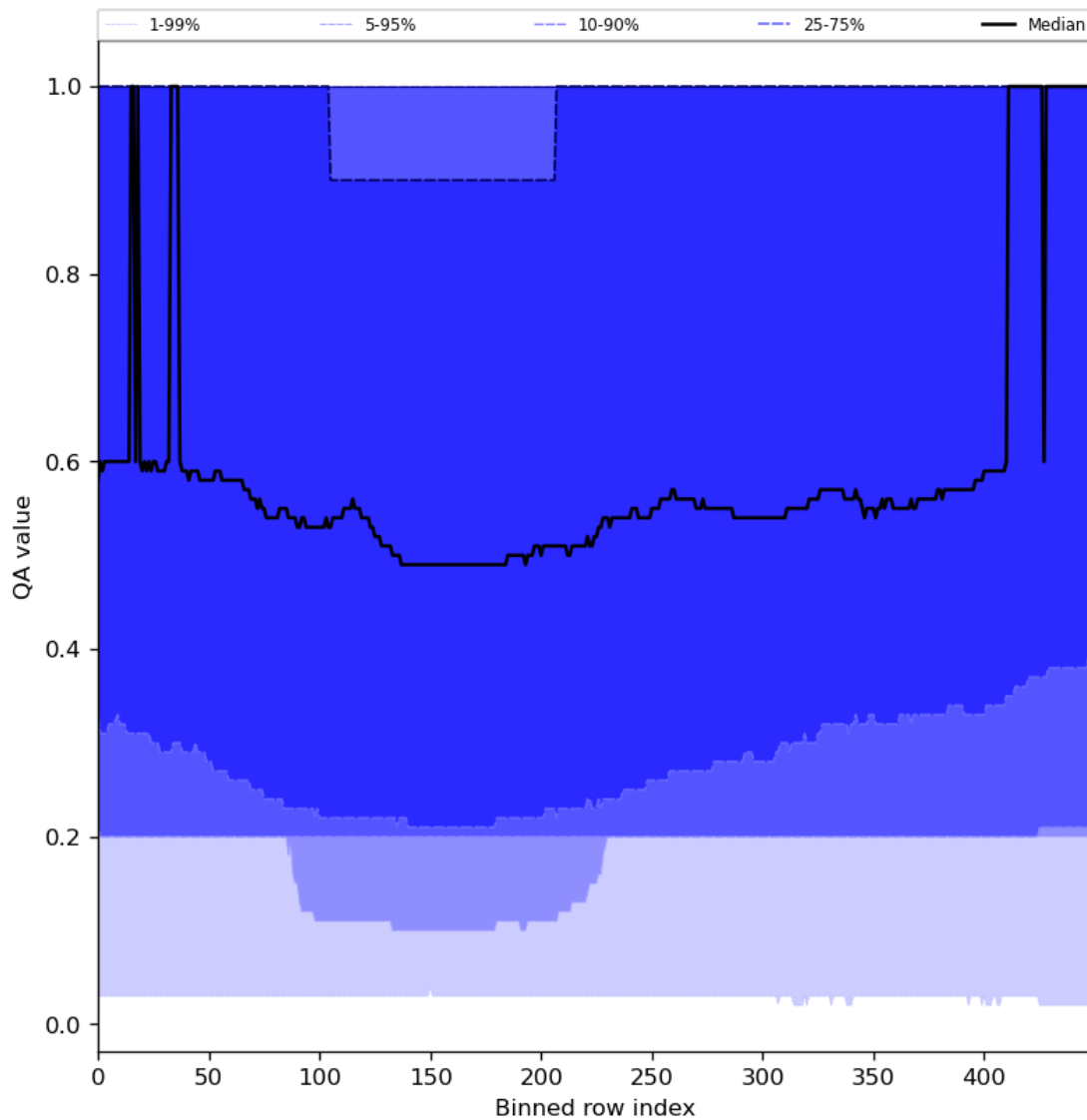
Figure 48: Along track statistics of “QA value” for 2024-03-31 to 2024-04-02
