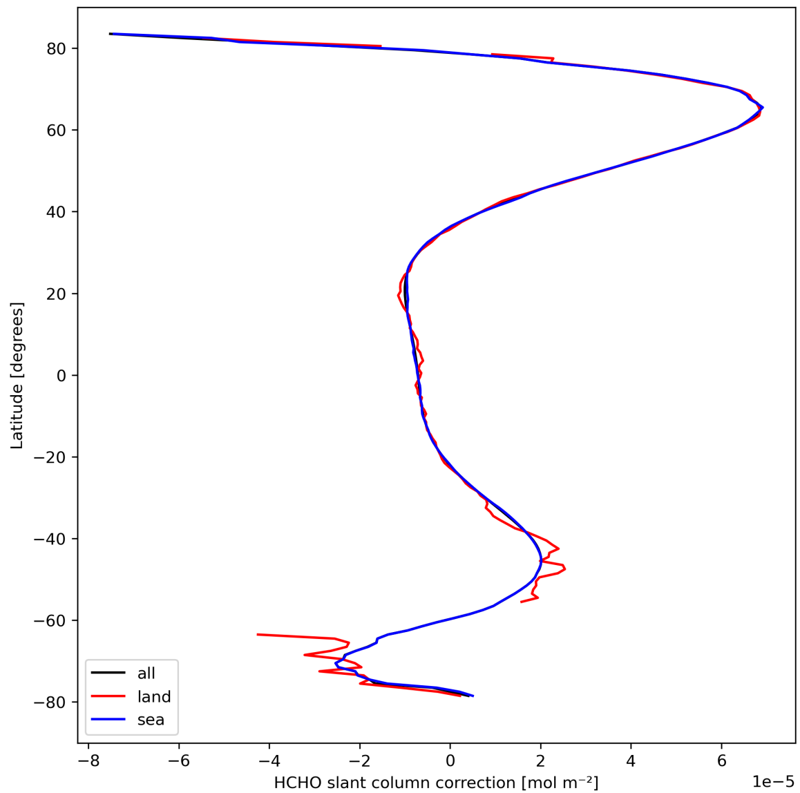
Figure 33: Zonal average of “HCHO slant column correction” for 2024-03-31 to 2024-04-02.
