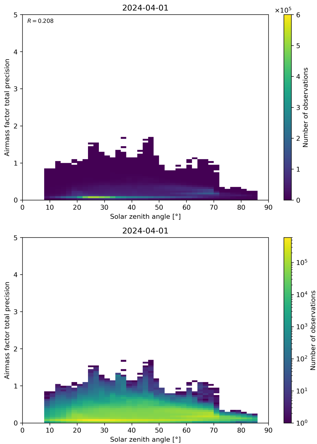
Figure 176: Scatter density plot of “Solar zenith angle” against “Airmass factor total precision” for 2024-03-31 to 2024-04-02.
