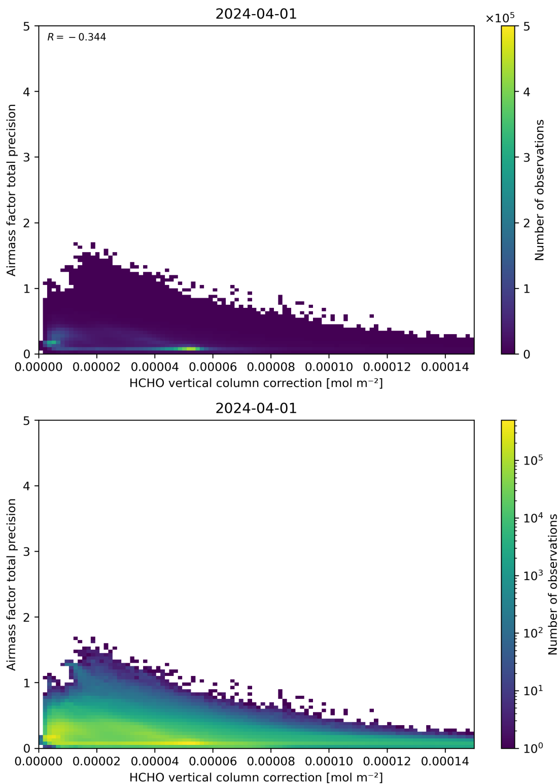
Figure 121: Scatter density plot of “HCHO vertical column correction” against “Airmass factor total precision” for 2024-03-31 to 2024-04-02.
