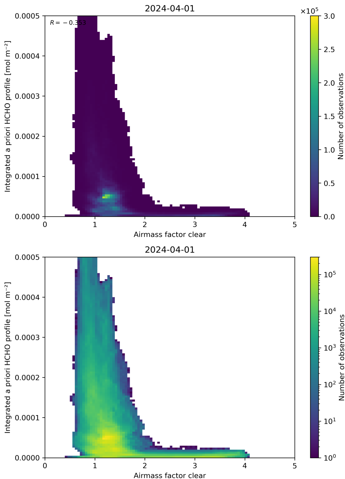
Figure 76: Scatter density plot of “Airmass factor clear” against “Integrated a priori HCHO profile” for 2024-03-31 to 2024-04-02.
