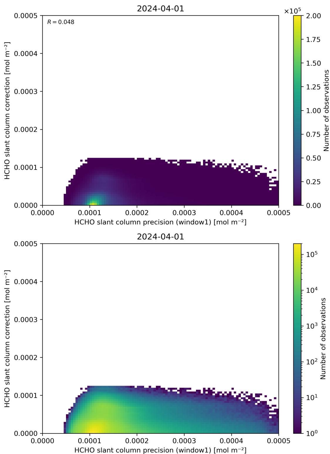
Figure 93: Scatter density plot of “HCHO slant column precision (window1)” against “HCHO slant column correction” for 2024-03-31 to 2024-04-02.
