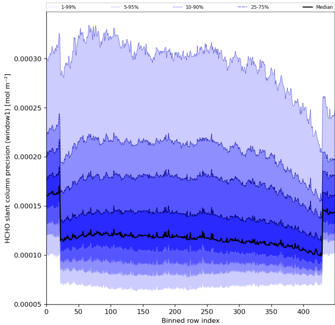
Figure 53: Along track statistics of “HCHO slant column precision (window1)” for 2024-03-31 to 2024-04-02
