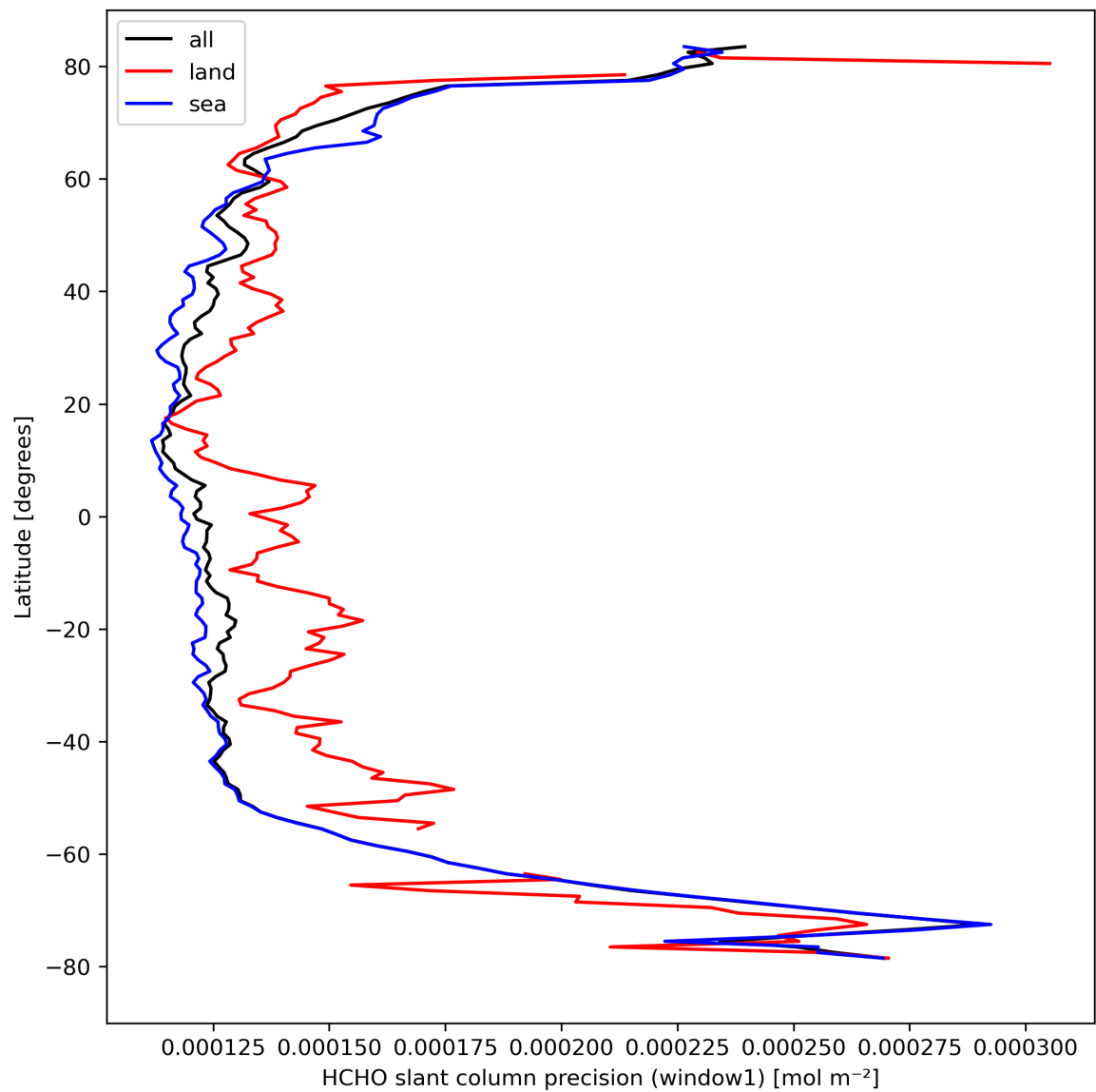
Figure 25: Zonal average of “HCHO slant column precision (window1)” for 2024-03-31 to 2024-04-02.
