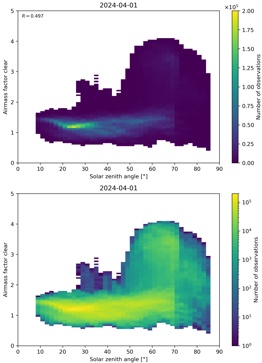
Figure 170: Scatter density plot of “Solar zenith angle” against “Airmass factor clear” for 2024-03-31 to 2024-04-02.
