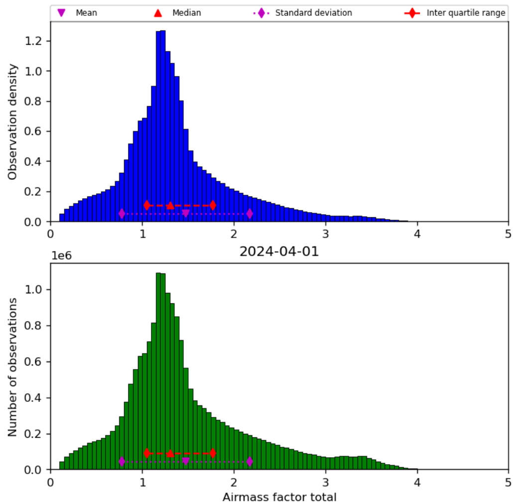
Figure 40: Histogram of “Airmass factor total” for 2024-03-31 to 2024-04-02
