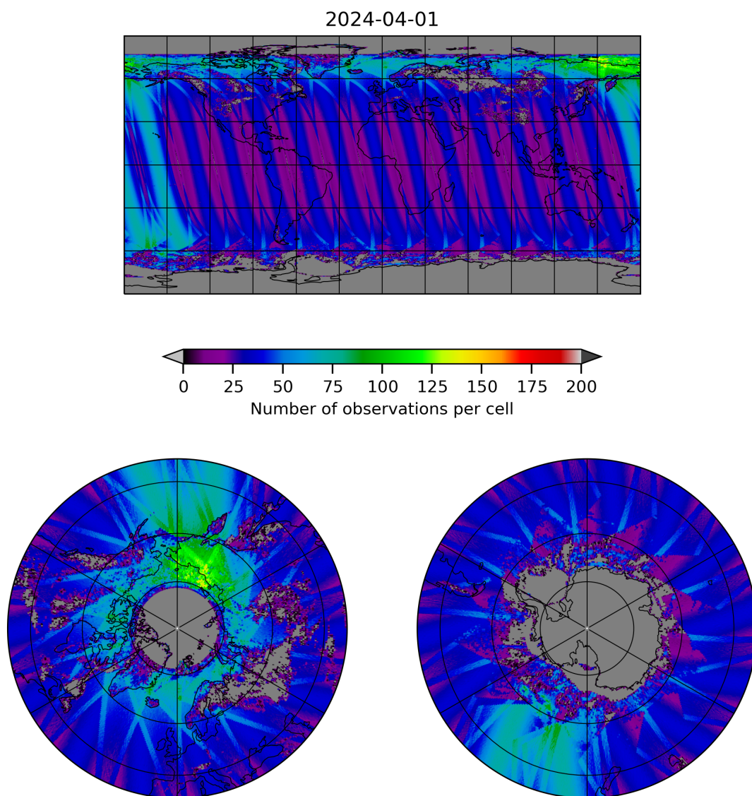
Figure 19: Map of the number of observations for 2024-03-31 to 2024-04-02
