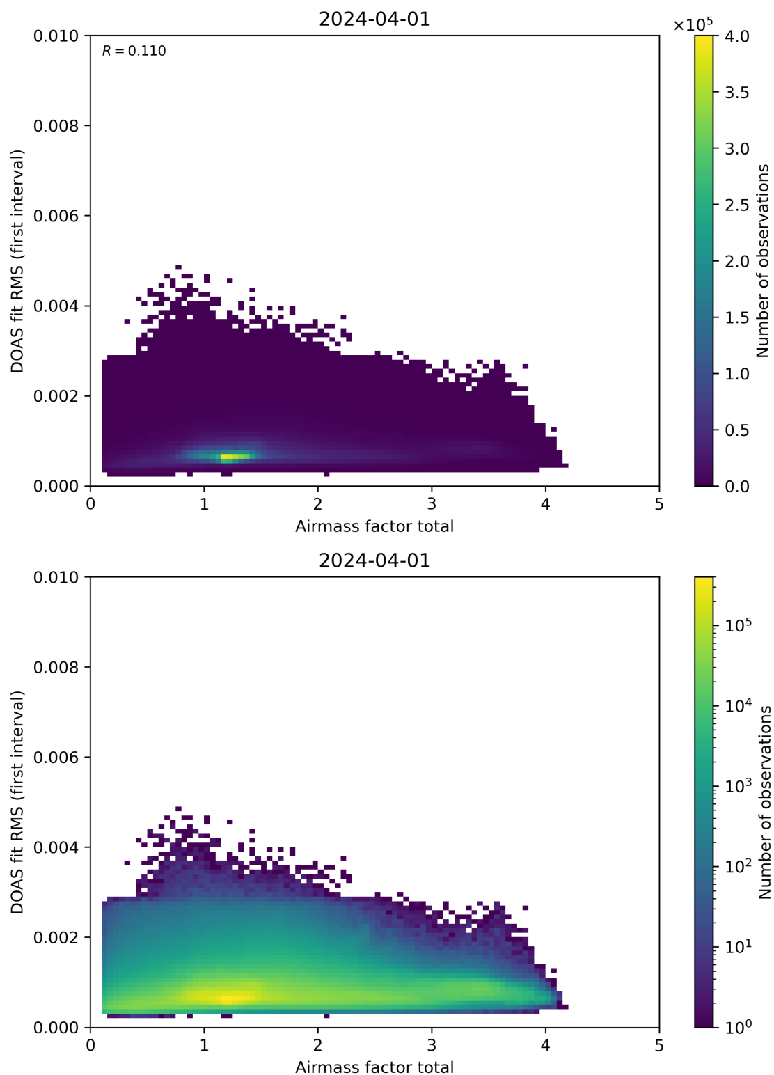
Figure 97: Scatter density plot of “Airmass factor total” against “DOAS fit RMS (first interval)” for 2024-03-31 to 2024-04-02.
