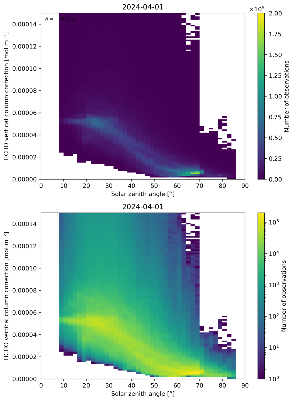
Figure 178: Scatter density plot of “Solar zenith angle” against “HCHO vertical column correction” for 2024-03-31 to 2024-04-02.
