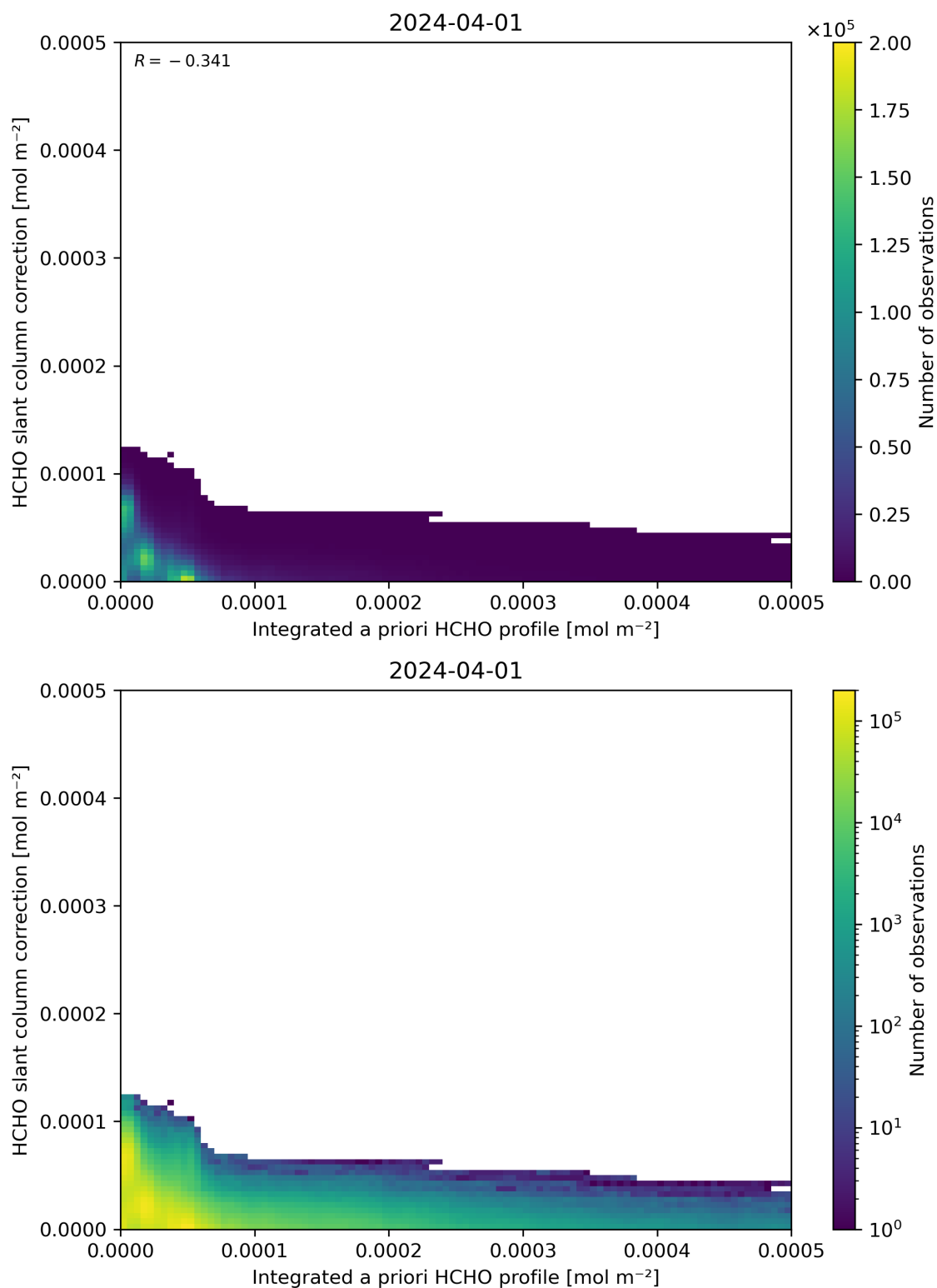
Figure 152: Scatter density plot of “Integrated a priori HCHO profile” against “HCHO slant column correction” for 2024-03-31 to 2024-04-02.
