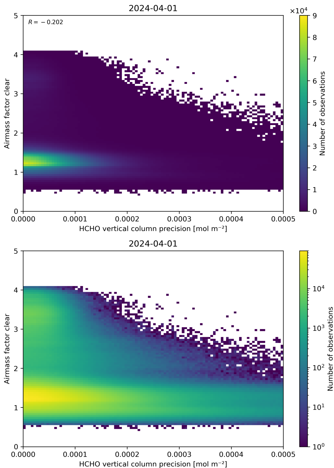
Figure 139: Scatter density plot of “HCHO vertical column precision” against “Airmass factor clear” for 2024-03-31 to 2024-04-02.
