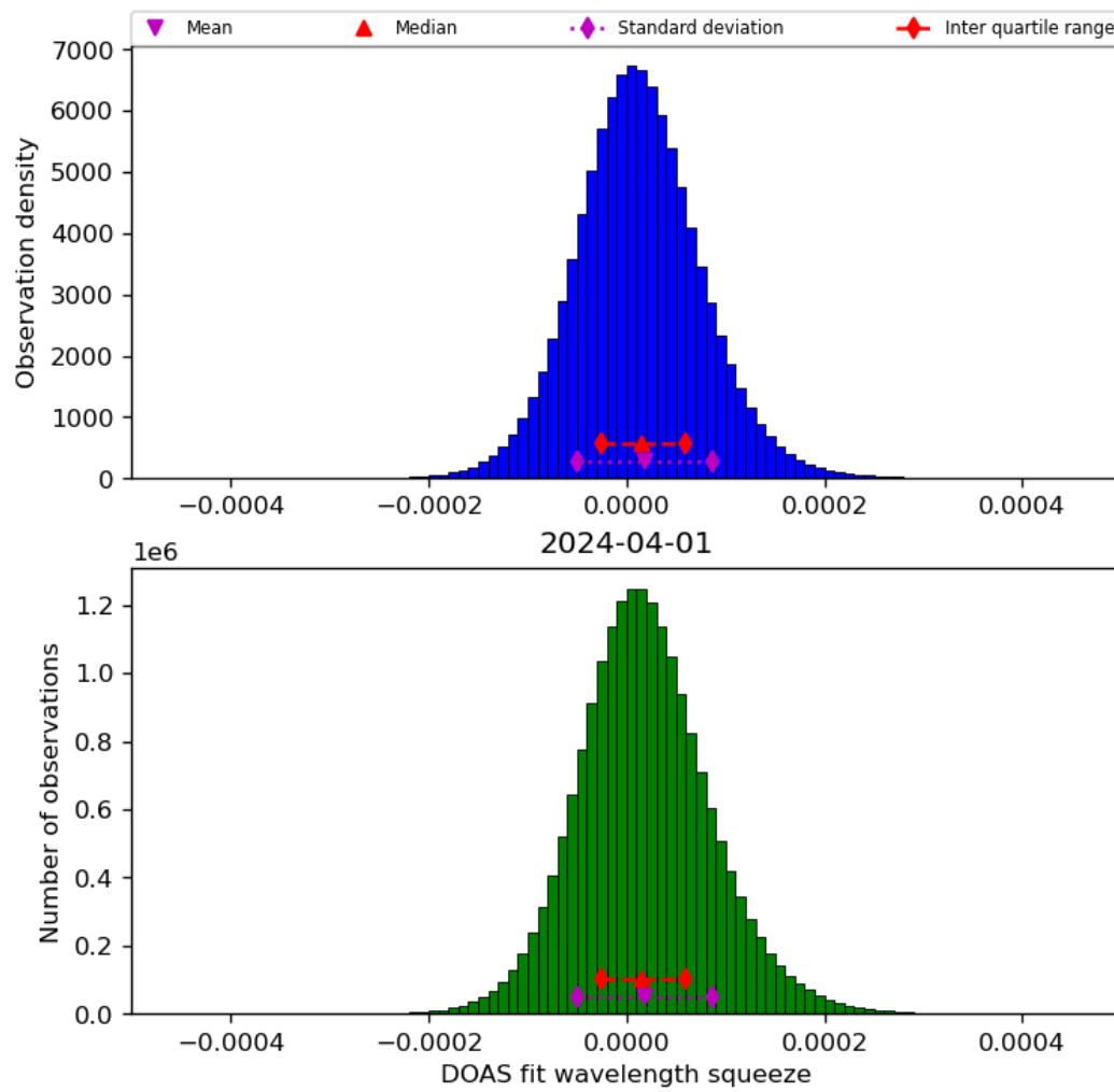
Figure 45: Histogram of “DOAS fit wavelength squeeze” for 2024-03-31 to 2024-04-02
