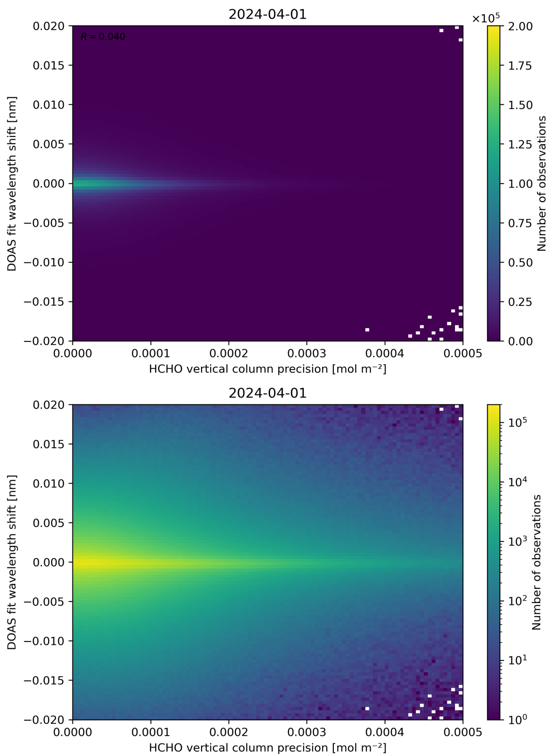
Figure 137: Scatter density plot of “HCHO vertical column precision” against “DOAS fit wavelength shift” for 2024-03-31 to 2024-04-02.
