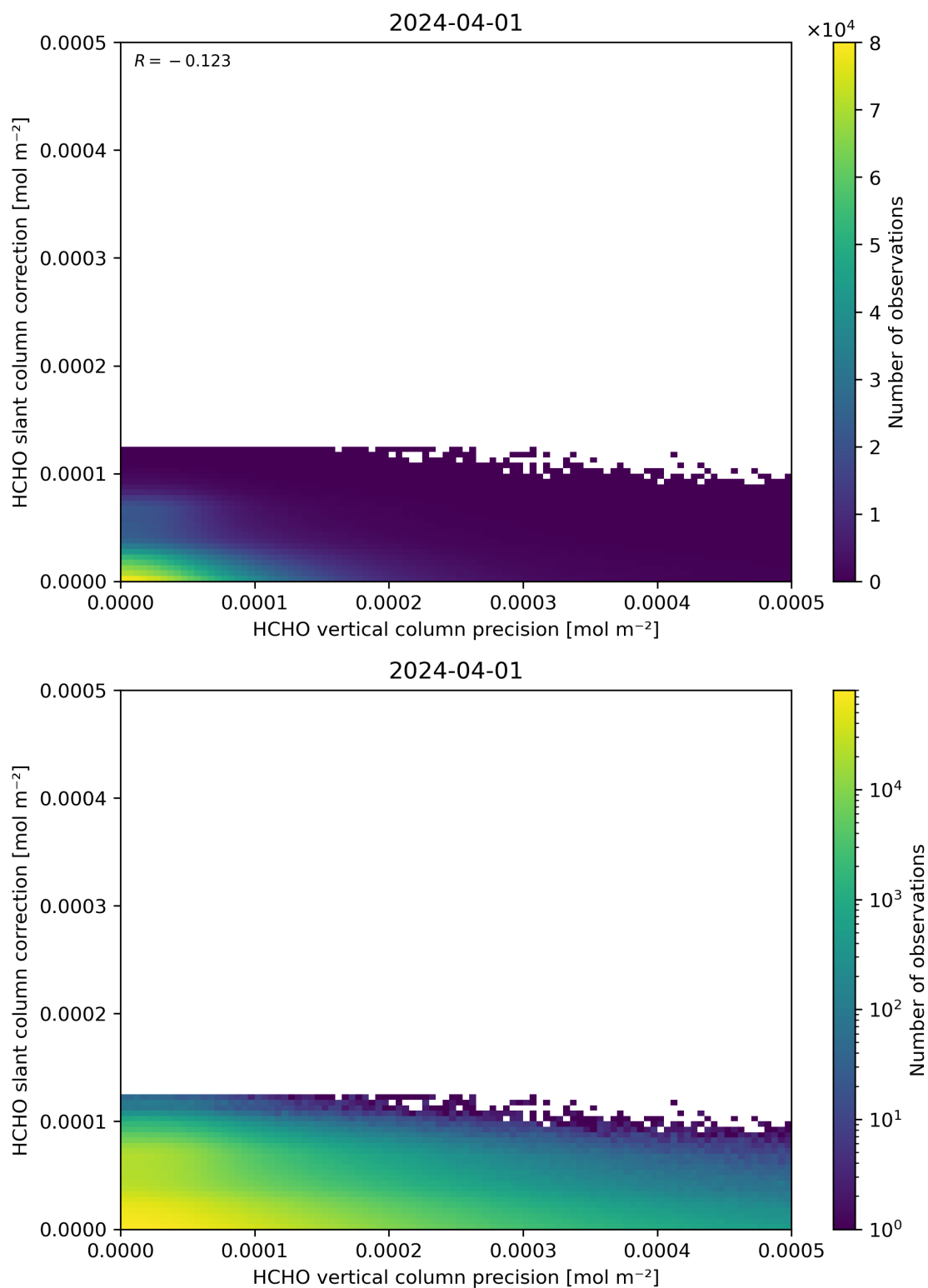
Figure 141: Scatter density plot of “HCHO vertical column precision” against “HCHO slant column correction” for 2024-03-31 to 2024-04-02.
