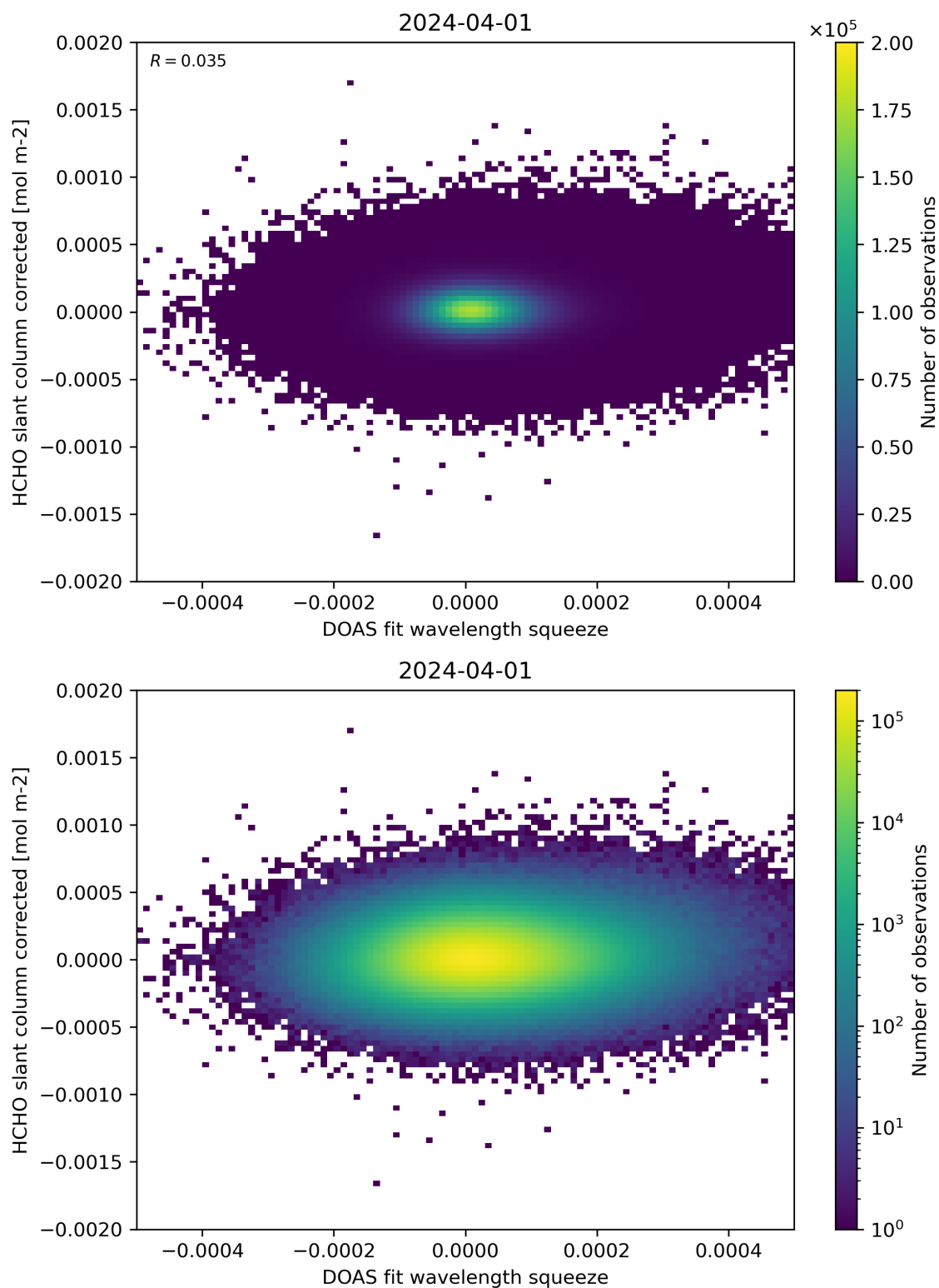
Figure 69: Scatter density plot of “DOAS fit wavelength squeeze” against “HCHO slant column corrected” for 2024-03-31 to 2024-04-02.
