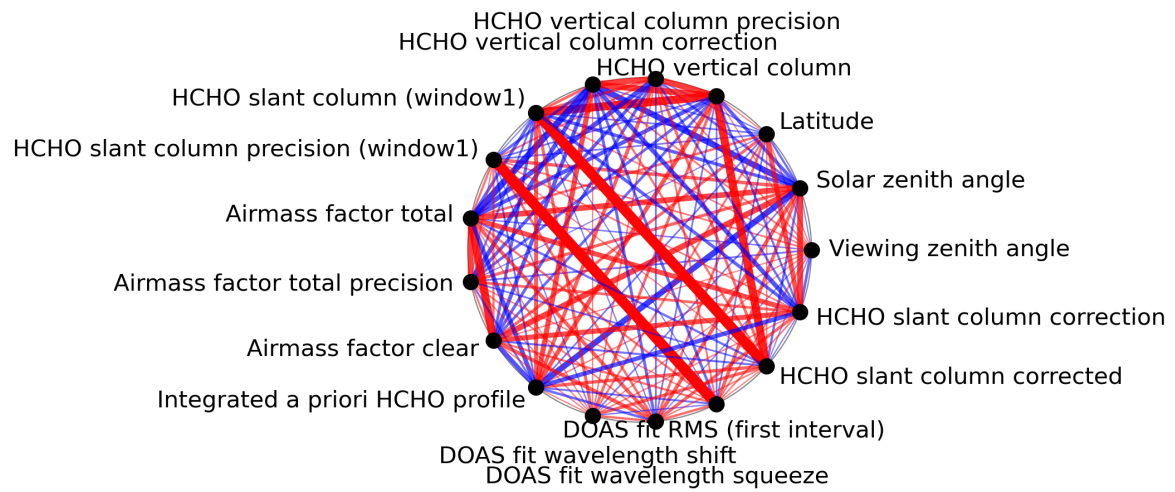
Figure 1: Map of correlation graph for 2024-03-31 to 2024-04-02.
