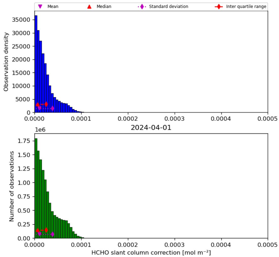
Figure 47: Histogram of “HCHO slant column correction” for 2024-03-31 to 2024-04-02
