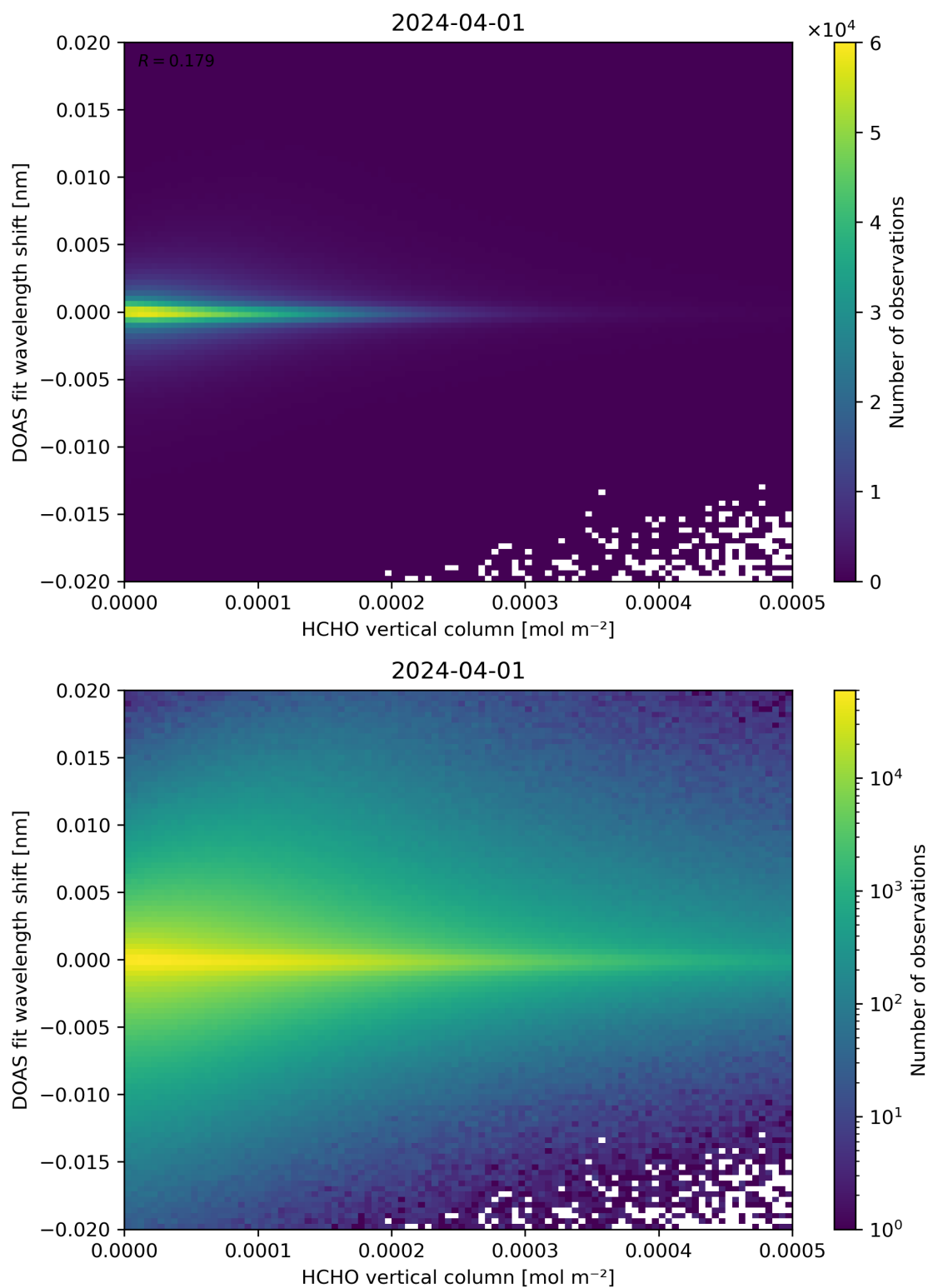
Figure 124: Scatter density plot of “HCHO vertical column” against “DOAS fit wavelength shift” for 2024-03-31 to 2024-04-02.
