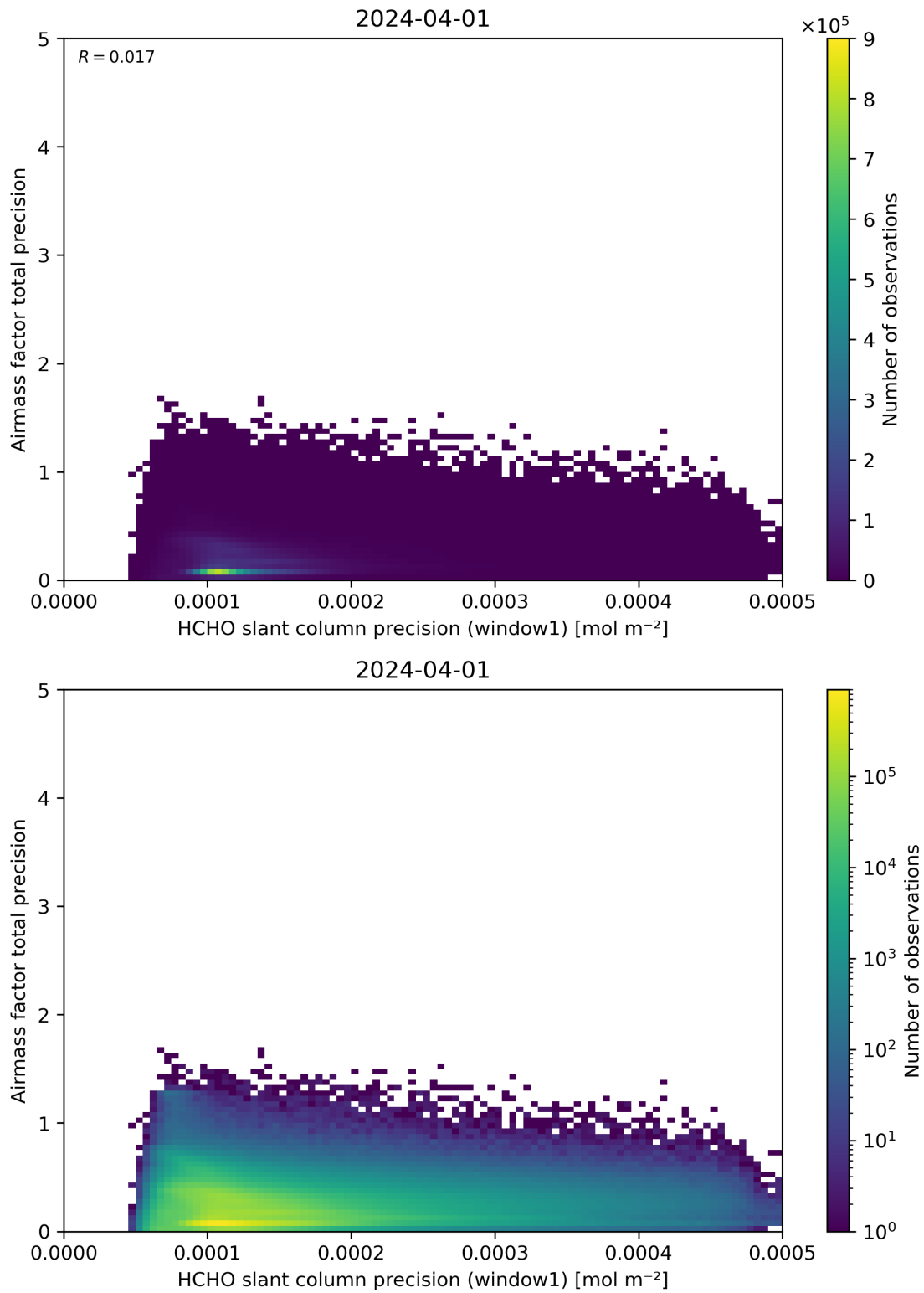
Figure 95: Scatter density plot of “HCHO slant column precision (window1)” against “Airmass factor total precision” for 2024-03-31 to 2024-04-02.
