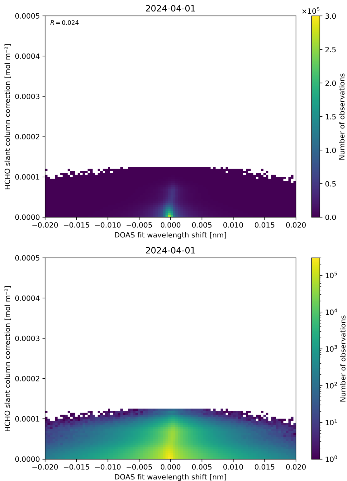
Figure 67: Scatter density plot of “DOAS fit wavelength shift” against “HCHO slant column correction” for 2024-03-31 to 2024-04-02.
