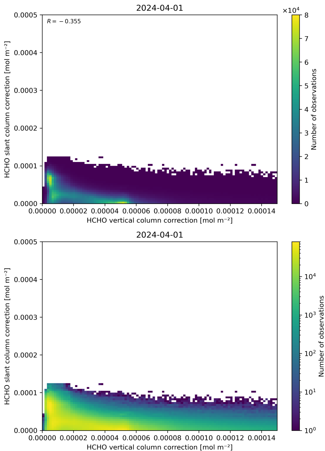
Figure 117: Scatter density plot of “HCHO vertical column correction” against “HCHO slant column correction” for 2024-03-31 to 2024-04-02.
