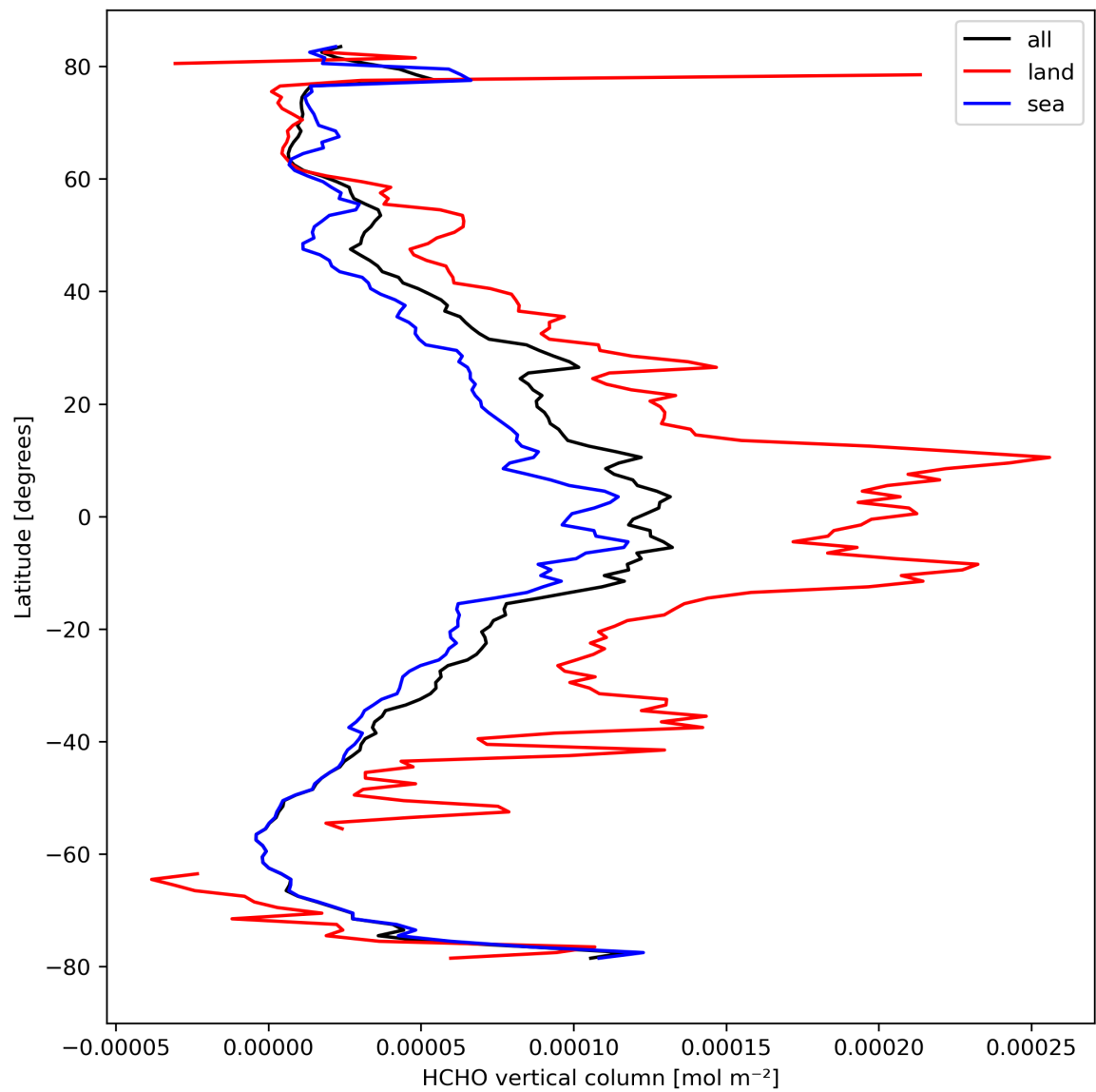
Figure 21: Zonal average of “HCHO vertical column” for 2024-03-31 to 2024-04-02.
