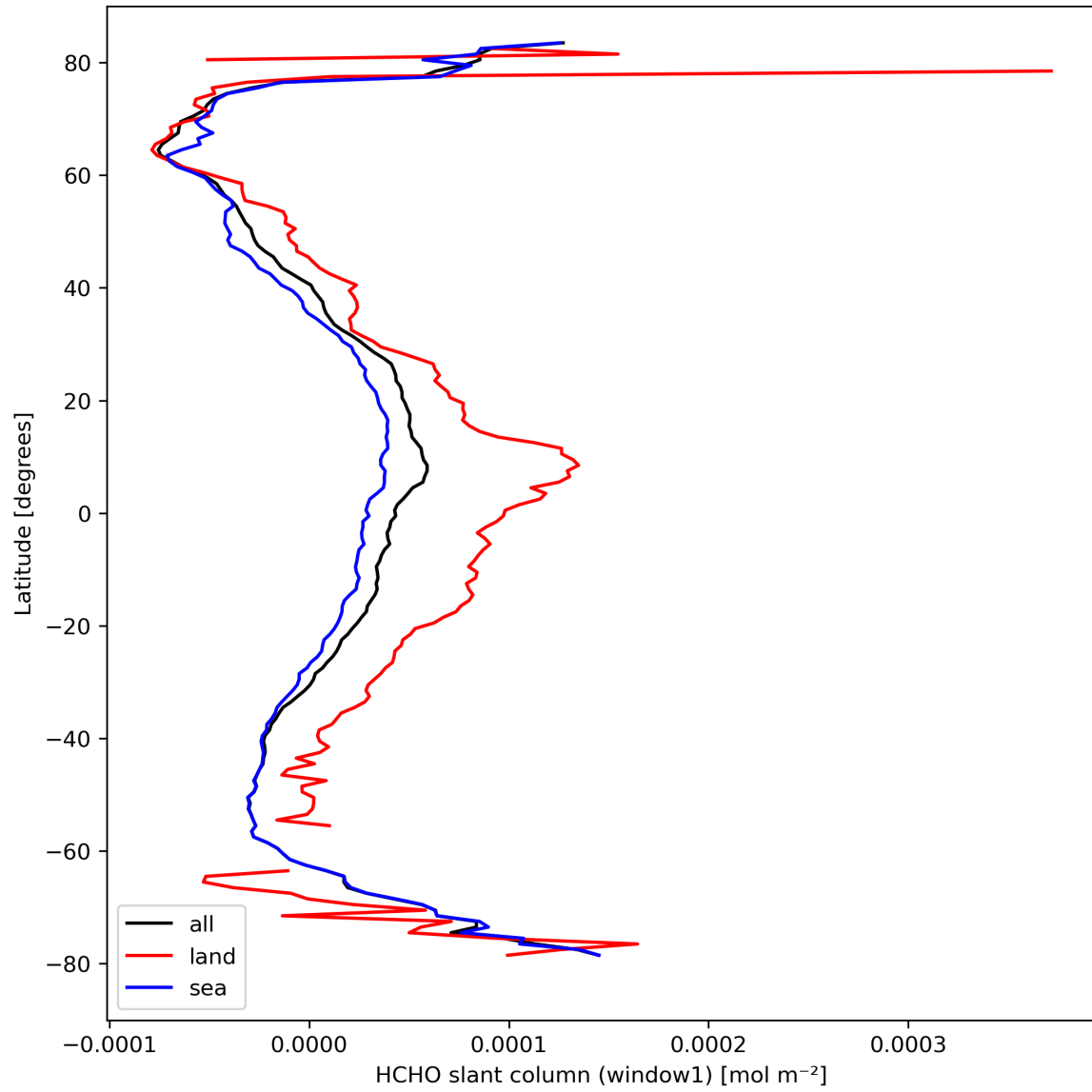
Figure 24: Zonal average of “HCHO slant column (window1)” for 2024-03-31 to 2024-04-02.
