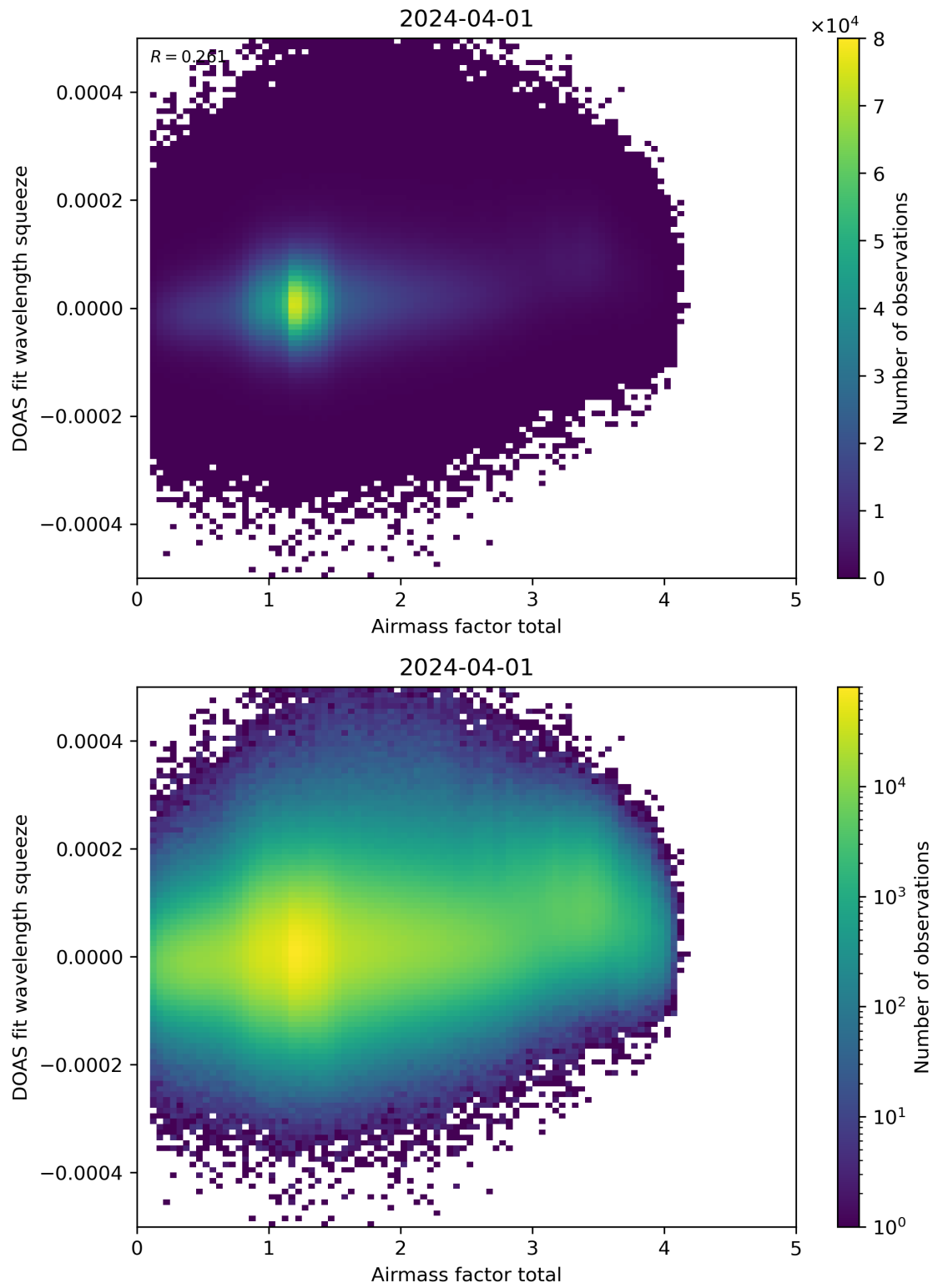
Figure 99: Scatter density plot of “Airmass factor total” against “DOAS fit wavelength squeeze” for 2024-03-31 to 2024-04-02.
