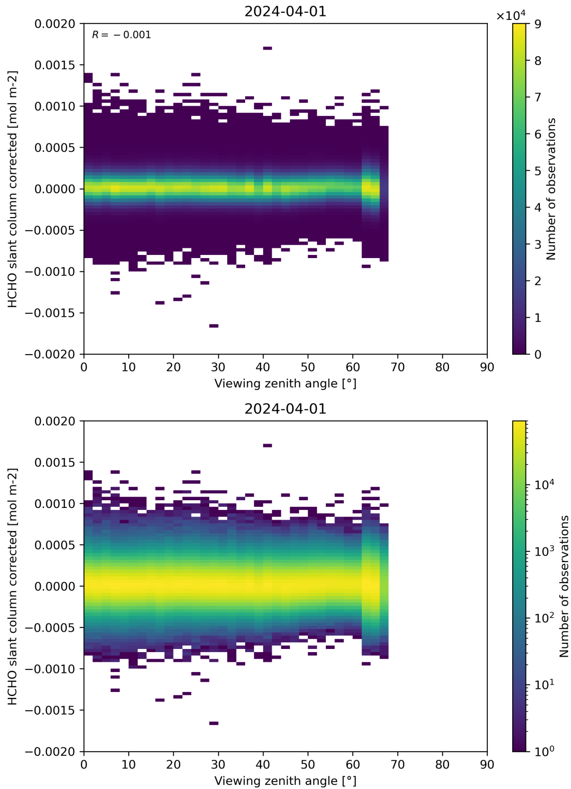
Figure 186: Scatter density plot of “Viewing zenith angle” against “HCHO slant column corrected” for 2024-03-31 to 2024-04-02.
