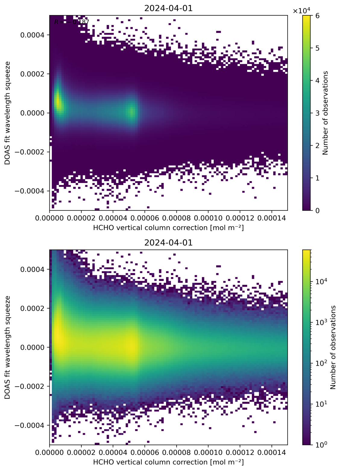
Figure 114: Scatter density plot of “HCHO vertical column correction” against “DOAS fit wavelength squeeze” for 2024-03-31 to 2024-04-02.
