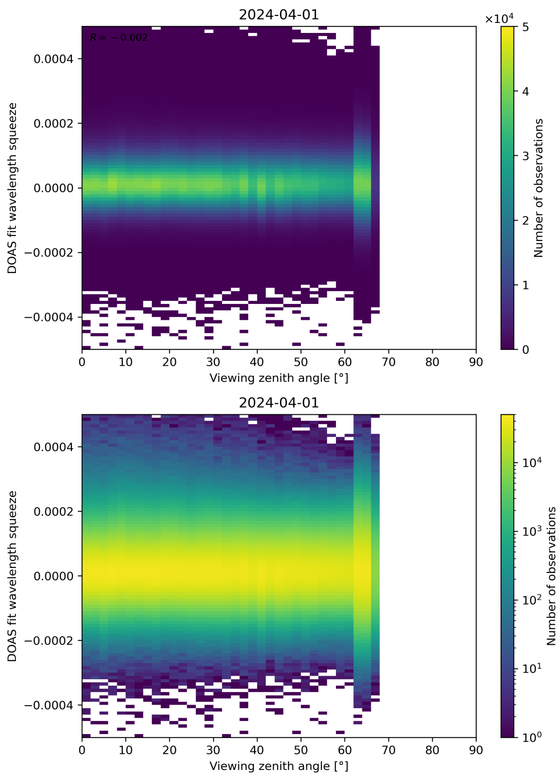
Figure 184: Scatter density plot of “Viewing zenith angle” against “DOAS fit wavelength squeeze” for 2024-03-31 to 2024-04-02.
