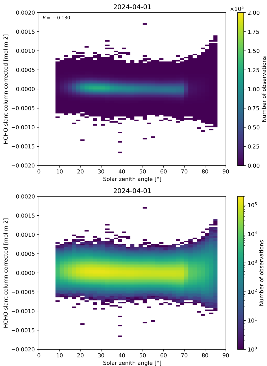
Figure 171: Scatter density plot of “Solar zenith angle” against “HCHO slant column corrected” for 2024-03-31 to 2024-04-02.
