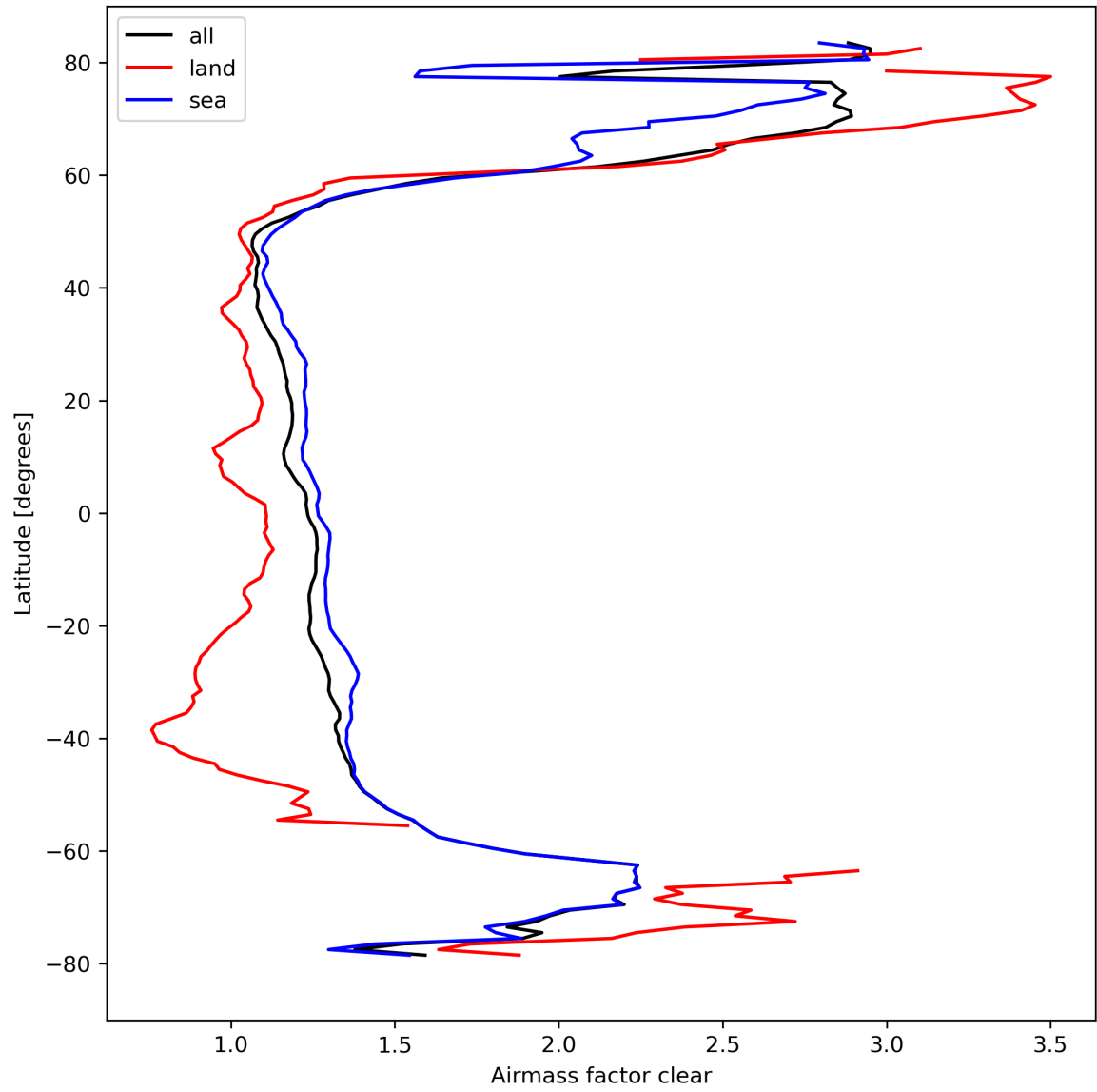
Figure 28: Zonal average of “Airmass factor clear” for 2024-03-31 to 2024-04-02.
