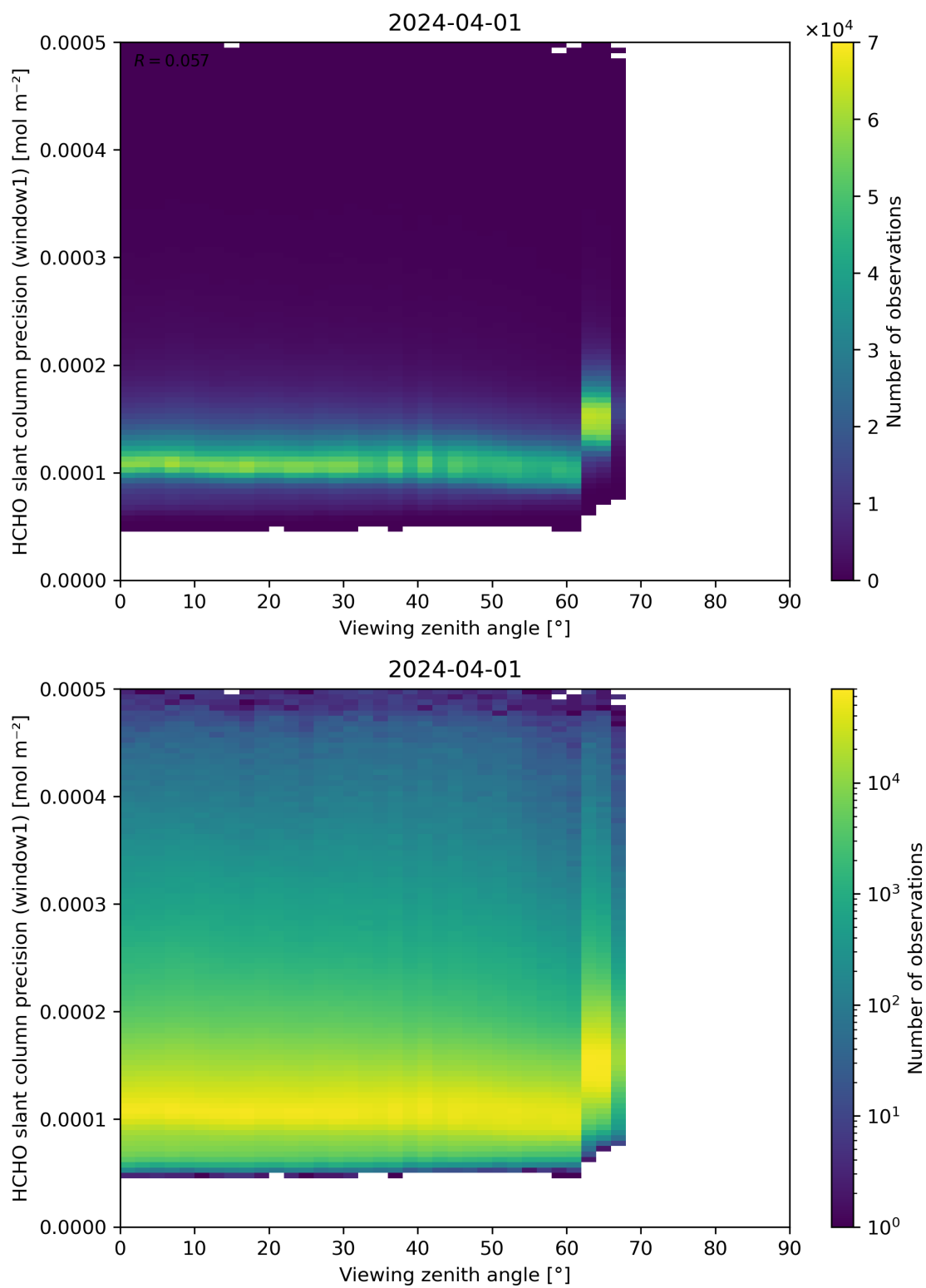
Figure 189: Scatter density plot of “Viewing zenith angle” against “HCHO slant column precision (window1)” for 2024-03-31 to 2024-04-02.
