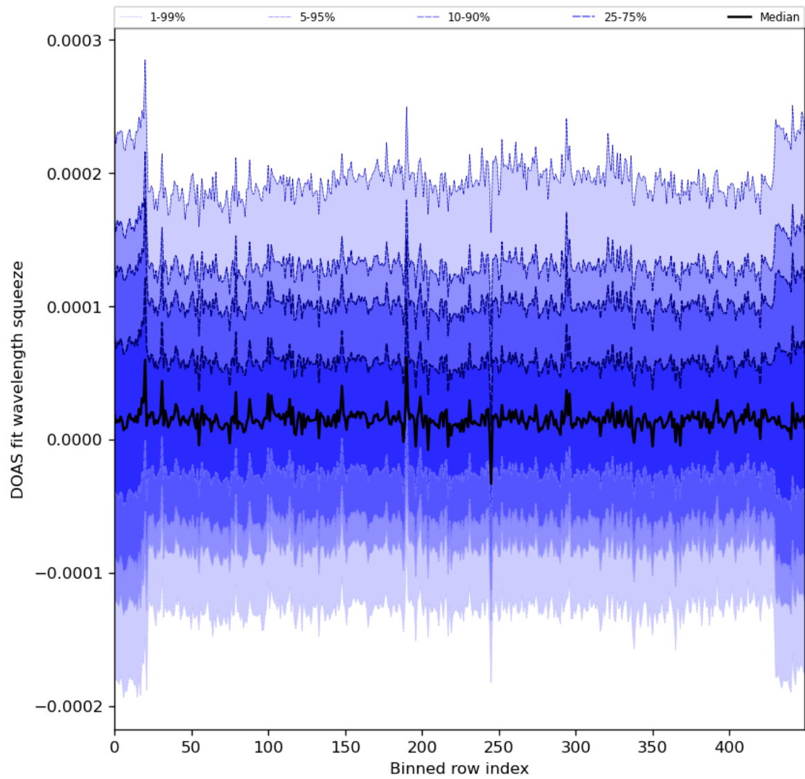
Figure 59: Along track statistics of “DOAS fit wavelength squeeze” for 2024-03-31 to 2024-04-02
