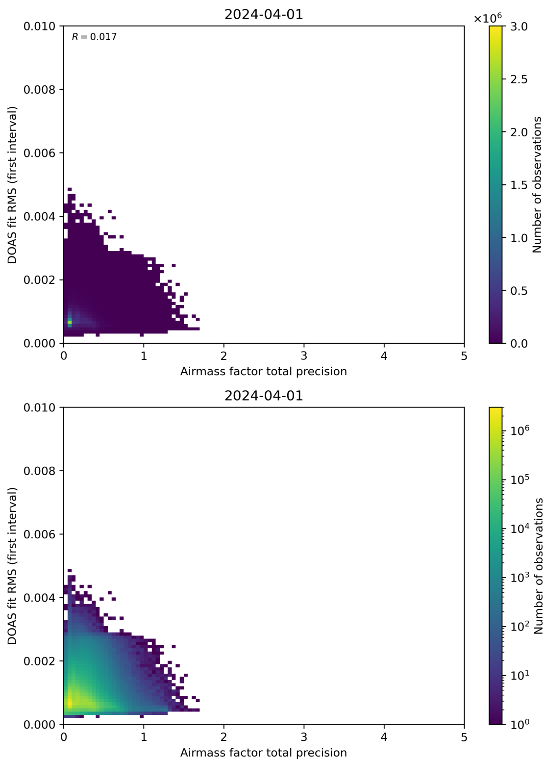
Figure 105: Scatter density plot of “Airmass factor total precision” against “DOAS fit RMS (first interval)” for 2024-03-31 to 2024-04-02.
