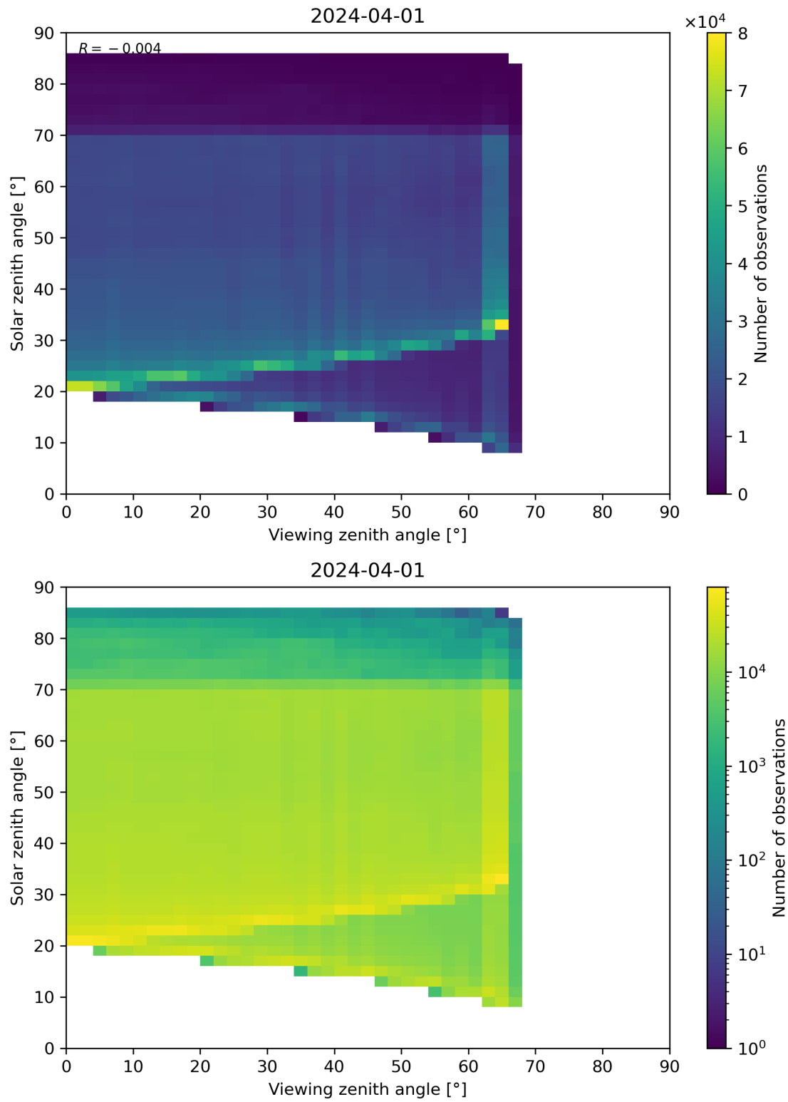
Figure 197: Scatter density plot of “Viewing zenith angle” against “Solar zenith angle” for 2024-03-31 to 2024-04-02.
