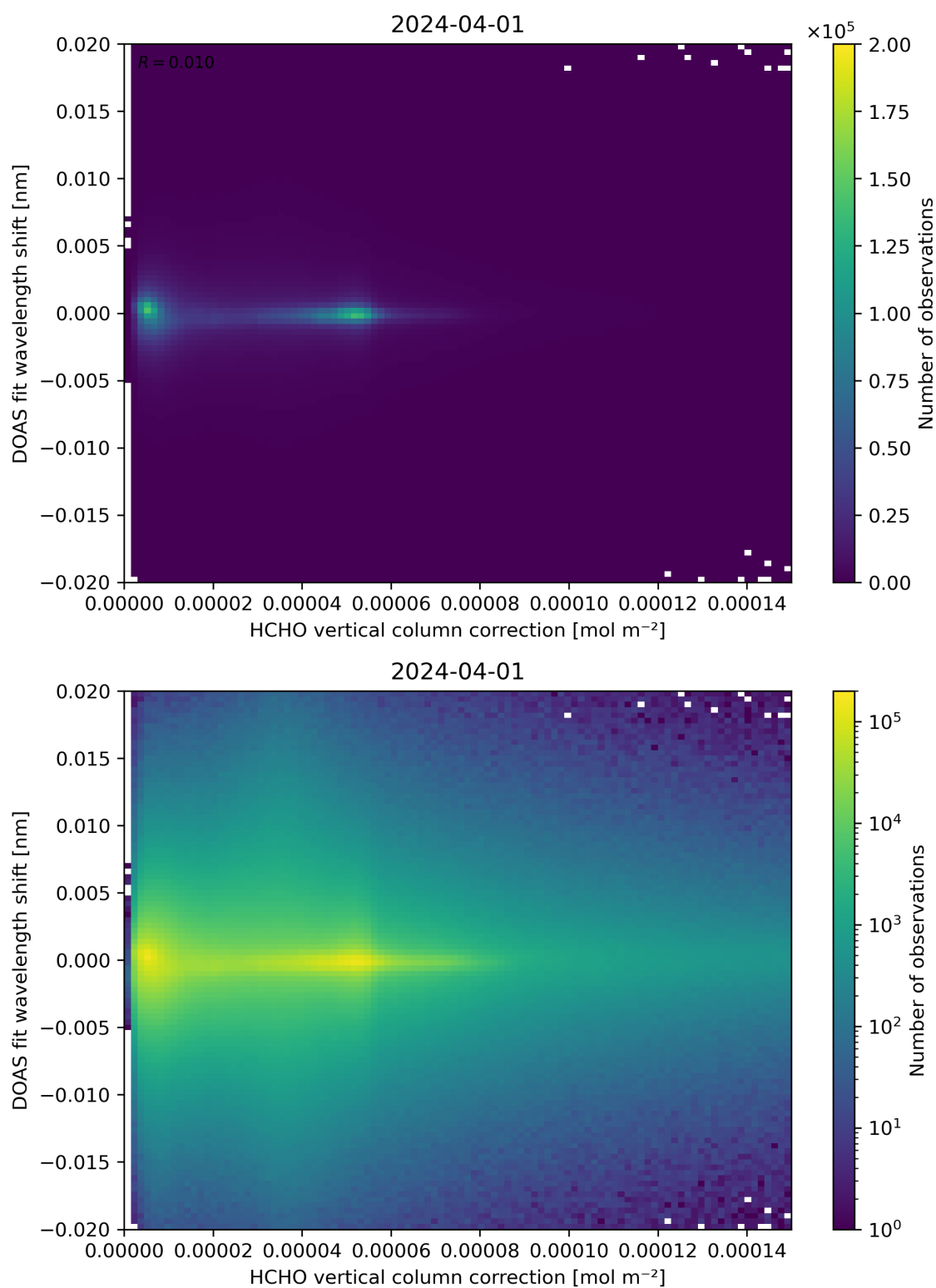
Figure 113: Scatter density plot of “HCHO vertical column correction” against “DOAS fit wavelength shift” for 2024-03-31 to 2024-04-02.
