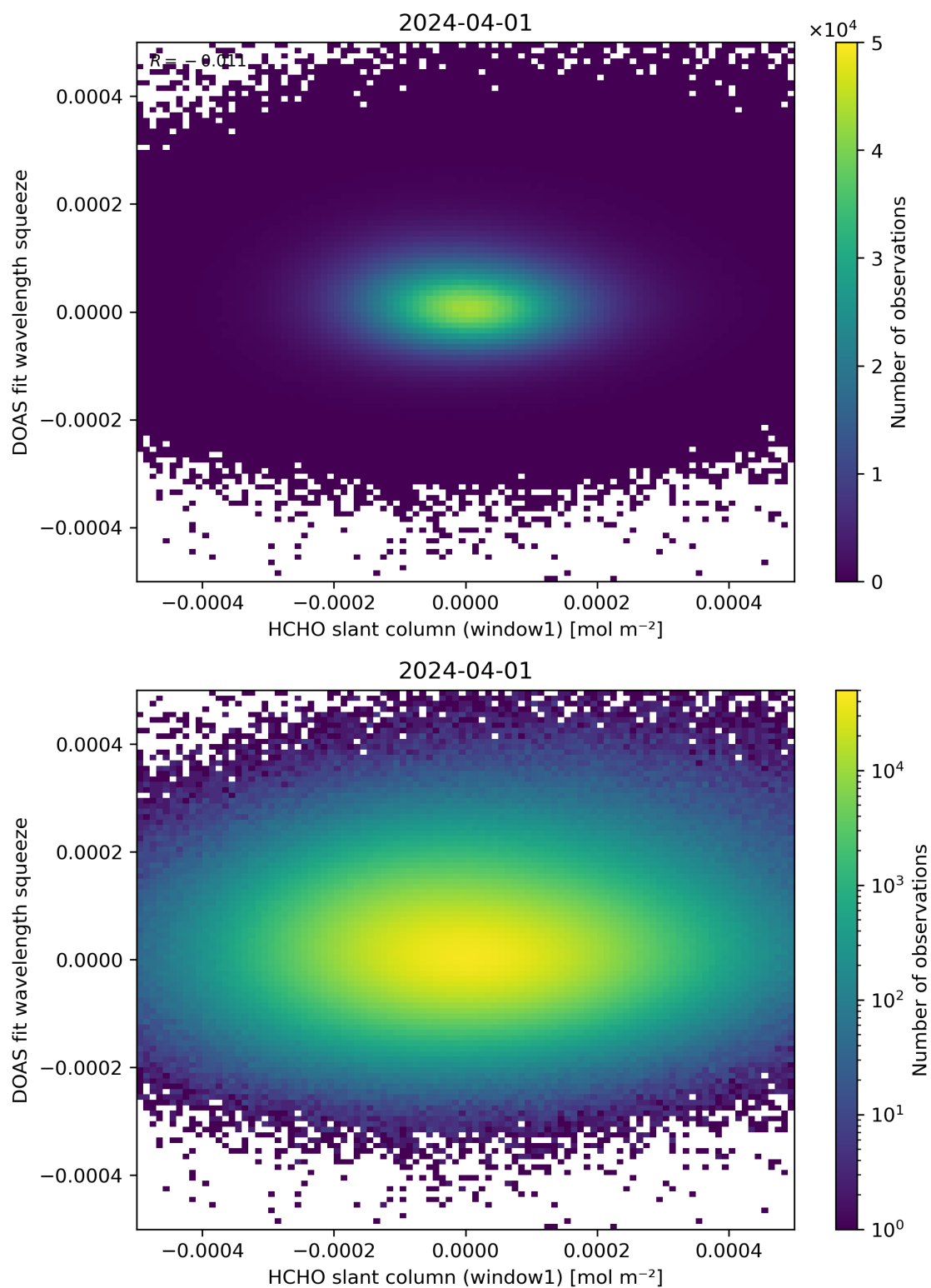
Figure 80: Scatter density plot of “HCHO slant column (window1)” against “DOAS fit wavelength squeeze” for 2024-03-31 to 2024-04-02.
