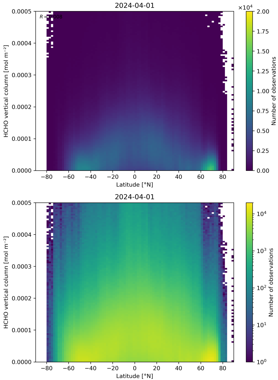
Figure 163: Scatter density plot of “Latitude” against “HCHO vertical column” for 2024-03-31 to 2024-04-02.
