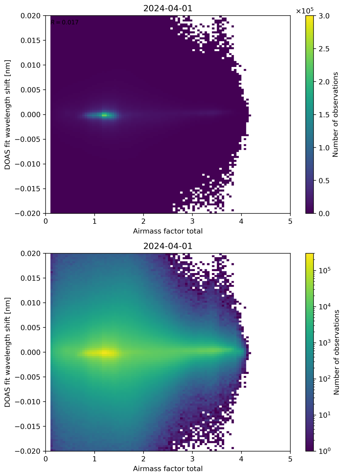
Figure 98: Scatter density plot of “Airmass factor total” against “DOAS fit wavelength shift” for 2024-03-31 to 2024-04-02.
