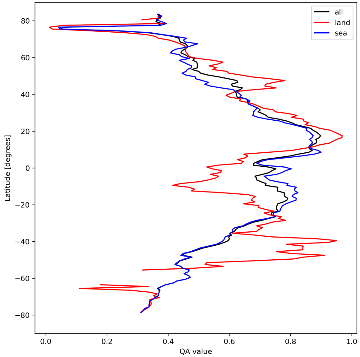
Figure 20: Zonal average of “QA value” for 2024-03-31 to 2024-04-02.
