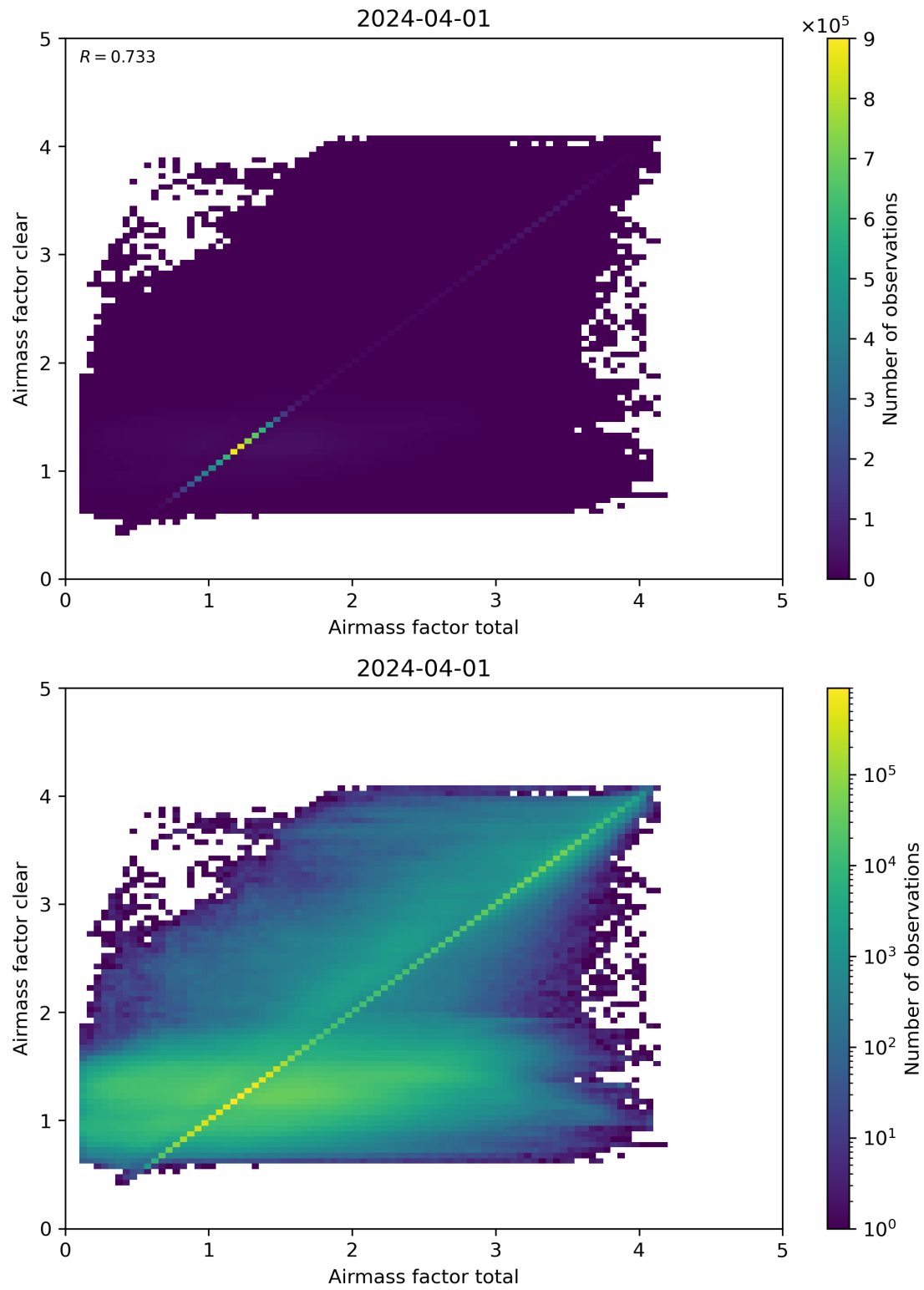
Figure 100: Scatter density plot of “Airmass factor total” against “Airmass factor clear” for 2024-03-31 to 2024-04-02.
