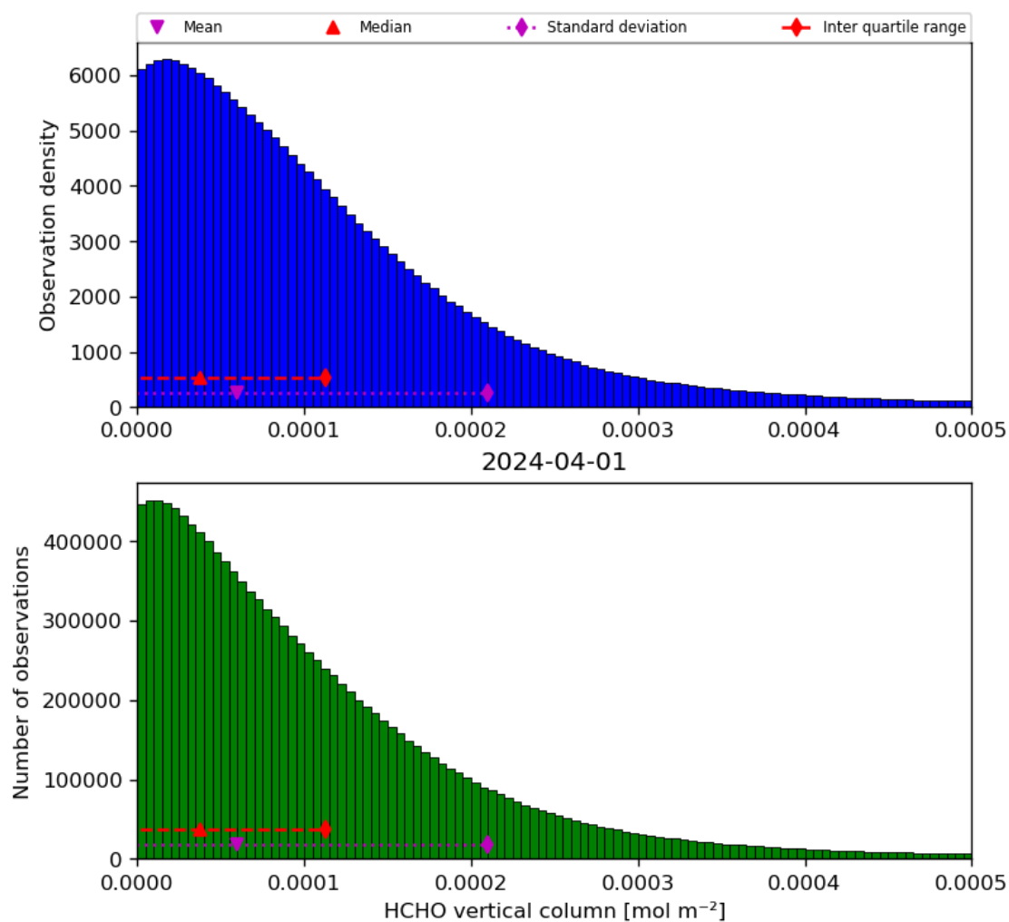
Figure 35: Histogram of “HCHO vertical column” for 2024-03-31 to 2024-04-02
