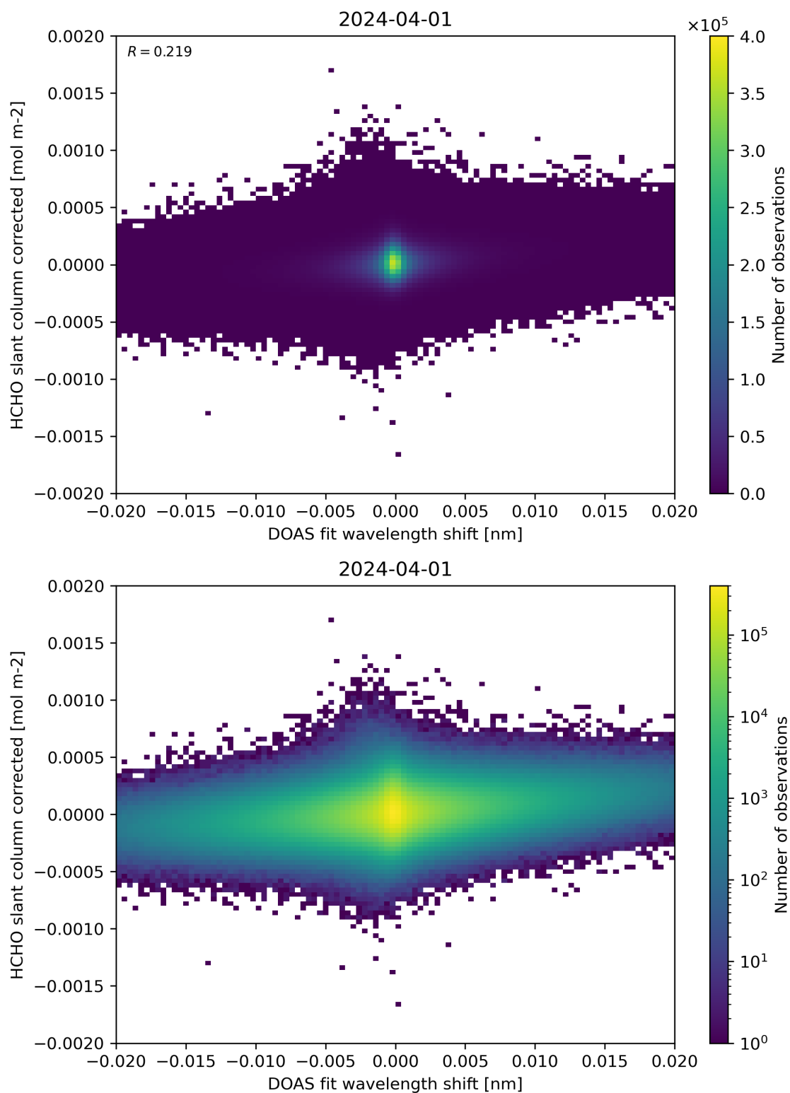
Figure 66: Scatter density plot of “DOAS fit wavelength shift” against “HCHO slant column corrected” for 2024-03-31 to 2024-04-02.
