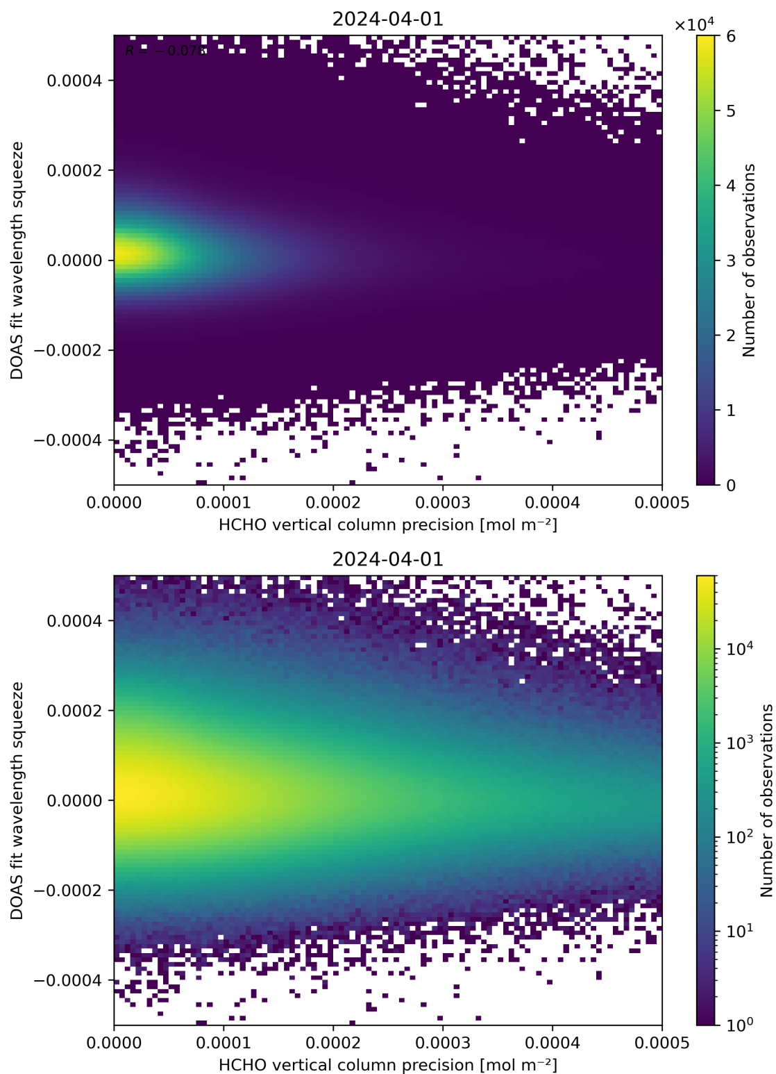
Figure 138: Scatter density plot of “HCHO vertical column precision” against “DOAS fit wavelength squeeze” for 2024-03-31 to 2024-04-02.
