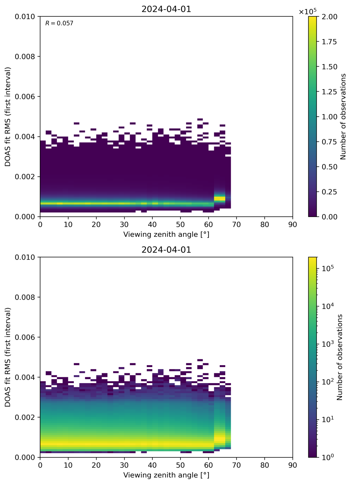
Figure 182: Scatter density plot of “Viewing zenith angle” against “DOAS fit RMS (first interval)” for 2024-03-31 to 2024-04-02.
