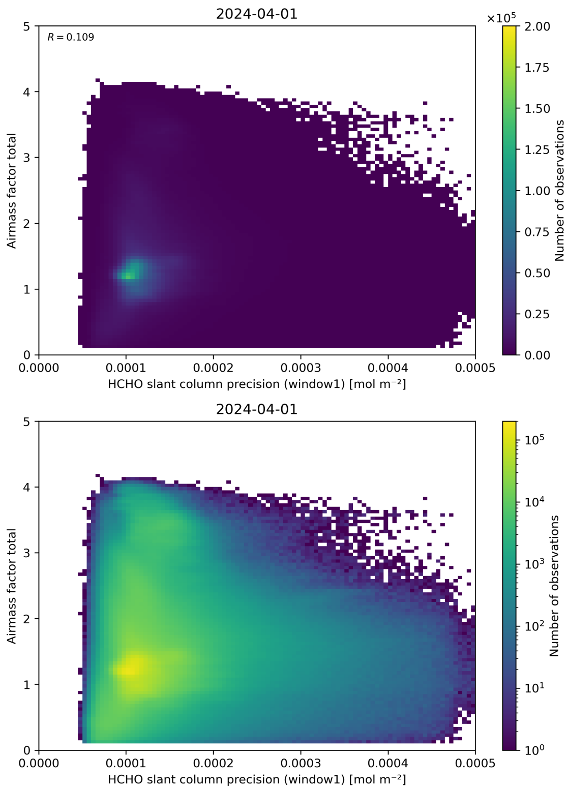
Figure 94: Scatter density plot of “HCHO slant column precision (window1)” against “Airmass factor total” for 2024-03-31 to 2024-04-02.
