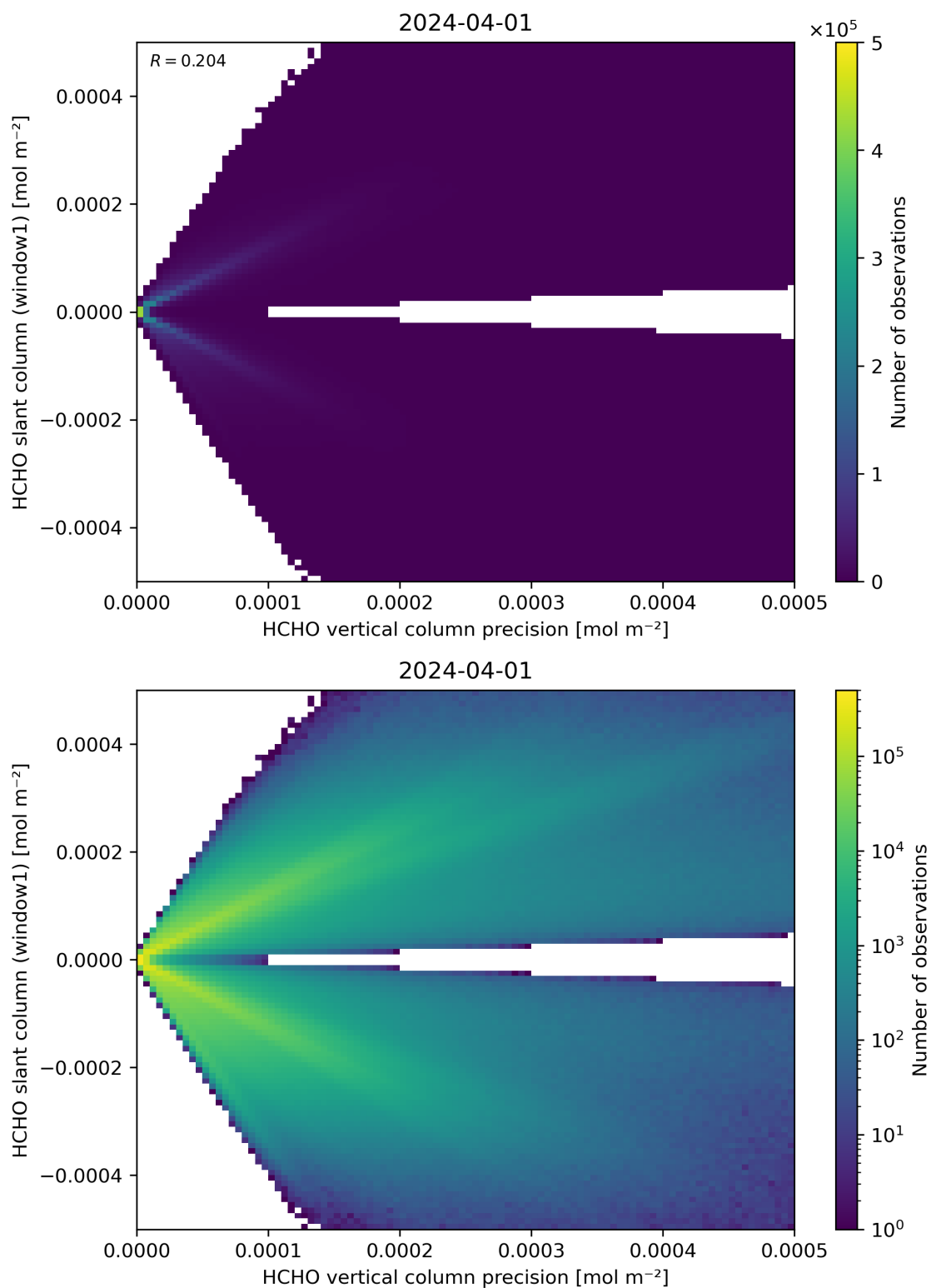
Figure 142: Scatter density plot of “HCHO vertical column precision” against “HCHO slant column (window1)” for 2024-03-31 to 2024-04-02.
