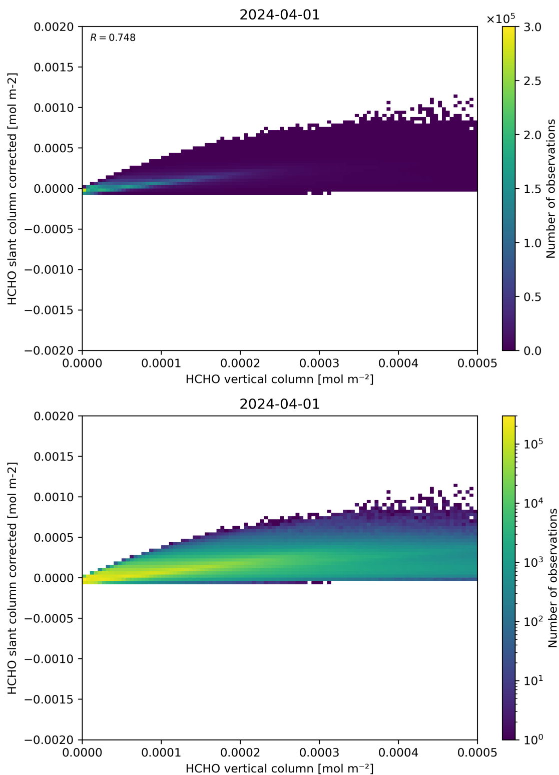
Figure 127: Scatter density plot of “HCHO vertical column” against “HCHO slant column corrected” for 2024-03-31 to 2024-04-02.
