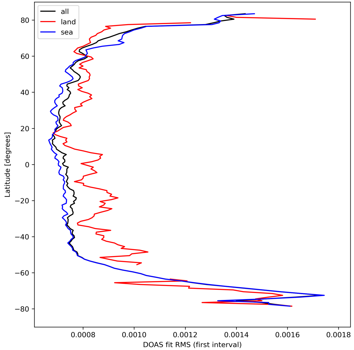
Figure 32: Zonal average of “DOAS fit RMS (first interval)” for 2024-03-31 to 2024-04-02.
