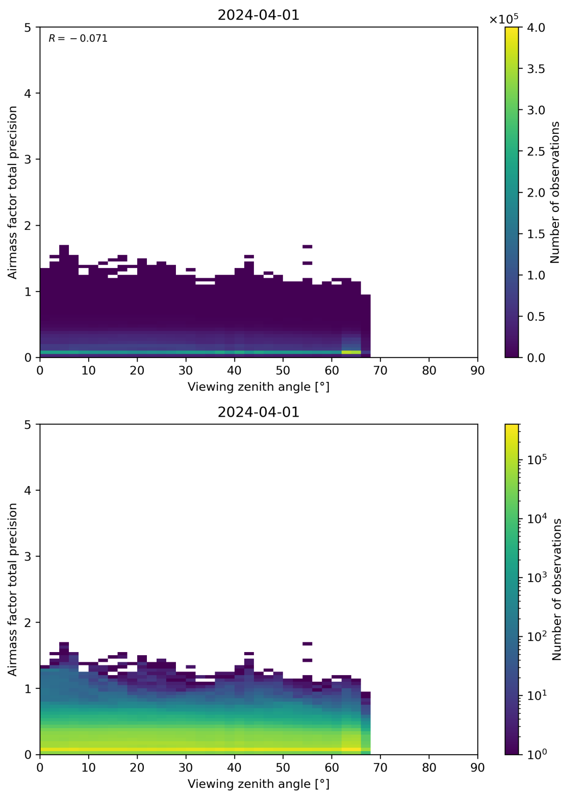
Figure 191: Scatter density plot of “Viewing zenith angle” against “Airmass factor total precision” for 2024-03-31 to 2024-04-02.
