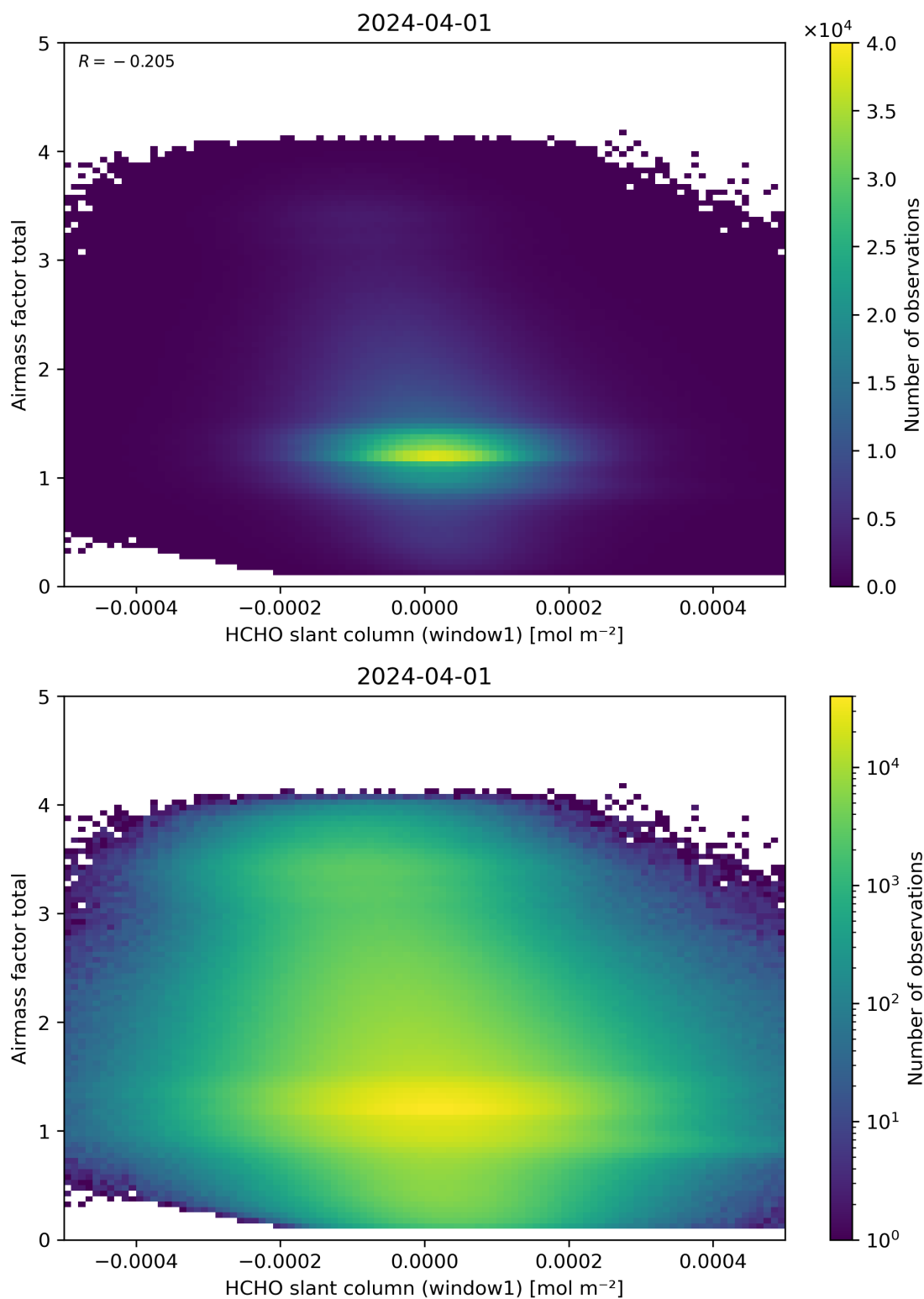
Figure 85: Scatter density plot of “HCHO slant column (window1)” against “Airmass factor total” for 2024-03-31 to 2024-04-02.
