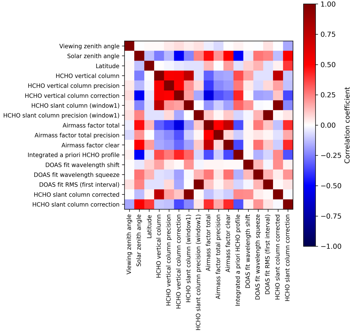
Figure 2: Map of correlation matrix for 2024-03-31 to 2024-04-02.
