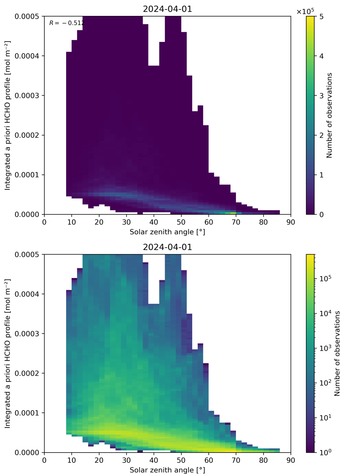
Figure 180: Scatter density plot of “Solar zenith angle” against “Integrated a priori HCHO profile” for 2024-03-31 to 2024-04-02.
