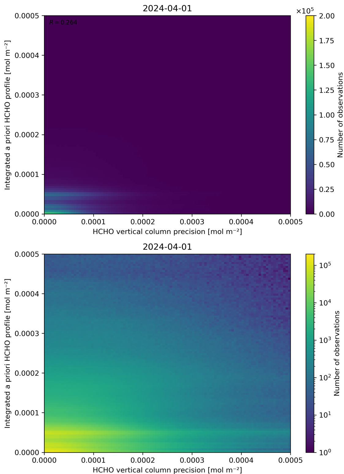
Figure 147: Scatter density plot of “HCHO vertical column precision” against “Integrated a priori HCHO profile” for 2024-03-31 to 2024-04-02.
