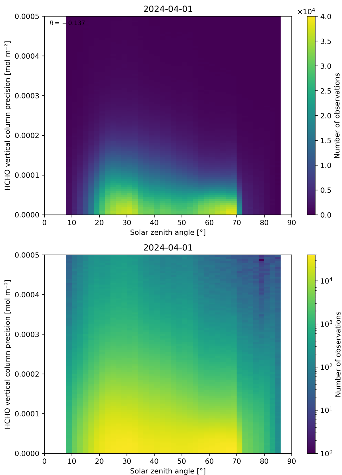
Figure 179: Scatter density plot of “Solar zenith angle” against “HCHO vertical column precision” for 2024-03-31 to 2024-04-02.
