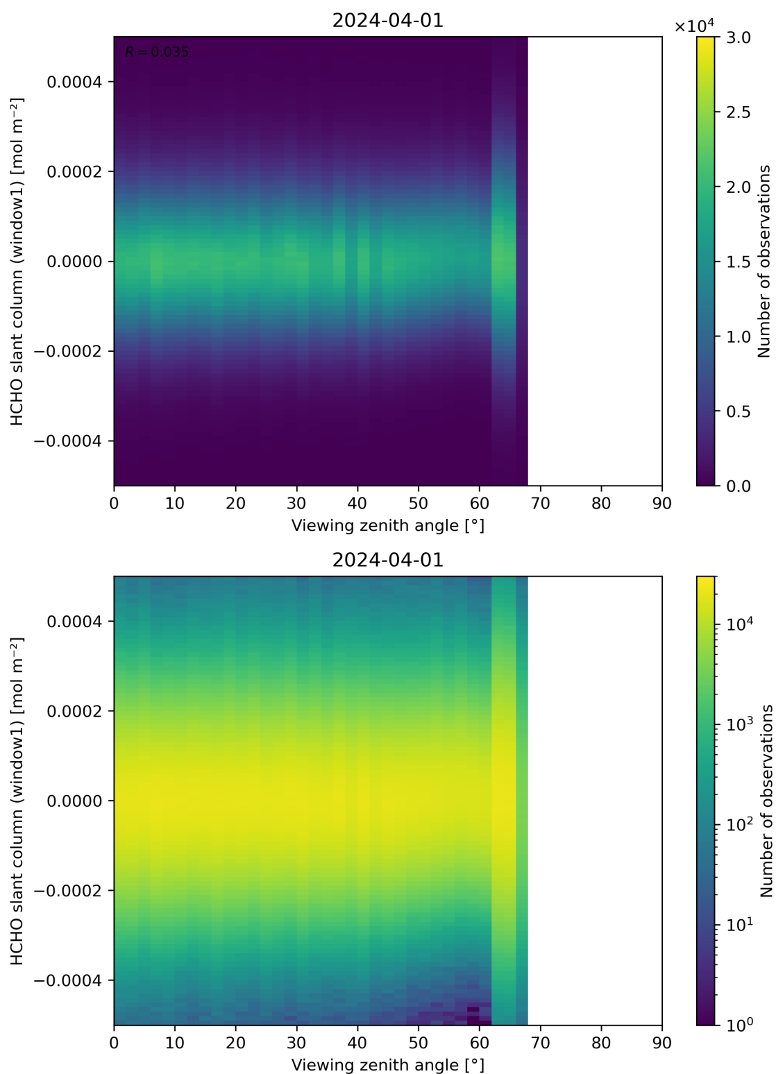
Figure 188: Scatter density plot of “Viewing zenith angle” against “HCHO slant column (window1)” for 2024-03-31 to 2024-04-02.
