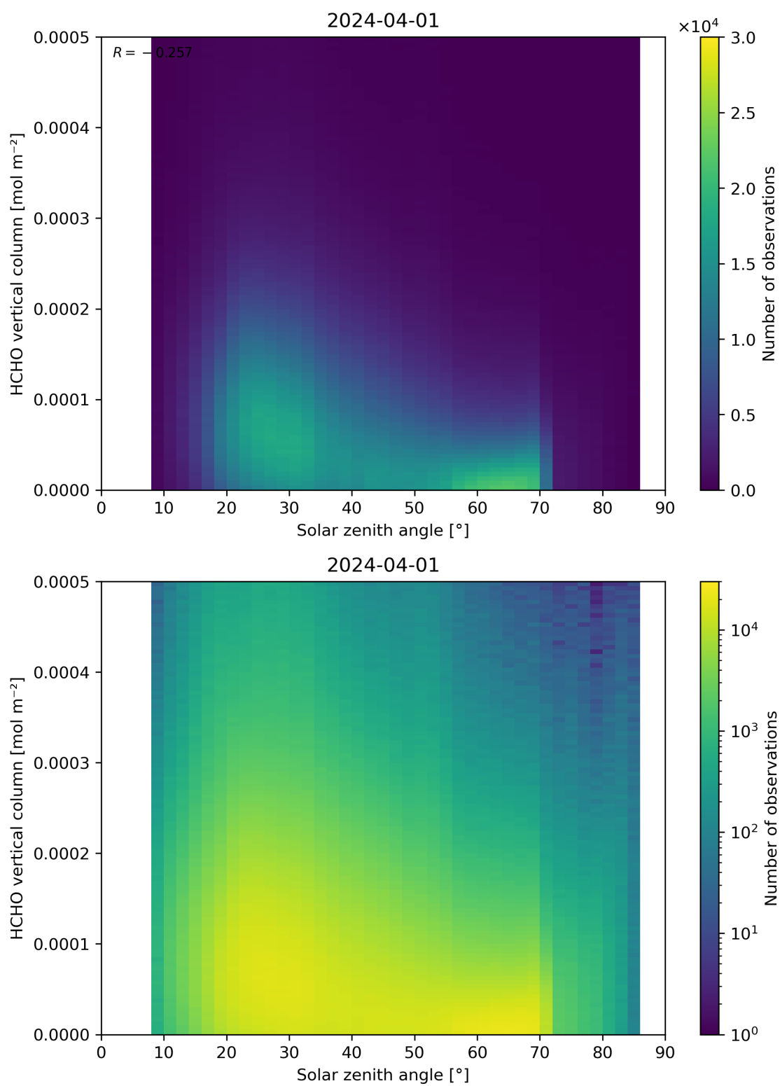
Figure 177: Scatter density plot of “Solar zenith angle” against “HCHO vertical column” for 2024-03-31 to 2024-04-02.
