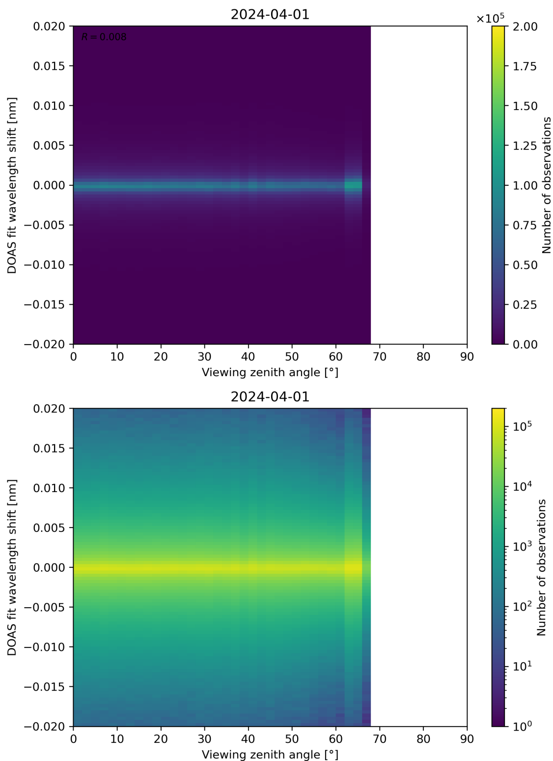
Figure 183: Scatter density plot of “Viewing zenith angle” against “DOAS fit wavelength shift” for 2024-03-31 to 2024-04-02.
