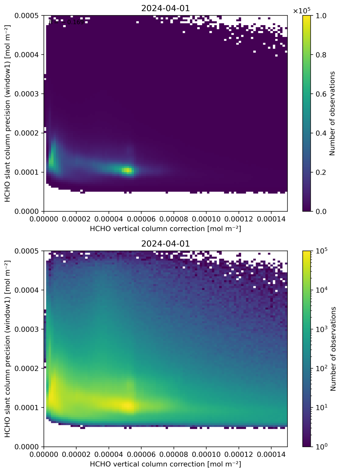
Figure 119: Scatter density plot of “HCHO vertical column correction” against “HCHO slant column precision (window1)” for 2024-03-31 to 2024-04-02.
