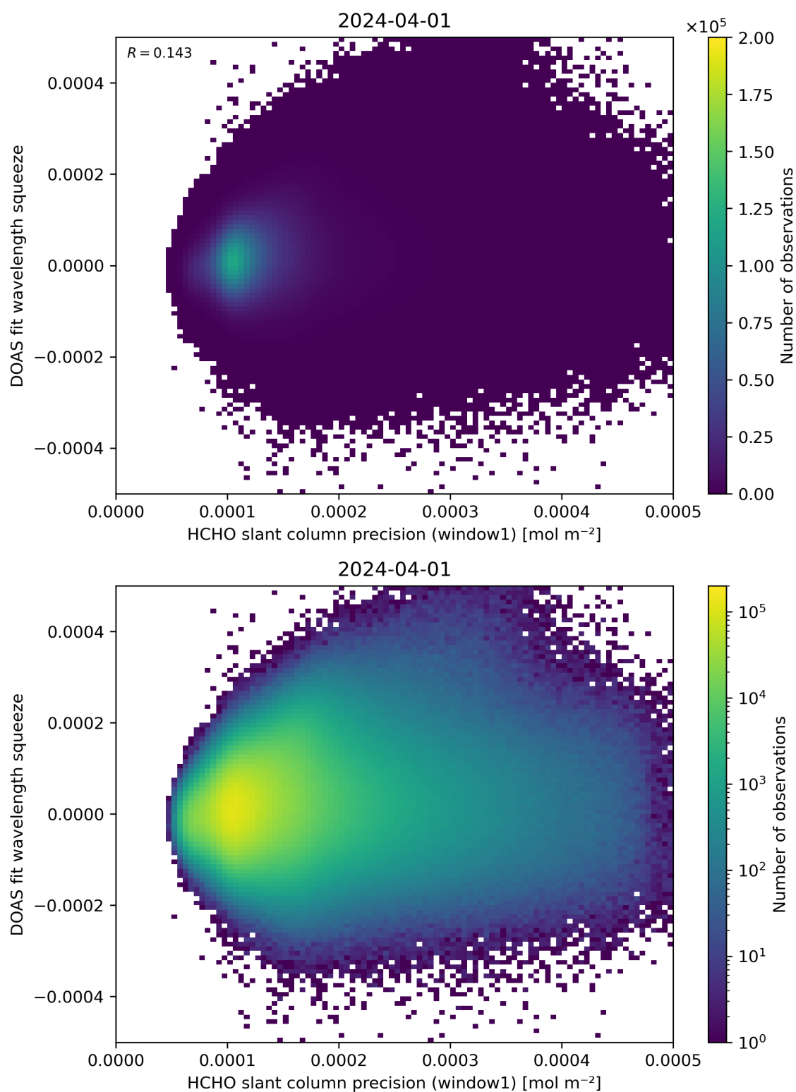
Figure 90: Scatter density plot of “HCHO slant column precision (window1)” against “DOAS fit wavelength squeeze” for 2024-03-31 to 2024-04-02.
