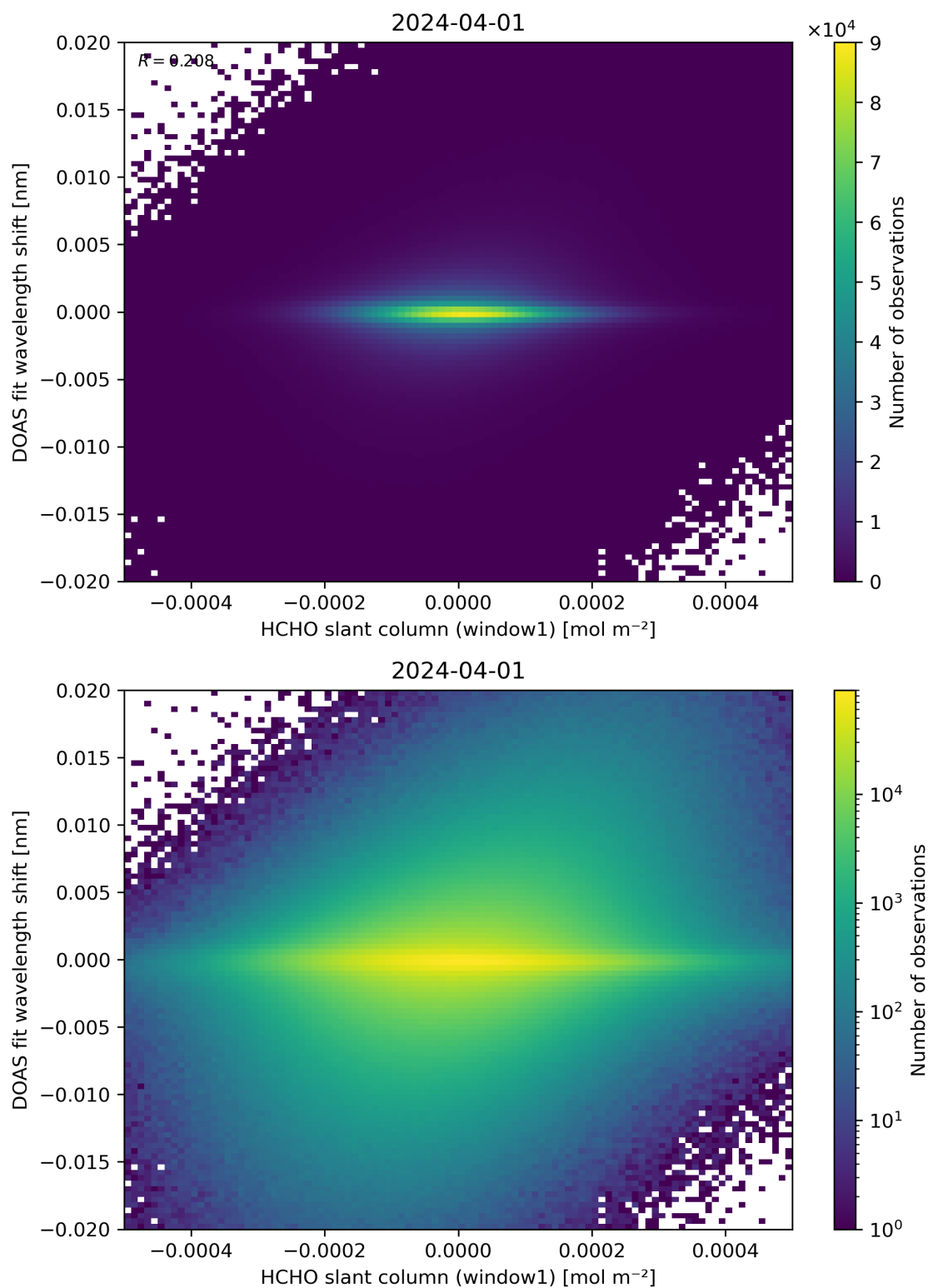
Figure 79: Scatter density plot of “HCHO slant column (window1)” against “DOAS fit wavelength shift” for 2024-03-31 to 2024-04-02.
