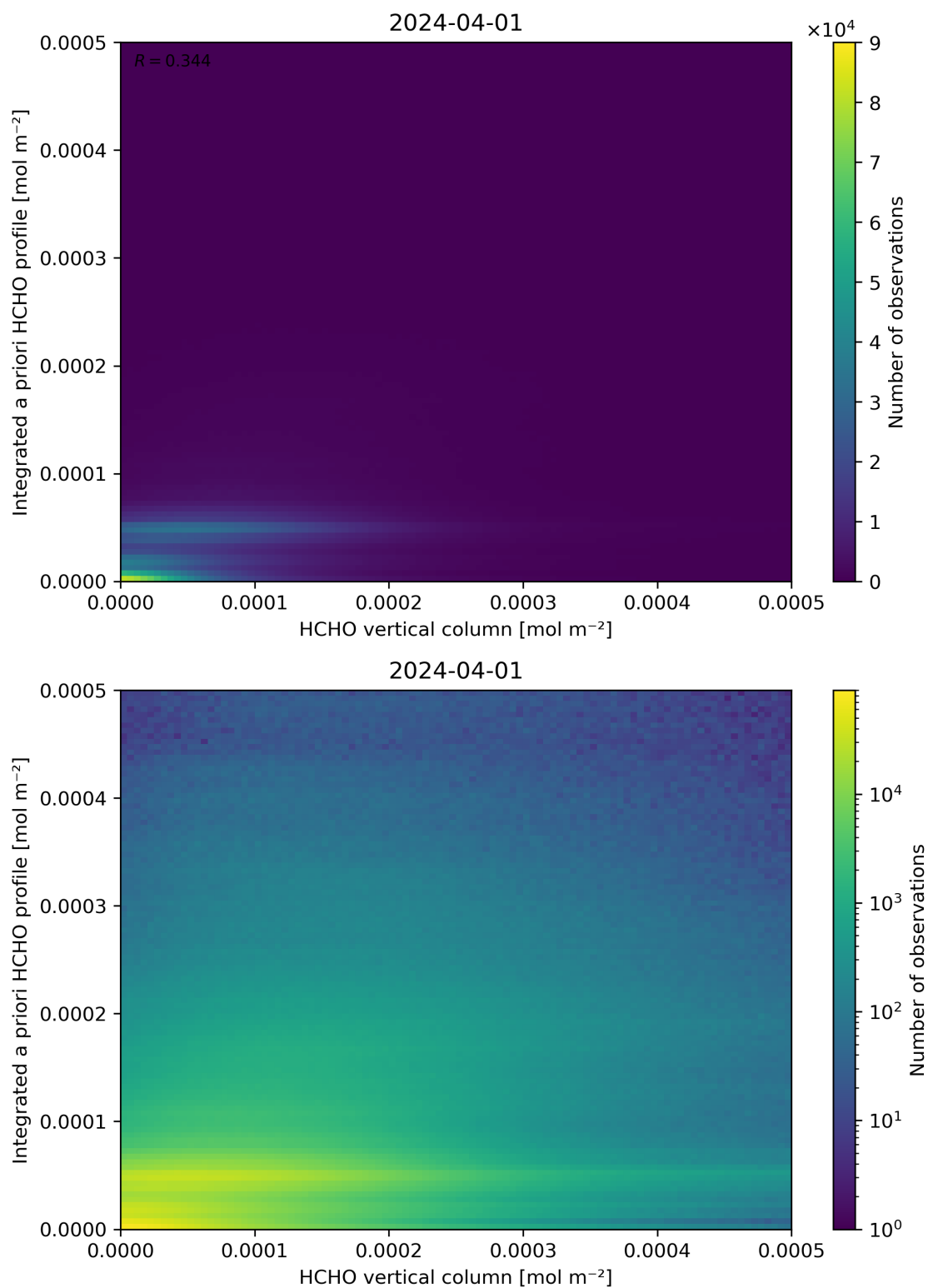
Figure 135: Scatter density plot of “HCHO vertical column” against “Integrated a priori HCHO profile” for 2024-03-31 to 2024-04-02.
