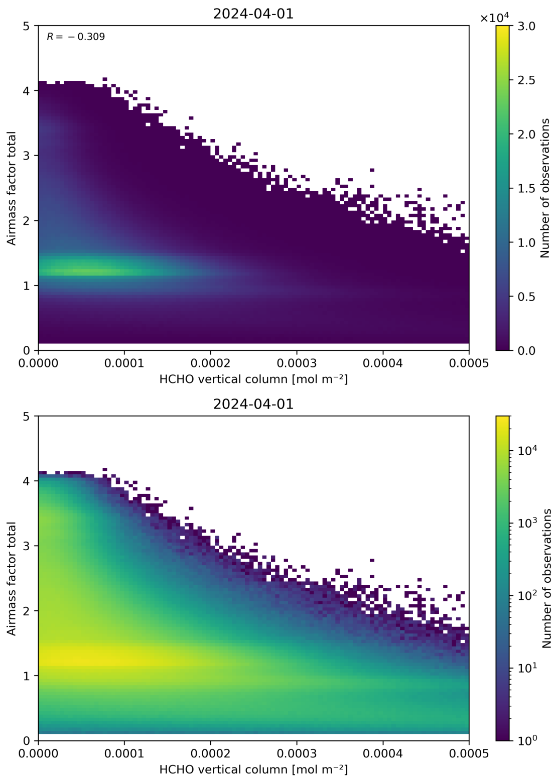
Figure 131: Scatter density plot of “HCHO vertical column” against “Airmass factor total” for 2024-03-31 to 2024-04-02.
