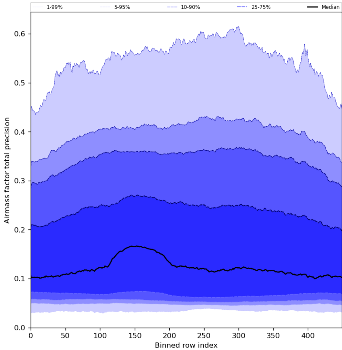
Figure 55: Along track statistics of “Airmass factor total precision” for 2024-03-31 to 2024-04-02
