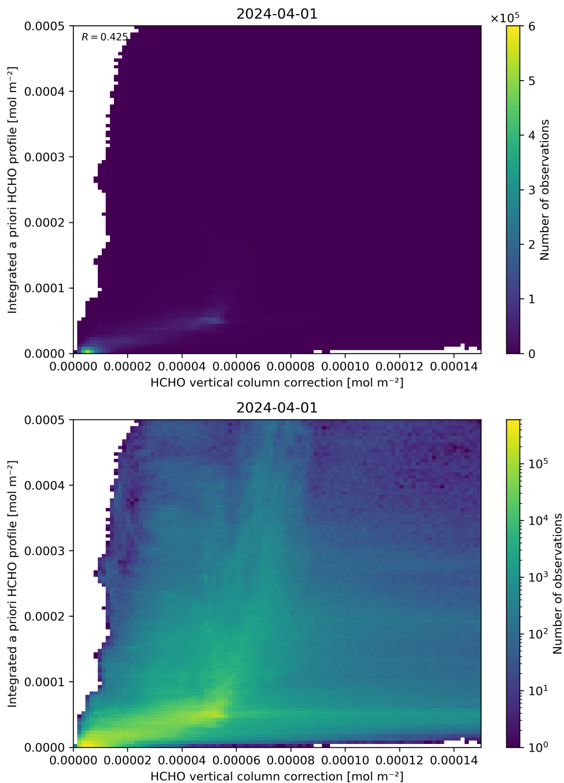
Figure 122: Scatter density plot of “HCHO vertical column correction” against “Integrated a priori HCHO profile” for 2024-03-31 to 2024-04-02.
