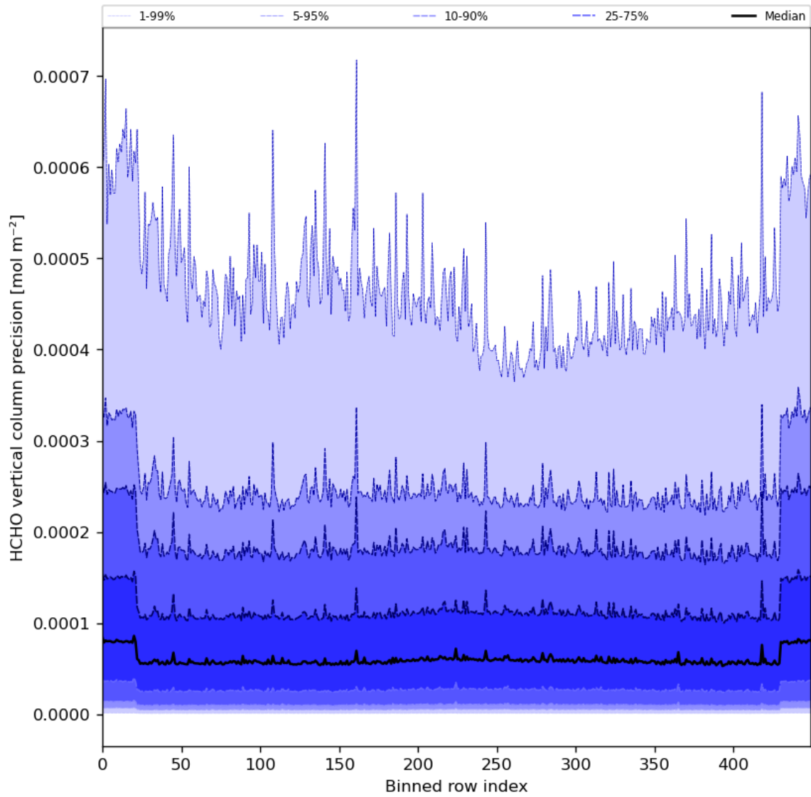
Figure 50: Along track statistics of “HCHO vertical column precision” for 2024-03-31 to 2024-04-02
