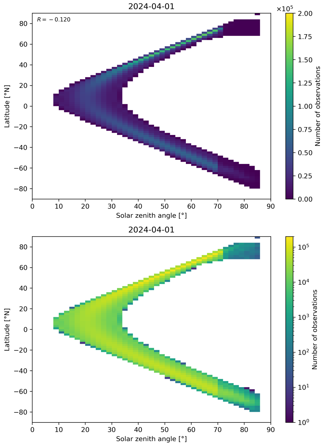
Figure 181: Scatter density plot of “Solar zenith angle” against “Latitude” for 2024-03-31 to 2024-04-02.
