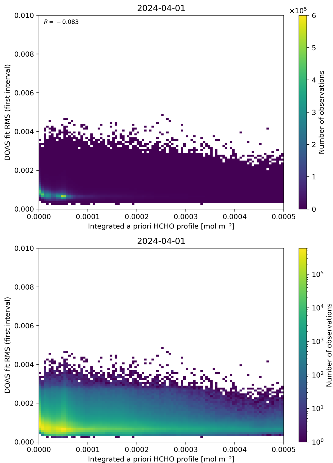
Figure 148: Scatter density plot of “Integrated a priori HCHO profile” against “DOAS fit RMS (first interval)” for 2024-03-31 to 2024-04-02.
