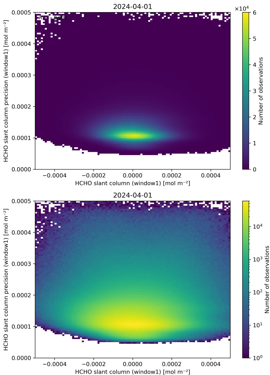
Figure 84: Scatter density plot of “HCHO slant column (window1)” against “HCHO slant column precision (window1)” for 2024-03-31 to 2024-04-02.
