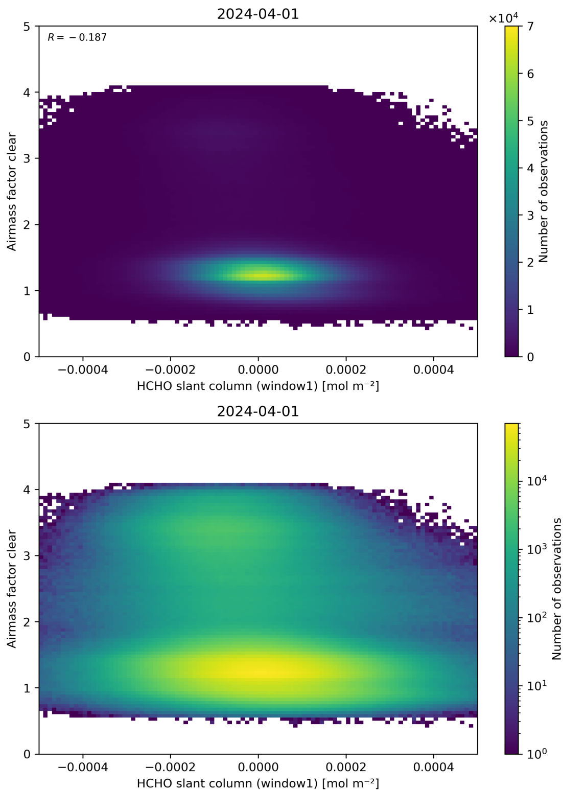
Figure 81: Scatter density plot of “HCHO slant column (window1)” against “Airmass factor clear” for 2024-03-31 to 2024-04-02.
