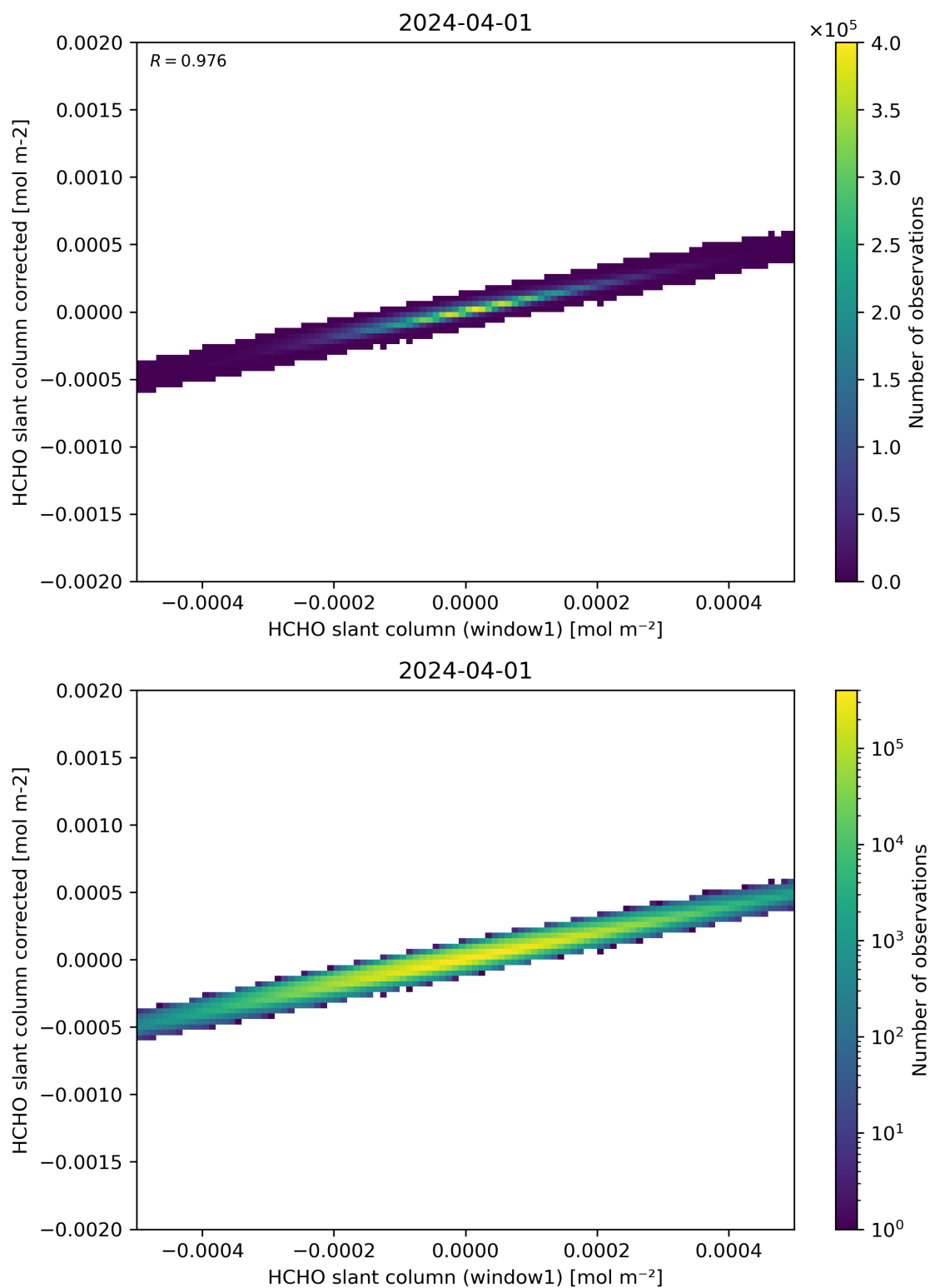
Figure 82: Scatter density plot of “HCHO slant column (window1)” against “HCHO slant column corrected” for 2024-03-31 to 2024-04-02.
