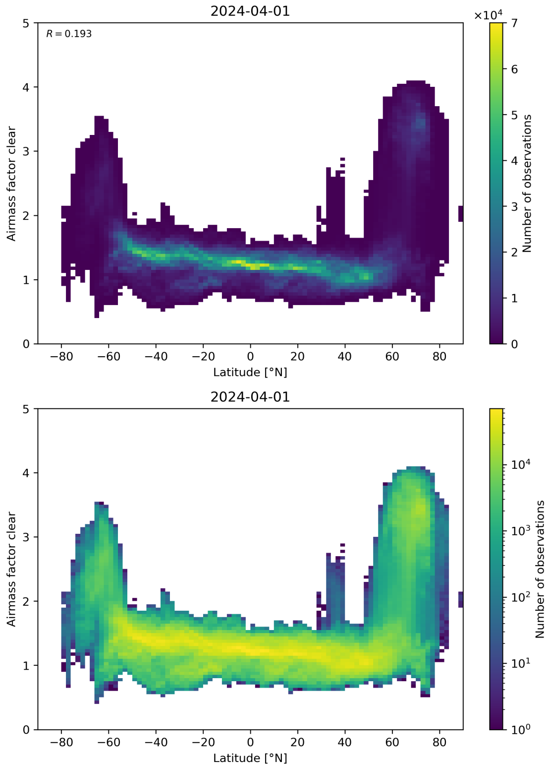
Figure 156: Scatter density plot of “Latitude” against “Airmass factor clear” for 2024-03-31 to 2024-04-02.
