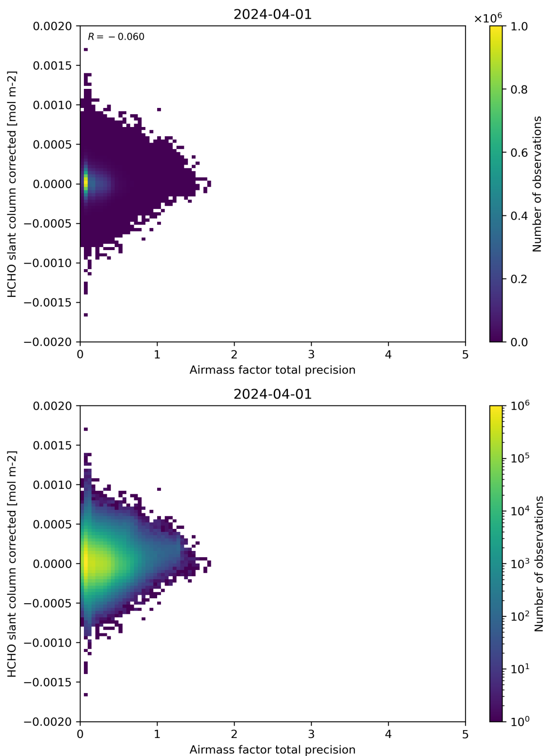
Figure 109: Scatter density plot of “Airmass factor total precision” against “HCHO slant column corrected” for 2024-03-31 to 2024-04-02.
