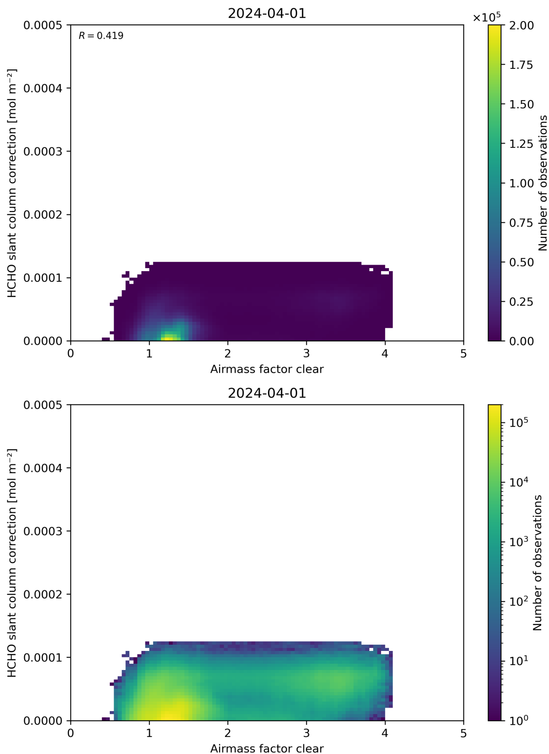
Figure 75: Scatter density plot of “Air mass factor clear” against “HCHO slant column correction” for 2024-03-31 to 2024-04-02.
