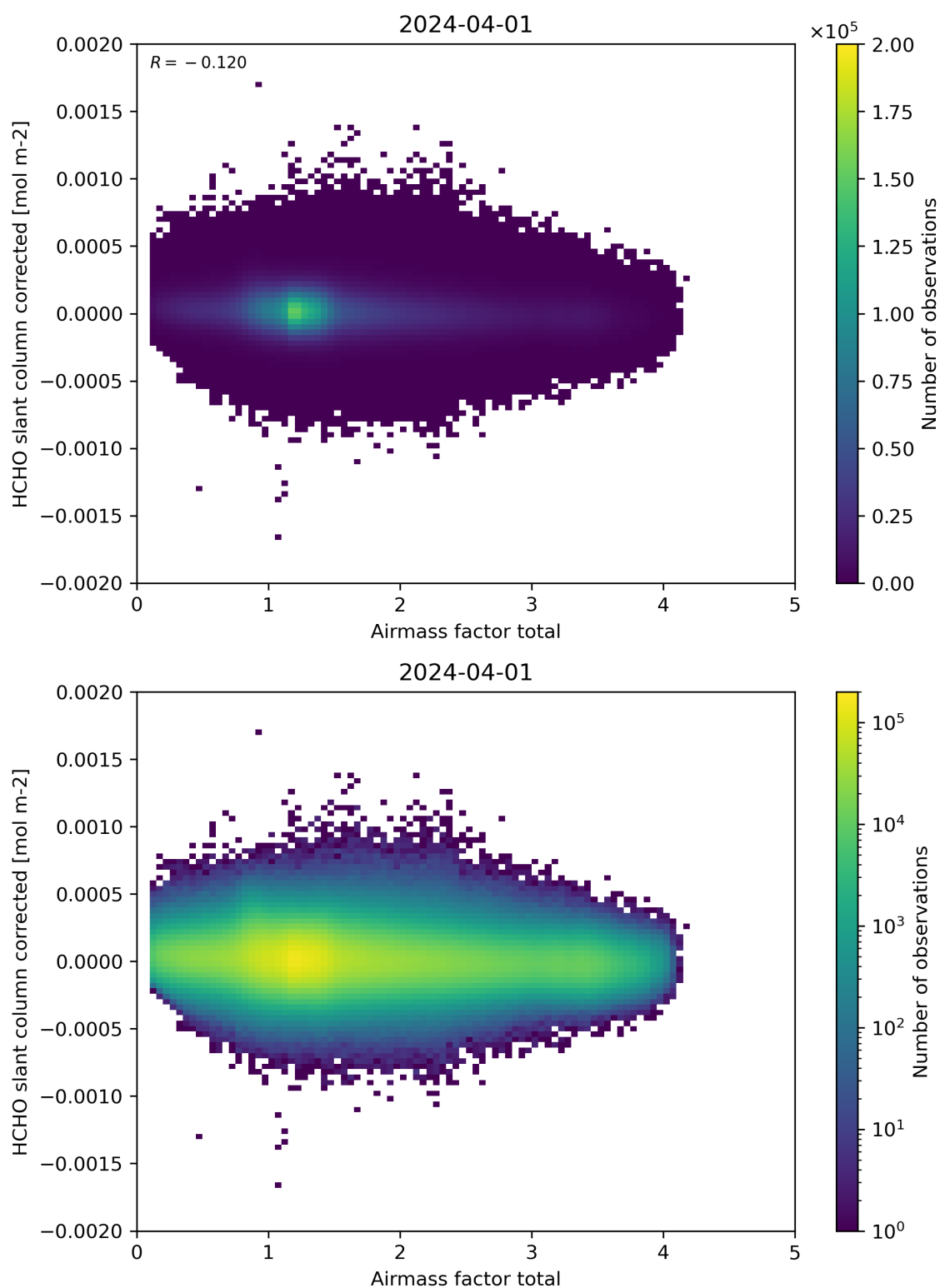
Figure 101: Scatter density plot of “Airmass factor total” against “HCHO slant column corrected” for 2024-03-31 to 2024-04-02.
