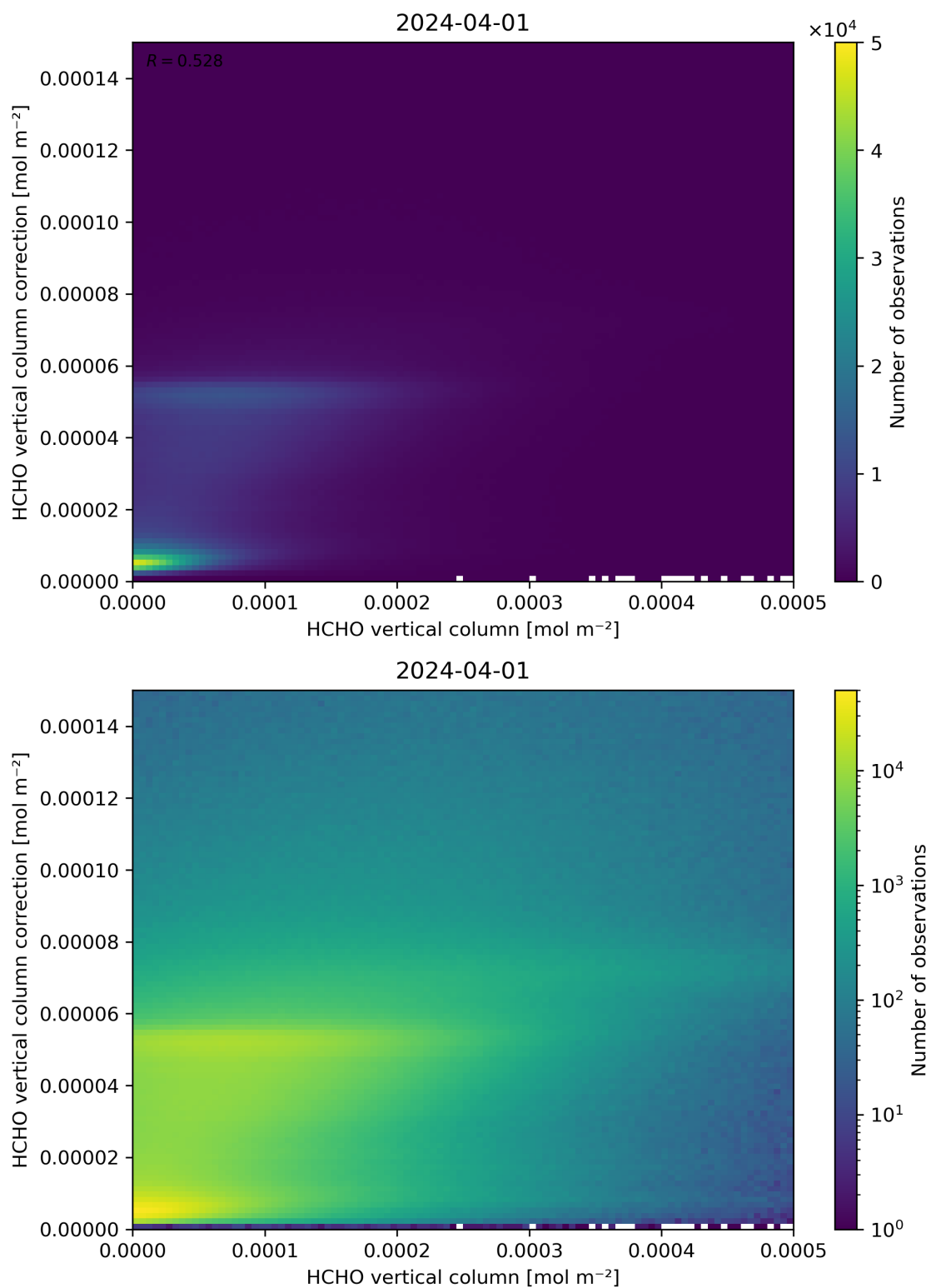
Figure 133: Scatter density plot of “HCHO vertical column” against “HCHO vertical column correction” for 2024-03-31 to 2024-04-02.
