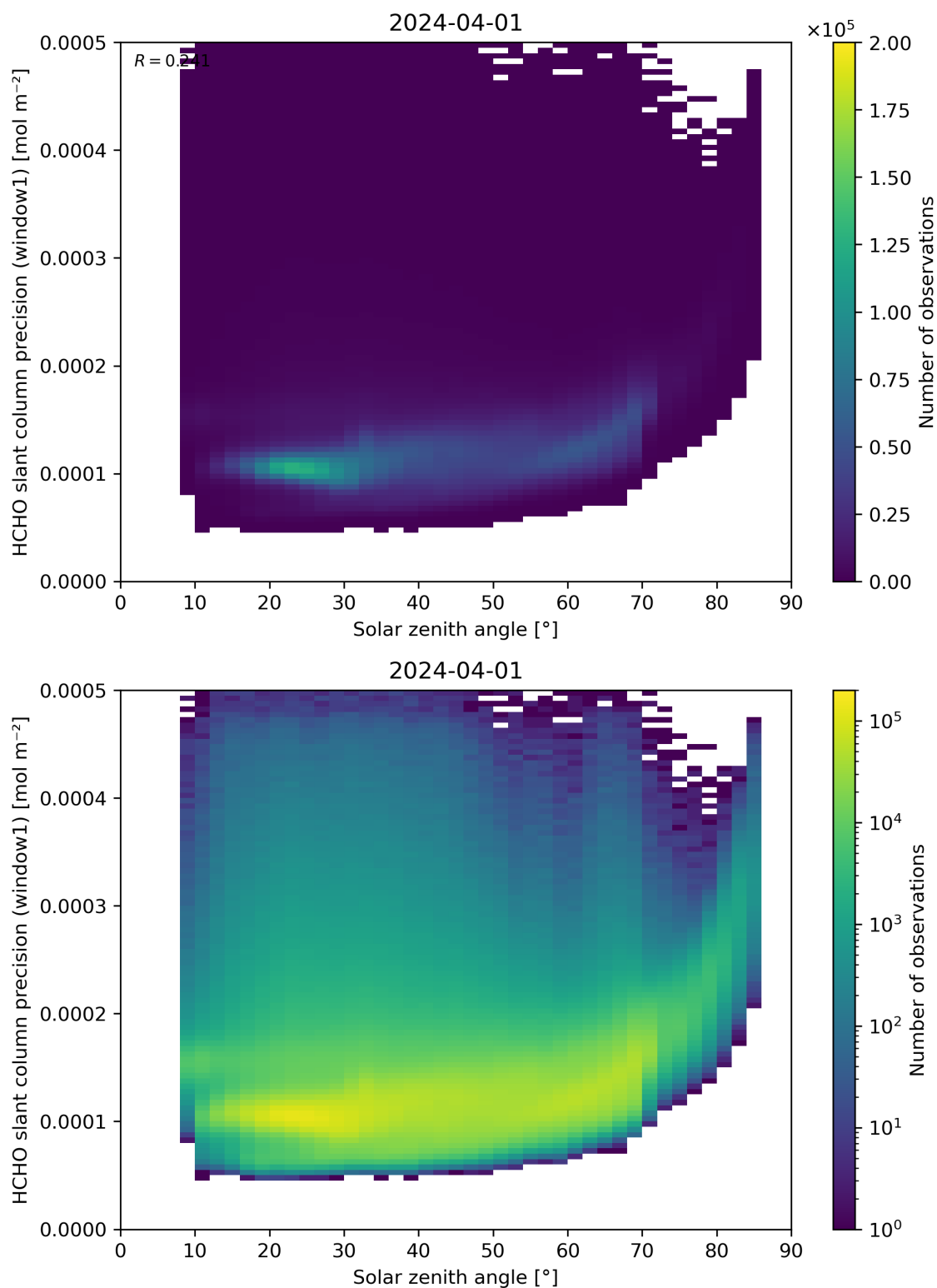
Figure 174: Scatter density plot of “Solar zenith angle” against “HCHO slant column precision (window1)” for 2024-03-31 to 2024-04-02.
