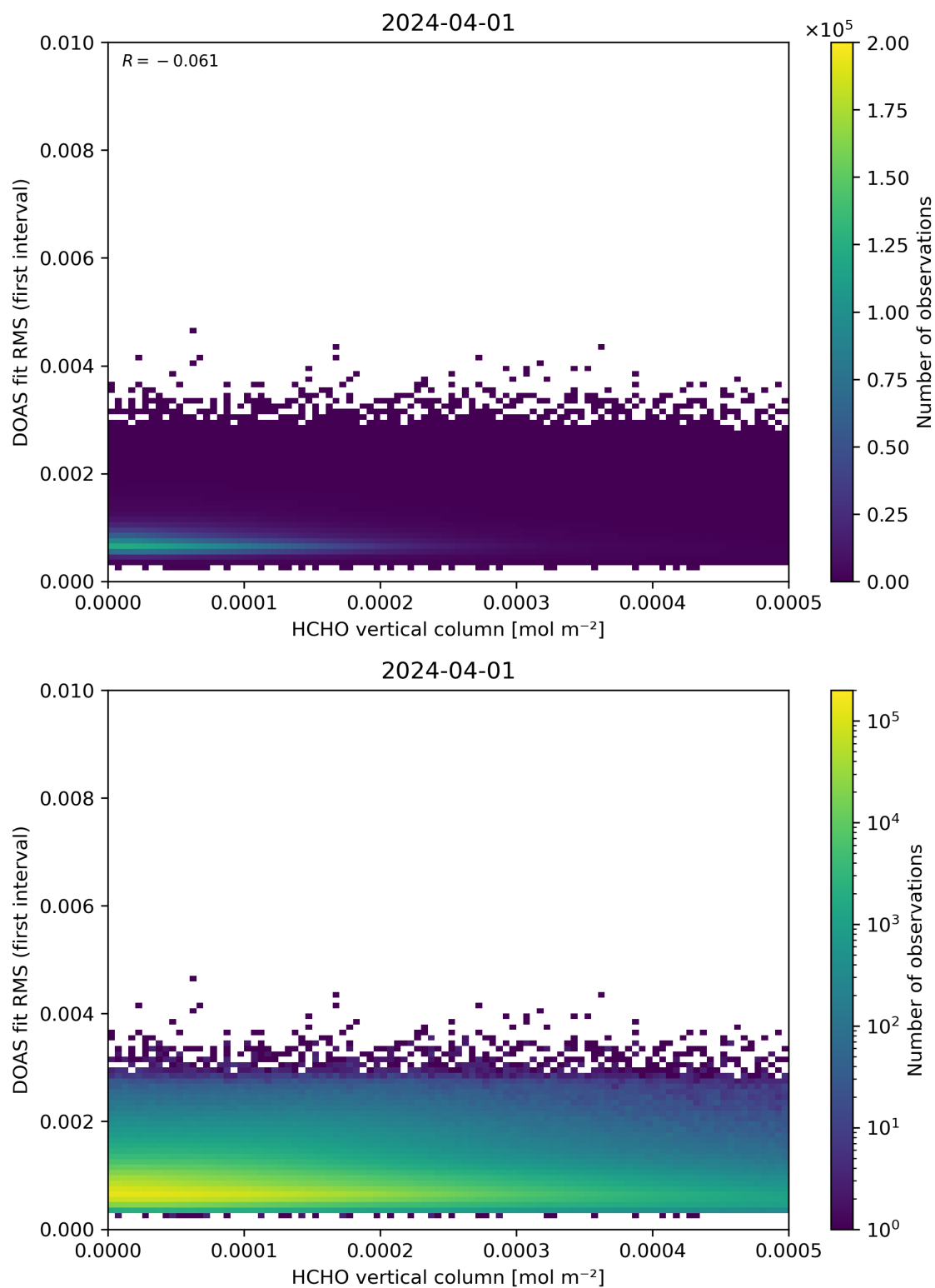
Figure 123: Scatter density plot of “HCHO vertical column” against “DOAS fit RMS (first interval)” for 2024-03-31 to 2024-04-02.
