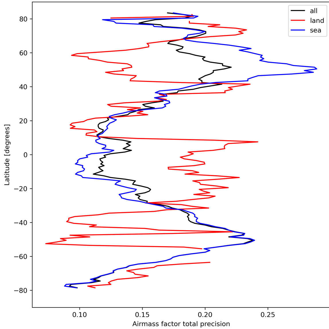
Figure 27: Zonal average of “Airmass factor total precision” for 2024-03-31 to 2024-04-02.
