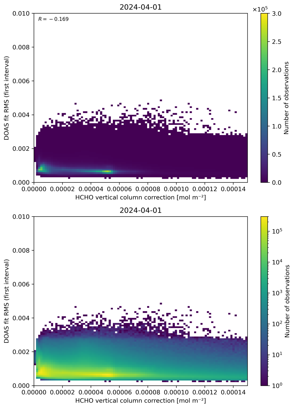
Figure 112: Scatter density plot of “HCHO vertical column correction” against “DOAS fit RMS (first interval)” for 2024-03-31 to 2024-04-02.
