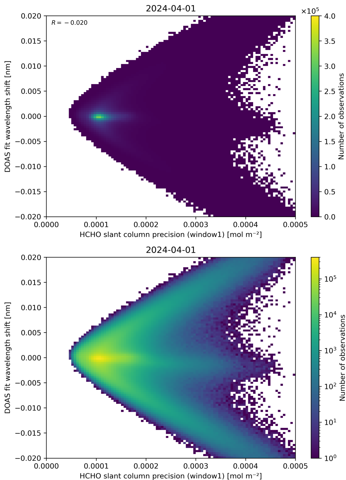
Figure 89: Scatter density plot of “HCHO slant column precision (window1)” against “DOAS fit wavelength shift” for 2024-03-31 to 2024-04-02.
