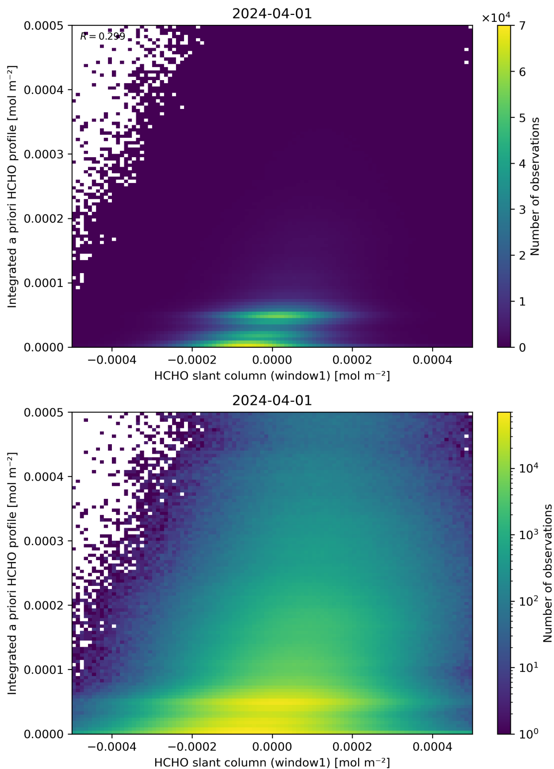
Figure 87: Scatter density plot of “HCHO slant column (window1)” against “Integrated a priori HCHO profile” for 2024-03-31 to 2024-04-02.
