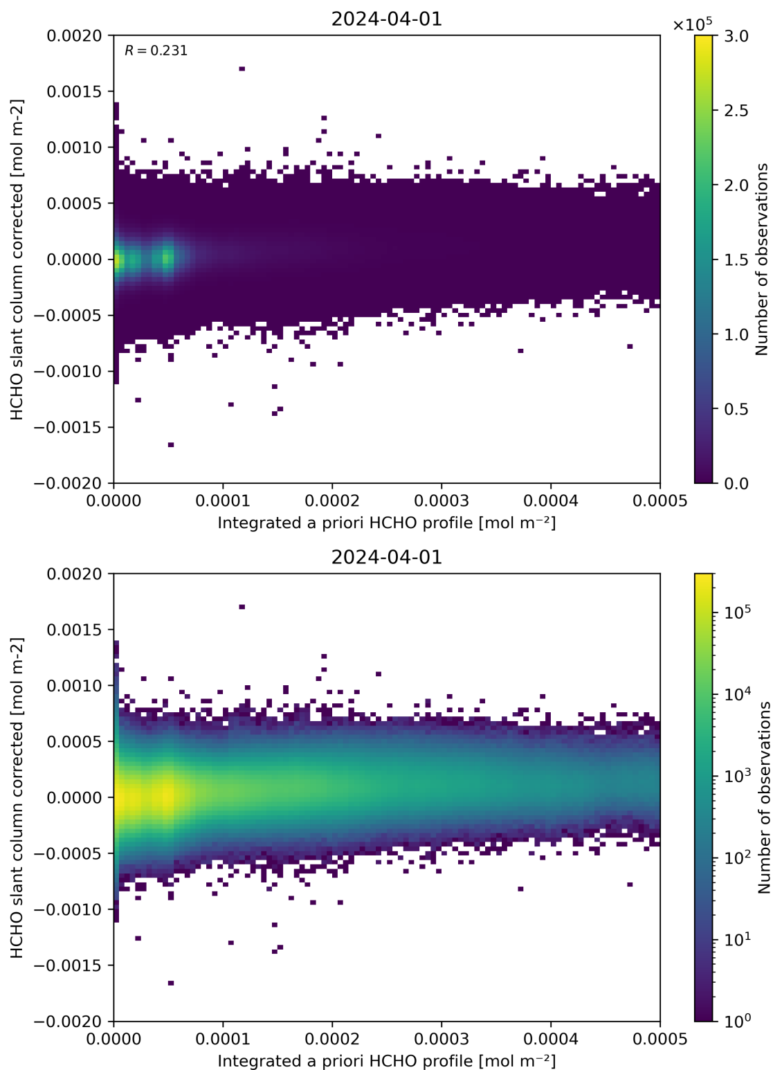
Figure 151: Scatter density plot of “Integrated a priori HCHO profile” against “HCHO slant column corrected” for 2024-03-31 to 2024-04-02.
