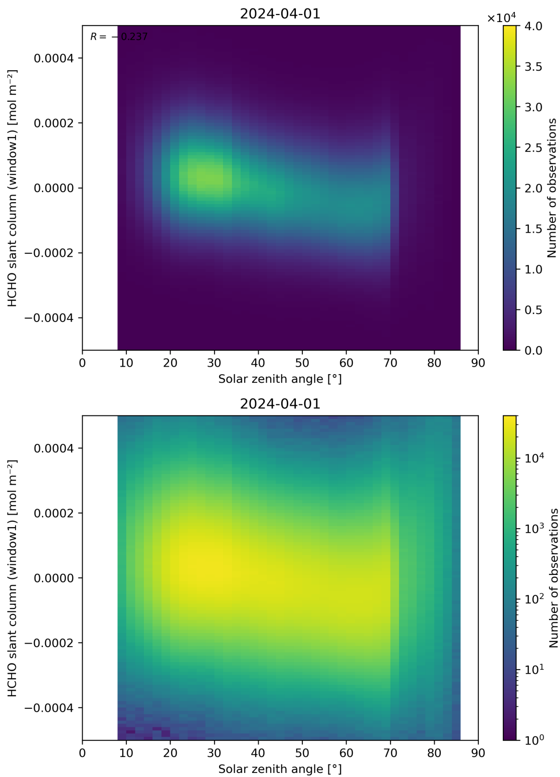
Figure 173: Scatter density plot of “Solar zenith angle” against “HCHO slant column (window1)” for 2024-03-31 to 2024-04-02.
