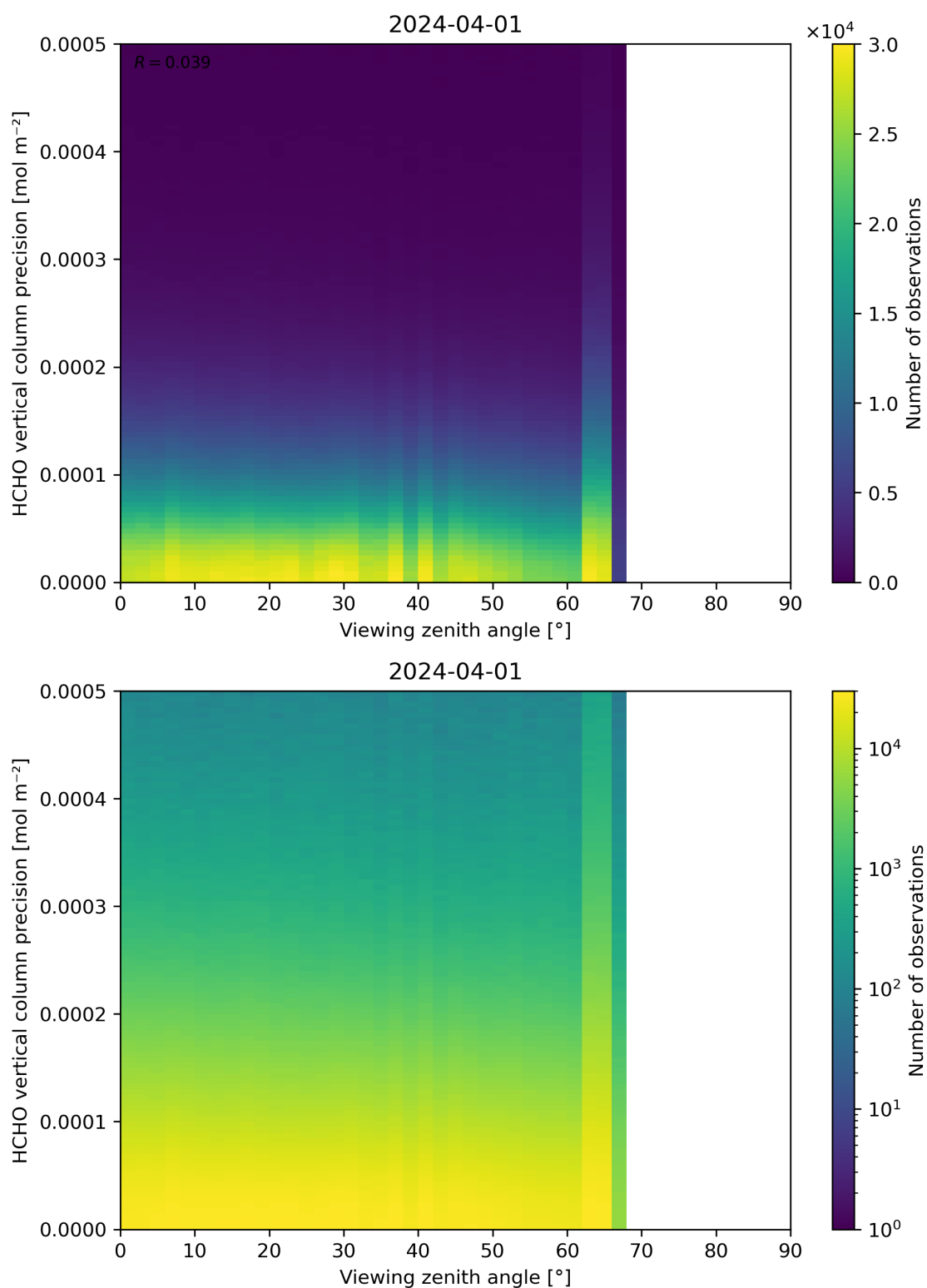
Figure 194: Scatter density plot of “Viewing zenith angle” against “HCHO vertical column precision” for 2024-03-31 to 2024-04-02.
