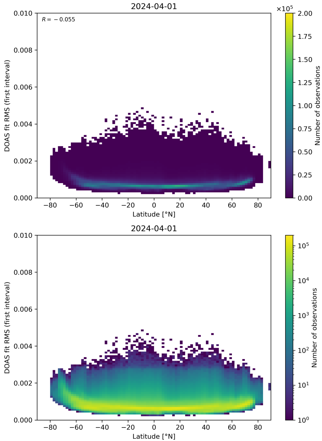
Figure 153: Scatter density plot of “Latitude” against “DOAS fit RMS (first interval)” for 2024-03-31 to 2024-04-02.
