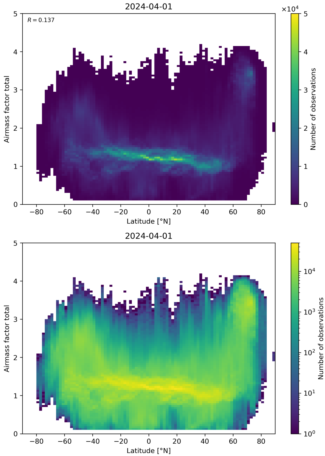
Figure 161: Scatter density plot of “Latitude” against “Airmass factor total” for 2024-03-31 to 2024-04-02.
