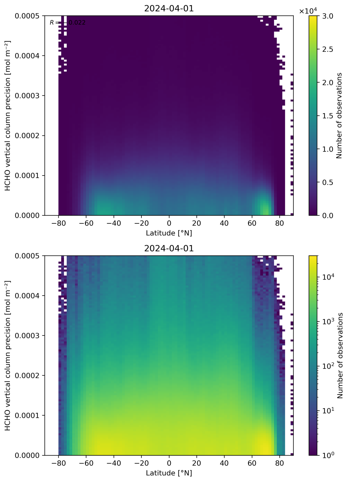
Figure 165: Scatter density plot of “Latitude” against “HCHO vertical column precision” for 2024-03-31 to 2024-04-02.
