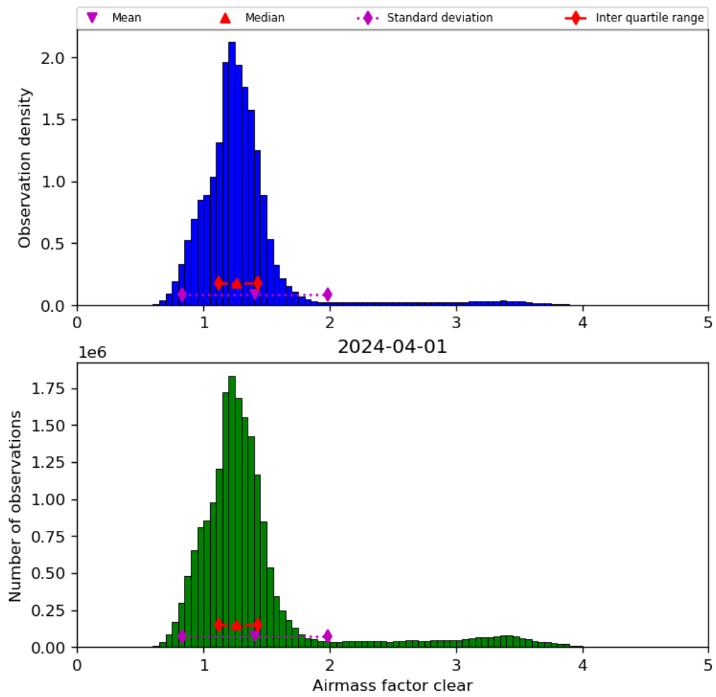
Figure 42: Histogram of “Airmass factor clear” for 2024-03-31 to 2024-04-02
