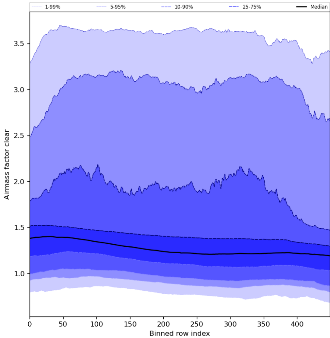
Figure 56: Along track statistics of “Airmass factor clear” for 2024-03-31 to 2024-04-02
