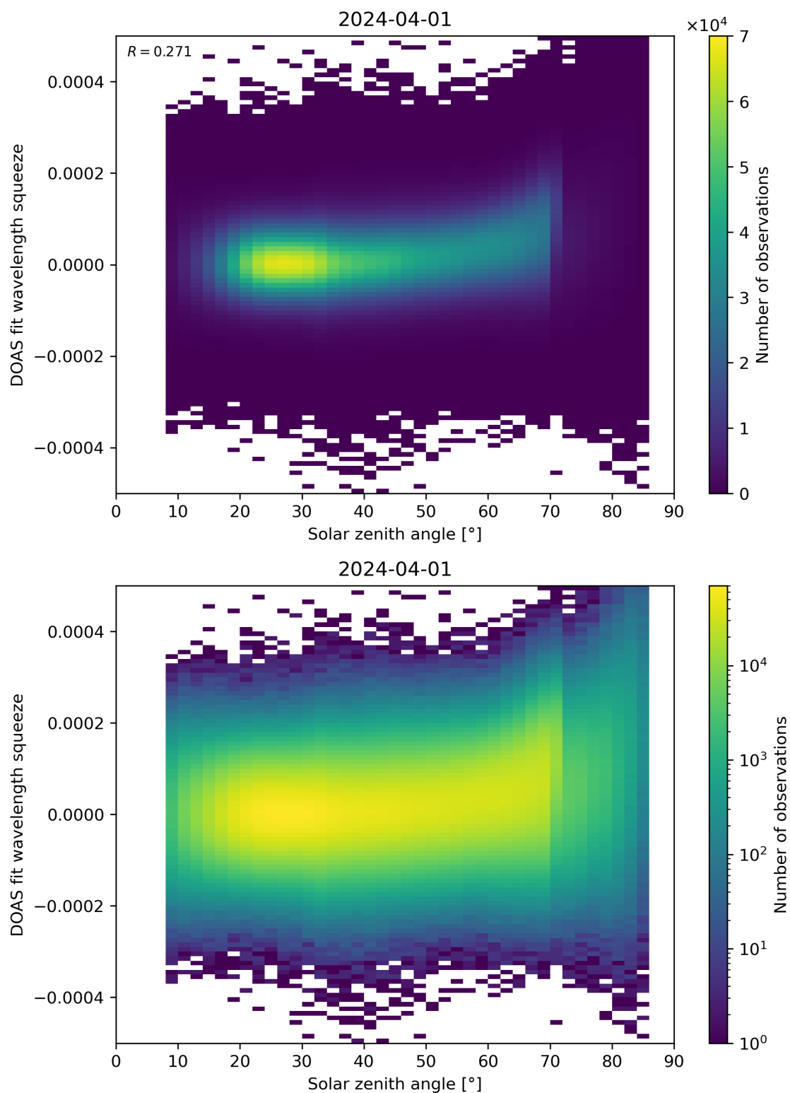
Figure 169: Scatter density plot of “Solar zenith angle” against “DOAS fit wavelength squeeze” for 2024-03-31 to 2024-04-02.
