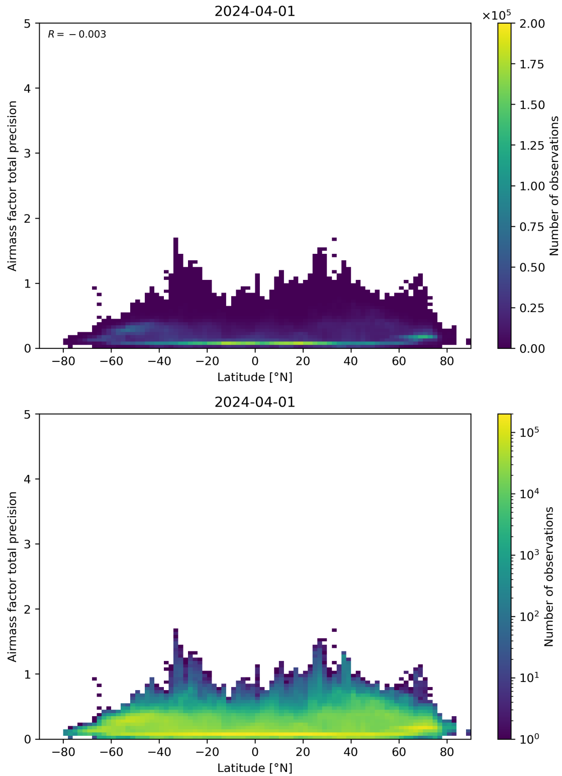
Figure 162: Scatter density plot of “Latitude” against “Airmass factor total precision” for 2024-03-31 to 2024-04-02.
