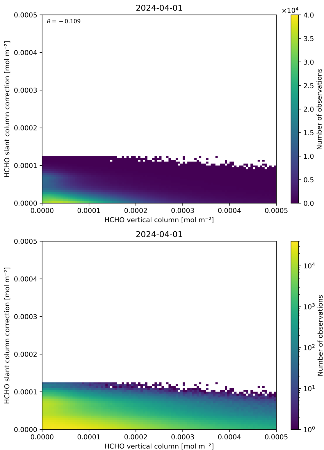
Figure 128: Scatter density plot of “HCHO vertical column” against “HCHO slant column correction” for 2024-03-31 to 2024-04-02.
