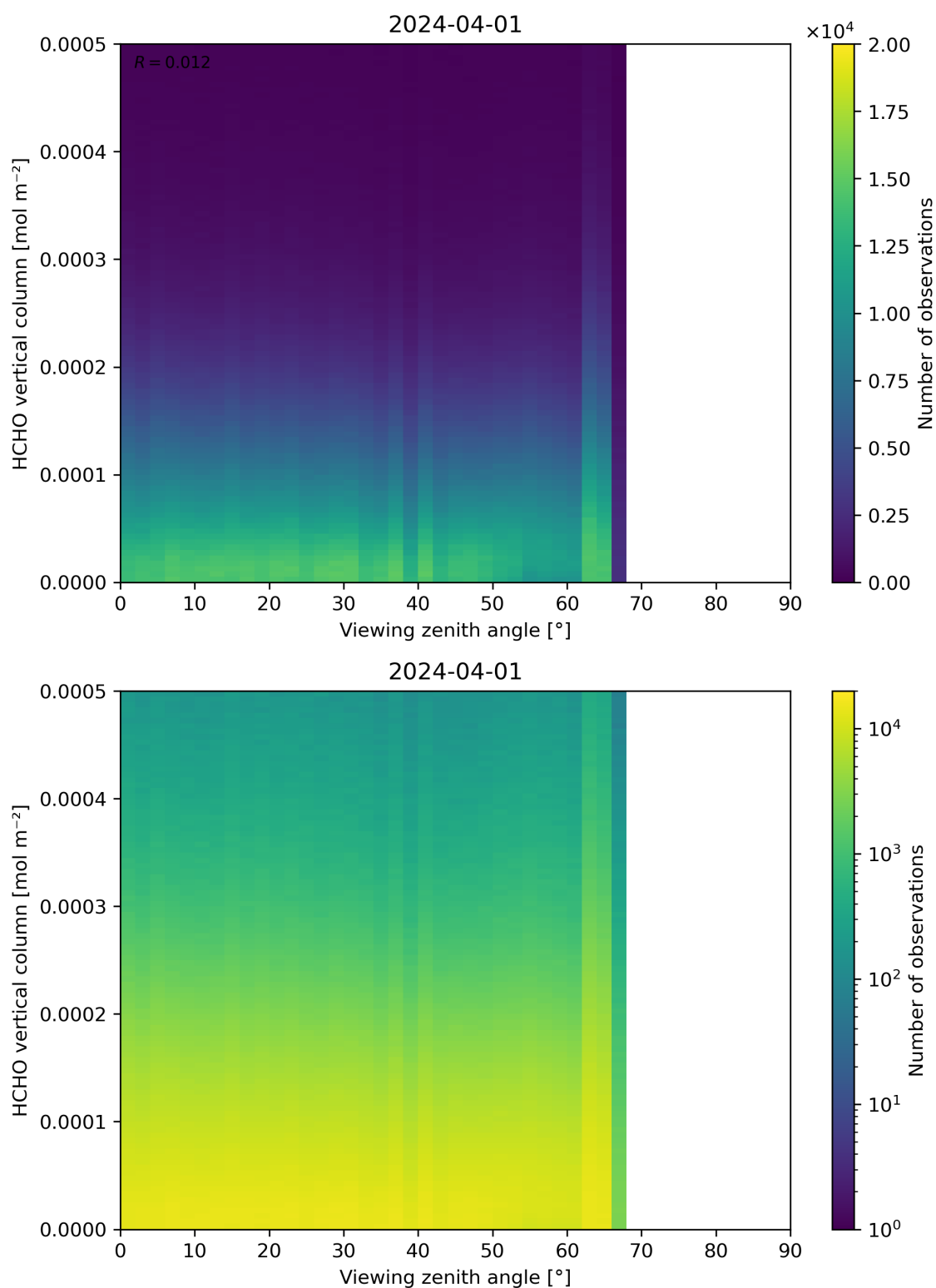
Figure 192: Scatter density plot of “Viewing zenith angle” against “HCHO vertical column” for 2024-03-31 to 2024-04-02.
