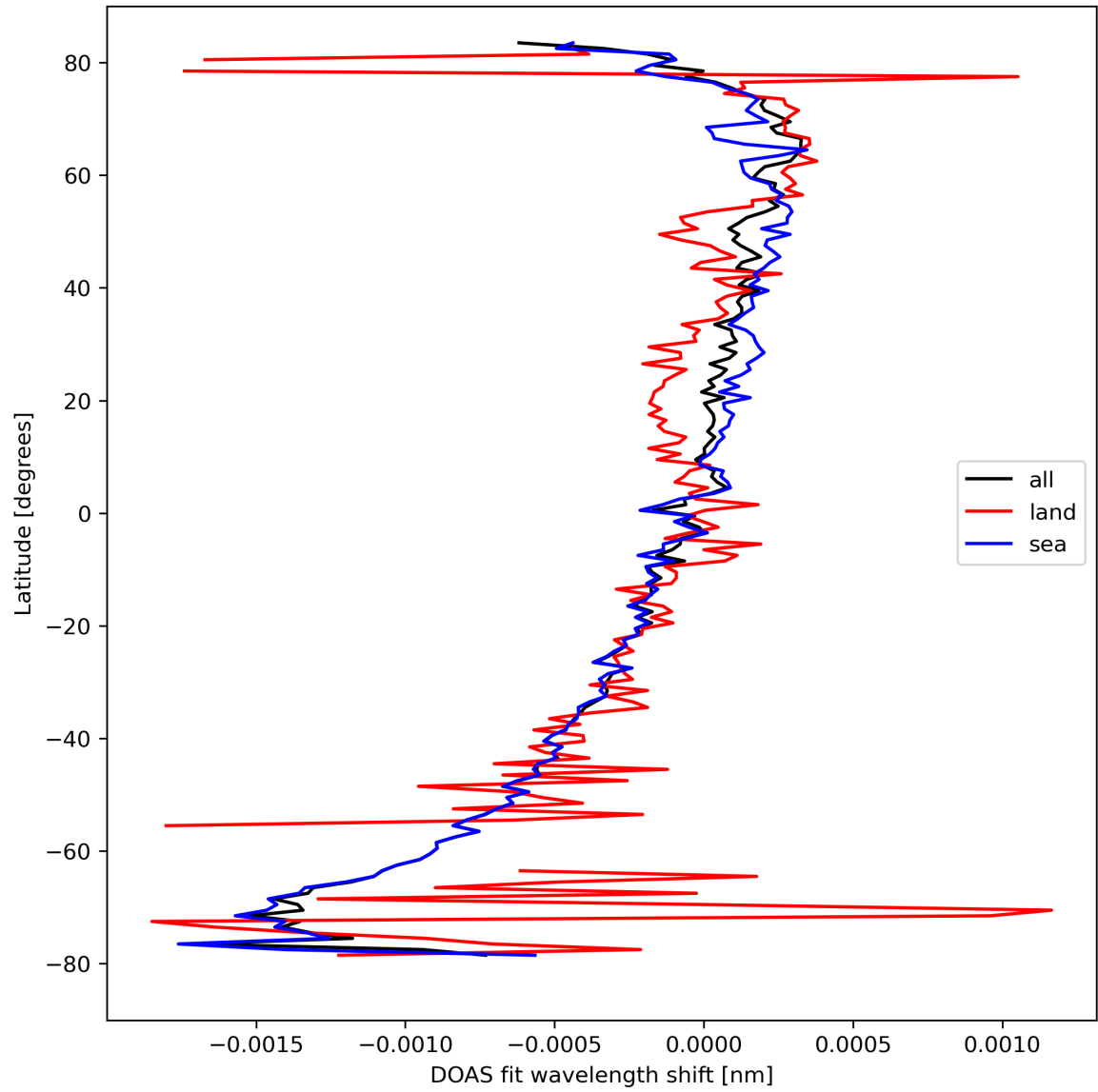
Figure 30: Zonal average of “DOAS fit wavelength shift” for 2024-03-31 to 2024-04-02.
