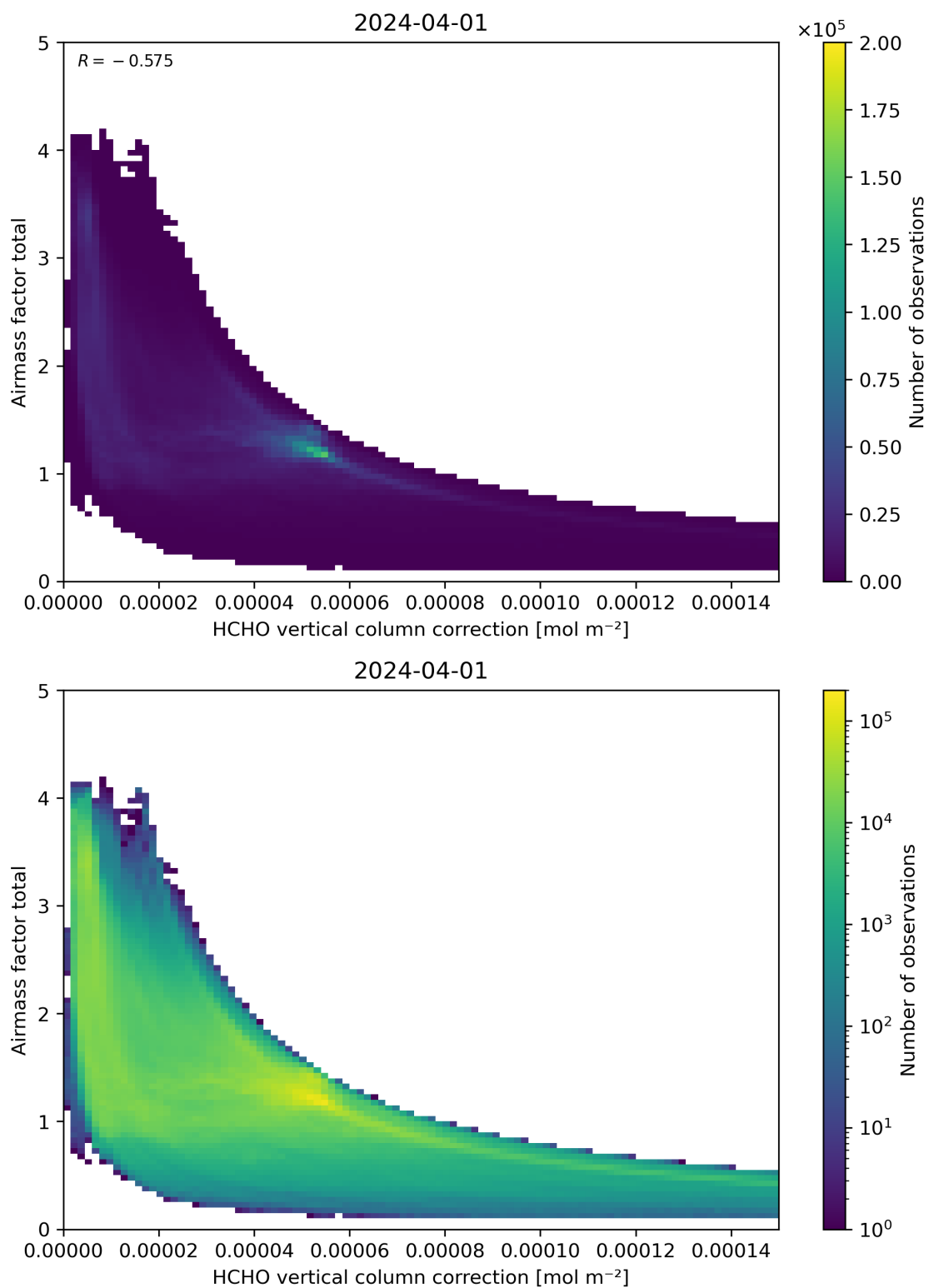
Figure 120: Scatter density plot of “HCHO vertical column correction” against “Airmass factor total” for 2024-03-31 to 2024-04-02.
