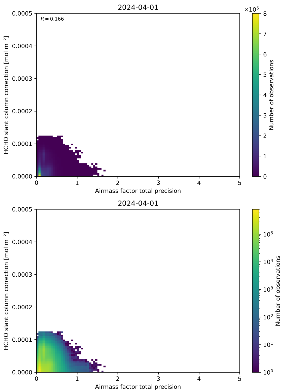
Figure 110: Scatter density plot of “Airmass factor total precision” against “HCHO slant column correction” for 2024-03-31 to 2024-04-02.
