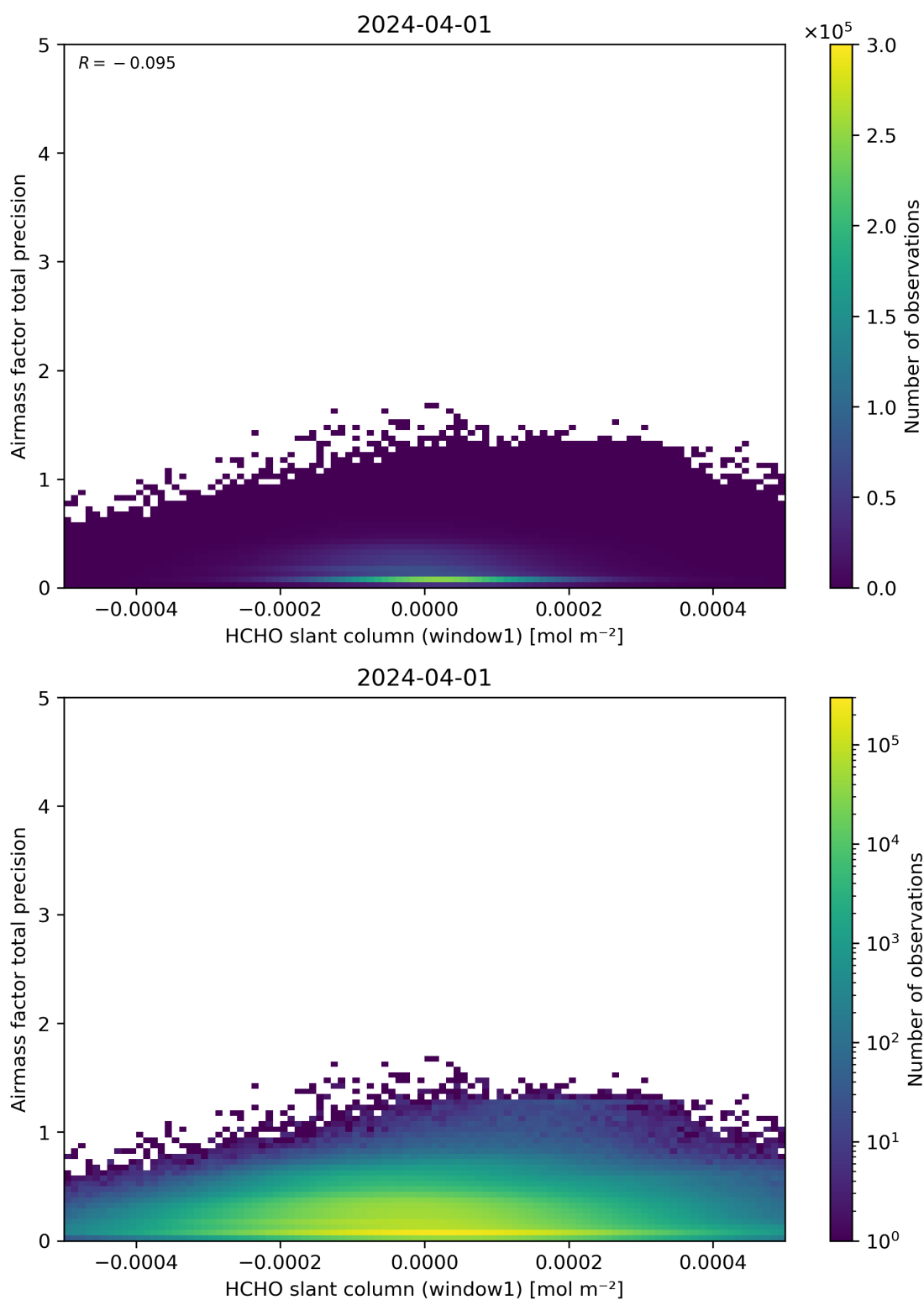
Figure 86: Scatter density plot of “HCHO slant column (window1)” against “Airmass factor total precision” for 2024-03-31 to 2024-04-02.
