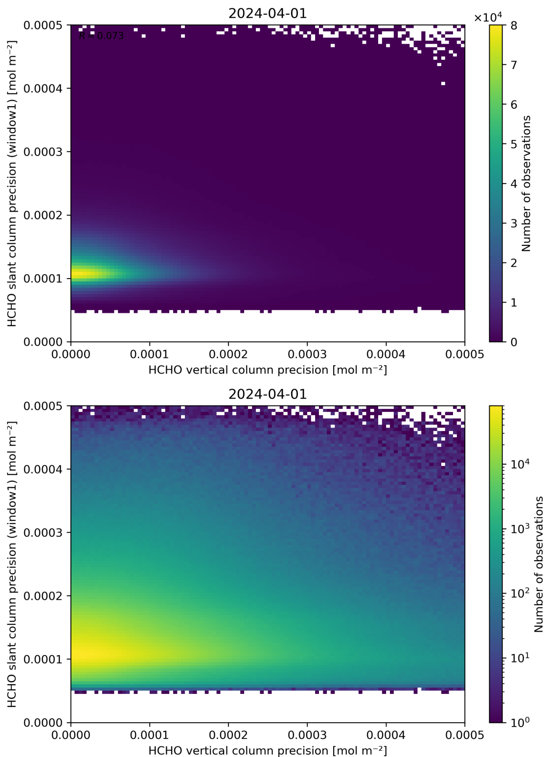
Figure 143: Scatter density plot of “HCHO vertical column precision” against “HCHO slant column precision (window1)” for 2024-03-31 to 2024-04-02.
