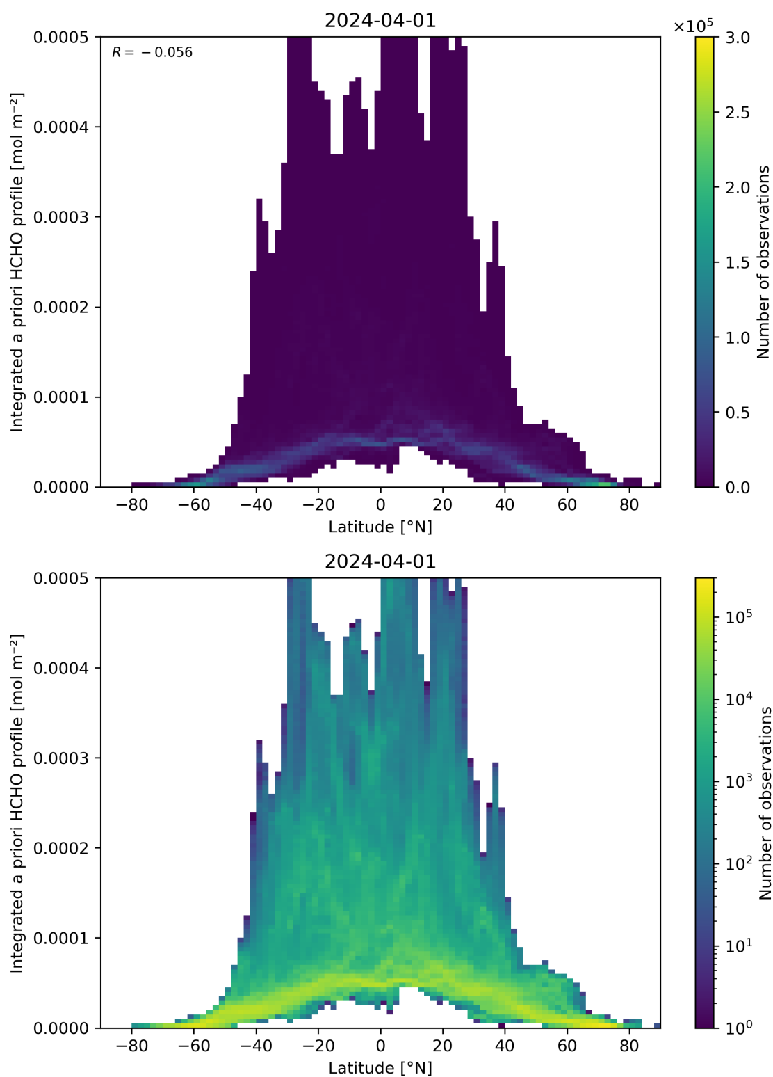
Figure 166: Scatter density plot of “Latitude” against “Integrated a priori HCHO profile” for 2024-03-31 to 2024-04-02.
