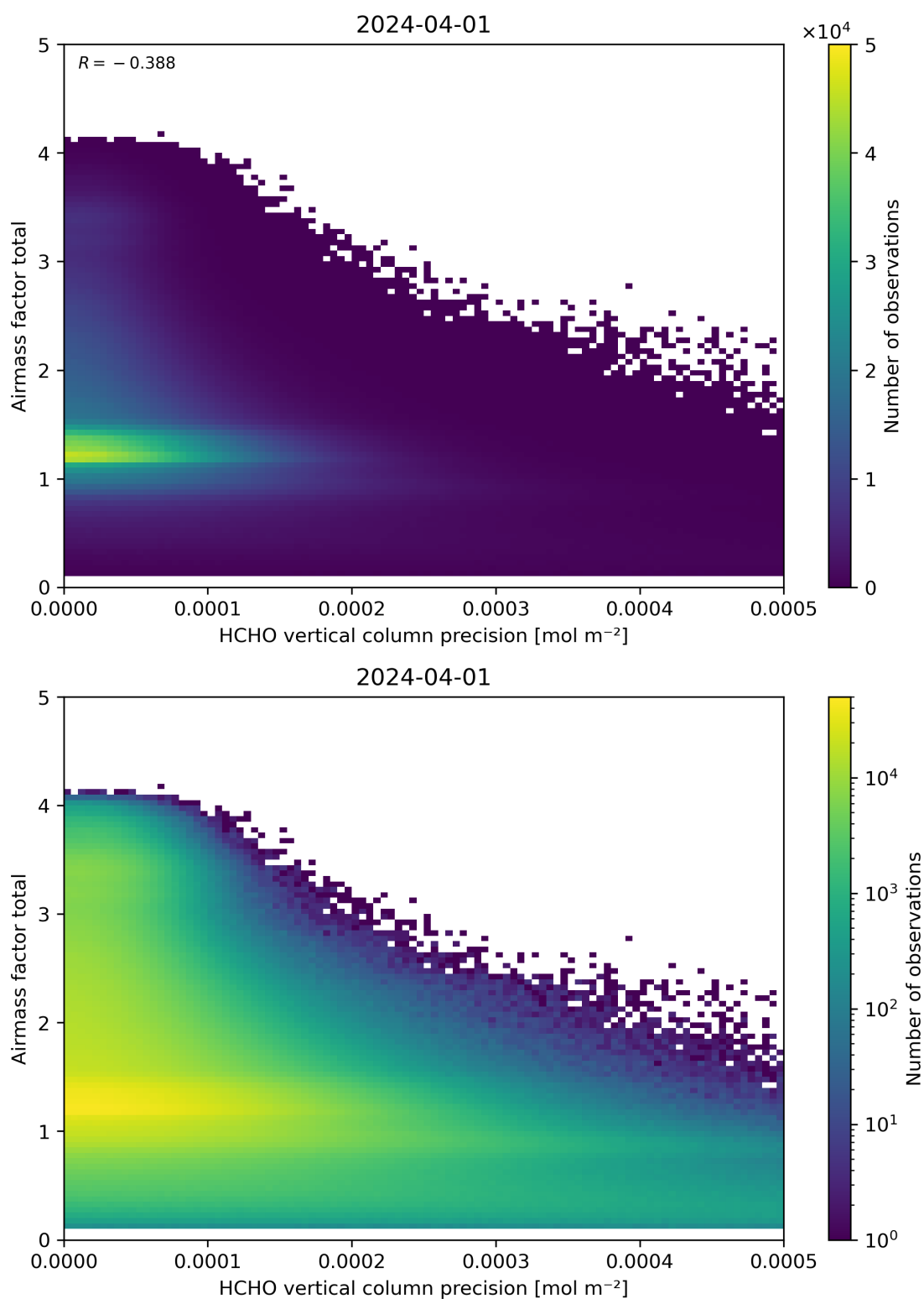
Figure 144: Scatter density plot of “HCHO vertical column precision” against “Airmass factor total” for 2024-03-31 to 2024-04-02.
