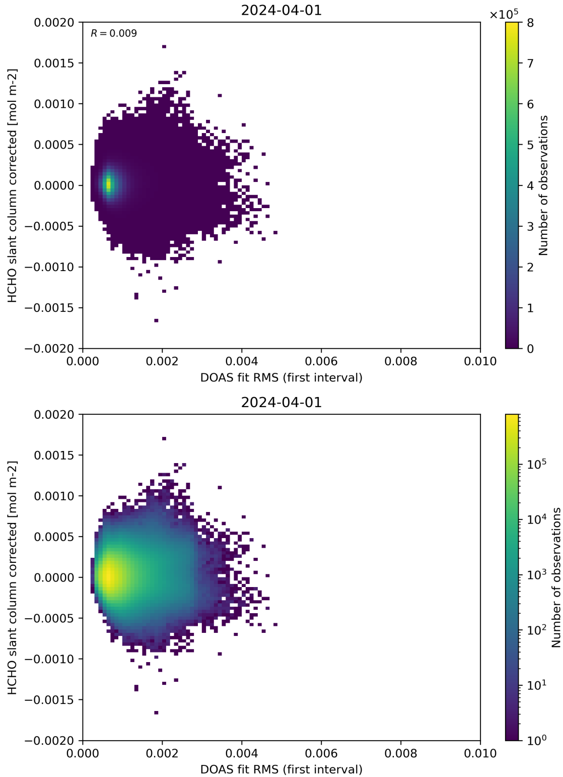
Figure 62: Scatter density plot of “DOAS fit RMS (first interval)” against “HCHO slant column corrected” for 2024-03-31 to 2024-04-02.
