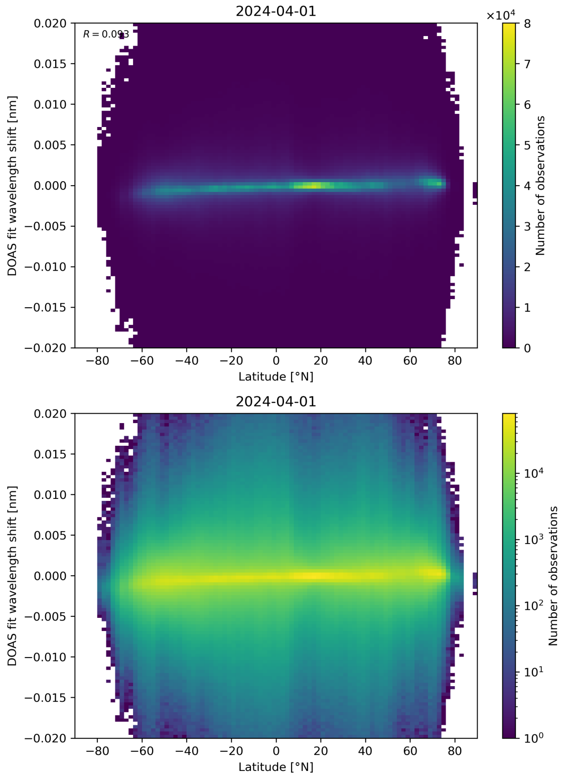
Figure 154: Scatter density plot of “Latitude” against “DOAS fit wavelength shift” for 2024-03-31 to 2024-04-02.
