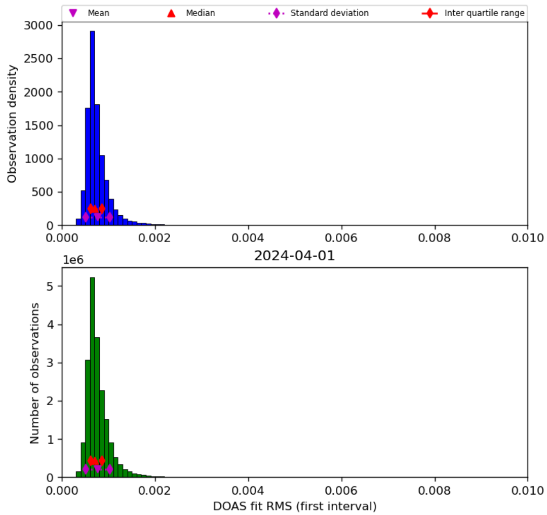
Figure 46: Histogram of “DOAS fit RMS (first interval)” for 2024-03-31 to 2024-04-02
