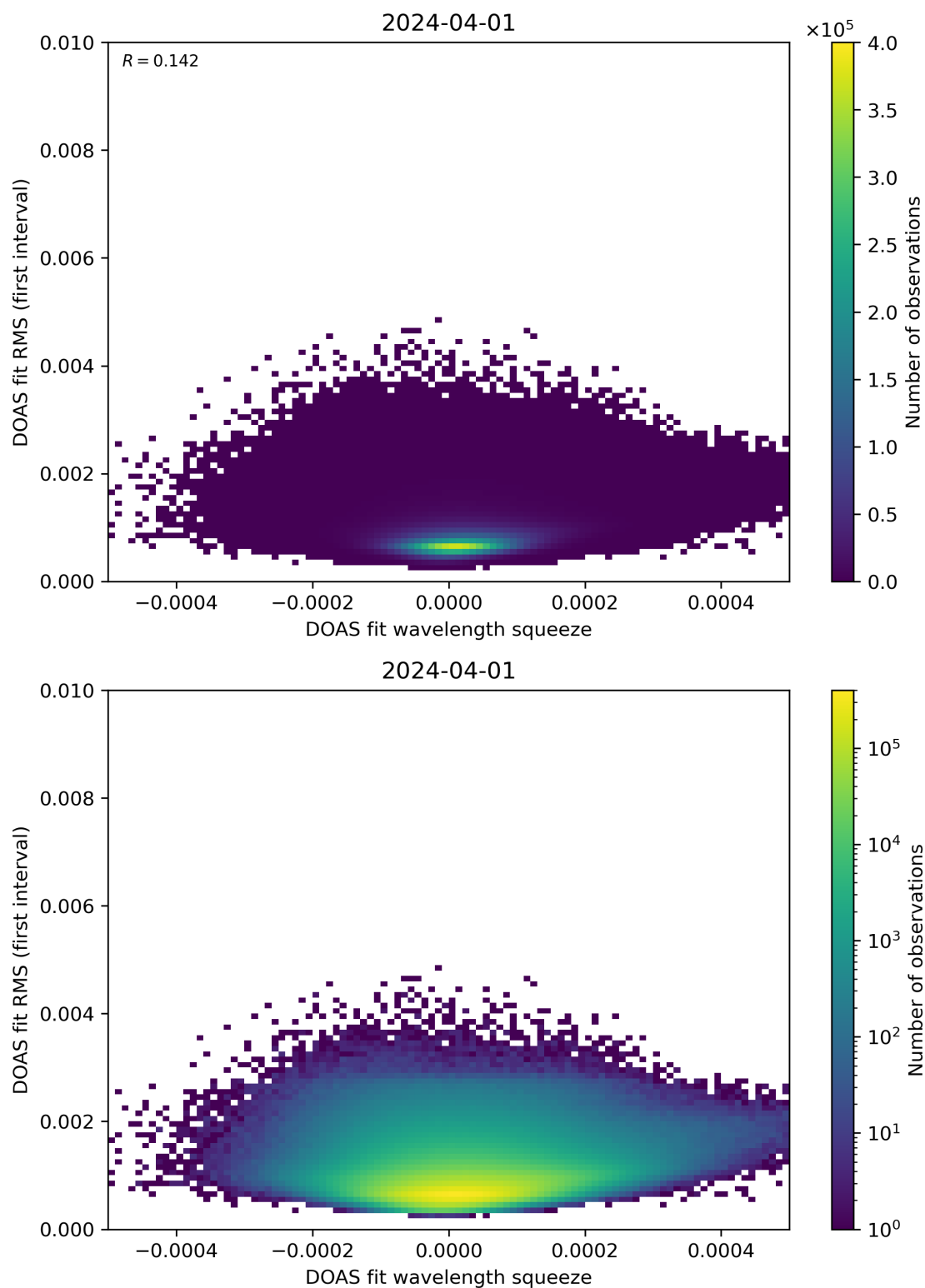
Figure 68: Scatter density plot of “DOAS fit wavelength squeeze” against “DOAS fit RMS (first interval)” for 2024-03-31 to 2024-04-02.
