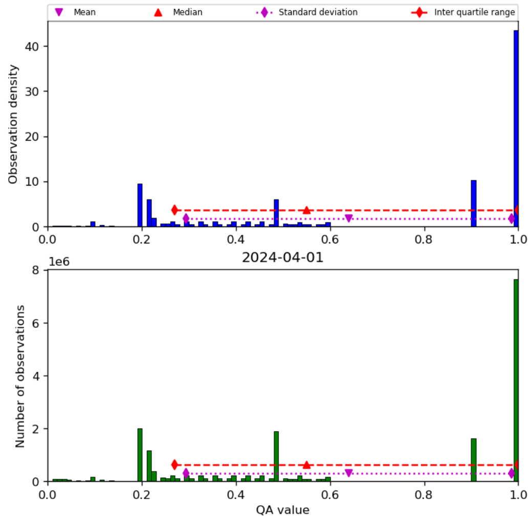
Figure 34: Histogram of “QA value” for 2024-03-31 to 2024-04-02
