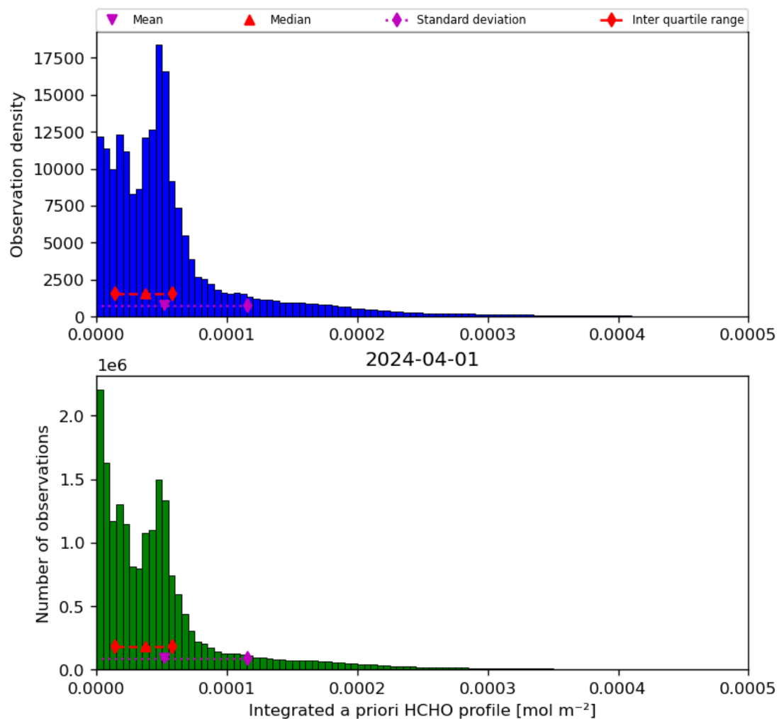
Figure 43: Histogram of “Integrated a priori HCHO profile” for 2024-03-31 to 2024-04-02
