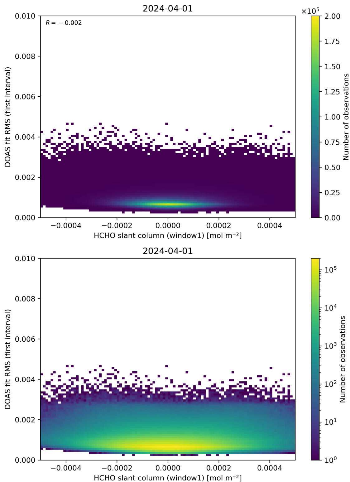
Figure 78: Scatter density plot of “HCHO slant column (window1)” against “DOAS fit RMS (first interval)” for 2024-03-31 to 2024-04-02.
