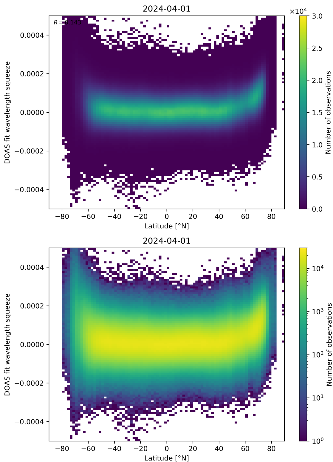
Figure 155: Scatter density plot of “Latitude” against “DOAS fit wavelength squeeze” for 2024-03-31 to 2024-04-02.
