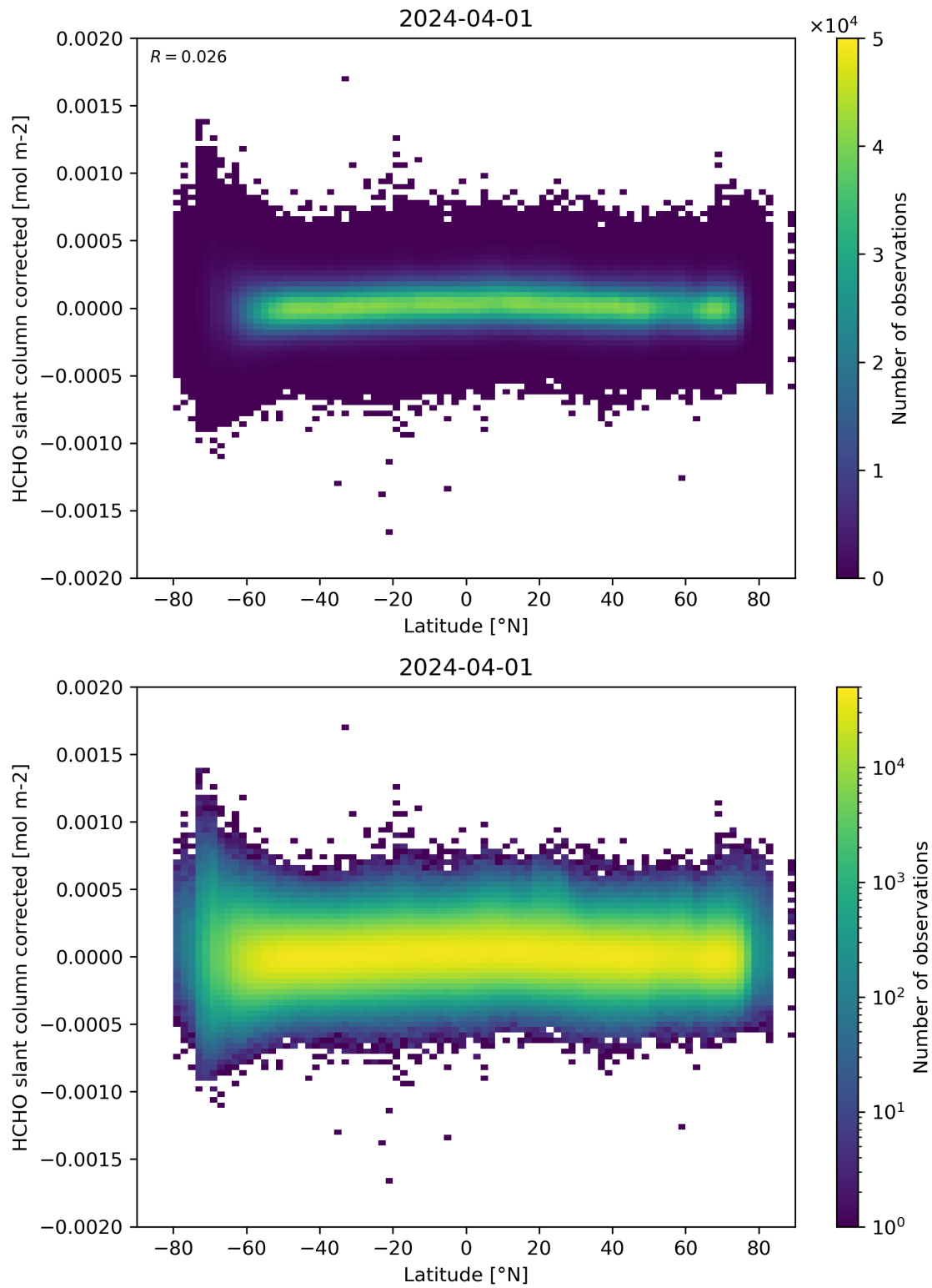
Figure 157: Scatter density plot of “Latitude” against “HCHO slant column corrected” for 2024-03-31 to 2024-04-02.
