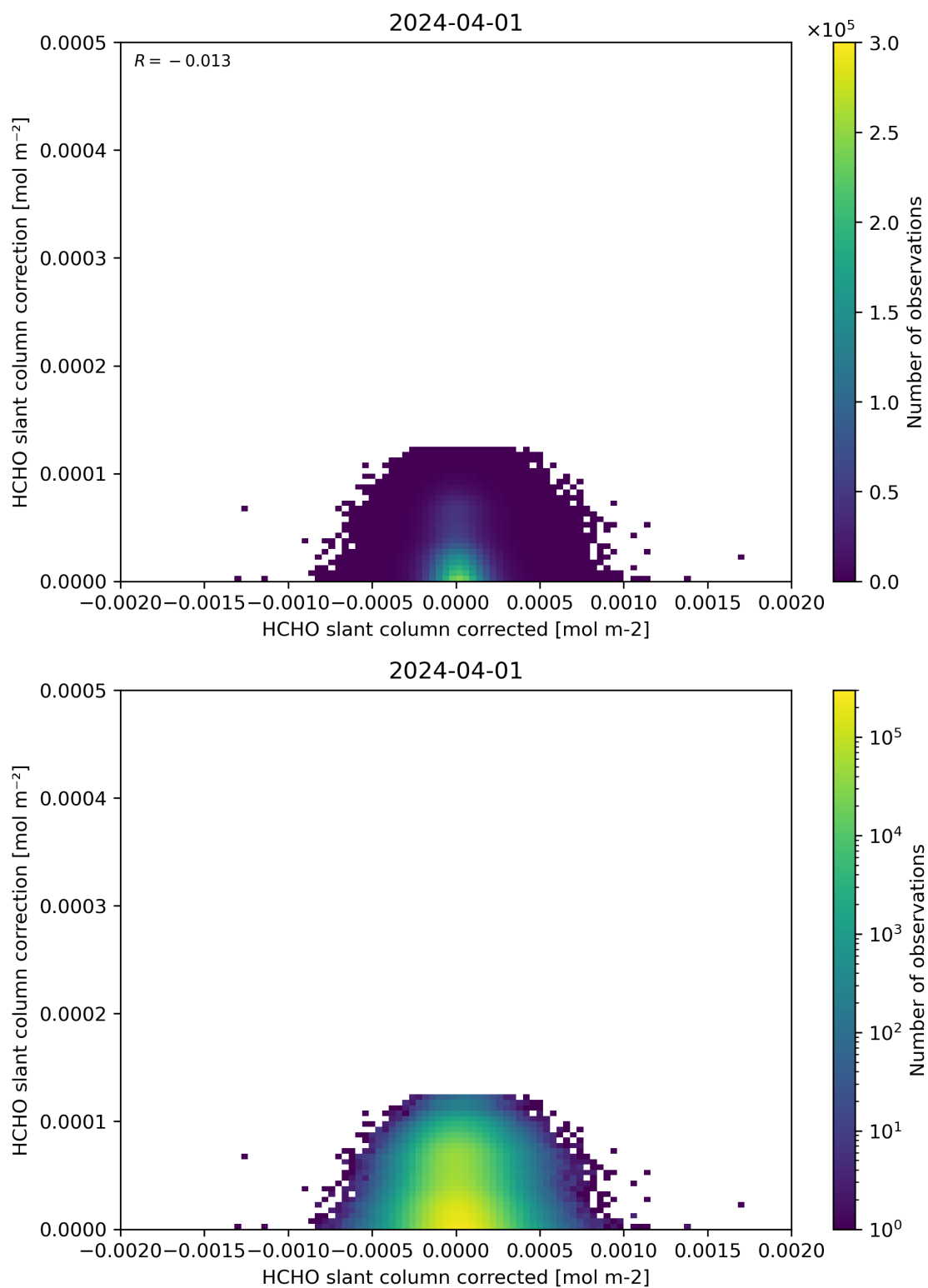
Figure 77: Scatter density plot of “HCHO slant column corrected” against “HCHO slant column correction” for 2024-03-31 to 2024-04-02.
