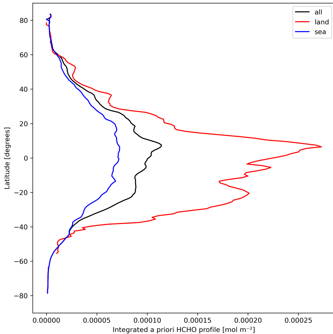
Figure 29: Zonal average of “Integrated a priori HCHO profile” for 2024-03-31 to 2024-04-02.
