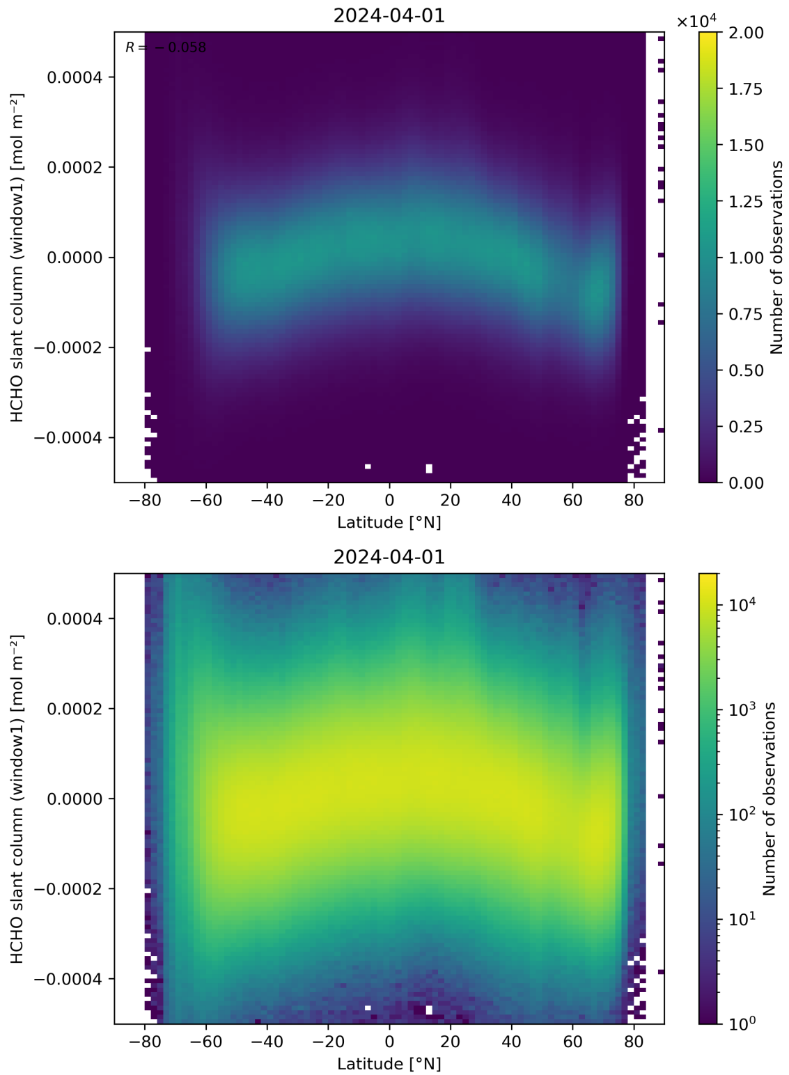
Figure 159: Scatter density plot of “Latitude” against “HCHO slant column (window1)” for 2024-03-31 to 2024-04-02.
