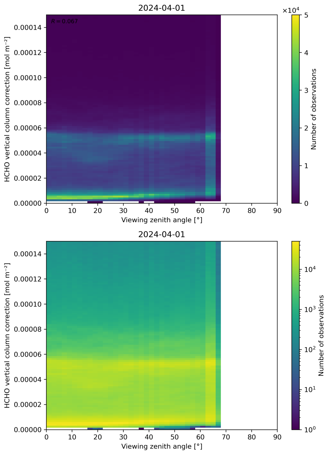
Figure 193: Scatter density plot of “Viewing zenith angle” against “HCHO vertical column correction” for 2024-03-31 to 2024-04-02.
