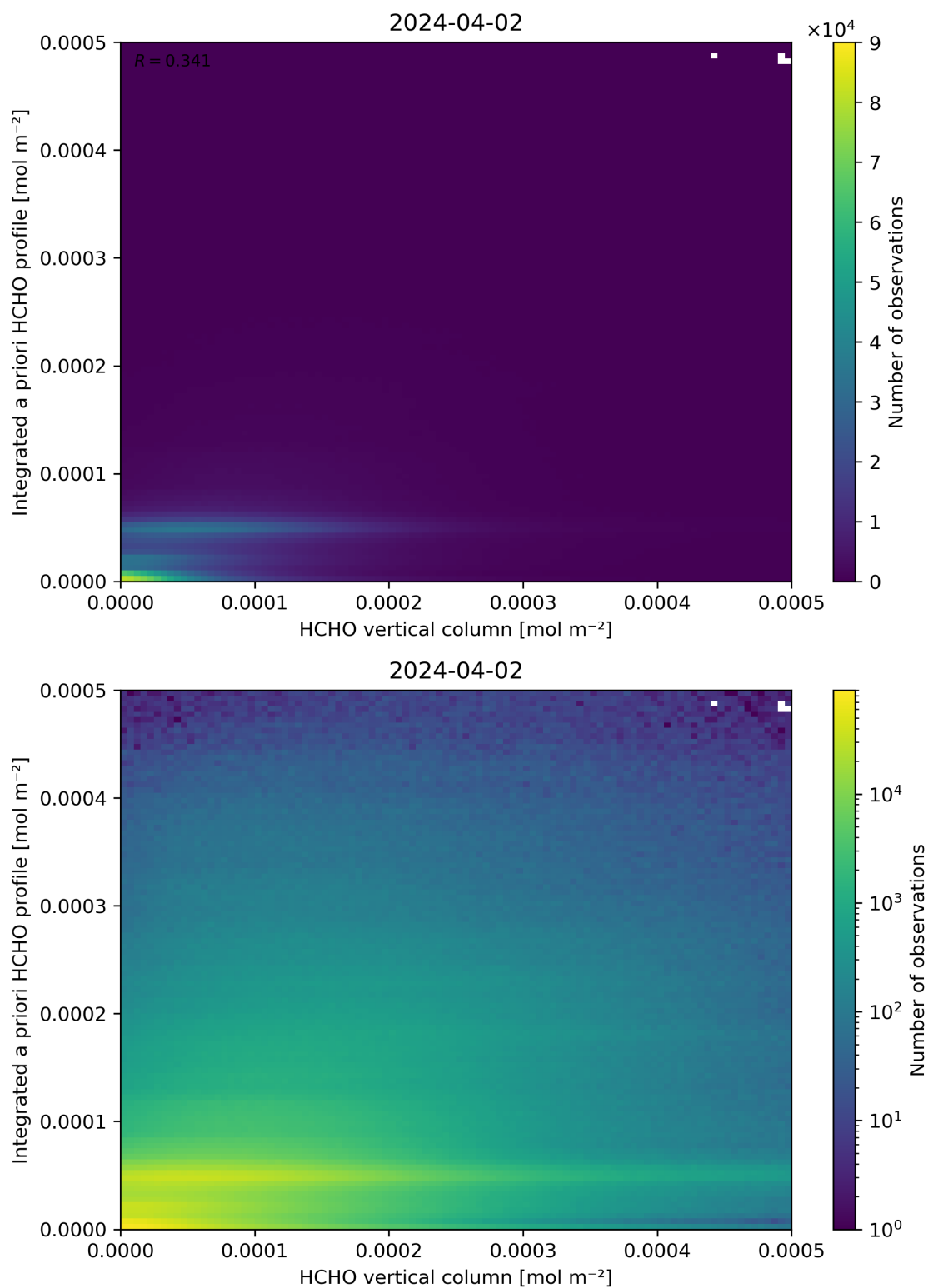
Figure 135: Scatter density plot of “HCHO vertical column” against “Integrated a priori HCHO profile” for 2024-04-01 to 2024-04-03.
