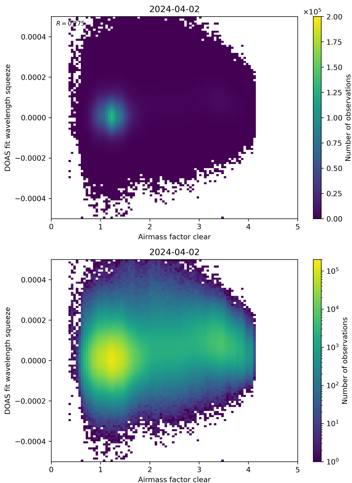
Figure 73: Scatter density plot of “Airmass factor clear” against “DOAS fit wavelength squeeze” for 2024-04-01 to 2024-04-03.
