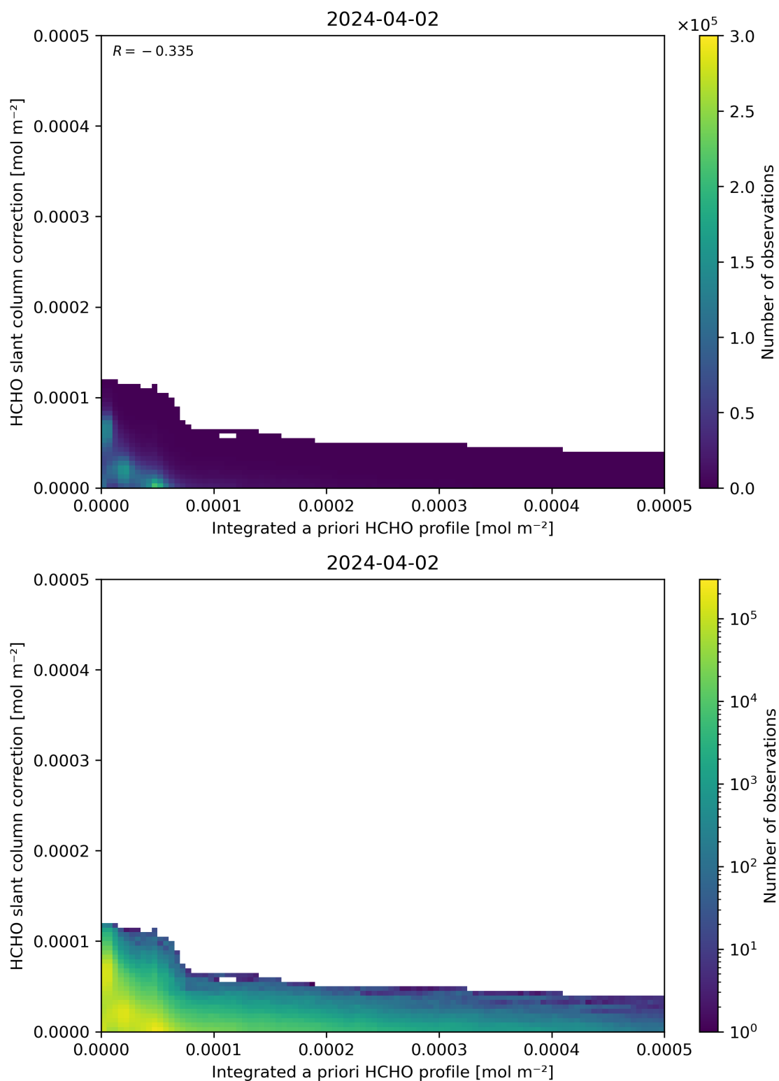
Figure 152: Scatter density plot of “Integrated a priori HCHO profile” against “HCHO slant column correction” for 2024-04-01 to 2024-04-03.
