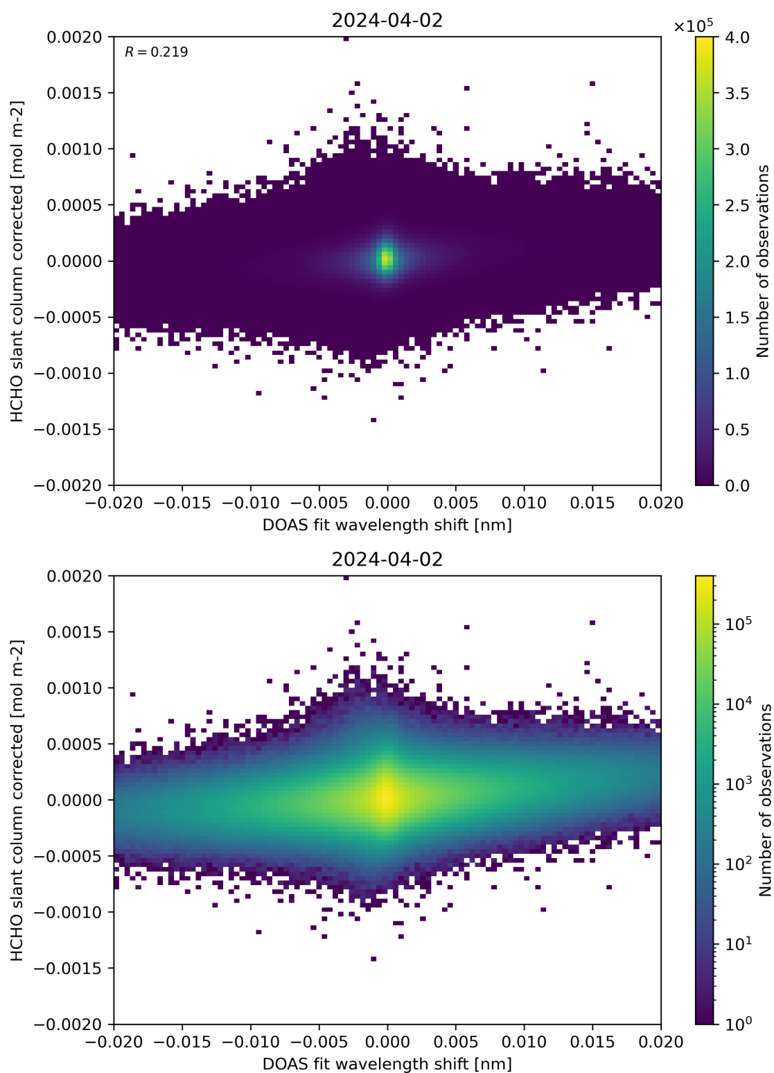
Figure 66: Scatter density plot of “DOAS fit wavelength shift” against “HCHO slant column corrected” for 2024-04-01 to 2024-04-03.
