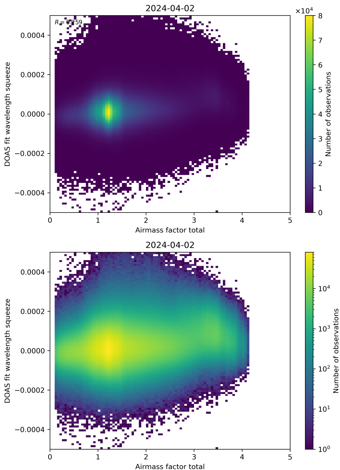
Figure 99: Scatter density plot of “Airmass factor total” against “DOAS fit wavelength squeeze” for 2024-04-01 to 2024-04-03.
