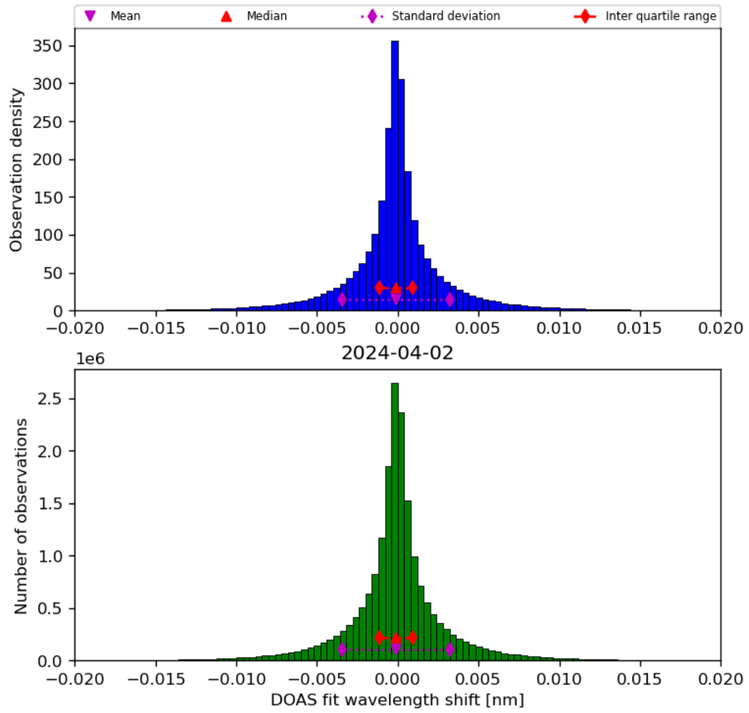
Figure 44: Histogram of “DOAS fit wavelength shift” for 2024-04-01 to 2024-04-03
