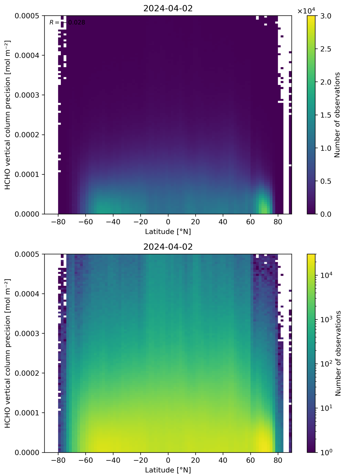
Figure 165: Scatter density plot of “Latitude” against “HCHO vertical column precision” for 2024-04-01 to 2024-04-03.
