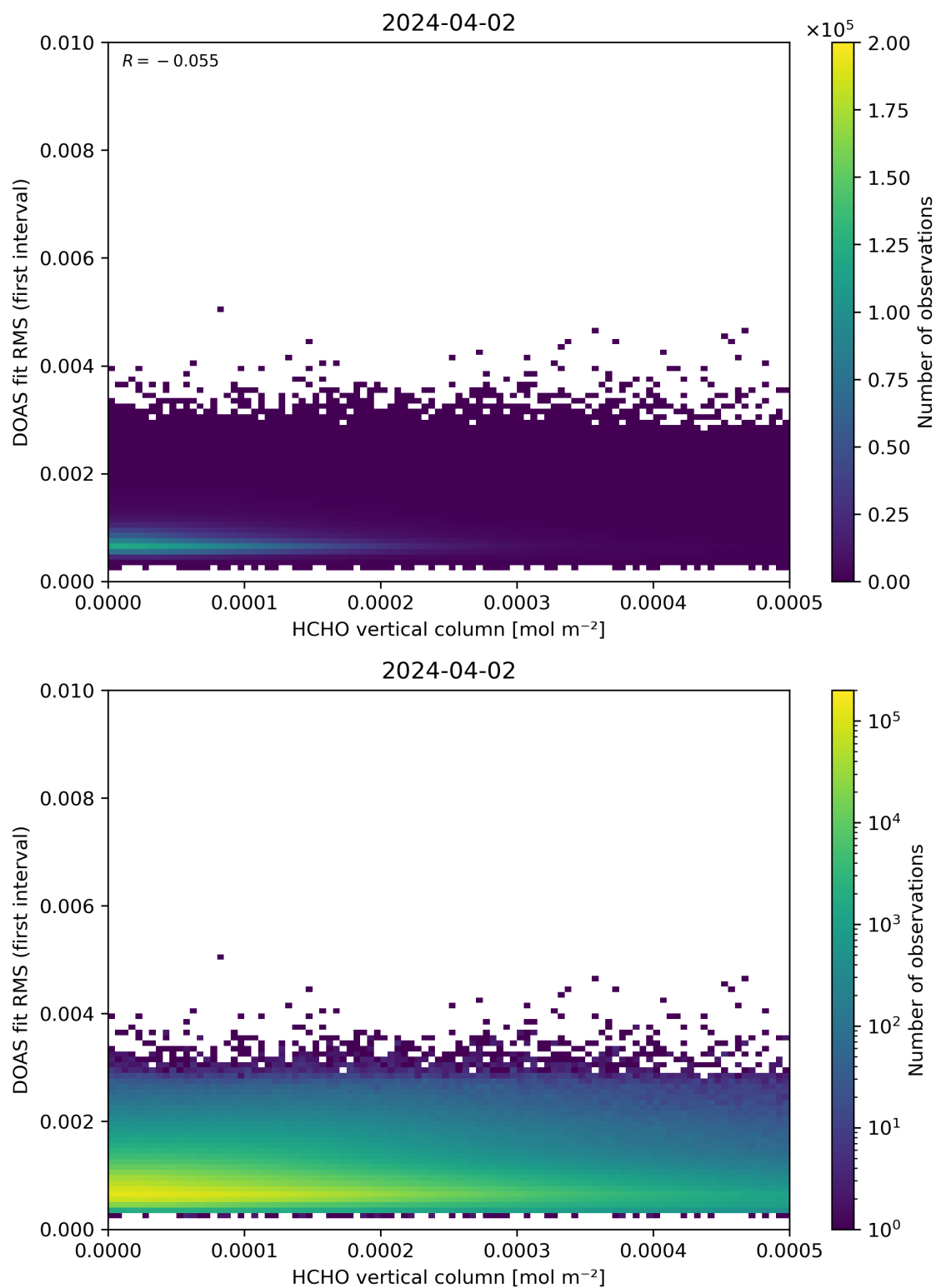
Figure 123: Scatter density plot of “HCHO vertical column” against “DOAS fit RMS (first interval)” for 2024-04-01 to 2024-04-03.
