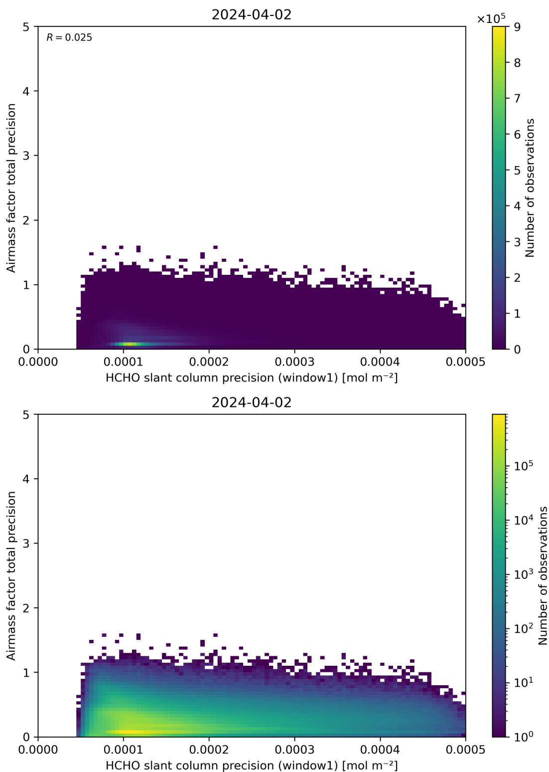
Figure 95: Scatter density plot of “HCHO slant column precision (window1)” against “Airmass factor total precision” for 2024-04-01 to 2024-04-03.
