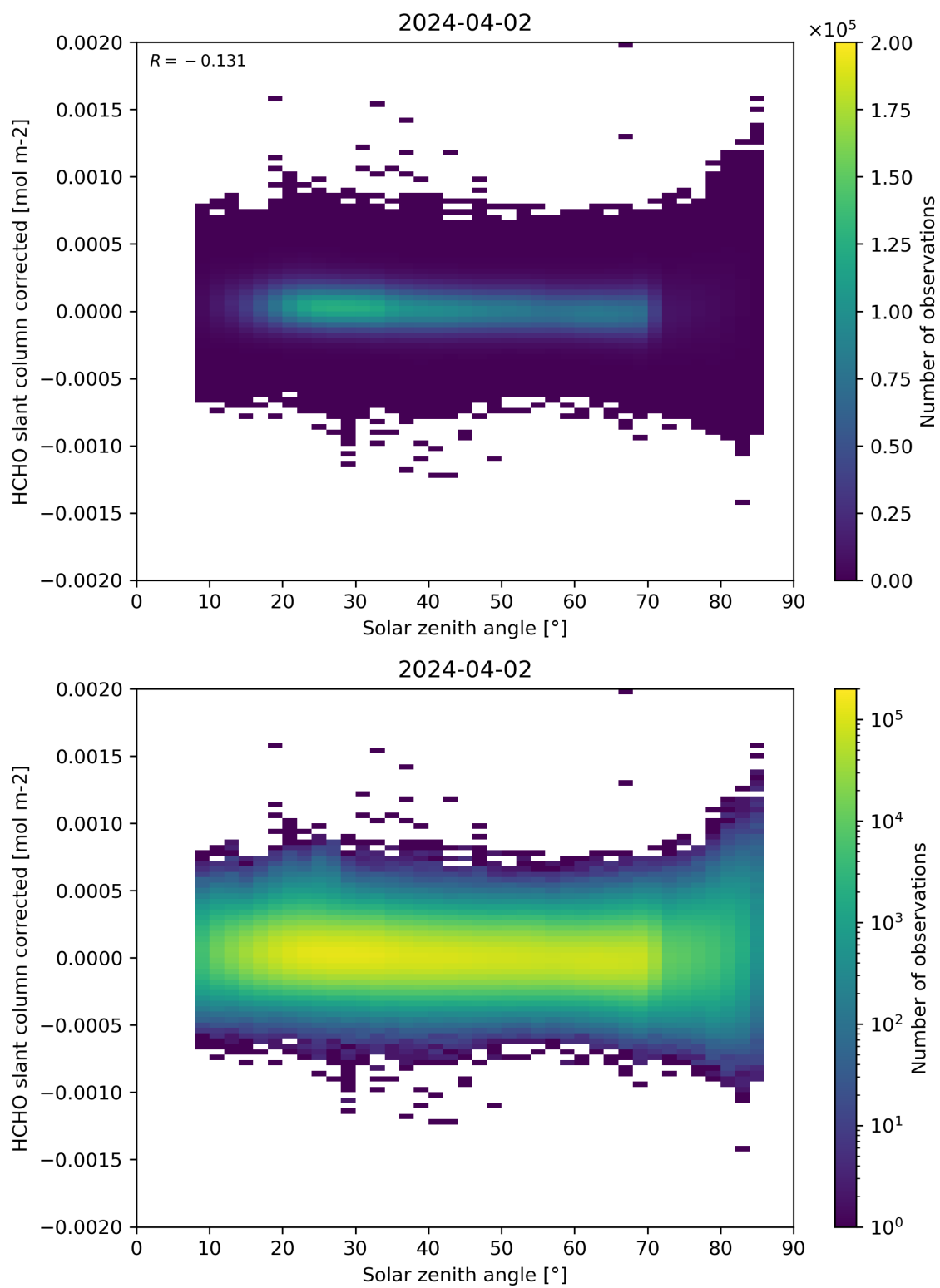
Figure 171: Scatter density plot of “Solar zenith angle” against “HCHO slant column corrected” for 2024-04-01 to 2024-04-03.
