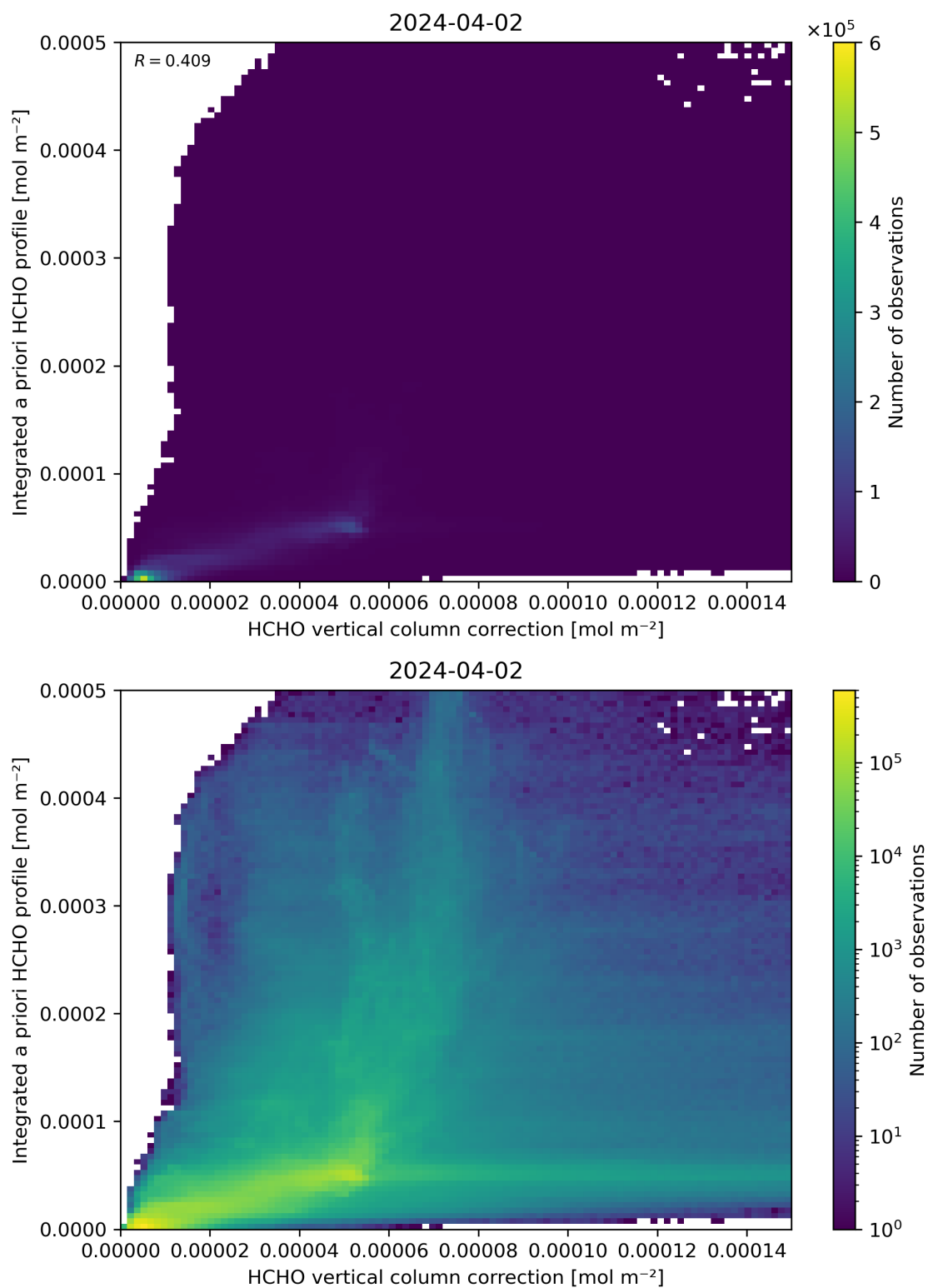
Figure 122: Scatter density plot of “HCHO vertical column correction” against “Integrated a priori HCHO profile” for 2024-04-01 to 2024-04-03.
