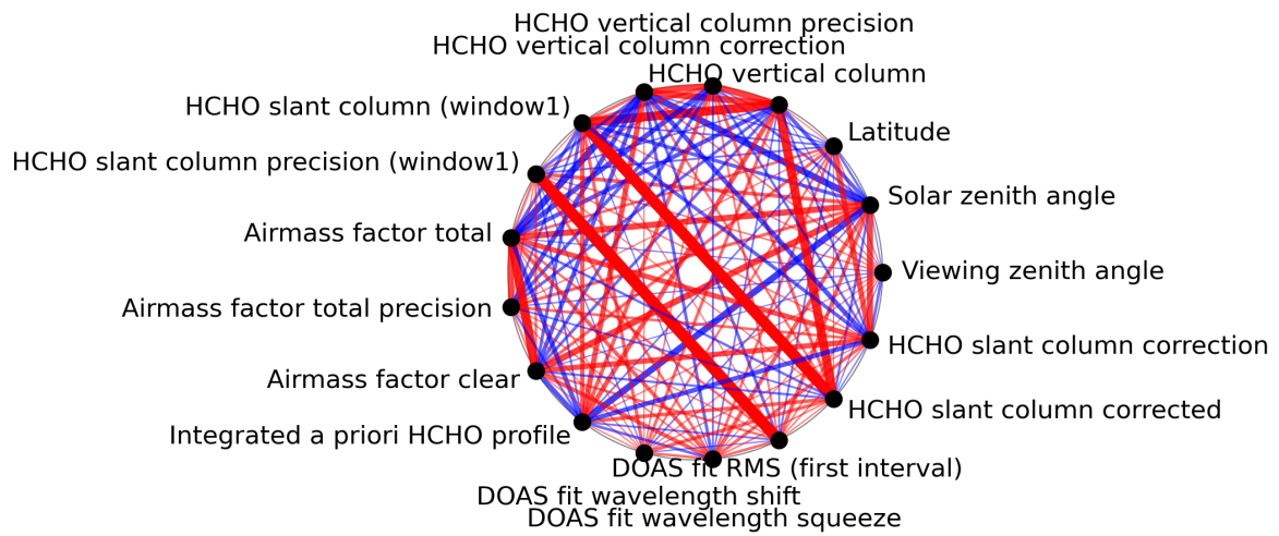
Figure 1: Map of correlation graph for 2024-04-01 to 2024-04-03.
