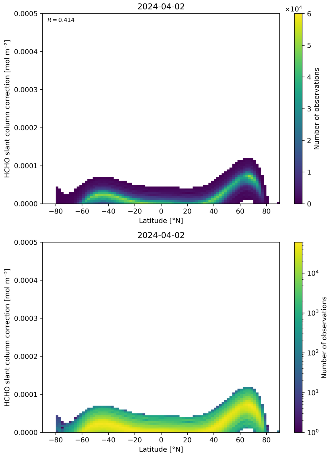
Figure 158: Scatter density plot of “Latitude” against “HCHO slant column correction” for 2024-04-01 to 2024-04-03.
