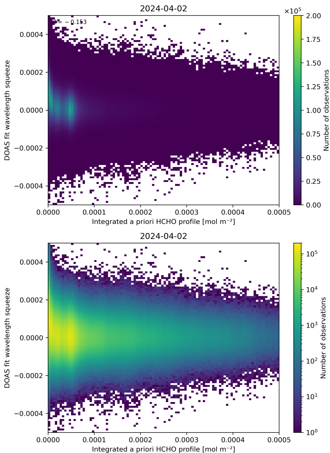
Figure 150: Scatter density plot of “Integrated a priori HCHO profile” against “DOAS fit wavelength squeeze” for 2024-04-01 to 2024-04-03.
