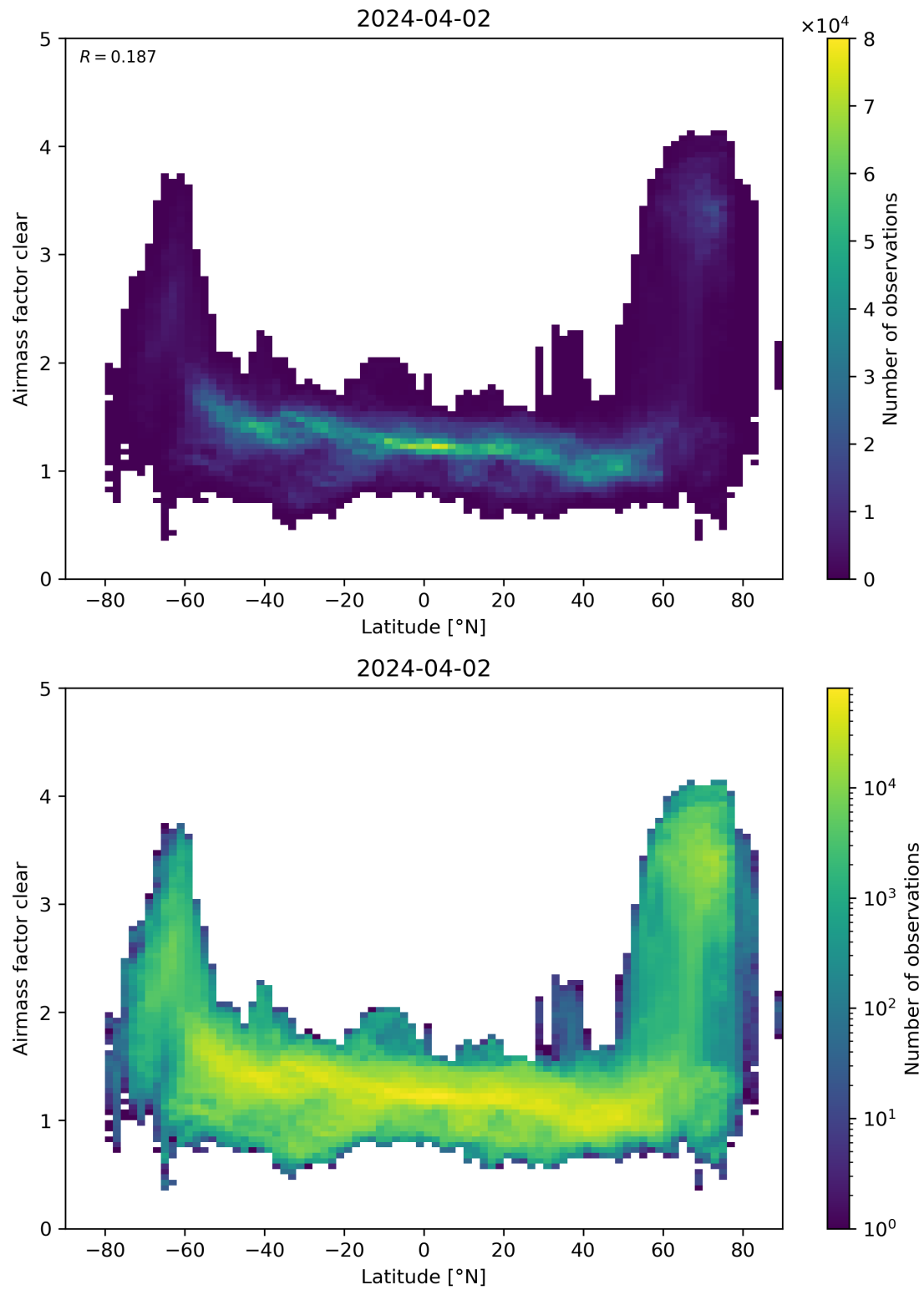
Figure 156: Scatter density plot of “Latitude” against “Airmass factor clear” for 2024-04-01 to 2024-04-03.
