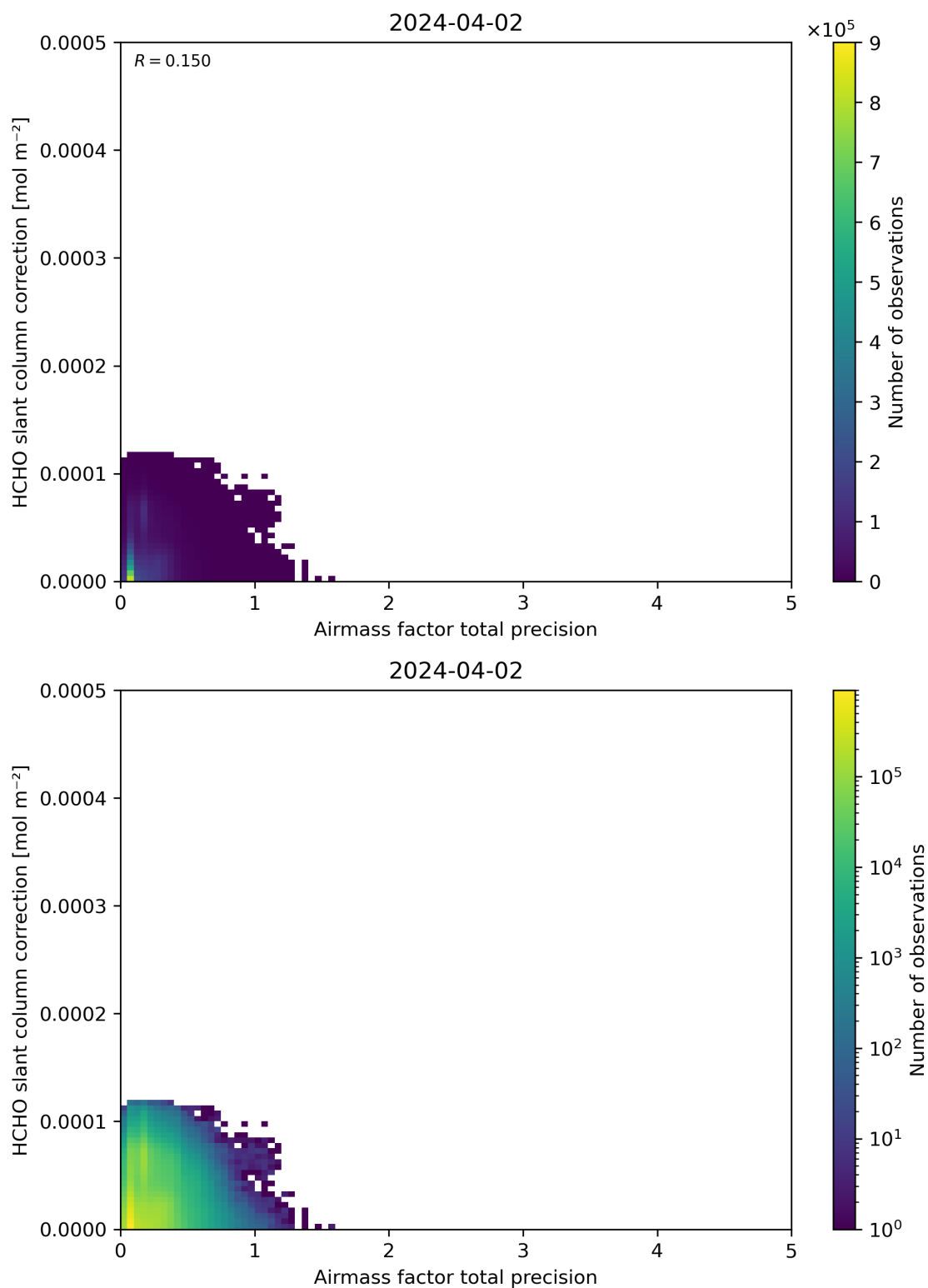
Figure 110: Scatter density plot of “Airmass factor total precision” against “HCHO slant column correction” for 2024-04-01 to 2024-04-03.
