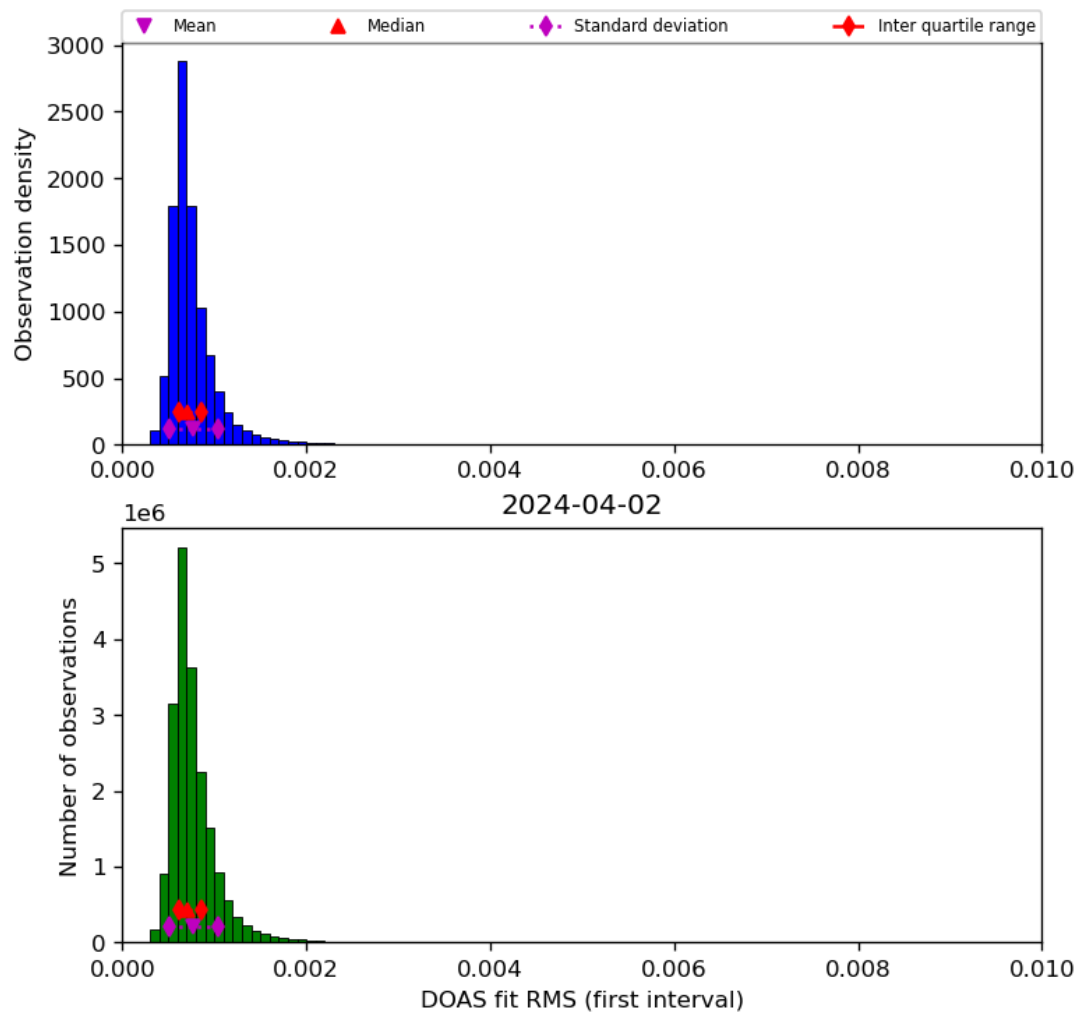
Figure 46: Histogram of “DOAS fit RMS (first interval)” for 2024-04-01 to 2024-04-03
