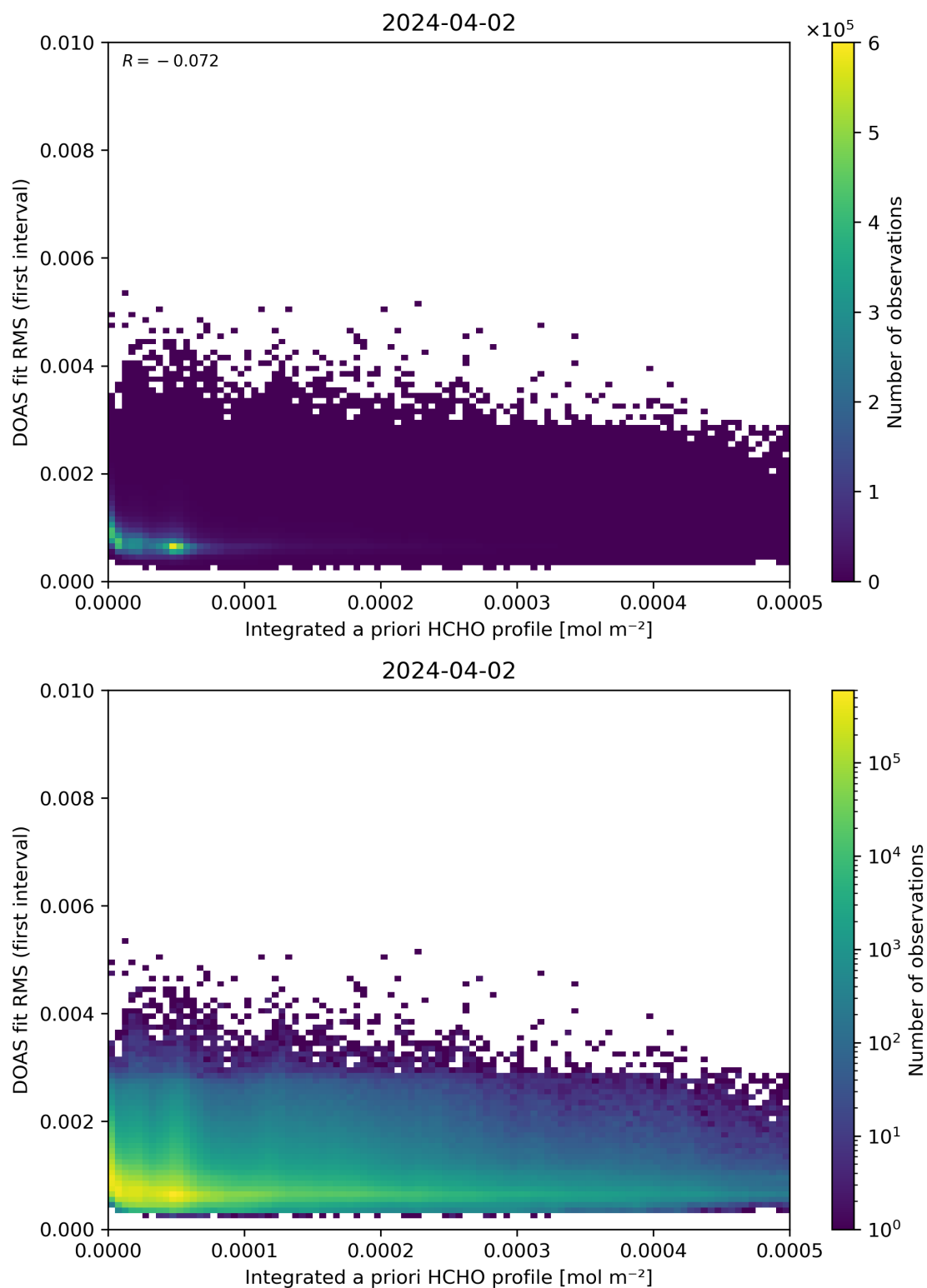
Figure 148: Scatter density plot of “Integrated a priori HCHO profile” against “DOAS fit RMS (first interval)” for 2024-04-01 to 2024-04-03.
