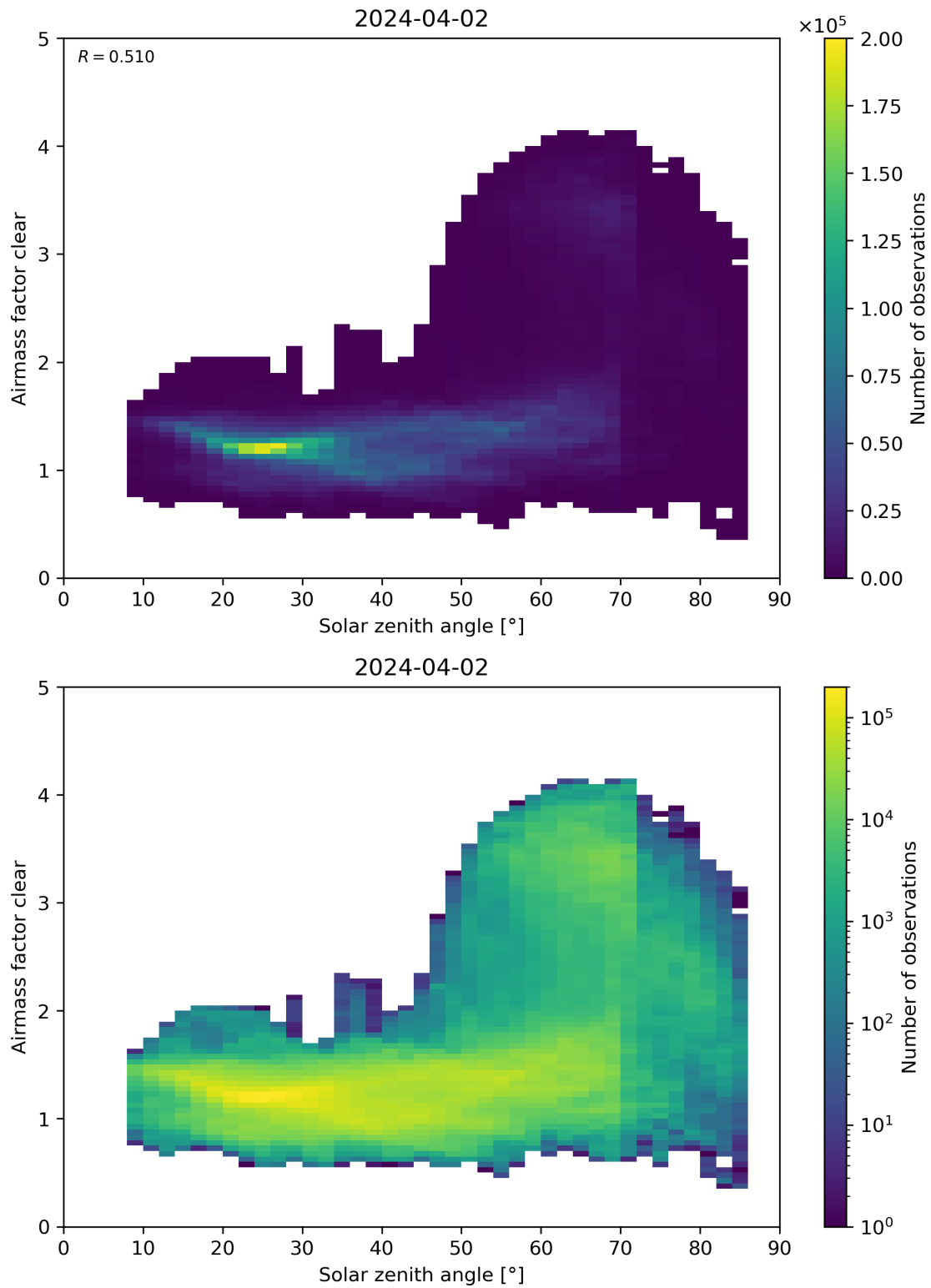
Figure 170: Scatter density plot of “Solar zenith angle” against “Airmass factor clear” for 2024-04-01 to 2024-04-03.
