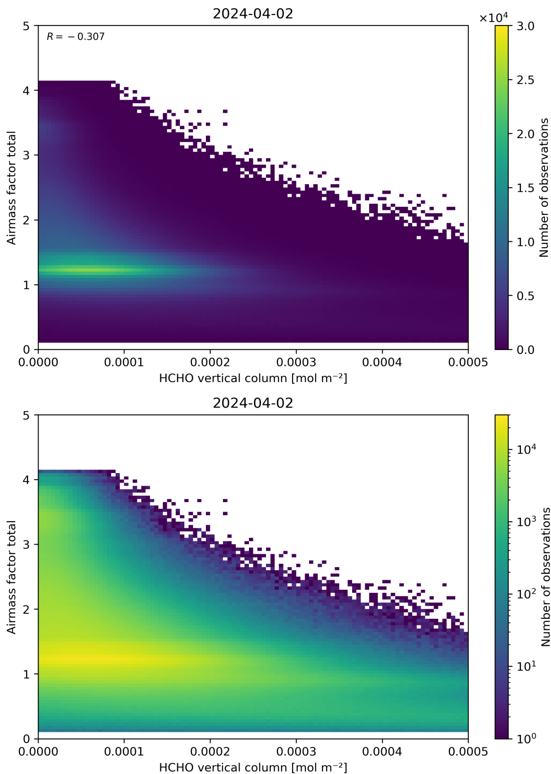
Figure 131: Scatter density plot of “HCHO vertical column” against “Airmass factor total” for 2024-04-01 to 2024-04-03.
