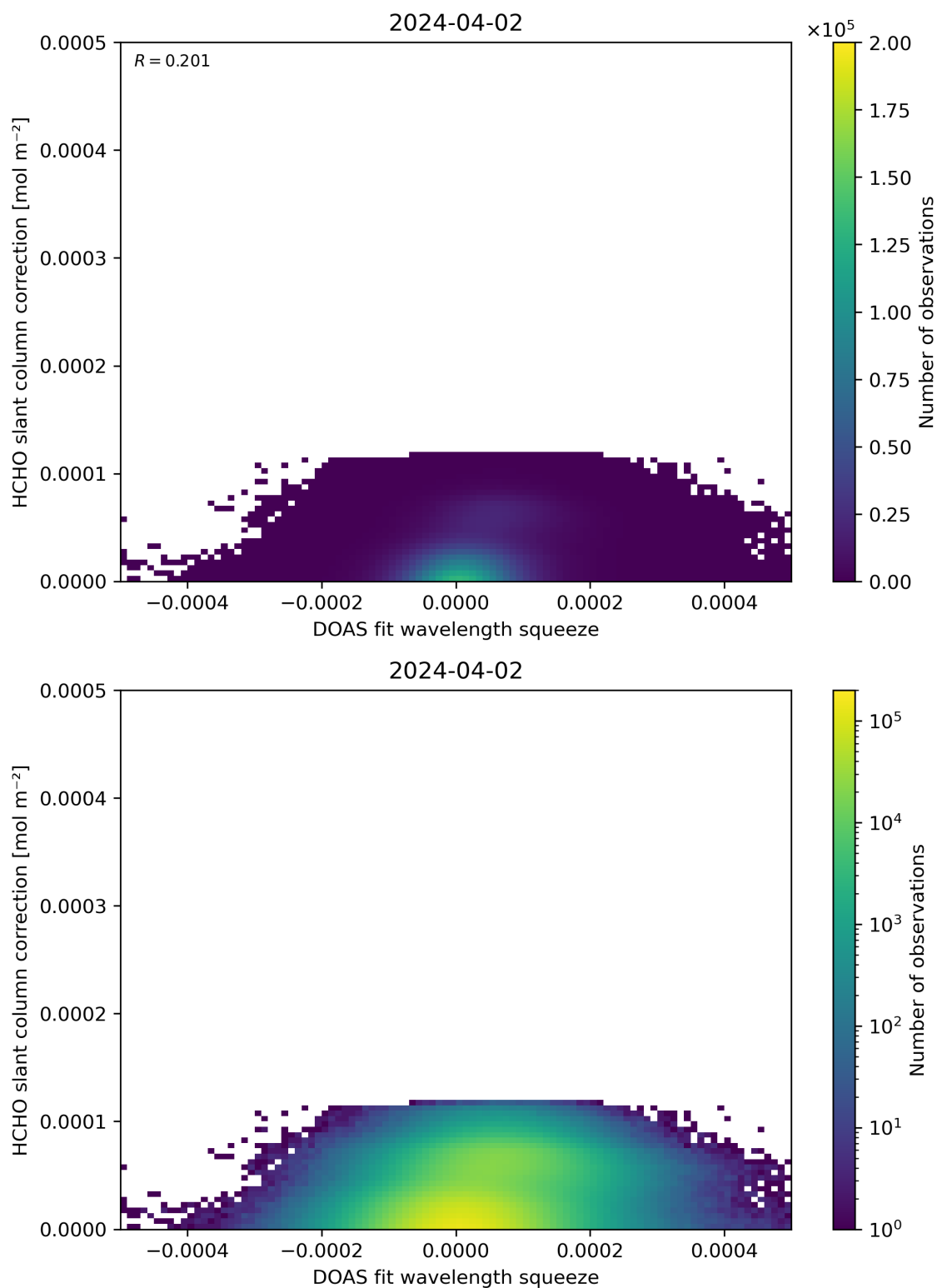
Figure 70: Scatter density plot of “DOAS fit wavelength squeeze” against “HCHO slant column correction” for 2024-04-01 to 2024-04-03.
