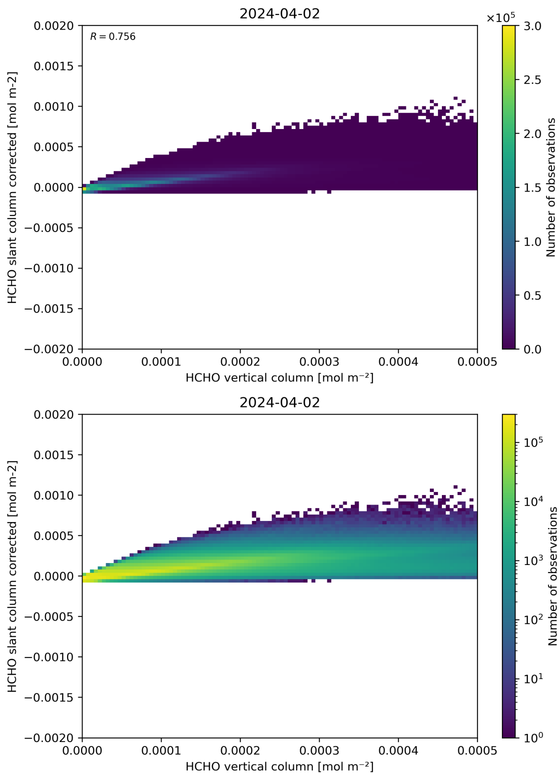
Figure 127: Scatter density plot of “HCHO vertical column” against “HCHO slant column corrected” for 2024-04-01 to 2024-04-03.
