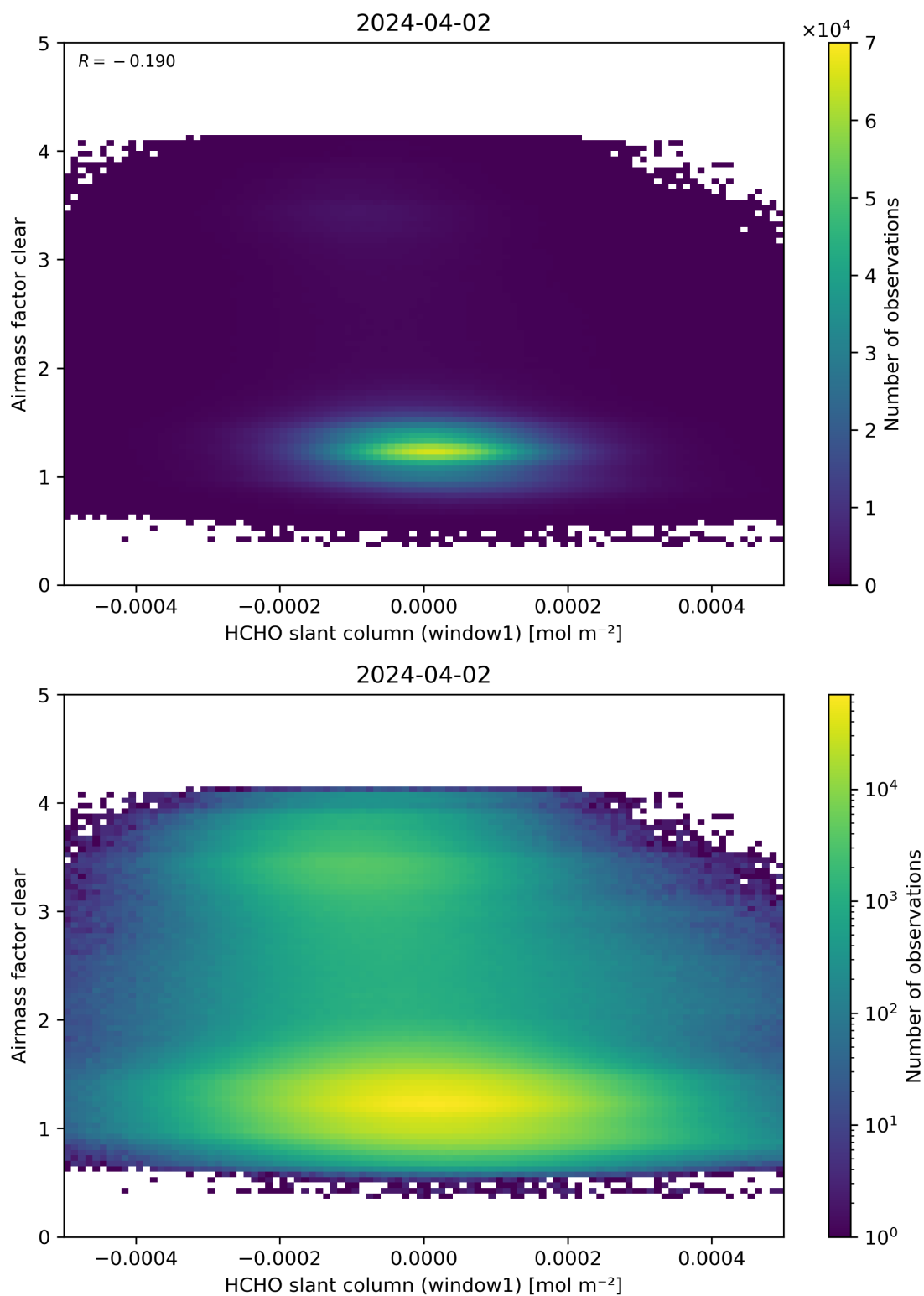
Figure 81: Scatter density plot of “HCHO slant column (window1)” against “Airmass factor clear” for 2024-04-01 to 2024-04-03.
