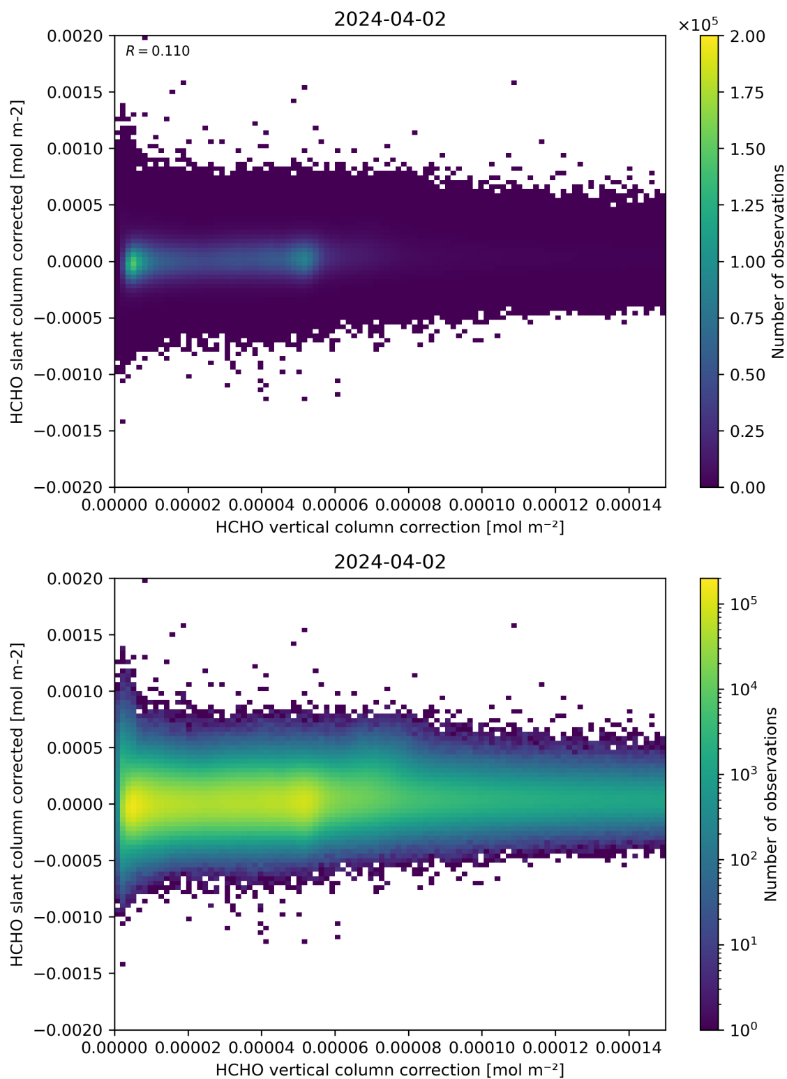
Figure 116: Scatter density plot of “HCHO vertical column correction” against “HCHO slant column corrected” for 2024-04-01 to 2024-04-03.
