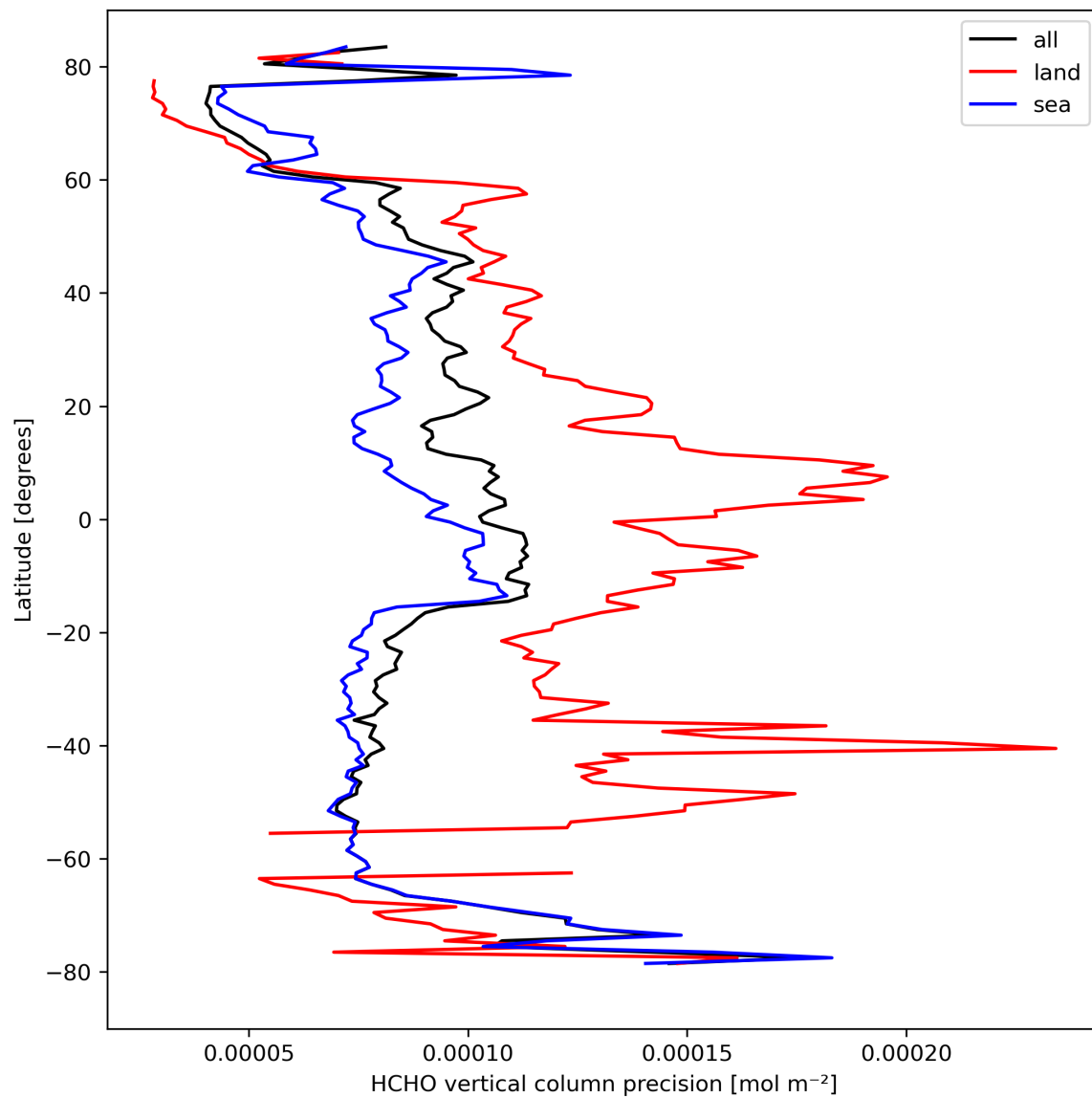
Figure 22: Zonal average of “HCHO vertical column precision” for 2024-04-01 to 2024-04-03.
