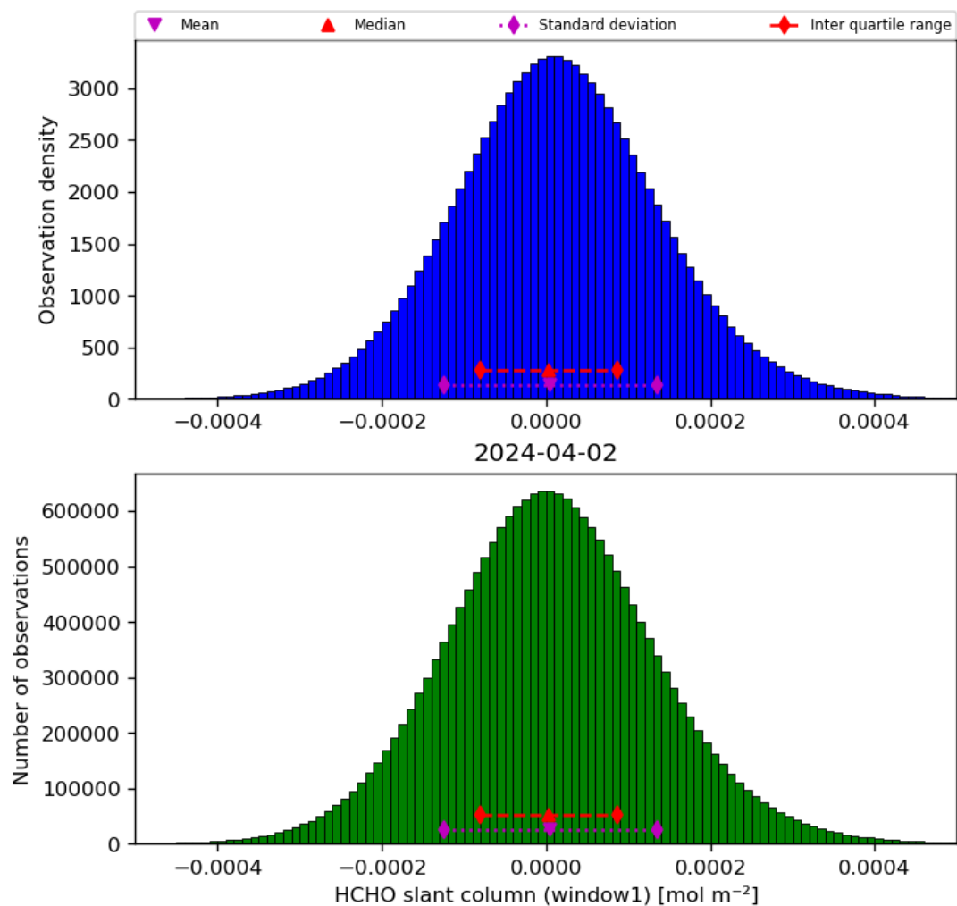
Figure 38: Histogram of “HCHO slant column (window1)” for 2024-04-01 to 2024-04-03
