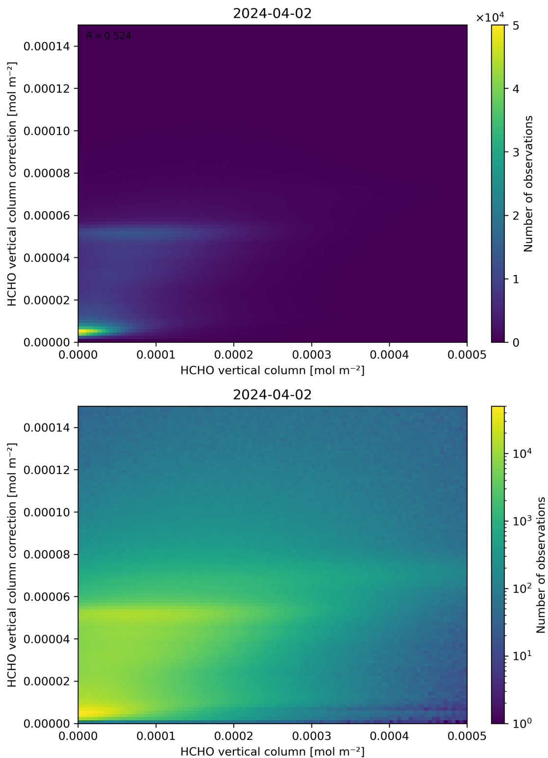
Figure 133: Scatter density plot of “HCHO vertical column” against “HCHO vertical column correction” for 2024-04-01 to 2024-04-03.
