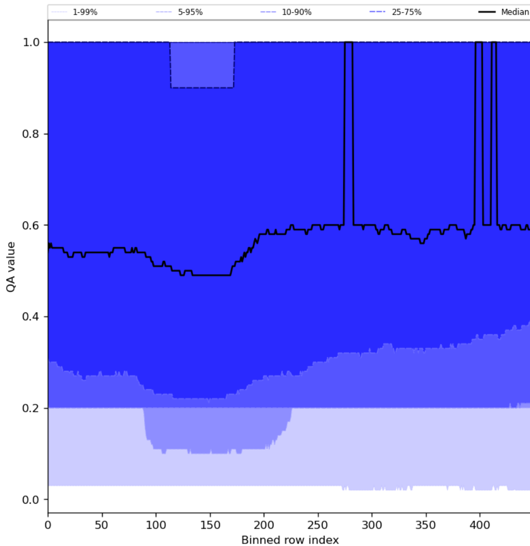
Figure 48: Along track statistics of "QA value" for 2024-04-01 to 2024-04-03
