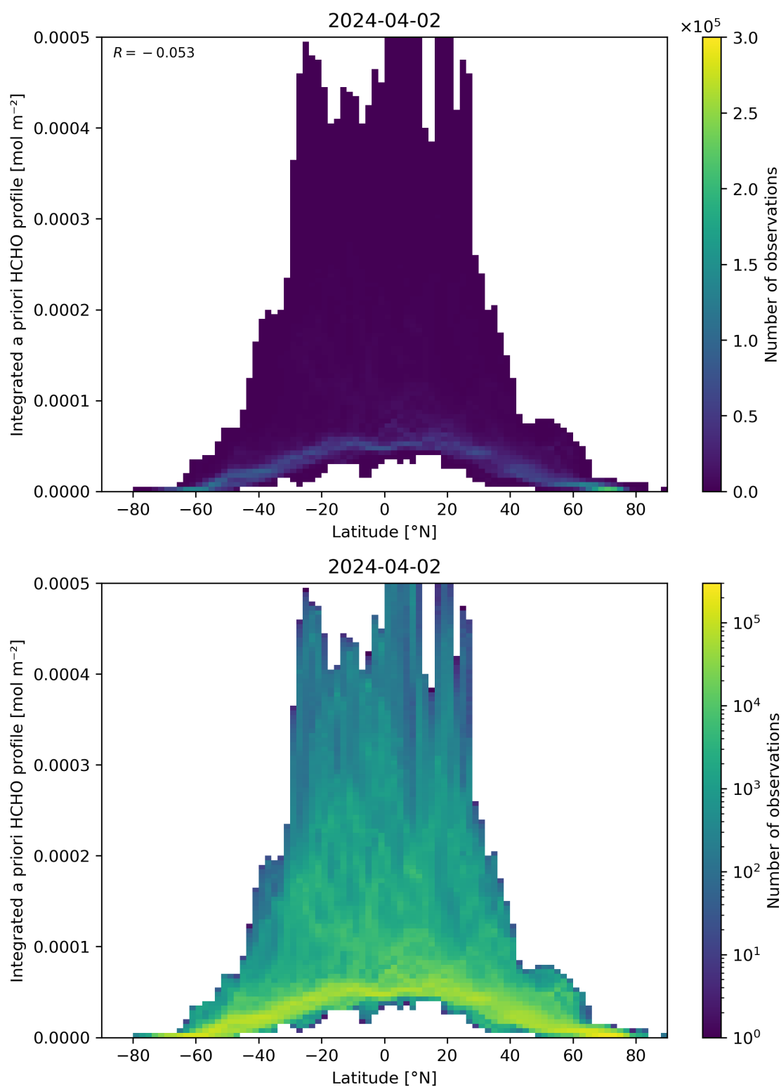
Figure 166: Scatter density plot of “Latitude” against “Integrated a priori HCHO profile” for 2024-04-01 to 2024-04-03.
