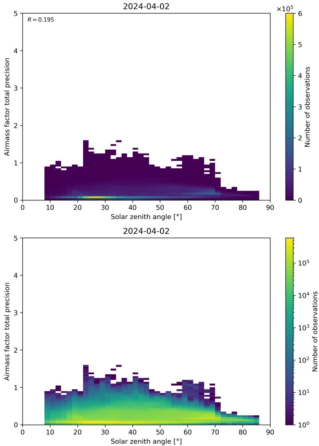
Figure 176: Scatter density plot of “Solar zenith angle” against “Airmass factor total precision” for 2024-04-01 to 2024-04-03.
