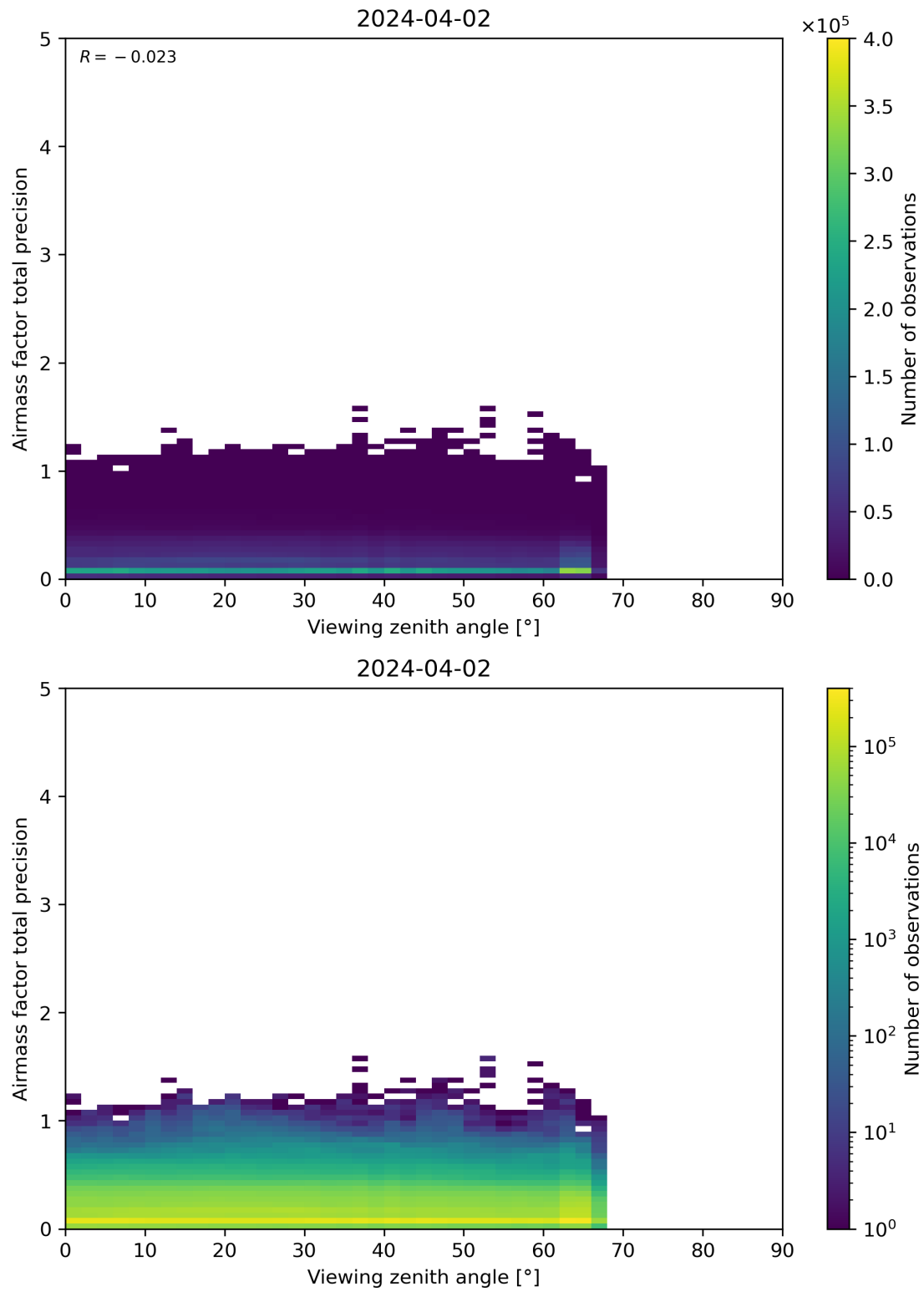
Figure 191: Scatter density plot of “Viewing zenith angle” against “Airmass factor total precision” for 2024-04-01 to 2024-04-03.
