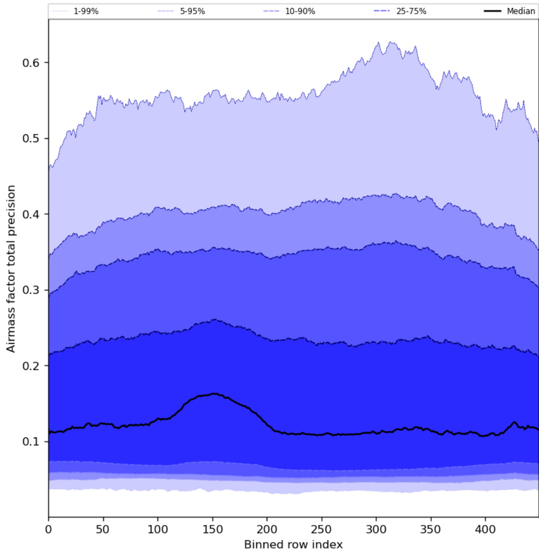
Figure 55: Along track statistics of “Airmass factor total precision” for 2024-04-01 to 2024-04-03
