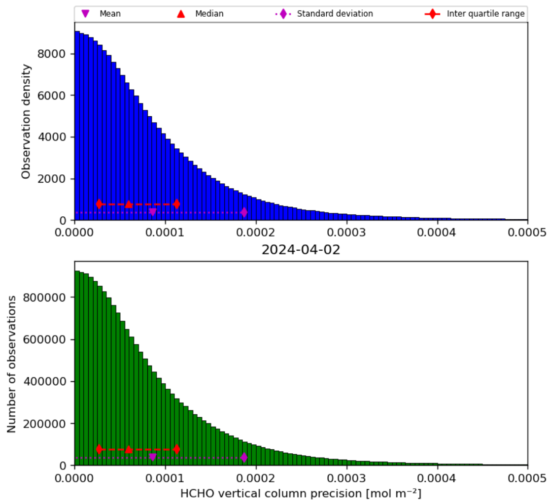
Figure 36: Histogram of “HCHO vertical column precision” for 2024-04-01 to 2024-04-03
