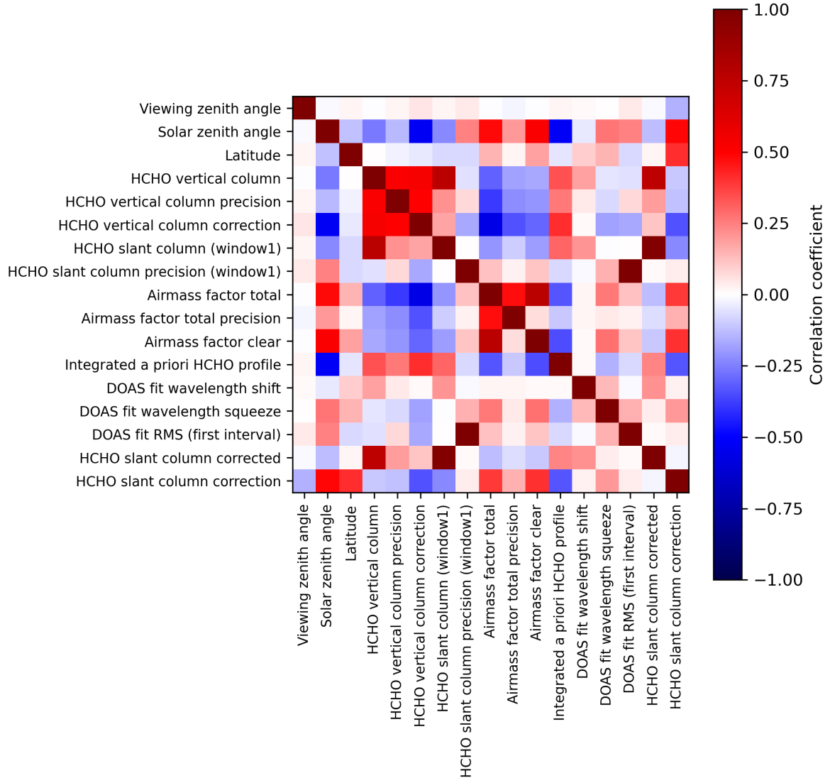
Figure 2: Map of correlation matrix for 2024-04-01 to 2024-04-03.
