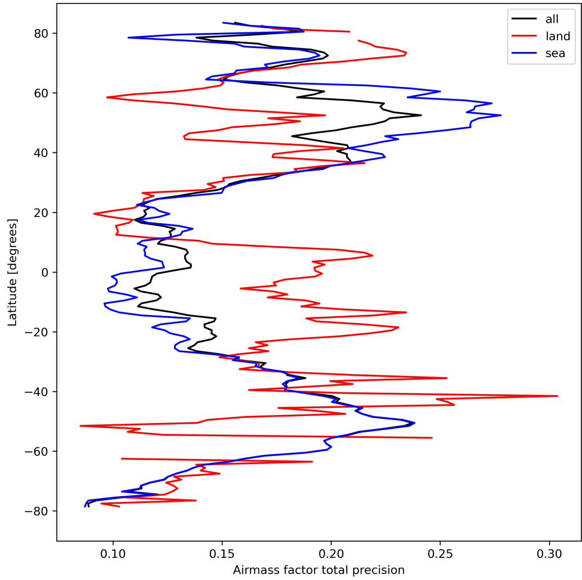
Figure 27: Zonal average of “Airmass factor total precision” for 2024-04-01 to 2024-04-03.
