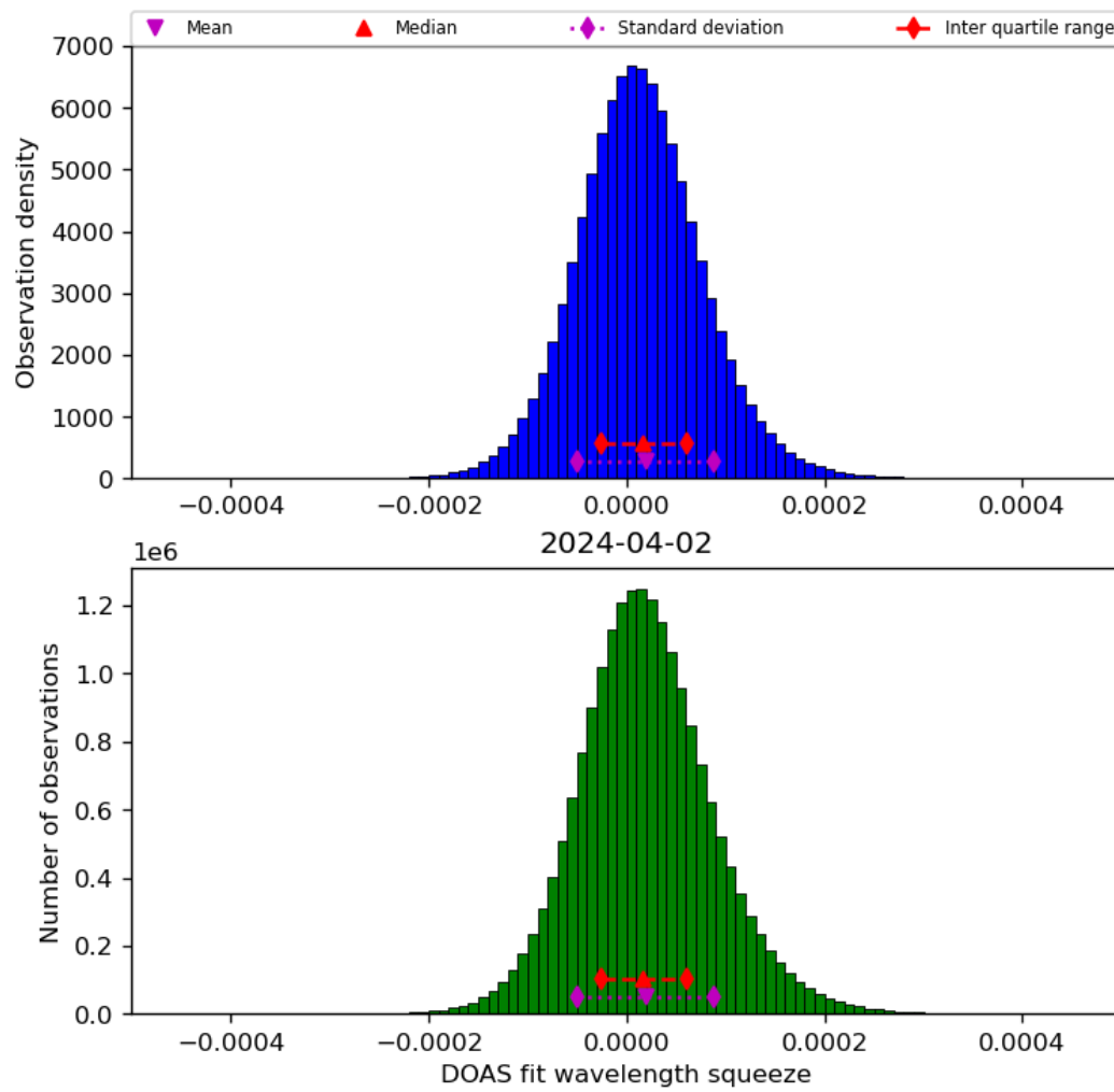
Figure 45: Histogram of “DOAS fit wavelength squeeze” for 2024-04-01 to 2024-04-03
