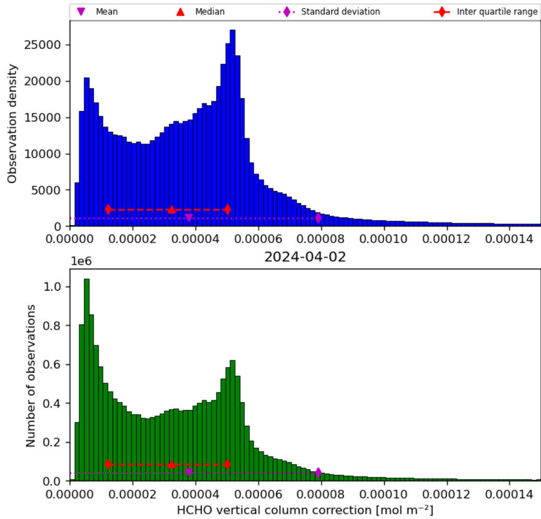
Figure 37: Histogram of “HCHO vertical column correction” for 2024-04-01 to 2024-04-03
