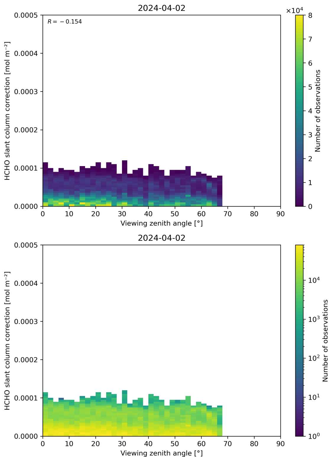
Figure 187: Scatter density plot of “Viewing zenith angle” against “HCHO slant column correction” for 2024-04-01 to 2024-04-03.
