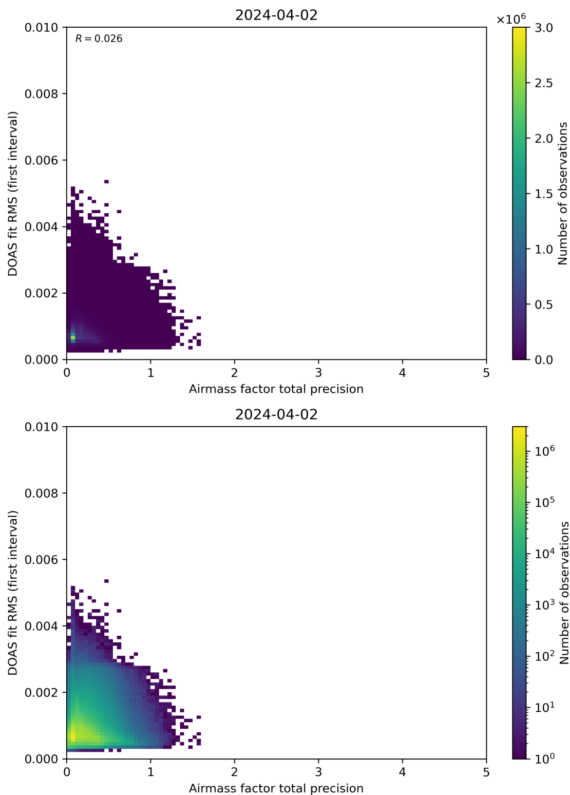
Figure 105: Scatter density plot of “Airmass factor total precision” against “DOAS fit RMS (first interval)” for 2024-04-01 to 2024-04-03.
