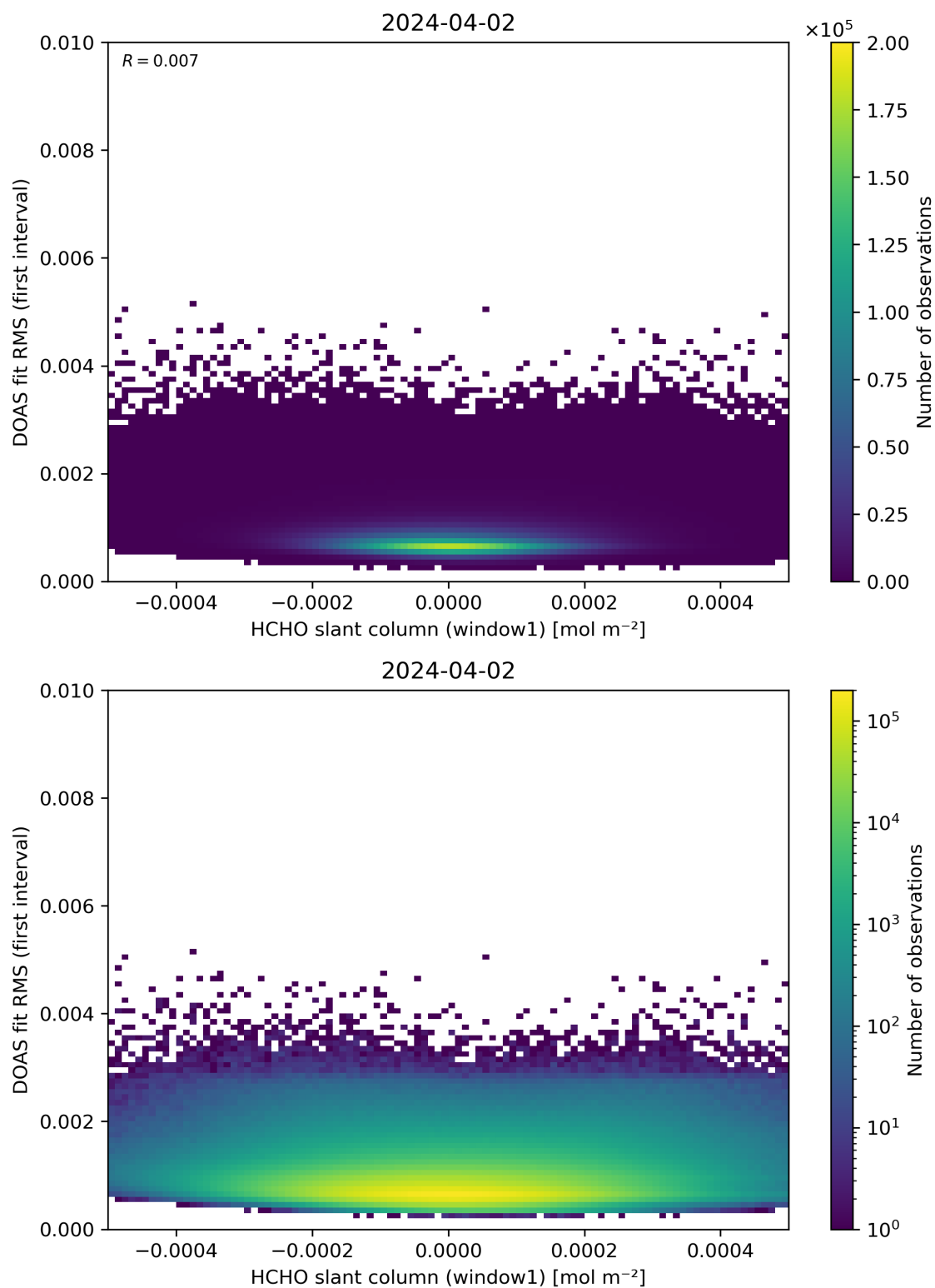
Figure 78: Scatter density plot of “HCHO slant column (window1)” against “DOAS fit RMS (first interval)” for 2024-04-01 to 2024-04-03.
