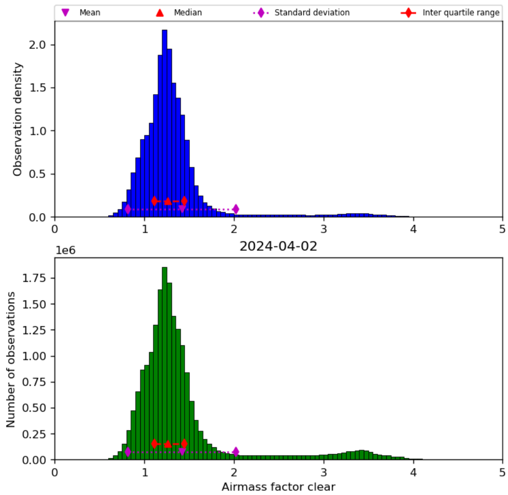
Figure 42: Histogram of “Airmass factor clear” for 2024-04-01 to 2024-04-03
