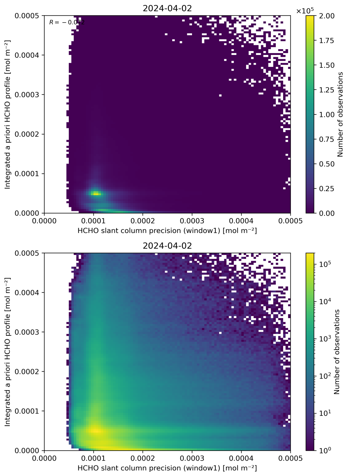
Figure 96: Scatter density plot of “HCHO slant column precision (window1)” against “Integrated a priori HCHO profile” for 2024-04-01 to 2024-04-03.
