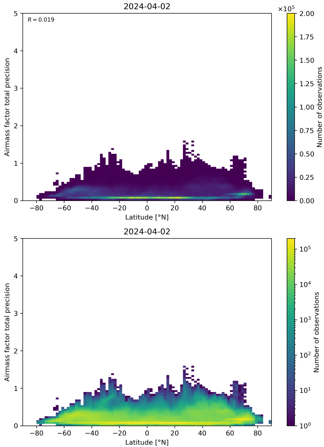
Figure 162: Scatter density plot of “Latitude” against “Airmass factor total precision” for 2024-04-01 to 2024-04-03.
