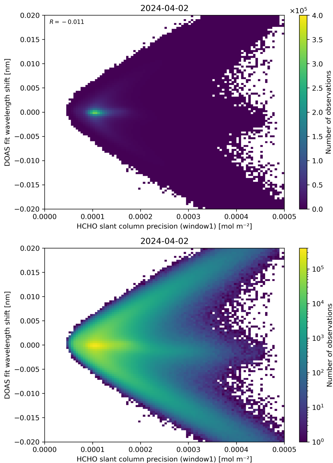
Figure 89: Scatter density plot of “HCHO slant column precision (window1)” against “DOAS fit wavelength shift” for 2024-04-01 to 2024-04-03.
