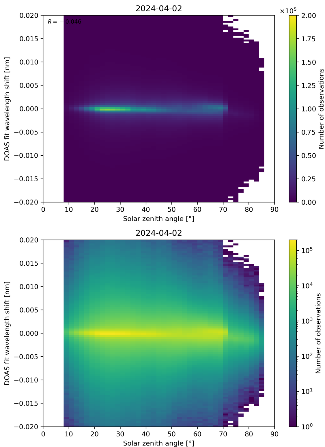
Figure 168: Scatter density plot of “Solar zenith angle” against “DOAS fit wavelength shift” for 2024-04-01 to 2024-04-03.
