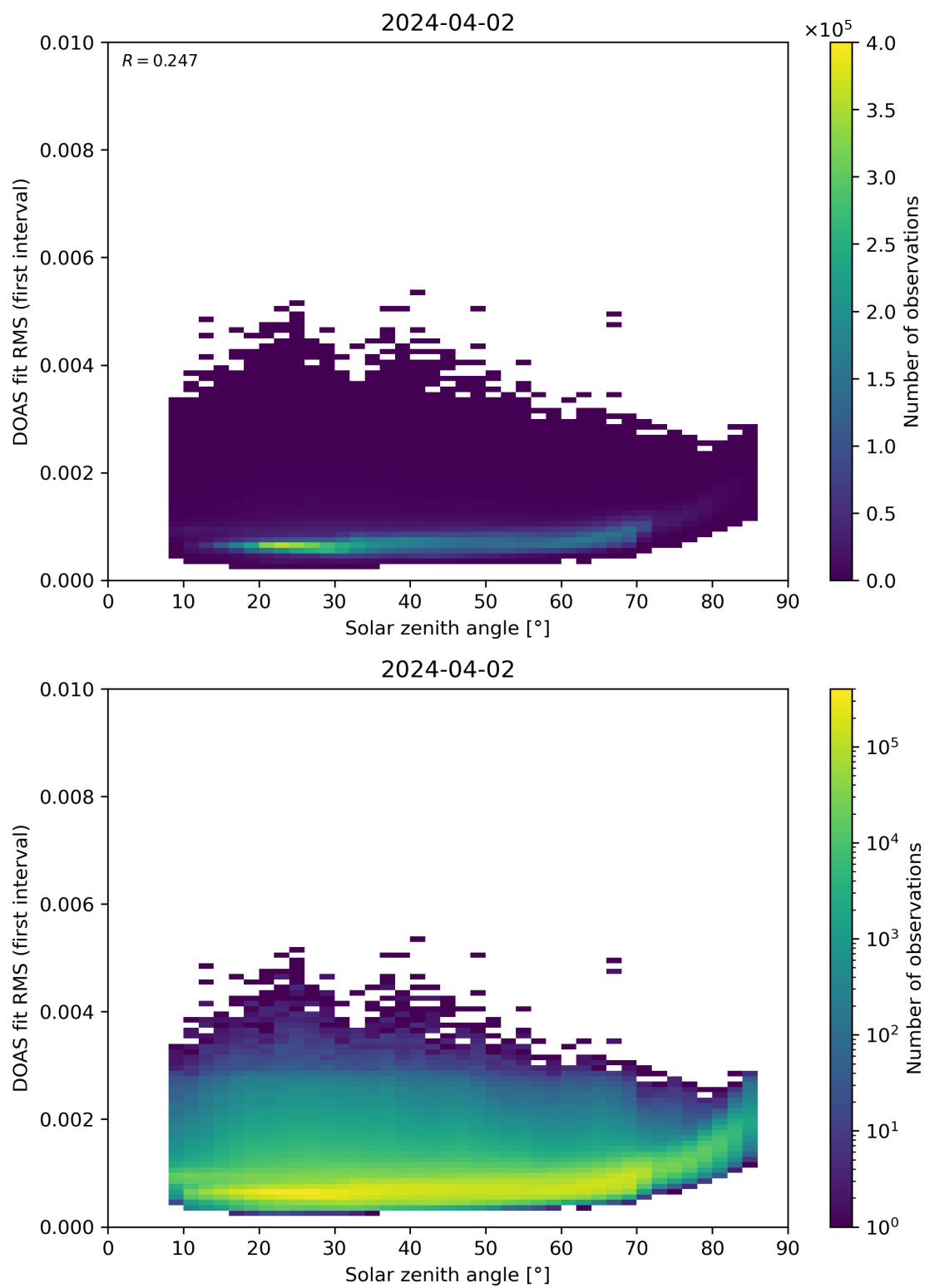
Figure 167: Scatter density plot of “Solar zenith angle” against “DOAS fit RMS (first interval)” for 2024-04-01 to 2024-04-03.
