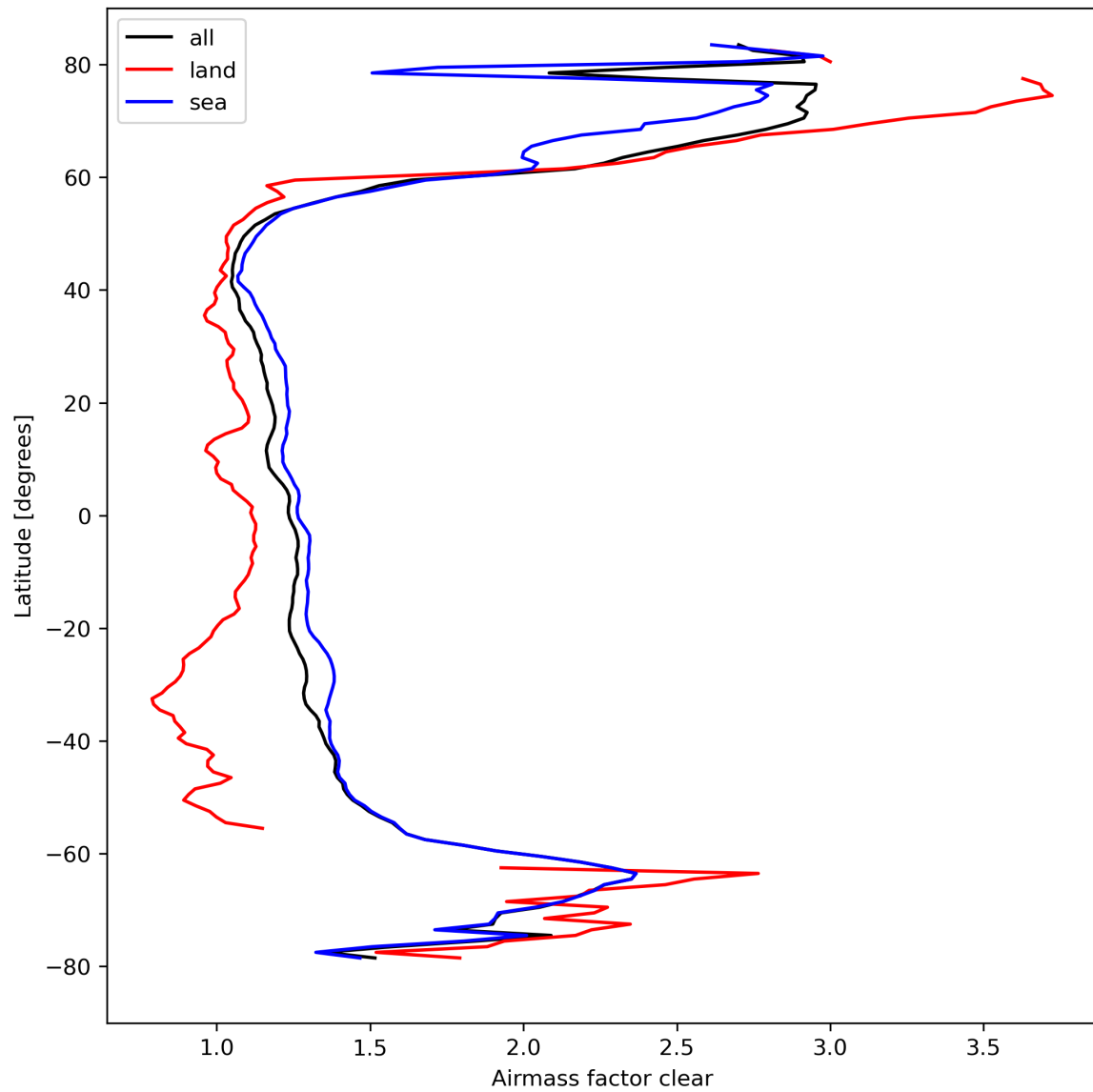
Figure 28: Zonal average of “Airmass factor clear” for 2024-04-01 to 2024-04-03.
