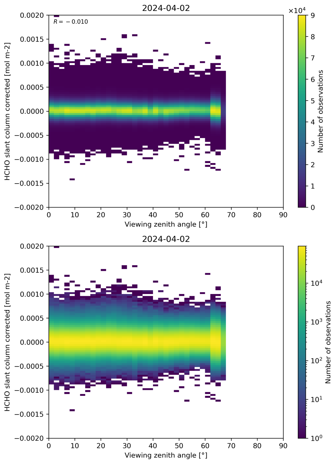
Figure 186: Scatter density plot of “Viewing zenith angle” against “HCHO slant column corrected” for 2024-04-01 to 2024-04-03.
