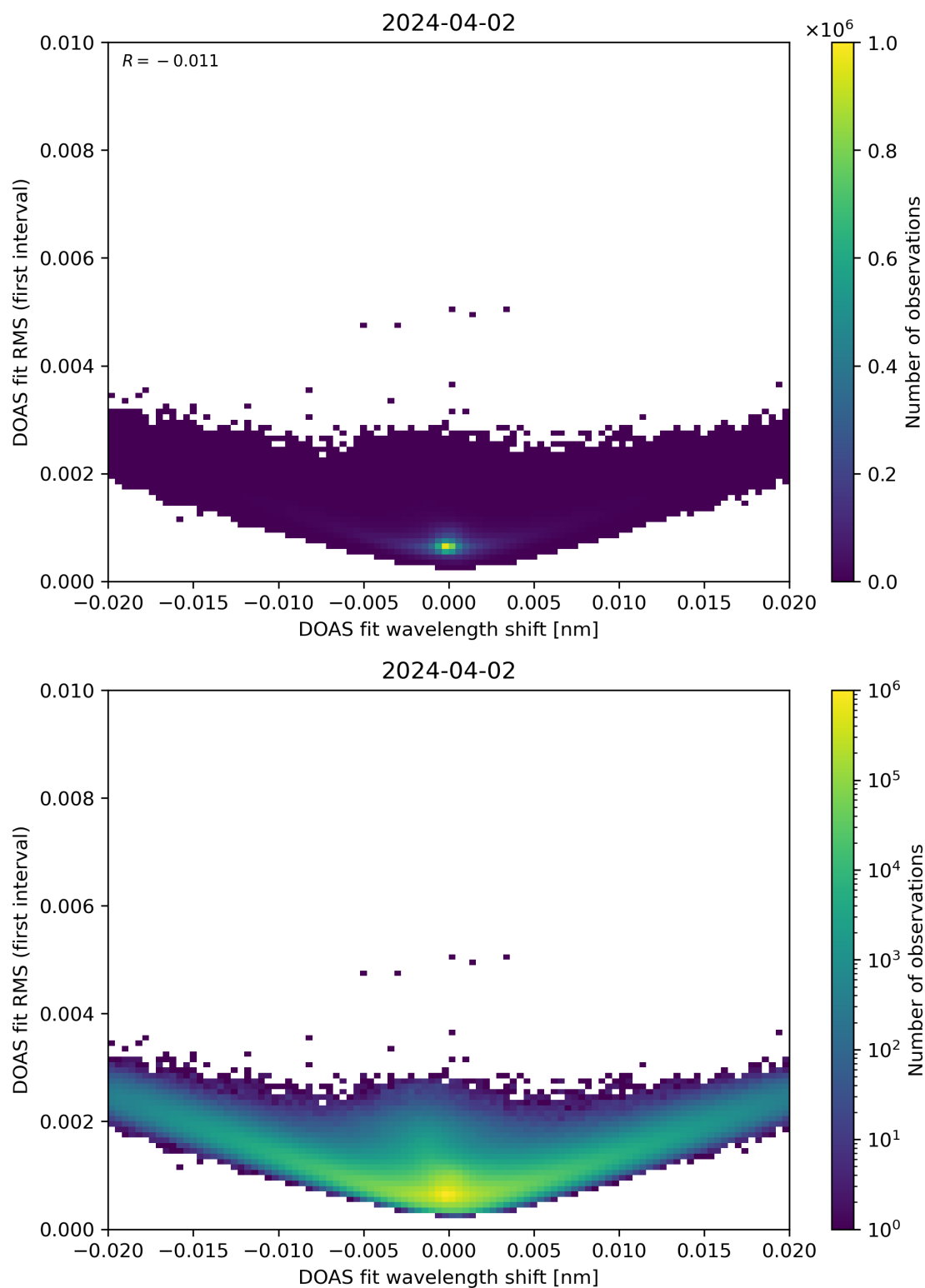
Figure 64: Scatter density plot of “DOAS fit wavelength shift” against “DOAS fit RMS (first interval)” for 2024-04-01 to 2024-04-03.
