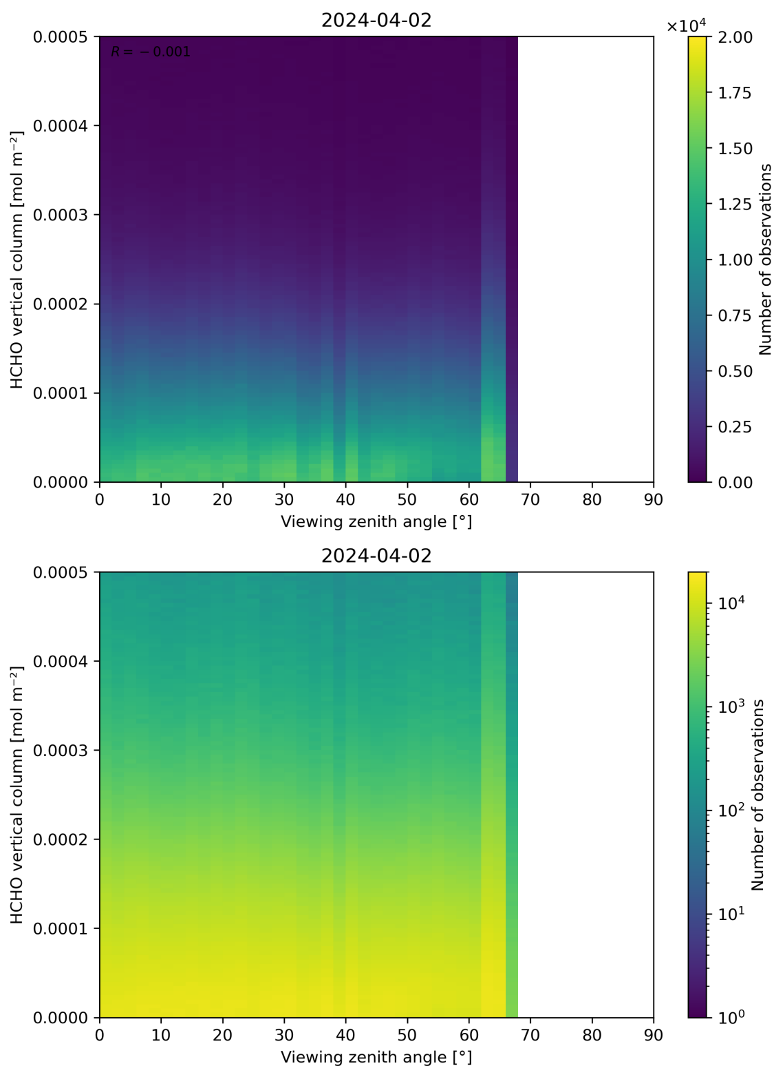
Figure 192: Scatter density plot of “Viewing zenith angle” against “HCHO vertical column” for 2024-04-01 to 2024-04-03.
