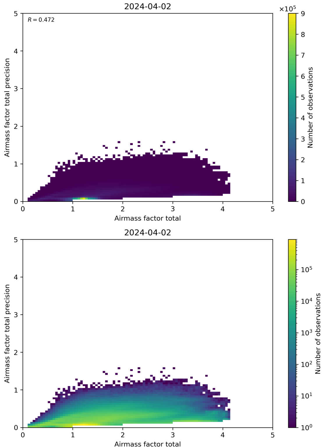
Figure 103: Scatter density plot of “Airmass factor total” against “Airmass factor total precision” for 2024-04-01 to 2024-04-03.
