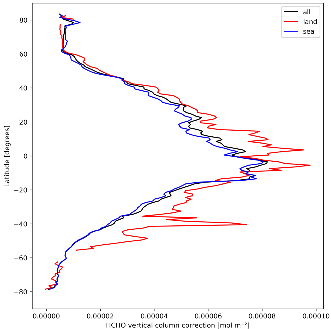
Figure 23: Zonal average of “HCHO vertical column correction” for 2024-04-01 to 2024-04-03.
