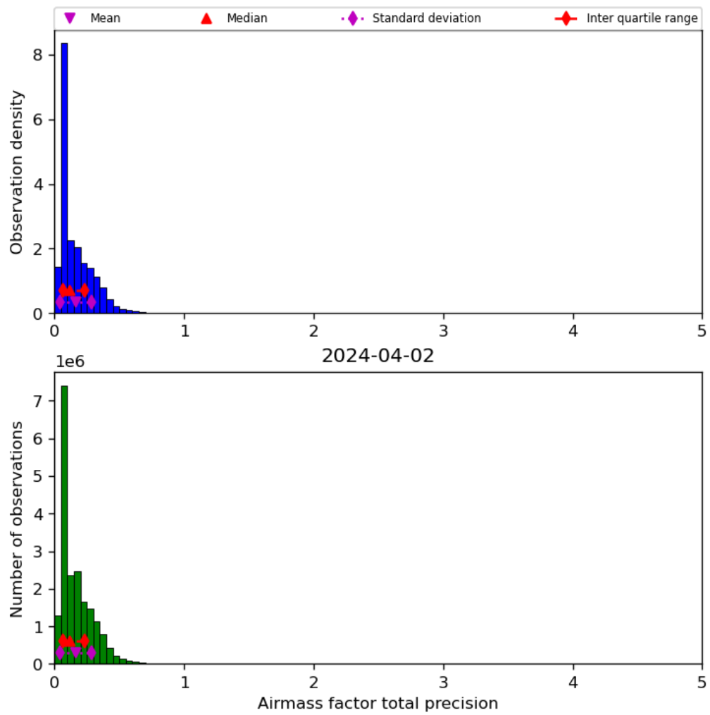
Figure 41: Histogram of "Airmass factor total precision" for 2024-04-01 to 2024-04-03
