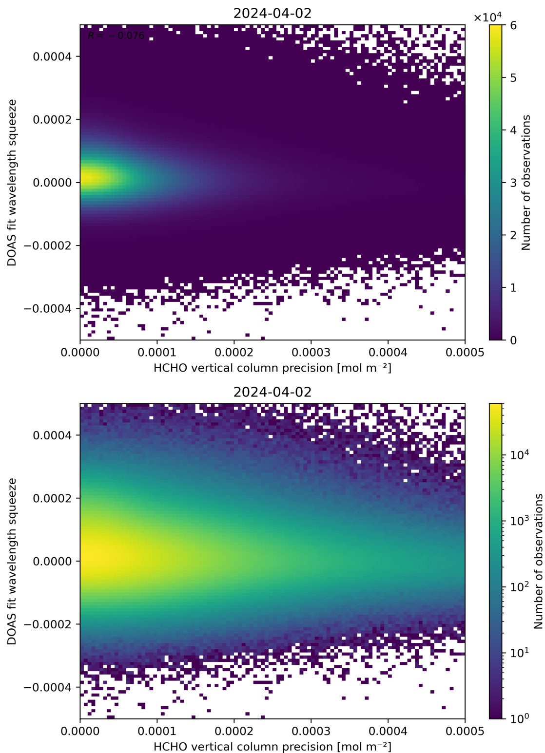
Figure 138: Scatter density plot of “HCHO vertical column precision” against “DOAS fit wavelength squeeze” for 2024-04-01 to 2024-04-03.
