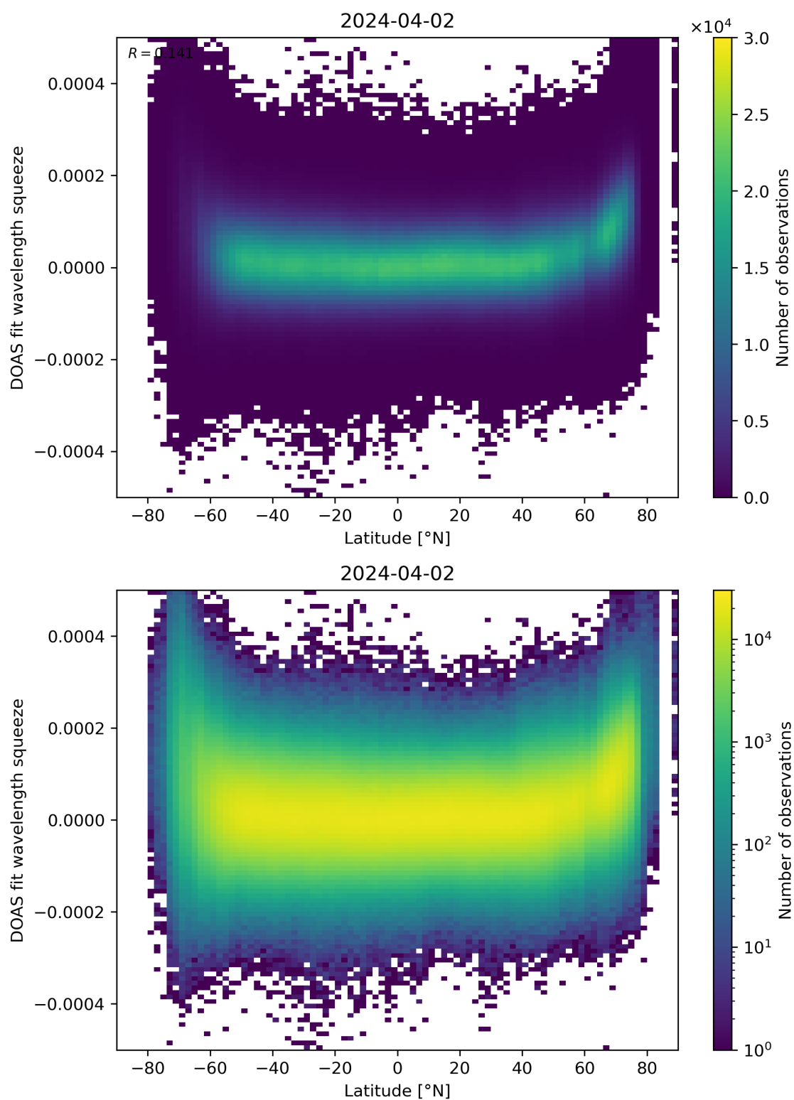
Figure 155: Scatter density plot of “Latitude” against “DOAS fit wavelength squeeze” for 2024-04-01 to 2024-04-03.
