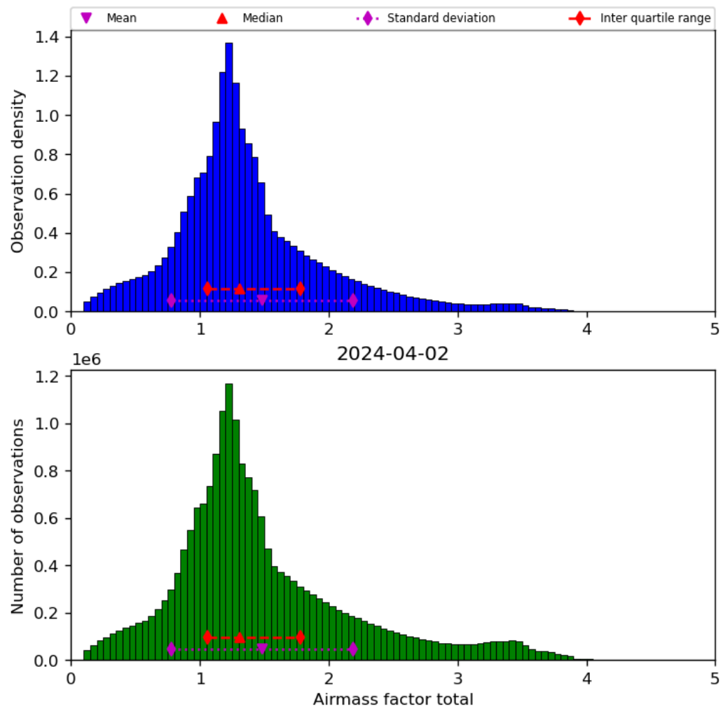
Figure 40: Histogram of “Airmass factor total” for 2024-04-01 to 2024-04-03
