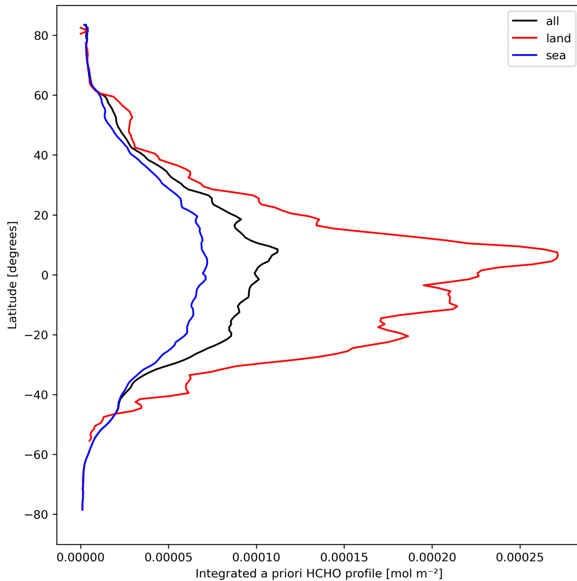
Figure 29: Zonal average of “Integrated a priori HCHO profile” for 2024-04-01 to 2024-04-03.
