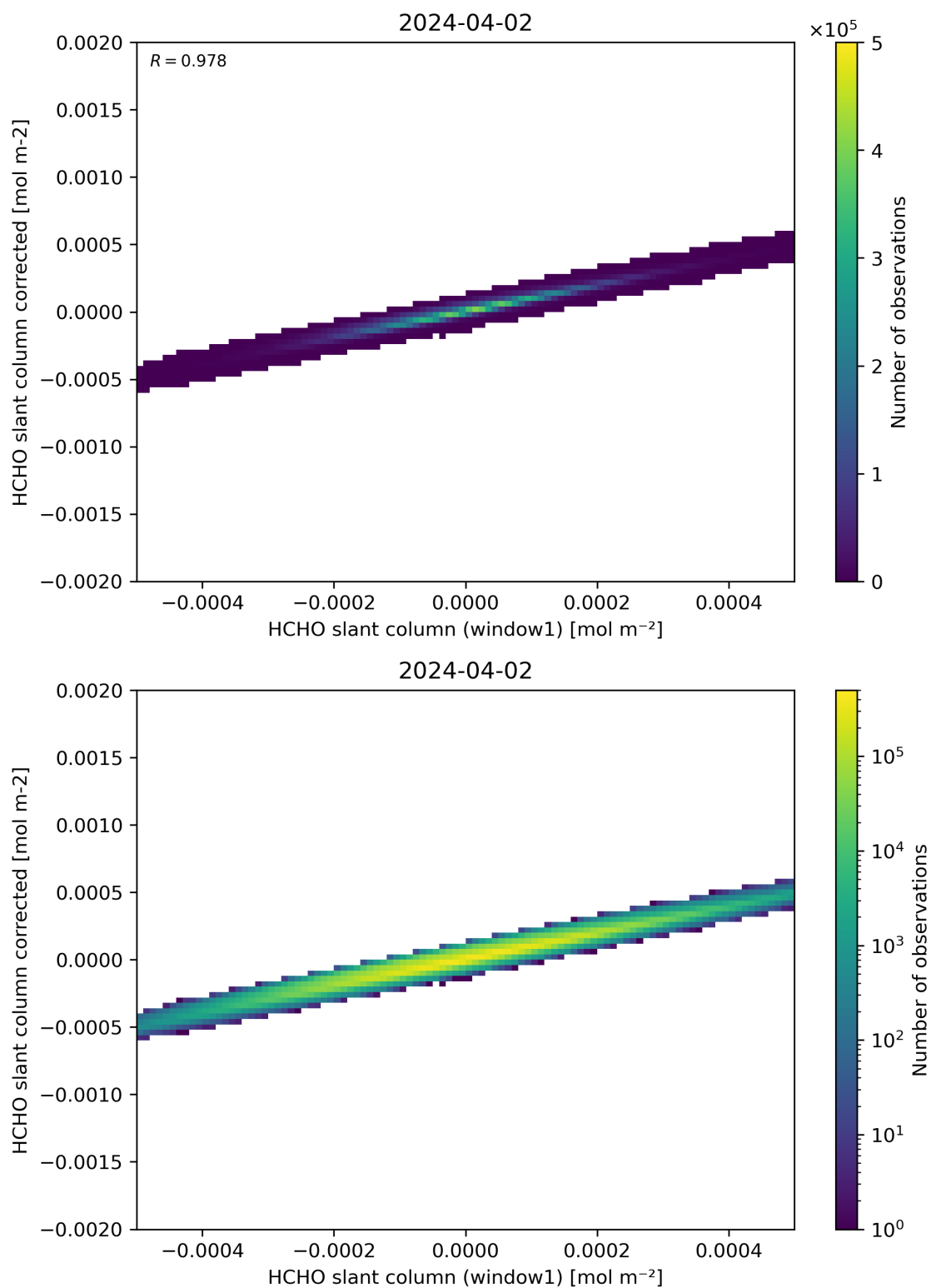
Figure 82: Scatter density plot of “HCHO slant column (window1)” against “HCHO slant column corrected” for 2024-04-01 to 2024-04-03.
