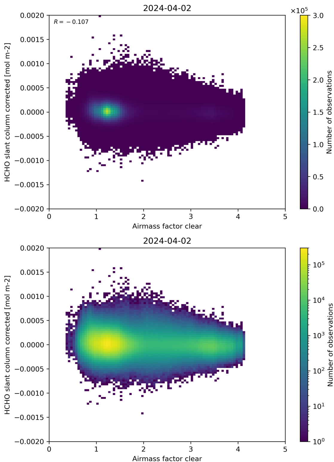
Figure 74: Scatter density plot of “Airmass factor clear” against “HCHO slant column corrected” for 2024-04-01 to 2024-04-03.
