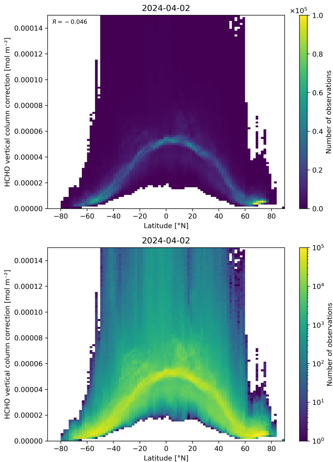
Figure 164: Scatter density plot of “Latitude” against “HCHO vertical column correction” for 2024-04-01 to 2024-04-03.
