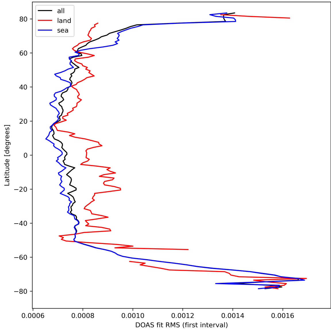
Figure 32: Zonal average of “DOAS fit RMS (first interval)” for 2024-04-01 to 2024-04-03.
