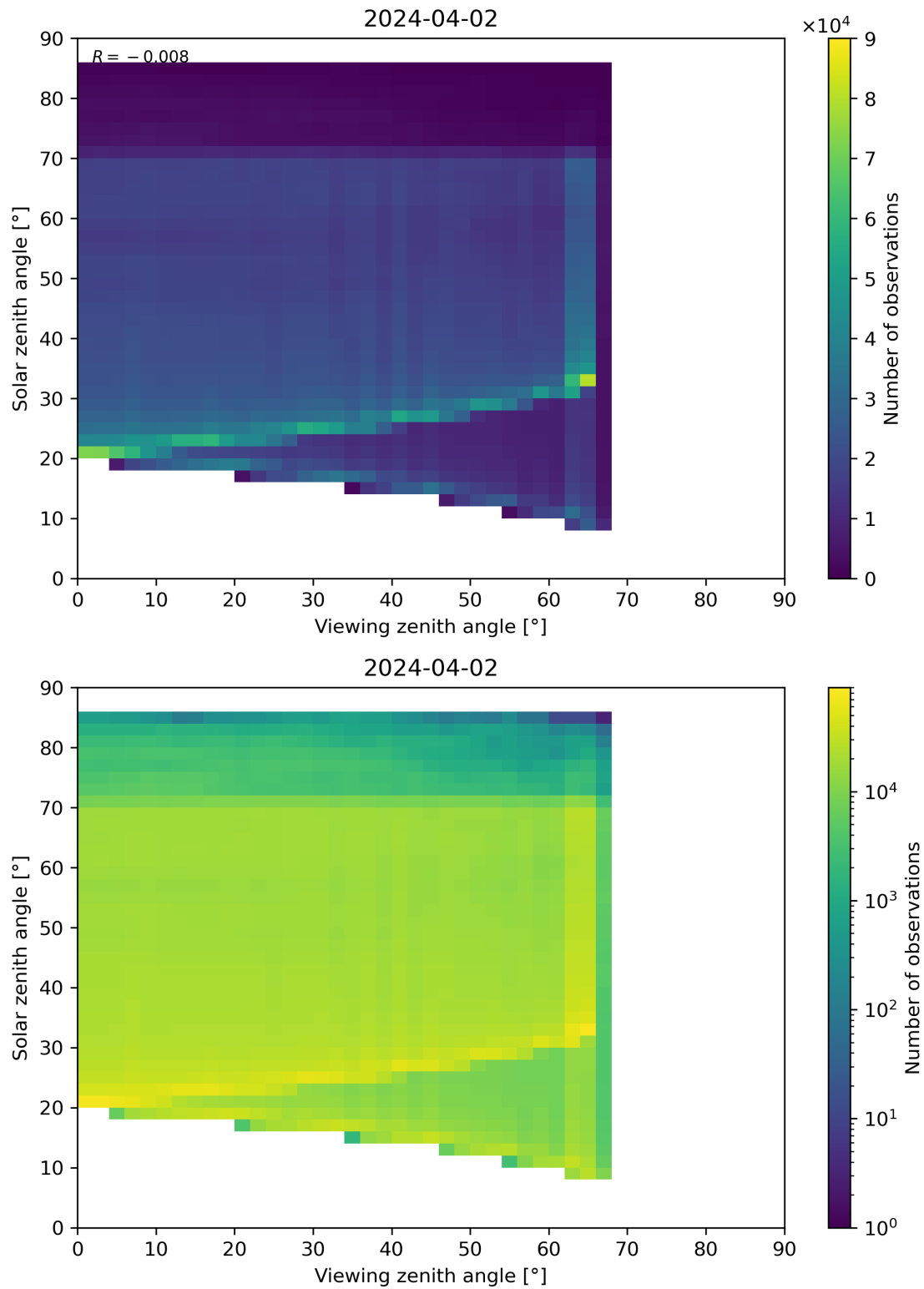
Figure 197: Scatter density plot of “Viewing zenith angle” against “Solar zenith angle” for 2024-04-01 to 2024-04-03.
