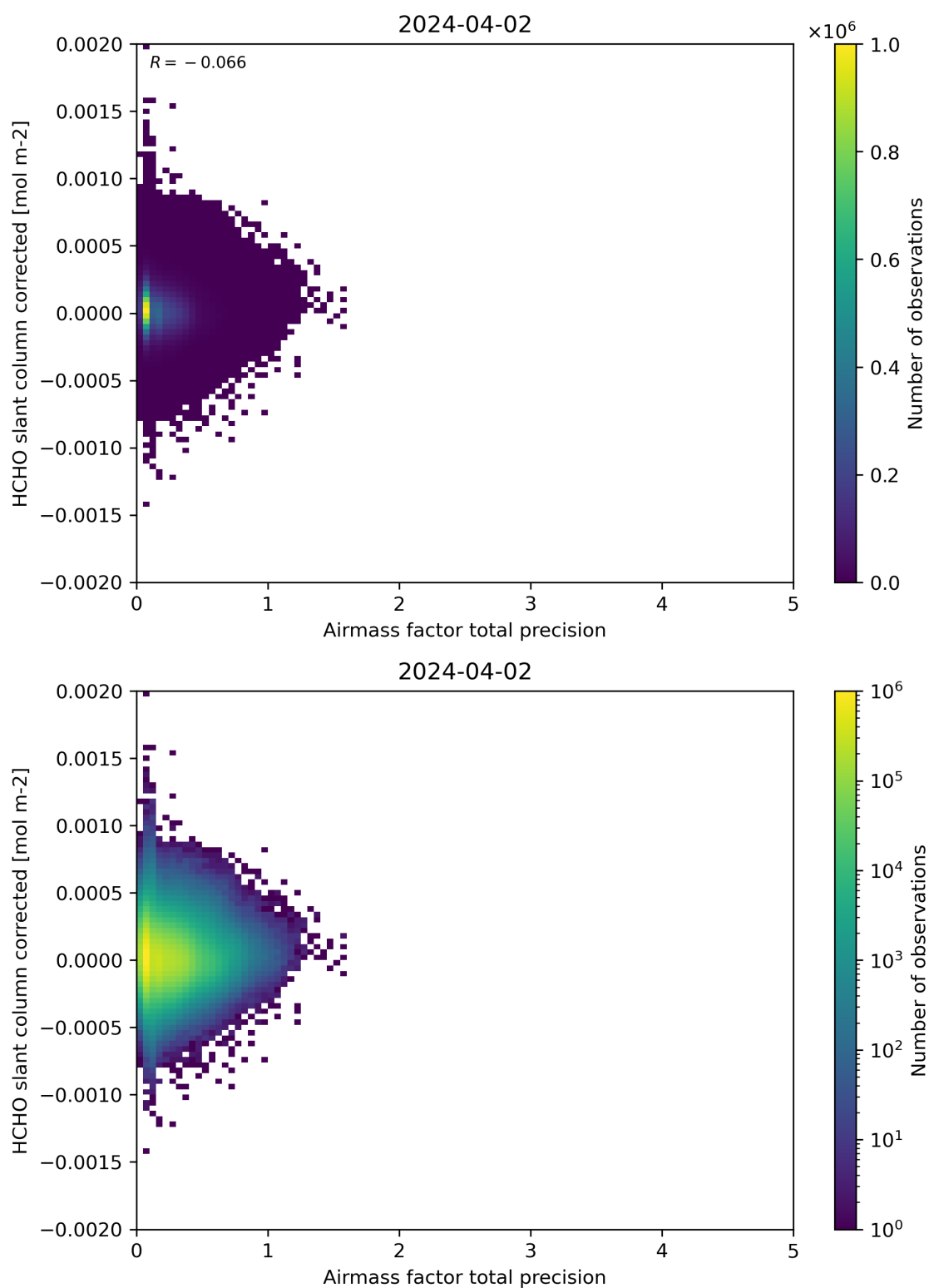
Figure 109: Scatter density plot of “Airmass factor total precision” against “HCHO slant column corrected” for 2024-04-01 to 2024-04-03.
