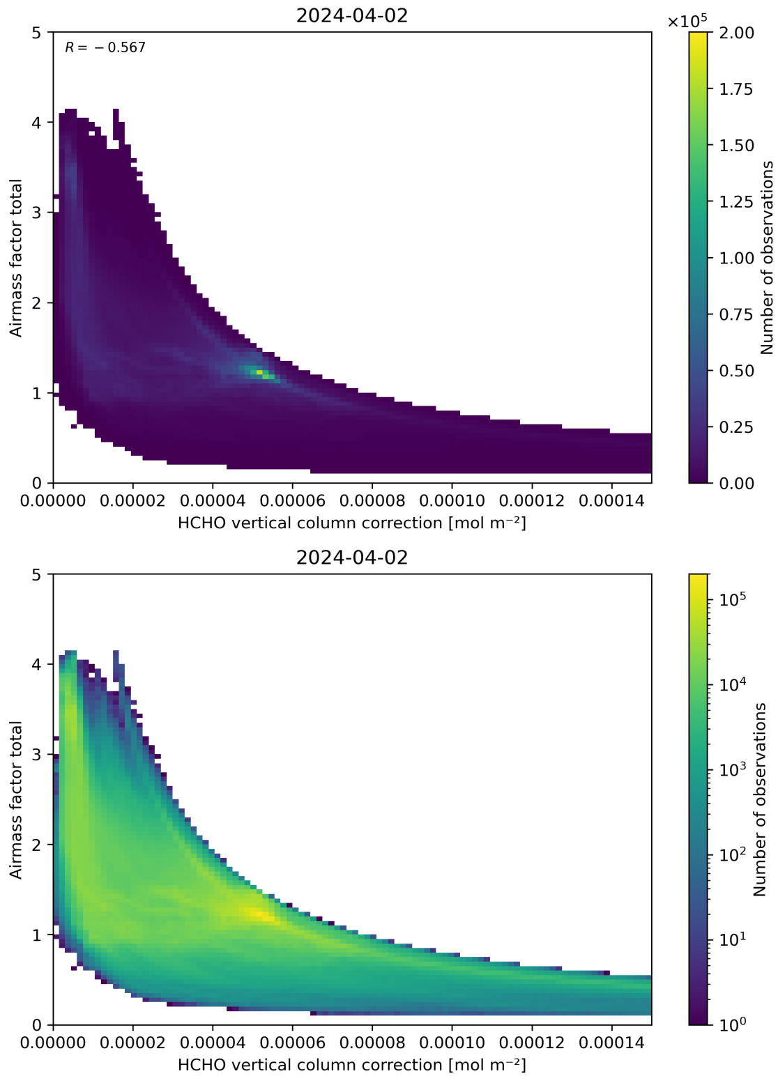
Figure 120: Scatter density plot of “HCHO vertical column correction” against “Airmass factor total” for 2024-04-01 to 2024-04-03.
