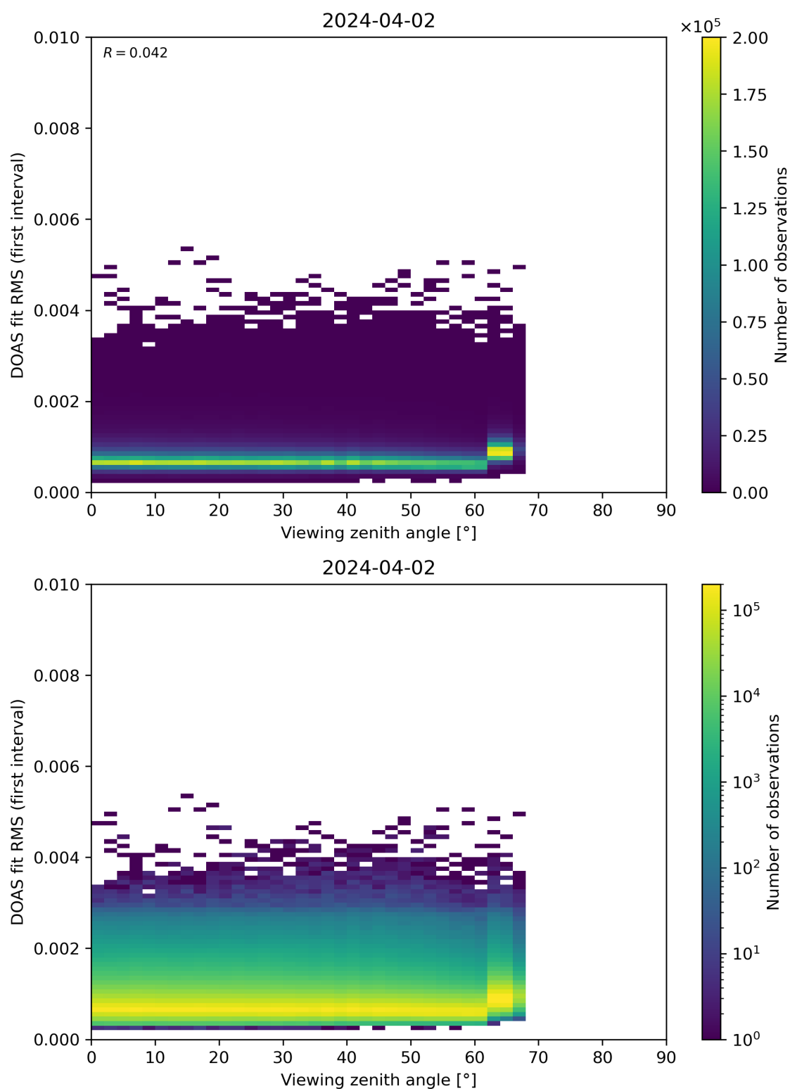
Figure 182: Scatter density plot of “Viewing zenith angle” against “DOAS fit RMS (first interval)” for 2024-04-01 to 2024-04-03.
