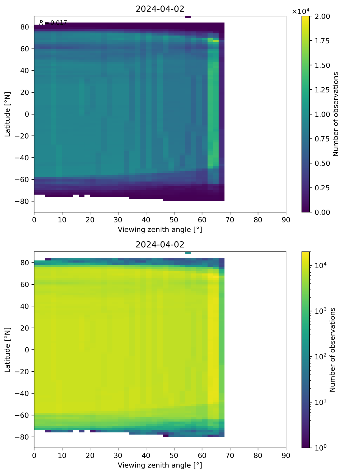
Figure 196: Scatter density plot of “Viewing zenith angle” against “Latitude” for 2024-04-01 to 2024-04-03.
