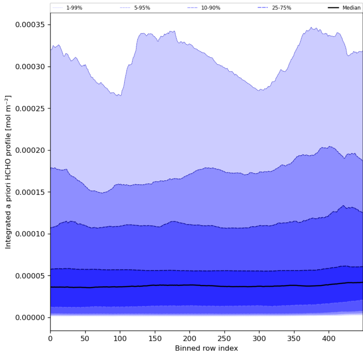
Figure 57: Along track statistics of "Integrated a priori HCHO profile" for 2024-04-01 to 2024-04-03
