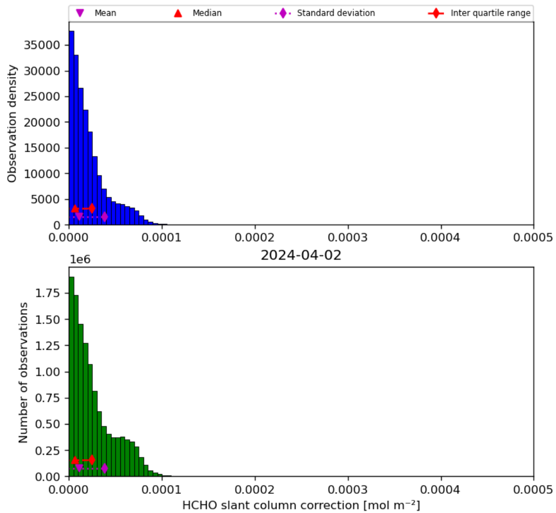
Figure 47: Histogram of “HCHO slant column correction” for 2024-04-01 to 2024-04-03
