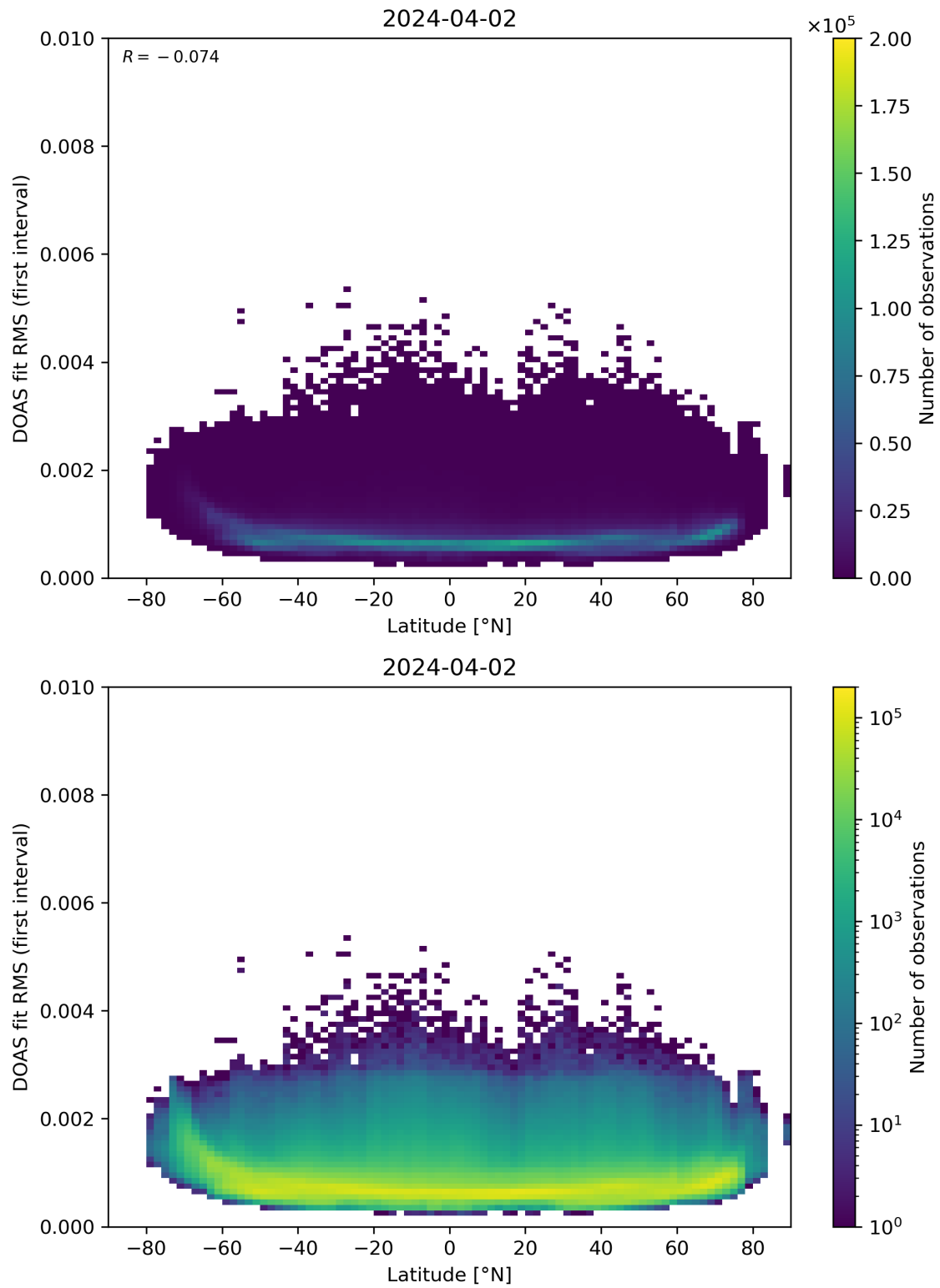
Figure 153: Scatter density plot of “Latitude” against “DOAS fit RMS (first interval)” for 2024-04-01 to 2024-04-03.
