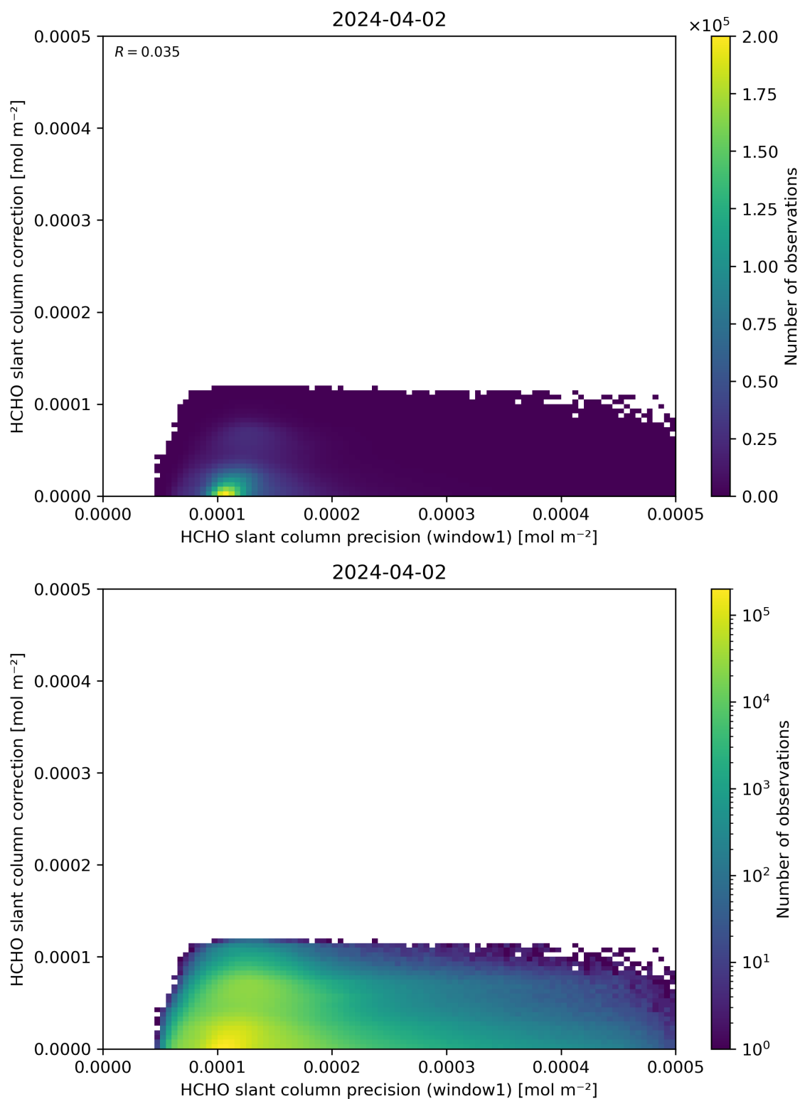
Figure 93: Scatter density plot of “HCHO slant column precision (window1)” against “HCHO slant column correction” for 2024-04-01 to 2024-04-03.
