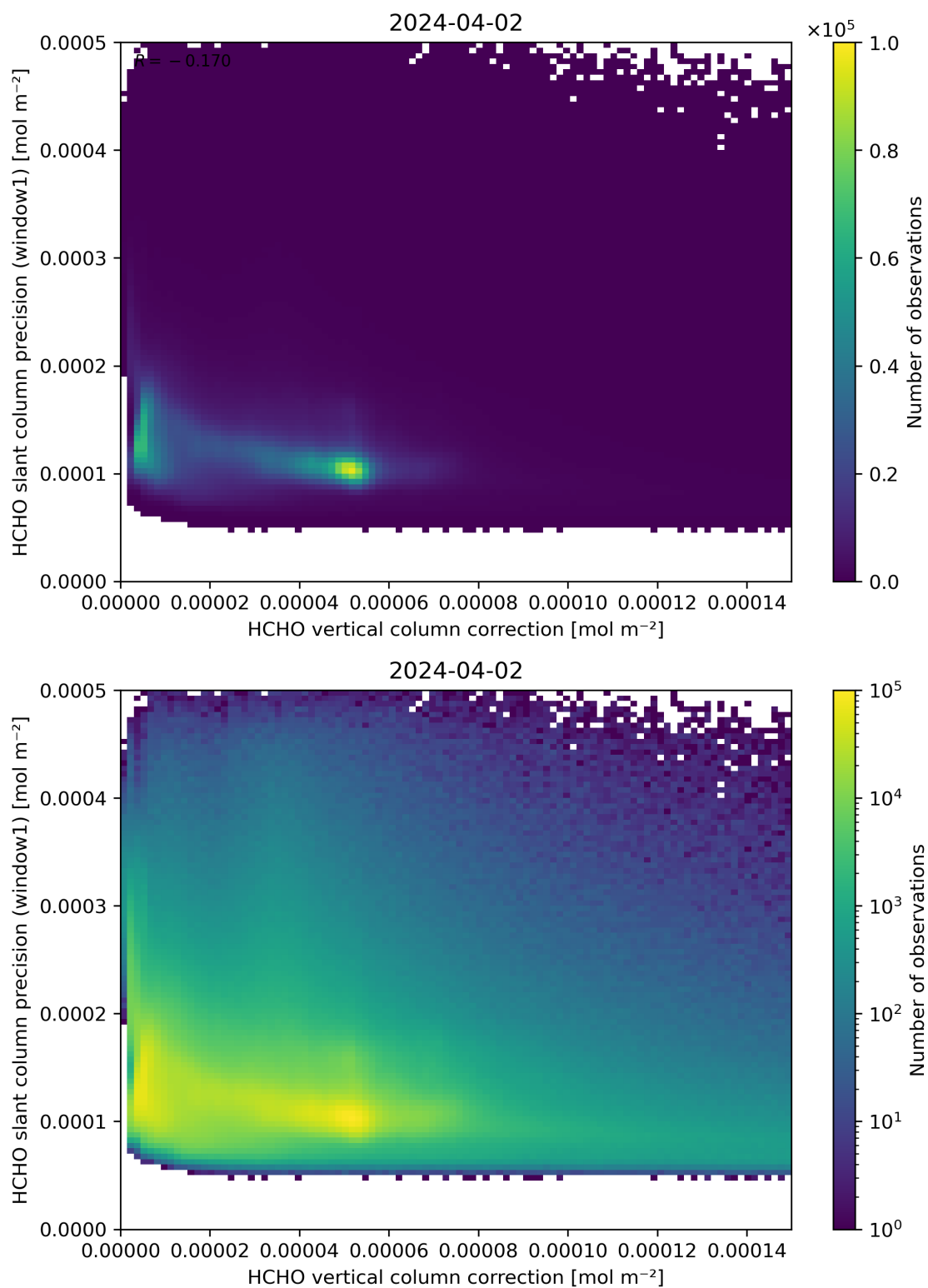
Figure 119: Scatter density plot of “HCHO vertical column correction” against “HCHO slant column precision (window1)” for 2024-04-01 to 2024-04-03.
