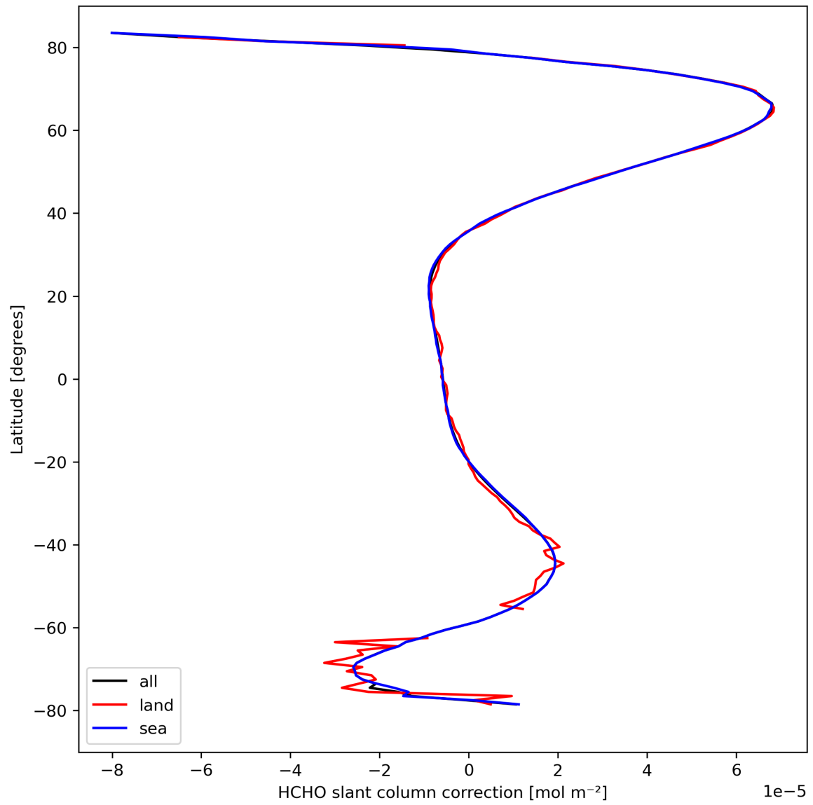
Figure 33: Zonal average of “HCHO slant column correction” for 2024-04-01 to 2024-04-03.
