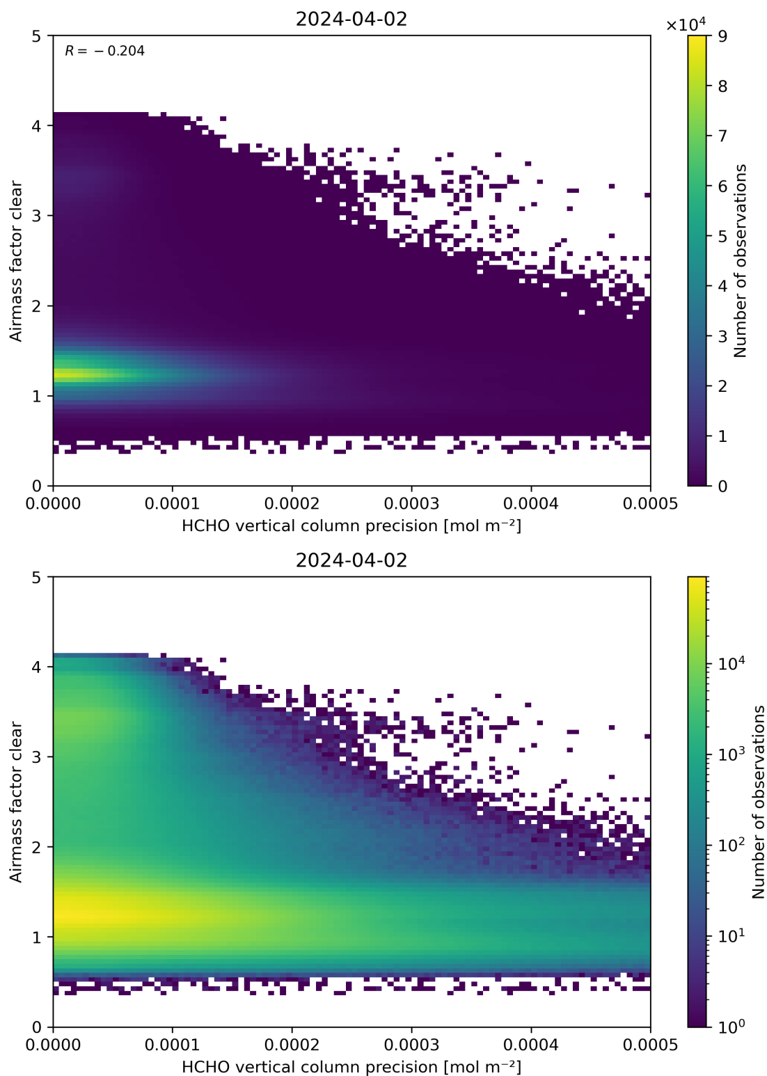
Figure 139: Scatter density plot of “HCHO vertical column precision” against “Airmass factor clear” for 2024-04-01 to 2024-04-03.
