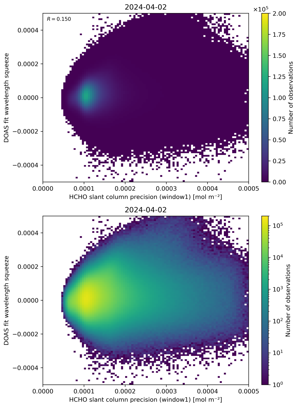
Figure 90: Scatter density plot of “HCHO slant column precision (window1)” against “DOAS fit wavelength squeeze” for 2024-04-01 to 2024-04-03.
