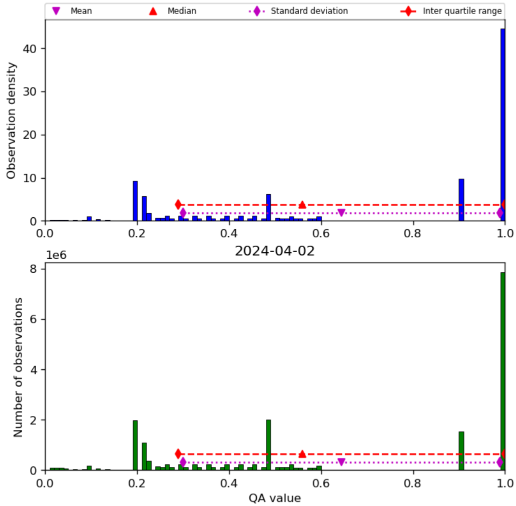
Figure 34: Histogram of “QA value” for 2024-04-01 to 2024-04-03
