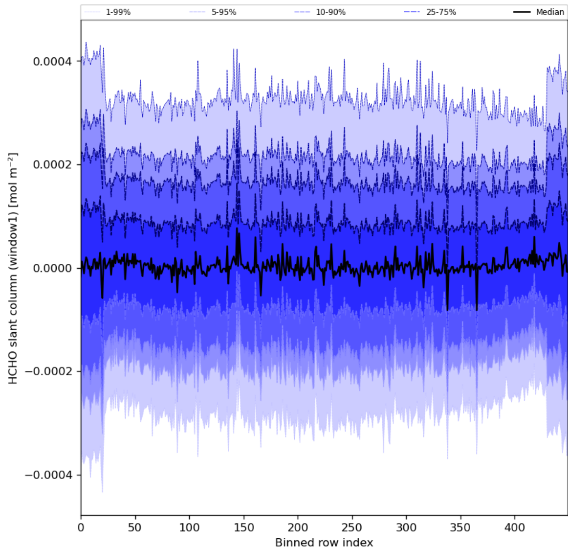
Figure 52: Along track statistics of “HCHO slant column (window1)” for 2024-04-01 to 2024-04-03
