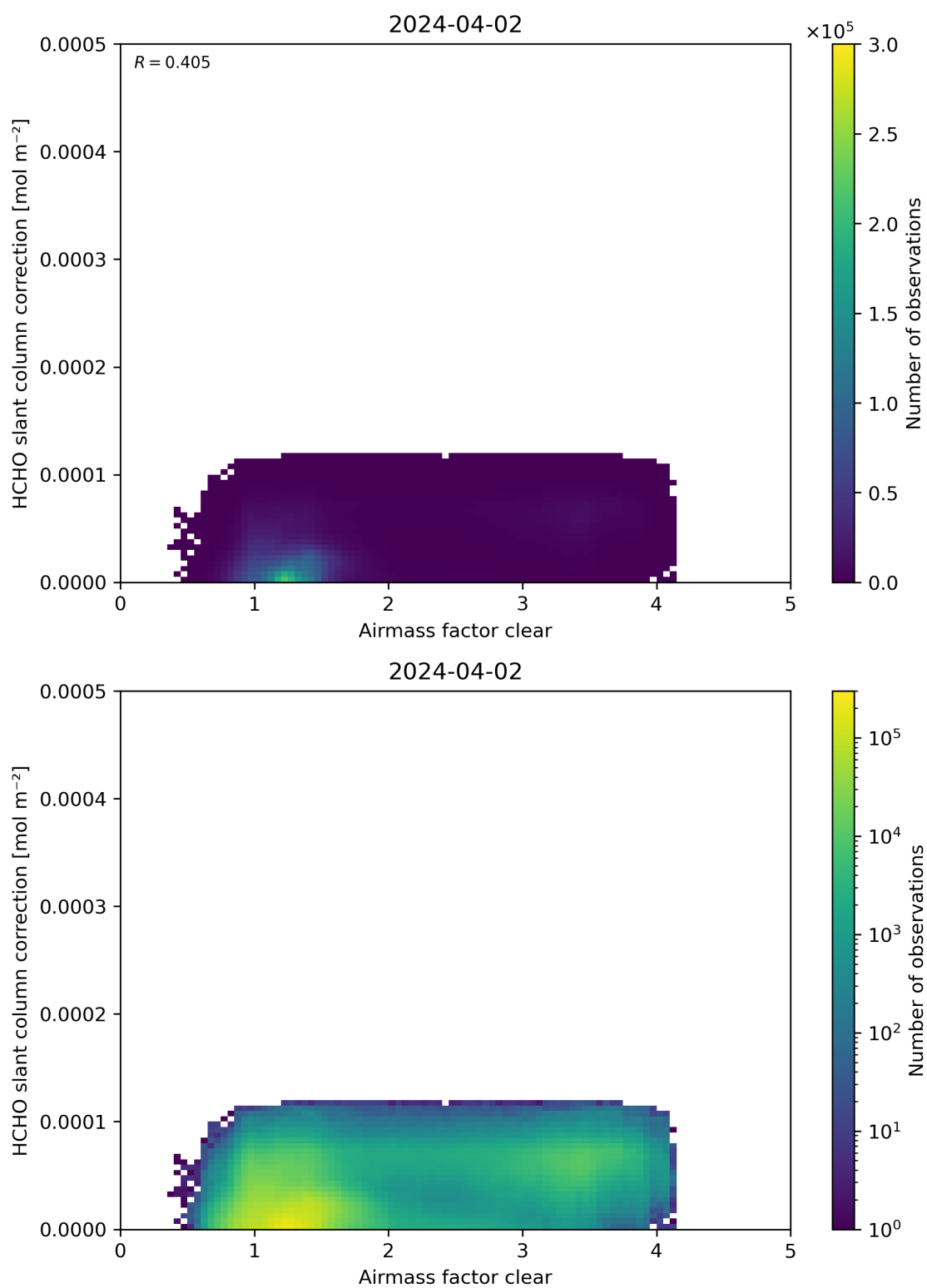
Figure 75: Scatter density plot of “Airmass factor clear” against “HCHO slant column correction” for 2024-04-01 to 2024-04-03.
