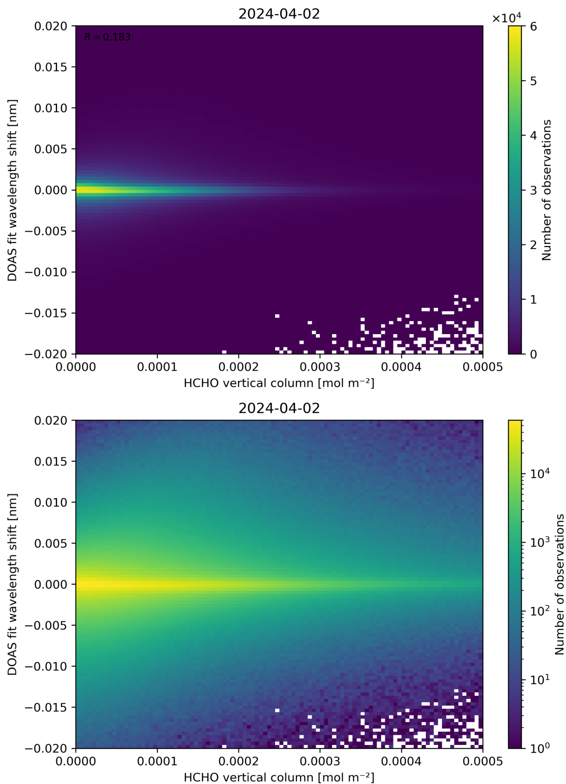
Figure 124: Scatter density plot of “HCHO vertical column” against “DOAS fit wavelength shift” for 2024-04-01 to 2024-04-03.
