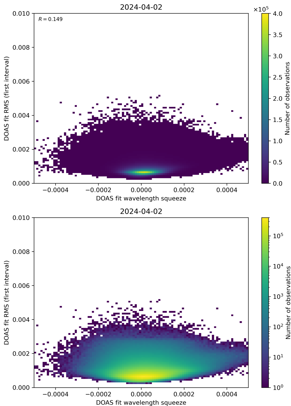
Figure 68: Scatter density plot of “DOAS fit wavelength squeeze” against “DOAS fit RMS (first interval)” for 2024-04-01 to 2024-04-03.
