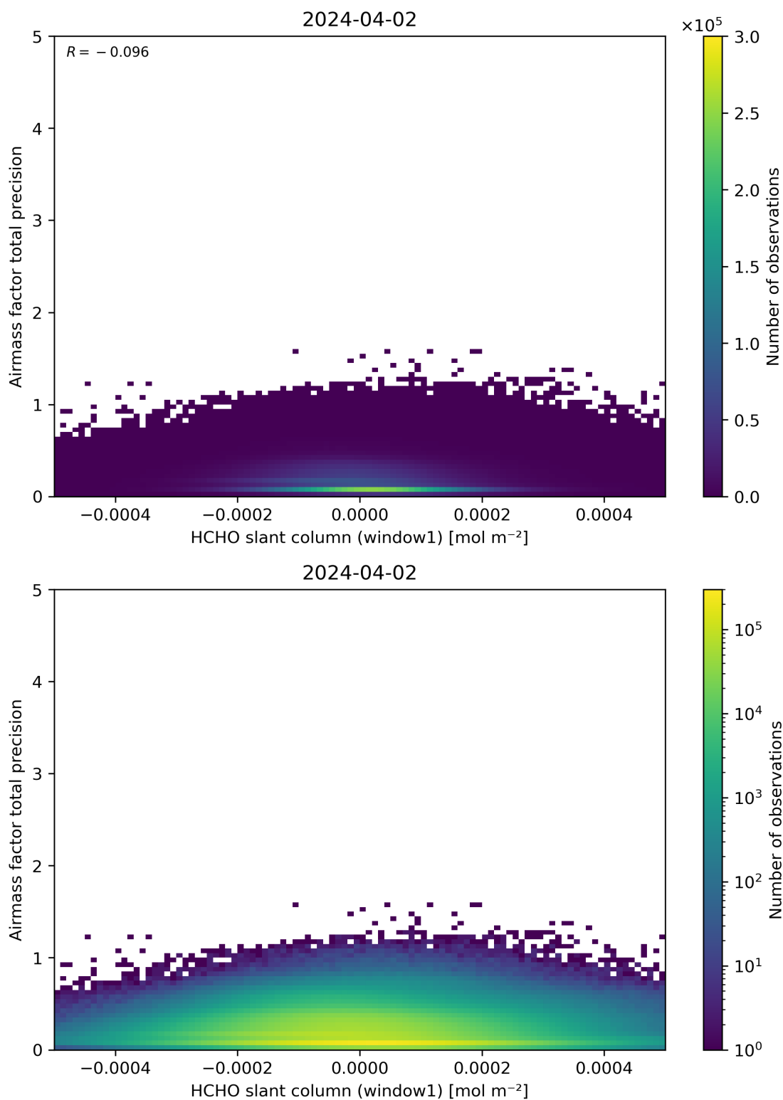
Figure 86: Scatter density plot of “HCHO slant column (window1)” against “Airmass factor total precision” for 2024-04-01 to 2024-04-03.
