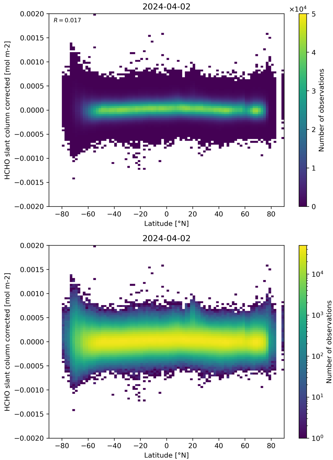
Figure 157: Scatter density plot of “Latitude” against “HCHO slant column corrected” for 2024-04-01 to 2024-04-03.
