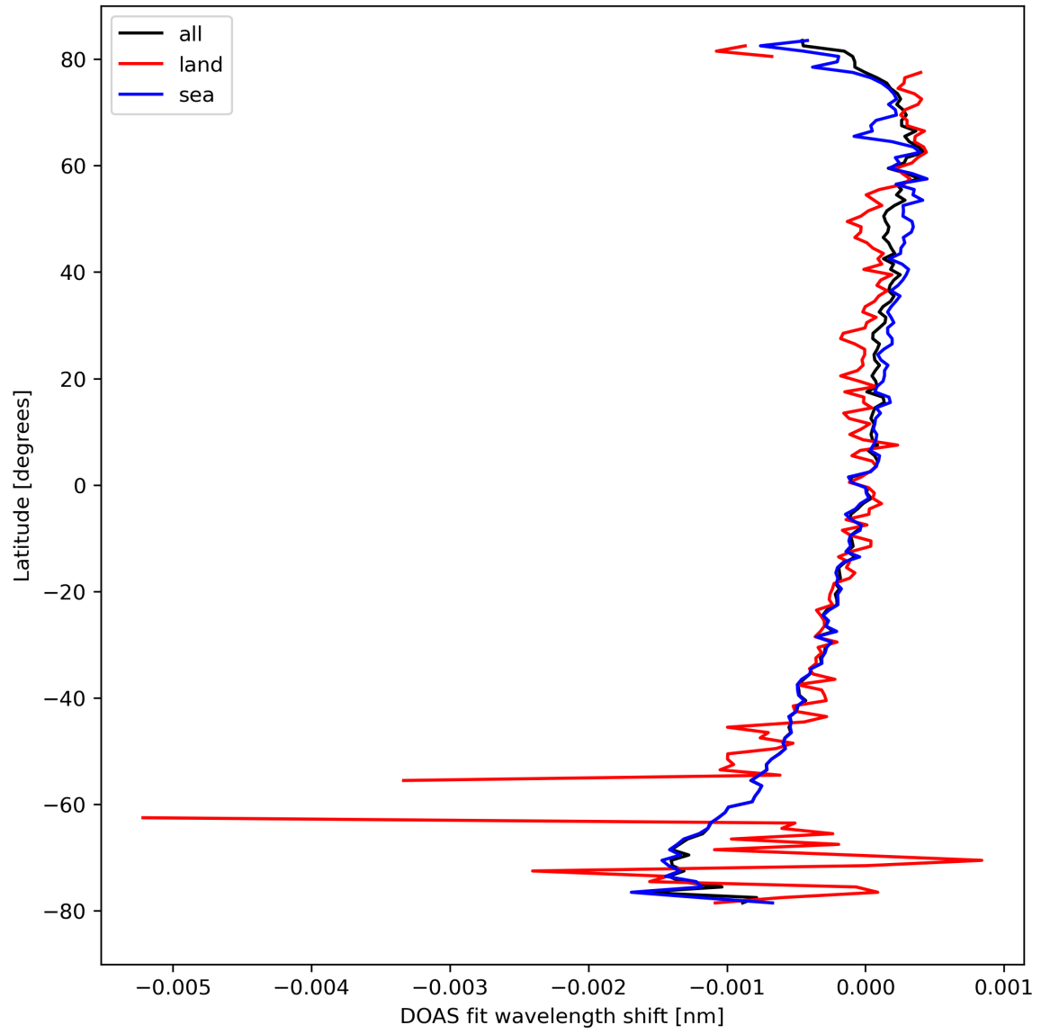
Figure 30: Zonal average of "DOAS fit wavelength shift" for 2024-04-01 to 2024-04-03.
