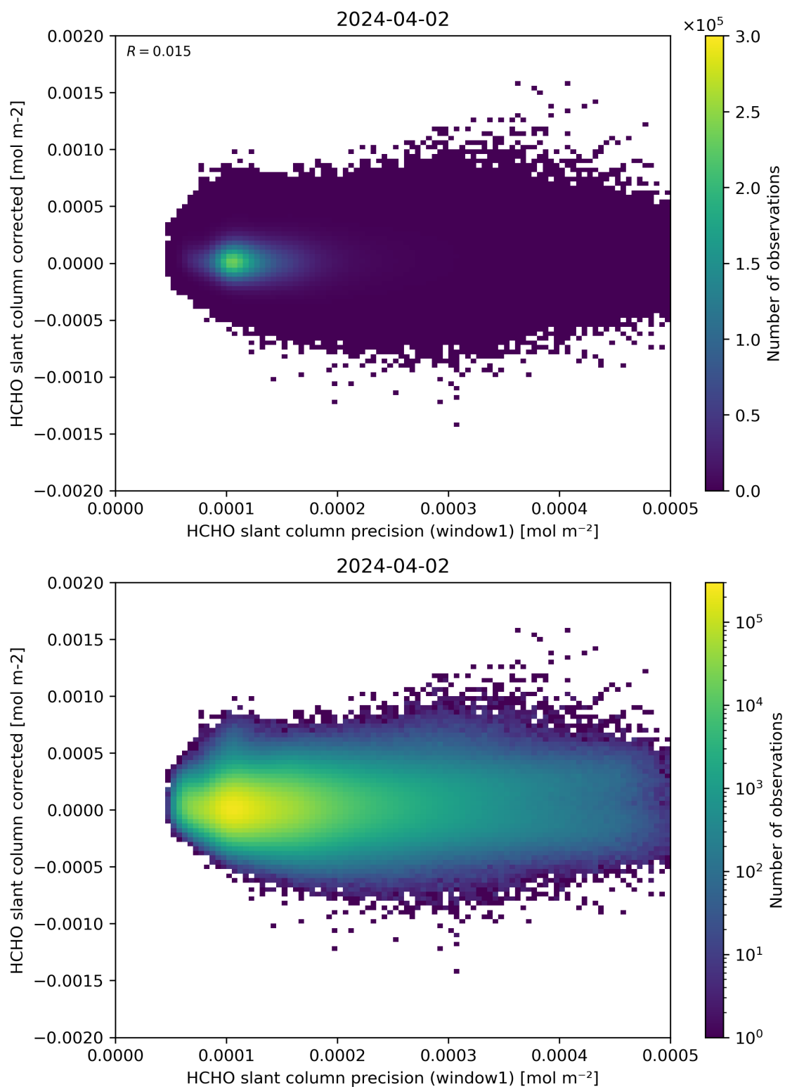
Figure 92: Scatter density plot of “HCHO slant column precision (window1)” against “HCHO slant column corrected” for 2024-04-01 to 2024-04-03.
