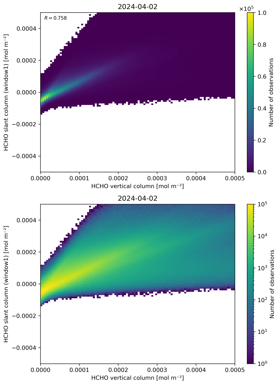
Figure 129: Scatter density plot of “HCHO vertical column” against “HCHO slant column (window1)” for 2024-04-01 to 2024-04-03.
