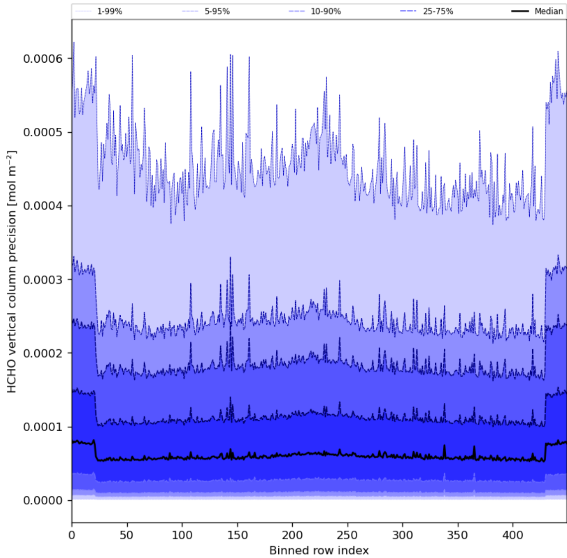
Figure 50: Along track statistics of “HCHO vertical column precision” for 2024-04-01 to 2024-04-03
