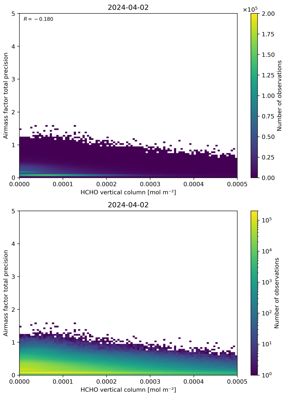
Figure 132: Scatter density plot of “HCHO vertical column” against “Airmass factor total precision” for 2024-04-01 to 2024-04-03.
