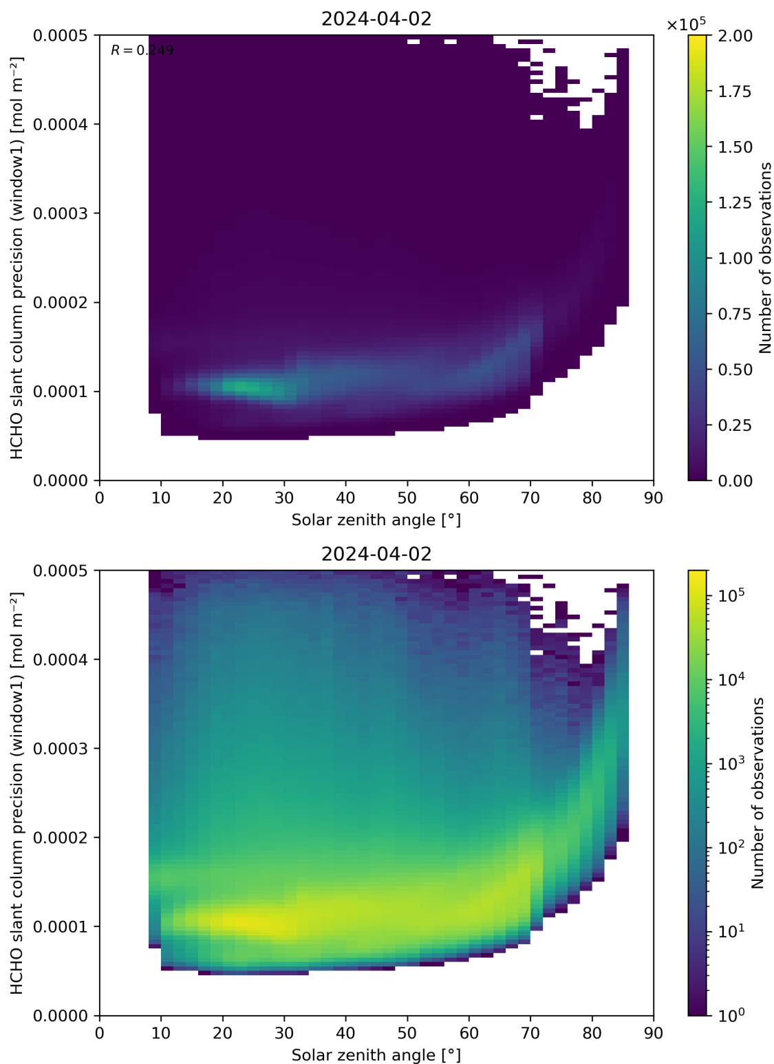
Figure 174: Scatter density plot of “Solar zenith angle” against “HCHO slant column precision (window1)” for 2024-04-01 to 2024-04-03.
