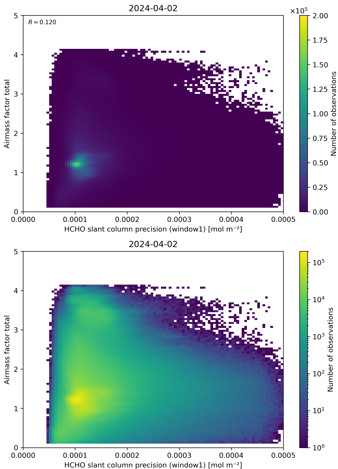
Figure 94: Scatter density plot of “HCHO slant column precision (window1)” against “Airmass factor total” for 2024-04-01 to 2024-04-03.
