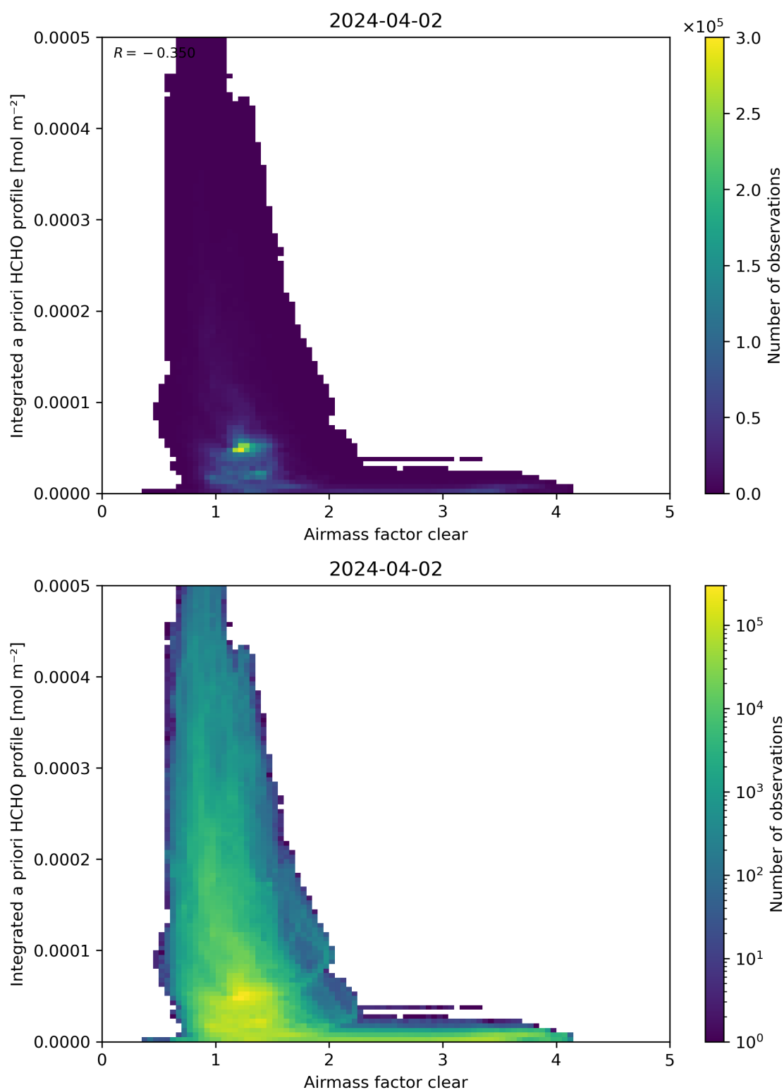
Figure 76: Scatter density plot of “Airmass factor clear” against “Integrated a priori HCHO profile” for 2024-04-01 to 2024-04-03.
