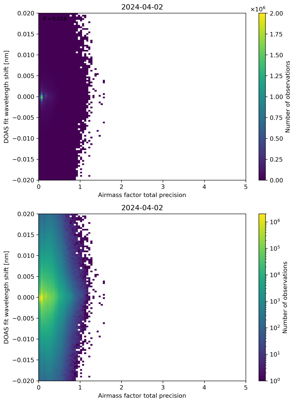
Figure 106: Scatter density plot of “Airmass factor total precision” against “DOAS fit wavelength shift” for 2024-04-01 to 2024-04-03.
