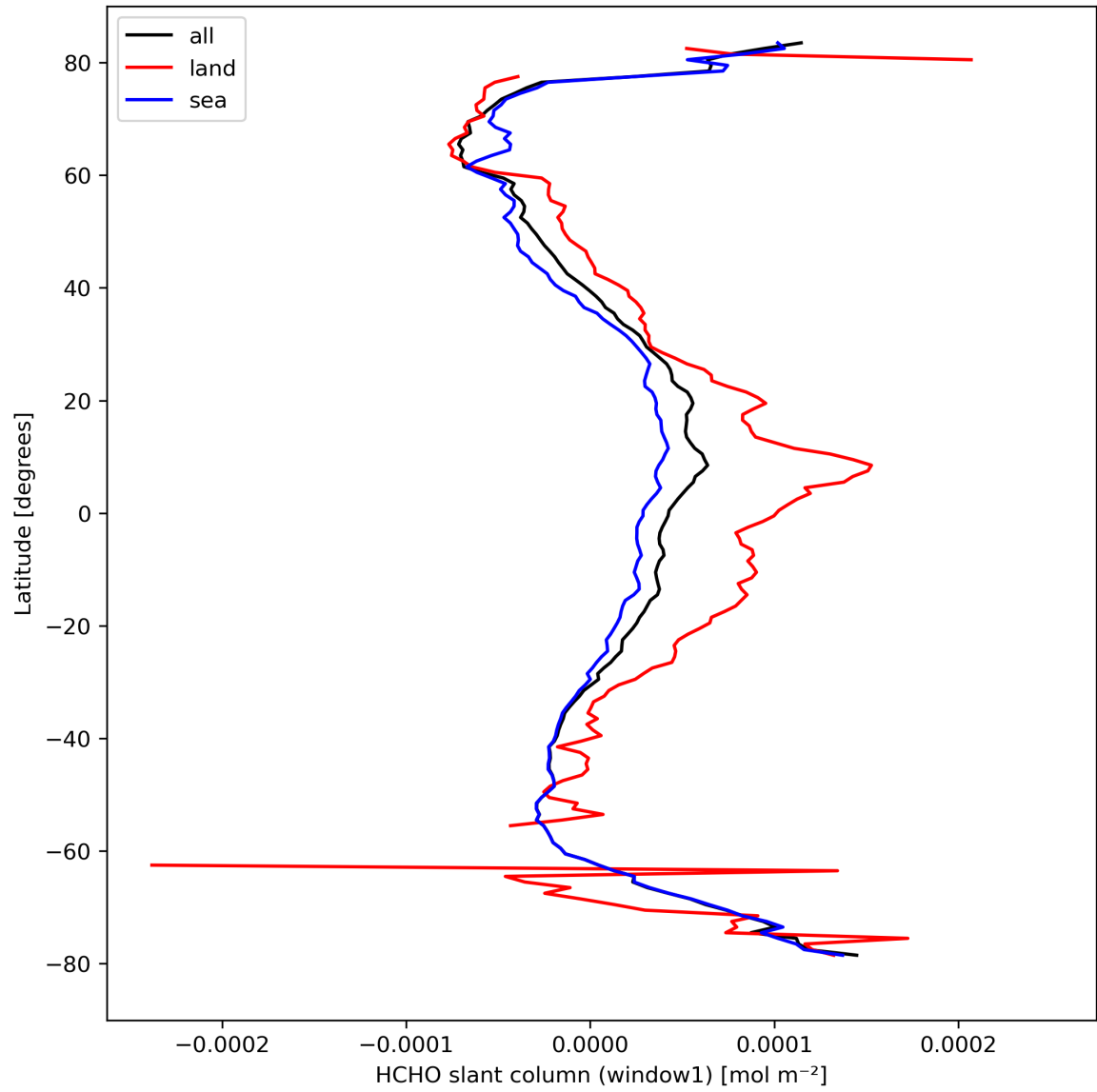
Figure 24: Zonal average of “HCHO slant column (window1)” for 2024-04-01 to 2024-04-03.
