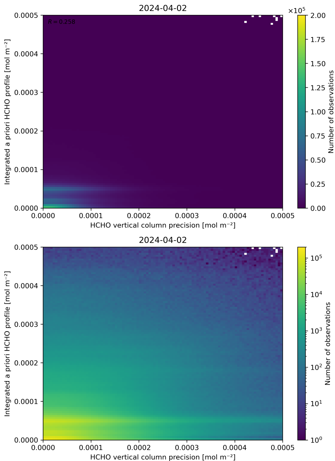
Figure 147: Scatter density plot of “HCHO vertical column precision” against “Integrated a priori HCHO profile” for 2024-04-01 to 2024-04-03.
