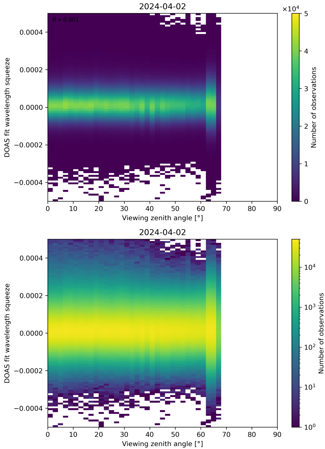
Figure 184: Scatter density plot of “Viewing zenith angle” against “DOAS fit wavelength squeeze” for 2024-04-01 to 2024-04-03.
