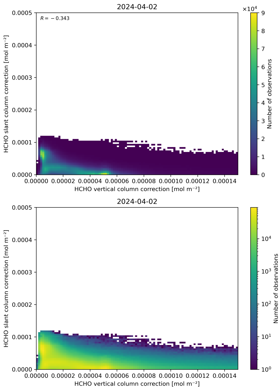
Figure 117: Scatter density plot of “HCHO vertical column correction” against “HCHO slant column correction” for 2024-04-01 to 2024-04-03.
