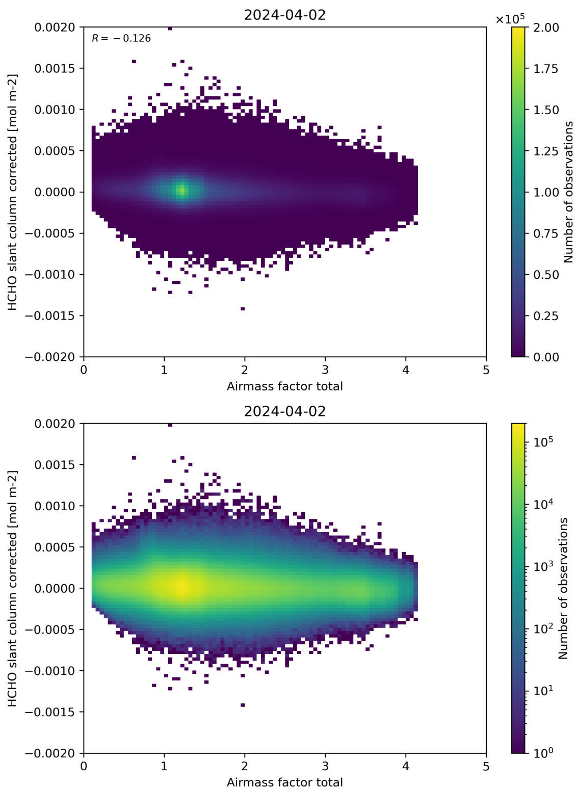
Figure 101: Scatter density plot of “Airmass factor total” against “HCHO slant column corrected” for 2024-04-01 to 2024-04-03.
