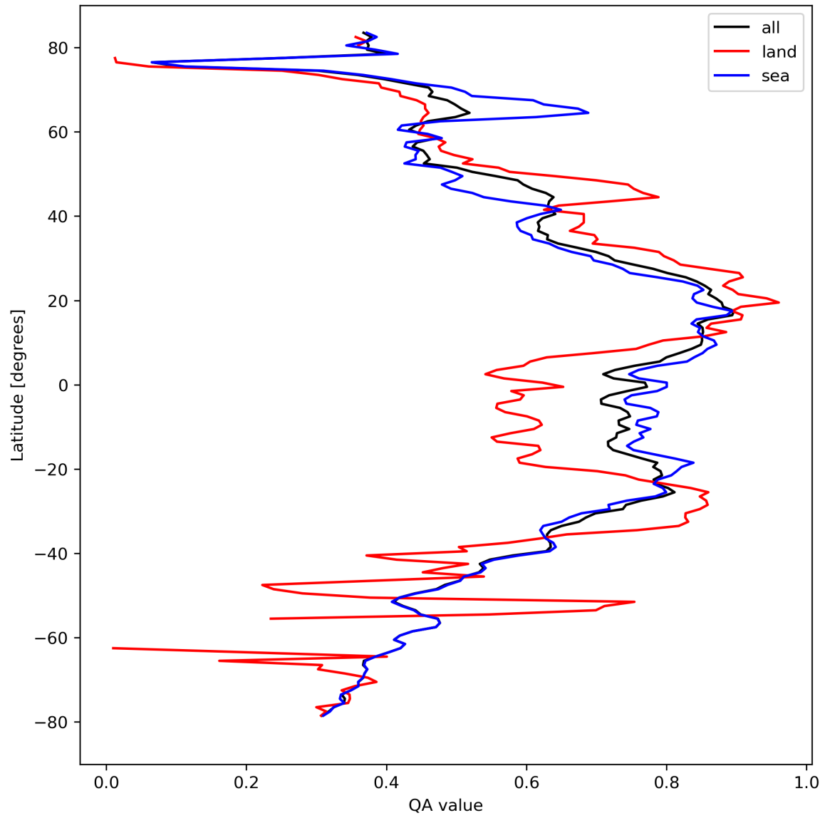
Figure 20: Zonal average of “QA value” for 2024-04-01 to 2024-04-03.
