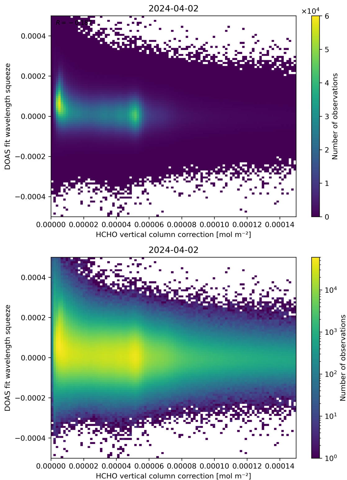
Figure 114: Scatter density plot of “HCHO vertical column correction” against “DOAS fit wavelength squeeze” for 2024-04-01 to 2024-04-03.
