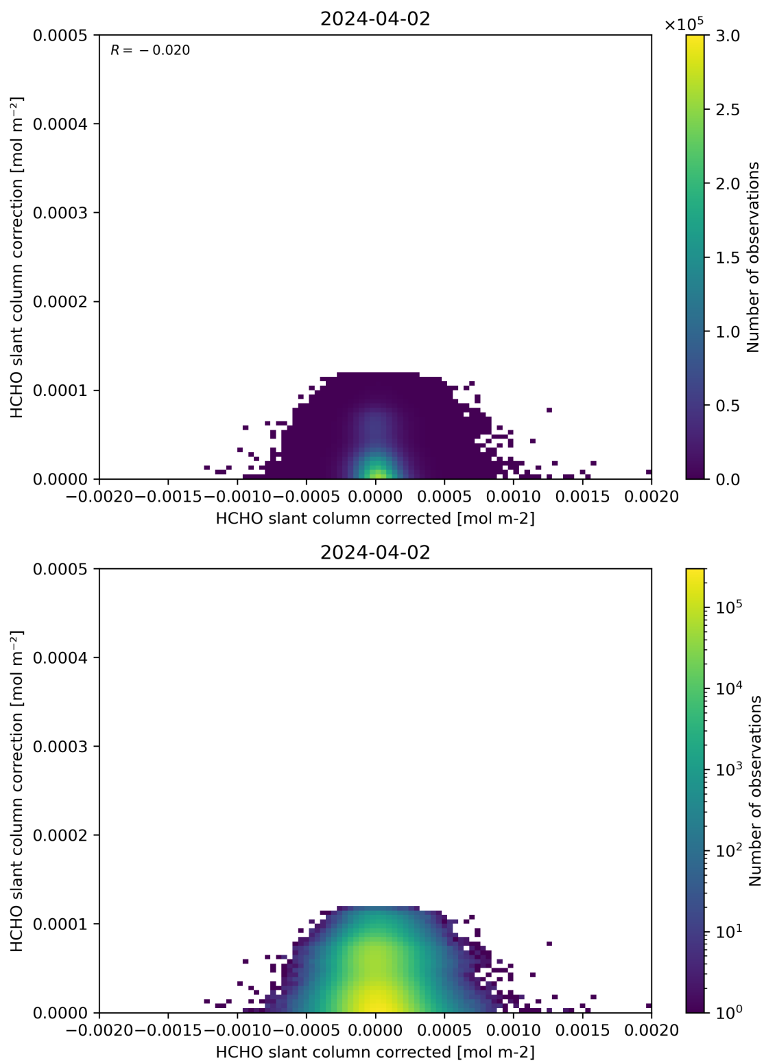
Figure 77: Scatter density plot of “HCHO slant column corrected” against “HCHO slant column correction” for 2024-04-01 to 2024-04-03.
