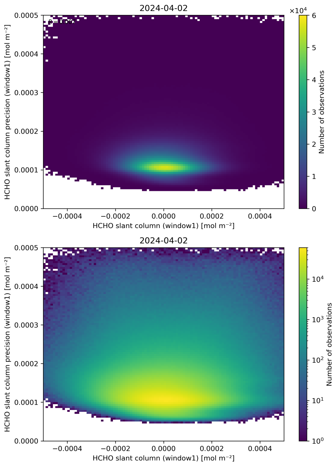
Figure 84: Scatter density plot of “HCHO slant column (window1)” against “HCHO slant column precision (window1)” for 2024-04-01 to 2024-04-03.
