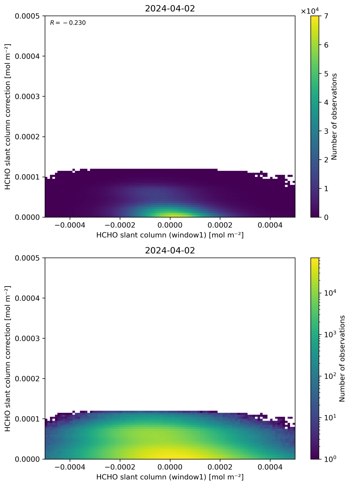
Figure 83: Scatter density plot of “HCHO slant column (window1)” against “HCHO slant column correction” for 2024-04-01 to 2024-04-03.
