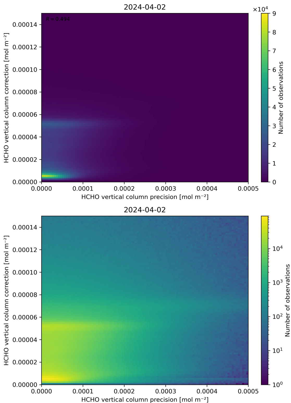
Figure 146: Scatter density plot of “HCHO vertical column precision” against “HCHO vertical column correction” for 2024-04-01 to 2024-04-03.
