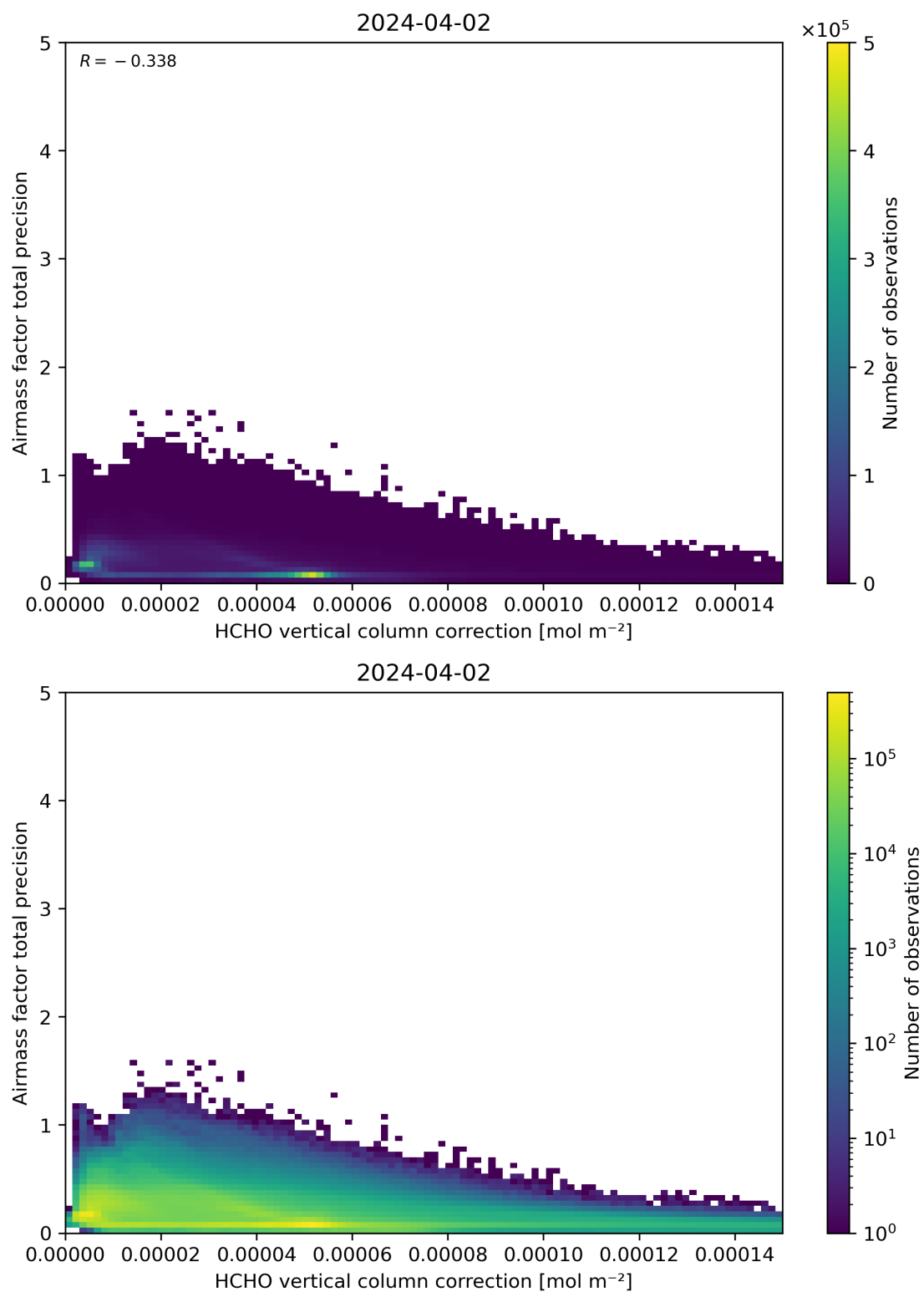
Figure 121: Scatter density plot of “HCHO vertical column correction” against “Airmass factor total precision” for 2024-04-01 to 2024-04-03.
