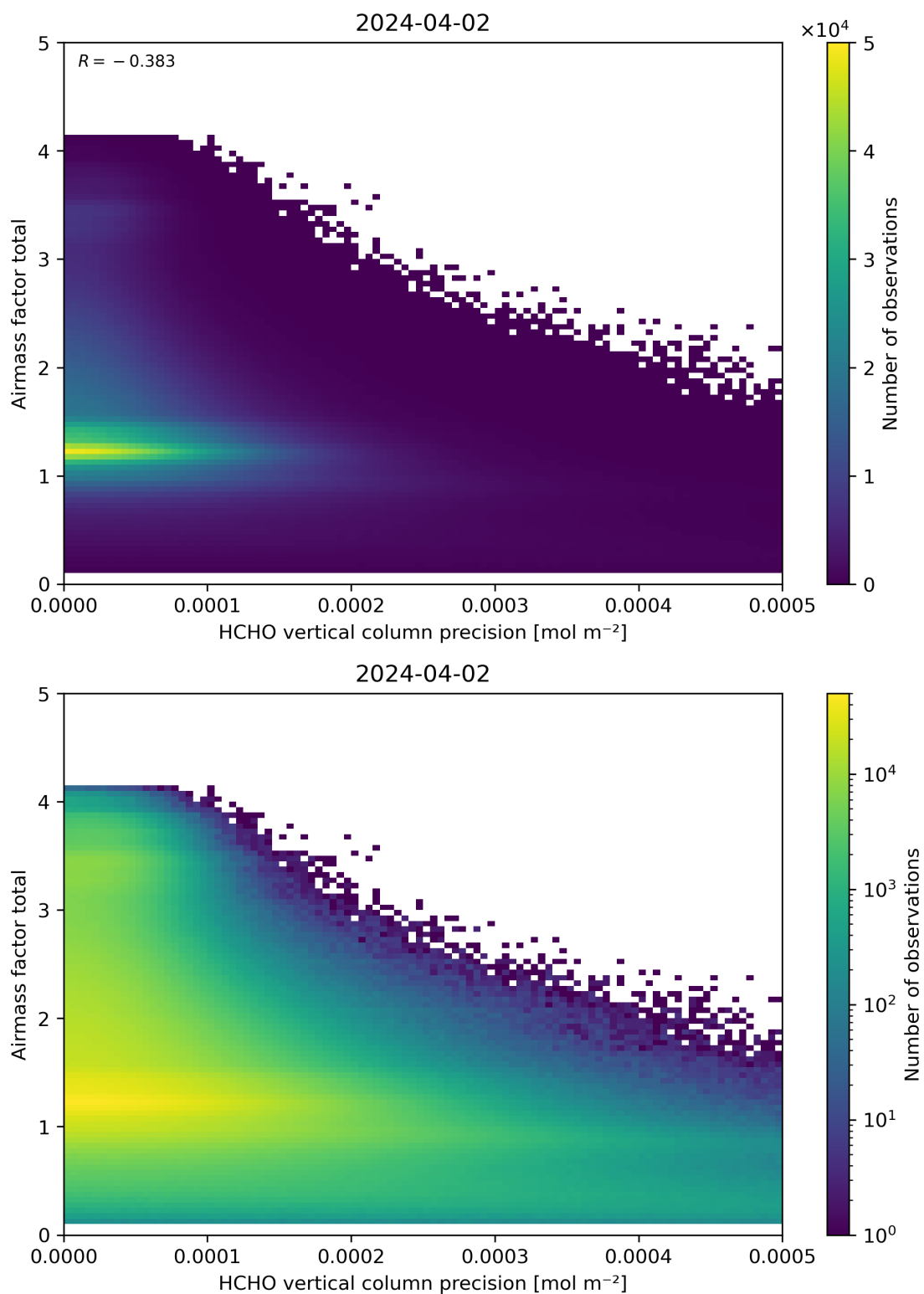
Figure 144: Scatter density plot of “HCHO vertical column precision” against “Airmass factor total” for 2024-04-01 to 2024-04-03.
