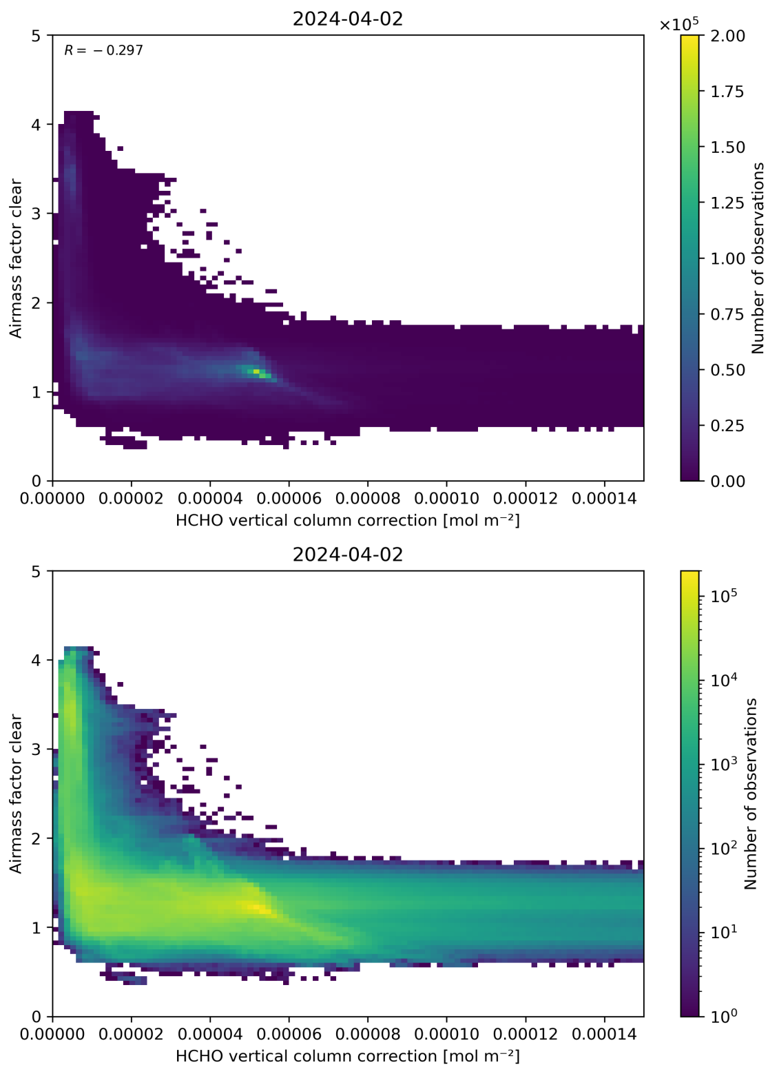
Figure 115: Scatter density plot of “HCHO vertical column correction” against “Airmass factor clear” for 2024-04-01 to 2024-04-03.
