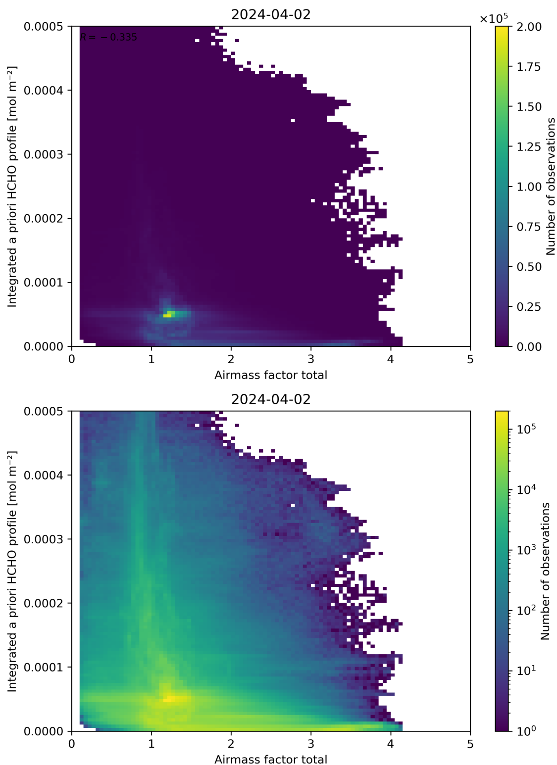
Figure 104: Scatter density plot of “Airmass factor total” against “Integrated a priori HCHO profile” for 2024-04-01 to 2024-04-03.
