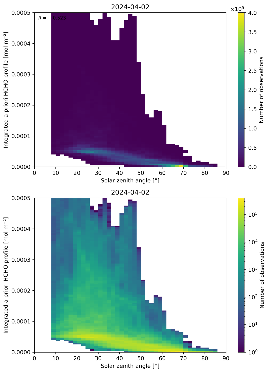
Figure 180: Scatter density plot of “Solar zenith angle” against “Integrated a priori HCHO profile” for 2024-04-01 to 2024-04-03.
