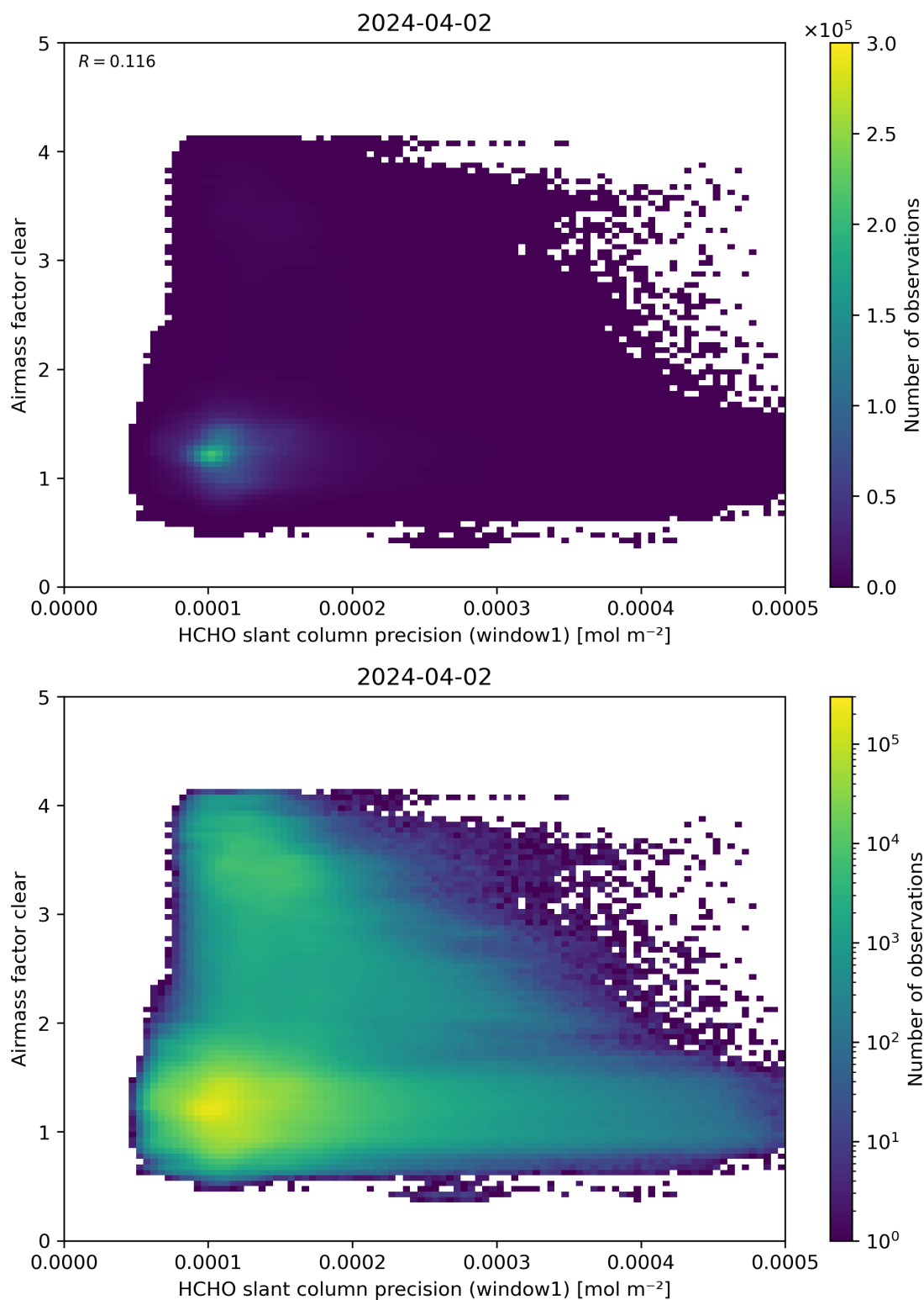
Figure 91: Scatter density plot of “HCHO slant column precision (window1)” against “Airmass factor clear” for 2024-04-01 to 2024-04-03.
