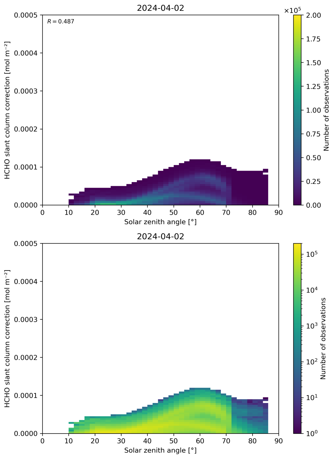
Figure 172: Scatter density plot of “Solar zenith angle” against “HCHO slant column correction” for 2024-04-01 to 2024-04-03.
