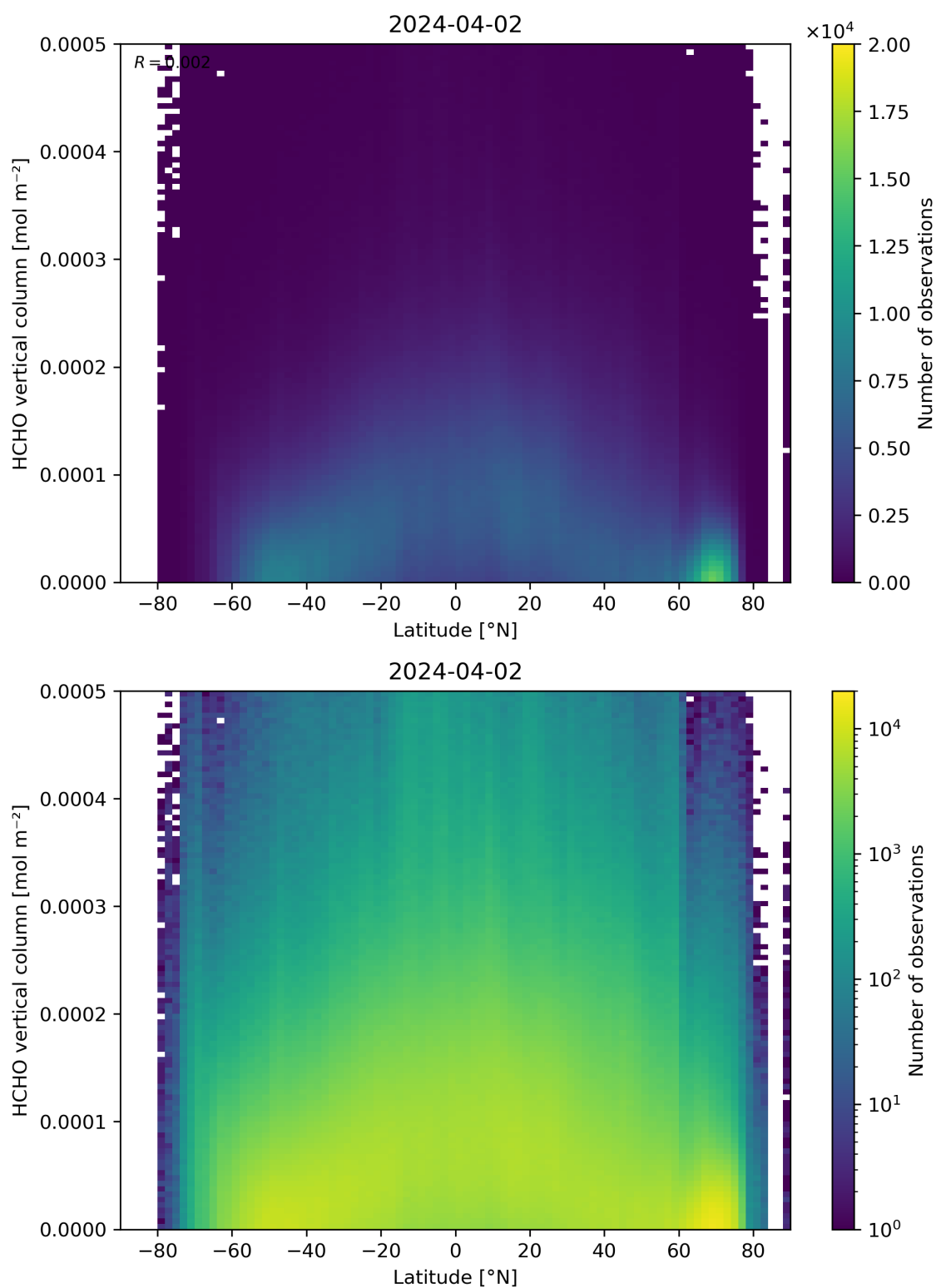
Figure 163: Scatter density plot of “Latitude” against “HCHO vertical column” for 2024-04-01 to 2024-04-03.
