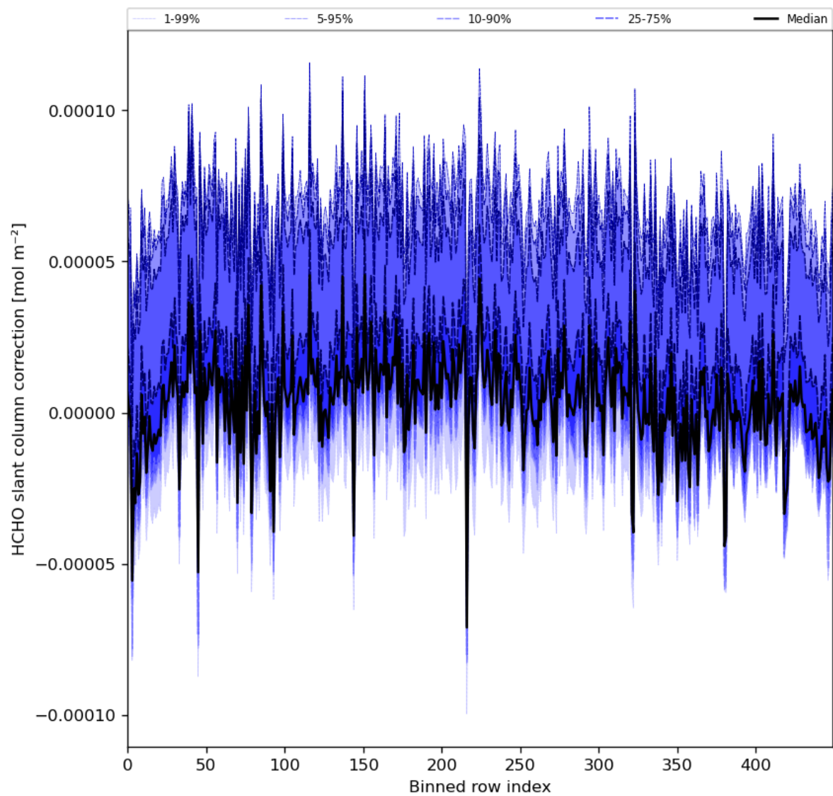
Figure 61: Along track statistics of “HCHO slant column correction” for 2024-04-01 to 2024-04-03
