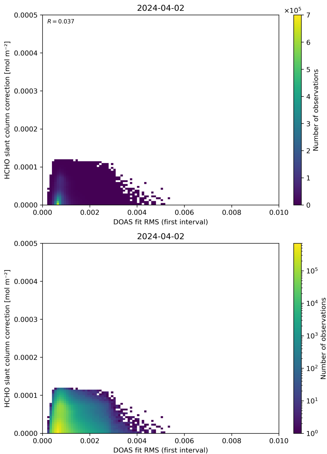
Figure 63: Scatter density plot of “DOAS fit RMS (first interval)” against “HCHO slant column correction” for 2024-04-01 to 2024-04-03.
