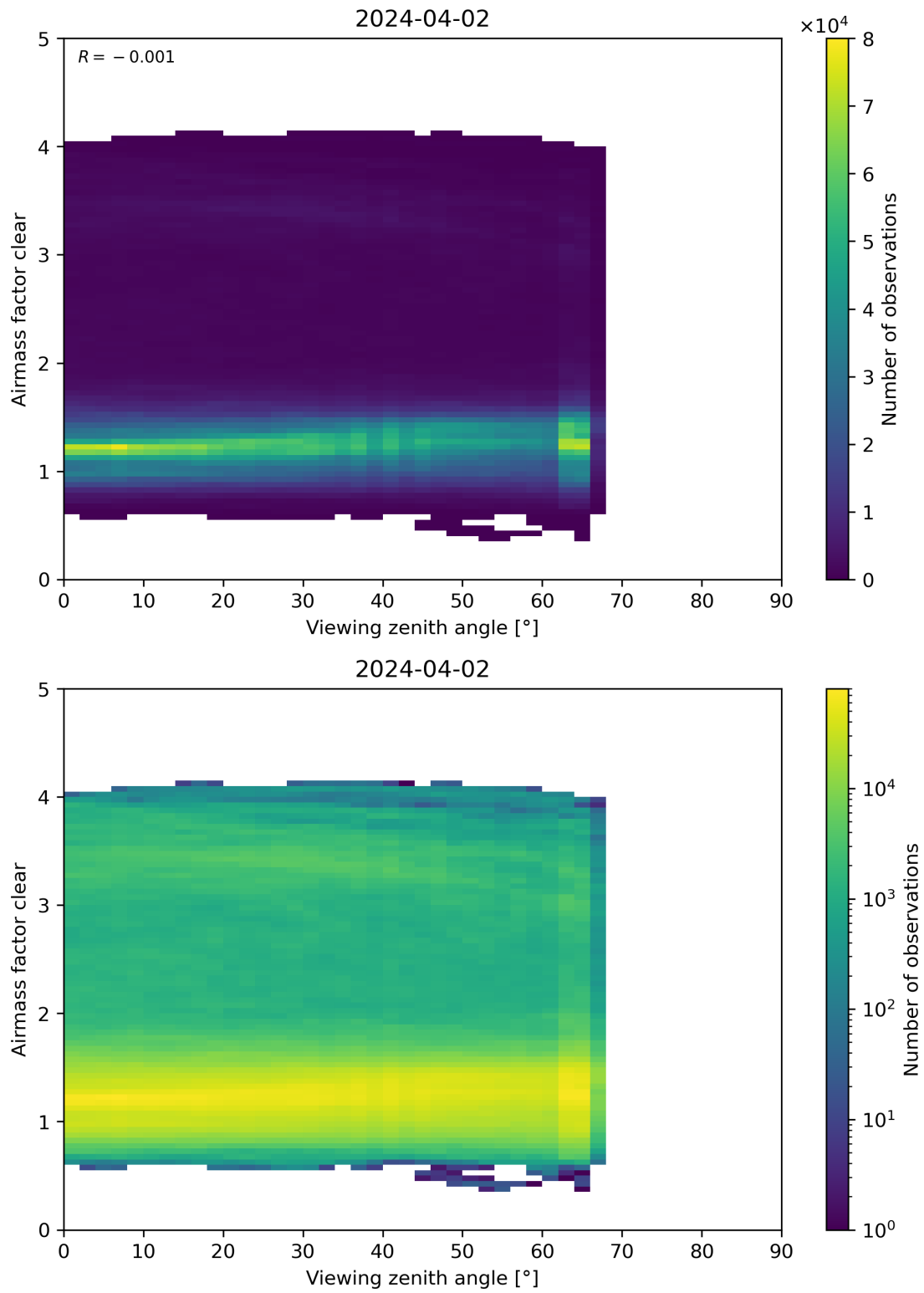
Figure 185: Scatter density plot of “Viewing zenith angle” against “Airmass factor clear” for 2024-04-01 to 2024-04-03.
