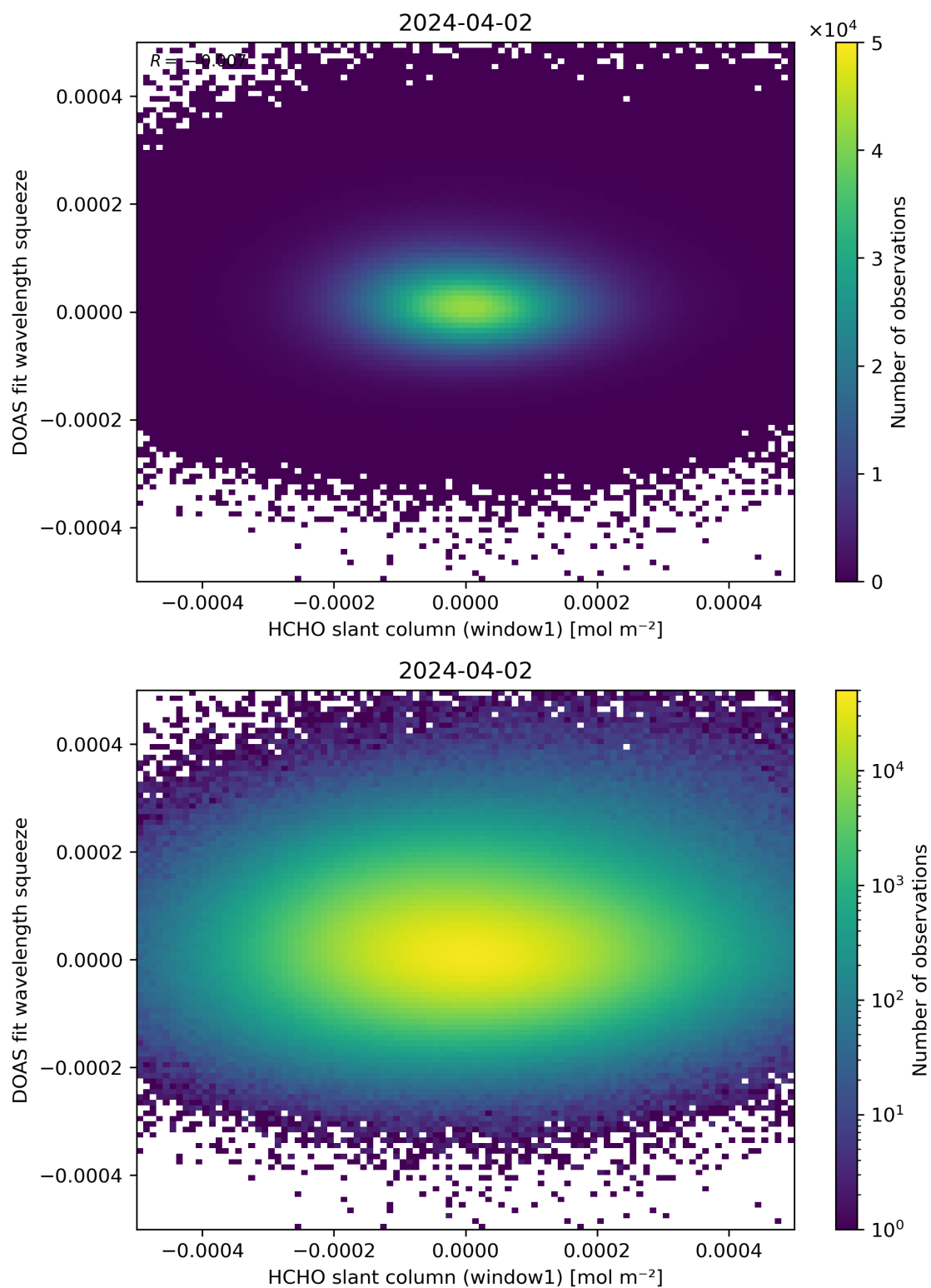
Figure 80: Scatter density plot of “HCHO slant column (window1)” against “DOAS fit wavelength squeeze” for 2024-04-01 to 2024-04-03.
