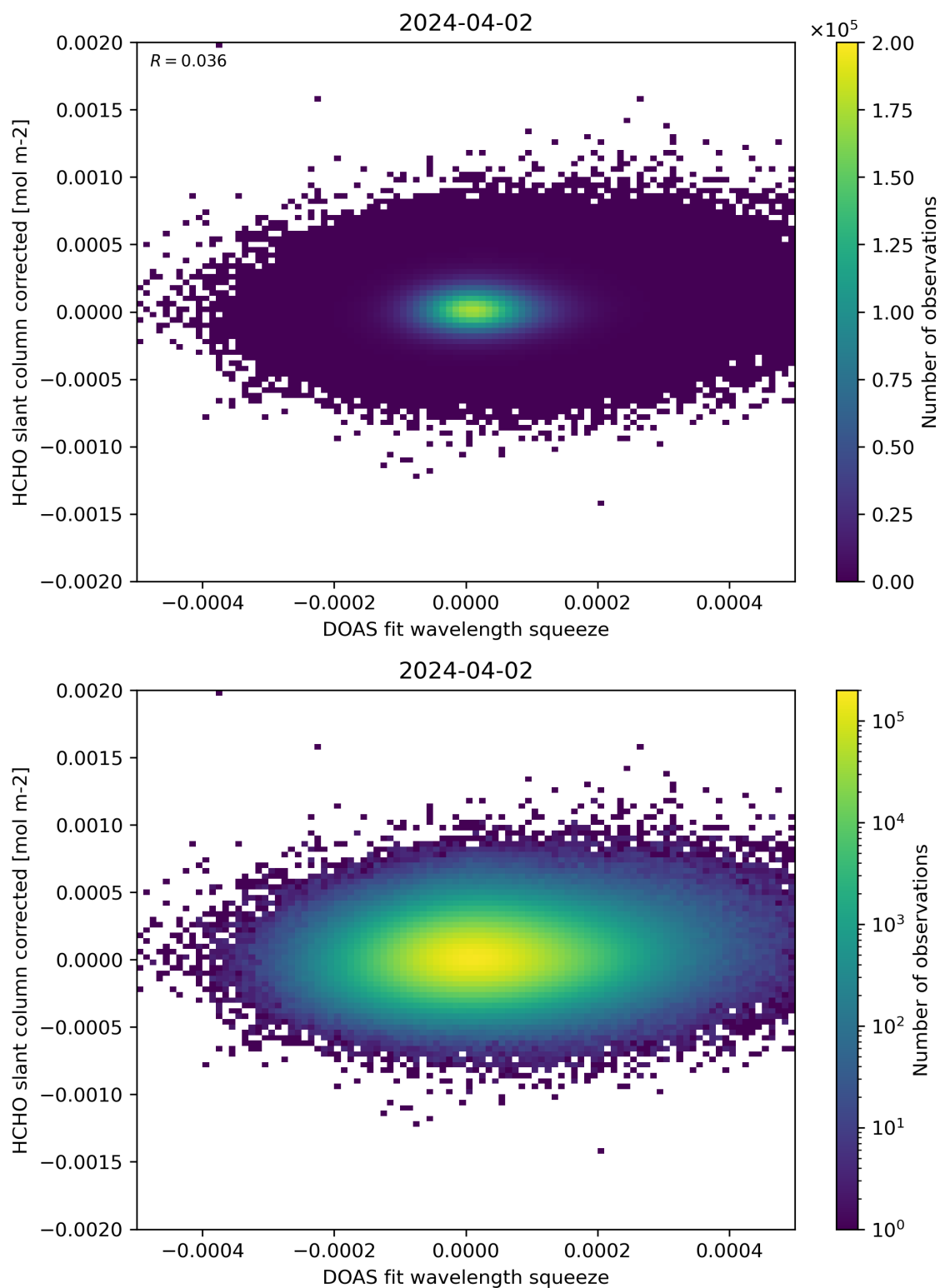
Figure 69: Scatter density plot of “DOAS fit wavelength squeeze” against “HCHO slant column corrected” for 2024-04-01 to 2024-04-03.
