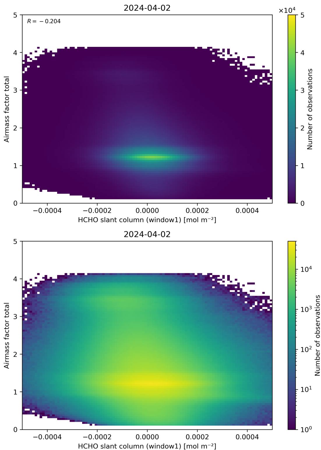
Figure 85: Scatter density plot of “HCHO slant column (window1)” against “Airmass factor total” for 2024-04-01 to 2024-04-03.
