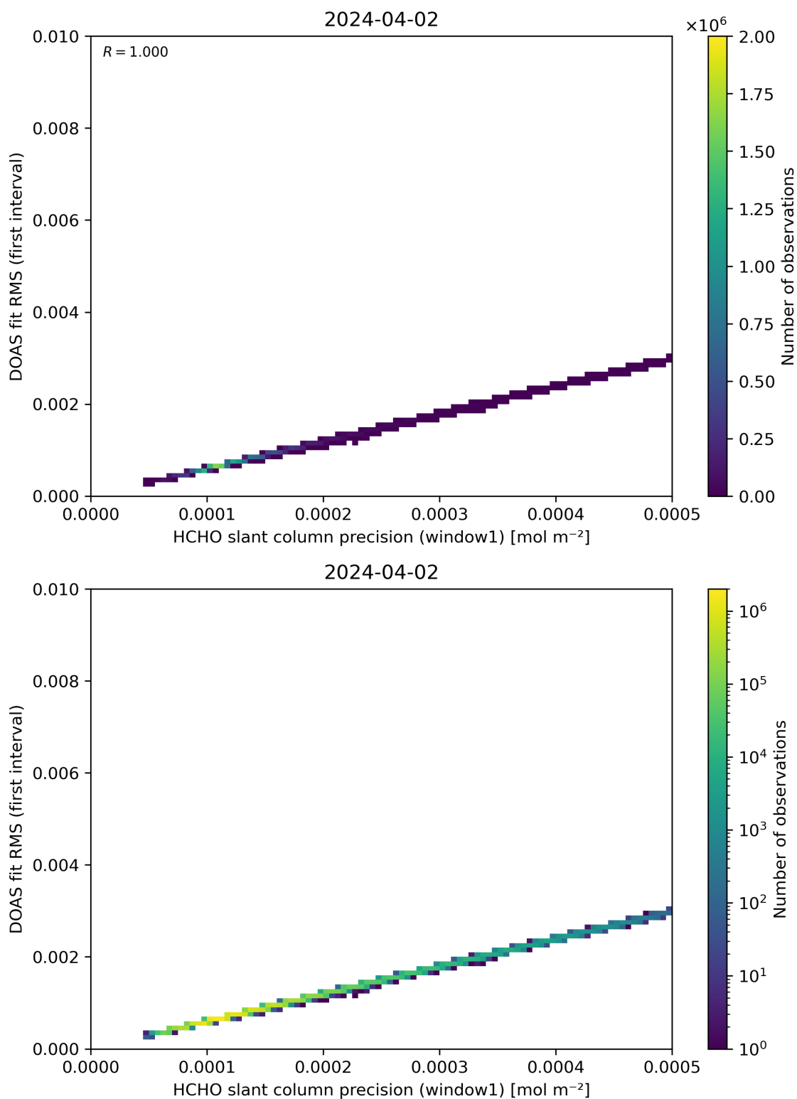
Figure 88: Scatter density plot of “HCHO slant column precision (window1)” against “DOAS fit RMS (first interval)” for 2024-04-01 to 2024-04-03.
