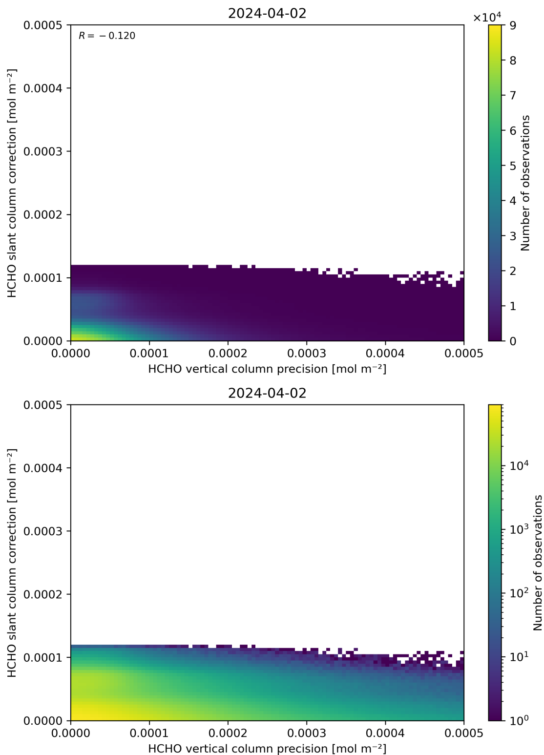
Figure 141: Scatter density plot of “HCHO vertical column precision” against “HCHO slant column correction” for 2024-04-01 to 2024-04-03.
