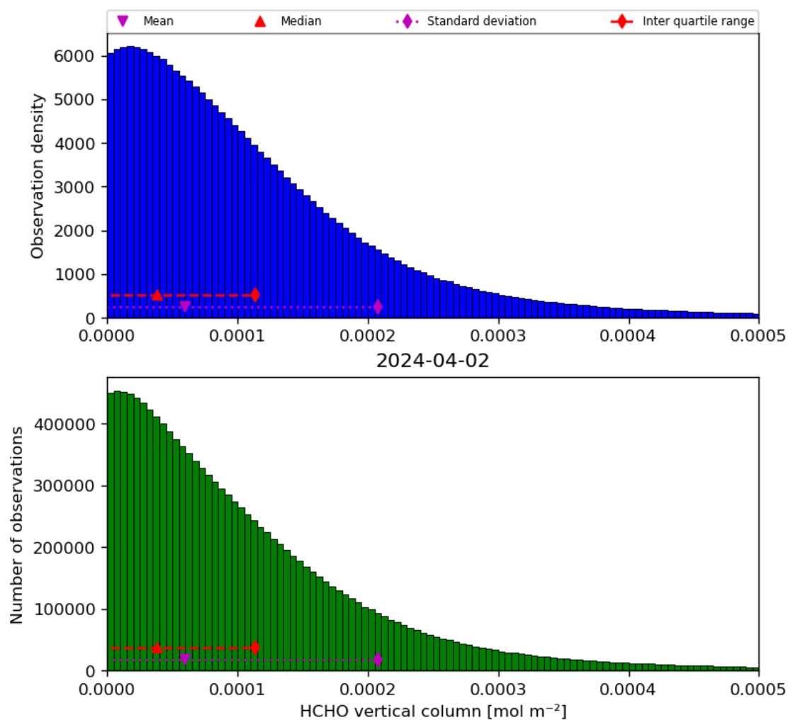
Figure 35: Histogram of “HCHO vertical column” for 2024-04-01 to 2024-04-03
