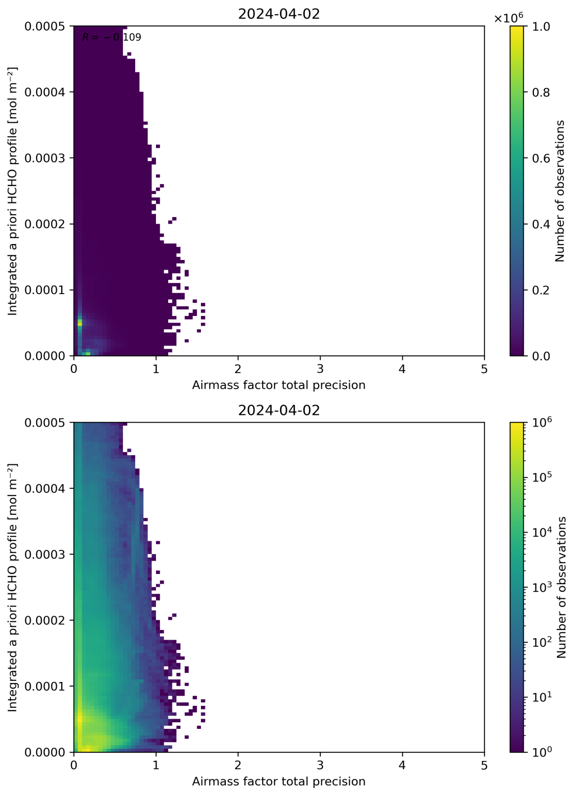
Figure 111: Scatter density plot of “Airmass factor total precision” against “Integrated a priori HCHO profile” for 2024-04-01 to 2024-04-03.
