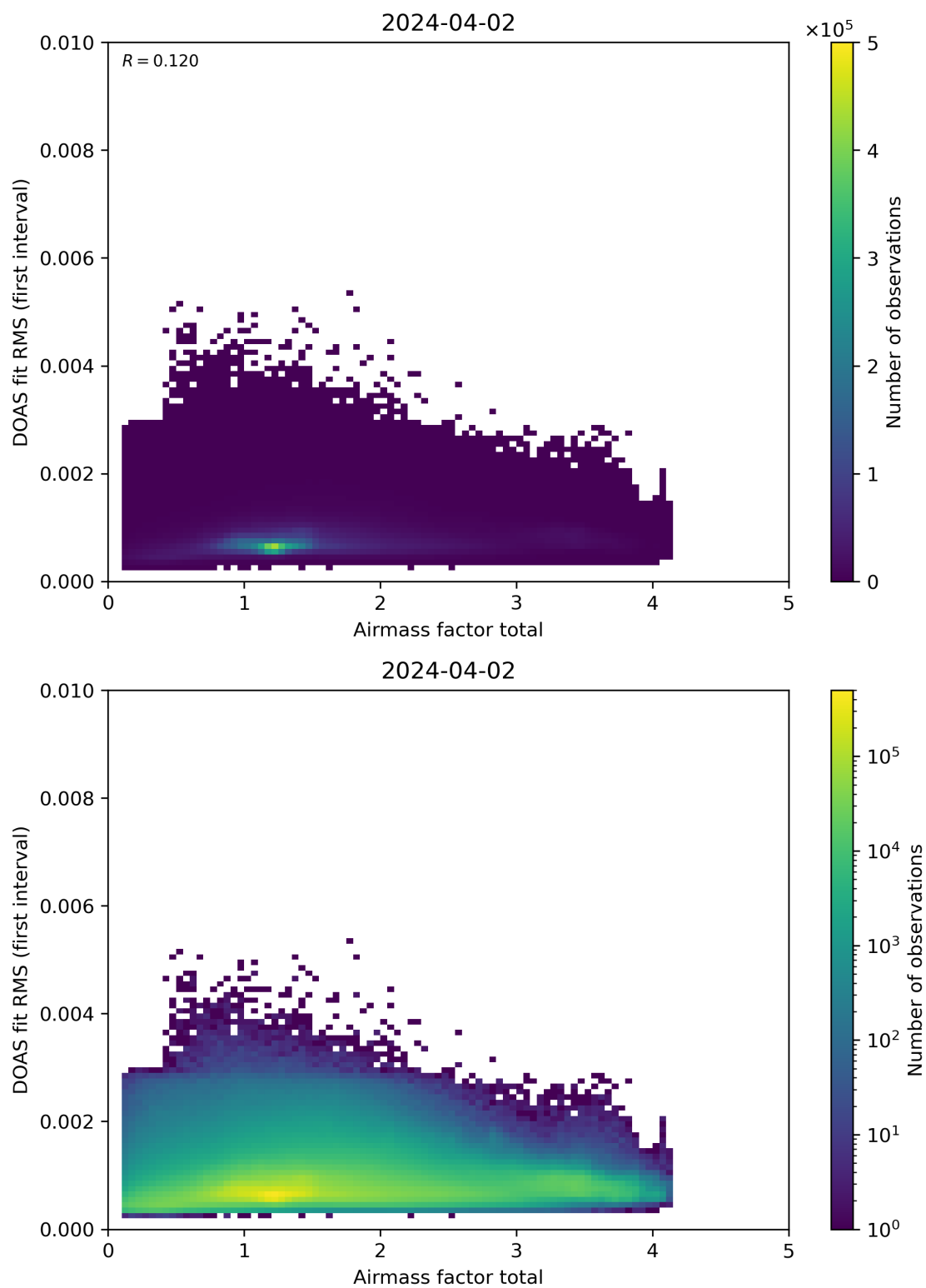
Figure 97: Scatter density plot of “Airmass factor total” against “DOAS fit RMS (first interval)” for 2024-04-01 to 2024-04-03.
