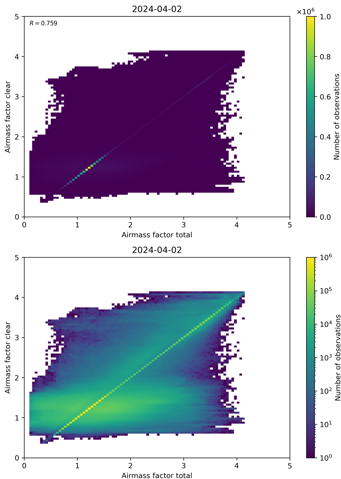
Figure 100: Scatter density plot of “Airmass factor total” against “Airmass factor clear” for 2024-04-01 to 2024-04-03.
