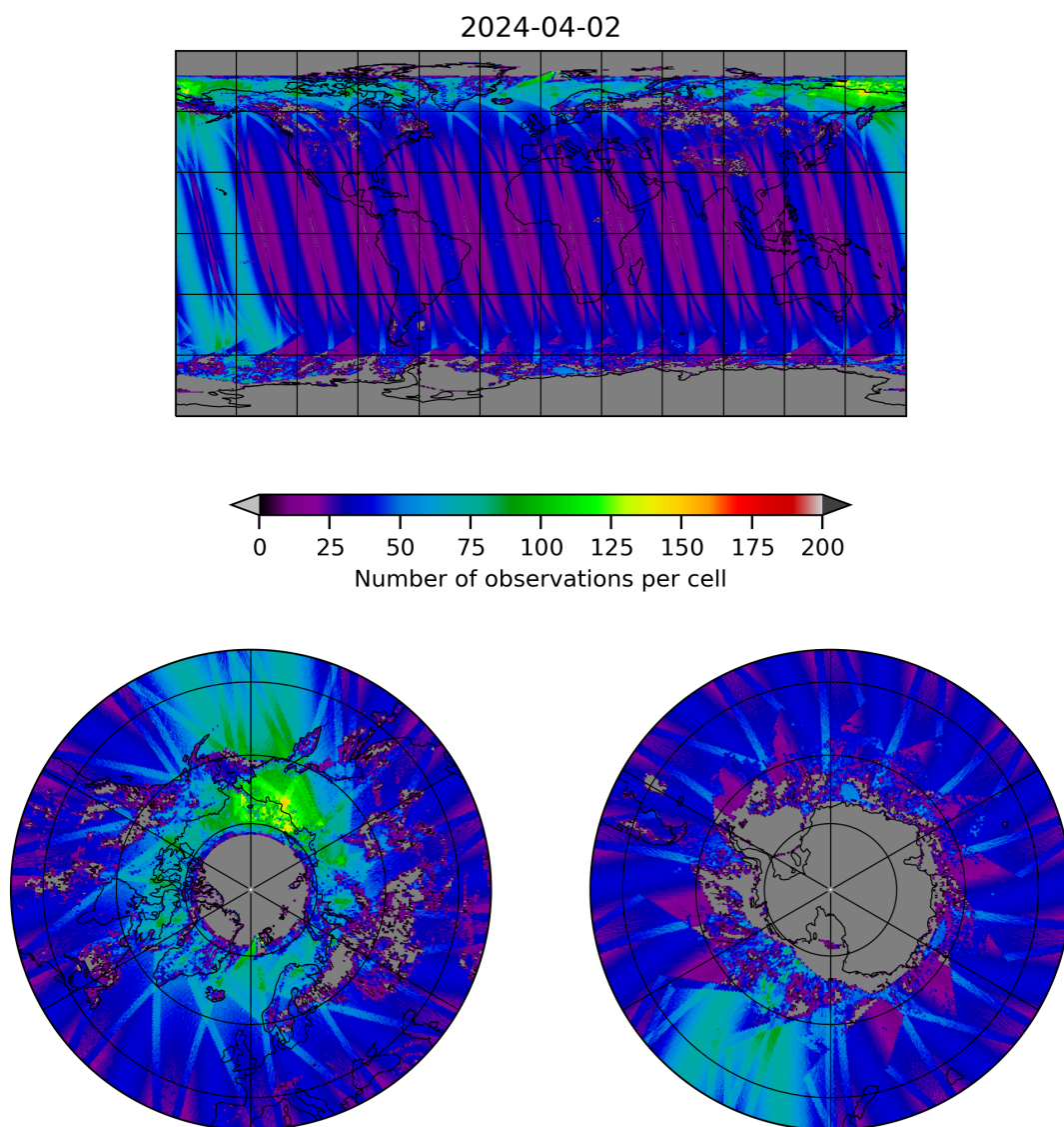
Figure 19: Map of the number of observations for 2024-04-01 to 2024-04-03
