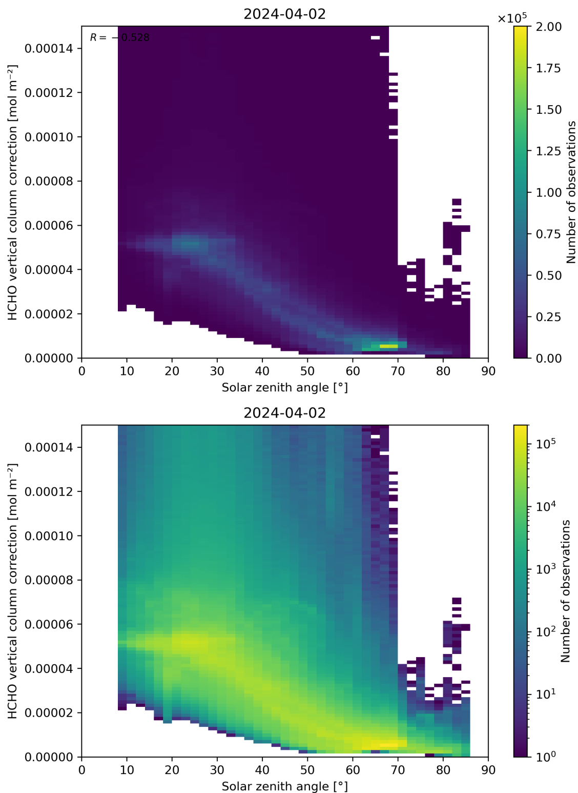
Figure 178: Scatter density plot of “Solar zenith angle” against “HCHO vertical column correction” for 2024-04-01 to 2024-04-03.
