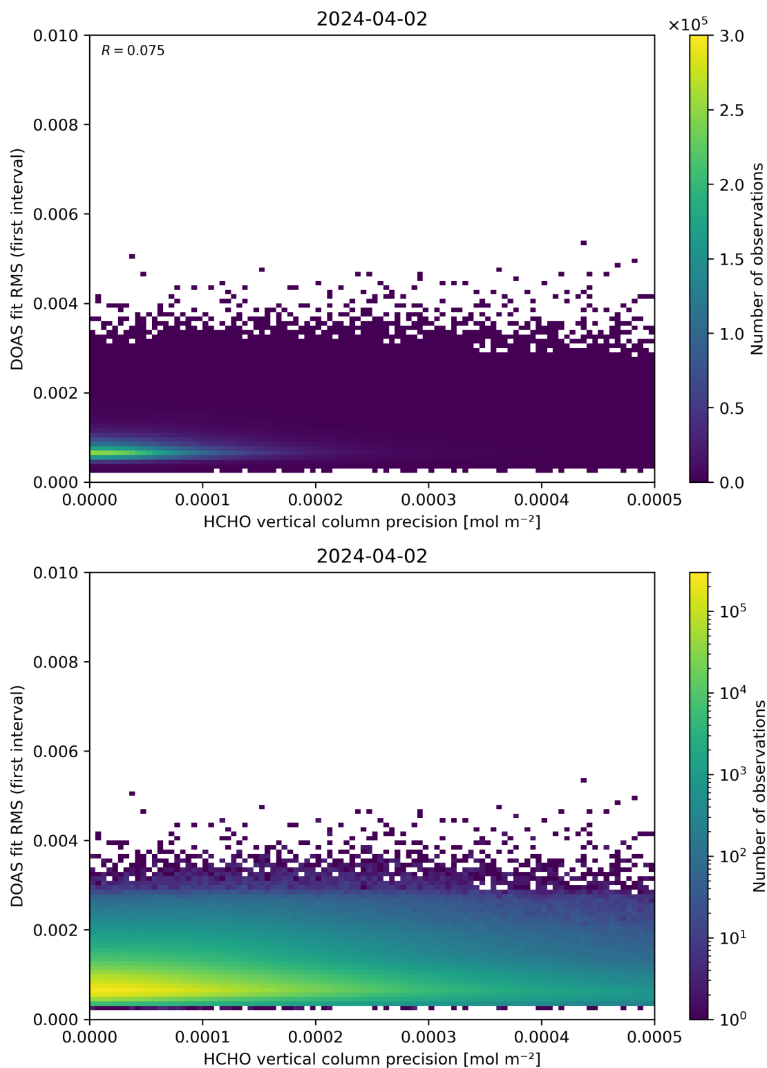
Figure 136: Scatter density plot of “HCHO vertical column precision” against “DOAS fit RMS (first interval)” for 2024-04-01 to 2024-04-03.
