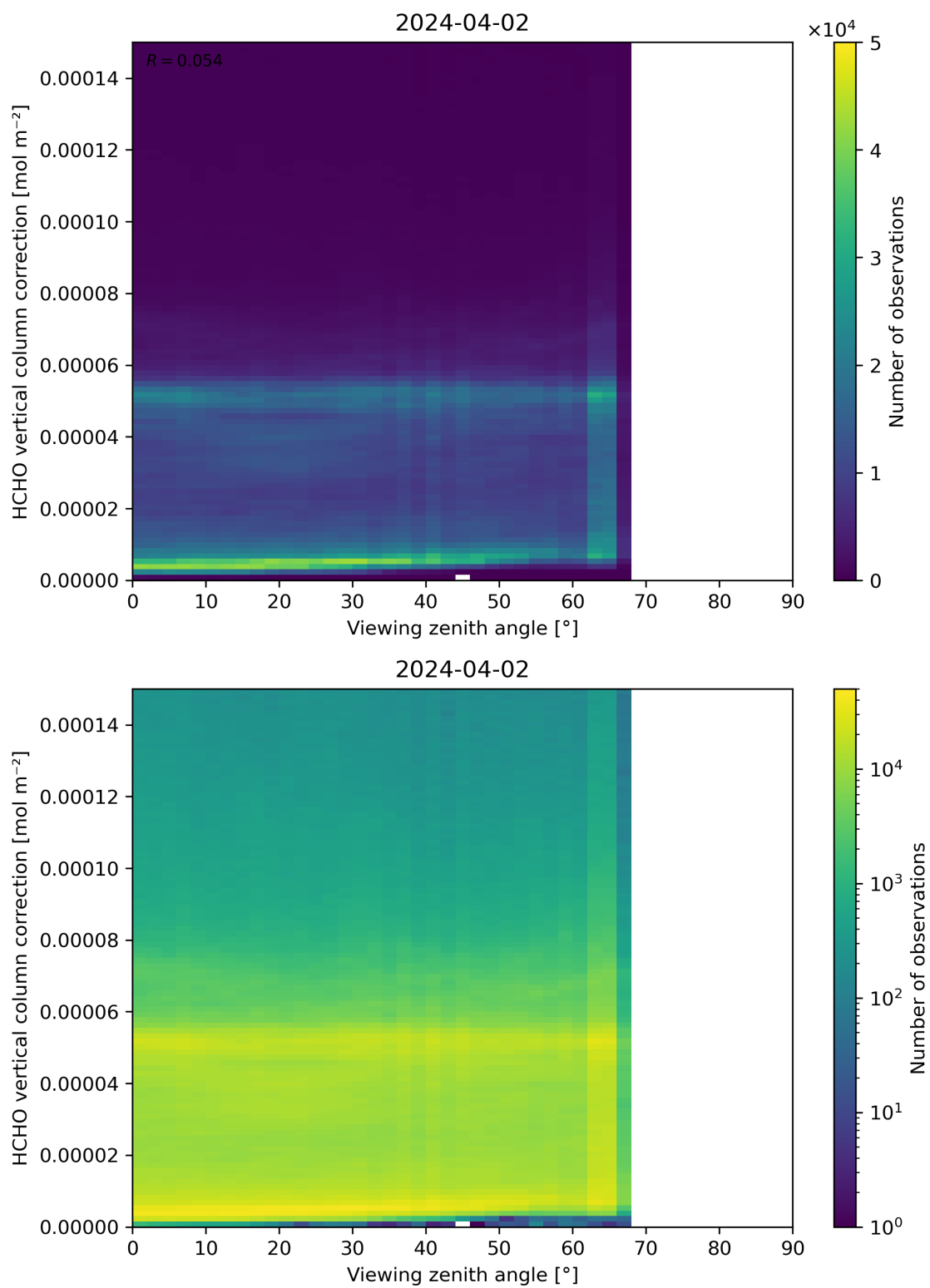
Figure 193: Scatter density plot of “Viewing zenith angle” against “HCHO vertical column correction” for 2024-04-01 to 2024-04-03.
