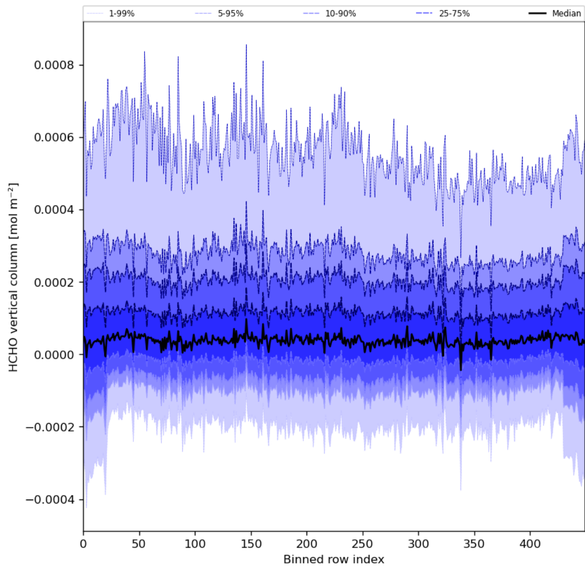
Figure 49: Along track statistics of “HCHO vertical column” for 2024-04-01 to 2024-04-03
