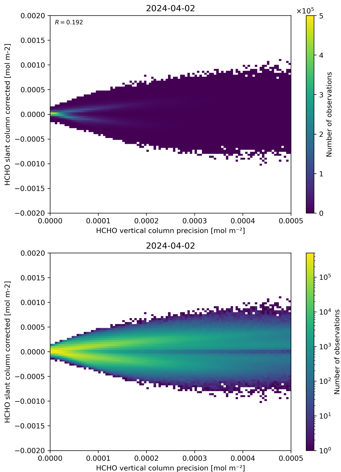
Figure 140: Scatter density plot of “HCHO vertical column precision” against “HCHO slant column corrected” for 2024-04-01 to 2024-04-03.
