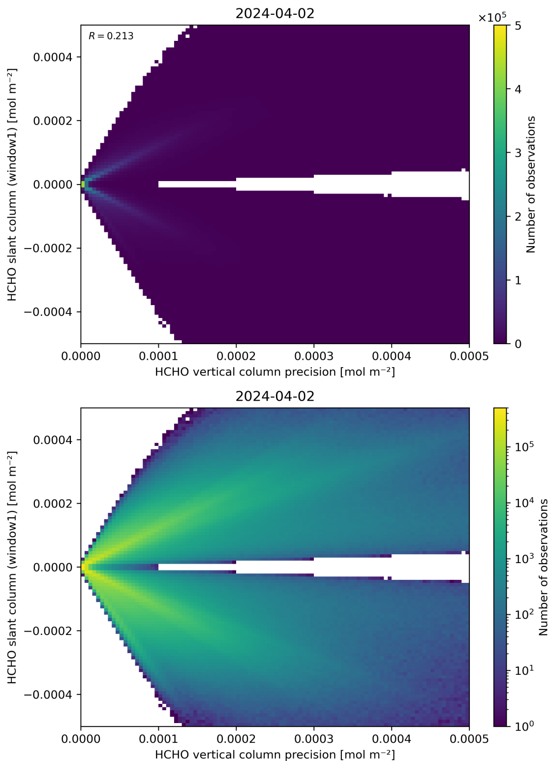
Figure 142: Scatter density plot of “HCHO vertical column precision” against “HCHO slant column (window1)” for 2024-04-01 to 2024-04-03.
