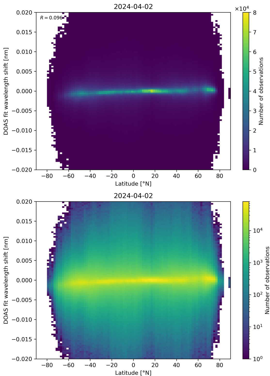
Figure 154: Scatter density plot of “Latitude” against “DOAS fit wavelength shift” for 2024-04-01 to 2024-04-03.
