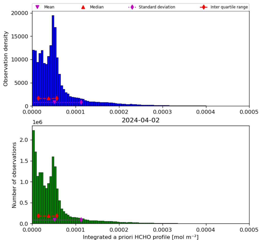
Figure 43: Histogram of “Integrated a priori HCHO profile” for 2024-04-01 to 2024-04-03
