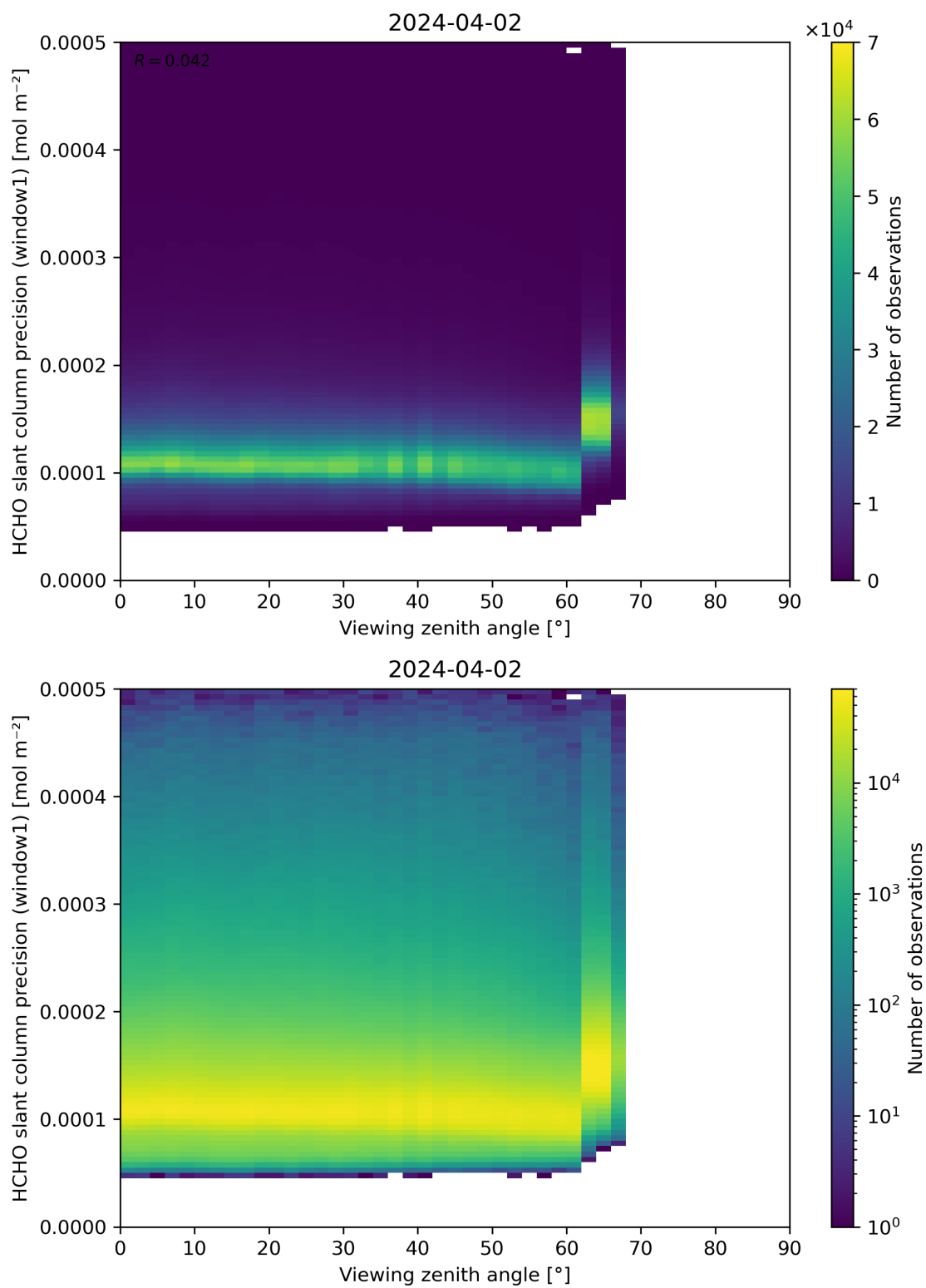
Figure 189: Scatter density plot of “Viewing zenith angle” against “HCHO slant column precision (window1)” for 2024-04-01 to 2024-04-03.
