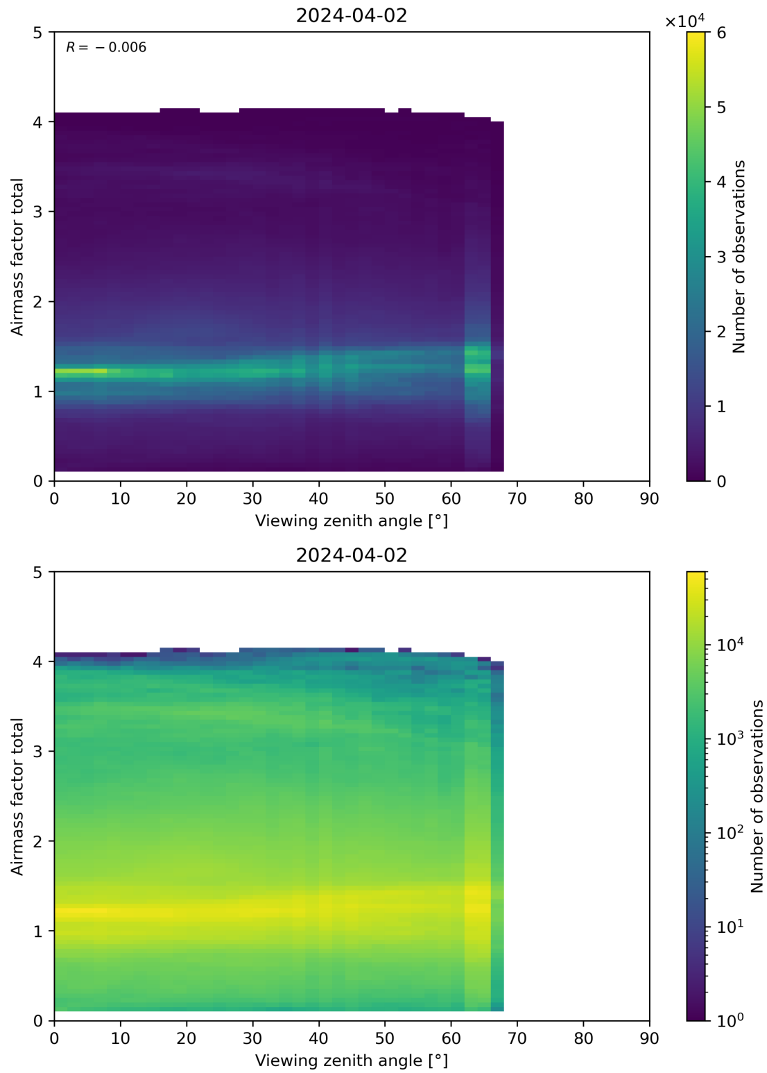
Figure 190: Scatter density plot of “Viewing zenith angle” against “Airmass factor total” for 2024-04-01 to 2024-04-03.
