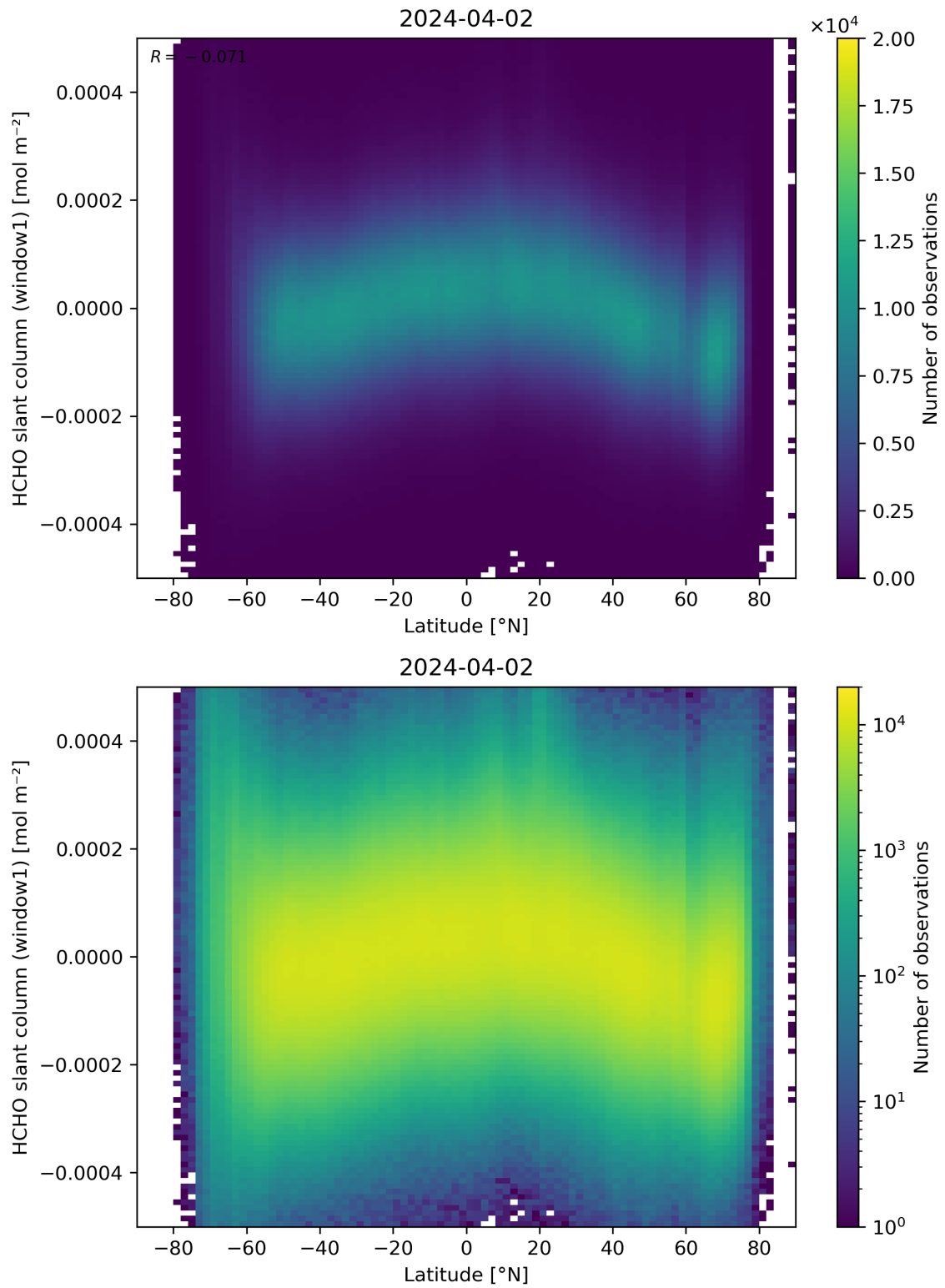
Figure 159: Scatter density plot of “Latitude” against “HCHO slant column (window1)” for 2024-04-01 to 2024-04-03.
