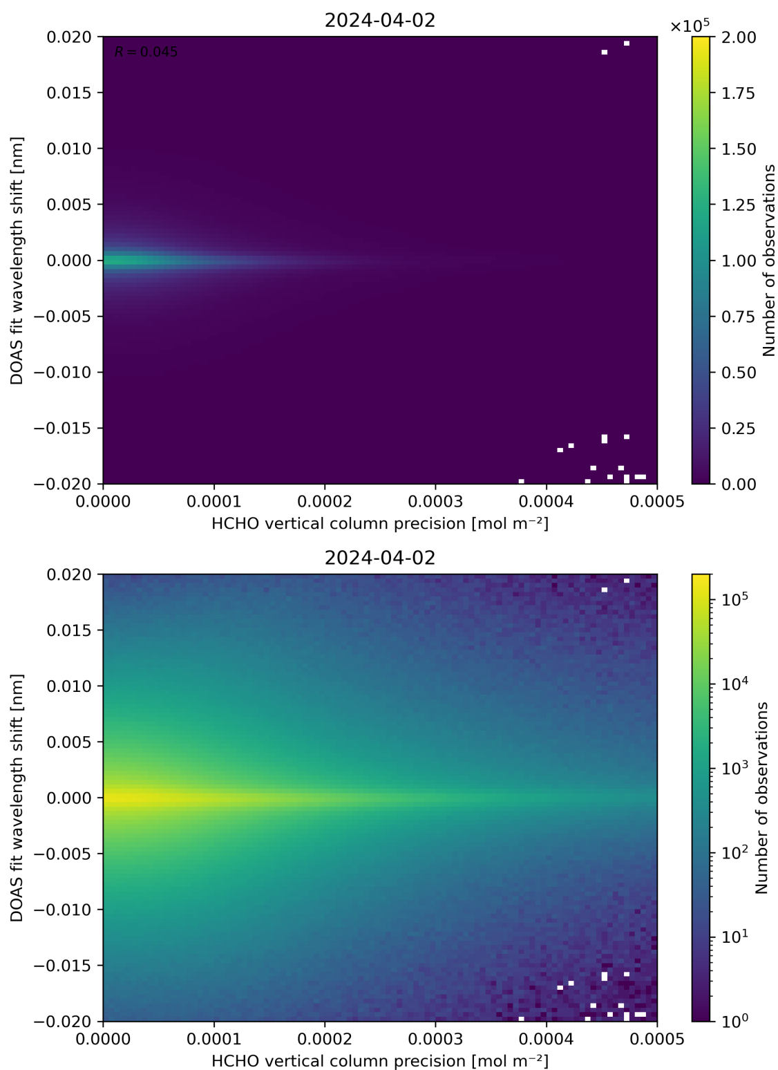
Figure 137: Scatter density plot of “HCHO vertical column precision” against “DOAS fit wavelength shift” for 2024-04-01 to 2024-04-03.
