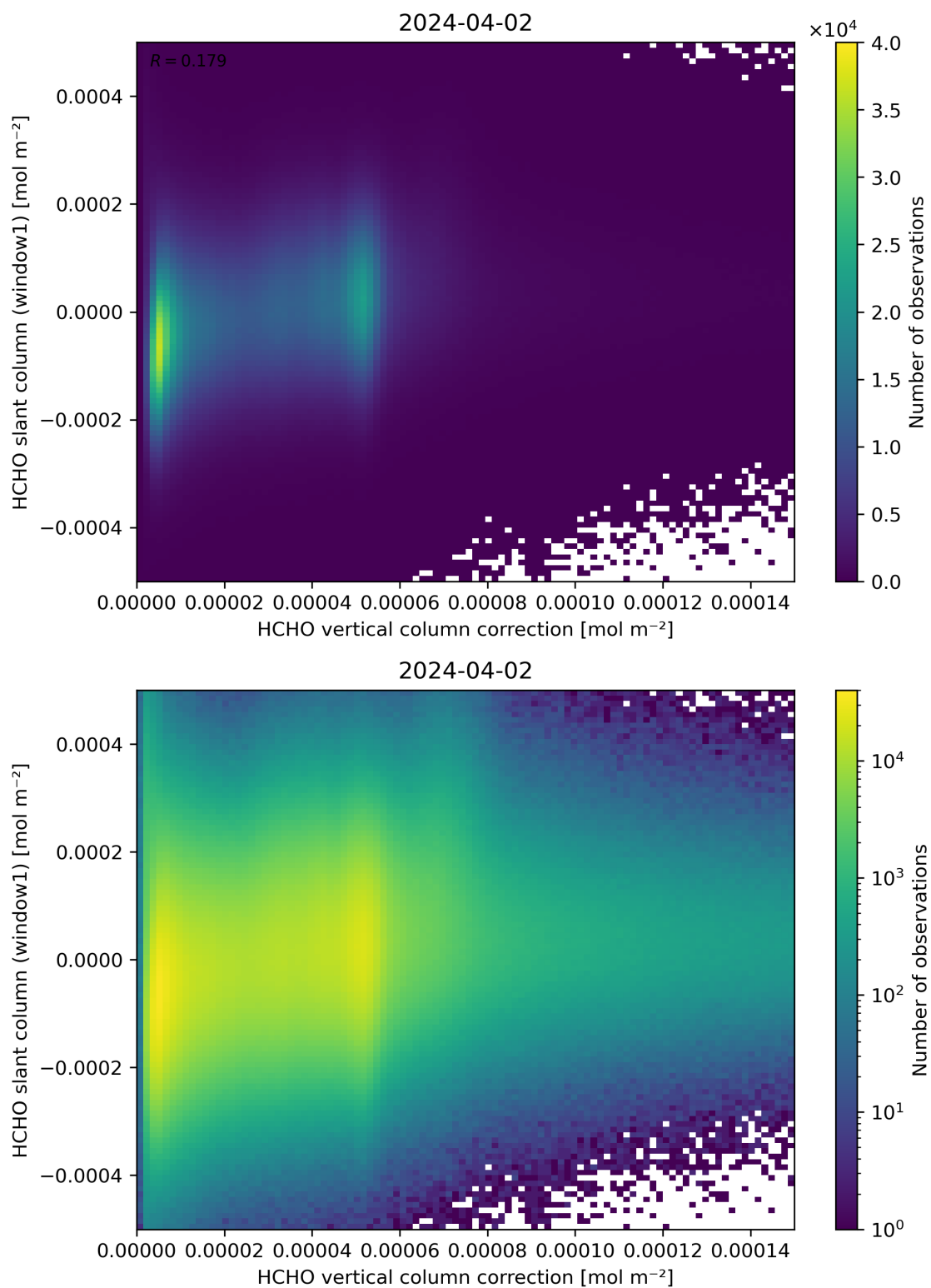
Figure 118: Scatter density plot of “HCHO vertical column correction” against “HCHO slant column (window1)” for 2024-04-01 to 2024-04-03.
