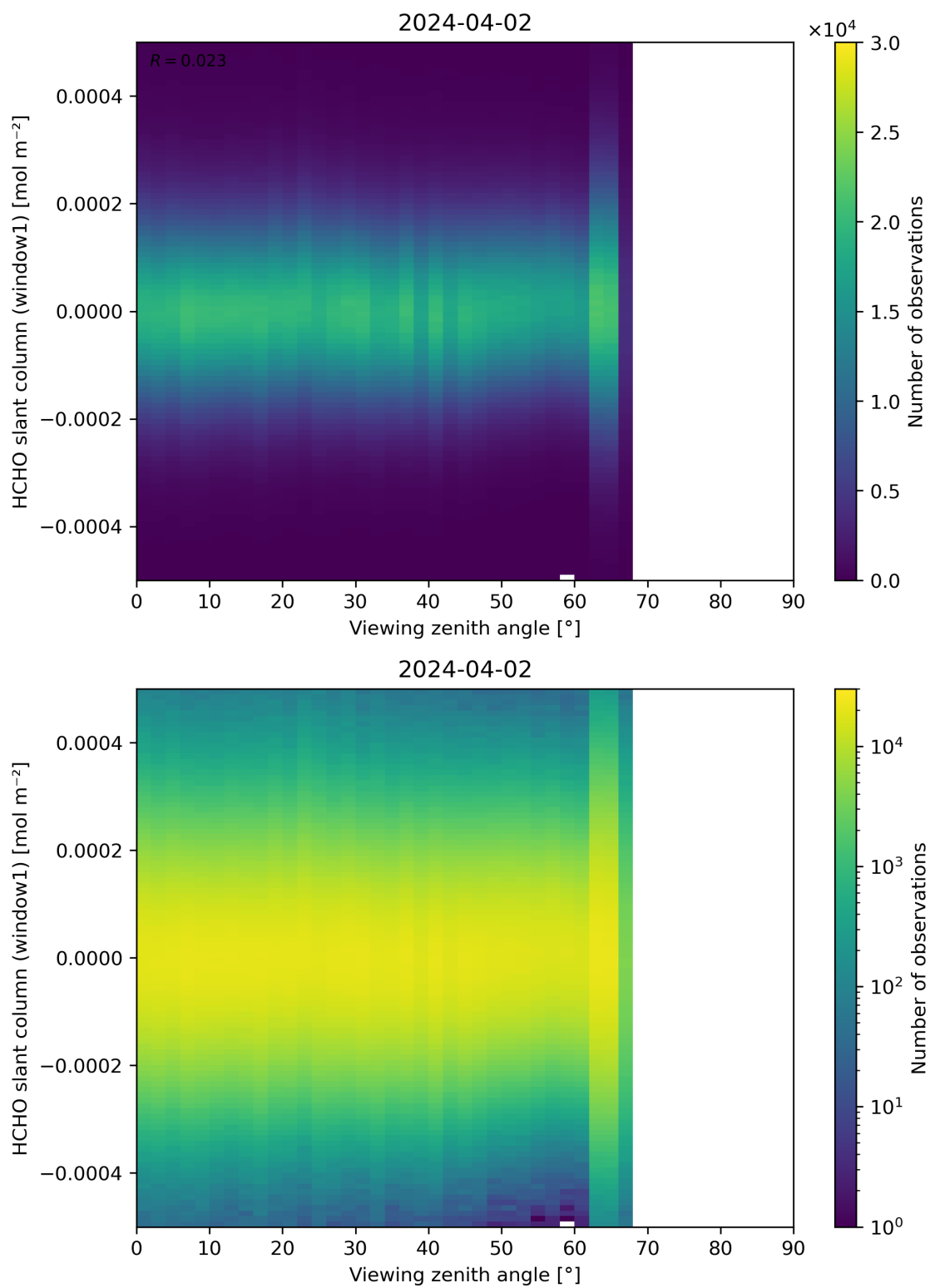
Figure 188: Scatter density plot of “Viewing zenith angle” against “HCHO slant column (window1)” for 2024-04-01 to 2024-04-03.
