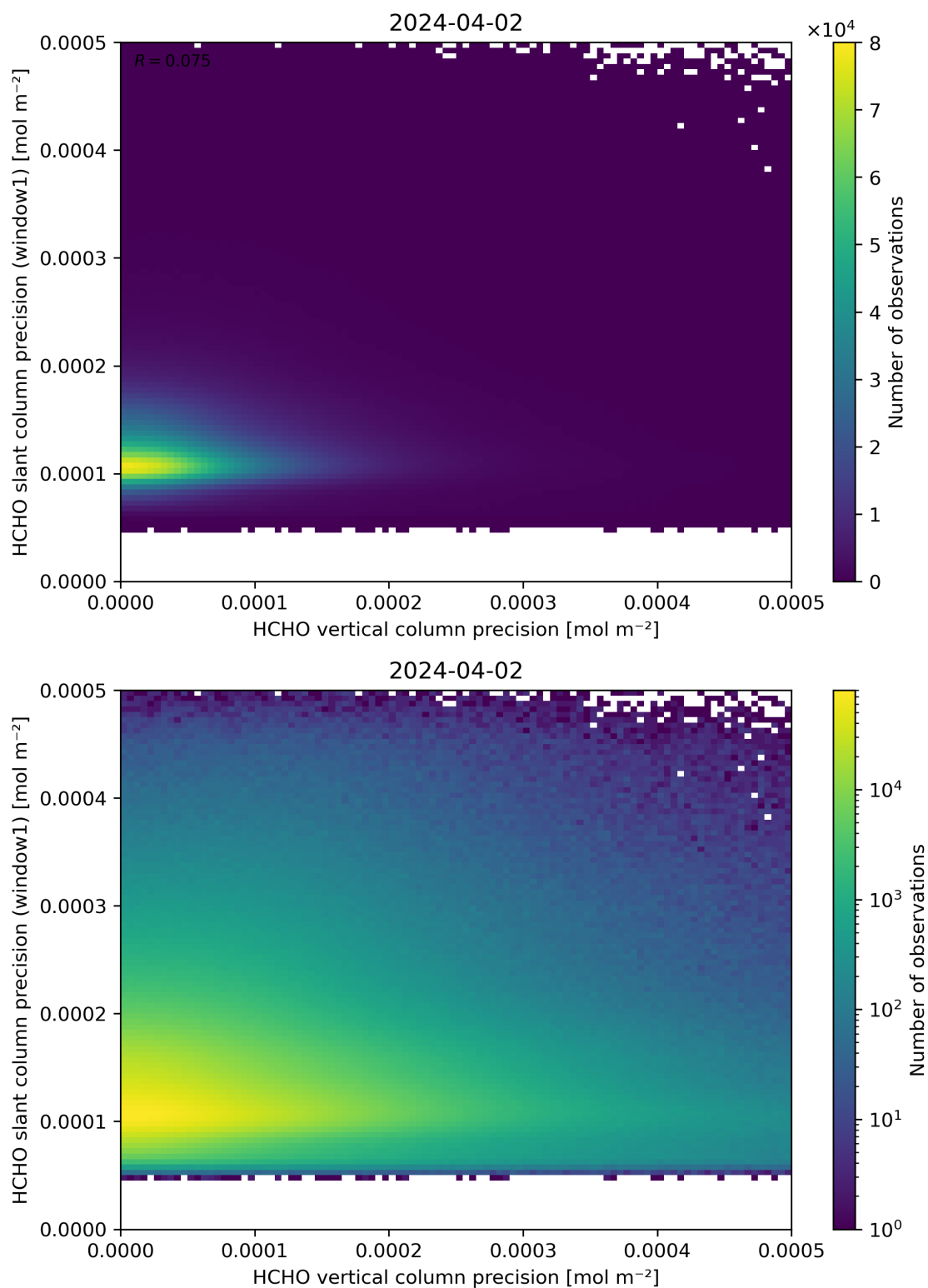
Figure 143: Scatter density plot of “HCHO vertical column precision” against “HCHO slant column precision (window1)” for 2024-04-01 to 2024-04-03.
