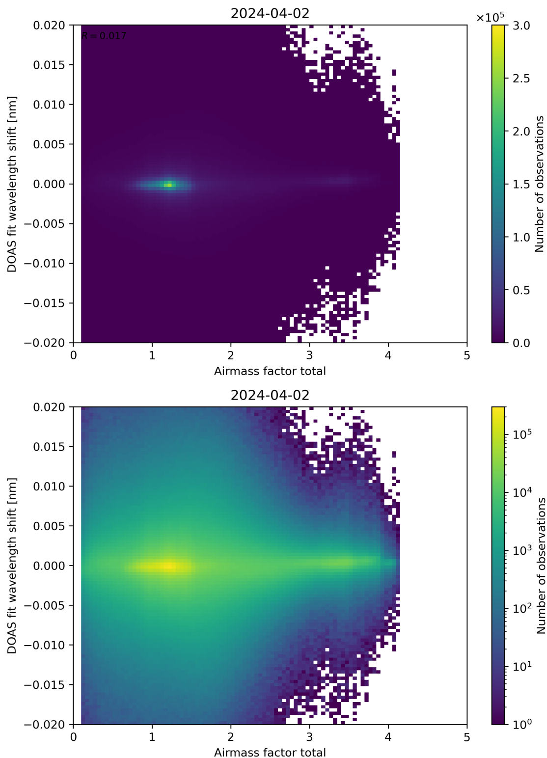
Figure 98: Scatter density plot of “Airmass factor total” against “DOAS fit wavelength shift” for 2024-04-01 to 2024-04-03.
