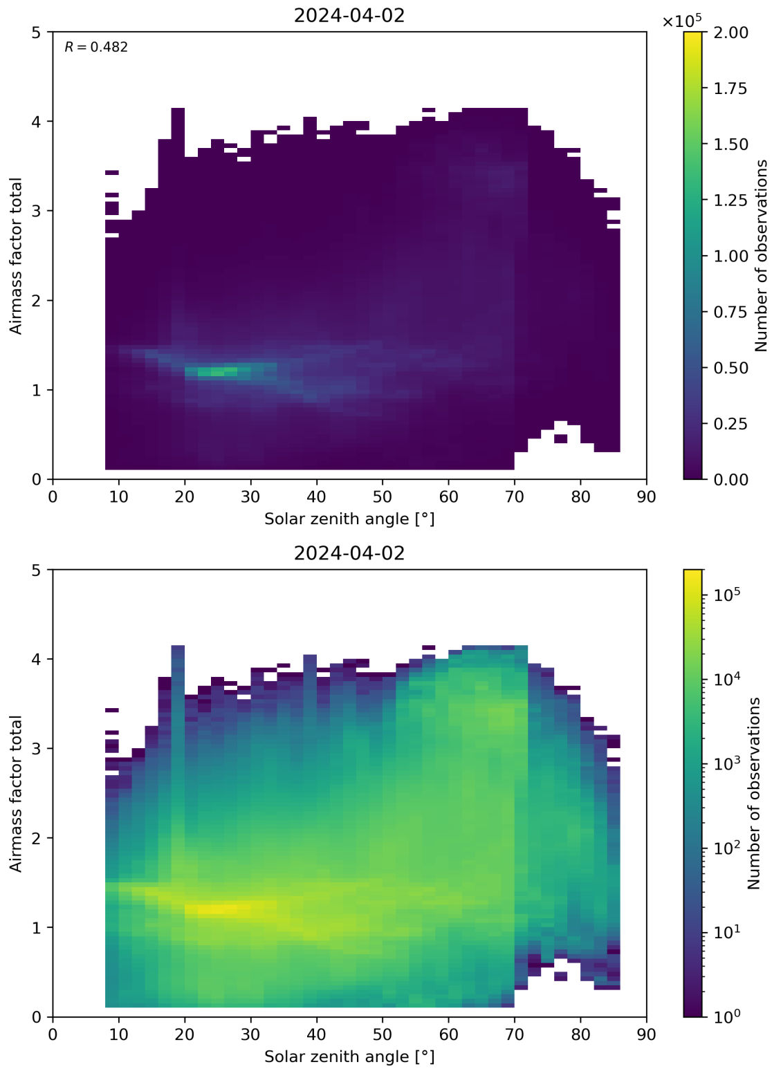
Figure 175: Scatter density plot of “Solar zenith angle” against “Airmass factor total” for 2024-04-01 to 2024-04-03.
