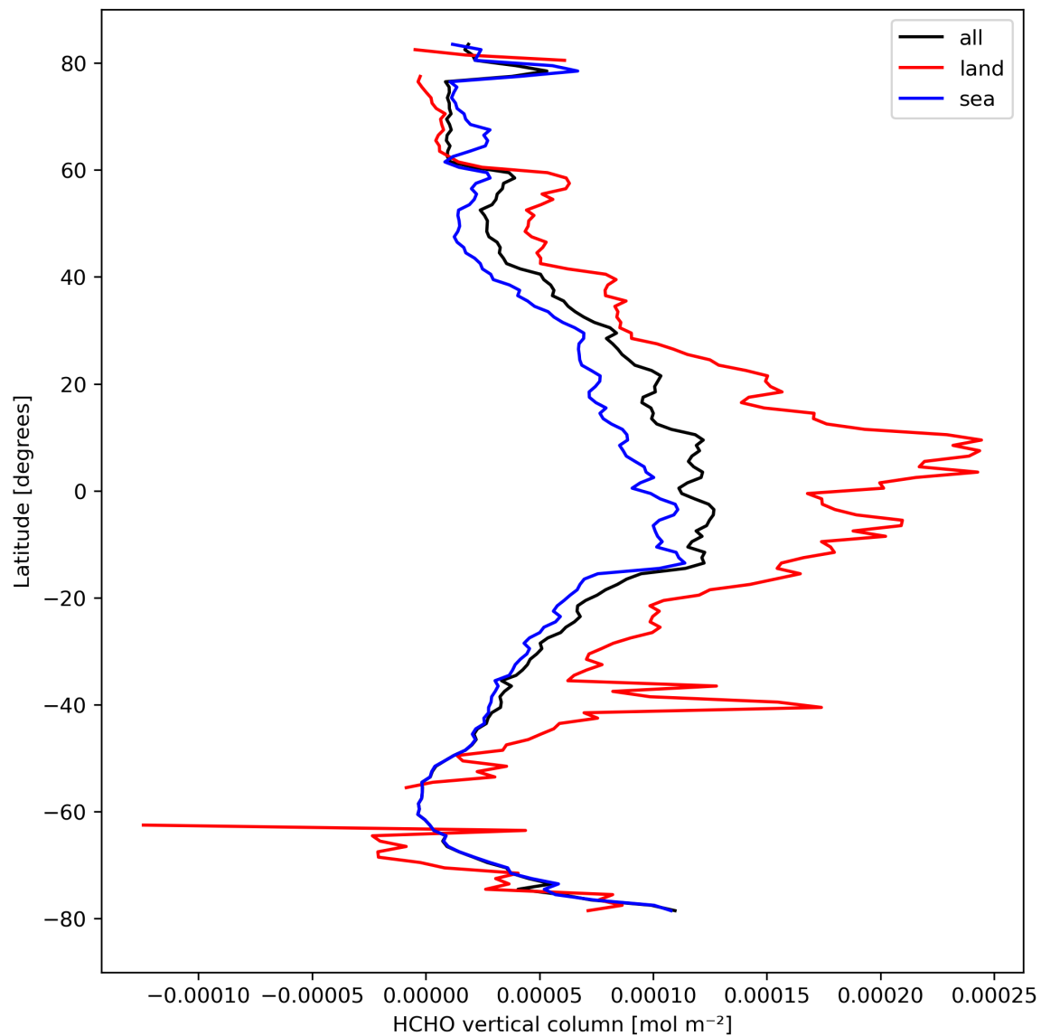
Figure 21: Zonal average of “HCHO vertical column” for 2024-04-01 to 2024-04-03.
