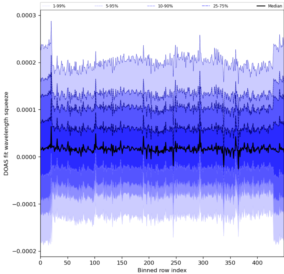
Figure 59: Along track statistics of “DOAS fit wavelength squeeze” for 2024-04-01 to 2024-04-03
