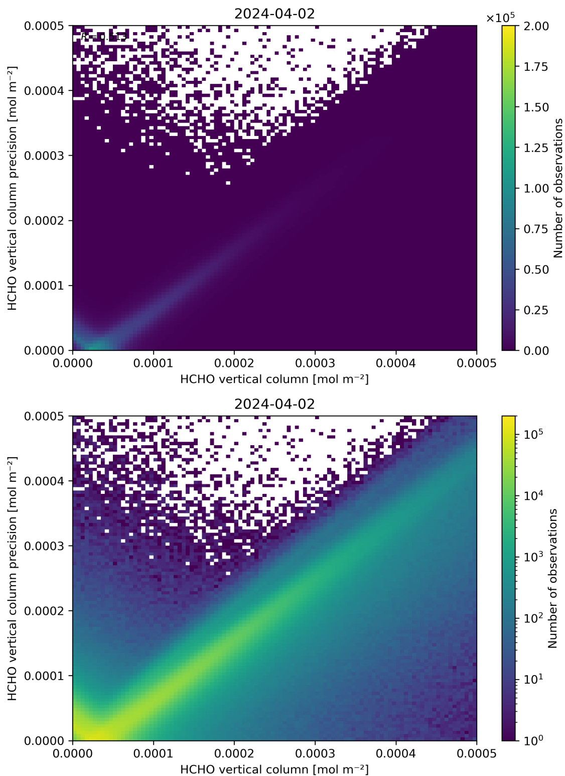
Figure 134: Scatter density plot of “HCHO vertical column” against “HCHO vertical column precision” for 2024-04-01 to 2024-04-03.
