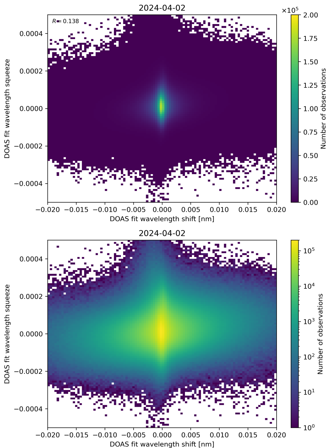
Figure 65: Scatter density plot of “DOAS fit wavelength shift” against “DOAS fit wavelength squeeze” for 2024-04-01 to 2024-04-03.
