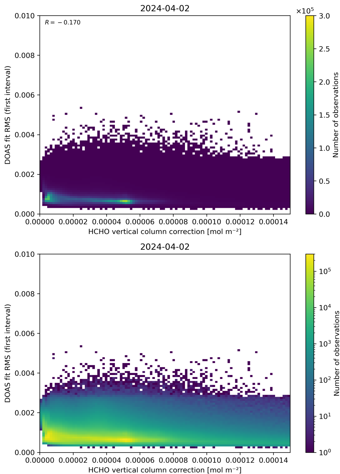
Figure 112: Scatter density plot of “HCHO vertical column correction” against “DOAS fit RMS (first interval)” for 2024-04-01 to 2024-04-03.
