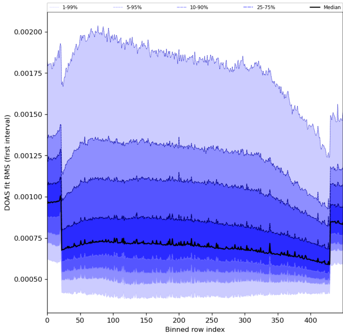
Figure 60: Along track statistics of “DOAS fit RMS (first interval)” for 2024-04-01 to 2024-04-03
