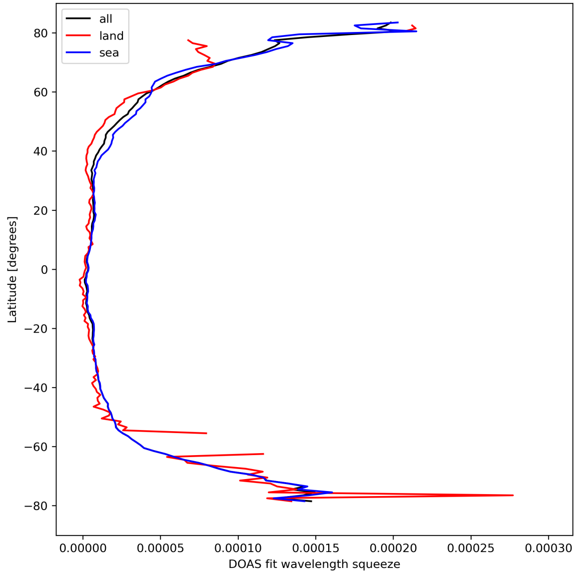
Figure 31: Zonal average of “DOAS fit wavelength squeeze” for 2024-04-01 to 2024-04-03.
