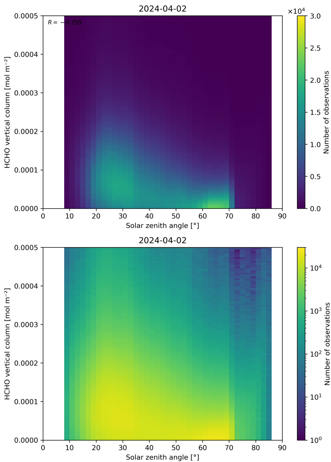
Figure 177: Scatter density plot of “Solar zenith angle” against “HCHO vertical column” for 2024-04-01 to 2024-04-03.
