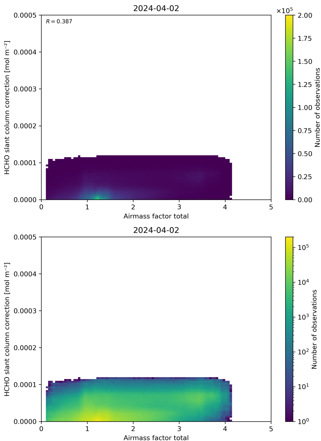
Figure 102: Scatter density plot of “Airmass factor total” against “HCHO slant column correction” for 2024-04-01 to 2024-04-03.
