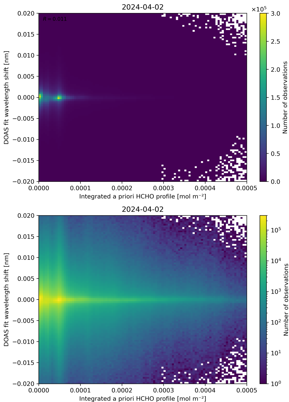
Figure 149: Scatter density plot of “Integrated a priori HCHO profile” against “DOAS fit wavelength shift” for 2024-04-01 to 2024-04-03.
