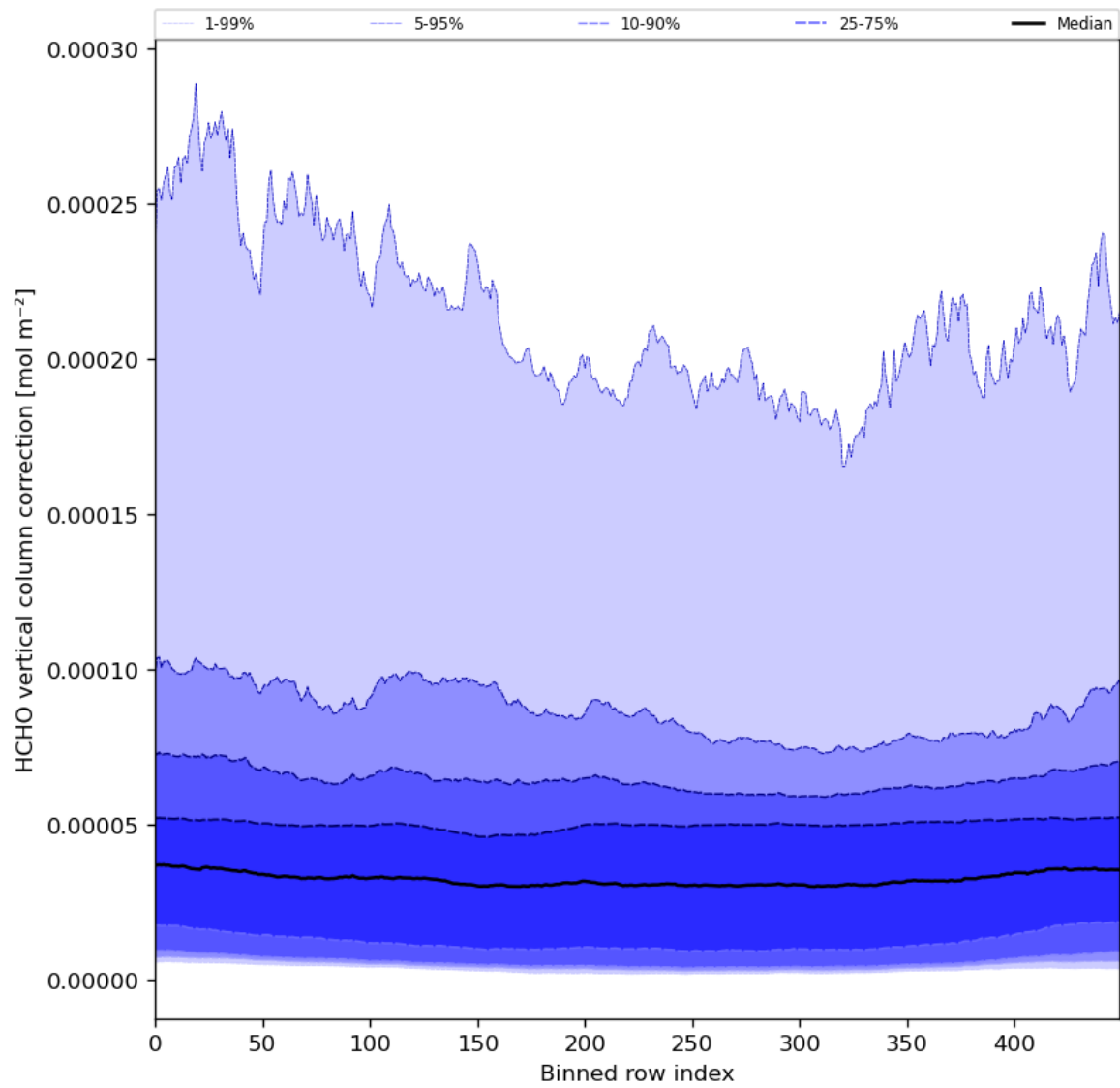
Figure 51: Along track statistics of “HCHO vertical column correction” for 2024-04-01 to 2024-04-03
