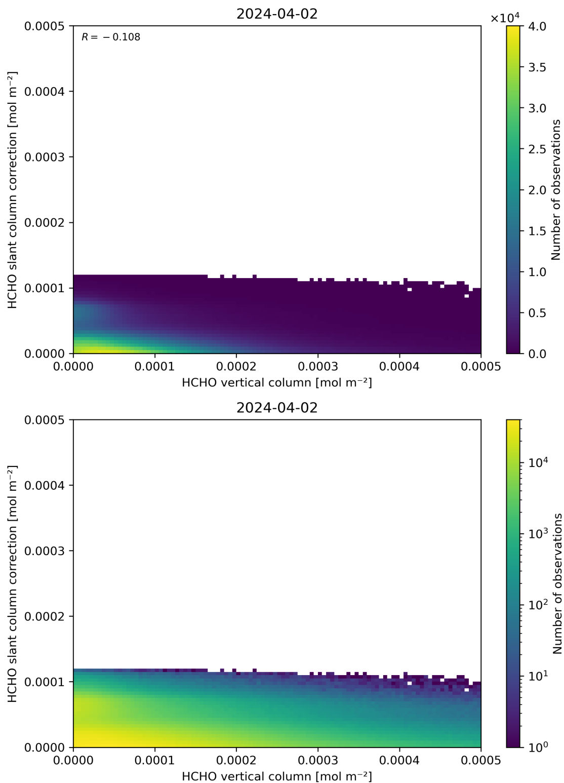
Figure 128: Scatter density plot of “HCHO vertical column” against “HCHO slant column correction” for 2024-04-01 to 2024-04-03.
