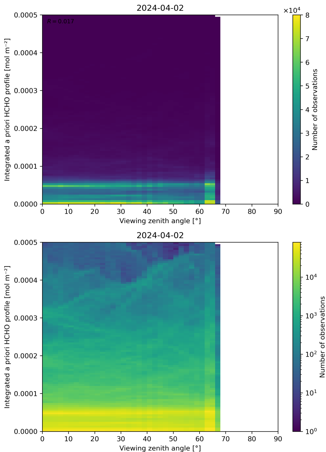
Figure 195: Scatter density plot of “Viewing zenith angle” against “Integrated a priori HCHO profile” for 2024-04-01 to 2024-04-03.
