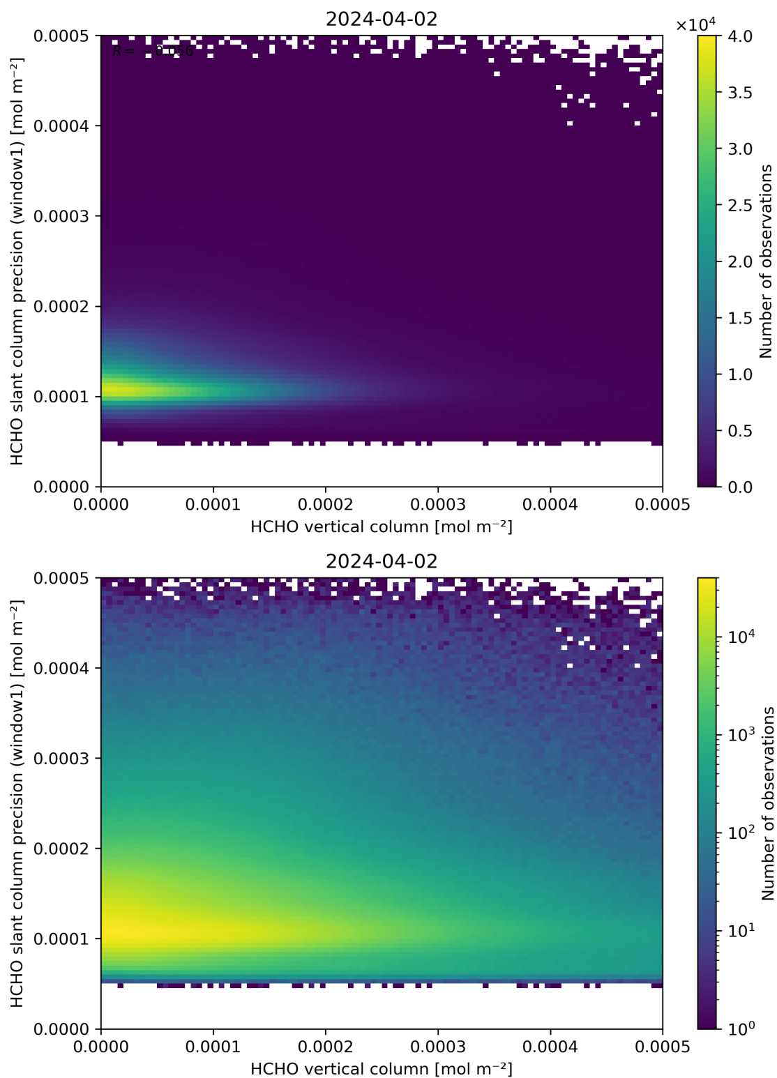
Figure 130: Scatter density plot of “HCHO vertical column” against “HCHO slant column precision (window1)” for 2024-04-01 to 2024-04-03.
