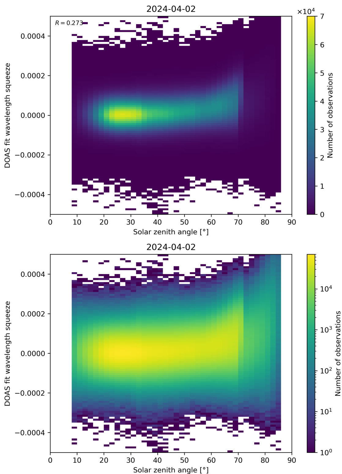
Figure 169: Scatter density plot of “Solar zenith angle” against “DOAS fit wavelength squeeze” for 2024-04-01 to 2024-04-03.
