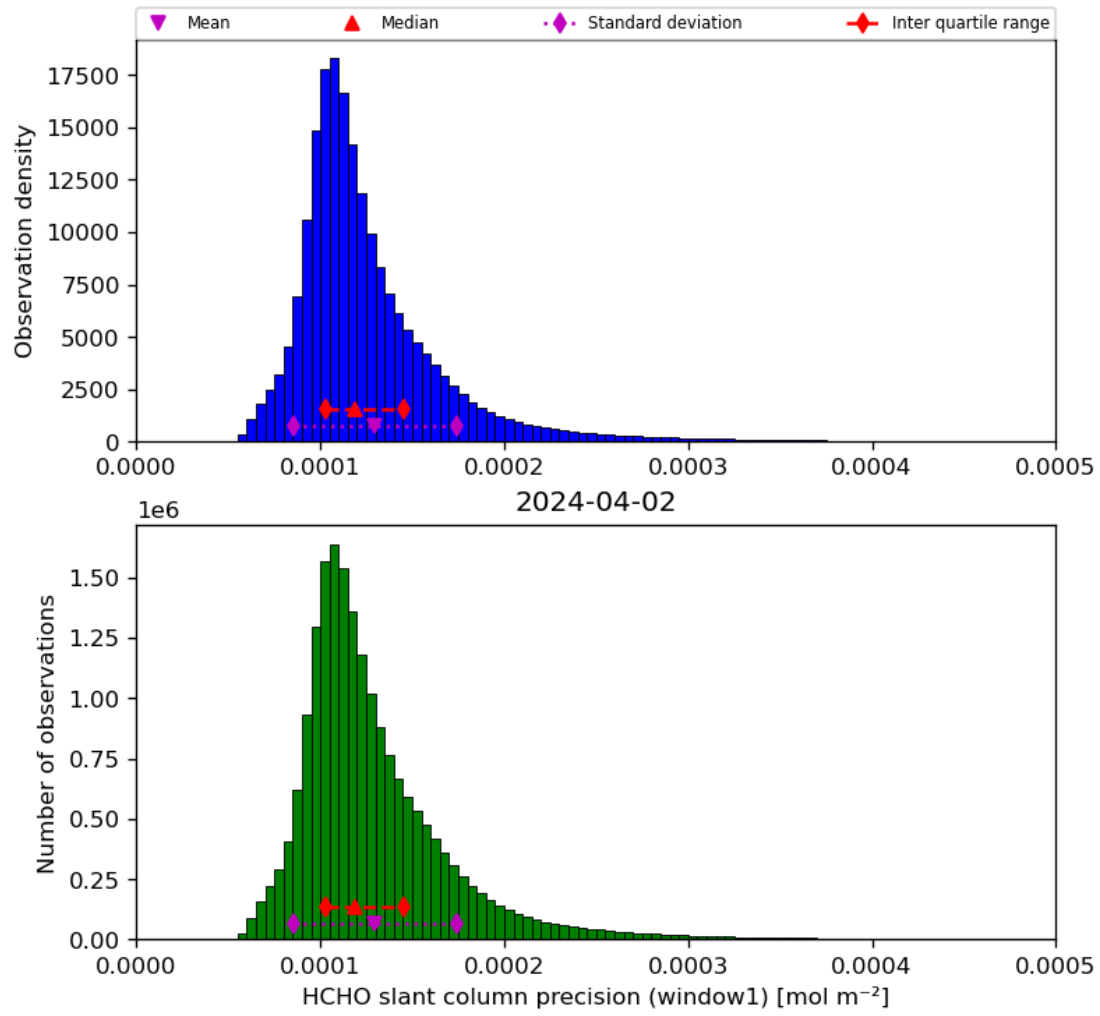
Figure 39: Histogram of “HCHO slant column precision (window1)” for 2024-04-01 to 2024-04-03
