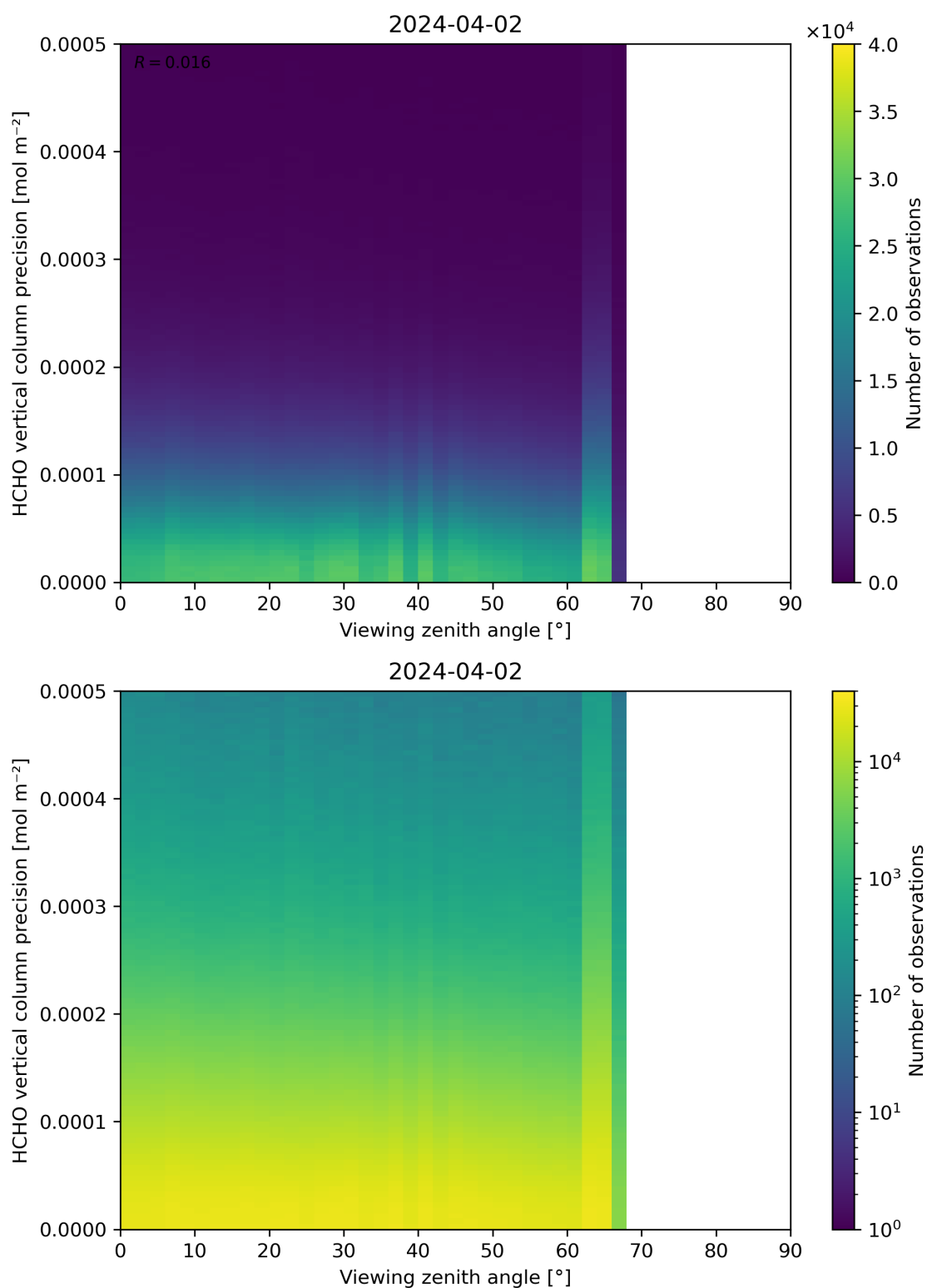
Figure 194: Scatter density plot of “Viewing zenith angle” against “HCHO vertical column precision” for 2024-04-01 to 2024-04-03.
