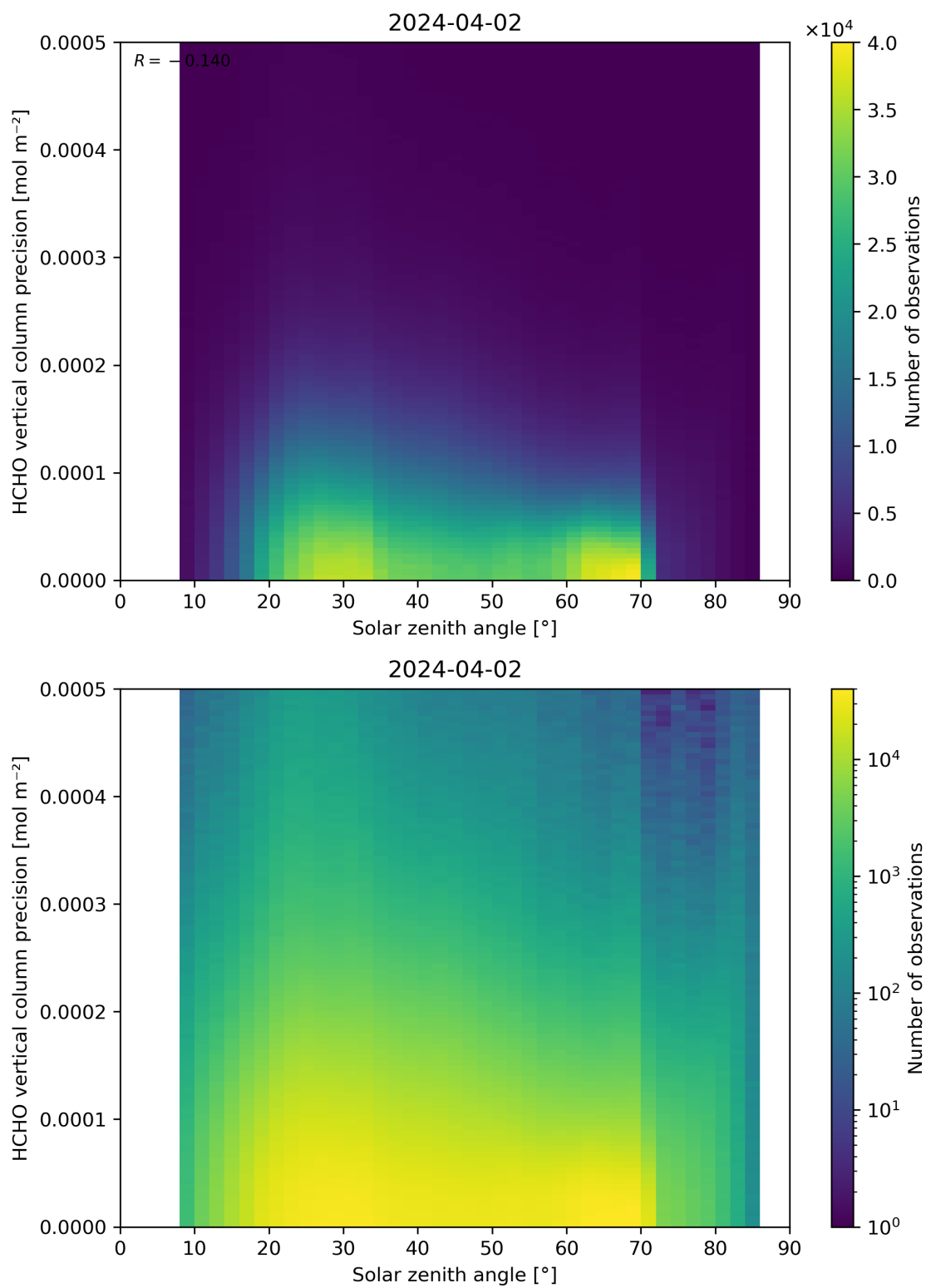
Figure 179: Scatter density plot of “Solar zenith angle” against “HCHO vertical column precision” for 2024-04-01 to 2024-04-03.
