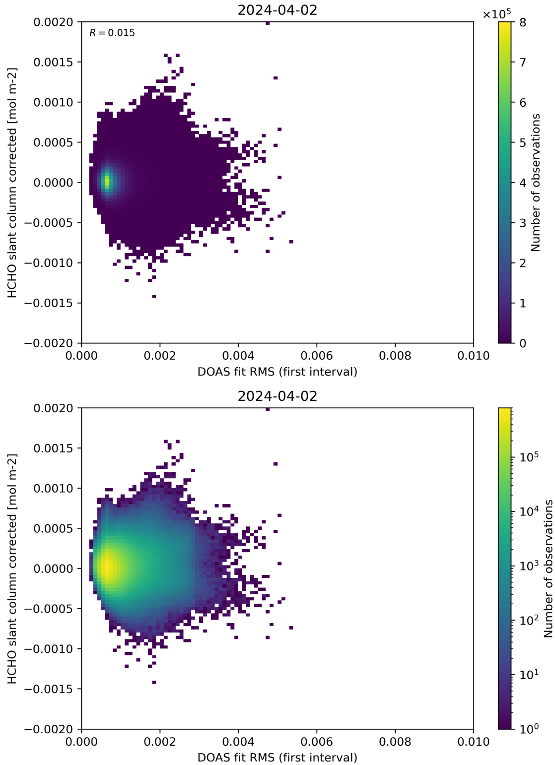
Figure 62: Scatter density plot of “DOAS fit RMS (first interval)” against “HCHO slant column corrected” for 2024-04-01 to 2024-04-03.
