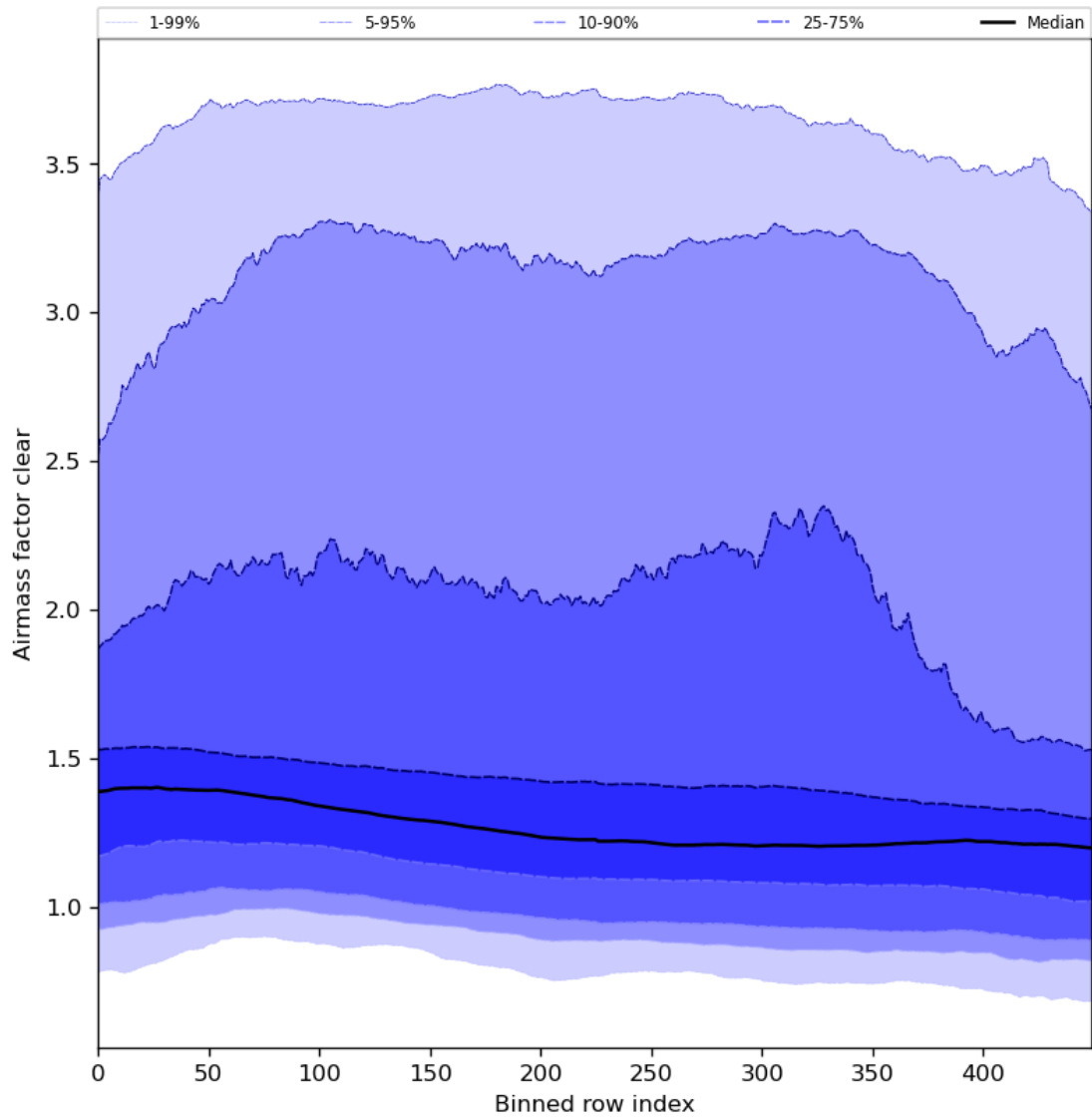
Figure 56: Along track statistics of “Airmass factor clear” for 2024-04-01 to 2024-04-03
