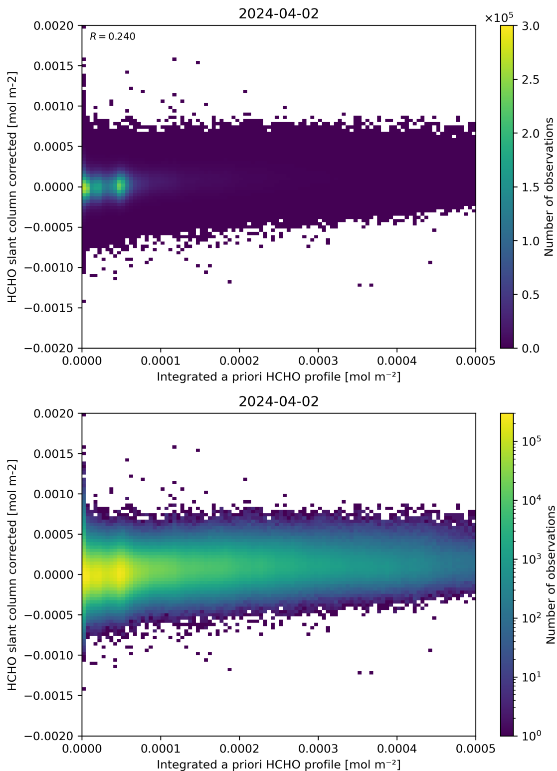
Figure 151: Scatter density plot of “Integrated a priori HCHO profile” against “HCHO slant column corrected” for 2024-04-01 to 2024-04-03.
