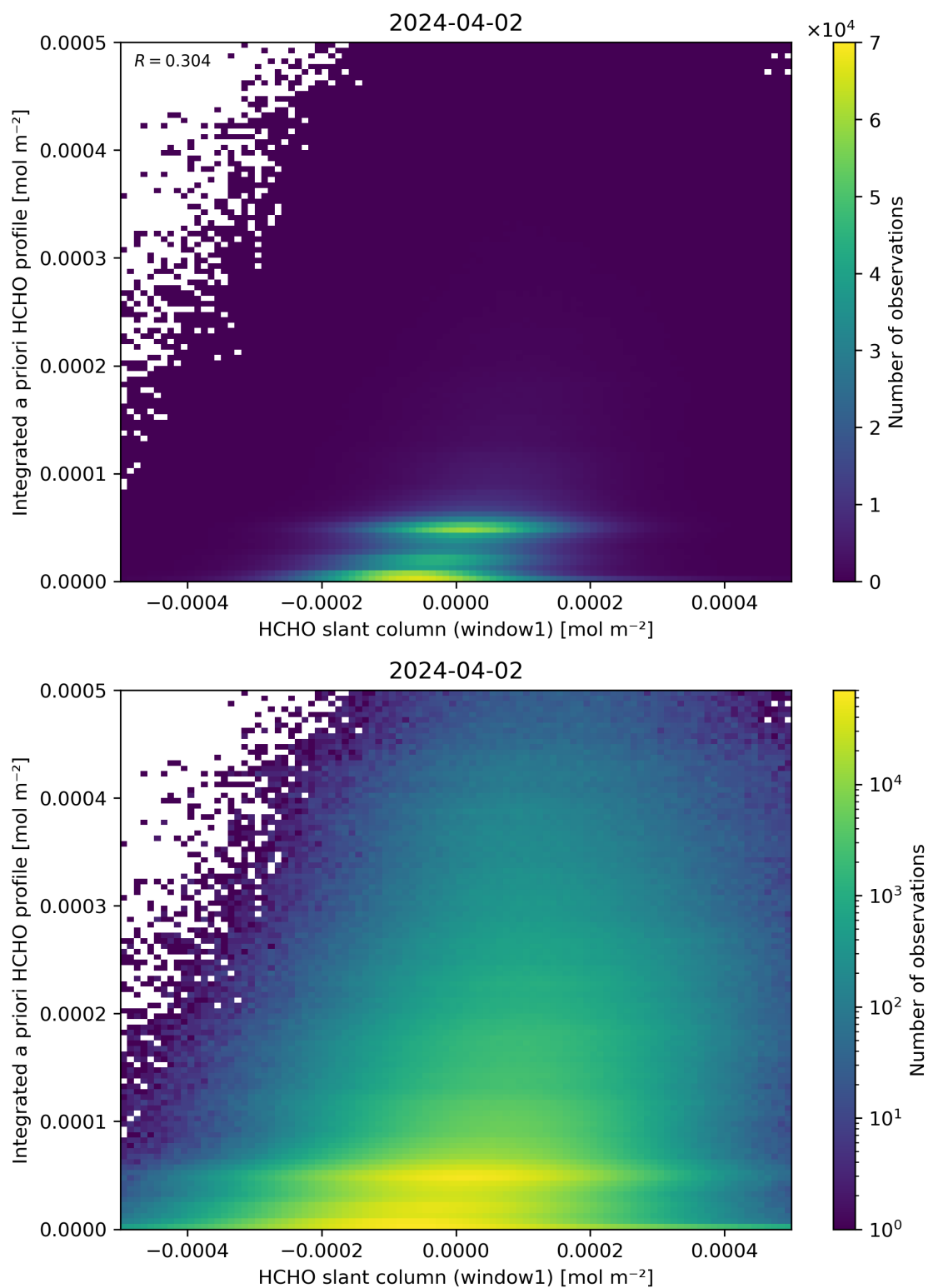
Figure 87: Scatter density plot of “HCHO slant column (window1)” against “Integrated a priori HCHO profile” for 2024-04-01 to 2024-04-03.
