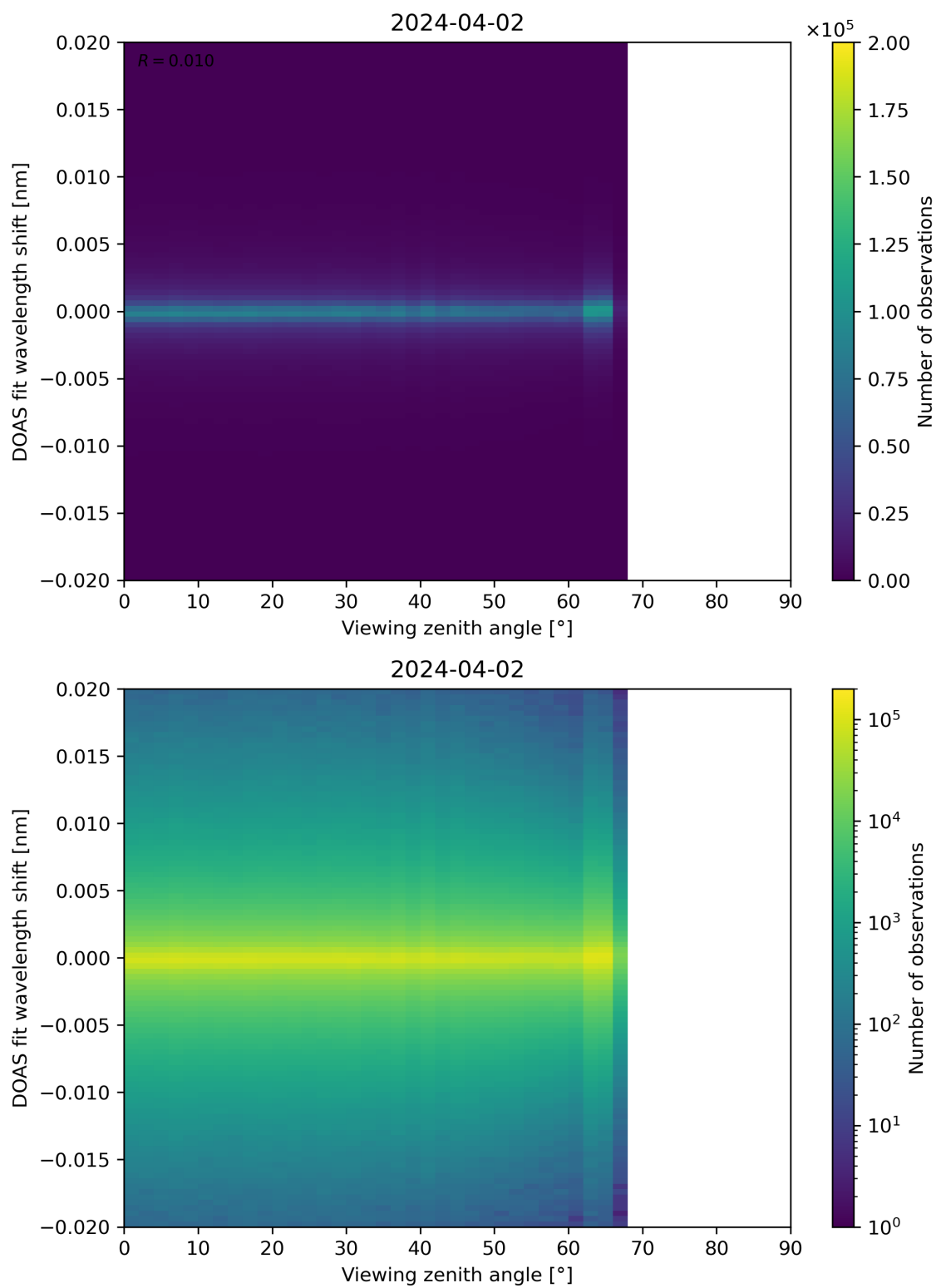
Figure 183: Scatter density plot of “Viewing zenith angle” against “DOAS fit wavelength shift” for 2024-04-01 to 2024-04-03.
