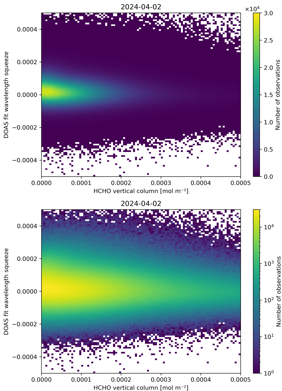
Figure 125: Scatter density plot of “HCHO vertical column” against “DOAS fit wavelength squeeze” for 2024-04-01 to 2024-04-03.
