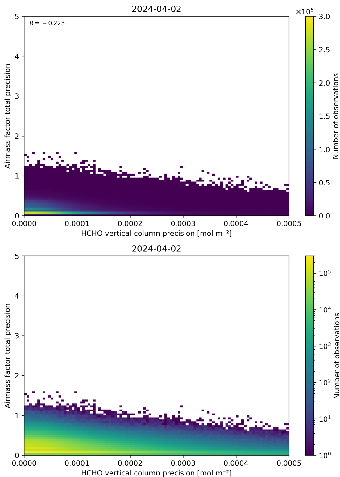
Figure 145: Scatter density plot of “HCHO vertical column precision” against “Airmass factor total precision” for 2024-04-01 to 2024-04-03.
