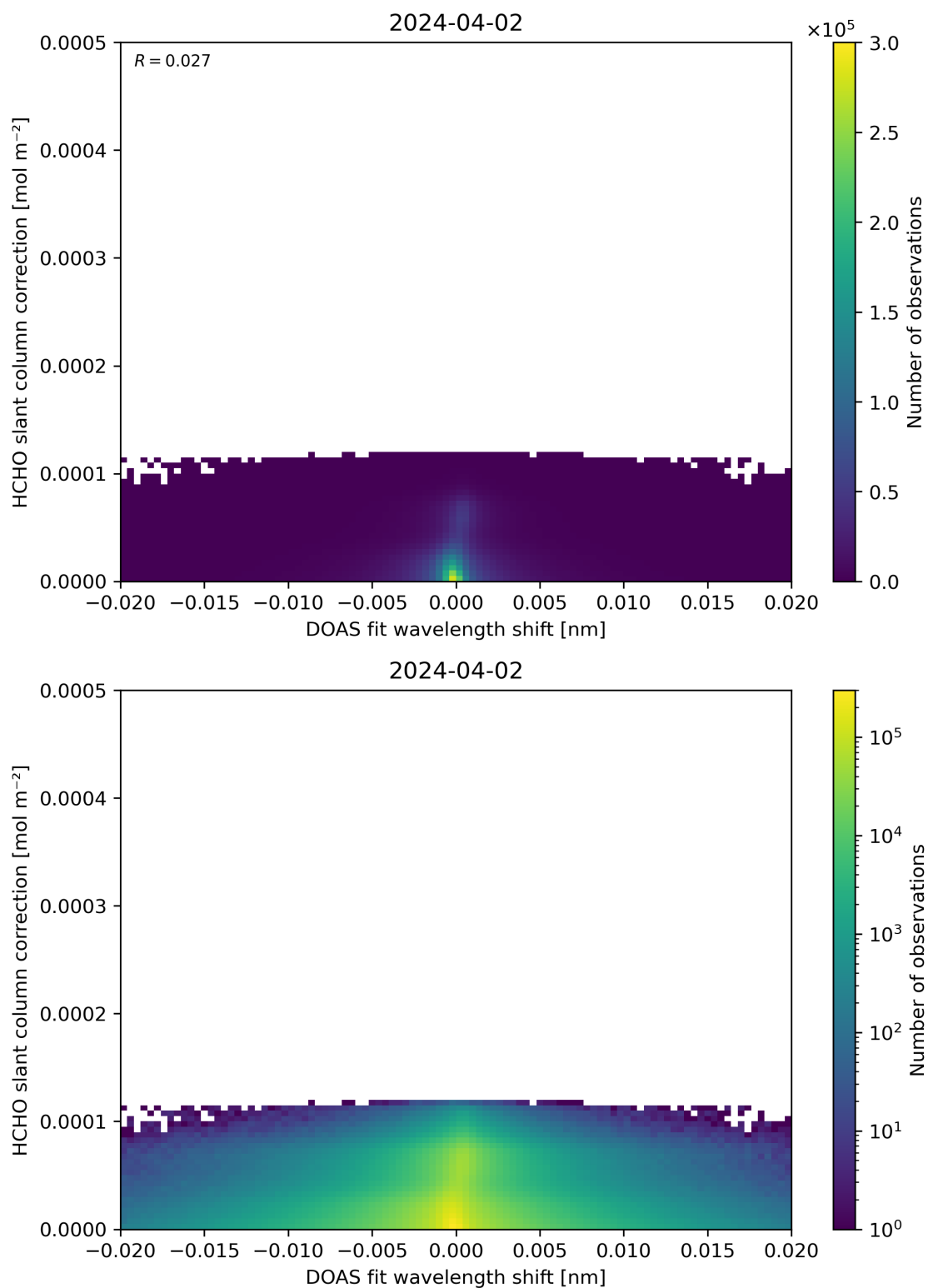
Figure 67: Scatter density plot of “DOAS fit wavelength shift” against “HCHO slant column correction” for 2024-04-01 to 2024-04-03.
