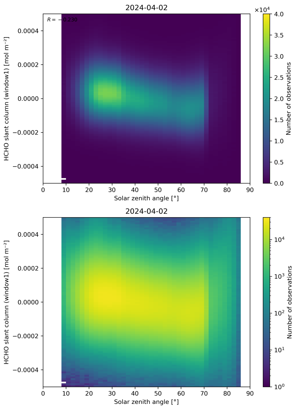
Figure 173: Scatter density plot of “Solar zenith angle” against “HCHO slant column (window1)” for 2024-04-01 to 2024-04-03.
