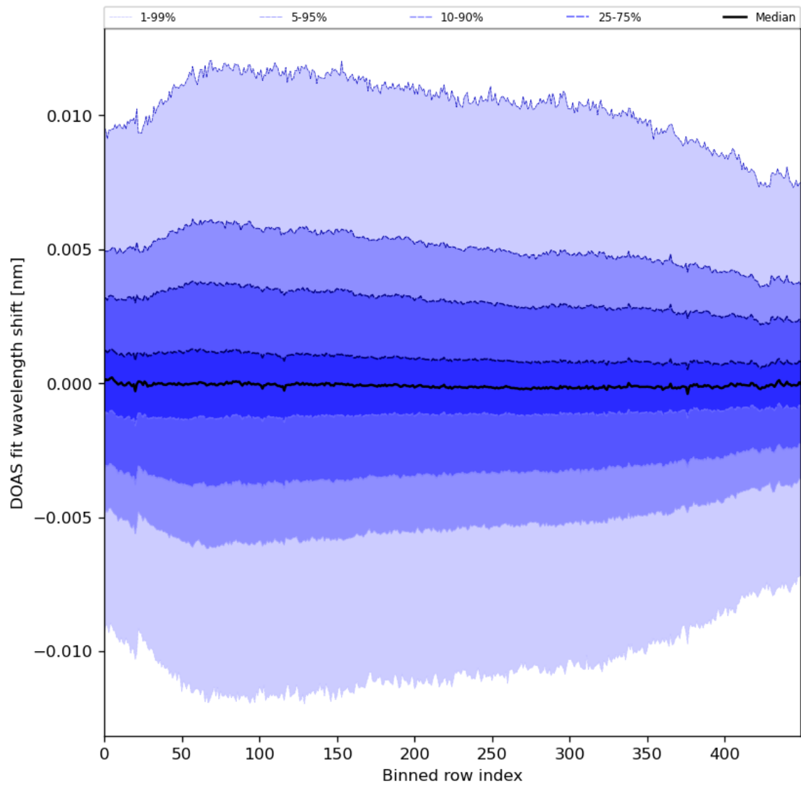
Figure 58: Along track statistics of “DOAS fit wavelength shift” for 2024-04-01 to 2024-04-03
