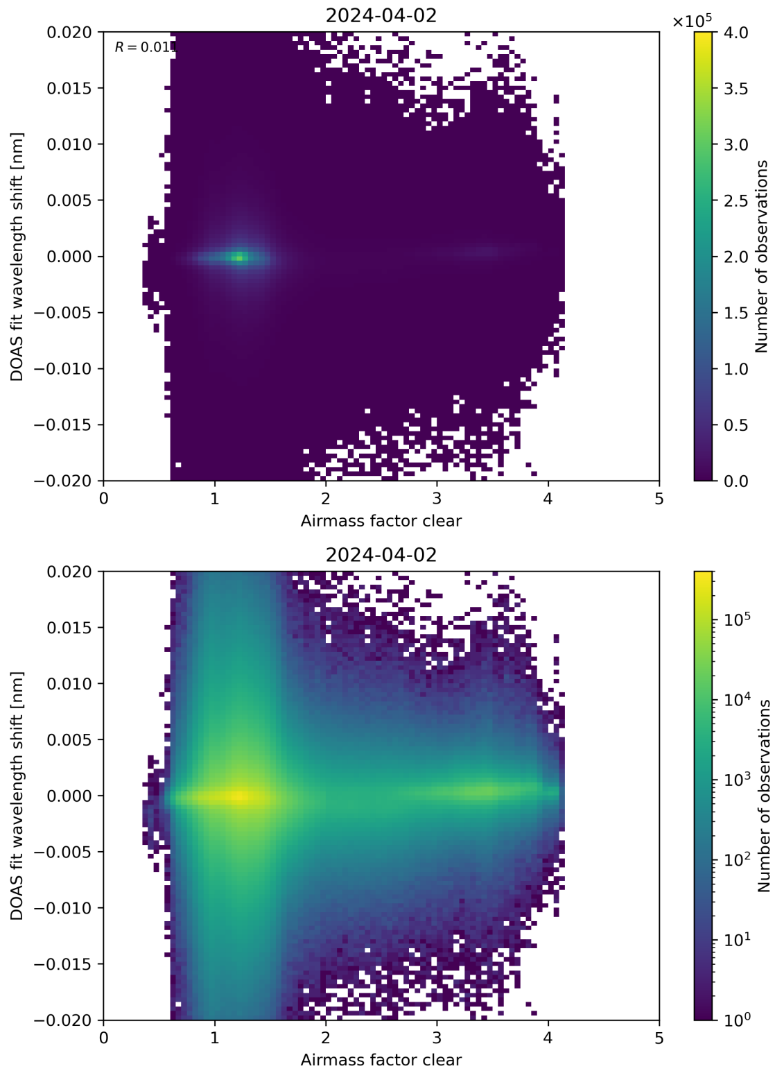
Figure 72: Scatter density plot of “Airmass factor clear” against “DOAS fit wavelength shift” for 2024-04-01 to 2024-04-03.
