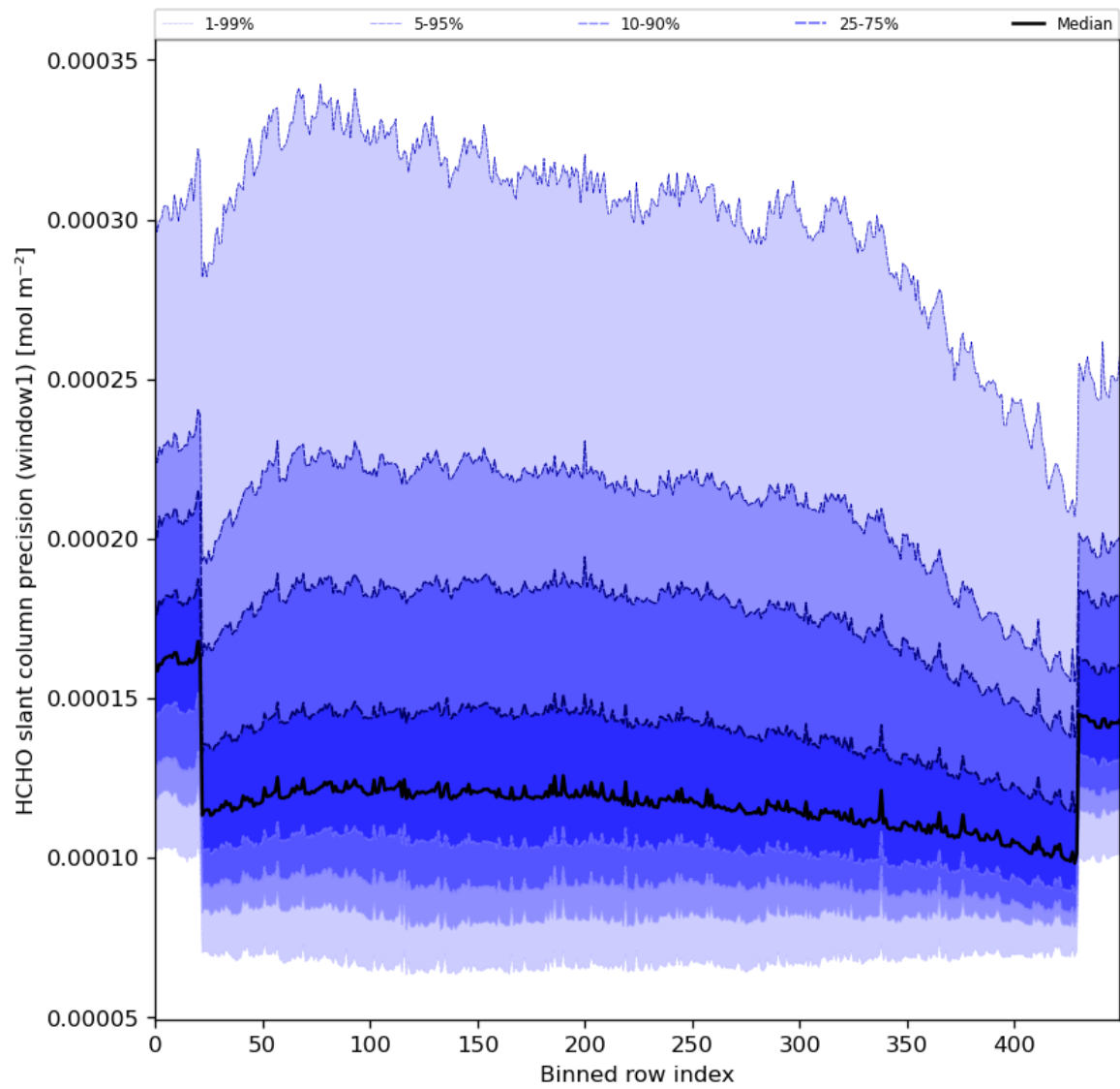
Figure 53: Along track statistics of "HCHO slant column precision (window1)" for 2024-04-01 to 2024-04-03
