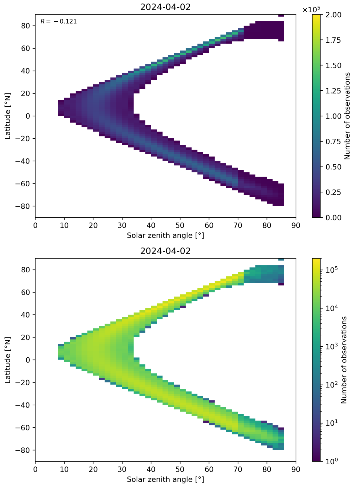
Figure 181: Scatter density plot of “Solar zenith angle” against “Latitude” for 2024-04-01 to 2024-04-03.
