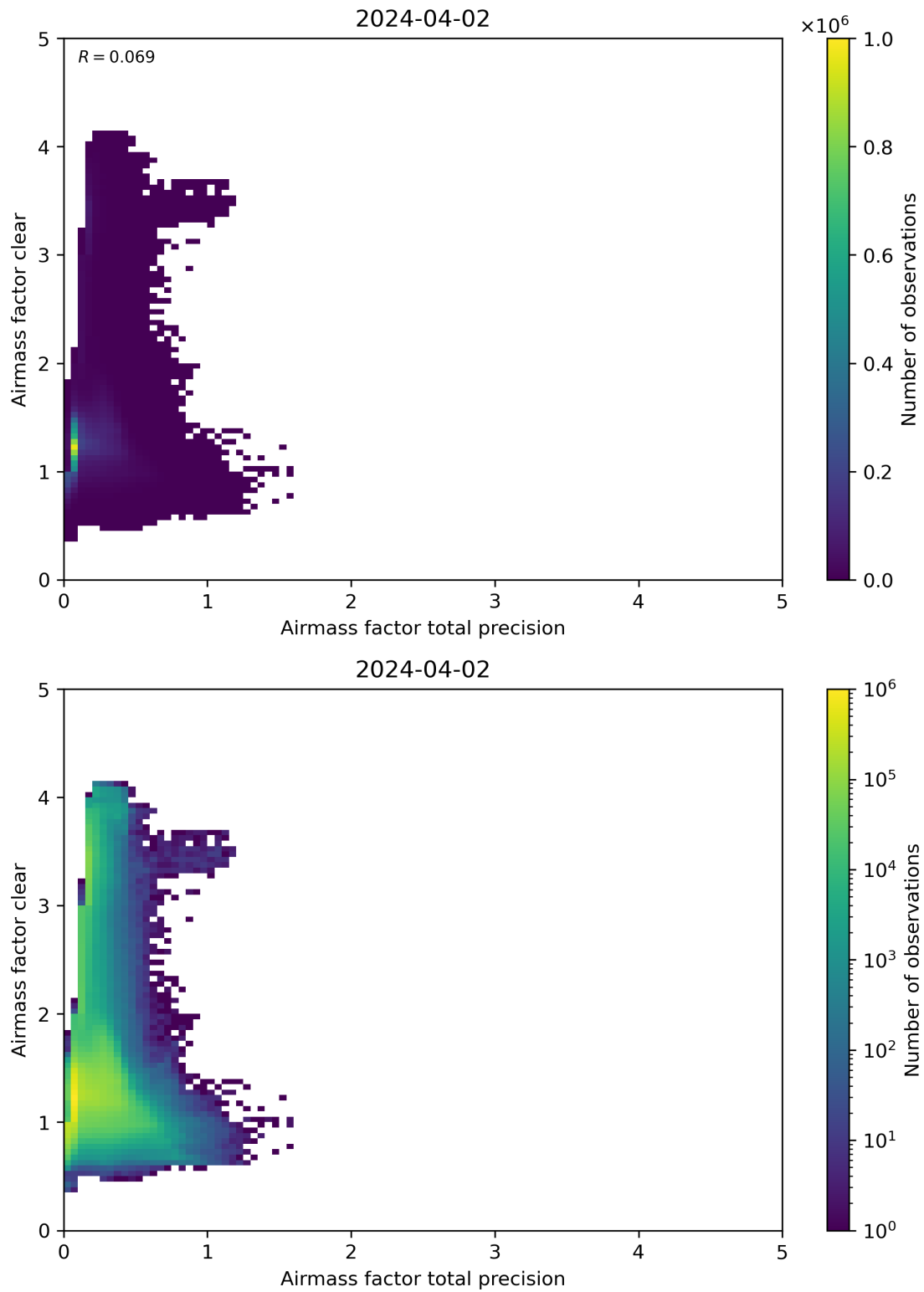
Figure 108: Scatter density plot of “Airmass factor total precision” against “Airmass factor clear” for 2024-04-01 to 2024-04-03.
