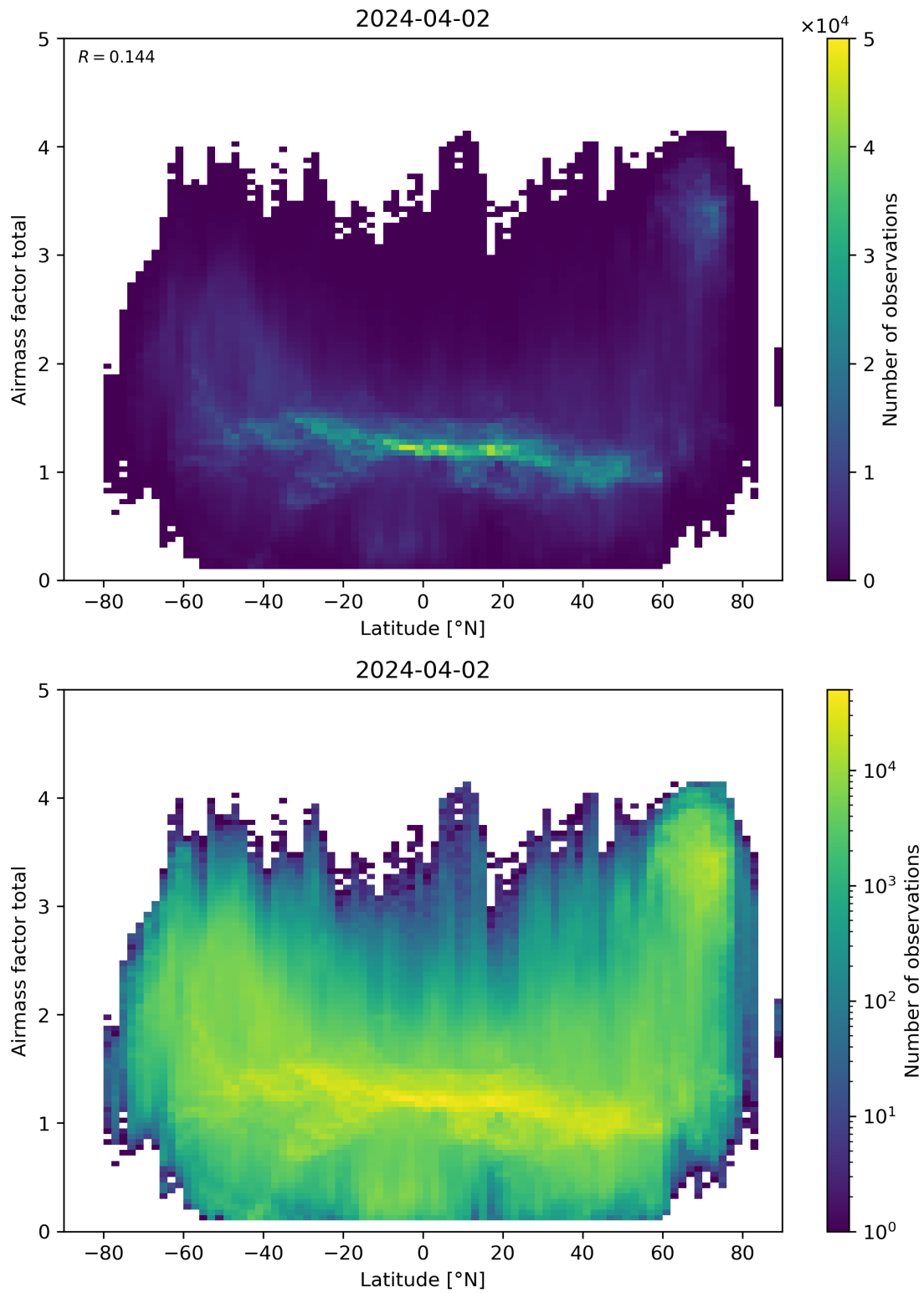
Figure 161: Scatter density plot of “Latitude” against “Airmass factor total” for 2024-04-01 to 2024-04-03.
