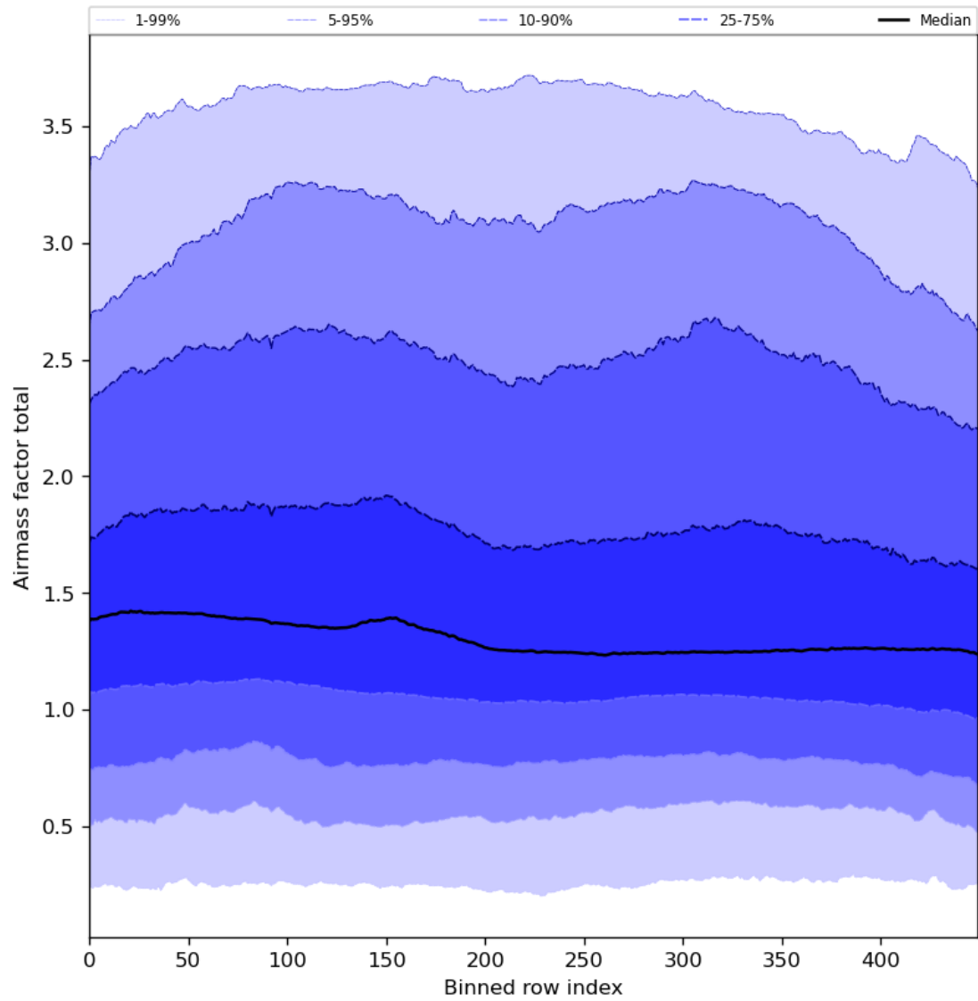
Figure 54: Along track statistics of “Airmass factor total” for 2024-04-01 to 2024-04-03
