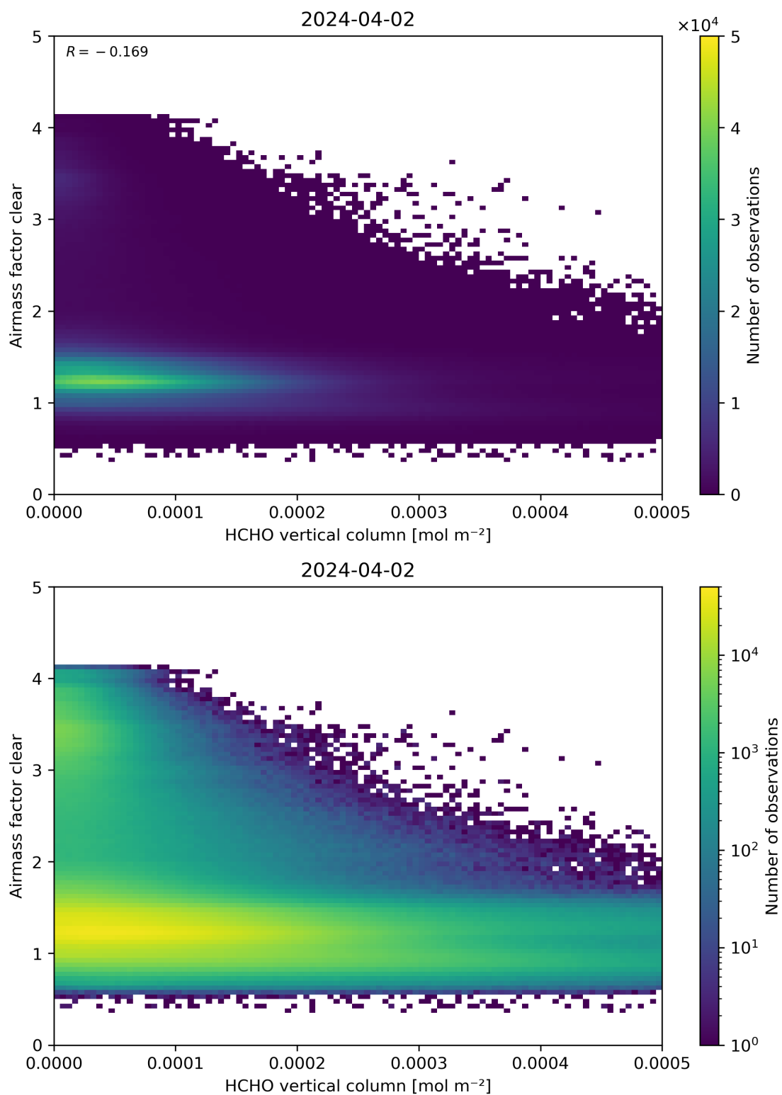
Figure 126: Scatter density plot of “HCHO vertical column” against “Airmass factor clear” for 2024-04-01 to 2024-04-03.
