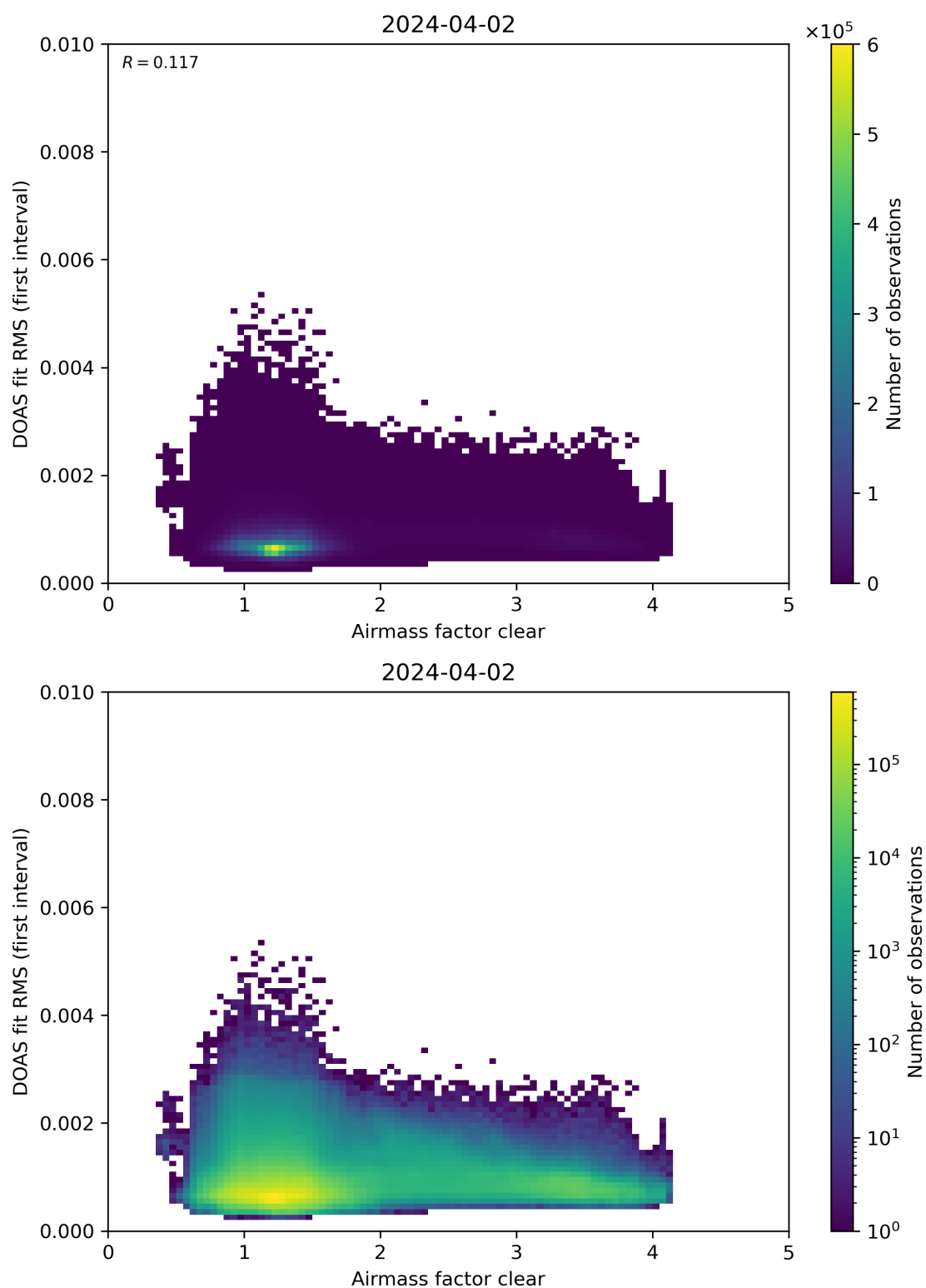
Figure 71: Scatter density plot of “Airmass factor clear” against “DOAS fit RMS (first interval)” for 2024-04-01 to 2024-04-03.
