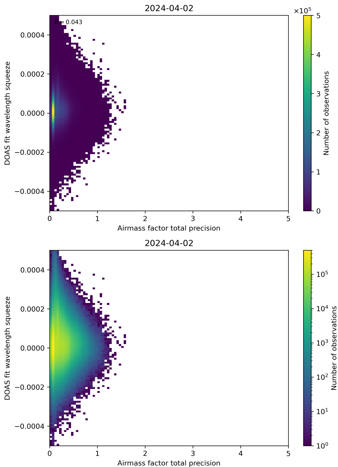
Figure 107: Scatter density plot of “Airmass factor total precision” against “DOAS fit wavelength squeeze” for 2024-04-01 to 2024-04-03.
