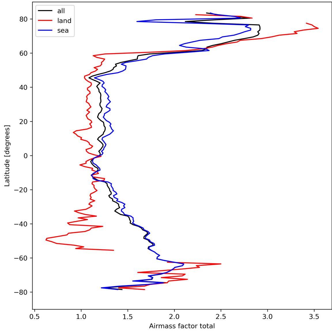
Figure 26: Zonal average of “Airmass factor total” for 2024-04-01 to 2024-04-03.
