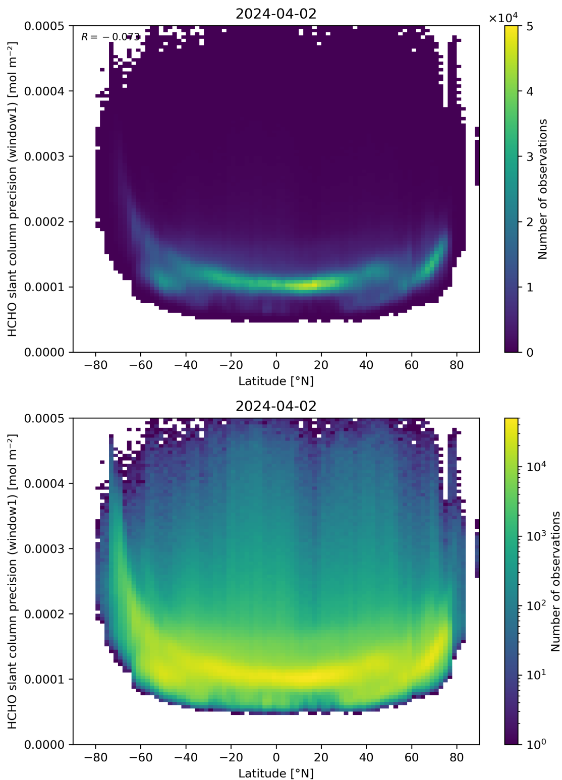
Figure 160: Scatter density plot of “Latitude” against “HCHO slant column precision (window1)” for 2024-04-01 to 2024-04-03.
