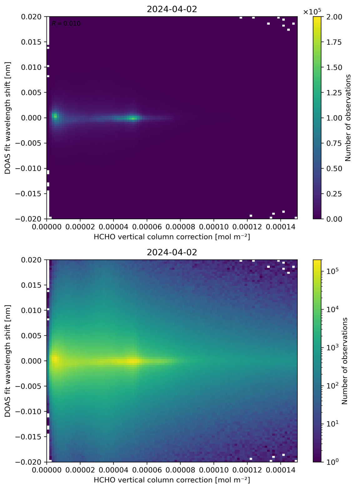
Figure 113: Scatter density plot of “HCHO vertical column correction” against “DOAS fit wavelength shift” for 2024-04-01 to 2024-04-03.
