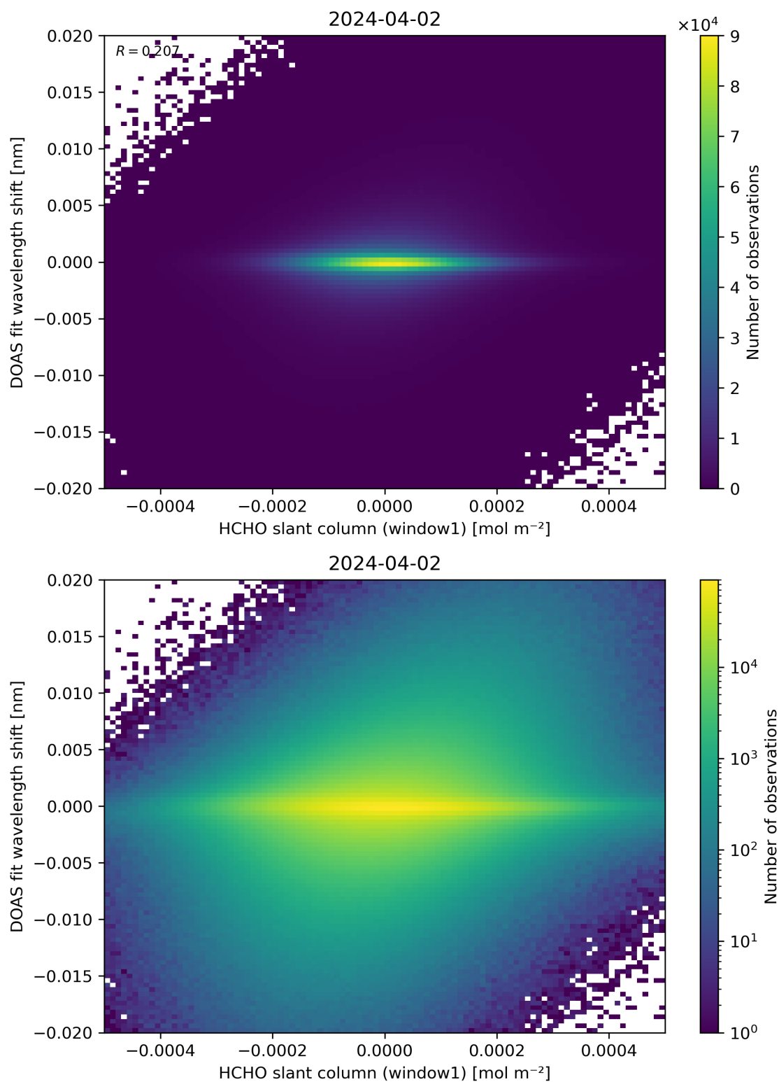
Figure 79: Scatter density plot of “HCHO slant column (window1)” against “DOAS fit wavelength shift” for 2024-04-01 to 2024-04-03.
