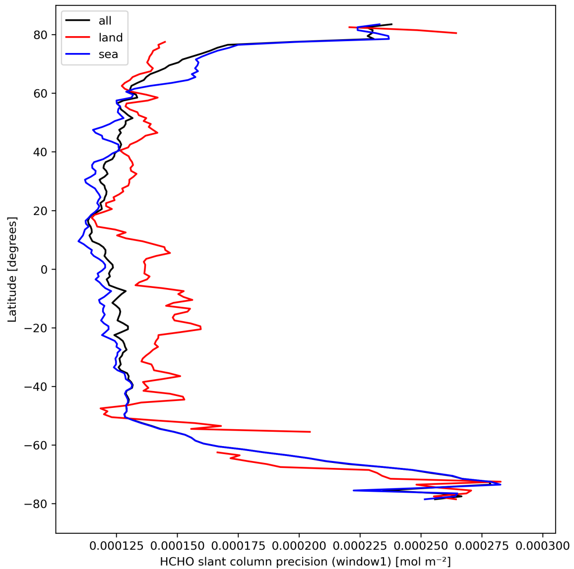
Figure 25: Zonal average of “HCHO slant column precision (window1)” for 2024-04-01 to 2024-04-03.
