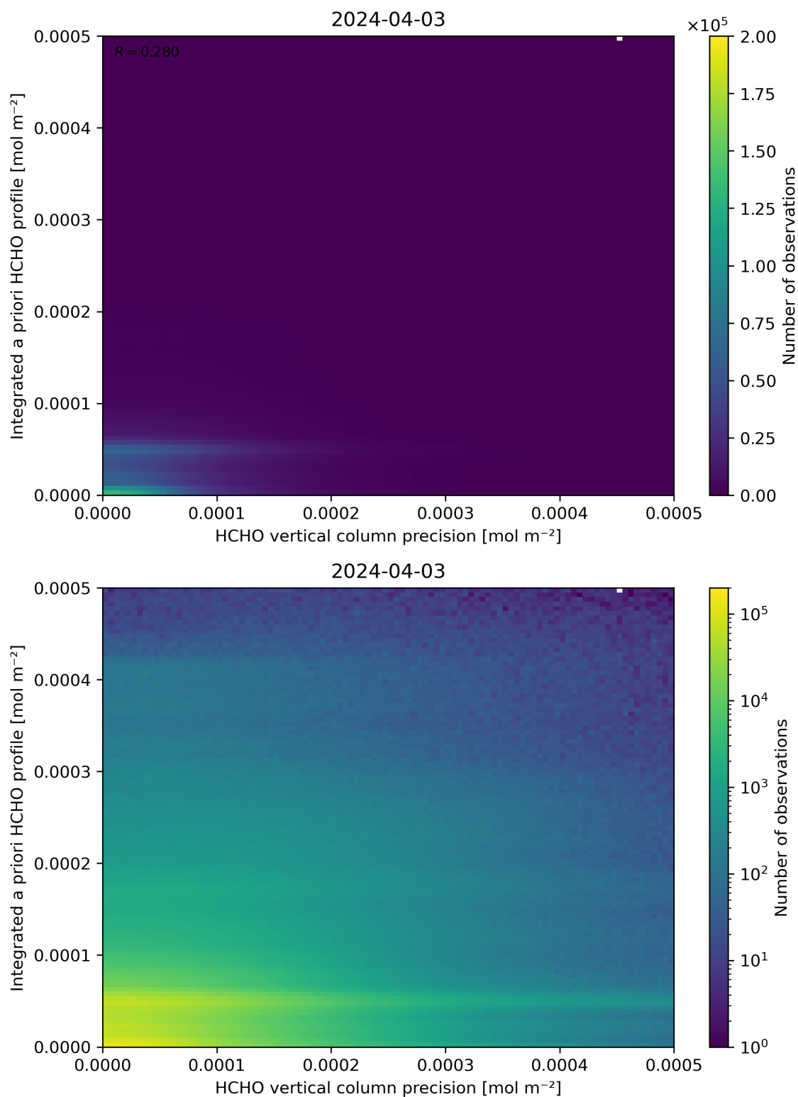
Figure 147: Scatter density plot of “HCHO vertical column precision” against “Integrated a priori HCHO profile” for 2024-04-02 to 2024-04-04.
