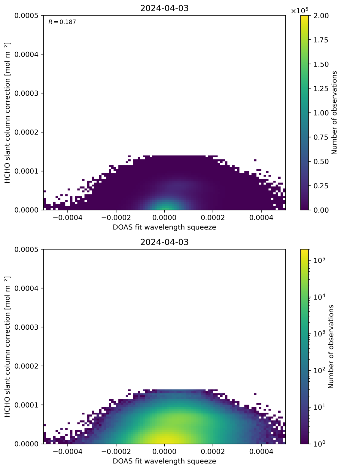
Figure 70: Scatter density plot of “DOAS fit wavelength squeeze” against “HCHO slant column correction” for 2024-04-02 to 2024-04-04.
