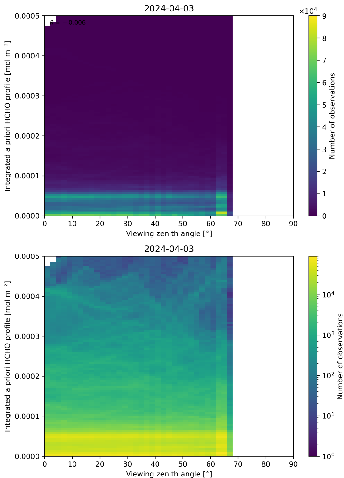
Figure 195: Scatter density plot of “Viewing zenith angle” against “Integrated a priori HCHO profile” for 2024-04-02 to 2024-04-04.
