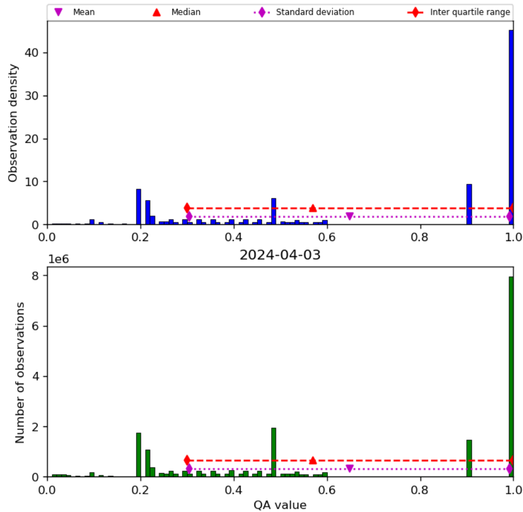
Figure 34: Histogram of “QA value” for 2024-04-02 to 2024-04-04
