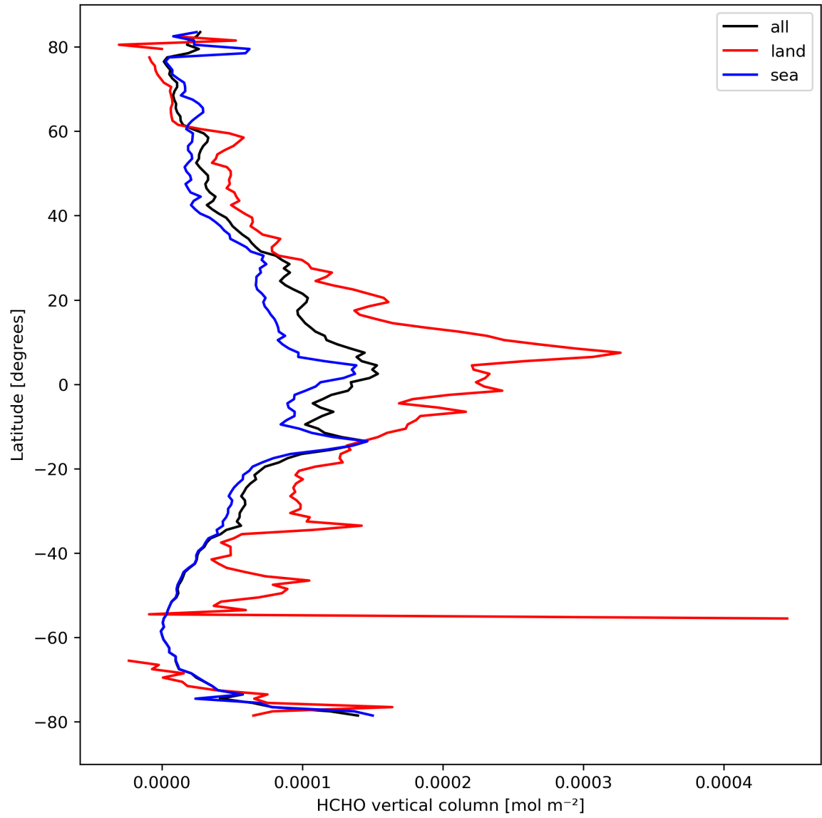
Figure 21: Zonal average of “HCHO vertical column” for 2024-04-02 to 2024-04-04.
