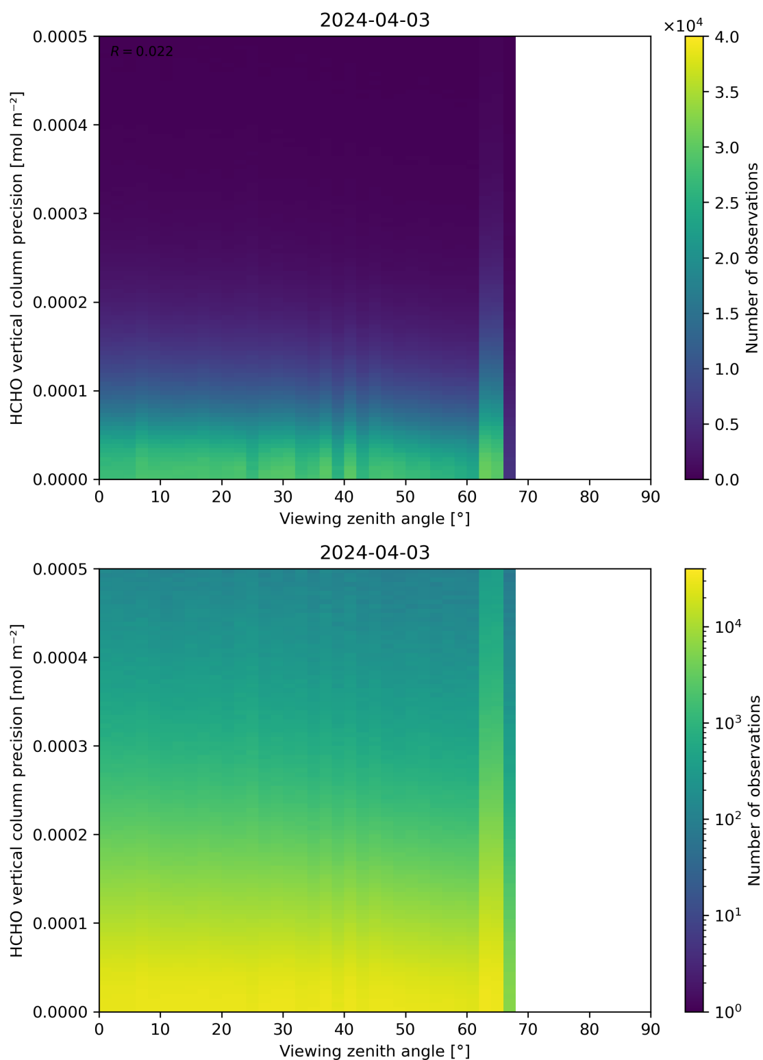
Figure 194: Scatter density plot of “Viewing zenith angle” against “HCHO vertical column precision” for 2024-04-02 to 2024-04-04.
