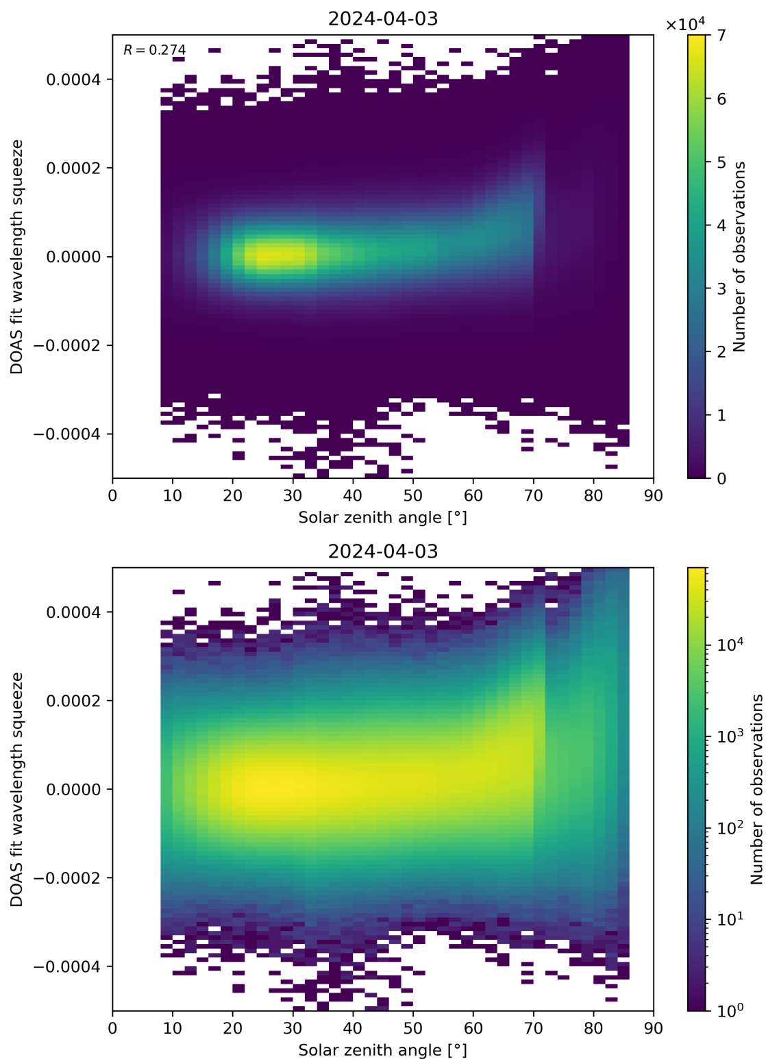
Figure 169: Scatter density plot of “Solar zenith angle” against “DOAS fit wavelength squeeze” for 2024-04-02 to 2024-04-04.
