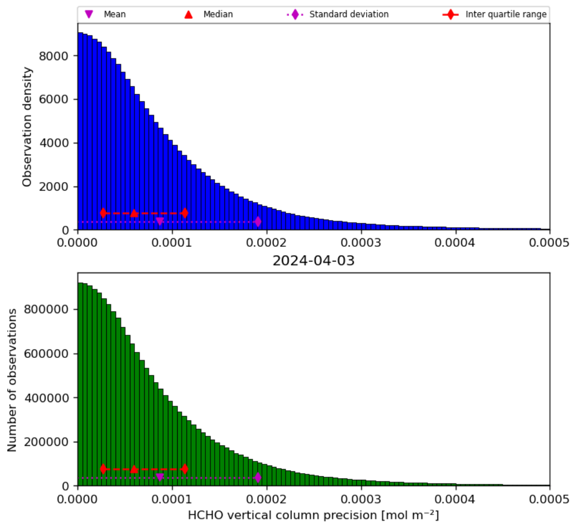
Figure 36: Histogram of “HCHO vertical column precision” for 2024-04-02 to 2024-04-04
