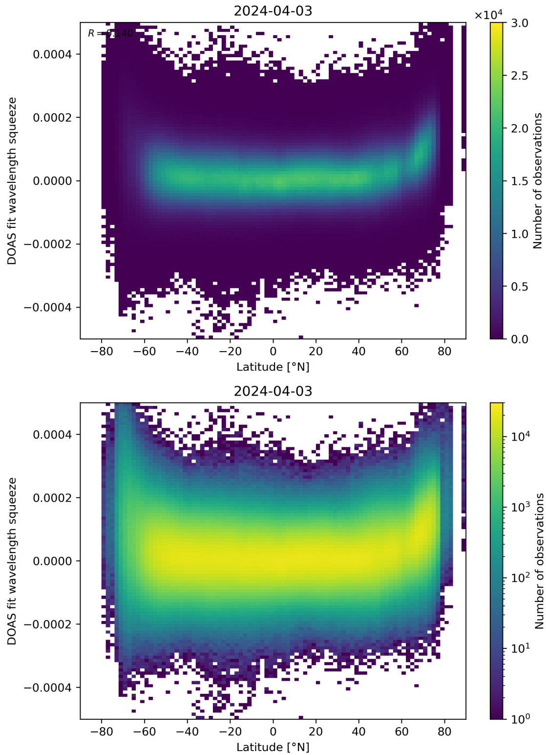
Figure 155: Scatter density plot of “Latitude” against “DOAS fit wavelength squeeze” for 2024-04-02 to 2024-04-04.
