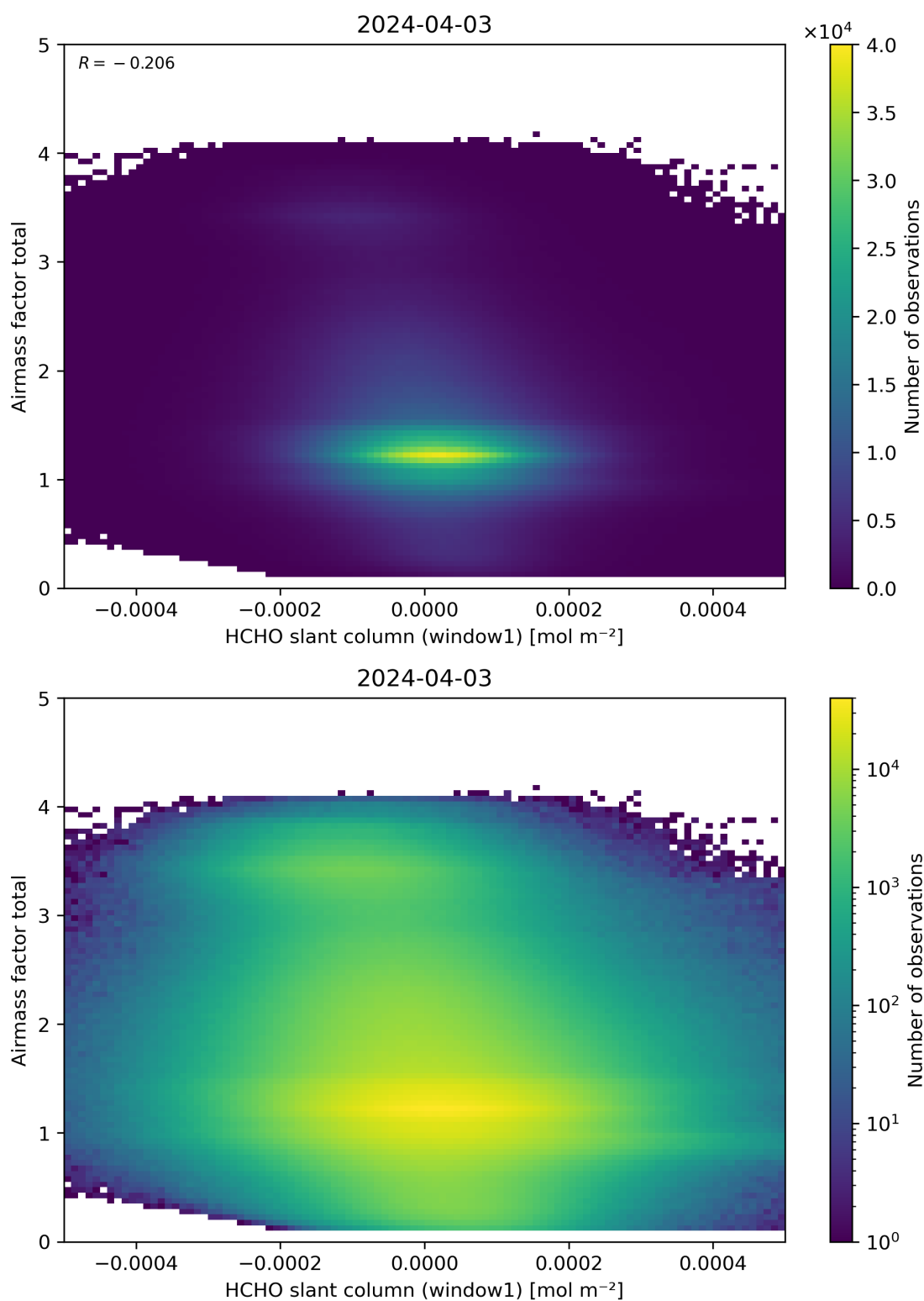
Figure 85: Scatter density plot of “HCHO slant column (window1)” against “Airmass factor total” for 2024-04-02 to 2024-04-04.
