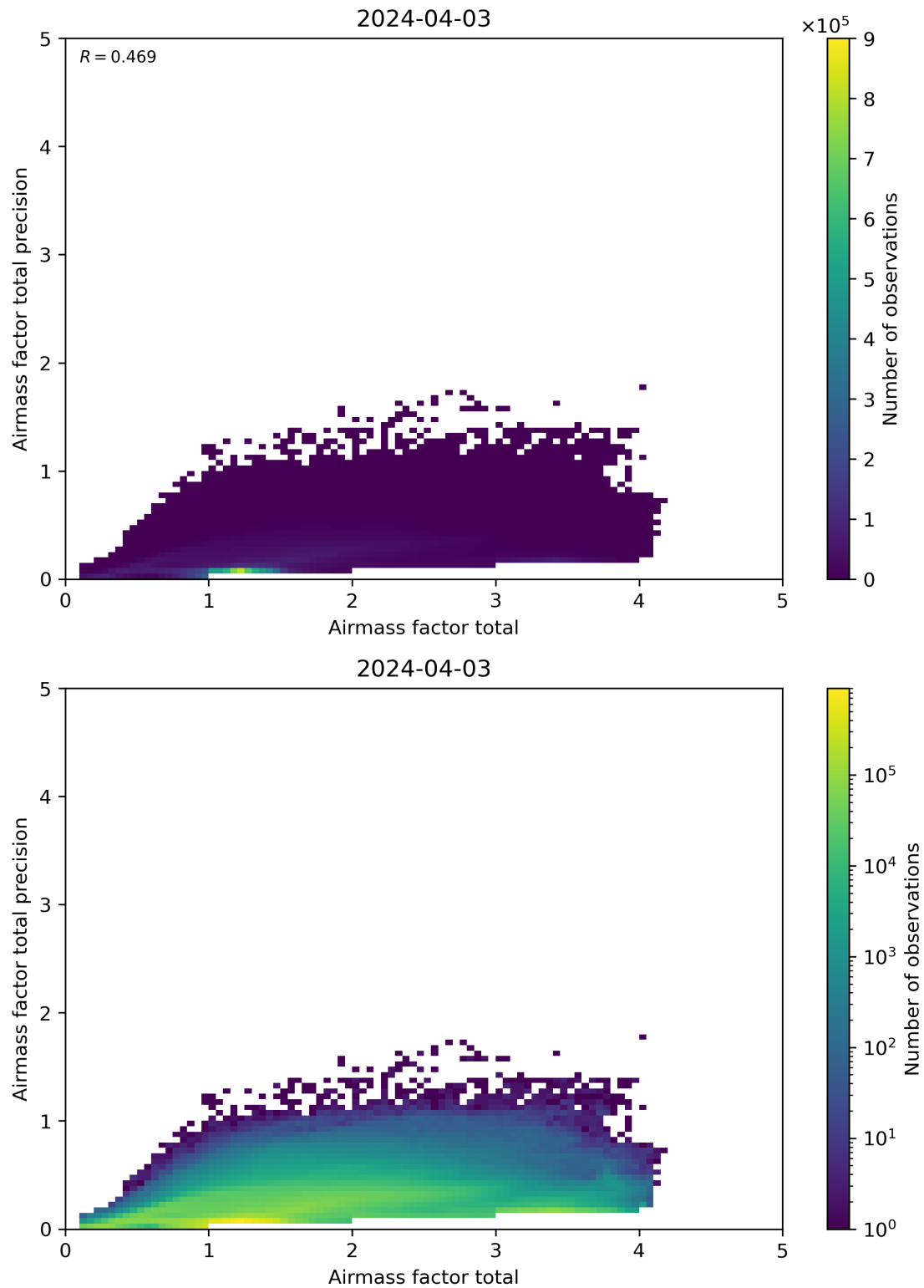
Figure 103: Scatter density plot of “Airmass factor total” against “Airmass factor total precision” for 2024-04-02 to 2024-04-04.
