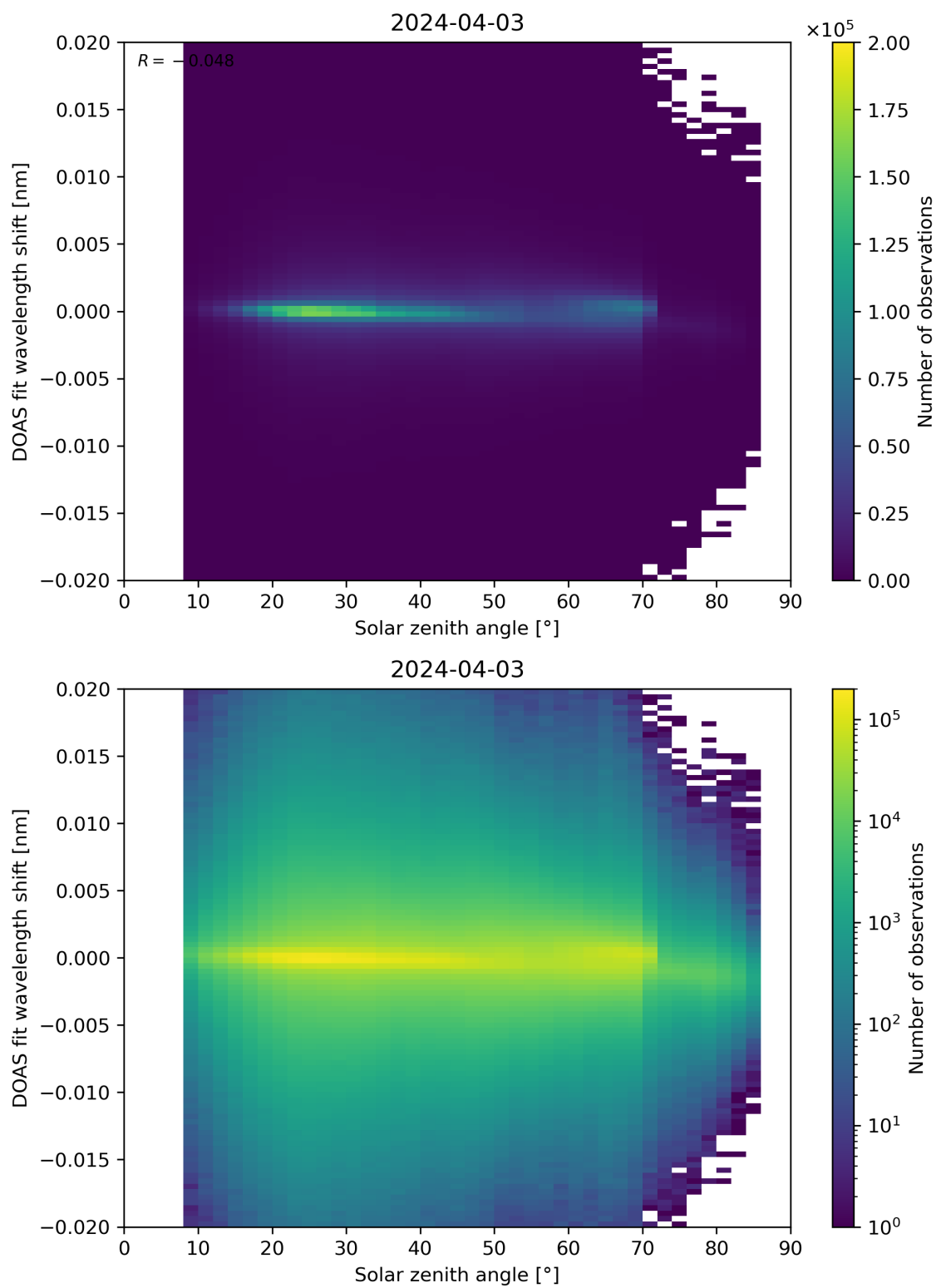
Figure 168: Scatter density plot of “Solar zenith angle” against “DOAS fit wavelength shift” for 2024-04-02 to 2024-04-04.
