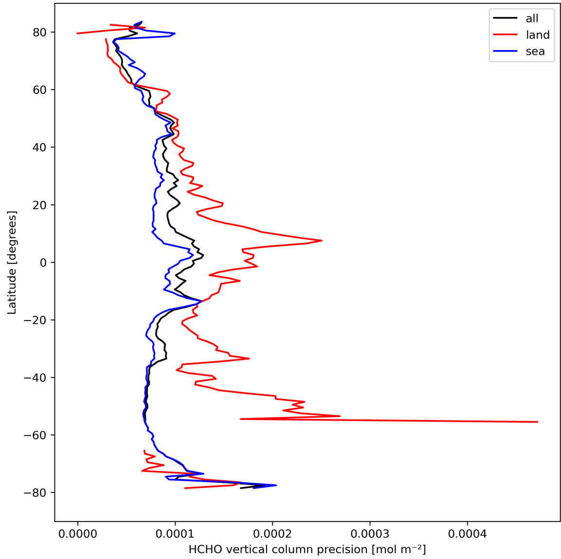
Figure 22: Zonal average of “HCHO vertical column precision” for 2024-04-02 to 2024-04-04.
