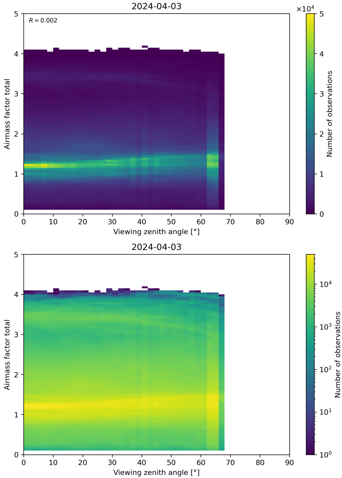
Figure 190: Scatter density plot of “Viewing zenith angle” against “Airmass factor total” for 2024-04-02 to 2024-04-04.
