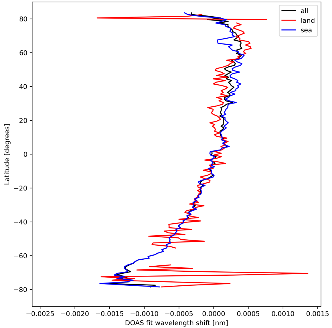
Figure 30: Zonal average of “DOAS fit wavelength shift” for 2024-04-02 to 2024-04-04.
