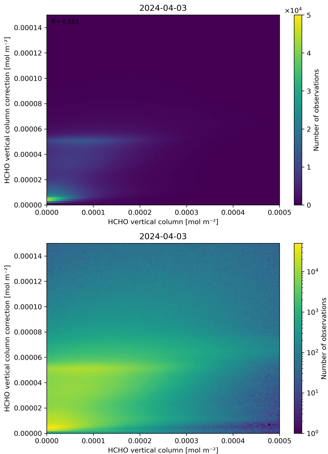
Figure 133: Scatter density plot of “HCHO vertical column” against “HCHO vertical column correction” for 2024-04-02 to 2024-04-04.
