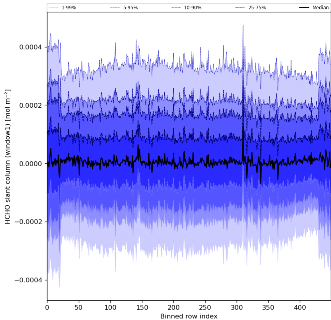
Figure 52: Along track statistics of “HCHO slant column (window1)” for 2024-04-02 to 2024-04-04
