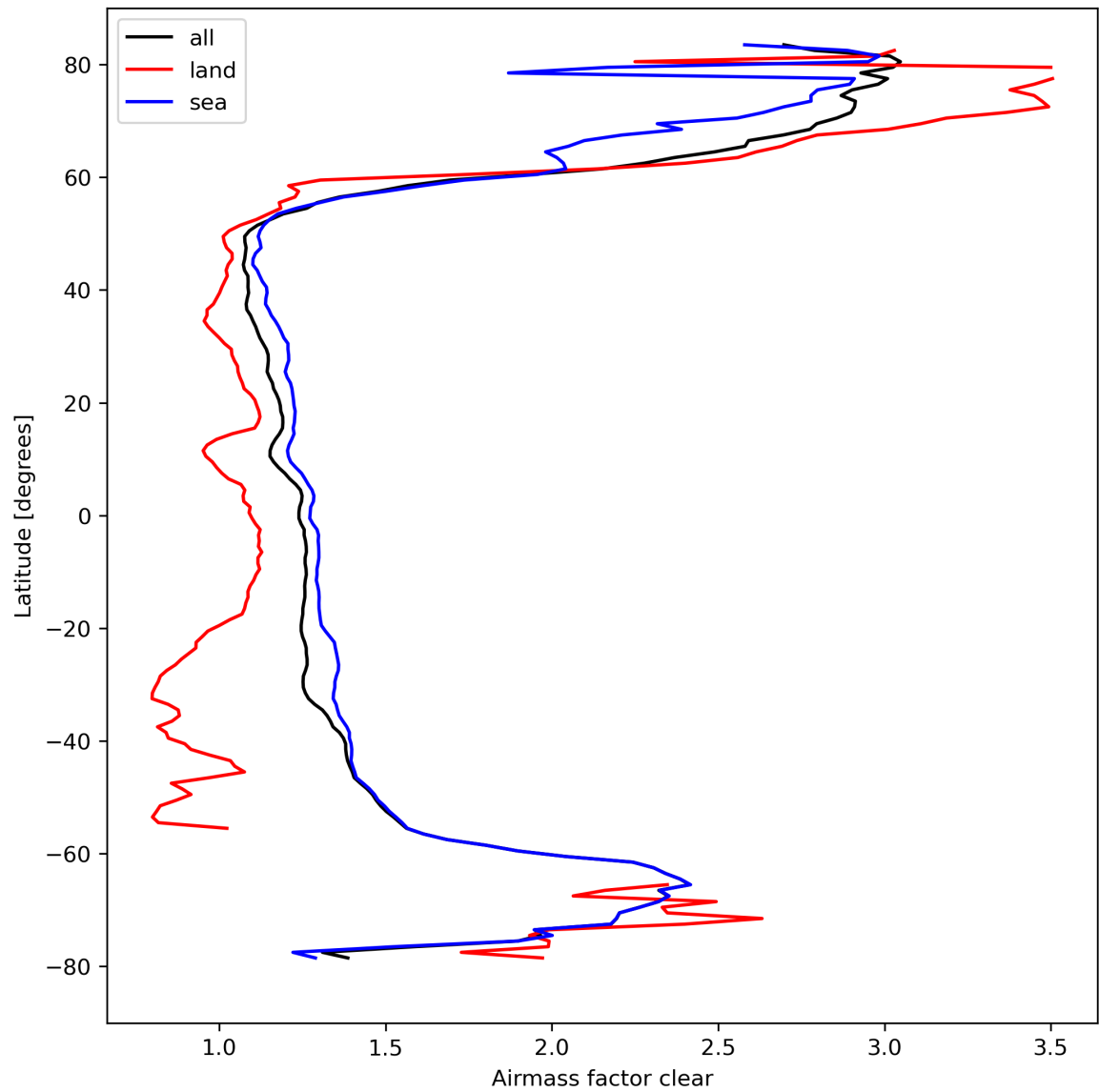
Figure 28: Zonal average of “Airmass factor clear” for 2024-04-02 to 2024-04-04.
