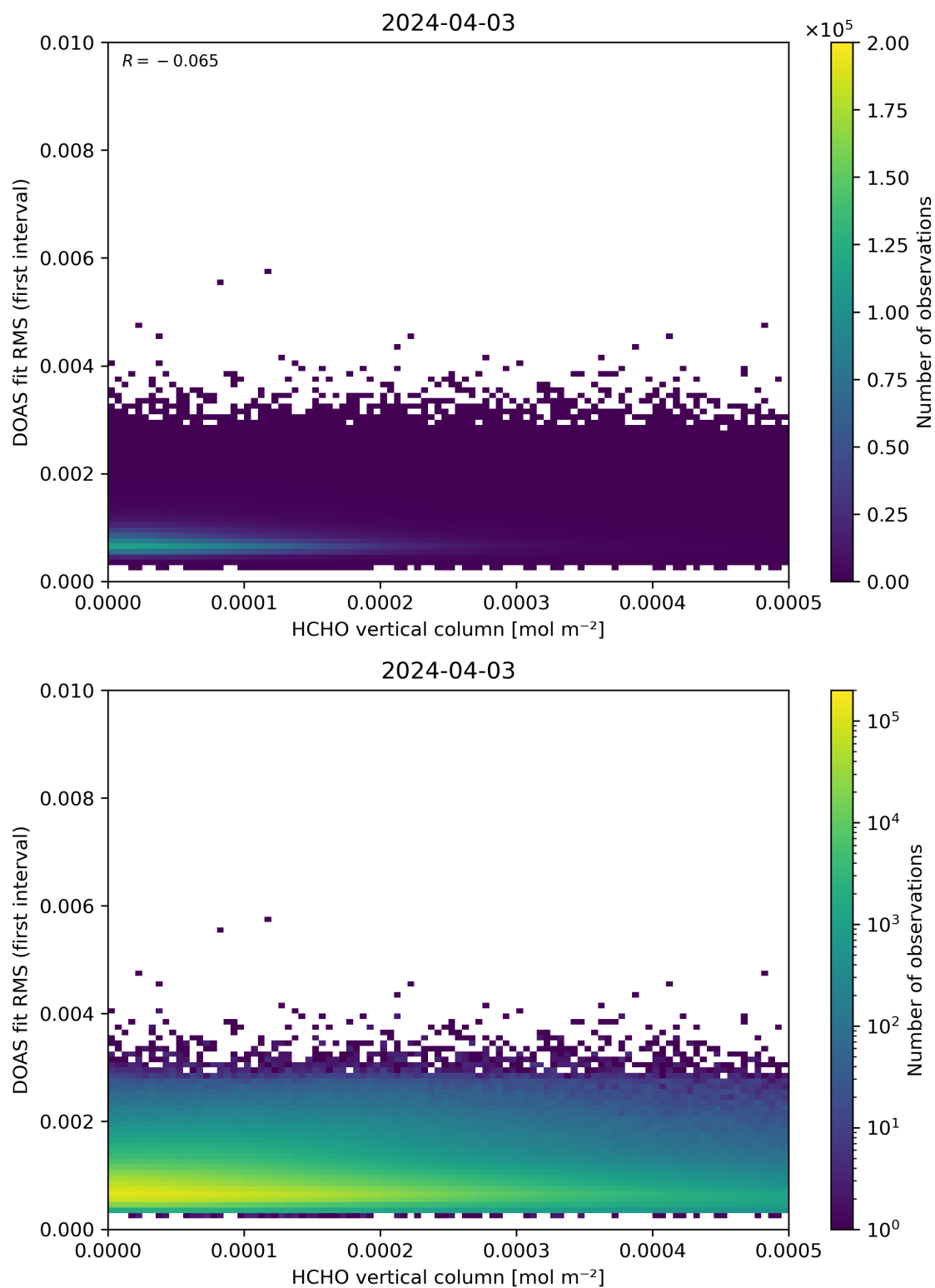
Figure 123: Scatter density plot of “HCHO vertical column” against “DOAS fit RMS (first interval)” for 2024-04-02 to 2024-04-04.
