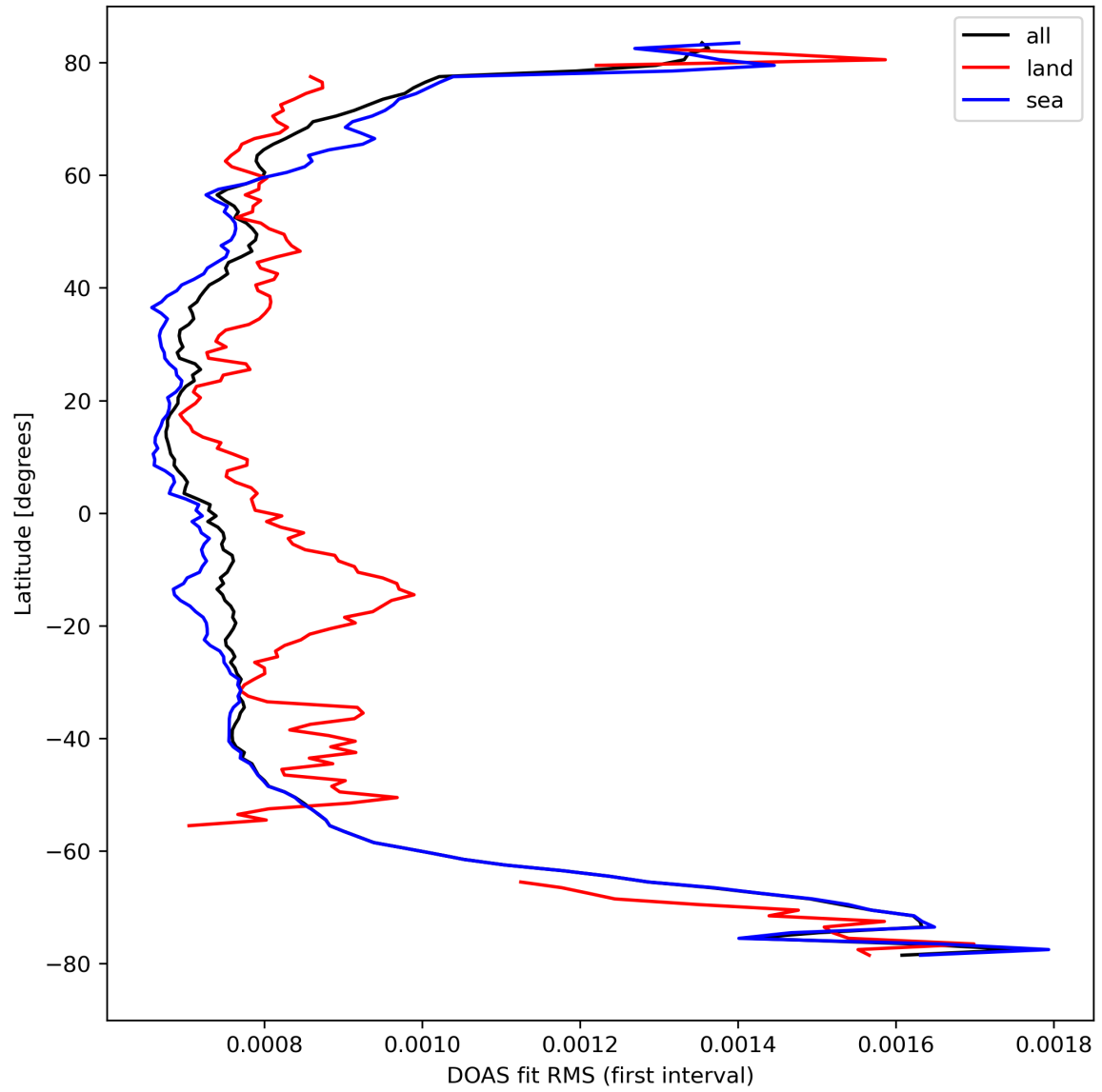
Figure 32: Zonal average of “DOAS fit RMS (first interval)” for 2024-04-02 to 2024-04-04.
