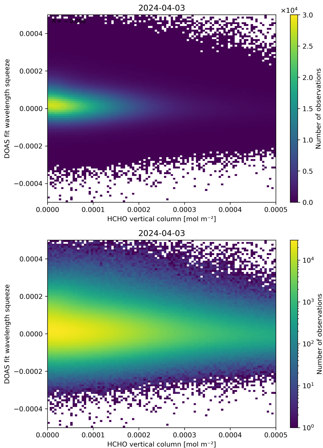
Figure 125: Scatter density plot of “HCHO vertical column” against “DOAS fit wavelength squeeze” for 2024-04-02 to 2024-04-04.
