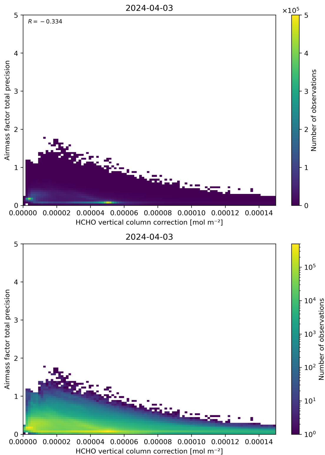
Figure 121: Scatter density plot of “HCHO vertical column correction” against “Airmass factor total precision” for 2024-04-02 to 2024-04-04.
