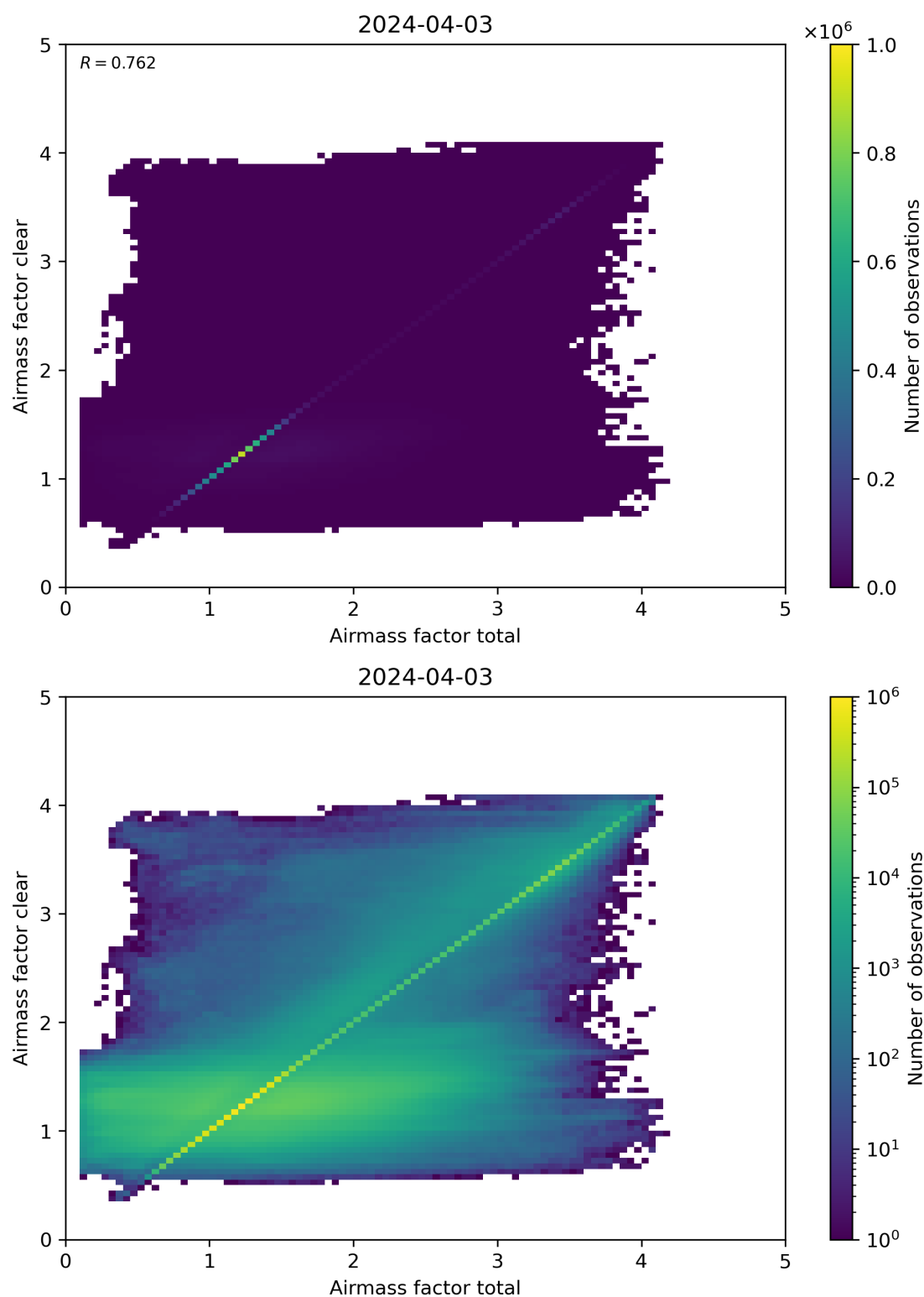
Figure 100: Scatter density plot of “Airmass factor total” against “Airmass factor clear” for 2024-04-02 to 2024-04-04.
