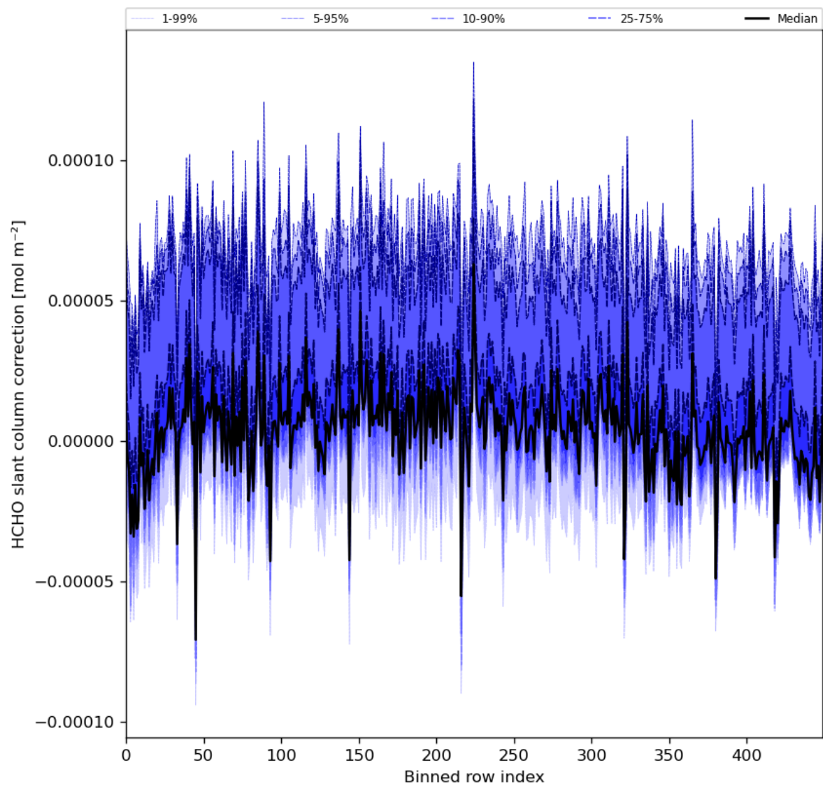
Figure 61: Along track statistics of “HCHO slant column correction” for 2024-04-02 to 2024-04-04
