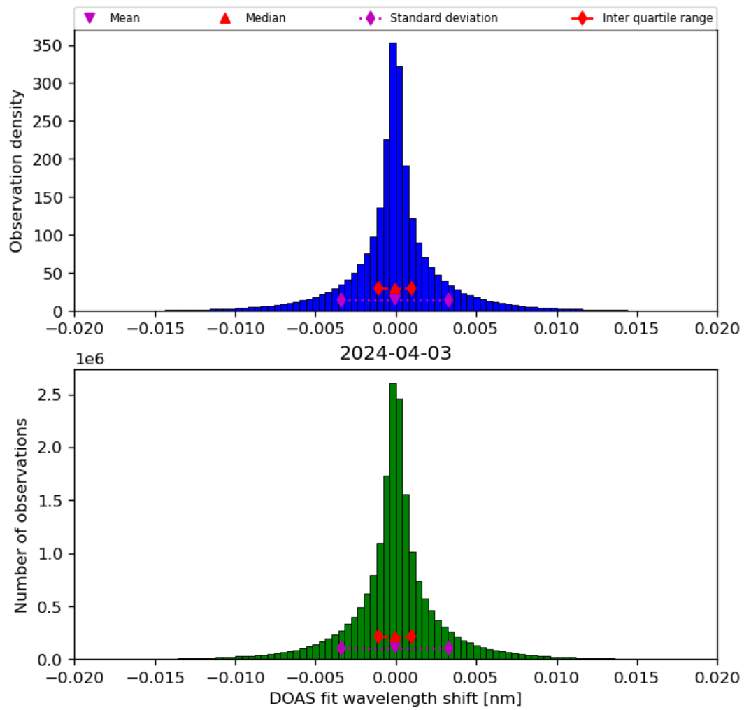
Figure 44: Histogram of “DOAS fit wavelength shift” for 2024-04-02 to 2024-04-04
