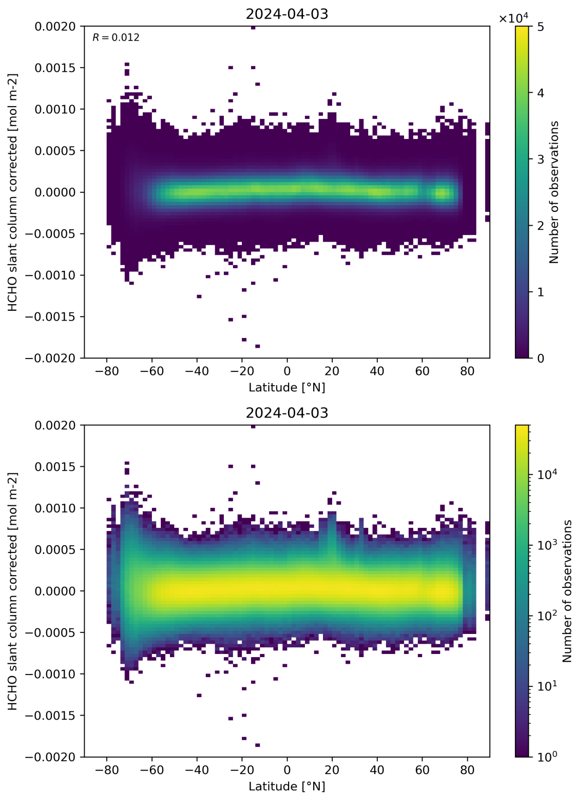
Figure 157: Scatter density plot of “Latitude” against “HCHO slant column corrected” for 2024-04-02 to 2024-04-04.
