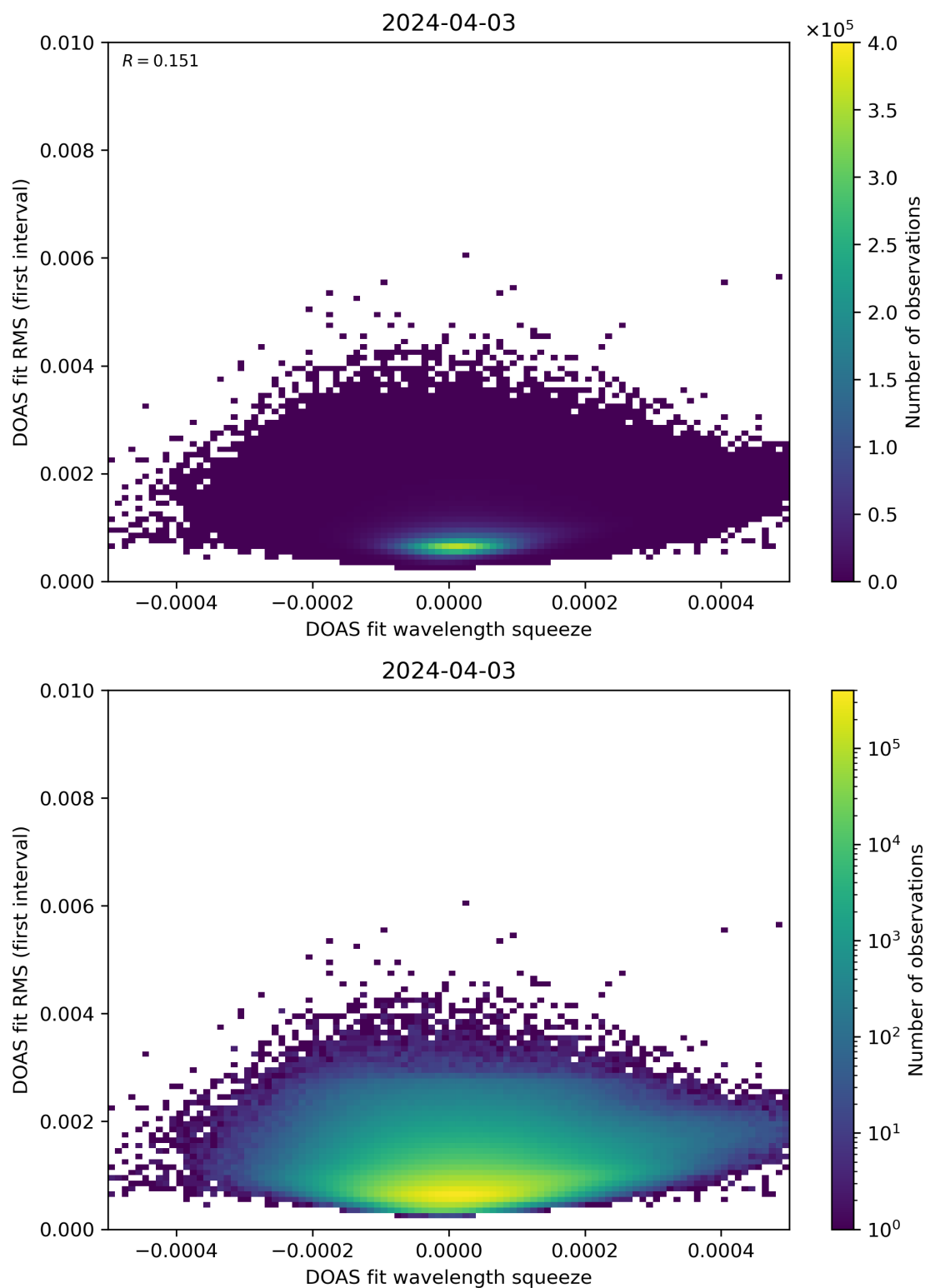
Figure 68: Scatter density plot of “DOAS fit wavelength squeeze” against “DOAS fit RMS (first interval)” for 2024-04-02 to 2024-04-04.
