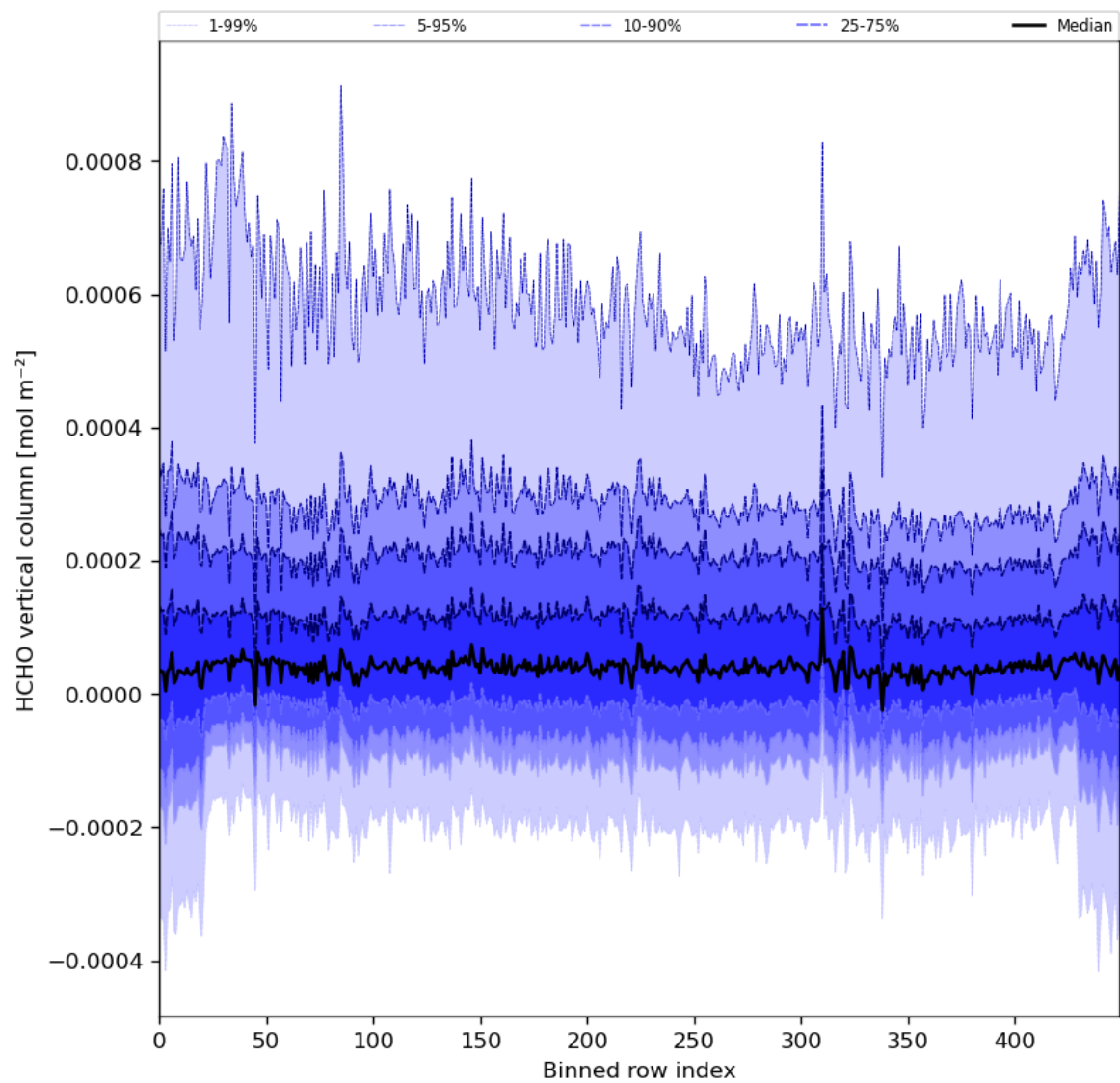
Figure 49: Along track statistics of “HCHO vertical column” for 2024-04-02 to 2024-04-04
