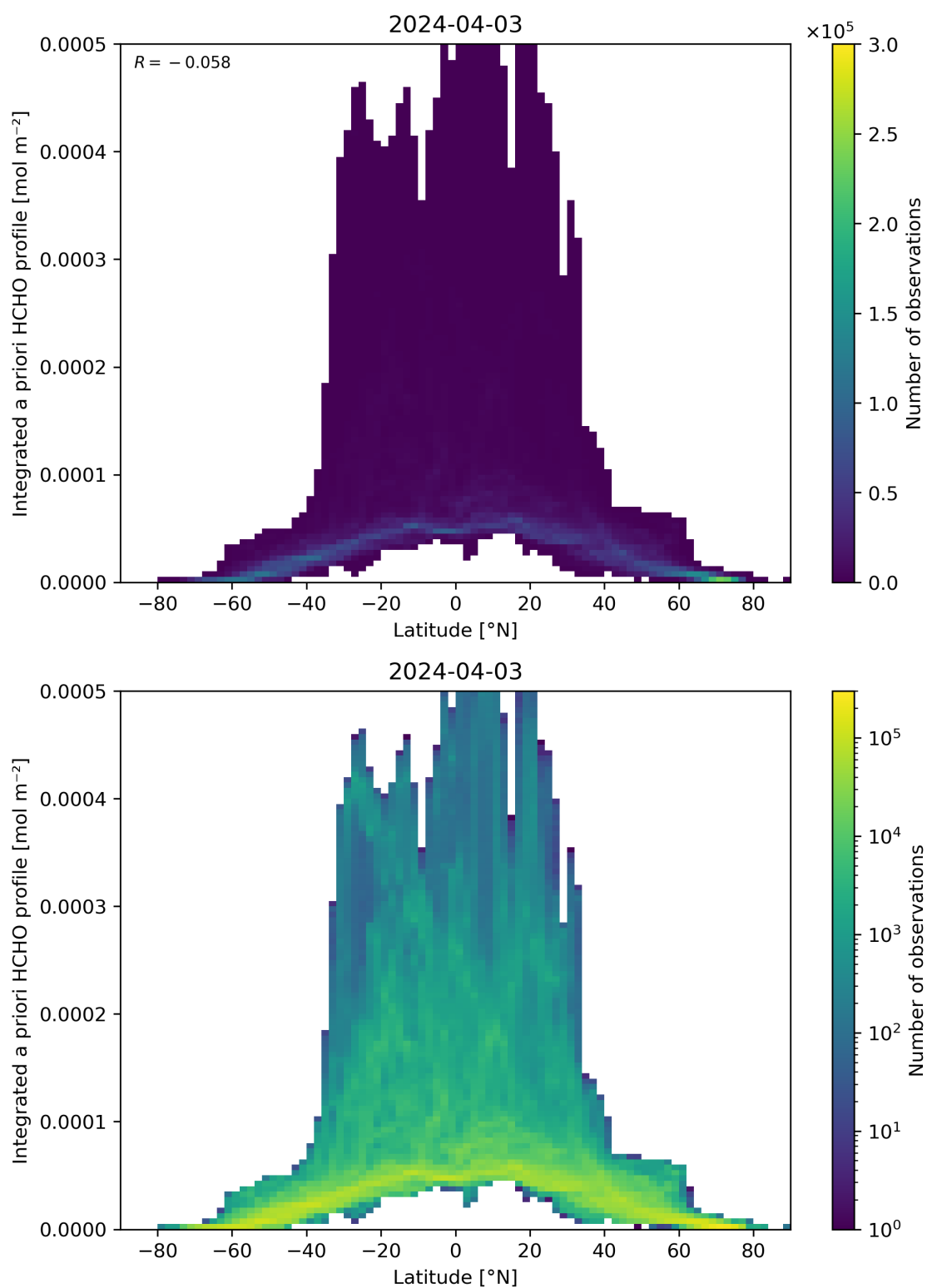
Figure 166: Scatter density plot of “Latitude” against “Integrated a priori HCHO profile” for 2024-04-02 to 2024-04-04.
