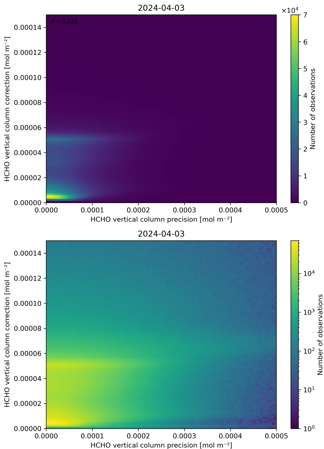
Figure 146: Scatter density plot of “HCHO vertical column precision” against “HCHO vertical column correction” for 2024-04-02 to 2024-04-04.
