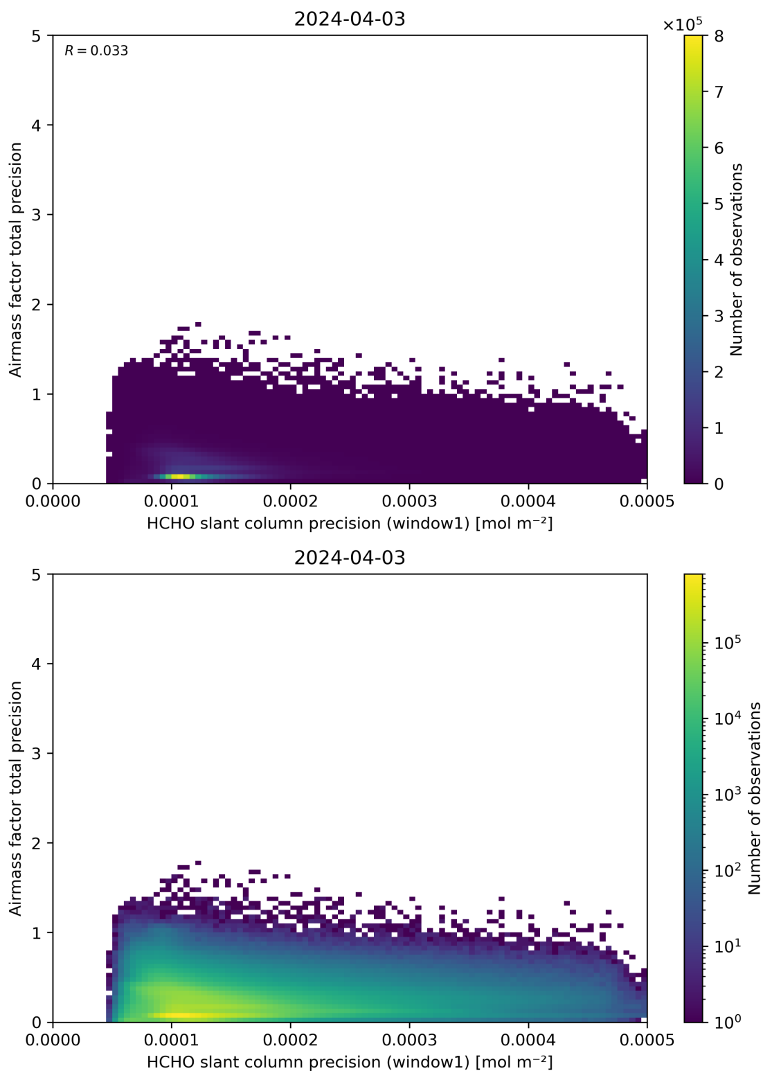
Figure 95: Scatter density plot of “HCHO slant column precision (window1)” against “Airmass factor total precision” for 2024-04-02 to 2024-04-04.
