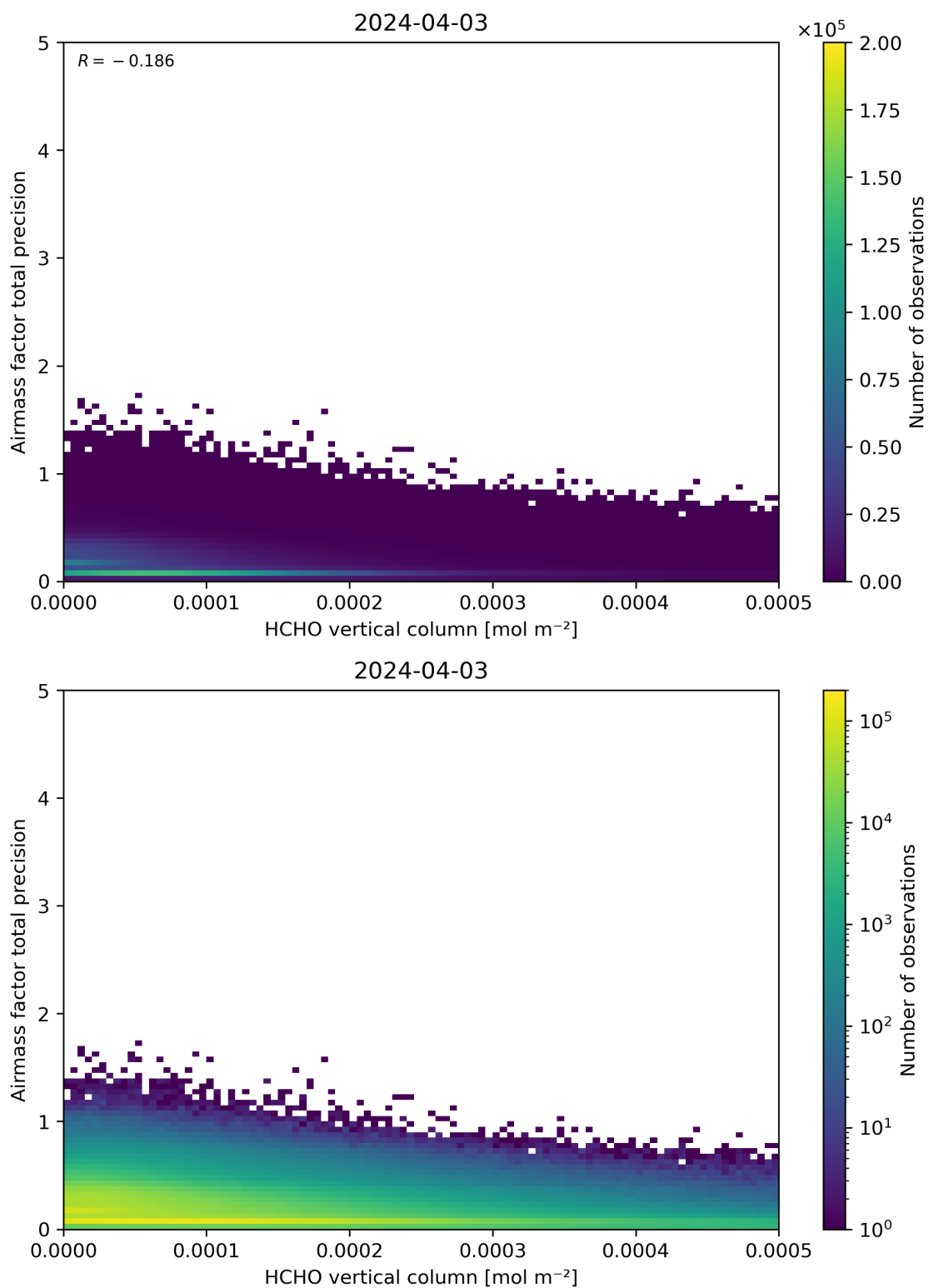
Figure 132: Scatter density plot of “HCHO vertical column” against “Airmass factor total precision” for 2024-04-02 to 2024-04-04.
