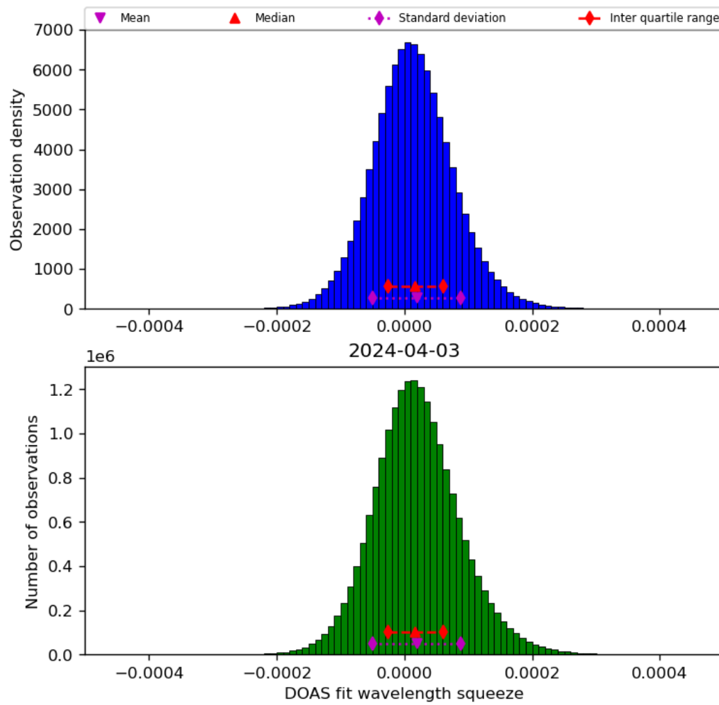
Figure 45: Histogram of “DOAS fit wavelength squeeze” for 2024-04-02 to 2024-04-04
