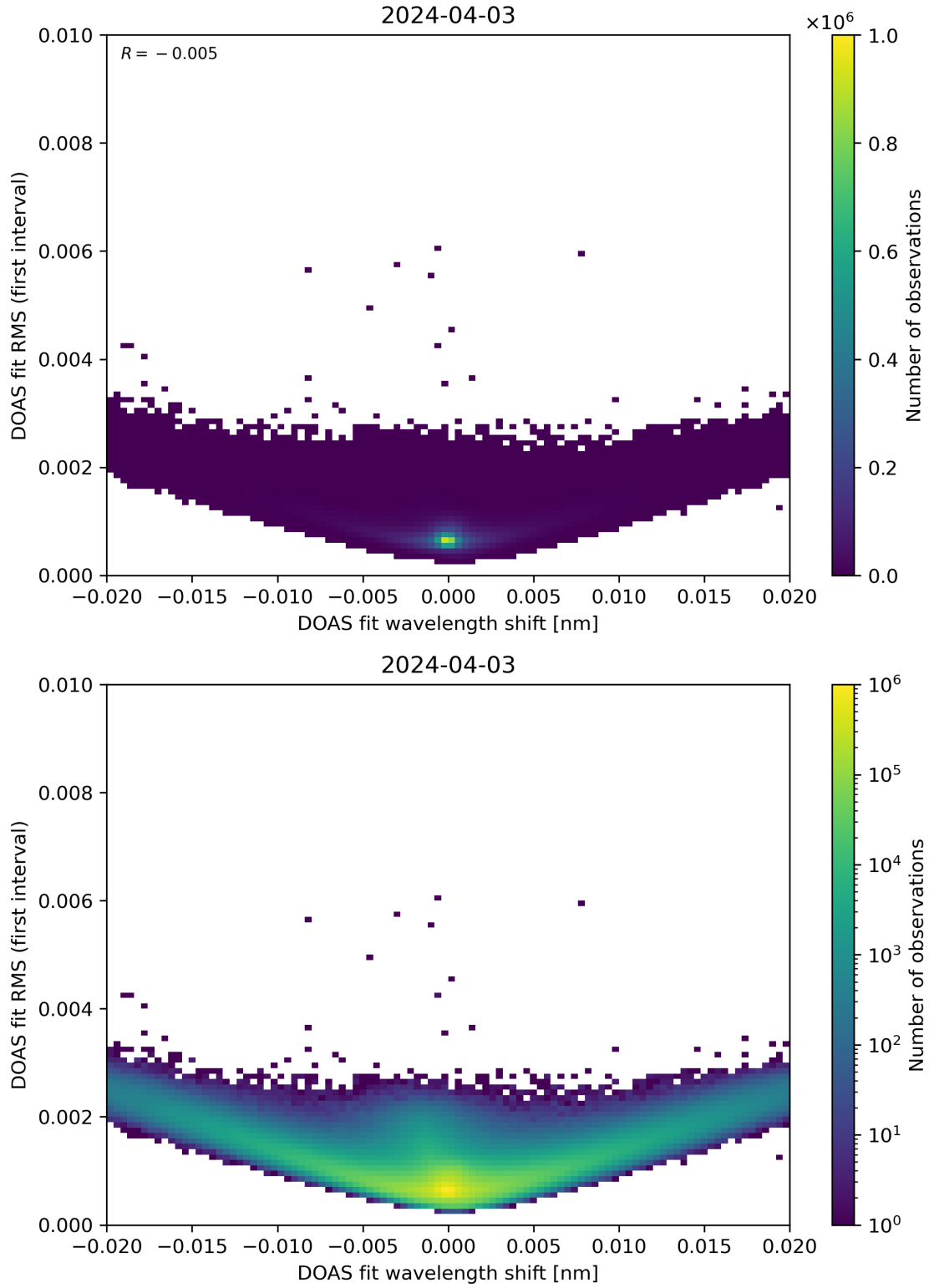
Figure 64: Scatter density plot of “DOAS fit wavelength shift” against “DOAS fit RMS (first interval)” for 2024-04-02 to 2024-04-04.
