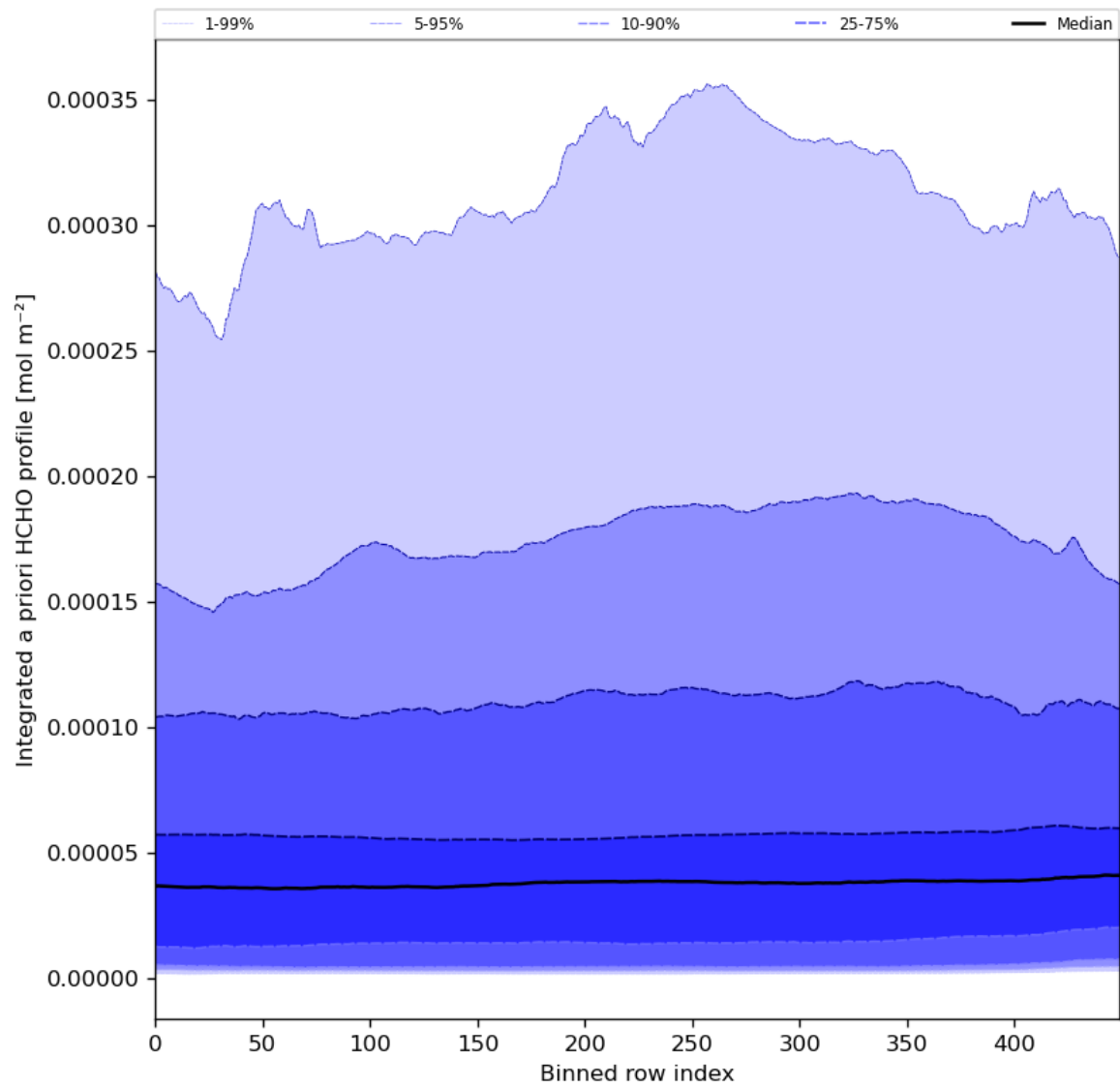
Figure 57: Along track statistics of “Integrated a priori HCHO profile” for 2024-04-02 to 2024-04-04
