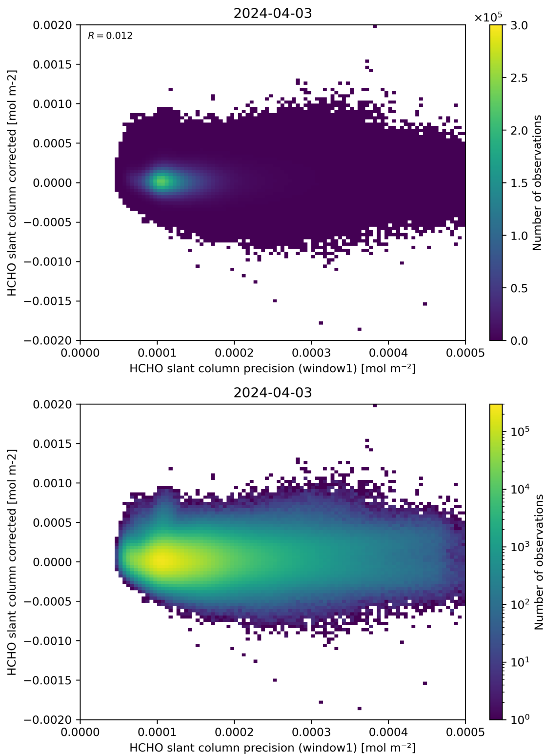
Figure 92: Scatter density plot of “HCHO slant column precision (window1)” against “HCHO slant column corrected” for 2024-04-02 to 2024-04-04.
