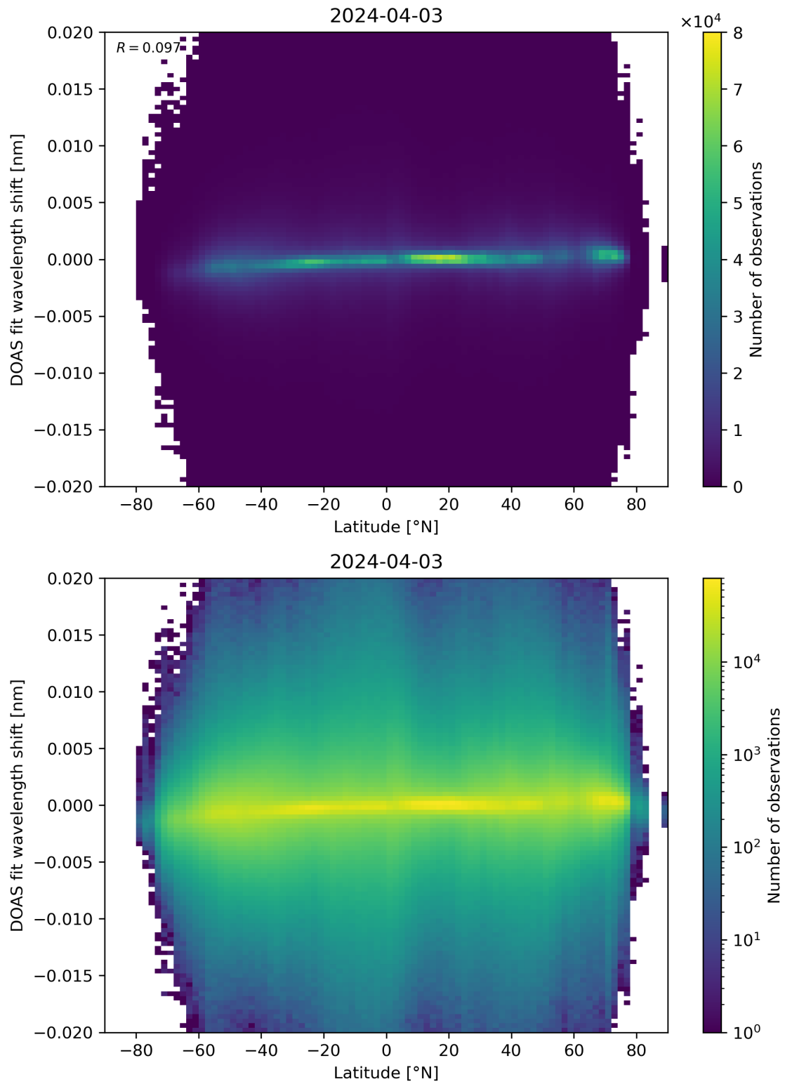
Figure 154: Scatter density plot of “Latitude” against “DOAS fit wavelength shift” for 2024-04-02 to 2024-04-04.
