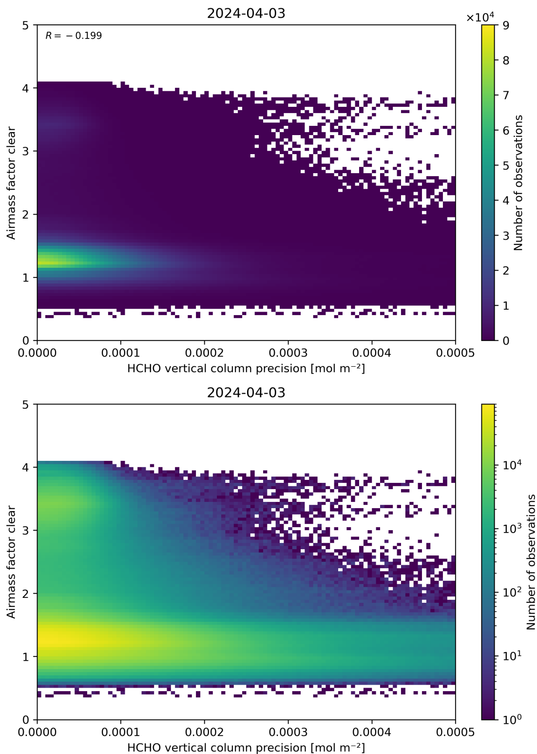
Figure 139: Scatter density plot of “HCHO vertical column precision” against “Airmass factor clear” for 2024-04-02 to 2024-04-04.
