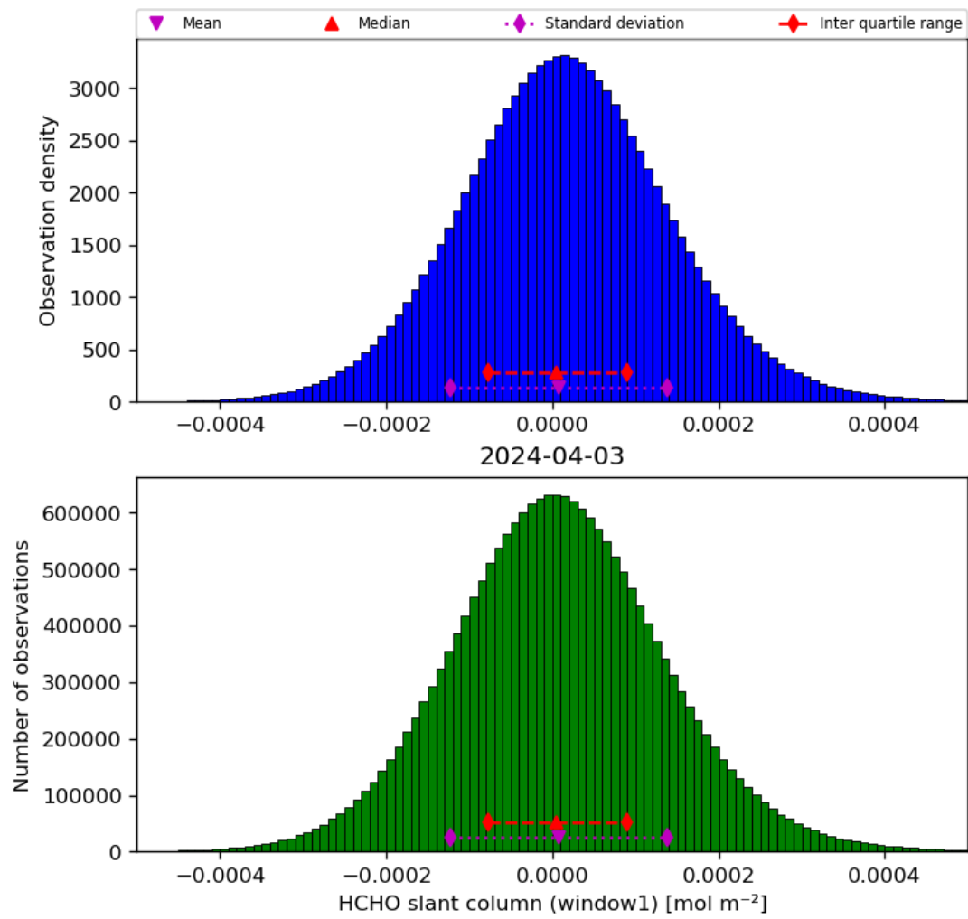
Figure 38: Histogram of “HCHO slant column (window1)” for 2024-04-02 to 2024-04-04
