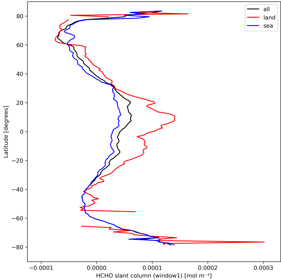
Figure 24: Zonal average of “HCHO slant column (window1)” for 2024-04-02 to 2024-04-04.
