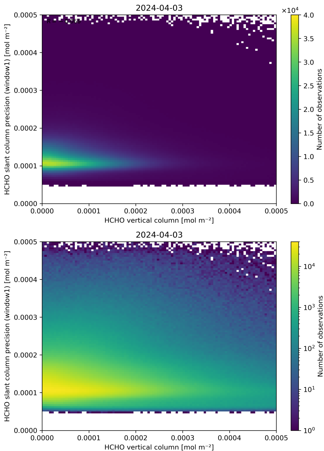
Figure 130: Scatter density plot of “HCHO vertical column” against “HCHO slant column precision (window1)” for 2024-04-02 to 2024-04-04.
