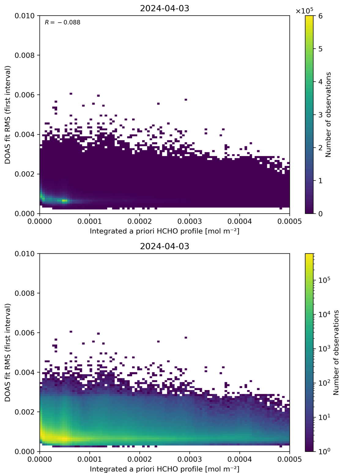
Figure 148: Scatter density plot of “Integrated a priori HCHO profile” against “DOAS fit RMS (first interval)” for 2024-04-02 to 2024-04-04.
