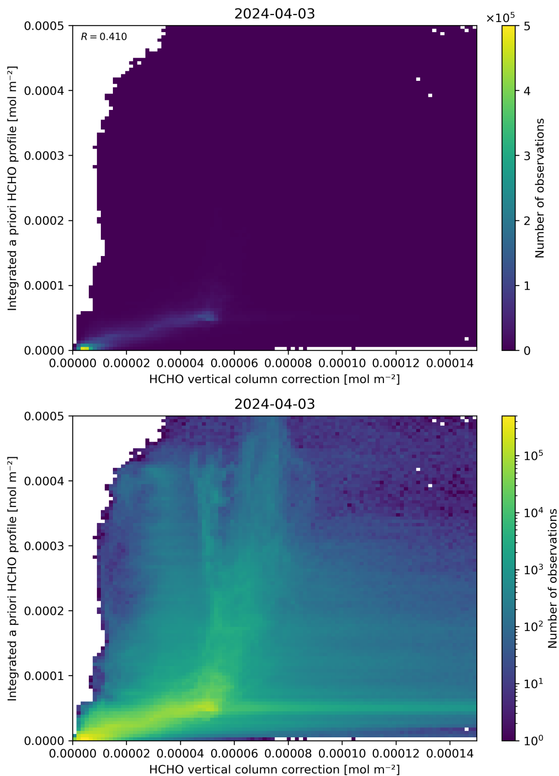
Figure 122: Scatter density plot of “HCHO vertical column correction” against “Integrated a priori HCHO profile” for 2024-04-02 to 2024-04-04.
