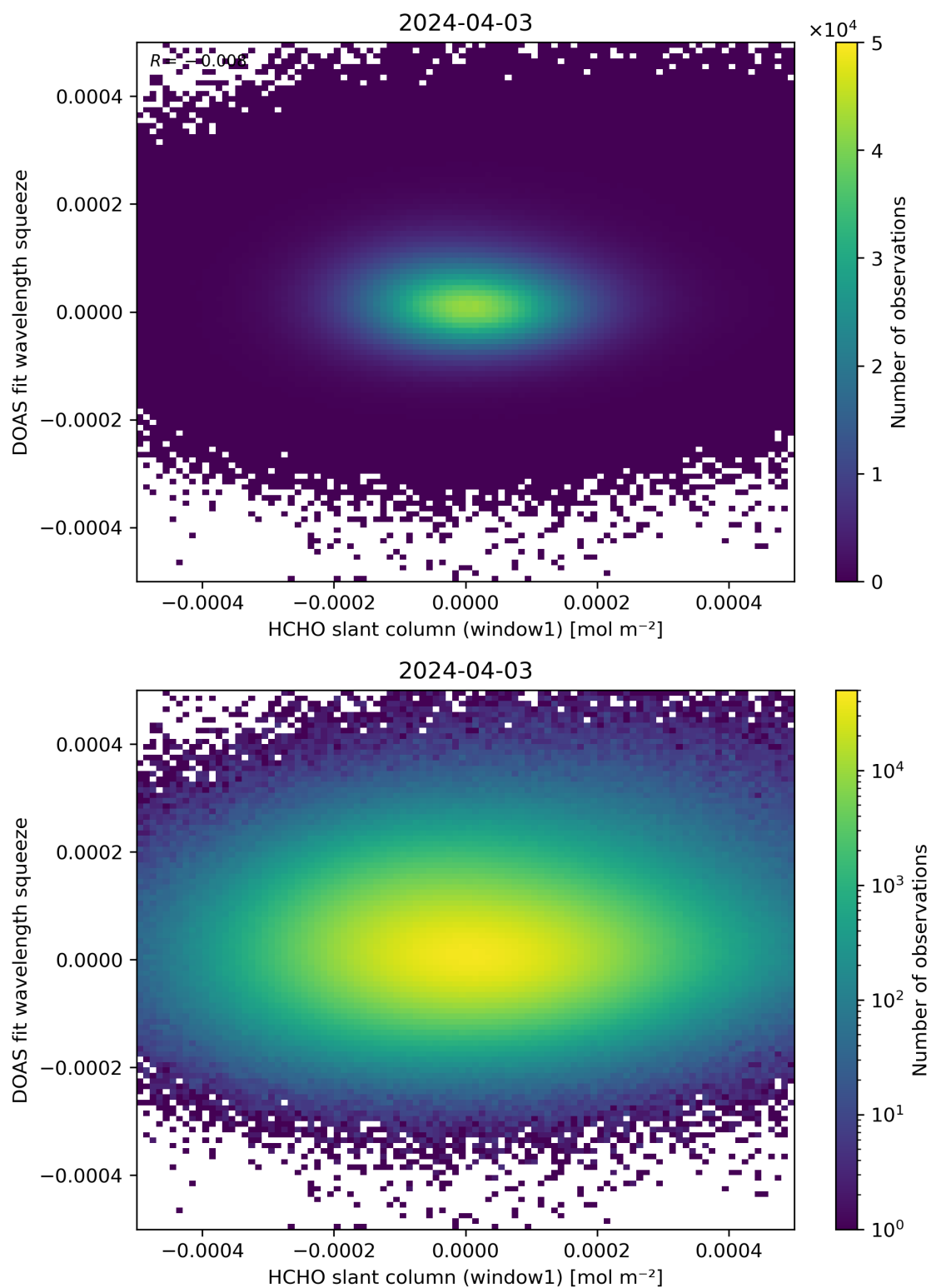
Figure 80: Scatter density plot of “HCHO slant column (window1)” against “DOAS fit wavelength squeeze” for 2024-04-02 to 2024-04-04.
