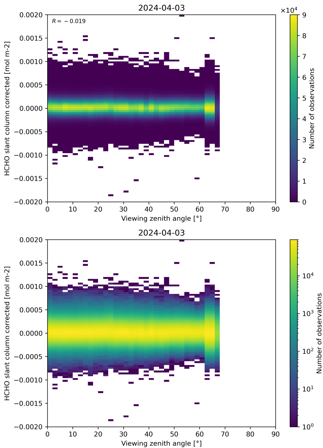
Figure 186: Scatter density plot of “Viewing zenith angle” against “HCHO slant column corrected” for 2024-04-02 to 2024-04-04.
