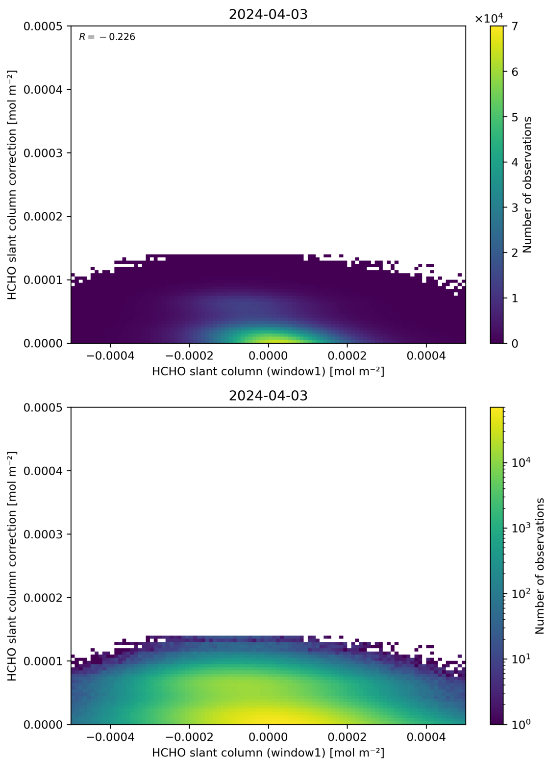
Figure 83: Scatter density plot of “HCHO slant column (window1)” against “HCHO slant column correction” for 2024-04-02 to 2024-04-04.
