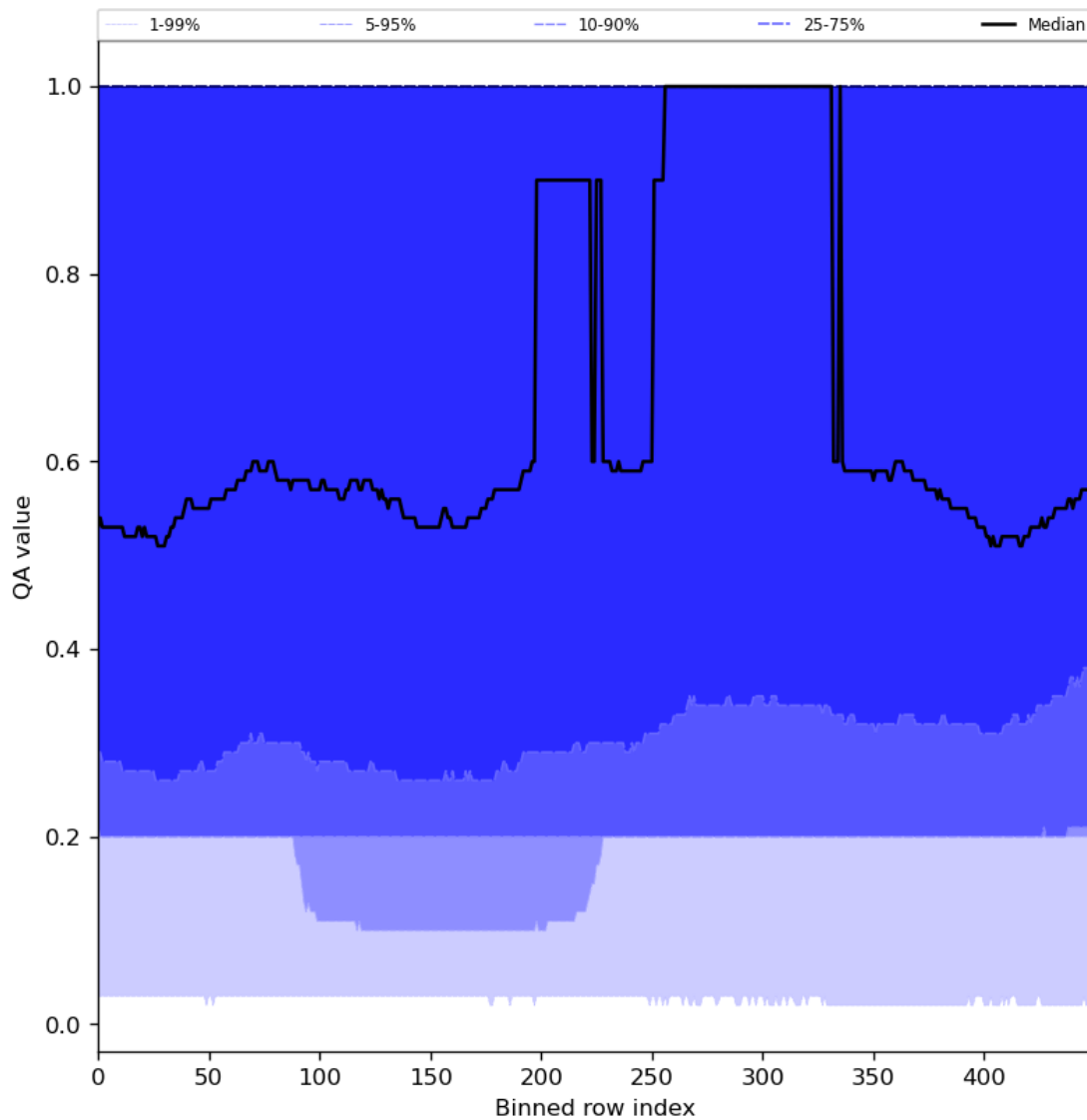
Figure 48: Along track statistics of “QA value” for 2024-04-02 to 2024-04-04
