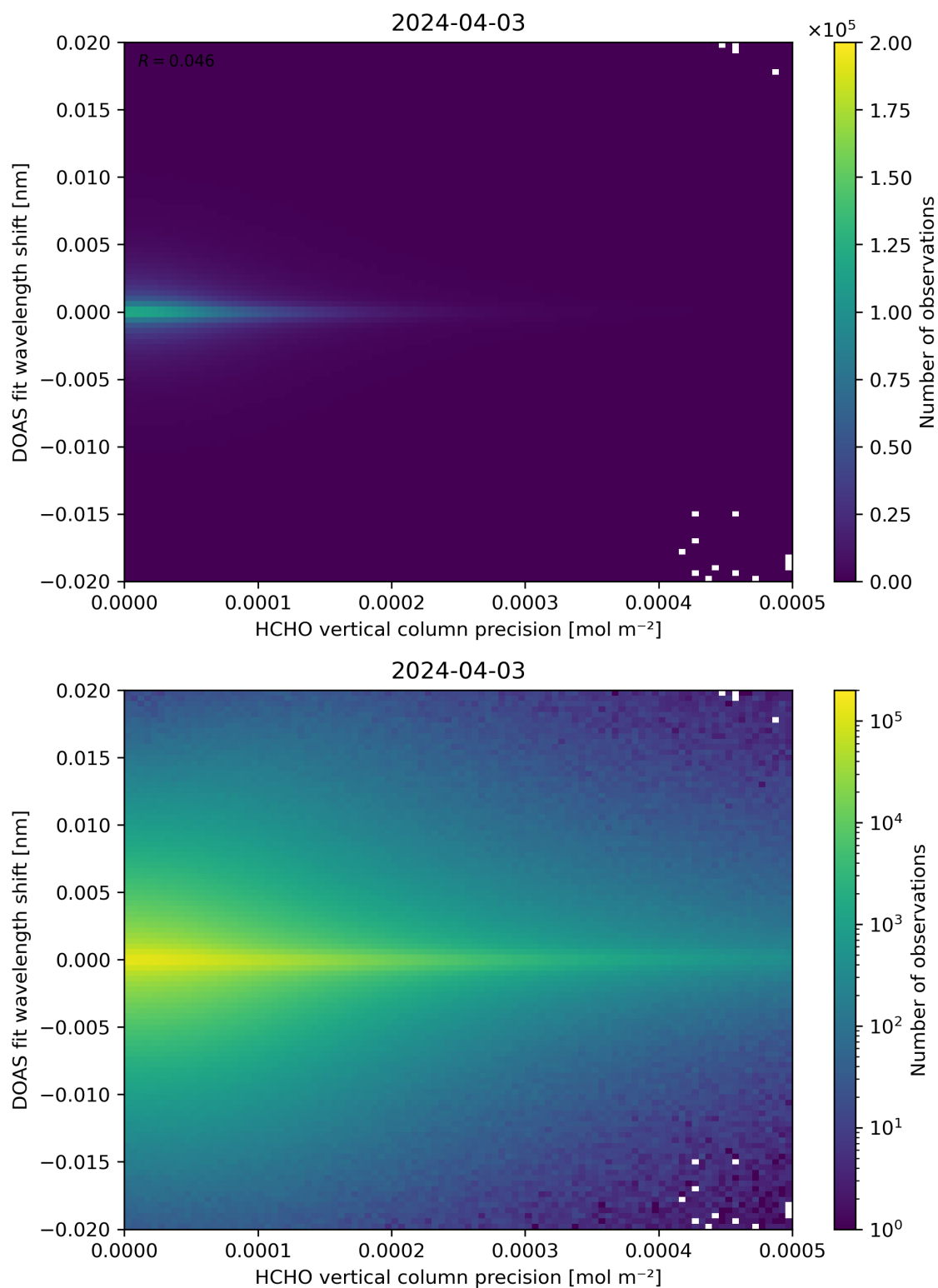
Figure 137: Scatter density plot of “HCHO vertical column precision” against “DOAS fit wavelength shift” for 2024-04-02 to 2024-04-04.
