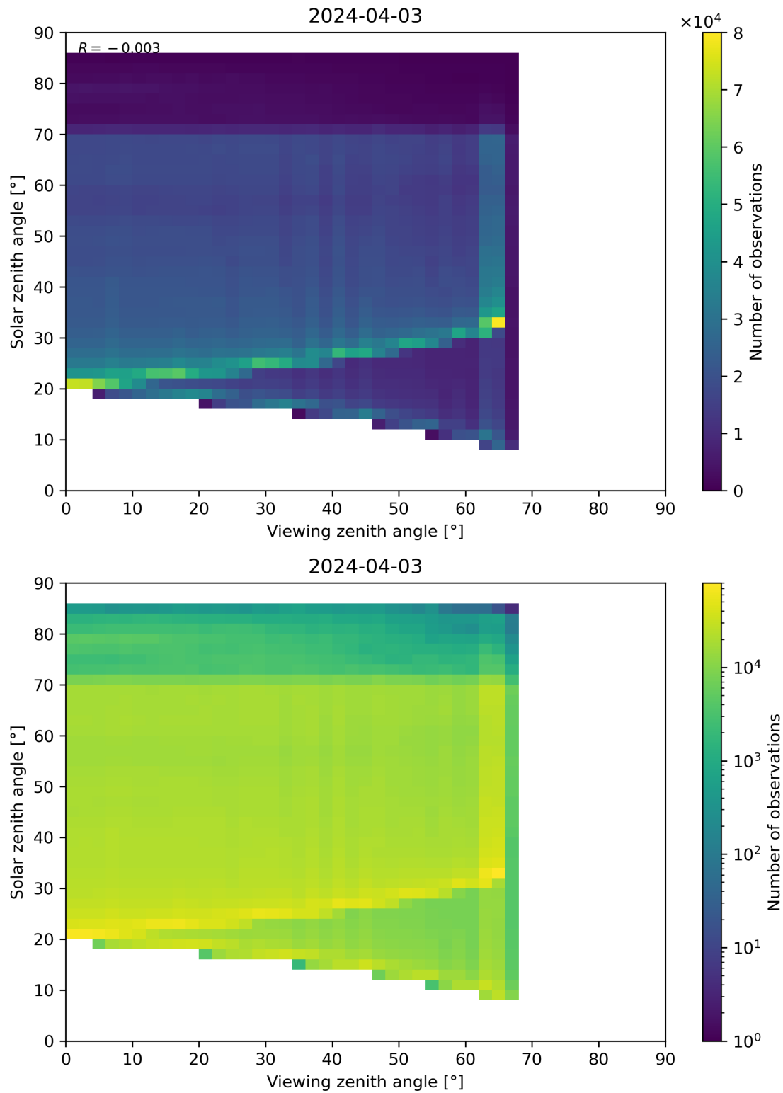
Figure 197: Scatter density plot of “Viewing zenith angle” against “Solar zenith angle” for 2024-04-02 to 2024-04-04.
