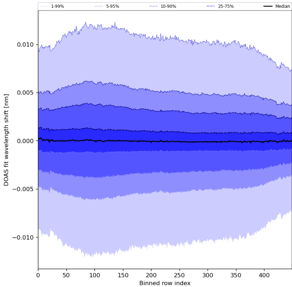
Figure 58: Along track statistics of “DOAS fit wavelength shift” for 2024-04-02 to 2024-04-04
