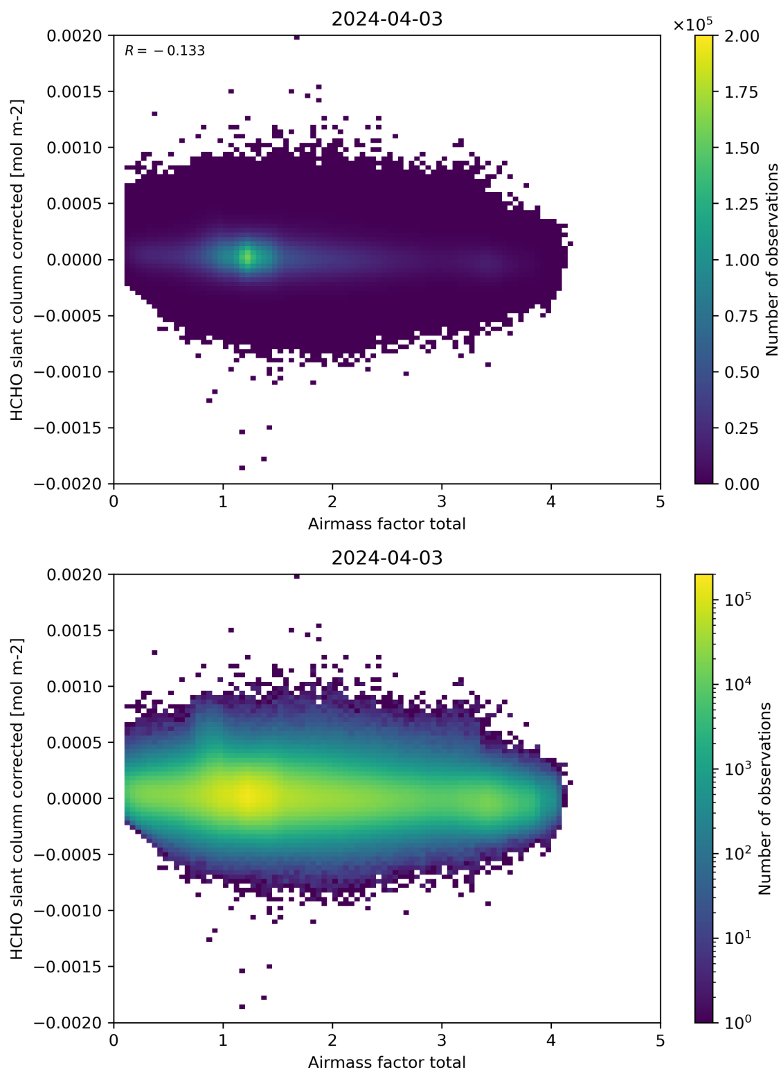
Figure 101: Scatter density plot of “Airmass factor total” against “HCHO slant column corrected” for 2024-04-02 to 2024-04-04.
