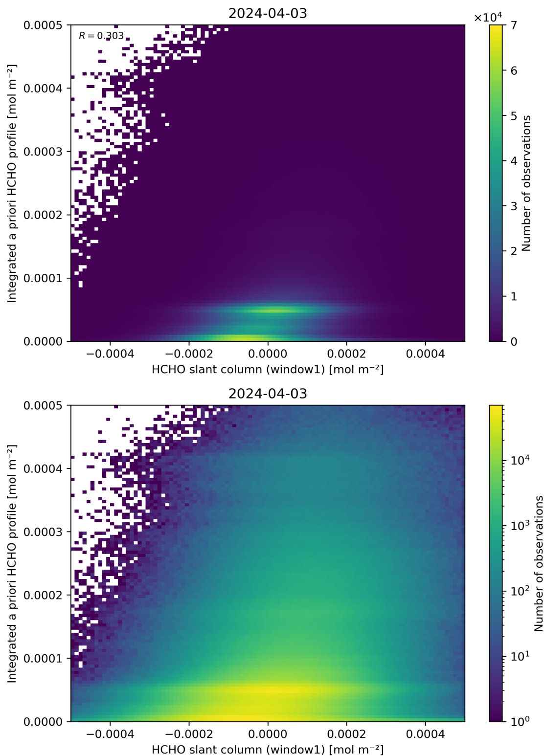
Figure 87: Scatter density plot of “HCHO slant column (window1)” against “Integrated a priori HCHO profile” for 2024-04-02 to 2024-04-04.
