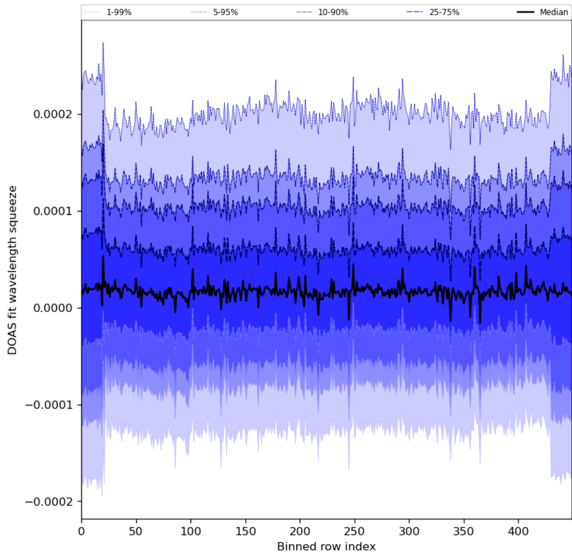
Figure 59: Along track statistics of “DOAS fit wavelength squeeze” for 2024-04-02 to 2024-04-04
