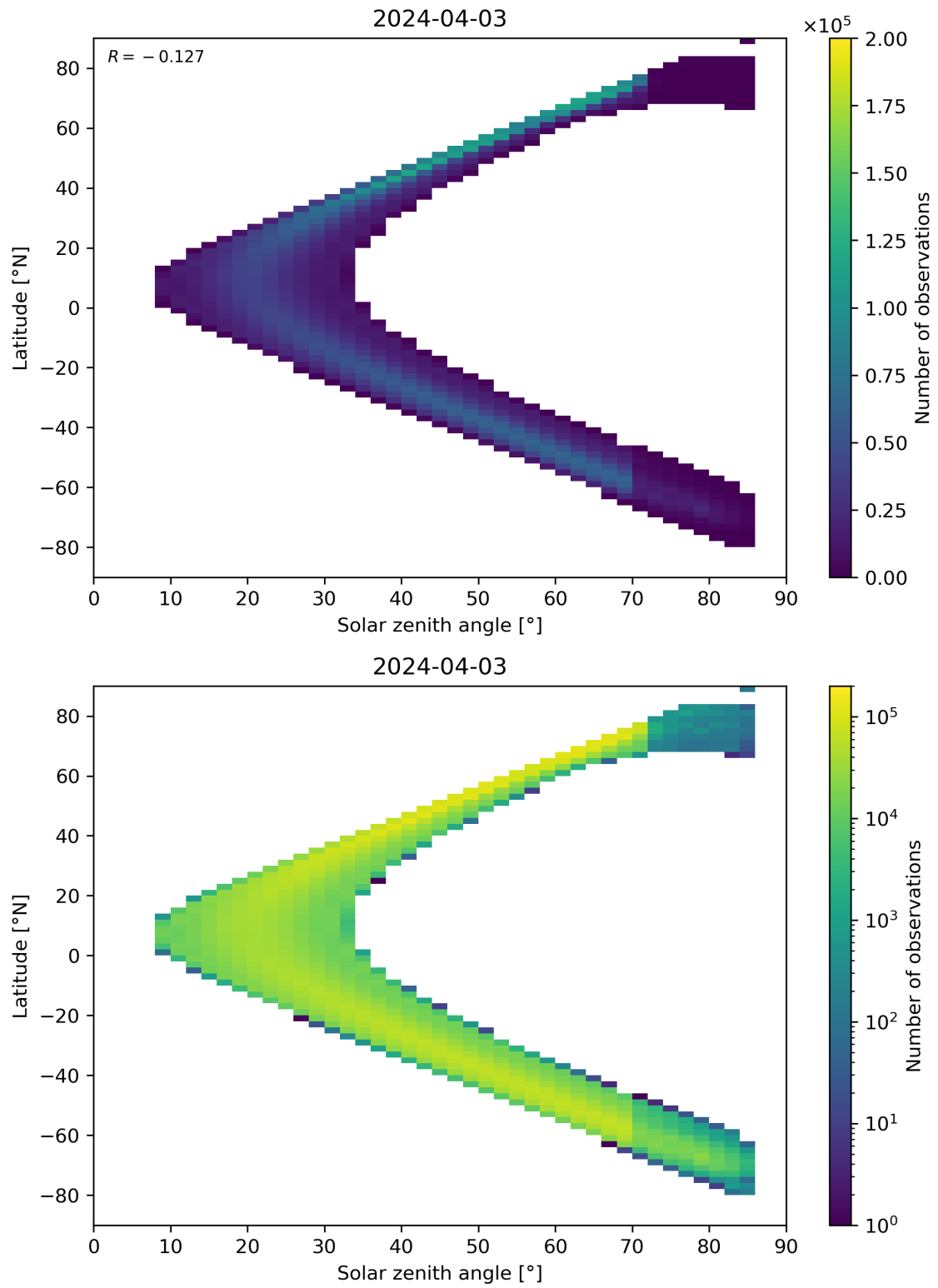
Figure 181: Scatter density plot of “Solar zenith angle” against “Latitude” for 2024-04-02 to 2024-04-04.
