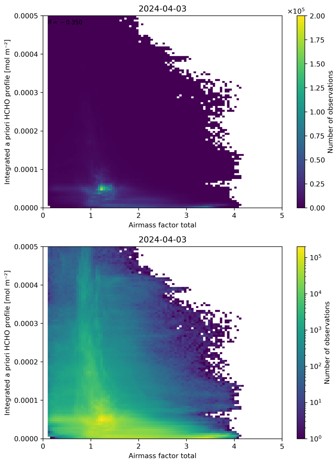
Figure 104: Scatter density plot of “Airmass factor total” against “Integrated a priori HCHO profile” for 2024-04-02 to 2024-04-04.
