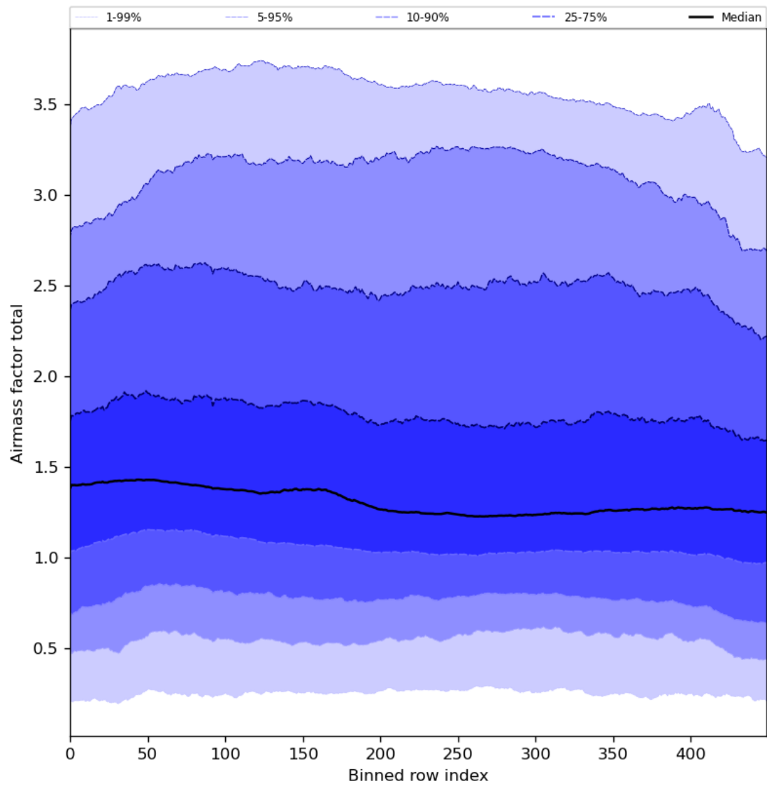
Figure 54: Along track statistics of “Airmass factor total” for 2024-04-02 to 2024-04-04
