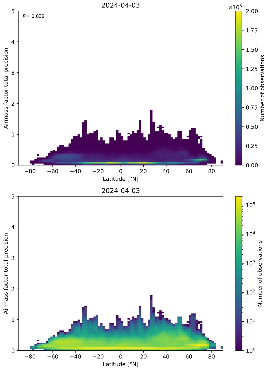
Figure 162: Scatter density plot of “Latitude” against “Airmass factor total precision” for 2024-04-02 to 2024-04-04.
