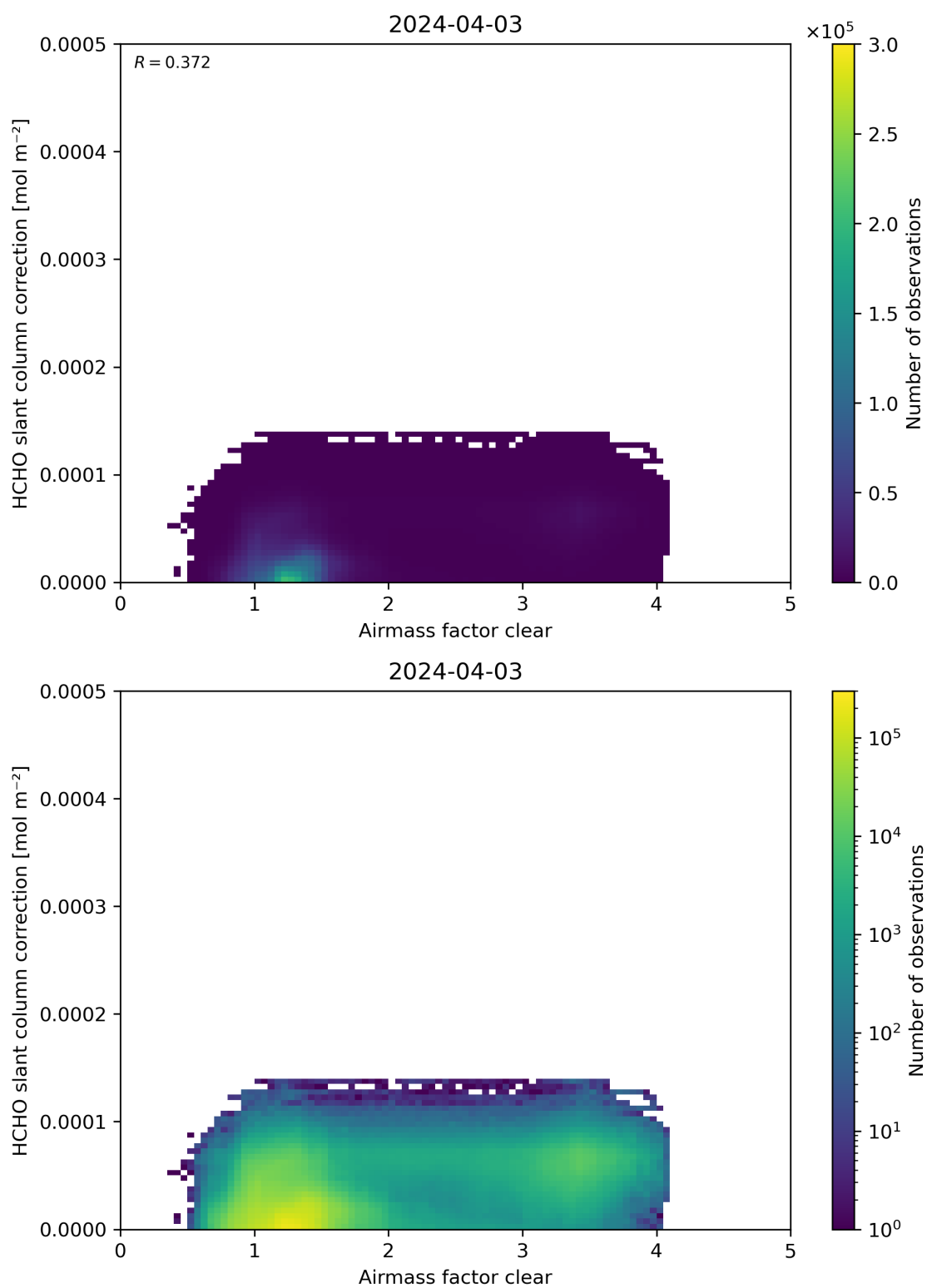
Figure 75: Scatter density plot of “Airmass factor clear” against “HCHO slant column correction” for 2024-04-02 to 2024-04-04.
