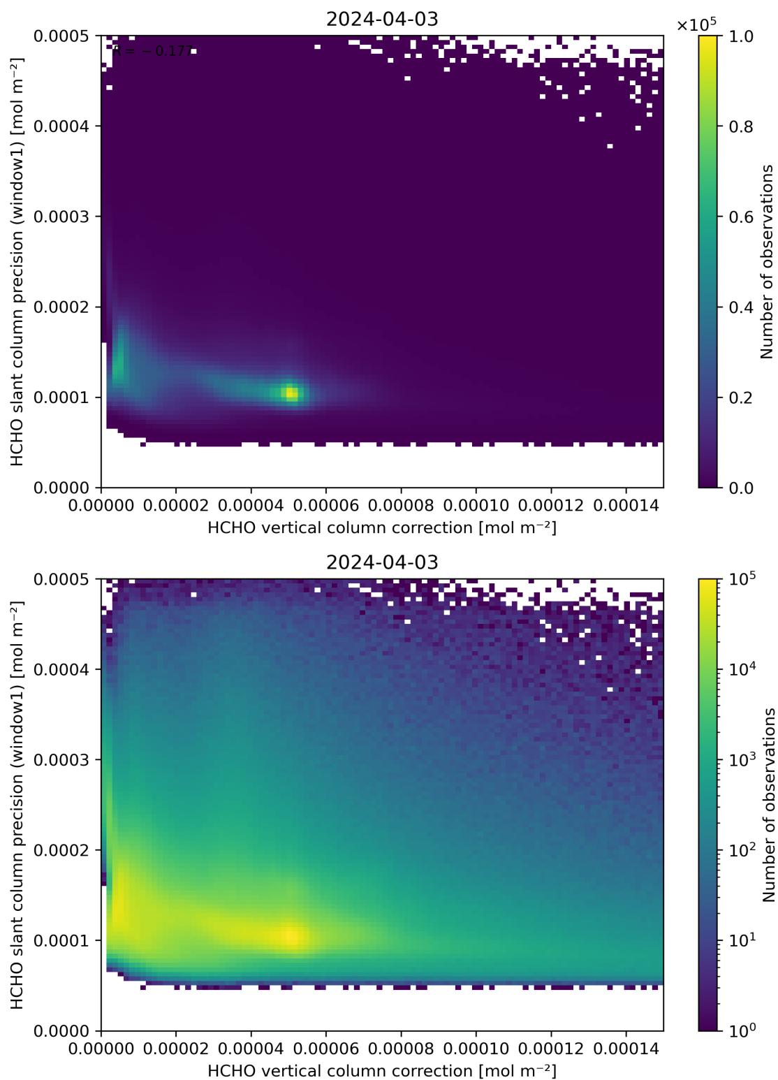
Figure 119: Scatter density plot of “HCHO vertical column correction” against “HCHO slant column precision (window1)” for 2024-04-02 to 2024-04-04.
