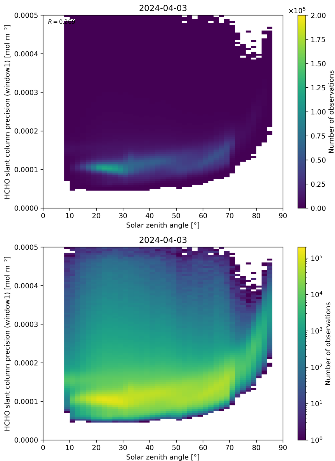
Figure 174: Scatter density plot of “Solar zenith angle” against “HCHO slant column precision (window1)” for 2024-04-02 to 2024-04-04.
