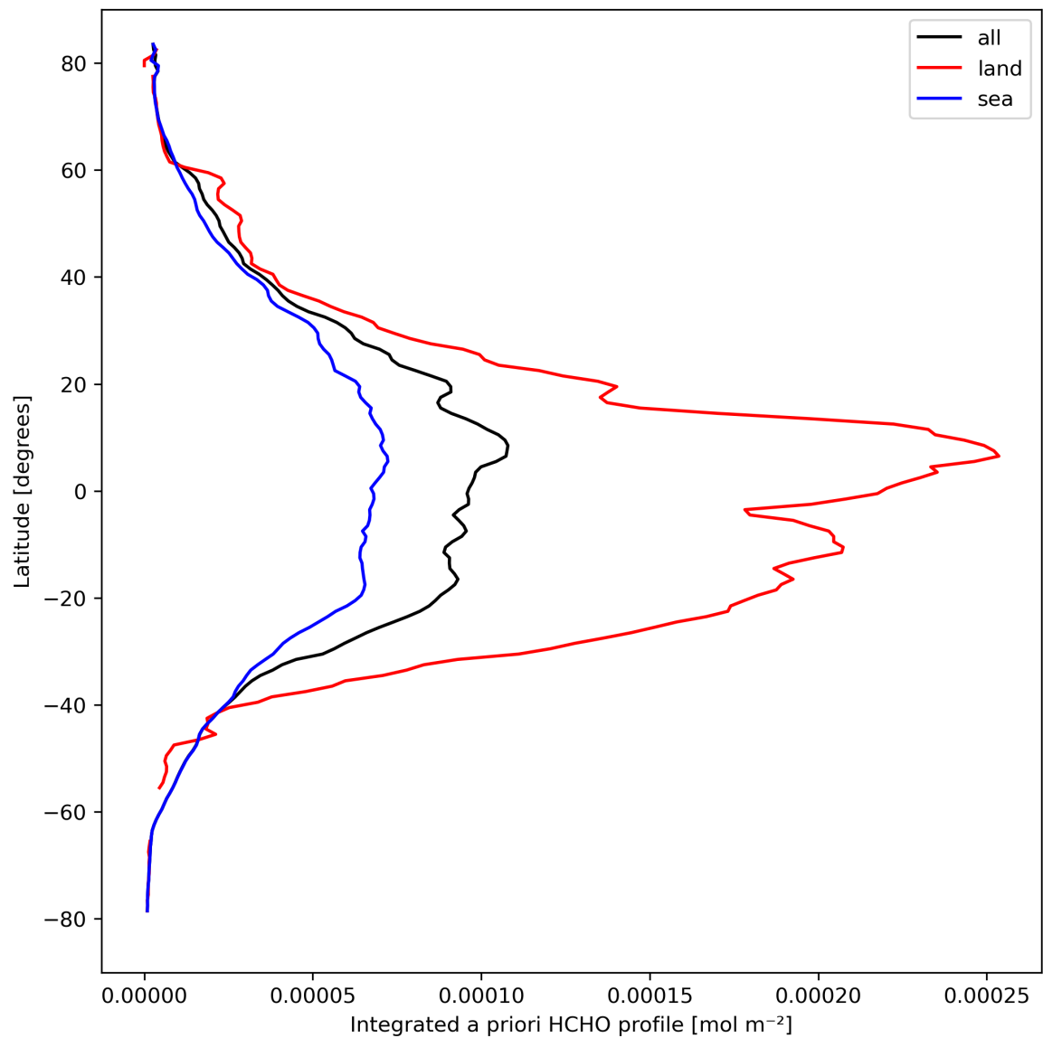
Figure 29: Zonal average of “Integrated a priori HCHO profile” for 2024-04-02 to 2024-04-04.
