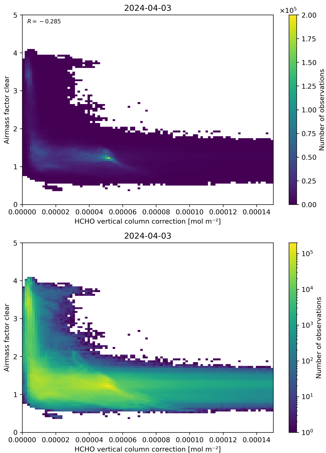
Figure 115: Scatter density plot of “HCHO vertical column correction” against “Airmass factor clear” for 2024-04-02 to 2024-04-04.
