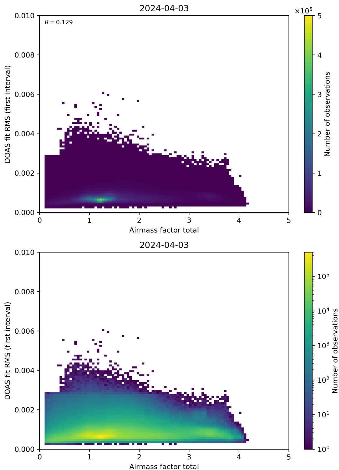
Figure 97: Scatter density plot of “Airmass factor total” against “DOAS fit RMS (first interval)” for 2024-04-02 to 2024-04-04.
