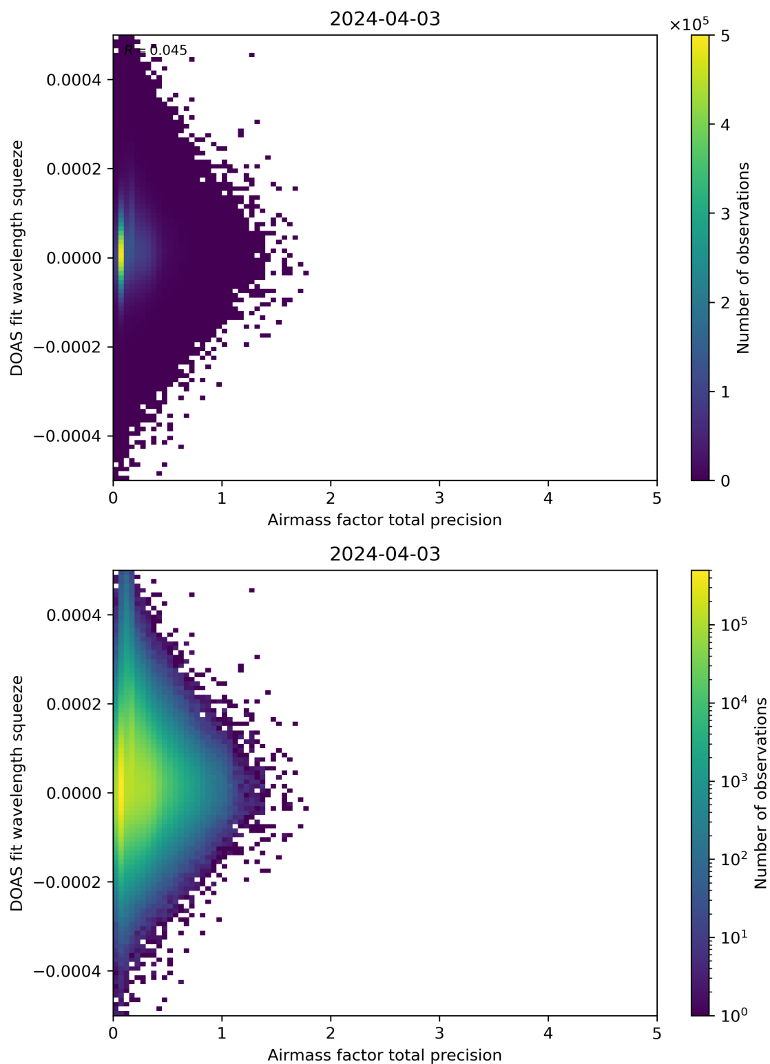
Figure 107: Scatter density plot of “Airmass factor total precision” against “DOAS fit wavelength squeeze” for 2024-04-02 to 2024-04-04.
