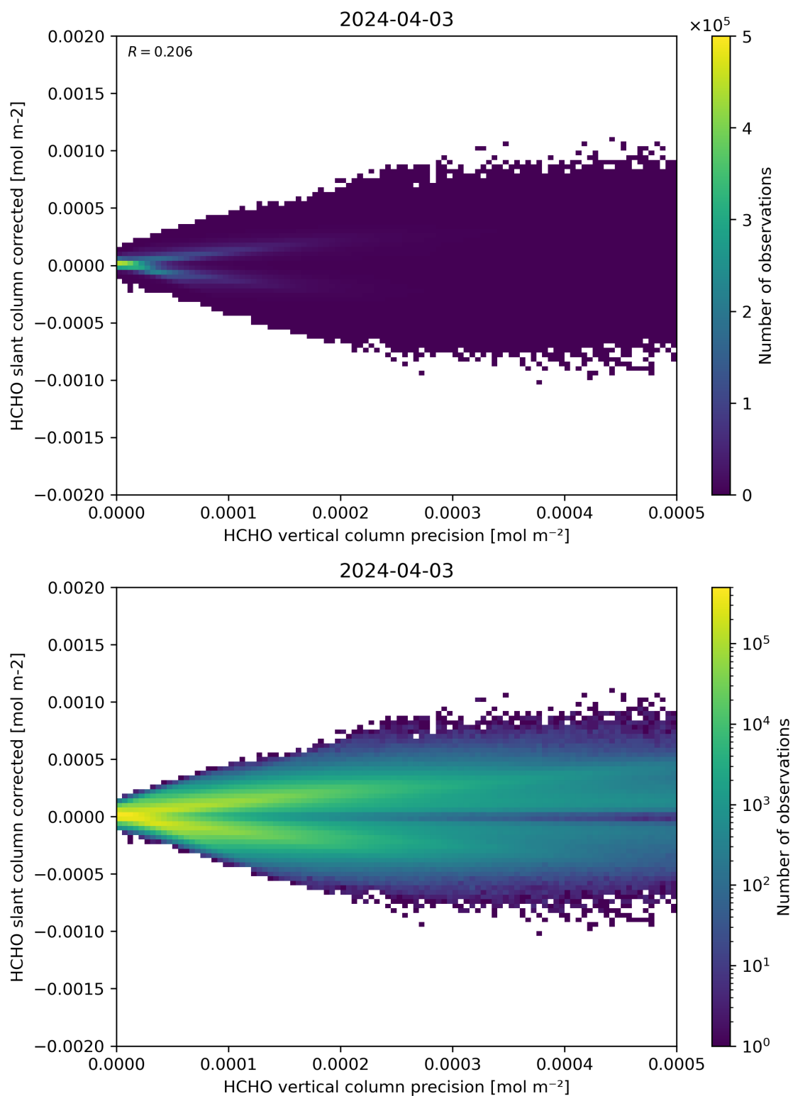
Figure 140: Scatter density plot of “HCHO vertical column precision” against “HCHO slant column corrected” for 2024-04-02 to 2024-04-04.
