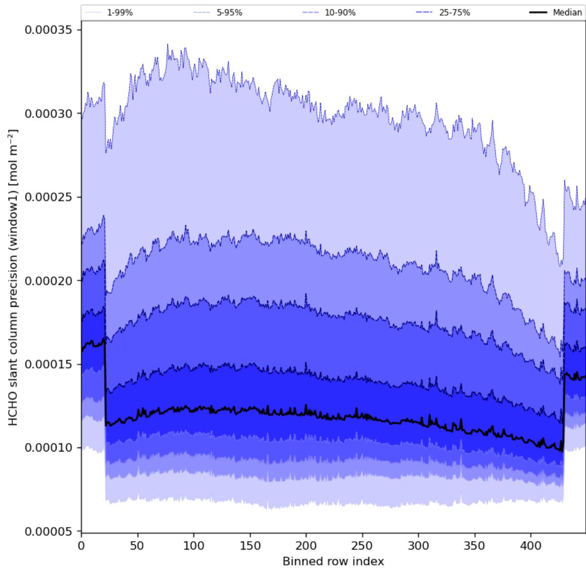
Figure 53: Along track statistics of “HCHO slant column precision (window1)” for 2024-04-02 to 2024-04-04
