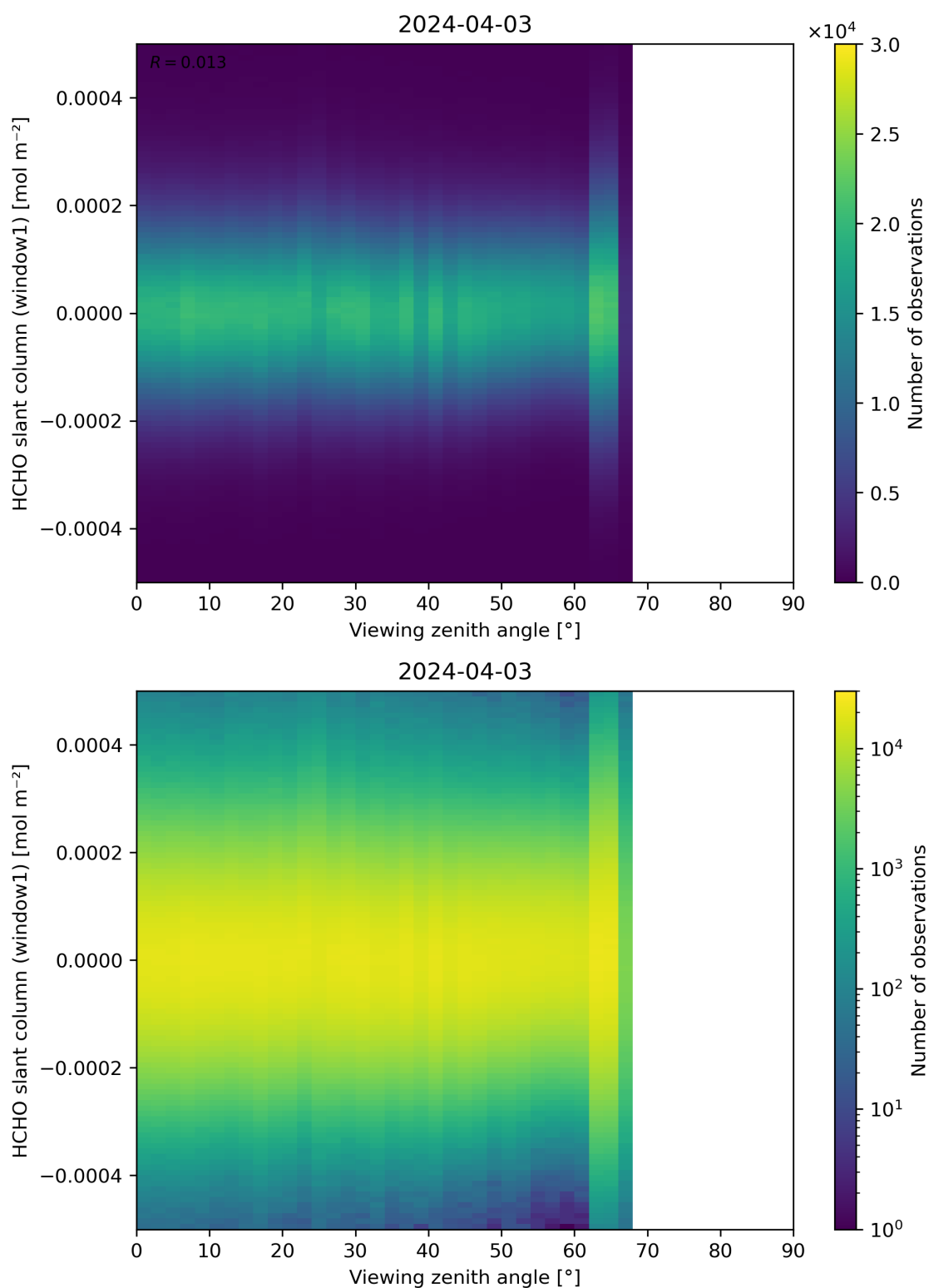
Figure 188: Scatter density plot of “Viewing zenith angle” against “HCHO slant column (window1)” for 2024-04-02 to 2024-04-04.
