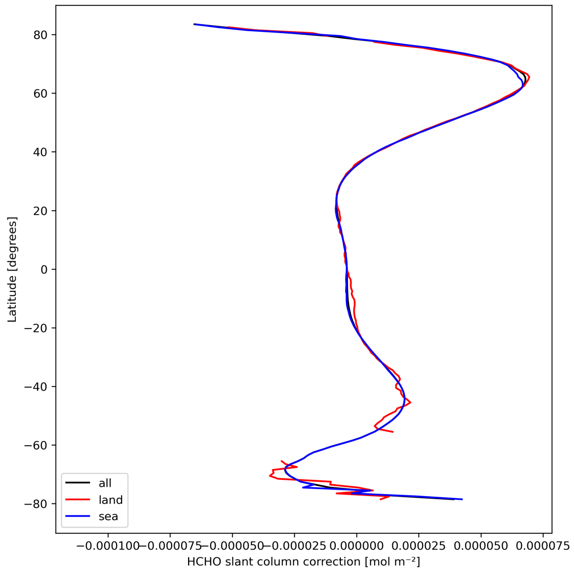
Figure 33: Zonal average of “HCHO slant column correction” for 2024-04-02 to 2024-04-04.
