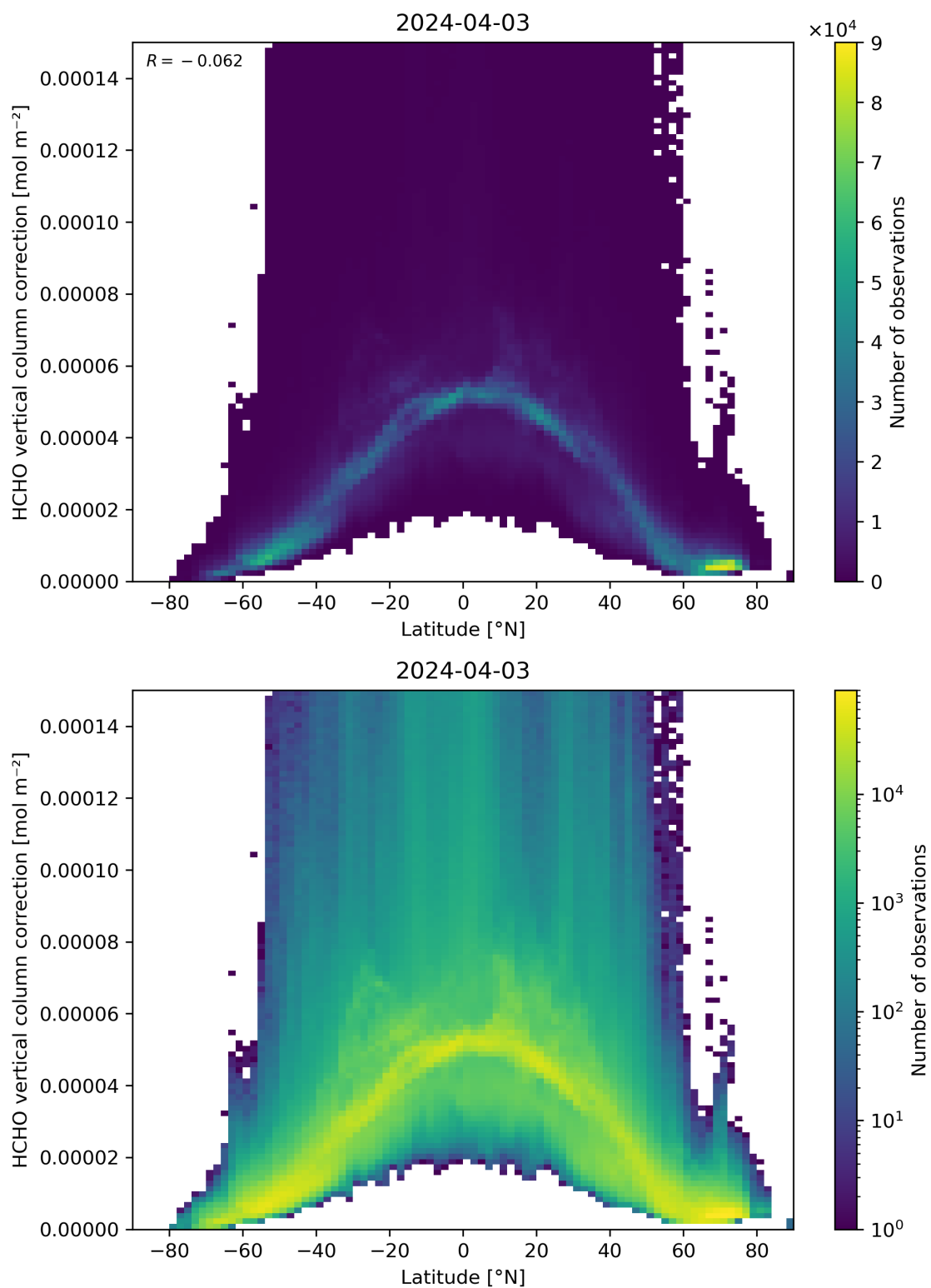
Figure 164: Scatter density plot of “Latitude” against “HCHO vertical column correction” for 2024-04-02 to 2024-04-04.
