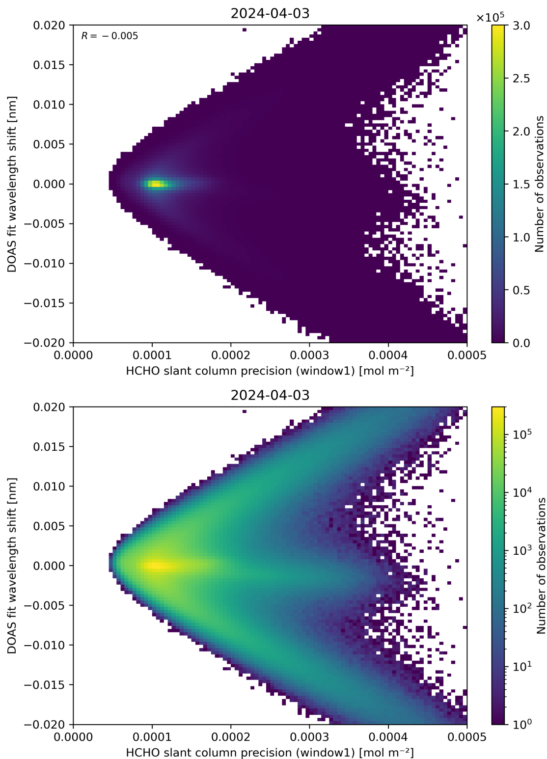
Figure 89: Scatter density plot of “HCHO slant column precision (window1)” against “DOAS fit wavelength shift” for 2024-04-02 to 2024-04-04.
