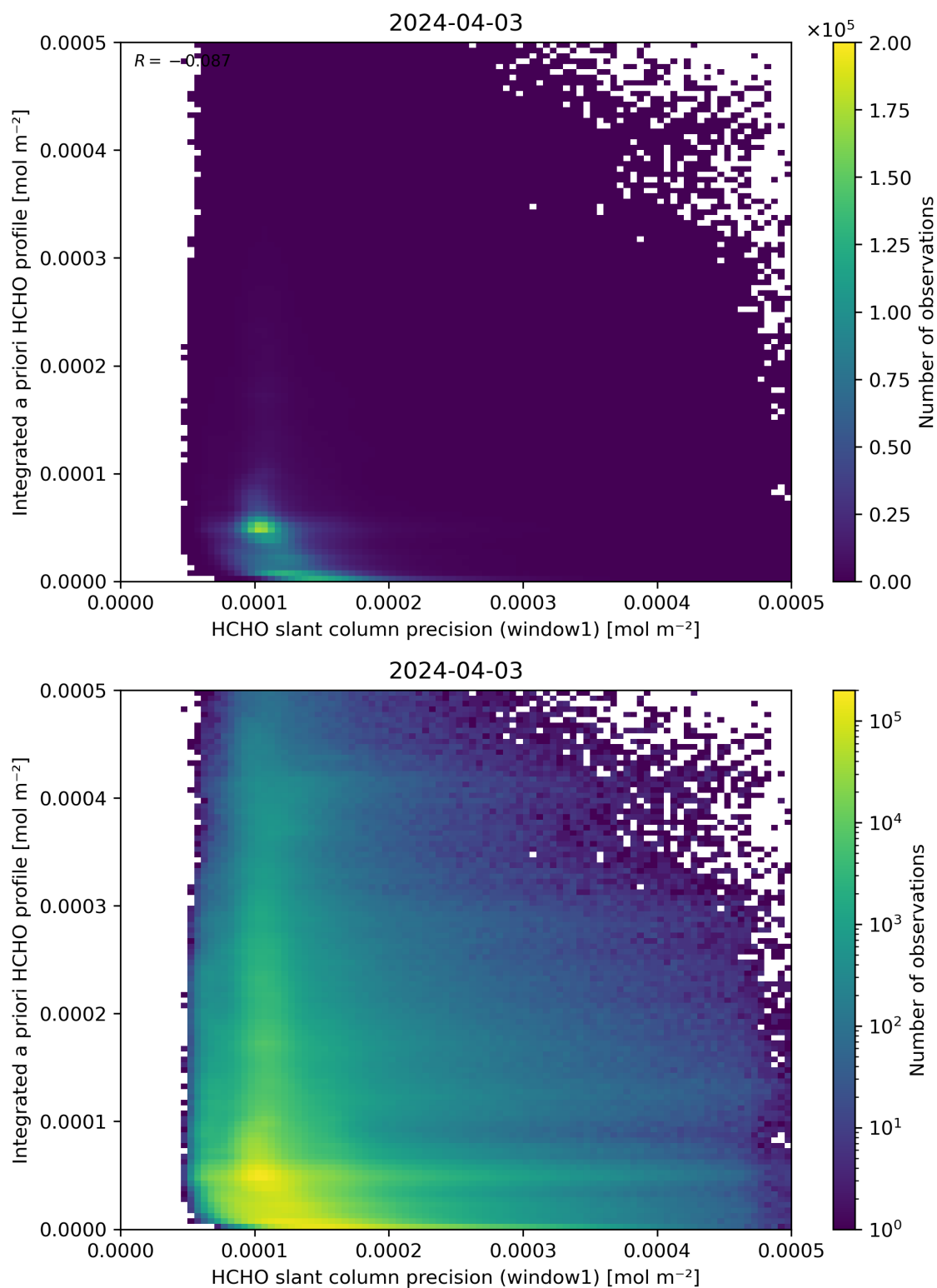
Figure 96: Scatter density plot of “HCHO slant column precision (window1)” against “Integrated a priori HCHO profile” for 2024-04-02 to 2024-04-04.
