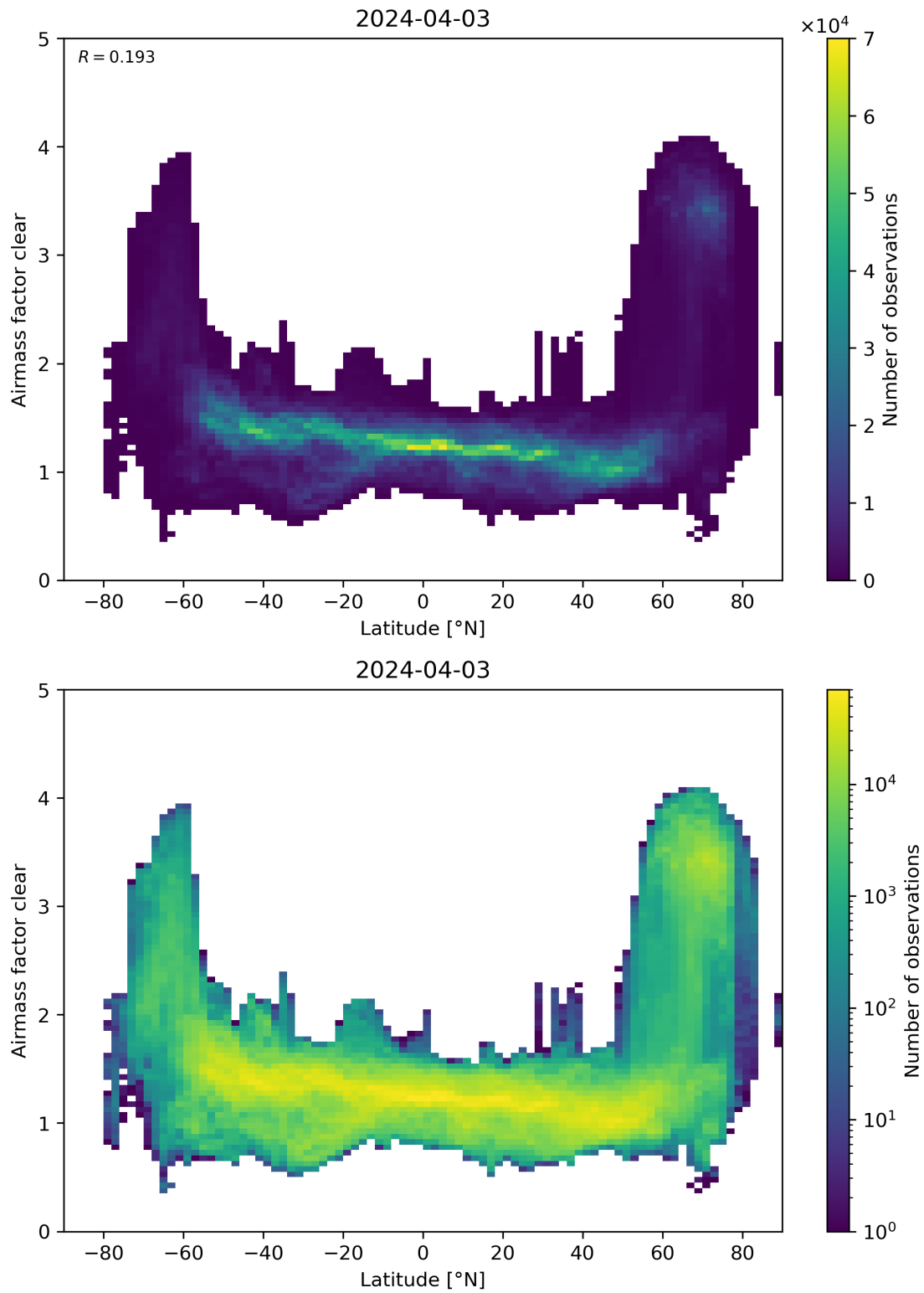
Figure 156: Scatter density plot of “Latitude” against “Airmass factor clear” for 2024-04-02 to 2024-04-04.
