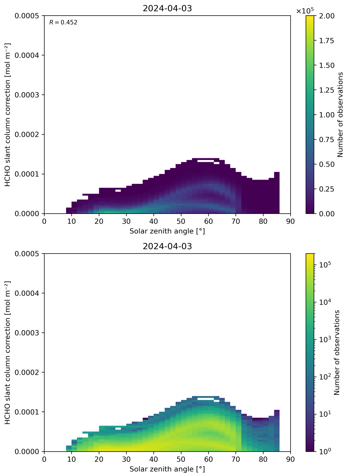
Figure 172: Scatter density plot of “Solar zenith angle” against “HCHO slant column correction” for 2024-04-02 to 2024-04-04.
