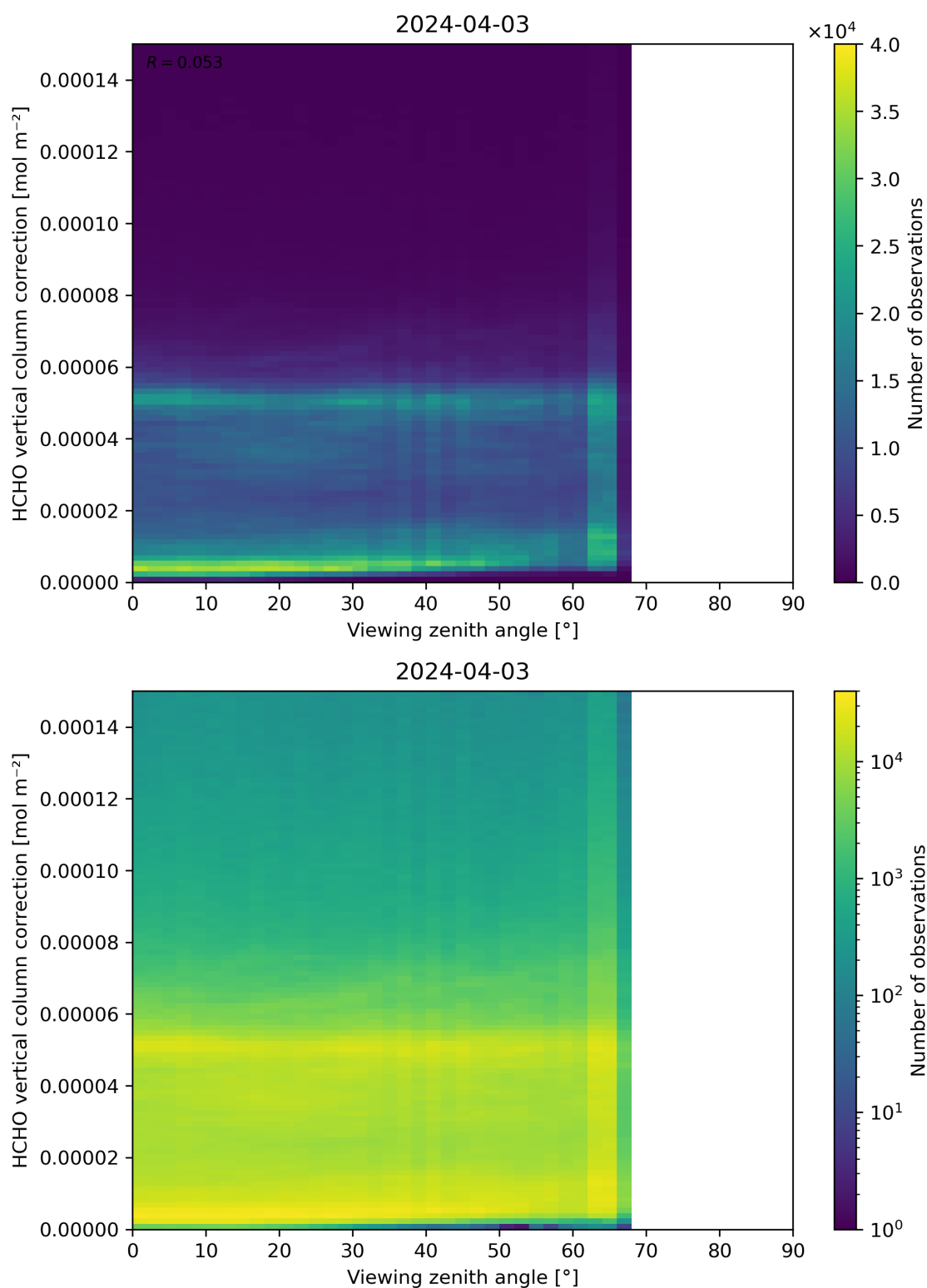
Figure 193: Scatter density plot of “Viewing zenith angle” against “HCHO vertical column correction” for 2024-04-02 to 2024-04-04.
