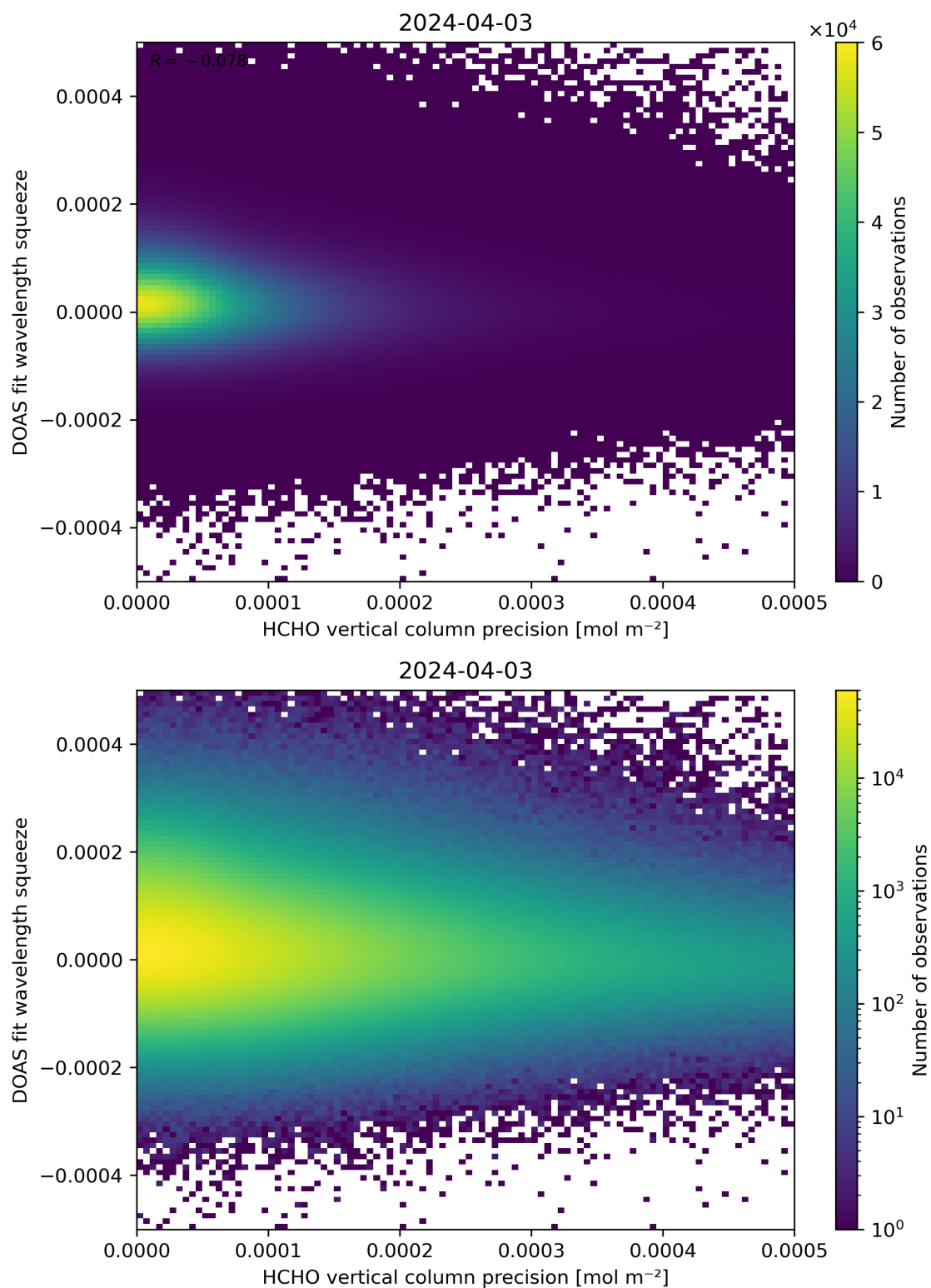
Figure 138: Scatter density plot of “HCHO vertical column precision” against “DOAS fit wavelength squeeze” for 2024-04-02 to 2024-04-04.
