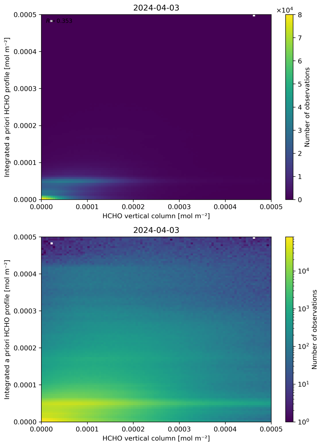
Figure 135: Scatter density plot of “HCHO vertical column” against “Integrated a priori HCHO profile” for 2024-04-02 to 2024-04-04.
