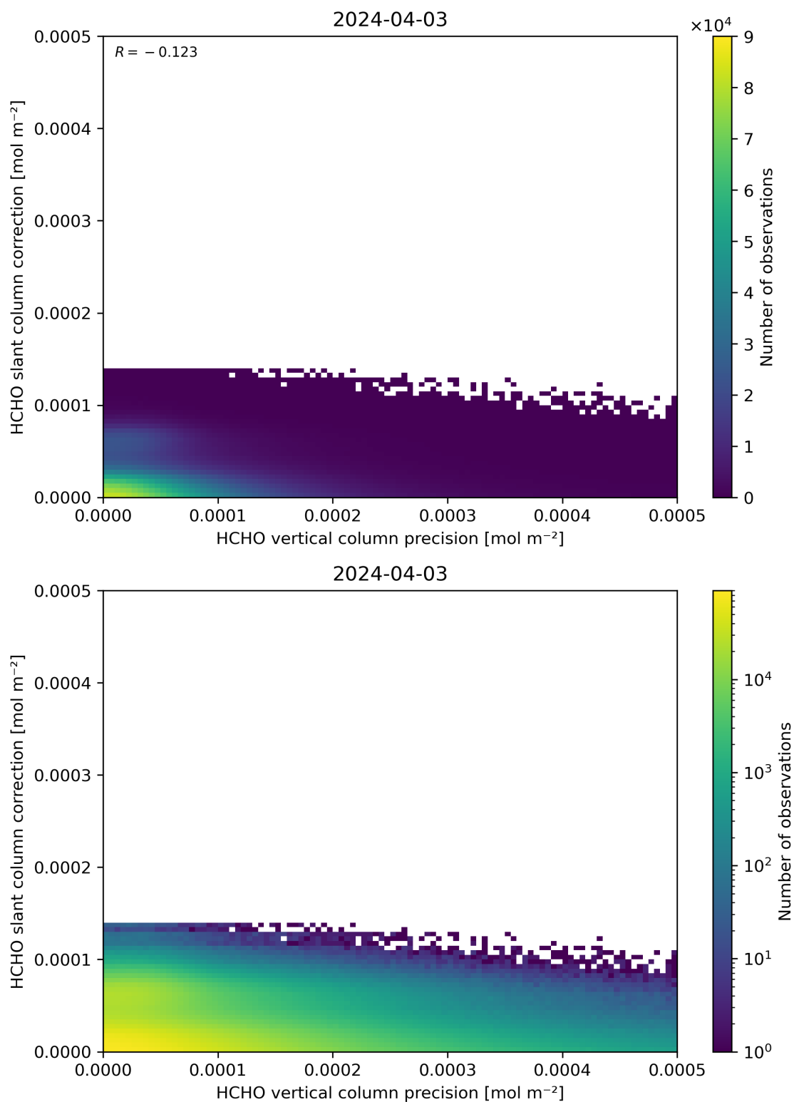
Figure 141: Scatter density plot of “HCHO vertical column precision” against “HCHO slant column correction” for 2024-04-02 to 2024-04-04.
