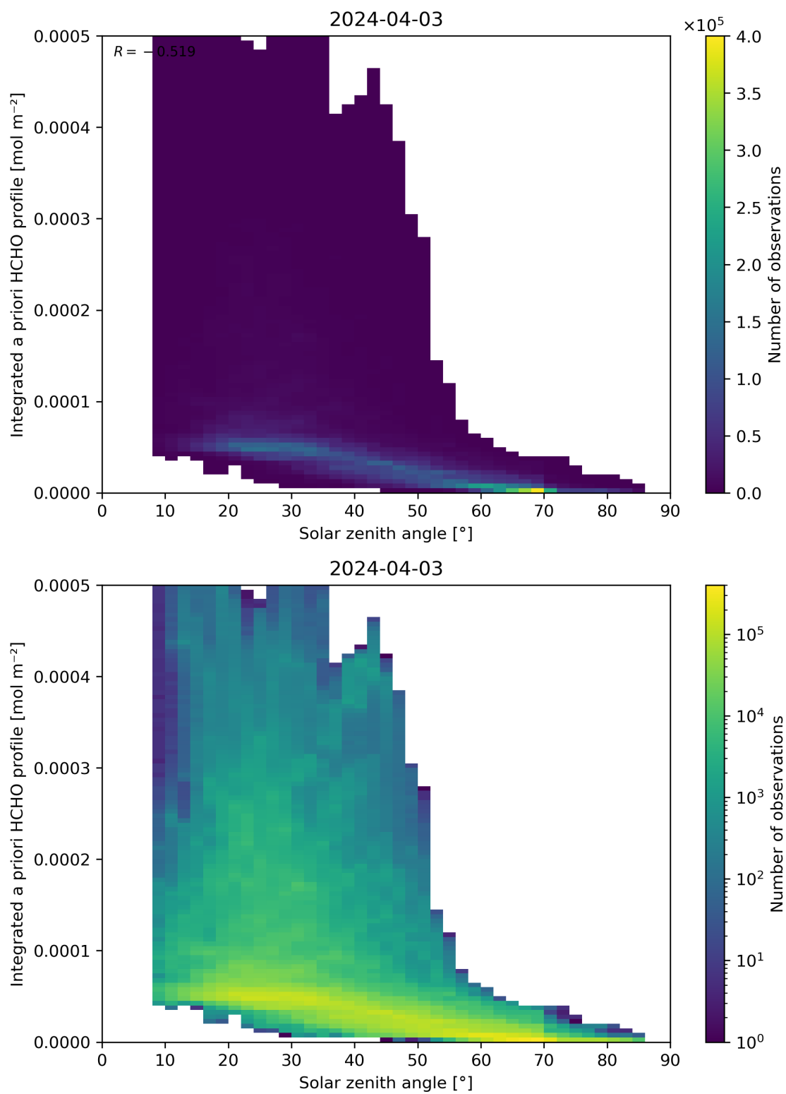
Figure 180: Scatter density plot of “Solar zenith angle” against “Integrated a priori HCHO profile” for 2024-04-02 to 2024-04-04.
