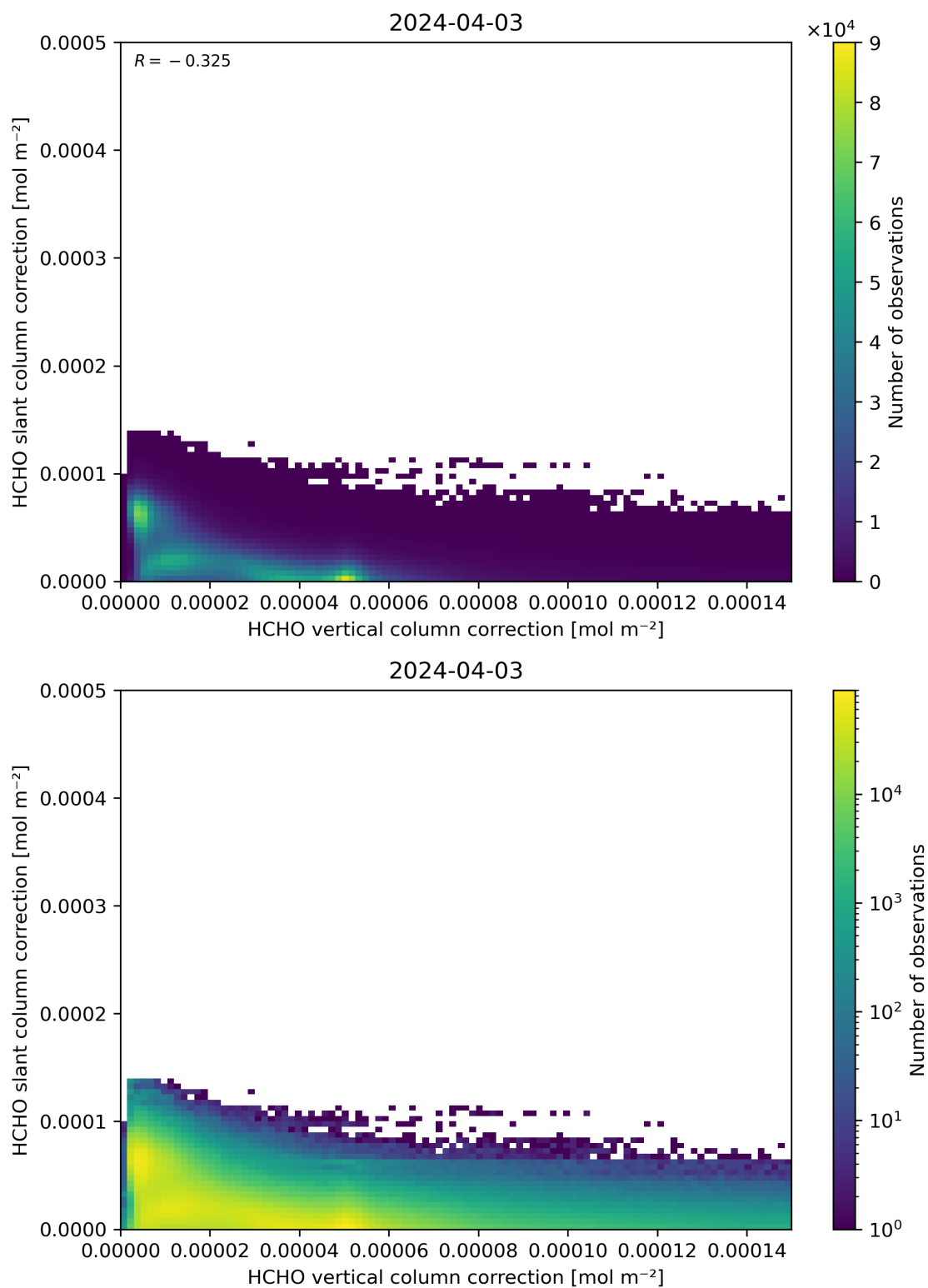
Figure 117: Scatter density plot of “HCHO vertical column correction” against “HCHO slant column correction” for 2024-04-02 to 2024-04-04.
