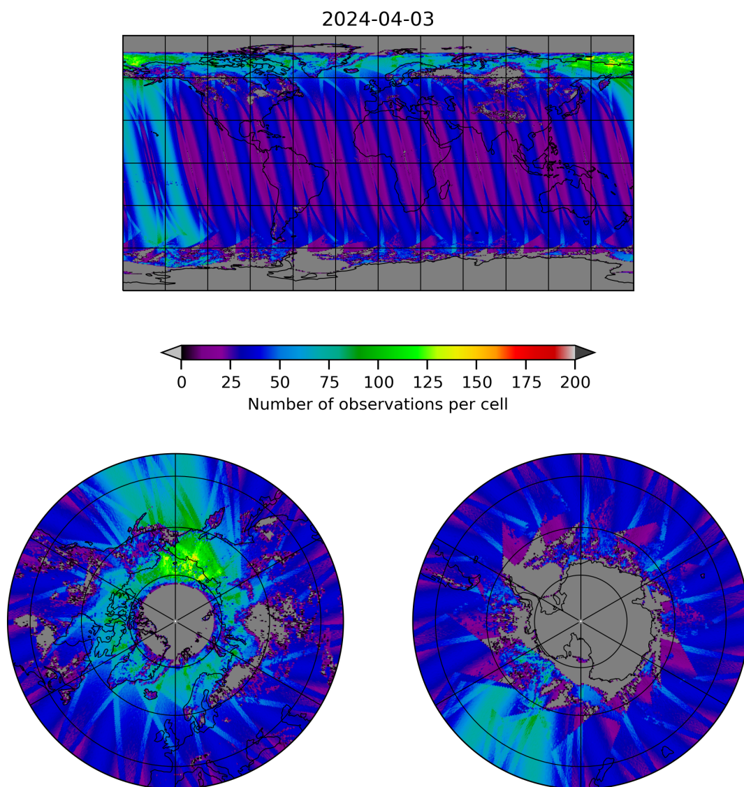
Figure 19: Map of the number of observations for 2024-04-02 to 2024-04-04
