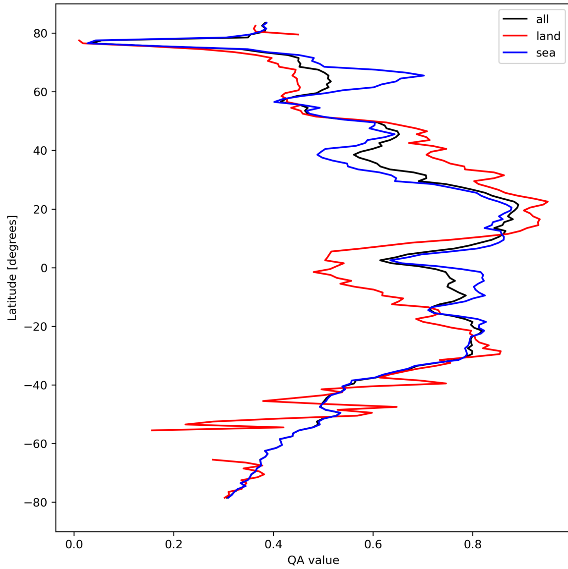
Figure 20: Zonal average of “QA value” for 2024-04-02 to 2024-04-04.
