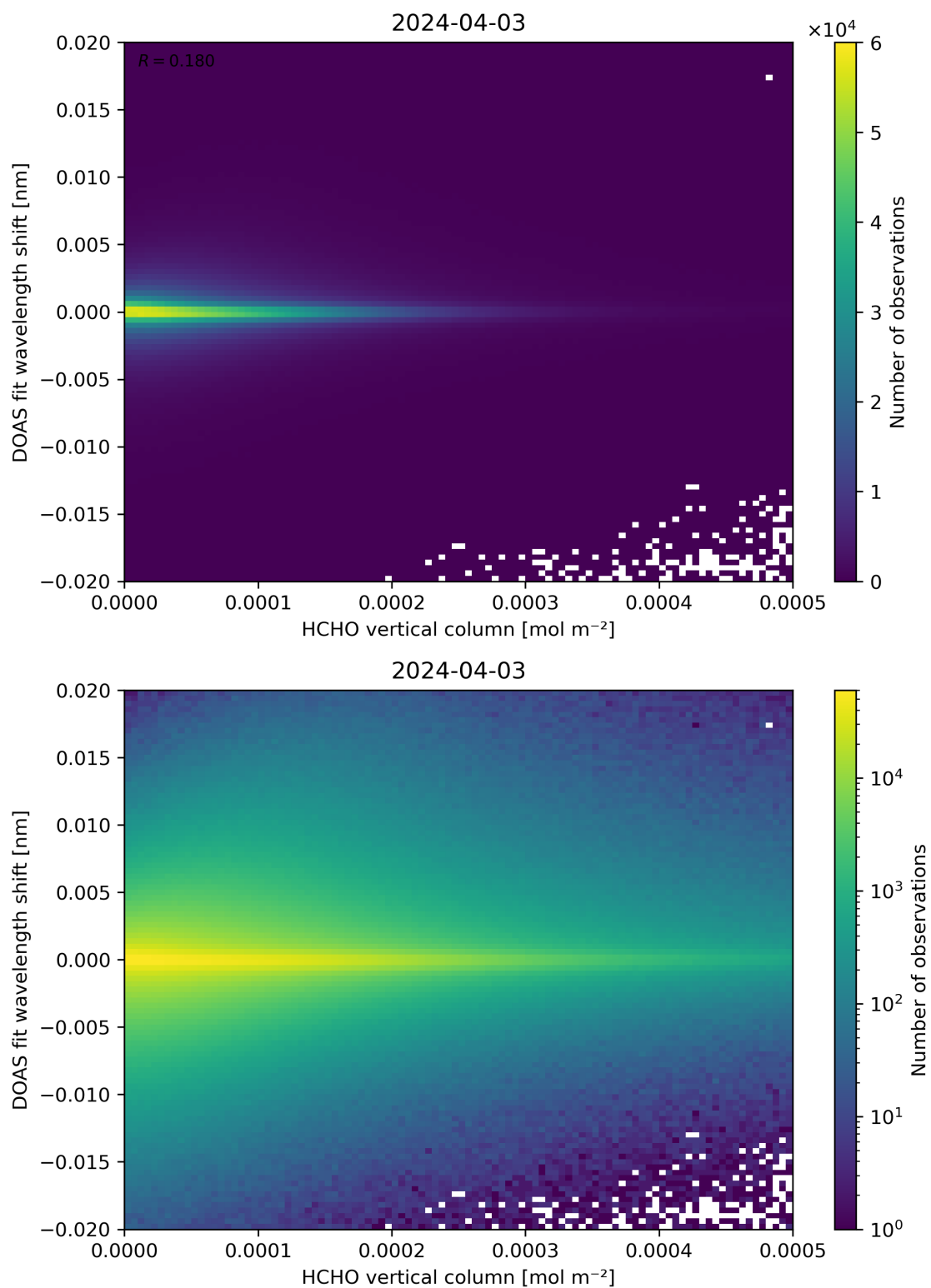
Figure 124: Scatter density plot of “HCHO vertical column” against “DOAS fit wavelength shift” for 2024-04-02 to 2024-04-04.
