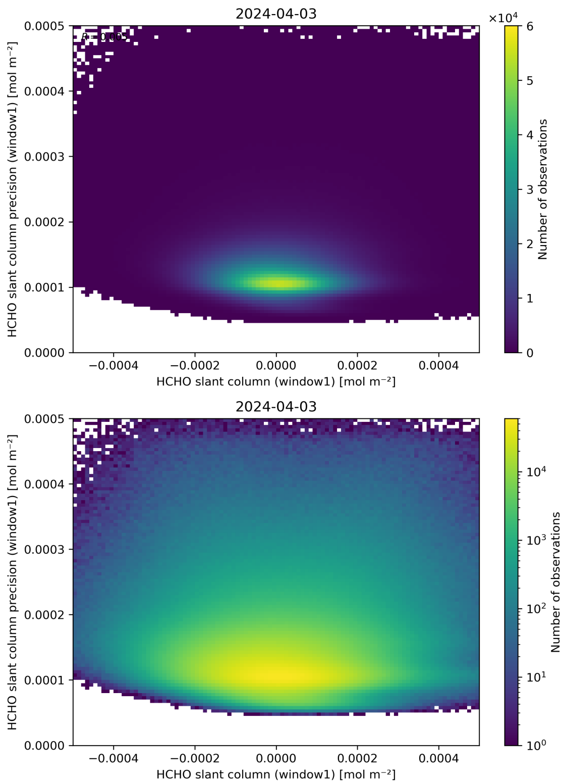
Figure 84: Scatter density plot of “HCHO slant column (window1)” against “HCHO slant column precision (window1)” for 2024-04-02 to 2024-04-04.
