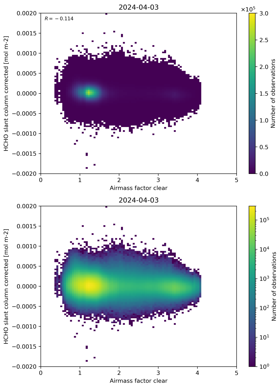
Figure 74: Scatter density plot of “Airmass factor clear” against “HCHO slant column corrected” for 2024-04-02 to 2024-04-04.
