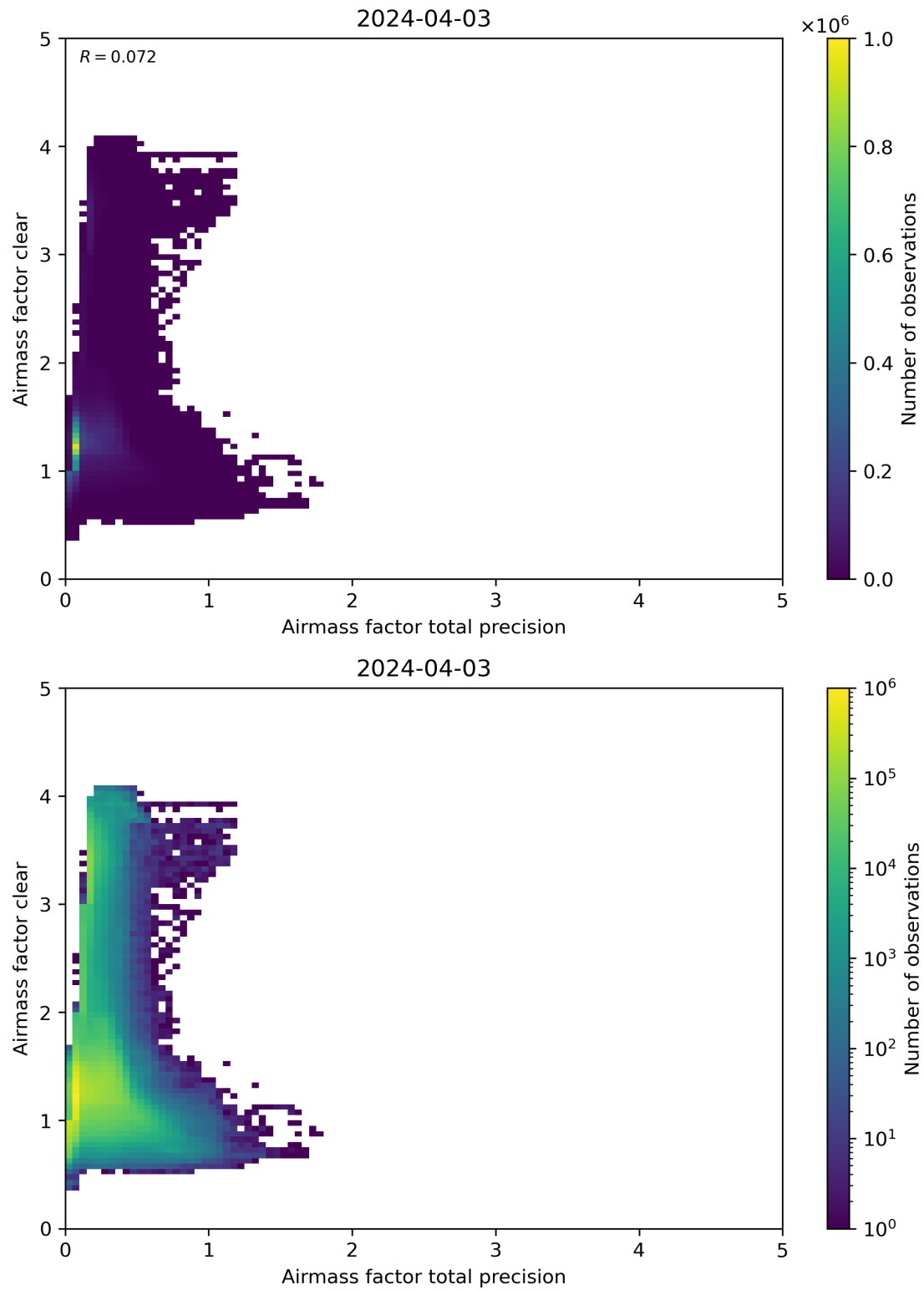
Figure 108: Scatter density plot of “Airmass factor total precision” against “Airmass factor clear” for 2024-04-02 to 2024-04-04.
