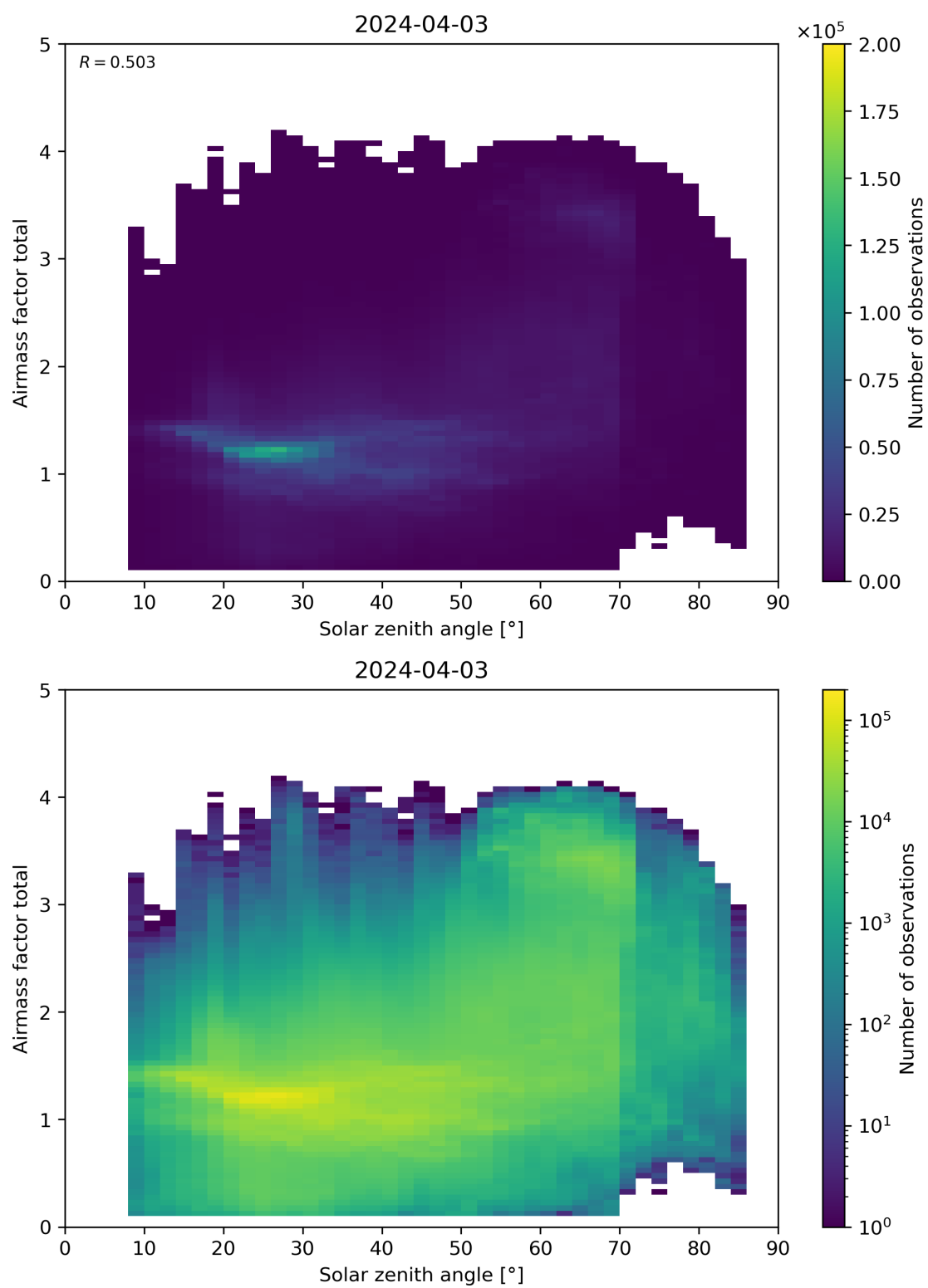
Figure 175: Scatter density plot of “Solar zenith angle” against “Airmass factor total” for 2024-04-02 to 2024-04-04.
