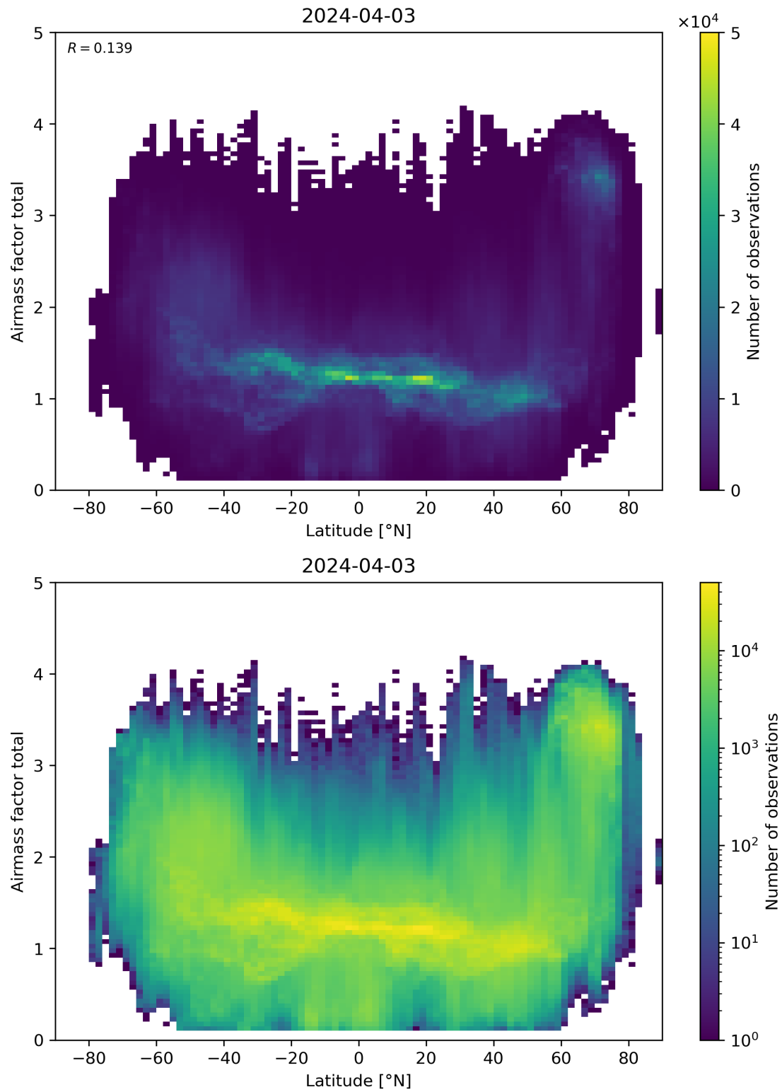
Figure 161: Scatter density plot of “Latitude” against “Airmass factor total” for 2024-04-02 to 2024-04-04.
