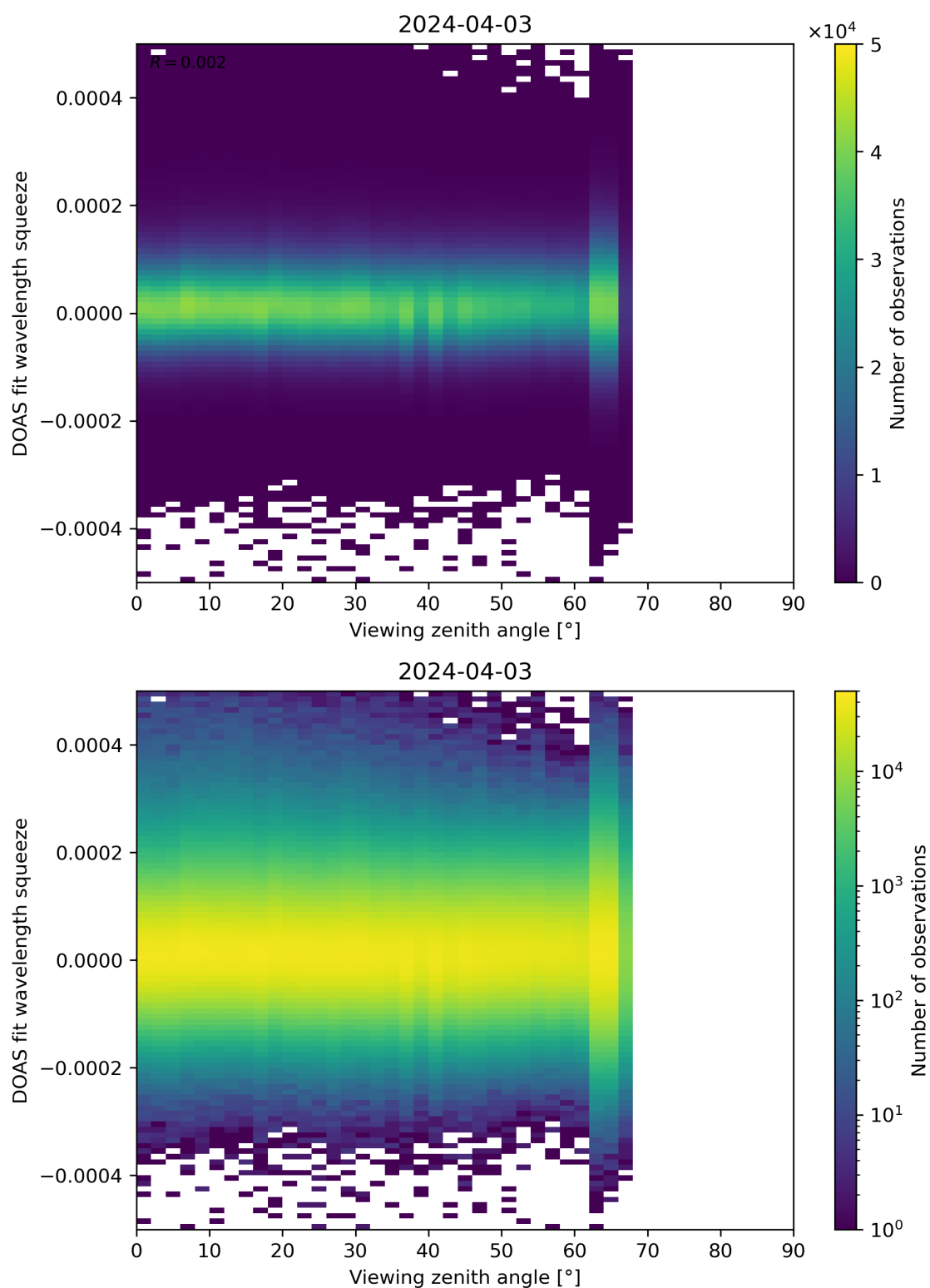
Figure 184: Scatter density plot of “Viewing zenith angle” against “DOAS fit wavelength squeeze” for 2024-04-02 to 2024-04-04.
