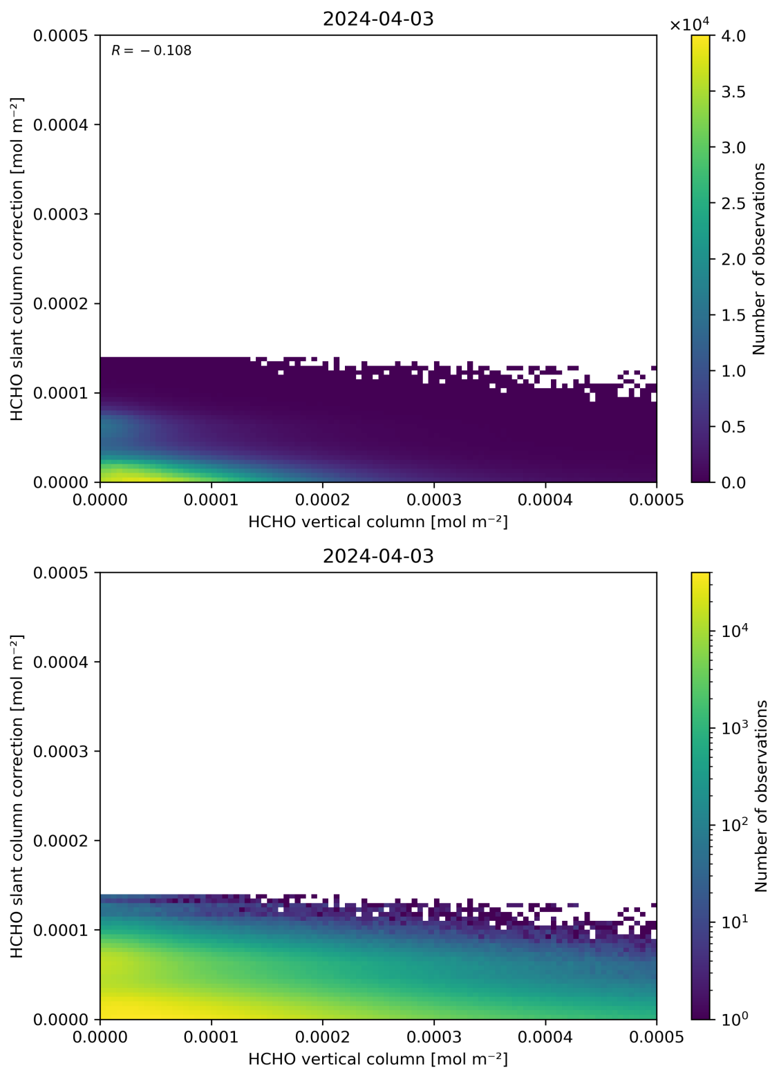
Figure 128: Scatter density plot of “HCHO vertical column” against “HCHO slant column correction” for 2024-04-02 to 2024-04-04.
