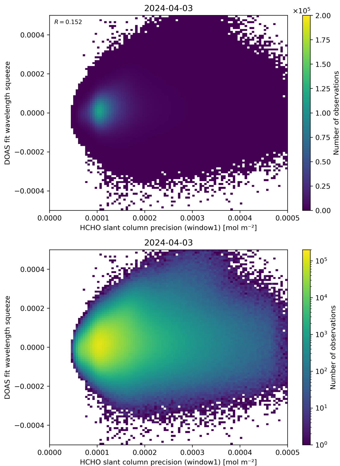
Figure 90: Scatter density plot of “HCHO slant column precision (window1)” against “DOAS fit wavelength squeeze” for 2024-04-02 to 2024-04-04.
