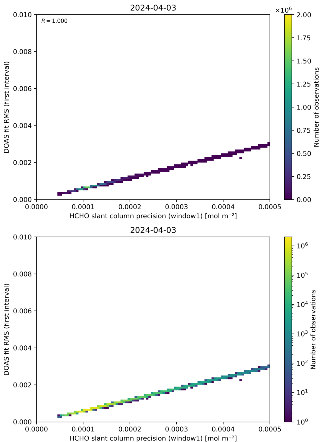
Figure 88: Scatter density plot of “HCHO slant column precision (window1)” against “DOAS fit RMS (first interval)” for 2024-04-02 to 2024-04-04.
