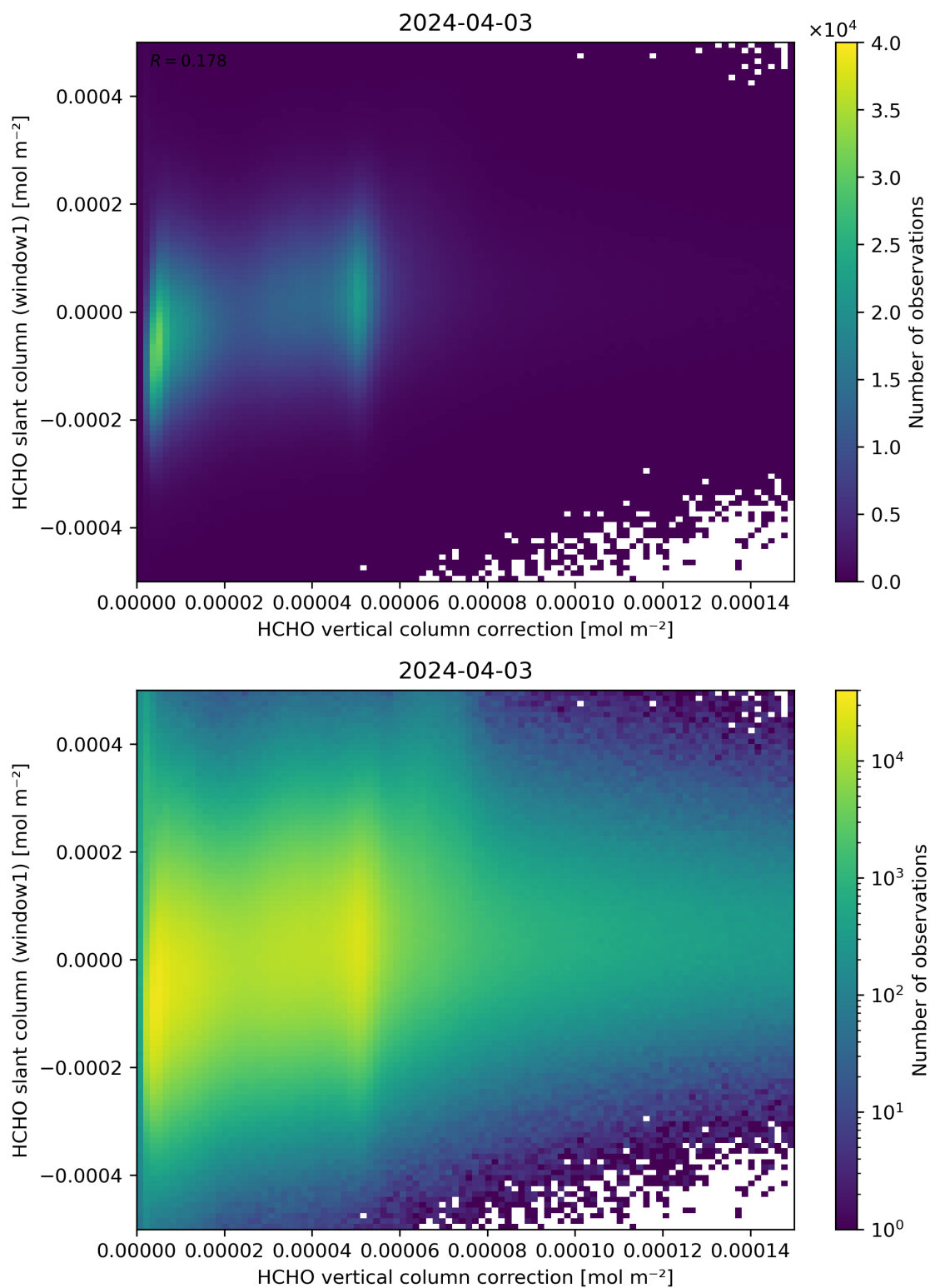
Figure 118: Scatter density plot of “HCHO vertical column correction” against “HCHO slant column (window1)” for 2024-04-02 to 2024-04-04.
