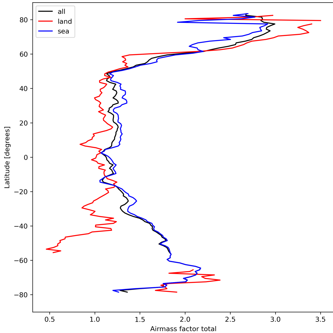
Figure 26: Zonal average of “Airmass factor total” for 2024-04-02 to 2024-04-04.
