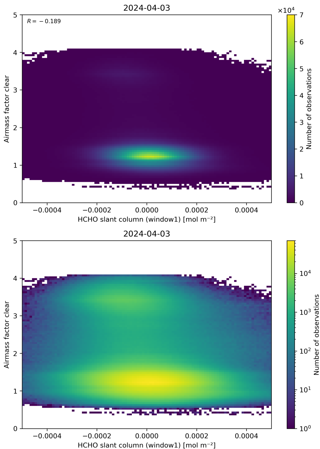
Figure 81: Scatter density plot of “HCHO slant column (window1)” against “Airmass factor clear” for 2024-04-02 to 2024-04-04.
