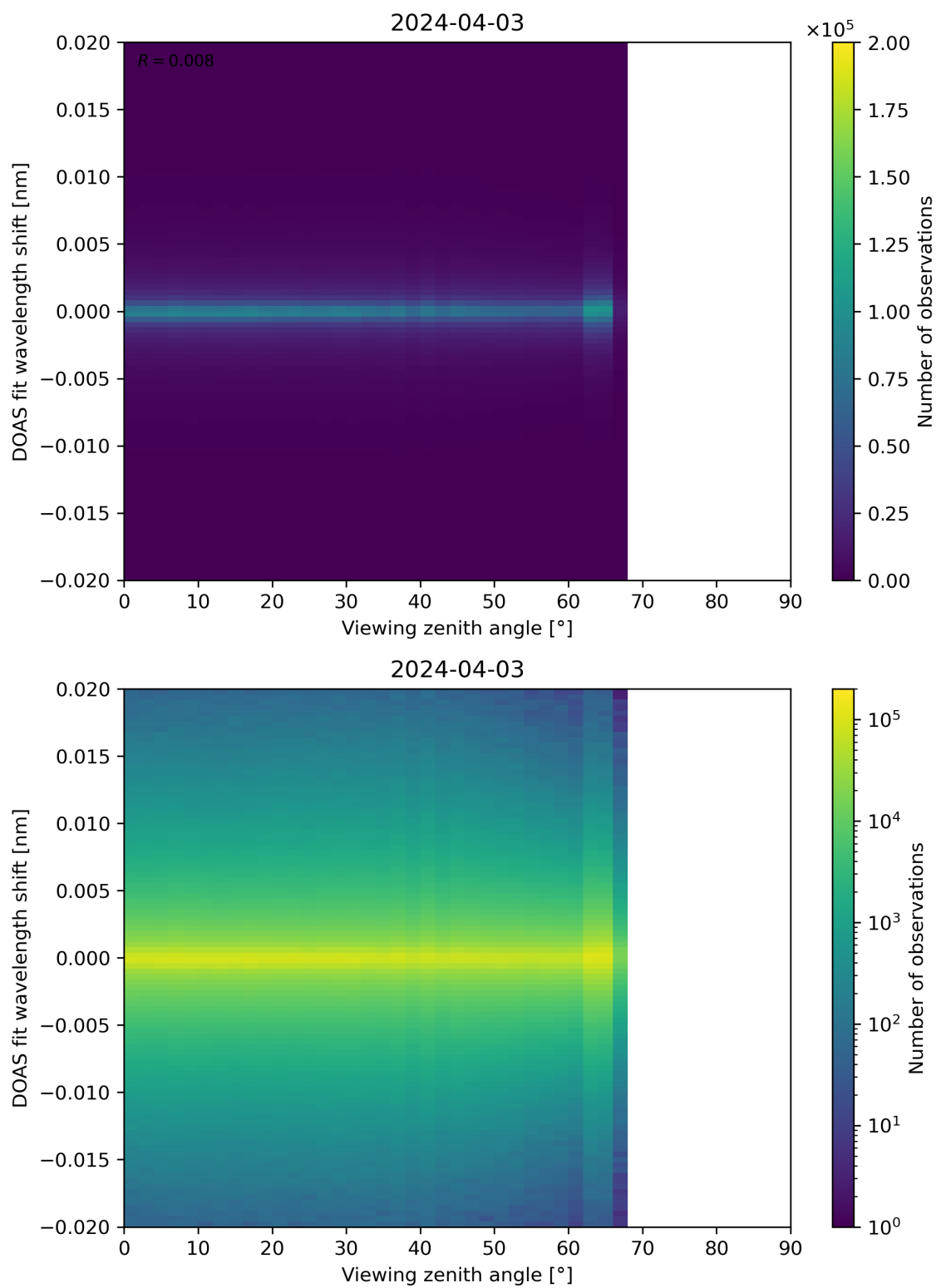
Figure 183: Scatter density plot of “Viewing zenith angle” against “DOAS fit wavelength shift” for 2024-04-02 to 2024-04-04.
