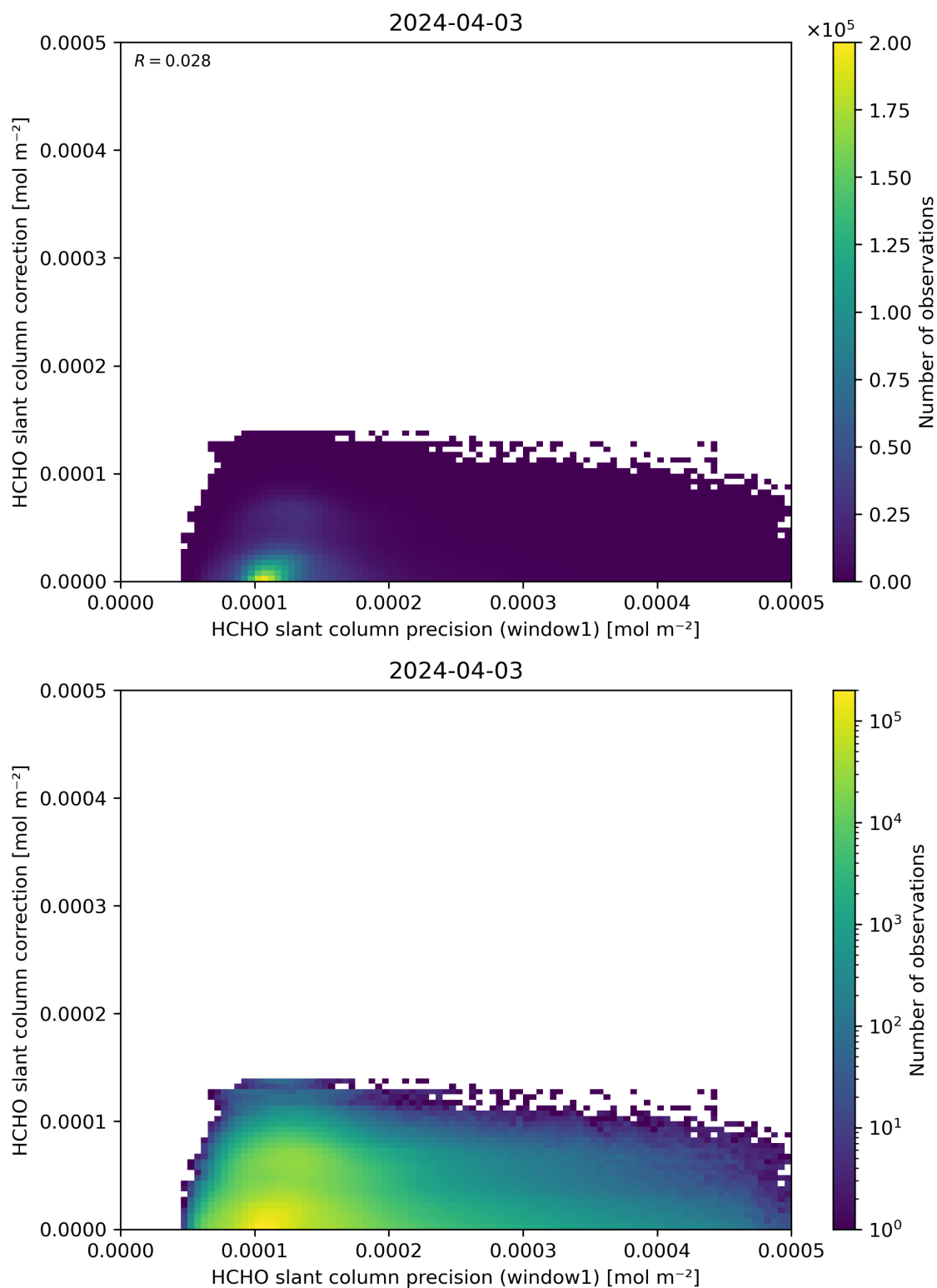
Figure 93: Scatter density plot of “HCHO slant column precision (window1)” against “HCHO slant column correction” for 2024-04-02 to 2024-04-04.
