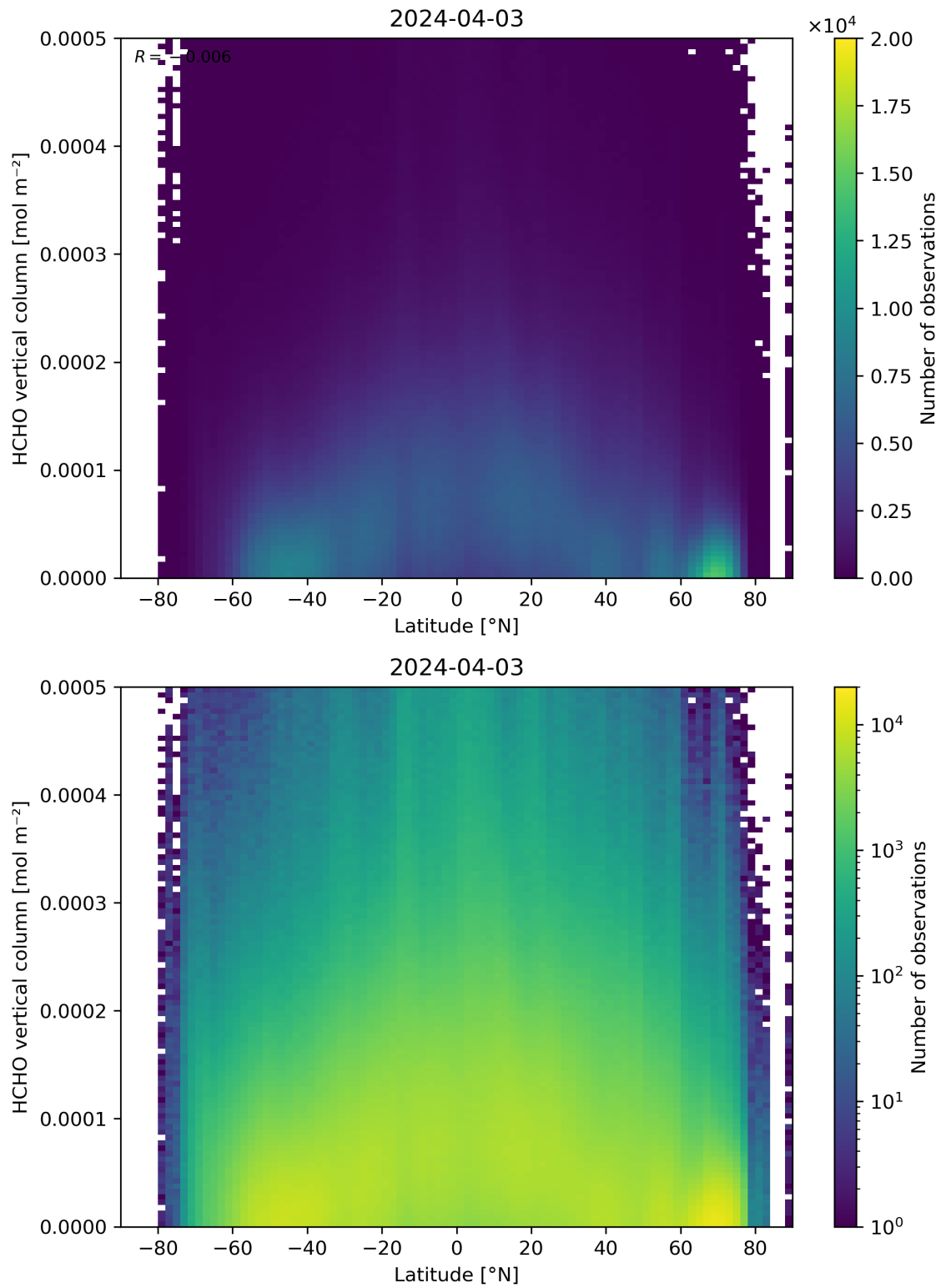
Figure 163: Scatter density plot of “Latitude” against “HCHO vertical column” for 2024-04-02 to 2024-04-04.
