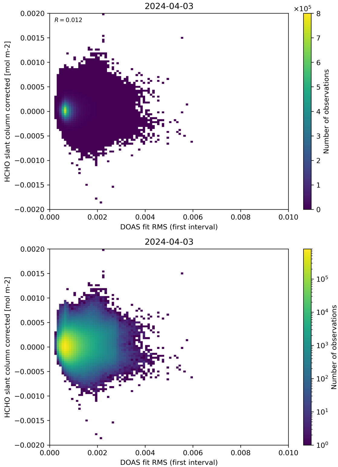
Figure 62: Scatter density plot of “DOAS fit RMS (first interval)” against “HCHO slant column corrected” for 2024-04-02 to 2024-04-04.
