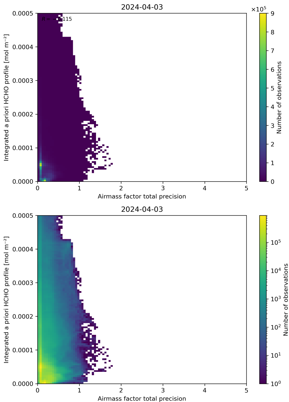
Figure 111: Scatter density plot of “Airmass factor total precision” against “Integrated a priori HCHO profile” for 2024-04-02 to 2024-04-04.
