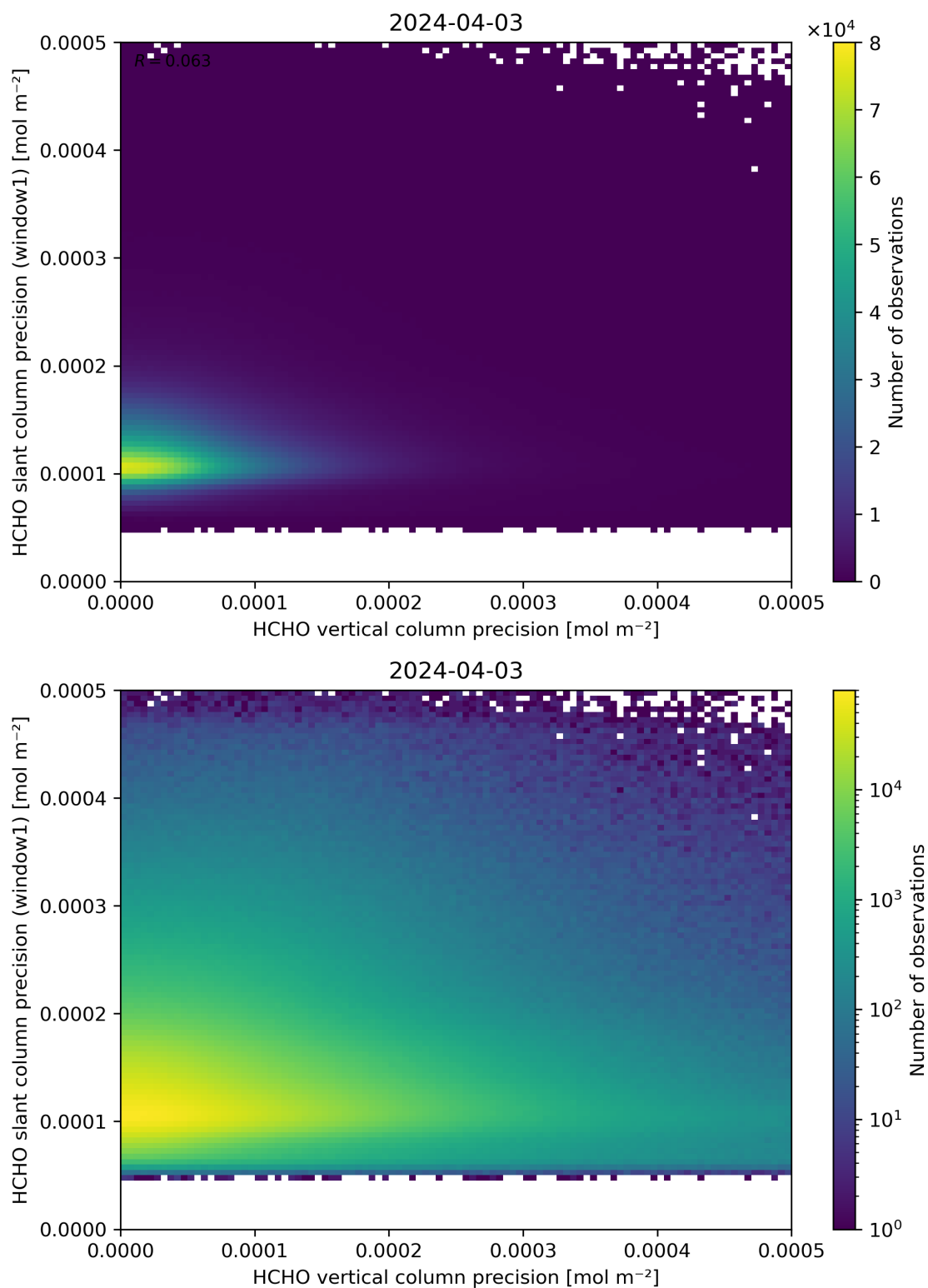
Figure 143: Scatter density plot of “HCHO vertical column precision” against “HCHO slant column precision (window1)” for 2024-04-02 to 2024-04-04.
