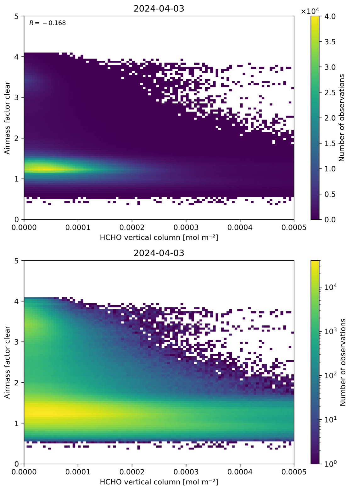
Figure 126: Scatter density plot of “HCHO vertical column” against “Airmass factor clear” for 2024-04-02 to 2024-04-04.
