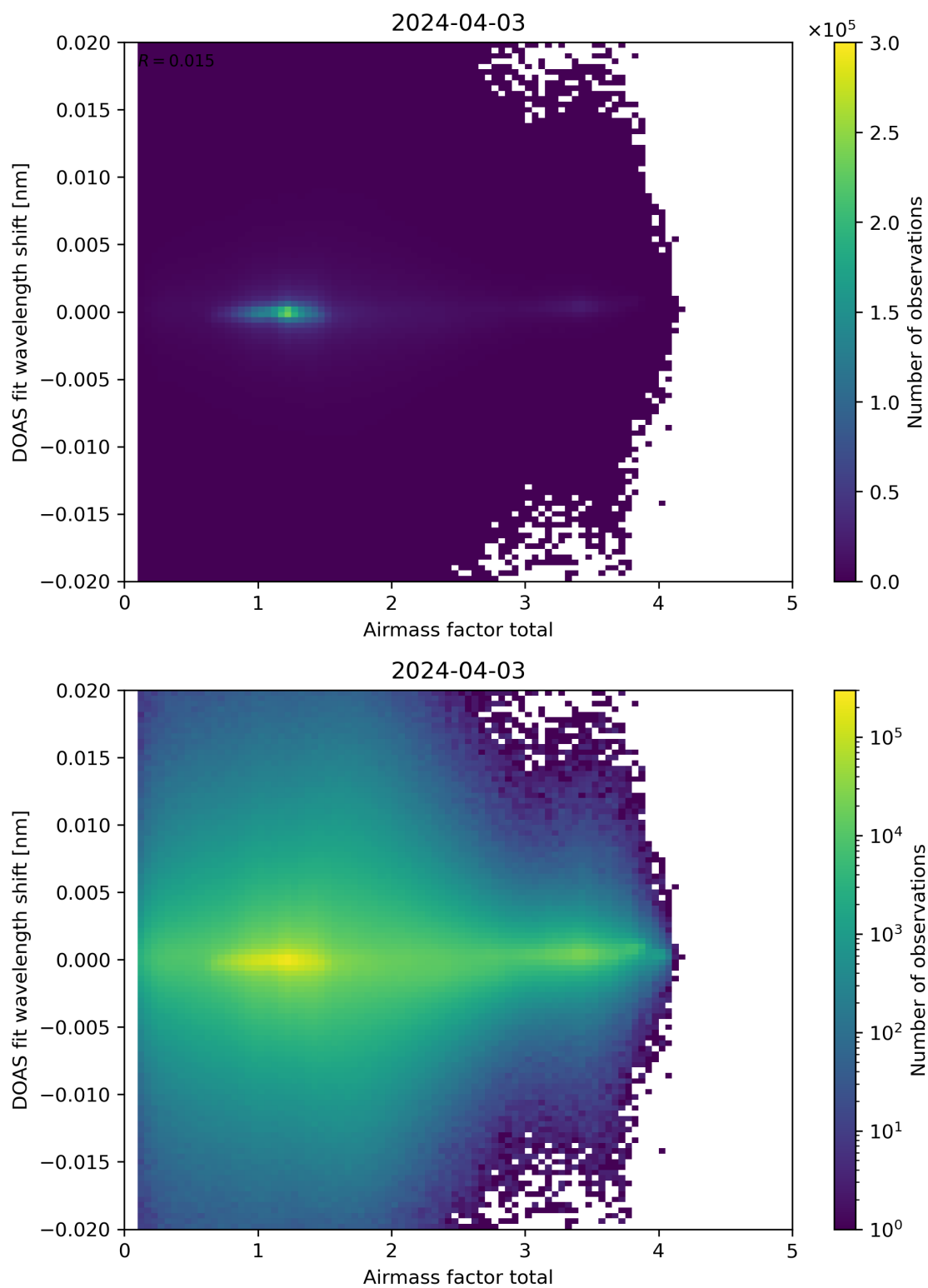
Figure 98: Scatter density plot of “Airmass factor total” against “DOAS fit wavelength shift” for 2024-04-02 to 2024-04-04.
