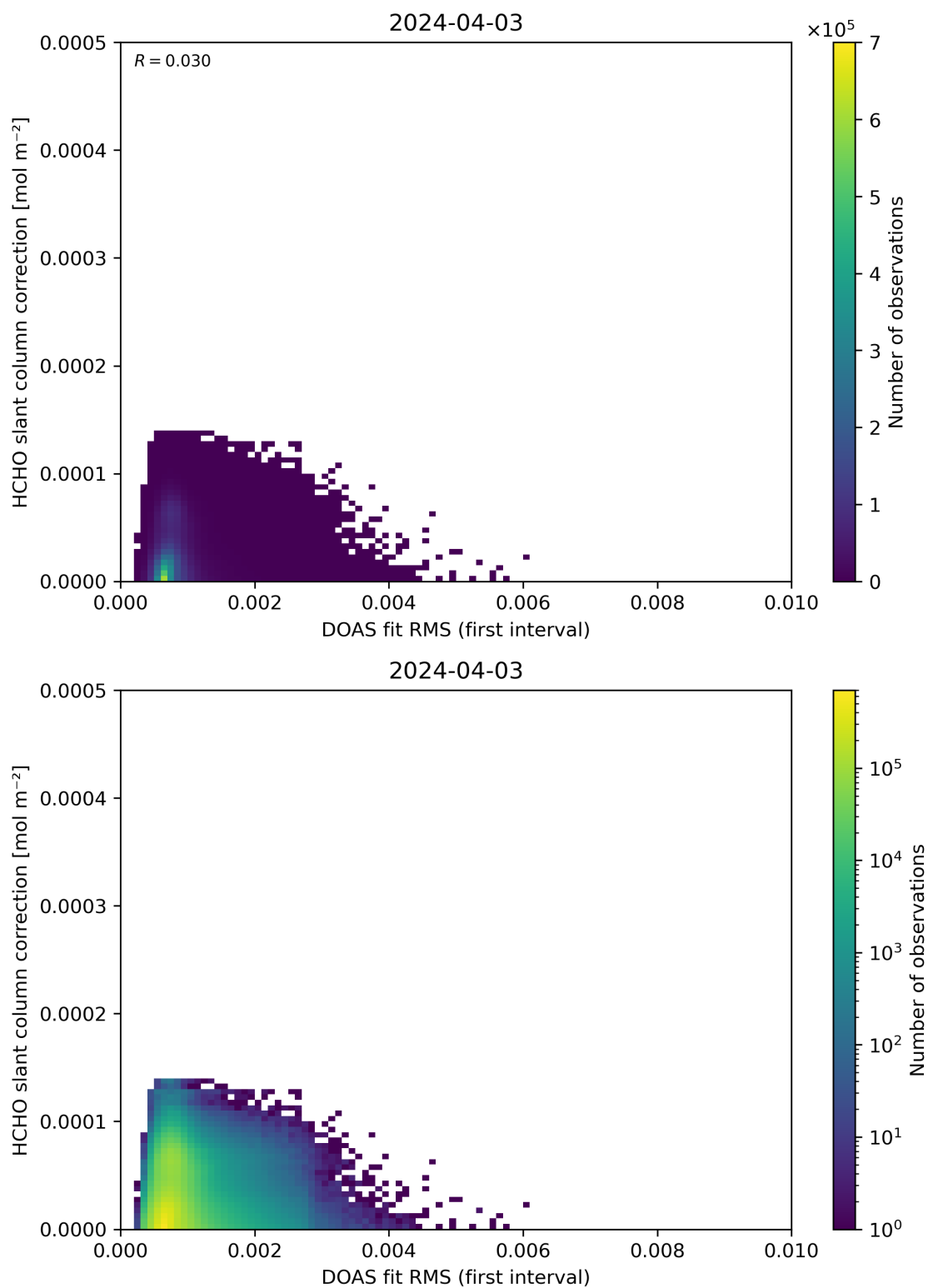
Figure 63: Scatter density plot of “DOAS fit RMS (first interval)” against “HCHO slant column correction” for 2024-04-02 to 2024-04-04.
