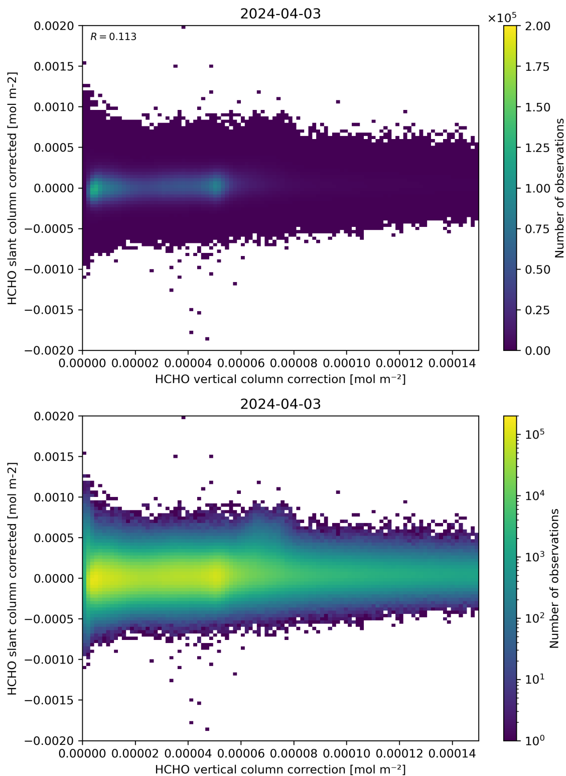
Figure 116: Scatter density plot of “HCHO vertical column correction” against “HCHO slant column corrected” for 2024-04-02 to 2024-04-04.
