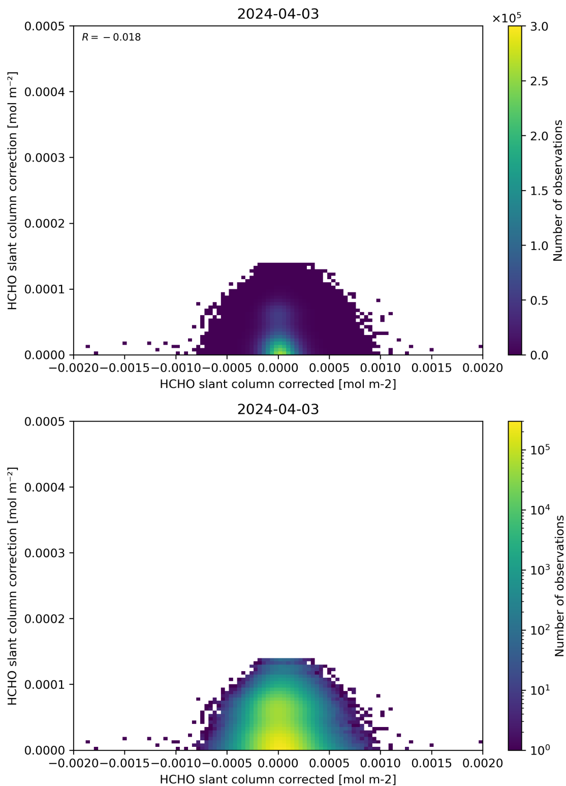
Figure 77: Scatter density plot of “HCHO slant column corrected” against “HCHO slant column correction” for 2024-04-02 to 2024-04-04.
