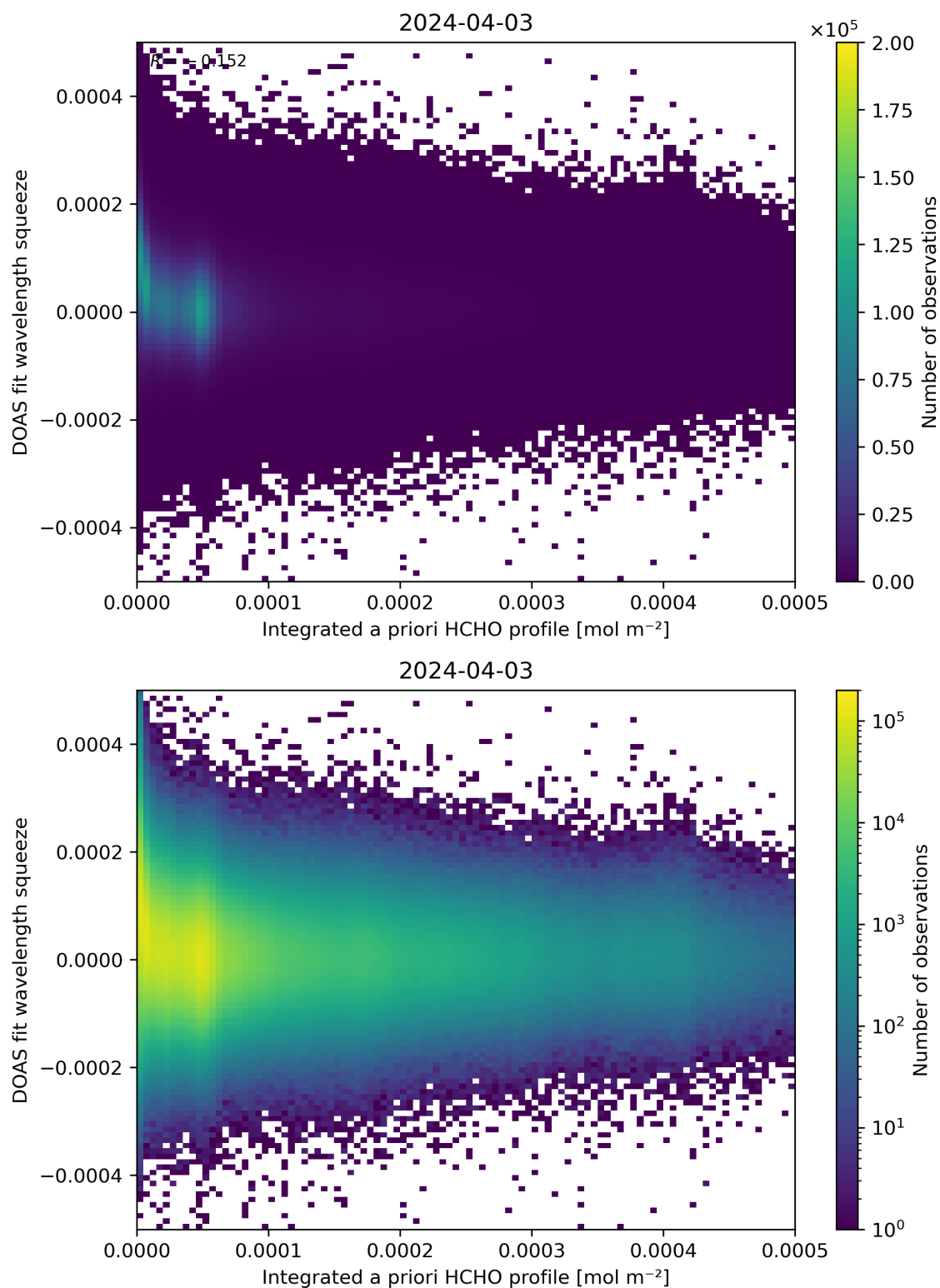
Figure 150: Scatter density plot of “Integrated a priori HCHO profile” against “DOAS fit wavelength squeeze” for 2024-04-02 to 2024-04-04.
