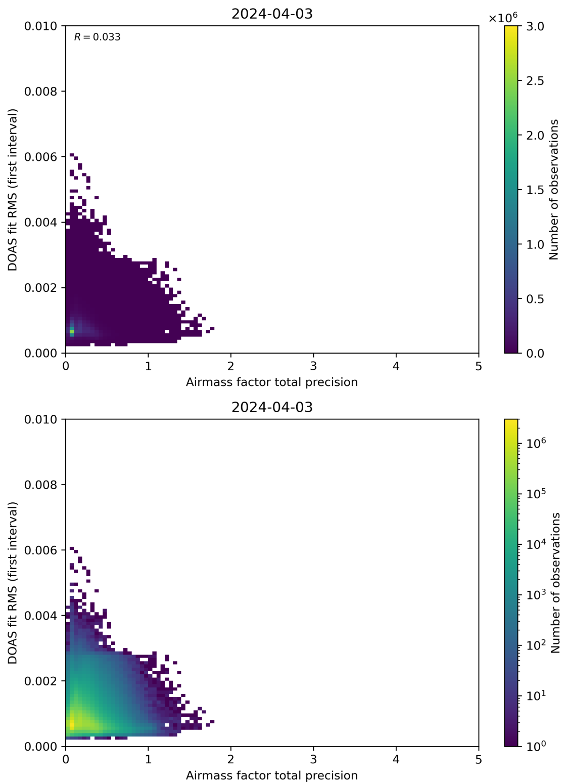
Figure 105: Scatter density plot of “Airmass factor total precision” against “DOAS fit RMS (first interval)” for 2024-04-02 to 2024-04-04.
