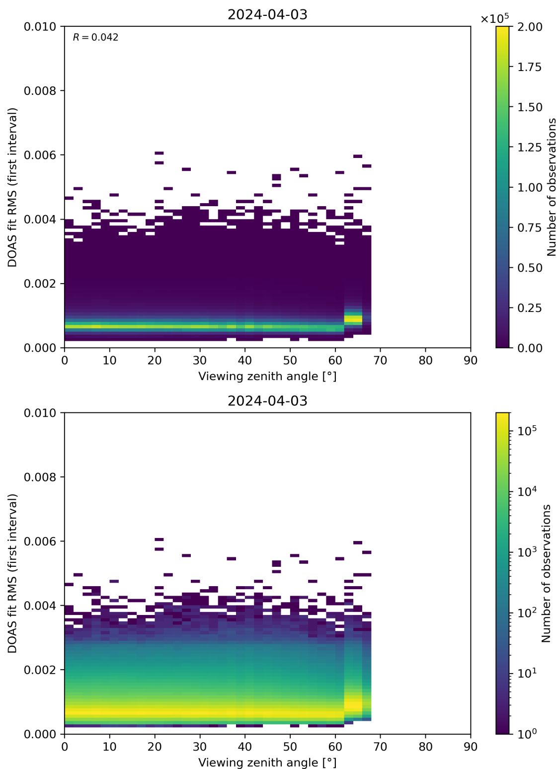
Figure 182: Scatter density plot of “Viewing zenith angle” against “DOAS fit RMS (first interval)” for 2024-04-02 to 2024-04-04.
