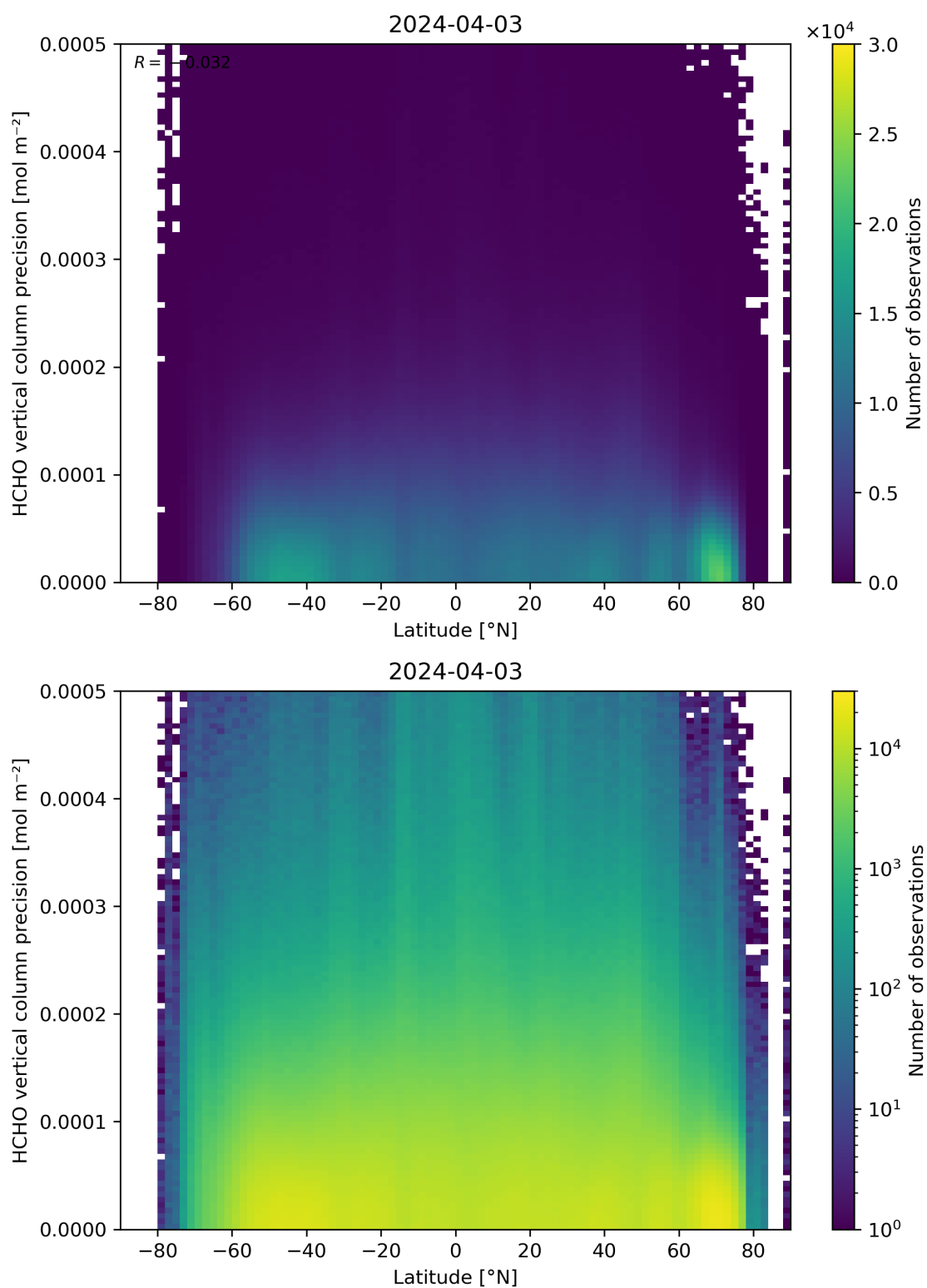
Figure 165: Scatter density plot of “Latitude” against “HCHO vertical column precision” for 2024-04-02 to 2024-04-04.
