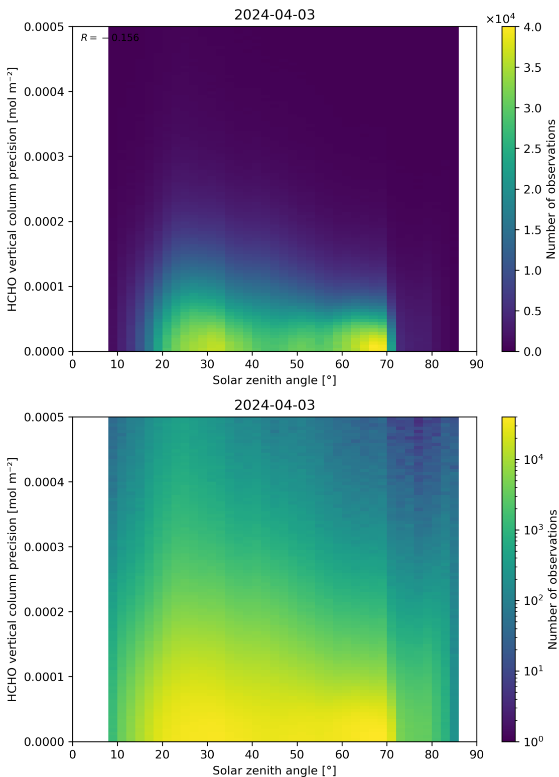
Figure 179: Scatter density plot of “Solar zenith angle” against “HCHO vertical column precision” for 2024-04-02 to 2024-04-04.
