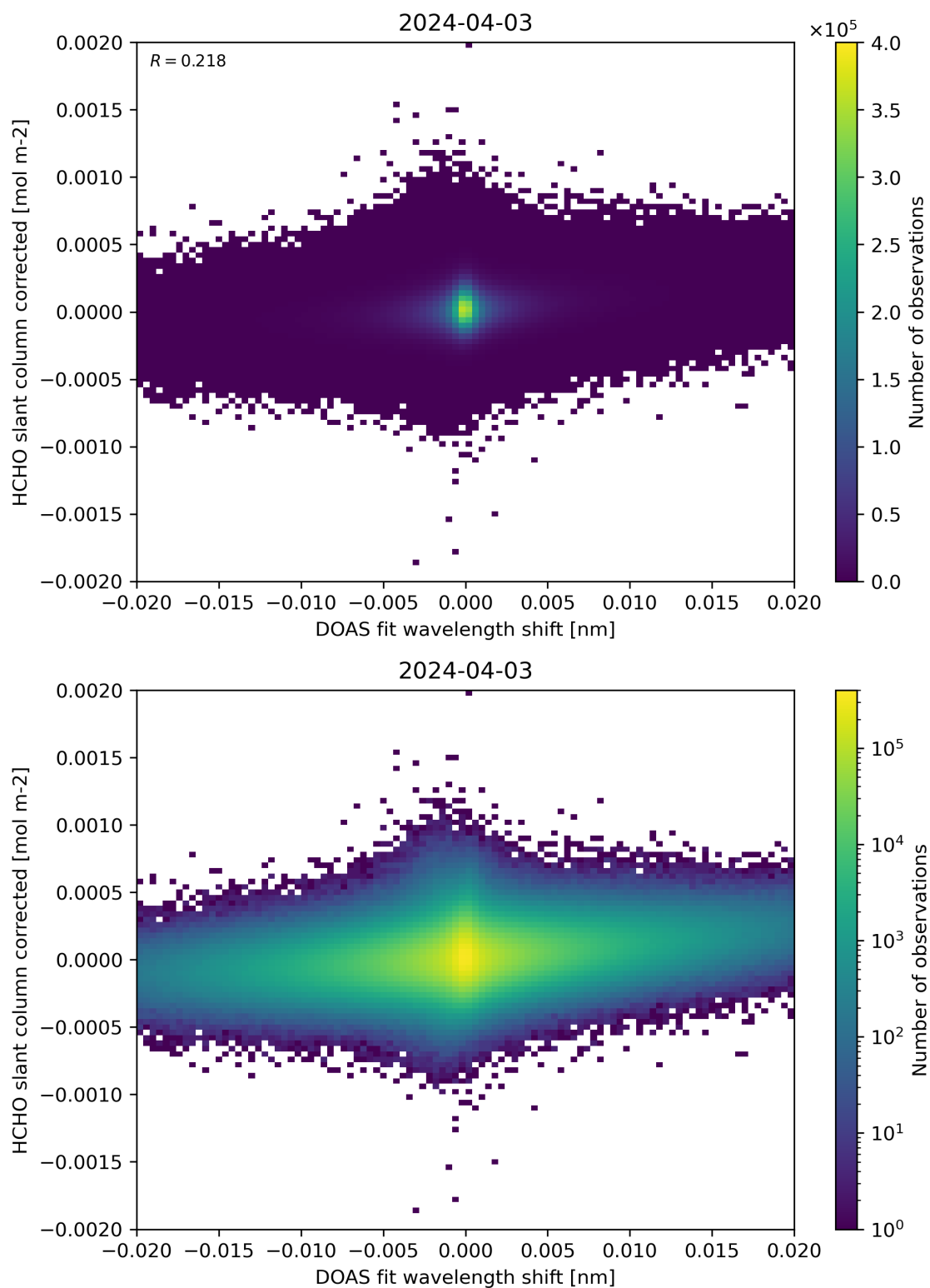
Figure 66: Scatter density plot of “DOAS fit wavelength shift” against “HCHO slant column corrected” for 2024-04-02 to 2024-04-04.
