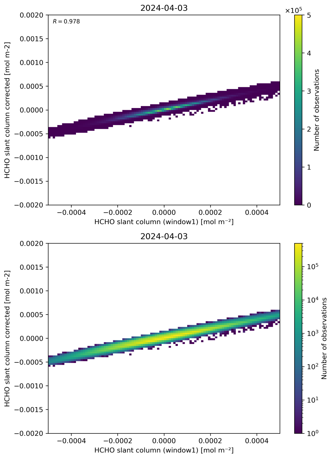
Figure 82: Scatter density plot of “HCHO slant column (window1)” against “HCHO slant column corrected” for 2024-04-02 to 2024-04-04.
