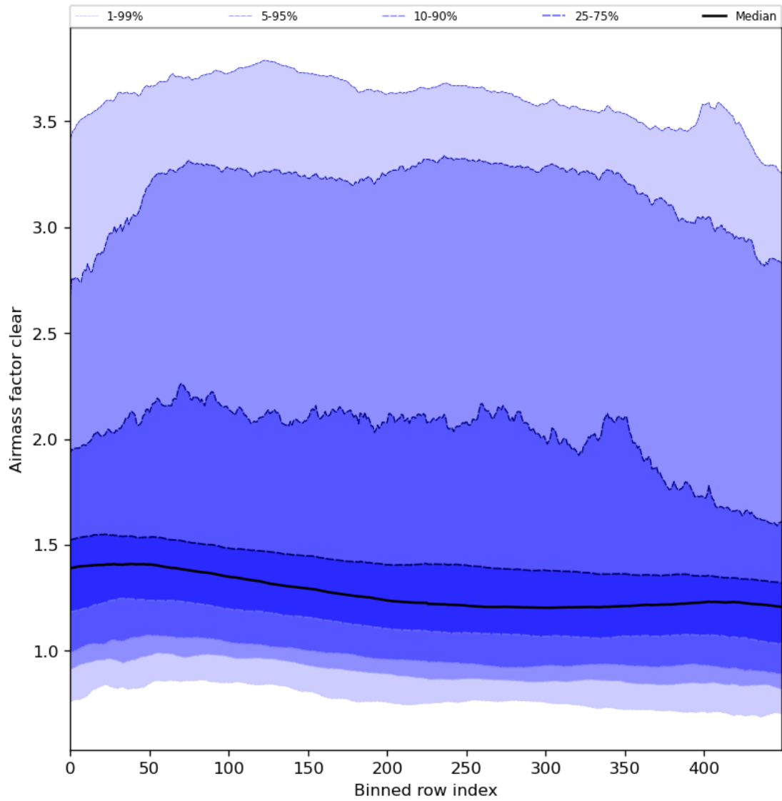
Figure 56: Along track statistics of “Airmass factor clear” for 2024-04-02 to 2024-04-04
