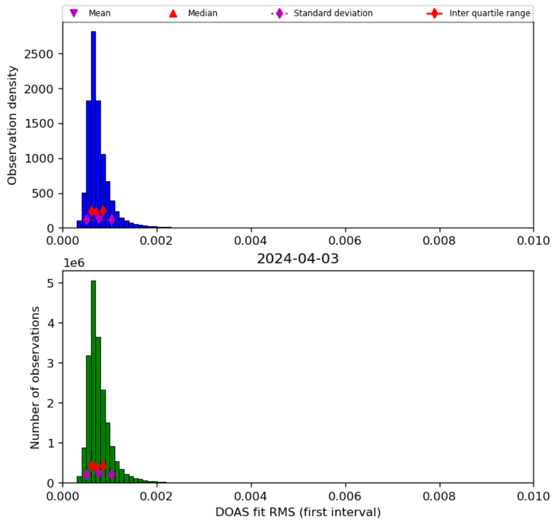
Figure 46: Histogram of “DOAS fit RMS (first interval)” for 2024-04-02 to 2024-04-04
