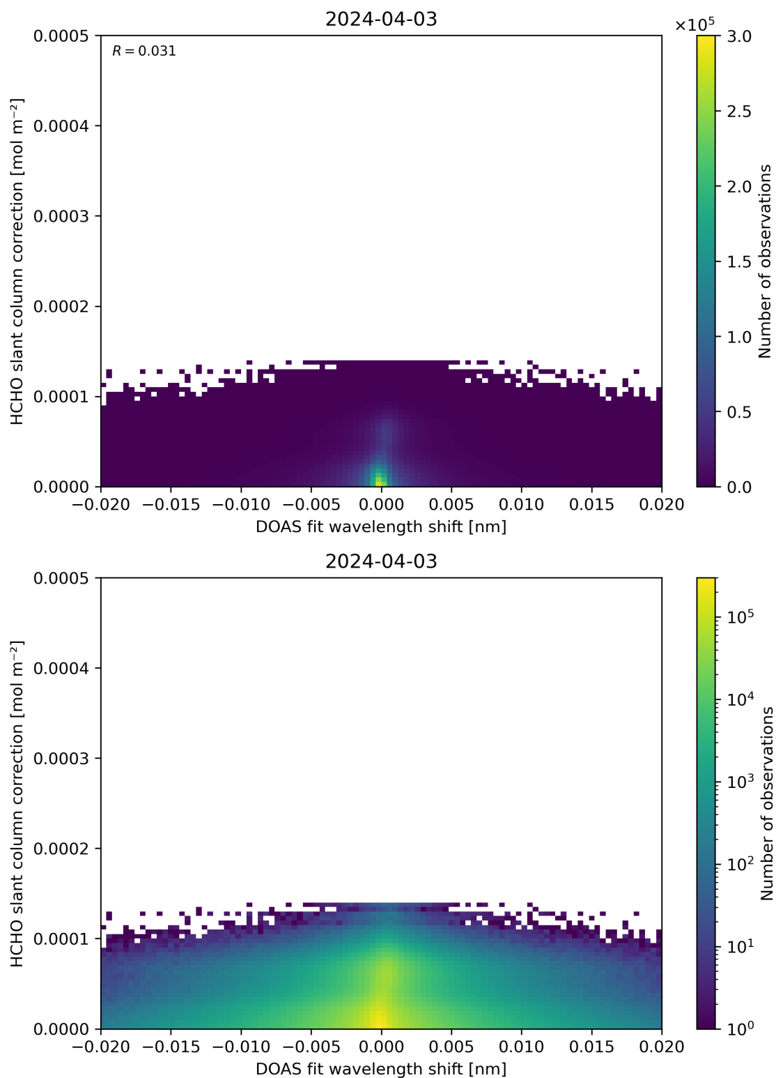
Figure 67: Scatter density plot of “DOAS fit wavelength shift” against “HCHO slant column correction” for 2024-04-02 to 2024-04-04.
