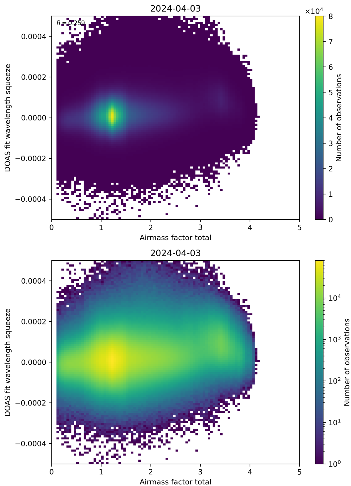
Figure 99: Scatter density plot of “Airmass factor total” against “DOAS fit wavelength squeeze” for 2024-04-02 to 2024-04-04.
