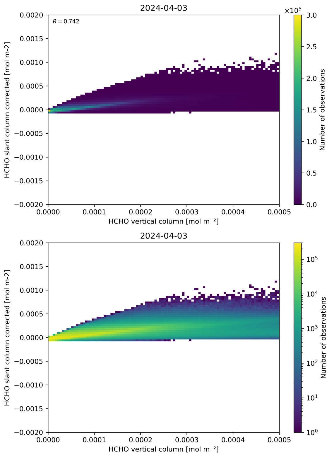
Figure 127: Scatter density plot of “HCHO vertical column” against “HCHO slant column corrected” for 2024-04-02 to 2024-04-04.
