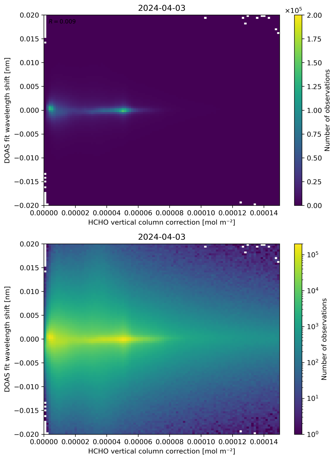
Figure 113: Scatter density plot of “HCHO vertical column correction” against “DOAS fit wavelength shift” for 2024-04-02 to 2024-04-04.
