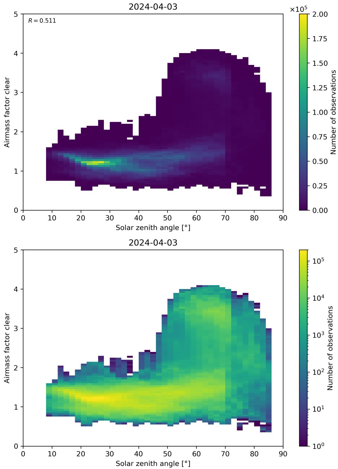
Figure 170: Scatter density plot of “Solar zenith angle” against “Airmass factor clear” for 2024-04-02 to 2024-04-04.
