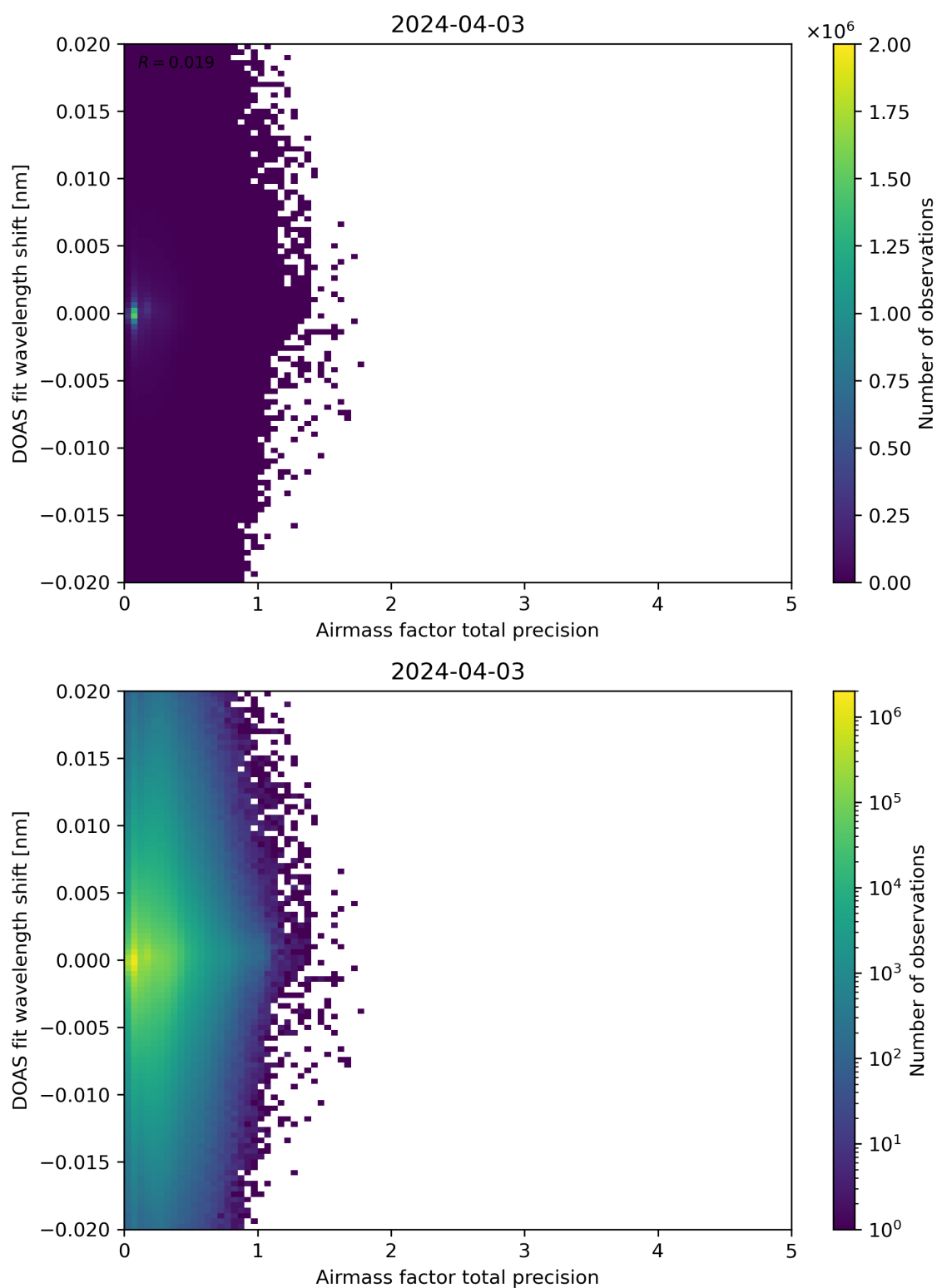
Figure 106: Scatter density plot of “Airmass factor total precision” against “DOAS fit wavelength shift” for 2024-04-02 to 2024-04-04.
