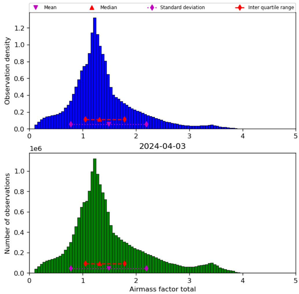
Figure 40: Histogram of “Airmass factor total” for 2024-04-02 to 2024-04-04
