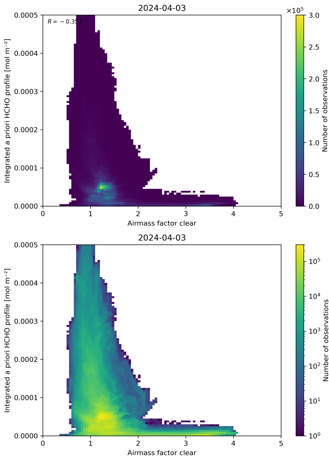
Figure 76: Scatter density plot of “Airmass factor clear” against “Integrated a priori HCHO profile” for 2024-04-02 to 2024-04-04.
