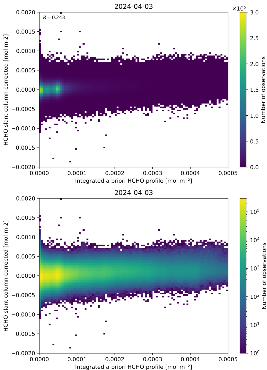
Figure 151: Scatter density plot of “Integrated a priori HCHO profile” against “HCHO slant column corrected” for 2024-04-02 to 2024-04-04.
