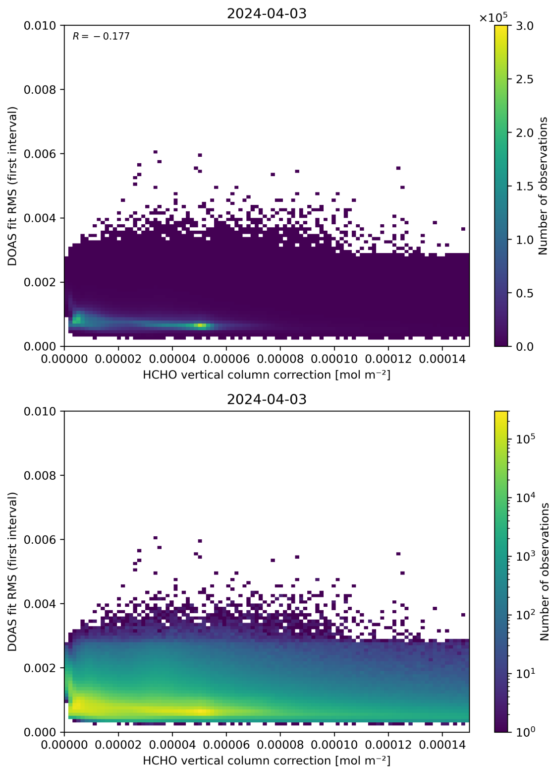
Figure 112: Scatter density plot of “HCHO vertical column correction” against “DOAS fit RMS (first interval)” for 2024-04-02 to 2024-04-04.
