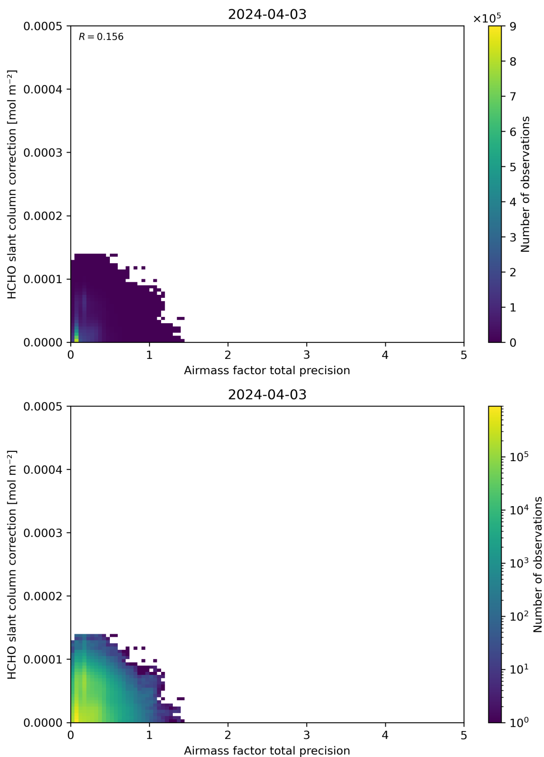
Figure 110: Scatter density plot of “Airmass factor total precision” against “HCHO slant column correction” for 2024-04-02 to 2024-04-04.
