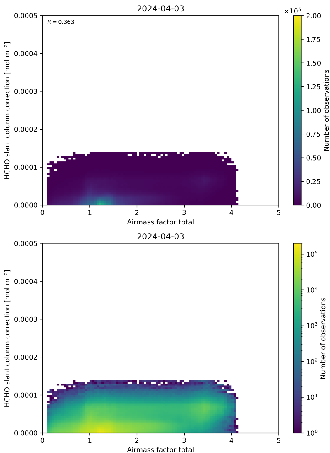
Figure 102: Scatter density plot of “Airmass factor total” against “HCHO slant column correction” for 2024-04-02 to 2024-04-04.
