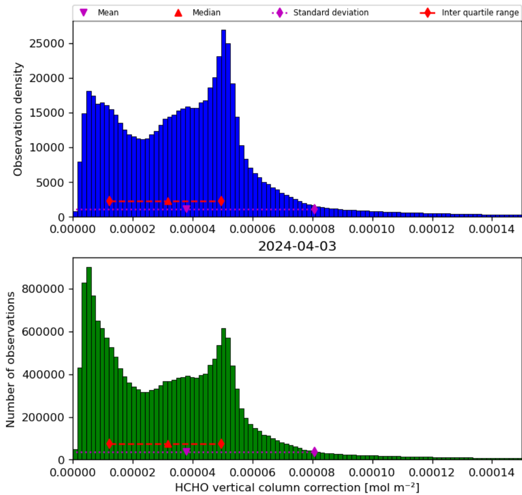
Figure 37: Histogram of “HCHO vertical column correction” for 2024-04-02 to 2024-04-04
