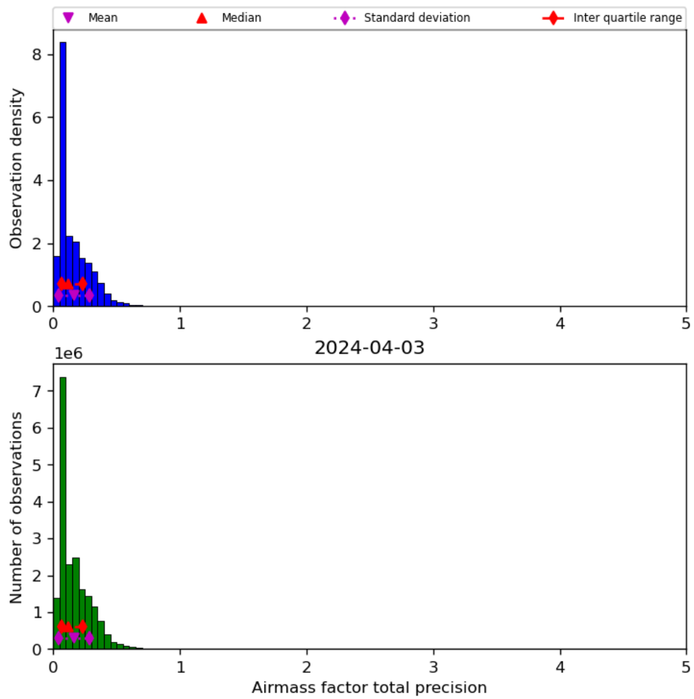
Figure 41: Histogram of “Airmass factor total precision” for 2024-04-02 to 2024-04-04
