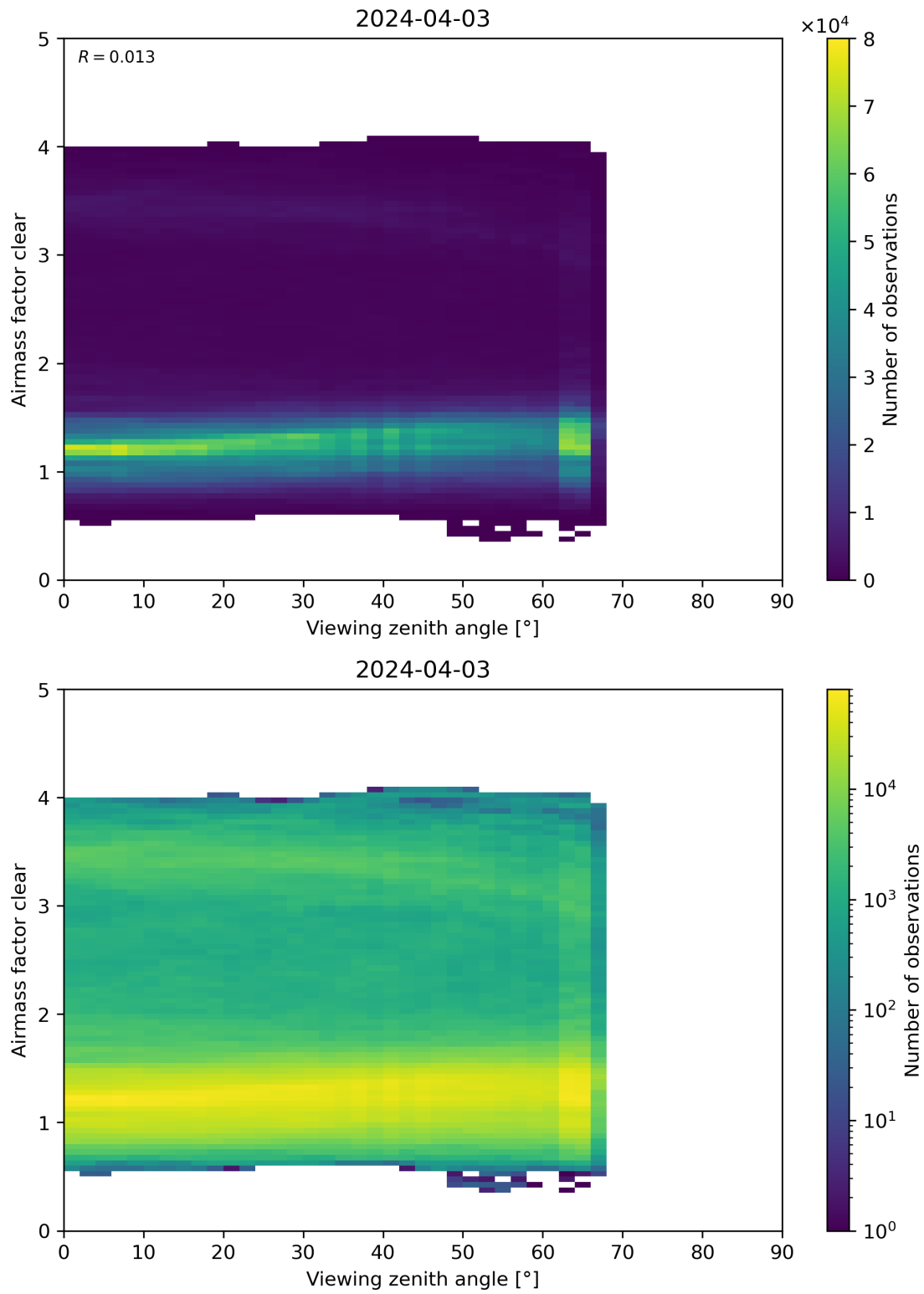
Figure 185: Scatter density plot of “Viewing zenith angle” against “Airmass factor clear” for 2024-04-02 to 2024-04-04.
