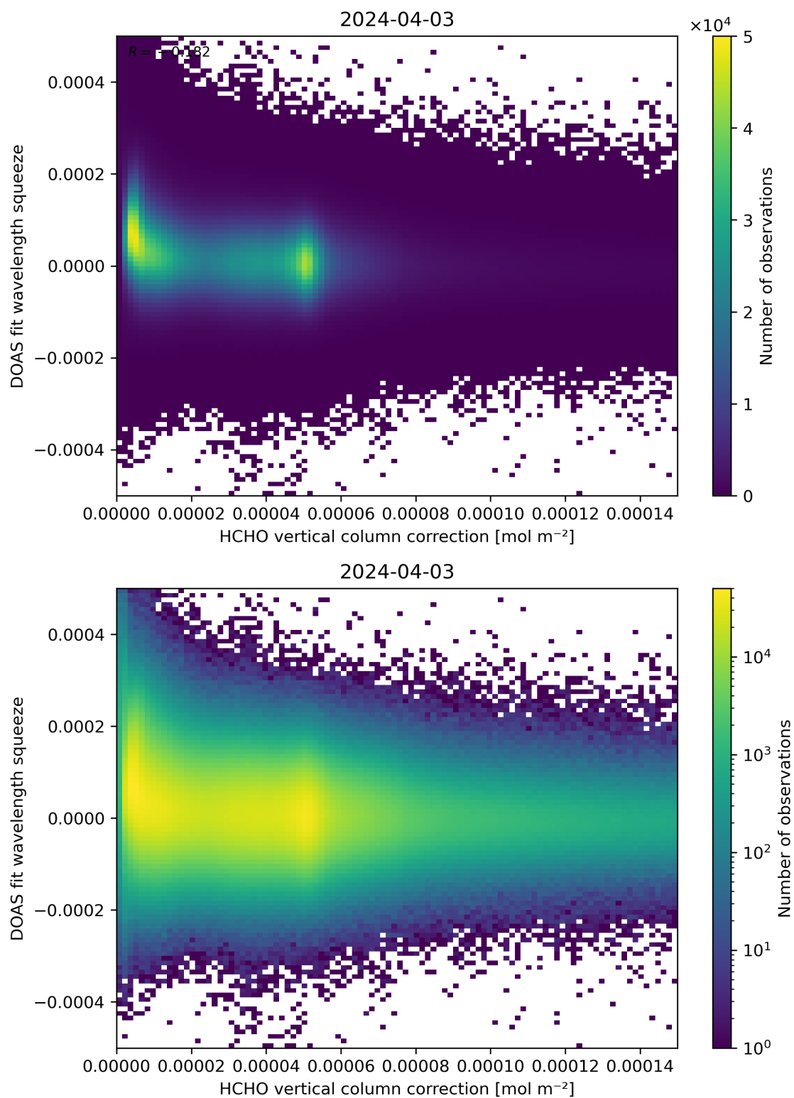
Figure 114: Scatter density plot of “HCHO vertical column correction” against “DOAS fit wavelength squeeze” for 2024-04-02 to 2024-04-04.
