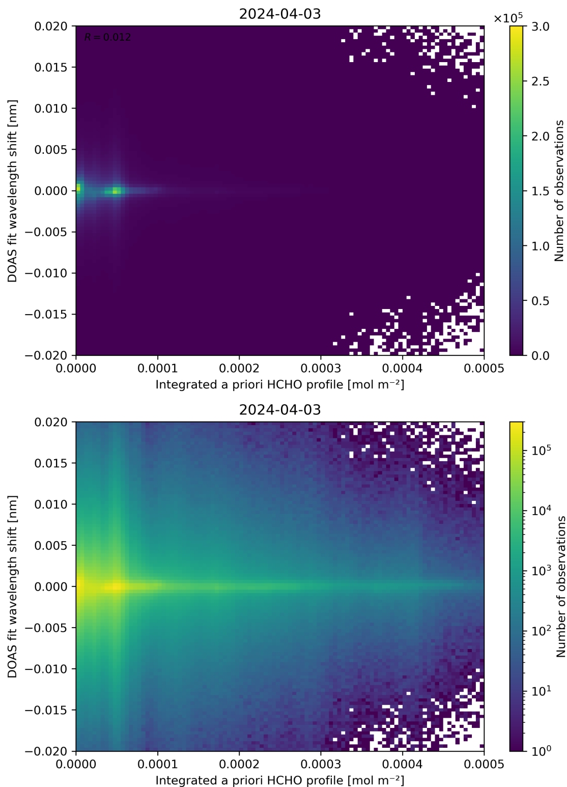
Figure 149: Scatter density plot of “Integrated a priori HCHO profile” against “DOAS fit wavelength shift” for 2024-04-02 to 2024-04-04.
