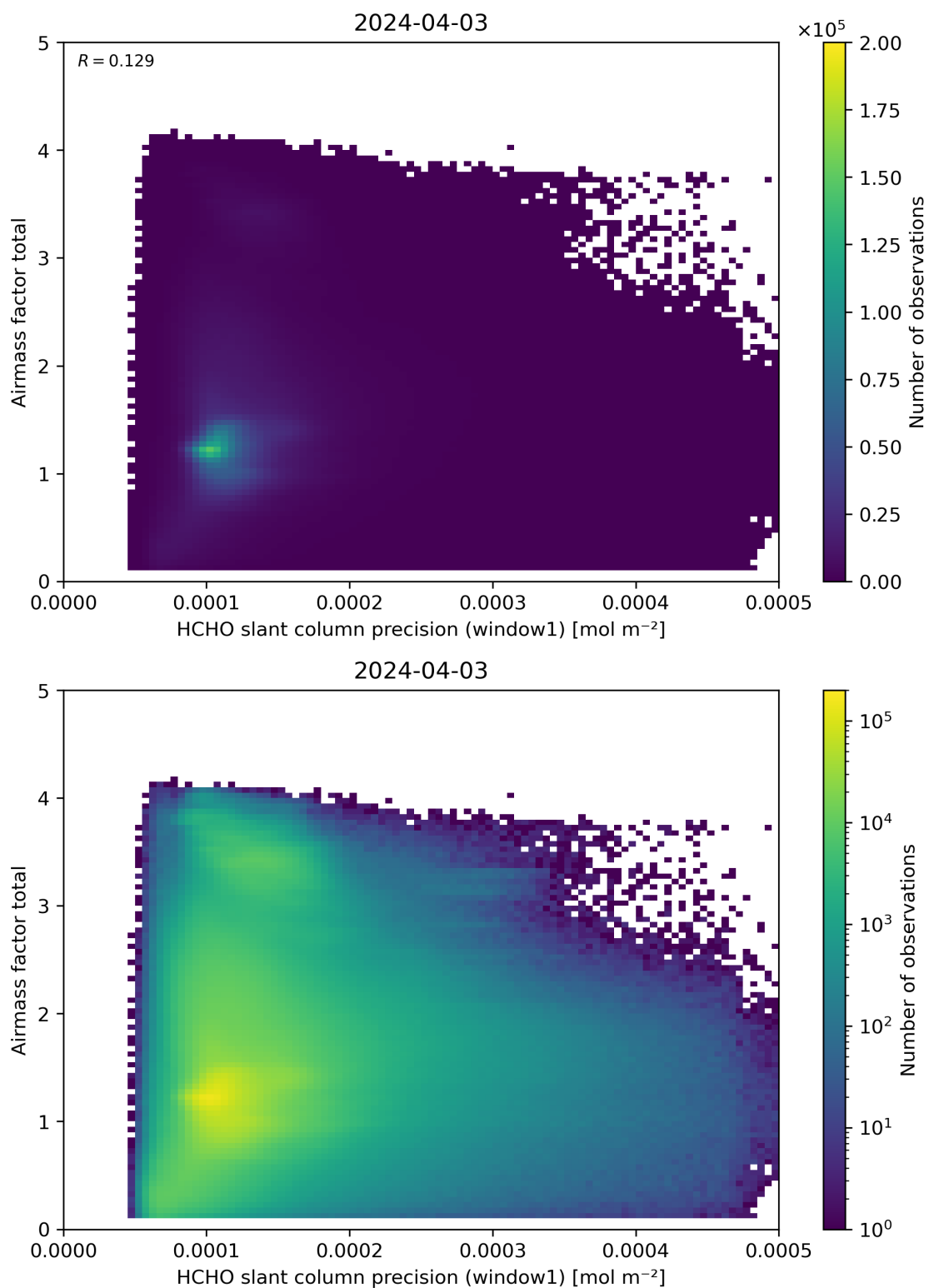
Figure 94: Scatter density plot of “HCHO slant column precision (window1)” against “Airmass factor total” for 2024-04-02 to 2024-04-04.
