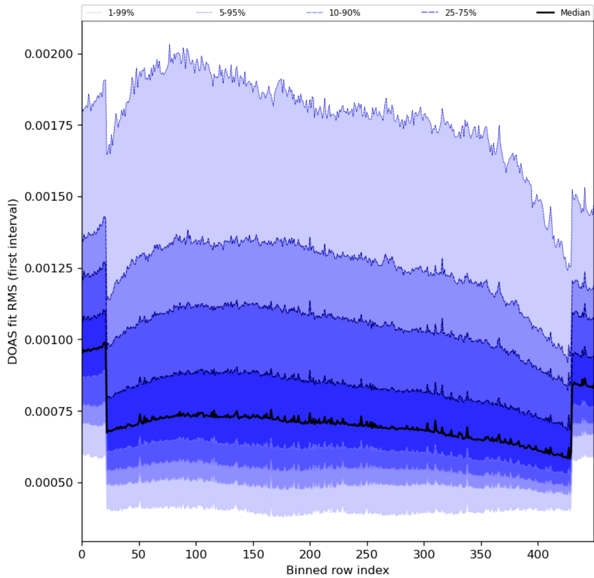
Figure 60: Along track statistics of “DOAS fit RMS (first interval)” for 2024-04-02 to 2024-04-04
