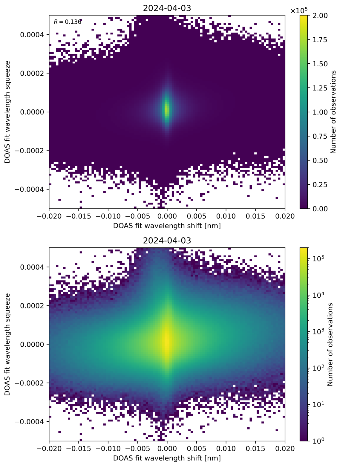
Figure 65: Scatter density plot of “DOAS fit wavelength shift” against “DOAS fit wavelength squeeze” for 2024-04-02 to 2024-04-04.
