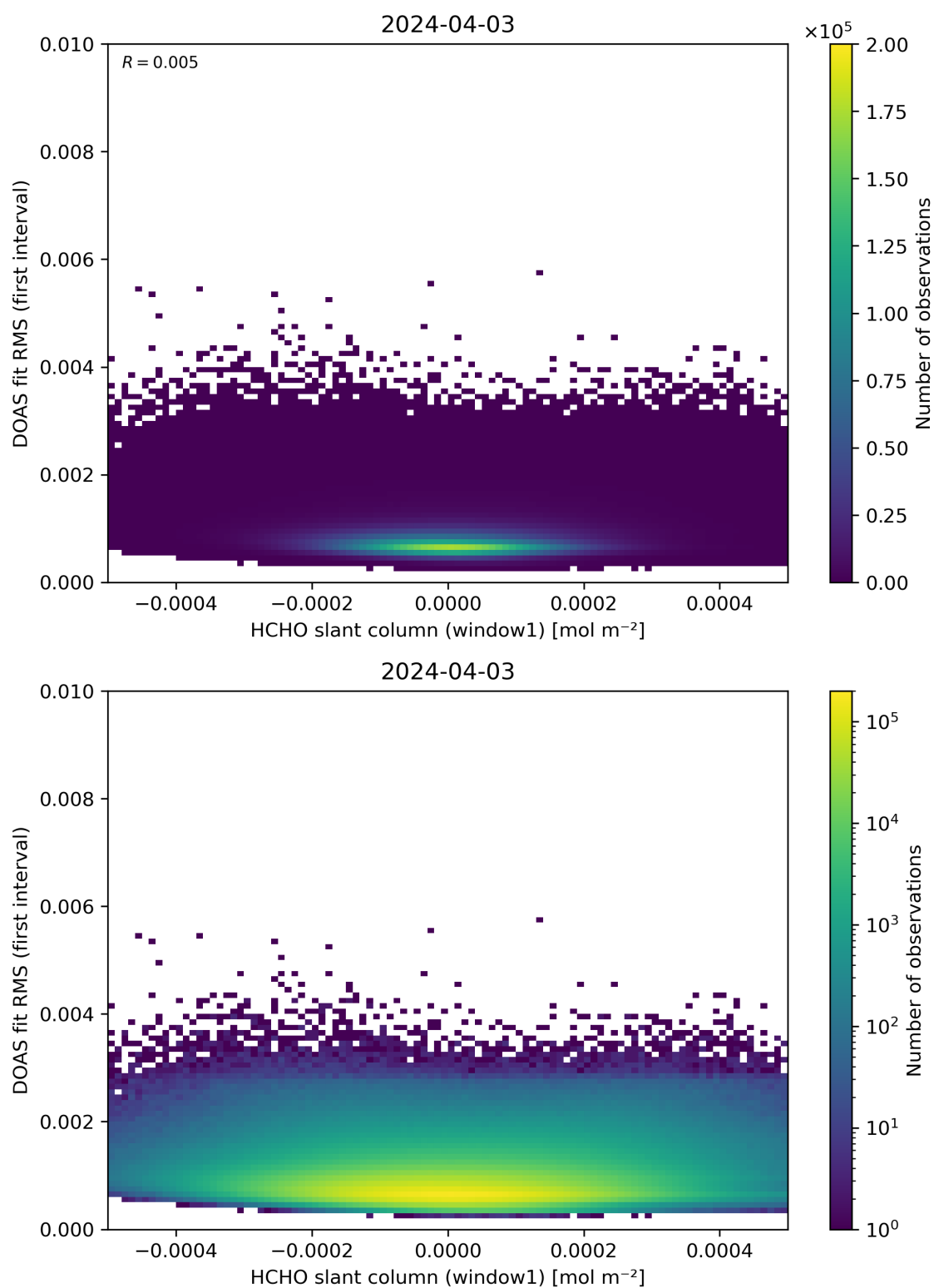
Figure 78: Scatter density plot of “HCHO slant column (window1)” against “DOAS fit RMS (first interval)” for 2024-04-02 to 2024-04-04.
