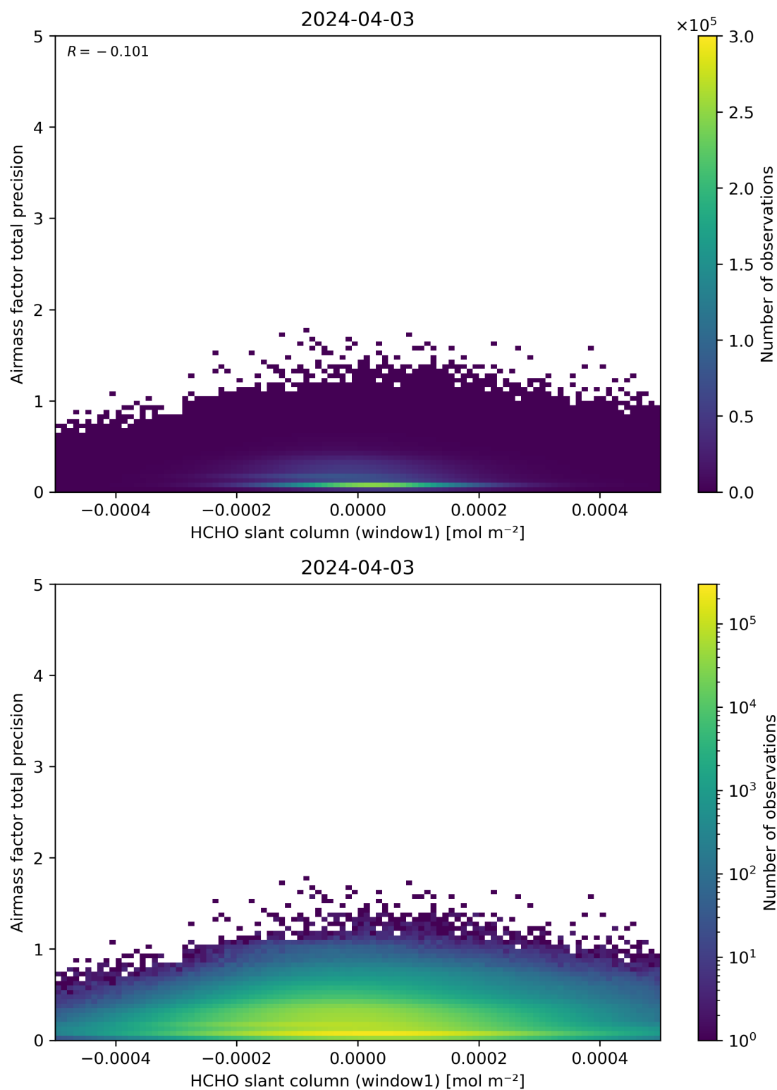
Figure 86: Scatter density plot of “HCHO slant column (window1)” against “Airmass factor total precision” for 2024-04-02 to 2024-04-04.
