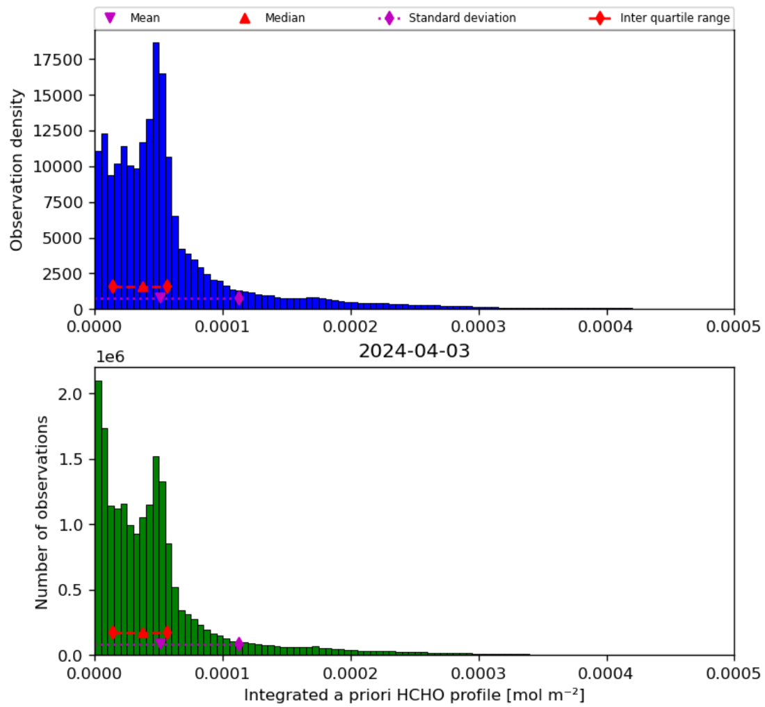
Figure 43: Histogram of “Integrated a priori HCHO profile” for 2024-04-02 to 2024-04-04
