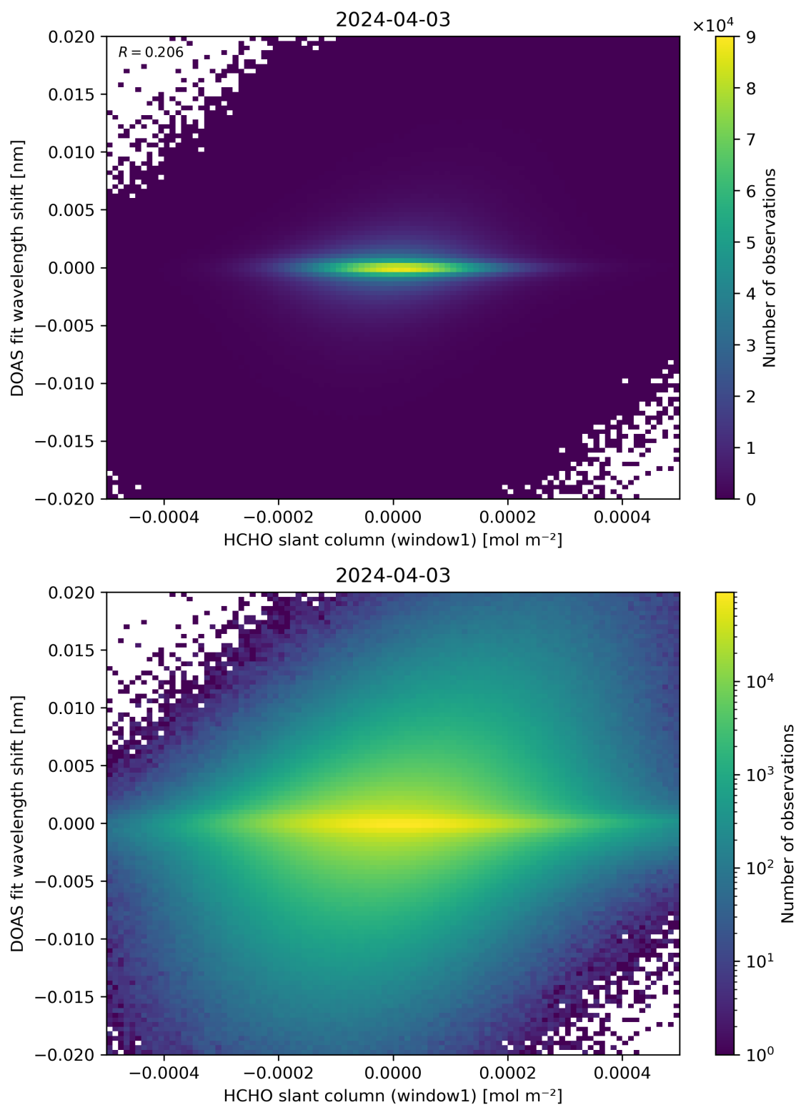
Figure 79: Scatter density plot of “HCHO slant column (window1)” against “DOAS fit wavelength shift” for 2024-04-02 to 2024-04-04.
