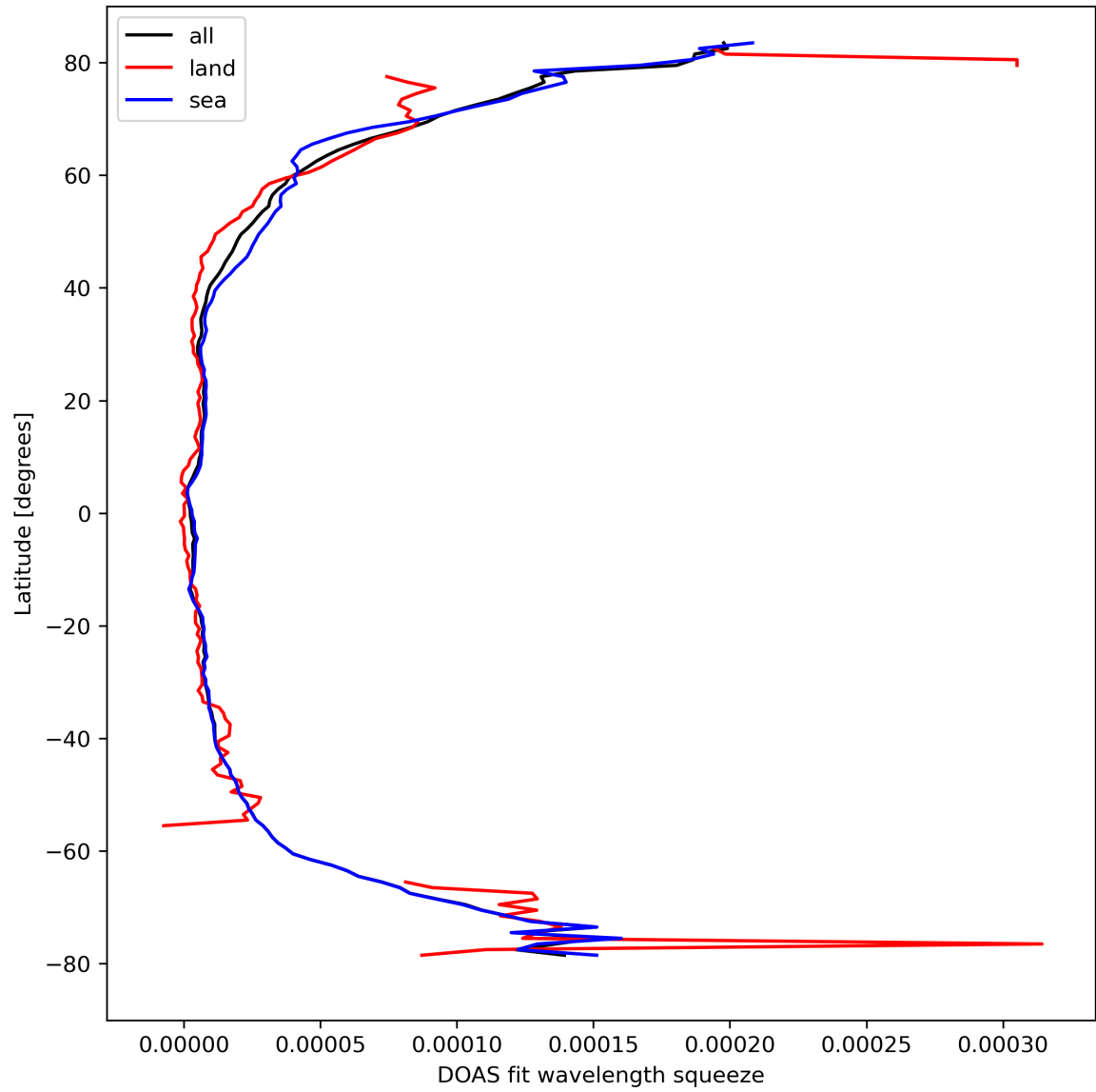
Figure 31: Zonal average of “DOAS fit wavelength squeeze” for 2024-04-02 to 2024-04-04.
