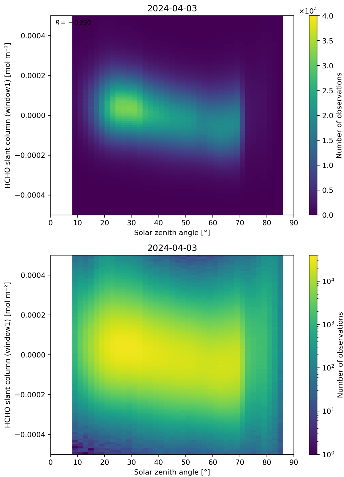
Figure 173: Scatter density plot of “Solar zenith angle” against “HCHO slant column (window1)” for 2024-04-02 to 2024-04-04.
