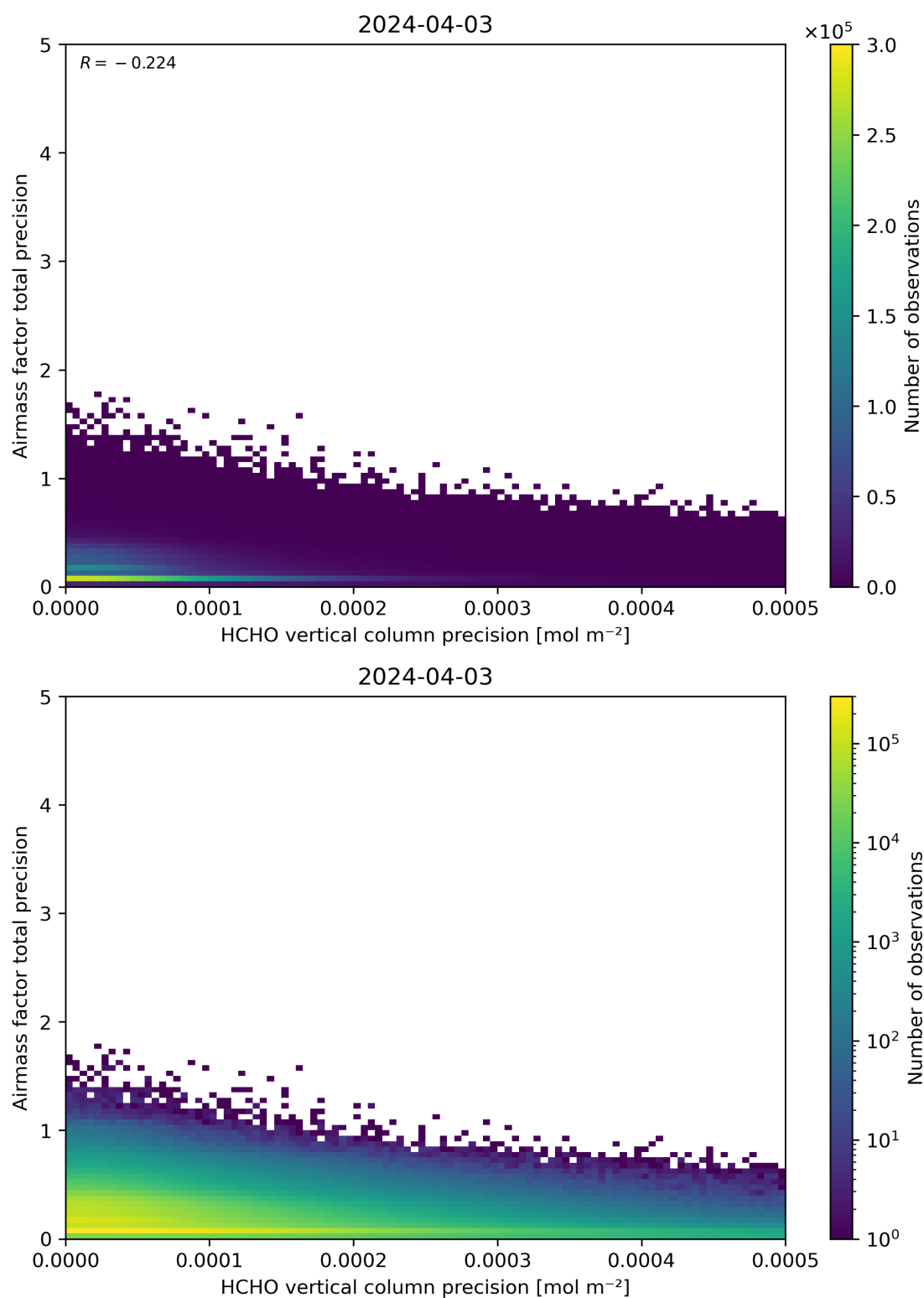
Figure 145: Scatter density plot of “HCHO vertical column precision” against “Airmass factor total precision” for 2024-04-02 to 2024-04-04.
