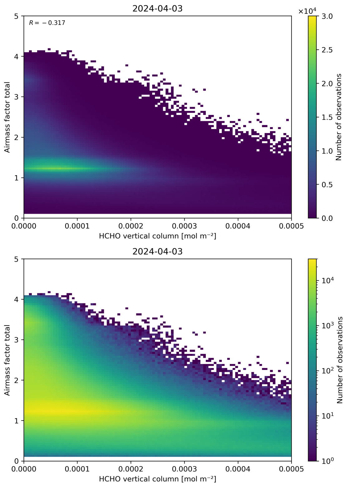
Figure 131: Scatter density plot of “HCHO vertical column” against “Airmass factor total” for 2024-04-02 to 2024-04-04.
