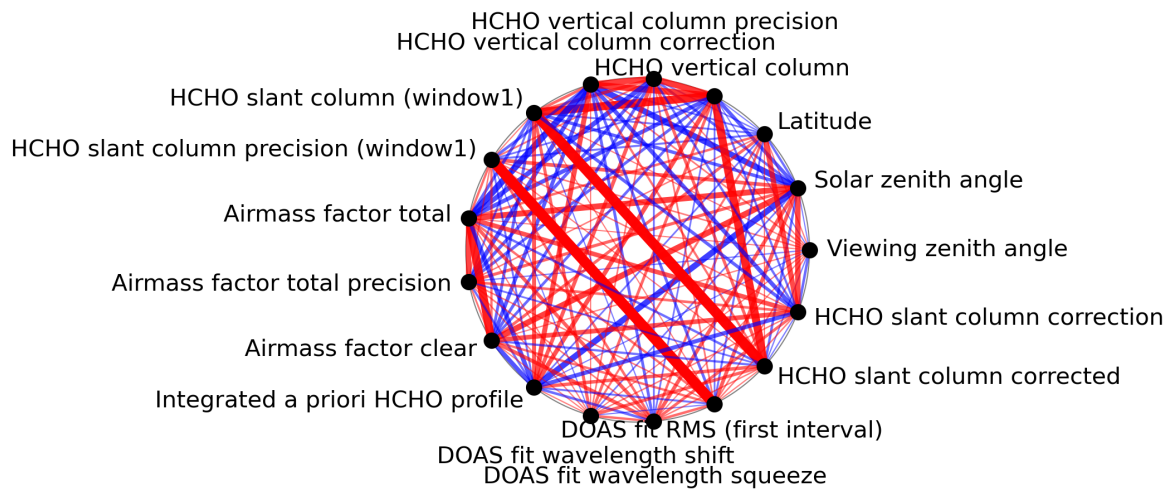
Figure 1: Map of correlation graph for 2024-04-02 to 2024-04-04.
