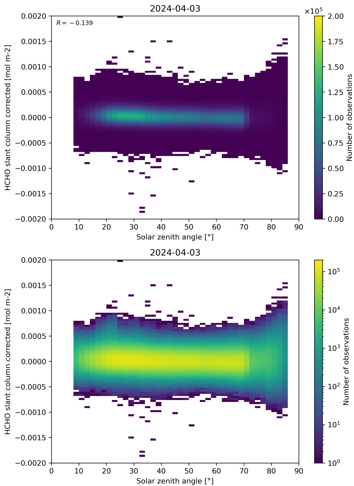
Figure 171: Scatter density plot of “Solar zenith angle” against “HCHO slant column corrected” for 2024-04-02 to 2024-04-04.
