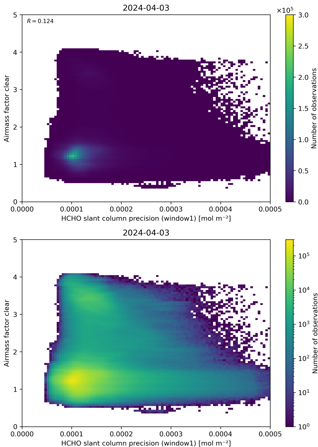
Figure 91: Scatter density plot of “HCHO slant column precision (window1)” against “Airmass factor clear” for 2024-04-02 to 2024-04-04.
