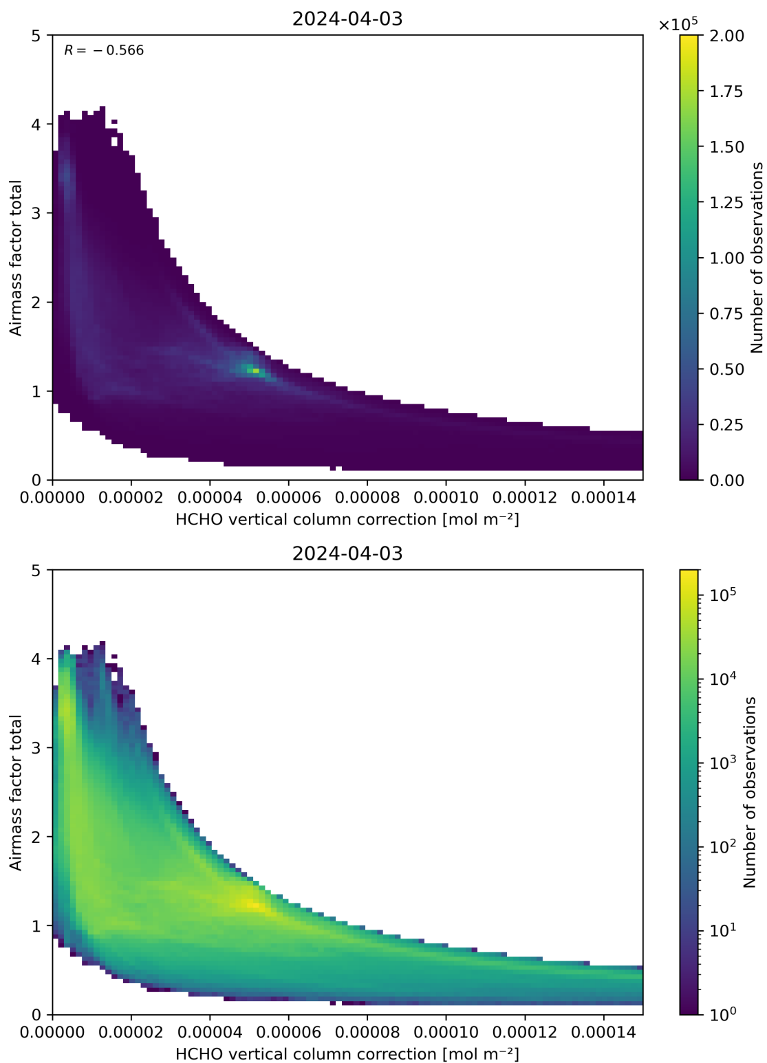
Figure 120: Scatter density plot of “HCHO vertical column correction” against “Airmass factor total” for 2024-04-02 to 2024-04-04.
