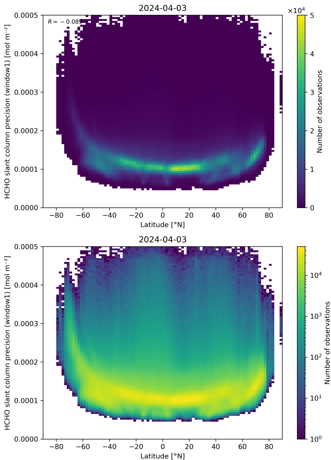
Figure 160: Scatter density plot of “Latitude” against “HCHO slant column precision (window1)” for 2024-04-02 to 2024-04-04.
