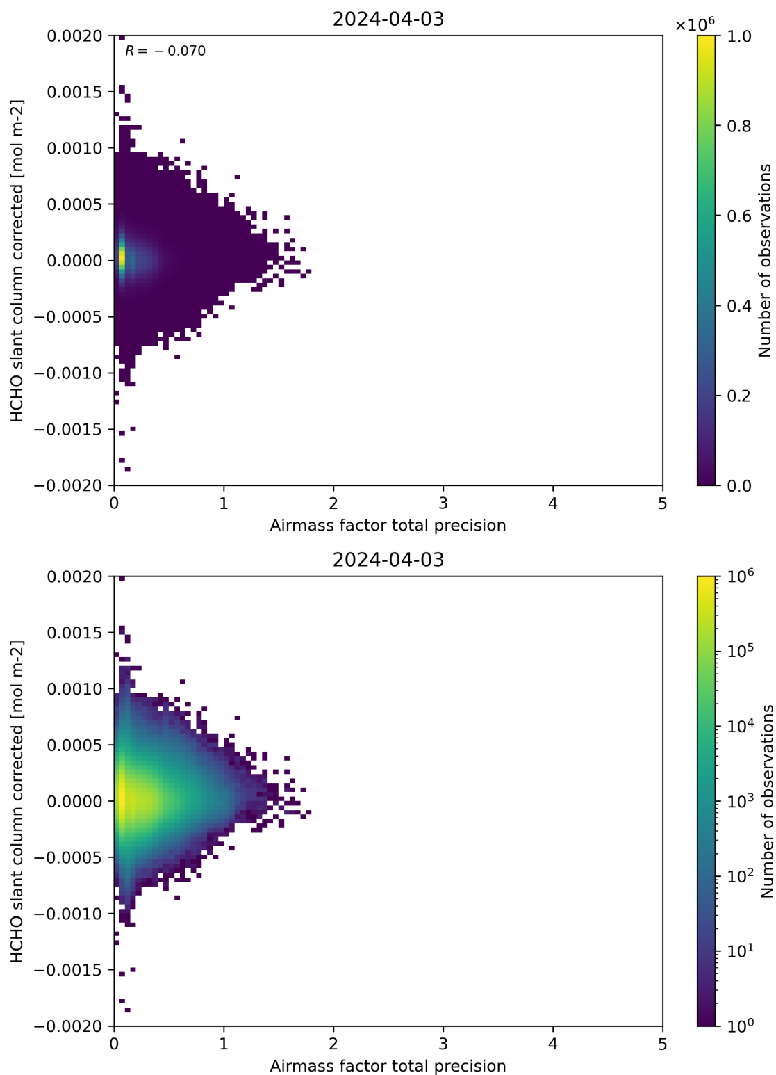
Figure 109: Scatter density plot of “Airmass factor total precision” against “HCHO slant column corrected” for 2024-04-02 to 2024-04-04.
