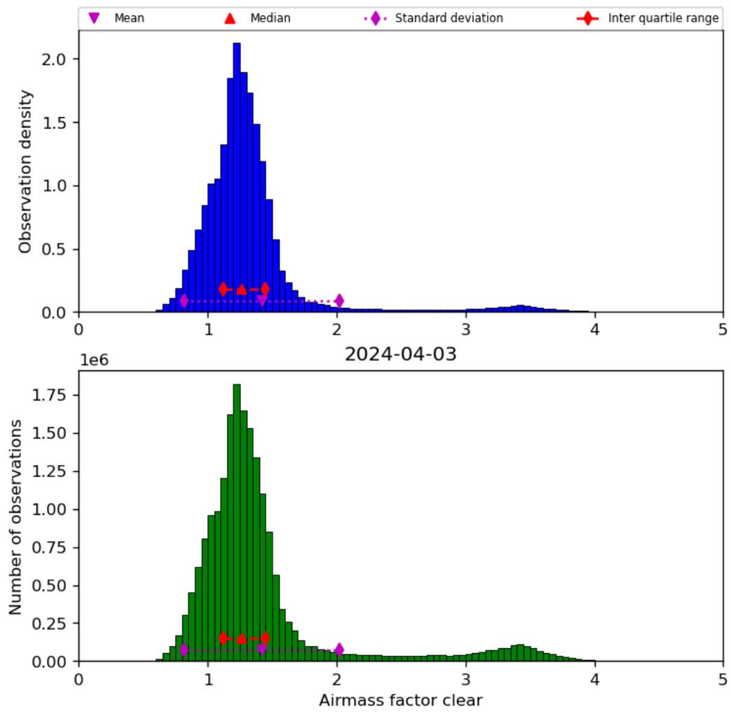
Figure 42: Histogram of “Airmass factor clear” for 2024-04-02 to 2024-04-04
