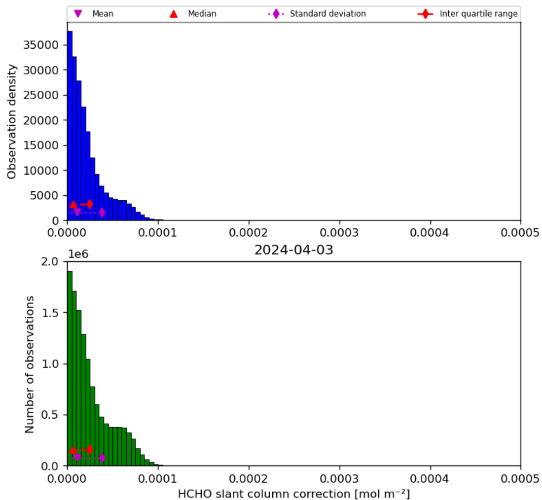
Figure 47: Histogram of “HCHO slant column correction” for 2024-04-02 to 2024-04-04
