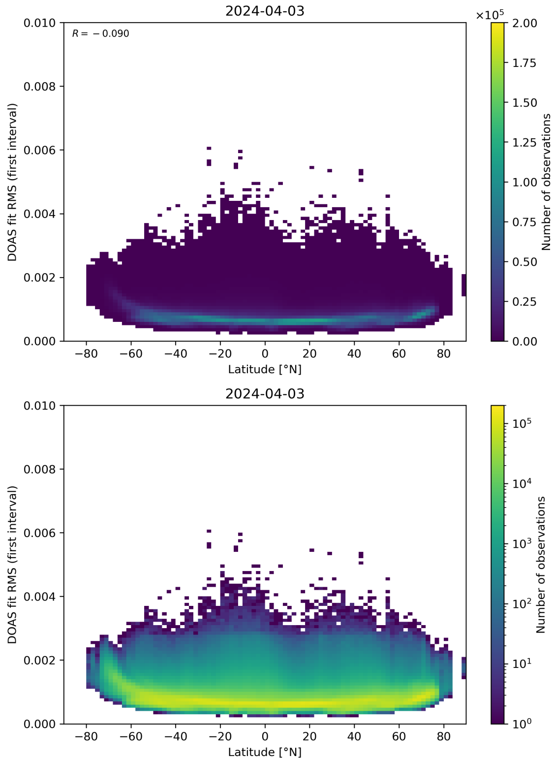
Figure 153: Scatter density plot of “Latitude” against “DOAS fit RMS (first interval)” for 2024-04-02 to 2024-04-04.
