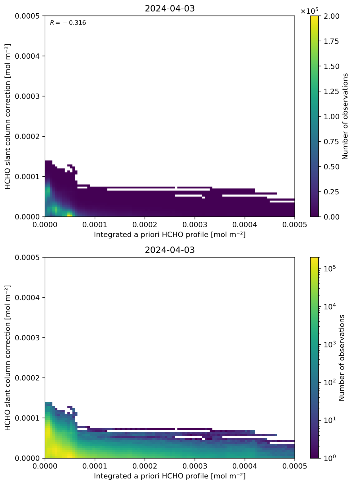
Figure 152: Scatter density plot of “Integrated a priori HCHO profile” against “HCHO slant column correction” for 2024-04-02 to 2024-04-04.
