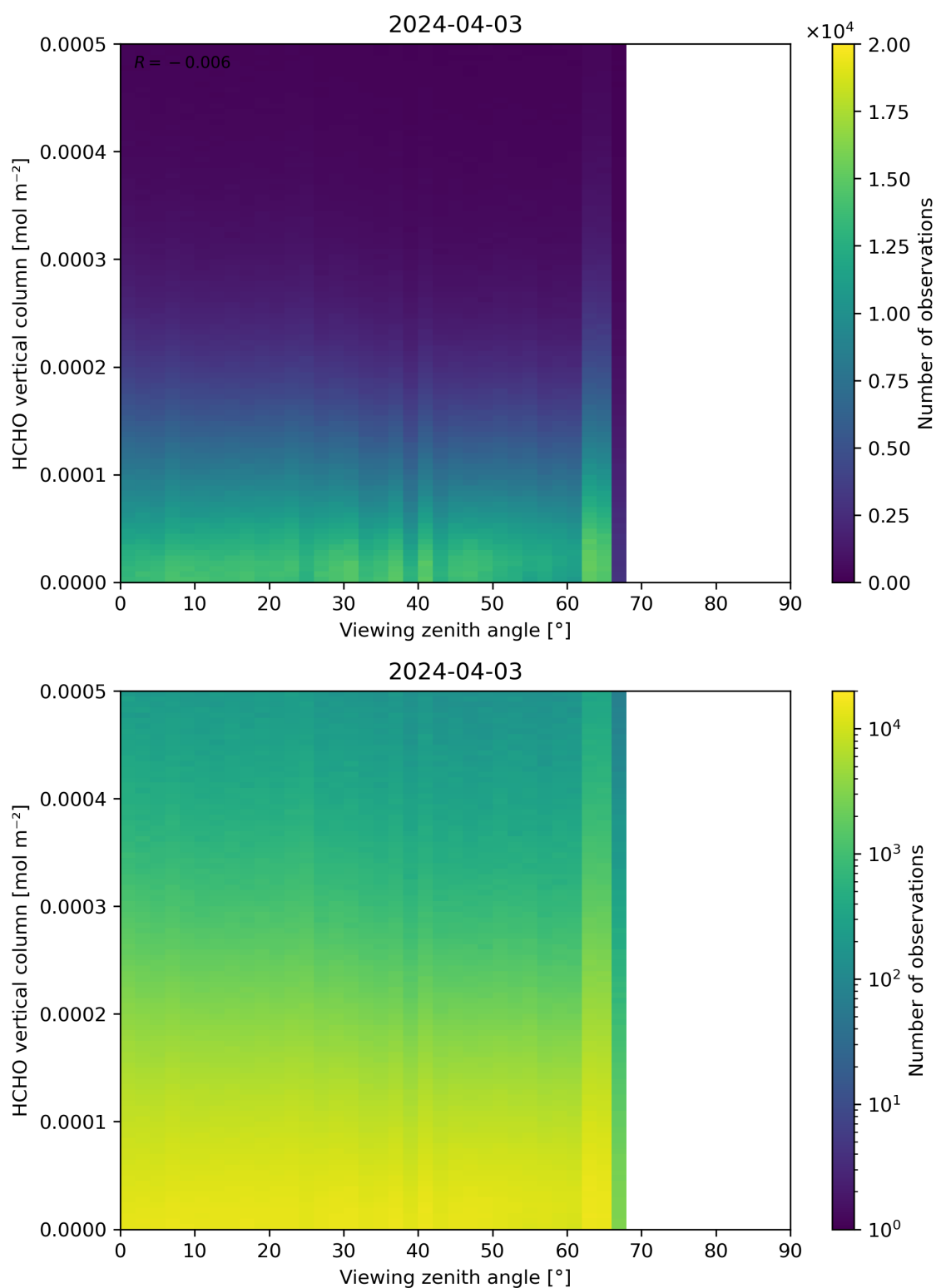
Figure 192: Scatter density plot of “Viewing zenith angle” against “HCHO vertical column” for 2024-04-02 to 2024-04-04.
