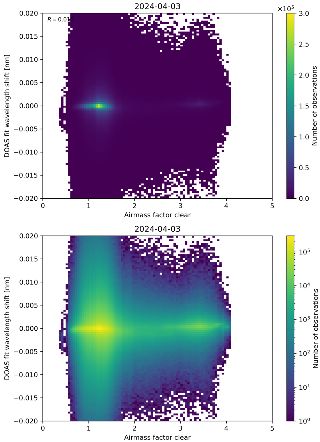
Figure 72: Scatter density plot of “Airmass factor clear” against “DOAS fit wavelength shift” for 2024-04-02 to 2024-04-04.
