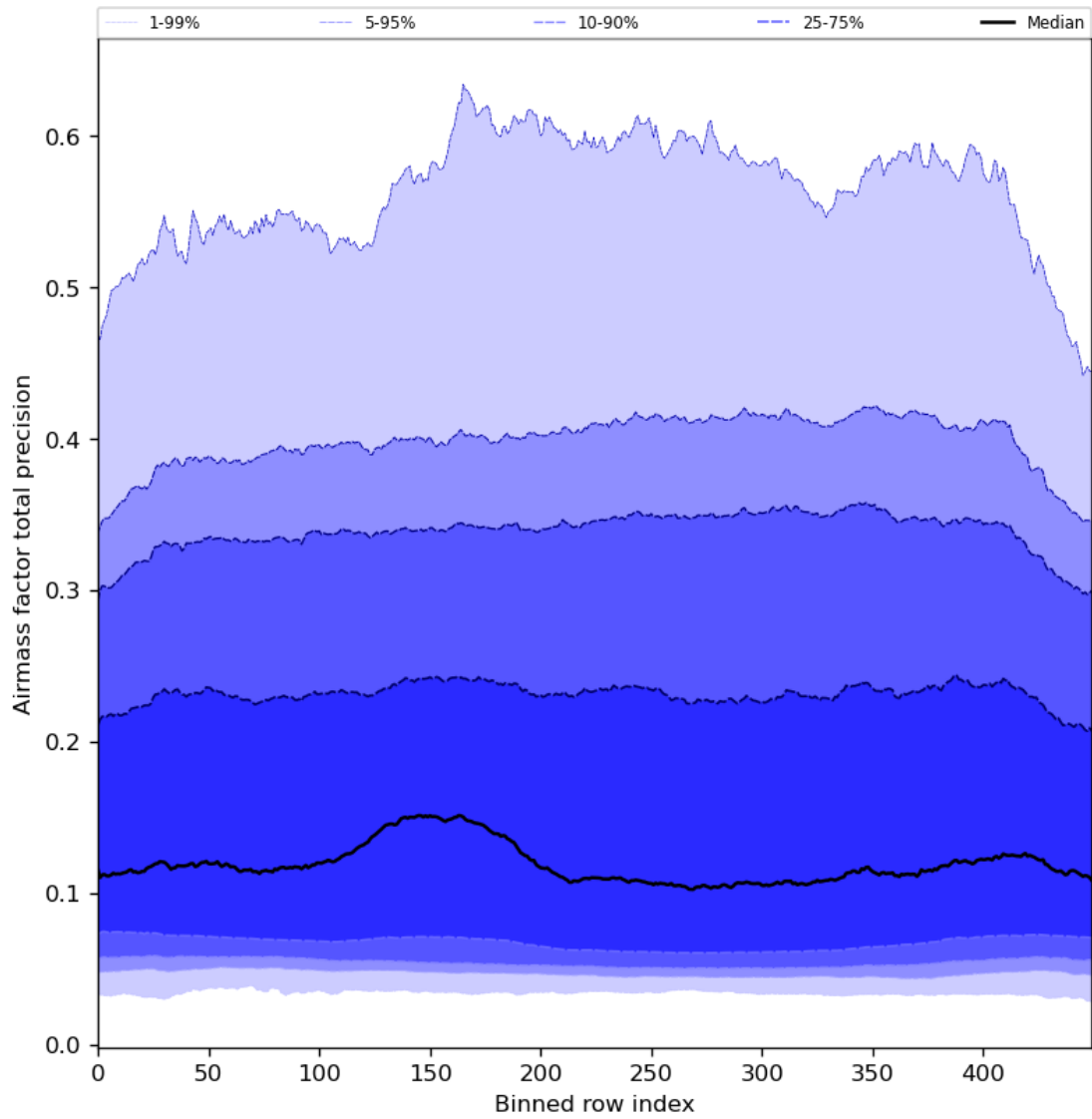
Figure 55: Along track statistics of “Airmass factor total precision” for 2024-04-02 to 2024-04-04
