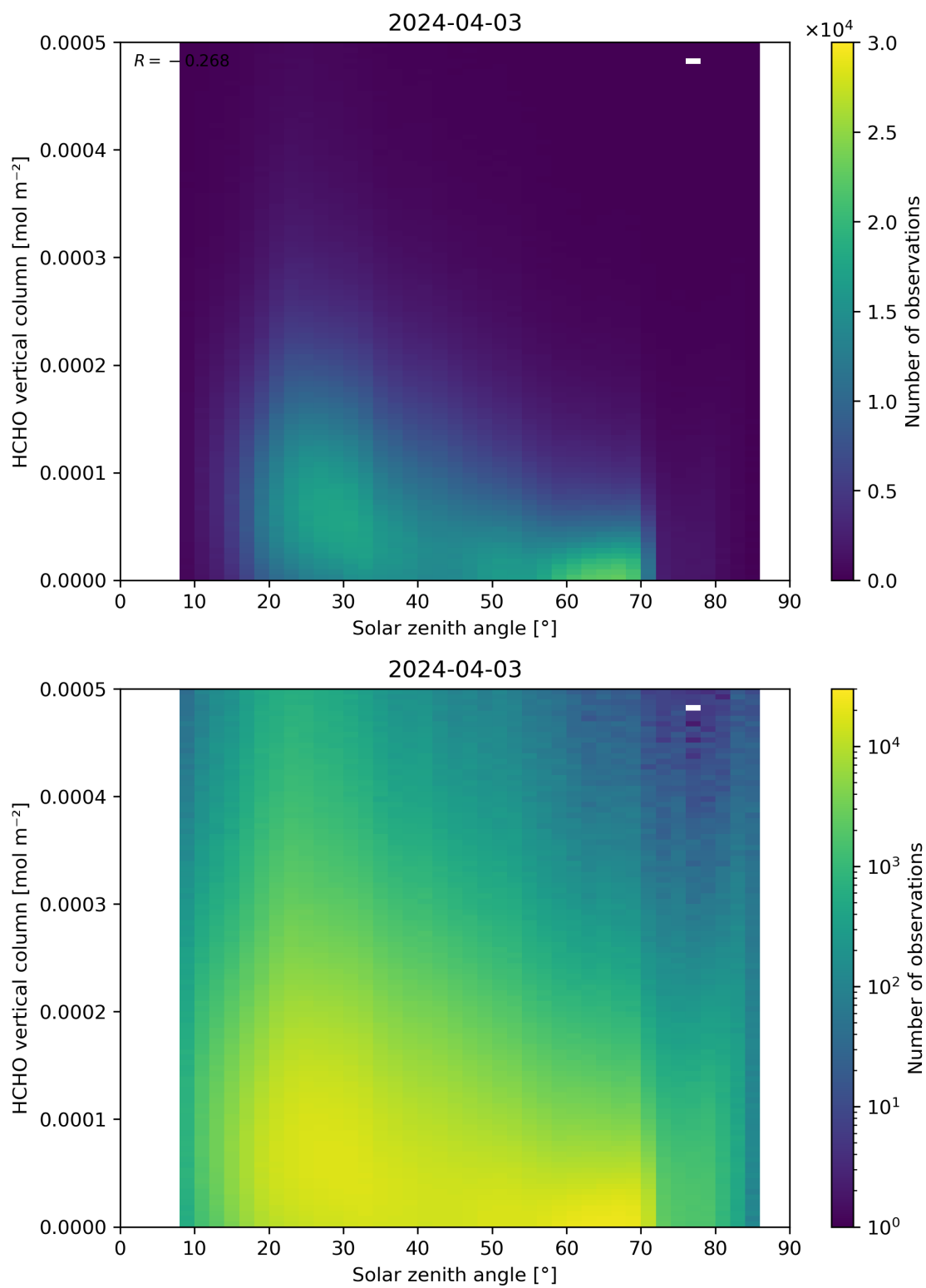
Figure 177: Scatter density plot of “Solar zenith angle” against “HCHO vertical column” for 2024-04-02 to 2024-04-04.
