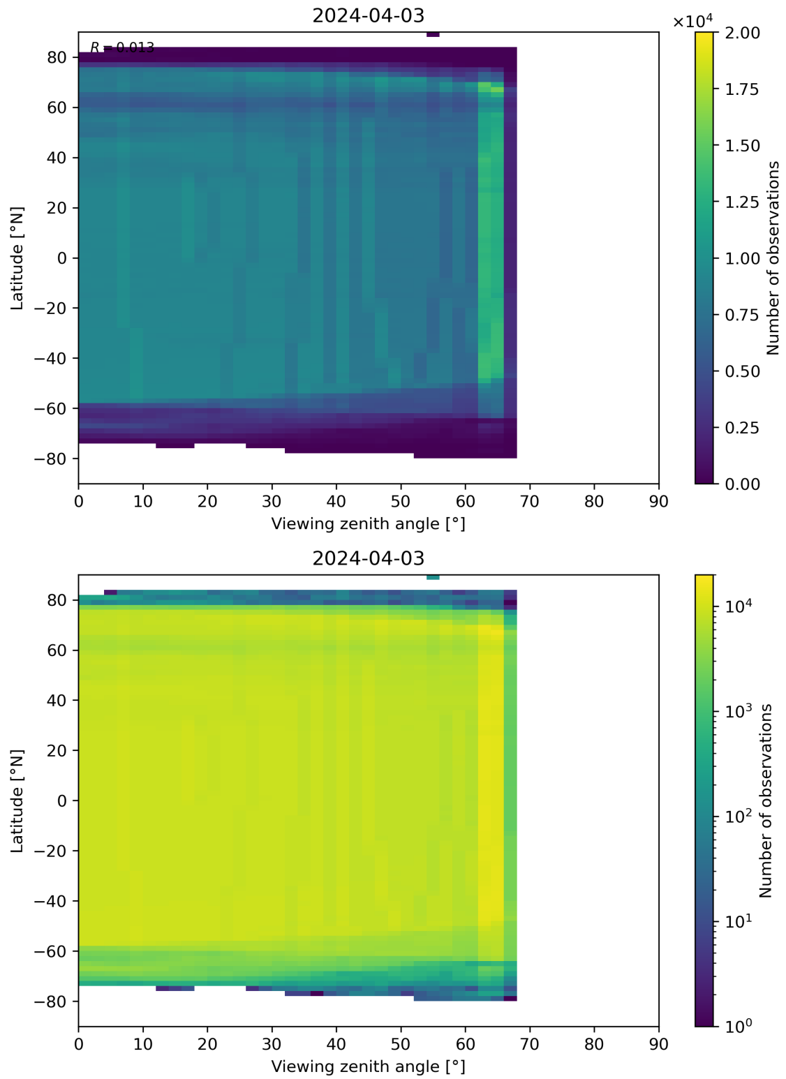
Figure 196: Scatter density plot of “Viewing zenith angle” against “Latitude” for 2024-04-02 to 2024-04-04.
