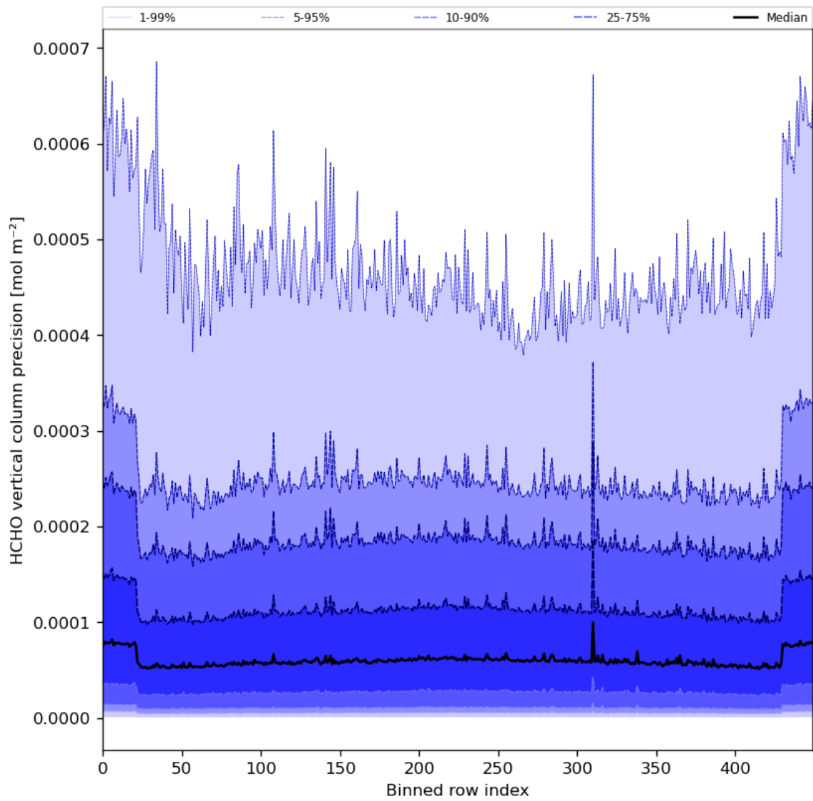
Figure 50: Along track statistics of "HCHO vertical column precision" for 2024-04-02 to 2024-04-04
