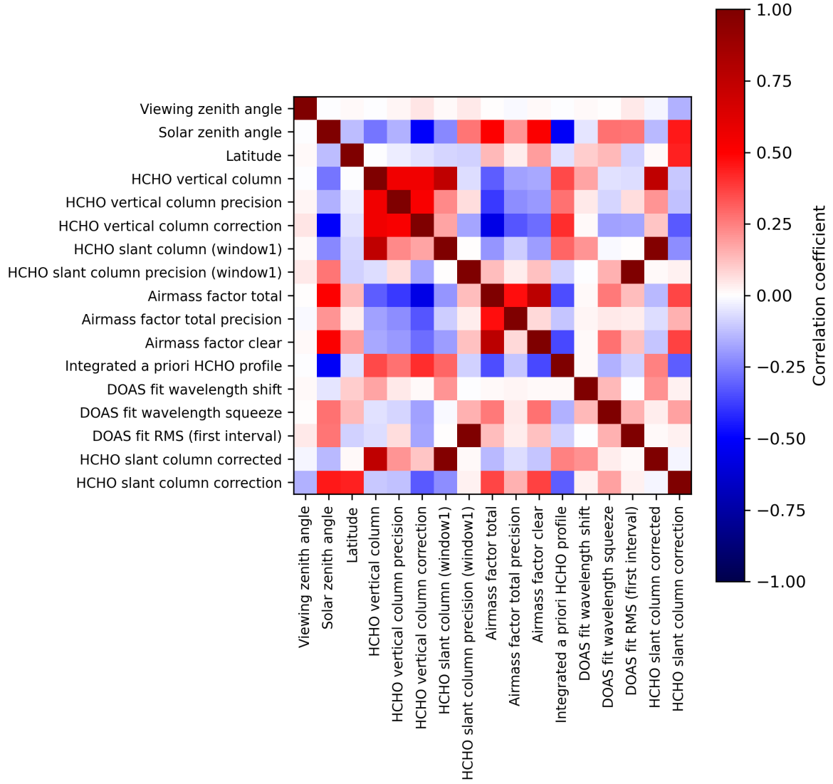
Figure 2: Map of correlation matrix for 2024-04-02 to 2024-04-04.
