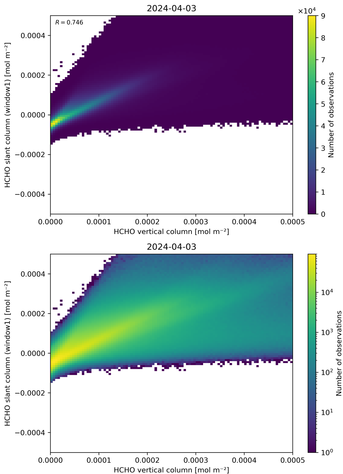
Figure 129: Scatter density plot of “HCHO vertical column” against “HCHO slant column (window1)” for 2024-04-02 to 2024-04-04.
