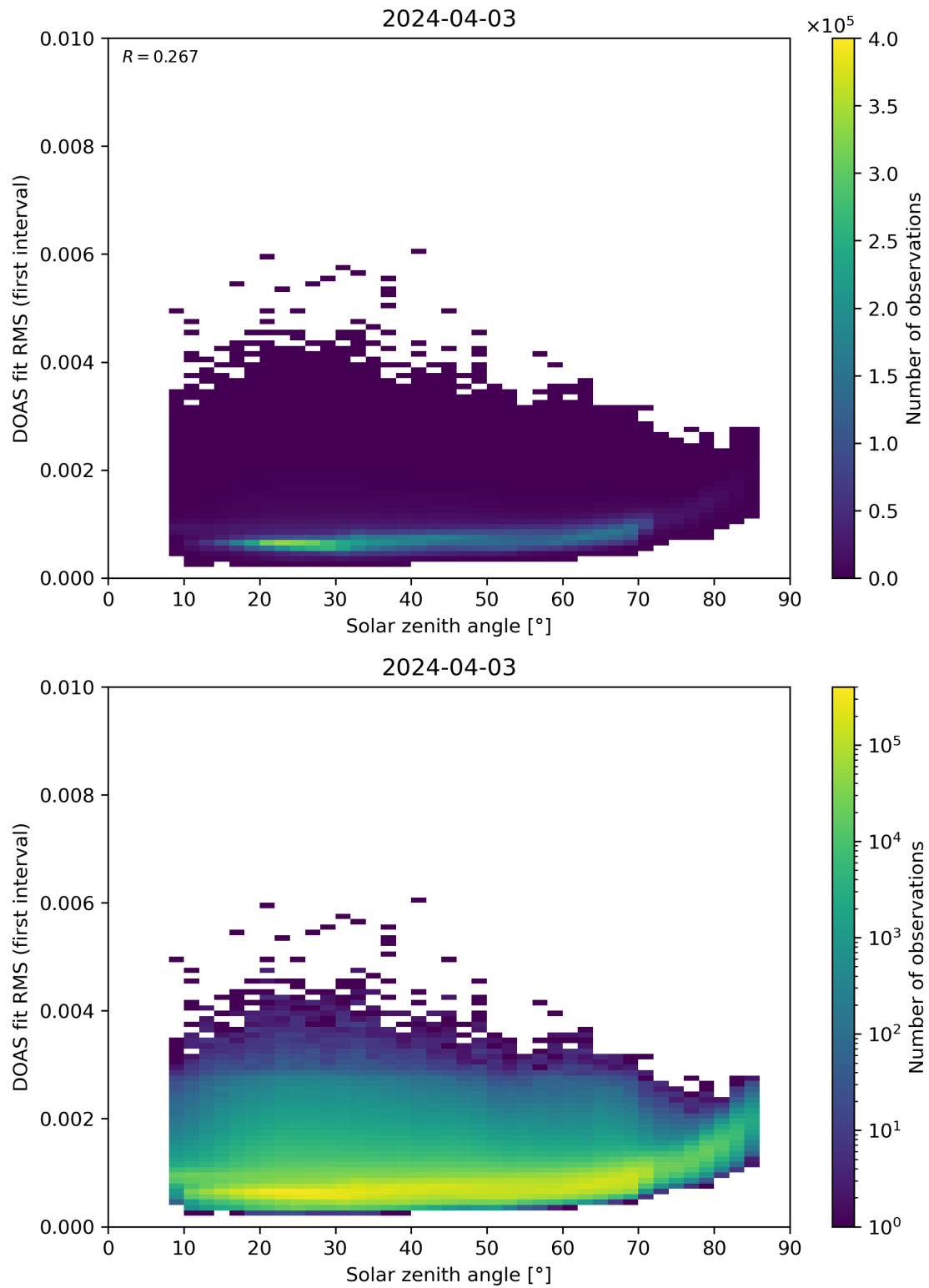
Figure 167: Scatter density plot of “Solar zenith angle” against “DOAS fit RMS (first interval)” for 2024-04-02 to 2024-04-04.
