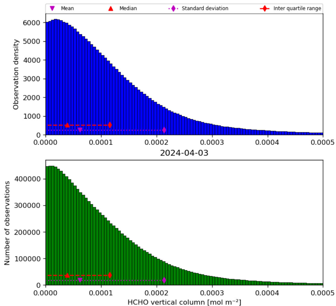
Figure 35: Histogram of “HCHO vertical column” for 2024-04-02 to 2024-04-04
