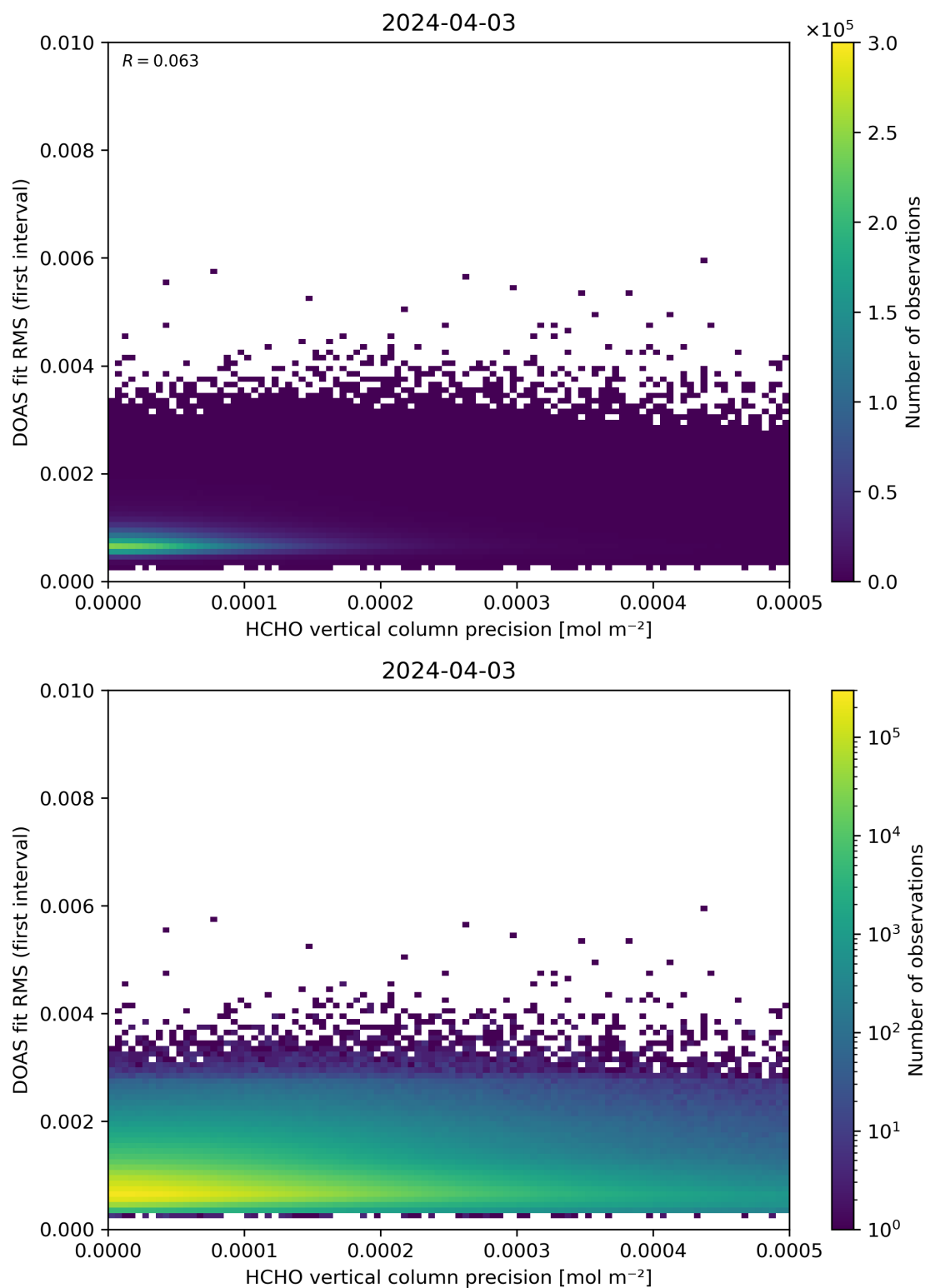
Figure 136: Scatter density plot of “HCHO vertical column precision” against “DOAS fit RMS (first interval)” for 2024-04-02 to 2024-04-04.
