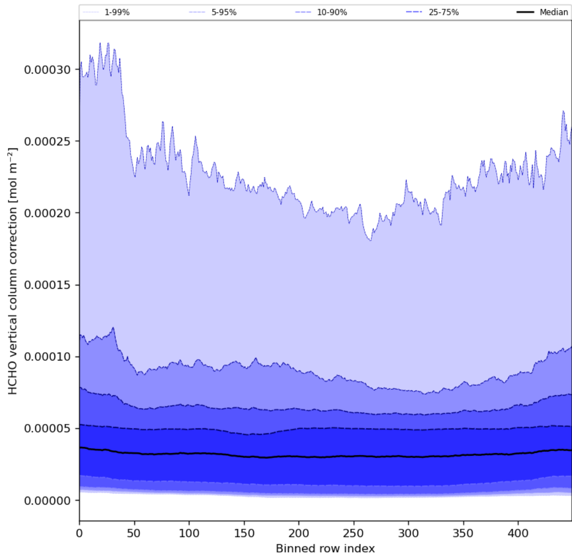
Figure 51: Along track statistics of “HCHO vertical column correction” for 2024-04-02 to 2024-04-04
