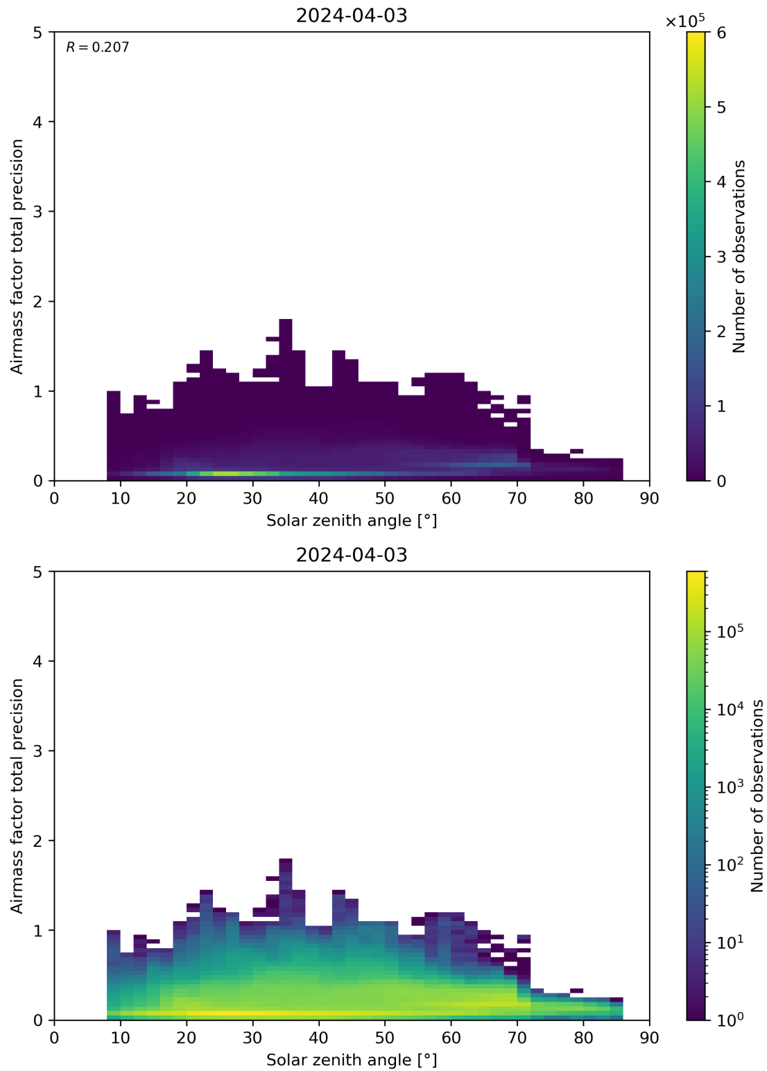
Figure 176: Scatter density plot of “Solar zenith angle” against “Airmass factor total precision” for 2024-04-02 to 2024-04-04.
