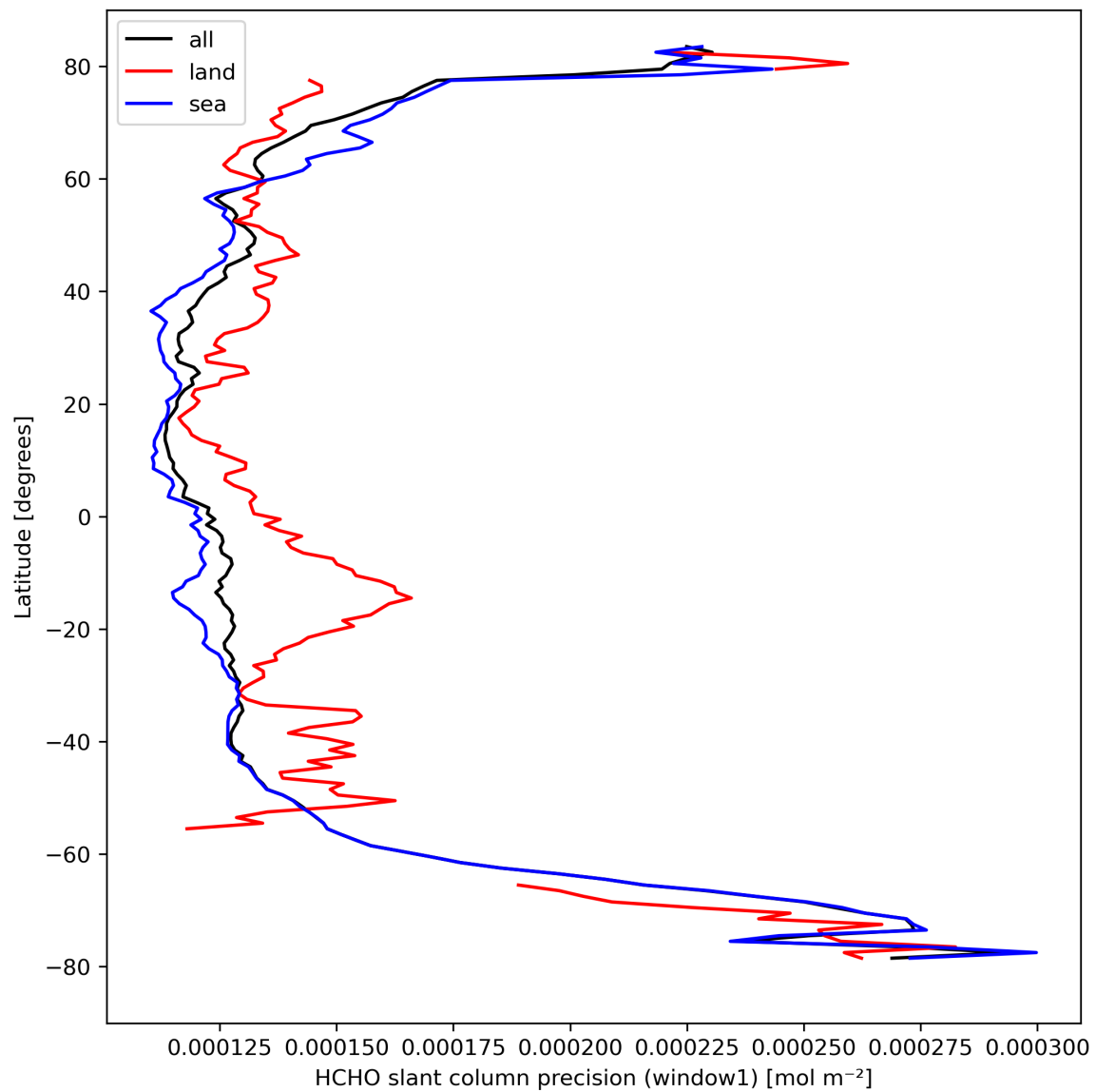
Figure 25: Zonal average of “HCHO slant column precision (window1)” for 2024-04-02 to 2024-04-04.
