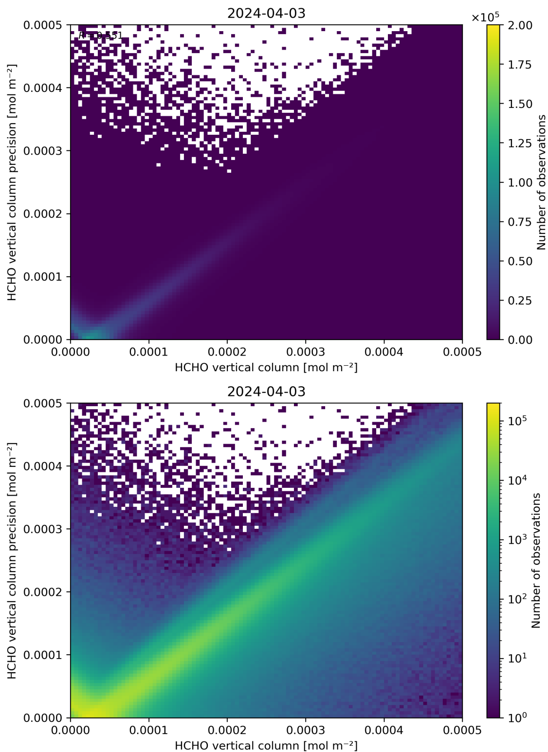
Figure 134: Scatter density plot of “HCHO vertical column” against “HCHO vertical column precision” for 2024-04-02 to 2024-04-04.
