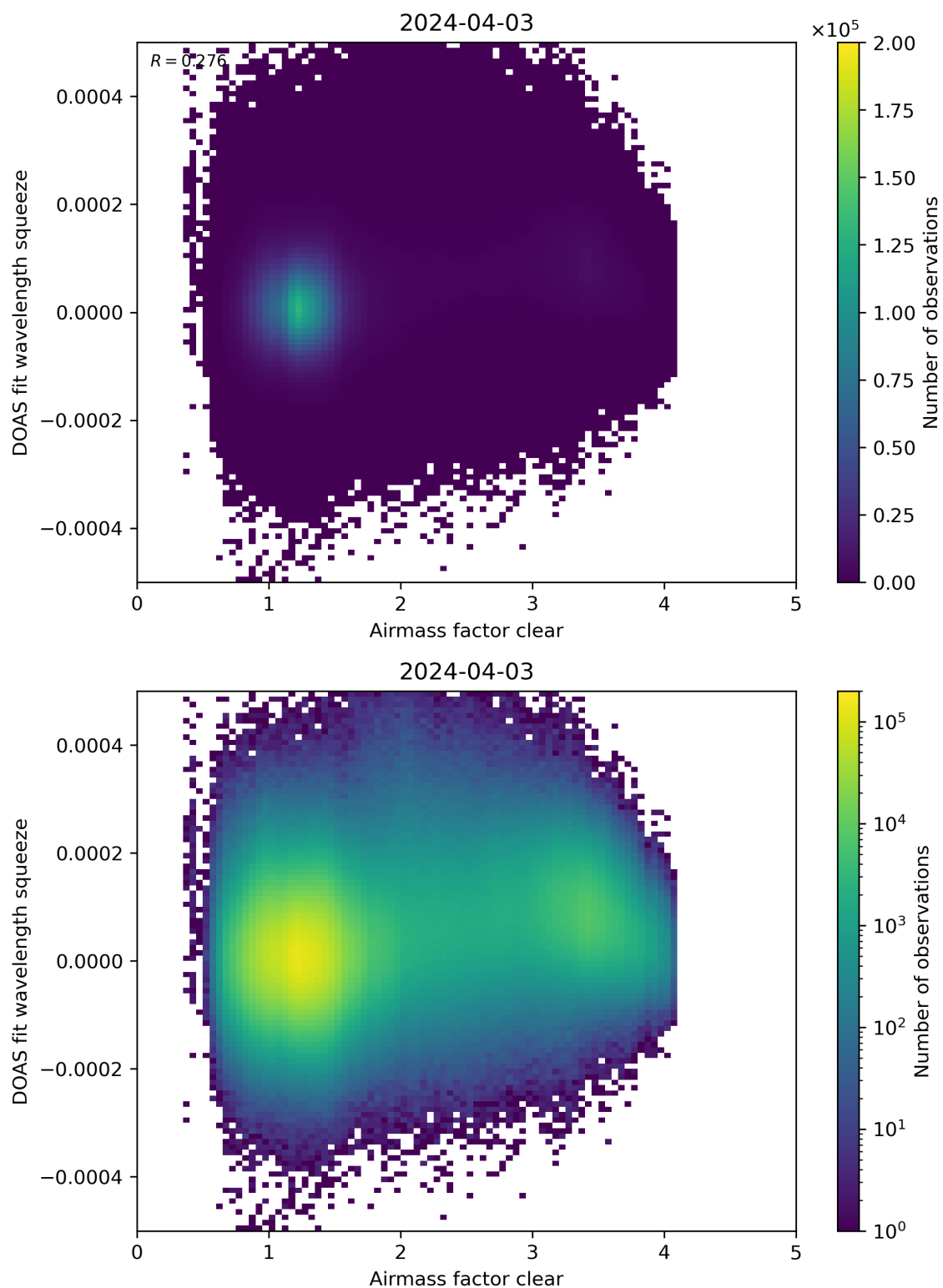
Figure 73: Scatter density plot of “Airmass factor clear” against “DOAS fit wavelength squeeze” for 2024-04-02 to 2024-04-04.
