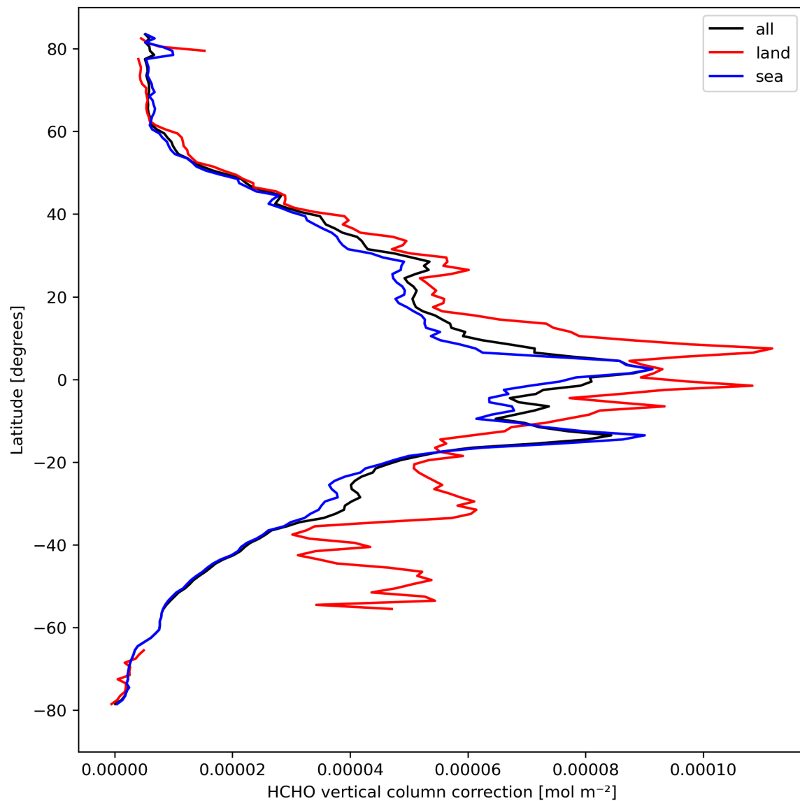
Figure 23: Zonal average of “HCHO vertical column correction” for 2024-04-02 to 2024-04-04.
