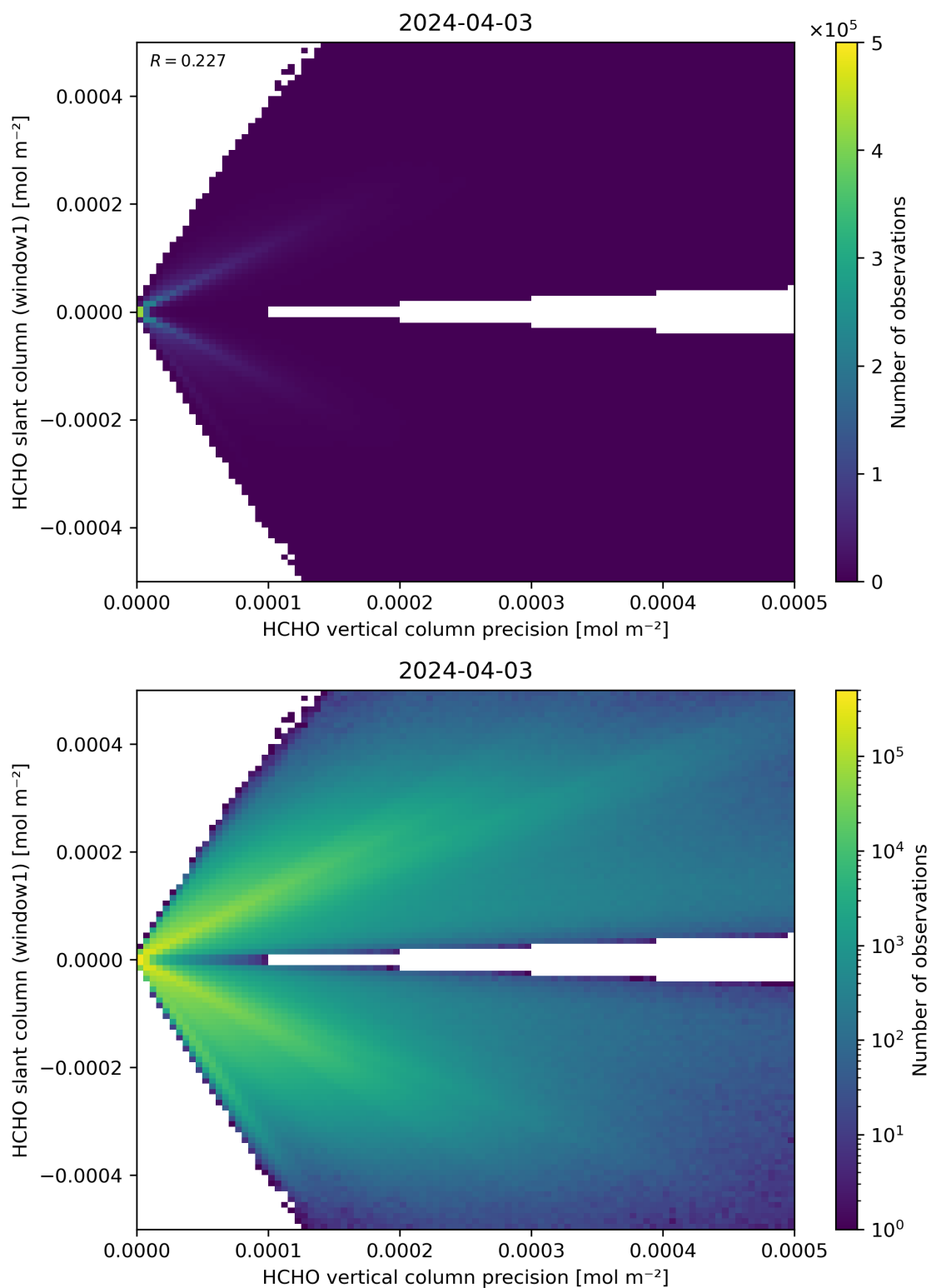
Figure 142: Scatter density plot of “HCHO vertical column precision” against “HCHO slant column (window1)” for 2024-04-02 to 2024-04-04.
