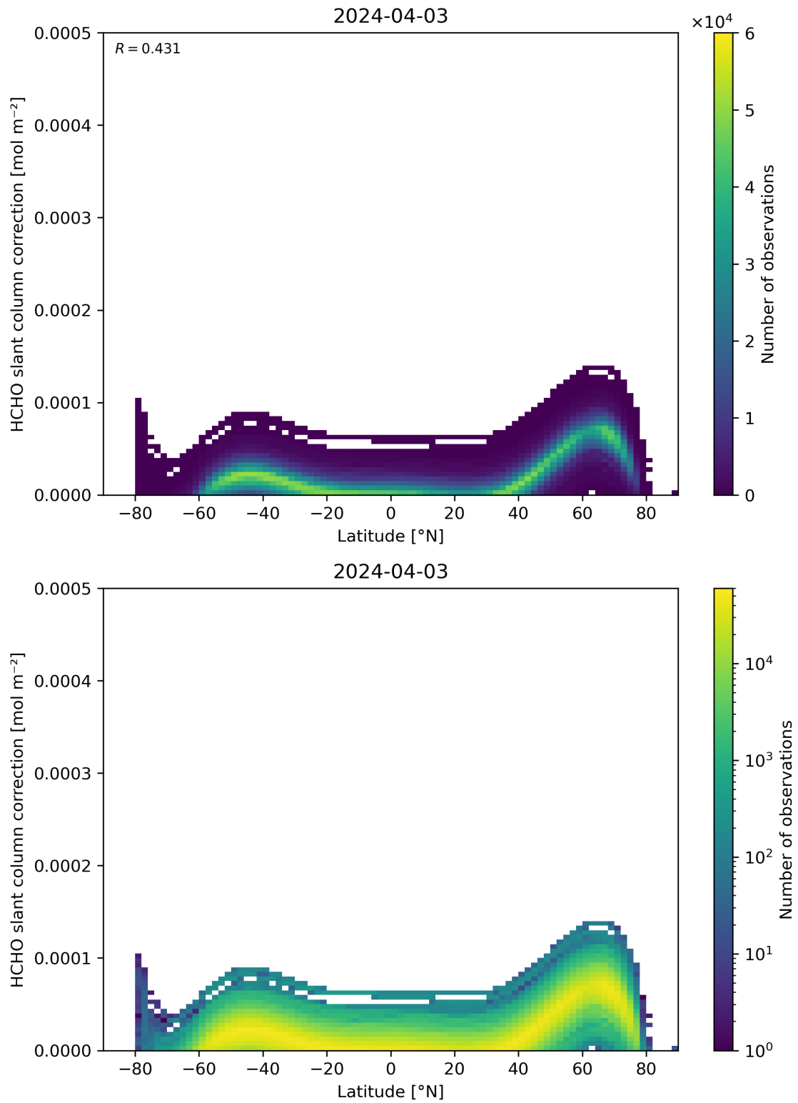
Figure 158: Scatter density plot of “Latitude” against “HCHO slant column correction” for 2024-04-02 to 2024-04-04.
