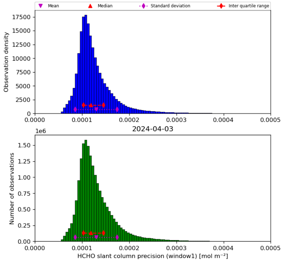
Figure 39: Histogram of “HCHO slant column precision (window1)” for 2024-04-02 to 2024-04-04
