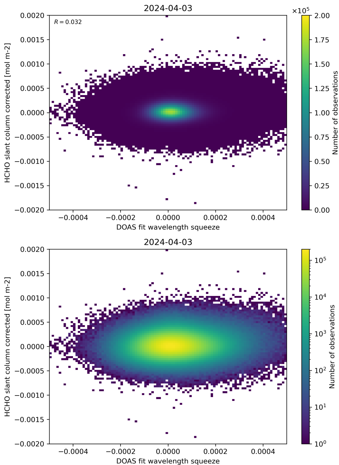
Figure 69: Scatter density plot of “DOAS fit wavelength squeeze” against “HCHO slant column corrected” for 2024-04-02 to 2024-04-04.
