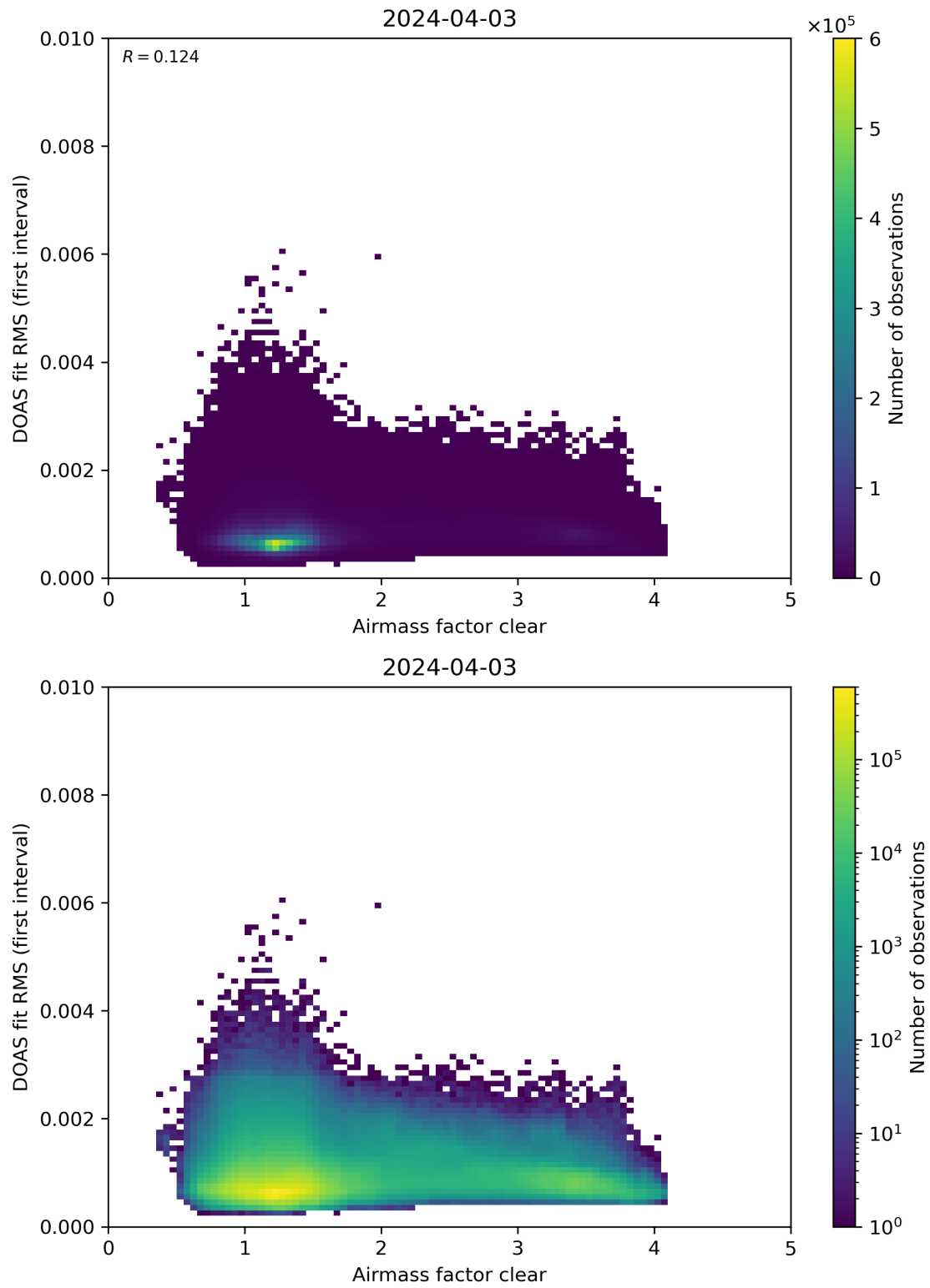
Figure 71: Scatter density plot of “Airmass factor clear” against “DOAS fit RMS (first interval)” for 2024-04-02 to 2024-04-04.
