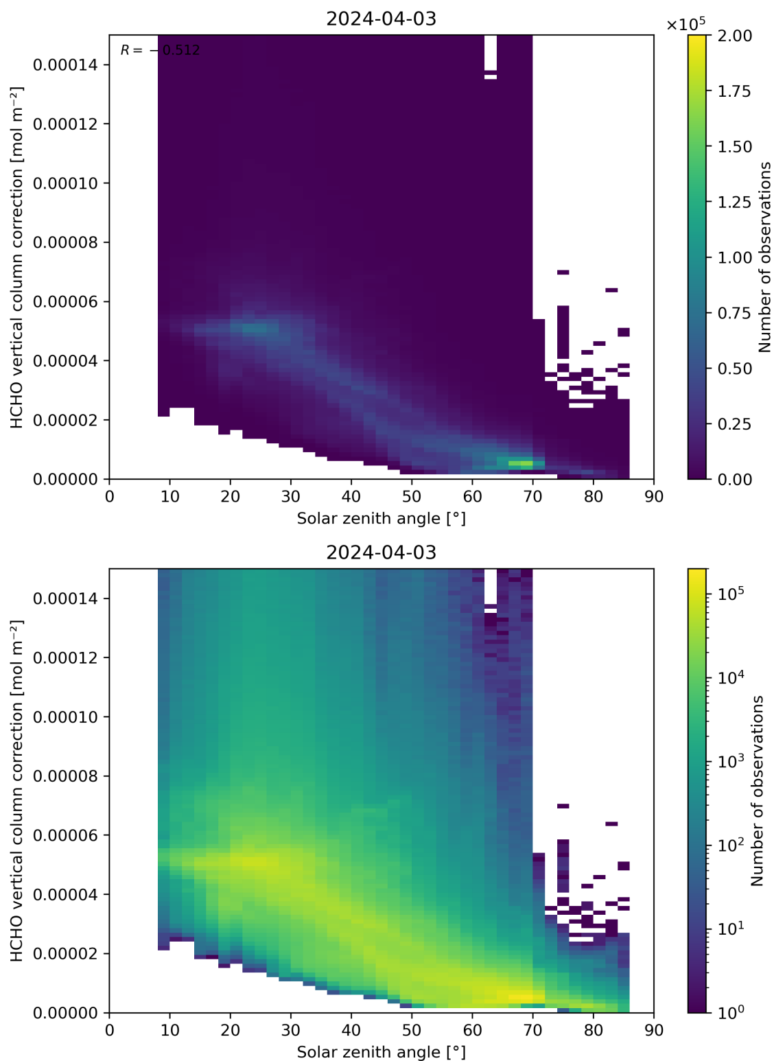
Figure 178: Scatter density plot of “Solar zenith angle” against “HCHO vertical column correction” for 2024-04-02 to 2024-04-04.
