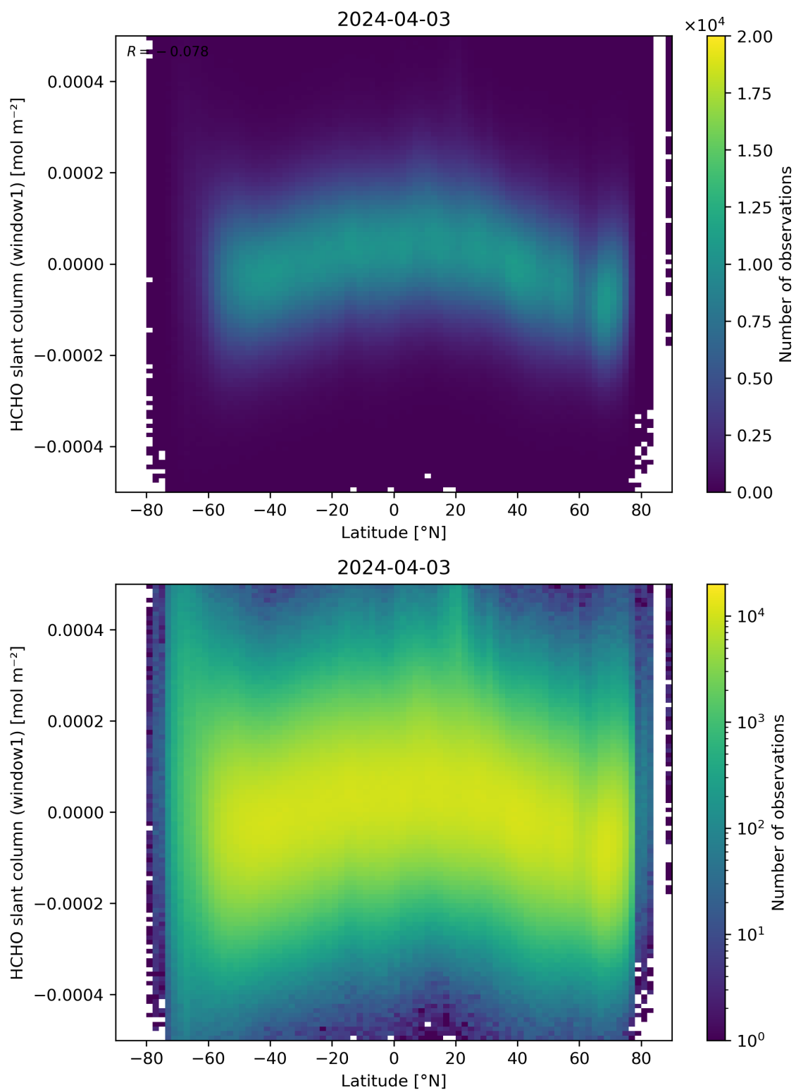
Figure 159: Scatter density plot of “Latitude” against “HCHO slant column (window1)” for 2024-04-02 to 2024-04-04.
