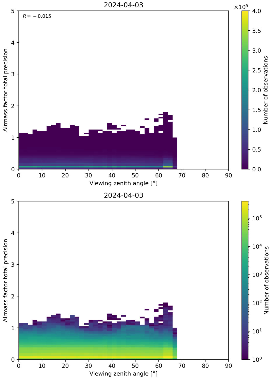
Figure 191: Scatter density plot of “Viewing zenith angle” against “Airmass factor total precision” for 2024-04-02 to 2024-04-04.
