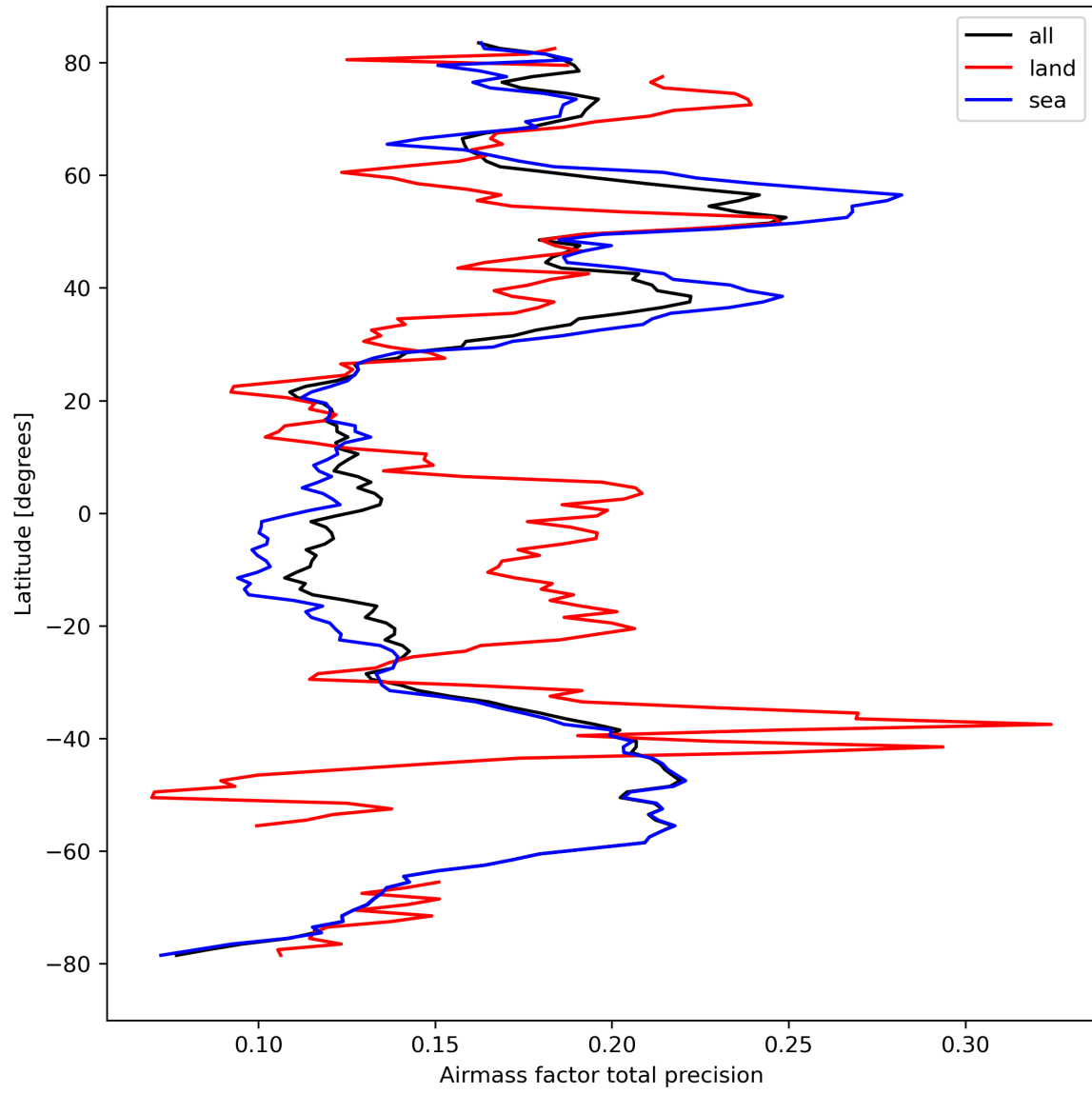
Figure 27: Zonal average of “Airmass factor total precision” for 2024-04-02 to 2024-04-04.
