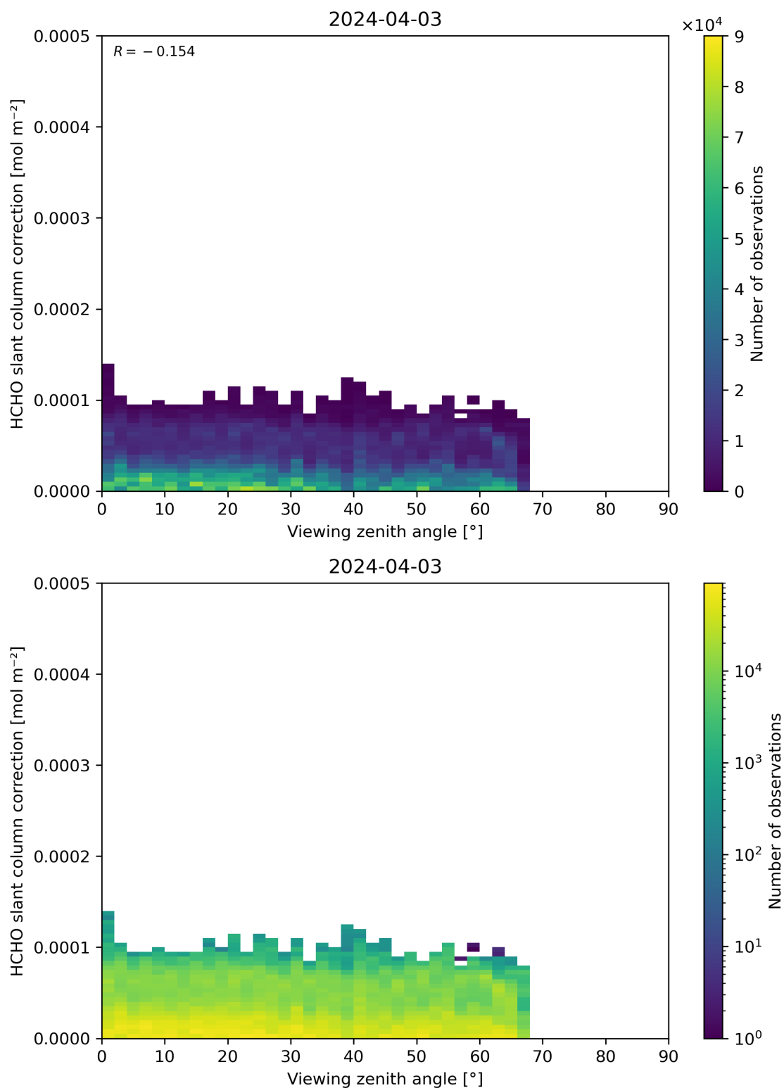
Figure 187: Scatter density plot of “Viewing zenith angle” against “HCHO slant column correction” for 2024-04-02 to 2024-04-04.
