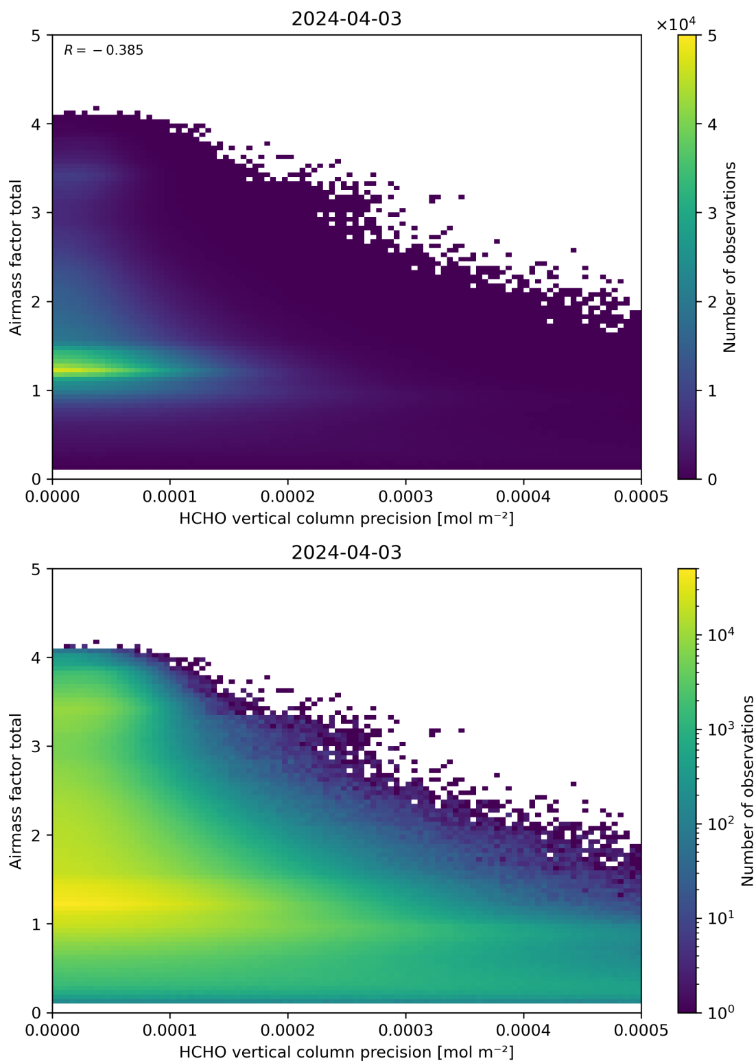
Figure 144: Scatter density plot of “HCHO vertical column precision” against “Airmass factor total” for 2024-04-02 to 2024-04-04.
