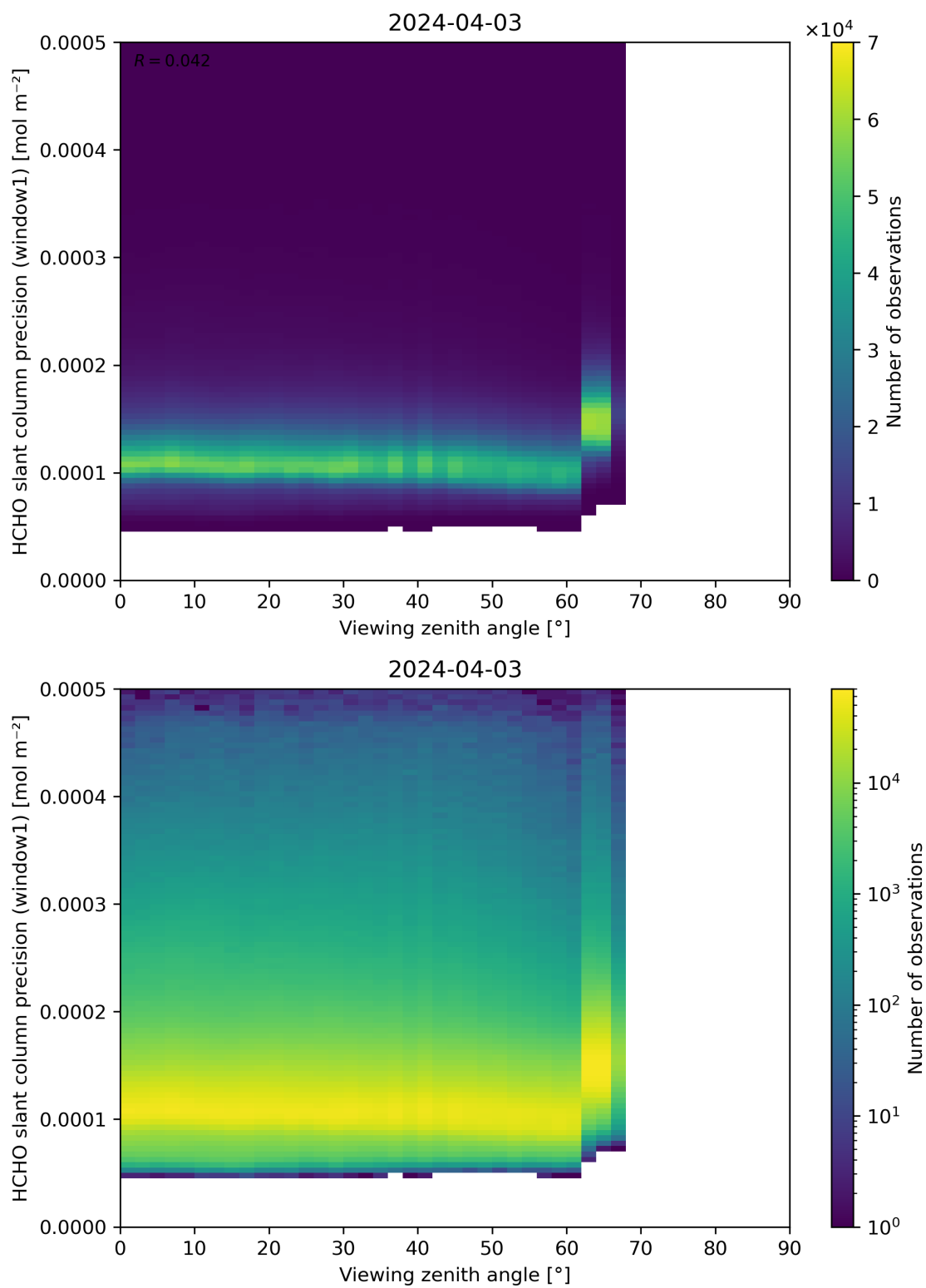
Figure 189: Scatter density plot of “Viewing zenith angle” against “HCHO slant column precision (window1)” for 2024-04-02 to 2024-04-04.
