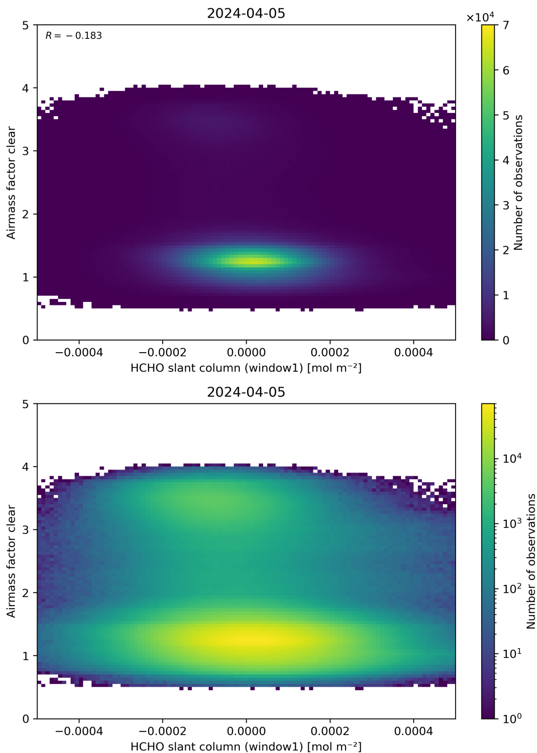
Figure 81: Scatter density plot of “HCHO slant column (window1)” against “Airmass factor clear” for 2024-04-05 to 2024-04-06.
