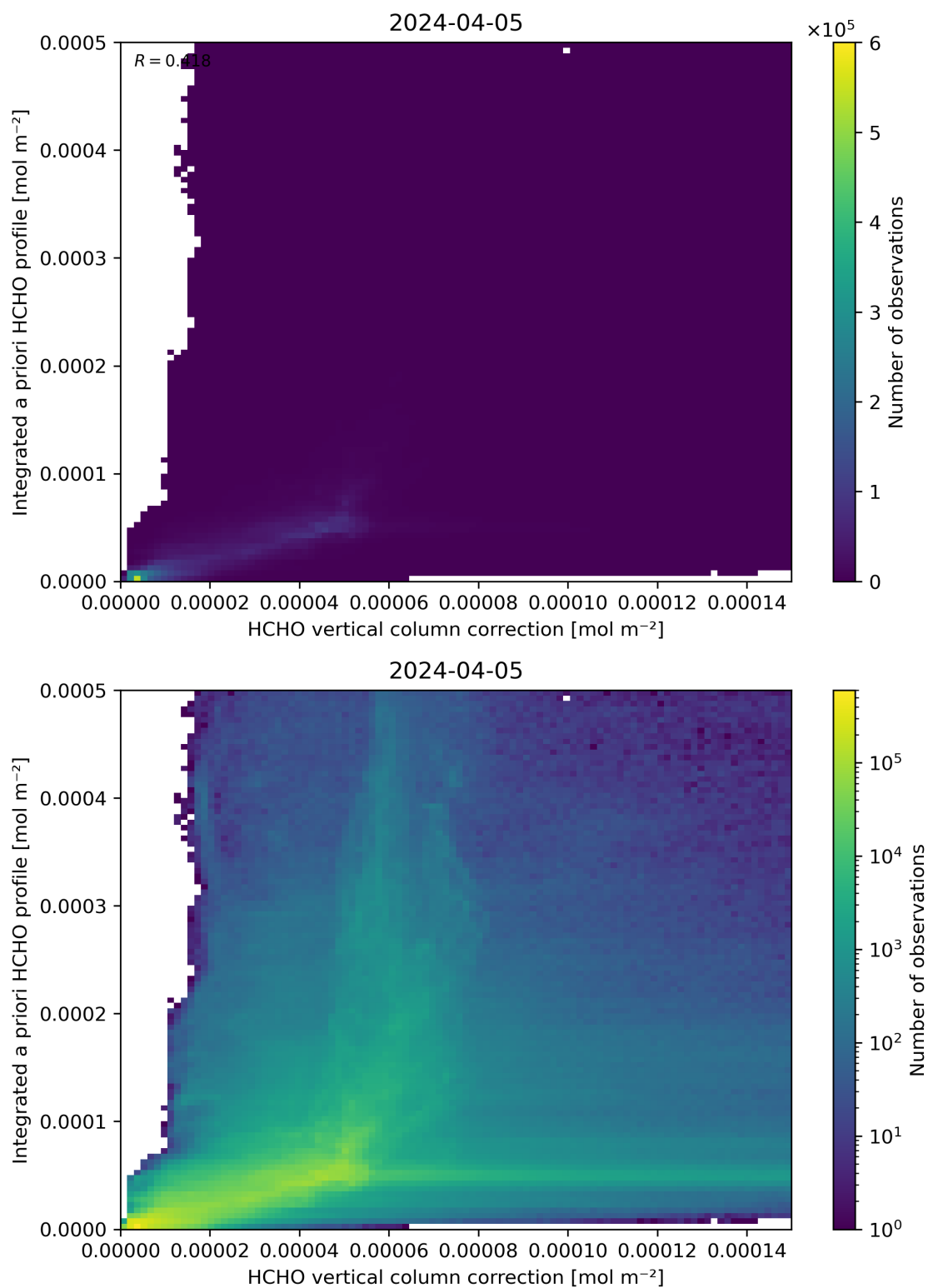
Figure 122: Scatter density plot of “HCHO vertical column correction” against “Integrated a priori HCHO profile” for 2024-04-05 to 2024-04-06.
