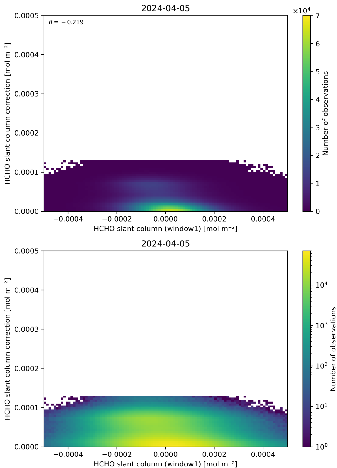
Figure 83: Scatter density plot of “HCHO slant column (window1)” against “HCHO slant column correction” for 2024-04-05 to 2024-04-06.
