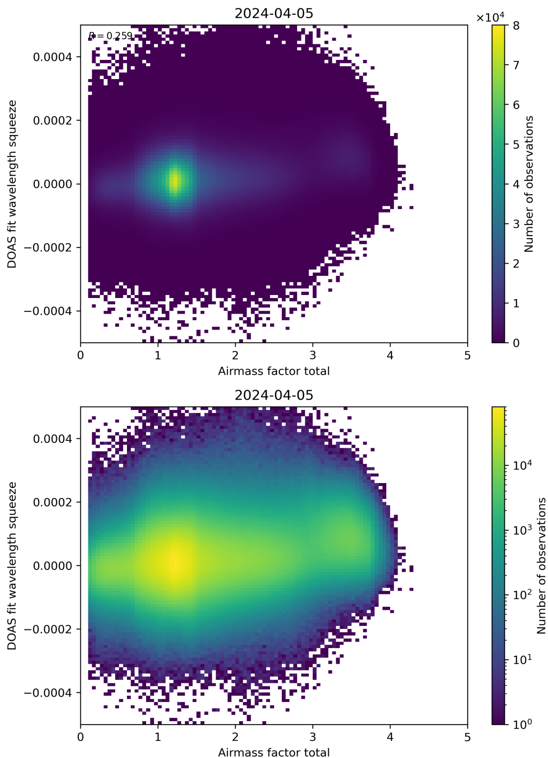
Figure 99: Scatter density plot of “Airmass factor total” against “DOAS fit wavelength squeeze” for 2024-04-05 to 2024-04-06.
