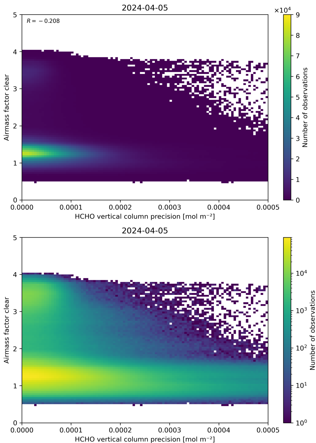
Figure 139: Scatter density plot of “HCHO vertical column precision” against “Airmass factor clear” for 2024-04-05 to 2024-04-06.
