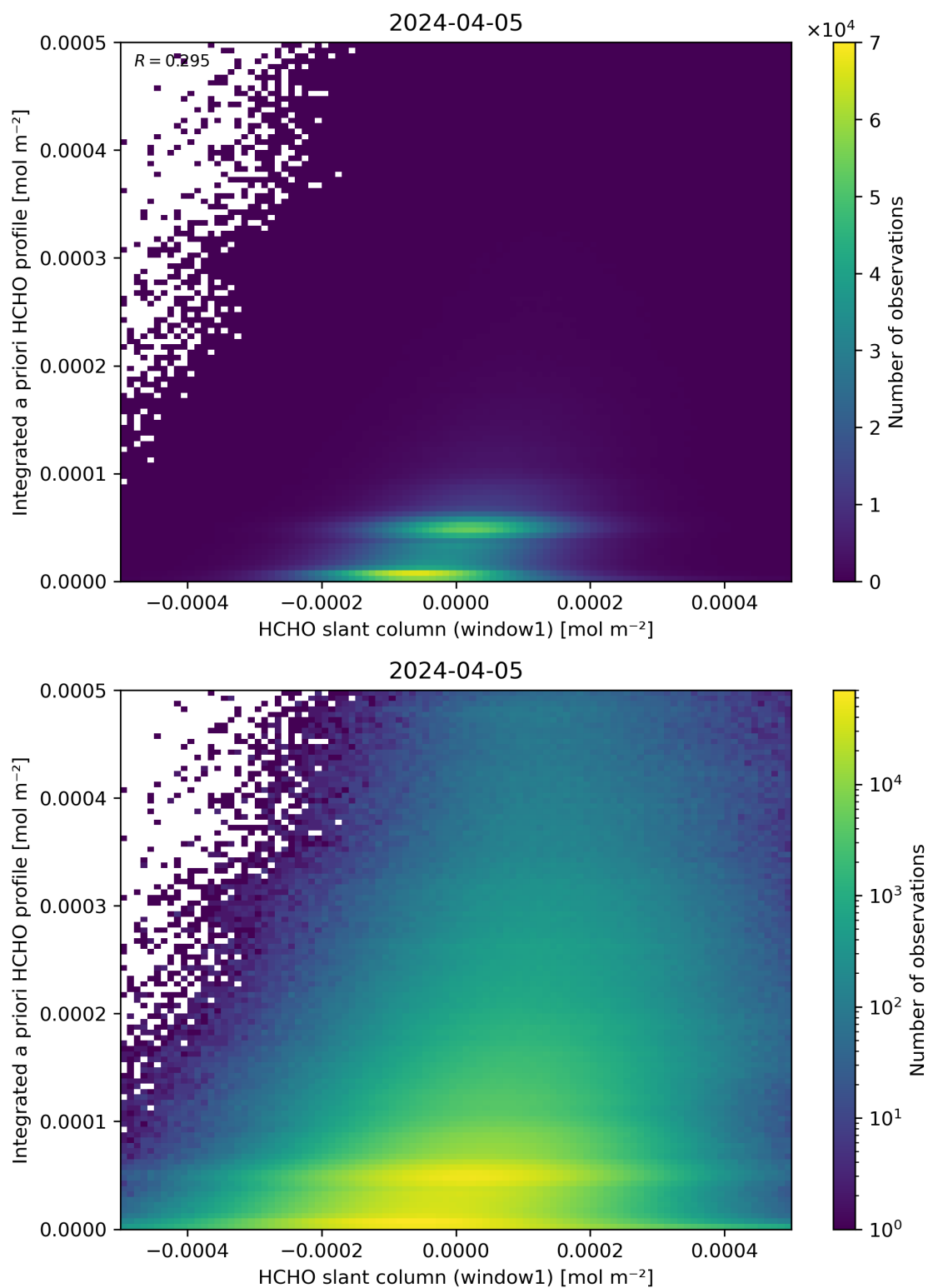
Figure 87: Scatter density plot of “HCHO slant column (window1)” against “Integrated a priori HCHO profile” for 2024-04-05 to 2024-04-06.
