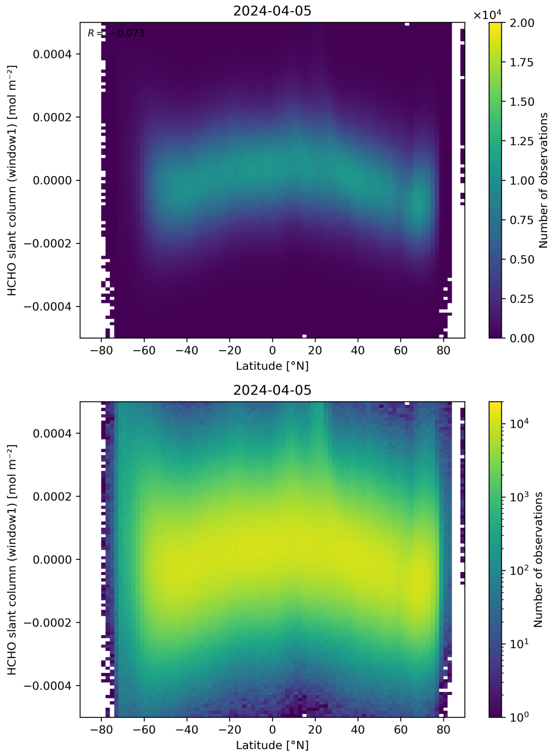
Figure 159: Scatter density plot of “Latitude” against “HCHO slant column (window1)” for 2024-04-05 to 2024-04-06.
