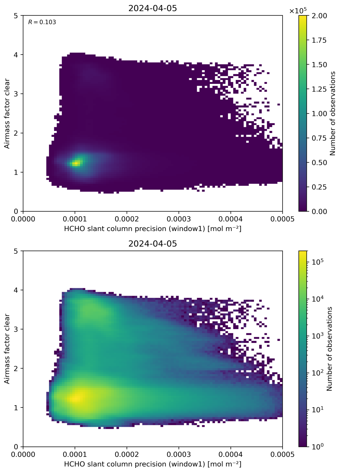
Figure 91: Scatter density plot of “HCHO slant column precision (window1)” against “Airmass factor clear” for 2024-04-05 to 2024-04-06.
