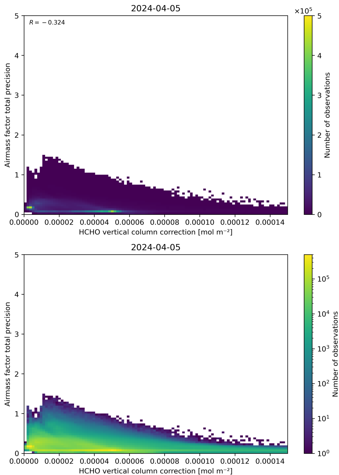
Figure 121: Scatter density plot of “HCHO vertical column correction” against “Airmass factor total precision” for 2024-04-05 to 2024-04-06.
