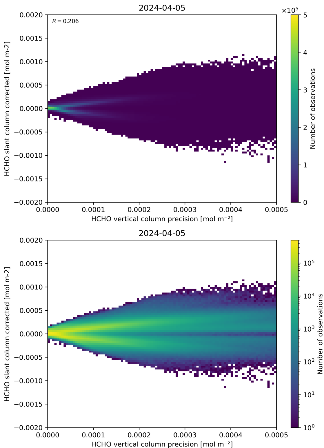
Figure 140: Scatter density plot of “HCHO vertical column precision” against “HCHO slant column corrected” for 2024-04-05 to 2024-04-06.
