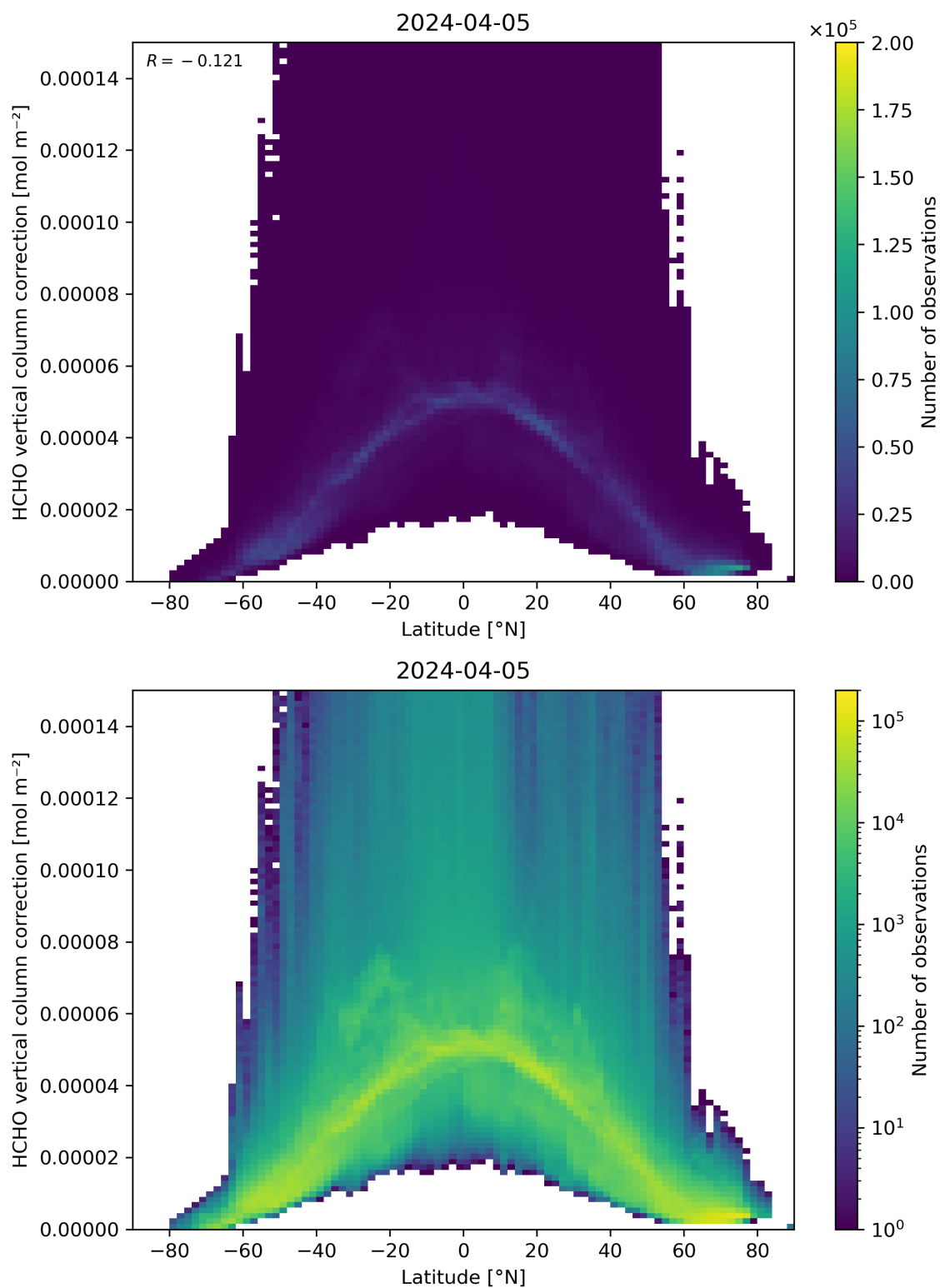
Figure 164: Scatter density plot of “Latitude” against “HCHO vertical column correction” for 2024-04-05 to 2024-04-06.
