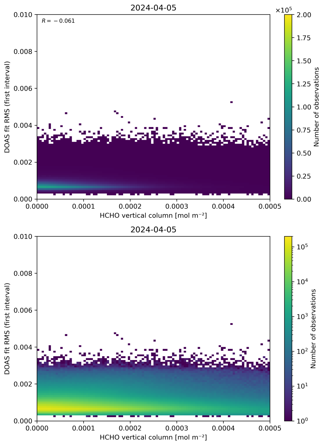
Figure 123: Scatter density plot of “HCHO vertical column” against “DOAS fit RMS (first interval)” for 2024-04-05 to 2024-04-06.
