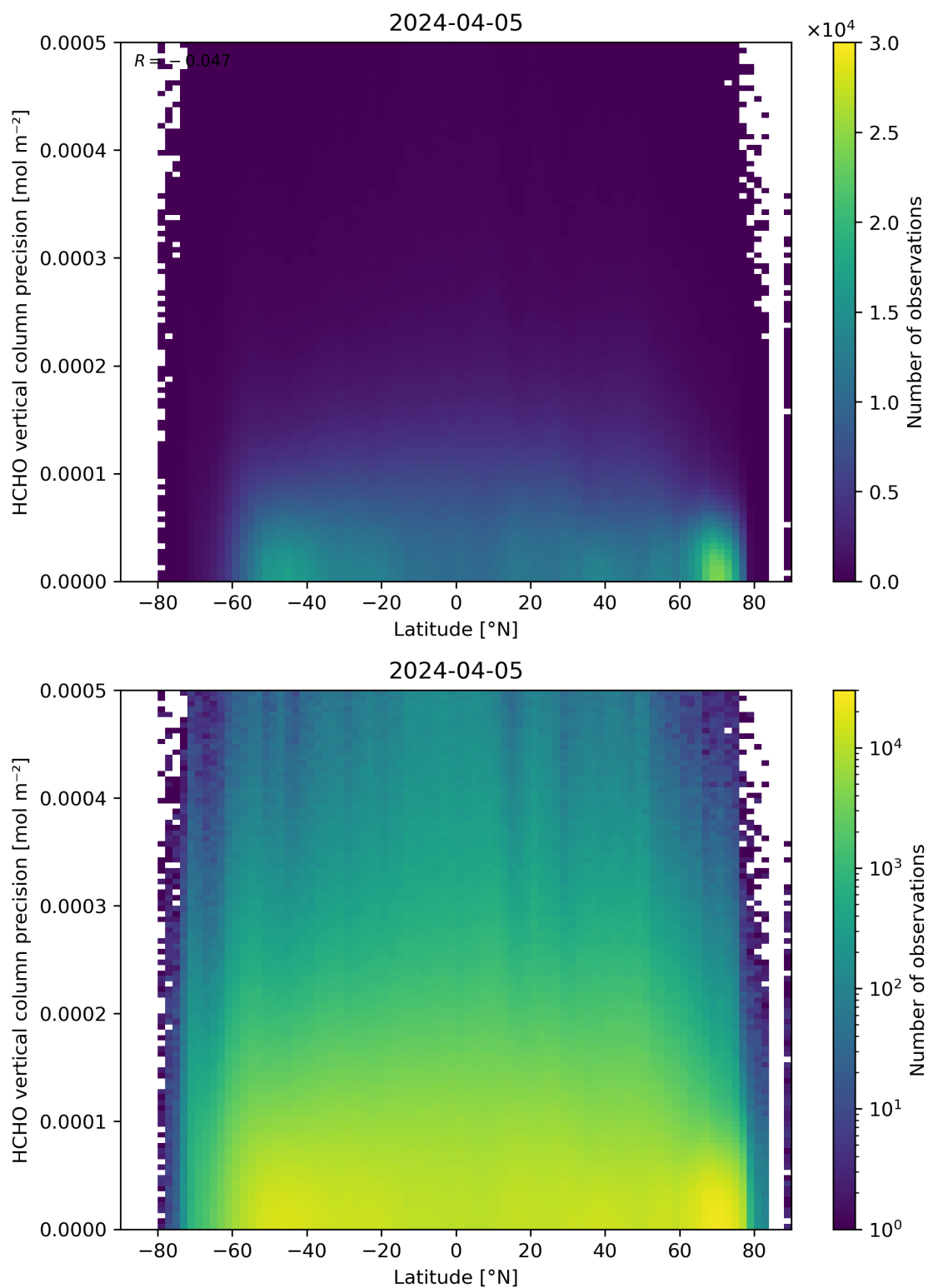
Figure 165: Scatter density plot of “Latitude” against “HCHO vertical column precision” for 2024-04-05 to 2024-04-06.
