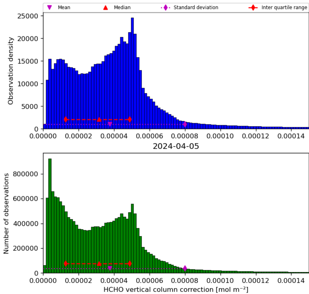
Figure 37: Histogram of “HCHO vertical column correction” for 2024-04-05 to 2024-04-06
