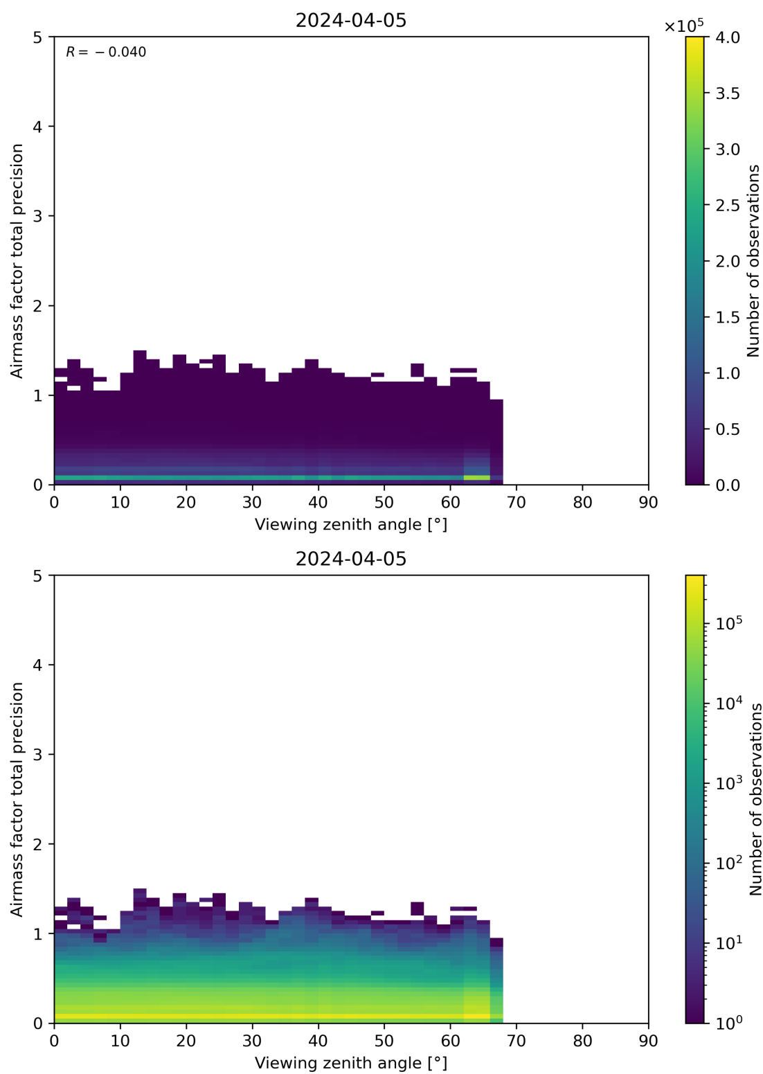
Figure 191: Scatter density plot of “Viewing zenith angle” against “Airmass factor total precision” for 2024-04-05 to 2024-04-06.
