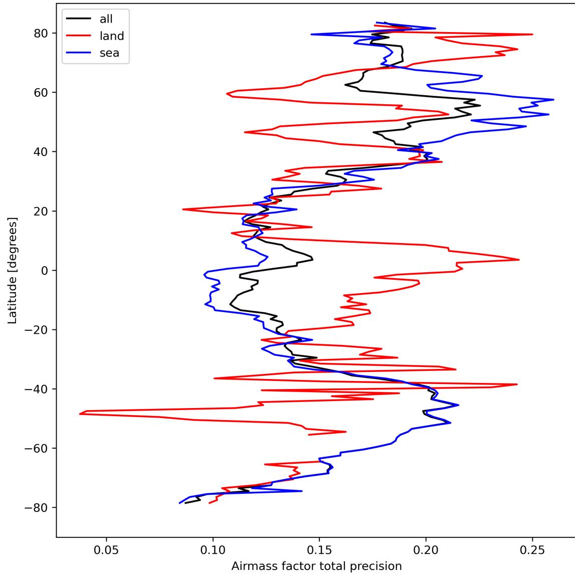
Figure 27: Zonal average of “Airmass factor total precision” for 2024-04-05 to 2024-04-06.
