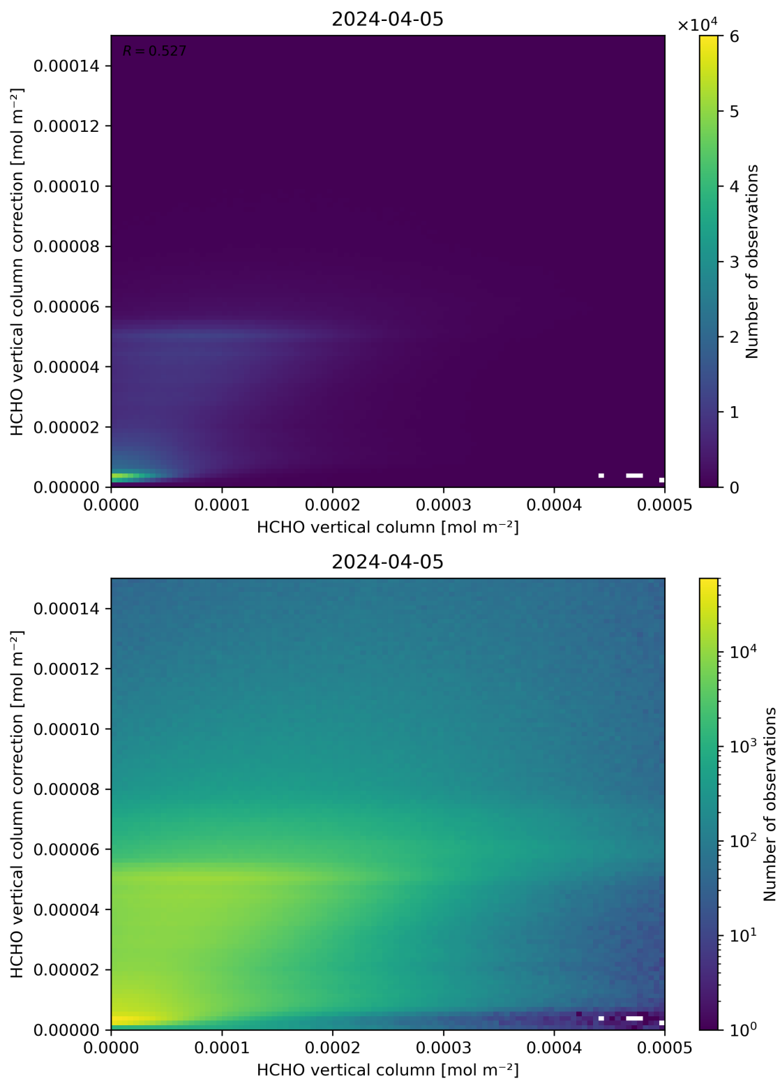
Figure 133: Scatter density plot of “HCHO vertical column” against “HCHO vertical column correction” for 2024-04-05 to 2024-04-06.
