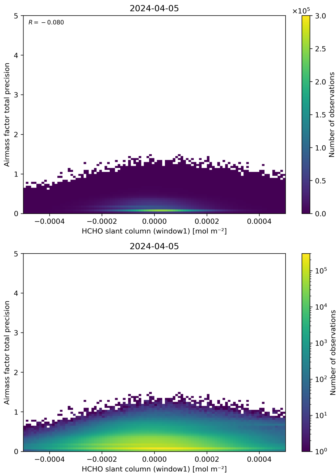
Figure 86: Scatter density plot of “HCHO slant column (window1)” against “Airmass factor total precision” for 2024-04-05 to 2024-04-06.
