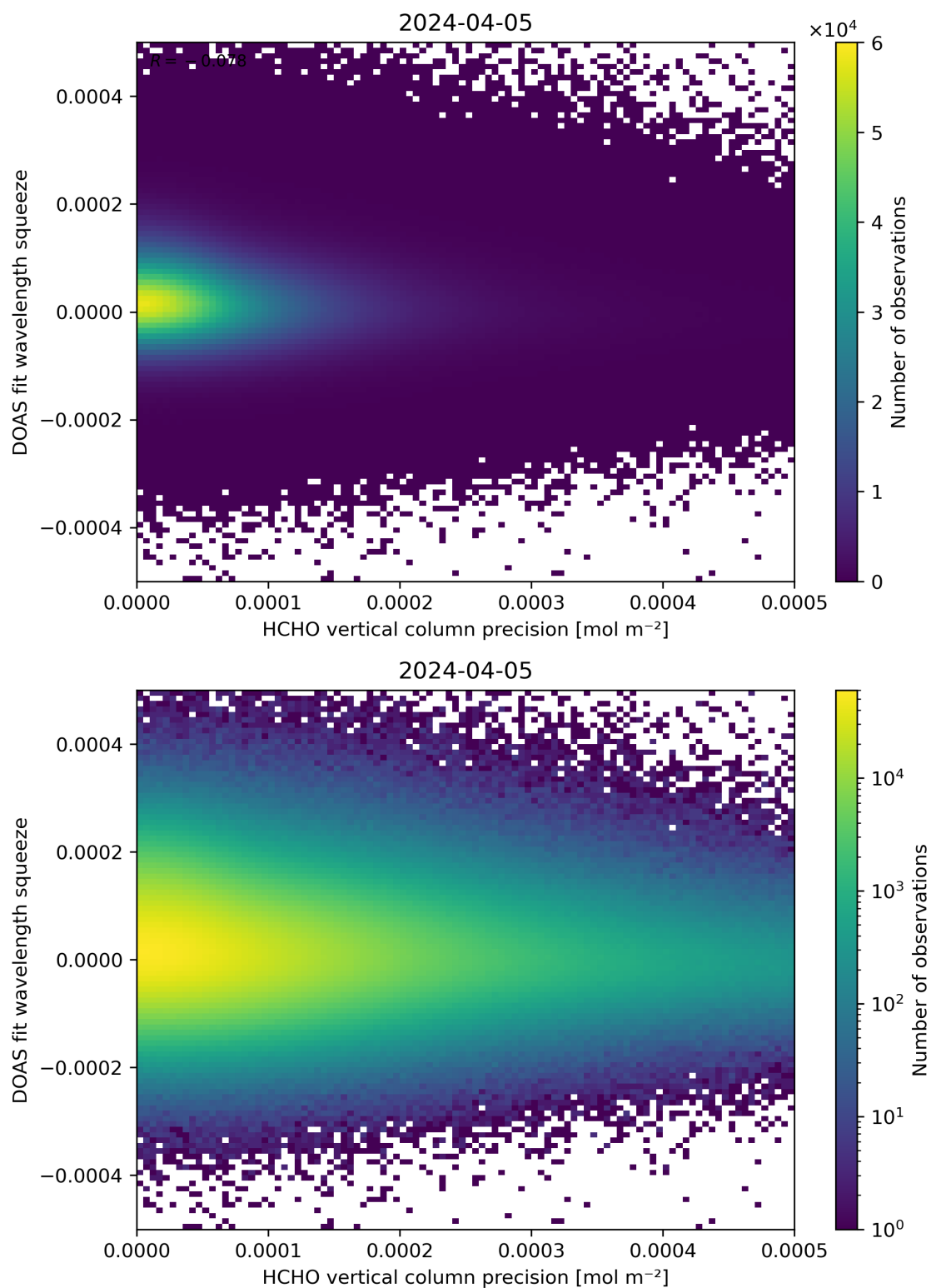
Figure 138: Scatter density plot of “HCHO vertical column precision” against “DOAS fit wavelength squeeze” for 2024-04-05 to 2024-04-06.
