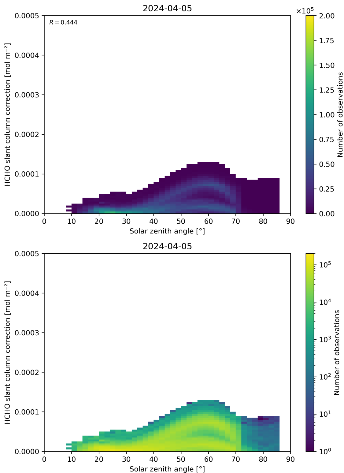
Figure 172: Scatter density plot of “Solar zenith angle” against “HCHO slant column correction” for 2024-04-05 to 2024-04-06.
