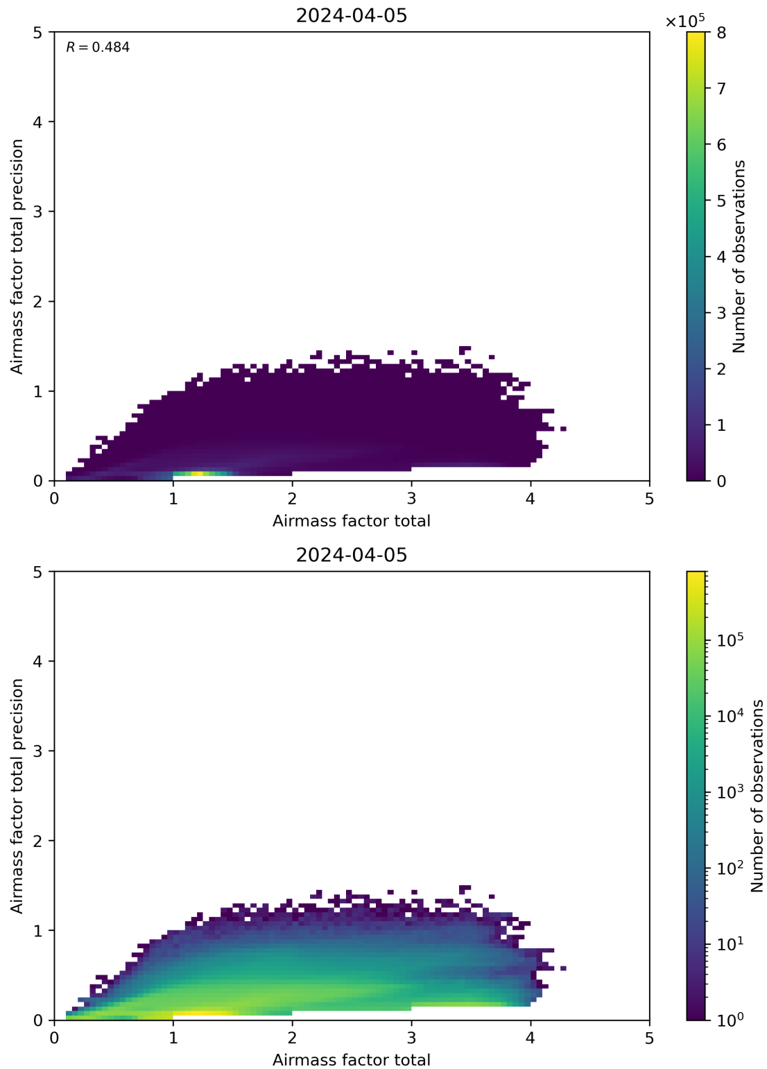
Figure 103: Scatter density plot of “Airmass factor total” against “Airmass factor total precision” for 2024-04-05 to 2024-04-06.
