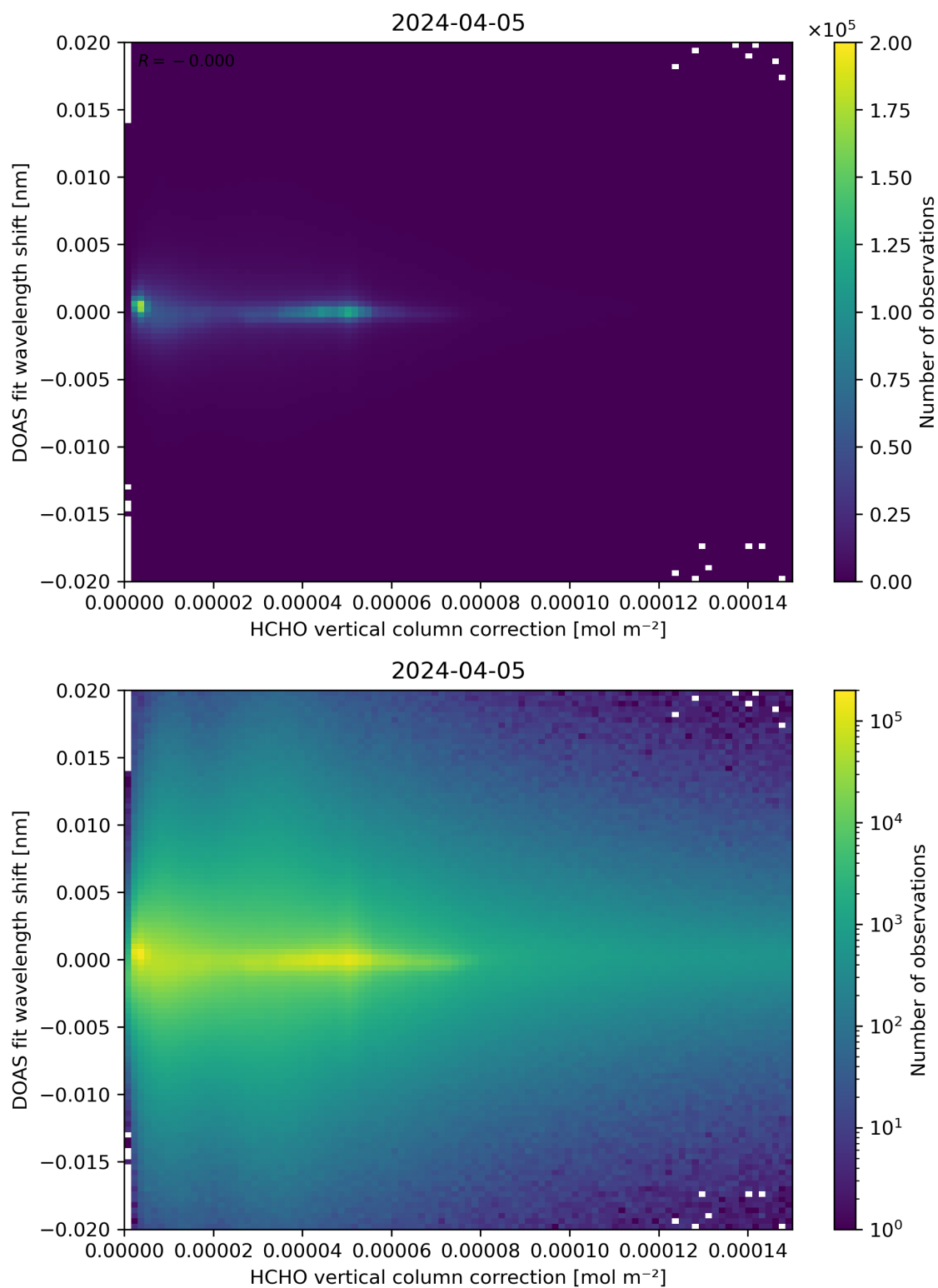
Figure 113: Scatter density plot of “HCHO vertical column correction” against “DOAS fit wavelength shift” for 2024-04-05 to 2024-04-06.
