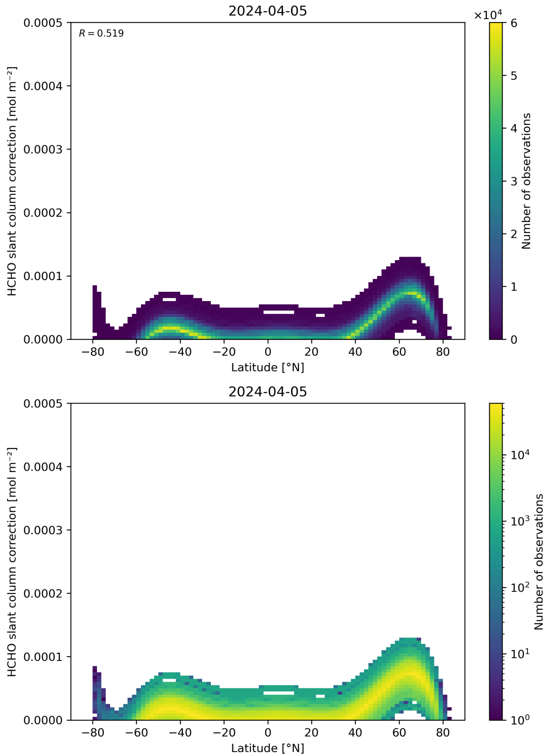
Figure 158: Scatter density plot of “Latitude” against “HCHO slant column correction” for 2024-04-05 to 2024-04-06.
