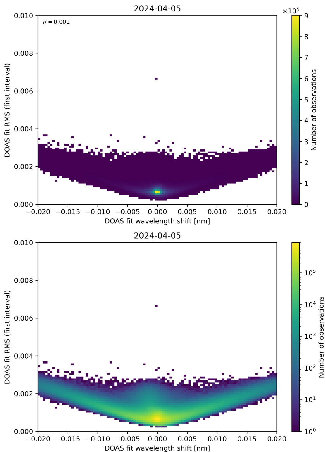
Figure 64: Scatter density plot of “DOAS fit wavelength shift” against “DOAS fit RMS (first interval)” for 2024-04-05 to 2024-04-06.
