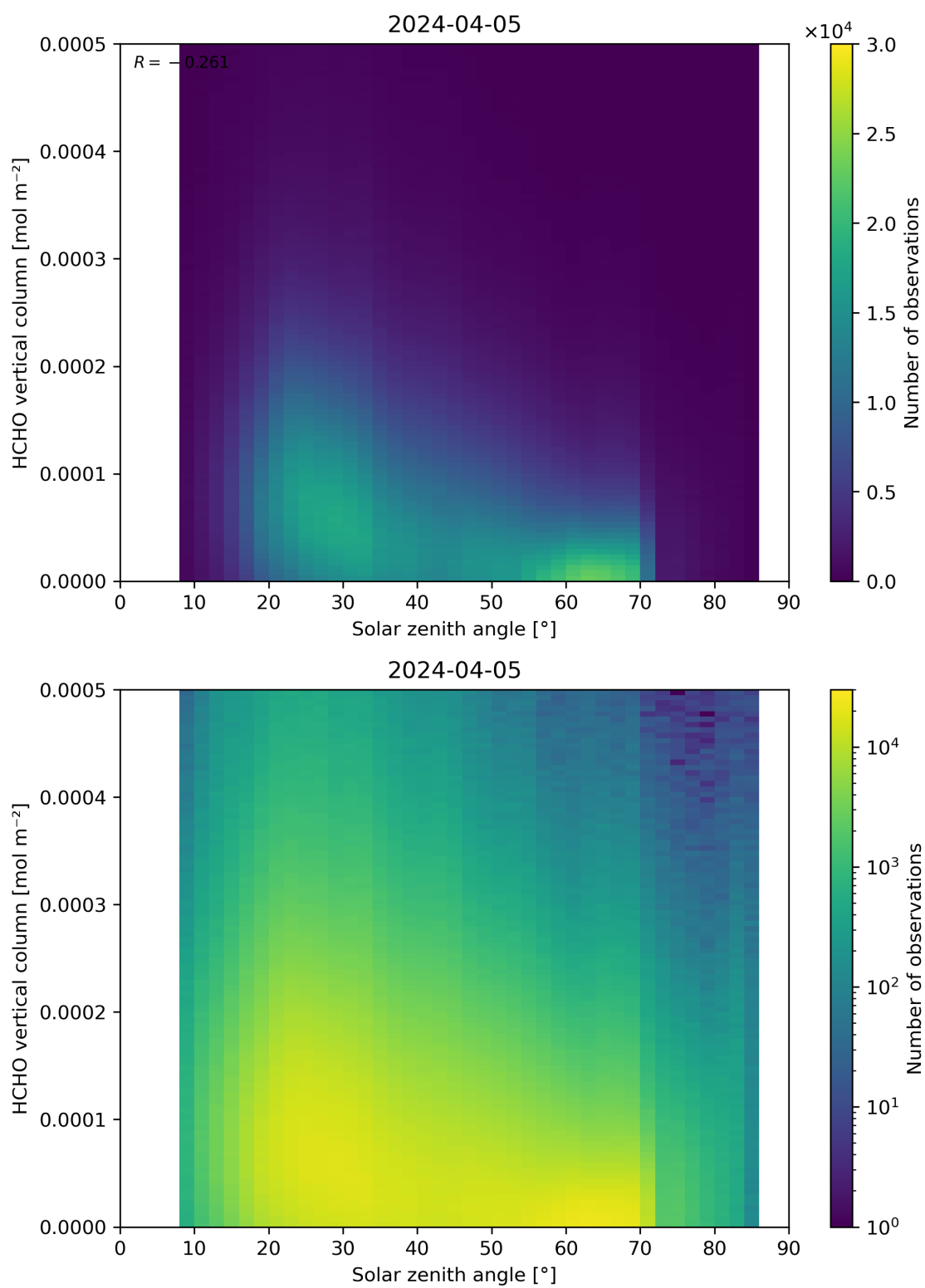
Figure 177: Scatter density plot of “Solar zenith angle” against “HCHO vertical column” for 2024-04-05 to 2024-04-06.
