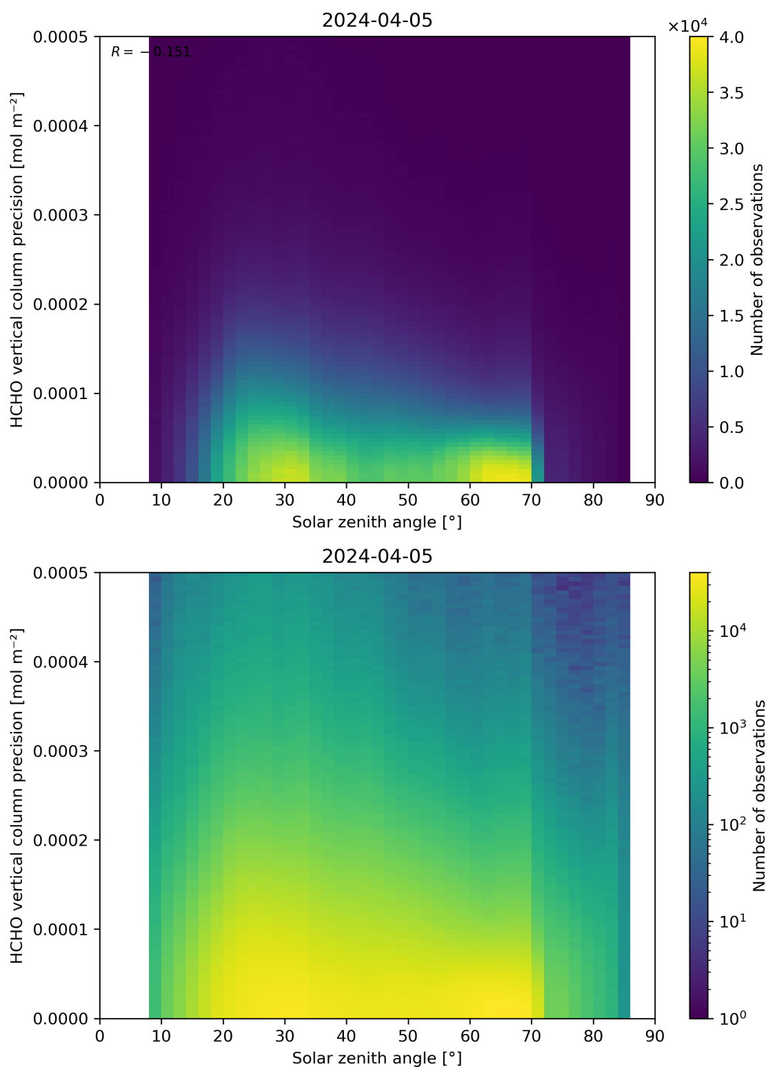
Figure 179: Scatter density plot of “Solar zenith angle” against “HCHO vertical column precision” for 2024-04-05 to 2024-04-06.
