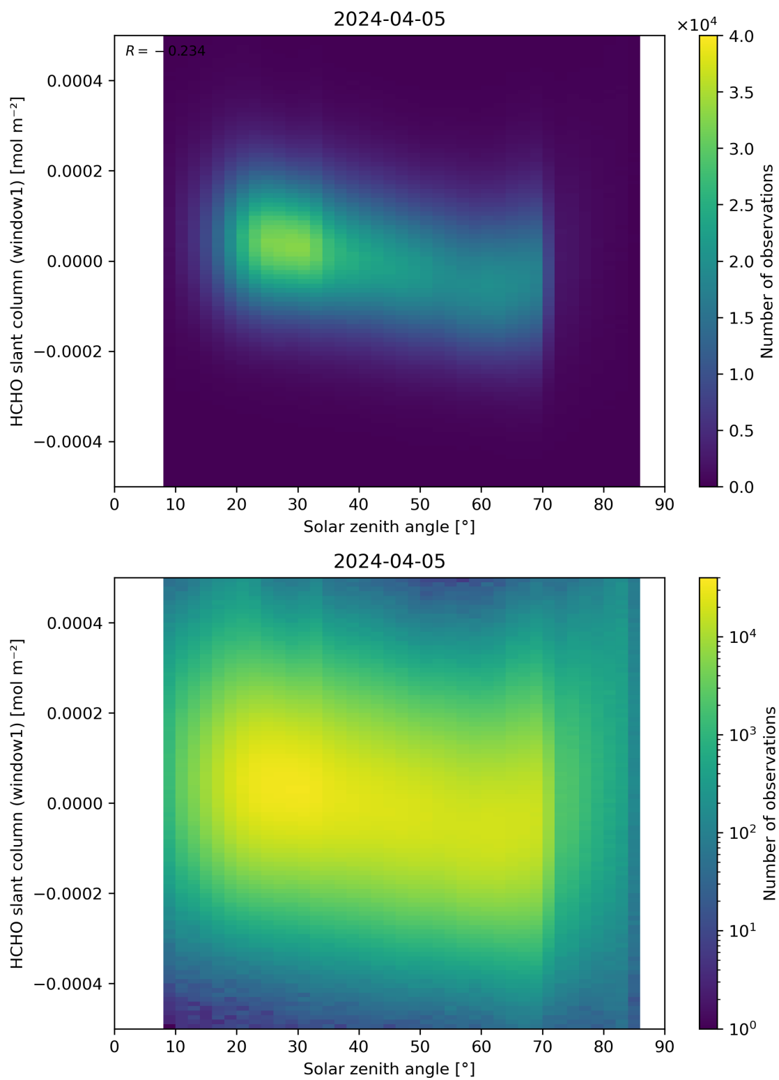
Figure 173: Scatter density plot of “Solar zenith angle” against “HCHO slant column (window1)” for 2024-04-05 to 2024-04-06.
