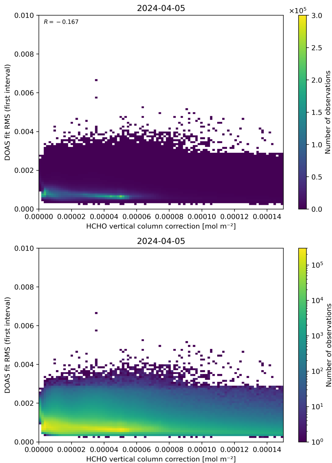
Figure 112: Scatter density plot of “HCHO vertical column correction” against “DOAS fit RMS (first interval)” for 2024-04-05 to 2024-04-06.
