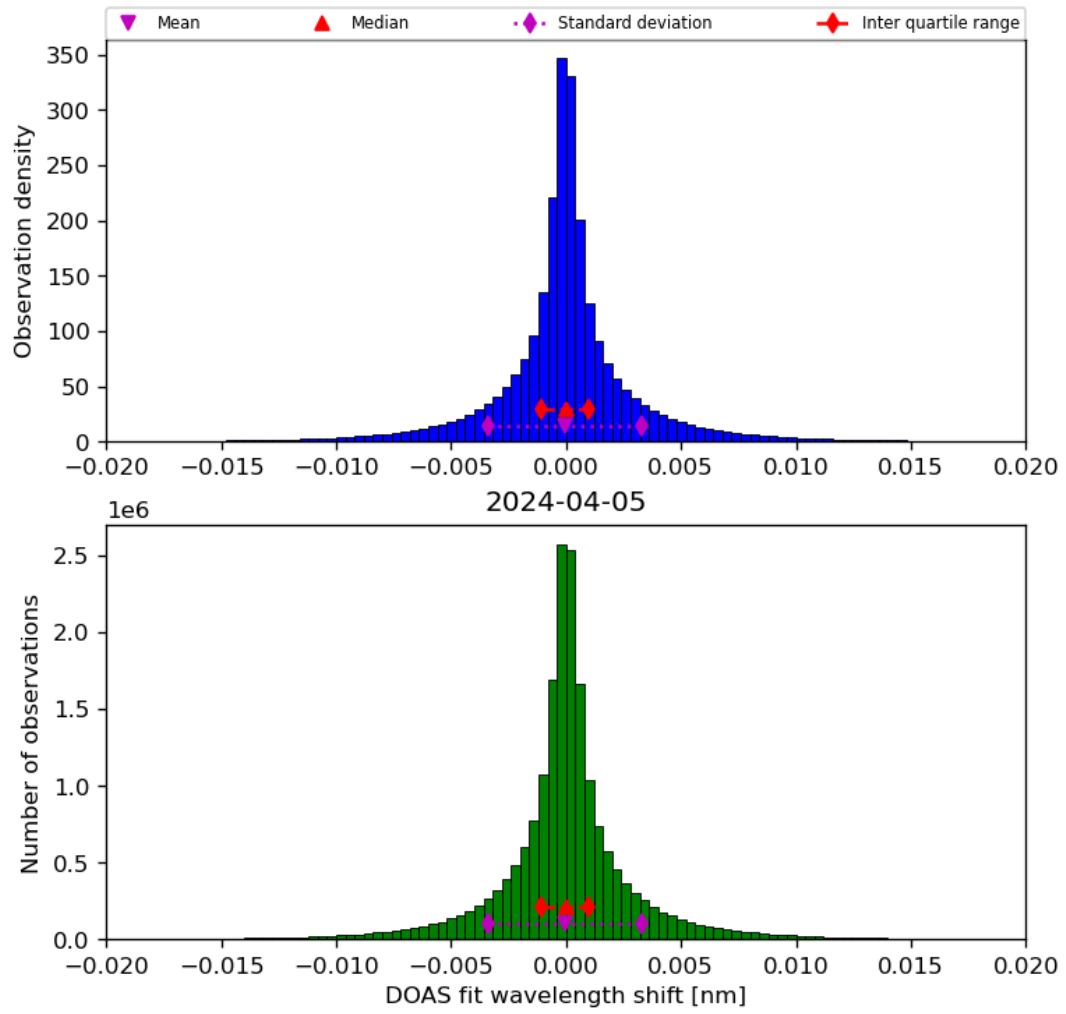
Figure 44: Histogram of “DOAS fit wavelength shift” for 2024-04-05 to 2024-04-06
