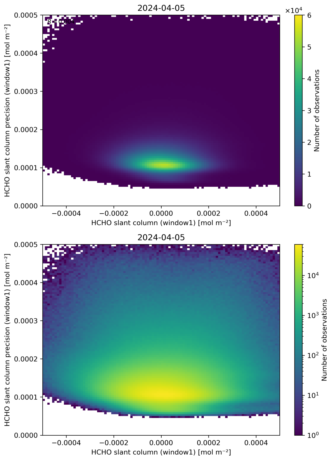
Figure 84: Scatter density plot of “HCHO slant column (window1)” against “HCHO slant column precision (window1)” for 2024-04-05 to 2024-04-06.
