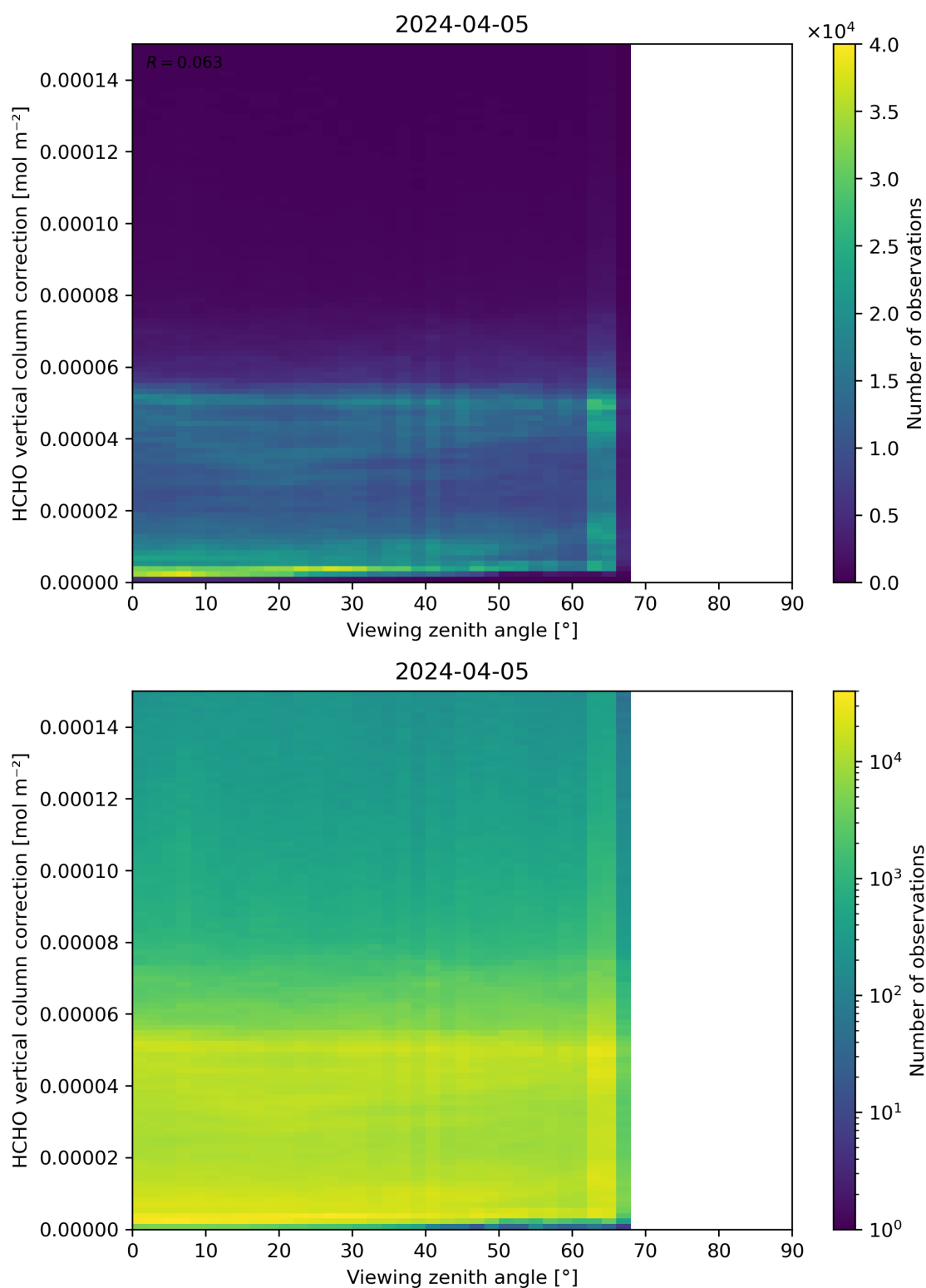
Figure 193: Scatter density plot of “Viewing zenith angle” against “HCHO vertical column correction” for 2024-04-05 to 2024-04-06.
