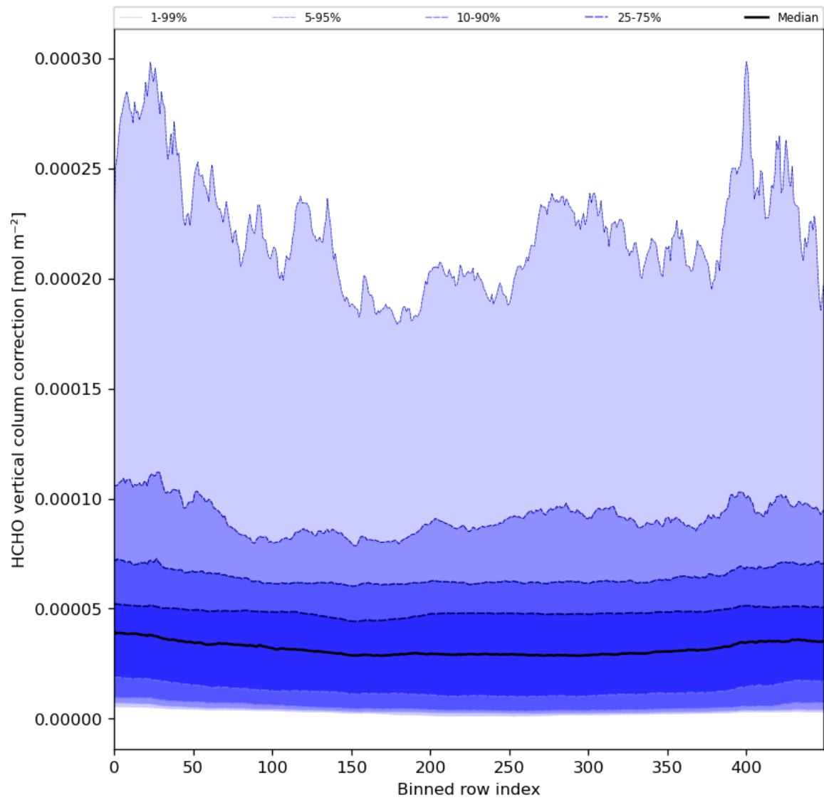
Figure 51: Along track statistics of “HCHO vertical column correction” for 2024-04-05 to 2024-04-06
