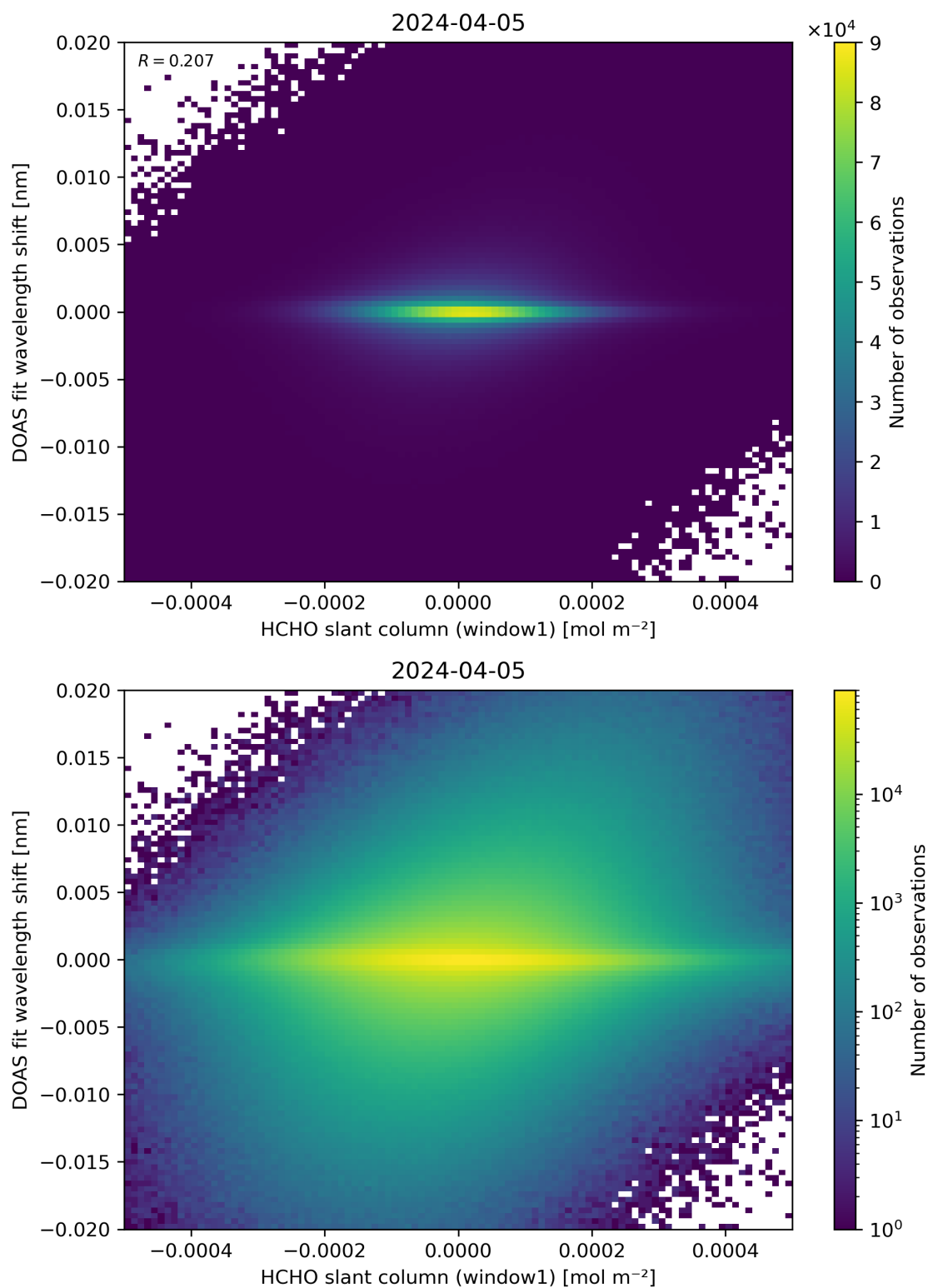
Figure 79: Scatter density plot of “HCHO slant column (window1)” against “DOAS fit wavelength shift” for 2024-04-05 to 2024-04-06.
