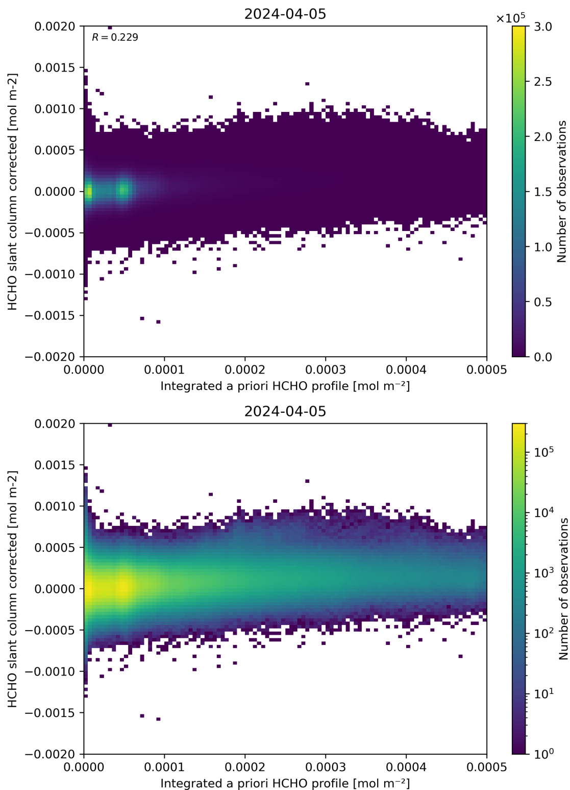
Figure 151: Scatter density plot of “Integrated a priori HCHO profile” against “HCHO slant column corrected” for 2024-04-05 to 2024-04-06.
