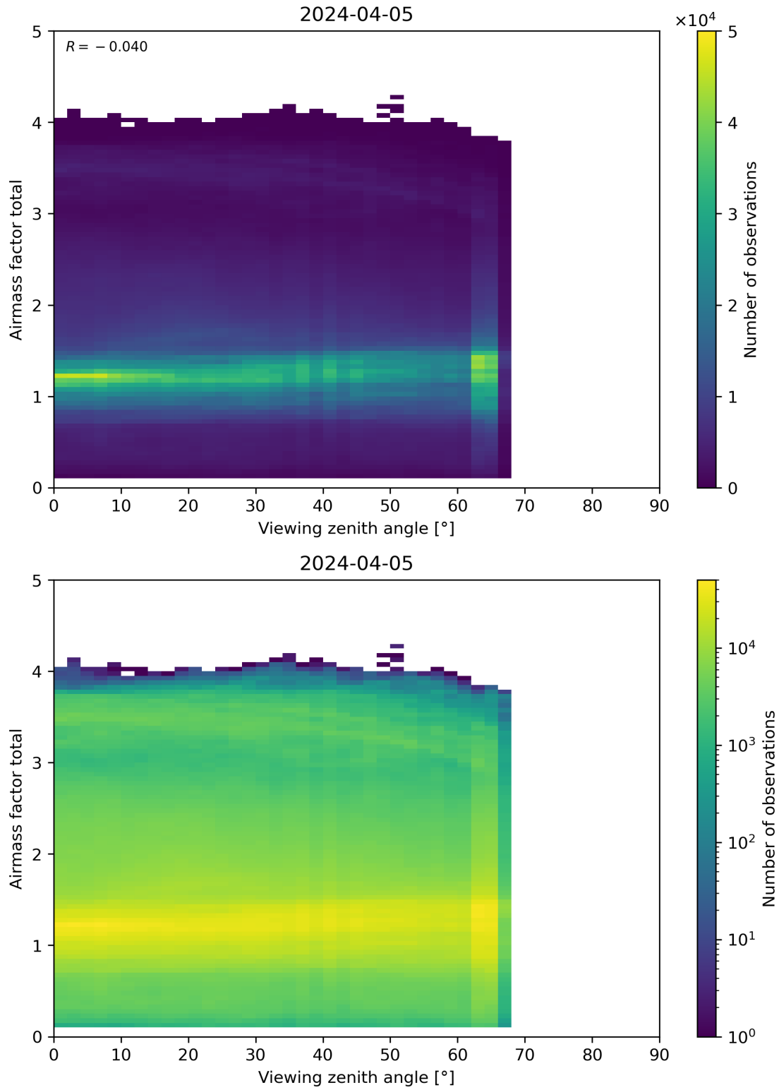
Figure 190: Scatter density plot of “Viewing zenith angle” against “Airmass factor total” for 2024-04-05 to 2024-04-06.
