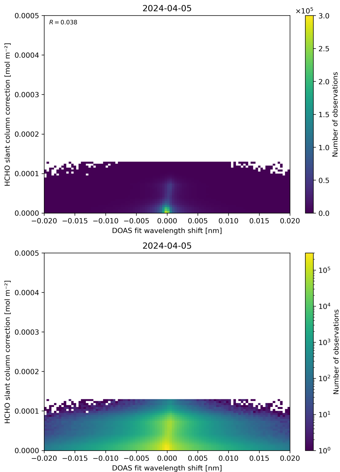
Figure 67: Scatter density plot of “DOAS fit wavelength shift” against “HCHO slant column correction” for 2024-04-05 to 2024-04-06.
