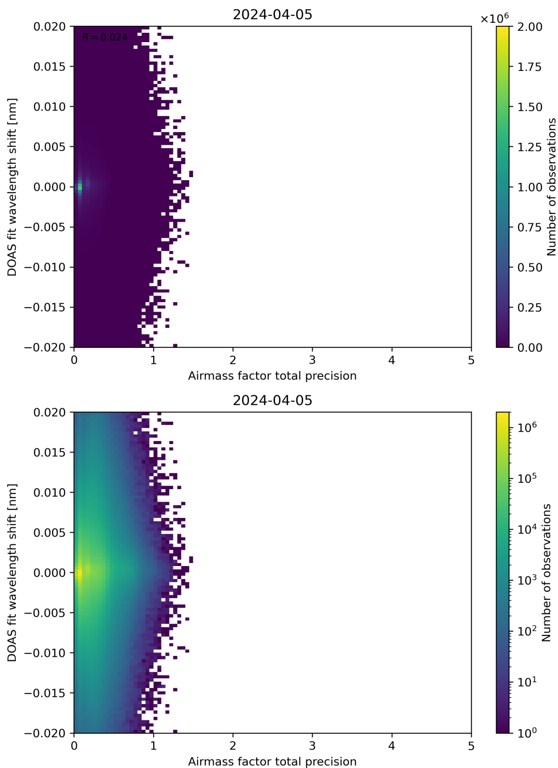
Figure 106: Scatter density plot of “Airmass factor total precision” against “DOAS fit wavelength shift” for 2024-04-05 to 2024-04-06.
