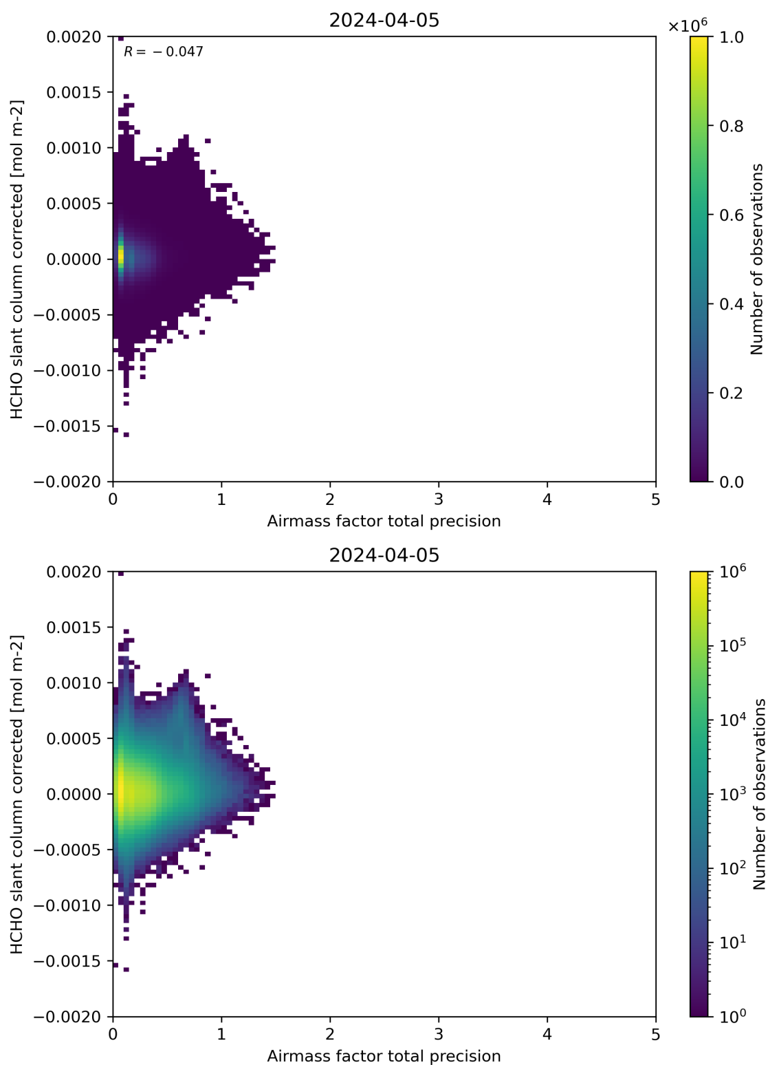
Figure 109: Scatter density plot of “Airmass factor total precision” against “HCHO slant column corrected” for 2024-04-05 to 2024-04-06.
