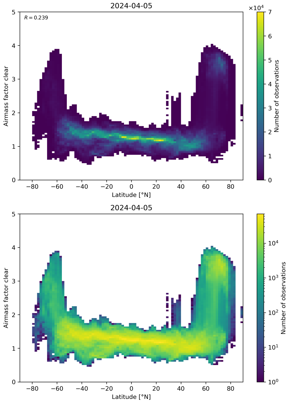
Figure 156: Scatter density plot of “Latitude” against “Airmass factor clear” for 2024-04-05 to 2024-04-06.
