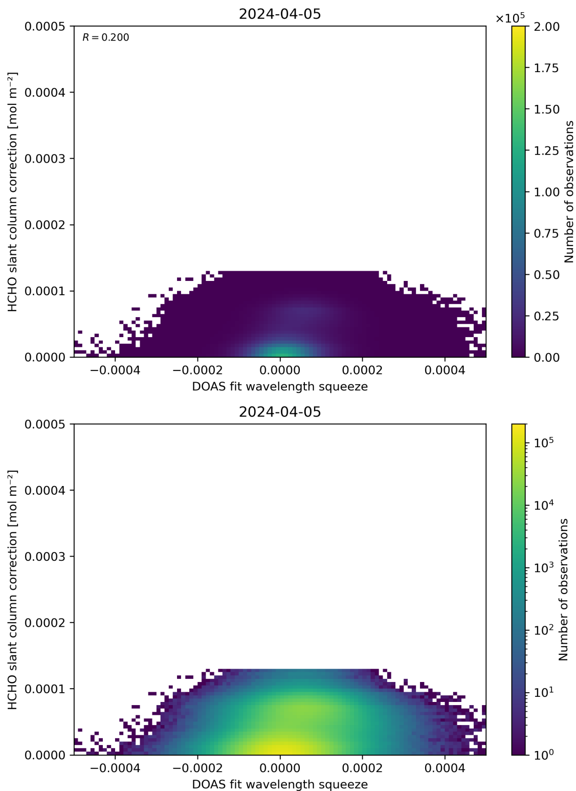
Figure 70: Scatter density plot of “DOAS fit wavelength squeeze” against “HCHO slant column correction” for 2024-04-05 to 2024-04-06.
