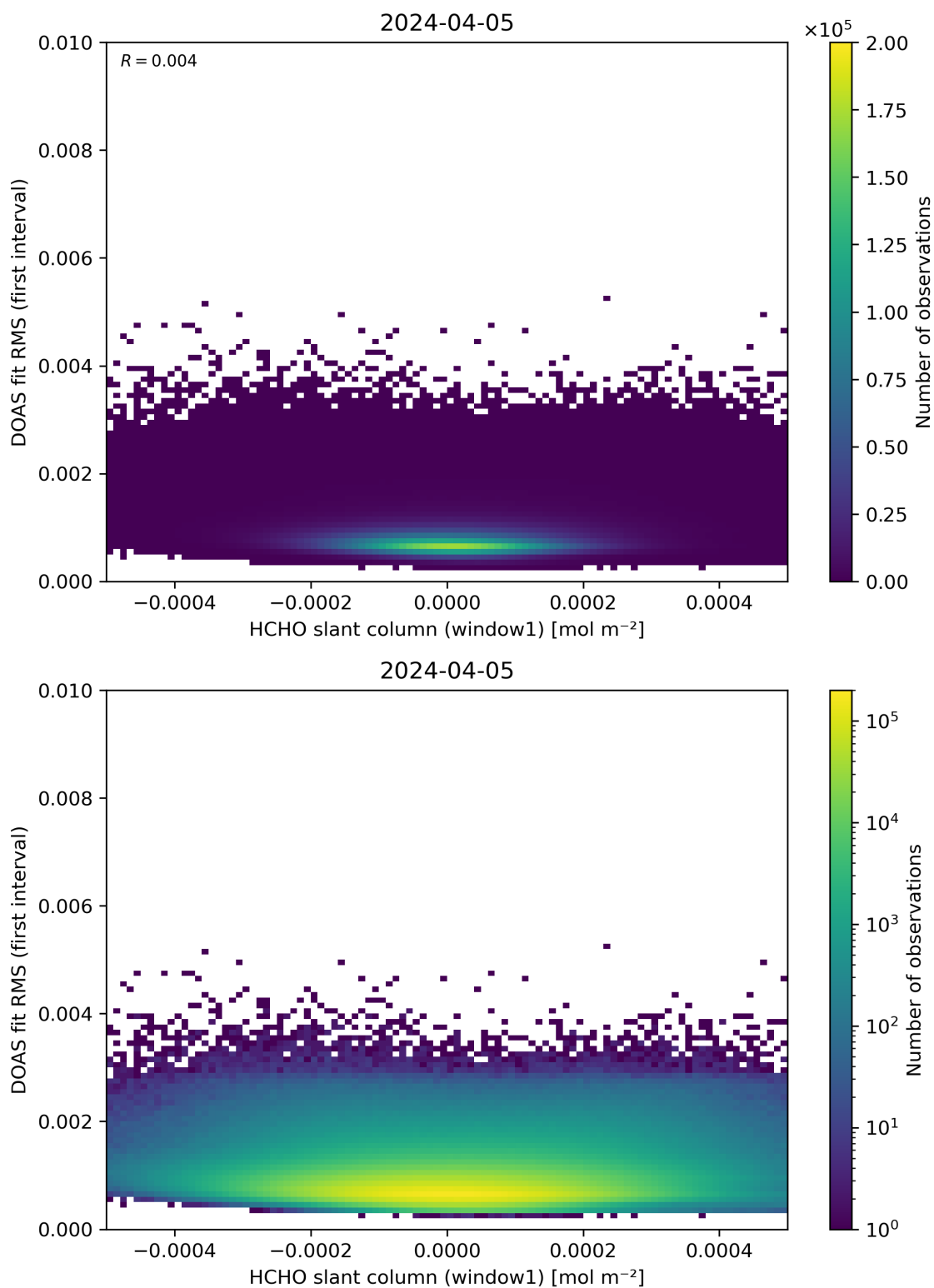
Figure 78: Scatter density plot of “HCHO slant column (window1)” against “DOAS fit RMS (first interval)” for 2024-04-05 to 2024-04-06.
