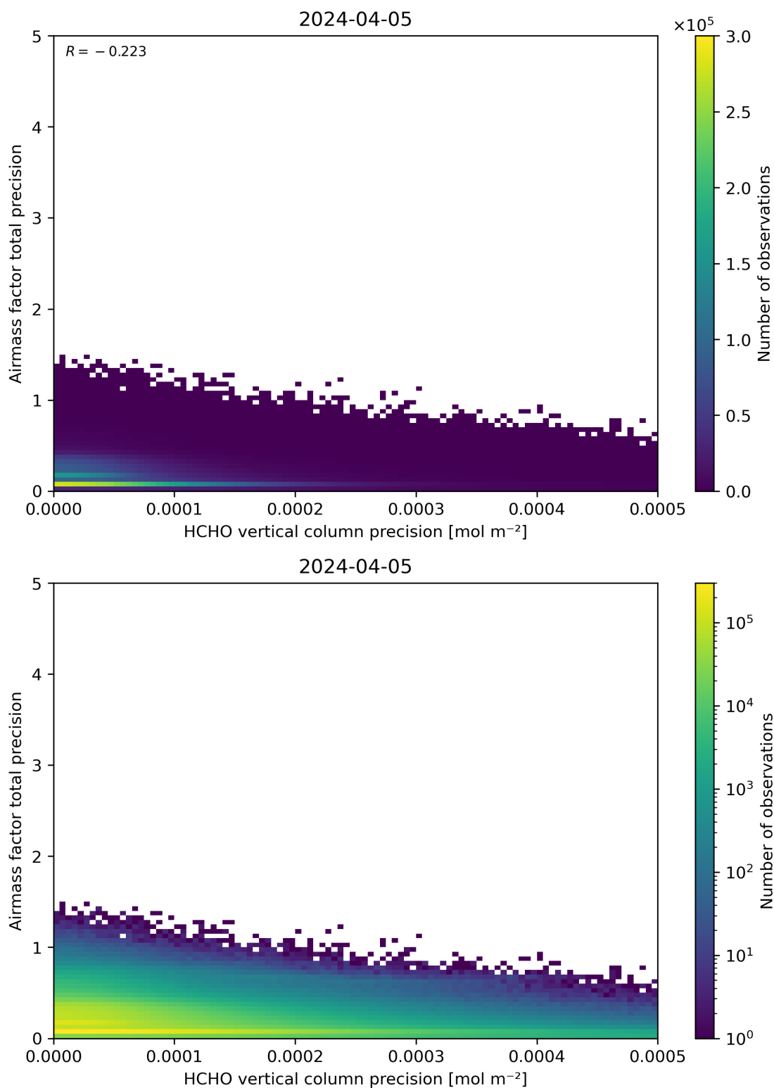
Figure 145: Scatter density plot of “HCHO vertical column precision” against “Airmass factor total precision” for 2024-04-05 to 2024-04-06.
