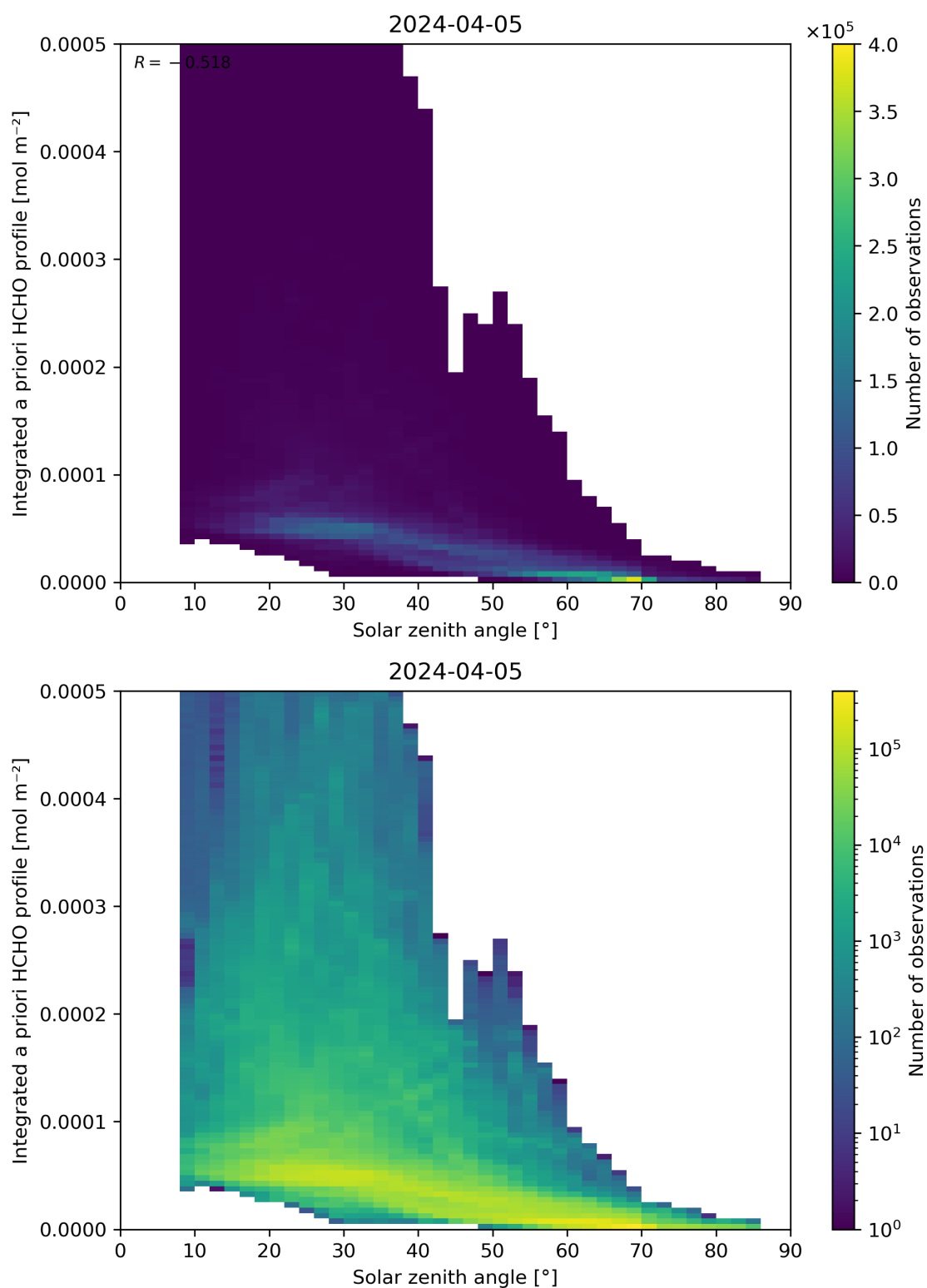
Figure 180: Scatter density plot of “Solar zenith angle” against “Integrated a priori HCHO profile” for 2024-04-05 to 2024-04-06.
