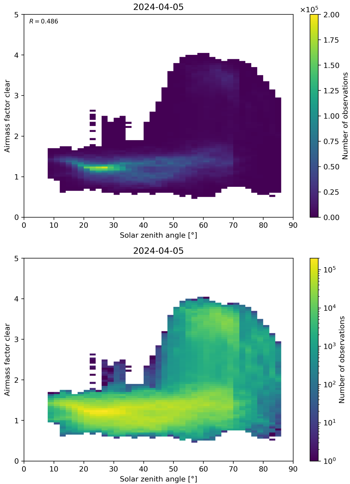
Figure 170: Scatter density plot of “Solar zenith angle” against “Airmass factor clear” for 2024-04-05 to 2024-04-06.
