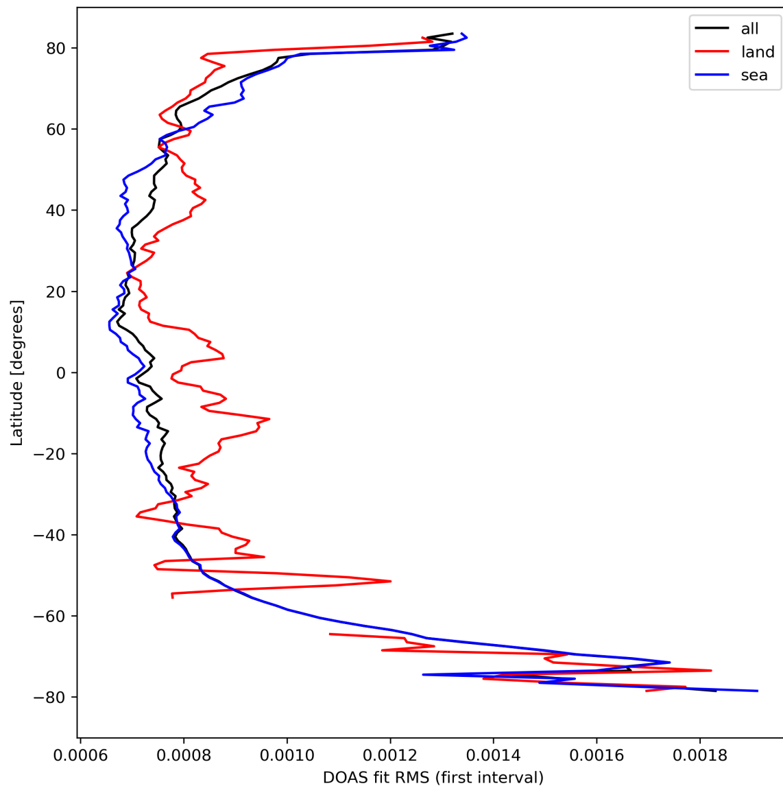
Figure 32: Zonal average of “DOAS fit RMS (first interval)” for 2024-04-05 to 2024-04-06.
