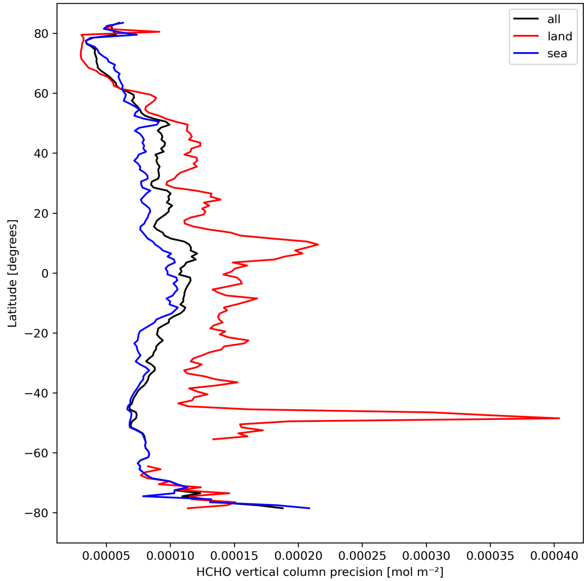
Figure 22: Zonal average of “HCHO vertical column precision” for 2024-04-05 to 2024-04-06.
