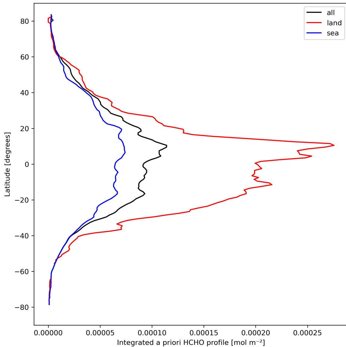
Figure 29: Zonal average of “Integrated a priori HCHO profile” for 2024-04-05 to 2024-04-06.
