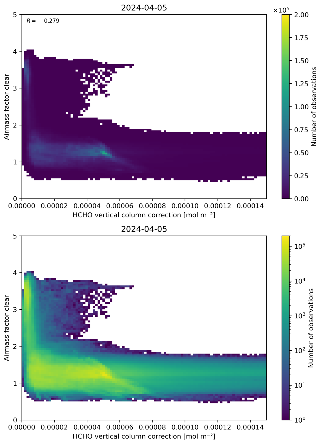
Figure 115: Scatter density plot of “HCHO vertical column correction” against “Airmass factor clear” for 2024-04-05 to 2024-04-06.
