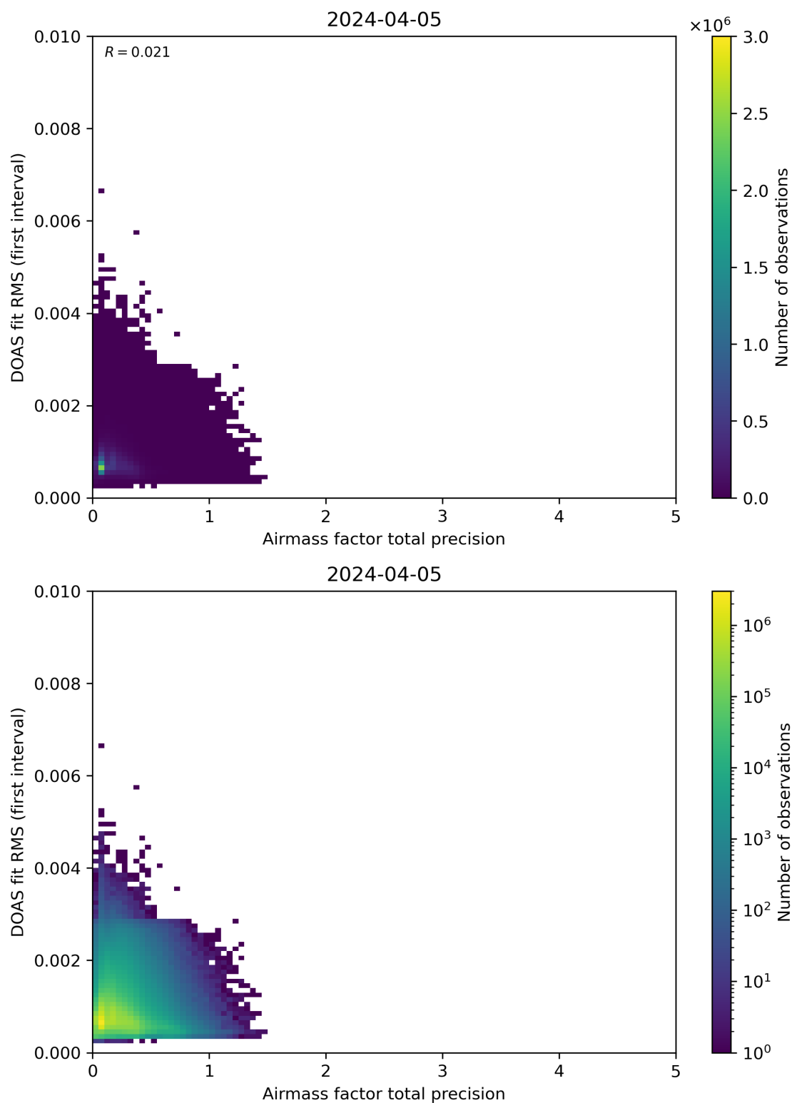
Figure 105: Scatter density plot of “Airmass factor total precision” against “DOAS fit RMS (first interval)” for 2024-04-05 to 2024-04-06.
