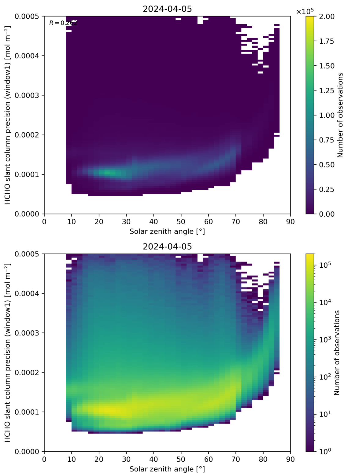
Figure 174: Scatter density plot of “Solar zenith angle” against “HCHO slant column precision (window1)” for 2024-04-05 to 2024-04-06.
