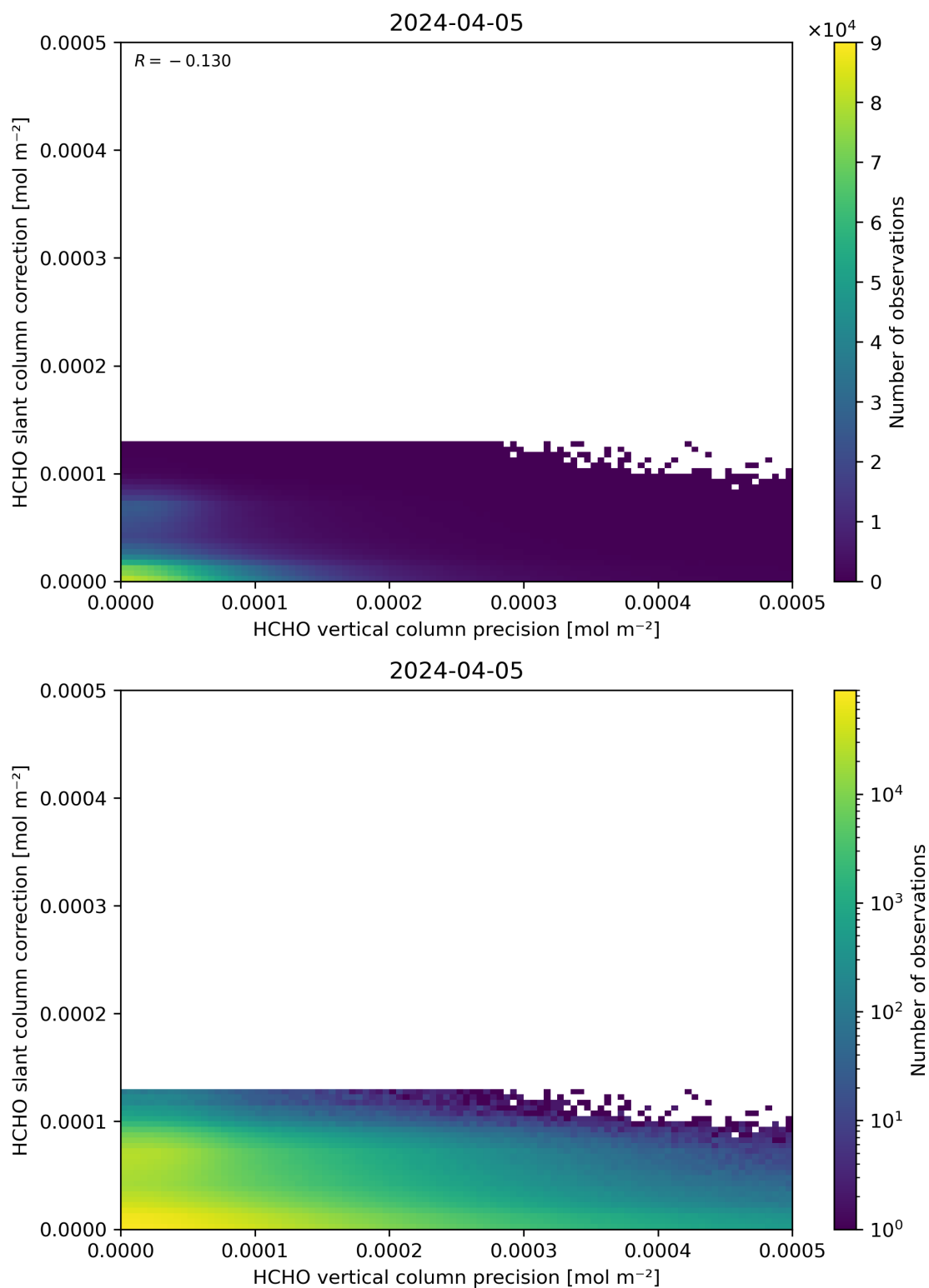
Figure 141: Scatter density plot of “HCHO vertical column precision” against “HCHO slant column correction” for 2024-04-05 to 2024-04-06.
