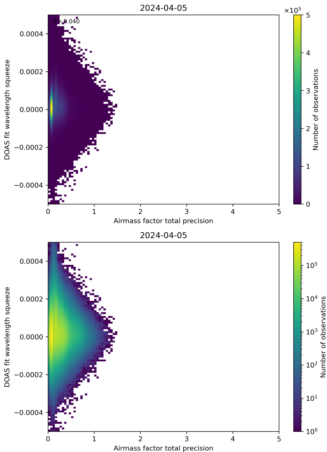
Figure 107: Scatter density plot of “Airmass factor total precision” against “DOAS fit wavelength squeeze” for 2024-04-05 to 2024-04-06.
