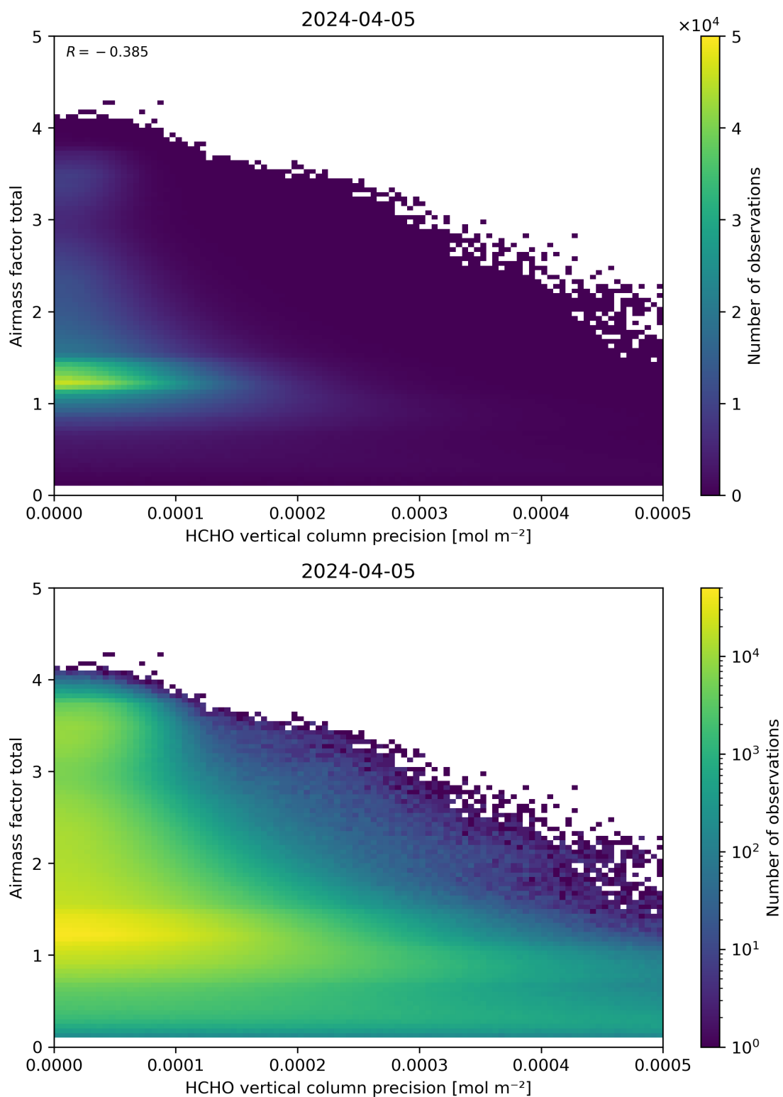
Figure 144: Scatter density plot of “HCHO vertical column precision” against “Airmass factor total” for 2024-04-05 to 2024-04-06.
