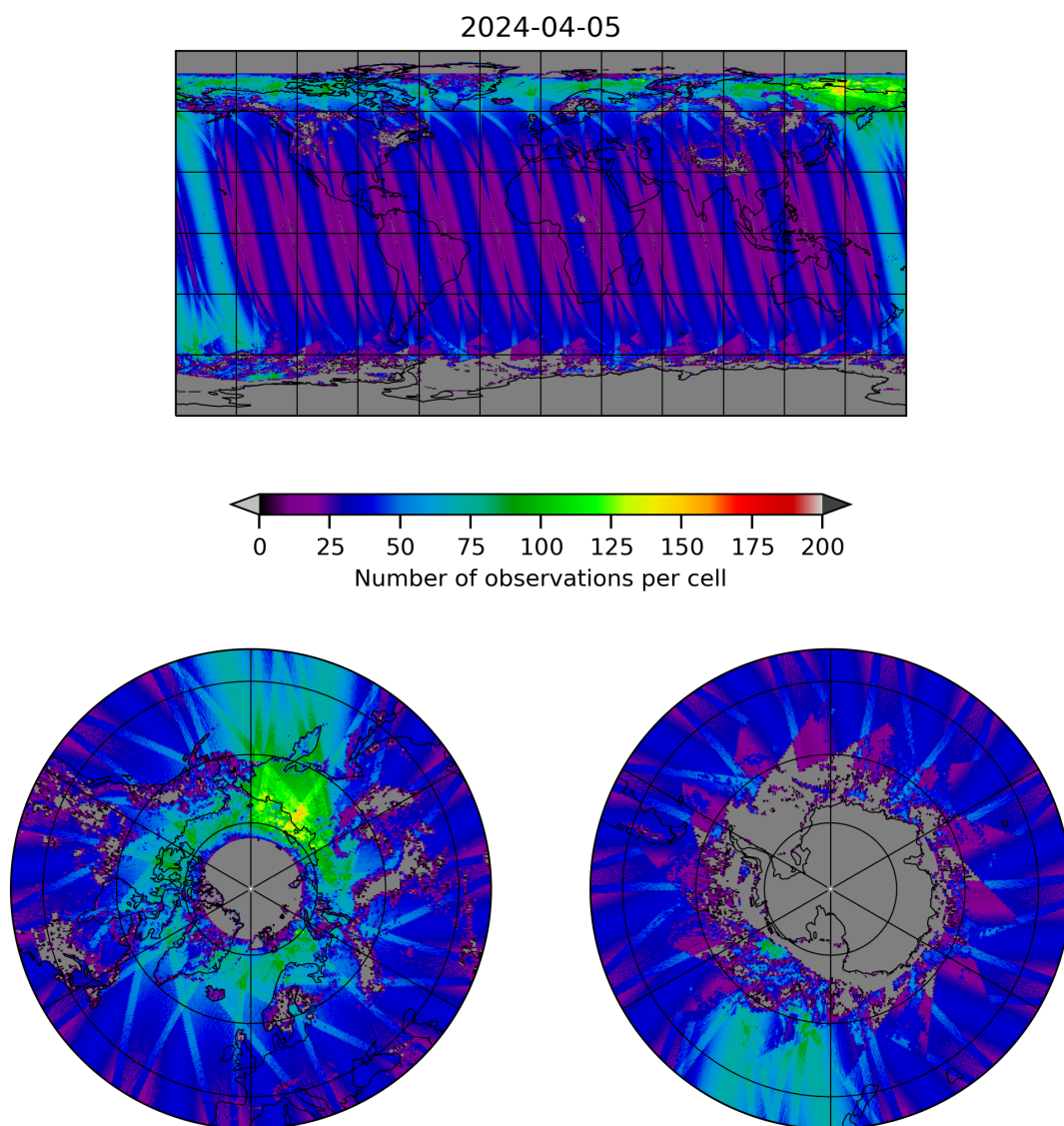
Figure 19: Map of the number of observations for 2024-04-05 to 2024-04-06
