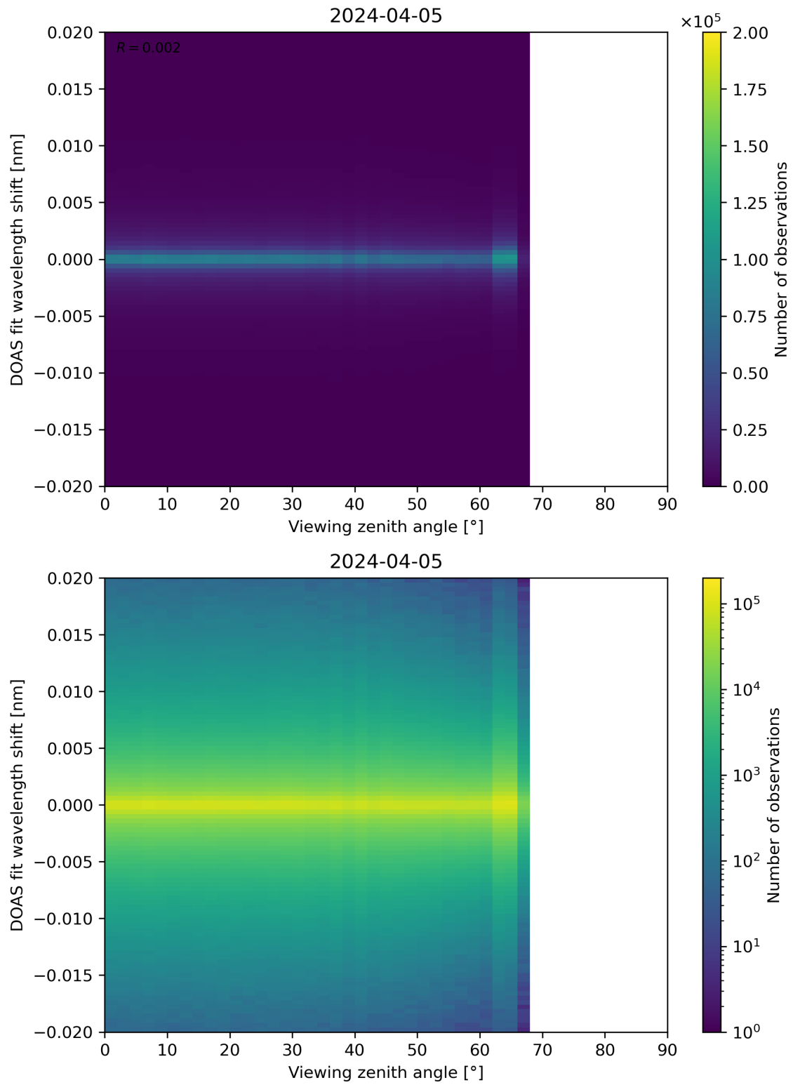
Figure 183: Scatter density plot of “Viewing zenith angle” against “DOAS fit wavelength shift” for 2024-04-05 to 2024-04-06.
