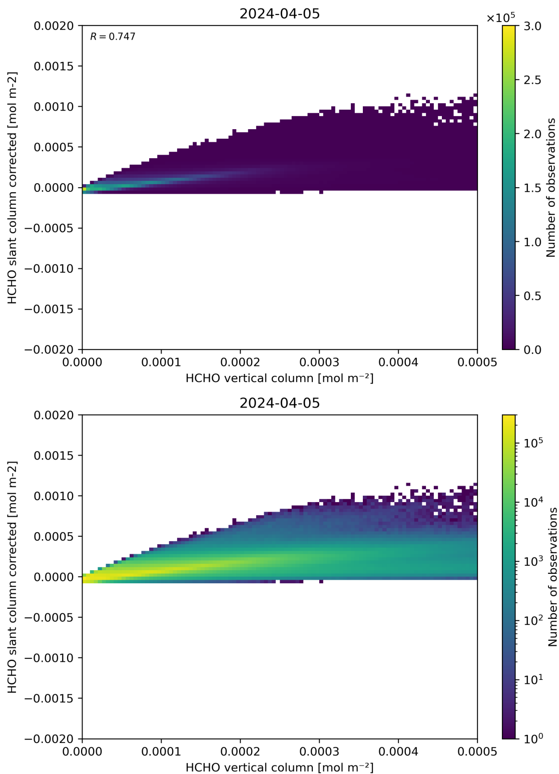
Figure 127: Scatter density plot of “HCHO vertical column” against “HCHO slant column corrected” for 2024-04-05 to 2024-04-06.
