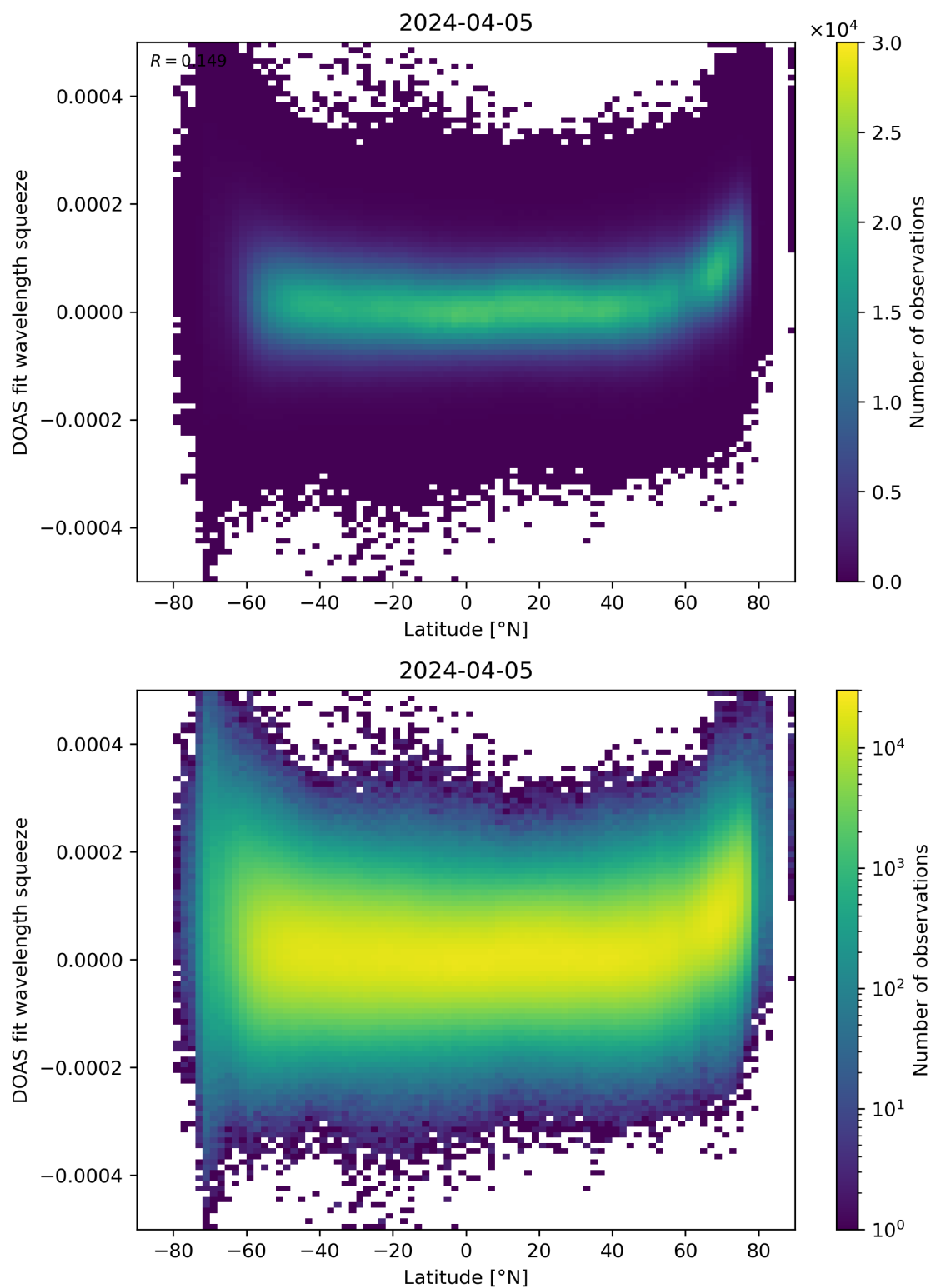
Figure 155: Scatter density plot of “Latitude” against “DOAS fit wavelength squeeze” for 2024-04-05 to 2024-04-06.
