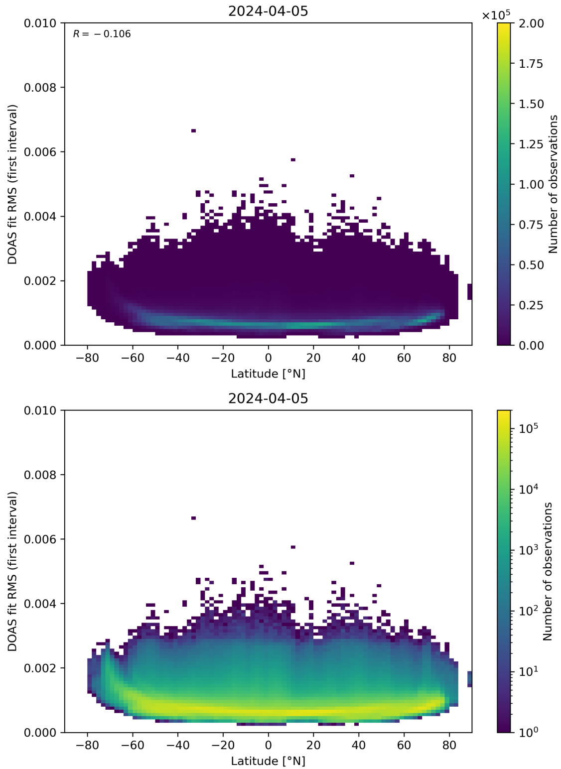
Figure 153: Scatter density plot of “Latitude” against “DOAS fit RMS (first interval)” for 2024-04-05 to 2024-04-06.
