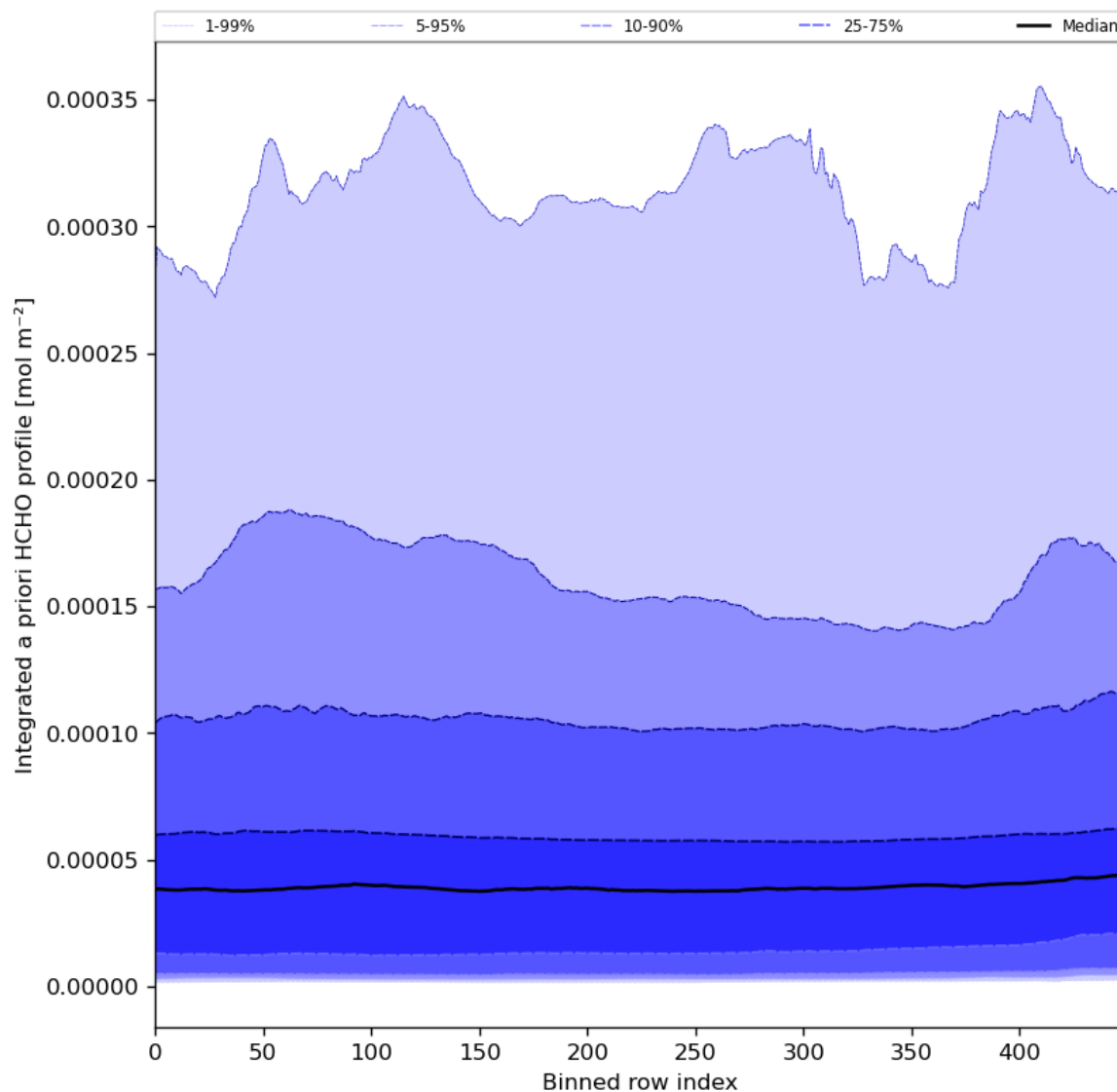
Figure 57: Along track statistics of “Integrated a priori HCHO profile” for 2024-04-05 to 2024-04-06
