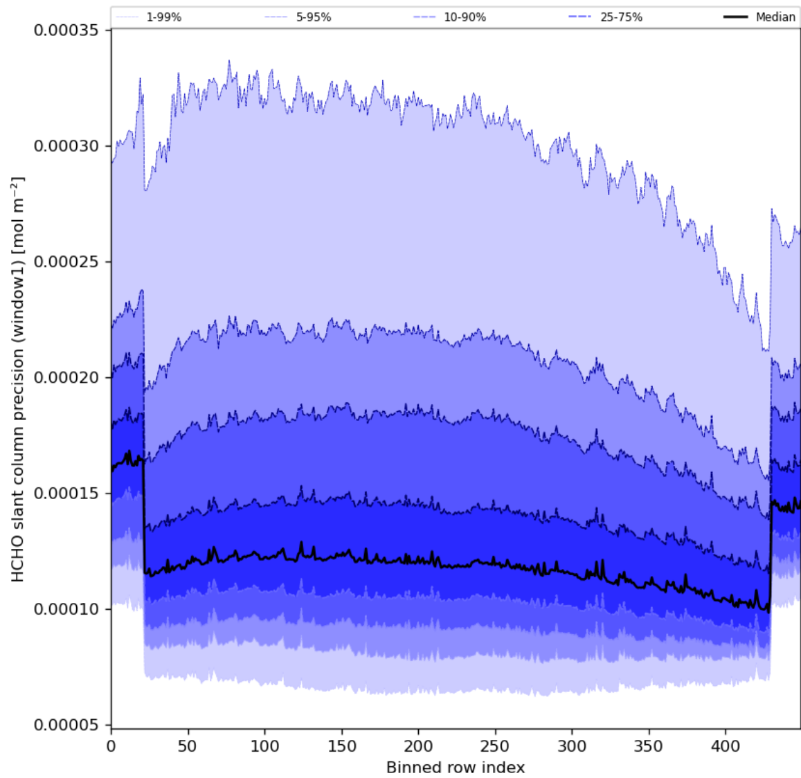
Figure 53: Along track statistics of “HCHO slant column precision (window1)” for 2024-04-05 to 2024-04-06
