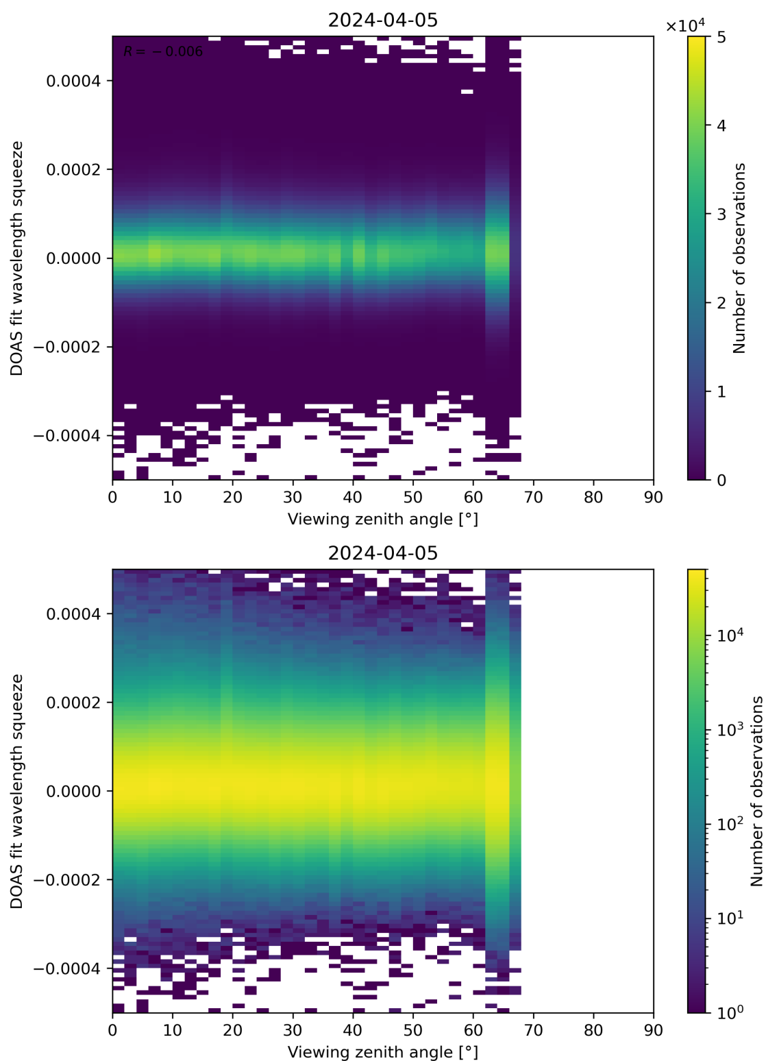
Figure 184: Scatter density plot of “Viewing zenith angle” against “DOAS fit wavelength squeeze” for 2024-04-05 to 2024-04-06.
