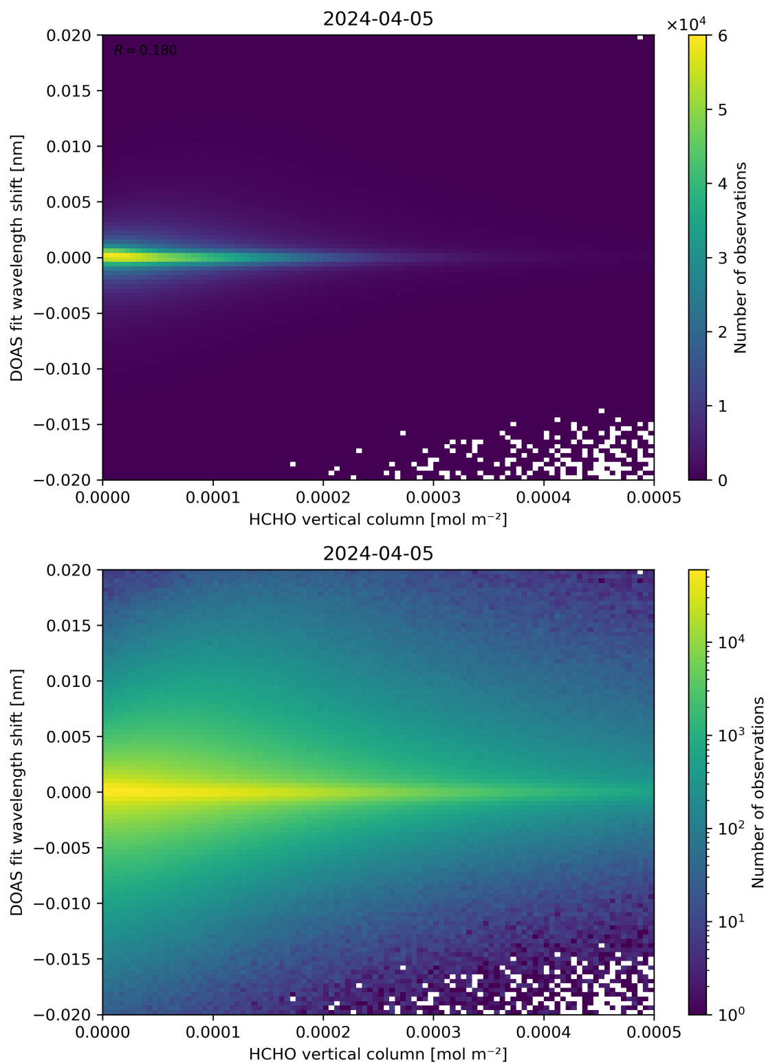
Figure 124: Scatter density plot of “HCHO vertical column” against “DOAS fit wavelength shift” for 2024-04-05 to 2024-04-06.
