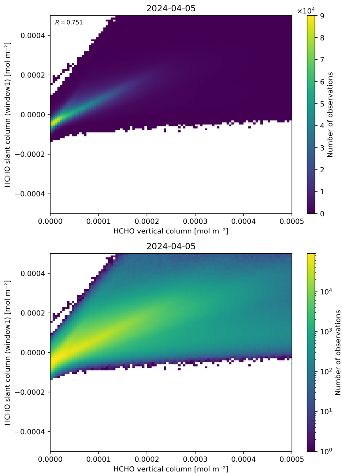
Figure 129: Scatter density plot of “HCHO vertical column” against “HCHO slant column (window1)” for 2024-04-05 to 2024-04-06.
