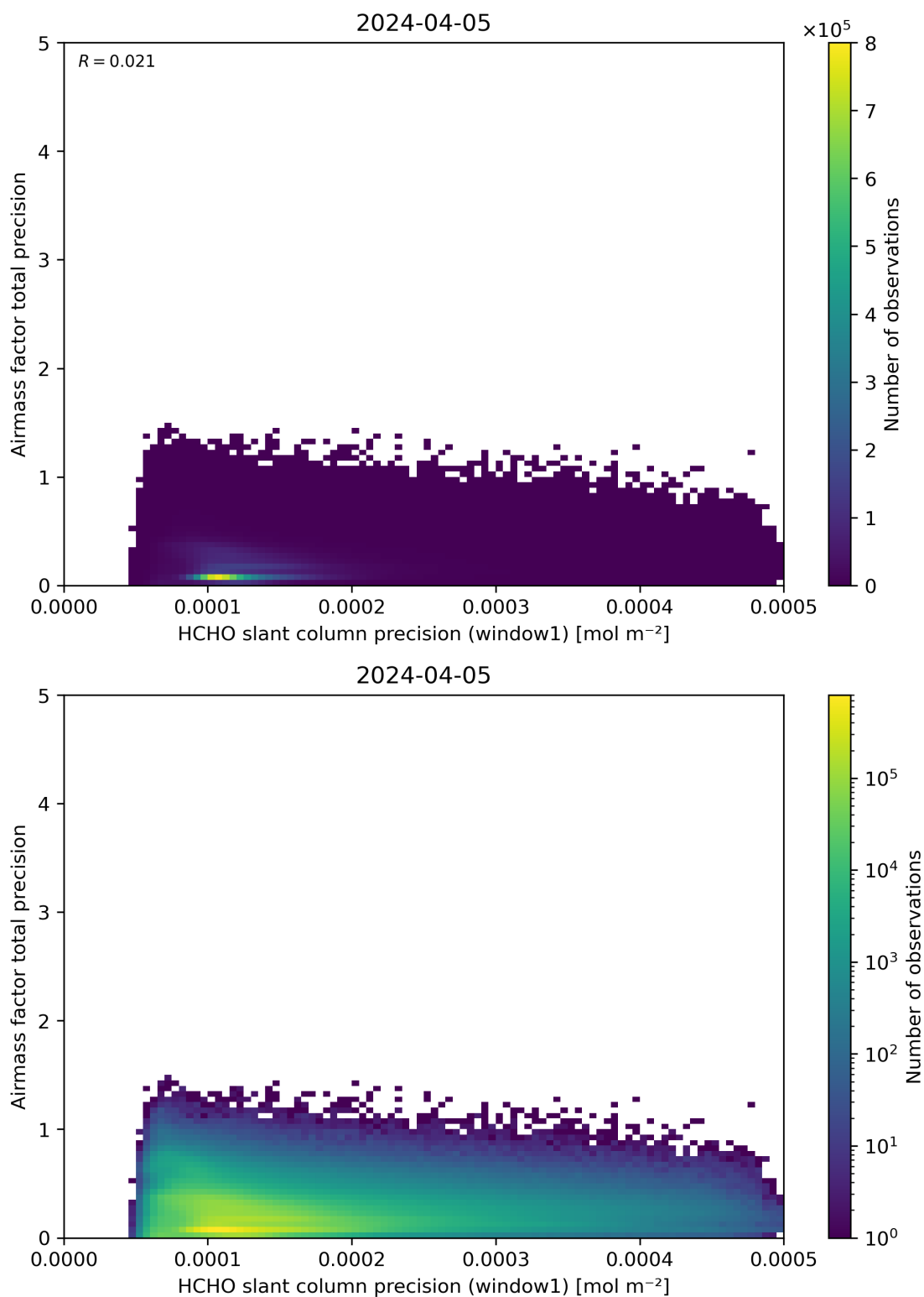
Figure 95: Scatter density plot of “HCHO slant column precision (window1)” against “Airmass factor total precision” for 2024-04-05 to 2024-04-06.
