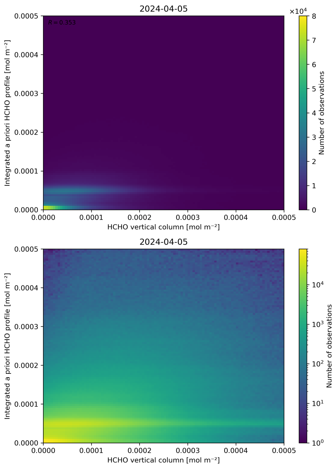
Figure 135: Scatter density plot of “HCHO vertical column” against “Integrated a priori HCHO profile” for 2024-04-05 to 2024-04-06.
