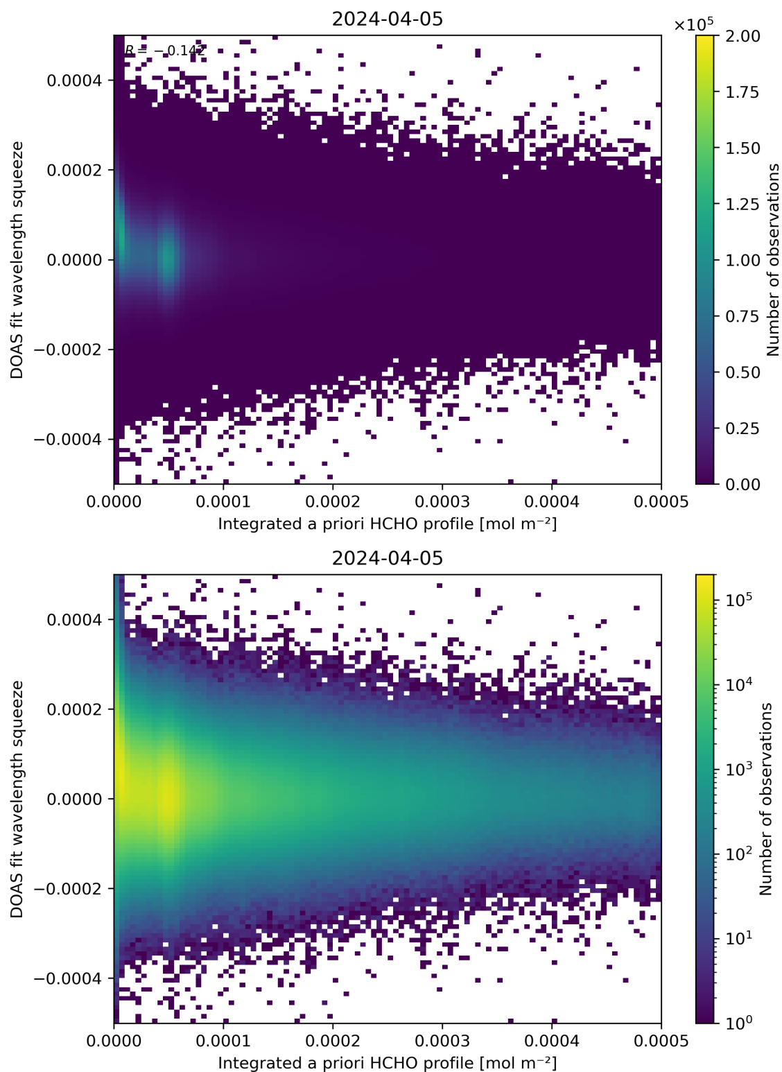
Figure 150: Scatter density plot of “Integrated a priori HCHO profile” against “DOAS fit wavelength squeeze” for 2024-04-05 to 2024-04-06.
