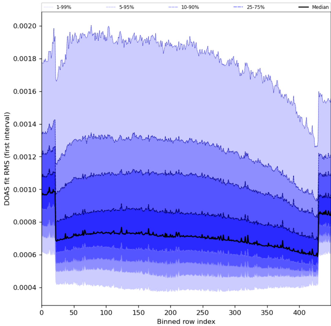
Figure 60: Along track statistics of “DOAS fit RMS (first interval)” for 2024-04-05 to 2024-04-06
