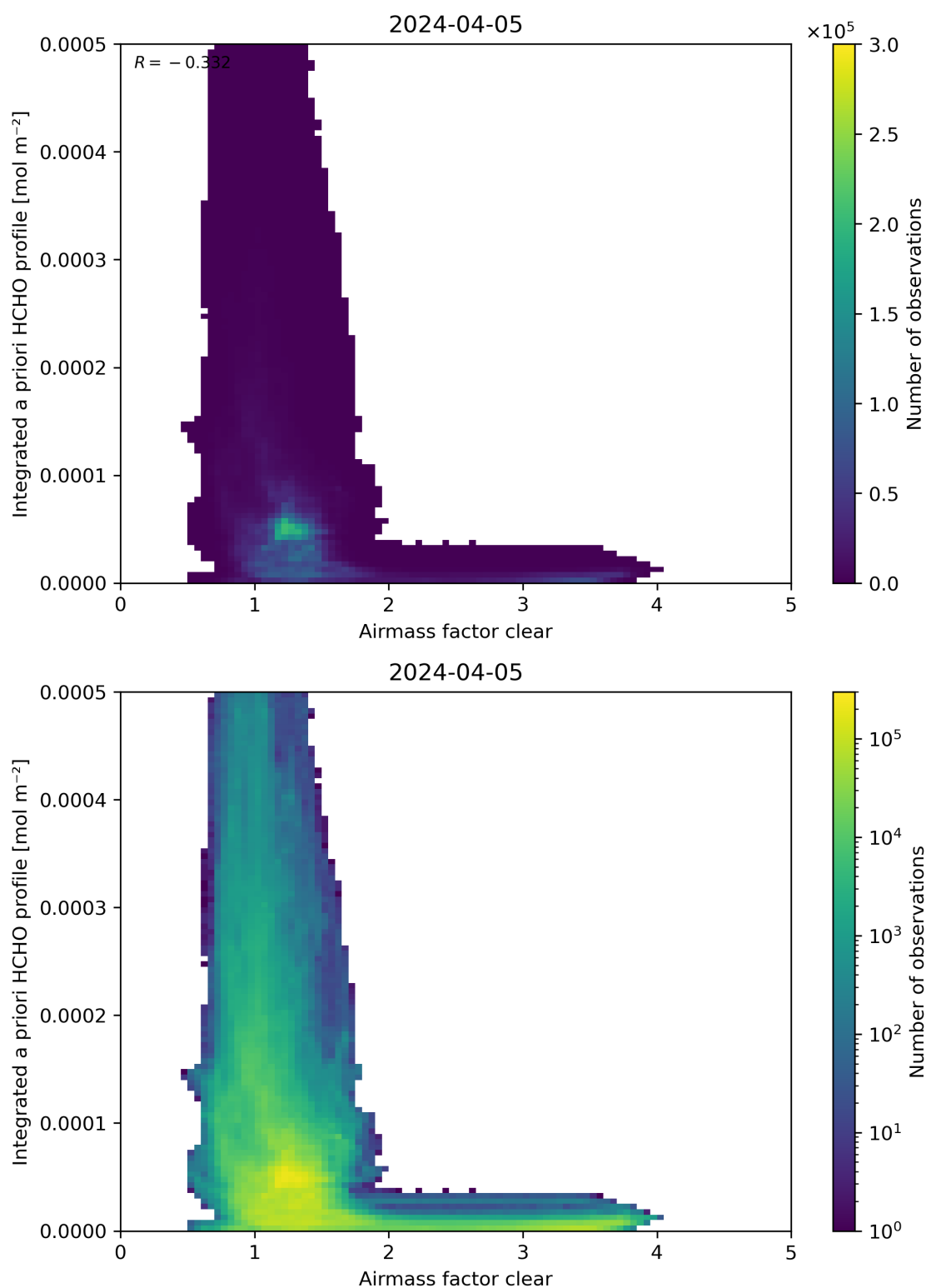
Figure 76: Scatter density plot of “Airmass factor clear” against “Integrated a priori HCHO profile” for 2024-04-05 to 2024-04-06.
