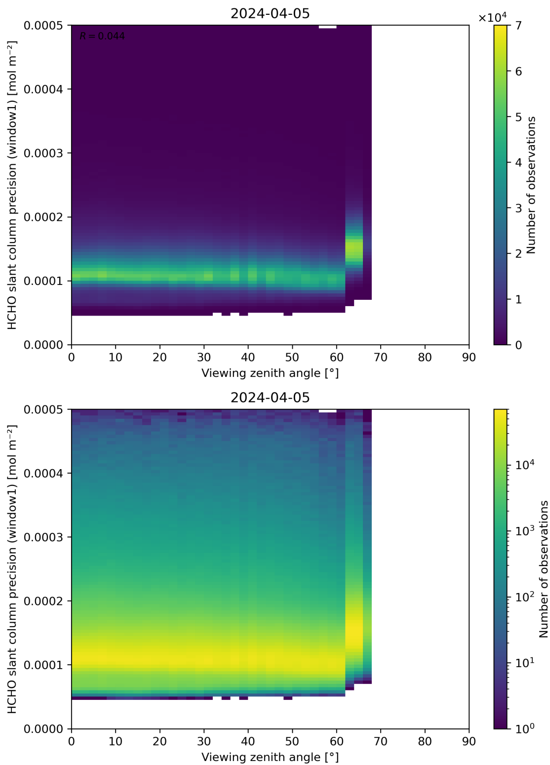
Figure 189: Scatter density plot of “Viewing zenith angle” against “HCHO slant column precision (window1)” for 2024-04-05 to 2024-04-06.
