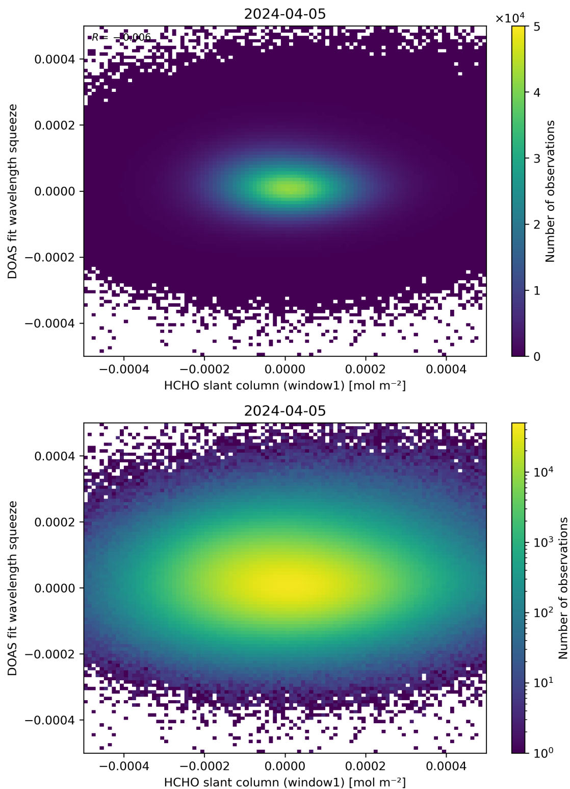
Figure 80: Scatter density plot of “HCHO slant column (window1)” against “DOAS fit wavelength squeeze” for 2024-04-05 to 2024-04-06.
