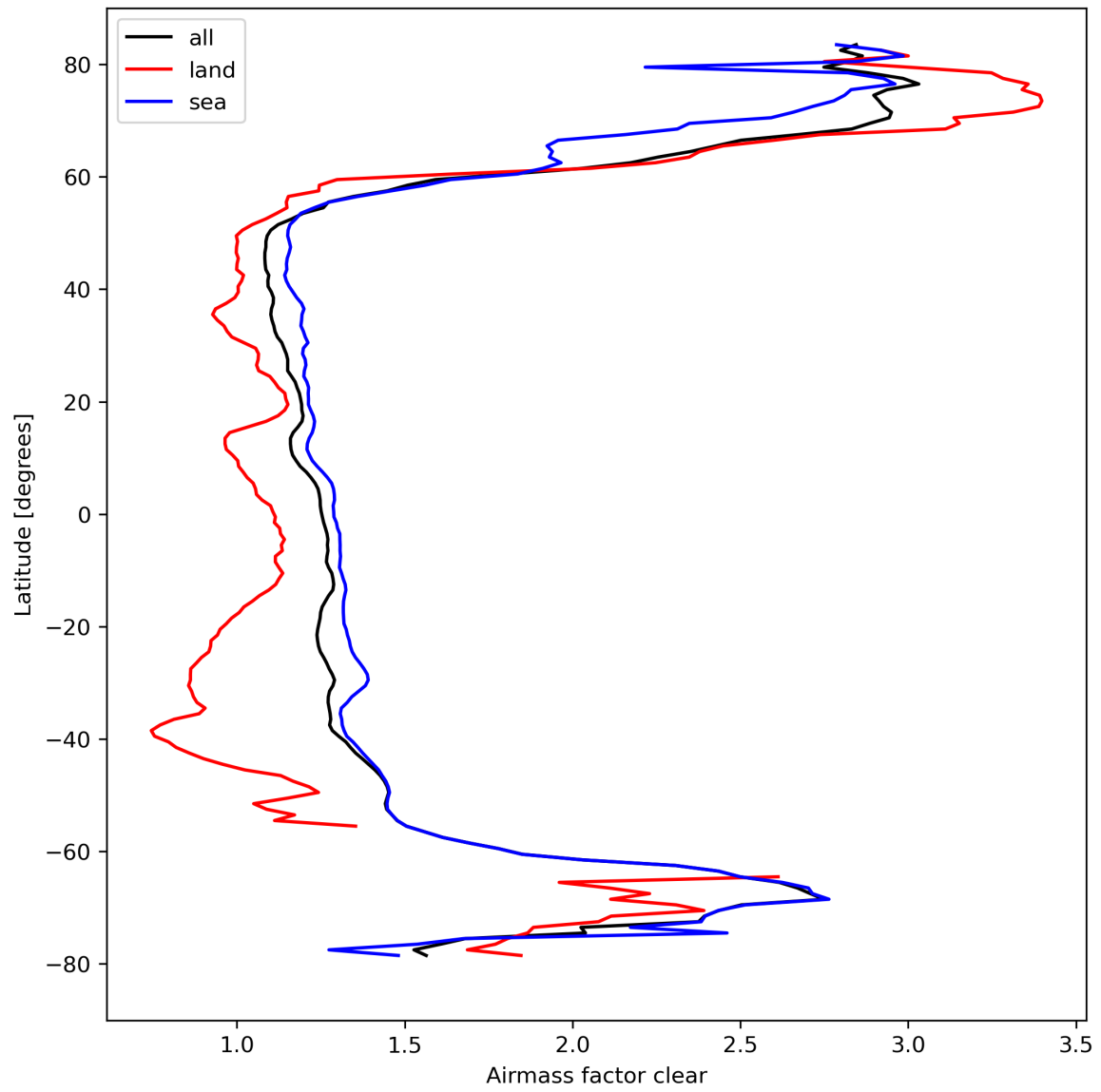
Figure 28: Zonal average of “Airmass factor clear” for 2024-04-05 to 2024-04-06.
