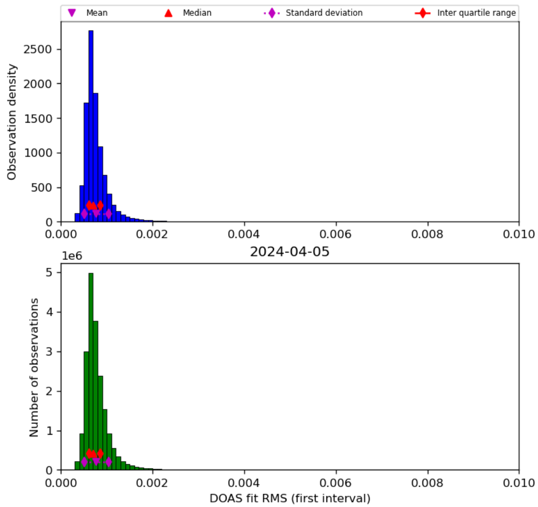
Figure 46: Histogram of “DOAS fit RMS (first interval)” for 2024-04-05 to 2024-04-06
