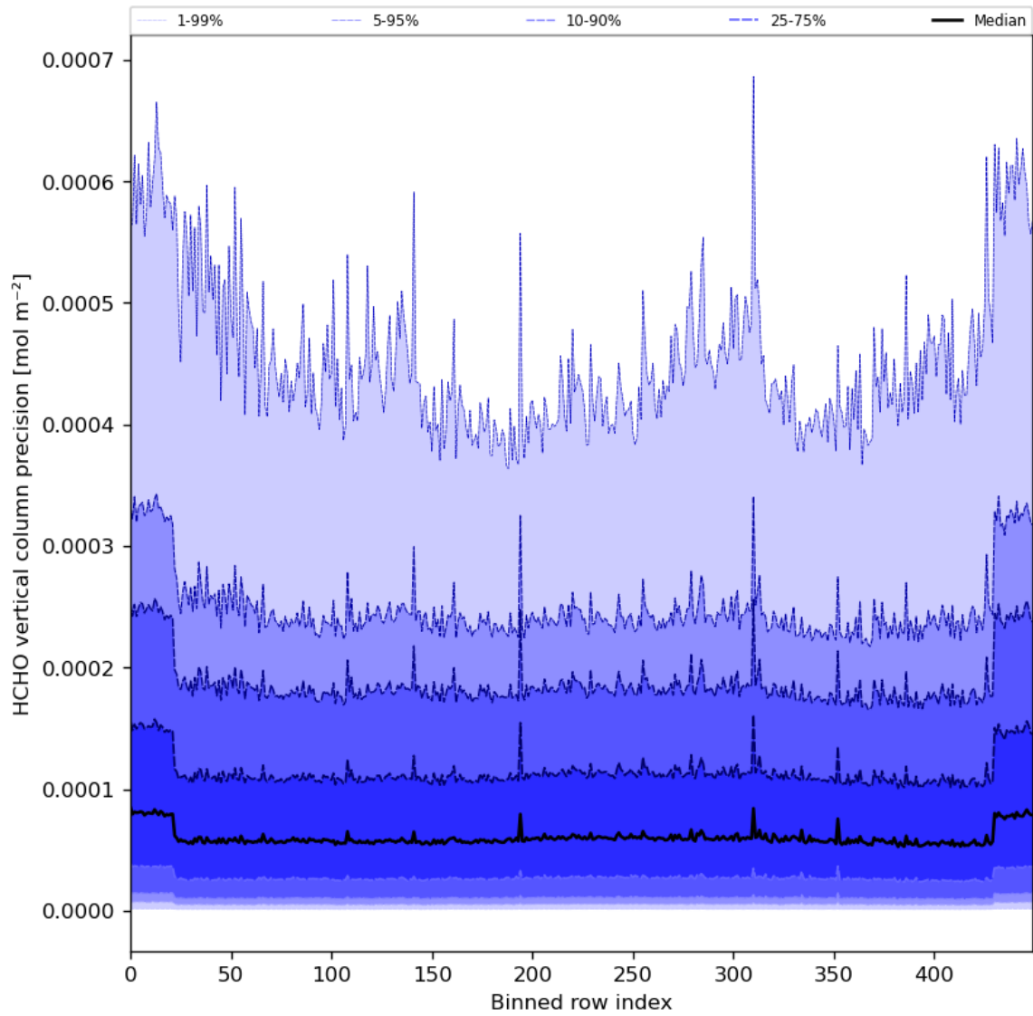
Figure 50: Along track statistics of “HCHO vertical column precision” for 2024-04-05 to 2024-04-06
