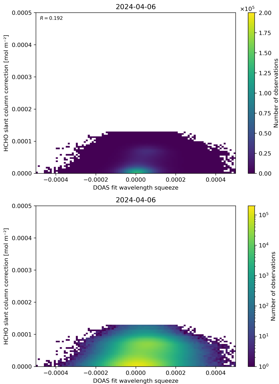
Figure 70: Scatter density plot of “DOAS fit wavelength squeeze” against “HCHO slant column correction” for 2024-04-05 to 2024-04-07.
