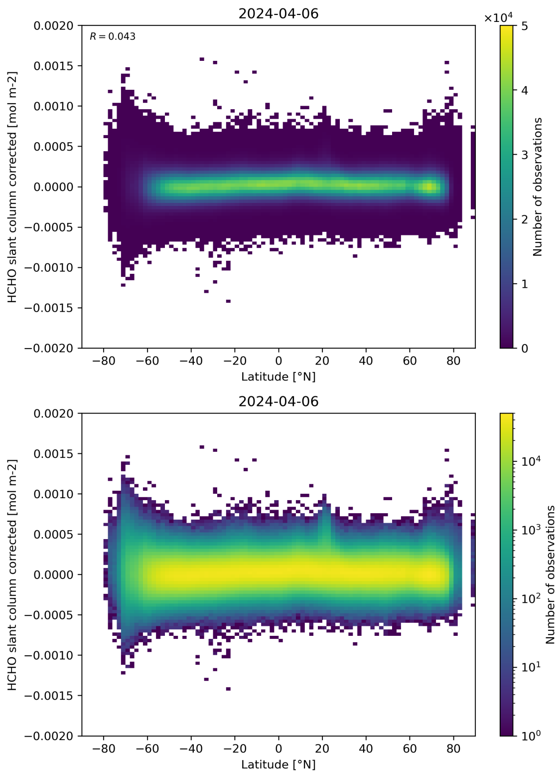
Figure 157: Scatter density plot of “Latitude” against “HCHO slant column corrected” for 2024-04-05 to 2024-04-07.
