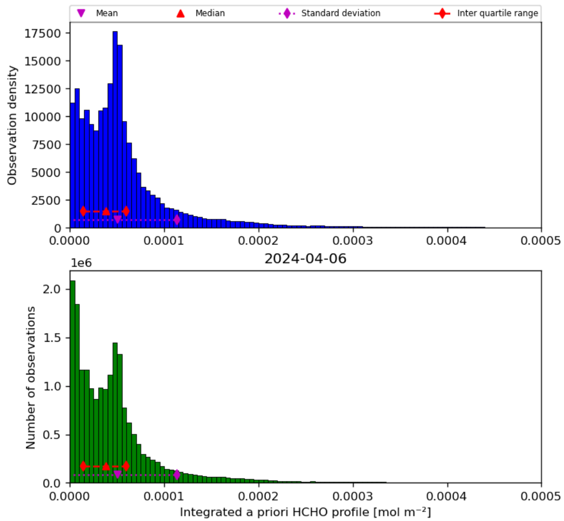
Figure 43: Histogram of “Integrated a priori HCHO profile” for 2024-04-05 to 2024-04-07
