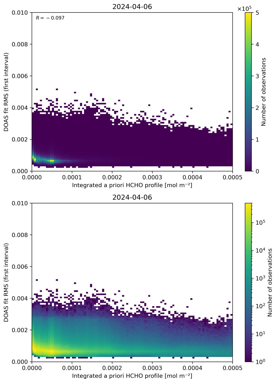
Figure 148: Scatter density plot of “Integrated a priori HCHO profile” against “DOAS fit RMS (first interval)” for 2024-04-05 to 2024-04-07.
