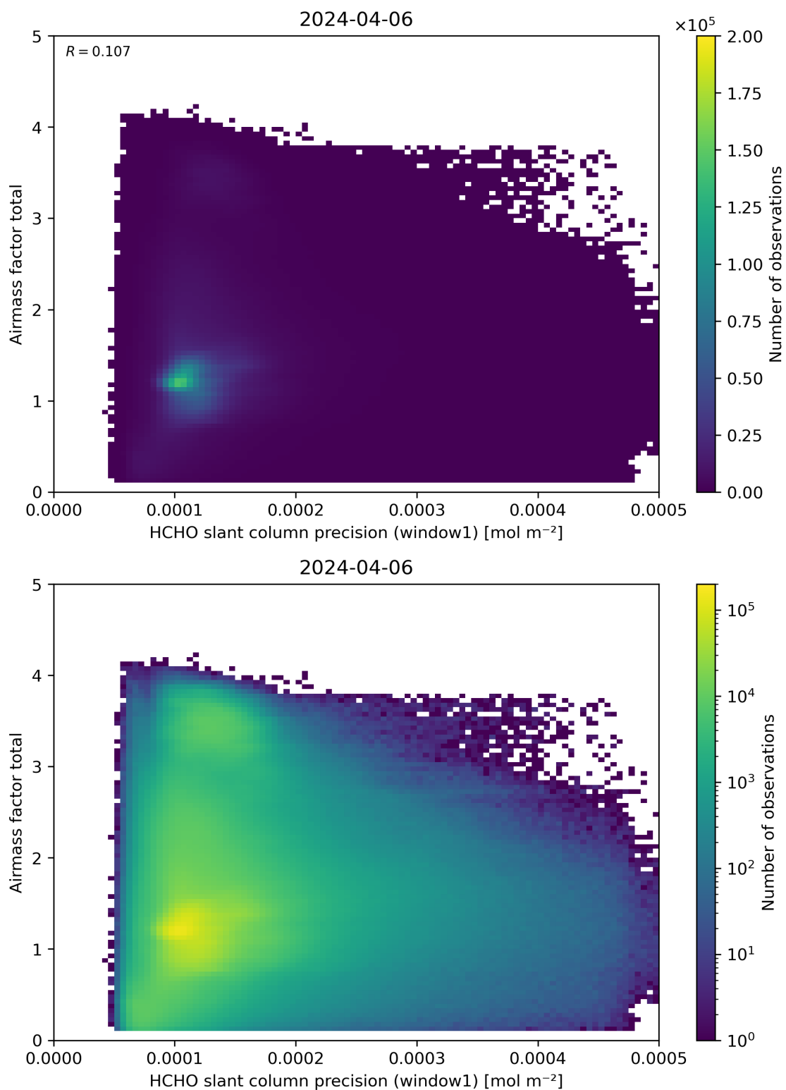
Figure 94: Scatter density plot of “HCHO slant column precision (window1)” against “Airmass factor total” for 2024-04-05 to 2024-04-07.
