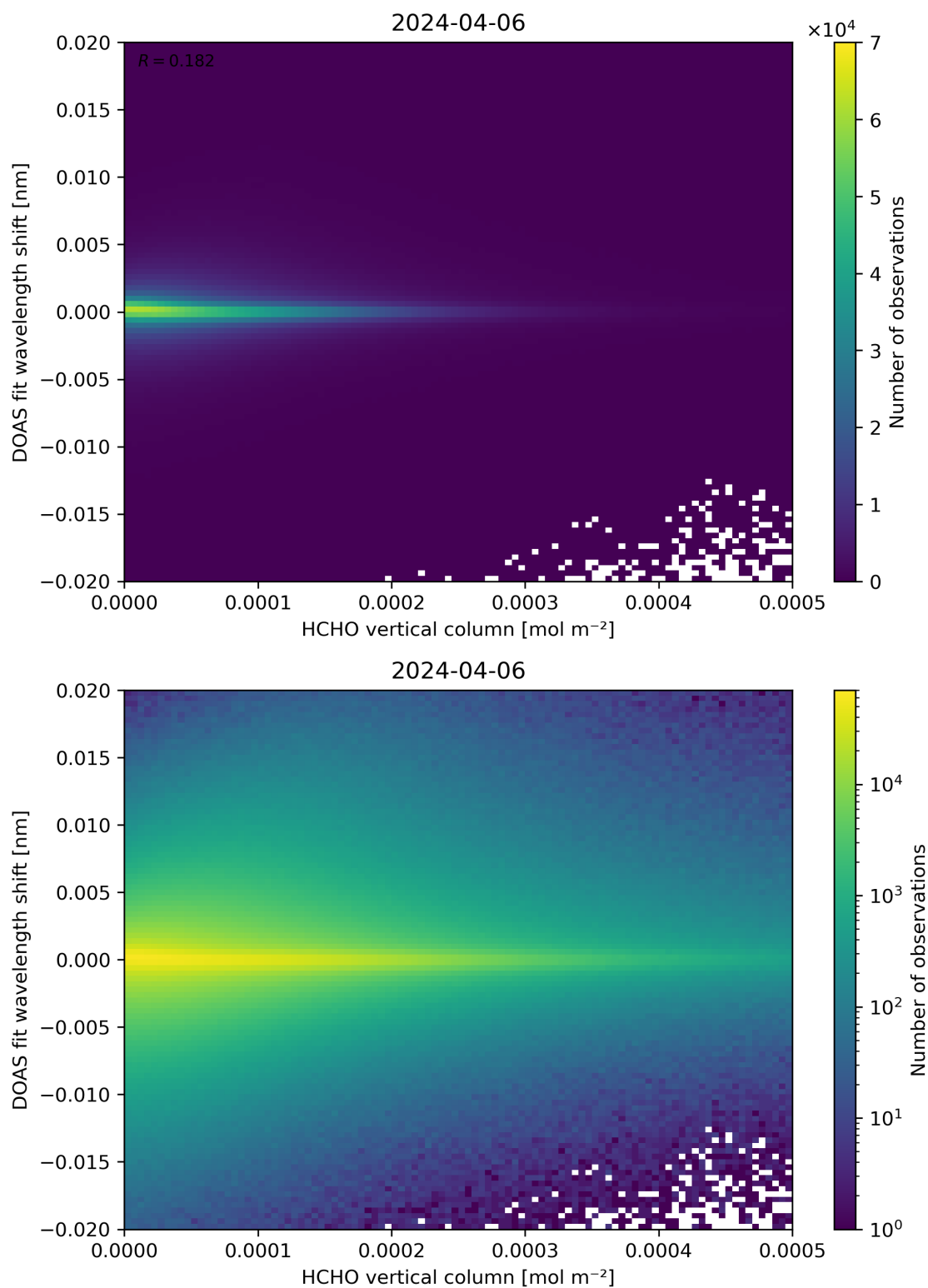
Figure 124: Scatter density plot of “HCHO vertical column” against “DOAS fit wavelength shift” for 2024-04-05 to 2024-04-07.
