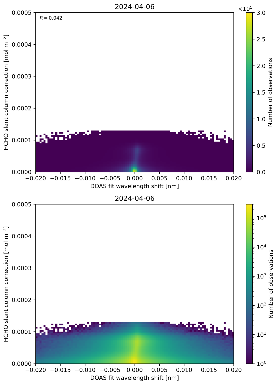
Figure 67: Scatter density plot of “DOAS fit wavelength shift” against “HCHO slant column correction” for 2024-04-05 to 2024-04-07.
