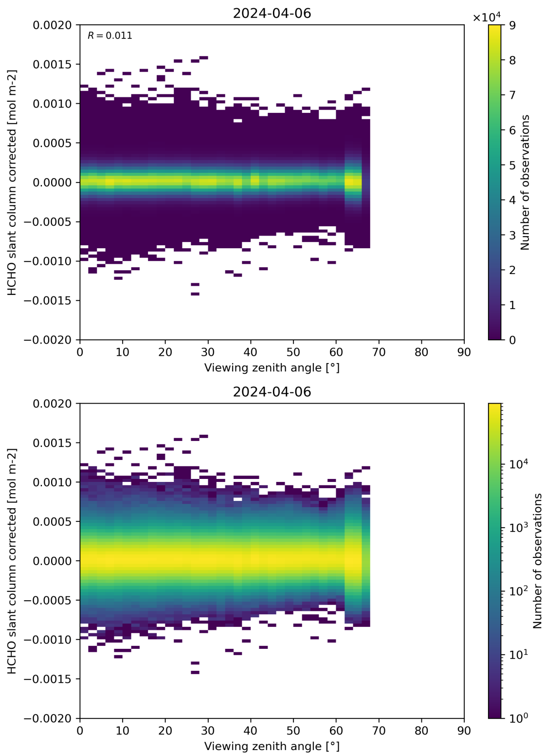
Figure 186: Scatter density plot of “Viewing zenith angle” against “HCHO slant column corrected” for 2024-04-05 to 2024-04-07.
