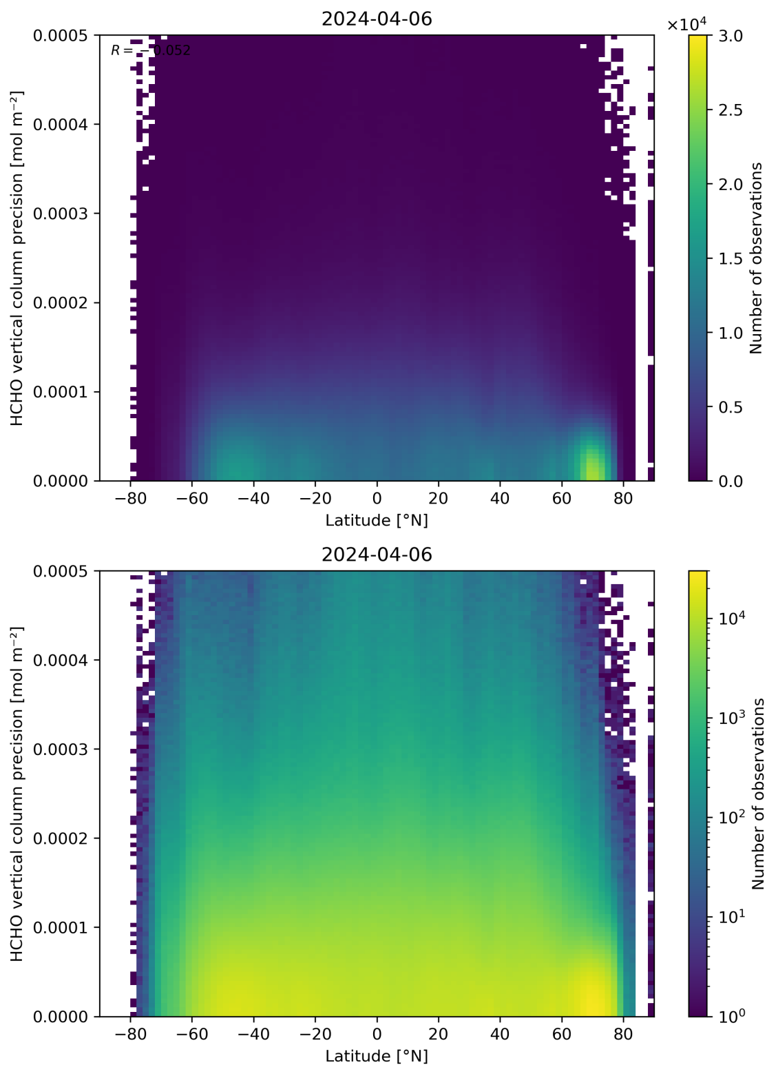
Figure 165: Scatter density plot of “Latitude” against “HCHO vertical column precision” for 2024-04-05 to 2024-04-07.
