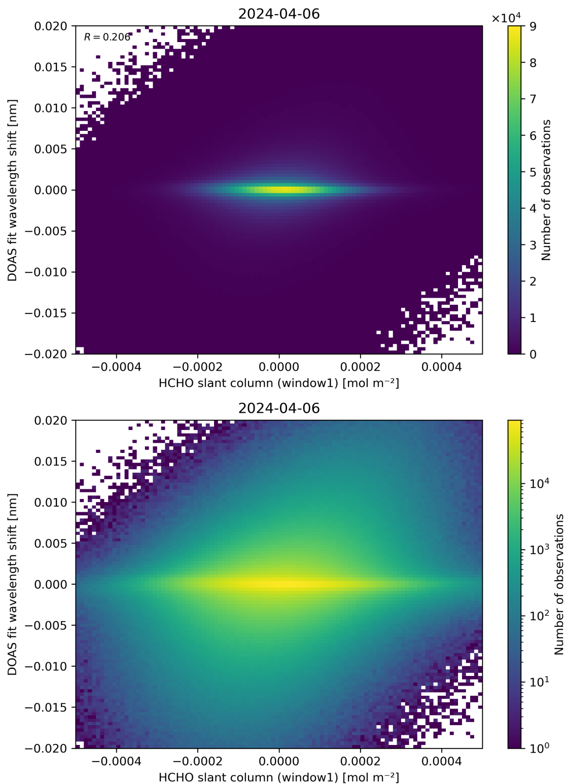
Figure 79: Scatter density plot of “HCHO slant column (window1)” against “DOAS fit wavelength shift” for 2024-04-05 to 2024-04-07.
