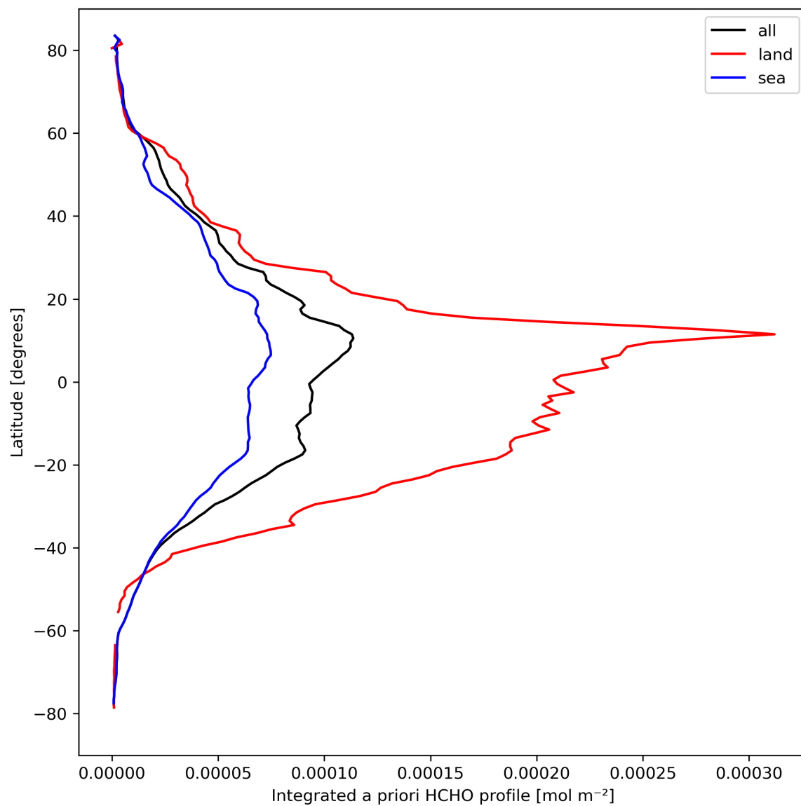
Figure 29: Zonal average of “Integrated a priori HCHO profile” for 2024-04-05 to 2024-04-07.
