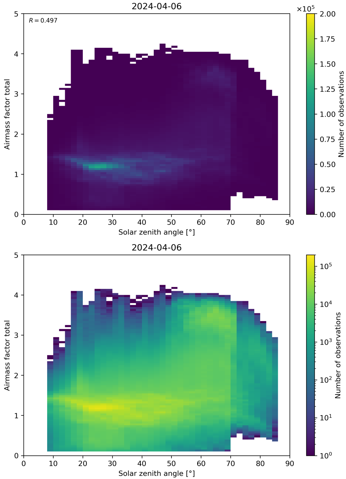
Figure 175: Scatter density plot of “Solar zenith angle” against “Airmass factor total” for 2024-04-05 to 2024-04-07.
