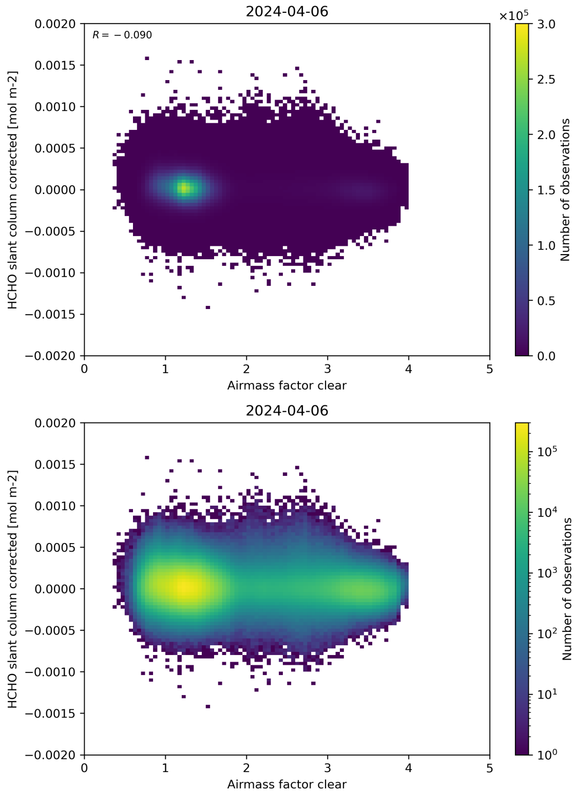
Figure 74: Scatter density plot of “Airmass factor clear” against “HCHO slant column corrected” for 2024-04-05 to 2024-04-07.
