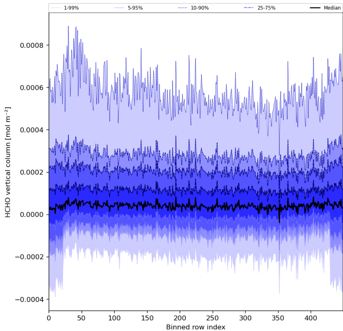
Figure 49: Along track statistics of “HCHO vertical column” for 2024-04-05 to 2024-04-07
