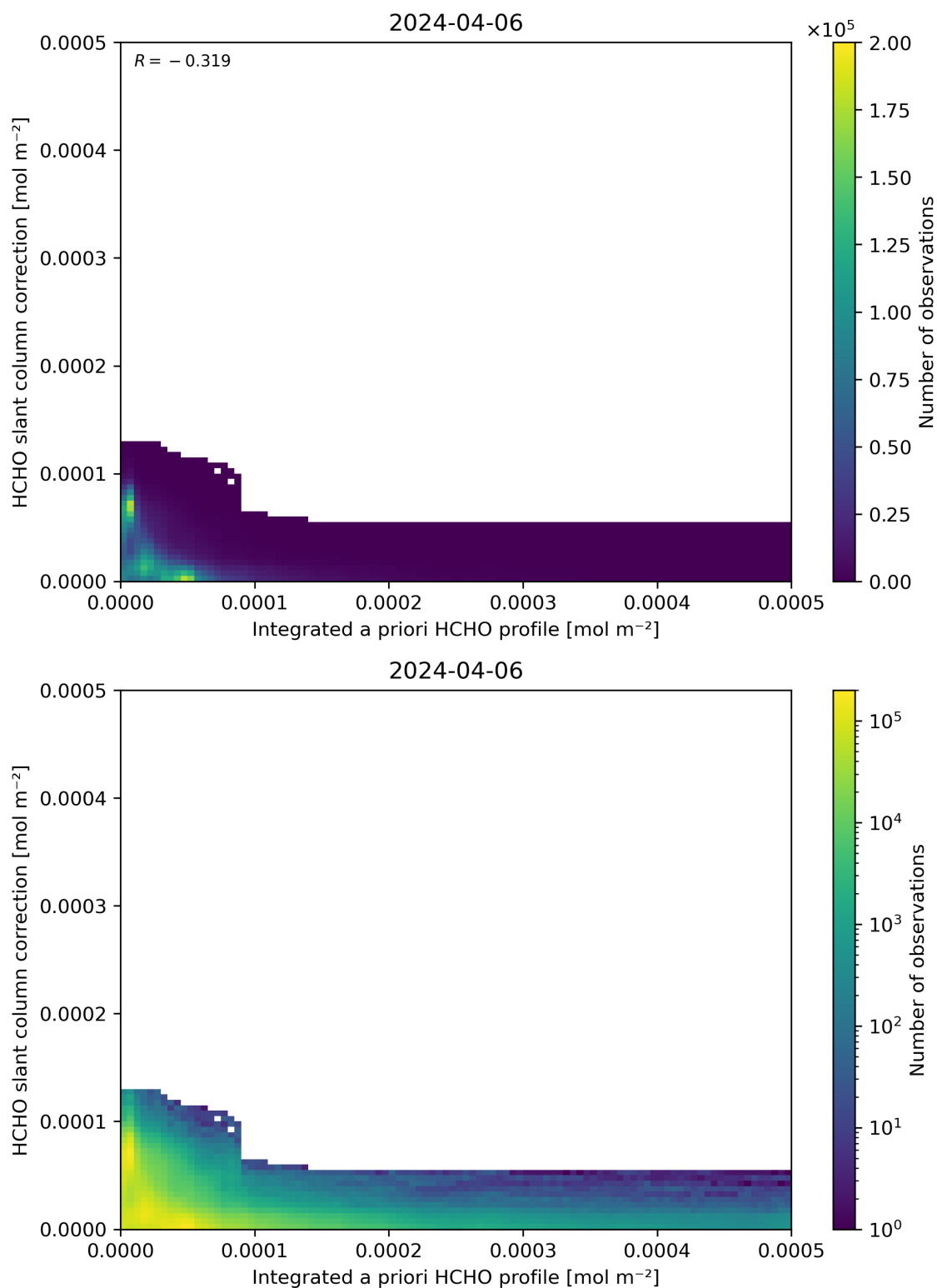
Figure 152: Scatter density plot of “Integrated a priori HCHO profile” against “HCHO slant column correction” for 2024-04-05 to 2024-04-07.
