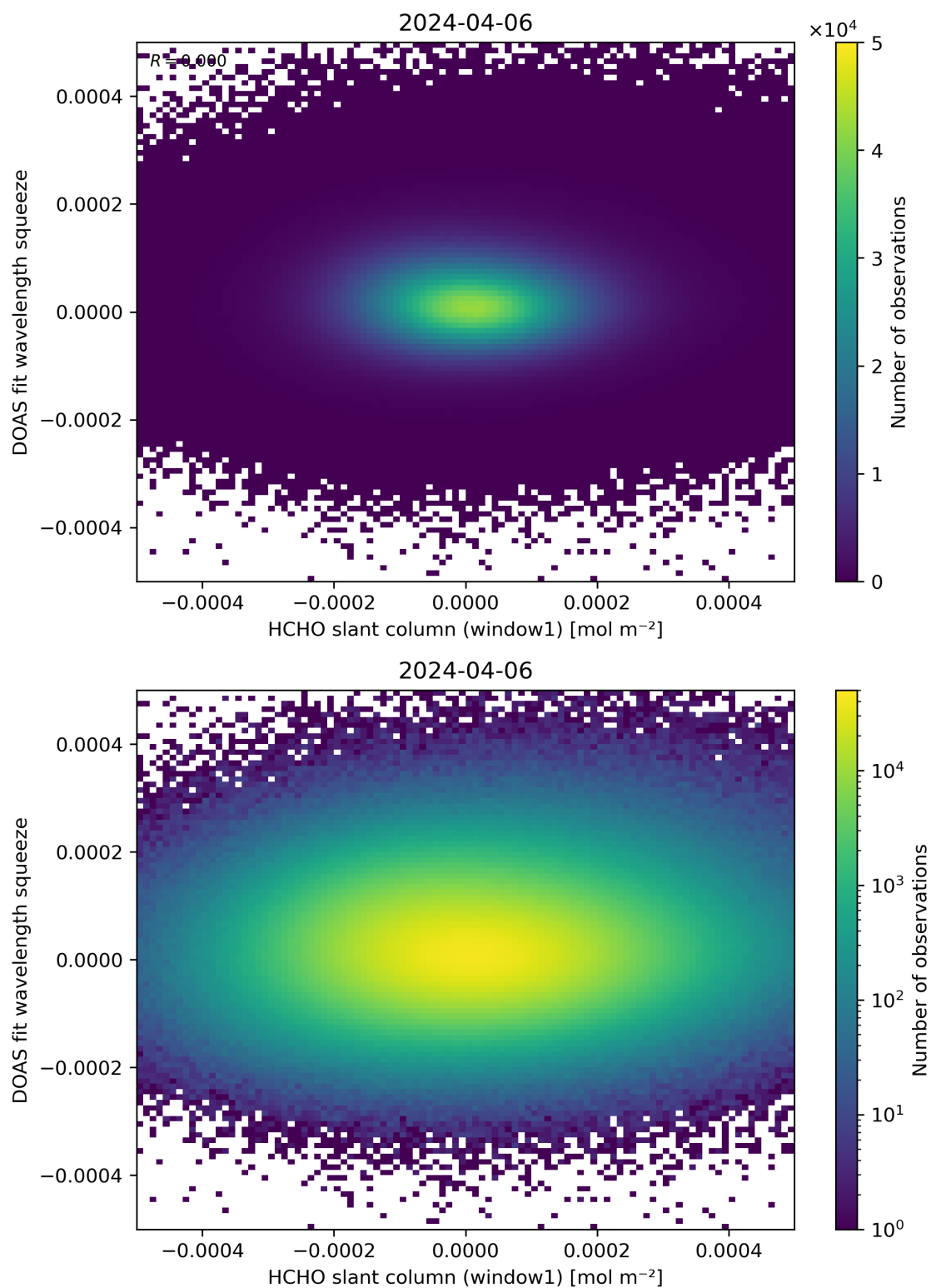
Figure 80: Scatter density plot of “HCHO slant column (window1)” against “DOAS fit wavelength squeeze” for 2024-04-05 to 2024-04-07.
