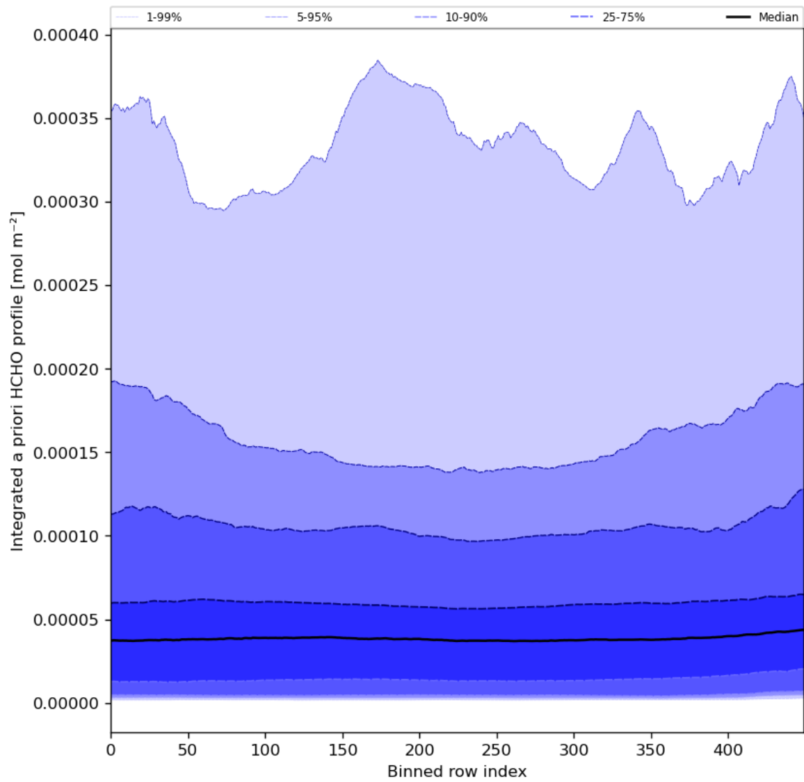
Figure 57: Along track statistics of “Integrated a priori HCHO profile” for 2024-04-05 to 2024-04-07
