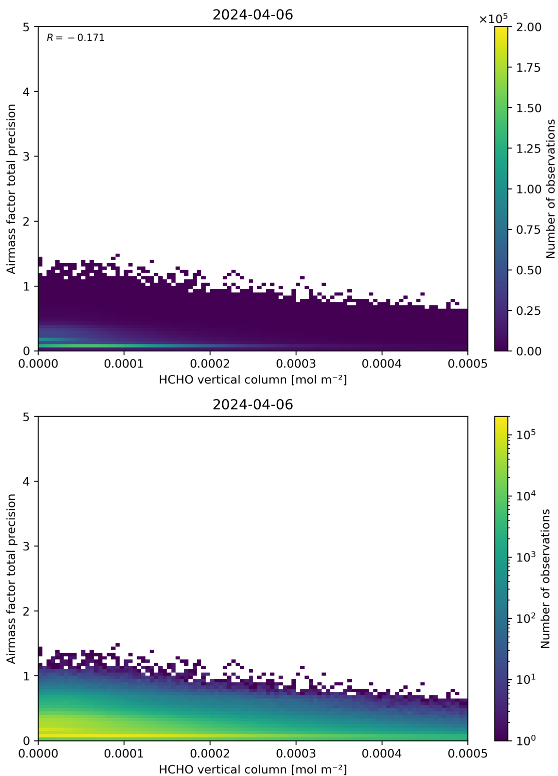
Figure 132: Scatter density plot of “HCHO vertical column” against “Airmass factor total precision” for 2024-04-05 to 2024-04-07.
