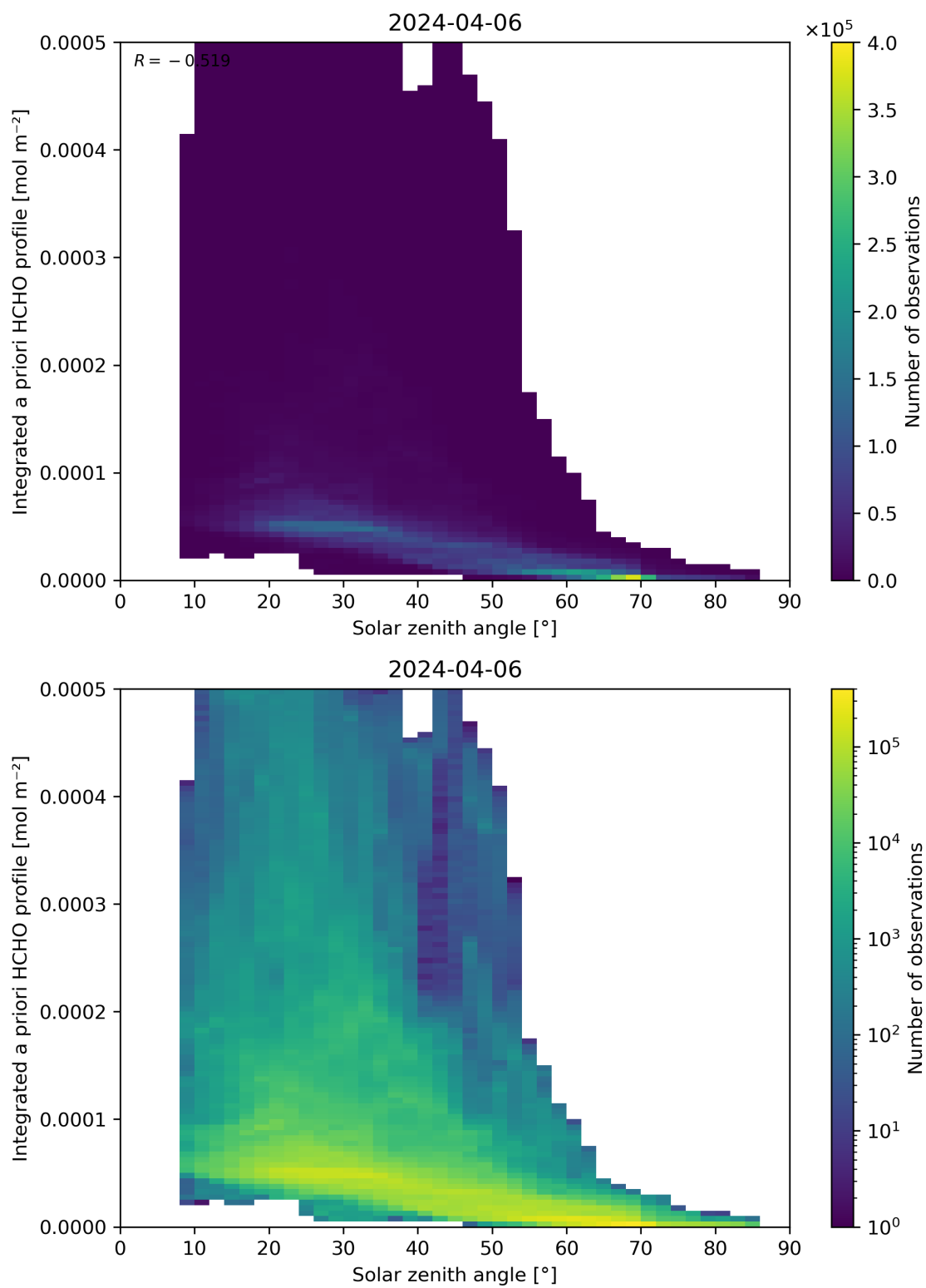
Figure 180: Scatter density plot of “Solar zenith angle” against “Integrated a priori HCHO profile” for 2024-04-05 to 2024-04-07.
