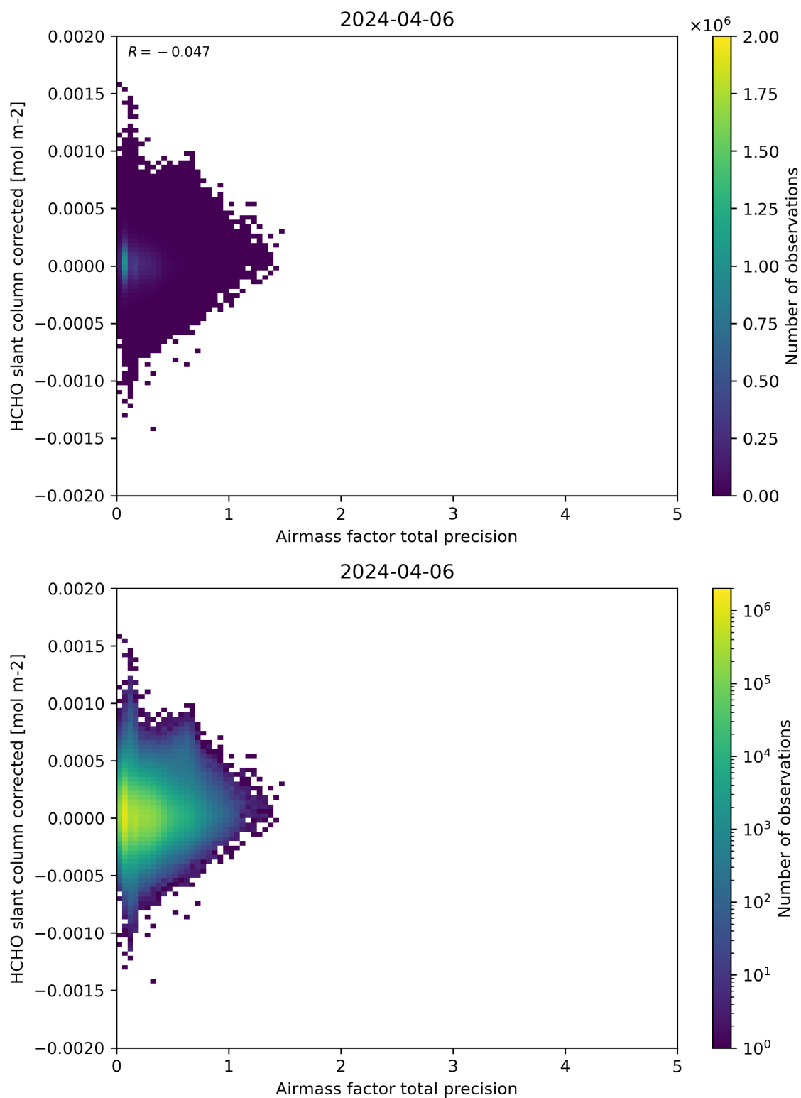
Figure 109: Scatter density plot of “Airmass factor total precision” against “HCHO slant column corrected” for 2024-04-05 to 2024-04-07.
