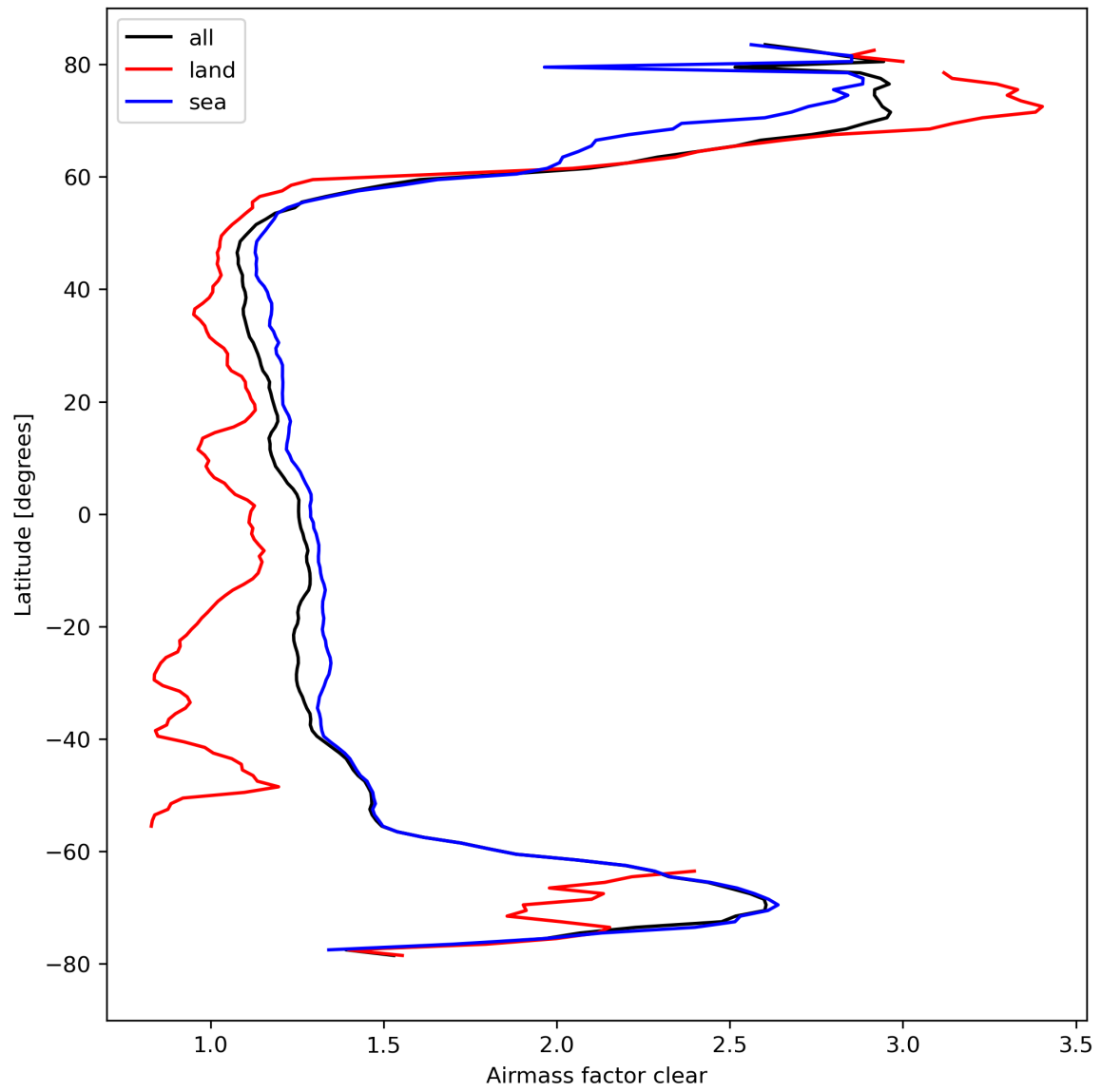
Figure 28: Zonal average of “Airmass factor clear” for 2024-04-05 to 2024-04-07.
