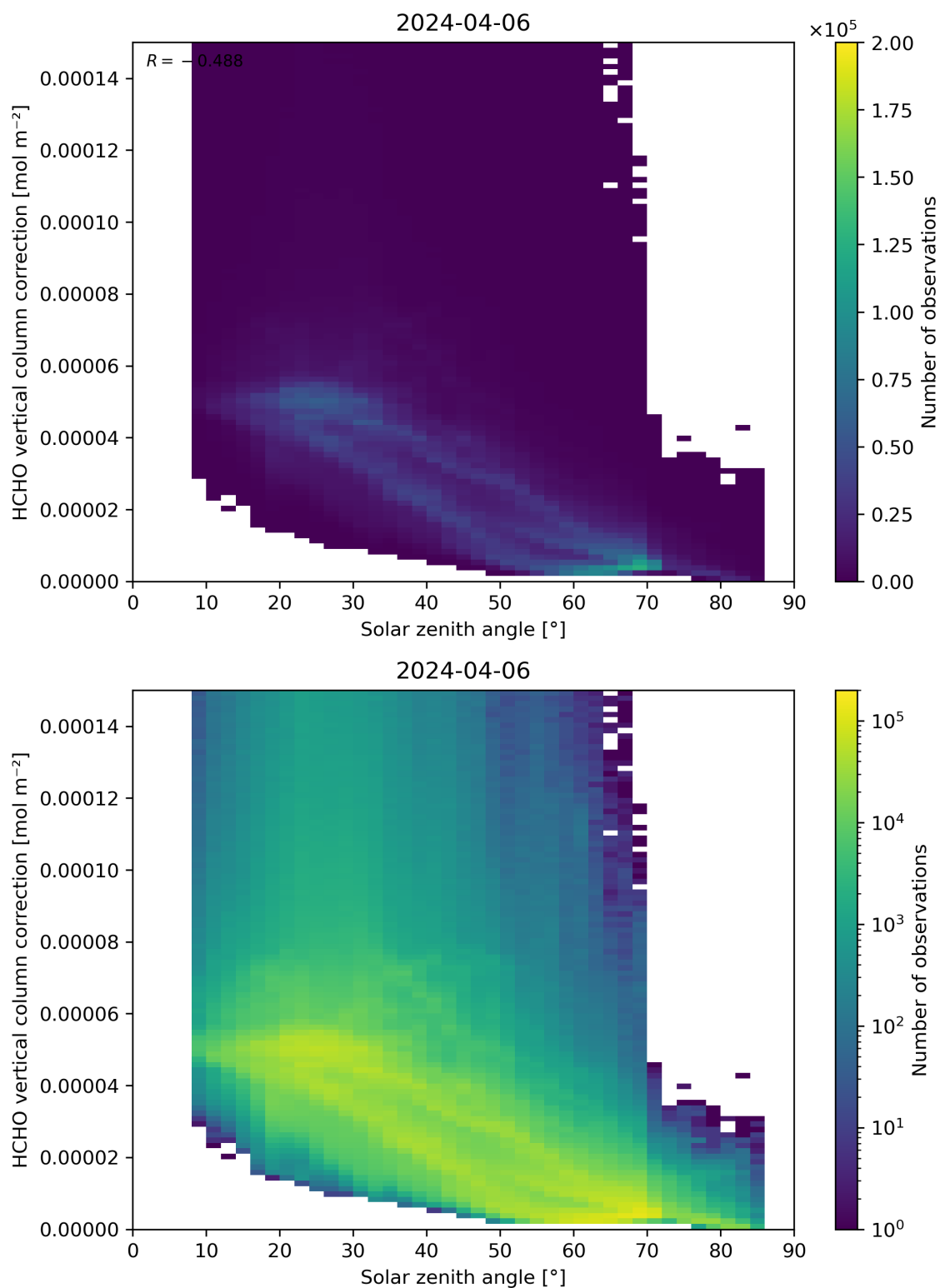
Figure 178: Scatter density plot of “Solar zenith angle” against “HCHO vertical column correction” for 2024-04-05 to 2024-04-07.
