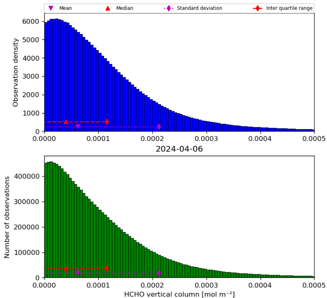
Figure 35: Histogram of “HCHO vertical column” for 2024-04-05 to 2024-04-07
