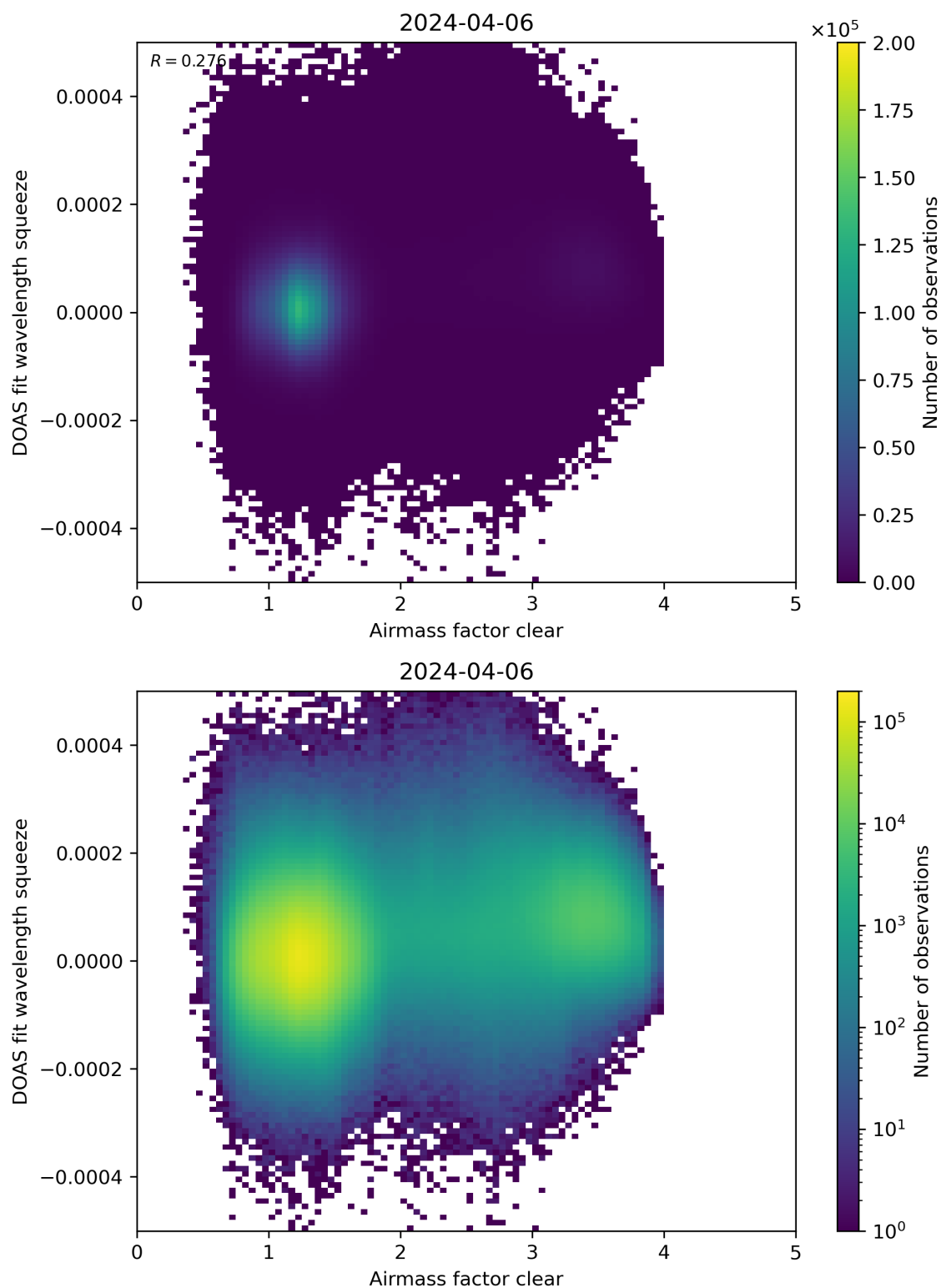
Figure 73: Scatter density plot of “Airmass factor clear” against “DOAS fit wavelength squeeze” for 2024-04-05 to 2024-04-07.
