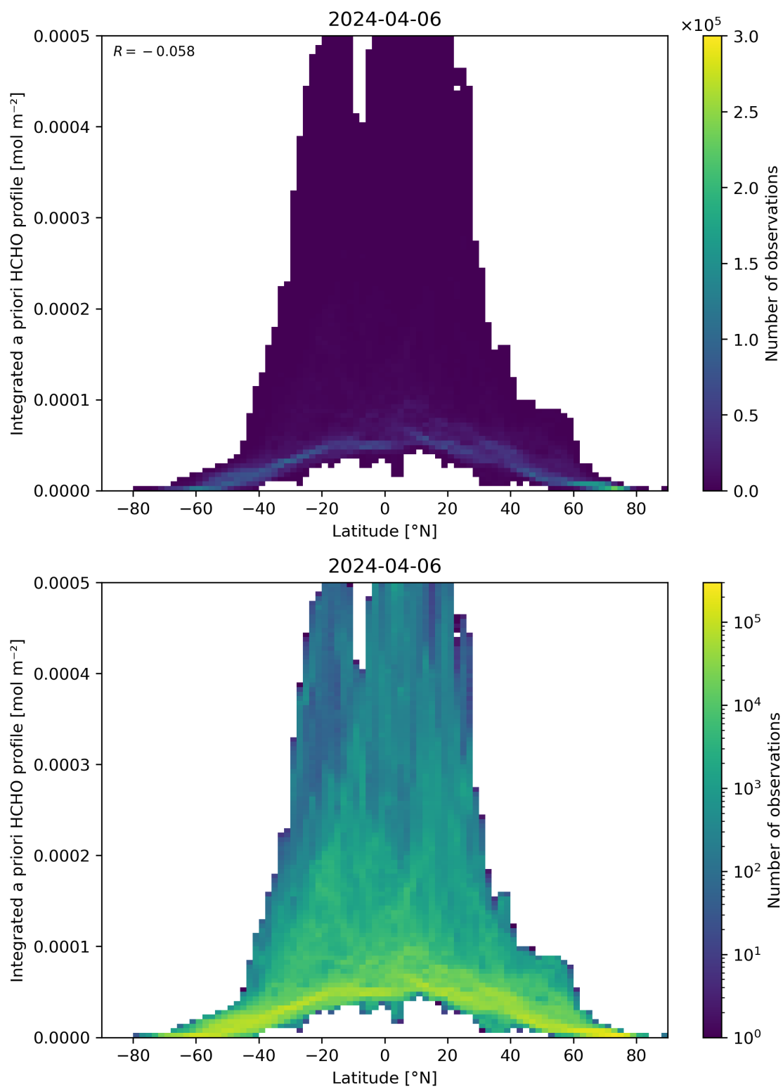
Figure 166: Scatter density plot of “Latitude” against “Integrated a priori HCHO profile” for 2024-04-05 to 2024-04-07.
