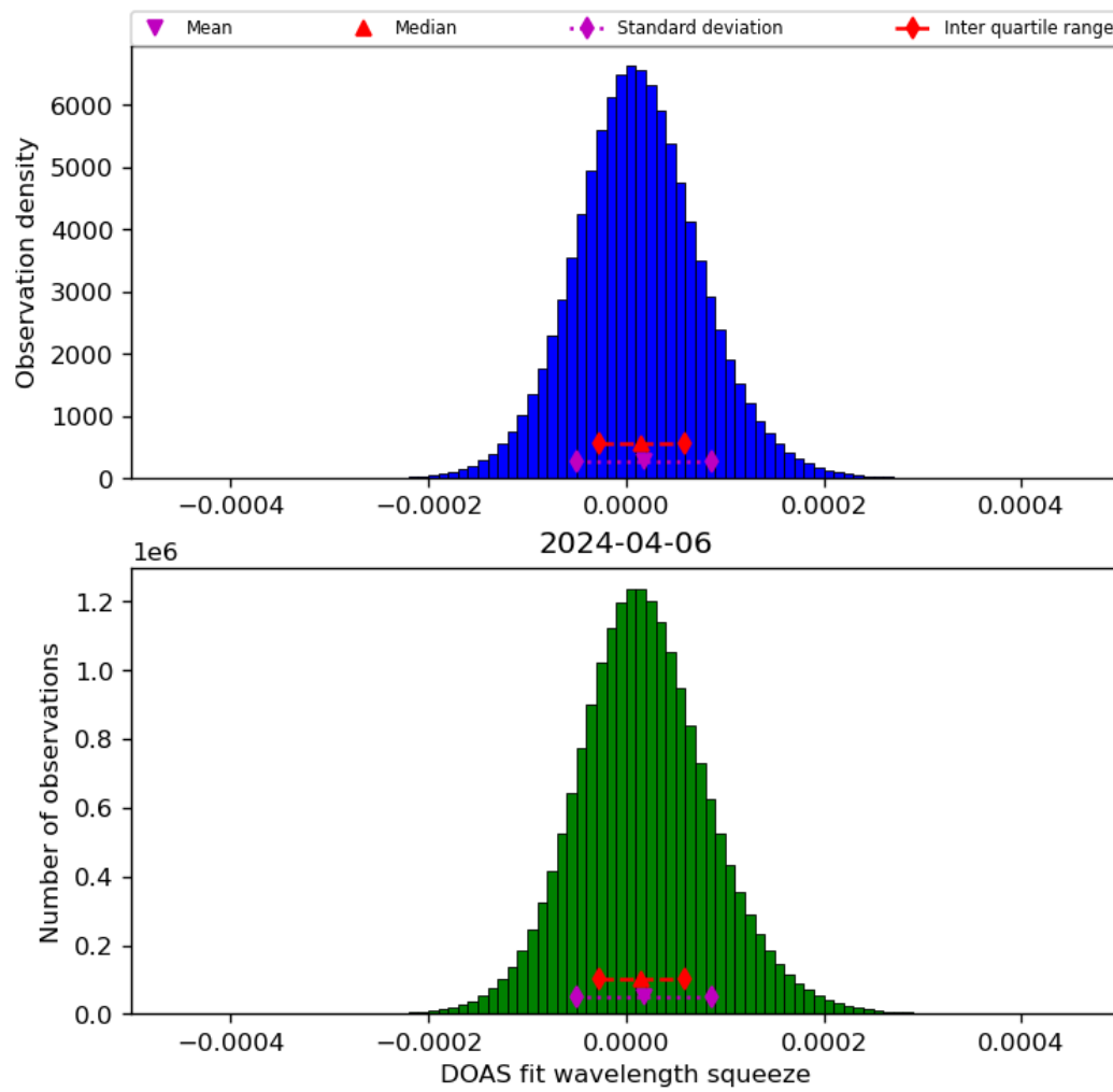
Figure 45: Histogram of “DOAS fit wavelength squeeze” for 2024-04-05 to 2024-04-07
