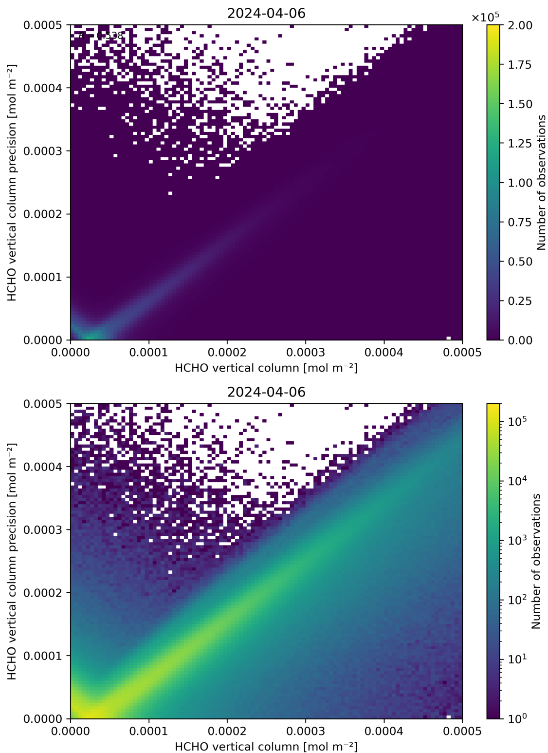
Figure 134: Scatter density plot of “HCHO vertical column” against “HCHO vertical column precision” for 2024-04-05 to 2024-04-07.
