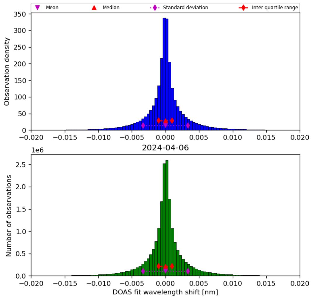
Figure 44: Histogram of “DOAS fit wavelength shift” for 2024-04-05 to 2024-04-07
