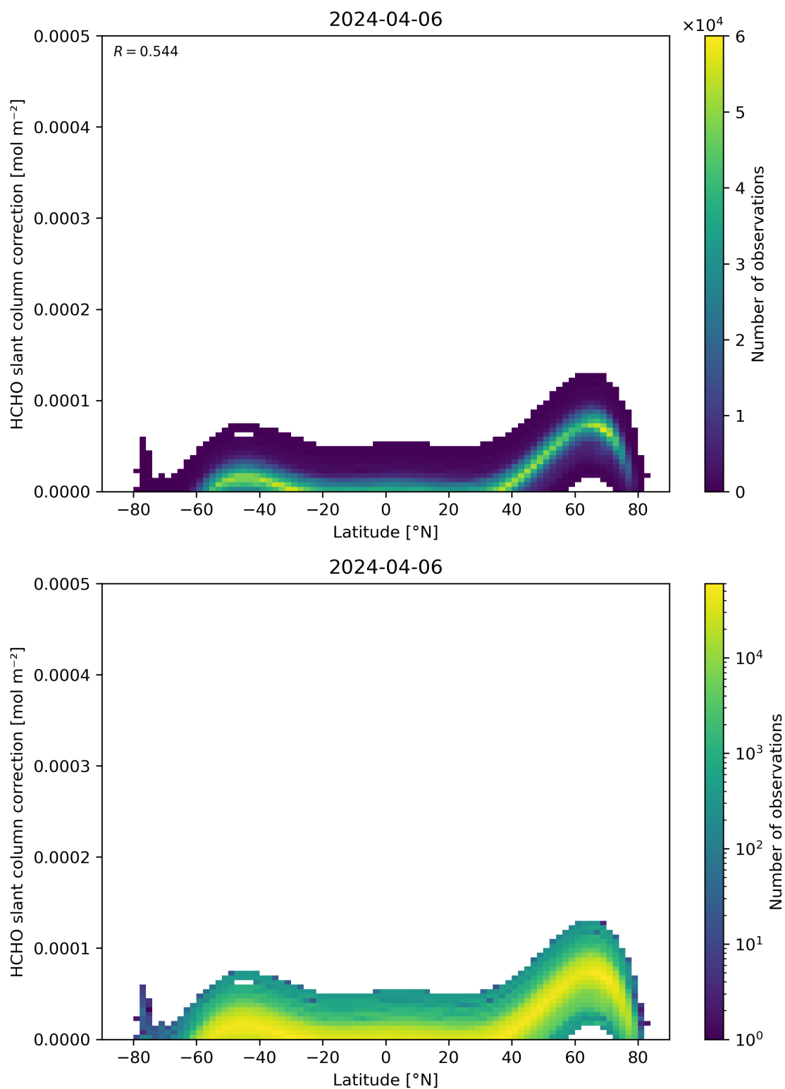
Figure 158: Scatter density plot of “Latitude” against “HCHO slant column correction” for 2024-04-05 to 2024-04-07.
