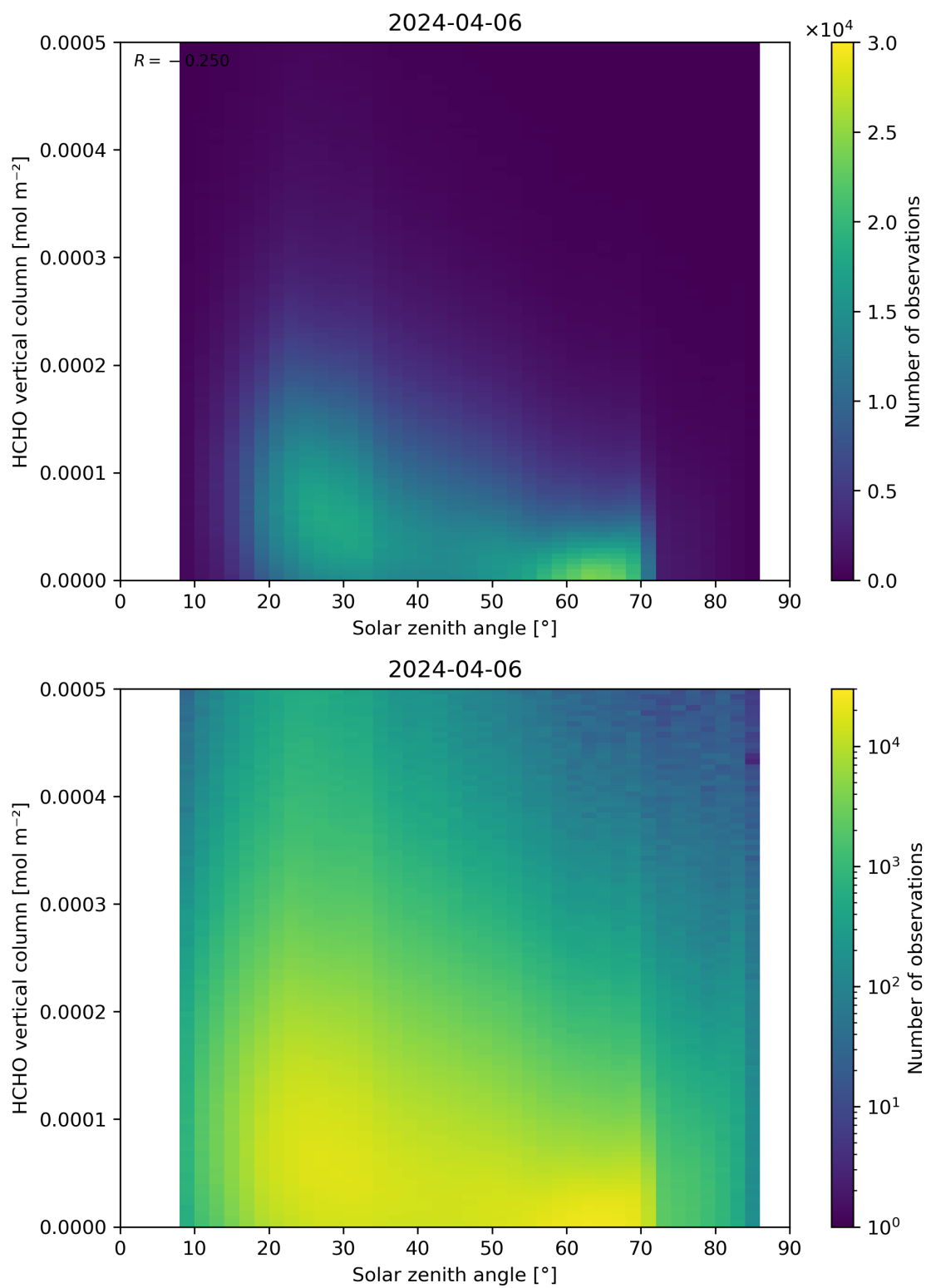
Figure 177: Scatter density plot of “Solar zenith angle” against “HCHO vertical column” for 2024-04-05 to 2024-04-07.
