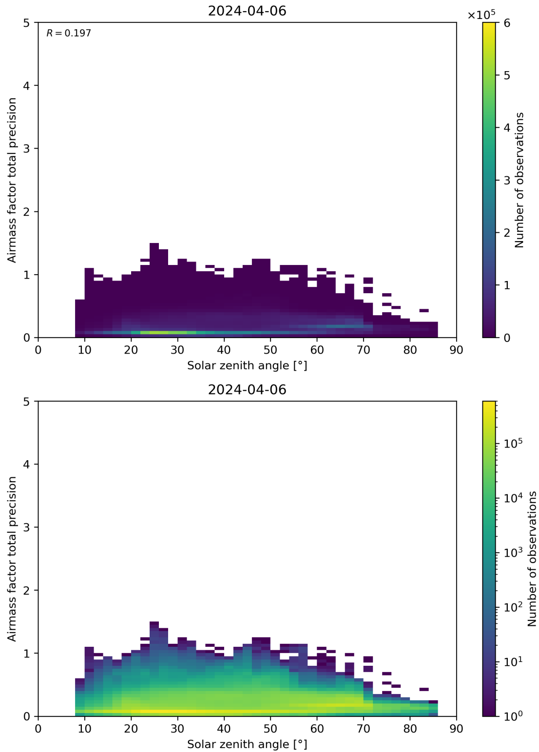
Figure 176: Scatter density plot of “Solar zenith angle” against “Airmass factor total precision” for 2024-04-05 to 2024-04-07.
