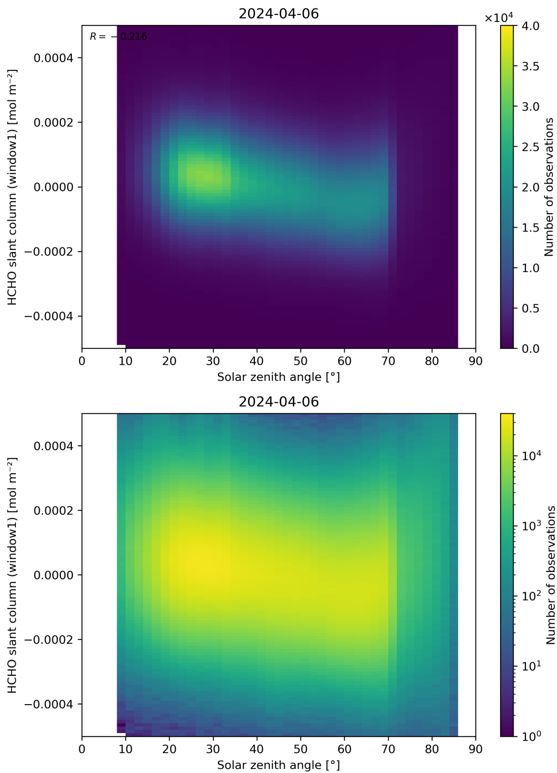
Figure 173: Scatter density plot of “Solar zenith angle” against “HCHO slant column (window1)” for 2024-04-05 to 2024-04-07.
