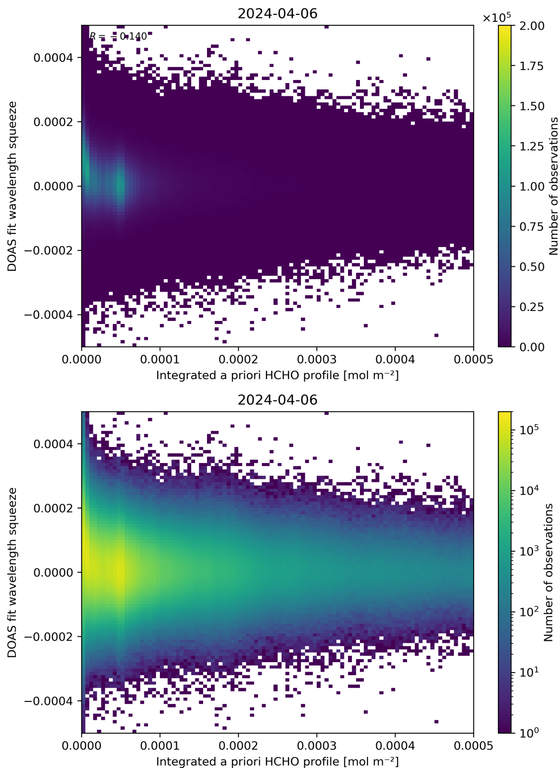
Figure 150: Scatter density plot of “Integrated a priori HCHO profile” against “DOAS fit wavelength squeeze” for 2024-04-05 to 2024-04-07.
