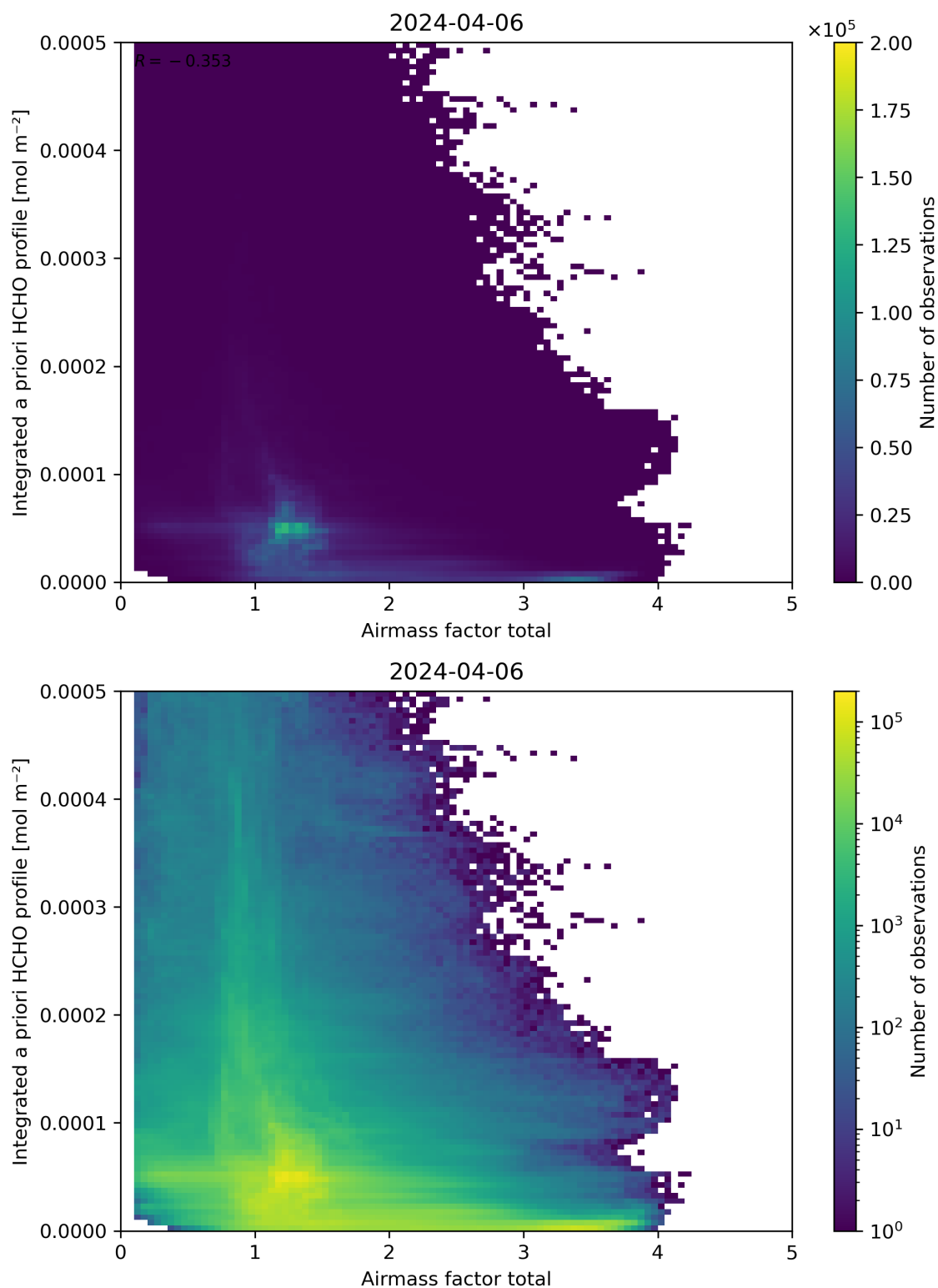
Figure 104: Scatter density plot of “Airmass factor total” against “Integrated a priori HCHO profile” for 2024-04-05 to 2024-04-07.
