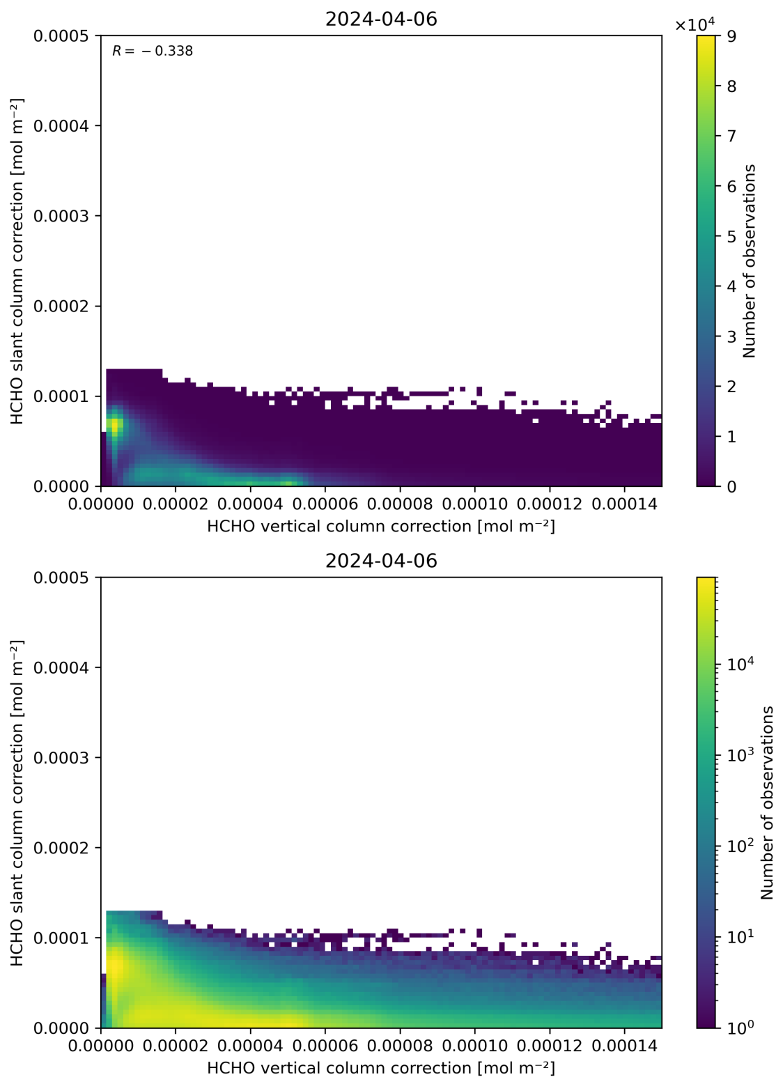
Figure 117: Scatter density plot of “HCHO vertical column correction” against “HCHO slant column correction” for 2024-04-05 to 2024-04-07.
