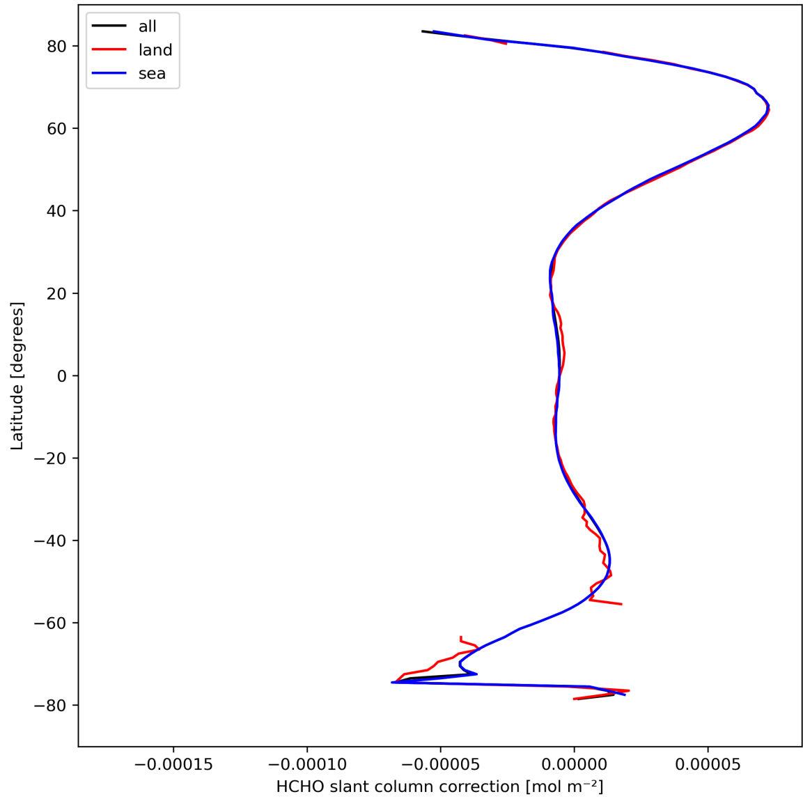
Figure 33: Zonal average of "HCHO slant column correction" for 2024-04-05 to 2024-04-07.
