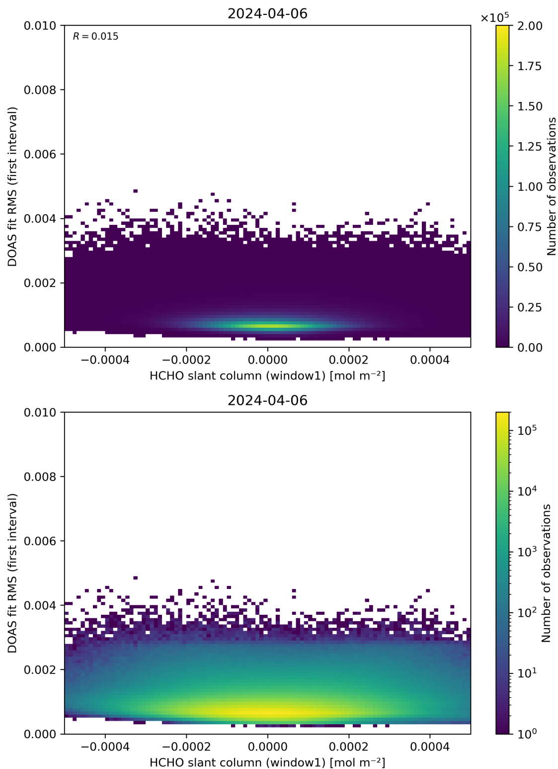
Figure 78: Scatter density plot of “HCHO slant column (window1)” against “DOAS fit RMS (first interval)” for 2024-04-05 to 2024-04-07.
