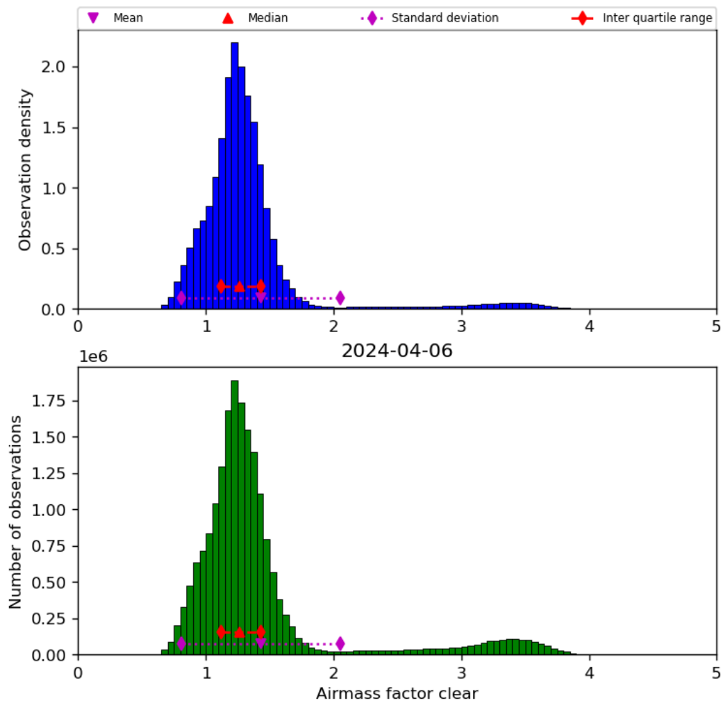
Figure 42: Histogram of “Airmass factor clear” for 2024-04-05 to 2024-04-07
