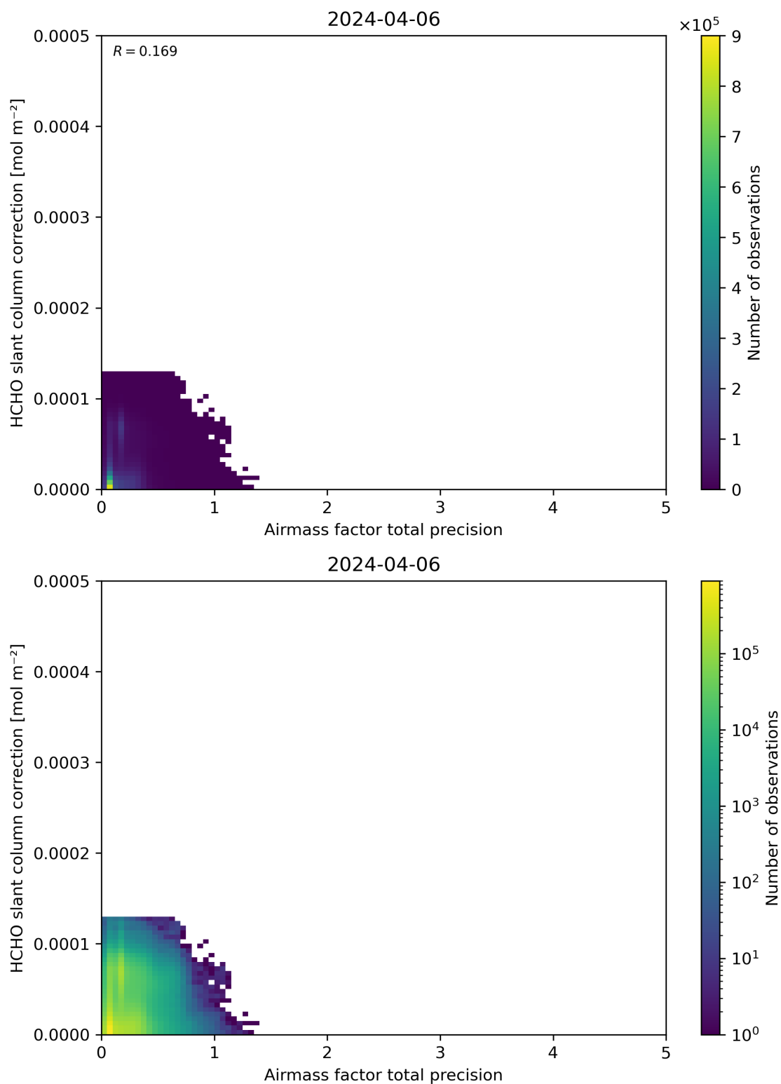
Figure 110: Scatter density plot of “Airmass factor total precision” against “HCHO slant column correction” for 2024-04-05 to 2024-04-07.
