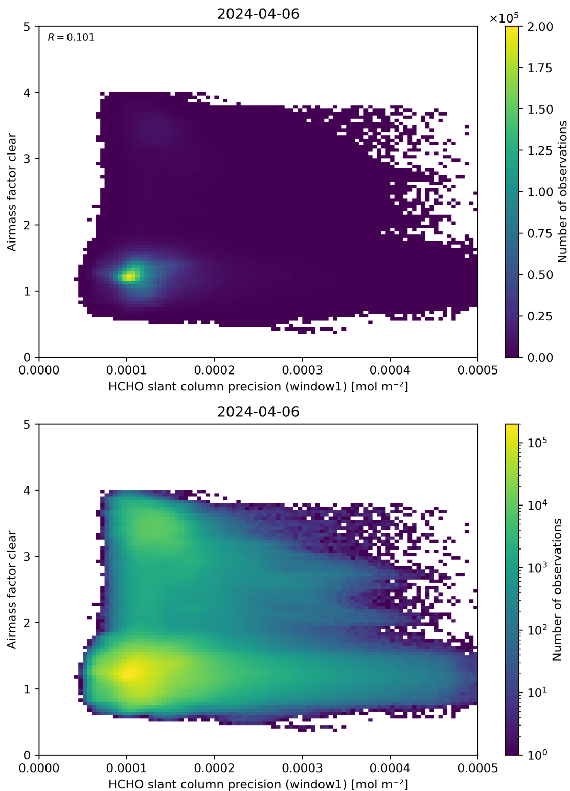
Figure 91: Scatter density plot of “HCHO slant column precision (window1)” against “Airmass factor clear” for 2024-04-05 to 2024-04-07.
