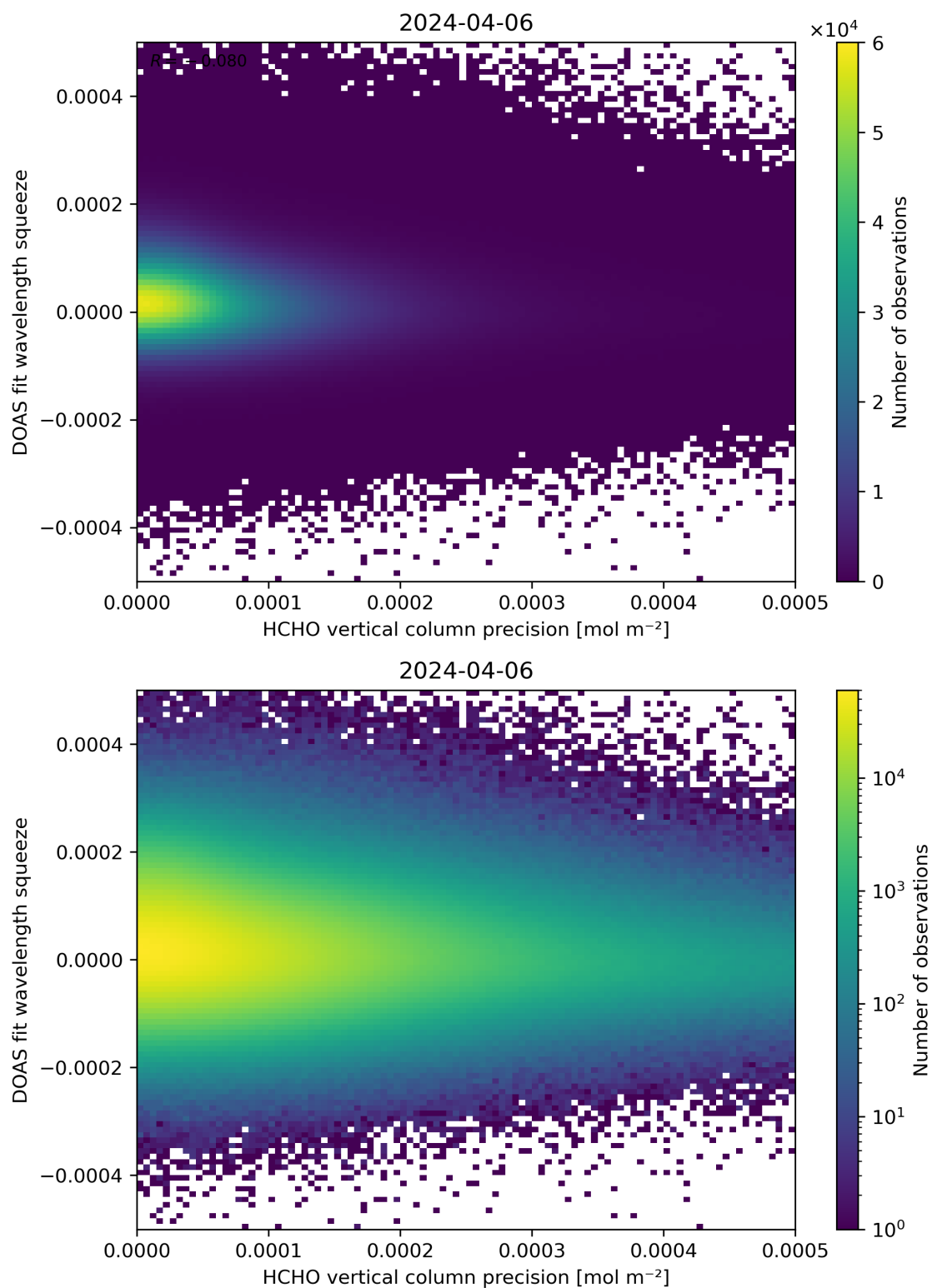
Figure 138: Scatter density plot of “HCHO vertical column precision” against “DOAS fit wavelength squeeze” for 2024-04-05 to 2024-04-07.
