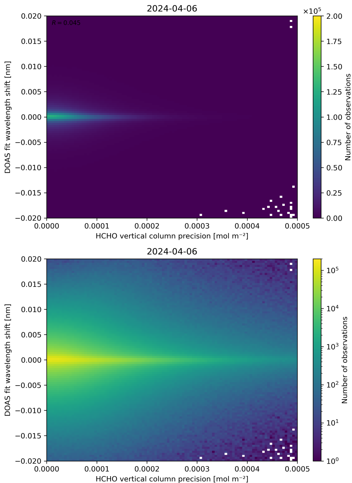
Figure 137: Scatter density plot of “HCHO vertical column precision” against “DOAS fit wavelength shift” for 2024-04-05 to 2024-04-07.
