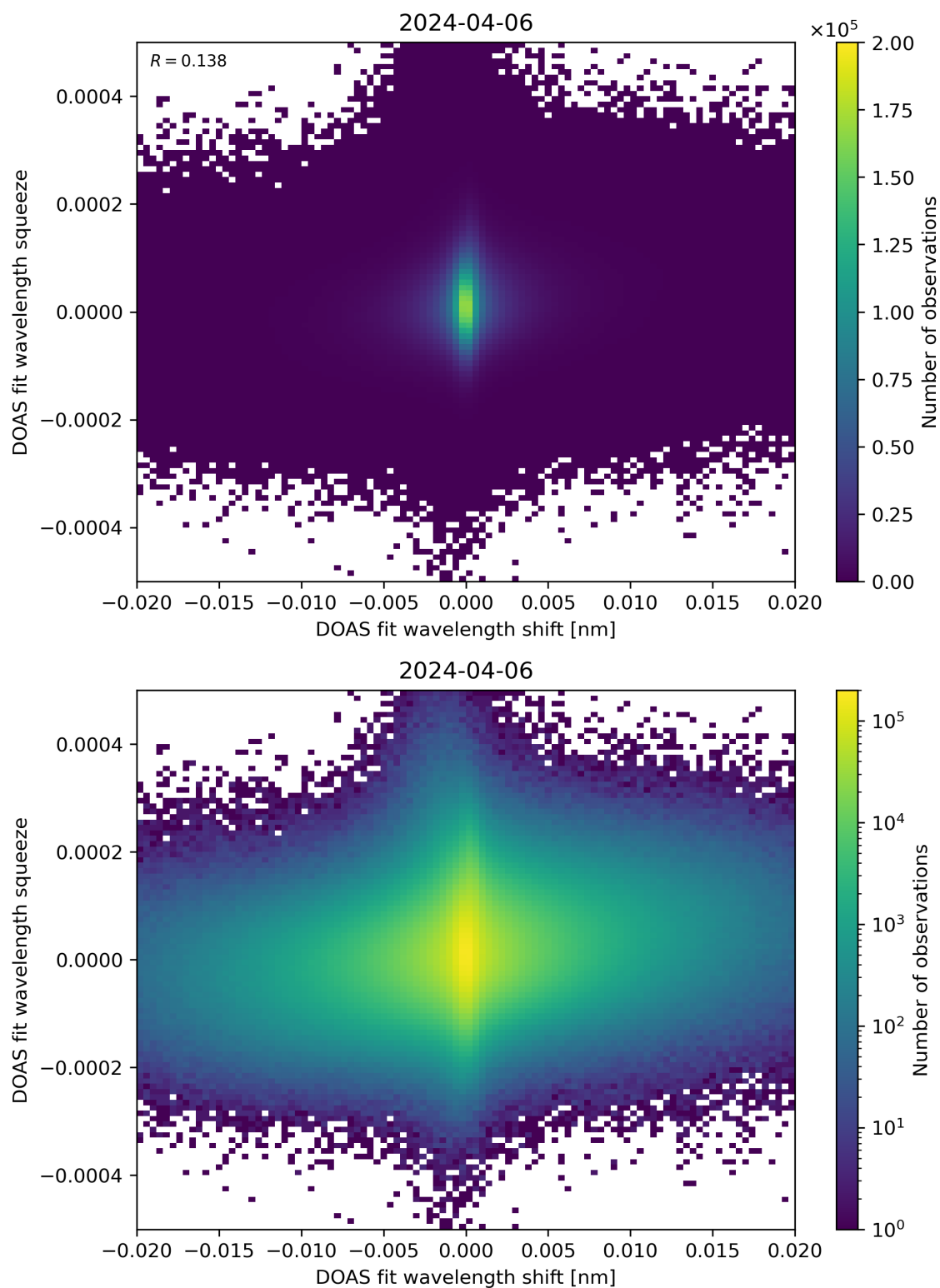
Figure 65: Scatter density plot of “DOAS fit wavelength shift” against “DOAS fit wavelength squeeze” for 2024-04-05 to 2024-04-07.
