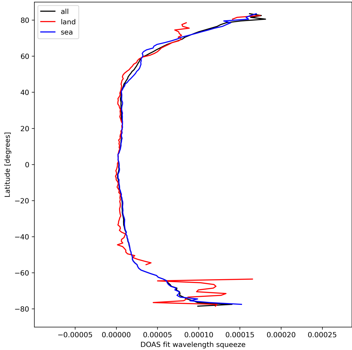
Figure 31: Zonal average of “DOAS fit wavelength squeeze” for 2024-04-05 to 2024-04-07.
