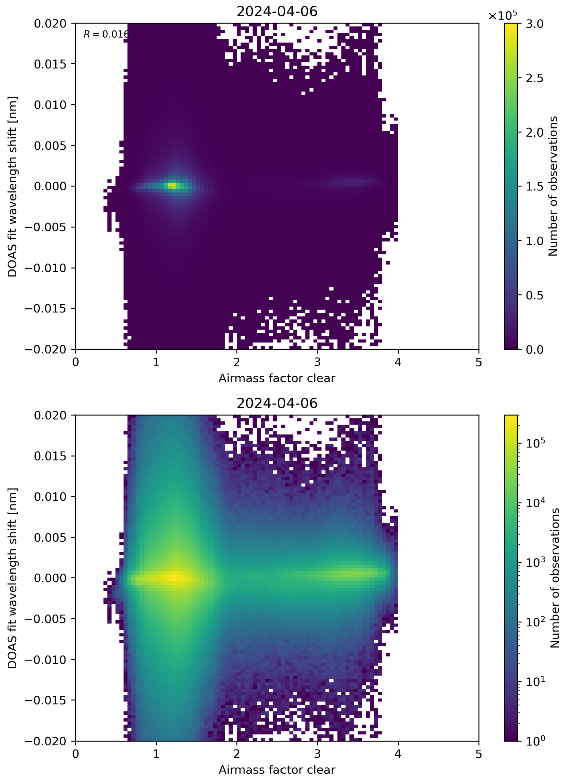
Figure 72: Scatter density plot of “Airmass factor clear” against “DOAS fit wavelength shift” for 2024-04-05 to 2024-04-07.
