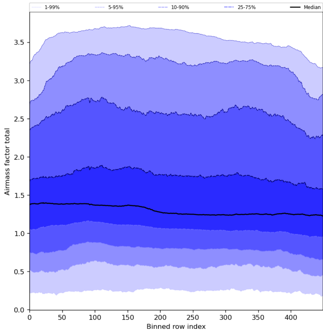
Figure 54: Along track statistics of “Airmass factor total” for 2024-04-05 to 2024-04-07
