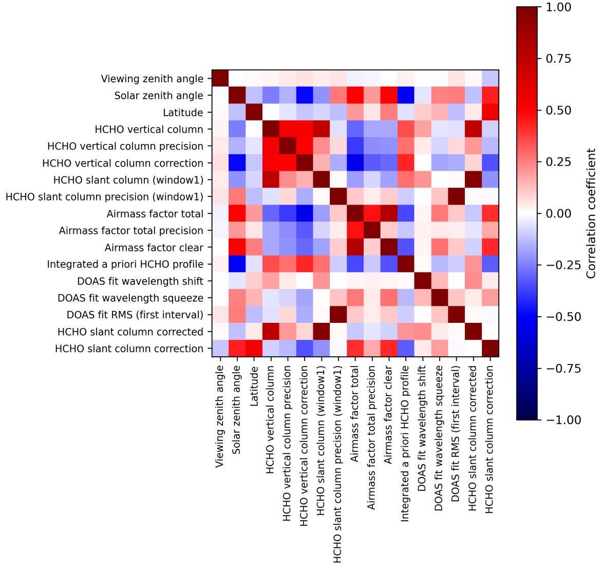
Figure 2: Map of correlation matrix for 2024-04-05 to 2024-04-07.
