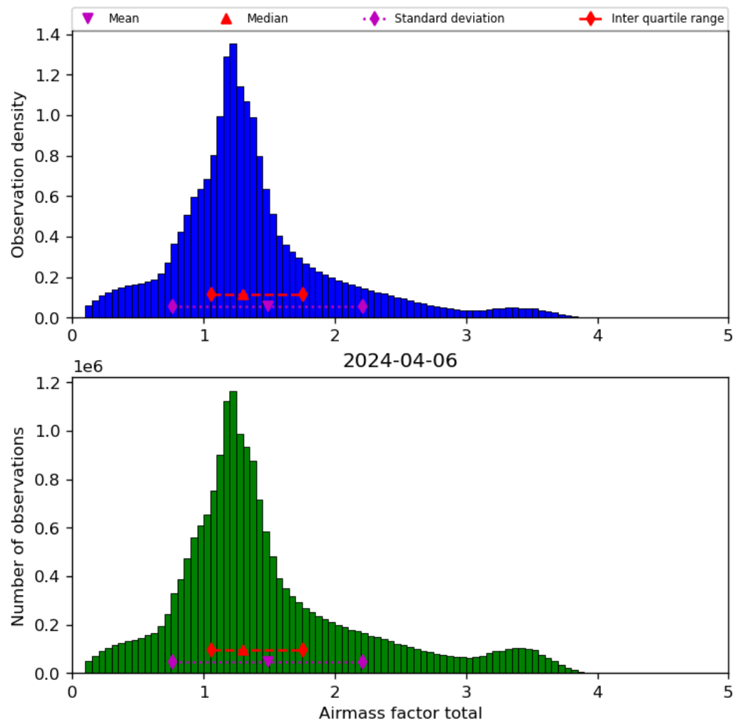
Figure 40: Histogram of “Airmass factor total” for 2024-04-05 to 2024-04-07
