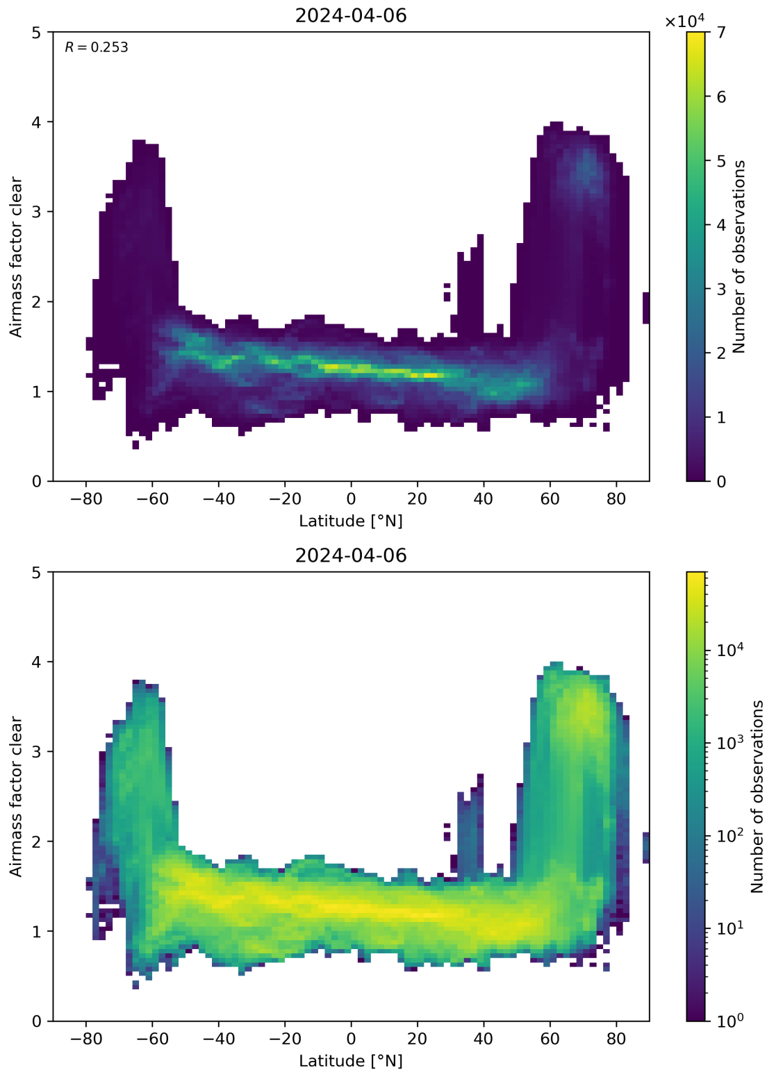
Figure 156: Scatter density plot of “Latitude” against “Airmass factor clear” for 2024-04-05 to 2024-04-07.
