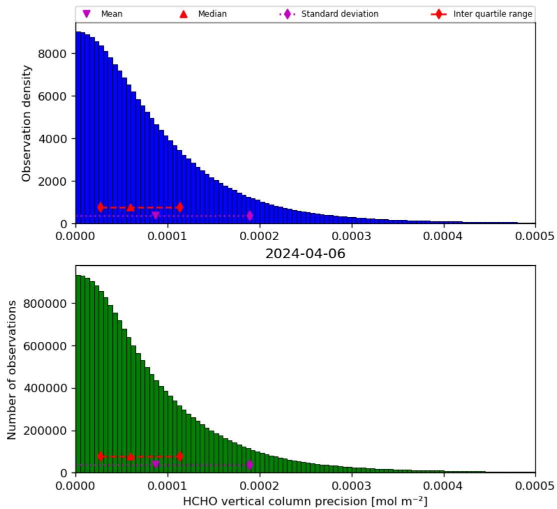
Figure 36: Histogram of “HCHO vertical column precision” for 2024-04-05 to 2024-04-07
