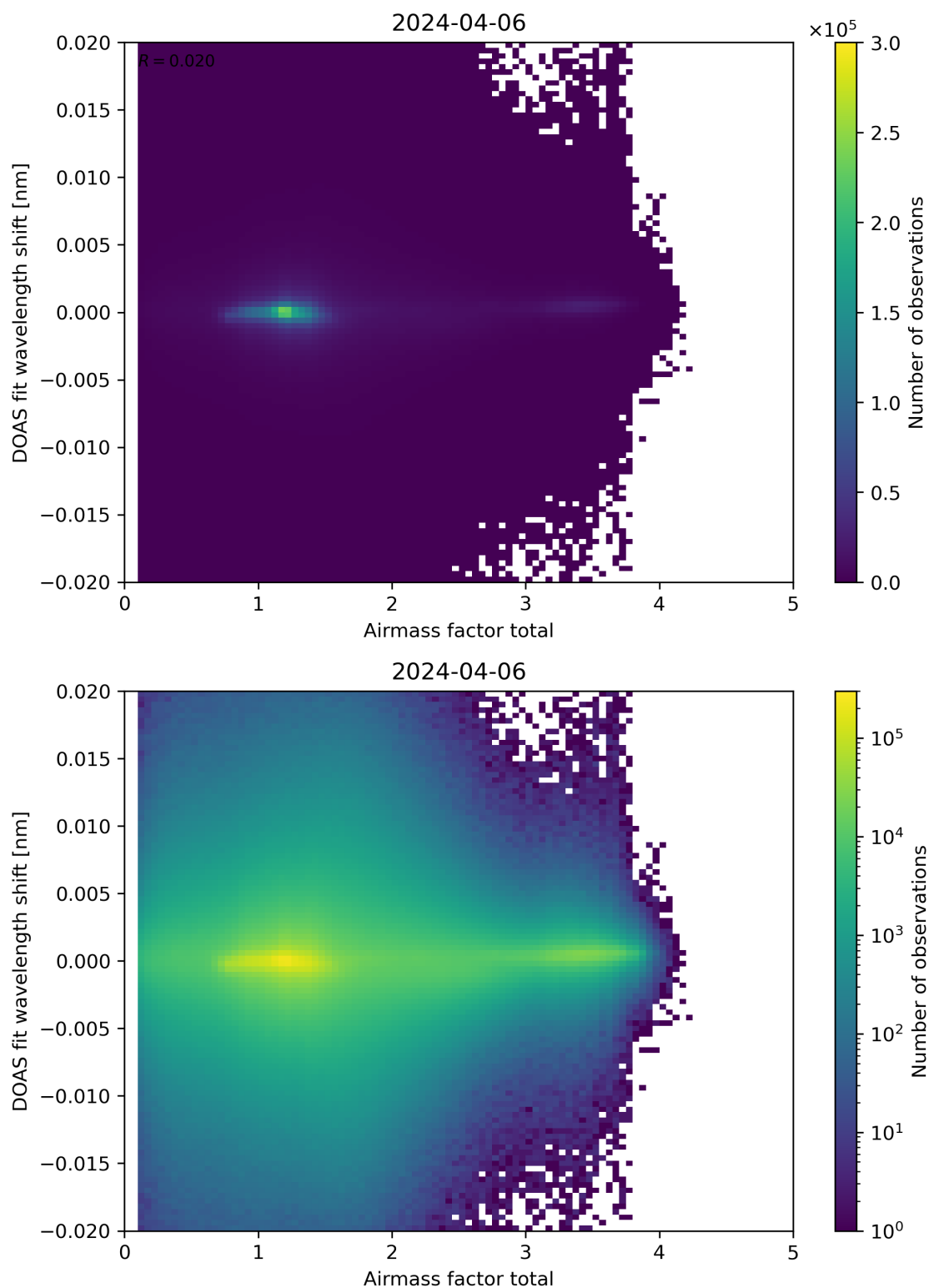
Figure 98: Scatter density plot of “Airmass factor total” against “DOAS fit wavelength shift” for 2024-04-05 to 2024-04-07.
