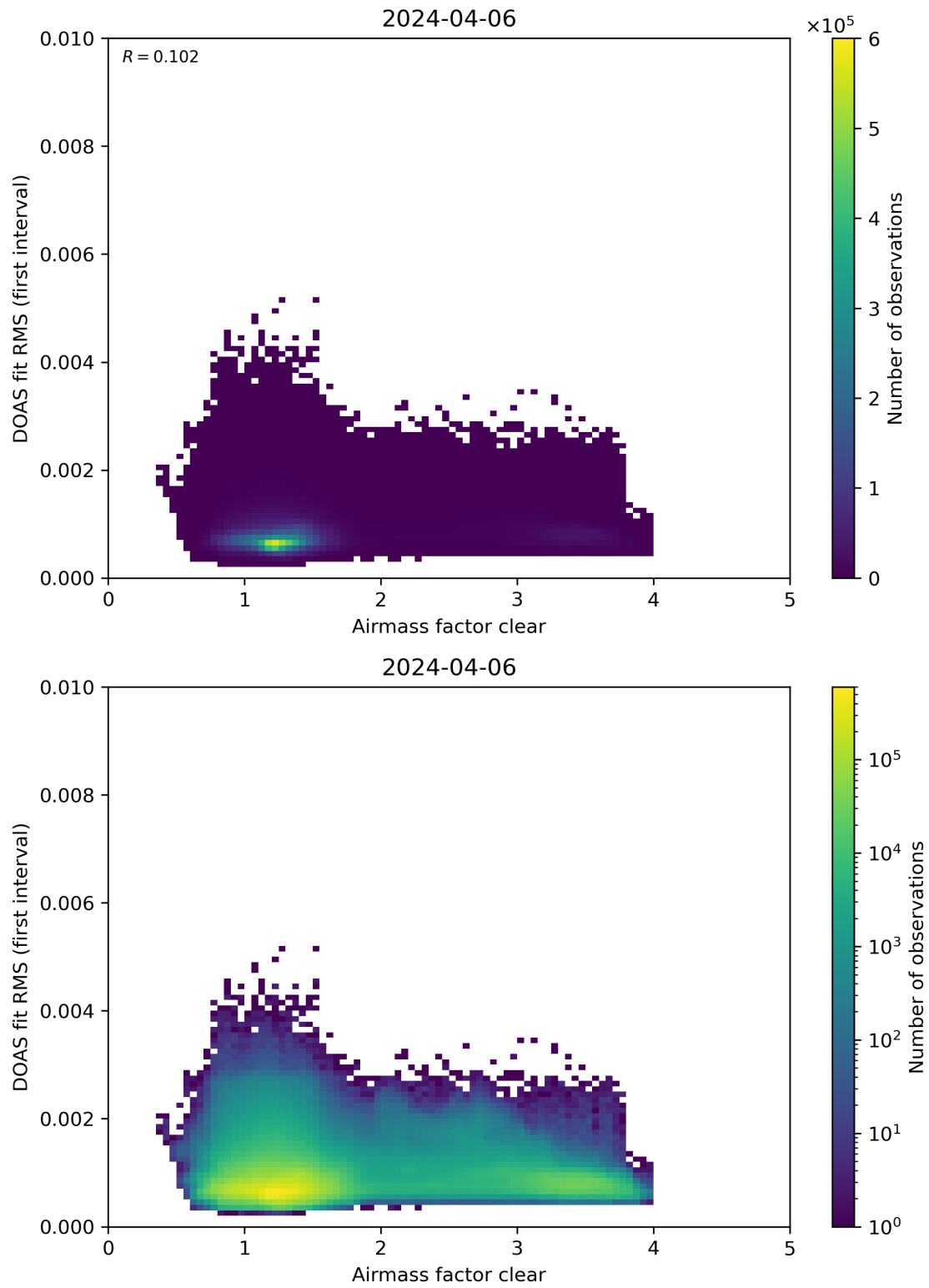
Figure 71: Scatter density plot of “Airmass factor clear” against “DOAS fit RMS (first interval)” for 2024-04-05 to 2024-04-07.
