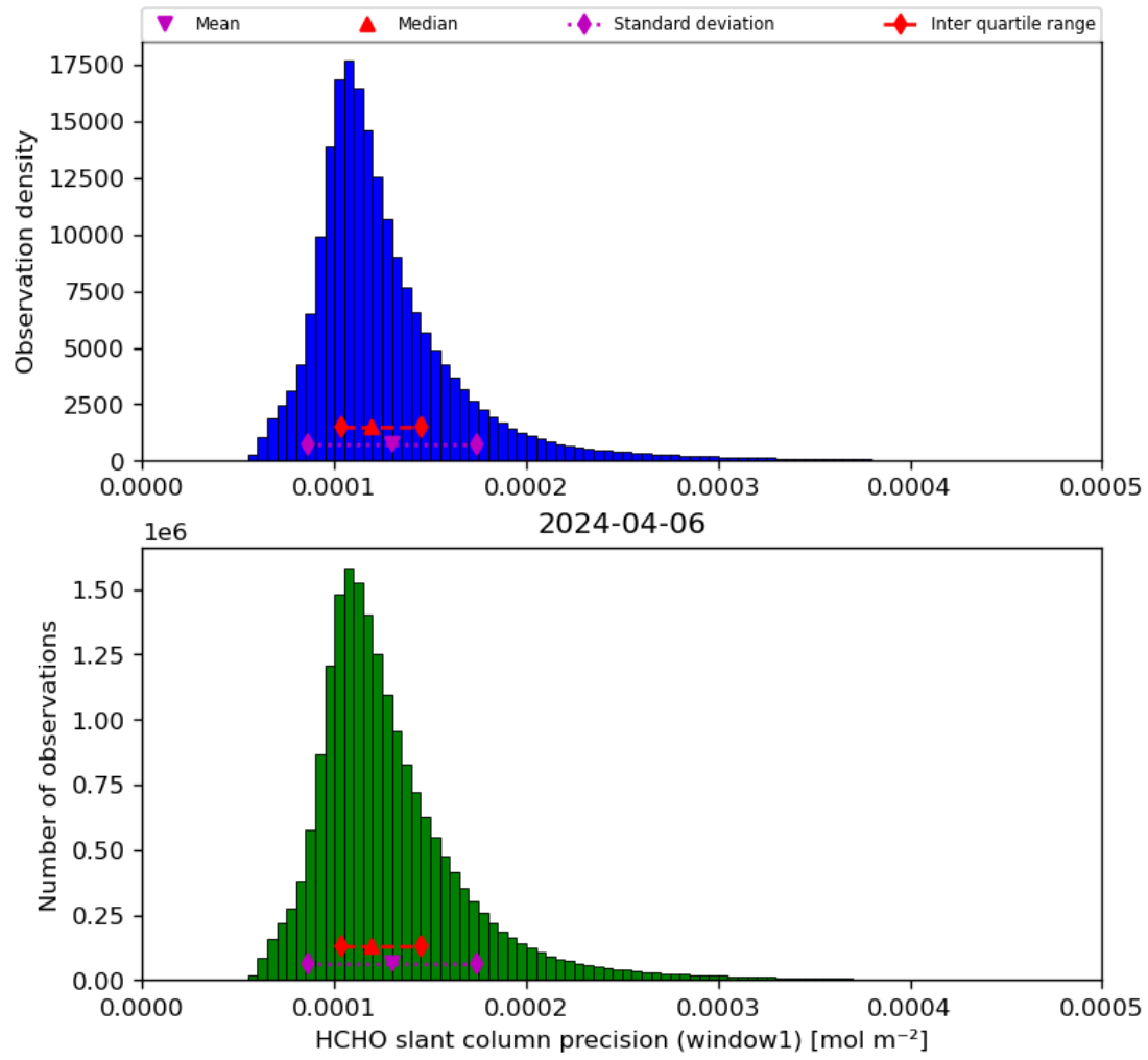
Figure 39: Histogram of “HCHO slant column precision (window1)” for 2024-04-05 to 2024-04-07
