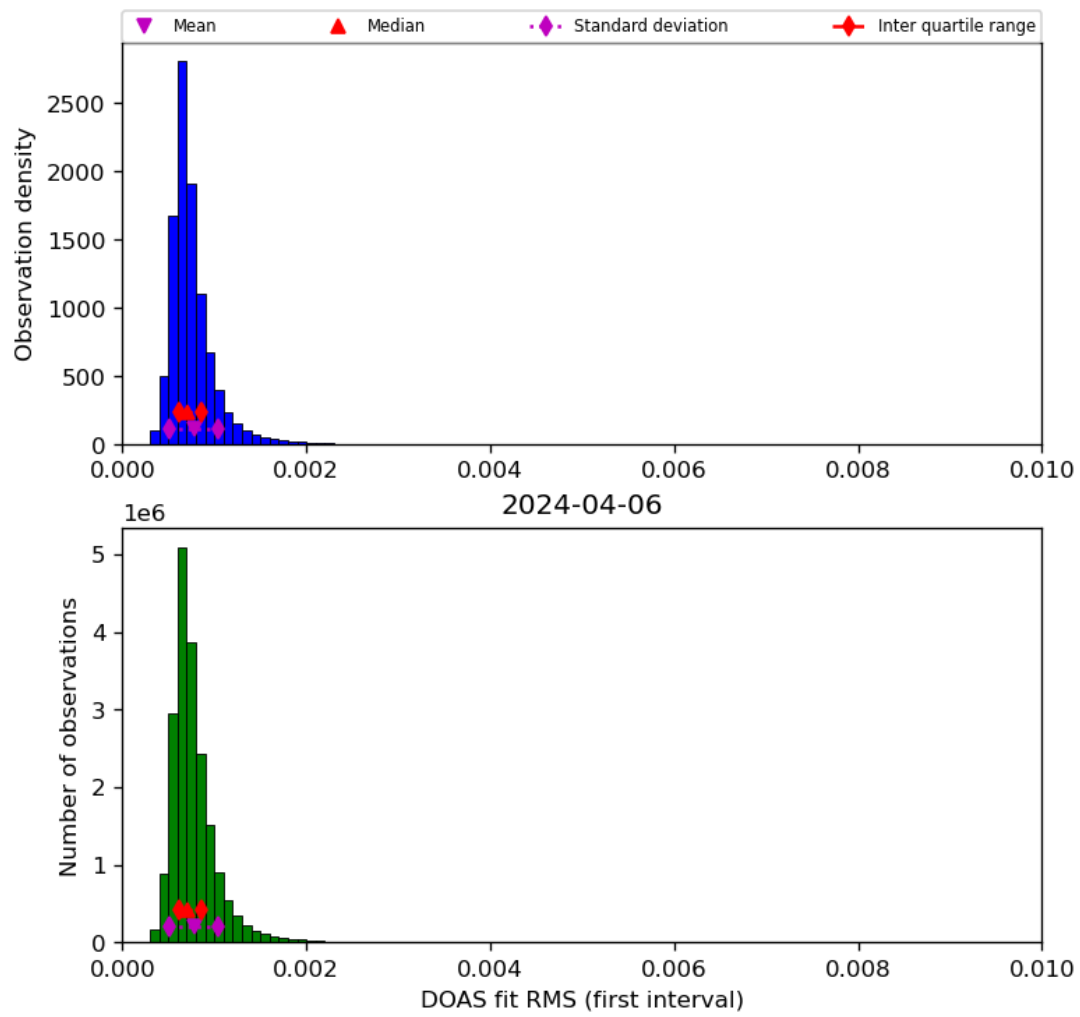
Figure 46: Histogram of “DOAS fit RMS (first interval)” for 2024-04-05 to 2024-04-07
