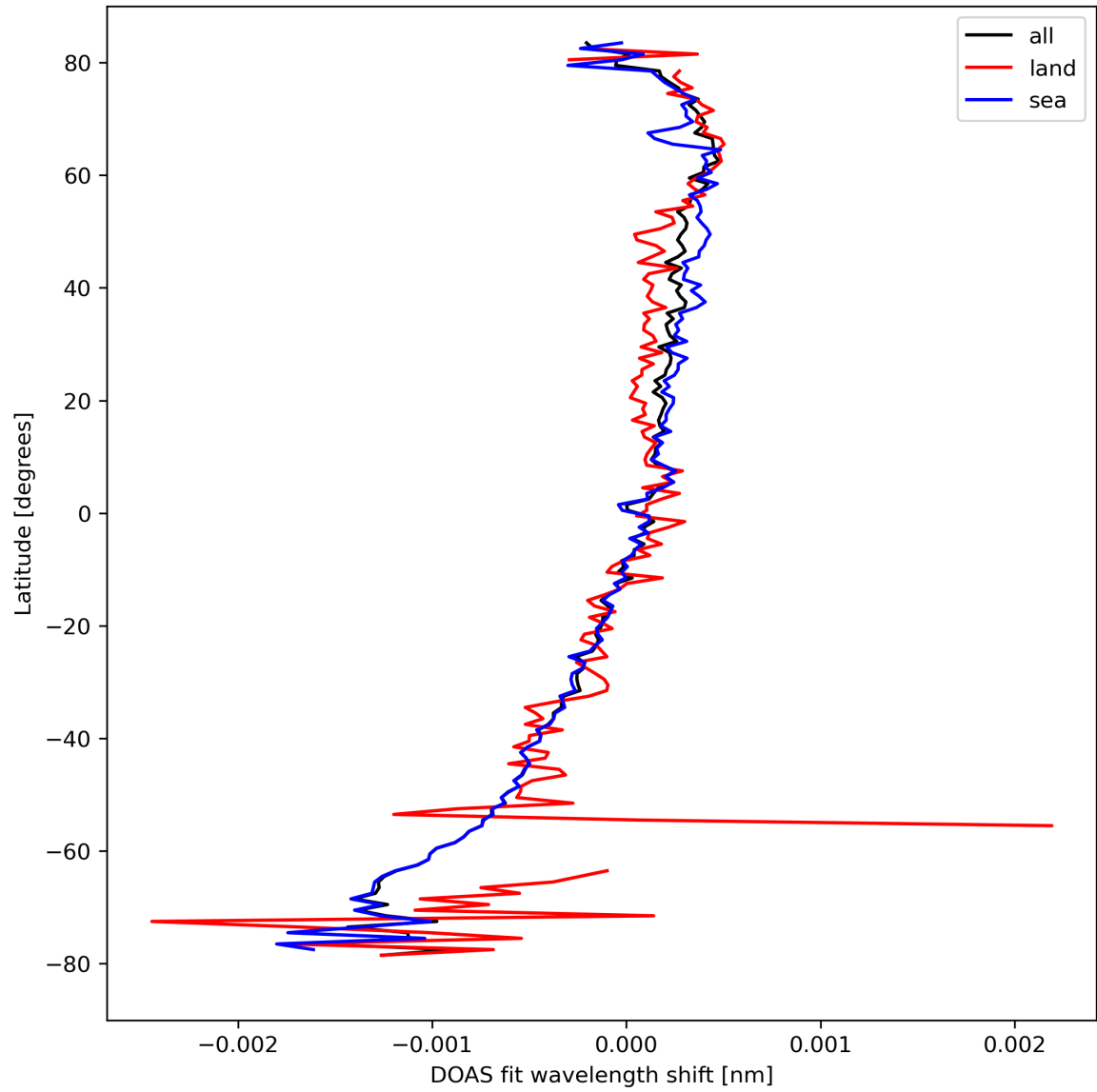
Figure 30: Zonal average of “DOAS fit wavelength shift” for 2024-04-05 to 2024-04-07.
