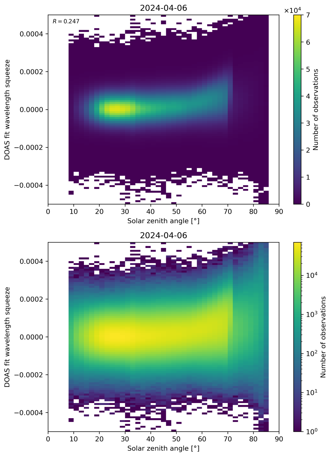
Figure 169: Scatter density plot of “Solar zenith angle” against “DOAS fit wavelength squeeze” for 2024-04-05 to 2024-04-07.
