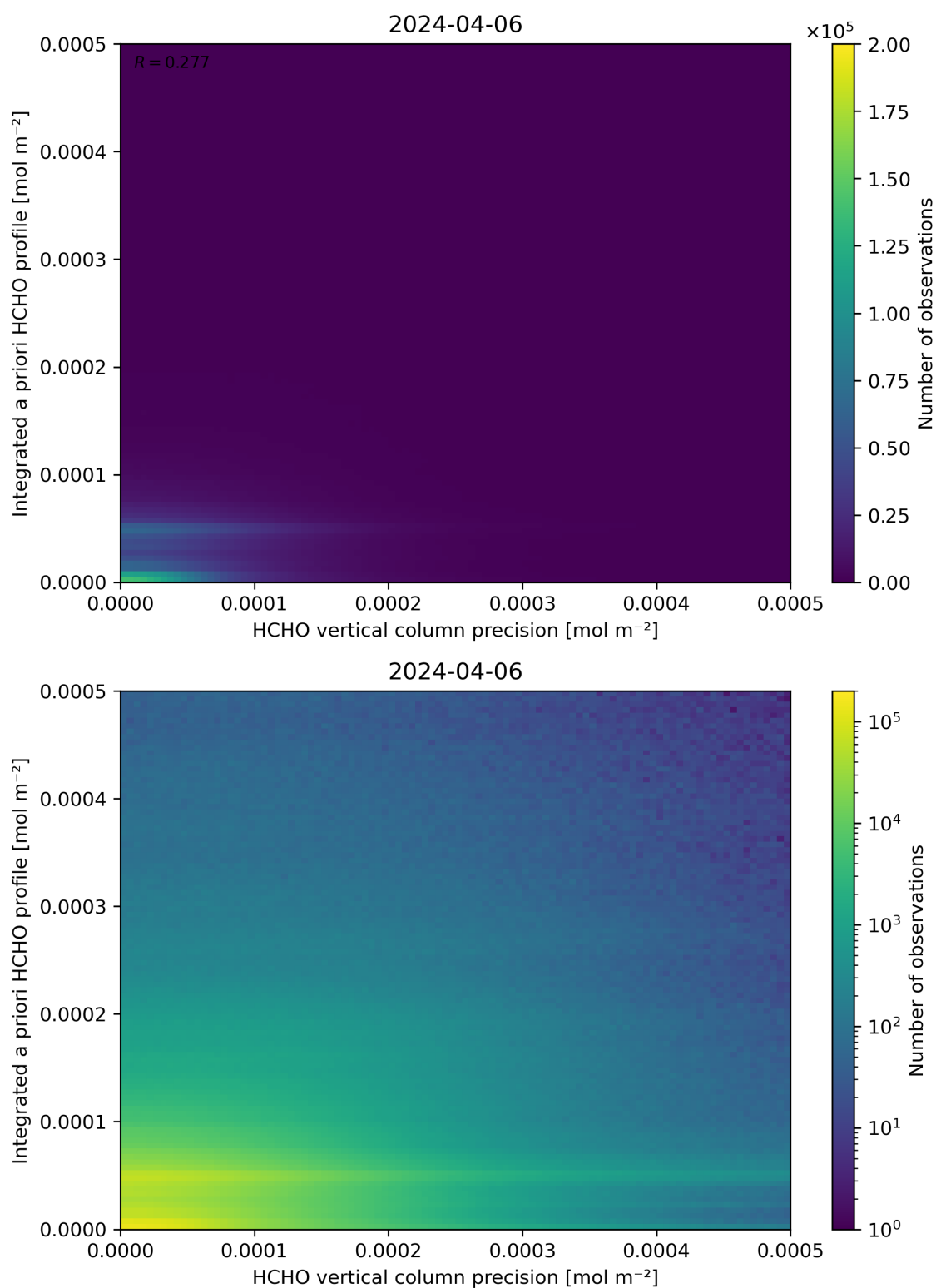
Figure 147: Scatter density plot of “HCHO vertical column precision” against “Integrated a priori HCHO profile” for 2024-04-05 to 2024-04-07.
