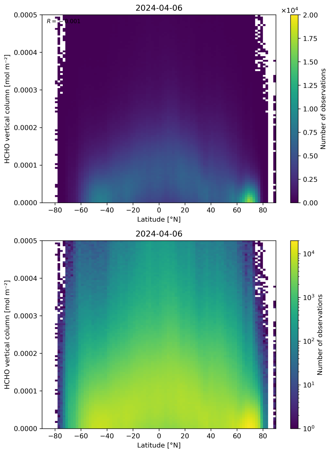
Figure 163: Scatter density plot of “Latitude” against “HCHO vertical column” for 2024-04-05 to 2024-04-07.
