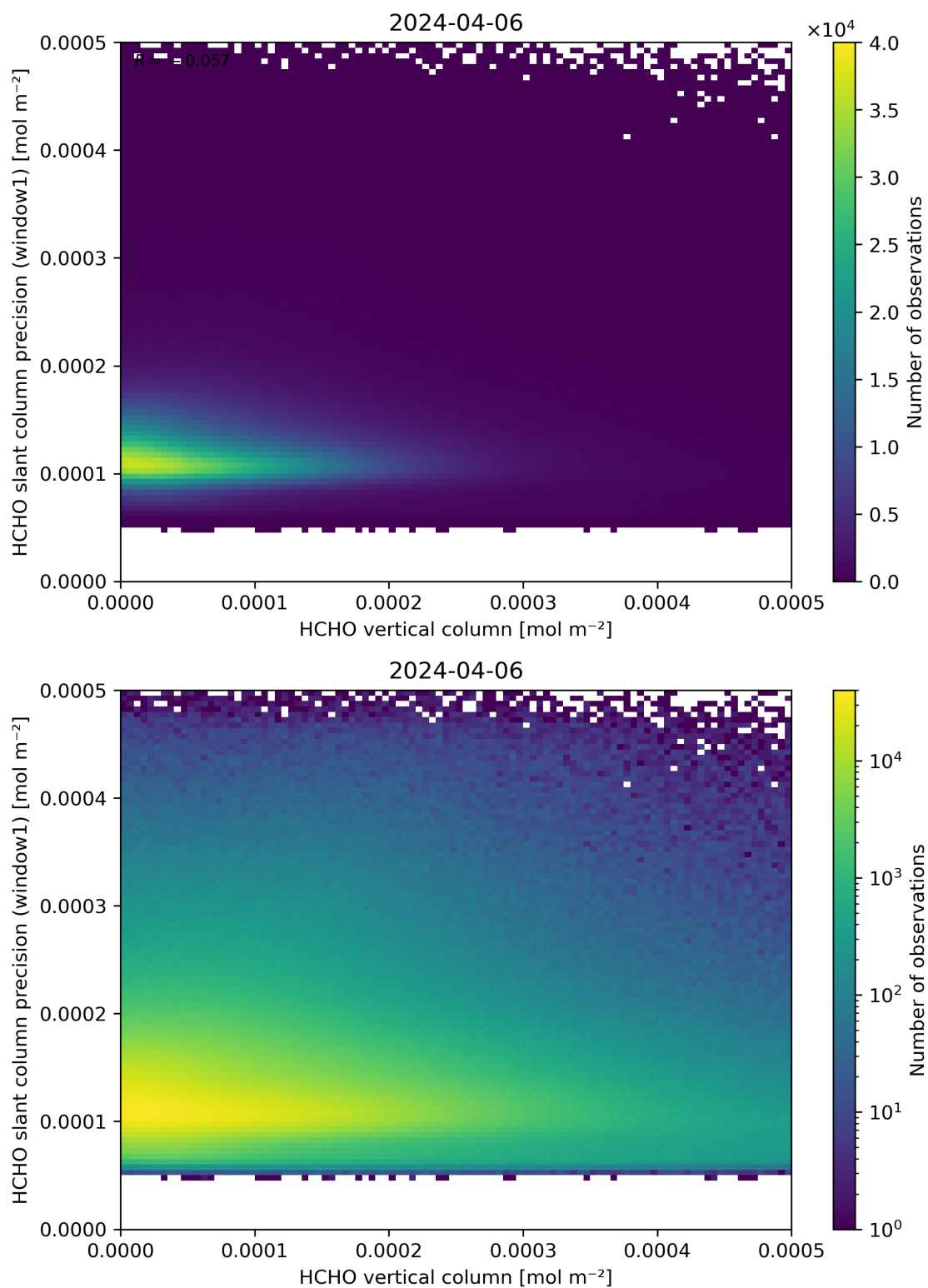
Figure 130: Scatter density plot of “HCHO vertical column” against “HCHO slant column precision (window1)” for 2024-04-05 to 2024-04-07.
