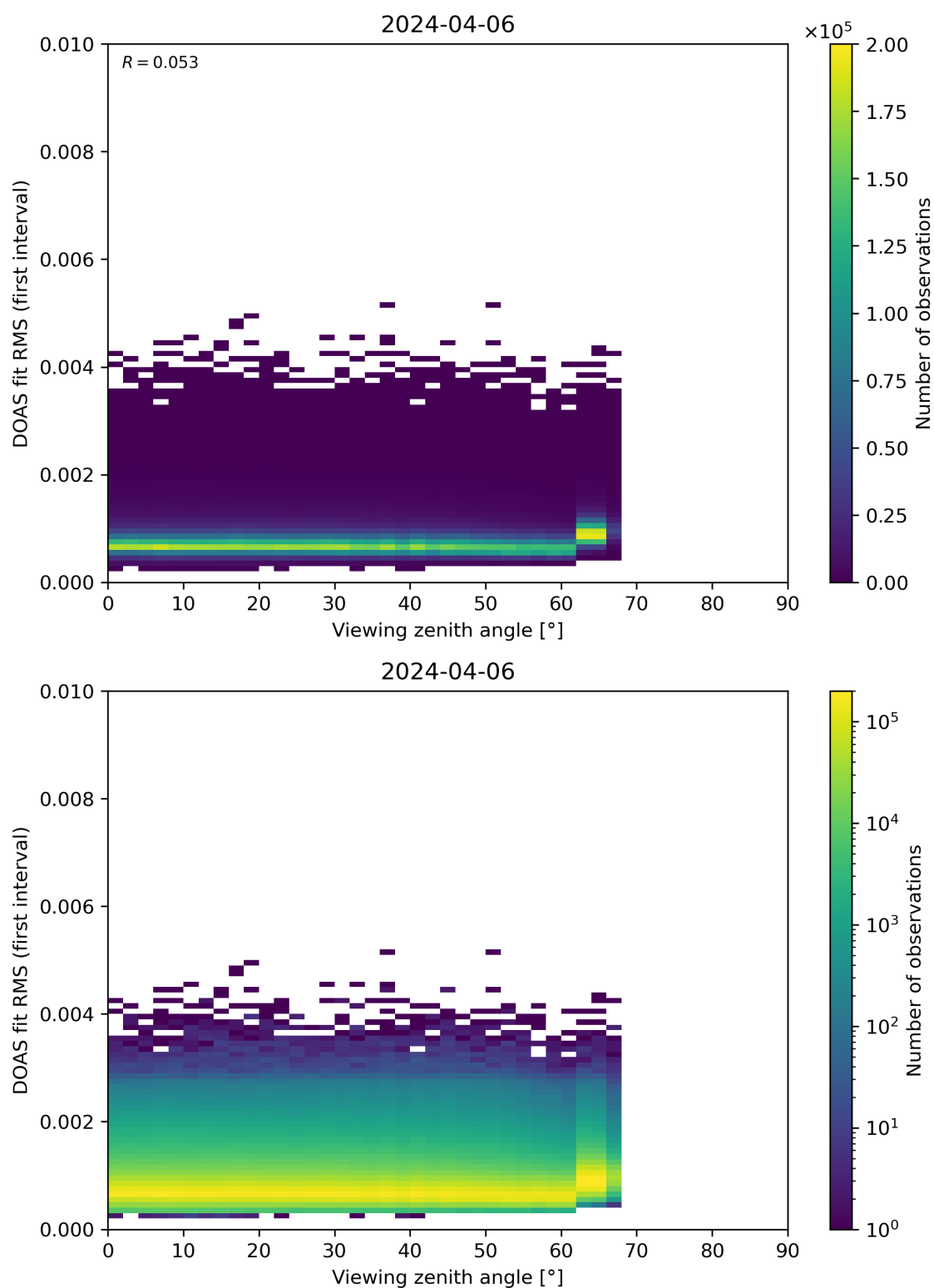
Figure 182: Scatter density plot of “Viewing zenith angle” against “DOAS fit RMS (first interval)” for 2024-04-05 to 2024-04-07.
