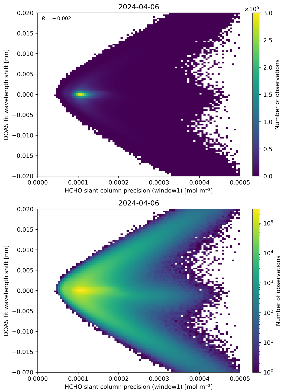
Figure 89: Scatter density plot of “HCHO slant column precision (window1)” against “DOAS fit wavelength shift” for 2024-04-05 to 2024-04-07.
