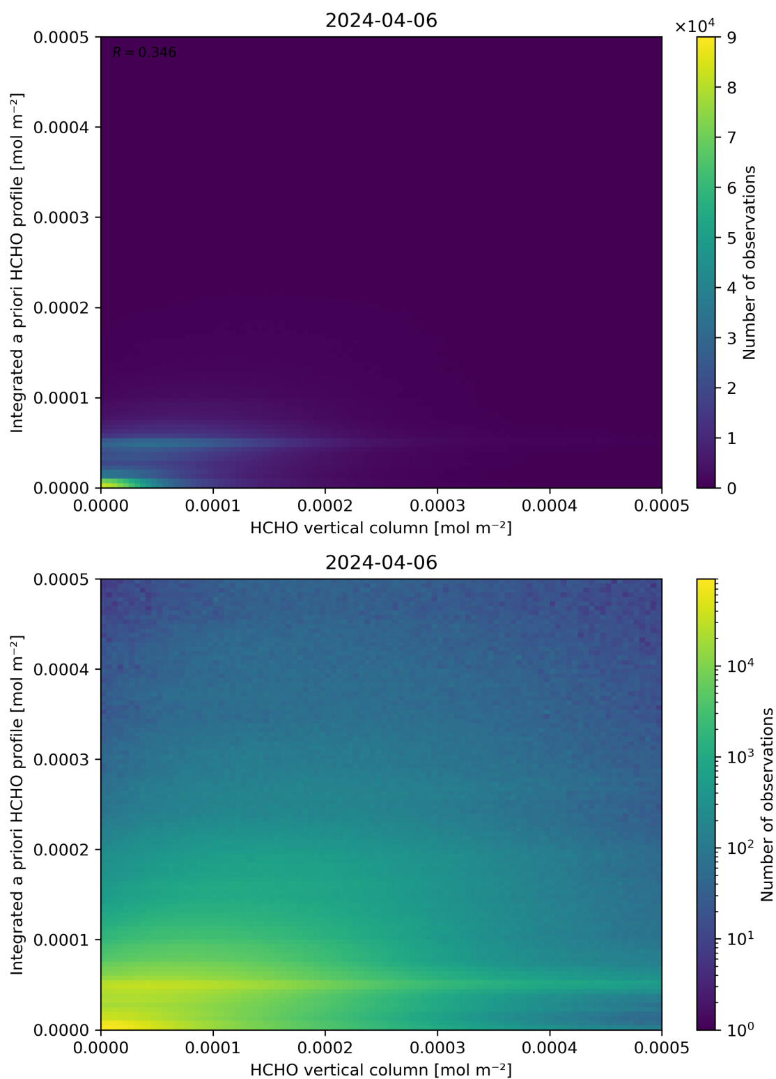
Figure 135: Scatter density plot of “HCHO vertical column” against “Integrated a priori HCHO profile” for 2024-04-05 to 2024-04-07.
