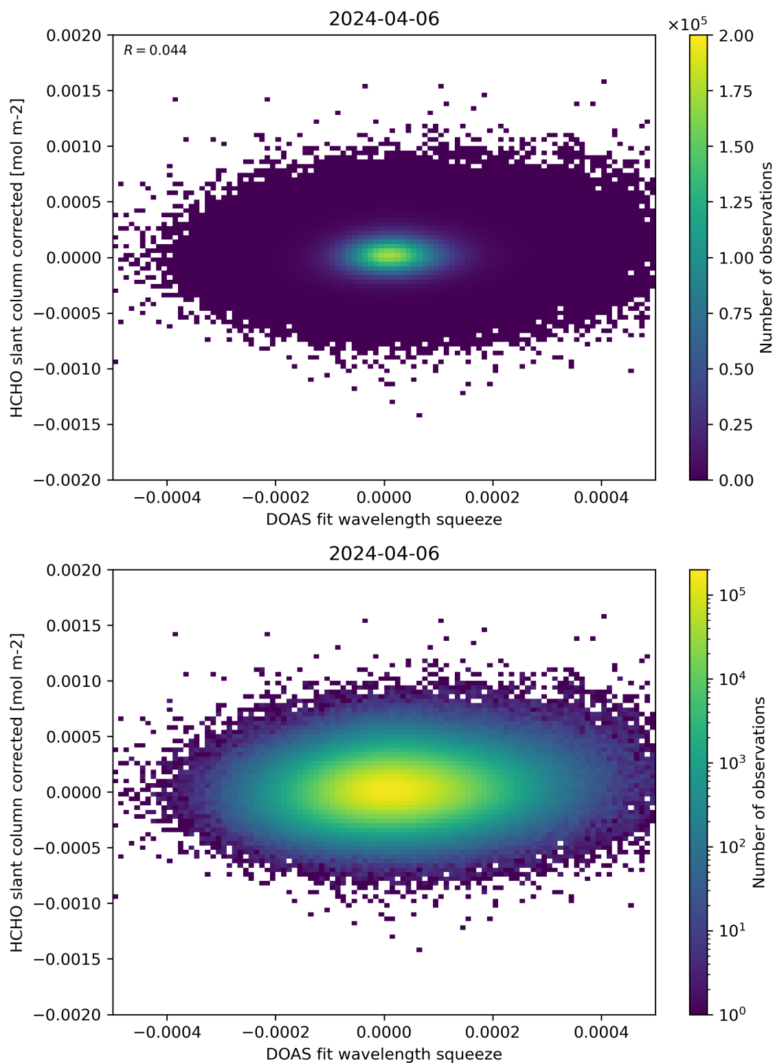
Figure 69: Scatter density plot of “DOAS fit wavelength squeeze” against “HCHO slant column corrected” for 2024-04-05 to 2024-04-07.
