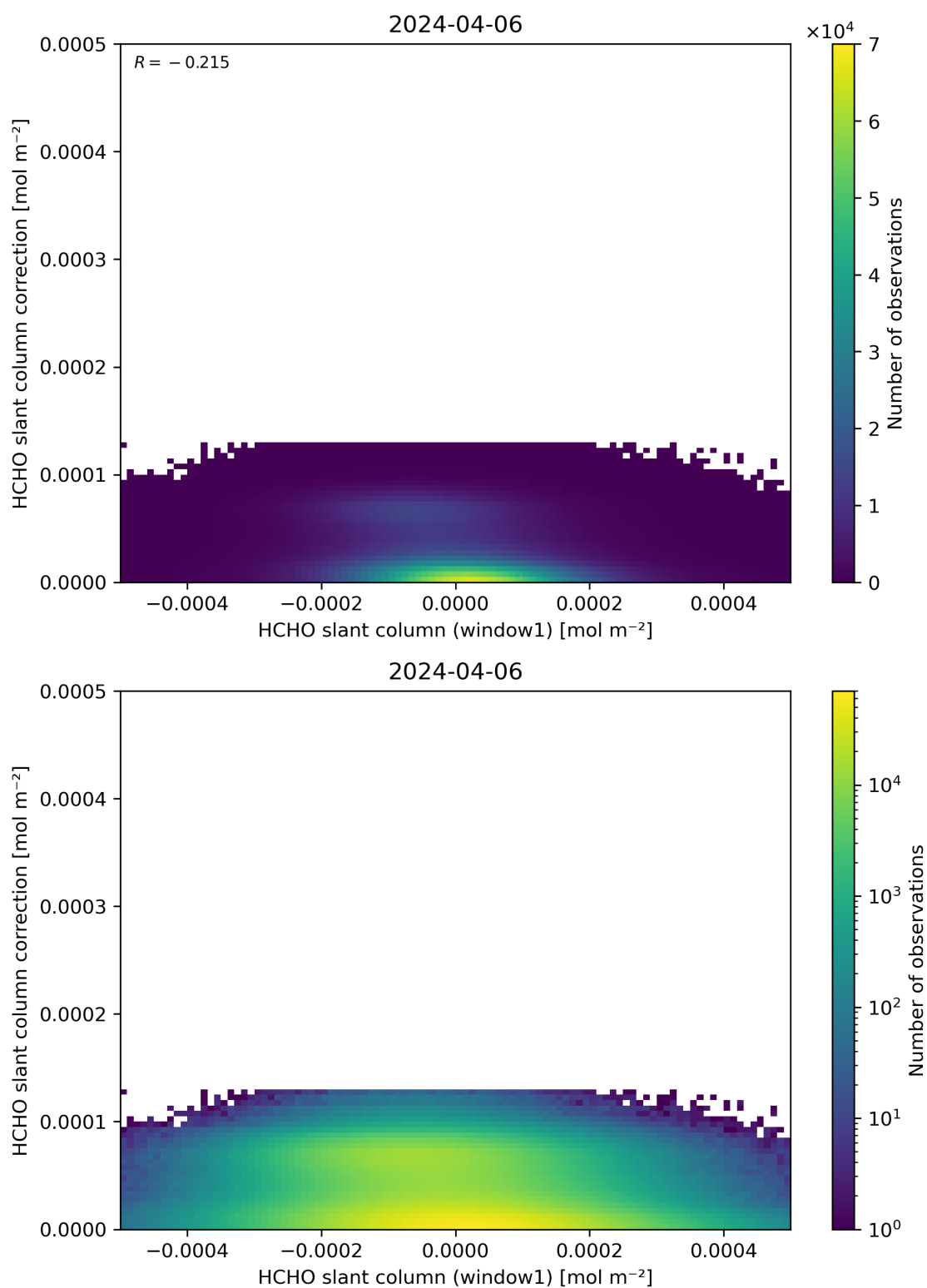
Figure 83: Scatter density plot of “HCHO slant column (window1)” against “HCHO slant column correction” for 2024-04-05 to 2024-04-07.
