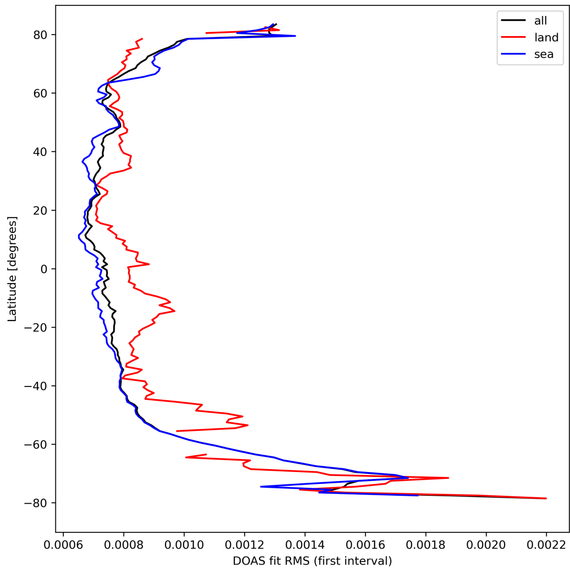
Figure 32: Zonal average of “DOAS fit RMS (first interval)” for 2024-04-05 to 2024-04-07.
