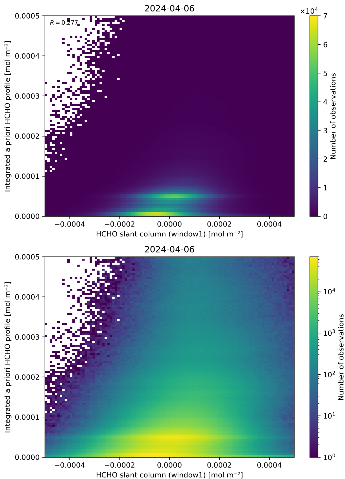
Figure 87: Scatter density plot of “HCHO slant column (window1)” against “Integrated a priori HCHO profile” for 2024-04-05 to 2024-04-07.
