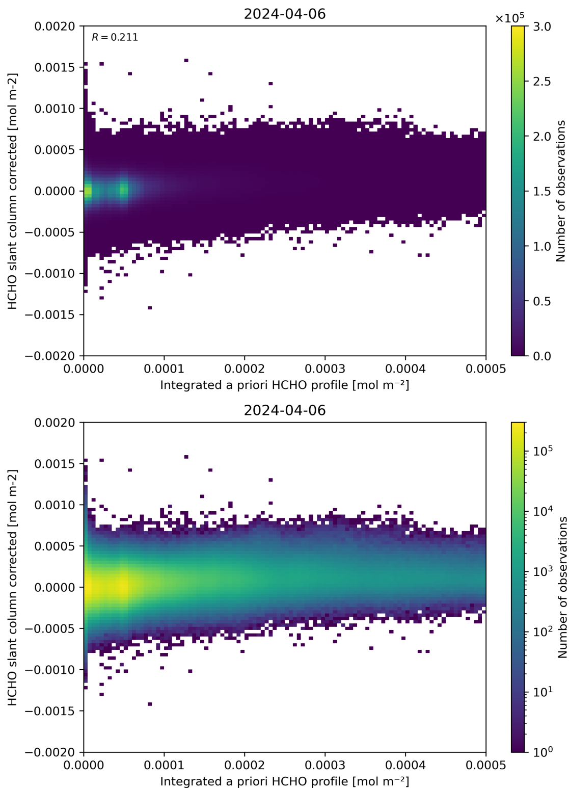
Figure 151: Scatter density plot of “Integrated a priori HCHO profile” against “HCHO slant column corrected” for 2024-04-05 to 2024-04-07.
