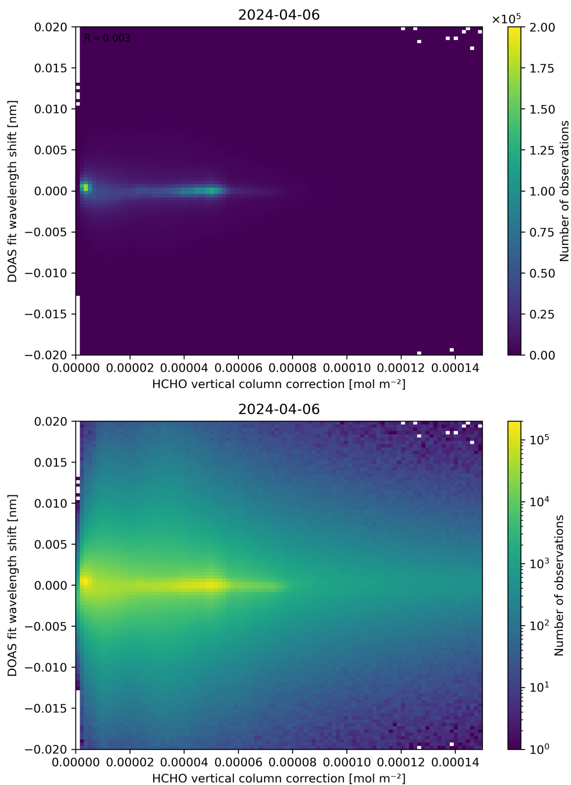
Figure 113: Scatter density plot of “HCHO vertical column correction” against “DOAS fit wavelength shift” for 2024-04-05 to 2024-04-07.
