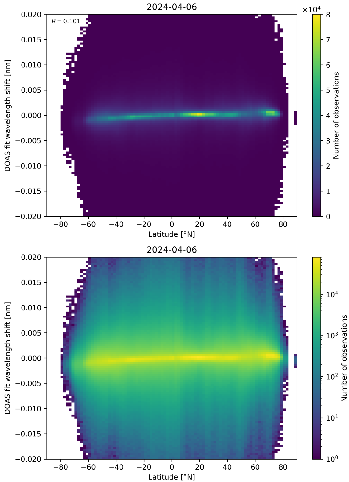
Figure 154: Scatter density plot of “Latitude” against “DOAS fit wavelength shift” for 2024-04-05 to 2024-04-07.
