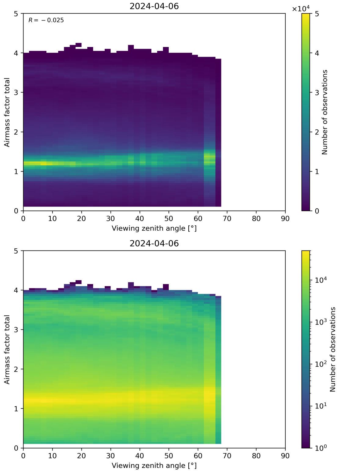
Figure 190: Scatter density plot of “Viewing zenith angle” against “Airmass factor total” for 2024-04-05 to 2024-04-07.
