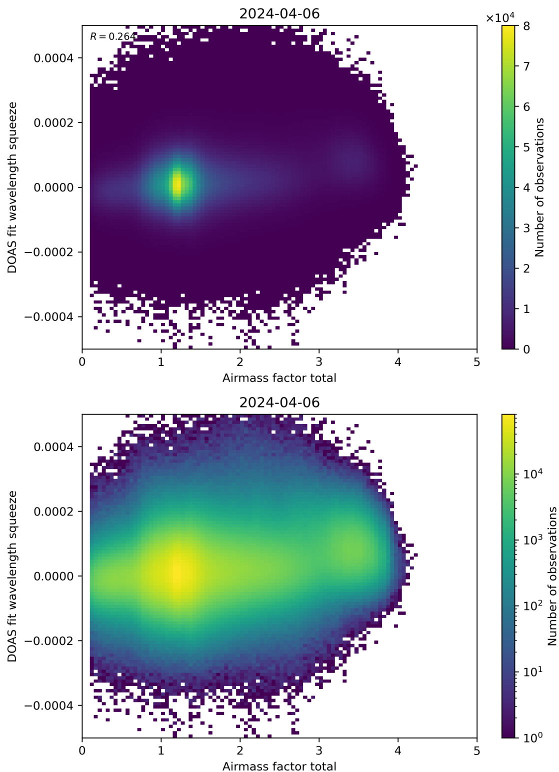
Figure 99: Scatter density plot of “Airmass factor total” against “DOAS fit wavelength squeeze” for 2024-04-05 to 2024-04-07.
