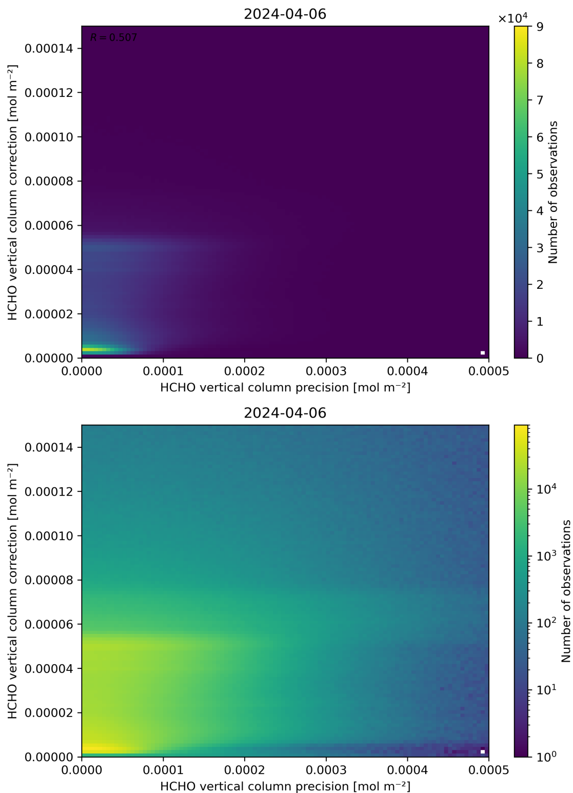
Figure 146: Scatter density plot of “HCHO vertical column precision” against “HCHO vertical column correction” for 2024-04-05 to 2024-04-07.
