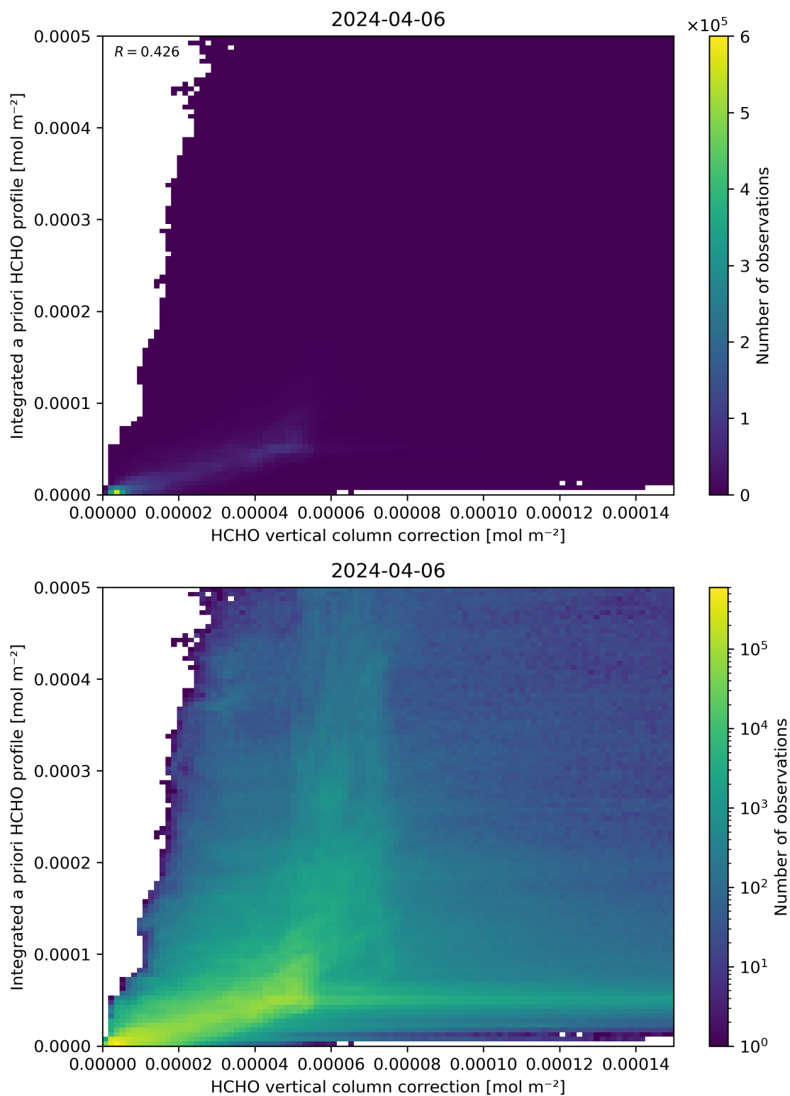
Figure 122: Scatter density plot of “HCHO vertical column correction” against “Integrated a priori HCHO profile” for 2024-04-05 to 2024-04-07.
