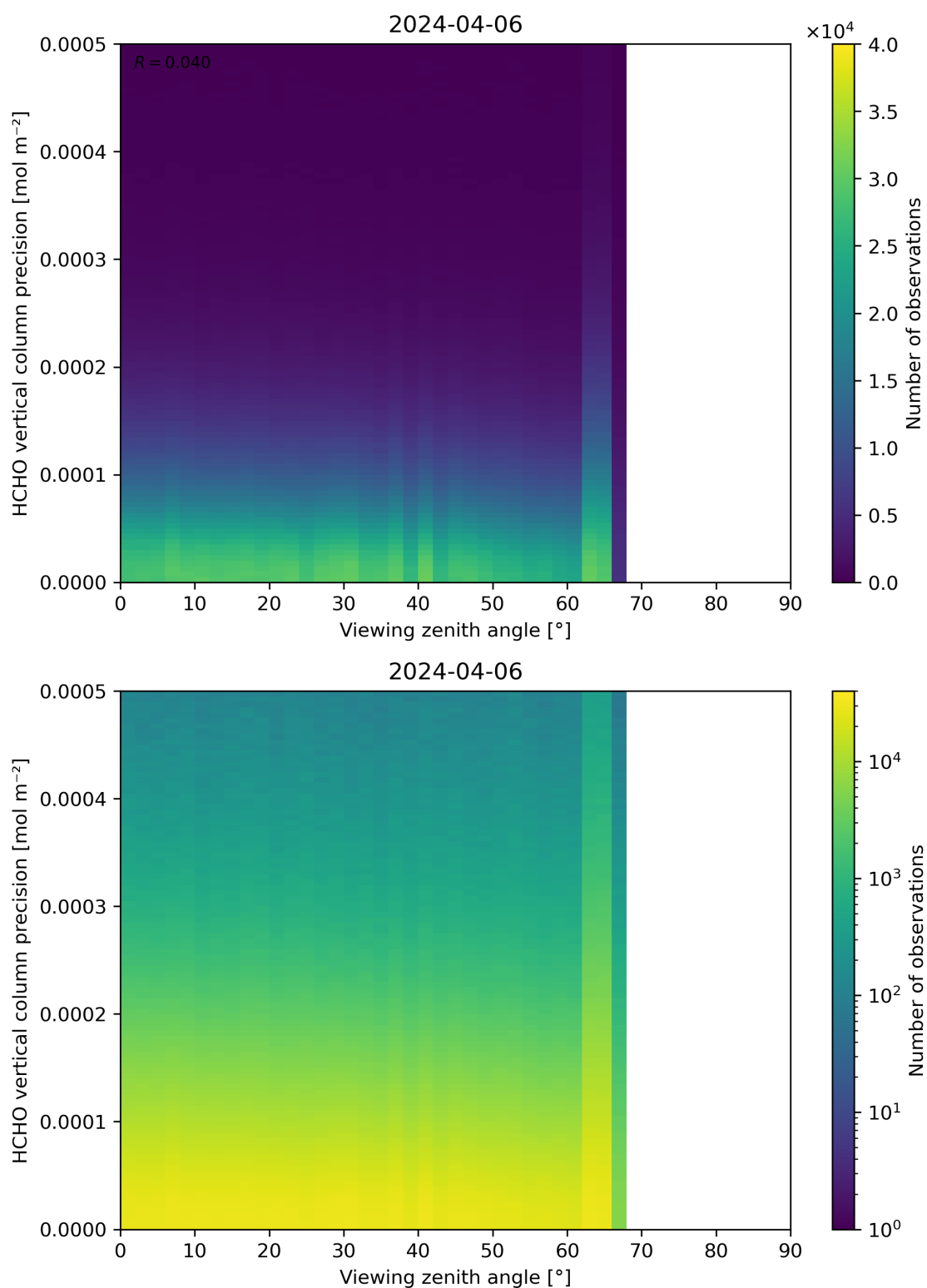
Figure 194: Scatter density plot of “Viewing zenith angle” against “HCHO vertical column precision” for 2024-04-05 to 2024-04-07.
