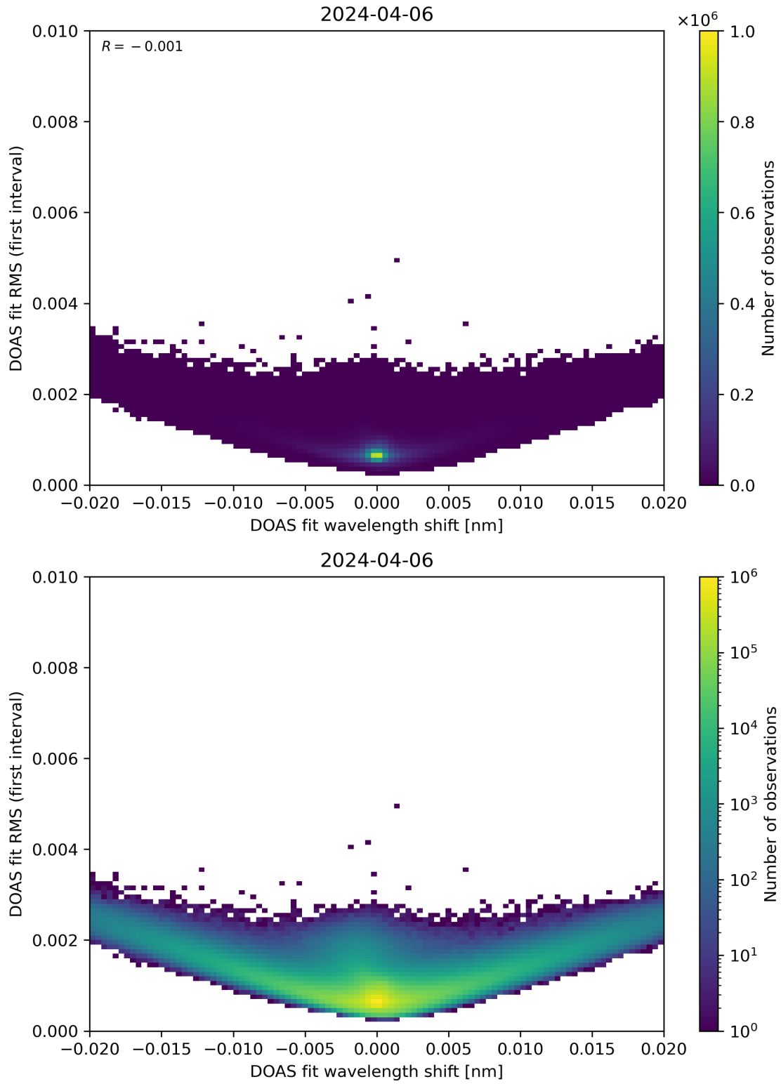
Figure 64: Scatter density plot of “DOAS fit wavelength shift” against “DOAS fit RMS (first interval)” for 2024-04-05 to 2024-04-07.
