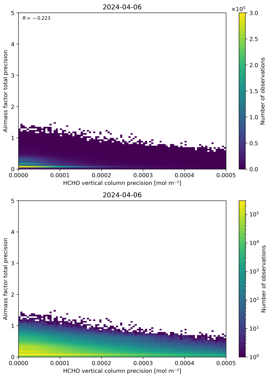
Figure 145: Scatter density plot of “HCHO vertical column precision” against “Airmass factor total precision” for 2024-04-05 to 2024-04-07.
