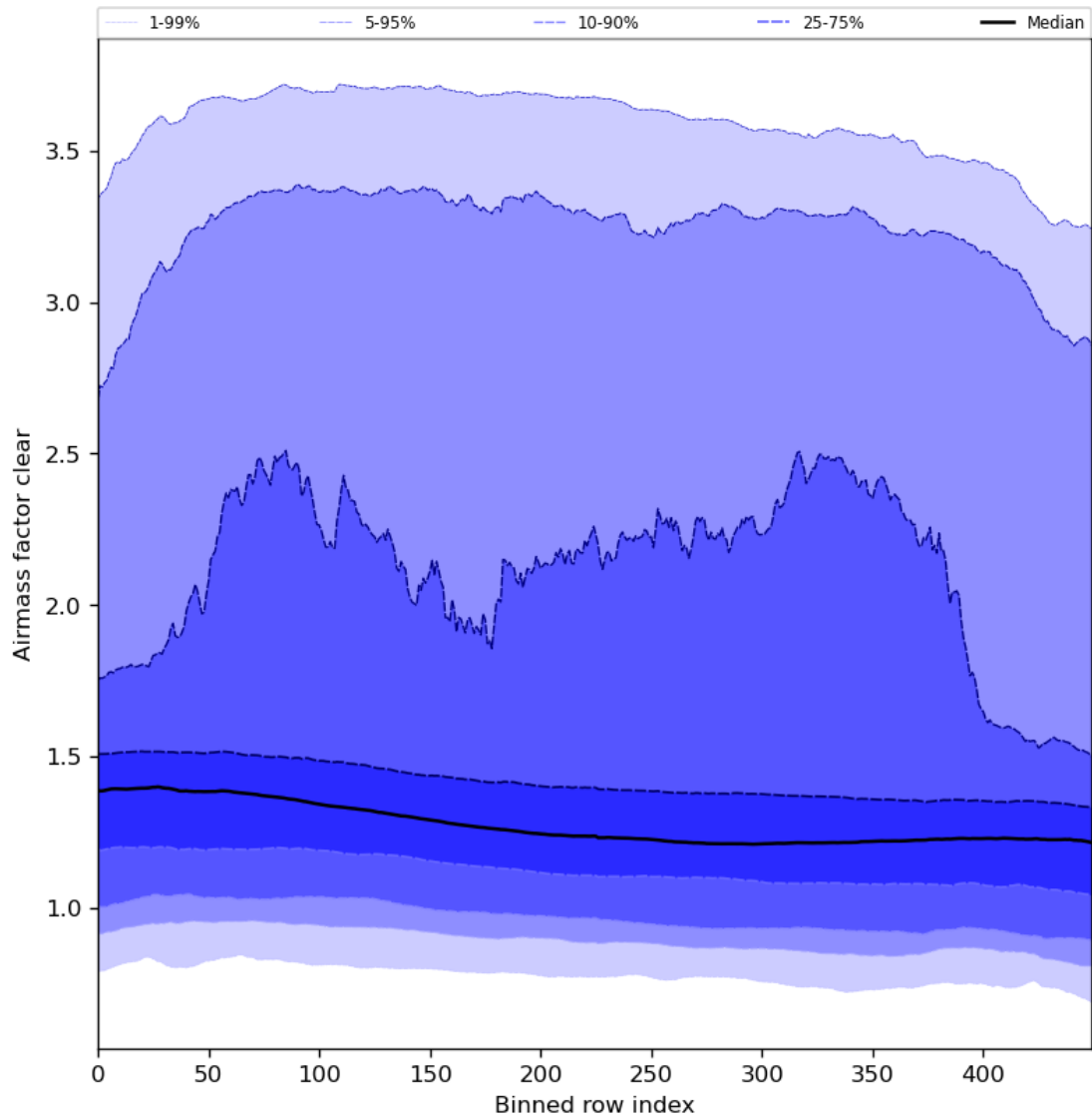
Figure 56: Along track statistics of “Airmass factor clear” for 2024-04-05 to 2024-04-07
