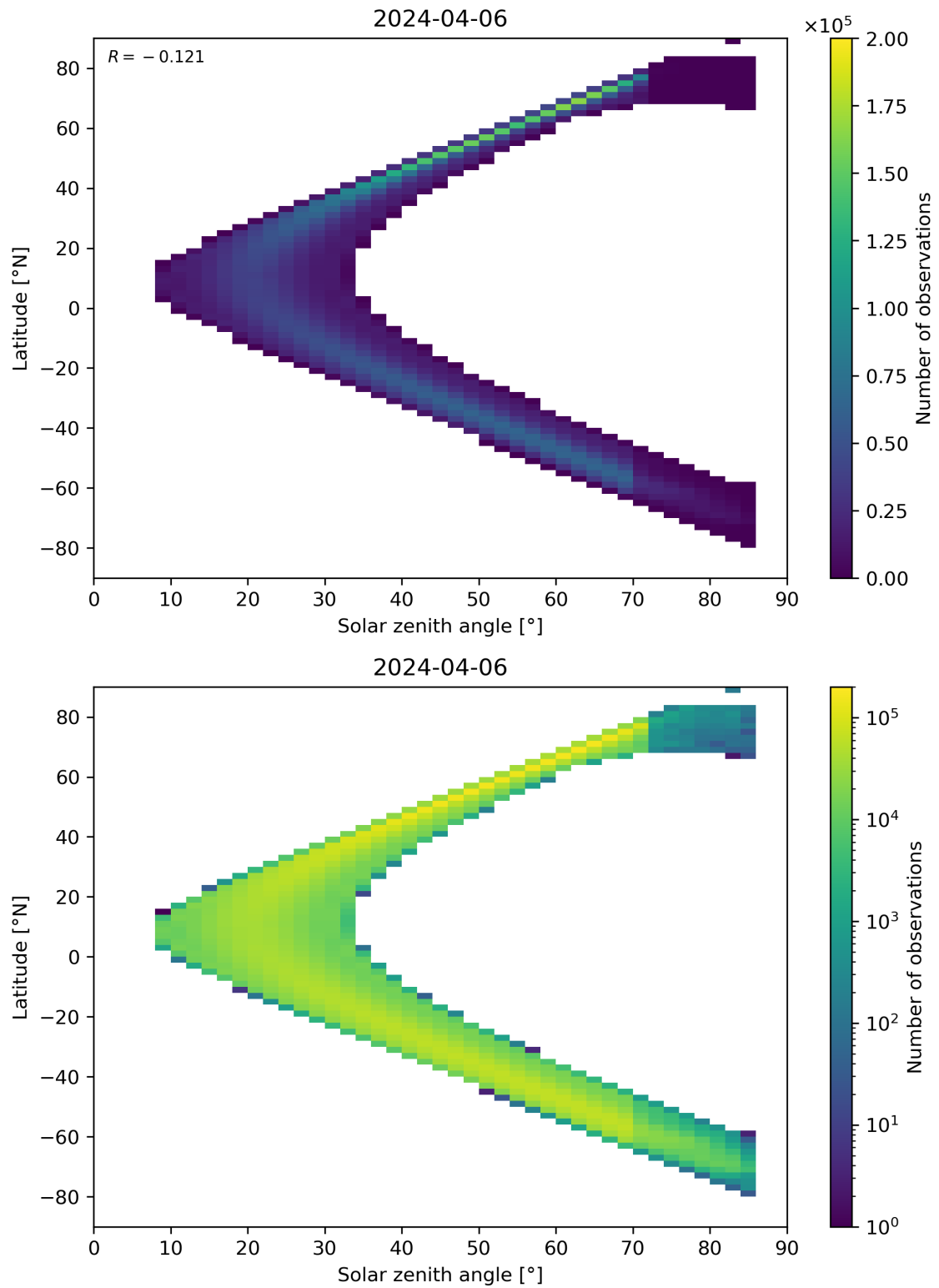
Figure 181: Scatter density plot of “Solar zenith angle” against “Latitude” for 2024-04-05 to 2024-04-07.
