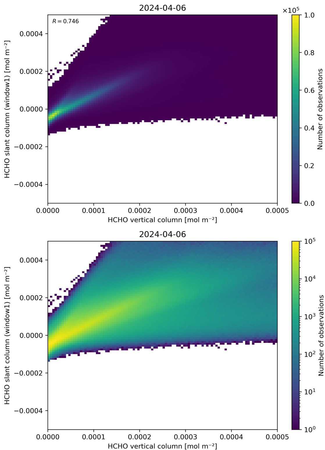
Figure 129: Scatter density plot of “HCHO vertical column” against “HCHO slant column (window1)” for 2024-04-05 to 2024-04-07.
