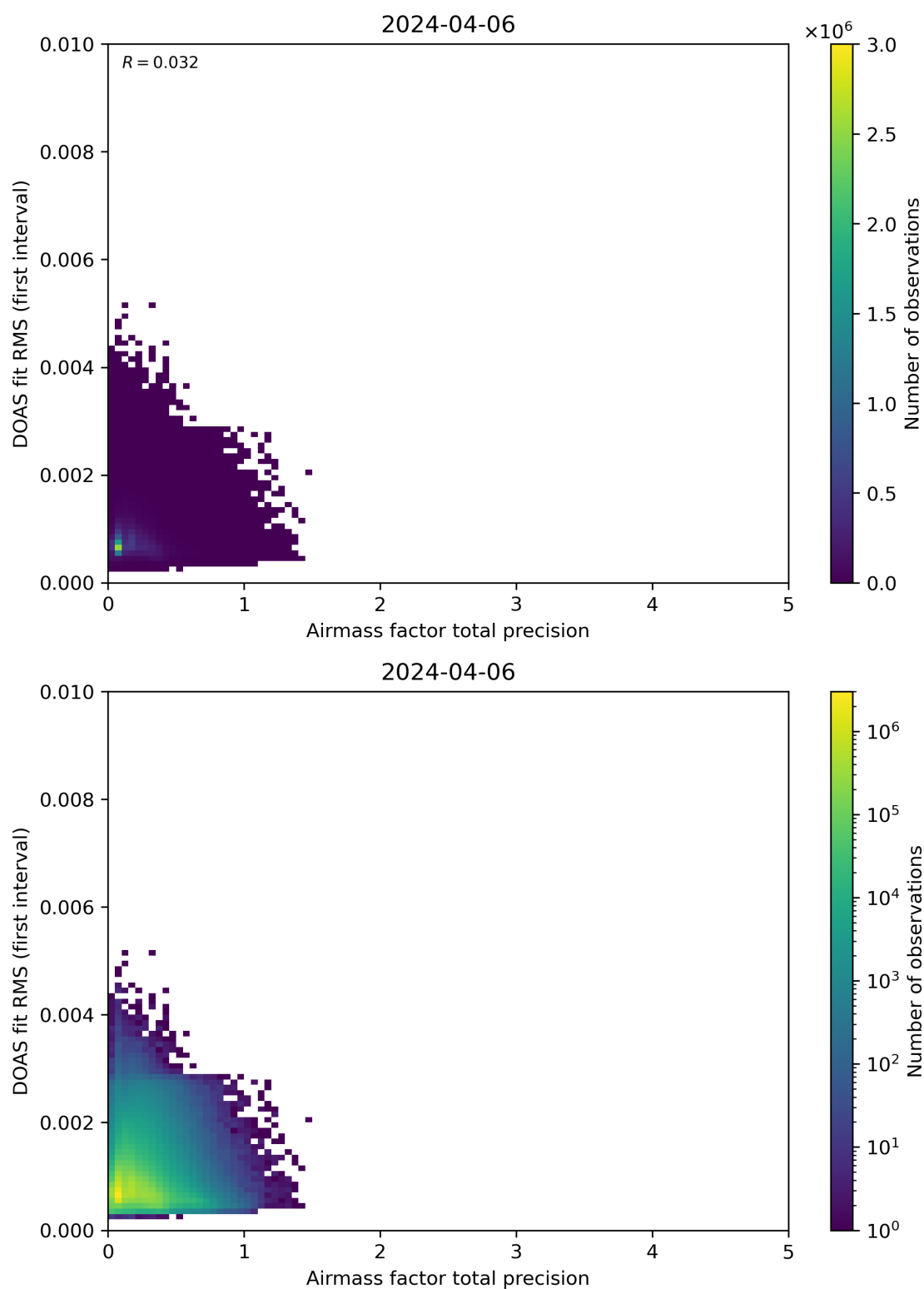
Figure 105: Scatter density plot of “Airmass factor total precision” against “DOAS fit RMS (first interval)” for 2024-04-05 to 2024-04-07.
