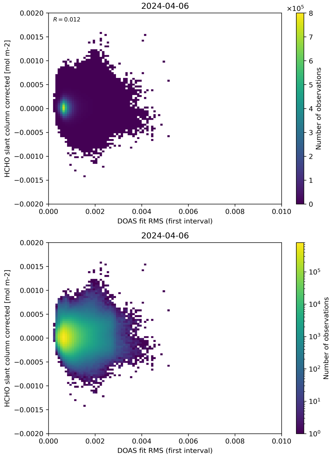
Figure 62: Scatter density plot of “DOAS fit RMS (first interval)” against “HCHO slant column corrected” for 2024-04-05 to 2024-04-07.
