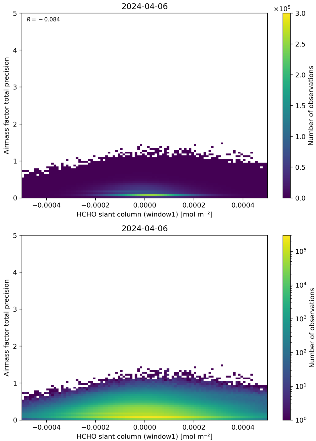
Figure 86: Scatter density plot of “HCHO slant column (window1)” against “Airmass factor total precision” for 2024-04-05 to 2024-04-07.
