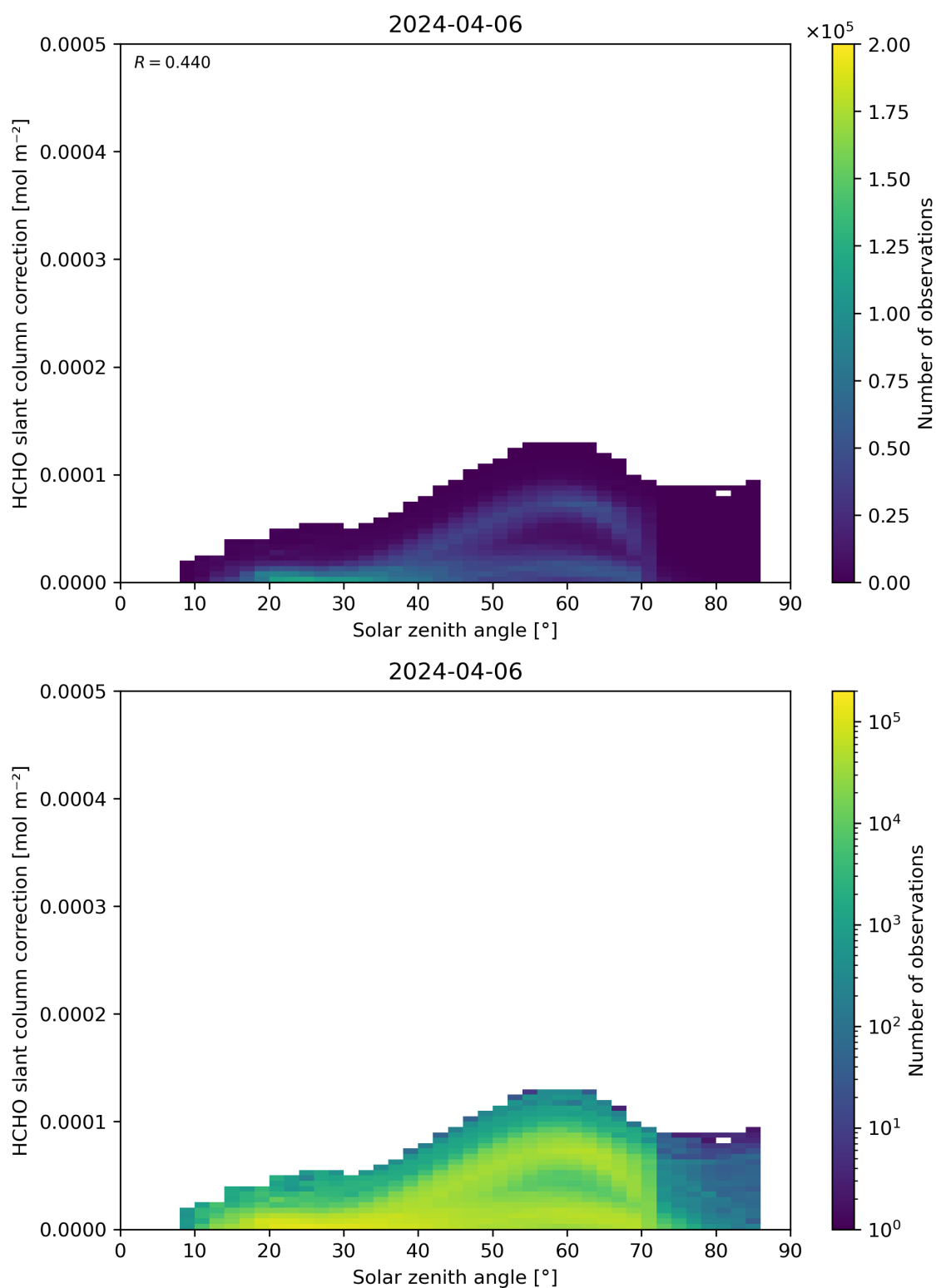
Figure 172: Scatter density plot of “Solar zenith angle” against “HCHO slant column correction” for 2024-04-05 to 2024-04-07.
