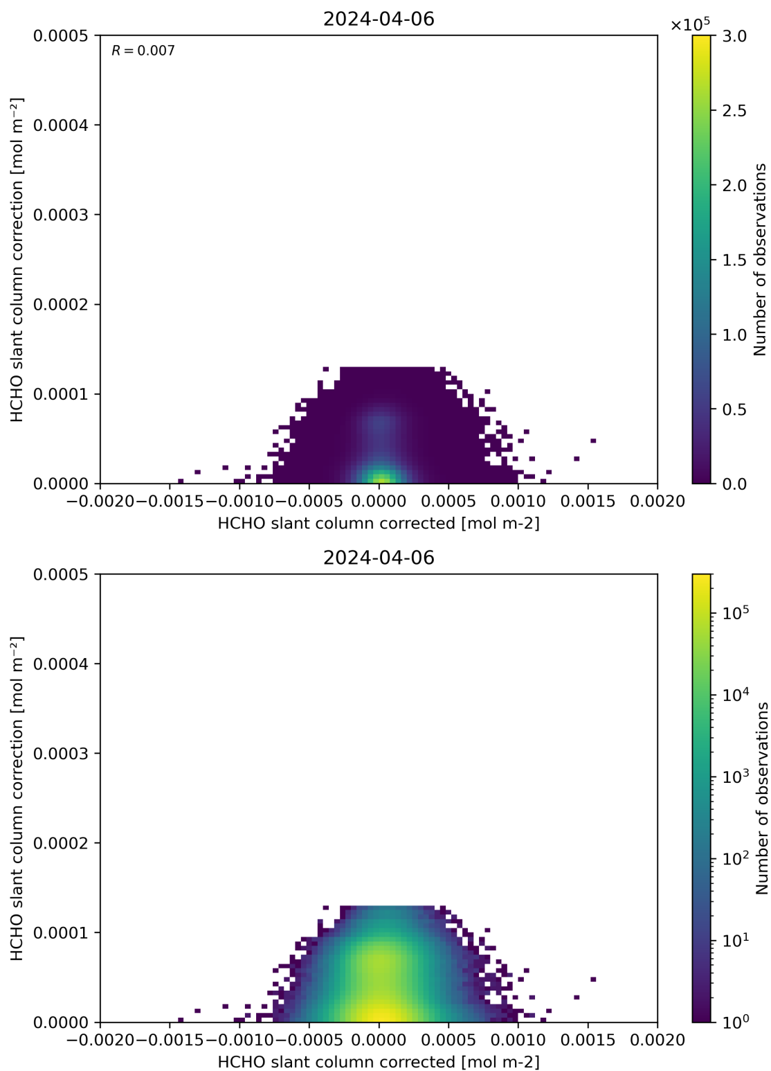
Figure 77: Scatter density plot of “HCHO slant column corrected” against “HCHO slant column correction” for 2024-04-05 to 2024-04-07.
