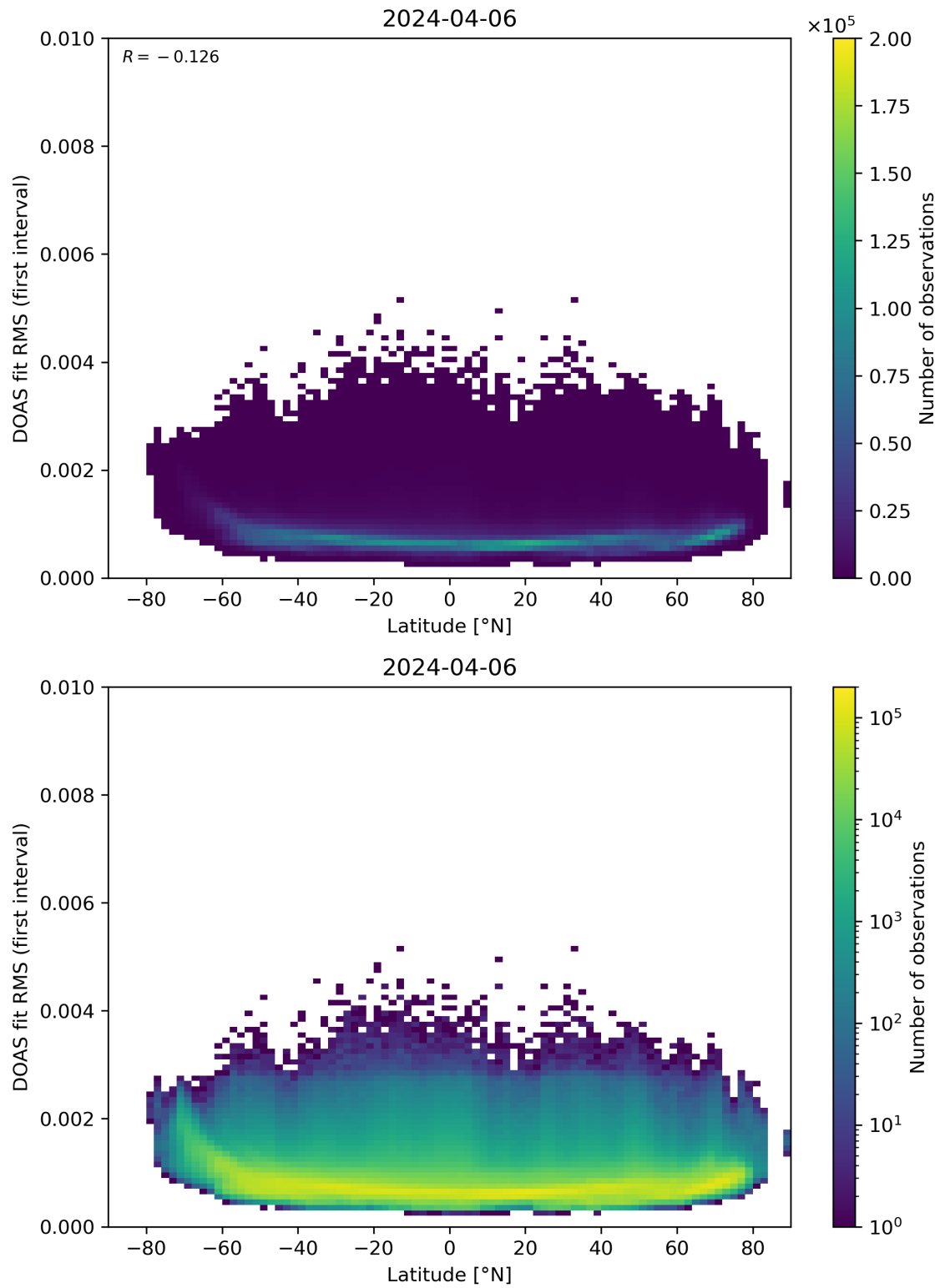
Figure 153: Scatter density plot of “Latitude” against “DOAS fit RMS (first interval)” for 2024-04-05 to 2024-04-07.
