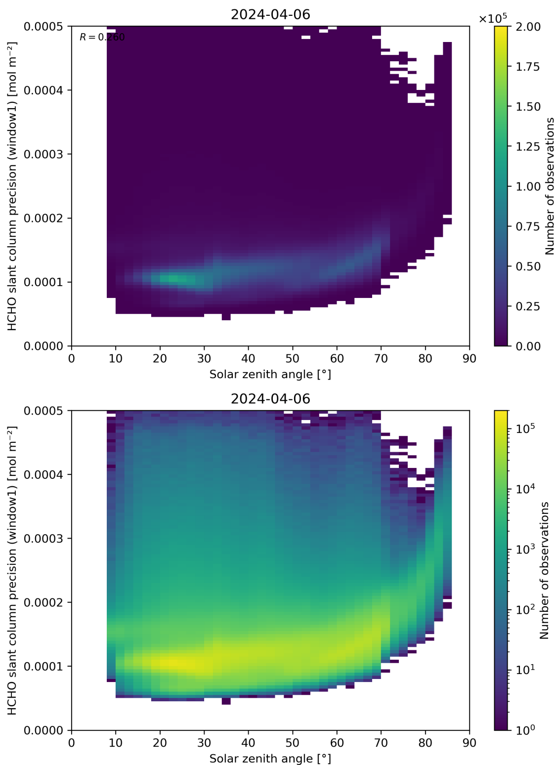
Figure 174: Scatter density plot of “Solar zenith angle” against “HCHO slant column precision (window1)” for 2024-04-05 to 2024-04-07.
