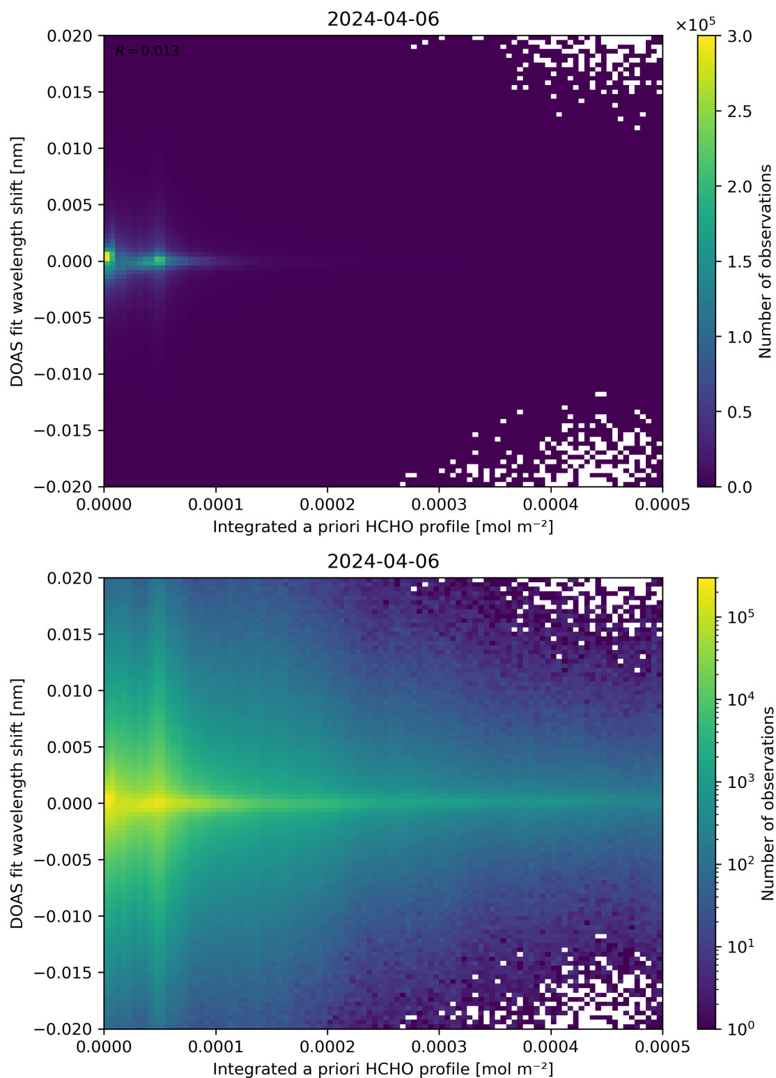
Figure 149: Scatter density plot of “Integrated a priori HCHO profile” against “DOAS fit wavelength shift” for 2024-04-05 to 2024-04-07.
