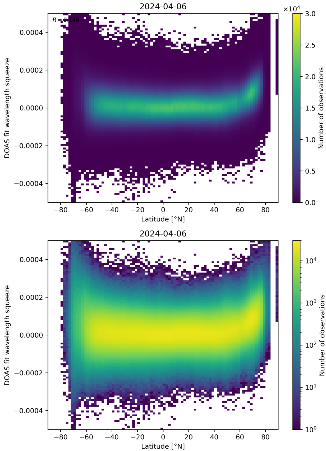
Figure 155: Scatter density plot of “Latitude” against “DOAS fit wavelength squeeze” for 2024-04-05 to 2024-04-07.
