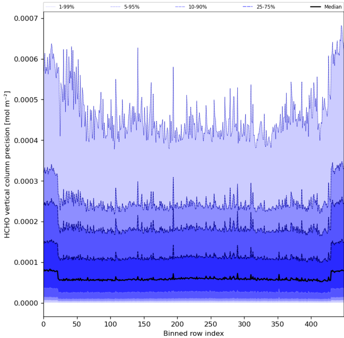
Figure 50: Along track statistics of “HCHO vertical column precision” for 2024-04-05 to 2024-04-07
