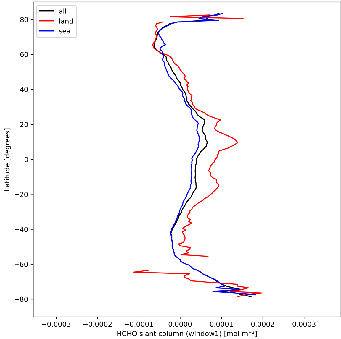
Figure 24: Zonal average of “HCHO slant column (window1)” for 2024-04-05 to 2024-04-07.
