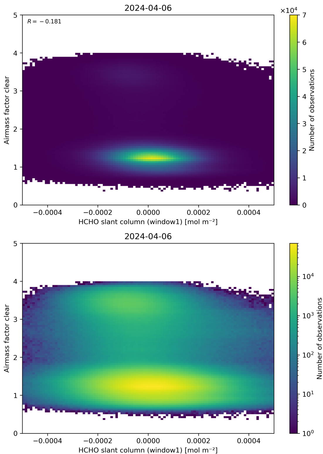
Figure 81: Scatter density plot of “HCHO slant column (window1)” against “Airmass factor clear” for 2024-04-05 to 2024-04-07.
