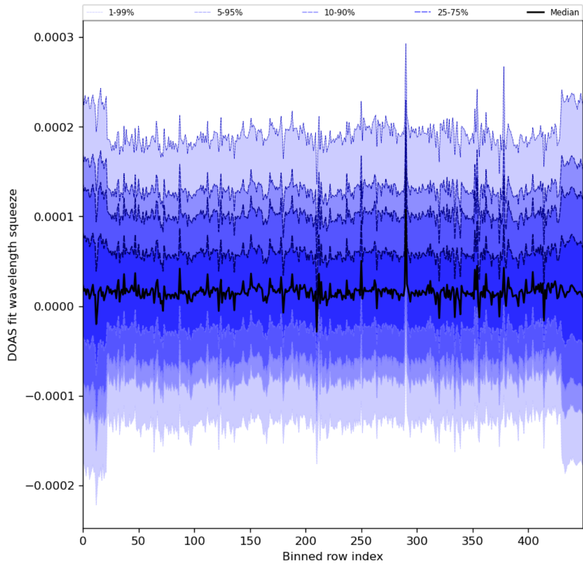
Figure 59: Along track statistics of “DOAS fit wavelength squeeze” for 2024-04-05 to 2024-04-07
