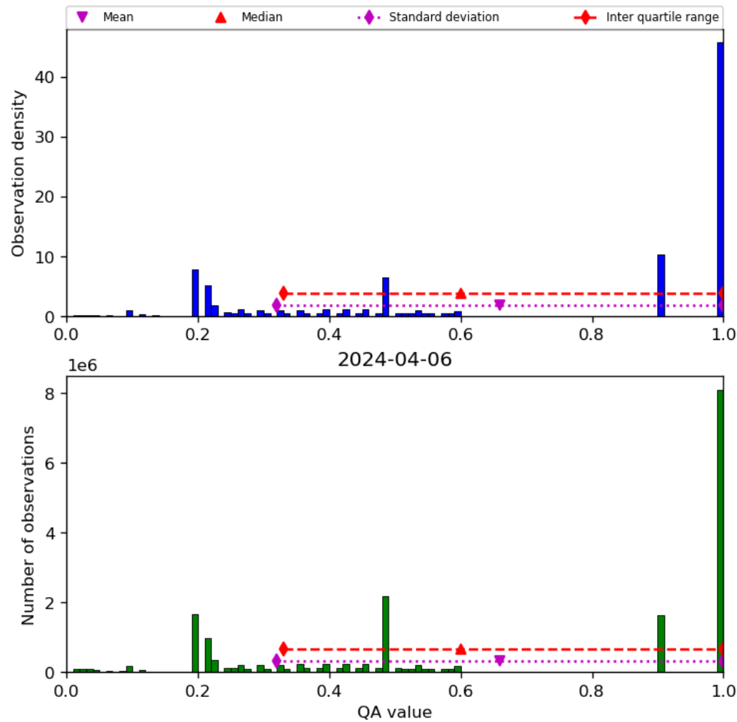
Figure 34: Histogram of “QA value” for 2024-04-05 to 2024-04-07
