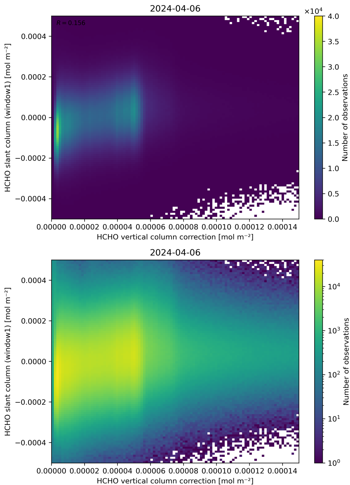
Figure 118: Scatter density plot of “HCHO vertical column correction” against “HCHO slant column (window1)” for 2024-04-05 to 2024-04-07.
