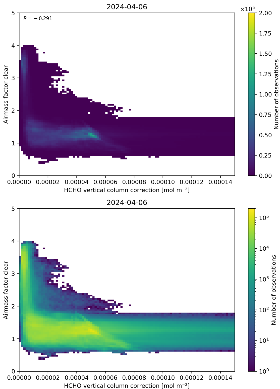
Figure 115: Scatter density plot of “HCHO vertical column correction” against “Airmass factor clear” for 2024-04-05 to 2024-04-07.
