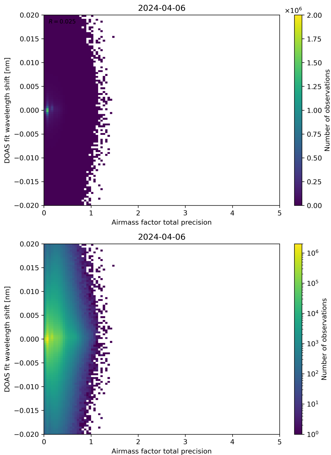
Figure 106: Scatter density plot of “Airmass factor total precision” against “DOAS fit wavelength shift” for 2024-04-05 to 2024-04-07.
