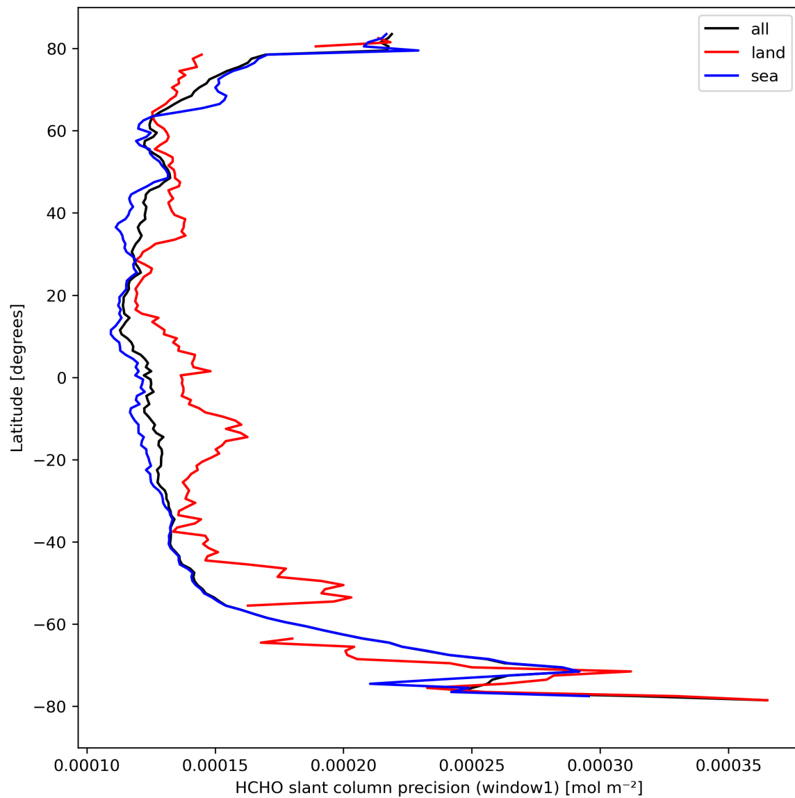
Figure 25: Zonal average of “HCHO slant column precision (window1)” for 2024-04-05 to 2024-04-07.
