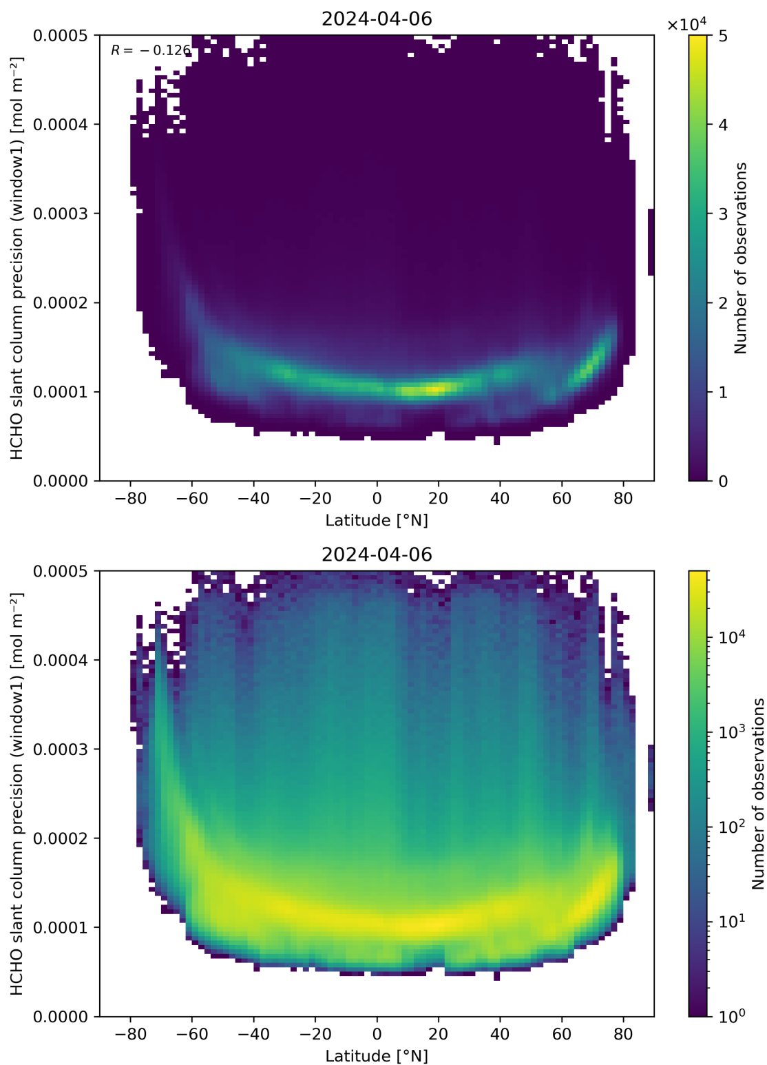
Figure 160: Scatter density plot of “Latitude” against “HCHO slant column precision (window1)” for 2024-04-05 to 2024-04-07.
