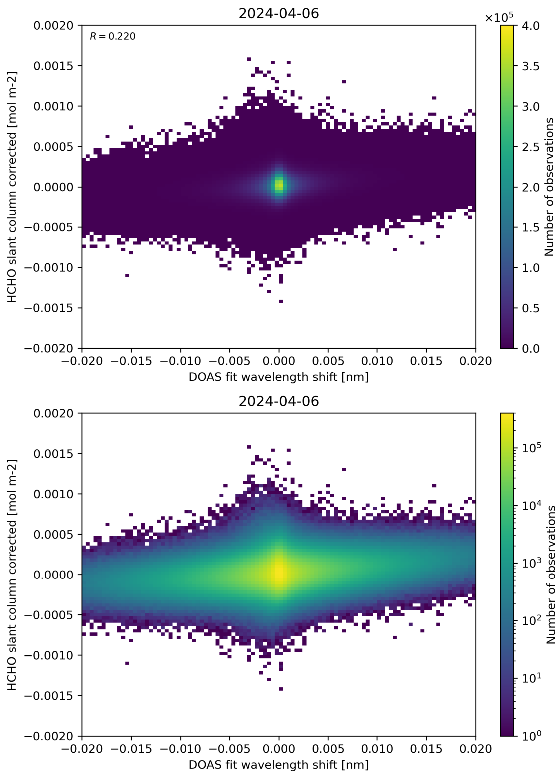
Figure 66: Scatter density plot of “DOAS fit wavelength shift” against “HCHO slant column corrected” for 2024-04-05 to 2024-04-07.
