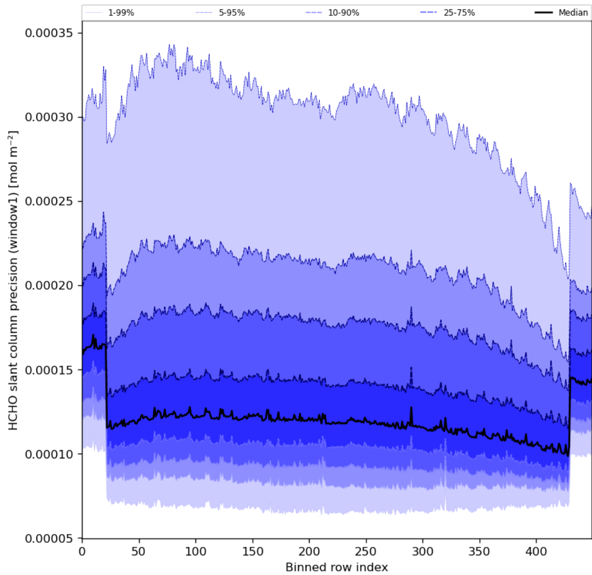
Figure 53: Along track statistics of “HCHO slant column precision (window1)” for 2024-04-05 to 2024-04-07
