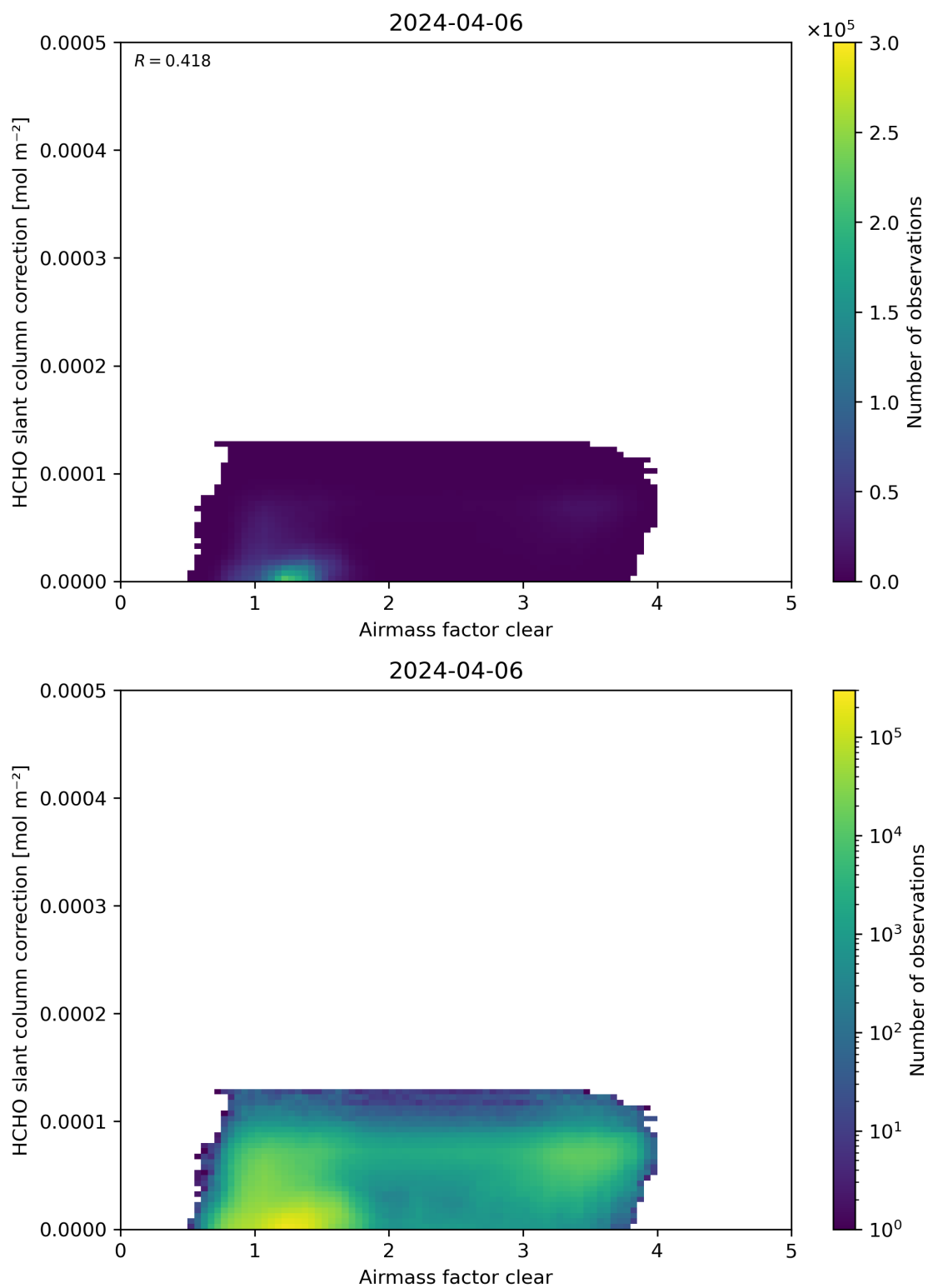
Figure 75: Scatter density plot of “Airmass factor clear” against “HCHO slant column correction” for 2024-04-05 to 2024-04-07.
