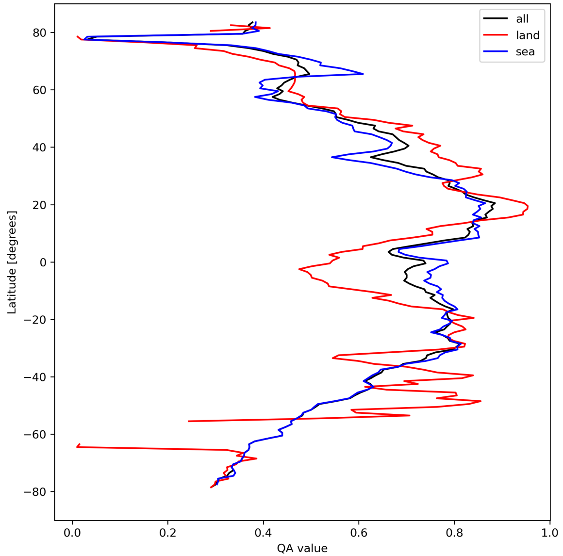
Figure 20: Zonal average of “QA value” for 2024-04-05 to 2024-04-07.
