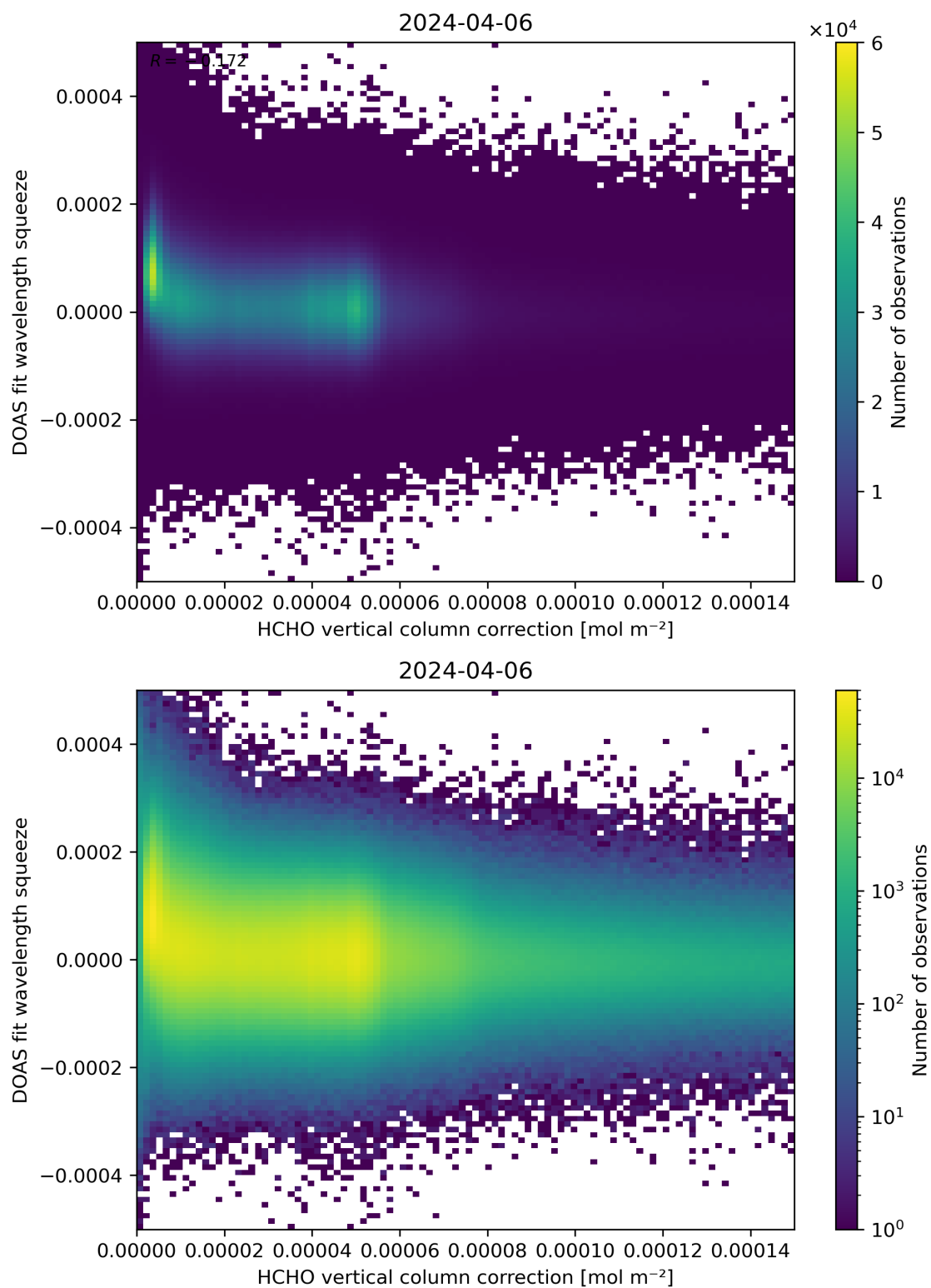
Figure 114: Scatter density plot of “HCHO vertical column correction” against “DOAS fit wavelength squeeze” for 2024-04-05 to 2024-04-07.
