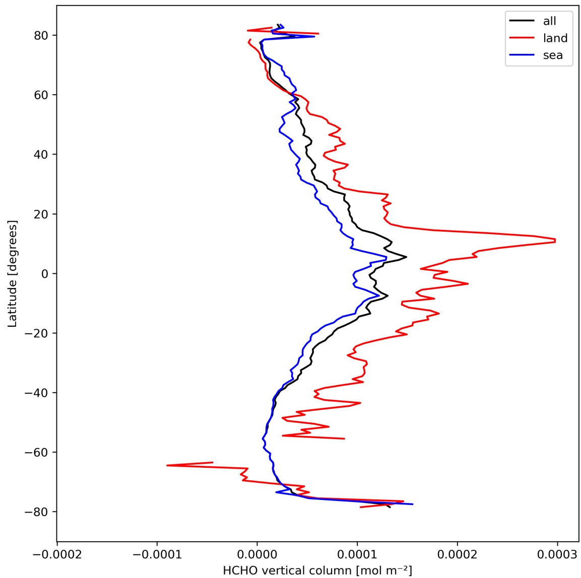
Figure 21: Zonal average of “HCHO vertical column” for 2024-04-05 to 2024-04-07.
