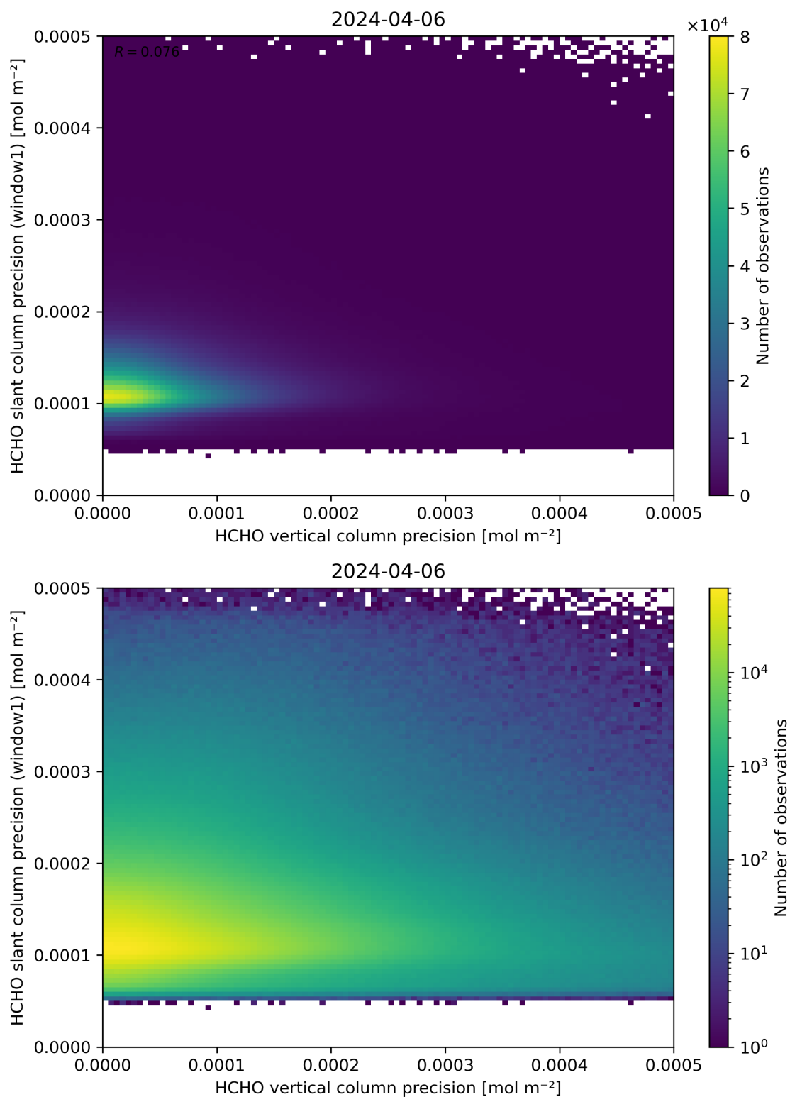
Figure 143: Scatter density plot of “HCHO vertical column precision” against “HCHO slant column precision (window1)” for 2024-04-05 to 2024-04-07.
