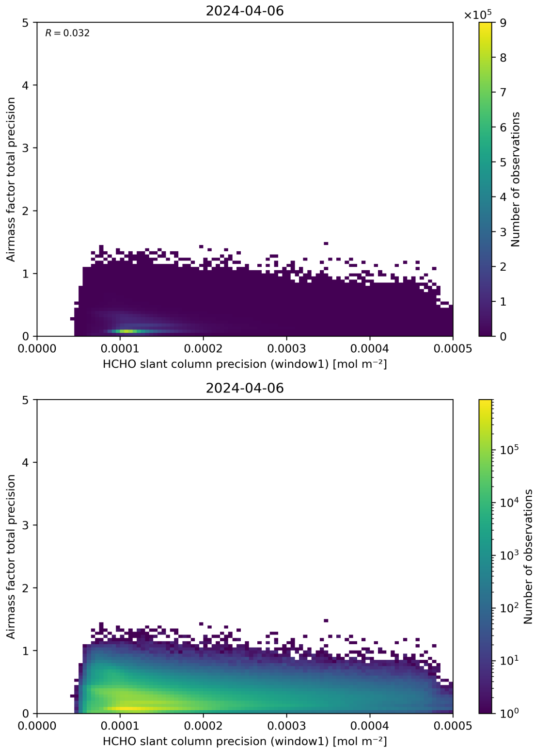
Figure 95: Scatter density plot of “HCHO slant column precision (window1)” against “Airmass factor total precision” for 2024-04-05 to 2024-04-07.
