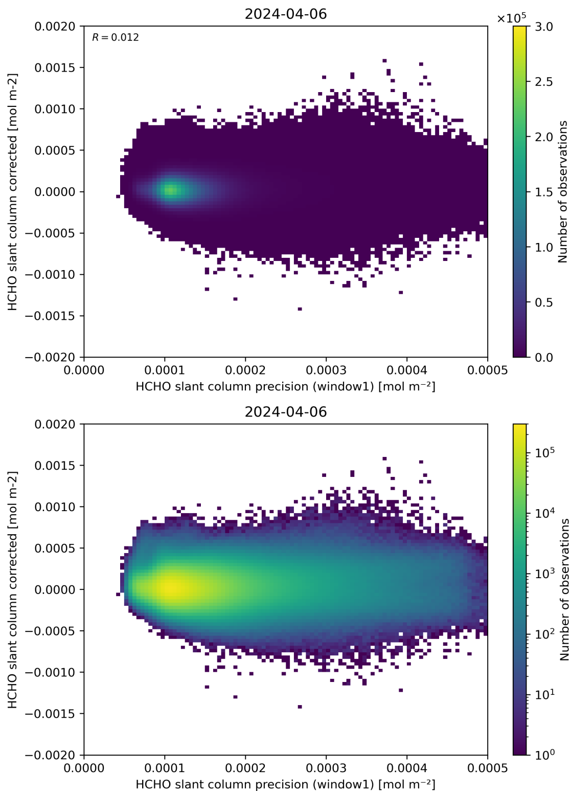
Figure 92: Scatter density plot of “HCHO slant column precision (window1)” against “HCHO slant column corrected” for 2024-04-05 to 2024-04-07.
