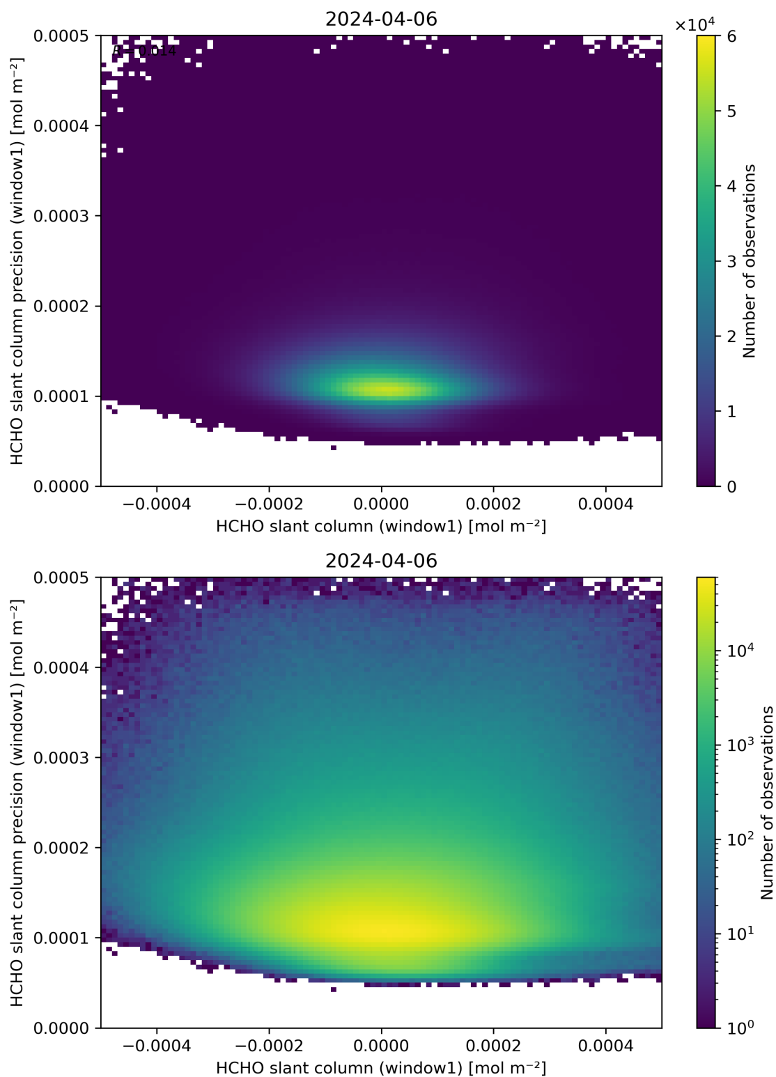
Figure 84: Scatter density plot of “HCHO slant column (window1)” against “HCHO slant column precision (window1)” for 2024-04-05 to 2024-04-07.
