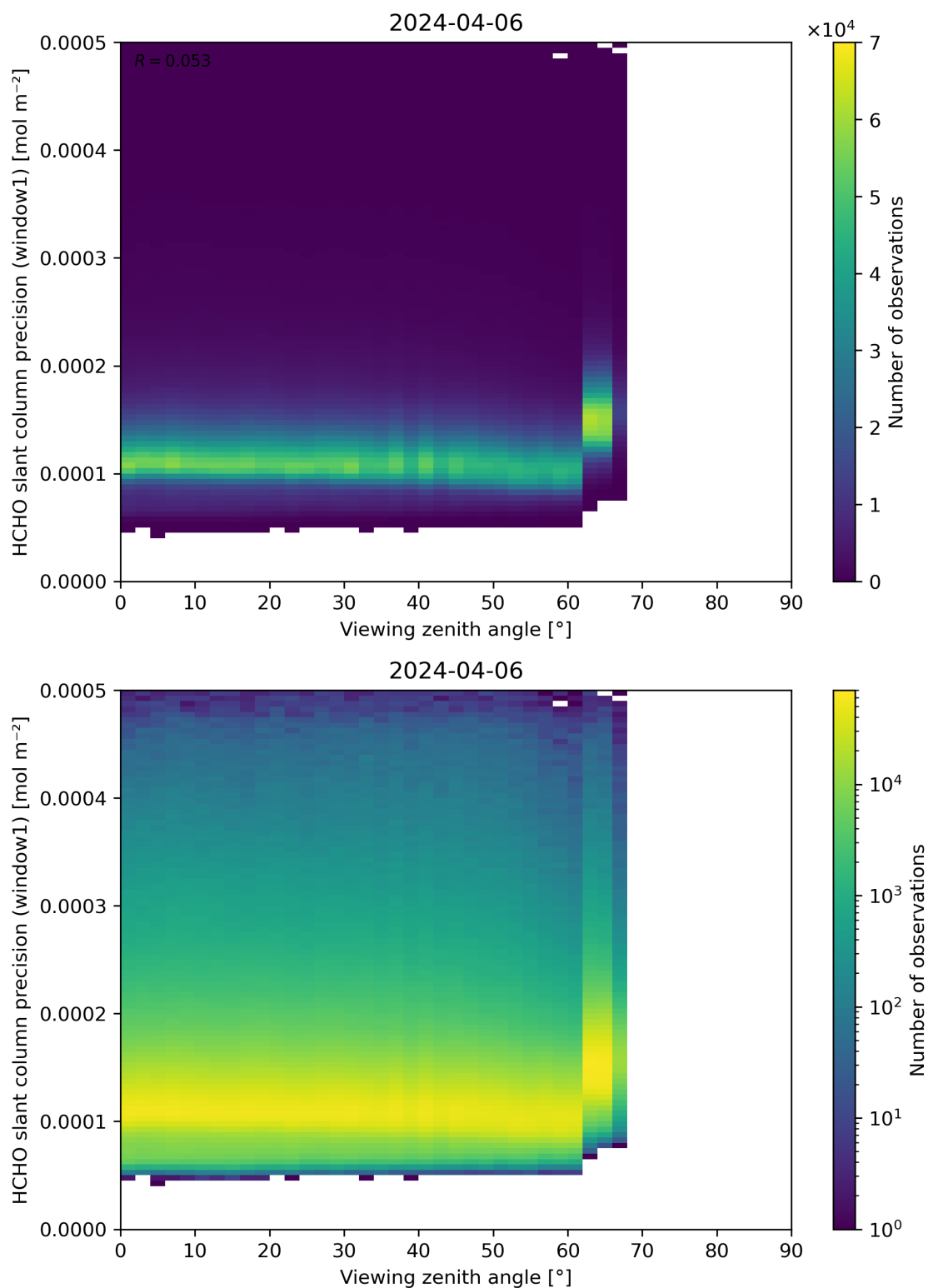
Figure 189: Scatter density plot of “Viewing zenith angle” against “HCHO slant column precision (window1)” for 2024-04-05 to 2024-04-07.
