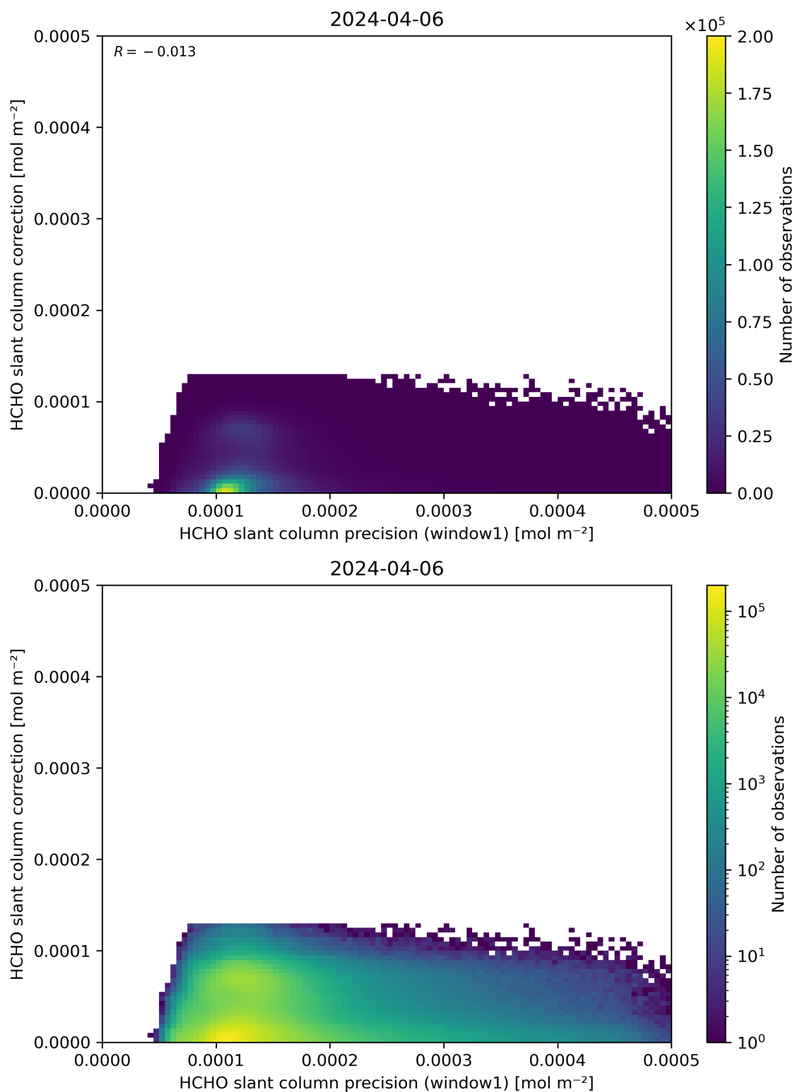
Figure 93: Scatter density plot of “HCHO slant column precision (window1)” against “HCHO slant column correction” for 2024-04-05 to 2024-04-07.
