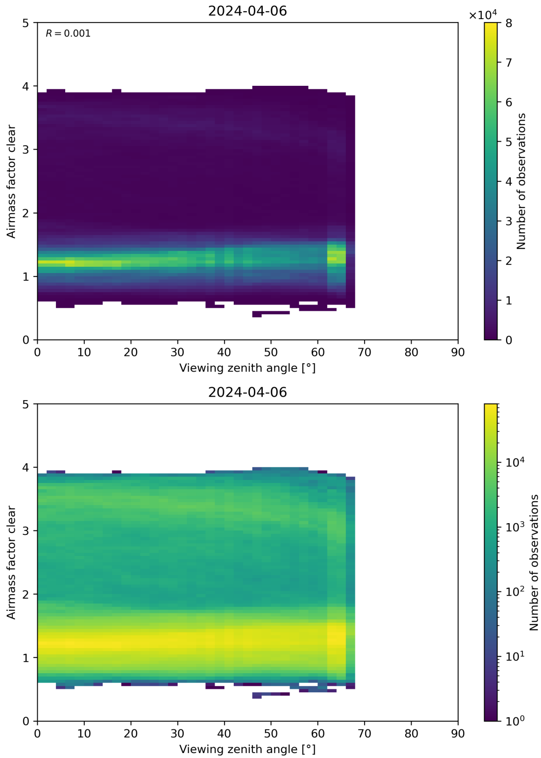
Figure 185: Scatter density plot of “Viewing zenith angle” against “Airmass factor clear” for 2024-04-05 to 2024-04-07.
