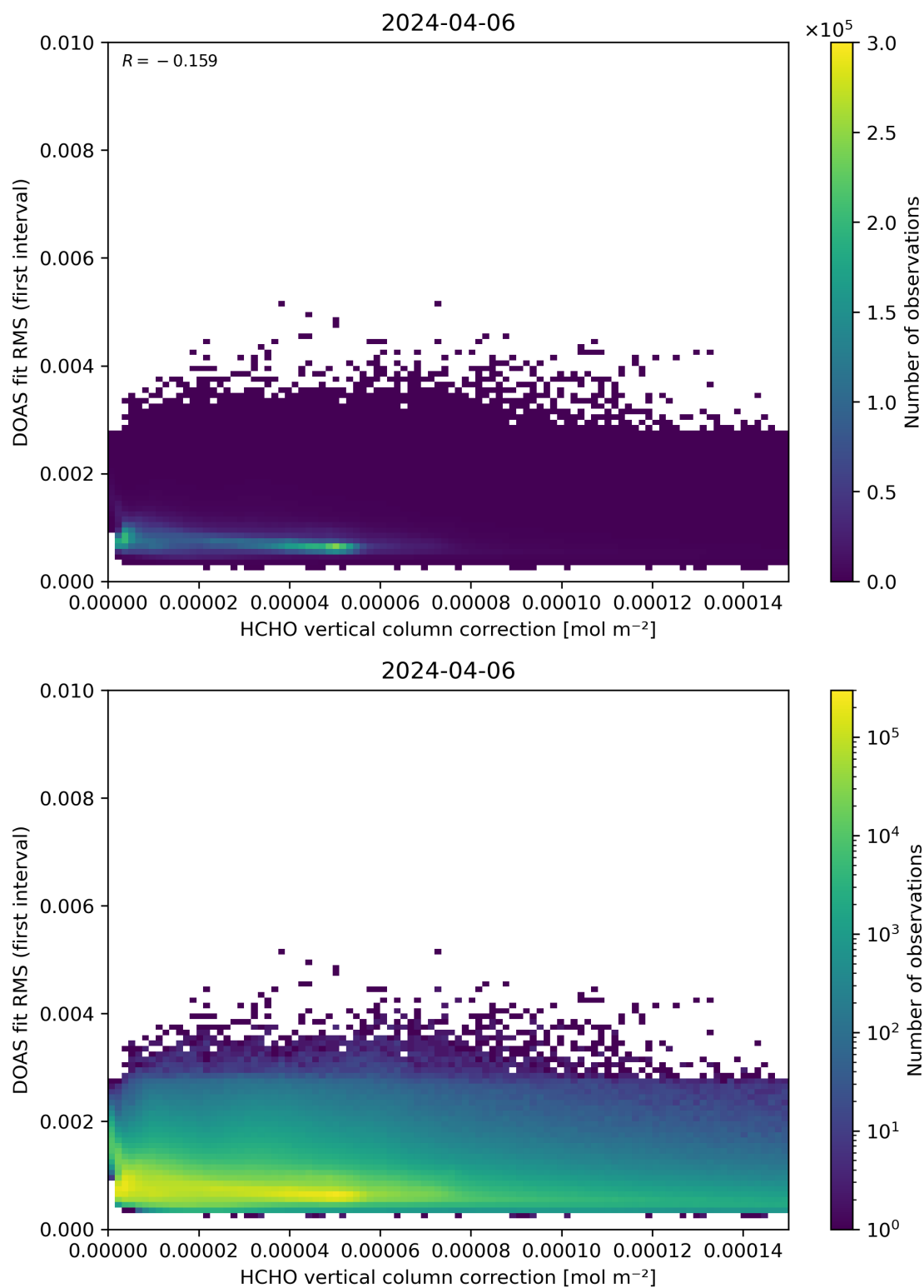
Figure 112: Scatter density plot of “HCHO vertical column correction” against “DOAS fit RMS (first interval)” for 2024-04-05 to 2024-04-07.
