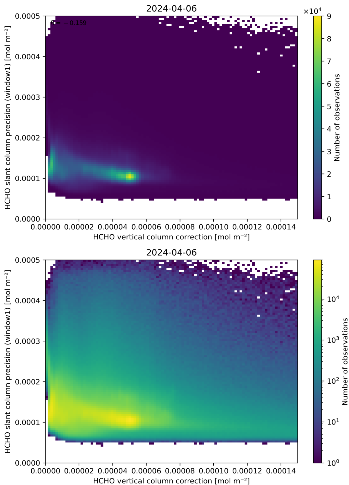
Figure 119: Scatter density plot of “HCHO vertical column correction” against “HCHO slant column precision (window1)” for 2024-04-05 to 2024-04-07.
