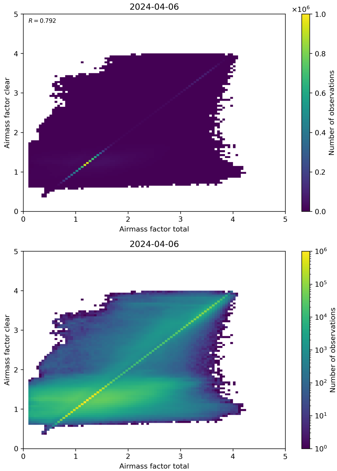
Figure 100: Scatter density plot of “Airmass factor total” against “Airmass factor clear” for 2024-04-05 to 2024-04-07.
