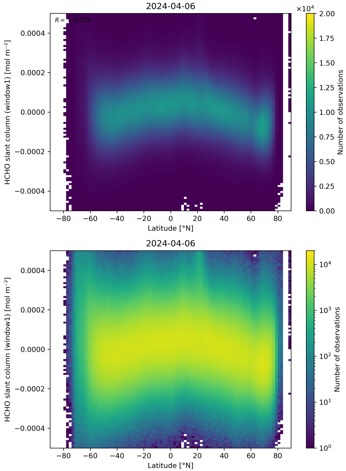
Figure 159: Scatter density plot of “Latitude” against “HCHO slant column (window1)” for 2024-04-05 to 2024-04-07.
