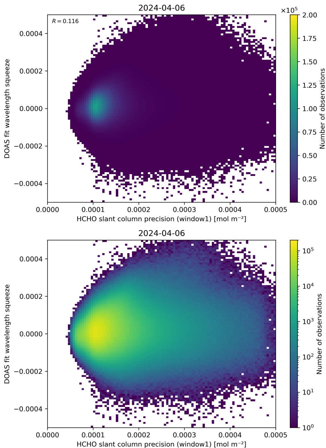
Figure 90: Scatter density plot of “HCHO slant column precision (window1)” against “DOAS fit wavelength squeeze” for 2024-04-05 to 2024-04-07.
