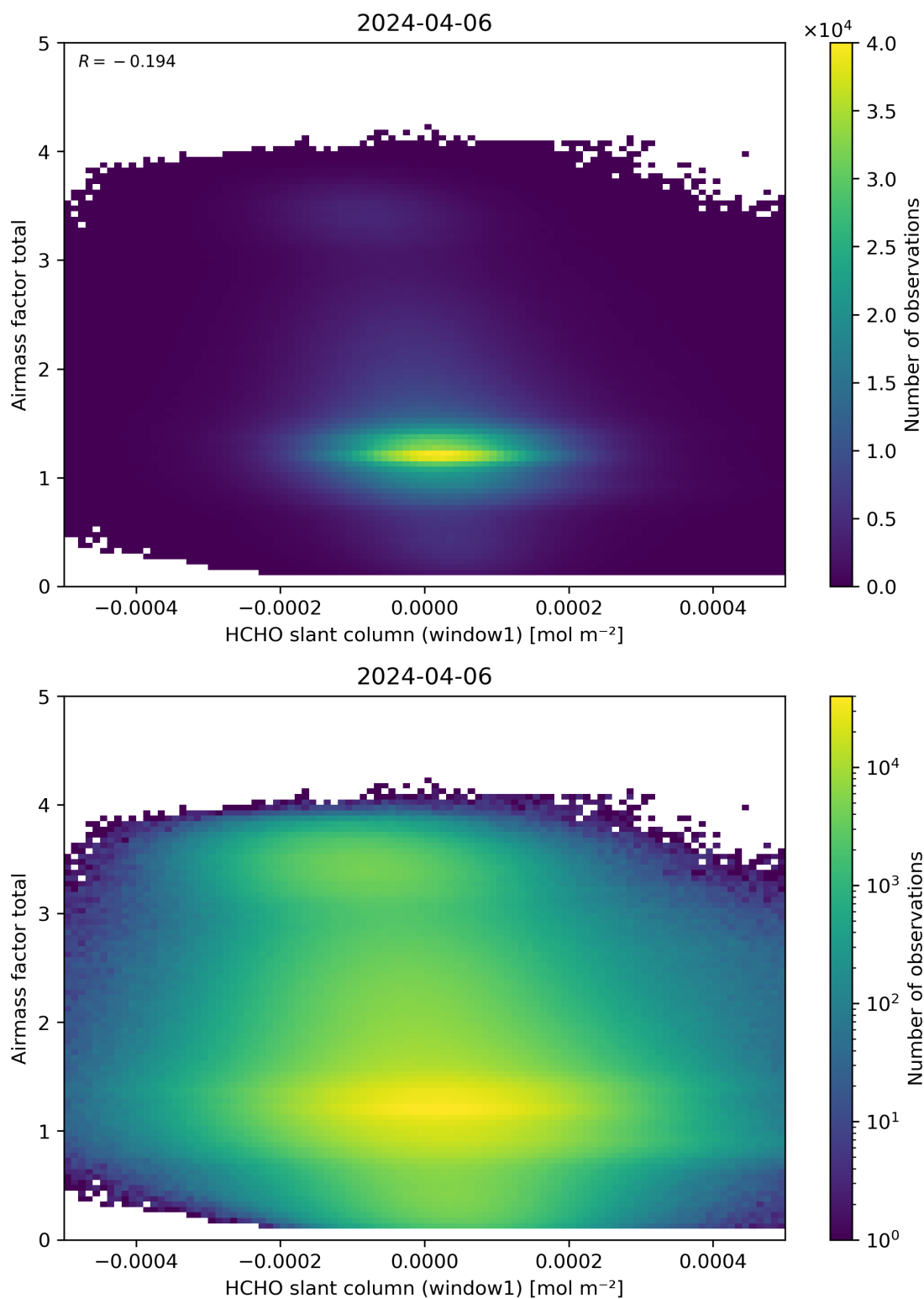
Figure 85: Scatter density plot of “HCHO slant column (window1)” against “Airmass factor total” for 2024-04-05 to 2024-04-07.
