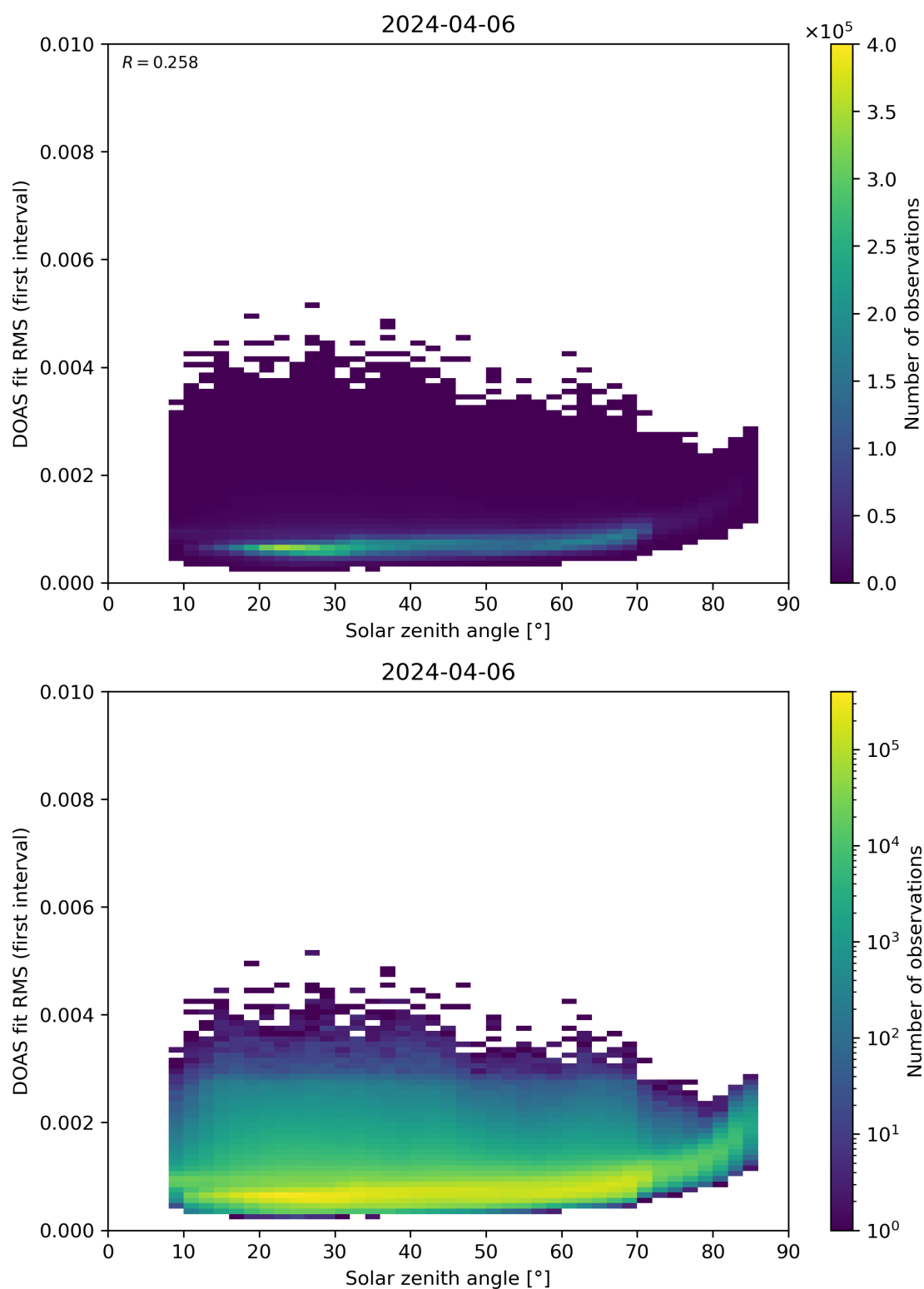
Figure 167: Scatter density plot of “Solar zenith angle” against “DOAS fit RMS (first interval)” for 2024-04-05 to 2024-04-07.
