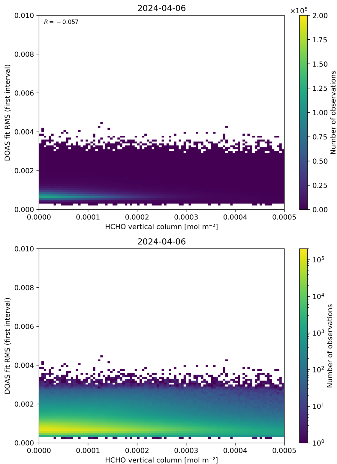
Figure 123: Scatter density plot of “HCHO vertical column” against “DOAS fit RMS (first interval)” for 2024-04-05 to 2024-04-07.
