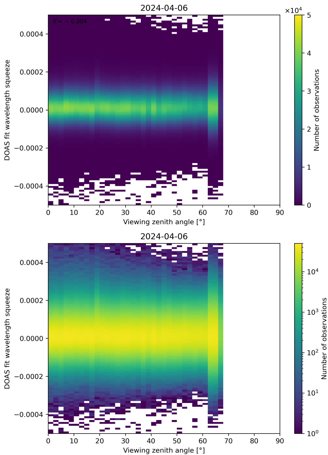
Figure 184: Scatter density plot of “Viewing zenith angle” against “DOAS fit wavelength squeeze” for 2024-04-05 to 2024-04-07.
