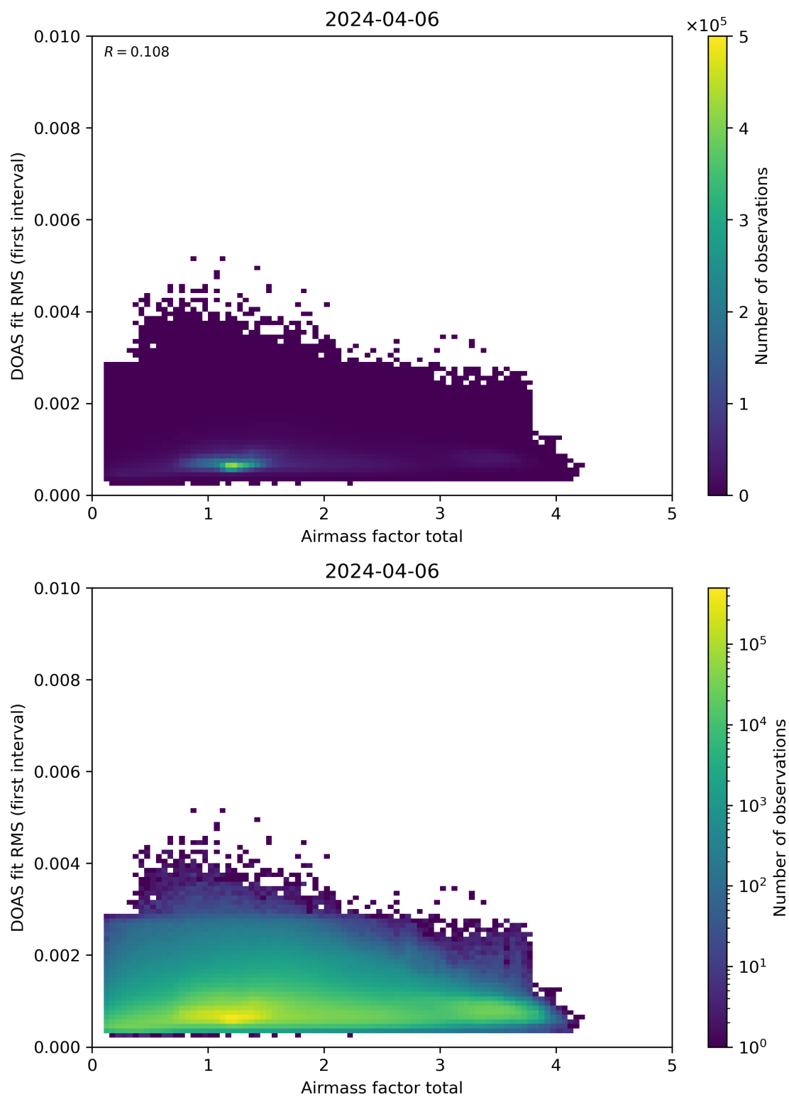
Figure 97: Scatter density plot of “Airmass factor total” against “DOAS fit RMS (first interval)” for 2024-04-05 to 2024-04-07.
