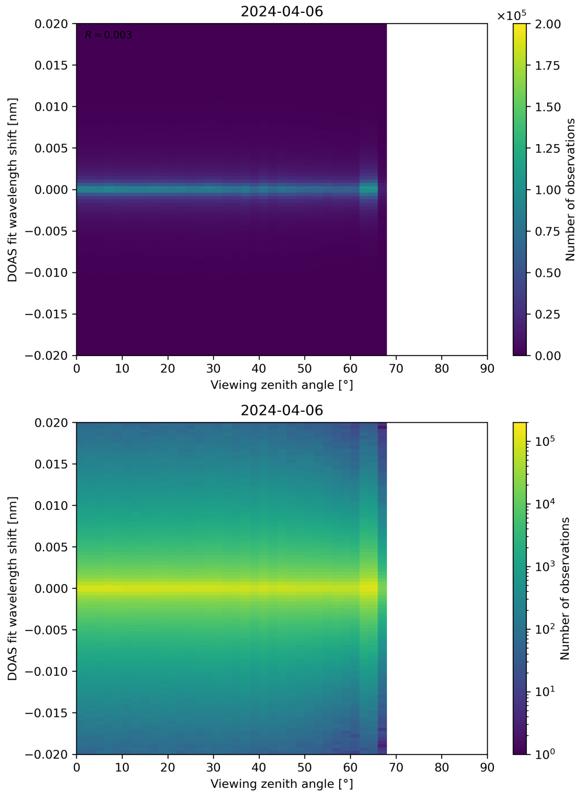
Figure 183: Scatter density plot of “Viewing zenith angle” against “DOAS fit wavelength shift” for 2024-04-05 to 2024-04-07.
