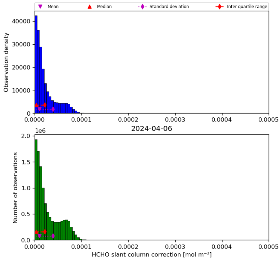
Figure 47: Histogram of “HCHO slant column correction” for 2024-04-05 to 2024-04-07
