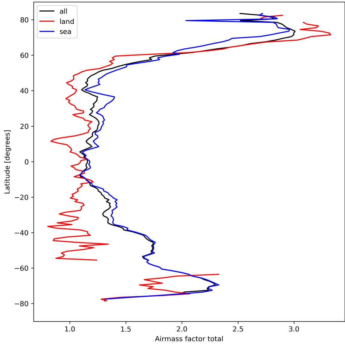
Figure 26: Zonal average of “Airmass factor total” for 2024-04-05 to 2024-04-07.
