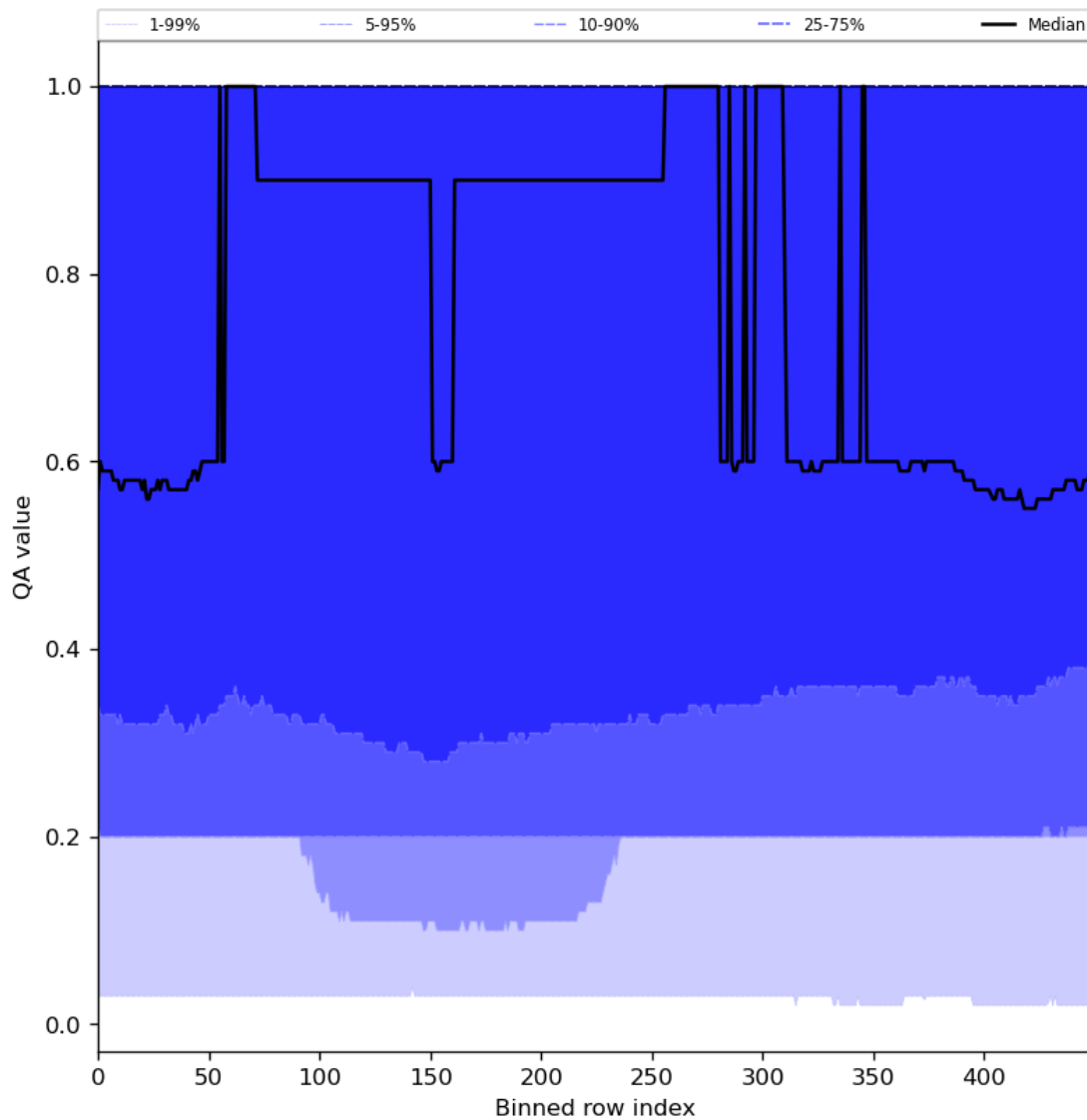
Figure 48: Along track statistics of “QA value” for 2024-04-05 to 2024-04-07
