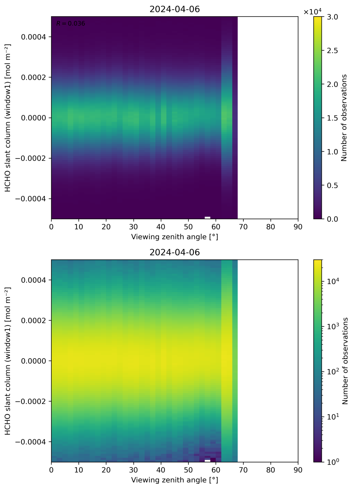
Figure 188: Scatter density plot of “Viewing zenith angle” against “HCHO slant column (window1)” for 2024-04-05 to 2024-04-07.
