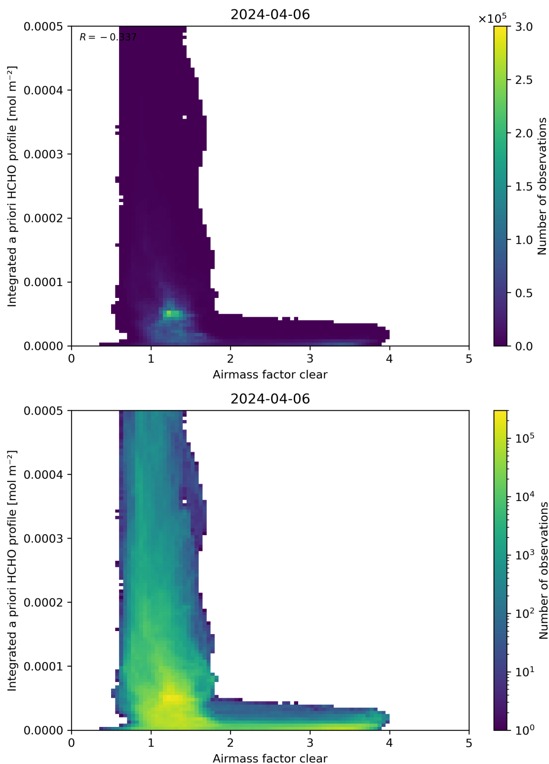
Figure 76: Scatter density plot of “Airmass factor clear” against “Integrated a priori HCHO profile” for 2024-04-05 to 2024-04-07.
