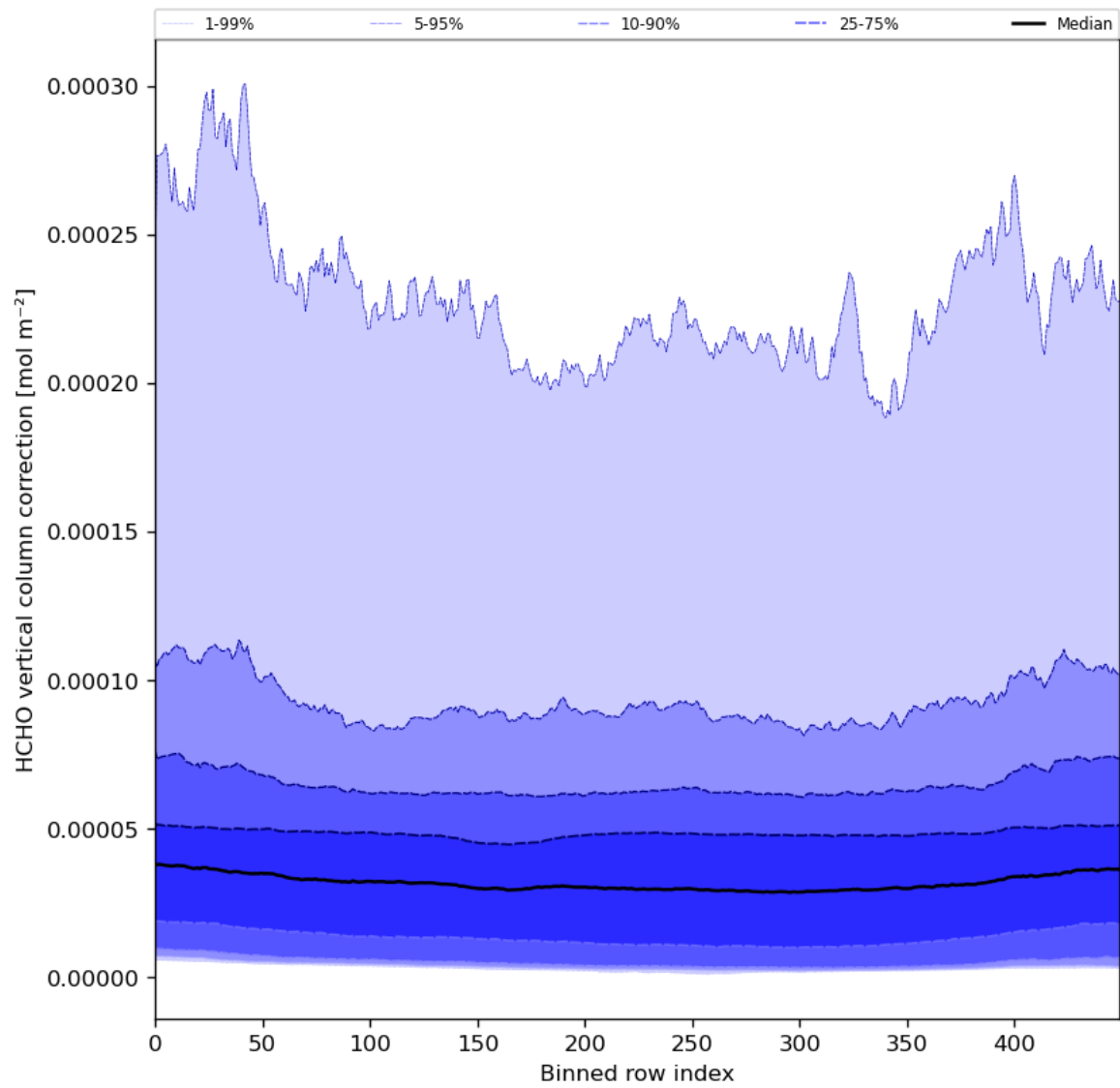
Figure 51: Along track statistics of "HCHO vertical column correction" for 2024-04-05 to 2024-04-07
