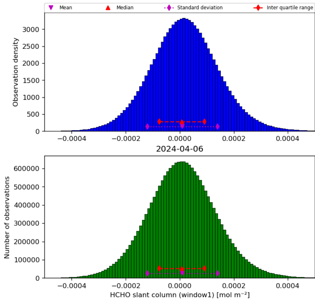
Figure 38: Histogram of “HCHO slant column (window1)” for 2024-04-05 to 2024-04-07
