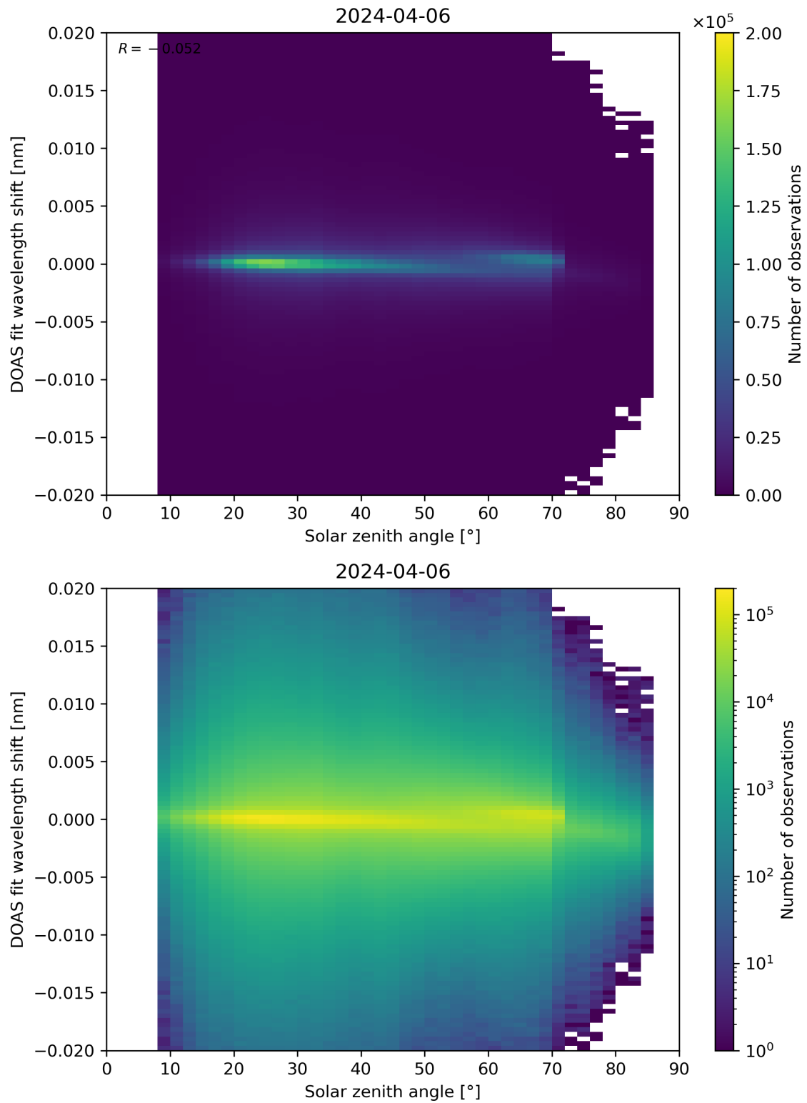
Figure 168: Scatter density plot of “Solar zenith angle” against “DOAS fit wavelength shift” for 2024-04-05 to 2024-04-07.
