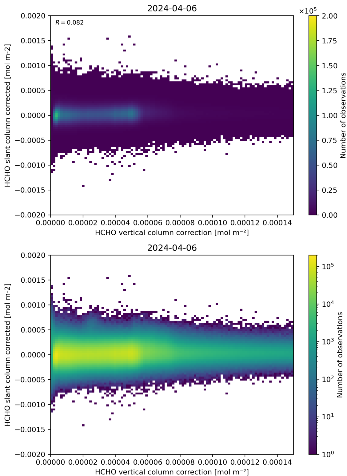
Figure 116: Scatter density plot of “HCHO vertical column correction” against “HCHO slant column corrected” for 2024-04-05 to 2024-04-07.
