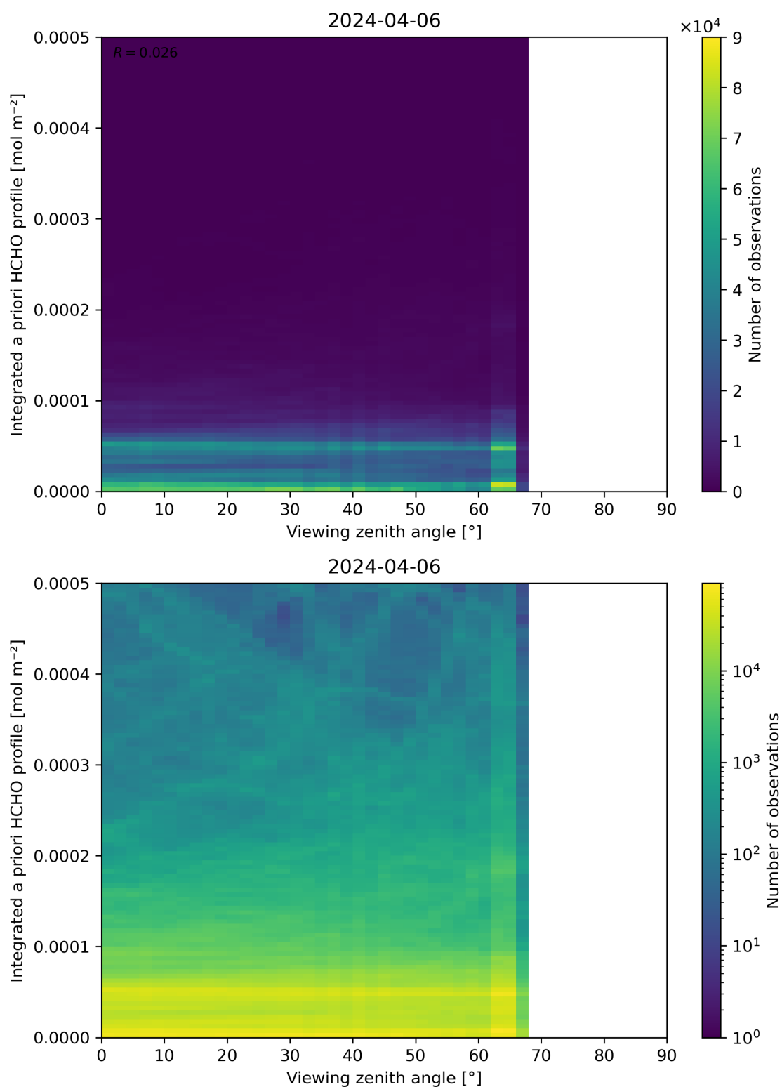
Figure 195: Scatter density plot of “Viewing zenith angle” against “Integrated a priori HCHO profile” for 2024-04-05 to 2024-04-07.
