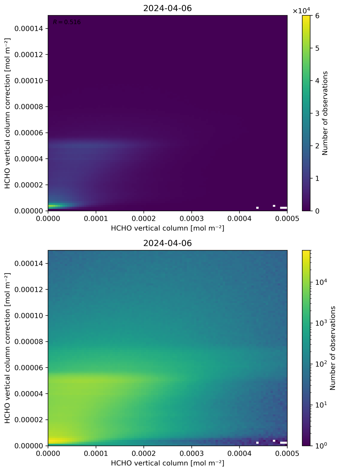
Figure 133: Scatter density plot of “HCHO vertical column” against “HCHO vertical column correction” for 2024-04-05 to 2024-04-07.
