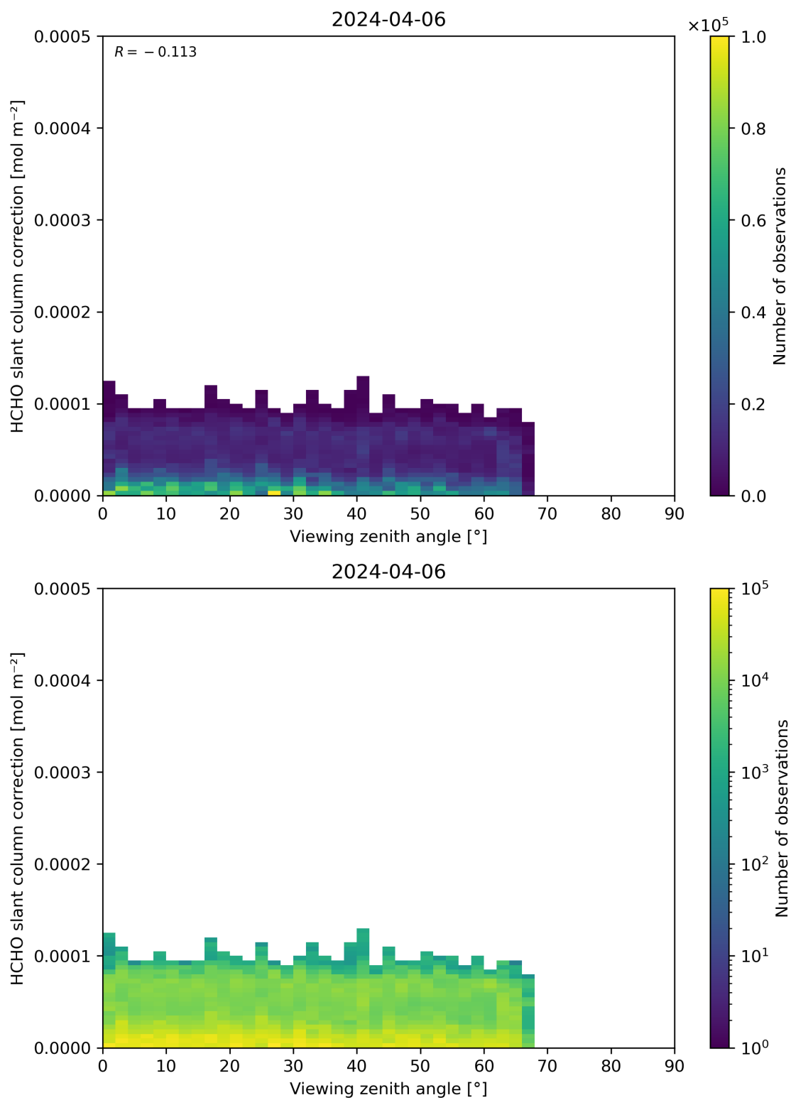
Figure 187: Scatter density plot of “Viewing zenith angle” against “HCHO slant column correction” for 2024-04-05 to 2024-04-07.
