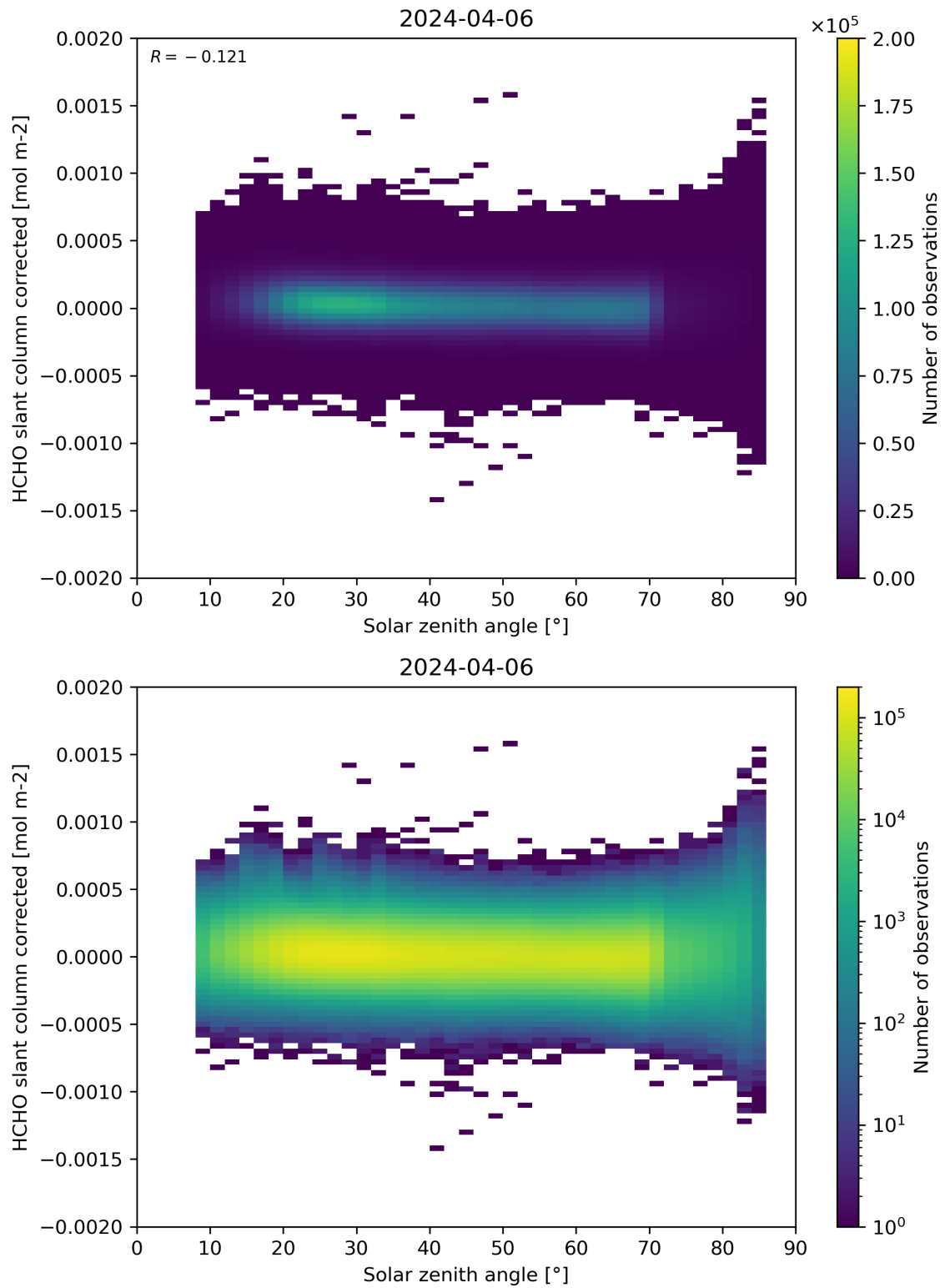
Figure 171: Scatter density plot of “Solar zenith angle” against “HCHO slant column corrected” for 2024-04-05 to 2024-04-07.
