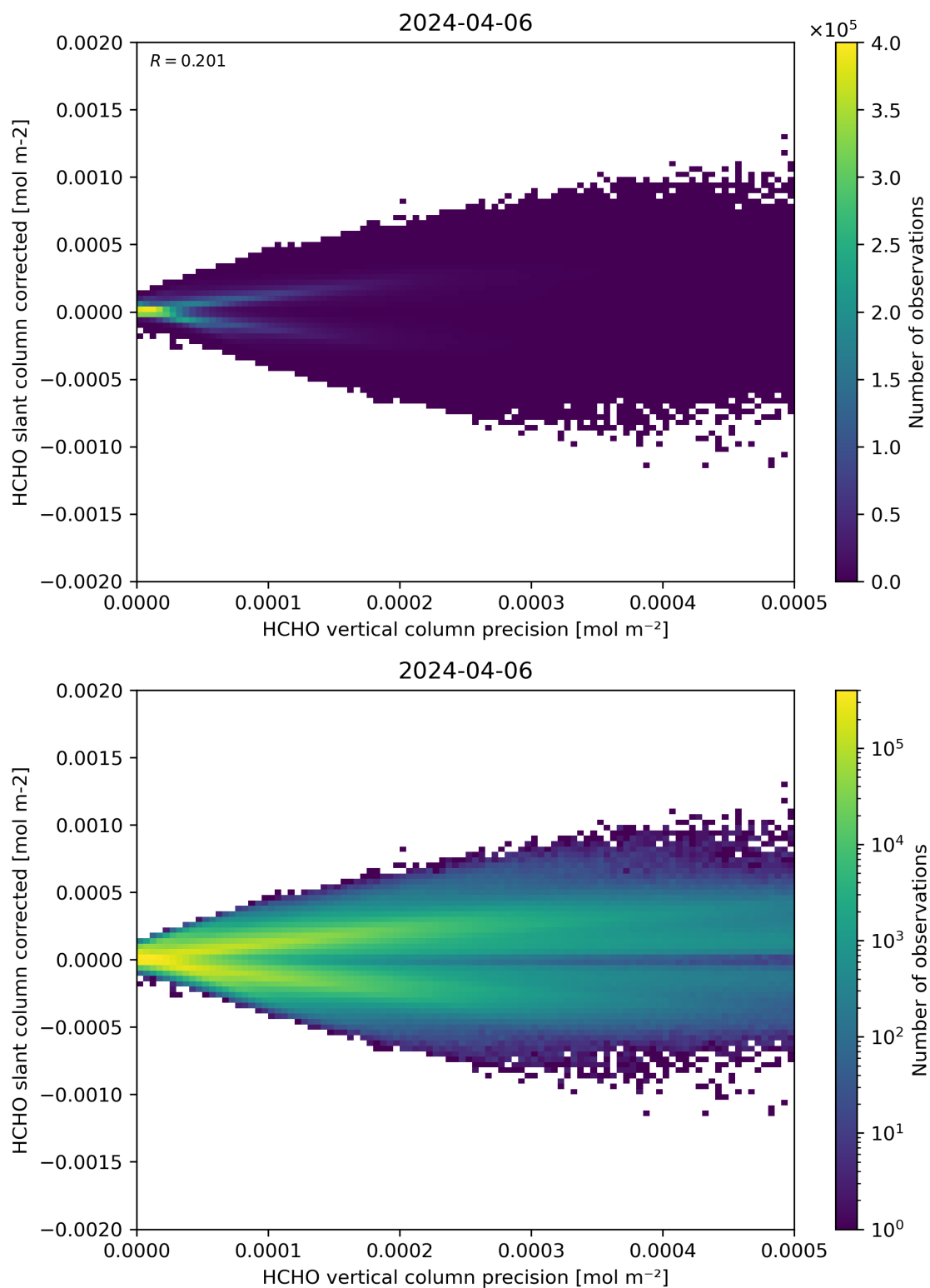
Figure 140: Scatter density plot of “HCHO vertical column precision” against “HCHO slant column corrected” for 2024-04-05 to 2024-04-07.
