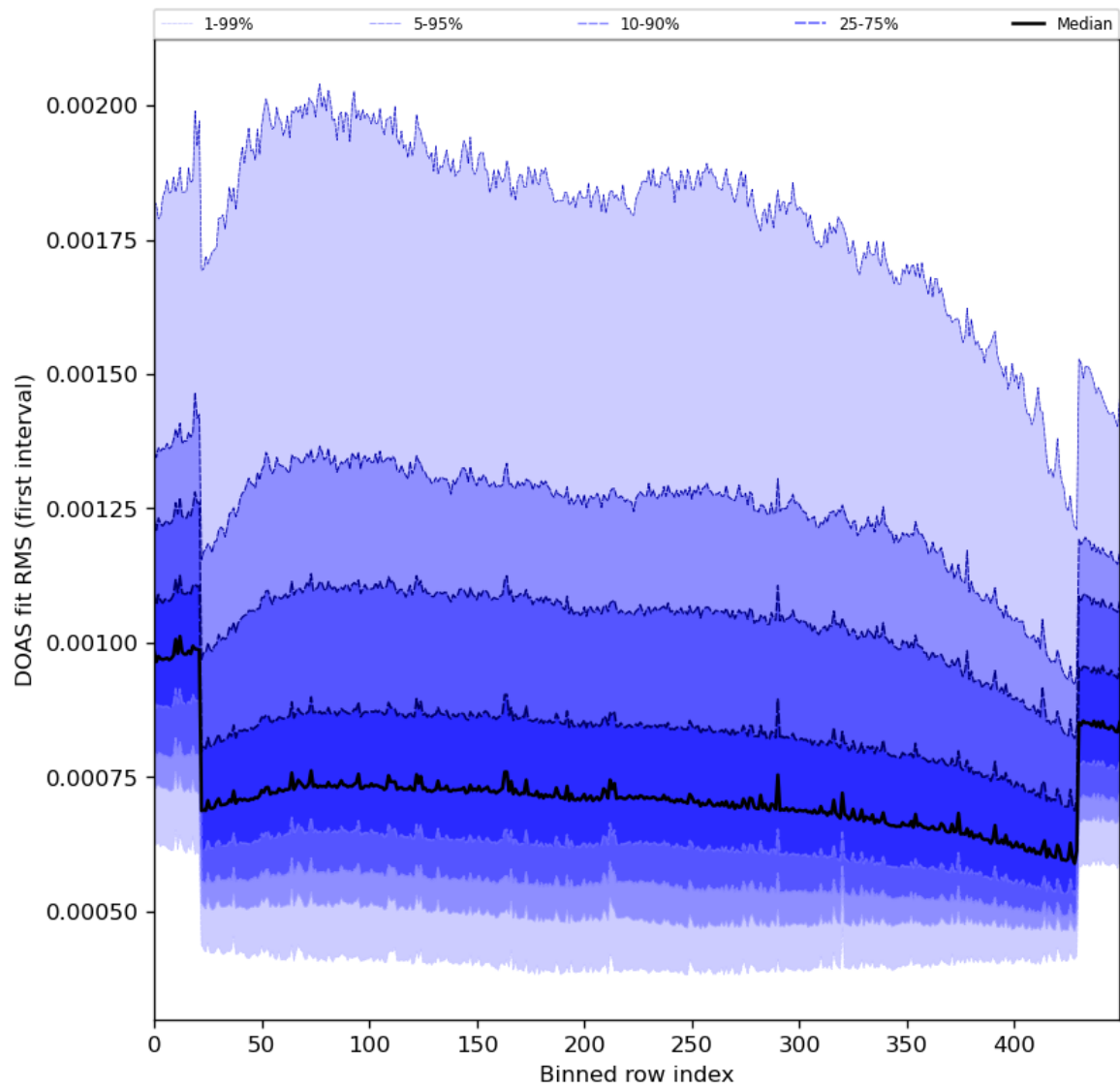
Figure 60: Along track statistics of “DOAS fit RMS (first interval)” for 2024-04-05 to 2024-04-07
