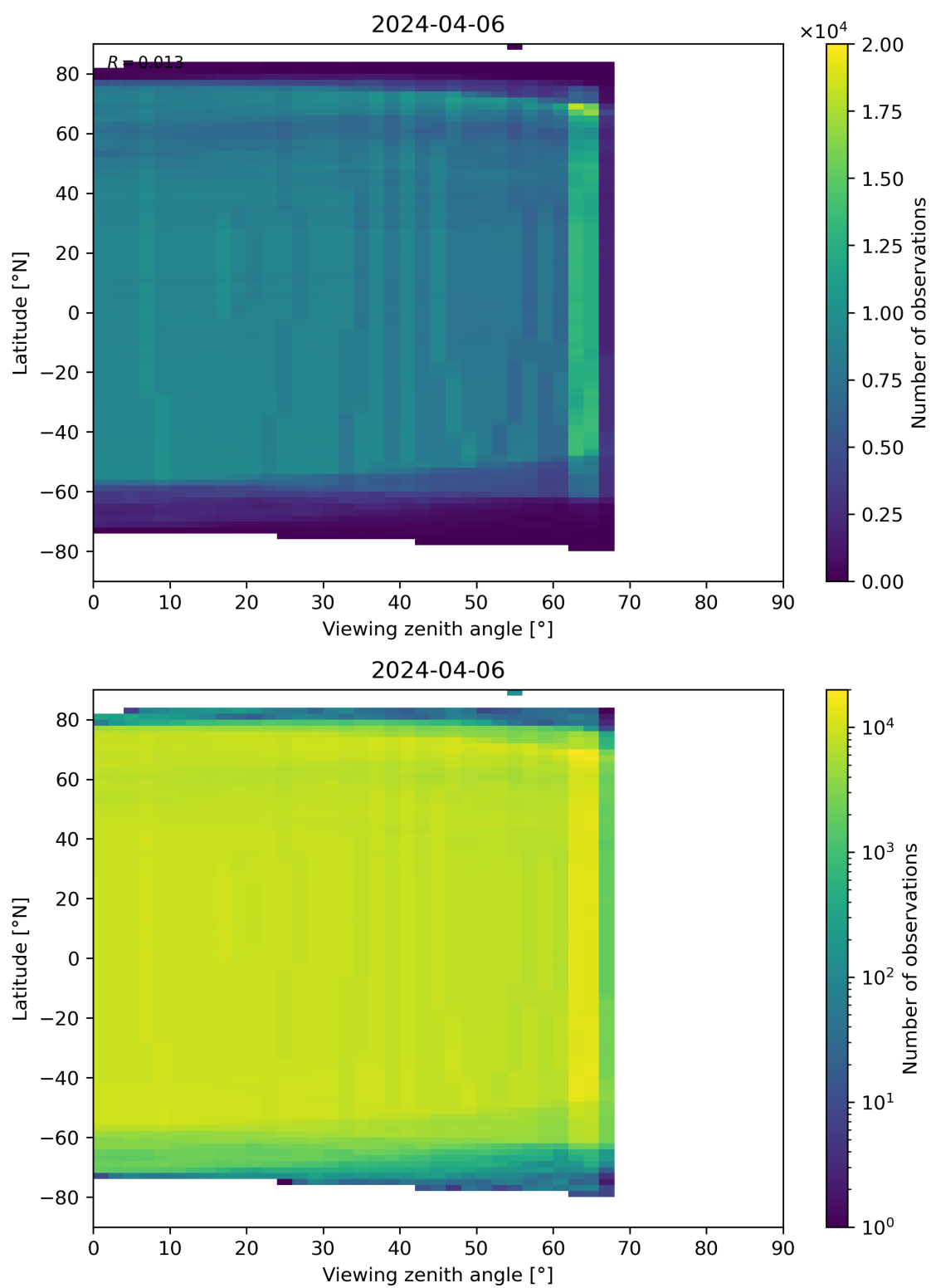
Figure 196: Scatter density plot of “Viewing zenith angle” against “Latitude” for 2024-04-05 to 2024-04-07.
