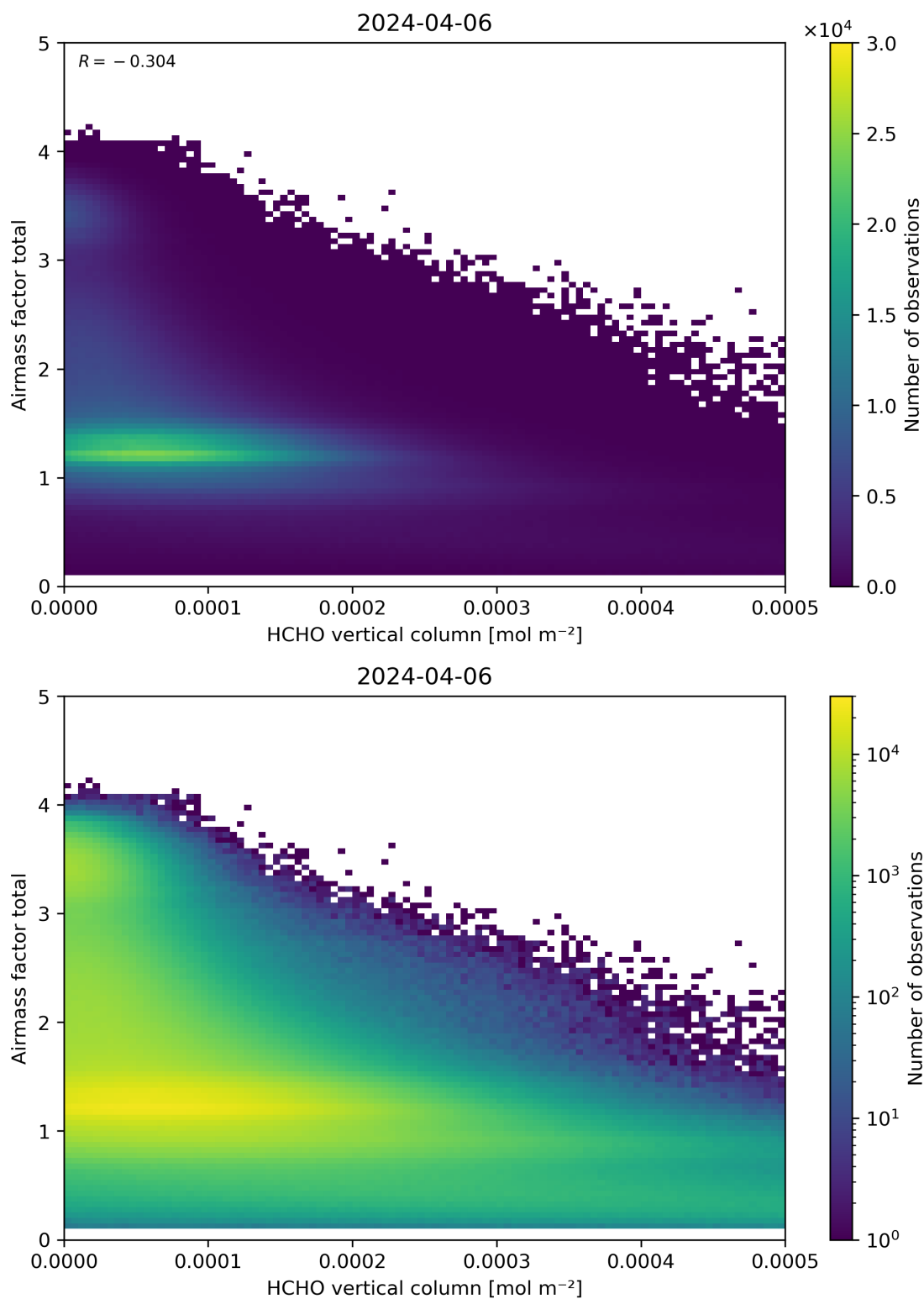
Figure 131: Scatter density plot of “HCHO vertical column” against “Airmass factor total” for 2024-04-05 to 2024-04-07.
