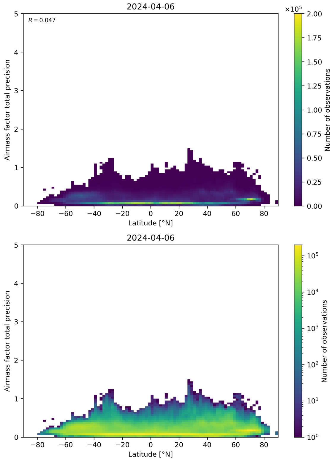
Figure 162: Scatter density plot of “Latitude” against “Airmass factor total precision” for 2024-04-05 to 2024-04-07.
