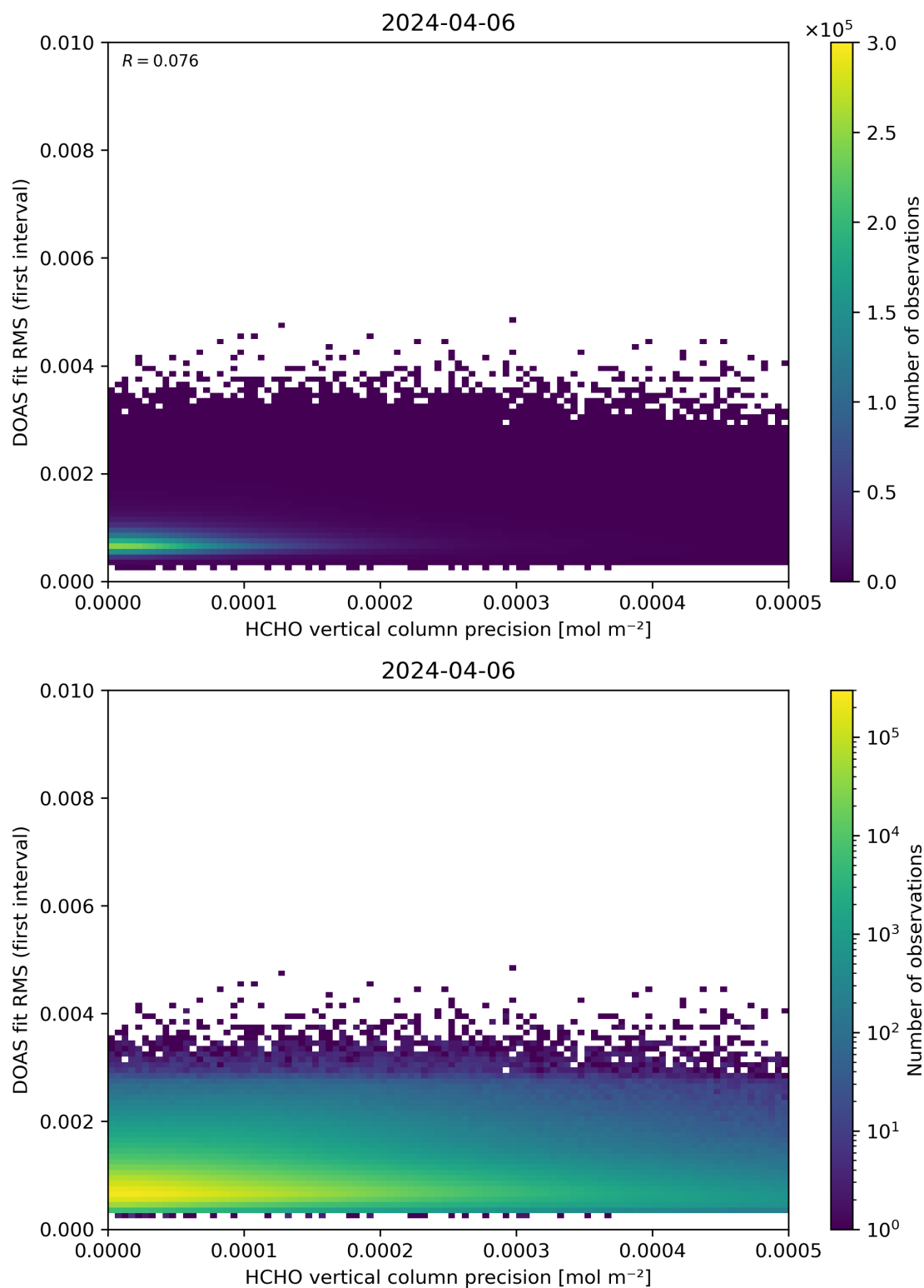
Figure 136: Scatter density plot of “HCHO vertical column precision” against “DOAS fit RMS (first interval)” for 2024-04-05 to 2024-04-07.
