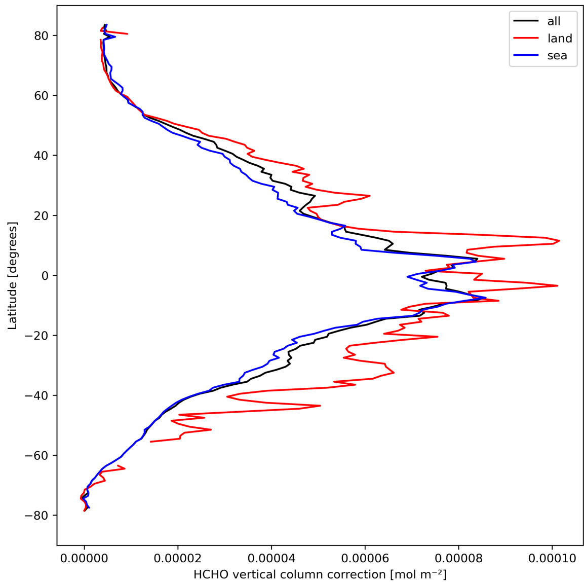
Figure 23: Zonal average of “HCHO vertical column correction” for 2024-04-05 to 2024-04-07.
