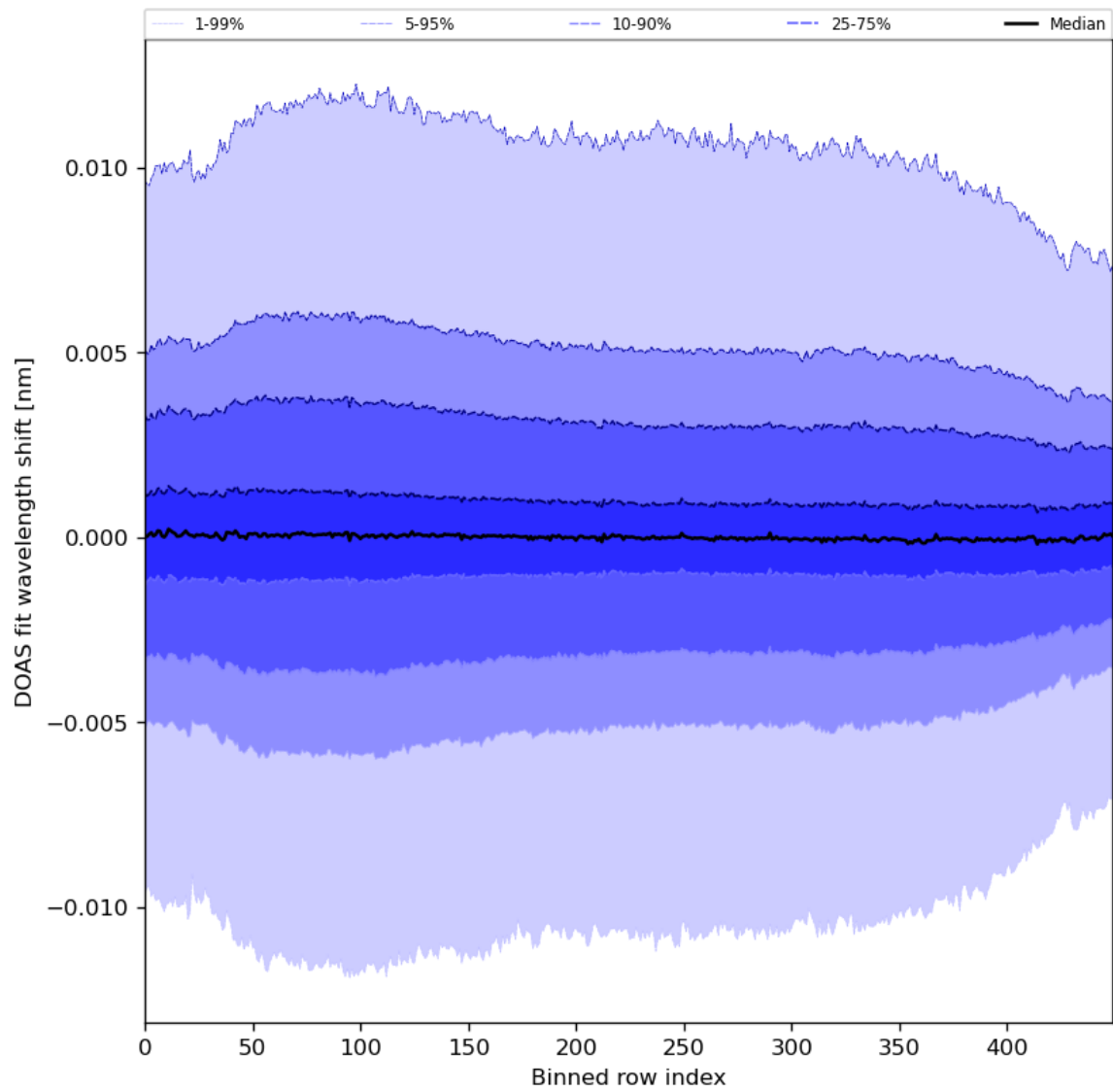
Figure 58: Along track statistics of “DOAS fit wavelength shift” for 2024-04-05 to 2024-04-07
