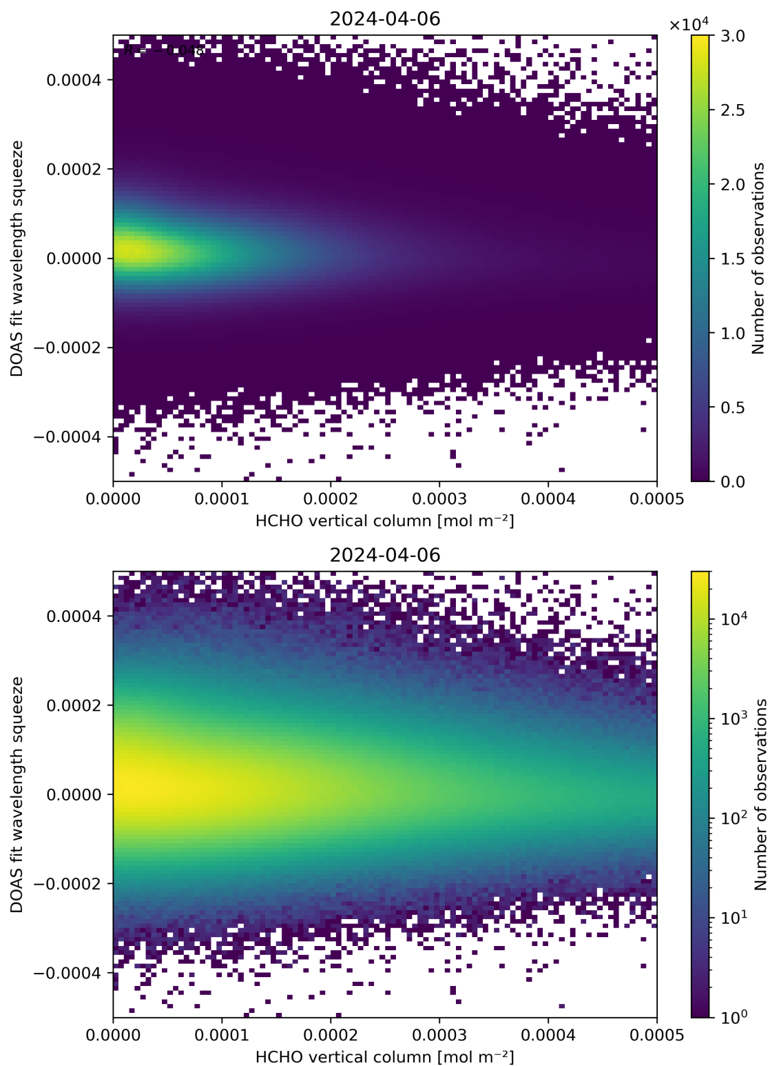
Figure 125: Scatter density plot of “HCHO vertical column” against “DOAS fit wavelength squeeze” for 2024-04-05 to 2024-04-07.
