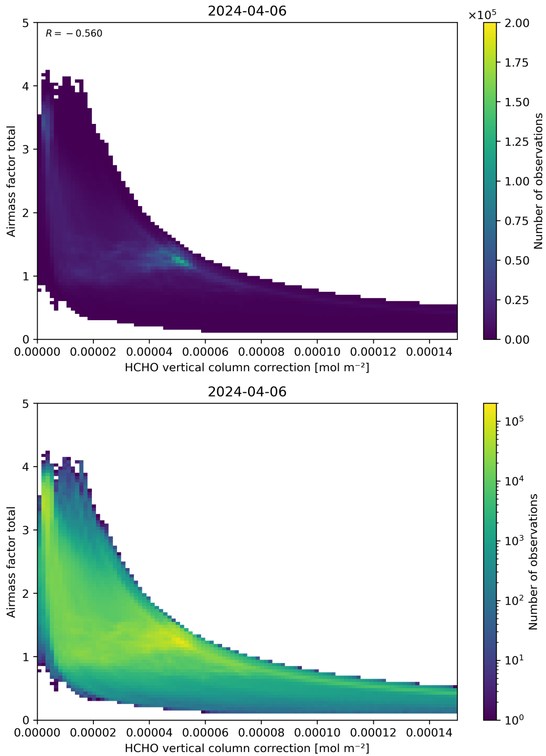
Figure 120: Scatter density plot of “HCHO vertical column correction” against “Airmass factor total” for 2024-04-05 to 2024-04-07.
