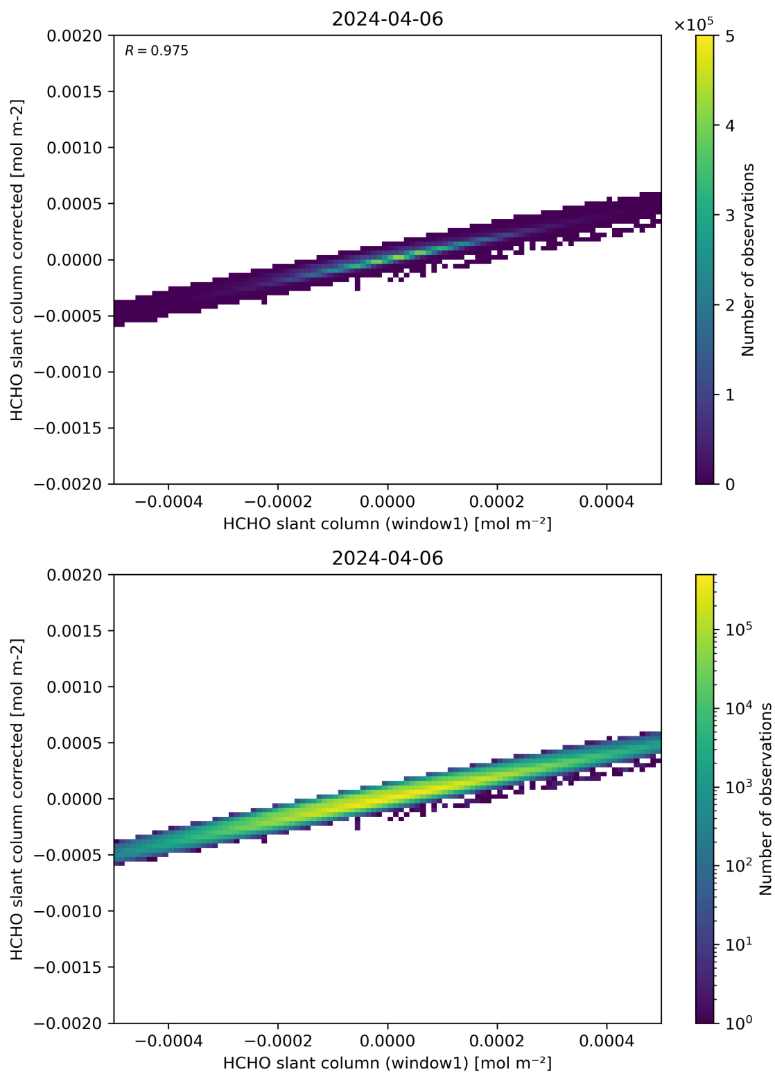
Figure 82: Scatter density plot of “HCHO slant column (window1)” against “HCHO slant column corrected” for 2024-04-05 to 2024-04-07.
