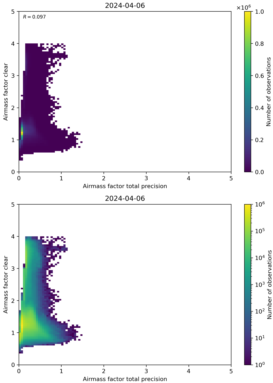
Figure 108: Scatter density plot of “Airmass factor total precision” against “Airmass factor clear” for 2024-04-05 to 2024-04-07.
