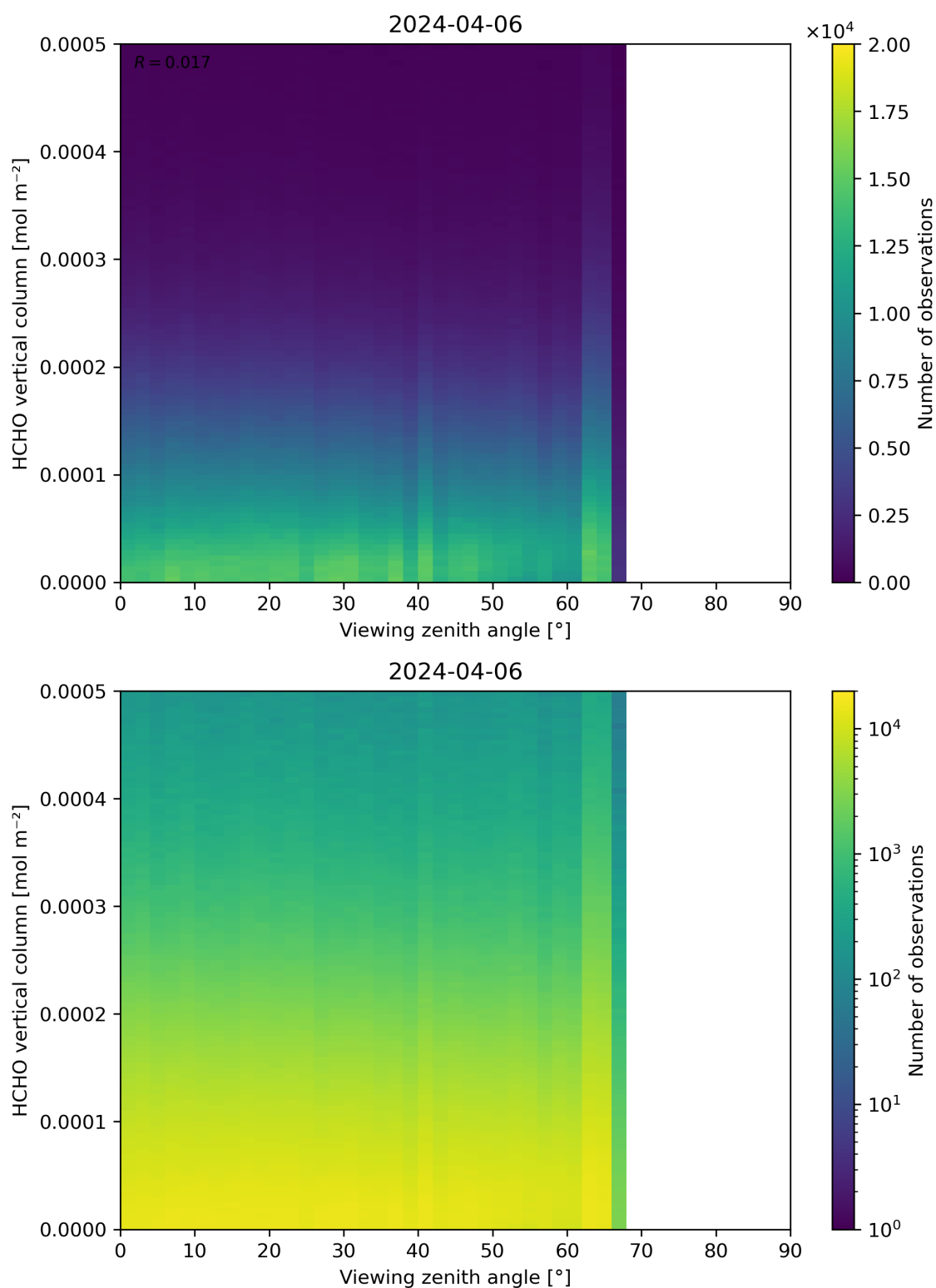
Figure 192: Scatter density plot of “Viewing zenith angle” against “HCHO vertical column” for 2024-04-05 to 2024-04-07.
