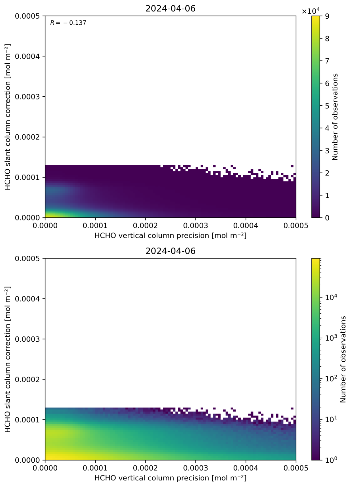
Figure 141: Scatter density plot of “HCHO vertical column precision” against “HCHO slant column correction” for 2024-04-05 to 2024-04-07.
