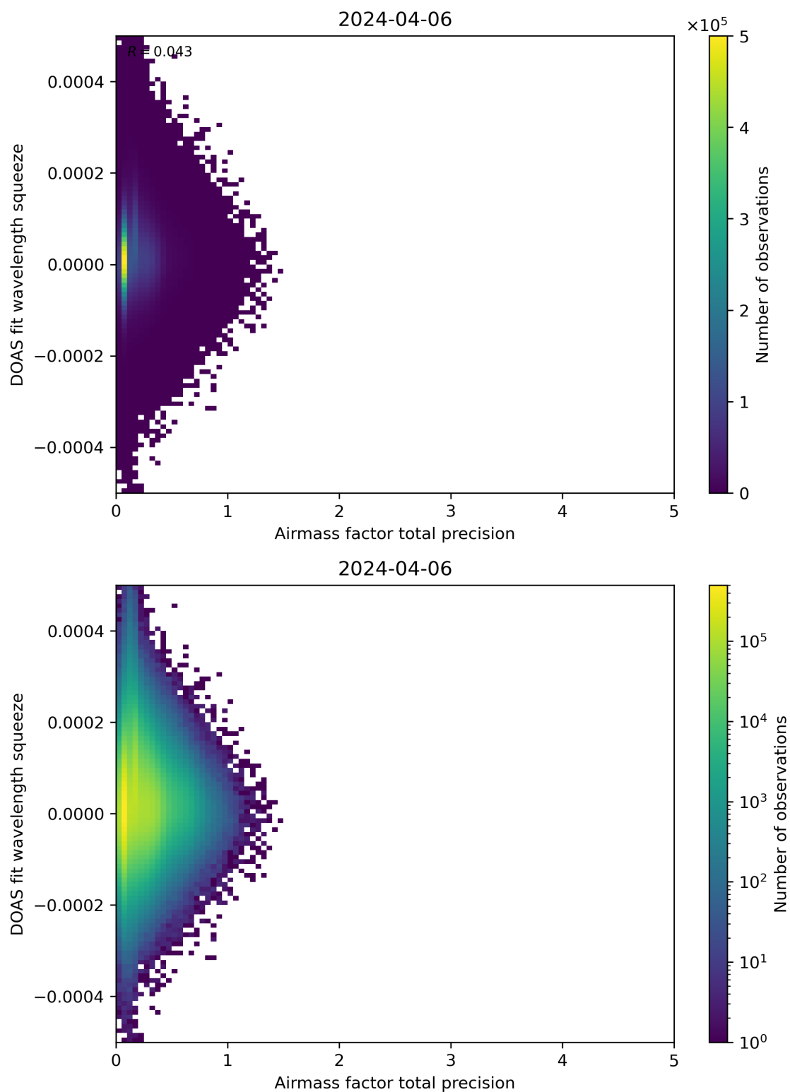
Figure 107: Scatter density plot of “Airmass factor total precision” against “DOAS fit wavelength squeeze” for 2024-04-05 to 2024-04-07.
