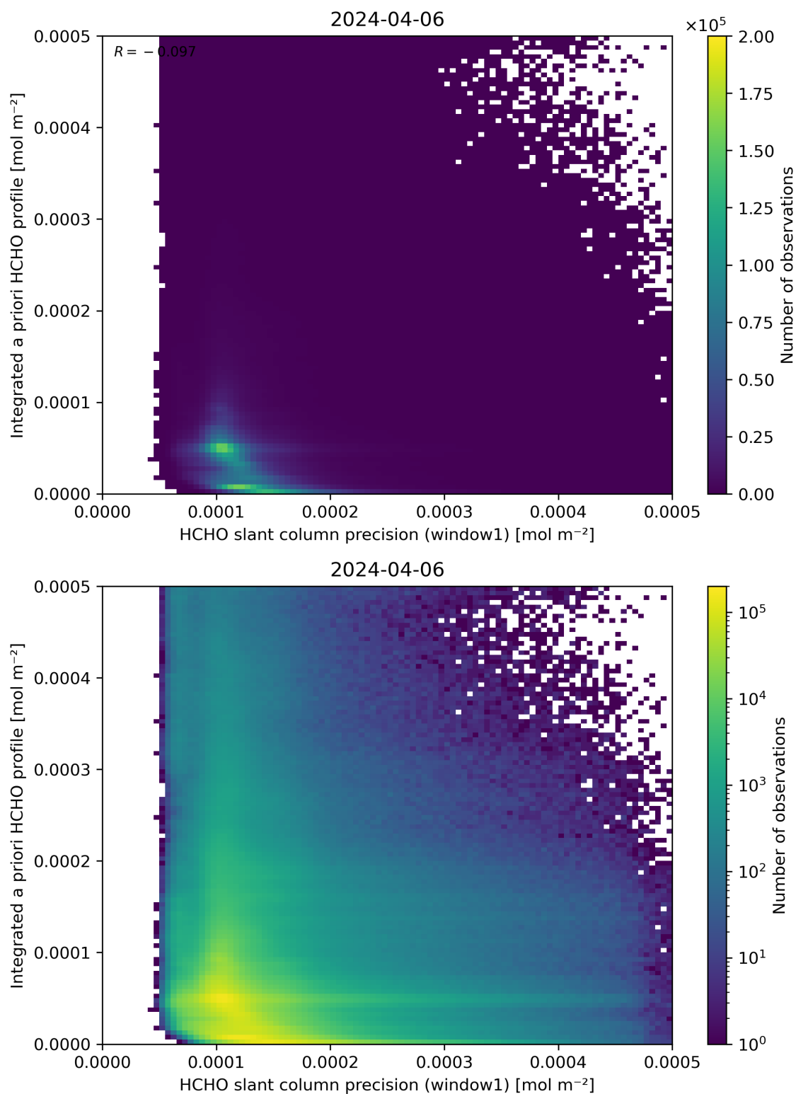
Figure 96: Scatter density plot of “HCHO slant column precision (window1)” against “Integrated a priori HCHO profile” for 2024-04-05 to 2024-04-07.
