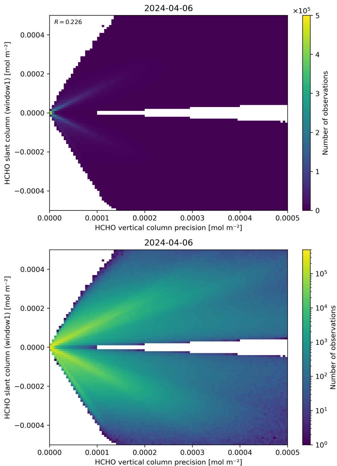
Figure 142: Scatter density plot of “HCHO vertical column precision” against “HCHO slant column (window1)” for 2024-04-05 to 2024-04-07.
