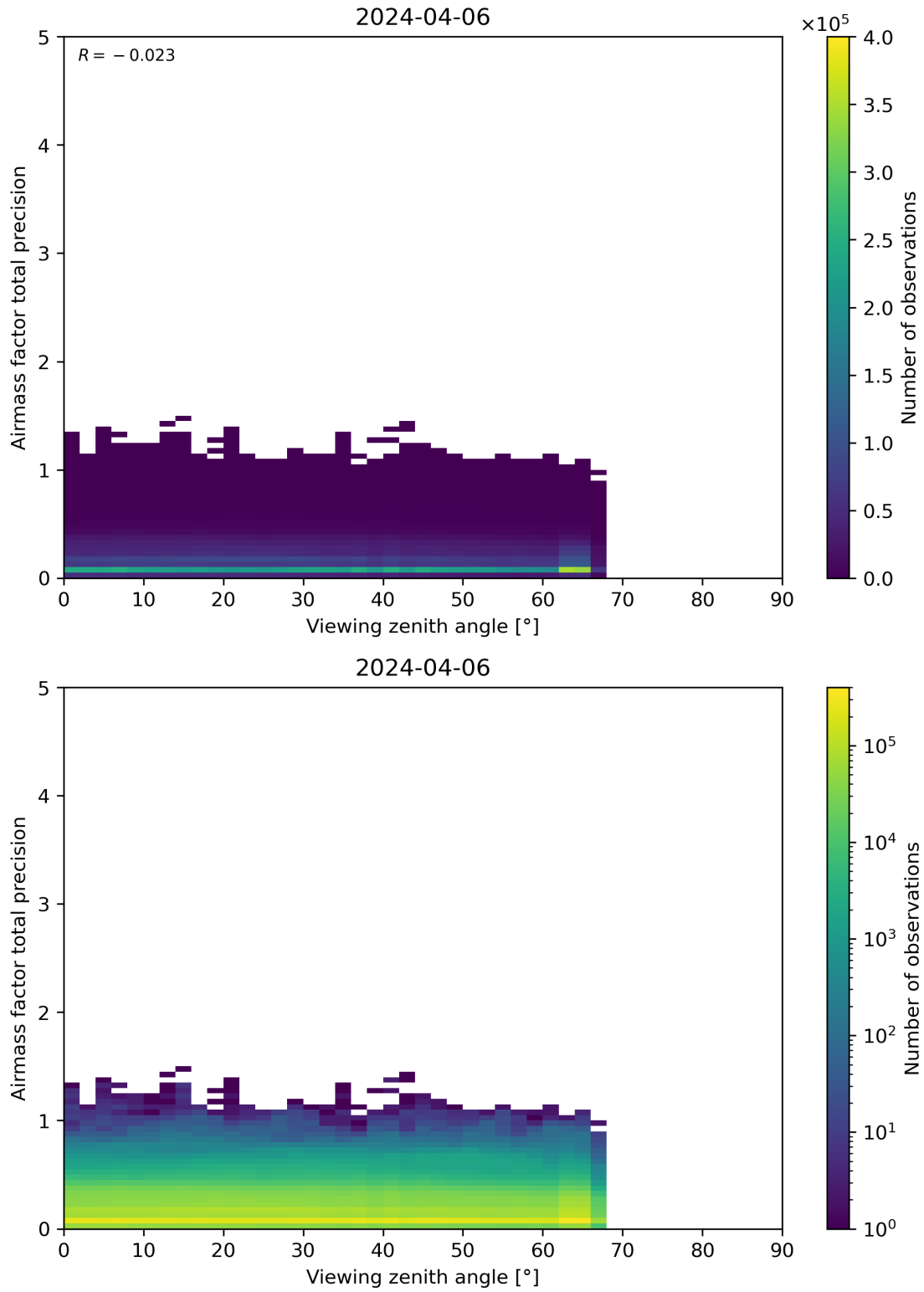
Figure 191: Scatter density plot of “Viewing zenith angle” against “Airmass factor total precision” for 2024-04-05 to 2024-04-07.
