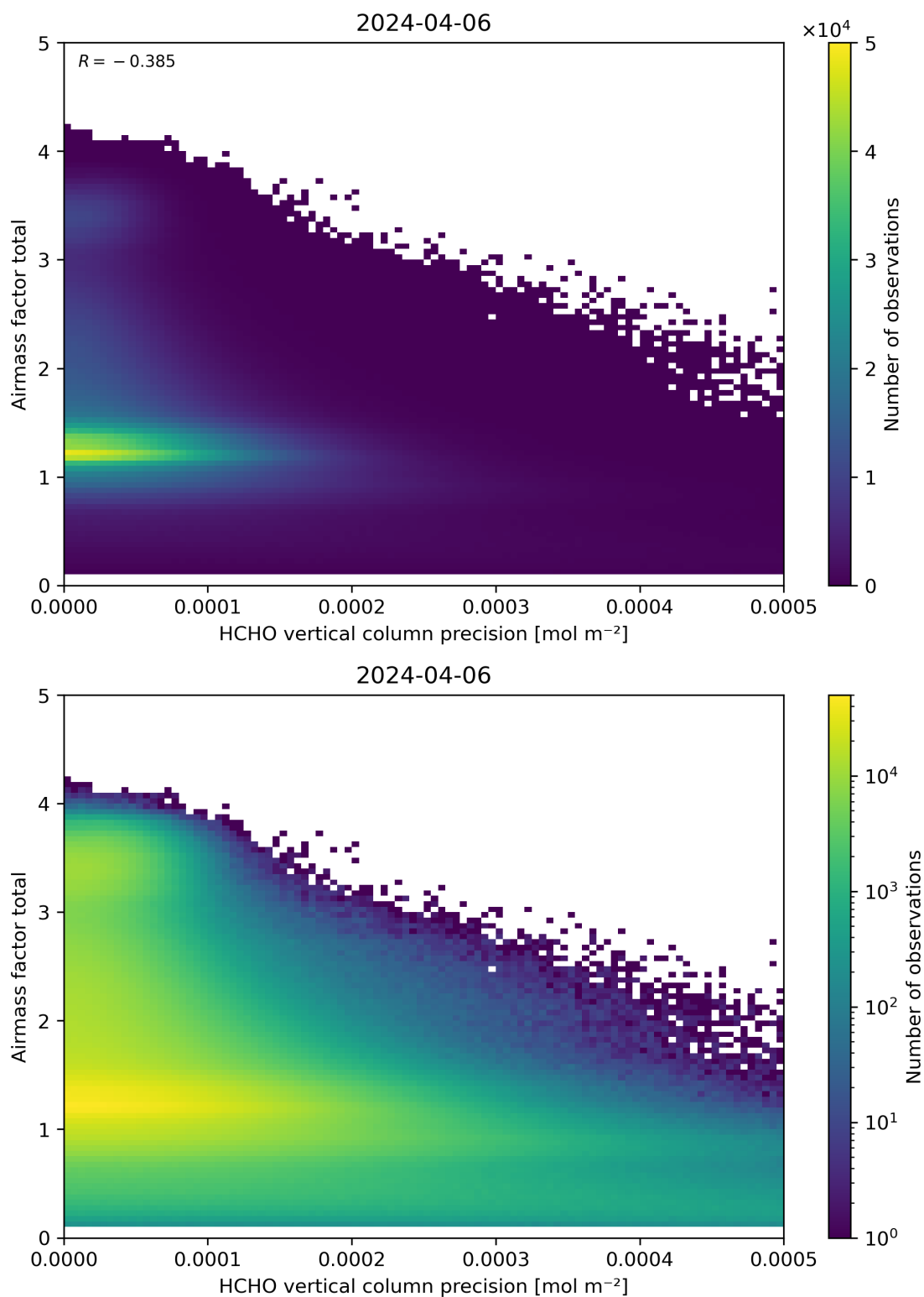
Figure 144: Scatter density plot of “HCHO vertical column precision” against “Airmass factor total” for 2024-04-05 to 2024-04-07.
