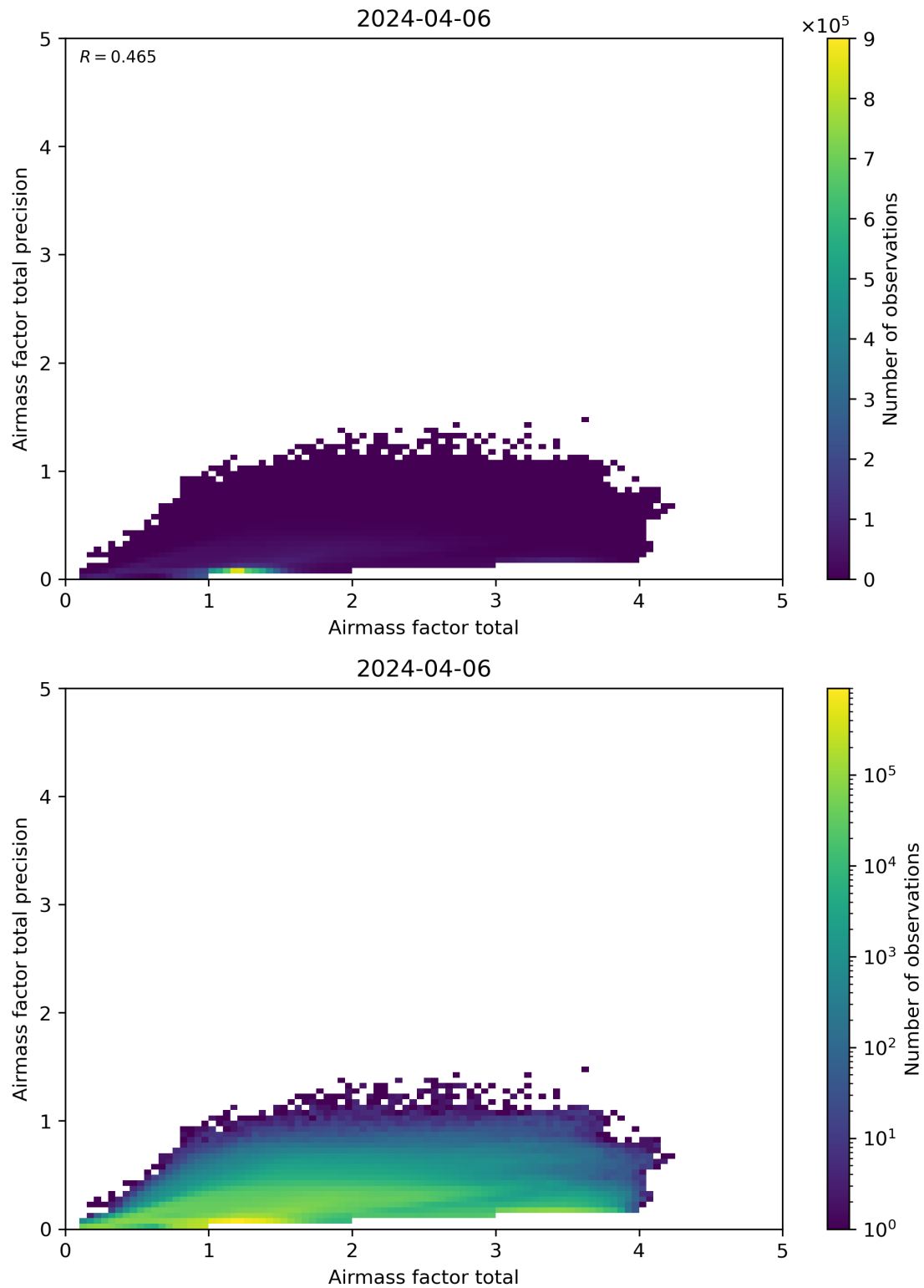
Figure 103: Scatter density plot of “Airmass factor total” against “Airmass factor total precision” for 2024-04-05 to 2024-04-07.
