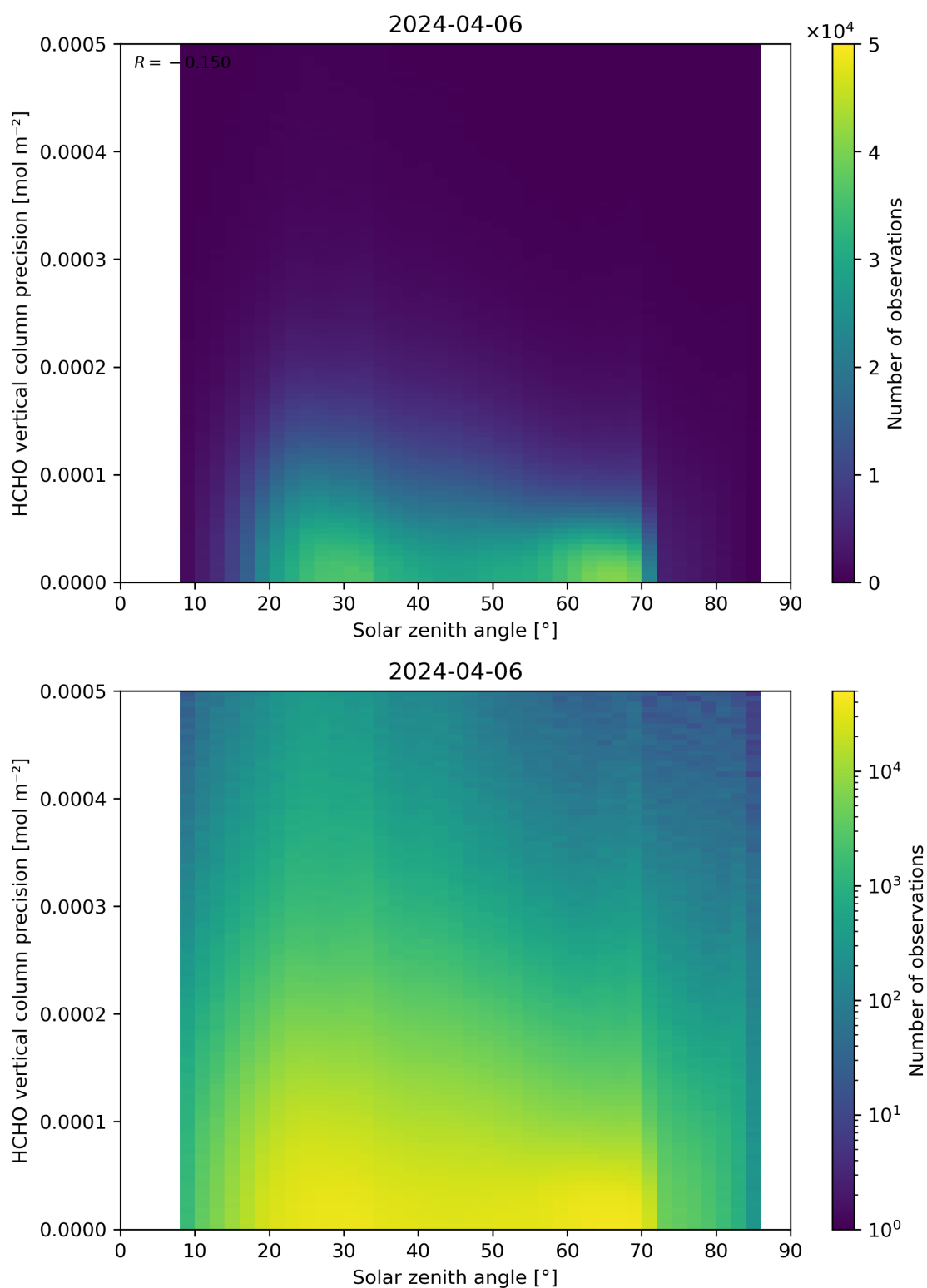
Figure 179: Scatter density plot of “Solar zenith angle” against “HCHO vertical column precision” for 2024-04-05 to 2024-04-07.
