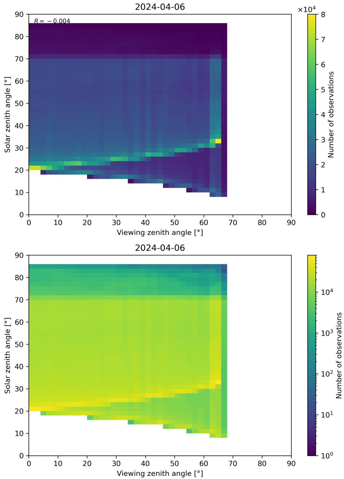
Figure 197: Scatter density plot of “Viewing zenith angle” against “Solar zenith angle” for 2024-04-05 to 2024-04-07.
