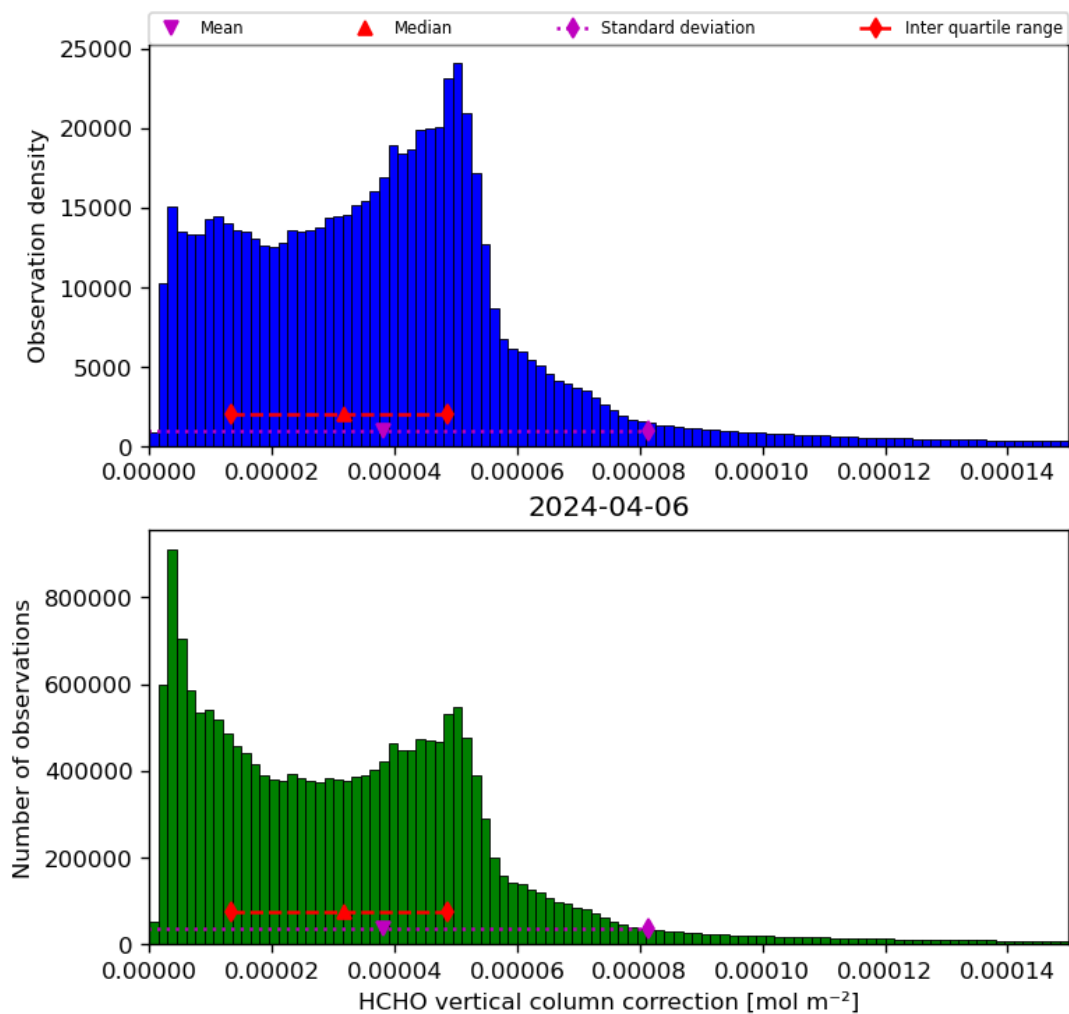
Figure 37: Histogram of “HCHO vertical column correction” for 2024-04-05 to 2024-04-07
