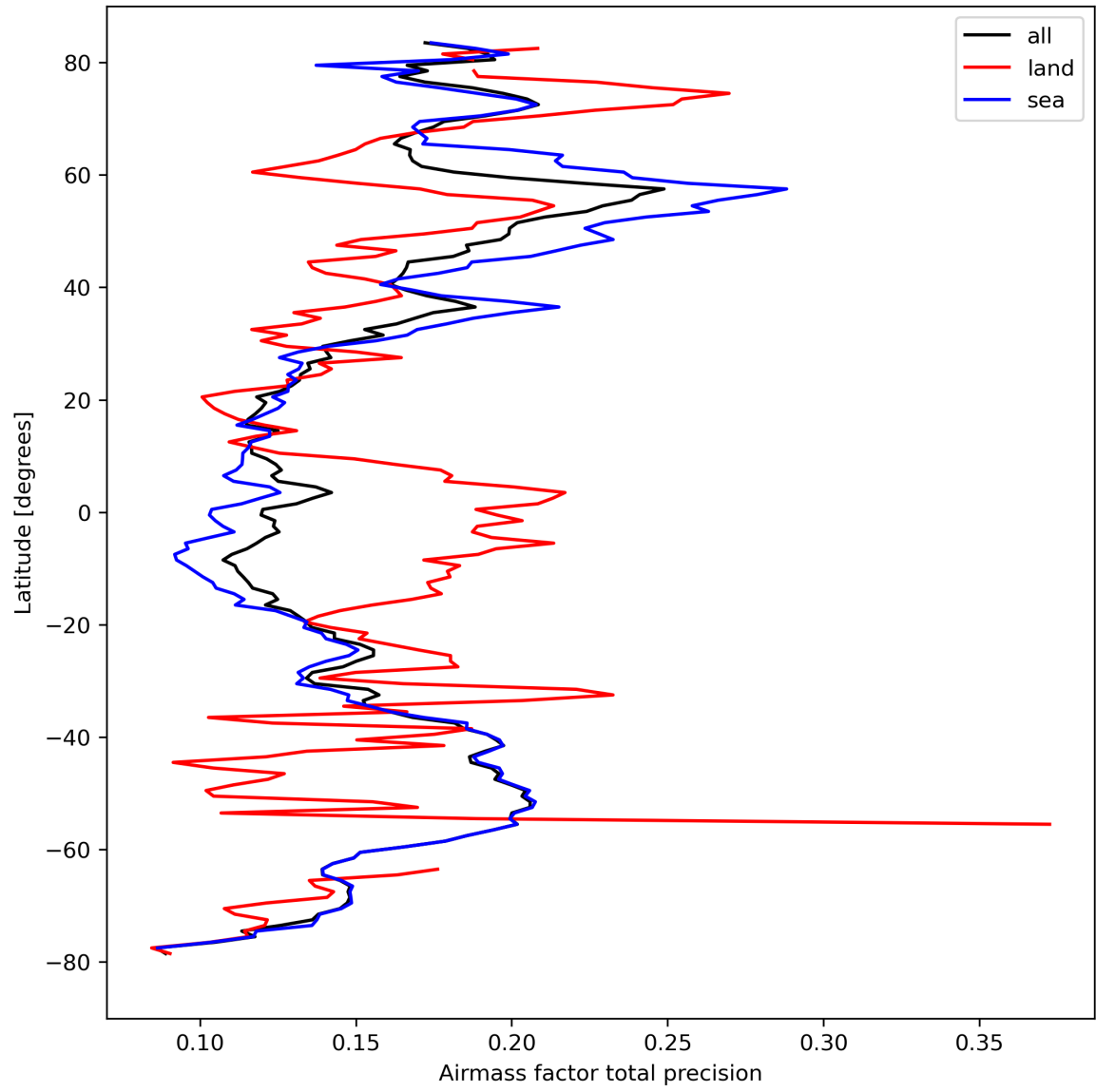
Figure 27: Zonal average of “Airmass factor total precision” for 2024-04-05 to 2024-04-07.
