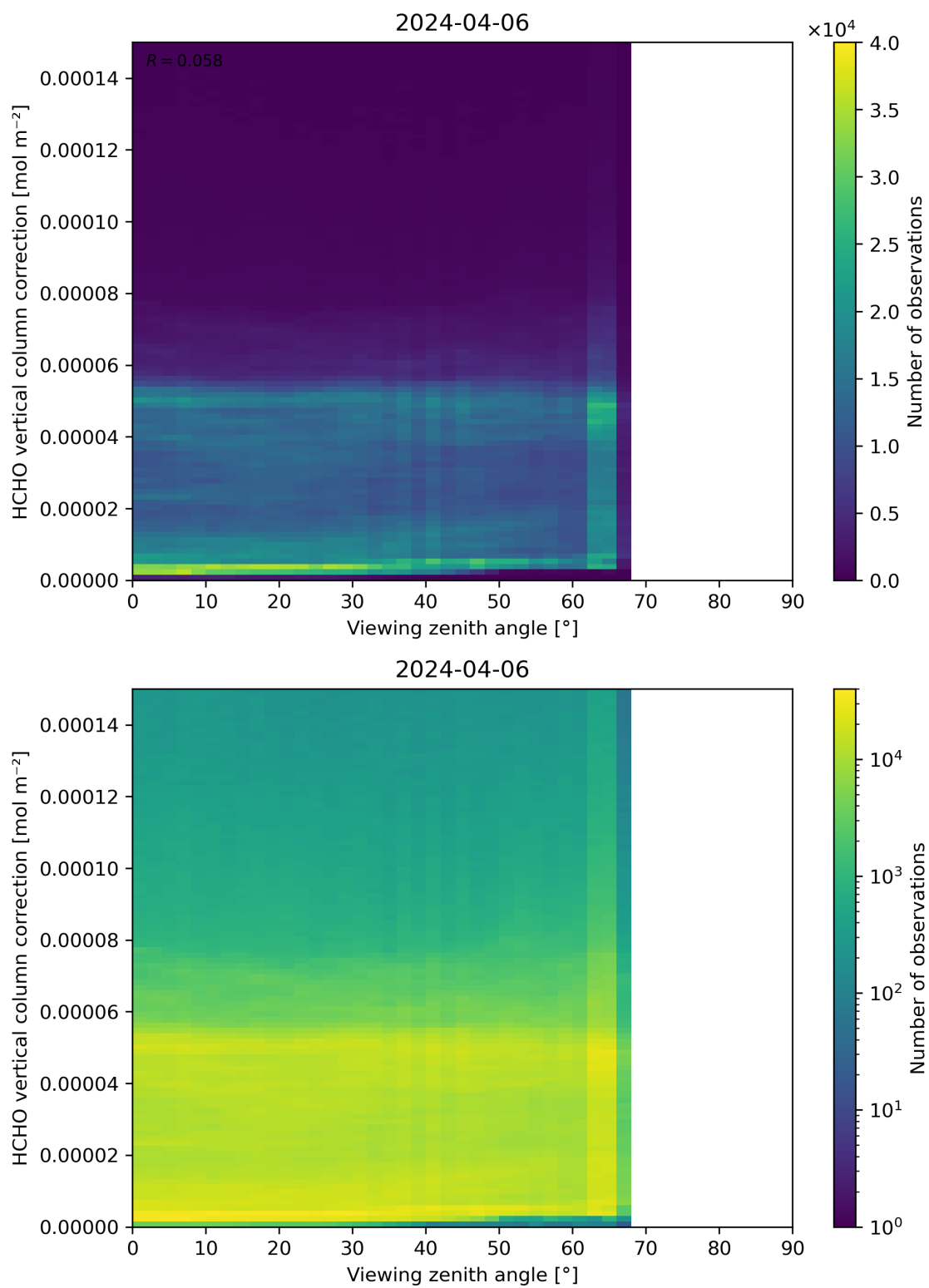
Figure 193: Scatter density plot of “Viewing zenith angle” against “HCHO vertical column correction” for 2024-04-05 to 2024-04-07.
