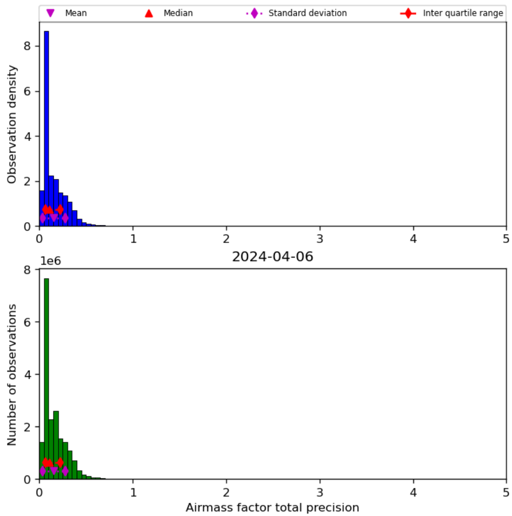
Figure 41: Histogram of “Airmass factor total precision” for 2024-04-05 to 2024-04-07
