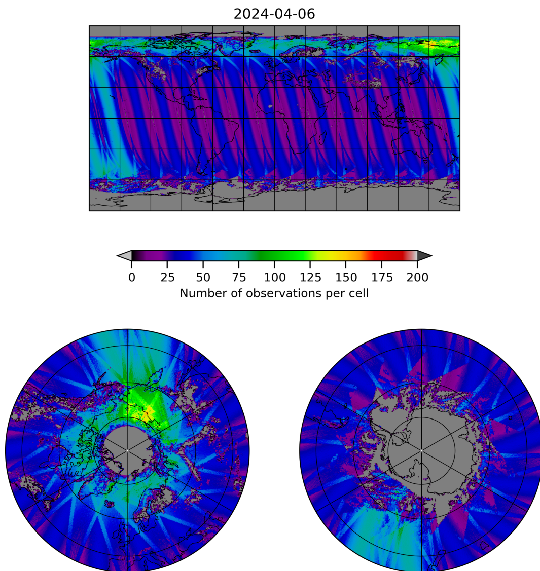
Figure 19: Map of the number of observations for 2024-04-05 to 2024-04-07
