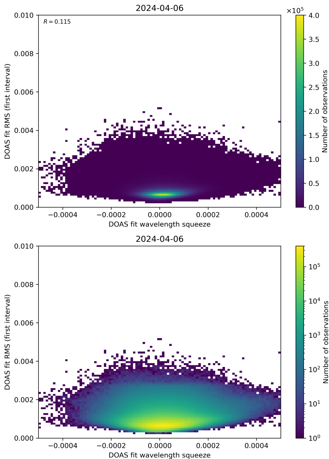
Figure 68: Scatter density plot of “DOAS fit wavelength squeeze” against “DOAS fit RMS (first interval)” for 2024-04-05 to 2024-04-07.
