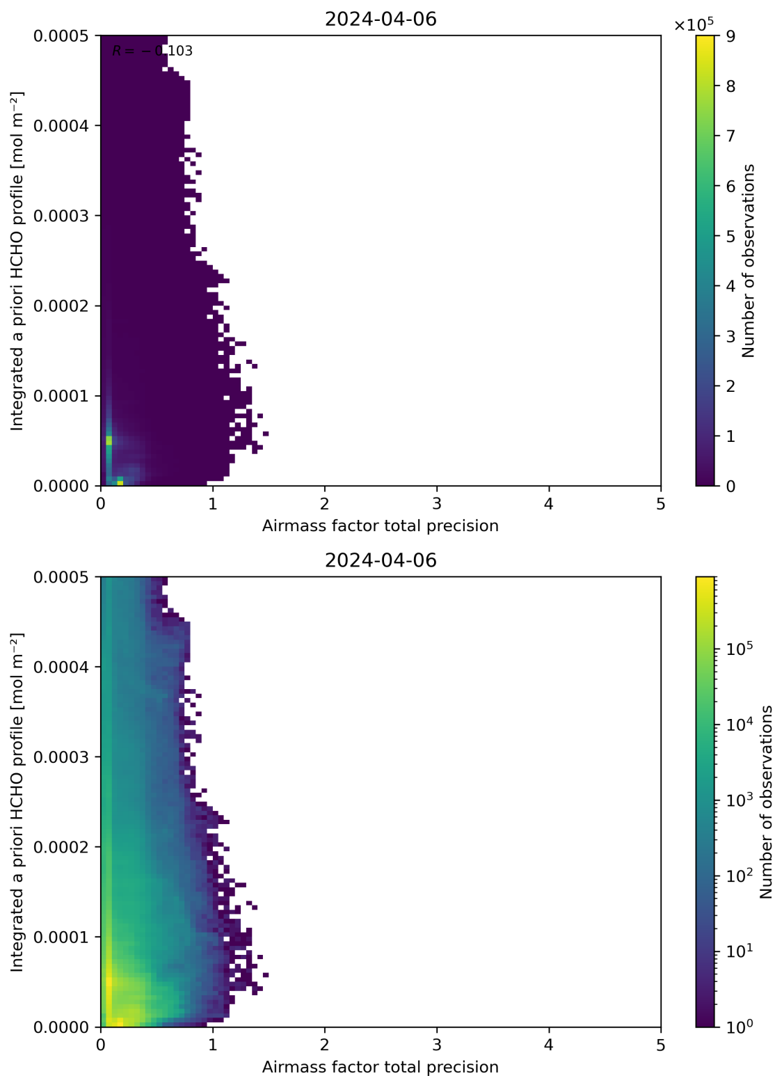
Figure 111: Scatter density plot of “Airmass factor total precision” against “Integrated a priori HCHO profile” for 2024-04-05 to 2024-04-07.
