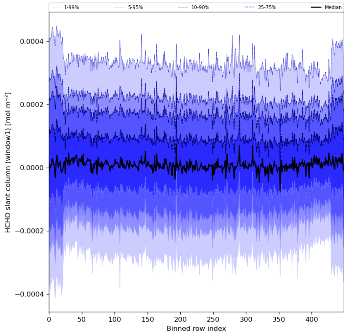
Figure 52: Along track statistics of “HCHO slant column (window1)” for 2024-04-05 to 2024-04-07
