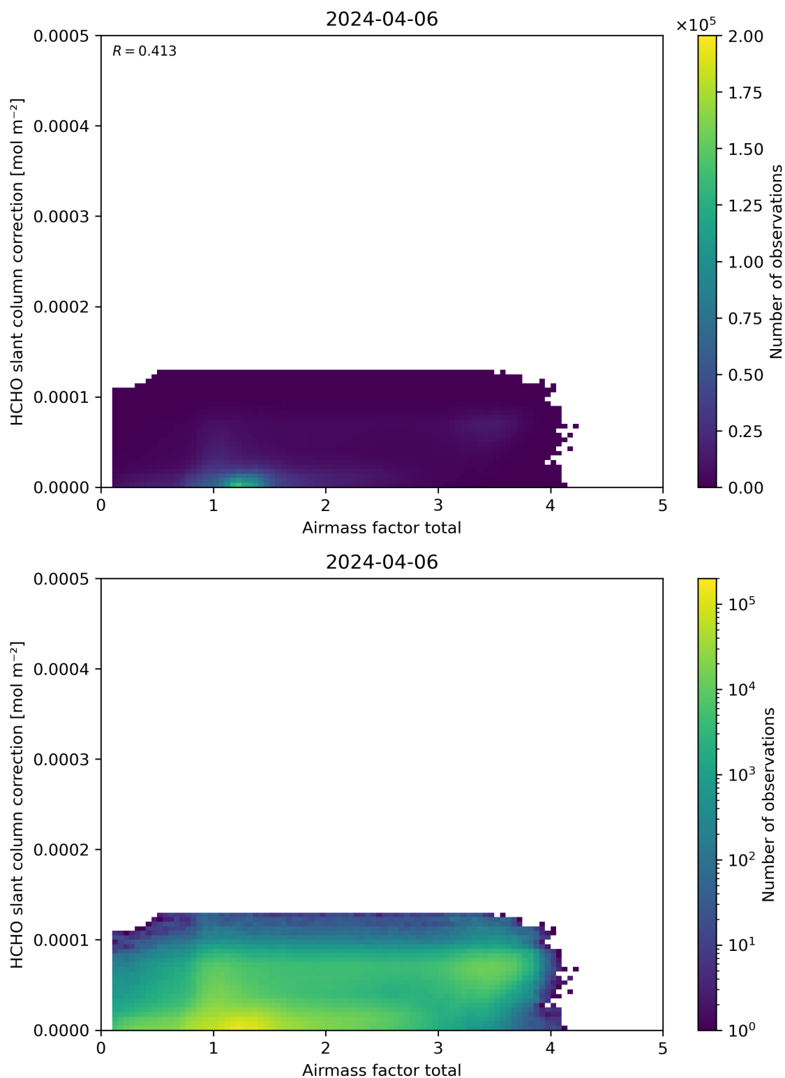
Figure 102: Scatter density plot of “Airmass factor total” against “HCHO slant column correction” for 2024-04-05 to 2024-04-07.
