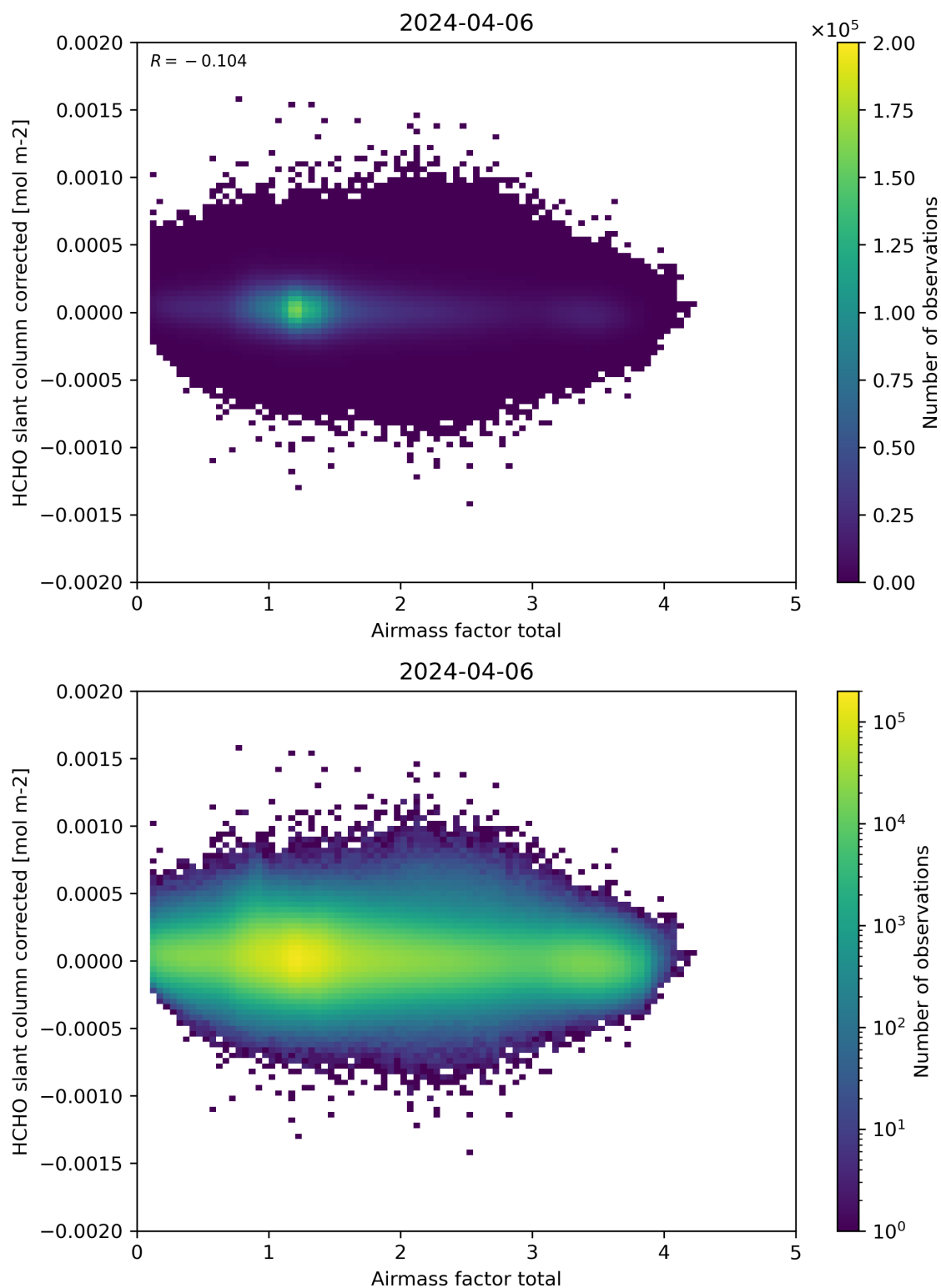
Figure 101: Scatter density plot of “Airmass factor total” against “HCHO slant column corrected” for 2024-04-05 to 2024-04-07.
