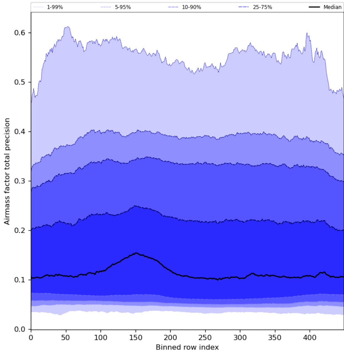
Figure 55: Along track statistics of “Airmass factor total precision” for 2024-04-05 to 2024-04-07
