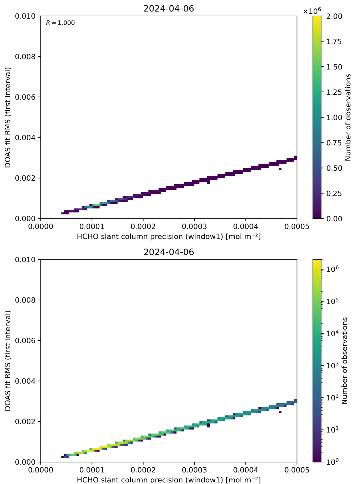
Figure 88: Scatter density plot of “HCHO slant column precision (window1)” against “DOAS fit RMS (first interval)” for 2024-04-05 to 2024-04-07.
