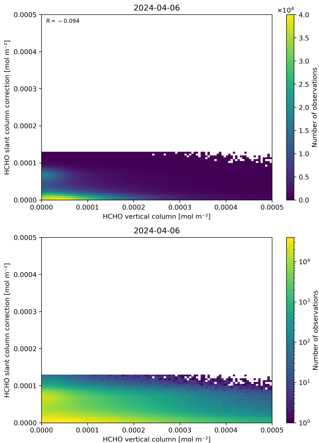
Figure 128: Scatter density plot of “HCHO vertical column” against “HCHO slant column correction” for 2024-04-05 to 2024-04-07.
