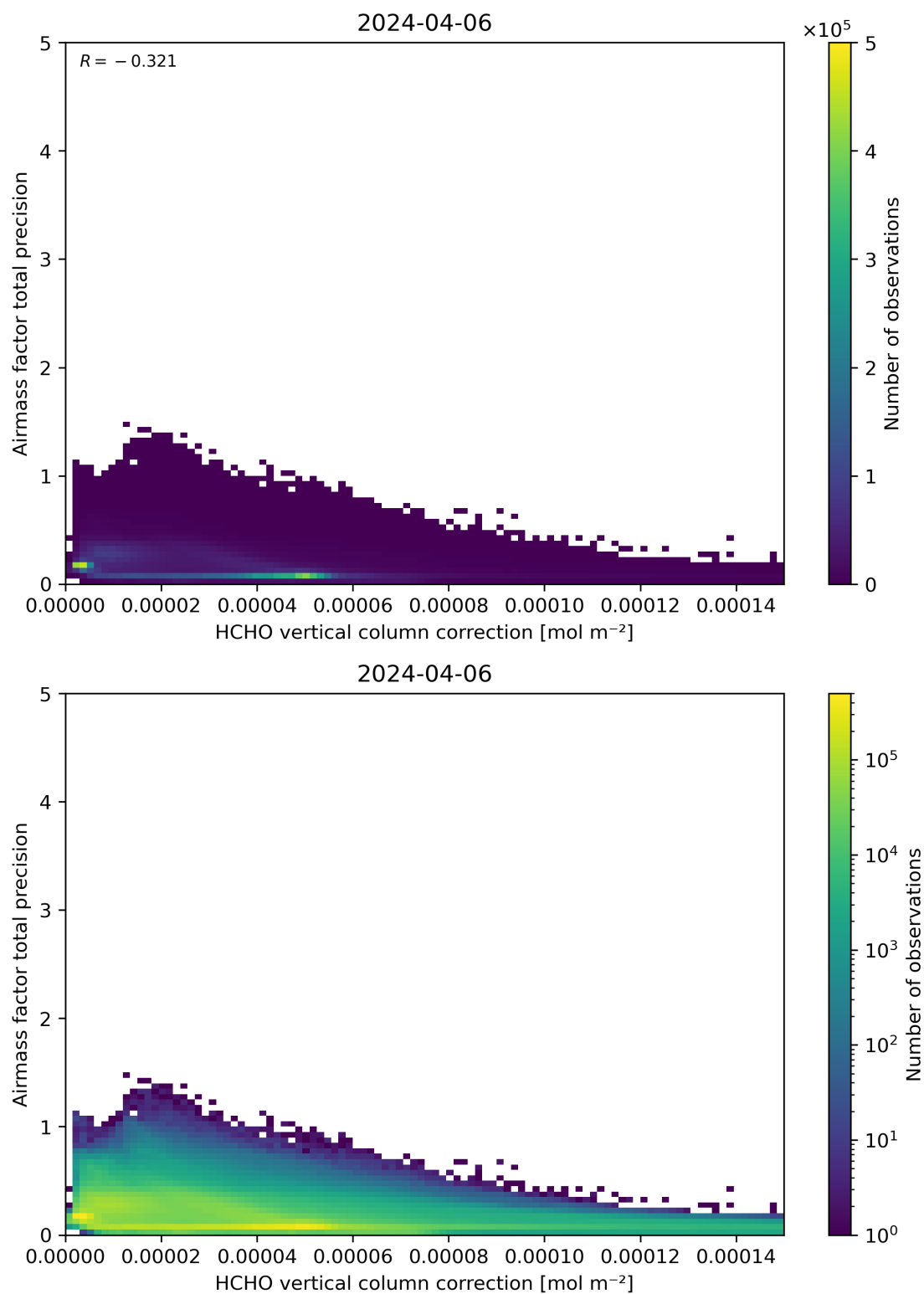
Figure 121: Scatter density plot of “HCHO vertical column correction” against “Airmass factor total precision” for 2024-04-05 to 2024-04-07.
