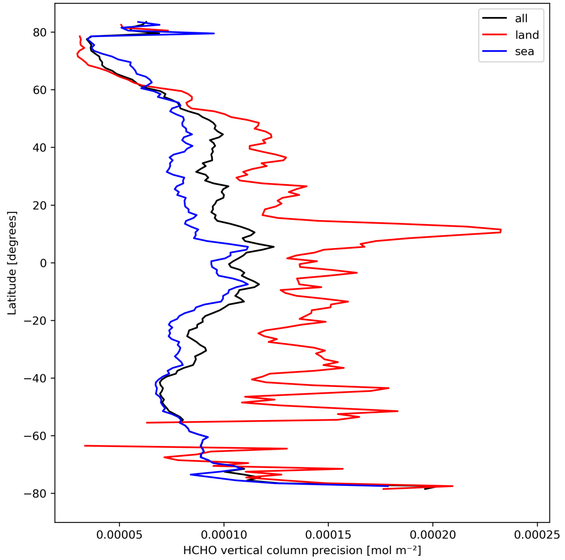
Figure 22: Zonal average of “HCHO vertical column precision” for 2024-04-05 to 2024-04-07.
