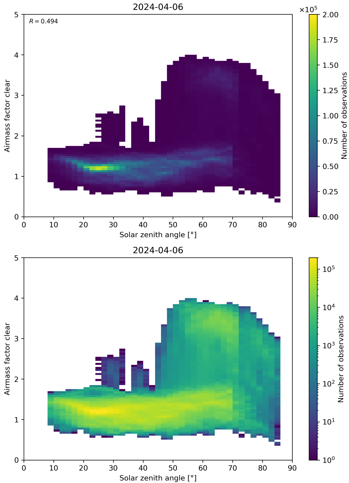
Figure 170: Scatter density plot of “Solar zenith angle” against “Airmass factor clear” for 2024-04-05 to 2024-04-07.
