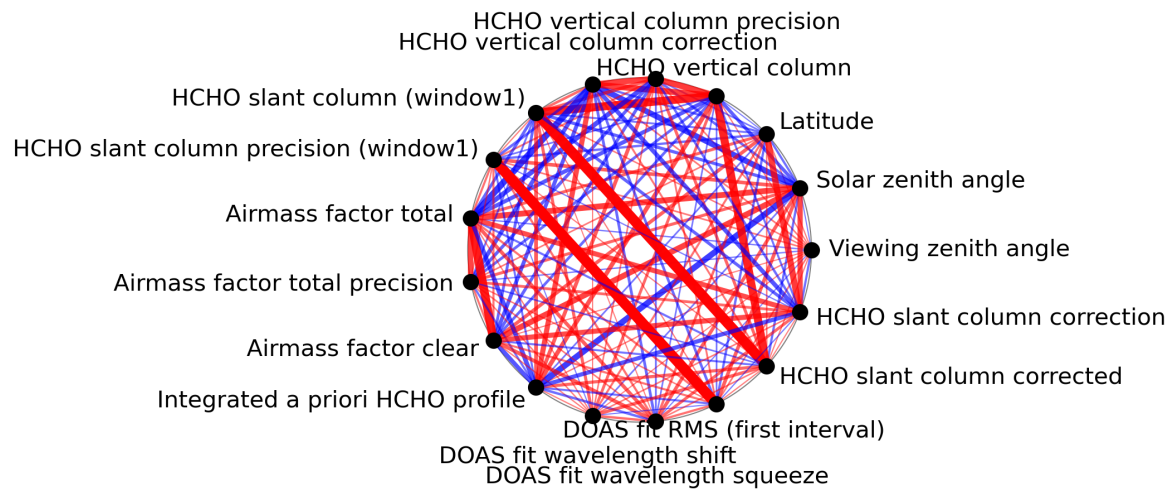
Figure 1: Map of correlation graph for 2024-04-05 to 2024-04-07.
