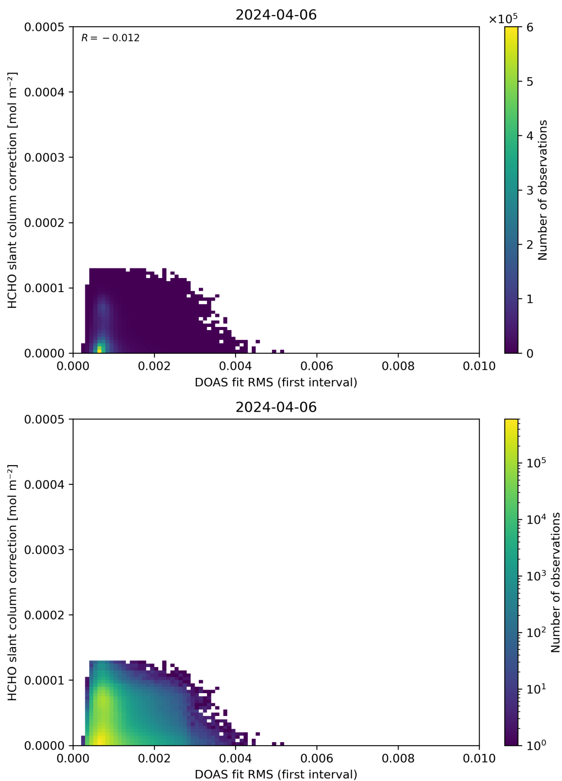
Figure 63: Scatter density plot of “DOAS fit RMS (first interval)” against “HCHO slant column correction” for 2024-04-05 to 2024-04-07.
