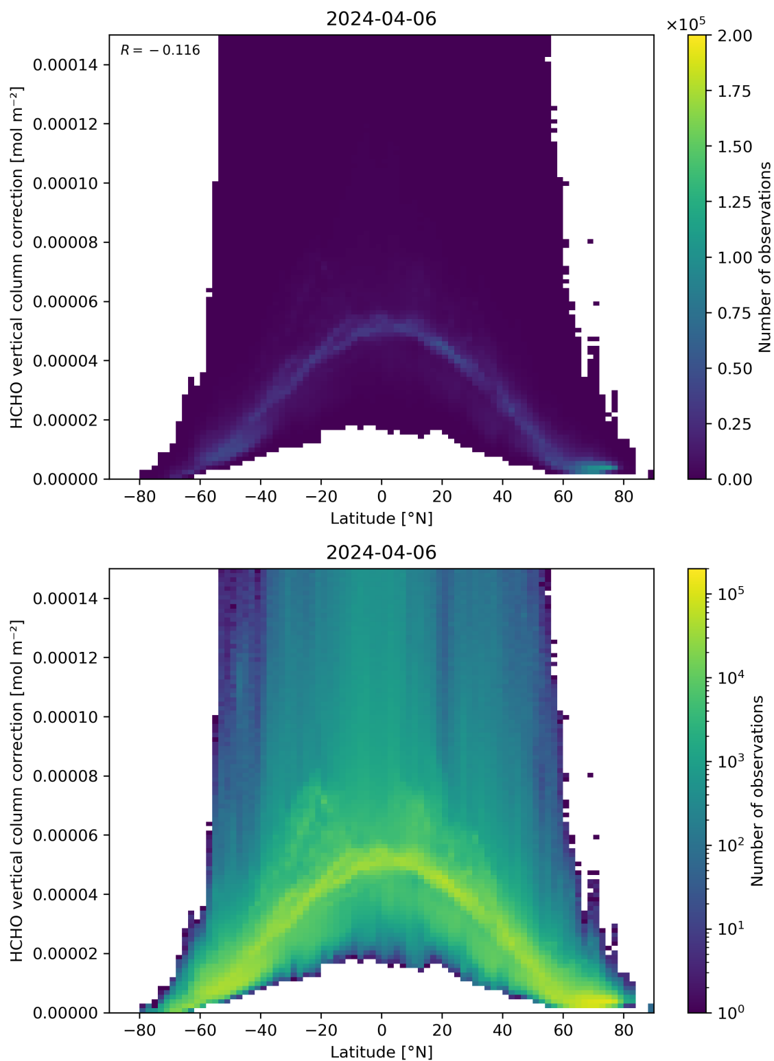
Figure 164: Scatter density plot of “Latitude” against “HCHO vertical column correction” for 2024-04-05 to 2024-04-07.
