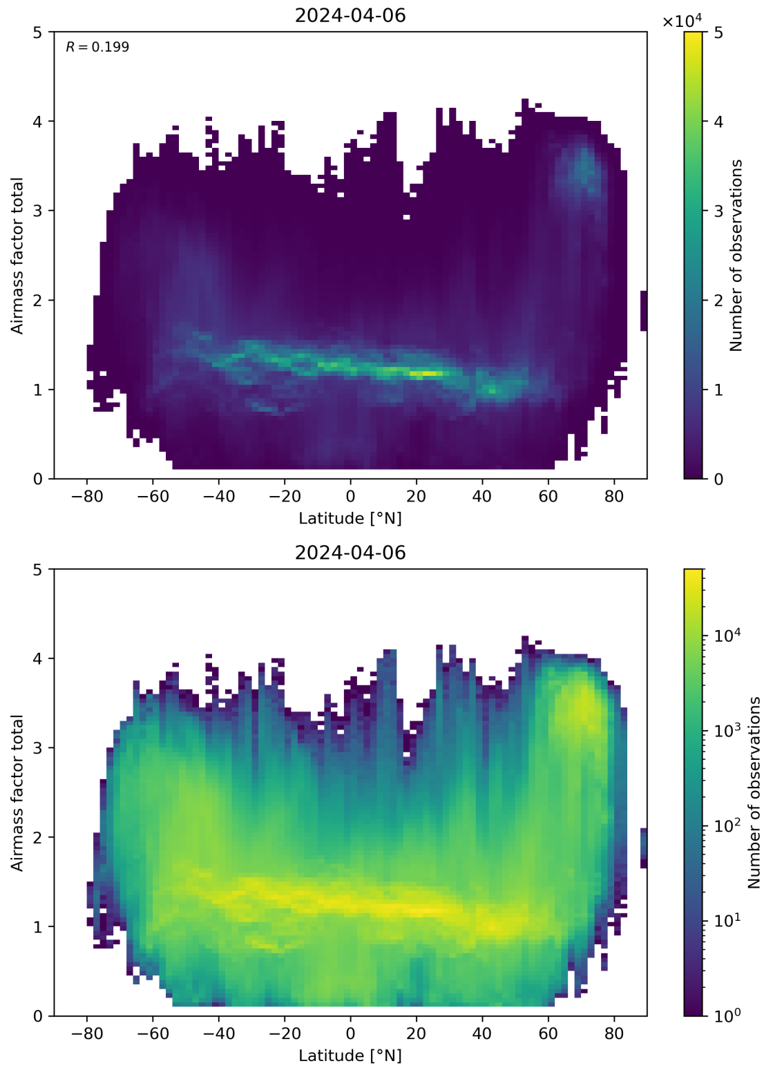
Figure 161: Scatter density plot of “Latitude” against “Airmass factor total” for 2024-04-05 to 2024-04-07.
