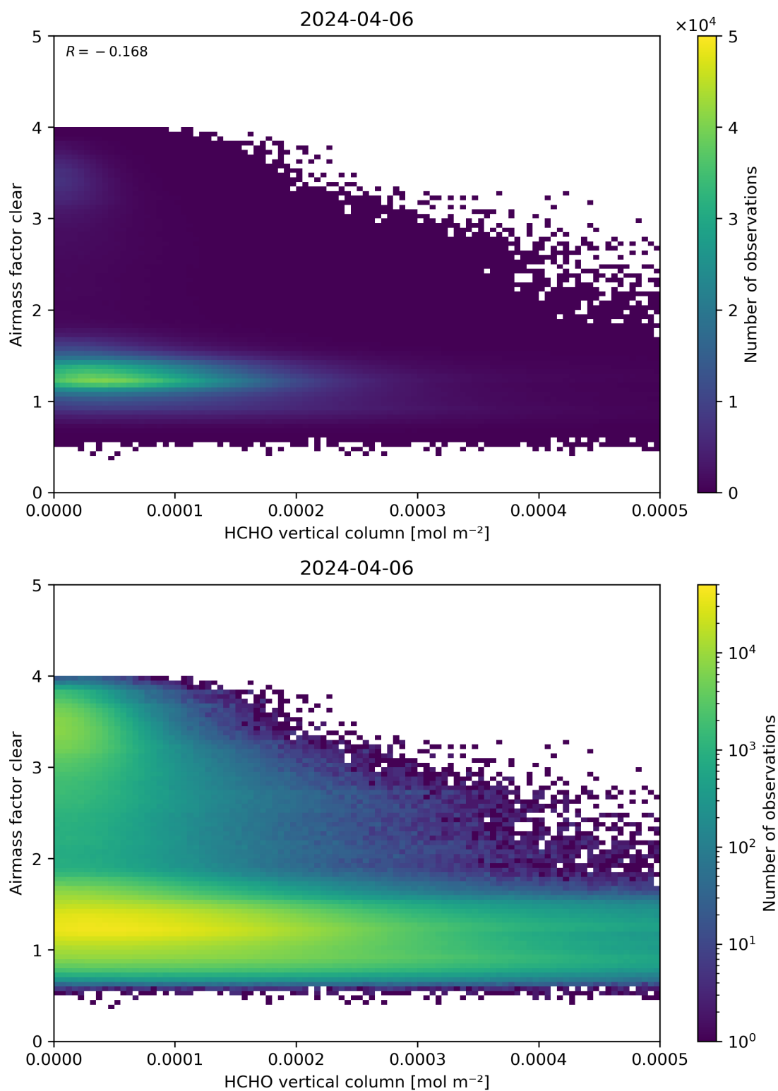
Figure 126: Scatter density plot of “HCHO vertical column” against “Airmass factor clear” for 2024-04-05 to 2024-04-07.
