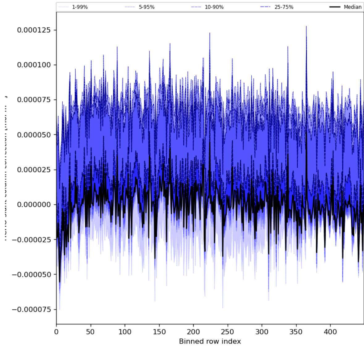
Figure 61: Along track statistics of “HCHO slant column correction” for 2024-04-05 to 2024-04-07
