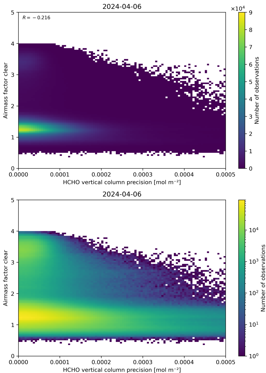
Figure 139: Scatter density plot of “HCHO vertical column precision” against “Airmass factor clear” for 2024-04-05 to 2024-04-07.
