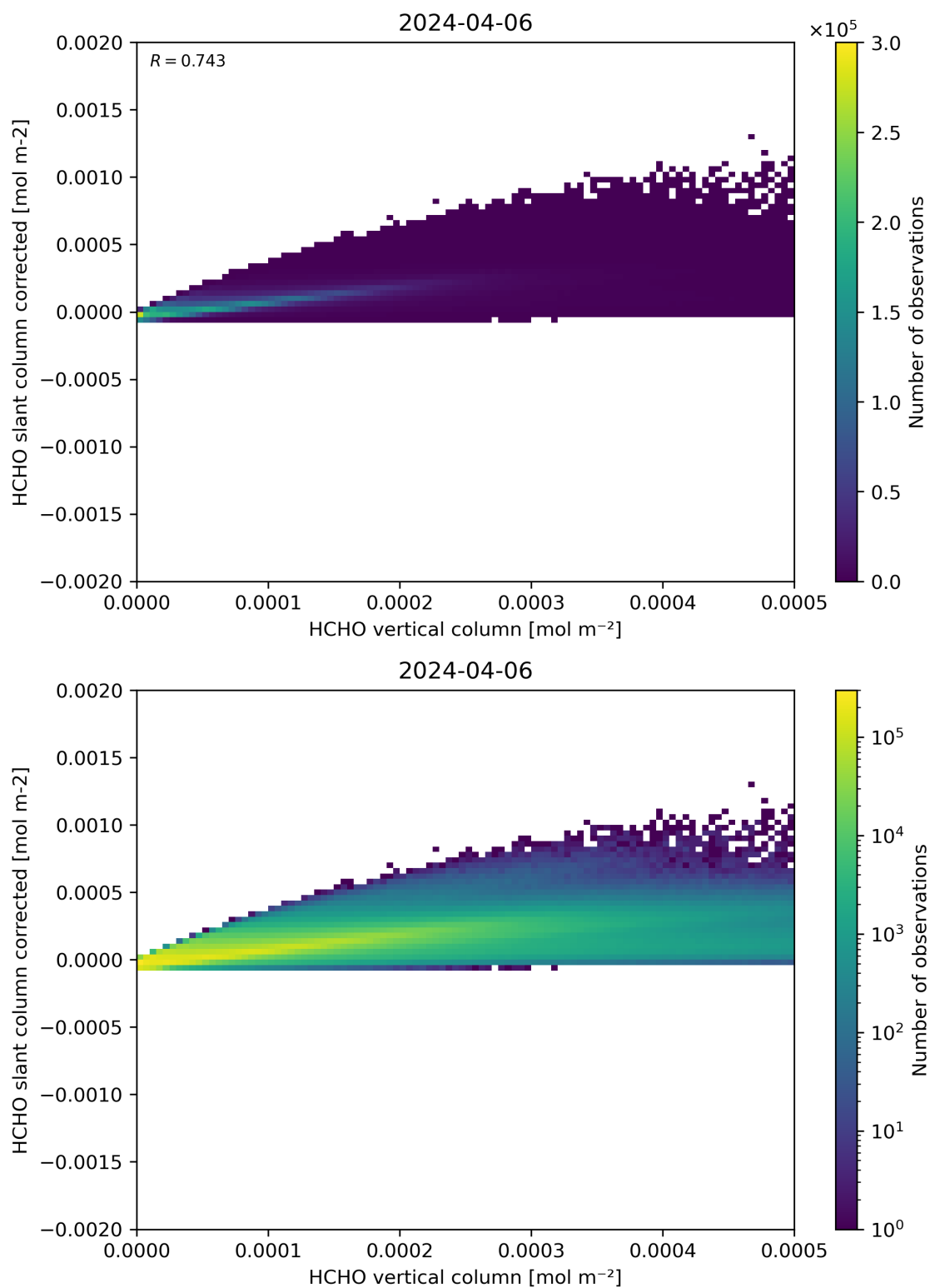
Figure 127: Scatter density plot of “HCHO vertical column” against “HCHO slant column corrected” for 2024-04-05 to 2024-04-07.
