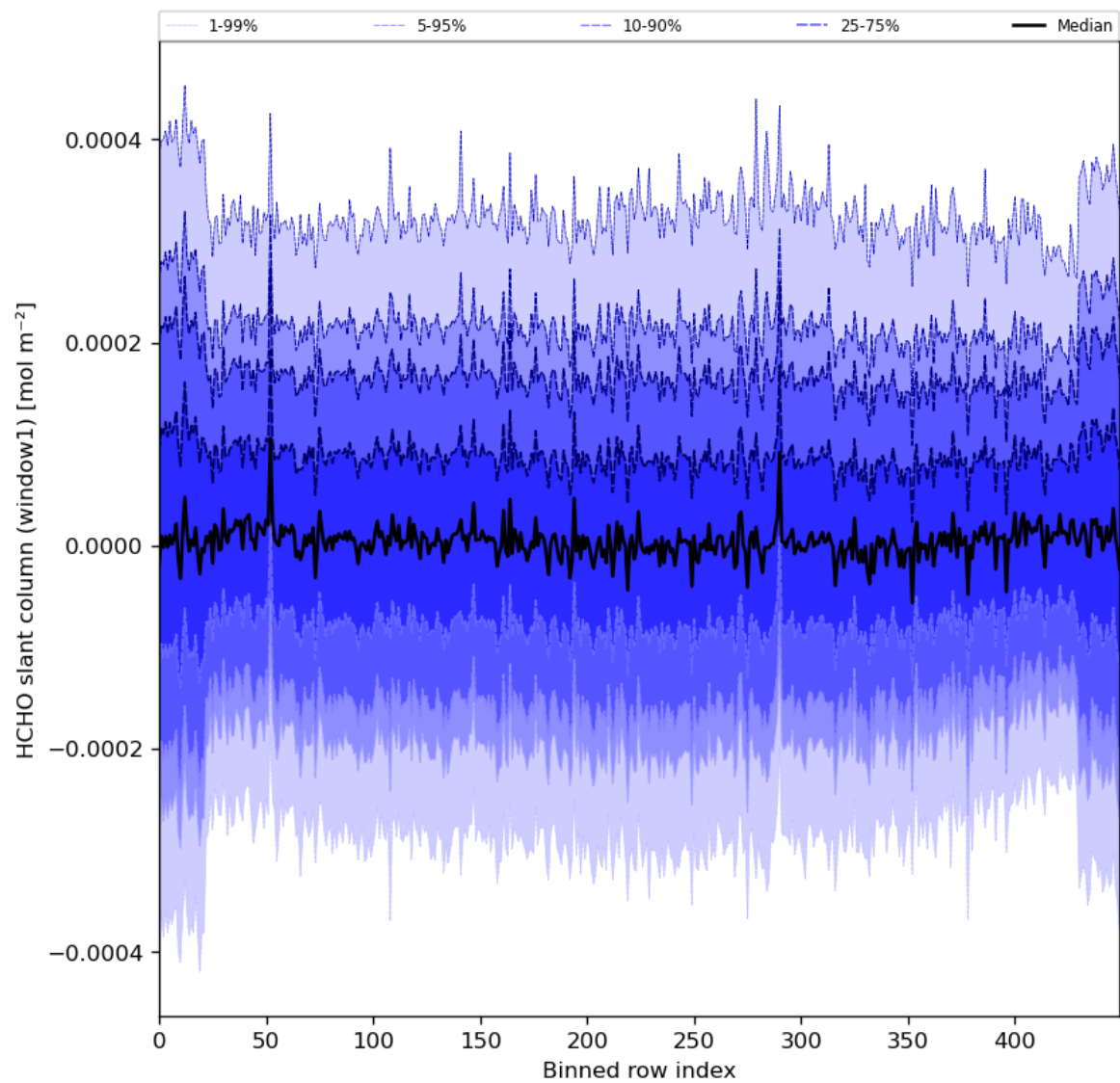
Figure 52: Along track statistics of “HCHO slant column (window1)” for 2024-04-06 to 2024-04-08
