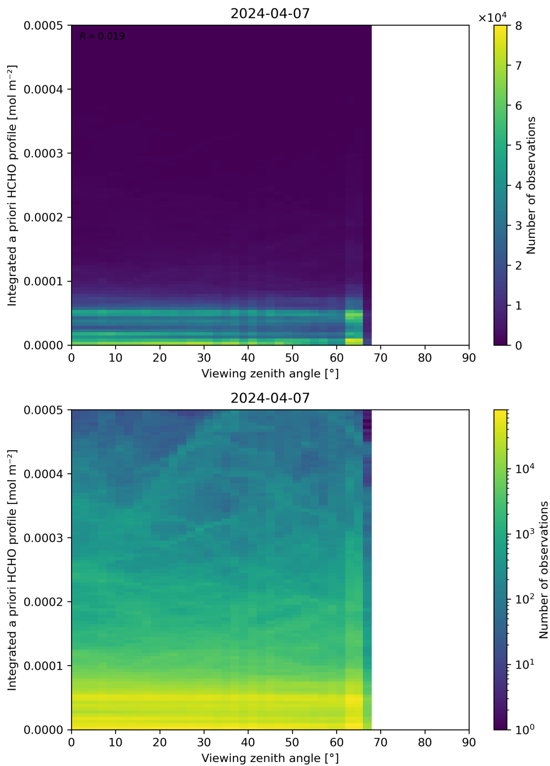
Figure 195: Scatter density plot of “Viewing zenith angle” against “Integrated a priori HCHO profile” for 2024-04-06 to 2024-04-08.
