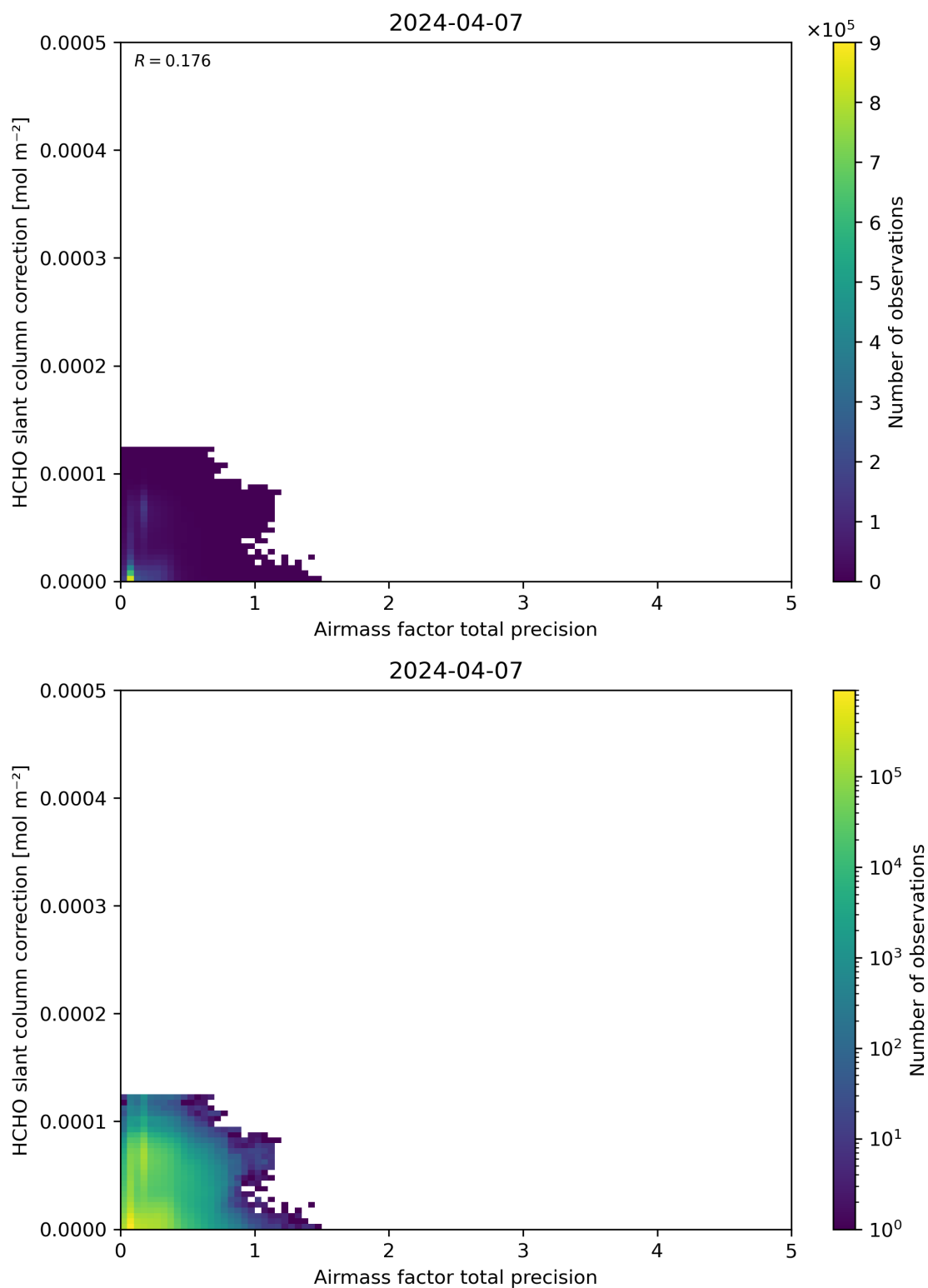
Figure 110: Scatter density plot of “Airmass factor total precision” against “HCHO slant column correction” for 2024-04-06 to 2024-04-08.
