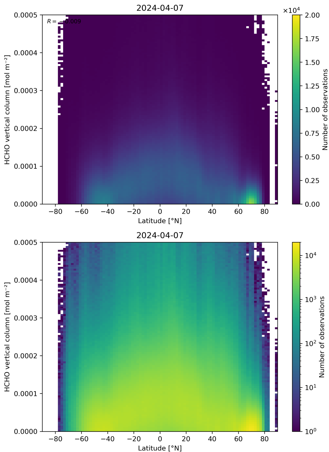
Figure 163: Scatter density plot of “Latitude” against “HCHO vertical column” for 2024-04-06 to 2024-04-08.
