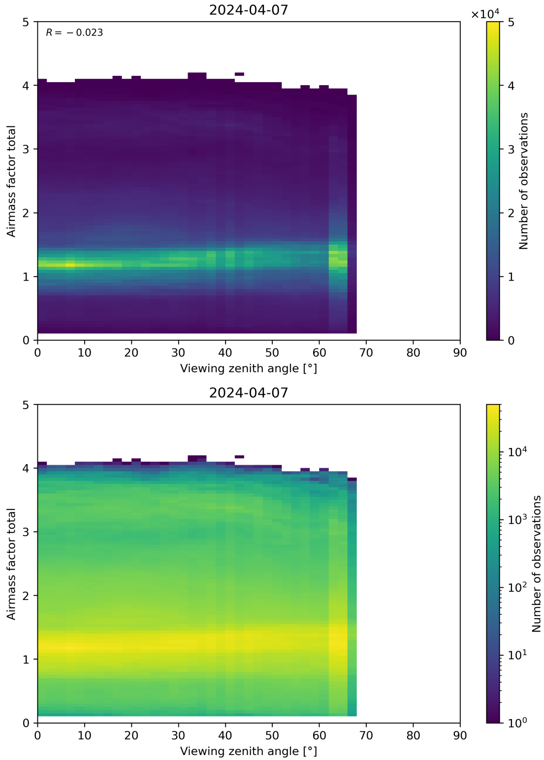
Figure 190: Scatter density plot of “Viewing zenith angle” against “Airmass factor total” for 2024-04-06 to 2024-04-08.
