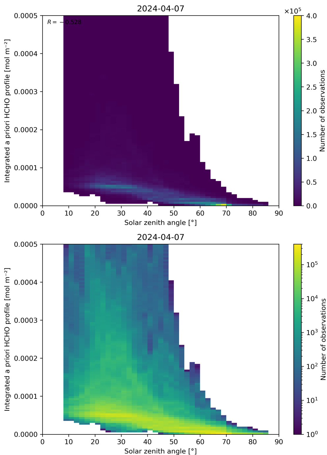
Figure 180: Scatter density plot of “Solar zenith angle” against “Integrated a priori HCHO profile” for 2024-04-06 to 2024-04-08.
