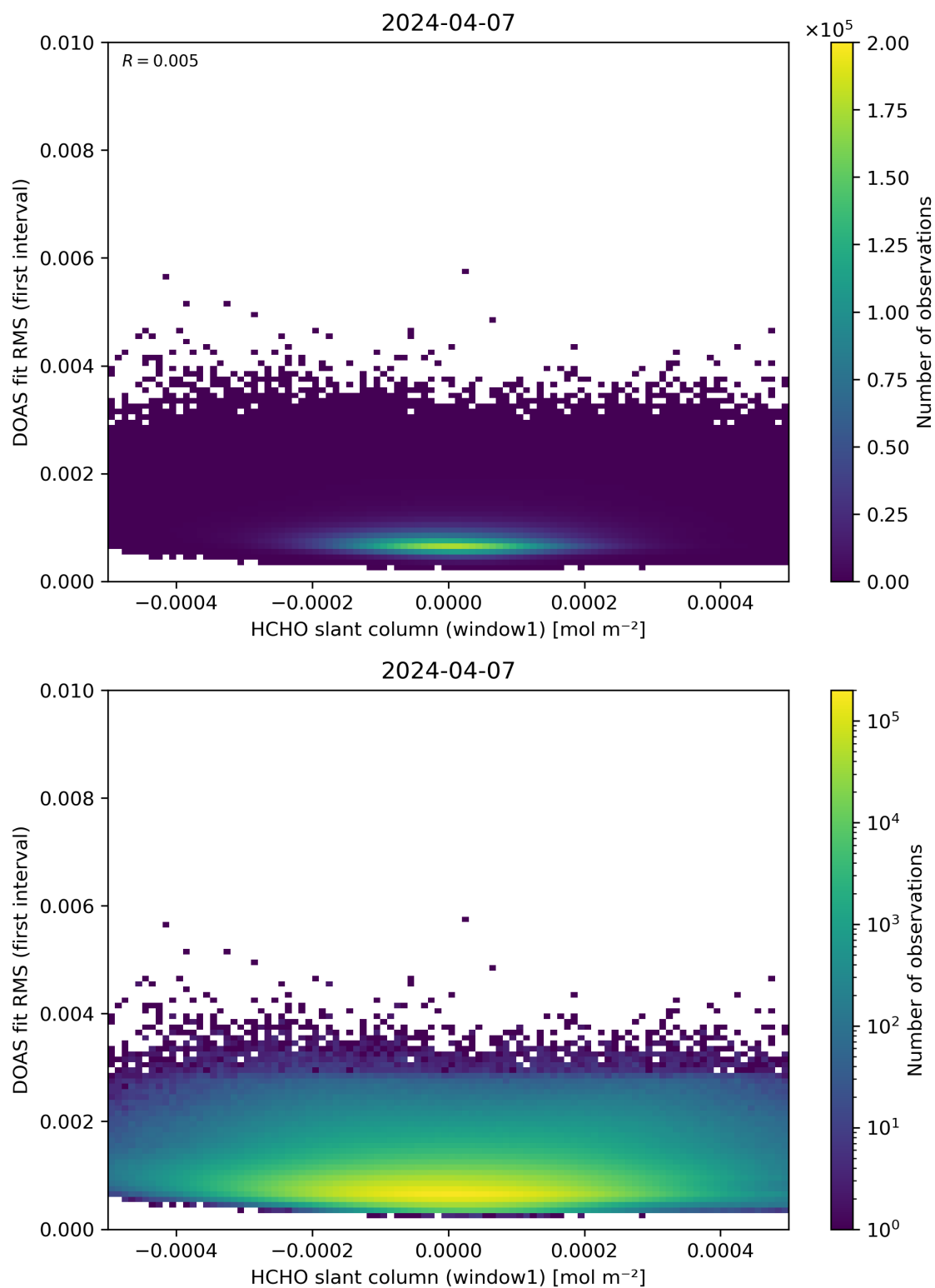
Figure 78: Scatter density plot of “HCHO slant column (window1)” against “DOAS fit RMS (first interval)” for 2024-04-06 to 2024-04-08.
