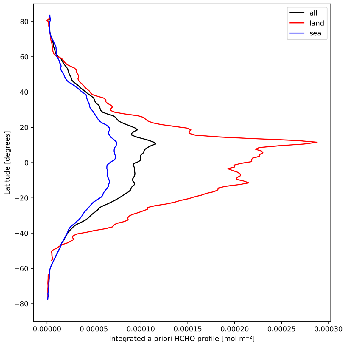
Figure 29: Zonal average of “Integrated a priori HCHO profile” for 2024-04-06 to 2024-04-08.
