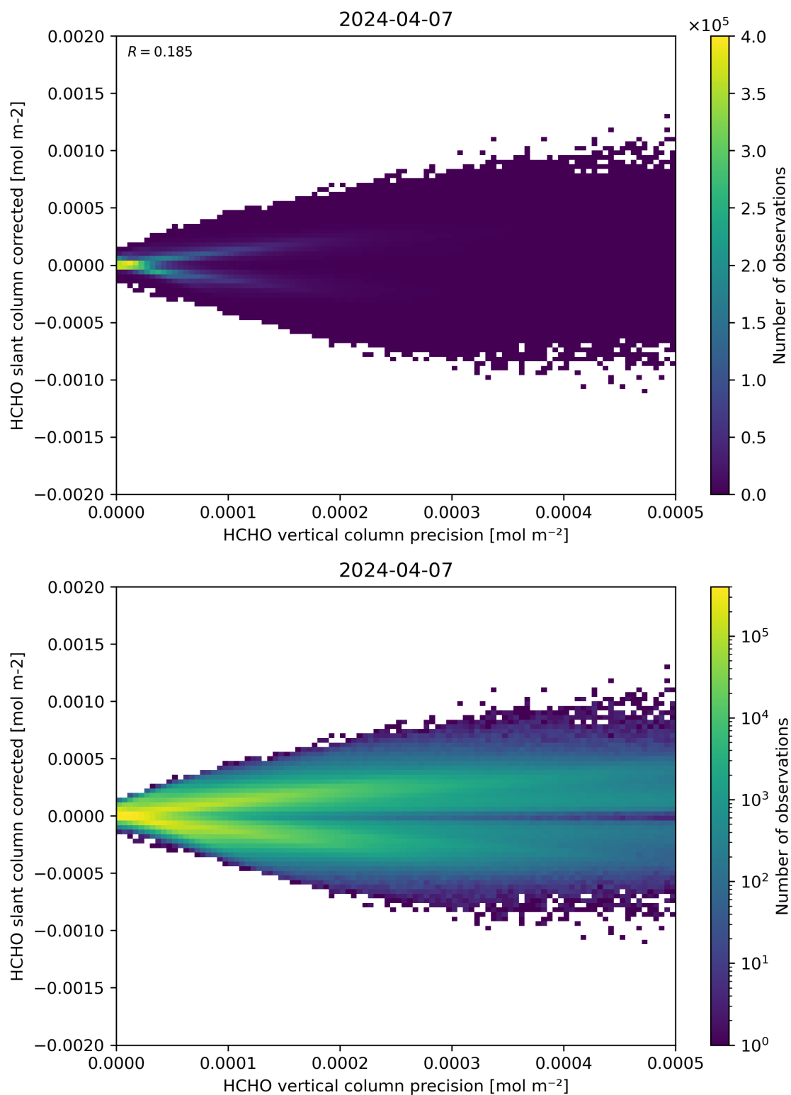
Figure 140: Scatter density plot of “HCHO vertical column precision” against “HCHO slant column corrected” for 2024-04-06 to 2024-04-08.
