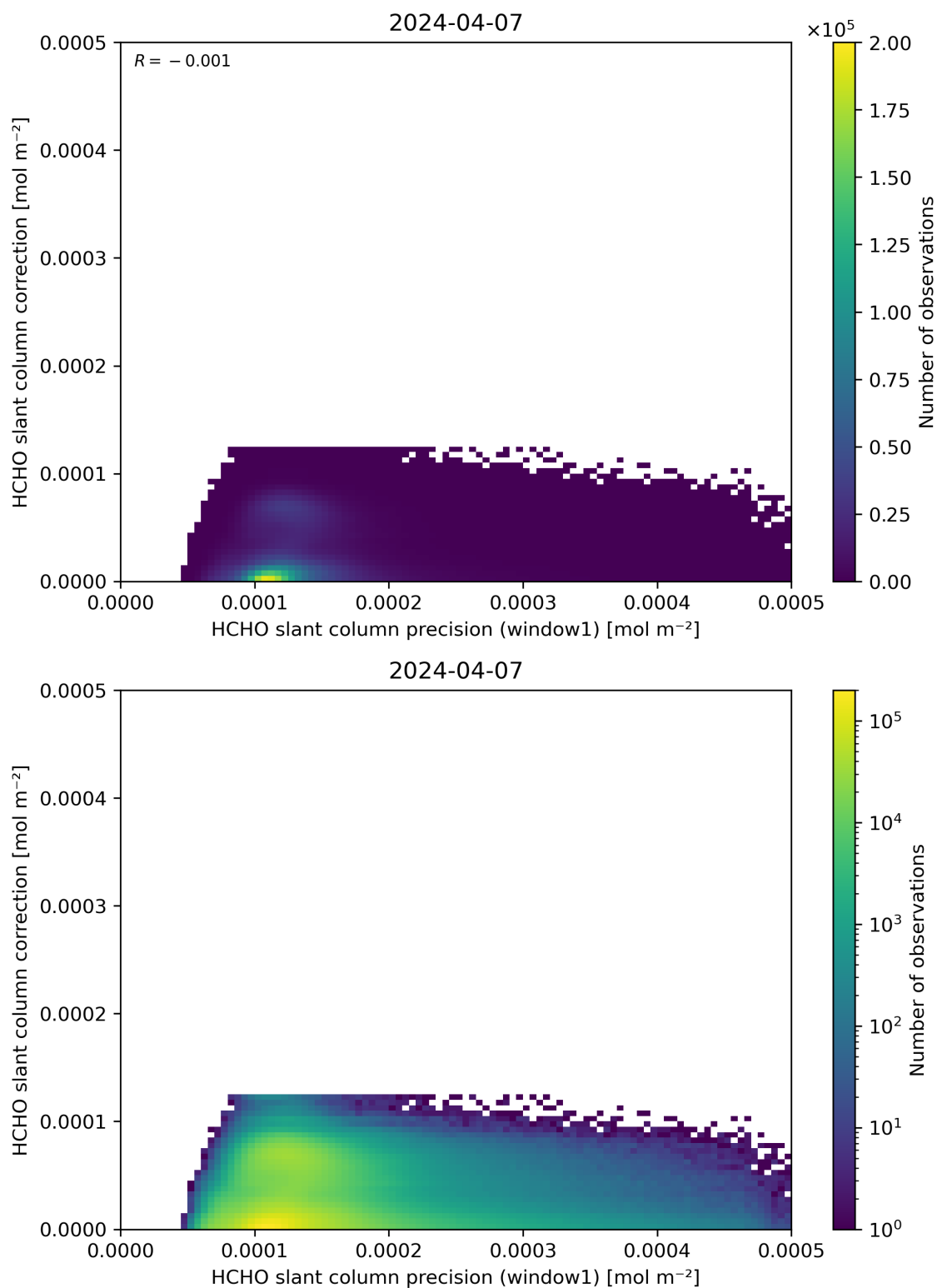
Figure 93: Scatter density plot of “HCHO slant column precision (window1)” against “HCHO slant column correction” for 2024-04-06 to 2024-04-08.
