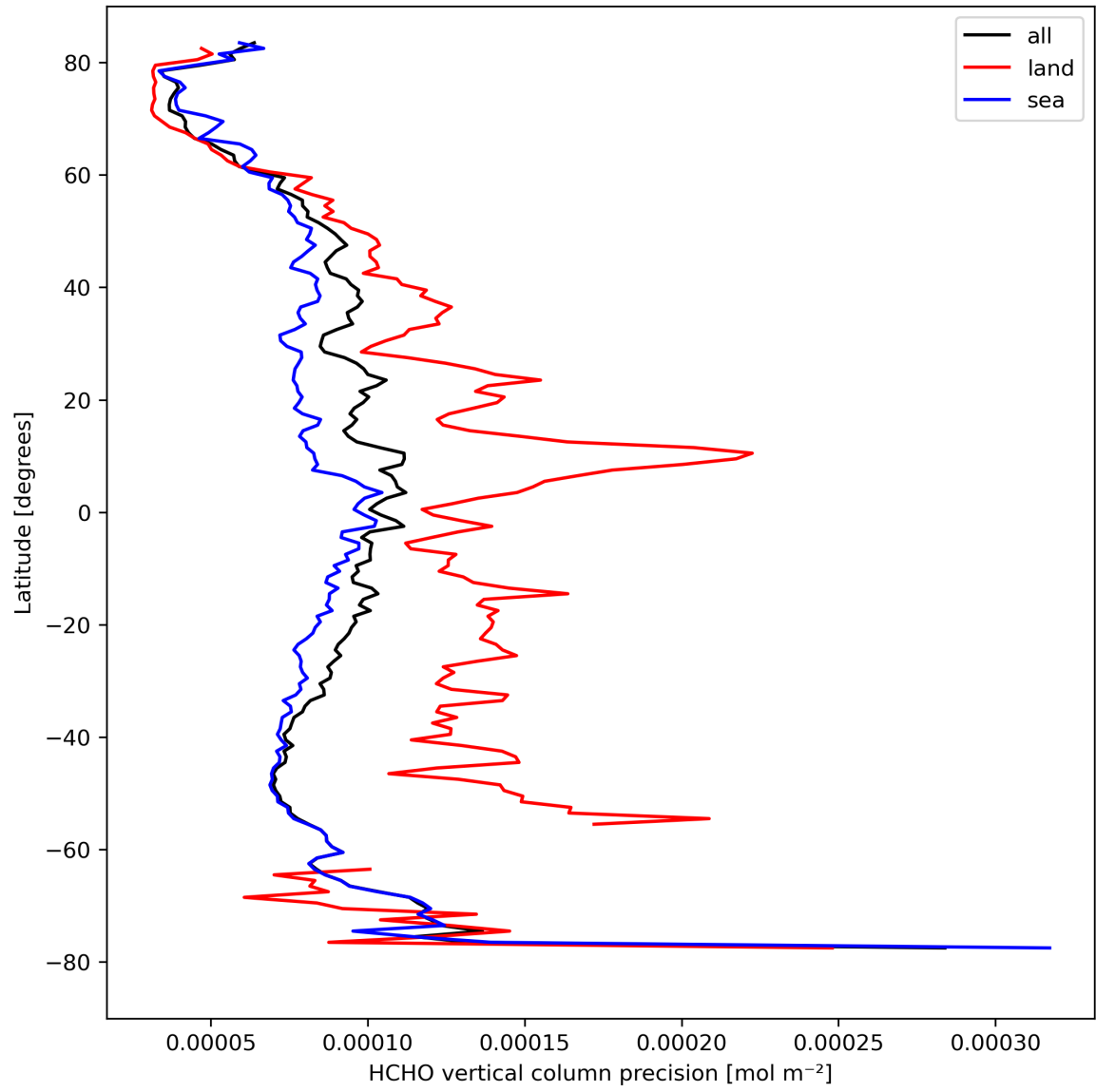
Figure 22: Zonal average of “HCHO vertical column precision” for 2024-04-06 to 2024-04-08.
