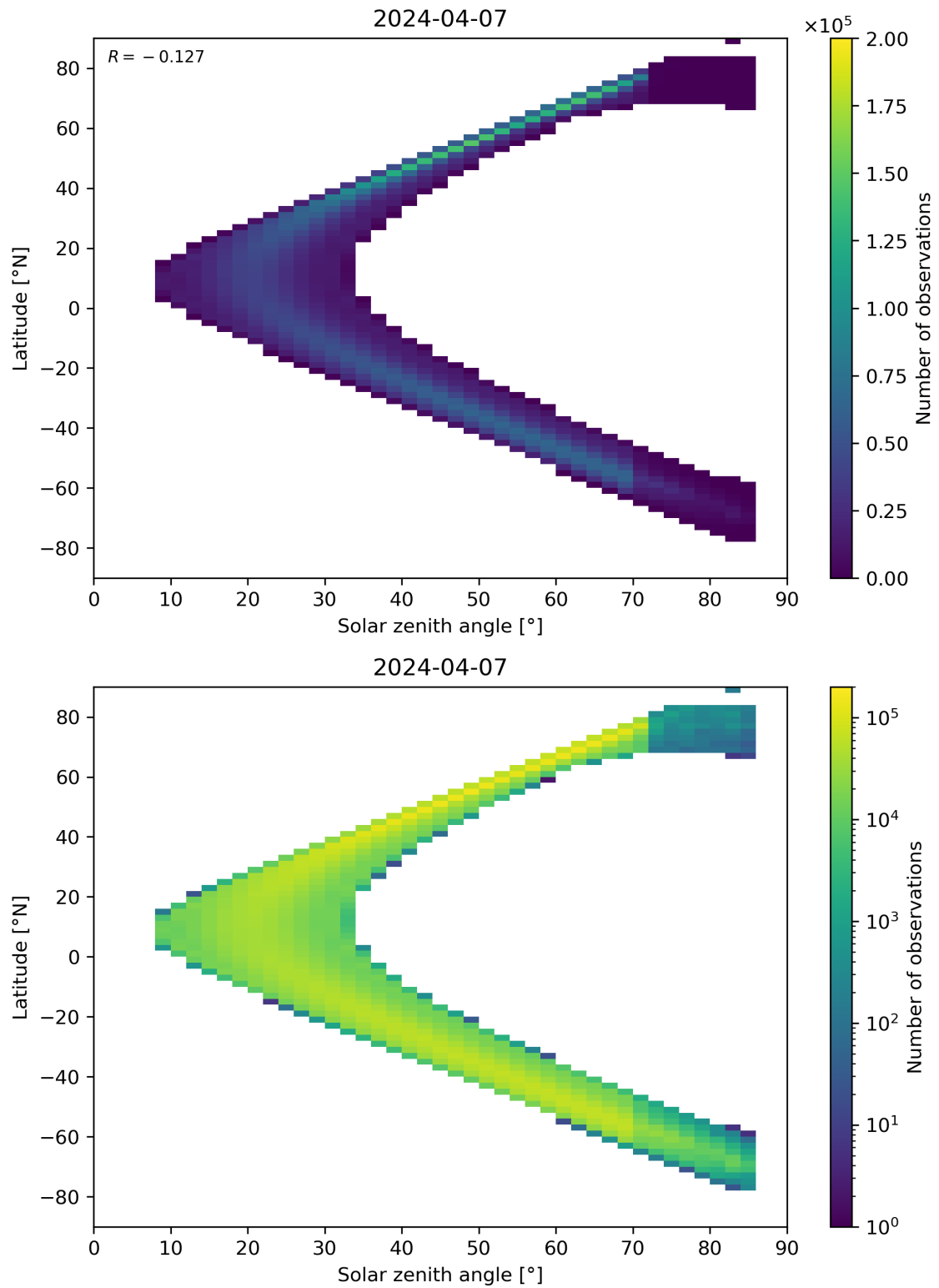
Figure 181: Scatter density plot of “Solar zenith angle” against “Latitude” for 2024-04-06 to 2024-04-08.
