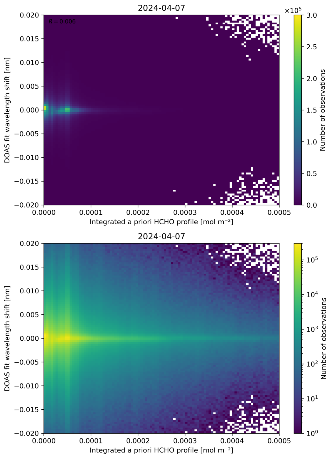
Figure 149: Scatter density plot of “Integrated a priori HCHO profile” against “DOAS fit wavelength shift” for 2024-04-06 to 2024-04-08.
