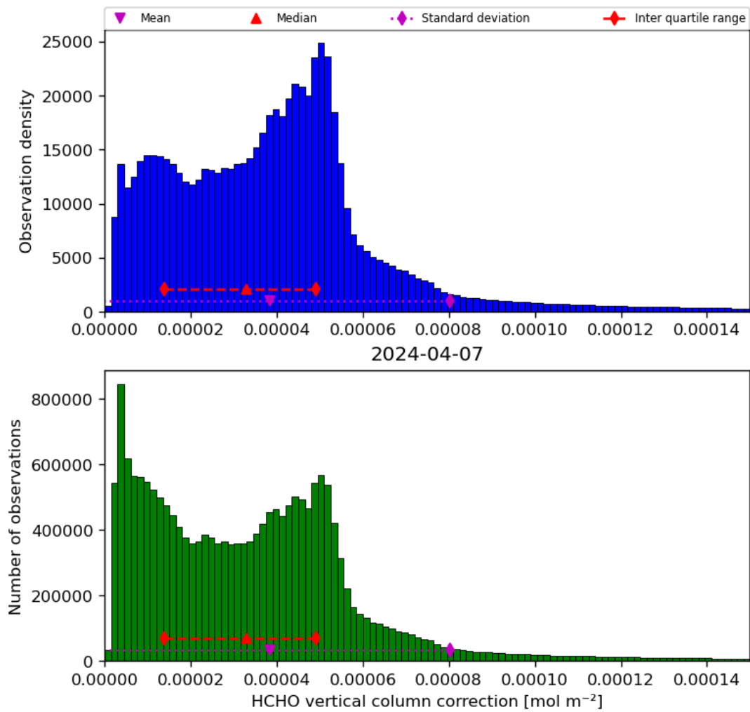
Figure 37: Histogram of “HCHO vertical column correction” for 2024-04-06 to 2024-04-08
