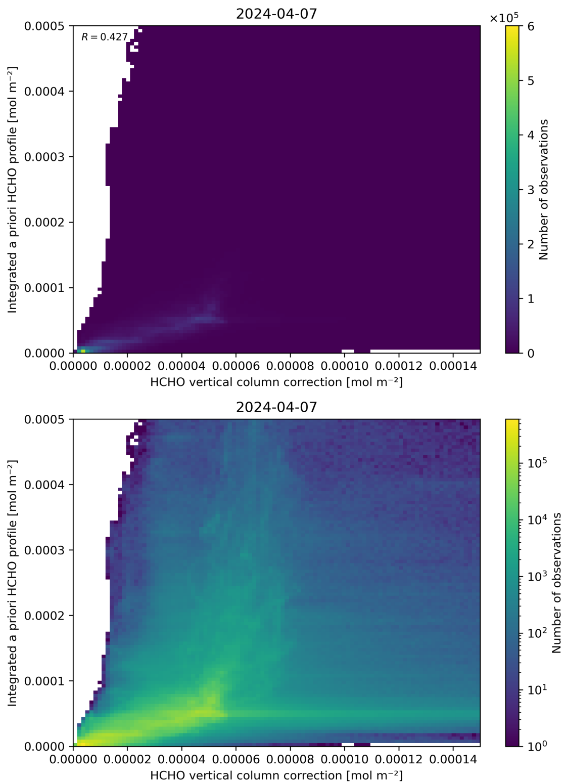
Figure 122: Scatter density plot of “HCHO vertical column correction” against “Integrated a priori HCHO profile” for 2024-04-06 to 2024-04-08.
