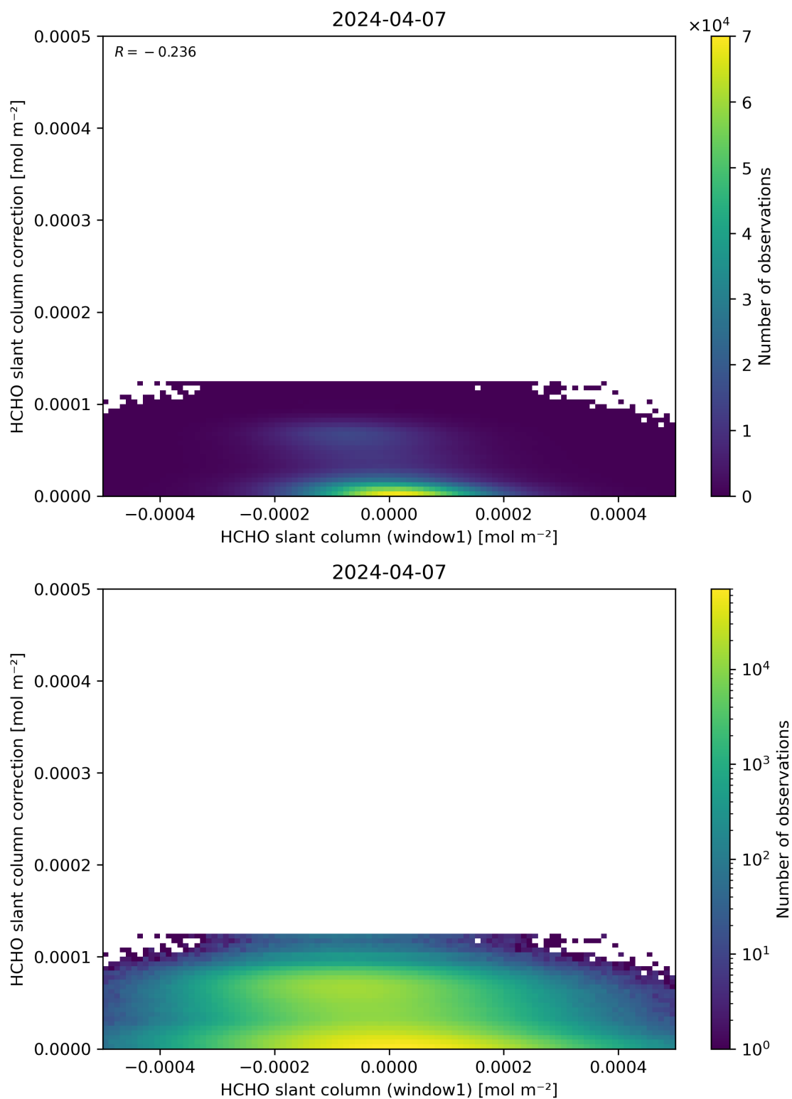
Figure 83: Scatter density plot of “HCHO slant column (window1)” against “HCHO slant column correction” for 2024-04-06 to 2024-04-08.
