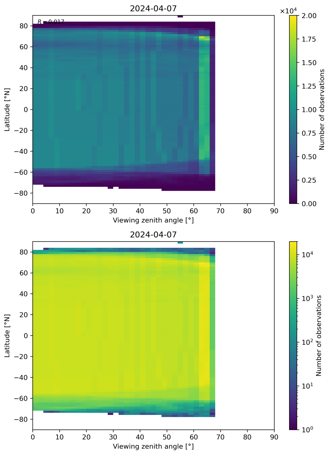
Figure 196: Scatter density plot of “Viewing zenith angle” against “Latitude” for 2024-04-06 to 2024-04-08.
