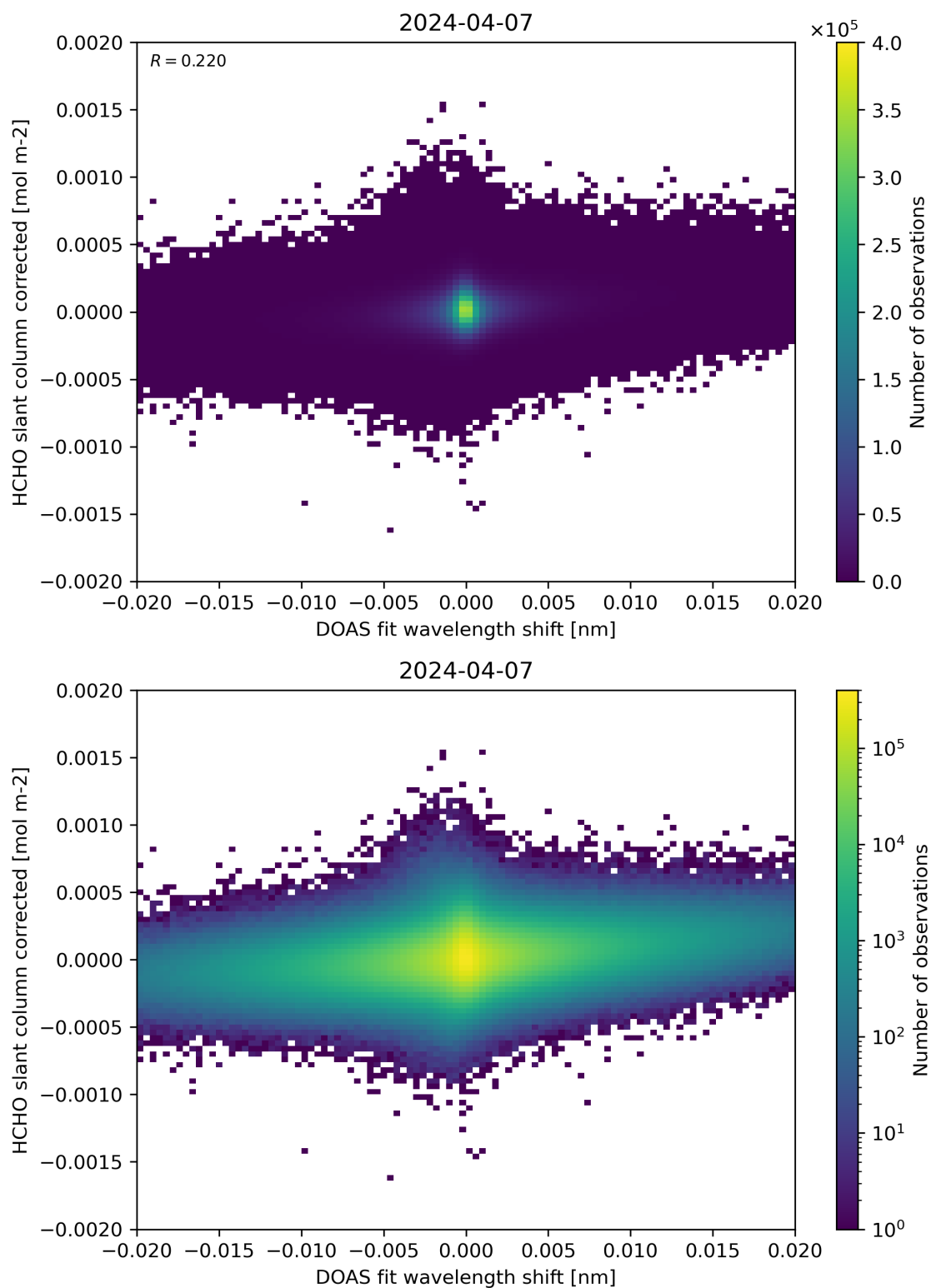
Figure 66: Scatter density plot of “DOAS fit wavelength shift” against “HCHO slant column corrected” for 2024-04-06 to 2024-04-08.
