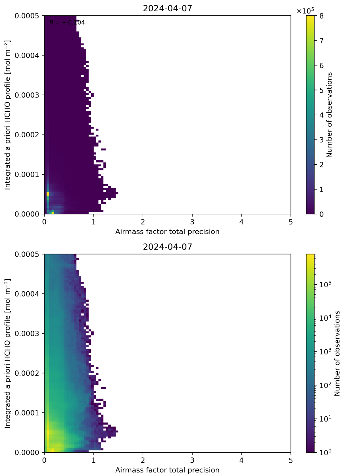
Figure 111: Scatter density plot of “Airmass factor total precision” against “Integrated a priori HCHO profile” for 2024-04-06 to 2024-04-08.
