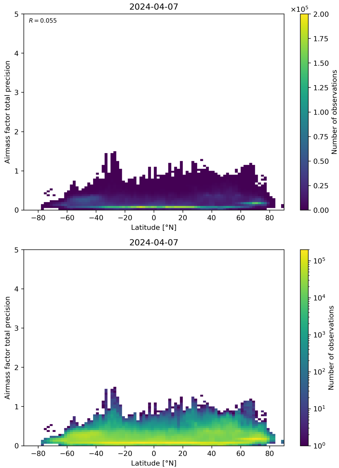
Figure 162: Scatter density plot of “Latitude” against “Airmass factor total precision” for 2024-04-06 to 2024-04-08.
