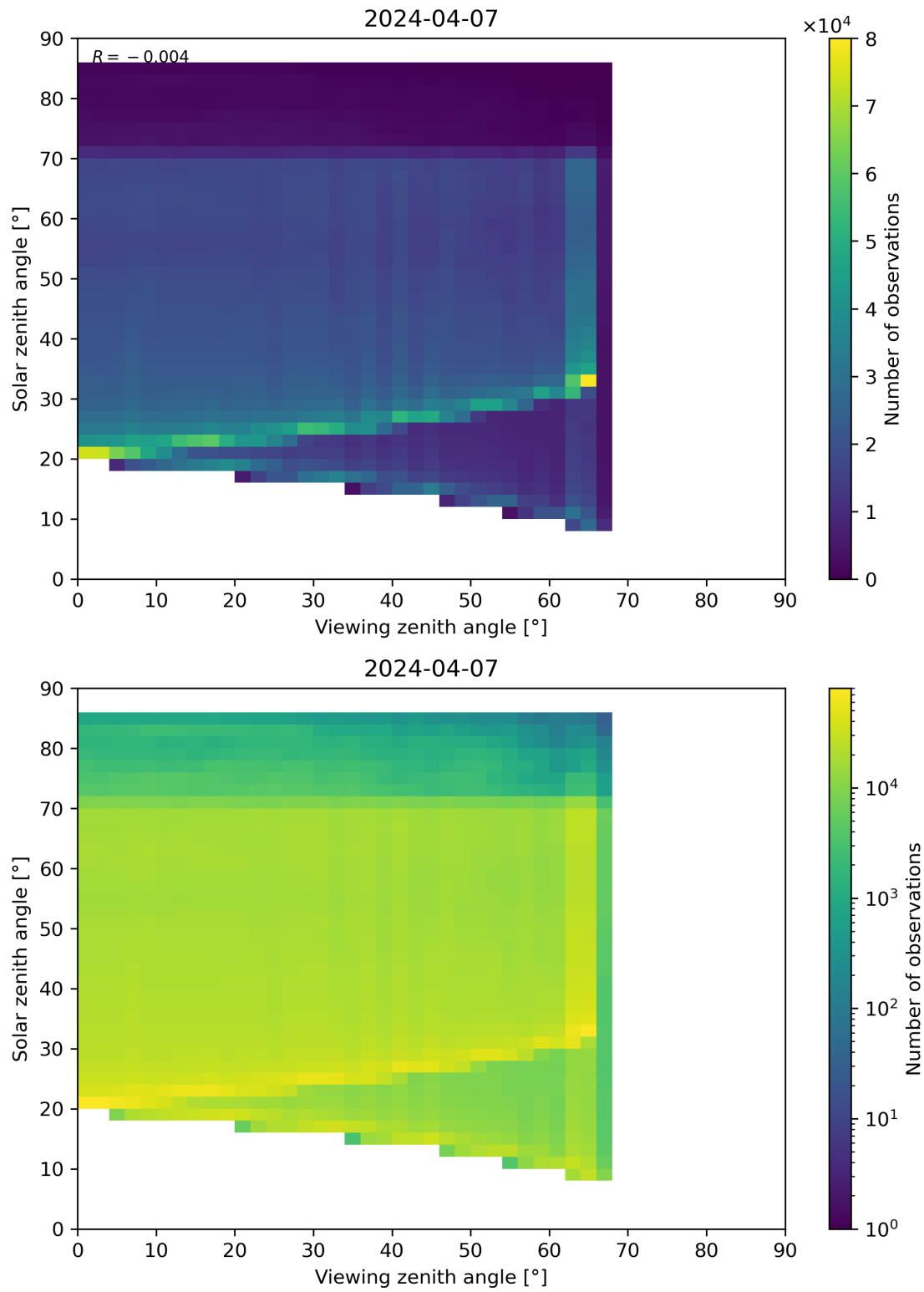
Figure 197: Scatter density plot of “Viewing zenith angle” against “Solar zenith angle” for 2024-04-06 to 2024-04-08.
