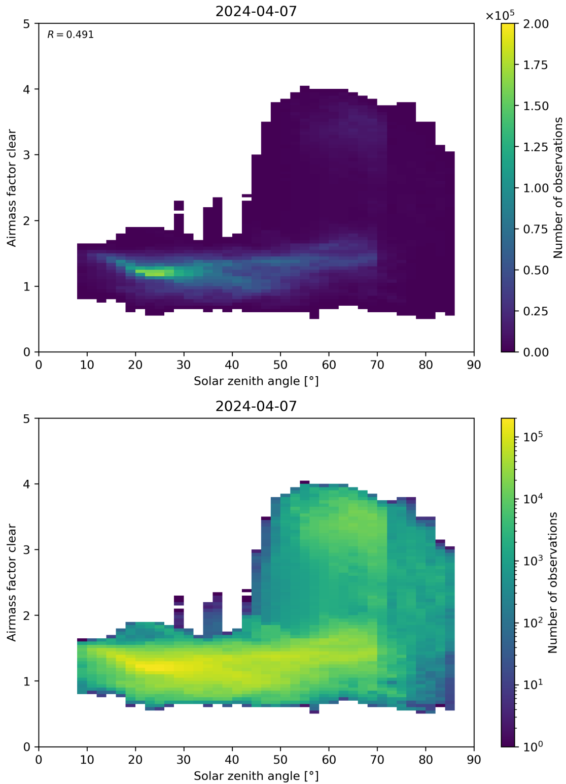
Figure 170: Scatter density plot of “Solar zenith angle” against “Airmass factor clear” for 2024-04-06 to 2024-04-08.
