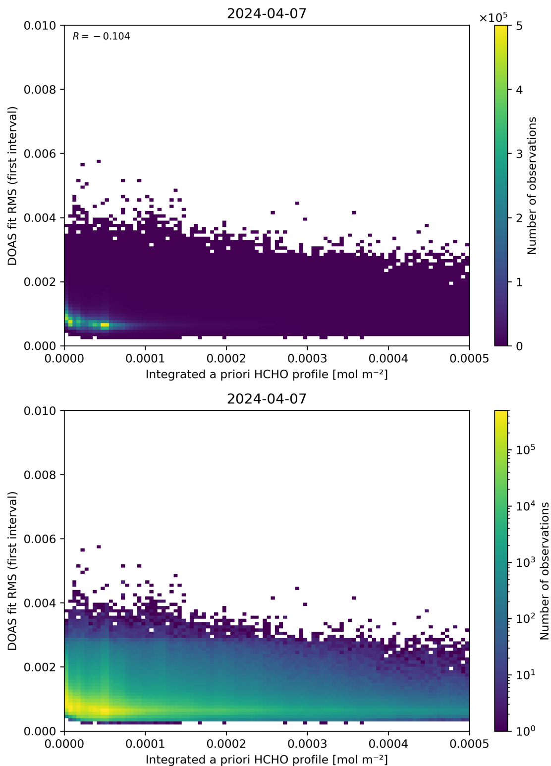
Figure 148: Scatter density plot of “Integrated a priori HCHO profile” against “DOAS fit RMS (first interval)” for 2024-04-06 to 2024-04-08.
