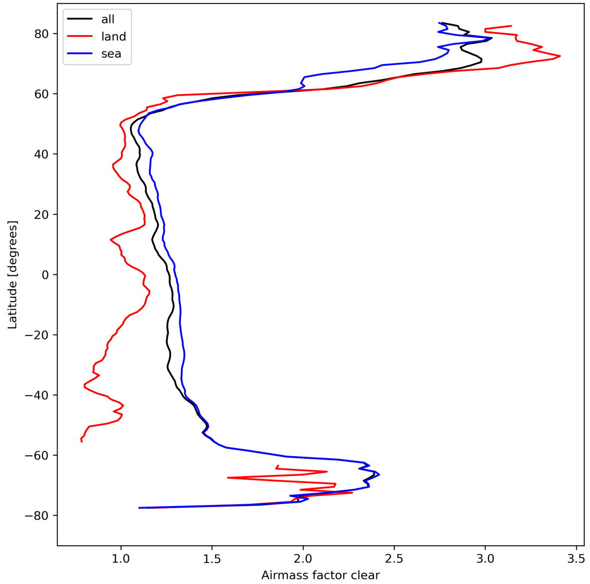
Figure 28: Zonal average of “Airmass factor clear” for 2024-04-06 to 2024-04-08.
