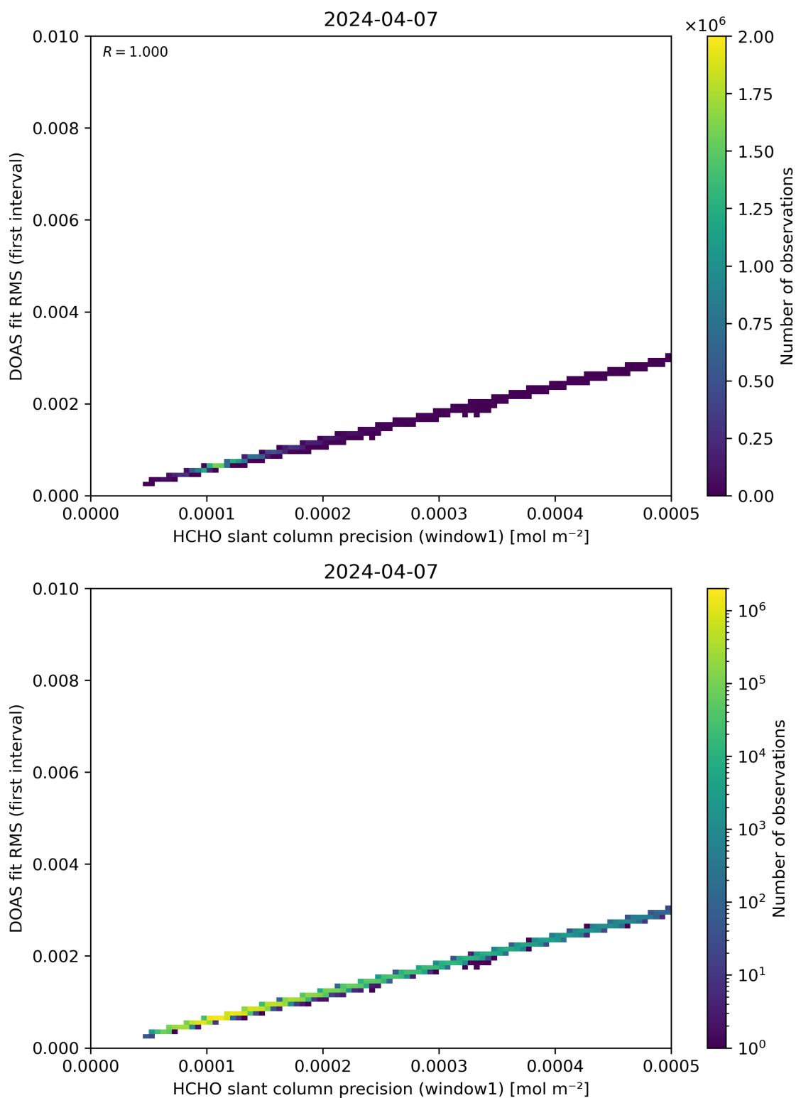
Figure 88: Scatter density plot of “HCHO slant column precision (window1)” against “DOAS fit RMS (first interval)” for 2024-04-06 to 2024-04-08.
