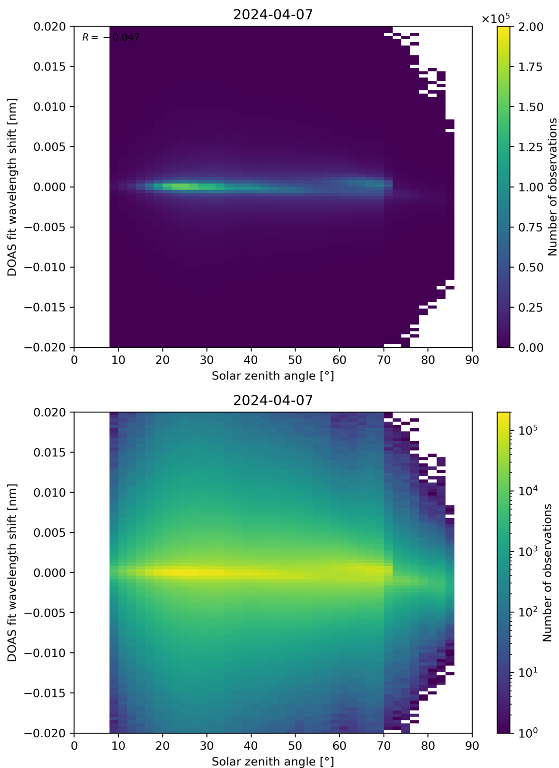
Figure 168: Scatter density plot of “Solar zenith angle” against “DOAS fit wavelength shift” for 2024-04-06 to 2024-04-08.
