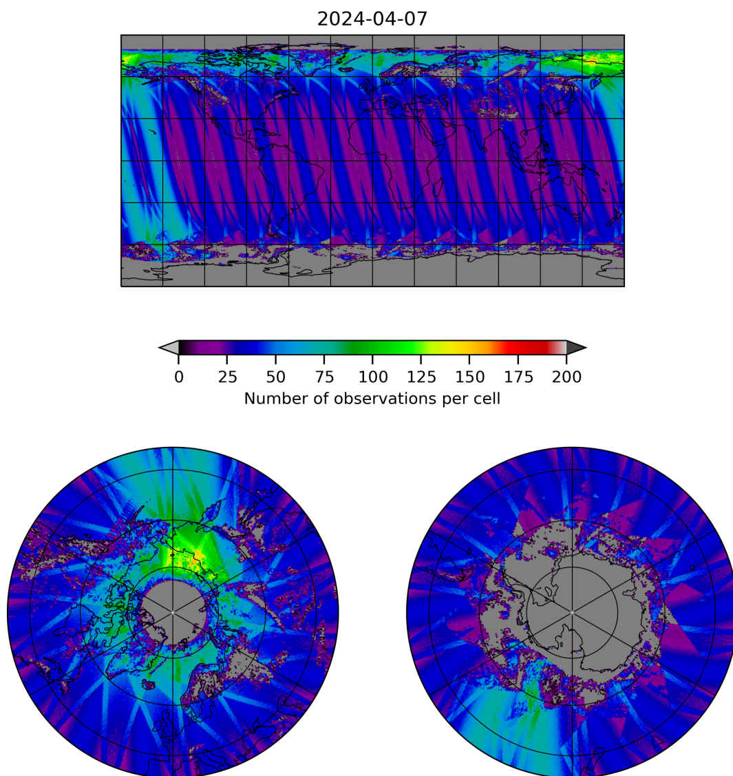
Figure 19: Map of the number of observations for 2024-04-06 to 2024-04-08
