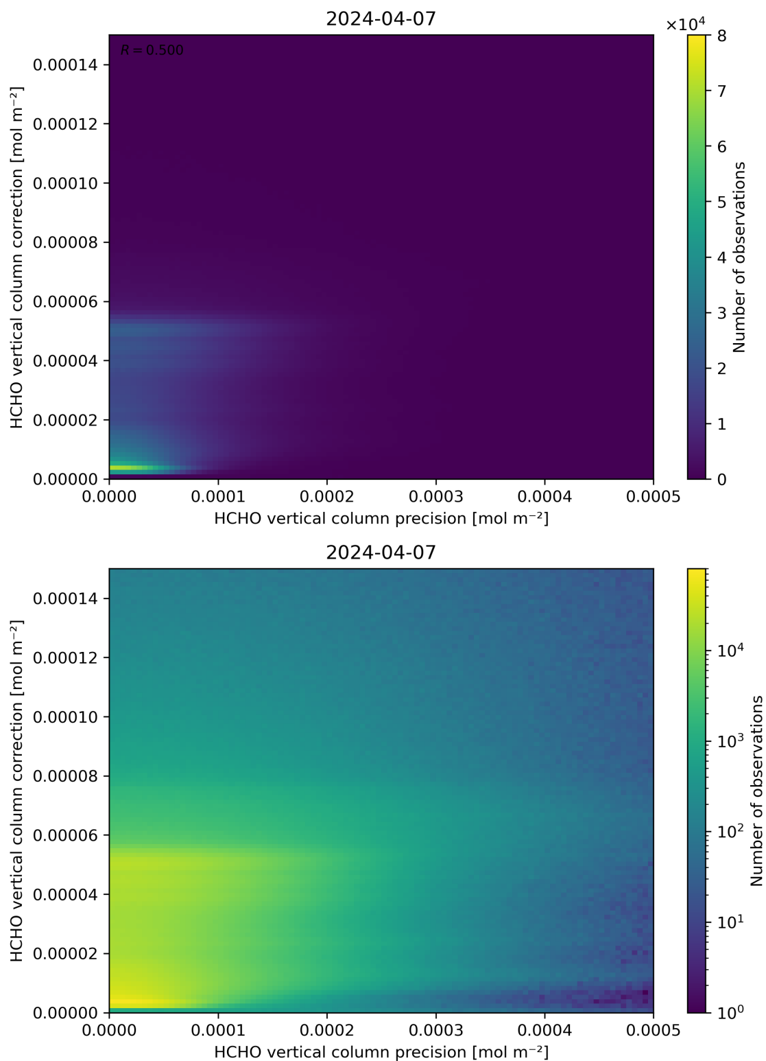
Figure 146: Scatter density plot of “HCHO vertical column precision” against “HCHO vertical column correction” for 2024-04-06 to 2024-04-08.
