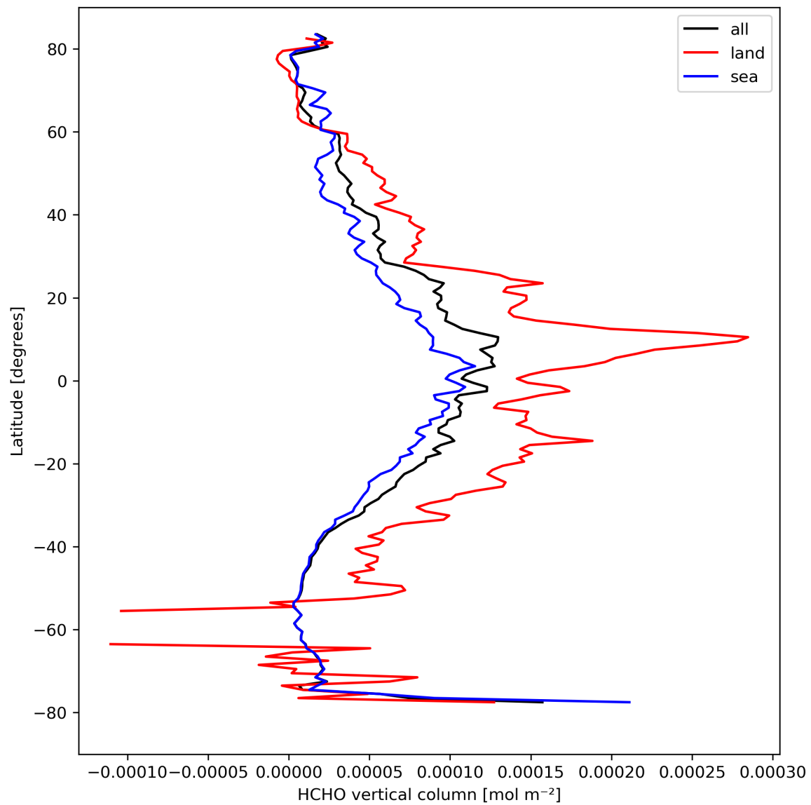
Figure 21: Zonal average of “HCHO vertical column” for 2024-04-06 to 2024-04-08.
