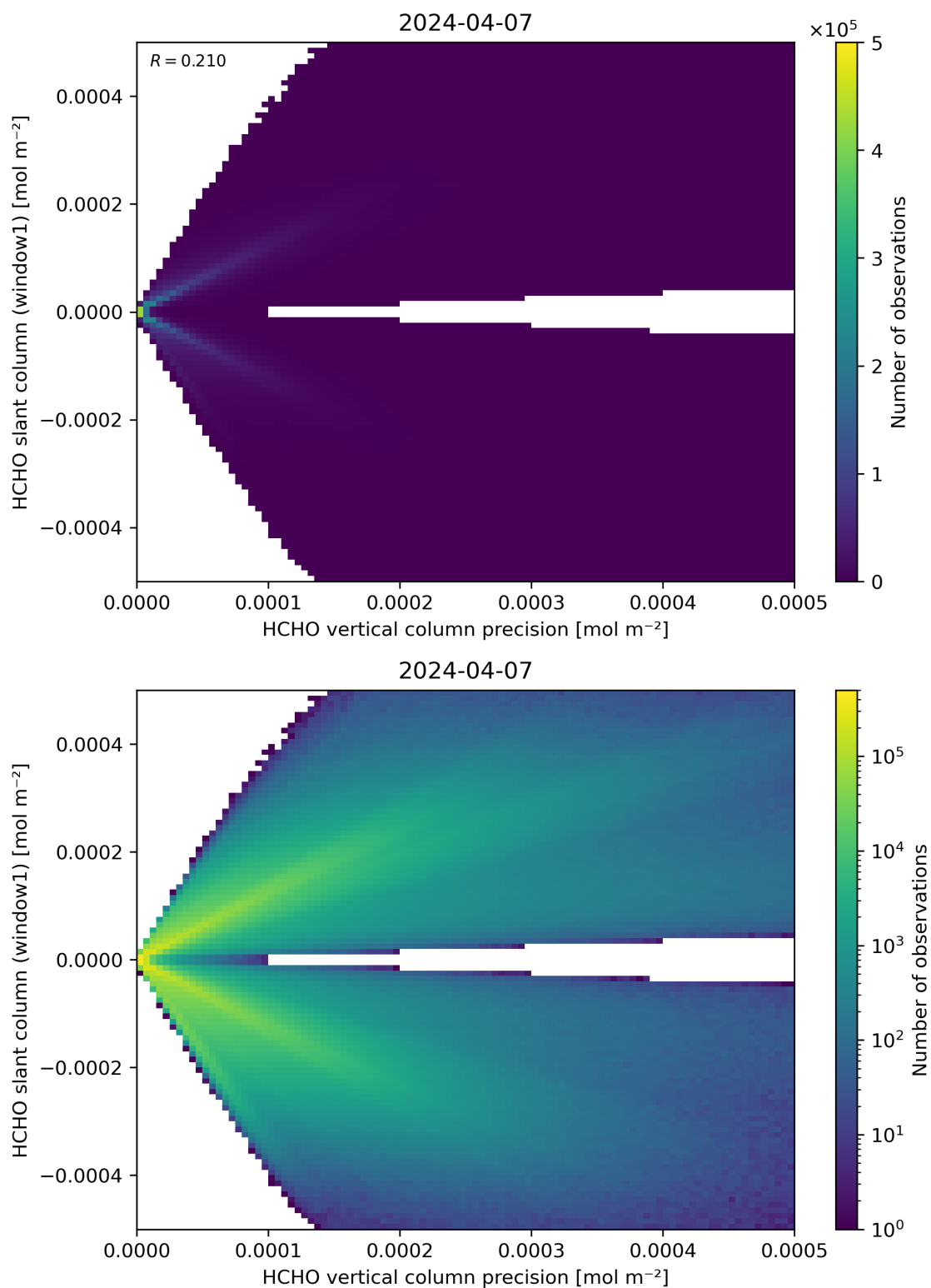
Figure 142: Scatter density plot of “HCHO vertical column precision” against “HCHO slant column (window1)” for 2024-04-06 to 2024-04-08.
