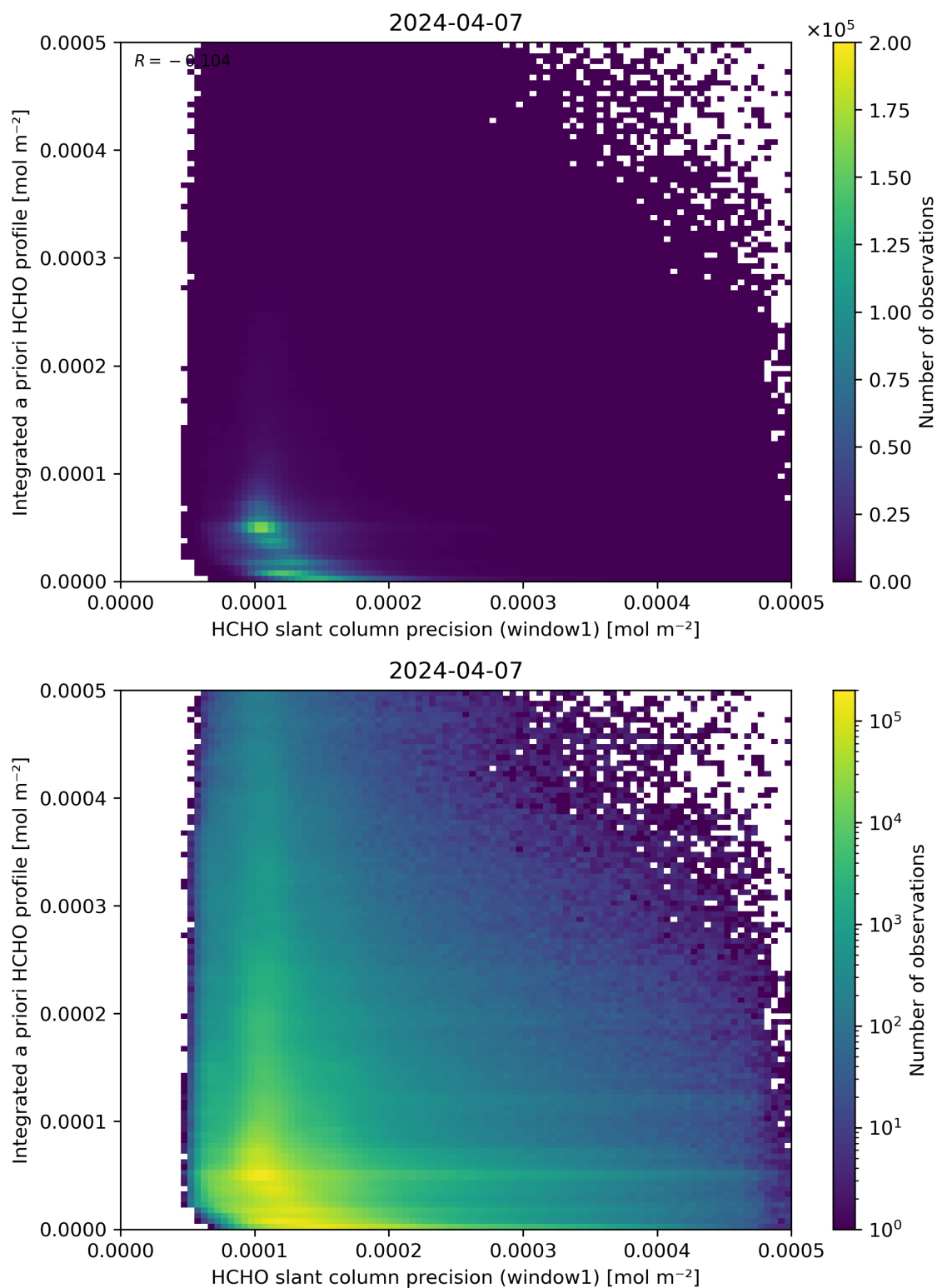
Figure 96: Scatter density plot of “HCHO slant column precision (window1)” against “Integrated a priori HCHO profile” for 2024-04-06 to 2024-04-08.
