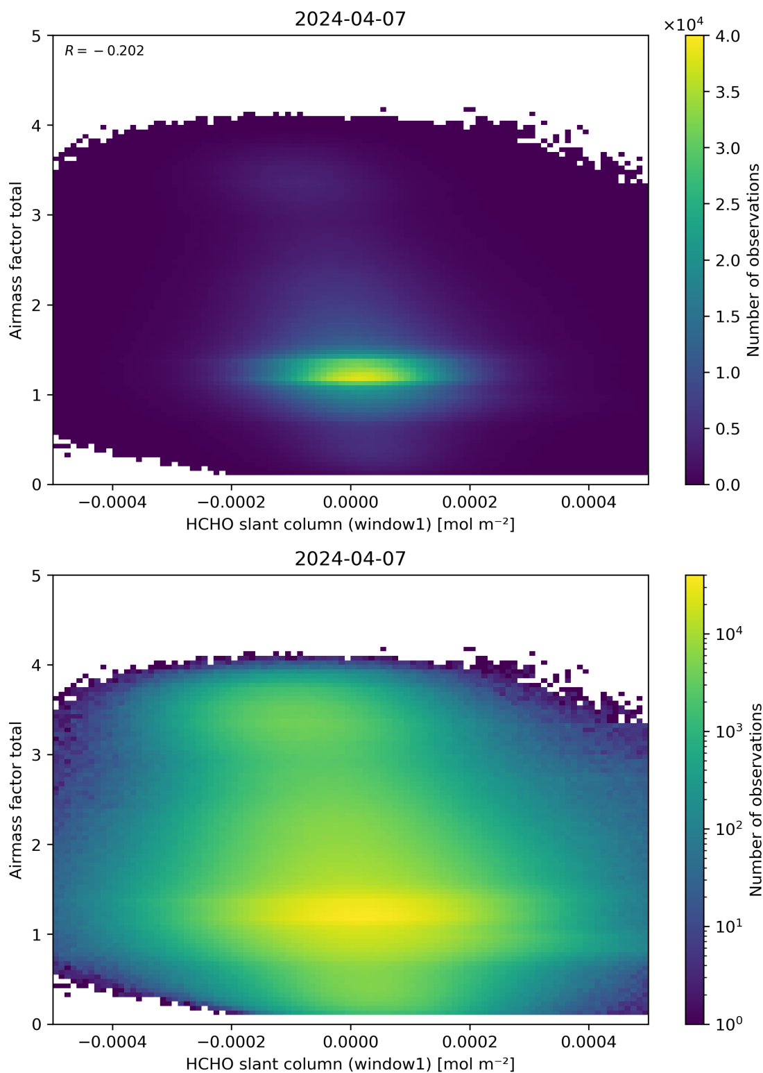
Figure 85: Scatter density plot of “HCHO slant column (window1)” against “Airmass factor total” for 2024-04-06 to 2024-04-08.
