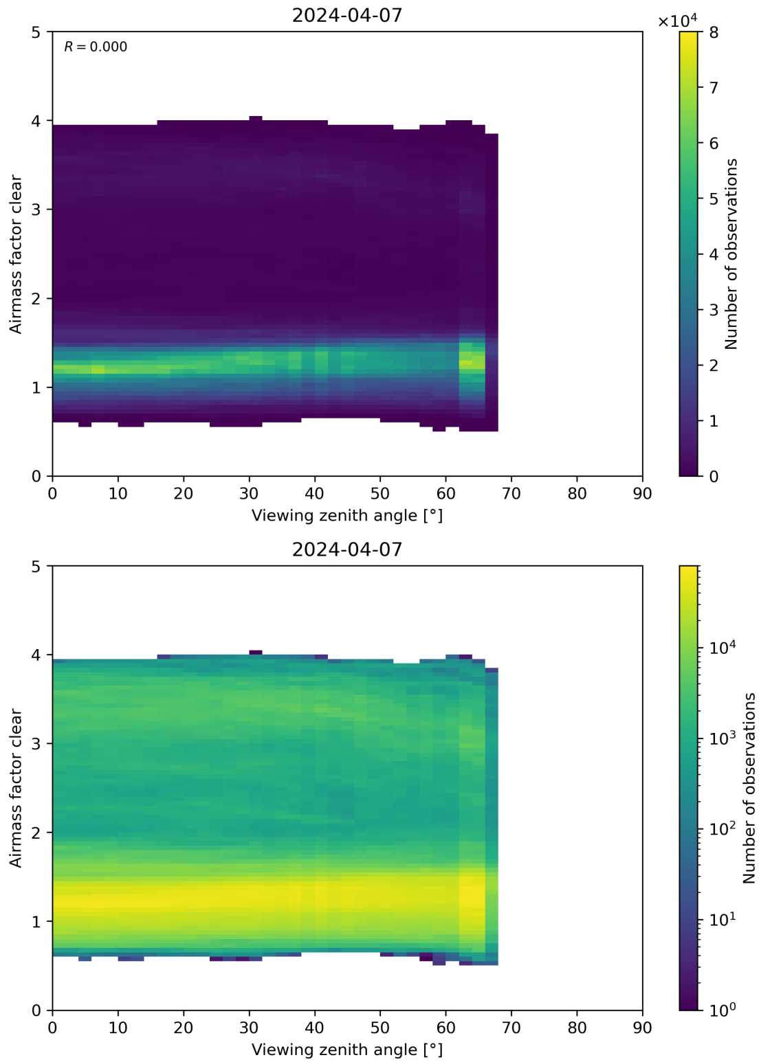
Figure 185: Scatter density plot of “Viewing zenith angle” against “Airmass factor clear” for 2024-04-06 to 2024-04-08.
