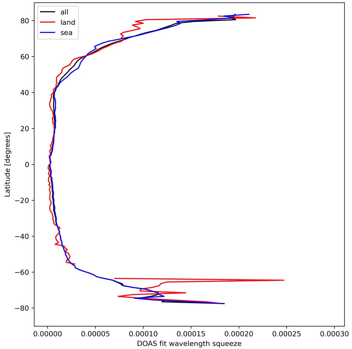
Figure 31: Zonal average of “DOAS fit wavelength squeeze” for 2024-04-06 to 2024-04-08.
