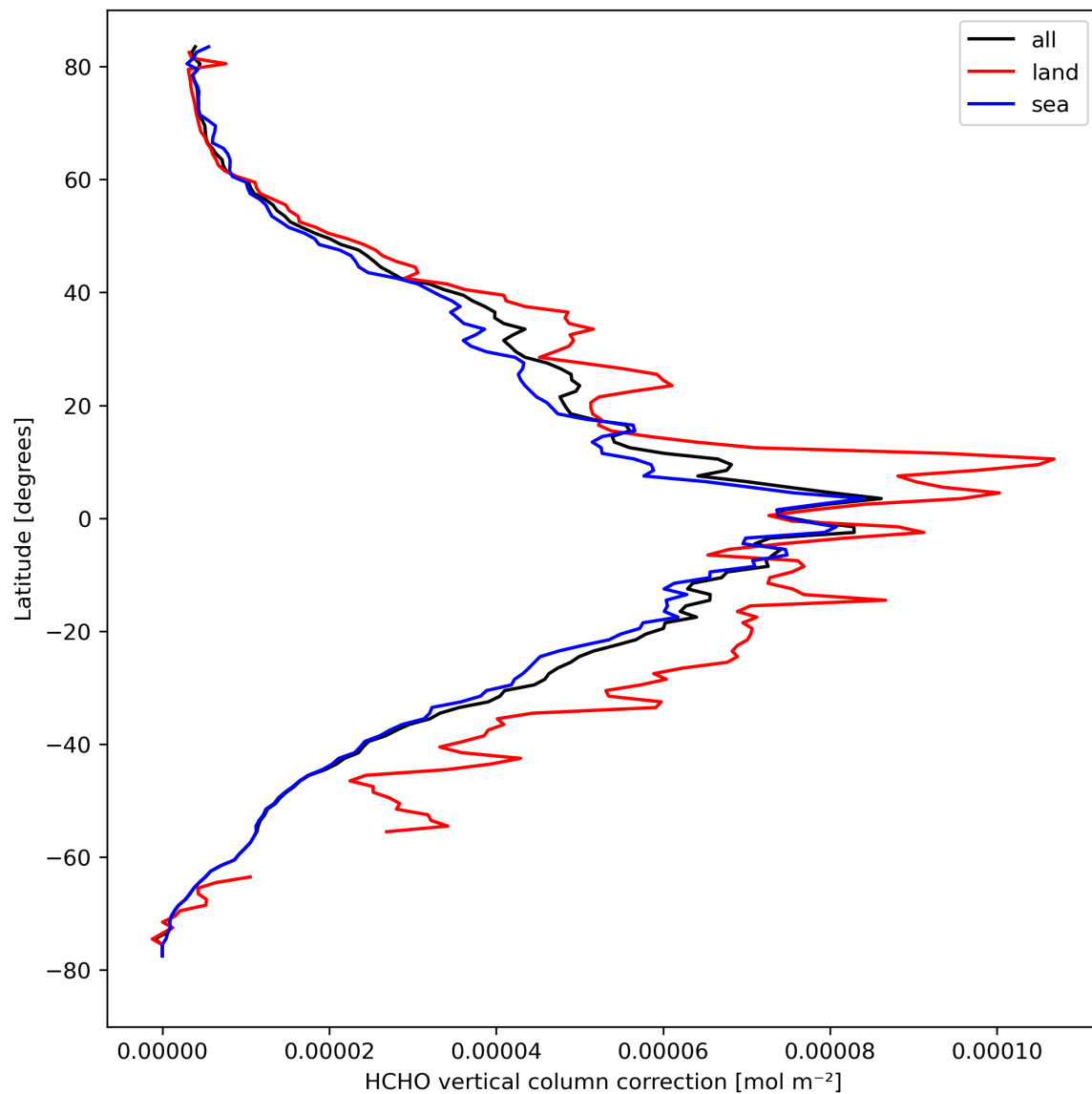
Figure 23: Zonal average of “HCHO vertical column correction” for 2024-04-06 to 2024-04-08.
