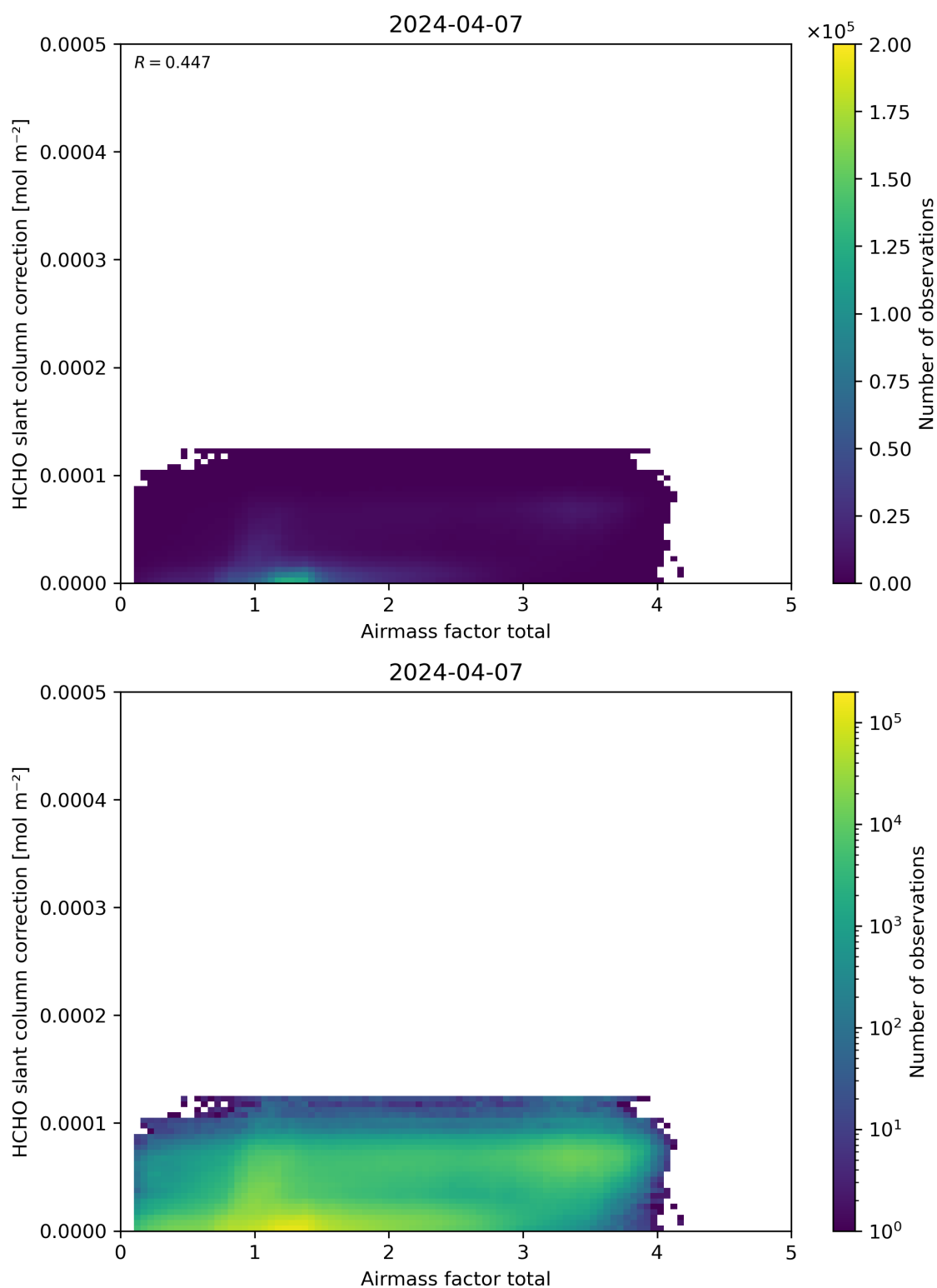
Figure 102: Scatter density plot of “Airmass factor total” against “HCHO slant column correction” for 2024-04-06 to 2024-04-08.
