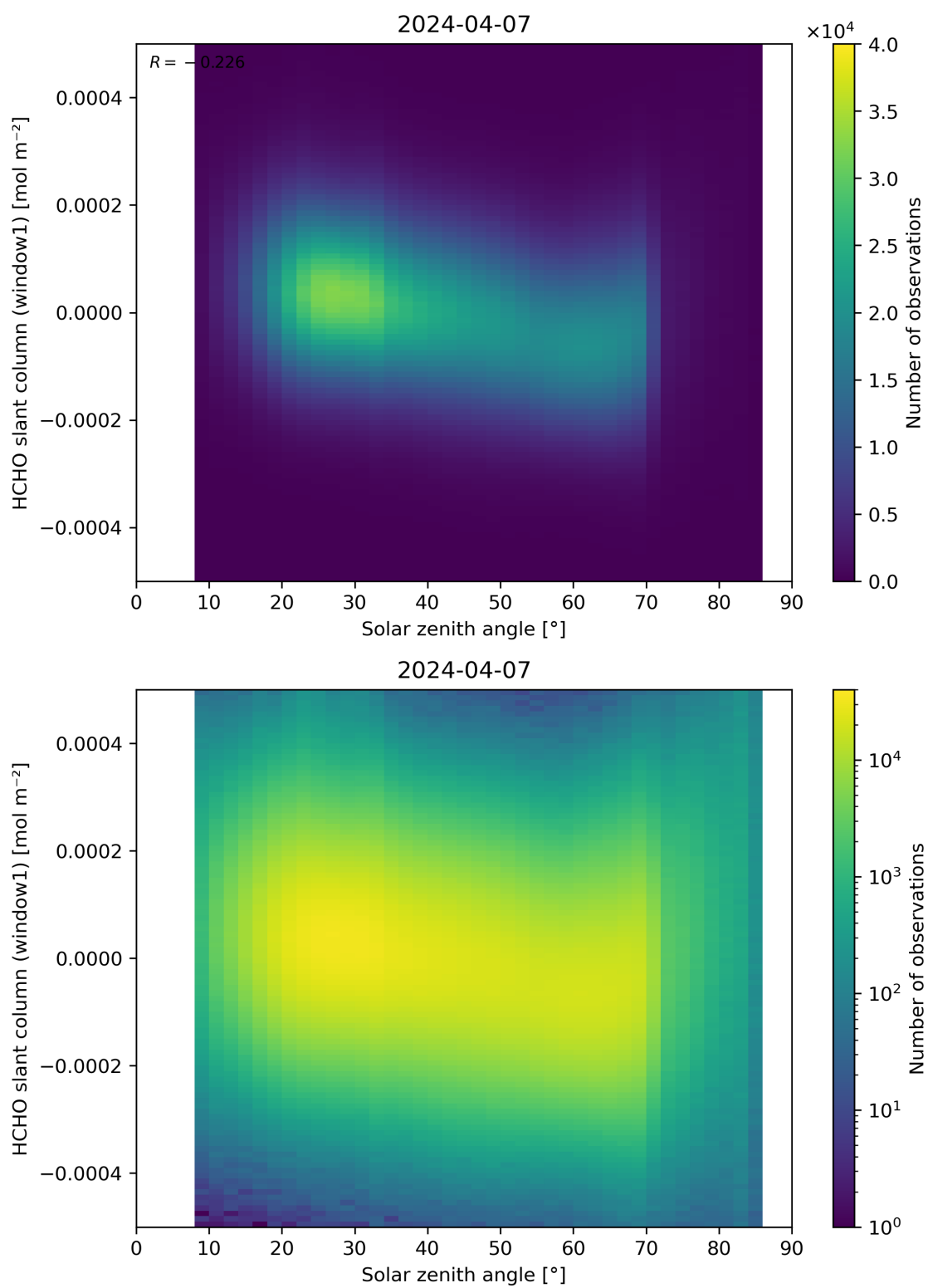
Figure 173: Scatter density plot of “Solar zenith angle” against “HCHO slant column (window1)” for 2024-04-06 to 2024-04-08.
