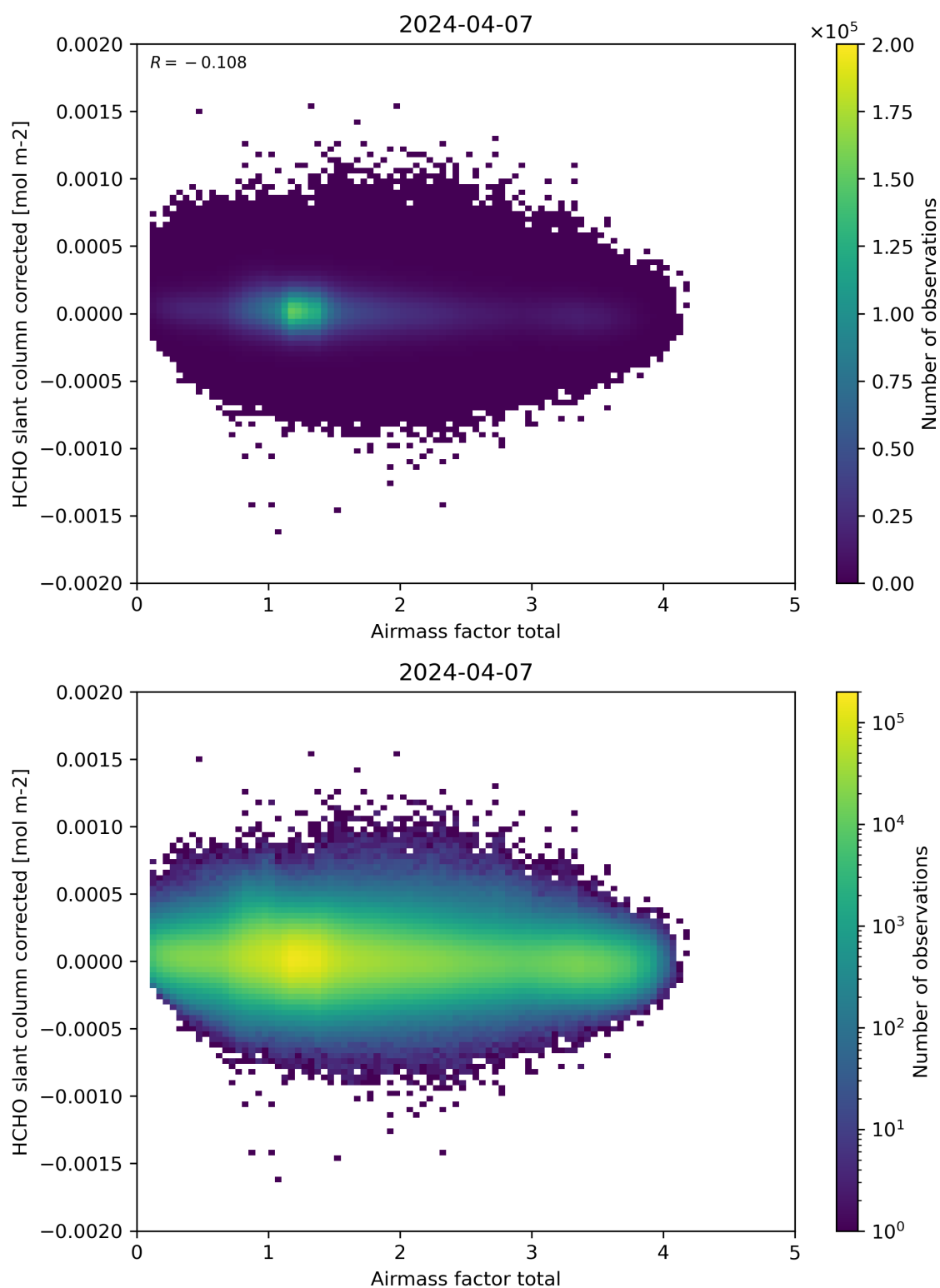
Figure 101: Scatter density plot of “Airmass factor total” against “HCHO slant column corrected” for 2024-04-06 to 2024-04-08.
