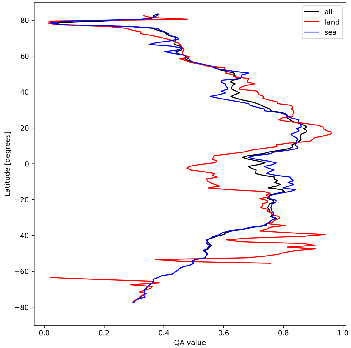
Figure 20: Zonal average of “QA value” for 2024-04-06 to 2024-04-08.
