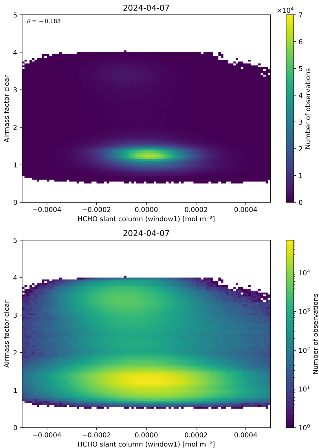
Figure 81: Scatter density plot of “HCHO slant column (window1)” against “Airmass factor clear” for 2024-04-06 to 2024-04-08.
