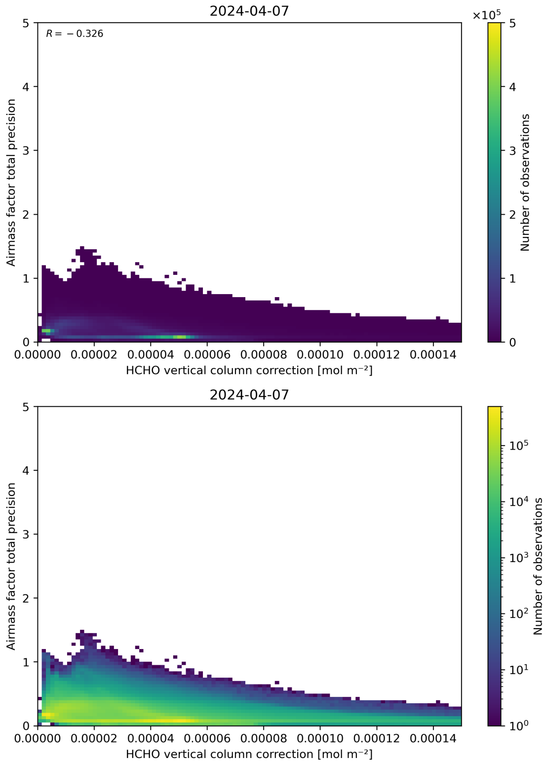
Figure 121: Scatter density plot of “HCHO vertical column correction” against “Airmass factor total precision” for 2024-04-06 to 2024-04-08.
