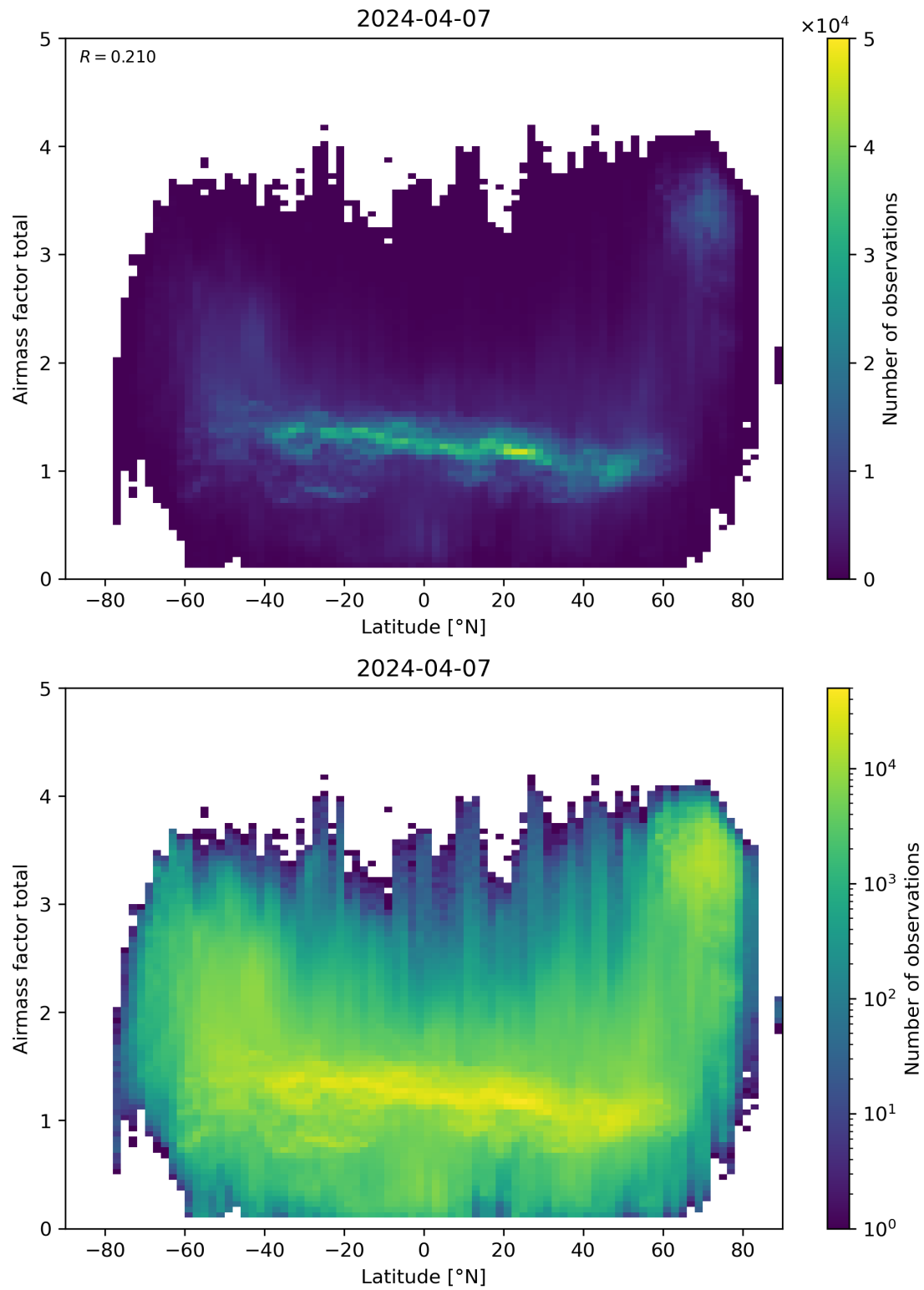
Figure 161: Scatter density plot of “Latitude” against “Airmass factor total” for 2024-04-06 to 2024-04-08.
