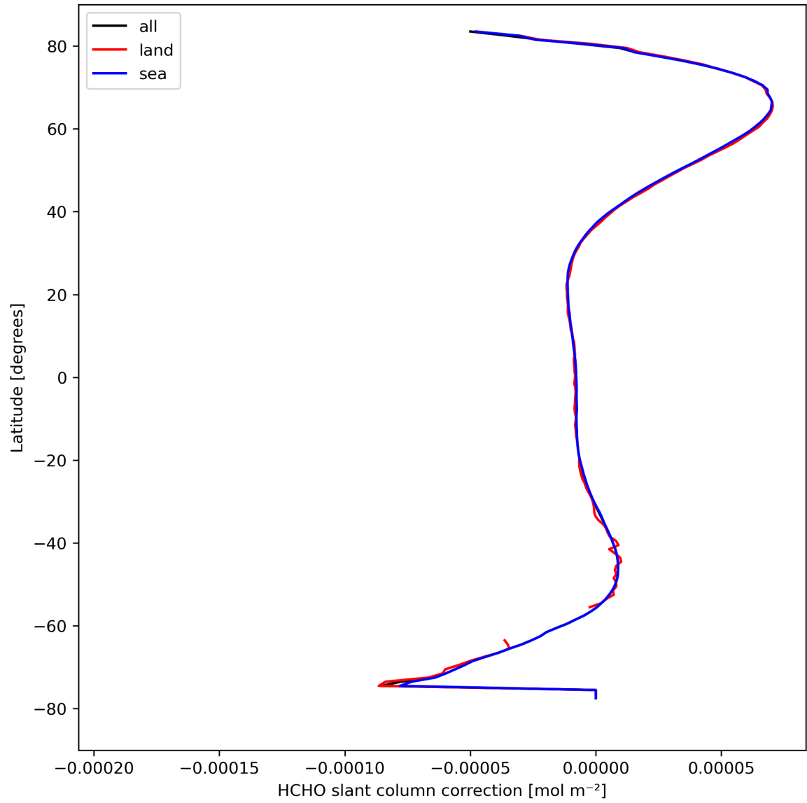
Figure 33: Zonal average of “HCHO slant column correction” for 2024-04-06 to 2024-04-08.
