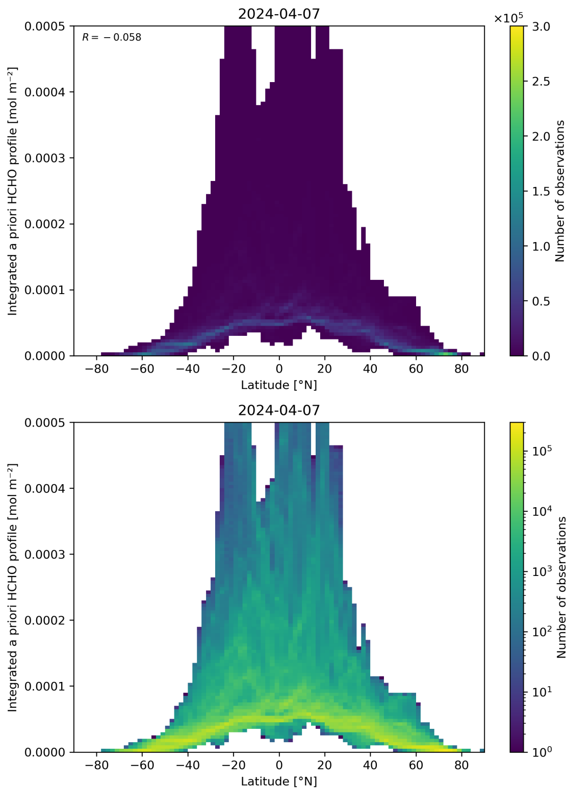
Figure 166: Scatter density plot of “Latitude” against “Integrated a priori HCHO profile” for 2024-04-06 to 2024-04-08.
