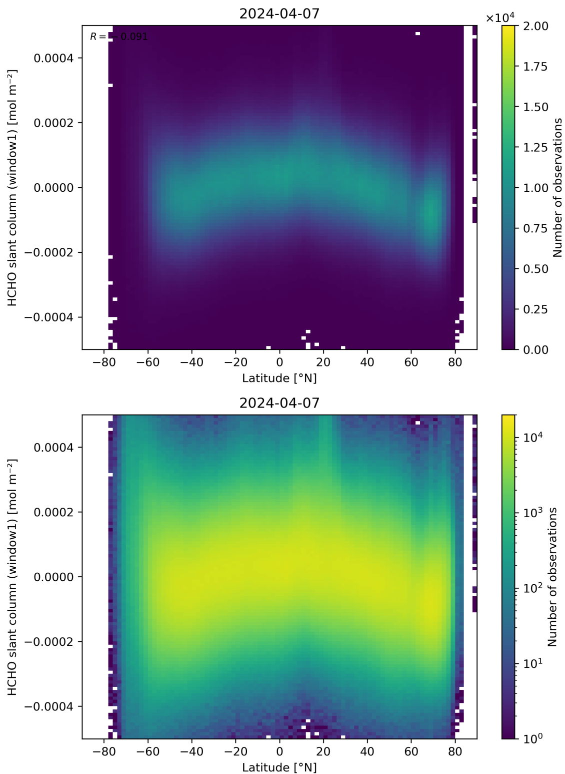
Figure 159: Scatter density plot of “Latitude” against “HCHO slant column (window1)” for 2024-04-06 to 2024-04-08.
