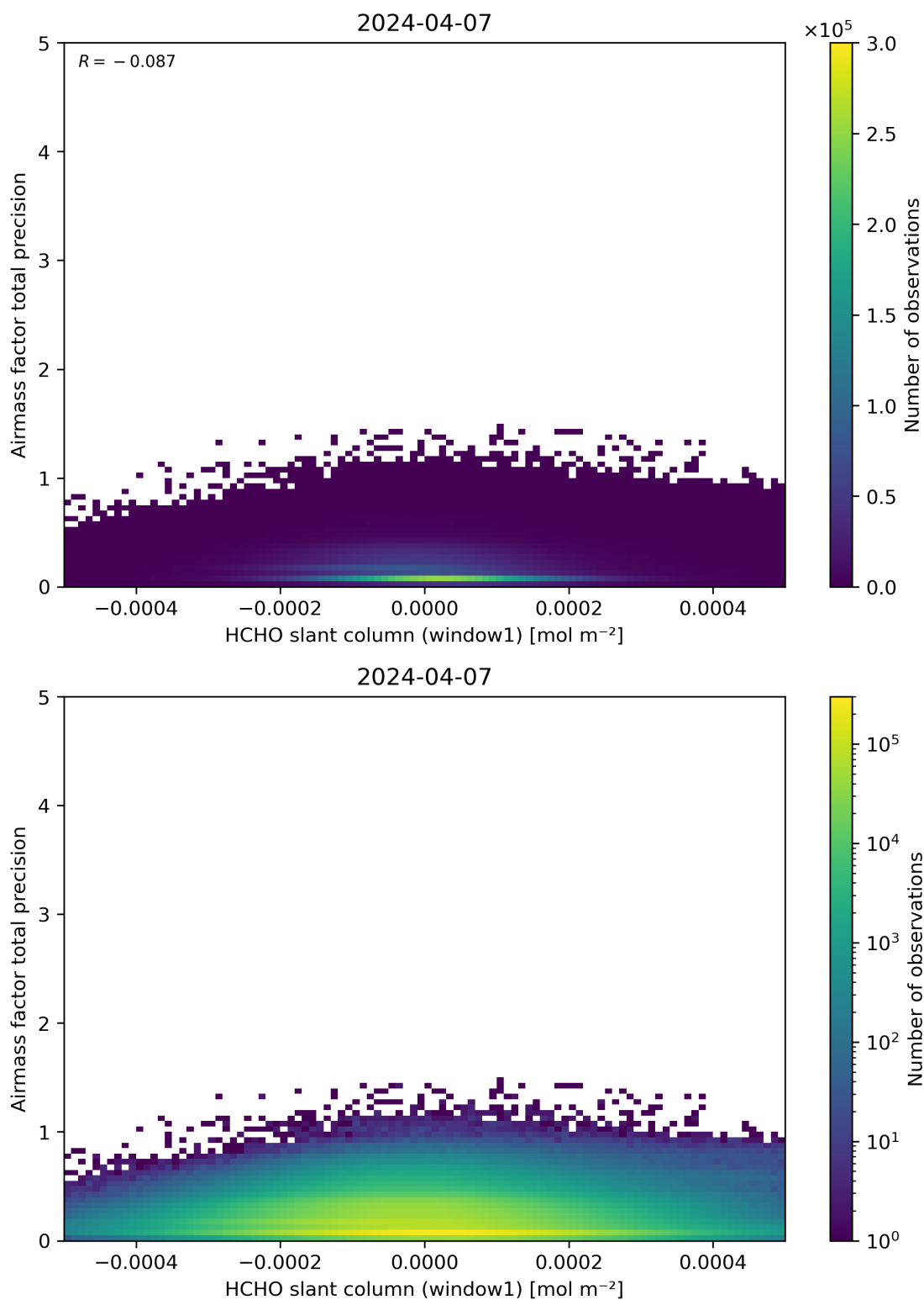
Figure 86: Scatter density plot of “HCHO slant column (window1)” against “Airmass factor total precision” for 2024-04-06 to 2024-04-08.
