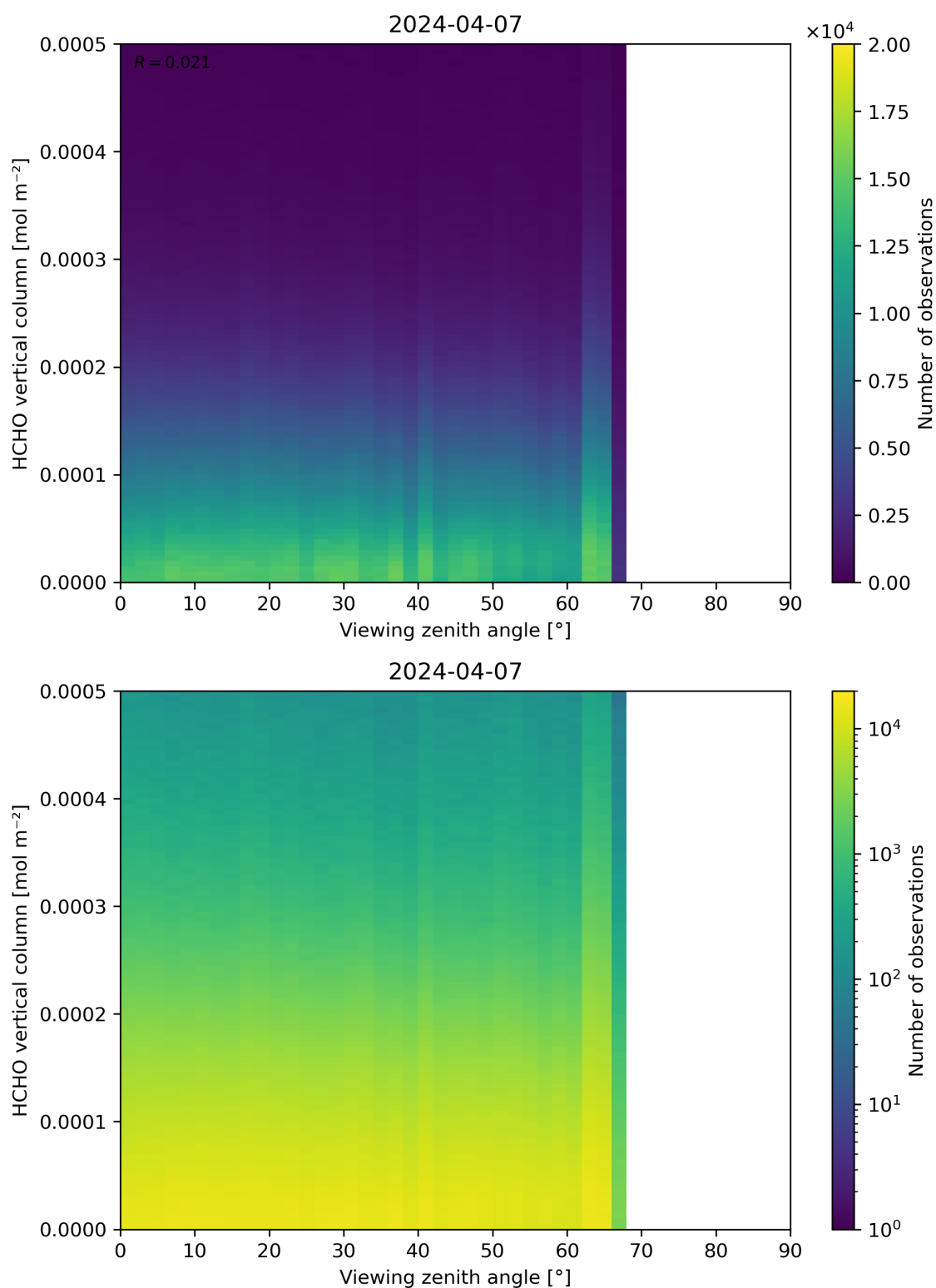
Figure 192: Scatter density plot of “Viewing zenith angle” against “HCHO vertical column” for 2024-04-06 to 2024-04-08.
