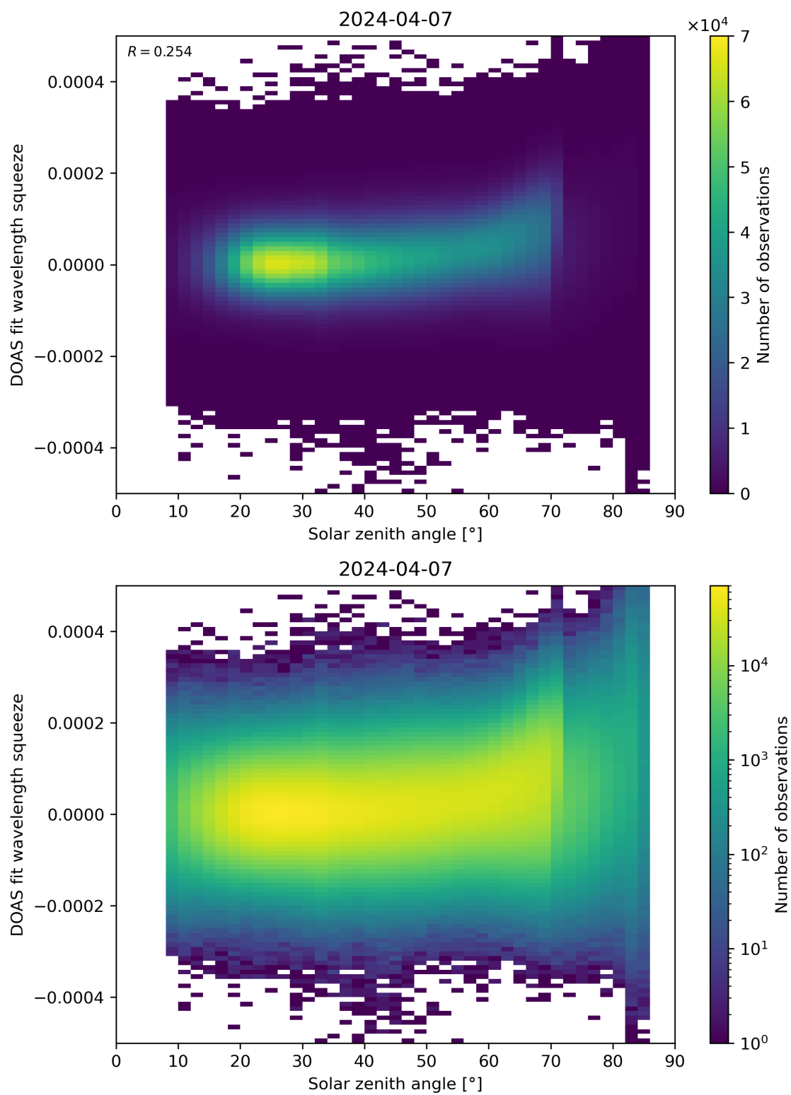
Figure 169: Scatter density plot of “Solar zenith angle” against “DOAS fit wavelength squeeze” for 2024-04-06 to 2024-04-08.
