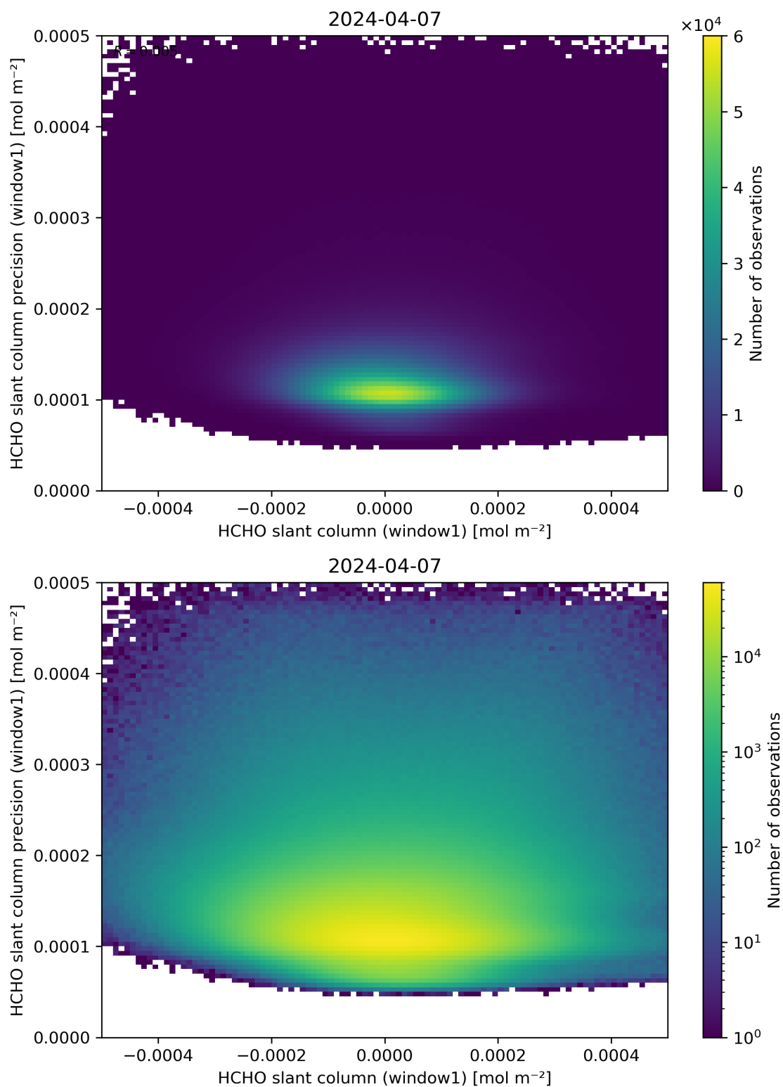
Figure 84: Scatter density plot of “HCHO slant column (window1)” against “HCHO slant column precision (window1)” for 2024-04-06 to 2024-04-08.
