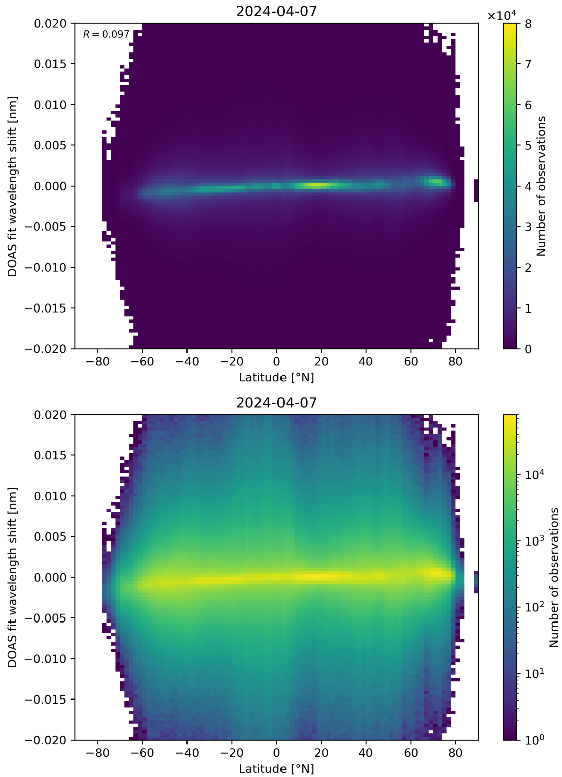
Figure 154: Scatter density plot of “Latitude” against “DOAS fit wavelength shift” for 2024-04-06 to 2024-04-08.
