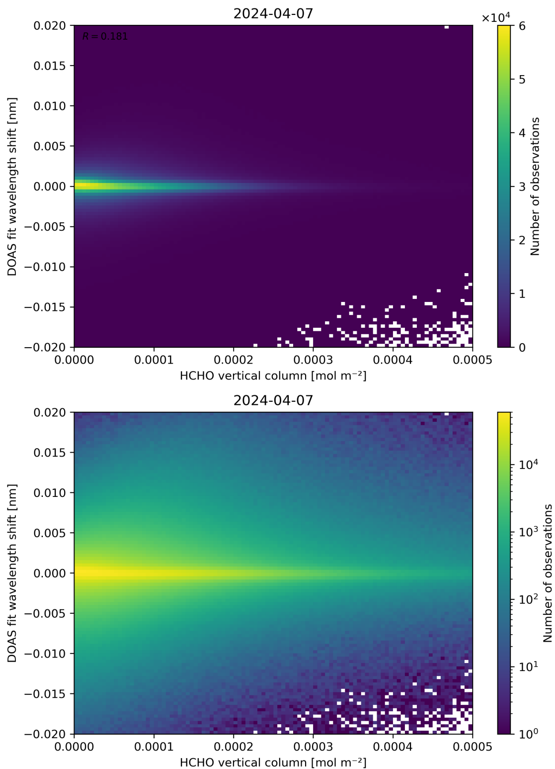
Figure 124: Scatter density plot of “HCHO vertical column” against “DOAS fit wavelength shift” for 2024-04-06 to 2024-04-08.
