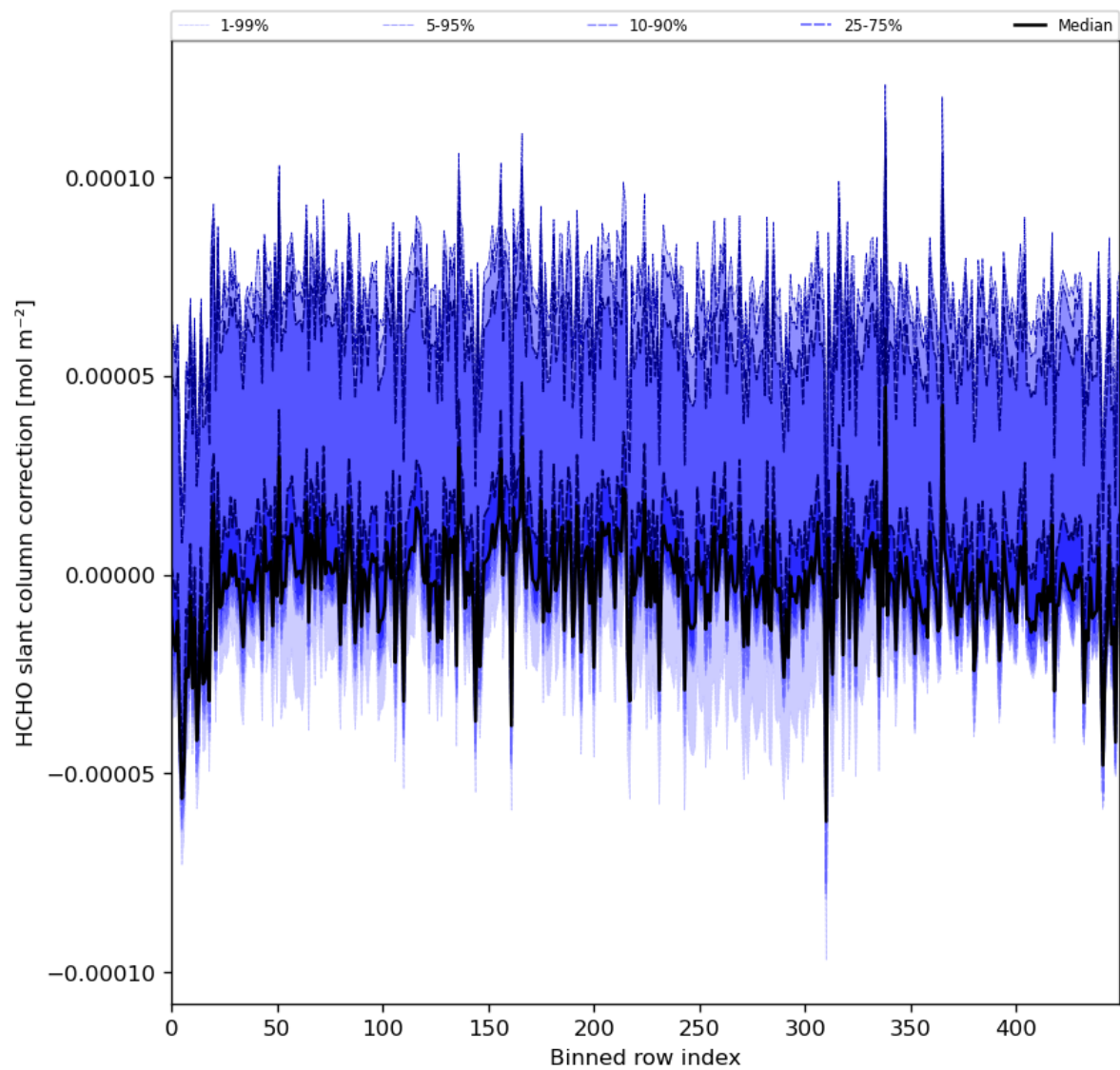
Figure 61: Along track statistics of “HCHO slant column correction” for 2024-04-06 to 2024-04-08
