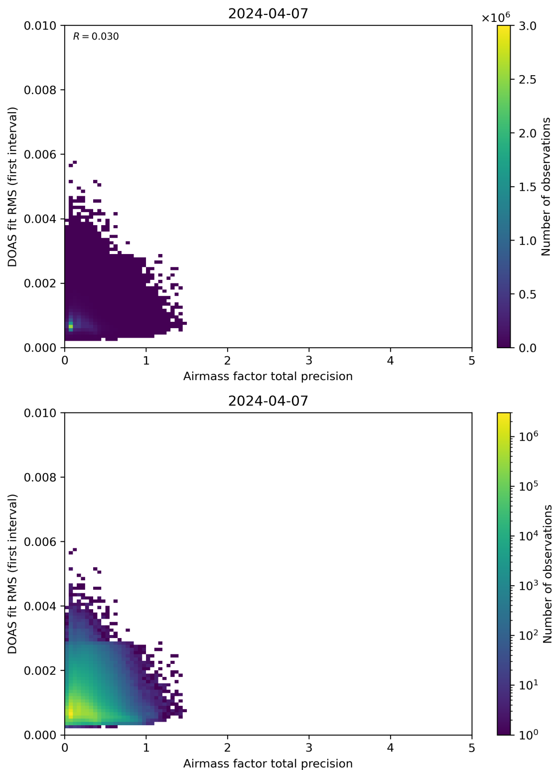
Figure 105: Scatter density plot of “Airmass factor total precision” against “DOAS fit RMS (first interval)” for 2024-04-06 to 2024-04-08.
