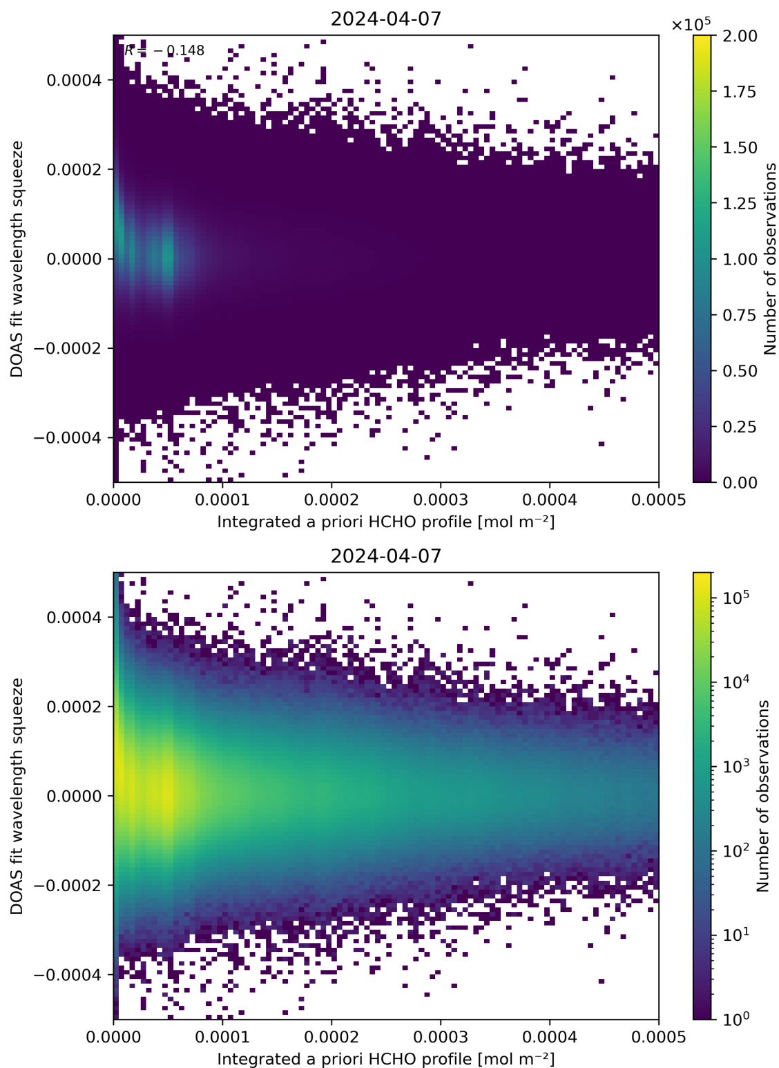
Figure 150: Scatter density plot of “Integrated a priori HCHO profile” against “DOAS fit wavelength squeeze” for 2024-04-06 to 2024-04-08.
