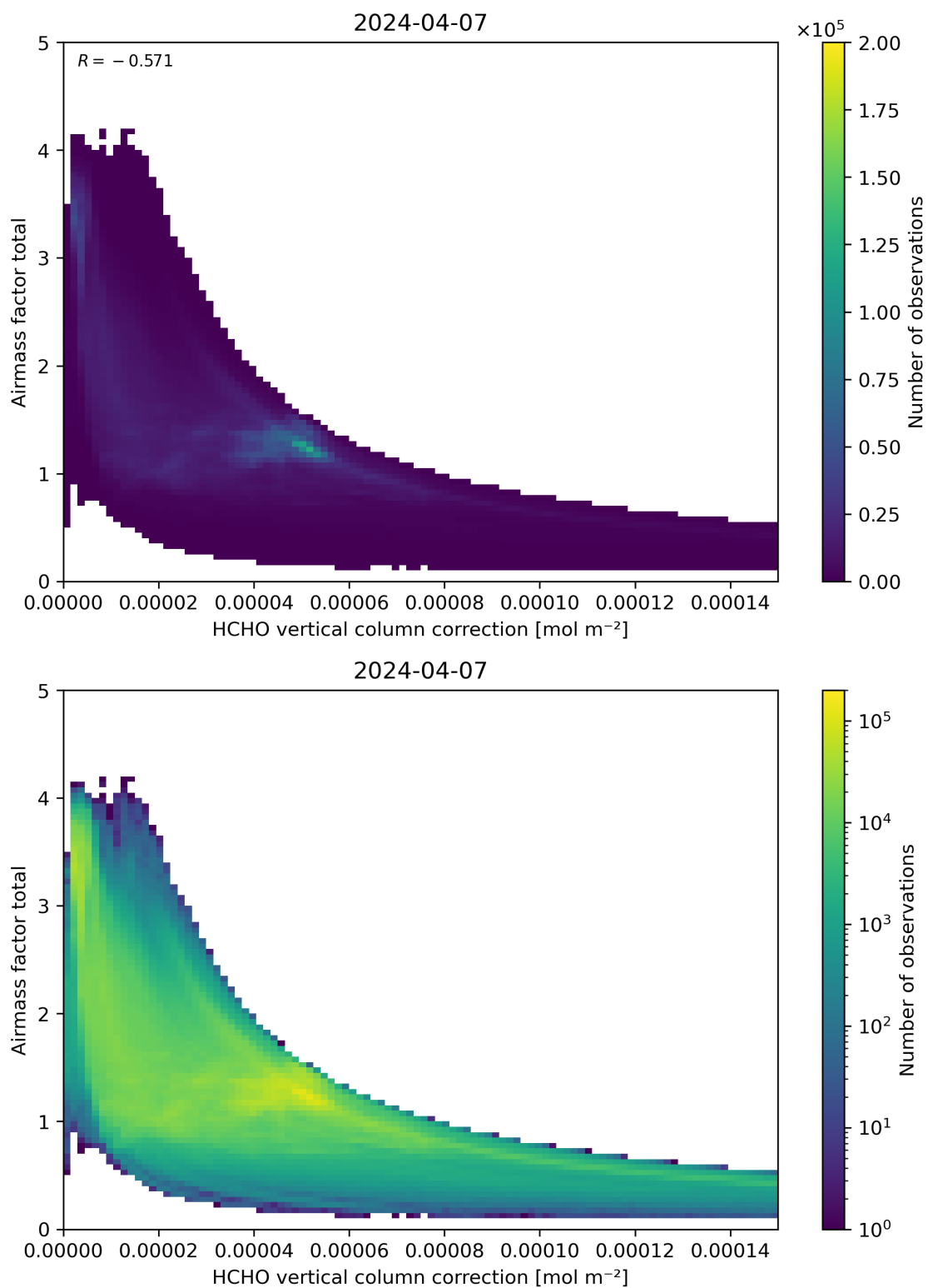
Figure 120: Scatter density plot of “HCHO vertical column correction” against “Airmass factor total” for 2024-04-06 to 2024-04-08.
