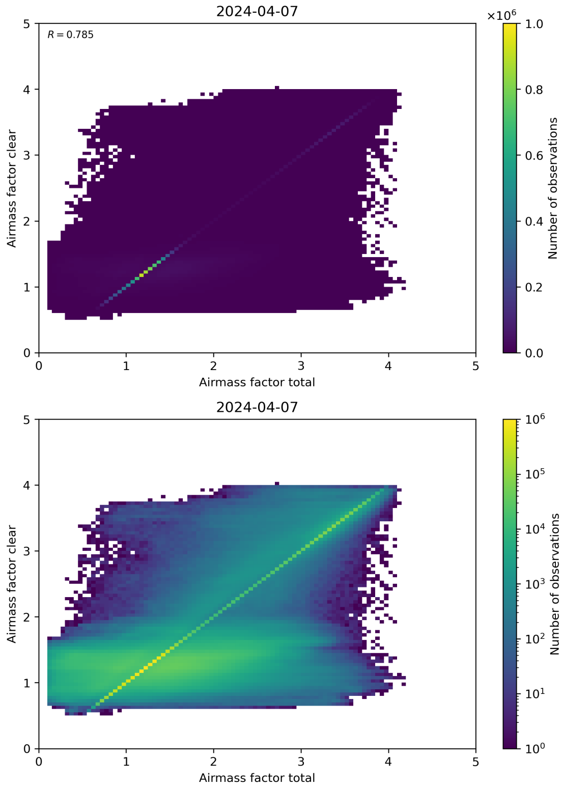
Figure 100: Scatter density plot of “Airmass factor total” against “Airmass factor clear” for 2024-04-06 to 2024-04-08.
