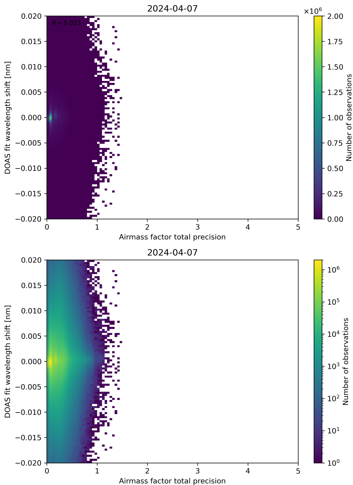
Figure 106: Scatter density plot of “Airmass factor total precision” against “DOAS fit wavelength shift” for 2024-04-06 to 2024-04-08.
