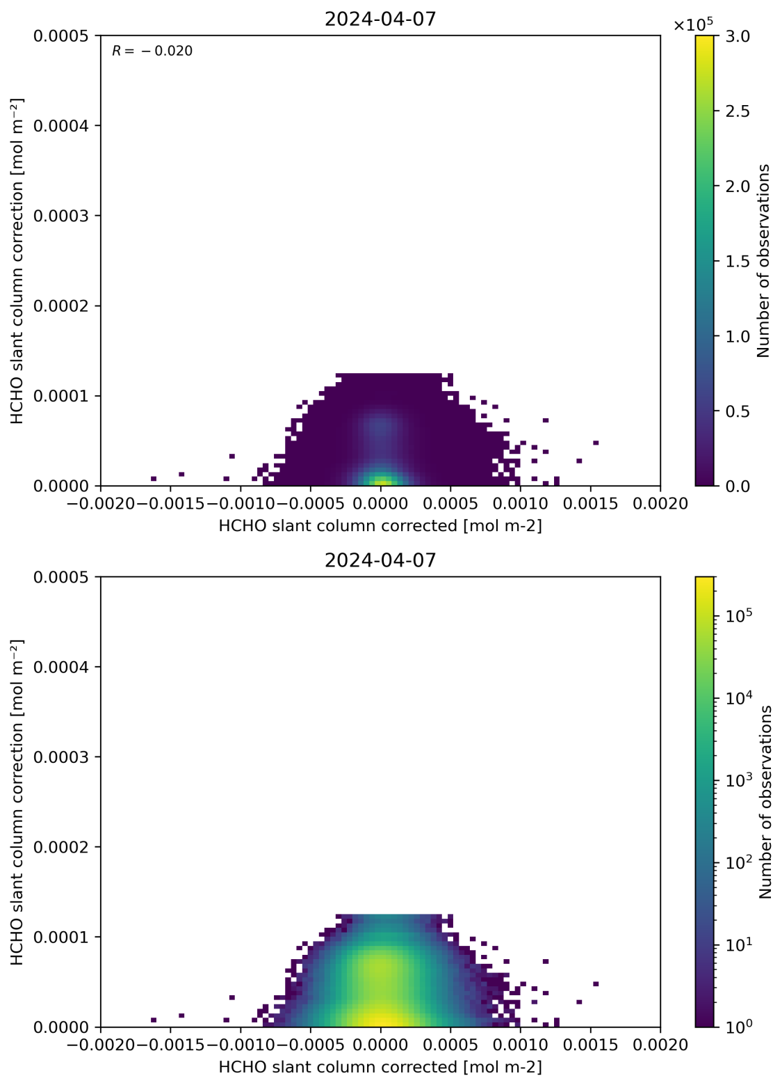
Figure 77: Scatter density plot of “HCHO slant column corrected” against “HCHO slant column correction” for 2024-04-06 to 2024-04-08.
