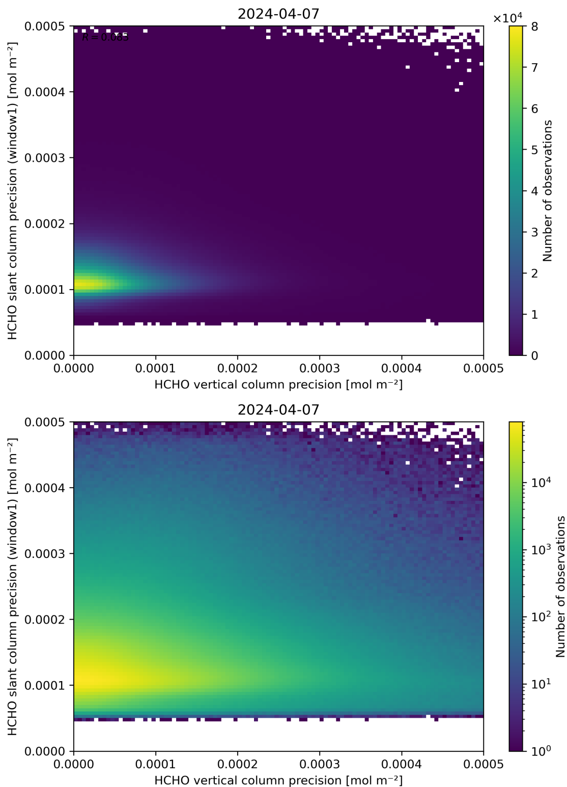
Figure 143: Scatter density plot of “HCHO vertical column precision” against “HCHO slant column precision (window1)” for 2024-04-06 to 2024-04-08.
