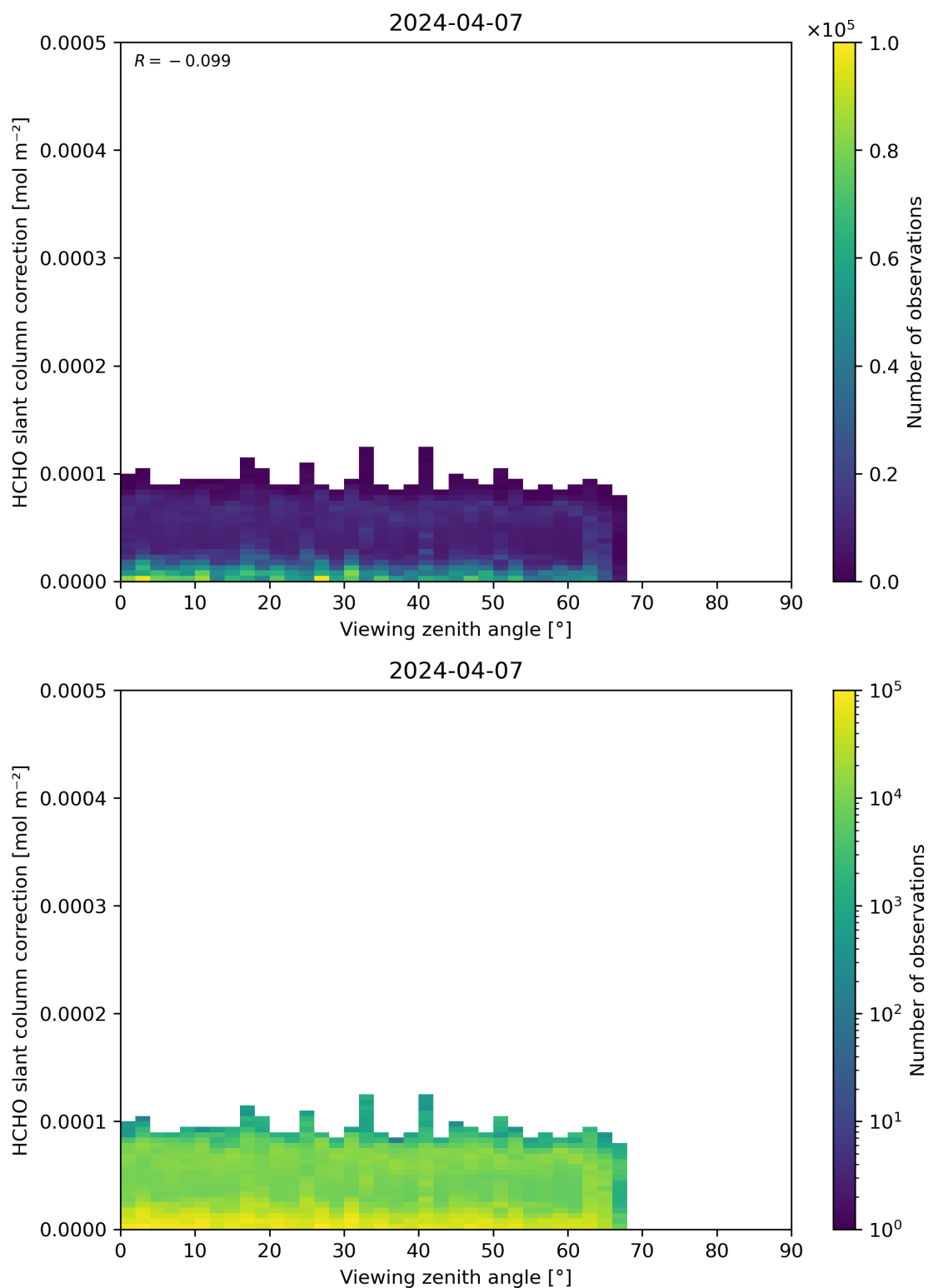
Figure 187: Scatter density plot of “Viewing zenith angle” against “HCHO slant column correction” for 2024-04-06 to 2024-04-08.
