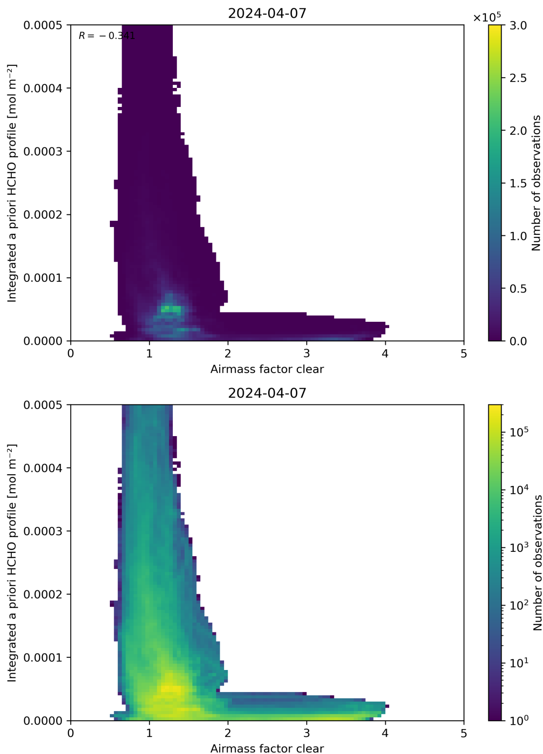
Figure 76: Scatter density plot of “Airmass factor clear” against “Integrated a priori HCHO profile” for 2024-04-06 to 2024-04-08.
