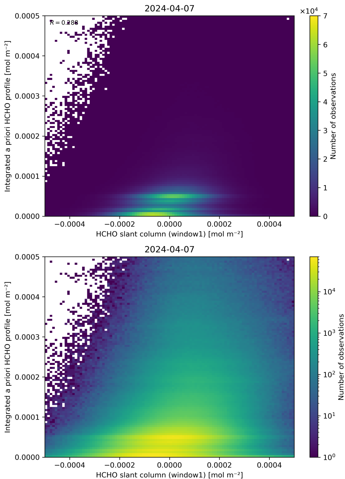
Figure 87: Scatter density plot of “HCHO slant column (window1)” against “Integrated a priori HCHO profile” for 2024-04-06 to 2024-04-08.
