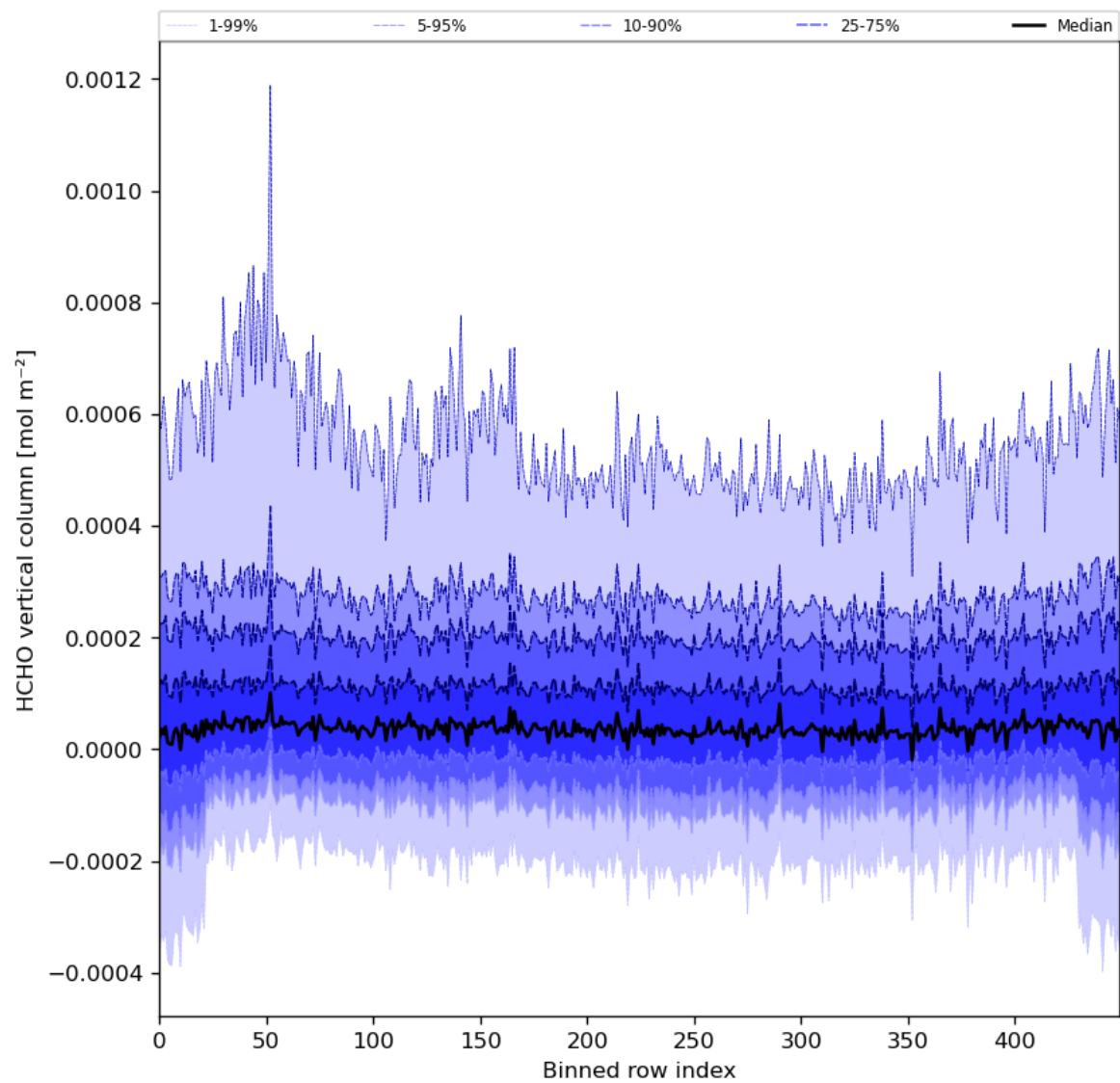
Figure 49: Along track statistics of “HCHO vertical column” for 2024-04-06 to 2024-04-08
