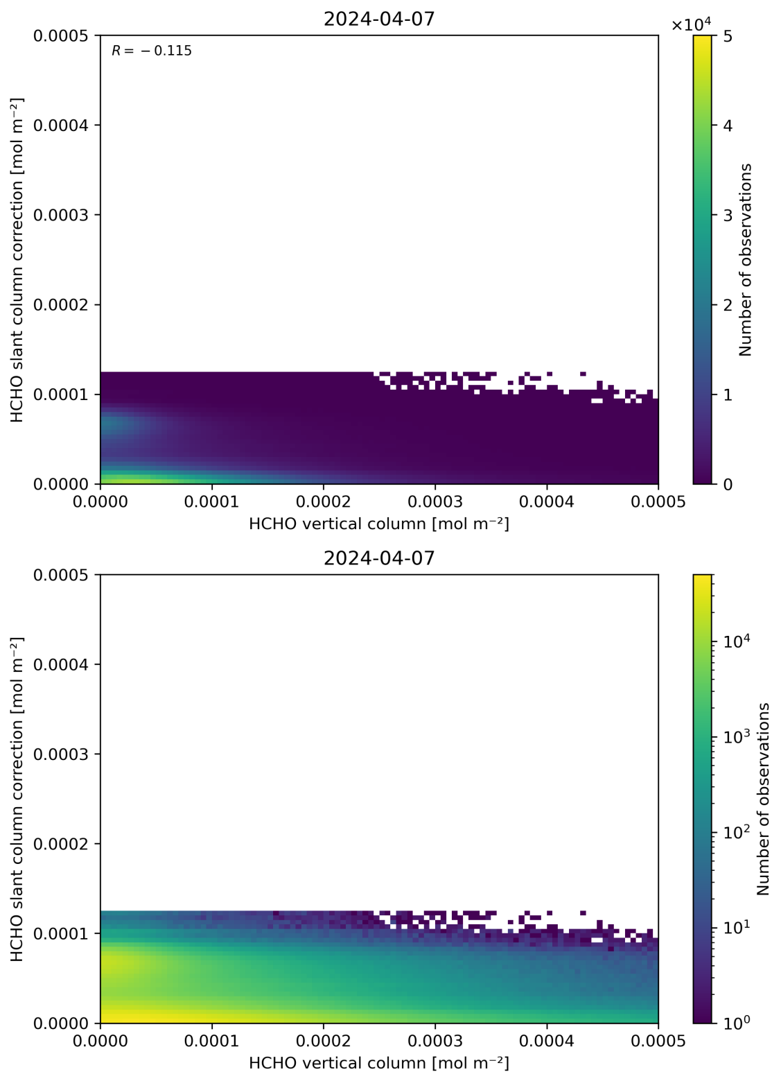
Figure 128: Scatter density plot of “HCHO vertical column” against “HCHO slant column correction” for 2024-04-06 to 2024-04-08.
