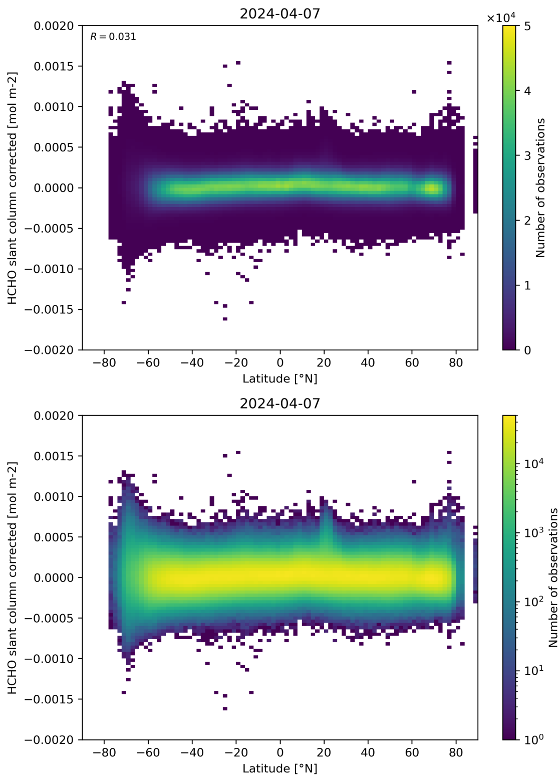
Figure 157: Scatter density plot of “Latitude” against “HCHO slant column corrected” for 2024-04-06 to 2024-04-08.
