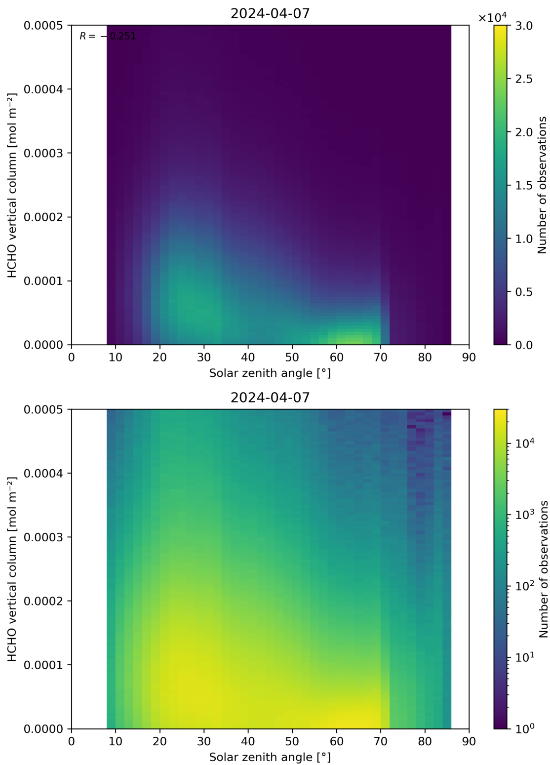
Figure 177: Scatter density plot of “Solar zenith angle” against “HCHO vertical column” for 2024-04-06 to 2024-04-08.
