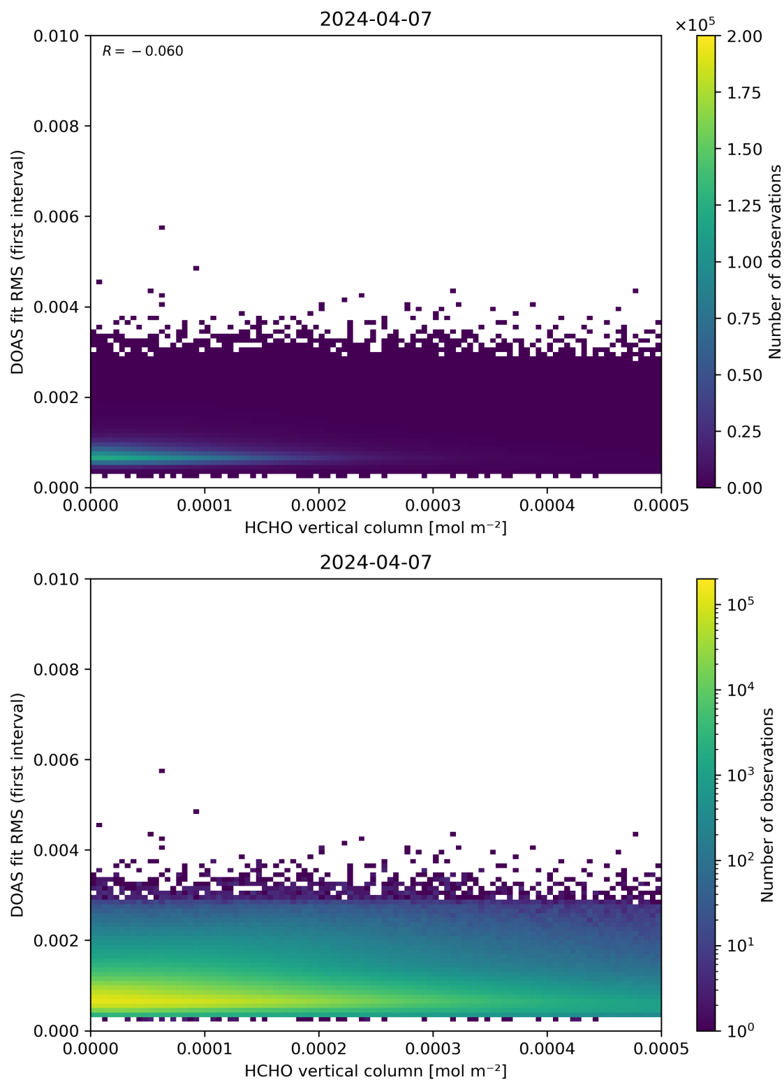
Figure 123: Scatter density plot of “HCHO vertical column” against “DOAS fit RMS (first interval)” for 2024-04-06 to 2024-04-08.
