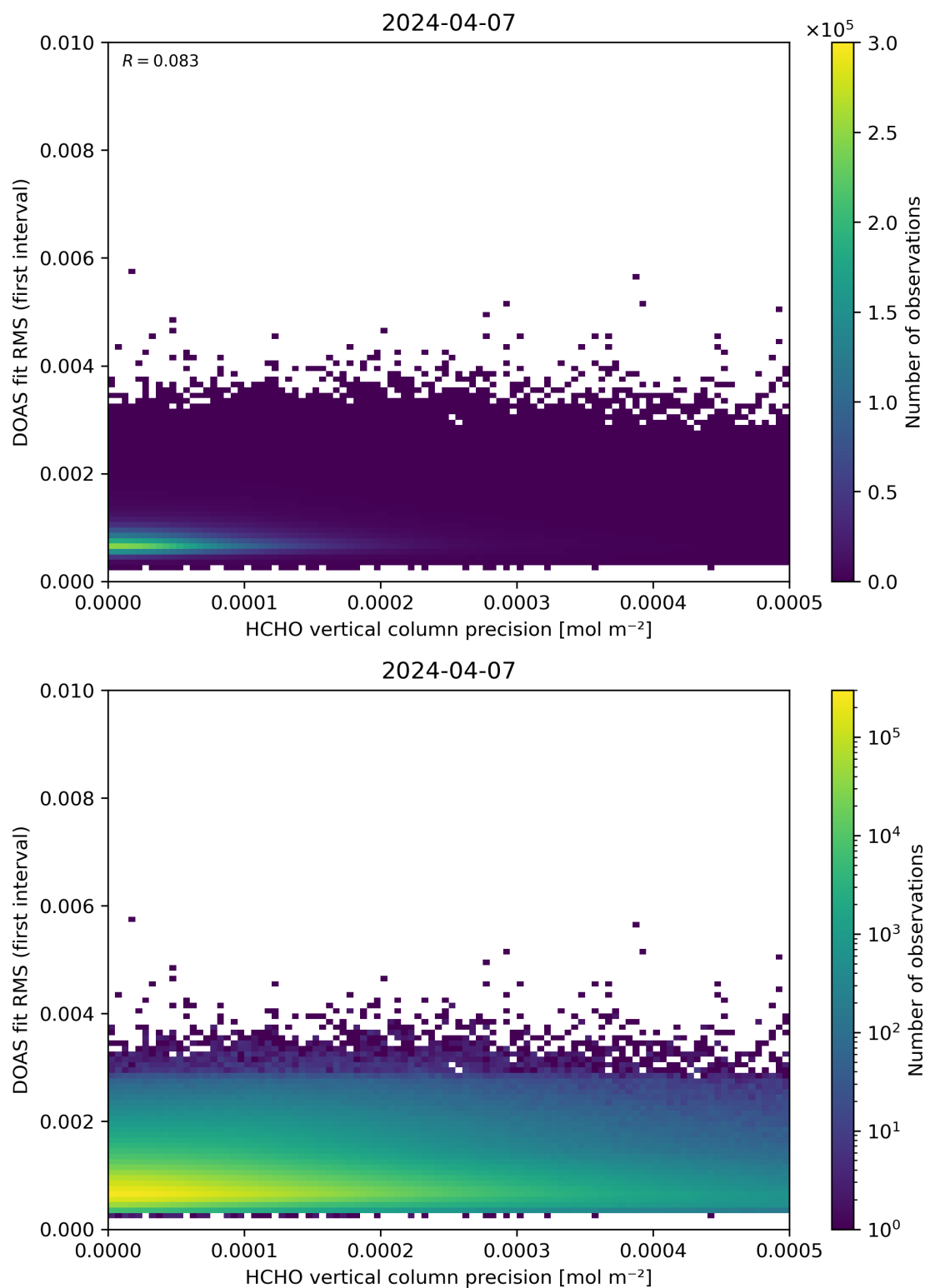
Figure 136: Scatter density plot of “HCHO vertical column precision” against “DOAS fit RMS (first interval)” for 2024-04-06 to 2024-04-08.
