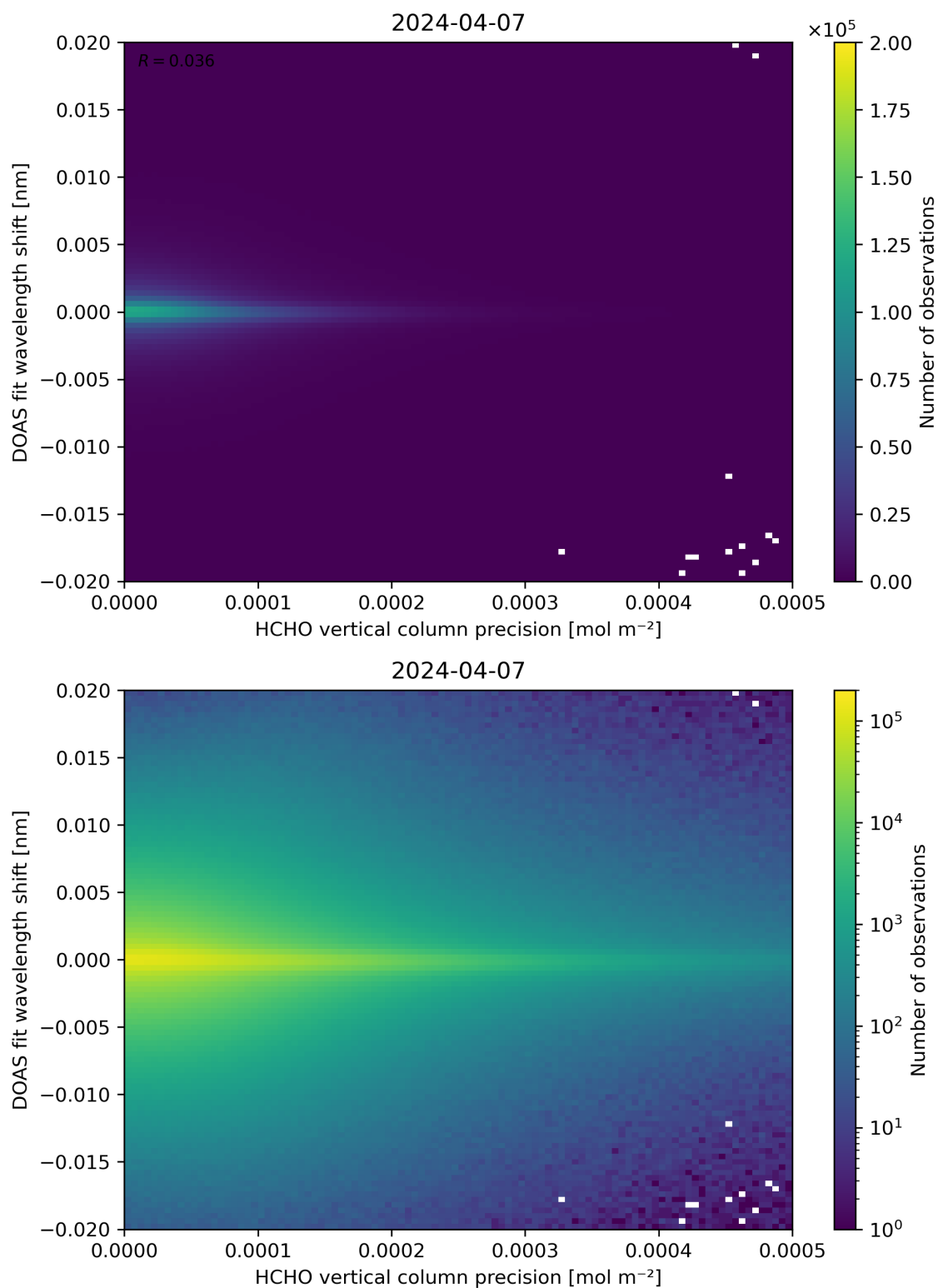
Figure 137: Scatter density plot of “HCHO vertical column precision” against “DOAS fit wavelength shift” for 2024-04-06 to 2024-04-08.
