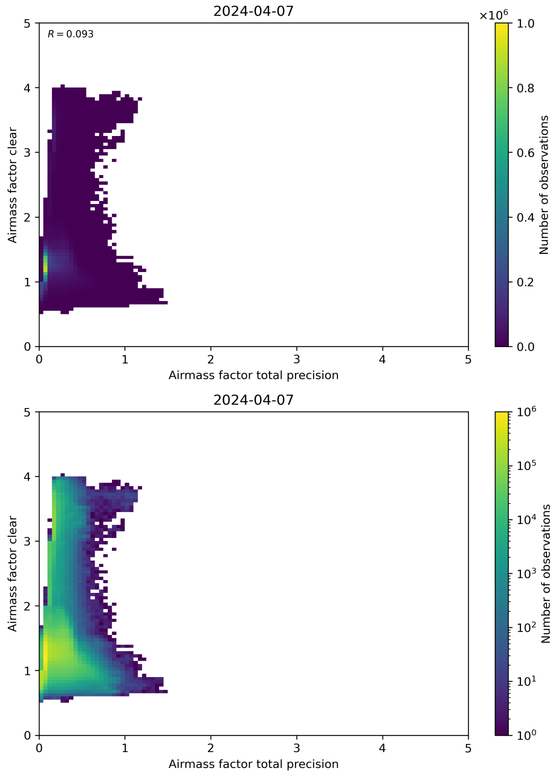
Figure 108: Scatter density plot of “Airmass factor total precision” against “Airmass factor clear” for 2024-04-06 to 2024-04-08.
