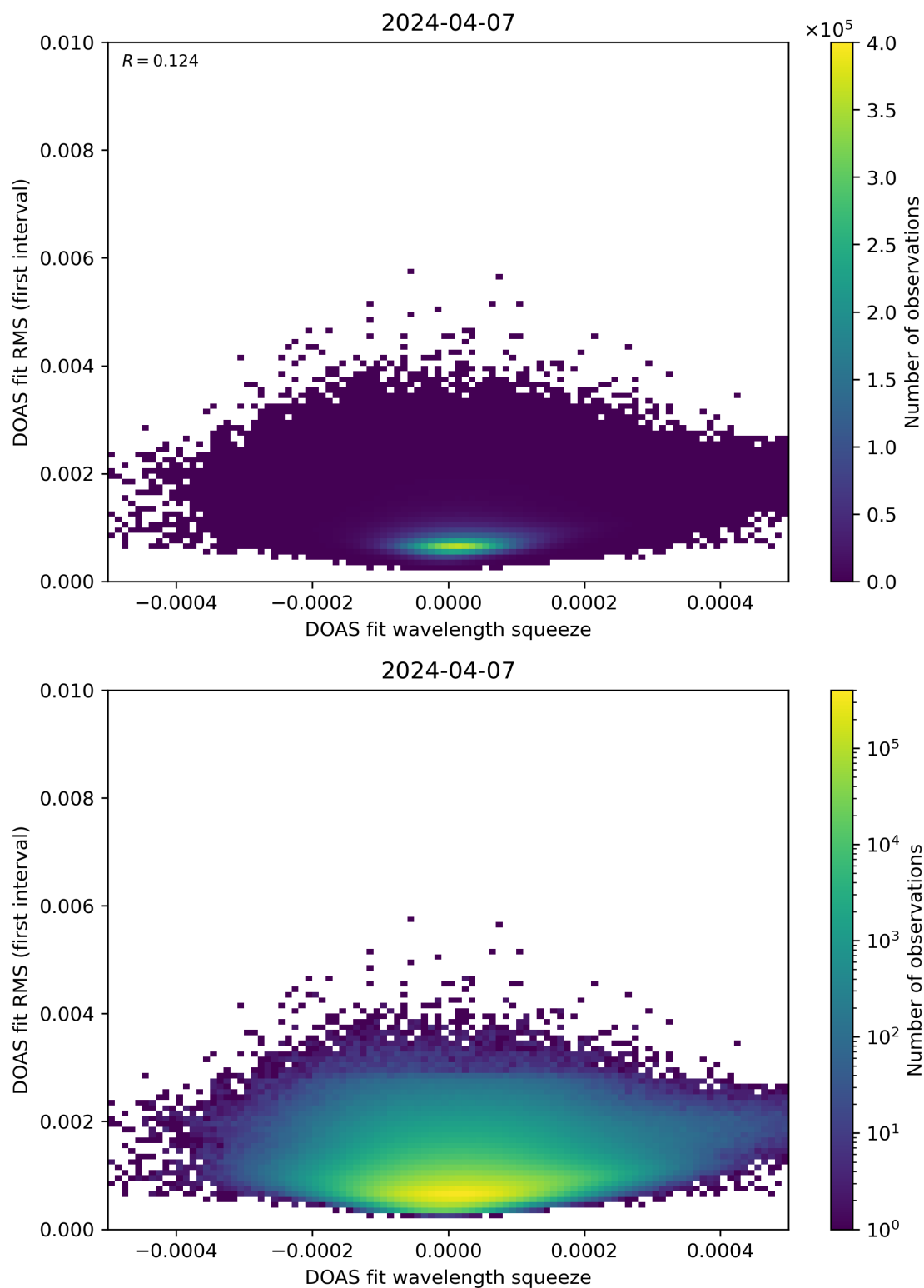
Figure 68: Scatter density plot of “DOAS fit wavelength squeeze” against “DOAS fit RMS (first interval)” for 2024-04-06 to 2024-04-08.
