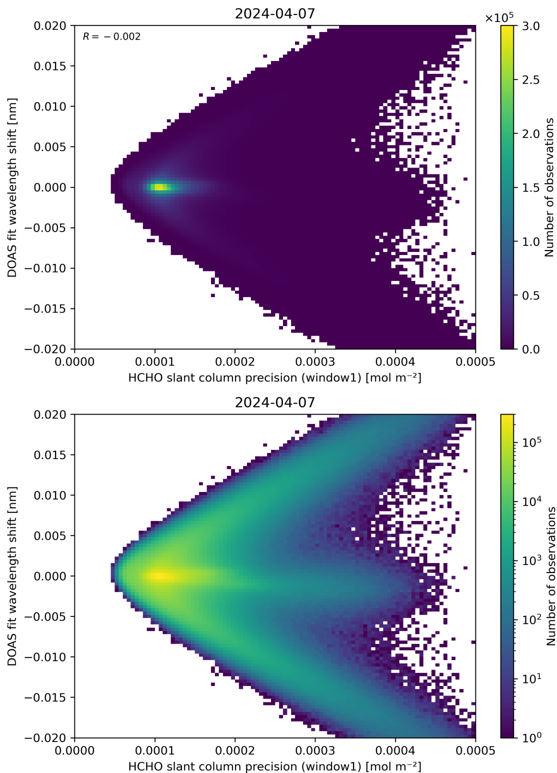
Figure 89: Scatter density plot of “HCHO slant column precision (window1)” against “DOAS fit wavelength shift” for 2024-04-06 to 2024-04-08.
