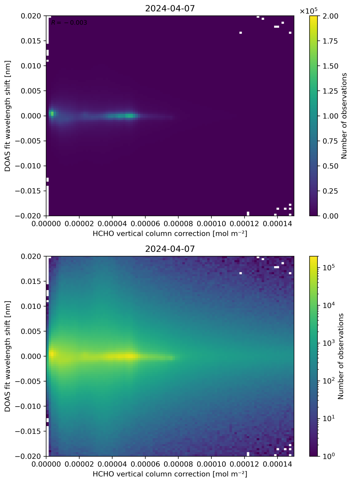
Figure 113: Scatter density plot of “HCHO vertical column correction” against “DOAS fit wavelength shift” for 2024-04-06 to 2024-04-08.
