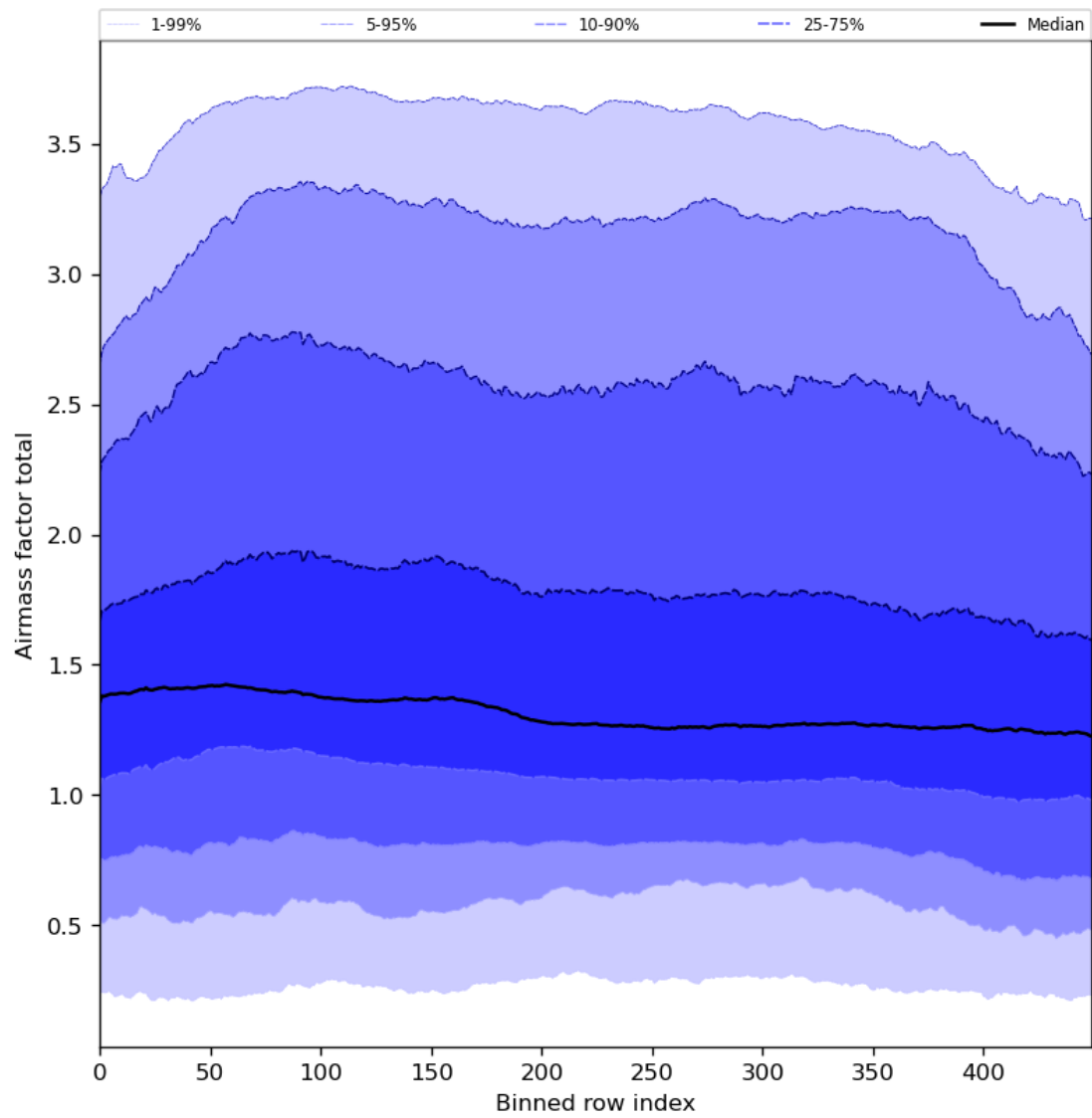
Figure 54: Along track statistics of “Airmass factor total” for 2024-04-06 to 2024-04-08
