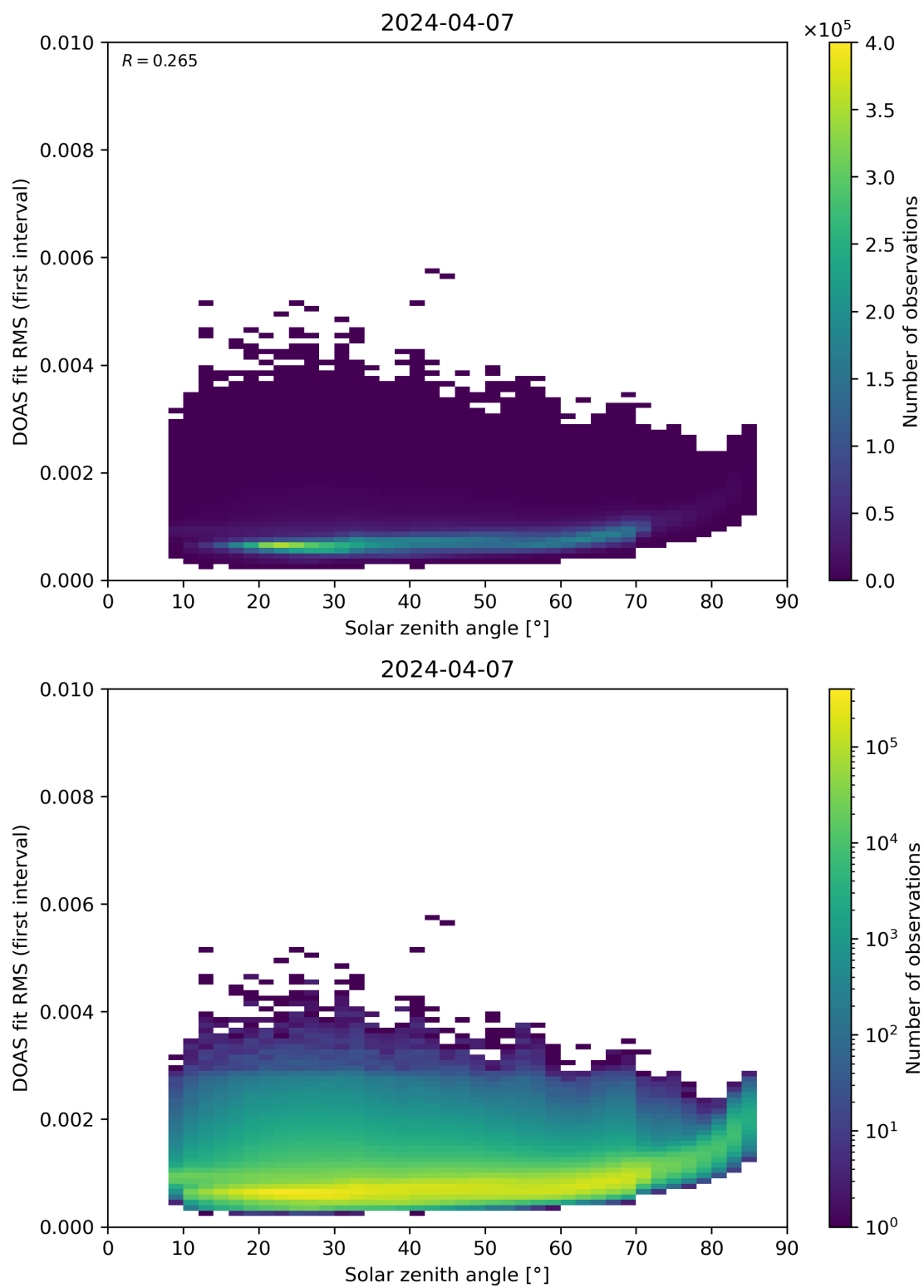
Figure 167: Scatter density plot of “Solar zenith angle” against “DOAS fit RMS (first interval)” for 2024-04-06 to 2024-04-08.
