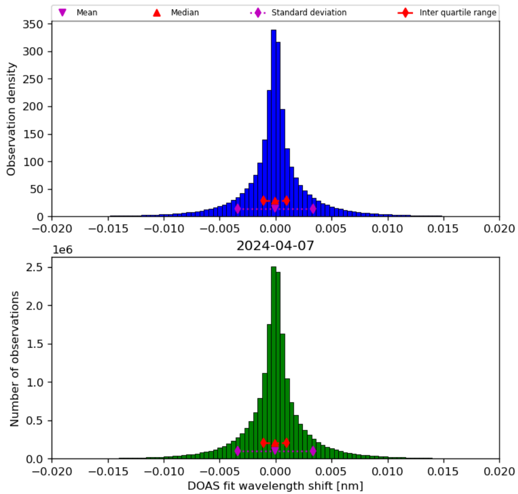
Figure 44: Histogram of “DOAS fit wavelength shift” for 2024-04-06 to 2024-04-08
