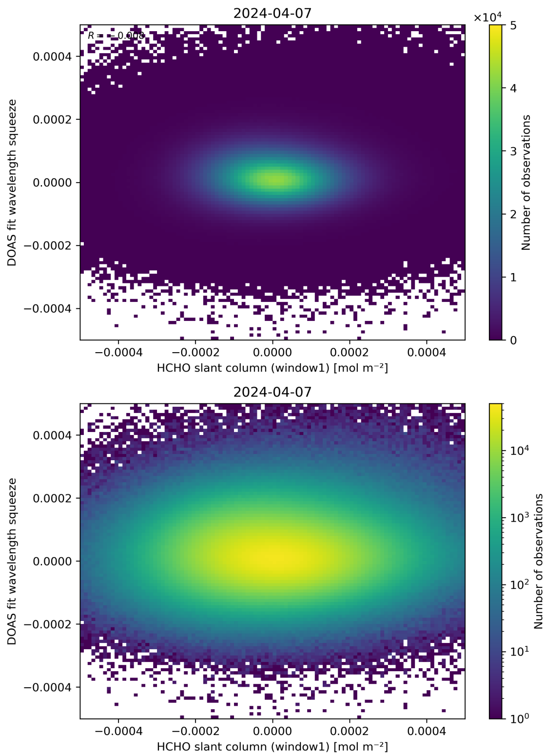
Figure 80: Scatter density plot of “HCHO slant column (window1)” against “DOAS fit wavelength squeeze” for 2024-04-06 to 2024-04-08.
