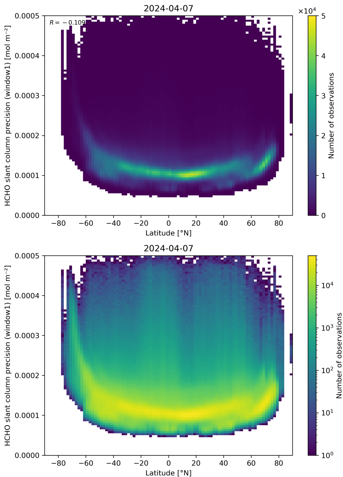
Figure 160: Scatter density plot of “Latitude” against “HCHO slant column precision (window1)” for 2024-04-06 to 2024-04-08.
