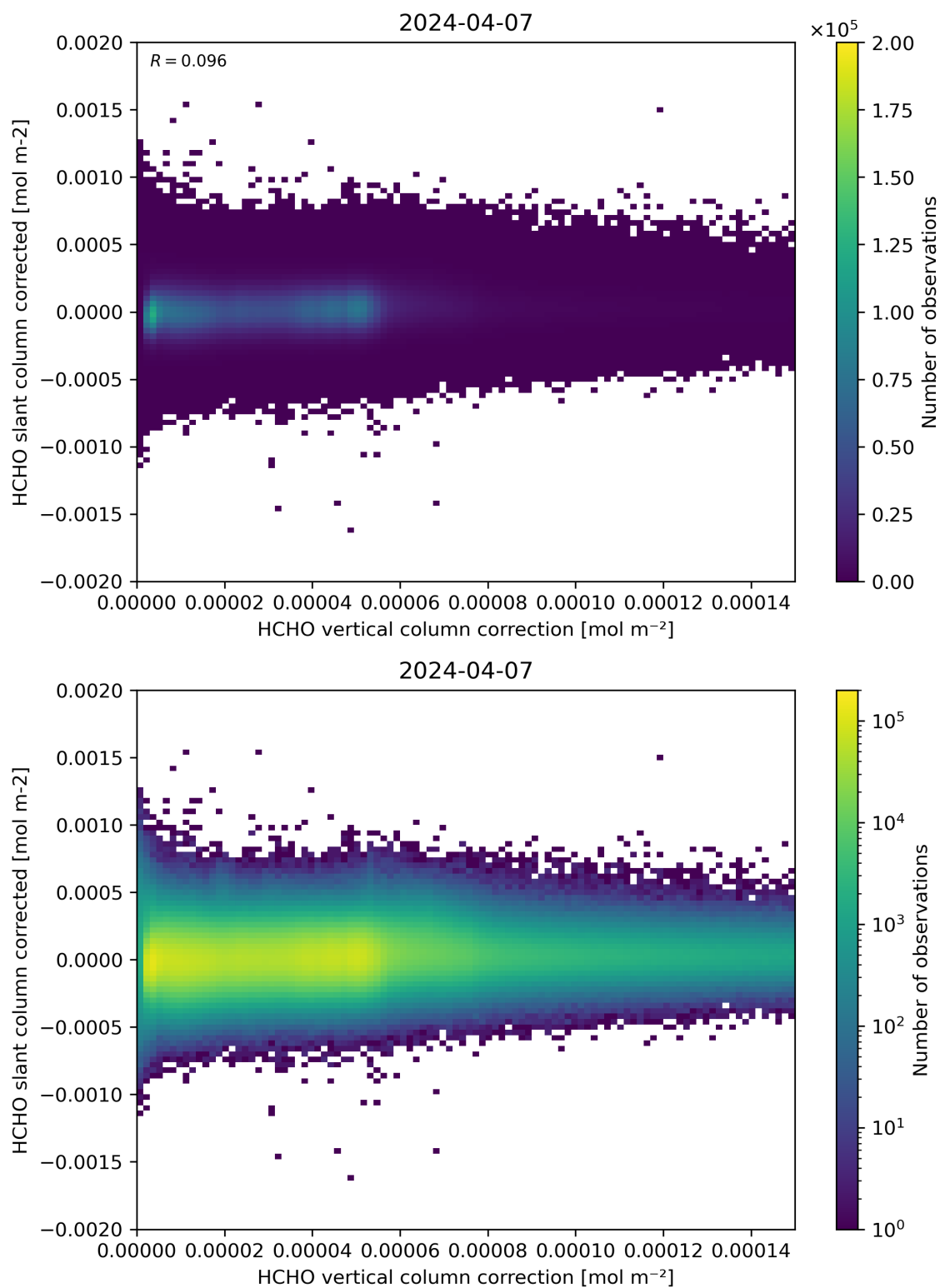
Figure 116: Scatter density plot of “HCHO vertical column correction” against “HCHO slant column corrected” for 2024-04-06 to 2024-04-08.
