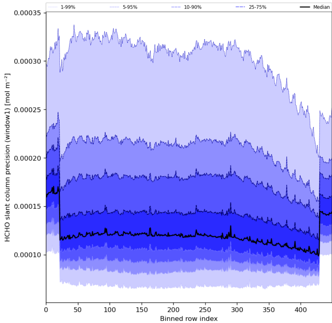
Figure 53: Along track statistics of “HCHO slant column precision (window1)” for 2024-04-06 to 2024-04-08
