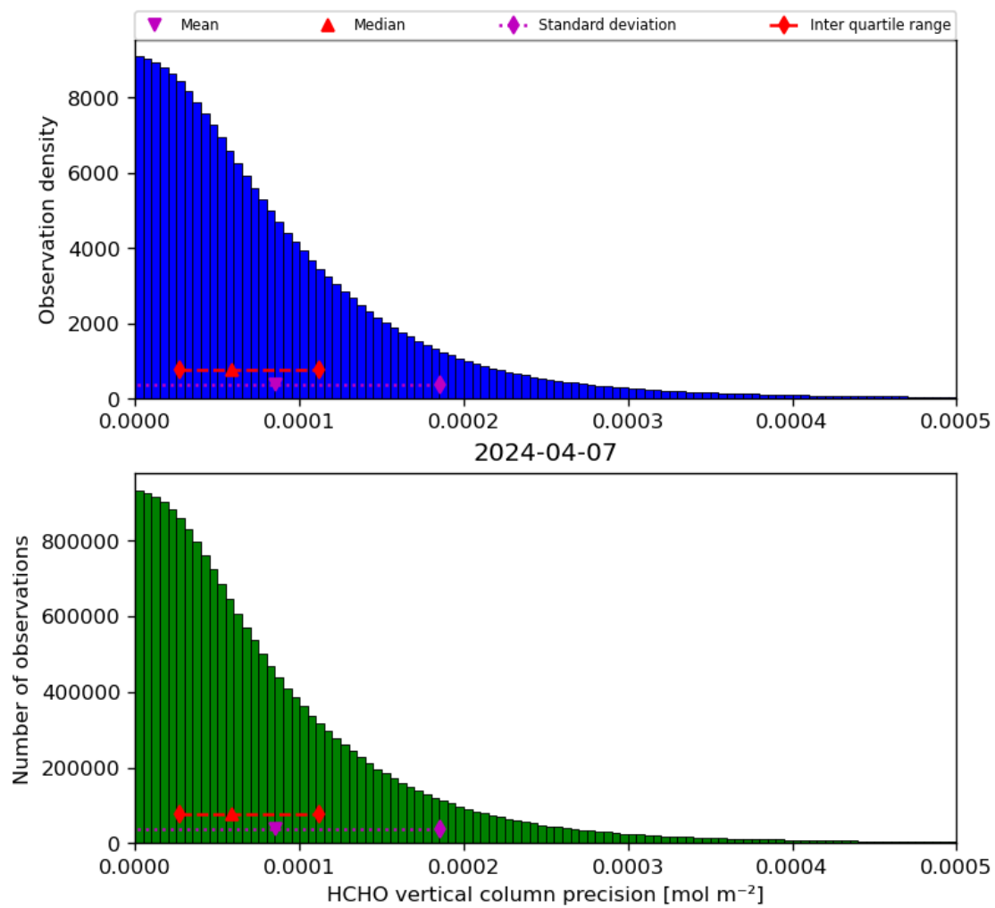
Figure 36: Histogram of “HCHO vertical column precision” for 2024-04-06 to 2024-04-08
