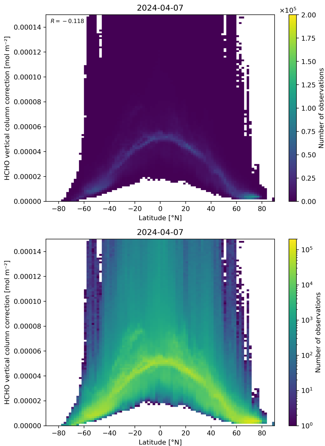
Figure 164: Scatter density plot of “Latitude” against “HCHO vertical column correction” for 2024-04-06 to 2024-04-08.
