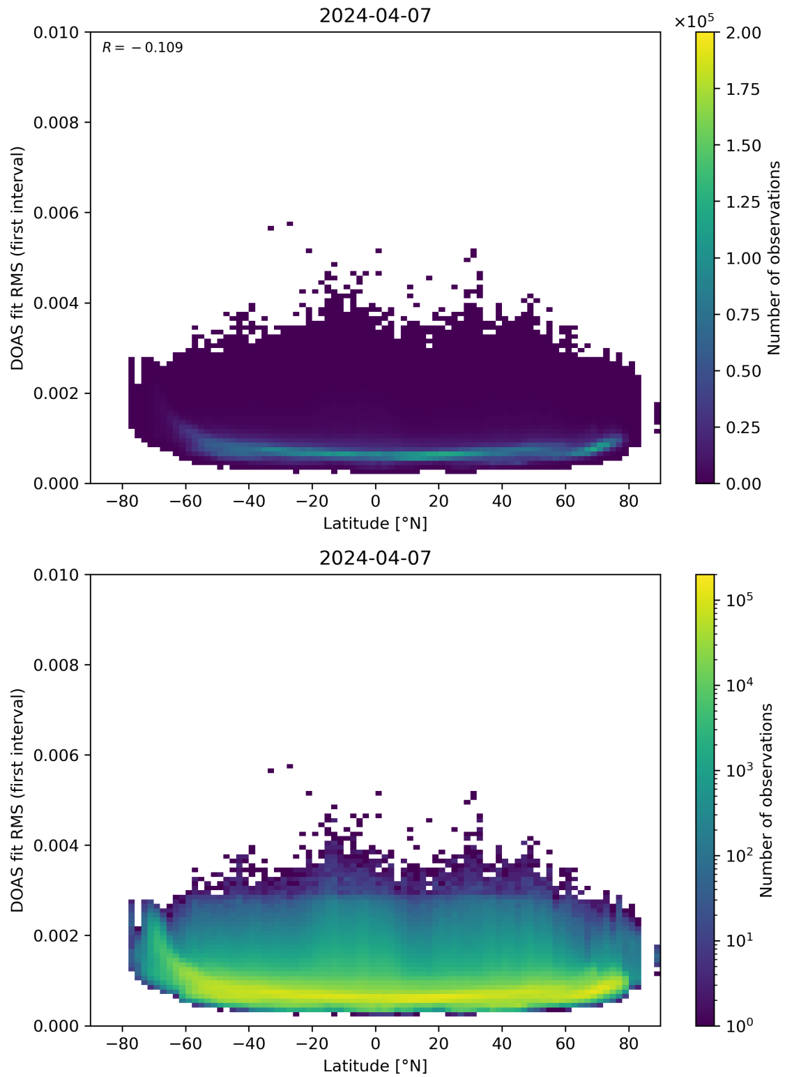
Figure 153: Scatter density plot of “Latitude” against “DOAS fit RMS (first interval)” for 2024-04-06 to 2024-04-08.
