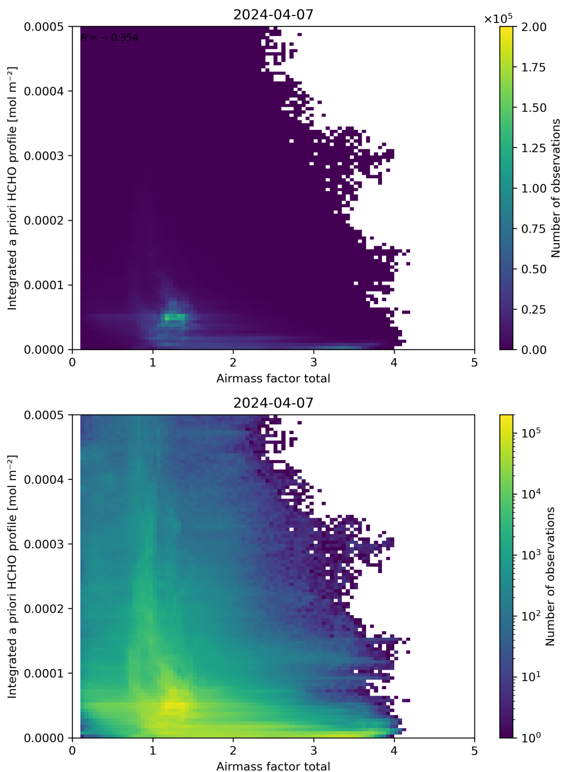
Figure 104: Scatter density plot of “Air mass factor total” against “Integrated a priori HCHO profile” for 2024-04-06 to 2024-04-08.
