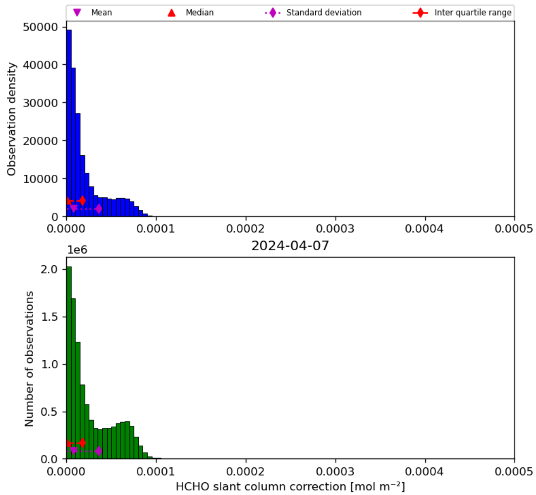
Figure 47: Histogram of “HCHO slant column correction” for 2024-04-06 to 2024-04-08
