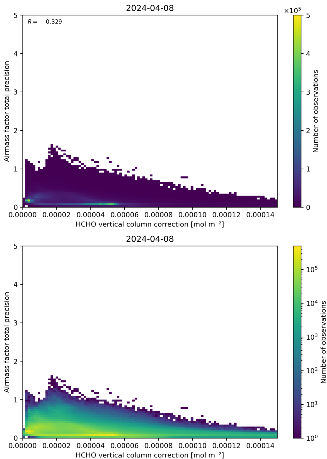
Figure 121: Scatter density plot of “HCHO vertical column correction” against “Airmass factor total precision” for 2024-04-07 to 2024-04-09.
