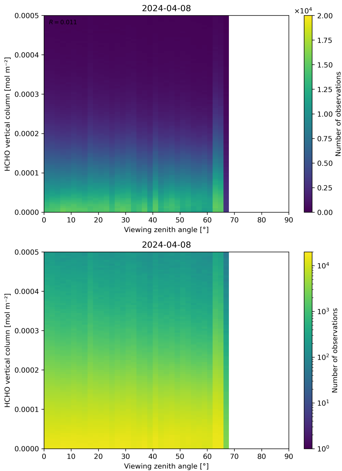
Figure 192: Scatter density plot of “Viewing zenith angle” against “HCHO vertical column” for 2024-04-07 to 2024-04-09.
