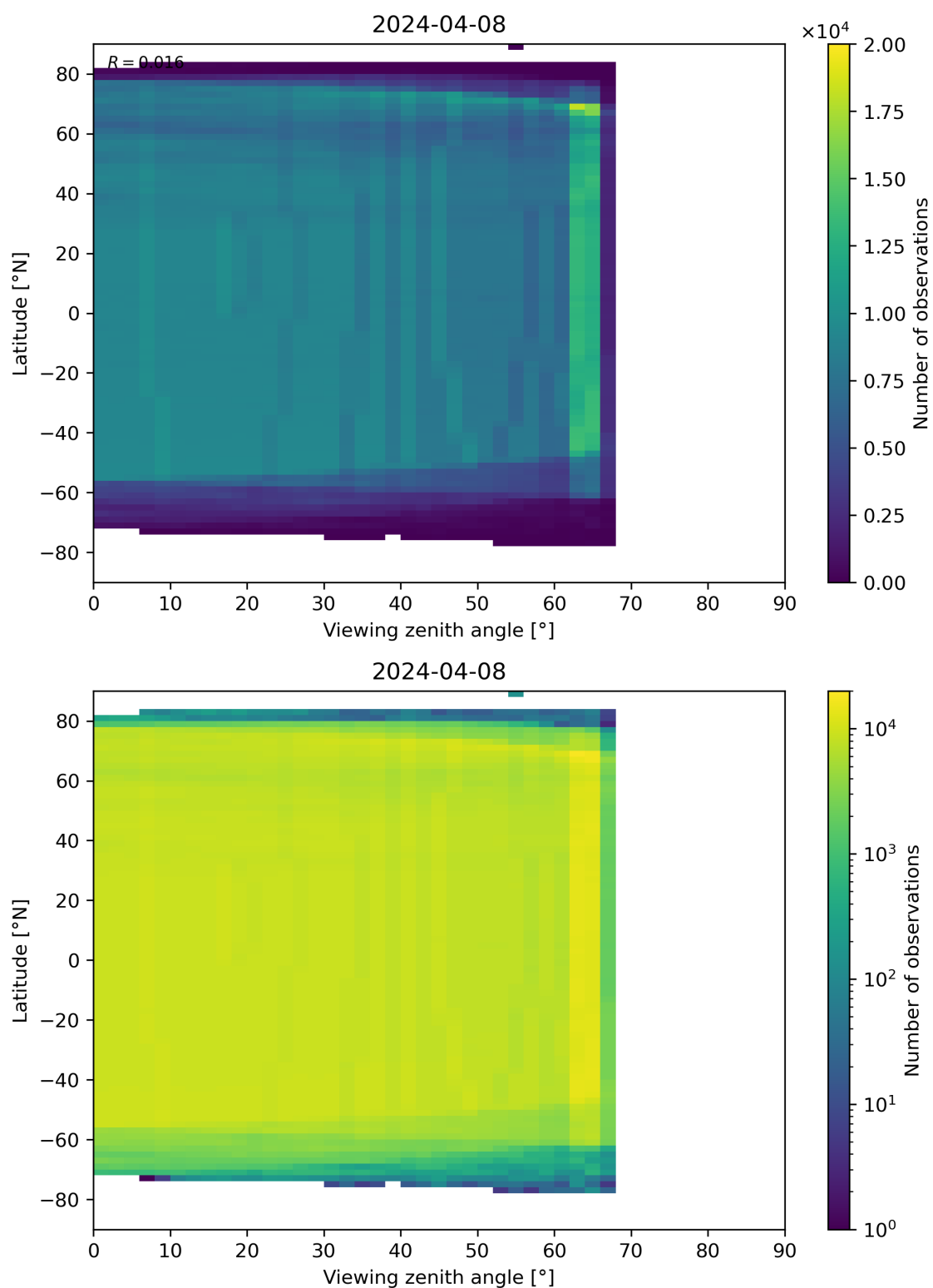
Figure 196: Scatter density plot of “Viewing zenith angle” against “Latitude” for 2024-04-07 to 2024-04-09.
