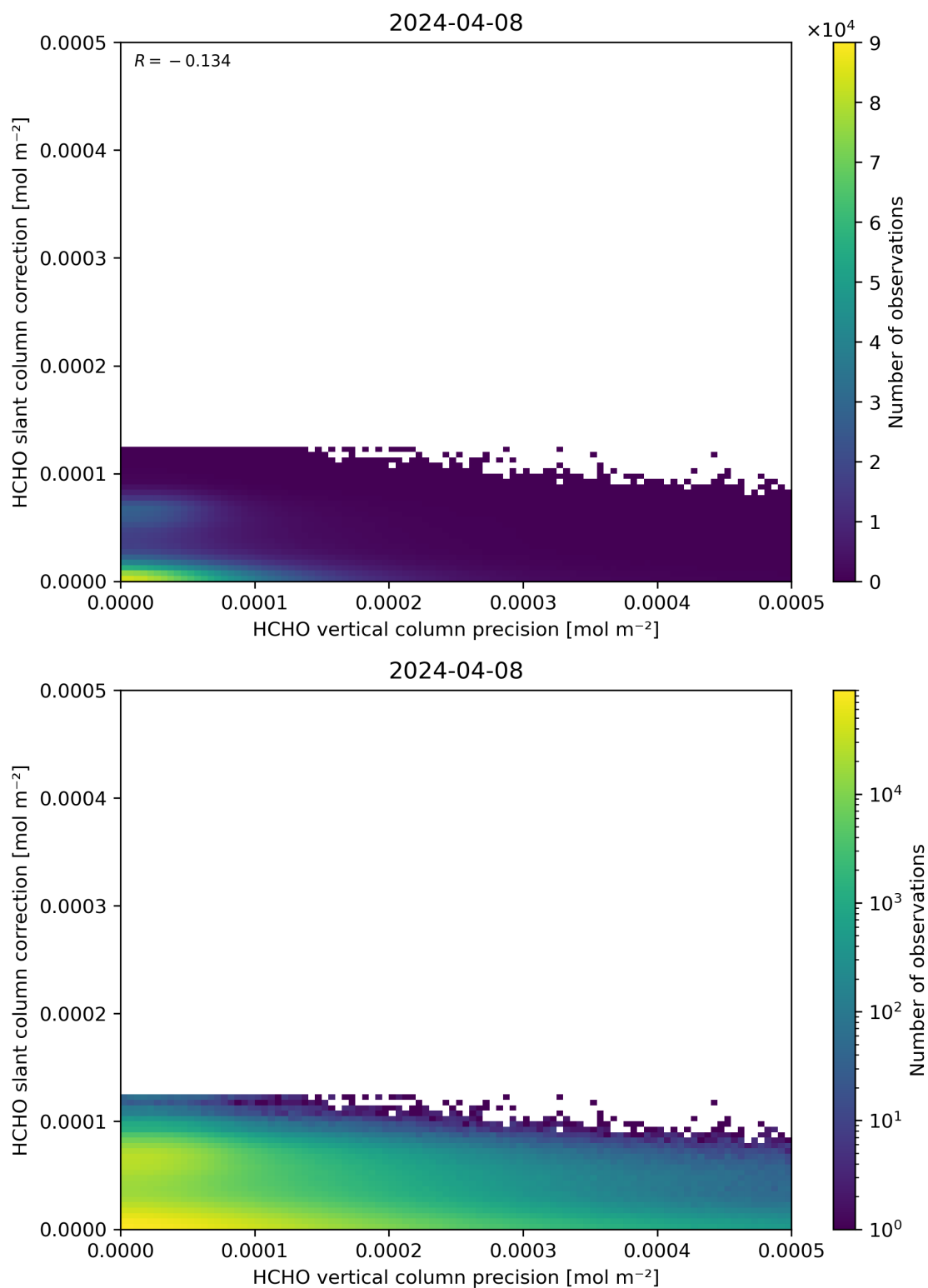
Figure 141: Scatter density plot of “HCHO vertical column precision” against “HCHO slant column correction” for 2024-04-07 to 2024-04-09.
