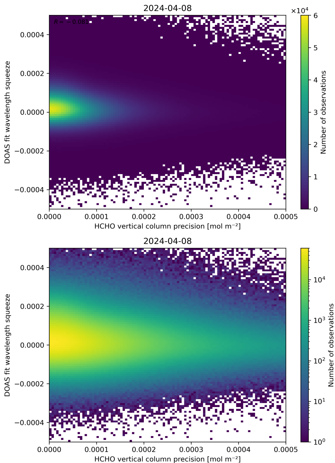
Figure 138: Scatter density plot of “HCHO vertical column precision” against “DOAS fit wavelength squeeze” for 2024-04-07 to 2024-04-09.
