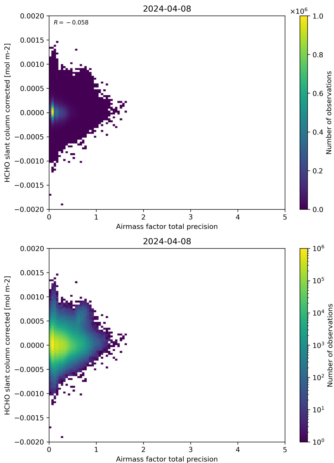
Figure 109: Scatter density plot of “Airmass factor total precision” against “HCHO slant column corrected” for 2024-04-07 to 2024-04-09.
