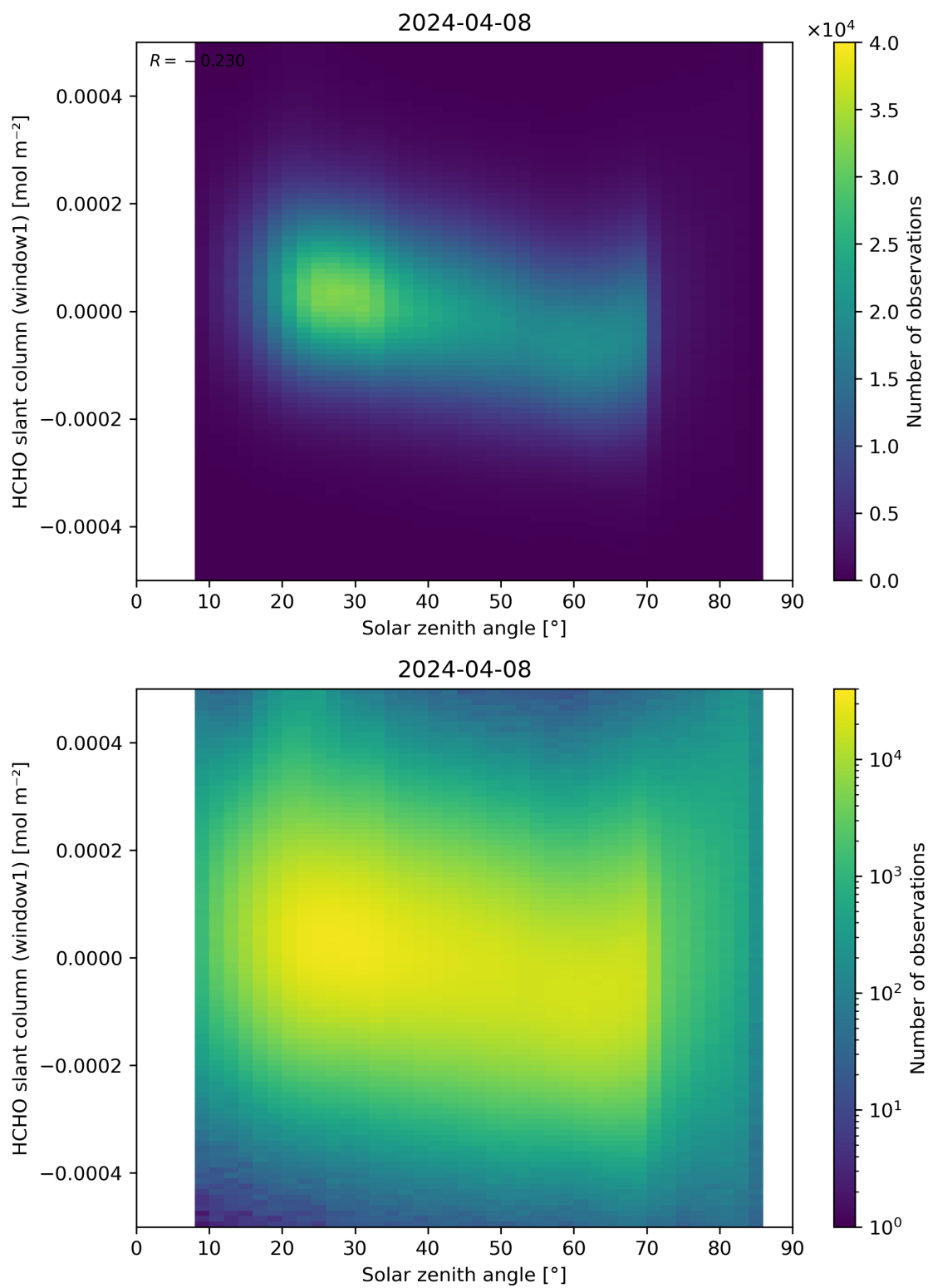
Figure 173: Scatter density plot of “Solar zenith angle” against “HCHO slant column (window1)” for 2024-04-07 to 2024-04-09.
