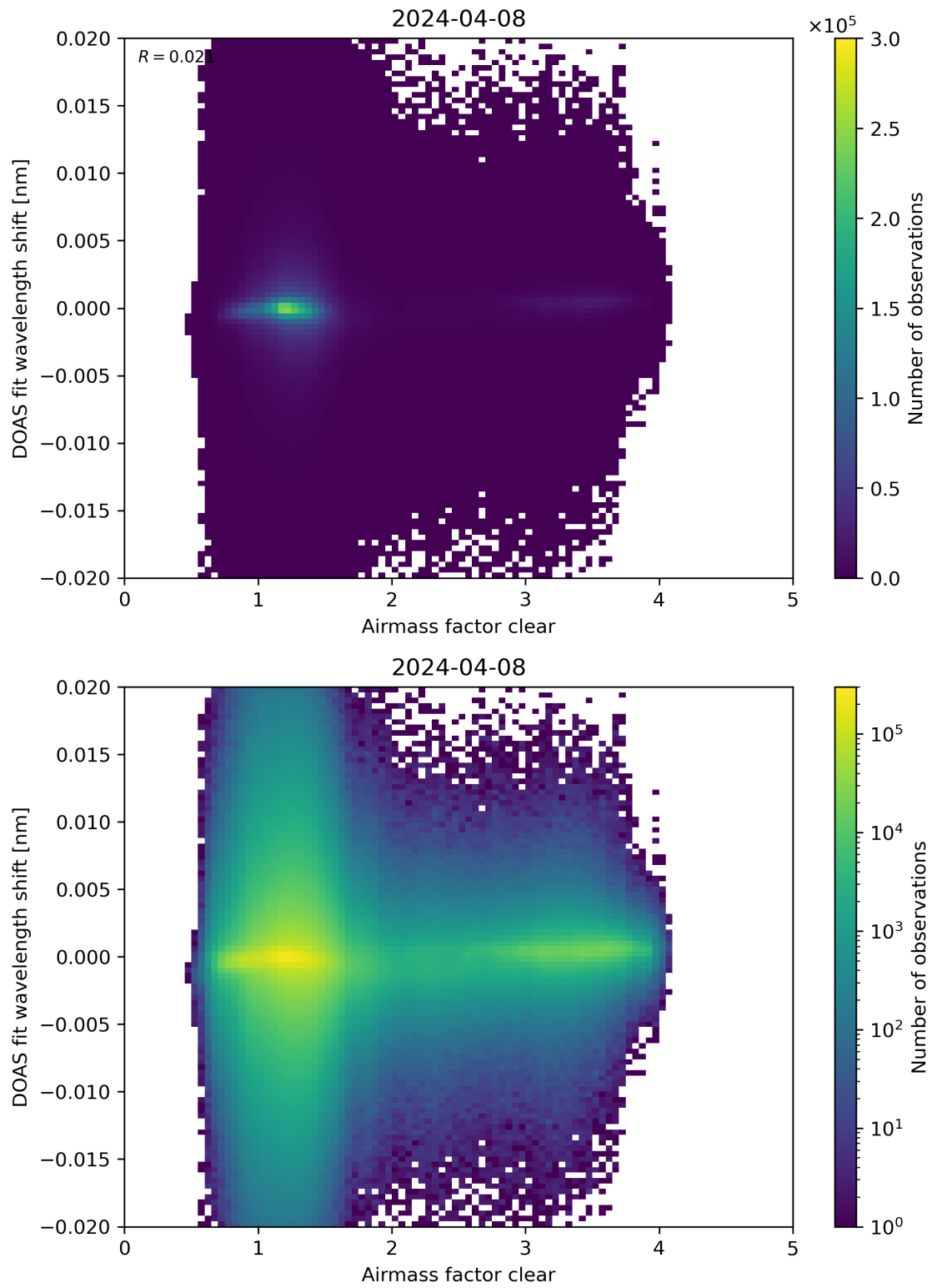
Figure 72: Scatter density plot of “Airmass factor clear” against “DOAS fit wavelength shift” for 2024-04-07 to 2024-04-09.
