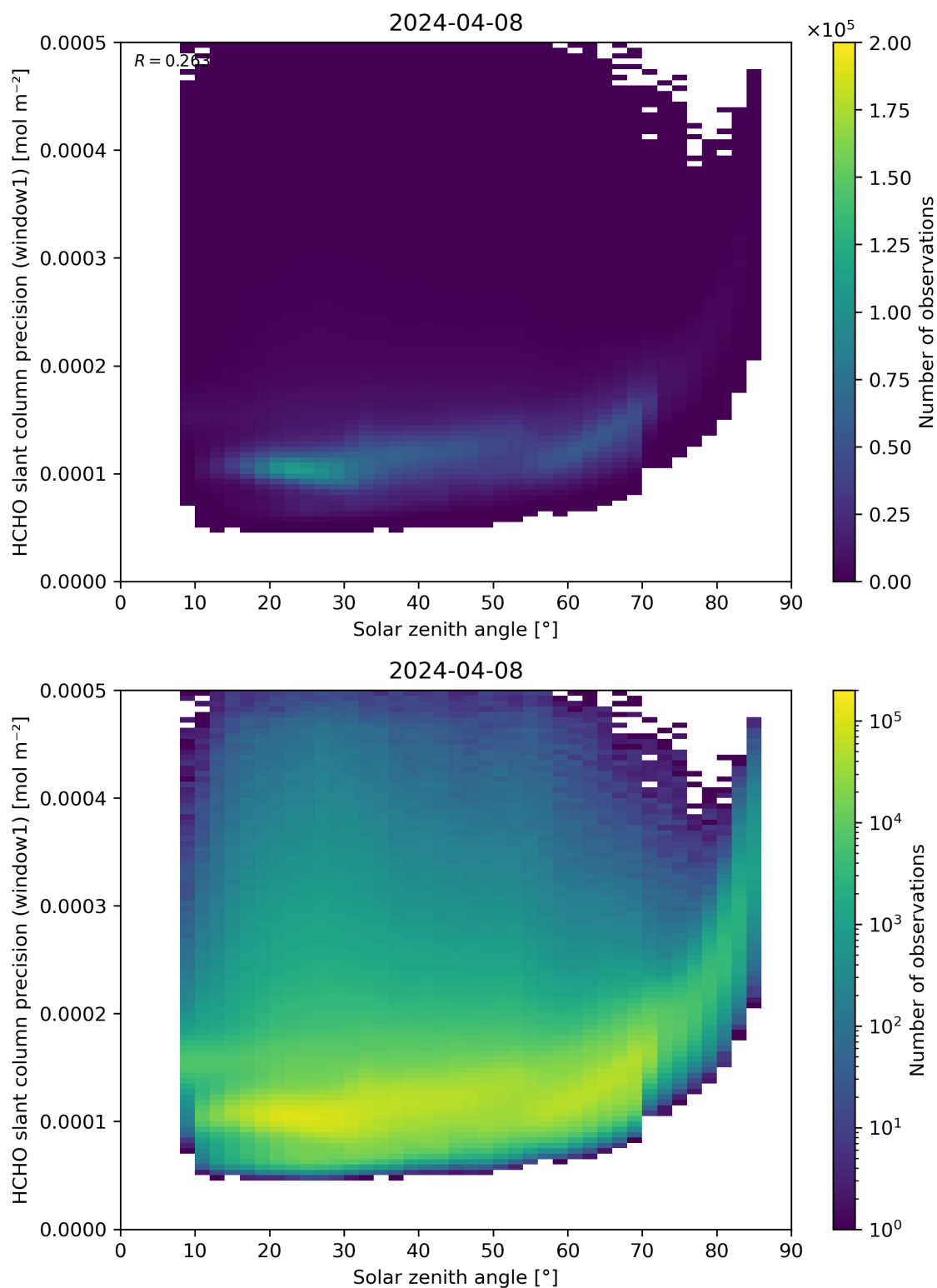
Figure 174: Scatter density plot of “Solar zenith angle” against “HCHO slant column precision (window1)” for 2024-04-07 to 2024-04-09.
