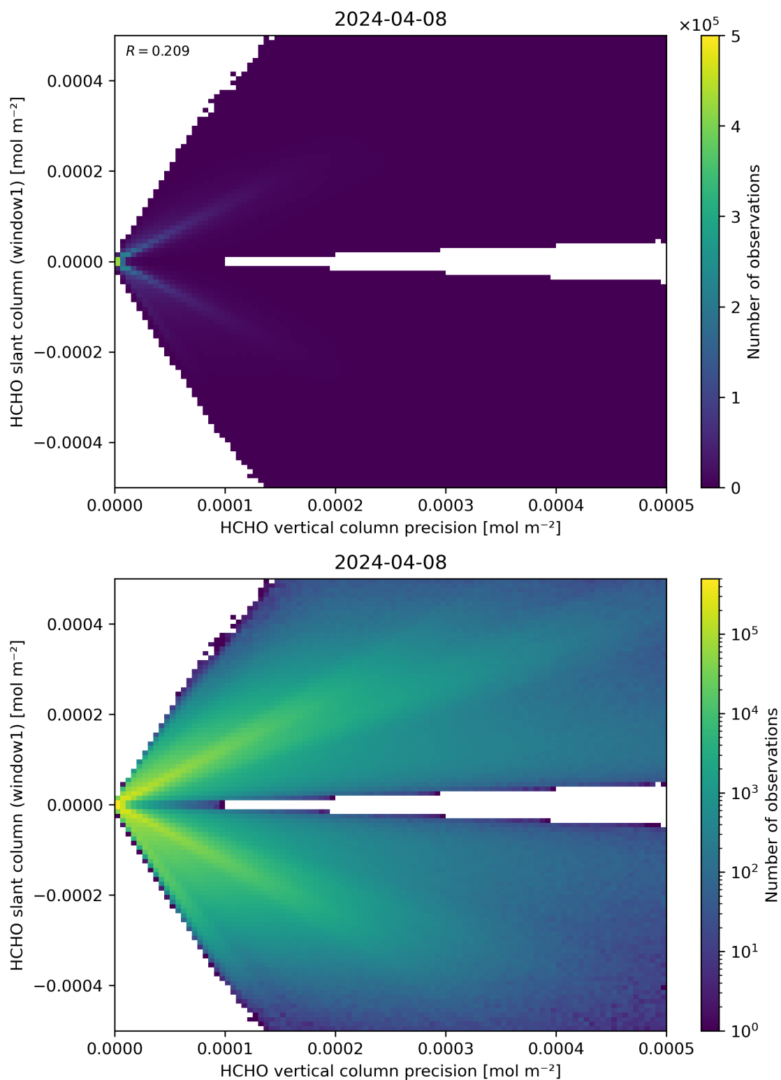
Figure 142: Scatter density plot of “HCHO vertical column precision” against “HCHO slant column (window1)” for 2024-04-07 to 2024-04-09.
