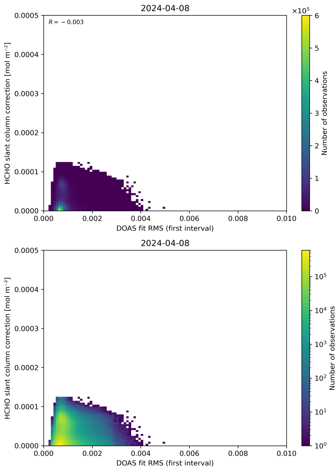
Figure 63: Scatter density plot of “DOAS fit RMS (first interval)” against “HCHO slant column correction” for 2024-04-07 to 2024-04-09.
