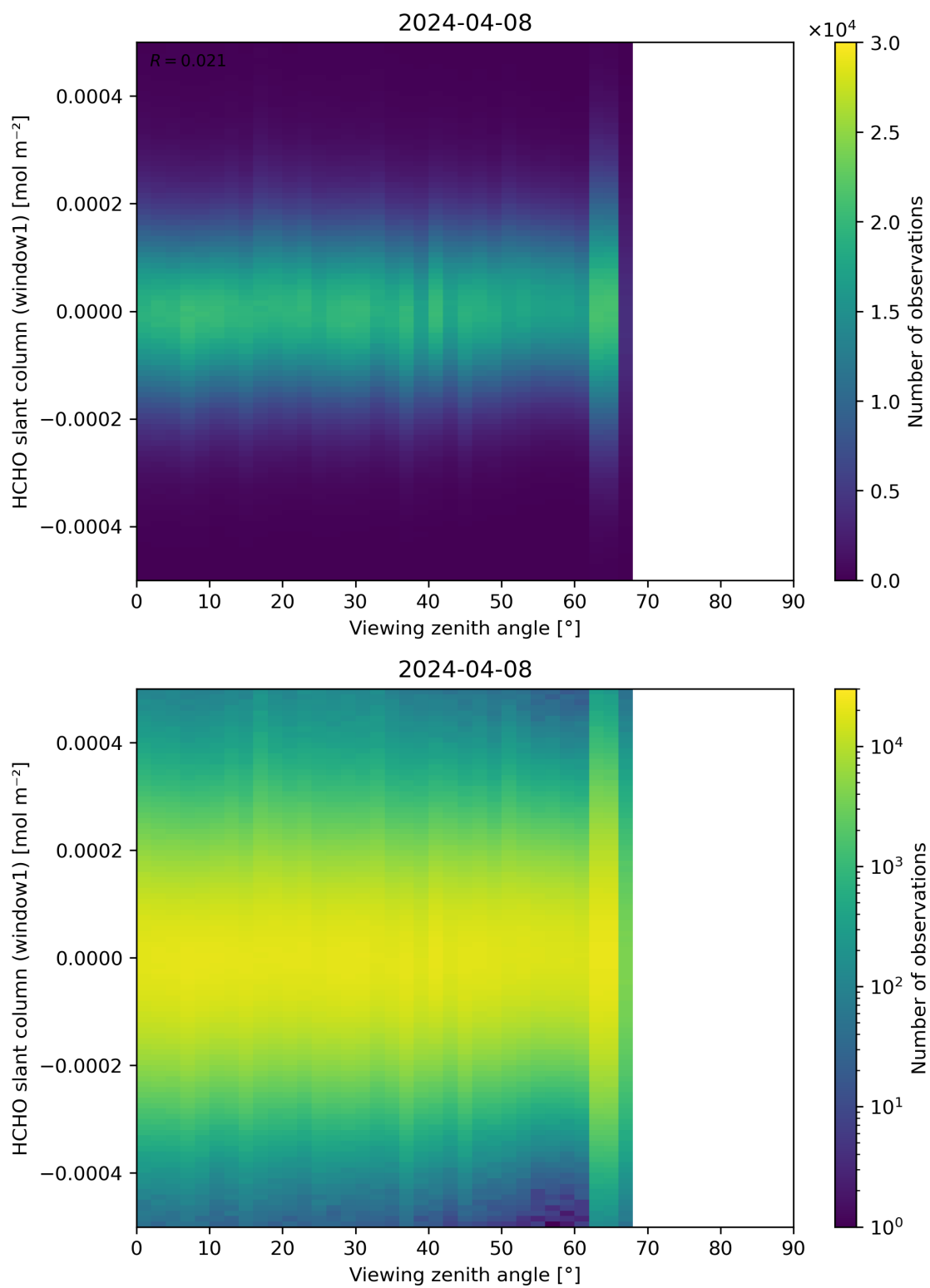
Figure 188: Scatter density plot of “Viewing zenith angle” against “HCHO slant column (window1)” for 2024-04-07 to 2024-04-09.
