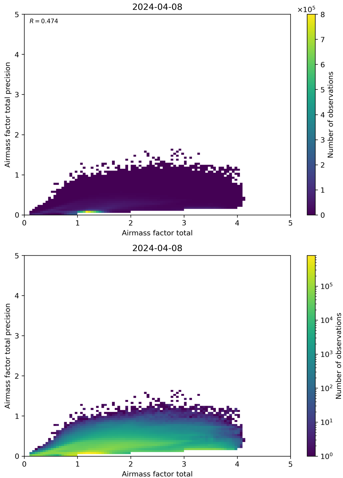
Figure 103: Scatter density plot of “Airmass factor total” against “Airmass factor total precision” for 2024-04-07 to 2024-04-09.
