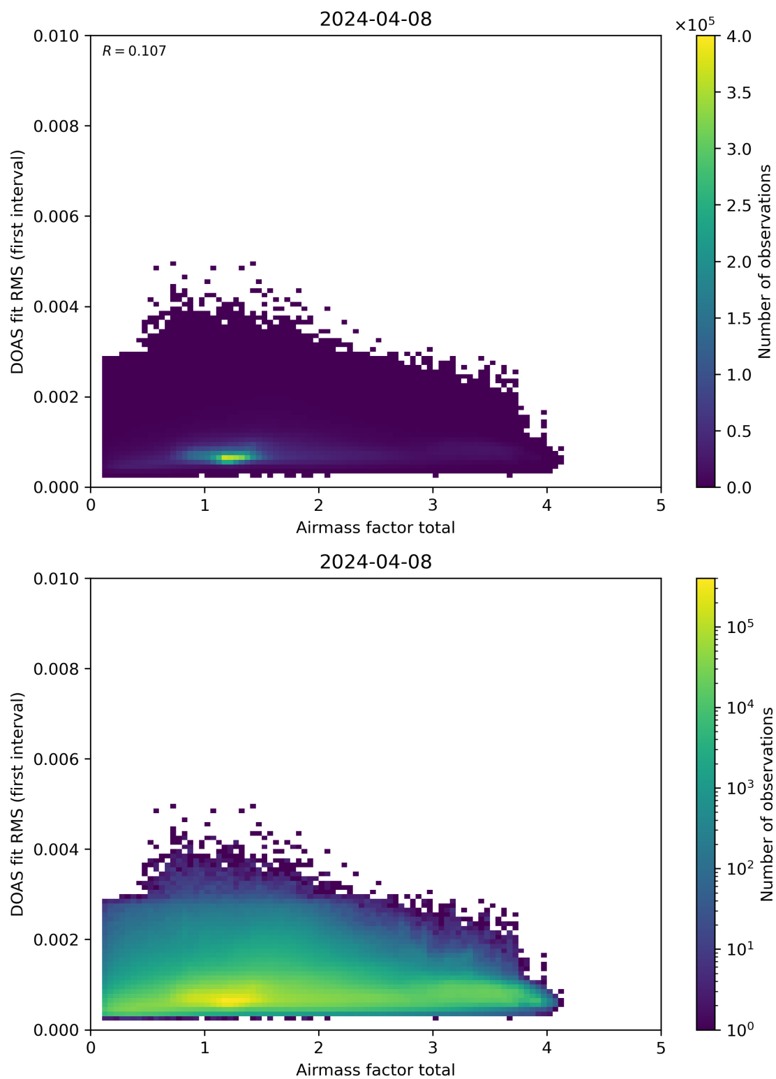
Figure 97: Scatter density plot of “Airmass factor total” against “DOAS fit RMS (first interval)” for 2024-04-07 to 2024-04-09.
