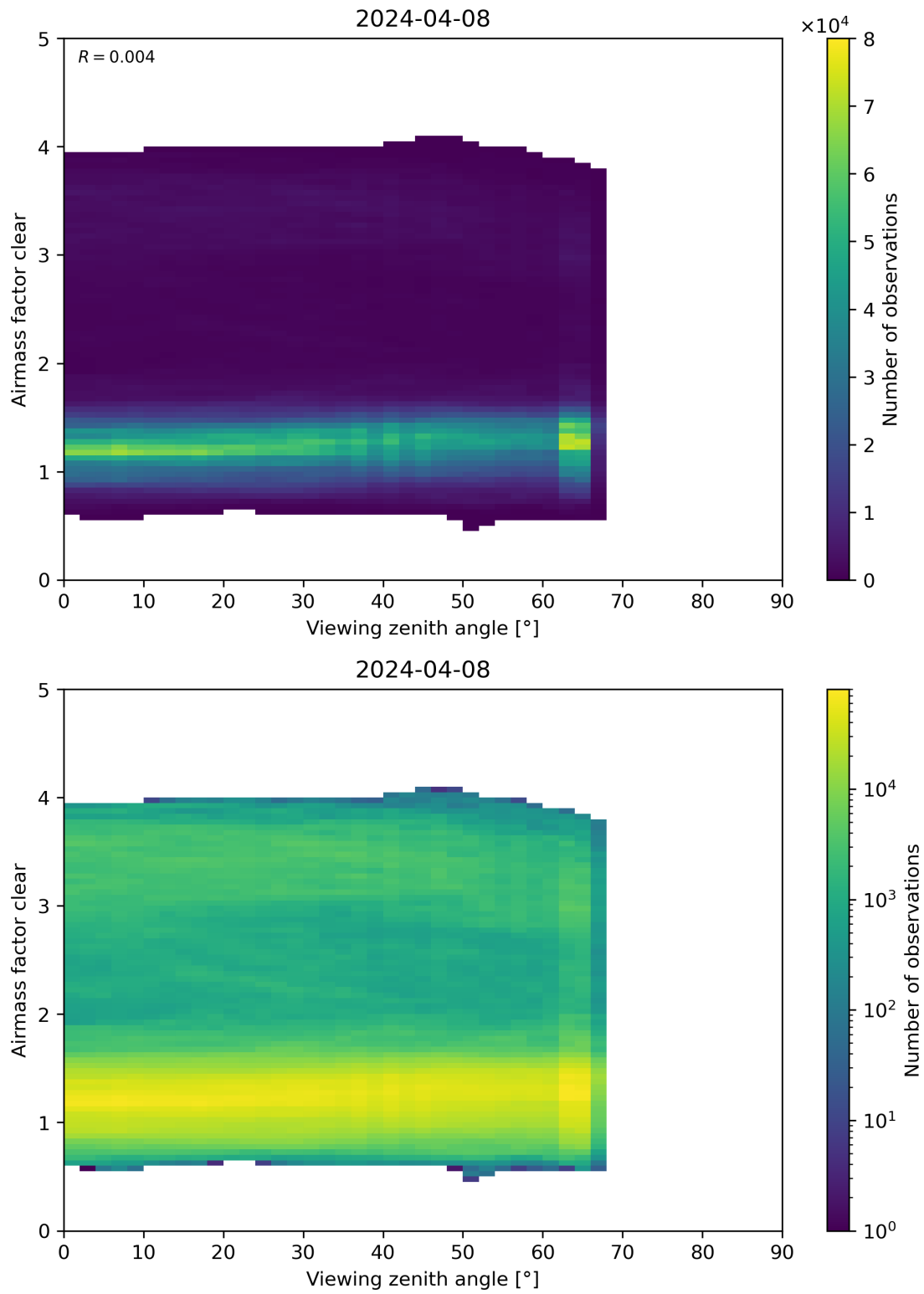
Figure 185: Scatter density plot of “Viewing zenith angle” against “Airmass factor clear” for 2024-04-07 to 2024-04-09.
