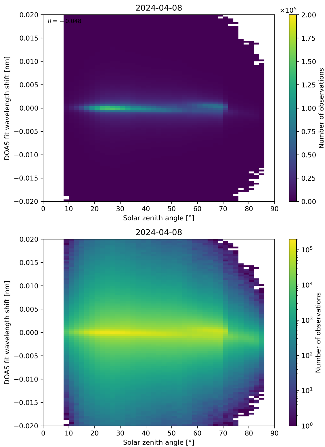
Figure 168: Scatter density plot of “Solar zenith angle” against “DOAS fit wavelength shift” for 2024-04-07 to 2024-04-09.
