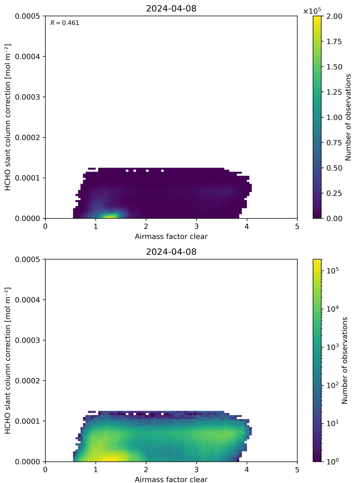
Figure 75: Scatter density plot of “Airmass factor clear” against “HCHO slant column correction” for 2024-04-07 to 2024-04-09.
