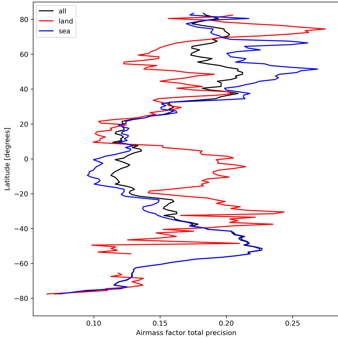
Figure 27: Zonal average of “Airmass factor total precision” for 2024-04-07 to 2024-04-09.
