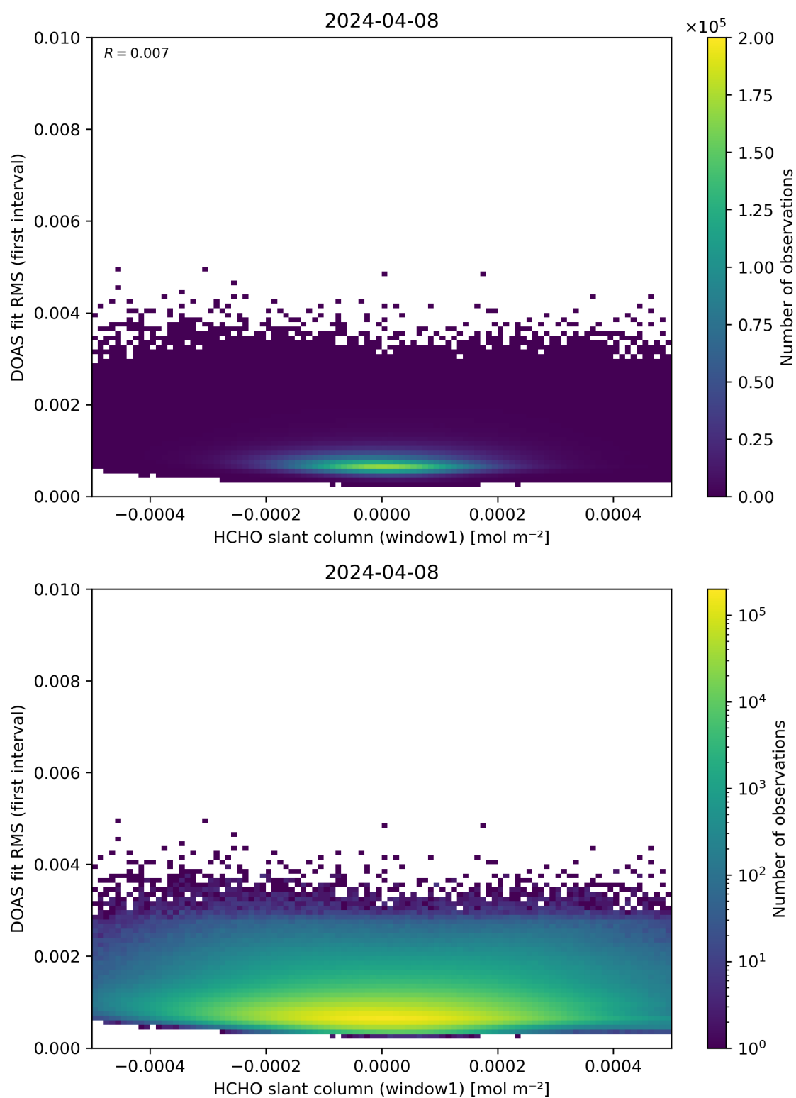
Figure 78: Scatter density plot of “HCHO slant column (window1)” against “DOAS fit RMS (first interval)” for 2024-04-07 to 2024-04-09.
