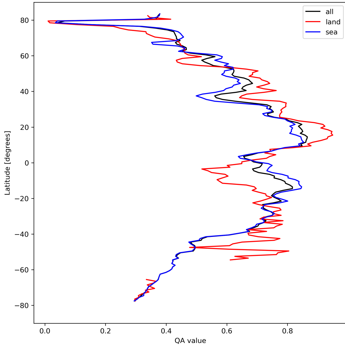
Figure 20: Zonal average of “QA value” for 2024-04-07 to 2024-04-09.
