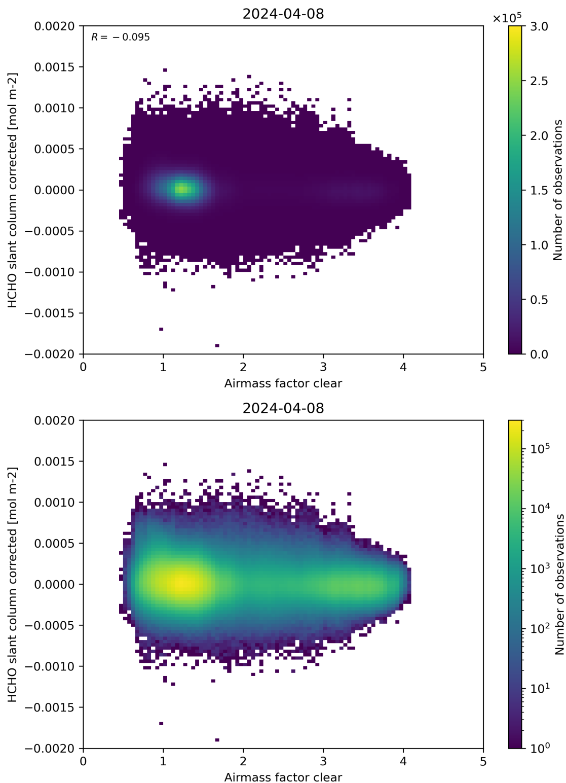
Figure 74: Scatter density plot of “Airmass factor clear” against “HCHO slant column corrected” for 2024-04-07 to 2024-04-09.
