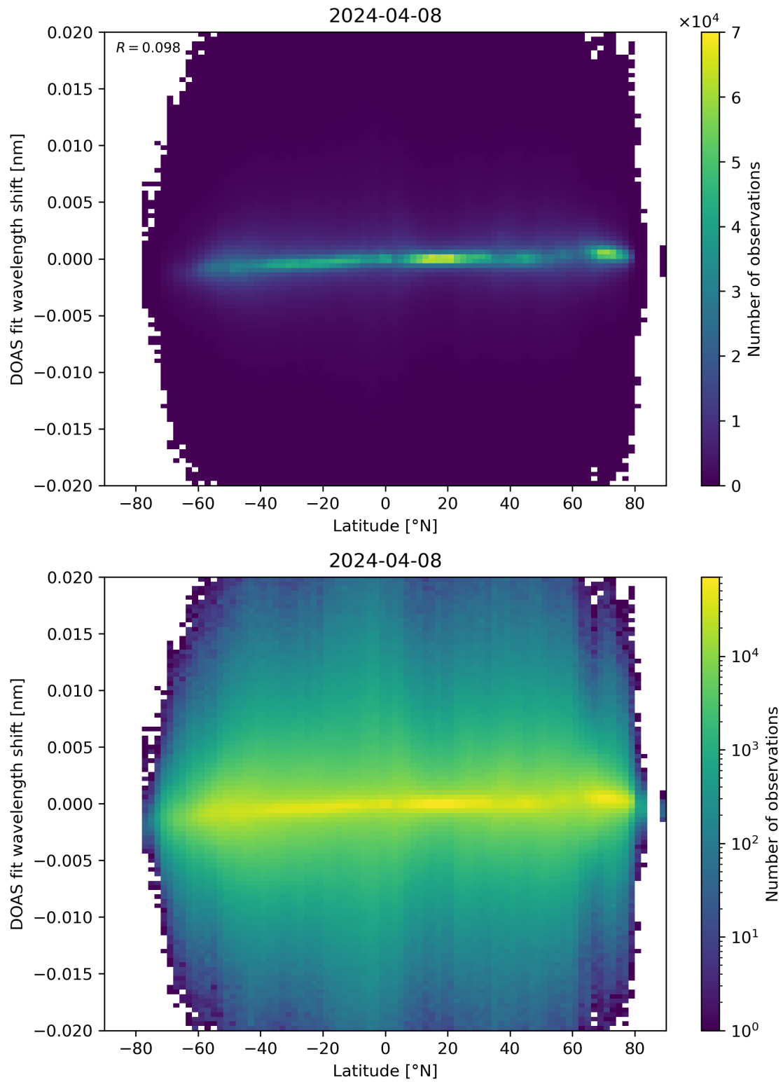
Figure 154: Scatter density plot of “Latitude” against “DOAS fit wavelength shift” for 2024-04-07 to 2024-04-09.
