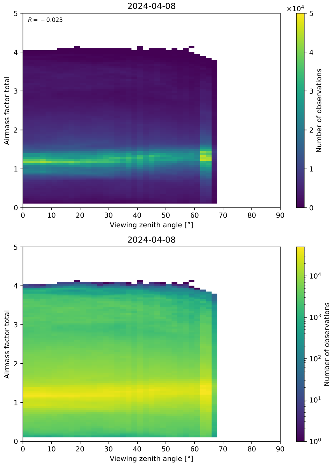
Figure 190: Scatter density plot of “Viewing zenith angle” against “Airmass factor total” for 2024-04-07 to 2024-04-09.
