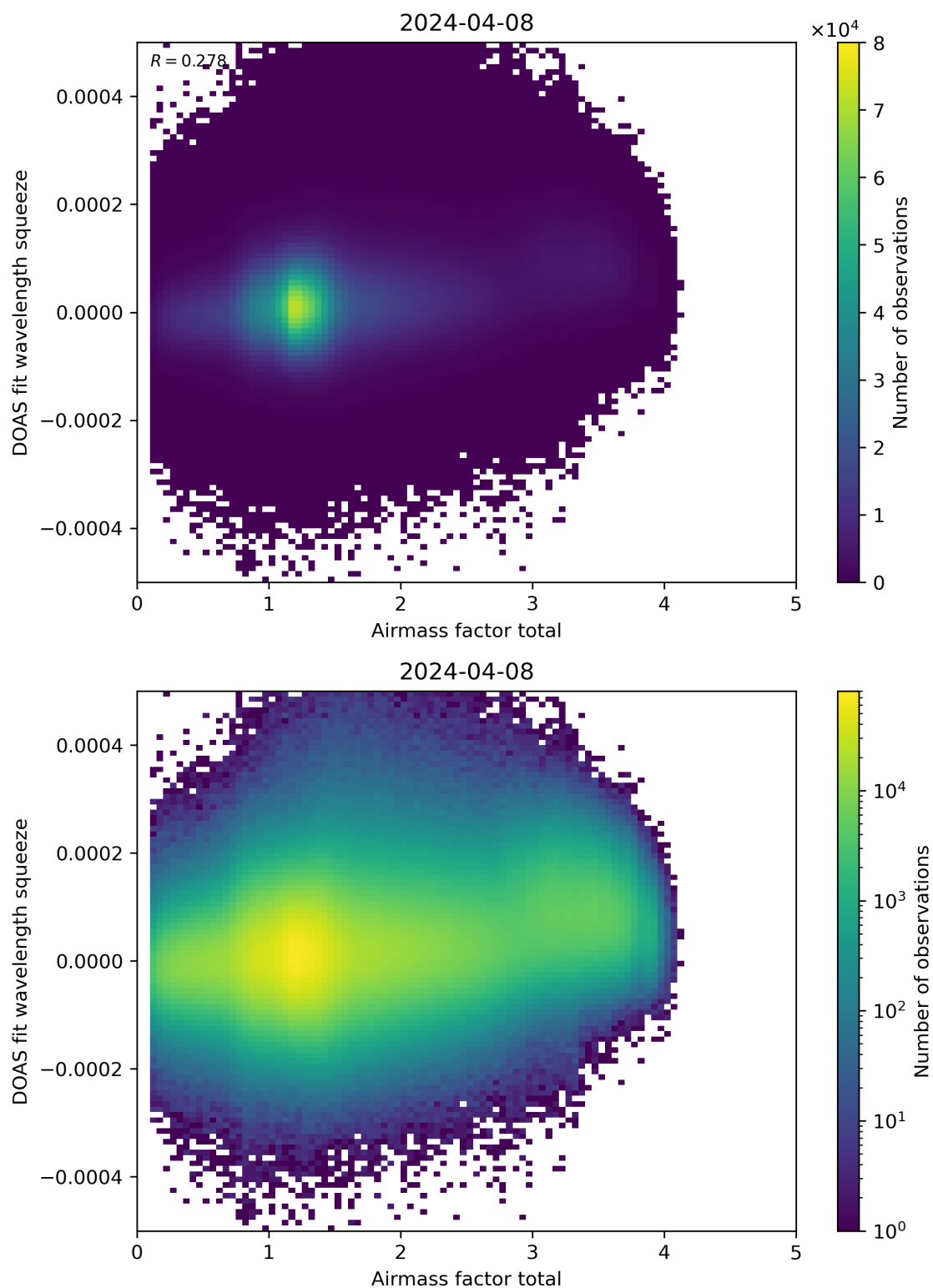
Figure 99: Scatter density plot of “Airmass factor total” against “DOAS fit wavelength squeeze” for 2024-04-07 to 2024-04-09.
