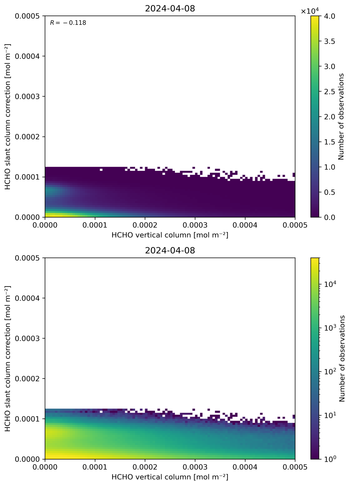
Figure 128: Scatter density plot of “HCHO vertical column” against “HCHO slant column correction” for 2024-04-07 to 2024-04-09.
