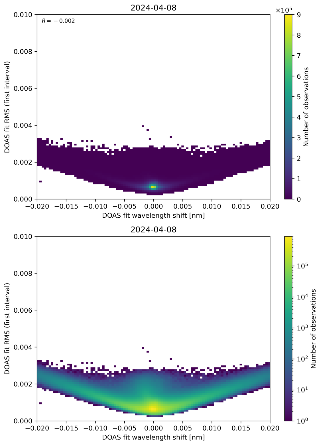
Figure 64: Scatter density plot of “DOAS fit wavelength shift” against “DOAS fit RMS (first interval)” for 2024-04-07 to 2024-04-09.
