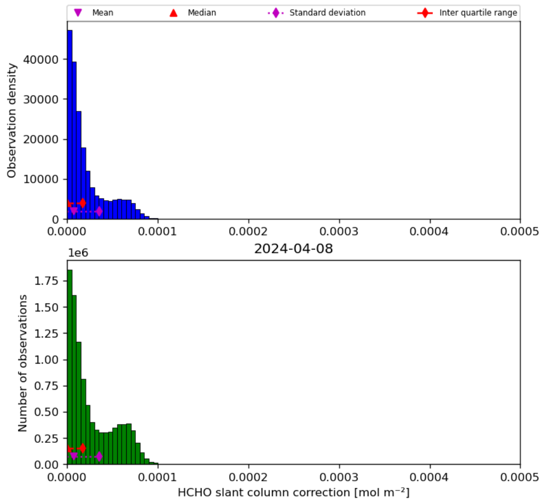
Figure 47: Histogram of “HCHO slant column correction” for 2024-04-07 to 2024-04-09
