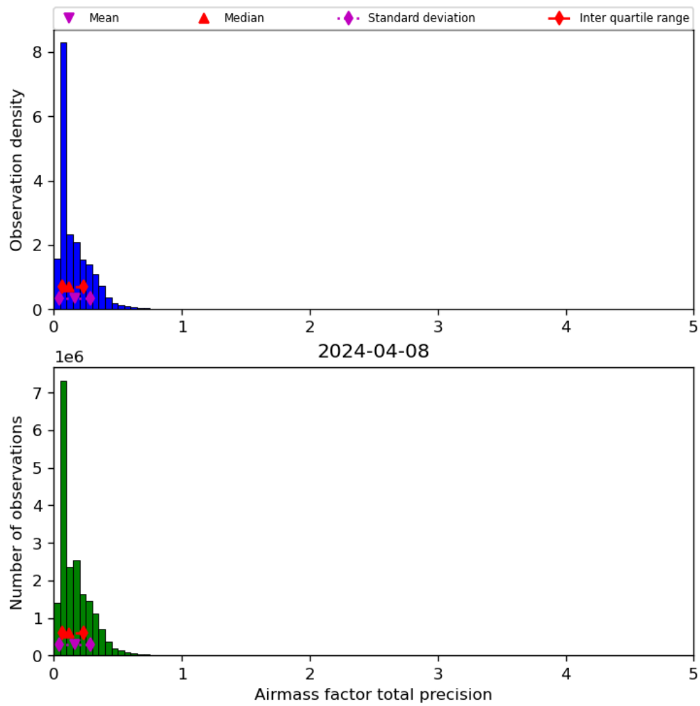
Figure 41: Histogram of "Airmass factor total precision" for 2024-04-07 to 2024-04-09
