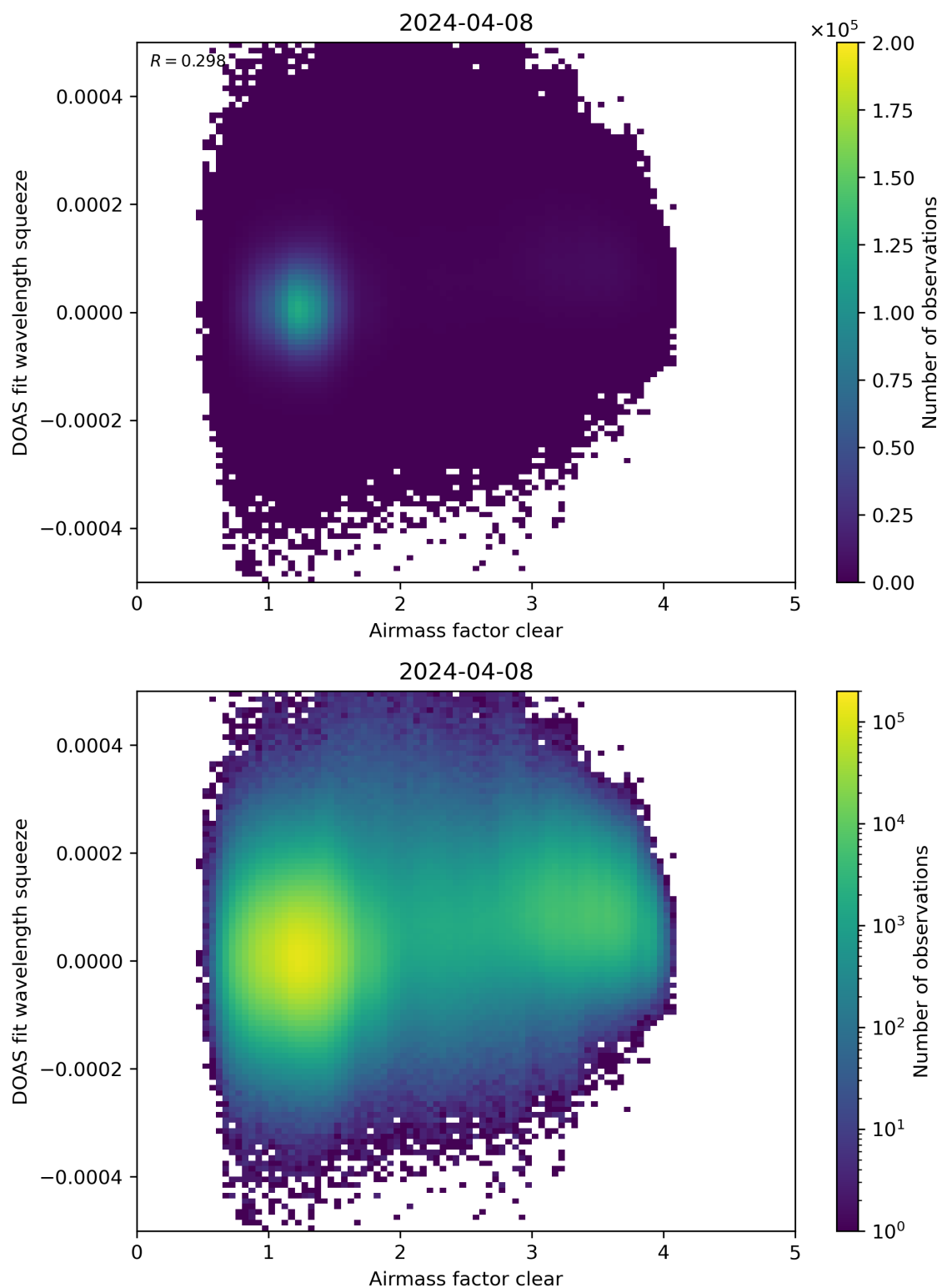
Figure 73: Scatter density plot of “Airmass factor clear” against “DOAS fit wavelength squeeze” for 2024-04-07 to 2024-04-09.
