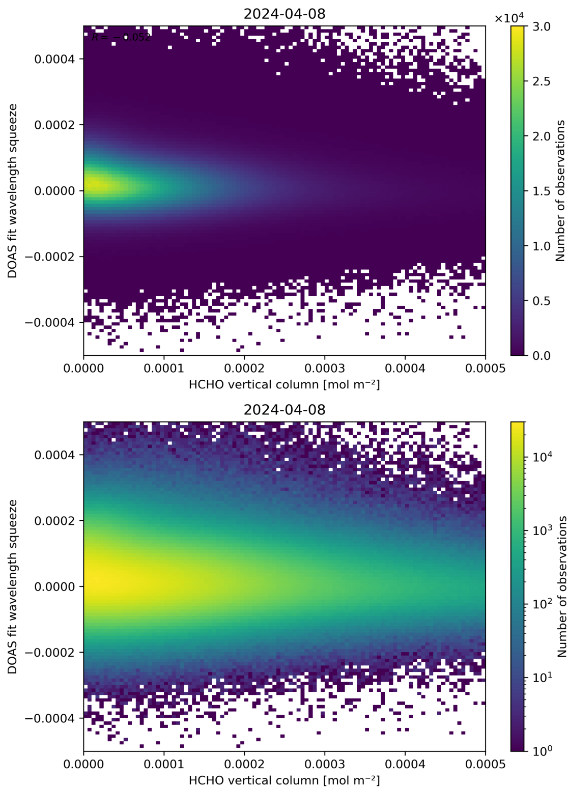
Figure 125: Scatter density plot of “HCHO vertical column” against “DOAS fit wavelength squeeze” for 2024-04-07 to 2024-04-09.
