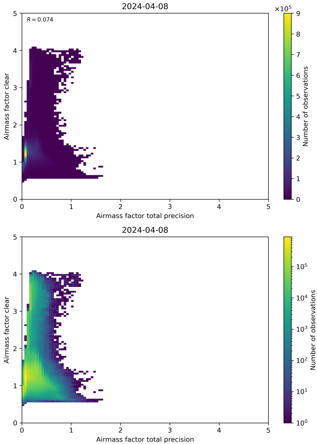
Figure 108: Scatter density plot of “Airmass factor total precision” against “Airmass factor clear” for 2024-04-07 to 2024-04-09.
