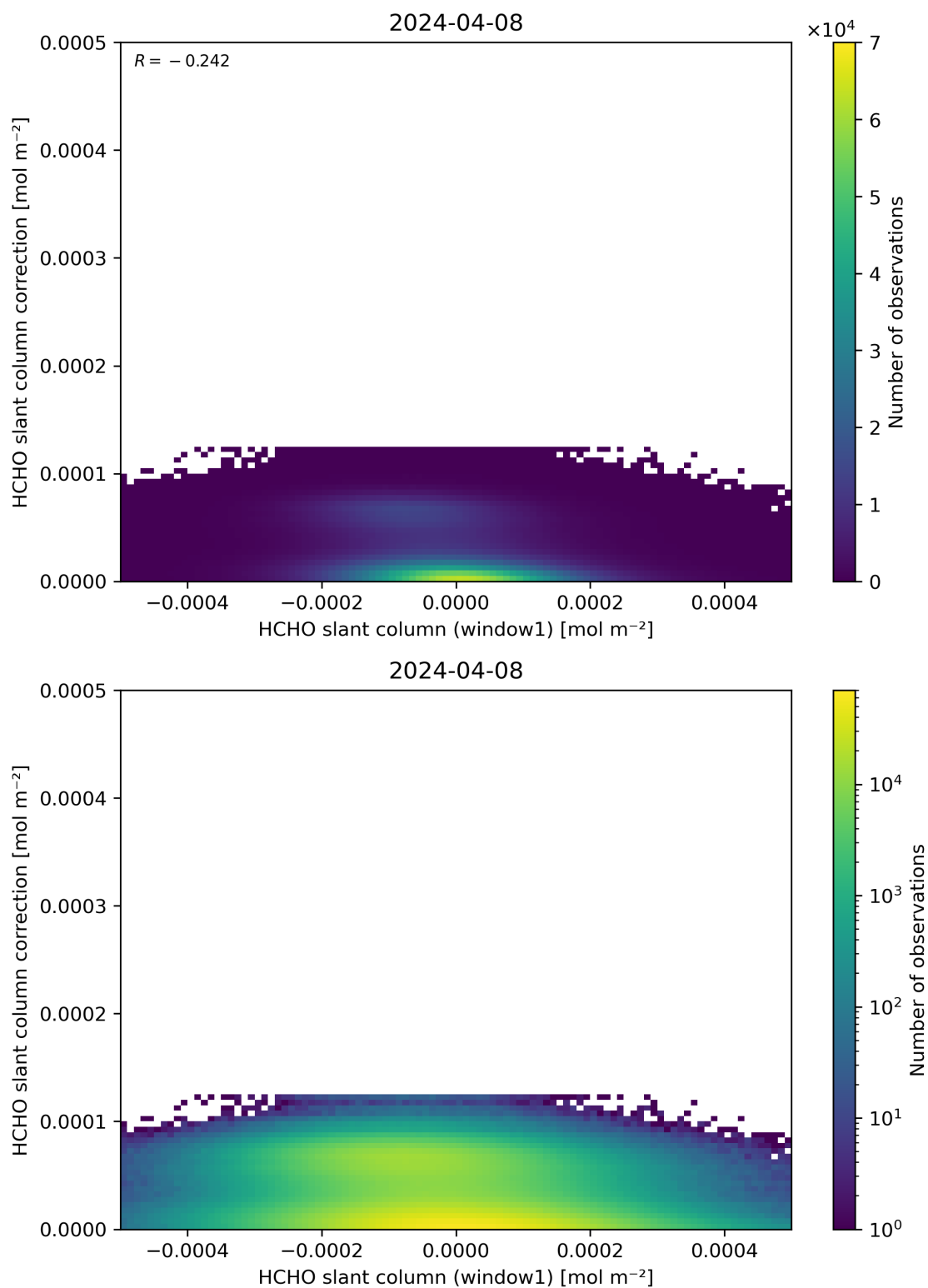
Figure 83: Scatter density plot of “HCHO slant column (window1)” against “HCHO slant column correction” for 2024-04-07 to 2024-04-09.
