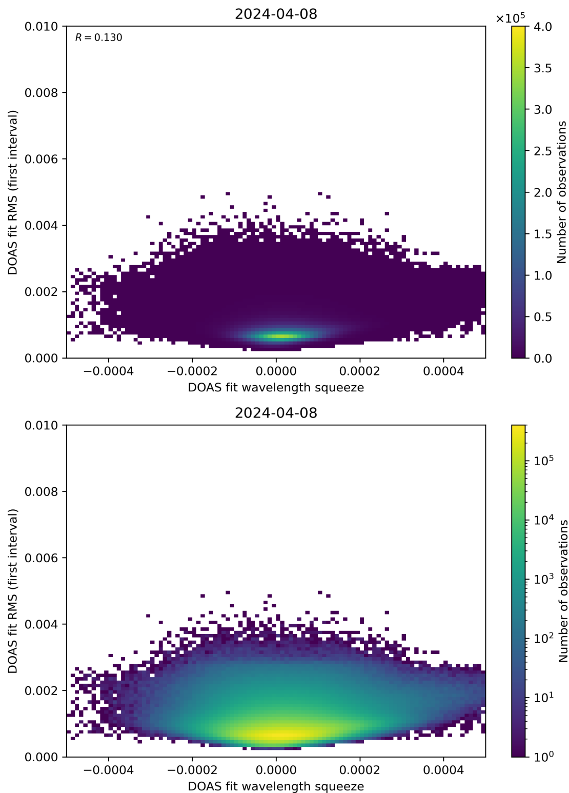
Figure 68: Scatter density plot of “DOAS fit wavelength squeeze” against “DOAS fit RMS (first interval)” for 2024-04-07 to 2024-04-09.
