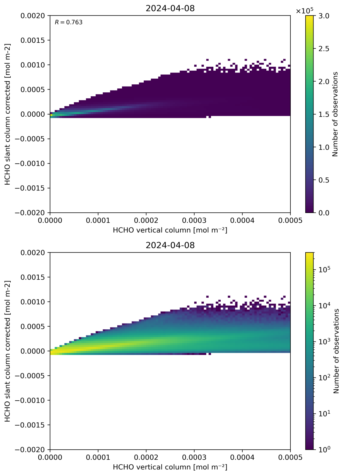
Figure 127: Scatter density plot of “HCHO vertical column” against “HCHO slant column corrected” for 2024-04-07 to 2024-04-09.
