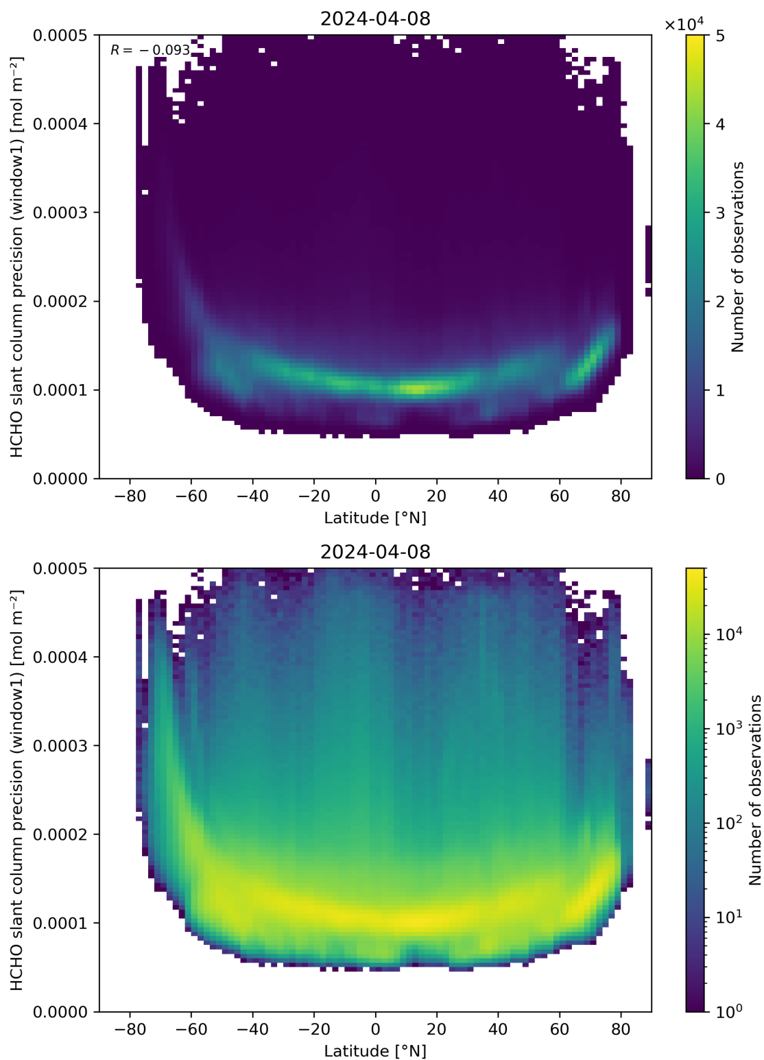
Figure 160: Scatter density plot of “Latitude” against “HCHO slant column precision (window1)” for 2024-04-07 to 2024-04-09.
