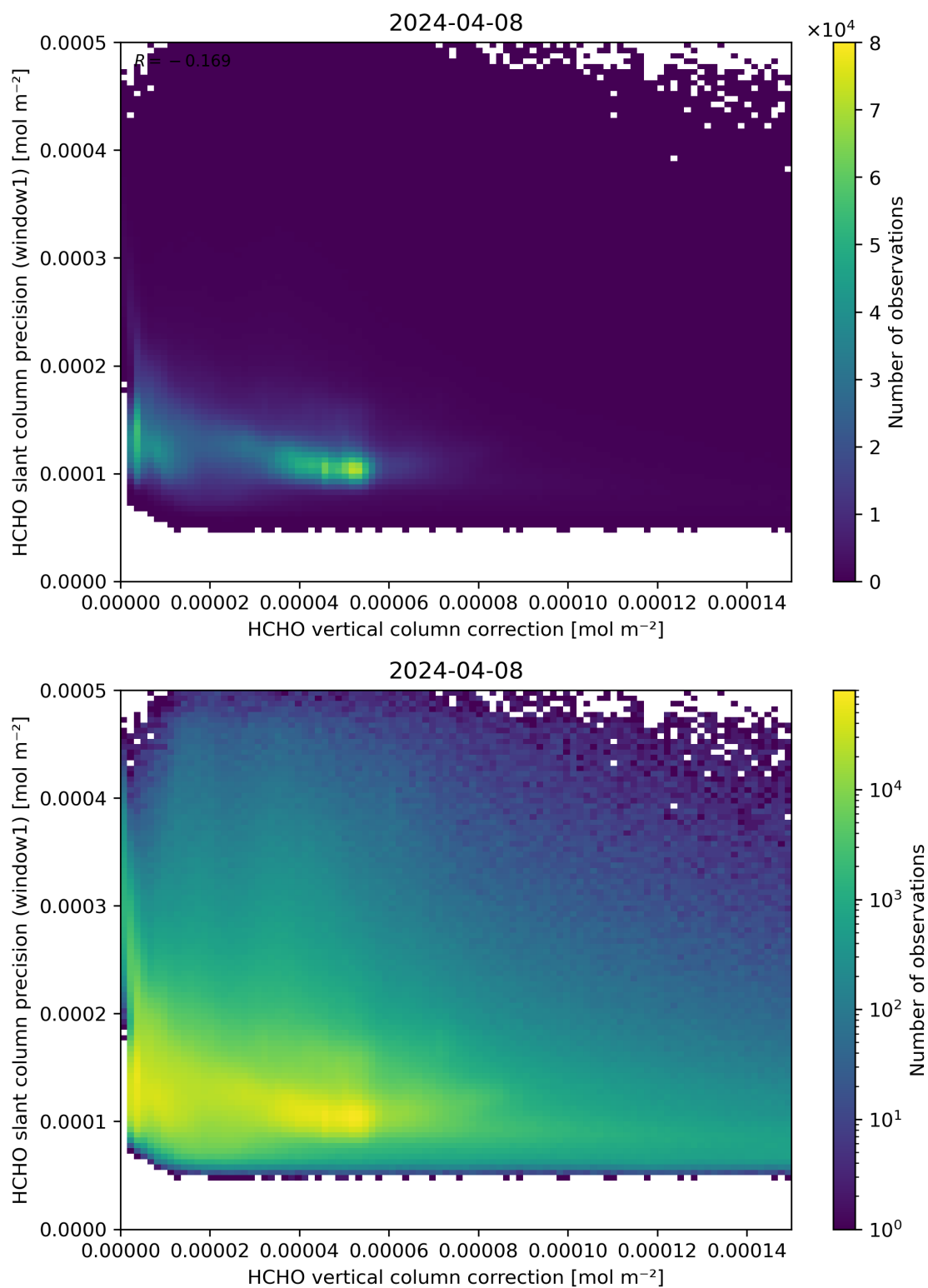
Figure 119: Scatter density plot of “HCHO vertical column correction” against “HCHO slant column precision (window1)” for 2024-04-07 to 2024-04-09.
