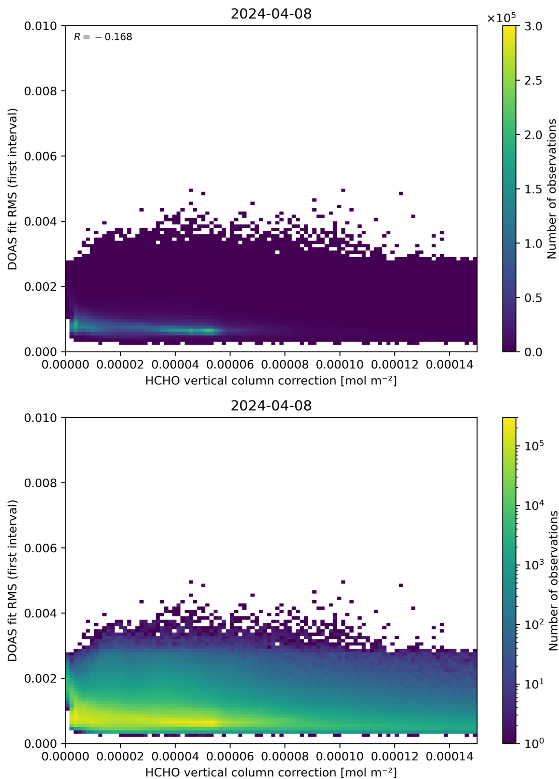
Figure 112: Scatter density plot of “HCHO vertical column correction” against “DOAS fit RMS (first interval)” for 2024-04-07 to 2024-04-09.
