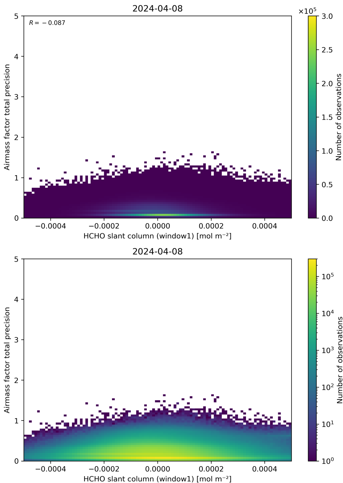
Figure 86: Scatter density plot of “HCHO slant column (window1)” against “Airmass factor total precision” for 2024-04-07 to 2024-04-09.
