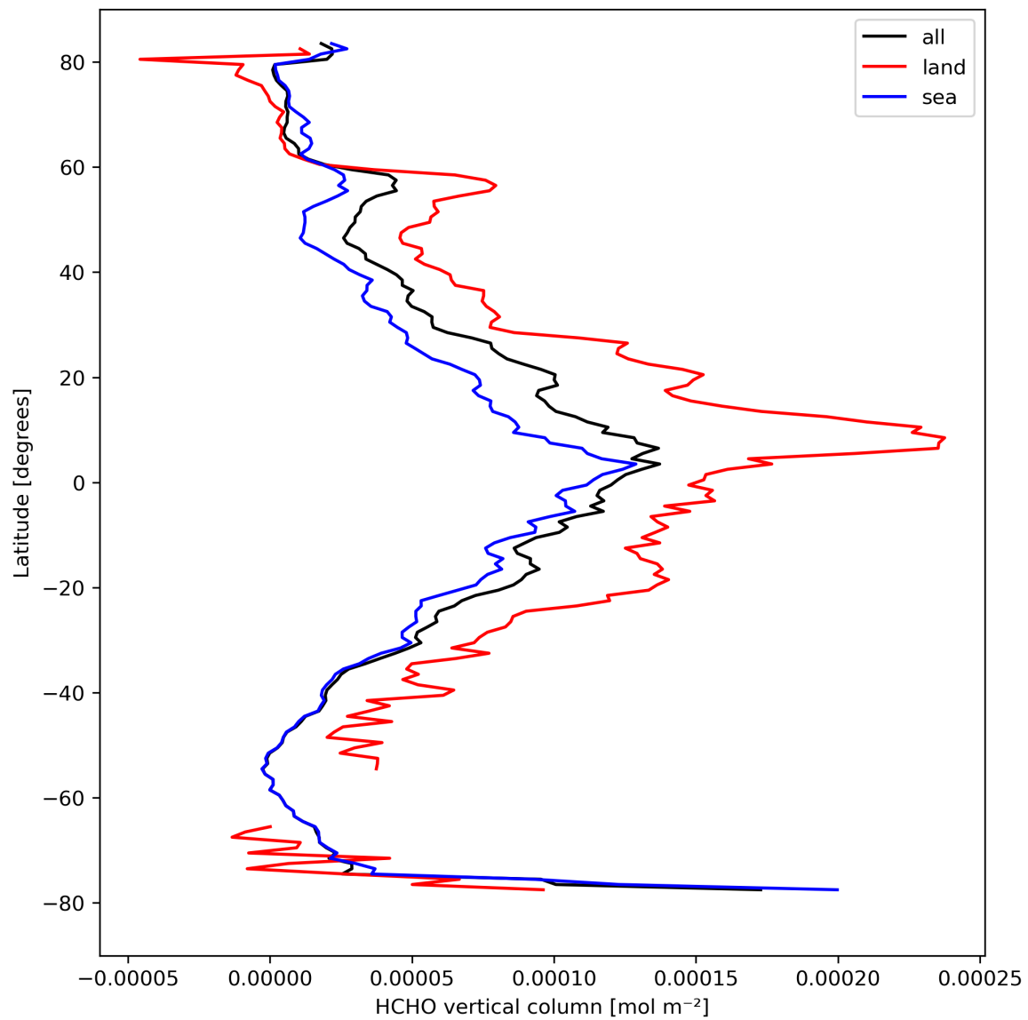
Figure 21: Zonal average of “HCHO vertical column” for 2024-04-07 to 2024-04-09.
