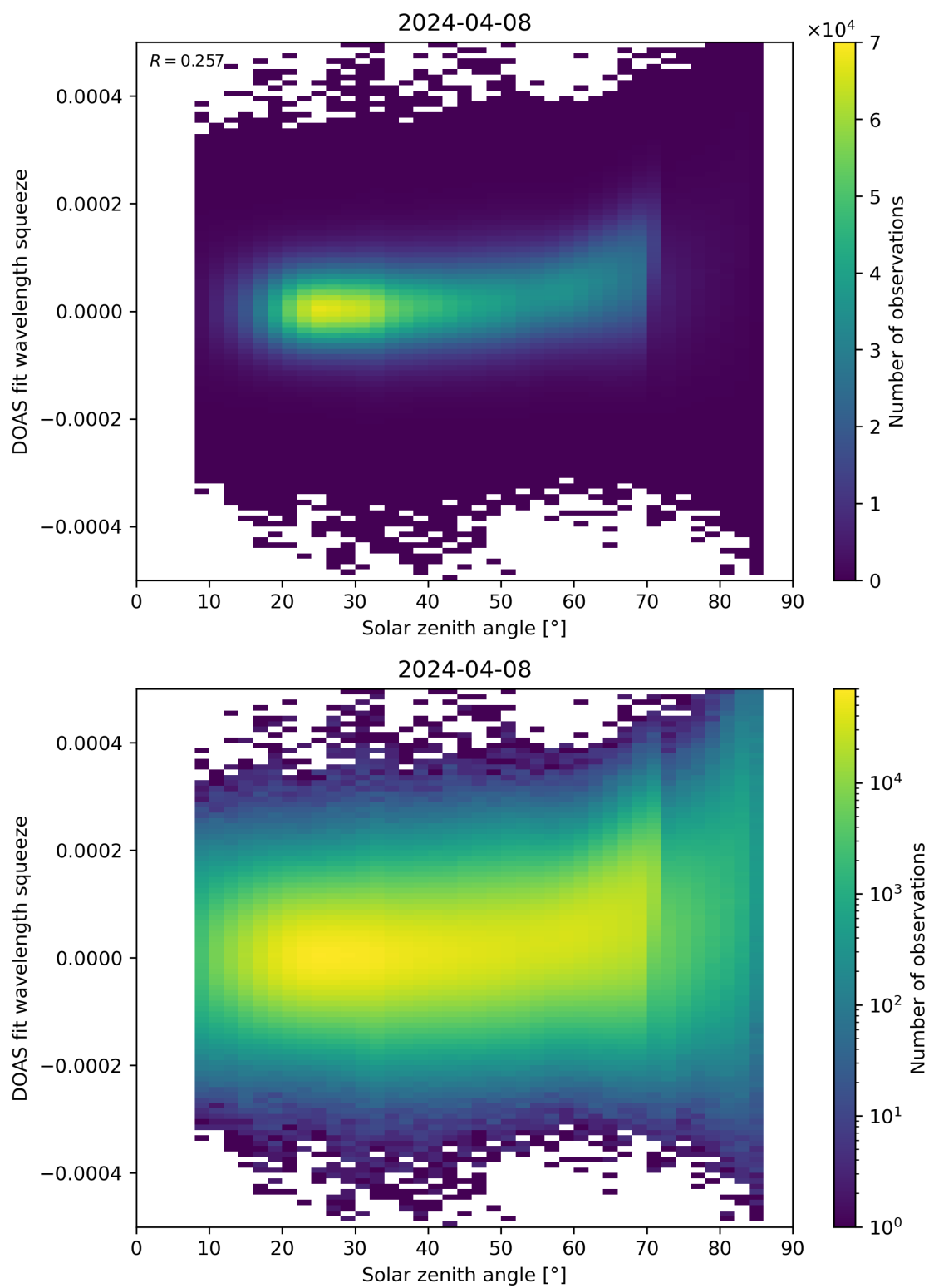
Figure 169: Scatter density plot of “Solar zenith angle” against “DOAS fit wavelength squeeze” for 2024-04-07 to 2024-04-09.
