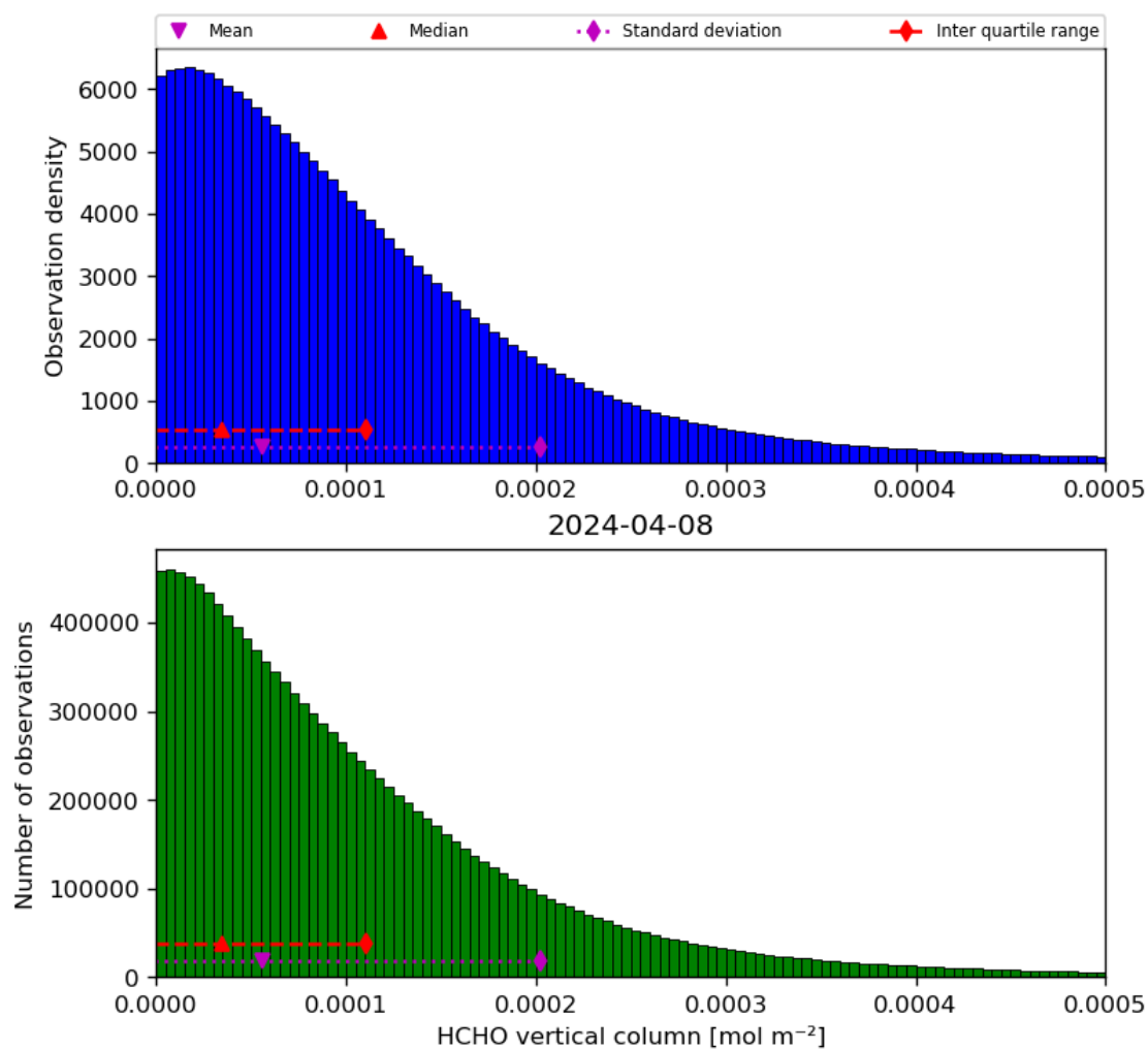
Figure 35: Histogram of “HCHO vertical column” for 2024-04-07 to 2024-04-09
