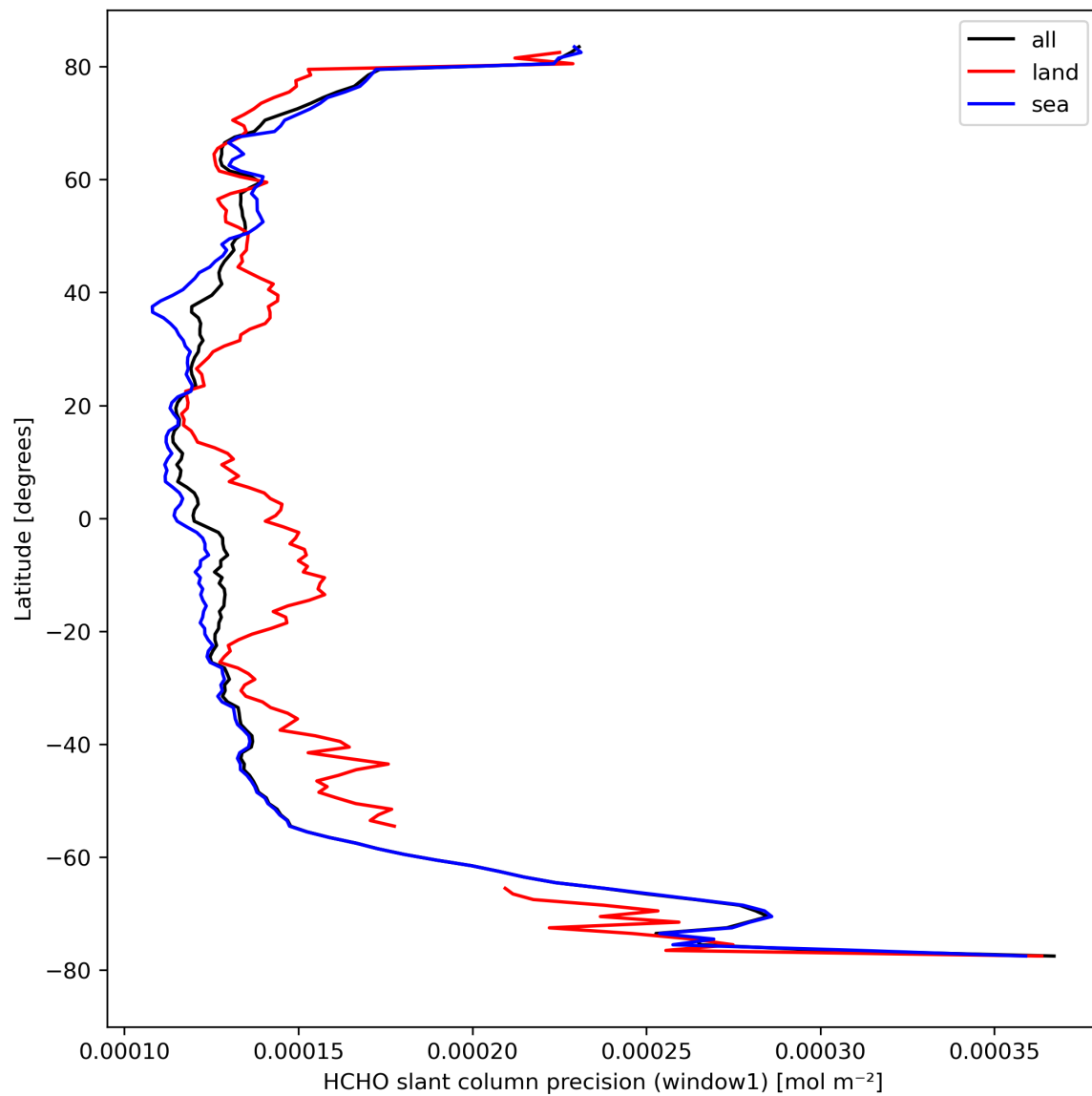
Figure 25: Zonal average of “HCHO slant column precision (window1)” for 2024-04-07 to 2024-04-09.
