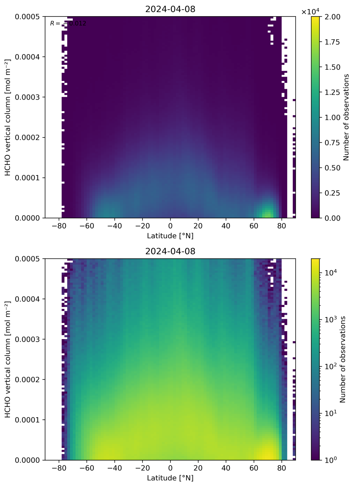
Figure 163: Scatter density plot of “Latitude” against “HCHO vertical column” for 2024-04-07 to 2024-04-09.
