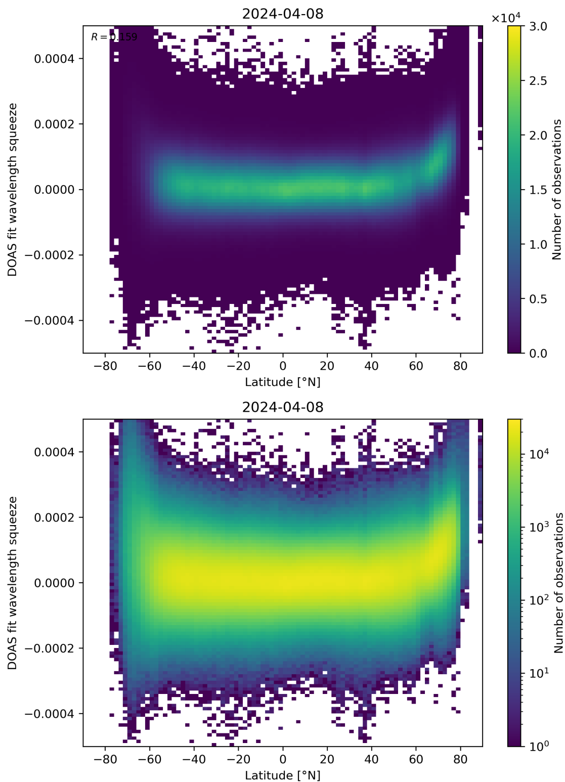
Figure 155: Scatter density plot of “Latitude” against “DOAS fit wavelength squeeze” for 2024-04-07 to 2024-04-09.
