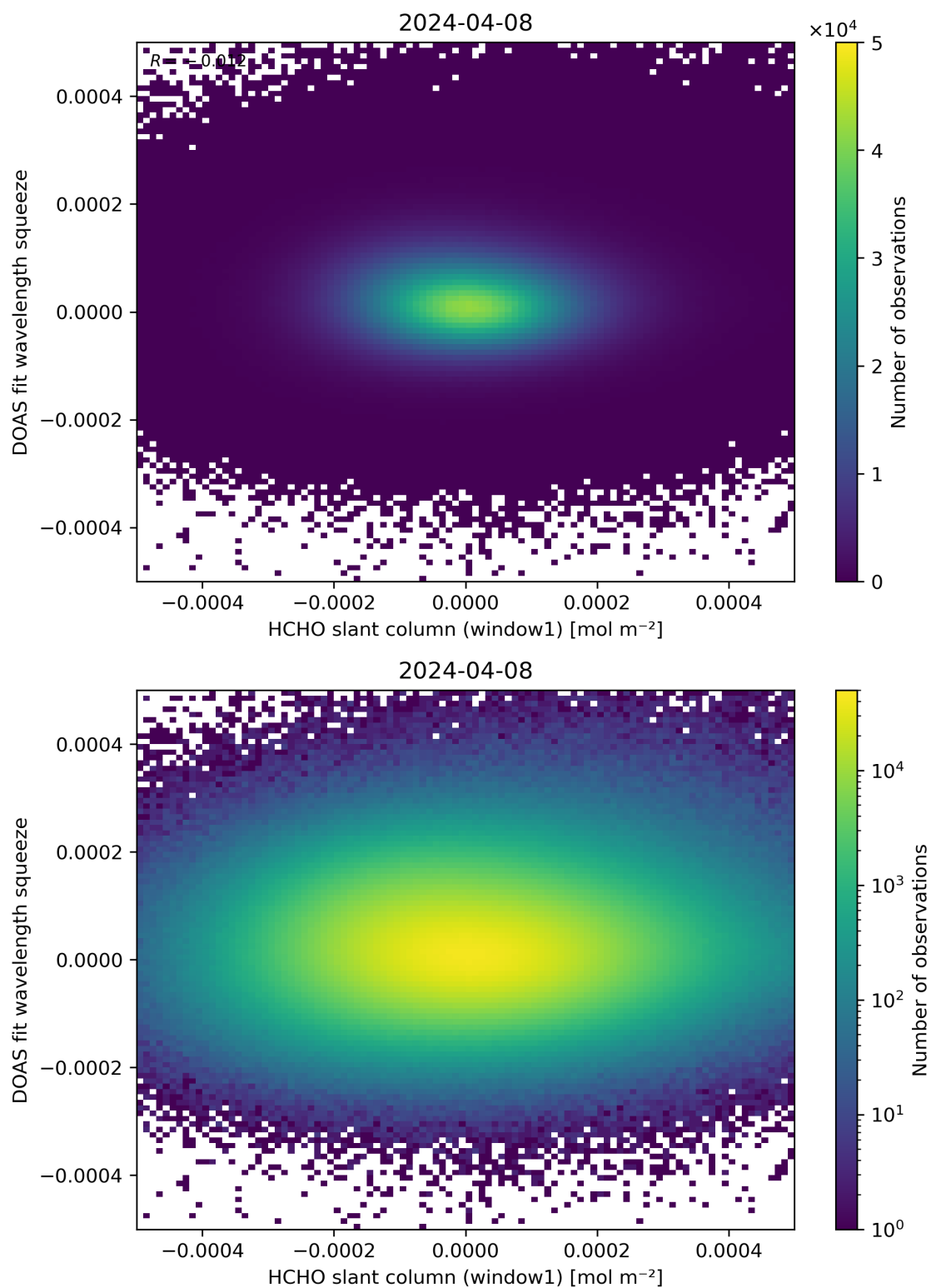
Figure 80: Scatter density plot of “HCHO slant column (window1)” against “DOAS fit wavelength squeeze” for 2024-04-07 to 2024-04-09.
