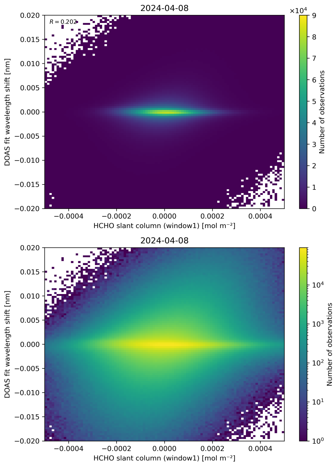
Figure 79: Scatter density plot of “HCHO slant column (window1)” against “DOAS fit wavelength shift” for 2024-04-07 to 2024-04-09.
