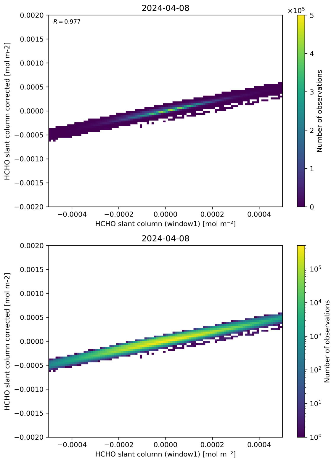
Figure 82: Scatter density plot of “HCHO slant column (window1)” against “HCHO slant column corrected” for 2024-04-07 to 2024-04-09.
