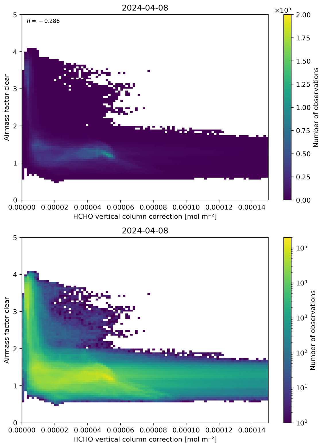
Figure 115: Scatter density plot of “HCHO vertical column correction” against “Airmass factor clear” for 2024-04-07 to 2024-04-09.
