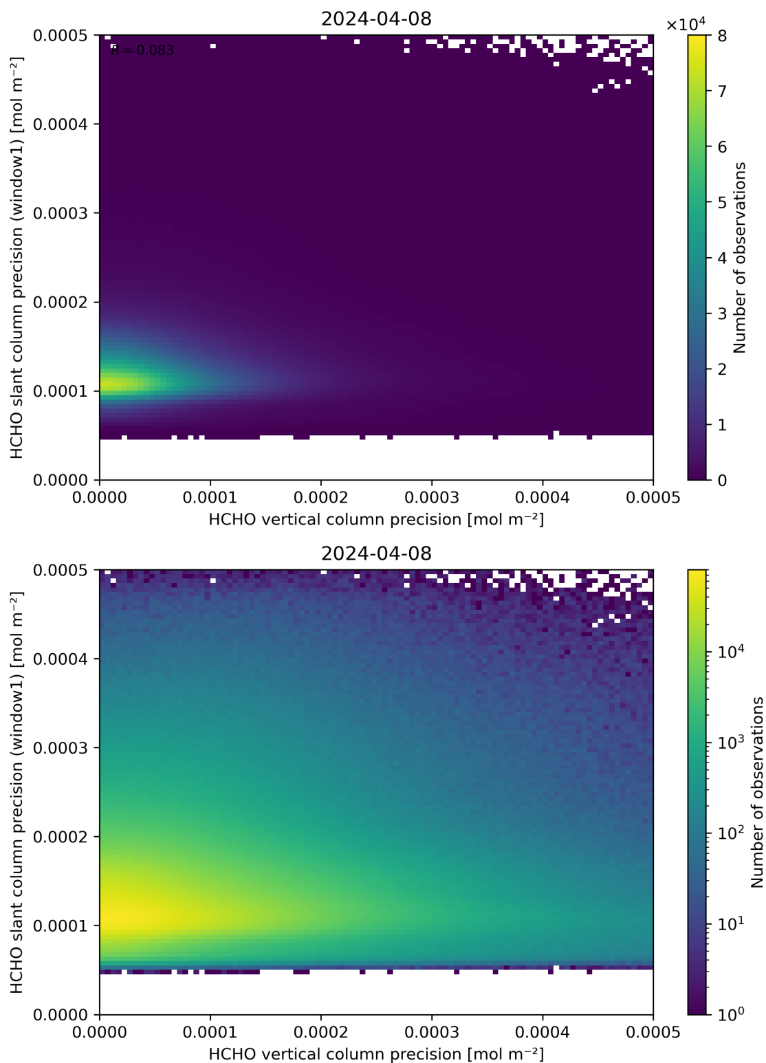
Figure 143: Scatter density plot of “HCHO vertical column precision” against “HCHO slant column precision (window1)” for 2024-04-07 to 2024-04-09.
