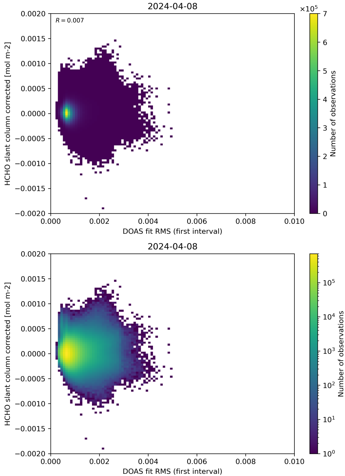
Figure 62: Scatter density plot of “DOAS fit RMS (first interval)” against “HCHO slant column corrected” for 2024-04-07 to 2024-04-09.
