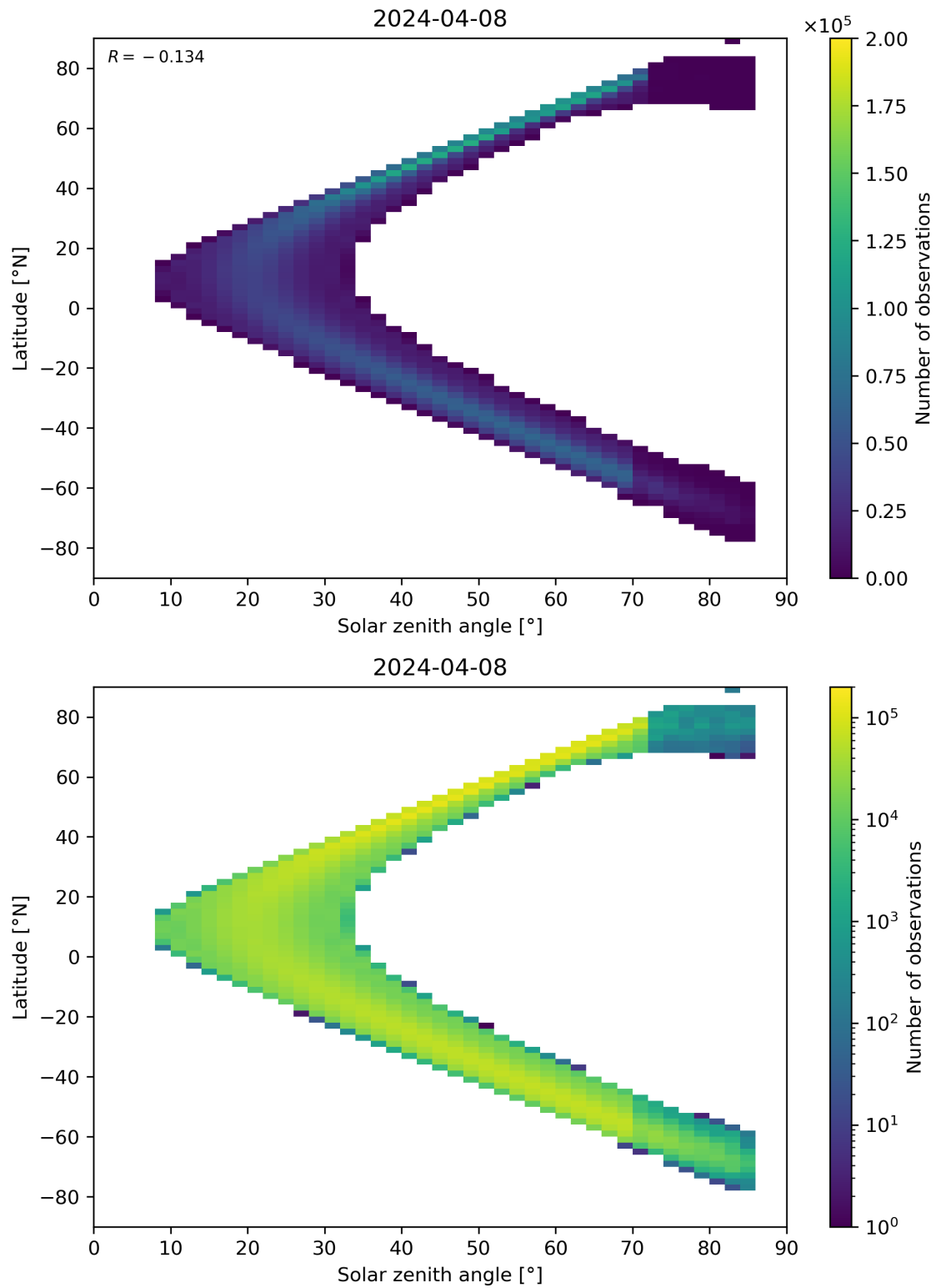
Figure 181: Scatter density plot of “Solar zenith angle” against “Latitude” for 2024-04-07 to 2024-04-09.
