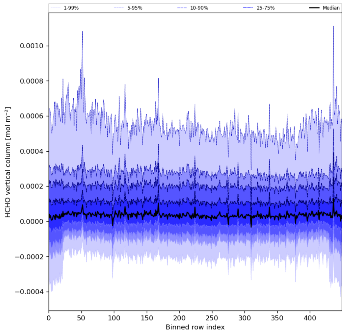
Figure 49: Along track statistics of “HCHO vertical column” for 2024-04-07 to 2024-04-09
