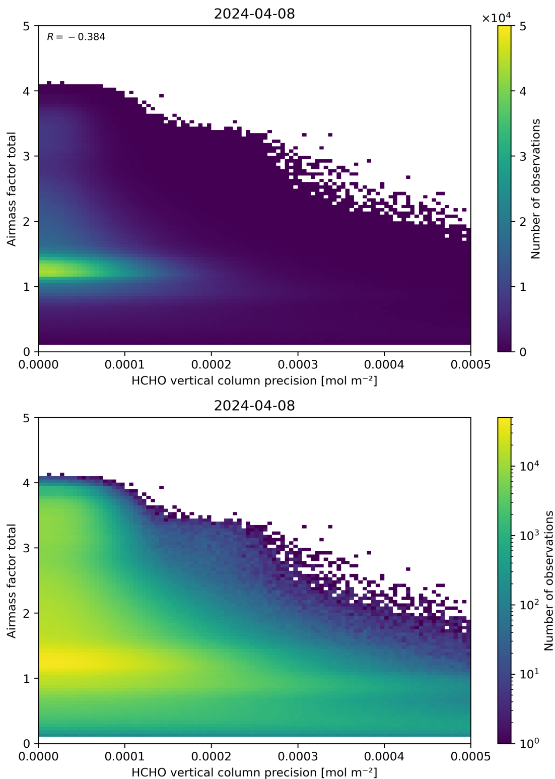
Figure 144: Scatter density plot of “HCHO vertical column precision” against “Airmass factor total” for 2024-04-07 to 2024-04-09.
