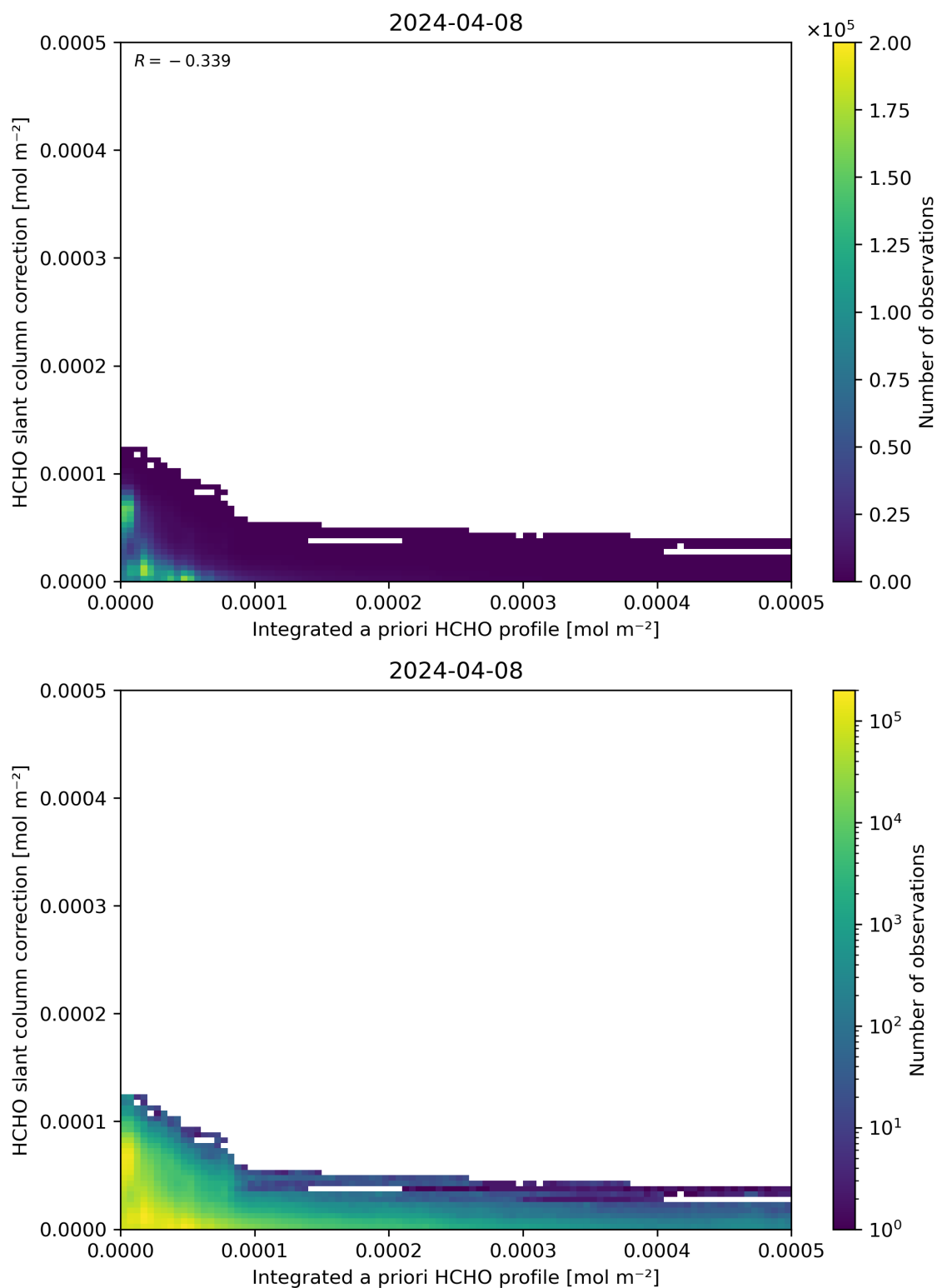
Figure 152: Scatter density plot of “Integrated a priori HCHO profile” against “HCHO slant column correction” for 2024-04-07 to 2024-04-09.
