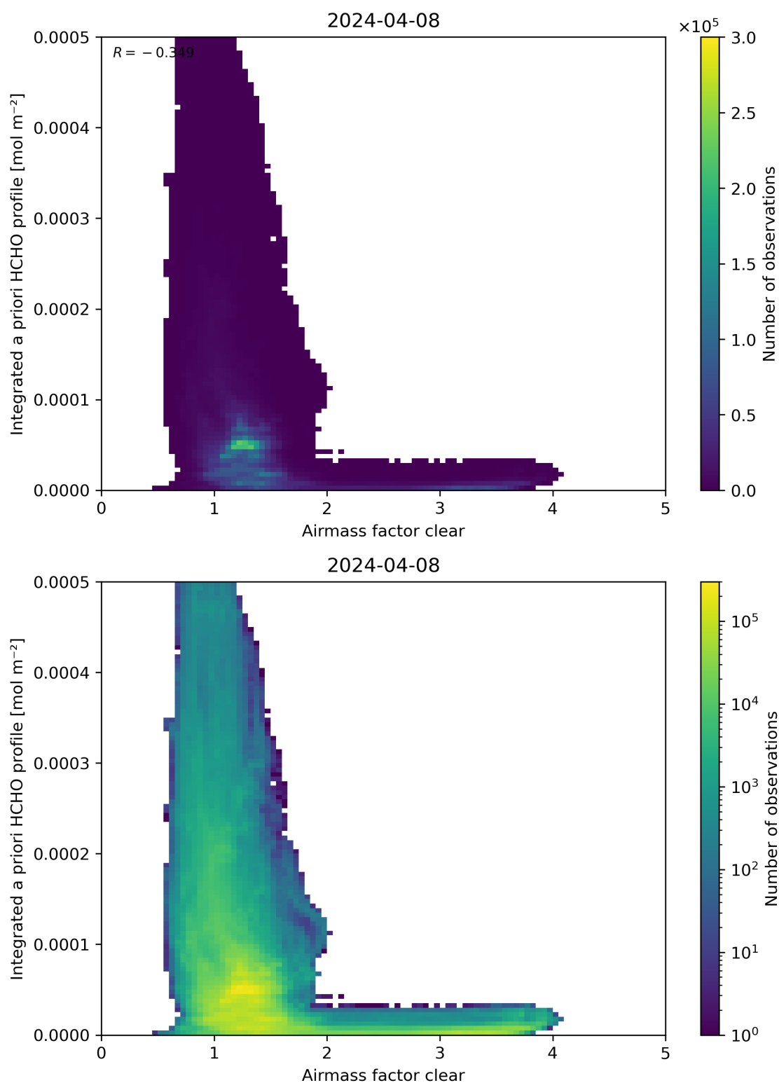
Figure 76: Scatter density plot of “Airmass factor clear” against “Integrated a priori HCHO profile” for 2024-04-07 to 2024-04-09.
