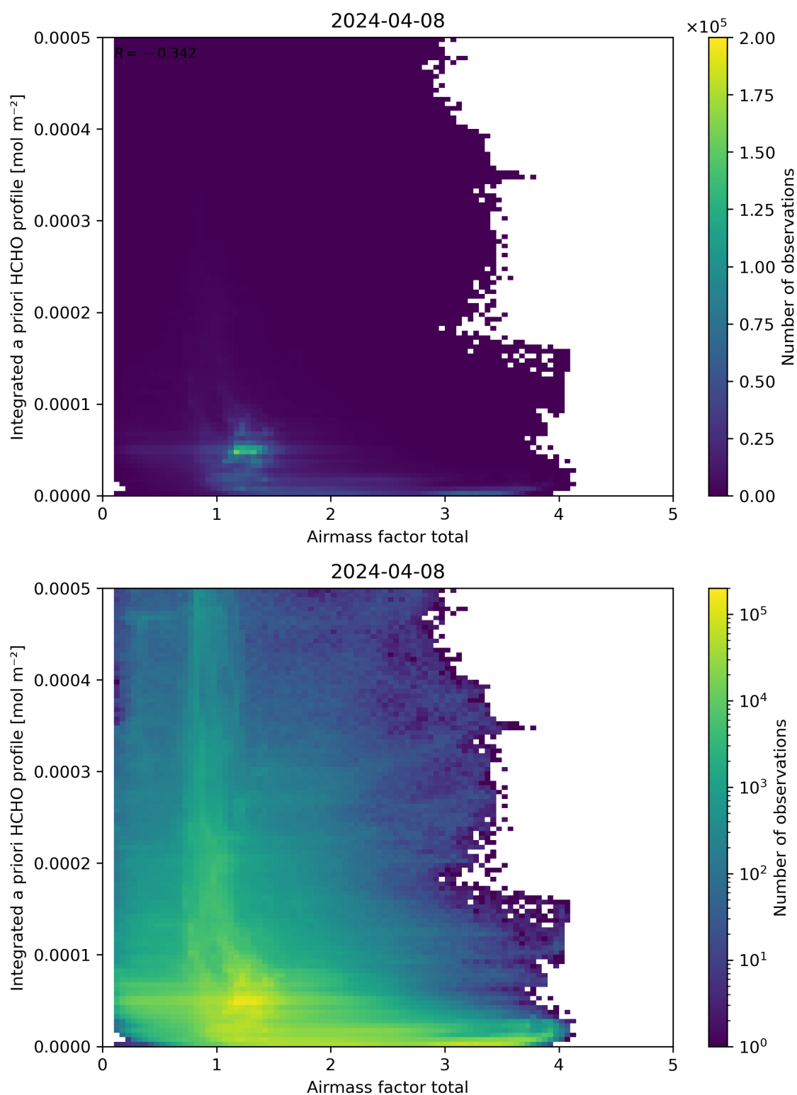
Figure 104: Scatter density plot of “Air mass factor total” against “Integrated a priori HCHO profile” for 2024-04-07 to 2024-04-09.
