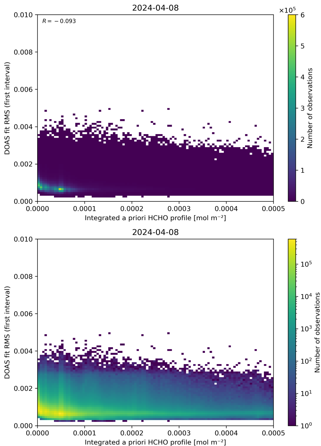
Figure 148: Scatter density plot of “Integrated a priori HCHO profile” against “DOAS fit RMS (first interval)” for 2024-04-07 to 2024-04-09.
