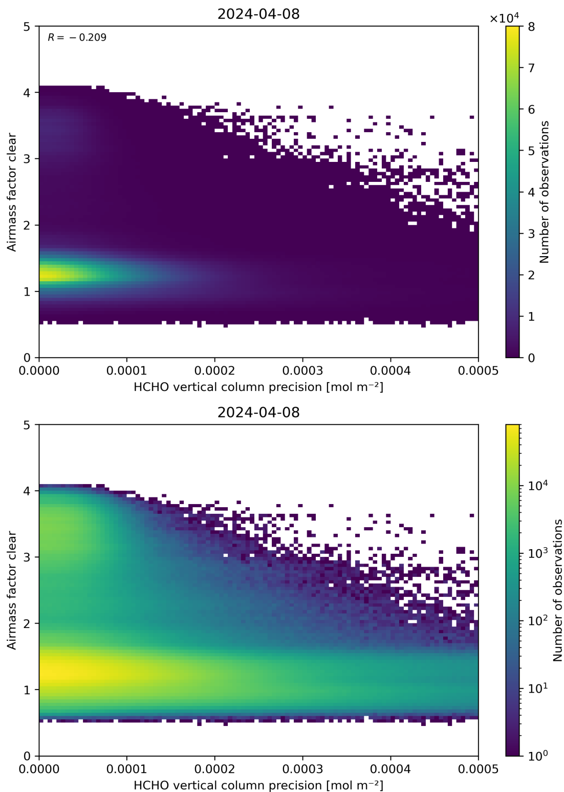
Figure 139: Scatter density plot of “HCHO vertical column precision” against “Airmass factor clear” for 2024-04-07 to 2024-04-09.
