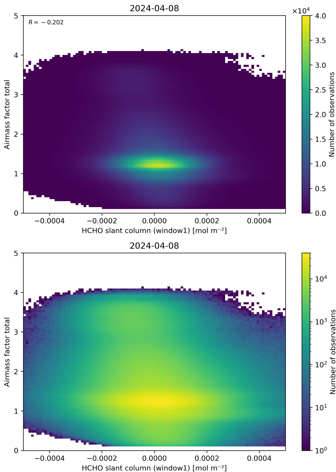
Figure 85: Scatter density plot of “HCHO slant column (window1)” against “Airmass factor total” for 2024-04-07 to 2024-04-09.
