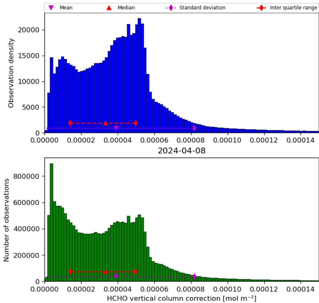
Figure 37: Histogram of “HCHO vertical column correction” for 2024-04-07 to 2024-04-09
