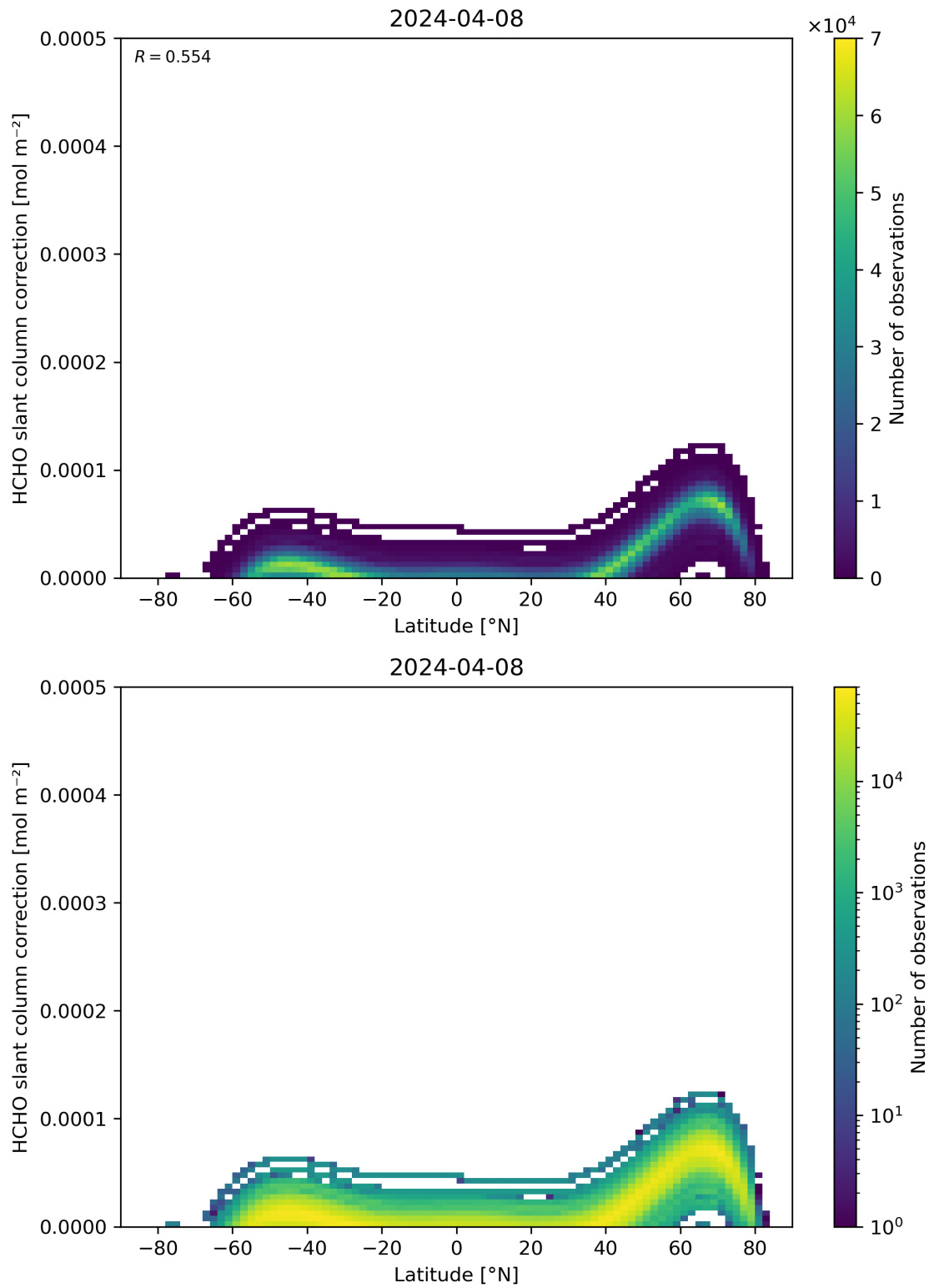
Figure 158: Scatter density plot of “Latitude” against “HCHO slant column correction” for 2024-04-07 to 2024-04-09.
