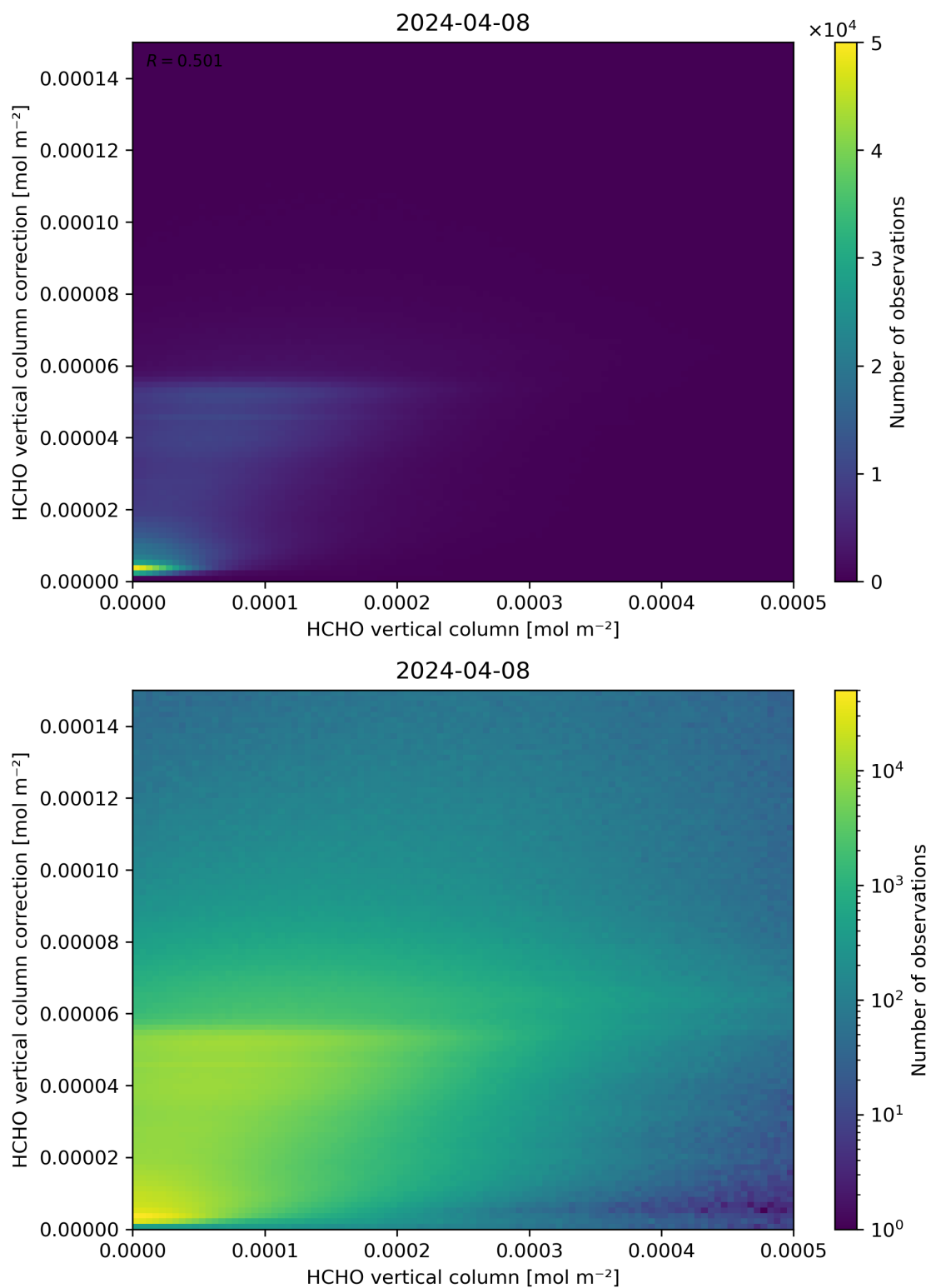
Figure 133: Scatter density plot of “HCHO vertical column” against “HCHO vertical column correction” for 2024-04-07 to 2024-04-09.
