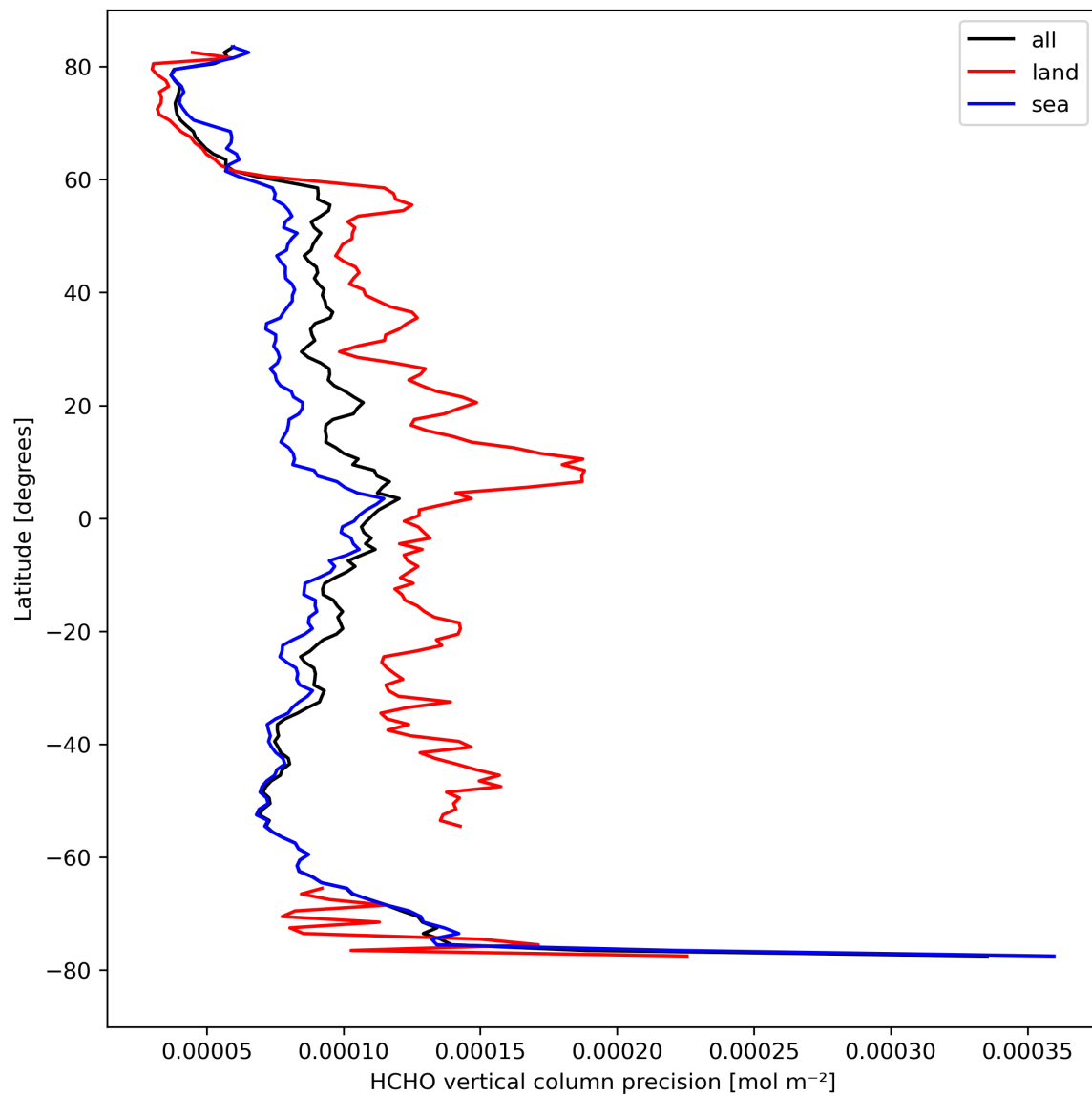
Figure 22: Zonal average of “HCHO vertical column precision” for 2024-04-07 to 2024-04-09.
