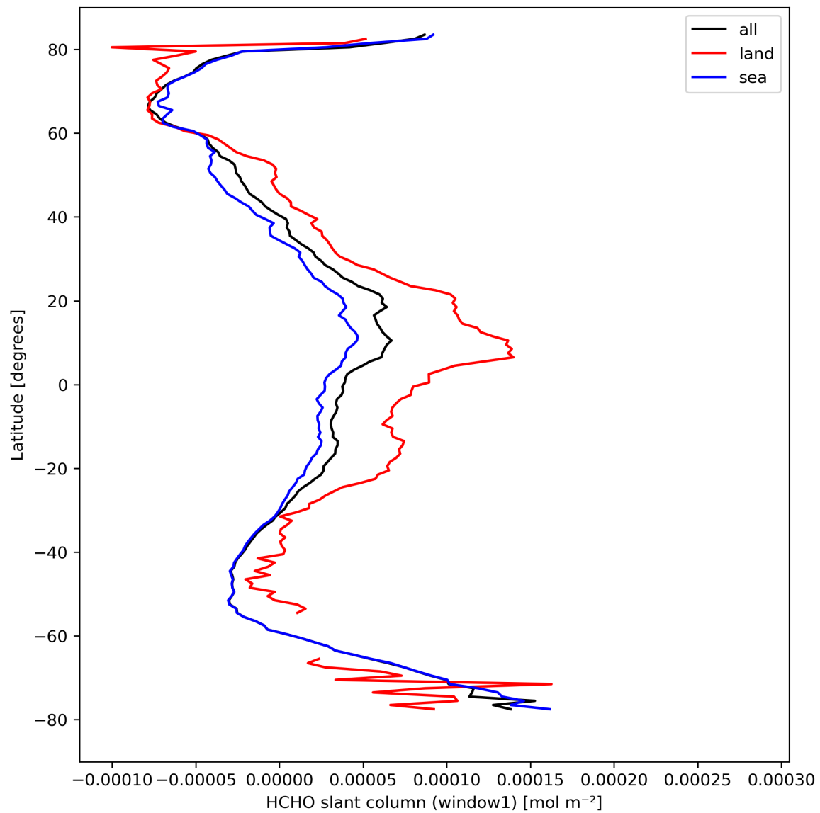
Figure 24: Zonal average of “HCHO slant column (window1)” for 2024-04-07 to 2024-04-09.
