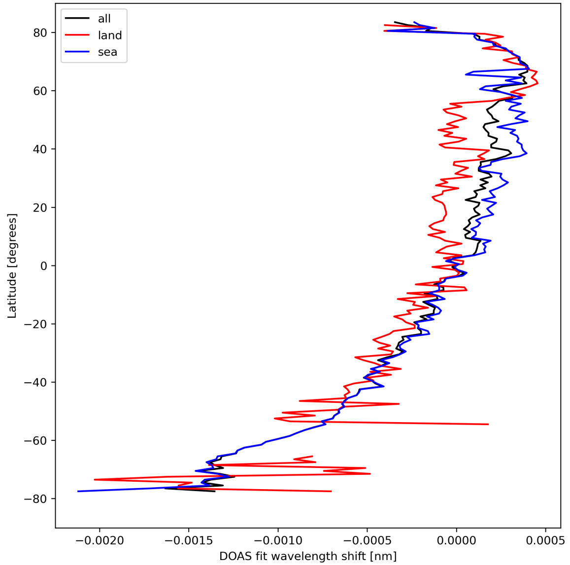
Figure 30: Zonal average of “DOAS fit wavelength shift” for 2024-04-07 to 2024-04-09.
