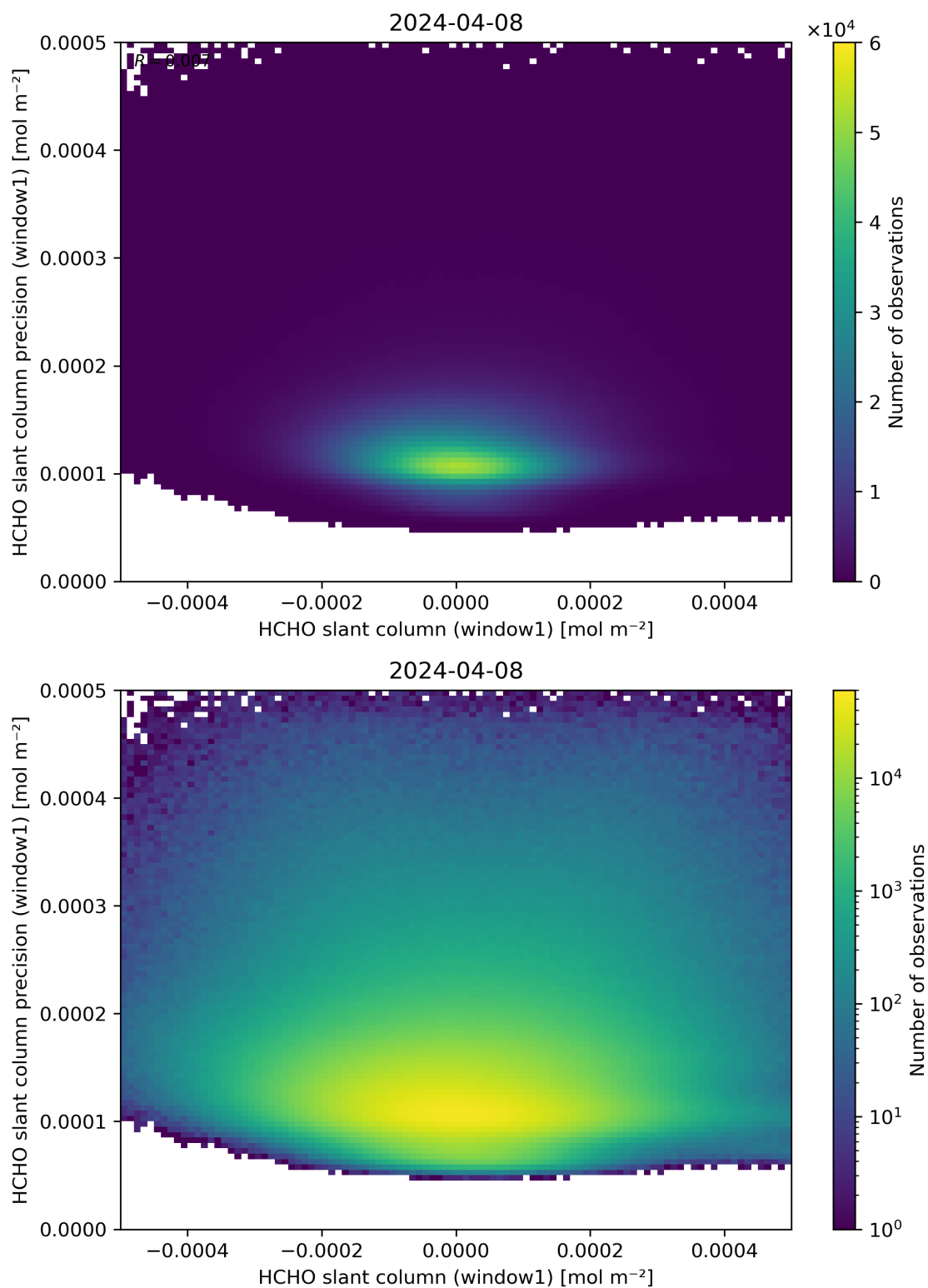
Figure 84: Scatter density plot of “HCHO slant column (window1)” against “HCHO slant column precision (window1)” for 2024-04-07 to 2024-04-09.
