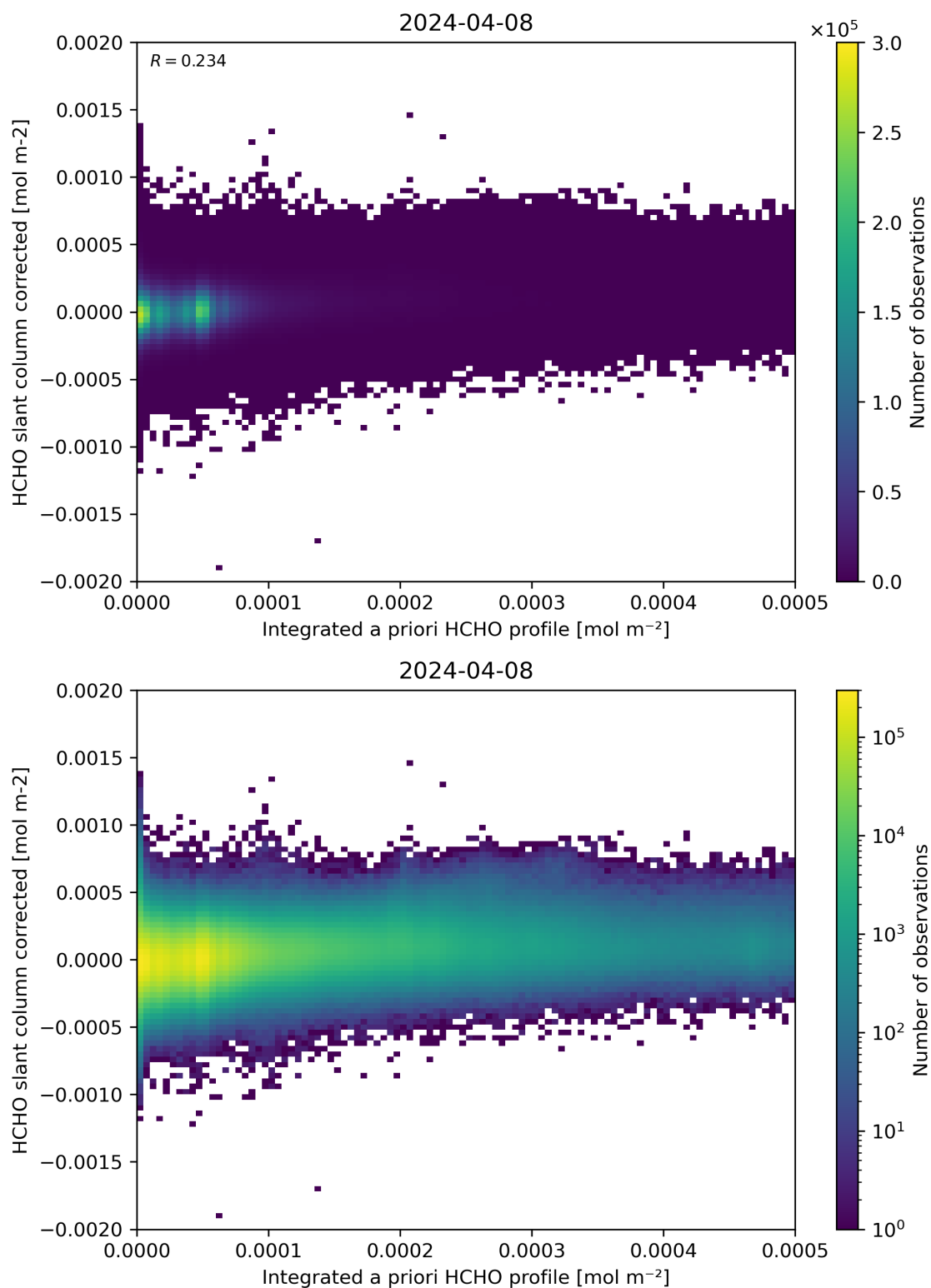
Figure 151: Scatter density plot of “Integrated a priori HCHO profile” against “HCHO slant column corrected” for 2024-04-07 to 2024-04-09.
