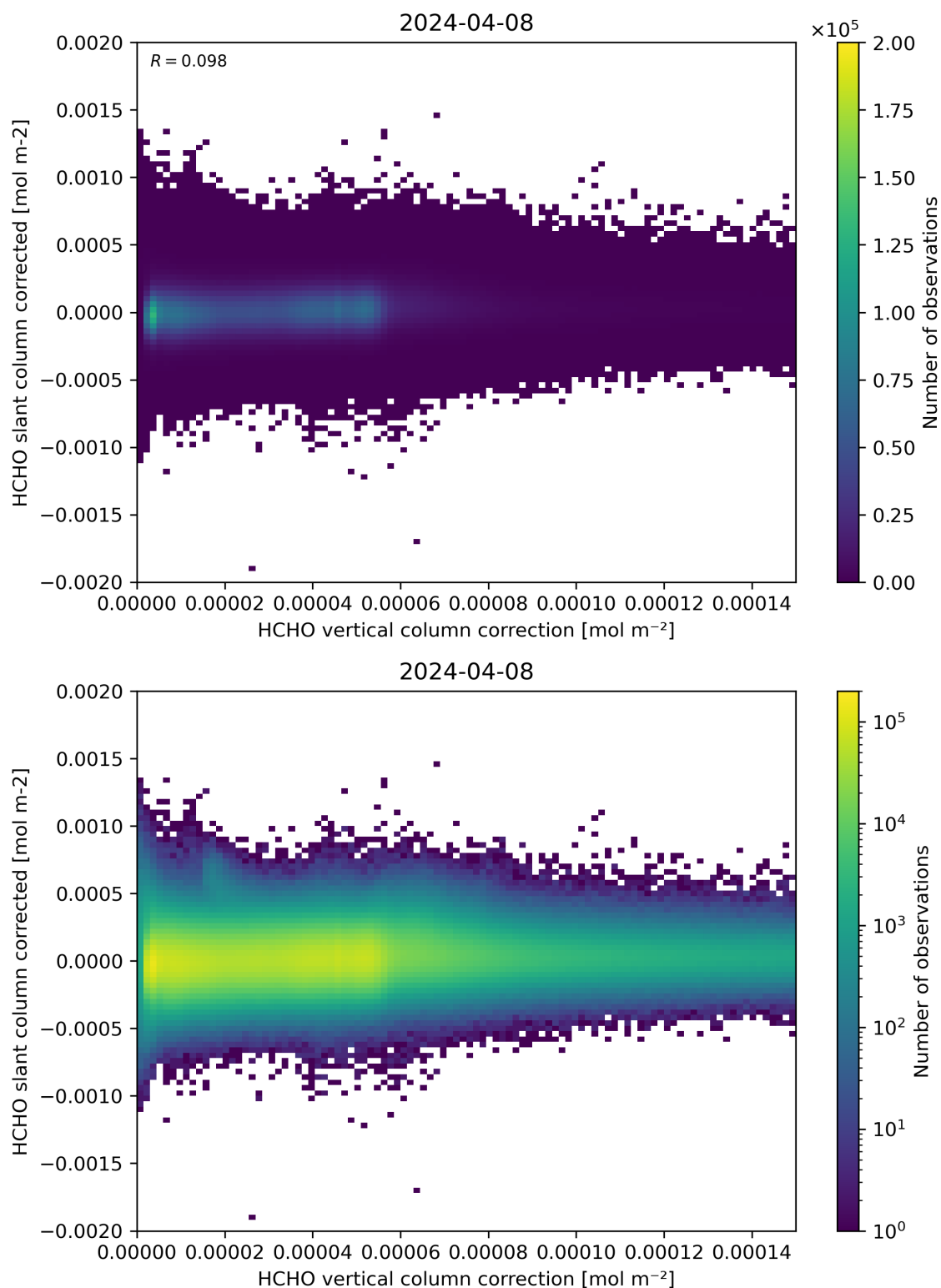
Figure 116: Scatter density plot of “HCHO vertical column correction” against “HCHO slant column corrected” for 2024-04-07 to 2024-04-09.
