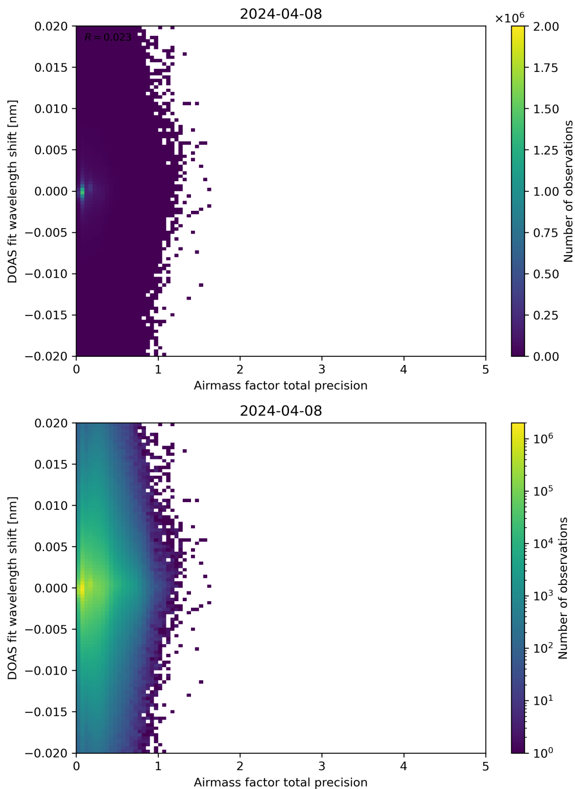
Figure 106: Scatter density plot of “Airmass factor total precision” against “DOAS fit wavelength shift” for 2024-04-07 to 2024-04-09.
