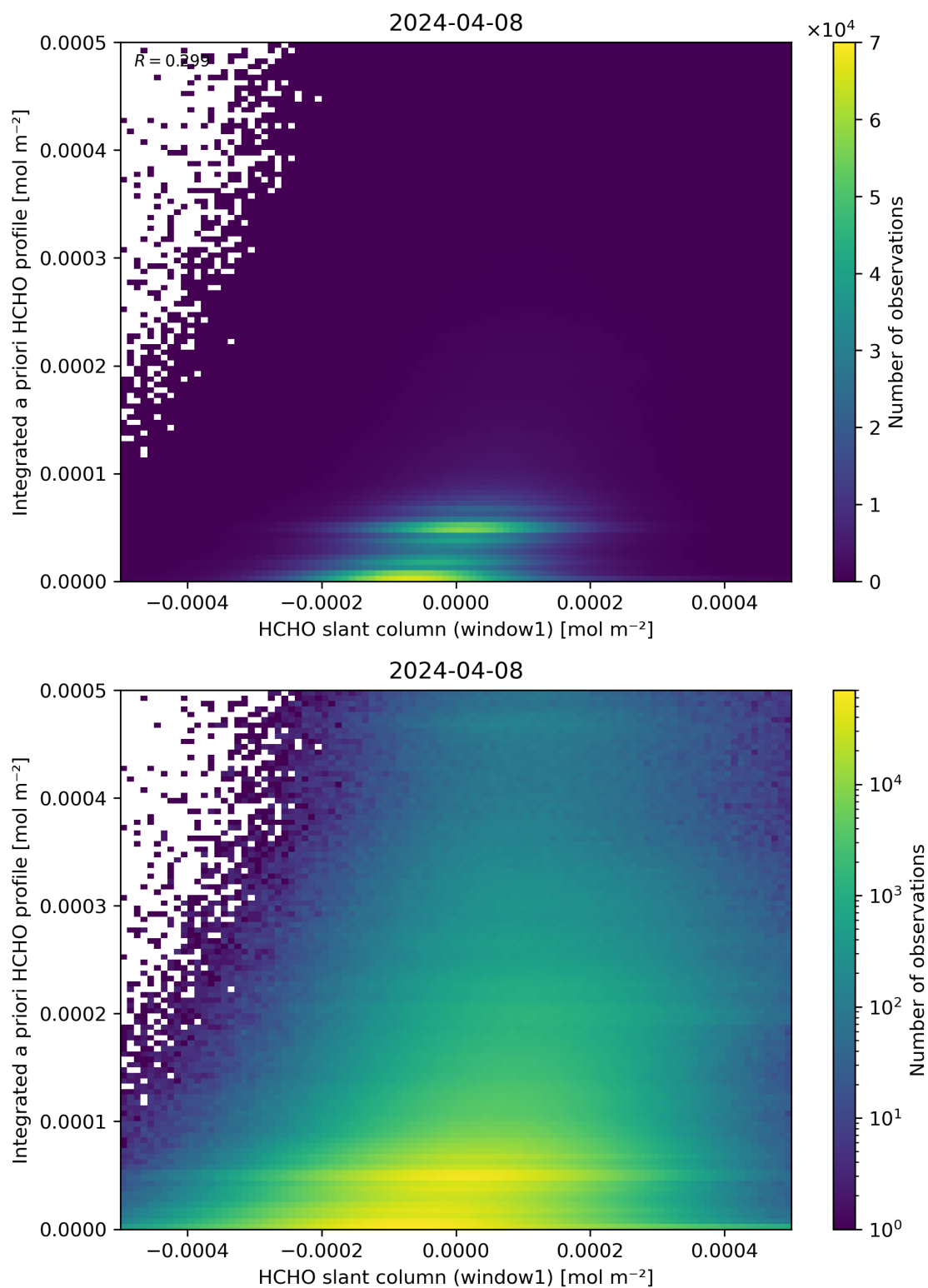
Figure 87: Scatter density plot of “HCHO slant column (window1)” against “Integrated a priori HCHO profile” for 2024-04-07 to 2024-04-09.
