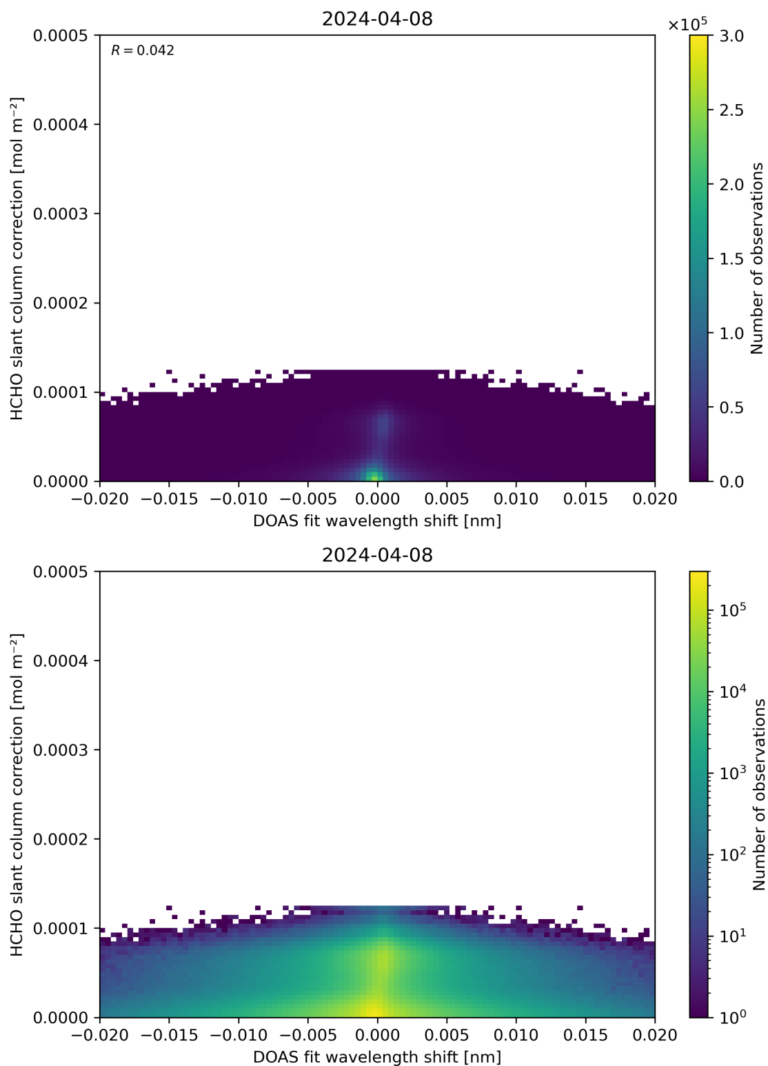
Figure 67: Scatter density plot of “DOAS fit wavelength shift” against “HCHO slant column correction” for 2024-04-07 to 2024-04-09.
