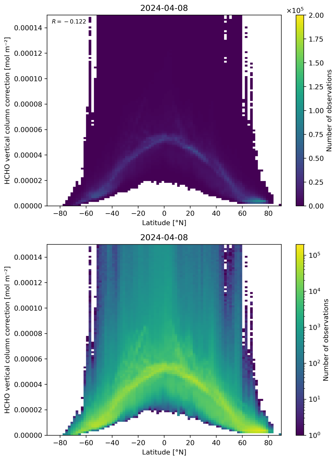
Figure 164: Scatter density plot of “Latitude” against “HCHO vertical column correction” for 2024-04-07 to 2024-04-09.
