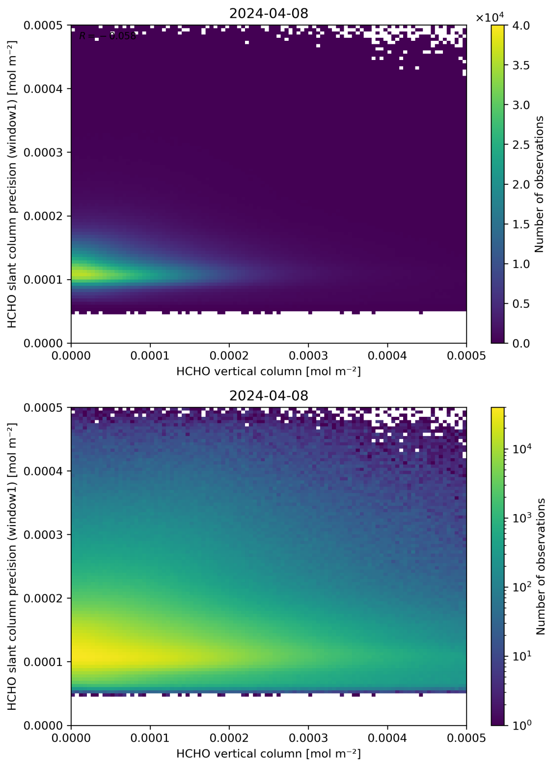
Figure 130: Scatter density plot of “HCHO vertical column” against “HCHO slant column precision (window1)” for 2024-04-07 to 2024-04-09.
