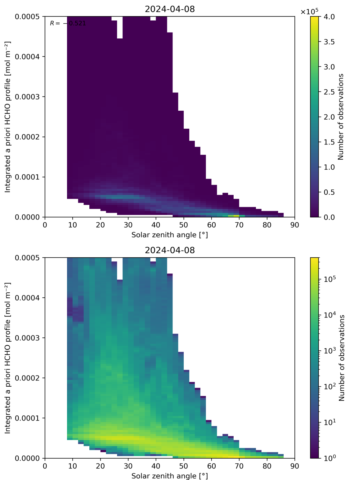
Figure 180: Scatter density plot of “Solar zenith angle” against “Integrated a priori HCHO profile” for 2024-04-07 to 2024-04-09.
