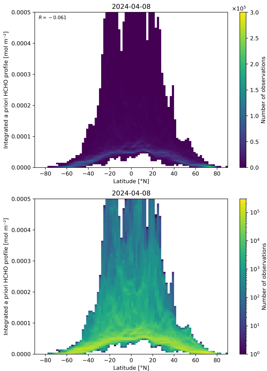
Figure 166: Scatter density plot of “Latitude” against “Integrated a priori HCHO profile” for 2024-04-07 to 2024-04-09.
