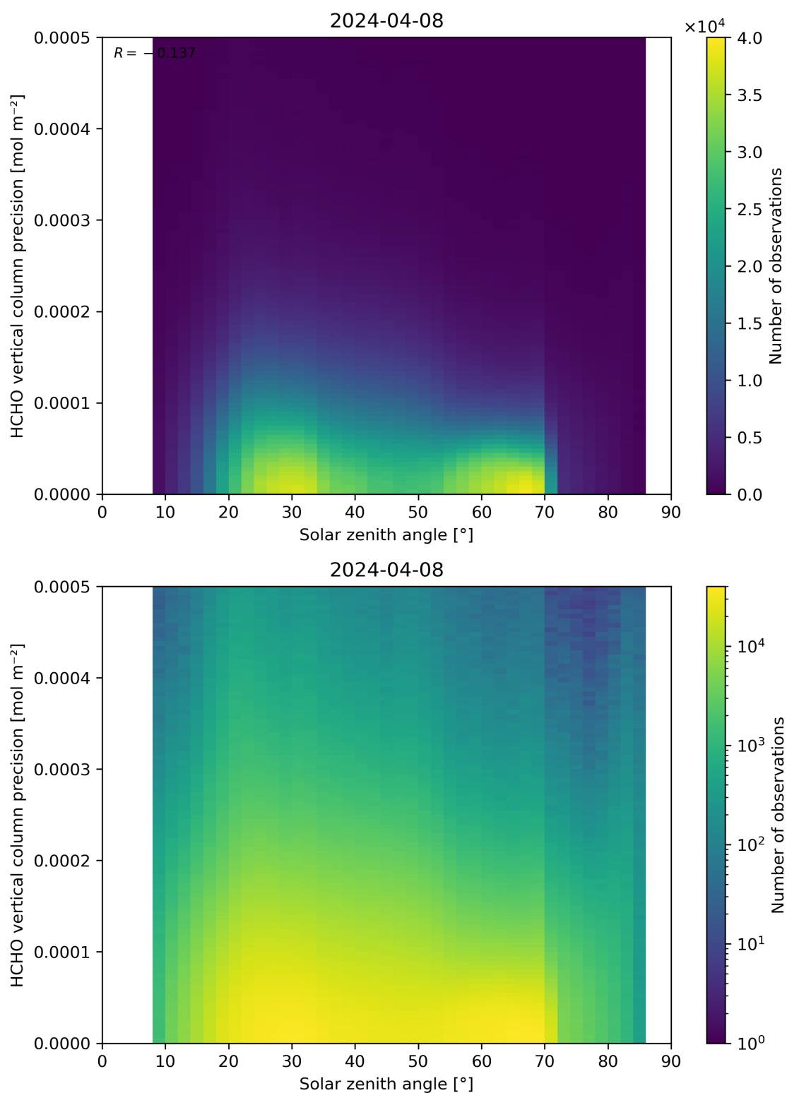
Figure 179: Scatter density plot of “Solar zenith angle” against “HCHO vertical column precision” for 2024-04-07 to 2024-04-09.
