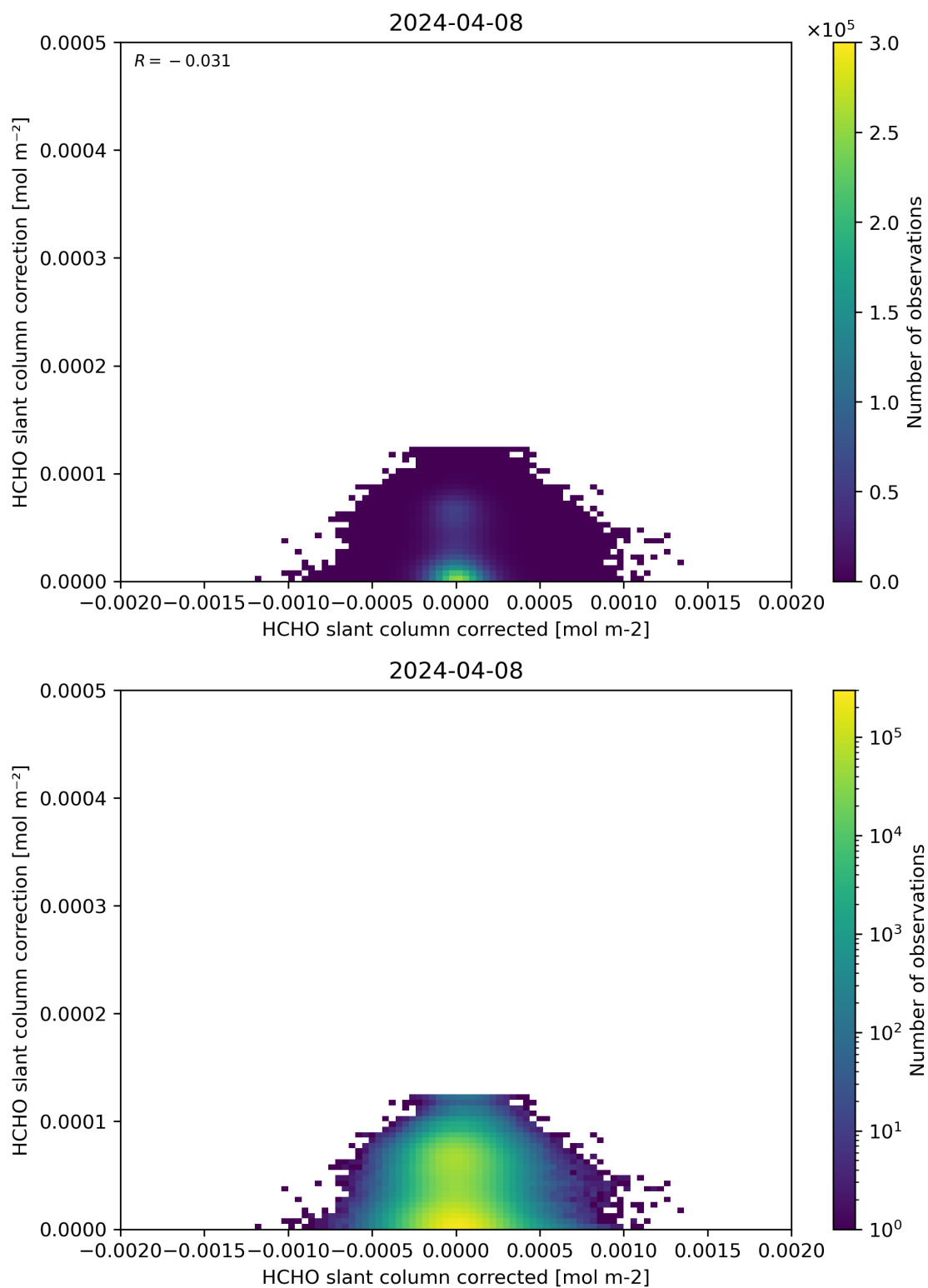
Figure 77: Scatter density plot of “HCHO slant column corrected” against “HCHO slant column correction” for 2024-04-07 to 2024-04-09.
