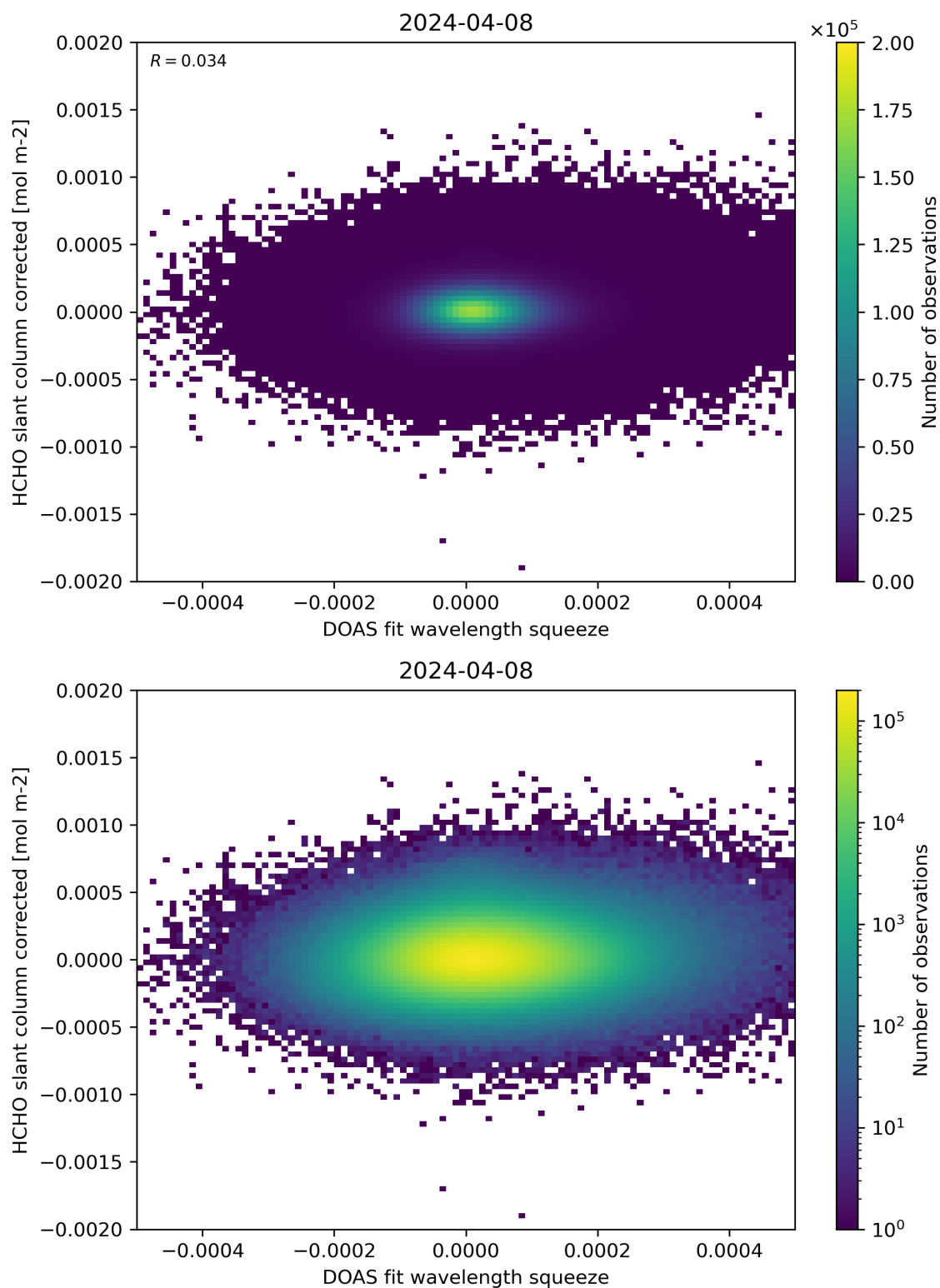
Figure 69: Scatter density plot of “DOAS fit wavelength squeeze” against “HCHO slant column corrected” for 2024-04-07 to 2024-04-09.
