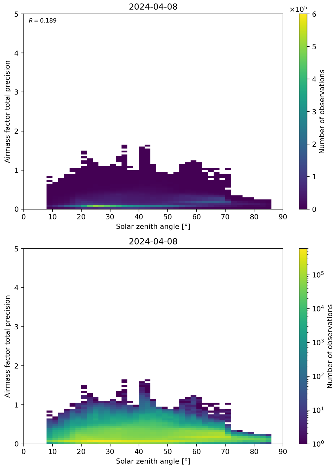
Figure 176: Scatter density plot of “Solar zenith angle” against “Airmass factor total precision” for 2024-04-07 to 2024-04-09.
