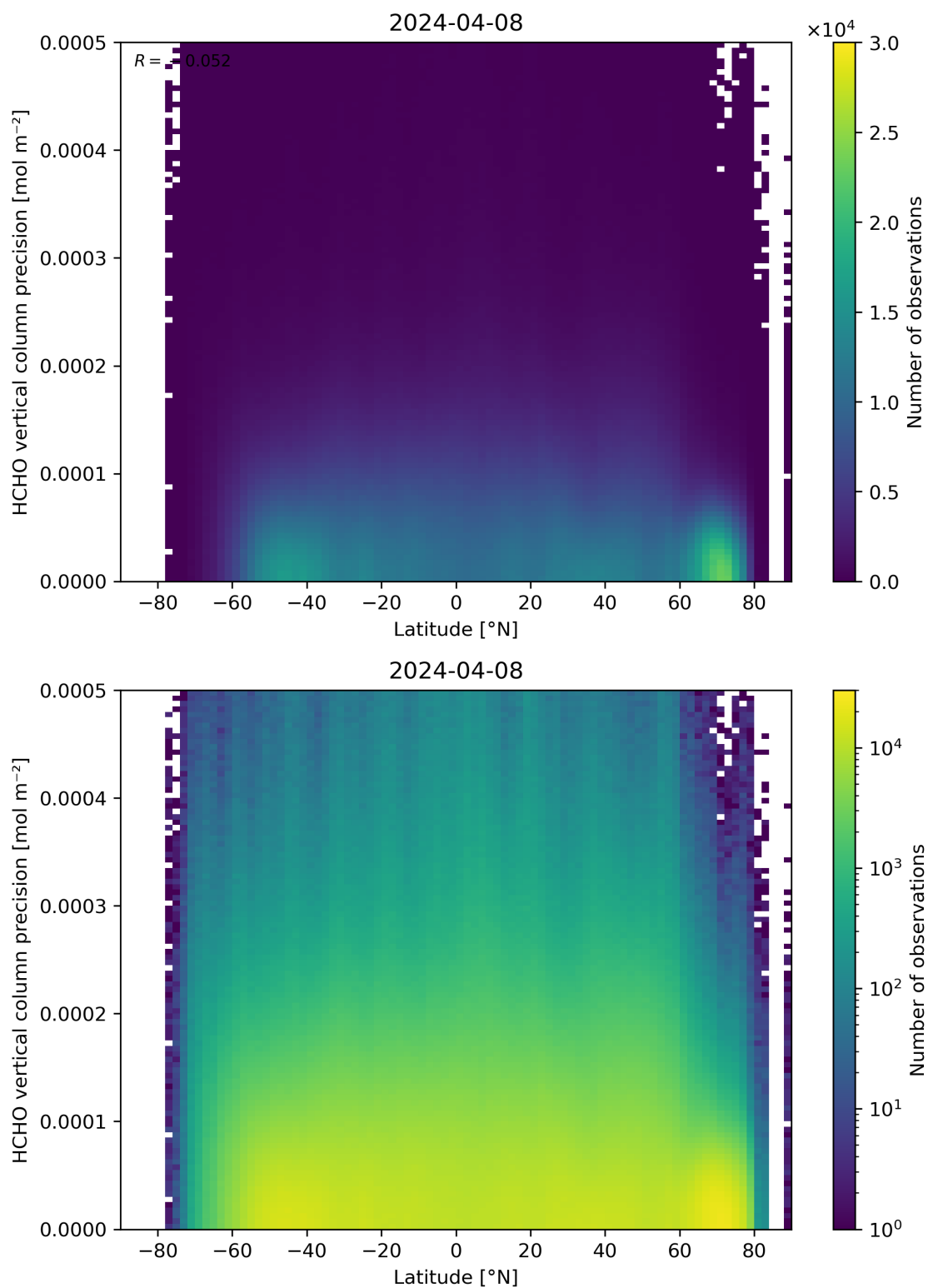
Figure 165: Scatter density plot of “Latitude” against “HCHO vertical column precision” for 2024-04-07 to 2024-04-09.
