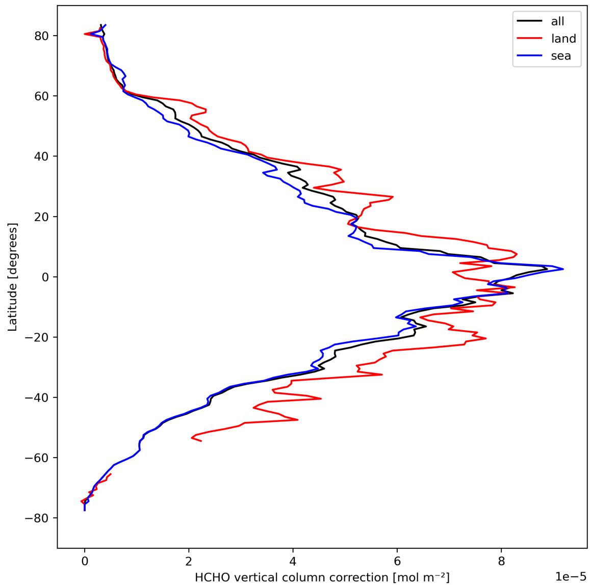
Figure 23: Zonal average of “HCHO vertical column correction” for 2024-04-07 to 2024-04-09.
