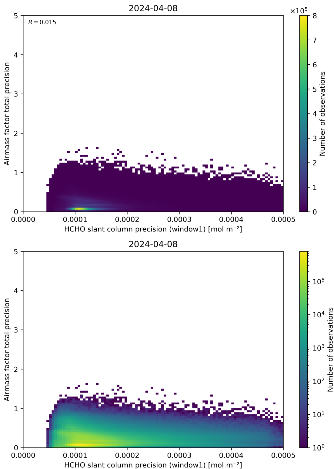
Figure 95: Scatter density plot of “HCHO slant column precision (window1)” against “Airmass factor total precision” for 2024-04-07 to 2024-04-09.
