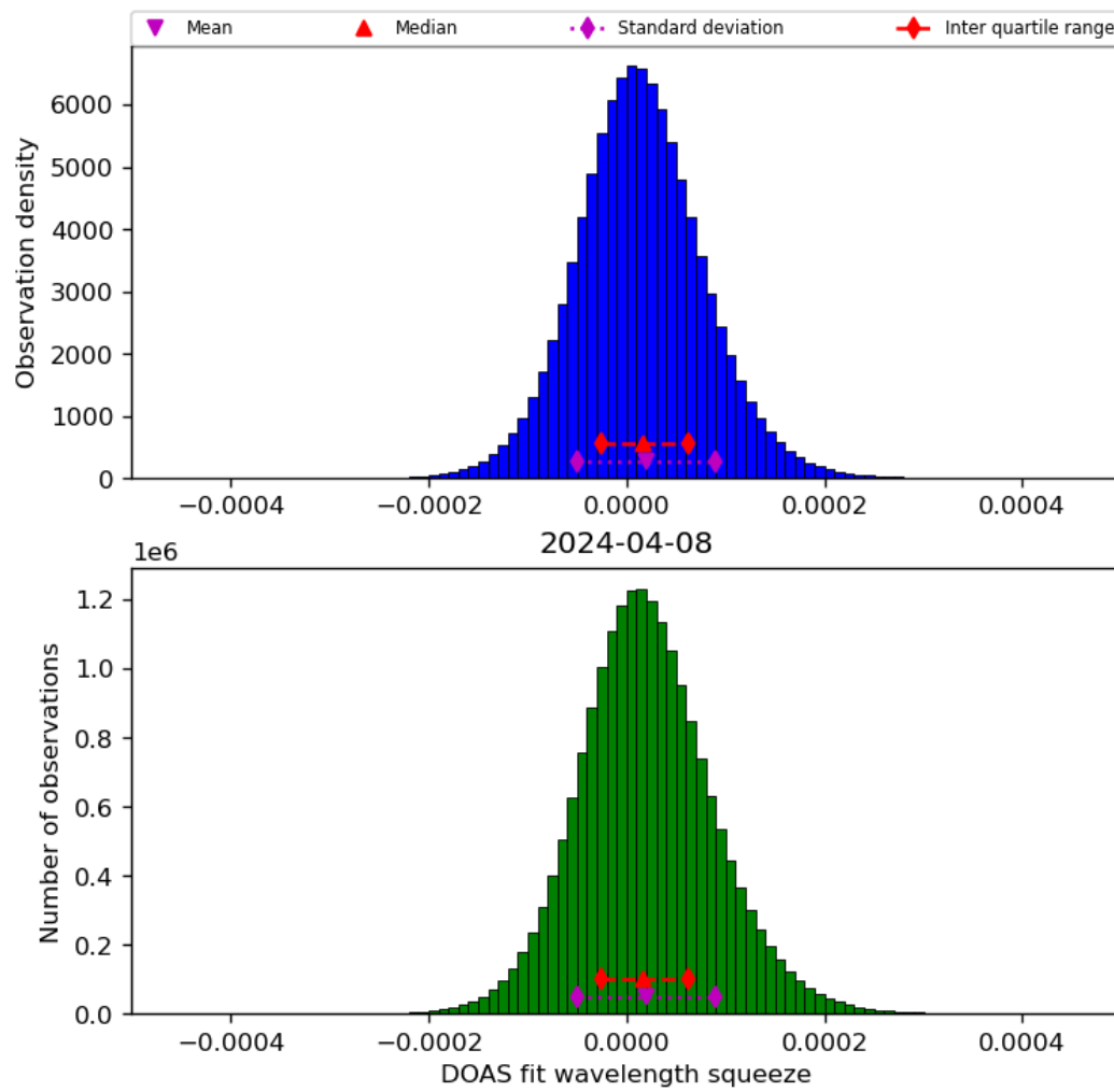
Figure 45: Histogram of “DOAS fit wavelength squeeze” for 2024-04-07 to 2024-04-09
