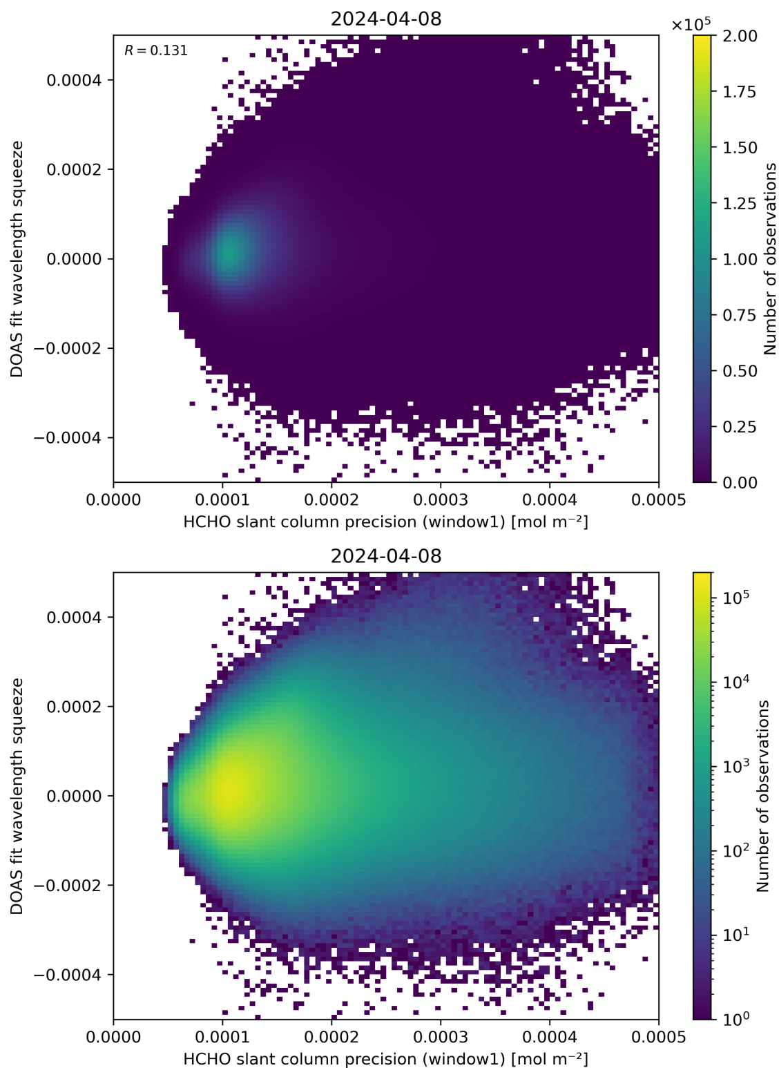
Figure 90: Scatter density plot of “HCHO slant column precision (window1)” against “DOAS fit wavelength squeeze” for 2024-04-07 to 2024-04-09.
