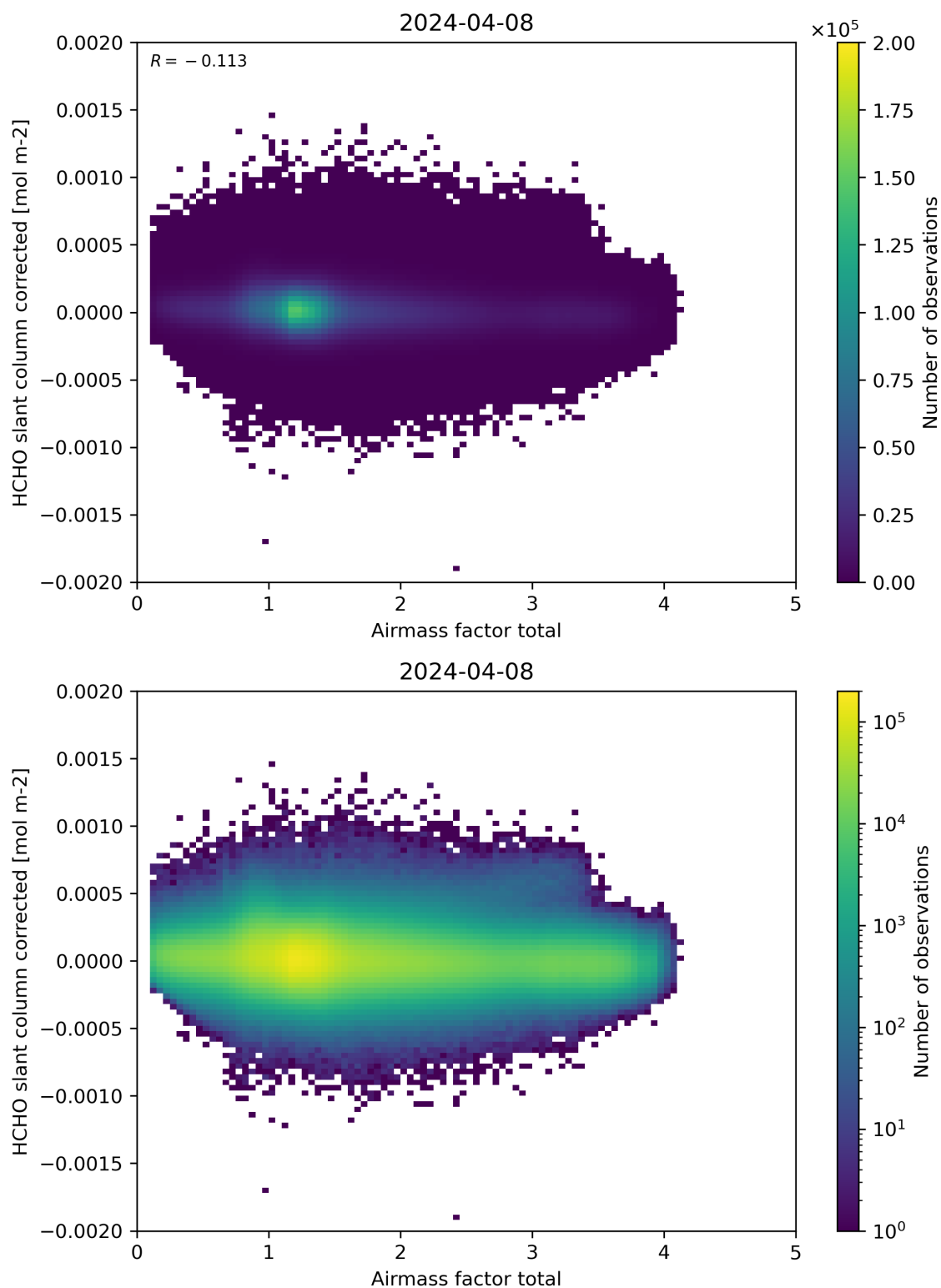
Figure 101: Scatter density plot of “Airmass factor total” against “HCHO slant column corrected” for 2024-04-07 to 2024-04-09.
