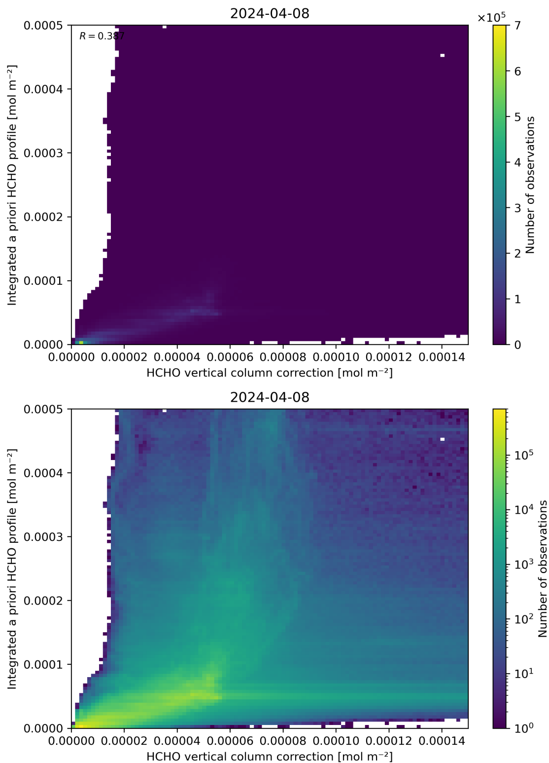
Figure 122: Scatter density plot of “HCHO vertical column correction” against “Integrated a priori HCHO profile” for 2024-04-07 to 2024-04-09.
