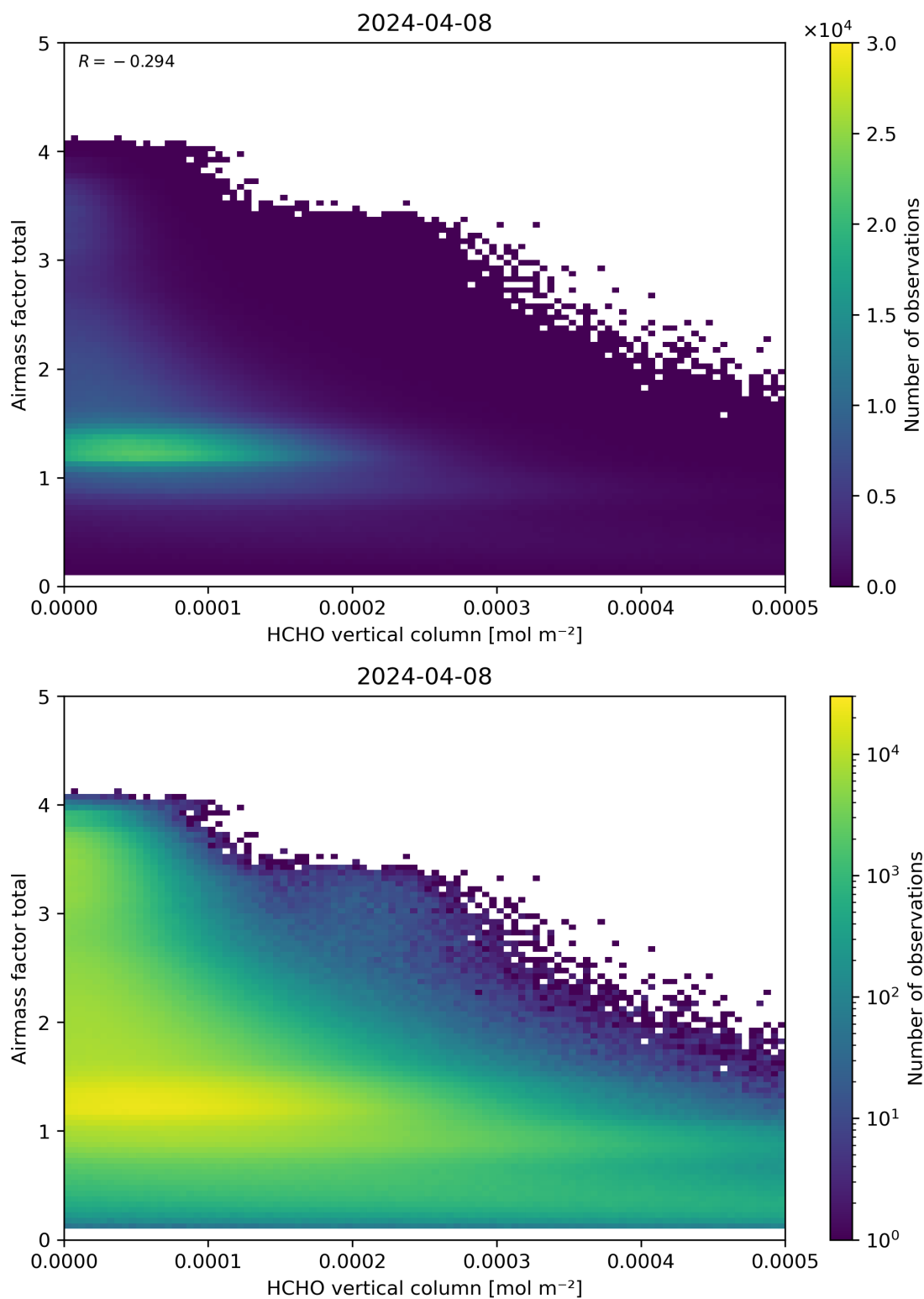
Figure 131: Scatter density plot of “HCHO vertical column” against “Airmass factor total” for 2024-04-07 to 2024-04-09.
