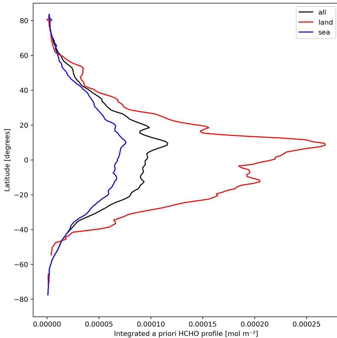
Figure 29: Zonal average of “Integrated a priori HCHO profile” for 2024-04-07 to 2024-04-09.
