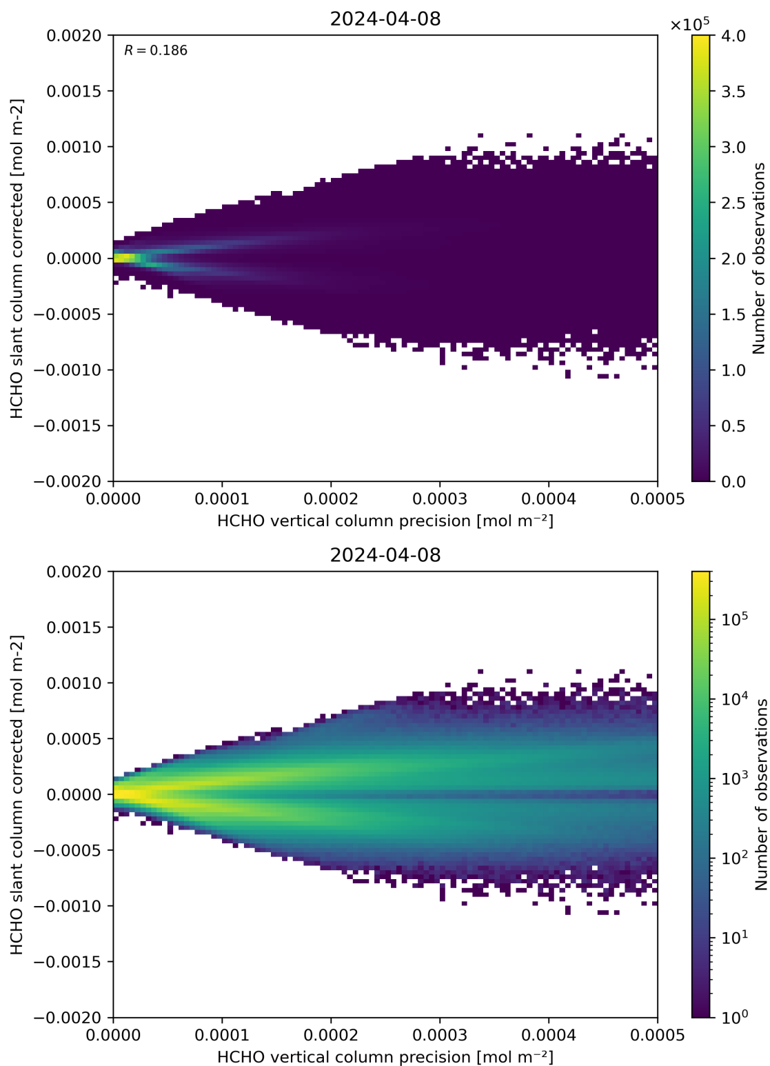
Figure 140: Scatter density plot of “HCHO vertical column precision” against “HCHO slant column corrected” for 2024-04-07 to 2024-04-09.
