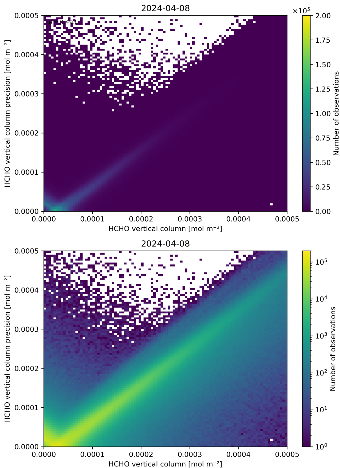
Figure 134: Scatter density plot of “HCHO vertical column” against “HCHO vertical column precision” for 2024-04-07 to 2024-04-09.
