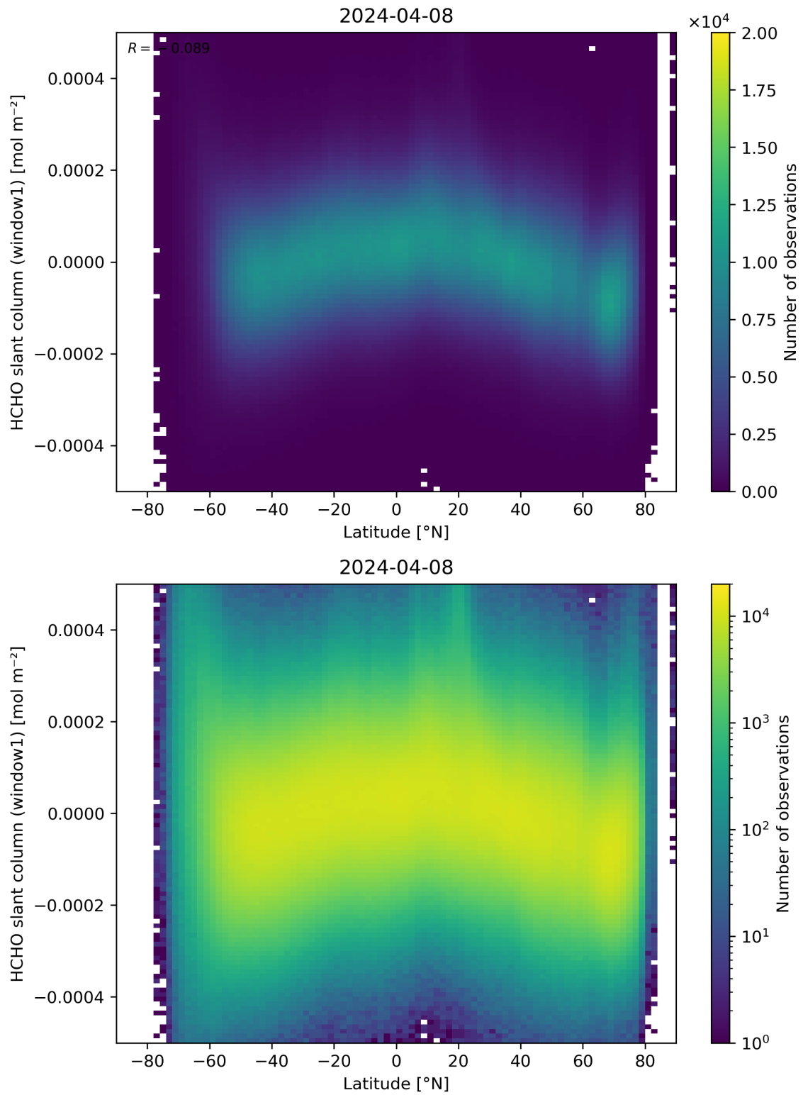
Figure 159: Scatter density plot of “Latitude” against “HCHO slant column (window1)” for 2024-04-07 to 2024-04-09.
