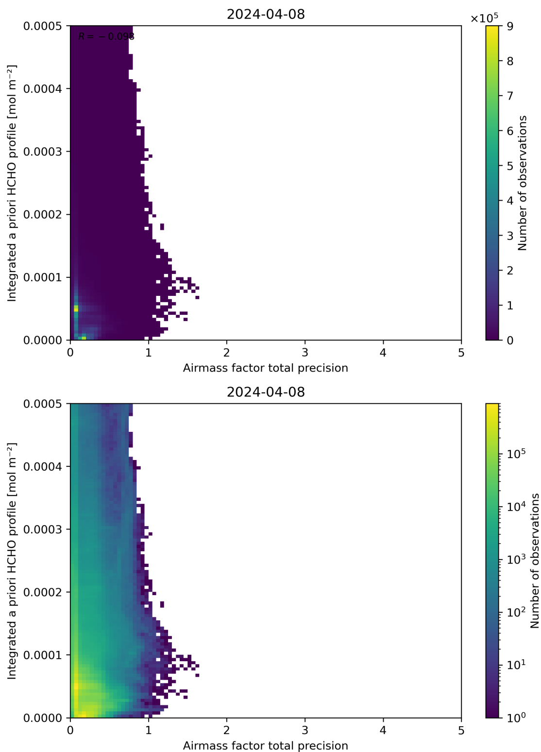
Figure 111: Scatter density plot of “Airmass factor total precision” against “Integrated a priori HCHO profile” for 2024-04-07 to 2024-04-09.
