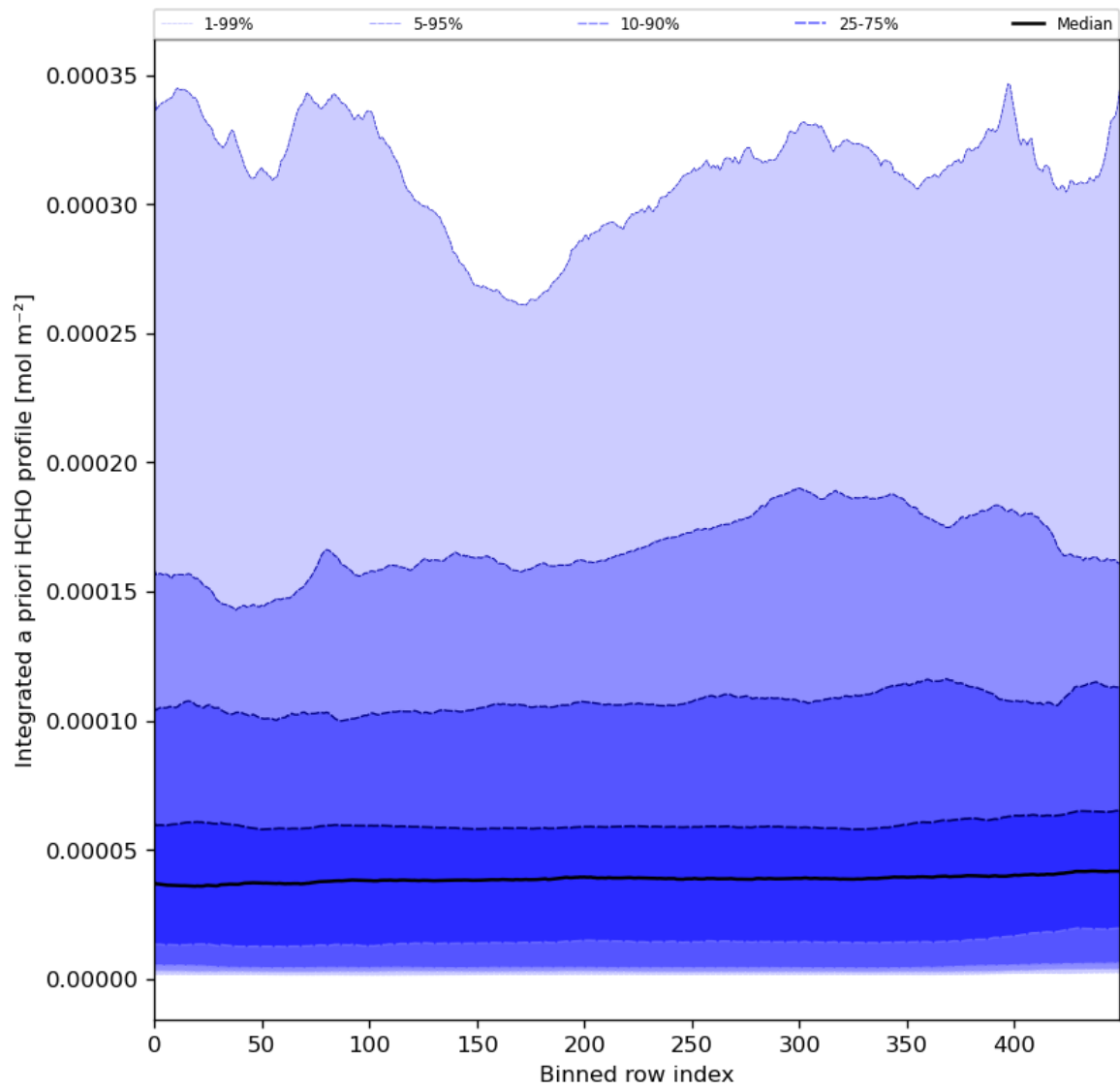
Figure 57: Along track statistics of “Integrated a priori HCHO profile” for 2024-04-07 to 2024-04-09
