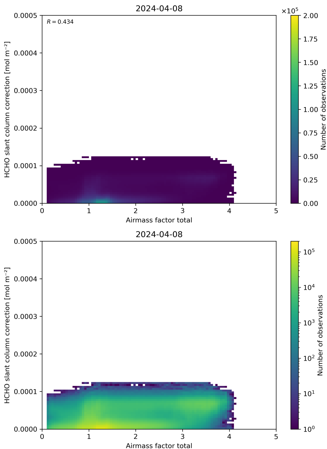
Figure 102: Scatter density plot of “Airmass factor total” against “HCHO slant column correction” for 2024-04-07 to 2024-04-09.
