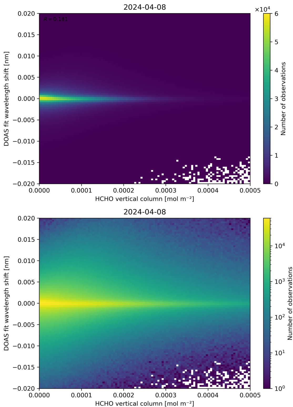
Figure 124: Scatter density plot of “HCHO vertical column” against “DOAS fit wavelength shift” for 2024-04-07 to 2024-04-09.
