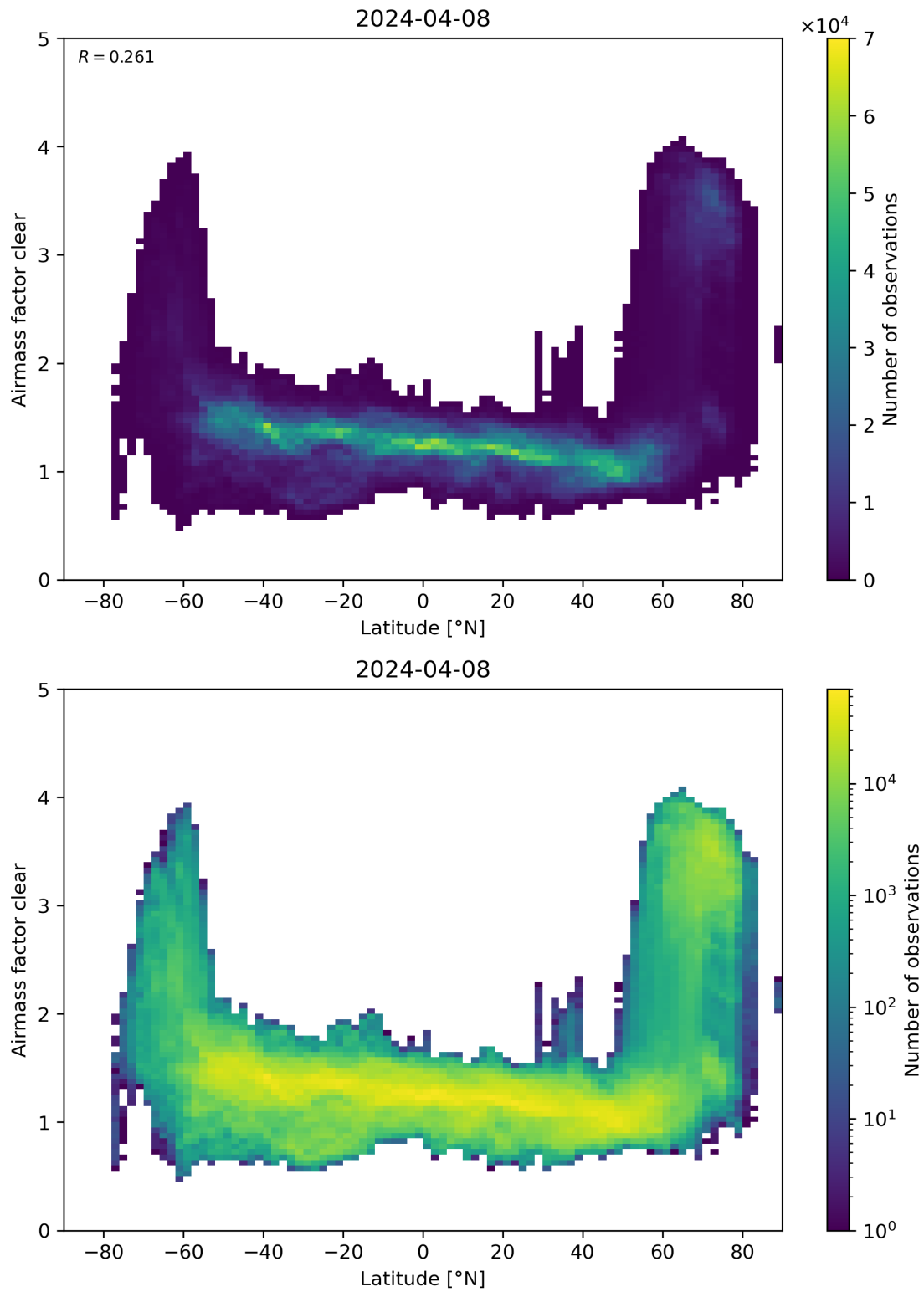
Figure 156: Scatter density plot of “Latitude” against “Airmass factor clear” for 2024-04-07 to 2024-04-09.
