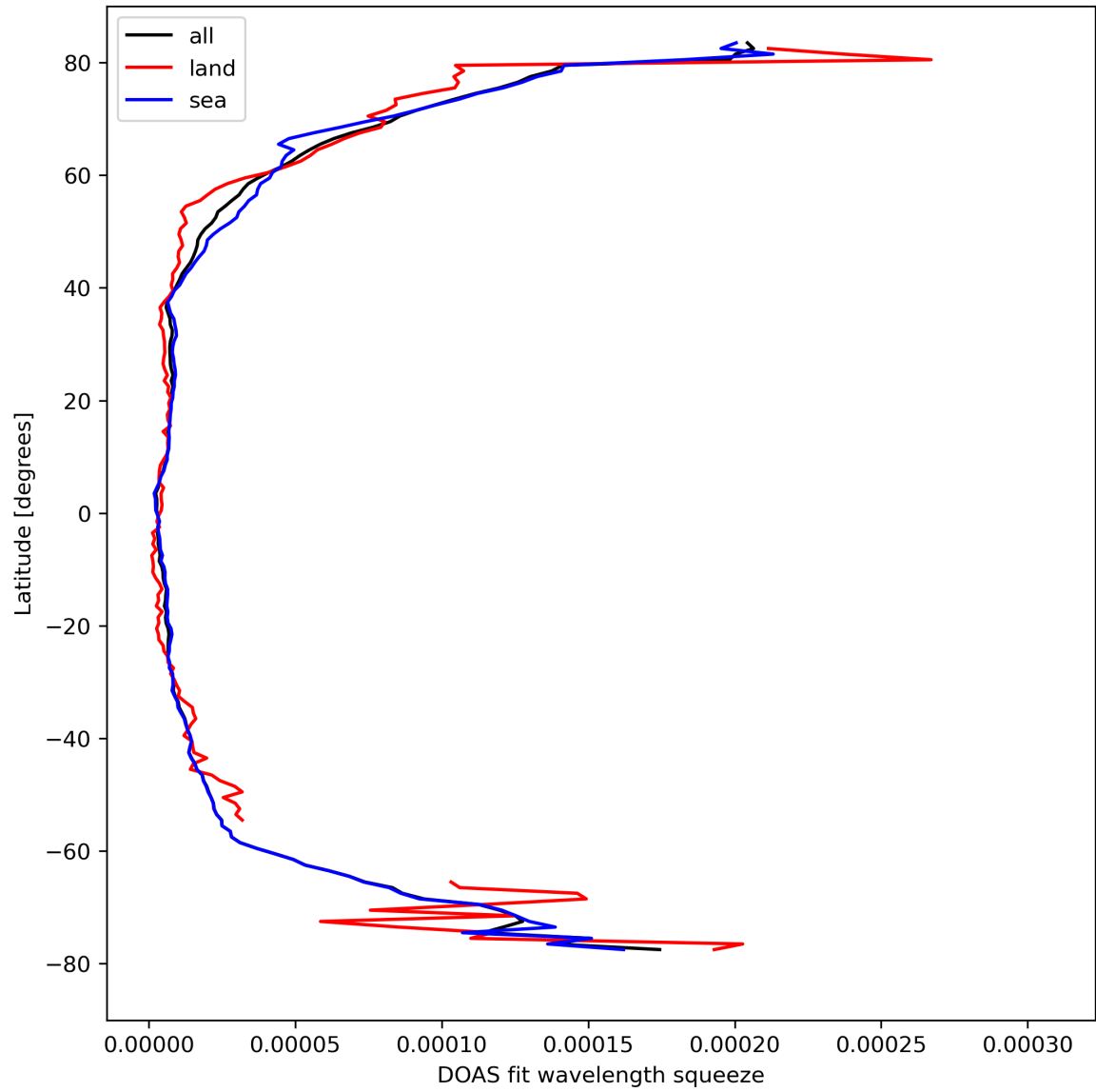
Figure 31: Zonal average of “DOAS fit wavelength squeeze” for 2024-04-07 to 2024-04-09.
