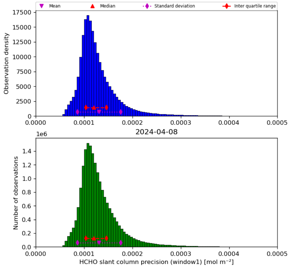
Figure 39: Histogram of “HCHO slant column precision (window1)” for 2024-04-07 to 2024-04-09
