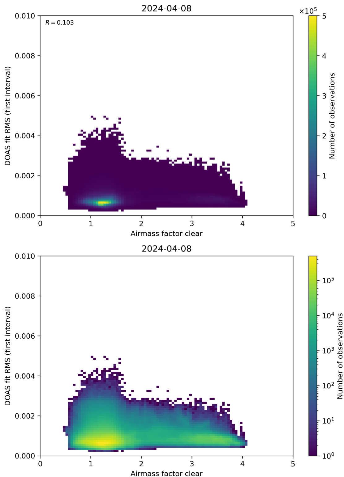
Figure 71: Scatter density plot of “Airmass factor clear” against “DOAS fit RMS (first interval)” for 2024-04-07 to 2024-04-09.
