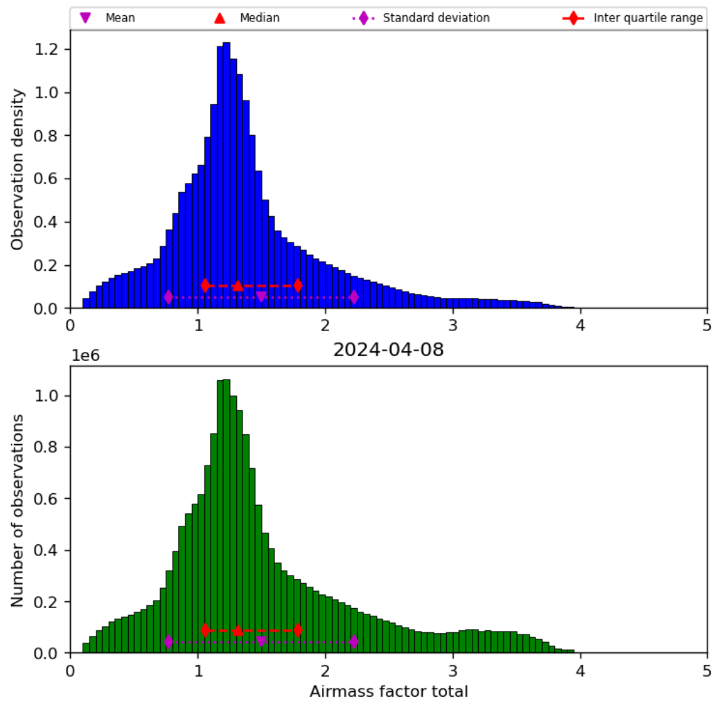
Figure 40: Histogram of “Airmass factor total” for 2024-04-07 to 2024-04-09
