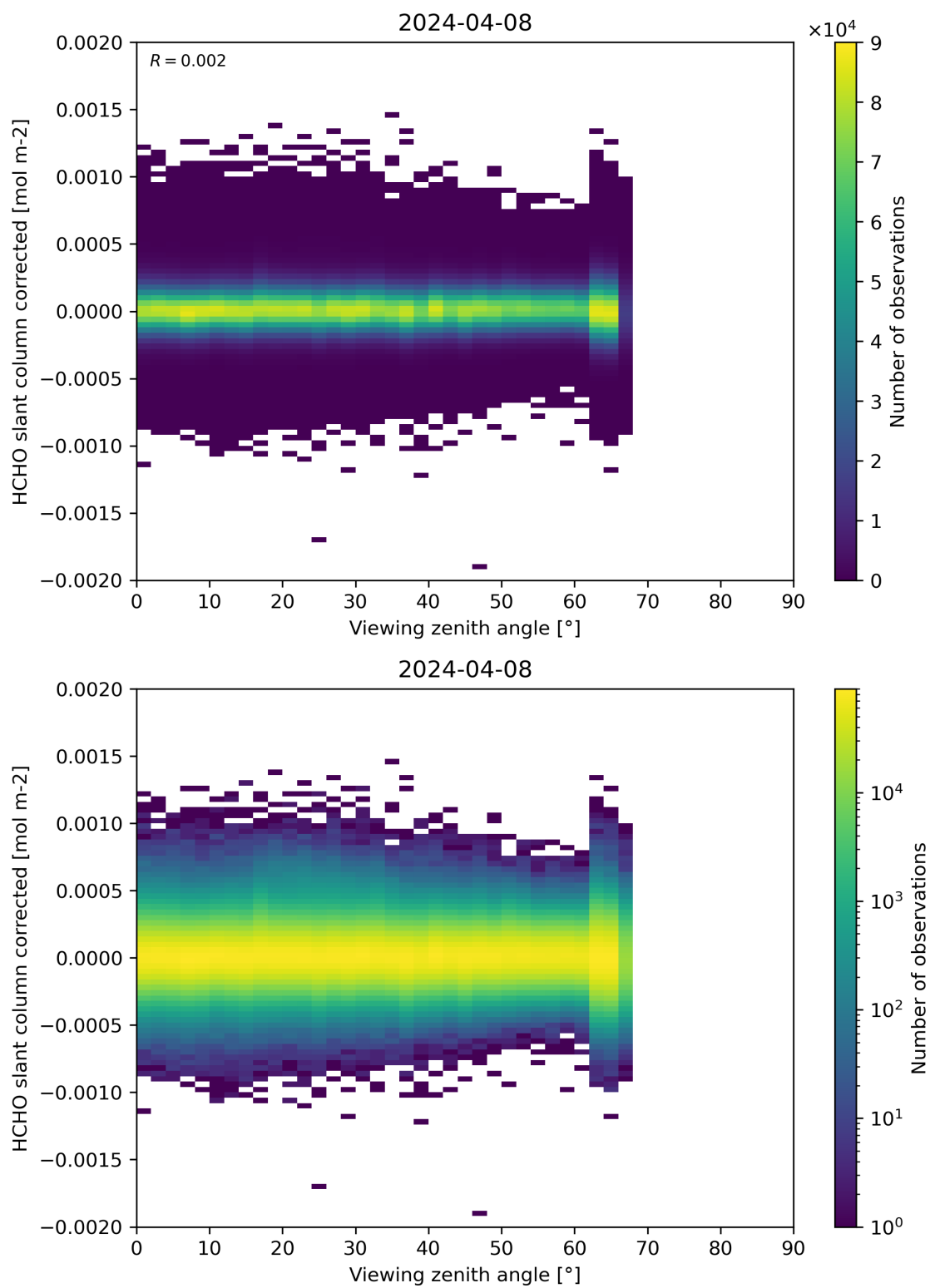
Figure 186: Scatter density plot of “Viewing zenith angle” against “HCHO slant column corrected” for 2024-04-07 to 2024-04-09.
