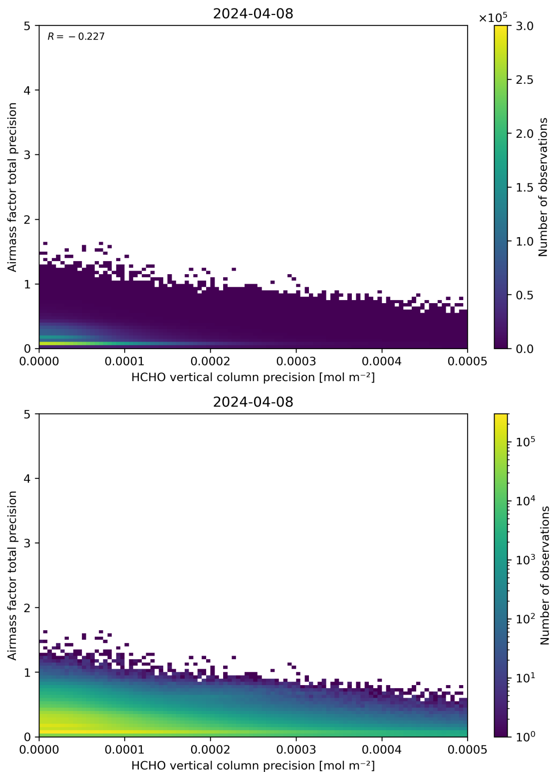
Figure 145: Scatter density plot of “HCHO vertical column precision” against “Airmass factor total precision” for 2024-04-07 to 2024-04-09.
