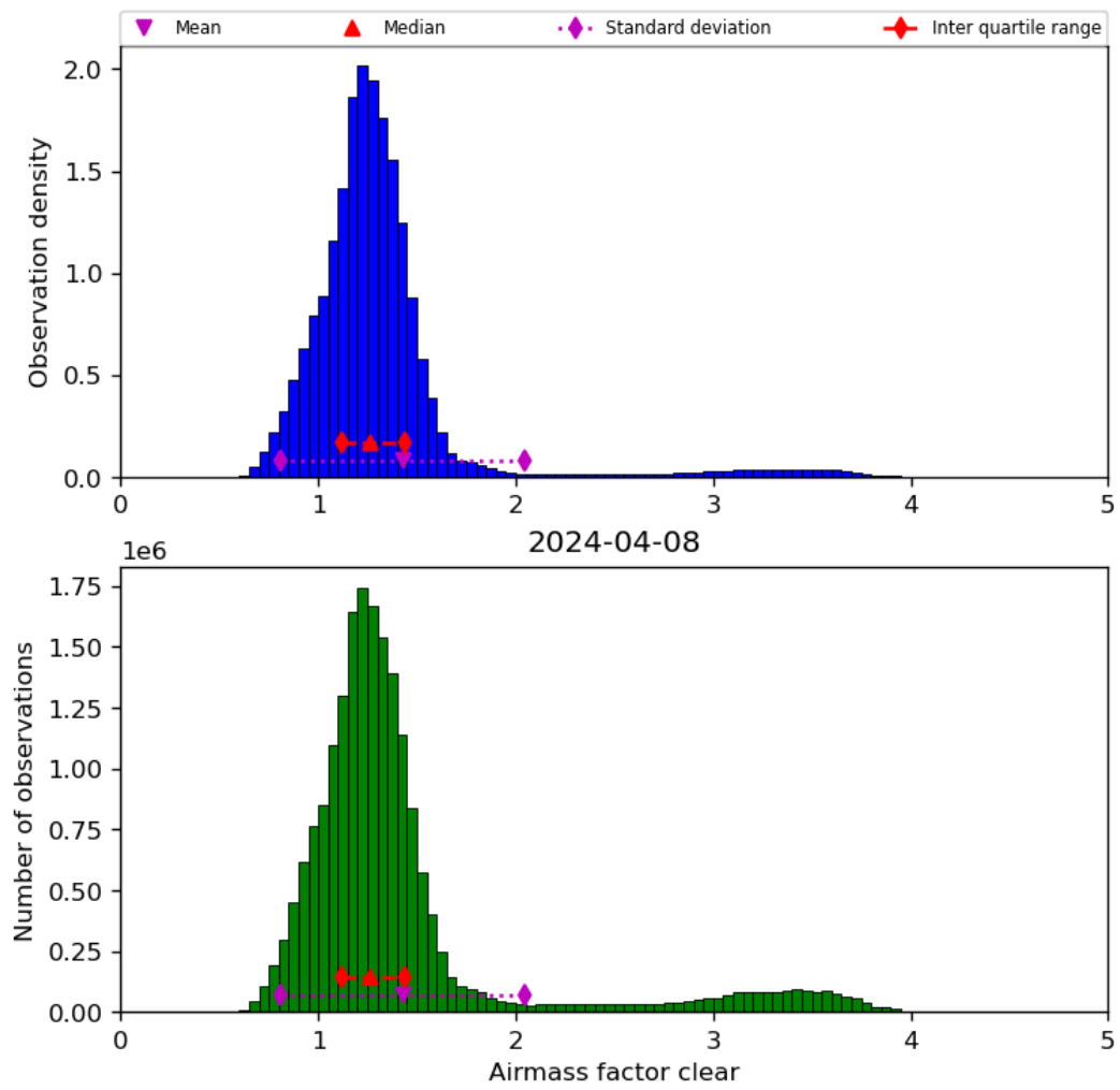
Figure 42: Histogram of “Airmass factor clear” for 2024-04-07 to 2024-04-09
