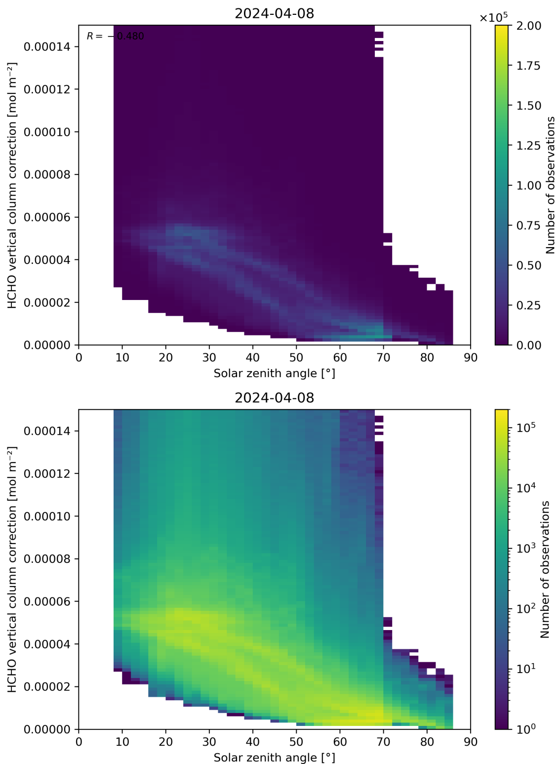
Figure 178: Scatter density plot of “Solar zenith angle” against “HCHO vertical column correction” for 2024-04-07 to 2024-04-09.
