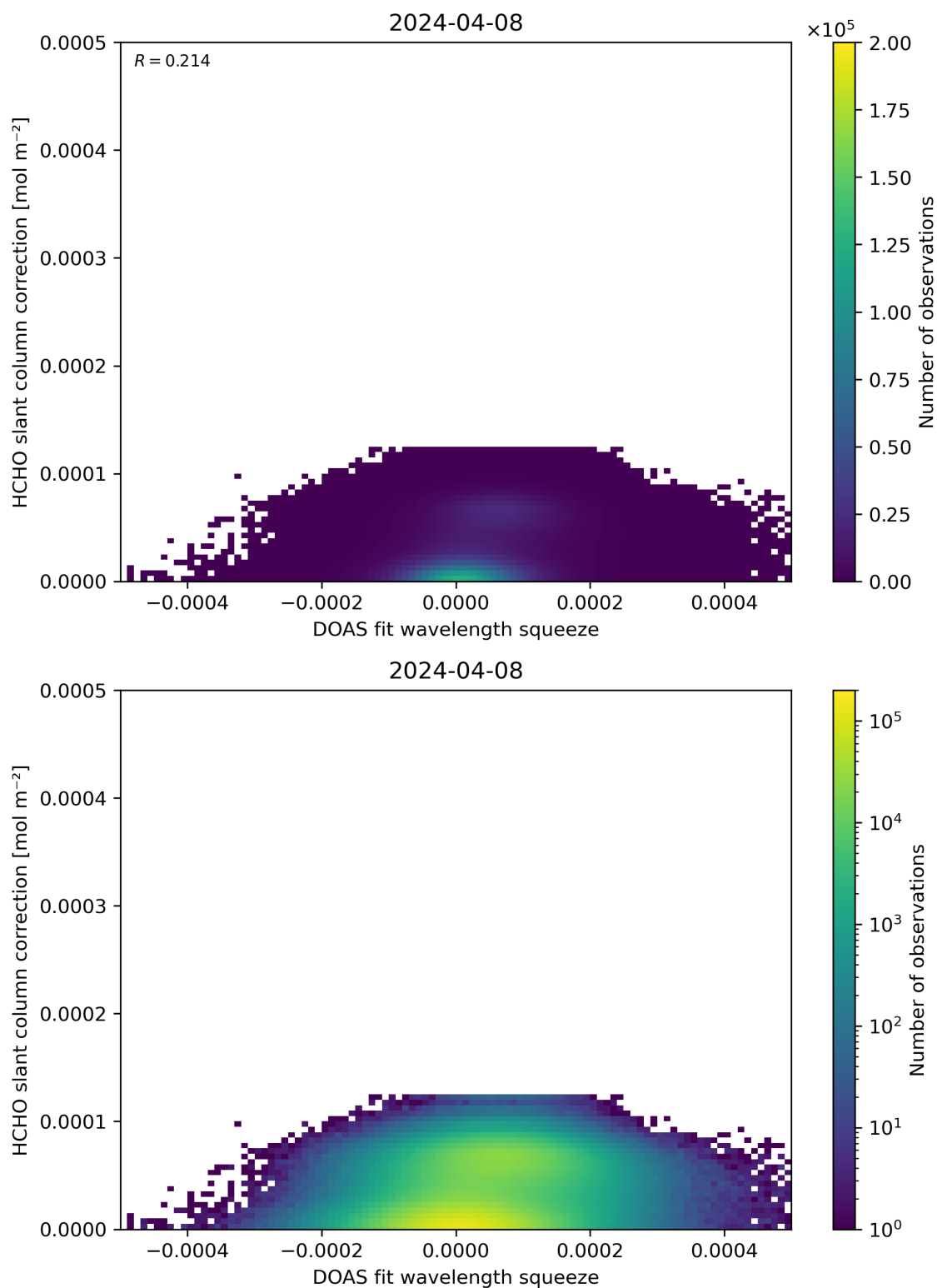
Figure 70: Scatter density plot of “DOAS fit wavelength squeeze” against “HCHO slant column correction” for 2024-04-07 to 2024-04-09.
