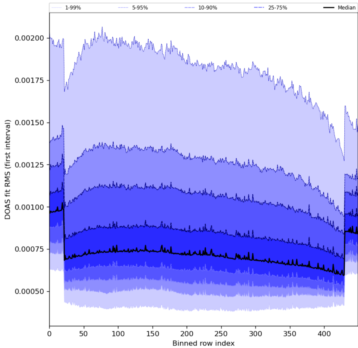
Figure 60: Along track statistics of “DOAS fit RMS (first interval)” for 2024-04-07 to 2024-04-09
