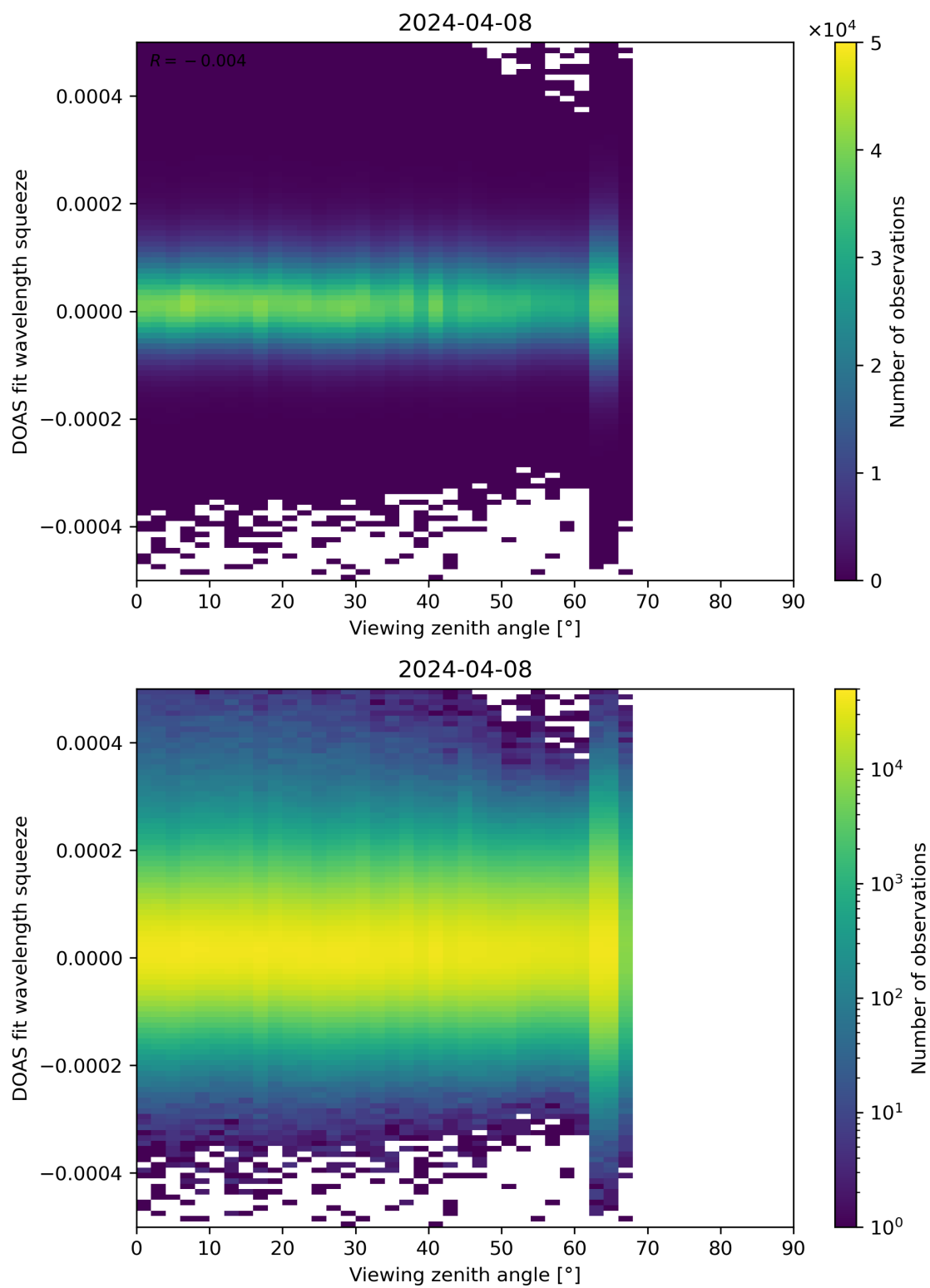
Figure 184: Scatter density plot of “Viewing zenith angle” against “DOAS fit wavelength squeeze” for 2024-04-07 to 2024-04-09.
