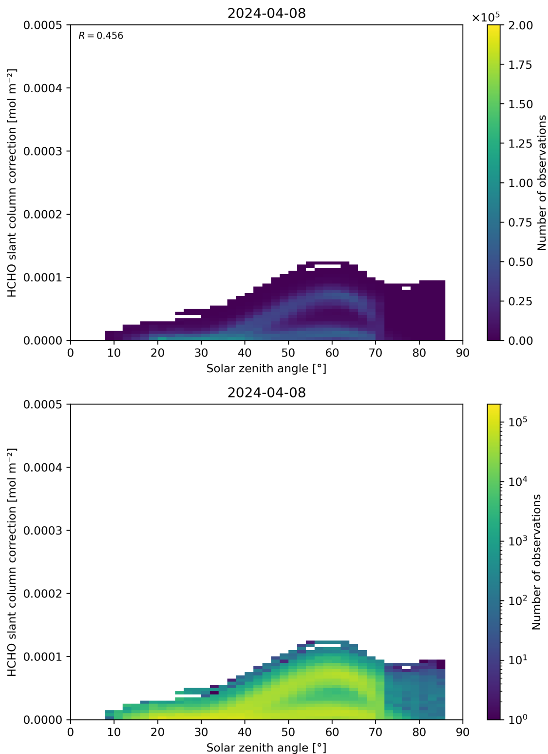
Figure 172: Scatter density plot of “Solar zenith angle” against “HCHO slant column correction” for 2024-04-07 to 2024-04-09.
