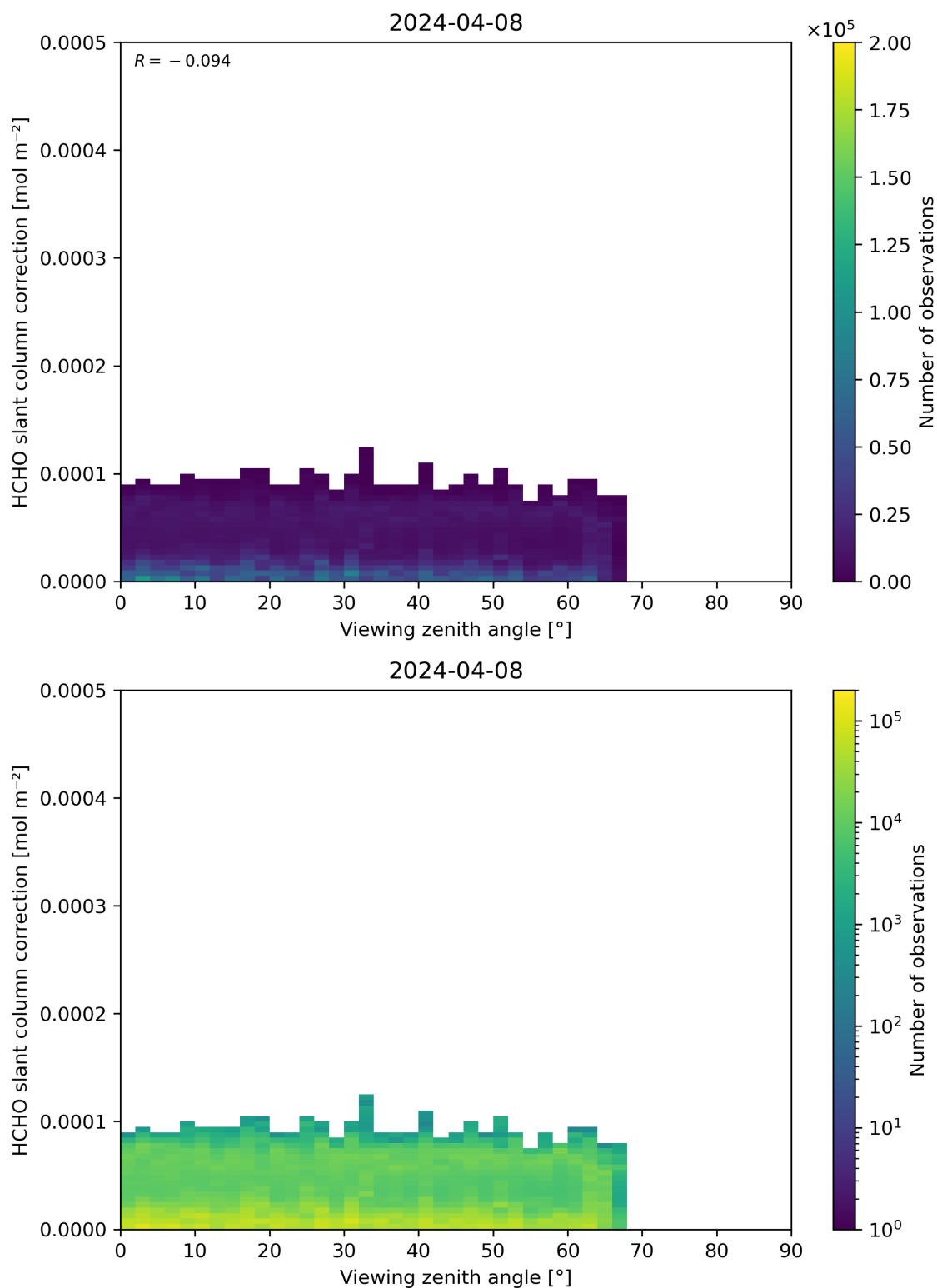
Figure 187: Scatter density plot of “Viewing zenith angle” against “HCHO slant column correction” for 2024-04-07 to 2024-04-09.
