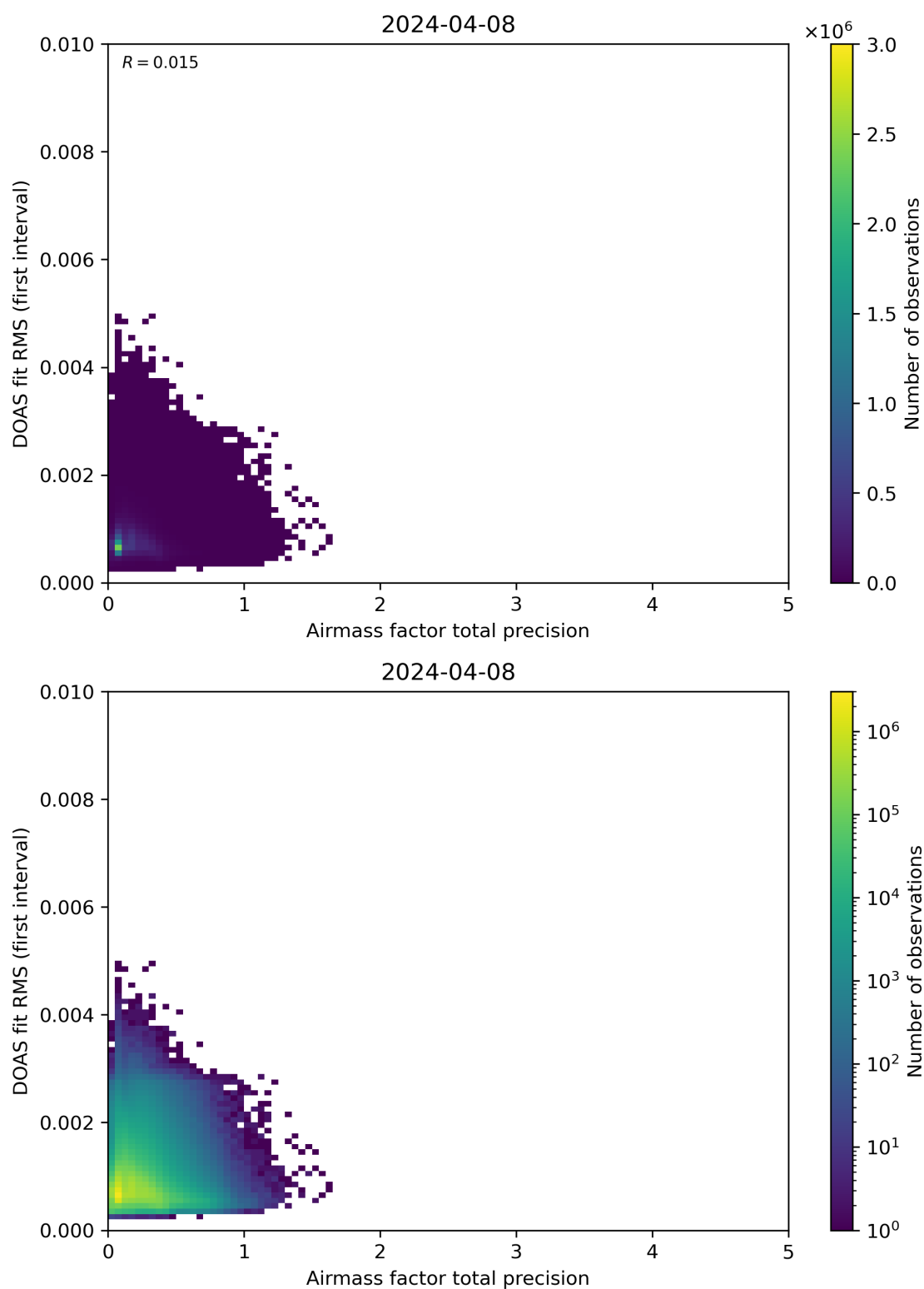
Figure 105: Scatter density plot of “Airmass factor total precision” against “DOAS fit RMS (first interval)” for 2024-04-07 to 2024-04-09.
