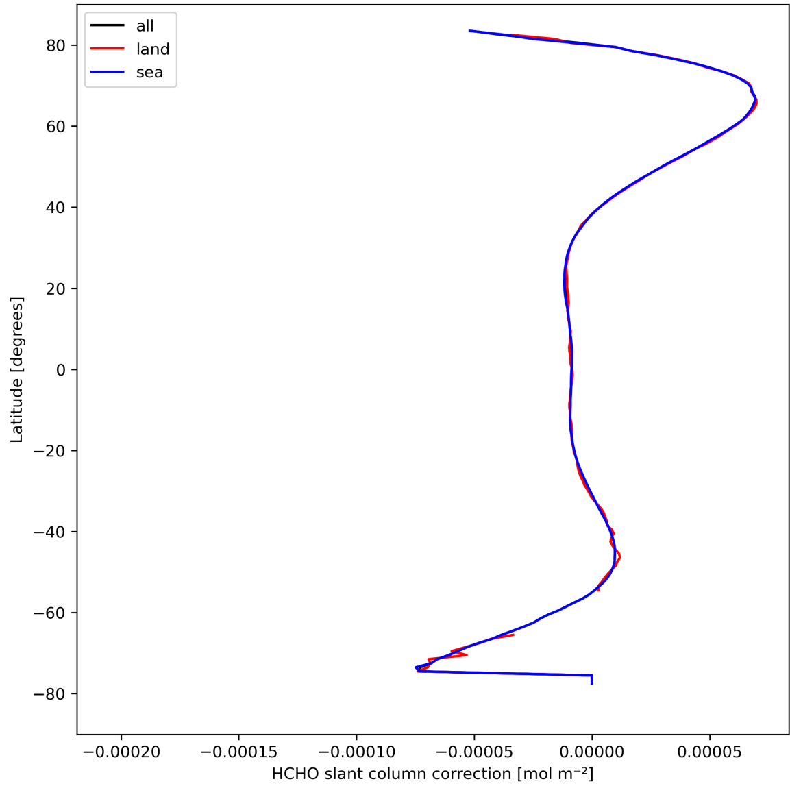
Figure 33: Zonal average of “HCHO slant column correction” for 2024-04-07 to 2024-04-09.
