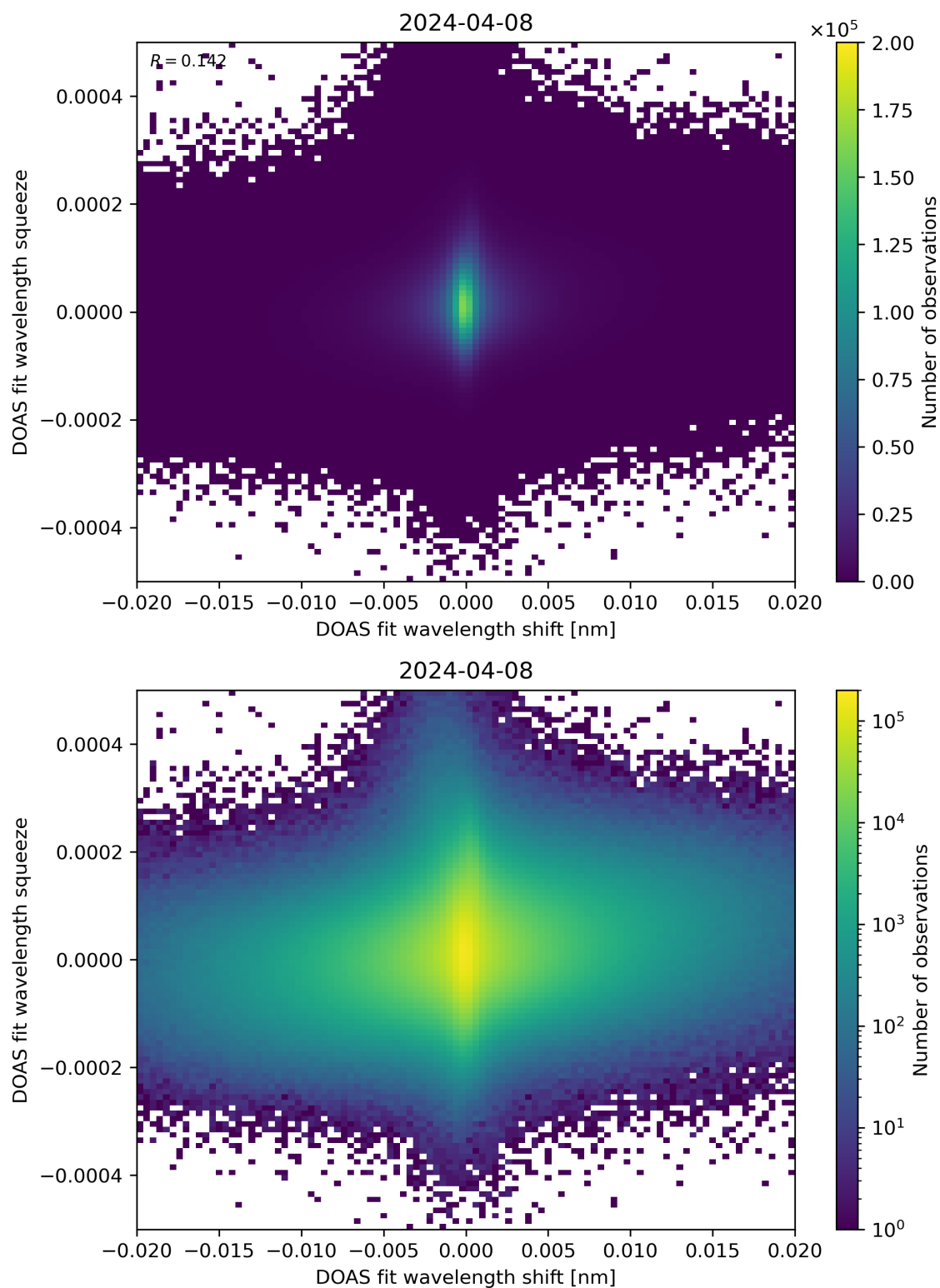
Figure 65: Scatter density plot of “DOAS fit wavelength shift” against “DOAS fit wavelength squeeze” for 2024-04-07 to 2024-04-09.
