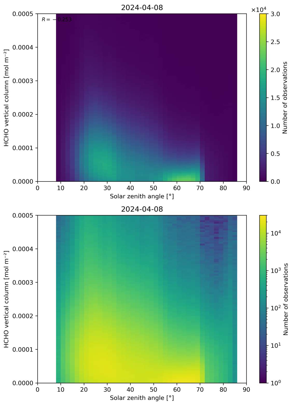
Figure 177: Scatter density plot of “Solar zenith angle” against “HCHO vertical column” for 2024-04-07 to 2024-04-09.
