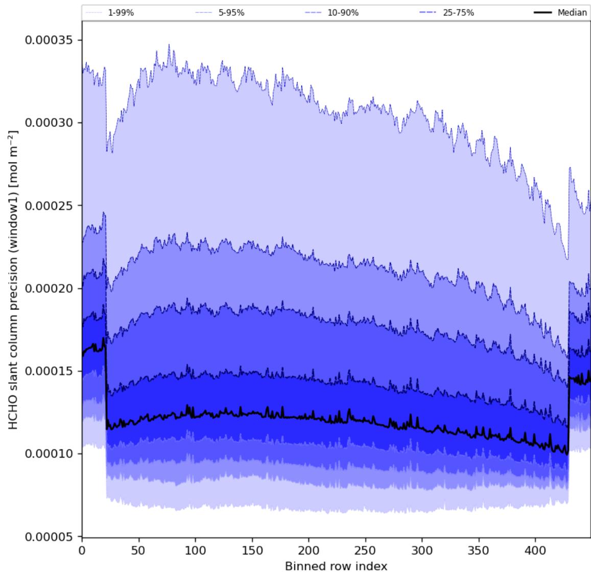
Figure 53: Along track statistics of “HCHO slant column precision (window1)” for 2024-04-07 to 2024-04-09
