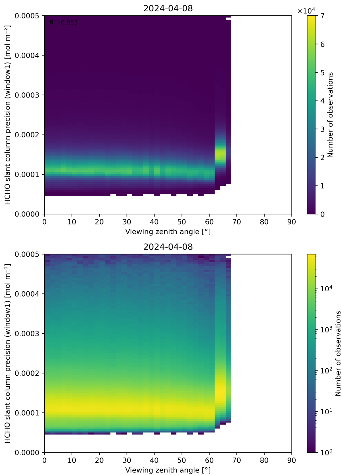
Figure 189: Scatter density plot of “Viewing zenith angle” against “HCHO slant column precision (window1)” for 2024-04-07 to 2024-04-09.
