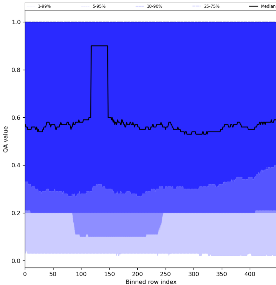
Figure 48: Along track statistics of “QA value” for 2024-04-07 to 2024-04-09
