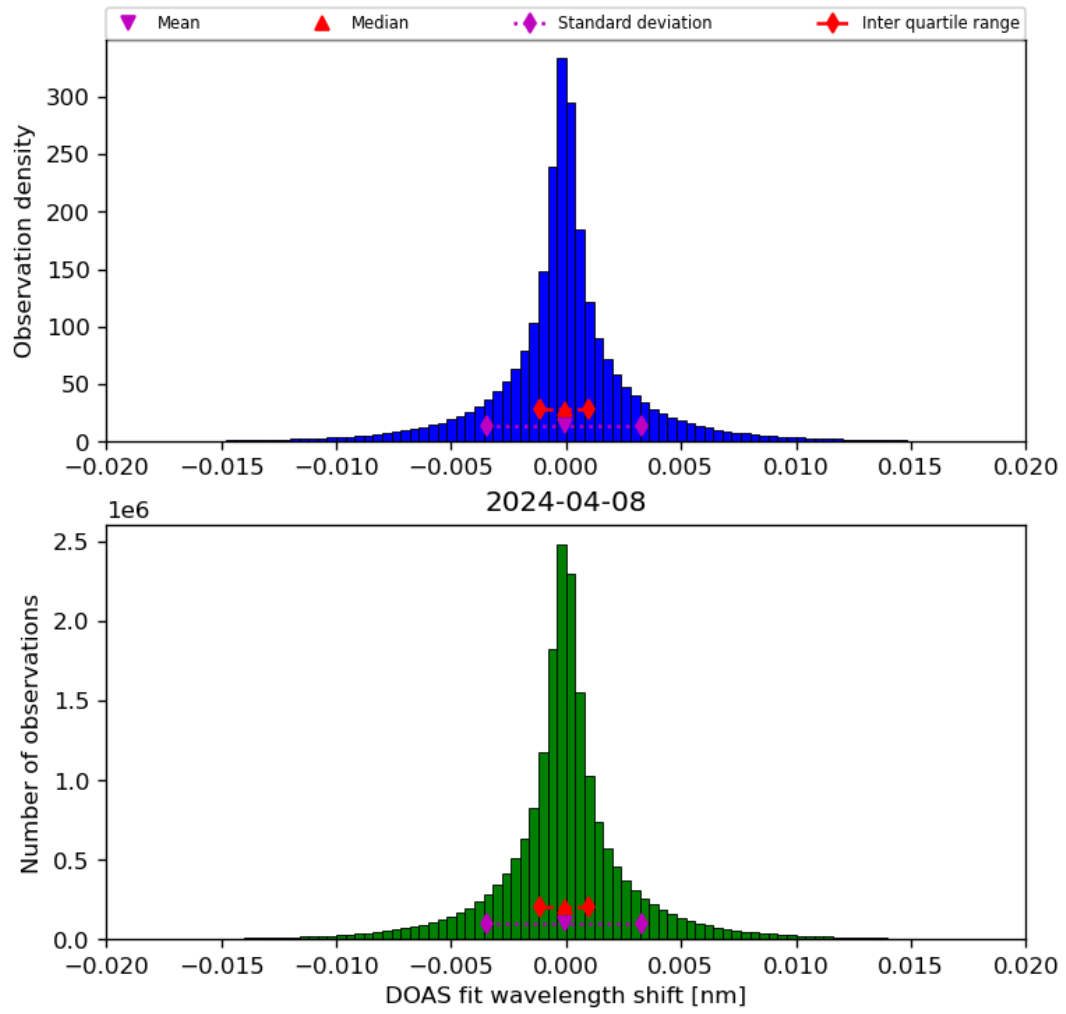
Figure 44: Histogram of “DOAS fit wavelength shift” for 2024-04-07 to 2024-04-09
