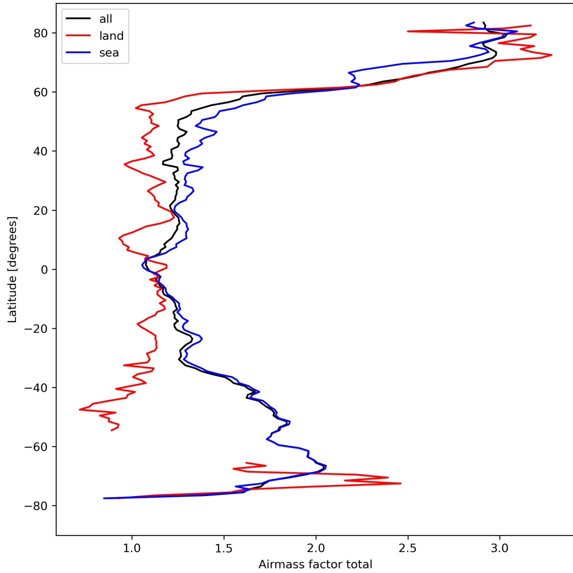
Figure 26: Zonal average of “Airmass factor total” for 2024-04-07 to 2024-04-09.
