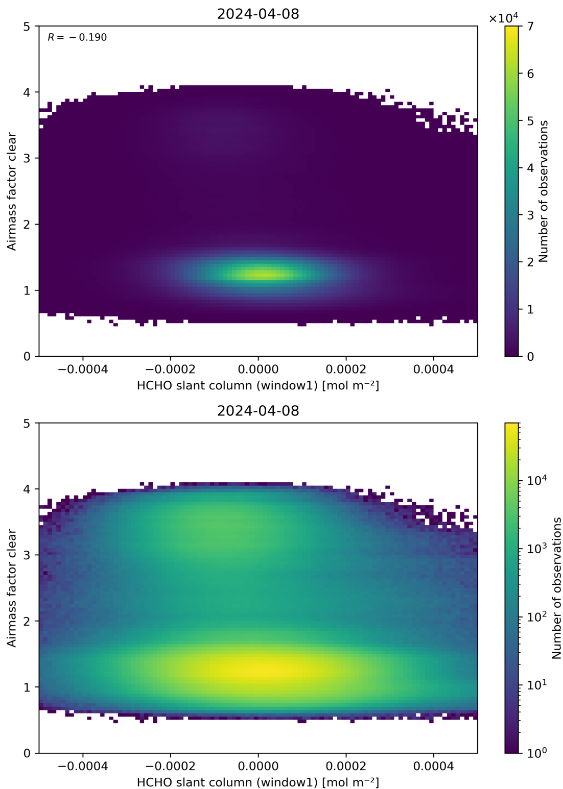
Figure 81: Scatter density plot of “HCHO slant column (window1)” against “Airmass factor clear” for 2024-04-07 to 2024-04-09.
