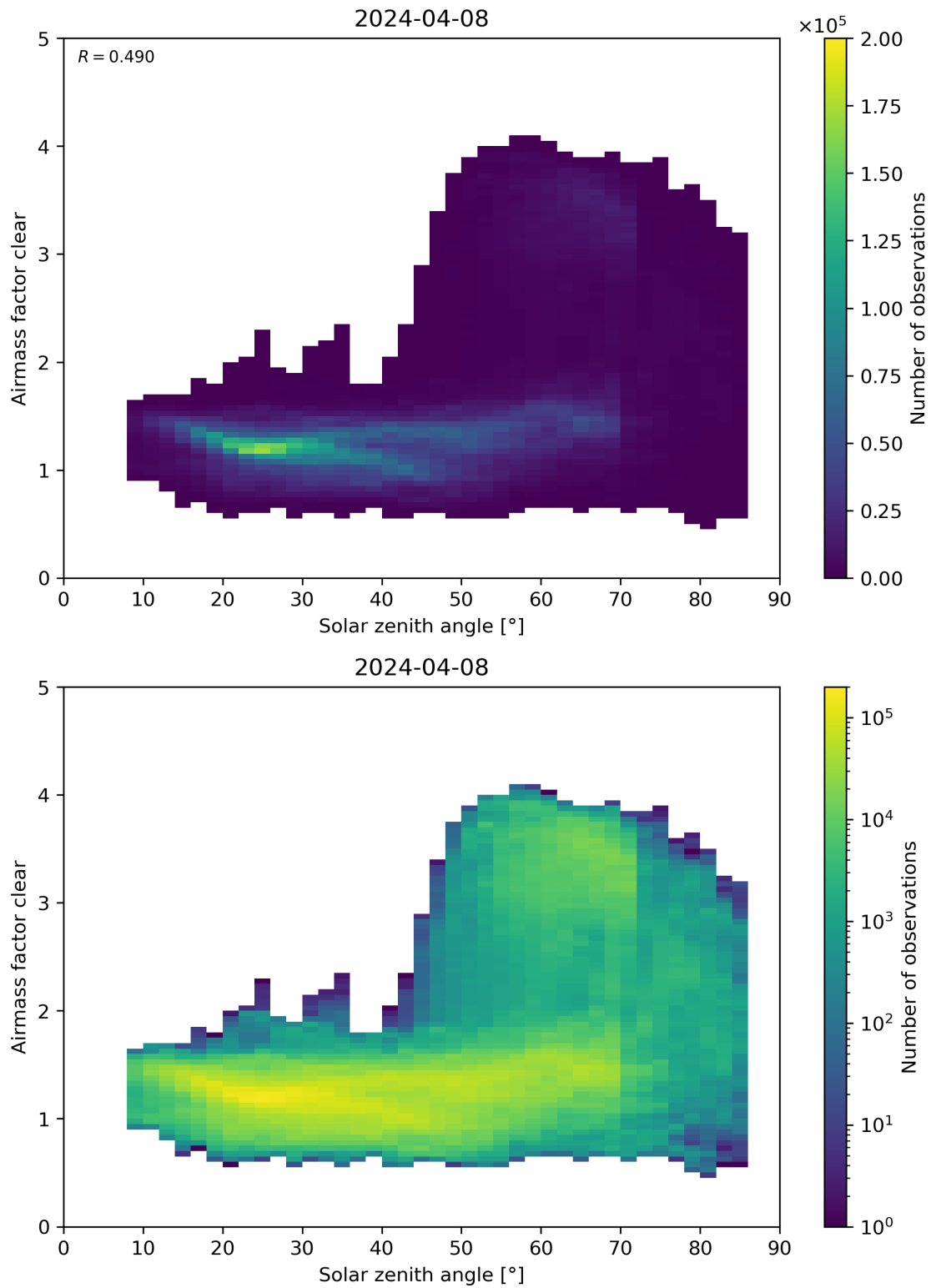
Figure 170: Scatter density plot of “Solar zenith angle” against “Airmass factor clear” for 2024-04-07 to 2024-04-09.
