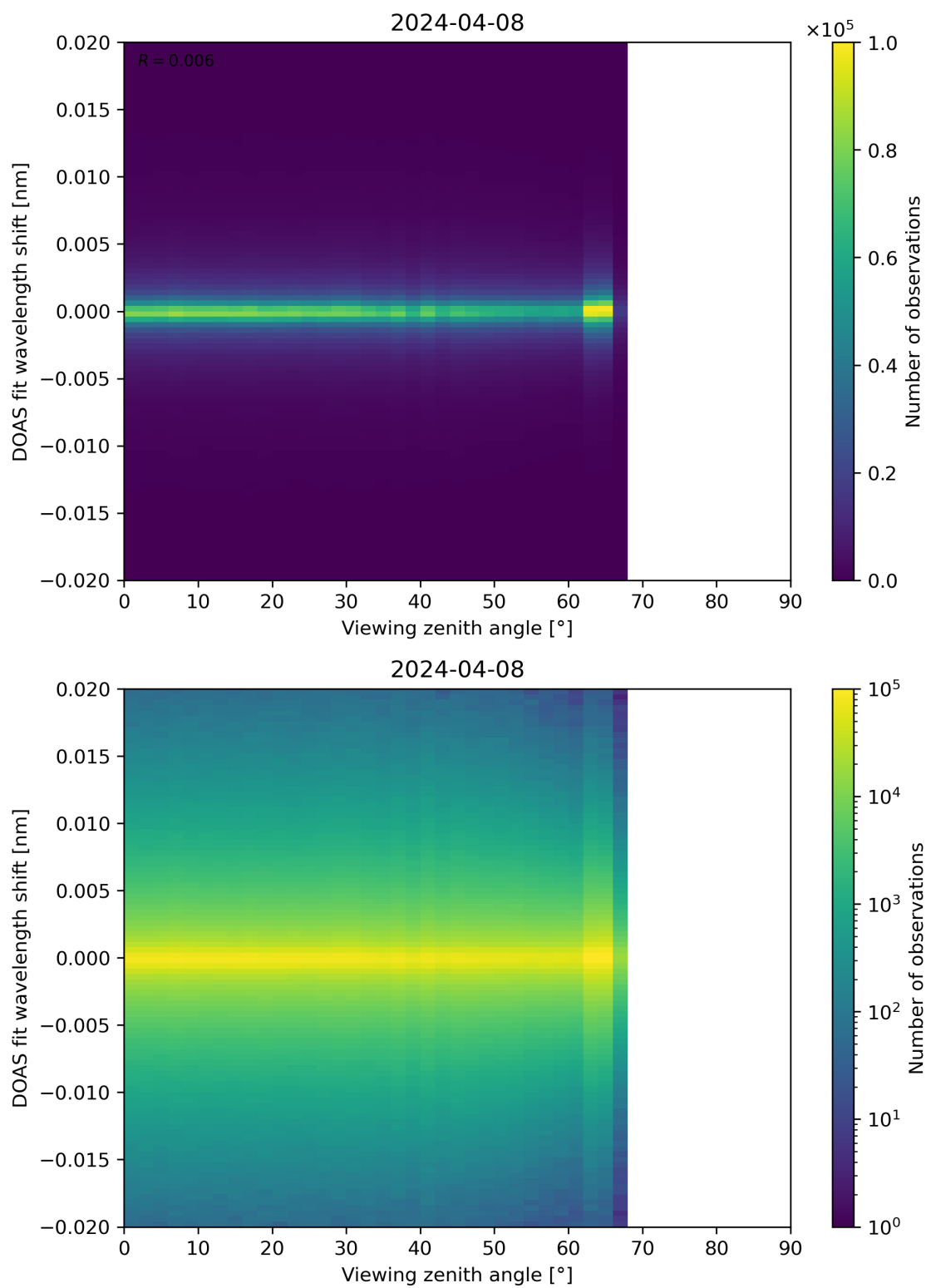
Figure 183: Scatter density plot of “Viewing zenith angle” against “DOAS fit wavelength shift” for 2024-04-07 to 2024-04-09.
