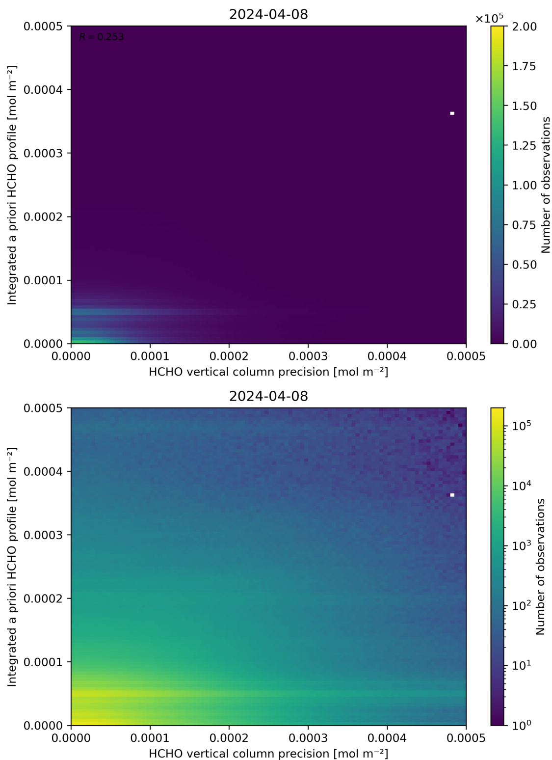
Figure 147: Scatter density plot of “HCHO vertical column precision” against “Integrated a priori HCHO profile” for 2024-04-07 to 2024-04-09.
