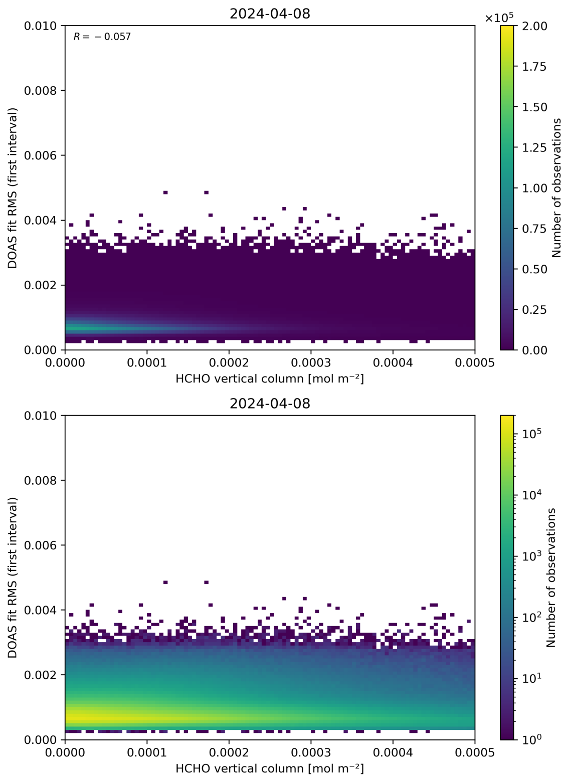
Figure 123: Scatter density plot of “HCHO vertical column” against “DOAS fit RMS (first interval)” for 2024-04-07 to 2024-04-09.
