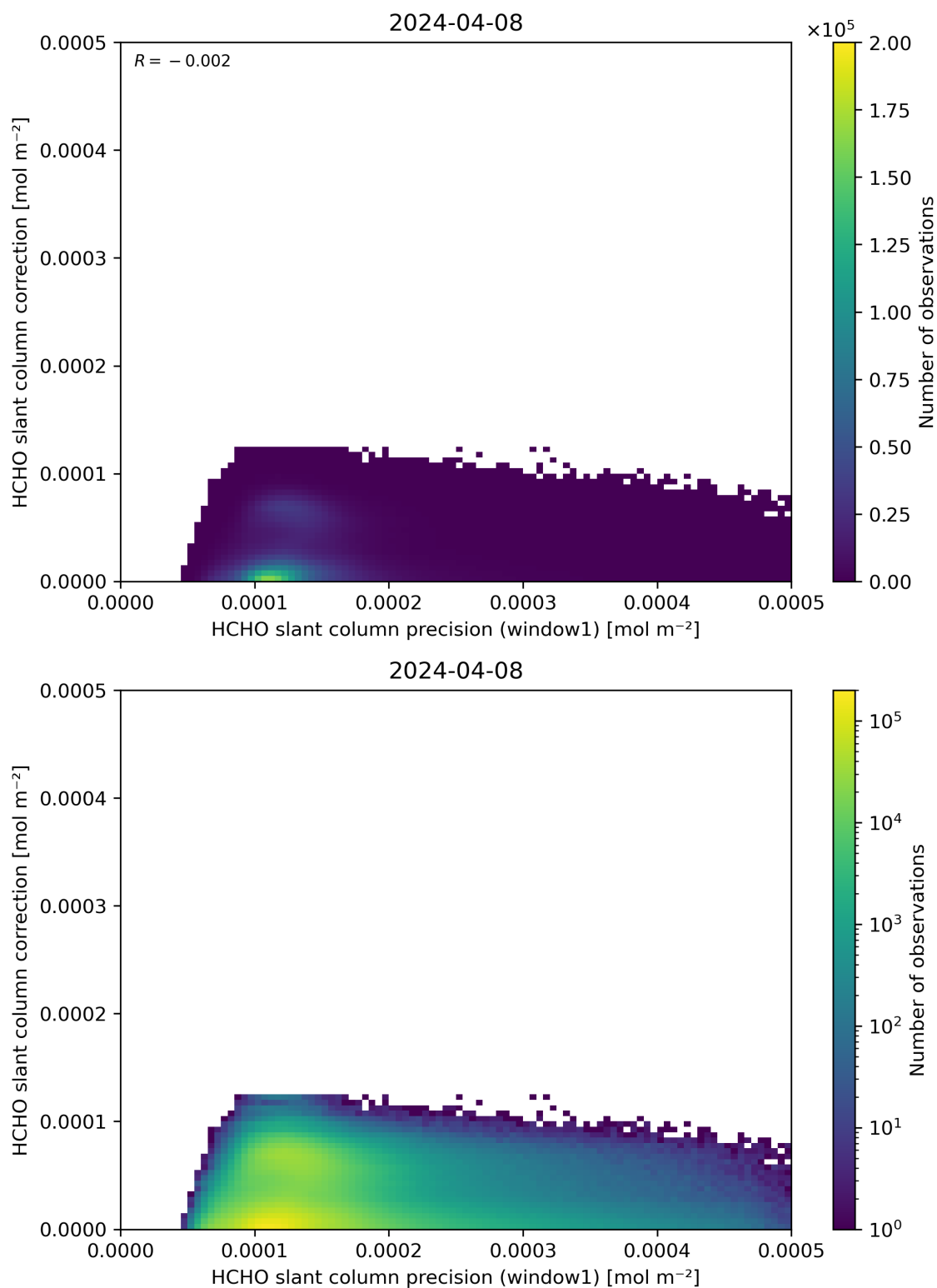
Figure 93: Scatter density plot of “HCHO slant column precision (window1)” against “HCHO slant column correction” for 2024-04-07 to 2024-04-09.
