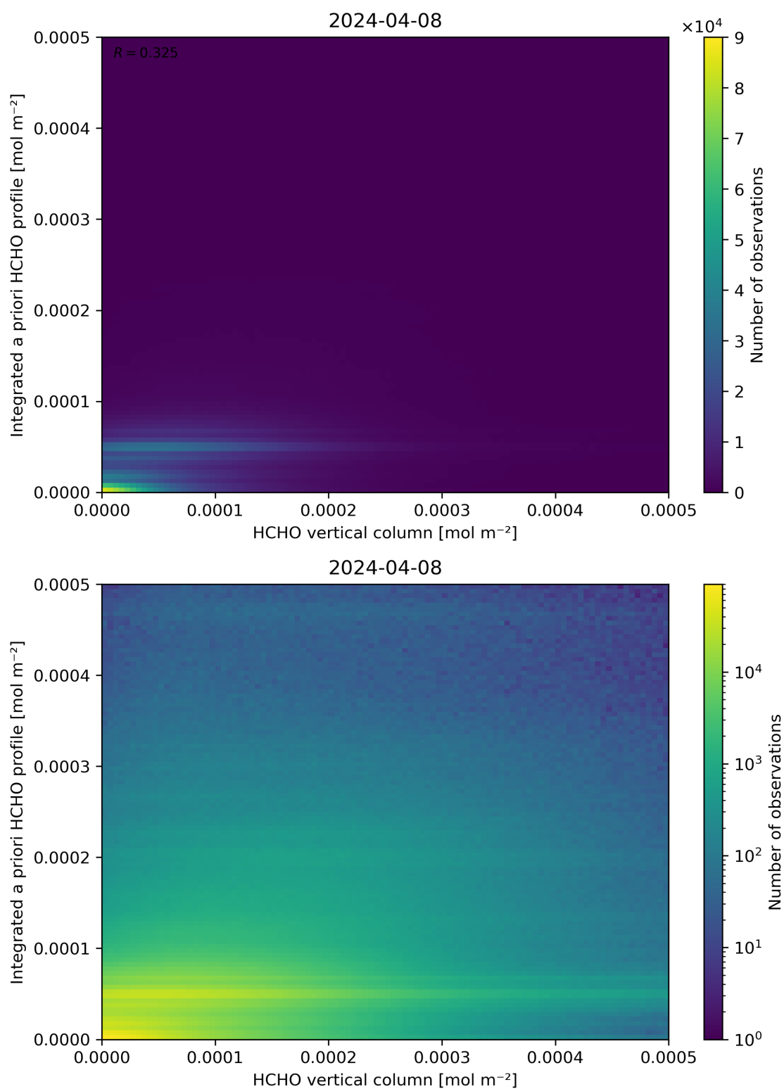
Figure 135: Scatter density plot of “HCHO vertical column” against “Integrated a priori HCHO profile” for 2024-04-07 to 2024-04-09.
