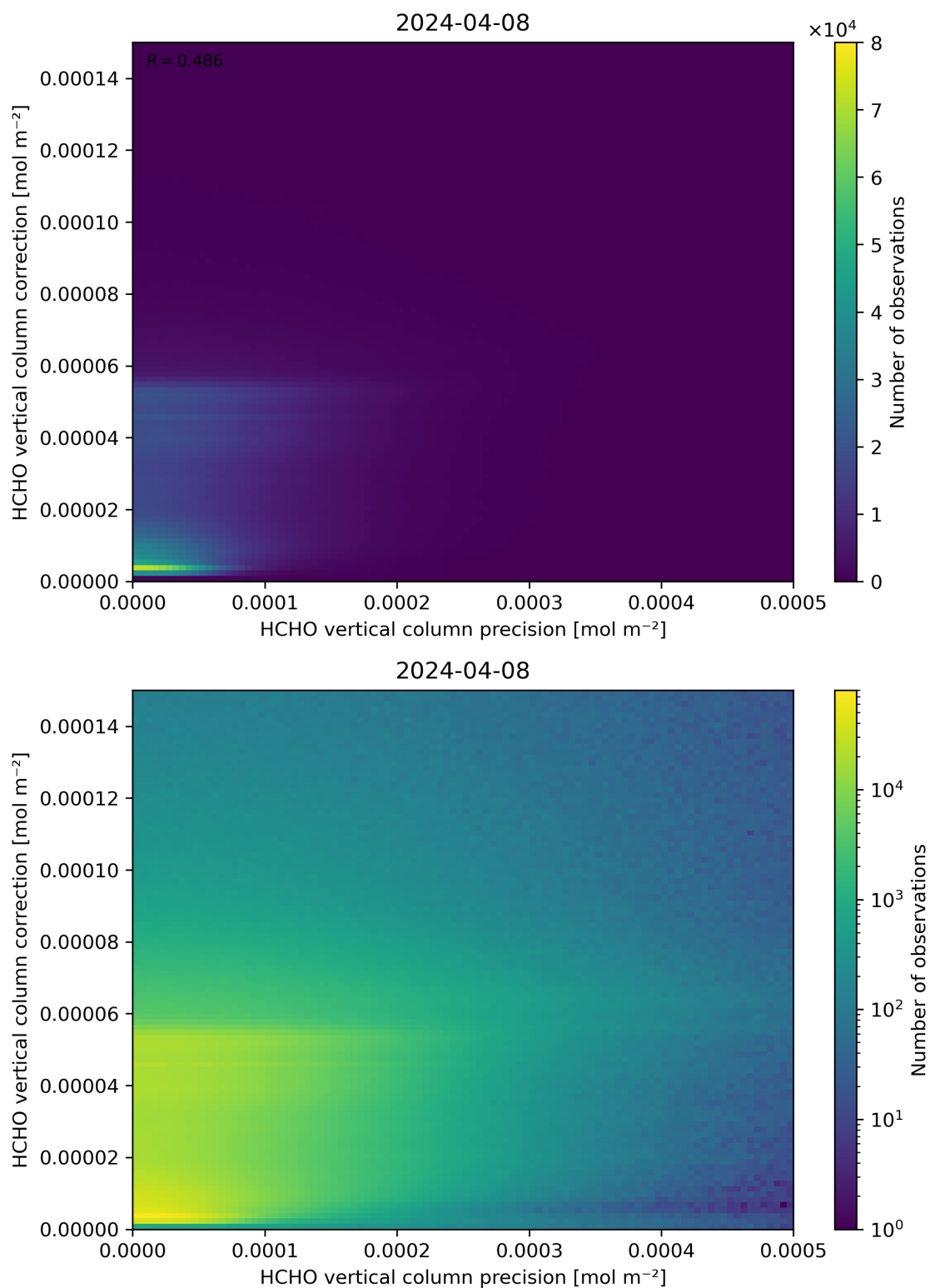
Figure 146: Scatter density plot of “HCHO vertical column precision” against “HCHO vertical column correction” for 2024-04-07 to 2024-04-09.
