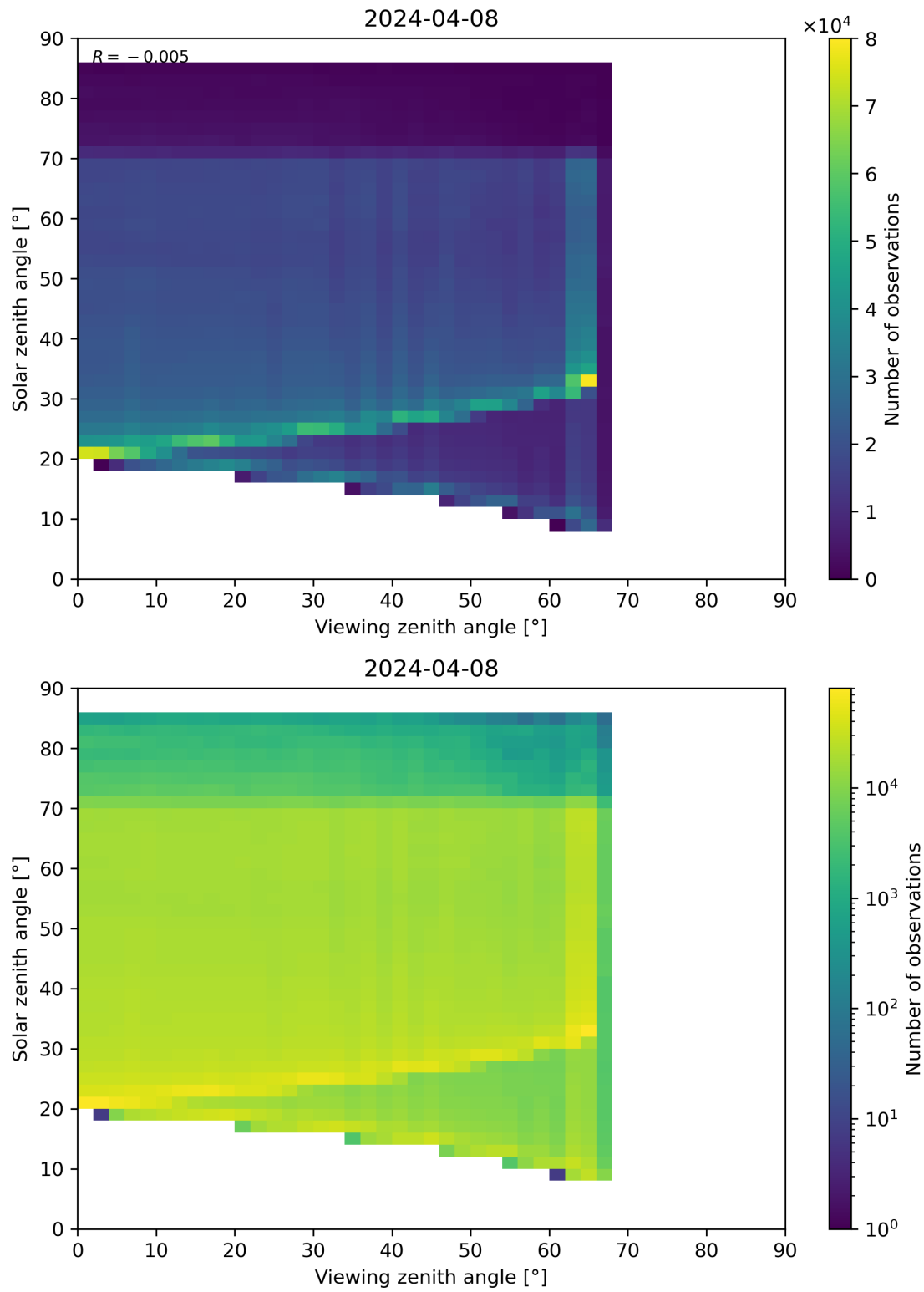
Figure 197: Scatter density plot of “Viewing zenith angle” against “Solar zenith angle” for 2024-04-07 to 2024-04-09.
