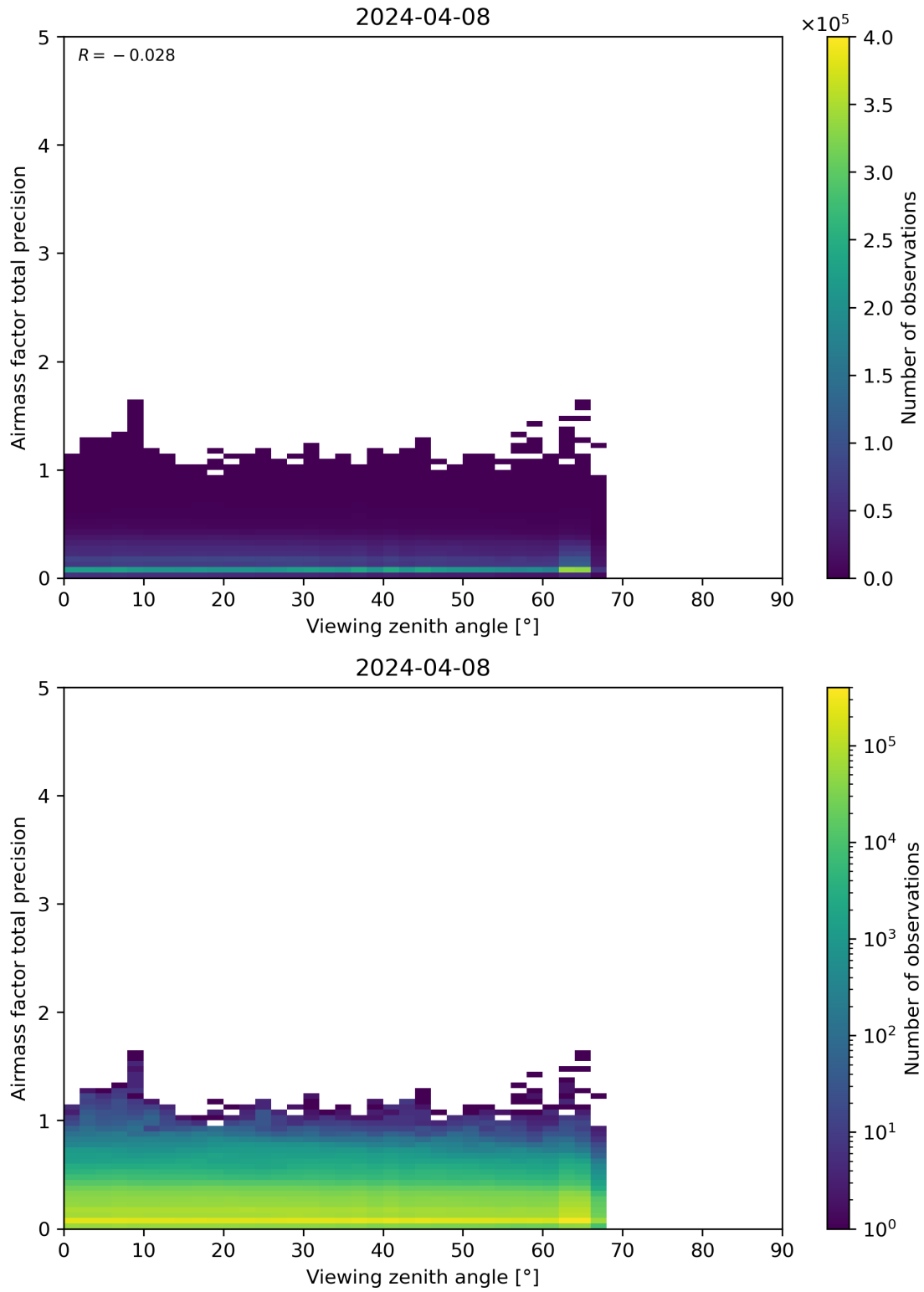
Figure 191: Scatter density plot of “Viewing zenith angle” against “Airmass factor total precision” for 2024-04-07 to 2024-04-09.
