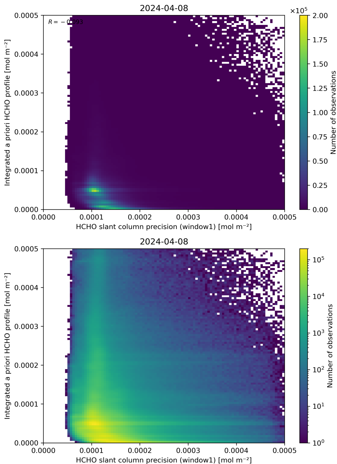
Figure 96: Scatter density plot of “HCHO slant column precision (window1)” against “Integrated a priori HCHO profile” for 2024-04-07 to 2024-04-09.
