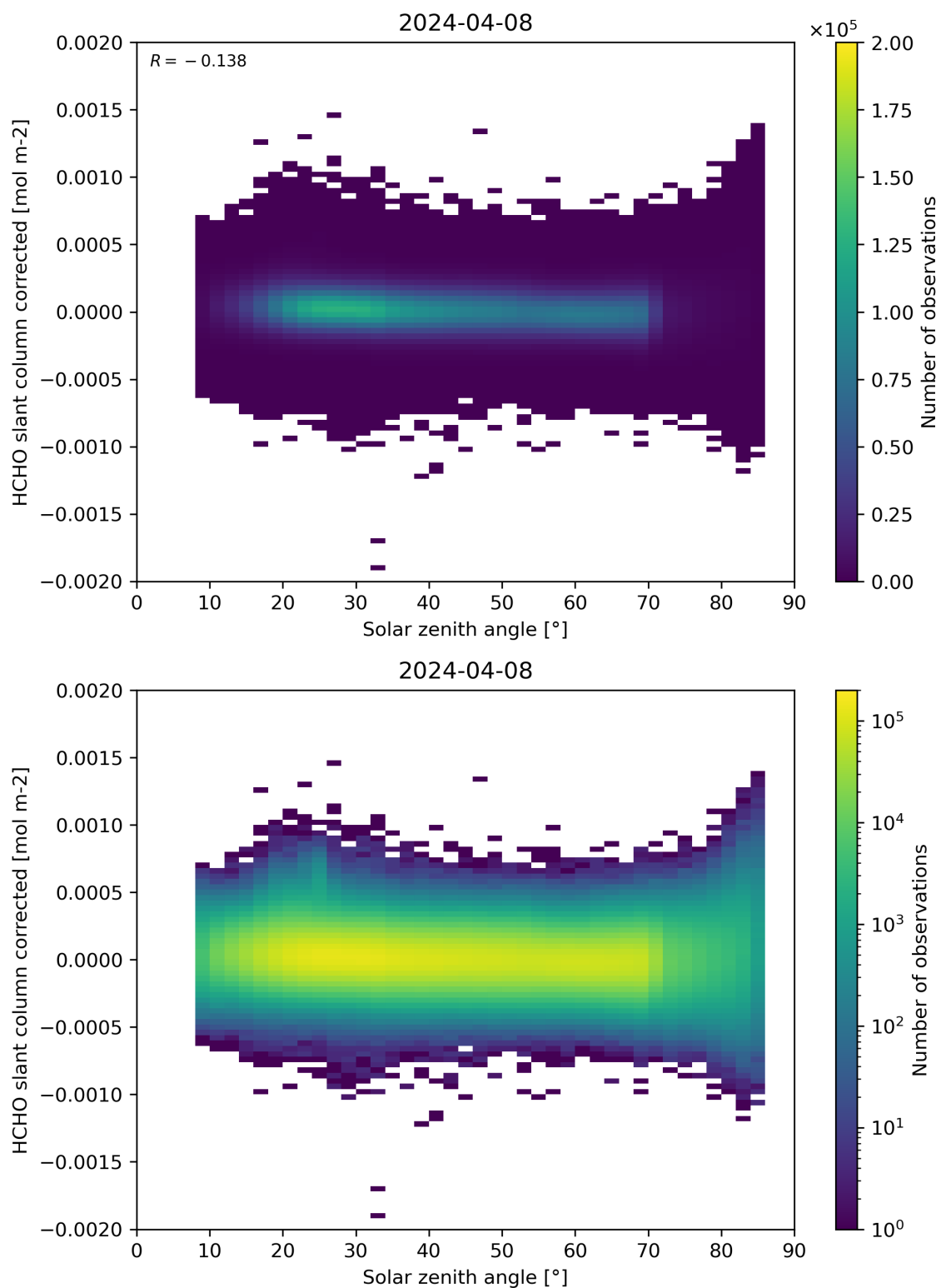
Figure 171: Scatter density plot of “Solar zenith angle” against “HCHO slant column corrected” for 2024-04-07 to 2024-04-09.
