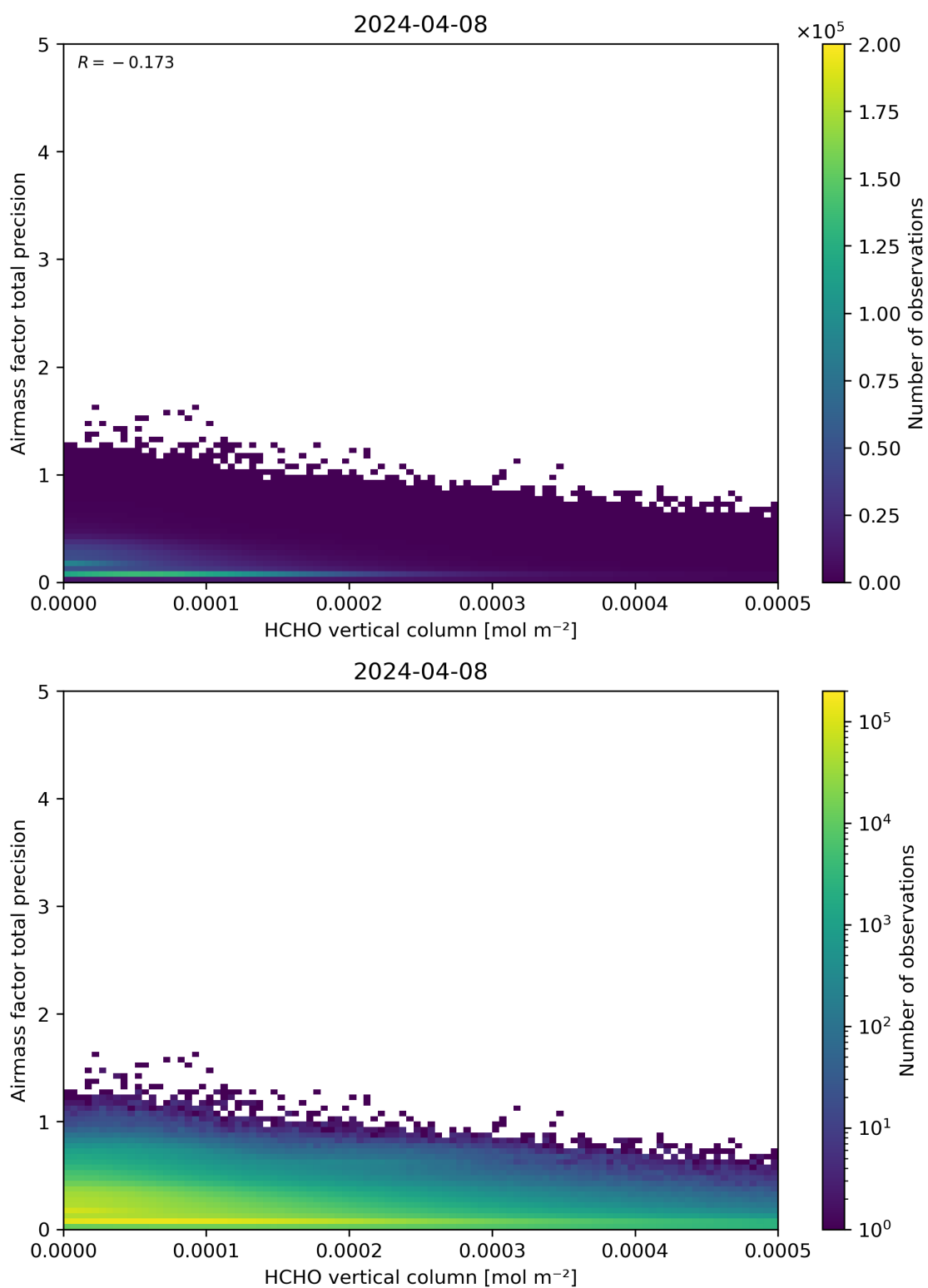
Figure 132: Scatter density plot of “HCHO vertical column” against “Airmass factor total precision” for 2024-04-07 to 2024-04-09.
