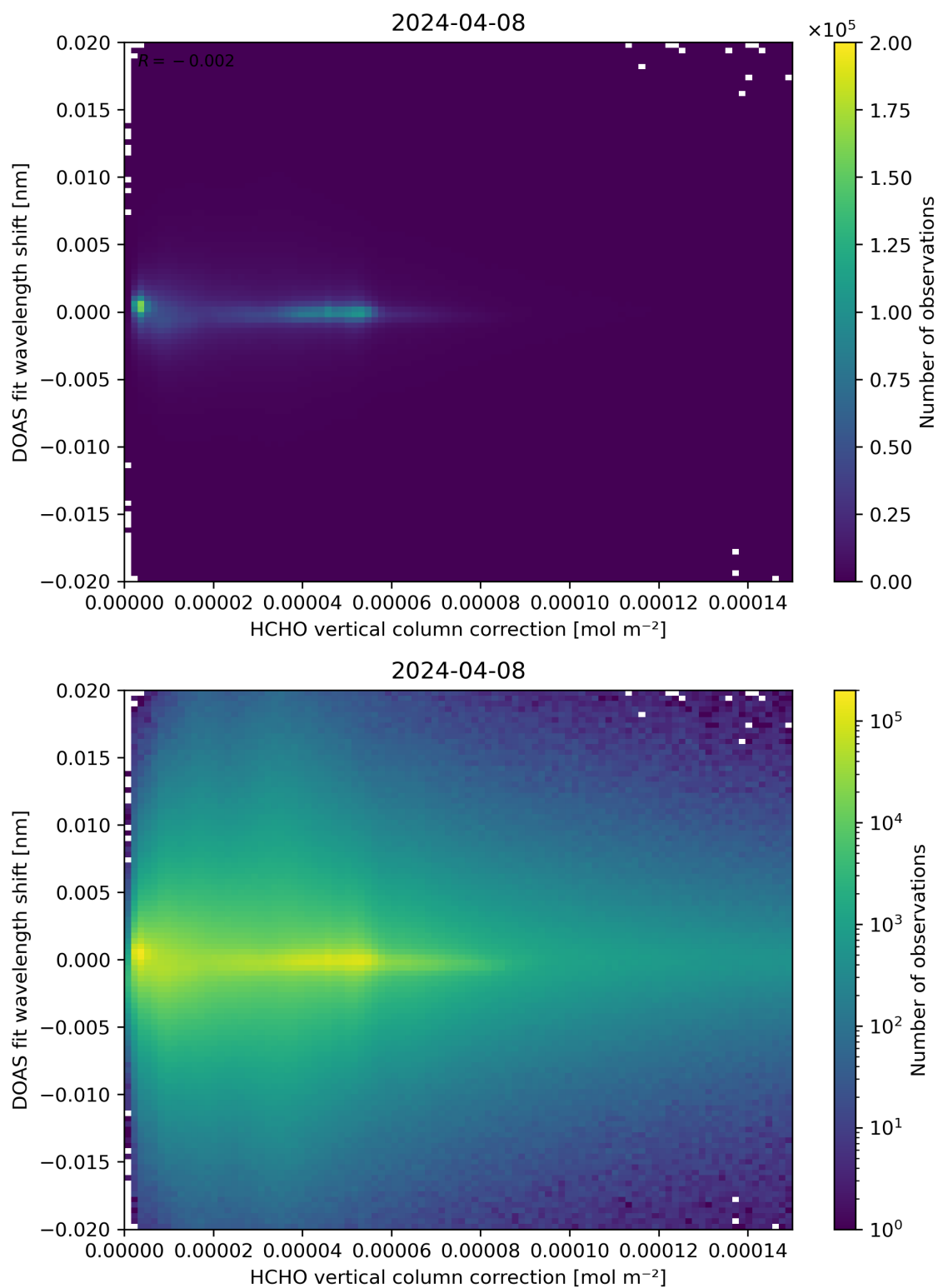
Figure 113: Scatter density plot of “HCHO vertical column correction” against “DOAS fit wavelength shift” for 2024-04-07 to 2024-04-09.
