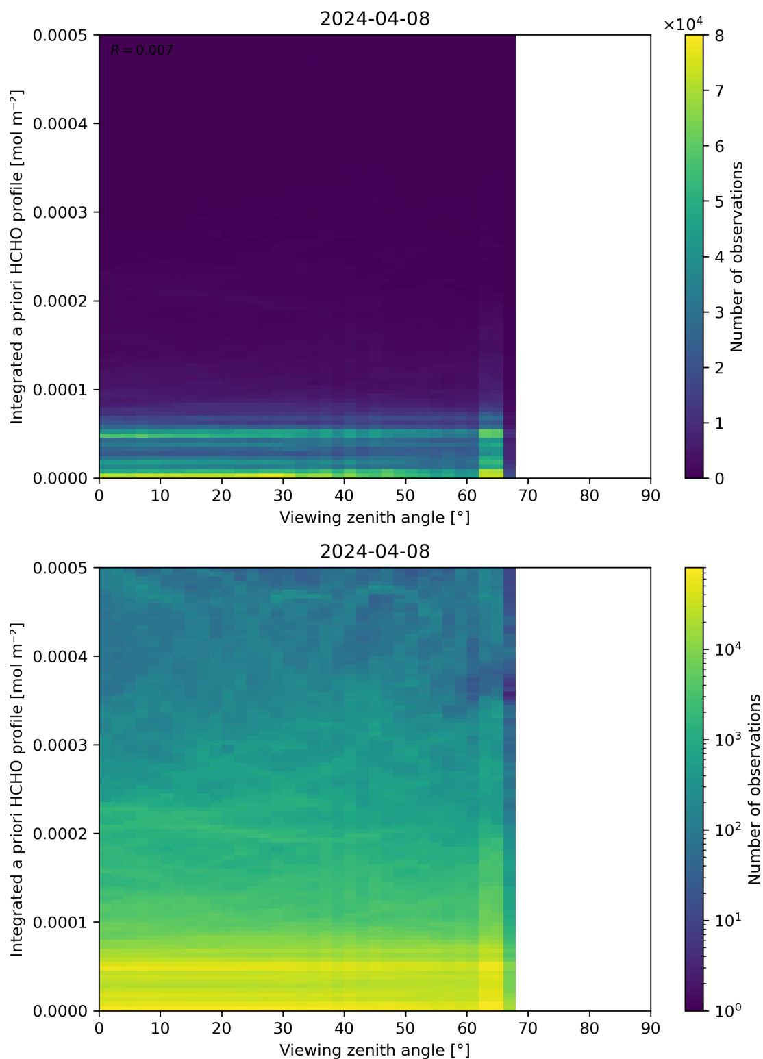
Figure 195: Scatter density plot of “Viewing zenith angle” against “Integrated a priori HCHO profile” for 2024-04-07 to 2024-04-09.
