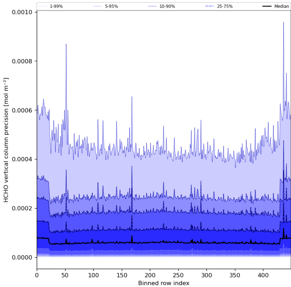
Figure 50: Along track statistics of “HCHO vertical column precision” for 2024-04-07 to 2024-04-09
