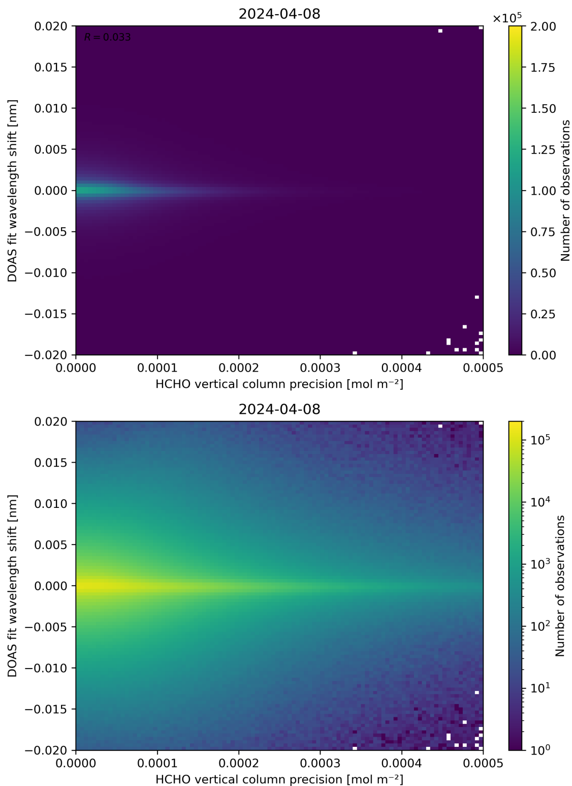
Figure 137: Scatter density plot of “HCHO vertical column precision” against “DOAS fit wavelength shift” for 2024-04-07 to 2024-04-09.
