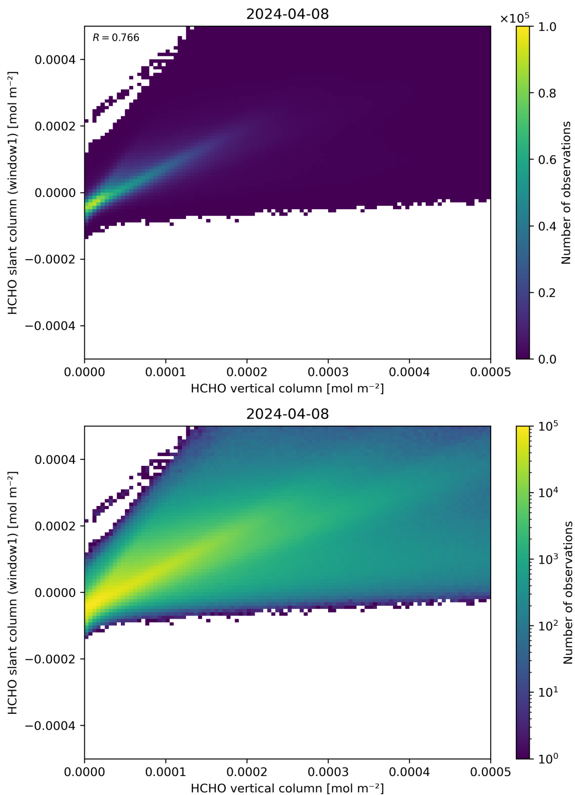
Figure 129: Scatter density plot of “HCHO vertical column” against “HCHO slant column (window1)” for 2024-04-07 to 2024-04-09.
