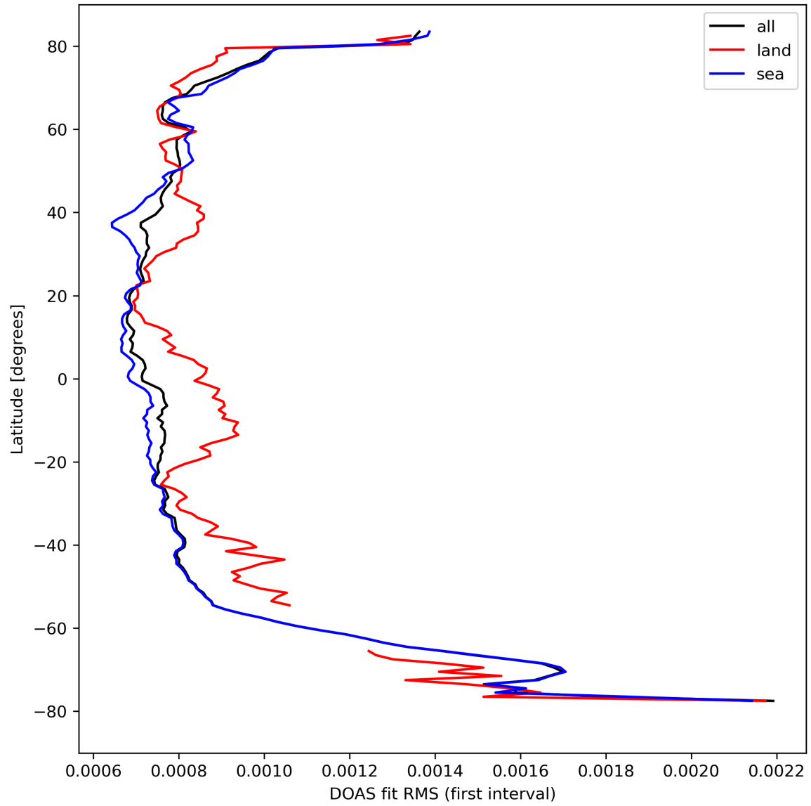
Figure 32: Zonal average of “DOAS fit RMS (first interval)” for 2024-04-07 to 2024-04-09.
