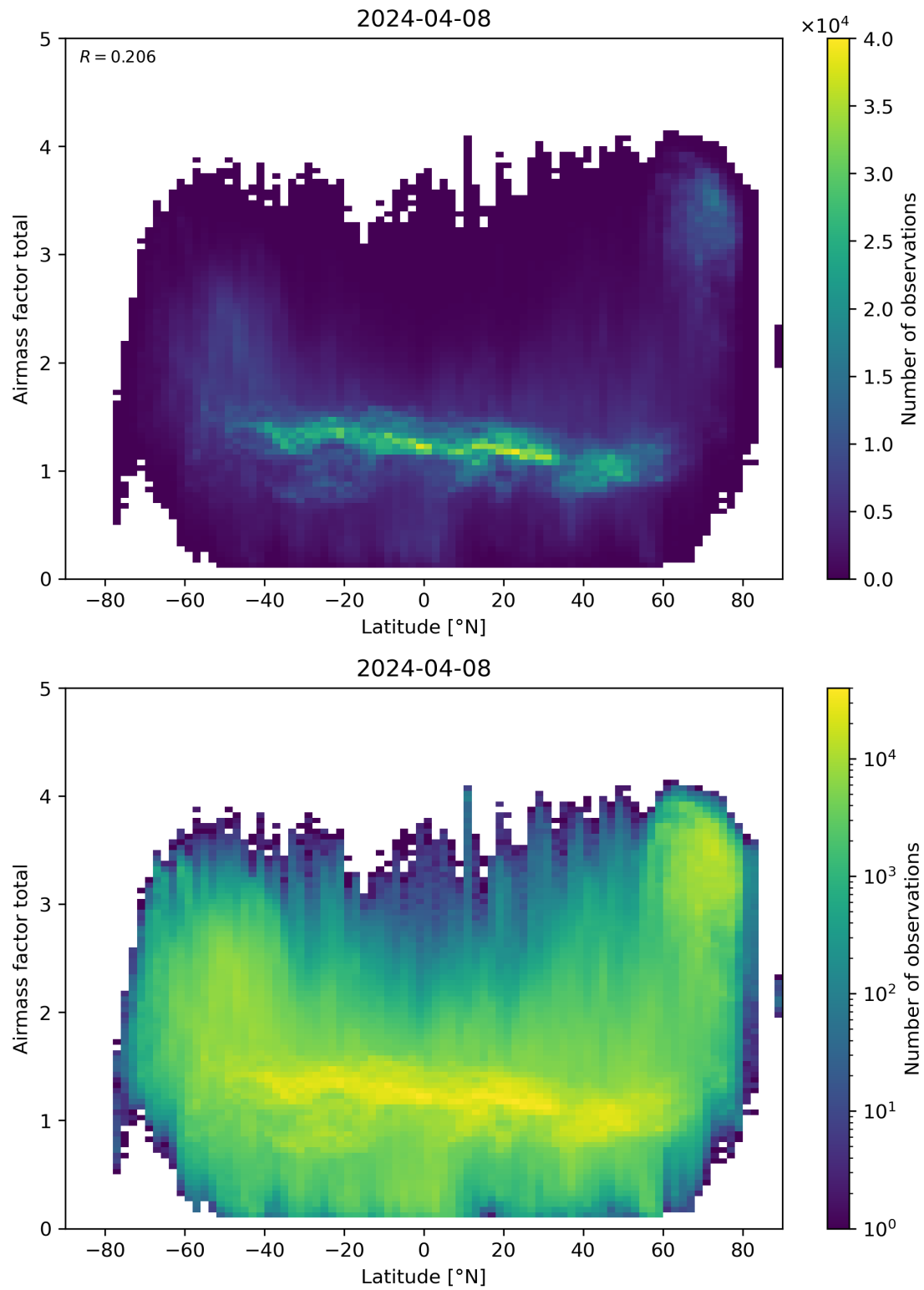
Figure 161: Scatter density plot of “Latitude” against “Airmass factor total” for 2024-04-07 to 2024-04-09.
