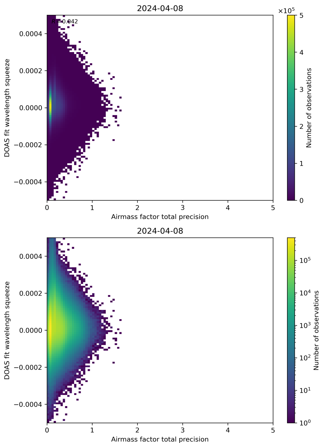
Figure 107: Scatter density plot of “Airmass factor total precision” against “DOAS fit wavelength squeeze” for 2024-04-07 to 2024-04-09.
