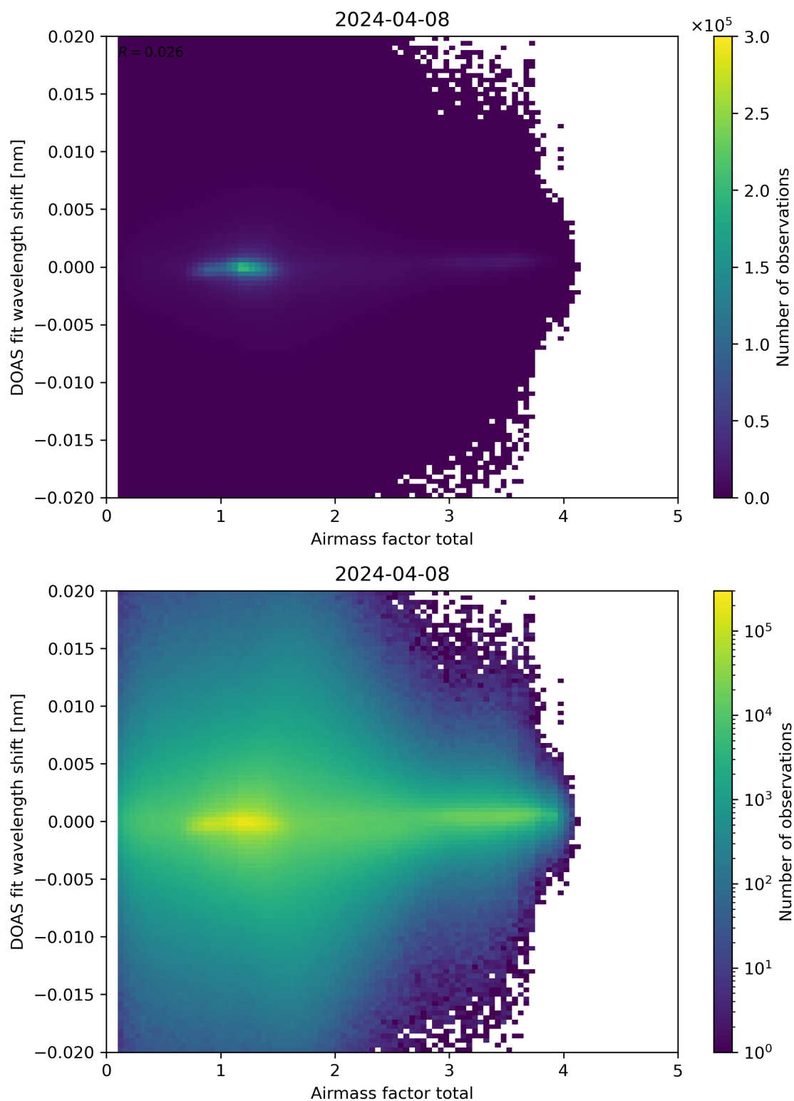
Figure 98: Scatter density plot of “Airmass factor total” against “DOAS fit wavelength shift” for 2024-04-07 to 2024-04-09.
