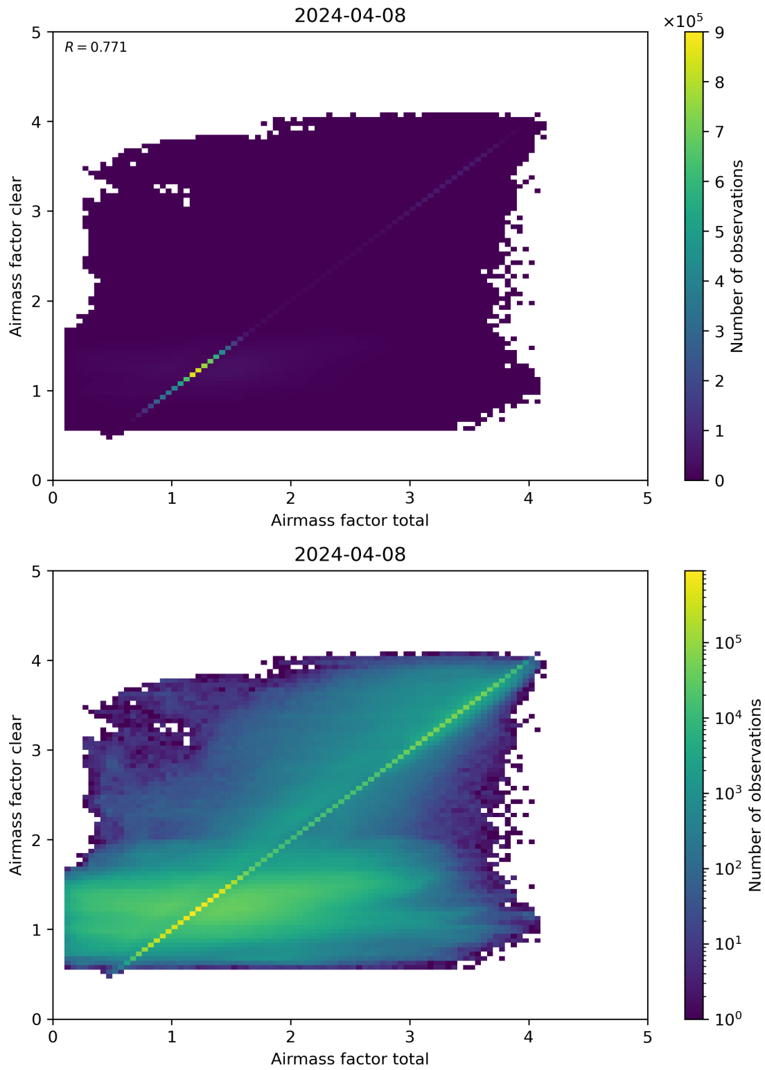
Figure 100: Scatter density plot of “Airmass factor total” against “Airmass factor clear” for 2024-04-07 to 2024-04-09.
