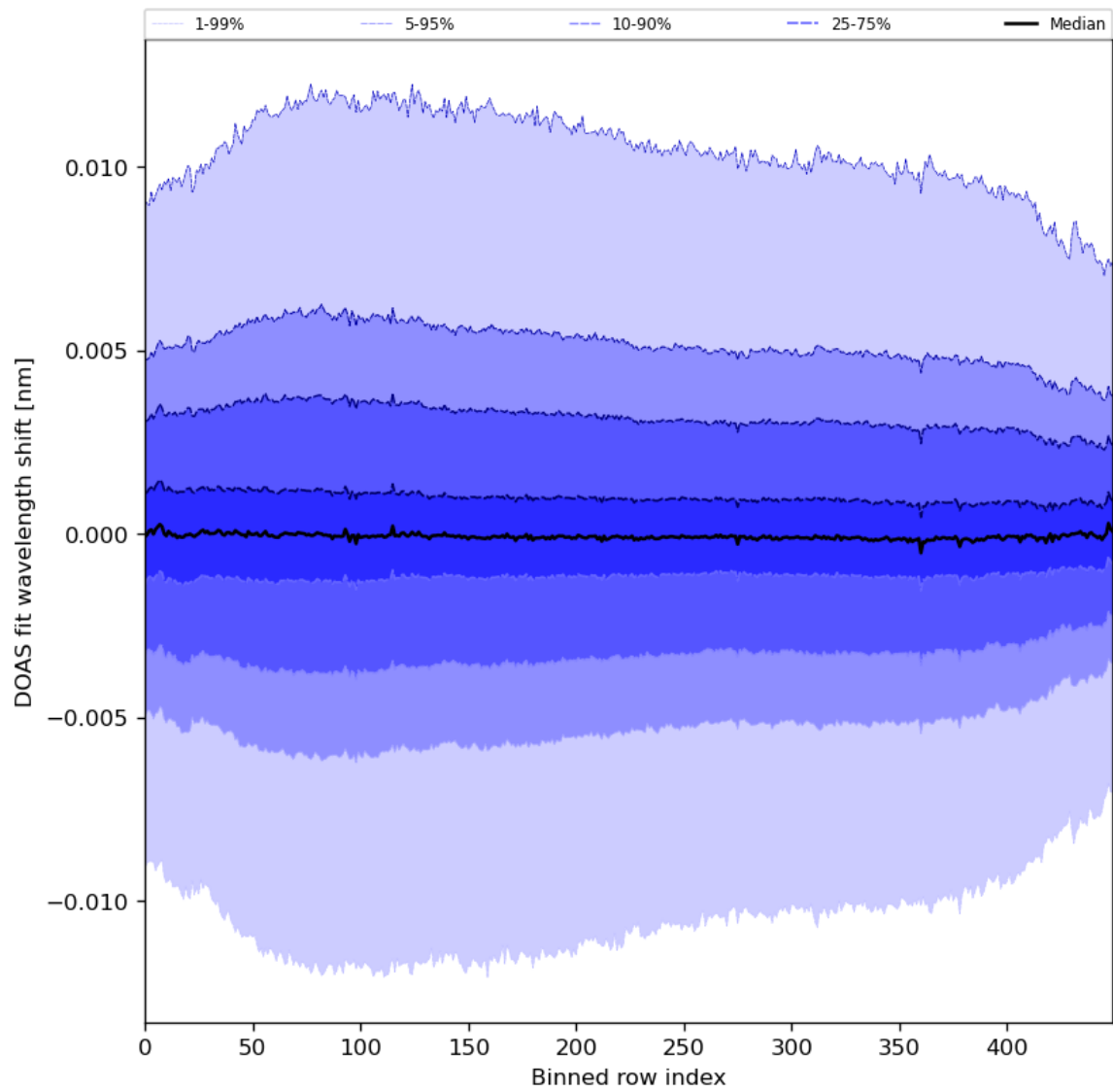
Figure 58: Along track statistics of “DOAS fit wavelength shift” for 2024-04-07 to 2024-04-09
