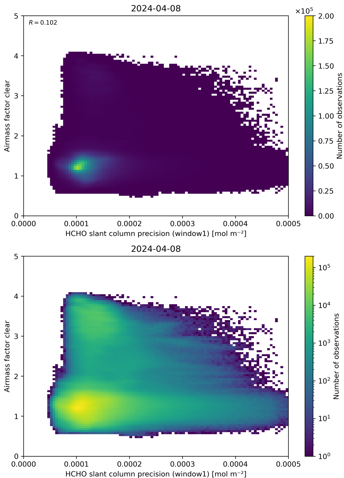
Figure 91: Scatter density plot of “HCHO slant column precision (window1)” against “Airmass factor clear” for 2024-04-07 to 2024-04-09.
