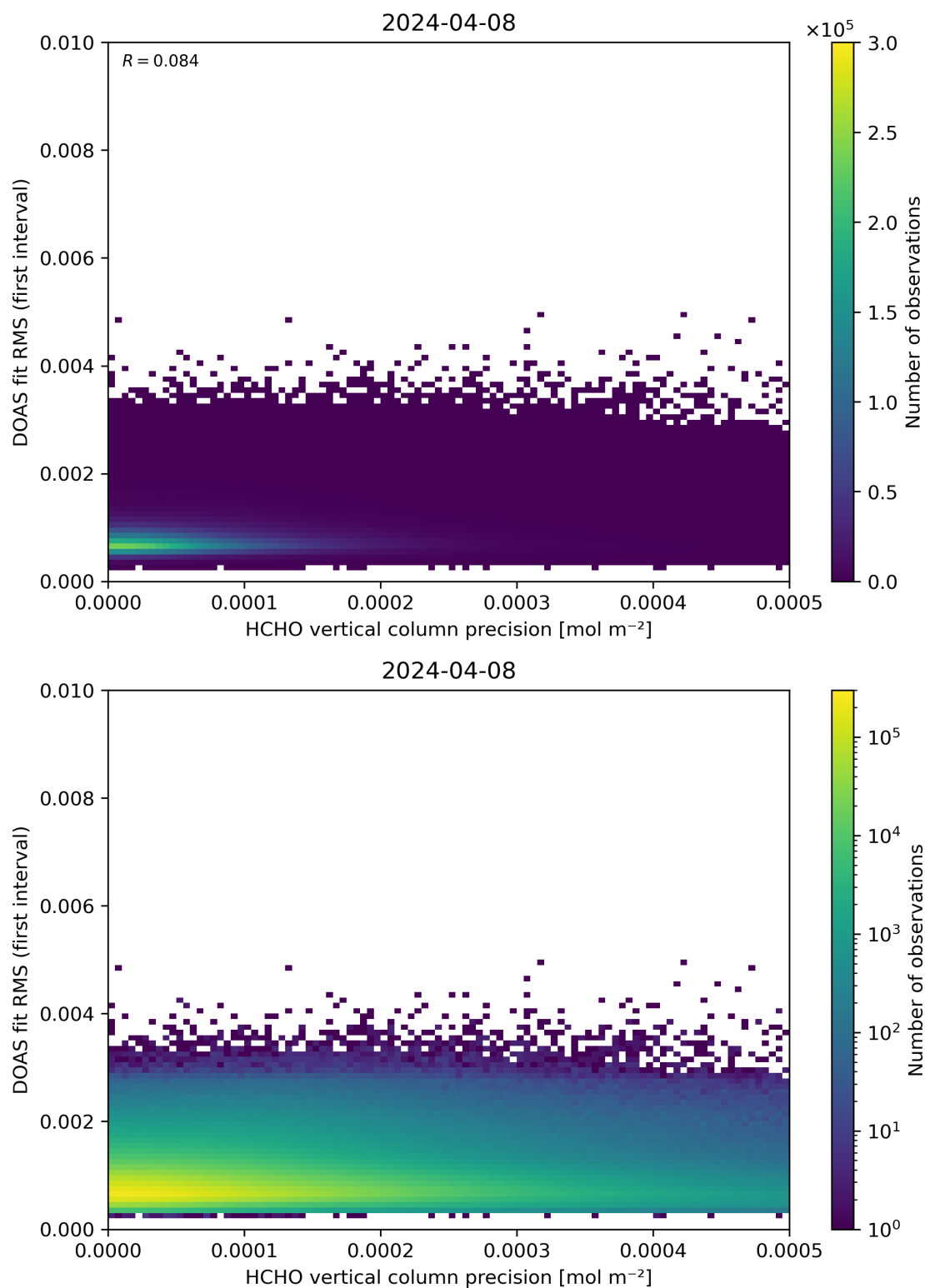
Figure 136: Scatter density plot of “HCHO vertical column precision” against “DOAS fit RMS (first interval)” for 2024-04-07 to 2024-04-09.
