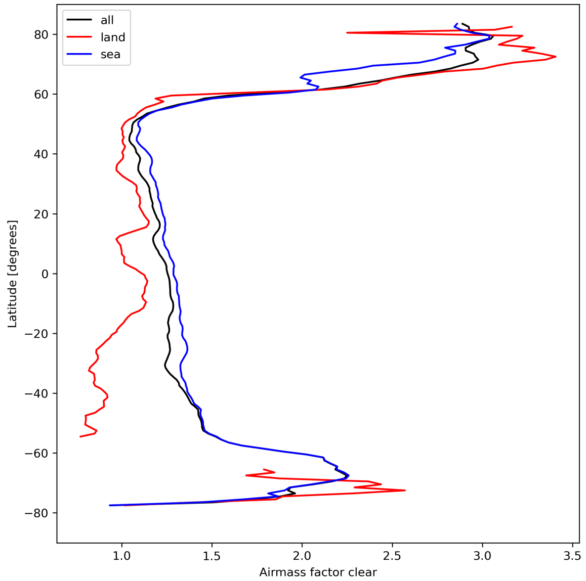
Figure 28: Zonal average of “Airmass factor clear” for 2024-04-07 to 2024-04-09.
