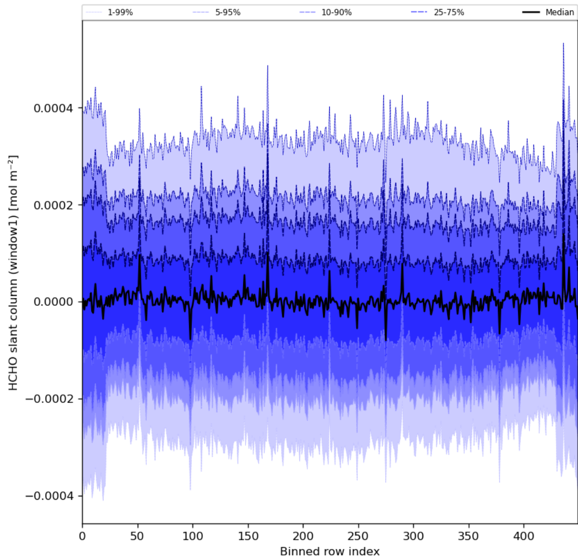
Figure 52: Along track statistics of “HCHO slant column (window1)” for 2024-04-07 to 2024-04-09
