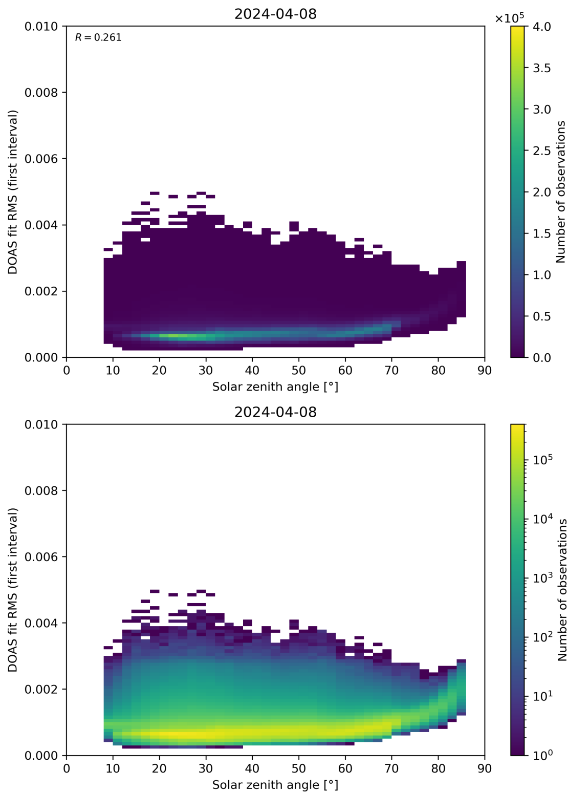
Figure 167: Scatter density plot of “Solar zenith angle” against “DOAS fit RMS (first interval)” for 2024-04-07 to 2024-04-09.
