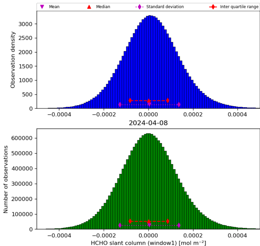
Figure 38: Histogram of “HCHO slant column (window1)” for 2024-04-07 to 2024-04-09
