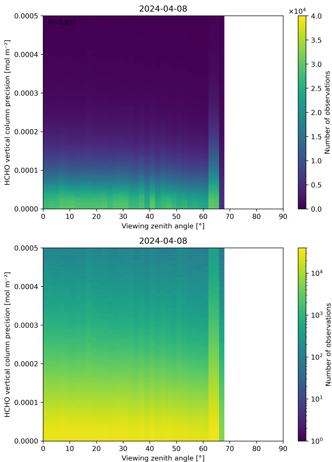
Figure 194: Scatter density plot of “Viewing zenith angle” against “HCHO vertical column precision” for 2024-04-07 to 2024-04-09.
