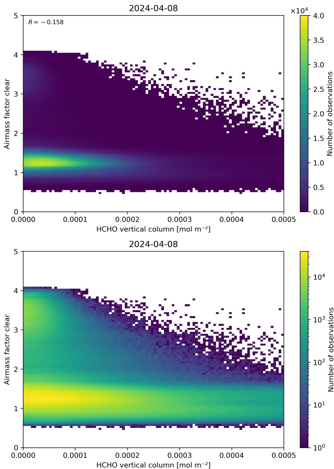
Figure 126: Scatter density plot of “HCHO vertical column” against “Airmass factor clear” for 2024-04-07 to 2024-04-09.
