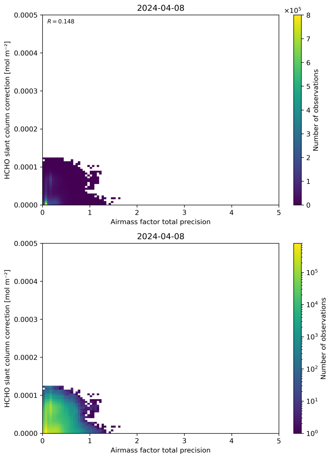
Figure 110: Scatter density plot of “Airmass factor total precision” against “HCHO slant column correction” for 2024-04-07 to 2024-04-09.
