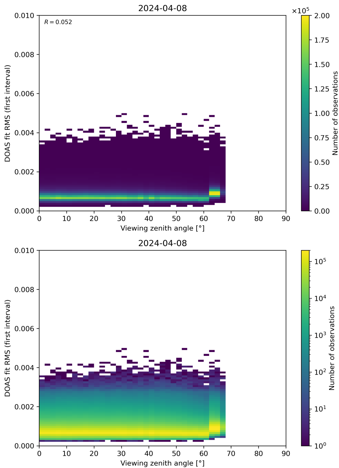
Figure 182: Scatter density plot of “Viewing zenith angle” against “DOAS fit RMS (first interval)” for 2024-04-07 to 2024-04-09.
