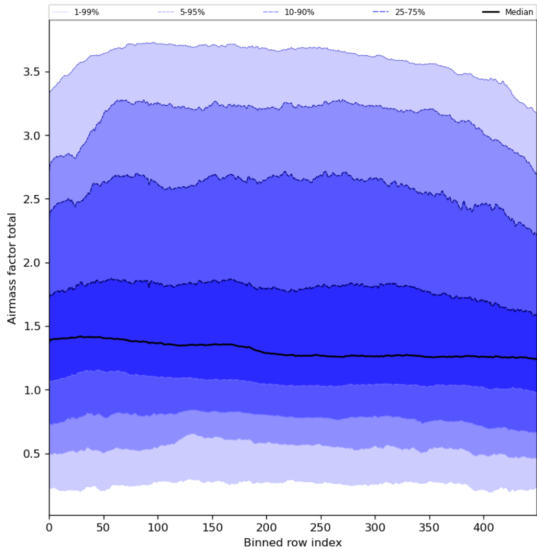
Figure 54: Along track statistics of “Airmass factor total” for 2024-04-07 to 2024-04-09
