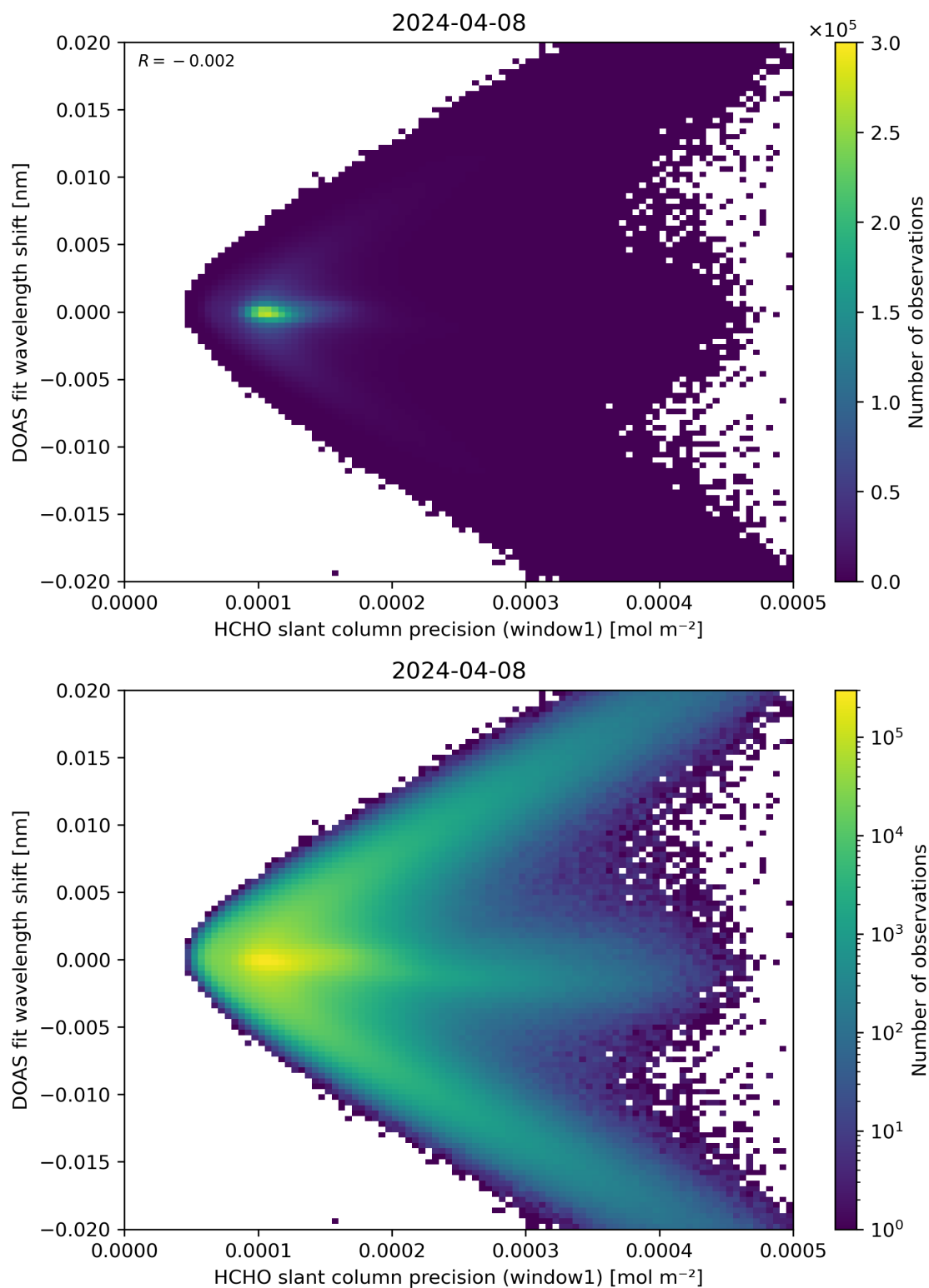
Figure 89: Scatter density plot of “HCHO slant column precision (window1)” against “DOAS fit wavelength shift” for 2024-04-07 to 2024-04-09.
