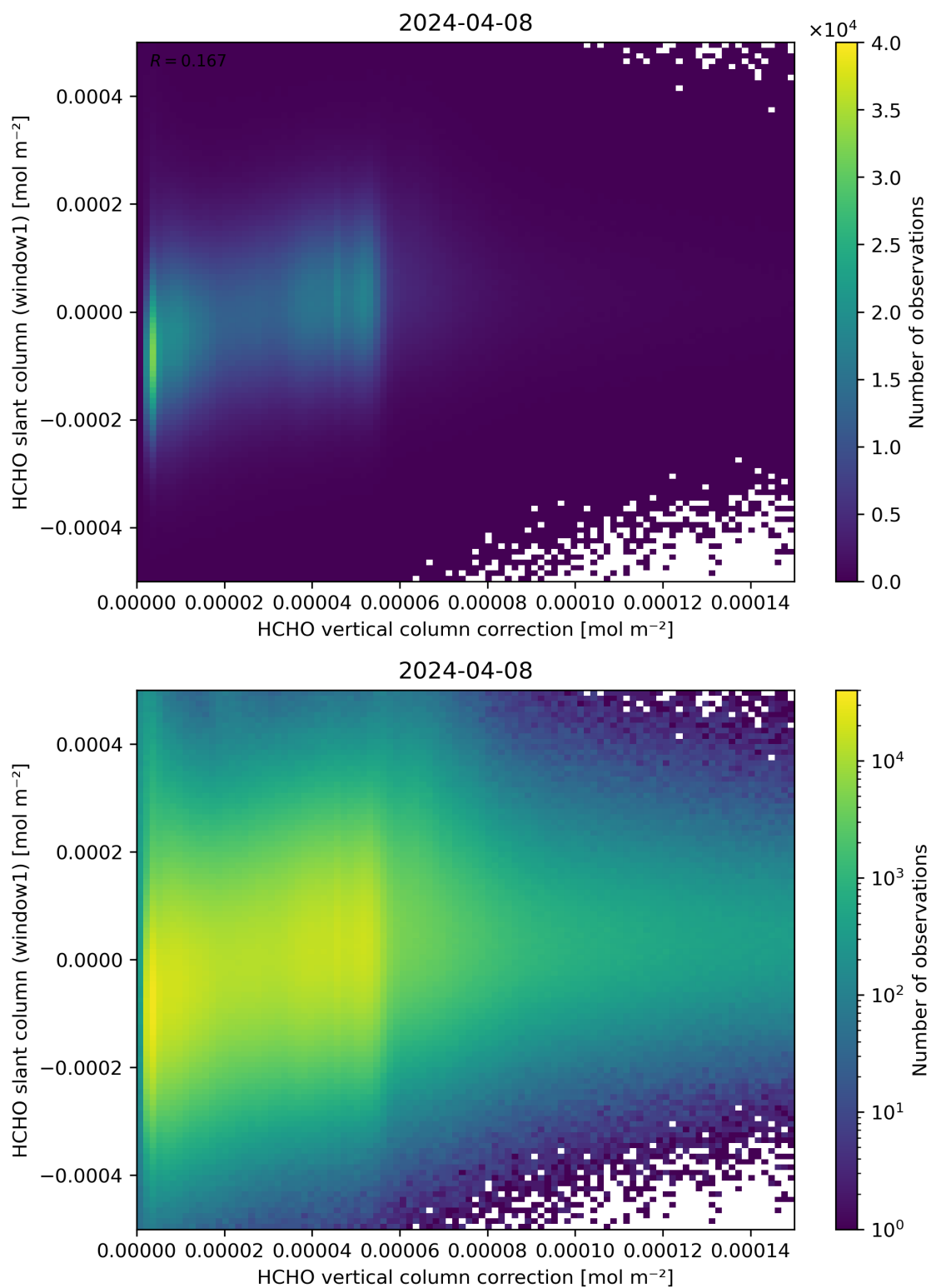
Figure 118: Scatter density plot of “HCHO vertical column correction” against “HCHO slant column (window1)” for 2024-04-07 to 2024-04-09.
