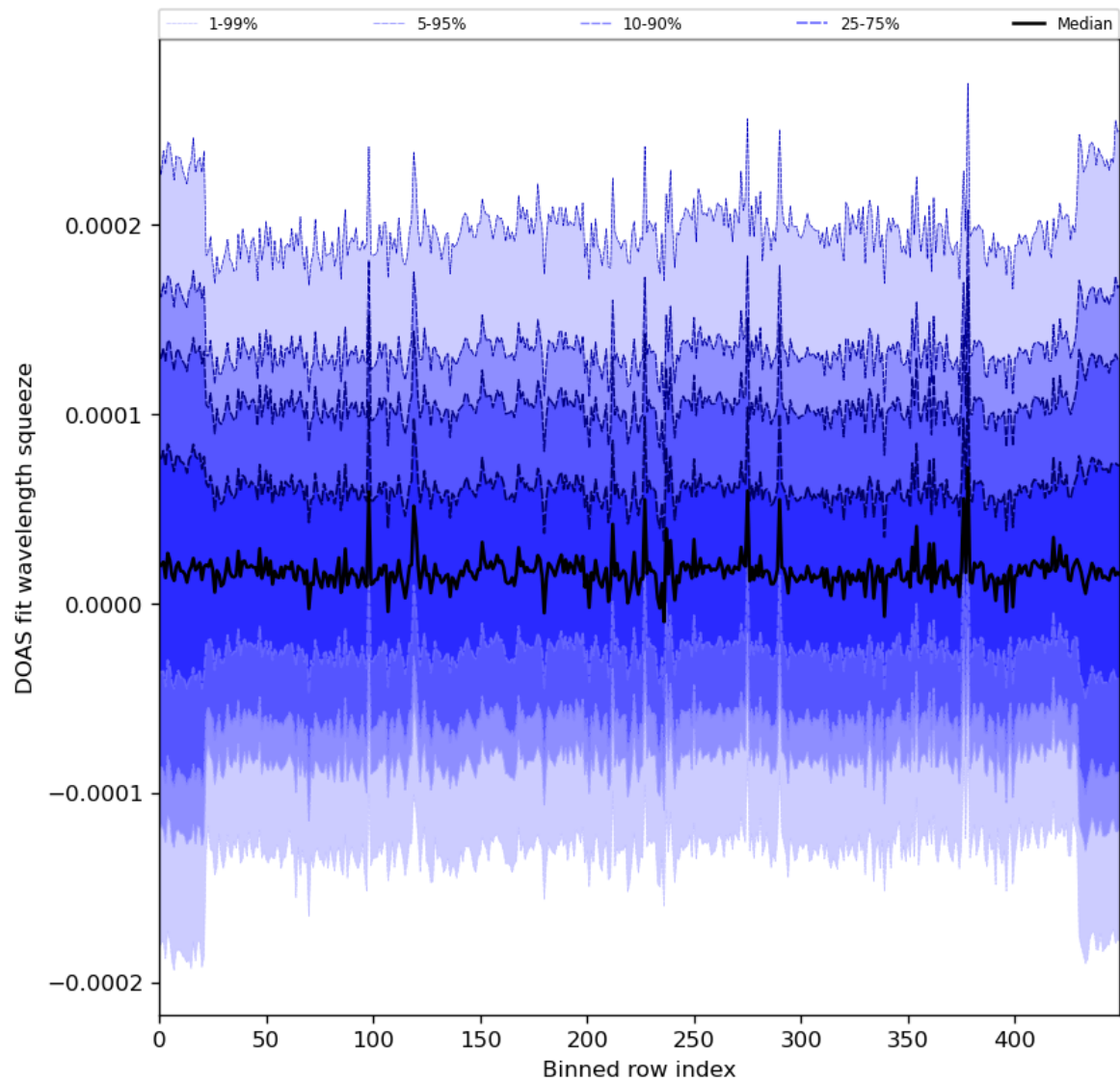
Figure 59: Along track statistics of “DOAS fit wavelength squeeze” for 2024-04-07 to 2024-04-09
