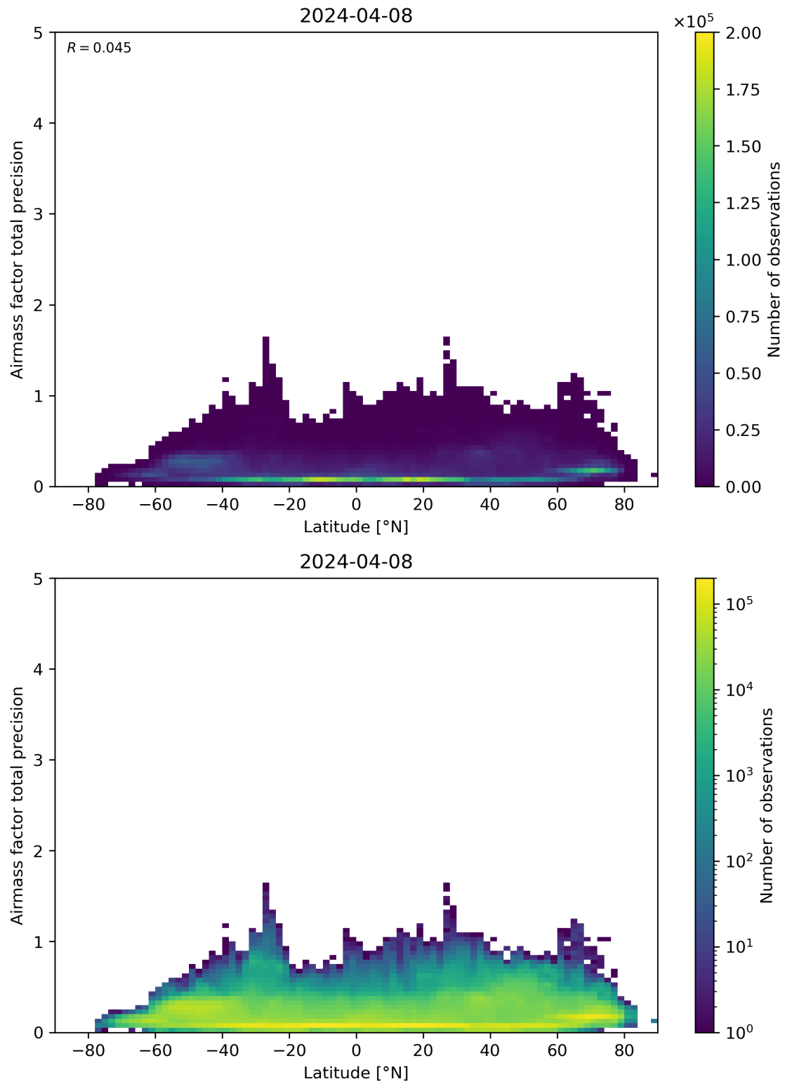
Figure 162: Scatter density plot of “Latitude” against “Airmass factor total precision” for 2024-04-07 to 2024-04-09.
