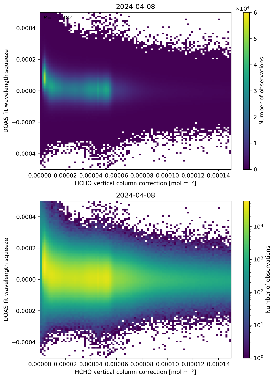
Figure 114: Scatter density plot of “HCHO vertical column correction” against “DOAS fit wavelength squeeze” for 2024-04-07 to 2024-04-09.
