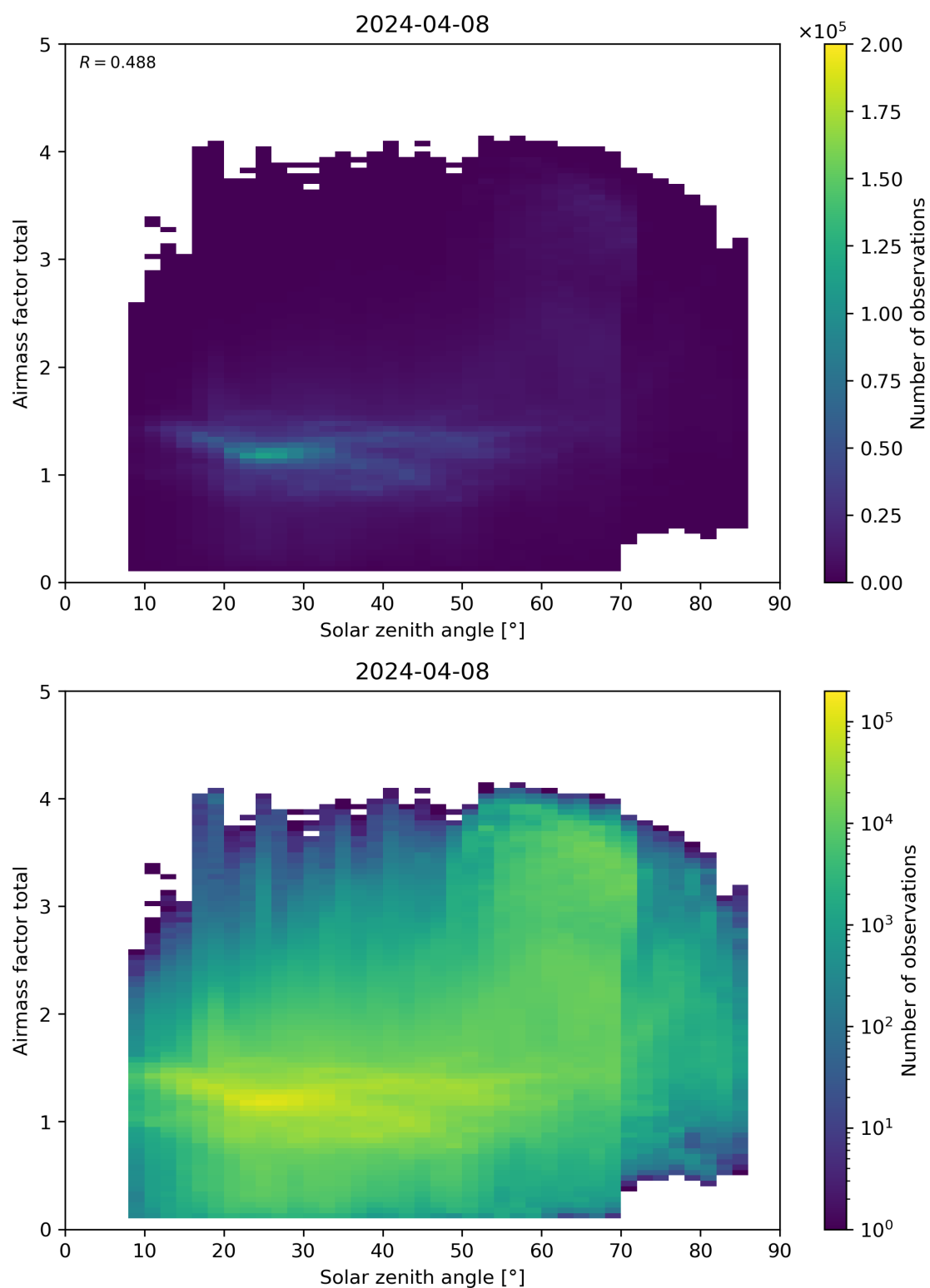
Figure 175: Scatter density plot of “Solar zenith angle” against “Airmass factor total” for 2024-04-07 to 2024-04-09.
