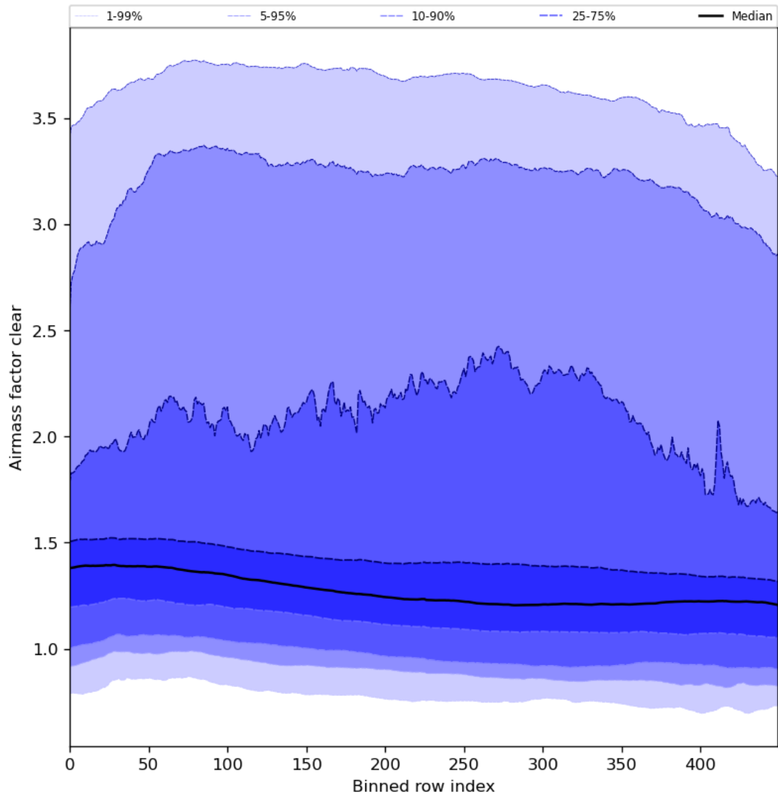
Figure 56: Along track statistics of “Airmass factor clear” for 2024-04-07 to 2024-04-09
