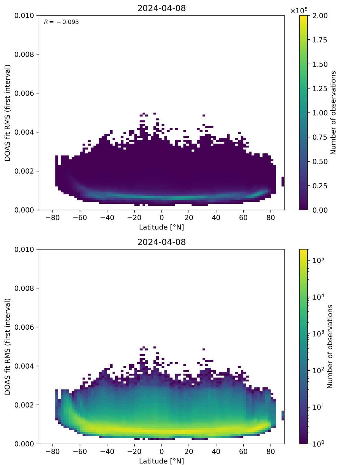
Figure 153: Scatter density plot of “Latitude” against “DOAS fit RMS (first interval)” for 2024-04-07 to 2024-04-09.
