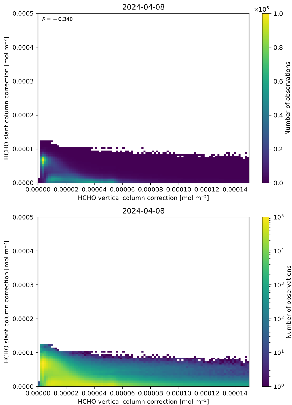
Figure 117: Scatter density plot of “HCHO vertical column correction” against “HCHO slant column correction” for 2024-04-07 to 2024-04-09.
