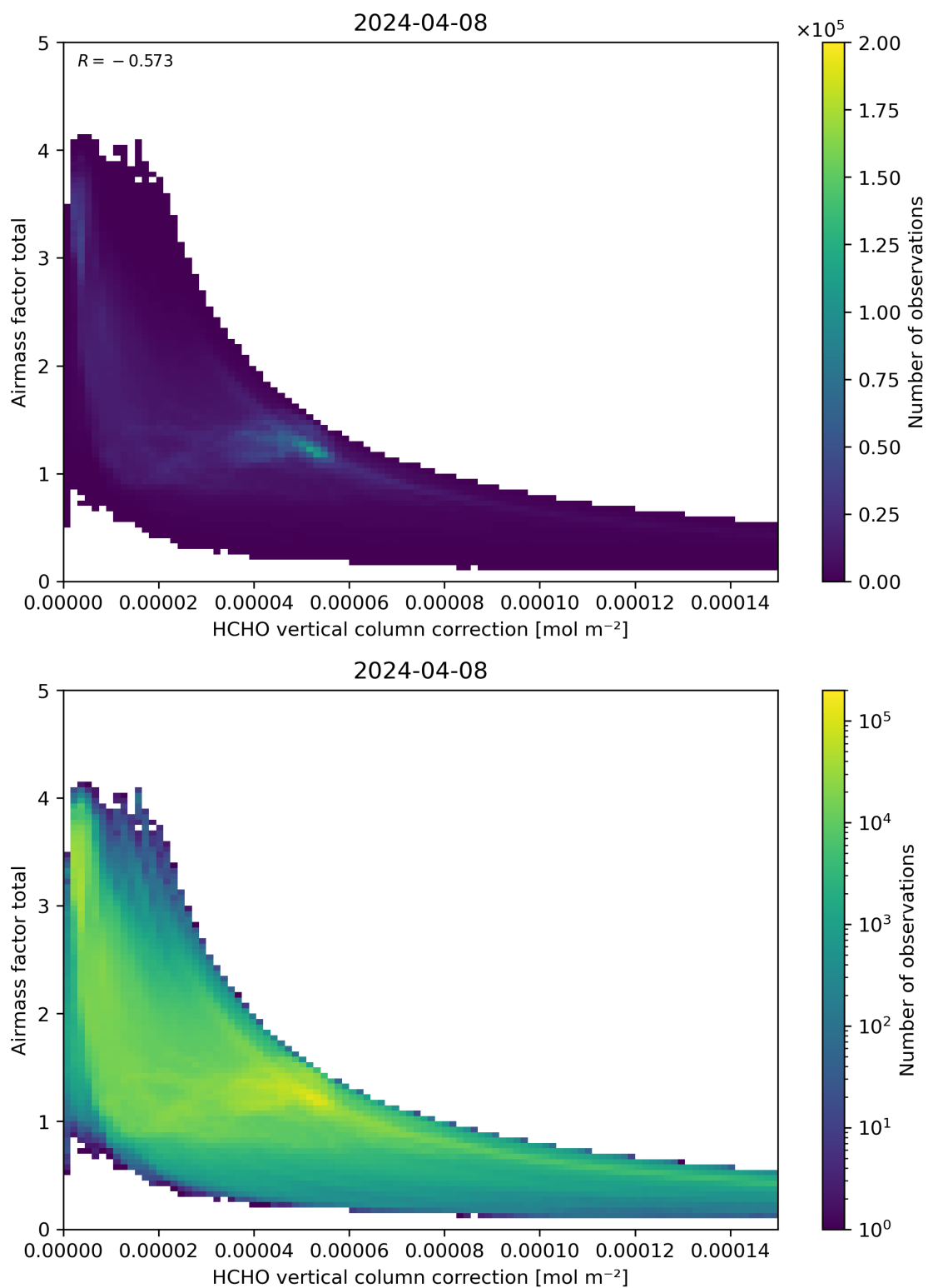
Figure 120: Scatter density plot of “HCHO vertical column correction” against “Airmass factor total” for 2024-04-07 to 2024-04-09.
