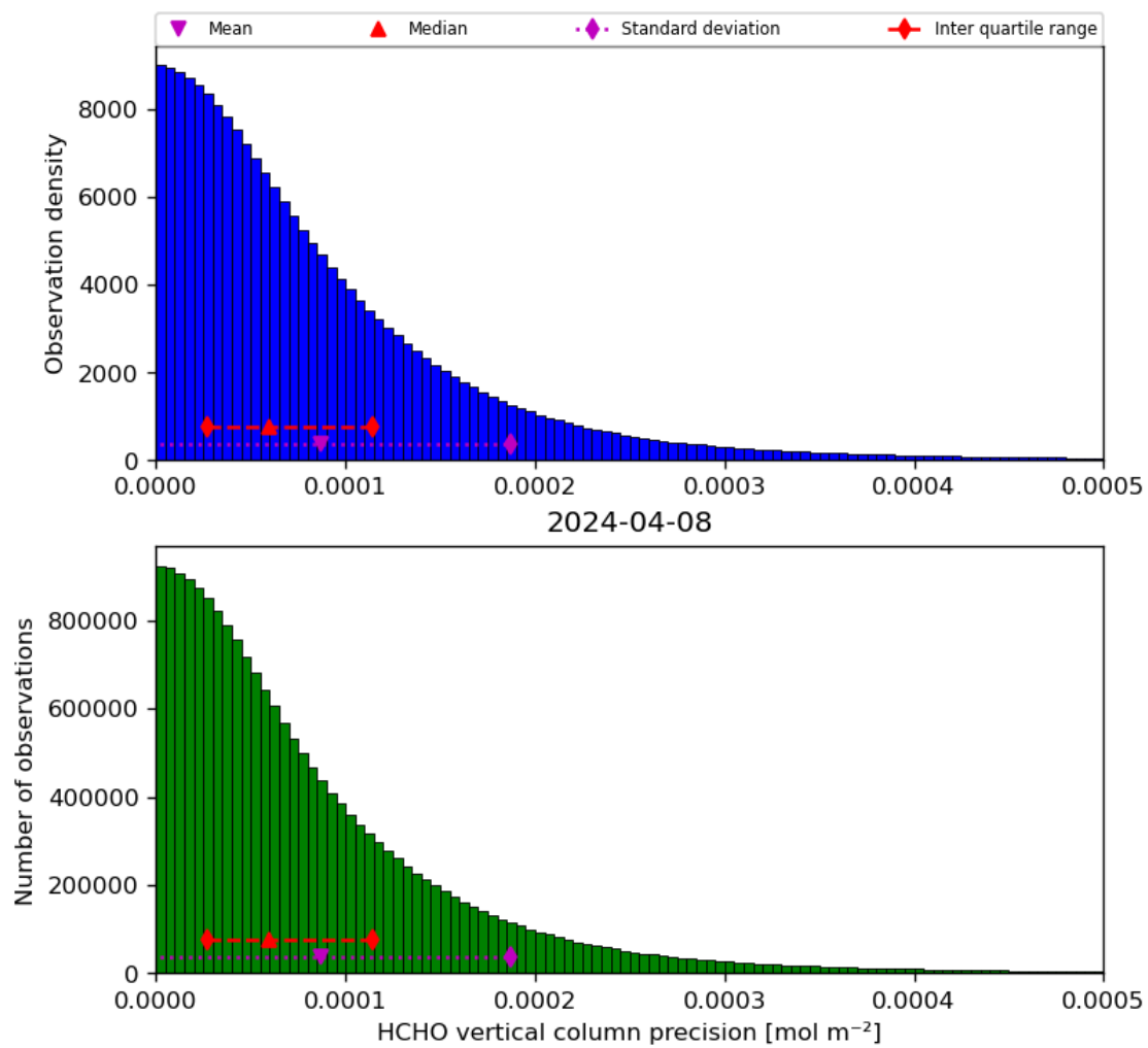
Figure 36: Histogram of “HCHO vertical column precision” for 2024-04-07 to 2024-04-09
