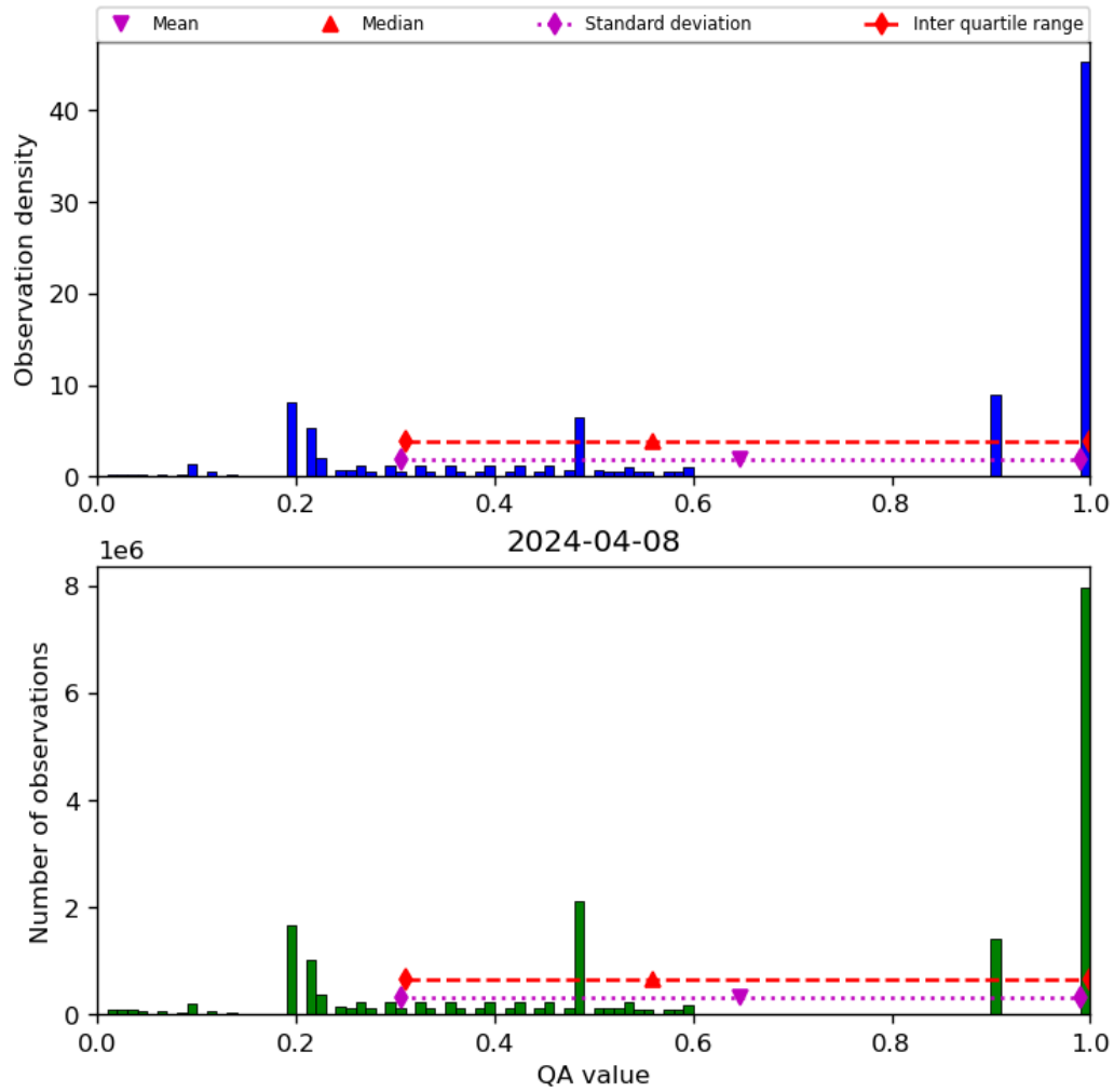
Figure 34: Histogram of “QA value” for 2024-04-07 to 2024-04-09
