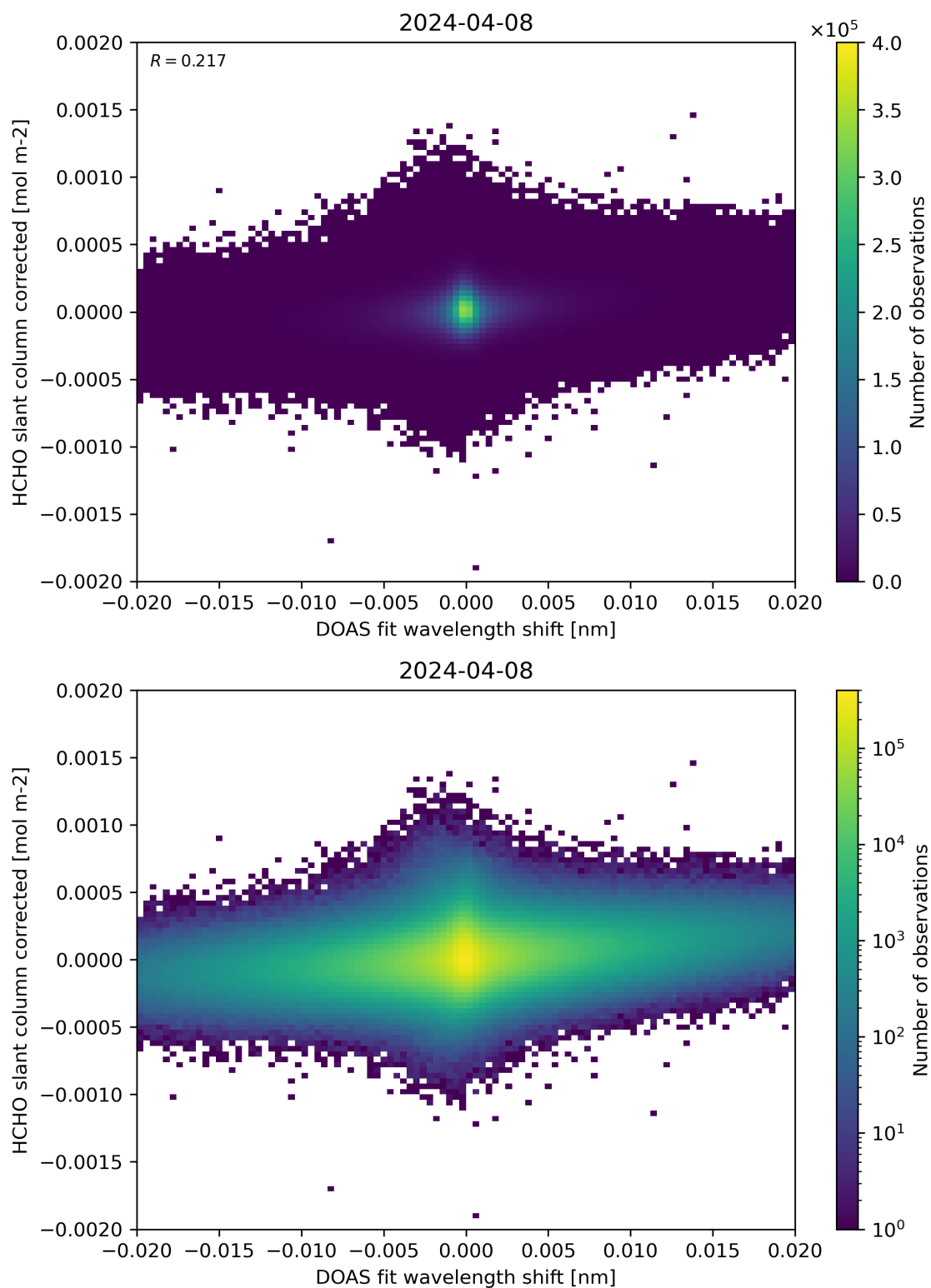
Figure 66: Scatter density plot of “DOAS fit wavelength shift” against “HCHO slant column corrected” for 2024-04-07 to 2024-04-09.
