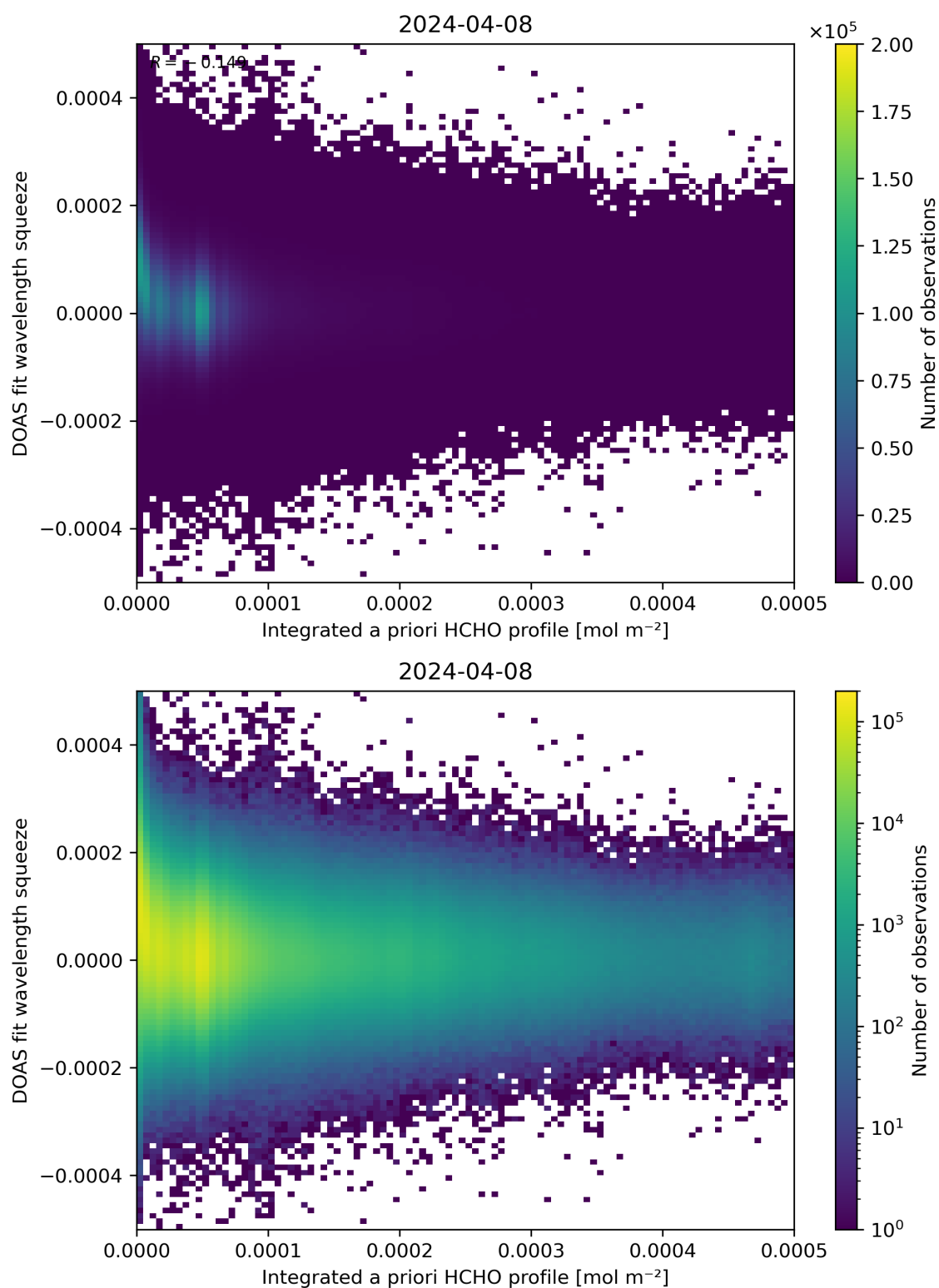
Figure 150: Scatter density plot of “Integrated a priori HCHO profile” against “DOAS fit wavelength squeeze” for 2024-04-07 to 2024-04-09.
