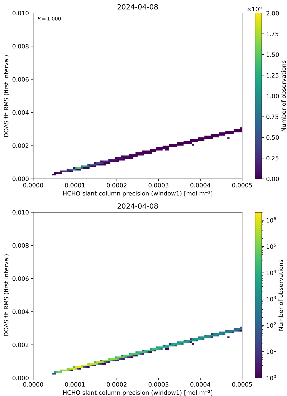
Figure 88: Scatter density plot of “HCHO slant column precision (window1)” against “DOAS fit RMS (first interval)” for 2024-04-07 to 2024-04-09.
