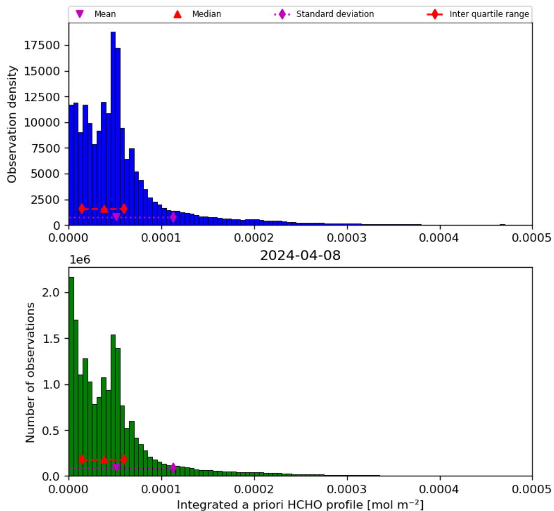
Figure 43: Histogram of “Integrated a priori HCHO profile” for 2024-04-07 to 2024-04-09
