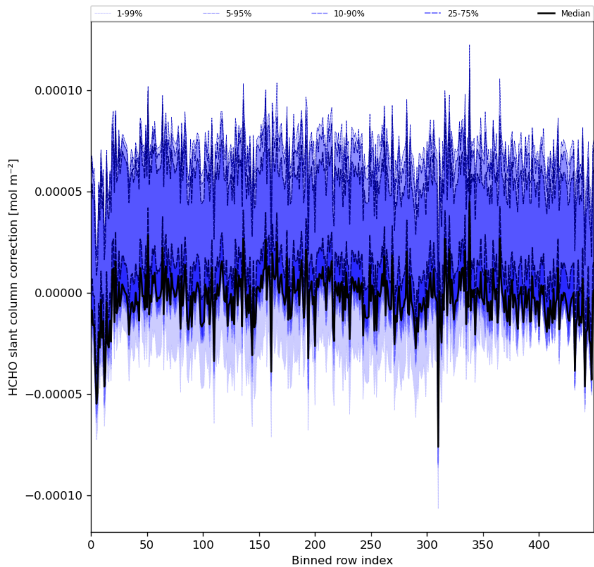
Figure 61: Along track statistics of “HCHO slant column correction” for 2024-04-07 to 2024-04-09
