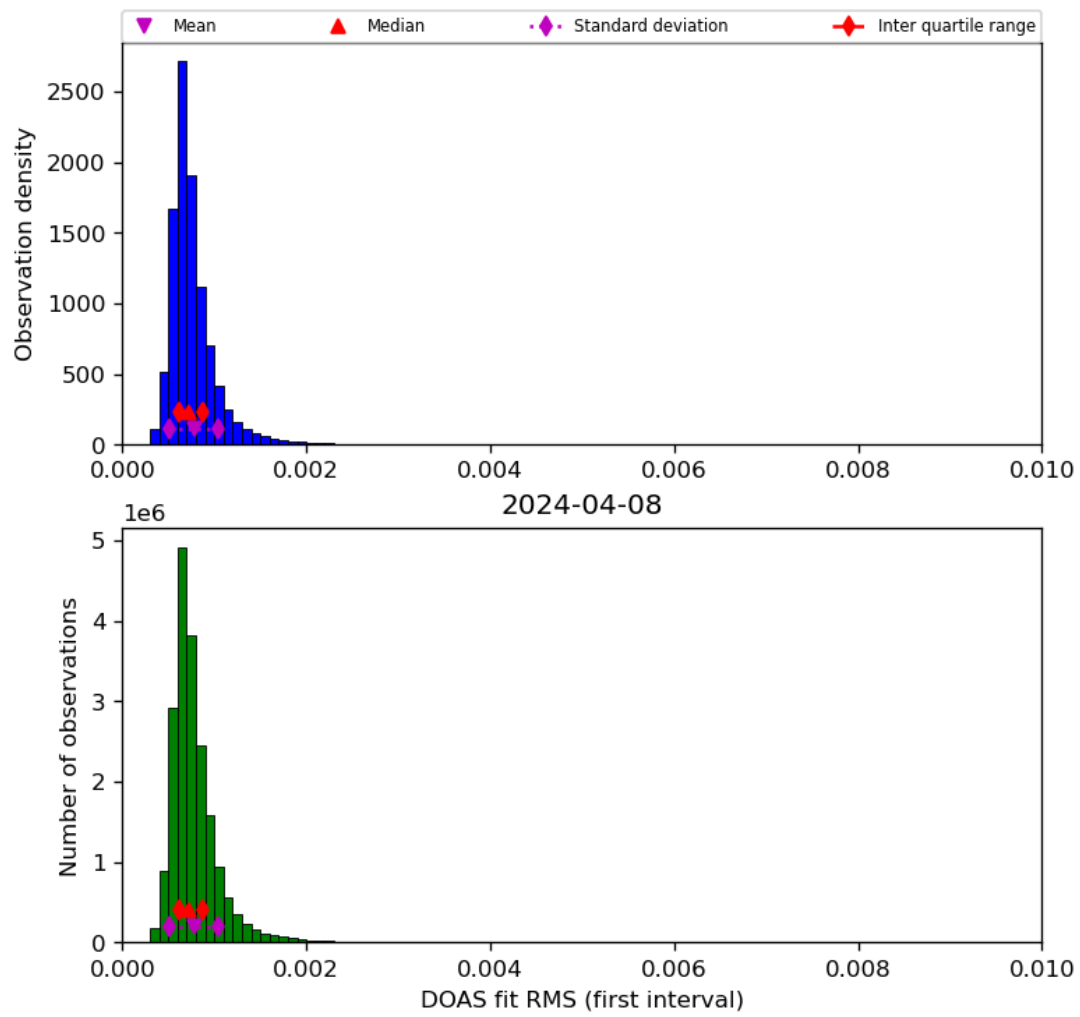
Figure 46: Histogram of “DOAS fit RMS (first interval)” for 2024-04-07 to 2024-04-09
