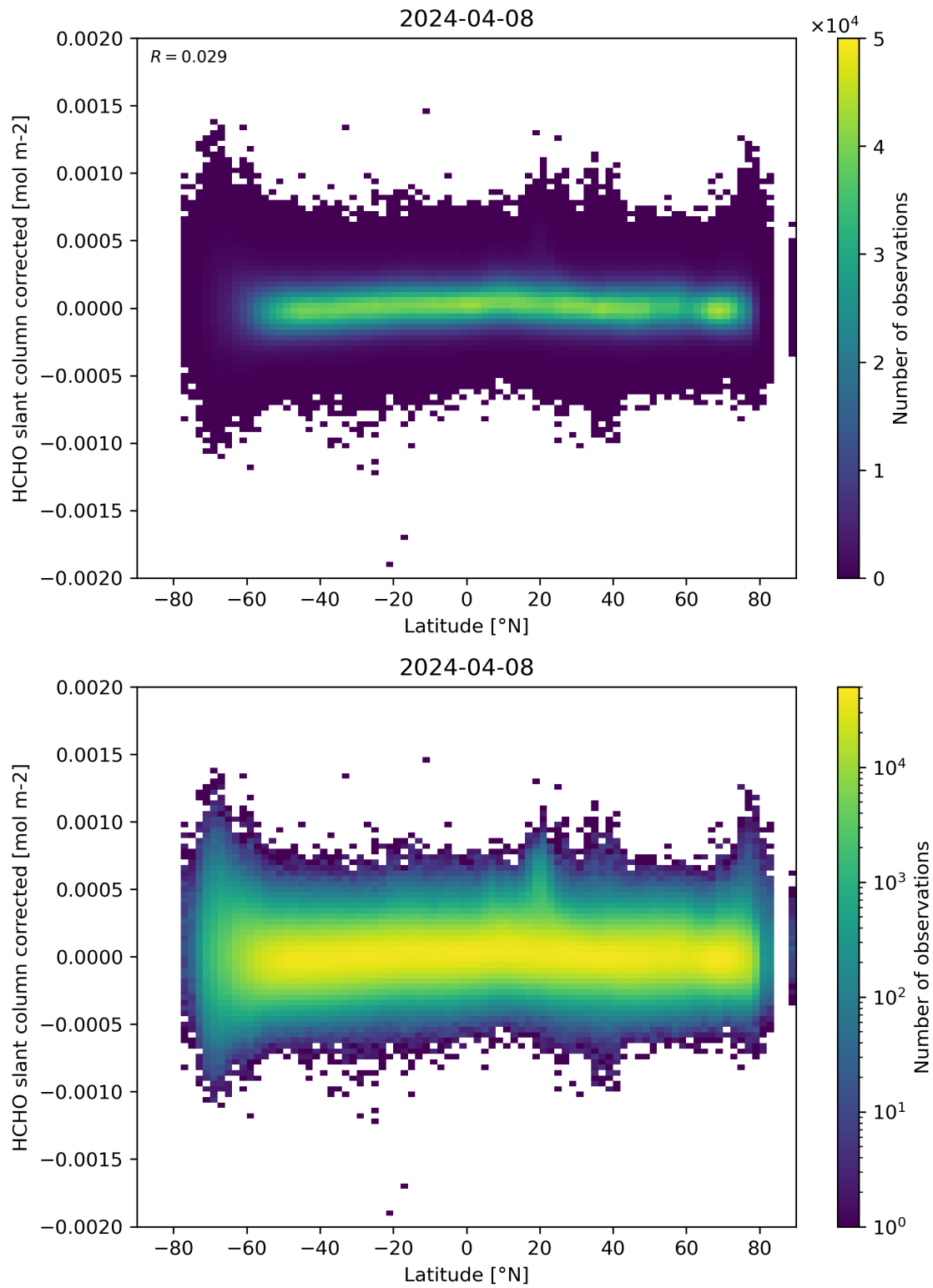
Figure 157: Scatter density plot of “Latitude” against “HCHO slant column corrected” for 2024-04-07 to 2024-04-09.
