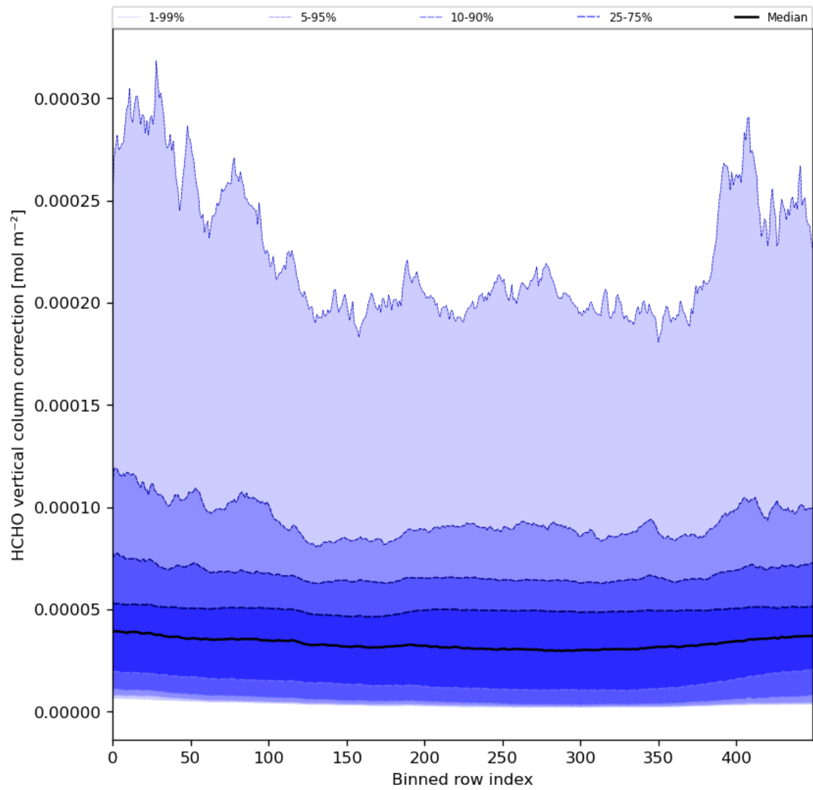
Figure 51: Along track statistics of “HCHO vertical column correction” for 2024-04-07 to 2024-04-09
