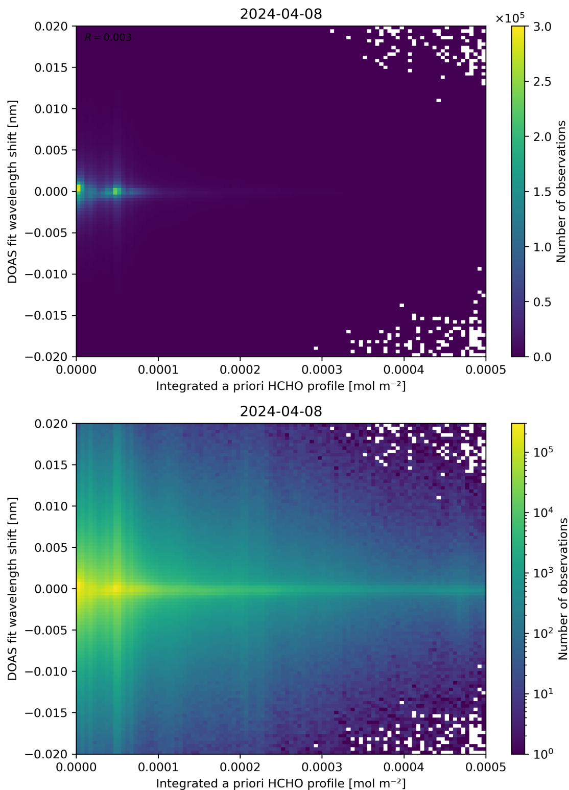
Figure 149: Scatter density plot of “Integrated a priori HCHO profile” against “DOAS fit wavelength shift” for 2024-04-07 to 2024-04-09.
