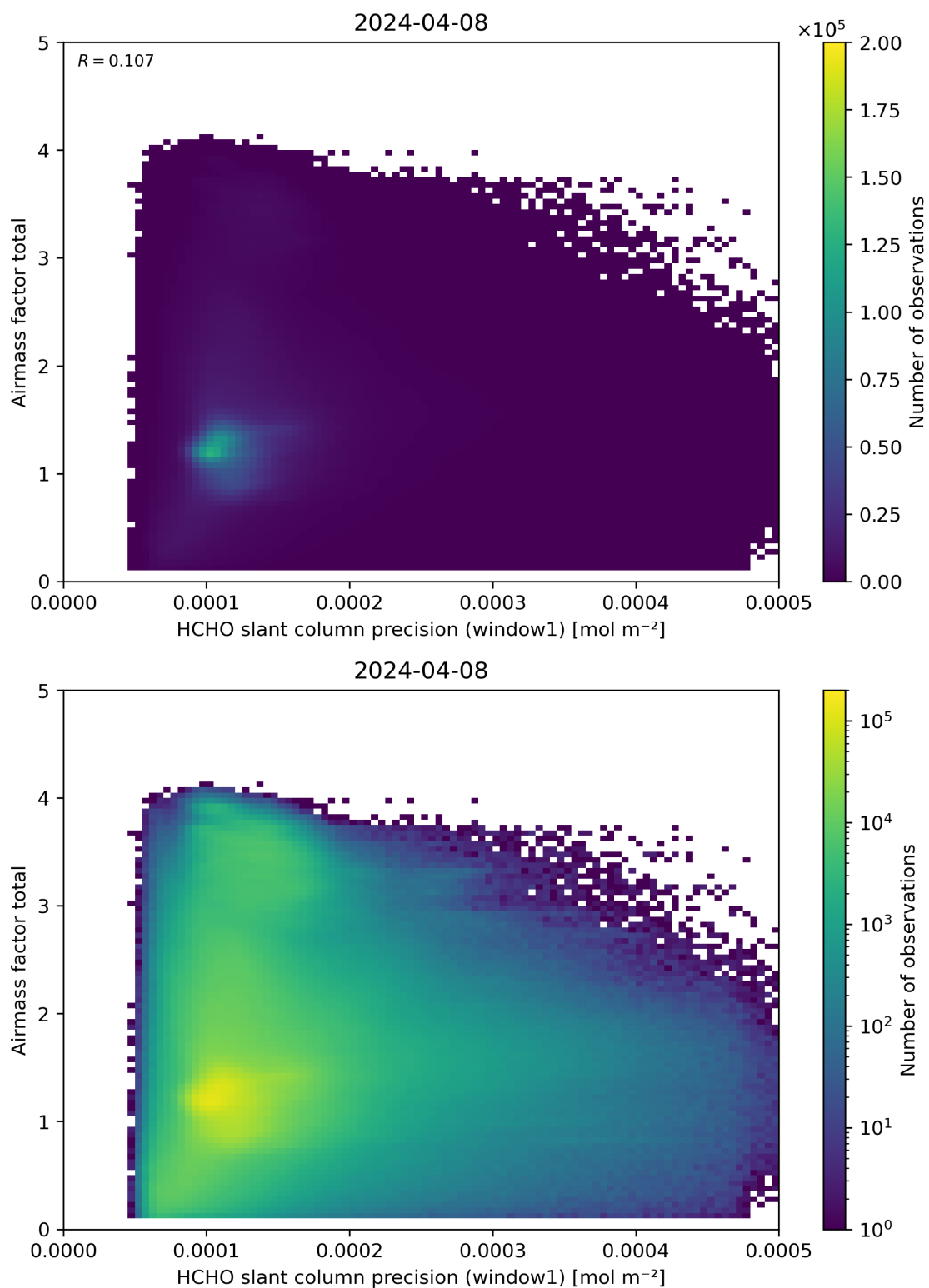
Figure 94: Scatter density plot of “HCHO slant column precision (window1)” against “Airmass factor total” for 2024-04-07 to 2024-04-09.
