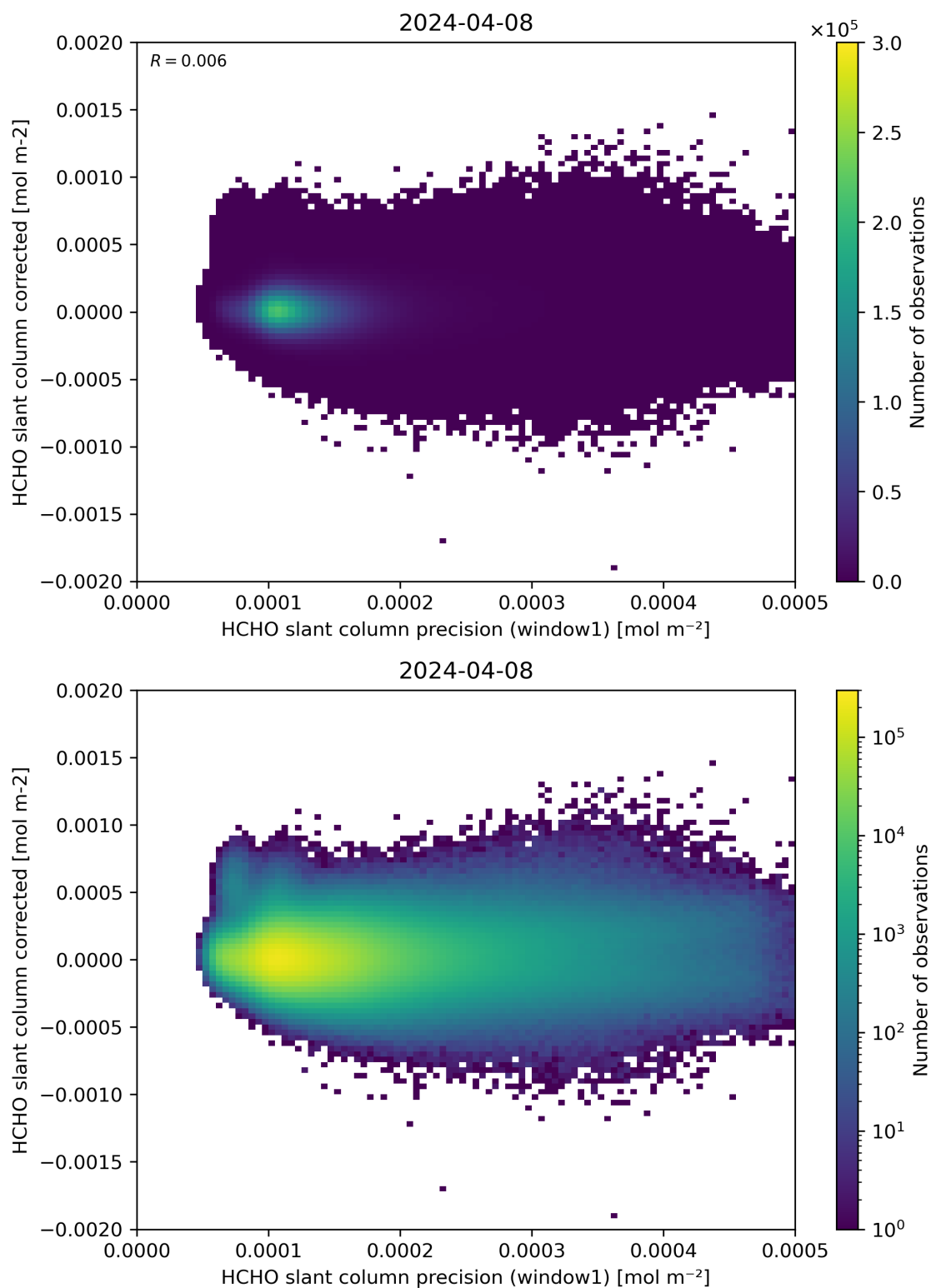
Figure 92: Scatter density plot of “HCHO slant column precision (window1)” against “HCHO slant column corrected” for 2024-04-07 to 2024-04-09.
