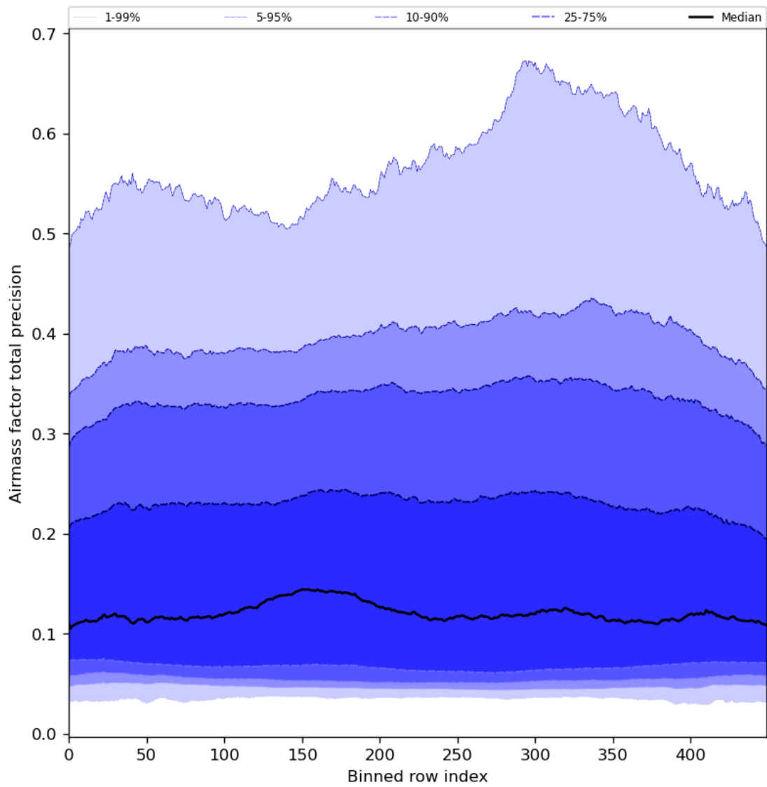
Figure 55: Along track statistics of “Airmass factor total precision” for 2024-04-07 to 2024-04-09
