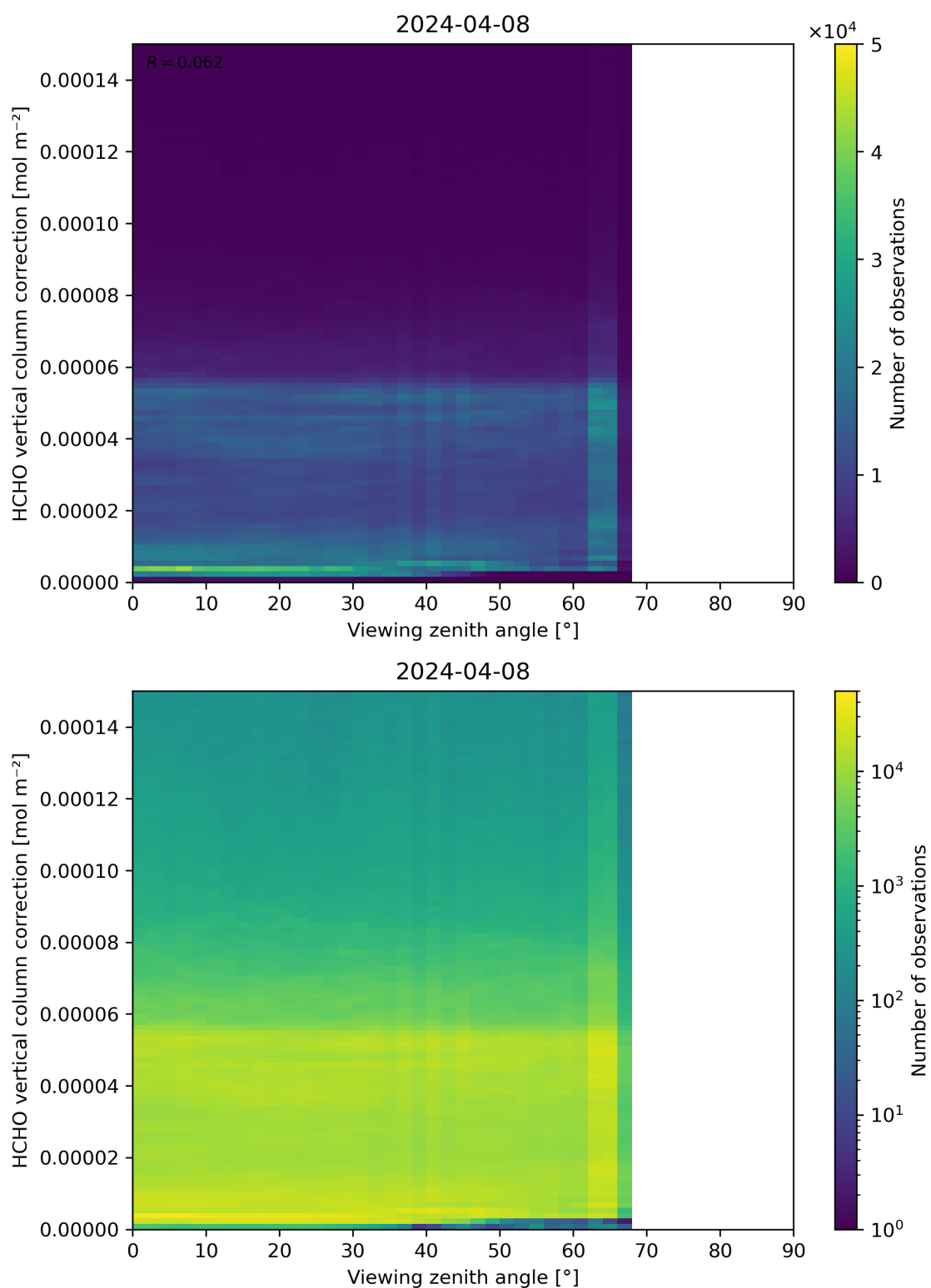
Figure 193: Scatter density plot of “Viewing zenith angle” against “HCHO vertical column correction” for 2024-04-07 to 2024-04-09.
