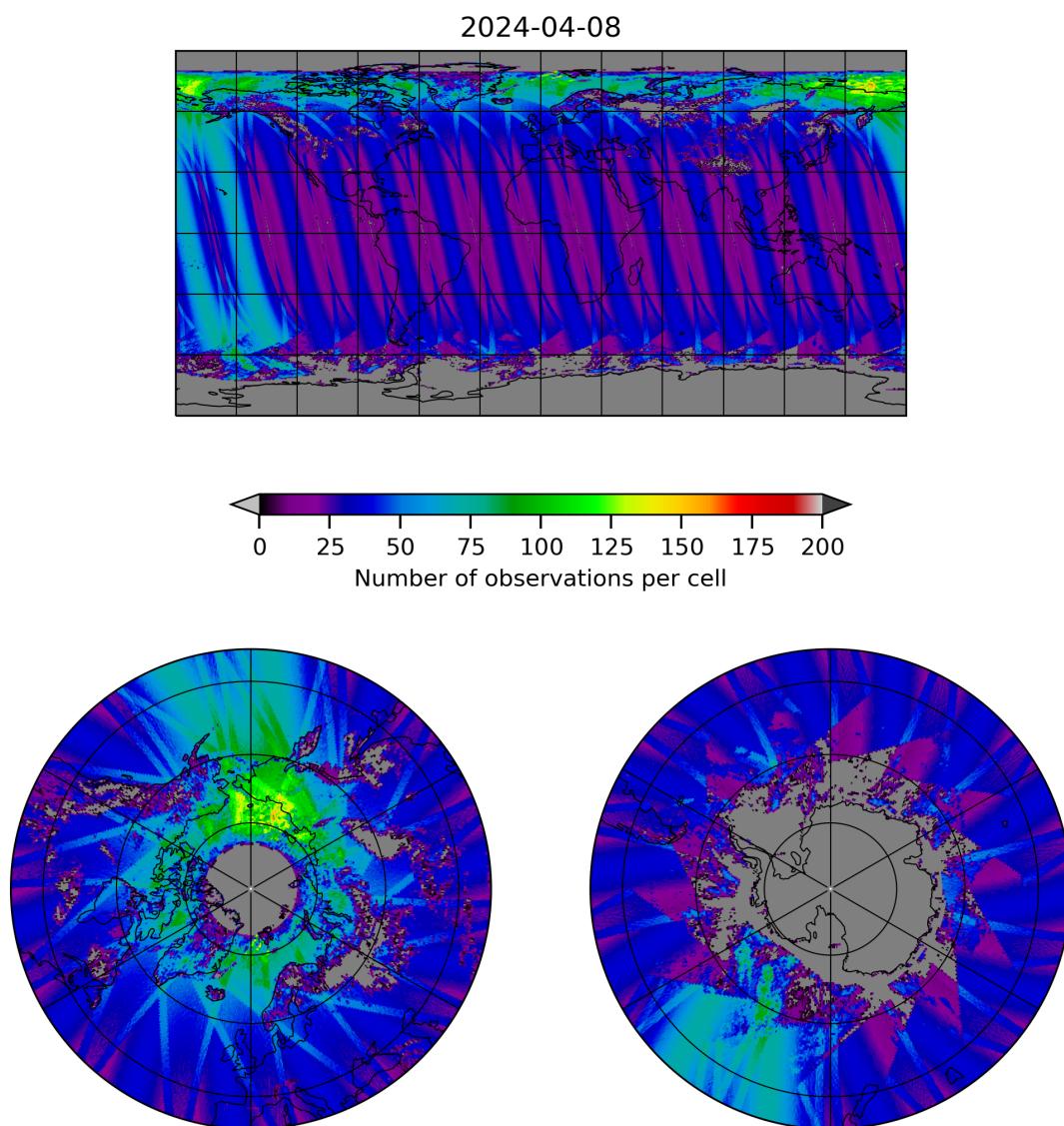
Figure 19: Map of the number of observations for 2024-04-07 to 2024-04-09
