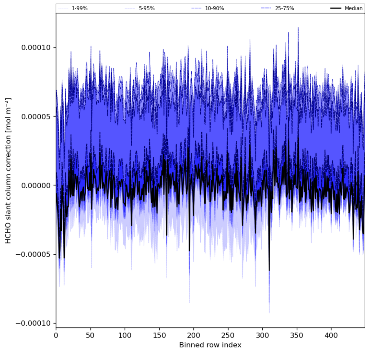
Figure 61: Along track statistics of “HCHO slant column correction” for 2024-04-08 to 2024-04-10
