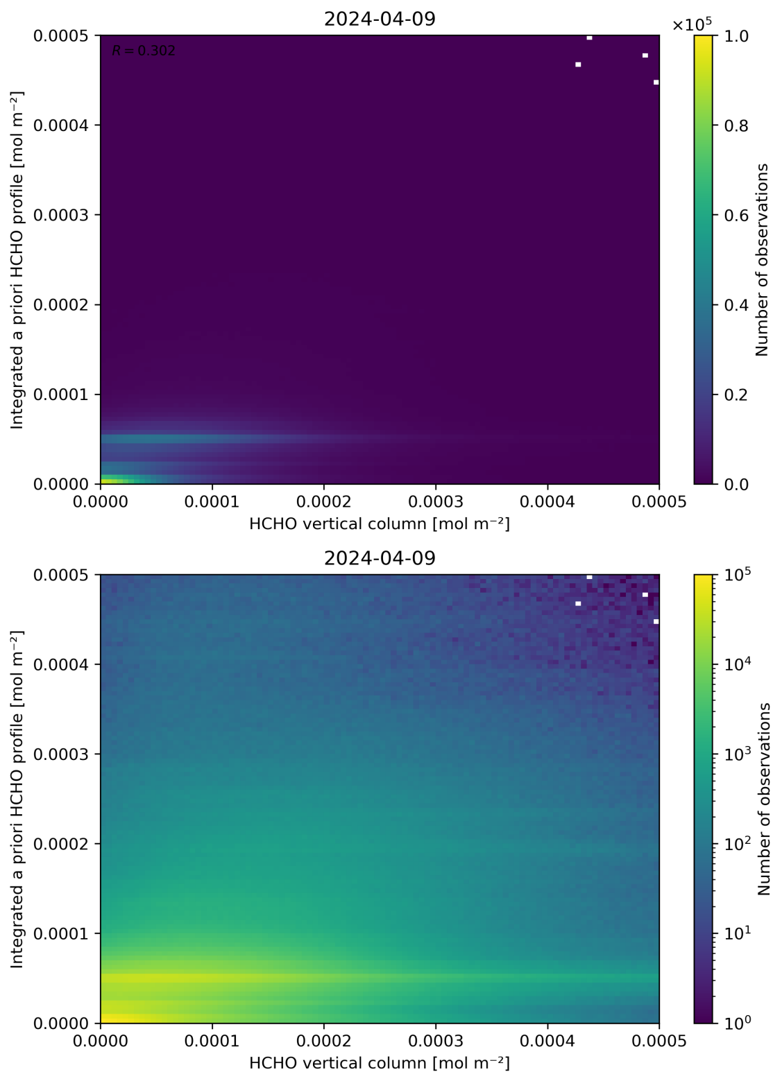
Figure 135: Scatter density plot of “HCHO vertical column” against “Integrated a priori HCHO profile” for 2024-04-08 to 2024-04-10.
