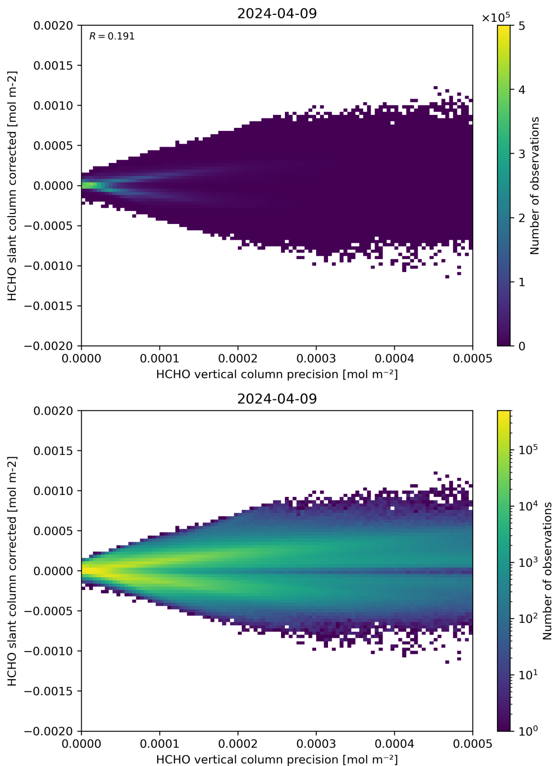
Figure 140: Scatter density plot of “HCHO vertical column precision” against “HCHO slant column corrected” for 2024-04-08 to 2024-04-10.
