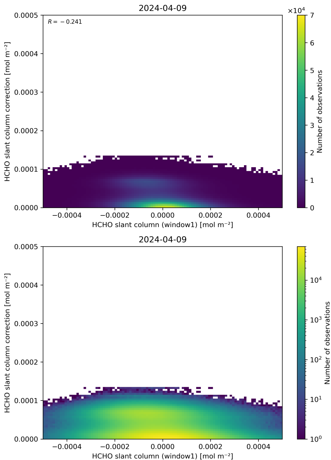
Figure 83: Scatter density plot of “HCHO slant column (window1)” against “HCHO slant column correction” for 2024-04-08 to 2024-04-10.
