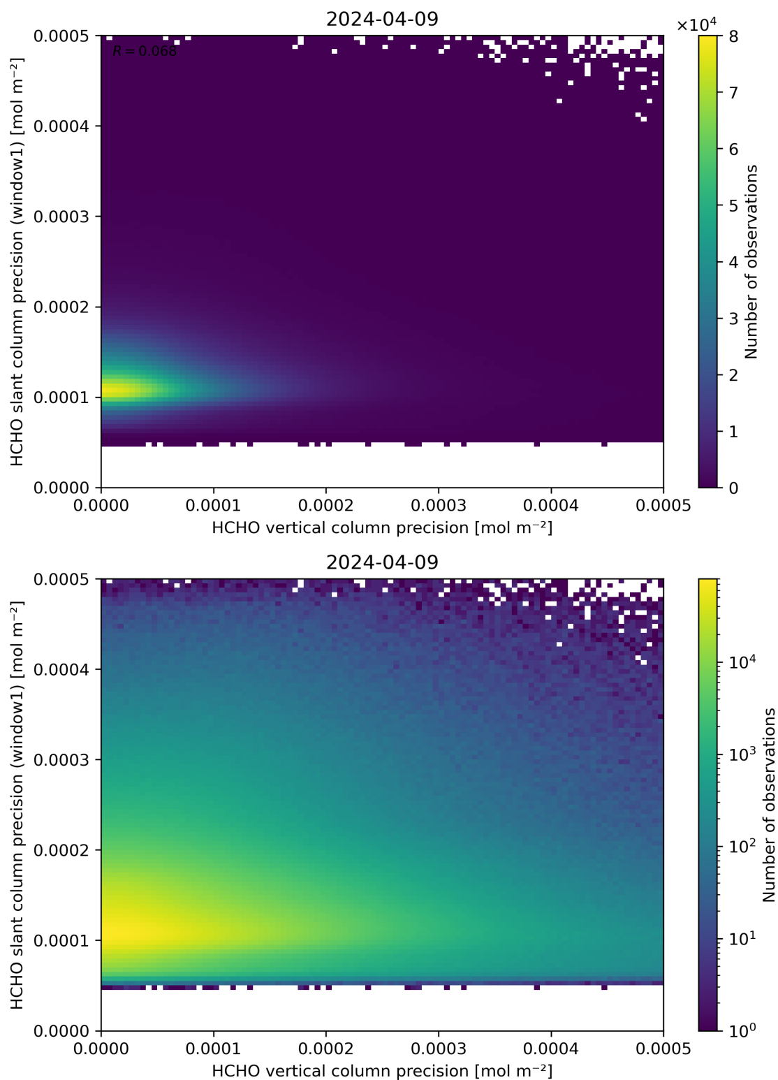
Figure 143: Scatter density plot of “HCHO vertical column precision” against “HCHO slant column precision (window1)” for 2024-04-08 to 2024-04-10.
