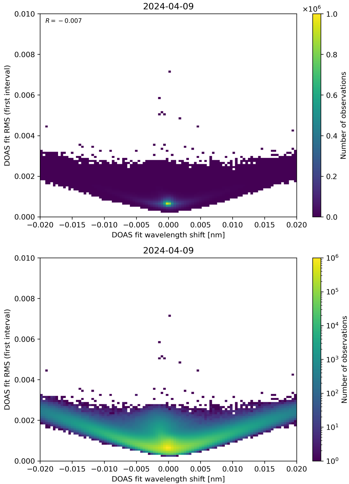
Figure 64: Scatter density plot of “DOAS fit wavelength shift” against “DOAS fit RMS (first interval)” for 2024-04-08 to 2024-04-10.
