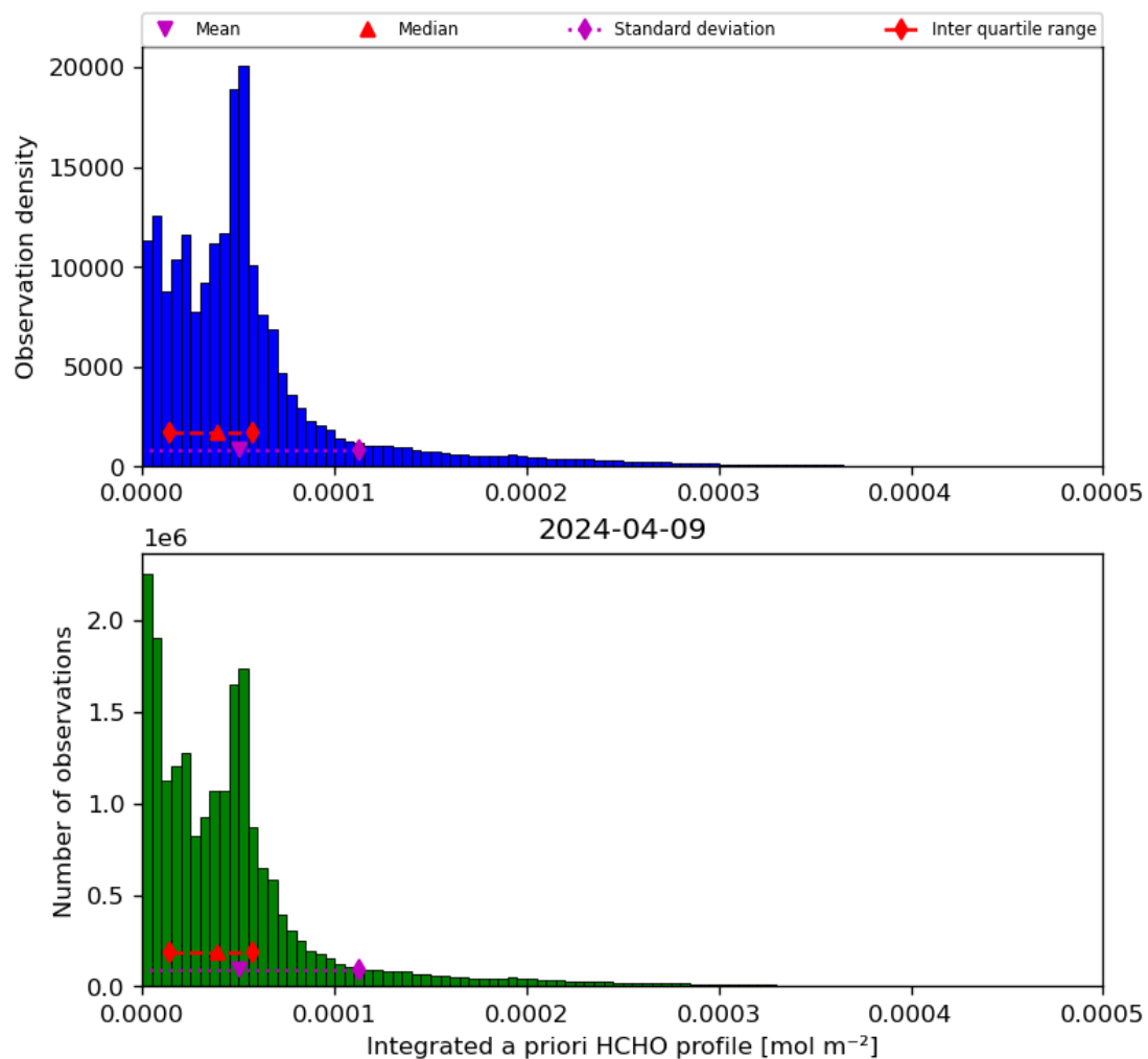
Figure 43: Histogram of “Integrated a priori HCHO profile” for 2024-04-08 to 2024-04-10
