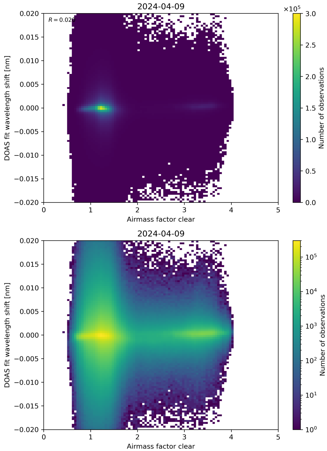
Figure 72: Scatter density plot of “Airmass factor clear” against “DOAS fit wavelength shift” for 2024-04-08 to 2024-04-10.
