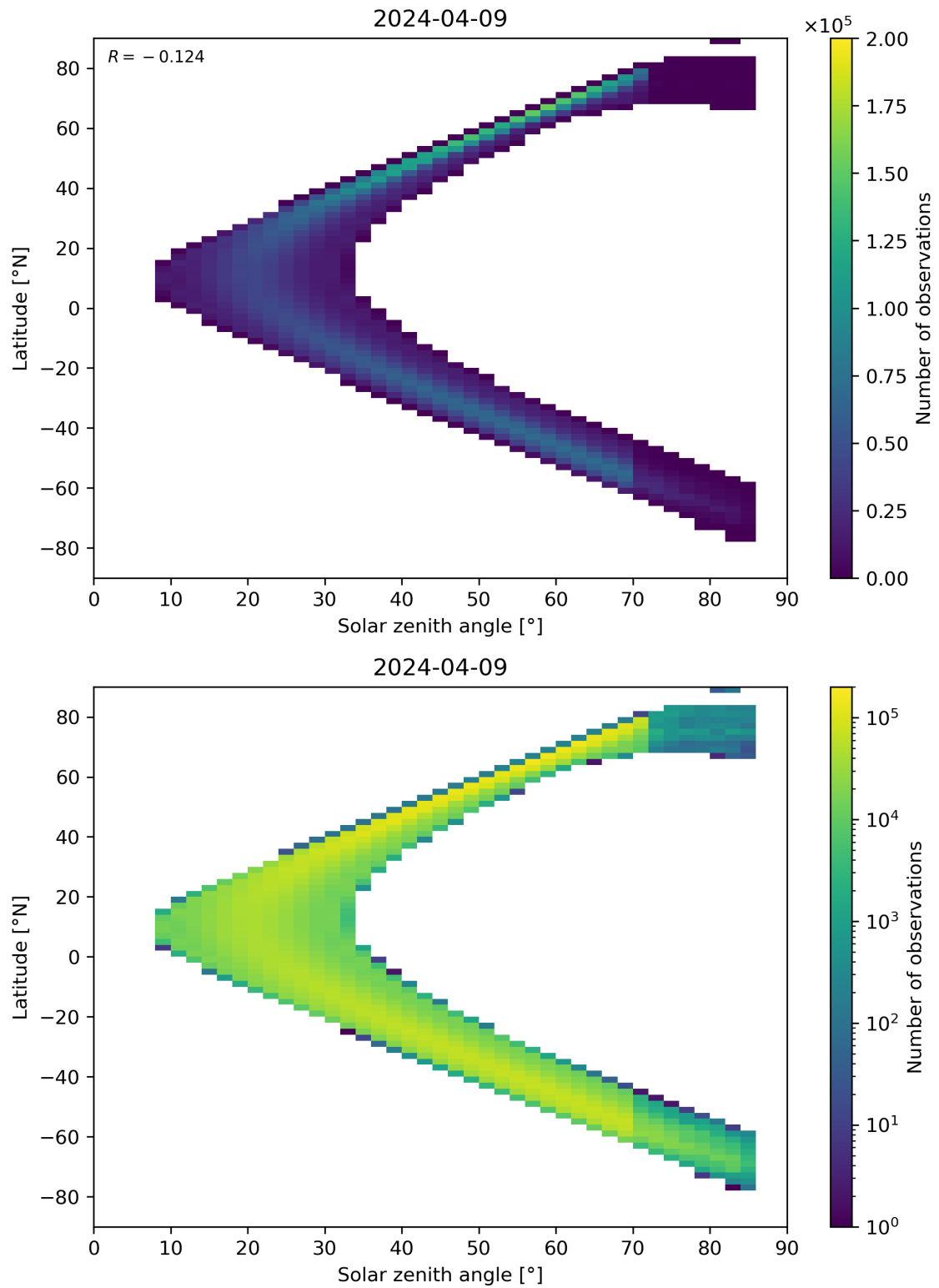
Figure 181: Scatter density plot of “Solar zenith angle” against “Latitude” for 2024-04-08 to 2024-04-10.
