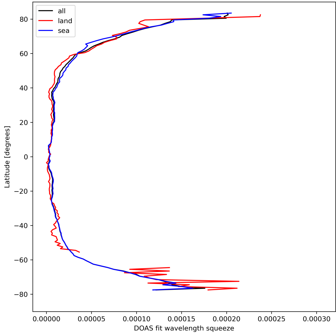
Figure 31: Zonal average of “DOAS fit wavelength squeeze” for 2024-04-08 to 2024-04-10.
