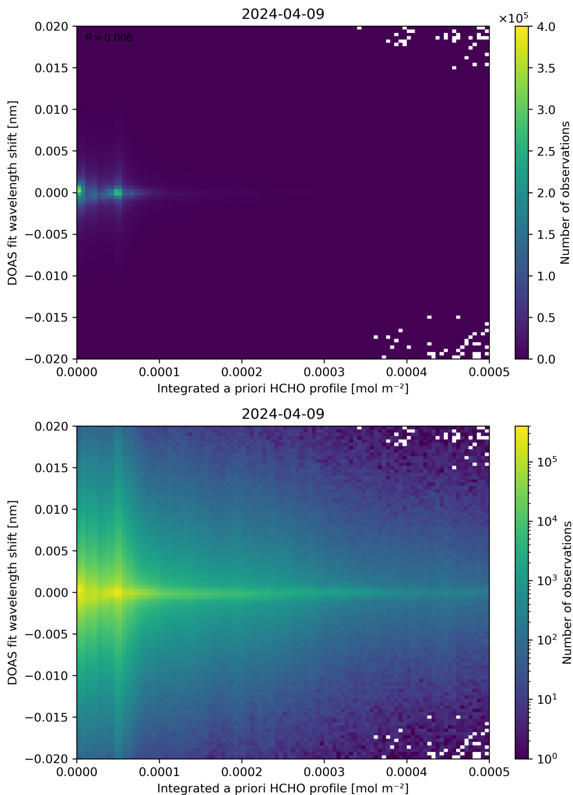
Figure 149: Scatter density plot of “Integrated a priori HCHO profile” against “DOAS fit wavelength shift” for 2024-04-08 to 2024-04-10.
