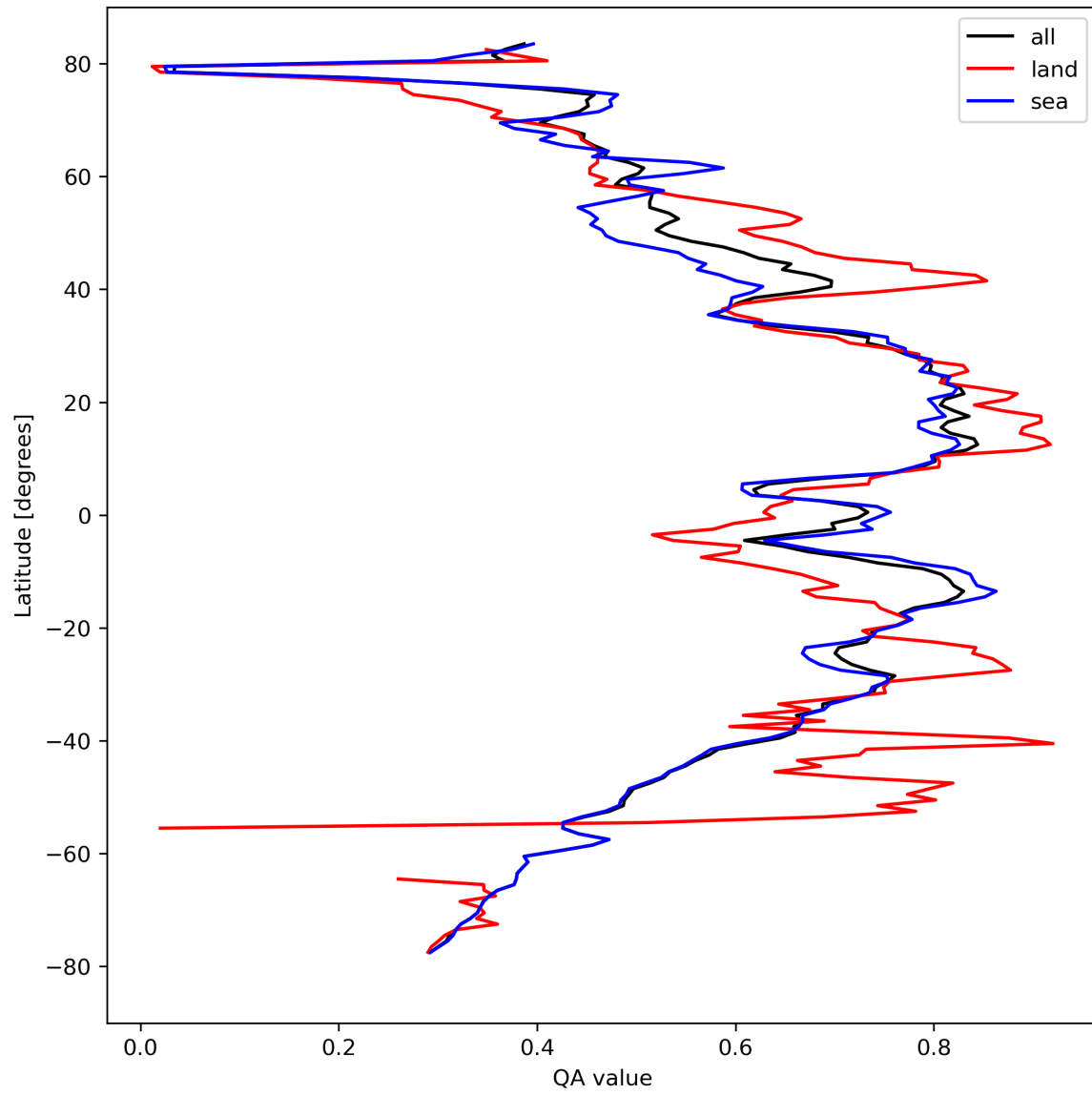
Figure 20: Zonal average of “QA value” for 2024-04-08 to 2024-04-10.
