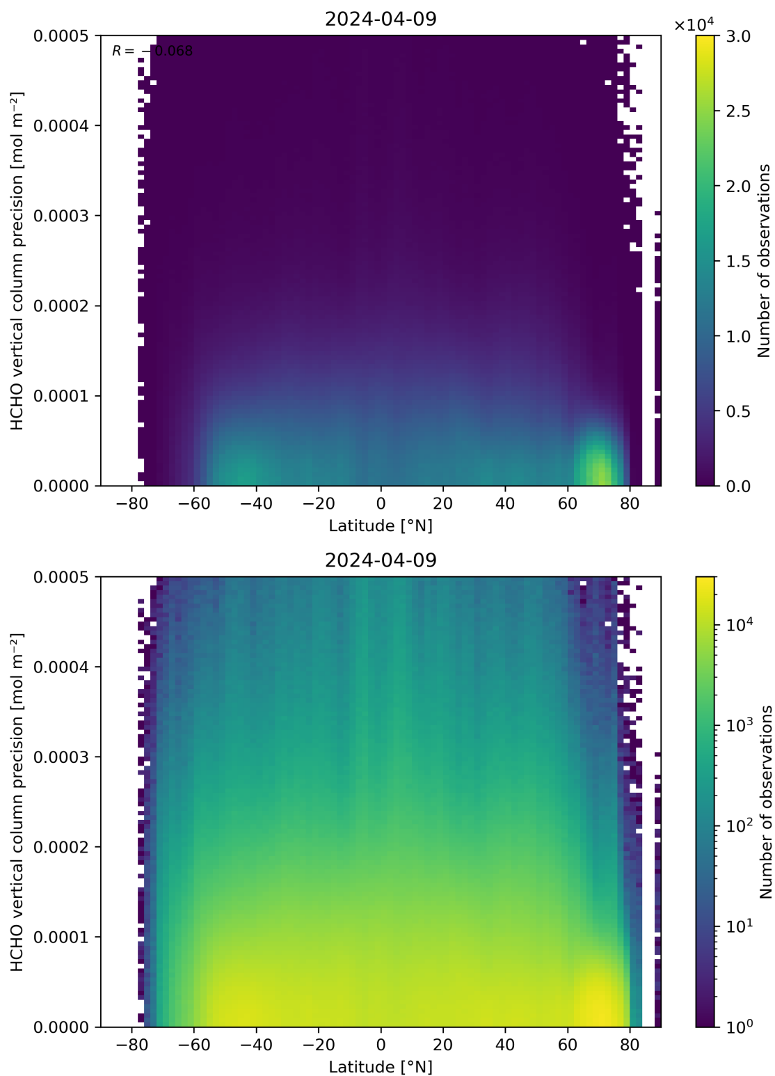
Figure 165: Scatter density plot of “Latitude” against “HCHO vertical column precision” for 2024-04-08 to 2024-04-10.
