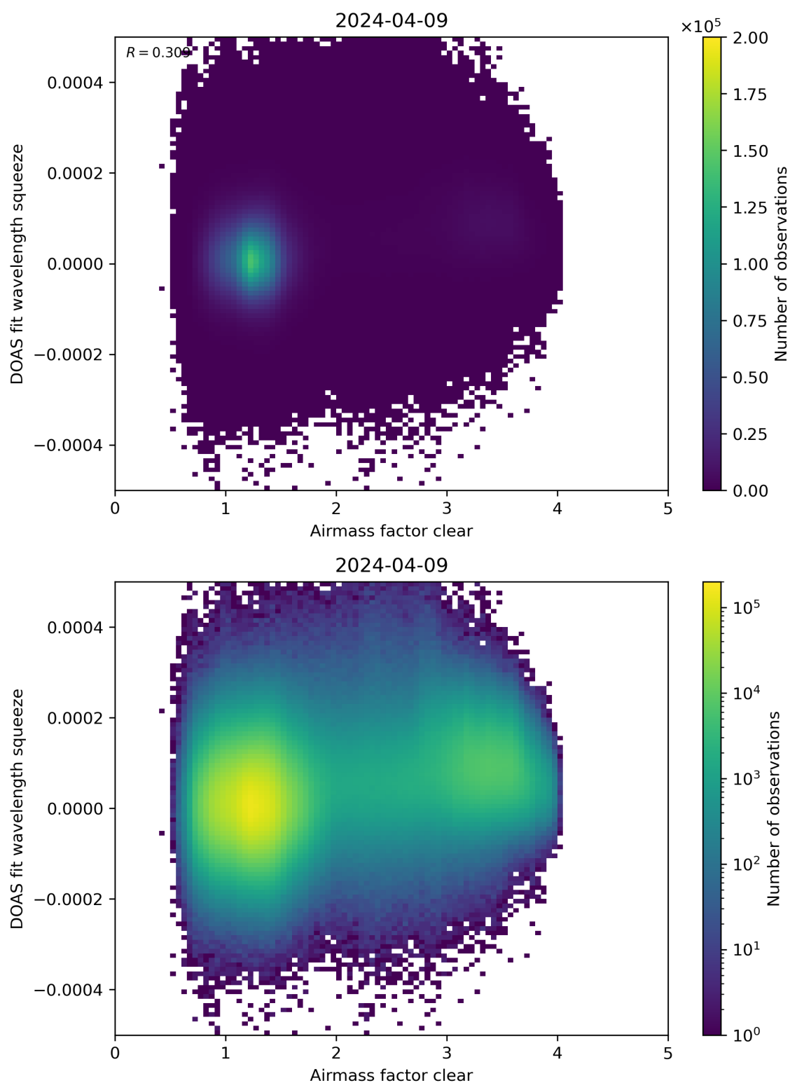
Figure 73: Scatter density plot of “Airmass factor clear” against “DOAS fit wavelength squeeze” for 2024-04-08 to 2024-04-10.
