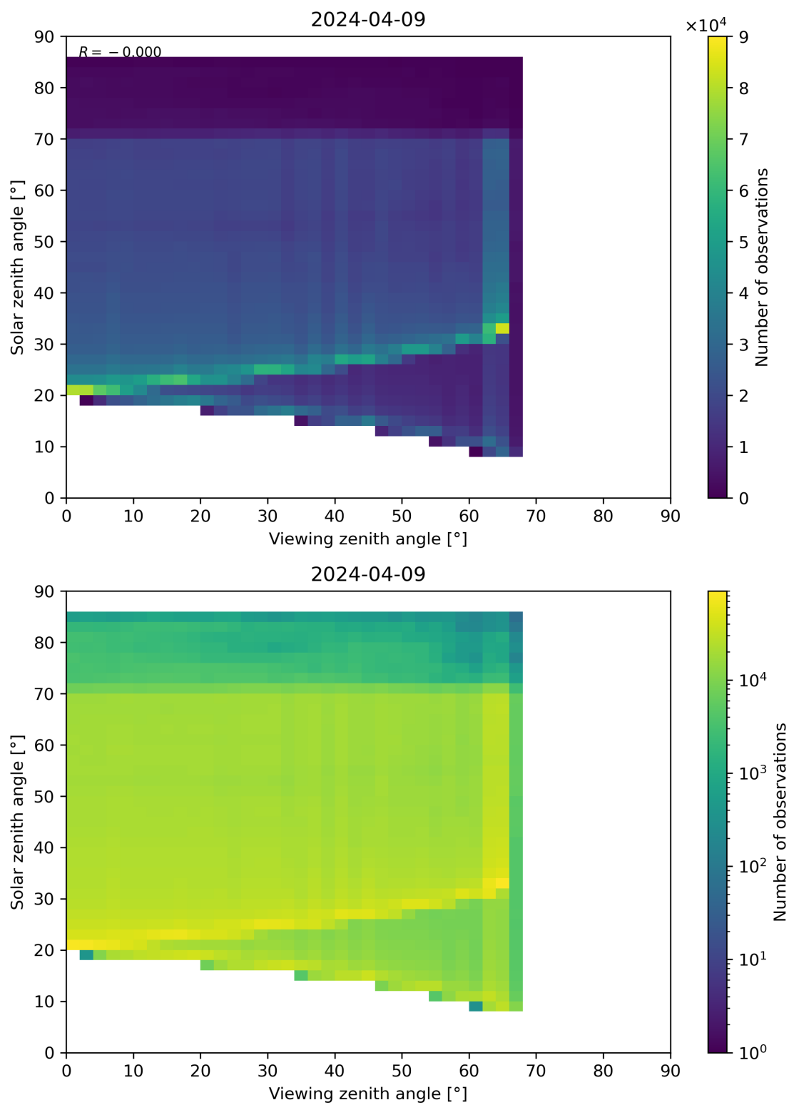
Figure 197: Scatter density plot of “Viewing zenith angle” against “Solar zenith angle” for 2024-04-08 to 2024-04-10.
