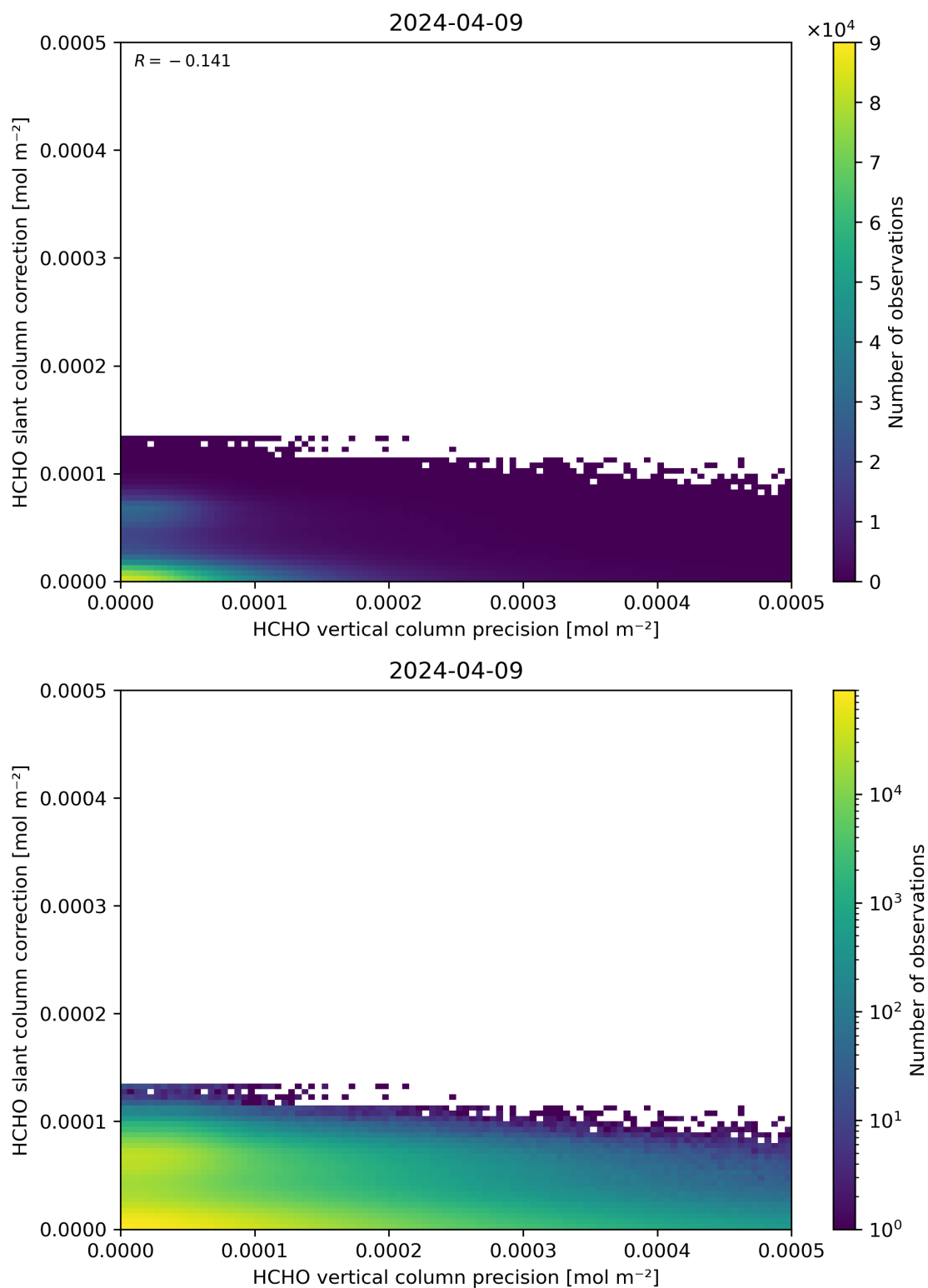
Figure 141: Scatter density plot of “HCHO vertical column precision” against “HCHO slant column correction” for 2024-04-08 to 2024-04-10.
