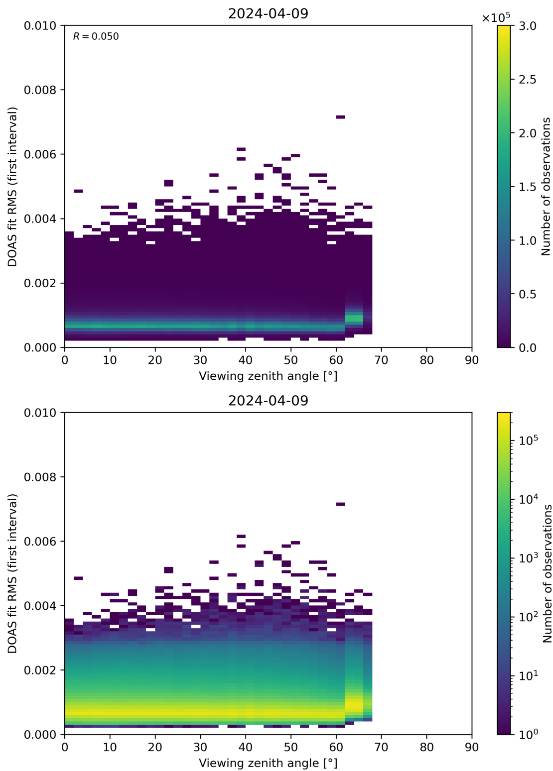
Figure 182: Scatter density plot of “Viewing zenith angle” against “DOAS fit RMS (first interval)” for 2024-04-08 to 2024-04-10.
