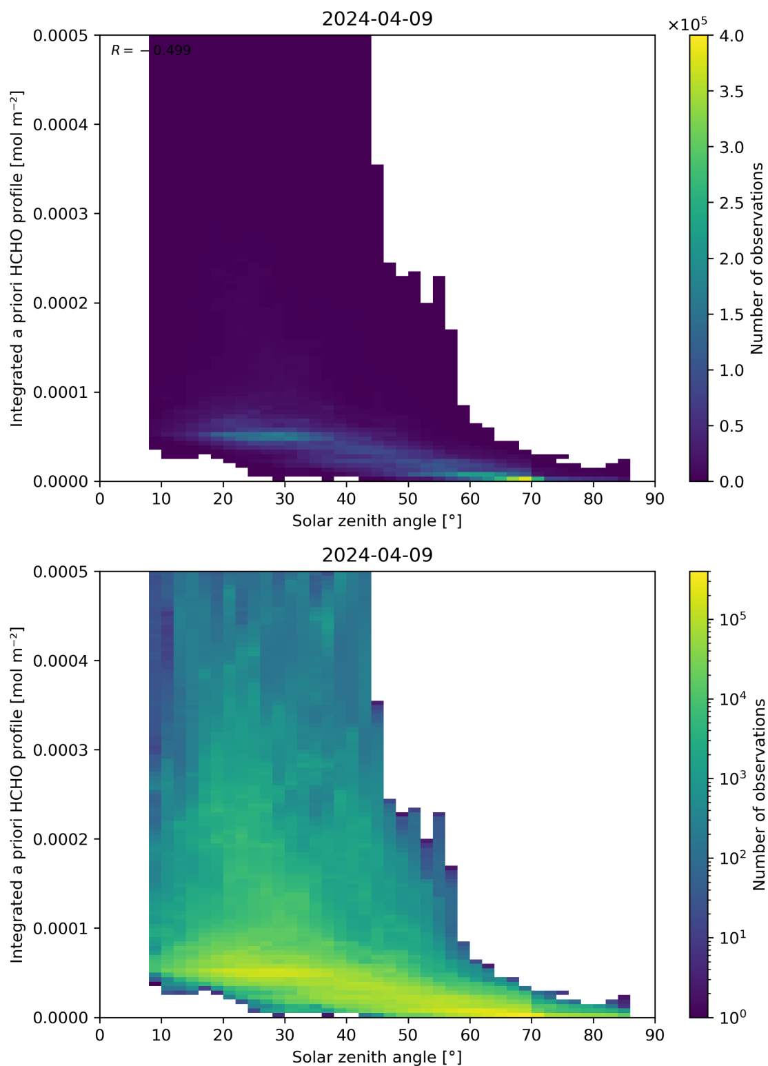
Figure 180: Scatter density plot of “Solar zenith angle” against “Integrated a priori HCHO profile” for 2024-04-08 to 2024-04-10.
