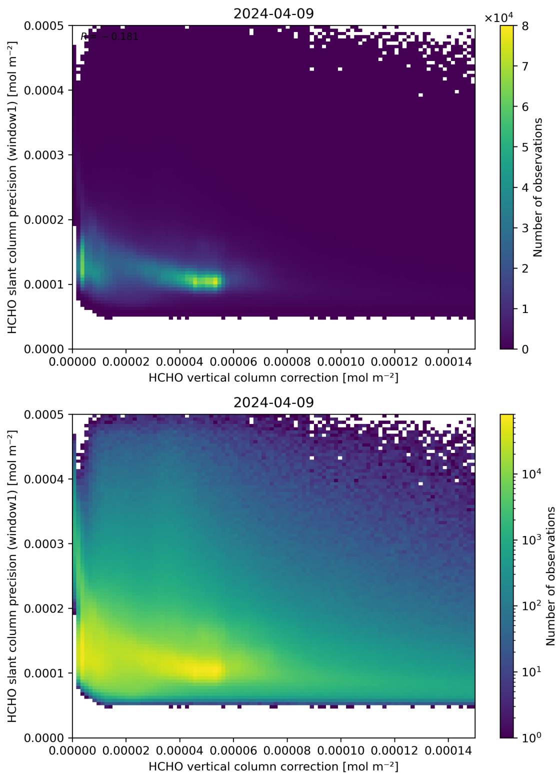
Figure 119: Scatter density plot of “HCHO vertical column correction” against “HCHO slant column precision (window1)” for 2024-04-08 to 2024-04-10.
