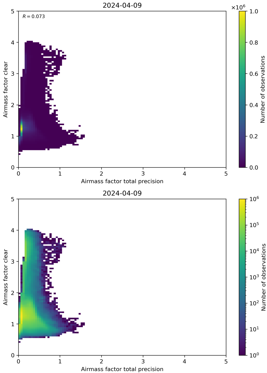
Figure 108: Scatter density plot of “Airmass factor total precision” against “Airmass factor clear” for 2024-04-08 to 2024-04-10.
