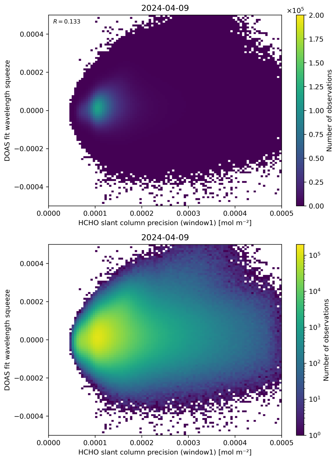
Figure 90: Scatter density plot of “HCHO slant column precision (window1)” against “DOAS fit wavelength squeeze” for 2024-04-08 to 2024-04-10.
