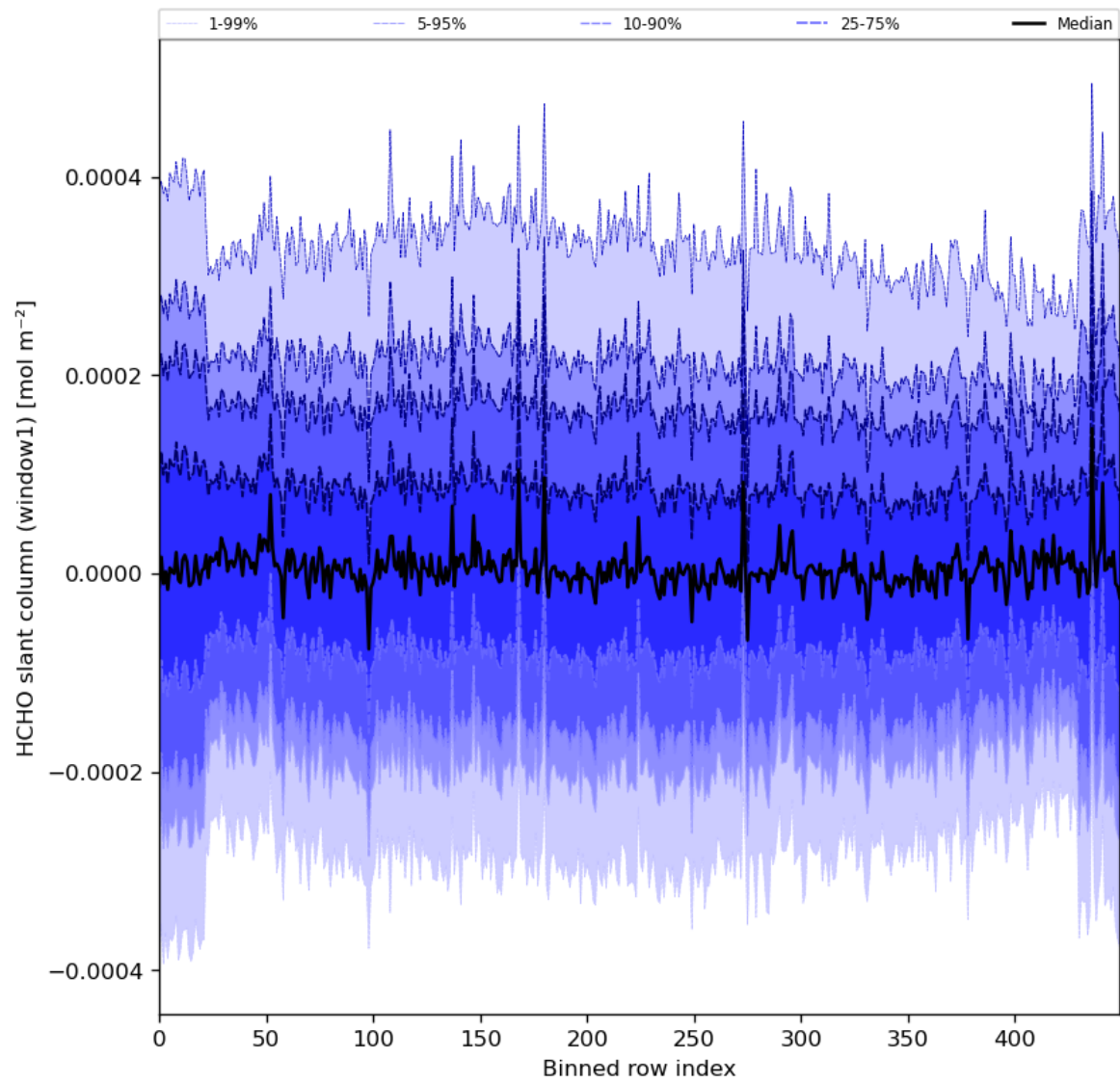
Figure 52: Along track statistics of “HCHO slant column (window1)” for 2024-04-08 to 2024-04-10
