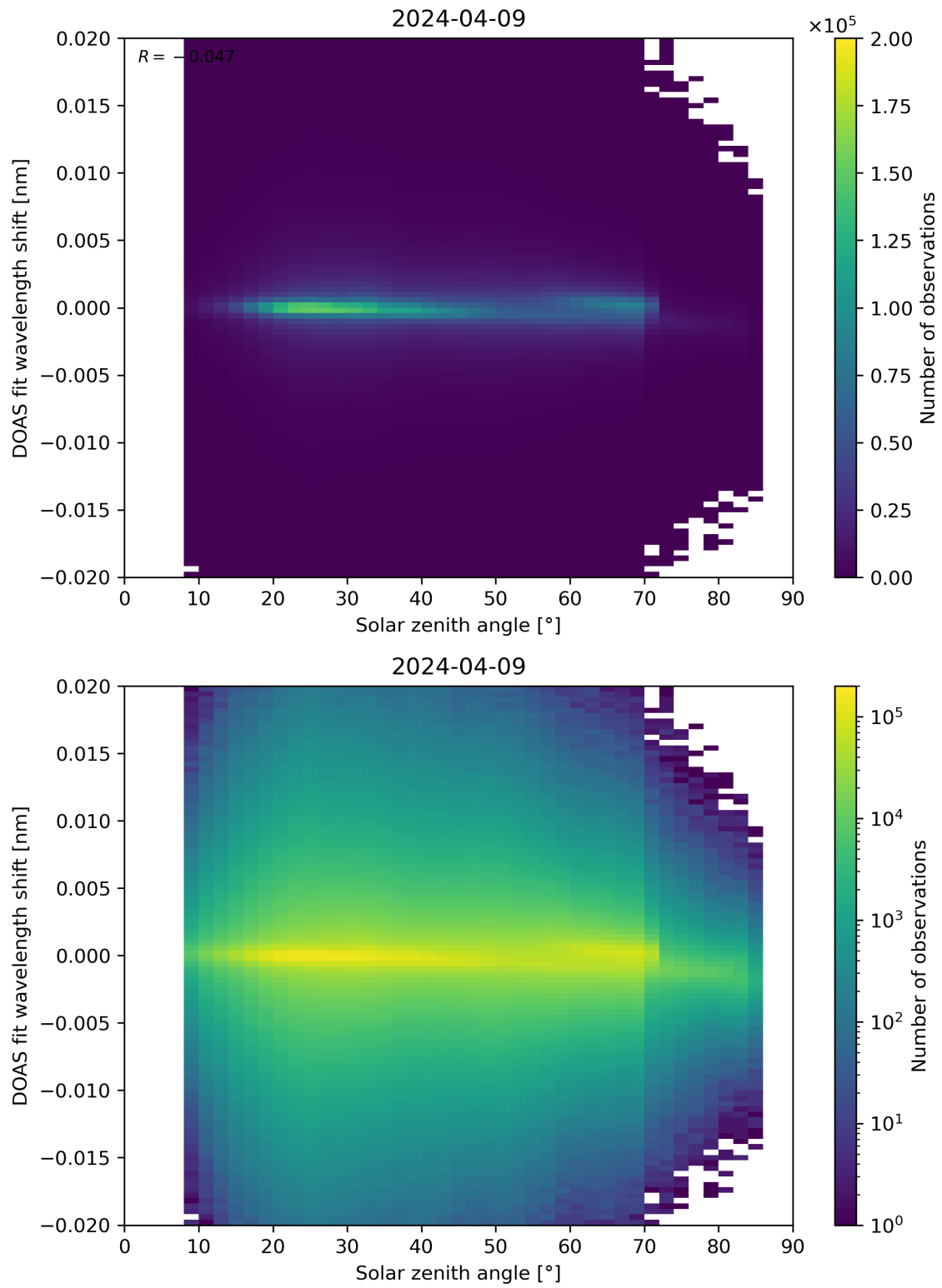
Figure 168: Scatter density plot of “Solar zenith angle” against “DOAS fit wavelength shift” for 2024-04-08 to 2024-04-10.
