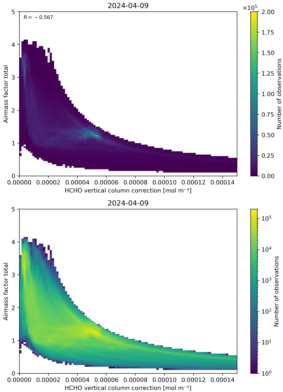
Figure 120: Scatter density plot of “HCHO vertical column correction” against “Airmass factor total” for 2024-04-08 to 2024-04-10.
