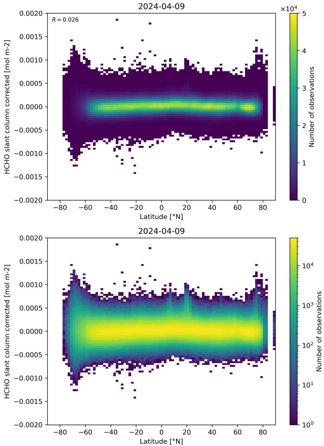
Figure 157: Scatter density plot of “Latitude” against “HCHO slant column corrected” for 2024-04-08 to 2024-04-10.
