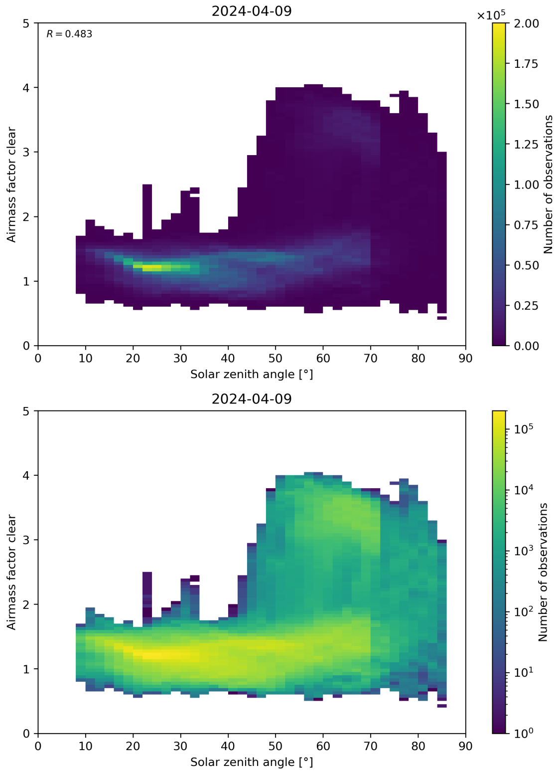
Figure 170: Scatter density plot of “Solar zenith angle” against “Airmass factor clear” for 2024-04-08 to 2024-04-10.
