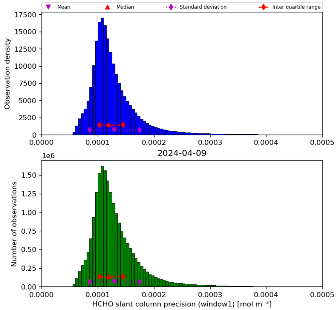
Figure 39: Histogram of “HCHO slant column precision (window1)” for 2024-04-08 to 2024-04-10
