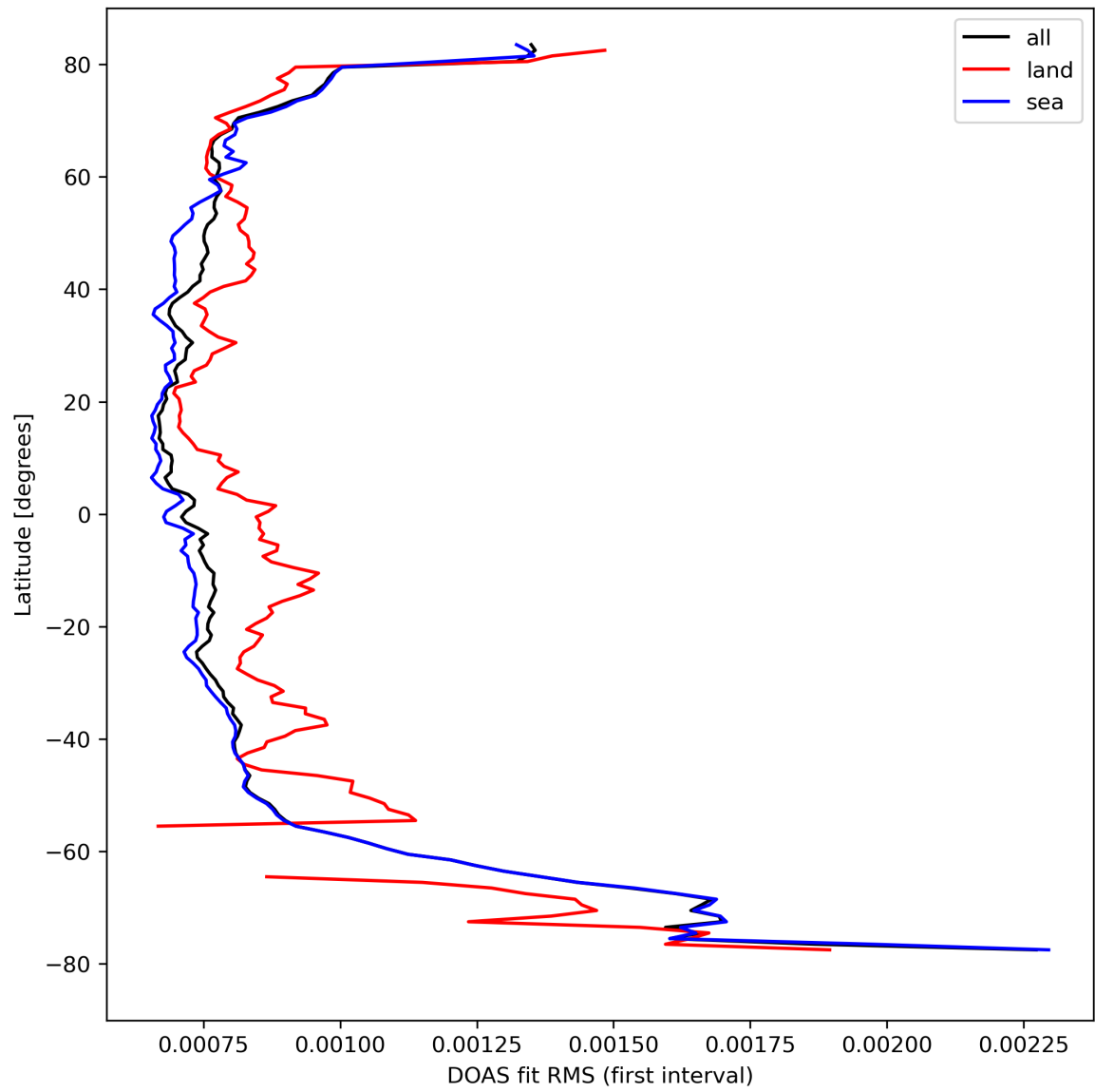
Figure 32: Zonal average of “DOAS fit RMS (first interval)” for 2024-04-08 to 2024-04-10.
