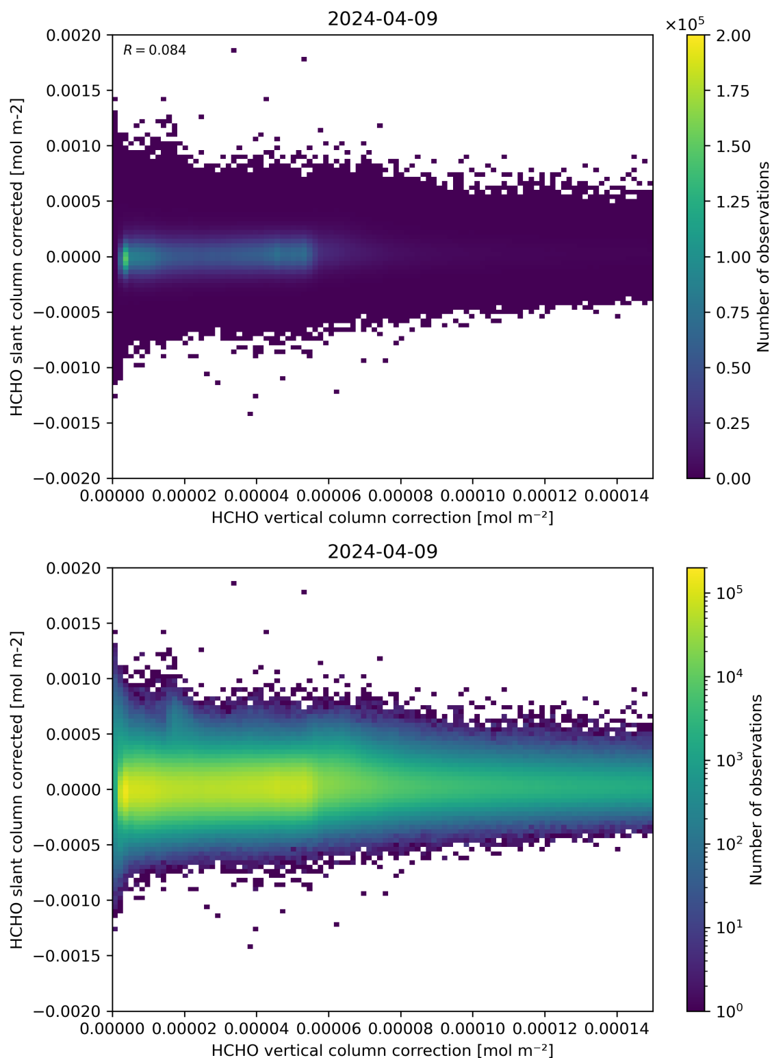
Figure 116: Scatter density plot of “HCHO vertical column correction” against “HCHO slant column corrected” for 2024-04-08 to 2024-04-10.
