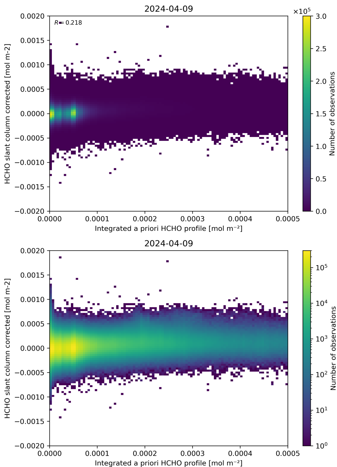
Figure 151: Scatter density plot of “Integrated a priori HCHO profile” against “HCHO slant column corrected” for 2024-04-08 to 2024-04-10.
