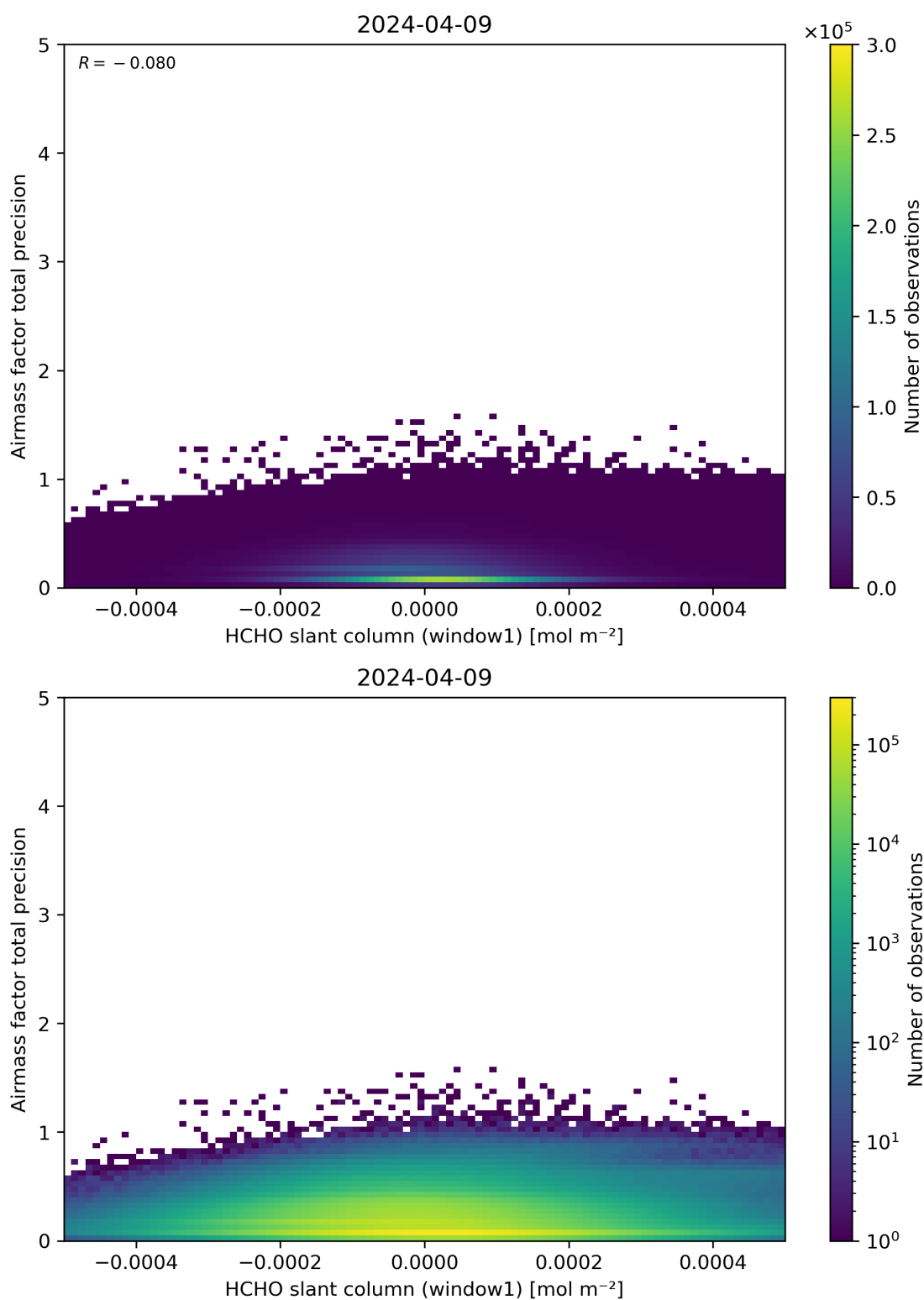
Figure 86: Scatter density plot of “HCHO slant column (window1)” against “Airmass factor total precision” for 2024-04-08 to 2024-04-10.
