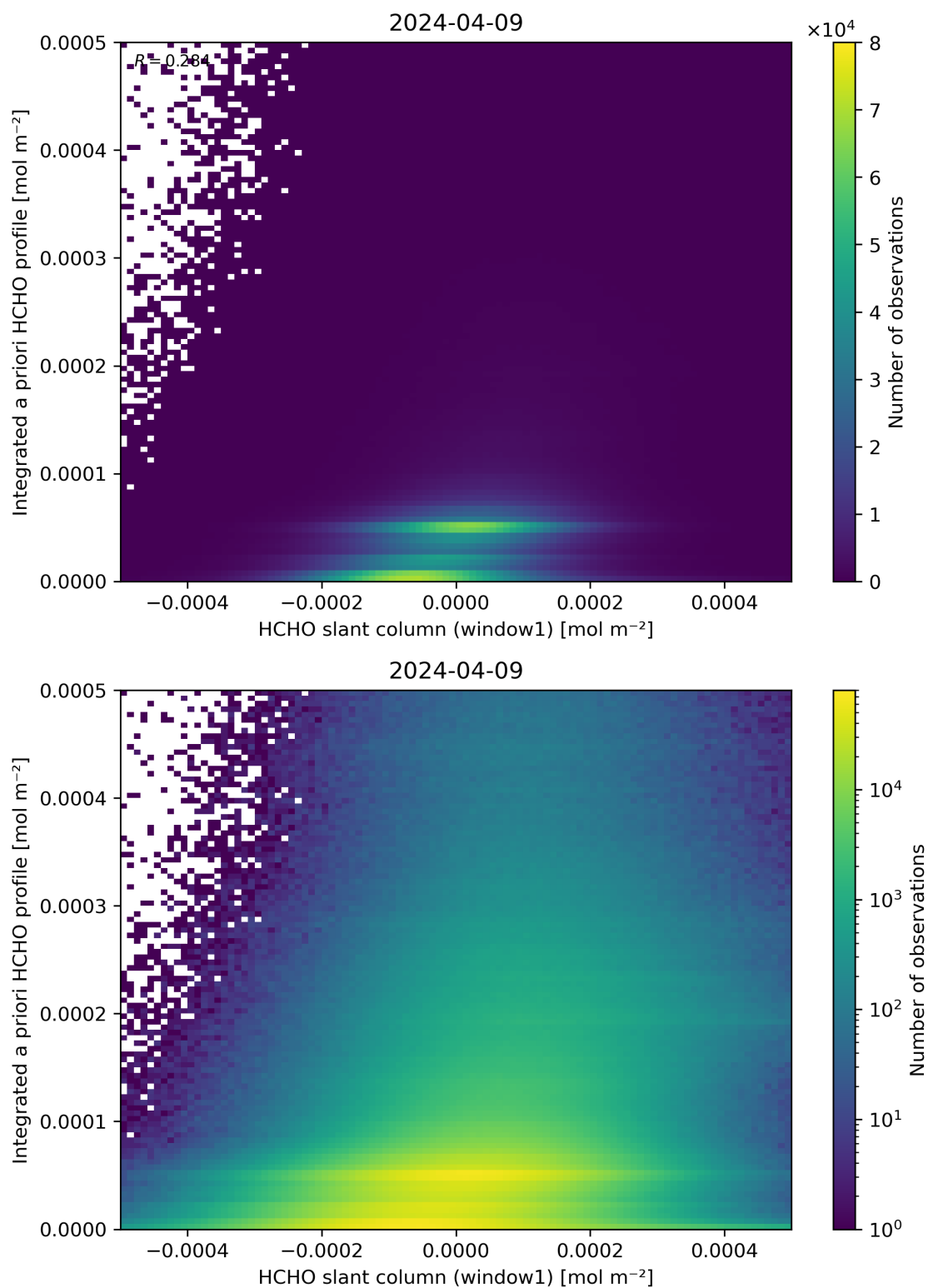
Figure 87: Scatter density plot of “HCHO slant column (window1)” against “Integrated a priori HCHO profile” for 2024-04-08 to 2024-04-10.
