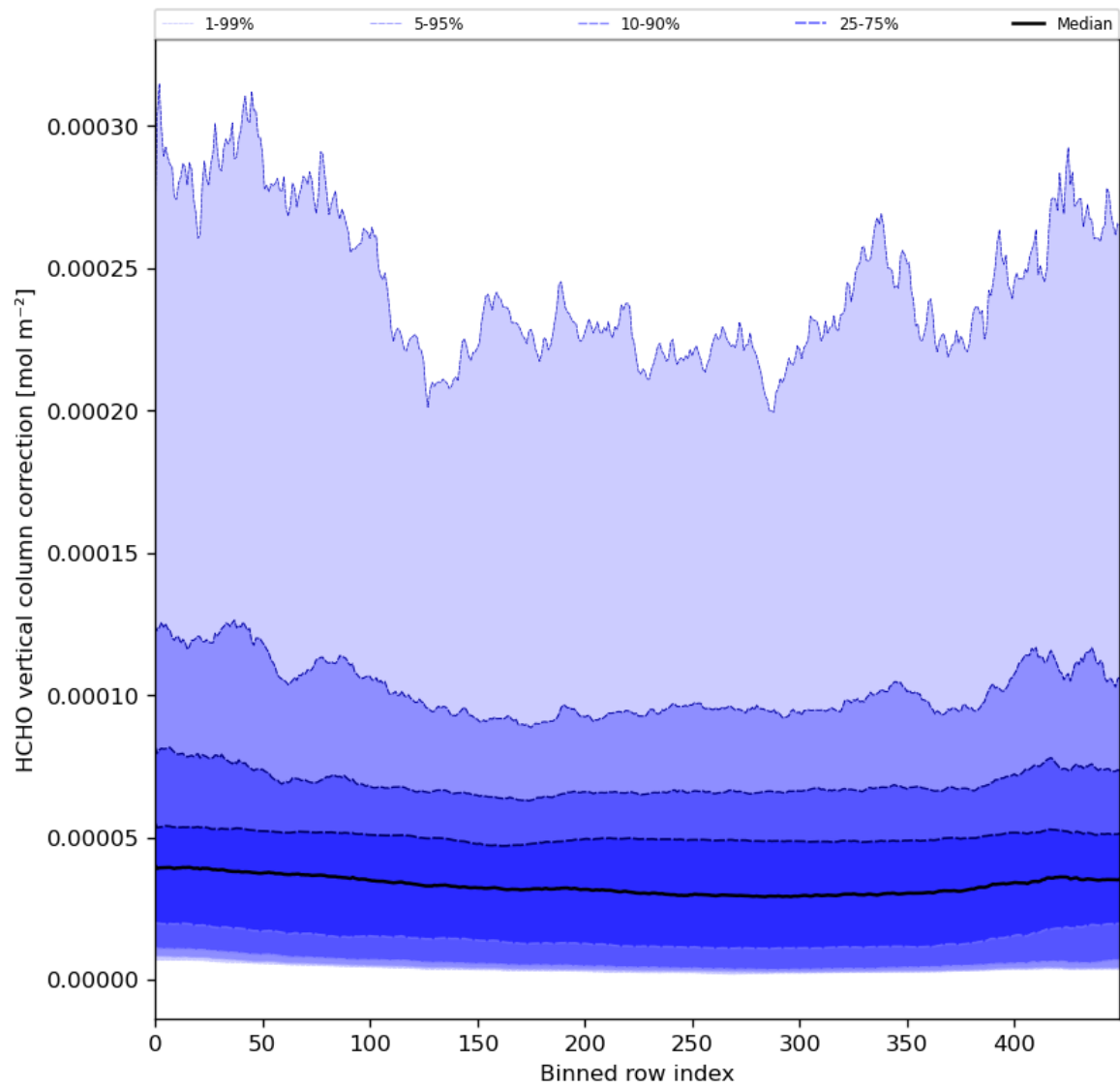
Figure 51: Along track statistics of “HCHO vertical column correction” for 2024-04-08 to 2024-04-10
