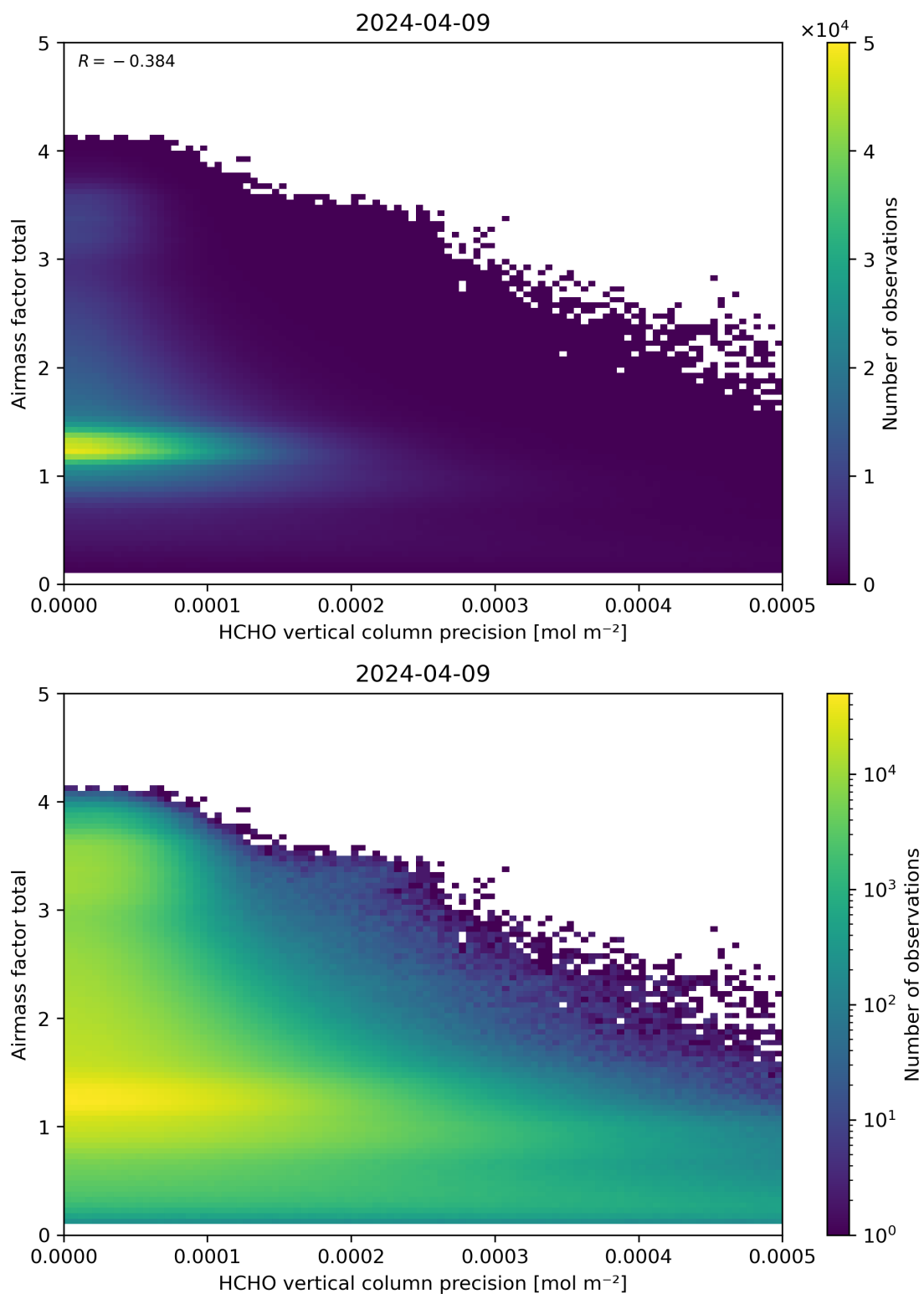
Figure 144: Scatter density plot of “HCHO vertical column precision” against “Airmass factor total” for 2024-04-08 to 2024-04-10.
