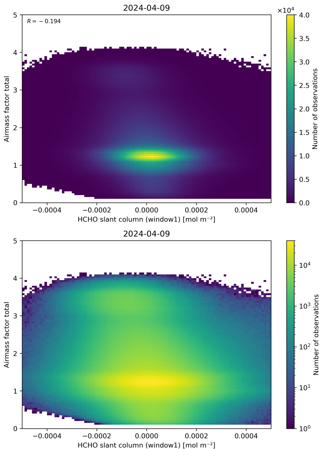
Figure 85: Scatter density plot of “HCHO slant column (window1)” against “Airmass factor total” for 2024-04-08 to 2024-04-10.
