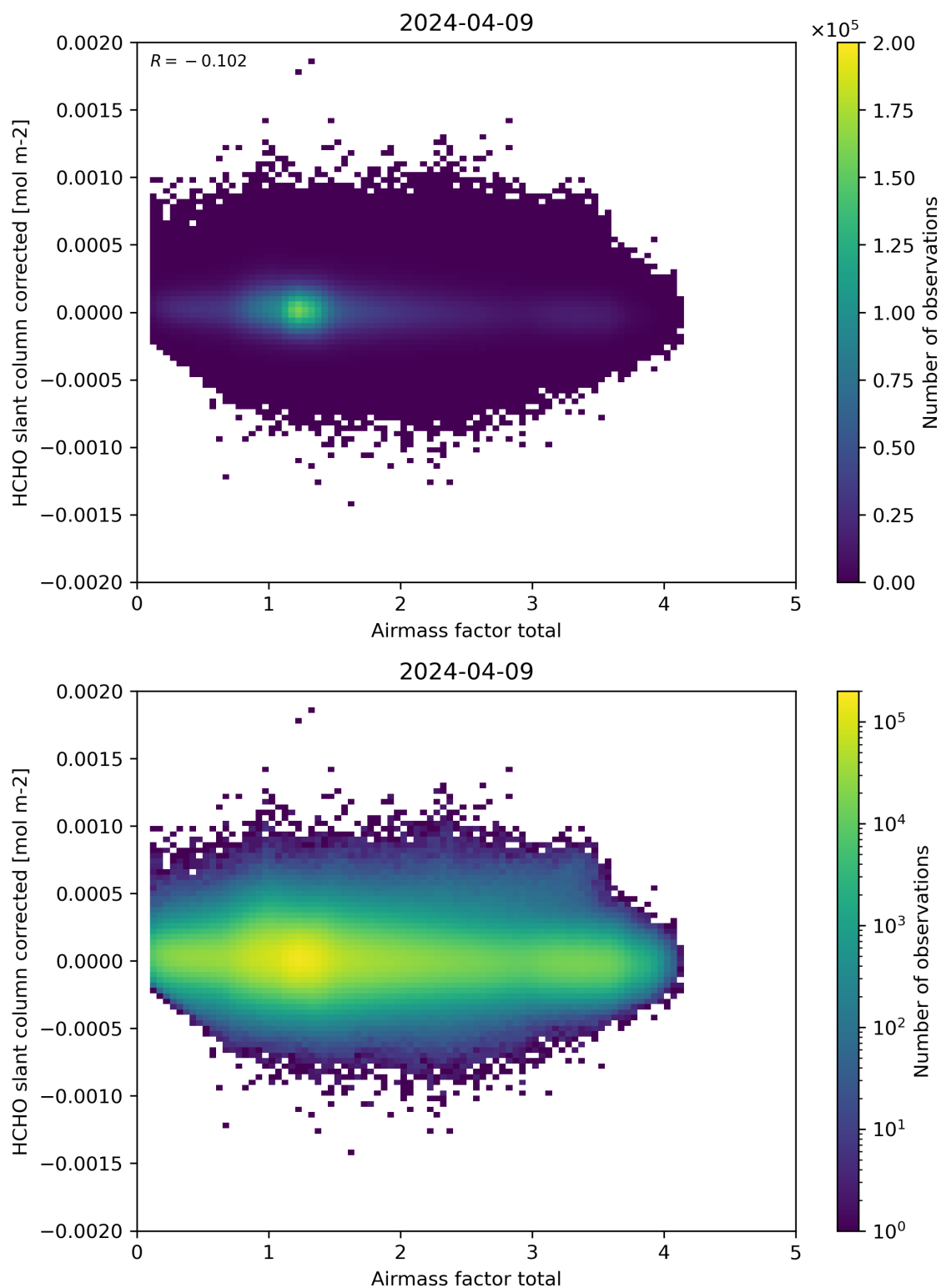
Figure 101: Scatter density plot of “Airmass factor total” against “HCHO slant column corrected” for 2024-04-08 to 2024-04-10.
