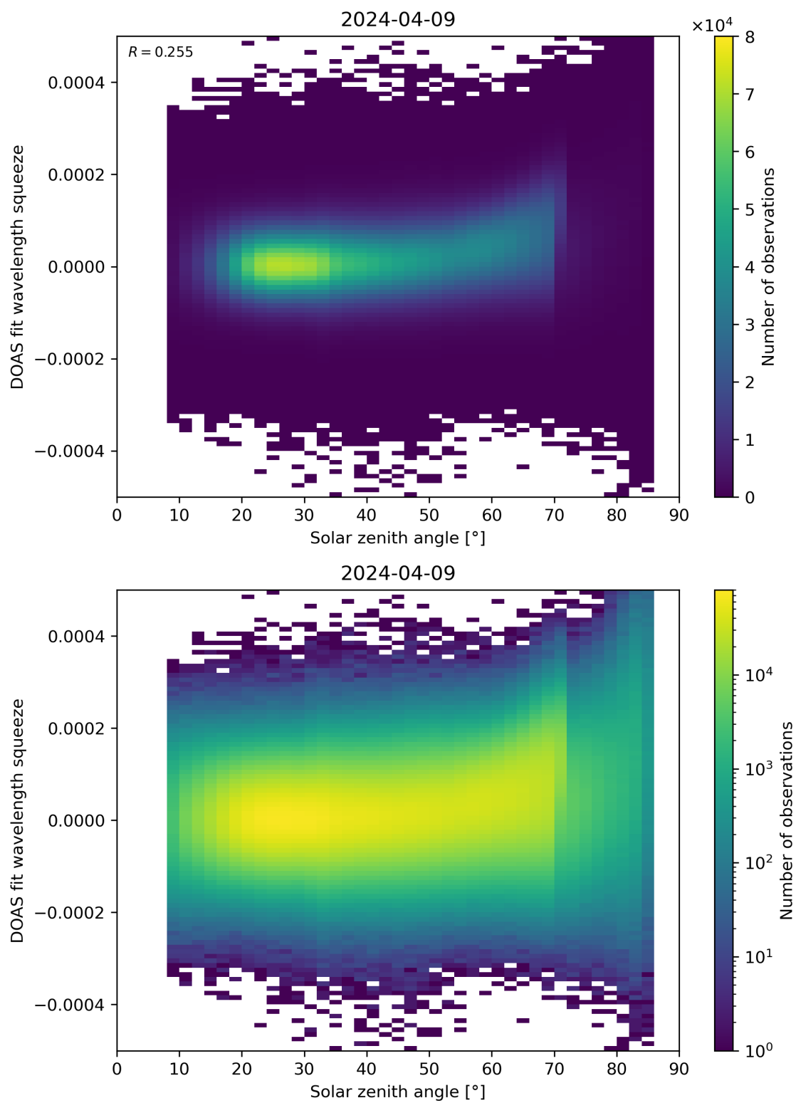
Figure 169: Scatter density plot of “Solar zenith angle” against “DOAS fit wavelength squeeze” for 2024-04-08 to 2024-04-10.
