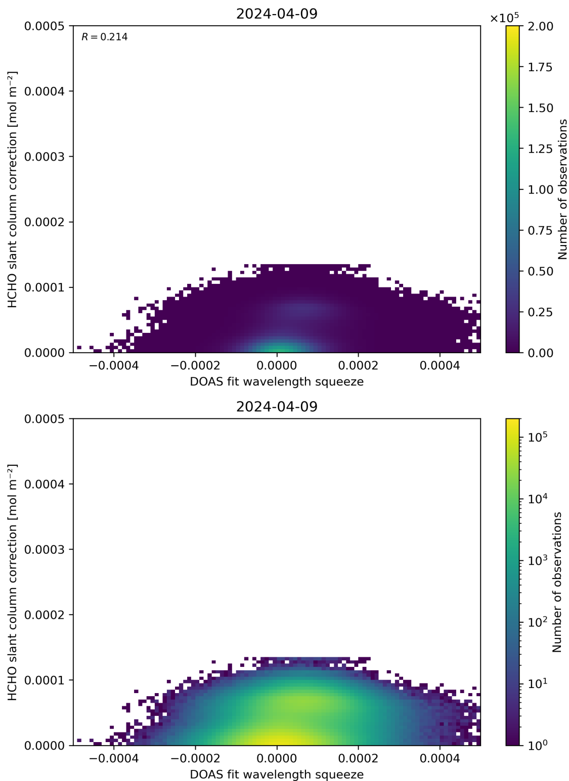
Figure 70: Scatter density plot of “DOAS fit wavelength squeeze” against “HCHO slant column correction” for 2024-04-08 to 2024-04-10.
