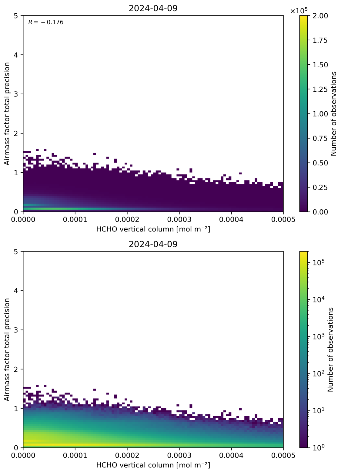
Figure 132: Scatter density plot of “HCHO vertical column” against “Airmass factor total precision” for 2024-04-08 to 2024-04-10.
