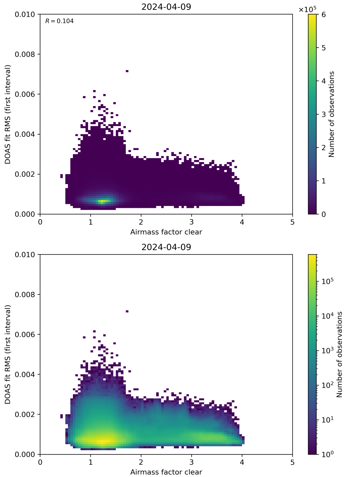
Figure 71: Scatter density plot of “Airmass factor clear” against “DOAS fit RMS (first interval)” for 2024-04-08 to 2024-04-10.
