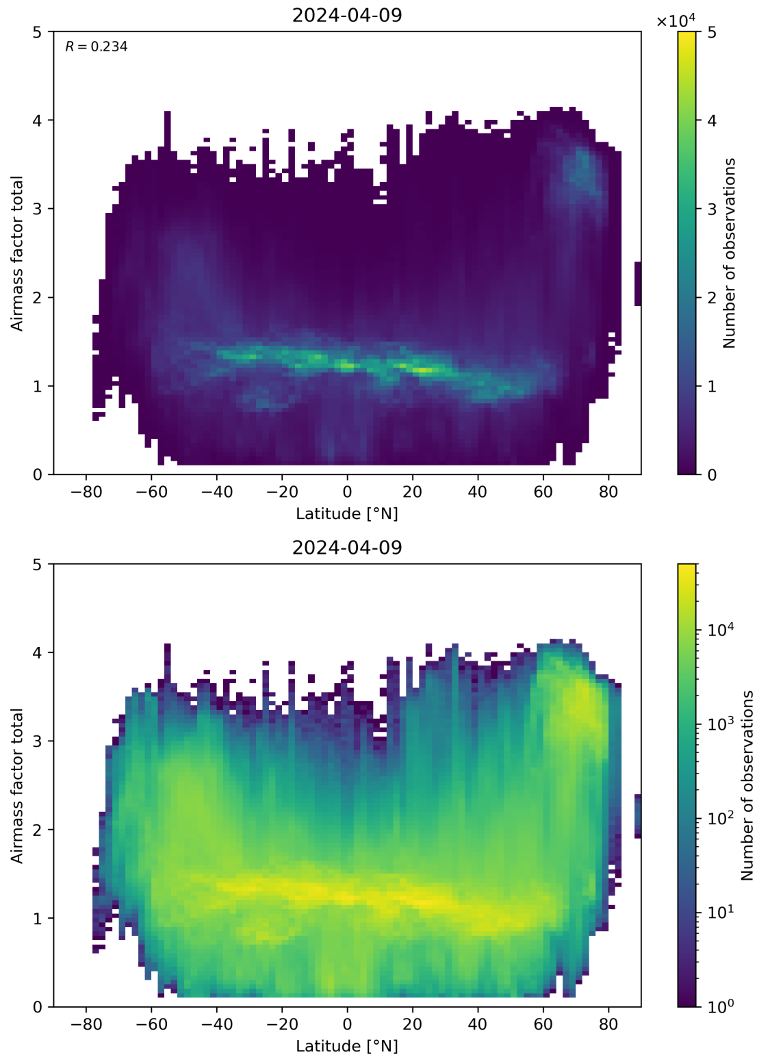
Figure 161: Scatter density plot of “Latitude” against “Airmass factor total” for 2024-04-08 to 2024-04-10.
