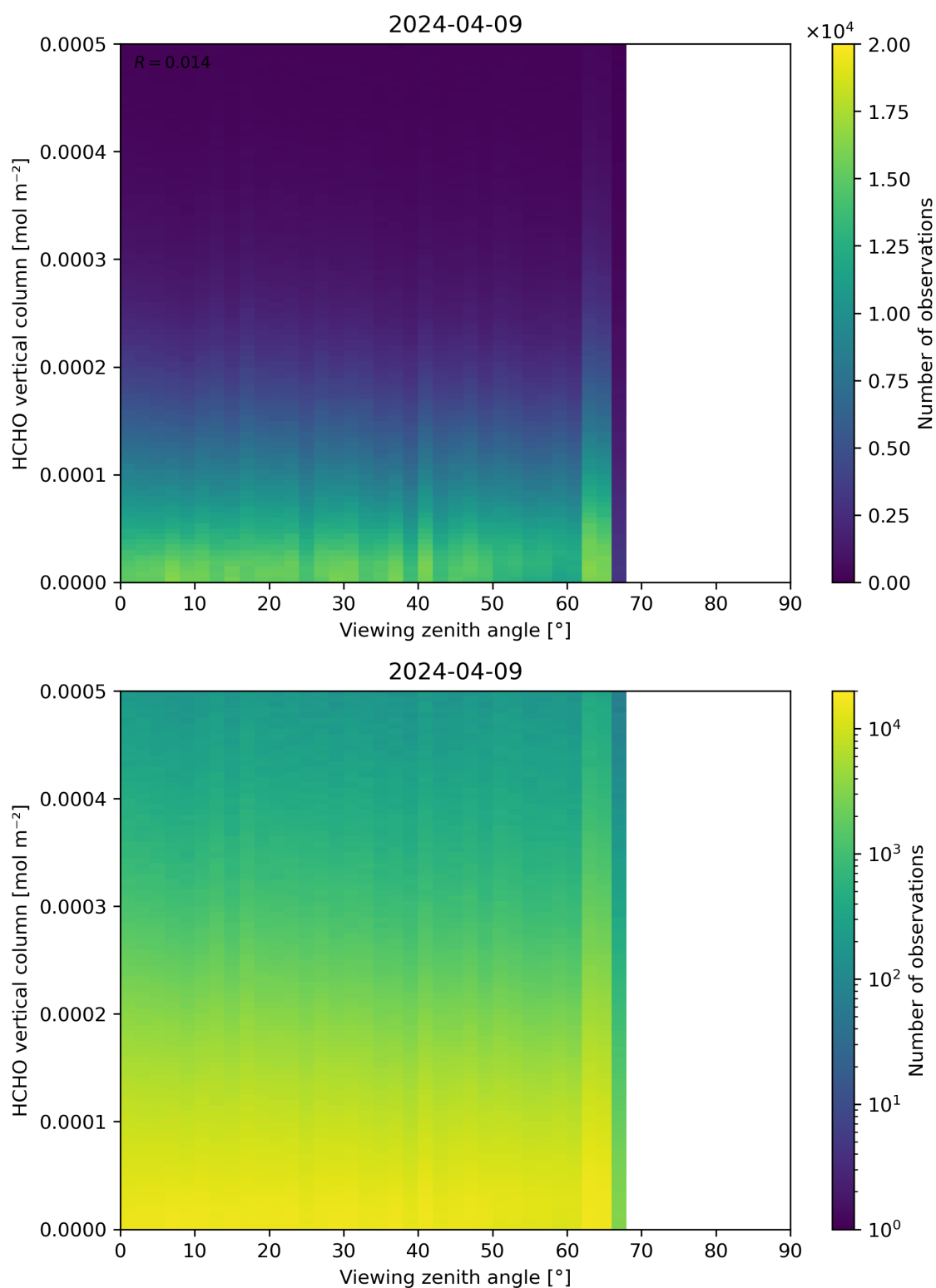
Figure 192: Scatter density plot of “Viewing zenith angle” against “HCHO vertical column” for 2024-04-08 to 2024-04-10.
