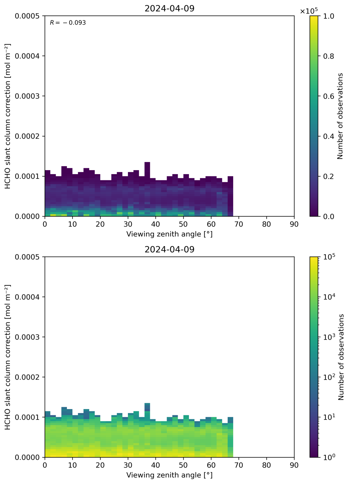
Figure 187: Scatter density plot of “Viewing zenith angle” against “HCHO slant column correction” for 2024-04-08 to 2024-04-10.
