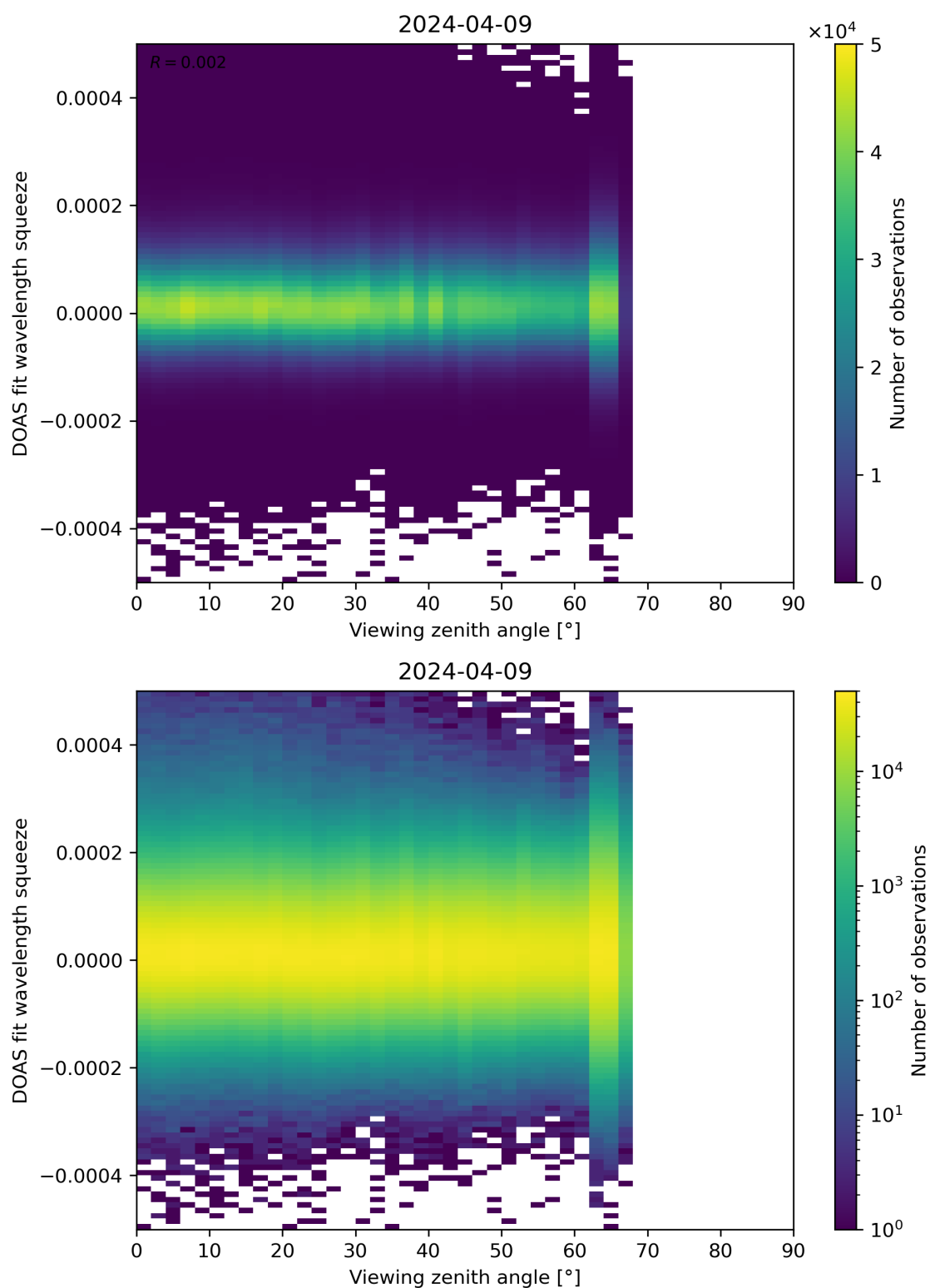
Figure 184: Scatter density plot of “Viewing zenith angle” against “DOAS fit wavelength squeeze” for 2024-04-08 to 2024-04-10.
