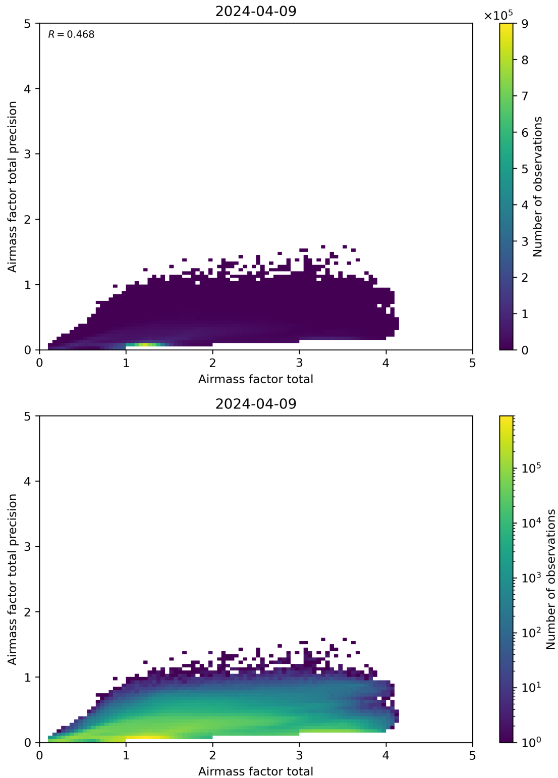
Figure 103: Scatter density plot of “Airmass factor total” against “Airmass factor total precision” for 2024-04-08 to 2024-04-10.
