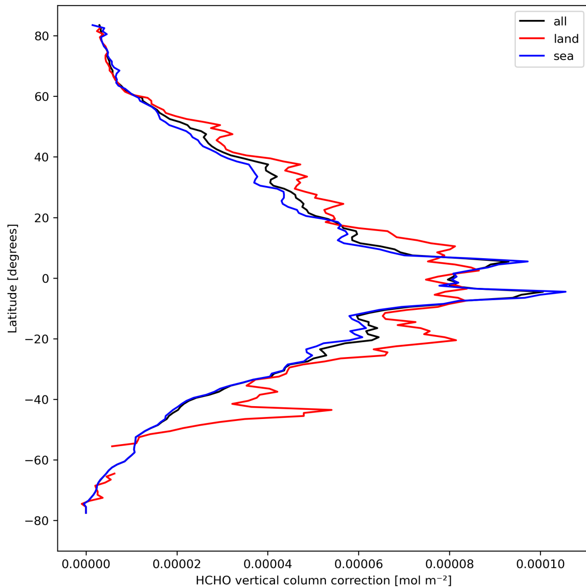
Figure 23: Zonal average of “HCHO vertical column correction” for 2024-04-08 to 2024-04-10.
