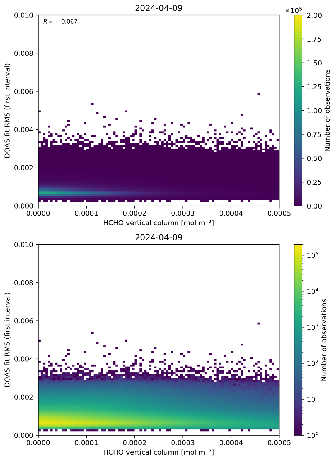
Figure 123: Scatter density plot of “HCHO vertical column” against “DOAS fit RMS (first interval)” for 2024-04-08 to 2024-04-10.
