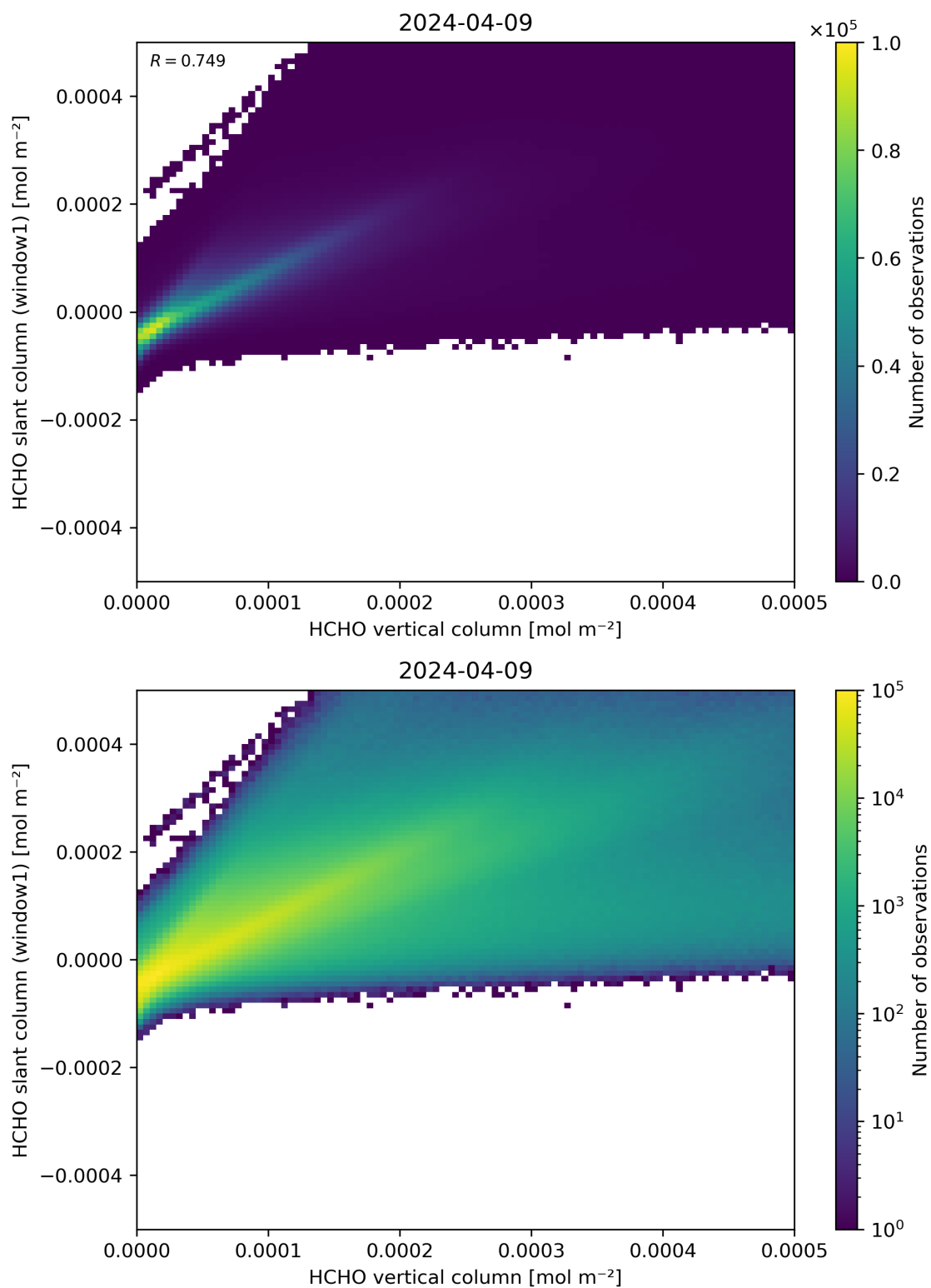
Figure 129: Scatter density plot of “HCHO vertical column” against “HCHO slant column (window1)” for 2024-04-08 to 2024-04-10.
