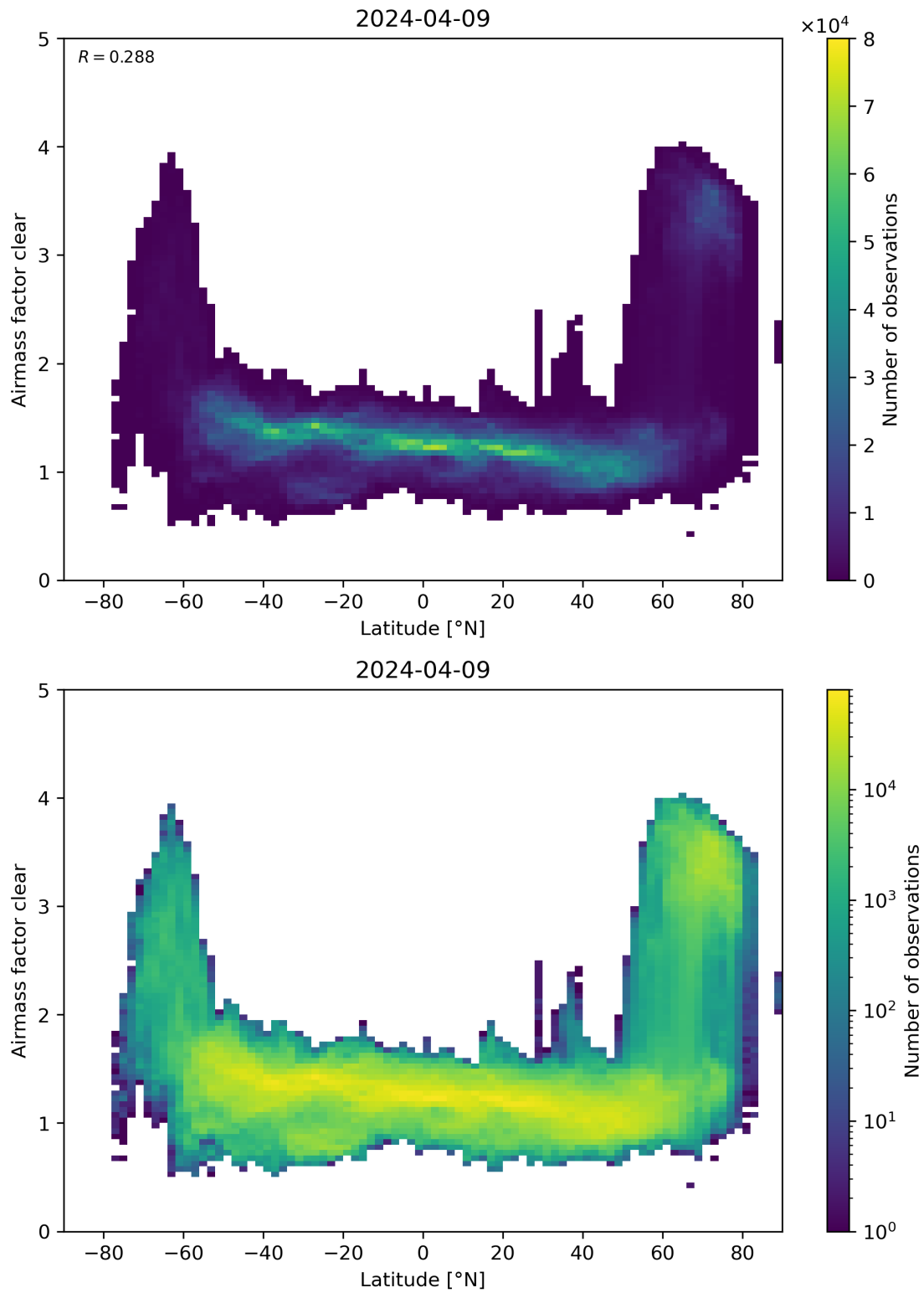
Figure 156: Scatter density plot of “Latitude” against “Airmass factor clear” for 2024-04-08 to 2024-04-10.
