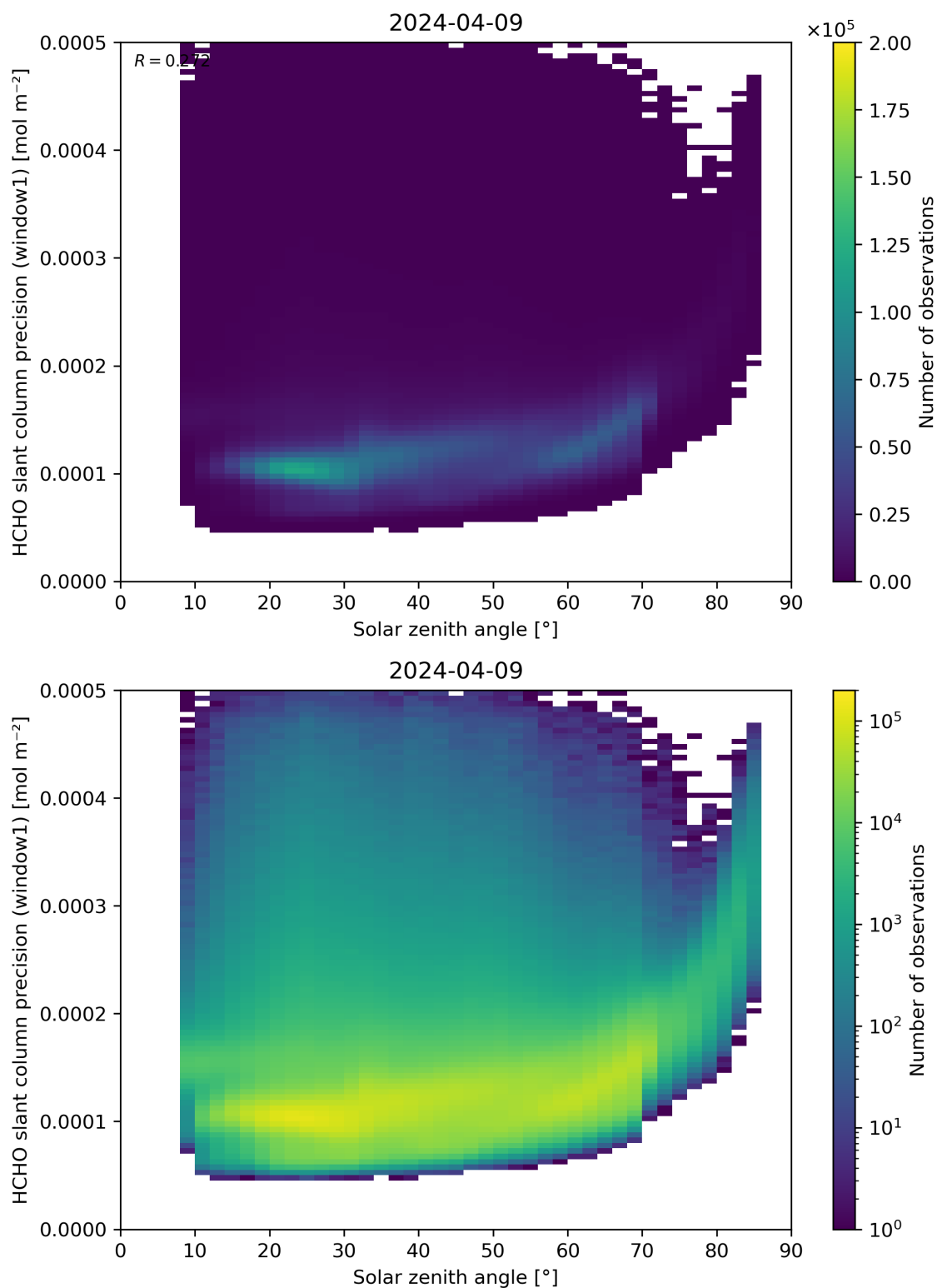
Figure 174: Scatter density plot of “Solar zenith angle” against “HCHO slant column precision (window1)” for 2024-04-08 to 2024-04-10.
