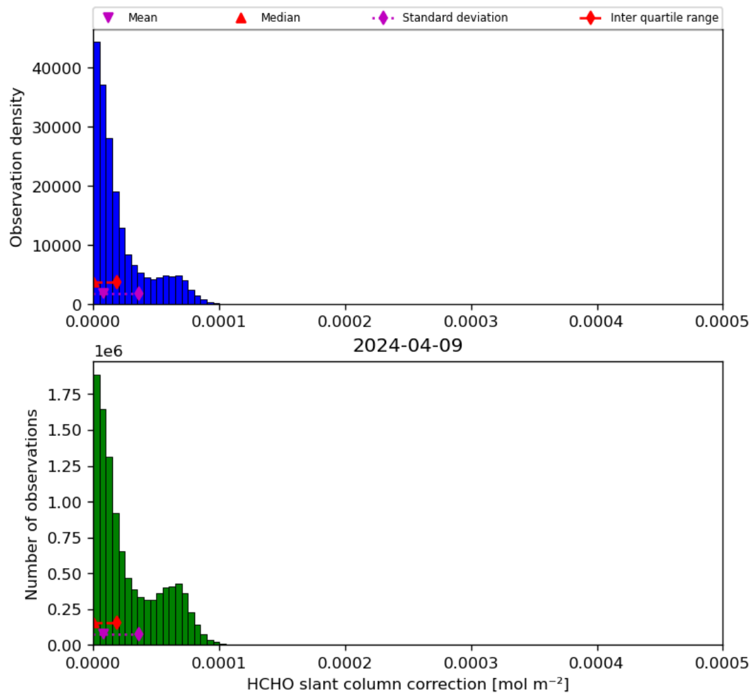
Figure 47: Histogram of “HCHO slant column correction” for 2024-04-08 to 2024-04-10
