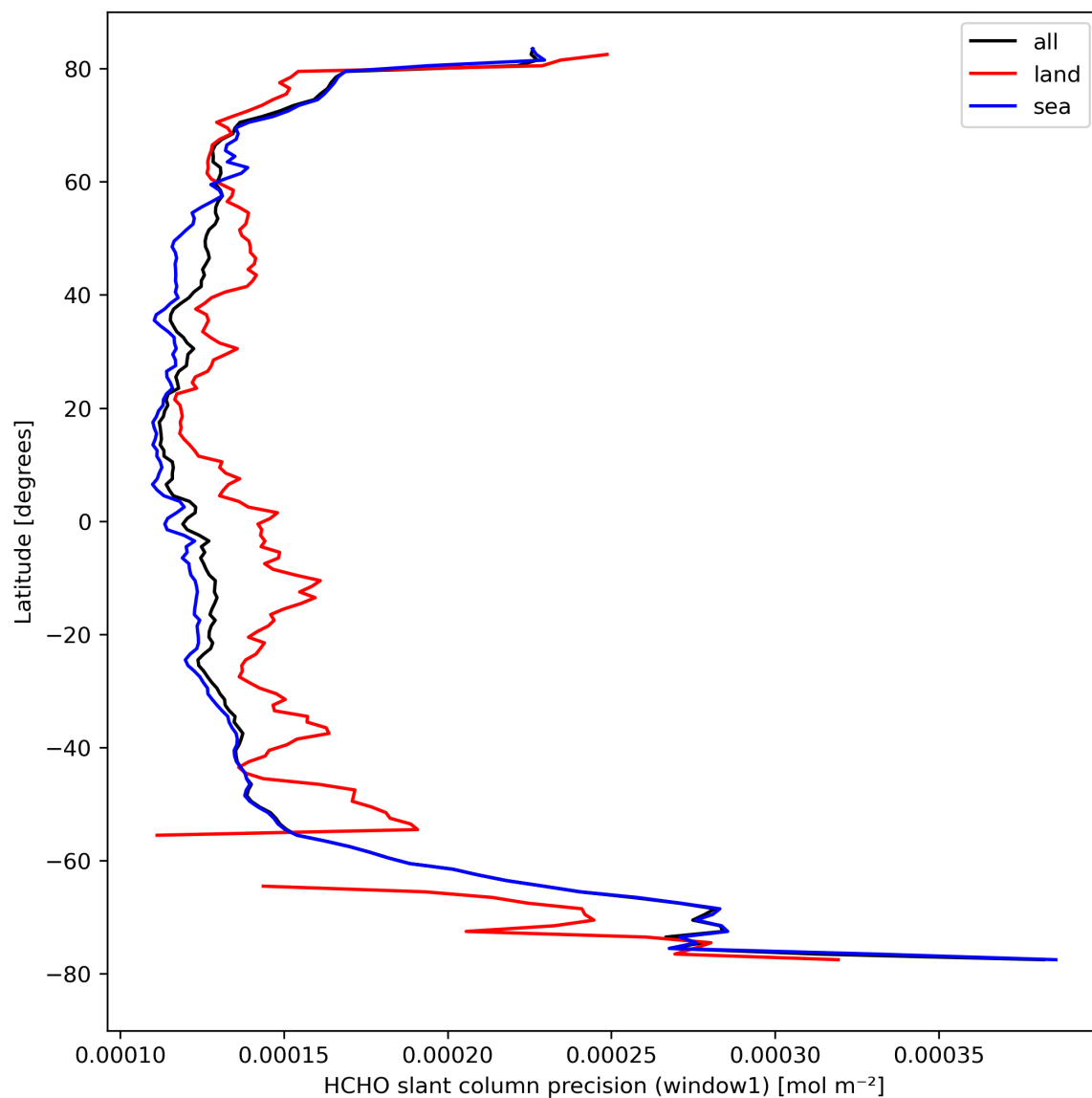
Figure 25: Zonal average of “HCHO slant column precision (window1)” for 2024-04-08 to 2024-04-10.
