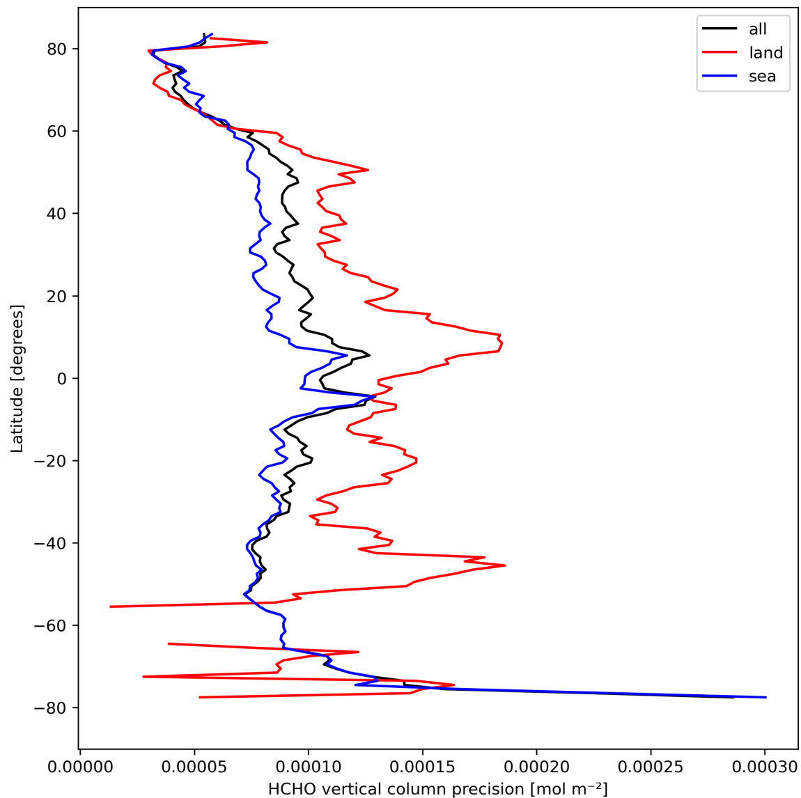
Figure 22: Zonal average of “HCHO vertical column precision” for 2024-04-08 to 2024-04-10.
