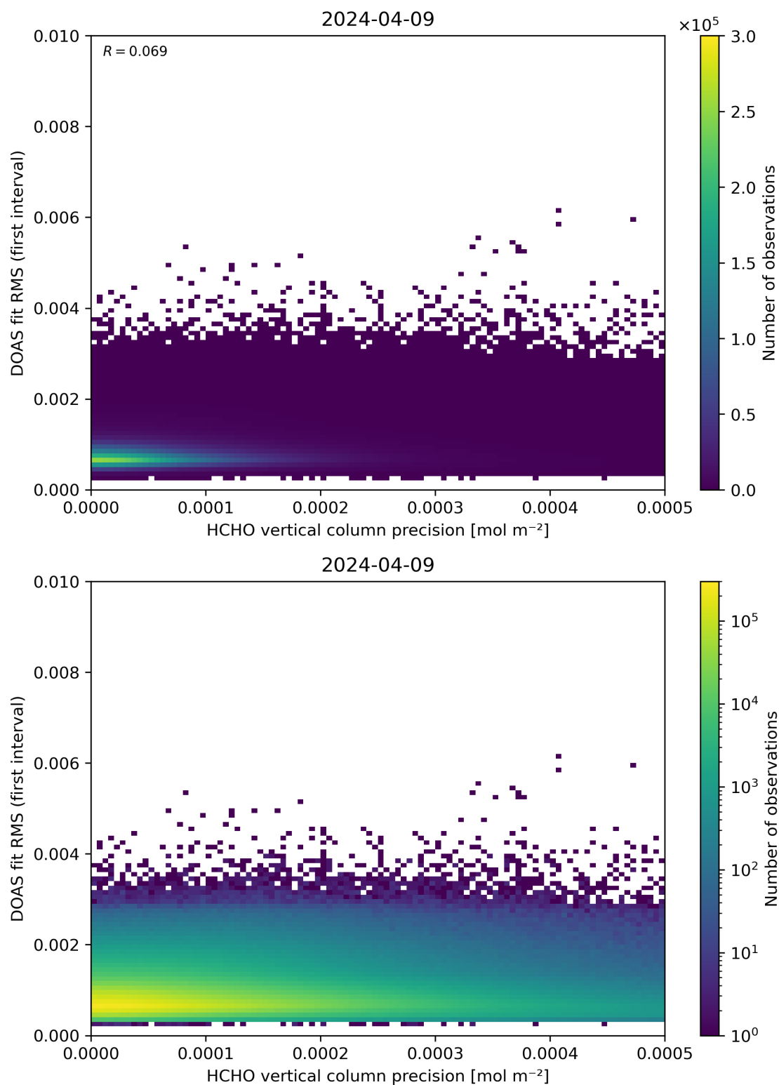
Figure 136: Scatter density plot of “HCHO vertical column precision” against “DOAS fit RMS (first interval)” for 2024-04-08 to 2024-04-10.
