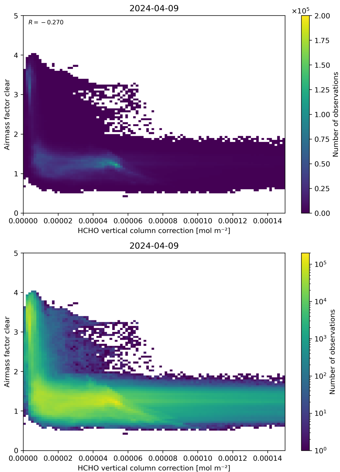
Figure 115: Scatter density plot of “HCHO vertical column correction” against “Airmass factor clear” for 2024-04-08 to 2024-04-10.
