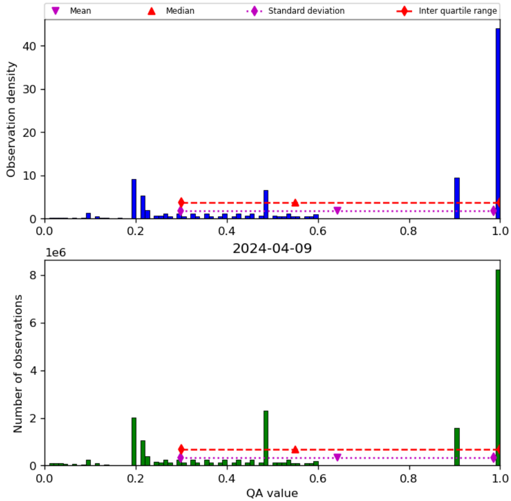
Figure 34: Histogram of “QA value” for 2024-04-08 to 2024-04-10
