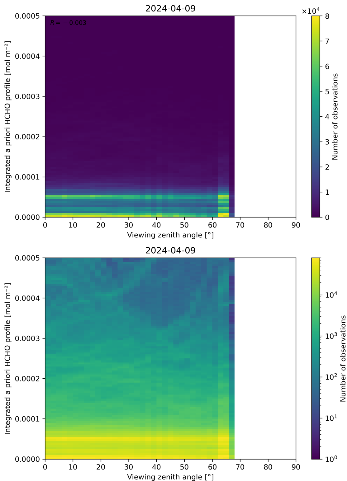
Figure 195: Scatter density plot of “Viewing zenith angle” against “Integrated a priori HCHO profile” for 2024-04-08 to 2024-04-10.
