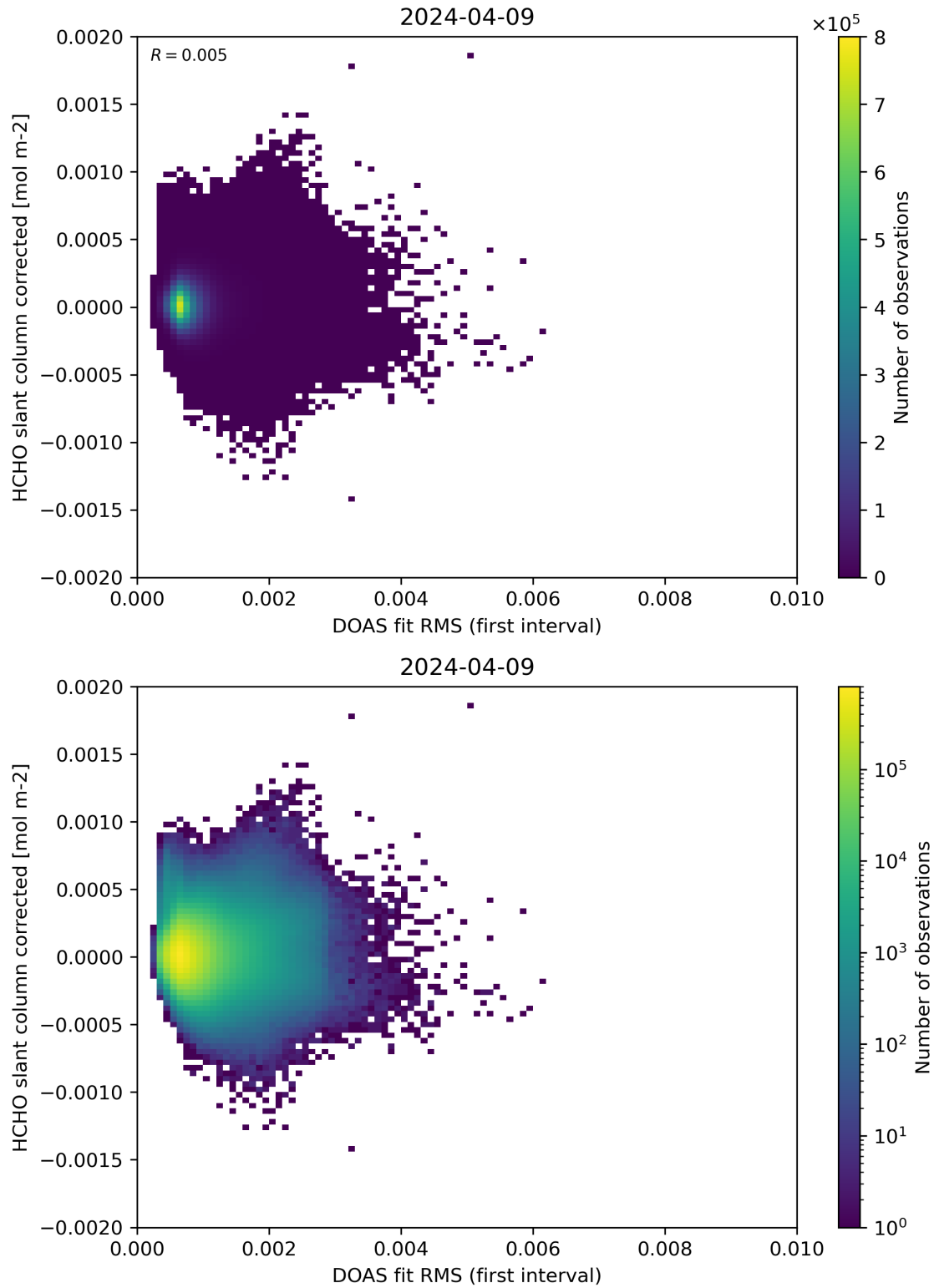
Figure 62: Scatter density plot of “DOAS fit RMS (first interval)” against “HCHO slant column corrected” for 2024-04-08 to 2024-04-10.
