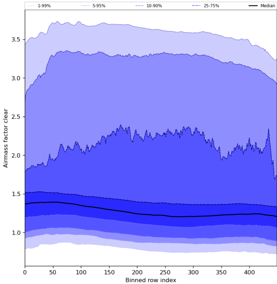
Figure 56: Along track statistics of “Airmass factor clear” for 2024-04-08 to 2024-04-10
