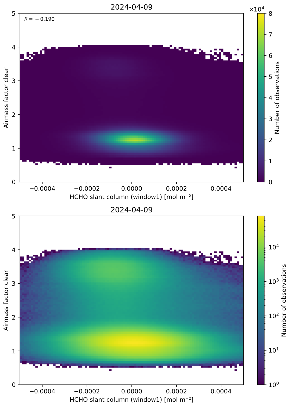
Figure 81: Scatter density plot of “HCHO slant column (window1)” against “Airmass factor clear” for 2024-04-08 to 2024-04-10.
