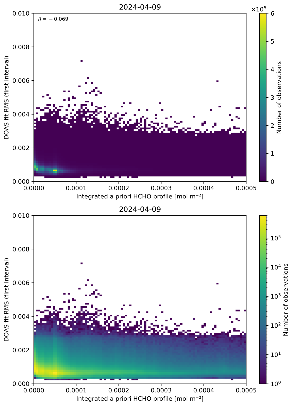
Figure 148: Scatter density plot of “Integrated a priori HCHO profile” against “DOAS fit RMS (first interval)” for 2024-04-08 to 2024-04-10.
