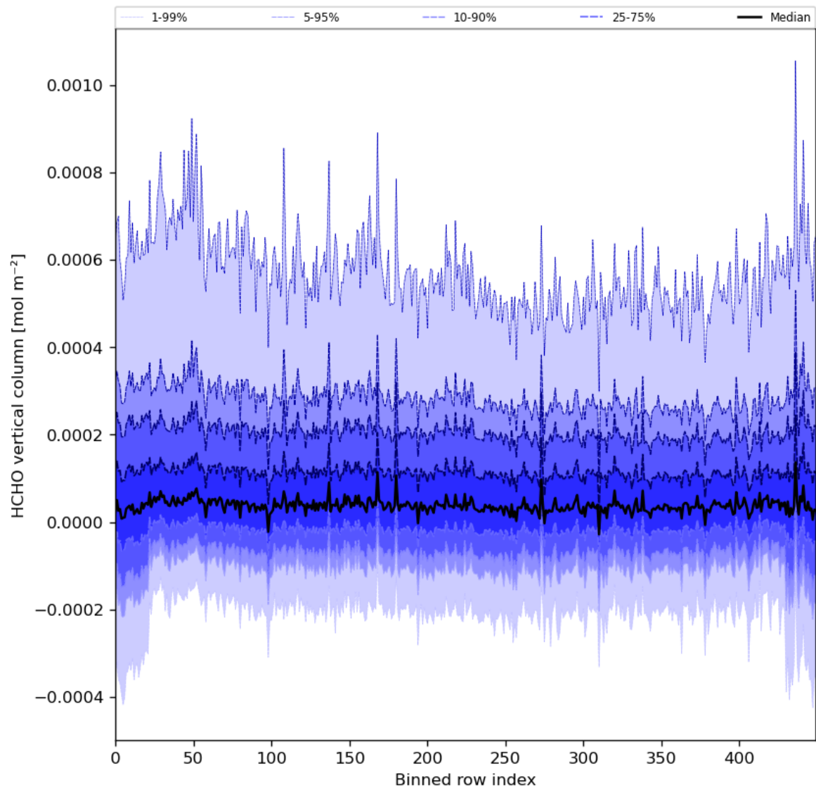
Figure 49: Along track statistics of “HCHO vertical column” for 2024-04-08 to 2024-04-10
