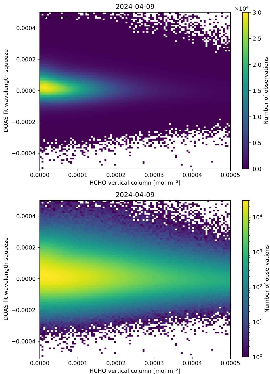
Figure 125: Scatter density plot of “HCHO vertical column” against “DOAS fit wavelength squeeze” for 2024-04-08 to 2024-04-10.
