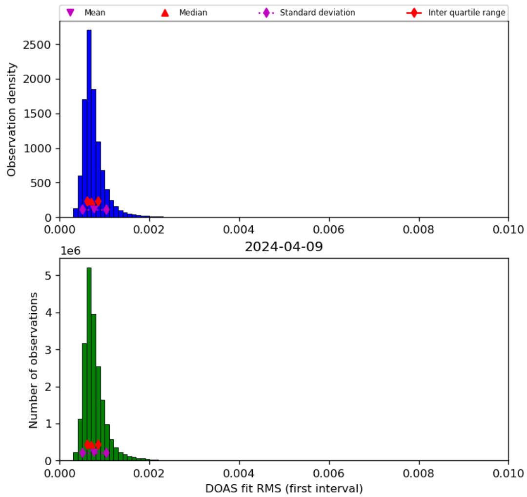
Figure 46: Histogram of “DOAS fit RMS (first interval)” for 2024-04-08 to 2024-04-10
