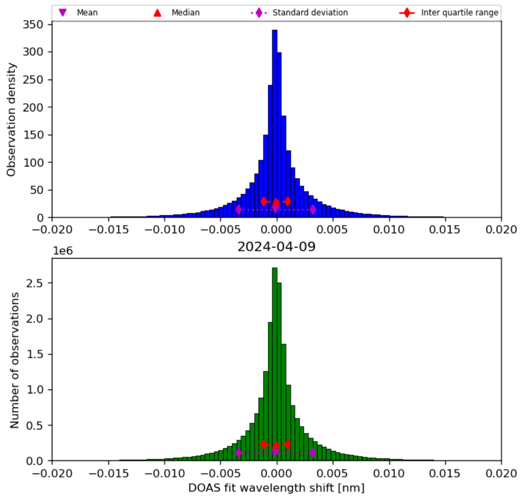
Figure 44: Histogram of “DOAS fit wavelength shift” for 2024-04-08 to 2024-04-10
