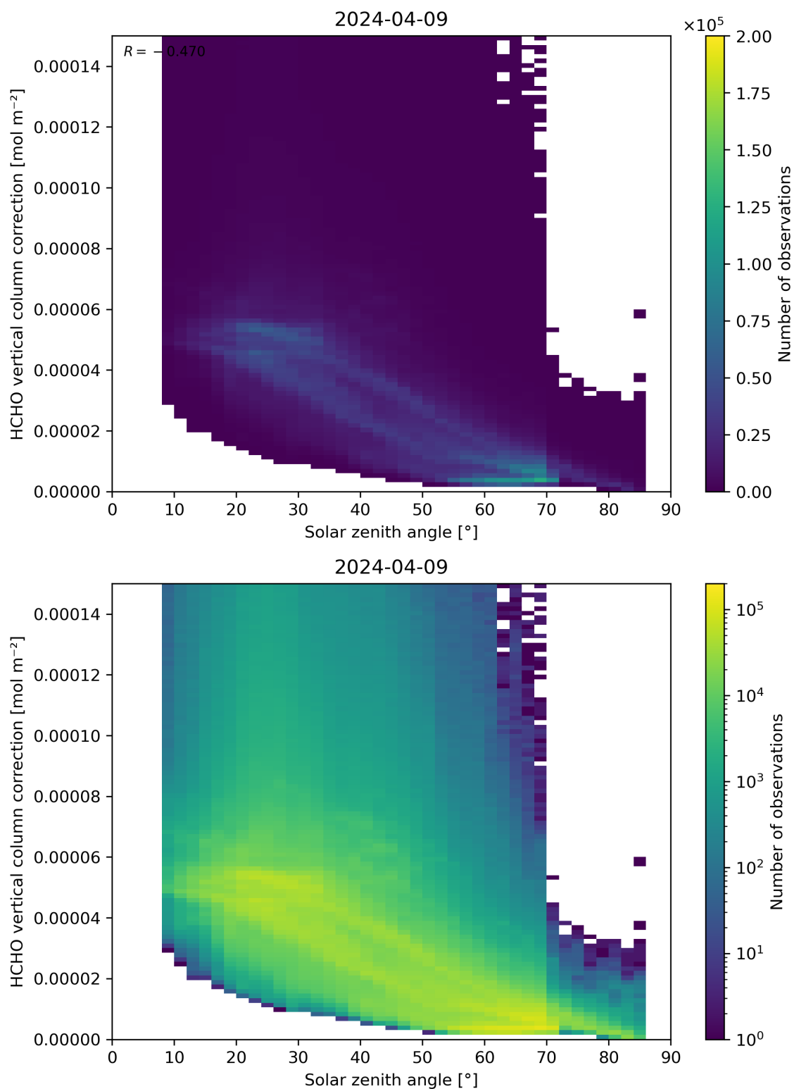
Figure 178: Scatter density plot of “Solar zenith angle” against “HCHO vertical column correction” for 2024-04-08 to 2024-04-10.
