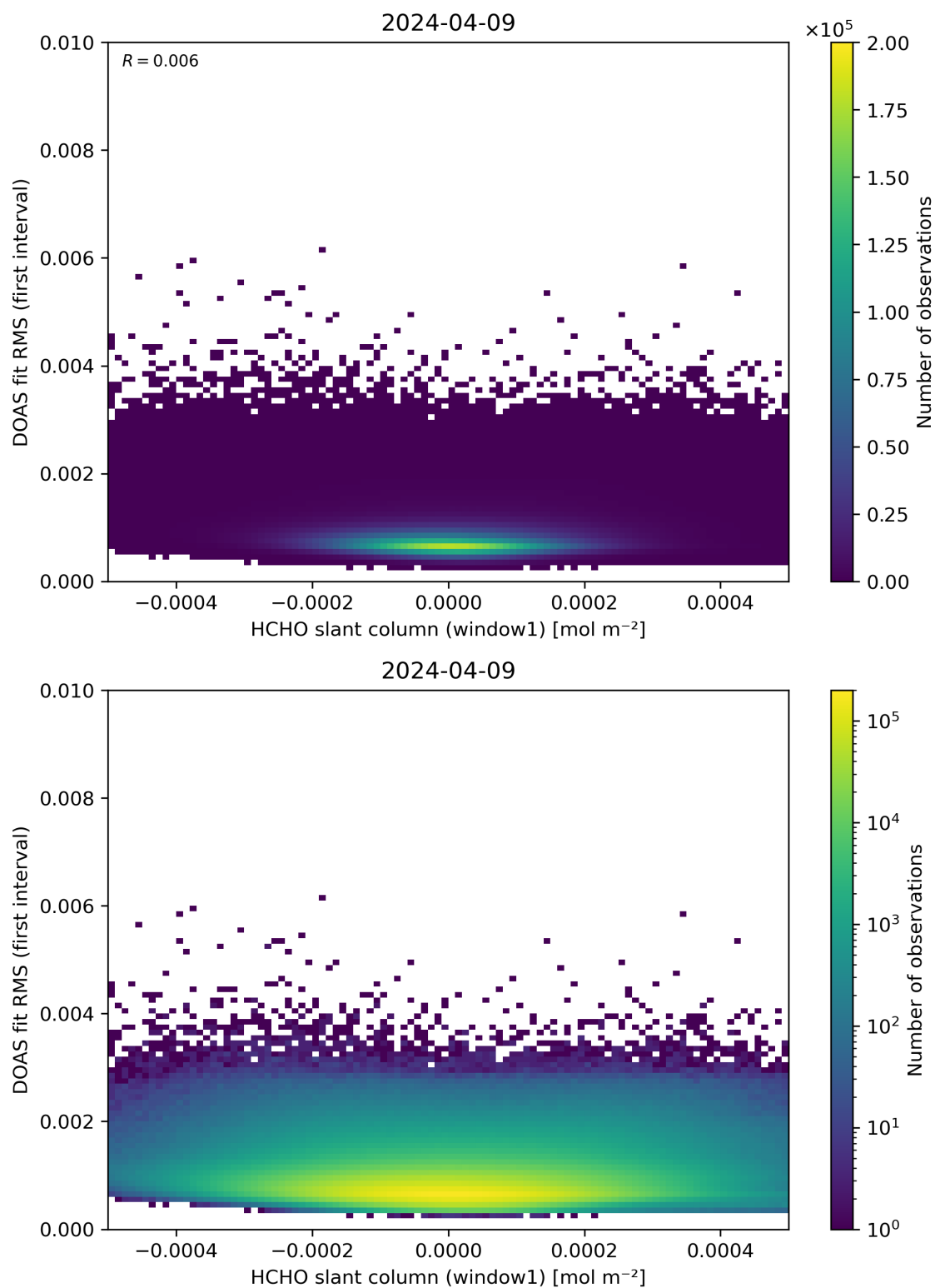
Figure 78: Scatter density plot of “HCHO slant column (window1)” against “DOAS fit RMS (first interval)” for 2024-04-08 to 2024-04-10.
