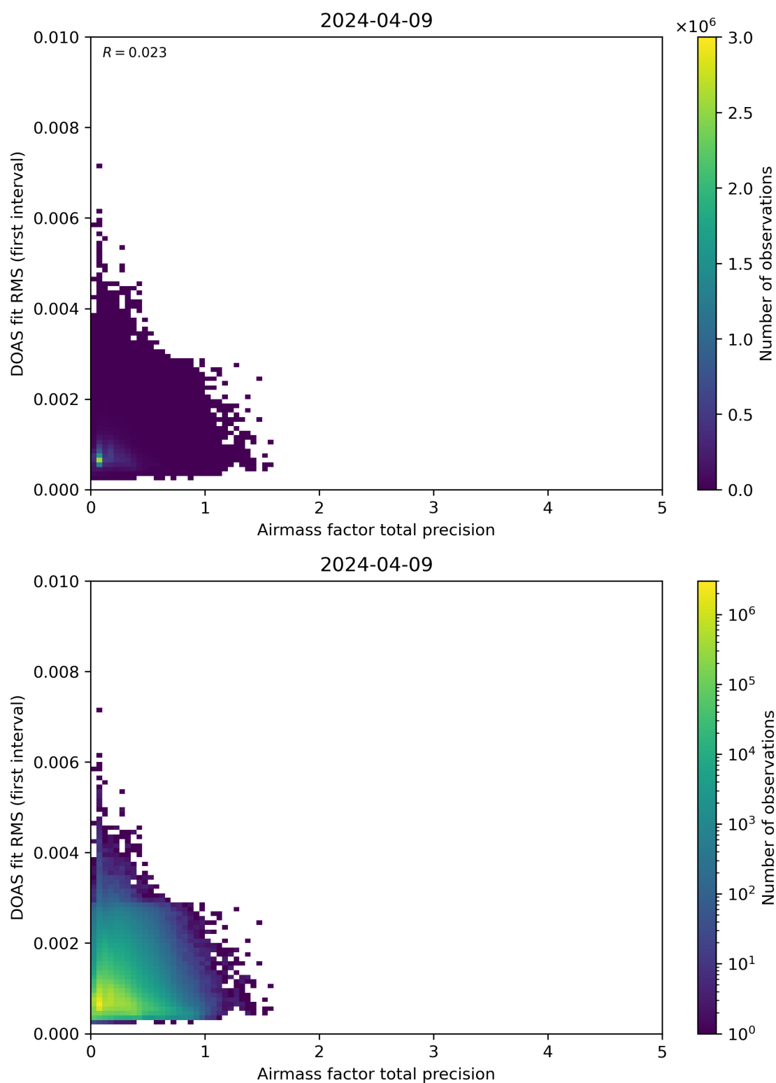
Figure 105: Scatter density plot of “Airmass factor total precision” against “DOAS fit RMS (first interval)” for 2024-04-08 to 2024-04-10.
