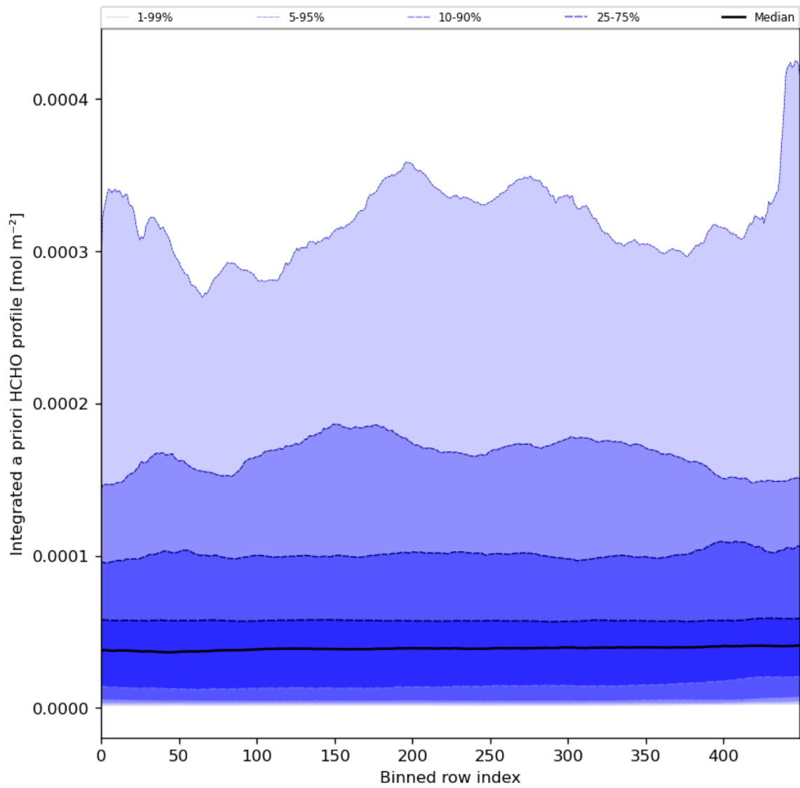
Figure 57: Along track statistics of “Integrated a priori HCHO profile” for 2024-04-08 to 2024-04-10
