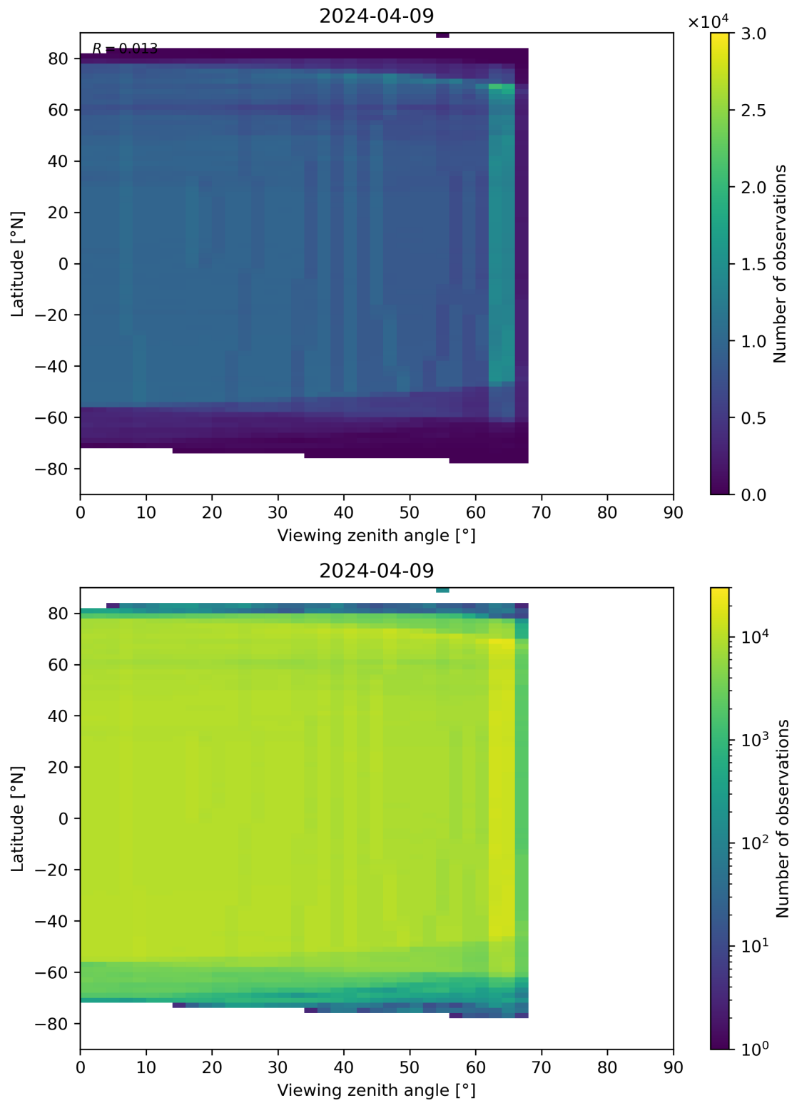
Figure 196: Scatter density plot of “Viewing zenith angle” against “Latitude” for 2024-04-08 to 2024-04-10.
