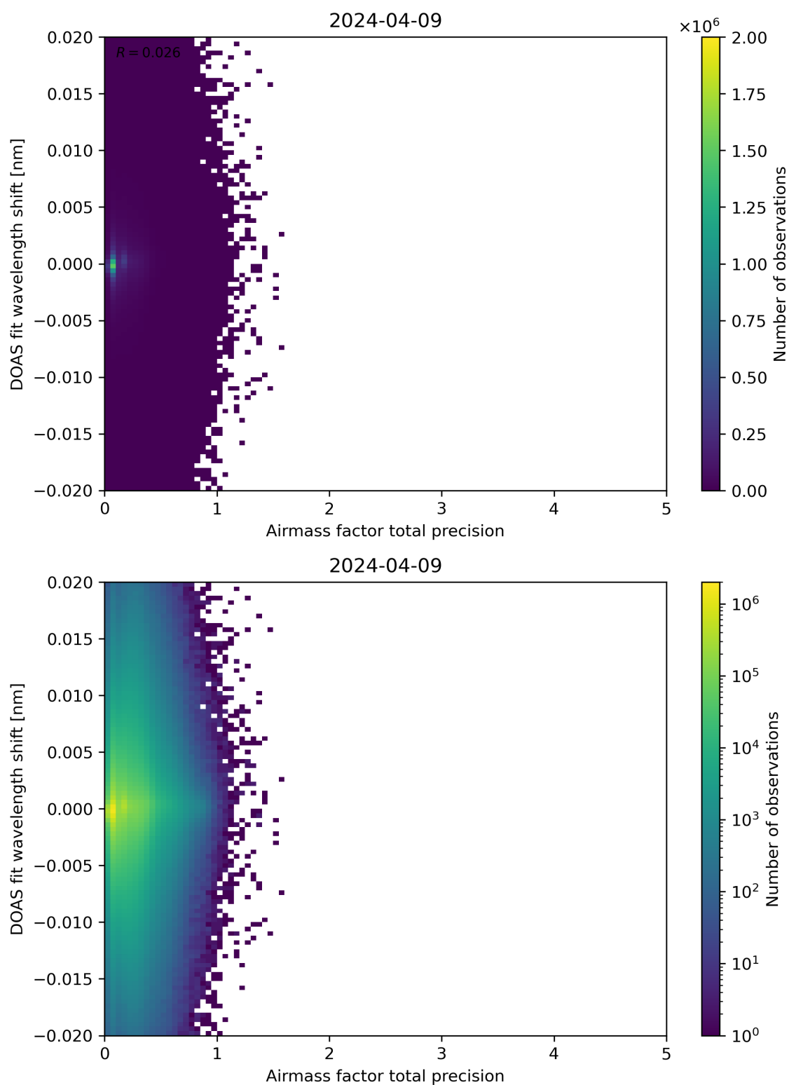
Figure 106: Scatter density plot of “Airmass factor total precision” against “DOAS fit wavelength shift” for 2024-04-08 to 2024-04-10.
