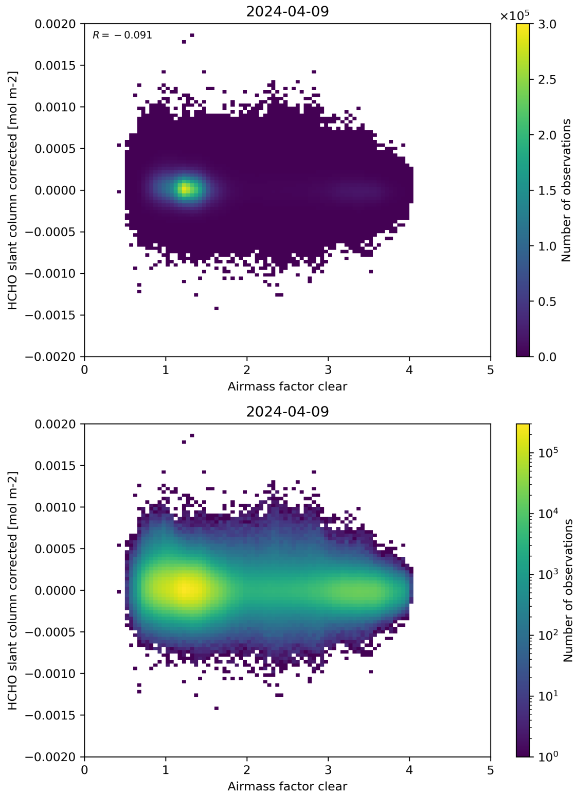
Figure 74: Scatter density plot of “Airmass factor clear” against “HCHO slant column corrected” for 2024-04-08 to 2024-04-10.
