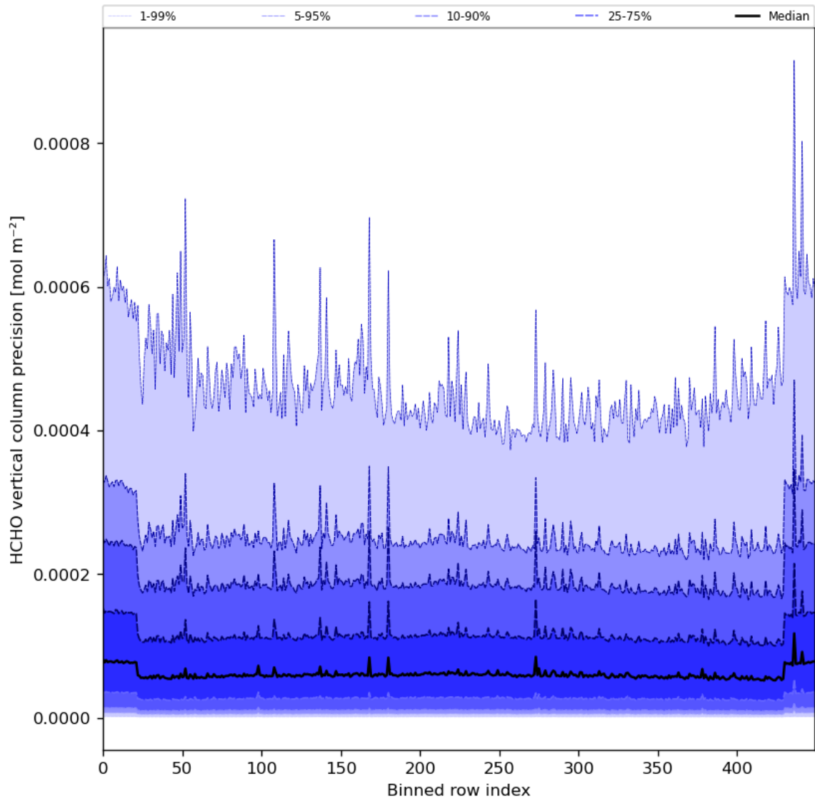
Figure 50: Along track statistics of “HCHO vertical column precision” for 2024-04-08 to 2024-04-10
