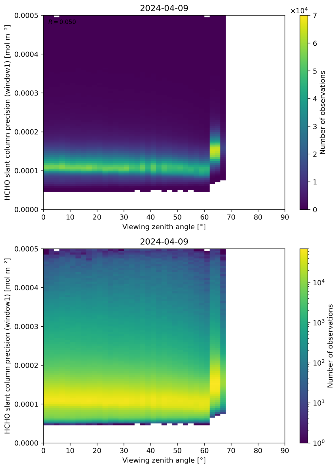
Figure 189: Scatter density plot of “Viewing zenith angle” against “HCHO slant column precision (window1)” for 2024-04-08 to 2024-04-10.
