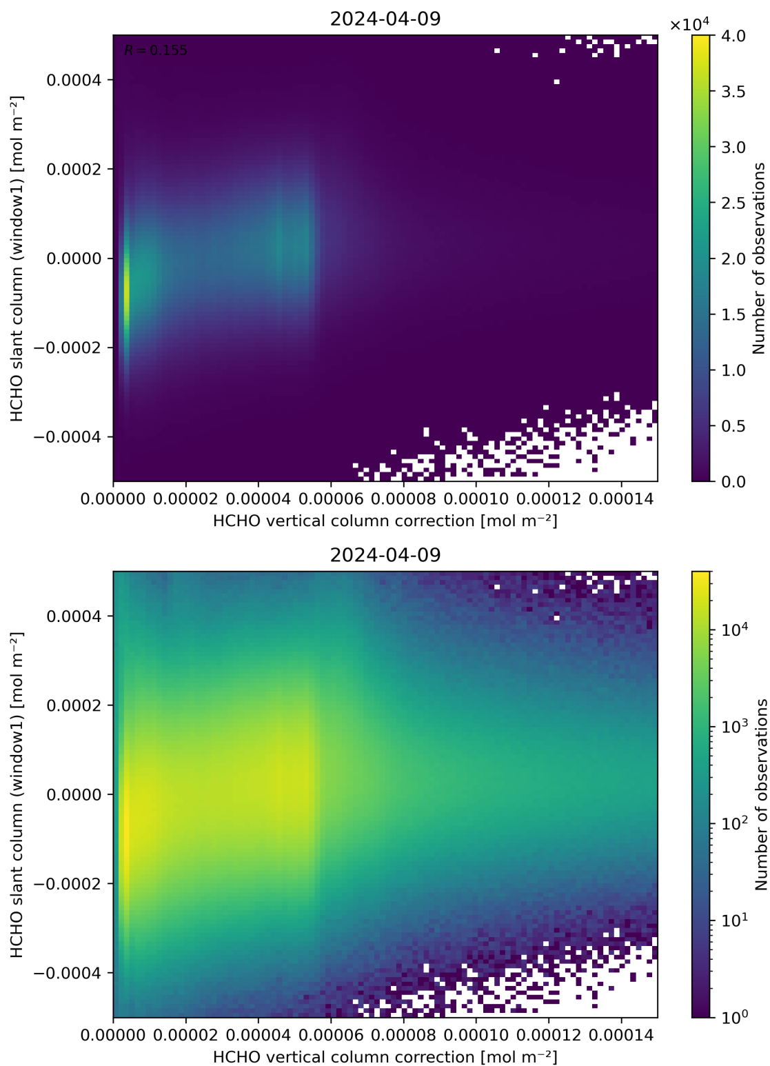
Figure 118: Scatter density plot of “HCHO vertical column correction” against “HCHO slant column (window1)” for 2024-04-08 to 2024-04-10.
