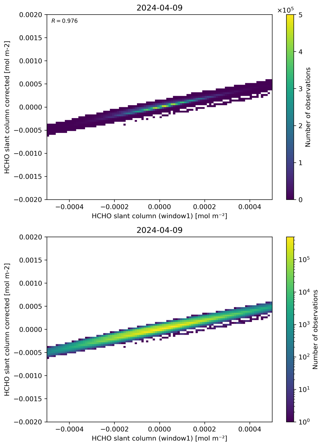
Figure 82: Scatter density plot of “HCHO slant column (window1)” against “HCHO slant column corrected” for 2024-04-08 to 2024-04-10.
