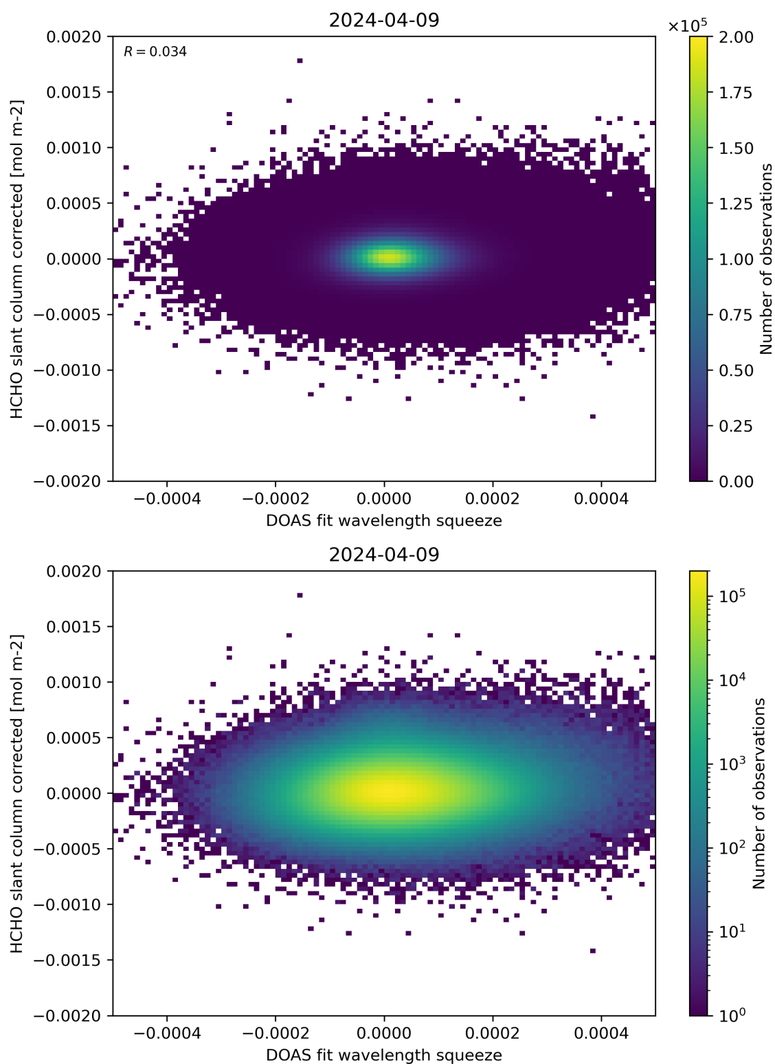
Figure 69: Scatter density plot of “DOAS fit wavelength squeeze” against “HCHO slant column corrected” for 2024-04-08 to 2024-04-10.
