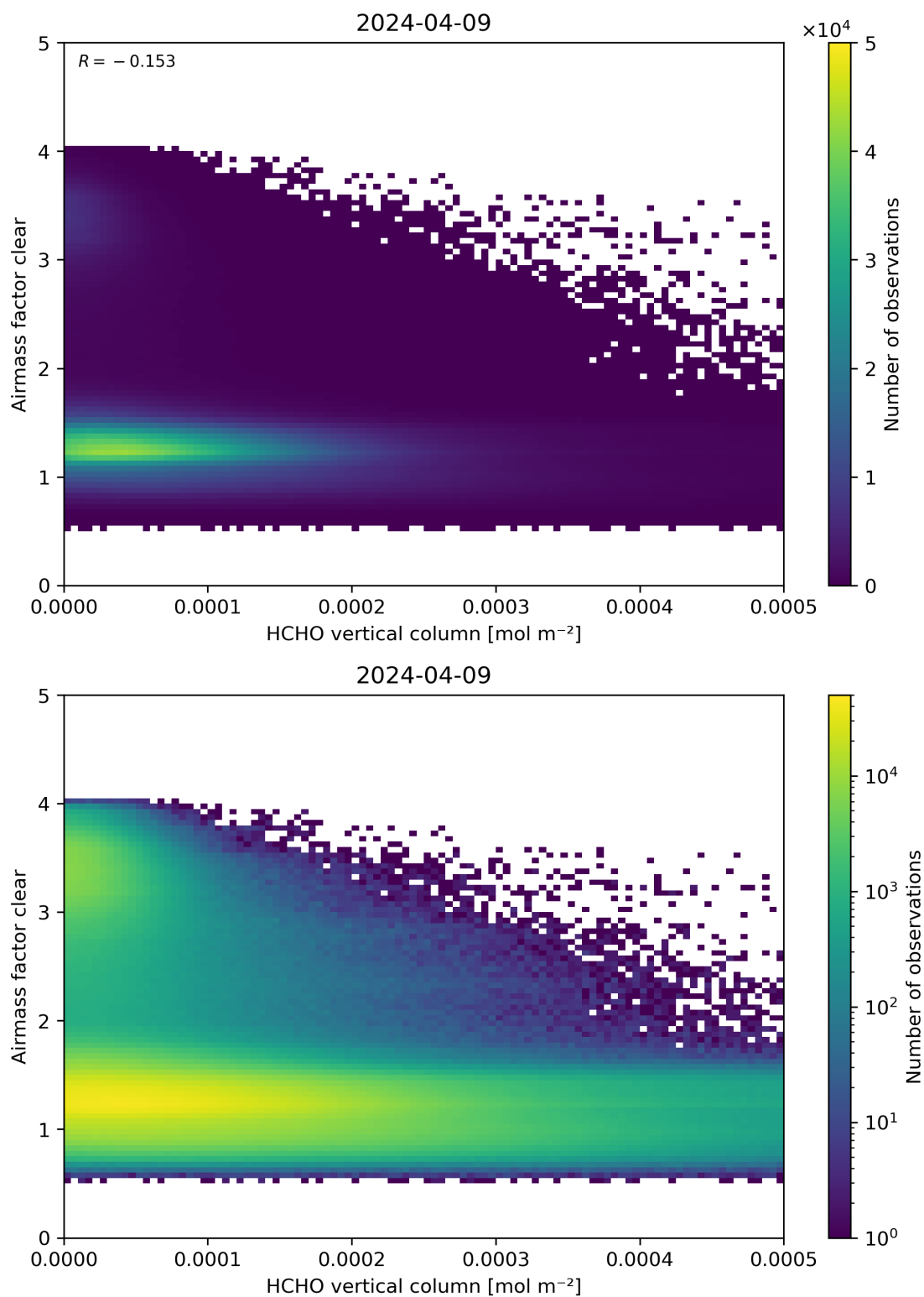
Figure 126: Scatter density plot of “HCHO vertical column” against “Airmass factor clear” for 2024-04-08 to 2024-04-10.
