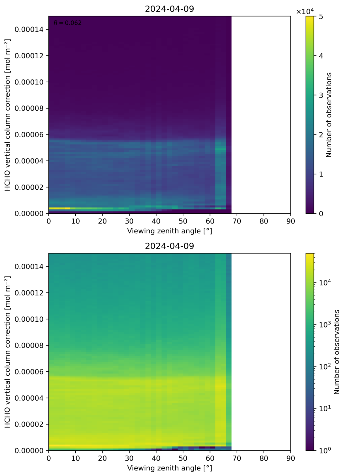
Figure 193: Scatter density plot of “Viewing zenith angle” against “HCHO vertical column correction” for 2024-04-08 to 2024-04-10.
