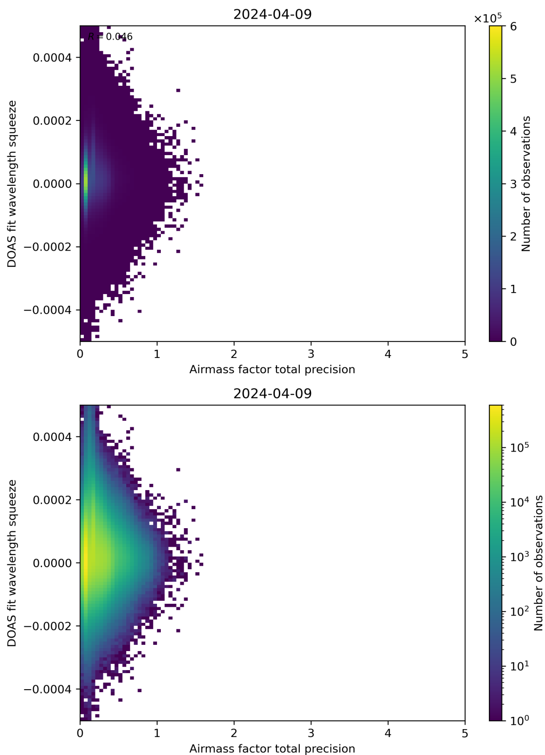
Figure 107: Scatter density plot of “Airmass factor total precision” against “DOAS fit wavelength squeeze” for 2024-04-08 to 2024-04-10.
