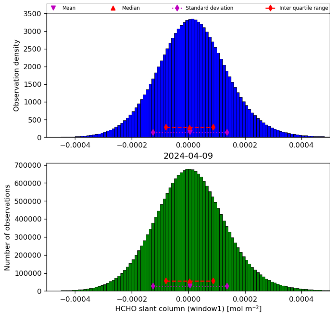
Figure 38: Histogram of “HCHO slant column (window1)” for 2024-04-08 to 2024-04-10
