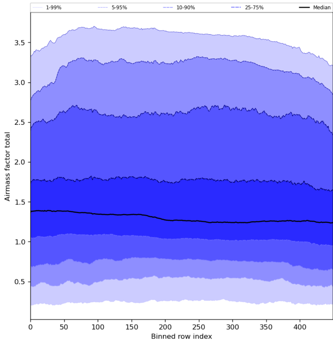
Figure 54: Along track statistics of “Airmass factor total” for 2024-04-08 to 2024-04-10
