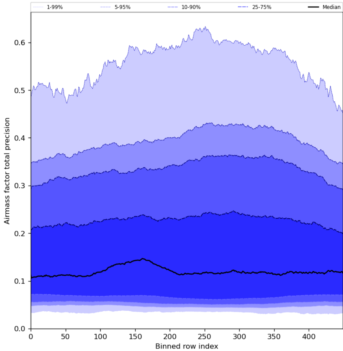
Figure 55: Along track statistics of “Airmass factor total precision” for 2024-04-08 to 2024-04-10
