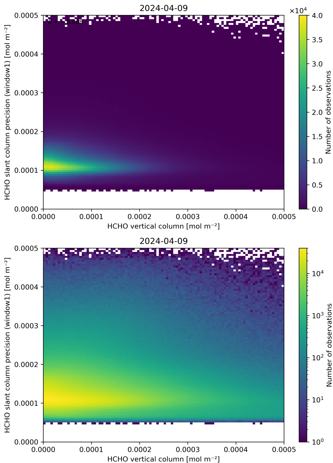
Figure 130: Scatter density plot of “HCHO vertical column” against “HCHO slant column precision (window1)” for 2024-04-08 to 2024-04-10.
