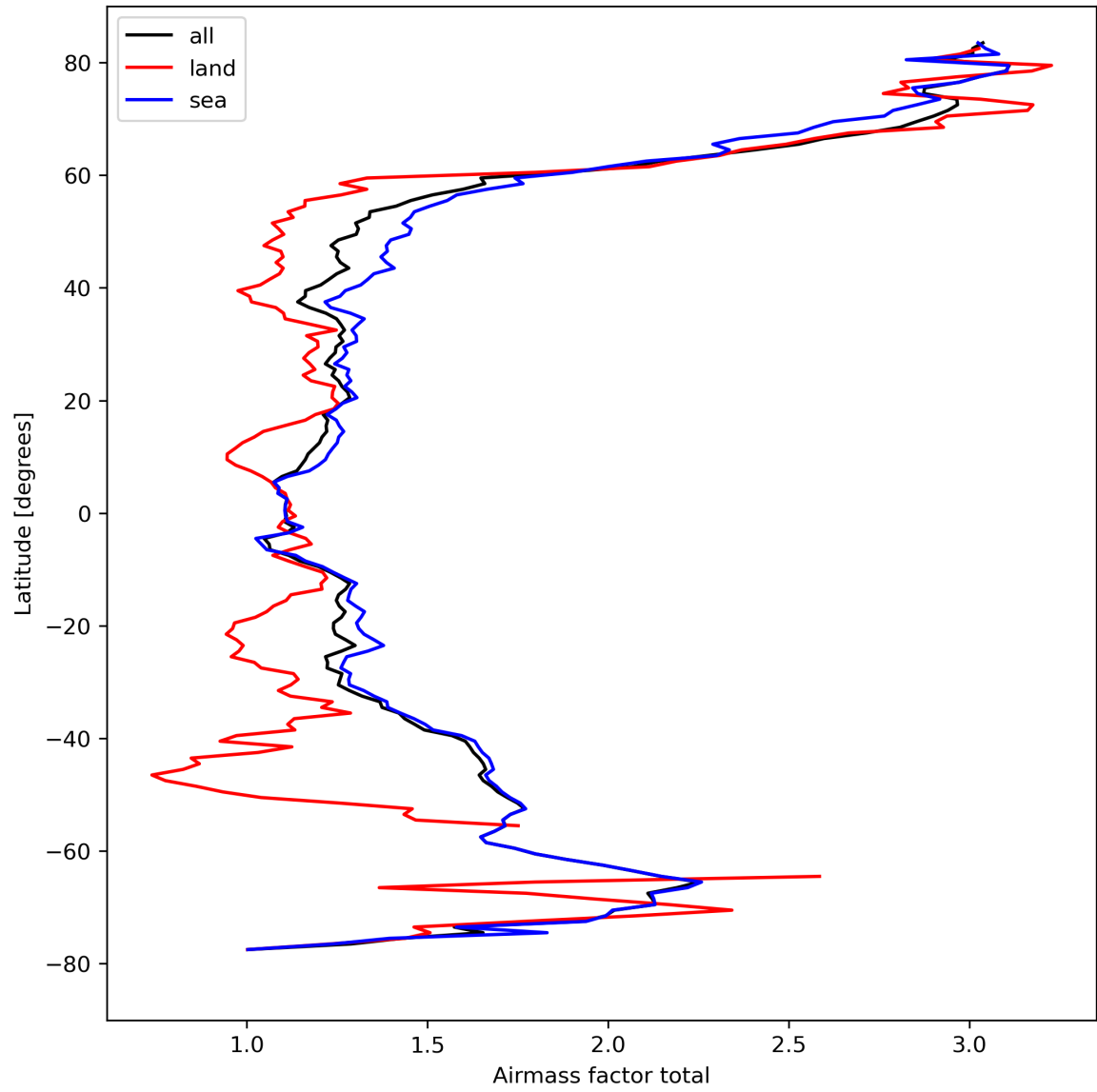
Figure 26: Zonal average of “Airmass factor total” for 2024-04-08 to 2024-04-10.
