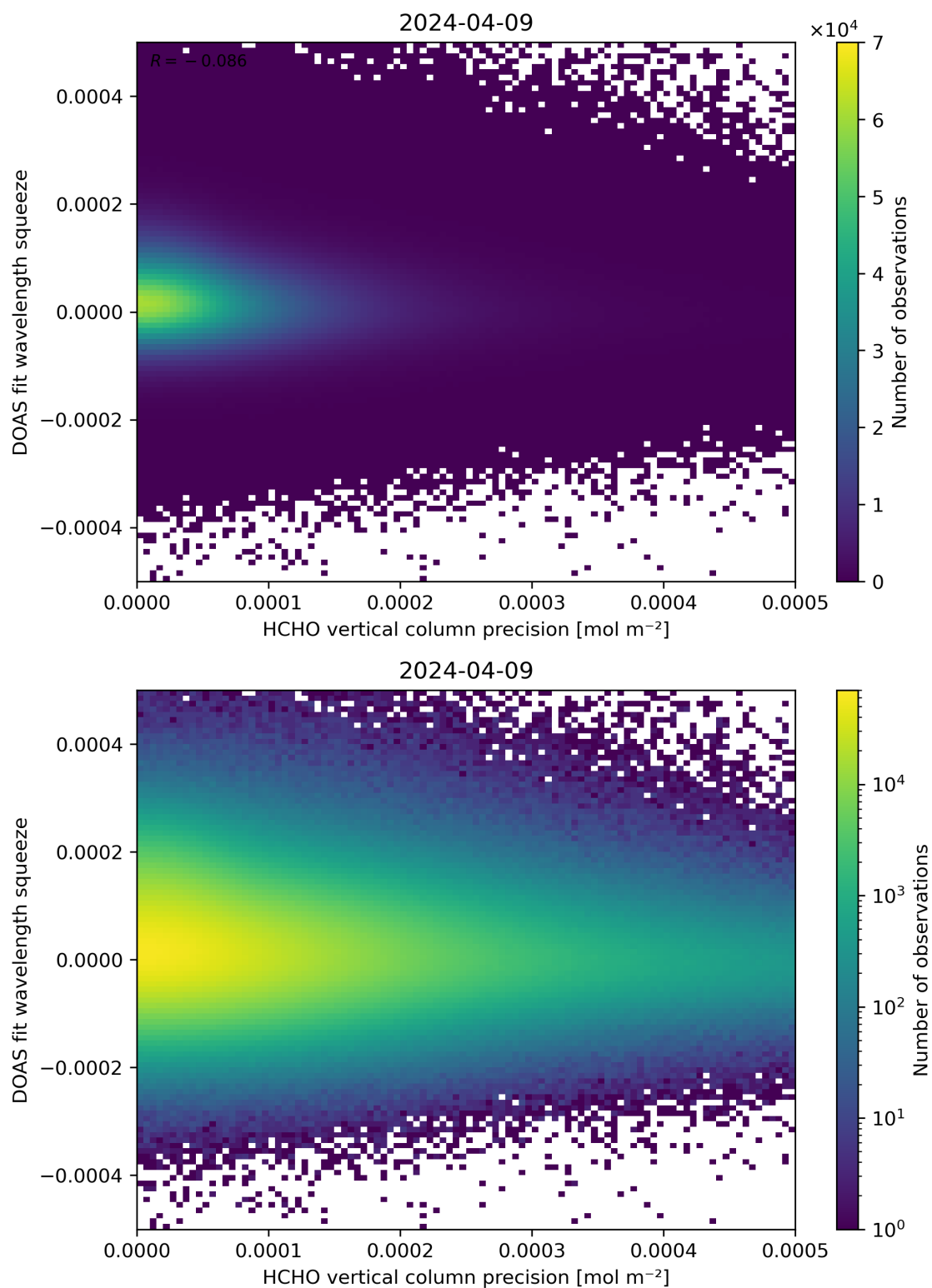
Figure 138: Scatter density plot of “HCHO vertical column precision” against “DOAS fit wavelength squeeze” for 2024-04-08 to 2024-04-10.
