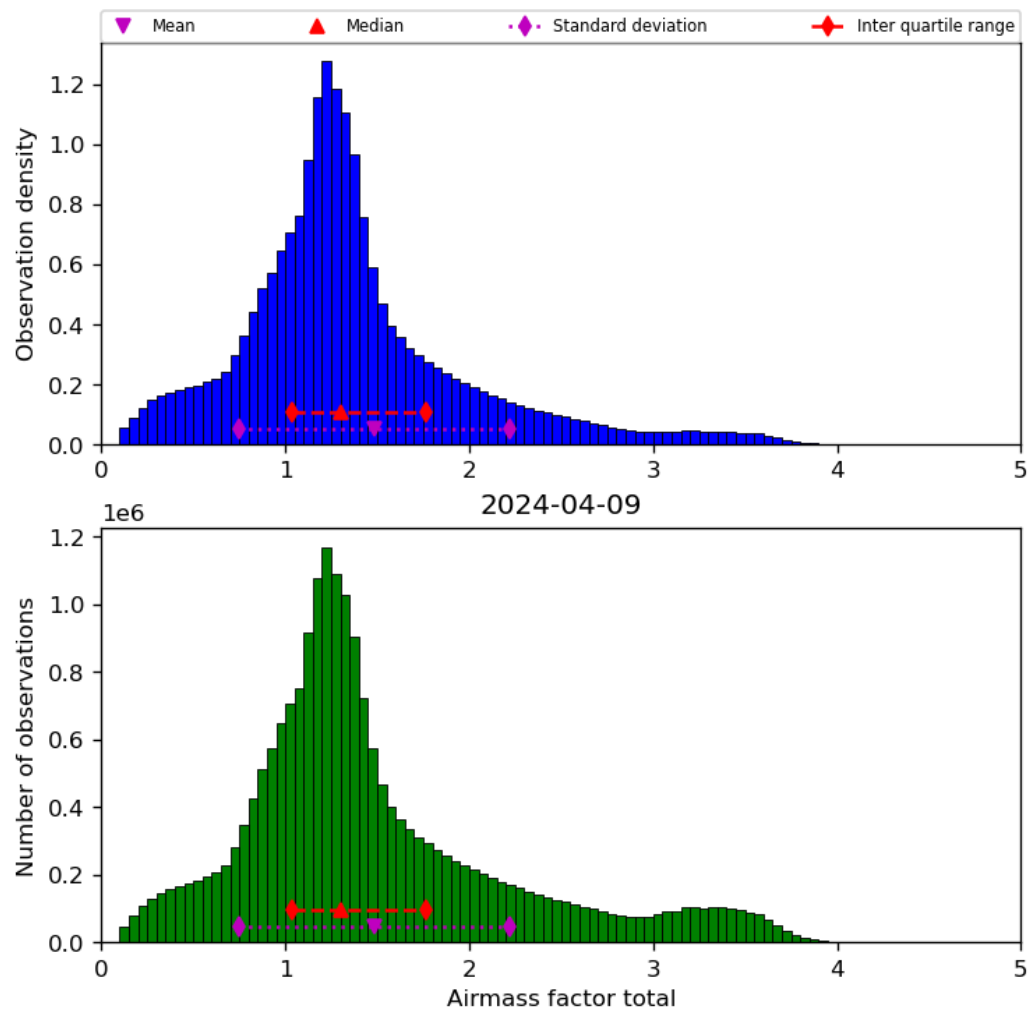
Figure 40: Histogram of “Airmass factor total” for 2024-04-08 to 2024-04-10
