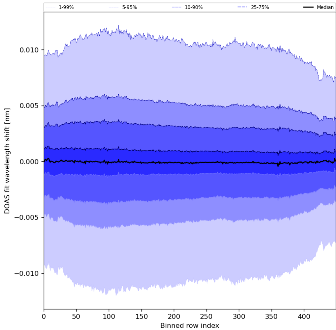
Figure 58: Along track statistics of “DOAS fit wavelength shift” for 2024-04-08 to 2024-04-10
