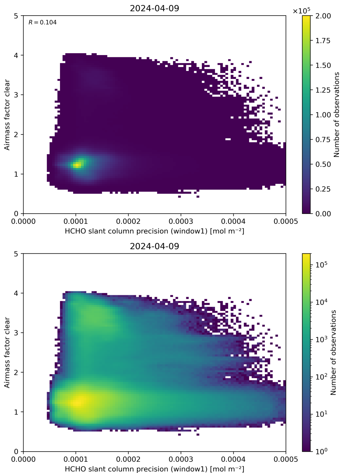
Figure 91: Scatter density plot of “HCHO slant column precision (window1)” against “Airmass factor clear” for 2024-04-08 to 2024-04-10.
