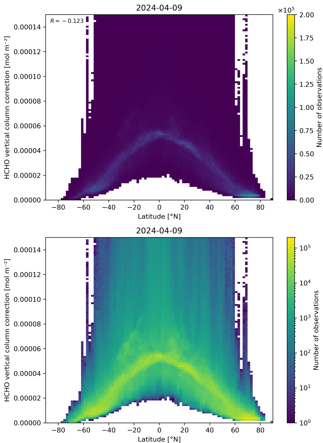
Figure 164: Scatter density plot of “Latitude” against “HCHO vertical column correction” for 2024-04-08 to 2024-04-10.
