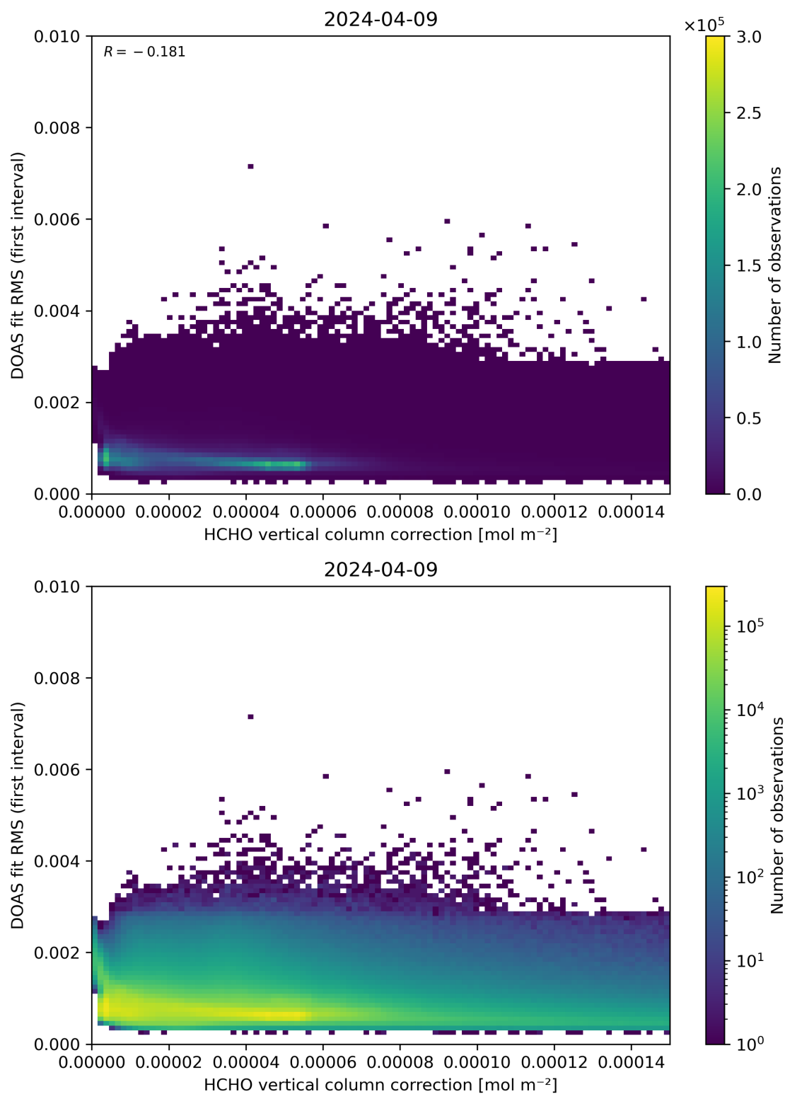
Figure 112: Scatter density plot of “HCHO vertical column correction” against “DOAS fit RMS (first interval)” for 2024-04-08 to 2024-04-10.
