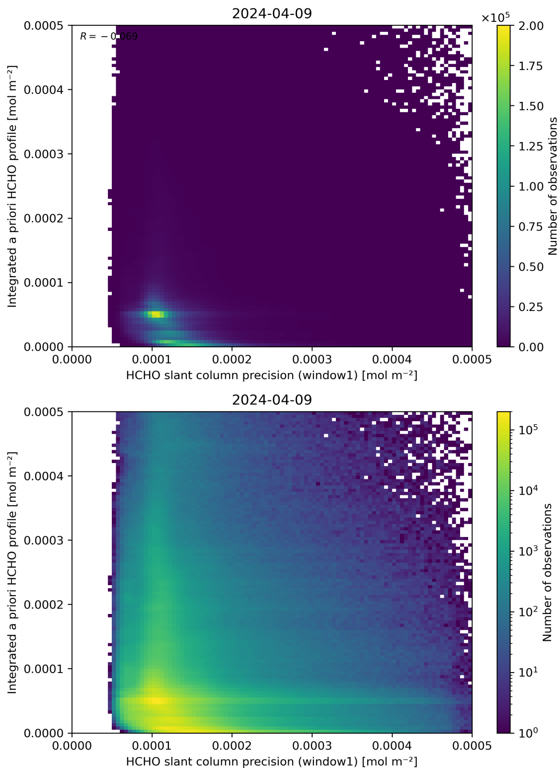
Figure 96: Scatter density plot of “HCHO slant column precision (window1)” against “Integrated a priori HCHO profile” for 2024-04-08 to 2024-04-10.
