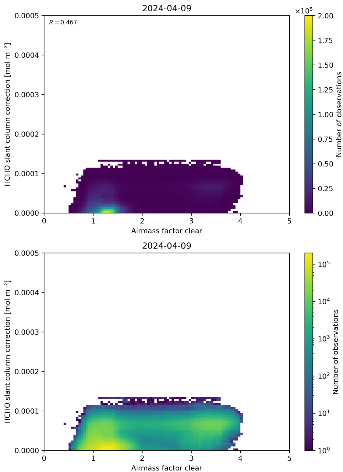
Figure 75: Scatter density plot of “Airmass factor clear” against “HCHO slant column correction” for 2024-04-08 to 2024-04-10.
