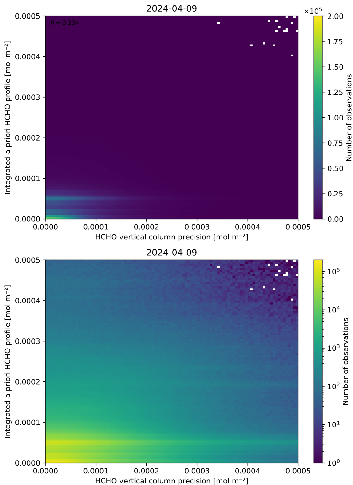
Figure 147: Scatter density plot of “HCHO vertical column precision” against “Integrated a priori HCHO profile” for 2024-04-08 to 2024-04-10.
