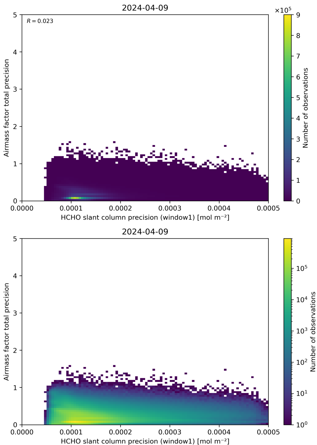
Figure 95: Scatter density plot of “HCHO slant column precision (window1)” against “Airmass factor total precision” for 2024-04-08 to 2024-04-10.
