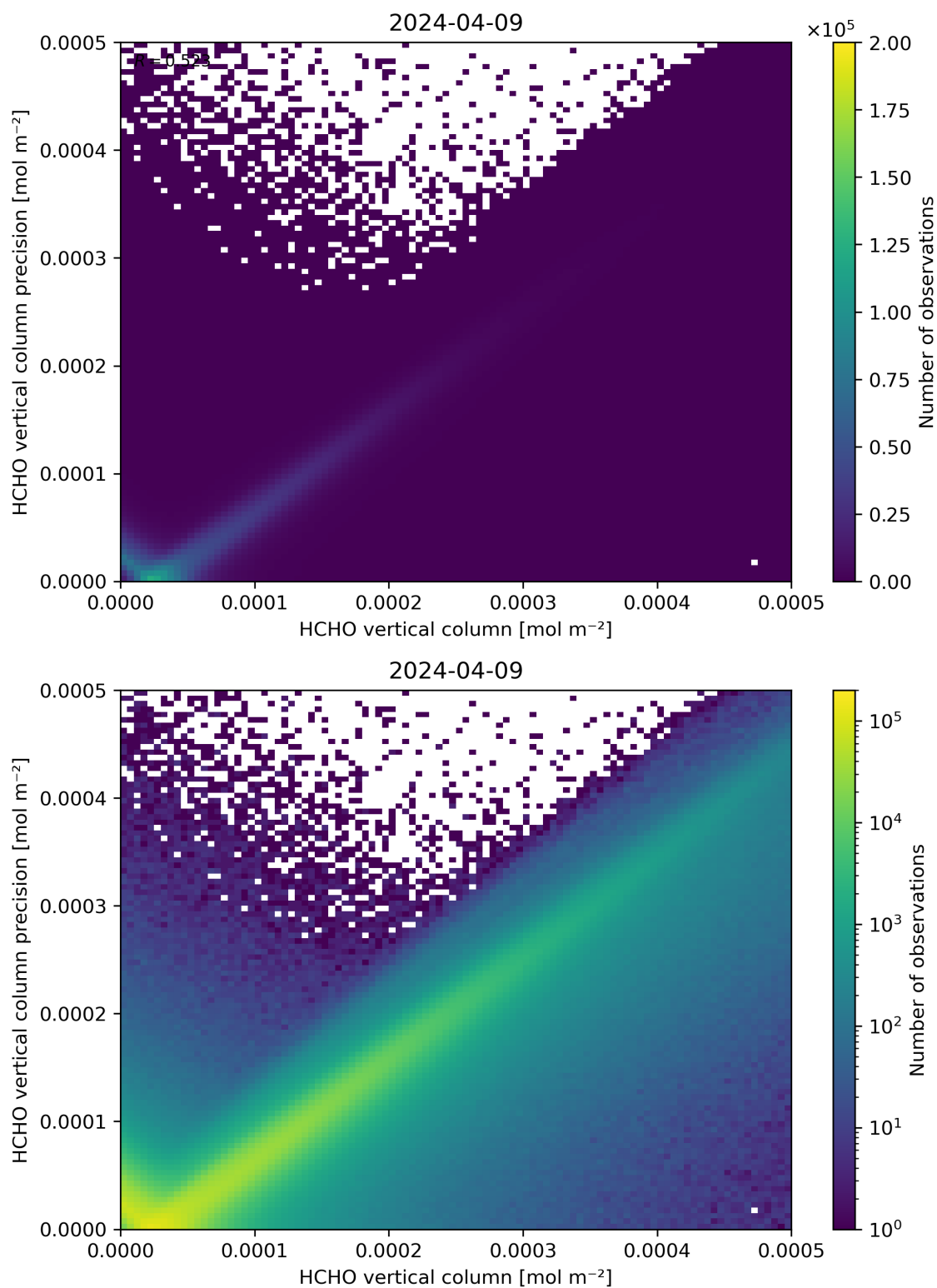
Figure 134: Scatter density plot of “HCHO vertical column” against “HCHO vertical column precision” for 2024-04-08 to 2024-04-10.
