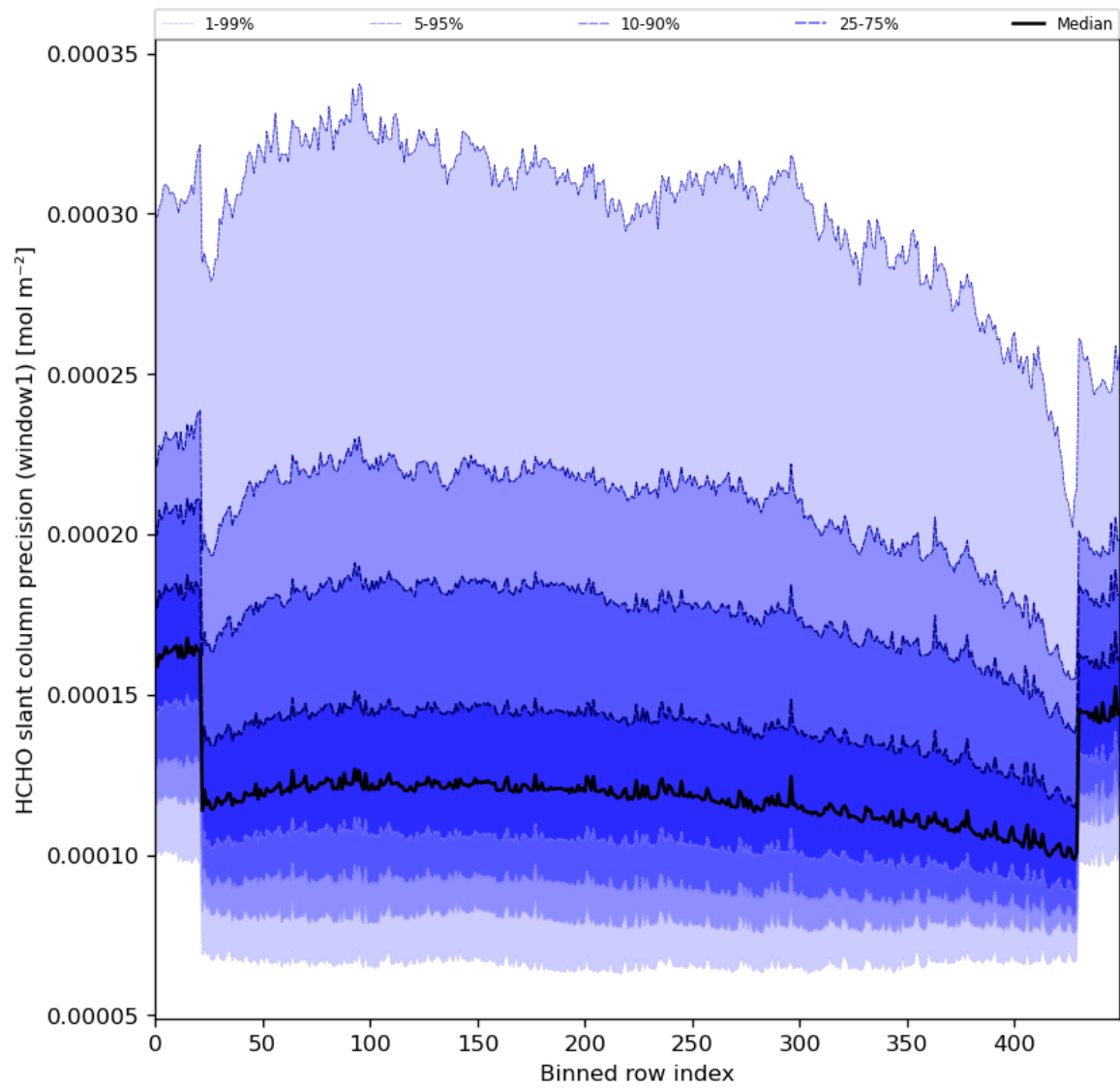
Figure 53: Along track statistics of “HCHO slant column precision (window1)” for 2024-04-08 to 2024-04-10
