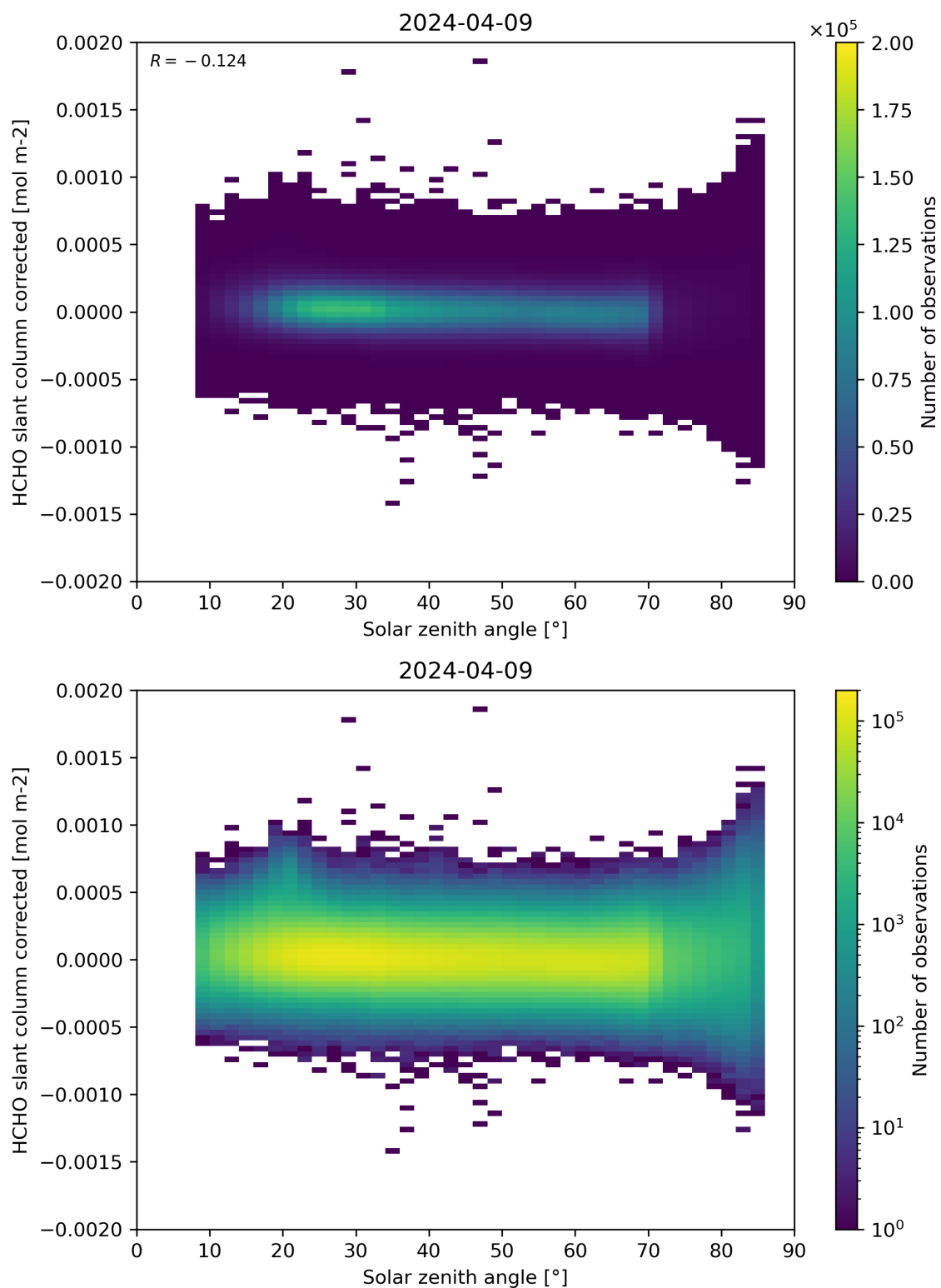
Figure 171: Scatter density plot of “Solar zenith angle” against “HCHO slant column corrected” for 2024-04-08 to 2024-04-10.
