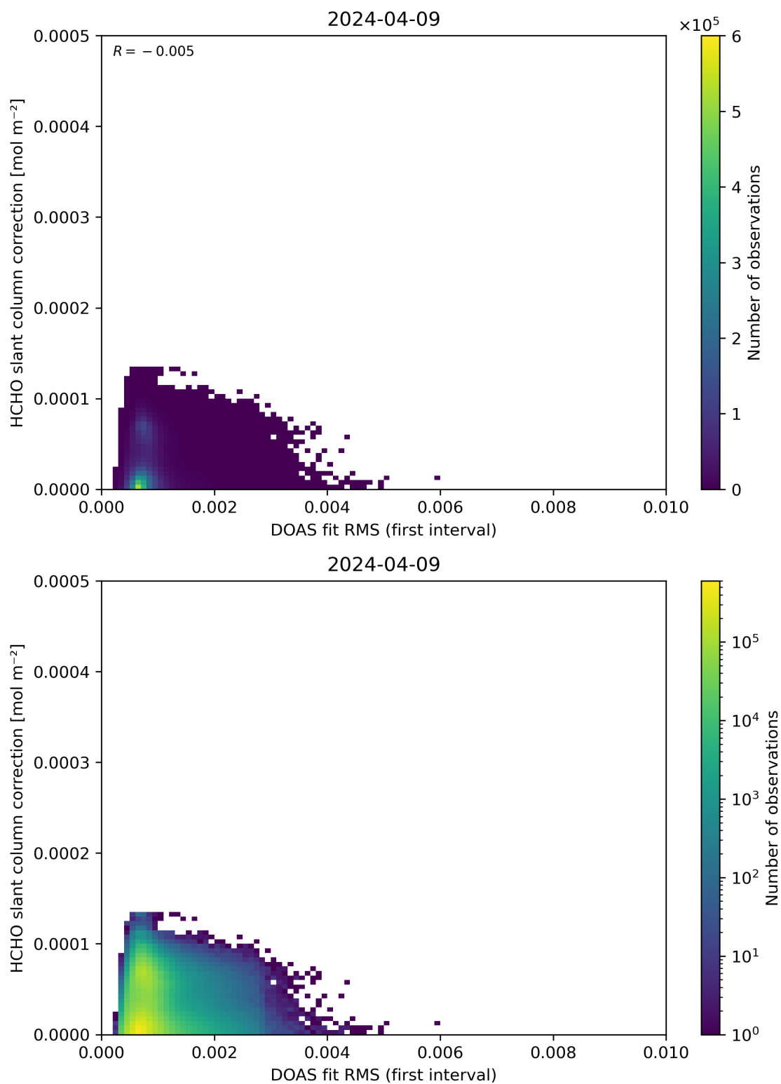
Figure 63: Scatter density plot of “DOAS fit RMS (first interval)” against “HCHO slant column correction” for 2024-04-08 to 2024-04-10.
