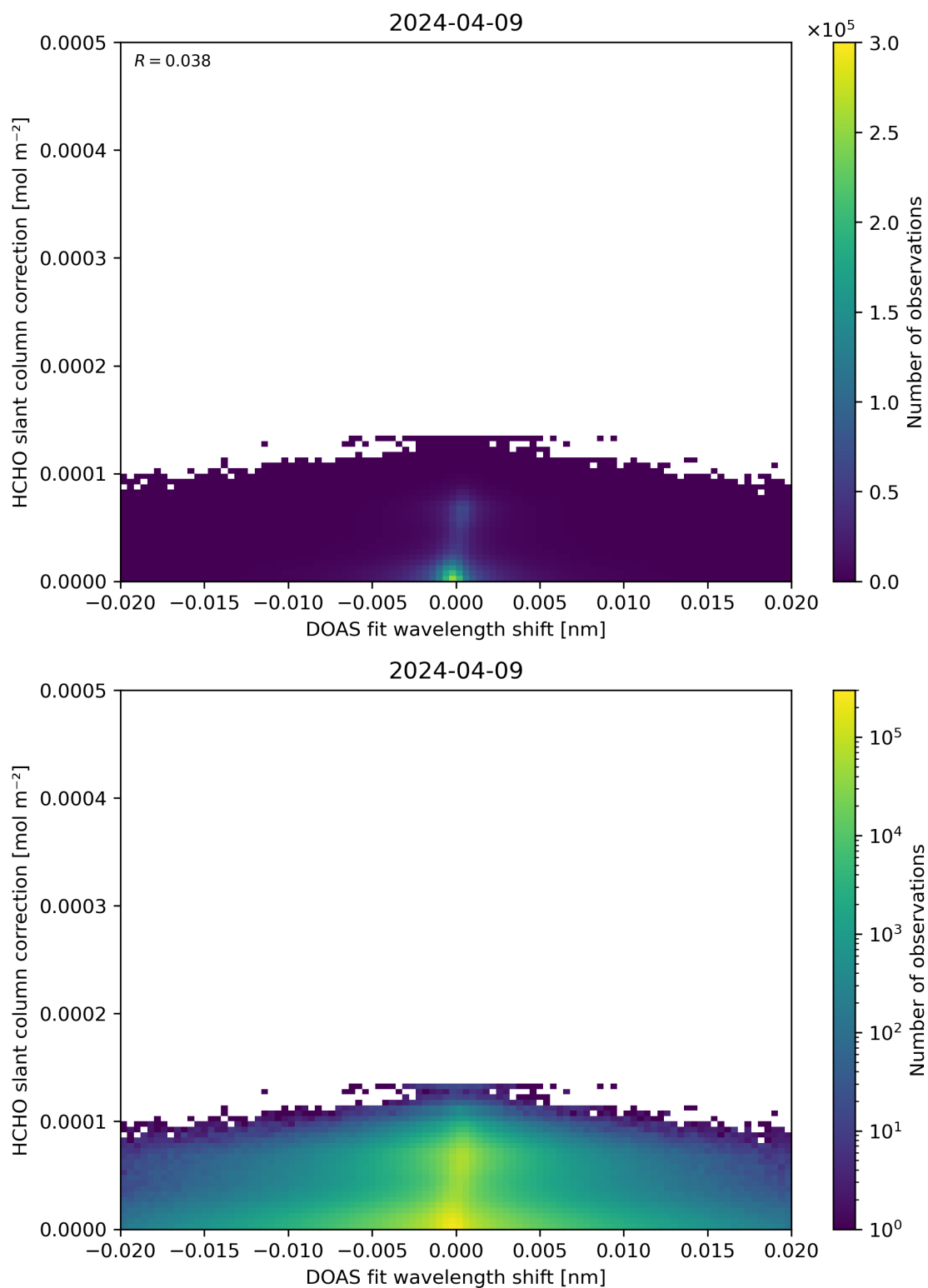
Figure 67: Scatter density plot of “DOAS fit wavelength shift” against “HCHO slant column correction” for 2024-04-08 to 2024-04-10.
