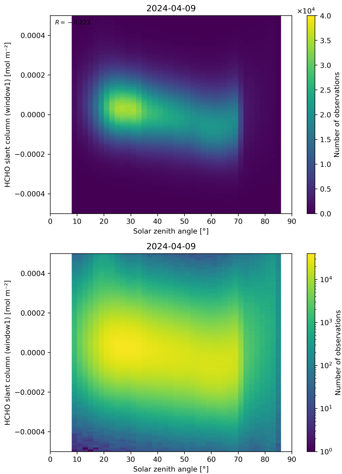
Figure 173: Scatter density plot of “Solar zenith angle” against “HCHO slant column (window1)” for 2024-04-08 to 2024-04-10.
