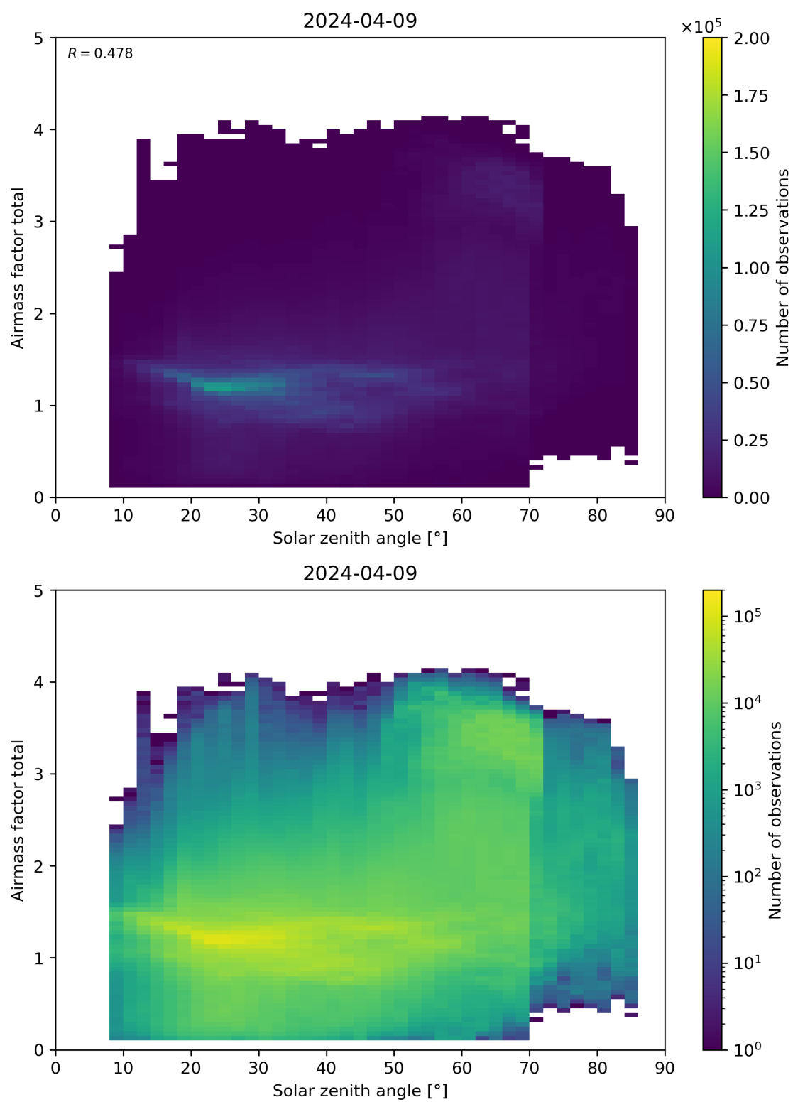
Figure 175: Scatter density plot of “Solar zenith angle” against “Airmass factor total” for 2024-04-08 to 2024-04-10.
