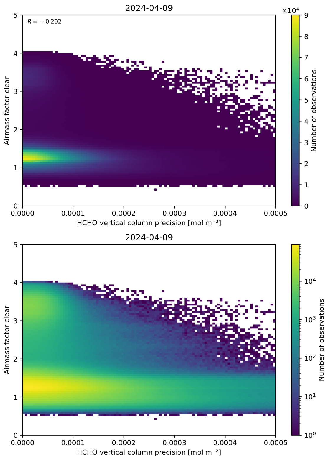
Figure 139: Scatter density plot of “HCHO vertical column precision” against “Airmass factor clear” for 2024-04-08 to 2024-04-10.
