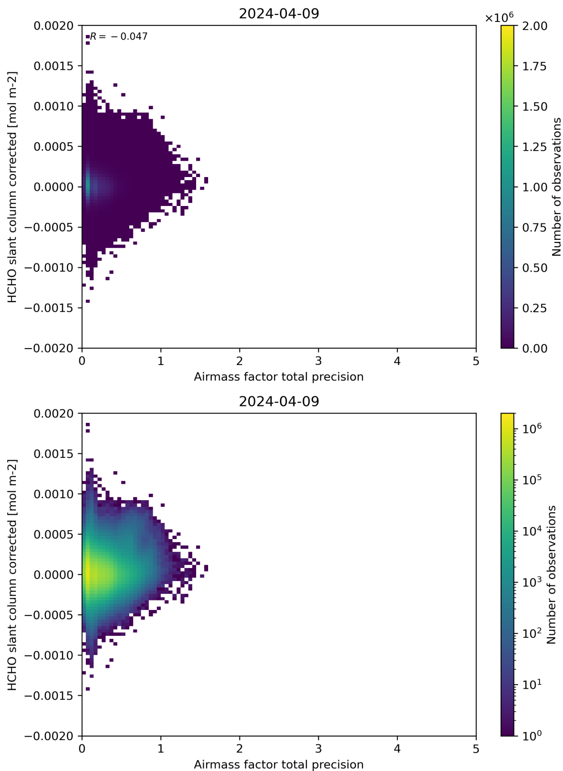
Figure 109: Scatter density plot of “Airmass factor total precision” against “HCHO slant column corrected” for 2024-04-08 to 2024-04-10.
