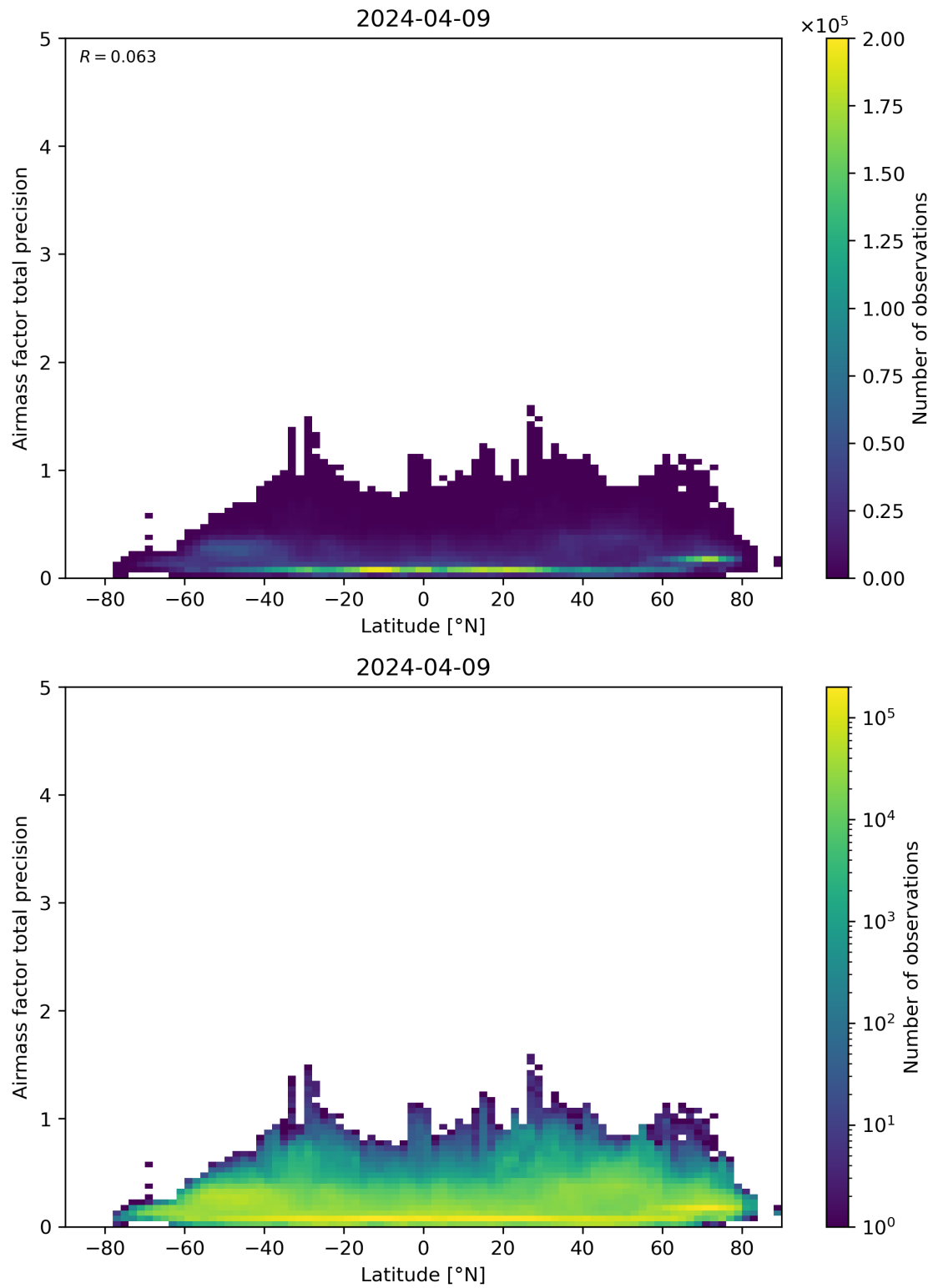
Figure 162: Scatter density plot of “Latitude” against “Airmass factor total precision” for 2024-04-08 to 2024-04-10.
