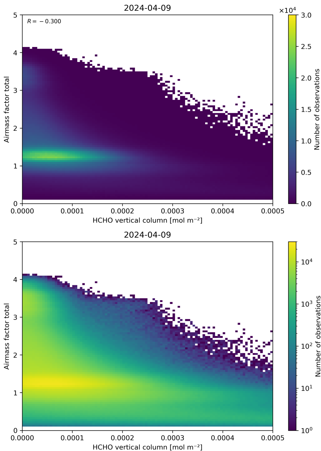
Figure 131: Scatter density plot of “HCHO vertical column” against “Airmass factor total” for 2024-04-08 to 2024-04-10.
