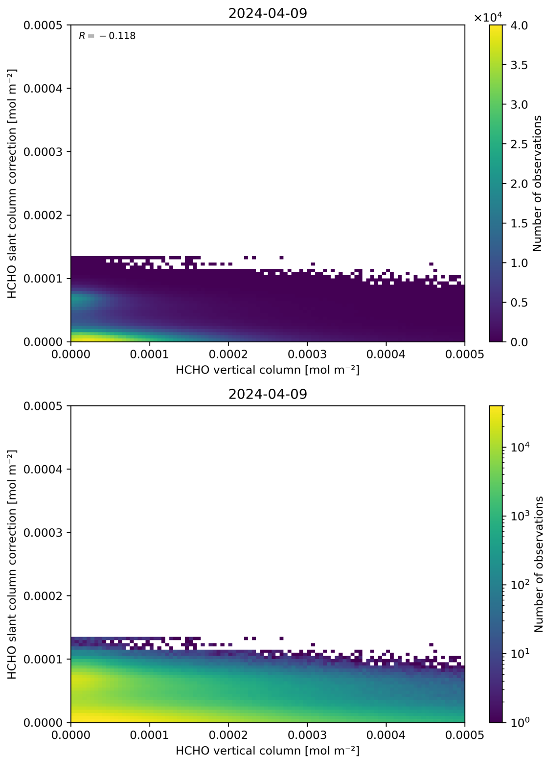
Figure 128: Scatter density plot of “HCHO vertical column” against “HCHO slant column correction” for 2024-04-08 to 2024-04-10.
