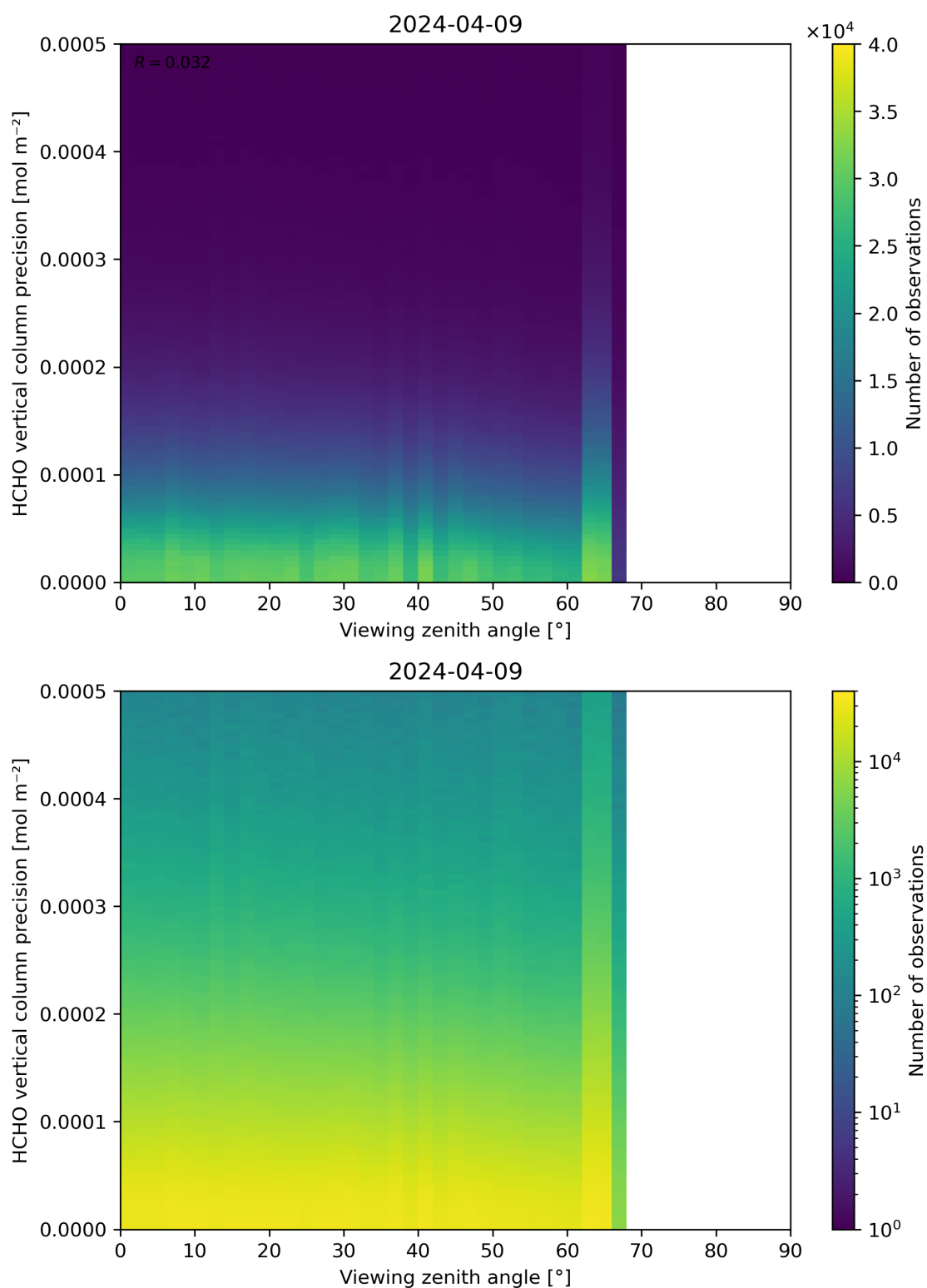
Figure 194: Scatter density plot of “Viewing zenith angle” against “HCHO vertical column precision” for 2024-04-08 to 2024-04-10.
