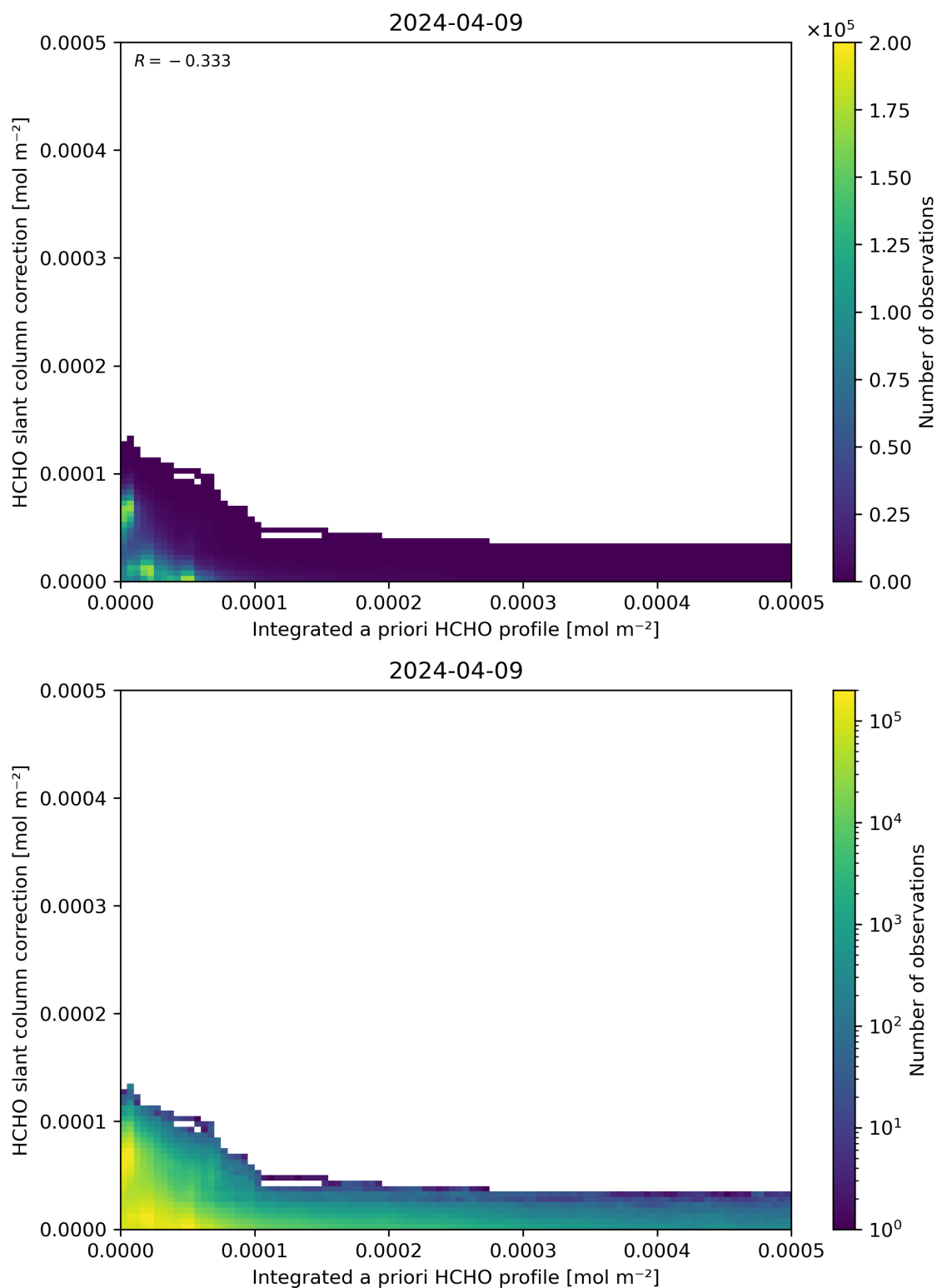
Figure 152: Scatter density plot of “Integrated a priori HCHO profile” against “HCHO slant column correction” for 2024-04-08 to 2024-04-10.
