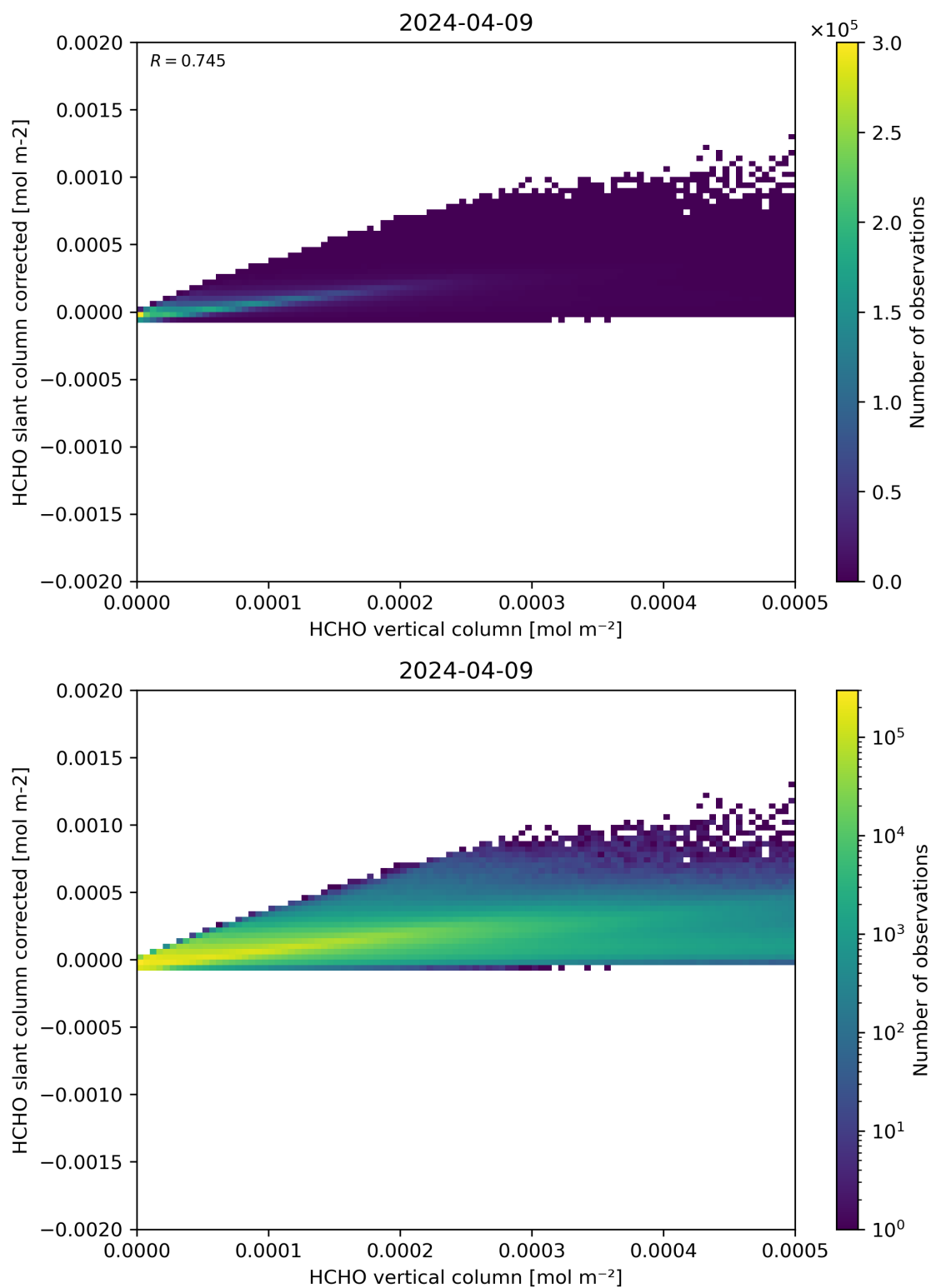
Figure 127: Scatter density plot of “HCHO vertical column” against “HCHO slant column corrected” for 2024-04-08 to 2024-04-10.
