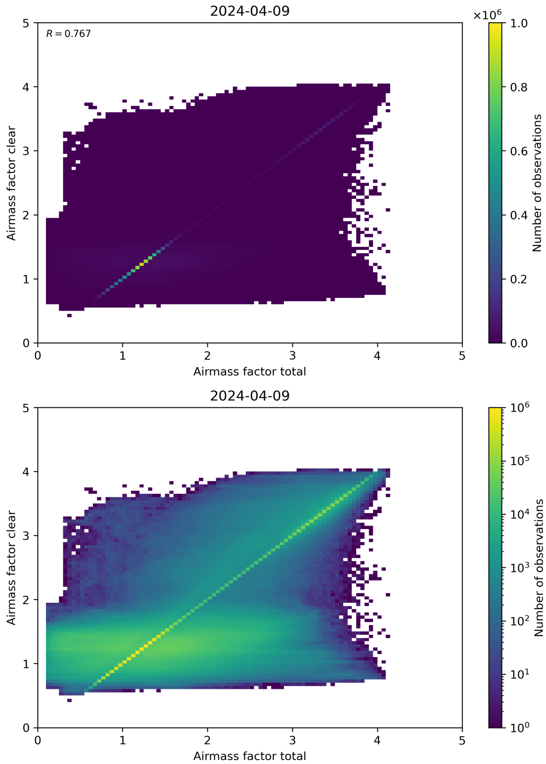
Figure 100: Scatter density plot of “Airmass factor total” against “Airmass factor clear” for 2024-04-08 to 2024-04-10.
