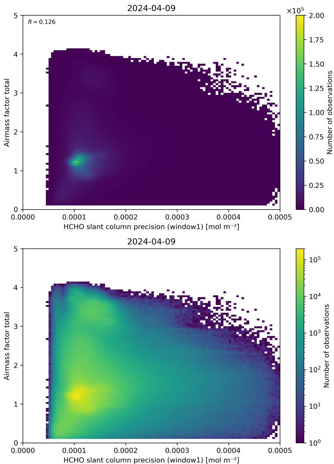
Figure 94: Scatter density plot of “HCHO slant column precision (window1)” against “Airmass factor total” for 2024-04-08 to 2024-04-10.
