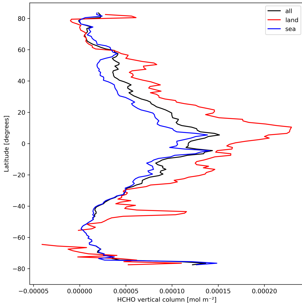
Figure 21: Zonal average of “HCHO vertical column” for 2024-04-08 to 2024-04-10.
