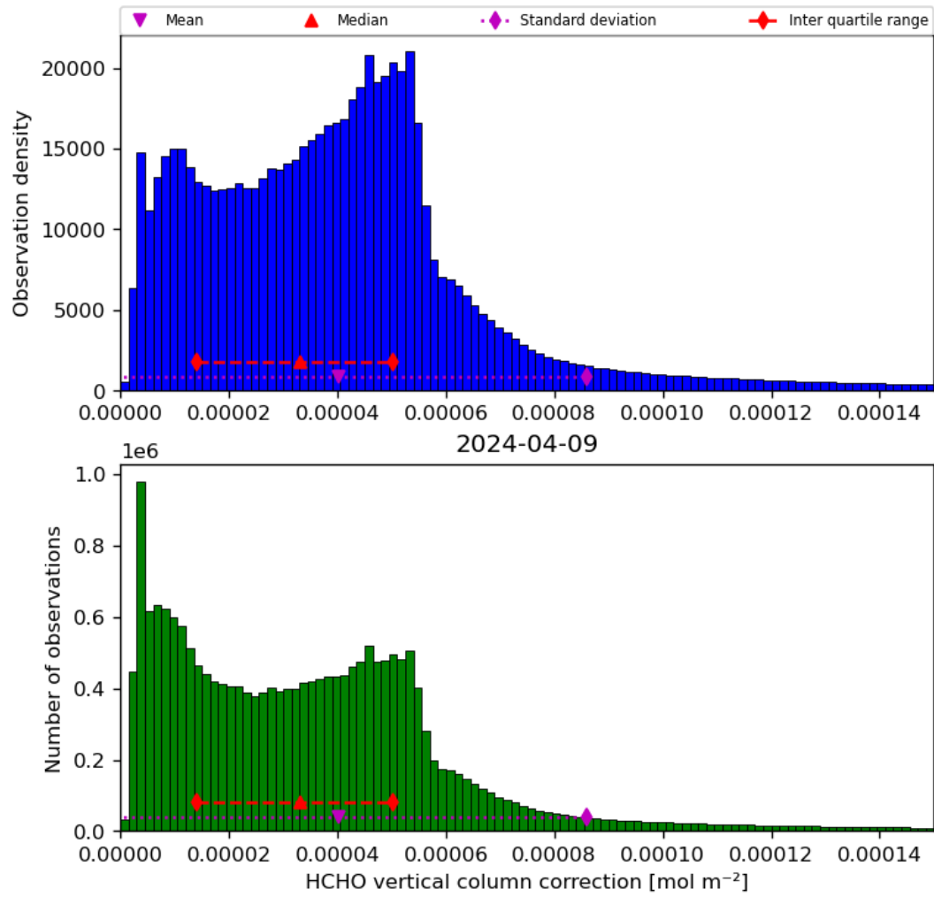
Figure 37: Histogram of “HCHO vertical column correction” for 2024-04-08 to 2024-04-10
