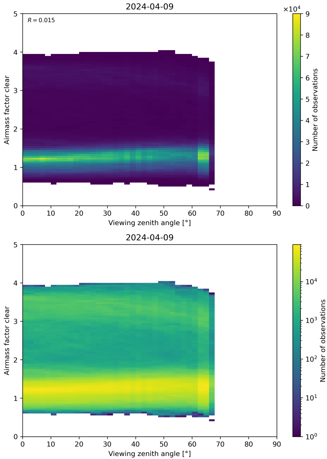
Figure 185: Scatter density plot of “Viewing zenith angle” against “Airmass factor clear” for 2024-04-08 to 2024-04-10.
