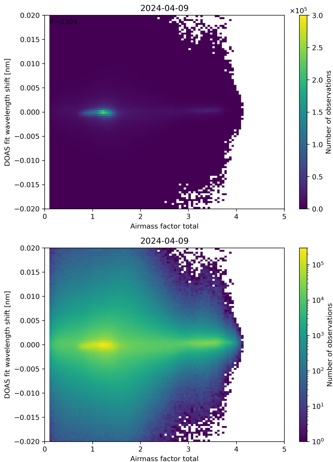
Figure 98: Scatter density plot of “Airmass factor total” against “DOAS fit wavelength shift” for 2024-04-08 to 2024-04-10.
