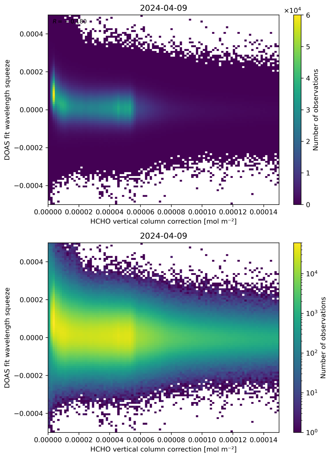
Figure 114: Scatter density plot of “HCHO vertical column correction” against “DOAS fit wavelength squeeze” for 2024-04-08 to 2024-04-10.
