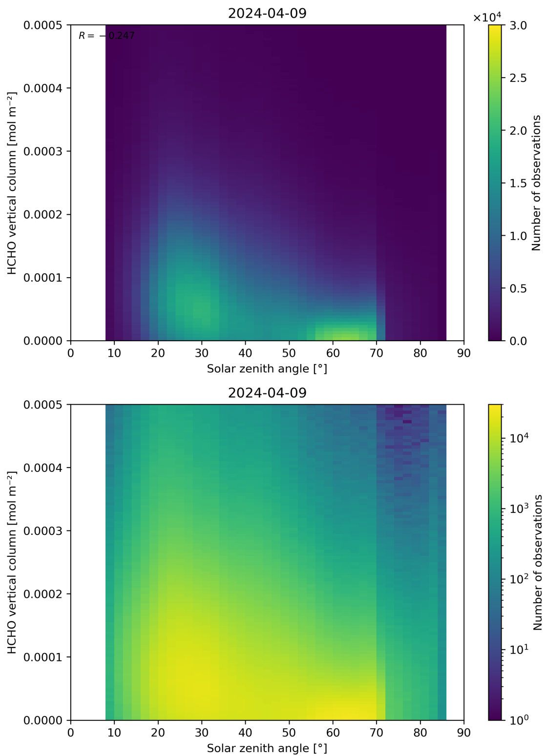
Figure 177: Scatter density plot of “Solar zenith angle” against “HCHO vertical column” for 2024-04-08 to 2024-04-10.
