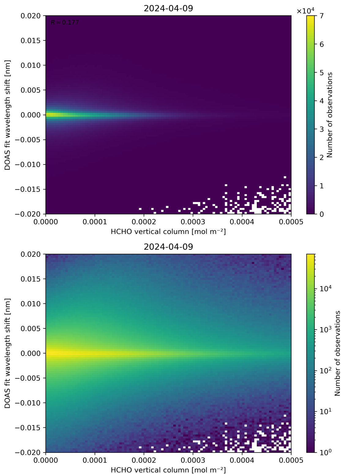
Figure 124: Scatter density plot of “HCHO vertical column” against “DOAS fit wavelength shift” for 2024-04-08 to 2024-04-10.
