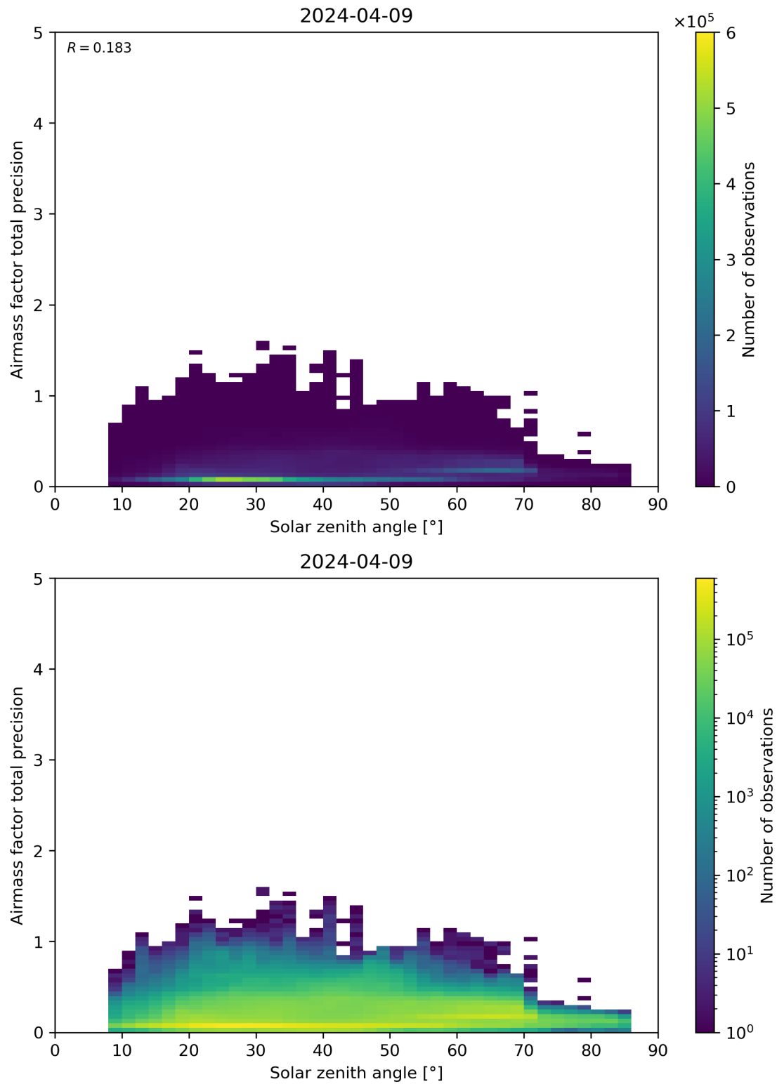
Figure 176: Scatter density plot of “Solar zenith angle” against “Airmass factor total precision” for 2024-04-08 to 2024-04-10.
