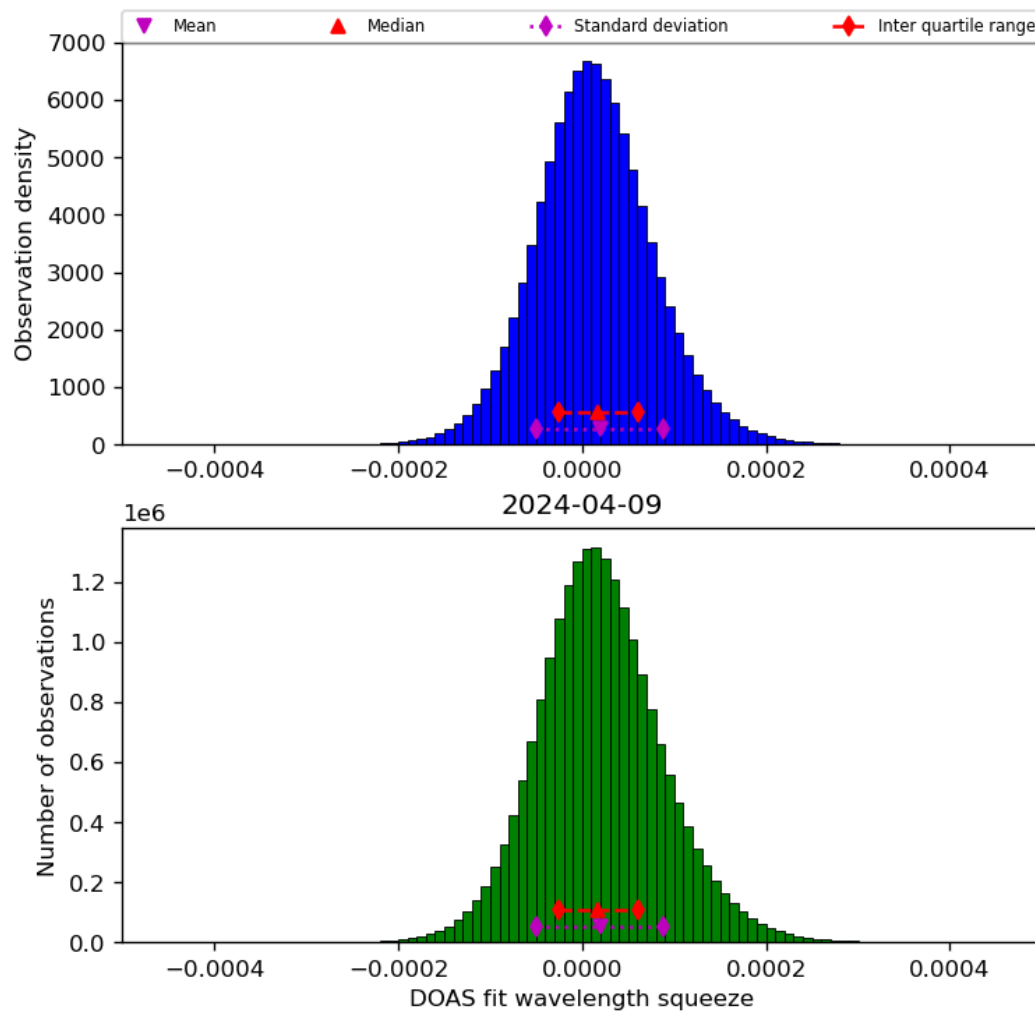
Figure 45: Histogram of “DOAS fit wavelength squeeze” for 2024-04-08 to 2024-04-10
