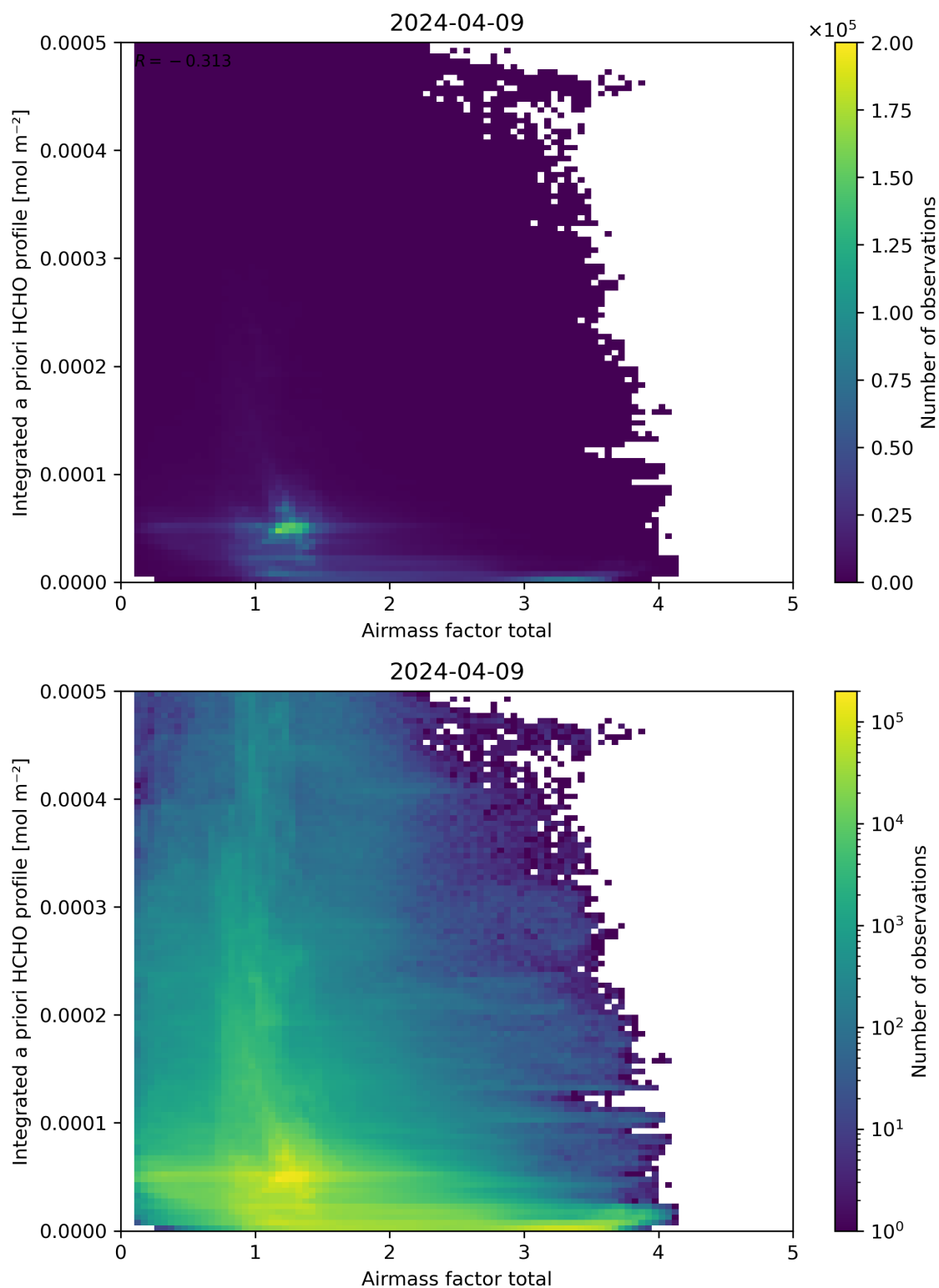
Figure 104: Scatter density plot of “Airmass factor total” against “Integrated a priori HCHO profile” for 2024-04-08 to 2024-04-10.
