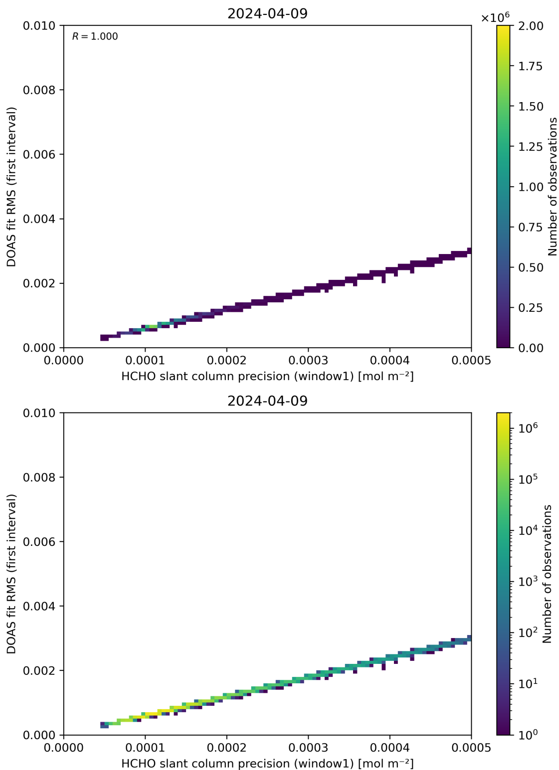
Figure 88: Scatter density plot of “HCHO slant column precision (window1)” against “DOAS fit RMS (first interval)” for 2024-04-08 to 2024-04-10.
