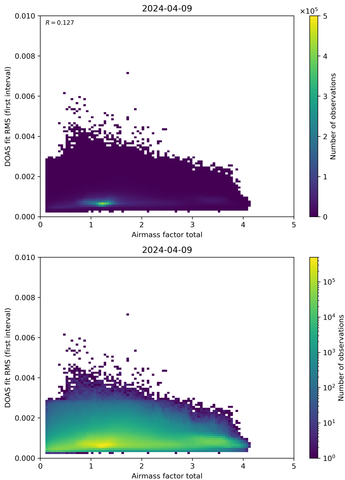
Figure 97: Scatter density plot of “Airmass factor total” against “DOAS fit RMS (first interval)” for 2024-04-08 to 2024-04-10.
