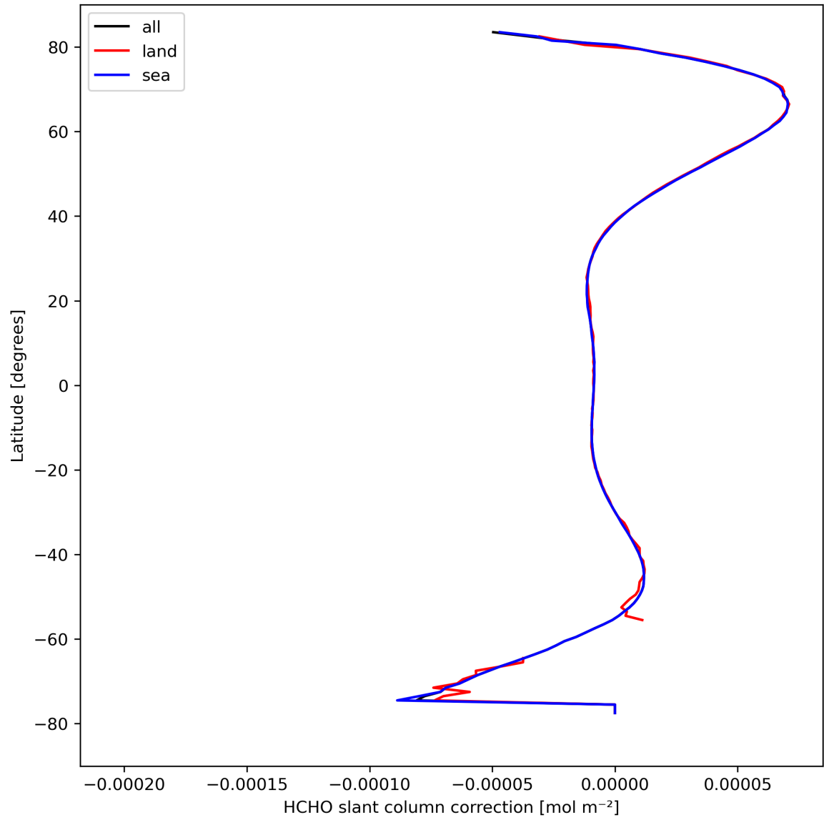
Figure 33: Zonal average of “HCHO slant column correction” for 2024-04-08 to 2024-04-10.
