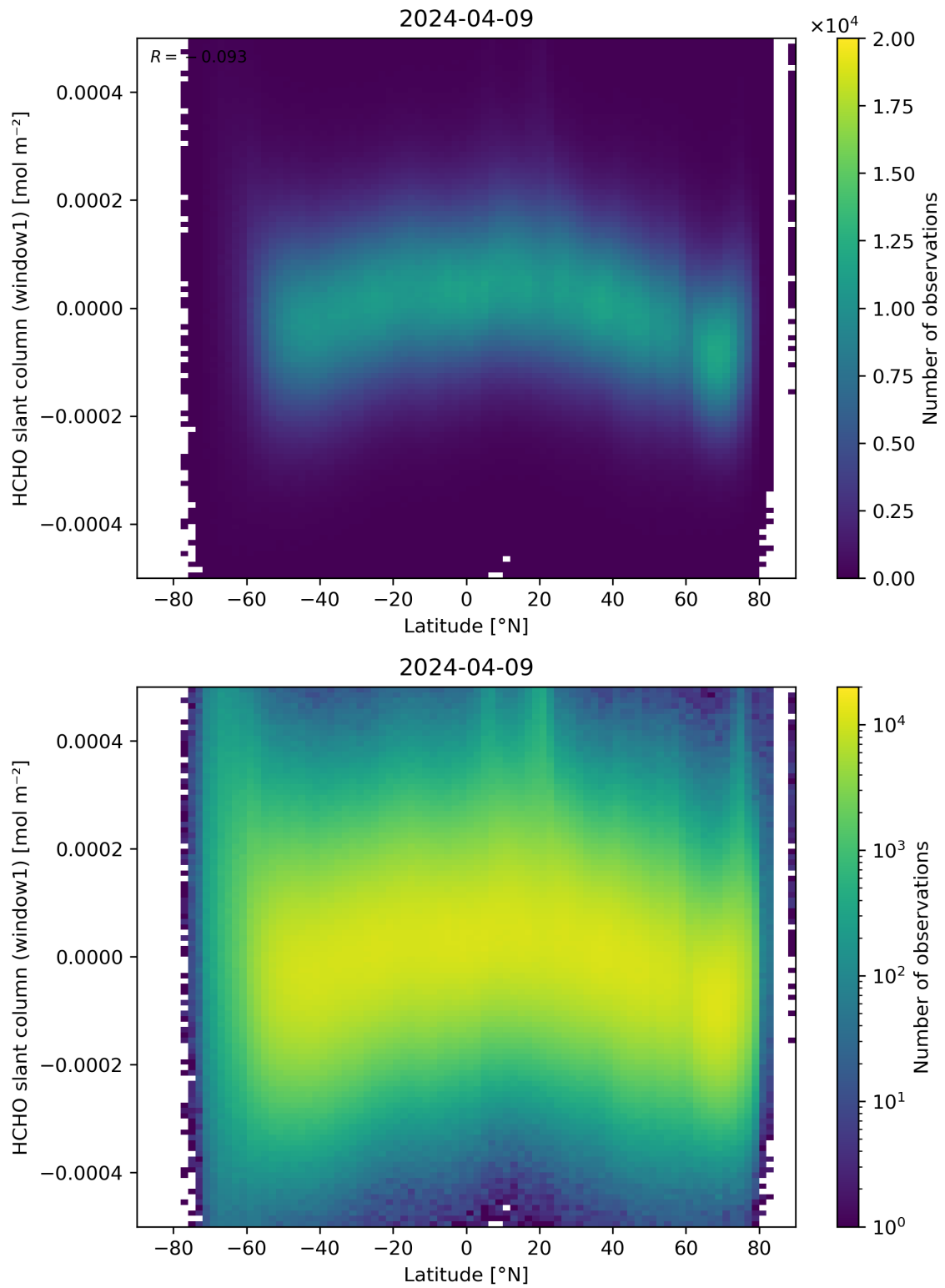
Figure 159: Scatter density plot of “Latitude” against “HCHO slant column (window1)” for 2024-04-08 to 2024-04-10.
