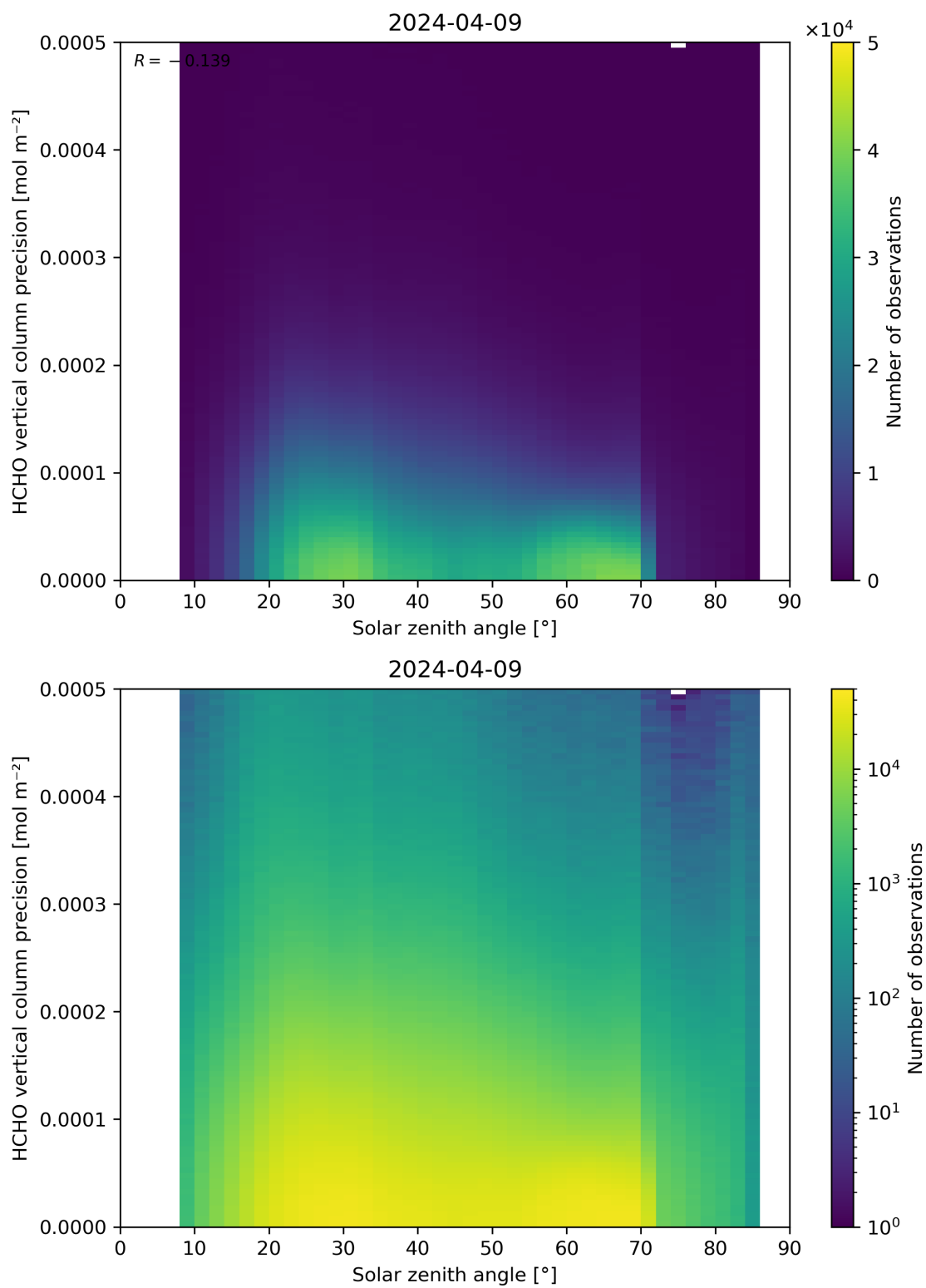
Figure 179: Scatter density plot of “Solar zenith angle” against “HCHO vertical column precision” for 2024-04-08 to 2024-04-10.
