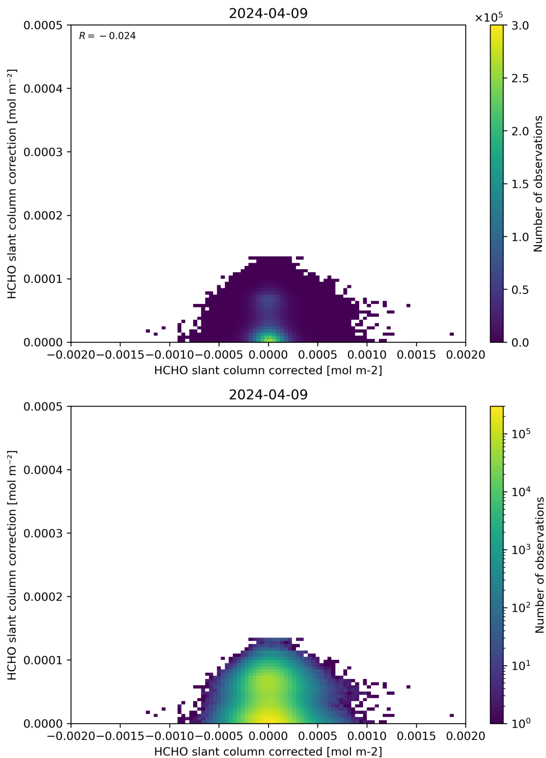
Figure 77: Scatter density plot of “HCHO slant column corrected” against “HCHO slant column correction” for 2024-04-08 to 2024-04-10.
