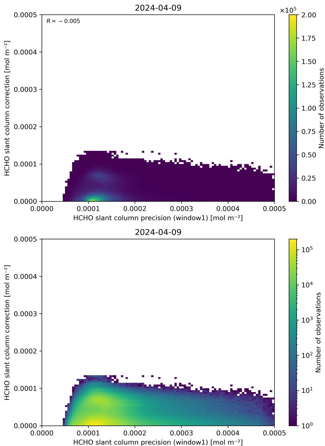
Figure 93: Scatter density plot of “HCHO slant column precision (window1)” against “HCHO slant column correction” for 2024-04-08 to 2024-04-10.
