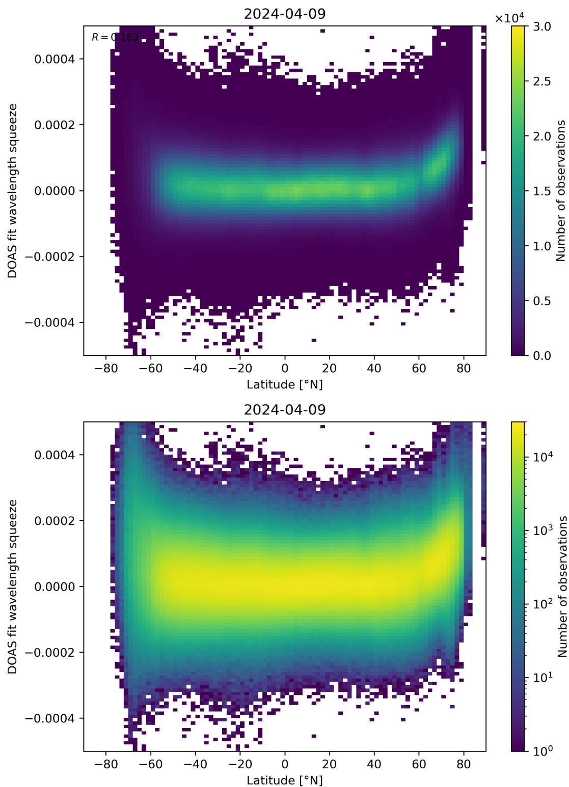
Figure 155: Scatter density plot of “Latitude” against “DOAS fit wavelength squeeze” for 2024-04-08 to 2024-04-10.
