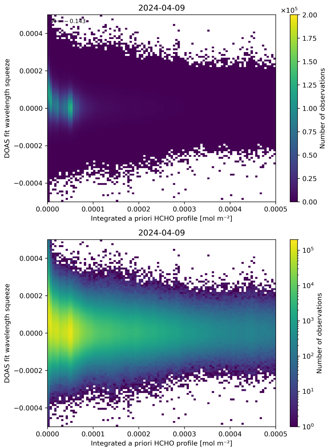
Figure 150: Scatter density plot of “Integrated a priori HCHO profile” against “DOAS fit wavelength squeeze” for 2024-04-08 to 2024-04-10.
