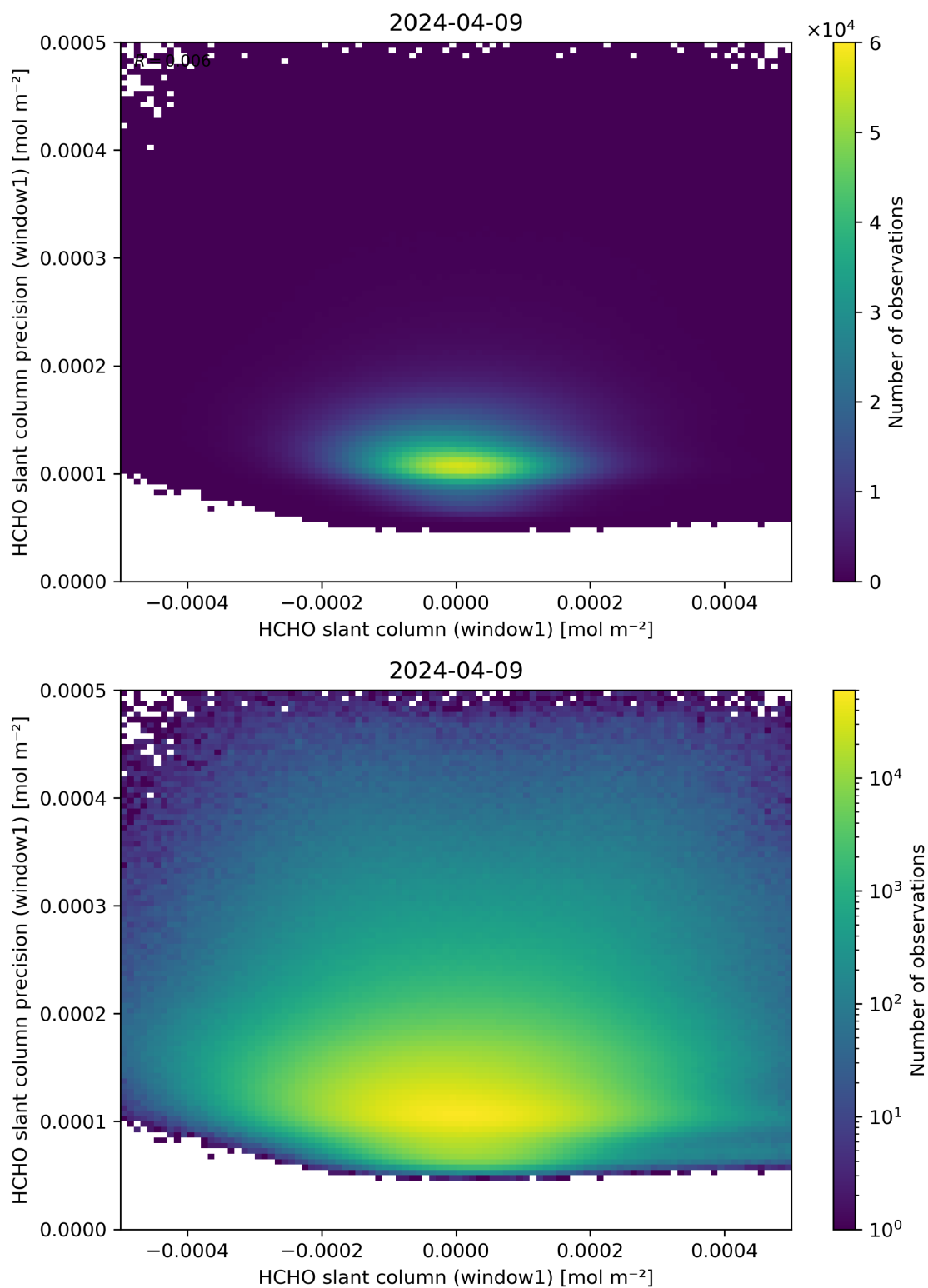
Figure 84: Scatter density plot of “HCHO slant column (window1)” against “HCHO slant column precision (window1)” for 2024-04-08 to 2024-04-10.
