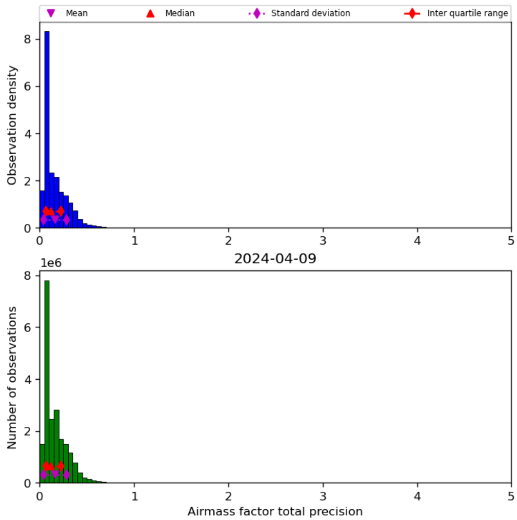
Figure 41: Histogram of “Airmass factor total precision” for 2024-04-08 to 2024-04-10
