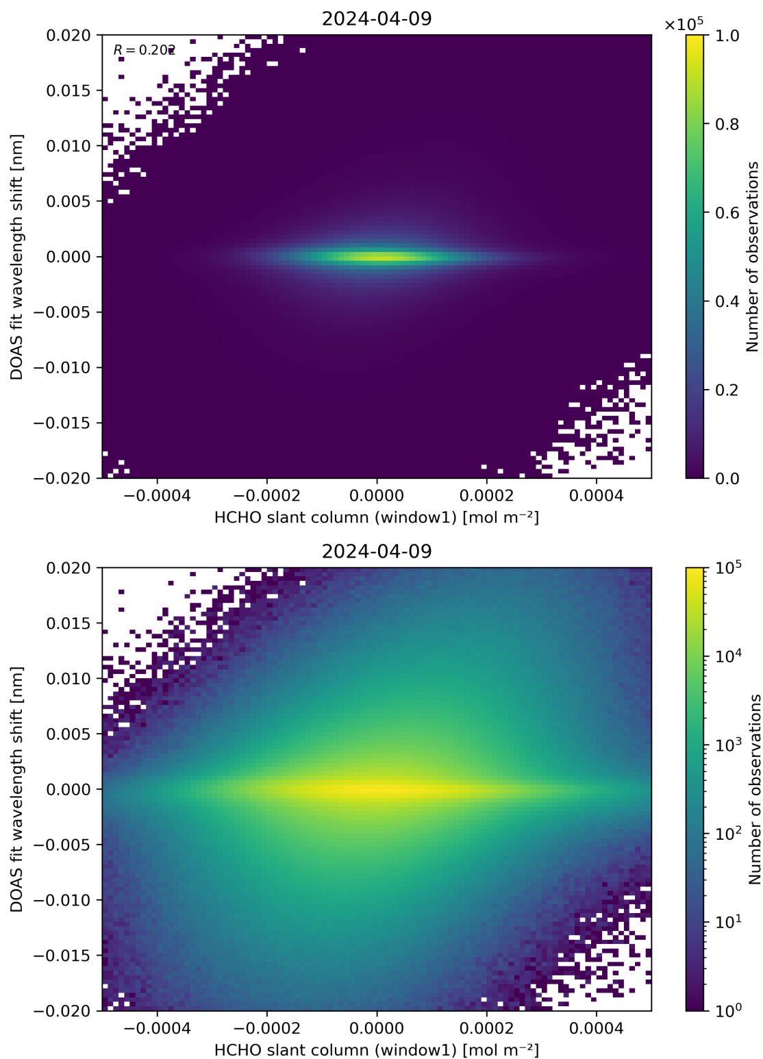
Figure 79: Scatter density plot of “HCHO slant column (window1)” against “DOAS fit wavelength shift” for 2024-04-08 to 2024-04-10.
