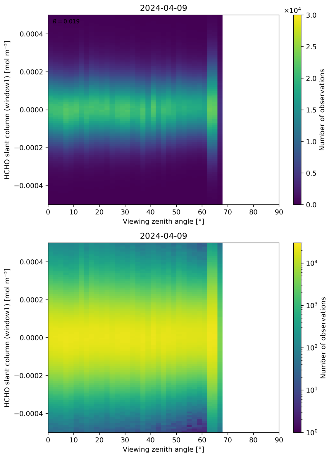
Figure 188: Scatter density plot of “Viewing zenith angle” against “HCHO slant column (window1)” for 2024-04-08 to 2024-04-10.
