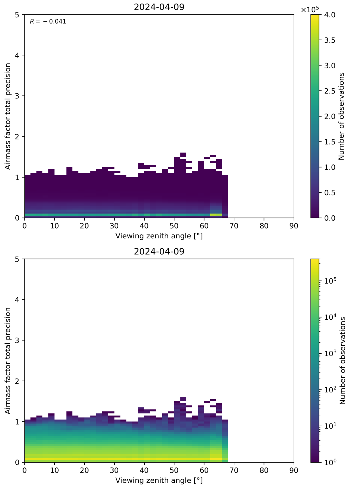
Figure 191: Scatter density plot of “Viewing zenith angle” against “Airmass factor total precision” for 2024-04-08 to 2024-04-10.
