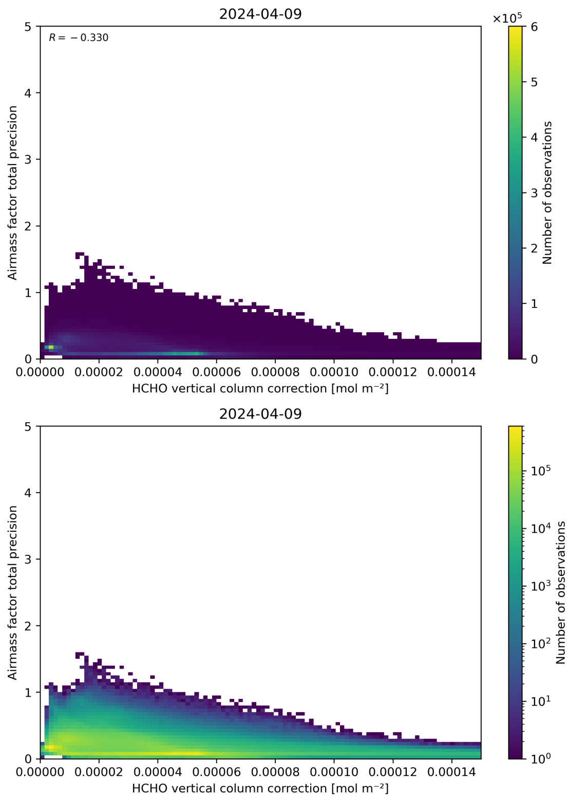
Figure 121: Scatter density plot of “HCHO vertical column correction” against “Airmass factor total precision” for 2024-04-08 to 2024-04-10.
