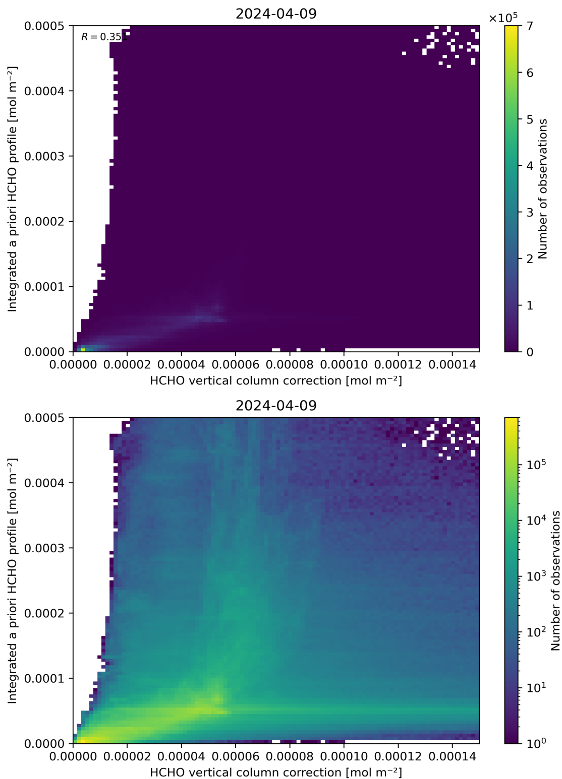
Figure 122: Scatter density plot of “HCHO vertical column correction” against “Integrated a priori HCHO profile” for 2024-04-08 to 2024-04-10.
