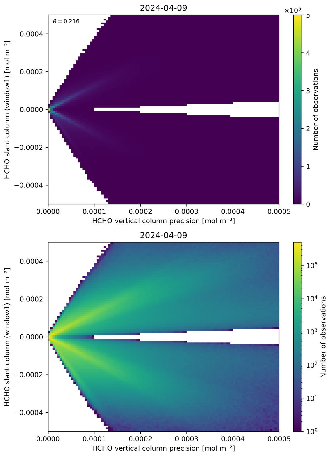
Figure 142: Scatter density plot of “HCHO vertical column precision” against “HCHO slant column (window1)” for 2024-04-08 to 2024-04-10.
