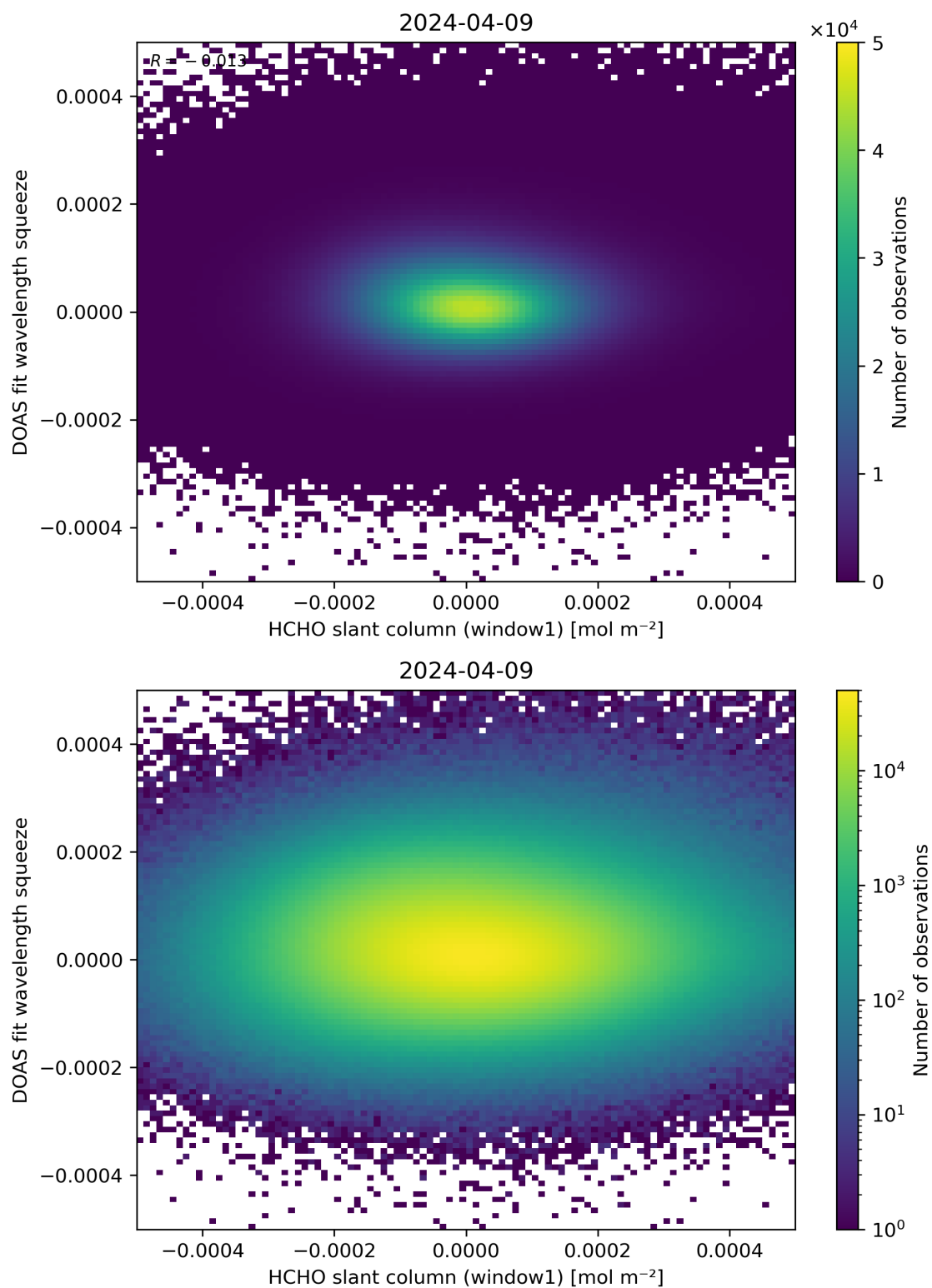
Figure 80: Scatter density plot of “HCHO slant column (window1)” against “DOAS fit wavelength squeeze” for 2024-04-08 to 2024-04-10.
