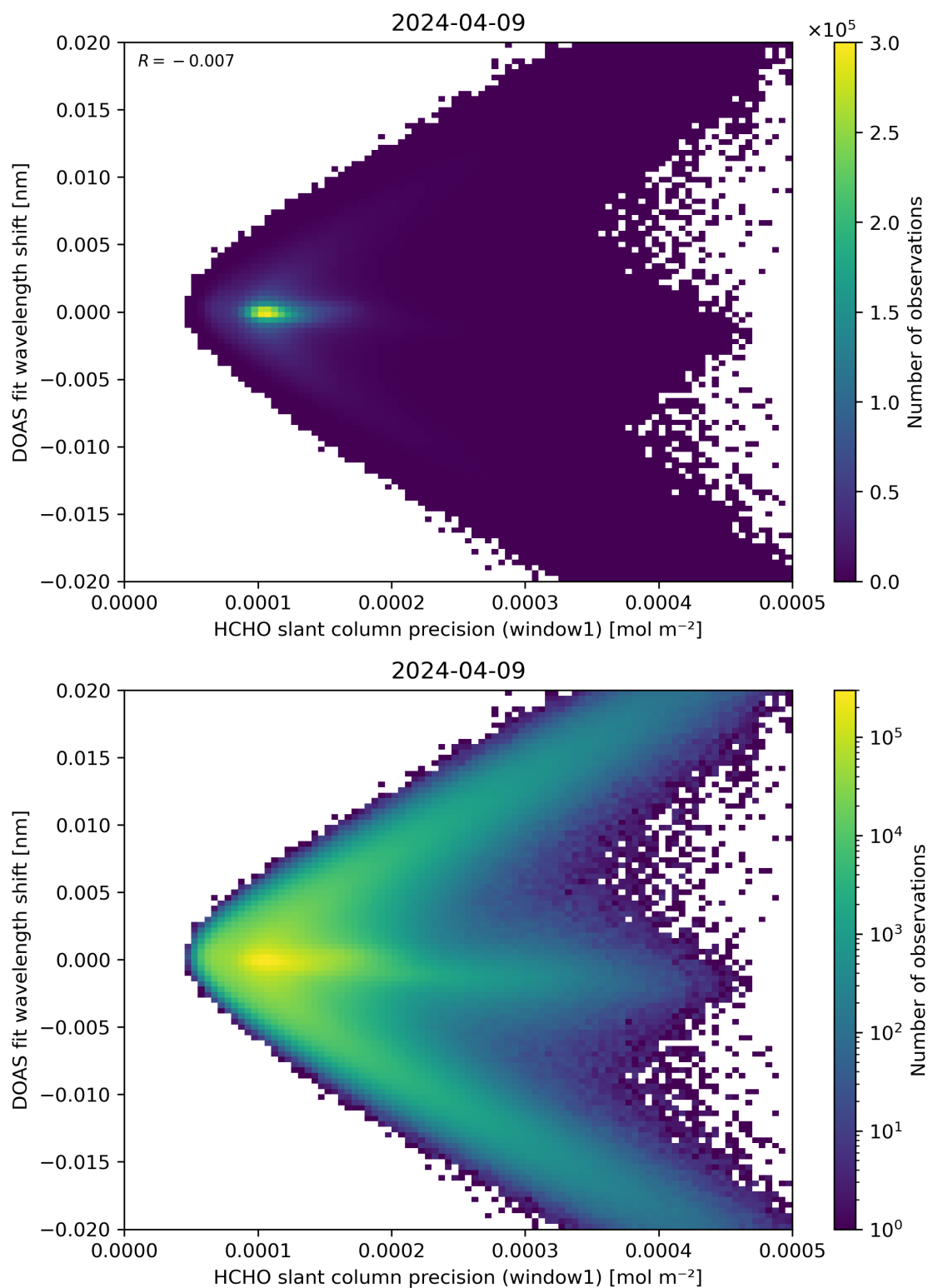
Figure 89: Scatter density plot of “HCHO slant column precision (window1)” against “DOAS fit wavelength shift” for 2024-04-08 to 2024-04-10.
