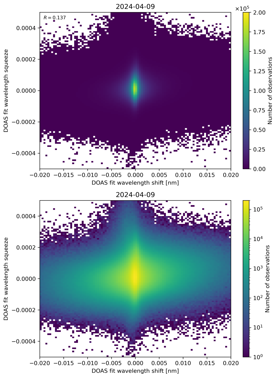
Figure 65: Scatter density plot of “DOAS fit wavelength shift” against “DOAS fit wavelength squeeze” for 2024-04-08 to 2024-04-10.
