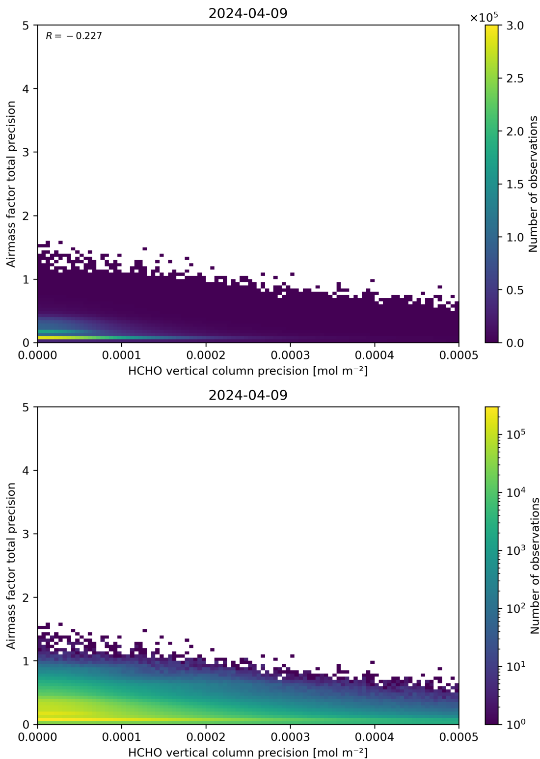
Figure 145: Scatter density plot of “HCHO vertical column precision” against “Airmass factor total precision” for 2024-04-08 to 2024-04-10.
