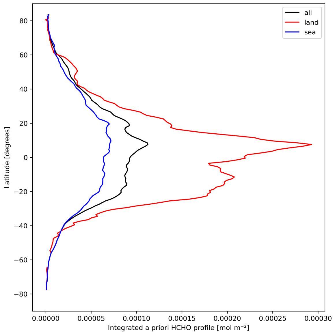
Figure 29: Zonal average of “Integrated a priori HCHO profile” for 2024-04-08 to 2024-04-10.
