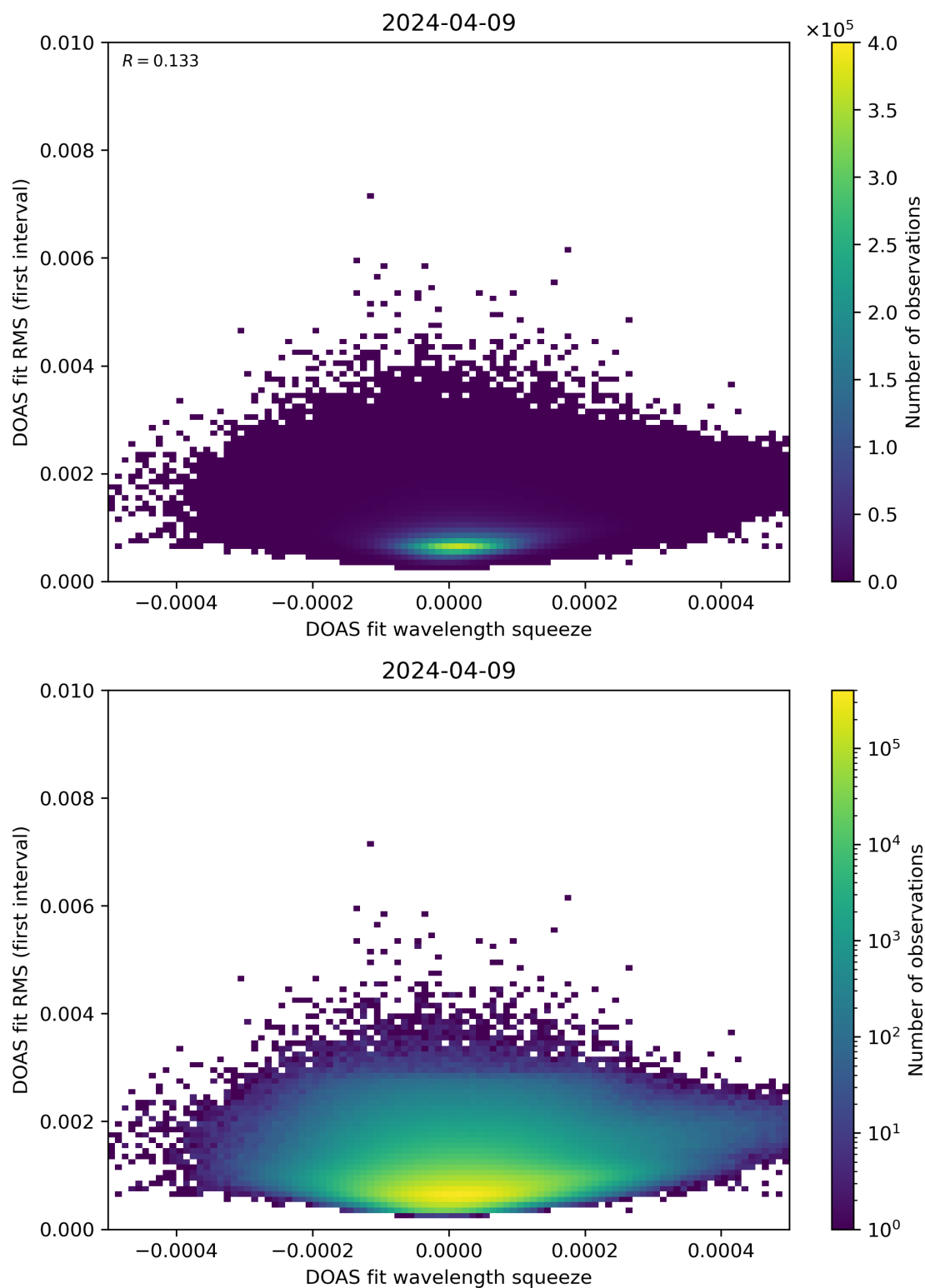
Figure 68: Scatter density plot of “DOAS fit wavelength squeeze” against “DOAS fit RMS (first interval)” for 2024-04-08 to 2024-04-10.
