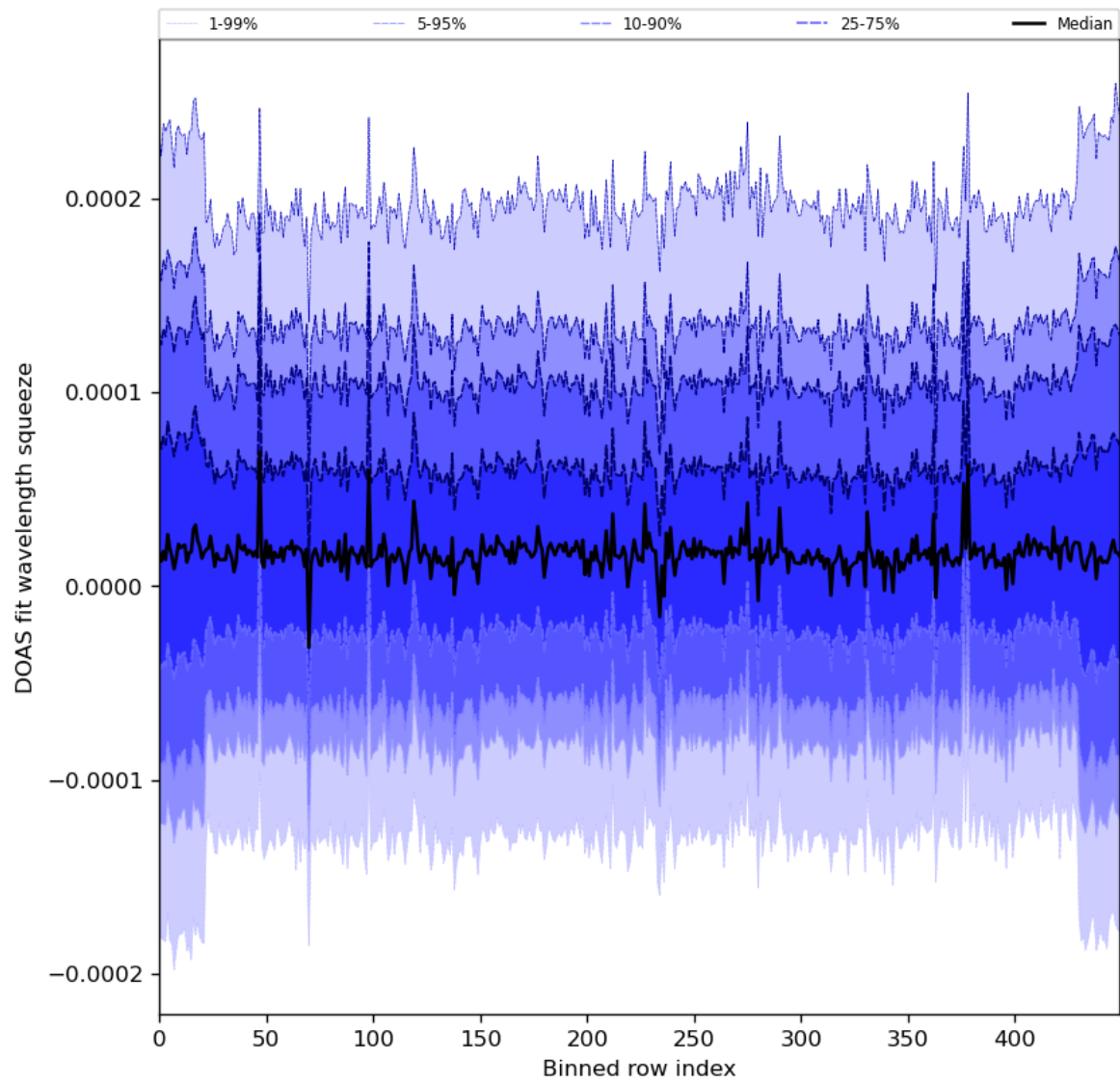
Figure 59: Along track statistics of “DOAS fit wavelength squeeze” for 2024-04-08 to 2024-04-10
