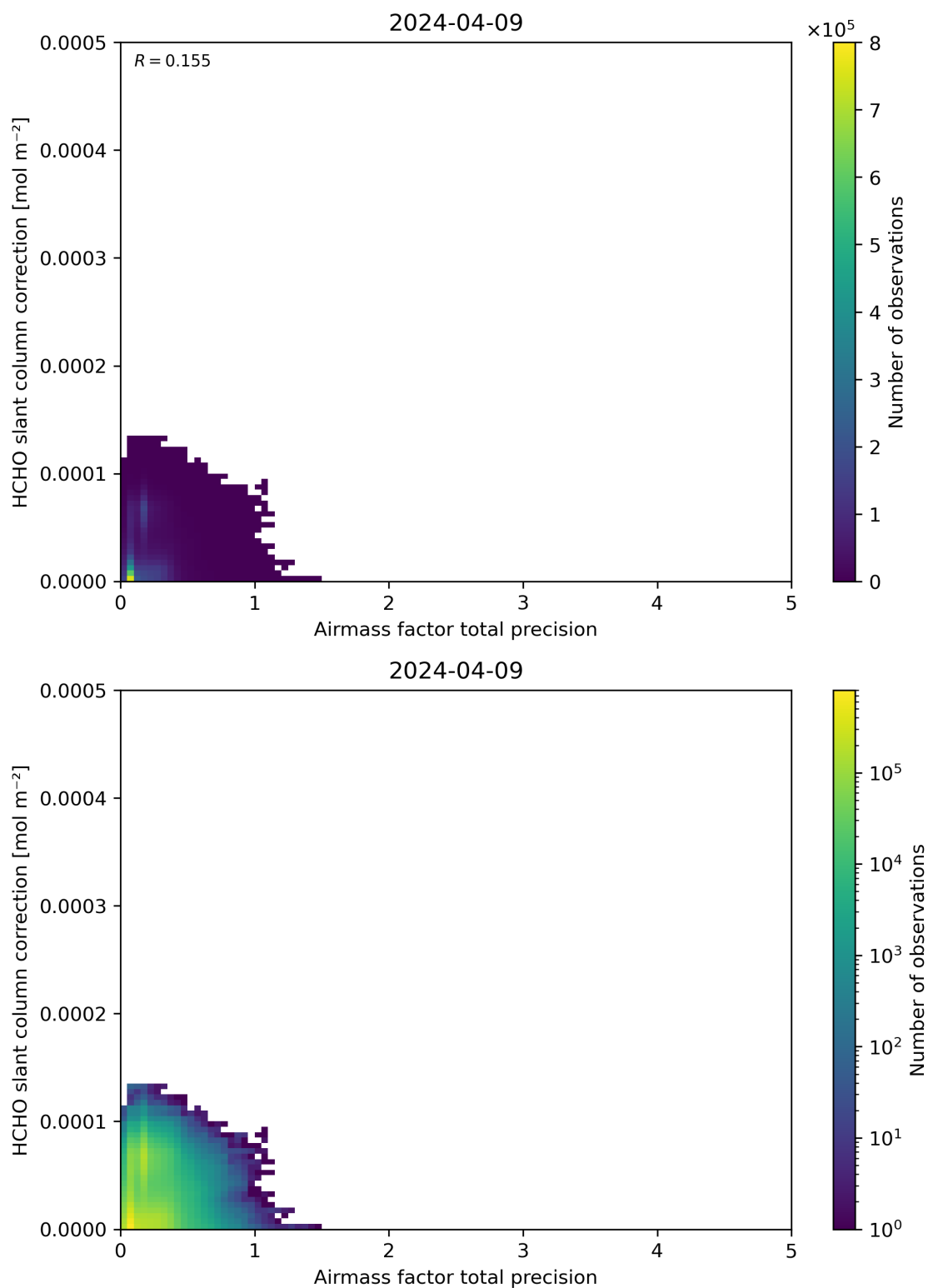
Figure 110: Scatter density plot of “Airmass factor total precision” against “HCHO slant column correction” for 2024-04-08 to 2024-04-10.
