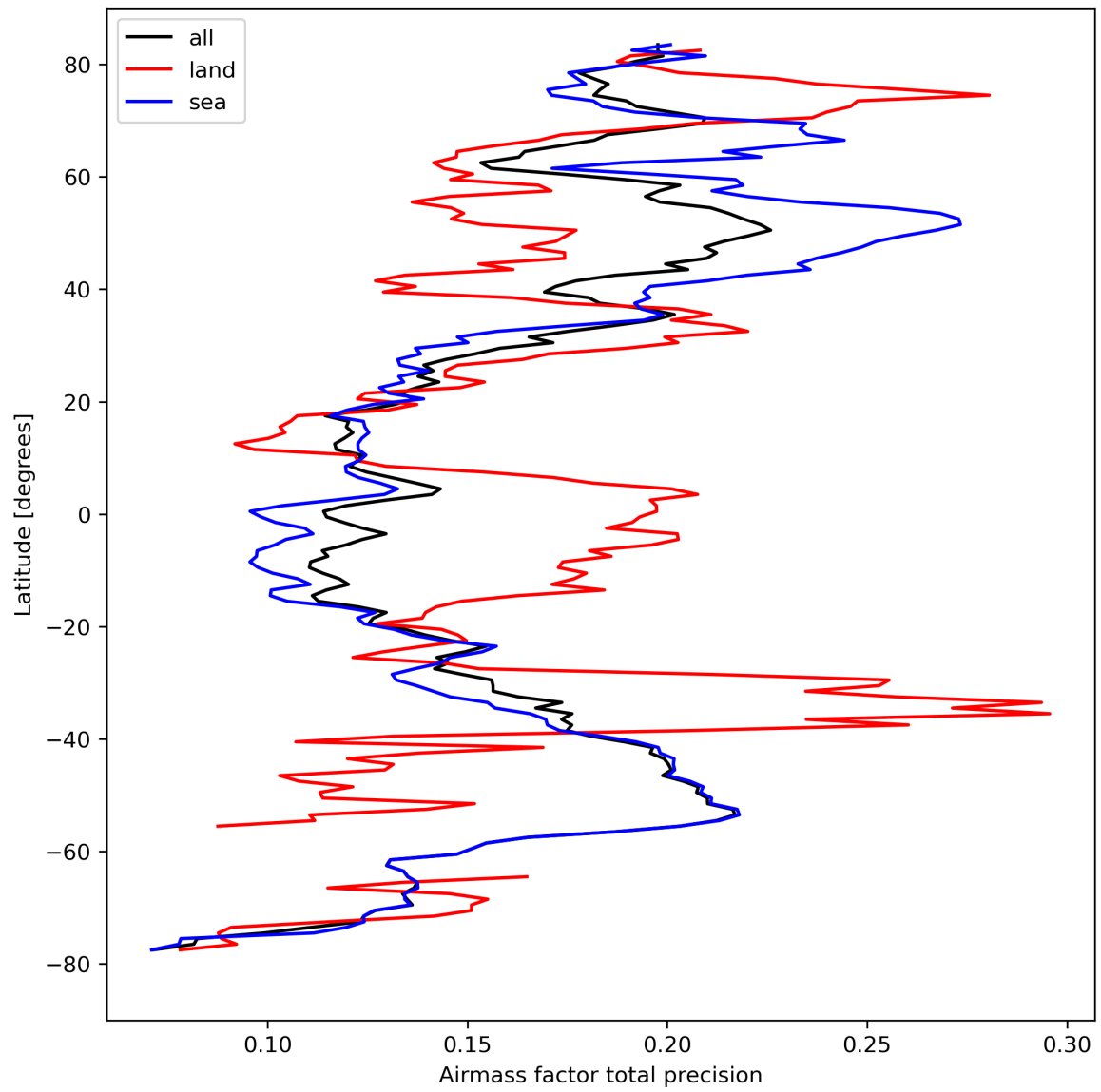
Figure 27: Zonal average of “Airmass factor total precision” for 2024-04-08 to 2024-04-10.
