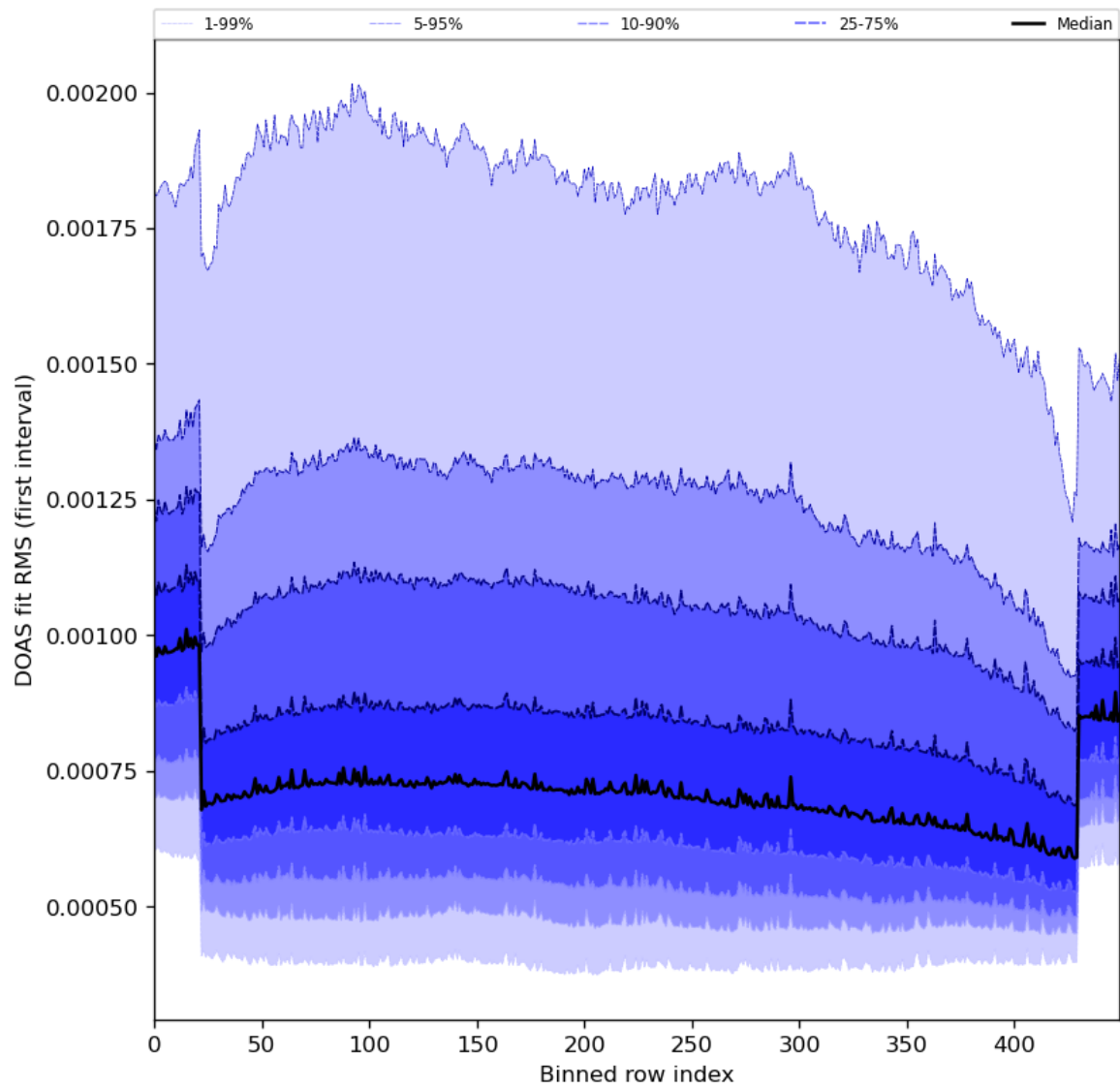
Figure 60: Along track statistics of “DOAS fit RMS (first interval)” for 2024-04-08 to 2024-04-10
