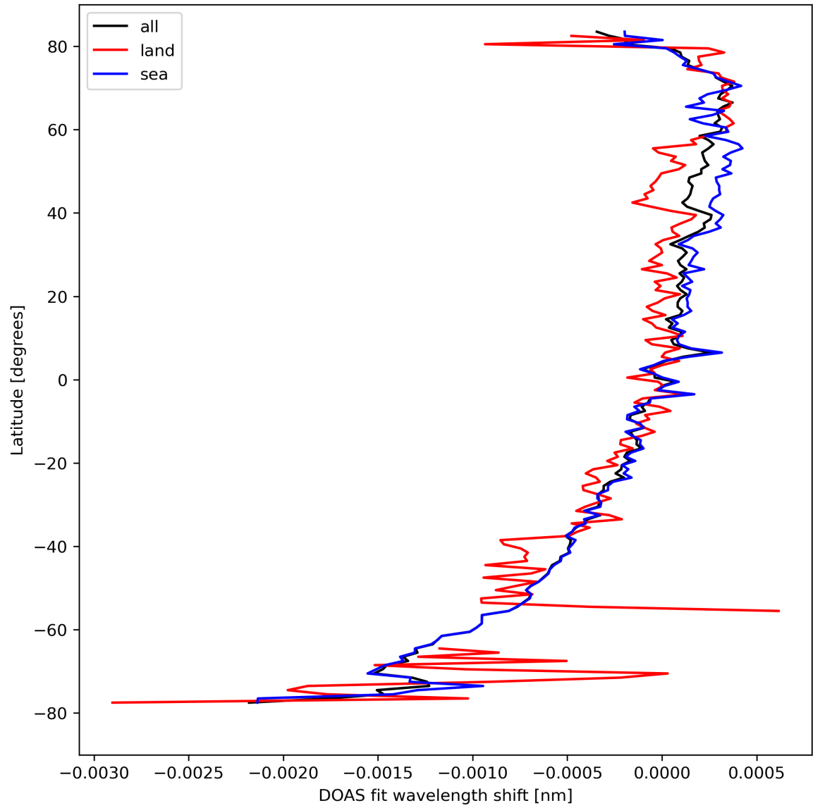
Figure 30: Zonal average of “DOAS fit wavelength shift” for 2024-04-08 to 2024-04-10.
