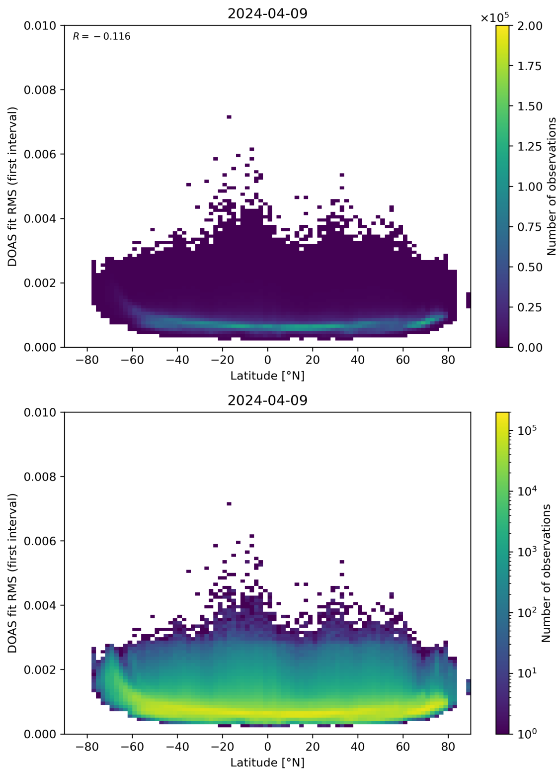
Figure 153: Scatter density plot of “Latitude” against “DOAS fit RMS (first interval)” for 2024-04-08 to 2024-04-10.
