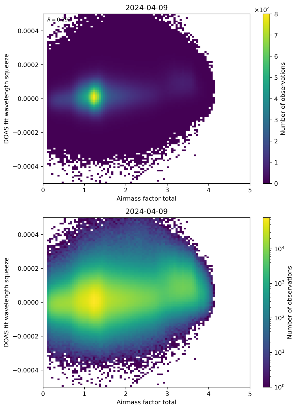
Figure 99: Scatter density plot of “Airmass factor total” against “DOAS fit wavelength squeeze” for 2024-04-08 to 2024-04-10.
