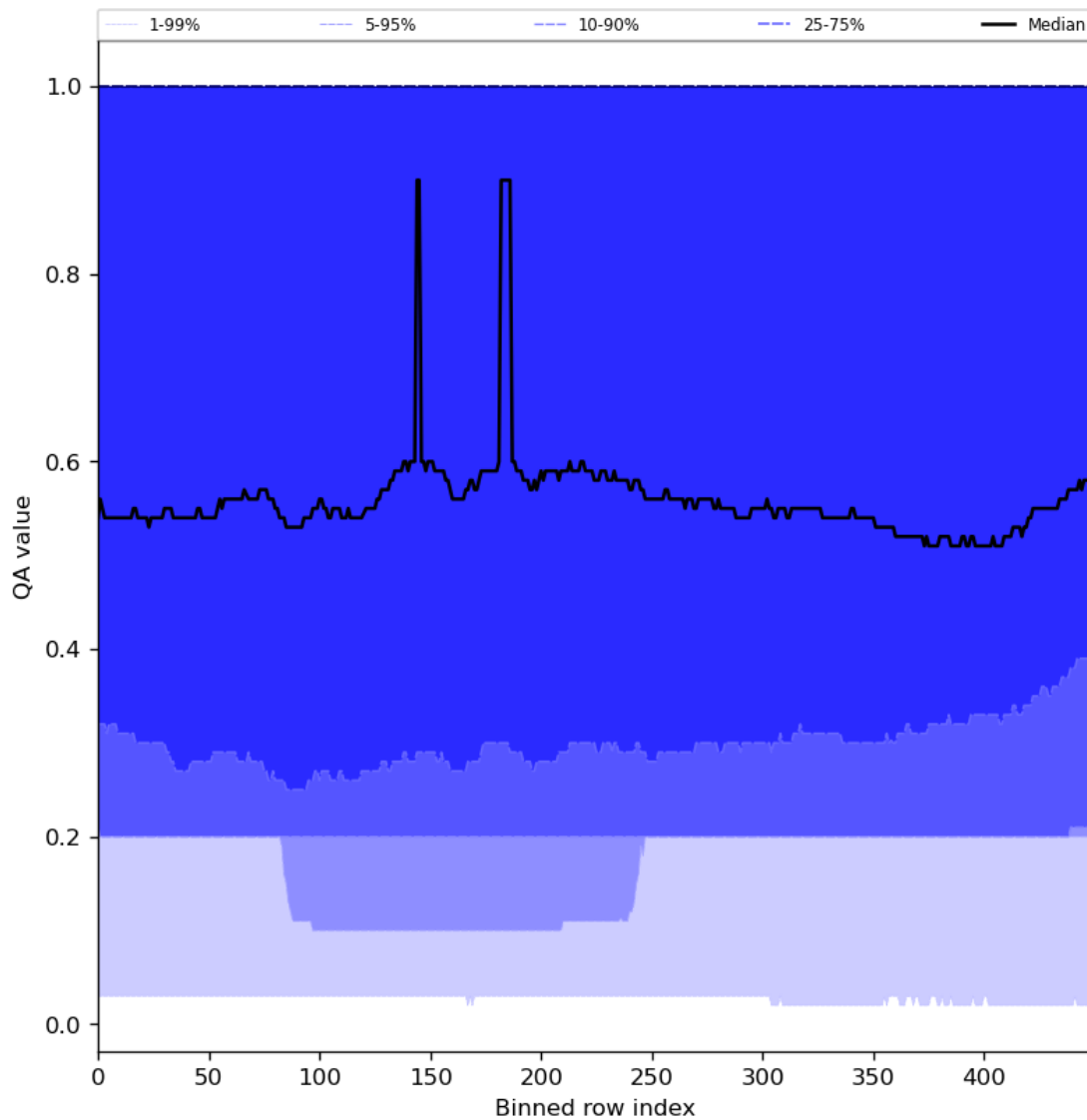
Figure 48: Along track statistics of “QA value” for 2024-04-08 to 2024-04-10
