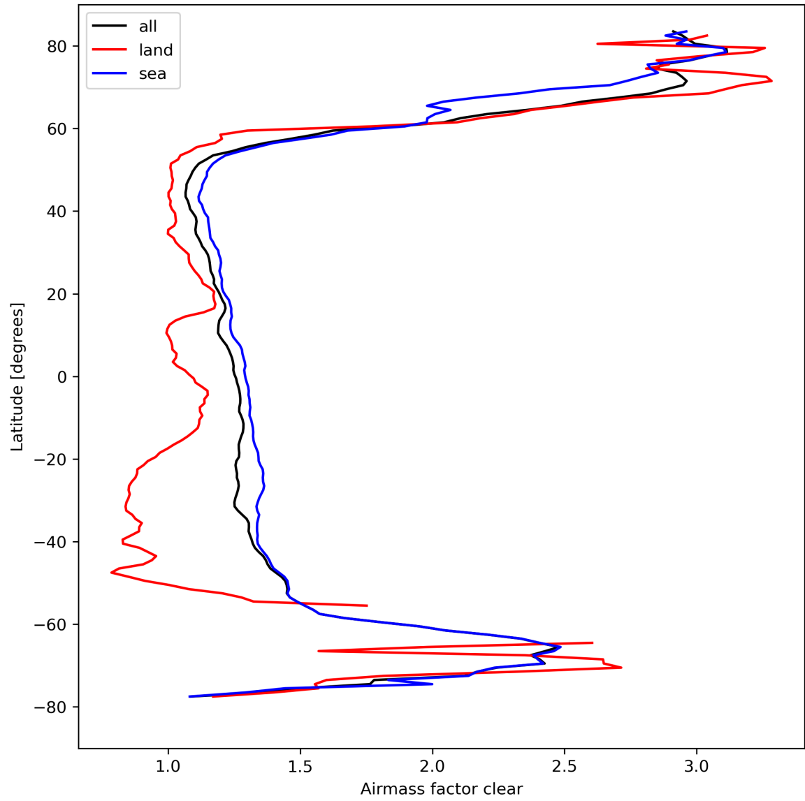
Figure 28: Zonal average of “Airmass factor clear” for 2024-04-08 to 2024-04-10.
