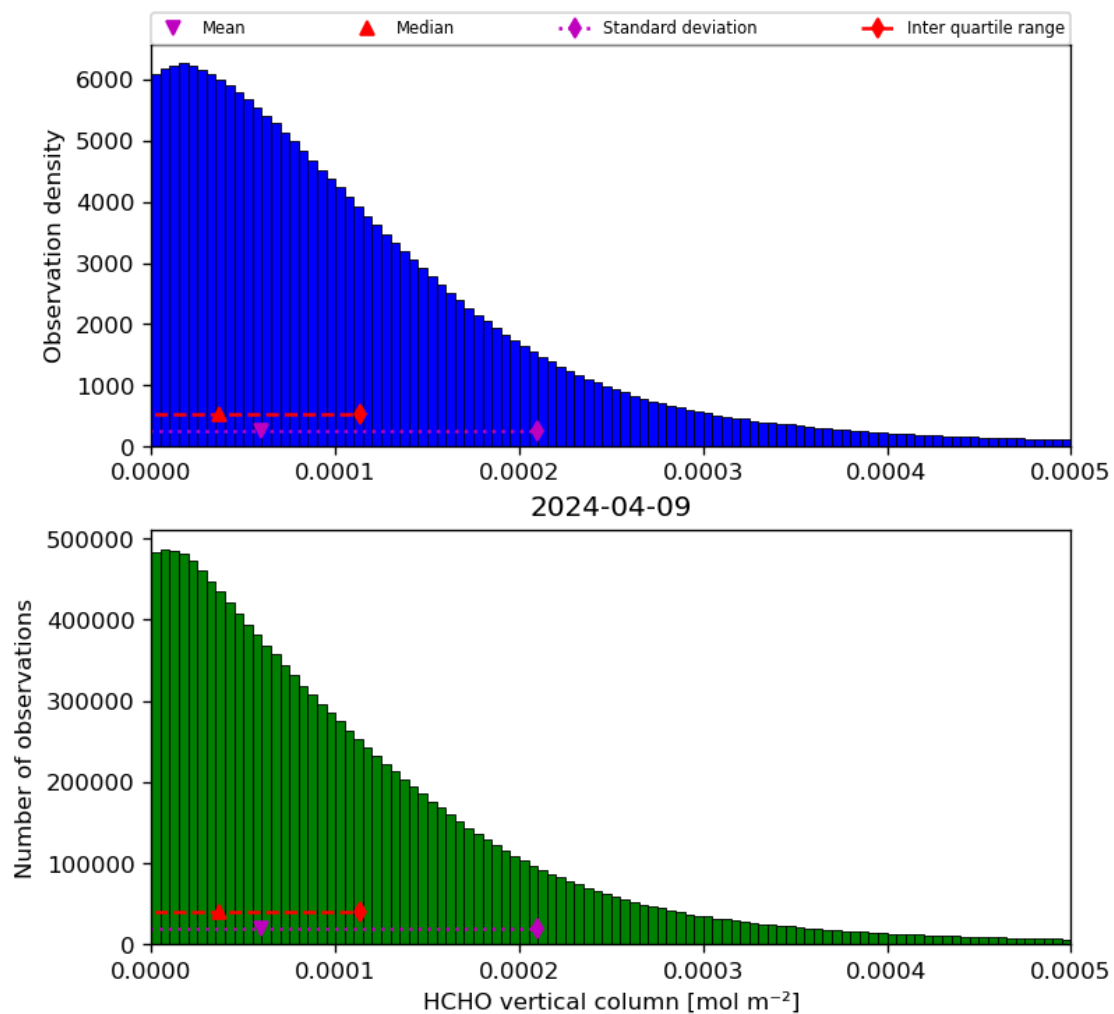
Figure 35: Histogram of “HCHO vertical column” for 2024-04-08 to 2024-04-10
