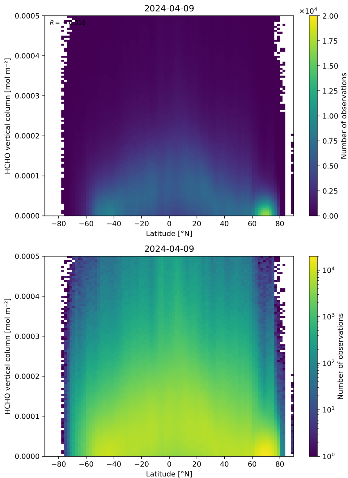
Figure 163: Scatter density plot of “Latitude” against “HCHO vertical column” for 2024-04-08 to 2024-04-10.
