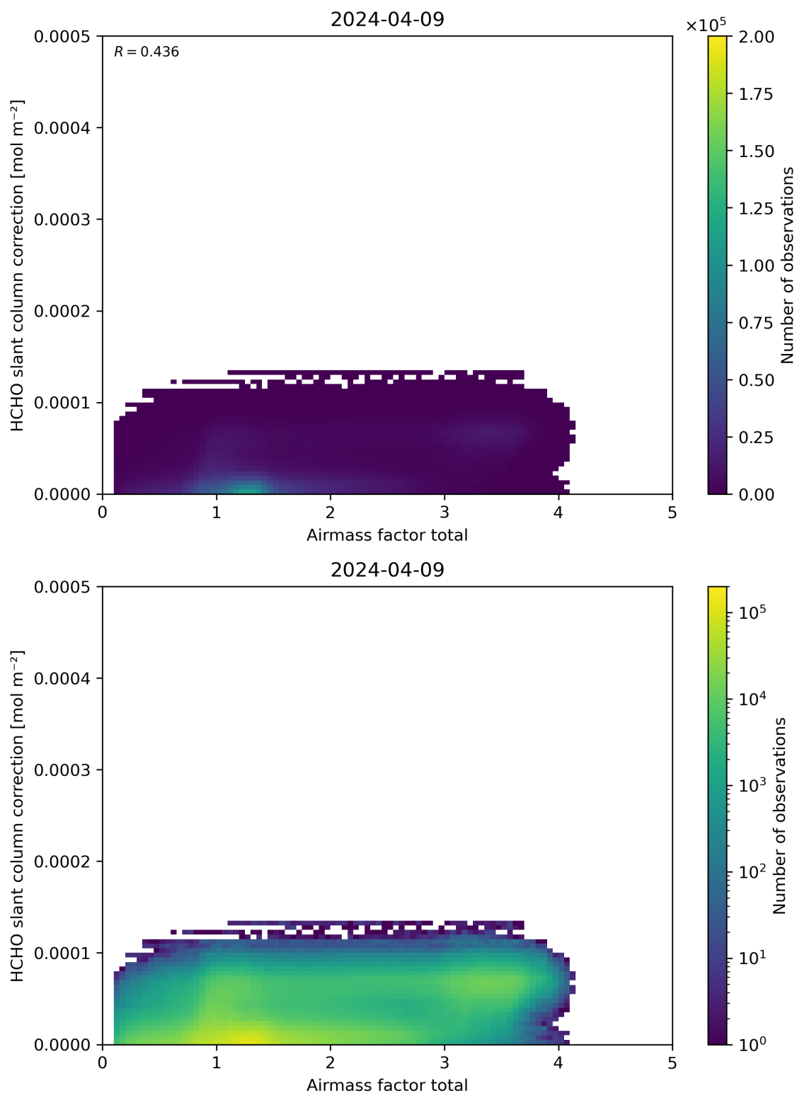
Figure 102: Scatter density plot of “Airmass factor total” against “HCHO slant column correction” for 2024-04-08 to 2024-04-10.
