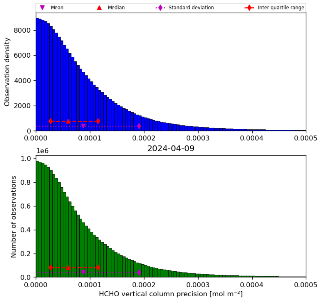
Figure 36: Histogram of “HCHO vertical column precision” for 2024-04-08 to 2024-04-10
