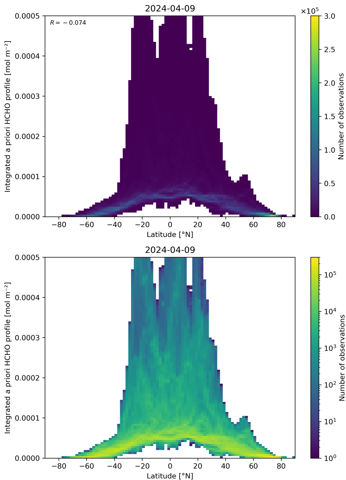
Figure 166: Scatter density plot of “Latitude” against “Integrated a priori HCHO profile” for 2024-04-08 to 2024-04-10.
