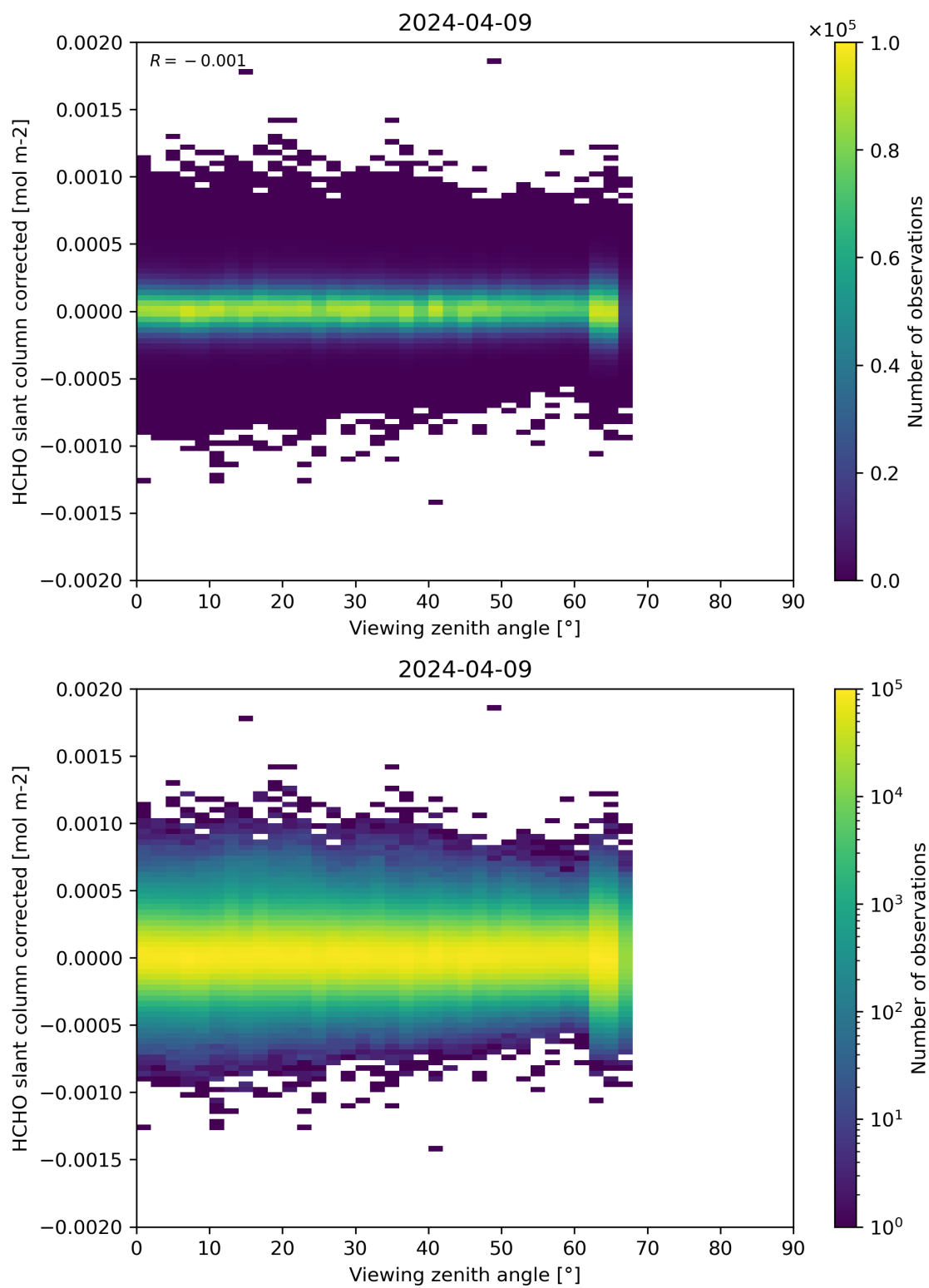
Figure 186: Scatter density plot of “Viewing zenith angle” against “HCHO slant column corrected” for 2024-04-08 to 2024-04-10.
