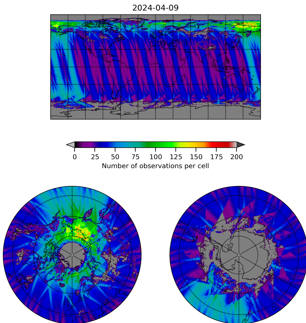
Figure 19: Map of the number of observations for 2024-04-08 to 2024-04-10
