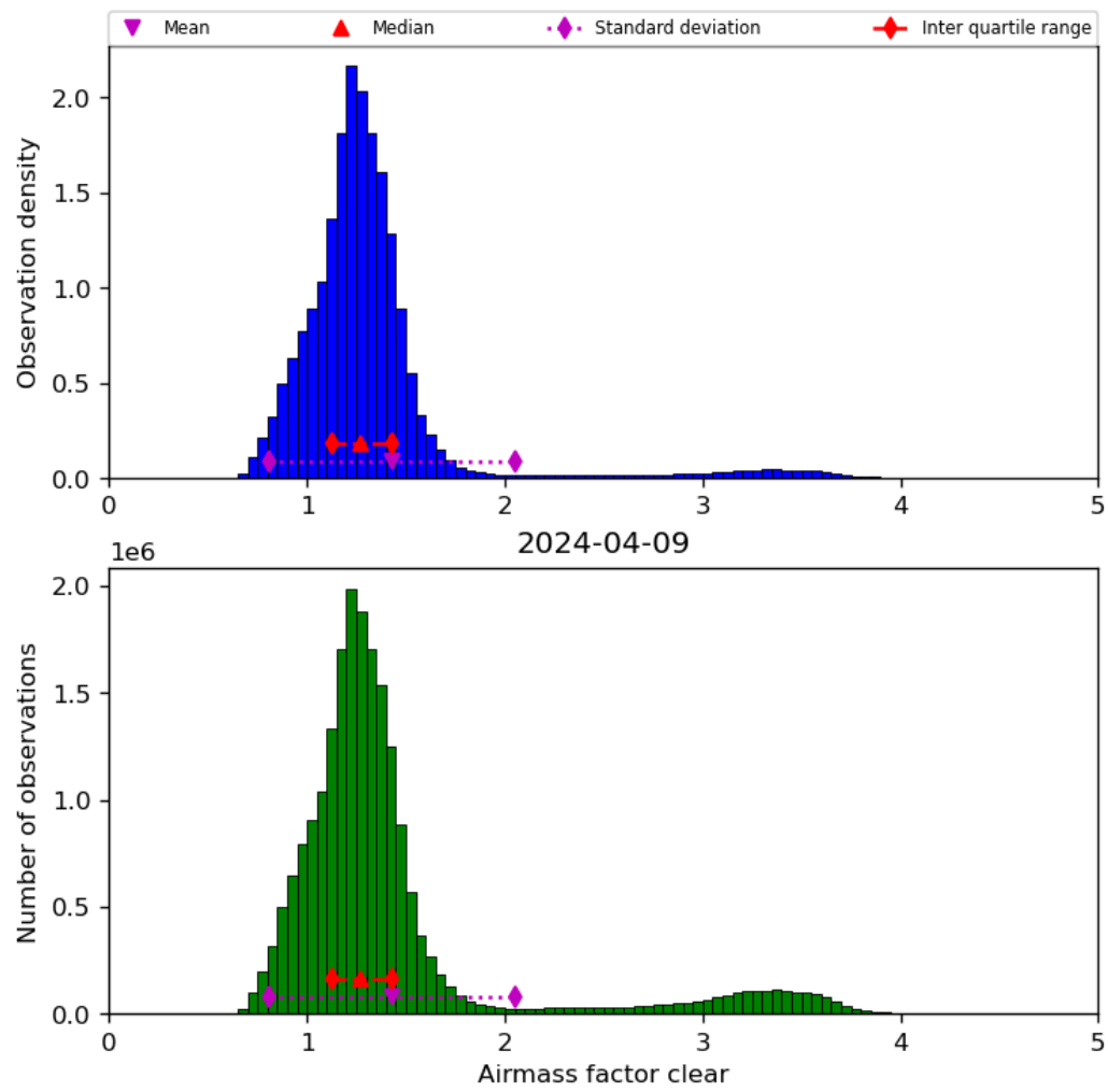
Figure 42: Histogram of “Airmass factor clear” for 2024-04-08 to 2024-04-10
