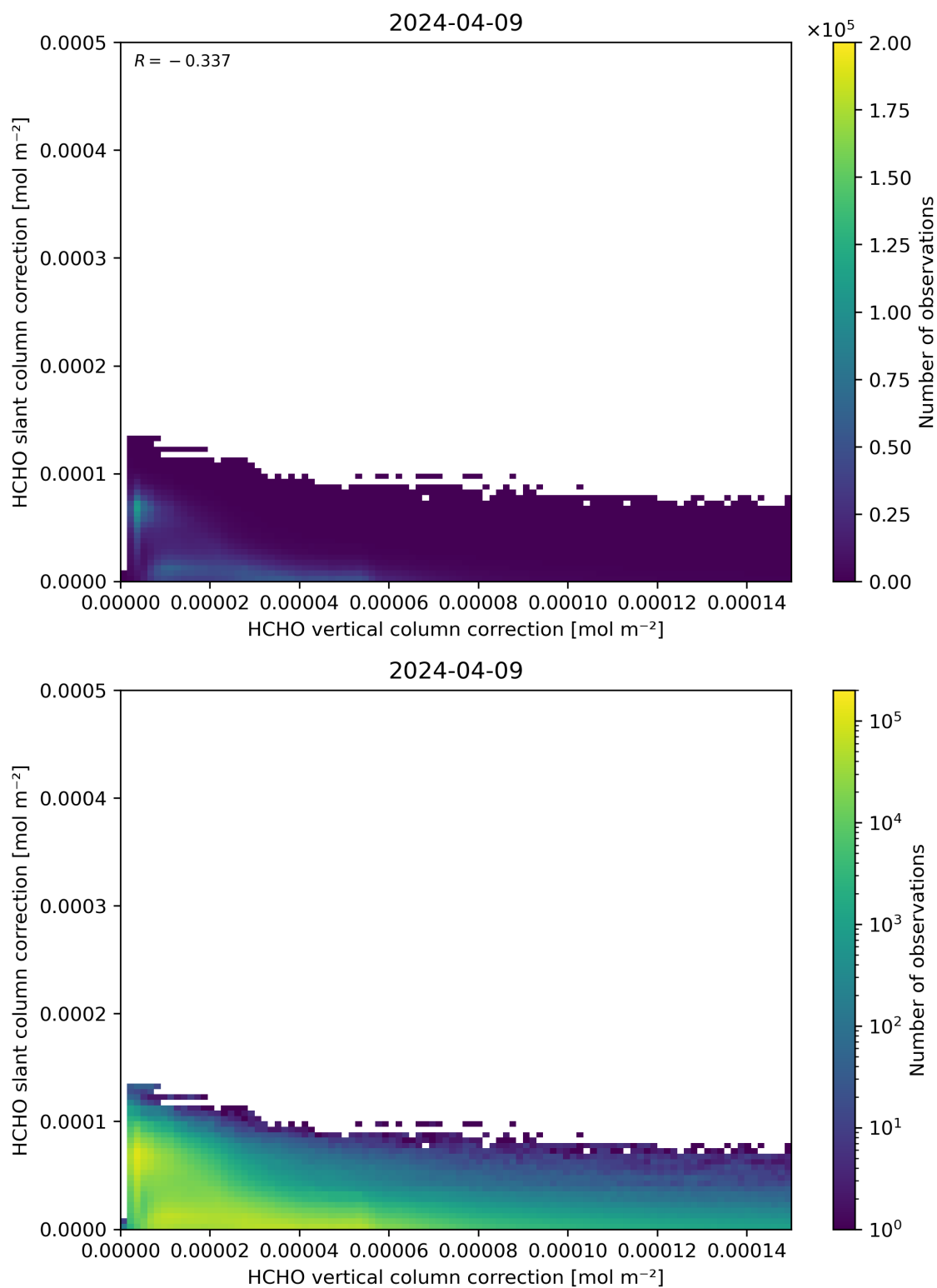
Figure 117: Scatter density plot of “HCHO vertical column correction” against “HCHO slant column correction” for 2024-04-08 to 2024-04-10.
