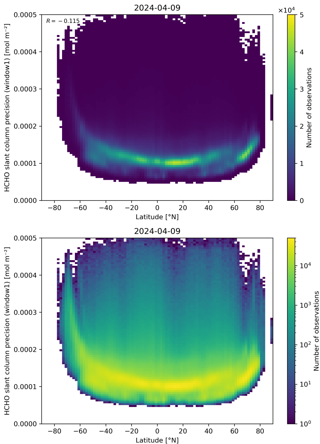
Figure 160: Scatter density plot of “Latitude” against “HCHO slant column precision (window1)” for 2024-04-08 to 2024-04-10.
