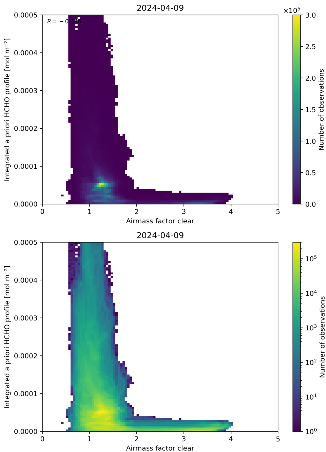
Figure 76: Scatter density plot of “Airmass factor clear” against “Integrated a priori HCHO profile” for 2024-04-08 to 2024-04-10.
