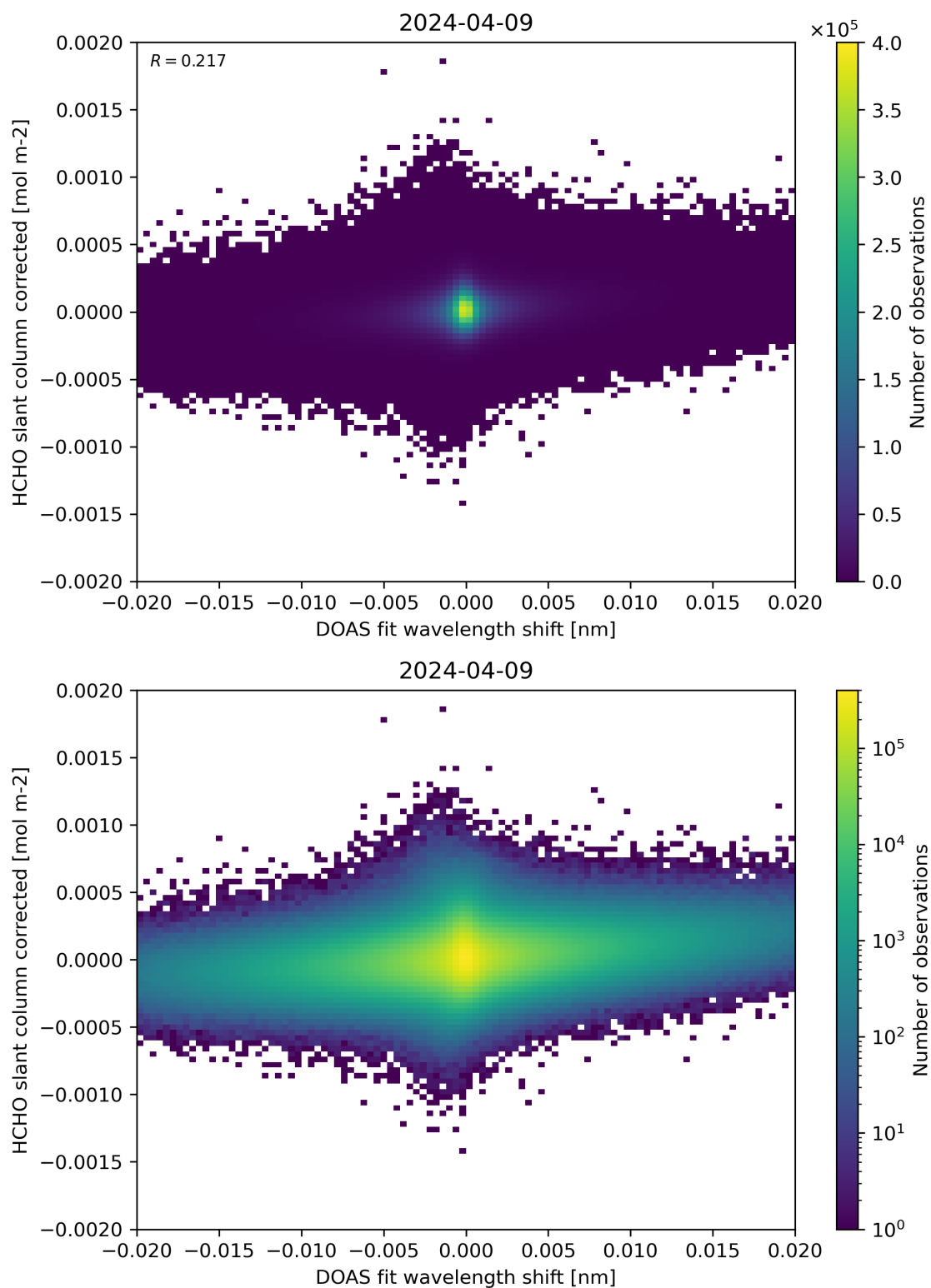
Figure 66: Scatter density plot of “DOAS fit wavelength shift” against “HCHO slant column corrected” for 2024-04-08 to 2024-04-10.
