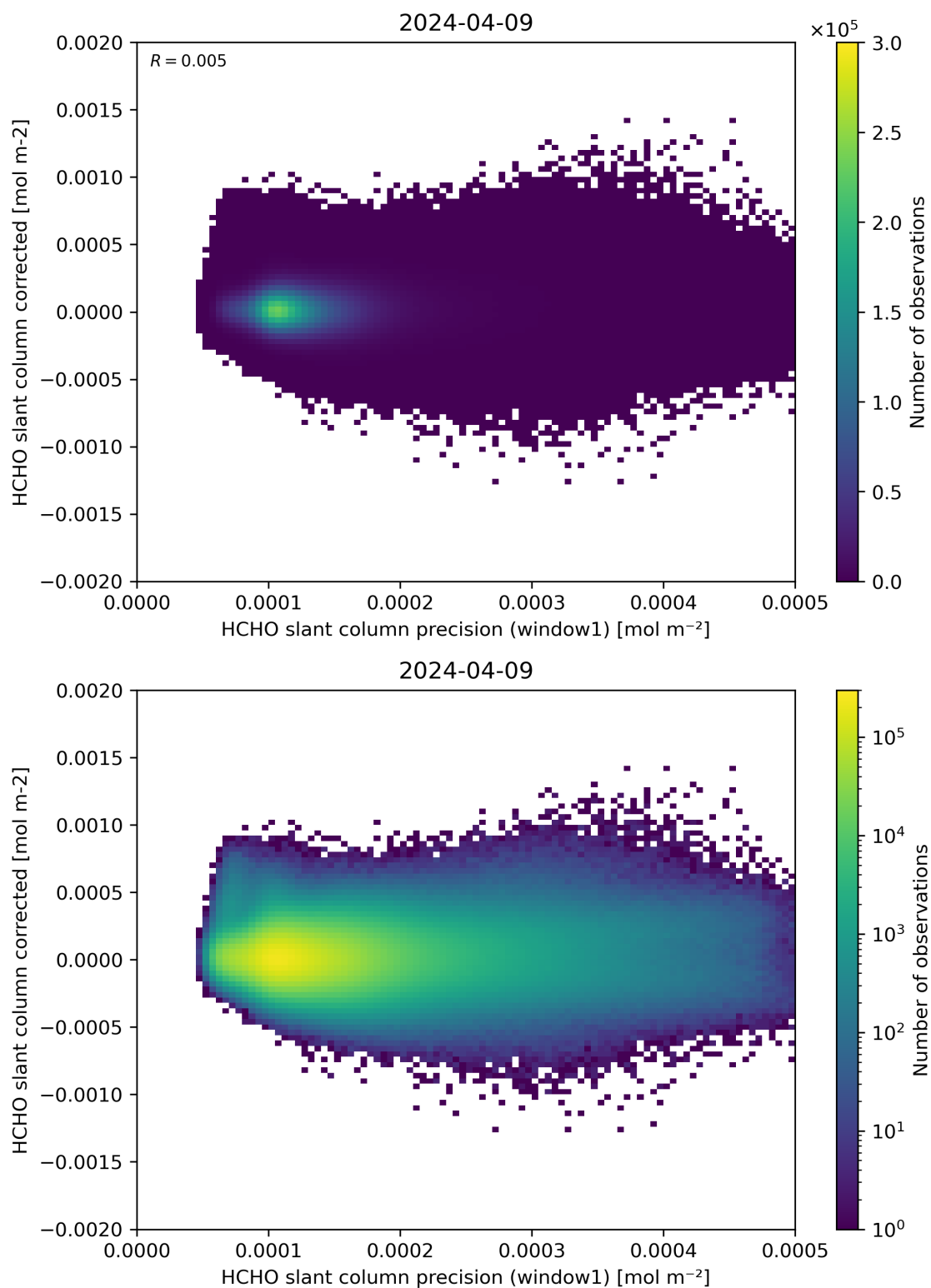
Figure 92: Scatter density plot of “HCHO slant column precision (window1)” against “HCHO slant column corrected” for 2024-04-08 to 2024-04-10.
