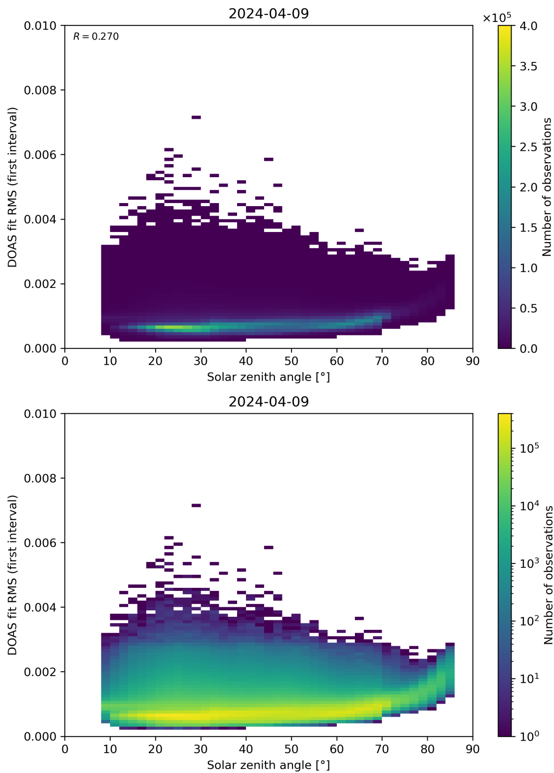
Figure 167: Scatter density plot of “Solar zenith angle” against “DOAS fit RMS (first interval)” for 2024-04-08 to 2024-04-10.
