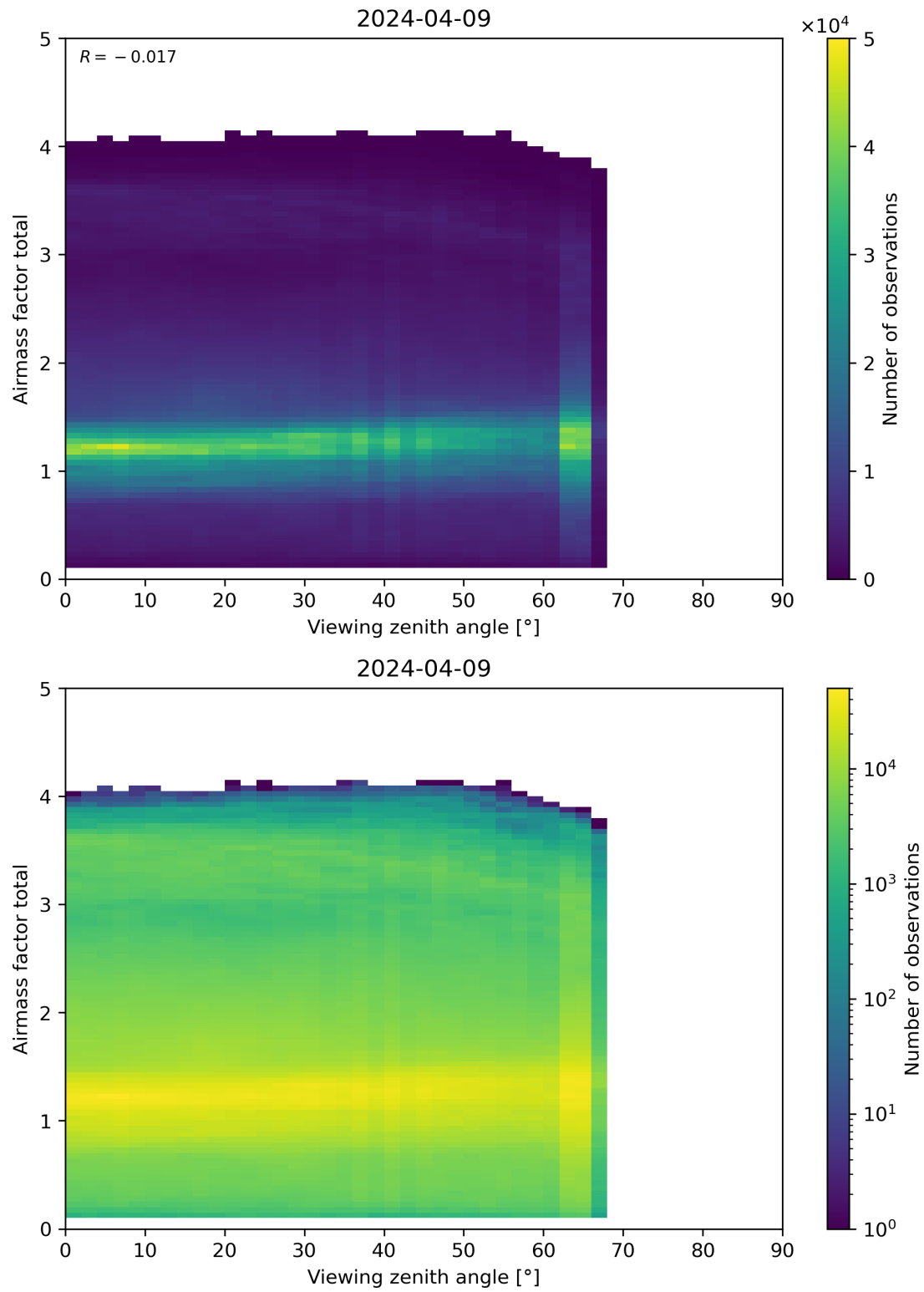
Figure 190: Scatter density plot of “Viewing zenith angle” against “Airmass factor total” for 2024-04-08 to 2024-04-10.
