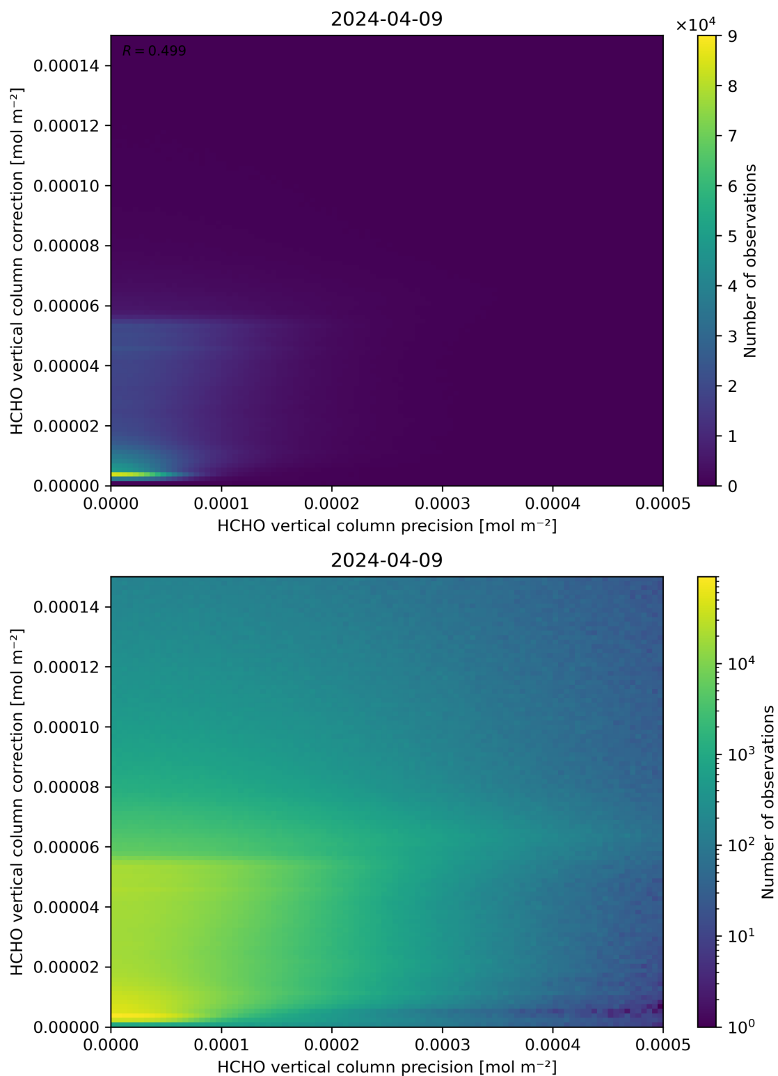
Figure 146: Scatter density plot of “HCHO vertical column precision” against “HCHO vertical column correction” for 2024-04-08 to 2024-04-10.
