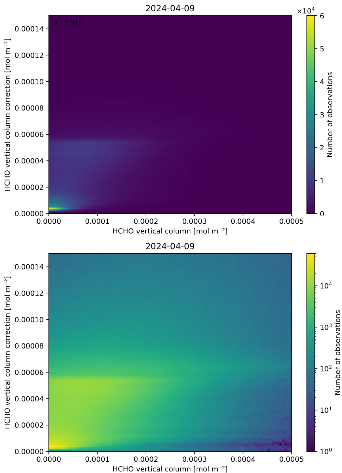
Figure 133: Scatter density plot of “HCHO vertical column” against “HCHO vertical column correction” for 2024-04-08 to 2024-04-10.
