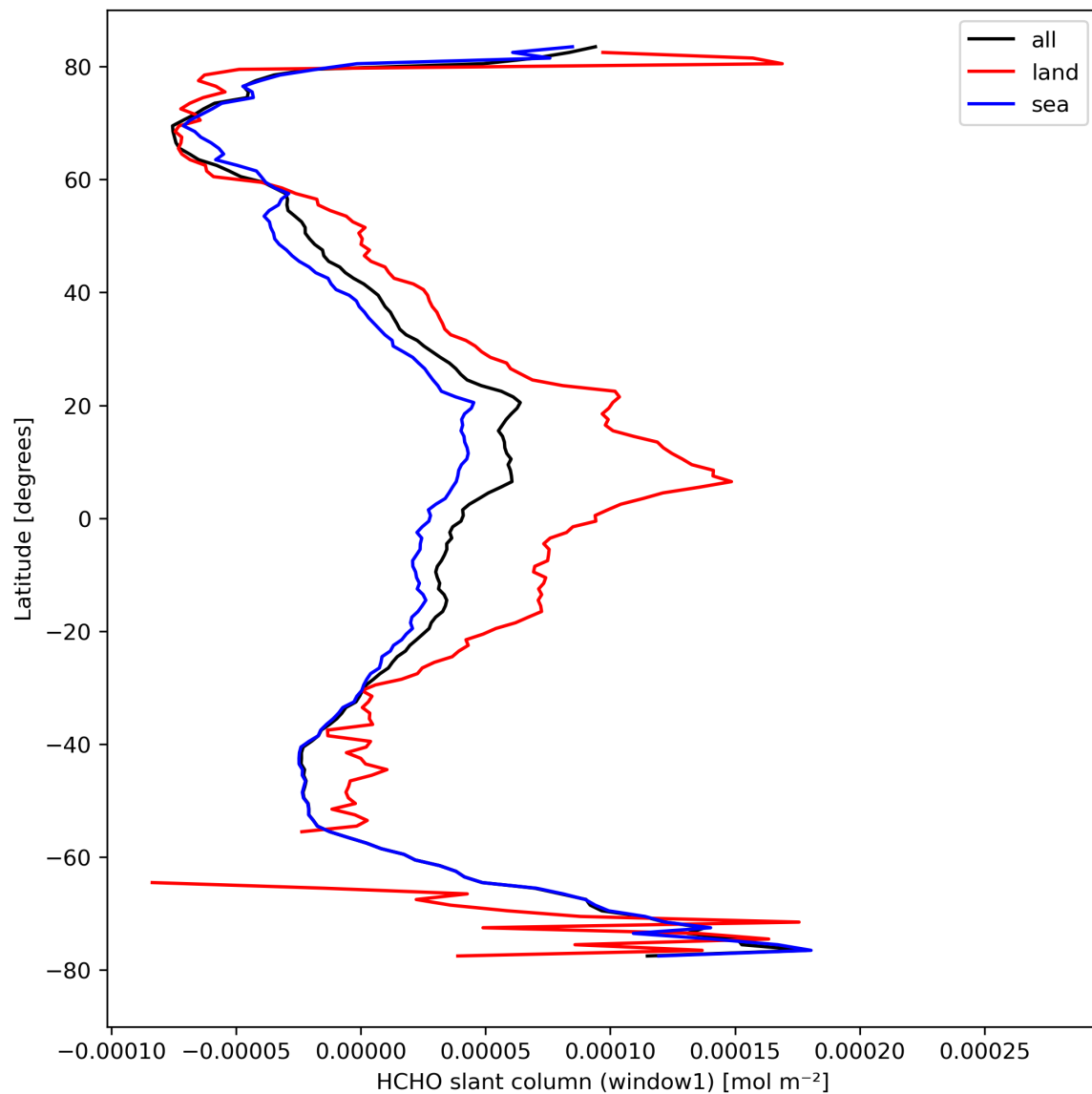
Figure 24: Zonal average of “HCHO slant column (window1)” for 2024-04-08 to 2024-04-10.
