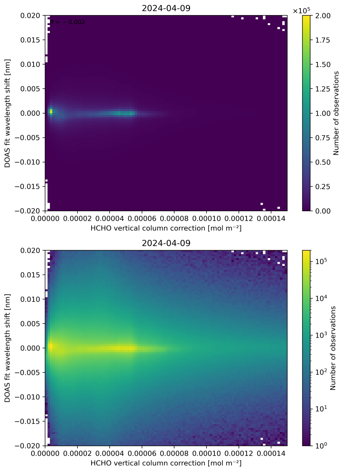
Figure 113: Scatter density plot of “HCHO vertical column correction” against “DOAS fit wavelength shift” for 2024-04-08 to 2024-04-10.
