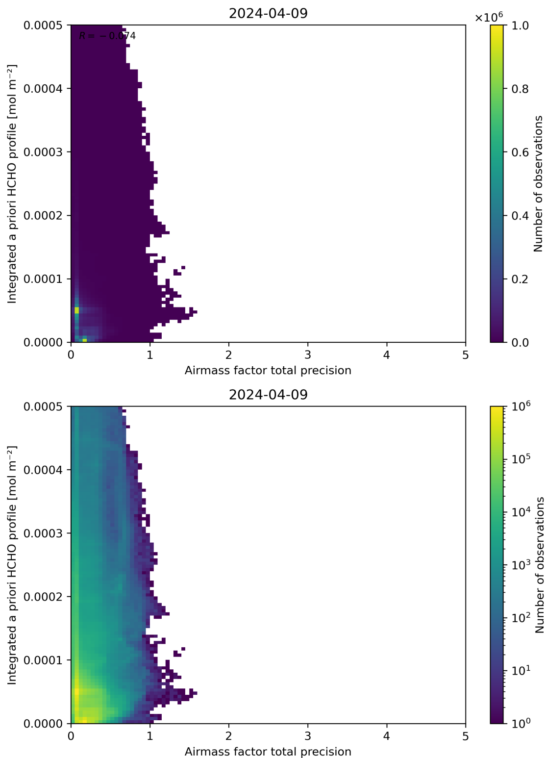
Figure 111: Scatter density plot of “Airmass factor total precision” against “Integrated a priori HCHO profile” for 2024-04-08 to 2024-04-10.
