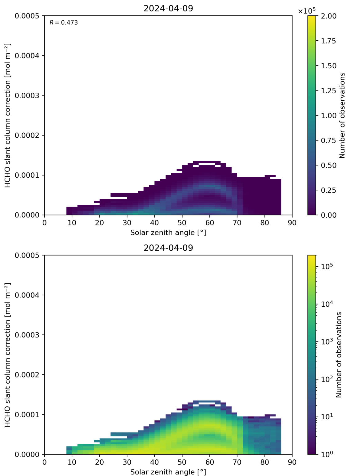
Figure 172: Scatter density plot of “Solar zenith angle” against “HCHO slant column correction” for 2024-04-08 to 2024-04-10.
