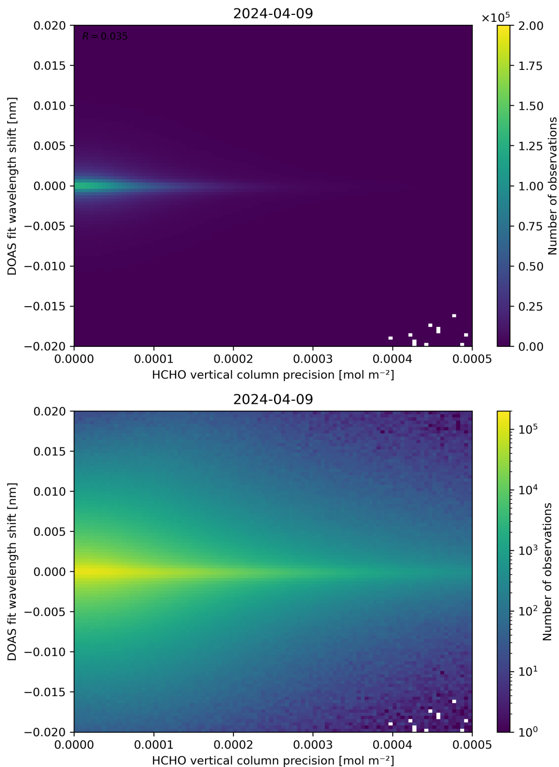
Figure 137: Scatter density plot of “HCHO vertical column precision” against “DOAS fit wavelength shift” for 2024-04-08 to 2024-04-10.
