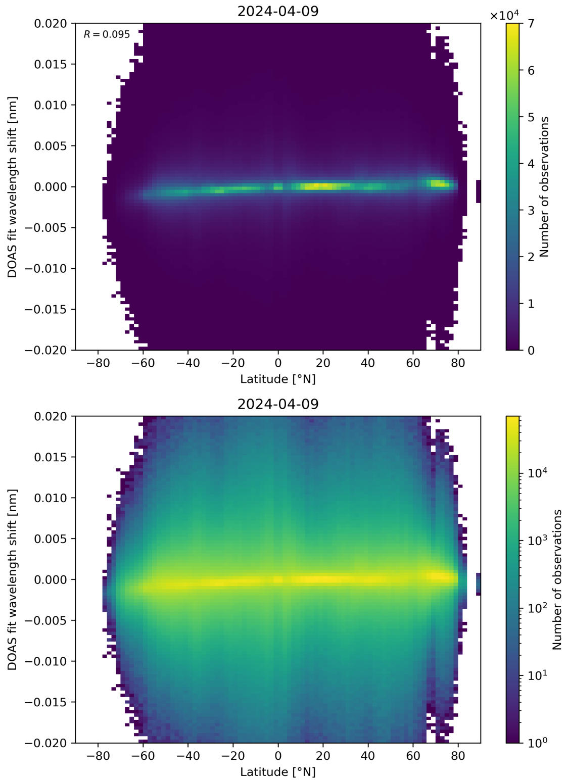
Figure 154: Scatter density plot of “Latitude” against “DOAS fit wavelength shift” for 2024-04-08 to 2024-04-10.
