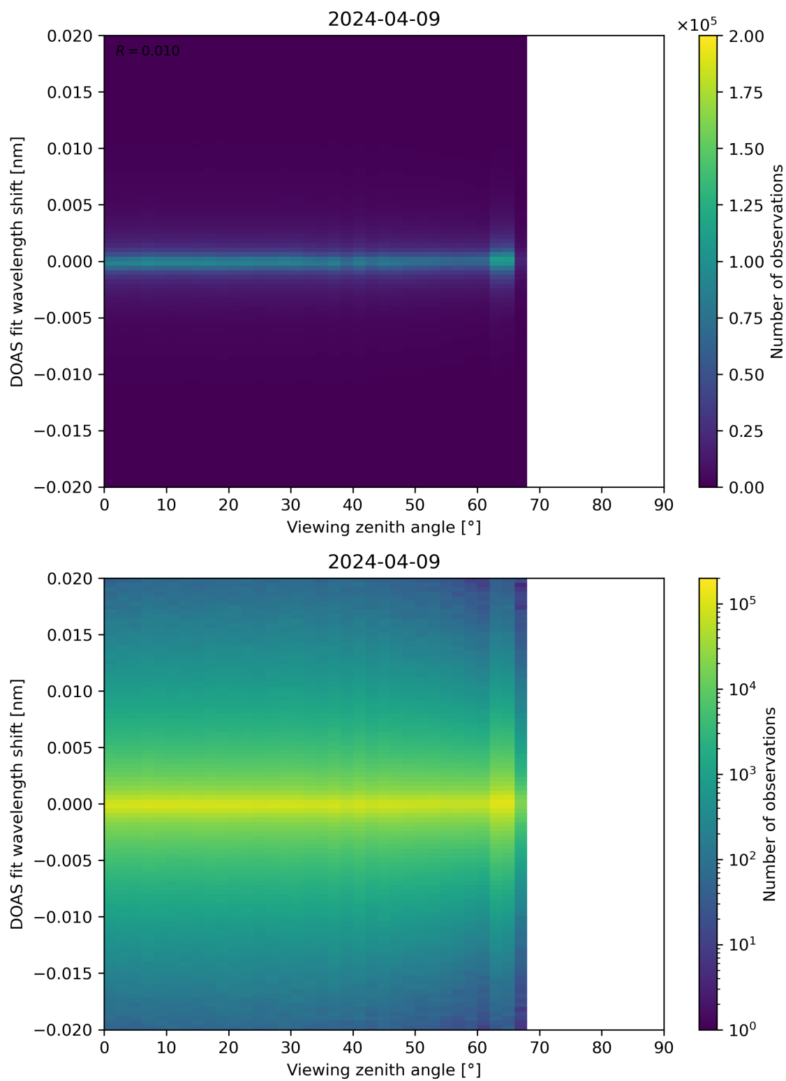
Figure 183: Scatter density plot of “Viewing zenith angle” against “DOAS fit wavelength shift” for 2024-04-08 to 2024-04-10.
