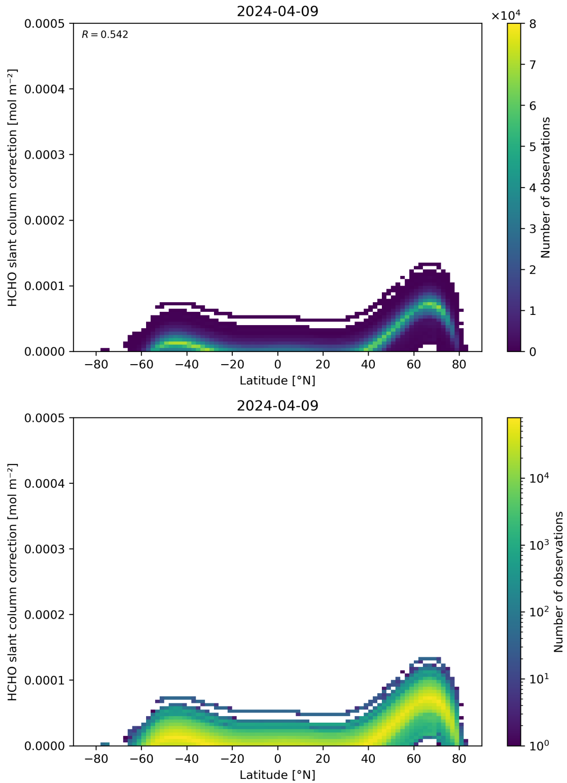
Figure 158: Scatter density plot of “Latitude” against “HCHO slant column correction” for 2024-04-08 to 2024-04-10.
