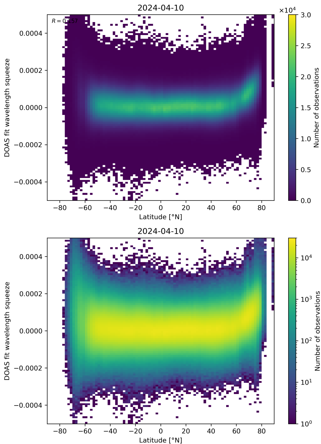
Figure 155: Scatter density plot of “Latitude” against “DOAS fit wavelength squeeze” for 2024-04-10 to 2024-04-11.
