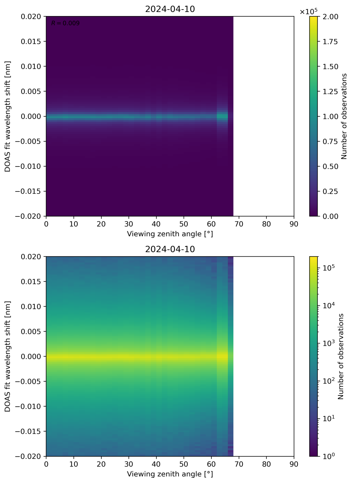
Figure 183: Scatter density plot of “Viewing zenith angle” against “DOAS fit wavelength shift” for 2024-04-10 to 2024-04-11.
