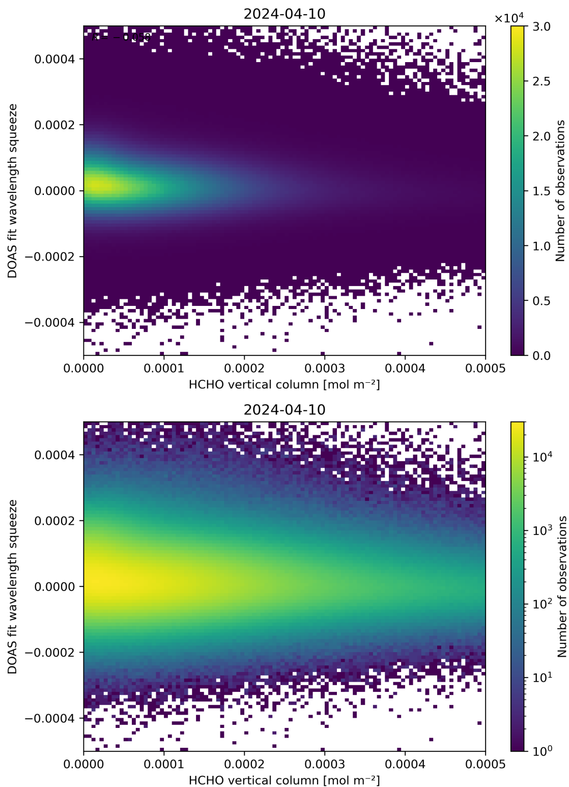
Figure 125: Scatter density plot of “HCHO vertical column” against “DOAS fit wavelength squeeze” for 2024-04-10 to 2024-04-11.
