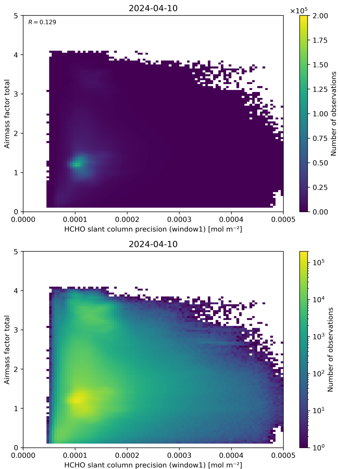
Figure 94: Scatter density plot of “HCHO slant column precision (window1)” against “Airmass factor total” for 2024-04-10 to 2024-04-11.
