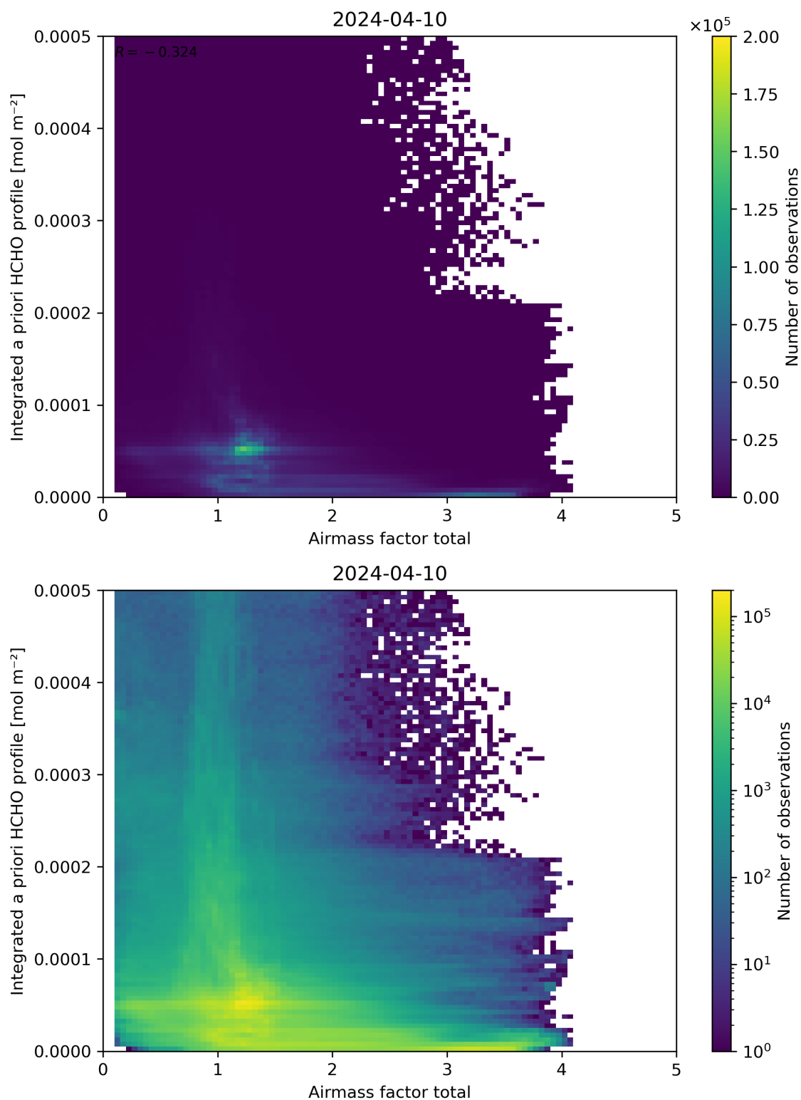
Figure 104: Scatter density plot of “Airmass factor total” against “Integrated a priori HCHO profile” for 2024-04-10 to 2024-04-11.
