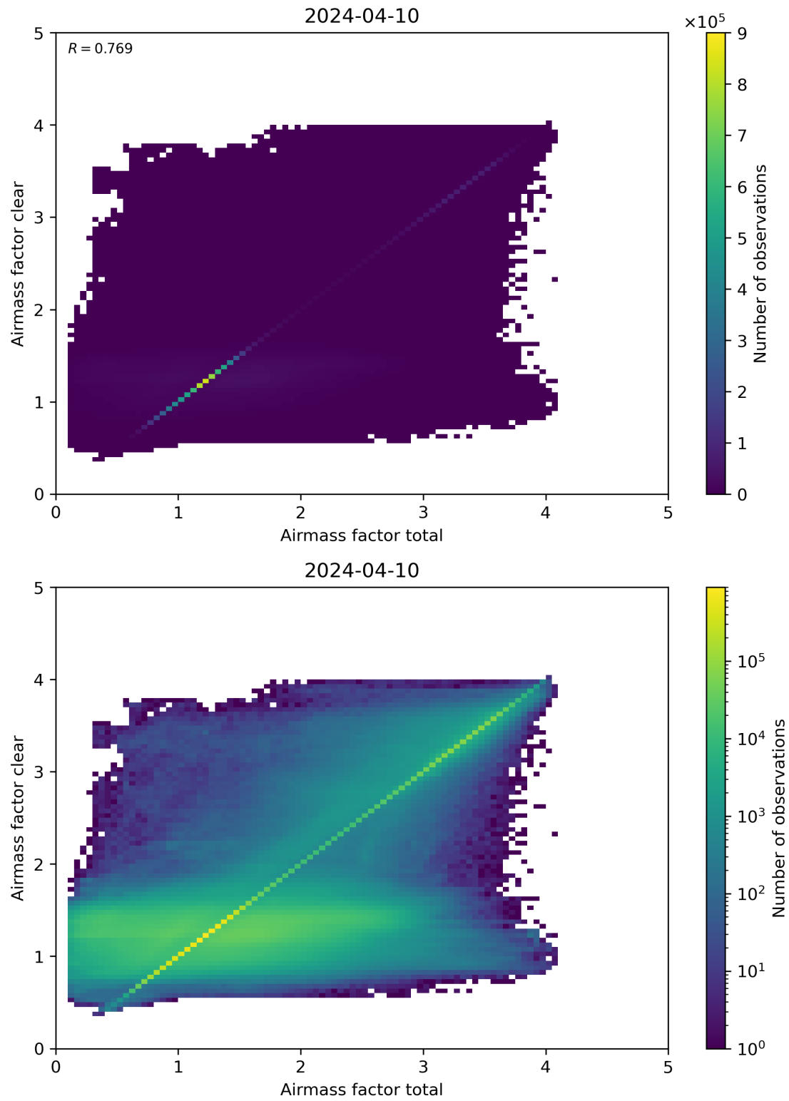
Figure 100: Scatter density plot of “Airmass factor total” against “Airmass factor clear” for 2024-04-10 to 2024-04-11.
