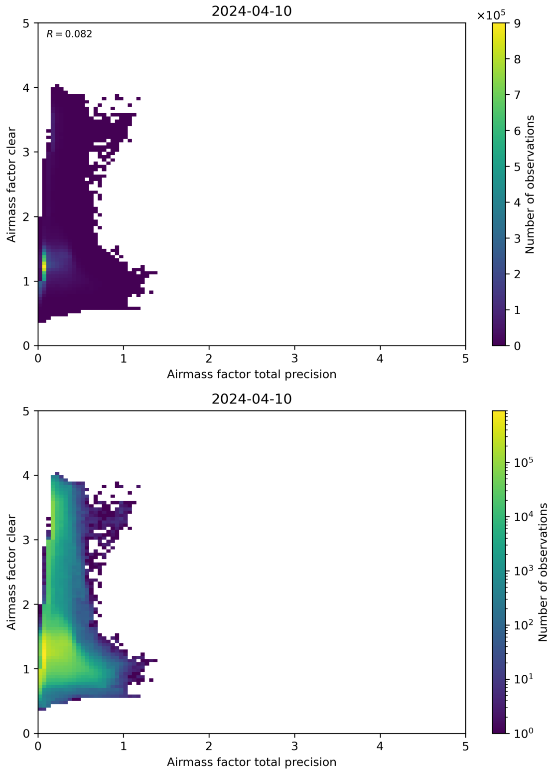
Figure 108: Scatter density plot of “Airmass factor total precision” against “Airmass factor clear” for 2024-04-10 to 2024-04-11.
