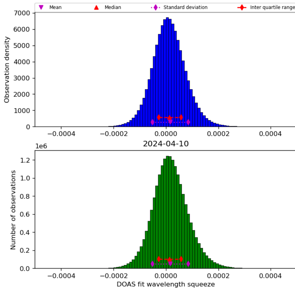
Figure 45: Histogram of “DOAS fit wavelength squeeze” for 2024-04-10 to 2024-04-11
