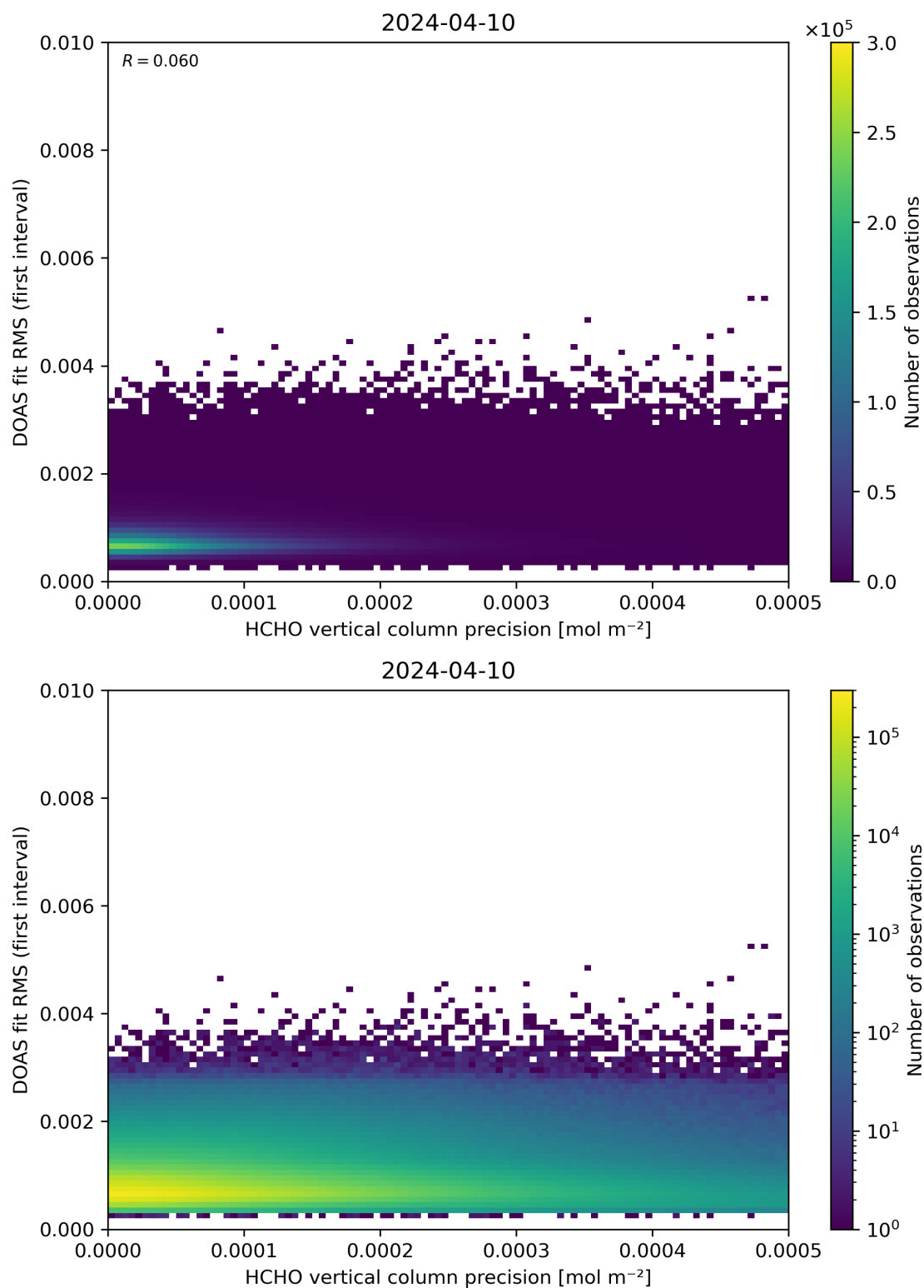
Figure 136: Scatter density plot of “HCHO vertical column precision” against “DOAS fit RMS (first interval)” for 2024-04-10 to 2024-04-11.
