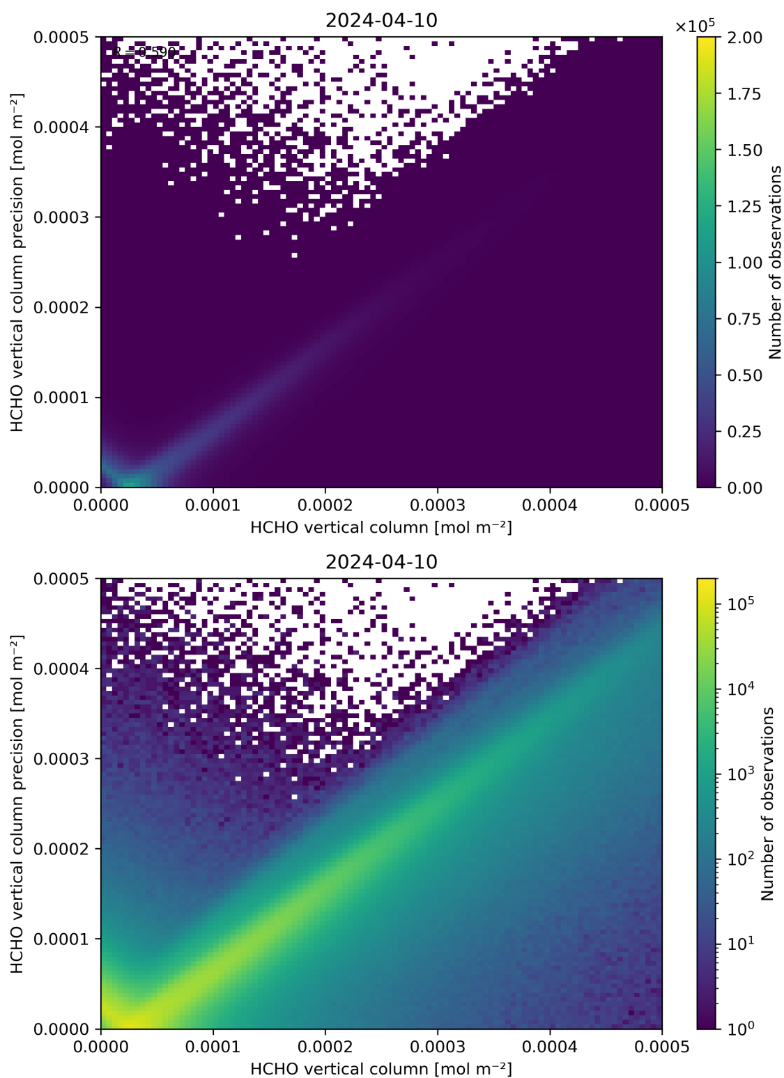
Figure 134: Scatter density plot of “HCHO vertical column” against “HCHO vertical column precision” for 2024-04-10 to 2024-04-11.
