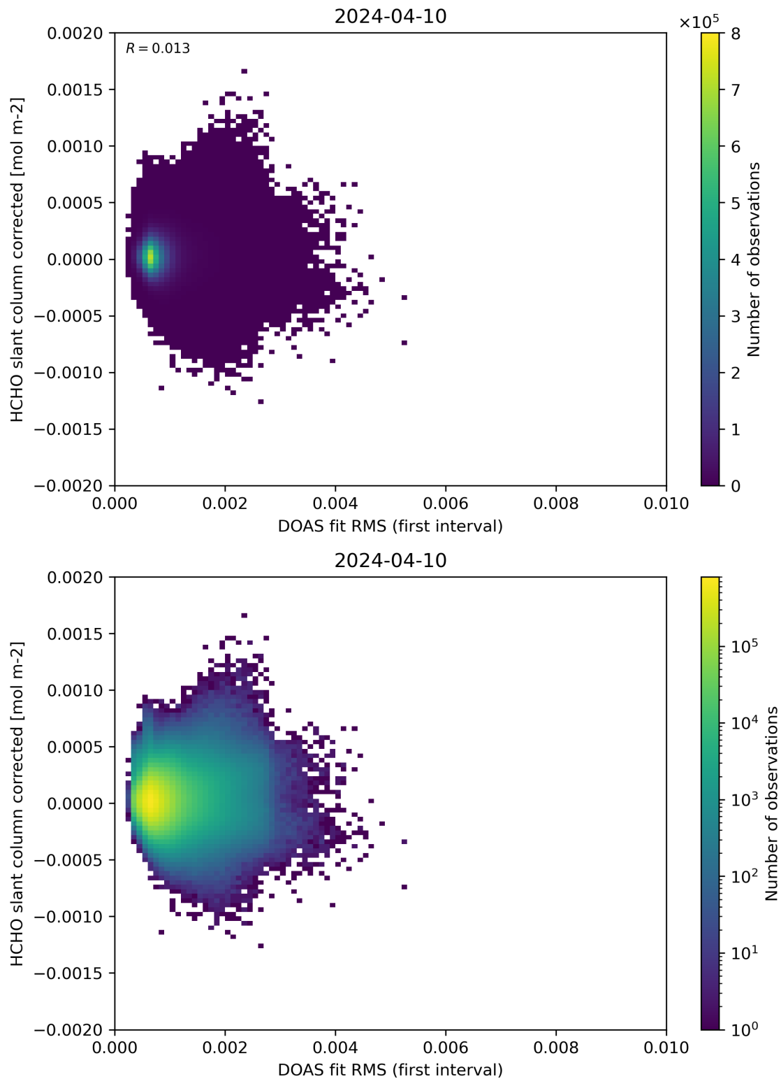
Figure 62: Scatter density plot of “DOAS fit RMS (first interval)” against “HCHO slant column corrected” for 2024-04-10 to 2024-04-11.
