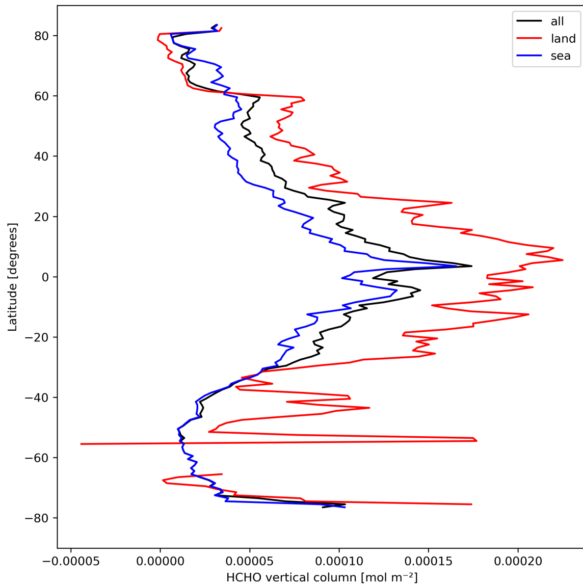
Figure 21: Zonal average of “HCHO vertical column” for 2024-04-10 to 2024-04-11.
