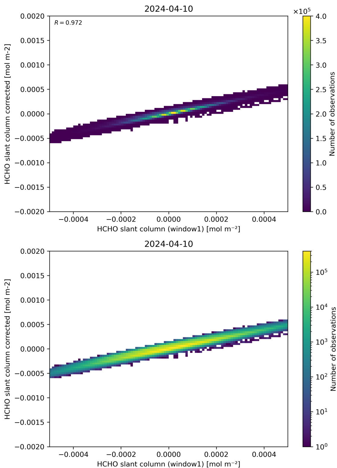
Figure 82: Scatter density plot of “HCHO slant column (window1)” against “HCHO slant column corrected” for 2024-04-10 to 2024-04-11.
