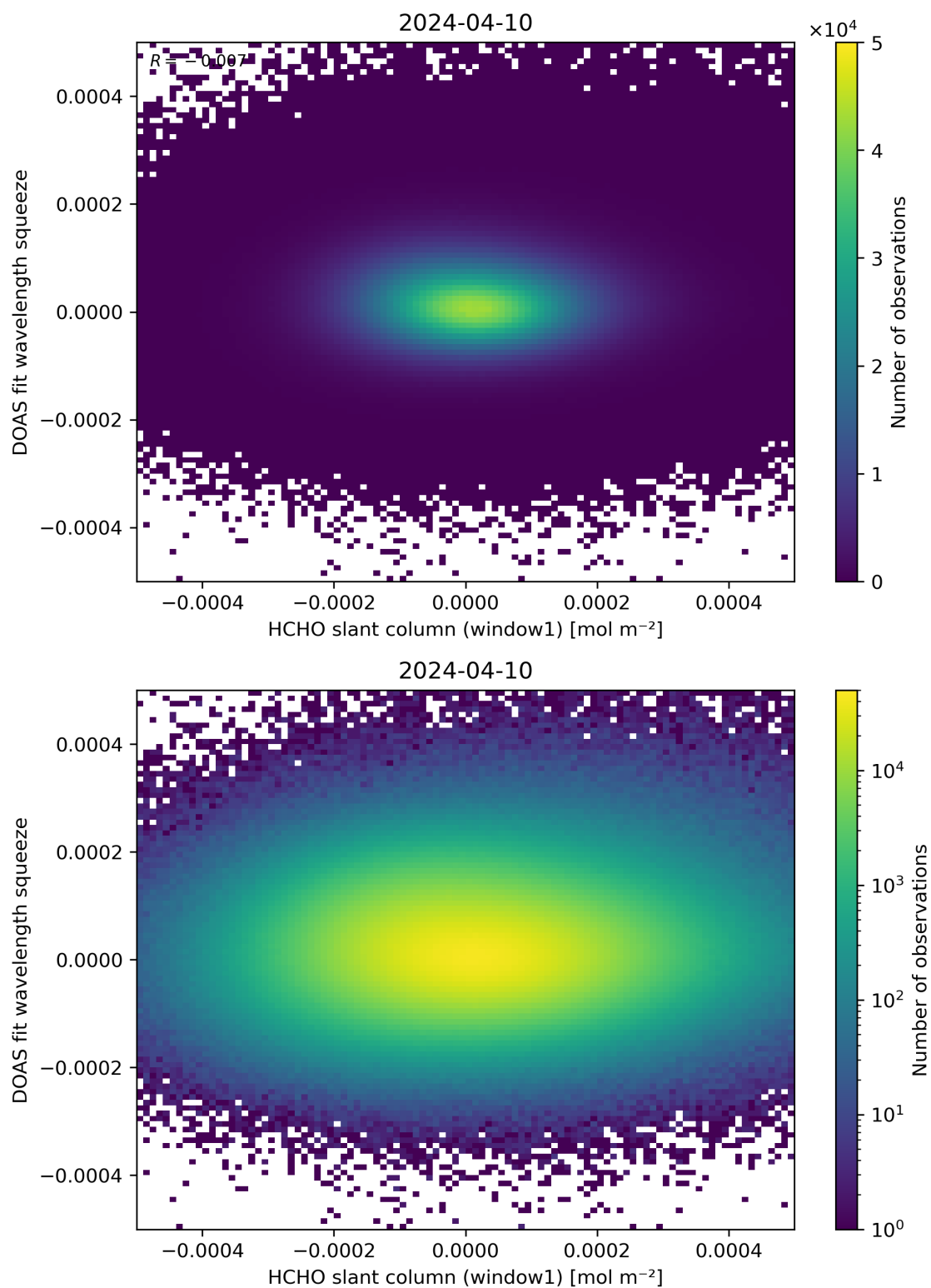
Figure 80: Scatter density plot of “HCHO slant column (window1)” against “DOAS fit wavelength squeeze” for 2024-04-10 to 2024-04-11.
