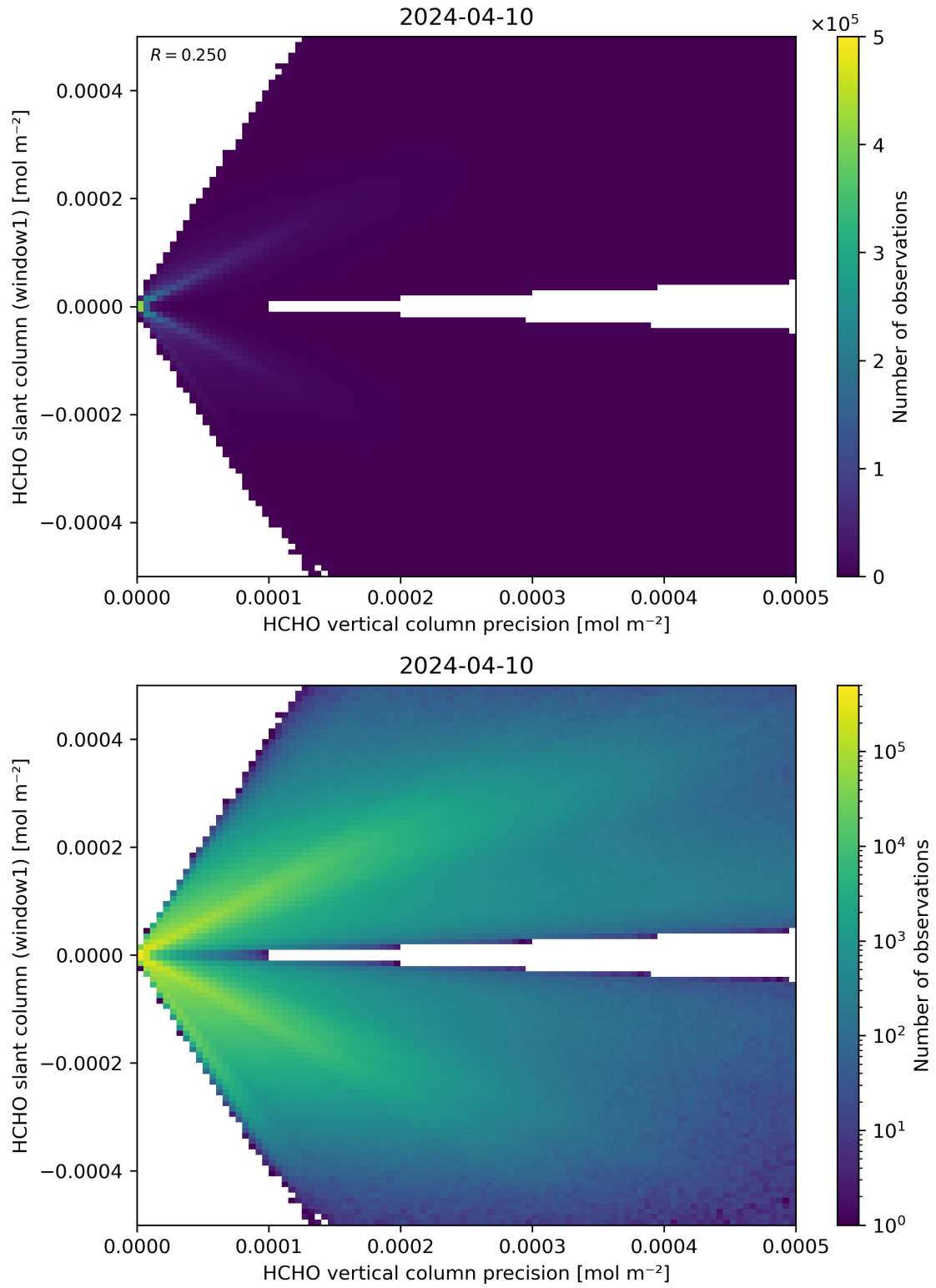
Figure 142: Scatter density plot of “HCHO vertical column precision” against “HCHO slant column (window1)” for 2024-04-10 to 2024-04-11.
