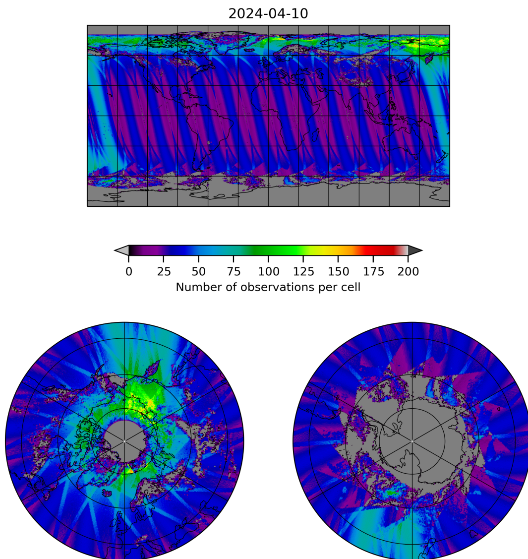
Figure 19: Map of the number of observations for 2024-04-10 to 2024-04-11
