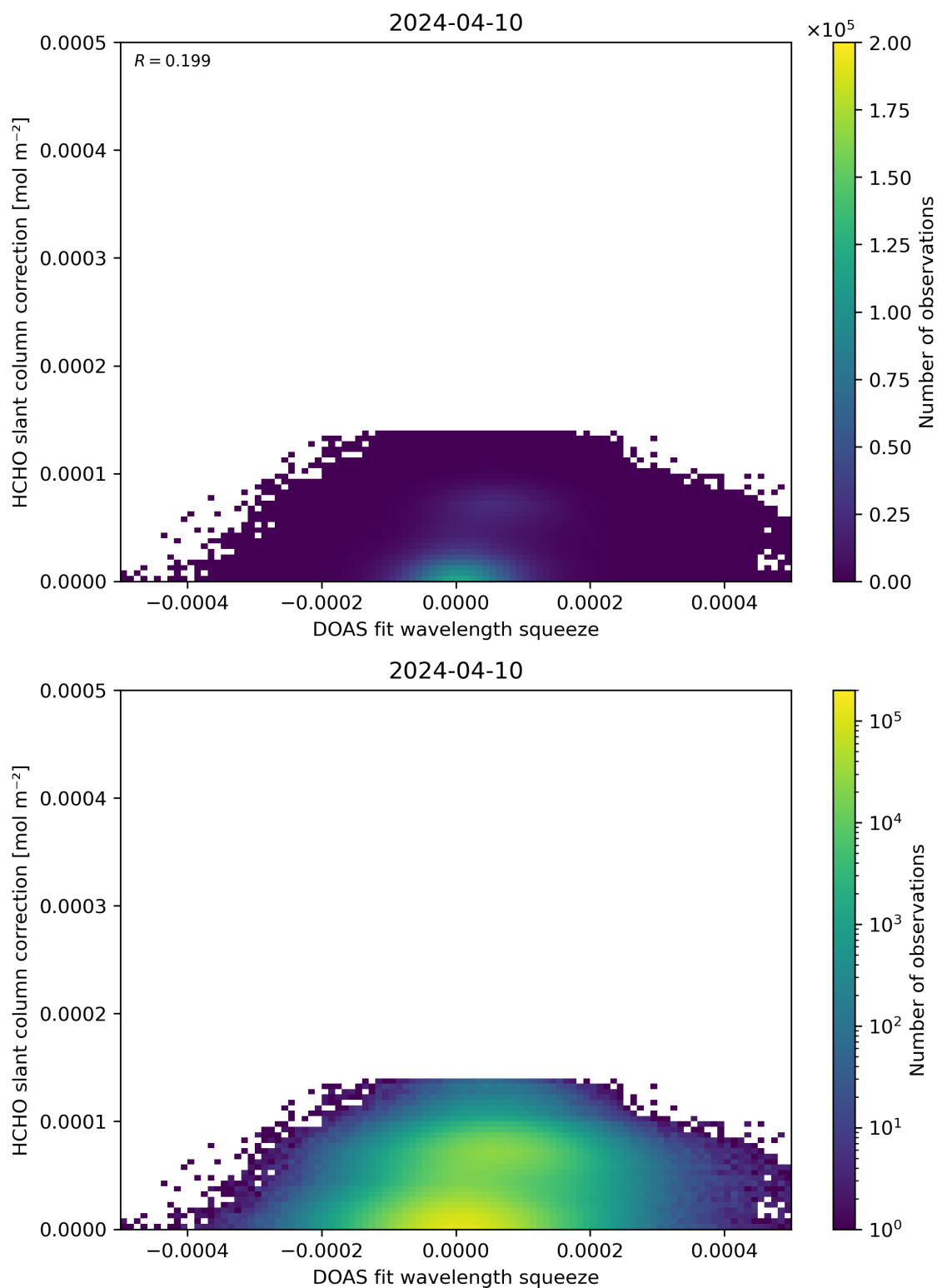
Figure 70: Scatter density plot of “DOAS fit wavelength squeeze” against “HCHO slant column correction” for 2024-04-10 to 2024-04-11.
