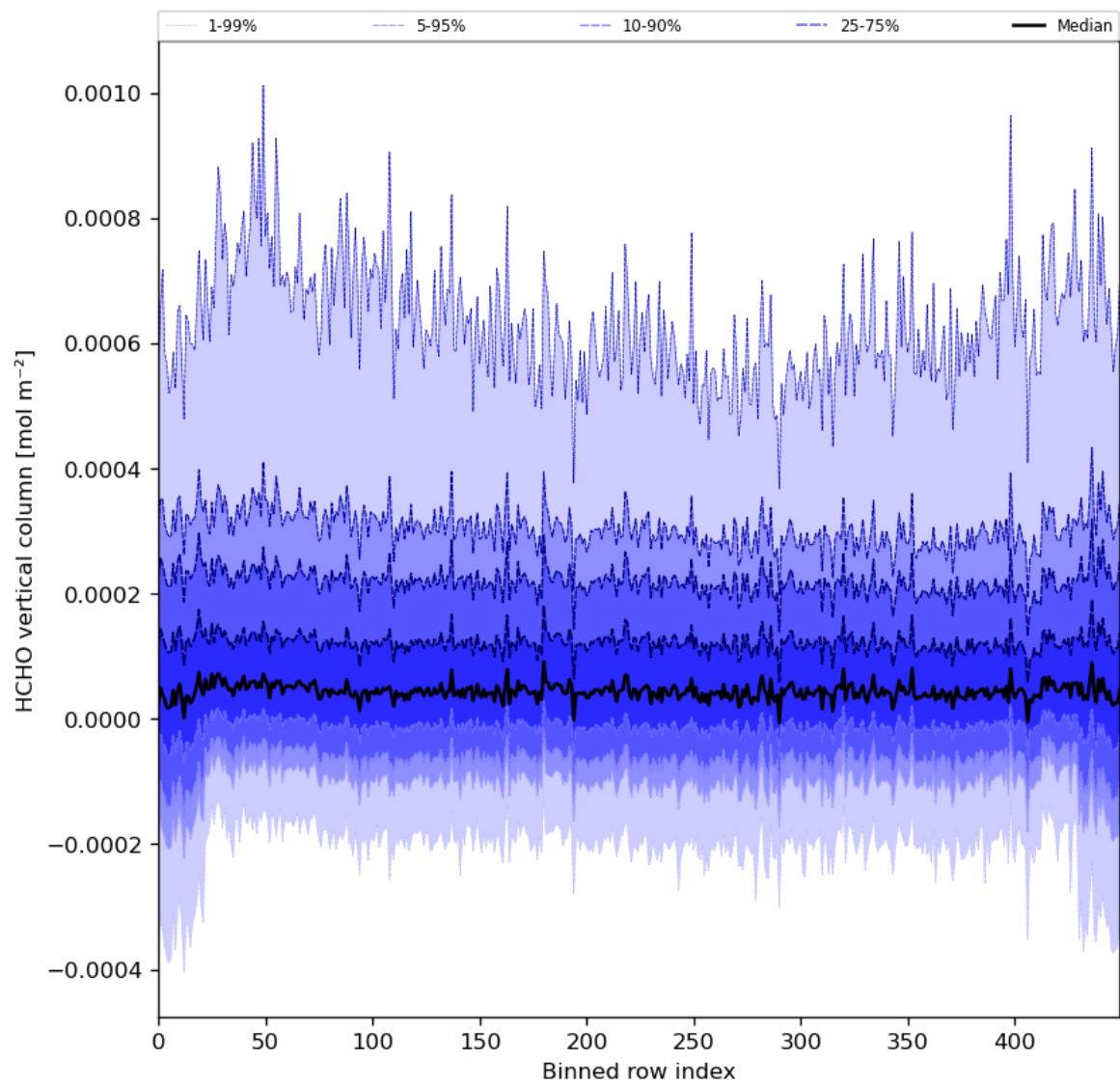
Figure 49: Along track statistics of “HCHO vertical column” for 2024-04-10 to 2024-04-11
