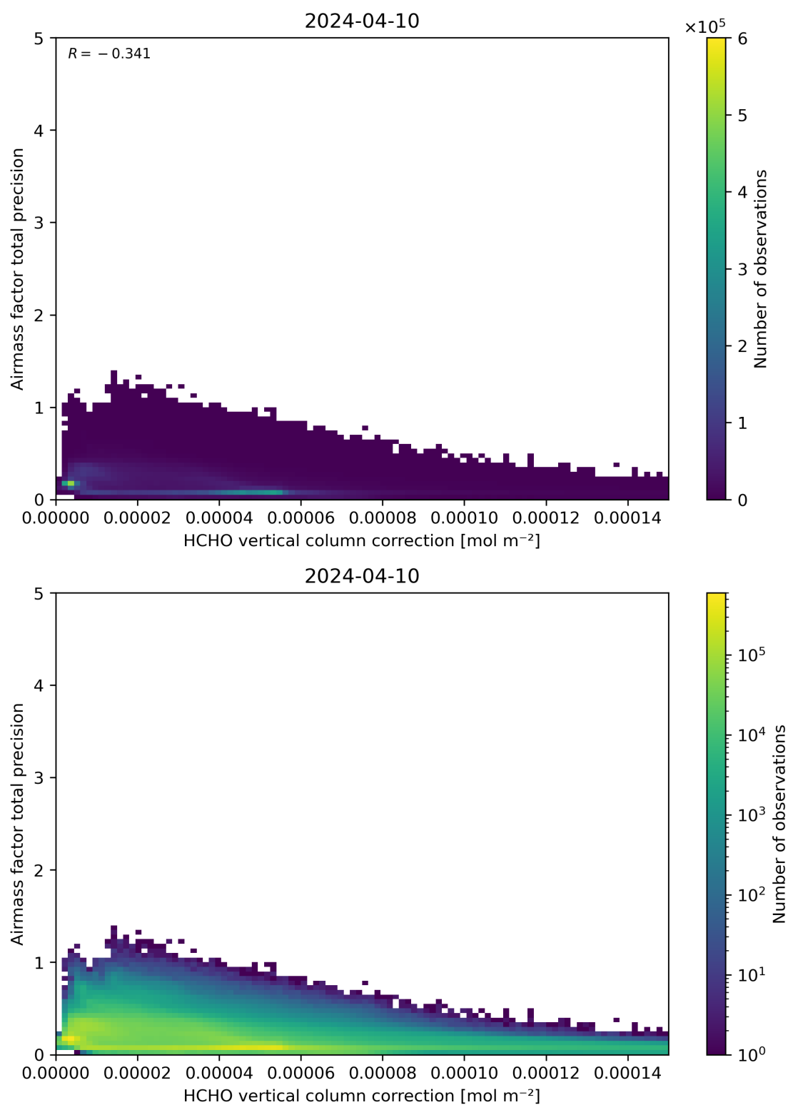
Figure 121: Scatter density plot of “HCHO vertical column correction” against “Airmass factor total precision” for 2024-04-10 to 2024-04-11.
