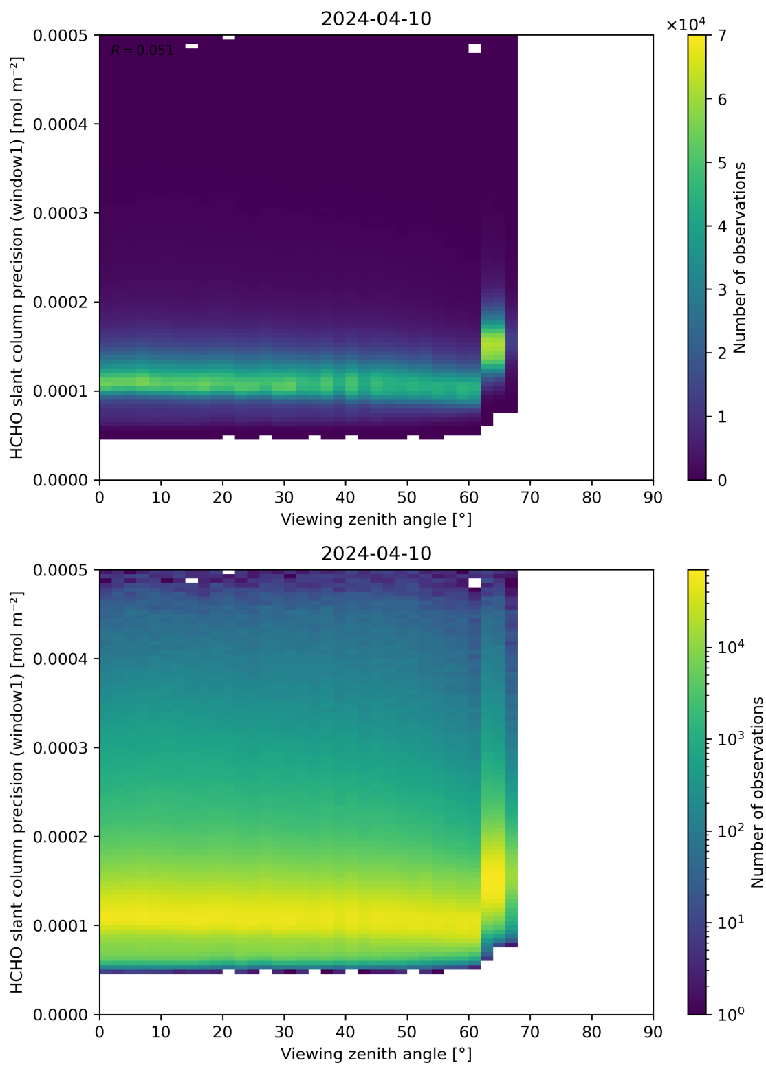
Figure 189: Scatter density plot of “Viewing zenith angle” against “HCHO slant column precision (window1)” for 2024-04-10 to 2024-04-11.
