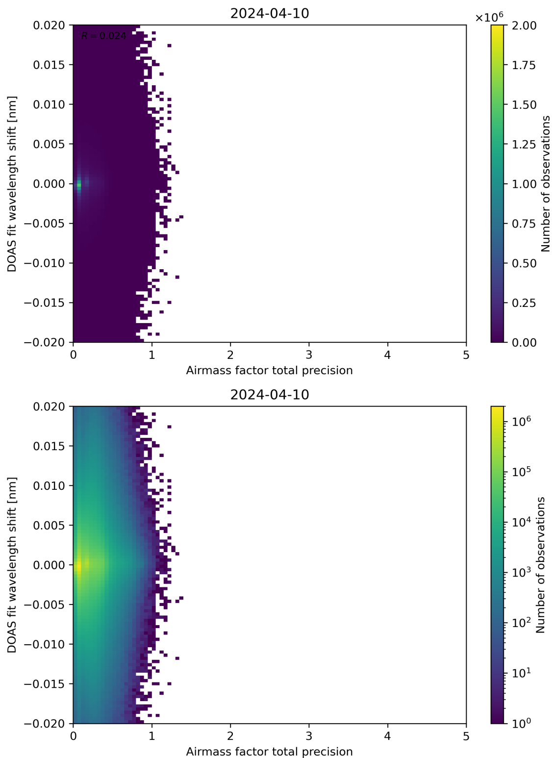
Figure 106: Scatter density plot of “Airmass factor total precision” against “DOAS fit wavelength shift” for 2024-04-10 to 2024-04-11.
