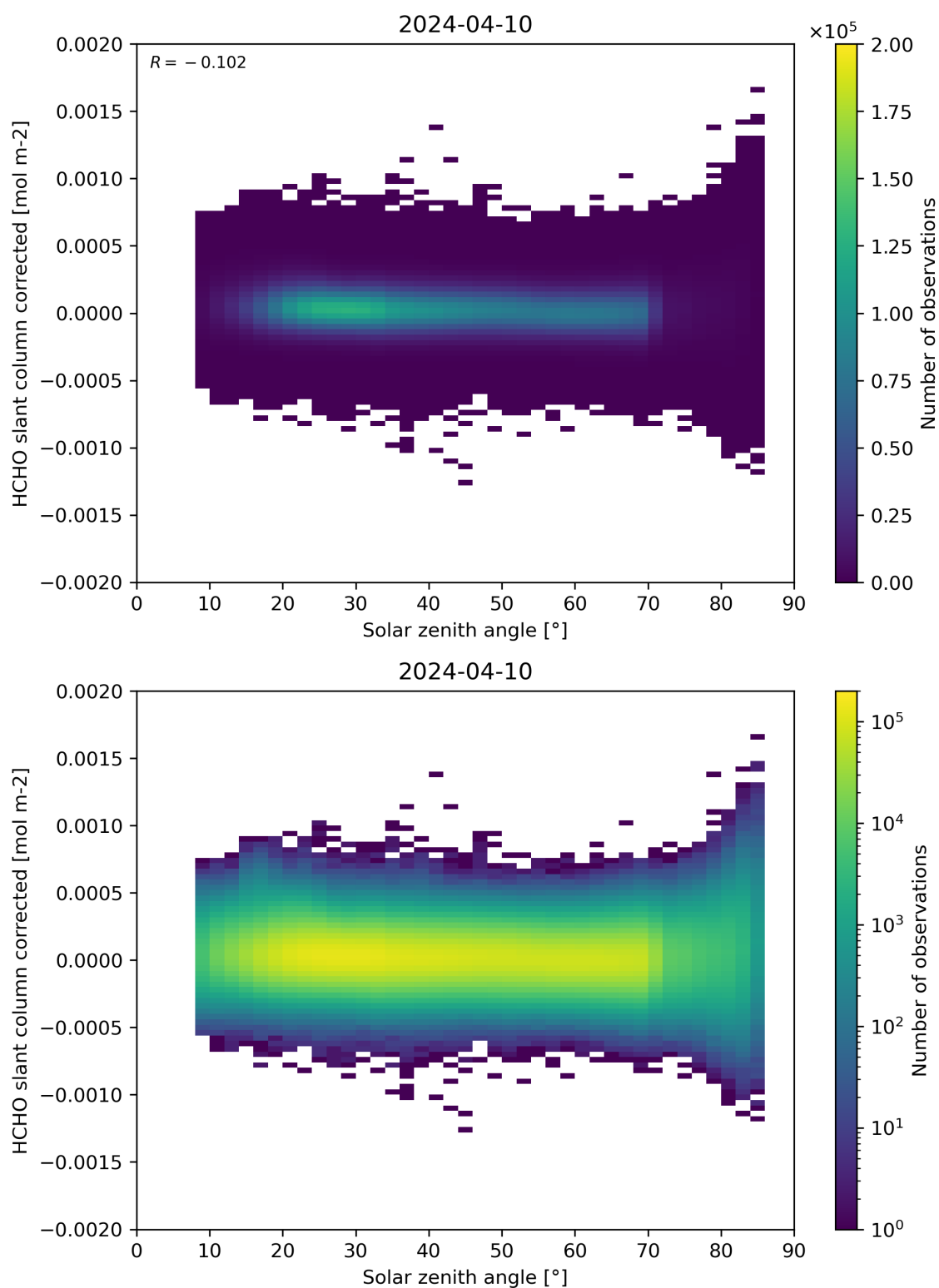
Figure 171: Scatter density plot of “Solar zenith angle” against “HCHO slant column corrected” for 2024-04-10 to 2024-04-11.
