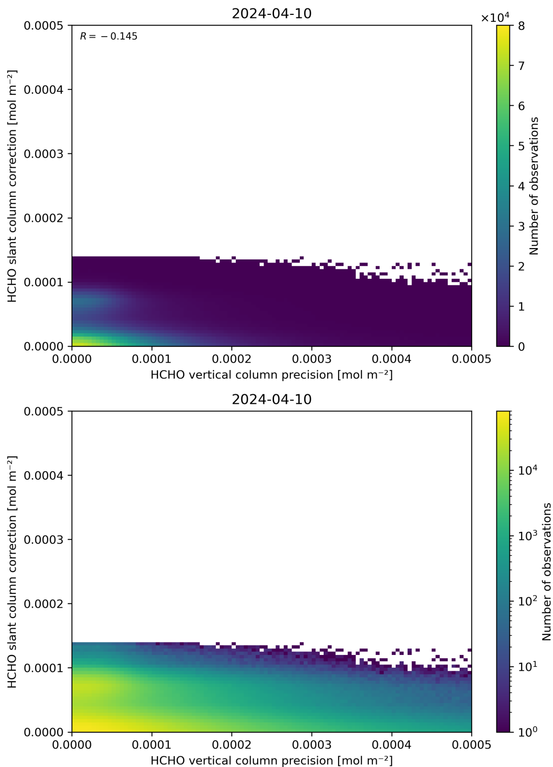
Figure 141: Scatter density plot of “HCHO vertical column precision” against “HCHO slant column correction” for 2024-04-10 to 2024-04-11.
