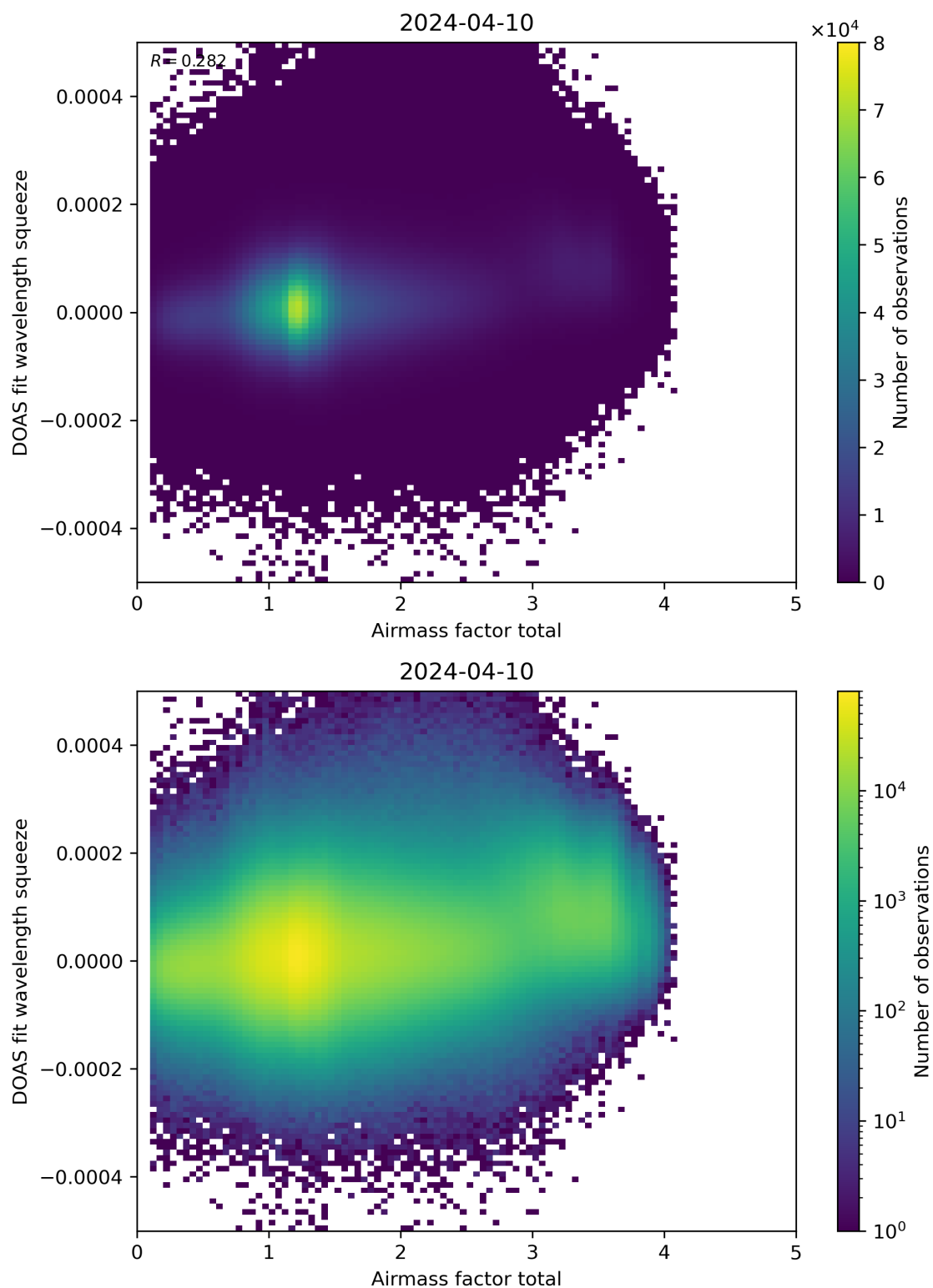
Figure 99: Scatter density plot of “Airmass factor total” against “DOAS fit wavelength squeeze” for 2024-04-10 to 2024-04-11.
