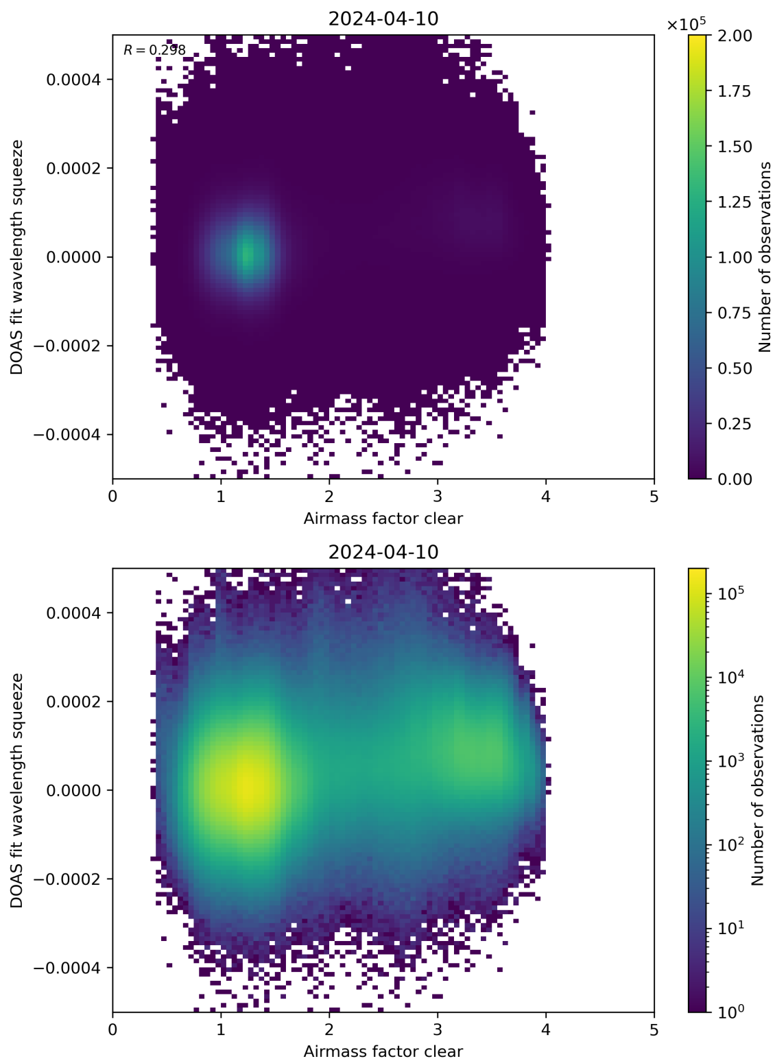
Figure 73: Scatter density plot of “Airmass factor clear” against “DOAS fit wavelength squeeze” for 2024-04-10 to 2024-04-11.
