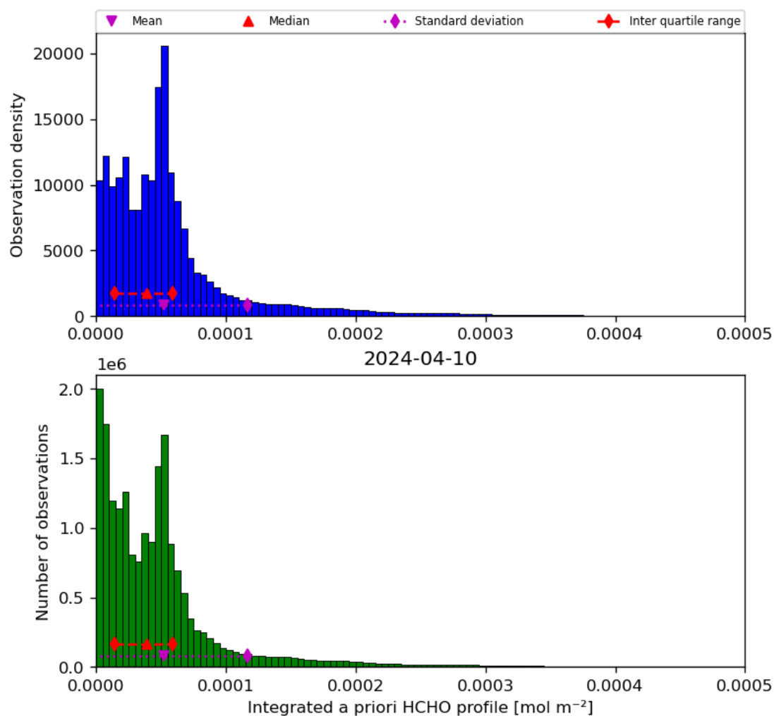
Figure 43: Histogram of “Integrated a priori HCHO profile” for 2024-04-10 to 2024-04-11
