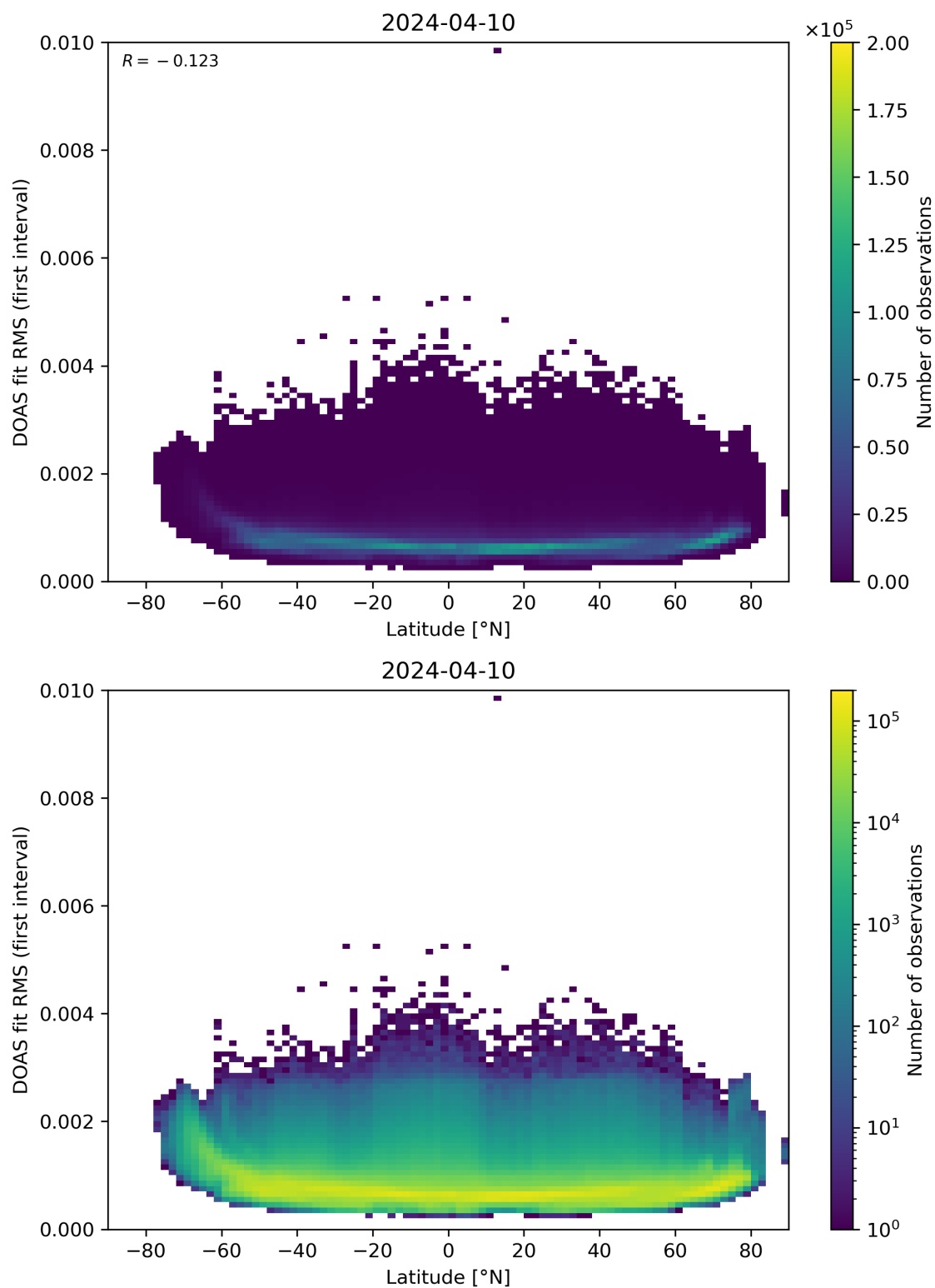
Figure 153: Scatter density plot of “Latitude” against “DOAS fit RMS (first interval)” for 2024-04-10 to 2024-04-11.
