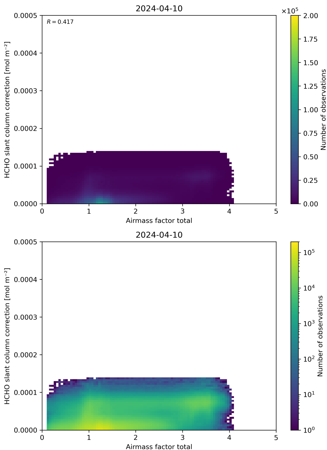
Figure 102: Scatter density plot of “Airmass factor total” against “HCHO slant column correction” for 2024-04-10 to 2024-04-11.
