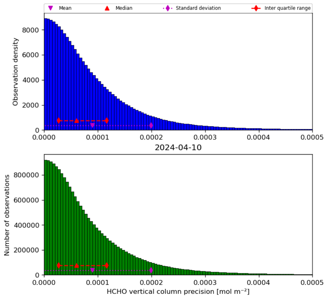
Figure 36: Histogram of “HCHO vertical column precision” for 2024-04-10 to 2024-04-11
