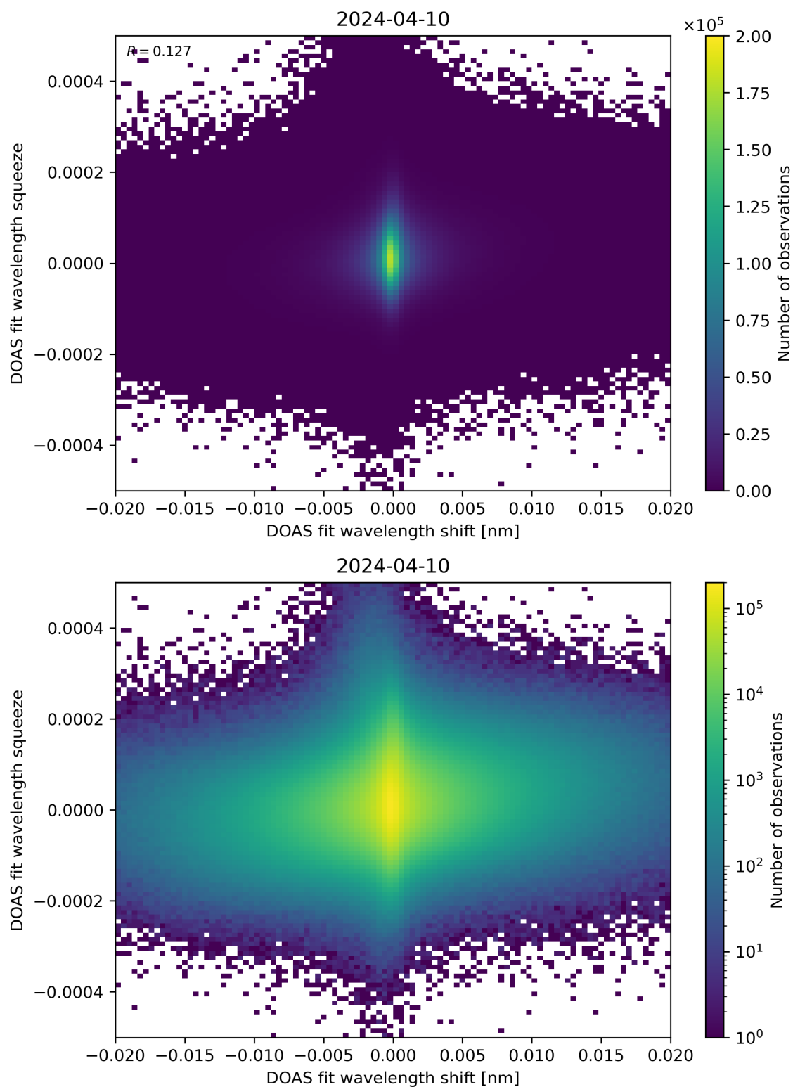
Figure 65: Scatter density plot of “DOAS fit wavelength shift” against “DOAS fit wavelength squeeze” for 2024-04-10 to 2024-04-11.
