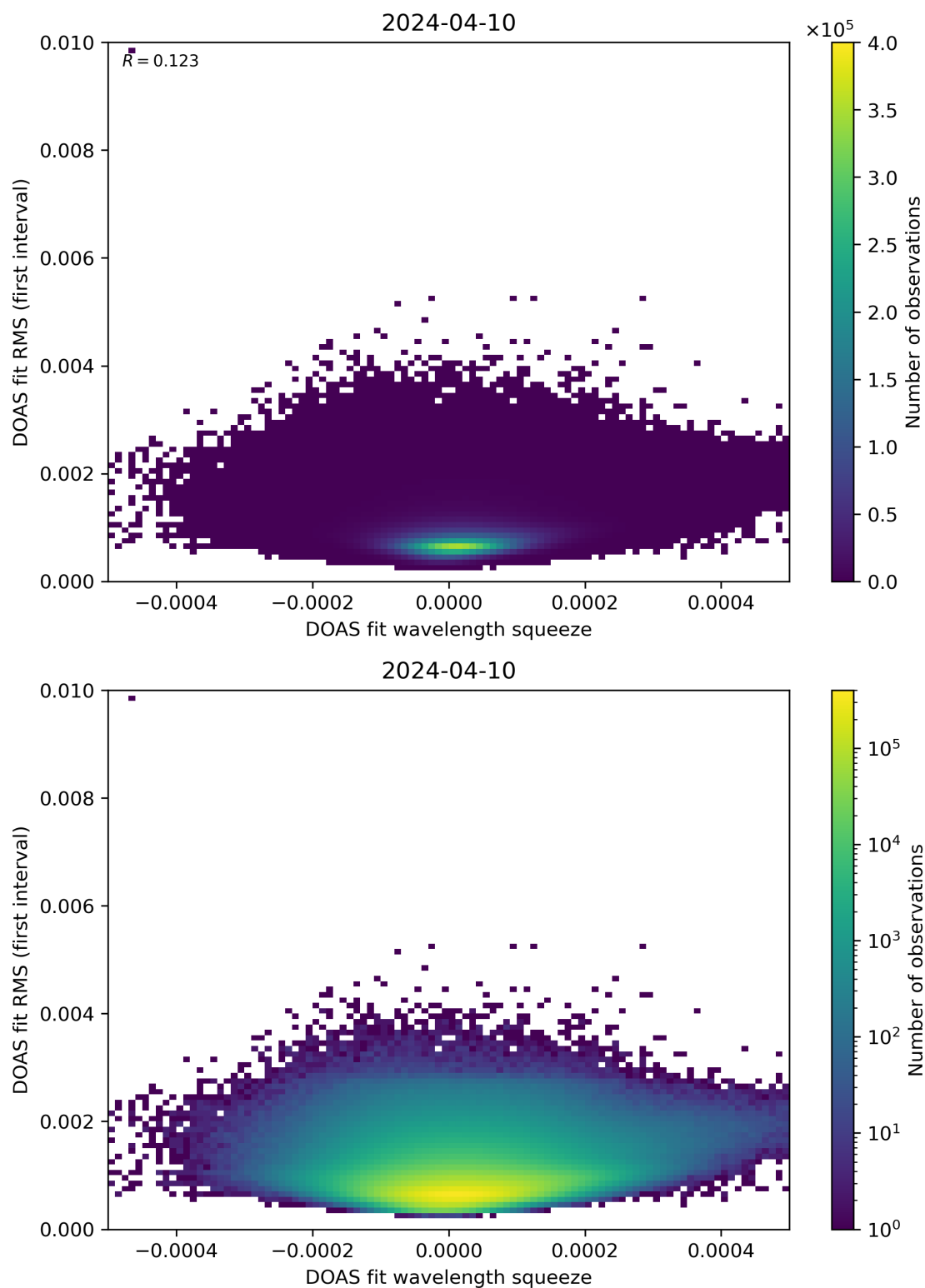
Figure 68: Scatter density plot of “DOAS fit wavelength squeeze” against “DOAS fit RMS (first interval)” for 2024-04-10 to 2024-04-11.
