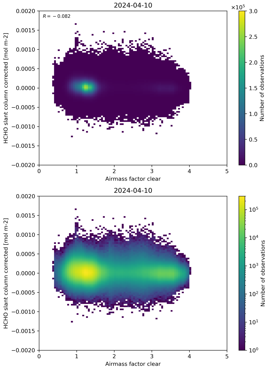
Figure 74: Scatter density plot of “Airmass factor clear” against “HCHO slant column corrected” for 2024-04-10 to 2024-04-11.
