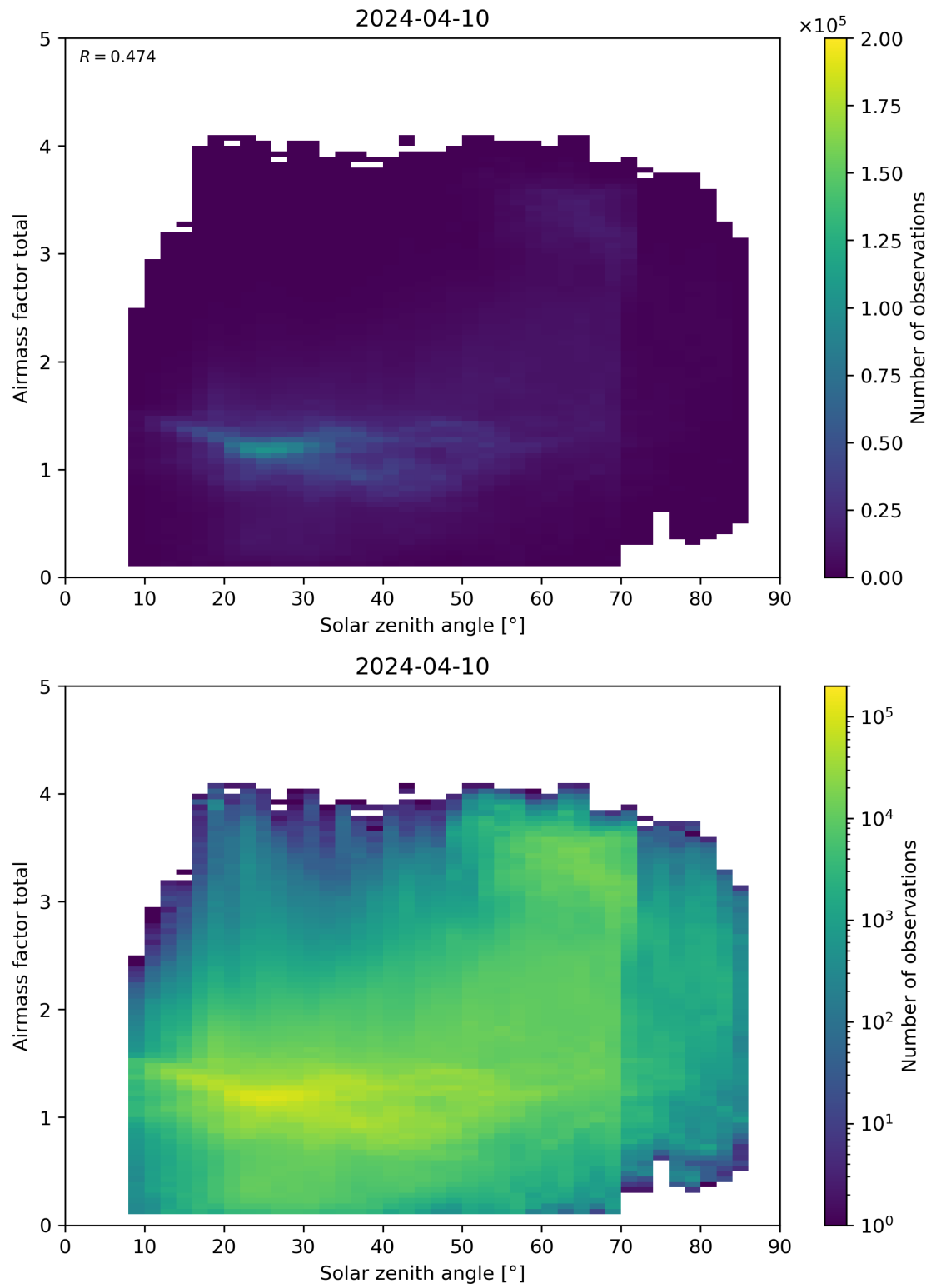
Figure 175: Scatter density plot of “Solar zenith angle” against “Airmass factor total” for 2024-04-10 to 2024-04-11.
