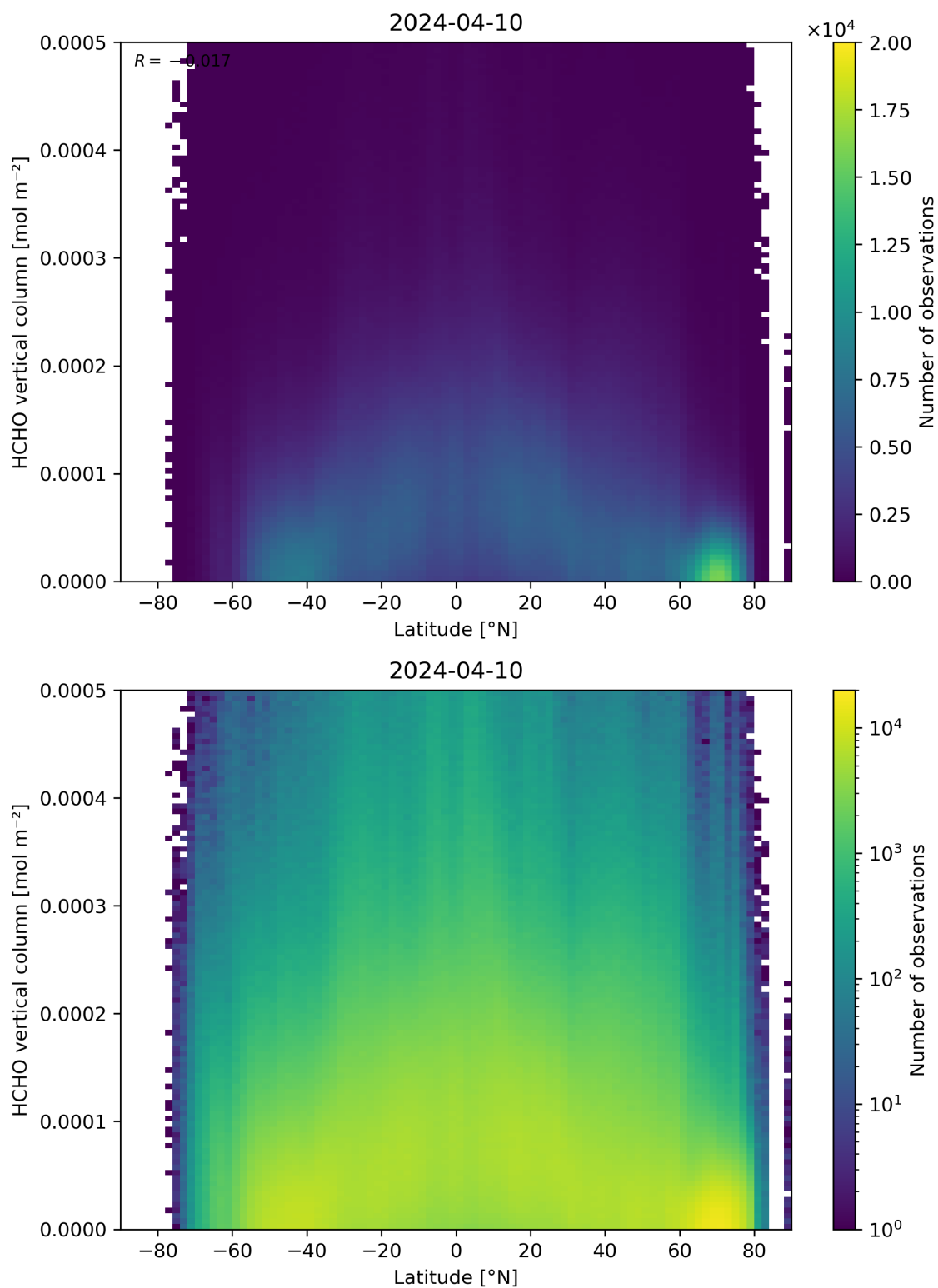
Figure 163: Scatter density plot of “Latitude” against “HCHO vertical column” for 2024-04-10 to 2024-04-11.
