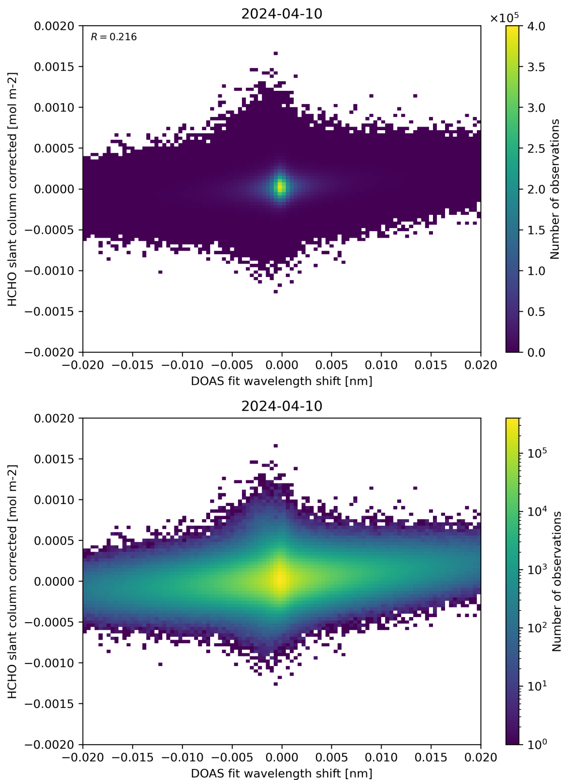
Figure 66: Scatter density plot of “DOAS fit wavelength shift” against “HCHO slant column corrected” for 2024-04-10 to 2024-04-11.
