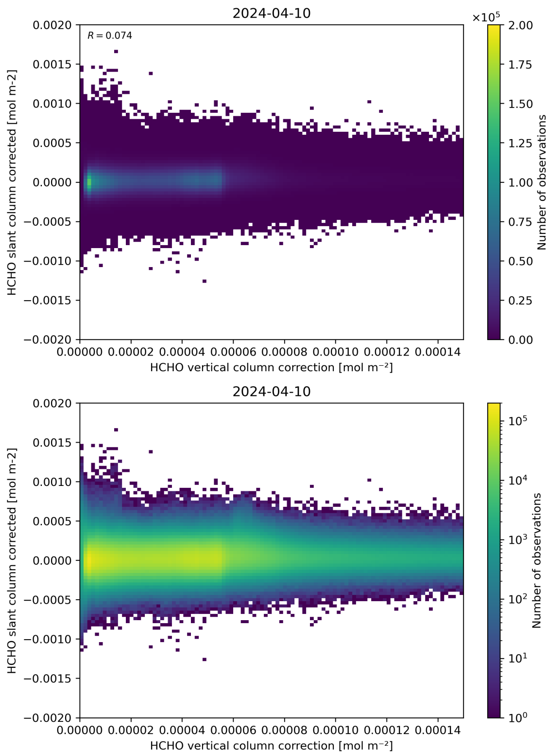
Figure 116: Scatter density plot of “HCHO vertical column correction” against “HCHO slant column corrected” for 2024-04-10 to 2024-04-11.
