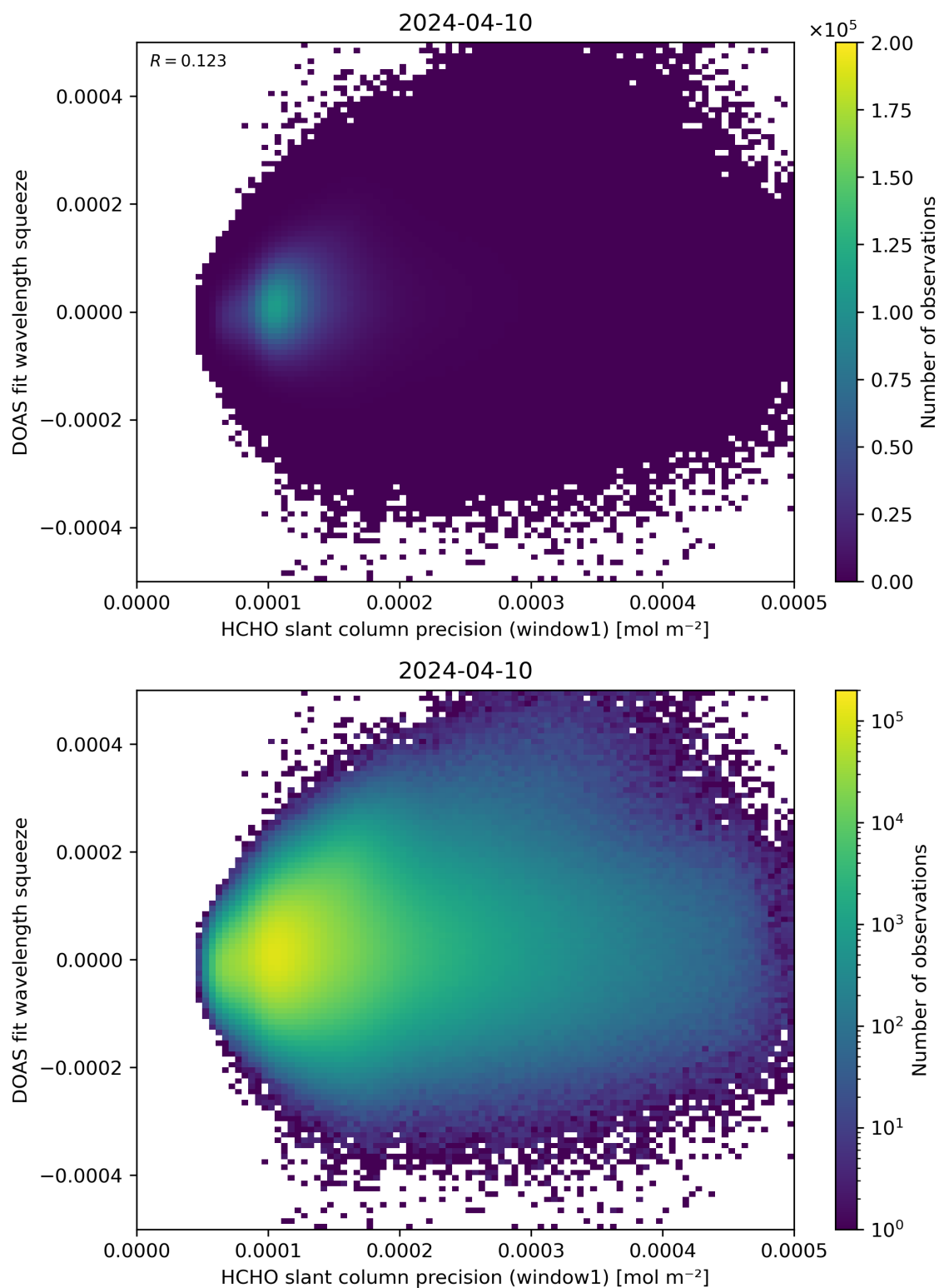
Figure 90: Scatter density plot of “HCHO slant column precision (window1)” against “DOAS fit wavelength squeeze” for 2024-04-10 to 2024-04-11.
