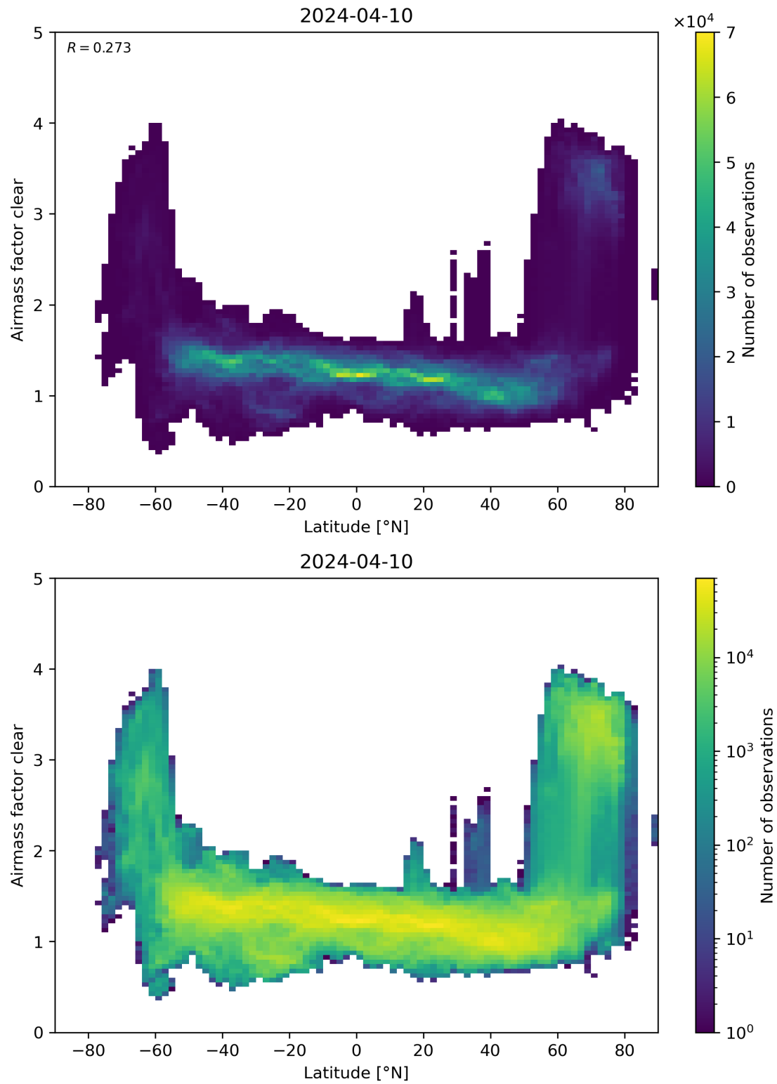
Figure 156: Scatter density plot of “Latitude” against “Airmass factor clear” for 2024-04-10 to 2024-04-11.
