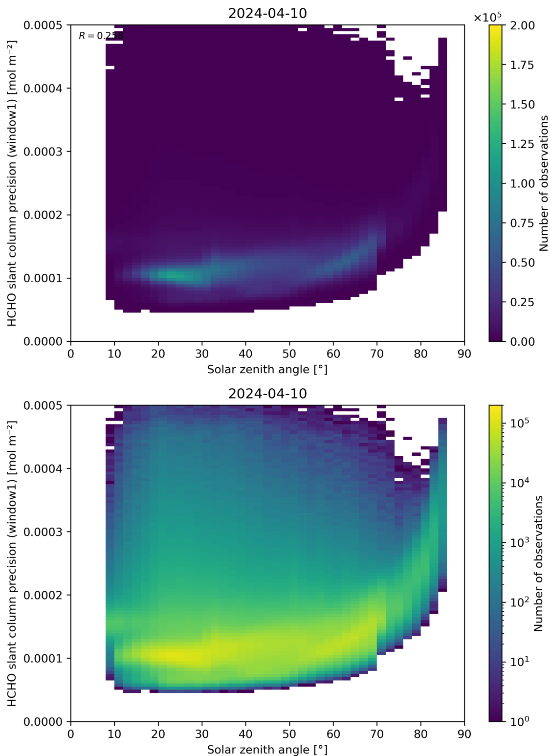
Figure 174: Scatter density plot of “Solar zenith angle” against “HCHO slant column precision (window1)” for 2024-04-10 to 2024-04-11.
