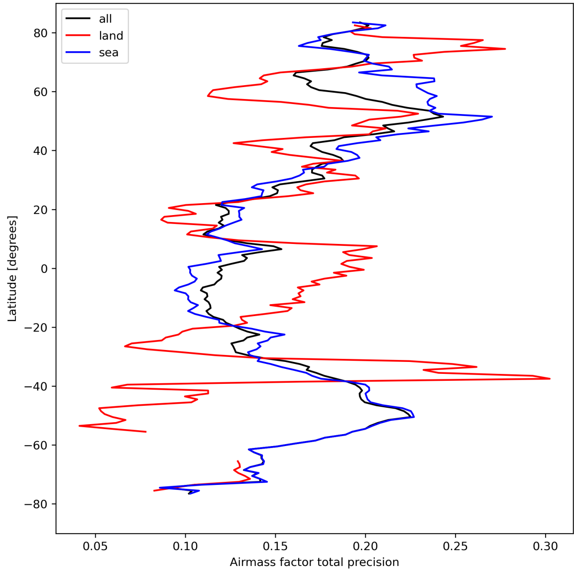
Figure 27: Zonal average of “Airmass factor total precision” for 2024-04-10 to 2024-04-11.
