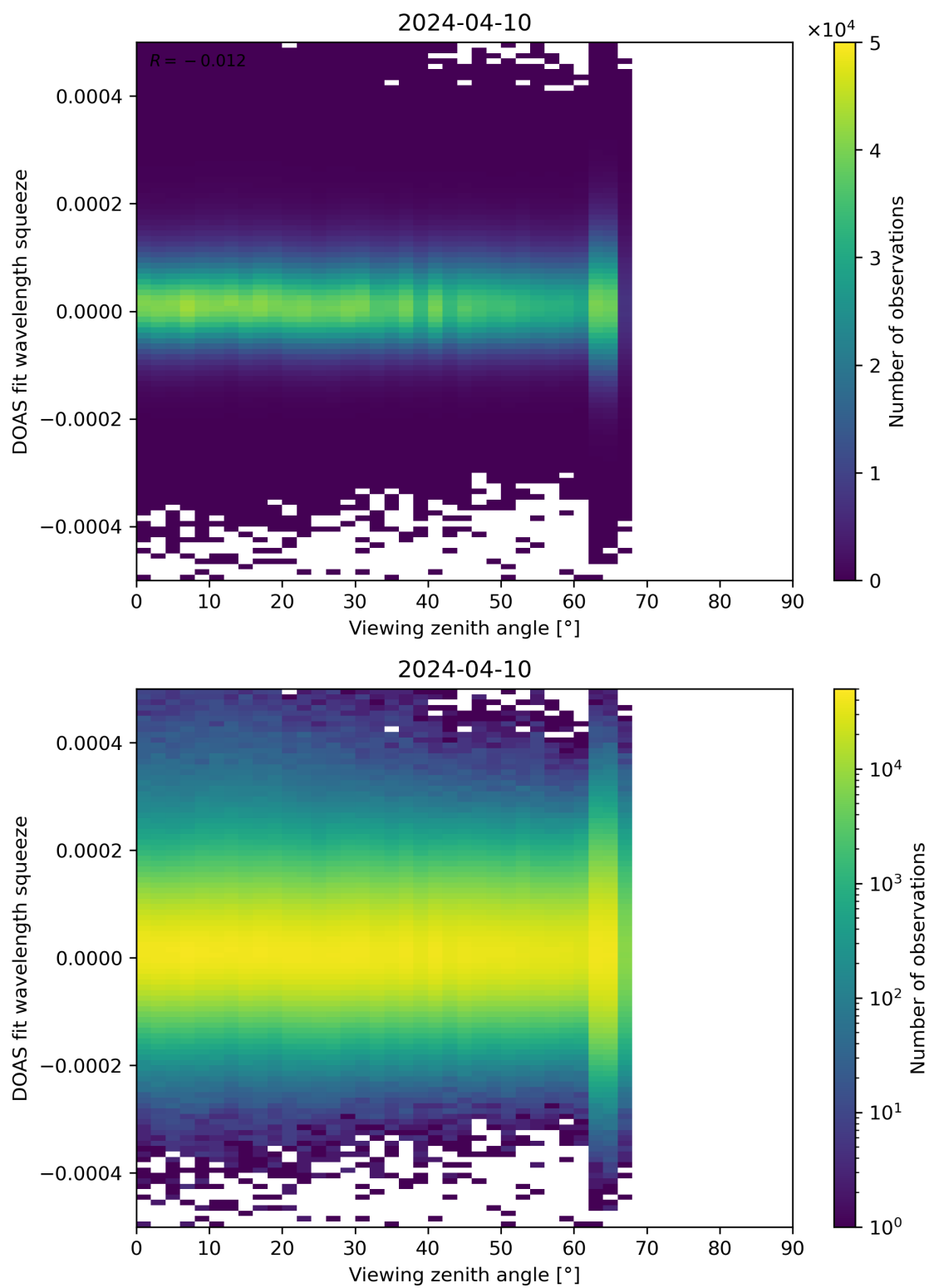
Figure 184: Scatter density plot of “Viewing zenith angle” against “DOAS fit wavelength squeeze” for 2024-04-10 to 2024-04-11.
