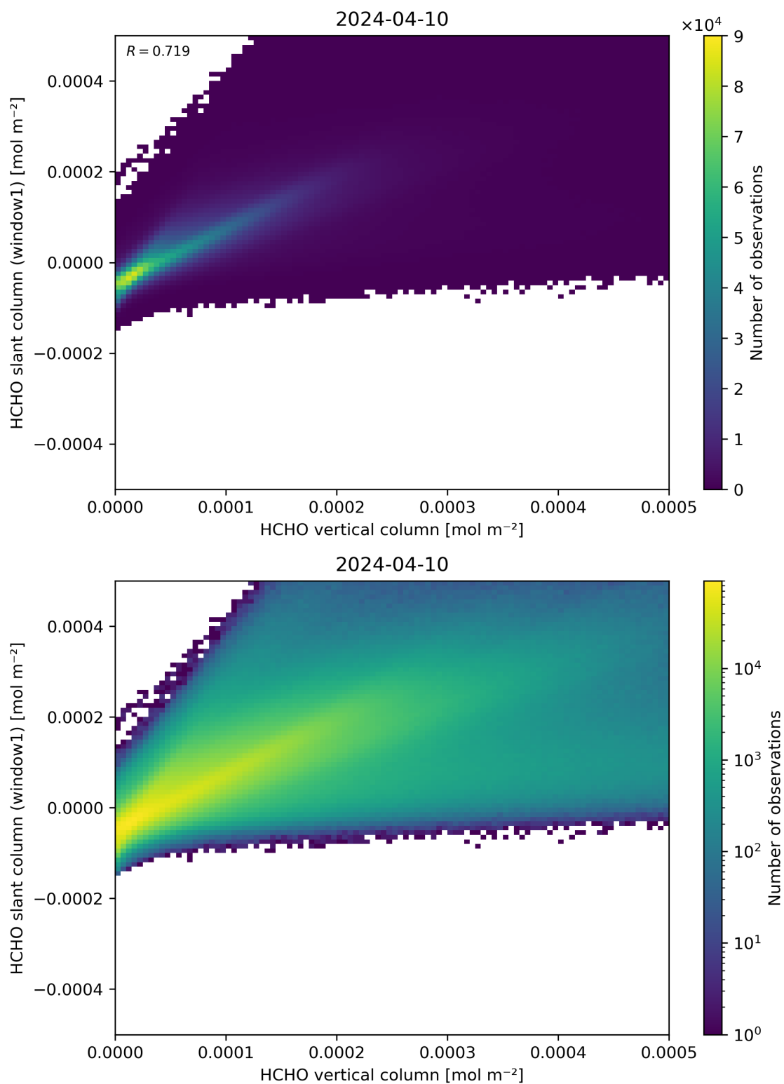
Figure 129: Scatter density plot of “HCHO vertical column” against “HCHO slant column (window1)” for 2024-04-10 to 2024-04-11.
