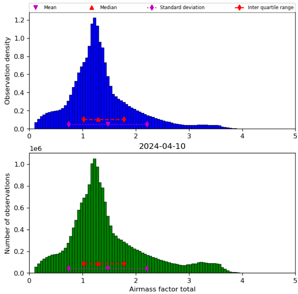
Figure 40: Histogram of “Airmass factor total” for 2024-04-10 to 2024-04-11
