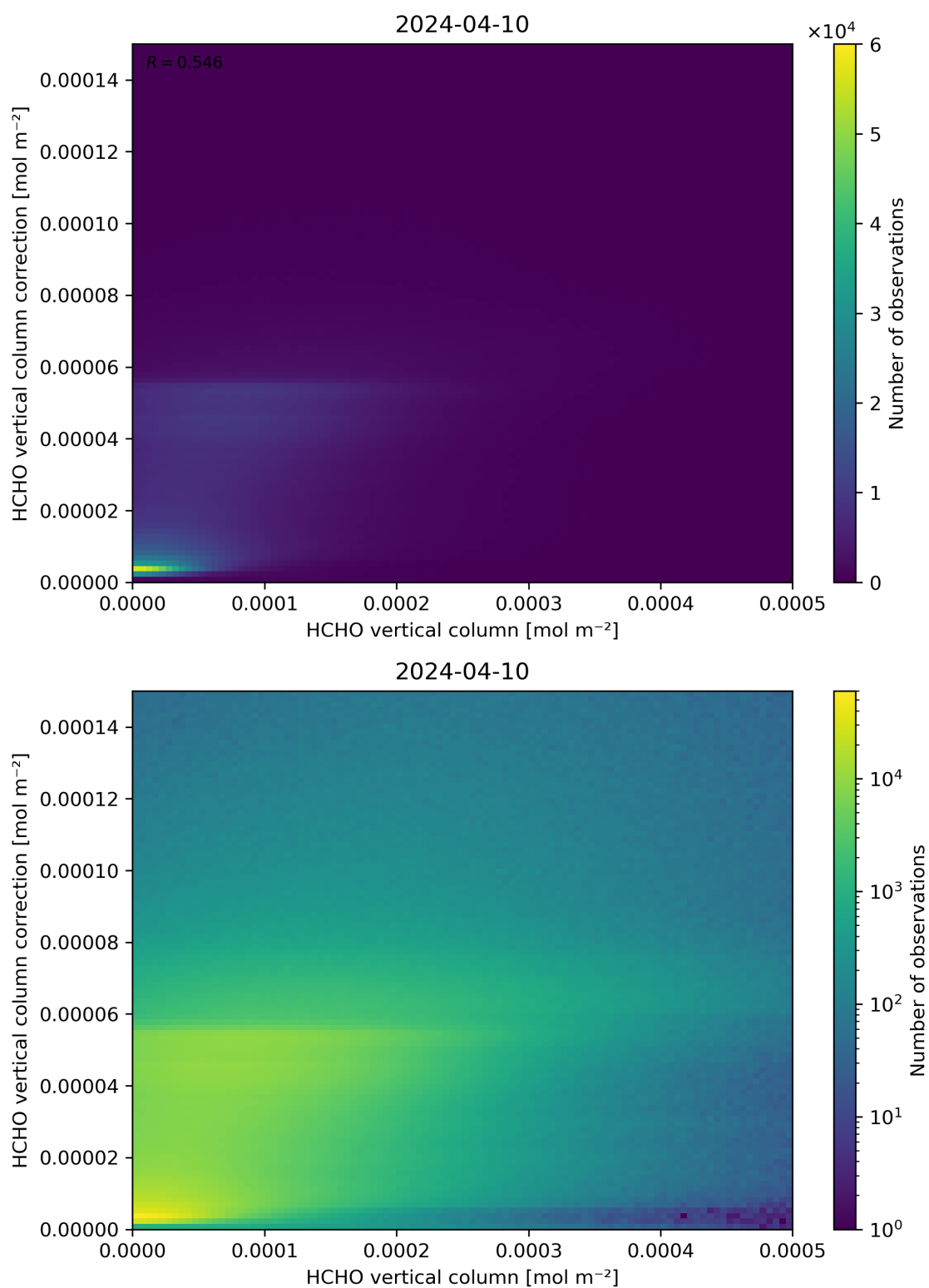
Figure 133: Scatter density plot of “HCHO vertical column” against “HCHO vertical column correction” for 2024-04-10 to 2024-04-11.
