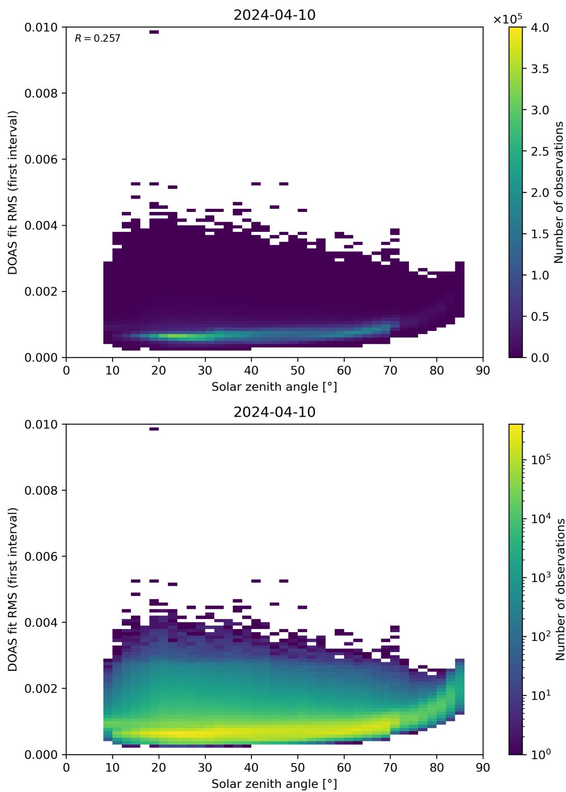
Figure 167: Scatter density plot of “Solar zenith angle” against “DOAS fit RMS (first interval)” for 2024-04-10 to 2024-04-11.
