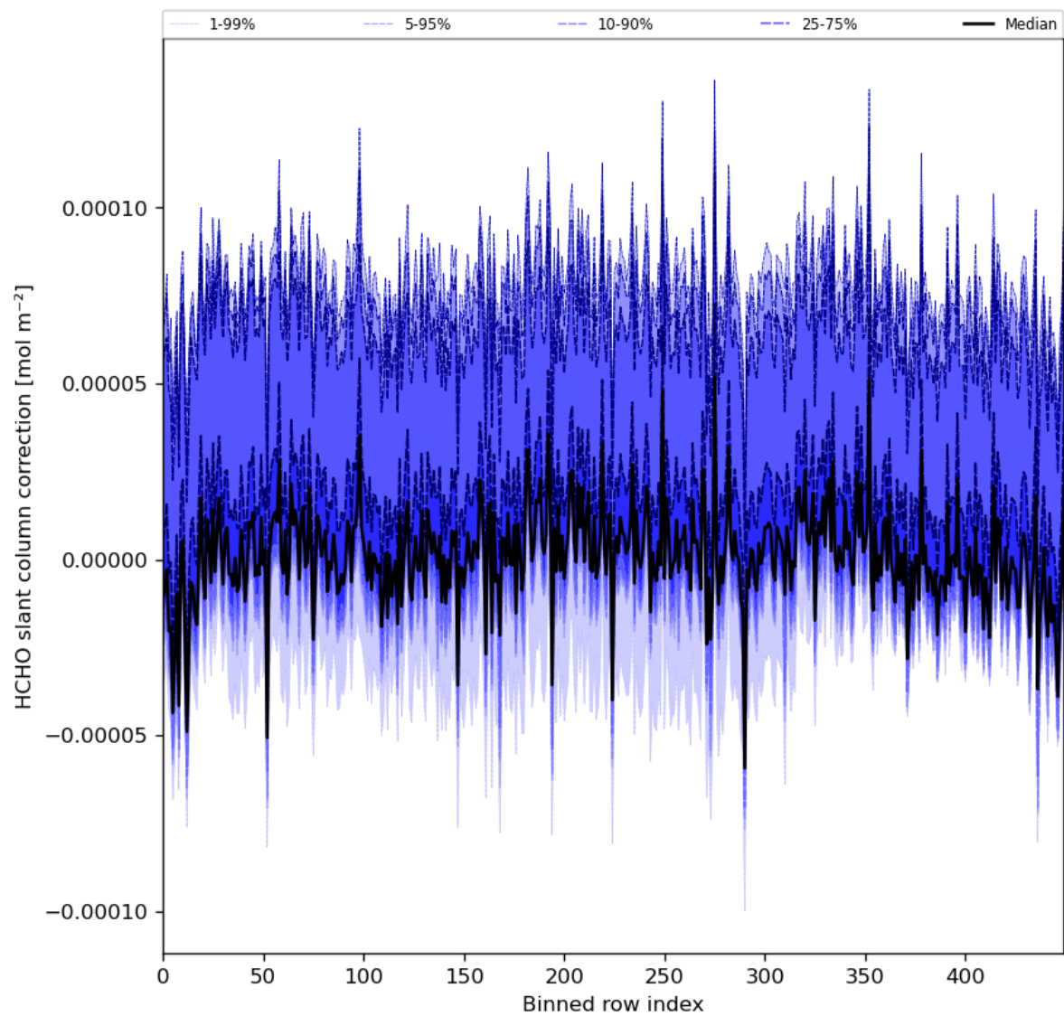
Figure 61: Along track statistics of “HCHO slant column correction” for 2024-04-10 to 2024-04-11
