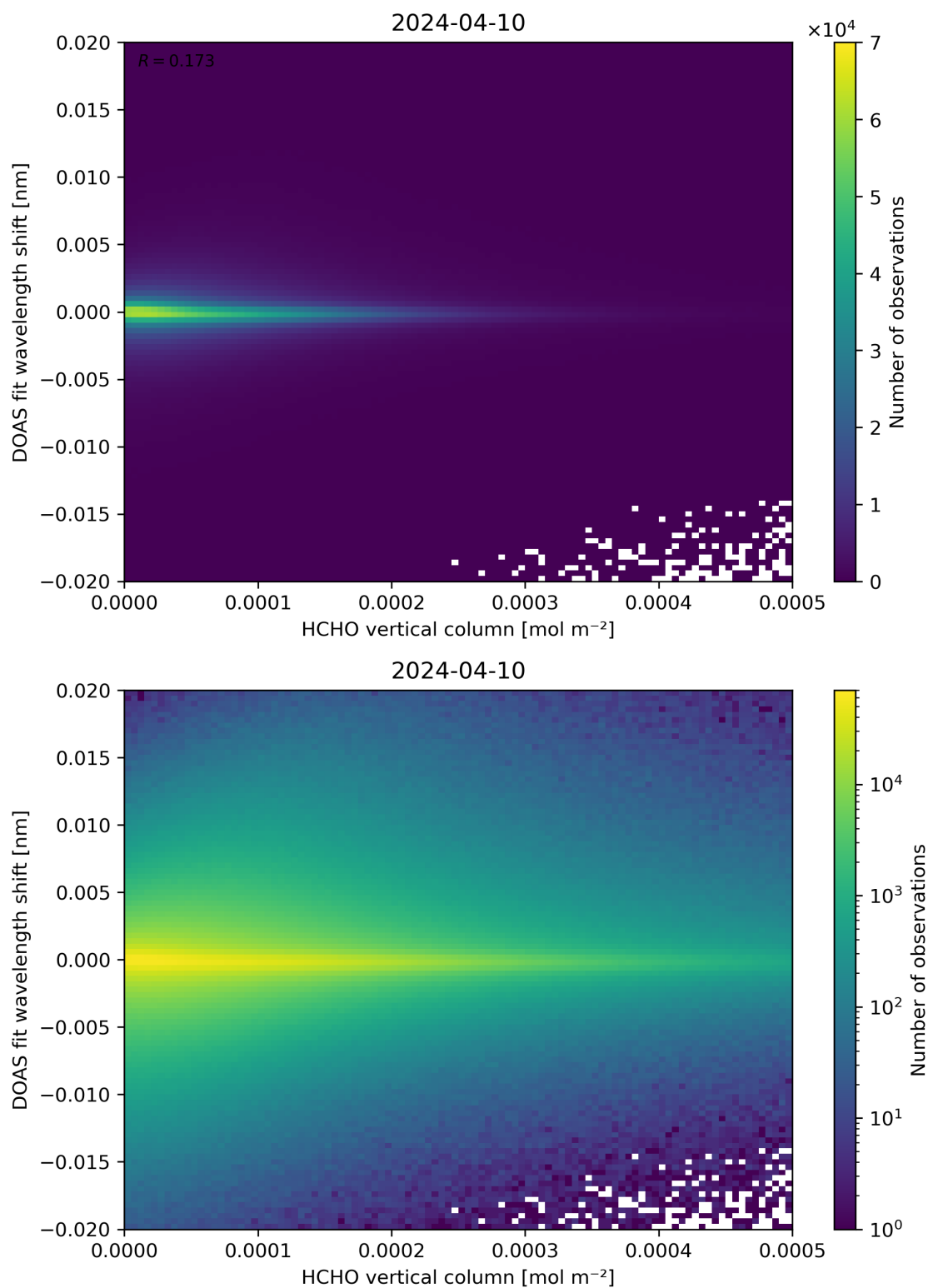
Figure 124: Scatter density plot of “HCHO vertical column” against “DOAS fit wavelength shift” for 2024-04-10 to 2024-04-11.
