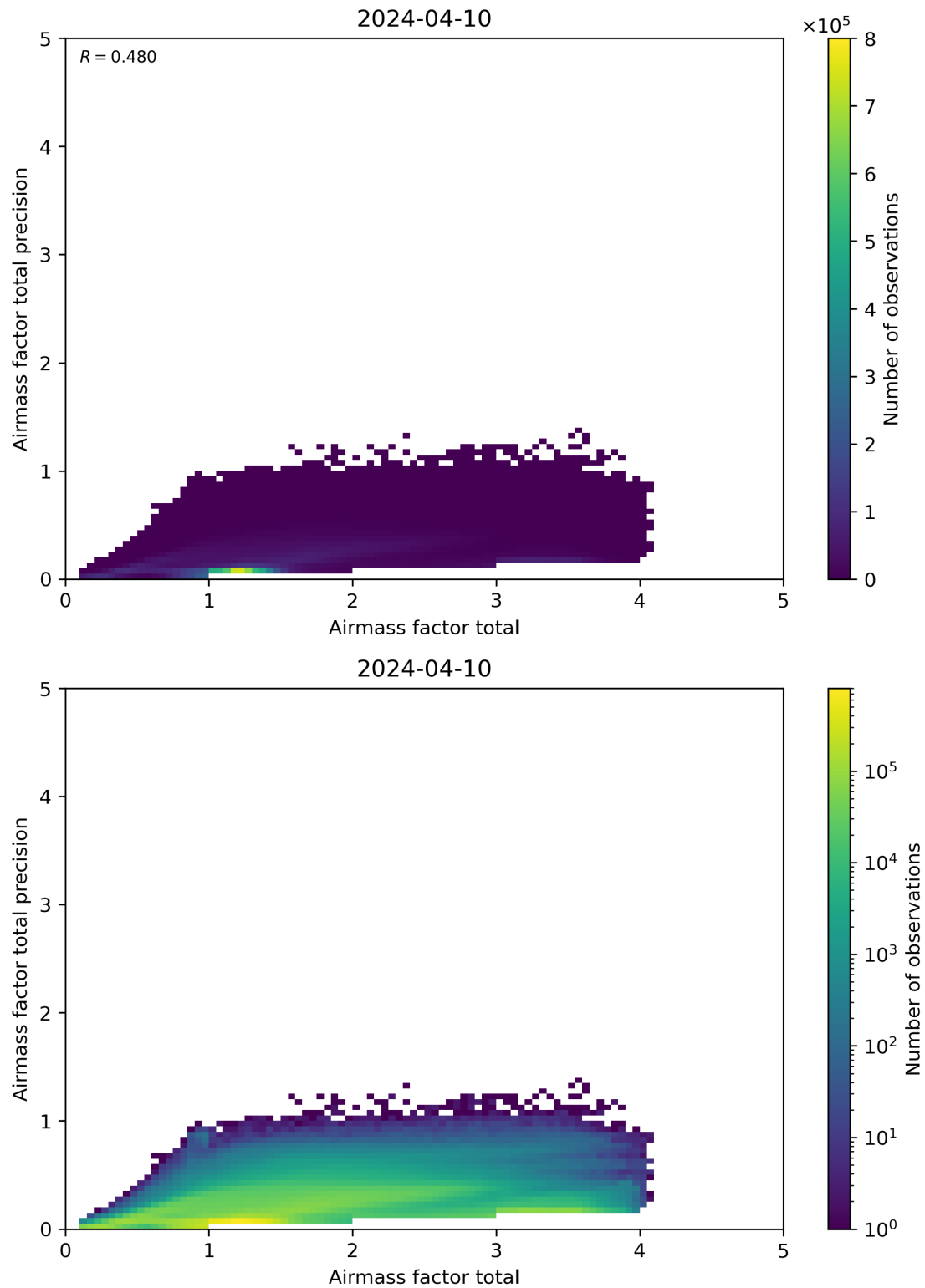
Figure 103: Scatter density plot of “Airmass factor total” against “Airmass factor total precision” for 2024-04-10 to 2024-04-11.
