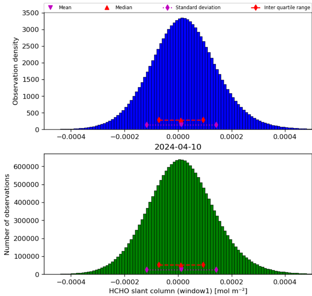
Figure 38: Histogram of “HCHO slant column (window1)” for 2024-04-10 to 2024-04-11
