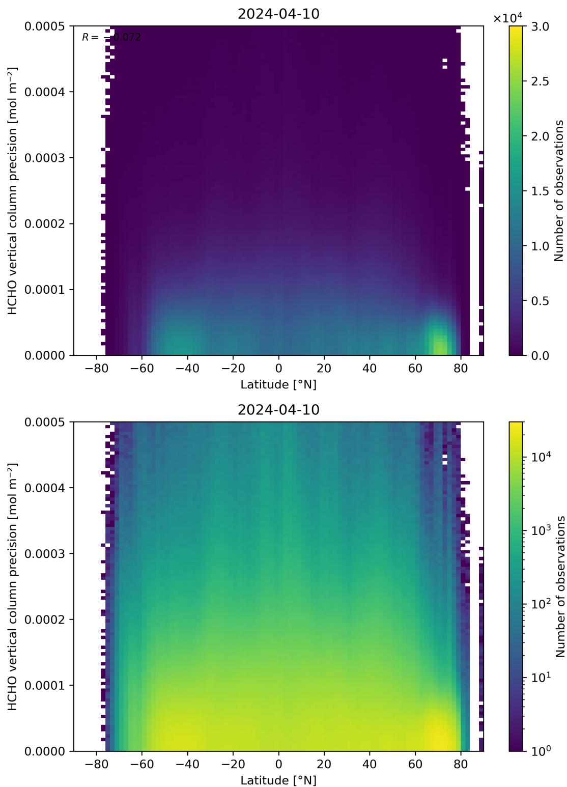
Figure 165: Scatter density plot of “Latitude” against “HCHO vertical column precision” for 2024-04-10 to 2024-04-11.
