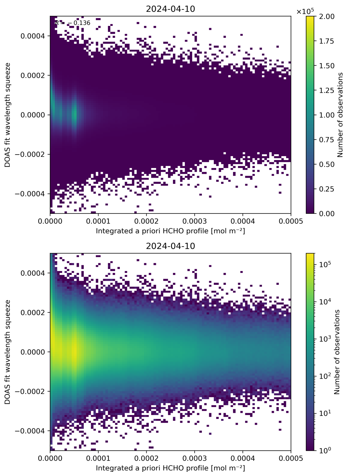
Figure 150: Scatter density plot of “Integrated a priori HCHO profile” against “DOAS fit wavelength squeeze” for 2024-04-10 to 2024-04-11.
