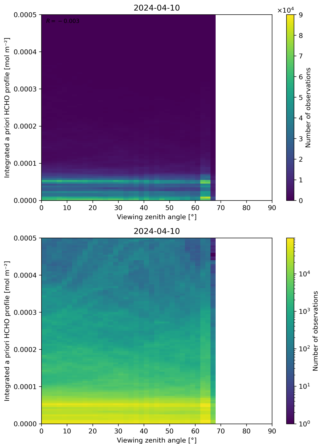
Figure 195: Scatter density plot of “Viewing zenith angle” against “Integrated a priori HCHO profile” for 2024-04-10 to 2024-04-11.
