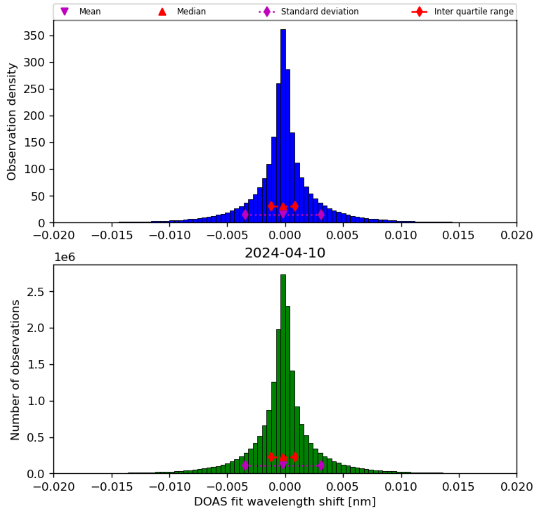
Figure 44: Histogram of “DOAS fit wavelength shift” for 2024-04-10 to 2024-04-11
