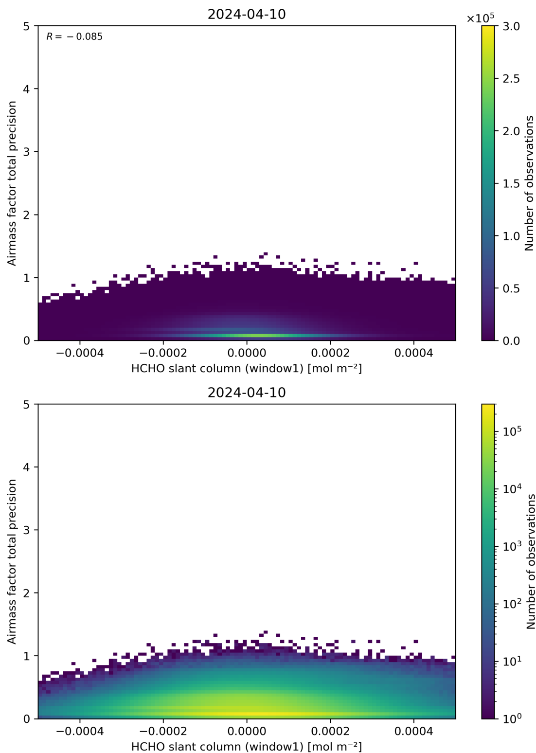
Figure 86: Scatter density plot of “HCHO slant column (window1)” against “Airmass factor total precision” for 2024-04-10 to 2024-04-11.
