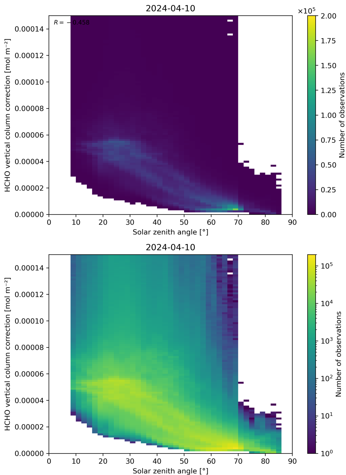
Figure 178: Scatter density plot of “Solar zenith angle” against “HCHO vertical column correction” for 2024-04-10 to 2024-04-11.
