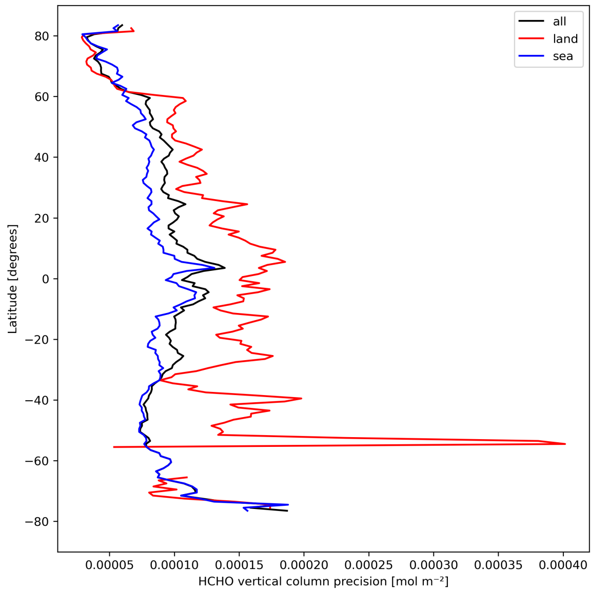
Figure 22: Zonal average of “HCHO vertical column precision” for 2024-04-10 to 2024-04-11.
