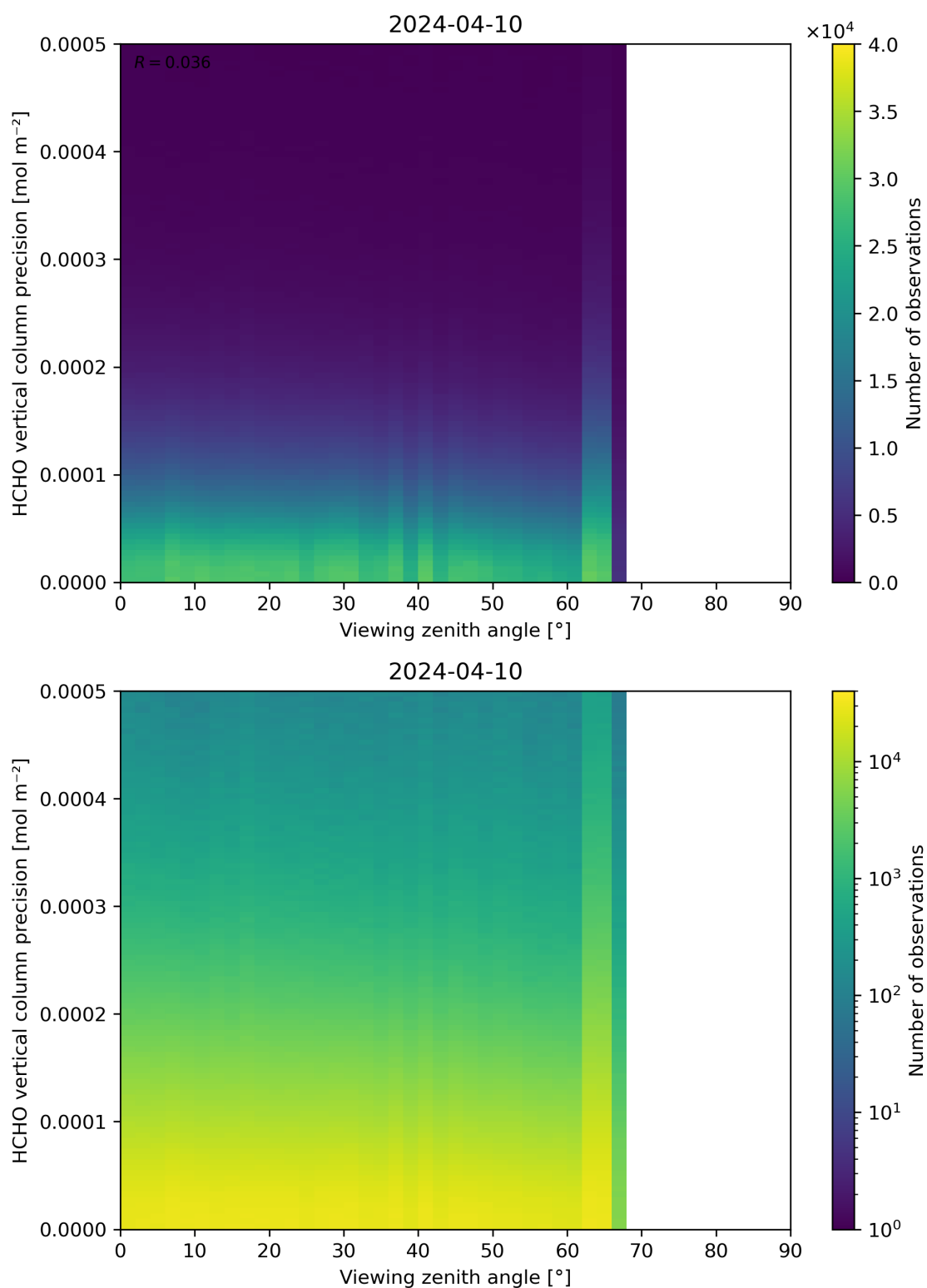
Figure 194: Scatter density plot of “Viewing zenith angle” against “HCHO vertical column precision” for 2024-04-10 to 2024-04-11.
