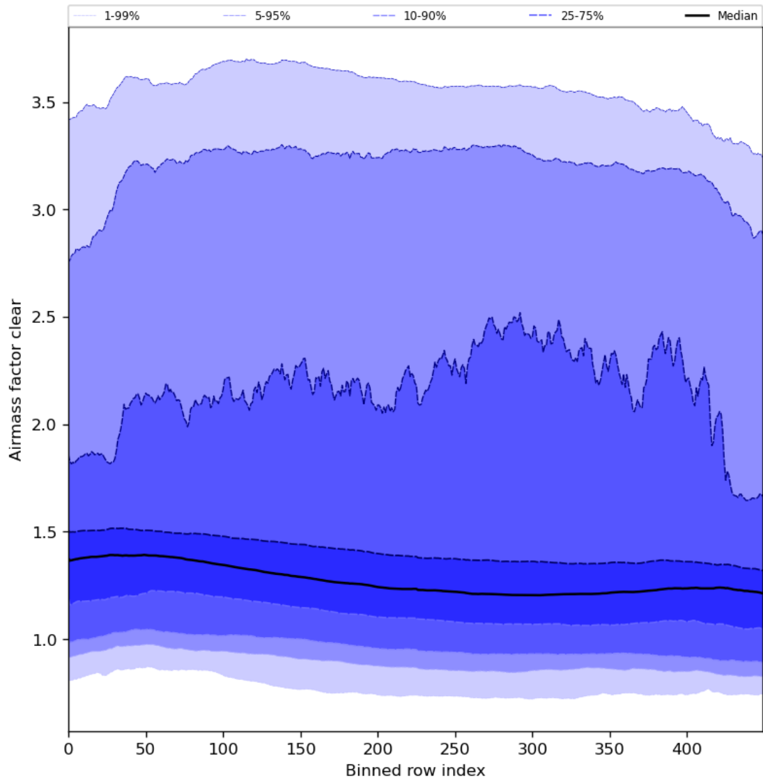
Figure 56: Along track statistics of “Airmass factor clear” for 2024-04-10 to 2024-04-11
