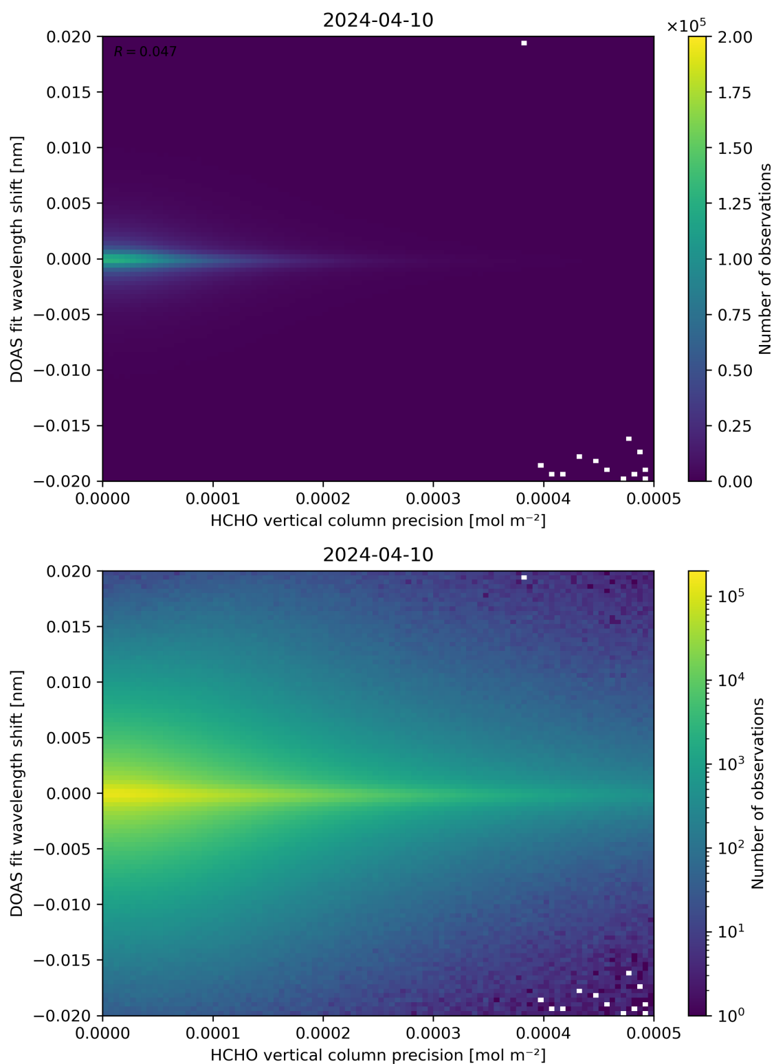
Figure 137: Scatter density plot of “HCHO vertical column precision” against “DOAS fit wavelength shift” for 2024-04-10 to 2024-04-11.
