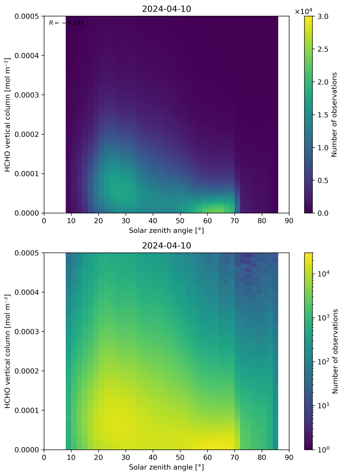
Figure 177: Scatter density plot of “Solar zenith angle” against “HCHO vertical column” for 2024-04-10 to 2024-04-11.
