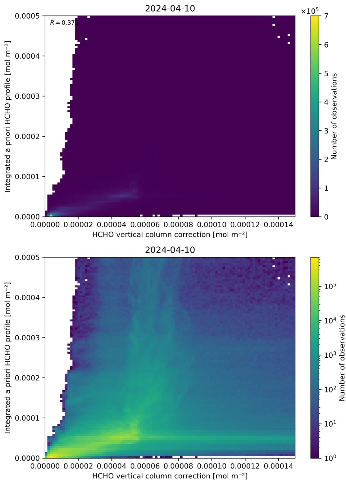
Figure 122: Scatter density plot of “HCHO vertical column correction” against “Integrated a priori HCHO profile” for 2024-04-10 to 2024-04-11.
