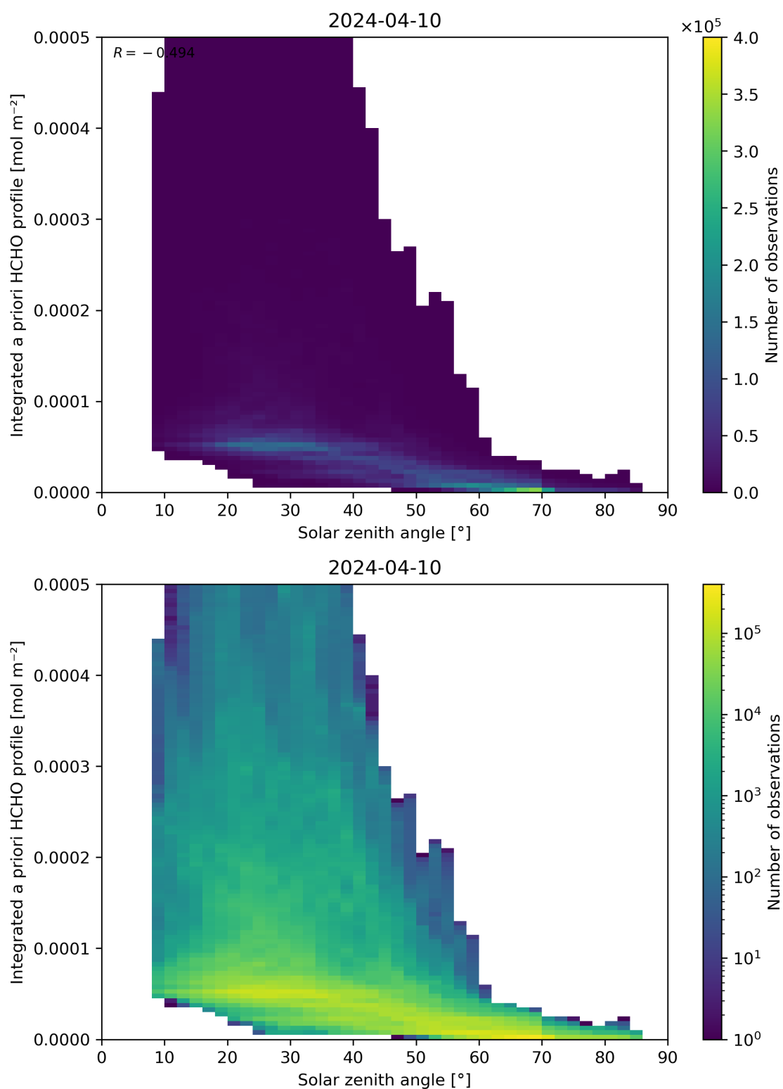
Figure 180: Scatter density plot of “Solar zenith angle” against “Integrated a priori HCHO profile” for 2024-04-10 to 2024-04-11.
