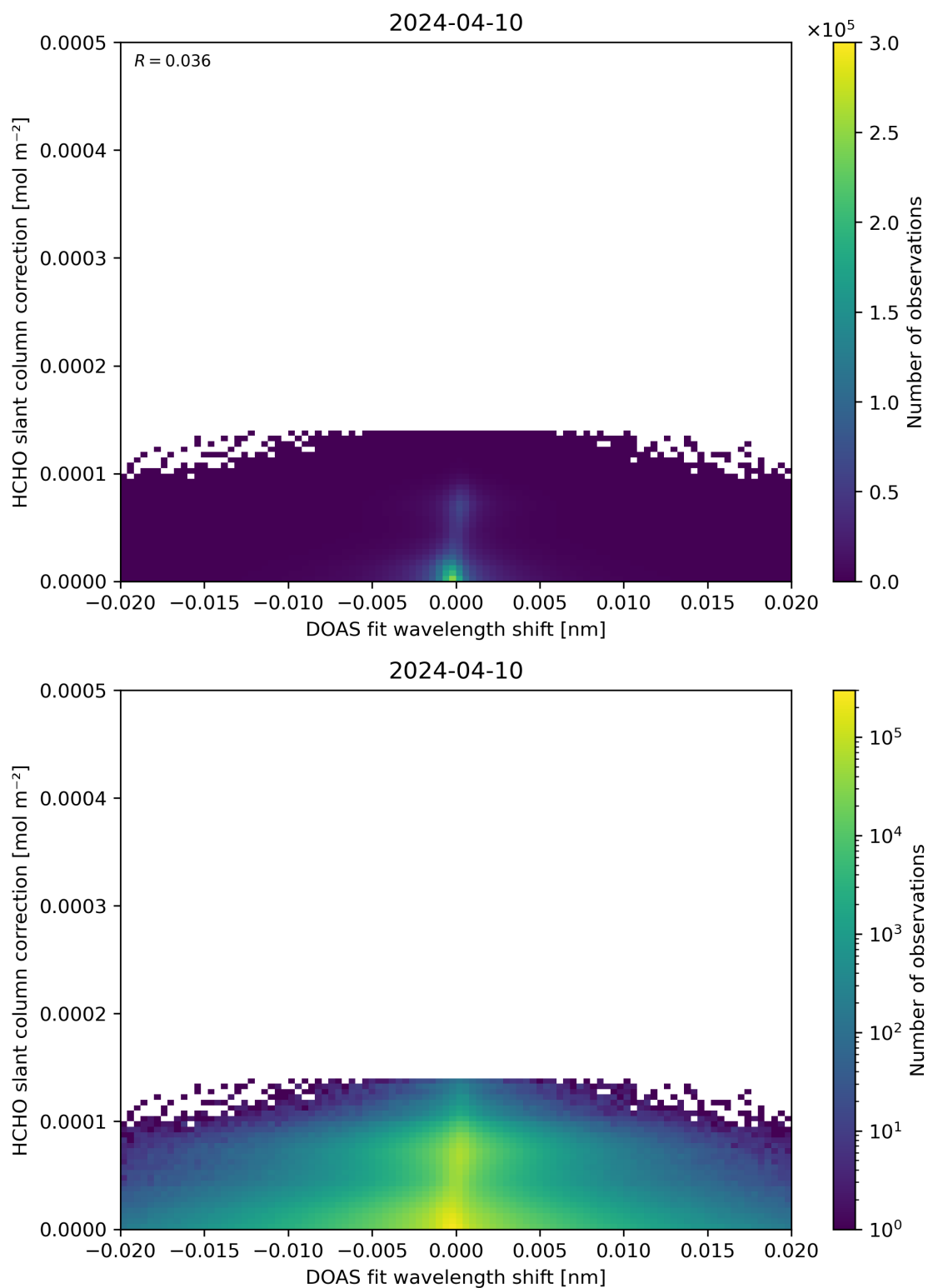
Figure 67: Scatter density plot of “DOAS fit wavelength shift” against “HCHO slant column correction” for 2024-04-10 to 2024-04-11.
