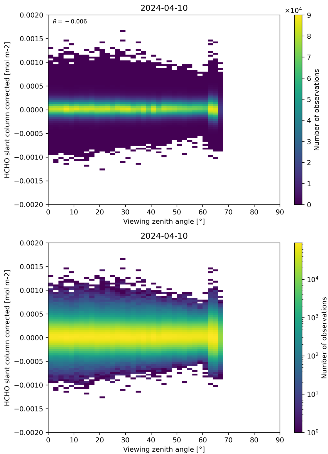
Figure 186: Scatter density plot of “Viewing zenith angle” against “HCHO slant column corrected” for 2024-04-10 to 2024-04-11.
