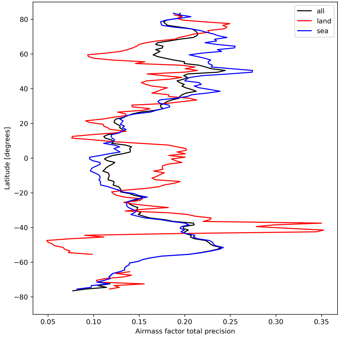
Figure 27: Zonal average of “Airmass factor total precision” for 2024-04-10 to 2024-04-12.
