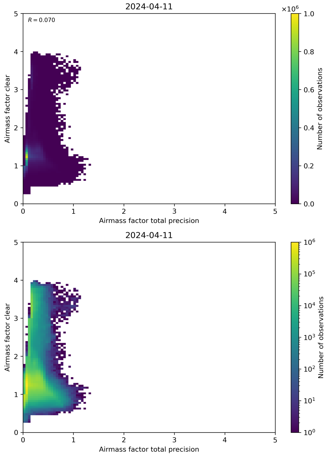
Figure 108: Scatter density plot of “Airmass factor total precision” against “Airmass factor clear” for 2024-04-10 to 2024-04-12.
