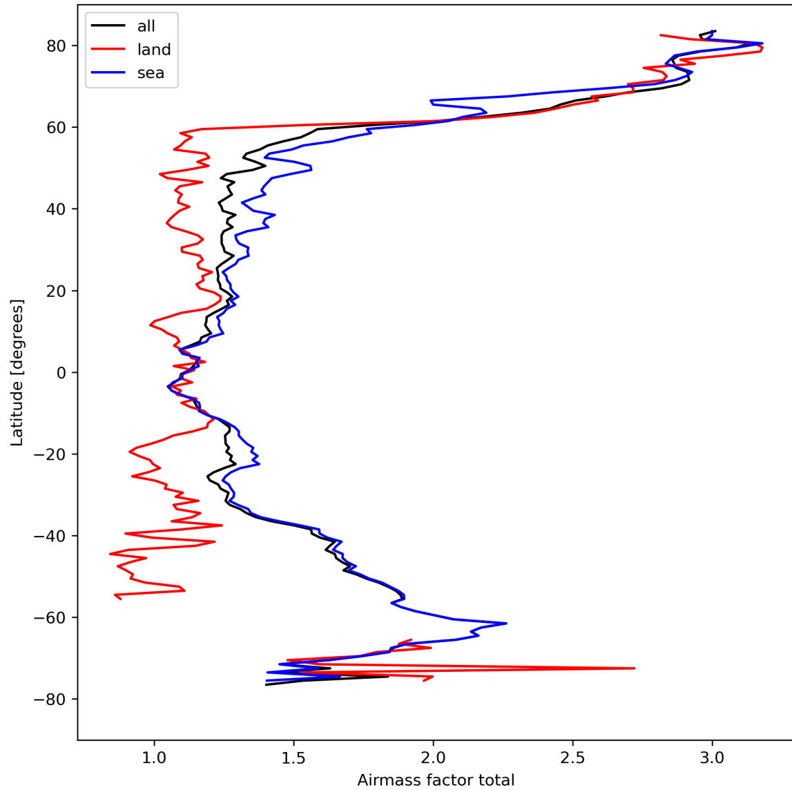
Figure 26: Zonal average of “Airmass factor total” for 2024-04-10 to 2024-04-12.
