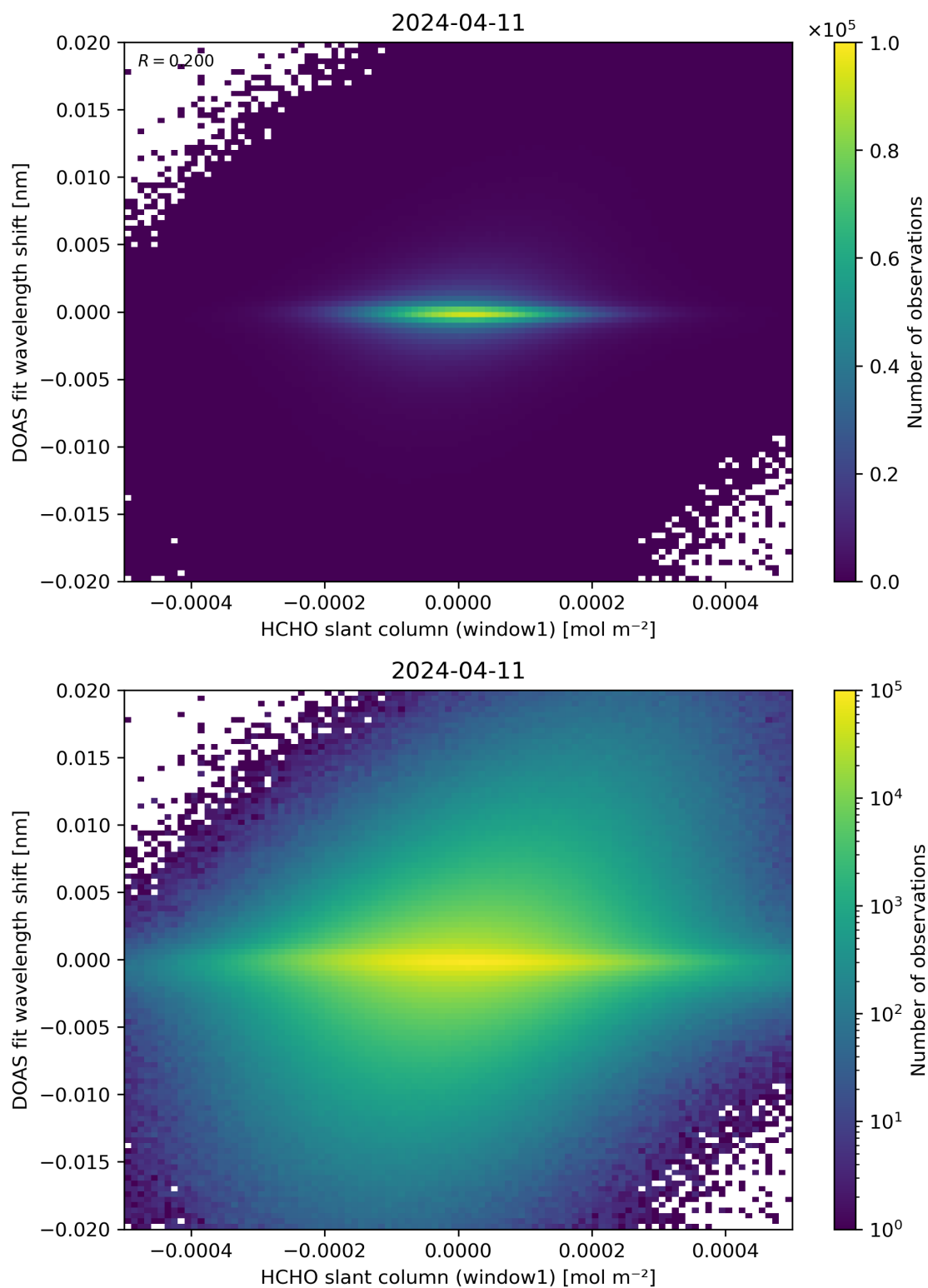
Figure 79: Scatter density plot of “HCHO slant column (window1)” against “DOAS fit wavelength shift” for 2024-04-10 to 2024-04-12.
