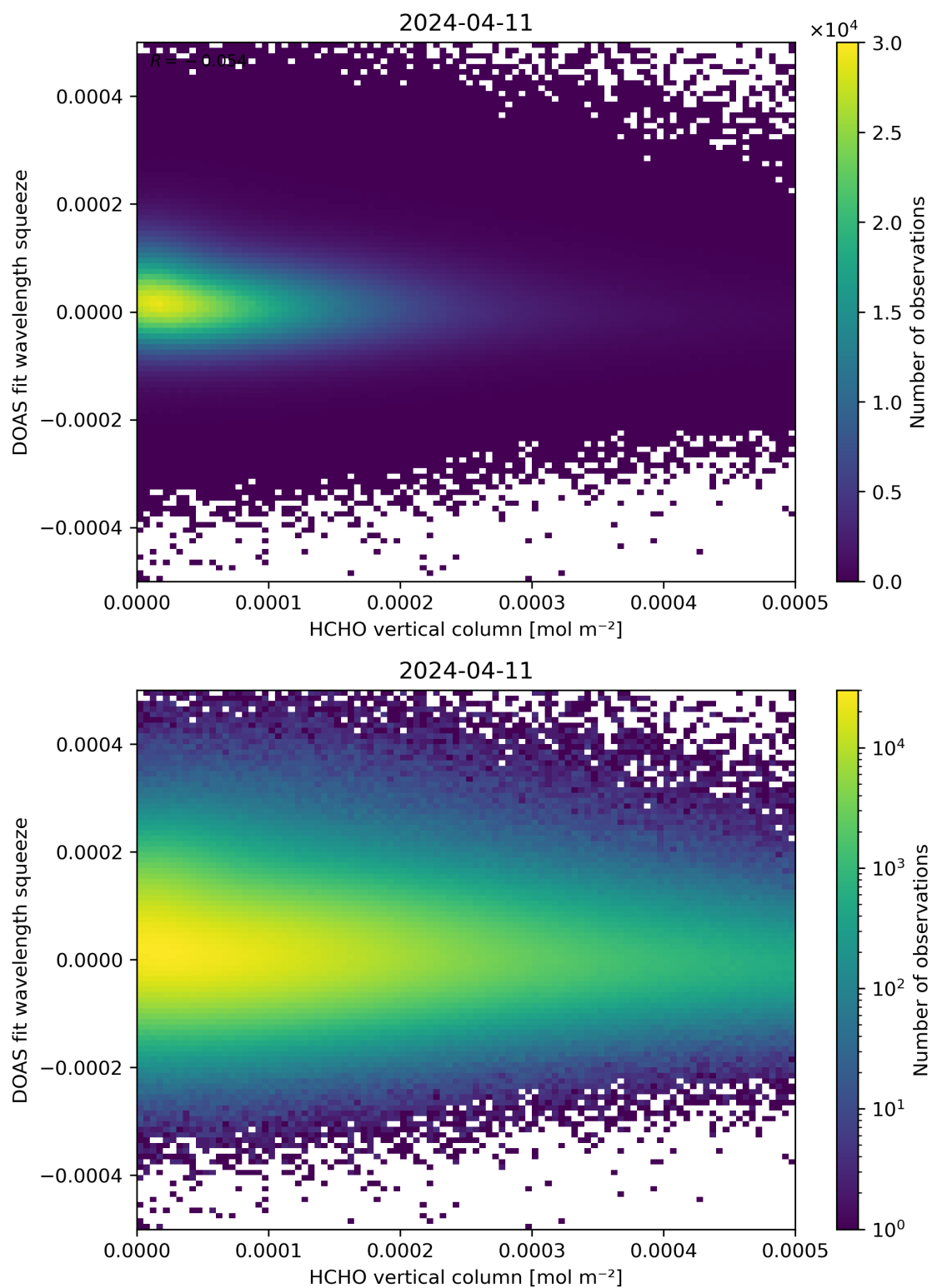
Figure 125: Scatter density plot of “HCHO vertical column” against “DOAS fit wavelength squeeze” for 2024-04-10 to 2024-04-12.
