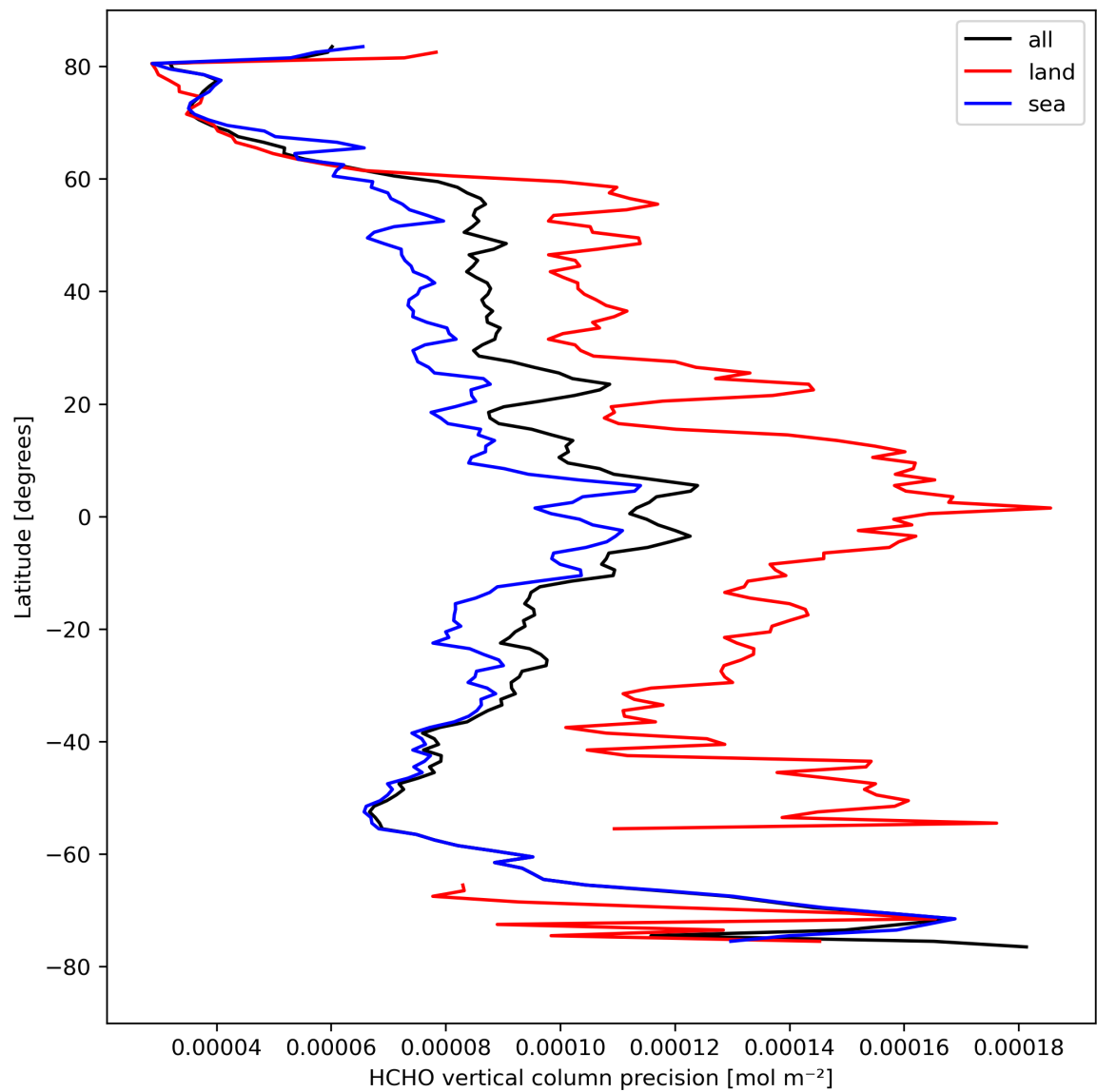
Figure 22: Zonal average of “HCHO vertical column precision” for 2024-04-10 to 2024-04-12.
