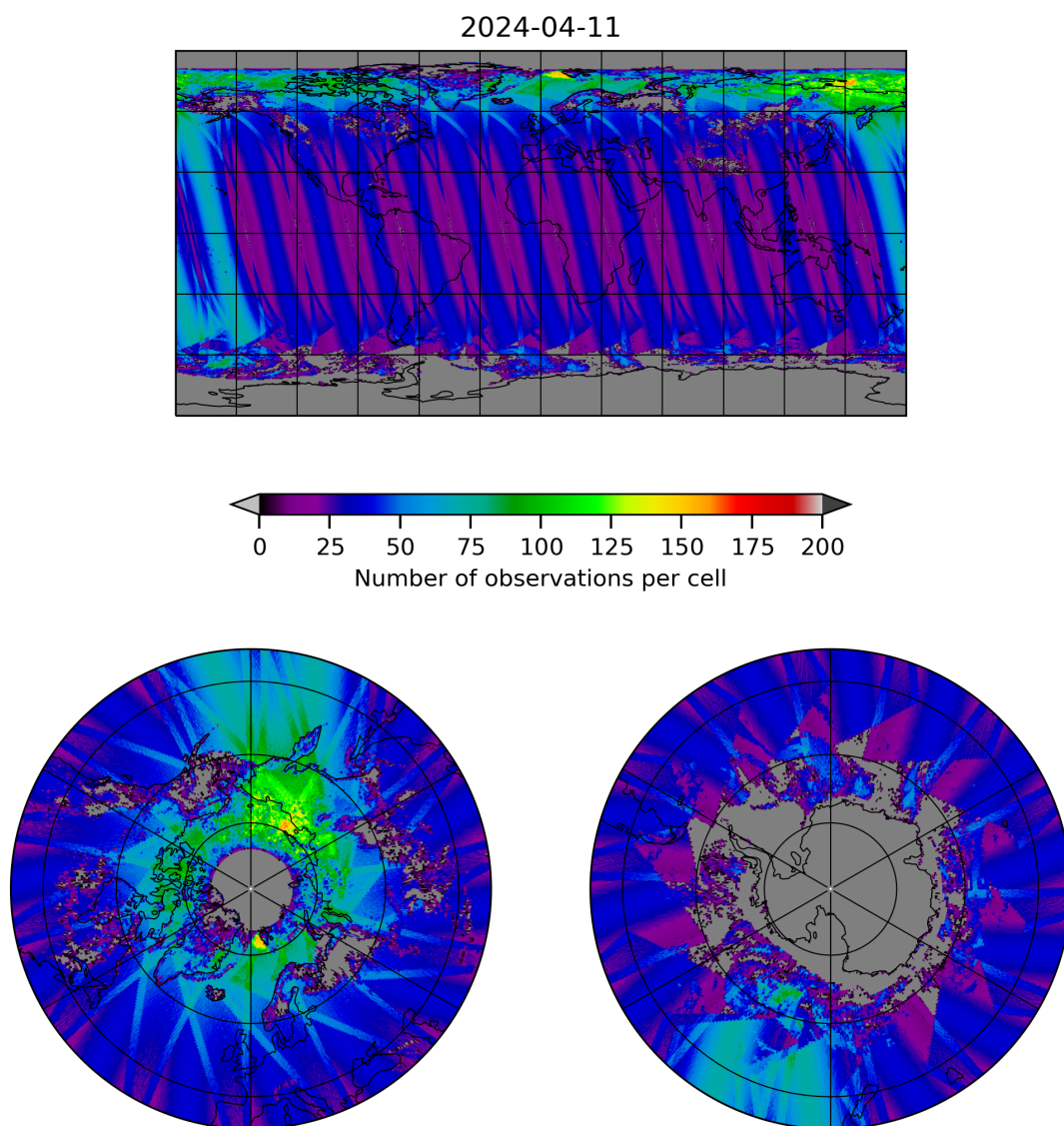
Figure 19: Map of the number of observations for 2024-04-10 to 2024-04-12
