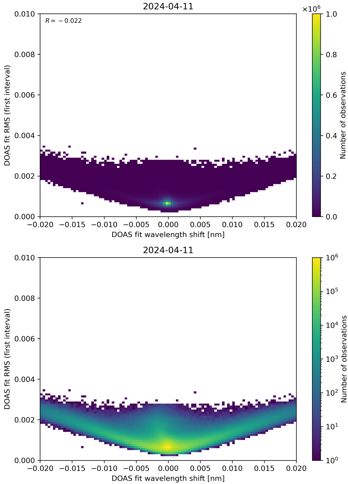
Figure 64: Scatter density plot of “DOAS fit wavelength shift” against “DOAS fit RMS (first interval)” for 2024-04-10 to 2024-04-12.
