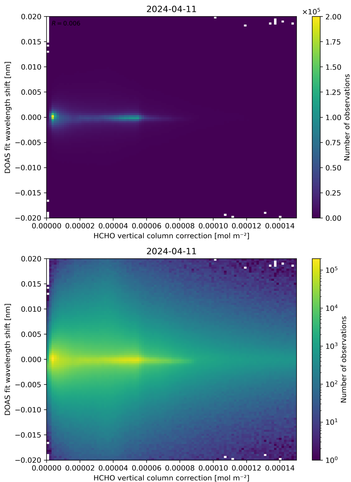
Figure 113: Scatter density plot of “HCHO vertical column correction” against “DOAS fit wavelength shift” for 2024-04-10 to 2024-04-12.
