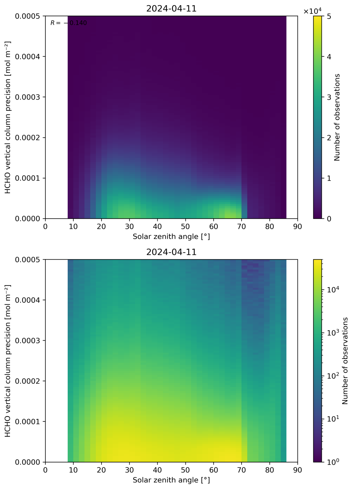
Figure 179: Scatter density plot of “Solar zenith angle” against “HCHO vertical column precision” for 2024-04-10 to 2024-04-12.
