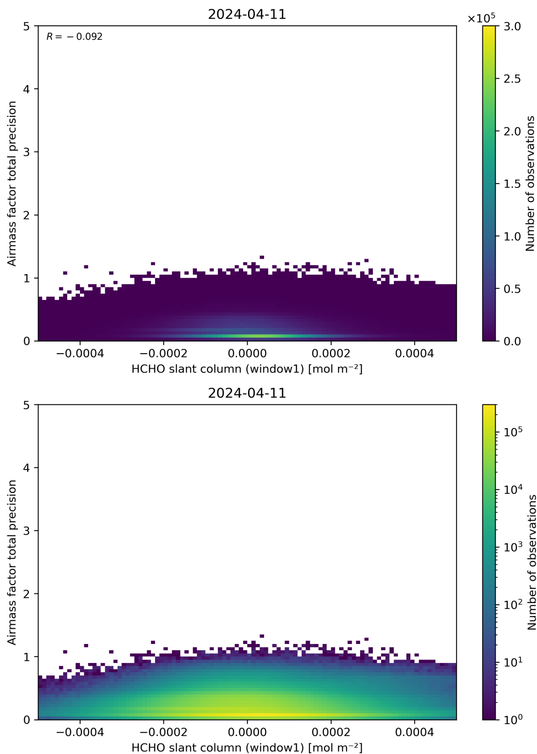
Figure 86: Scatter density plot of “HCHO slant column (window1)” against “Airmass factor total precision” for 2024-04-10 to 2024-04-12.
