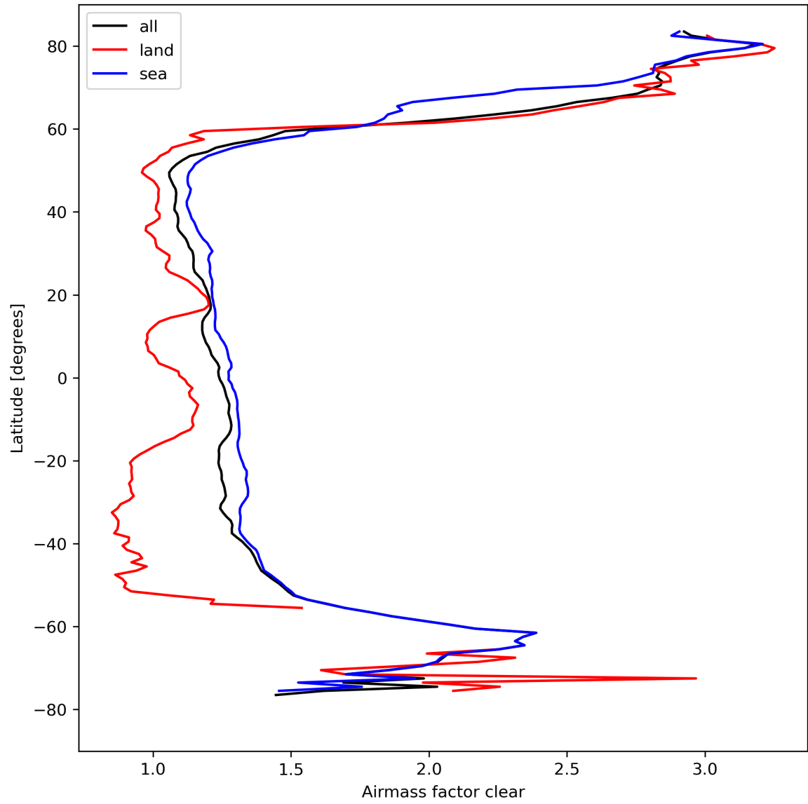
Figure 28: Zonal average of “Airmass factor clear” for 2024-04-10 to 2024-04-12.
