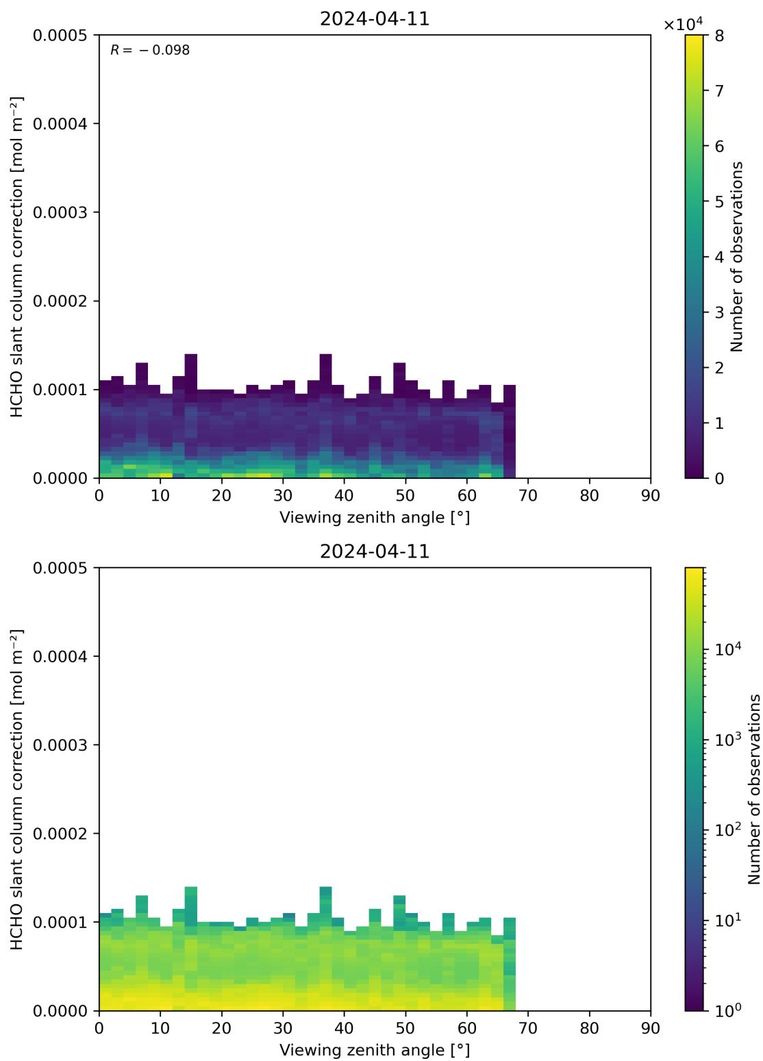
Figure 187: Scatter density plot of “Viewing zenith angle” against “HCHO slant column correction” for 2024-04-10 to 2024-04-12.
