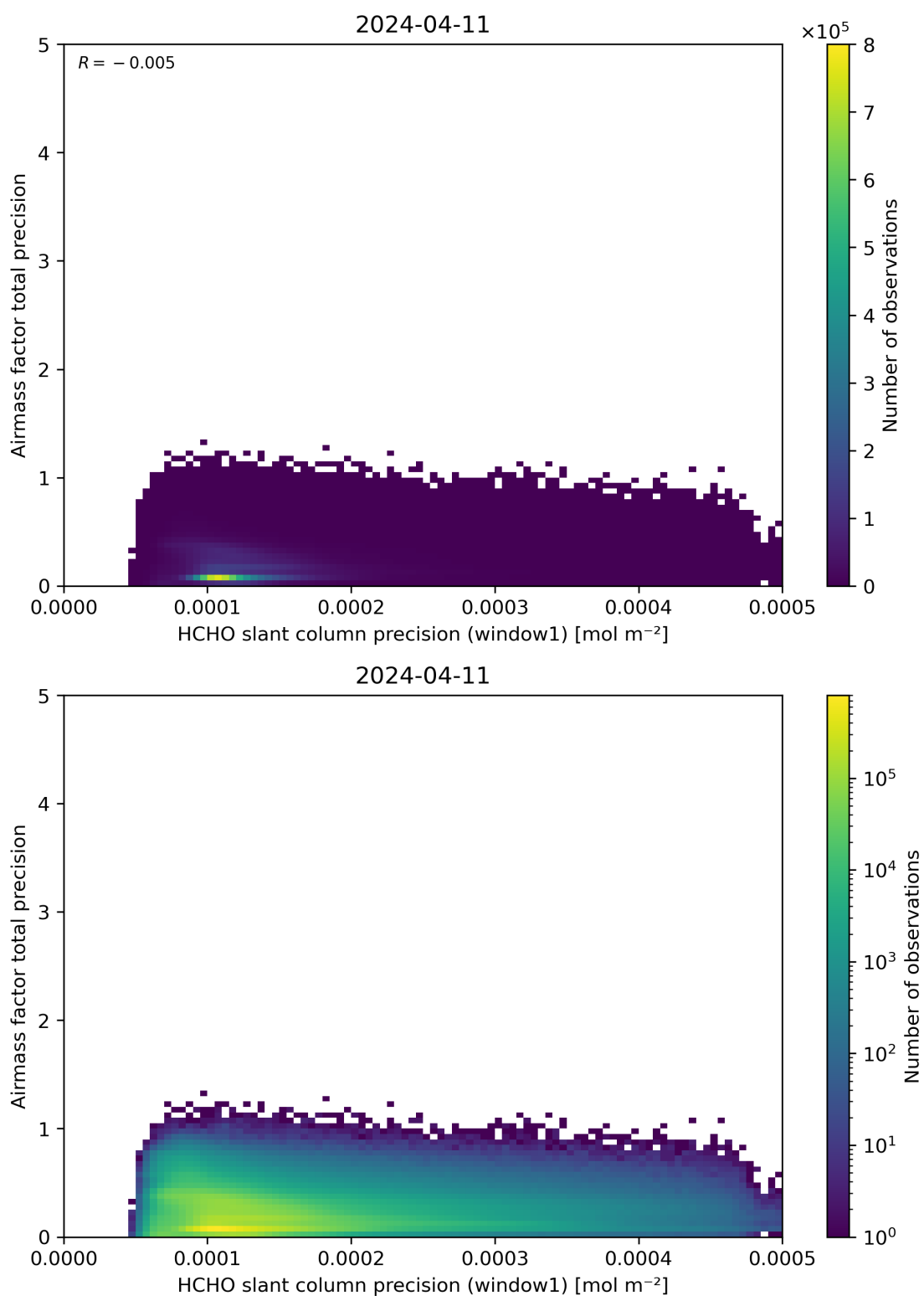
Figure 95: Scatter density plot of “HCHO slant column precision (window1)” against “Airmass factor total precision” for 2024-04-10 to 2024-04-12.
