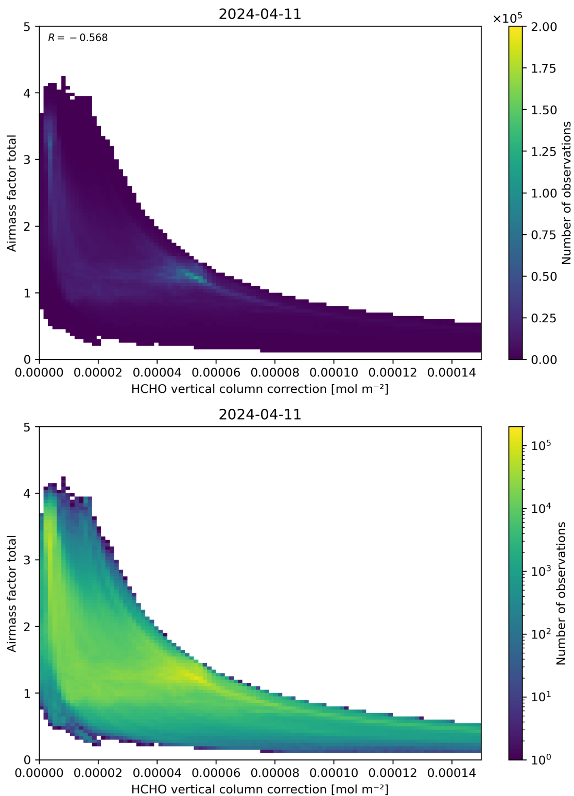
Figure 120: Scatter density plot of “HCHO vertical column correction” against “Airmass factor total” for 2024-04-10 to 2024-04-12.
