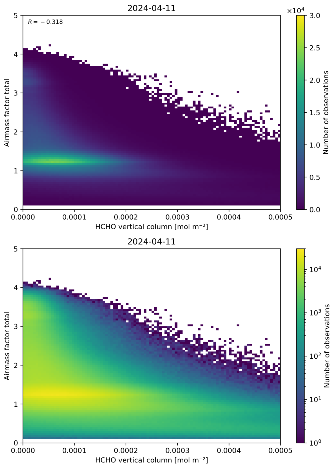
Figure 131: Scatter density plot of “HCHO vertical column” against “Airmass factor total” for 2024-04-10 to 2024-04-12.
