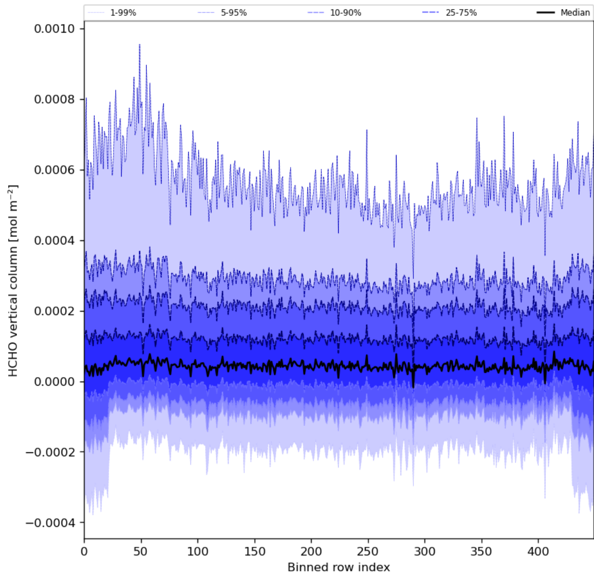
Figure 49: Along track statistics of “HCHO vertical column” for 2024-04-10 to 2024-04-12
