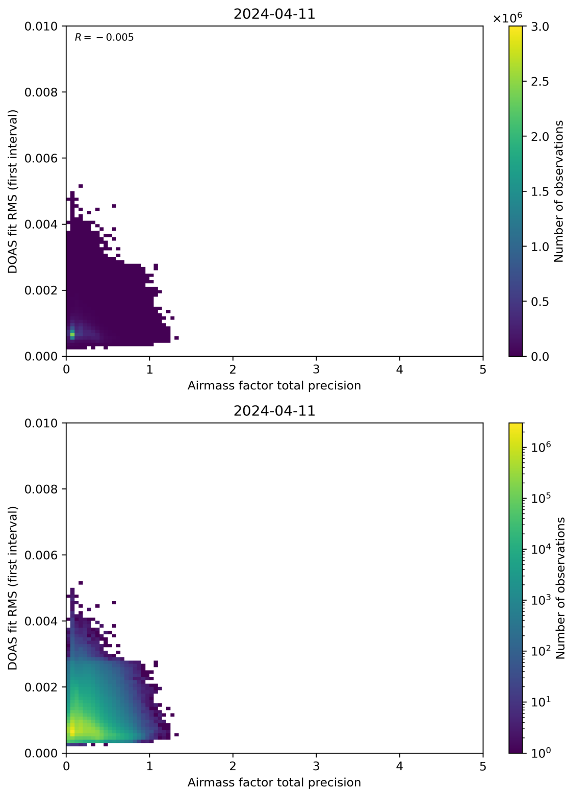
Figure 105: Scatter density plot of “Airmass factor total precision” against “DOAS fit RMS (first interval)” for 2024-04-10 to 2024-04-12.
