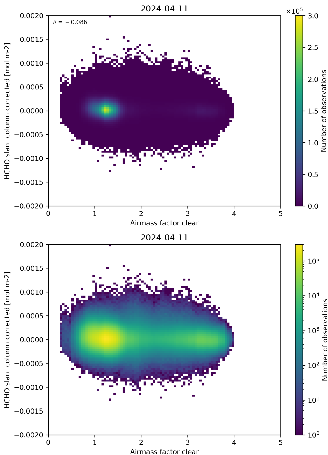
Figure 74: Scatter density plot of “Airmass factor clear” against “HCHO slant column corrected” for 2024-04-10 to 2024-04-12.
