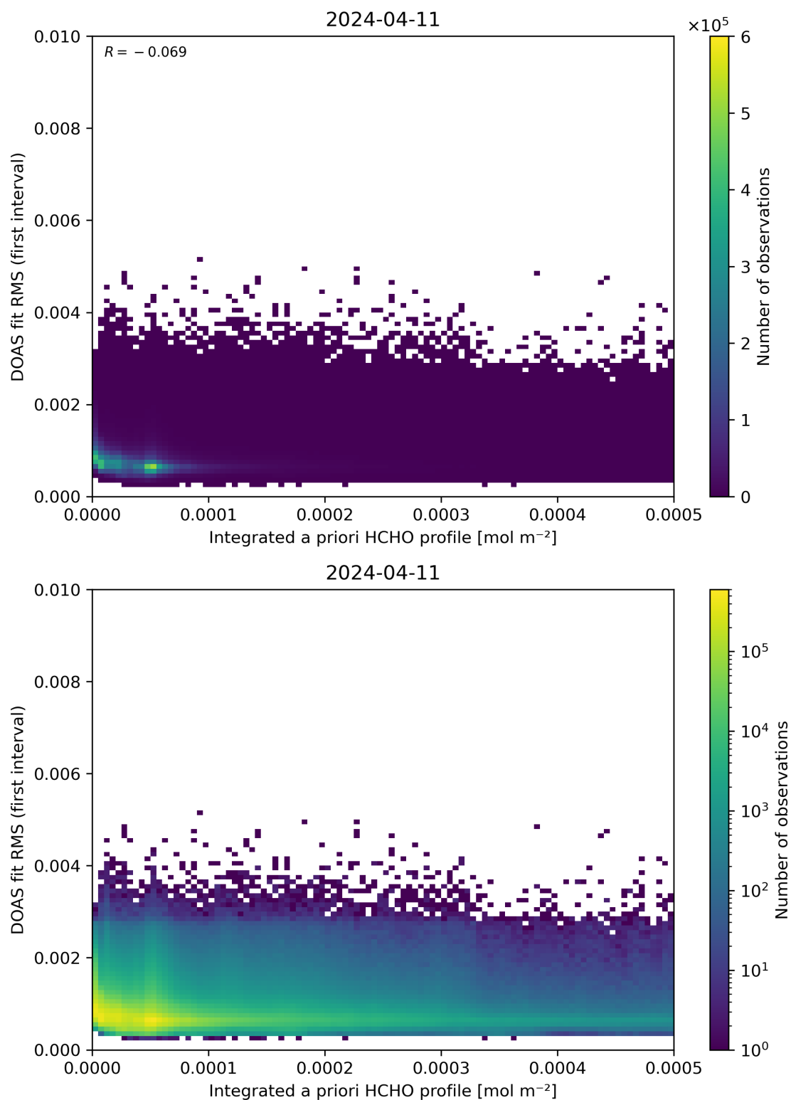
Figure 148: Scatter density plot of “Integrated a priori HCHO profile” against “DOAS fit RMS (first interval)” for 2024-04-10 to 2024-04-12.
