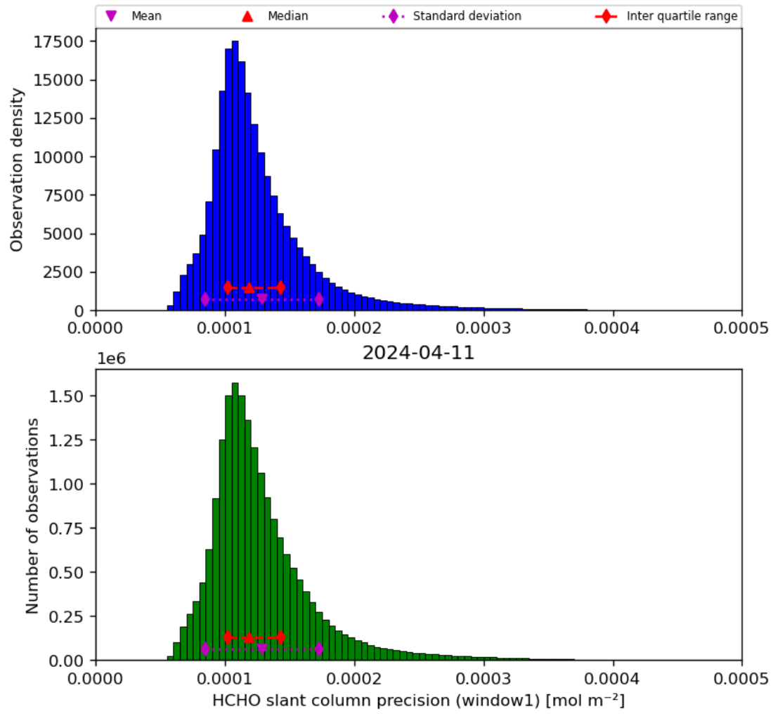
Figure 39: Histogram of “HCHO slant column precision (window1)” for 2024-04-10 to 2024-04-12
