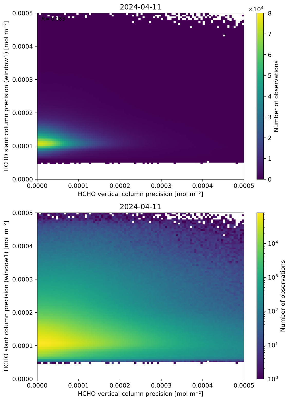
Figure 143: Scatter density plot of “HCHO vertical column precision” against “HCHO slant column precision (window1)” for 2024-04-10 to 2024-04-12.
