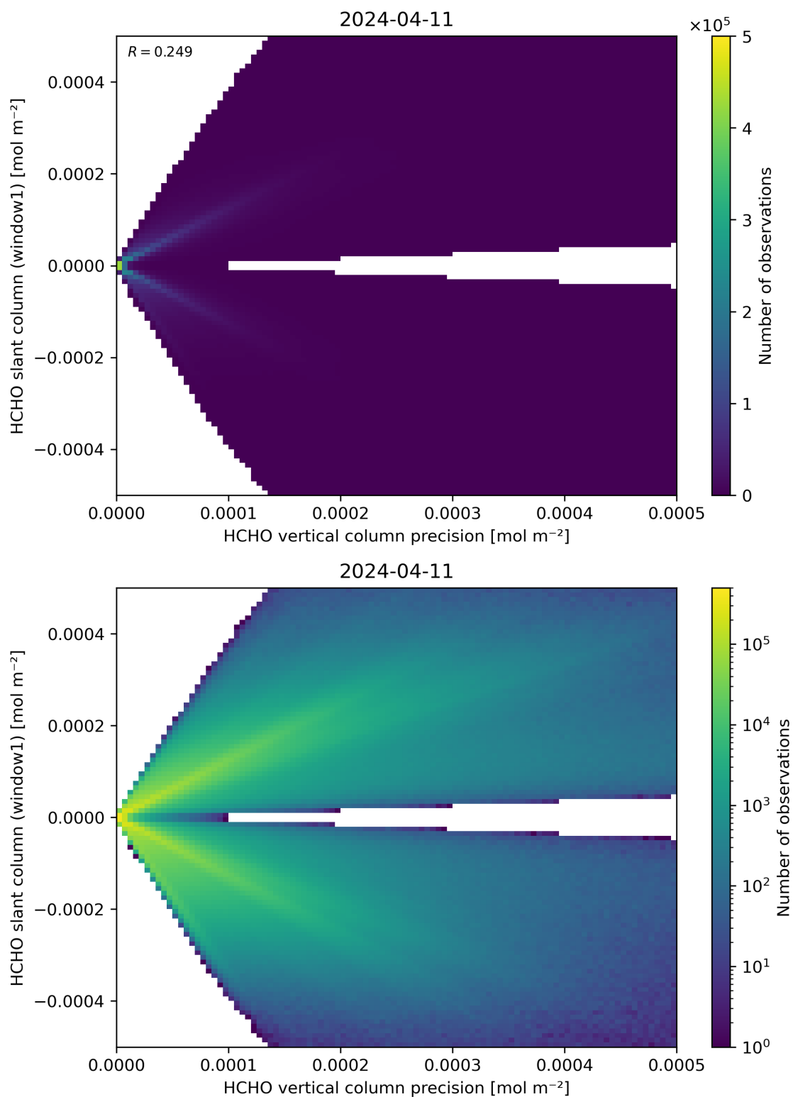
Figure 142: Scatter density plot of “HCHO vertical column precision” against “HCHO slant column (window1)” for 2024-04-10 to 2024-04-12.
