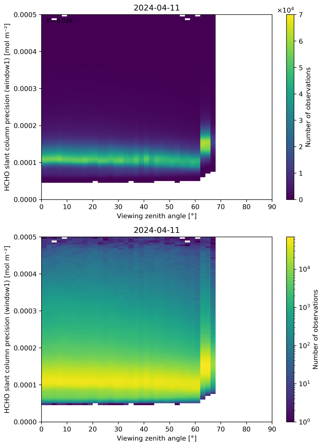
Figure 189: Scatter density plot of “Viewing zenith angle” against “HCHO slant column precision (window1)” for 2024-04-10 to 2024-04-12.
