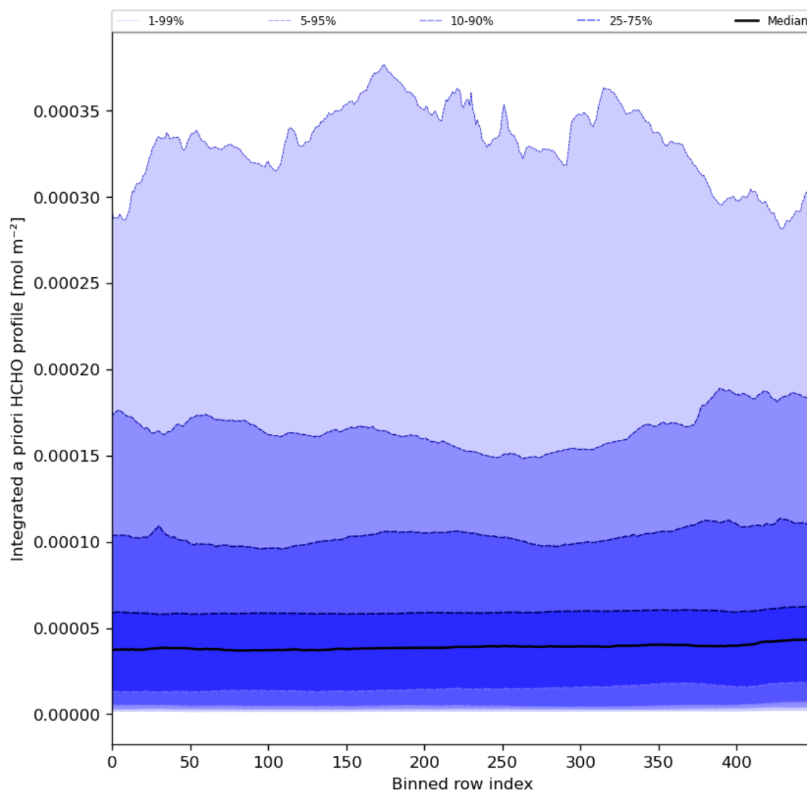
Figure 57: Along track statistics of "Integrated a priori HCHO profile" for 2024-04-10 to 2024-04-12
