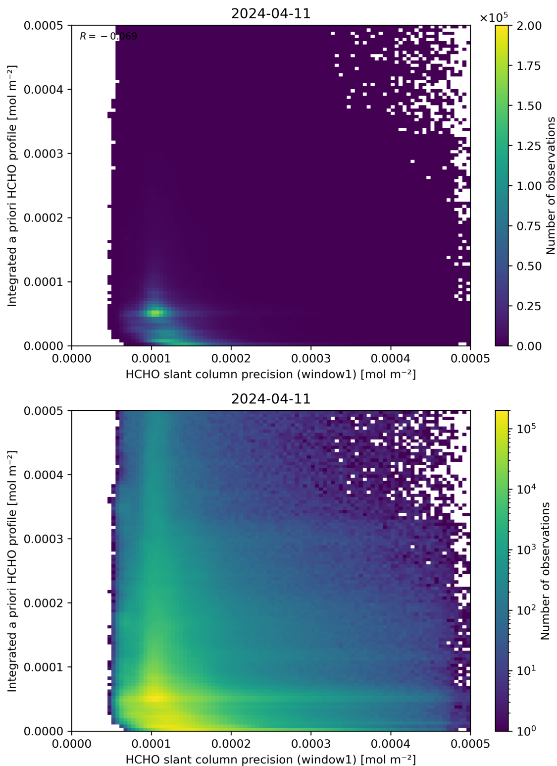
Figure 96: Scatter density plot of “HCHO slant column precision (window1)” against “Integrated a priori HCHO profile” for 2024-04-10 to 2024-04-12.
