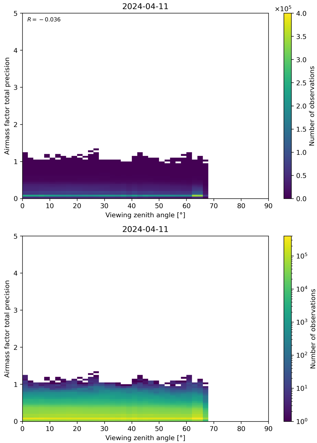
Figure 191: Scatter density plot of “Viewing zenith angle” against “Airmass factor total precision” for 2024-04-10 to 2024-04-12.
