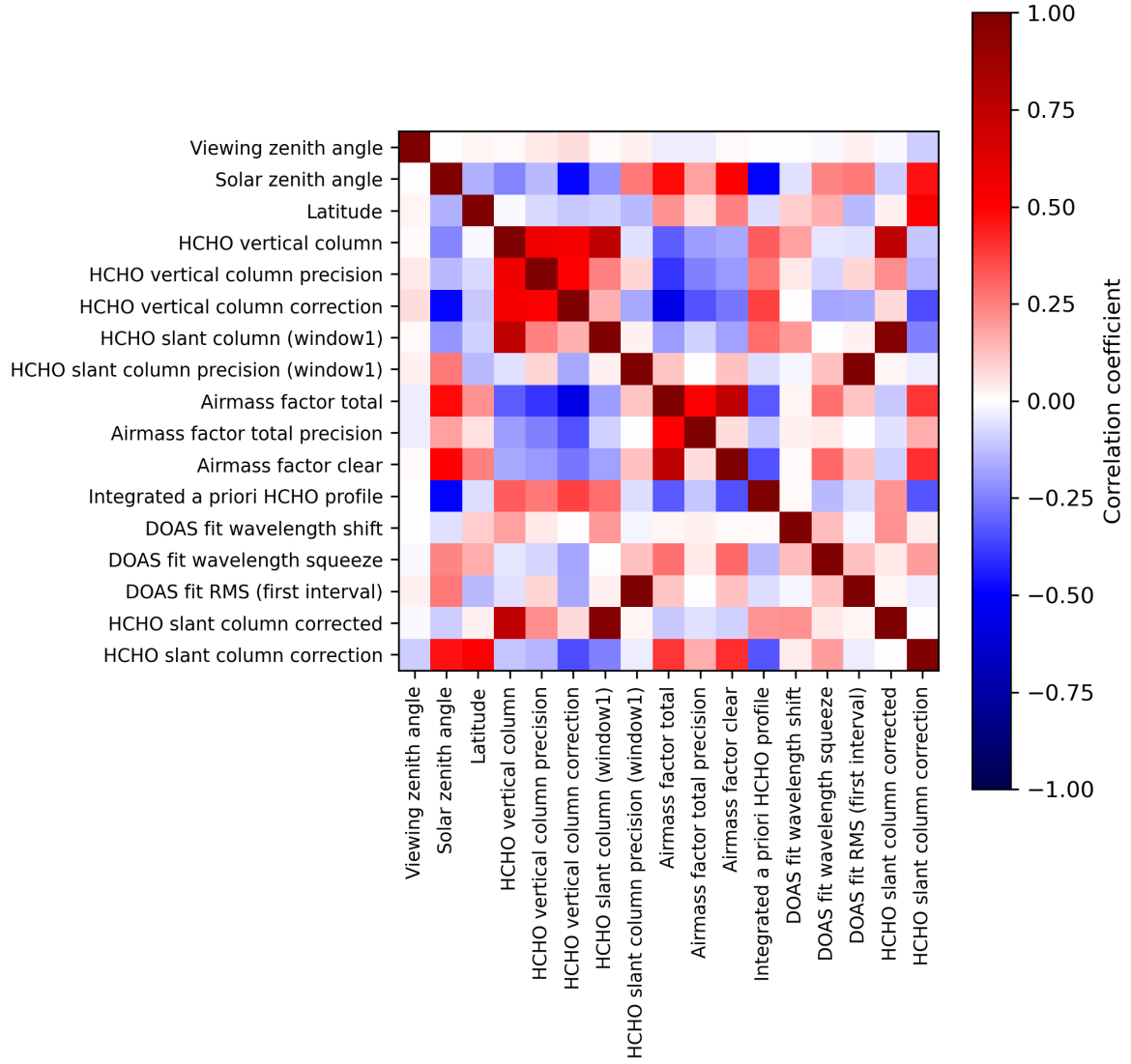
Figure 2: Map of correlation matrix for 2024-04-10 to 2024-04-12.
