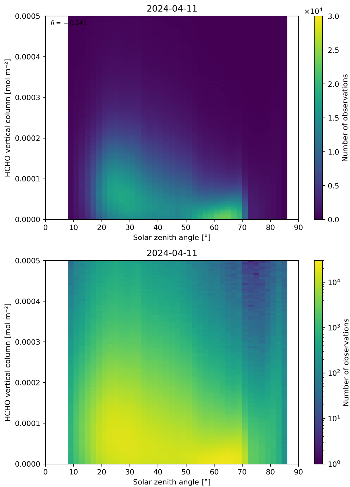
Figure 177: Scatter density plot of “Solar zenith angle” against “HCHO vertical column” for 2024-04-10 to 2024-04-12.
