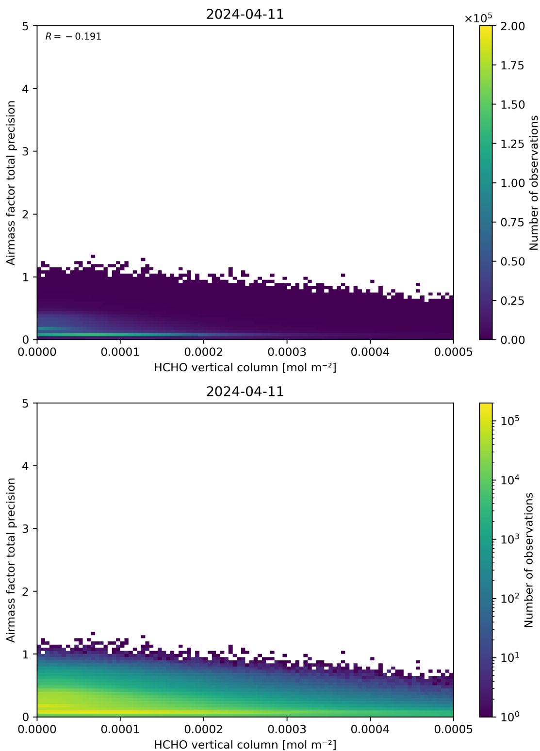
Figure 132: Scatter density plot of “HCHO vertical column” against “Airmass factor total precision” for 2024-04-10 to 2024-04-12.
