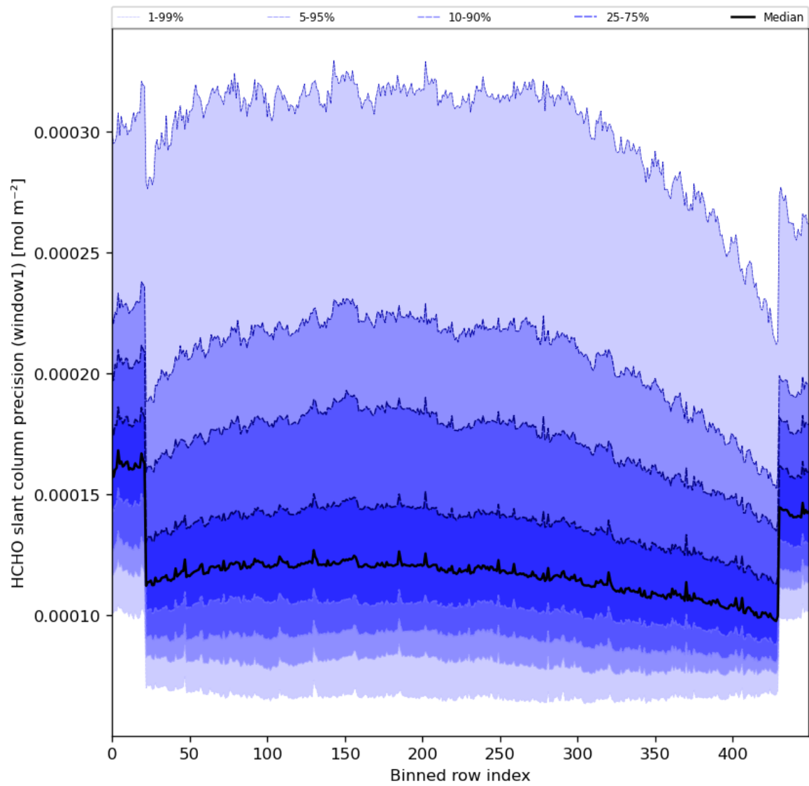
Figure 53: Along track statistics of “HCHO slant column precision (window1)” for 2024-04-10 to 2024-04-12
