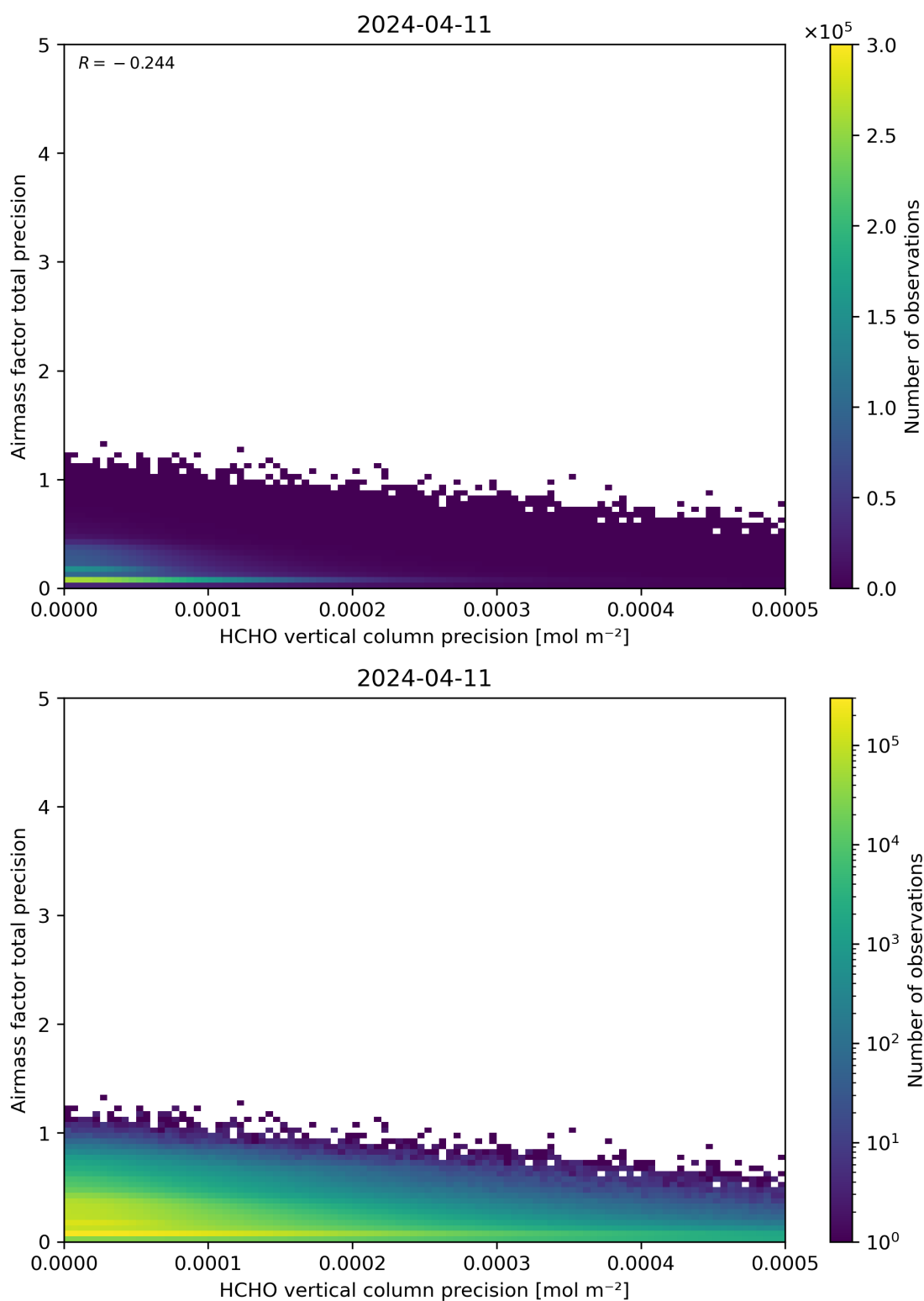
Figure 145: Scatter density plot of “HCHO vertical column precision” against “Airmass factor total precision” for 2024-04-10 to 2024-04-12.
