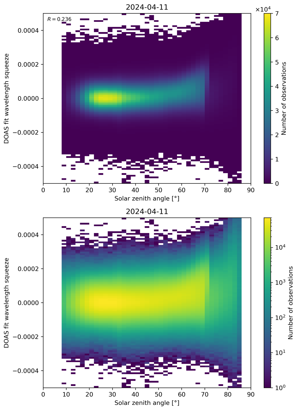
Figure 169: Scatter density plot of “Solar zenith angle” against “DOAS fit wavelength squeeze” for 2024-04-10 to 2024-04-12.
