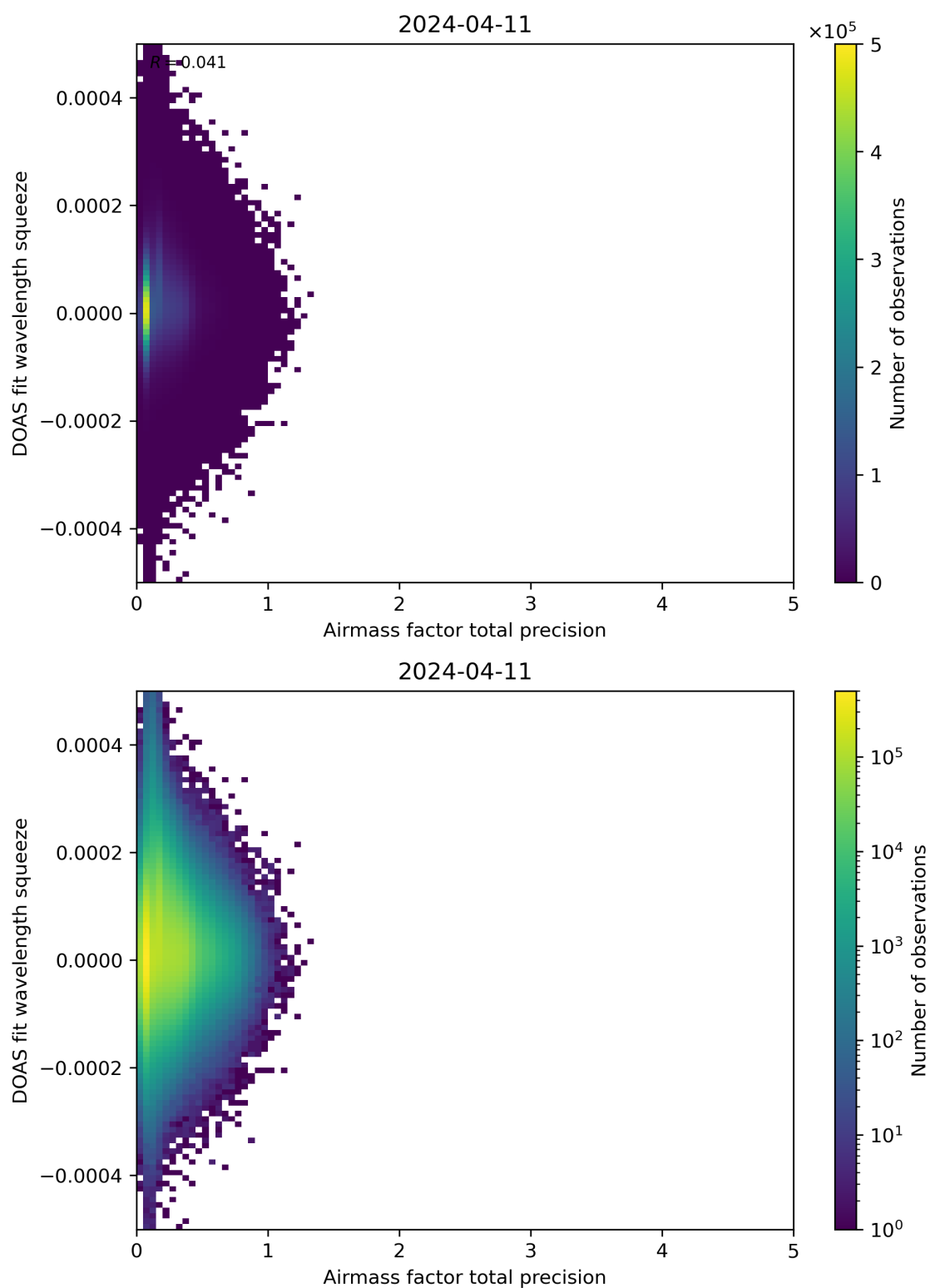
Figure 107: Scatter density plot of “Airmass factor total precision” against “DOAS fit wavelength squeeze” for 2024-04-10 to 2024-04-12.
