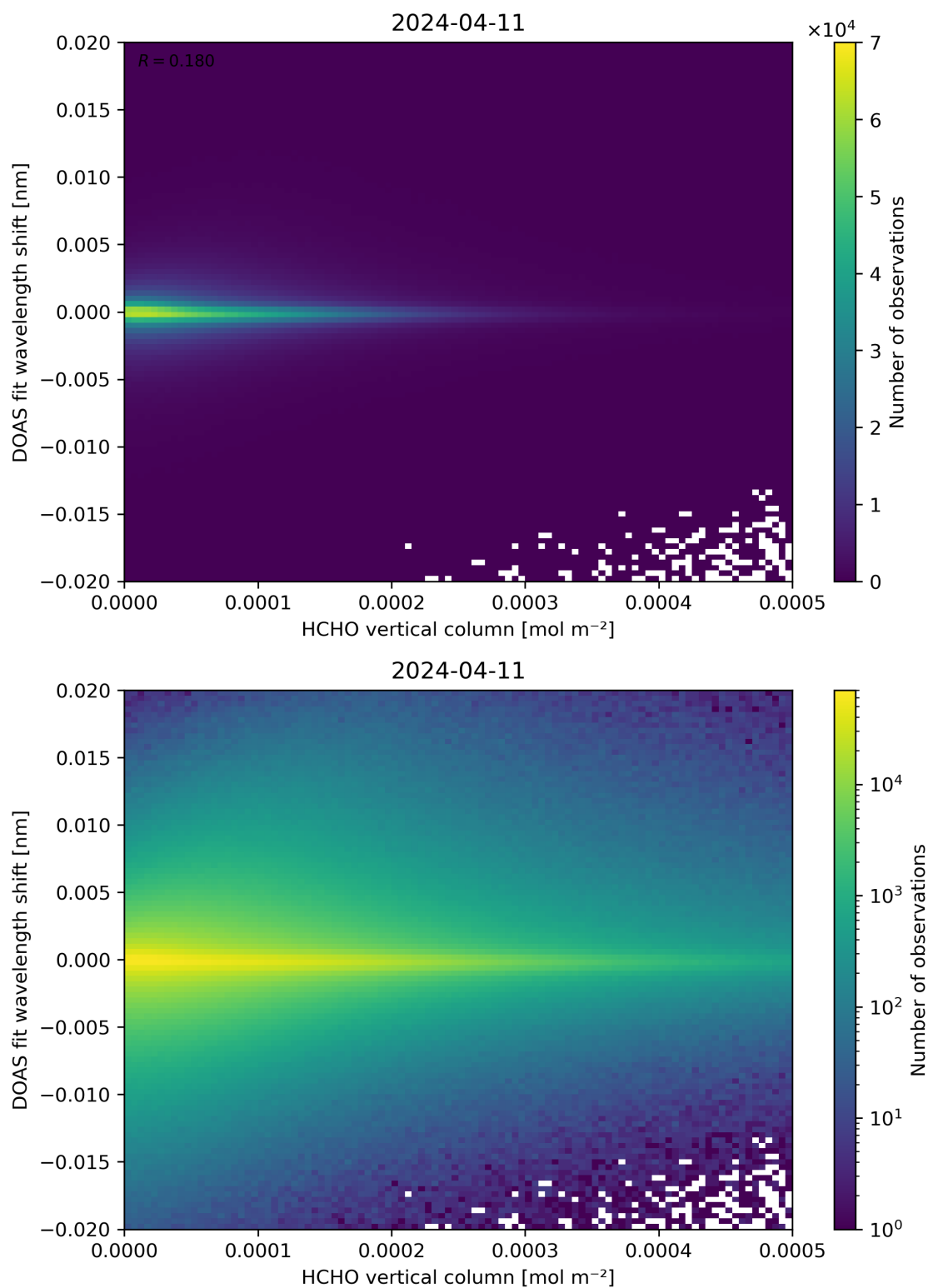
Figure 124: Scatter density plot of “HCHO vertical column” against “DOAS fit wavelength shift” for 2024-04-10 to 2024-04-12.
