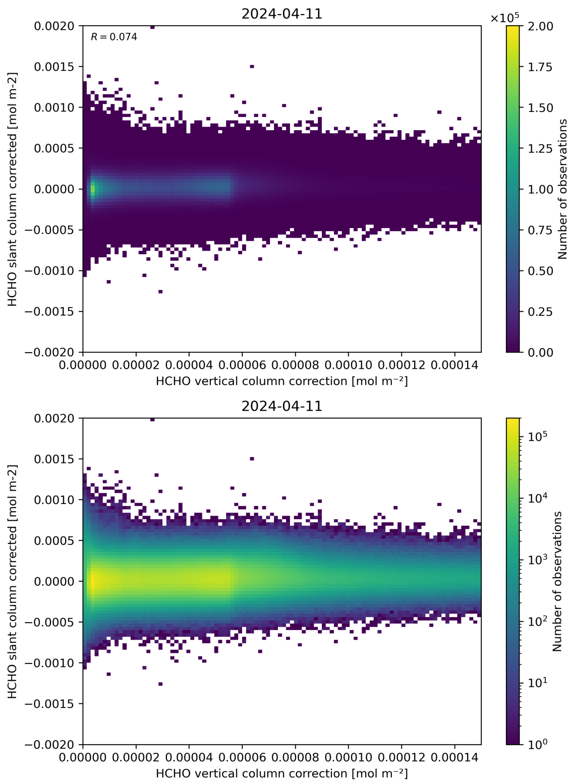
Figure 116: Scatter density plot of “HCHO vertical column correction” against “HCHO slant column corrected” for 2024-04-10 to 2024-04-12.
