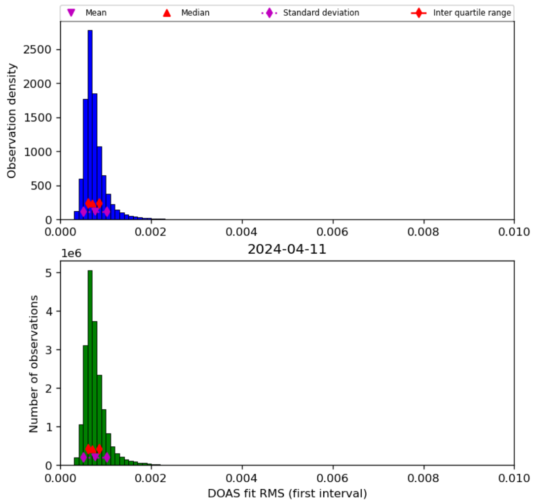
Figure 46: Histogram of “DOAS fit RMS (first interval)” for 2024-04-10 to 2024-04-12
