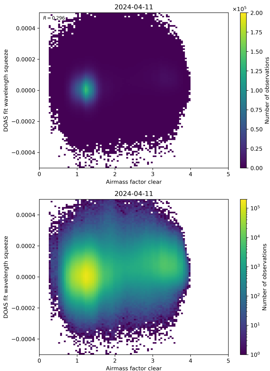
Figure 73: Scatter density plot of “Airmass factor clear” against “DOAS fit wavelength squeeze” for 2024-04-10 to 2024-04-12.
