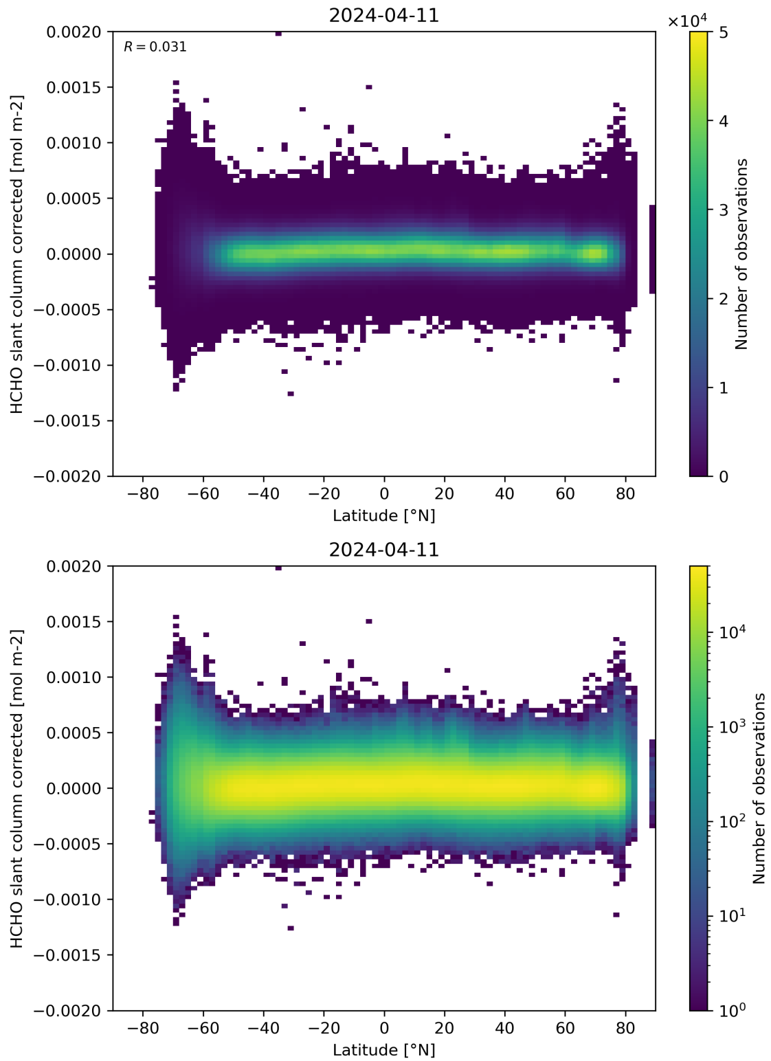
Figure 157: Scatter density plot of “Latitude” against “HCHO slant column corrected” for 2024-04-10 to 2024-04-12.
