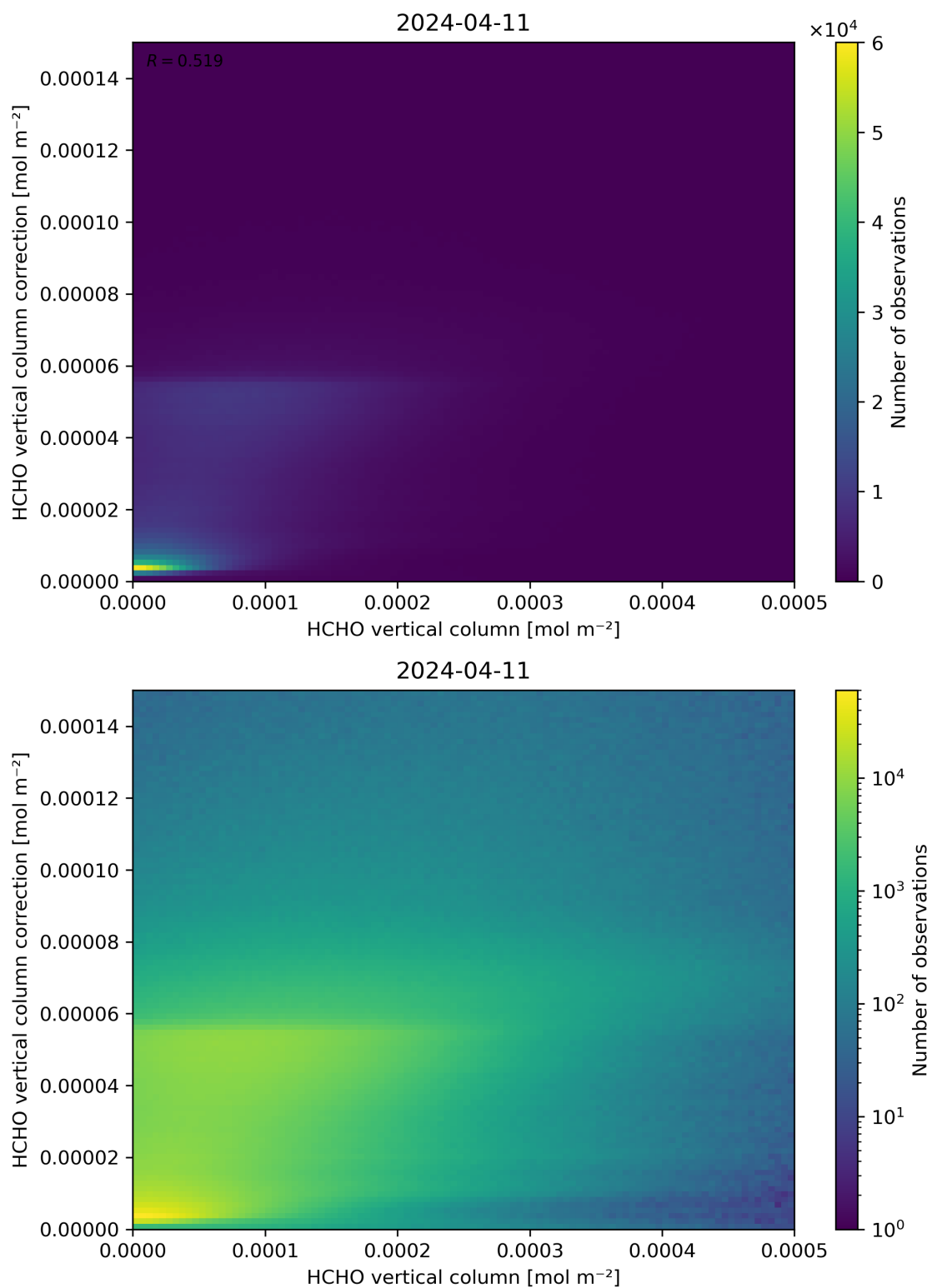
Figure 133: Scatter density plot of “HCHO vertical column” against “HCHO vertical column correction” for 2024-04-10 to 2024-04-12.
