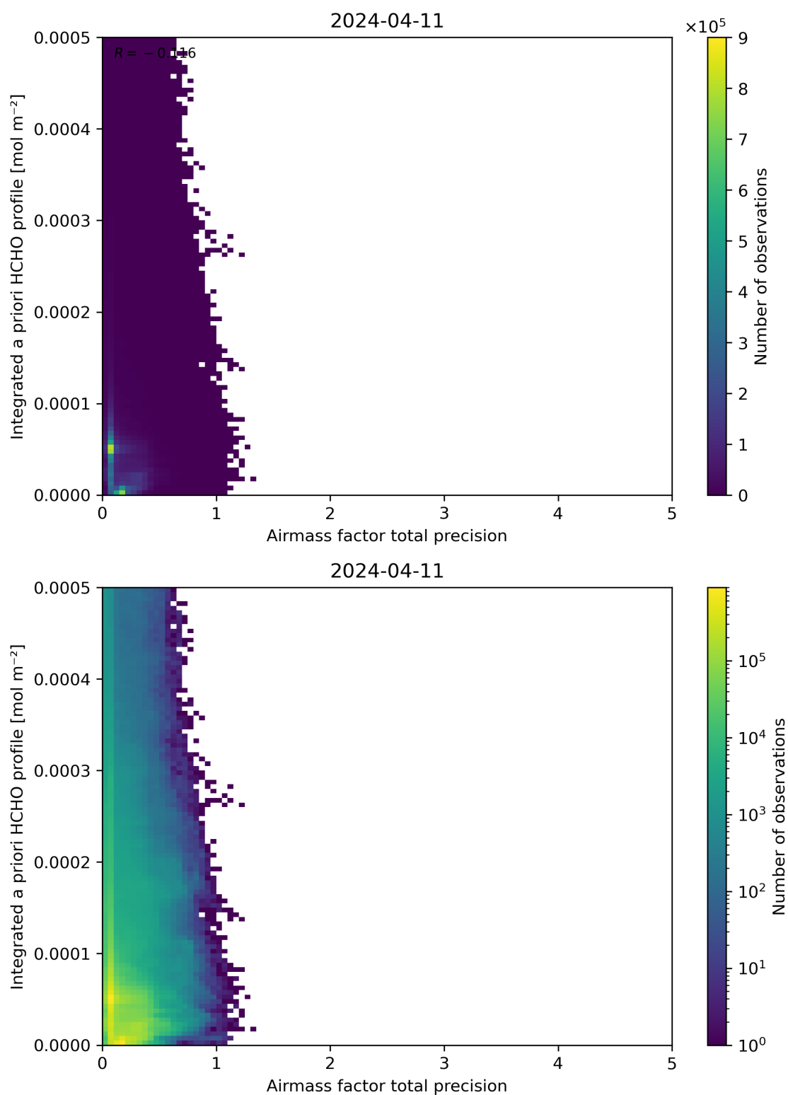
Figure 111: Scatter density plot of “Airmass factor total precision” against “Integrated a priori HCHO profile” for 2024-04-10 to 2024-04-12.
