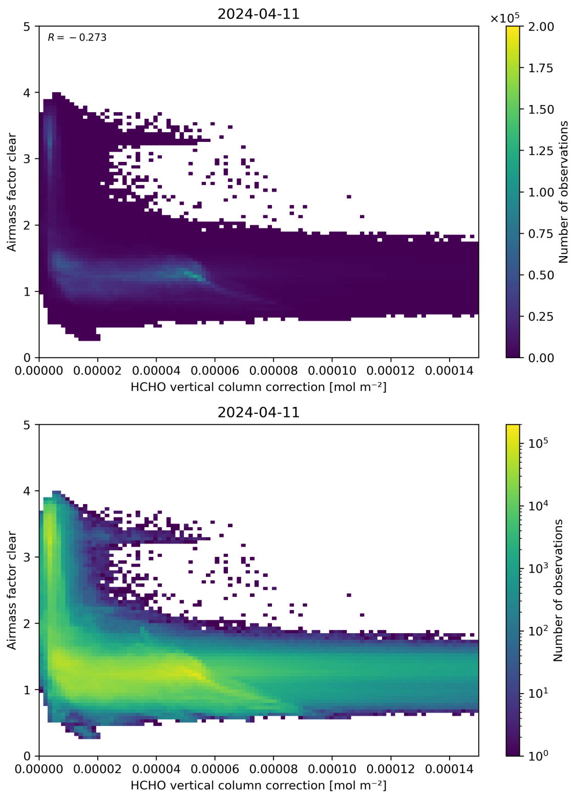
Figure 115: Scatter density plot of “HCHO vertical column correction” against “Airmass factor clear” for 2024-04-10 to 2024-04-12.
