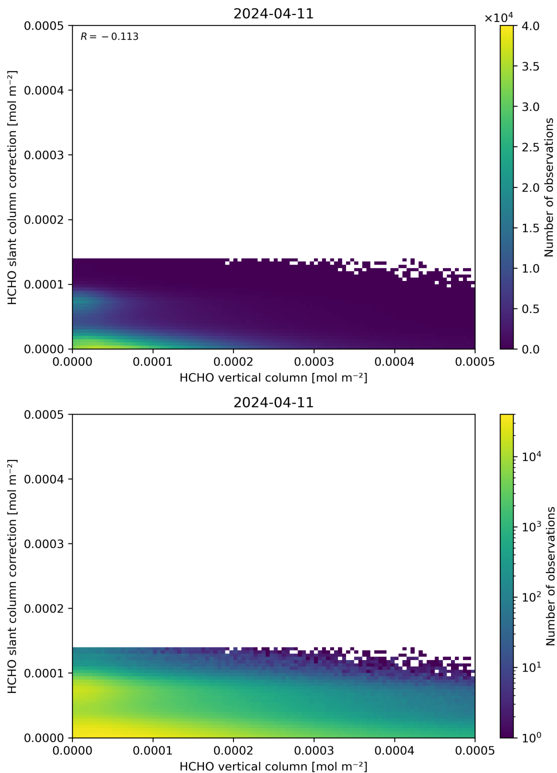
Figure 128: Scatter density plot of “HCHO vertical column” against “HCHO slant column correction” for 2024-04-10 to 2024-04-12.
