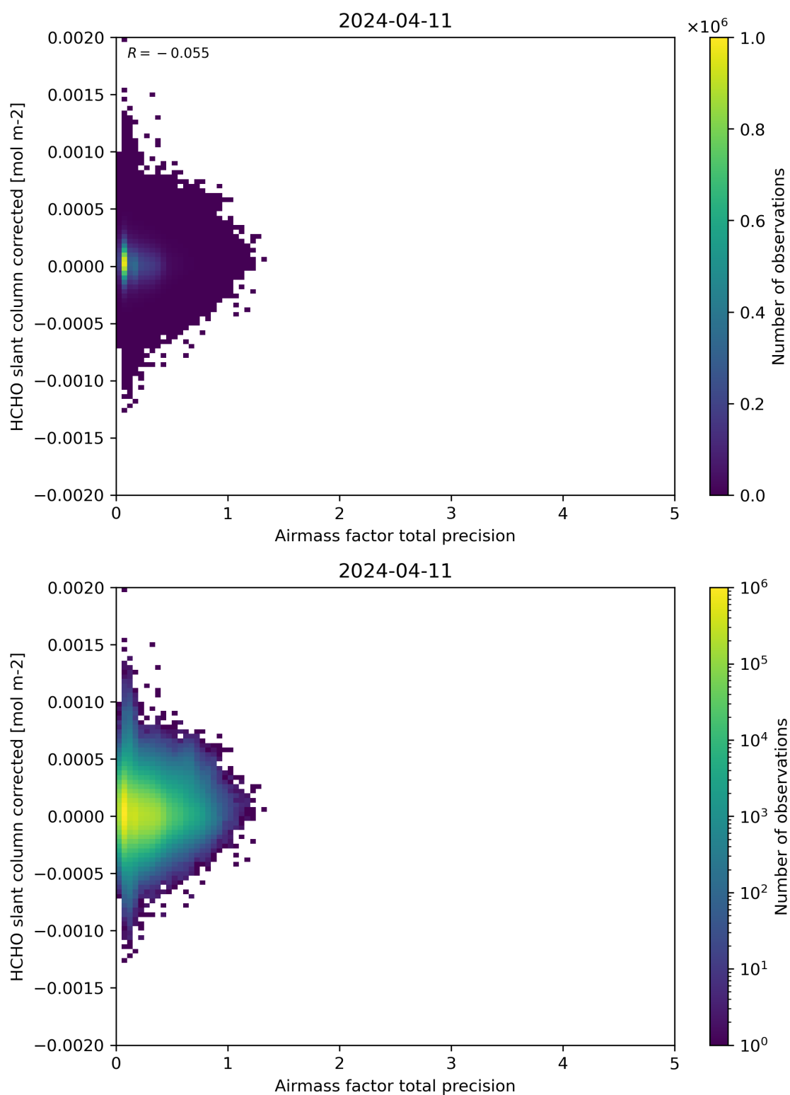
Figure 109: Scatter density plot of “Airmass factor total precision” against “HCHO slant column corrected” for 2024-04-10 to 2024-04-12.
