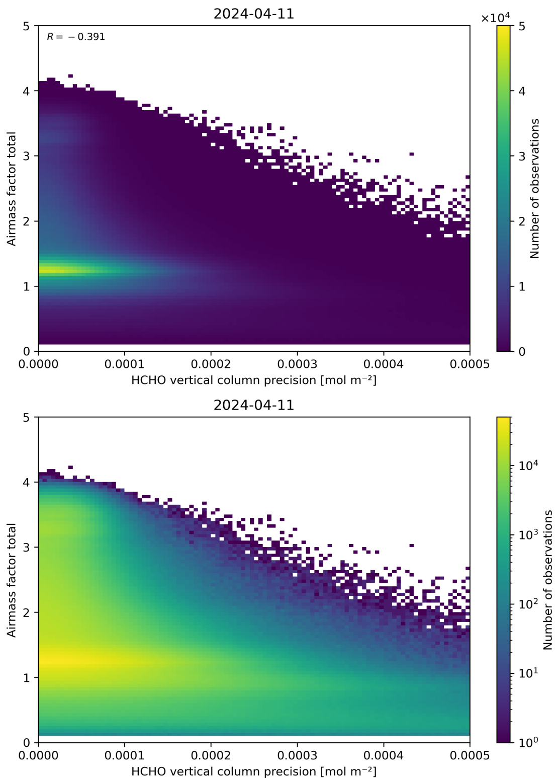
Figure 144: Scatter density plot of “HCHO vertical column precision” against “Airmass factor total” for 2024-04-10 to 2024-04-12.
