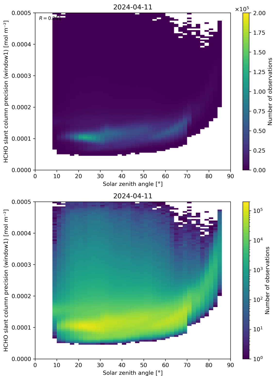
Figure 174: Scatter density plot of “Solar zenith angle” against “HCHO slant column precision (window1)” for 2024-04-10 to 2024-04-12.
