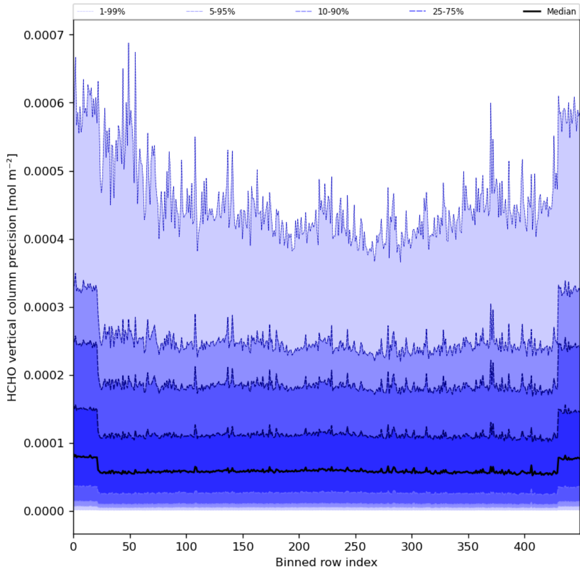
Figure 50: Along track statistics of “HCHO vertical column precision” for 2024-04-10 to 2024-04-12
