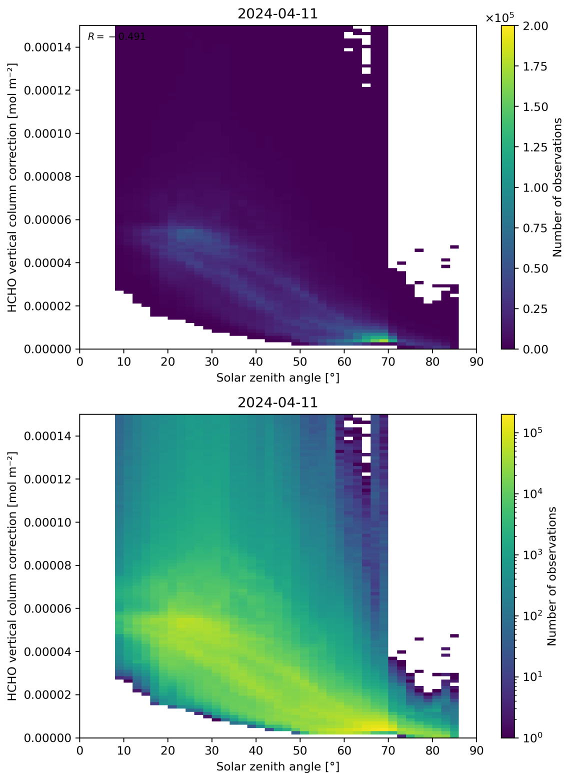
Figure 178: Scatter density plot of “Solar zenith angle” against “HCHO vertical column correction” for 2024-04-10 to 2024-04-12.
