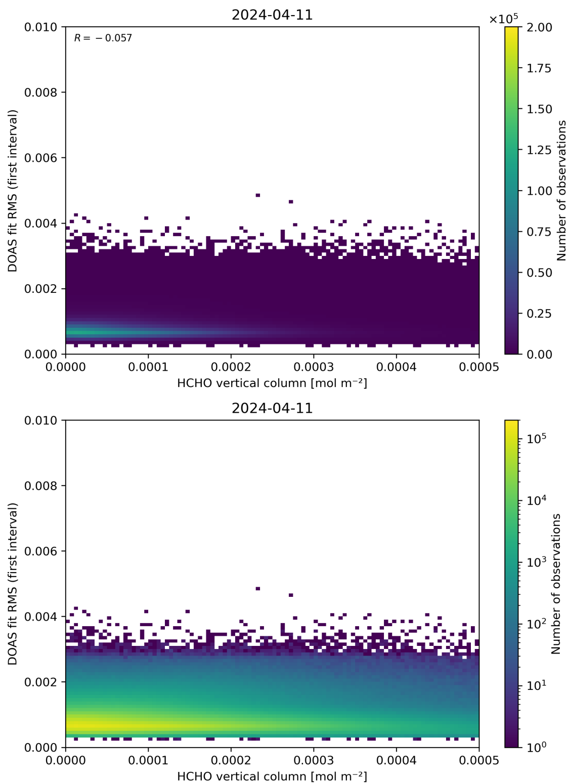
Figure 123: Scatter density plot of “HCHO vertical column” against “DOAS fit RMS (first interval)” for 2024-04-10 to 2024-04-12.
