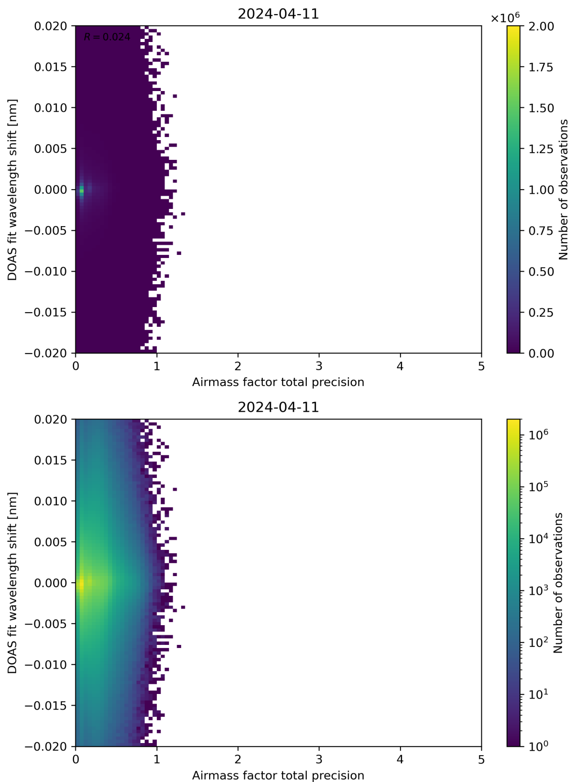
Figure 106: Scatter density plot of “Airmass factor total precision” against “DOAS fit wavelength shift” for 2024-04-10 to 2024-04-12.
