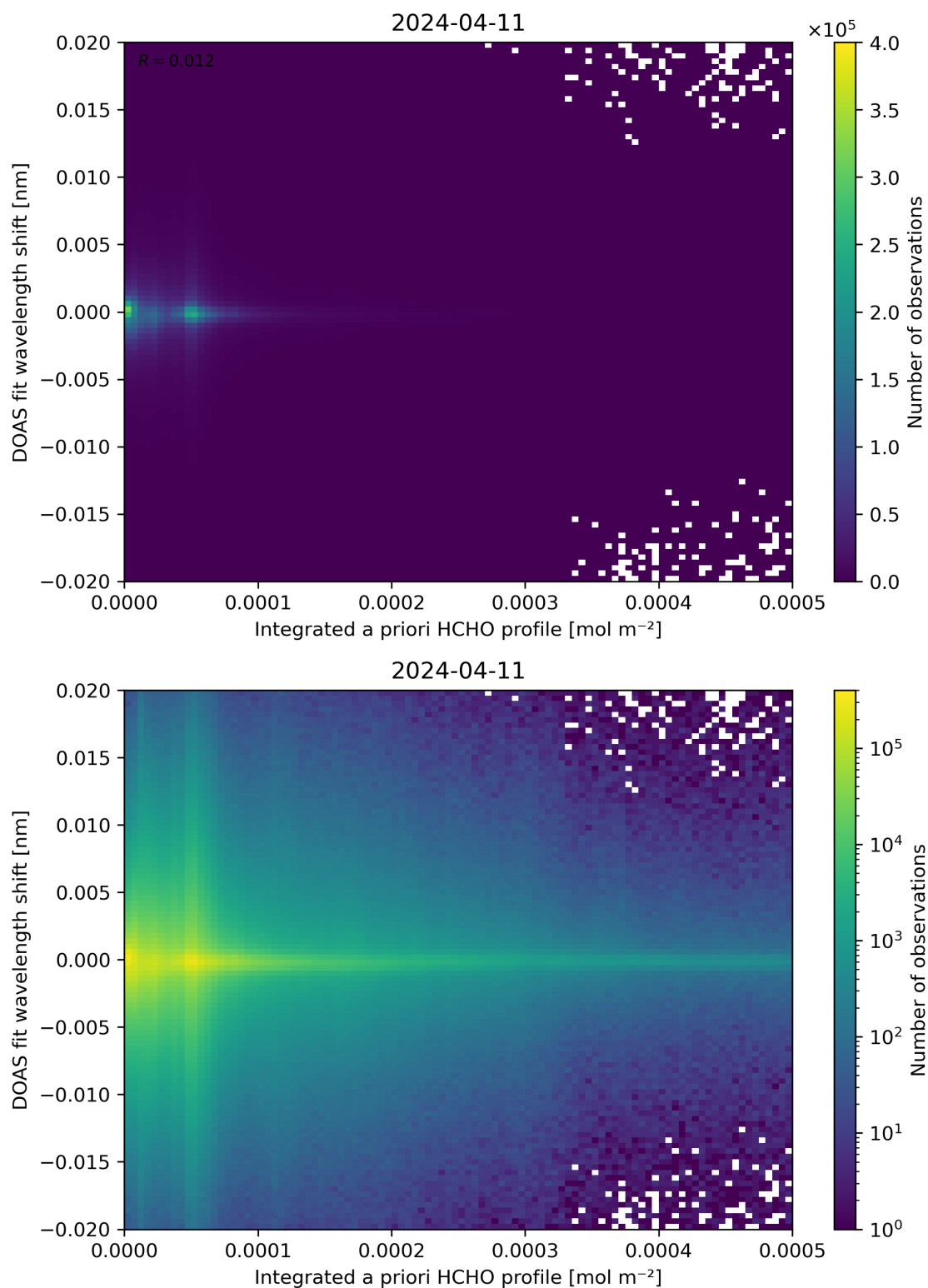
Figure 149: Scatter density plot of “Integrated a priori HCHO profile” against “DOAS fit wavelength shift” for 2024-04-10 to 2024-04-12.
