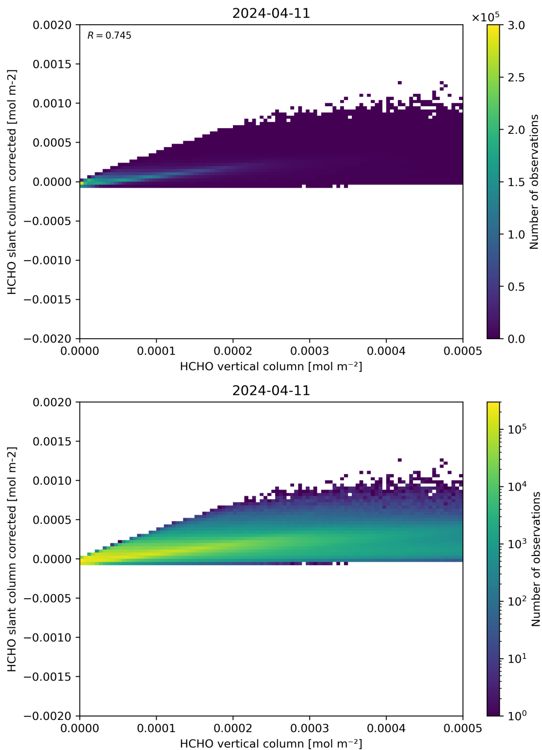
Figure 127: Scatter density plot of “HCHO vertical column” against “HCHO slant column corrected” for 2024-04-10 to 2024-04-12.
