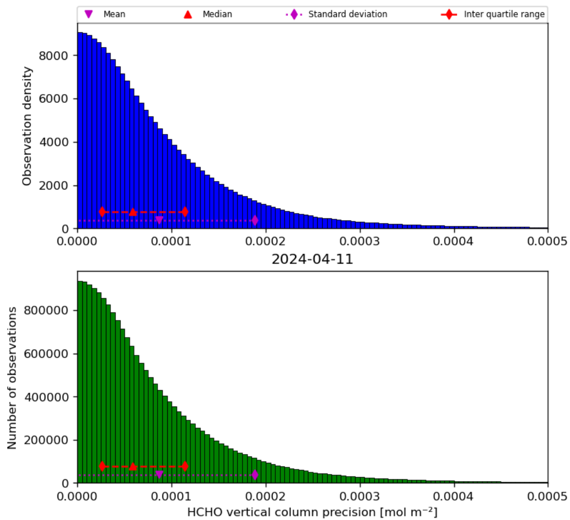
Figure 36: Histogram of “HCHO vertical column precision” for 2024-04-10 to 2024-04-12
