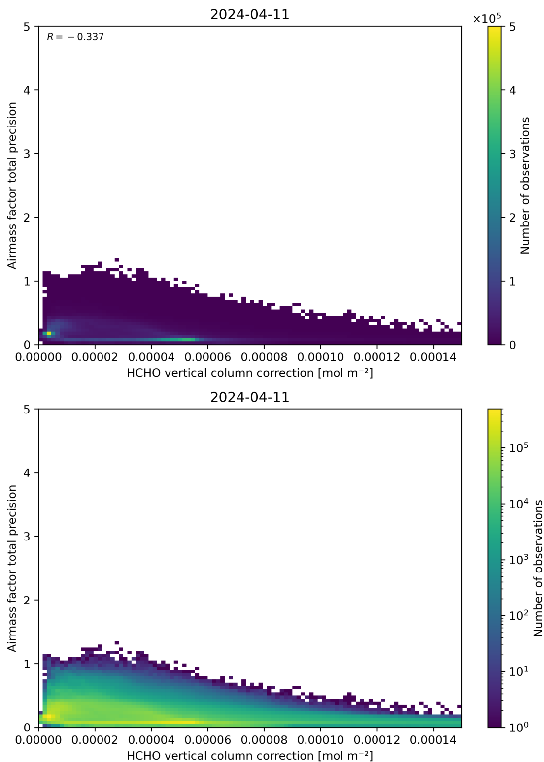
Figure 121: Scatter density plot of “HCHO vertical column correction” against “Airmass factor total precision” for 2024-04-10 to 2024-04-12.
