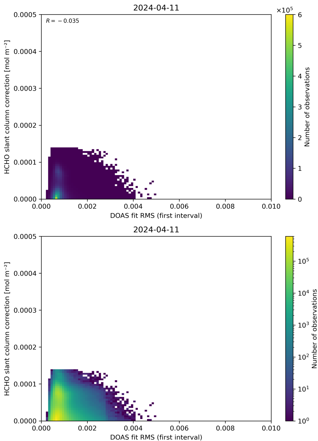
Figure 63: Scatter density plot of “DOAS fit RMS (first interval)” against “HCHO slant column correction” for 2024-04-10 to 2024-04-12.
