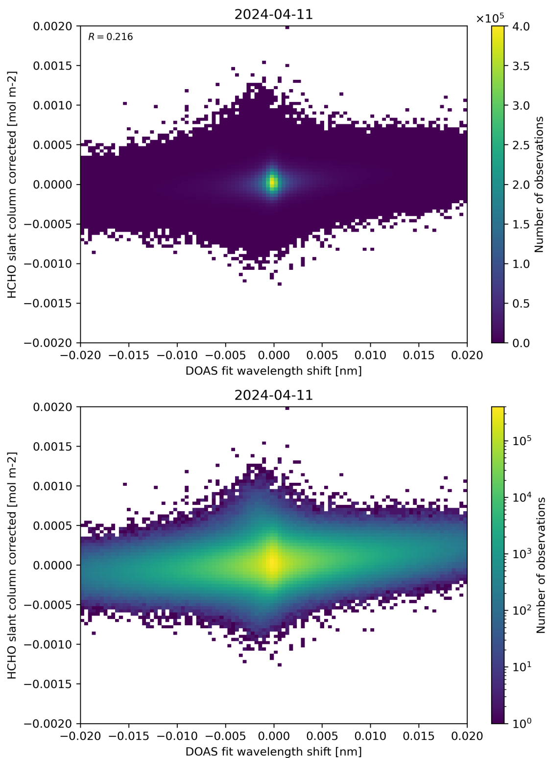
Figure 66: Scatter density plot of “DOAS fit wavelength shift” against “HCHO slant column corrected” for 2024-04-10 to 2024-04-12.
