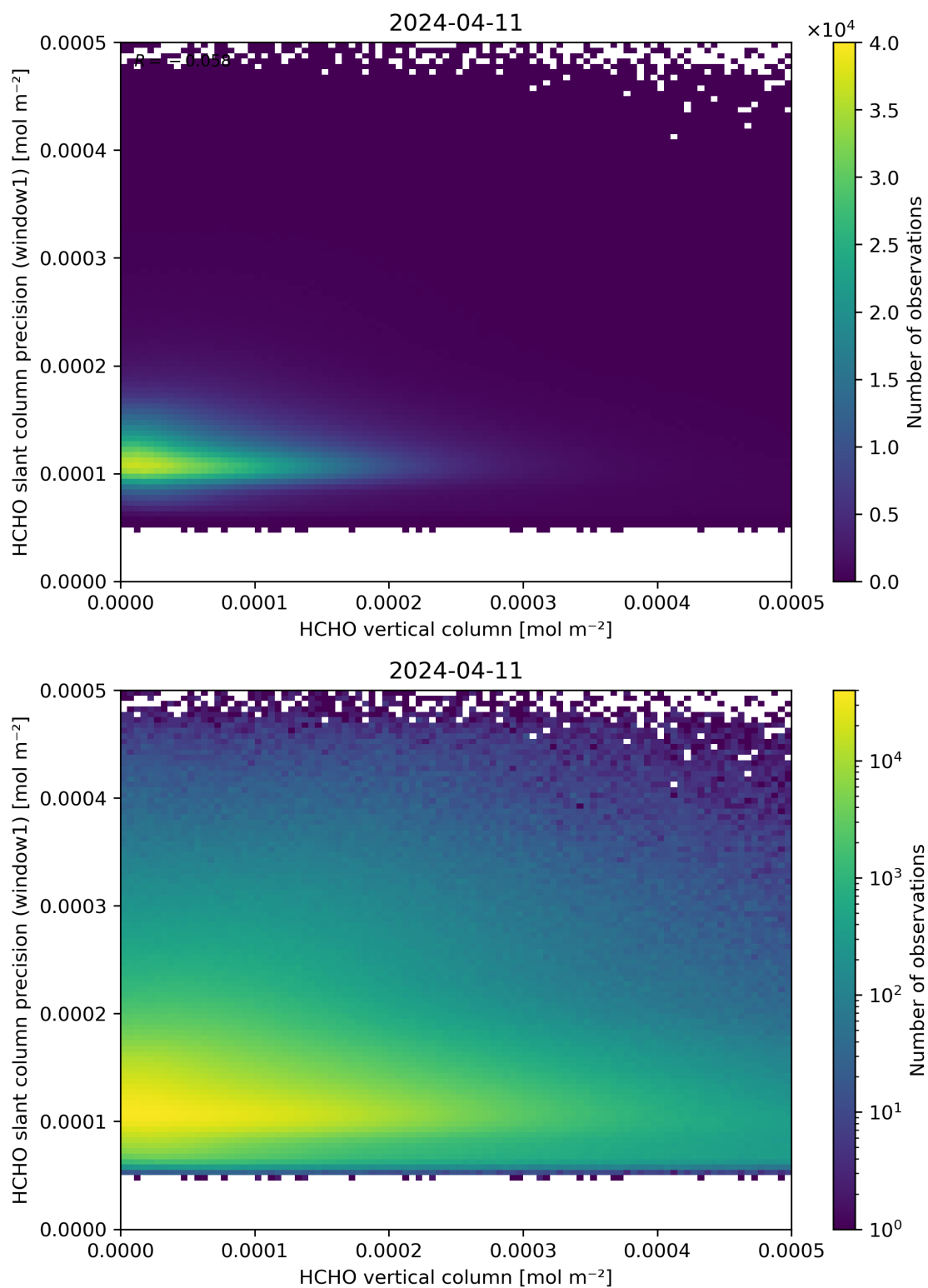
Figure 130: Scatter density plot of “HCHO vertical column” against “HCHO slant column precision (window1)” for 2024-04-10 to 2024-04-12.
