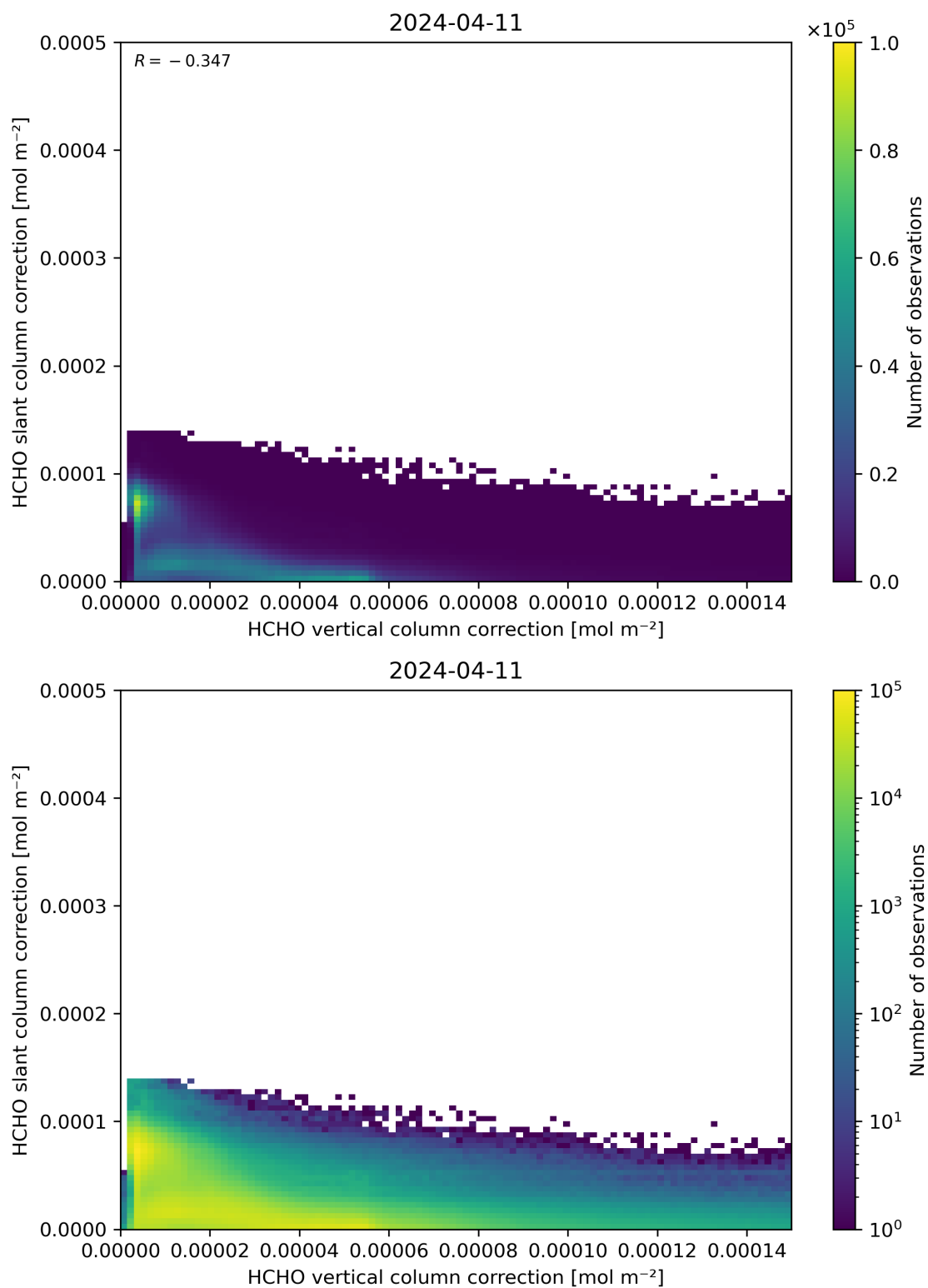
Figure 117: Scatter density plot of “HCHO vertical column correction” against “HCHO slant column correction” for 2024-04-10 to 2024-04-12.
