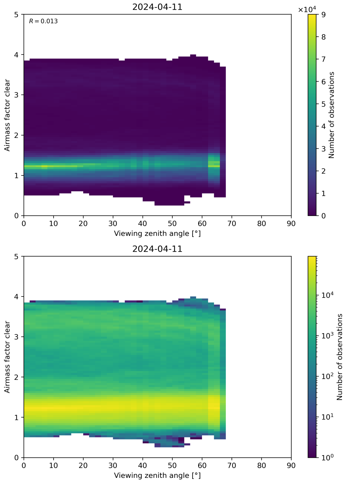
Figure 185: Scatter density plot of “Viewing zenith angle” against “Airmass factor clear” for 2024-04-10 to 2024-04-12.
