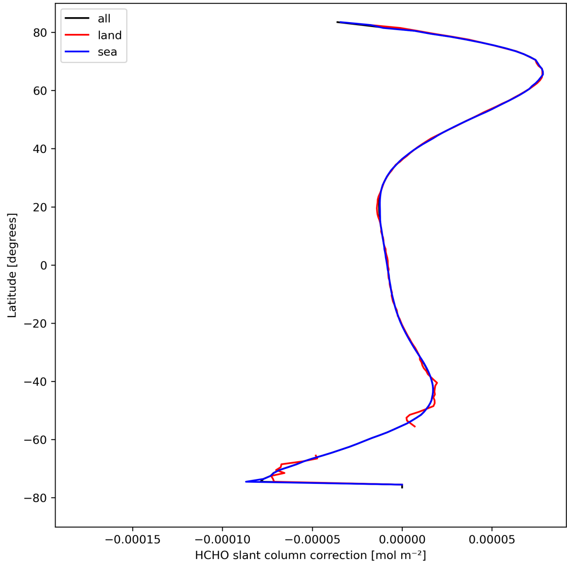
Figure 33: Zonal average of “HCHO slant column correction” for 2024-04-10 to 2024-04-12.
