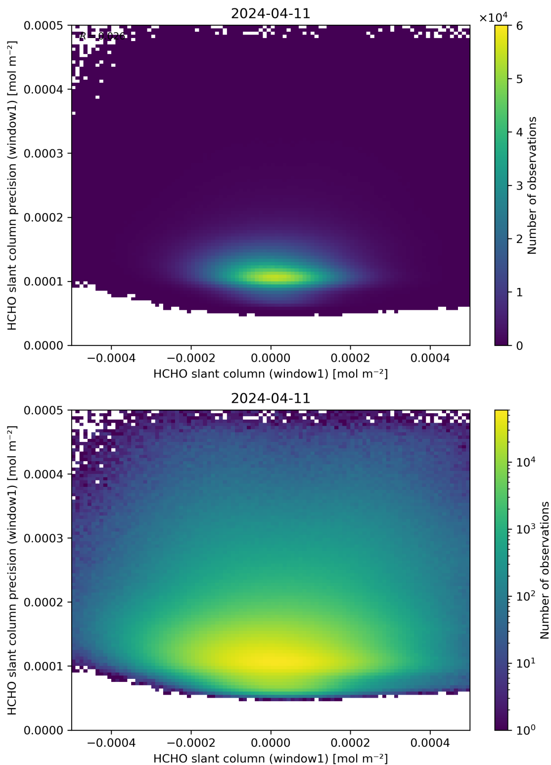
Figure 84: Scatter density plot of “HCHO slant column (window1)” against “HCHO slant column precision (window1)” for 2024-04-10 to 2024-04-12.
