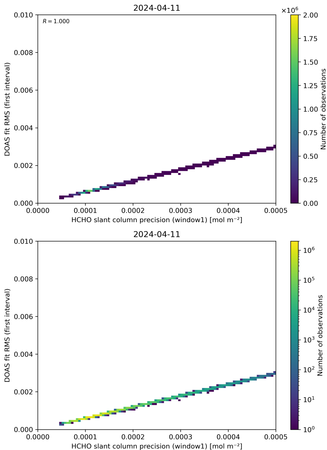
Figure 88: Scatter density plot of “HCHO slant column precision (window1)” against “DOAS fit RMS (first interval)” for 2024-04-10 to 2024-04-12.
