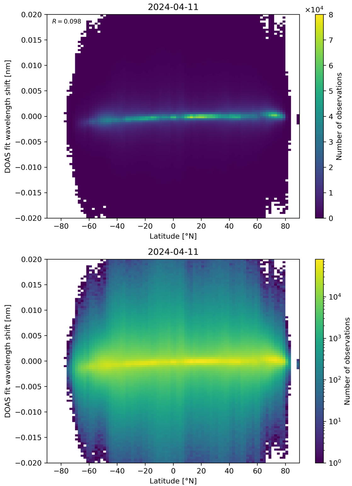
Figure 154: Scatter density plot of “Latitude” against “DOAS fit wavelength shift” for 2024-04-10 to 2024-04-12.
