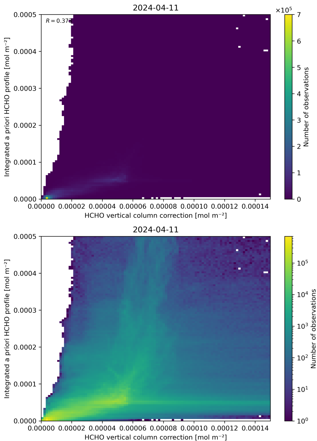
Figure 122: Scatter density plot of “HCHO vertical column correction” against “Integrated a priori HCHO profile” for 2024-04-10 to 2024-04-12.
