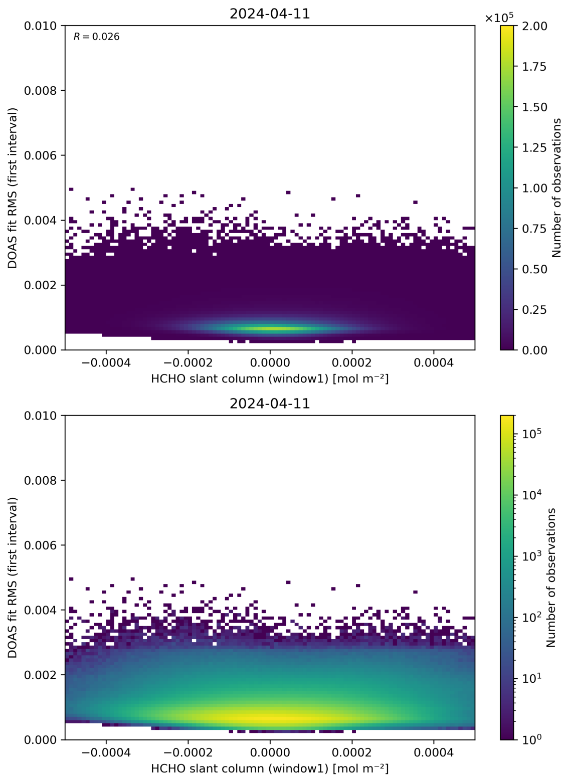
Figure 78: Scatter density plot of “HCHO slant column (window1)” against “DOAS fit RMS (first interval)” for 2024-04-10 to 2024-04-12.
