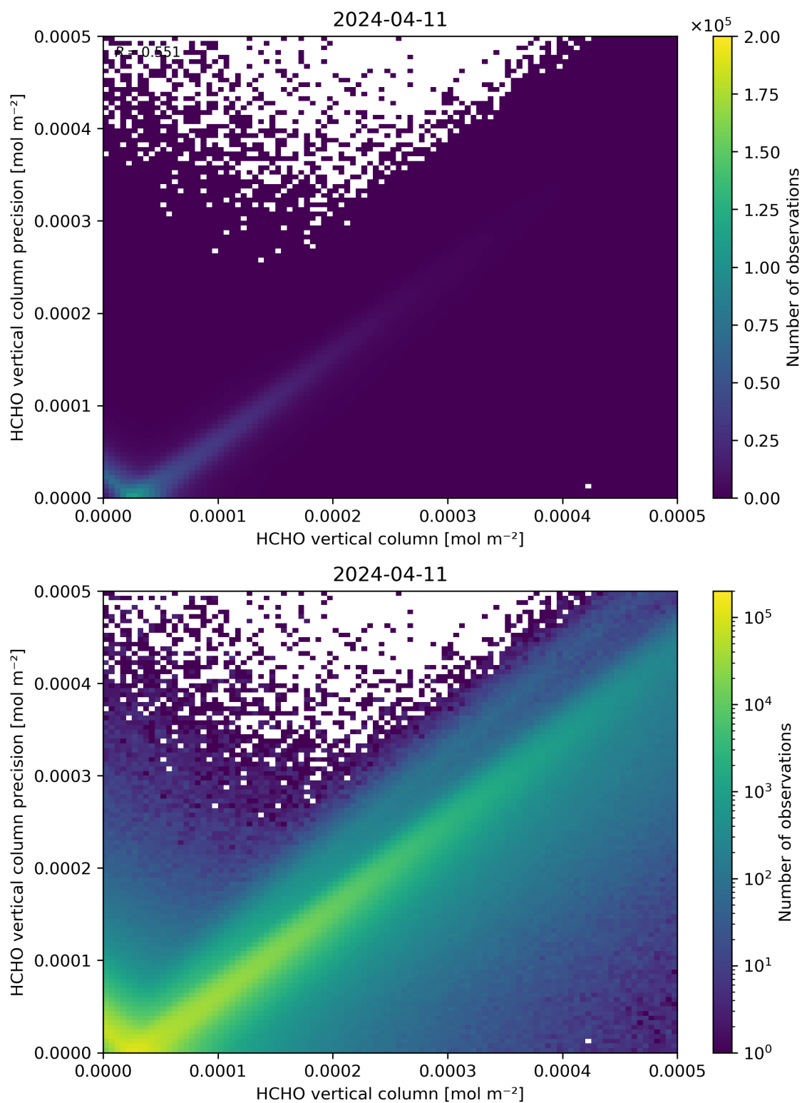
Figure 134: Scatter density plot of “HCHO vertical column” against “HCHO vertical column precision” for 2024-04-10 to 2024-04-12.
