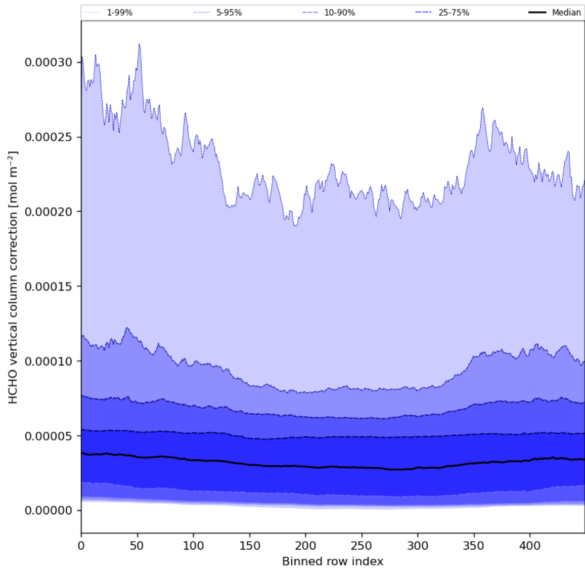
Figure 51: Along track statistics of “HCHO vertical column correction” for 2024-04-10 to 2024-04-12
