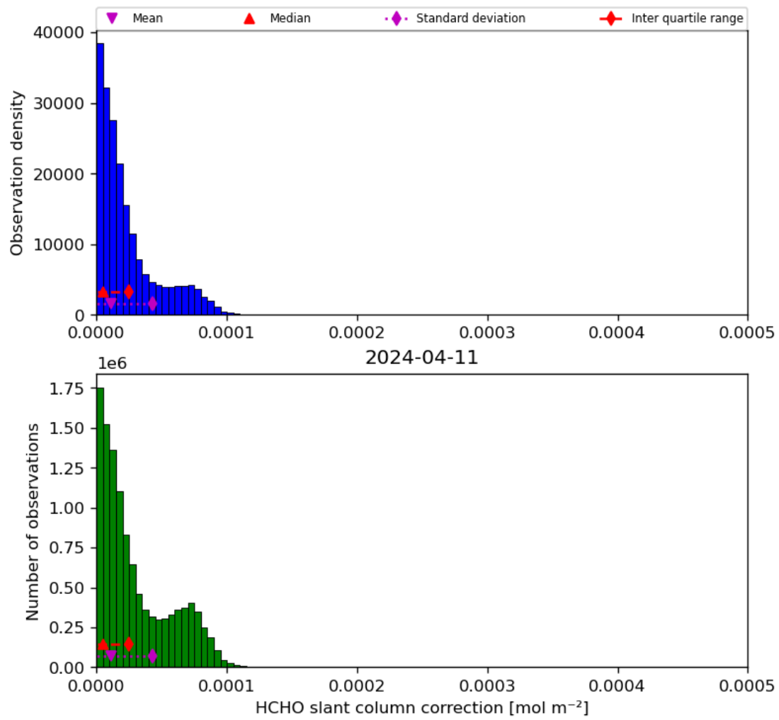
Figure 47: Histogram of “HCHO slant column correction” for 2024-04-10 to 2024-04-12
