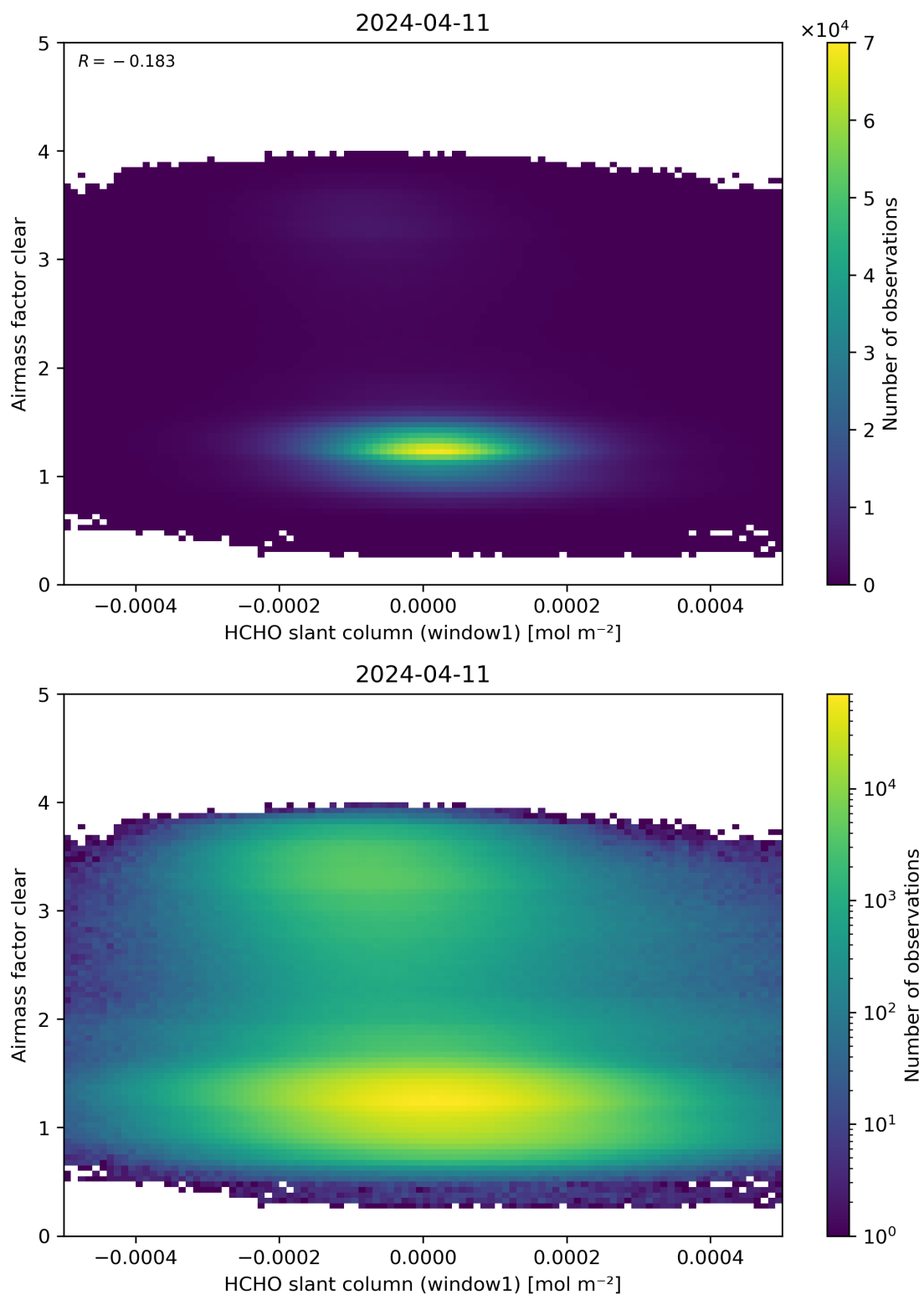
Figure 81: Scatter density plot of “HCHO slant column (window1)” against “Airmass factor clear” for 2024-04-10 to 2024-04-12.
