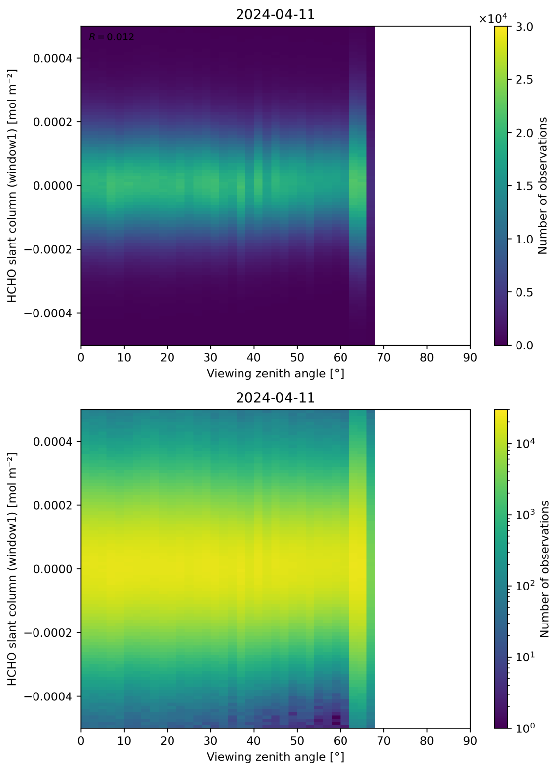
Figure 188: Scatter density plot of “Viewing zenith angle” against “HCHO slant column (window1)” for 2024-04-10 to 2024-04-12.
