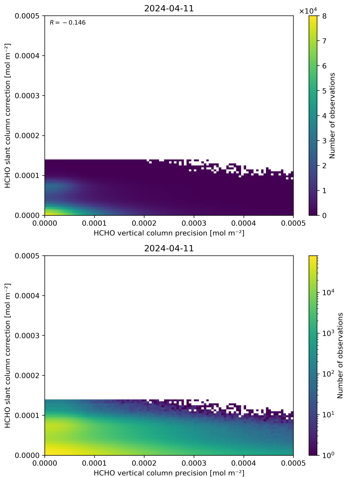
Figure 141: Scatter density plot of “HCHO vertical column precision” against “HCHO slant column correction” for 2024-04-10 to 2024-04-12.
