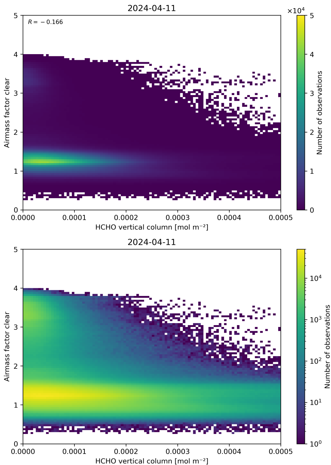
Figure 126: Scatter density plot of “HCHO vertical column” against “Airmass factor clear” for 2024-04-10 to 2024-04-12.
