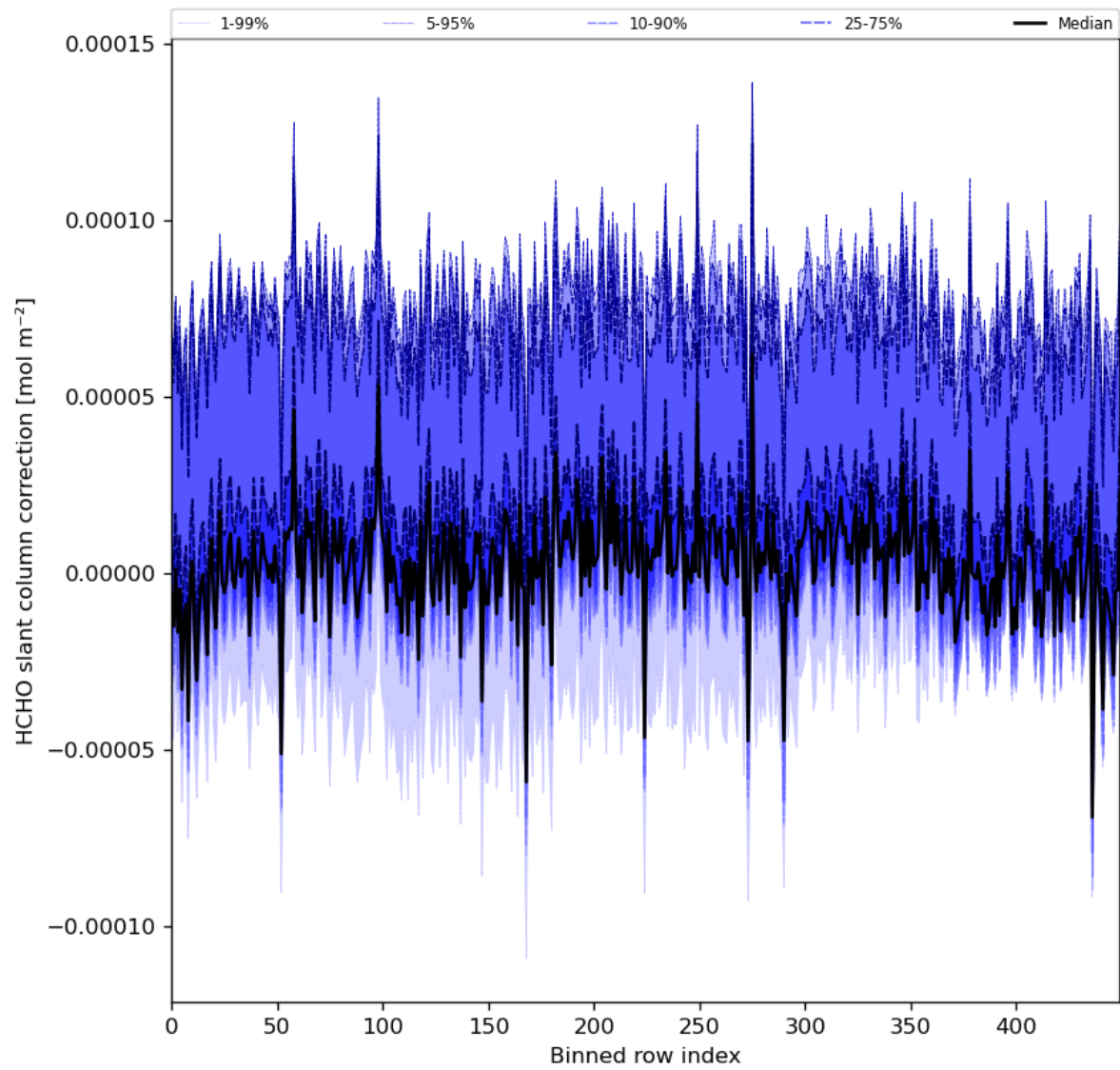
Figure 61: Along track statistics of “HCHO slant column correction” for 2024-04-10 to 2024-04-12
