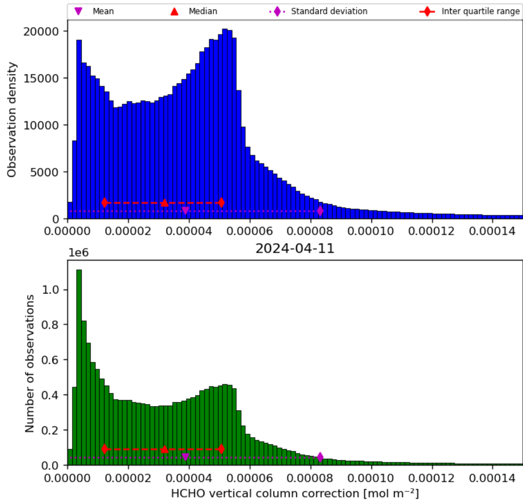
Figure 37: Histogram of “HCHO vertical column correction” for 2024-04-10 to 2024-04-12
