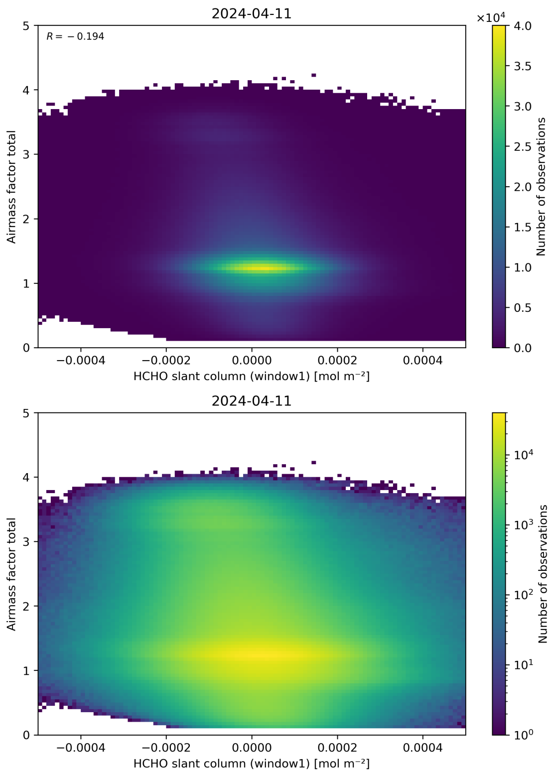
Figure 85: Scatter density plot of “HCHO slant column (window1)” against “Airmass factor total” for 2024-04-10 to 2024-04-12.
