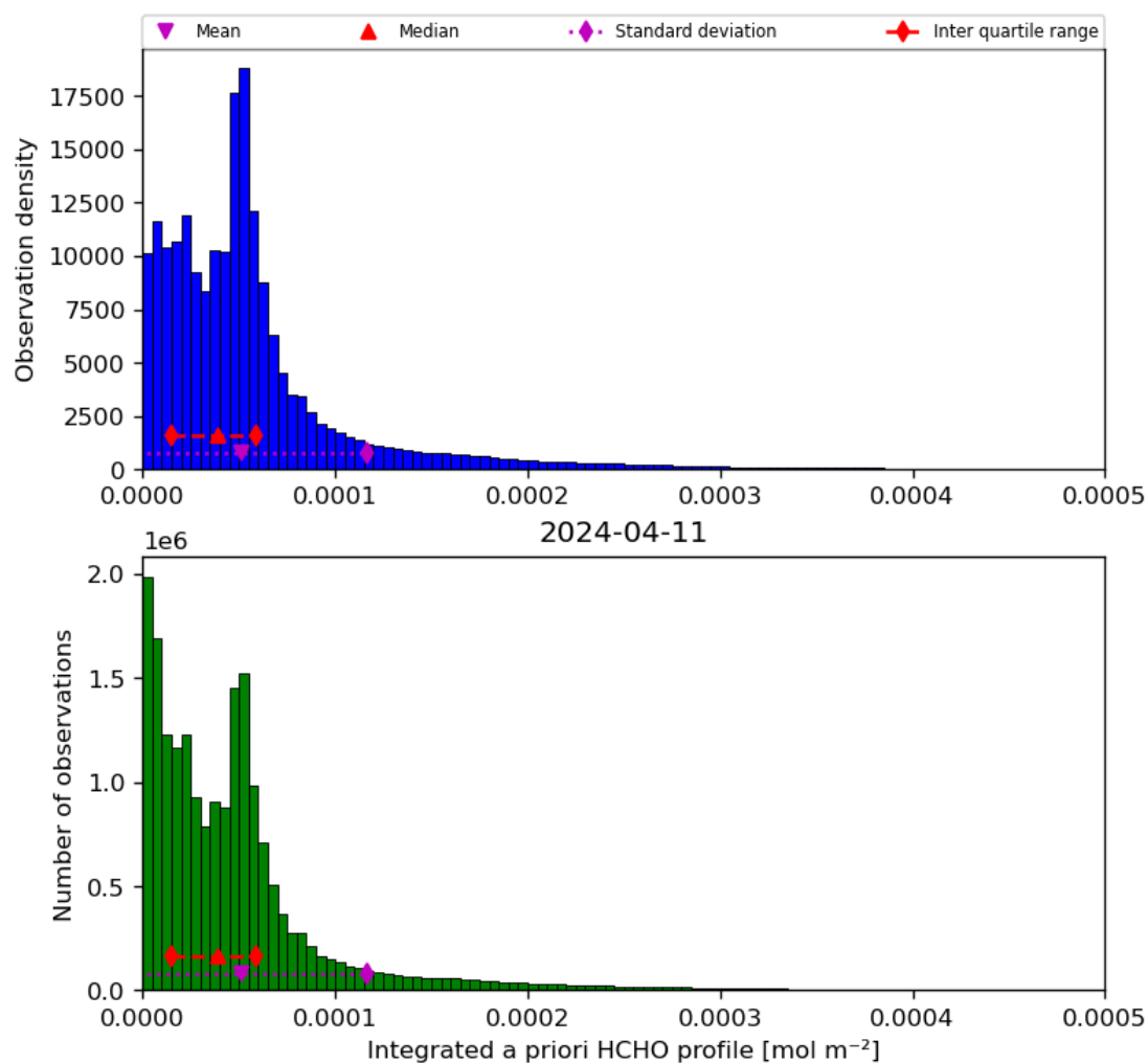
Figure 43: Histogram of “Integrated a priori HCHO profile” for 2024-04-10 to 2024-04-12
