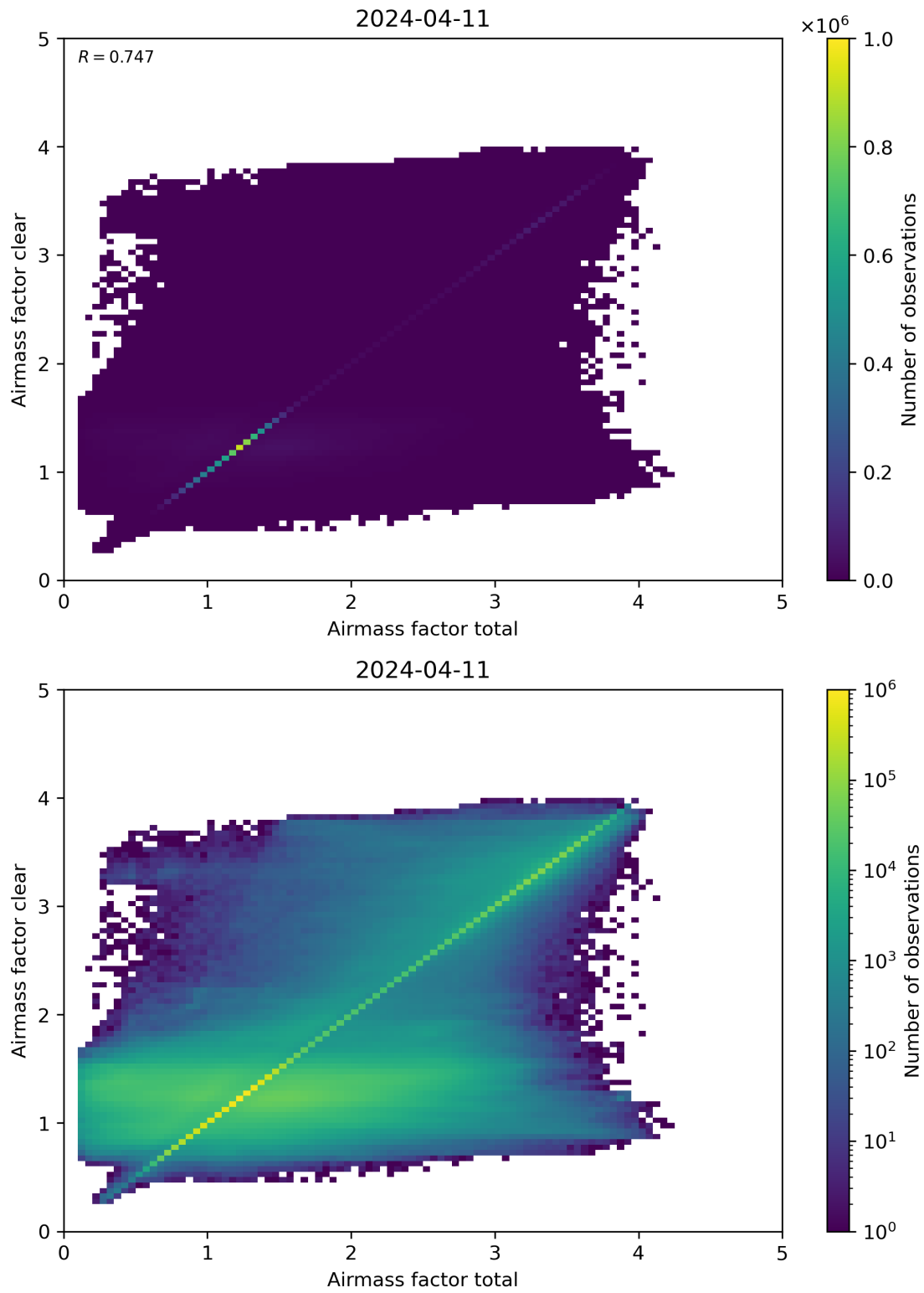
Figure 100: Scatter density plot of “Airmass factor total” against “Airmass factor clear” for 2024-04-10 to 2024-04-12.
