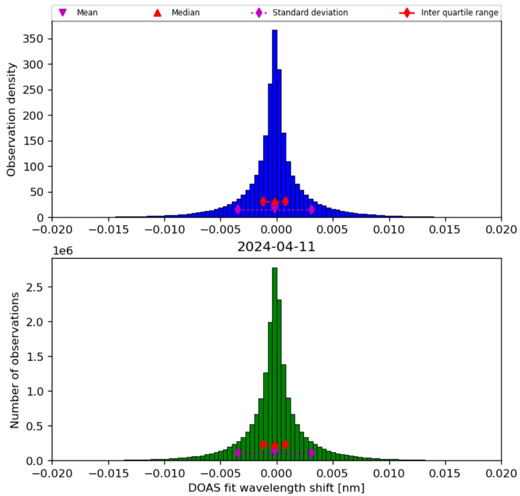
Figure 44: Histogram of “DOAS fit wavelength shift” for 2024-04-10 to 2024-04-12
