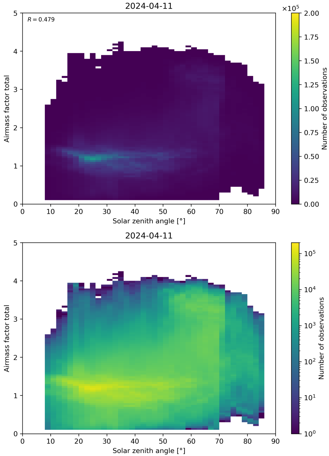
Figure 175: Scatter density plot of “Solar zenith angle” against “Airmass factor total” for 2024-04-10 to 2024-04-12.
