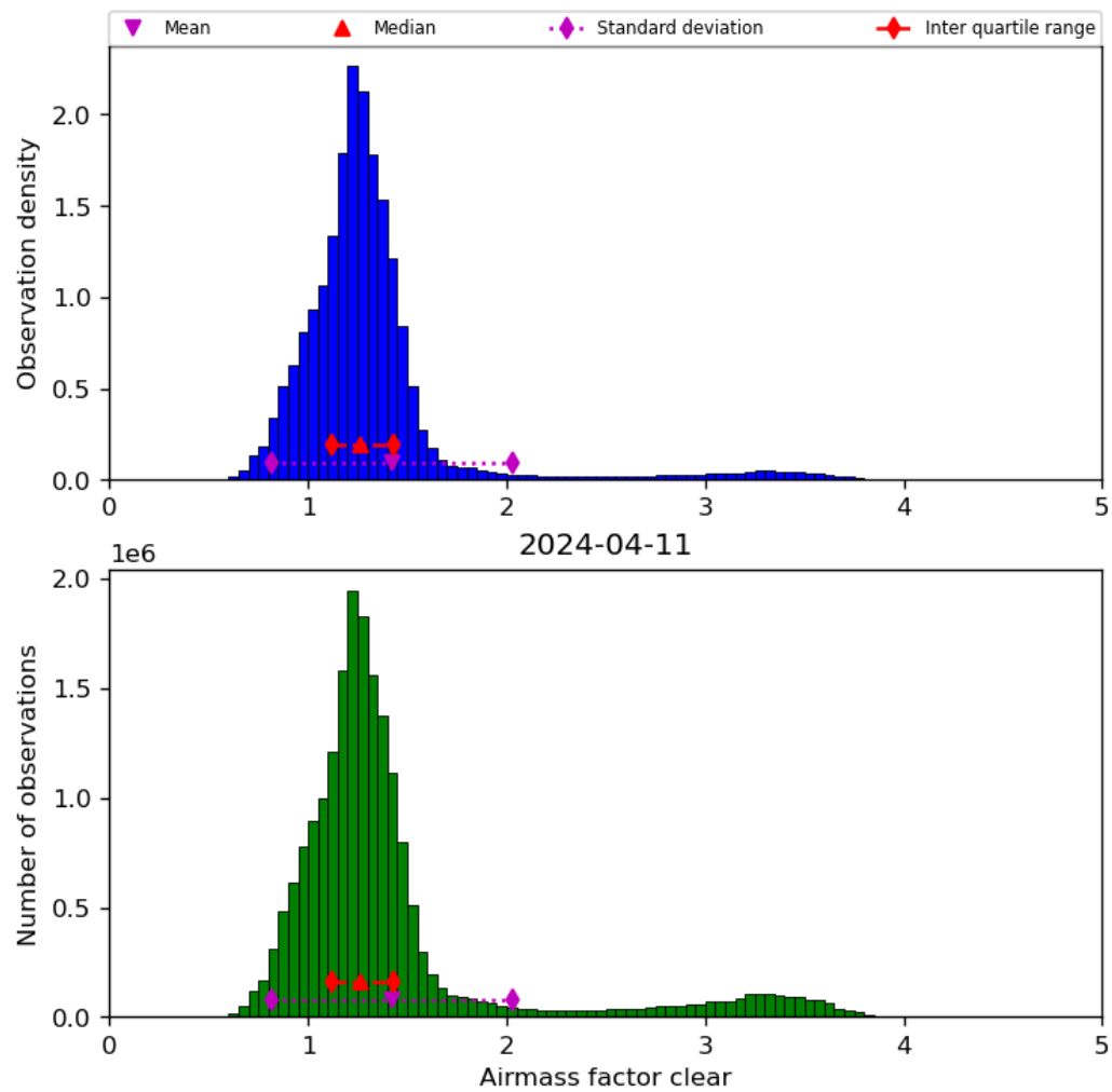
Figure 42: Histogram of “Airmass factor clear” for 2024-04-10 to 2024-04-12
