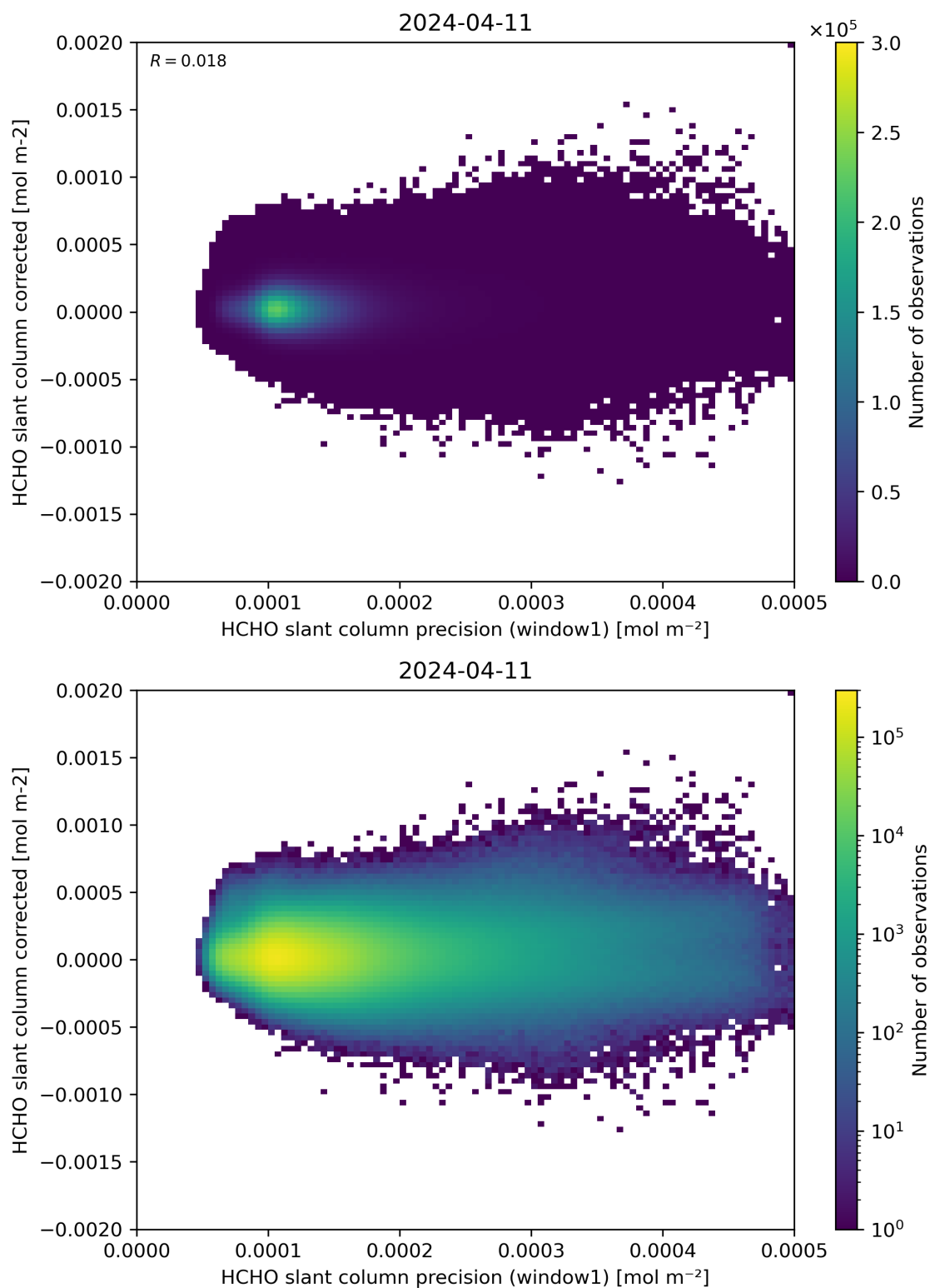
Figure 92: Scatter density plot of “HCHO slant column precision (window1)” against “HCHO slant column corrected” for 2024-04-10 to 2024-04-12.
