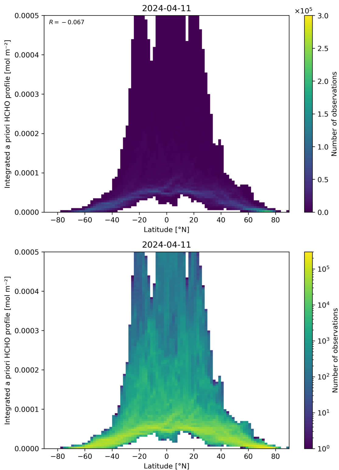
Figure 166: Scatter density plot of “Latitude” against “Integrated a priori HCHO profile” for 2024-04-10 to 2024-04-12.
