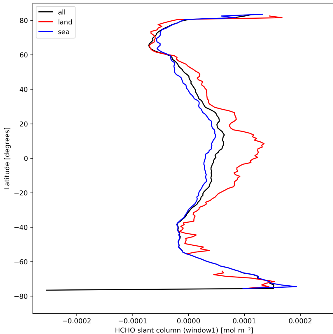
Figure 24: Zonal average of “HCHO slant column (window1)” for 2024-04-10 to 2024-04-12.
