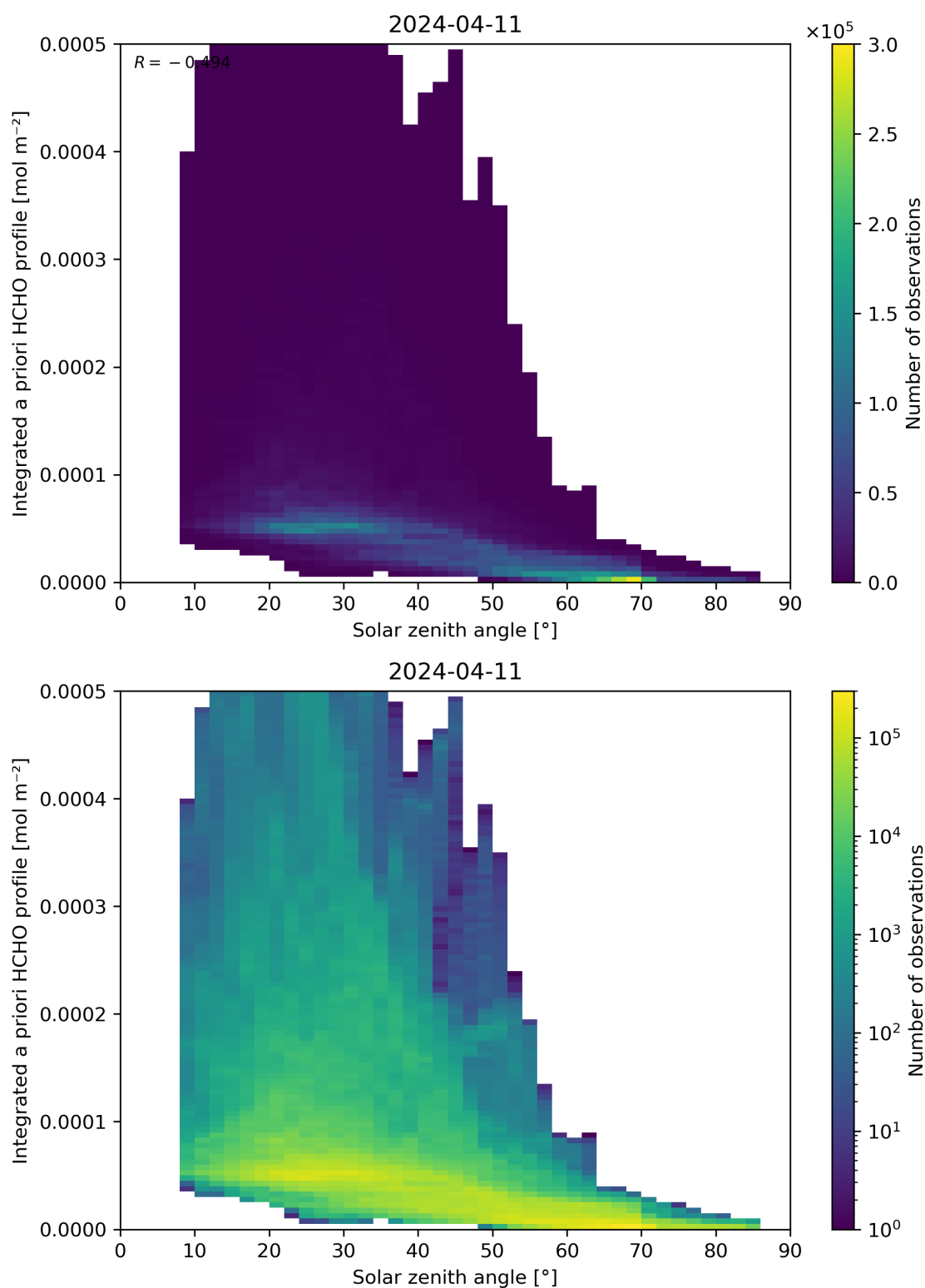
Figure 180: Scatter density plot of “Solar zenith angle” against “Integrated a priori HCHO profile” for 2024-04-10 to 2024-04-12.
