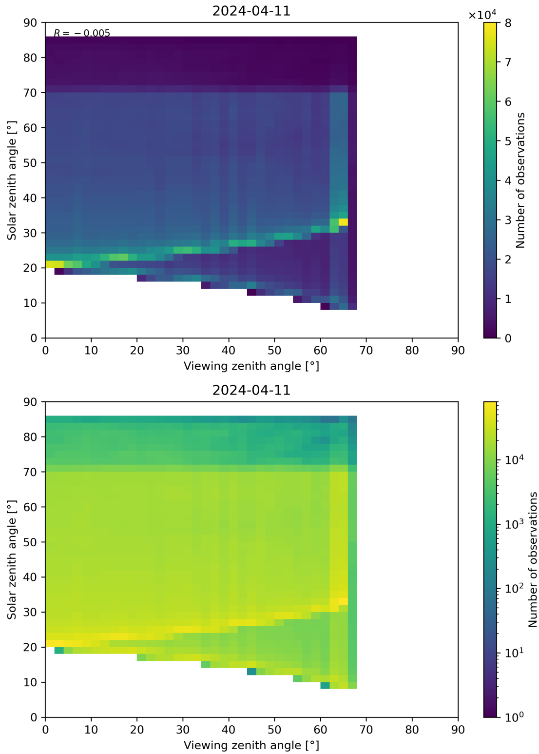
Figure 197: Scatter density plot of “Viewing zenith angle” against “Solar zenith angle” for 2024-04-10 to 2024-04-12.
