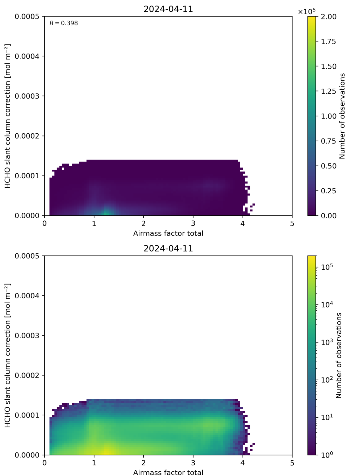
Figure 102: Scatter density plot of “Airmass factor total” against “HCHO slant column correction” for 2024-04-10 to 2024-04-12.
