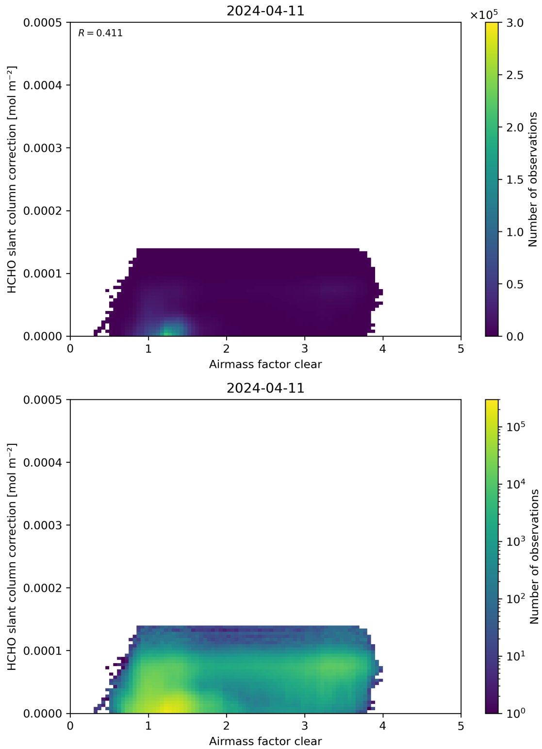
Figure 75: Scatter density plot of “Airmass factor clear” against “HCHO slant column correction” for 2024-04-10 to 2024-04-12.
