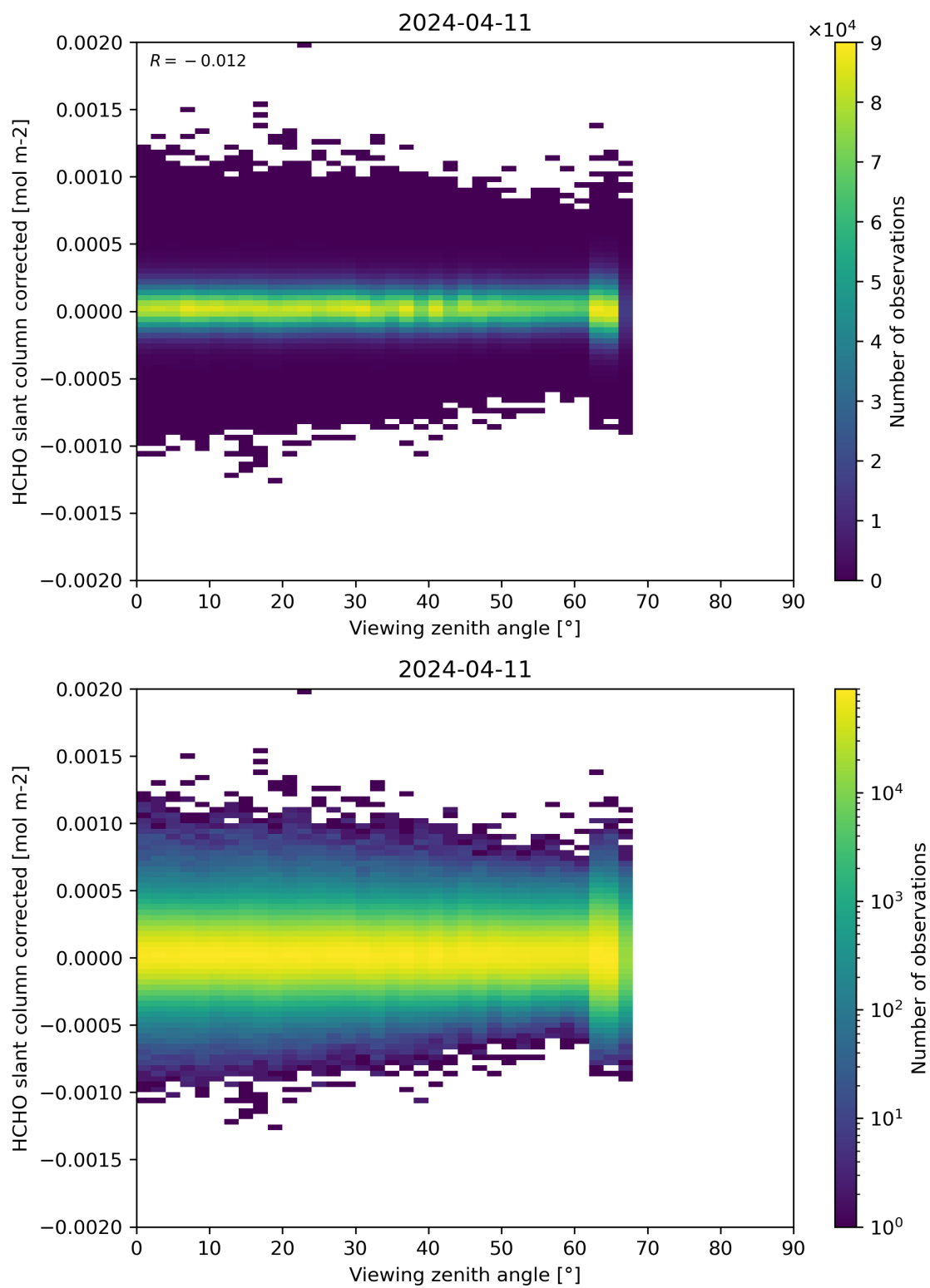
Figure 186: Scatter density plot of “Viewing zenith angle” against “HCHO slant column corrected” for 2024-04-10 to 2024-04-12.
