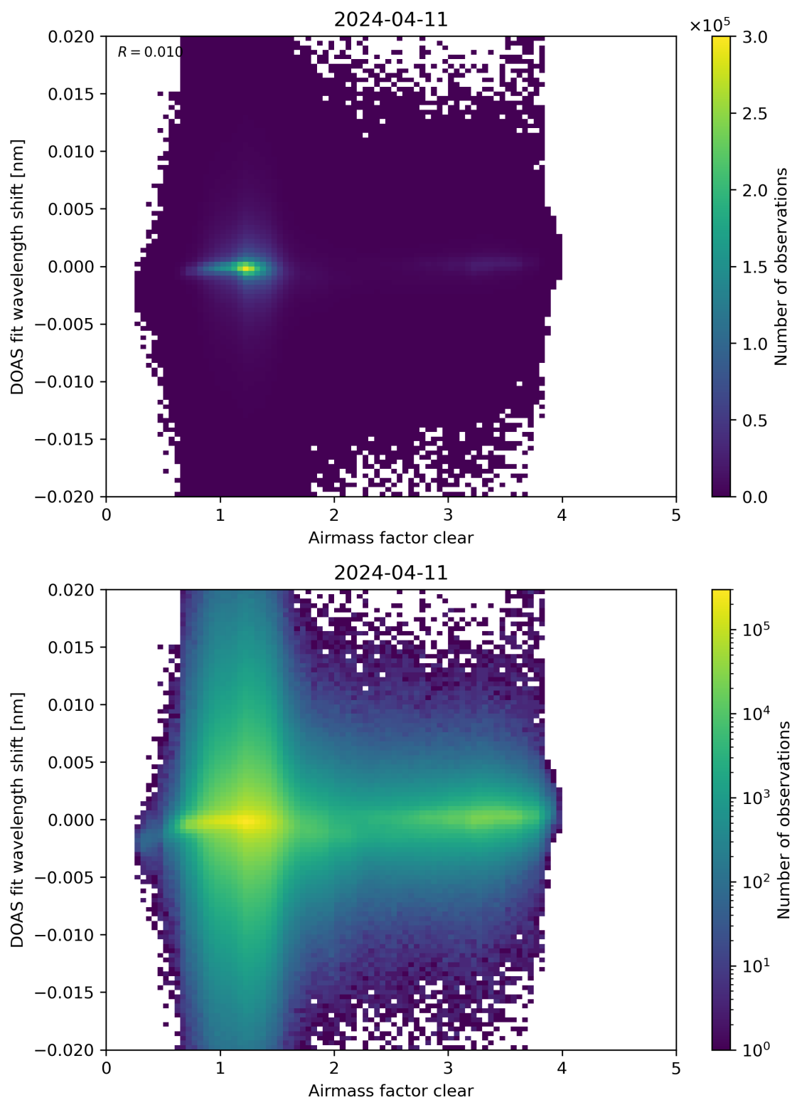
Figure 72: Scatter density plot of “Airmass factor clear” against “DOAS fit wavelength shift” for 2024-04-10 to 2024-04-12.
