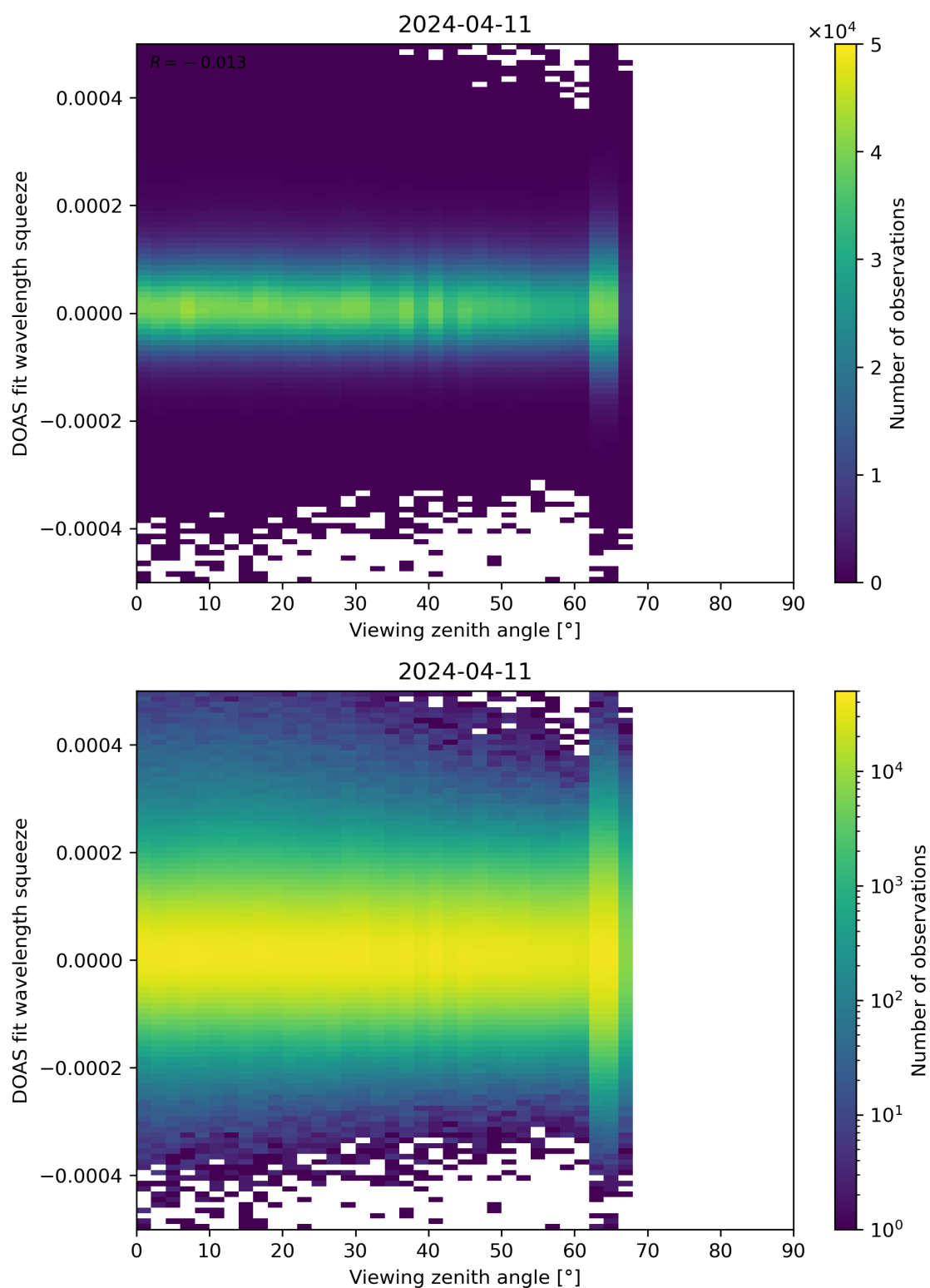
Figure 184: Scatter density plot of “Viewing zenith angle” against “DOAS fit wavelength squeeze” for 2024-04-10 to 2024-04-12.
