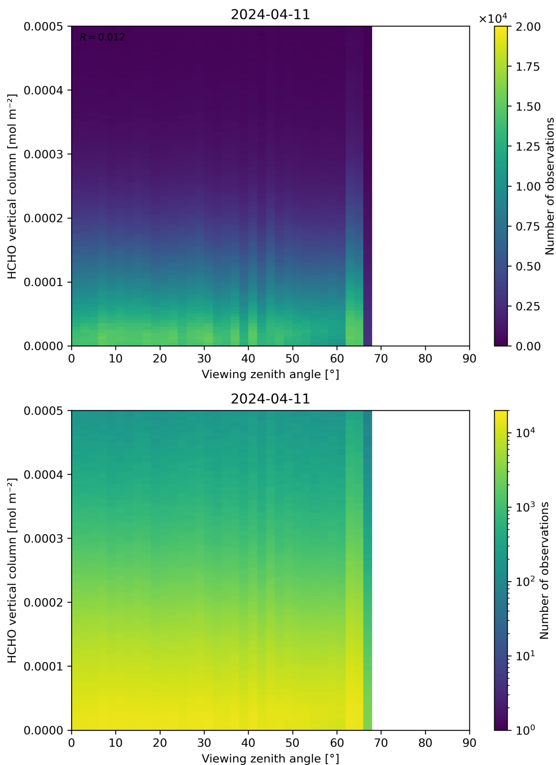
Figure 192: Scatter density plot of “Viewing zenith angle” against “HCHO vertical column” for 2024-04-10 to 2024-04-12.
