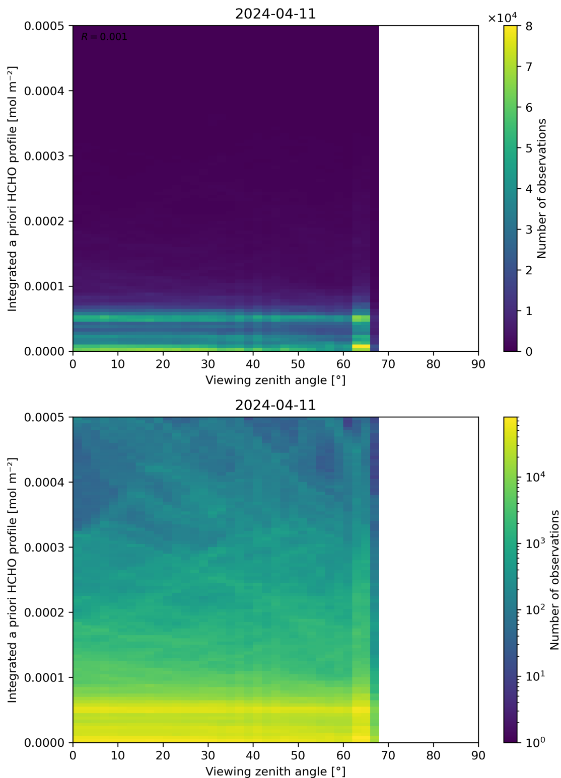
Figure 195: Scatter density plot of “Viewing zenith angle” against “Integrated a priori HCHO profile” for 2024-04-10 to 2024-04-12.
