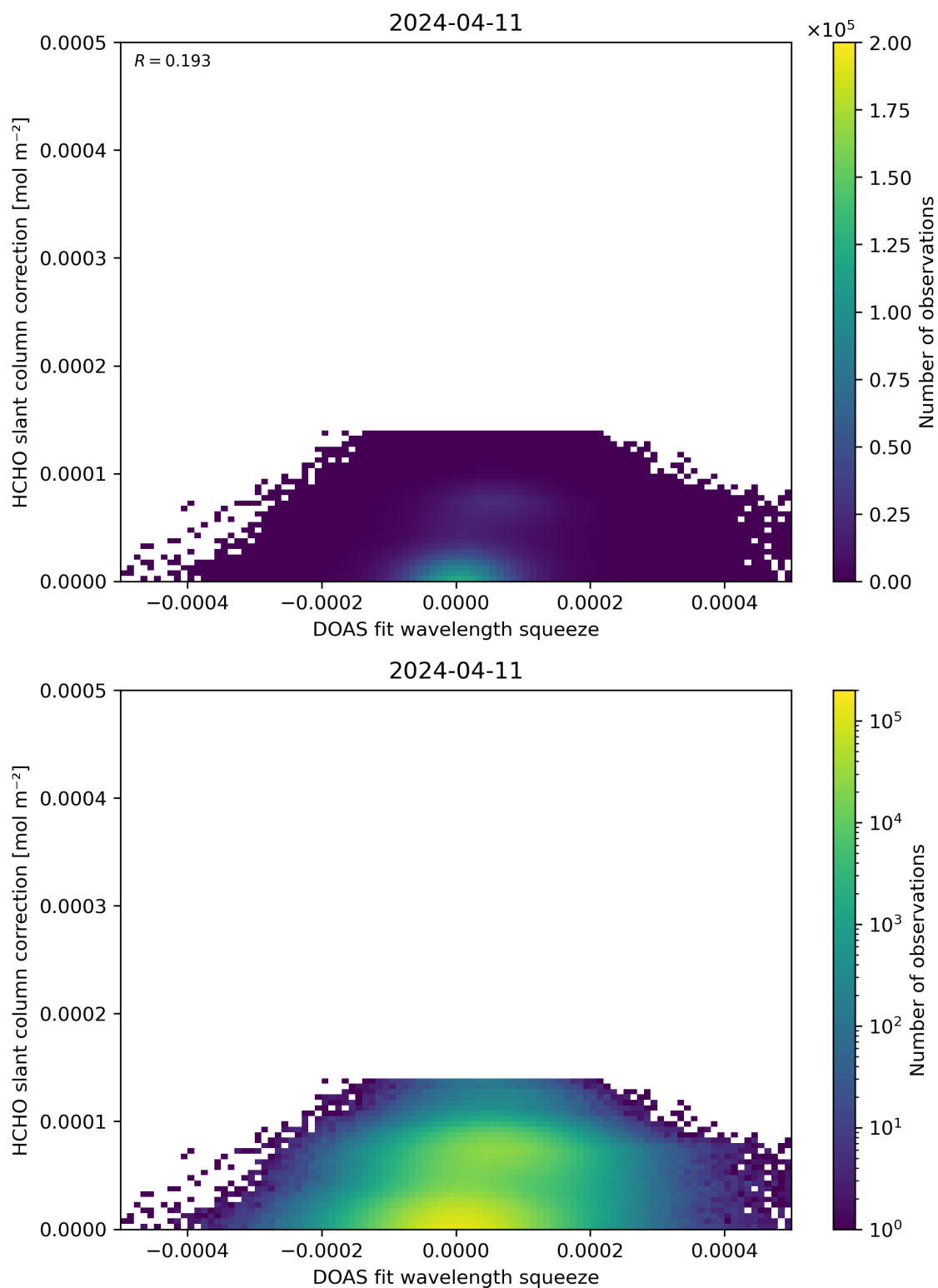
Figure 70: Scatter density plot of “DOAS fit wavelength squeeze” against “HCHO slant column correction” for 2024-04-10 to 2024-04-12.
