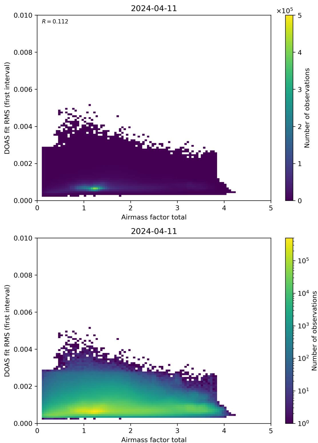
Figure 97: Scatter density plot of “Airmass factor total” against “DOAS fit RMS (first interval)” for 2024-04-10 to 2024-04-12.
