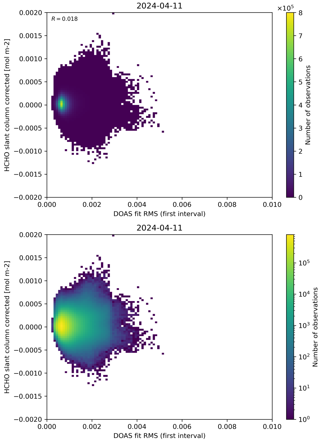
Figure 62: Scatter density plot of “DOAS fit RMS (first interval)” against “HCHO slant column corrected” for 2024-04-10 to 2024-04-12.
