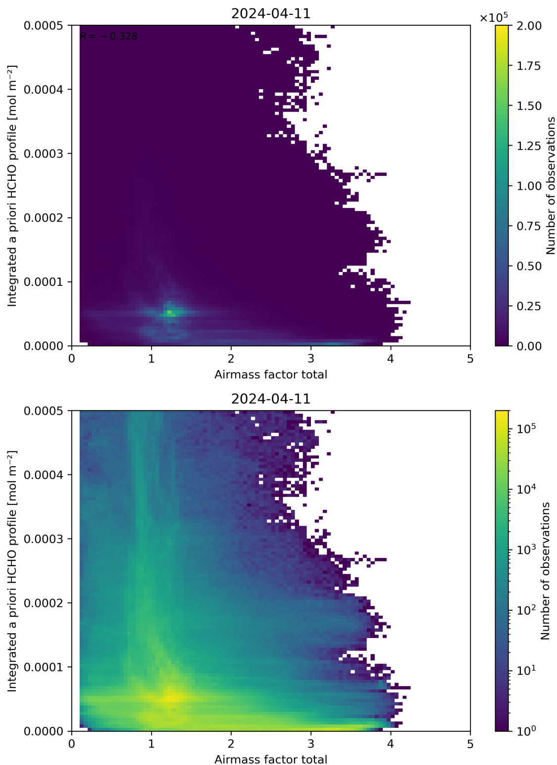
Figure 104: Scatter density plot of “Airmass factor total” against “Integrated a priori HCHO profile” for 2024-04-10 to 2024-04-12.
