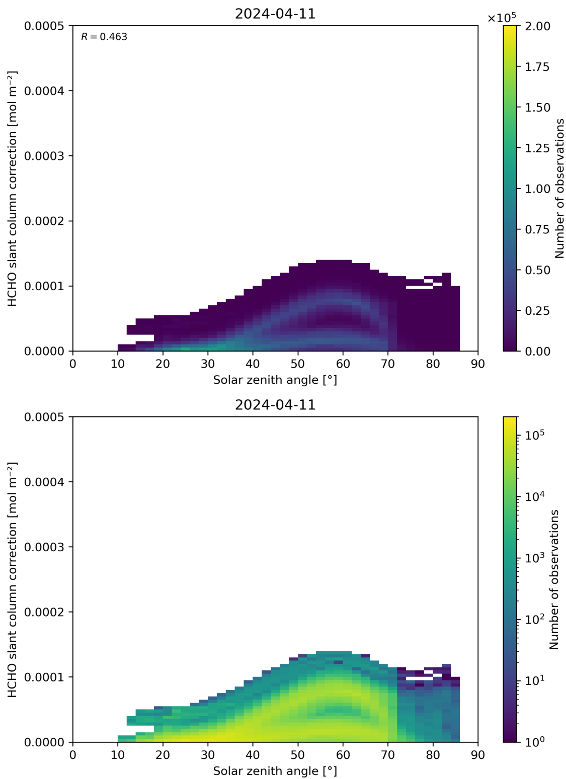
Figure 172: Scatter density plot of “Solar zenith angle” against “HCHO slant column correction” for 2024-04-10 to 2024-04-12.
