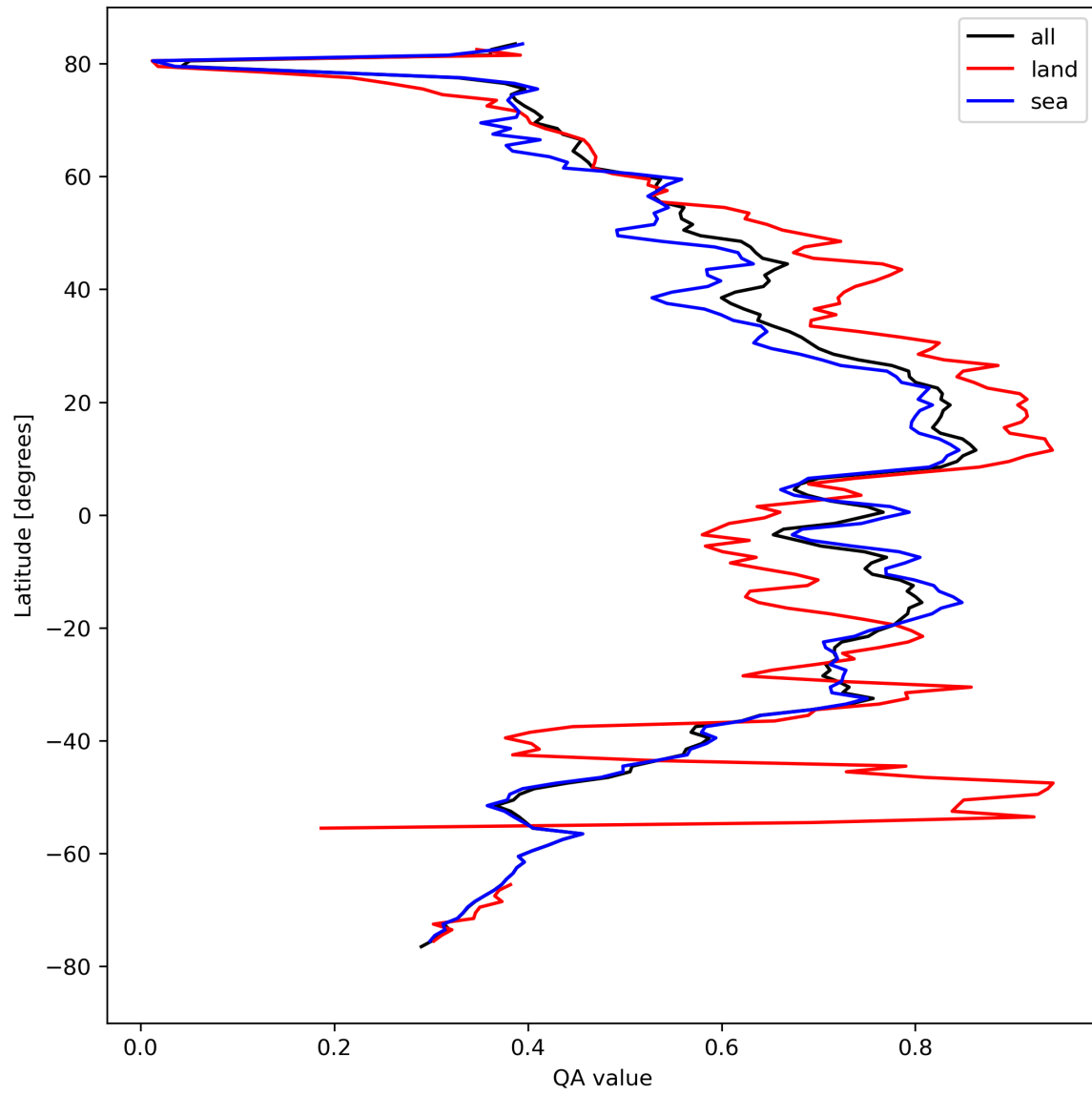
Figure 20: Zonal average of “QA value” for 2024-04-10 to 2024-04-12.
