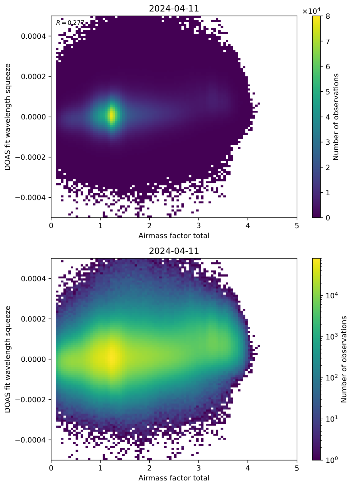
Figure 99: Scatter density plot of “Airmass factor total” against “DOAS fit wavelength squeeze” for 2024-04-10 to 2024-04-12.
