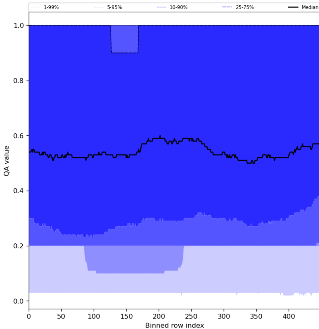
Figure 48: Along track statistics of “QA value” for 2024-04-10 to 2024-04-12
