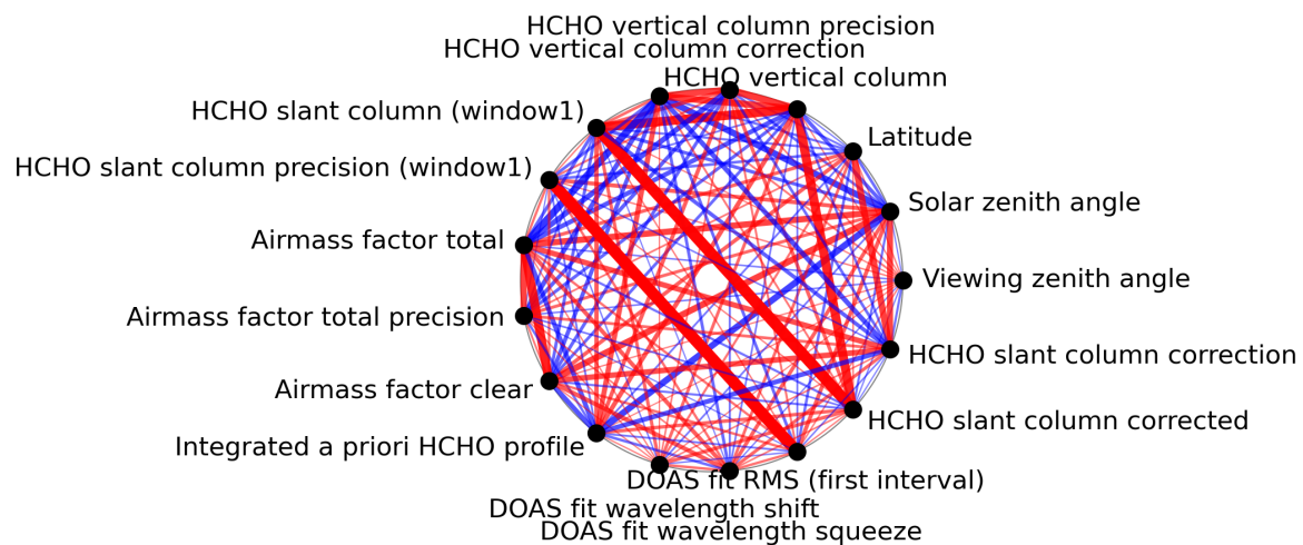
Figure 1: Map of correlation graph for 2024-04-10 to 2024-04-12.
