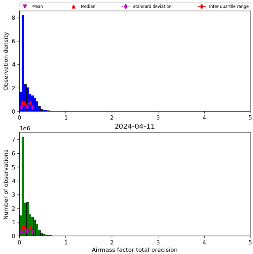
Figure 41: Histogram of “Airmass factor total precision” for 2024-04-10 to 2024-04-12
