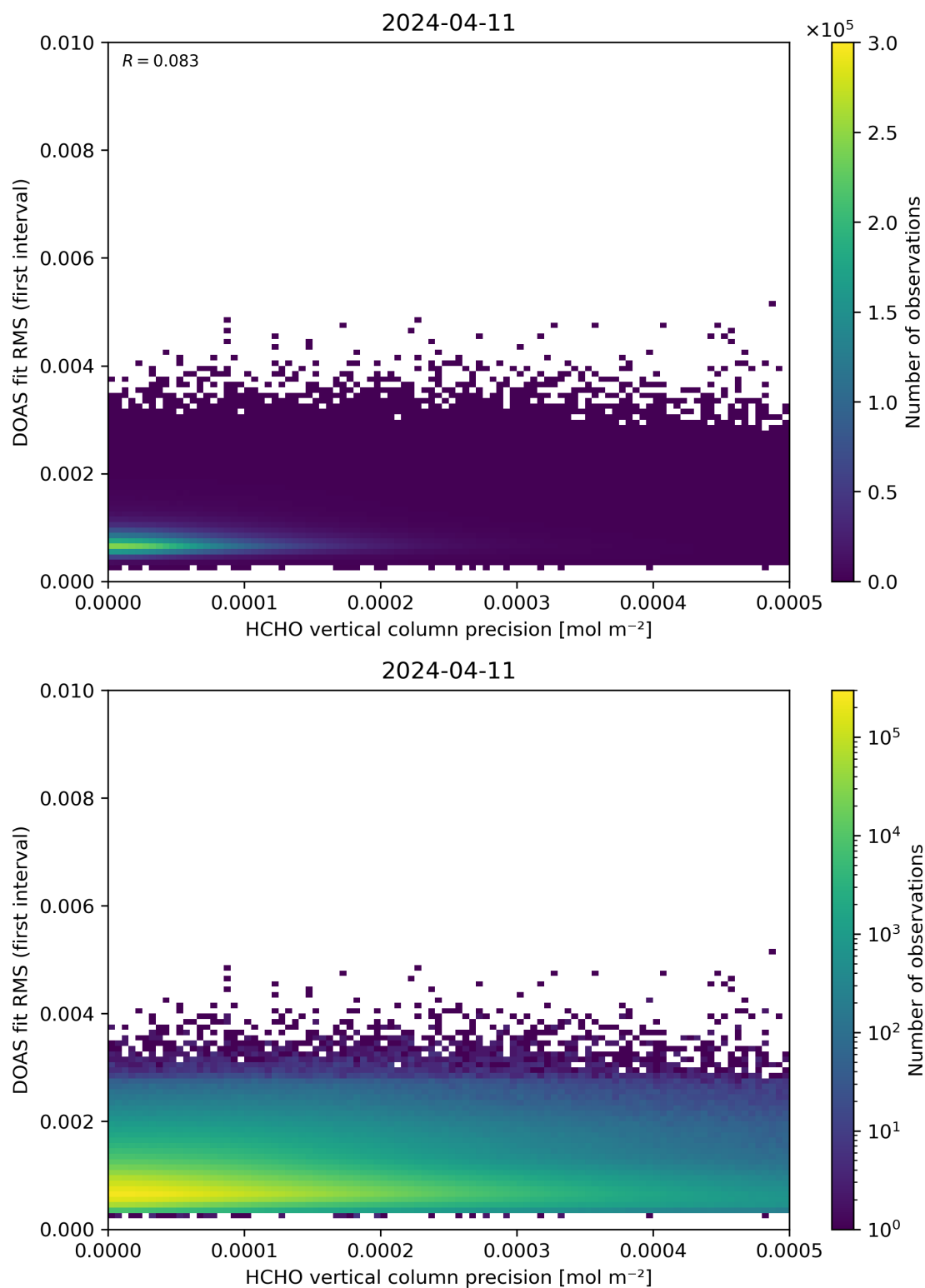
Figure 136: Scatter density plot of “HCHO vertical column precision” against “DOAS fit RMS (first interval)” for 2024-04-10 to 2024-04-12.
