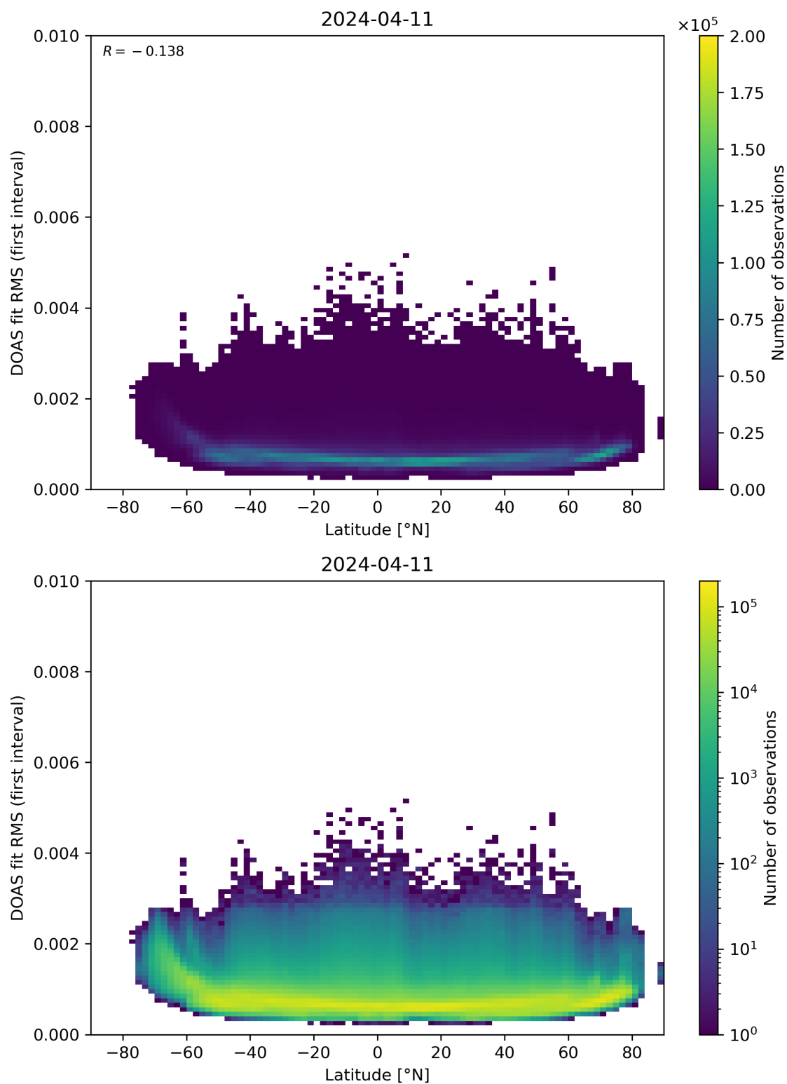
Figure 153: Scatter density plot of “Latitude” against “DOAS fit RMS (first interval)” for 2024-04-10 to 2024-04-12.
