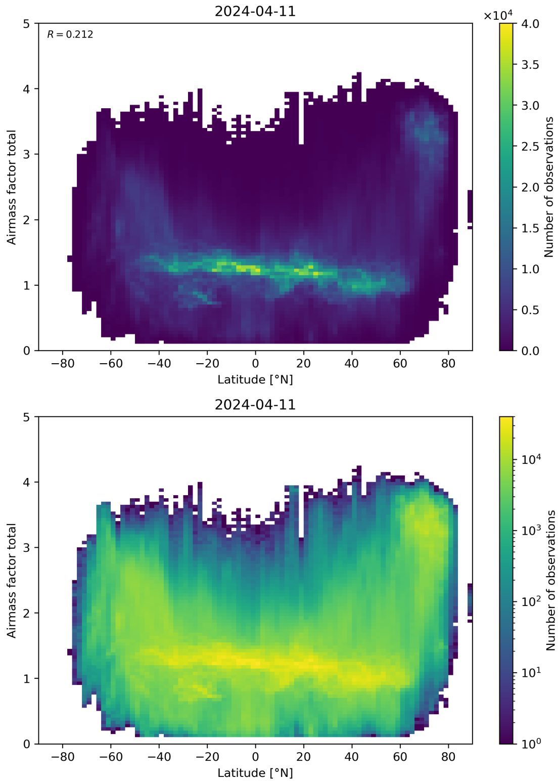
Figure 161: Scatter density plot of “Latitude” against “Airmass factor total” for 2024-04-10 to 2024-04-12.
