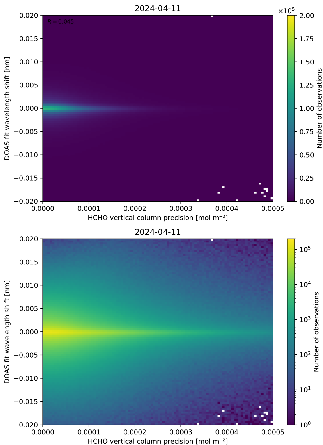
Figure 137: Scatter density plot of “HCHO vertical column precision” against “DOAS fit wavelength shift” for 2024-04-10 to 2024-04-12.
