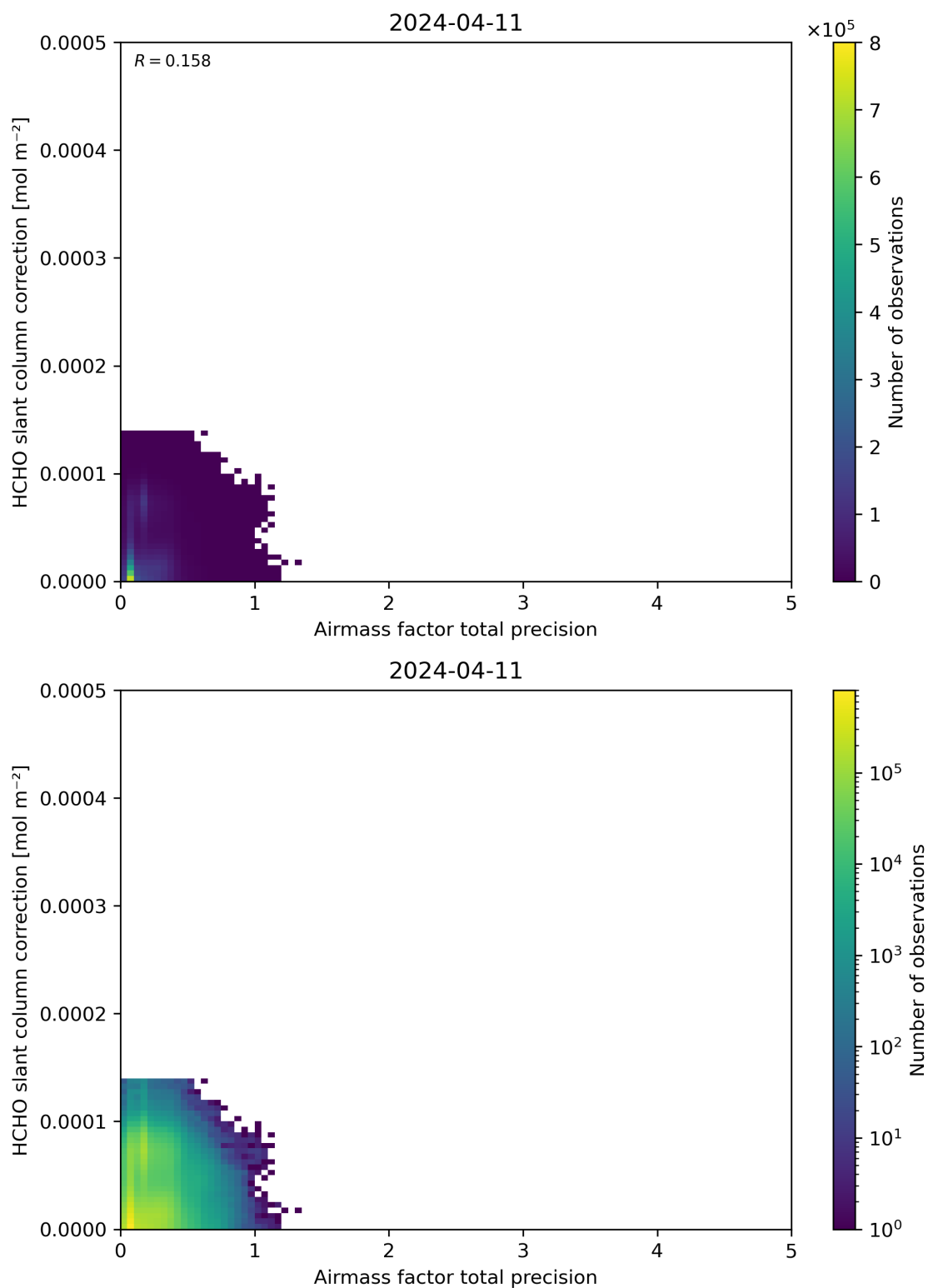
Figure 110: Scatter density plot of “Airmass factor total precision” against “HCHO slant column correction” for 2024-04-10 to 2024-04-12.
