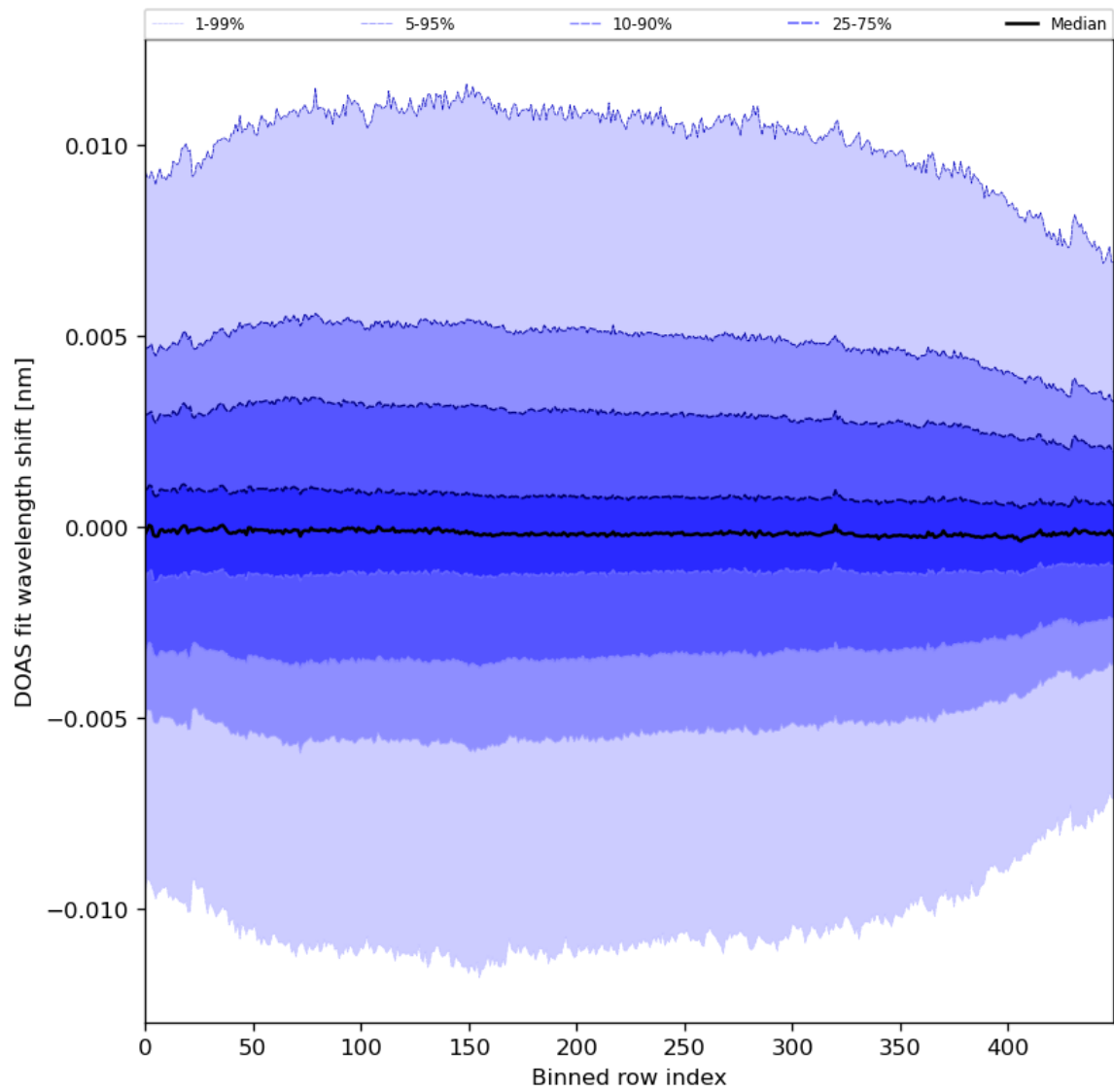
Figure 58: Along track statistics of “DOAS fit wavelength shift” for 2024-04-10 to 2024-04-12
