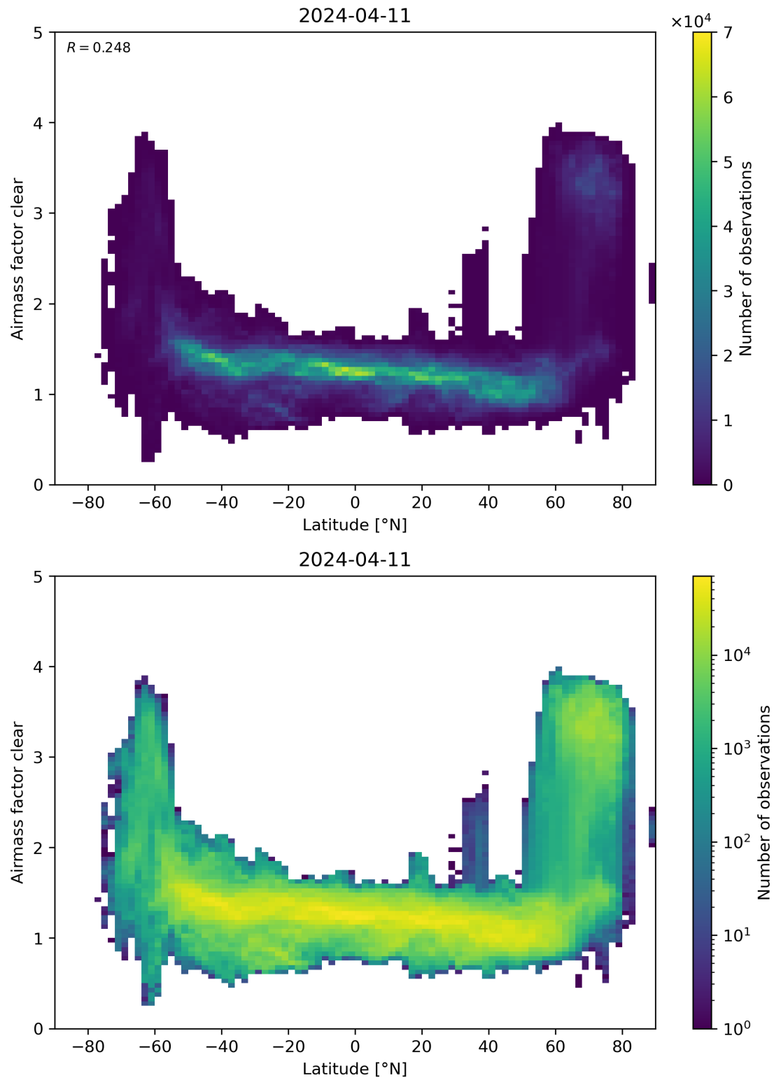
Figure 156: Scatter density plot of “Latitude” against “Airmass factor clear” for 2024-04-10 to 2024-04-12.
