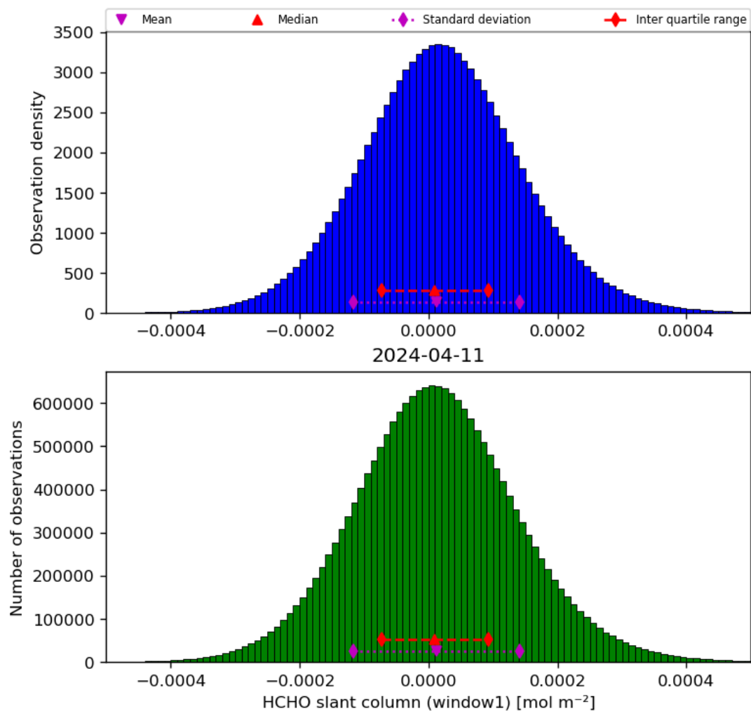
Figure 38: Histogram of “HCHO slant column (window1)” for 2024-04-10 to 2024-04-12
