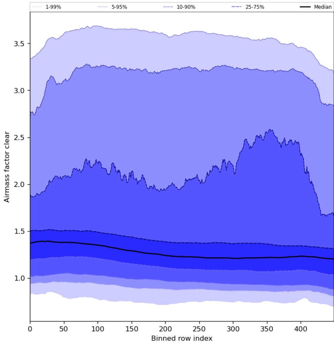
Figure 56: Along track statistics of “Airmass factor clear” for 2024-04-10 to 2024-04-12
