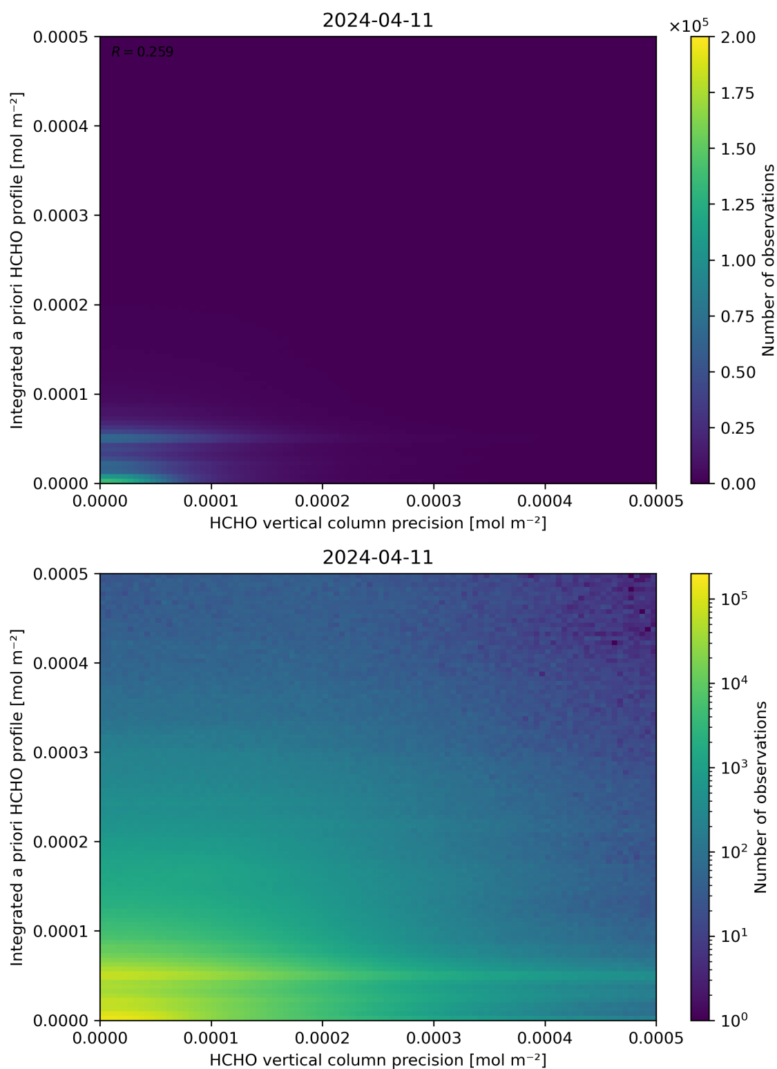
Figure 147: Scatter density plot of “HCHO vertical column precision” against “Integrated a priori HCHO profile” for 2024-04-10 to 2024-04-12.
