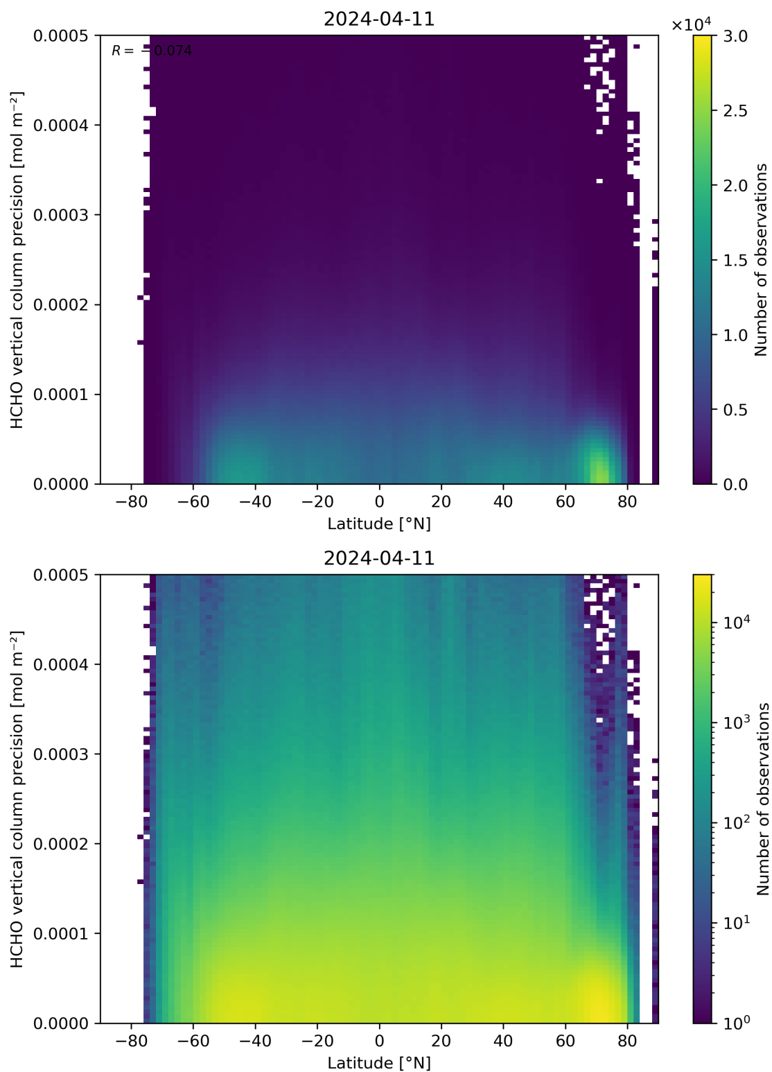
Figure 165: Scatter density plot of “Latitude” against “HCHO vertical column precision” for 2024-04-10 to 2024-04-12.
