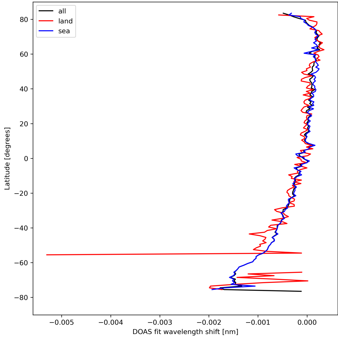
Figure 30: Zonal average of “DOAS fit wavelength shift” for 2024-04-10 to 2024-04-12.
