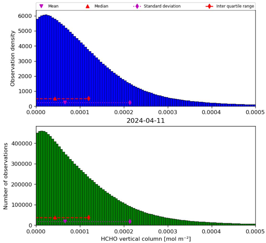
Figure 35: Histogram of “HCHO vertical column” for 2024-04-10 to 2024-04-12
