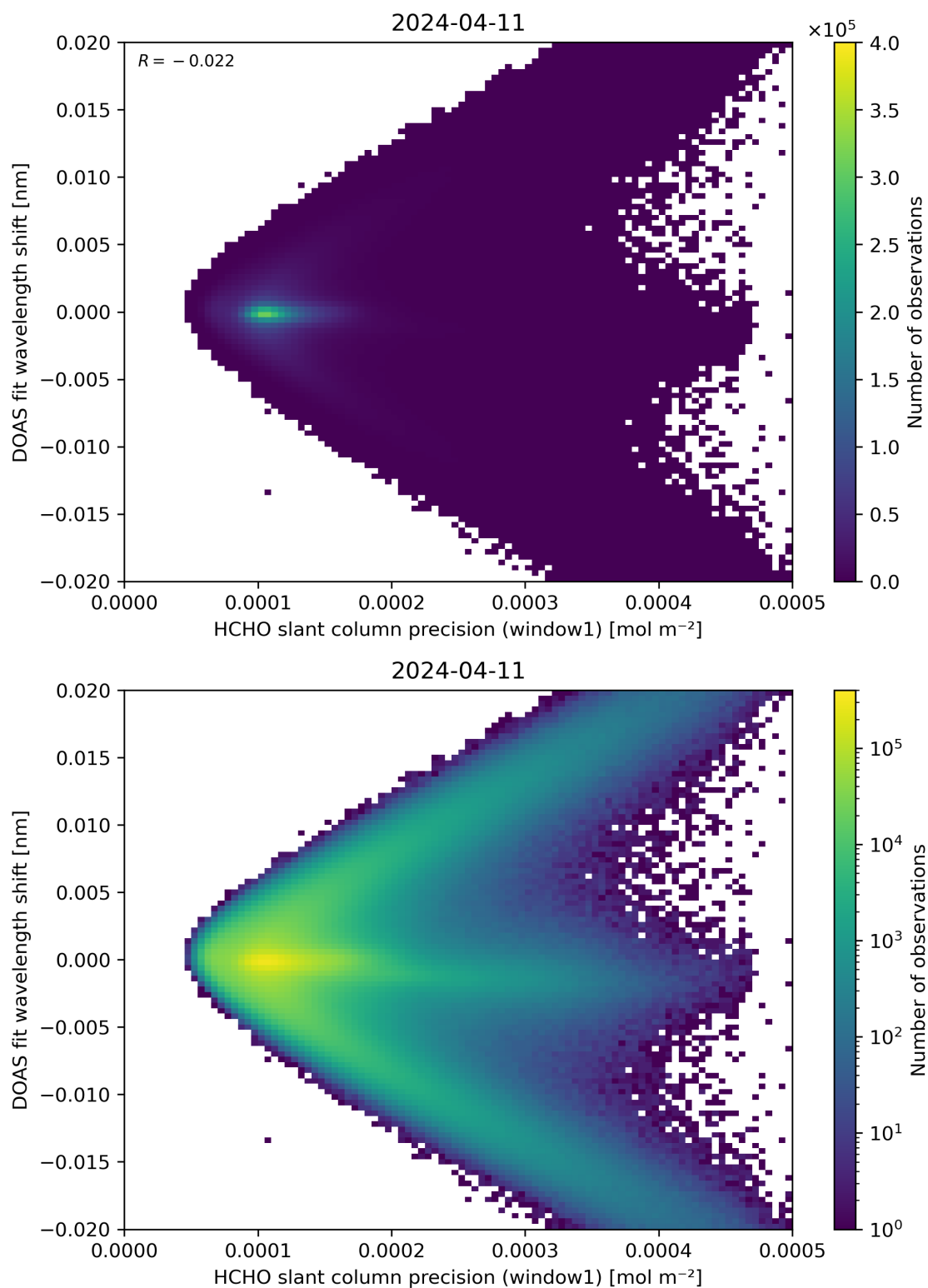
Figure 89: Scatter density plot of “HCHO slant column precision (window1)” against “DOAS fit wavelength shift” for 2024-04-10 to 2024-04-12.
