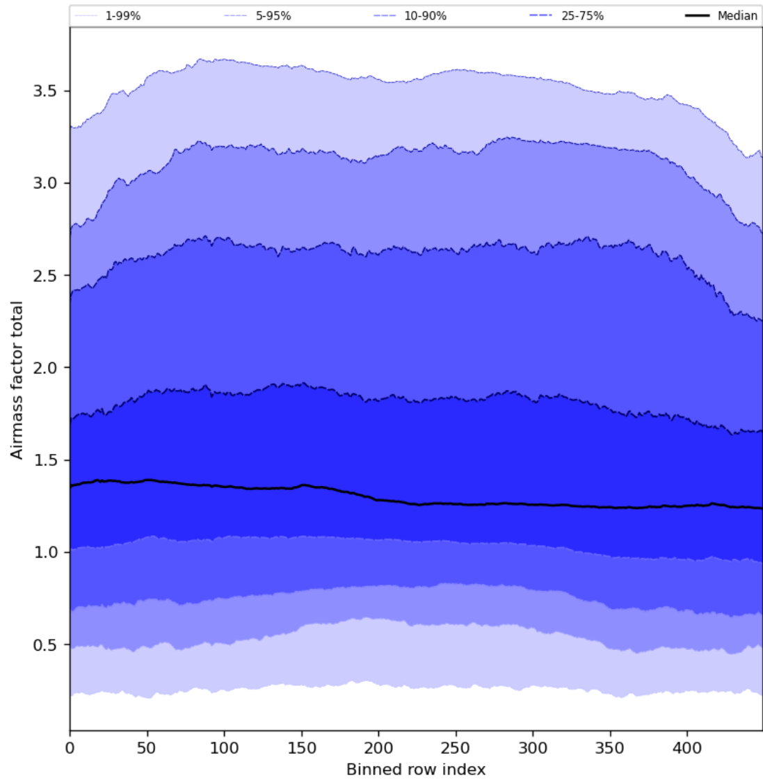
Figure 54: Along track statistics of “Airmass factor total” for 2024-04-10 to 2024-04-12
