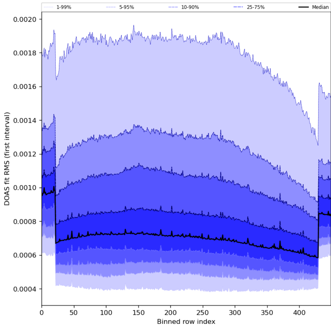
Figure 60: Along track statistics of “DOAS fit RMS (first interval)” for 2024-04-10 to 2024-04-12
