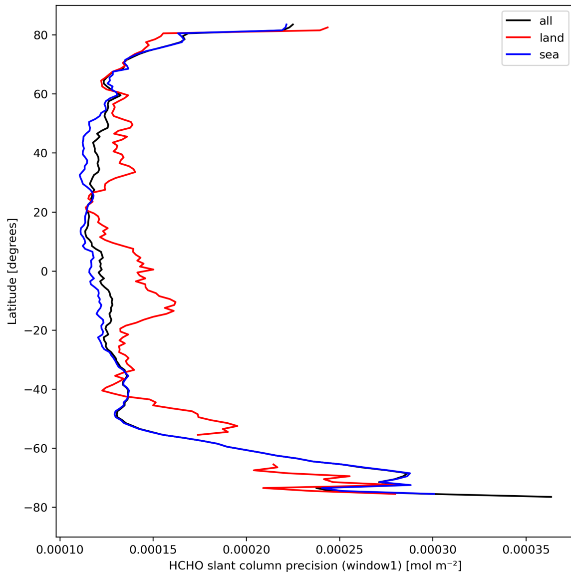
Figure 25: Zonal average of “HCHO slant column precision (window1)” for 2024-04-10 to 2024-04-12.
