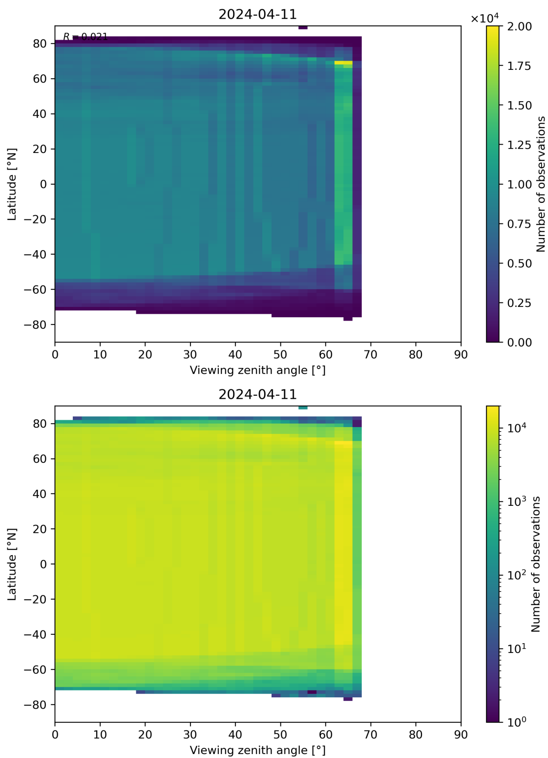
Figure 196: Scatter density plot of “Viewing zenith angle” against “Latitude” for 2024-04-10 to 2024-04-12.
