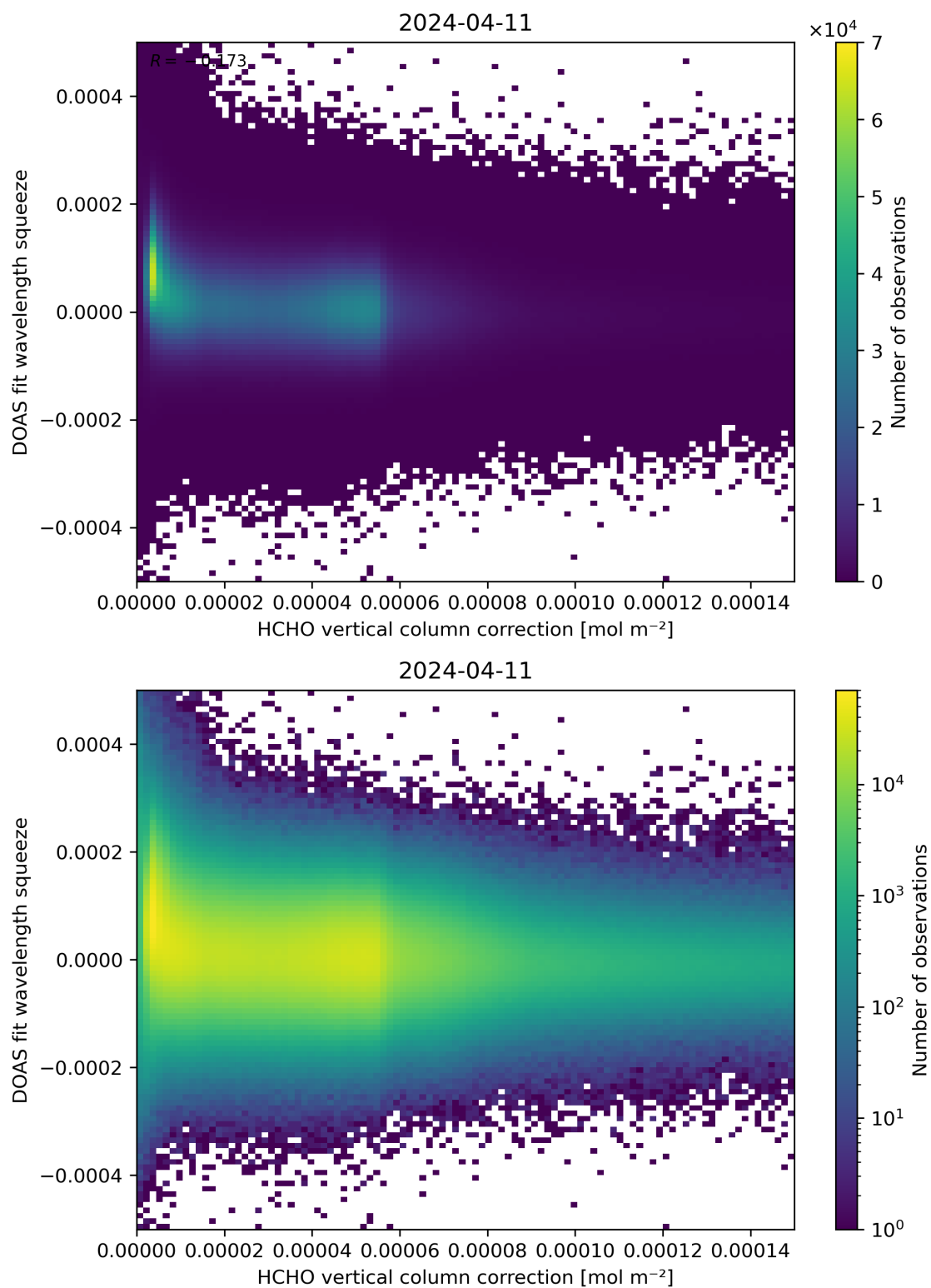
Figure 114: Scatter density plot of “HCHO vertical column correction” against “DOAS fit wavelength squeeze” for 2024-04-10 to 2024-04-12.
