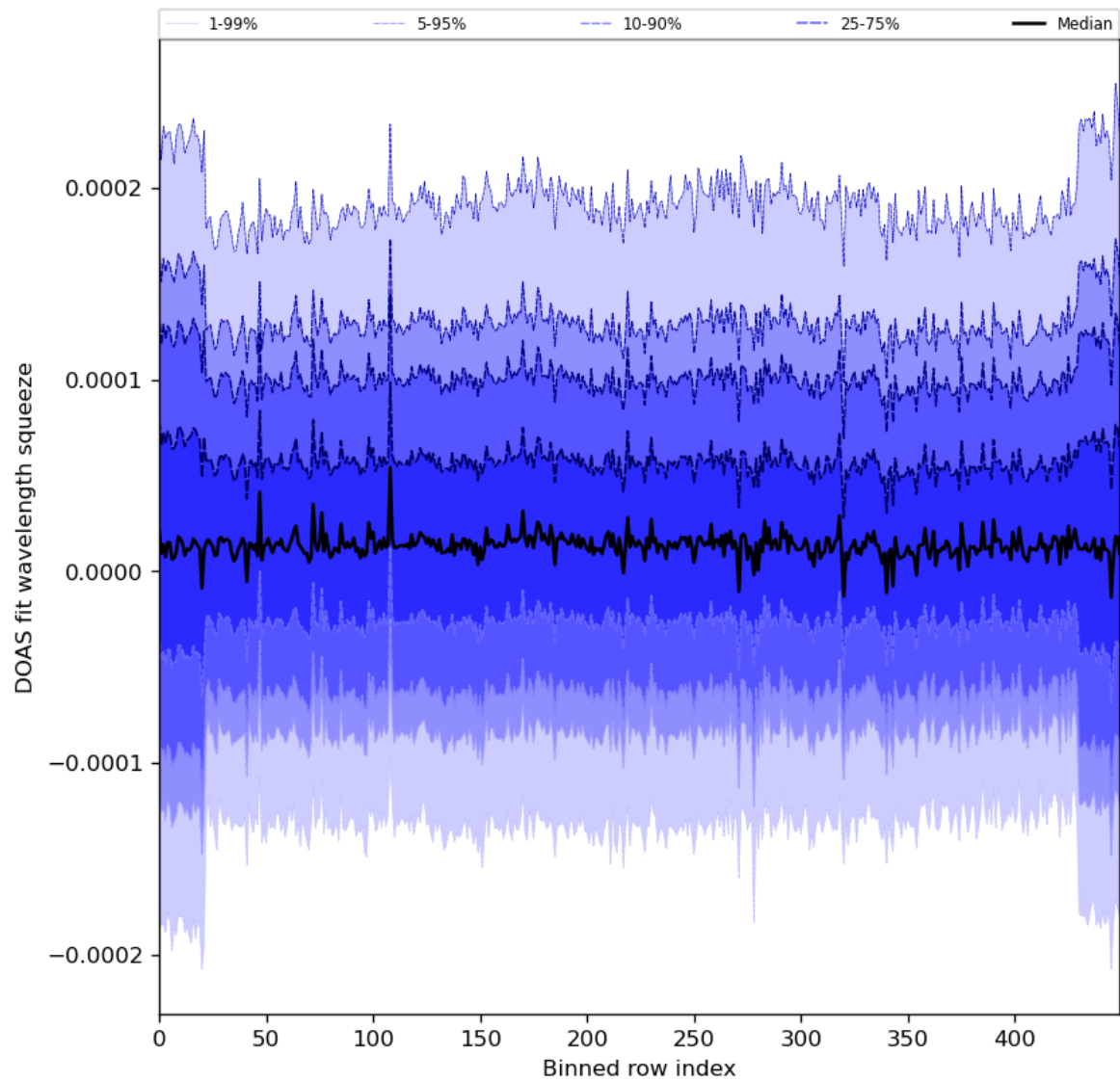
Figure 59: Along track statistics of “DOAS fit wavelength squeeze” for 2024-04-10 to 2024-04-12
