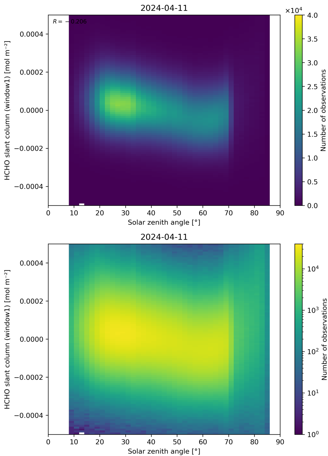
Figure 173: Scatter density plot of “Solar zenith angle” against “HCHO slant column (window1)” for 2024-04-10 to 2024-04-12.
