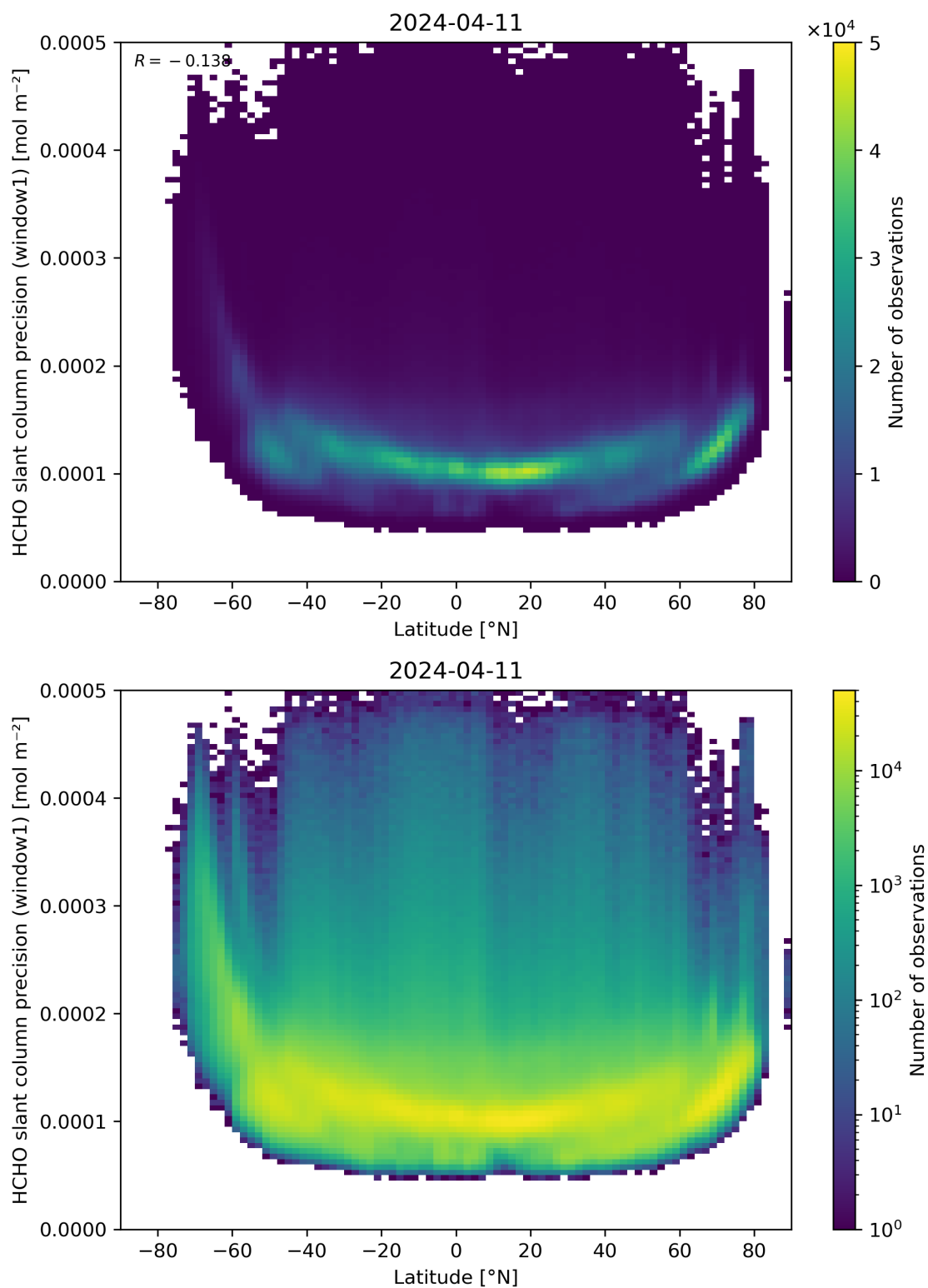
Figure 160: Scatter density plot of “Latitude” against “HCHO slant column precision (window1)” for 2024-04-10 to 2024-04-12.
