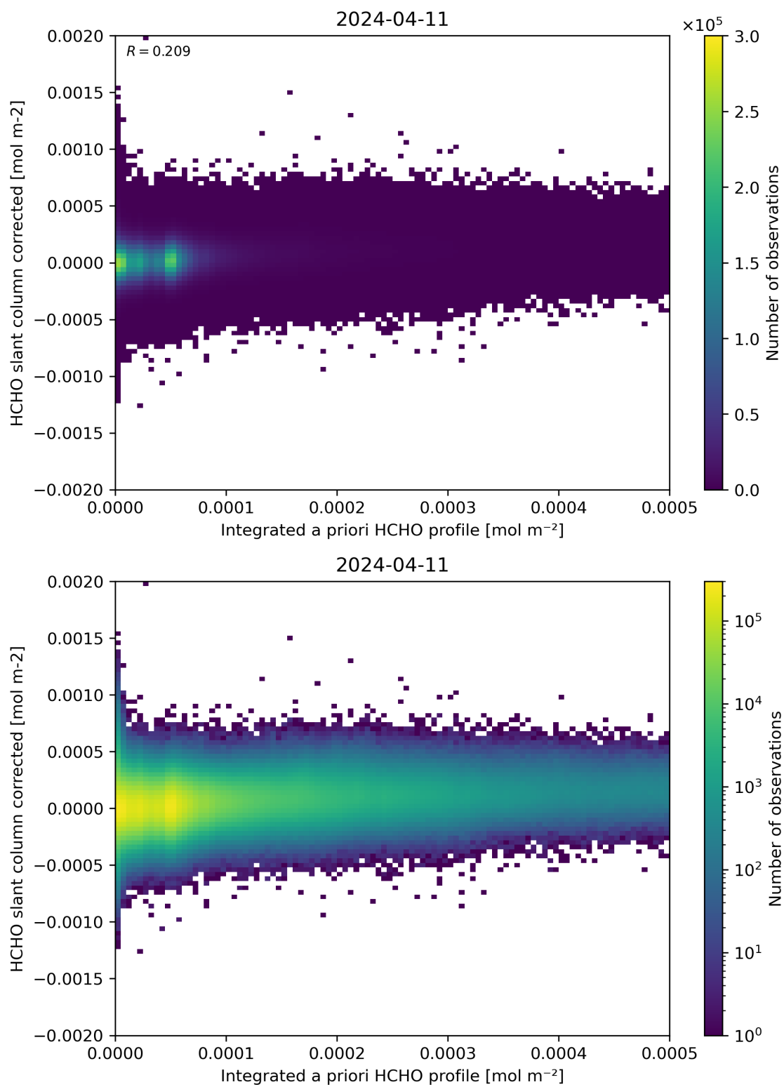
Figure 151: Scatter density plot of “Integrated a priori HCHO profile” against “HCHO slant column corrected” for 2024-04-10 to 2024-04-12.
