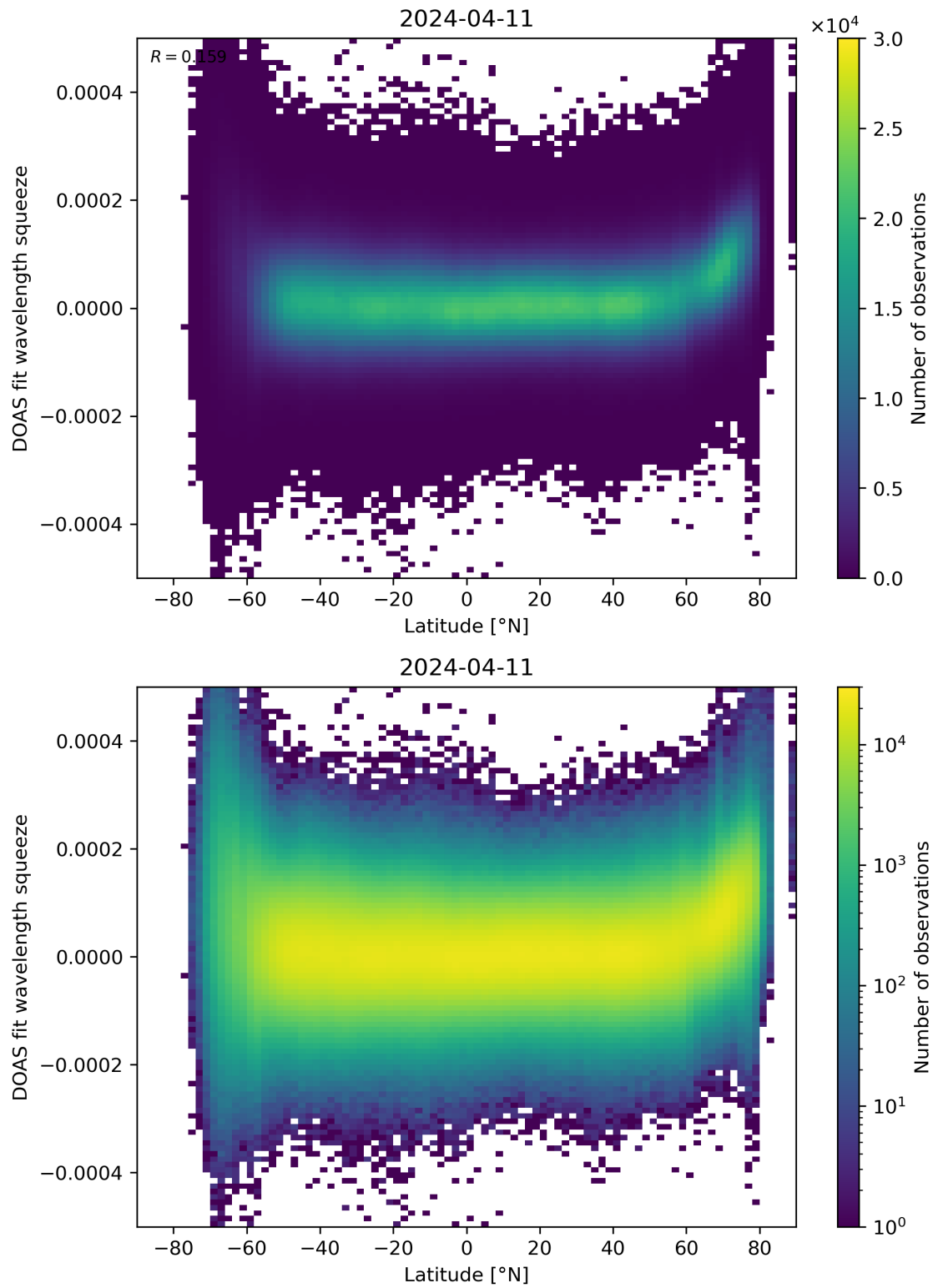
Figure 155: Scatter density plot of “Latitude” against “DOAS fit wavelength squeeze” for 2024-04-10 to 2024-04-12.
