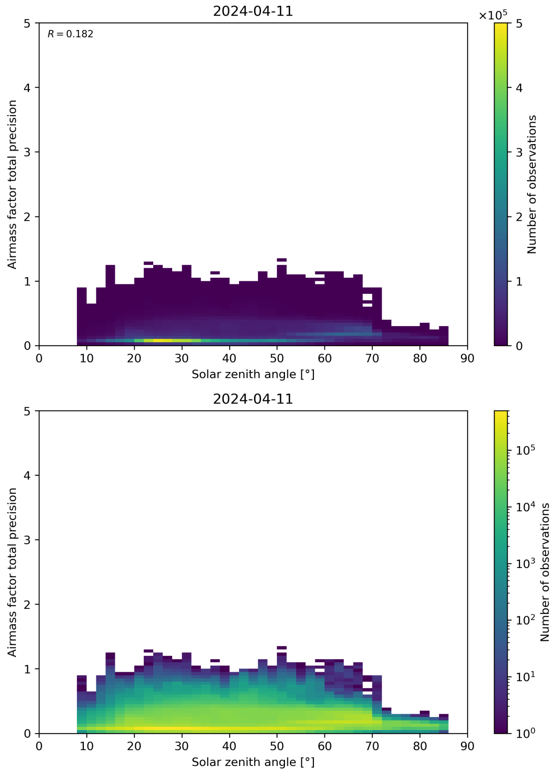
Figure 176: Scatter density plot of “Solar zenith angle” against “Airmass factor total precision” for 2024-04-10 to 2024-04-12.
