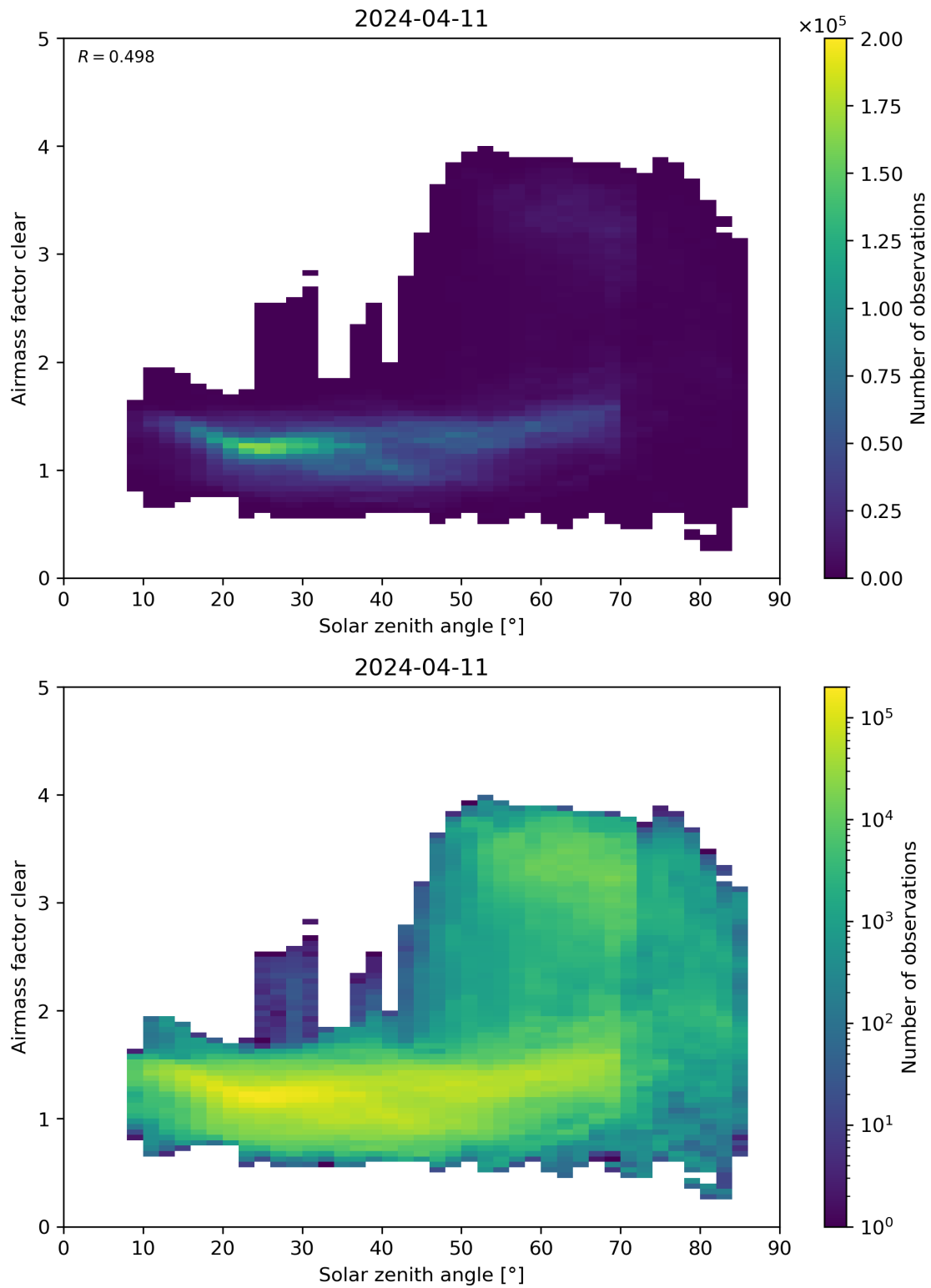
Figure 170: Scatter density plot of “Solar zenith angle” against “Airmass factor clear” for 2024-04-10 to 2024-04-12.
