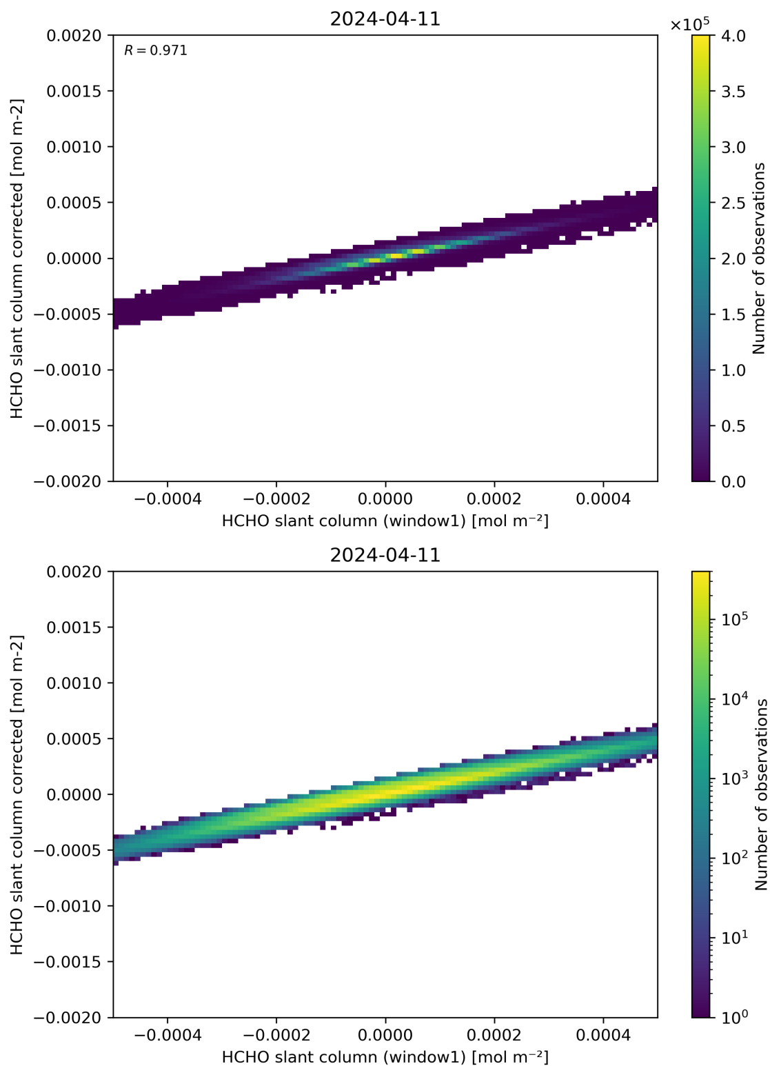
Figure 82: Scatter density plot of “HCHO slant column (window1)” against “HCHO slant column corrected” for 2024-04-10 to 2024-04-12.
