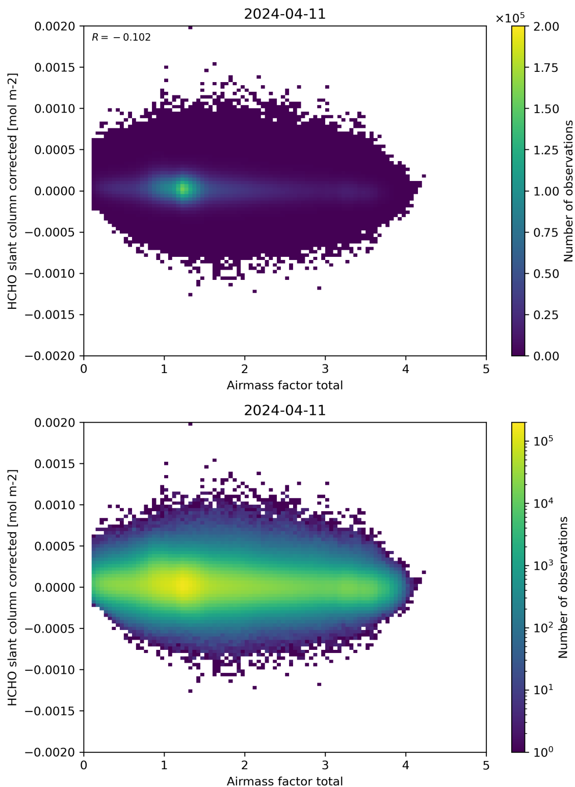
Figure 101: Scatter density plot of “Airmass factor total” against “HCHO slant column corrected” for 2024-04-10 to 2024-04-12.
