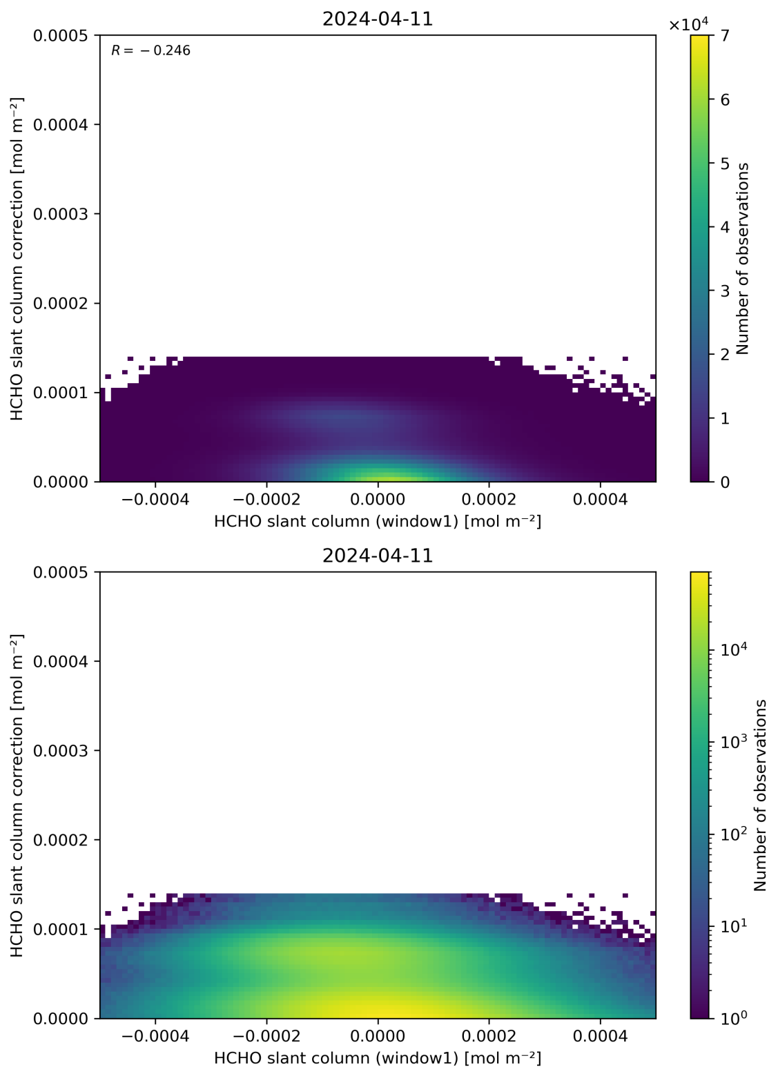
Figure 83: Scatter density plot of “HCHO slant column (window1)” against “HCHO slant column correction” for 2024-04-10 to 2024-04-12.
