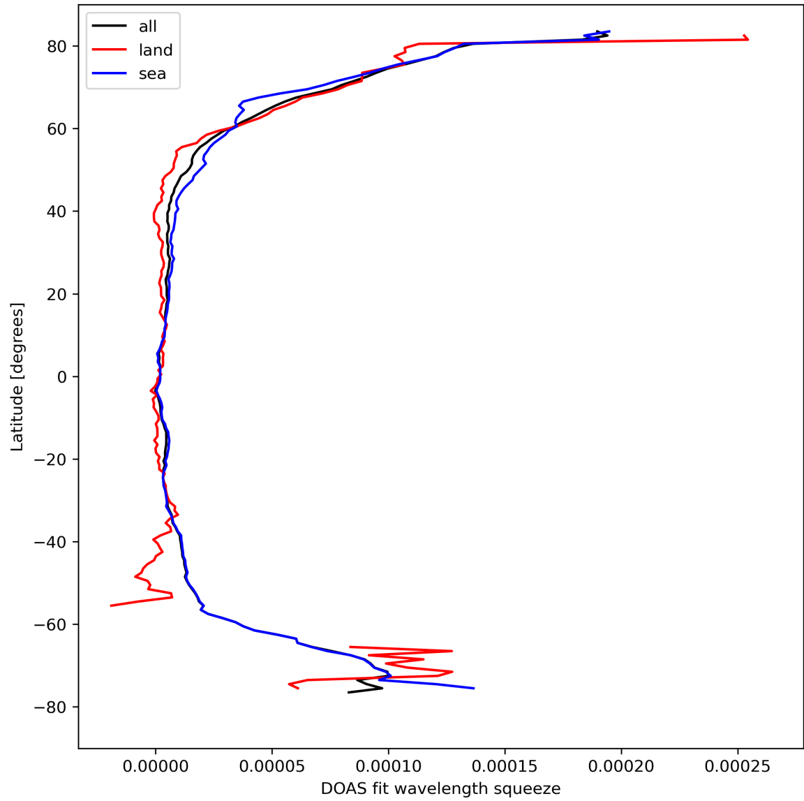
Figure 31: Zonal average of “DOAS fit wavelength squeeze” for 2024-04-10 to 2024-04-12.
