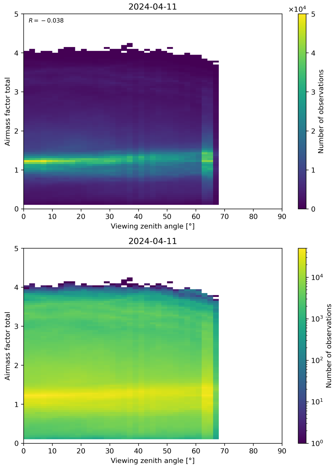
Figure 190: Scatter density plot of “Viewing zenith angle” against “Airmass factor total” for 2024-04-10 to 2024-04-12.
