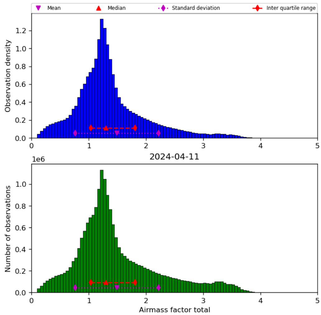
Figure 40: Histogram of “Airmass factor total” for 2024-04-10 to 2024-04-12
