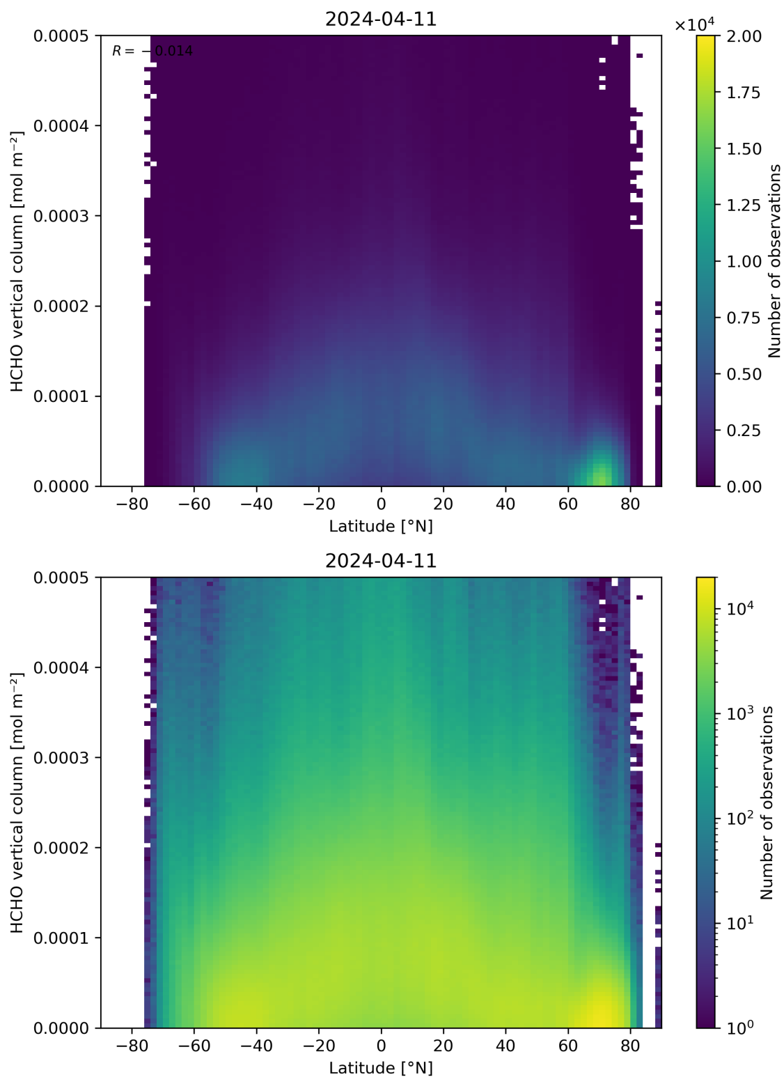
Figure 163: Scatter density plot of “Latitude” against “HCHO vertical column” for 2024-04-10 to 2024-04-12.
