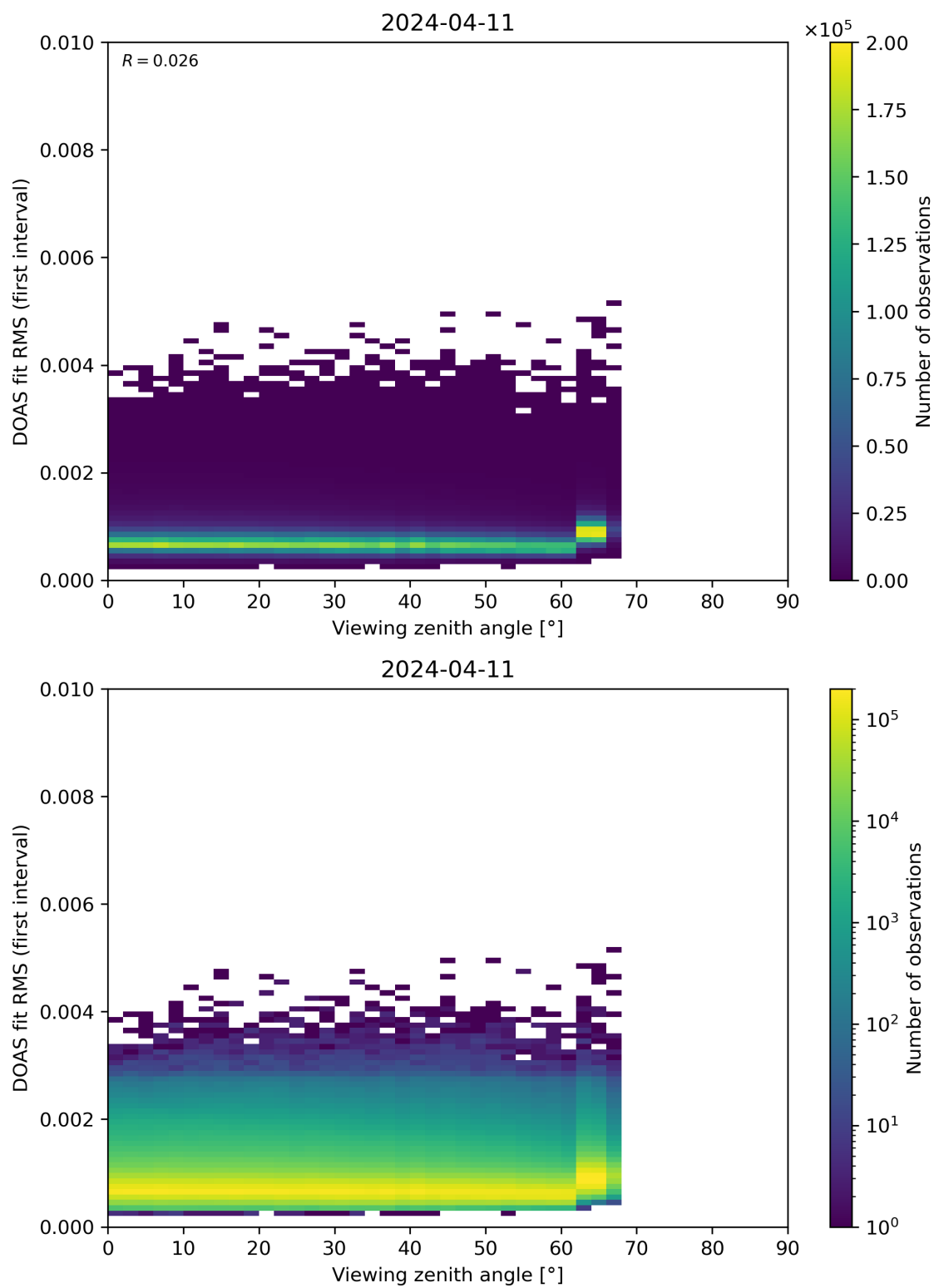
Figure 182: Scatter density plot of “Viewing zenith angle” against “DOAS fit RMS (first interval)” for 2024-04-10 to 2024-04-12.
