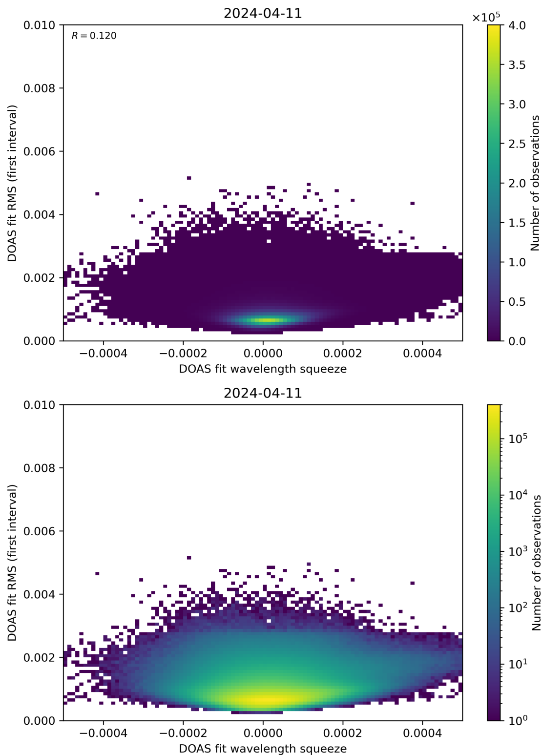
Figure 68: Scatter density plot of “DOAS fit wavelength squeeze” against “DOAS fit RMS (first interval)” for 2024-04-10 to 2024-04-12.
