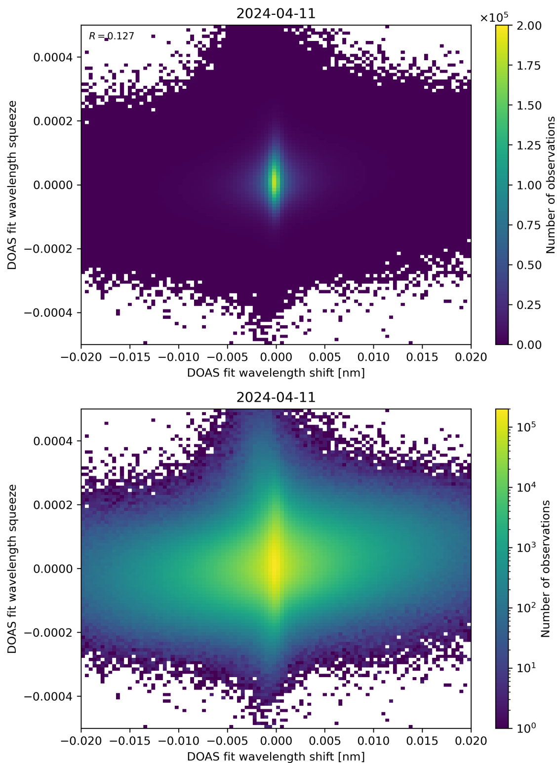
Figure 65: Scatter density plot of “DOAS fit wavelength shift” against “DOAS fit wavelength squeeze” for 2024-04-10 to 2024-04-12.
