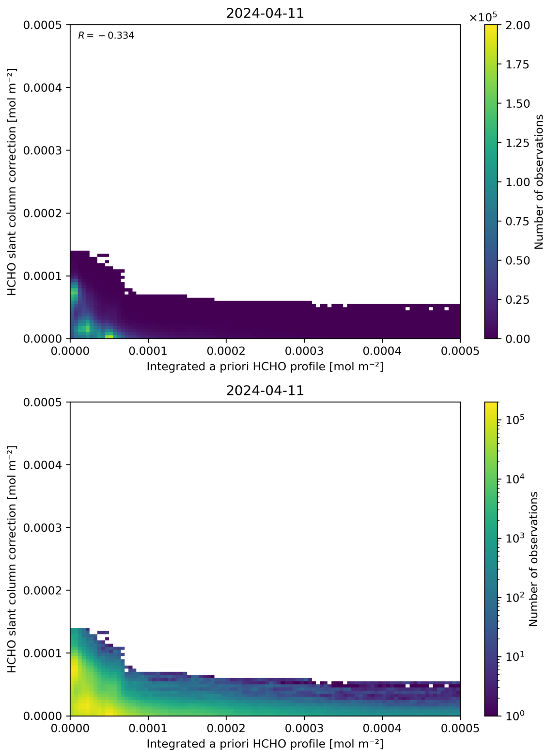
Figure 152: Scatter density plot of “Integrated a priori HCHO profile” against “HCHO slant column correction” for 2024-04-10 to 2024-04-12.
