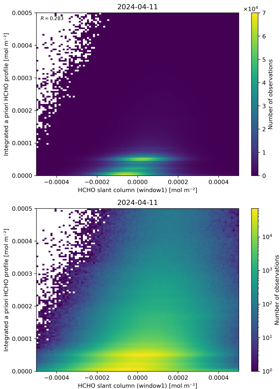
Figure 87: Scatter density plot of “HCHO slant column (window1)” against “Integrated a priori HCHO profile” for 2024-04-10 to 2024-04-12.
