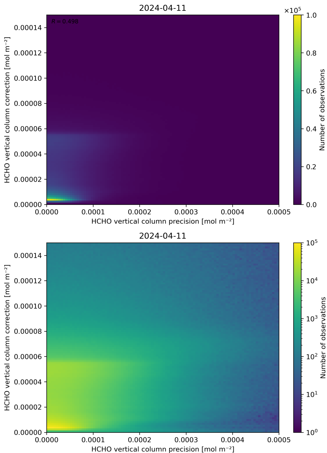
Figure 146: Scatter density plot of “HCHO vertical column precision” against “HCHO vertical column correction” for 2024-04-10 to 2024-04-12.
