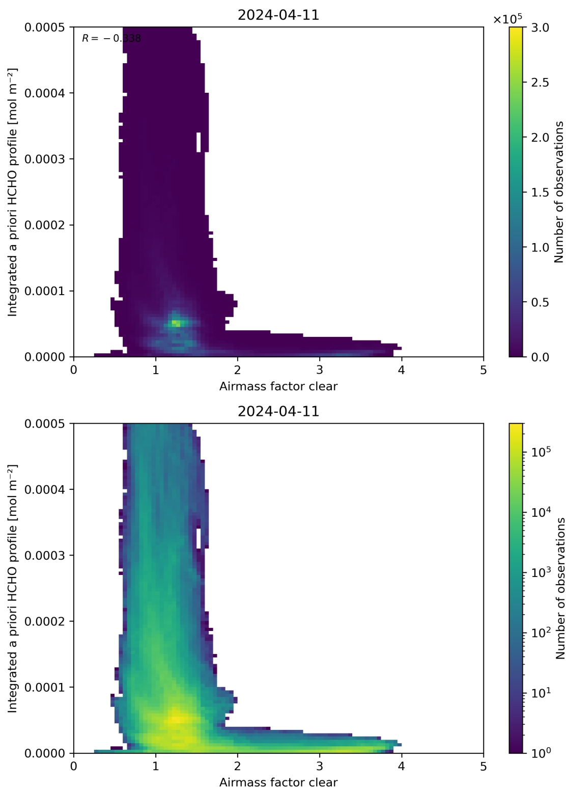
Figure 76: Scatter density plot of “Airmass factor clear” against “Integrated a priori HCHO profile” for 2024-04-10 to 2024-04-12.
