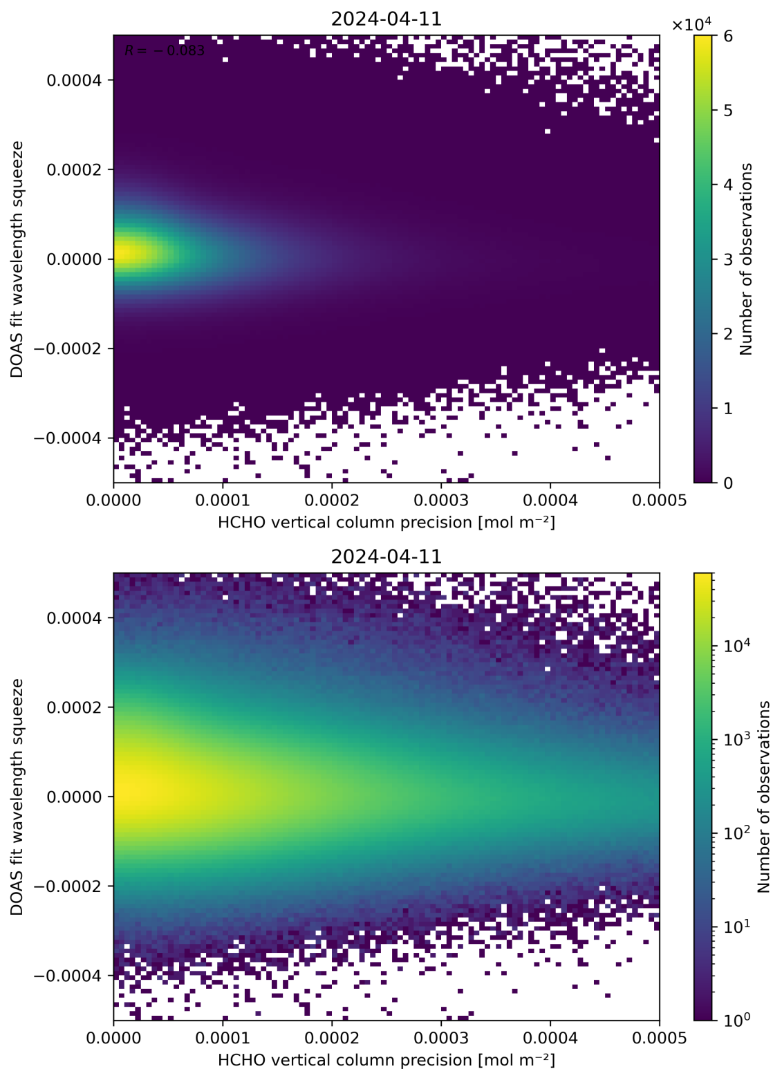
Figure 138: Scatter density plot of “HCHO vertical column precision” against “DOAS fit wavelength squeeze” for 2024-04-10 to 2024-04-12.
