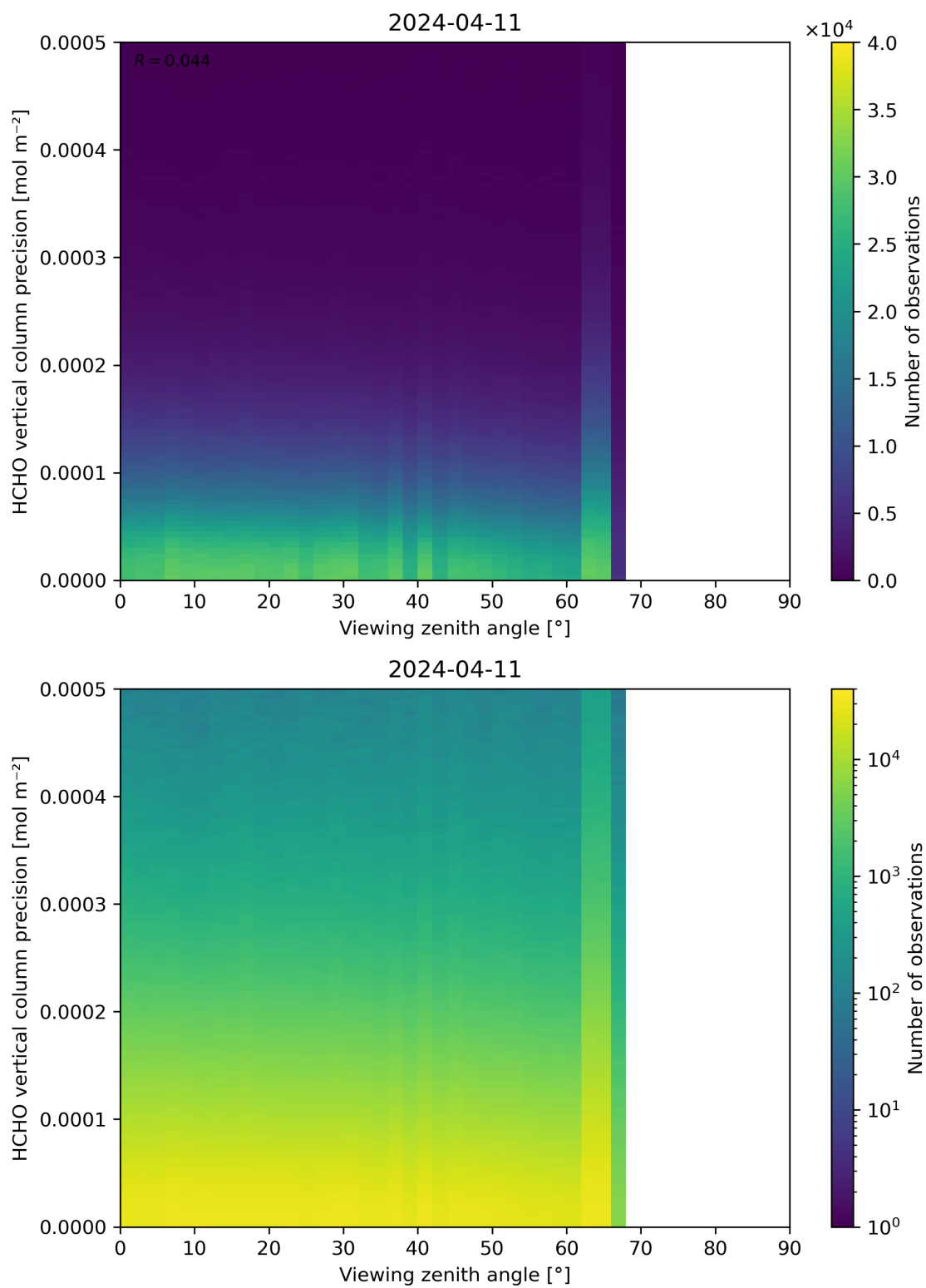
Figure 194: Scatter density plot of “Viewing zenith angle” against “HCHO vertical column precision” for 2024-04-10 to 2024-04-12.
