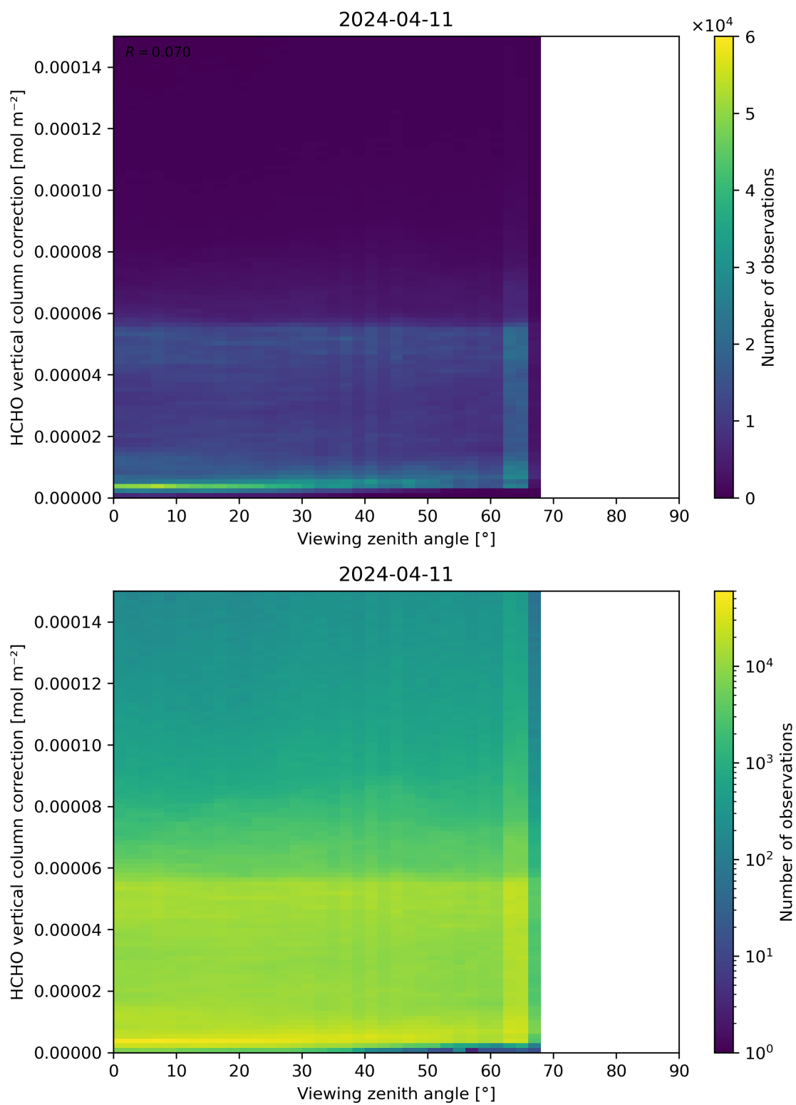
Figure 193: Scatter density plot of “Viewing zenith angle” against “HCHO vertical column correction” for 2024-04-10 to 2024-04-12.
