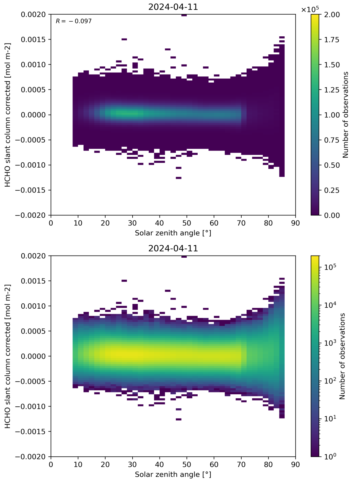
Figure 171: Scatter density plot of “Solar zenith angle” against “HCHO slant column corrected” for 2024-04-10 to 2024-04-12.
