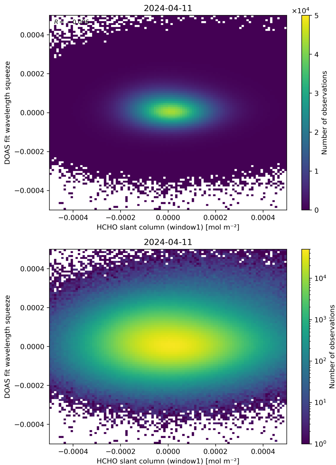
Figure 80: Scatter density plot of “HCHO slant column (window1)” against “DOAS fit wavelength squeeze” for 2024-04-10 to 2024-04-12.
