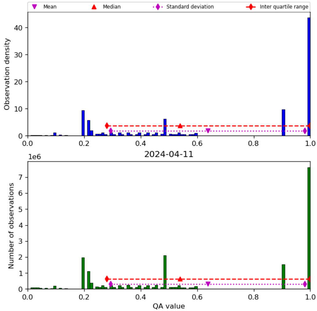
Figure 34: Histogram of “QA value” for 2024-04-10 to 2024-04-12
