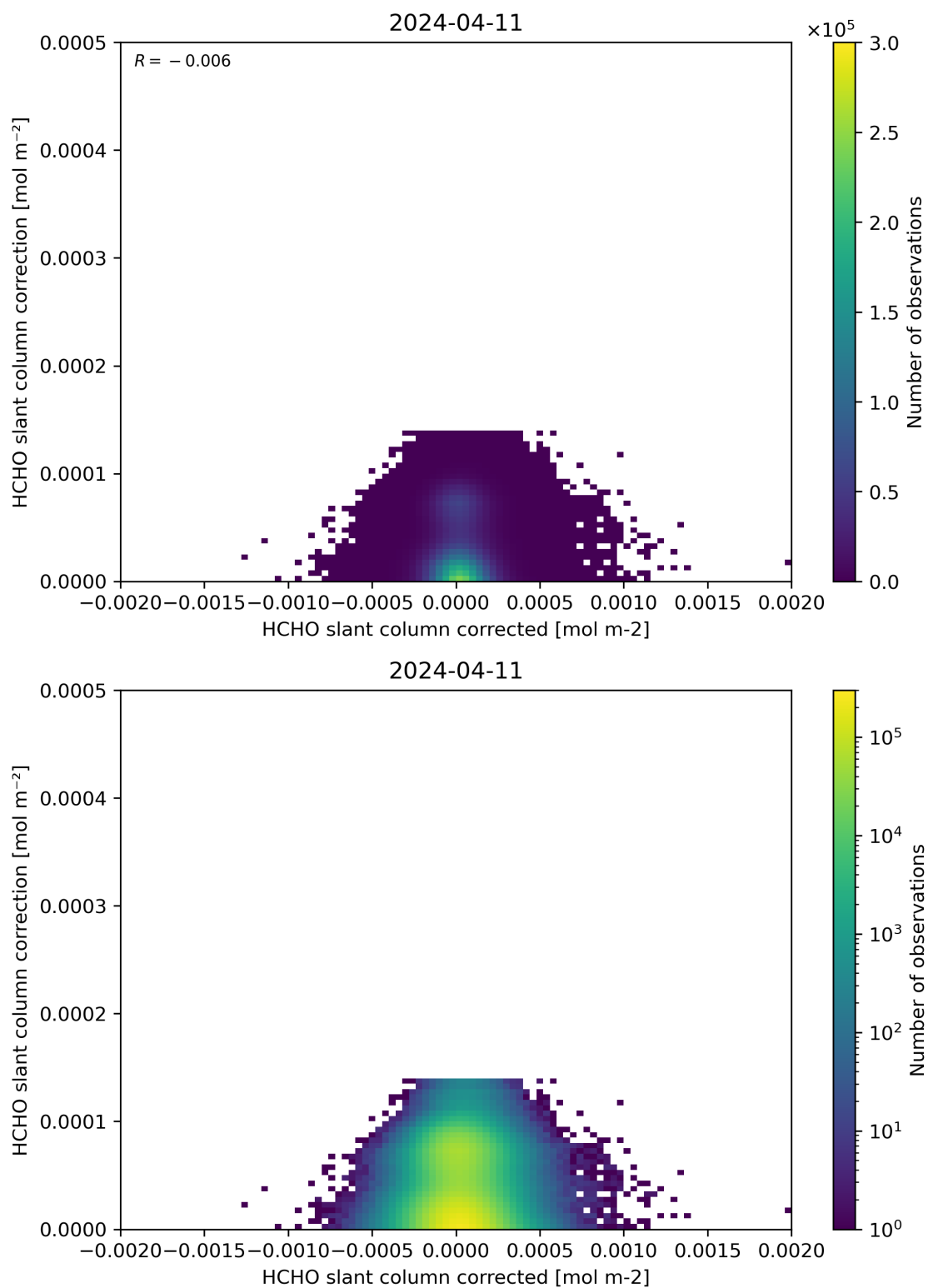
Figure 77: Scatter density plot of “HCHO slant column corrected” against “HCHO slant column correction” for 2024-04-10 to 2024-04-12.
