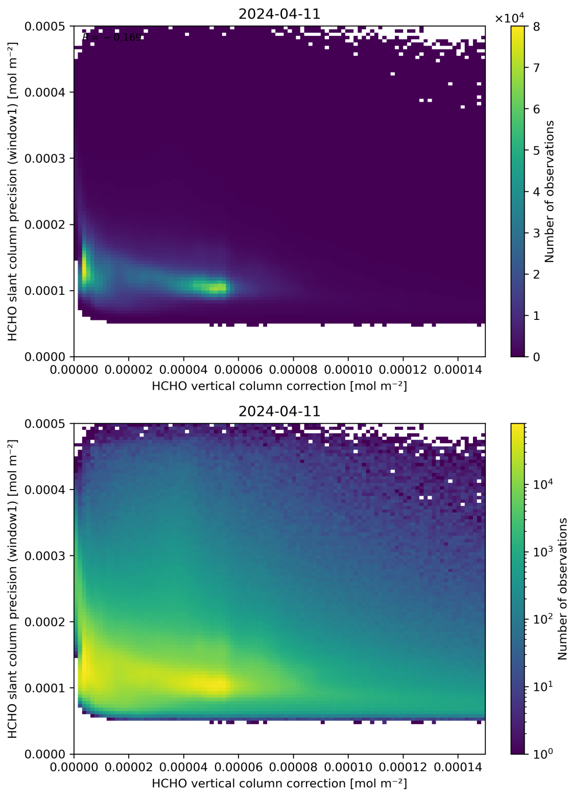
Figure 119: Scatter density plot of “HCHO vertical column correction” against “HCHO slant column precision (window1)” for 2024-04-10 to 2024-04-12.
