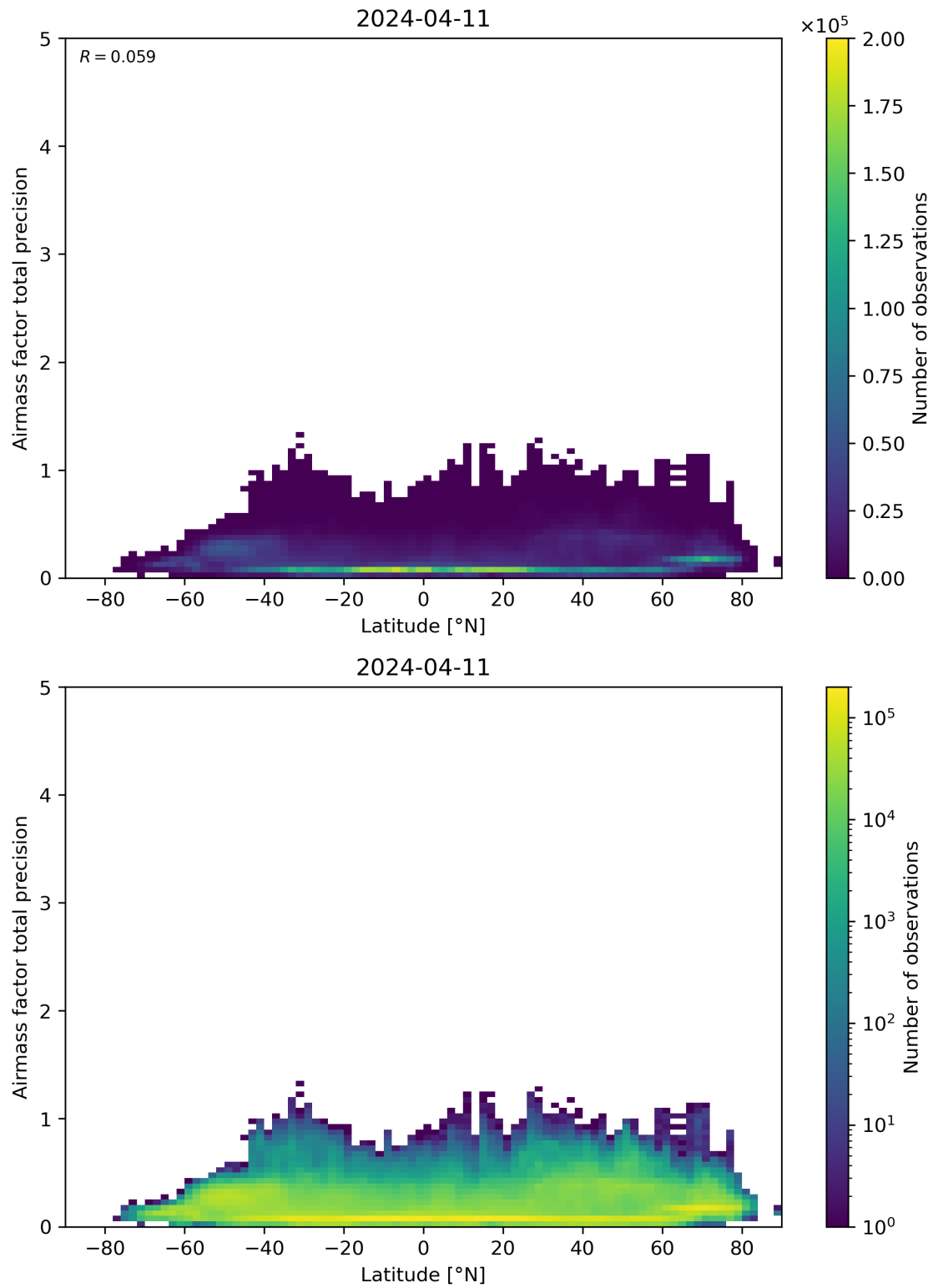
Figure 162: Scatter density plot of “Latitude” against “Airmass factor total precision” for 2024-04-10 to 2024-04-12.
