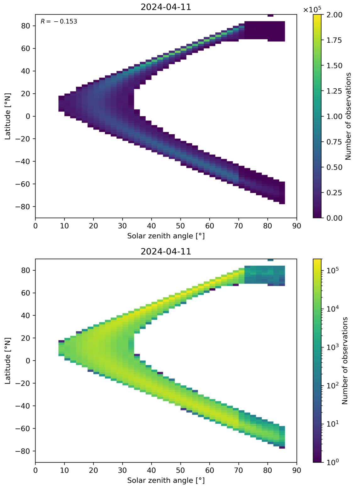
Figure 181: Scatter density plot of “Solar zenith angle” against “Latitude” for 2024-04-10 to 2024-04-12.
