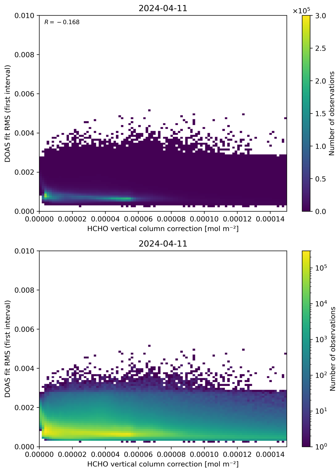
Figure 112: Scatter density plot of “HCHO vertical column correction” against “DOAS fit RMS (first interval)” for 2024-04-10 to 2024-04-12.
