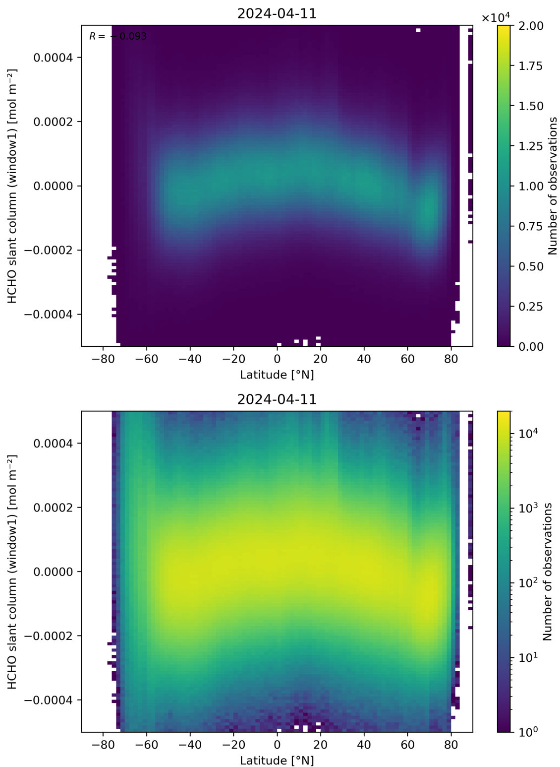
Figure 159: Scatter density plot of “Latitude” against “HCHO slant column (window1)” for 2024-04-10 to 2024-04-12.
