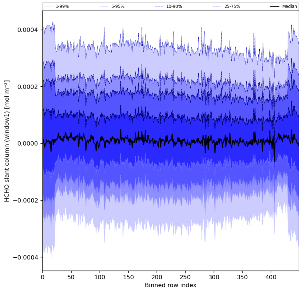
Figure 52: Along track statistics of “HCHO slant column (window1)” for 2024-04-10 to 2024-04-12
