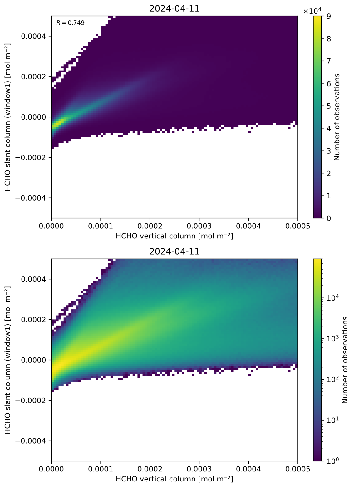
Figure 129: Scatter density plot of “HCHO vertical column” against “HCHO slant column (window1)” for 2024-04-10 to 2024-04-12.
