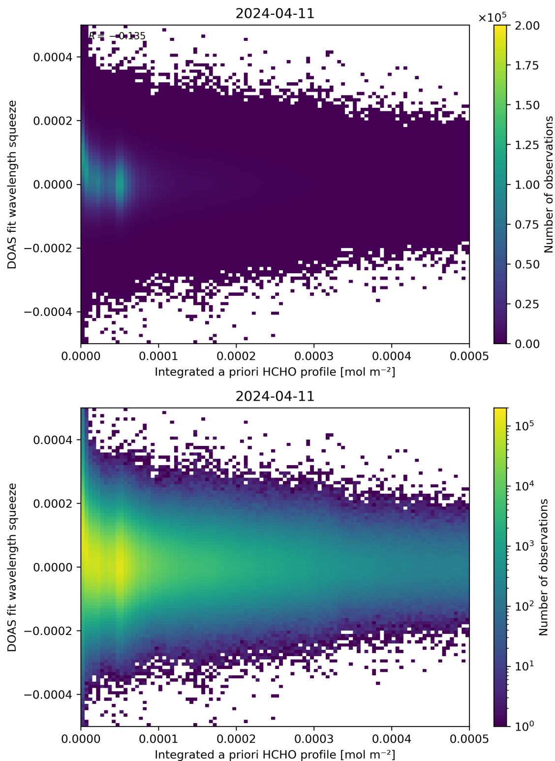
Figure 150: Scatter density plot of “Integrated a priori HCHO profile” against “DOAS fit wavelength squeeze” for 2024-04-10 to 2024-04-12.
