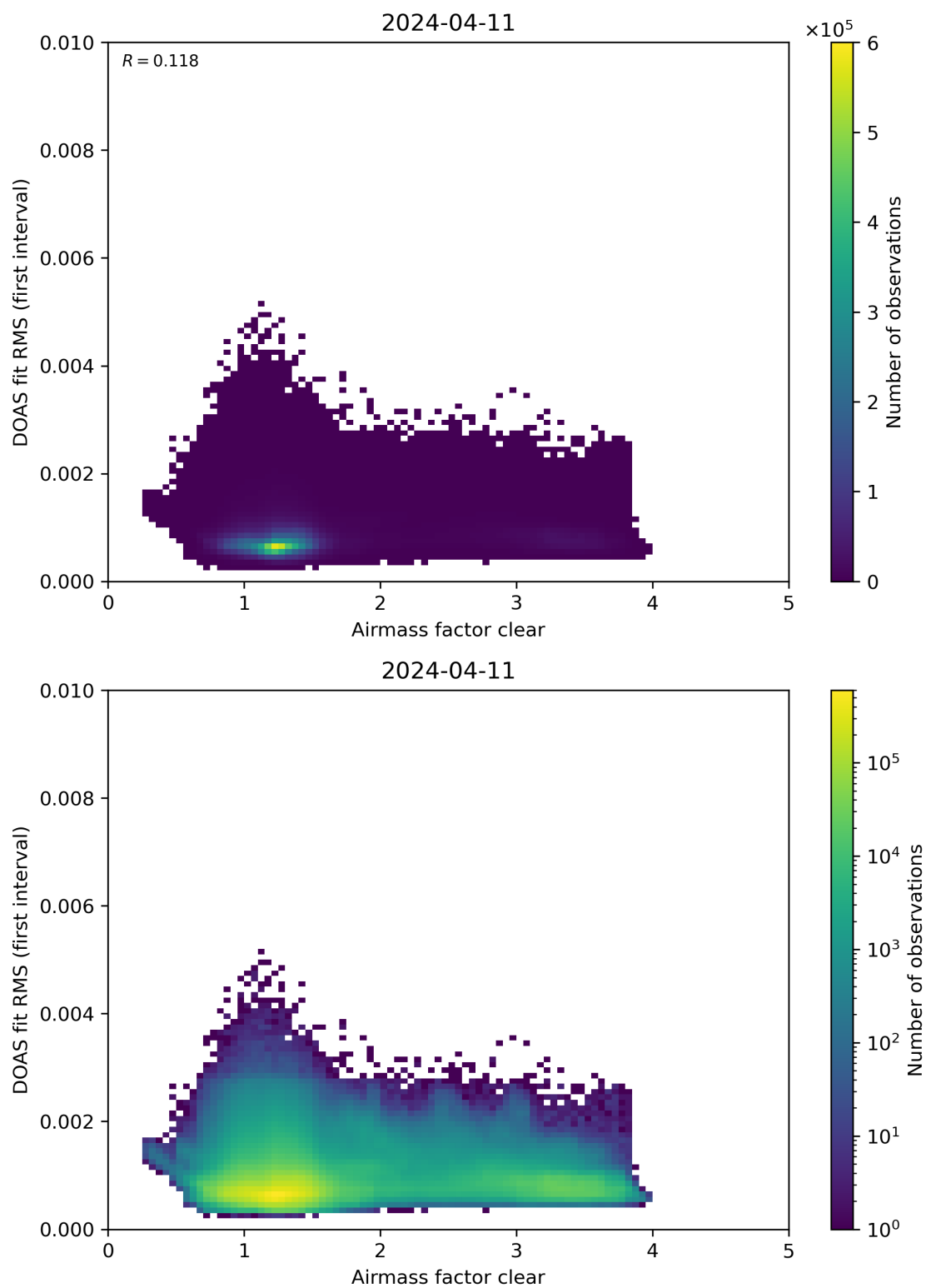
Figure 71: Scatter density plot of “Airmass factor clear” against “DOAS fit RMS (first interval)” for 2024-04-10 to 2024-04-12.
