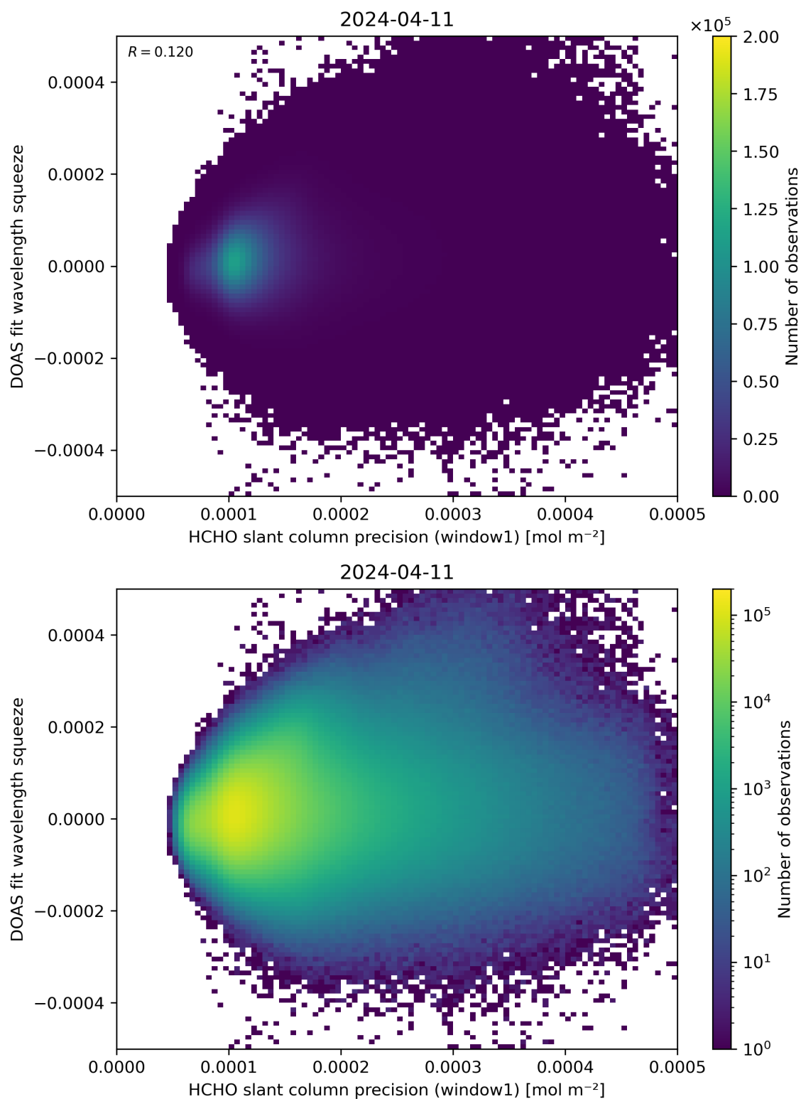
Figure 90: Scatter density plot of “HCHO slant column precision (window1)” against “DOAS fit wavelength squeeze” for 2024-04-10 to 2024-04-12.
