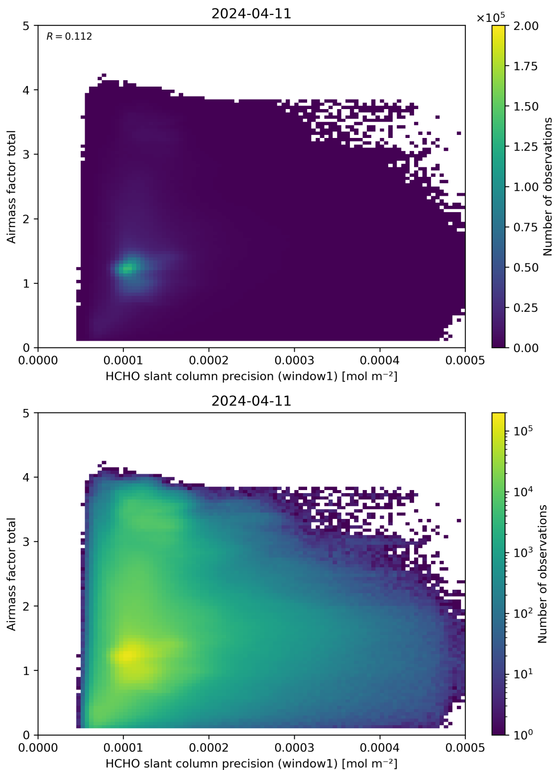
Figure 94: Scatter density plot of “HCHO slant column precision (window1)” against “Airmass factor total” for 2024-04-10 to 2024-04-12.
