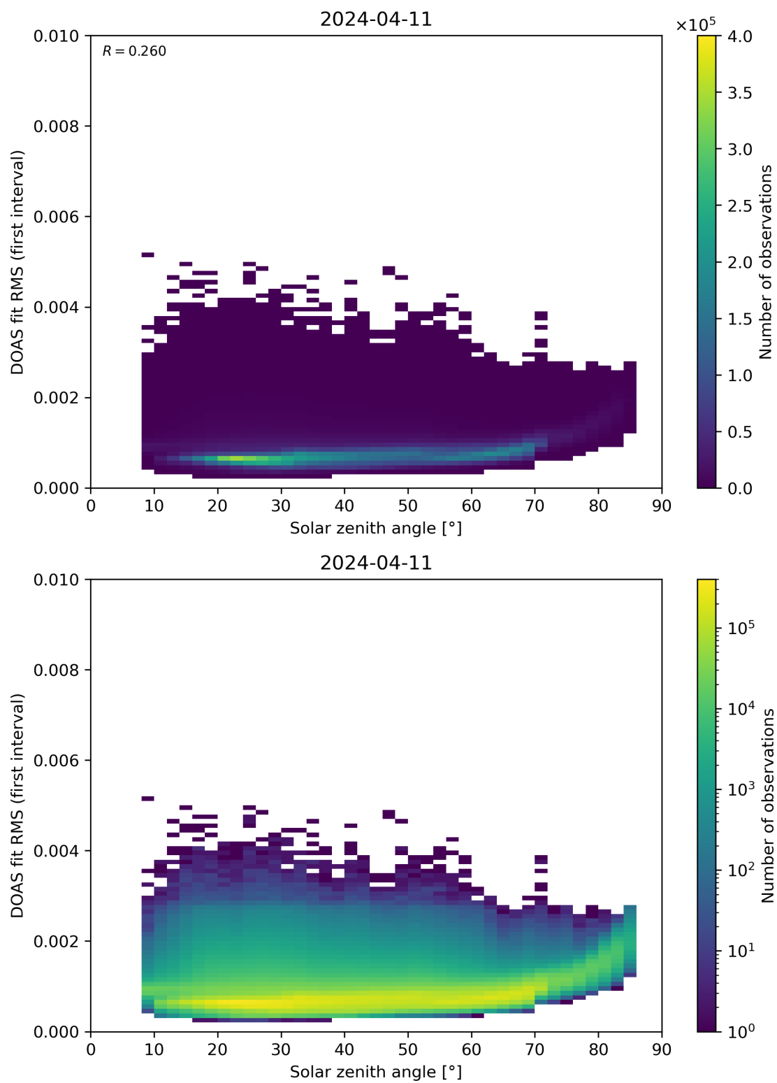
Figure 167: Scatter density plot of “Solar zenith angle” against “DOAS fit RMS (first interval)” for 2024-04-10 to 2024-04-12.
