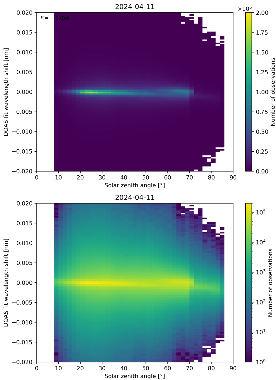
Figure 168: Scatter density plot of “Solar zenith angle” against “DOAS fit wavelength shift” for 2024-04-10 to 2024-04-12.
