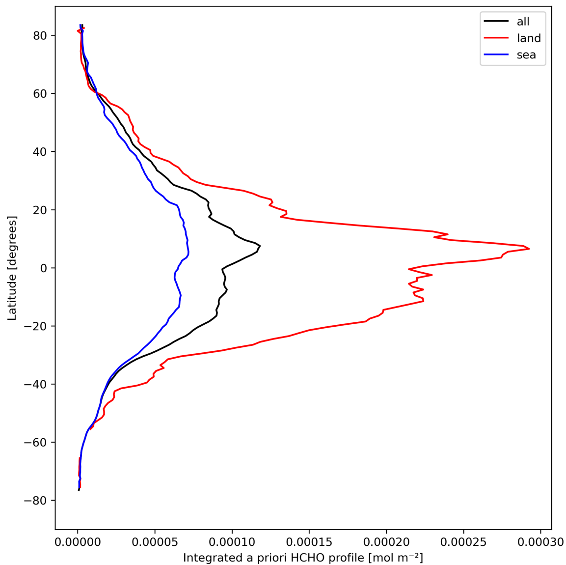
Figure 29: Zonal average of “Integrated a priori HCHO profile” for 2024-04-10 to 2024-04-12.
