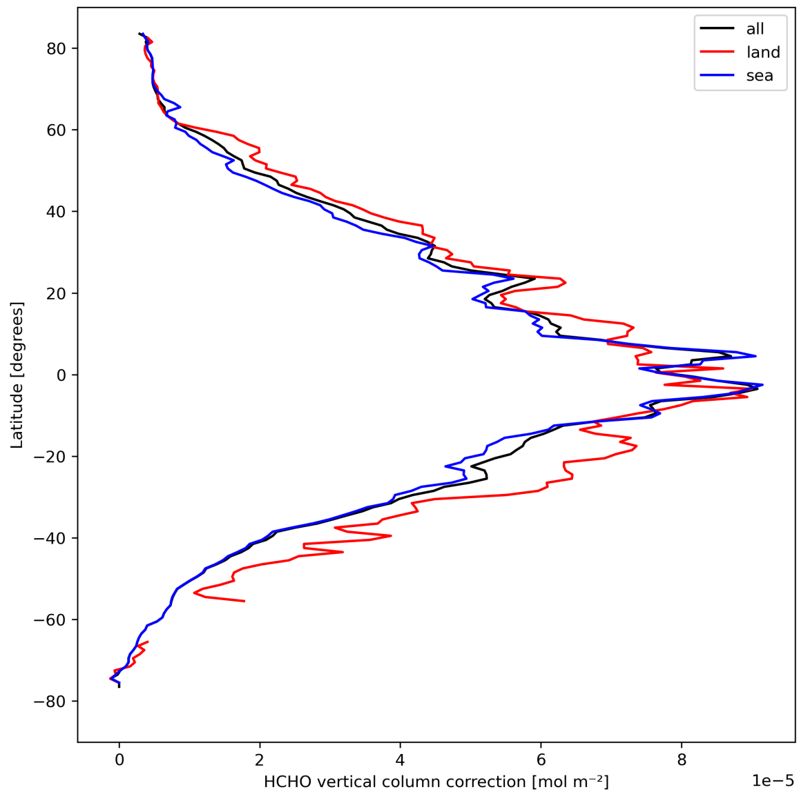
Figure 23: Zonal average of “HCHO vertical column correction” for 2024-04-10 to 2024-04-12.
