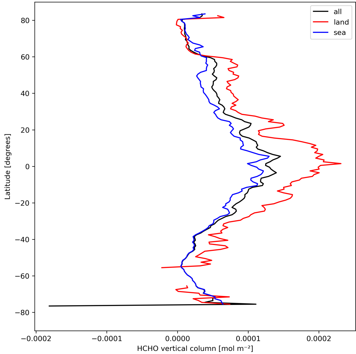
Figure 21: Zonal average of “HCHO vertical column” for 2024-04-10 to 2024-04-12.
