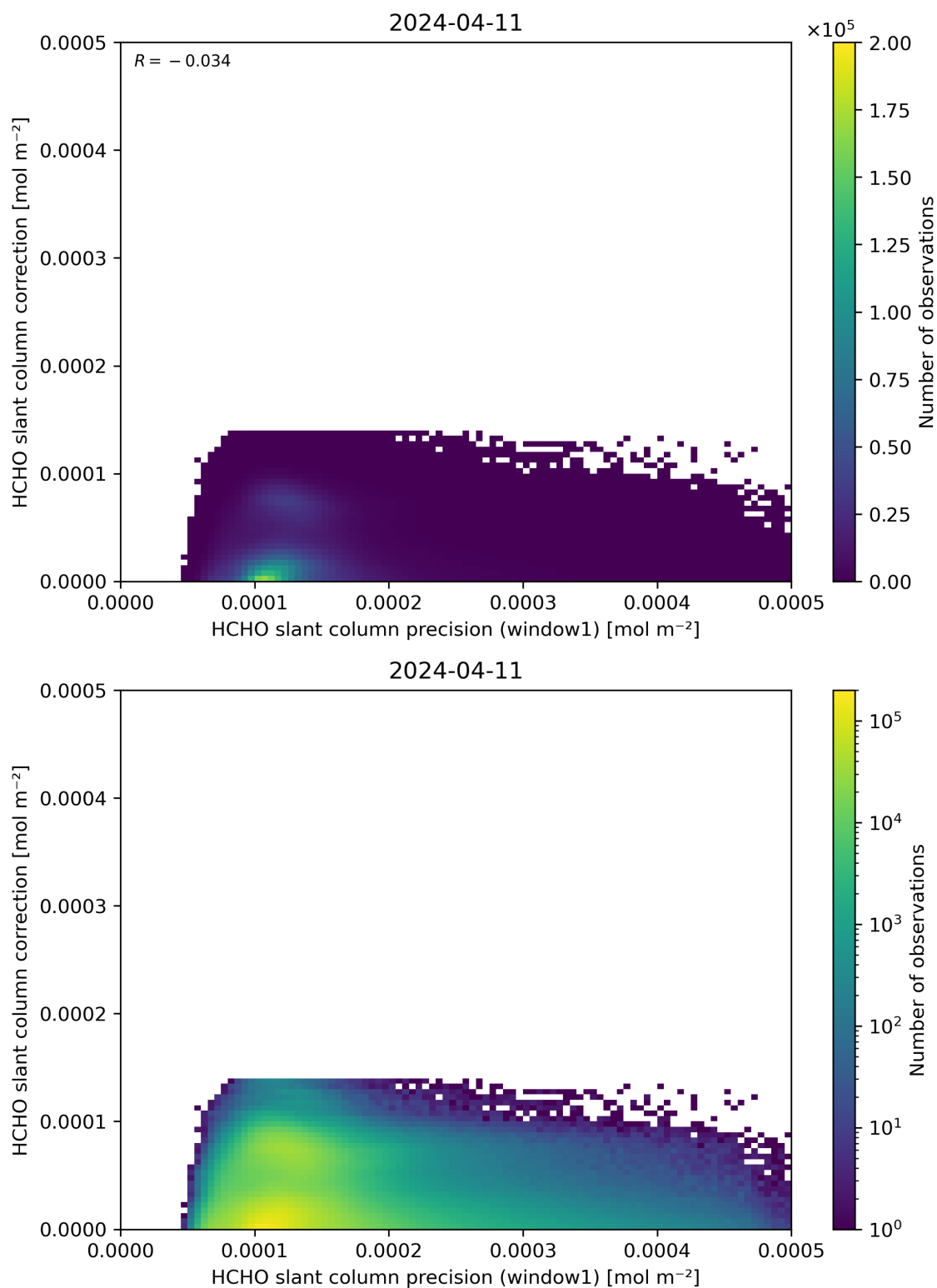
Figure 93: Scatter density plot of “HCHO slant column precision (window1)” against “HCHO slant column correction” for 2024-04-10 to 2024-04-12.
