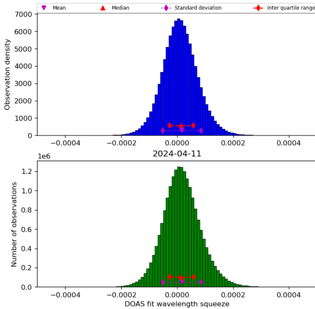
Figure 45: Histogram of “DOAS fit wavelength squeeze” for 2024-04-10 to 2024-04-12
