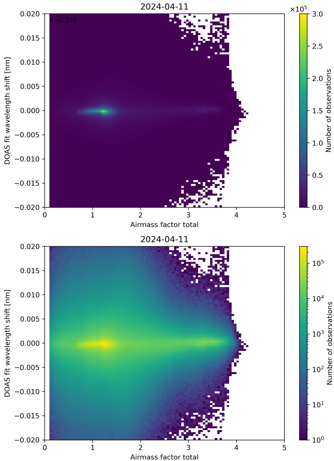
Figure 98: Scatter density plot of “Airmass factor total” against “DOAS fit wavelength shift” for 2024-04-10 to 2024-04-12.
