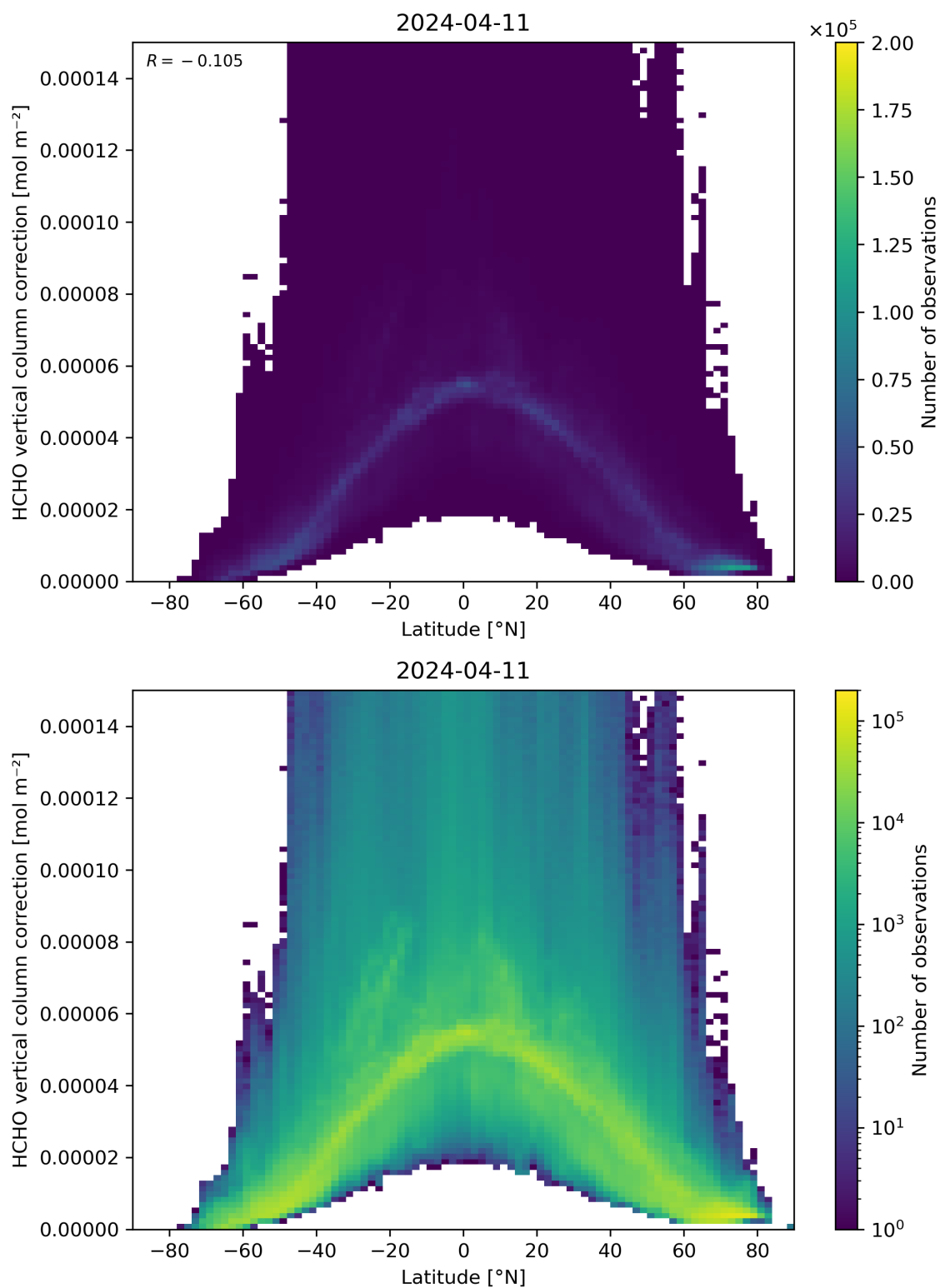
Figure 164: Scatter density plot of “Latitude” against “HCHO vertical column correction” for 2024-04-10 to 2024-04-12.
