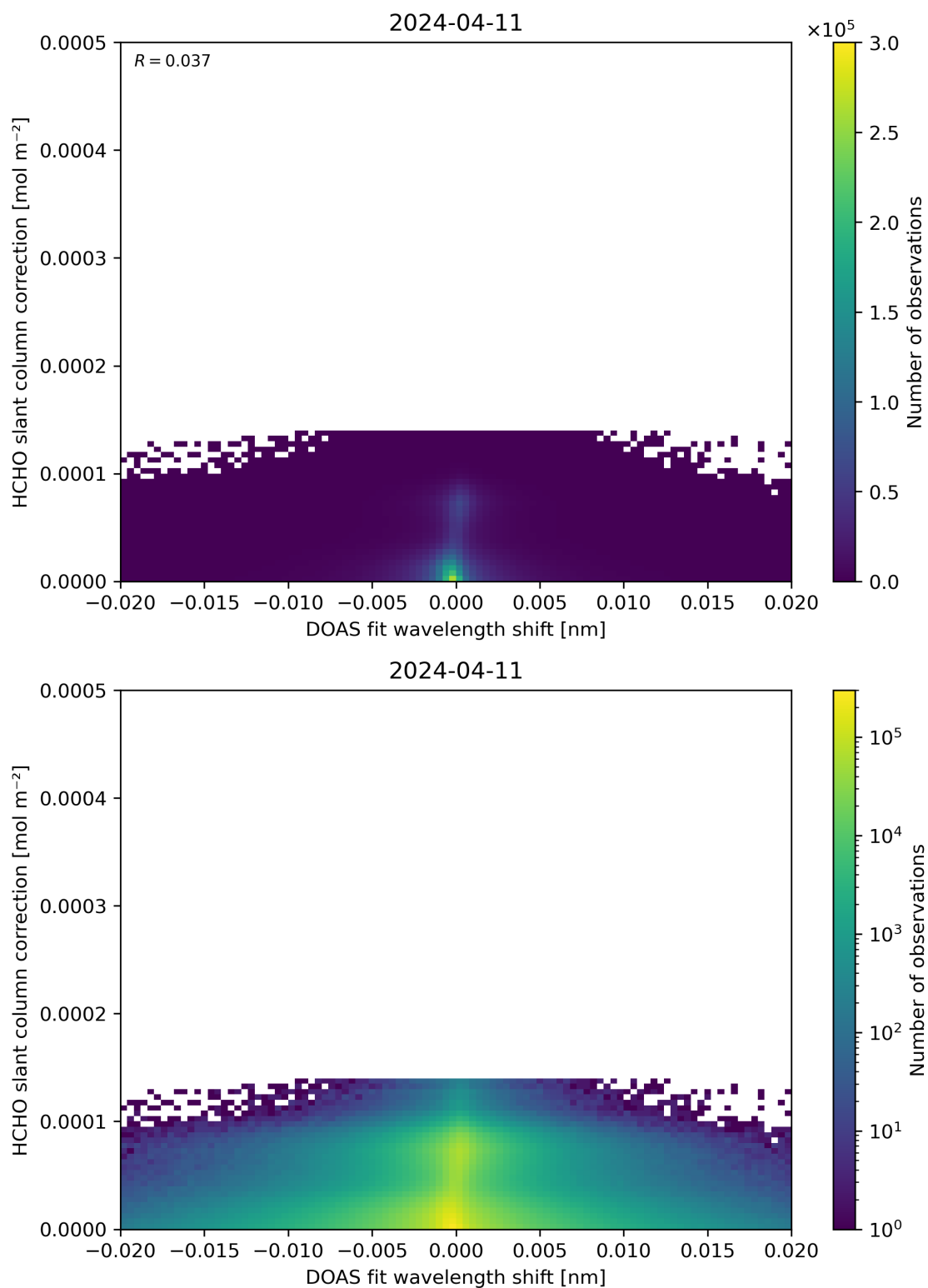
Figure 67: Scatter density plot of “DOAS fit wavelength shift” against “HCHO slant column correction” for 2024-04-10 to 2024-04-12.
