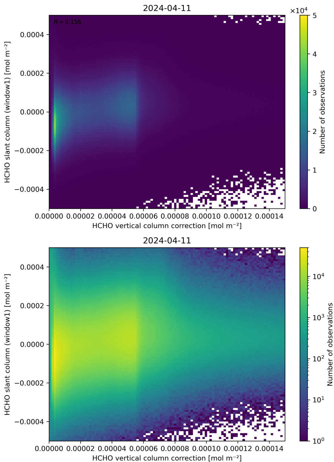
Figure 118: Scatter density plot of “HCHO vertical column correction” against “HCHO slant column (window1)” for 2024-04-10 to 2024-04-12.
