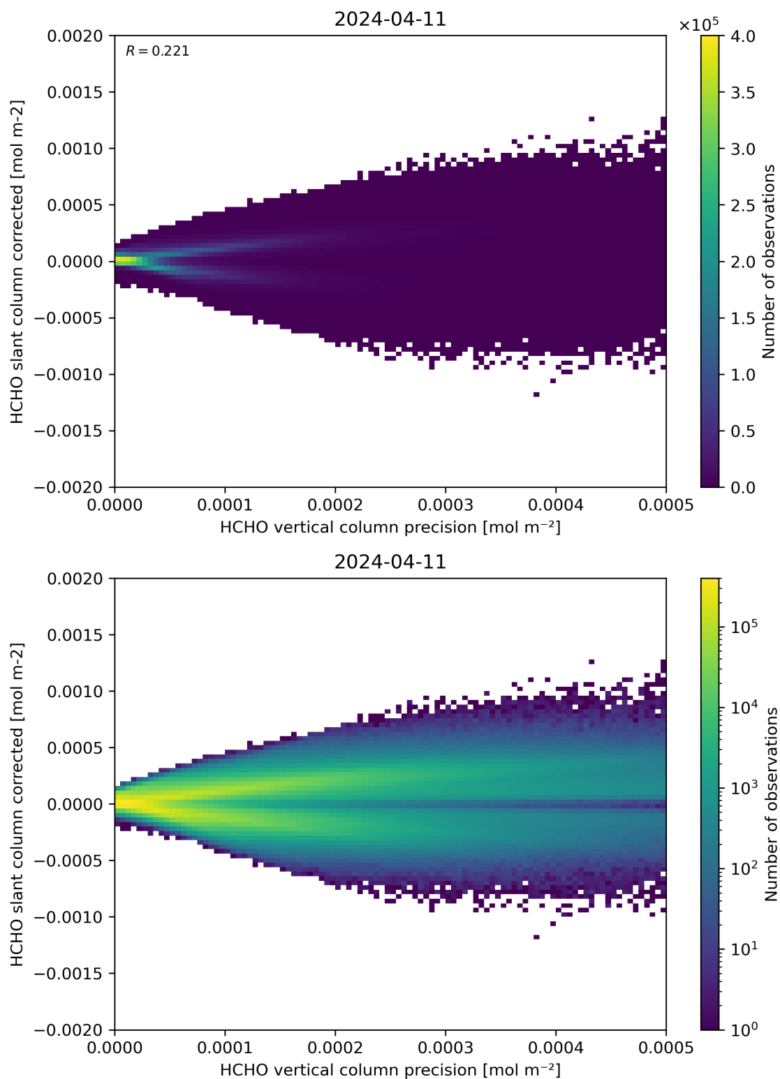
Figure 140: Scatter density plot of “HCHO vertical column precision” against “HCHO slant column corrected” for 2024-04-10 to 2024-04-12.
