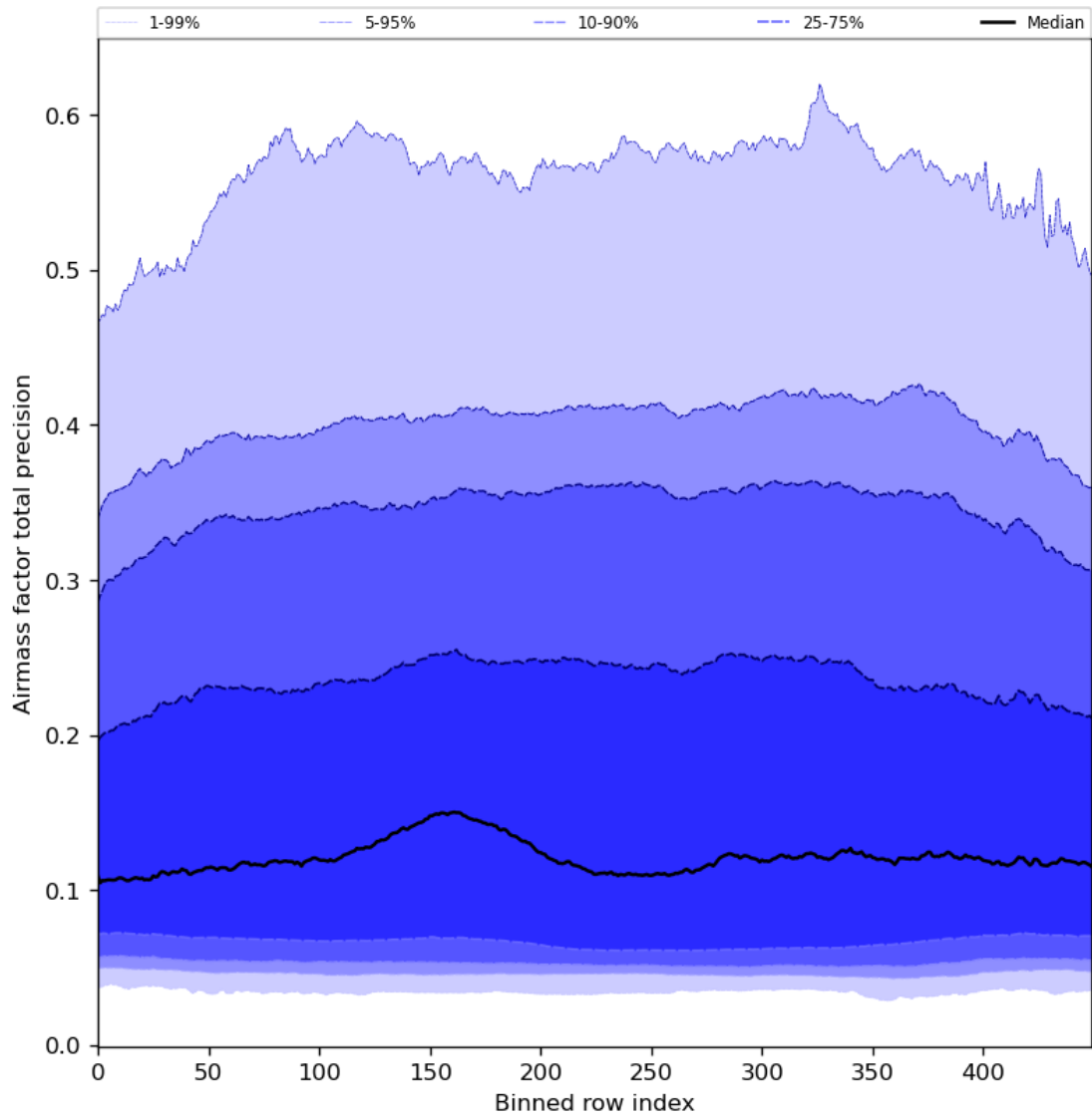
Figure 55: Along track statistics of “Airmass factor total precision” for 2024-04-10 to 2024-04-12
