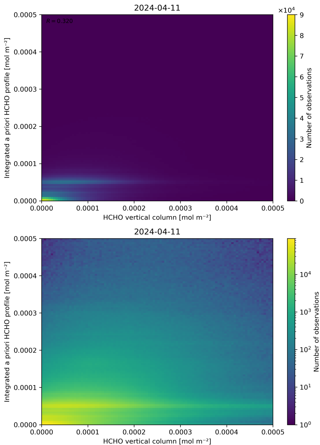
Figure 135: Scatter density plot of “HCHO vertical column” against “Integrated a priori HCHO profile” for 2024-04-10 to 2024-04-12.
