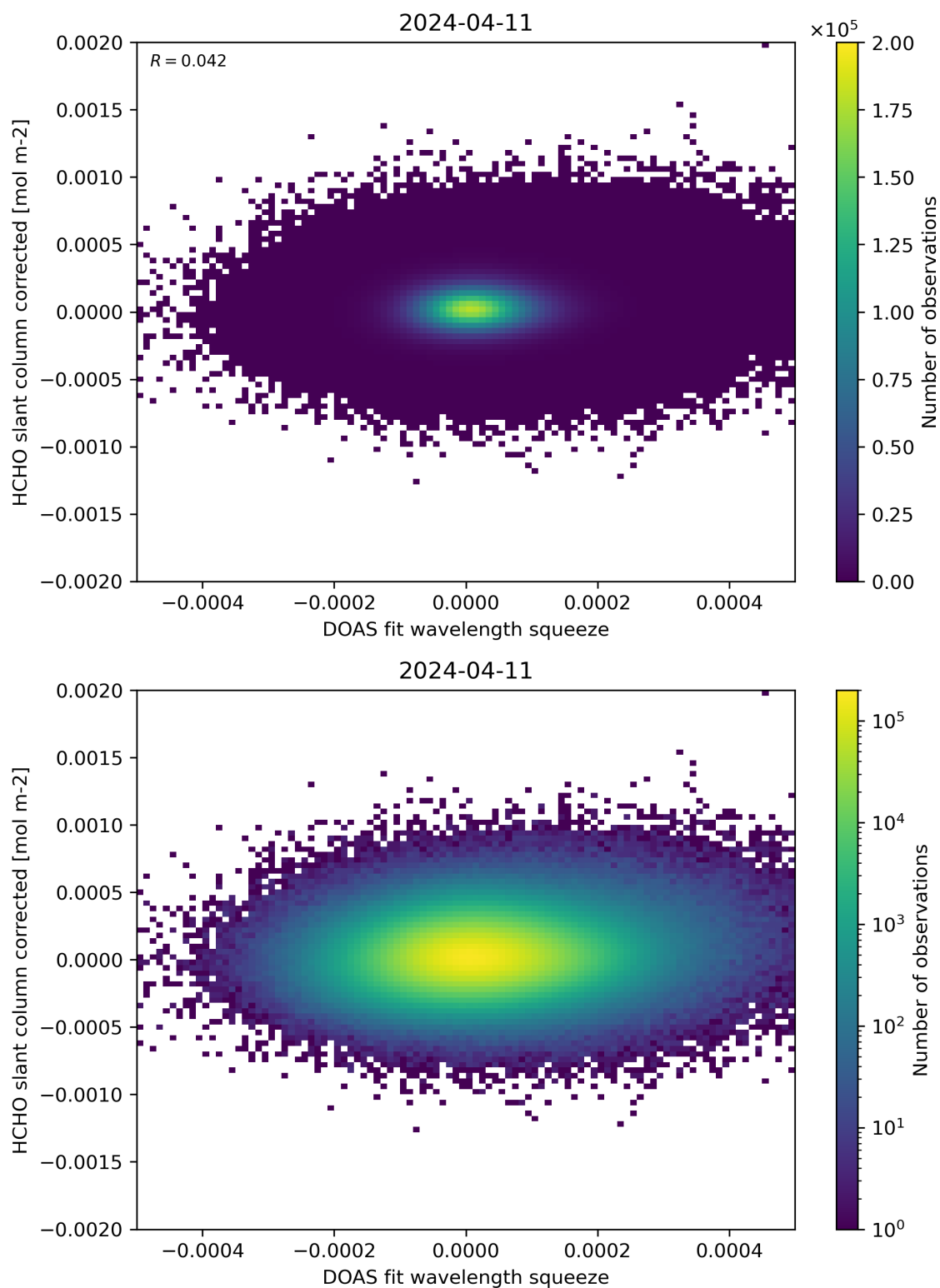
Figure 69: Scatter density plot of “DOAS fit wavelength squeeze” against “HCHO slant column corrected” for 2024-04-10 to 2024-04-12.
