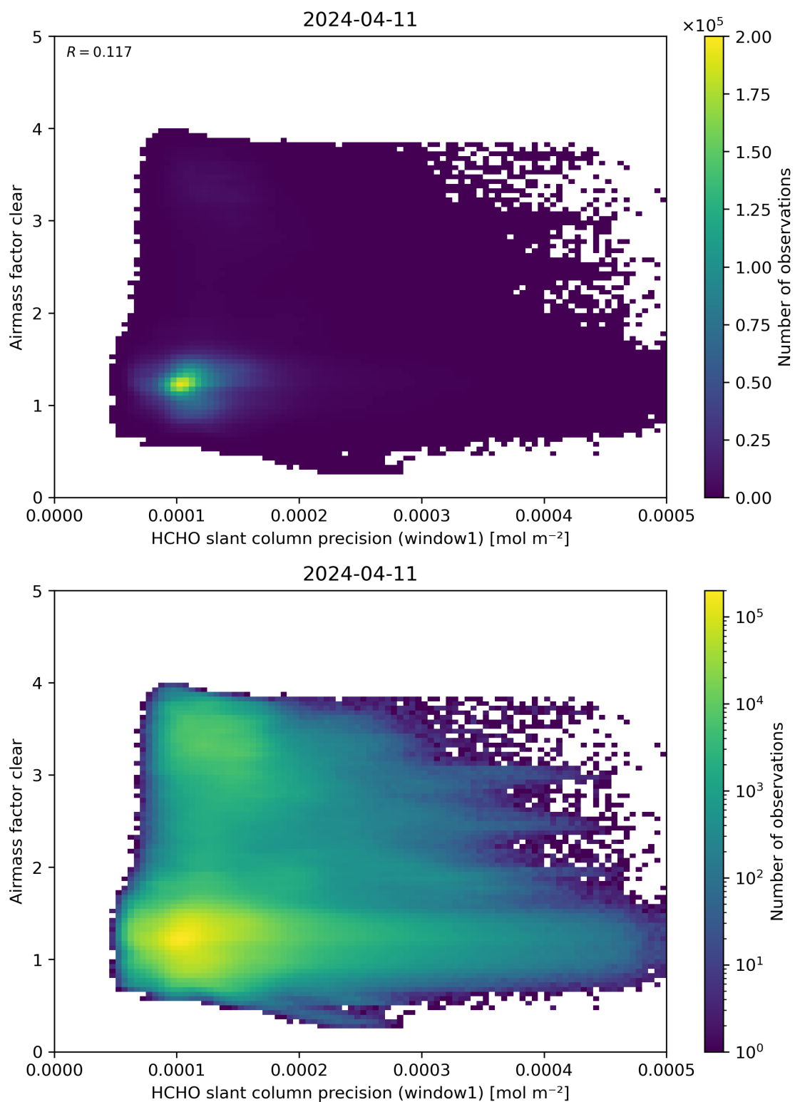
Figure 91: Scatter density plot of “HCHO slant column precision (window1)” against “Airmass factor clear” for 2024-04-10 to 2024-04-12.
