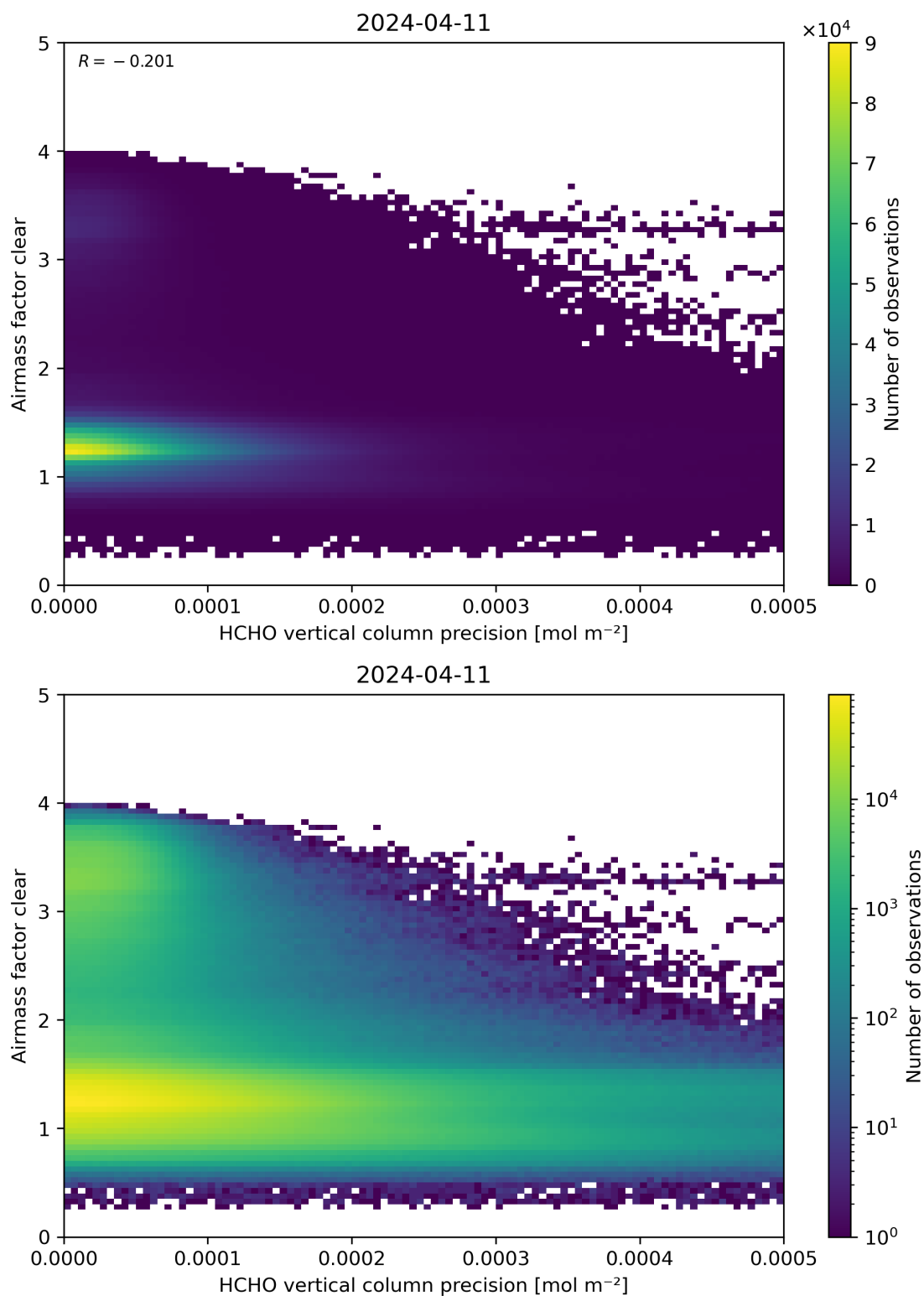
Figure 139: Scatter density plot of “HCHO vertical column precision” against “Airmass factor clear” for 2024-04-10 to 2024-04-12.
