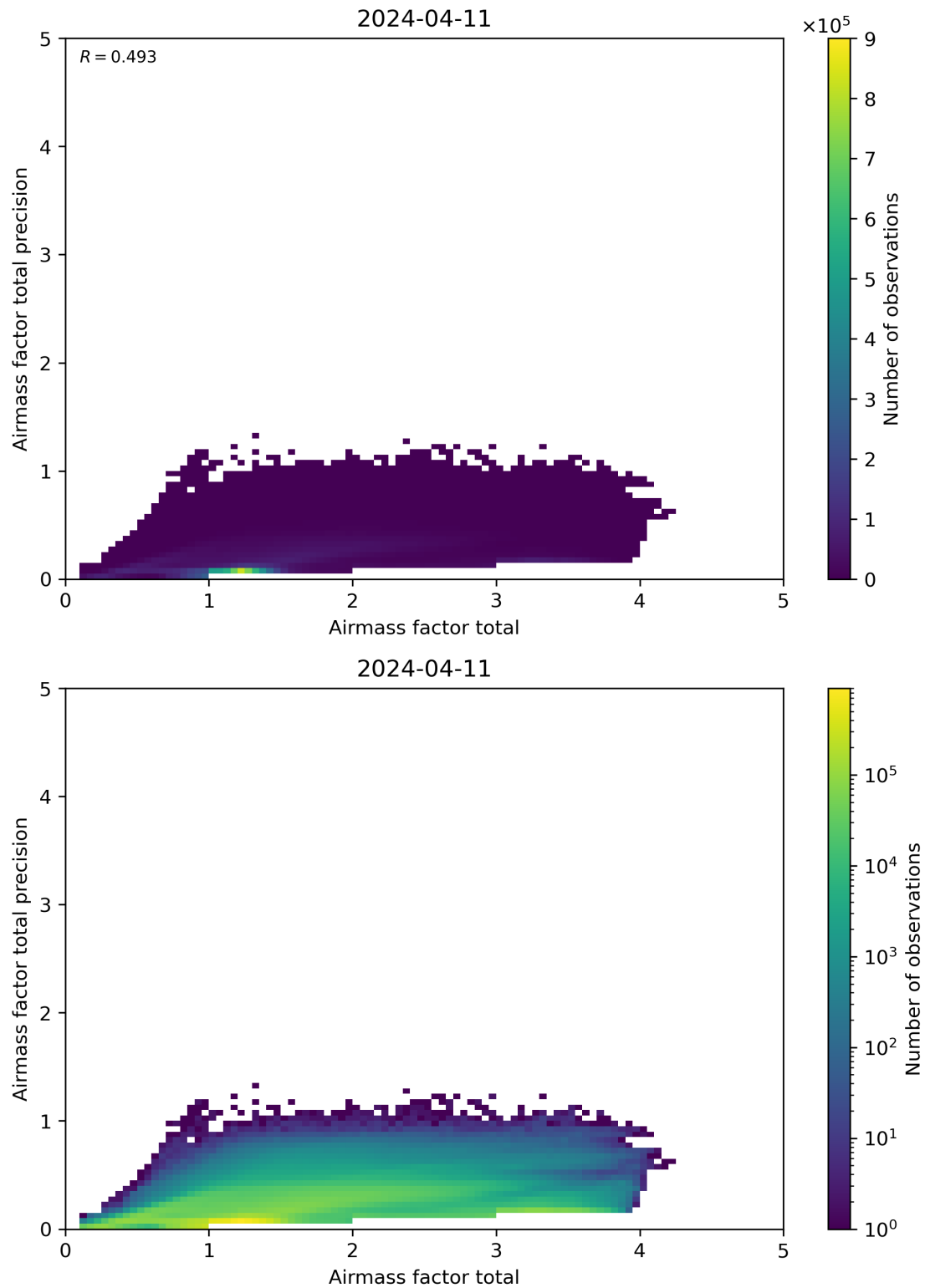
Figure 103: Scatter density plot of “Airmass factor total” against “Airmass factor total precision” for 2024-04-10 to 2024-04-12.
