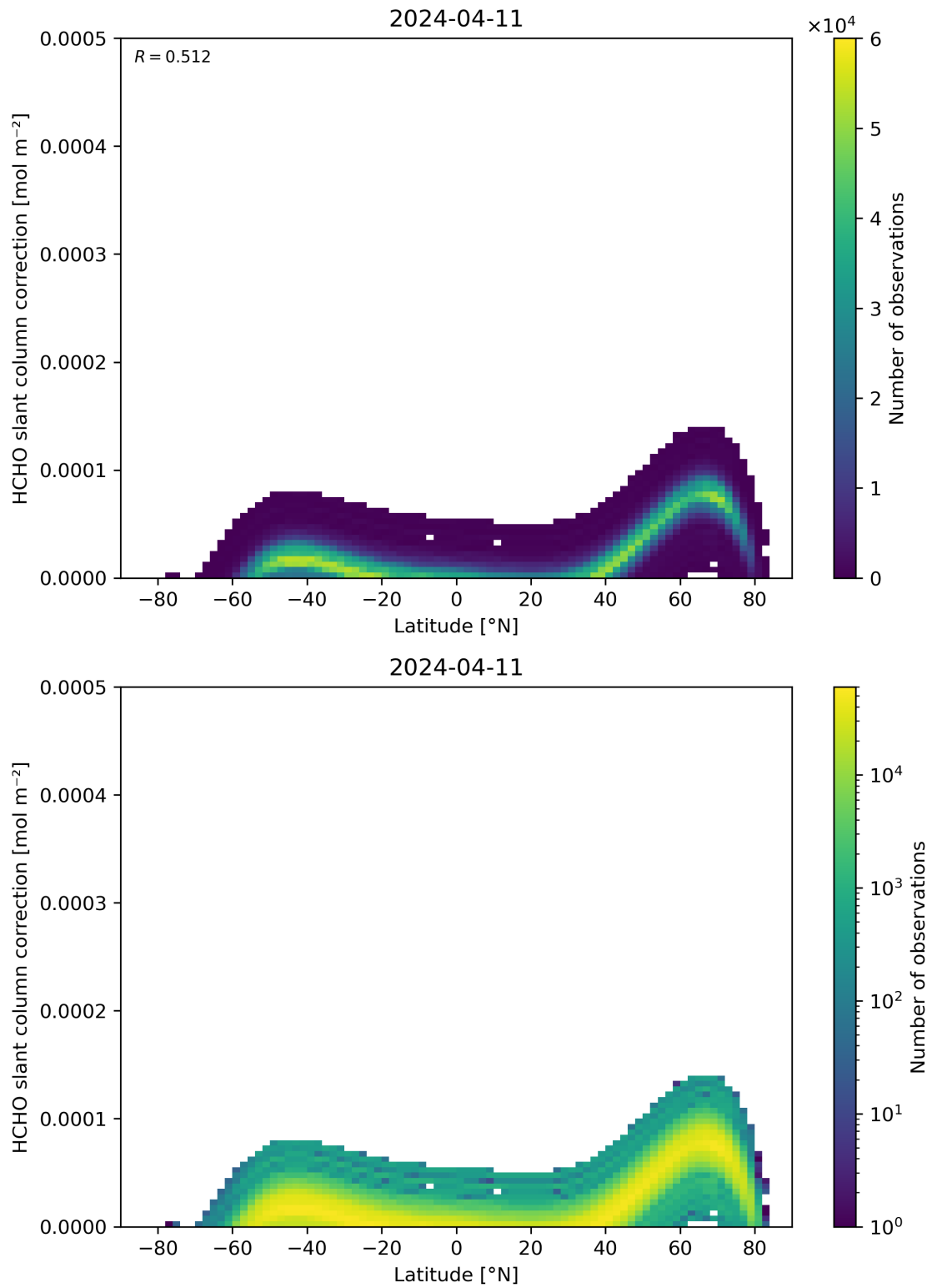
Figure 158: Scatter density plot of “Latitude” against “HCHO slant column correction” for 2024-04-10 to 2024-04-12.
