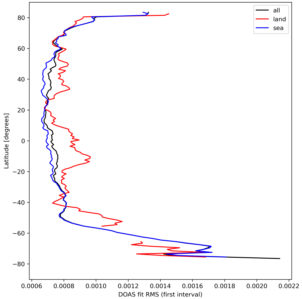
Figure 32: Zonal average of “DOAS fit RMS (first interval)” for 2024-04-10 to 2024-04-12.
