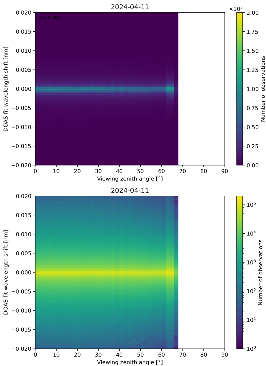
Figure 183: Scatter density plot of “Viewing zenith angle” against “DOAS fit wavelength shift” for 2024-04-10 to 2024-04-12.
