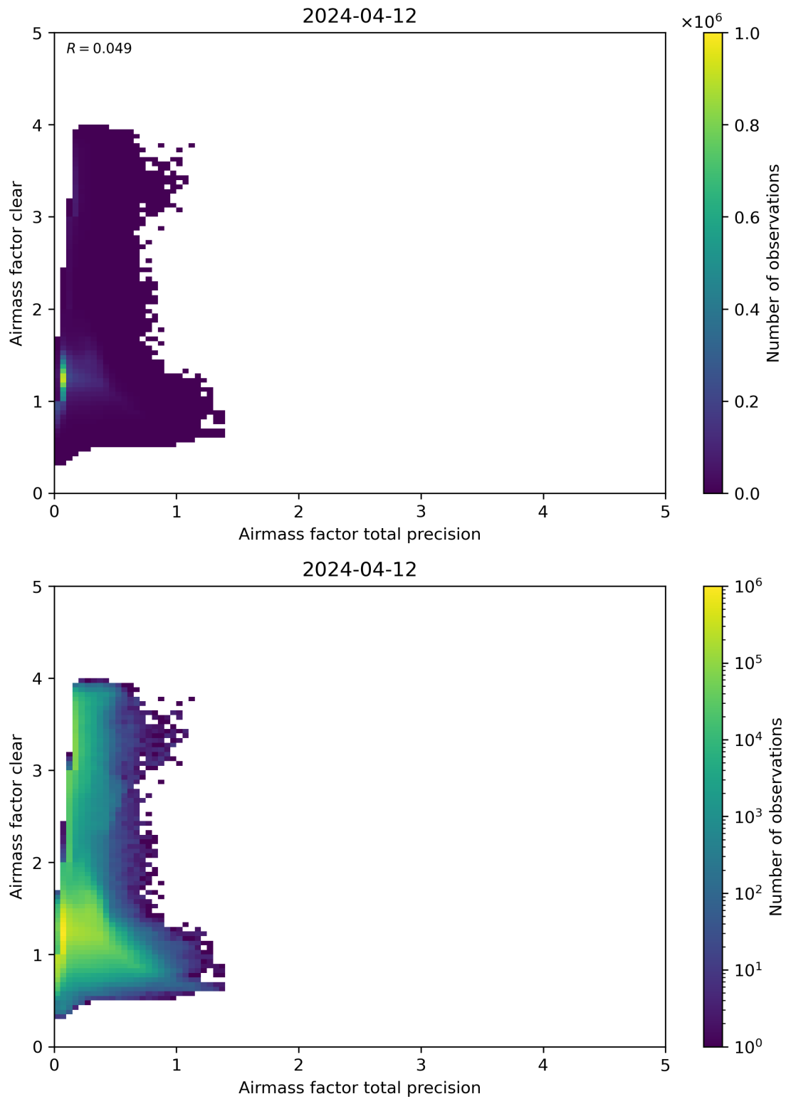
Figure 108: Scatter density plot of “Airmass factor total precision” against “Airmass factor clear” for 2024-04-11 to 2024-04-13.
