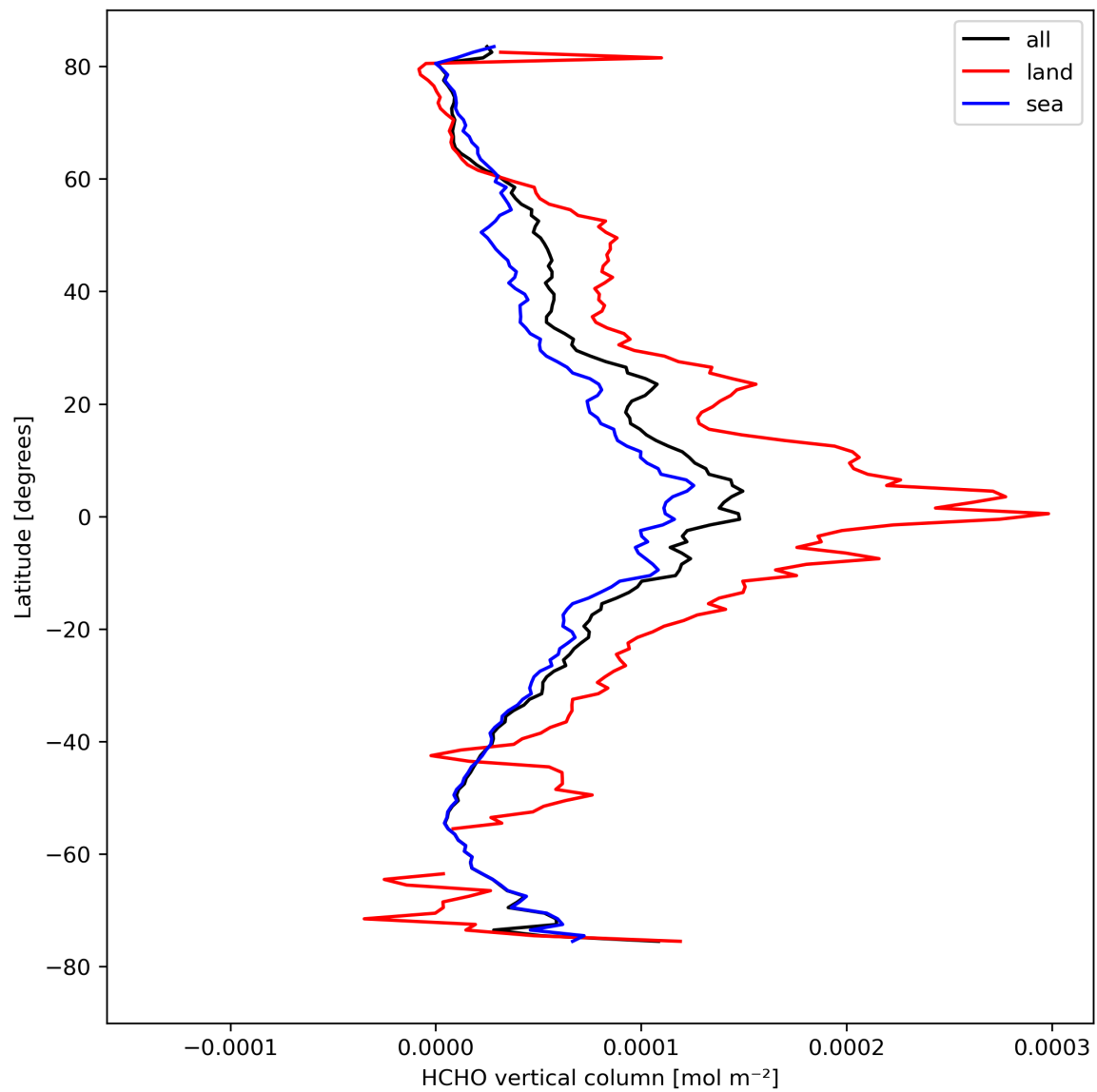
Figure 21: Zonal average of “HCHO vertical column” for 2024-04-11 to 2024-04-13.
