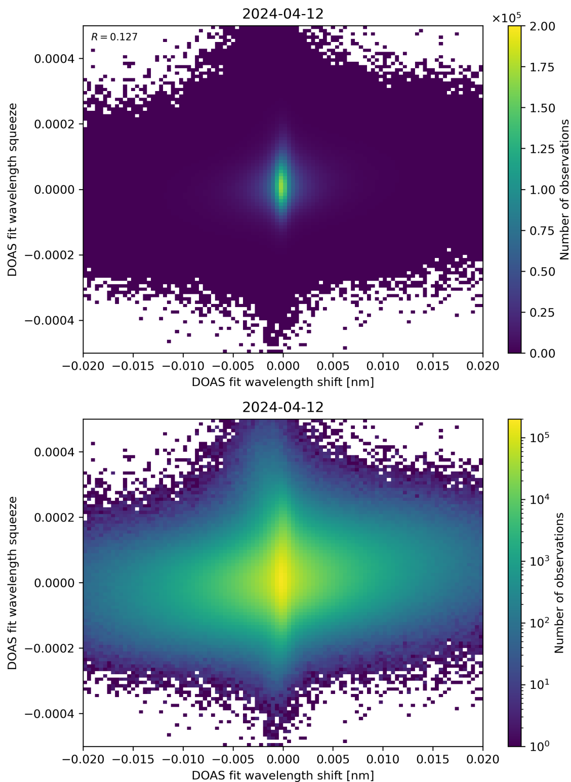
Figure 65: Scatter density plot of “DOAS fit wavelength shift” against “DOAS fit wavelength squeeze” for 2024-04-11 to 2024-04-13.
