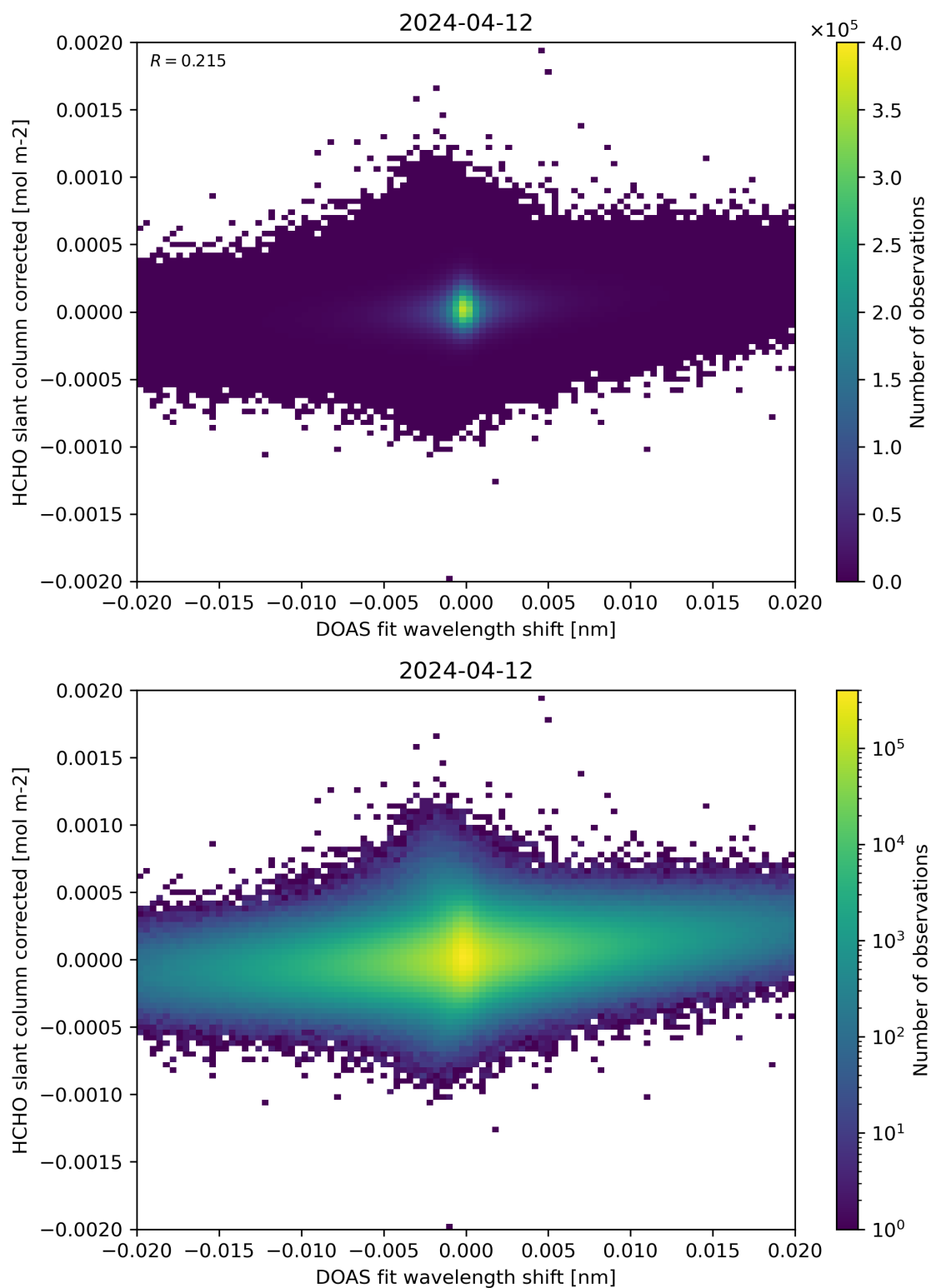
Figure 66: Scatter density plot of “DOAS fit wavelength shift” against “HCHO slant column corrected” for 2024-04-11 to 2024-04-13.
