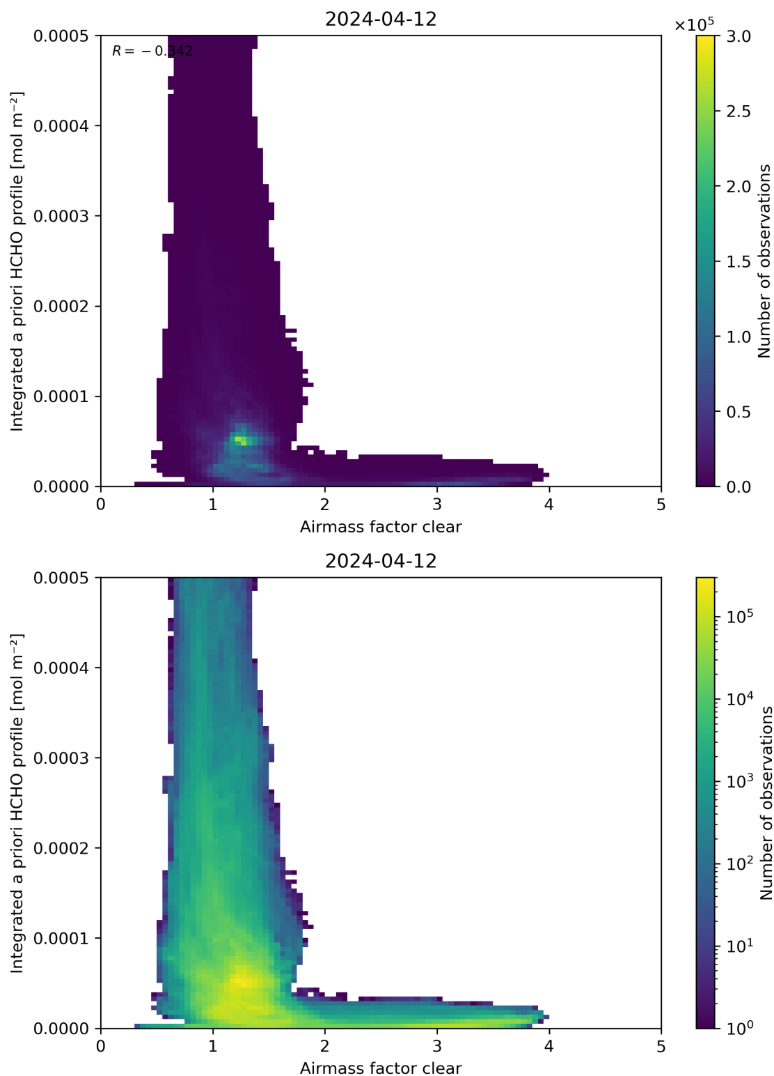
Figure 76: Scatter density plot of “Airmass factor clear” against “Integrated a priori HCHO profile” for 2024-04-11 to 2024-04-13.
