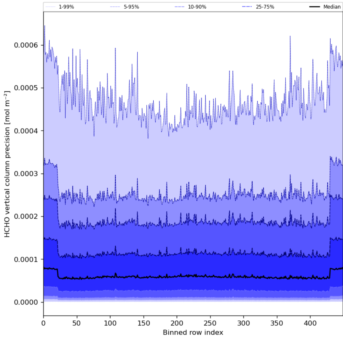
Figure 50: Along track statistics of “HCHO vertical column precision” for 2024-04-11 to 2024-04-13
