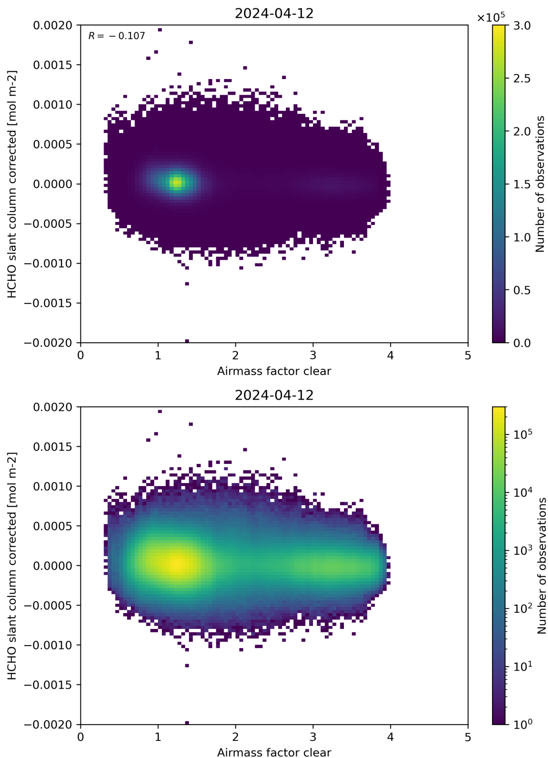
Figure 74: Scatter density plot of “Airmass factor clear” against “HCHO slant column corrected” for 2024-04-11 to 2024-04-13.
