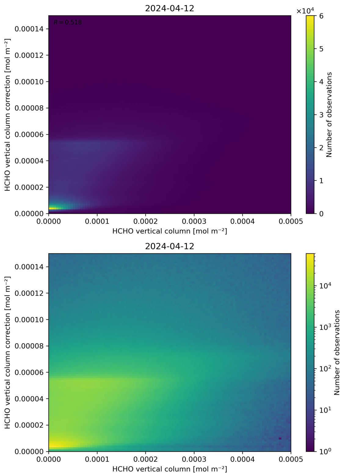
Figure 133: Scatter density plot of “HCHO vertical column” against “HCHO vertical column correction” for 2024-04-11 to 2024-04-13.
