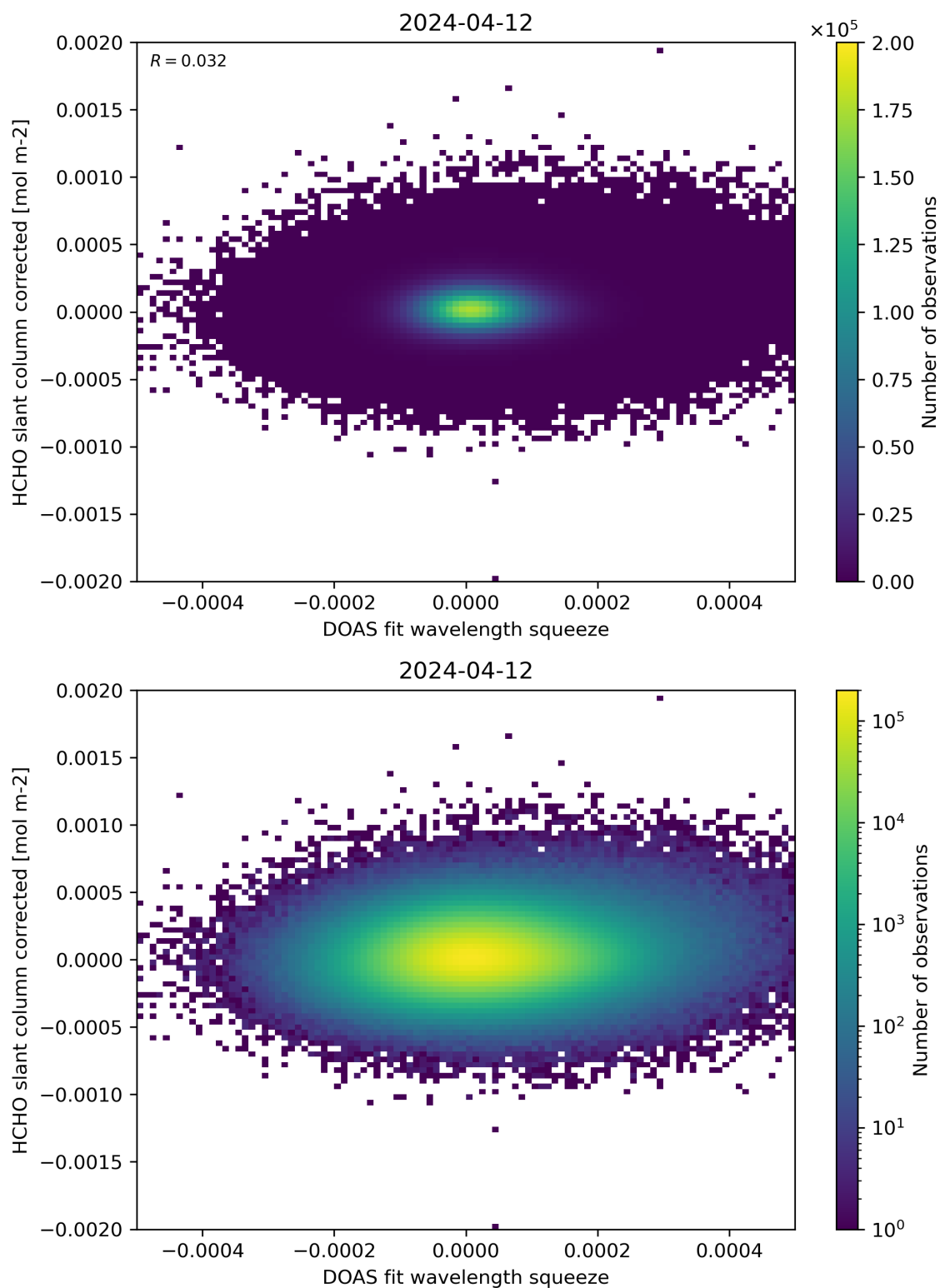
Figure 69: Scatter density plot of “DOAS fit wavelength squeeze” against “HCHO slant column corrected” for 2024-04-11 to 2024-04-13.
