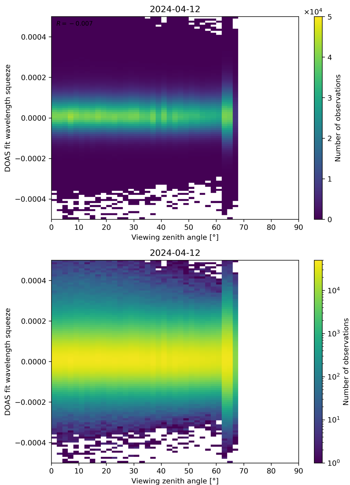
Figure 184: Scatter density plot of “Viewing zenith angle” against “DOAS fit wavelength squeeze” for 2024-04-11 to 2024-04-13.
