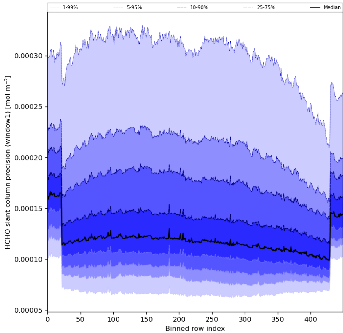
Figure 53: Along track statistics of “HCHO slant column precision (window1)” for 2024-04-11 to 2024-04-13
