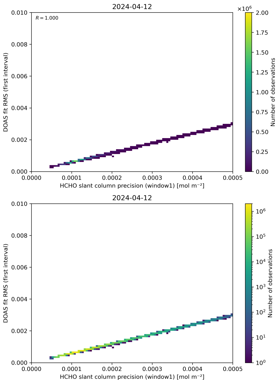
Figure 88: Scatter density plot of “HCHO slant column precision (window1)” against “DOAS fit RMS (first interval)” for 2024-04-11 to 2024-04-13.
