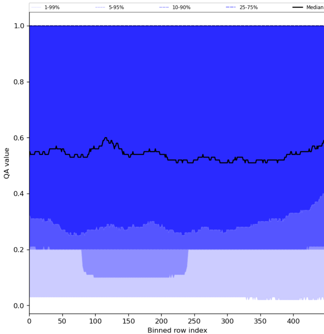
Figure 48: Along track statistics of “QA value” for 2024-04-11 to 2024-04-13
