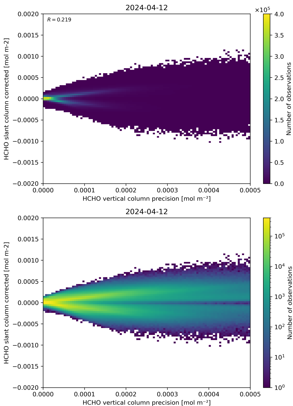
Figure 140: Scatter density plot of “HCHO vertical column precision” against “HCHO slant column corrected” for 2024-04-11 to 2024-04-13.
