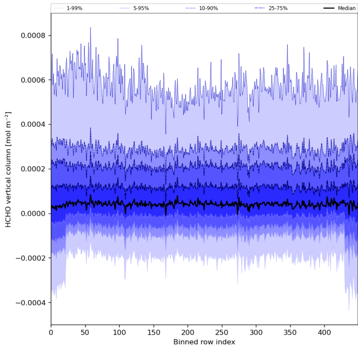
Figure 49: Along track statistics of “HCHO vertical column” for 2024-04-11 to 2024-04-13
