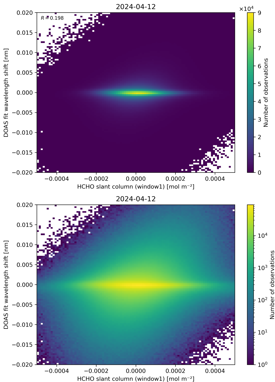
Figure 79: Scatter density plot of “HCHO slant column (window1)” against “DOAS fit wavelength shift” for 2024-04-11 to 2024-04-13.
