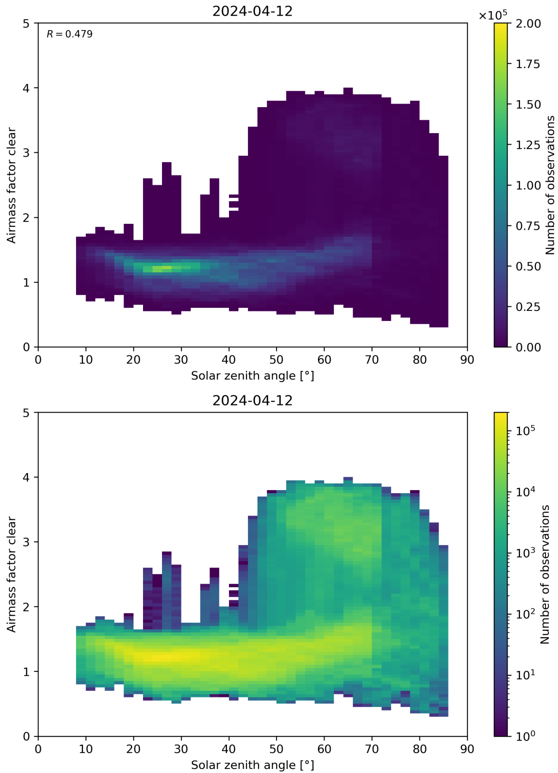
Figure 170: Scatter density plot of “Solar zenith angle” against “Airmass factor clear” for 2024-04-11 to 2024-04-13.
