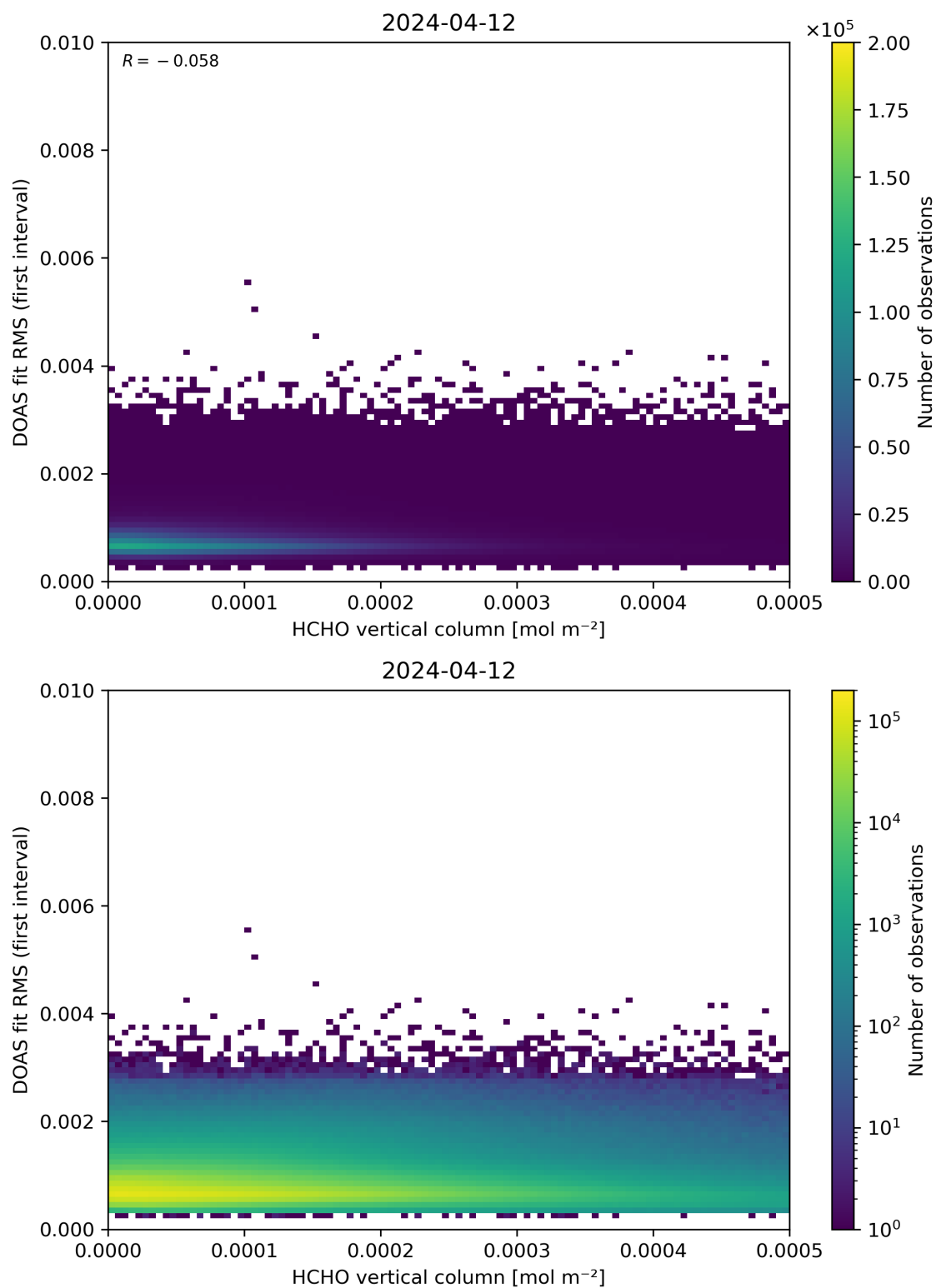
Figure 123: Scatter density plot of “HCHO vertical column” against “DOAS fit RMS (first interval)” for 2024-04-11 to 2024-04-13.
