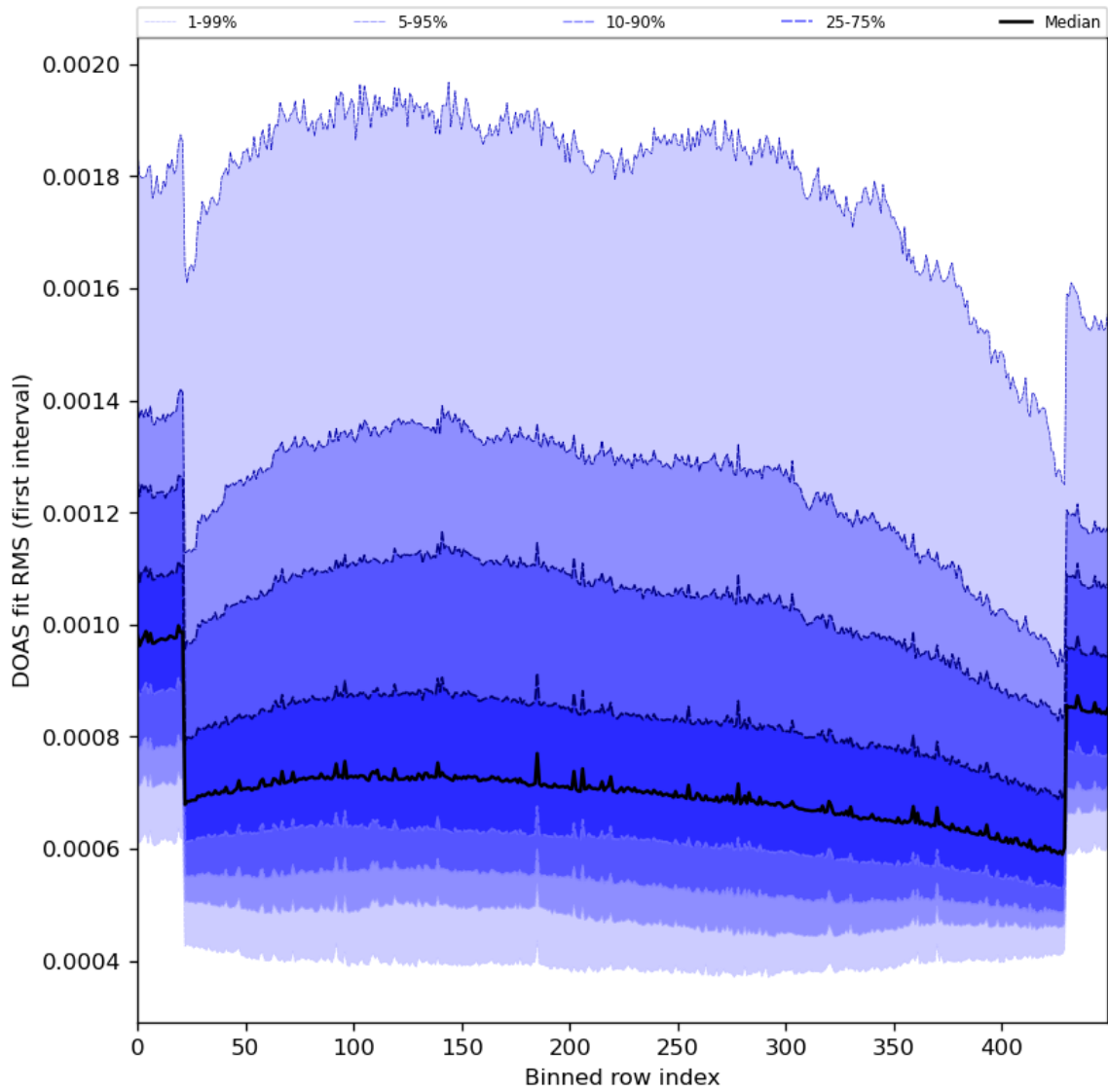
Figure 60: Along track statistics of “DOAS fit RMS (first interval)” for 2024-04-11 to 2024-04-13
