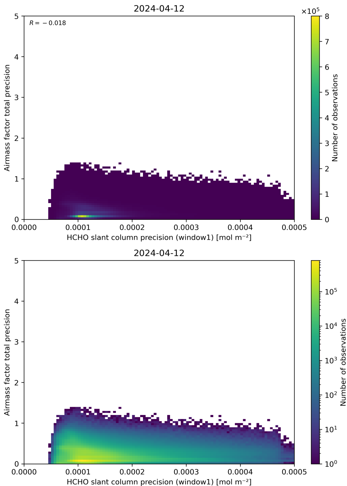
Figure 95: Scatter density plot of “HCHO slant column precision (window1)” against “Airmass factor total precision” for 2024-04-11 to 2024-04-13.
