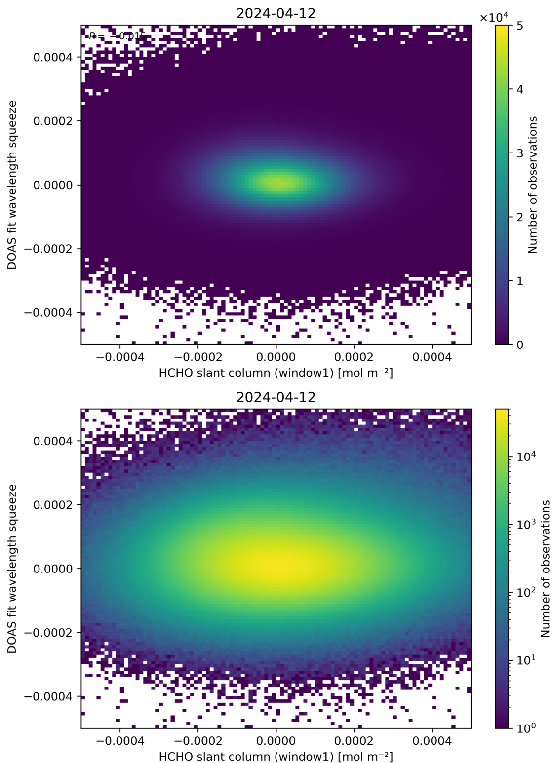
Figure 80: Scatter density plot of “HCHO slant column (window1)” against “DOAS fit wavelength squeeze” for 2024-04-11 to 2024-04-13.
