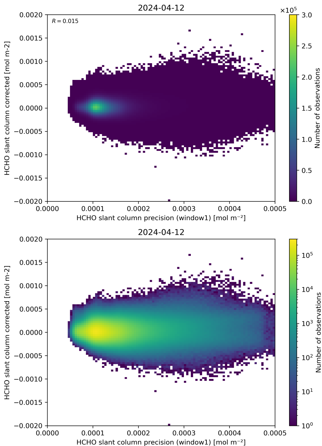
Figure 92: Scatter density plot of “HCHO slant column precision (window1)” against “HCHO slant column corrected” for 2024-04-11 to 2024-04-13.
