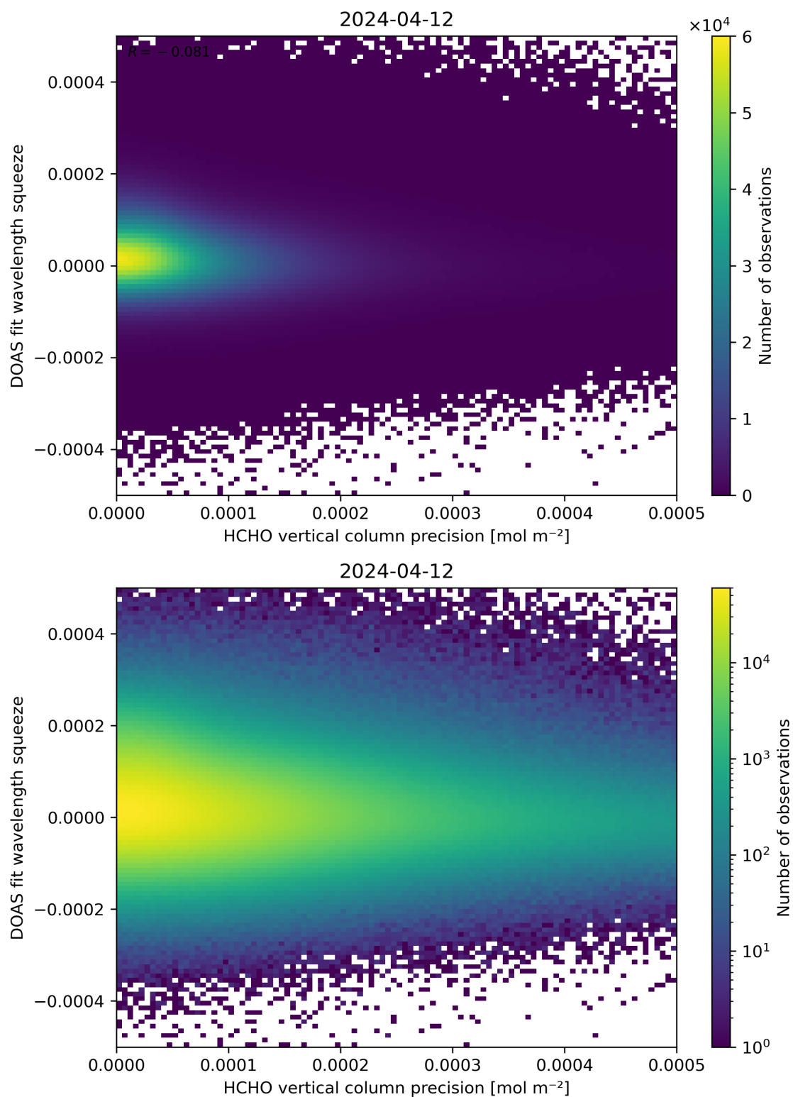
Figure 138: Scatter density plot of “HCHO vertical column precision” against “DOAS fit wavelength squeeze” for 2024-04-11 to 2024-04-13.
