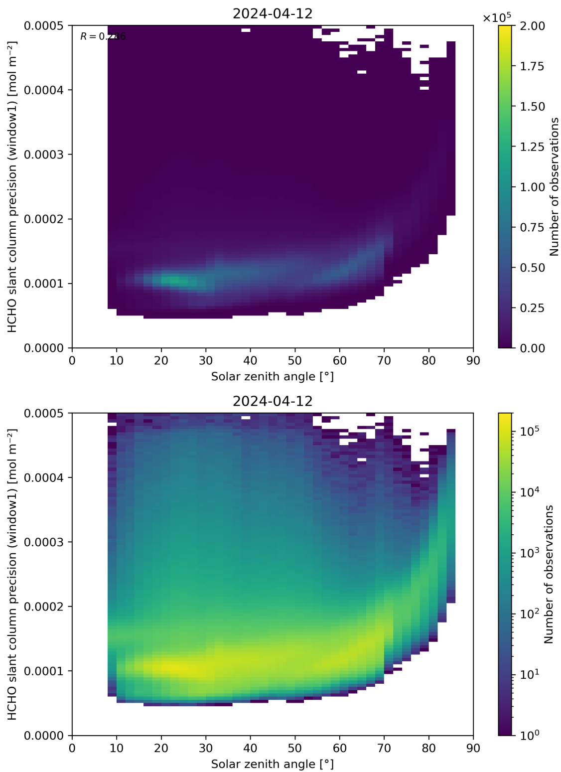
Figure 174: Scatter density plot of “Solar zenith angle” against “HCHO slant column precision (window1)” for 2024-04-11 to 2024-04-13.
