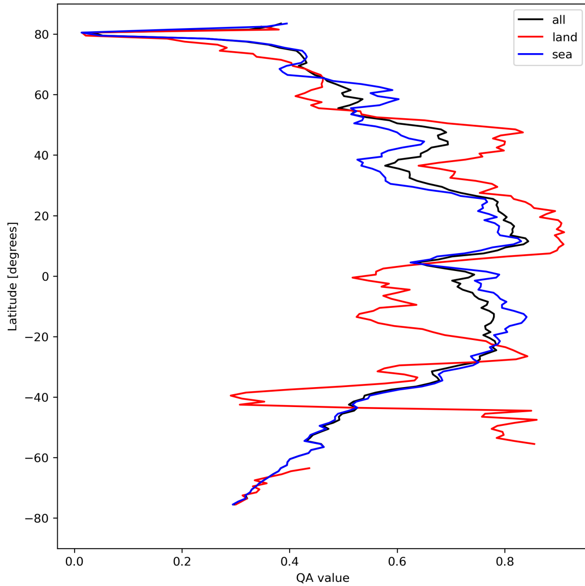
Figure 20: Zonal average of “QA value” for 2024-04-11 to 2024-04-13.
