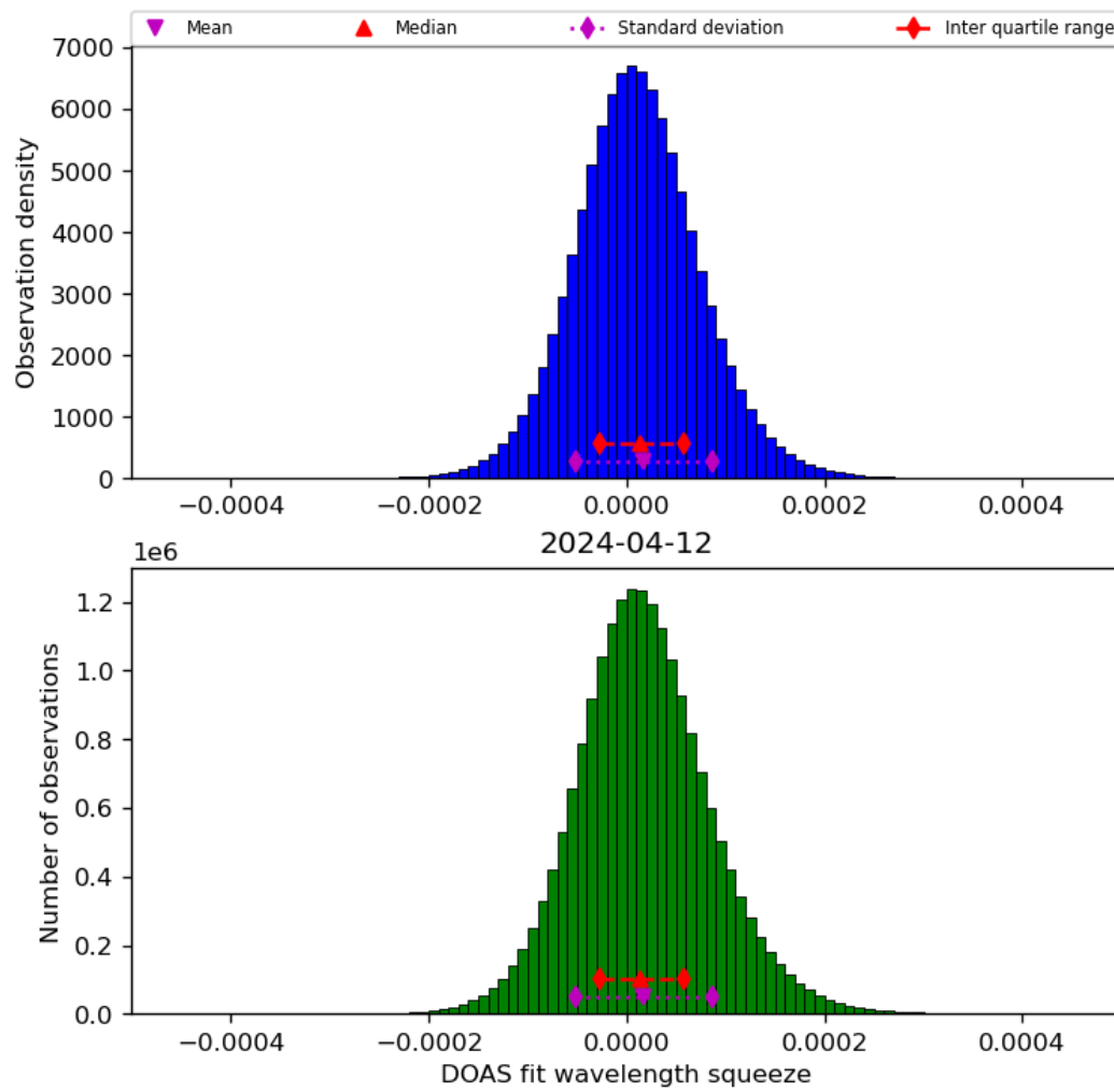
Figure 45: Histogram of “DOAS fit wavelength squeeze” for 2024-04-11 to 2024-04-13
