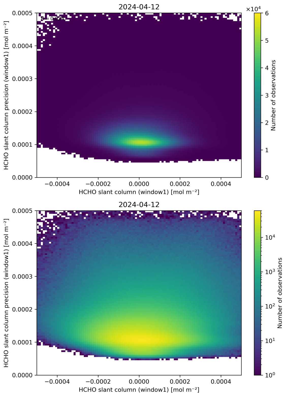
Figure 84: Scatter density plot of “HCHO slant column (window1)” against “HCHO slant column precision (window1)” for 2024-04-11 to 2024-04-13.
