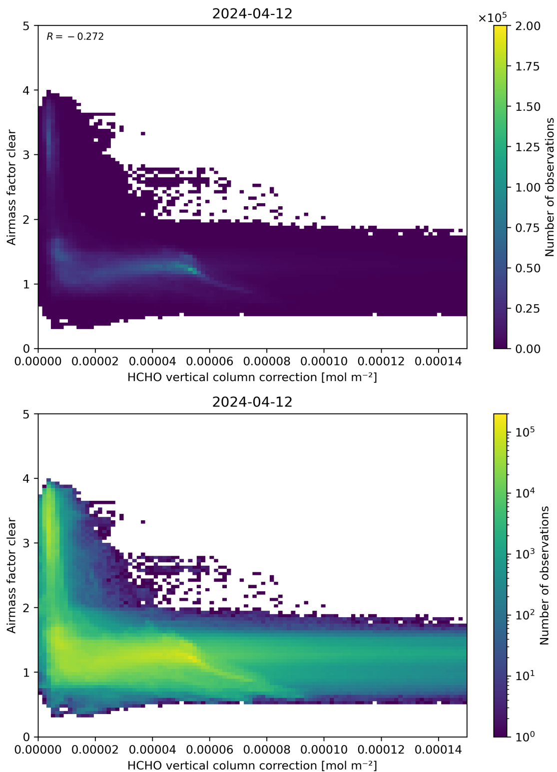
Figure 115: Scatter density plot of “HCHO vertical column correction” against “Airmass factor clear” for 2024-04-11 to 2024-04-13.
