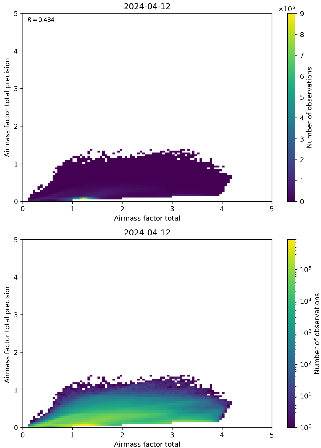
Figure 103: Scatter density plot of “Airmass factor total” against “Airmass factor total precision” for 2024-04-11 to 2024-04-13.
