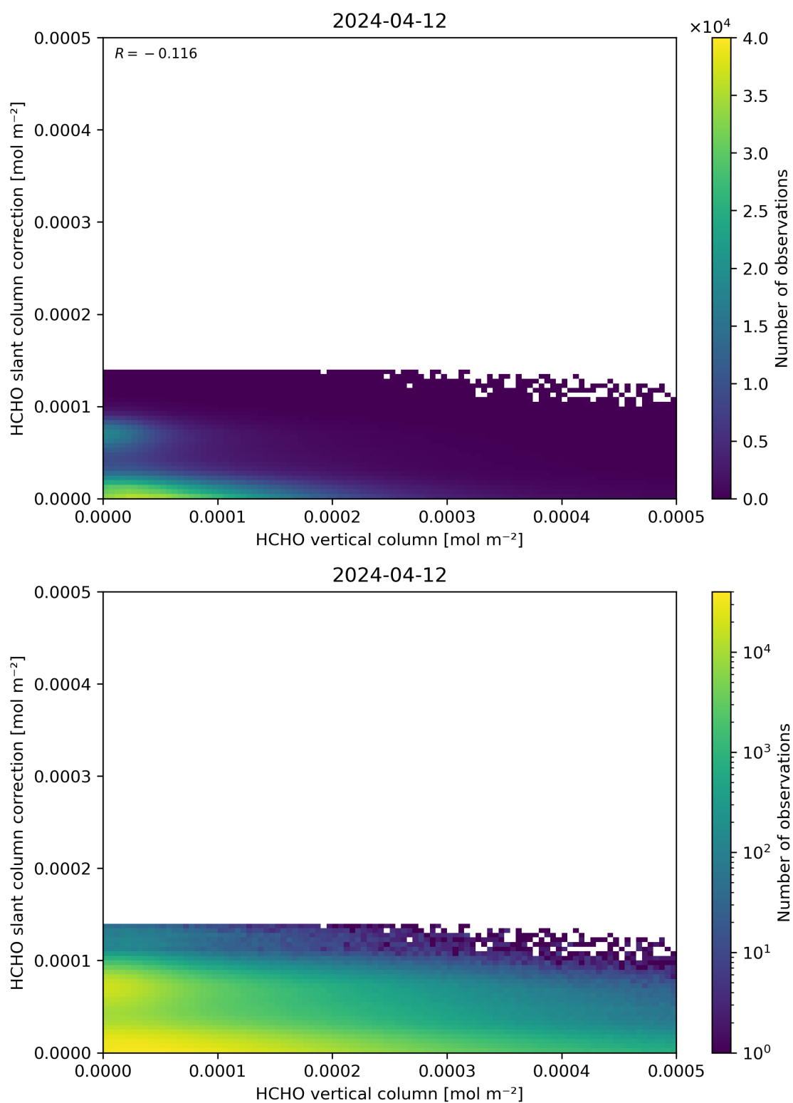
Figure 128: Scatter density plot of “HCHO vertical column” against “HCHO slant column correction” for 2024-04-11 to 2024-04-13.
