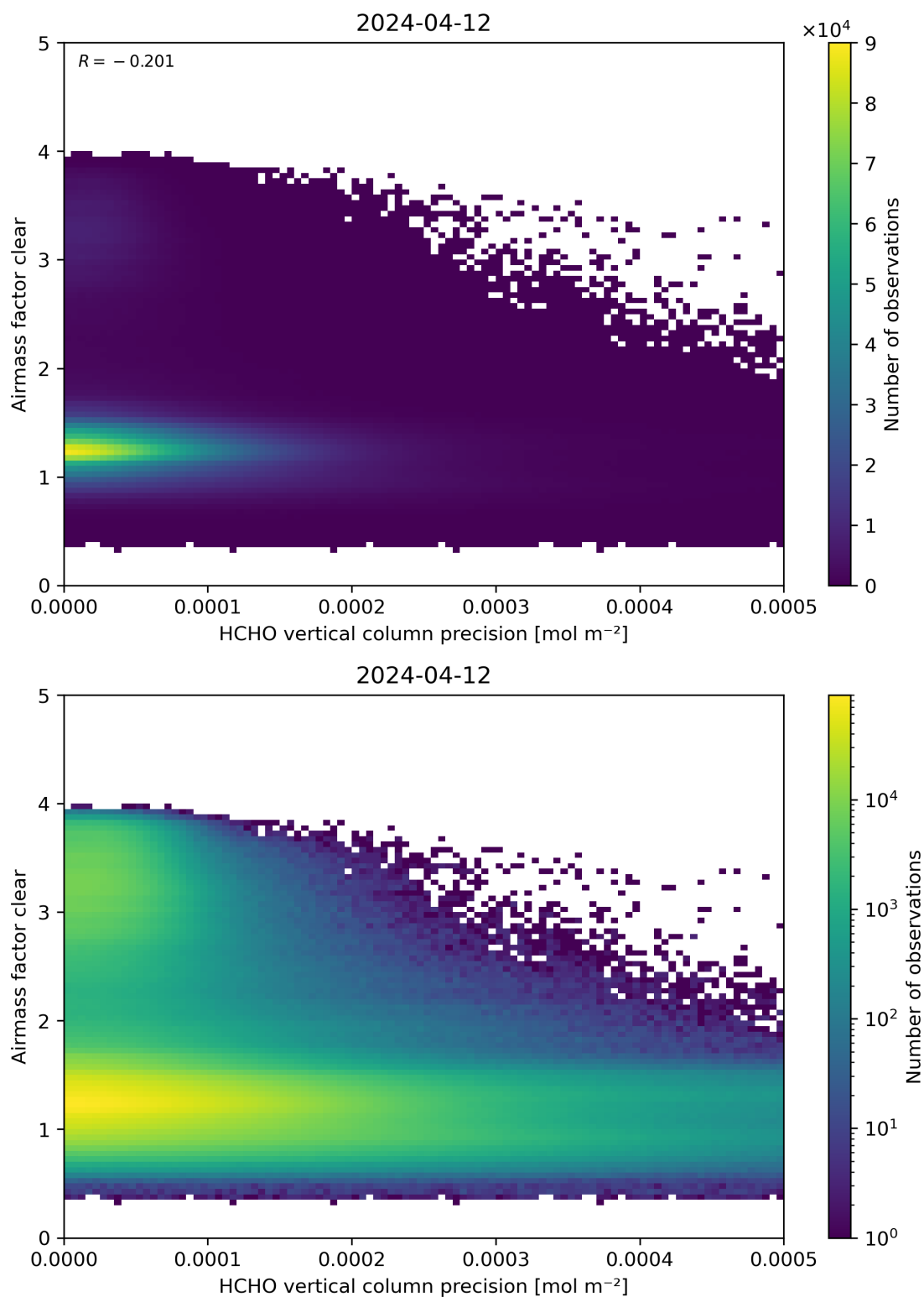
Figure 139: Scatter density plot of “HCHO vertical column precision” against “Airmass factor clear” for 2024-04-11 to 2024-04-13.
