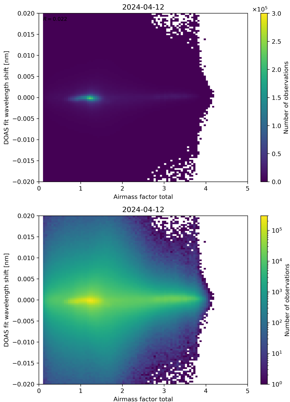
Figure 98: Scatter density plot of “Airmass factor total” against “DOAS fit wavelength shift” for 2024-04-11 to 2024-04-13.
