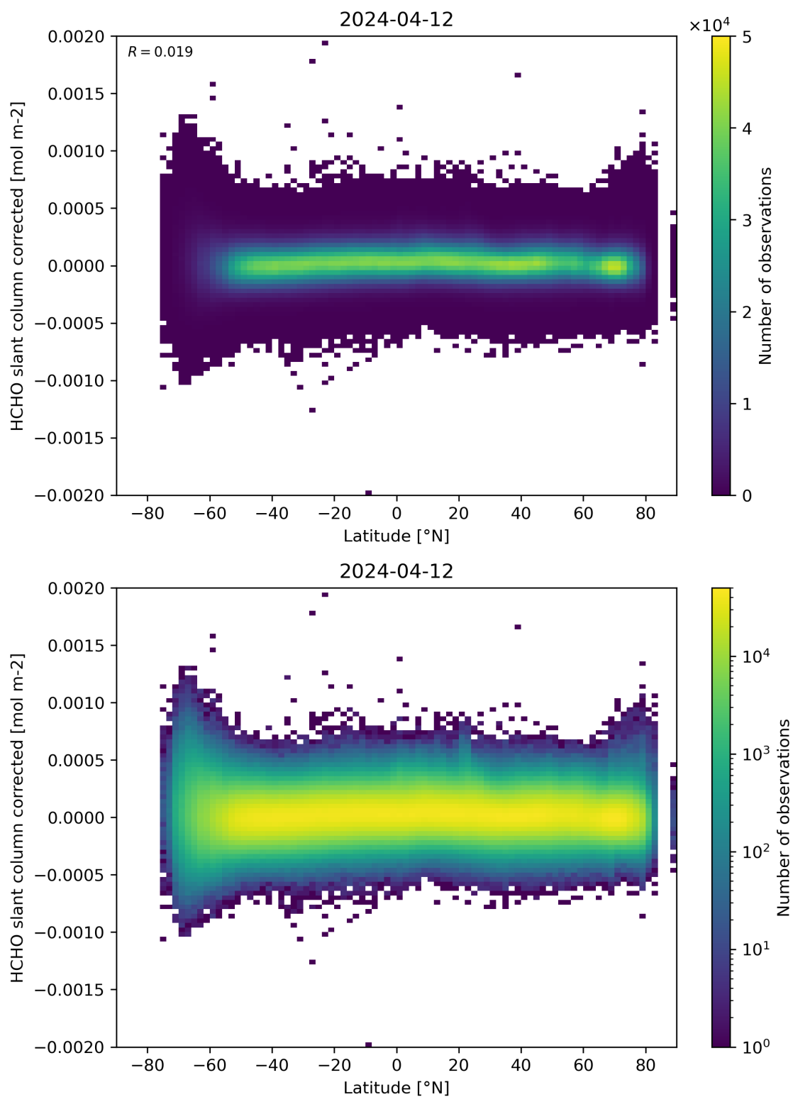
Figure 157: Scatter density plot of “Latitude” against “HCHO slant column corrected” for 2024-04-11 to 2024-04-13.
