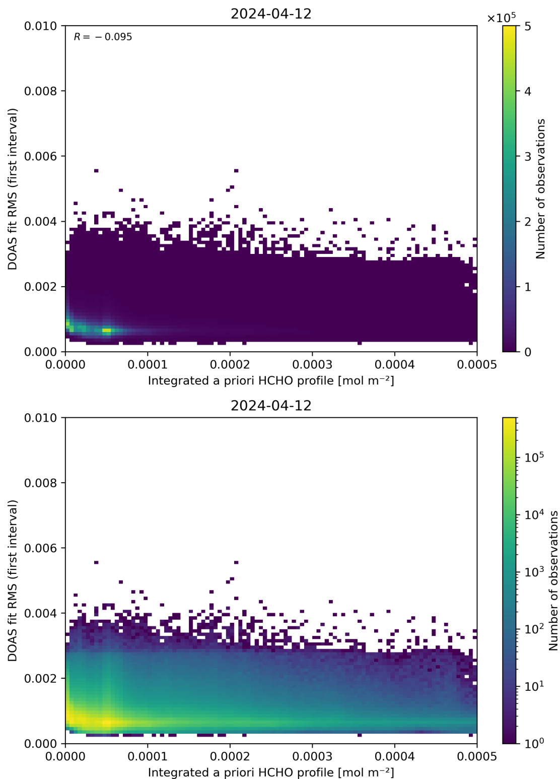
Figure 148: Scatter density plot of “Integrated a priori HCHO profile” against “DOAS fit RMS (first interval)” for 2024-04-11 to 2024-04-13.
