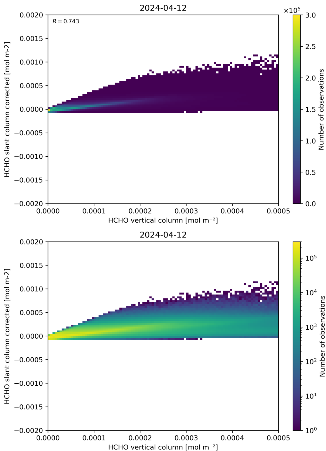
Figure 127: Scatter density plot of “HCHO vertical column” against “HCHO slant column corrected” for 2024-04-11 to 2024-04-13.
