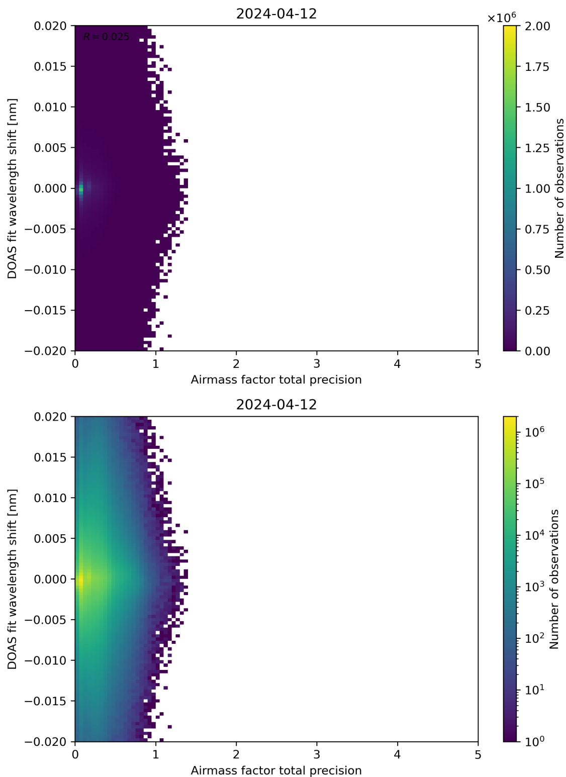
Figure 106: Scatter density plot of “Airmass factor total precision” against “DOAS fit wavelength shift” for 2024-04-11 to 2024-04-13.
