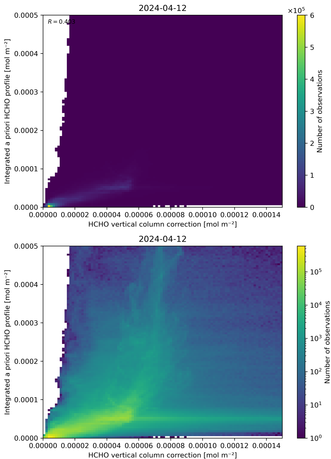
Figure 122: Scatter density plot of “HCHO vertical column correction” against “Integrated a priori HCHO profile” for 2024-04-11 to 2024-04-13.
