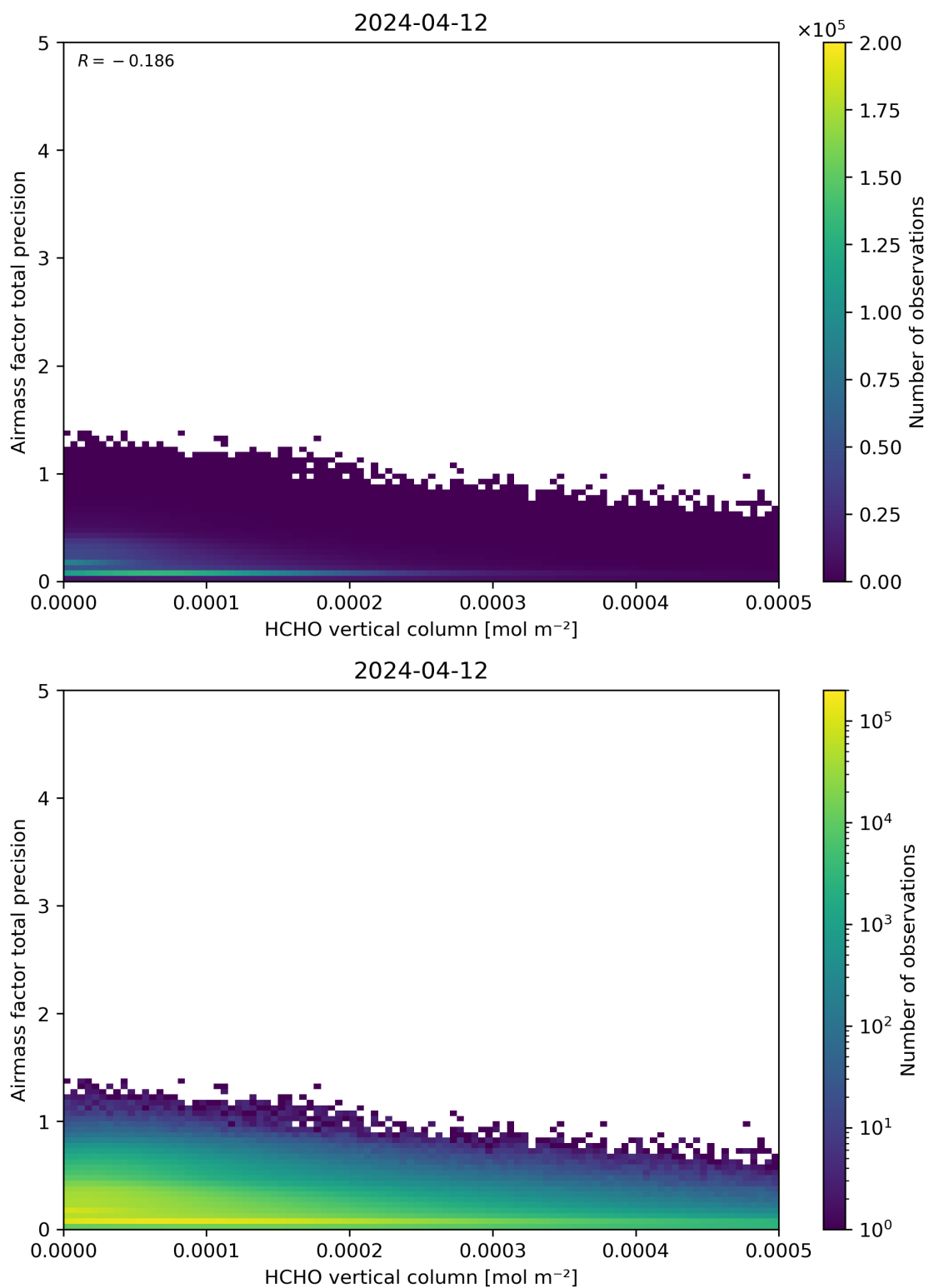
Figure 132: Scatter density plot of “HCHO vertical column” against “Airmass factor total precision” for 2024-04-11 to 2024-04-13.
