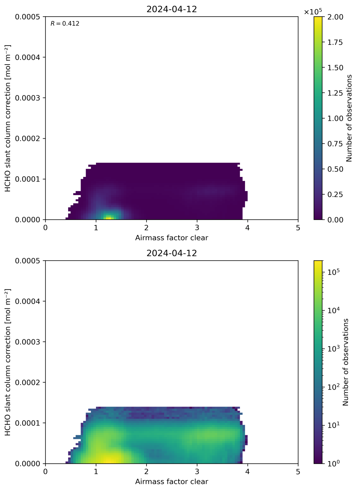
Figure 75: Scatter density plot of “Airmass factor clear” against “HCHO slant column correction” for 2024-04-11 to 2024-04-13.
