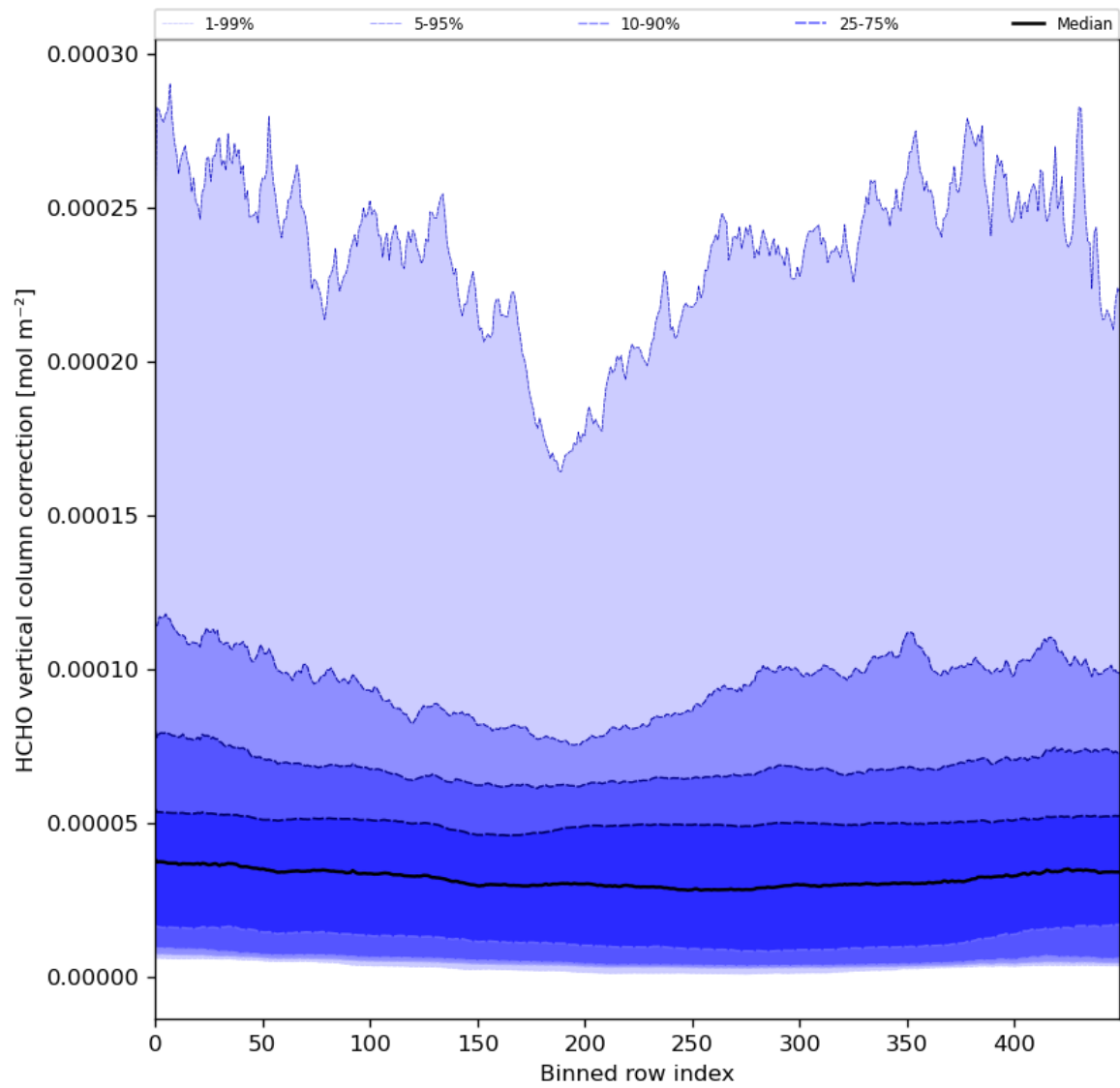
Figure 51: Along track statistics of “HCHO vertical column correction” for 2024-04-11 to 2024-04-13
