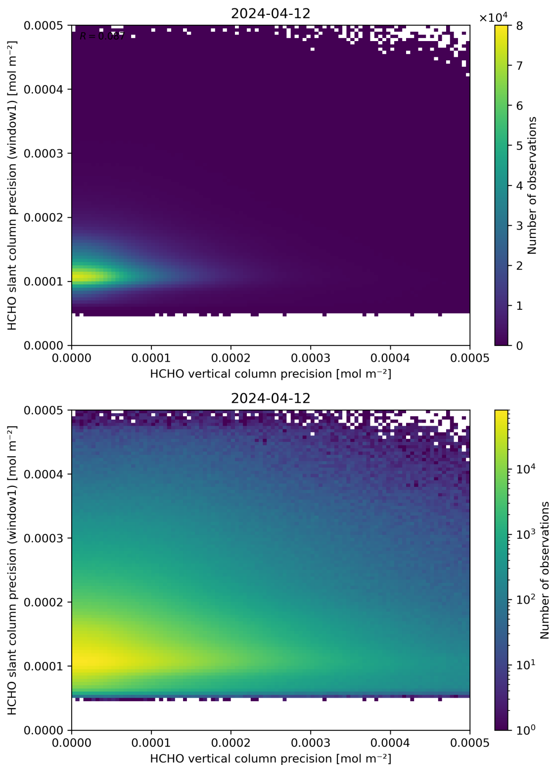
Figure 143: Scatter density plot of “HCHO vertical column precision” against “HCHO slant column precision (window1)” for 2024-04-11 to 2024-04-13.
