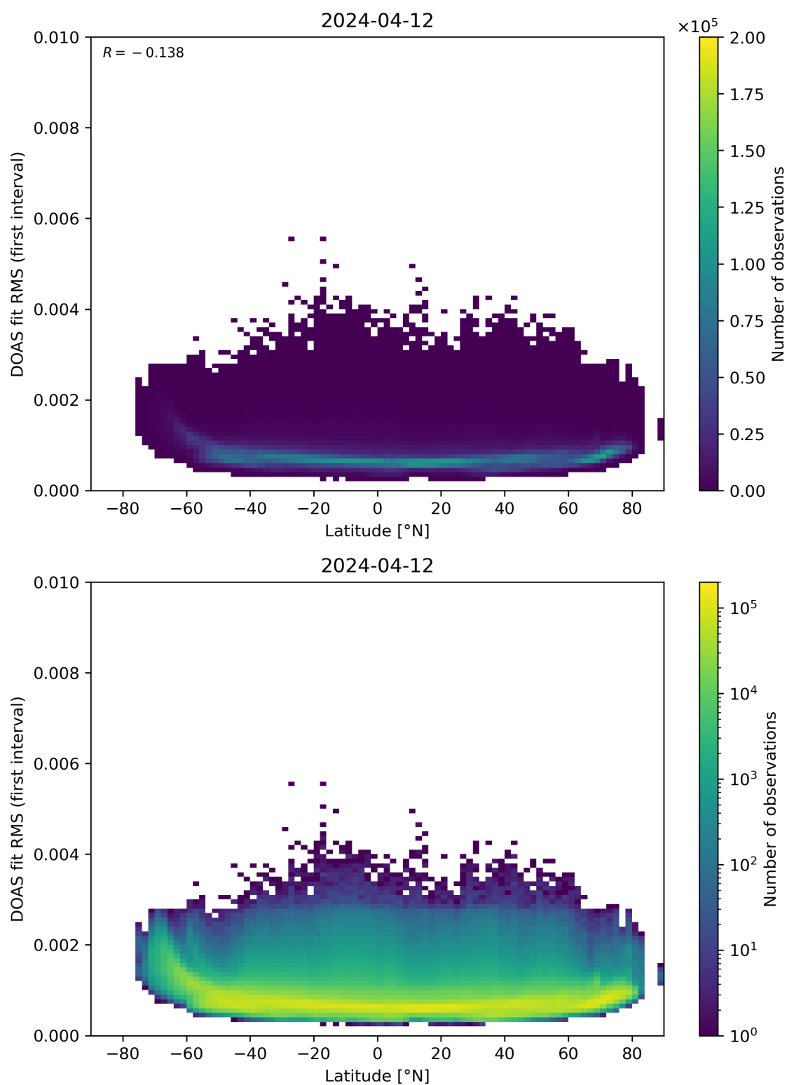
Figure 153: Scatter density plot of “Latitude” against “DOAS fit RMS (first interval)” for 2024-04-11 to 2024-04-13.
