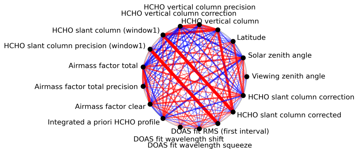
Figure 1: Map of correlation graph for 2024-04-11 to 2024-04-13.
