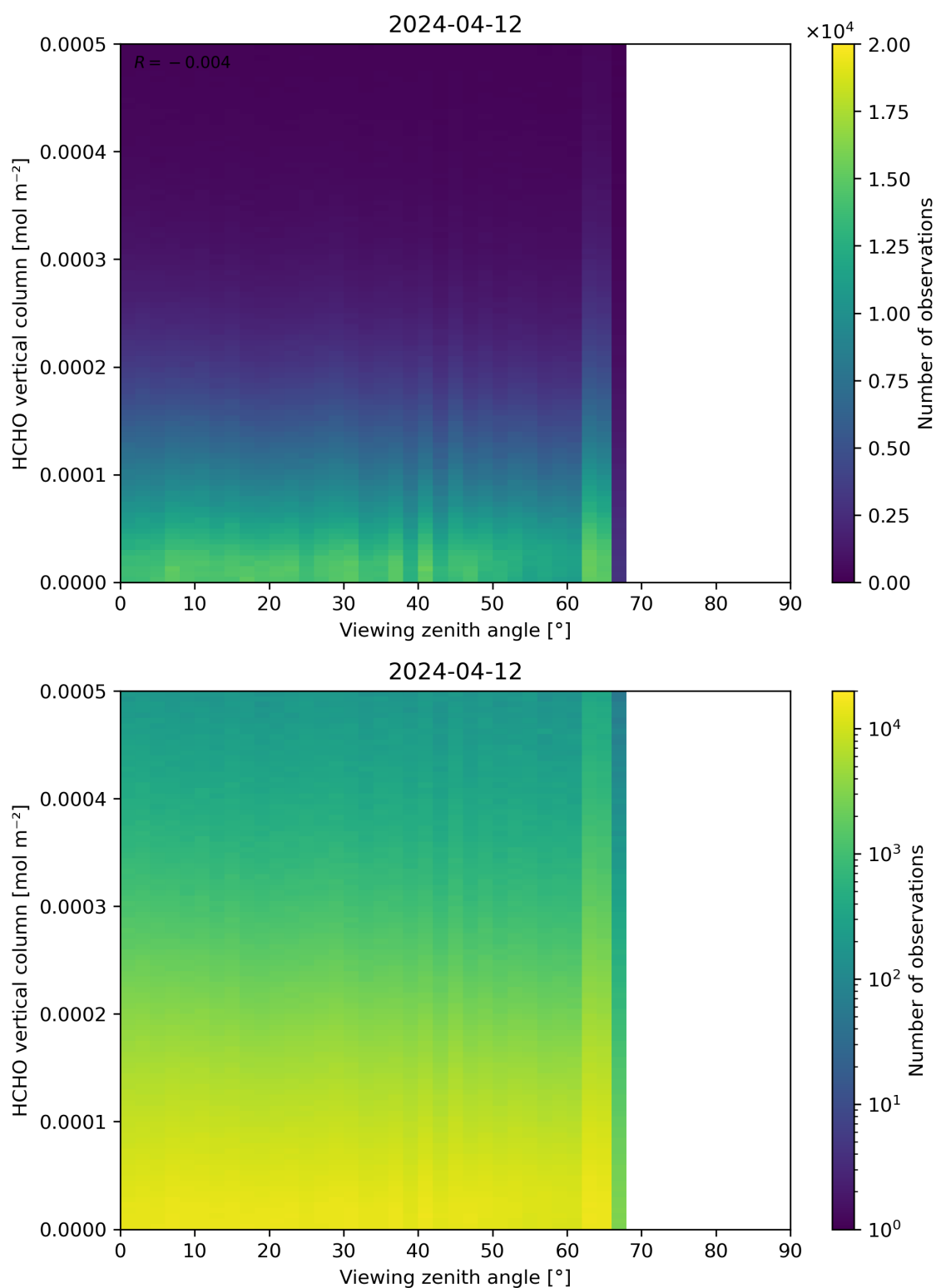
Figure 192: Scatter density plot of “Viewing zenith angle” against “HCHO vertical column” for 2024-04-11 to 2024-04-13.
