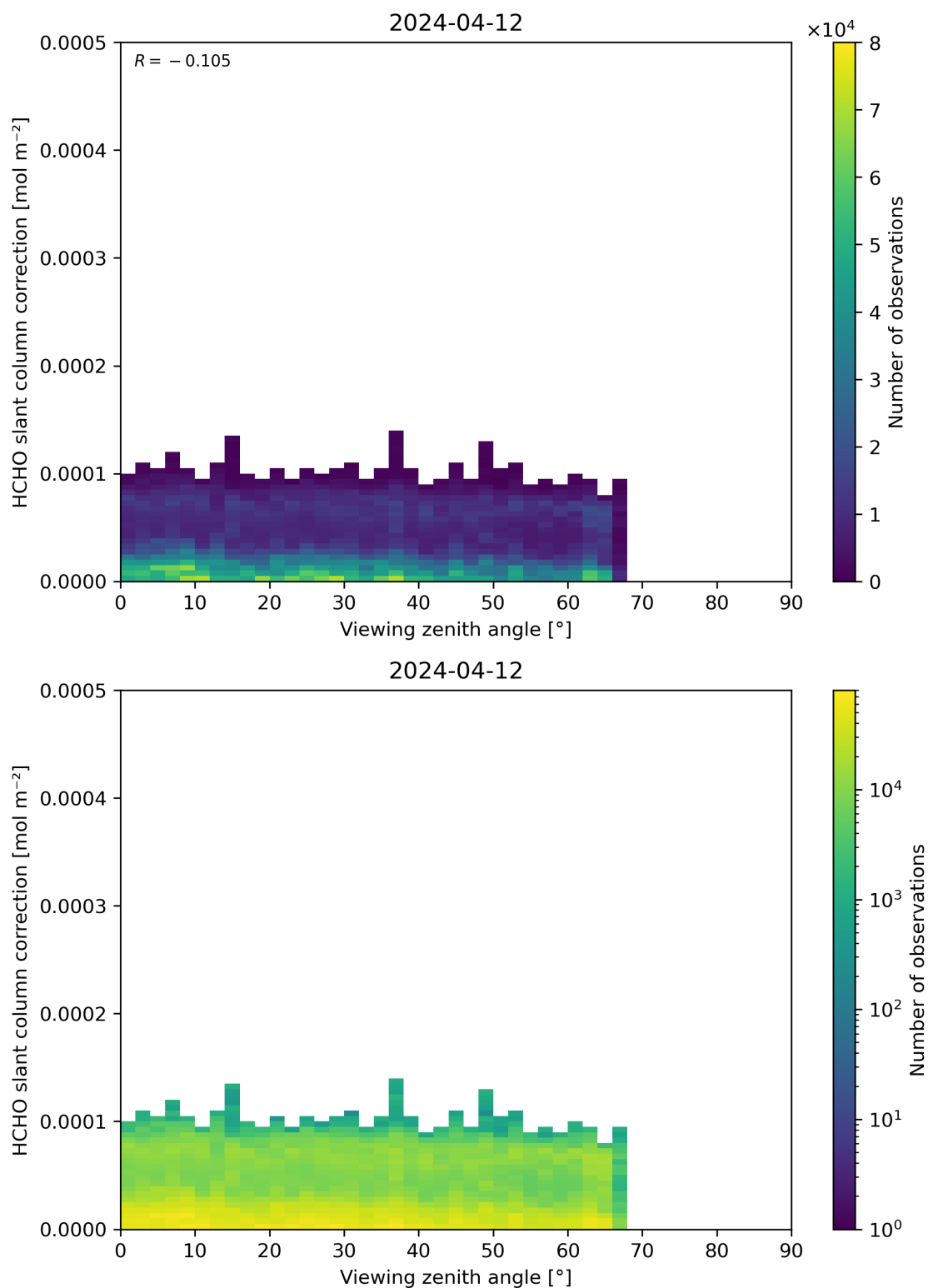
Figure 187: Scatter density plot of “Viewing zenith angle” against “HCHO slant column correction” for 2024-04-11 to 2024-04-13.
