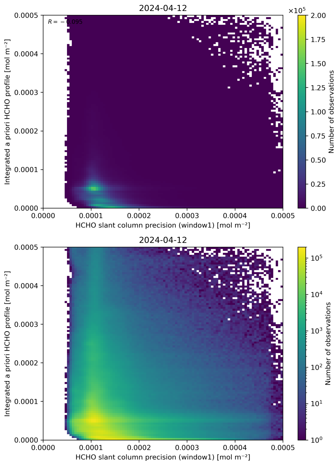
Figure 96: Scatter density plot of “HCHO slant column precision (window1)” against “Integrated a priori HCHO profile” for 2024-04-11 to 2024-04-13.
