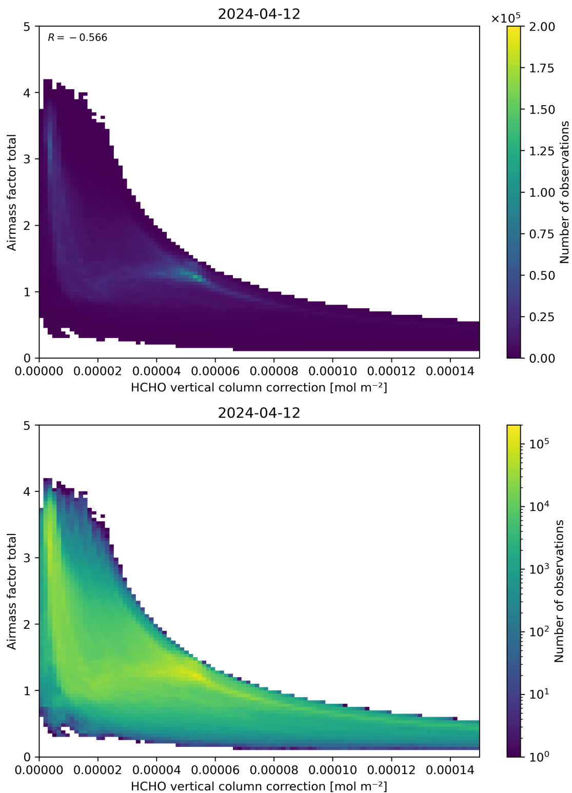
Figure 120: Scatter density plot of “HCHO vertical column correction” against “Airmass factor total” for 2024-04-11 to 2024-04-13.
