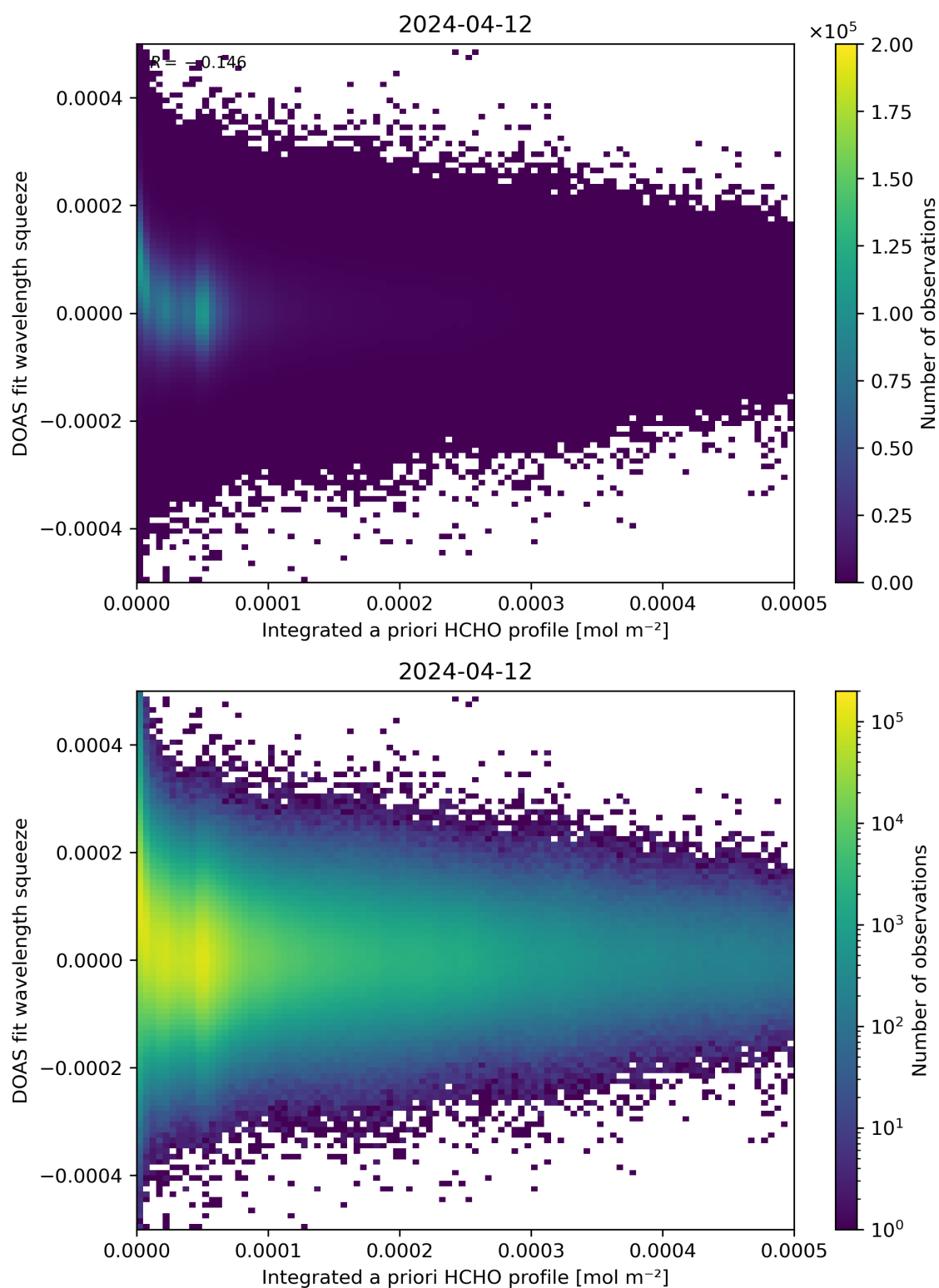
Figure 150: Scatter density plot of “Integrated a priori HCHO profile” against “DOAS fit wavelength squeeze” for 2024-04-11 to 2024-04-13.
