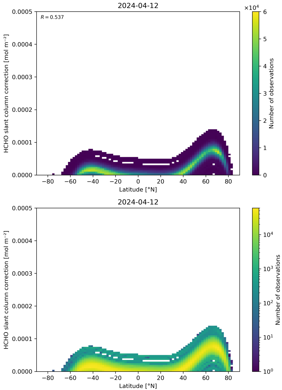
Figure 158: Scatter density plot of “Latitude” against “HCHO slant column correction” for 2024-04-11 to 2024-04-13.
