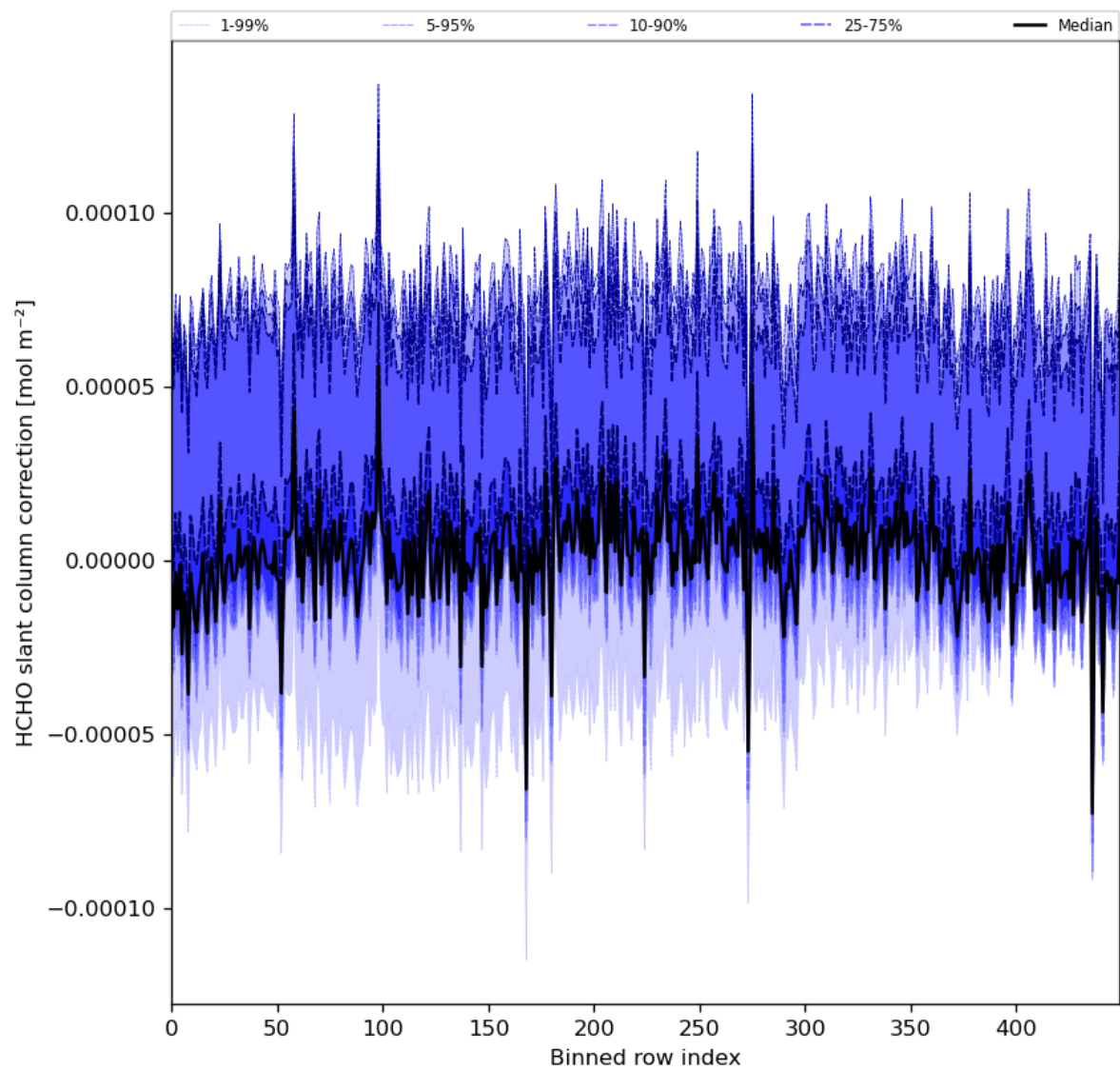
Figure 61: Along track statistics of “HCHO slant column correction” for 2024-04-11 to 2024-04-13
