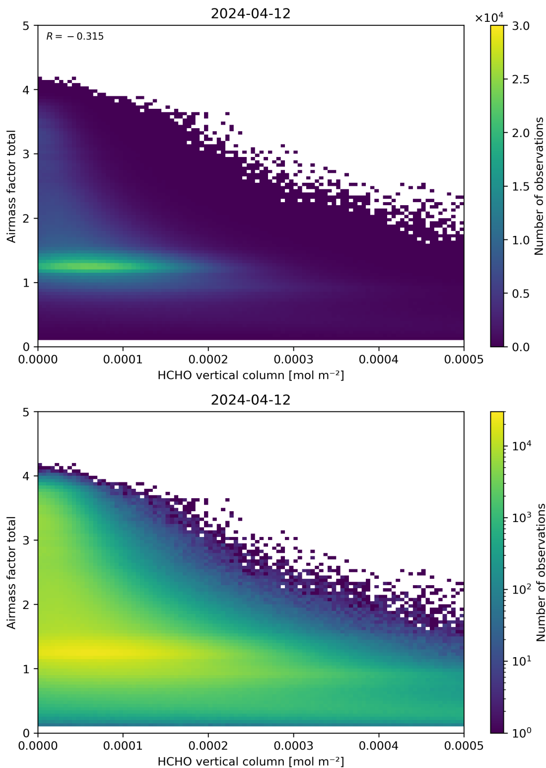
Figure 131: Scatter density plot of “HCHO vertical column” against “Airmass factor total” for 2024-04-11 to 2024-04-13.
