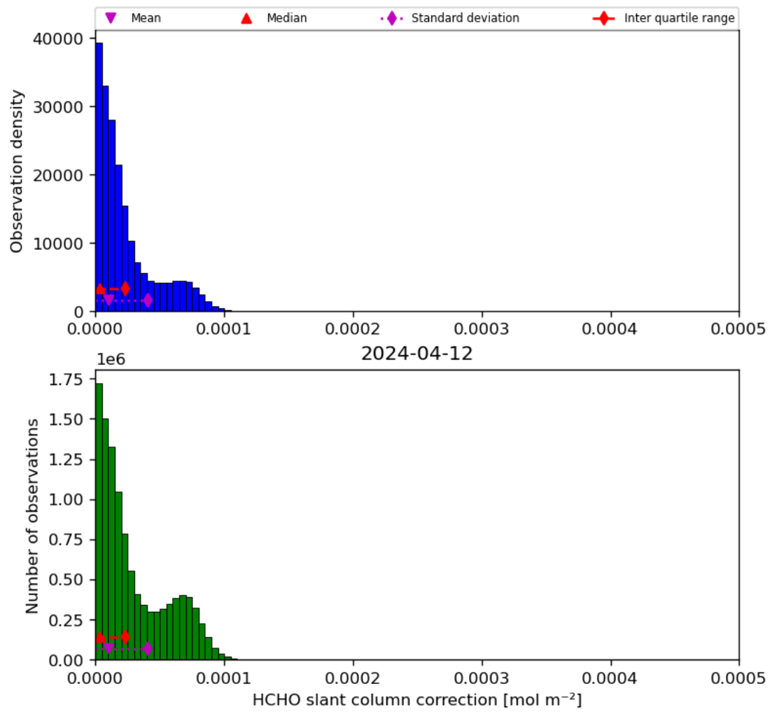
Figure 47: Histogram of “HCHO slant column correction” for 2024-04-11 to 2024-04-13
