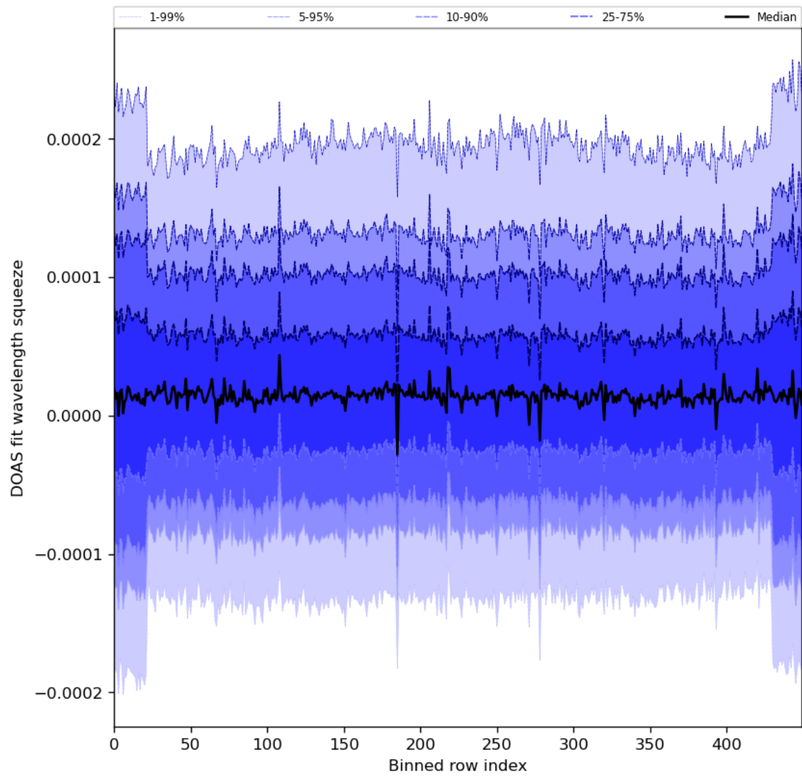
Figure 59: Along track statistics of “DOAS fit wavelength squeeze” for 2024-04-11 to 2024-04-13
