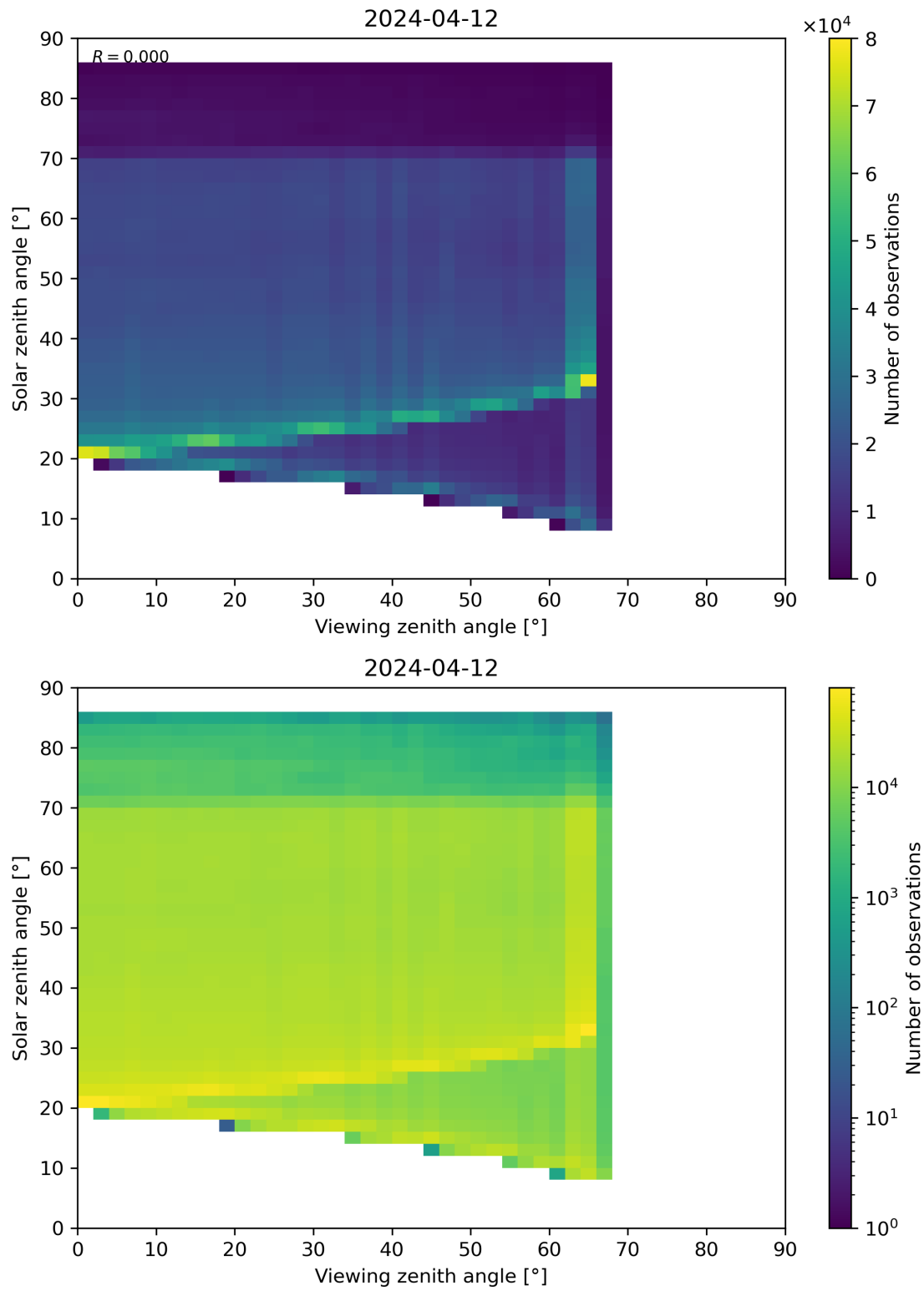
Figure 197: Scatter density plot of “Viewing zenith angle” against “Solar zenith angle” for 2024-04-11 to 2024-04-13.
