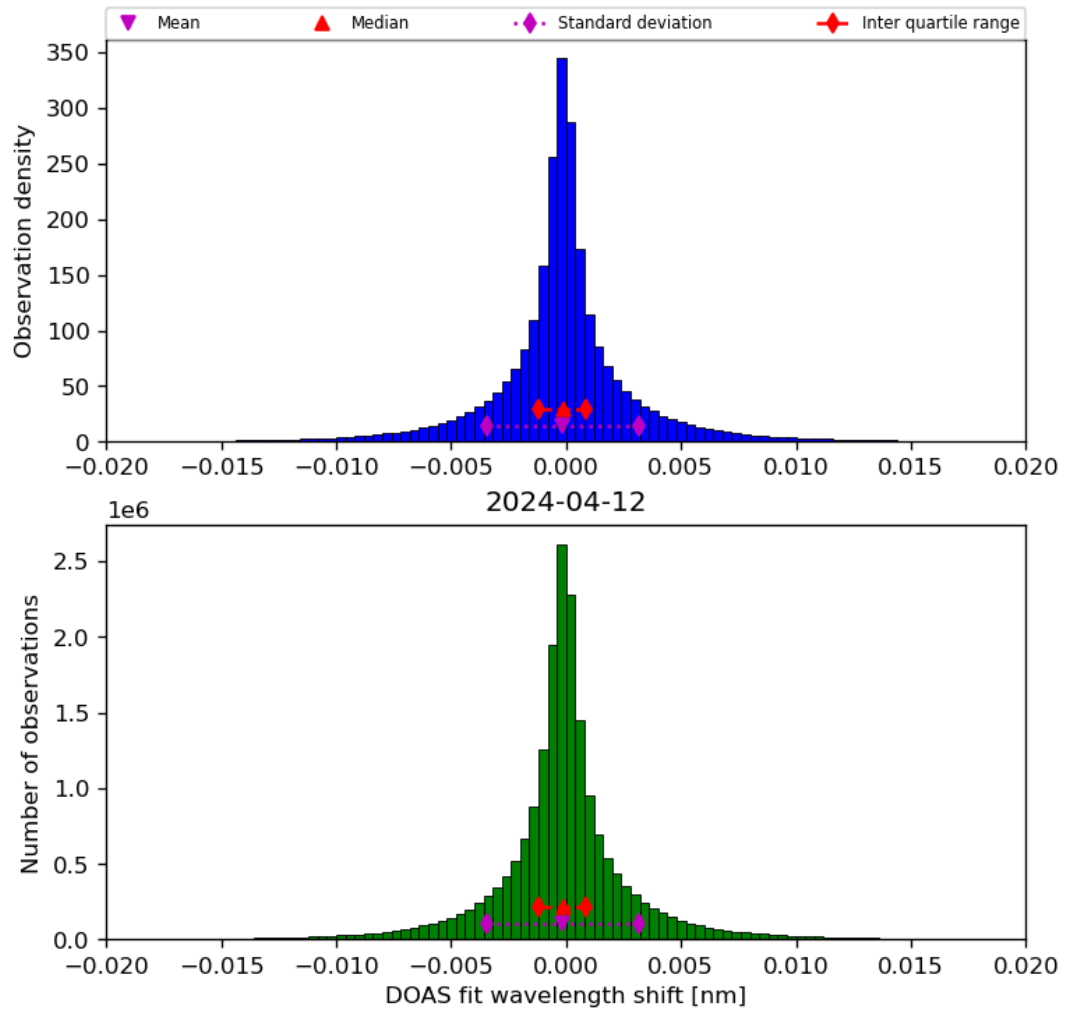
Figure 44: Histogram of “DOAS fit wavelength shift” for 2024-04-11 to 2024-04-13
