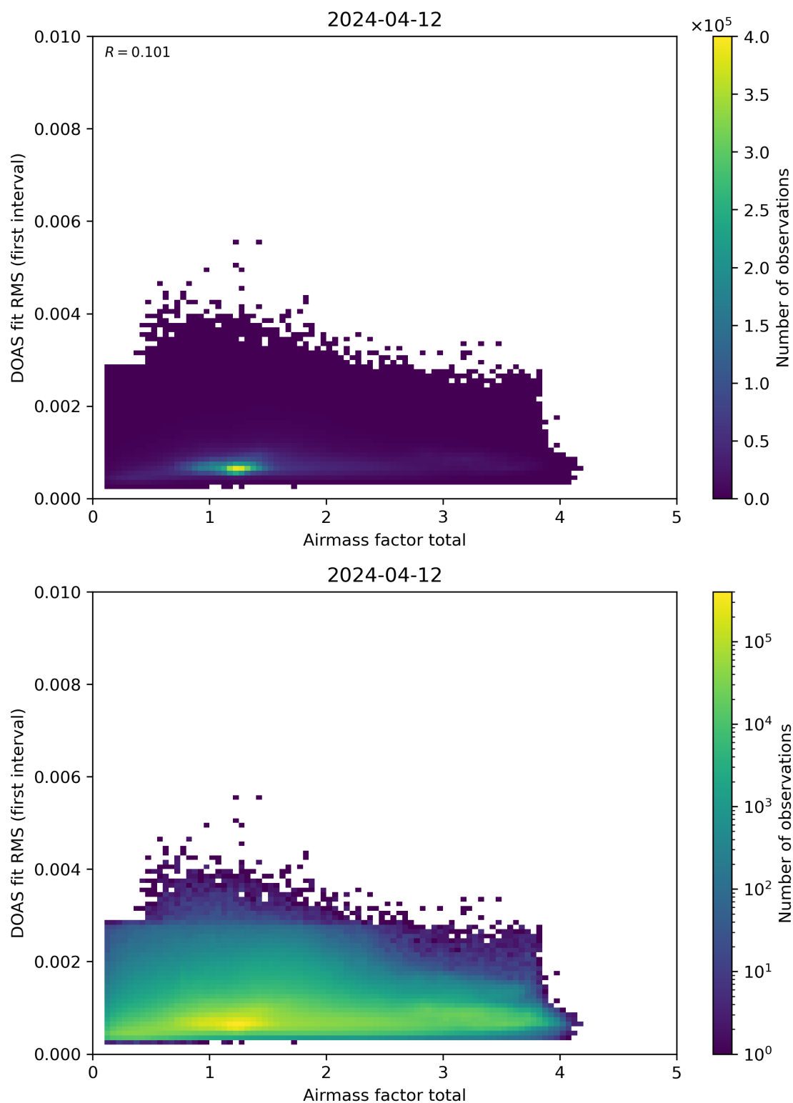
Figure 97: Scatter density plot of “Airmass factor total” against “DOAS fit RMS (first interval)” for 2024-04-11 to 2024-04-13.
