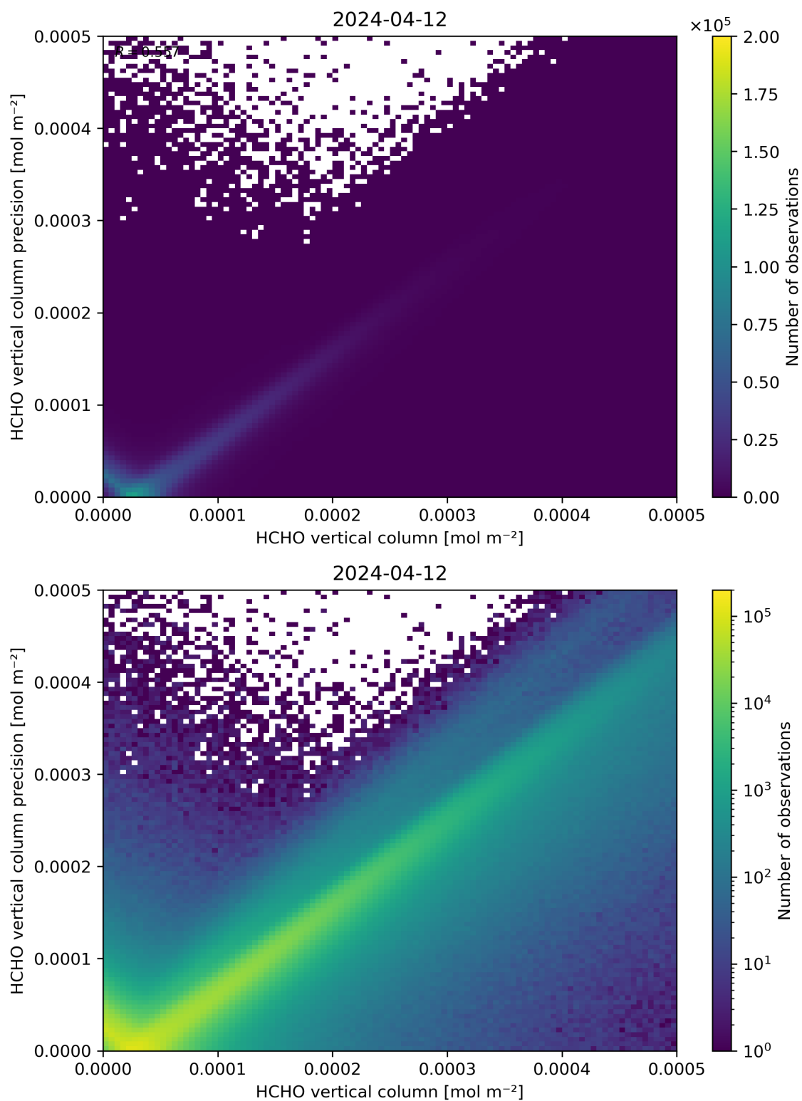
Figure 134: Scatter density plot of “HCHO vertical column” against “HCHO vertical column precision” for 2024-04-11 to 2024-04-13.
