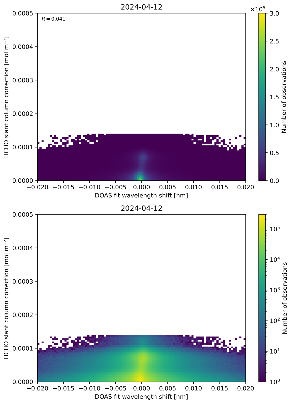
Figure 67: Scatter density plot of “DOAS fit wavelength shift” against “HCHO slant column correction” for 2024-04-11 to 2024-04-13.
