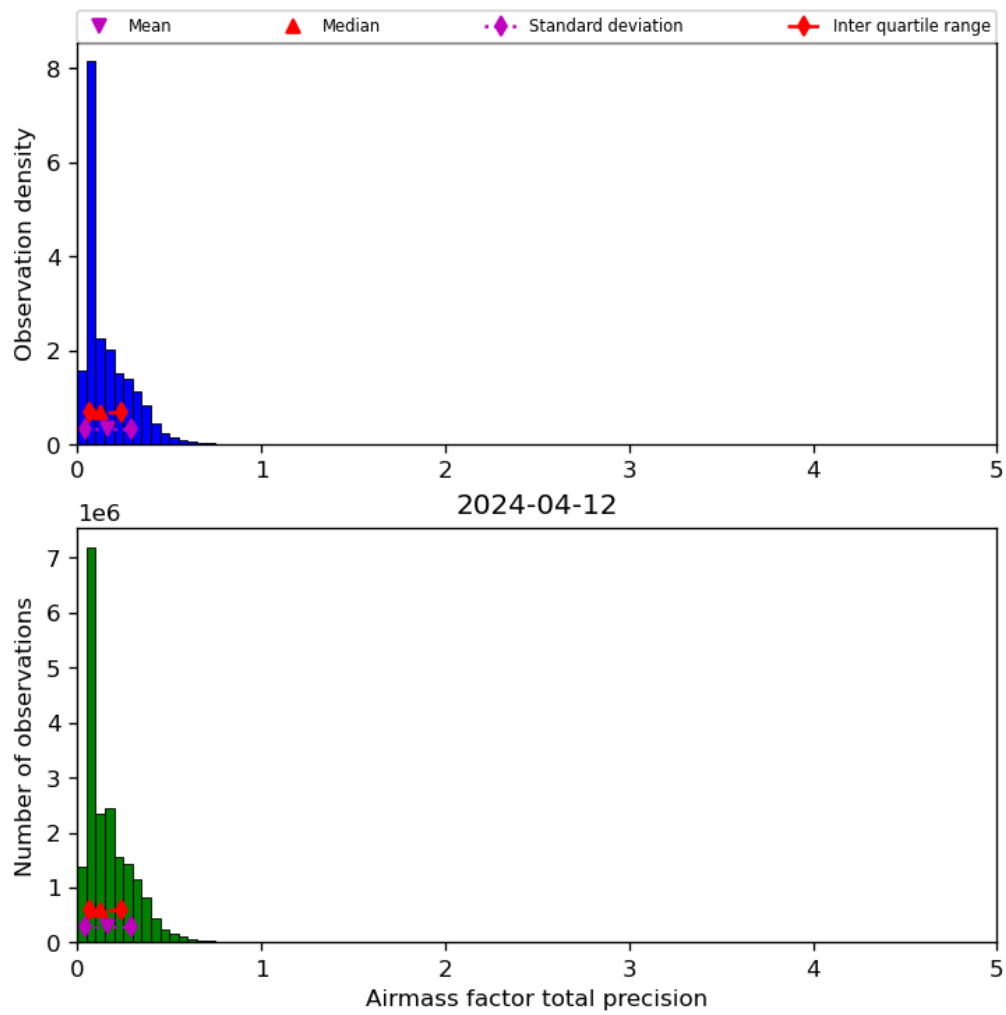
Figure 41: Histogram of “Airmass factor total precision” for 2024-04-11 to 2024-04-13
