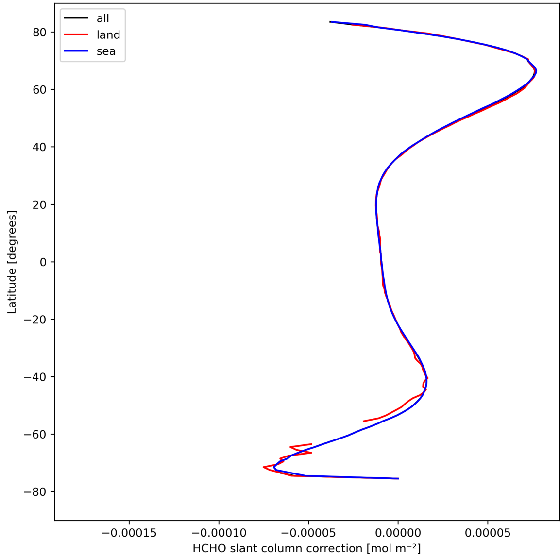
Figure 33: Zonal average of "HCHO slant column correction" for 2024-04-11 to 2024-04-13.
