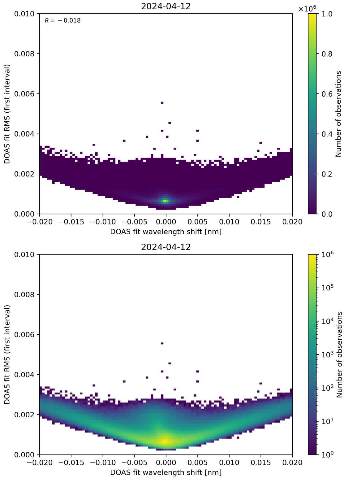
Figure 64: Scatter density plot of “DOAS fit wavelength shift” against “DOAS fit RMS (first interval)” for 2024-04-11 to 2024-04-13.
