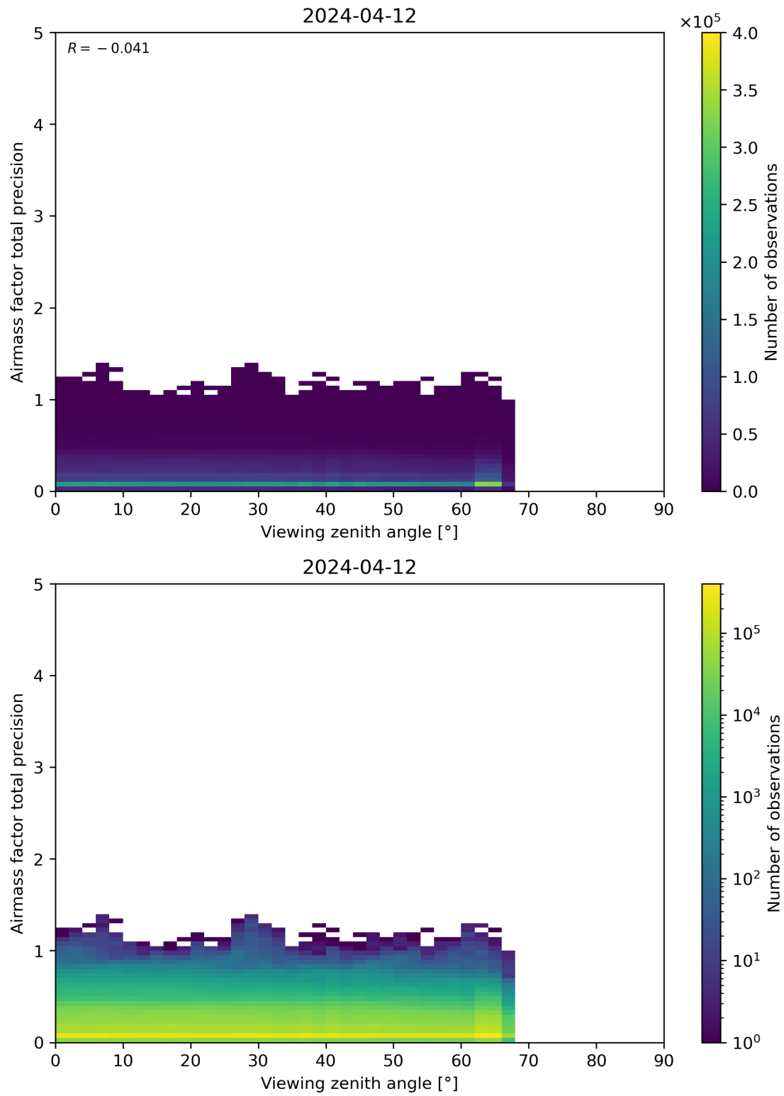
Figure 191: Scatter density plot of “Viewing zenith angle” against “Airmass factor total precision” for 2024-04-11 to 2024-04-13.
