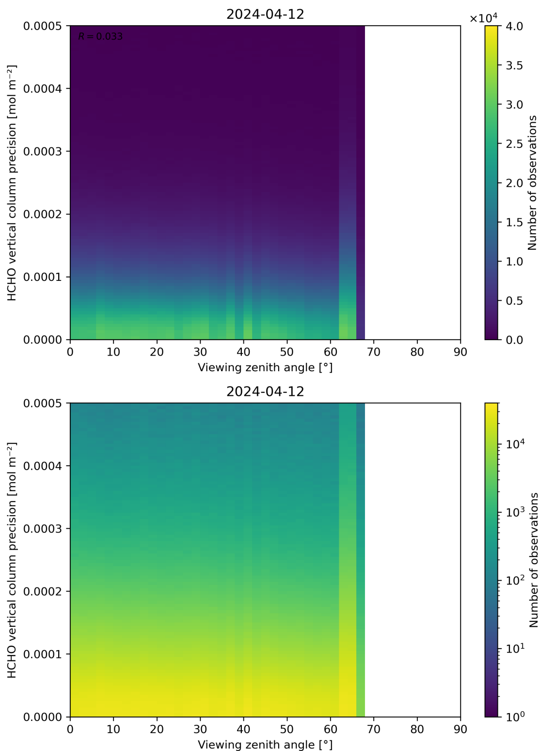
Figure 194: Scatter density plot of “Viewing zenith angle” against “HCHO vertical column precision” for 2024-04-11 to 2024-04-13.
