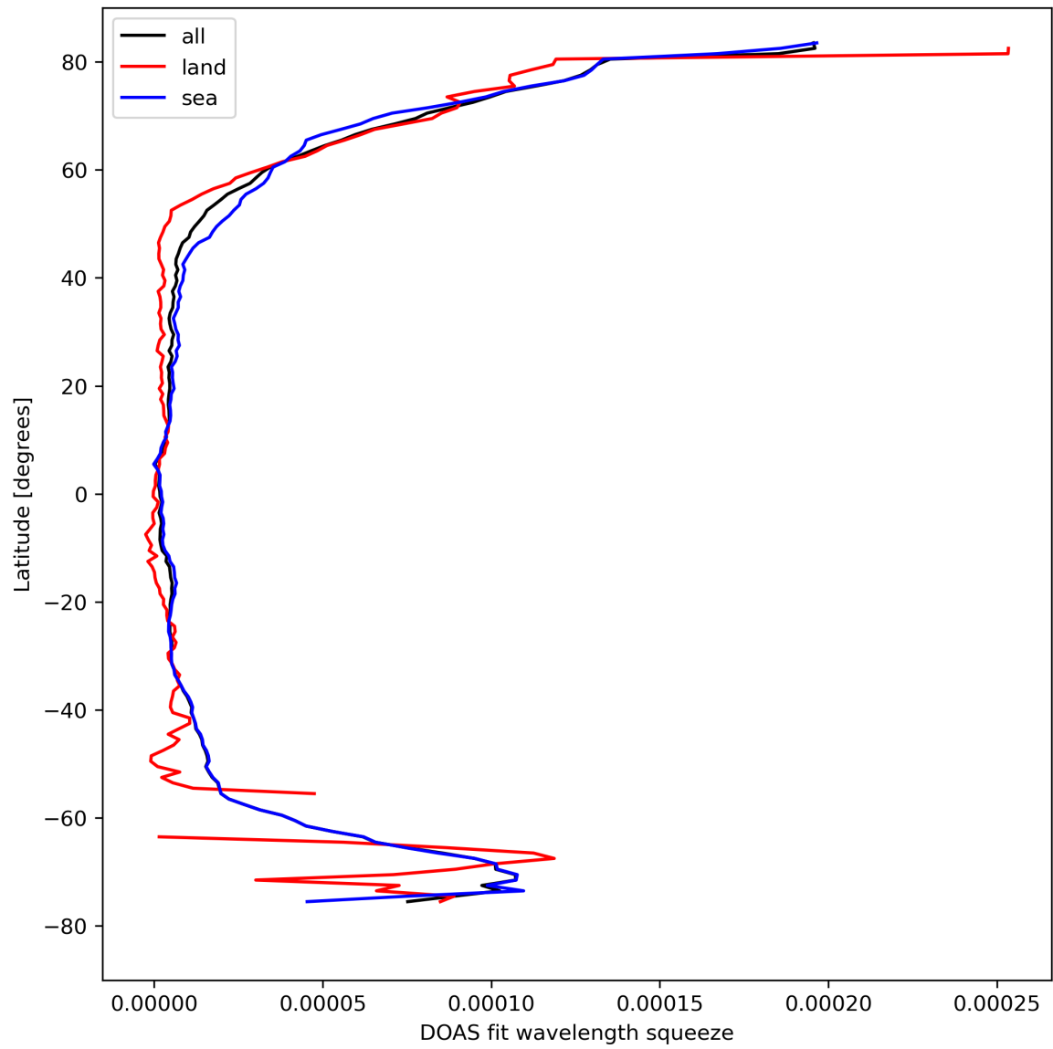
Figure 31: Zonal average of “DOAS fit wavelength squeeze” for 2024-04-11 to 2024-04-13.
