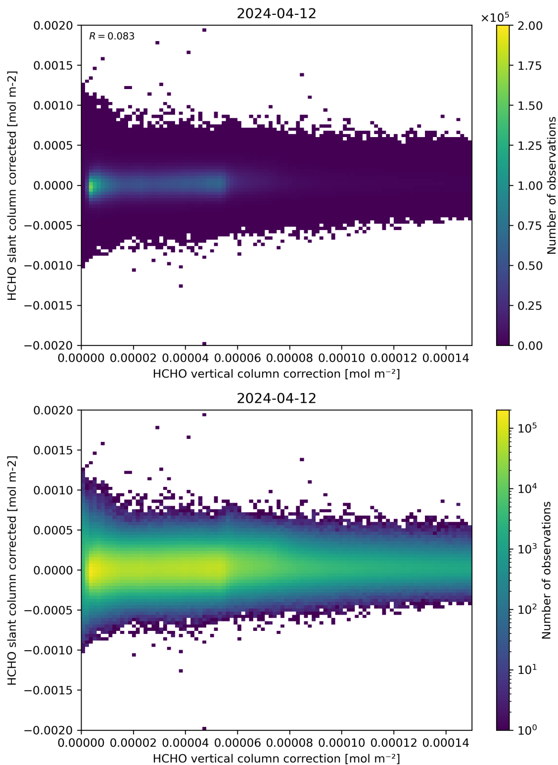
Figure 116: Scatter density plot of “HCHO vertical column correction” against “HCHO slant column corrected” for 2024-04-11 to 2024-04-13.
