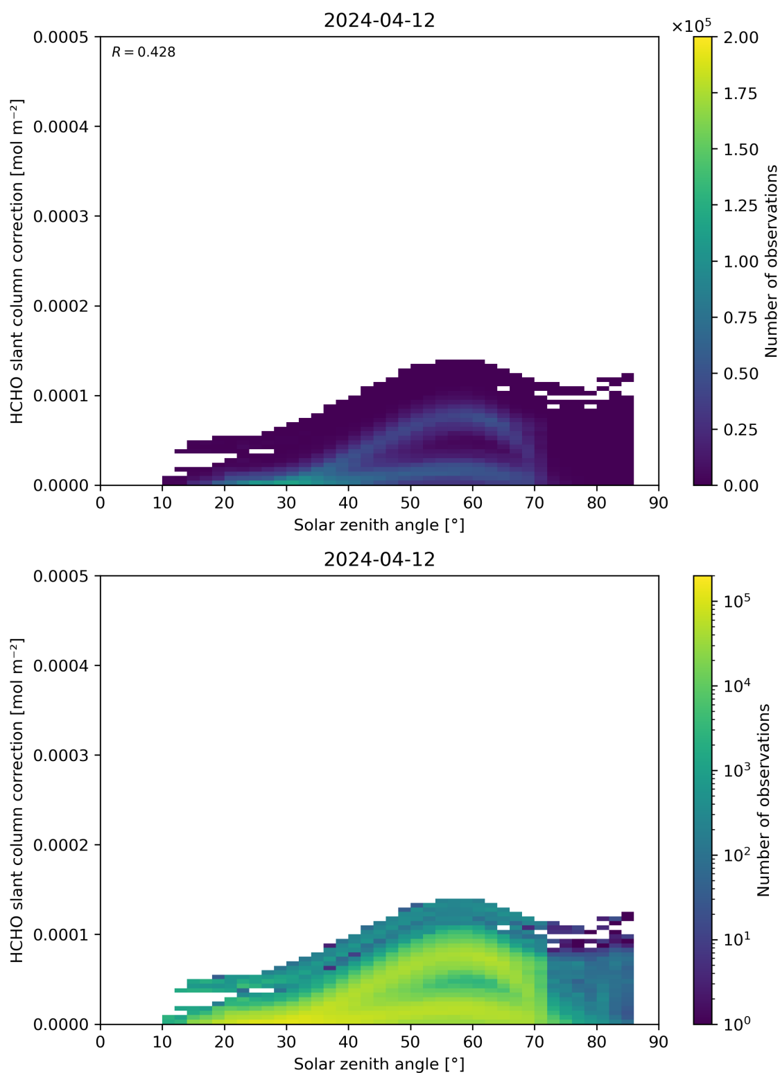
Figure 172: Scatter density plot of “Solar zenith angle” against “HCHO slant column correction” for 2024-04-11 to 2024-04-13.
