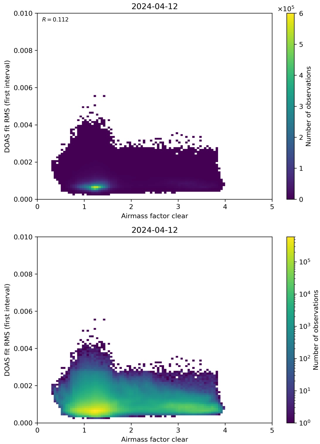
Figure 71: Scatter density plot of “Airmass factor clear” against “DOAS fit RMS (first interval)” for 2024-04-11 to 2024-04-13.
