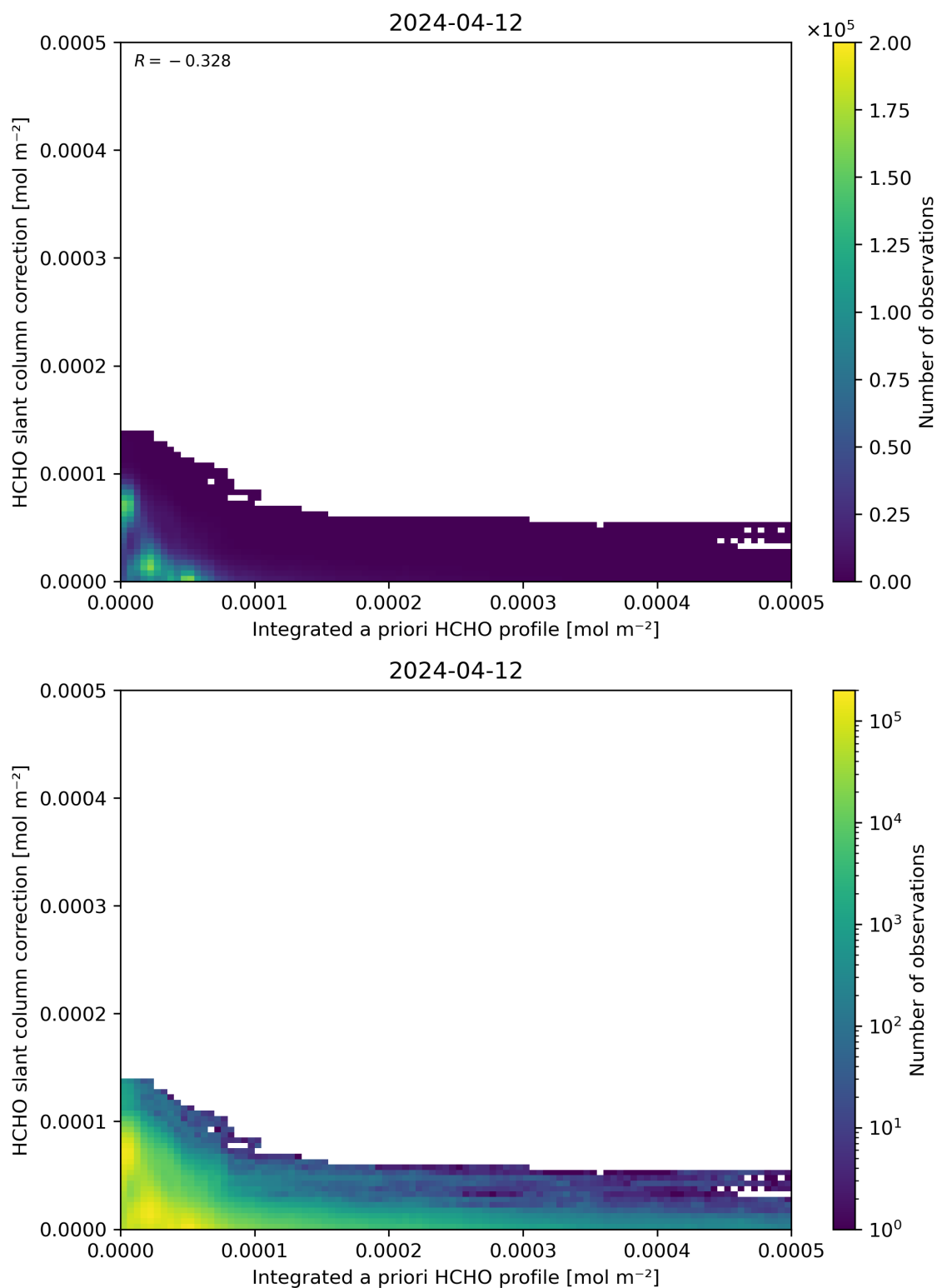
Figure 152: Scatter density plot of “Integrated a priori HCHO profile” against “HCHO slant column correction” for 2024-04-11 to 2024-04-13.
