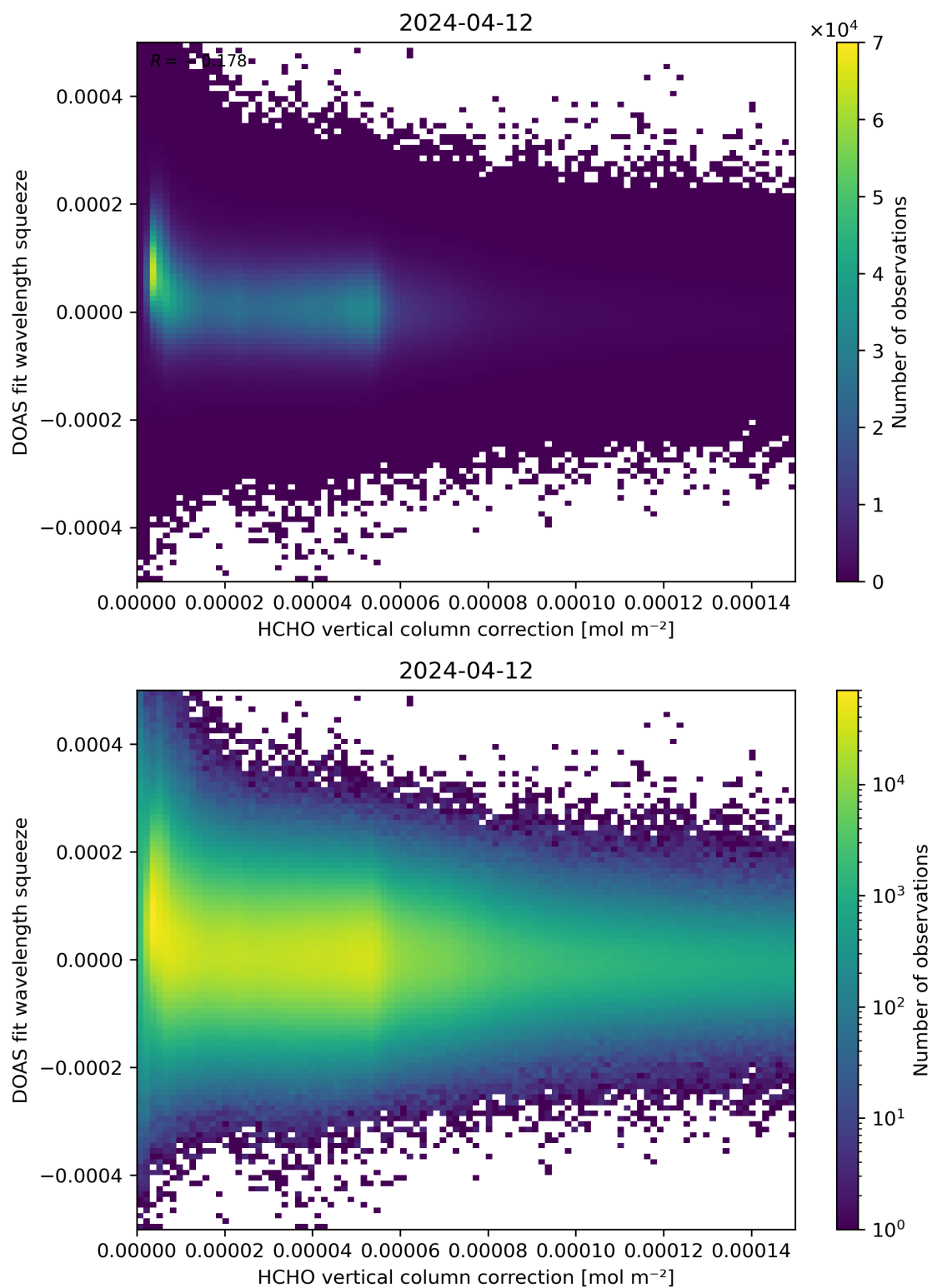
Figure 114: Scatter density plot of “HCHO vertical column correction” against “DOAS fit wavelength squeeze” for 2024-04-11 to 2024-04-13.
