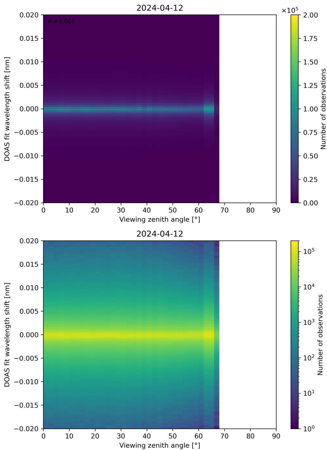
Figure 183: Scatter density plot of “Viewing zenith angle” against “DOAS fit wavelength shift” for 2024-04-11 to 2024-04-13.
