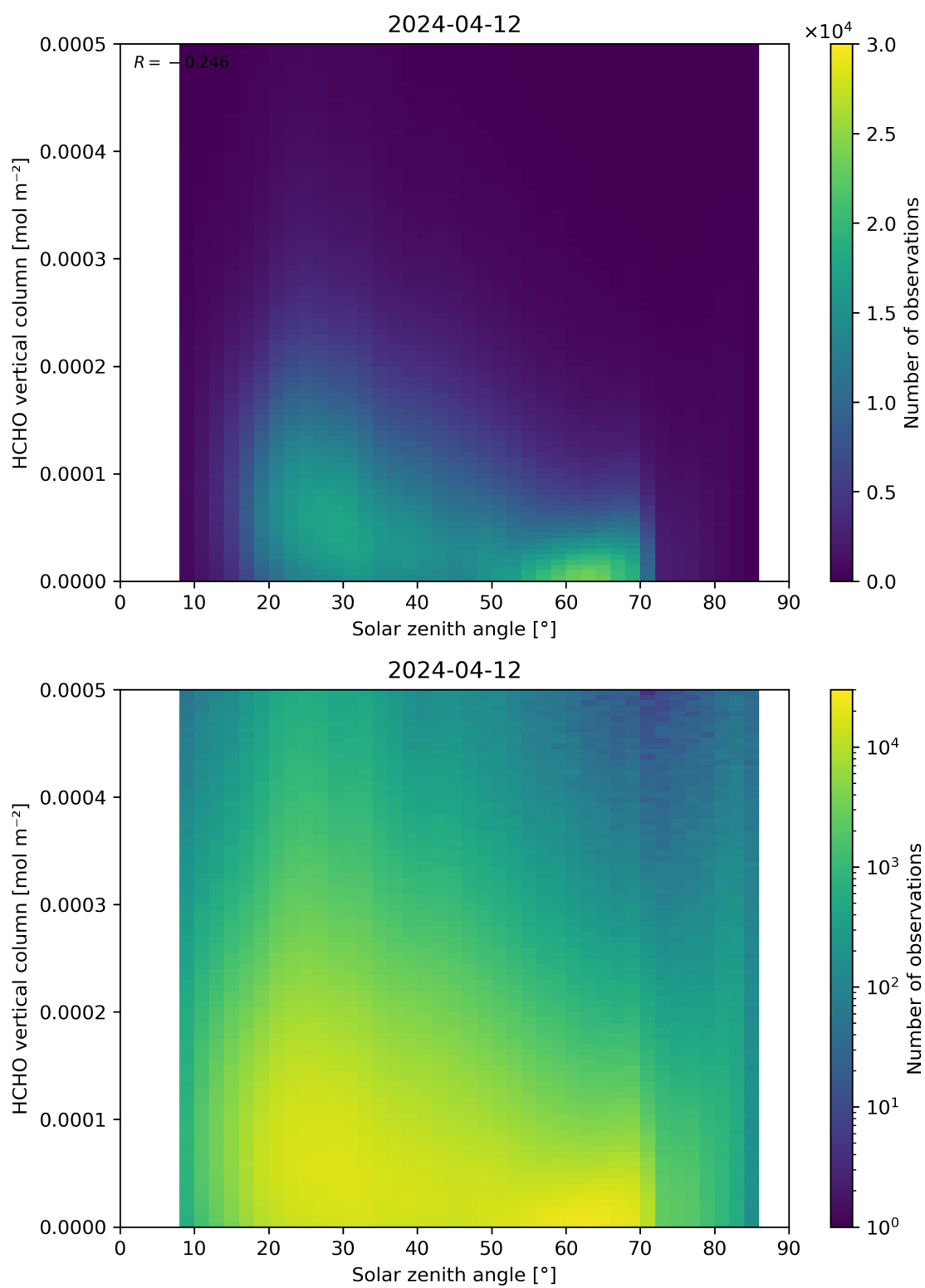
Figure 177: Scatter density plot of “Solar zenith angle” against “HCHO vertical column” for 2024-04-11 to 2024-04-13.
