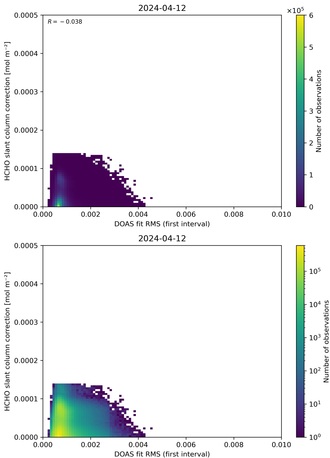
Figure 63: Scatter density plot of “DOAS fit RMS (first interval)” against “HCHO slant column correction” for 2024-04-11 to 2024-04-13.
