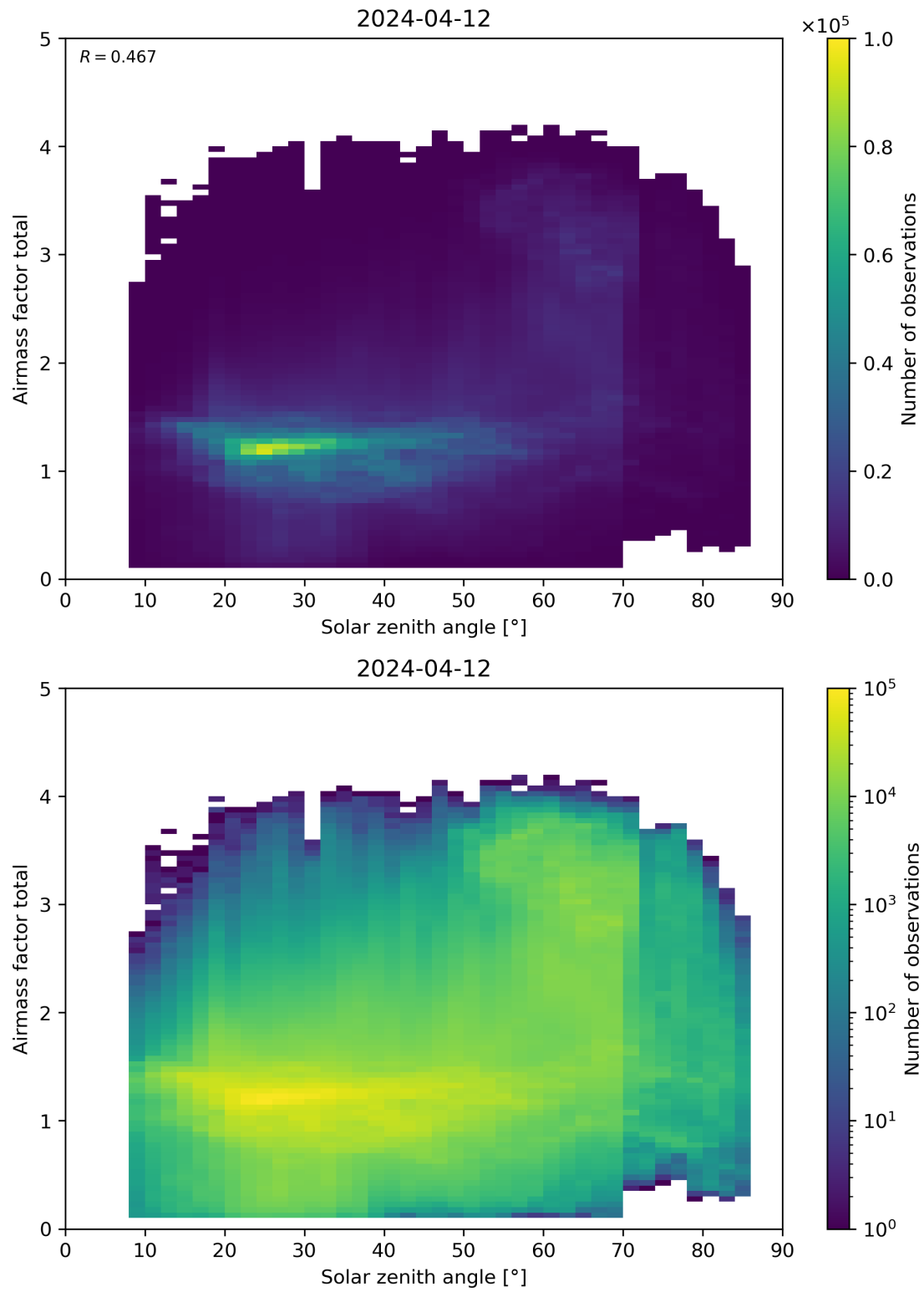
Figure 175: Scatter density plot of “Solar zenith angle” against “Airmass factor total” for 2024-04-11 to 2024-04-13.
