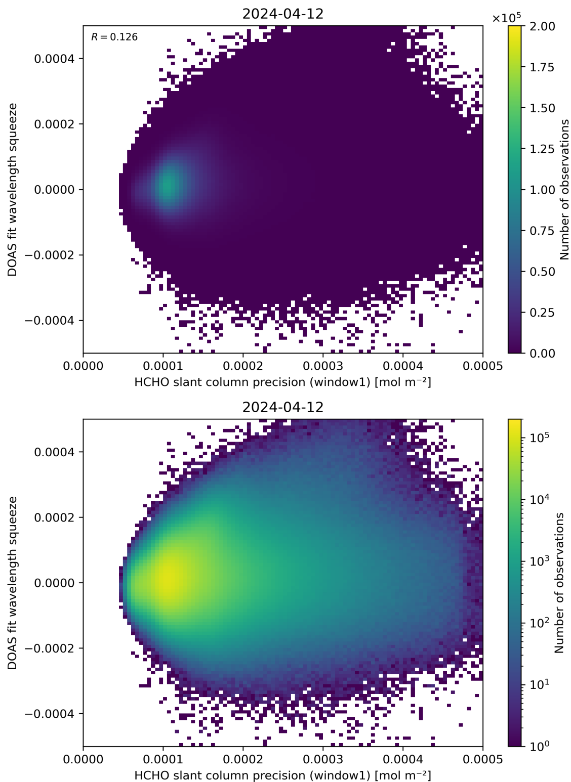
Figure 90: Scatter density plot of “HCHO slant column precision (window1)” against “DOAS fit wavelength squeeze” for 2024-04-11 to 2024-04-13.
