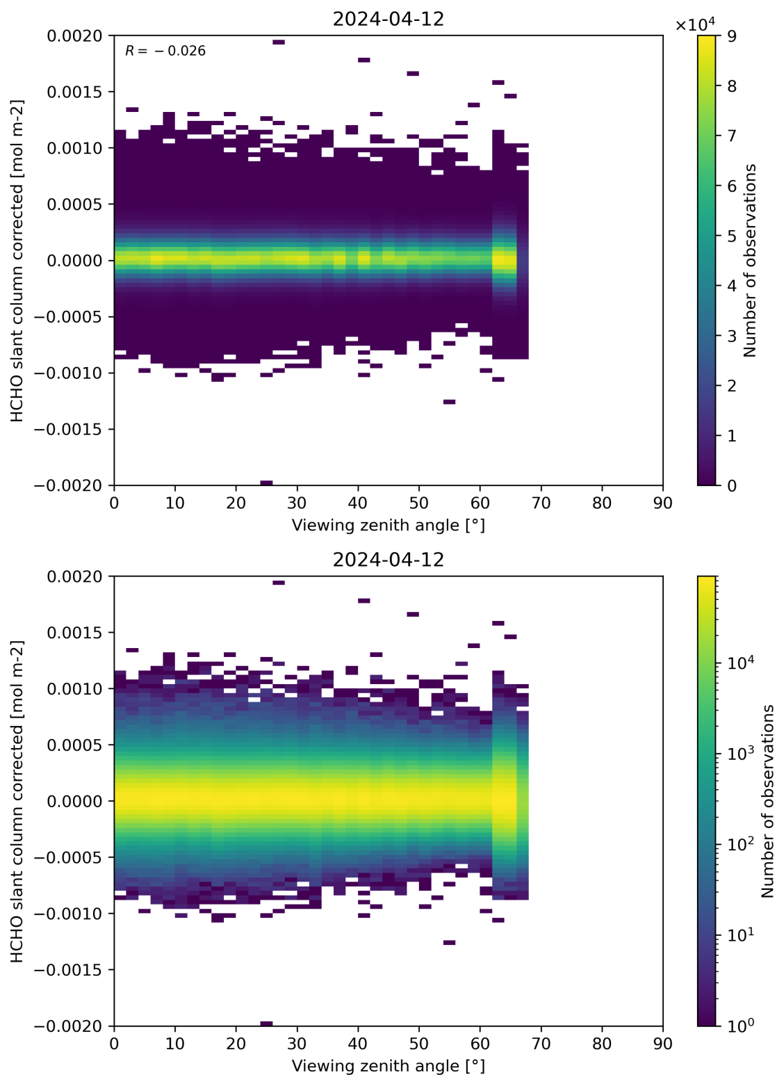
Figure 186: Scatter density plot of “Viewing zenith angle” against “HCHO slant column corrected” for 2024-04-11 to 2024-04-13.
