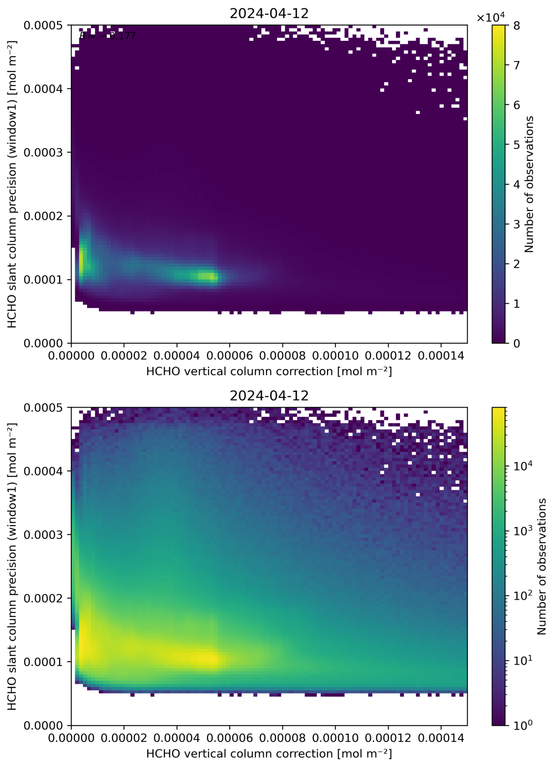
Figure 119: Scatter density plot of “HCHO vertical column correction” against “HCHO slant column precision (window1)” for 2024-04-11 to 2024-04-13.
