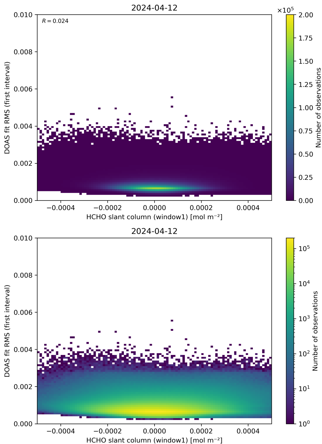
Figure 78: Scatter density plot of “HCHO slant column (window1)” against “DOAS fit RMS (first interval)” for 2024-04-11 to 2024-04-13.
