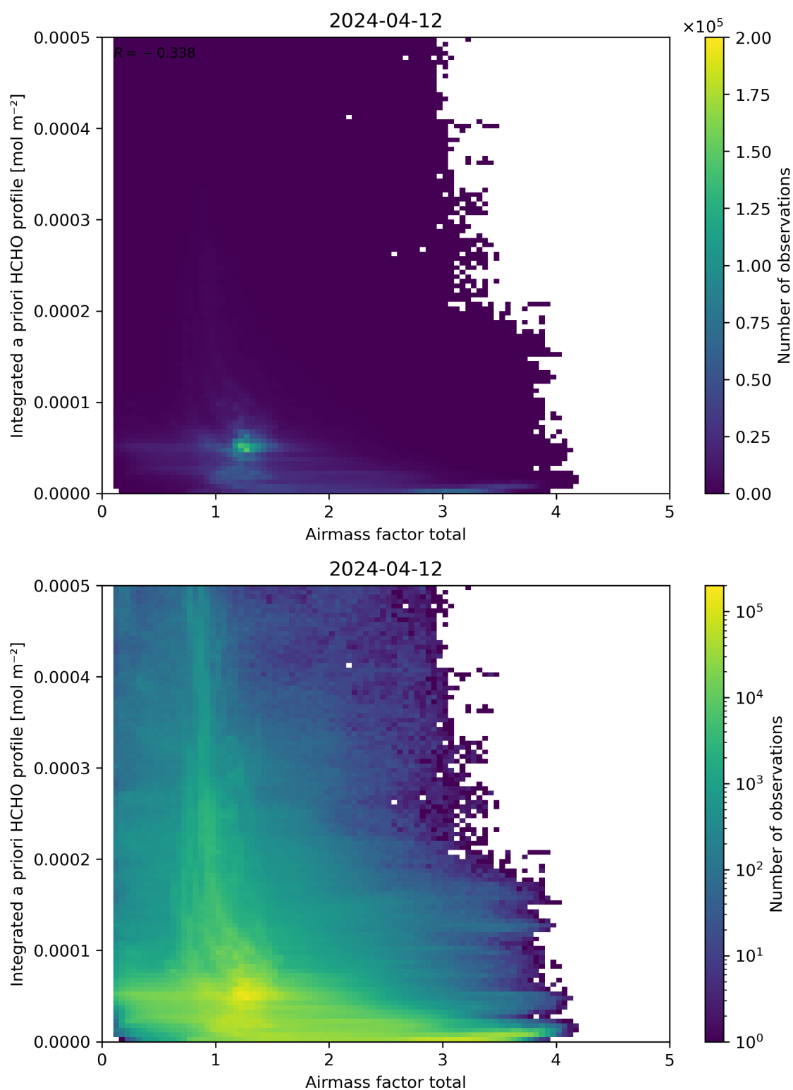
Figure 104: Scatter density plot of “Airmass factor total” against “Integrated a priori HCHO profile” for 2024-04-11 to 2024-04-13.
