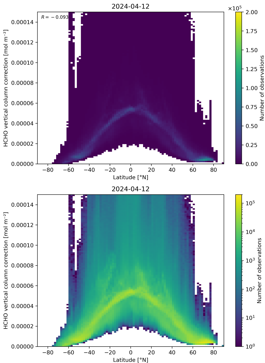
Figure 164: Scatter density plot of “Latitude” against “HCHO vertical column correction” for 2024-04-11 to 2024-04-13.
