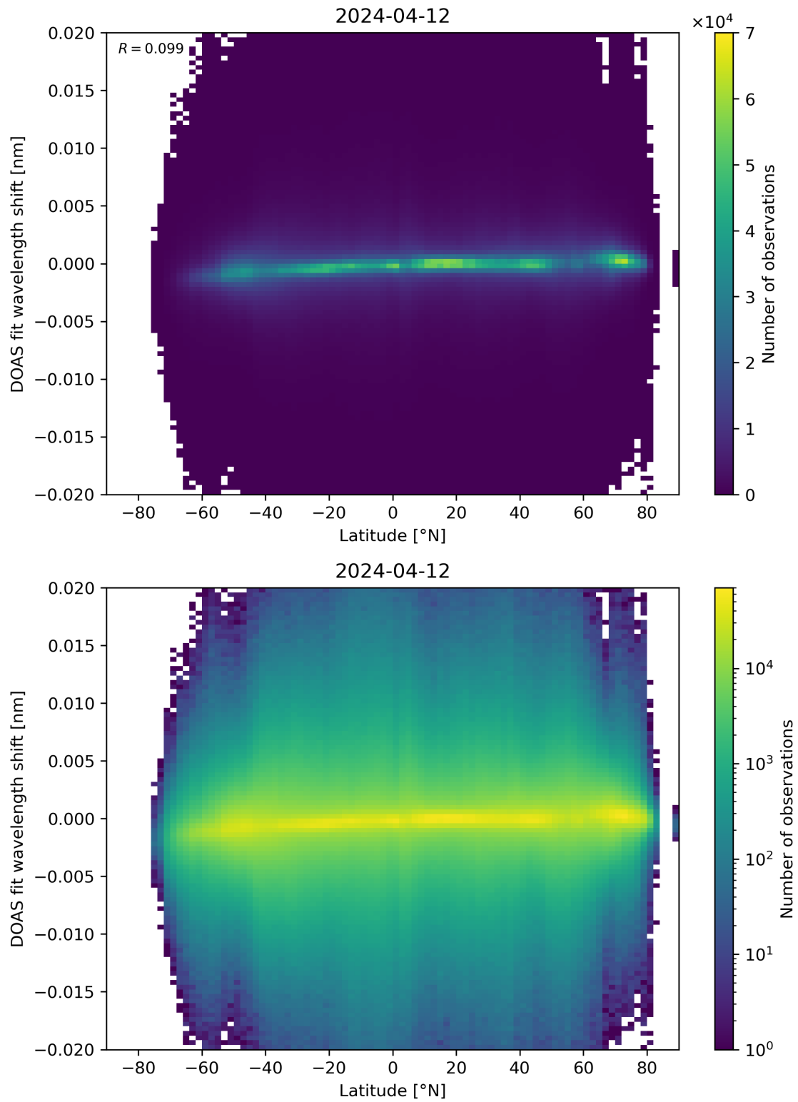
Figure 154: Scatter density plot of “Latitude” against “DOAS fit wavelength shift” for 2024-04-11 to 2024-04-13.
