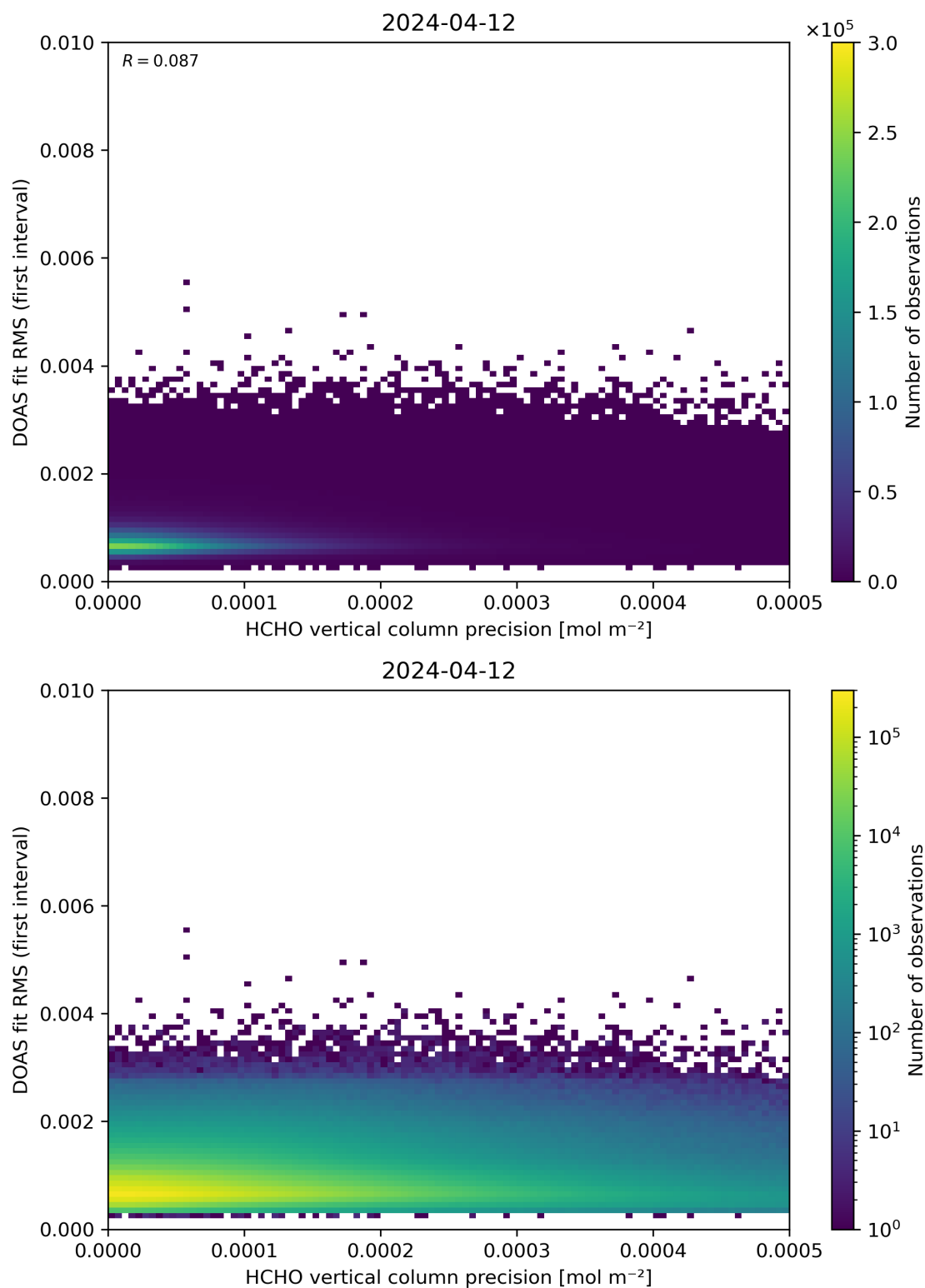
Figure 136: Scatter density plot of “HCHO vertical column precision” against “DOAS fit RMS (first interval)” for 2024-04-11 to 2024-04-13.
