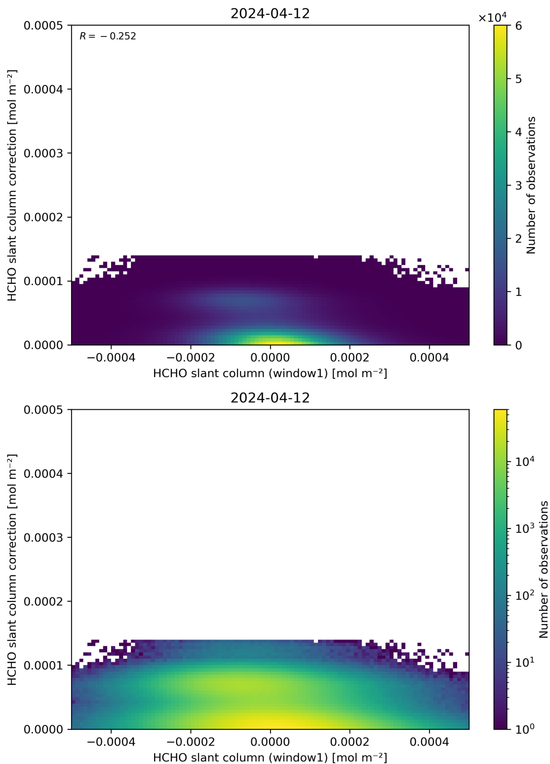
Figure 83: Scatter density plot of “HCHO slant column (window1)” against “HCHO slant column correction” for 2024-04-11 to 2024-04-13.
