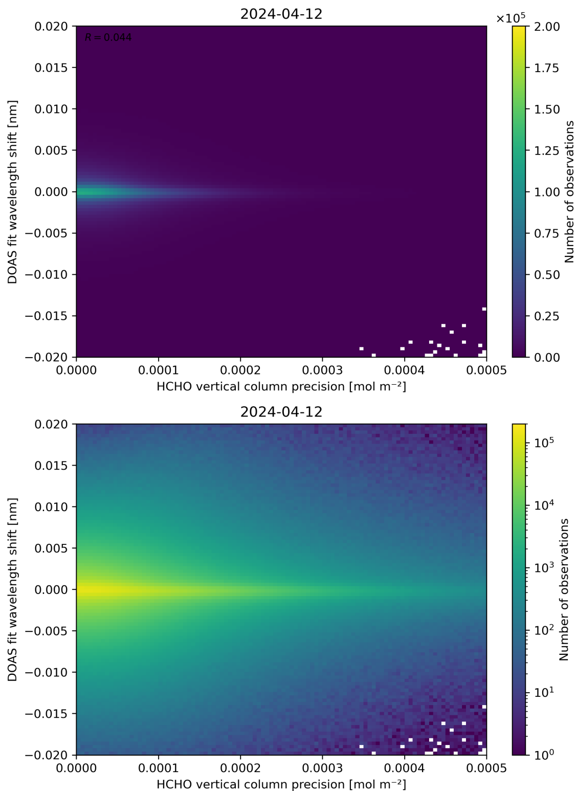
Figure 137: Scatter density plot of “HCHO vertical column precision” against “DOAS fit wavelength shift” for 2024-04-11 to 2024-04-13.
