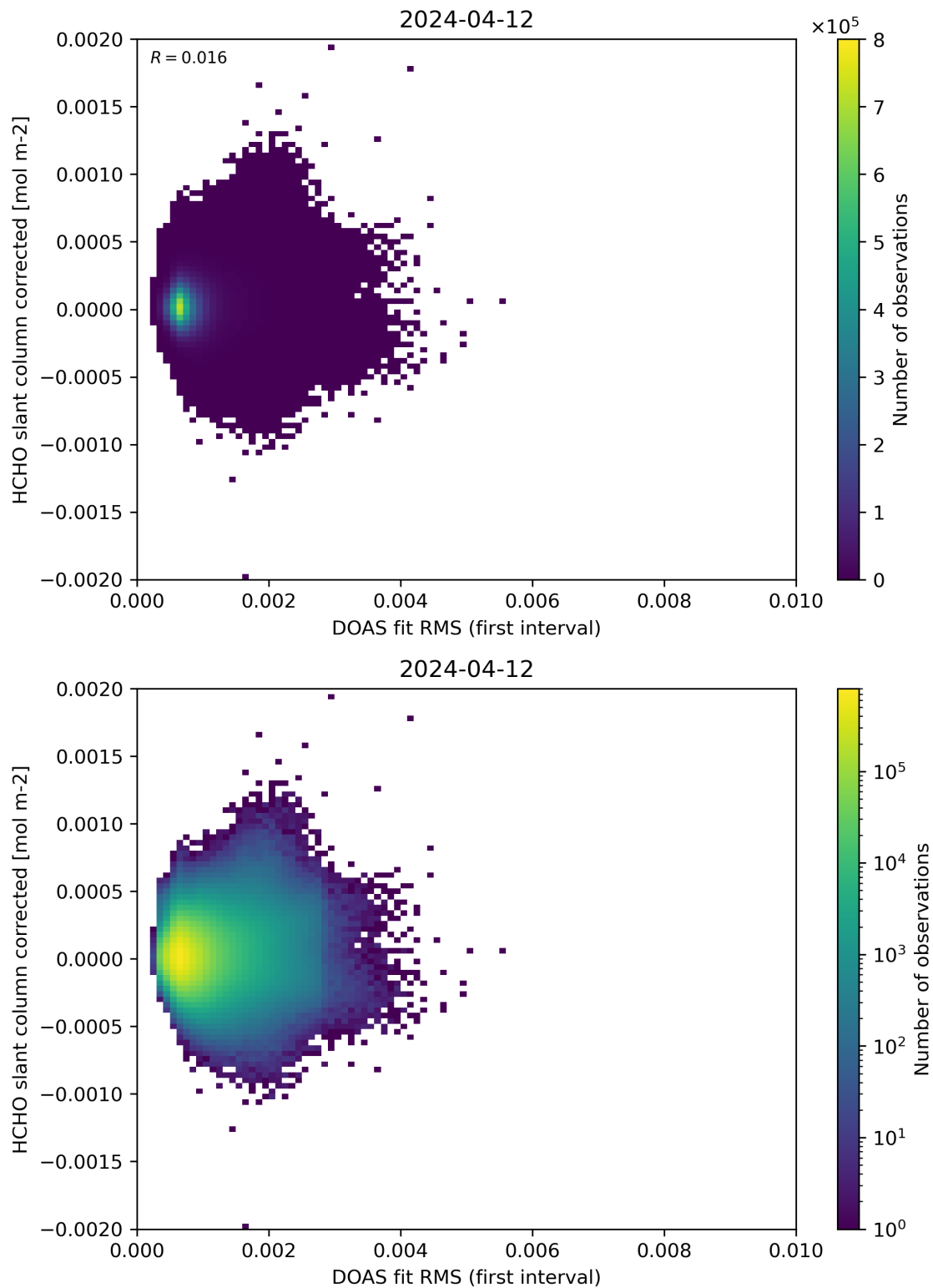
Figure 62: Scatter density plot of “DOAS fit RMS (first interval)” against “HCHO slant column corrected” for 2024-04-11 to 2024-04-13.
