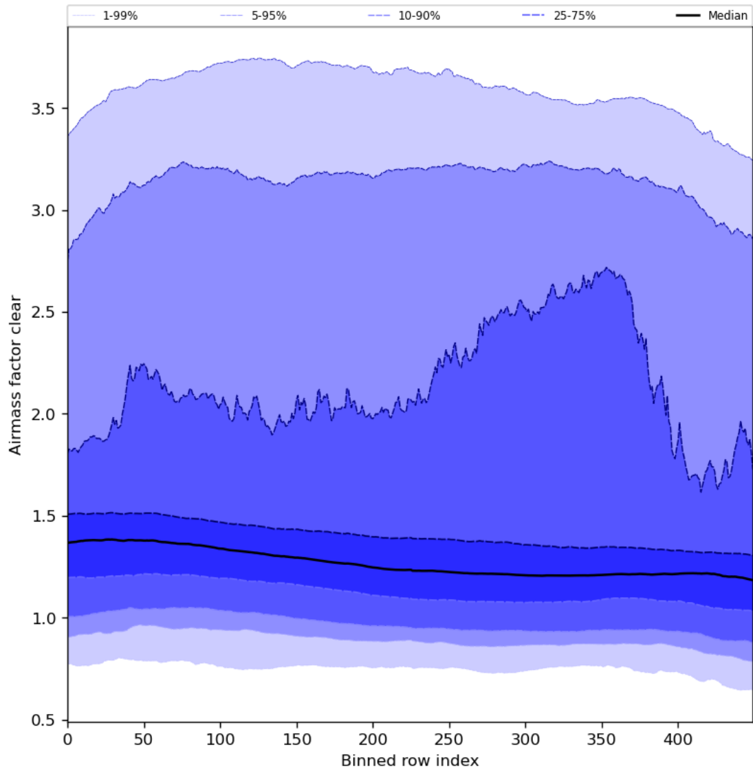
Figure 56: Along track statistics of “Airmass factor clear” for 2024-04-11 to 2024-04-13
