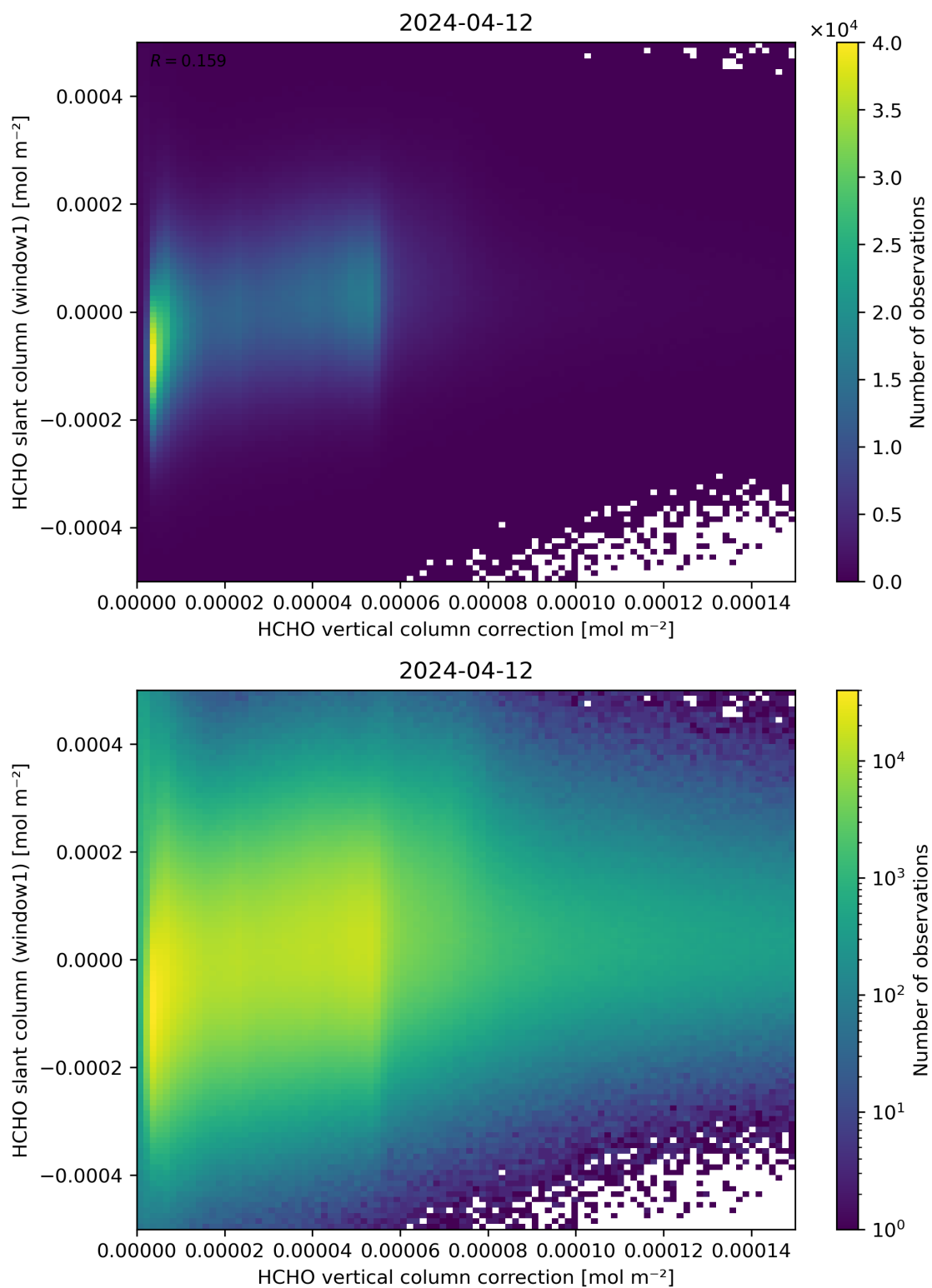
Figure 118: Scatter density plot of “HCHO vertical column correction” against “HCHO slant column (window1)” for 2024-04-11 to 2024-04-13.
