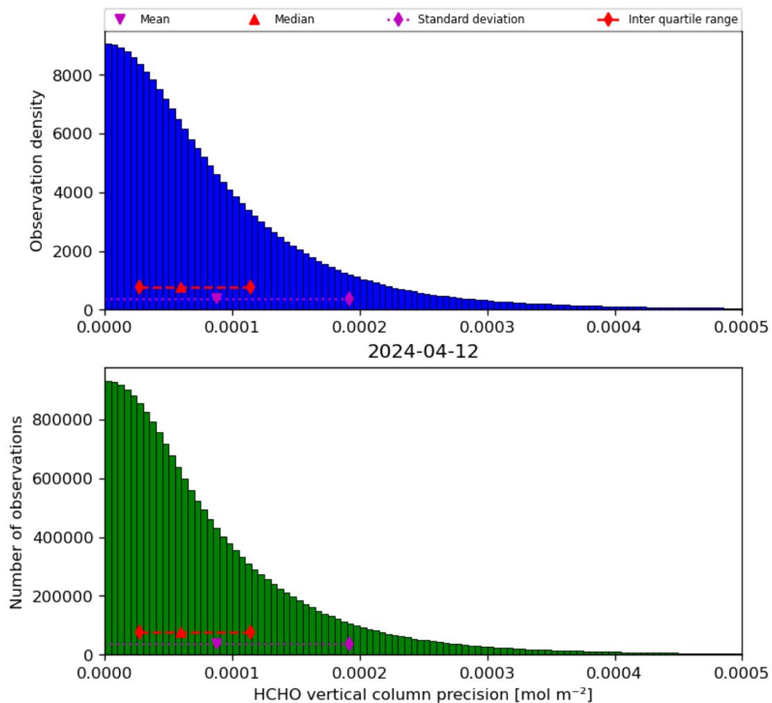
Figure 36: Histogram of “HCHO vertical column precision” for 2024-04-11 to 2024-04-13
