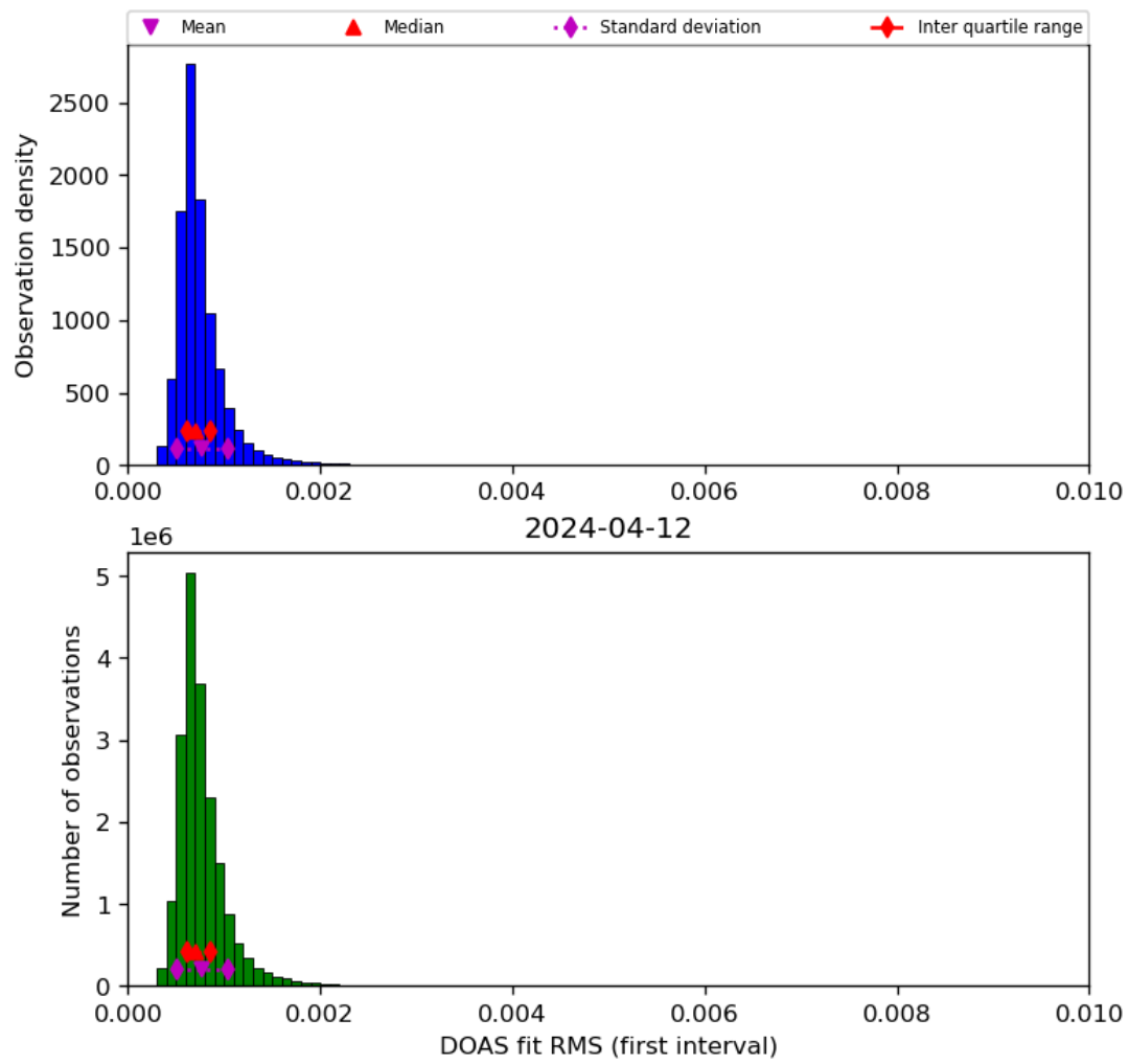
Figure 46: Histogram of “DOAS fit RMS (first interval)” for 2024-04-11 to 2024-04-13
