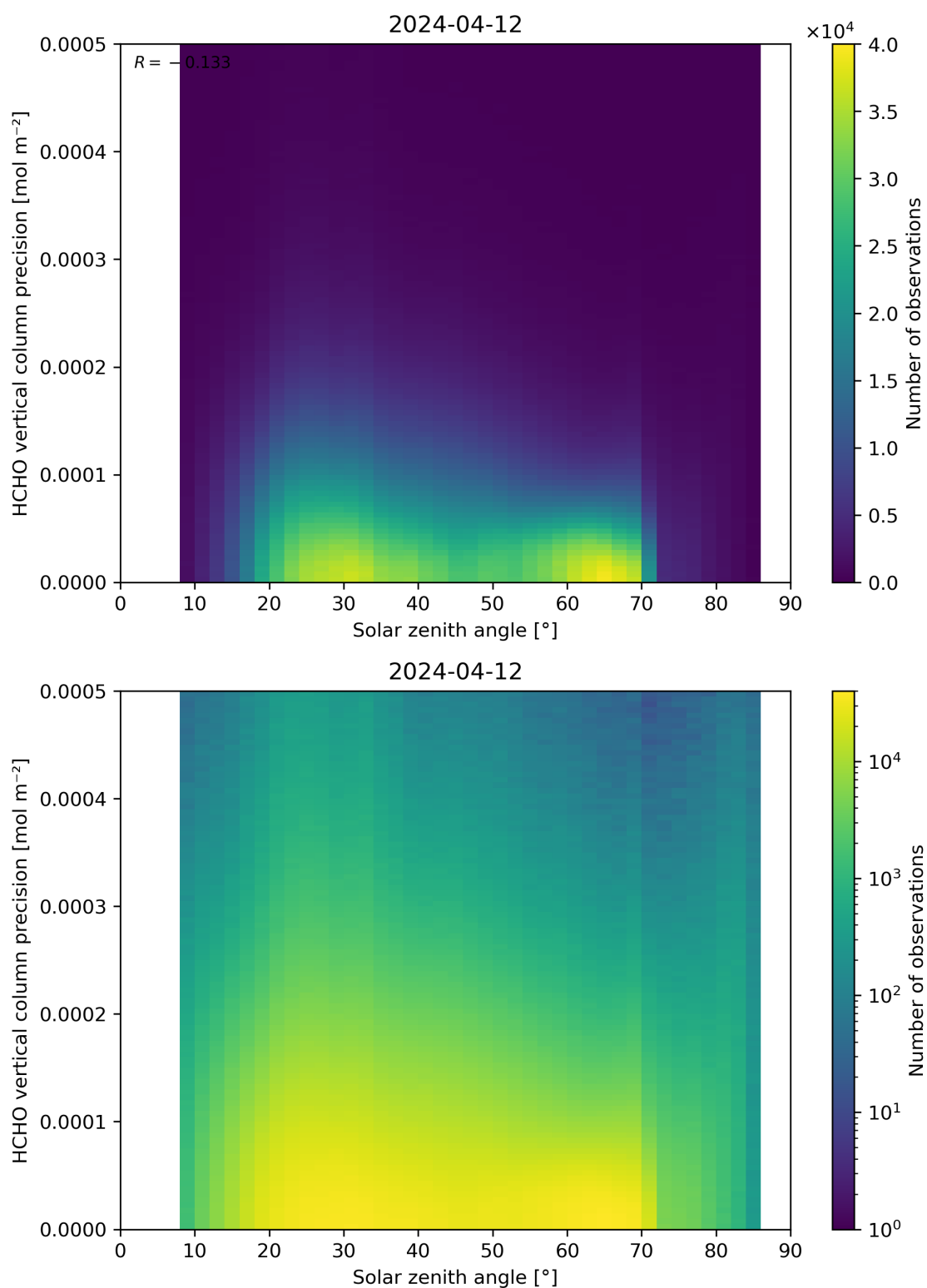
Figure 179: Scatter density plot of “Solar zenith angle” against “HCHO vertical column precision” for 2024-04-11 to 2024-04-13.
