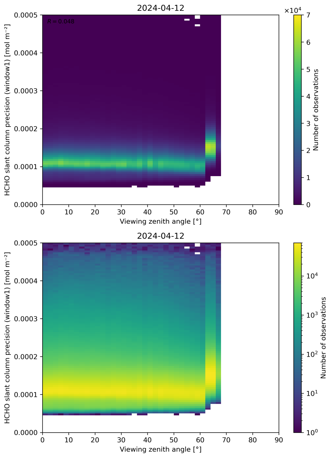
Figure 189: Scatter density plot of “Viewing zenith angle” against “HCHO slant column precision (window1)” for 2024-04-11 to 2024-04-13.
