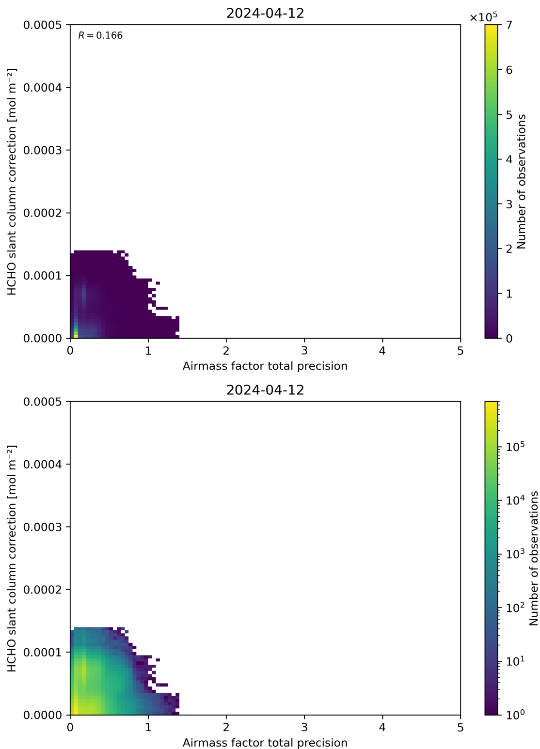
Figure 110: Scatter density plot of “Airmass factor total precision” against “HCHO slant column correction” for 2024-04-11 to 2024-04-13.
