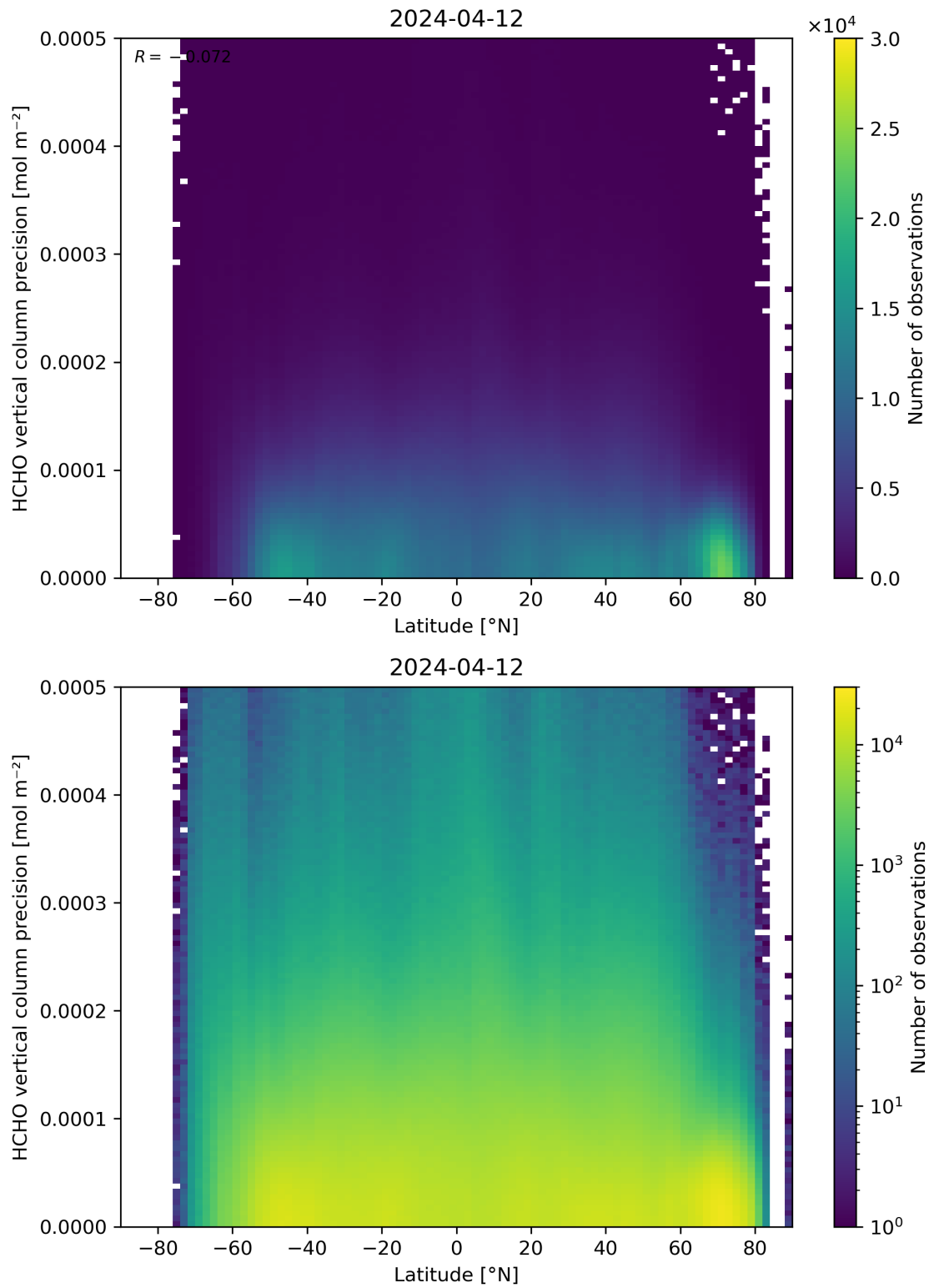
Figure 165: Scatter density plot of “Latitude” against “HCHO vertical column precision” for 2024-04-11 to 2024-04-13.
