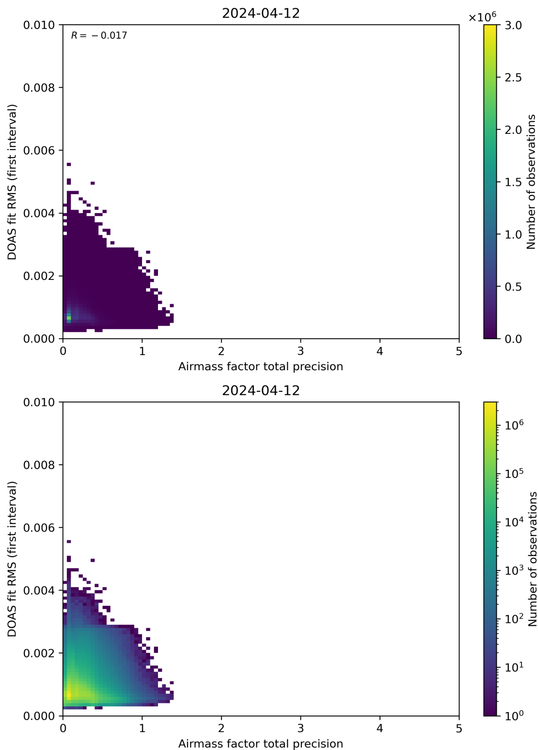
Figure 105: Scatter density plot of “Airmass factor total precision” against “DOAS fit RMS (first interval)” for 2024-04-11 to 2024-04-13.
