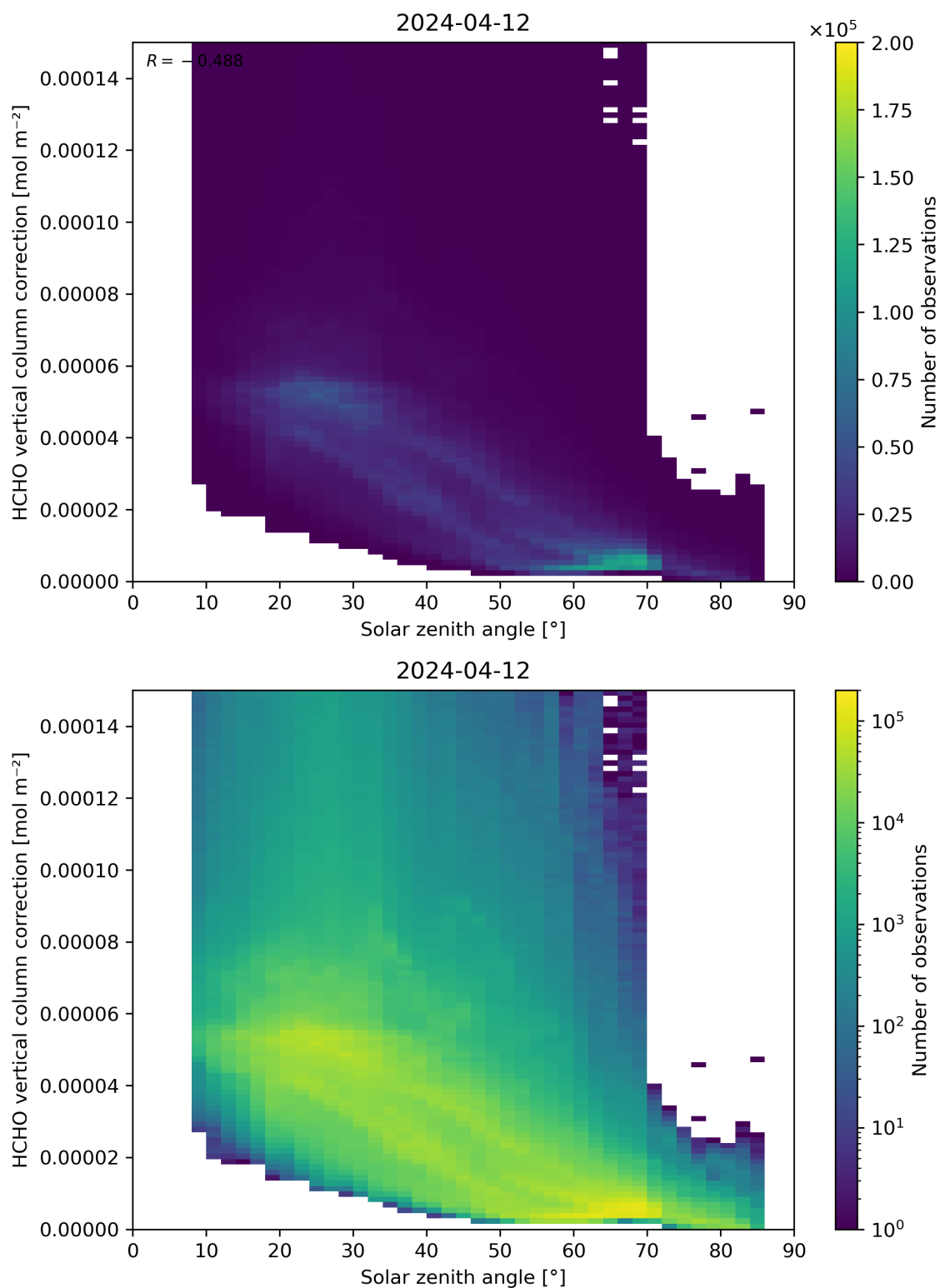
Figure 178: Scatter density plot of “Solar zenith angle” against “HCHO vertical column correction” for 2024-04-11 to 2024-04-13.
