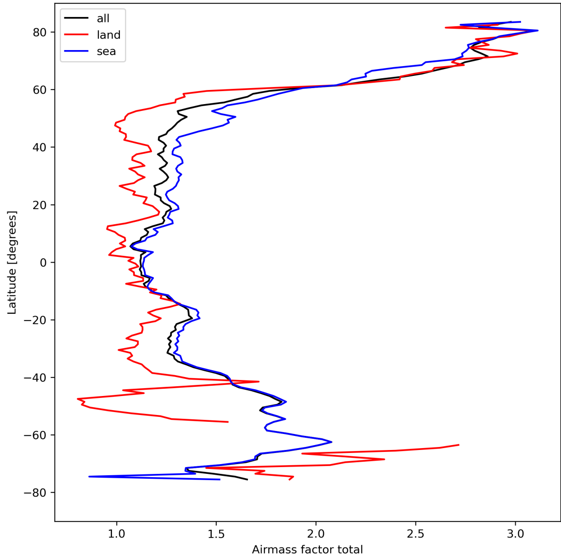
Figure 26: Zonal average of “Airmass factor total” for 2024-04-11 to 2024-04-13.
