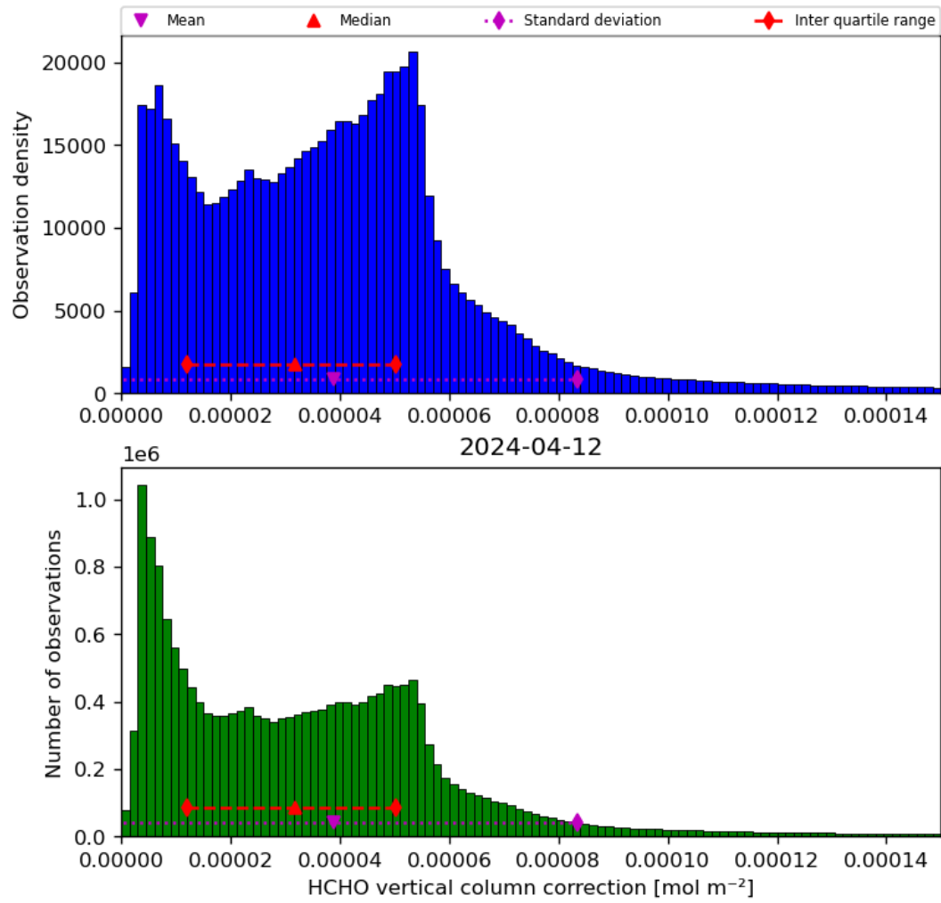
Figure 37: Histogram of “HCHO vertical column correction” for 2024-04-11 to 2024-04-13
