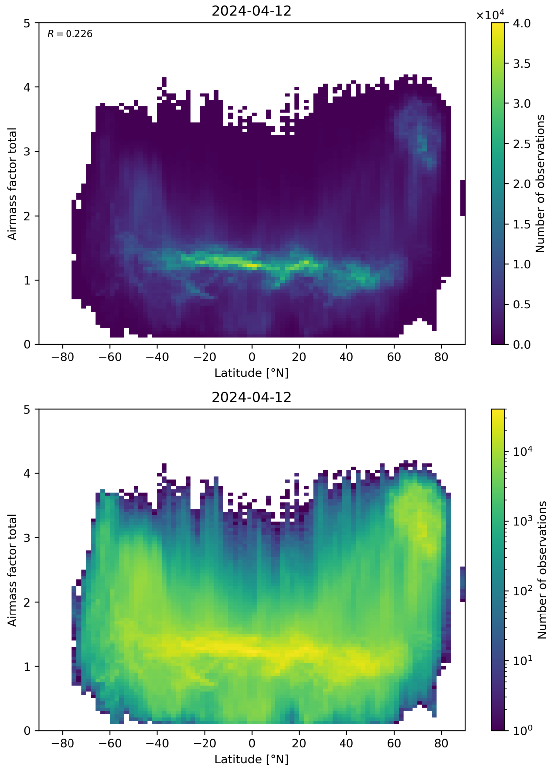
Figure 161: Scatter density plot of “Latitude” against “Airmass factor total” for 2024-04-11 to 2024-04-13.
