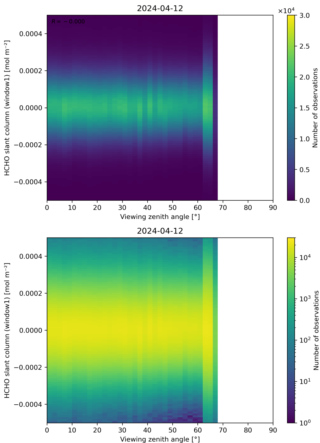
Figure 188: Scatter density plot of “Viewing zenith angle” against “HCHO slant column (window1)” for 2024-04-11 to 2024-04-13.
