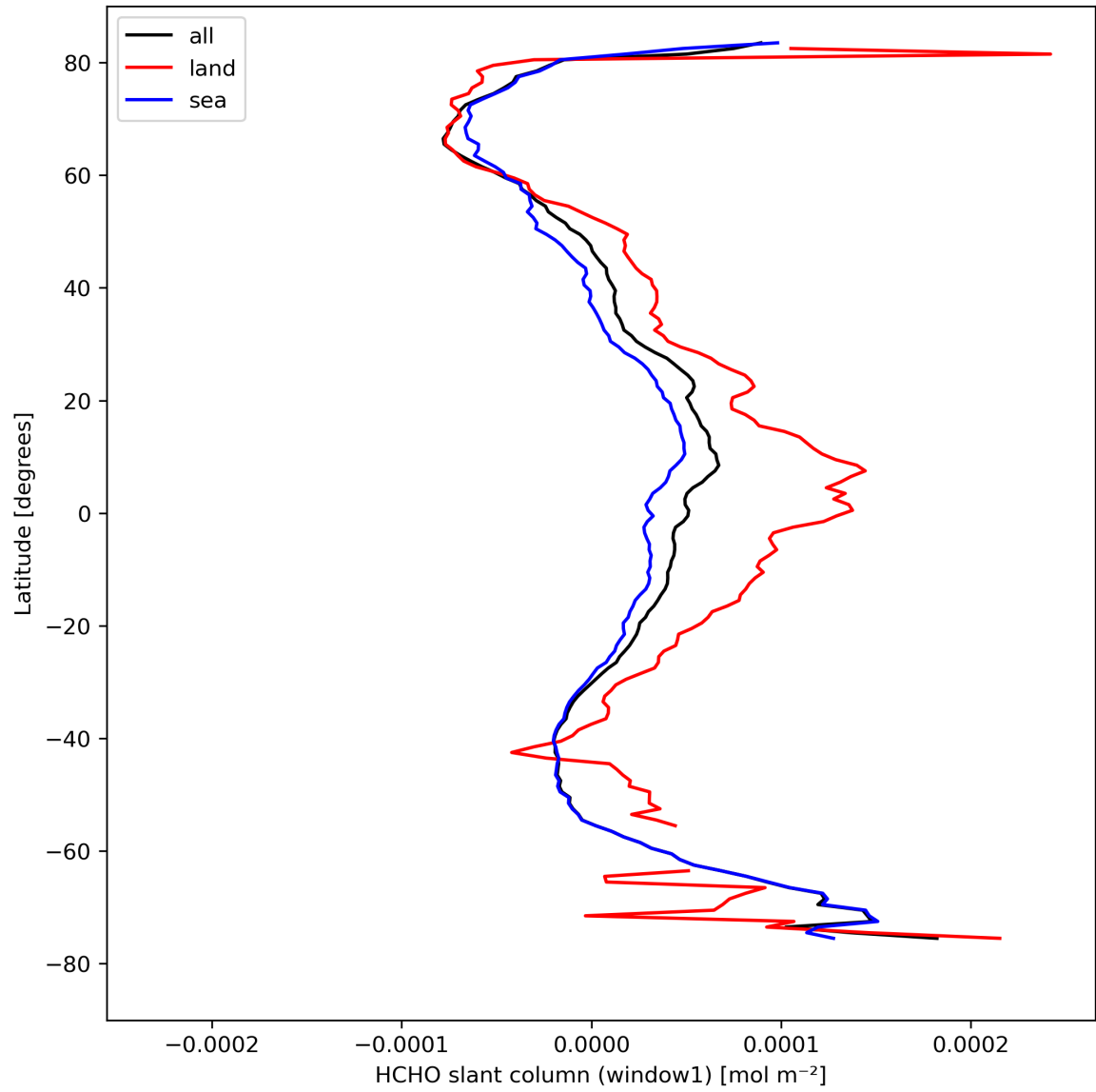
Figure 24: Zonal average of “HCHO slant column (window1)” for 2024-04-11 to 2024-04-13.
