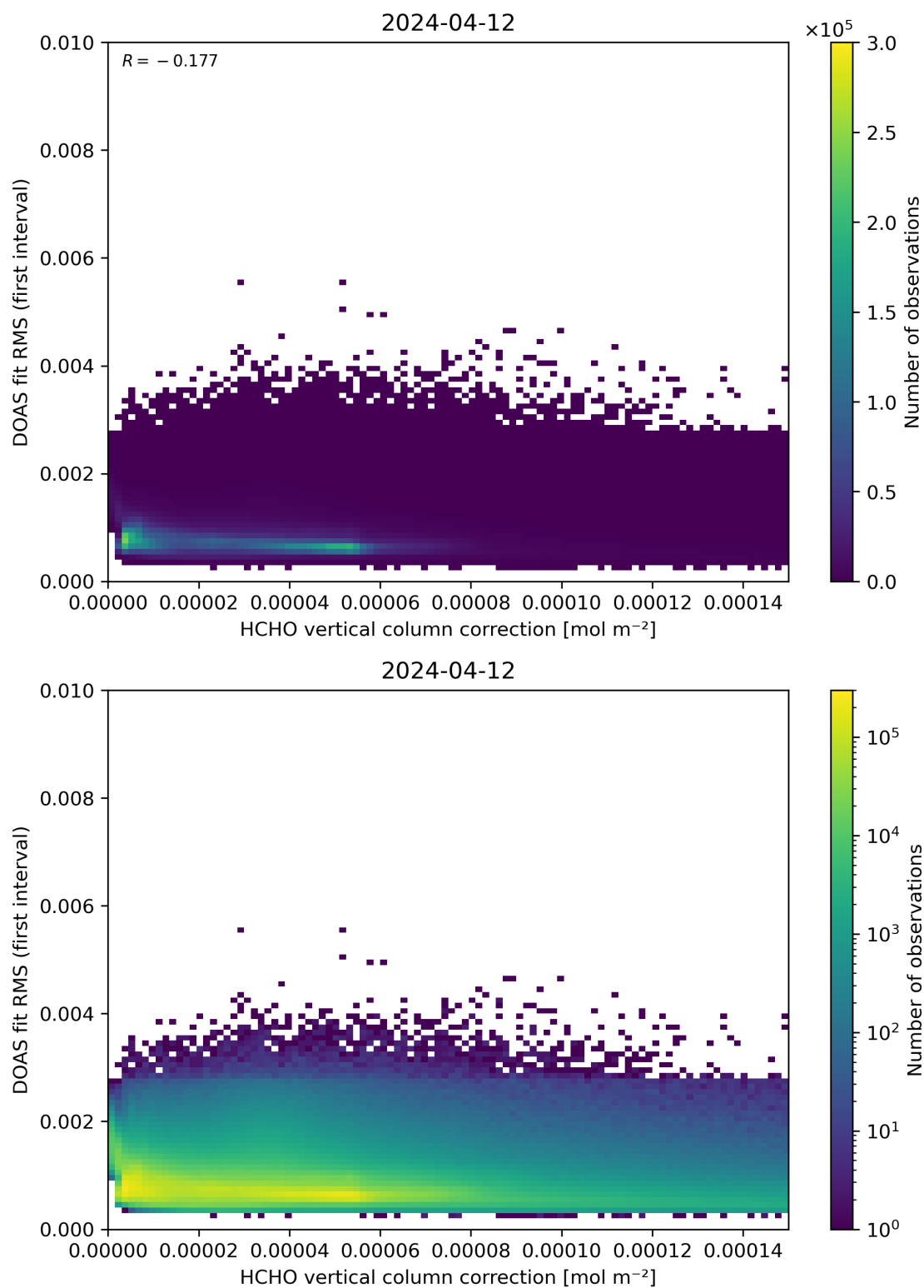
Figure 112: Scatter density plot of “HCHO vertical column correction” against “DOAS fit RMS (first interval)” for 2024-04-11 to 2024-04-13.
