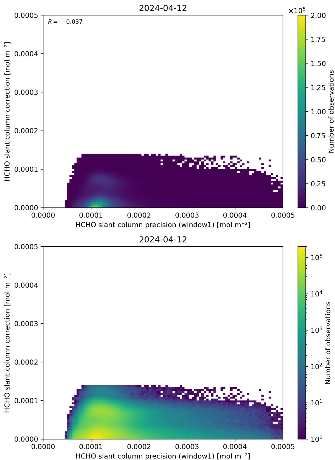
Figure 93: Scatter density plot of “HCHO slant column precision (window1)” against “HCHO slant column correction” for 2024-04-11 to 2024-04-13.
