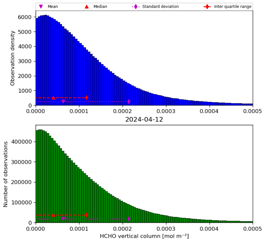
Figure 35: Histogram of “HCHO vertical column” for 2024-04-11 to 2024-04-13
