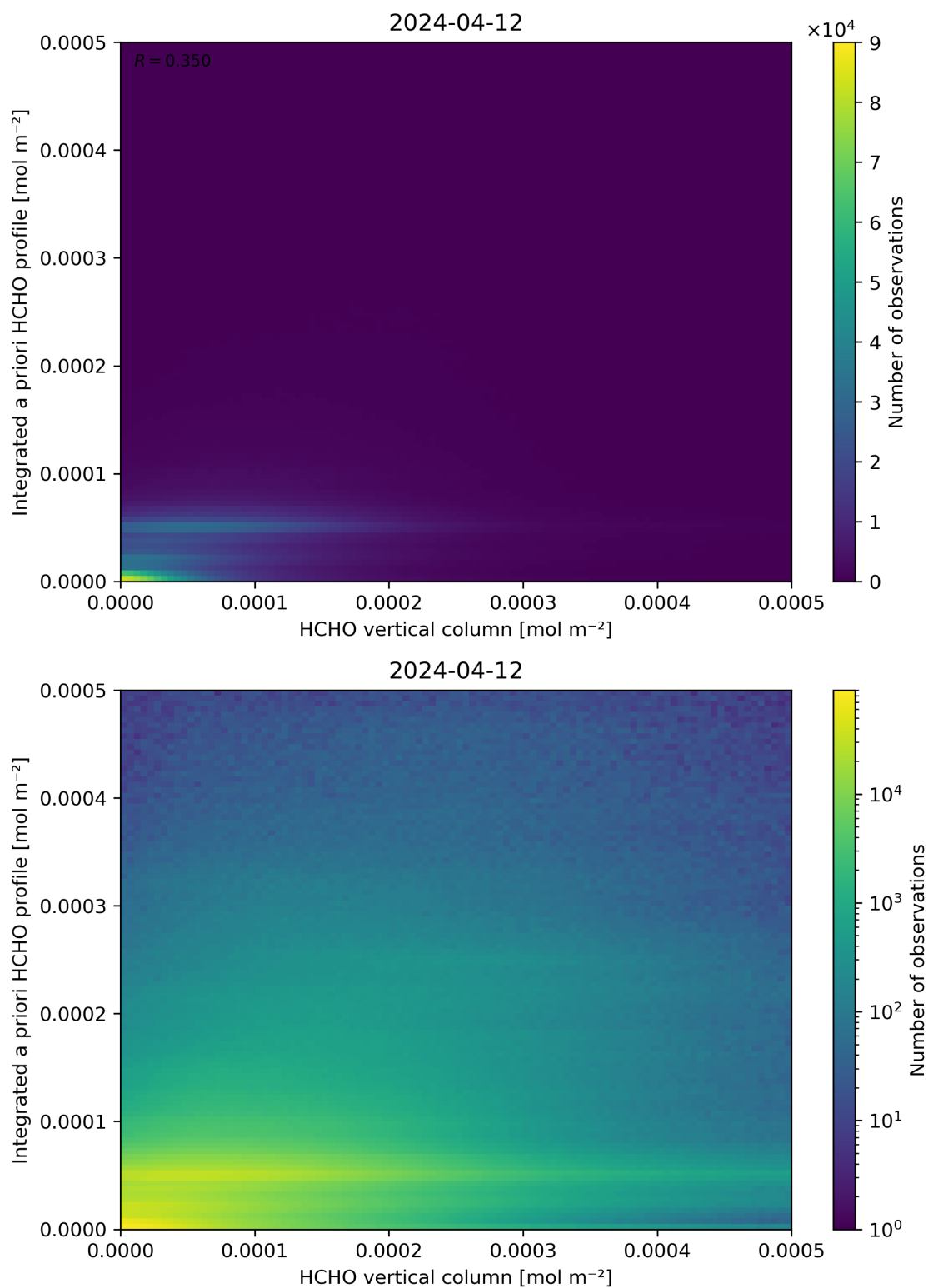
Figure 135: Scatter density plot of “HCHO vertical column” against “Integrated a priori HCHO profile” for 2024-04-11 to 2024-04-13.
