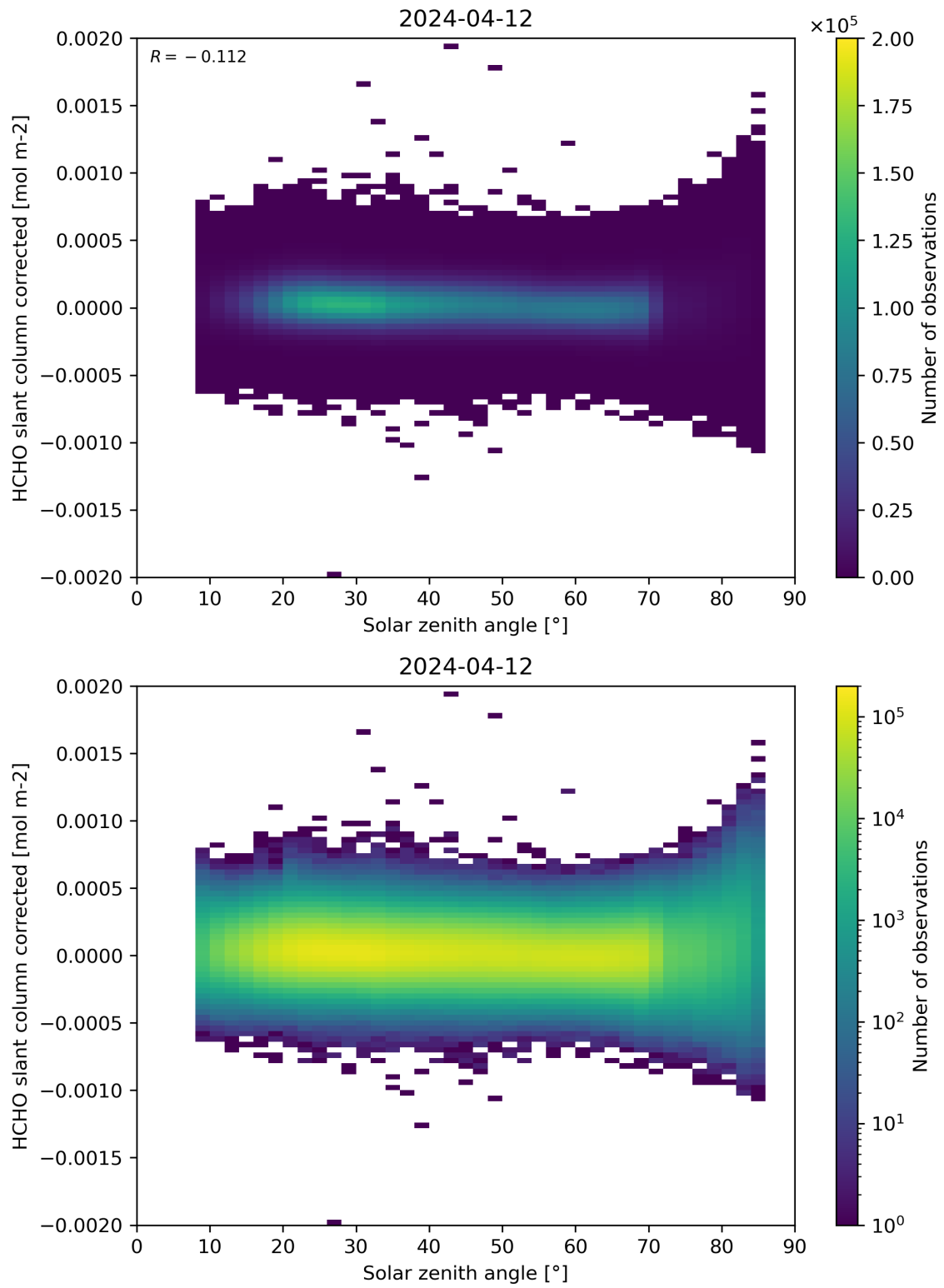
Figure 171: Scatter density plot of “Solar zenith angle” against “HCHO slant column corrected” for 2024-04-11 to 2024-04-13.
