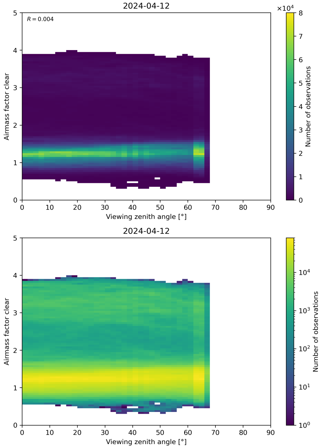
Figure 185: Scatter density plot of “Viewing zenith angle” against “Airmass factor clear” for 2024-04-11 to 2024-04-13.
