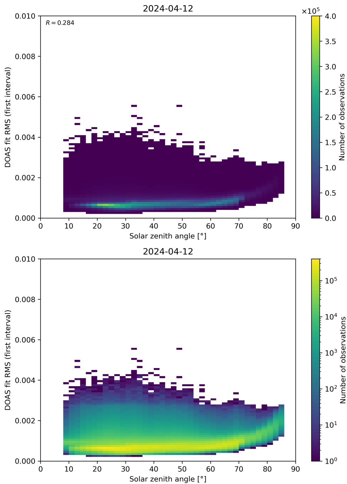
Figure 167: Scatter density plot of “Solar zenith angle” against “DOAS fit RMS (first interval)” for 2024-04-11 to 2024-04-13.
