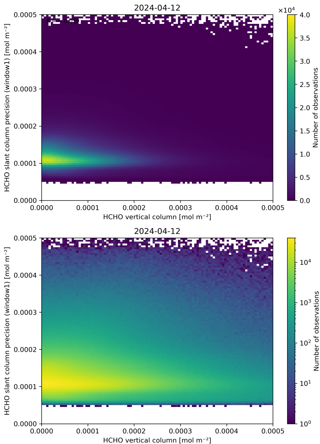
Figure 130: Scatter density plot of “HCHO vertical column” against “HCHO slant column precision (window1)” for 2024-04-11 to 2024-04-13.
