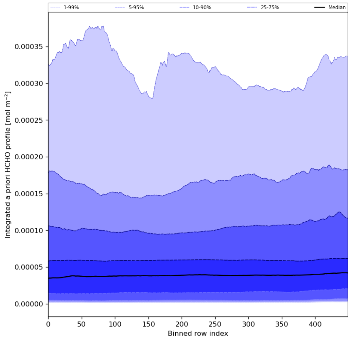
Figure 57: Along track statistics of “Integrated a priori HCHO profile” for 2024-04-11 to 2024-04-13
