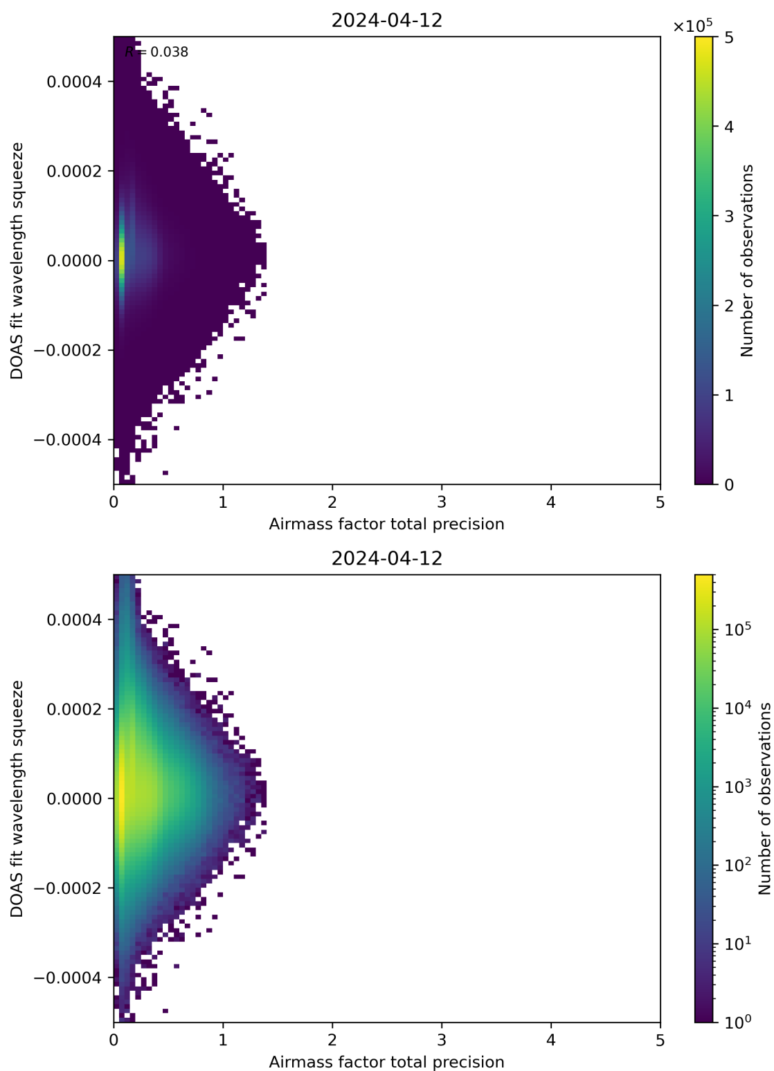
Figure 107: Scatter density plot of “Airmass factor total precision” against “DOAS fit wavelength squeeze” for 2024-04-11 to 2024-04-13.
