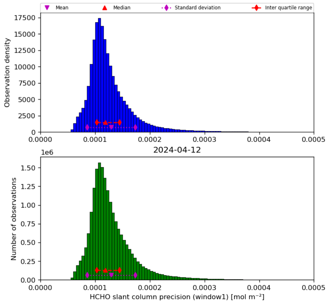
Figure 39: Histogram of “HCHO slant column precision (window1)” for 2024-04-11 to 2024-04-13
