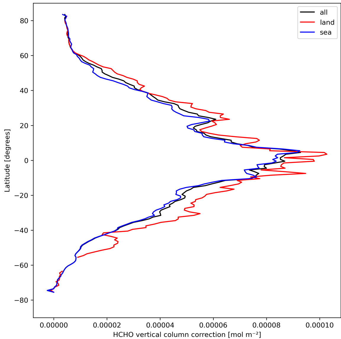
Figure 23: Zonal average of “HCHO vertical column correction” for 2024-04-11 to 2024-04-13.
