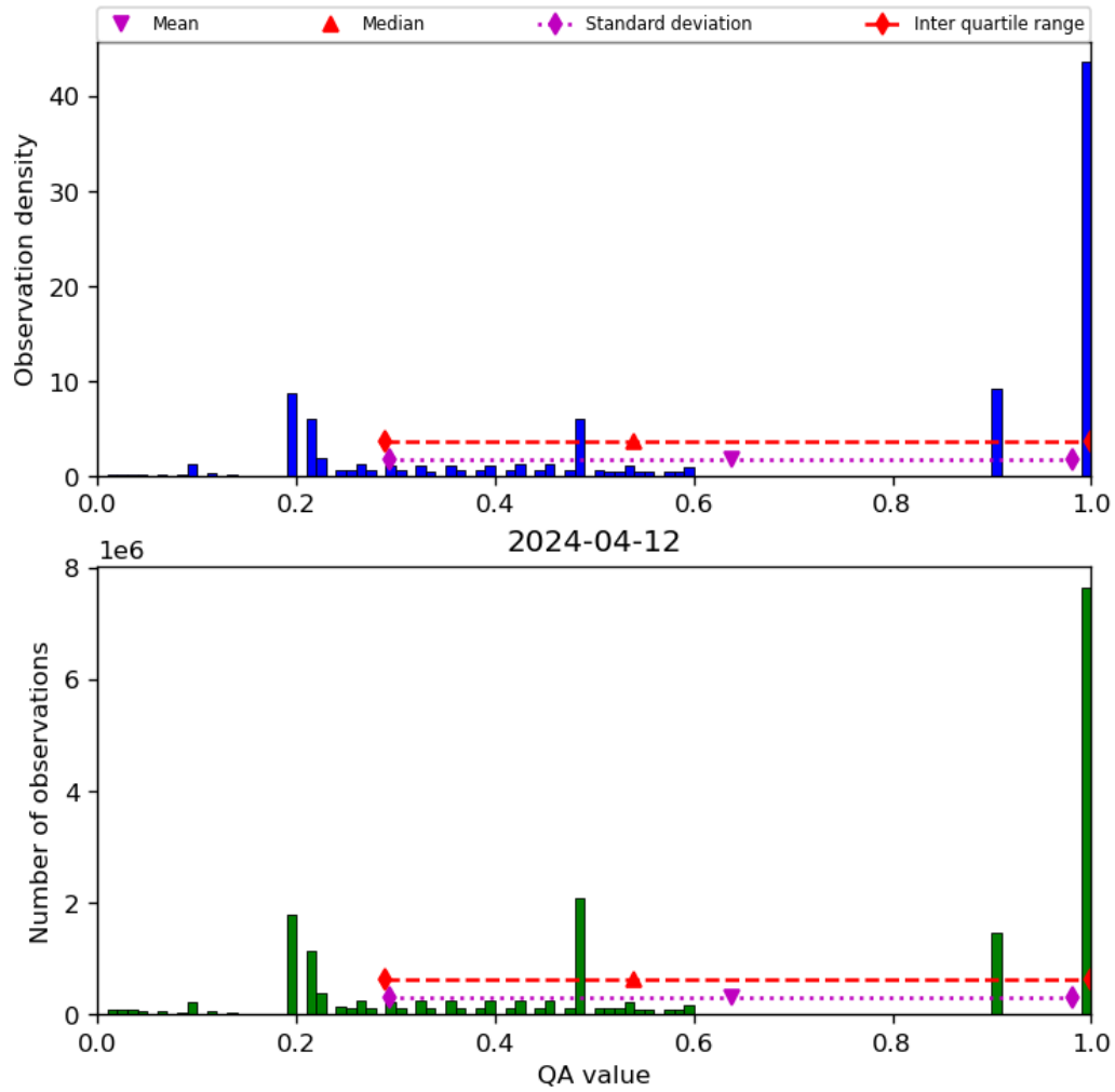
Figure 34: Histogram of “QA value” for 2024-04-11 to 2024-04-13
