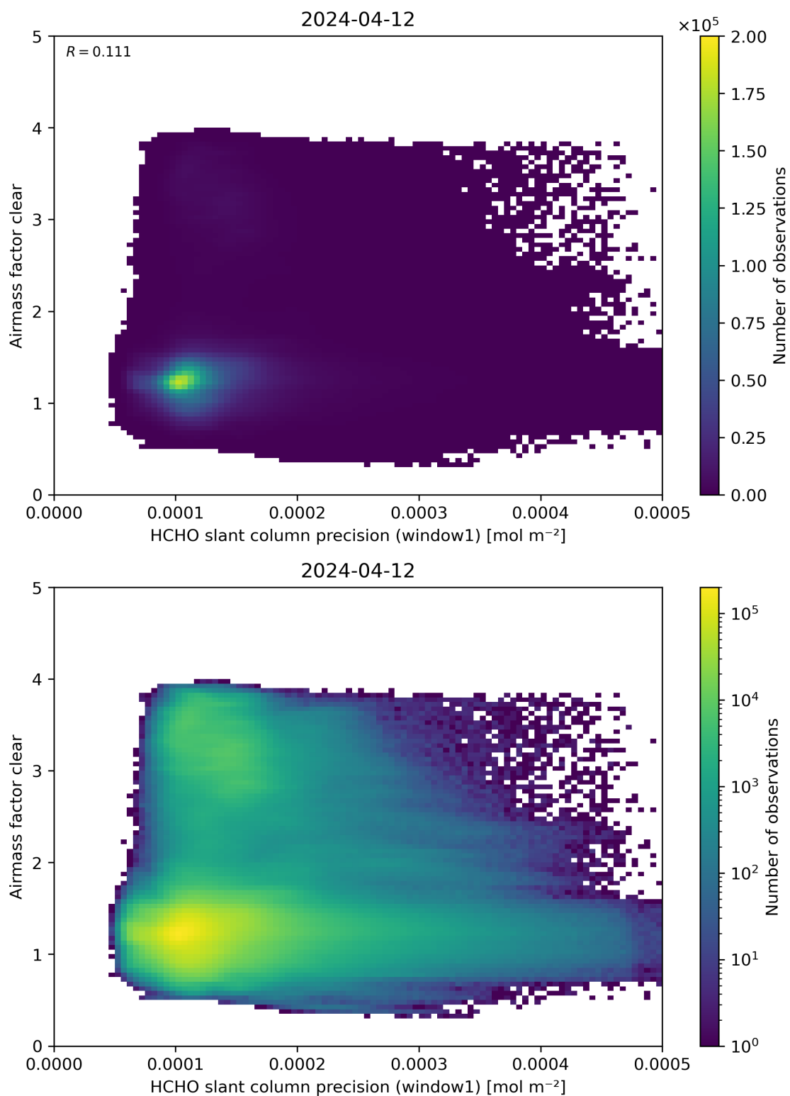
Figure 91: Scatter density plot of “HCHO slant column precision (window1)” against “Airmass factor clear” for 2024-04-11 to 2024-04-13.
