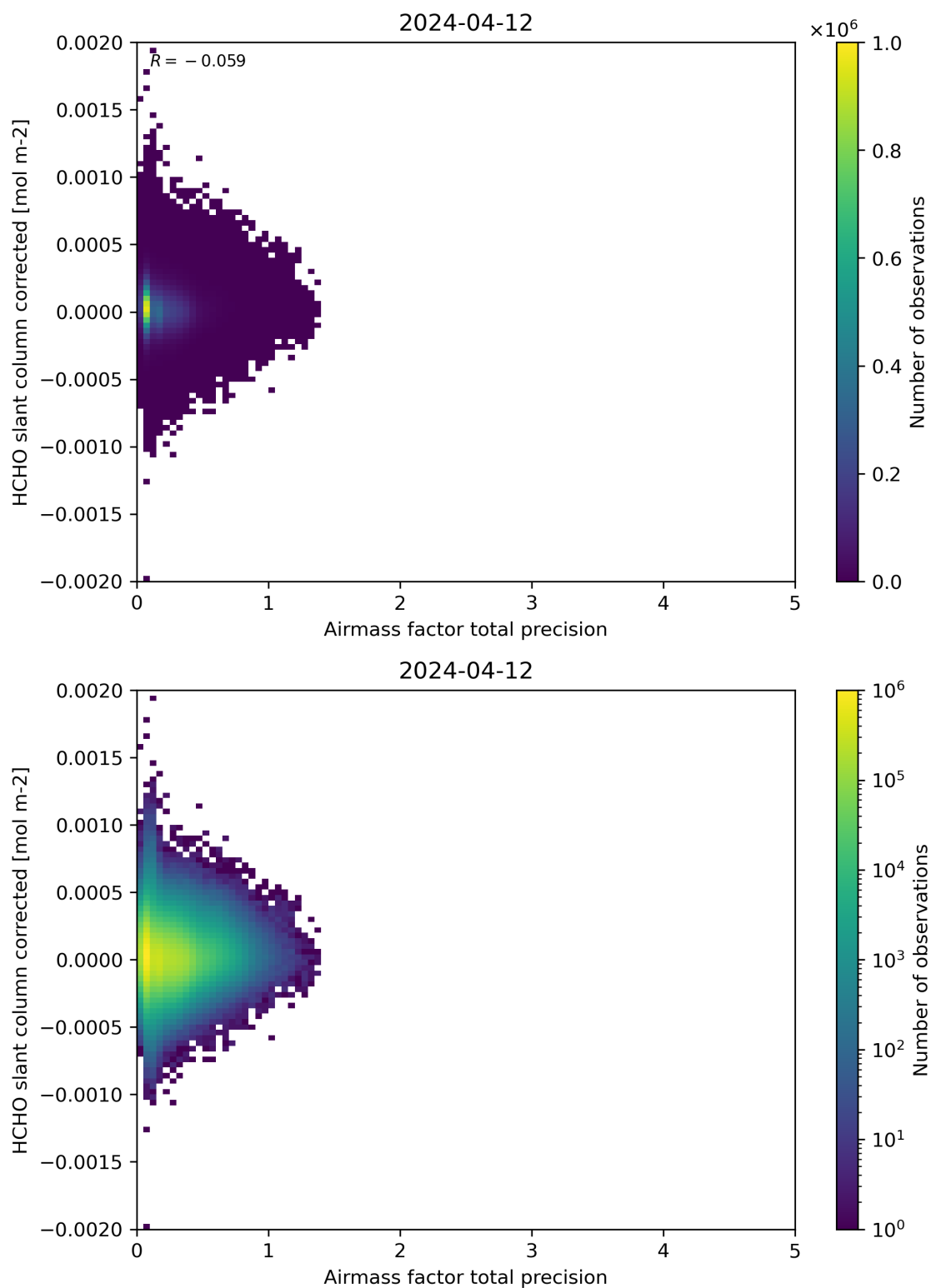
Figure 109: Scatter density plot of “Airmass factor total precision” against “HCHO slant column corrected” for 2024-04-11 to 2024-04-13.
