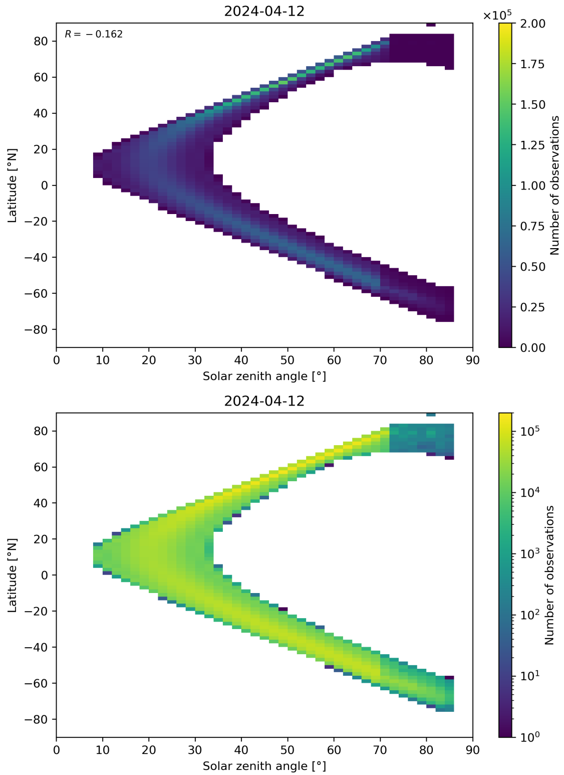
Figure 181: Scatter density plot of “Solar zenith angle” against “Latitude” for 2024-04-11 to 2024-04-13.
