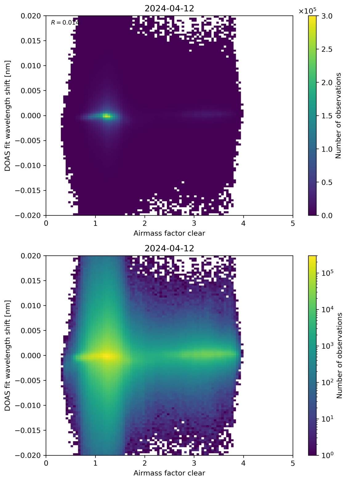
Figure 72: Scatter density plot of “Airmass factor clear” against “DOAS fit wavelength shift” for 2024-04-11 to 2024-04-13.
