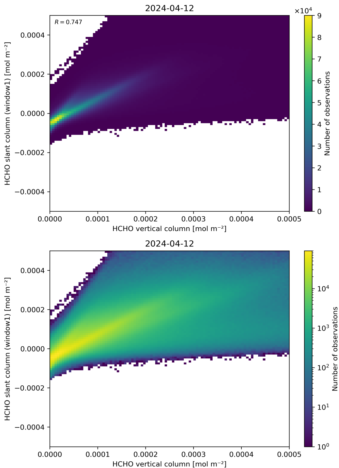
Figure 129: Scatter density plot of “HCHO vertical column” against “HCHO slant column (window1)” for 2024-04-11 to 2024-04-13.
