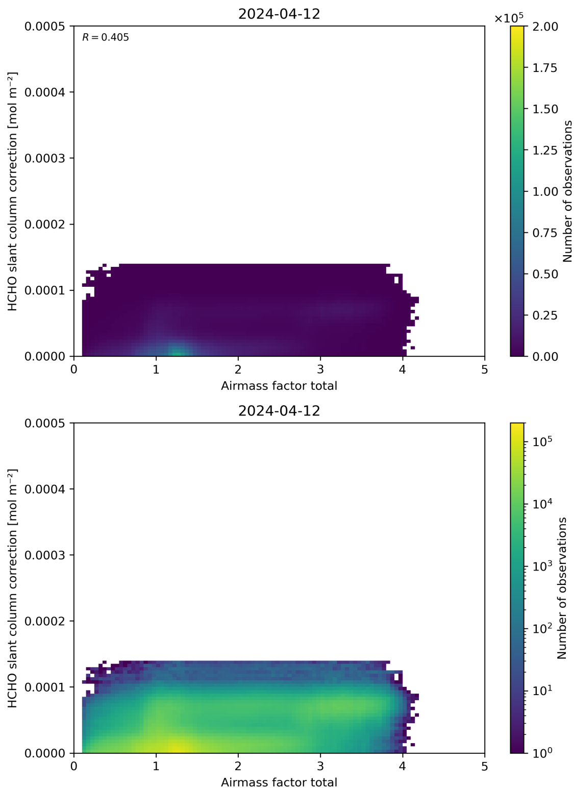
Figure 102: Scatter density plot of “Airmass factor total” against “HCHO slant column correction” for 2024-04-11 to 2024-04-13.
