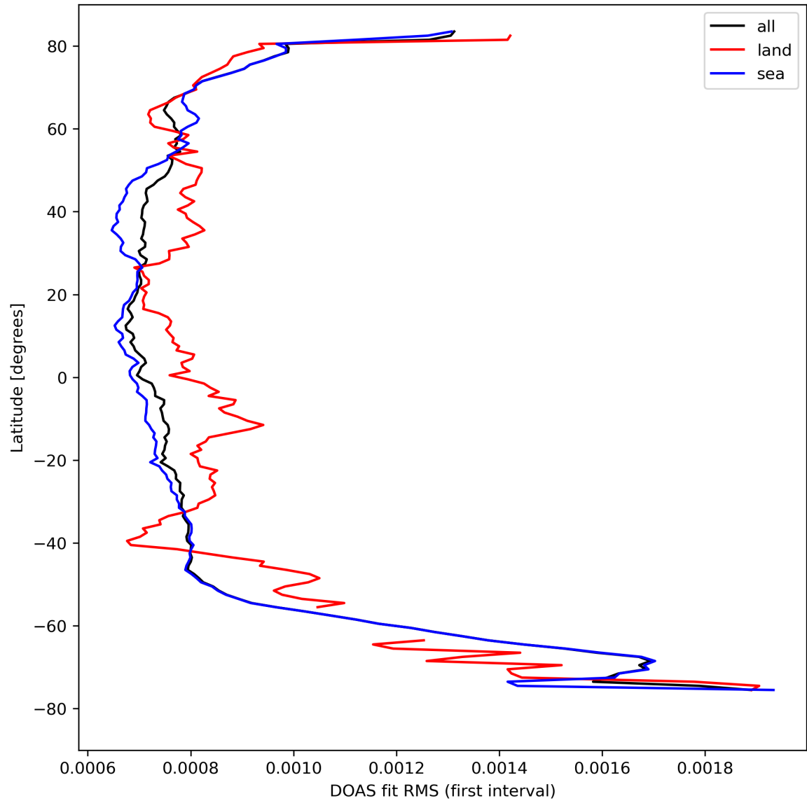
Figure 32: Zonal average of “DOAS fit RMS (first interval)” for 2024-04-11 to 2024-04-13.
