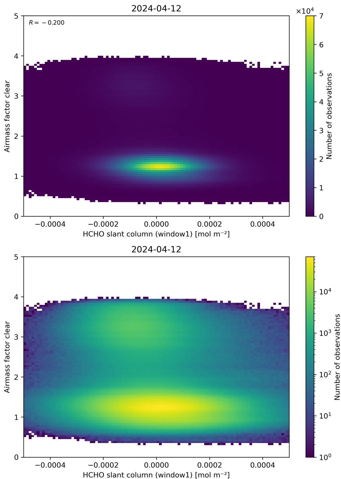
Figure 81: Scatter density plot of “HCHO slant column (window1)” against “Airmass factor clear” for 2024-04-11 to 2024-04-13.
