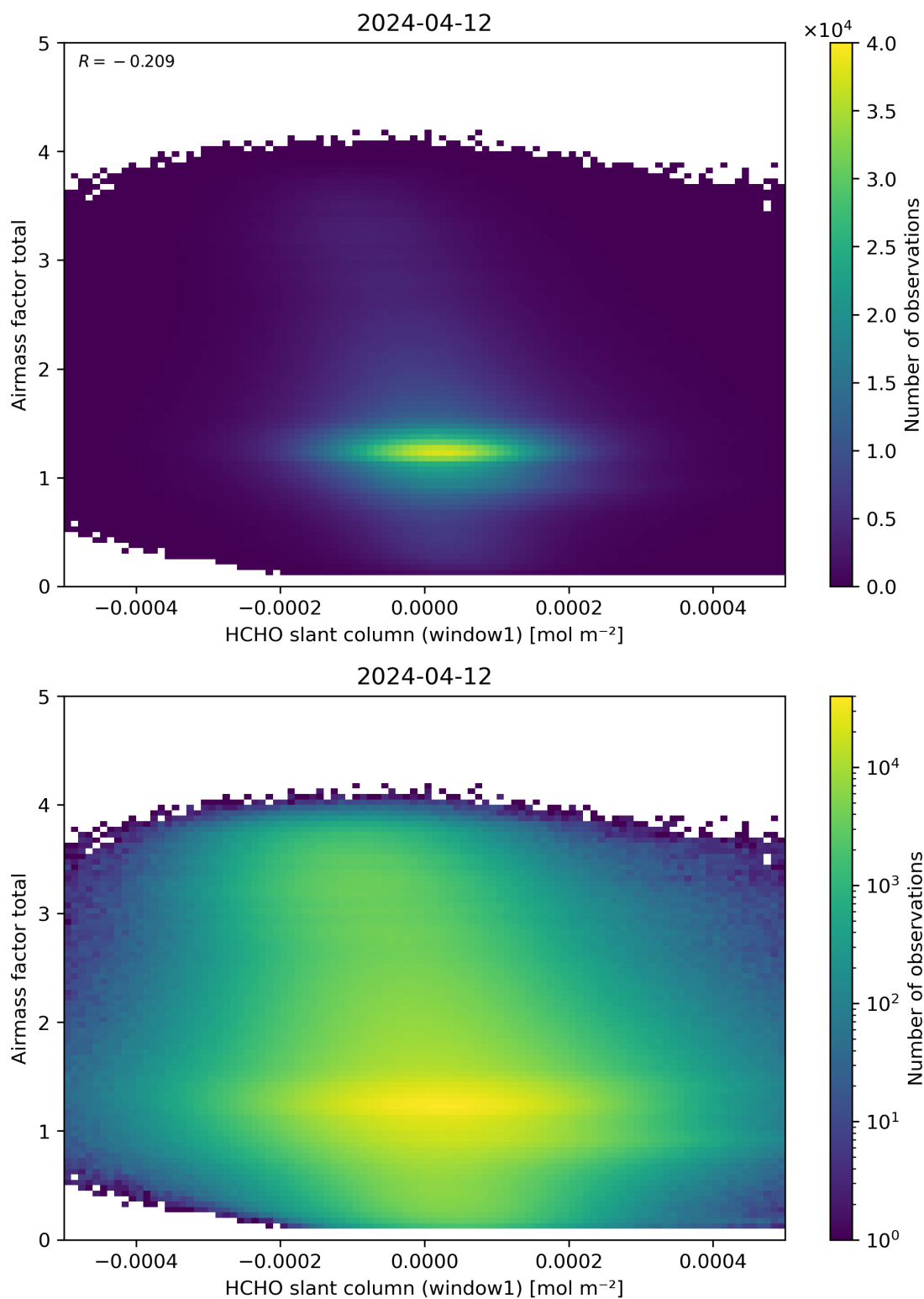
Figure 85: Scatter density plot of “HCHO slant column (window1)” against “Airmass factor total” for 2024-04-11 to 2024-04-13.
