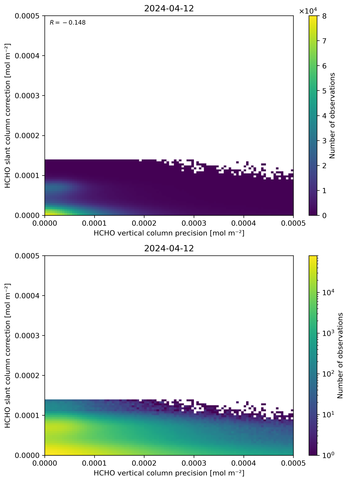
Figure 141: Scatter density plot of “HCHO vertical column precision” against “HCHO slant column correction” for 2024-04-11 to 2024-04-13.
