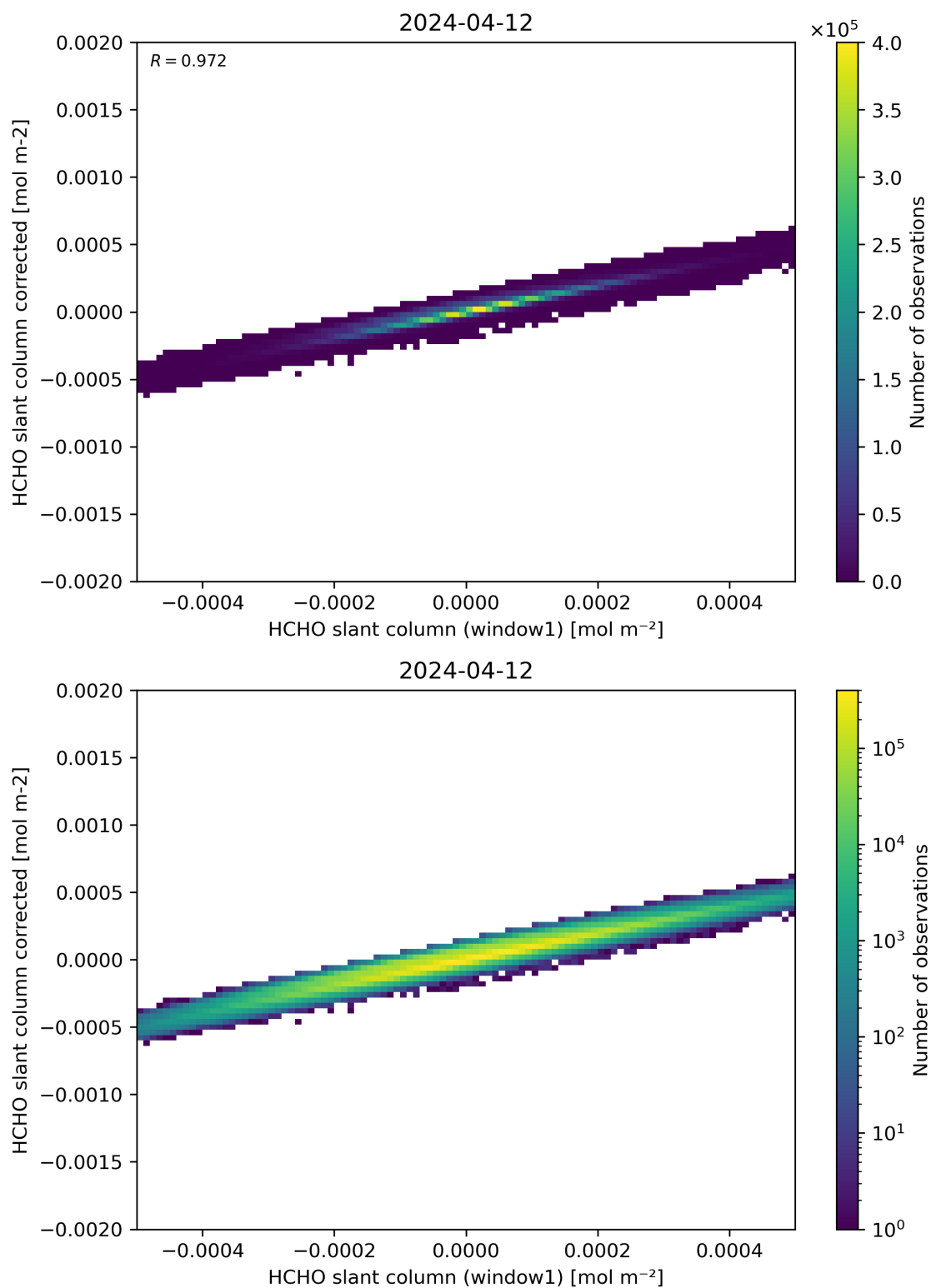
Figure 82: Scatter density plot of “HCHO slant column (window1)” against “HCHO slant column corrected” for 2024-04-11 to 2024-04-13.
