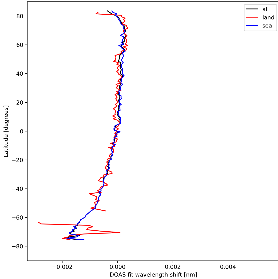
Figure 30: Zonal average of “DOAS fit wavelength shift” for 2024-04-11 to 2024-04-13.
