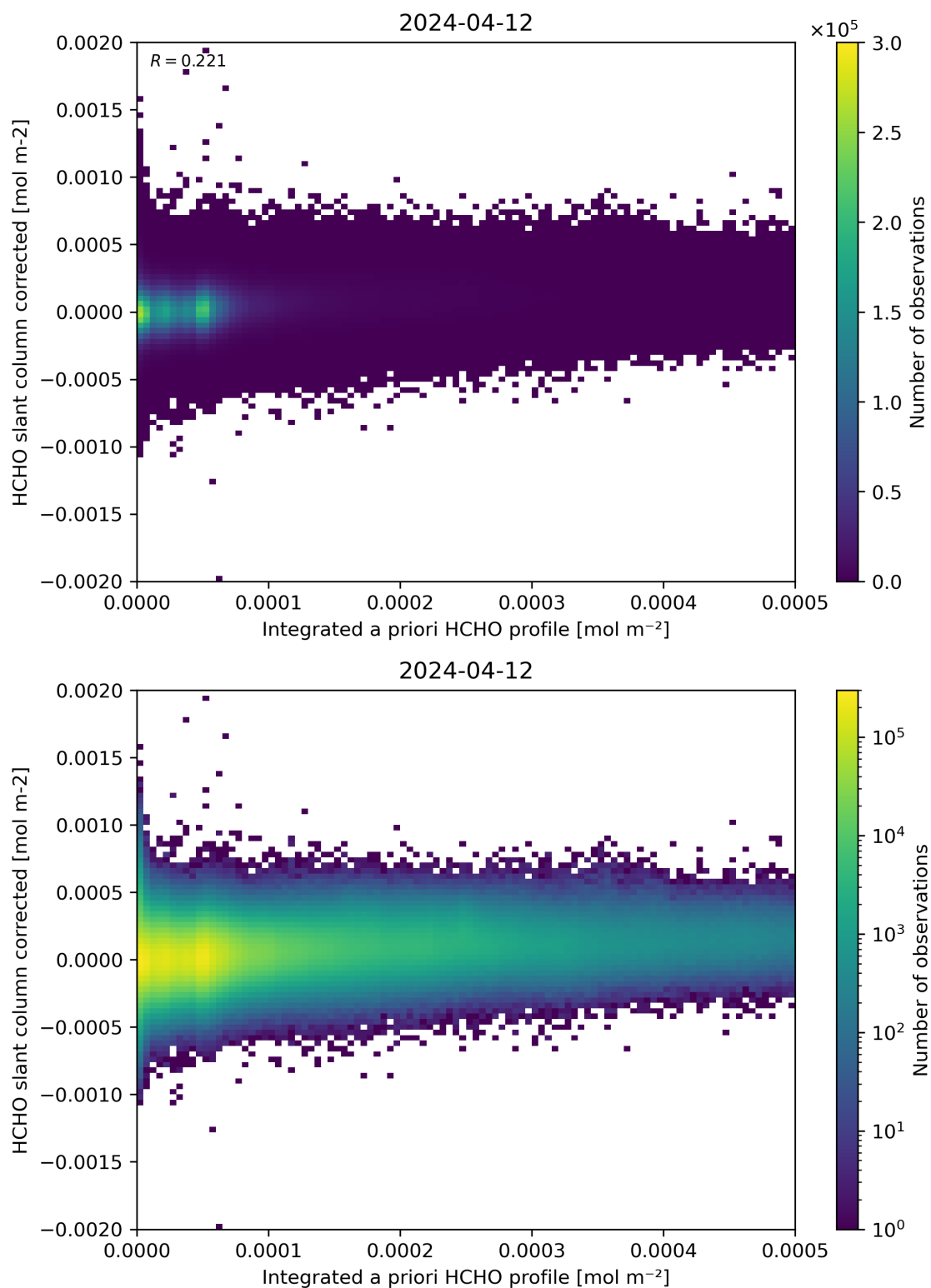
Figure 151: Scatter density plot of “Integrated a priori HCHO profile” against “HCHO slant column corrected” for 2024-04-11 to 2024-04-13.
