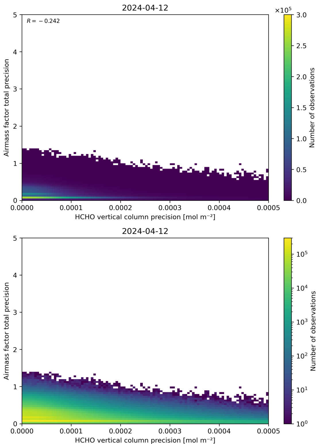
Figure 145: Scatter density plot of “HCHO vertical column precision” against “Airmass factor total precision” for 2024-04-11 to 2024-04-13.
