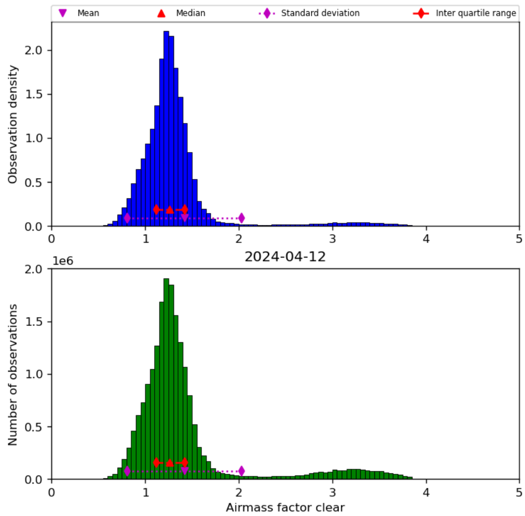
Figure 42: Histogram of “Airmass factor clear” for 2024-04-11 to 2024-04-13
