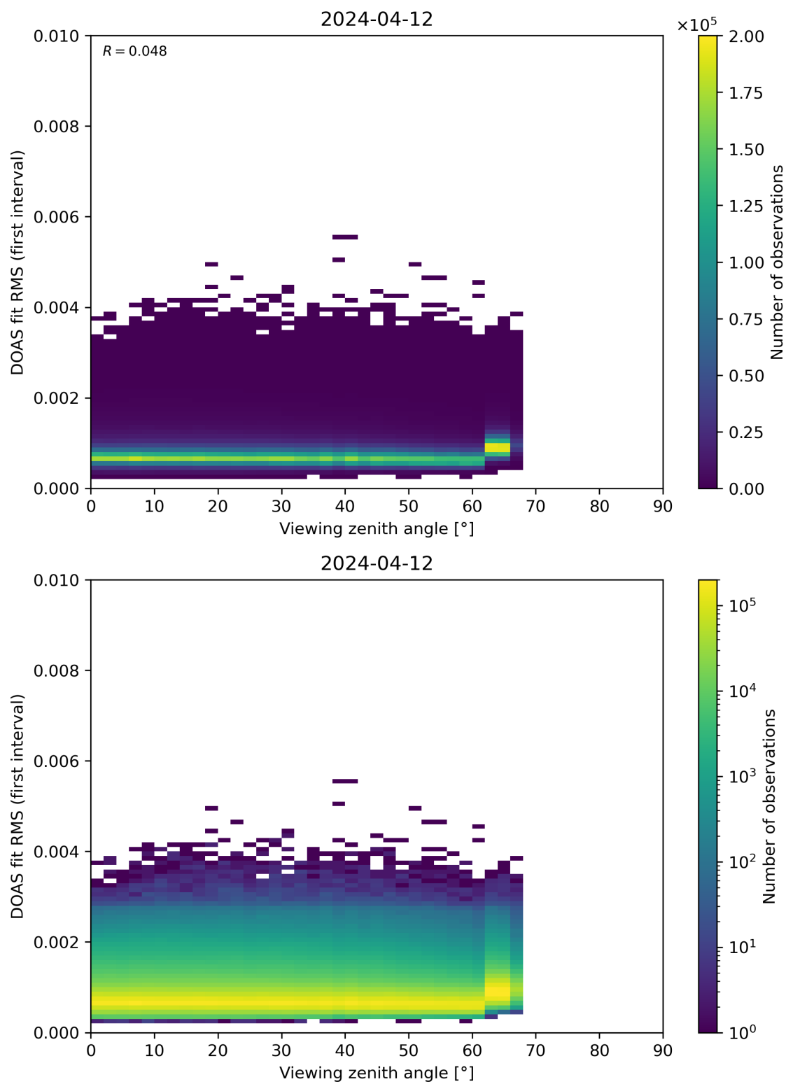
Figure 182: Scatter density plot of “Viewing zenith angle” against “DOAS fit RMS (first interval)” for 2024-04-11 to 2024-04-13.
