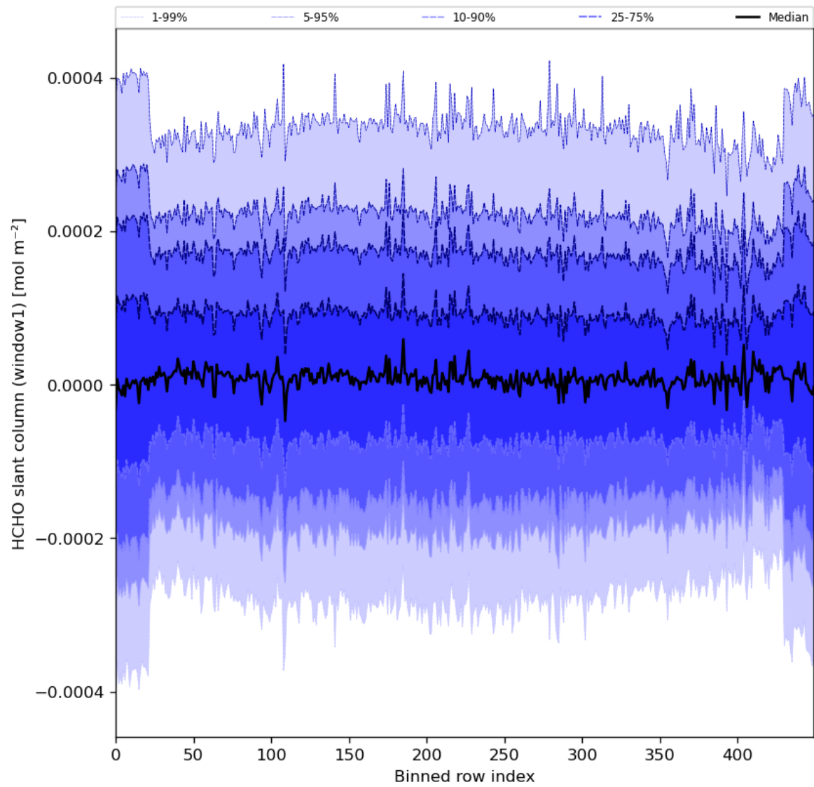
Figure 52: Along track statistics of “HCHO slant column (window1)” for 2024-04-11 to 2024-04-13
