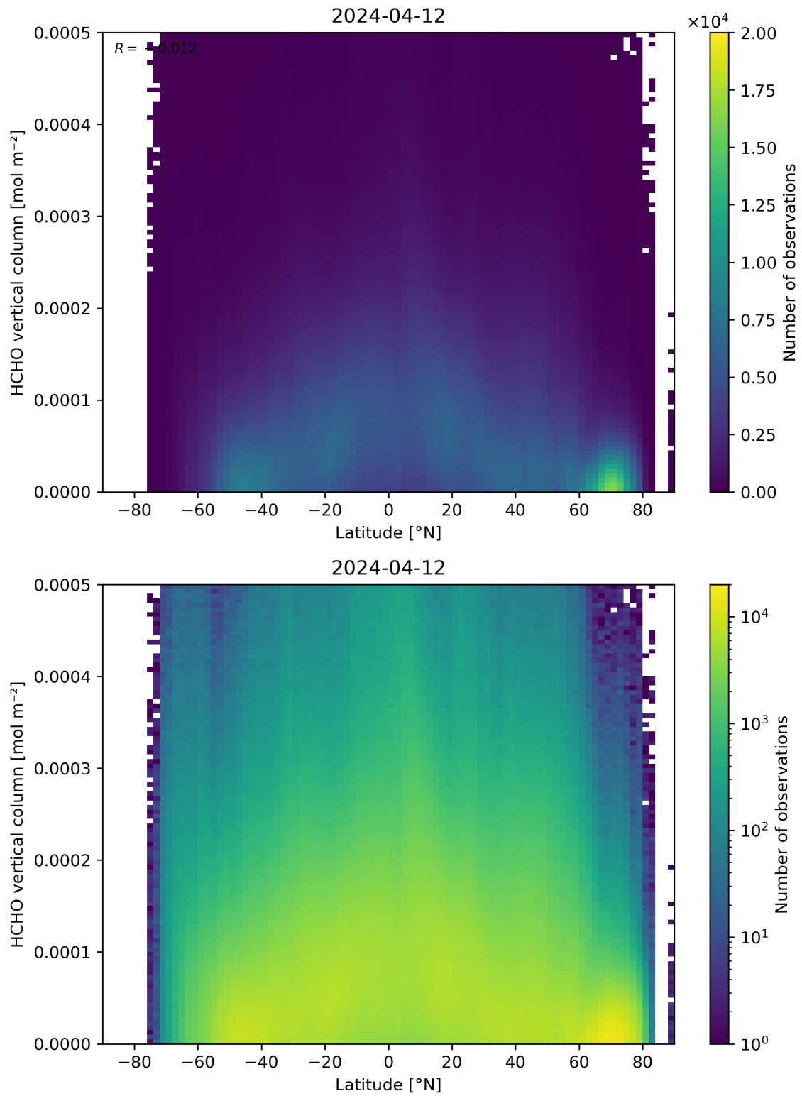
Figure 163: Scatter density plot of “Latitude” against “HCHO vertical column” for 2024-04-11 to 2024-04-13.
