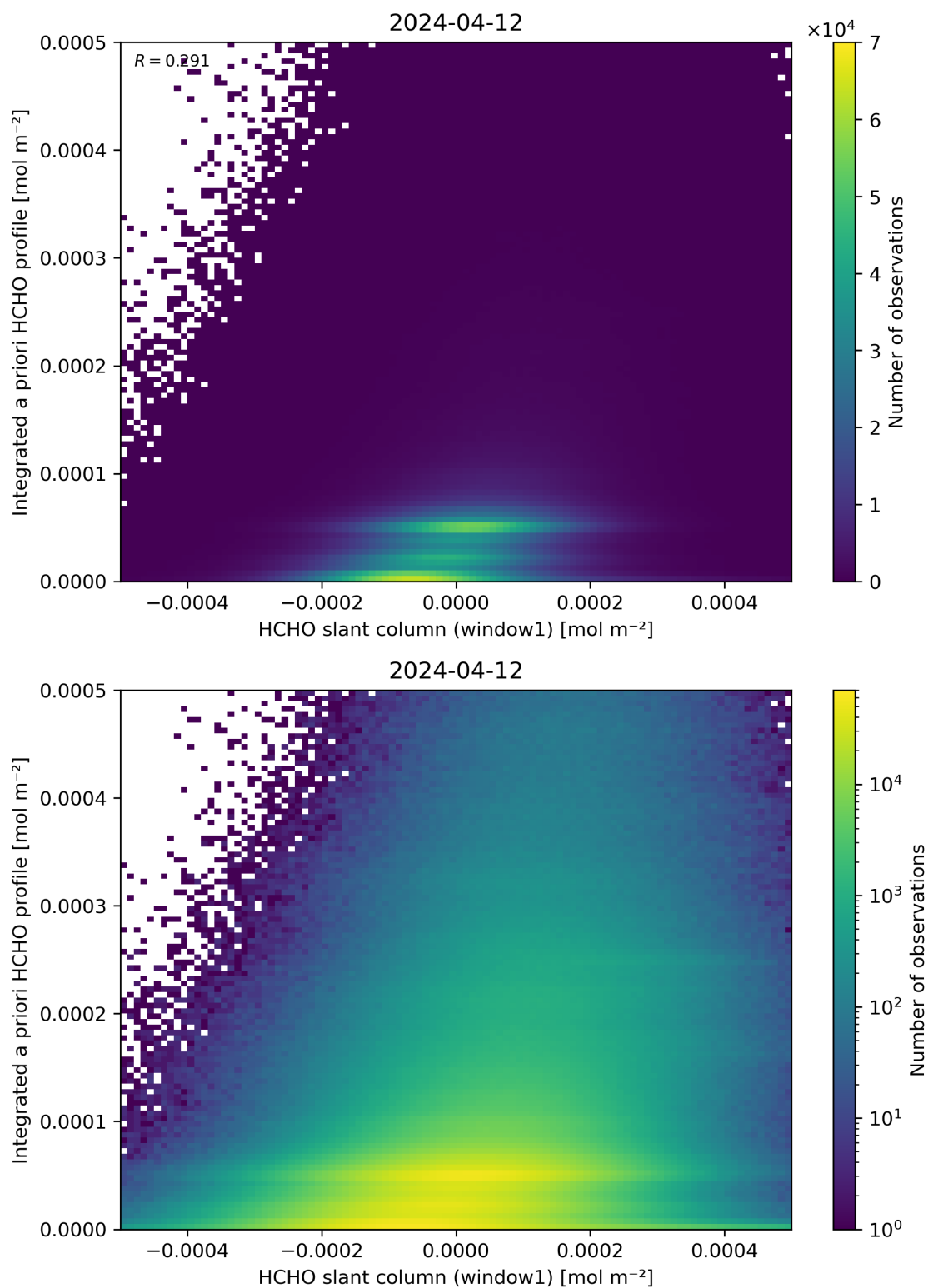
Figure 87: Scatter density plot of “HCHO slant column (window1)” against “Integrated a priori HCHO profile” for 2024-04-11 to 2024-04-13.
