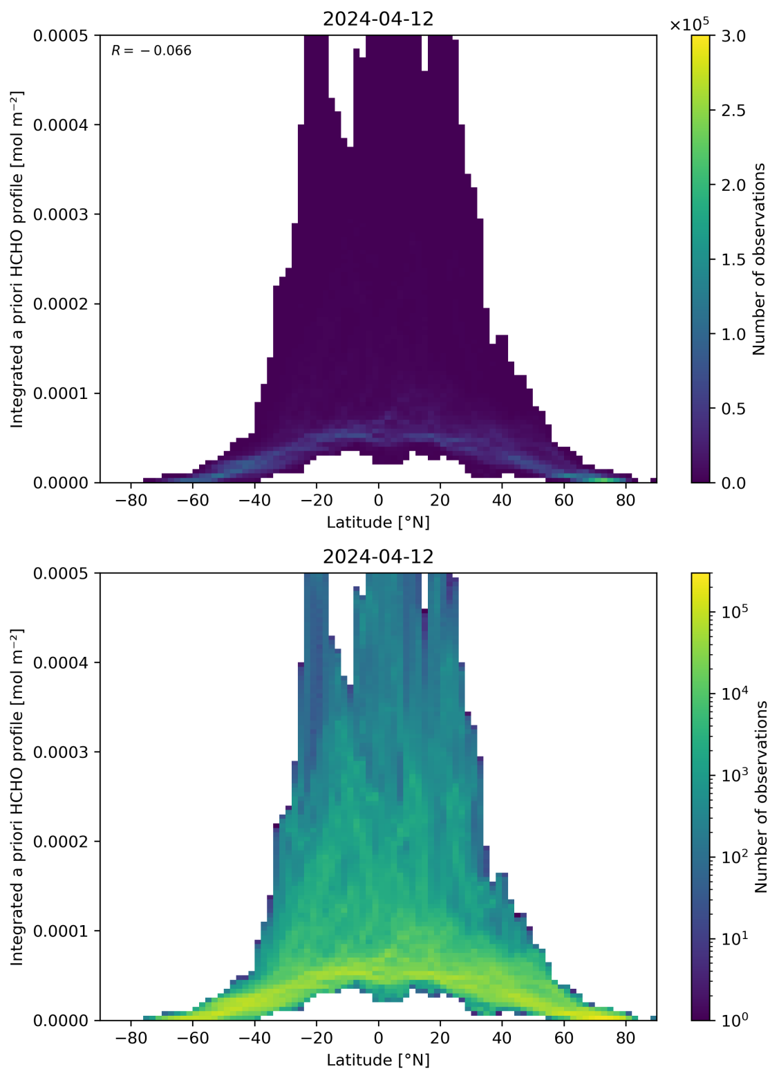
Figure 166: Scatter density plot of “Latitude” against “Integrated a priori HCHO profile” for 2024-04-11 to 2024-04-13.
