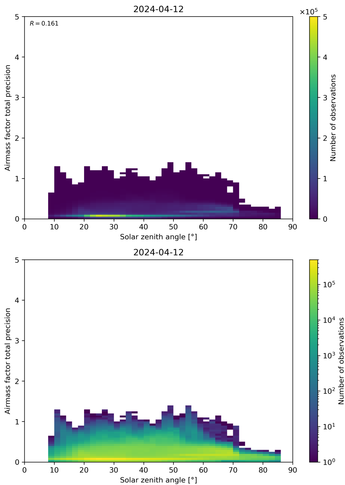
Figure 176: Scatter density plot of “Solar zenith angle” against “Airmass factor total precision” for 2024-04-11 to 2024-04-13.
