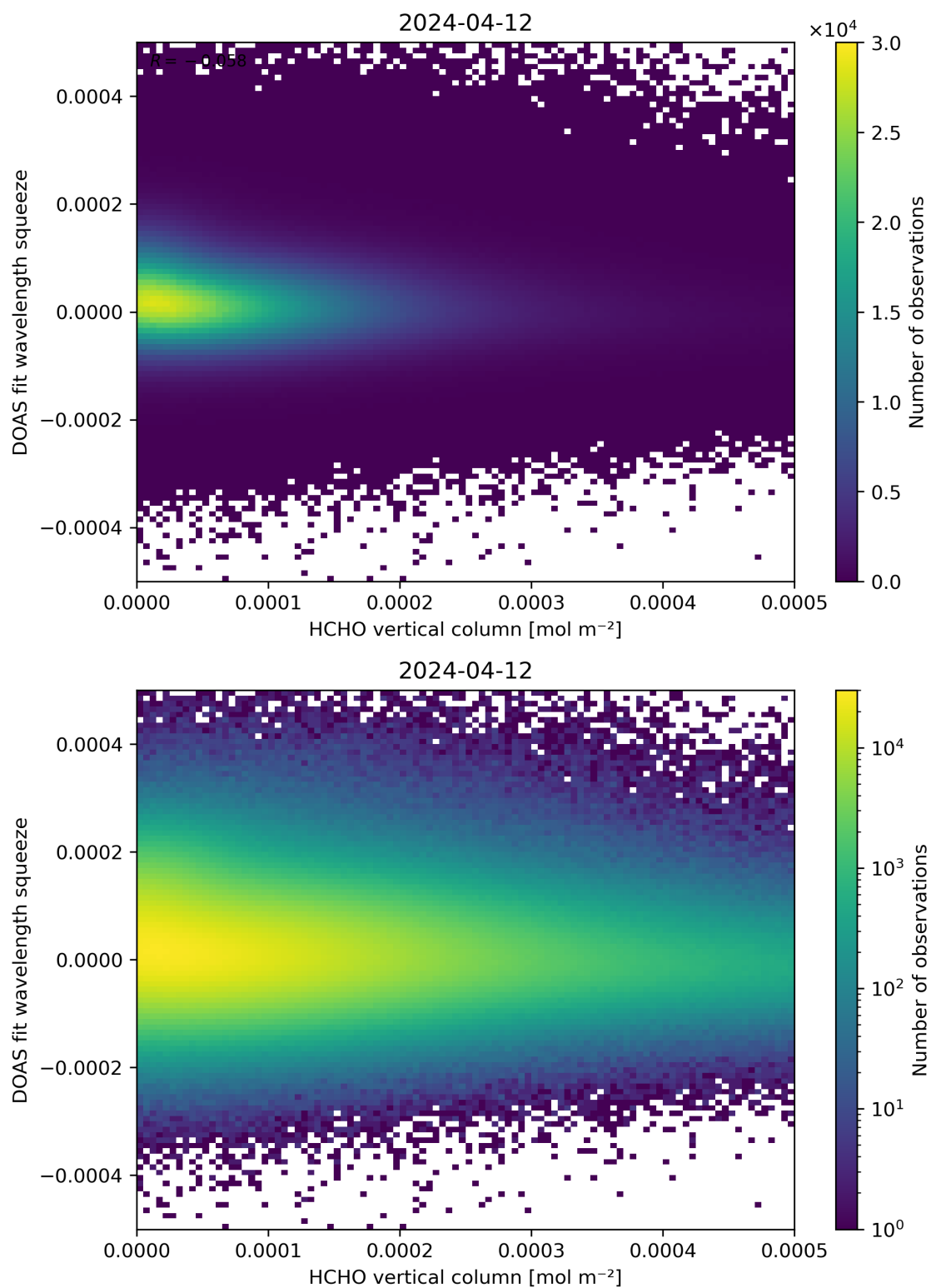
Figure 125: Scatter density plot of “HCHO vertical column” against “DOAS fit wavelength squeeze” for 2024-04-11 to 2024-04-13.
