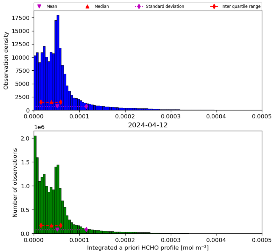
Figure 43: Histogram of “Integrated a priori HCHO profile” for 2024-04-11 to 2024-04-13
