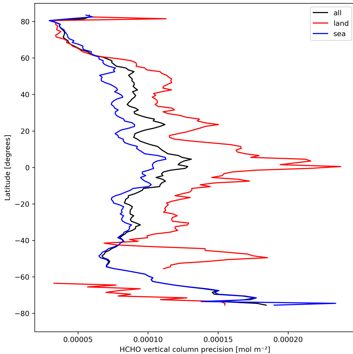
Figure 22: Zonal average of “HCHO vertical column precision” for 2024-04-11 to 2024-04-13.
