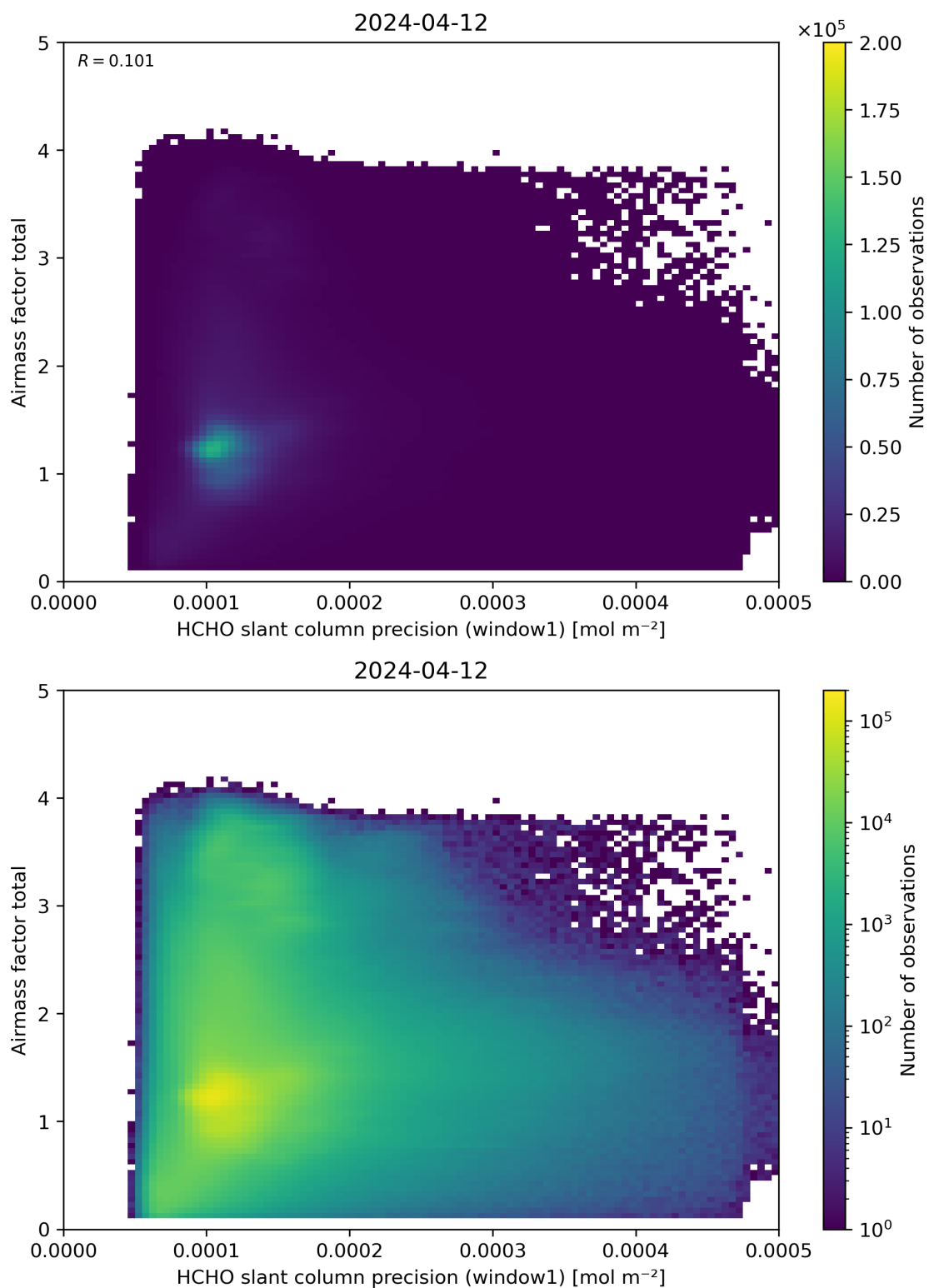
Figure 94: Scatter density plot of “HCHO slant column precision (window1)” against “Airmass factor total” for 2024-04-11 to 2024-04-13.
