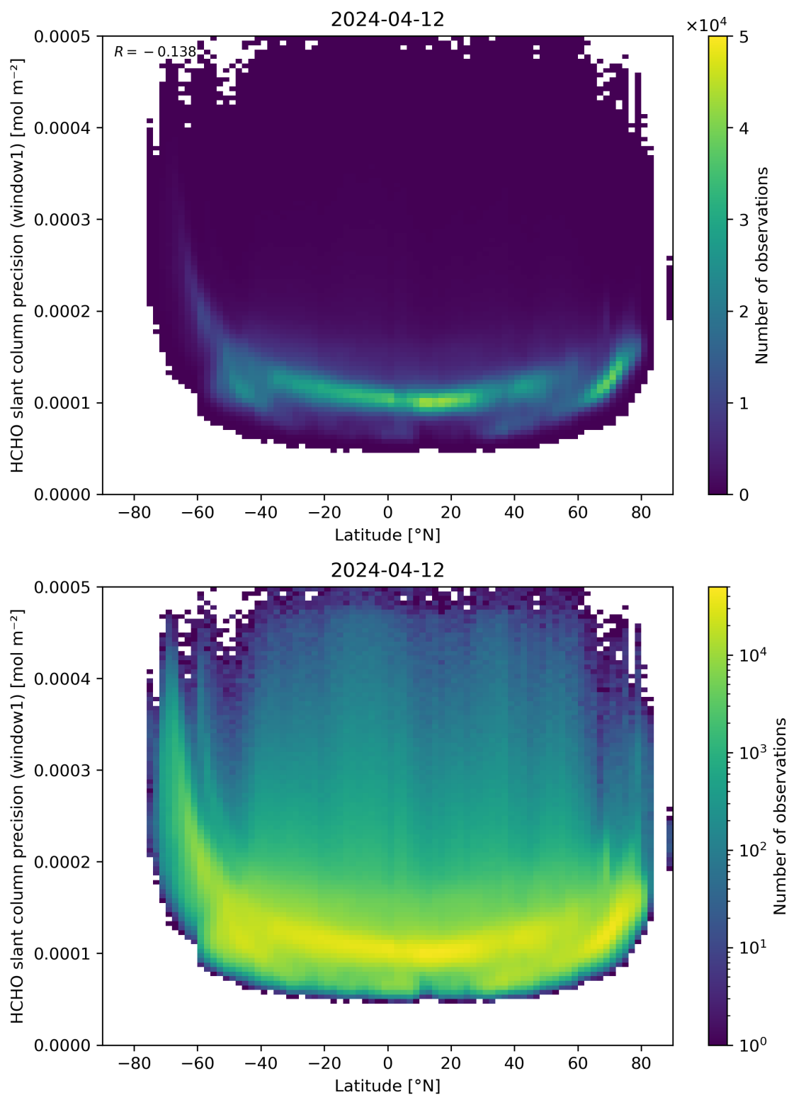
Figure 160: Scatter density plot of “Latitude” against “HCHO slant column precision (window1)” for 2024-04-11 to 2024-04-13.
