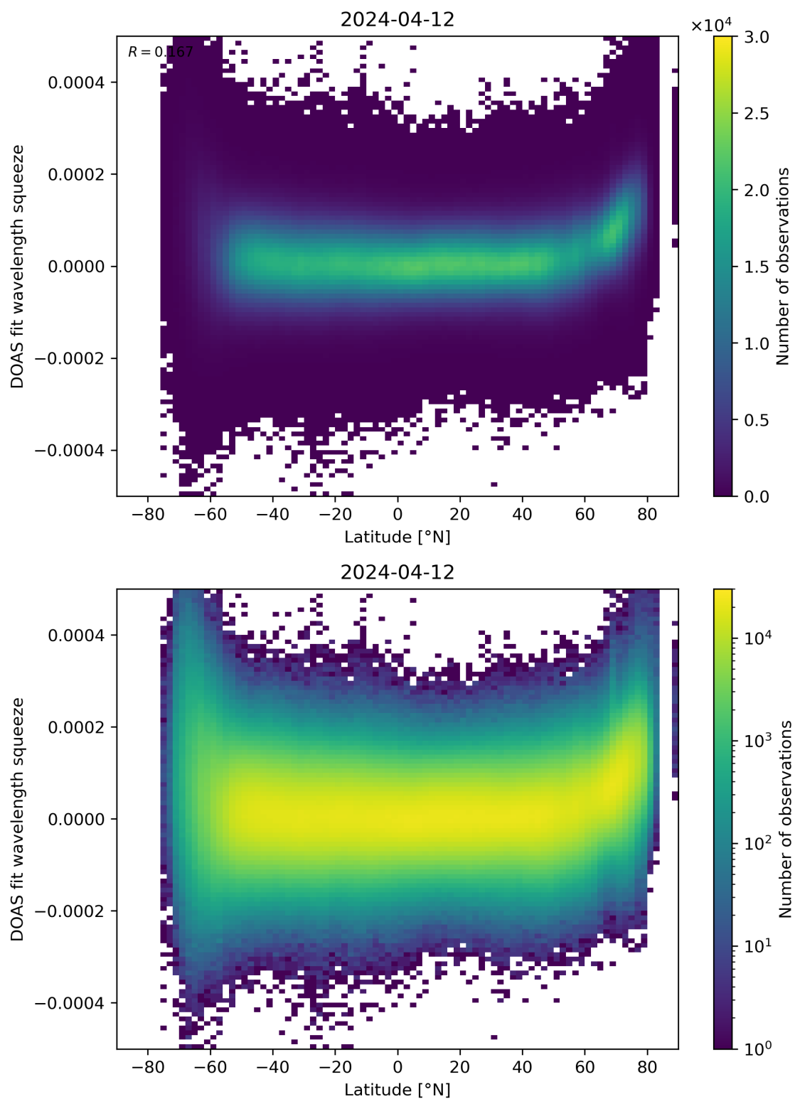
Figure 155: Scatter density plot of “Latitude” against “DOAS fit wavelength squeeze” for 2024-04-11 to 2024-04-13.
