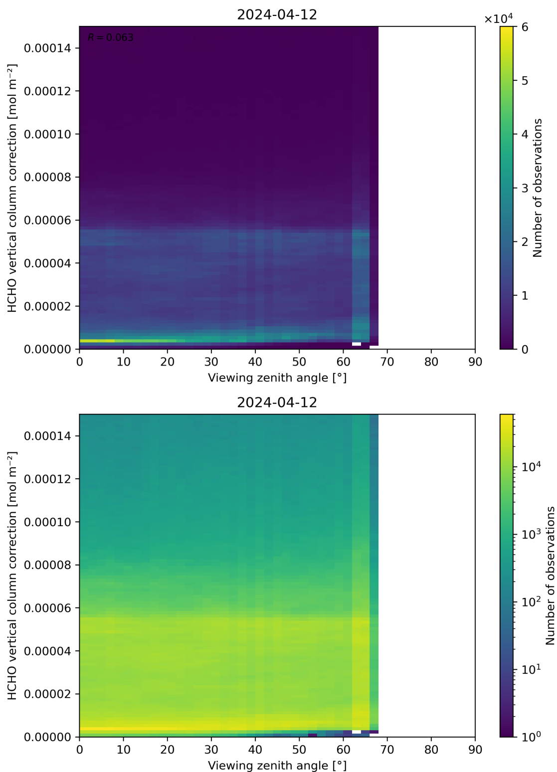
Figure 193: Scatter density plot of “Viewing zenith angle” against “HCHO vertical column correction” for 2024-04-11 to 2024-04-13.
