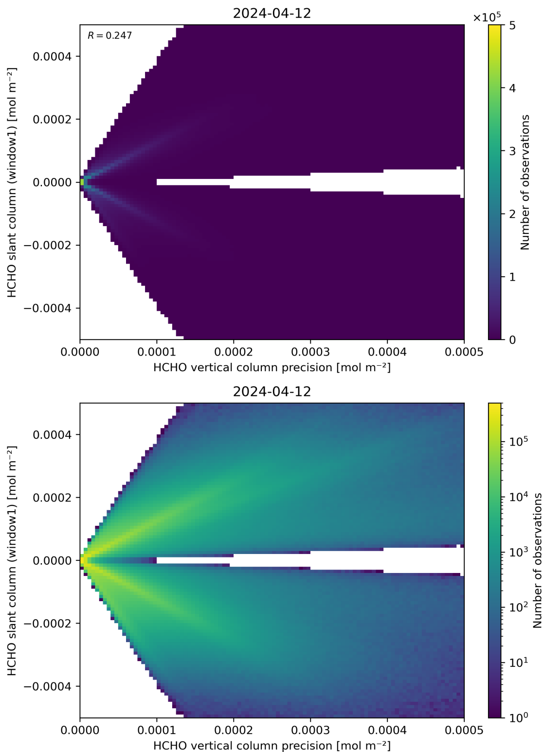
Figure 142: Scatter density plot of “HCHO vertical column precision” against “HCHO slant column (window1)” for 2024-04-11 to 2024-04-13.
