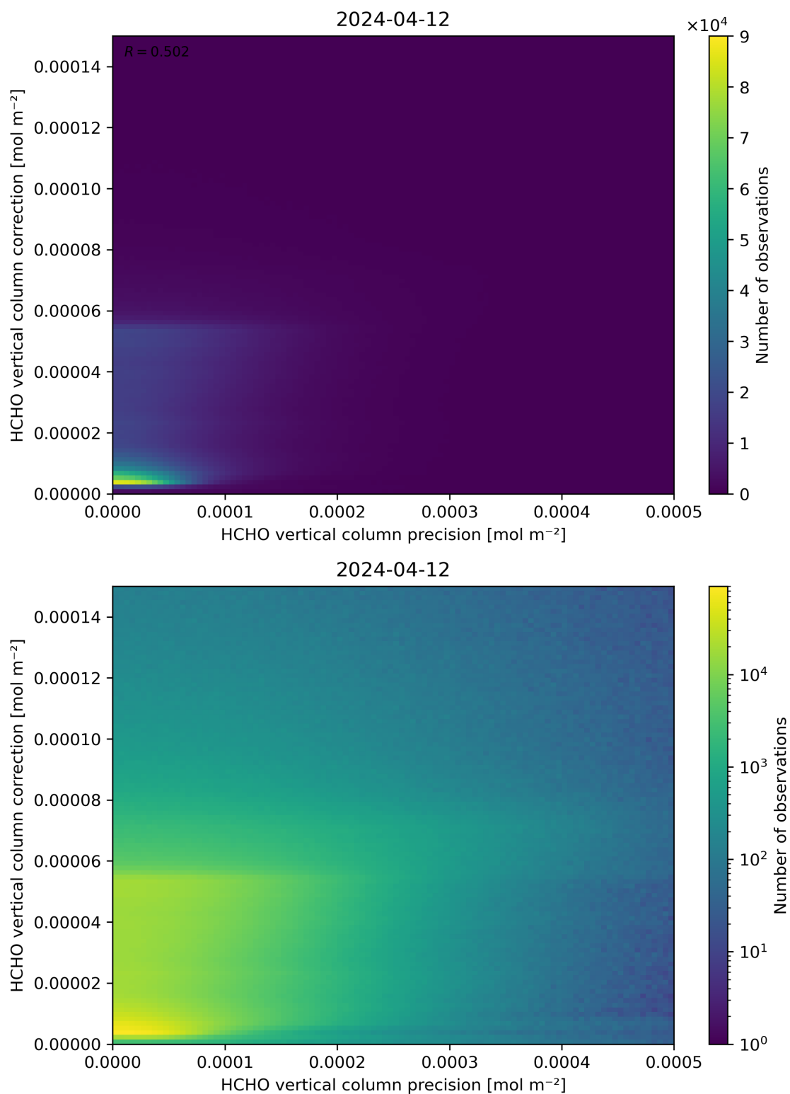
Figure 146: Scatter density plot of “HCHO vertical column precision” against “HCHO vertical column correction” for 2024-04-11 to 2024-04-13.
