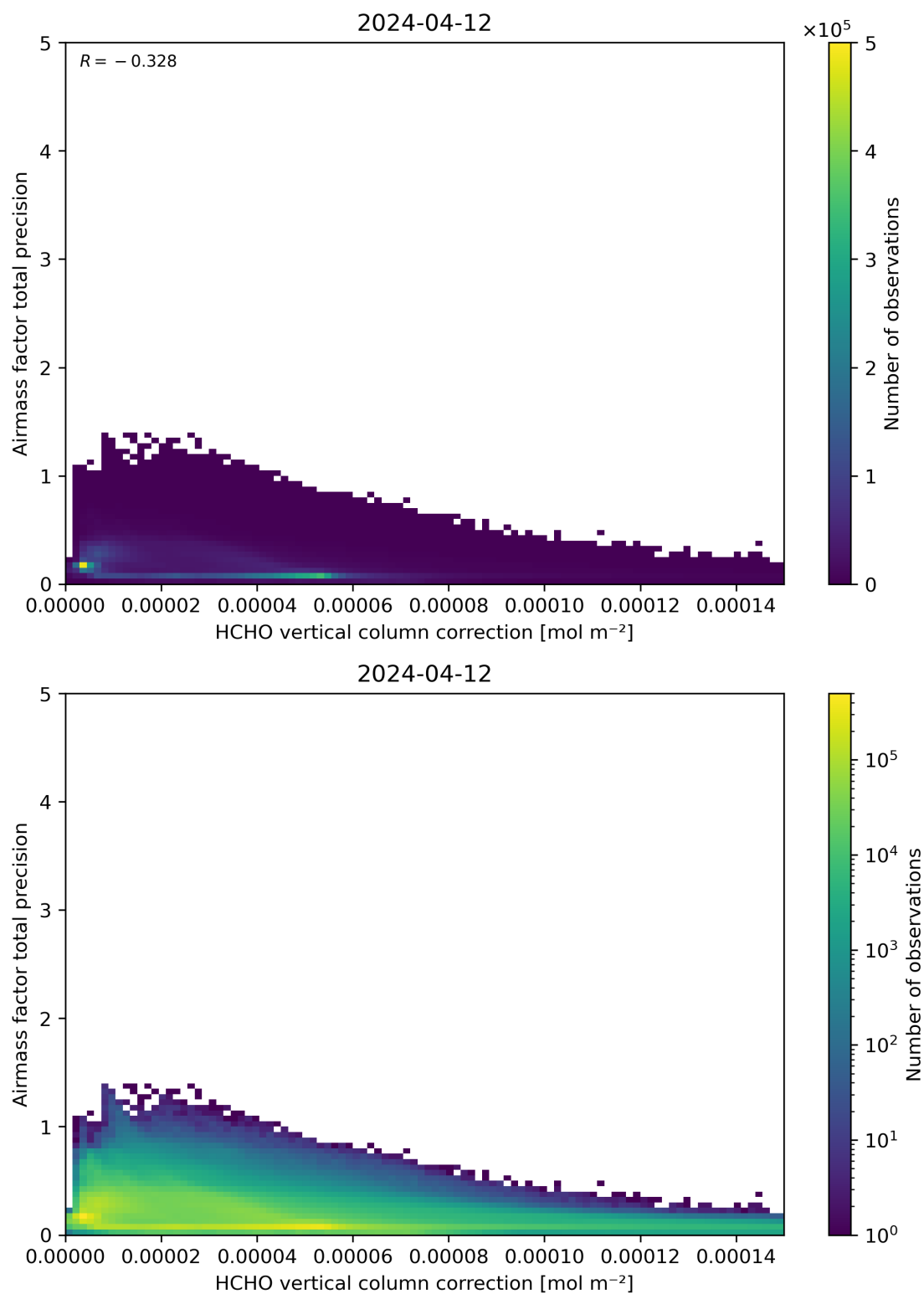
Figure 121: Scatter density plot of “HCHO vertical column correction” against “Airmass factor total precision” for 2024-04-11 to 2024-04-13.
