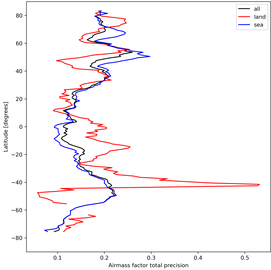
Figure 27: Zonal average of “Airmass factor total precision” for 2024-04-11 to 2024-04-13.
