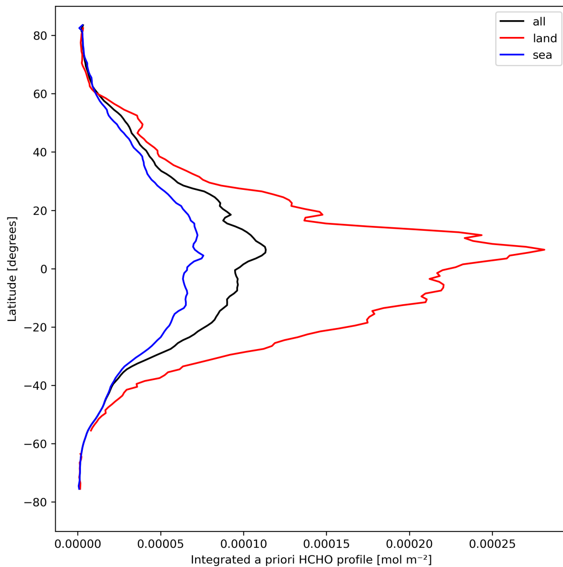
Figure 29: Zonal average of “Integrated a priori HCHO profile” for 2024-04-11 to 2024-04-13.
