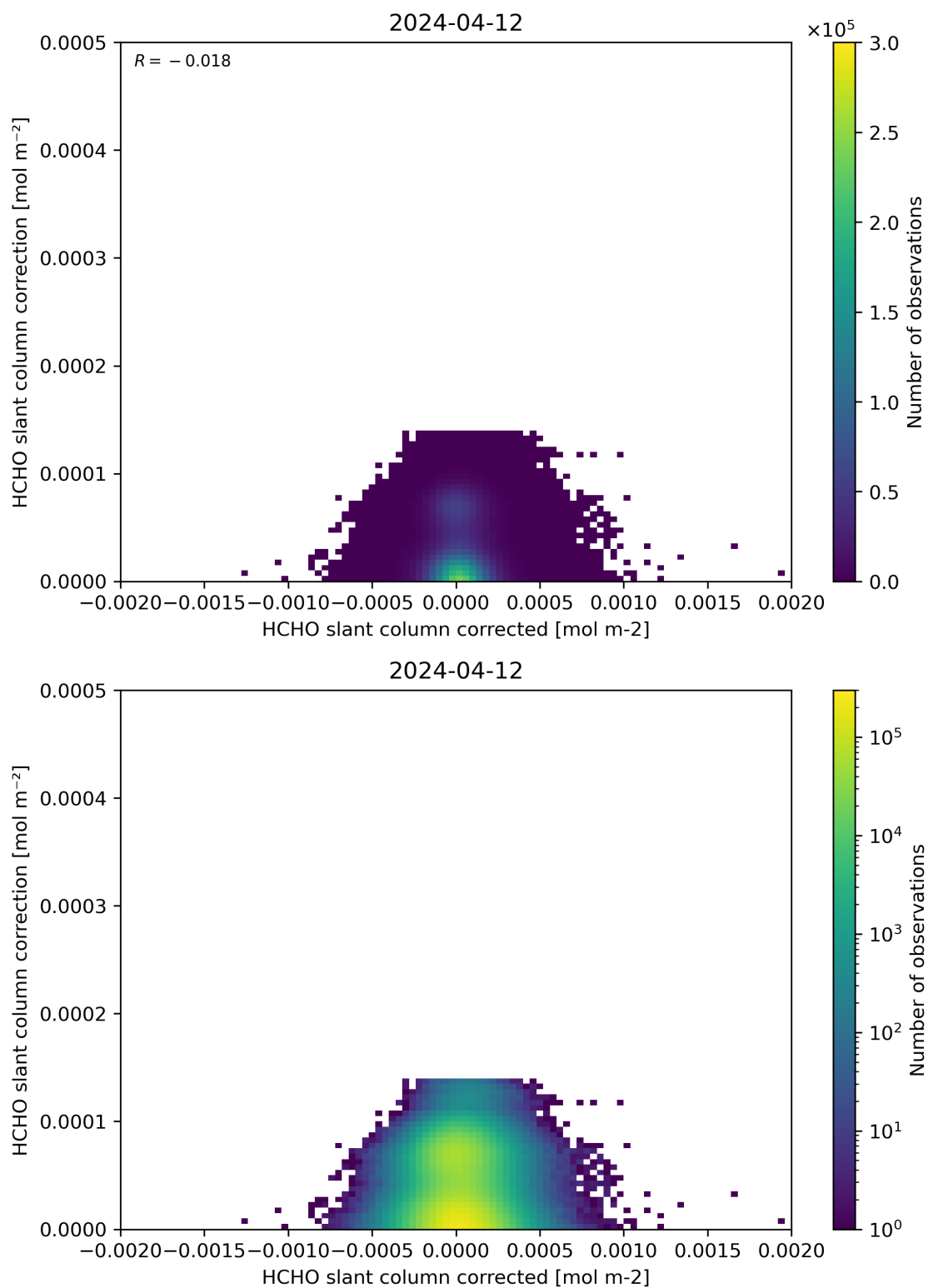
Figure 77: Scatter density plot of “HCHO slant column corrected” against “HCHO slant column correction” for 2024-04-11 to 2024-04-13.
