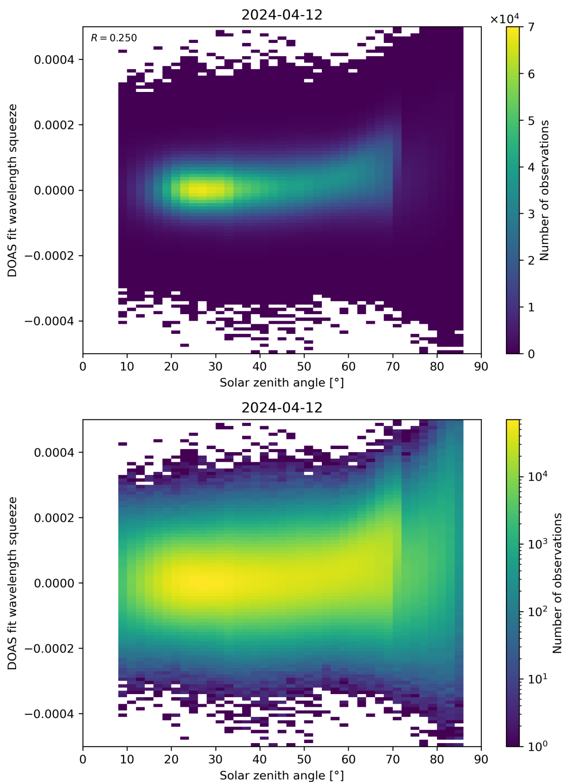
Figure 169: Scatter density plot of “Solar zenith angle” against “DOAS fit wavelength squeeze” for 2024-04-11 to 2024-04-13.
