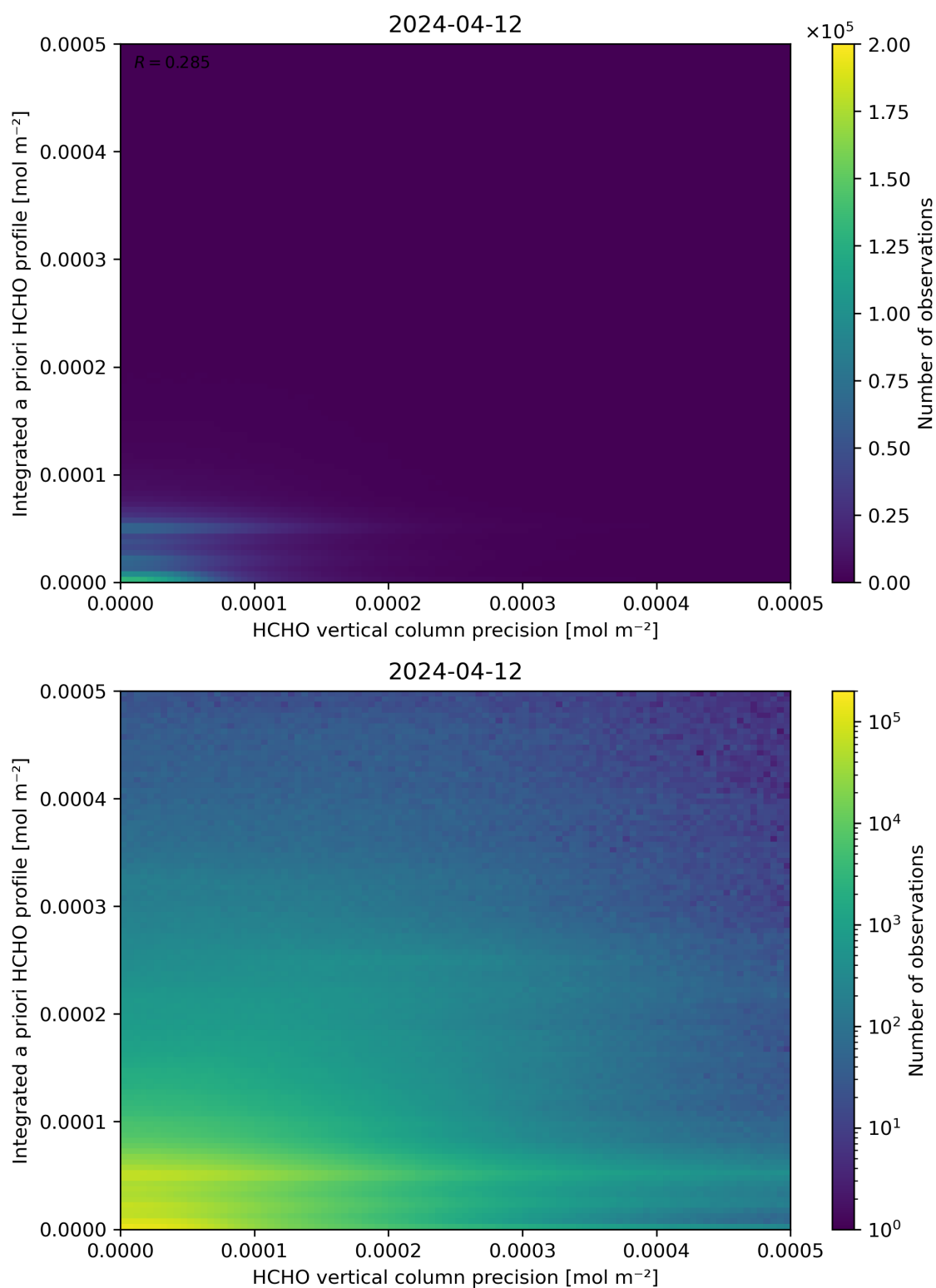
Figure 147: Scatter density plot of “HCHO vertical column precision” against “Integrated a priori HCHO profile” for 2024-04-11 to 2024-04-13.
