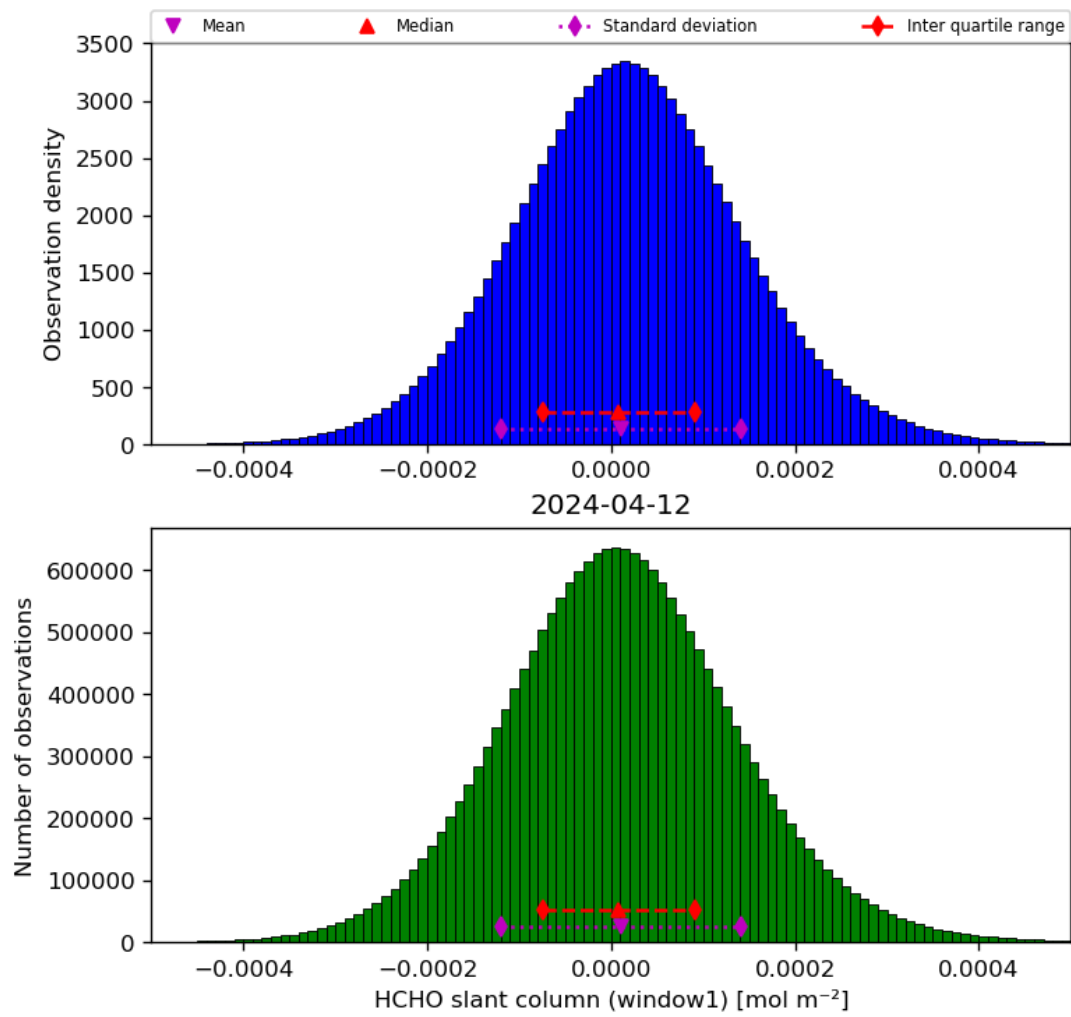
Figure 38: Histogram of “HCHO slant column (window1)” for 2024-04-11 to 2024-04-13
