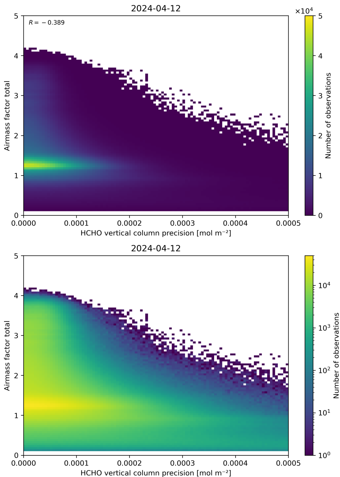
Figure 144: Scatter density plot of “HCHO vertical column precision” against “Airmass factor total” for 2024-04-11 to 2024-04-13.
