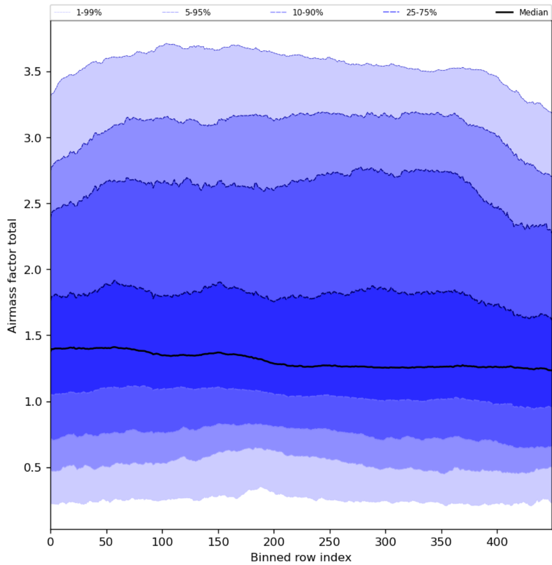
Figure 54: Along track statistics of “Airmass factor total” for 2024-04-11 to 2024-04-13
