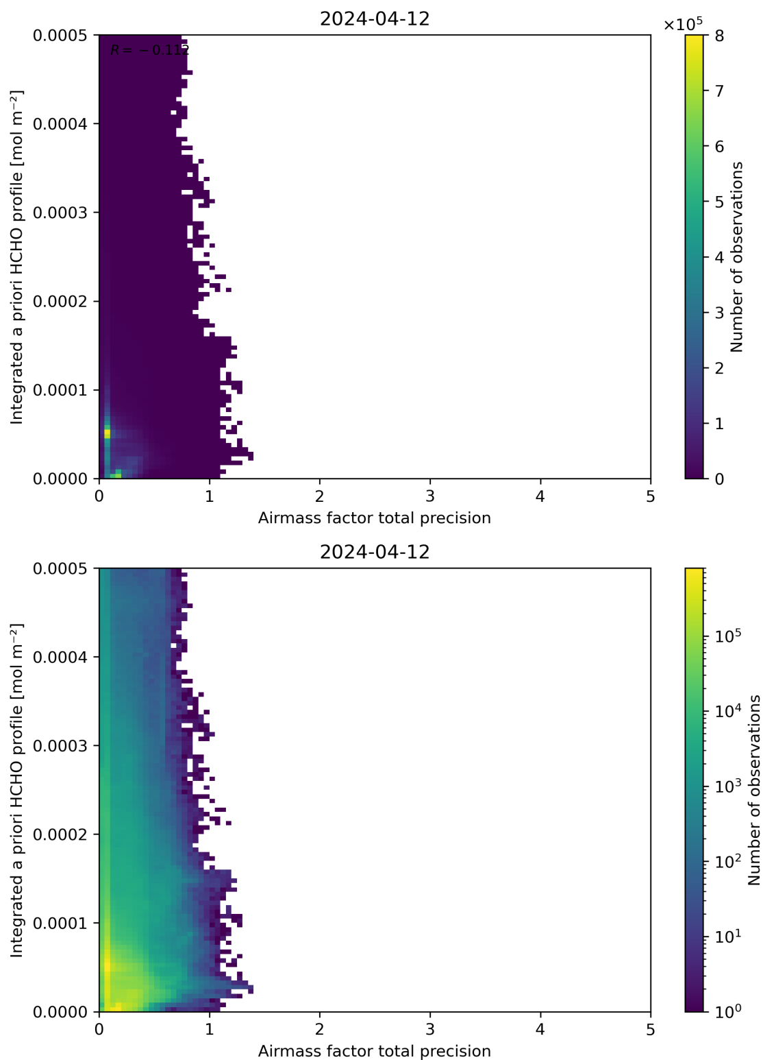
Figure 111: Scatter density plot of “Airmass factor total precision” against “Integrated a priori HCHO profile” for 2024-04-11 to 2024-04-13.
