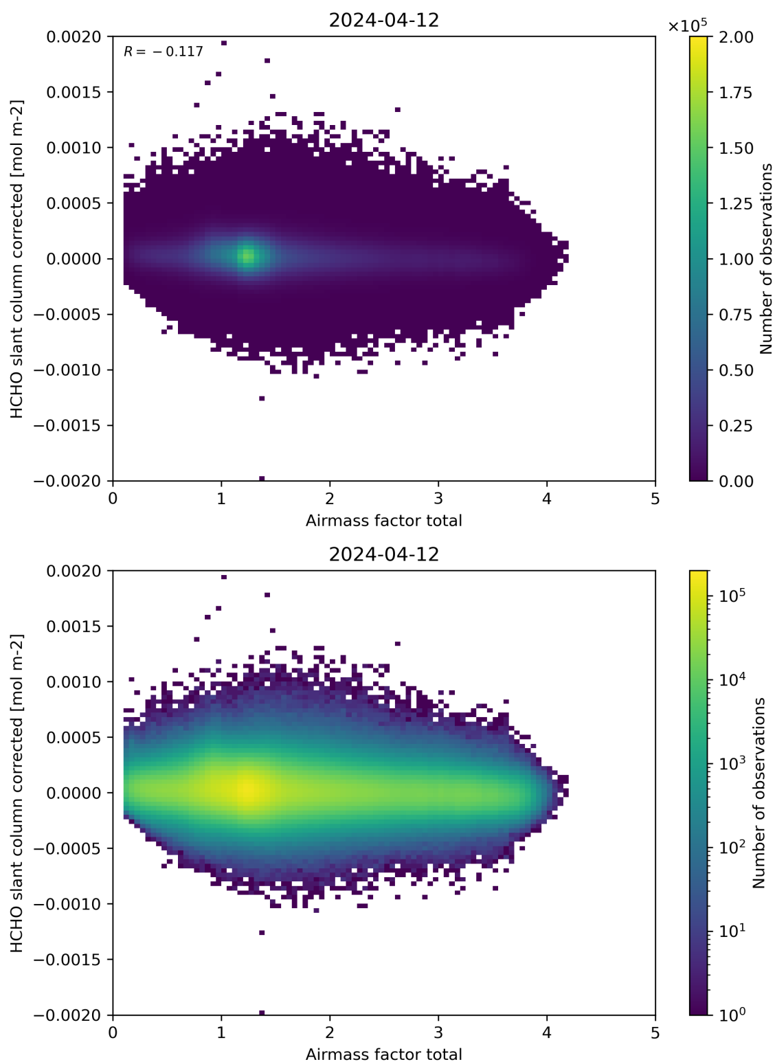
Figure 101: Scatter density plot of “Airmass factor total” against “HCHO slant column corrected” for 2024-04-11 to 2024-04-13.
