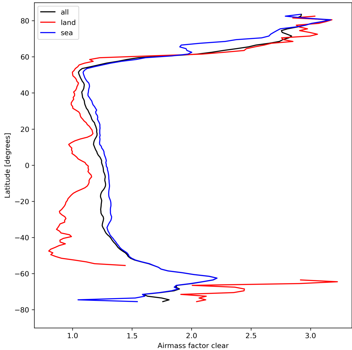
Figure 28: Zonal average of “Airmass factor clear” for 2024-04-11 to 2024-04-13.
