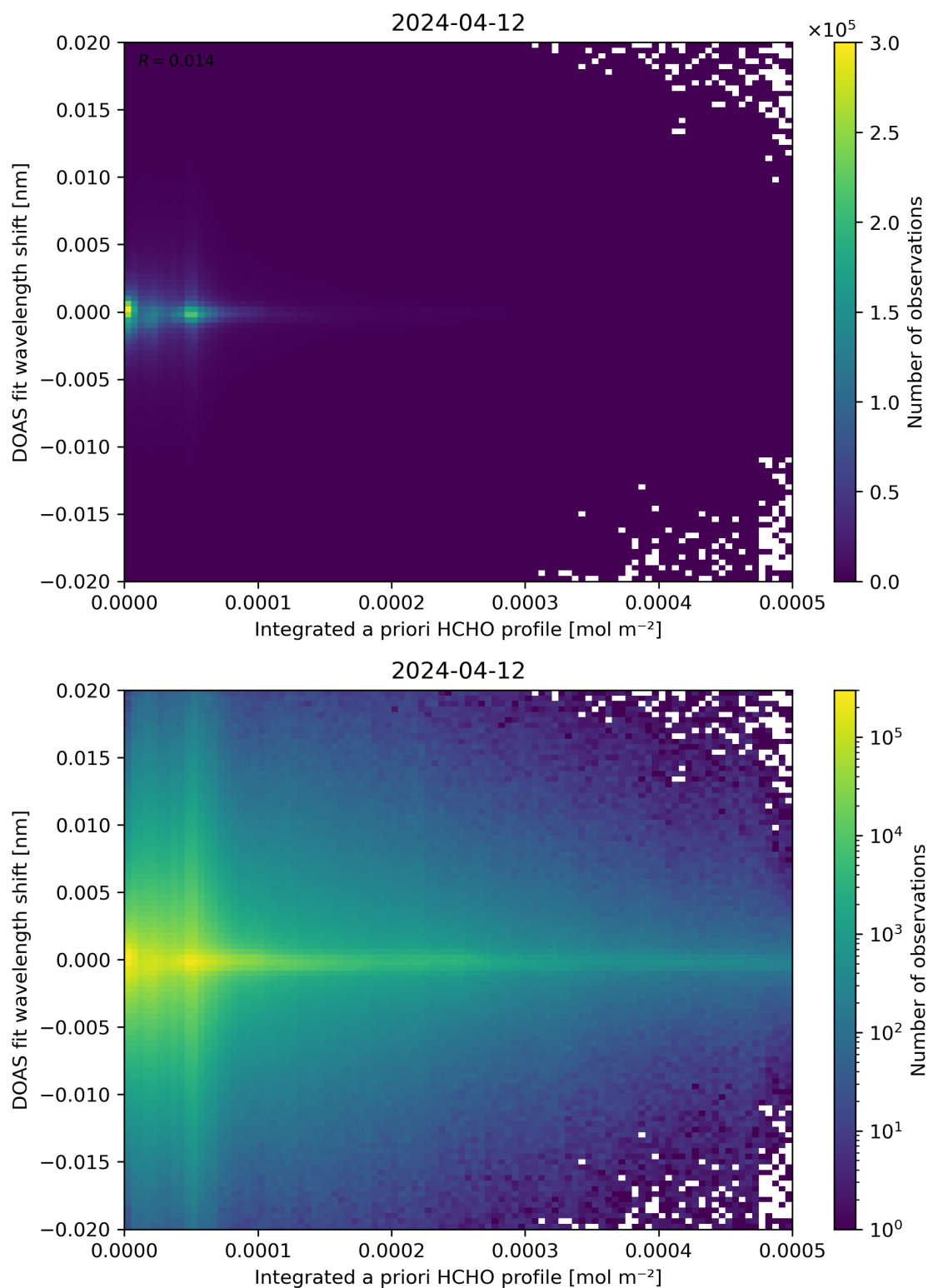
Figure 149: Scatter density plot of “Integrated a priori HCHO profile” against “DOAS fit wavelength shift” for 2024-04-11 to 2024-04-13.
