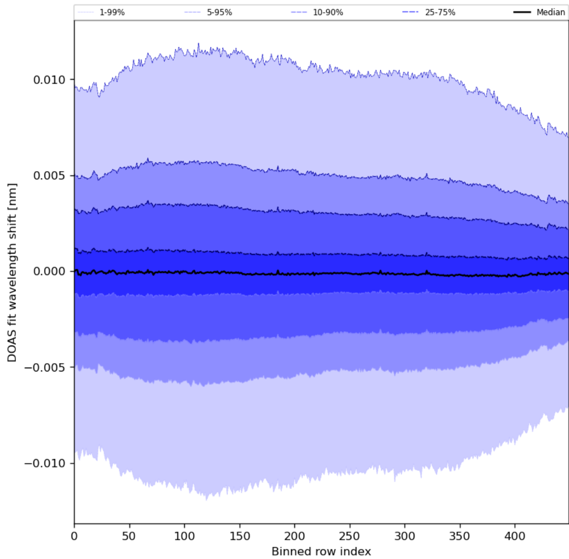
Figure 58: Along track statistics of “DOAS fit wavelength shift” for 2024-04-11 to 2024-04-13
