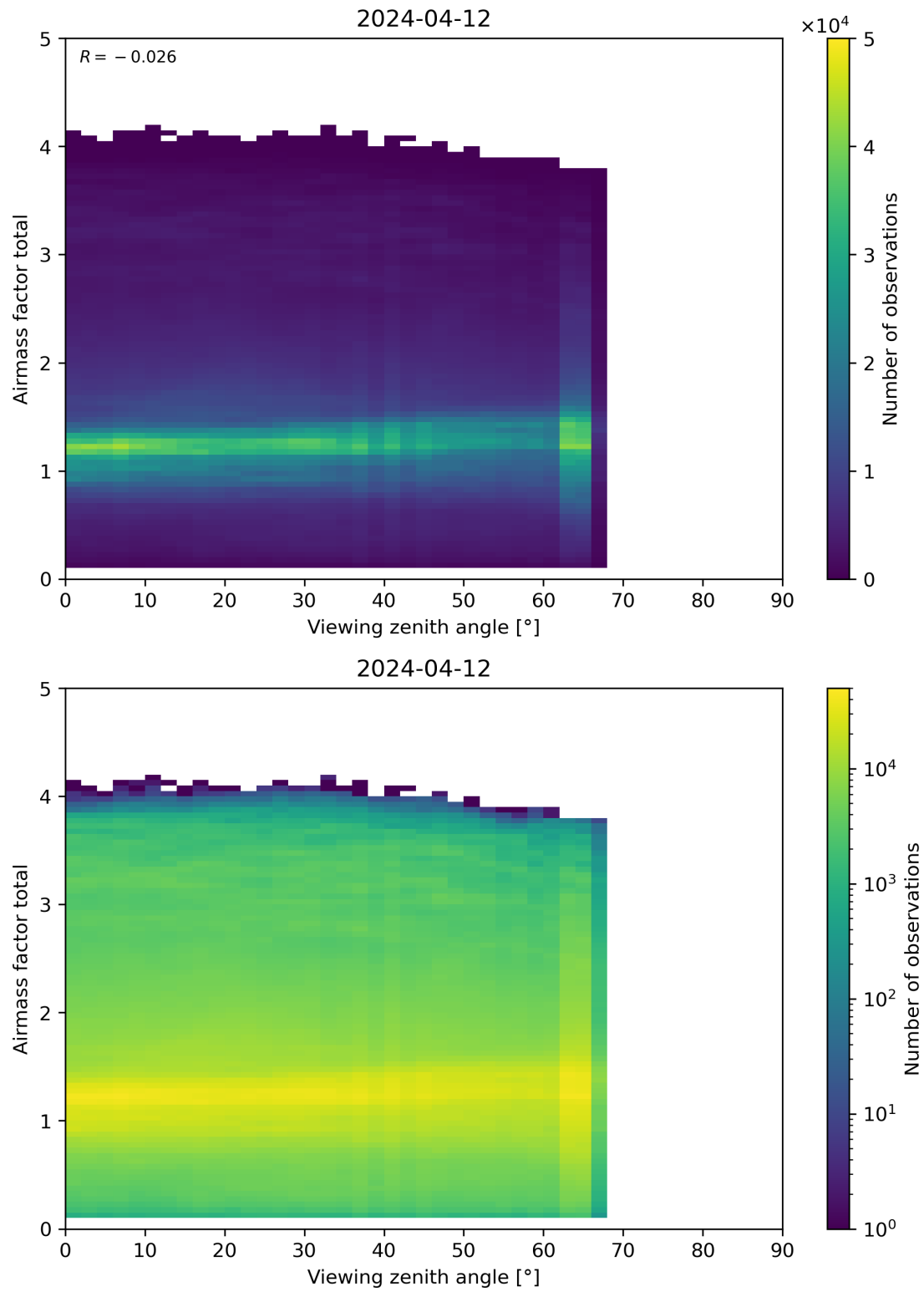
Figure 190: Scatter density plot of “Viewing zenith angle” against “Airmass factor total” for 2024-04-11 to 2024-04-13.
