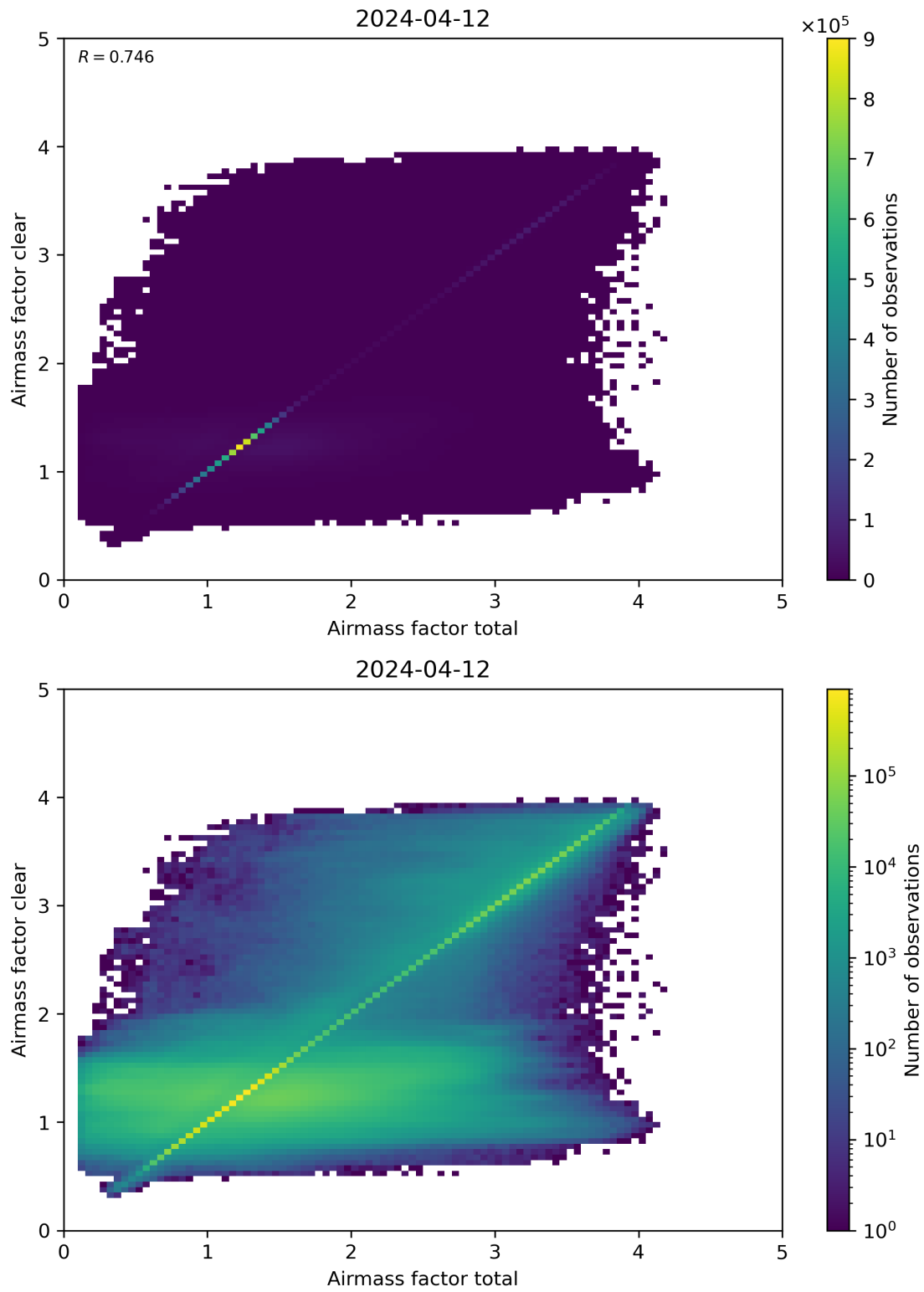
Figure 100: Scatter density plot of “Airmass factor total” against “Airmass factor clear” for 2024-04-11 to 2024-04-13.
