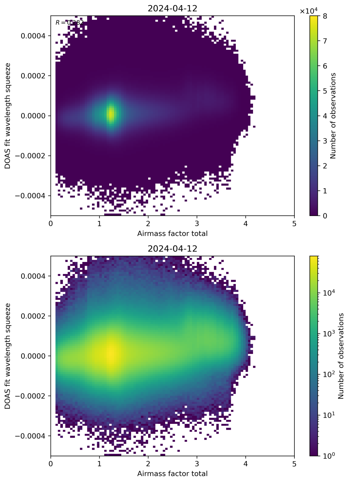
Figure 99: Scatter density plot of “Airmass factor total” against “DOAS fit wavelength squeeze” for 2024-04-11 to 2024-04-13.
