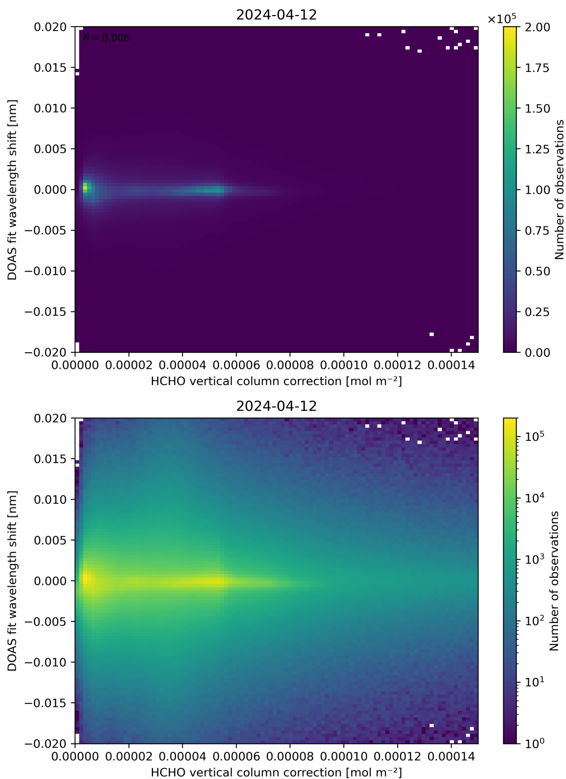
Figure 113: Scatter density plot of “HCHO vertical column correction” against “DOAS fit wavelength shift” for 2024-04-11 to 2024-04-13.
