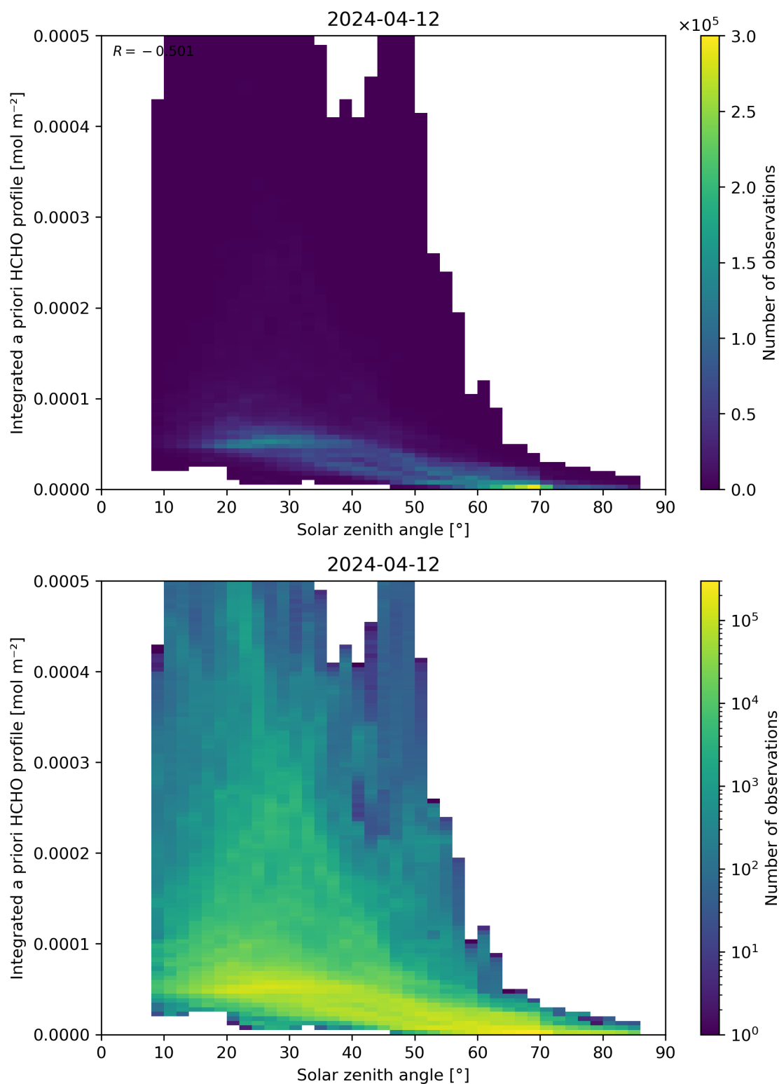
Figure 180: Scatter density plot of “Solar zenith angle” against “Integrated a priori HCHO profile” for 2024-04-11 to 2024-04-13.
