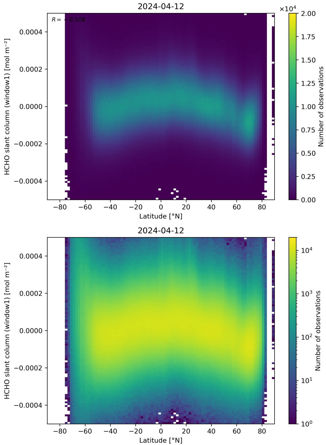
Figure 159: Scatter density plot of “Latitude” against “HCHO slant column (window1)” for 2024-04-11 to 2024-04-13.
