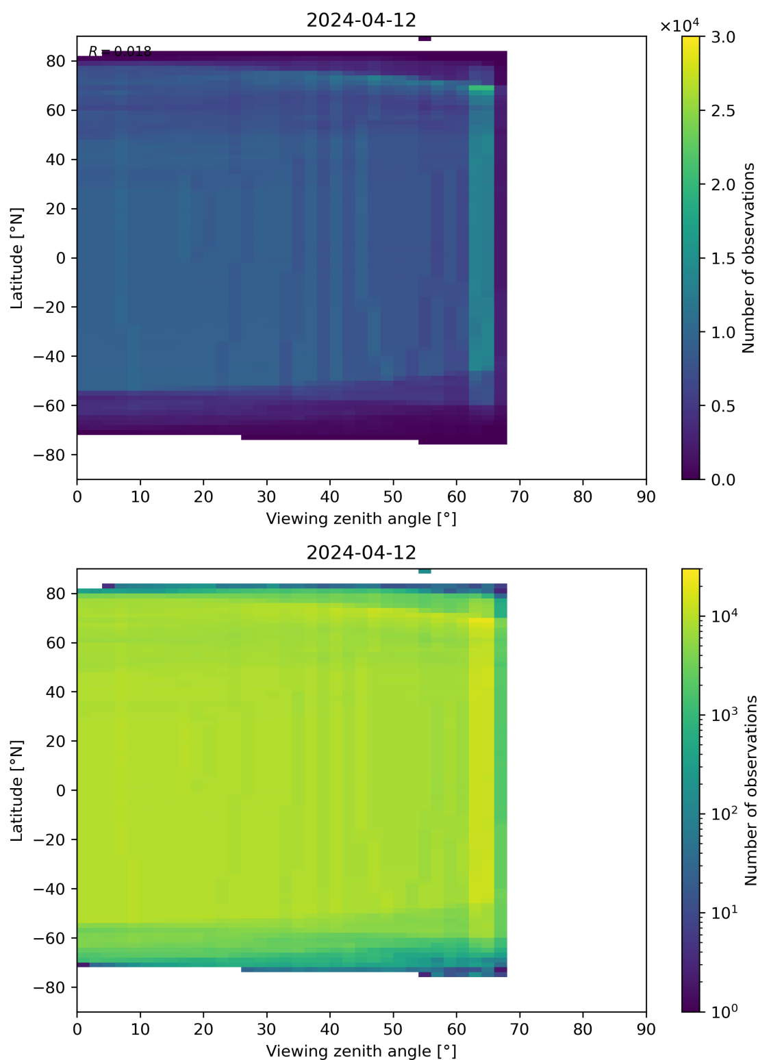
Figure 196: Scatter density plot of “Viewing zenith angle” against “Latitude” for 2024-04-11 to 2024-04-13.
