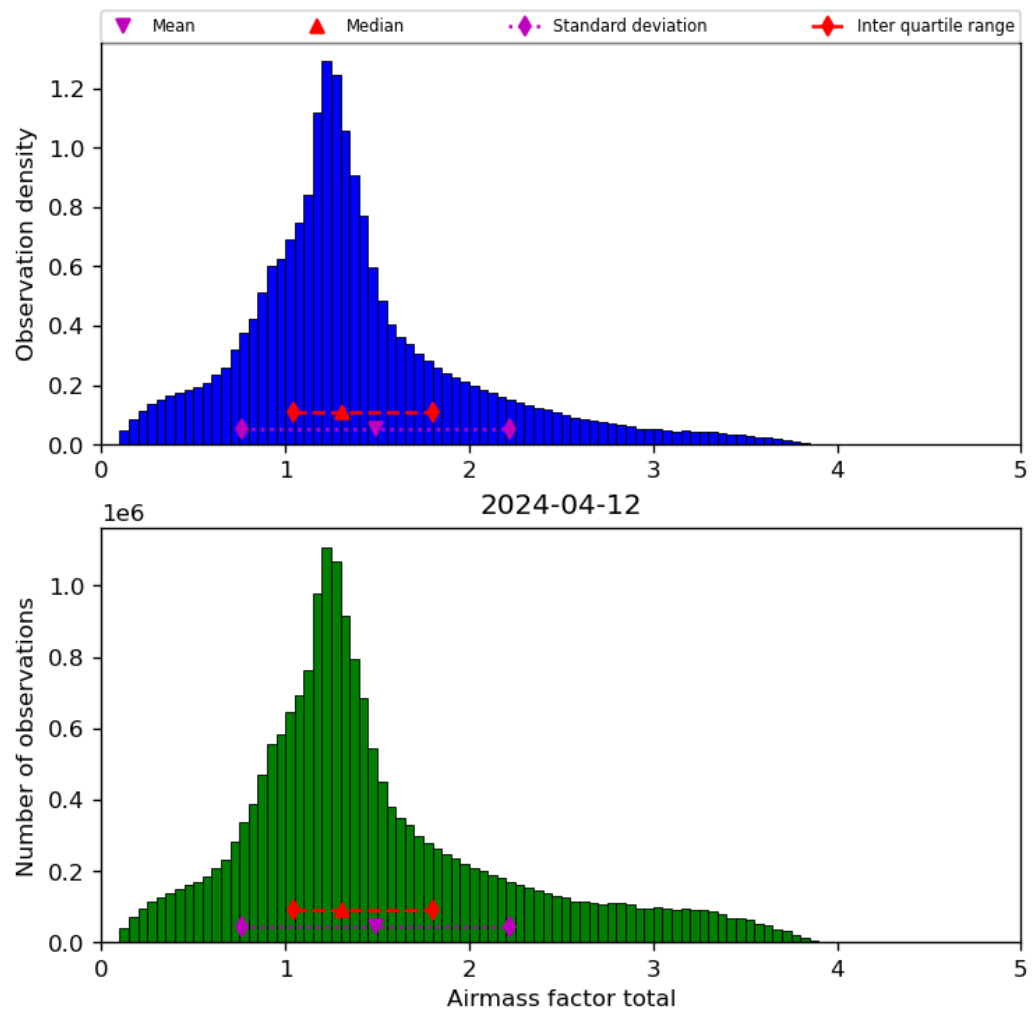
Figure 40: Histogram of “Airmass factor total” for 2024-04-11 to 2024-04-13
