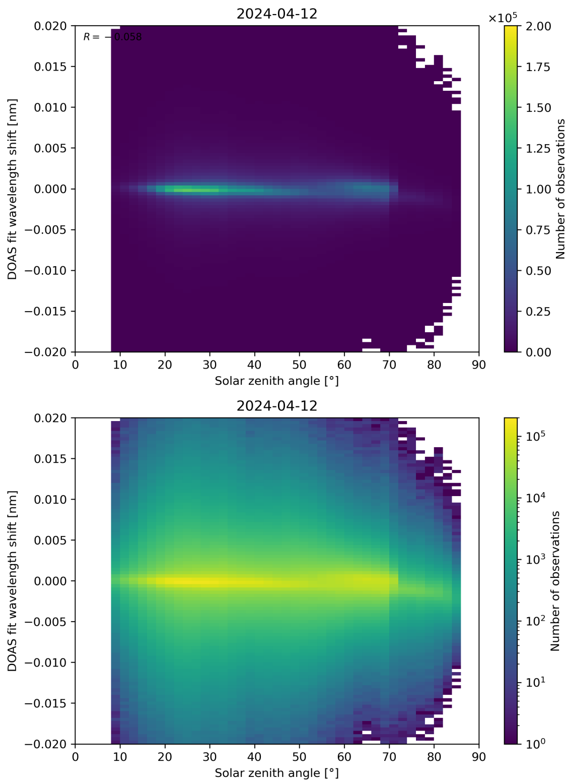
Figure 168: Scatter density plot of “Solar zenith angle” against “DOAS fit wavelength shift” for 2024-04-11 to 2024-04-13.
