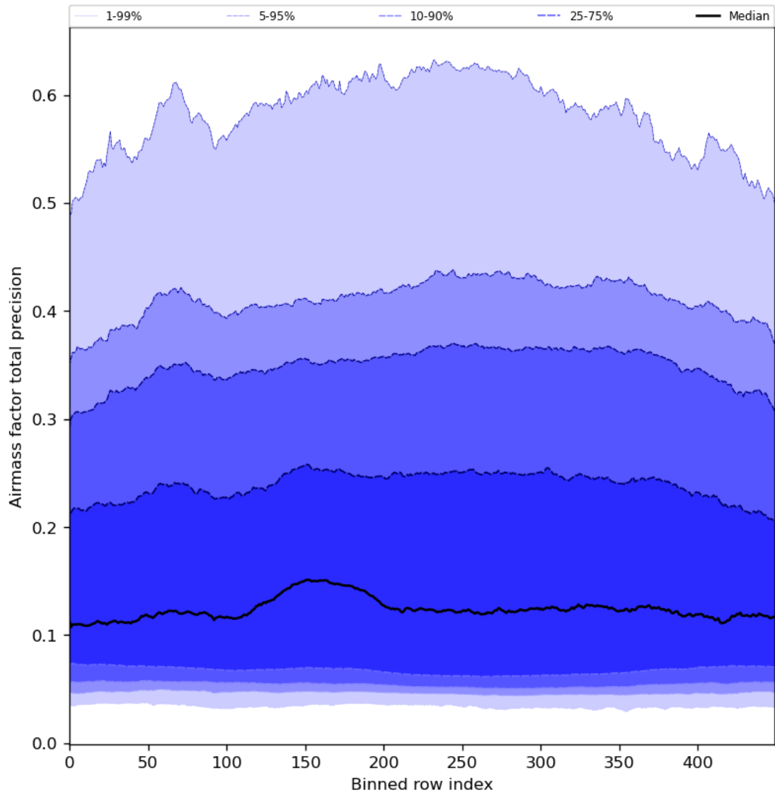
Figure 55: Along track statistics of “Airmass factor total precision” for 2024-04-11 to 2024-04-13
