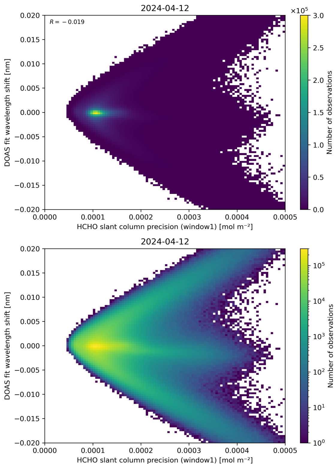
Figure 89: Scatter density plot of “HCHO slant column precision (window1)” against “DOAS fit wavelength shift” for 2024-04-11 to 2024-04-13.
