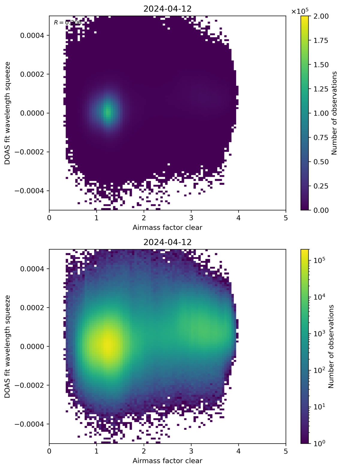
Figure 73: Scatter density plot of “Airmass factor clear” against “DOAS fit wavelength squeeze” for 2024-04-11 to 2024-04-13.
