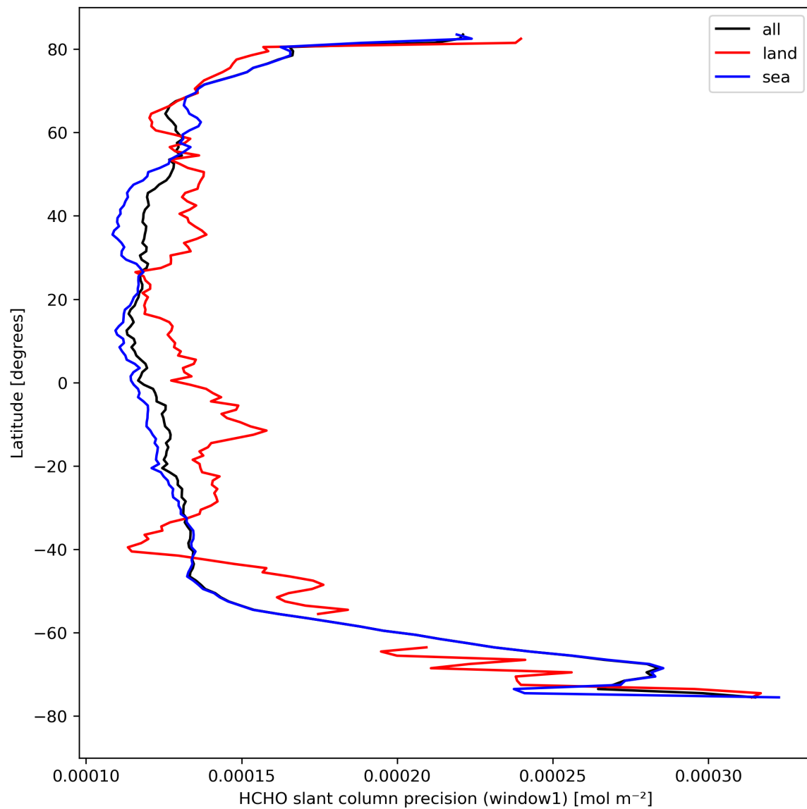
Figure 25: Zonal average of “HCHO slant column precision (window1)” for 2024-04-11 to 2024-04-13.
