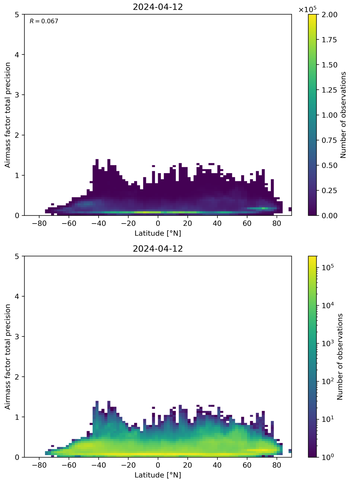
Figure 162: Scatter density plot of “Latitude” against “Airmass factor total precision” for 2024-04-11 to 2024-04-13.
