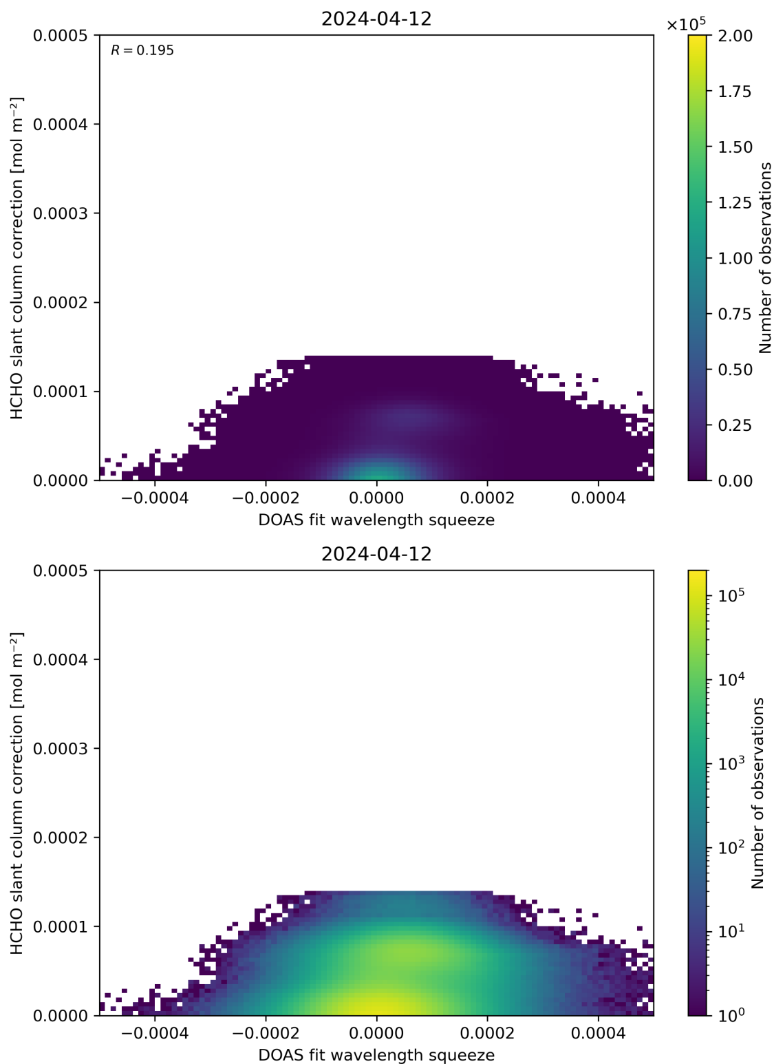
Figure 70: Scatter density plot of “DOAS fit wavelength squeeze” against “HCHO slant column correction” for 2024-04-11 to 2024-04-13.
