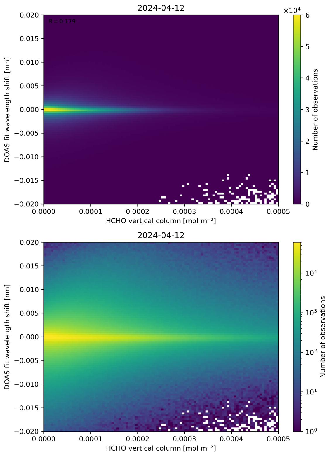
Figure 124: Scatter density plot of “HCHO vertical column” against “DOAS fit wavelength shift” for 2024-04-11 to 2024-04-13.
