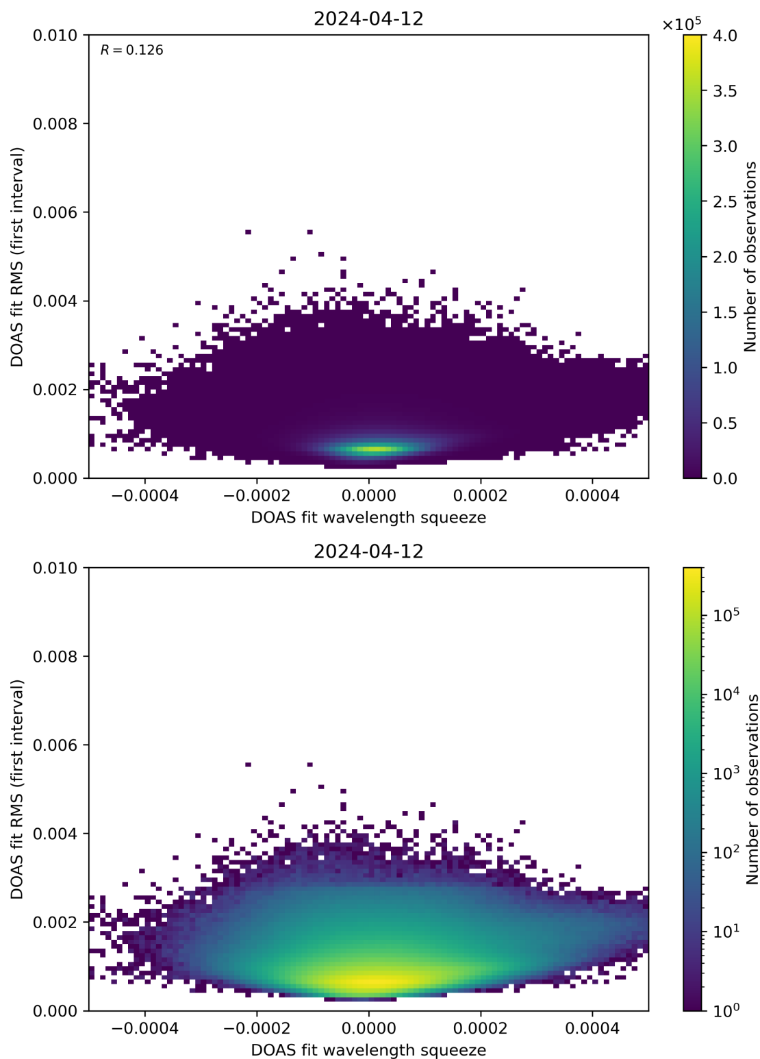
Figure 68: Scatter density plot of “DOAS fit wavelength squeeze” against “DOAS fit RMS (first interval)” for 2024-04-11 to 2024-04-13.
