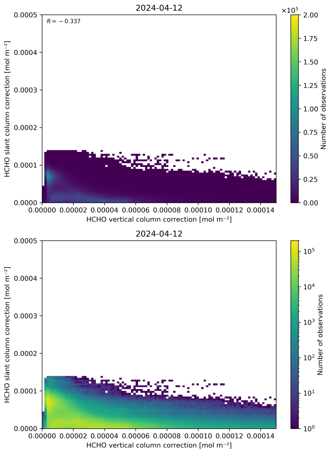
Figure 117: Scatter density plot of “HCHO vertical column correction” against “HCHO slant column correction” for 2024-04-11 to 2024-04-13.
