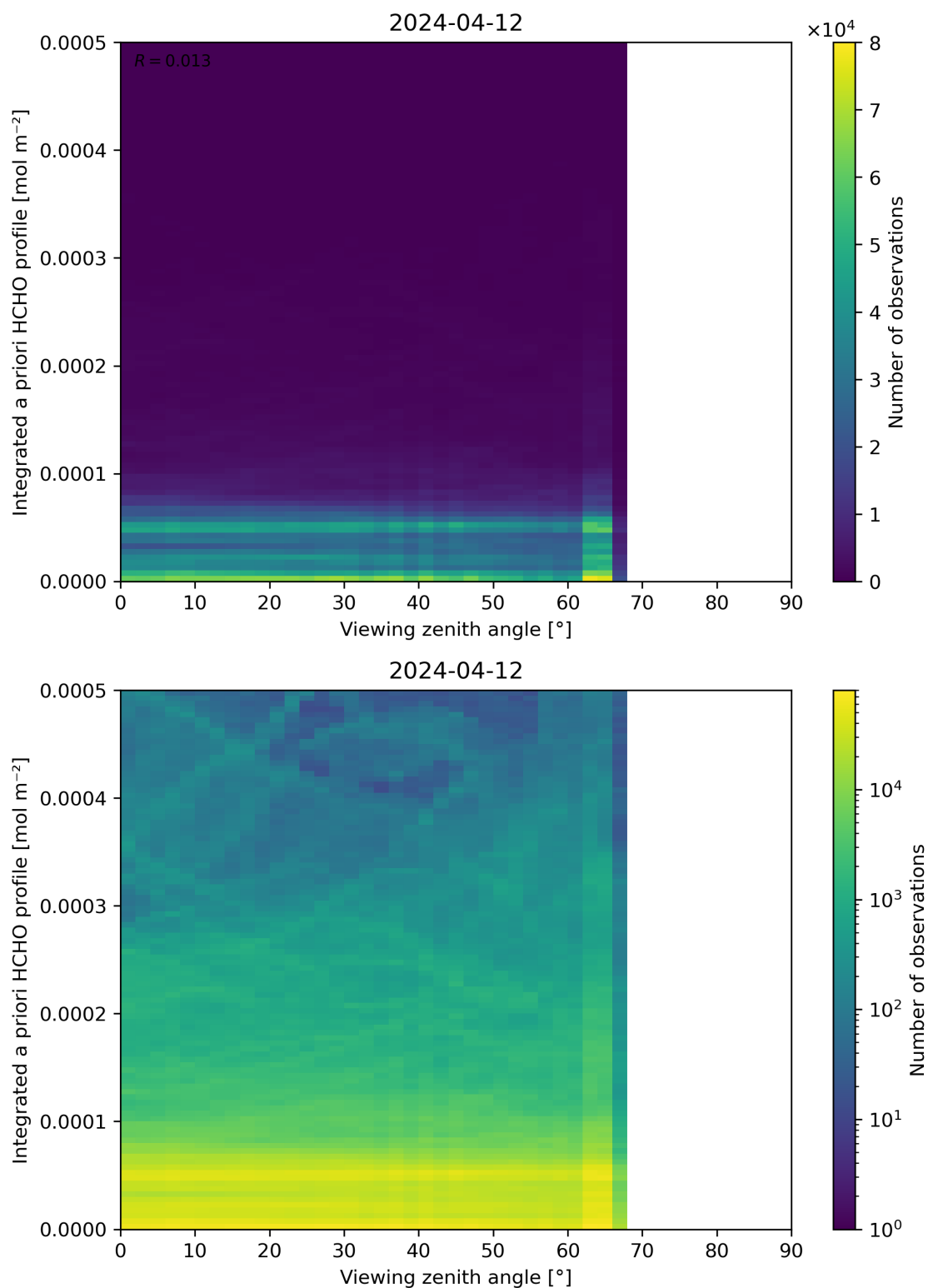
Figure 195: Scatter density plot of “Viewing zenith angle” against “Integrated a priori HCHO profile” for 2024-04-11 to 2024-04-13.
