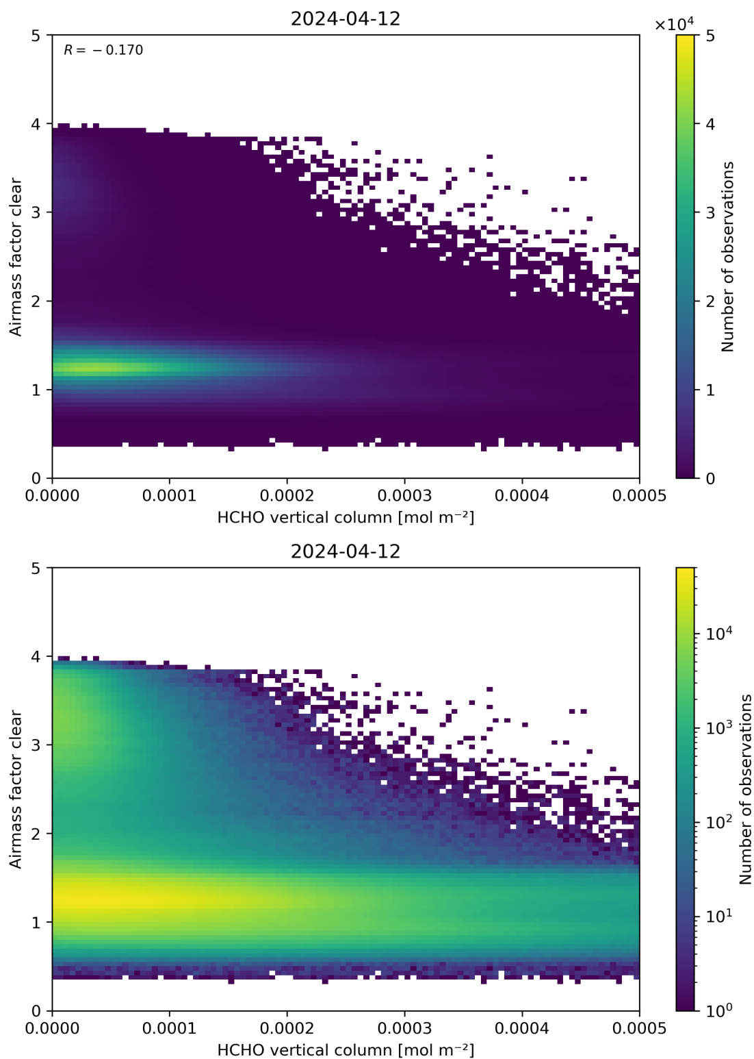
Figure 126: Scatter density plot of “HCHO vertical column” against “Airmass factor clear” for 2024-04-11 to 2024-04-13.
