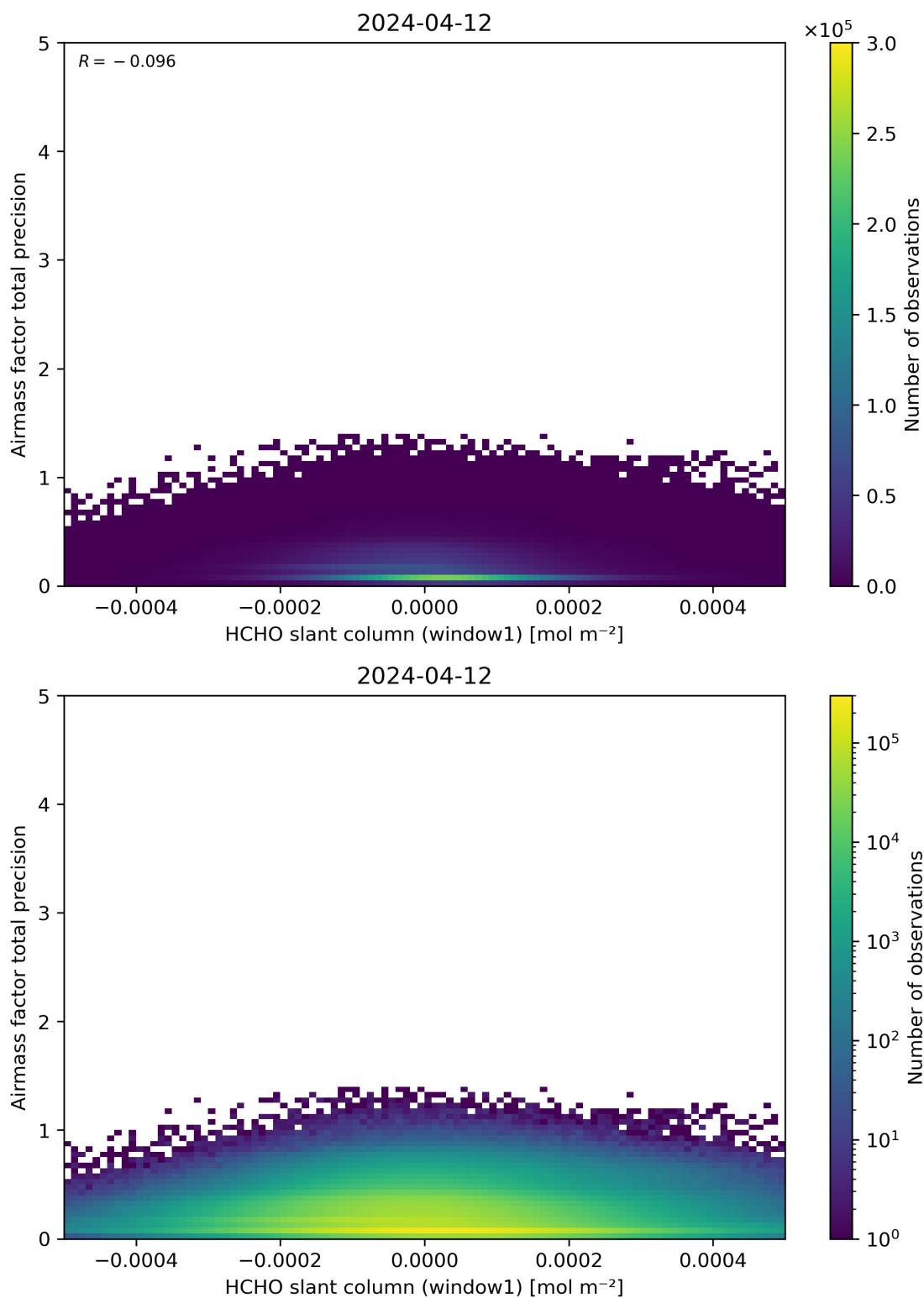
Figure 86: Scatter density plot of “HCHO slant column (window1)” against “Airmass factor total precision” for 2024-04-11 to 2024-04-13.
