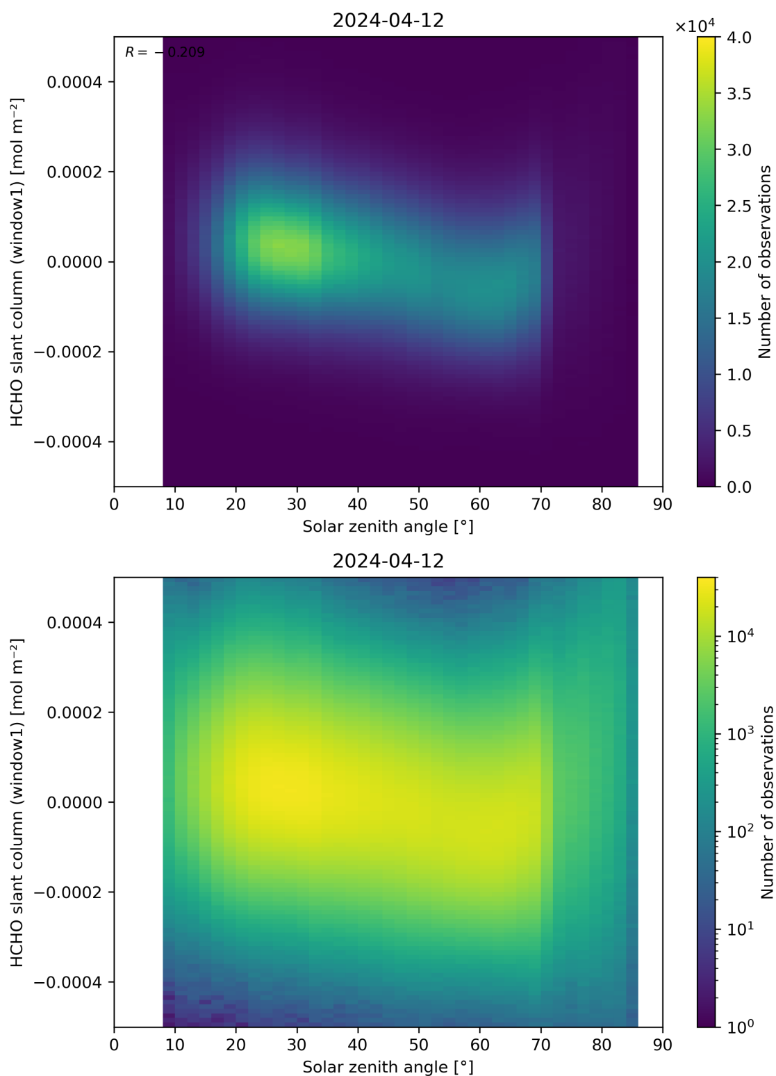
Figure 173: Scatter density plot of “Solar zenith angle” against “HCHO slant column (window1)” for 2024-04-11 to 2024-04-13.
