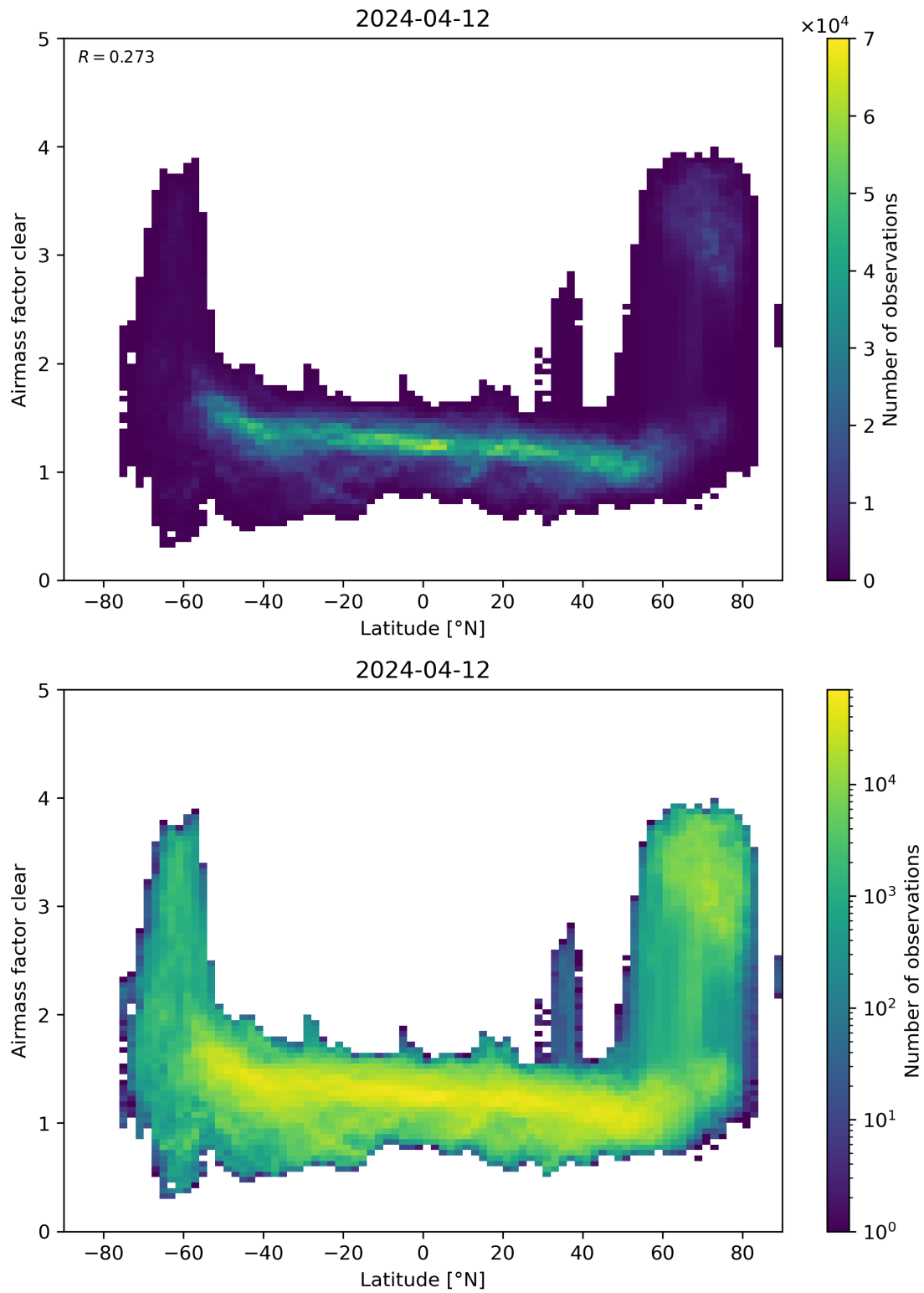
Figure 156: Scatter density plot of “Latitude” against “Airmass factor clear” for 2024-04-11 to 2024-04-13.
