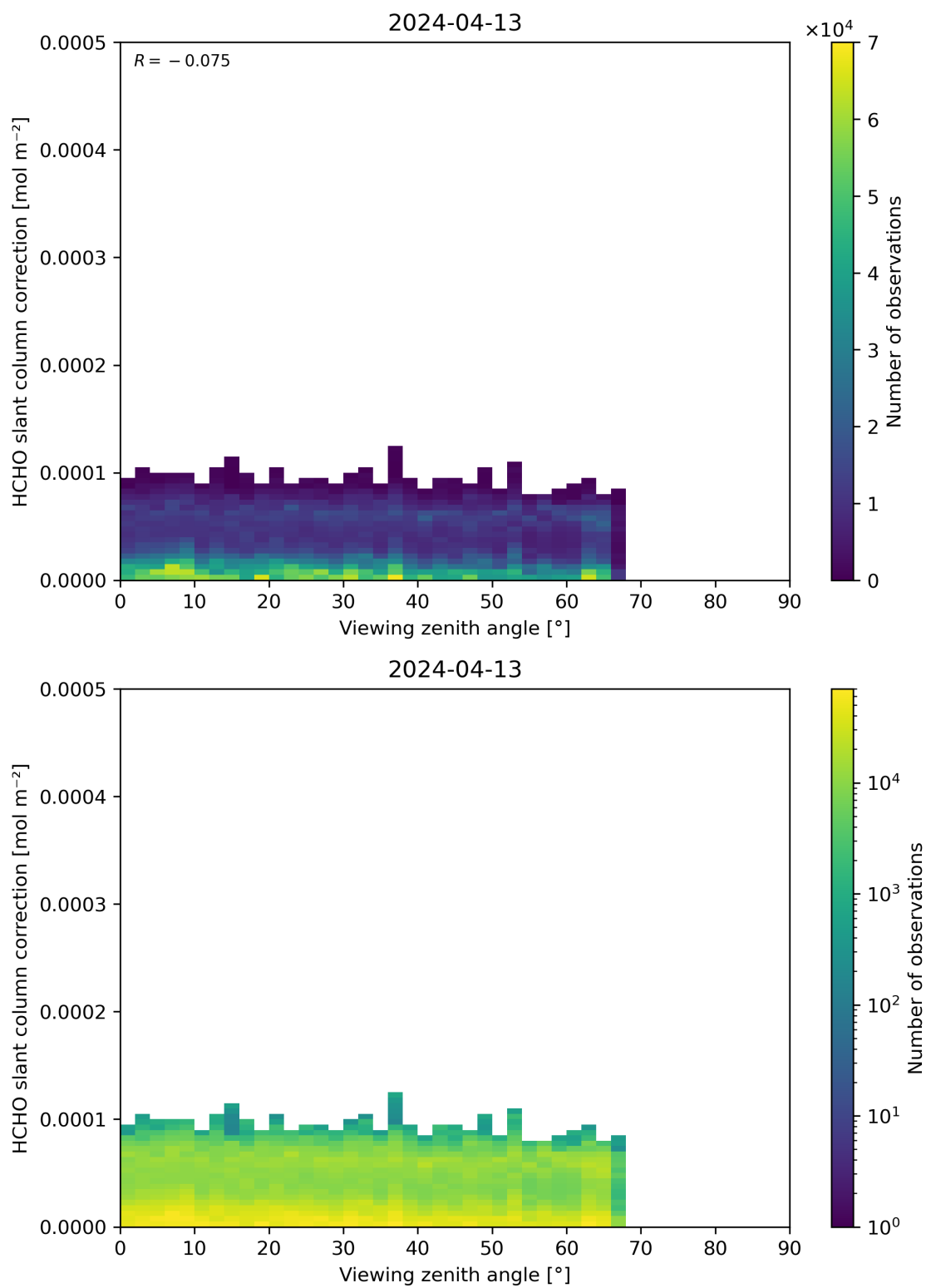
Figure 187: Scatter density plot of “Viewing zenith angle” against “HCHO slant column correction” for 2024-04-12 to 2024-04-14.
