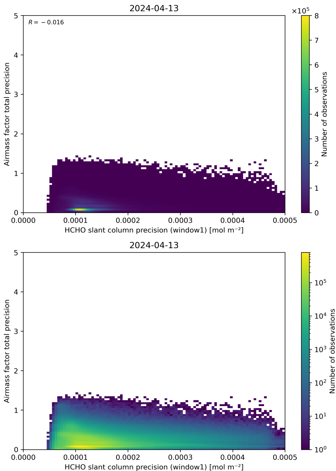
Figure 95: Scatter density plot of “HCHO slant column precision (window1)” against “Airmass factor total precision” for 2024-04-12 to 2024-04-14.
