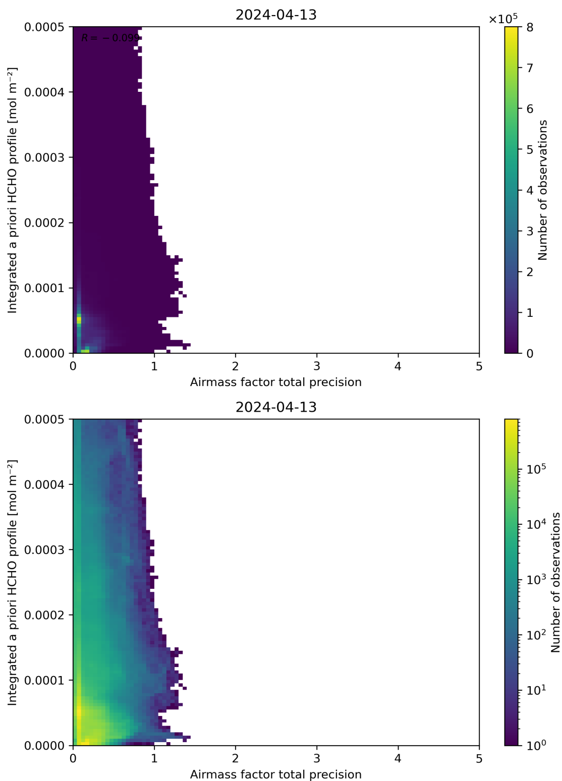
Figure 111: Scatter density plot of “Airmass factor total precision” against “Integrated a priori HCHO profile” for 2024-04-12 to 2024-04-14.
