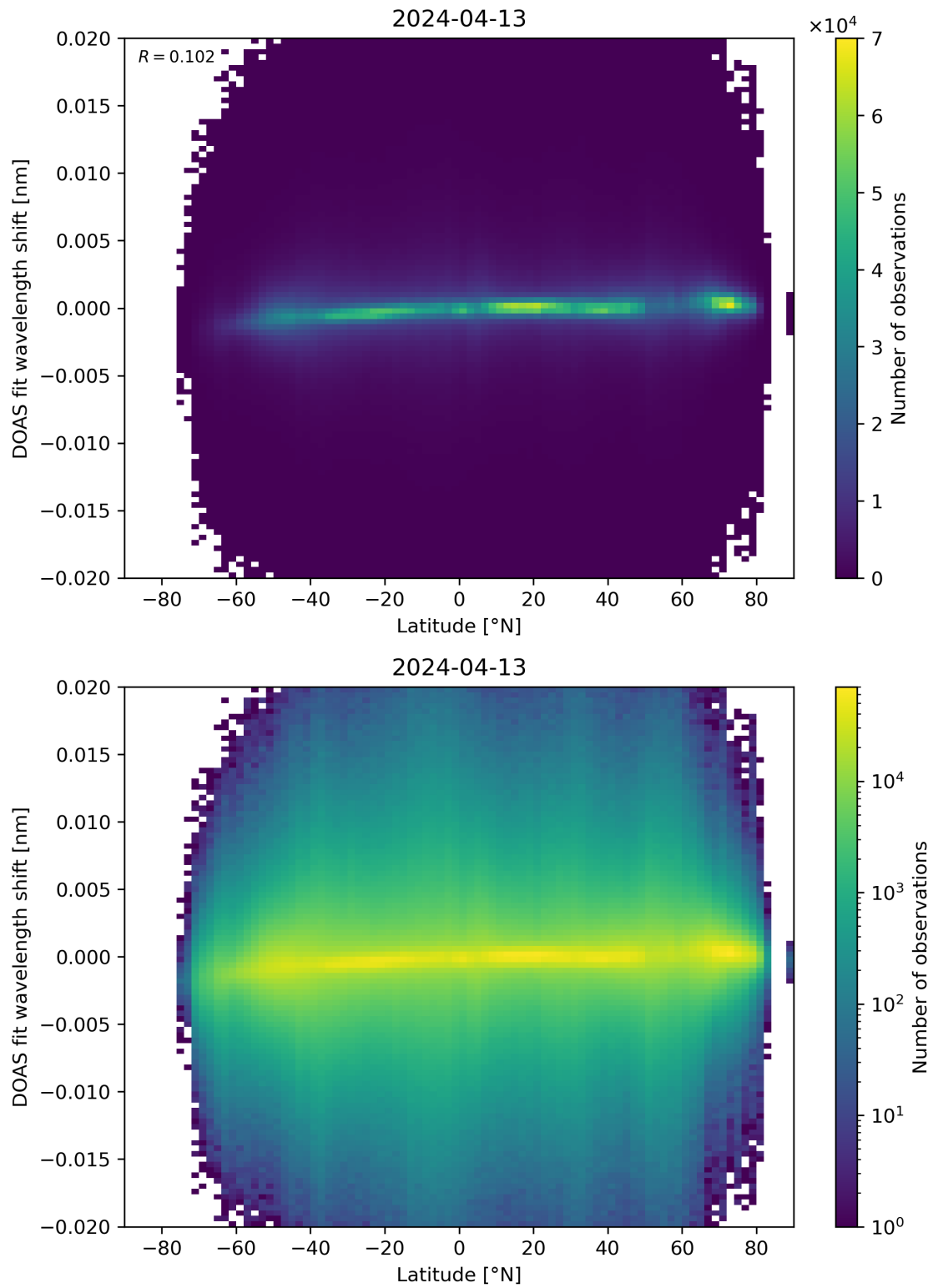
Figure 154: Scatter density plot of “Latitude” against “DOAS fit wavelength shift” for 2024-04-12 to 2024-04-14.
