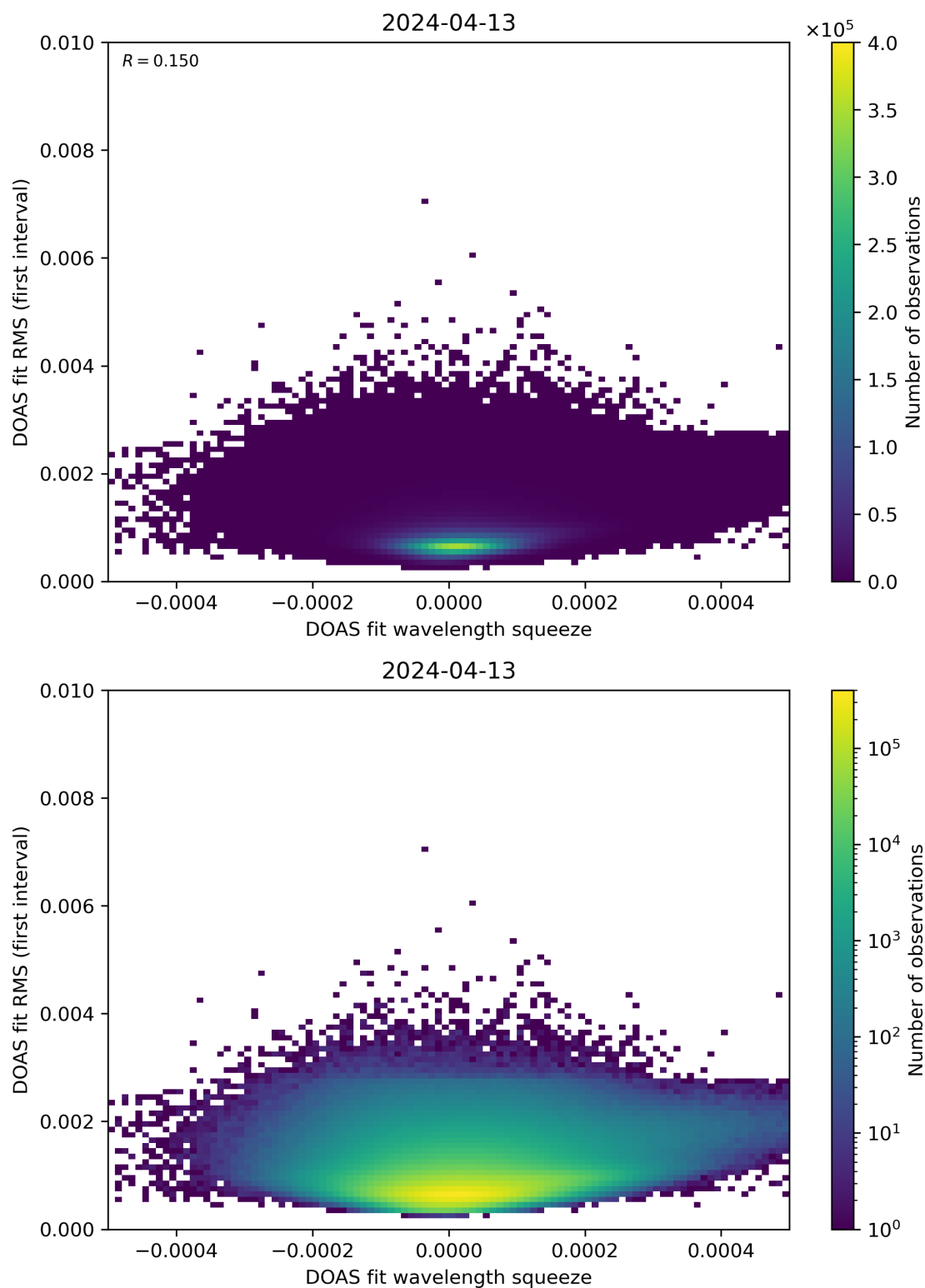
Figure 68: Scatter density plot of “DOAS fit wavelength squeeze” against “DOAS fit RMS (first interval)” for 2024-04-12 to 2024-04-14.
