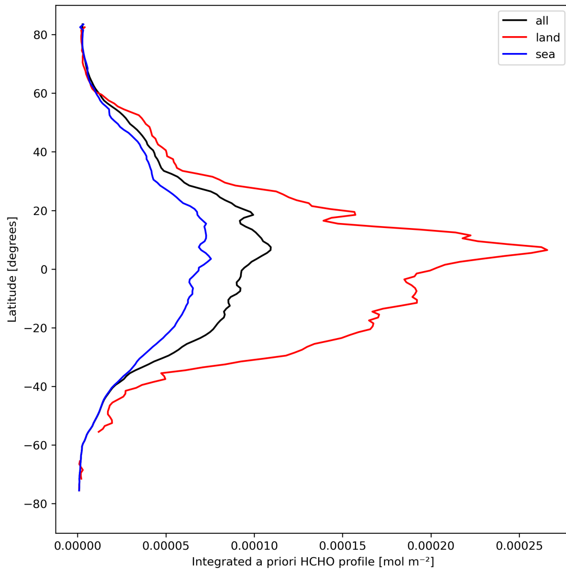
Figure 29: Zonal average of “Integrated a priori HCHO profile” for 2024-04-12 to 2024-04-14.
