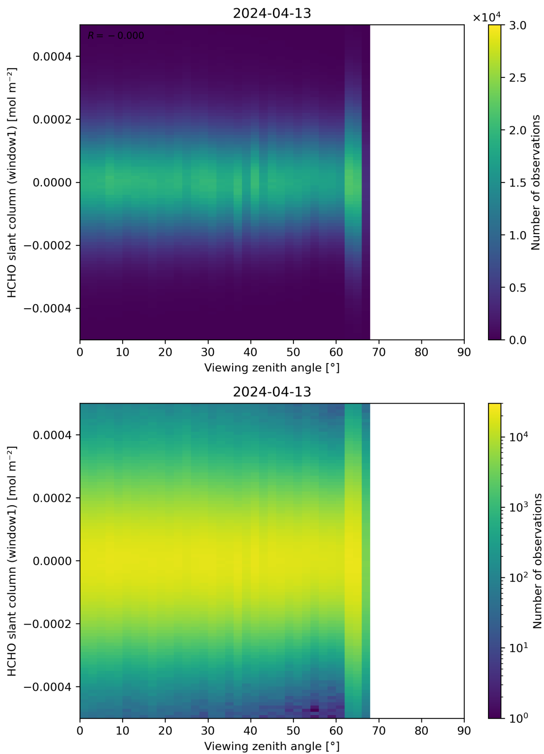
Figure 188: Scatter density plot of “Viewing zenith angle” against “HCHO slant column (window1)” for 2024-04-12 to 2024-04-14.
