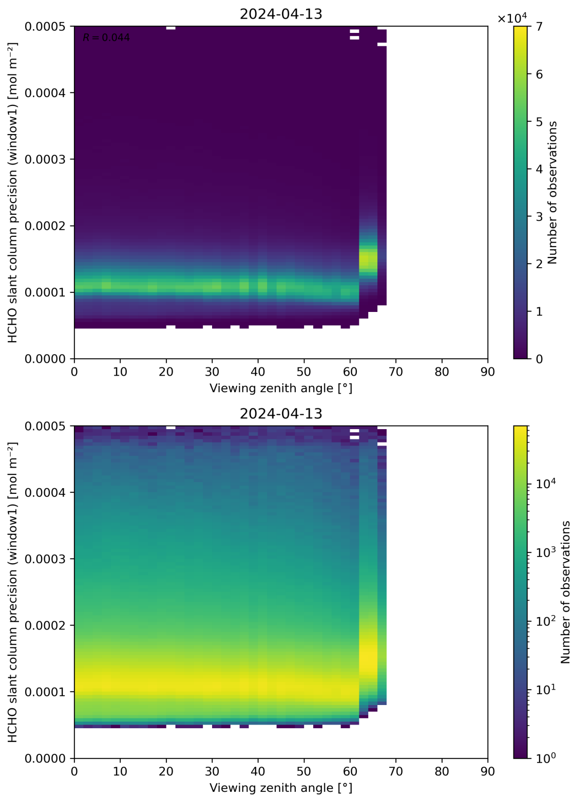
Figure 189: Scatter density plot of “Viewing zenith angle” against “HCHO slant column precision (window1)” for 2024-04-12 to 2024-04-14.
