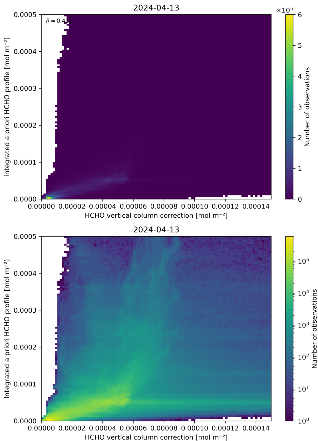
Figure 122: Scatter density plot of “HCHO vertical column correction” against “Integrated a priori HCHO profile” for 2024-04-12 to 2024-04-14.
