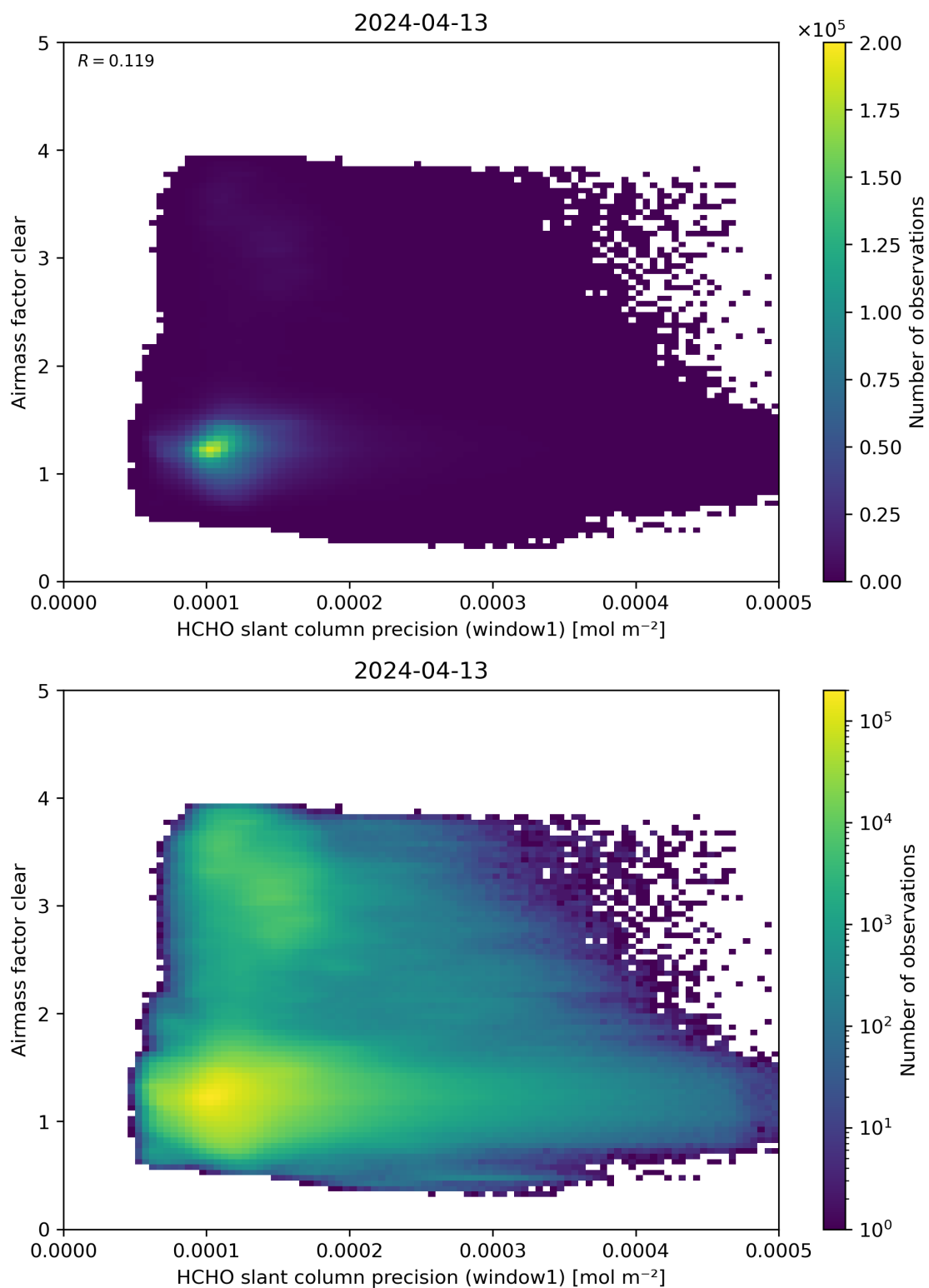
Figure 91: Scatter density plot of “HCHO slant column precision (window1)” against “Airmass factor clear” for 2024-04-12 to 2024-04-14.
