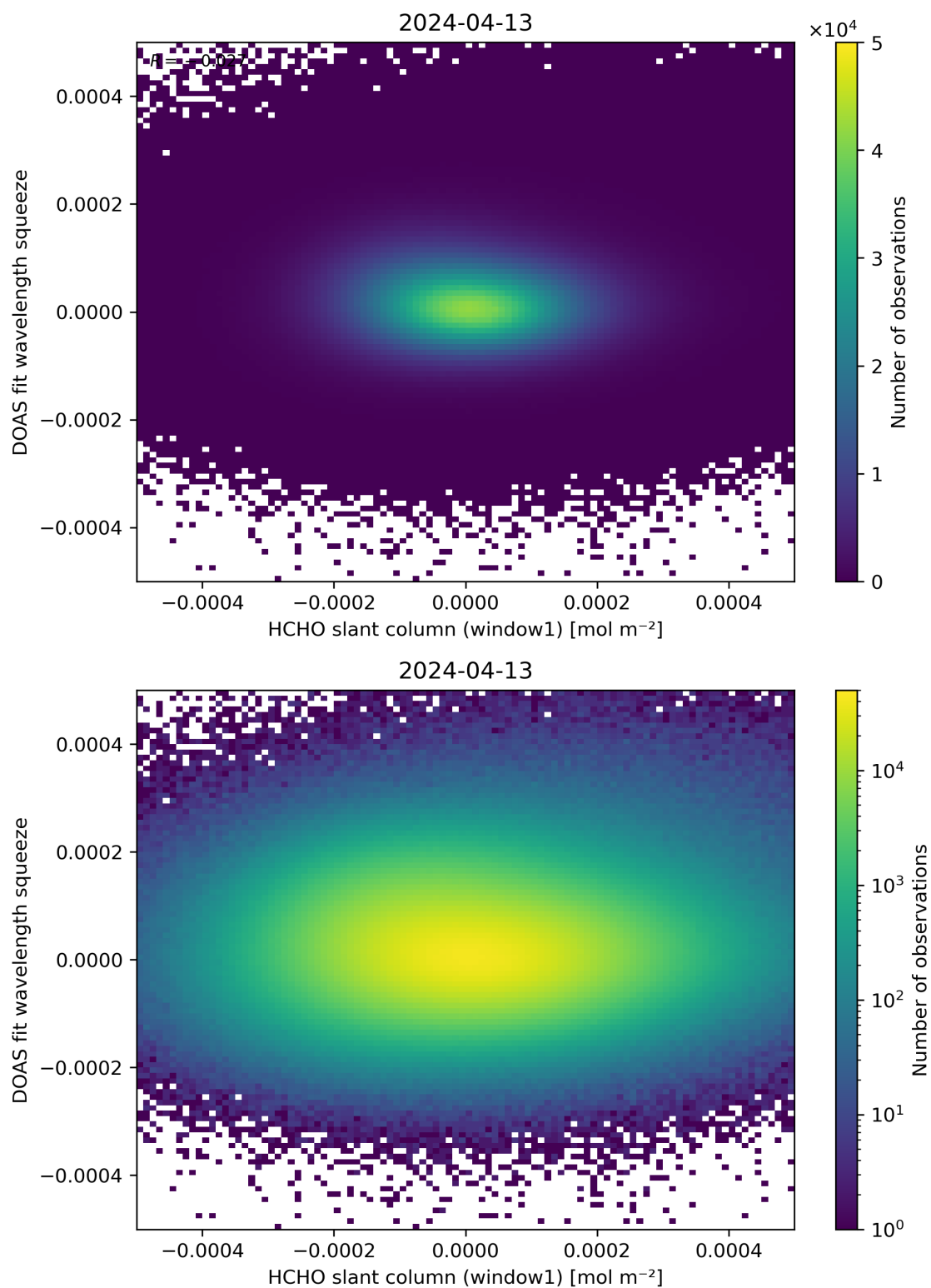
Figure 80: Scatter density plot of “HCHO slant column (window1)” against “DOAS fit wavelength squeeze” for 2024-04-12 to 2024-04-14.
