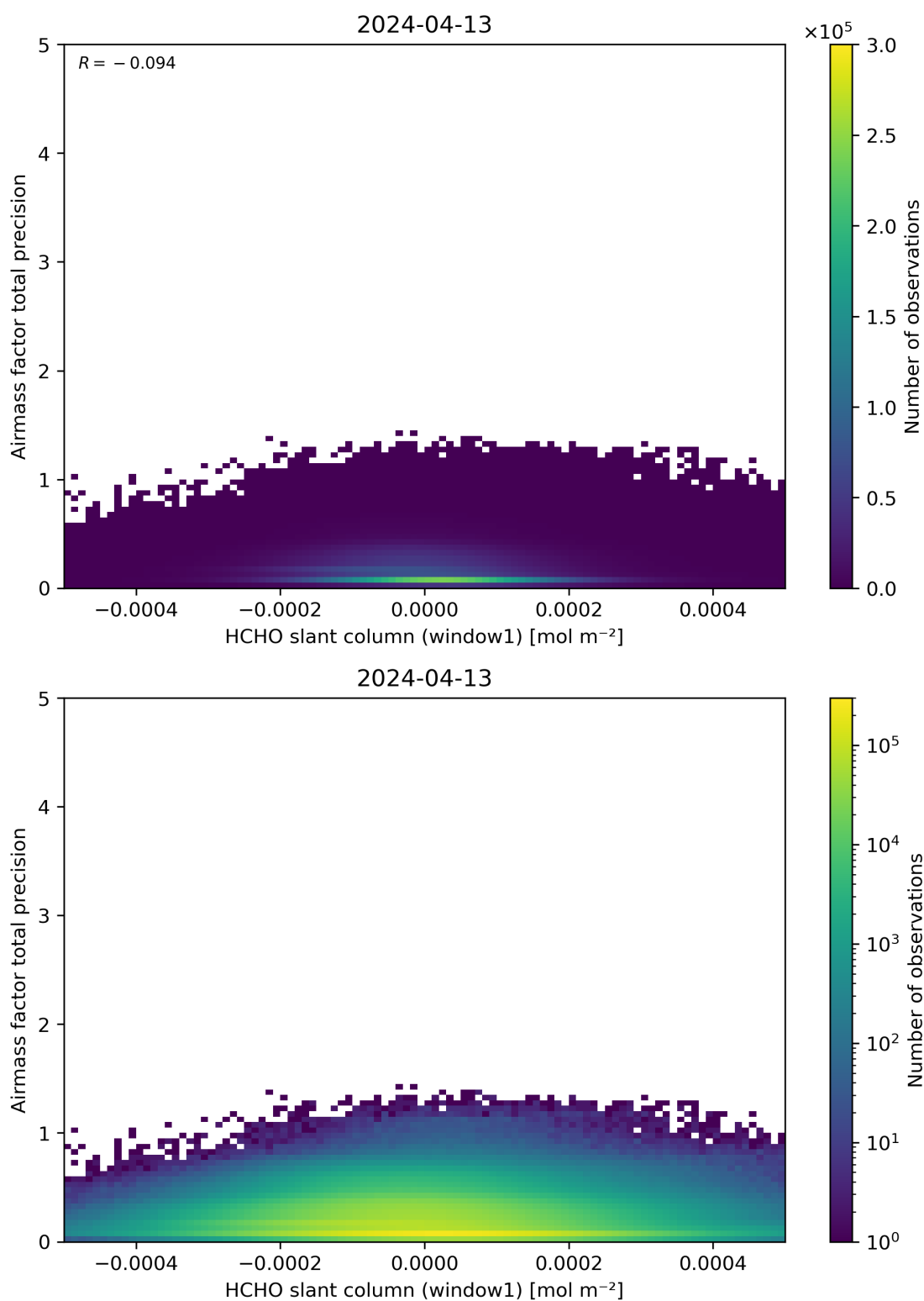
Figure 86: Scatter density plot of “HCHO slant column (window1)” against “Airmass factor total precision” for 2024-04-12 to 2024-04-14.
