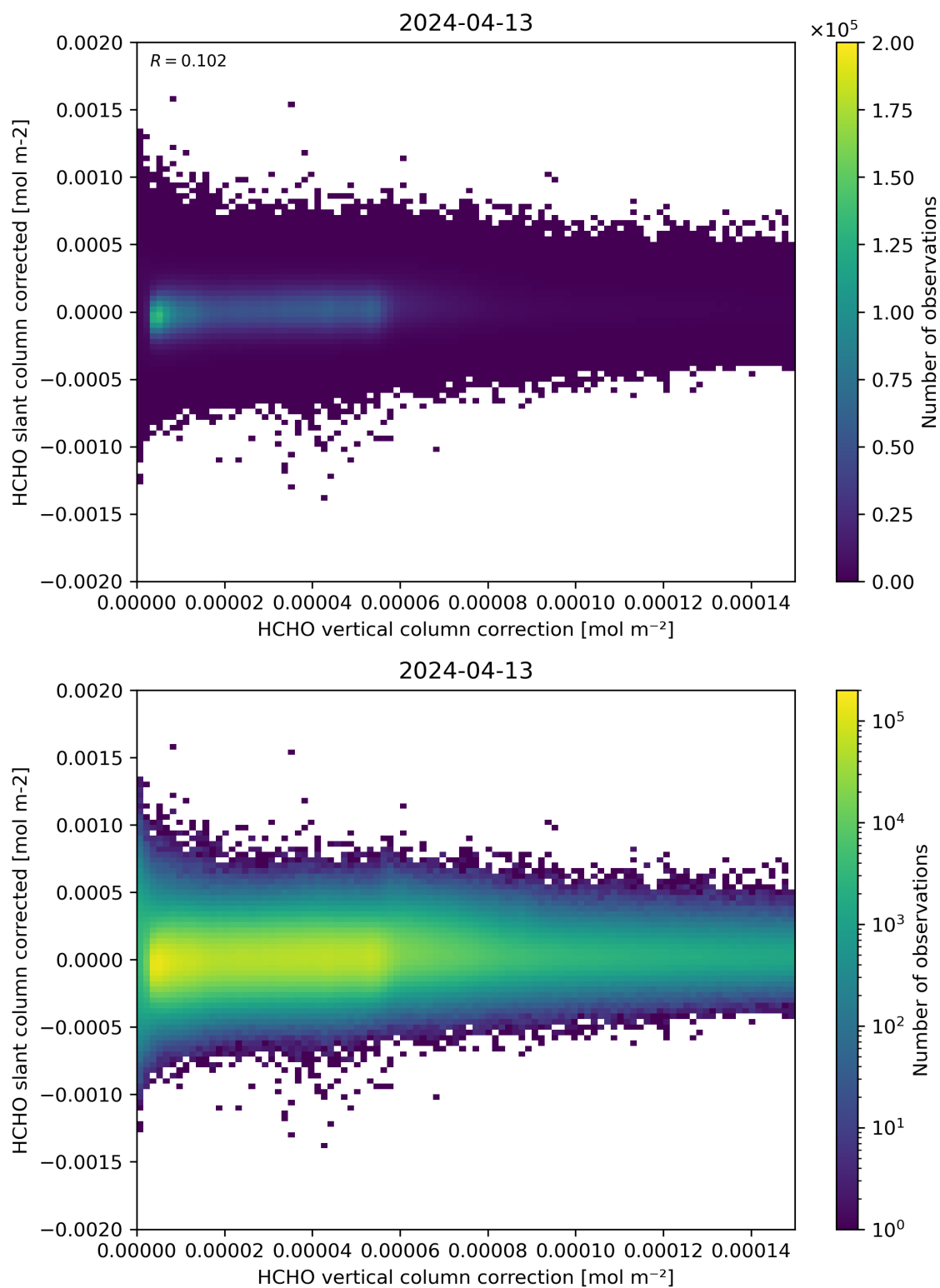
Figure 116: Scatter density plot of “HCHO vertical column correction” against “HCHO slant column corrected” for 2024-04-12 to 2024-04-14.
