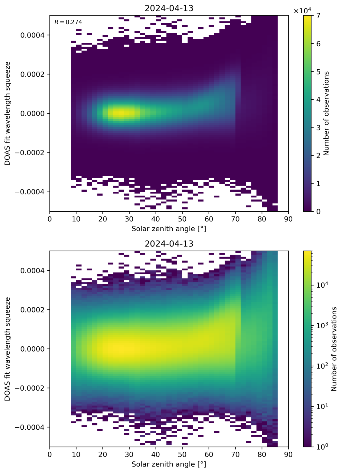
Figure 169: Scatter density plot of “Solar zenith angle” against “DOAS fit wavelength squeeze” for 2024-04-12 to 2024-04-14.
