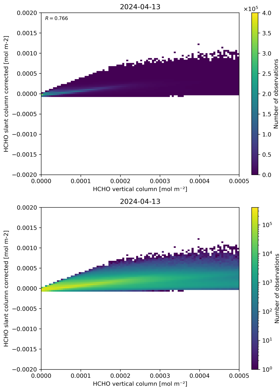
Figure 127: Scatter density plot of “HCHO vertical column” against “HCHO slant column corrected” for 2024-04-12 to 2024-04-14.
