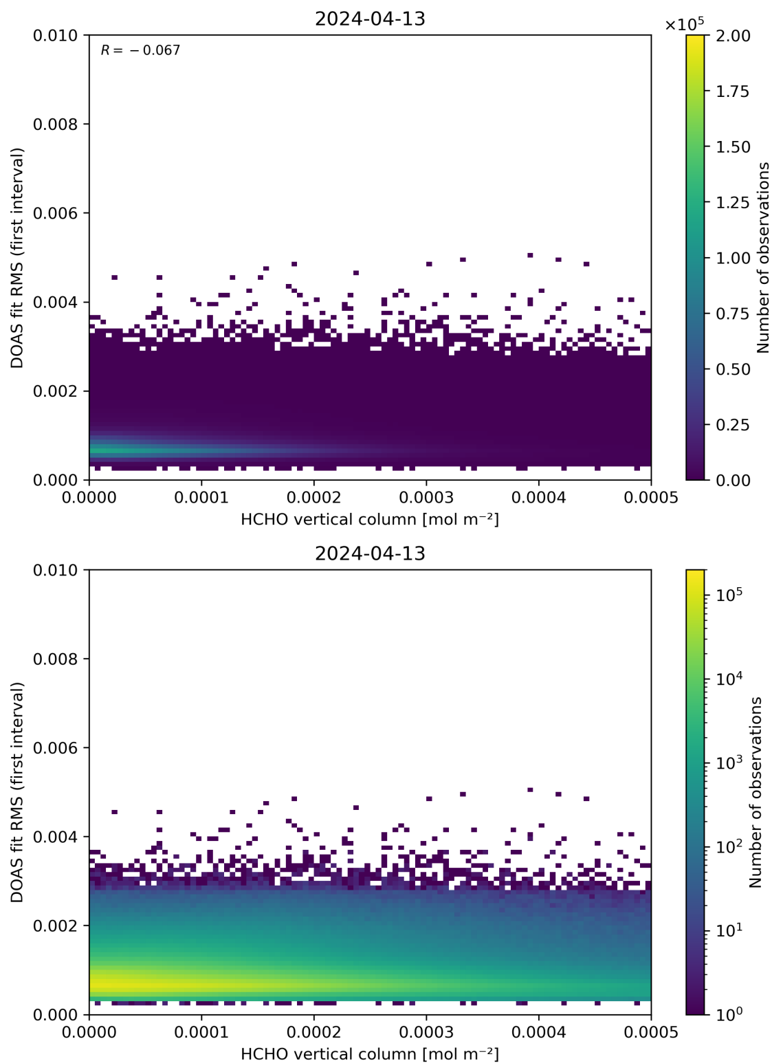
Figure 123: Scatter density plot of “HCHO vertical column” against “DOAS fit RMS (first interval)” for 2024-04-12 to 2024-04-14.
