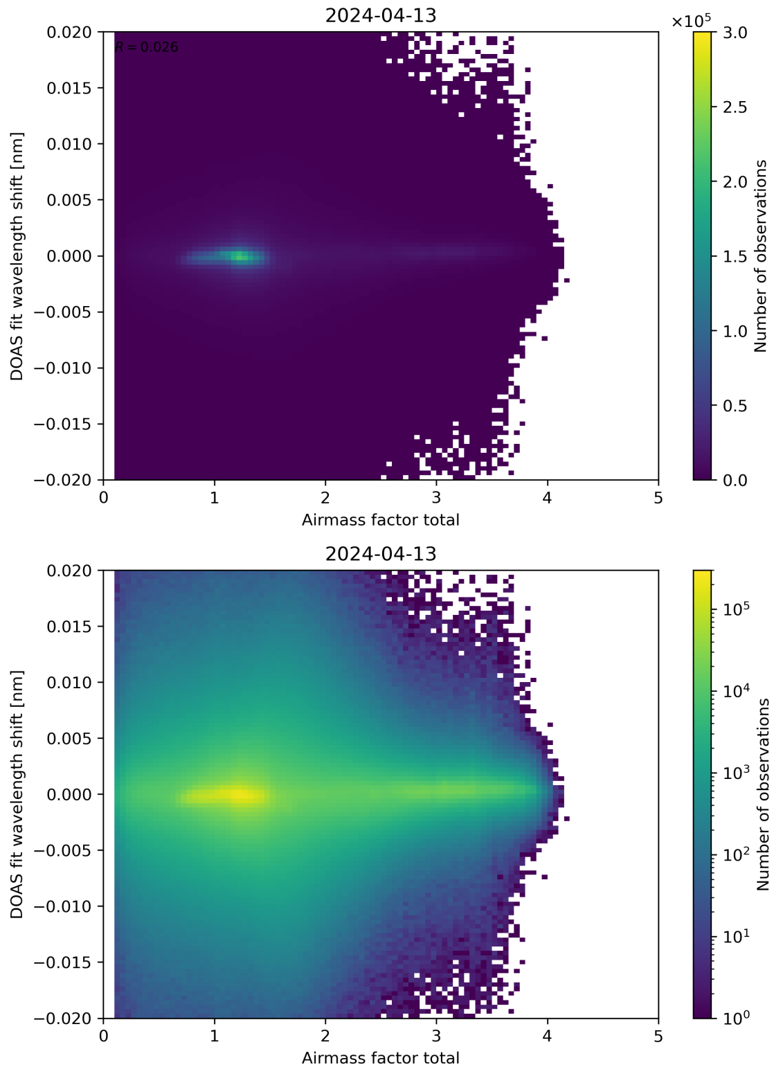
Figure 98: Scatter density plot of “Airmass factor total” against “DOAS fit wavelength shift” for 2024-04-12 to 2024-04-14.
