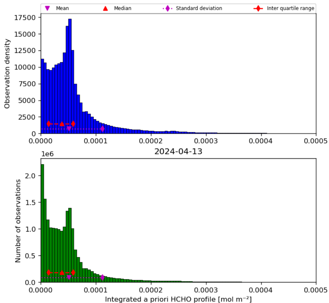
Figure 43: Histogram of “Integrated a priori HCHO profile” for 2024-04-12 to 2024-04-14
