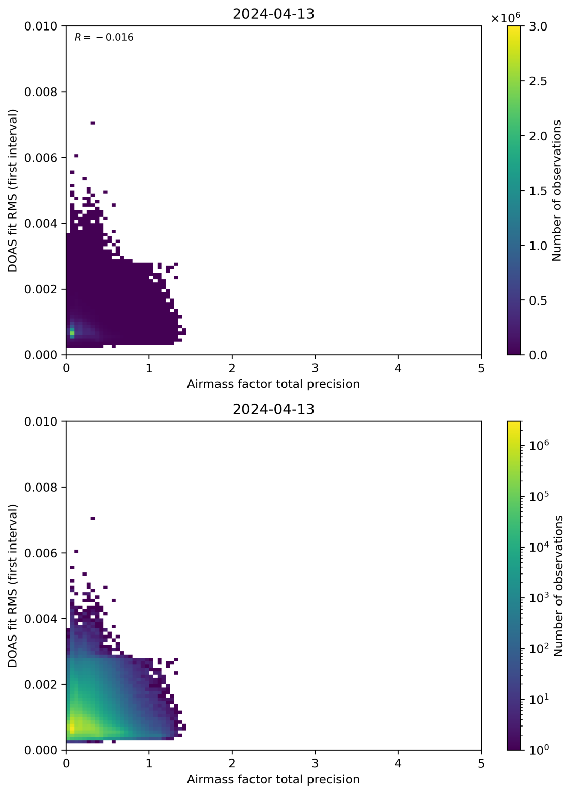
Figure 105: Scatter density plot of “Airmass factor total precision” against “DOAS fit RMS (first interval)” for 2024-04-12 to 2024-04-14.
