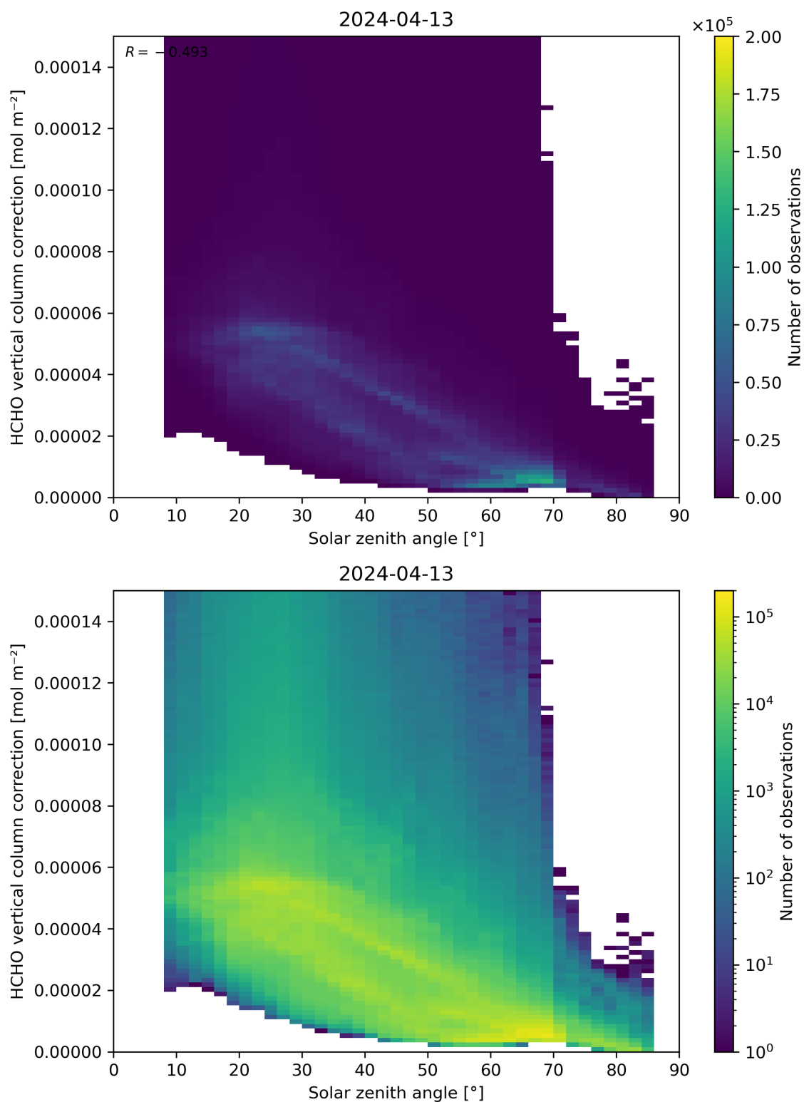
Figure 178: Scatter density plot of “Solar zenith angle” against “HCHO vertical column correction” for 2024-04-12 to 2024-04-14.
