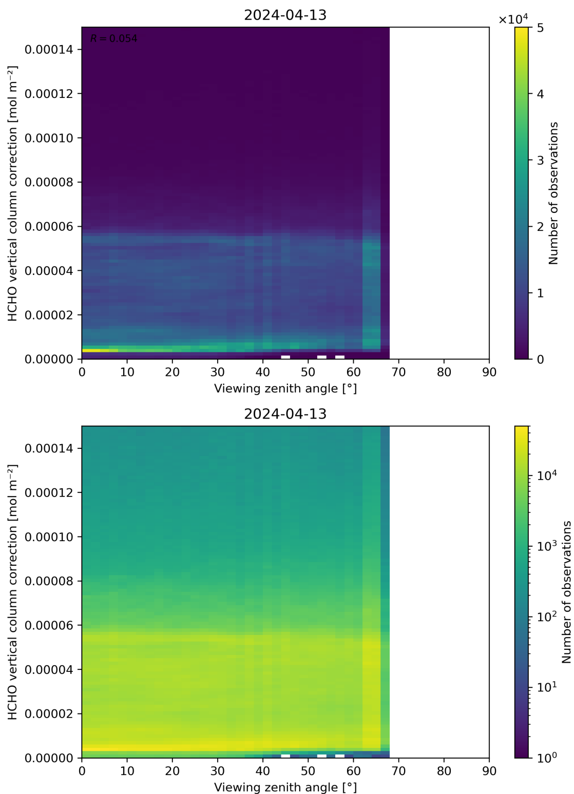
Figure 193: Scatter density plot of “Viewing zenith angle” against “HCHO vertical column correction” for 2024-04-12 to 2024-04-14.
