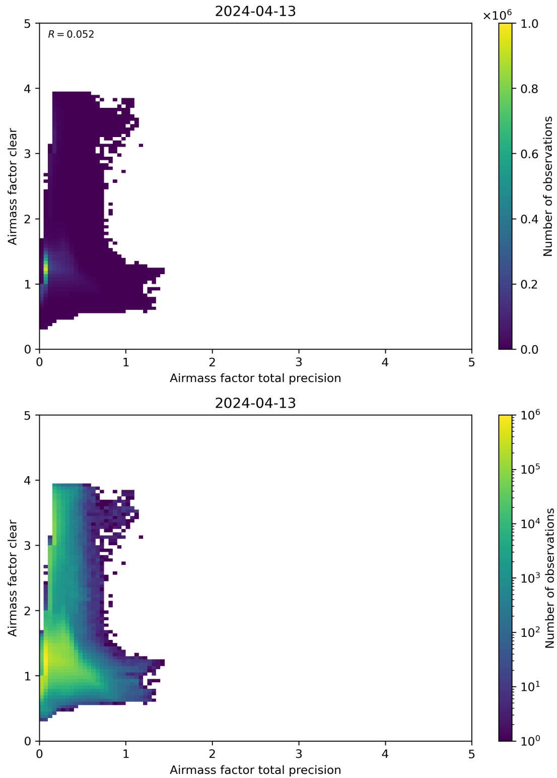
Figure 108: Scatter density plot of “Airmass factor total precision” against “Airmass factor clear” for 2024-04-12 to 2024-04-14.
