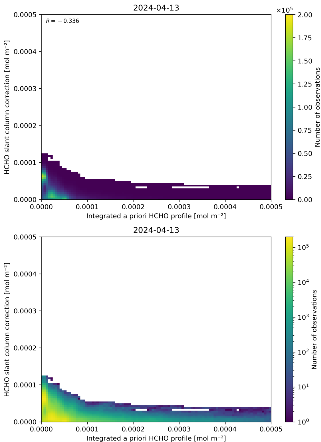
Figure 152: Scatter density plot of “Integrated a priori HCHO profile” against “HCHO slant column correction” for 2024-04-12 to 2024-04-14.
