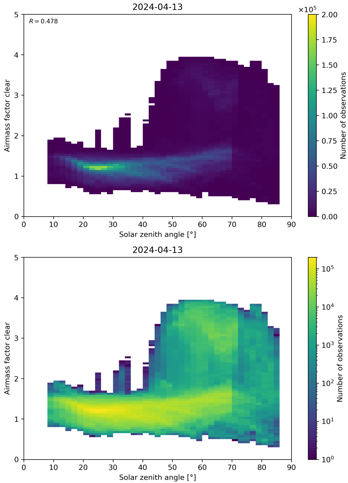
Figure 170: Scatter density plot of “Solar zenith angle” against “Airmass factor clear” for 2024-04-12 to 2024-04-14.
