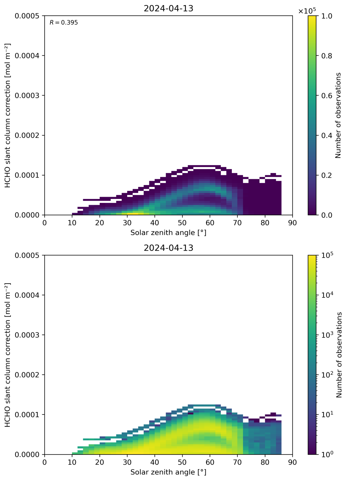
Figure 172: Scatter density plot of “Solar zenith angle” against “HCHO slant column correction” for 2024-04-12 to 2024-04-14.
