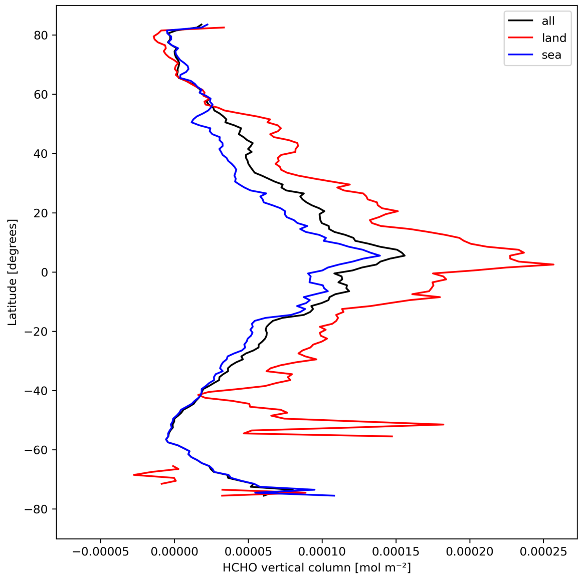
Figure 21: Zonal average of “HCHO vertical column” for 2024-04-12 to 2024-04-14.
