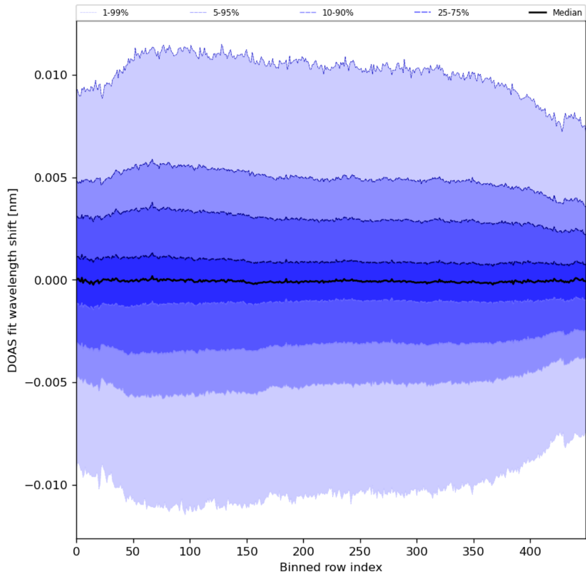
Figure 58: Along track statistics of “DOAS fit wavelength shift” for 2024-04-12 to 2024-04-14
