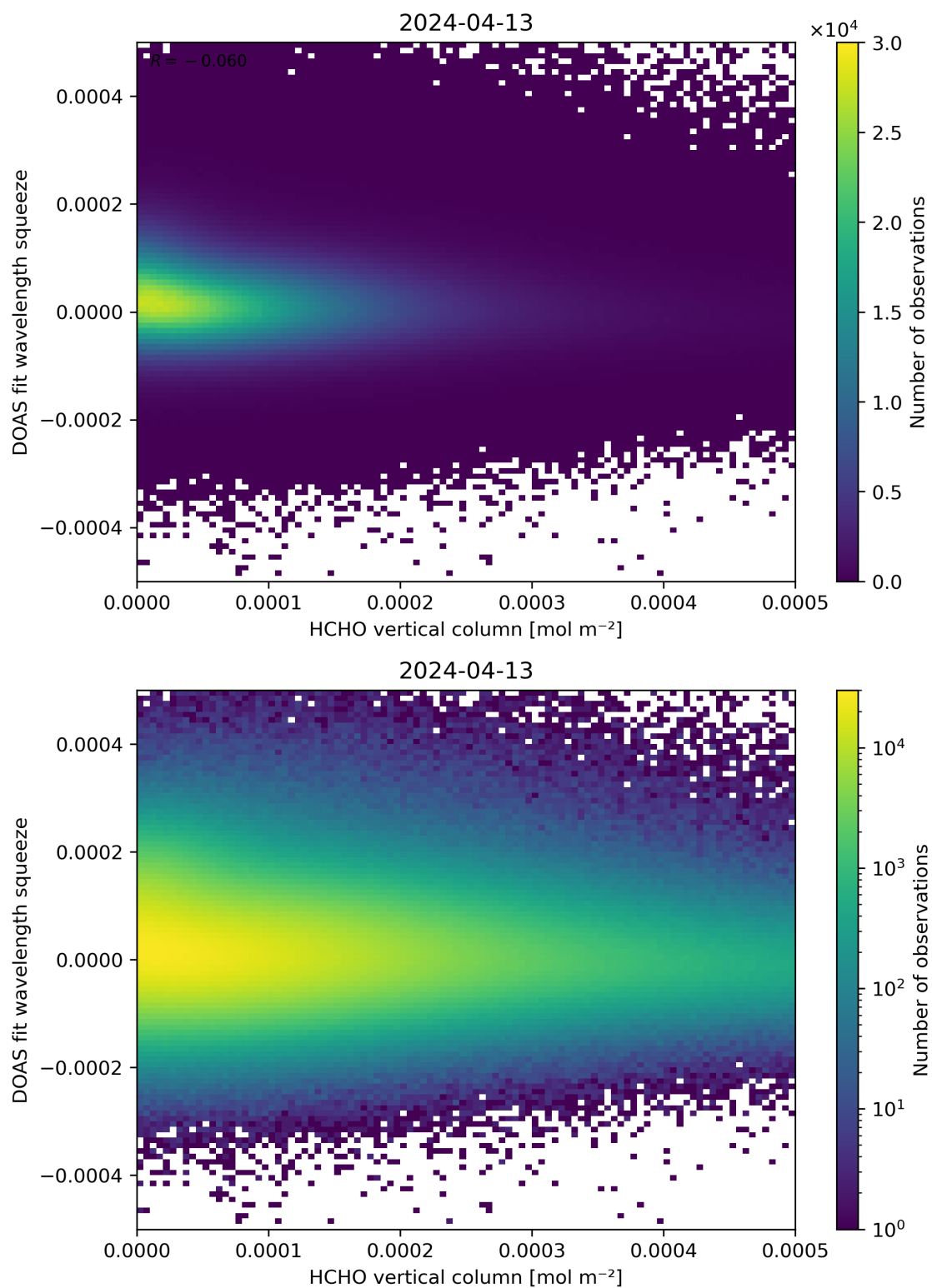
Figure 125: Scatter density plot of “HCHO vertical column” against “DOAS fit wavelength squeeze” for 2024-04-12 to 2024-04-14.
