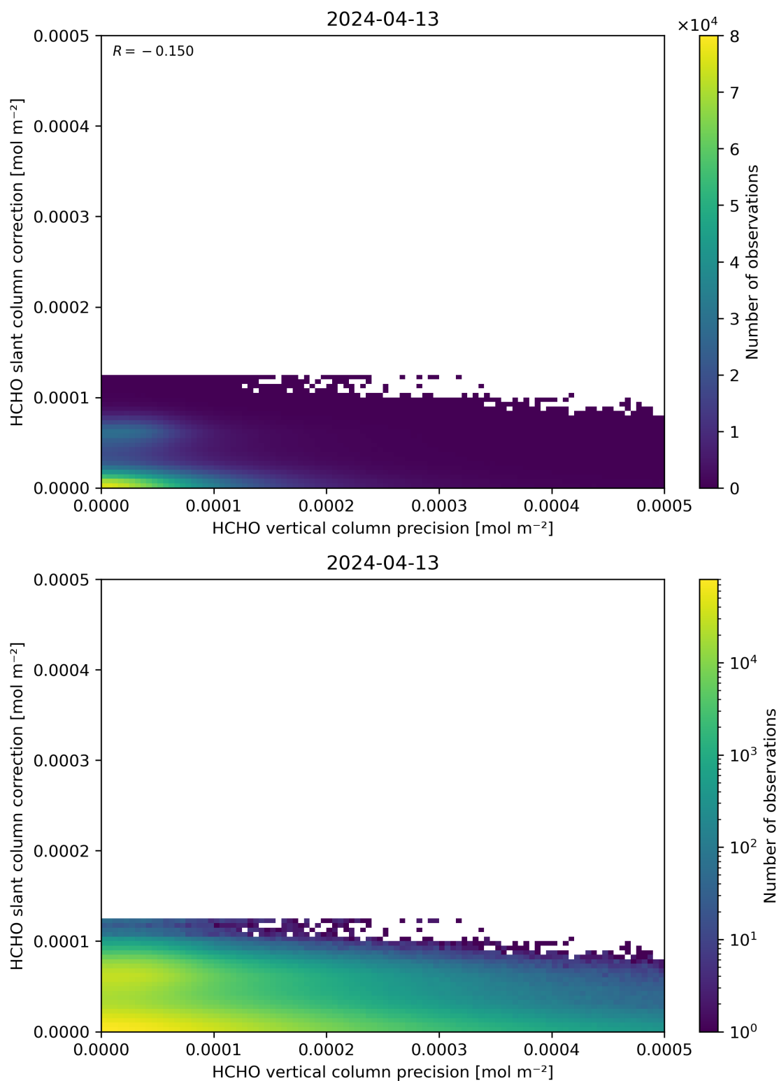
Figure 141: Scatter density plot of “HCHO vertical column precision” against “HCHO slant column correction” for 2024-04-12 to 2024-04-14.
