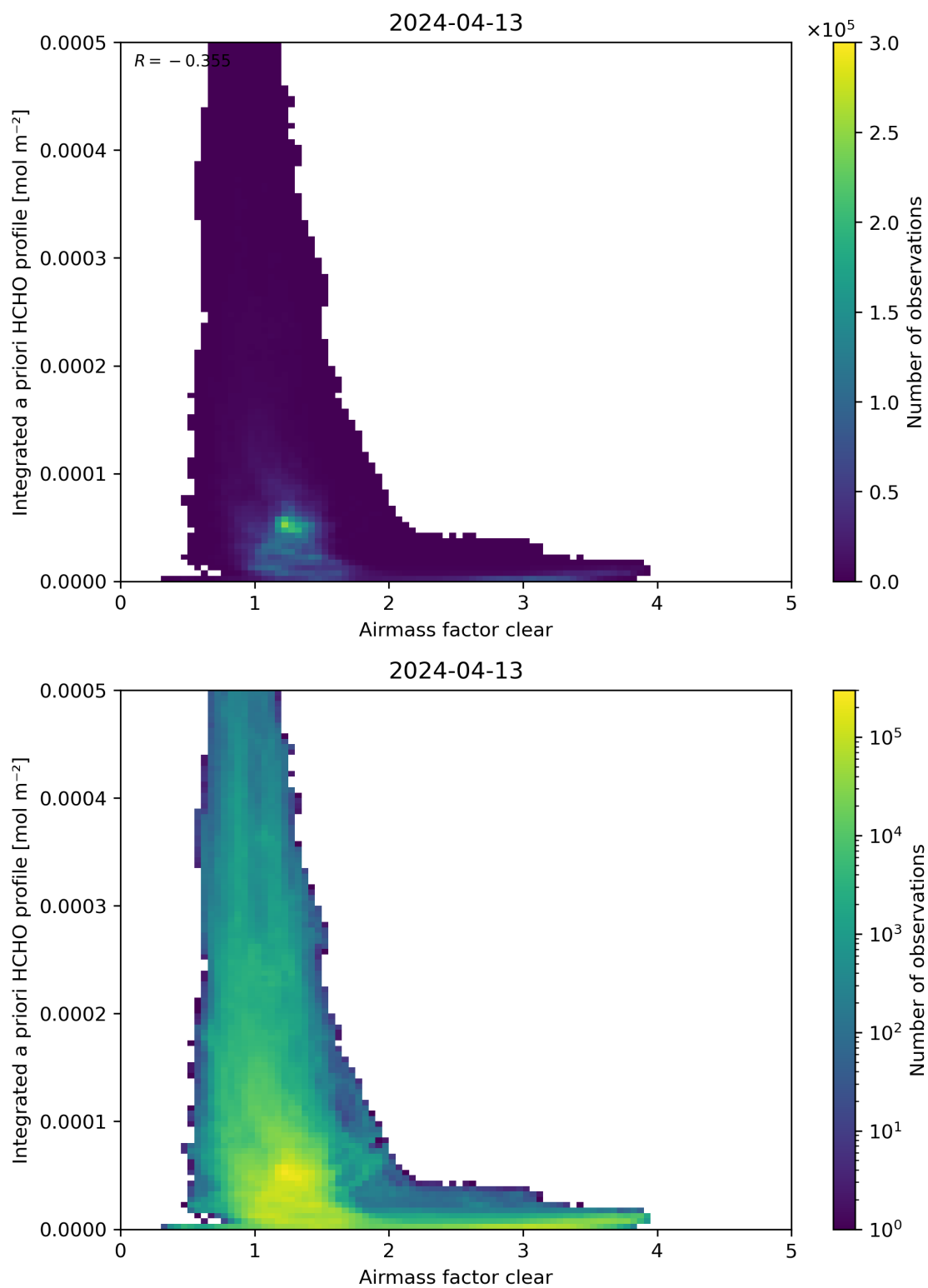
Figure 76: Scatter density plot of “Airmass factor clear” against “Integrated a priori HCHO profile” for 2024-04-12 to 2024-04-14.
