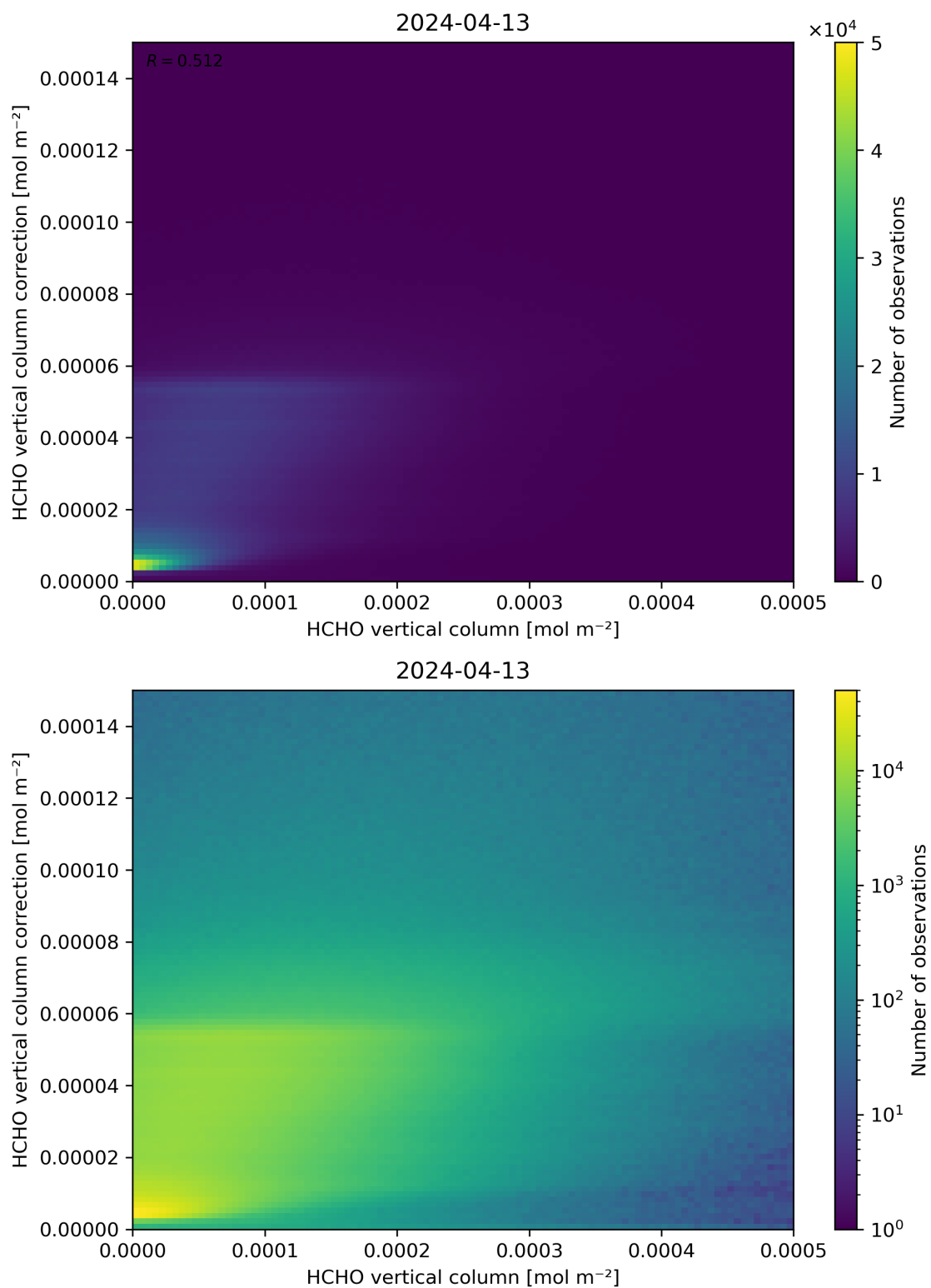
Figure 133: Scatter density plot of “HCHO vertical column” against “HCHO vertical column correction” for 2024-04-12 to 2024-04-14.
