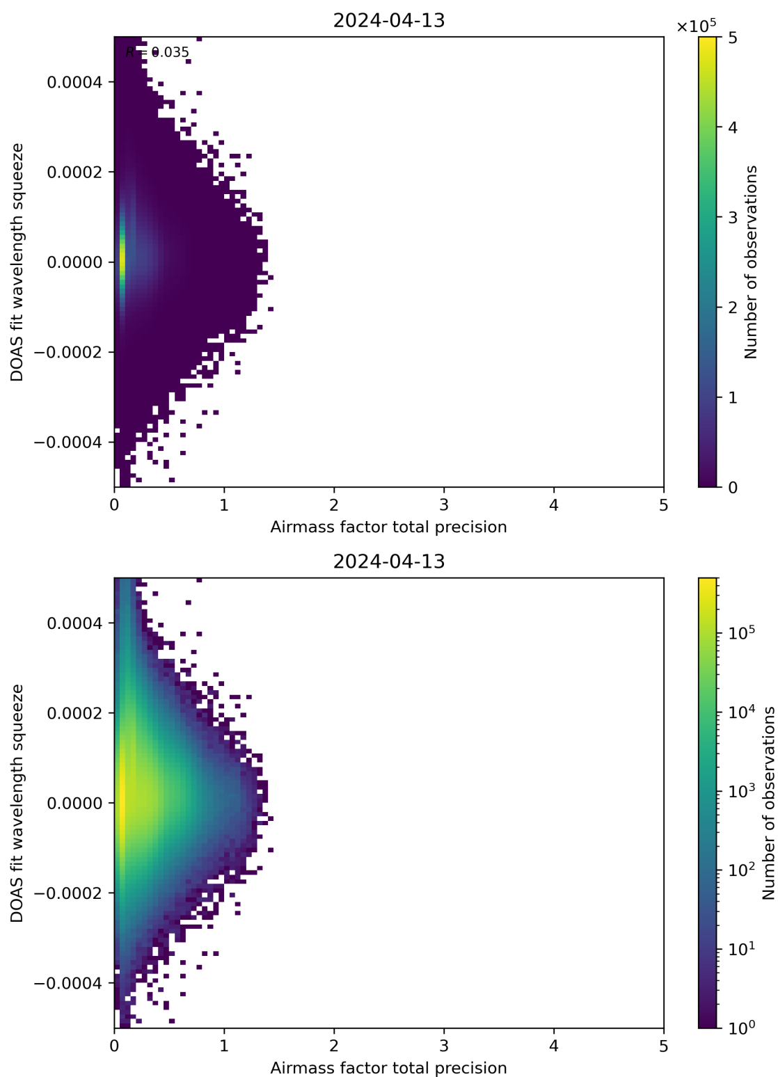
Figure 107: Scatter density plot of “Airmass factor total precision” against “DOAS fit wavelength squeeze” for 2024-04-12 to 2024-04-14.
