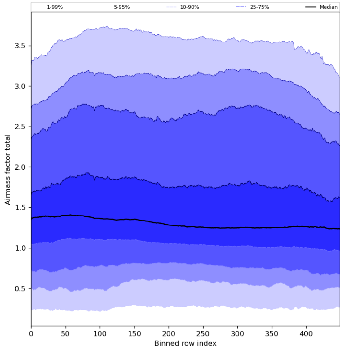
Figure 54: Along track statistics of “Airmass factor total” for 2024-04-12 to 2024-04-14
