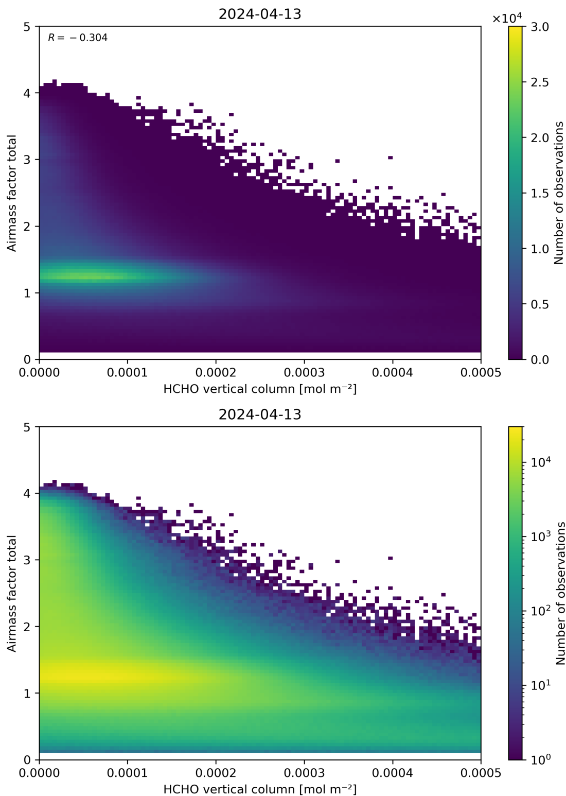
Figure 131: Scatter density plot of “HCHO vertical column” against “Airmass factor total” for 2024-04-12 to 2024-04-14.
