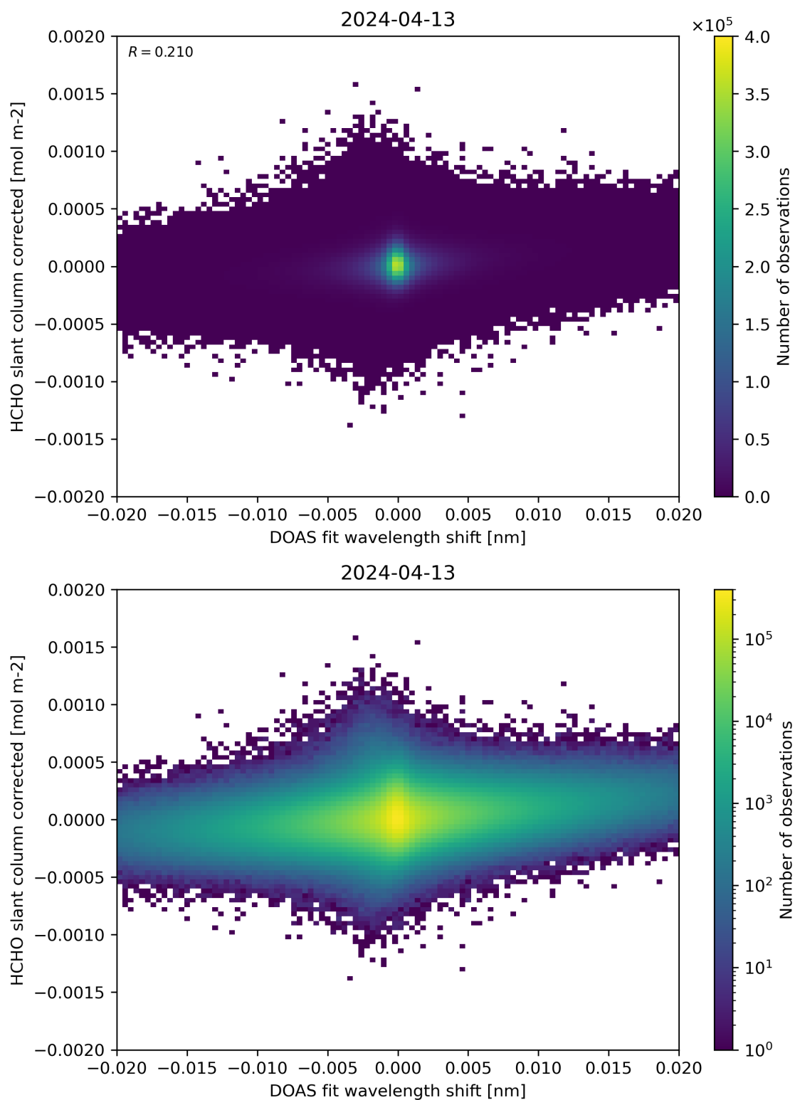
Figure 66: Scatter density plot of “DOAS fit wavelength shift” against “HCHO slant column corrected” for 2024-04-12 to 2024-04-14.
