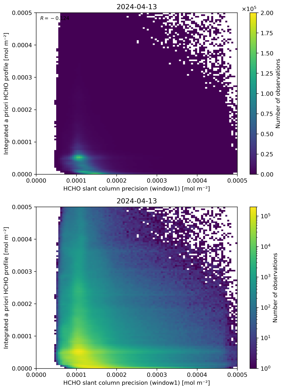
Figure 96: Scatter density plot of “HCHO slant column precision (window1)” against “Integrated a priori HCHO profile” for 2024-04-12 to 2024-04-14.
