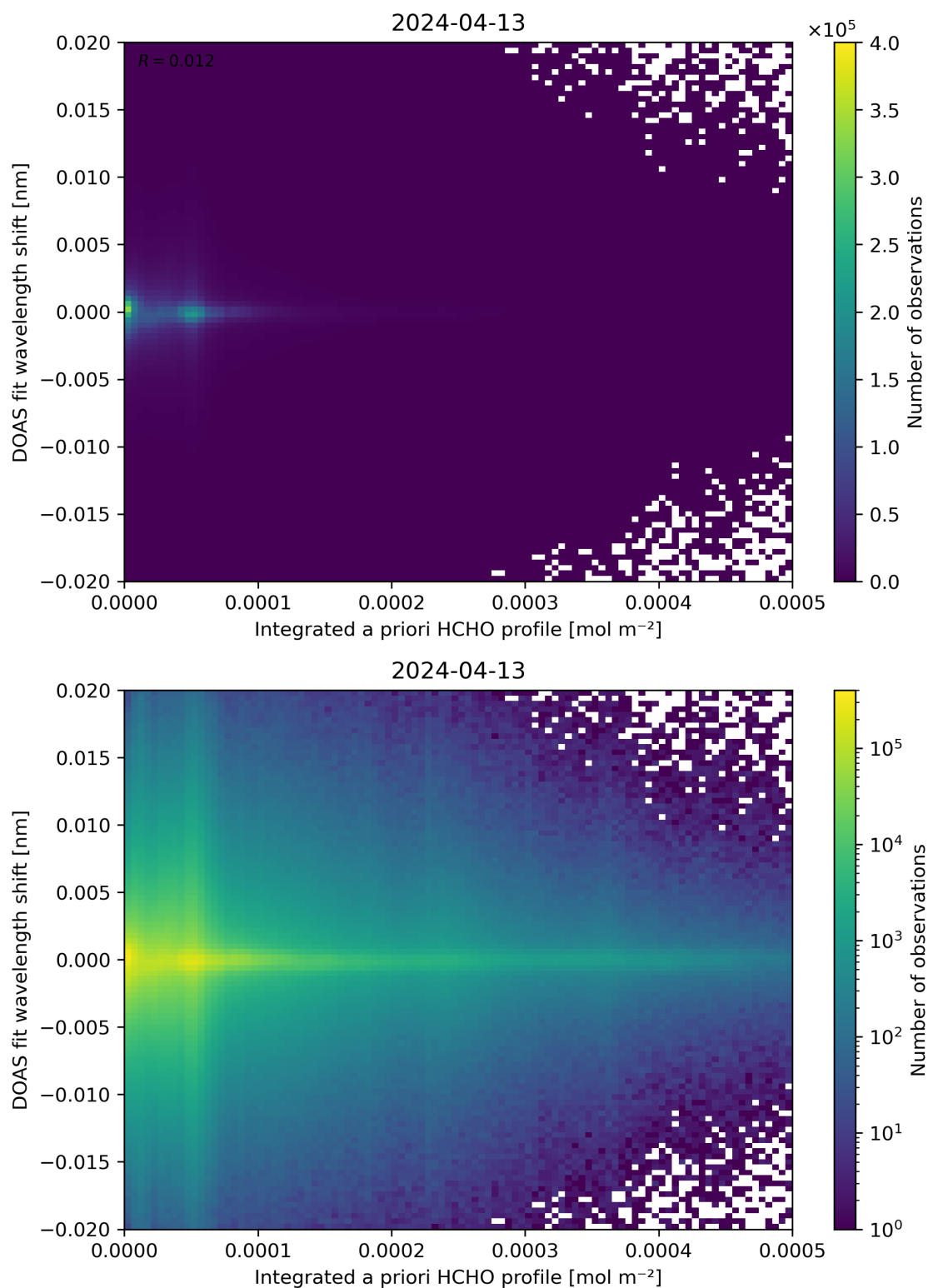
Figure 149: Scatter density plot of “Integrated a priori HCHO profile” against “DOAS fit wavelength shift” for 2024-04-12 to 2024-04-14.
