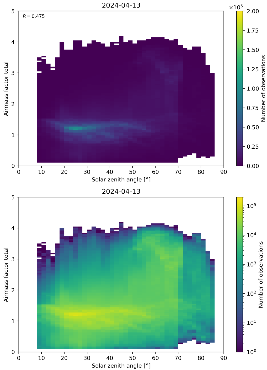
Figure 175: Scatter density plot of “Solar zenith angle” against “Airmass factor total” for 2024-04-12 to 2024-04-14.
