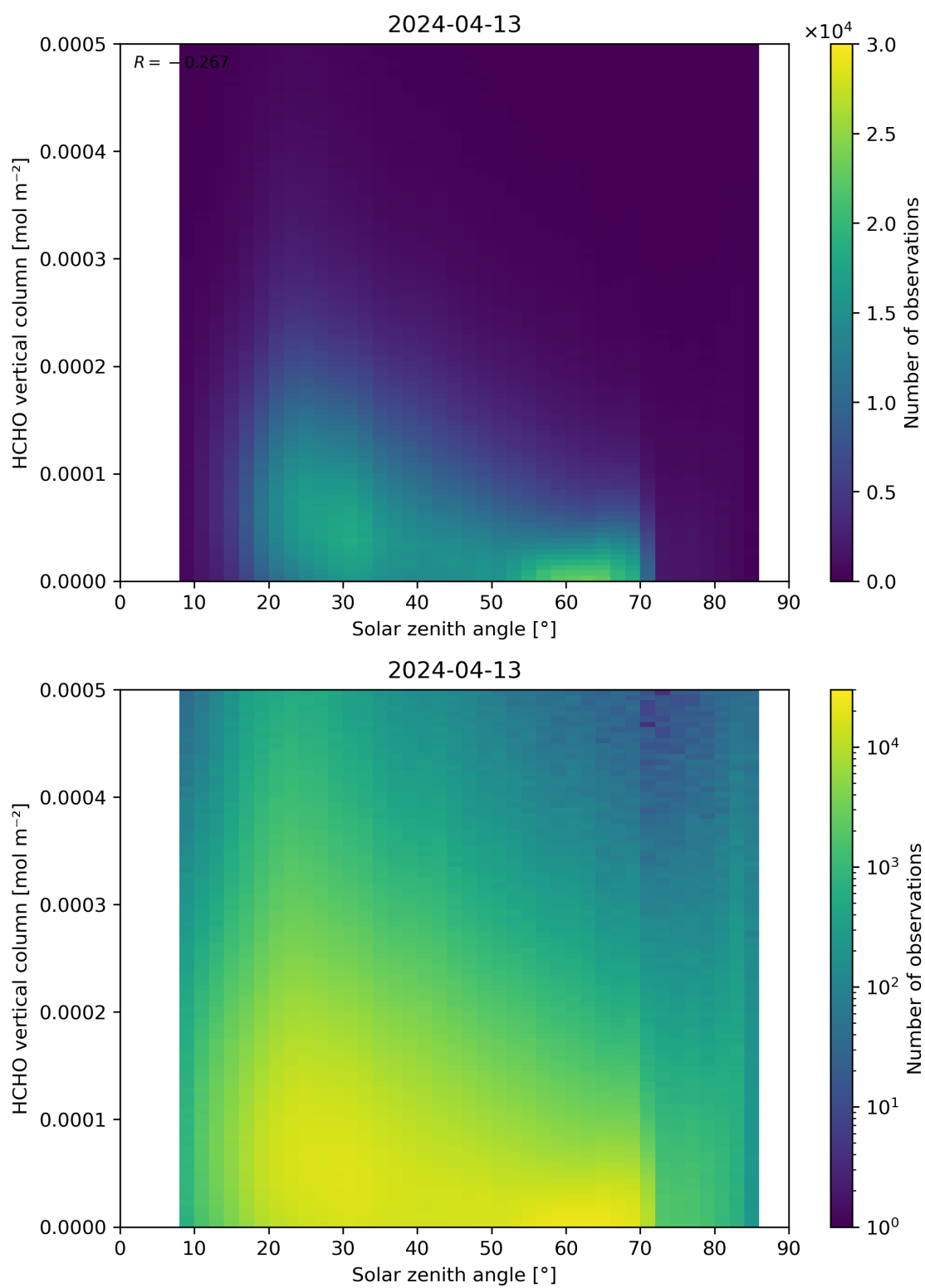
Figure 177: Scatter density plot of “Solar zenith angle” against “HCHO vertical column” for 2024-04-12 to 2024-04-14.
