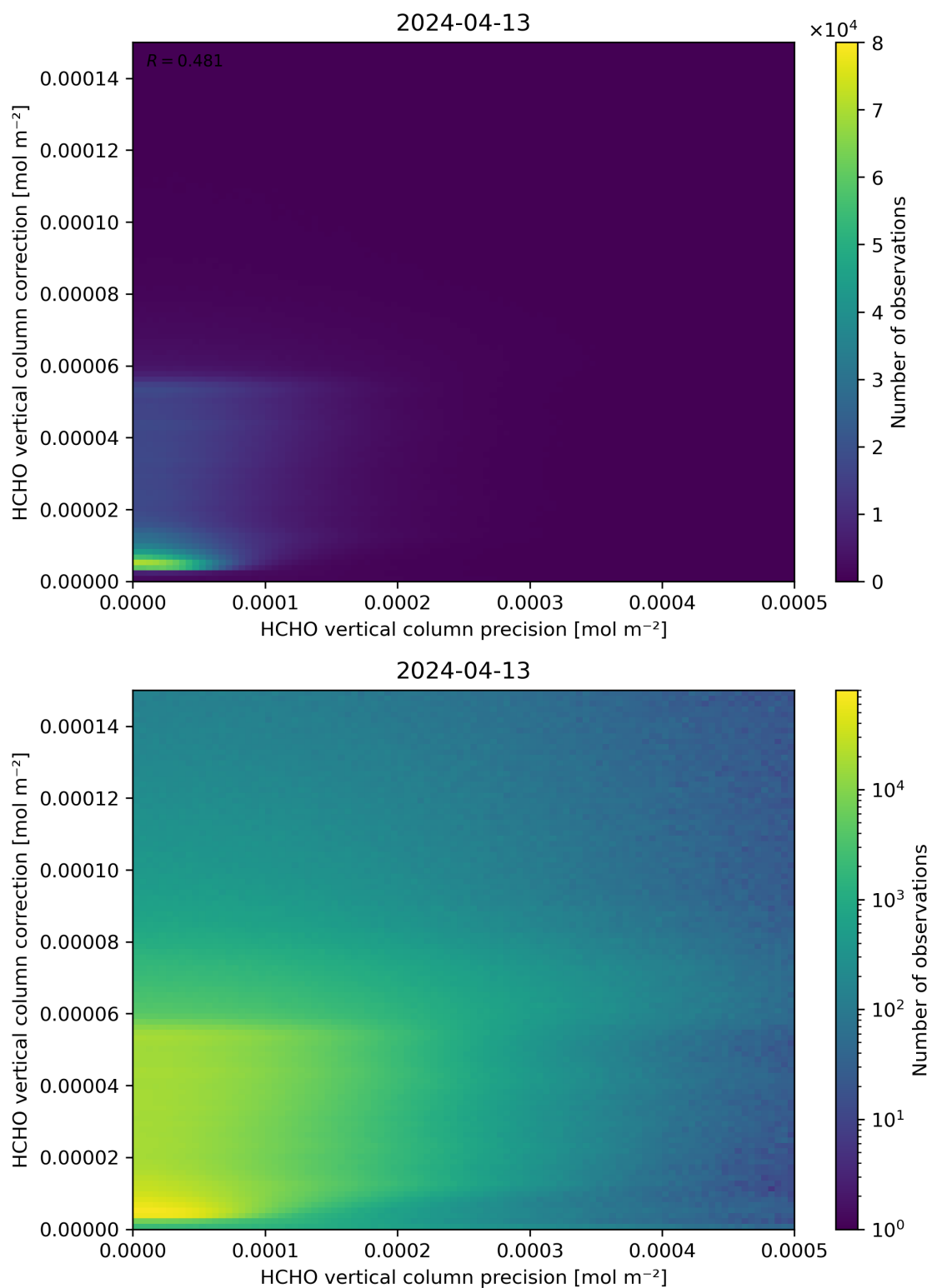
Figure 146: Scatter density plot of “HCHO vertical column precision” against “HCHO vertical column correction” for 2024-04-12 to 2024-04-14.
