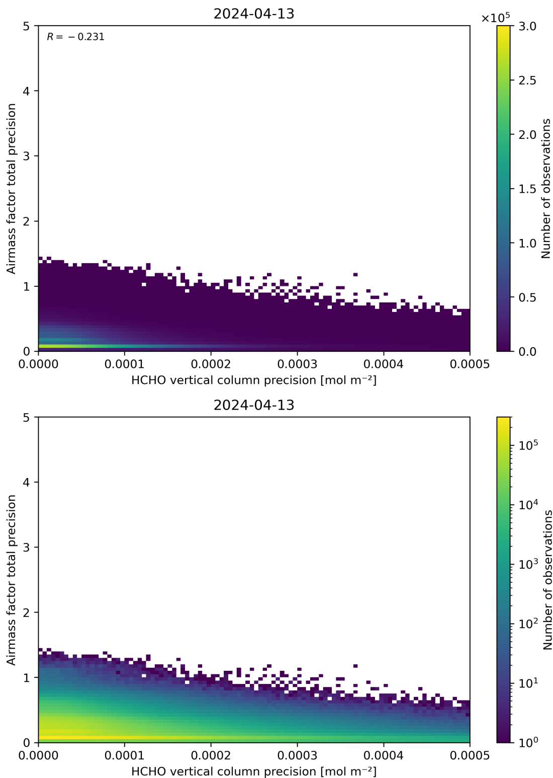
Figure 145: Scatter density plot of “HCHO vertical column precision” against “Airmass factor total precision” for 2024-04-12 to 2024-04-14.
