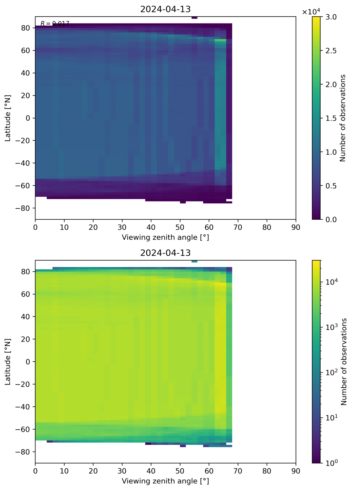
Figure 196: Scatter density plot of “Viewing zenith angle” against “Latitude” for 2024-04-12 to 2024-04-14.
