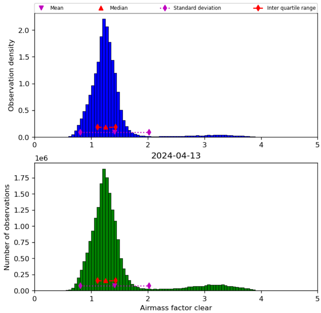
Figure 42: Histogram of “Airmass factor clear” for 2024-04-12 to 2024-04-14
