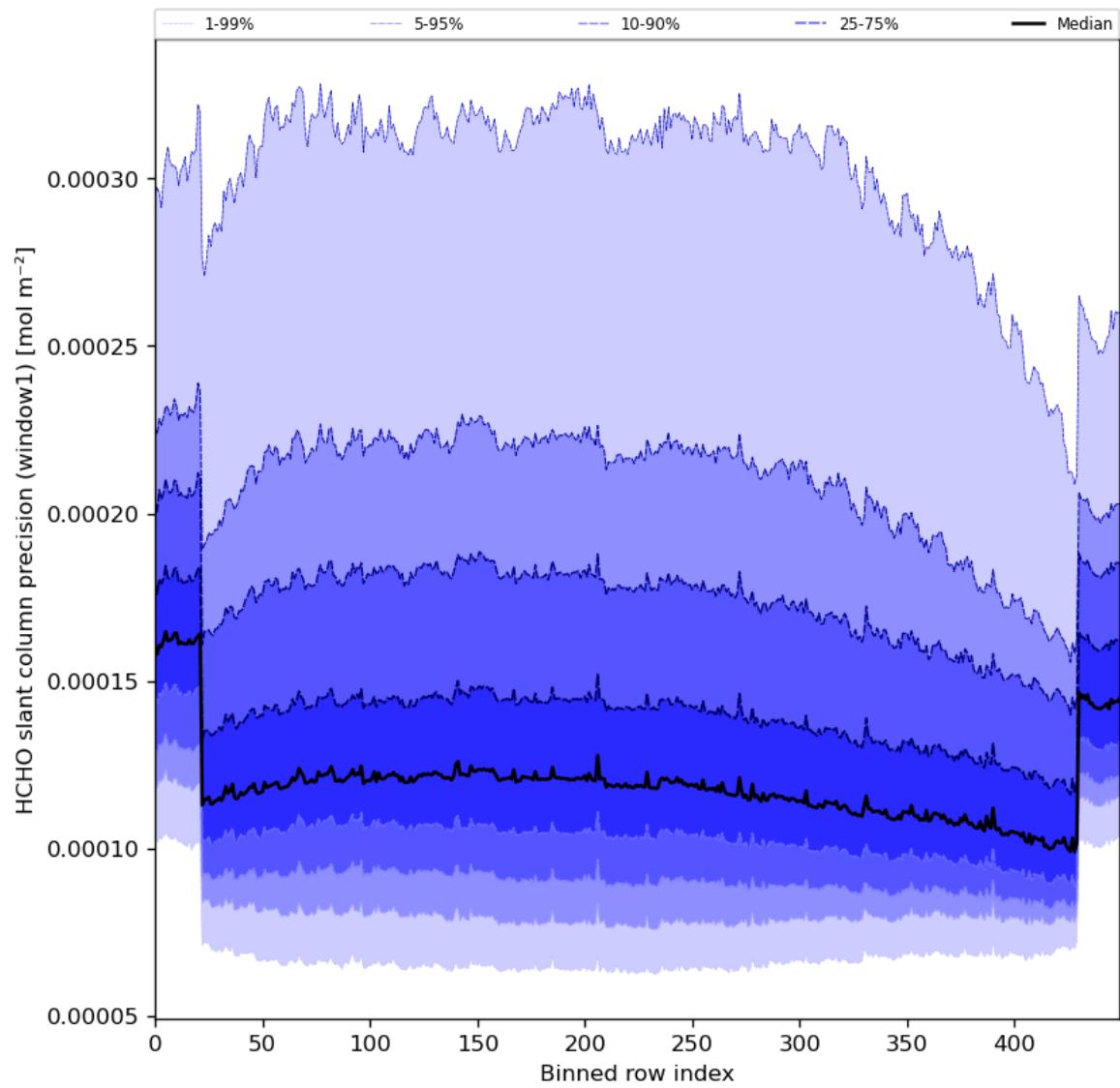
Figure 53: Along track statistics of “HCHO slant column precision (window1)” for 2024-04-12 to 2024-04-14
