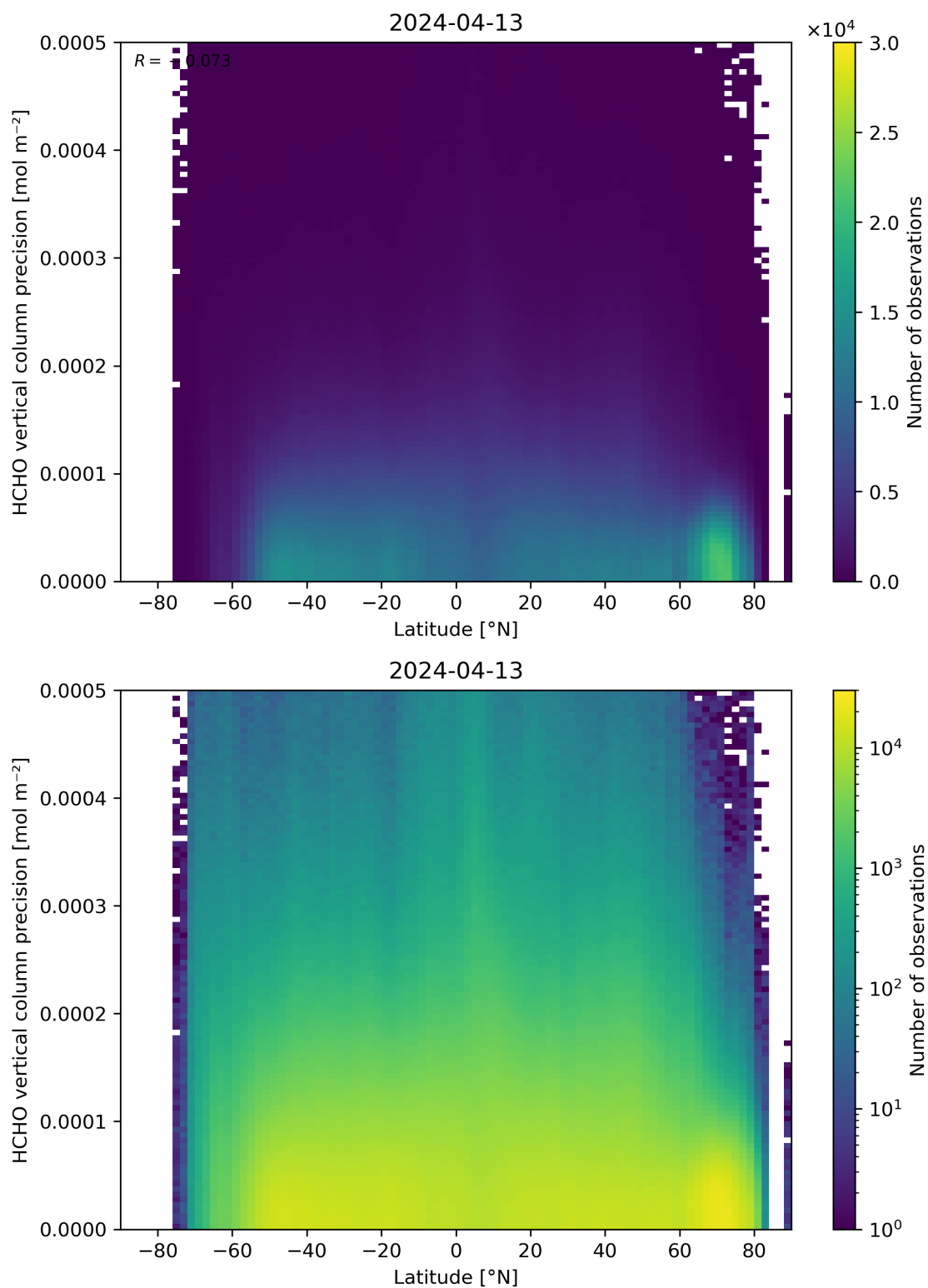
Figure 165: Scatter density plot of “Latitude” against “HCHO vertical column precision” for 2024-04-12 to 2024-04-14.
