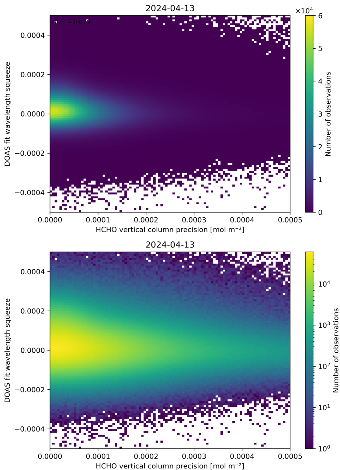
Figure 138: Scatter density plot of “HCHO vertical column precision” against “DOAS fit wavelength squeeze” for 2024-04-12 to 2024-04-14.
