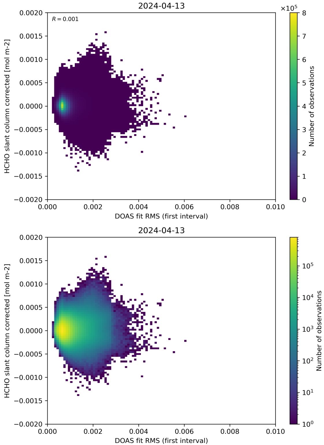
Figure 62: Scatter density plot of “DOAS fit RMS (first interval)” against “HCHO slant column corrected” for 2024-04-12 to 2024-04-14.
