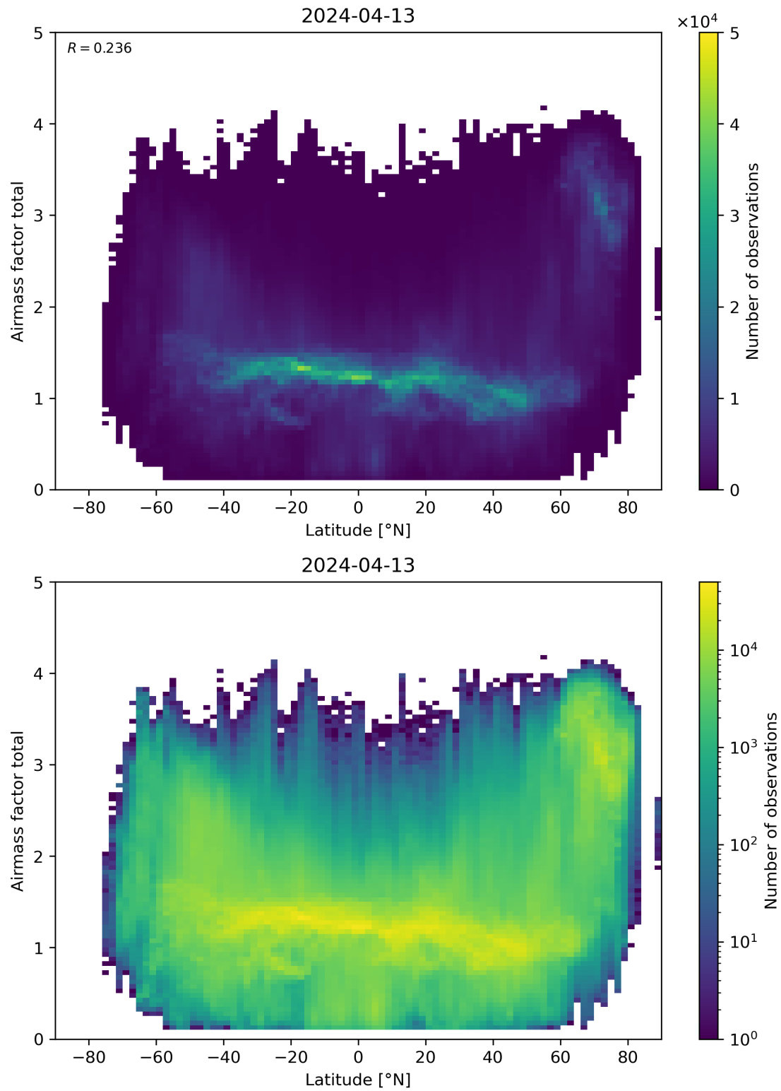
Figure 161: Scatter density plot of “Latitude” against “Airmass factor total” for 2024-04-12 to 2024-04-14.
