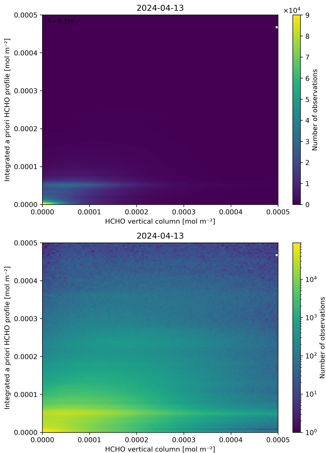
Figure 135: Scatter density plot of “HCHO vertical column” against “Integrated a priori HCHO profile” for 2024-04-12 to 2024-04-14.
