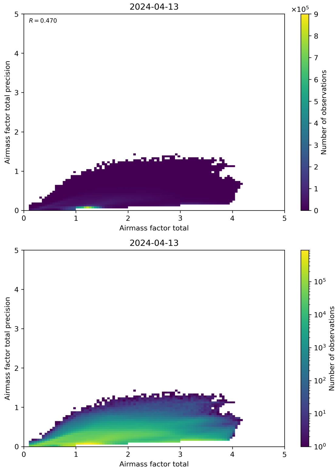
Figure 103: Scatter density plot of “Airmass factor total” against “Airmass factor total precision” for 2024-04-12 to 2024-04-14.
