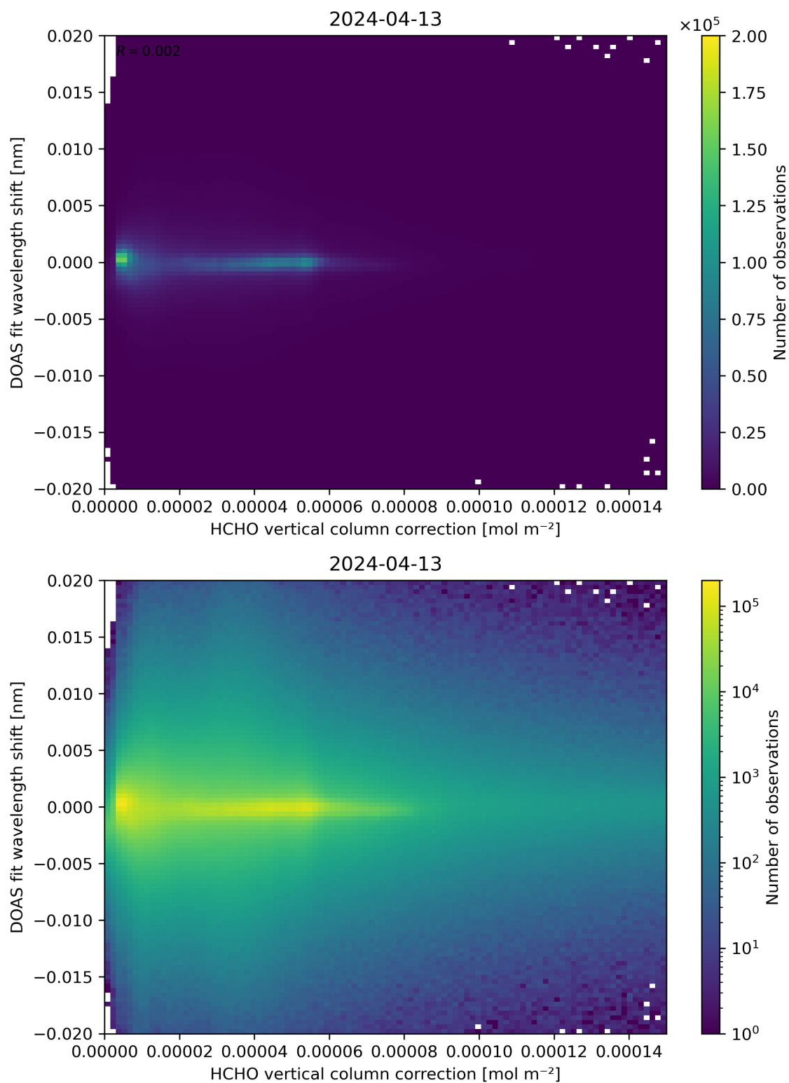
Figure 113: Scatter density plot of “HCHO vertical column correction” against “DOAS fit wavelength shift” for 2024-04-12 to 2024-04-14.
