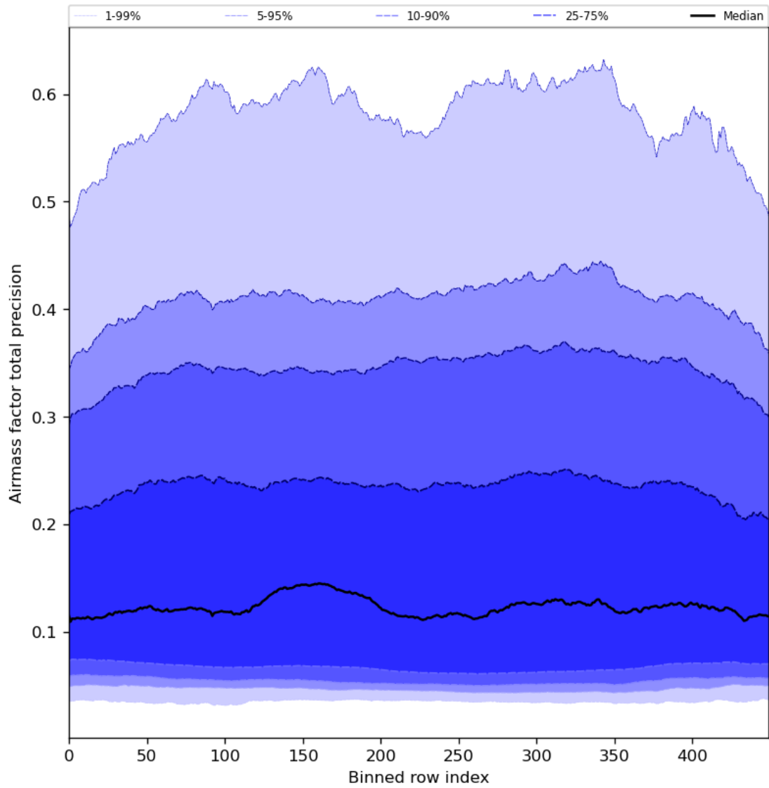
Figure 55: Along track statistics of “Airmass factor total precision” for 2024-04-12 to 2024-04-14
