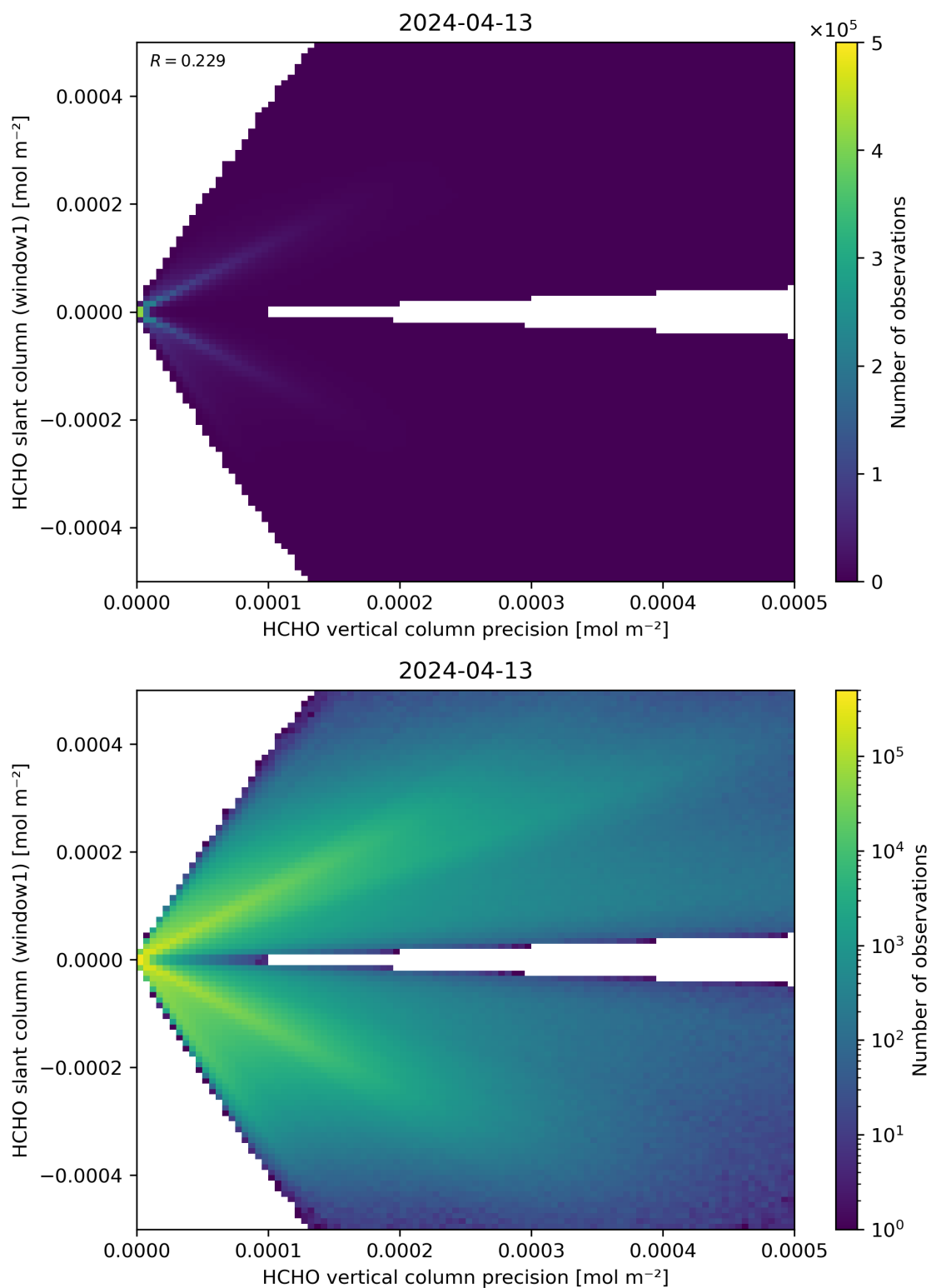
Figure 142: Scatter density plot of “HCHO vertical column precision” against “HCHO slant column (window1)” for 2024-04-12 to 2024-04-14.
