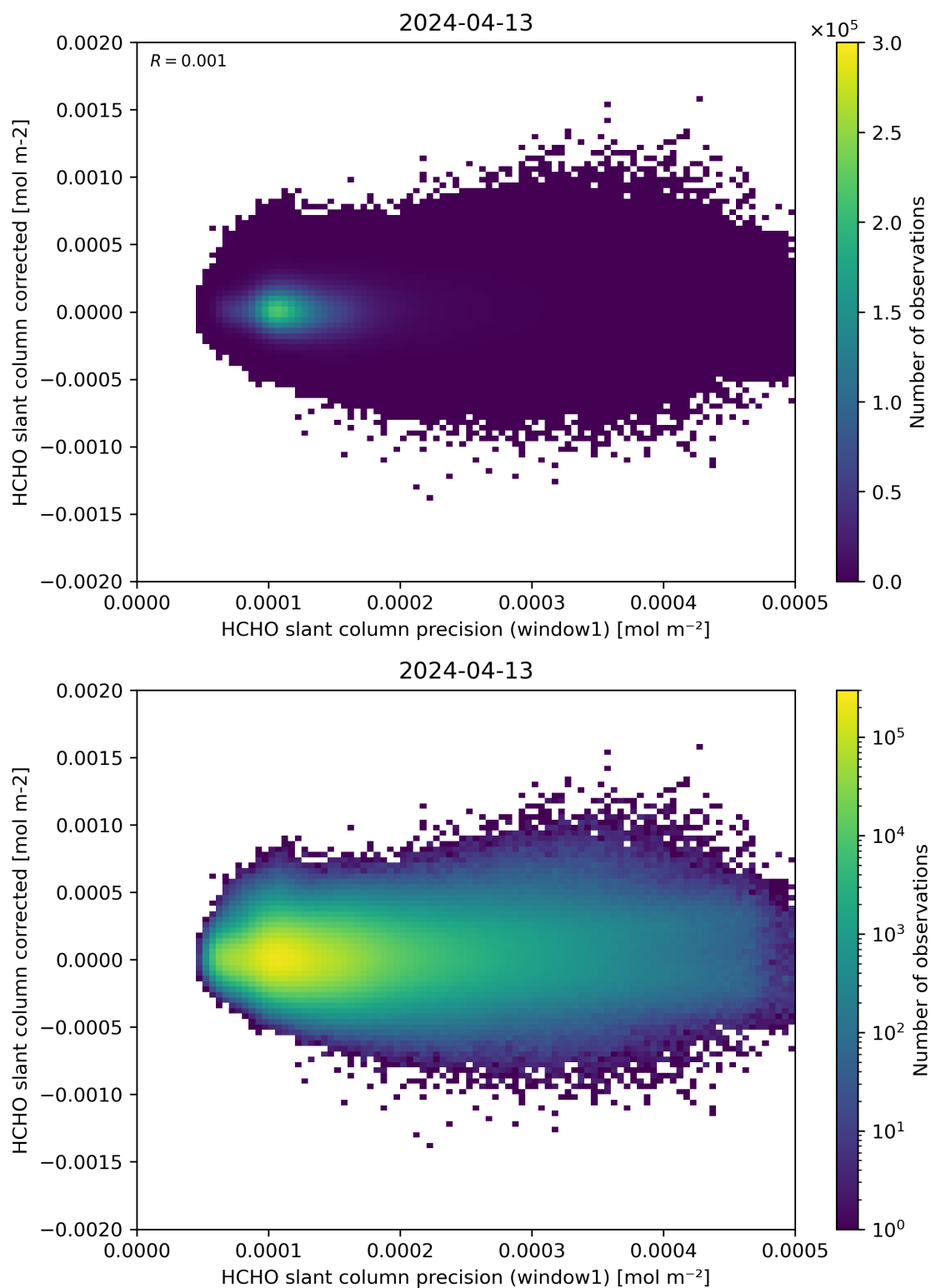
Figure 92: Scatter density plot of “HCHO slant column precision (window1)” against “HCHO slant column corrected” for 2024-04-12 to 2024-04-14.
