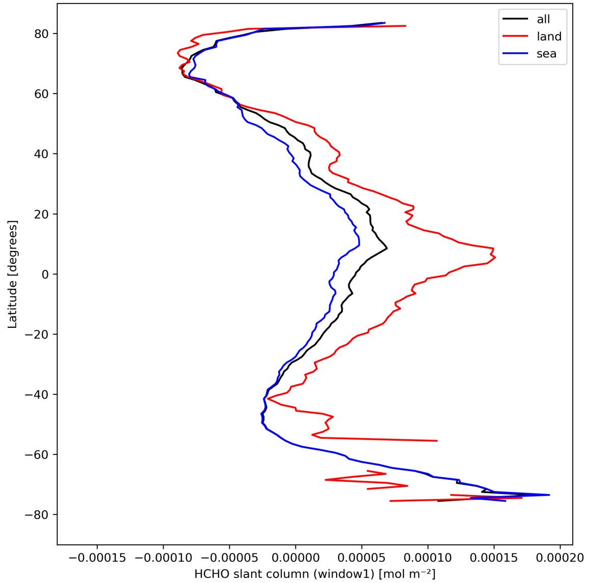
Figure 24: Zonal average of “HCHO slant column (window1)” for 2024-04-12 to 2024-04-14.
