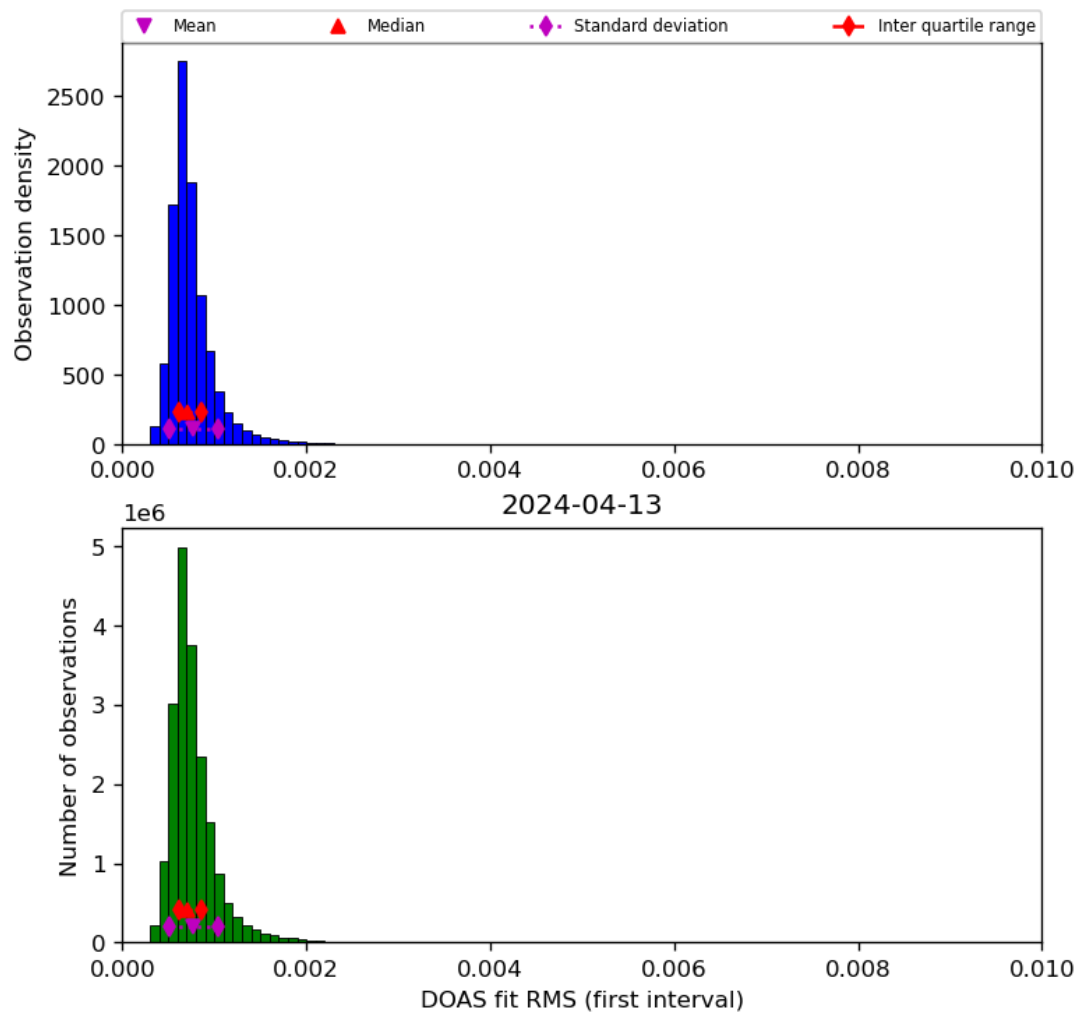
Figure 46: Histogram of “DOAS fit RMS (first interval)” for 2024-04-12 to 2024-04-14
