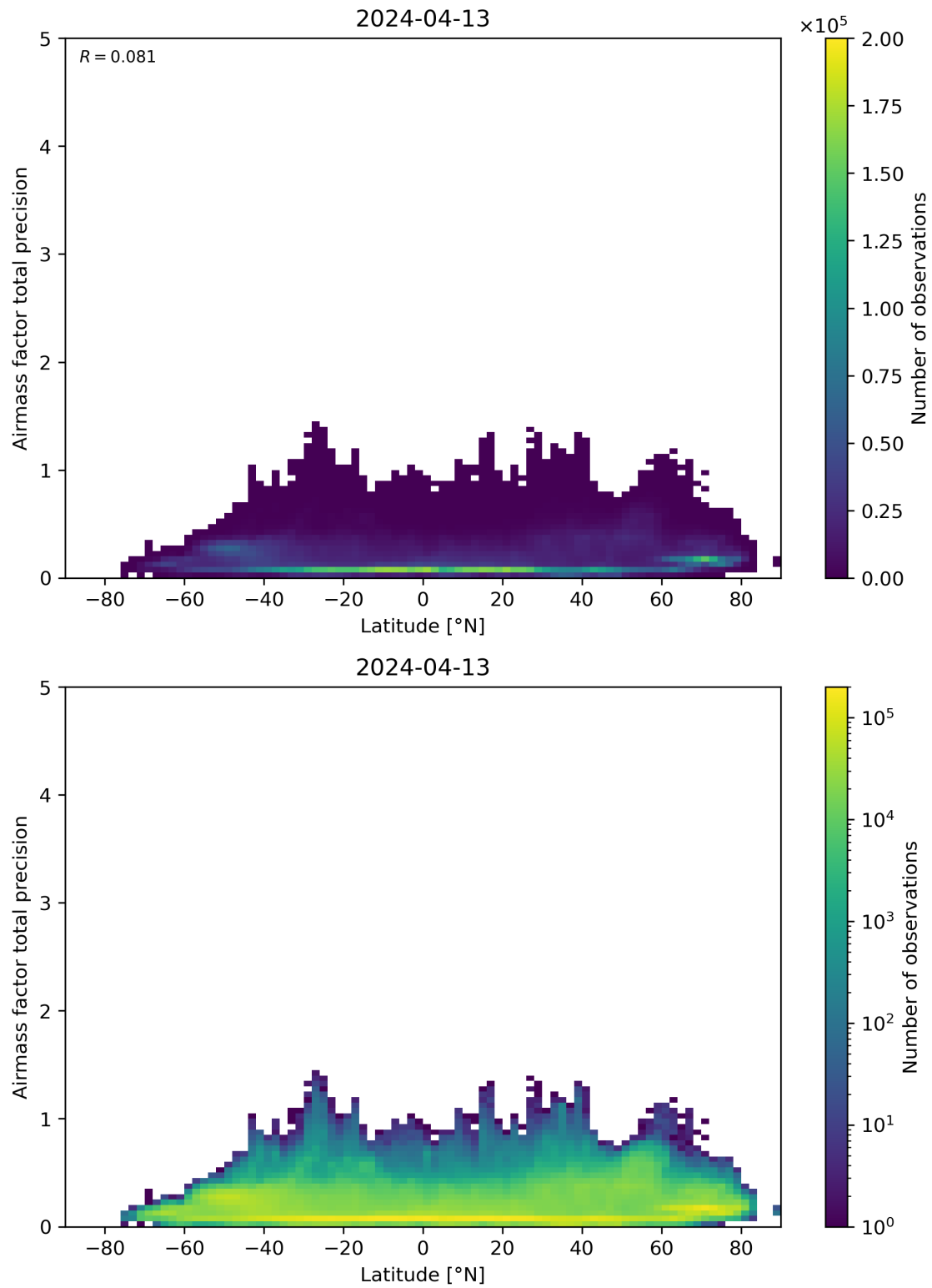
Figure 162: Scatter density plot of “Latitude” against “Airmass factor total precision” for 2024-04-12 to 2024-04-14.
