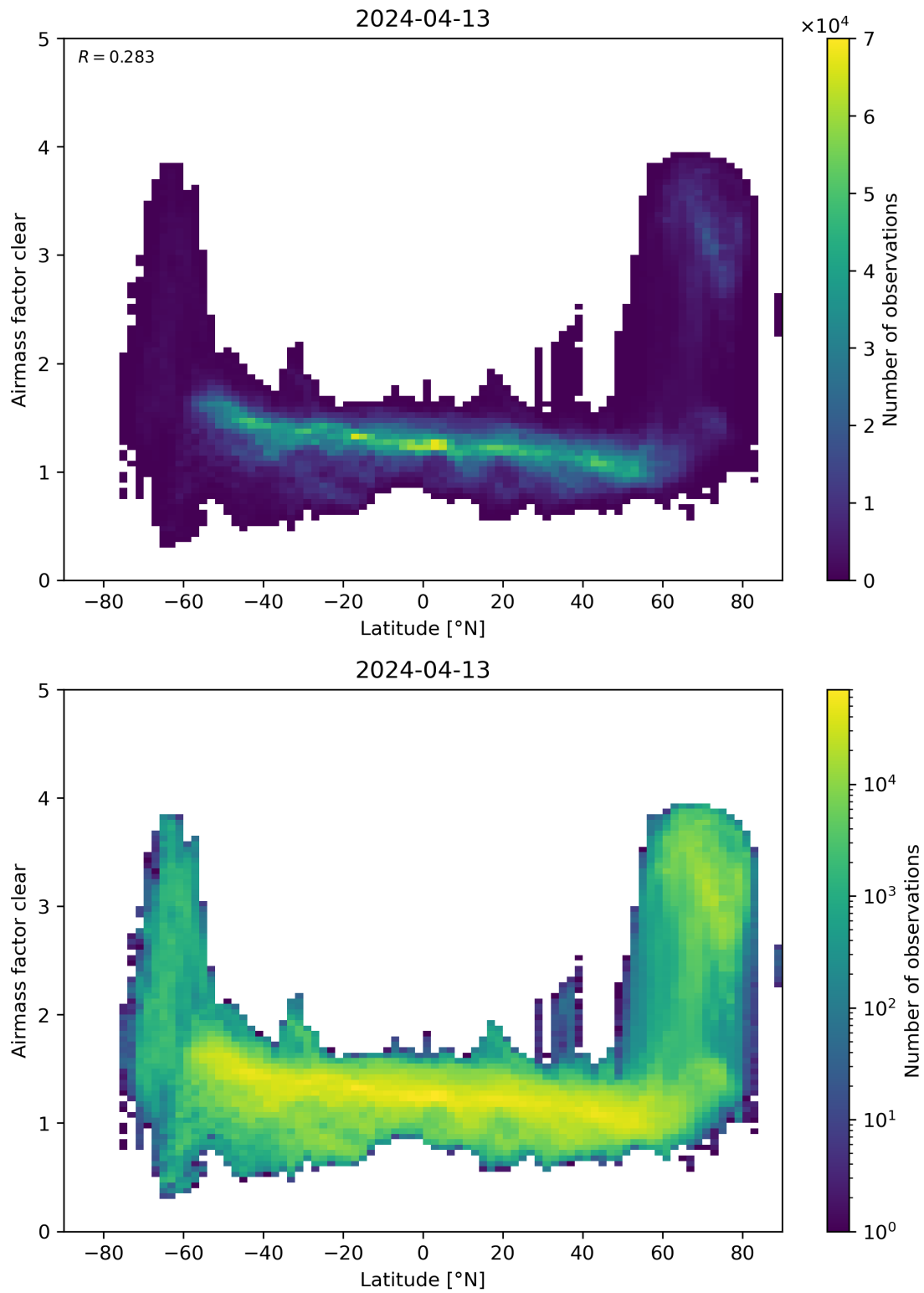
Figure 156: Scatter density plot of “Latitude” against “Airmass factor clear” for 2024-04-12 to 2024-04-14.
