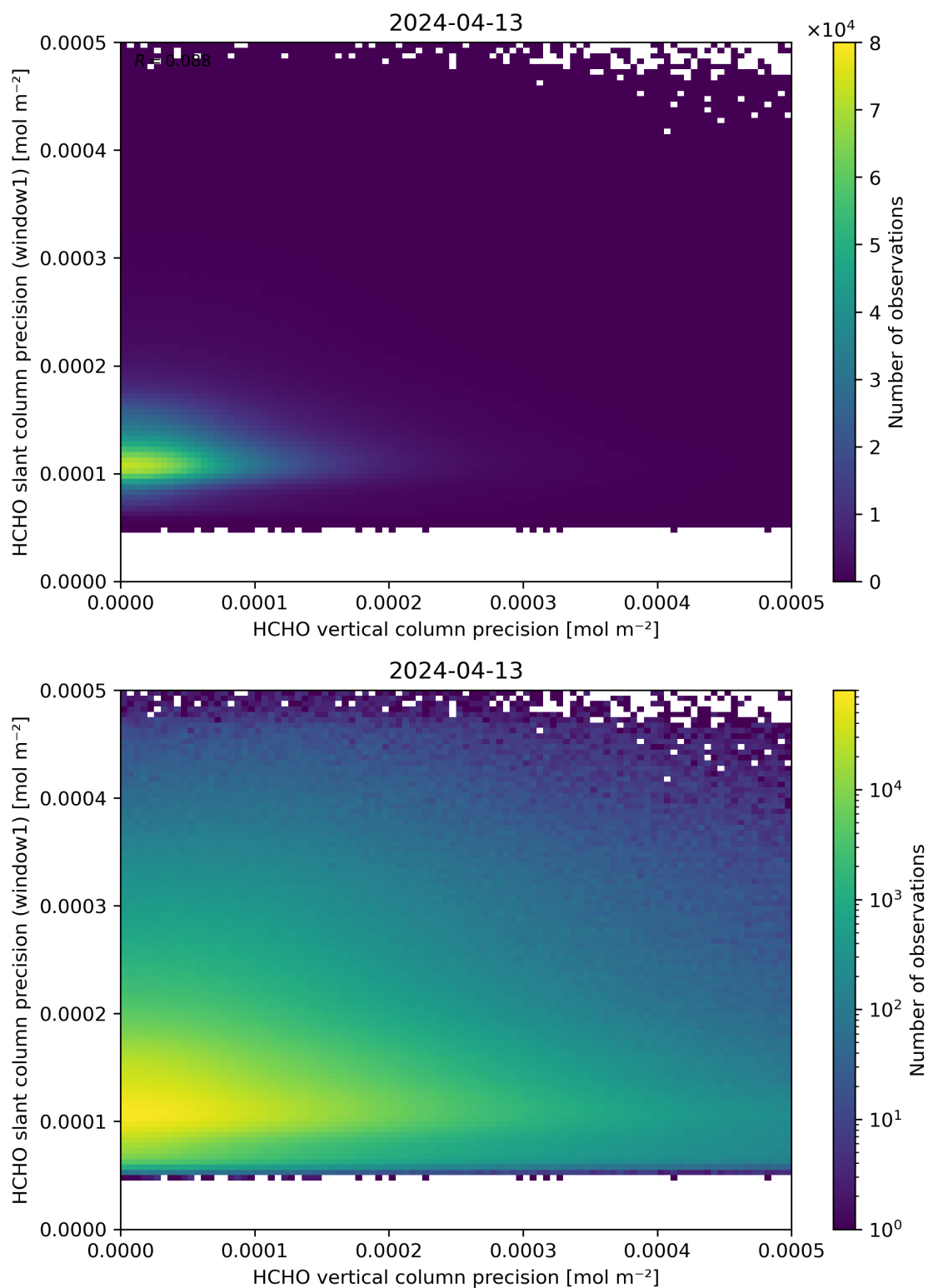
Figure 143: Scatter density plot of “HCHO vertical column precision” against “HCHO slant column precision (window1)” for 2024-04-12 to 2024-04-14.
