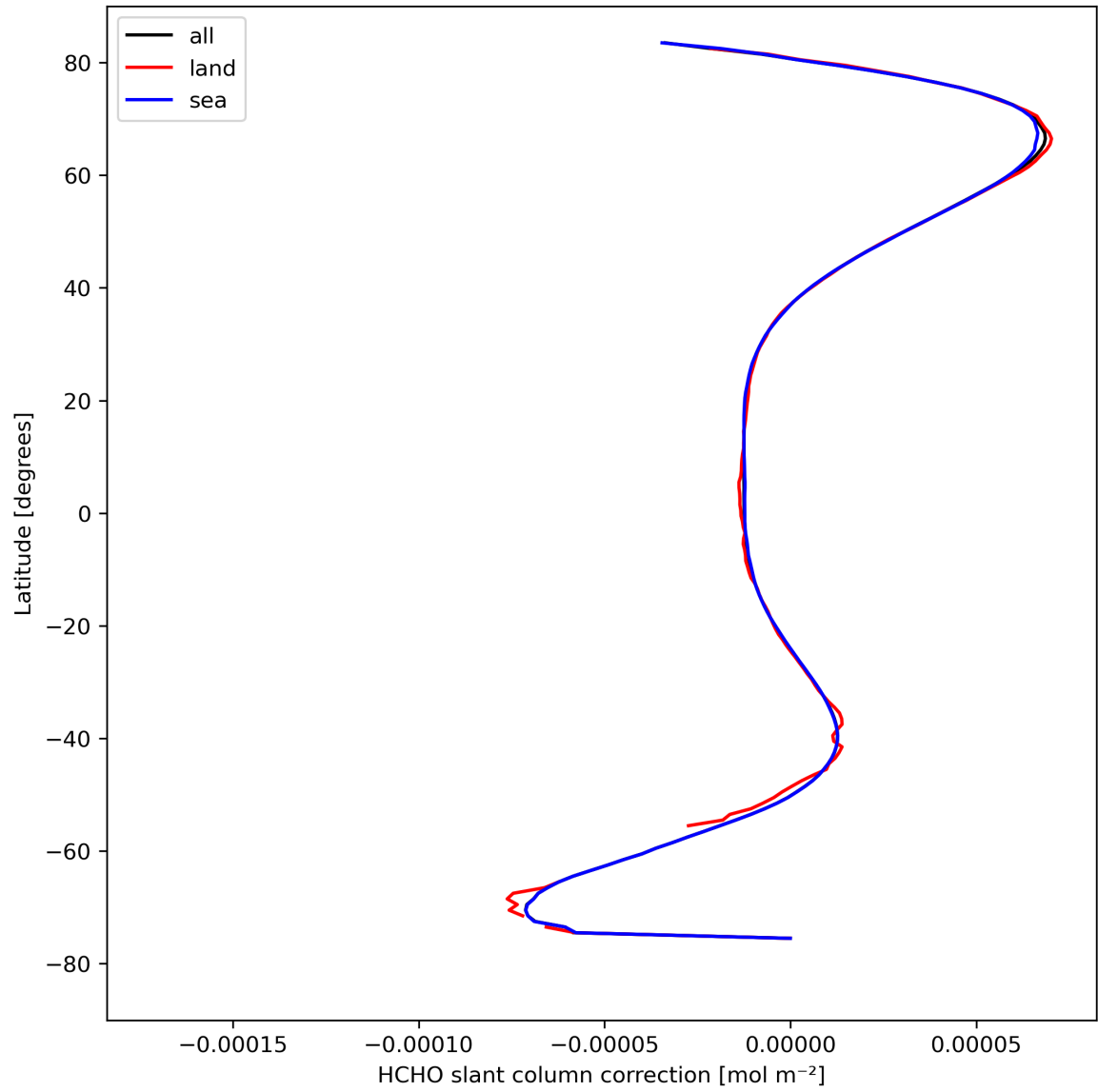
Figure 33: Zonal average of "HCHO slant column correction" for 2024-04-12 to 2024-04-14.
