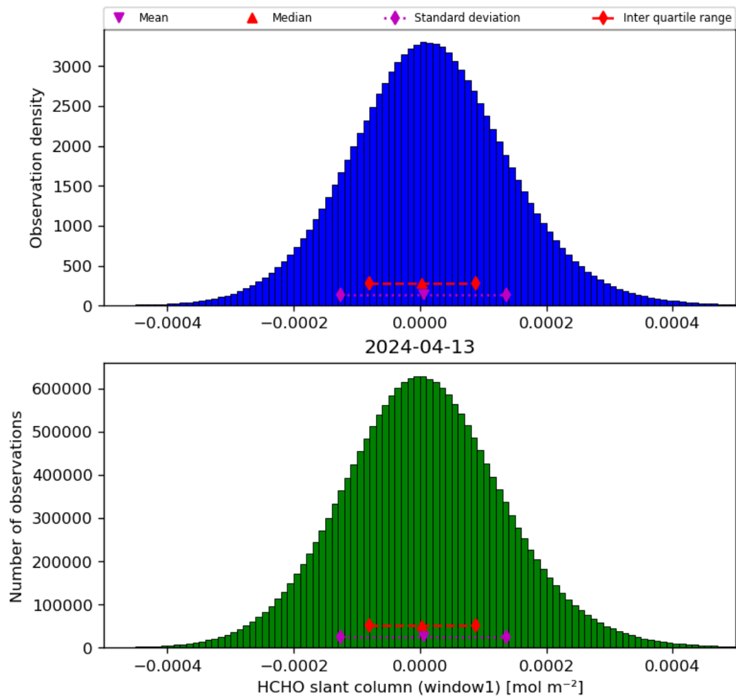
Figure 38: Histogram of “HCHO slant column (window1)” for 2024-04-12 to 2024-04-14
