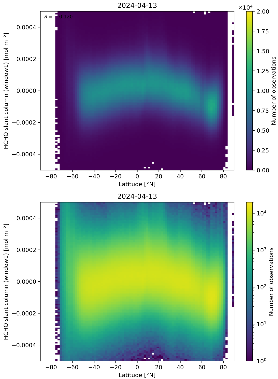
Figure 159: Scatter density plot of “Latitude” against “HCHO slant column (window1)” for 2024-04-12 to 2024-04-14.
