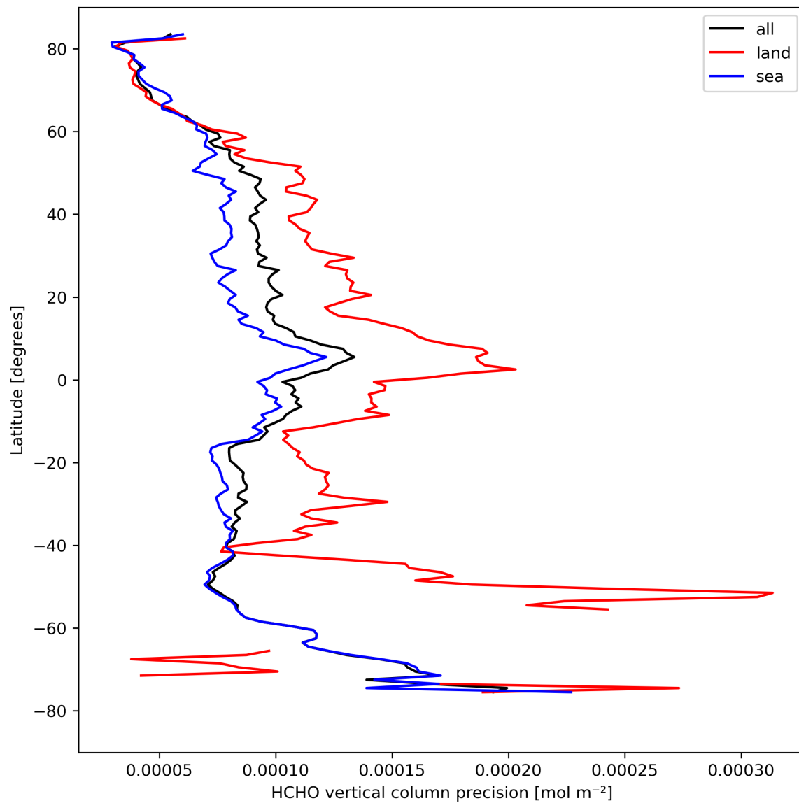
Figure 22: Zonal average of “HCHO vertical column precision” for 2024-04-12 to 2024-04-14.
