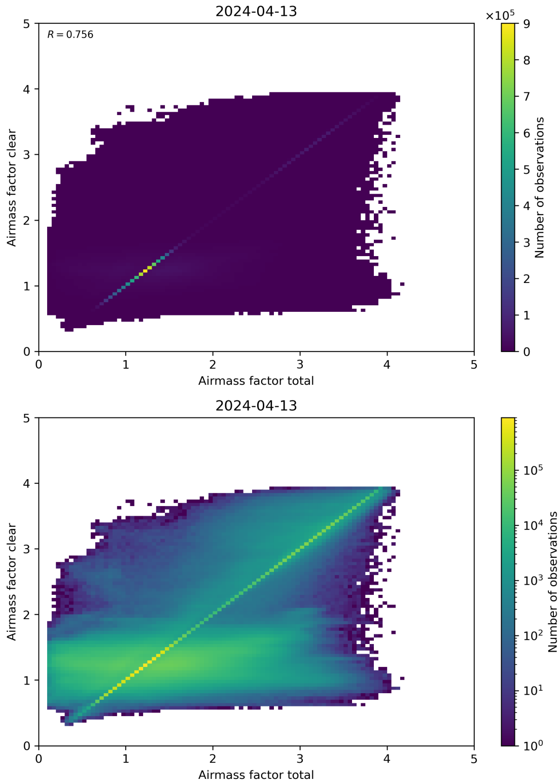
Figure 100: Scatter density plot of “Airmass factor total” against “Airmass factor clear” for 2024-04-12 to 2024-04-14.
