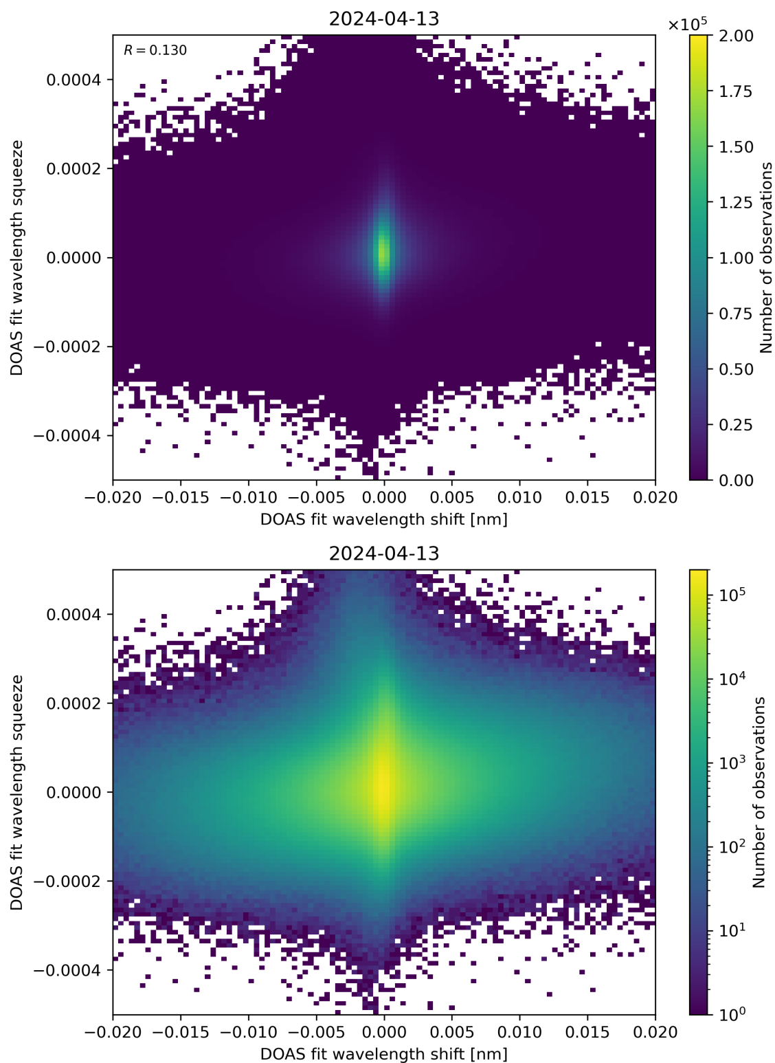
Figure 65: Scatter density plot of “DOAS fit wavelength shift” against “DOAS fit wavelength squeeze” for 2024-04-12 to 2024-04-14.
