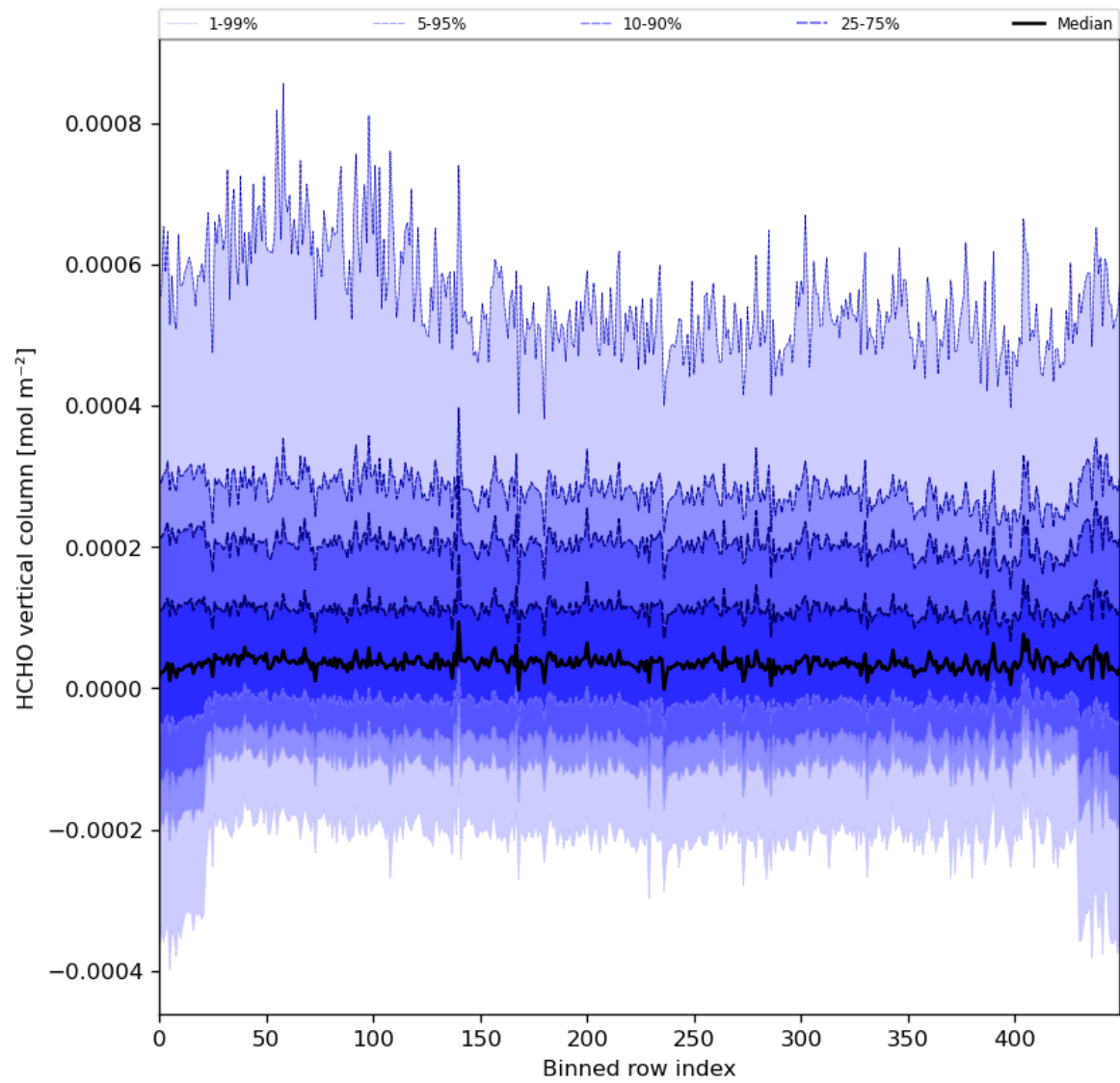
Figure 49: Along track statistics of “HCHO vertical column” for 2024-04-12 to 2024-04-14
