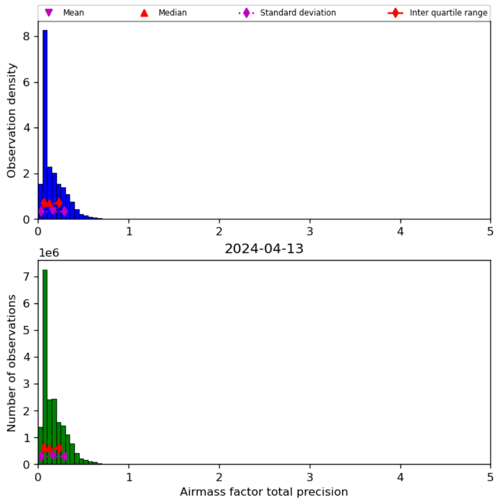
Figure 41: Histogram of “Airmass factor total precision” for 2024-04-12 to 2024-04-14
