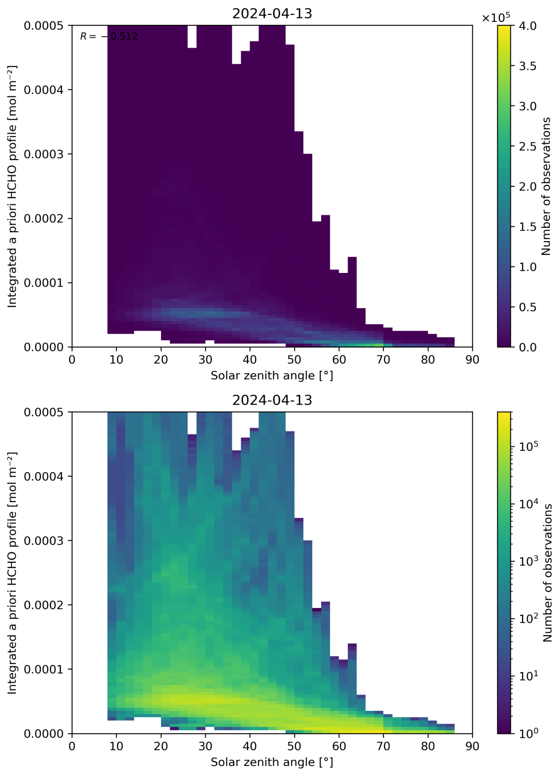
Figure 180: Scatter density plot of “Solar zenith angle” against “Integrated a priori HCHO profile” for 2024-04-12 to 2024-04-14.
