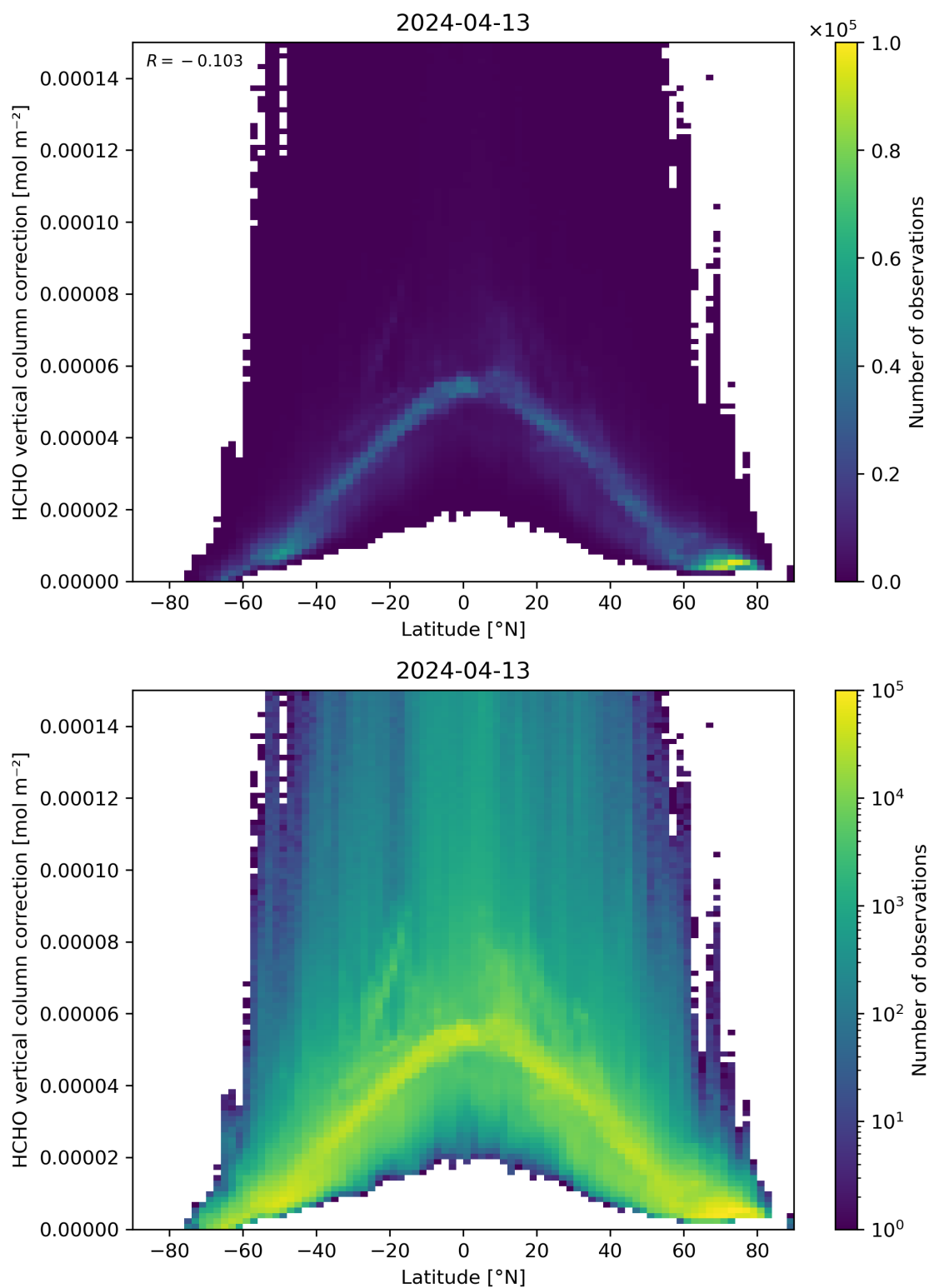
Figure 164: Scatter density plot of “Latitude” against “HCHO vertical column correction” for 2024-04-12 to 2024-04-14.
