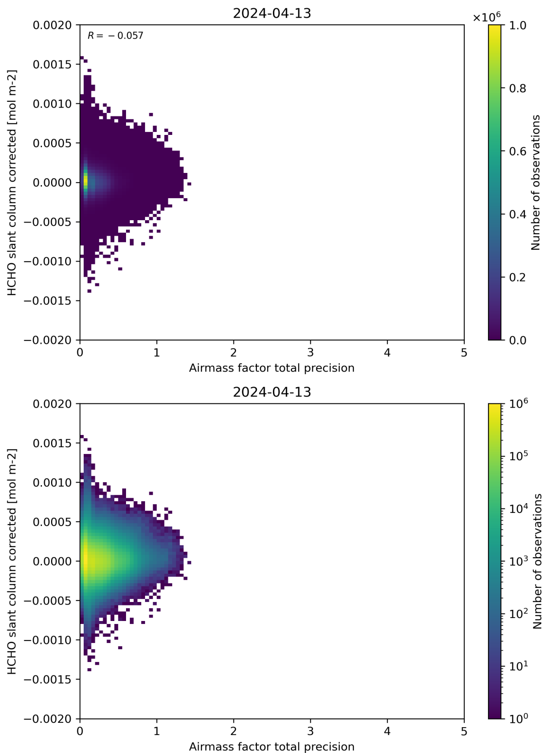
Figure 109: Scatter density plot of “Airmass factor total precision” against “HCHO slant column corrected” for 2024-04-12 to 2024-04-14.
