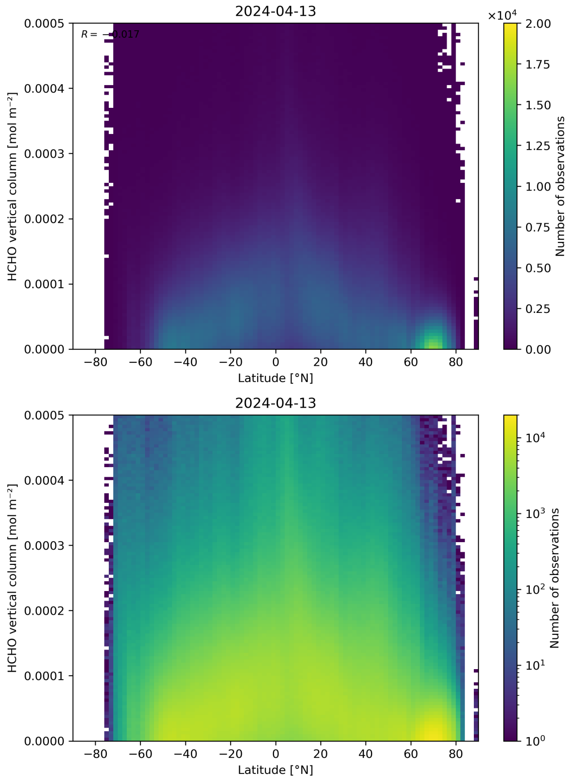
Figure 163: Scatter density plot of “Latitude” against “HCHO vertical column” for 2024-04-12 to 2024-04-14.
