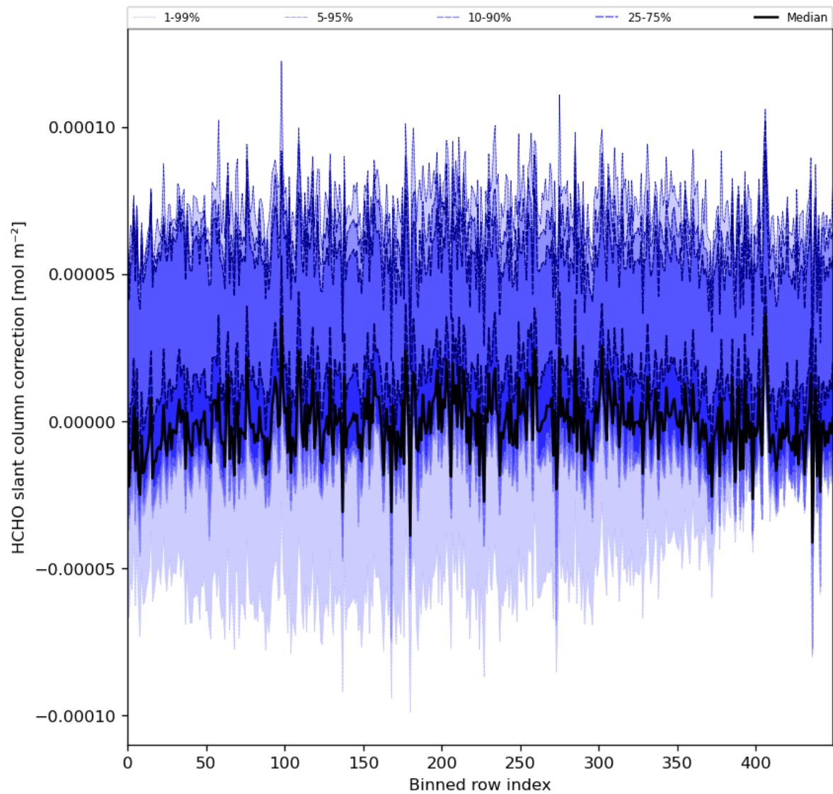
Figure 61: Along track statistics of “HCHO slant column correction” for 2024-04-12 to 2024-04-14
