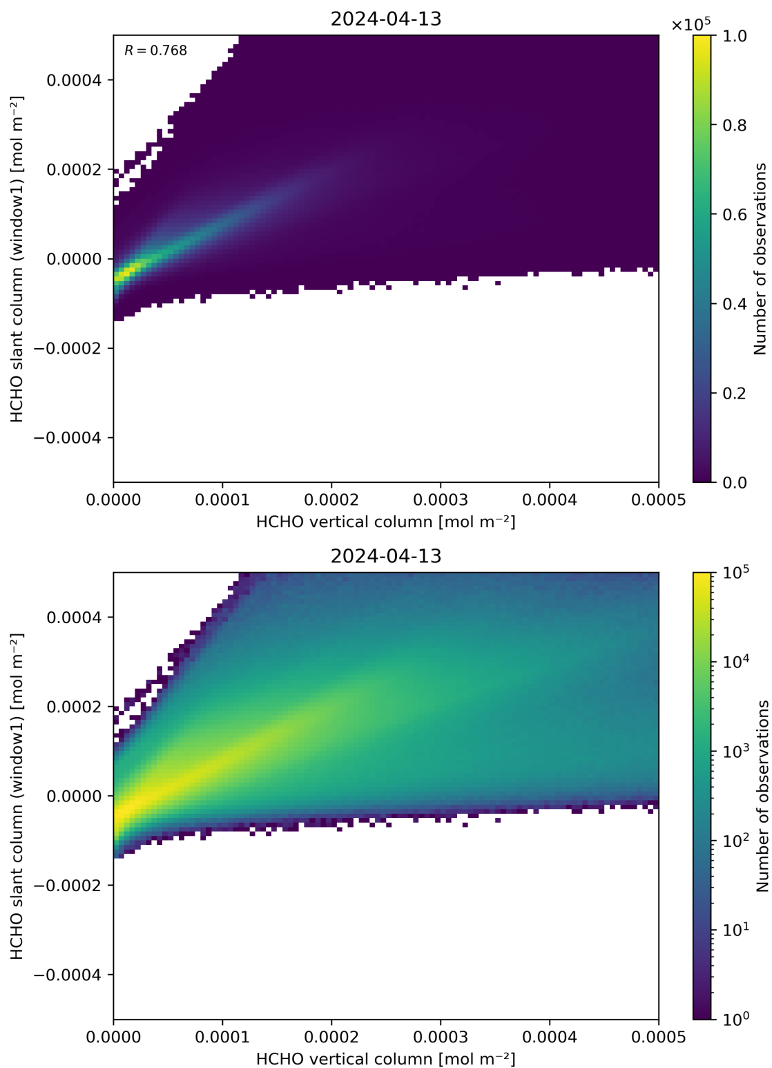
Figure 129: Scatter density plot of “HCHO vertical column” against “HCHO slant column (window1)” for 2024-04-12 to 2024-04-14.
