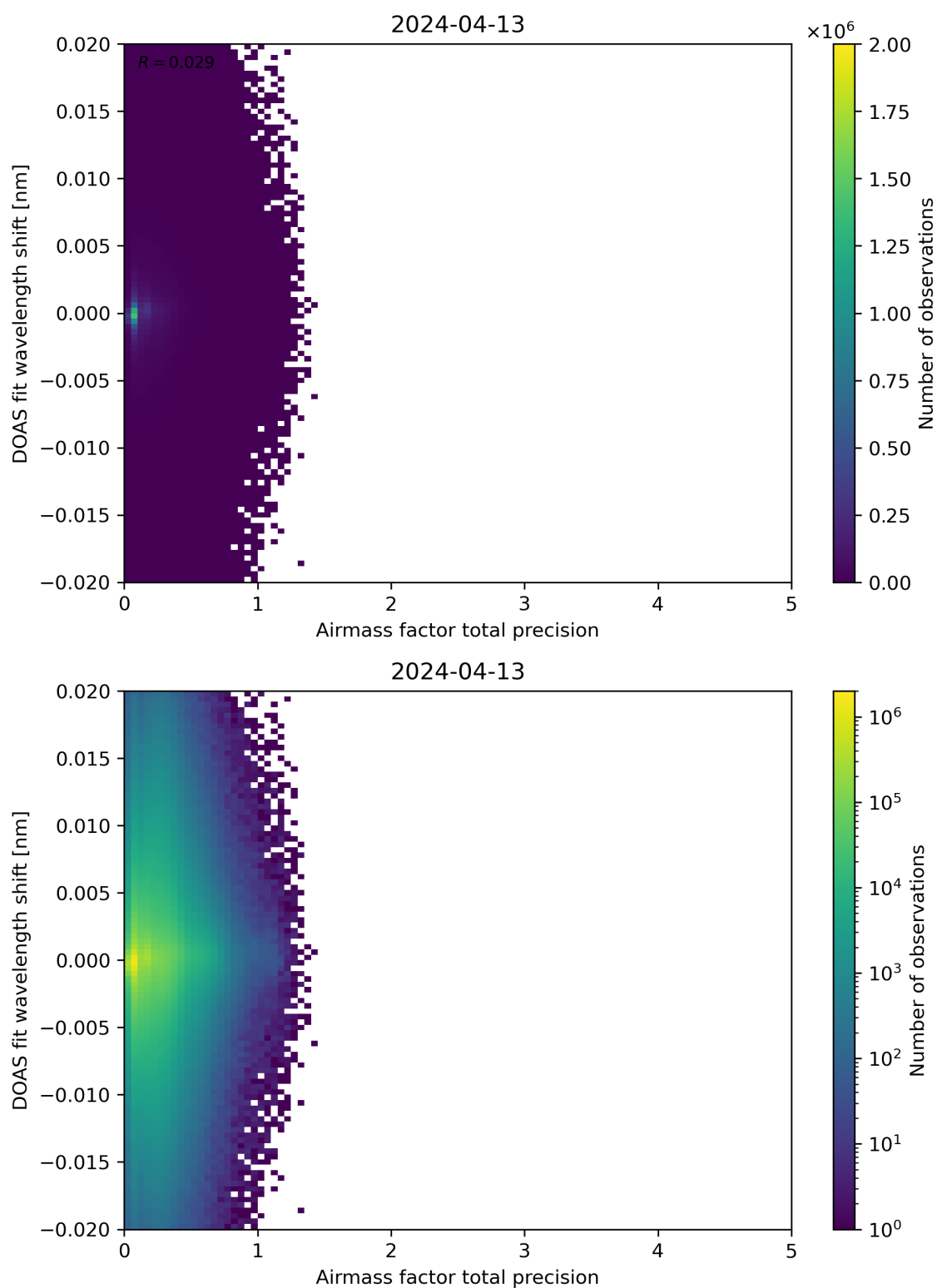
Figure 106: Scatter density plot of “Airmass factor total precision” against “DOAS fit wavelength shift” for 2024-04-12 to 2024-04-14.
