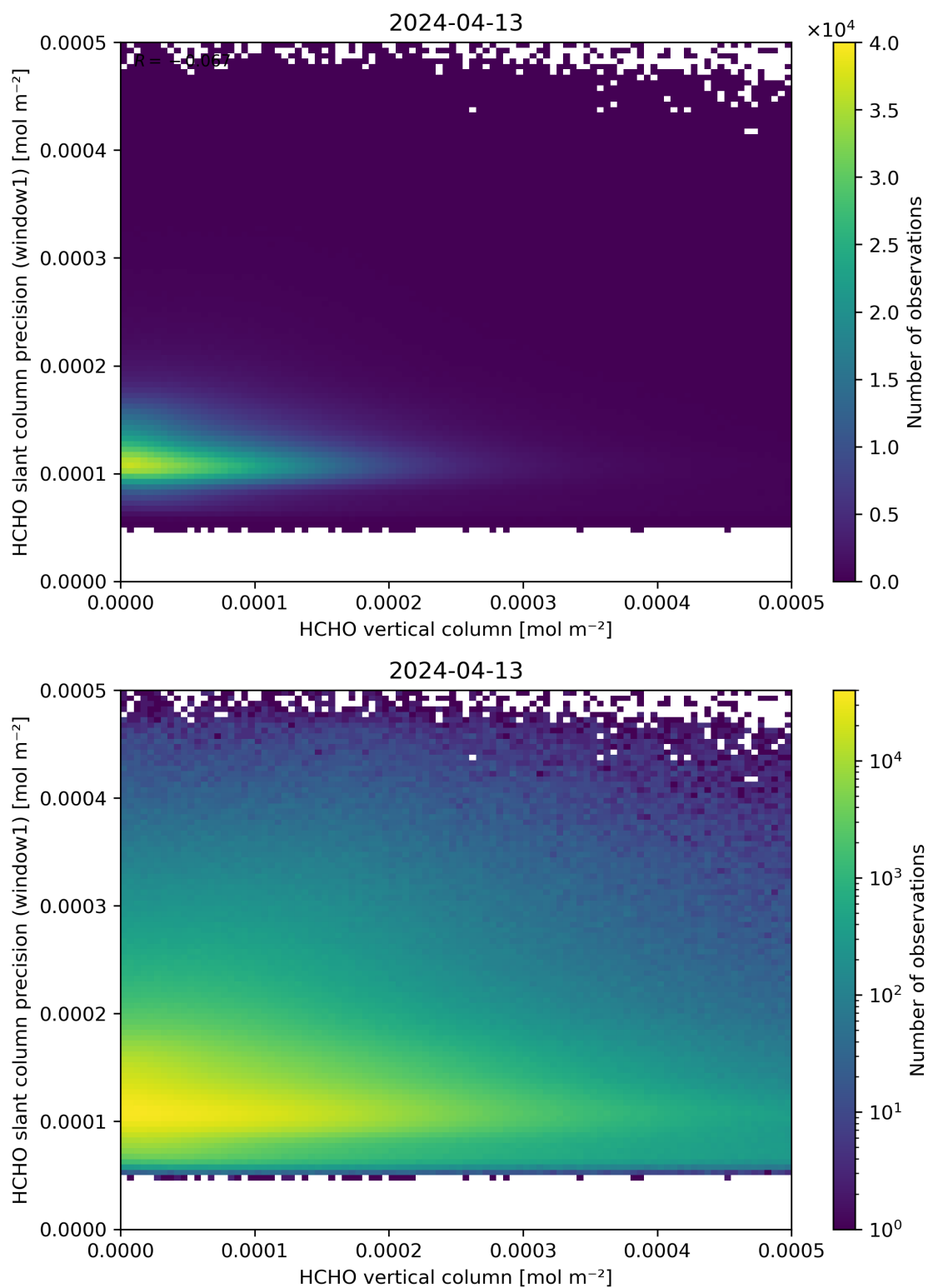
Figure 130: Scatter density plot of “HCHO vertical column” against “HCHO slant column precision (window1)” for 2024-04-12 to 2024-04-14.
