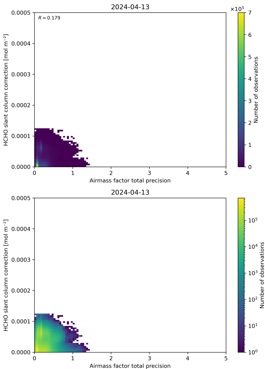
Figure 110: Scatter density plot of “Airmass factor total precision” against “HCHO slant column correction” for 2024-04-12 to 2024-04-14.
