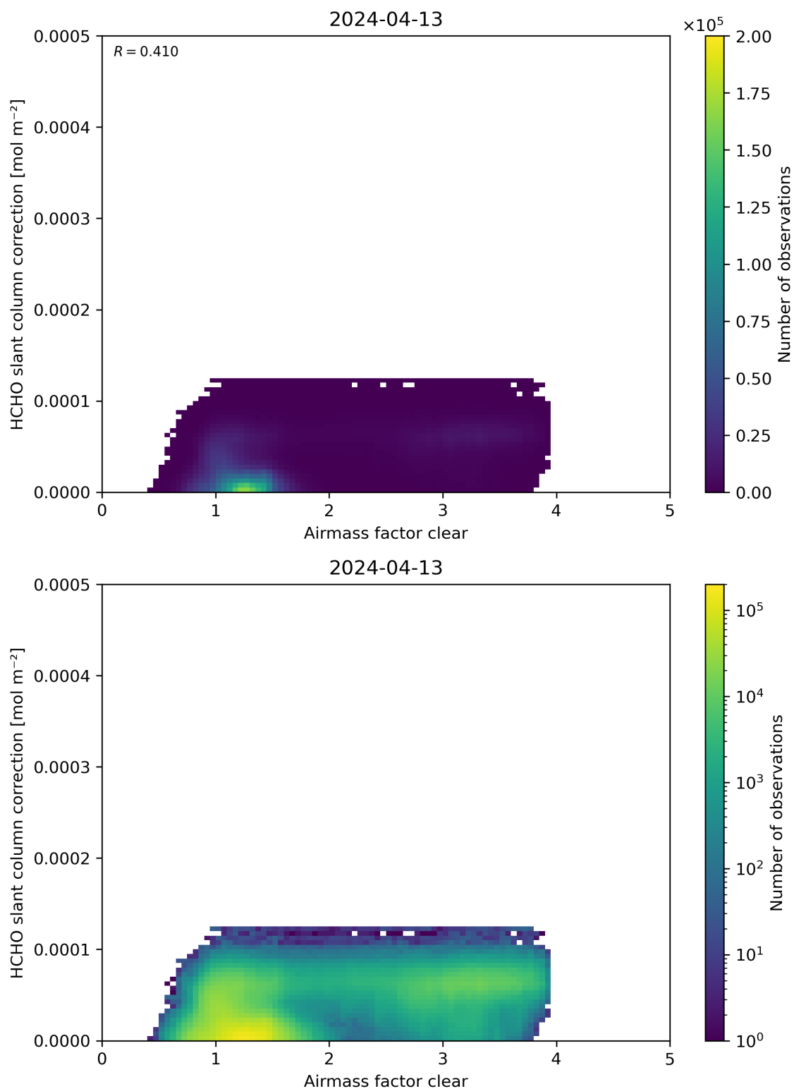
Figure 75: Scatter density plot of “Airmass factor clear” against “HCHO slant column correction” for 2024-04-12 to 2024-04-14.
