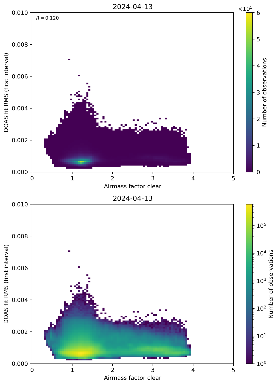
Figure 71: Scatter density plot of “Airmass factor clear” against “DOAS fit RMS (first interval)” for 2024-04-12 to 2024-04-14.
