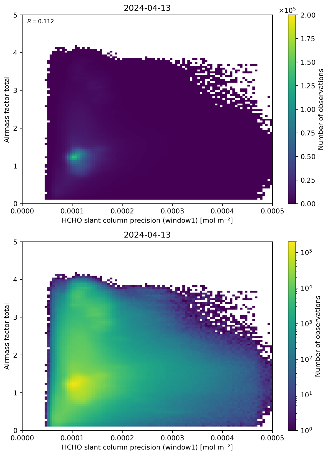
Figure 94: Scatter density plot of “HCHO slant column precision (window1)” against “Airmass factor total” for 2024-04-12 to 2024-04-14.
