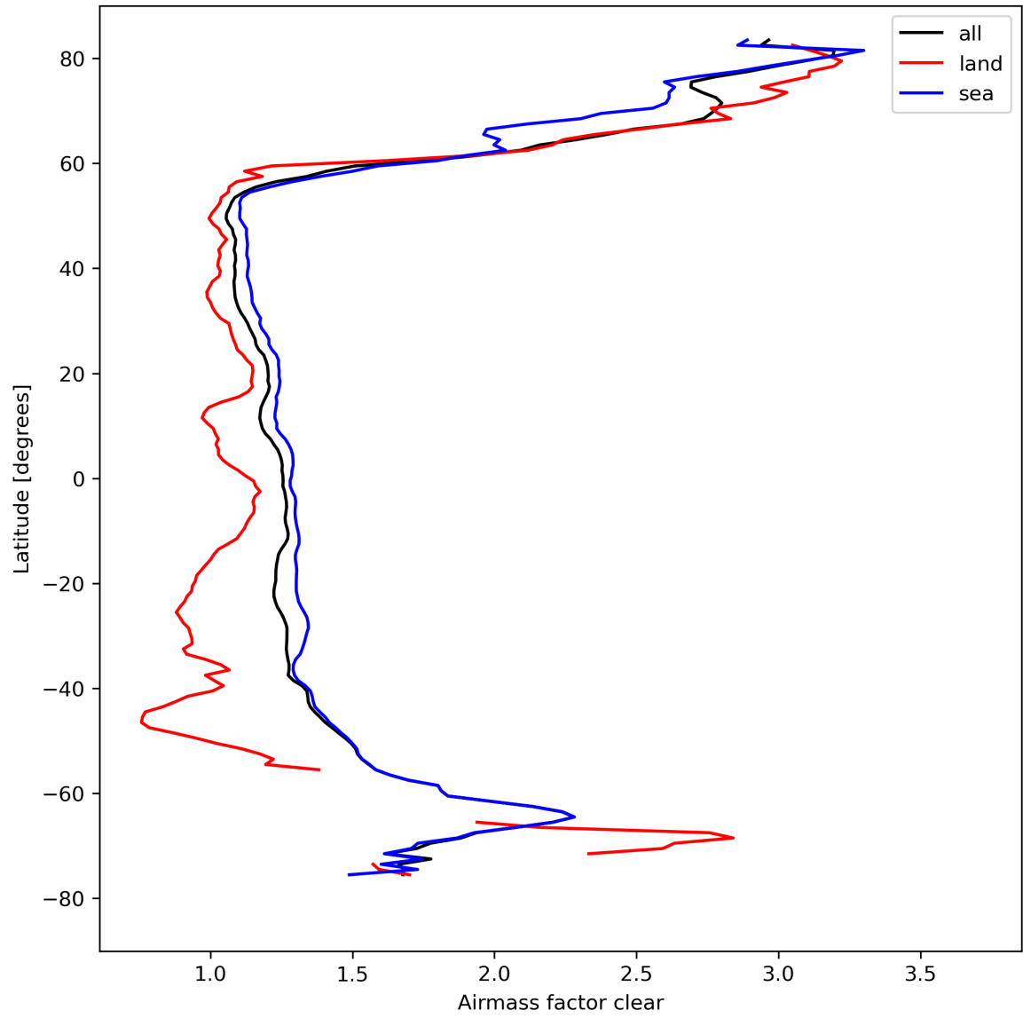
Figure 28: Zonal average of “Airmass factor clear” for 2024-04-12 to 2024-04-14.
