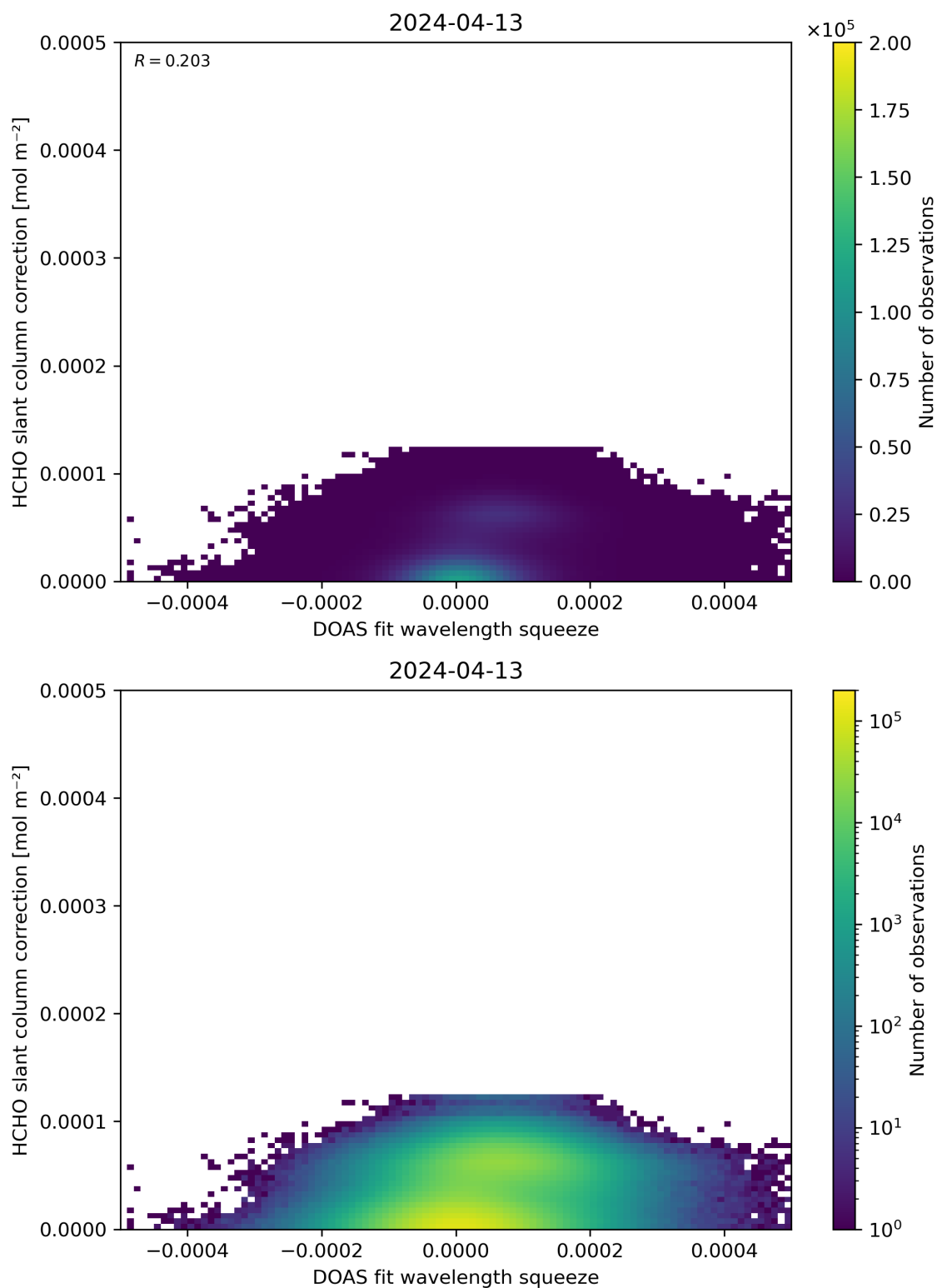
Figure 70: Scatter density plot of “DOAS fit wavelength squeeze” against “HCHO slant column correction” for 2024-04-12 to 2024-04-14.
