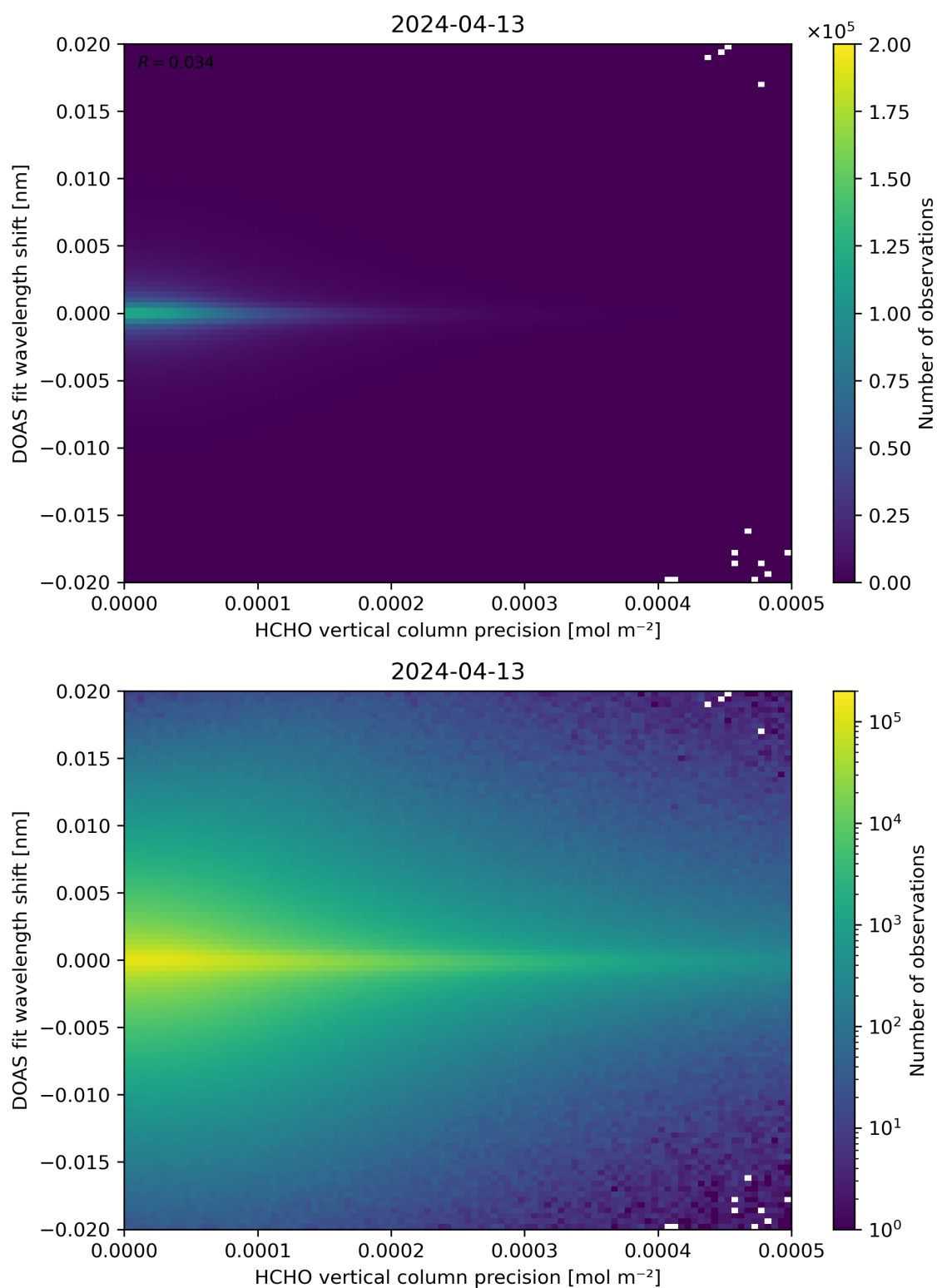
Figure 137: Scatter density plot of “HCHO vertical column precision” against “DOAS fit wavelength shift” for 2024-04-12 to 2024-04-14.
