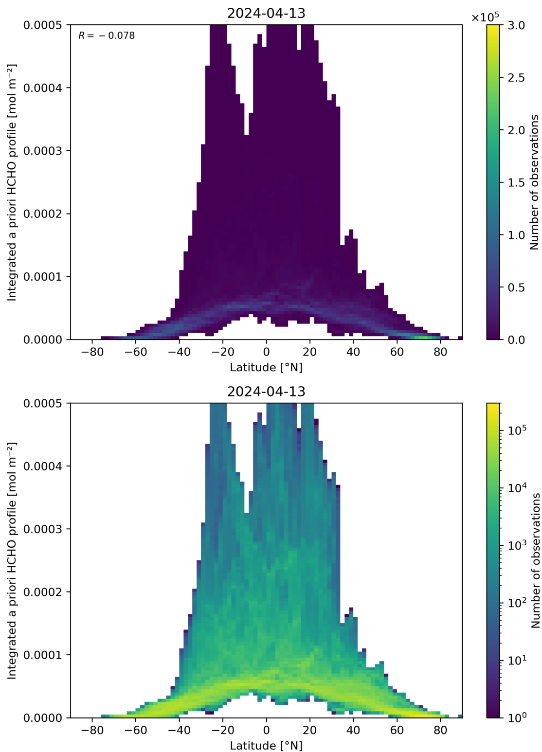
Figure 166: Scatter density plot of “Latitude” against “Integrated a priori HCHO profile” for 2024-04-12 to 2024-04-14.
