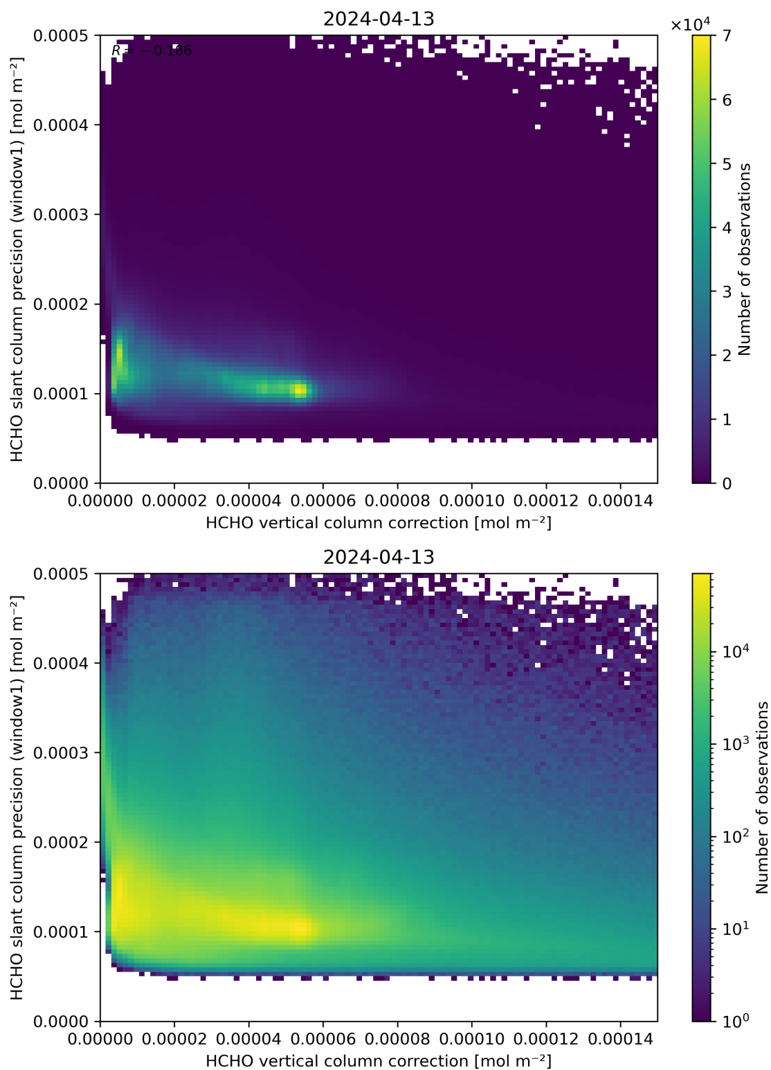
Figure 119: Scatter density plot of “HCHO vertical column correction” against “HCHO slant column precision (window1)” for 2024-04-12 to 2024-04-14.
