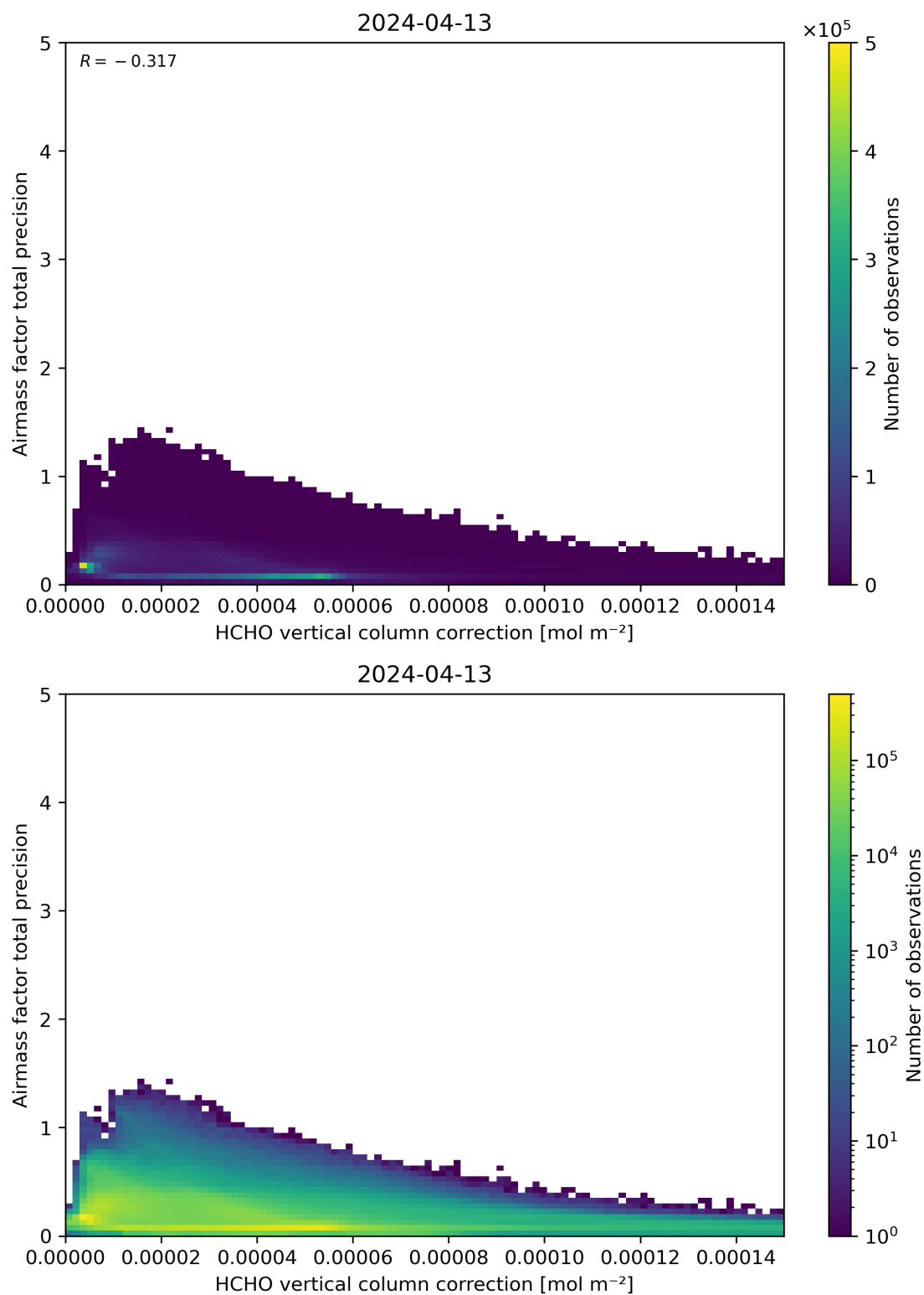
Figure 121: Scatter density plot of “HCHO vertical column correction” against “Airmass factor total precision” for 2024-04-12 to 2024-04-14.
