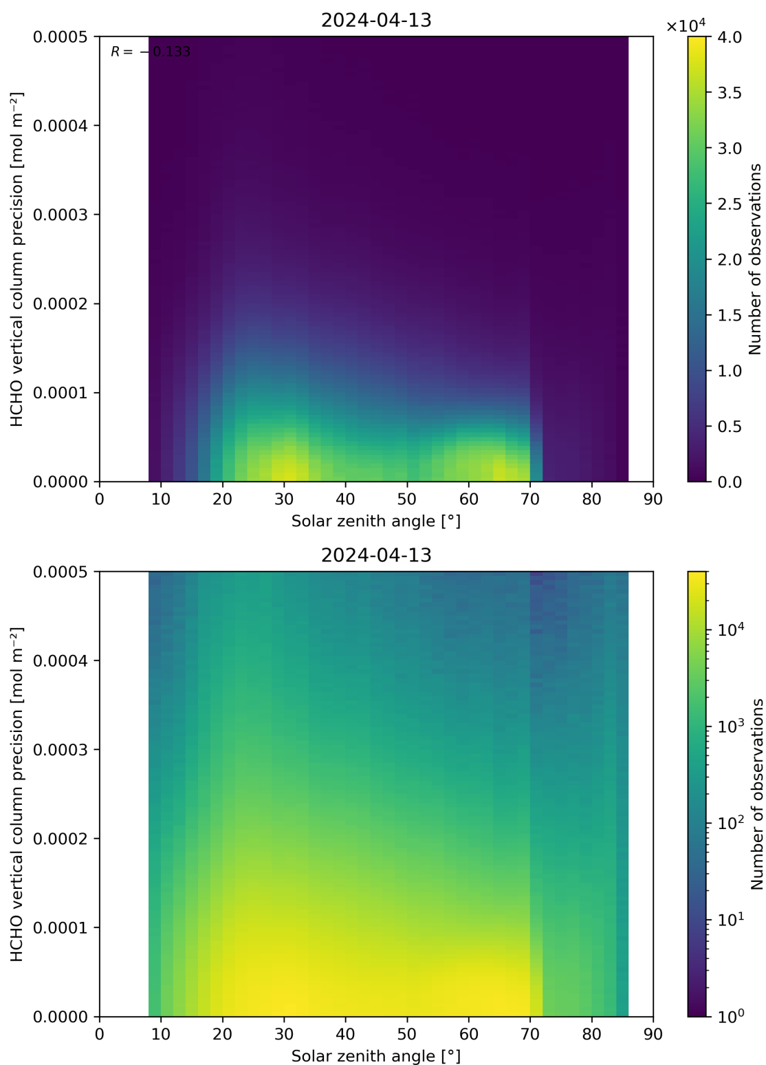
Figure 179: Scatter density plot of “Solar zenith angle” against “HCHO vertical column precision” for 2024-04-12 to 2024-04-14.
