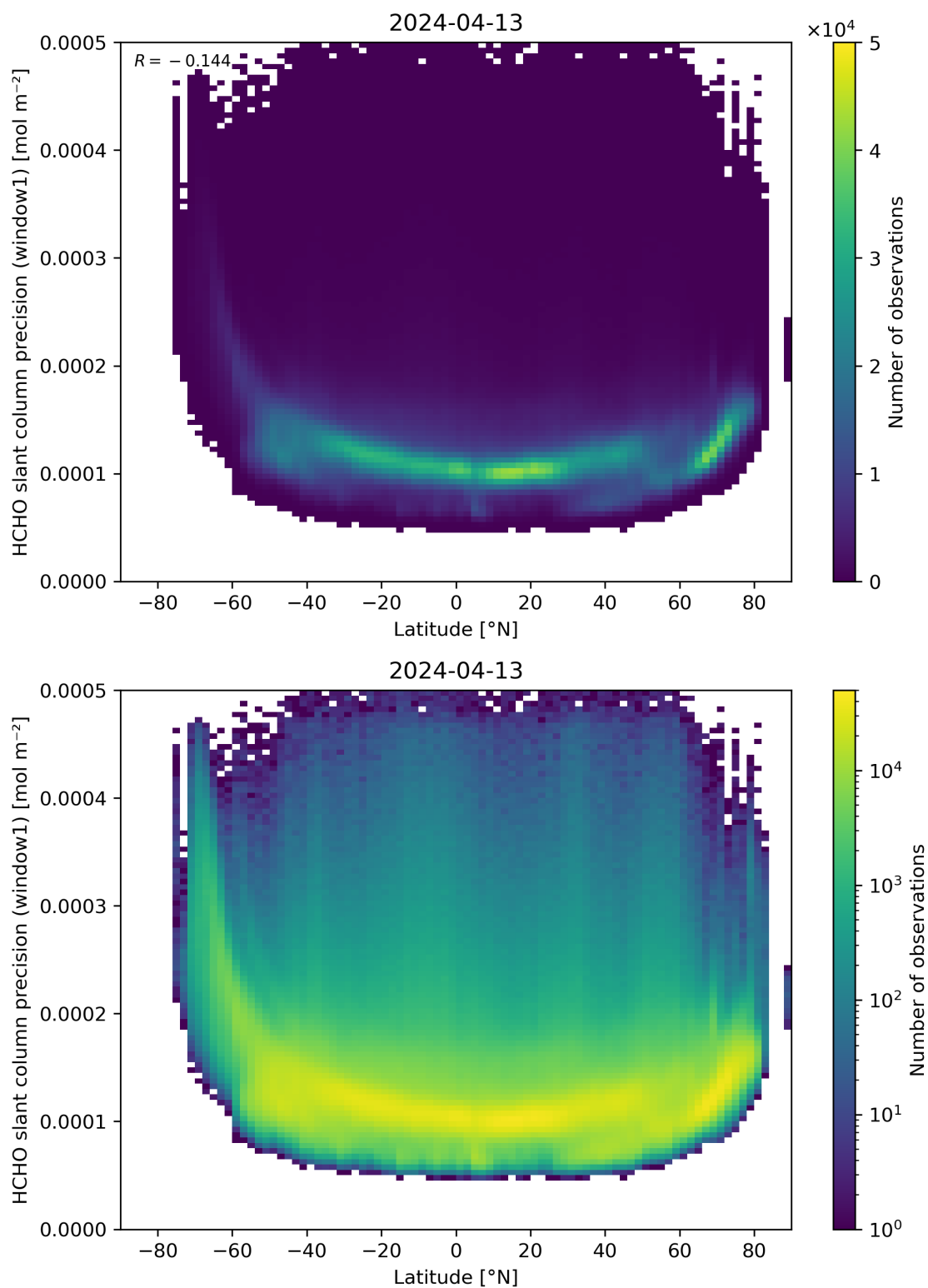
Figure 160: Scatter density plot of “Latitude” against “HCHO slant column precision (window1)” for 2024-04-12 to 2024-04-14.
