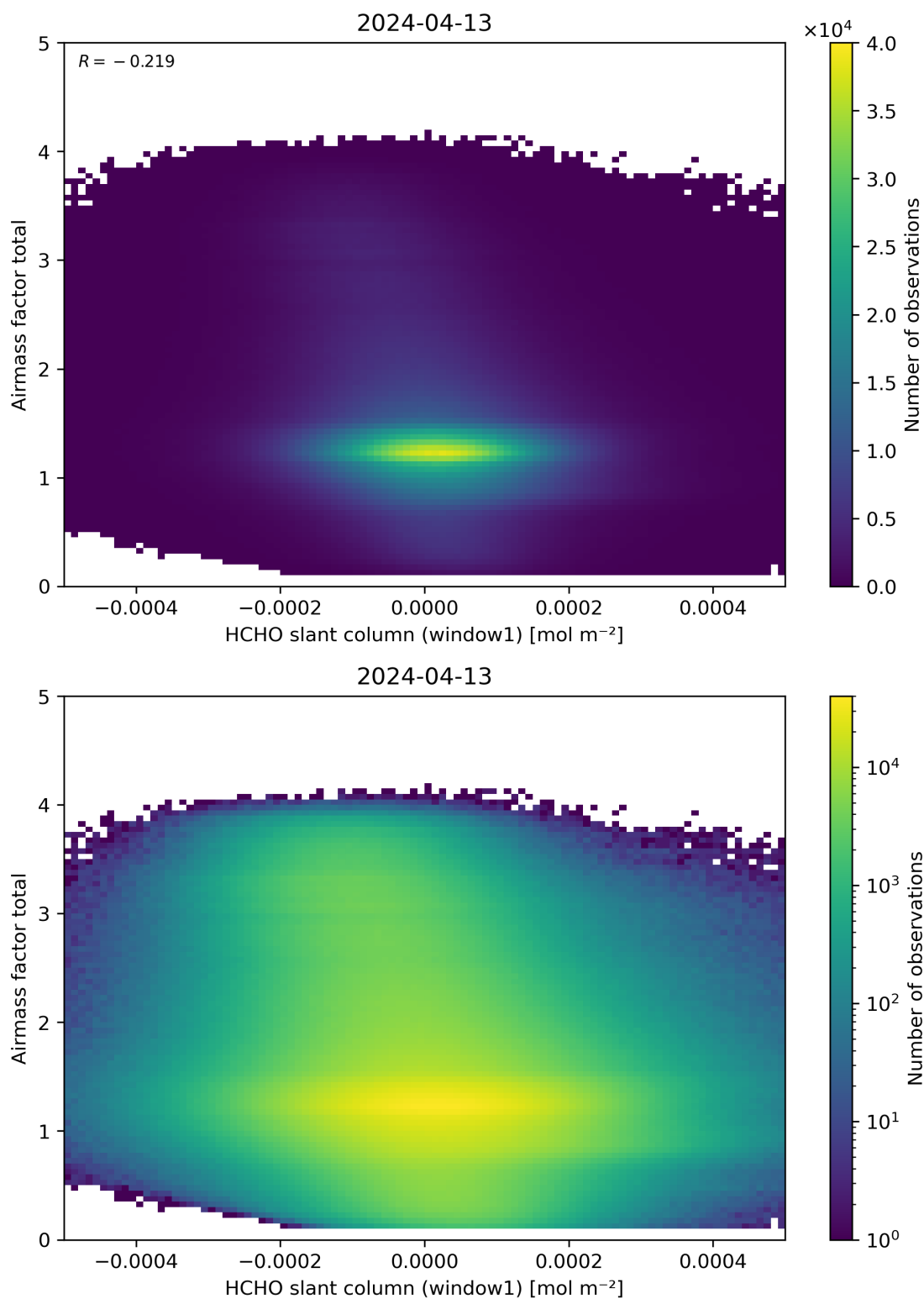
Figure 85: Scatter density plot of “HCHO slant column (window1)” against “Airmass factor total” for 2024-04-12 to 2024-04-14.
