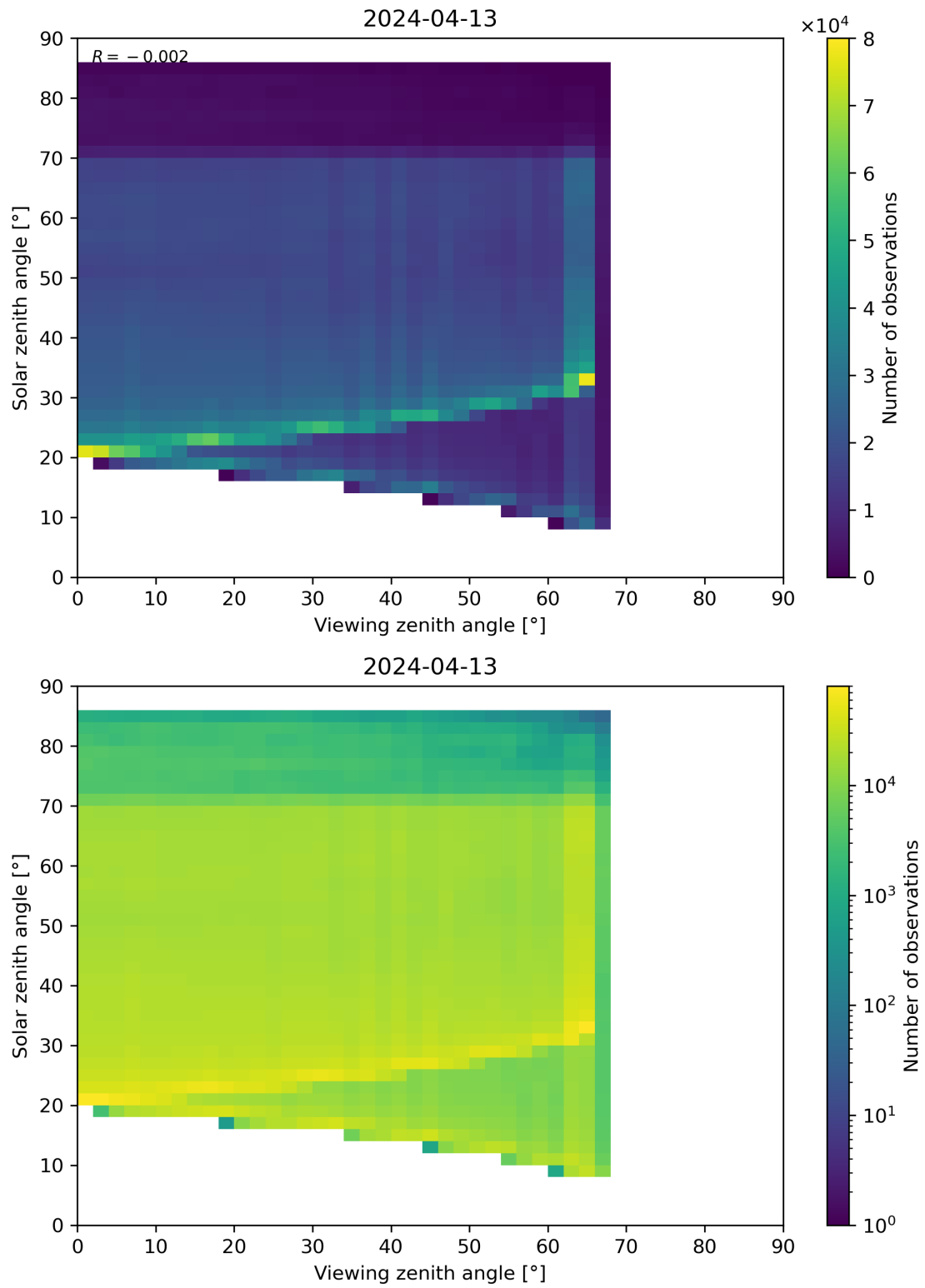
Figure 197: Scatter density plot of “Viewing zenith angle” against “Solar zenith angle” for 2024-04-12 to 2024-04-14.
