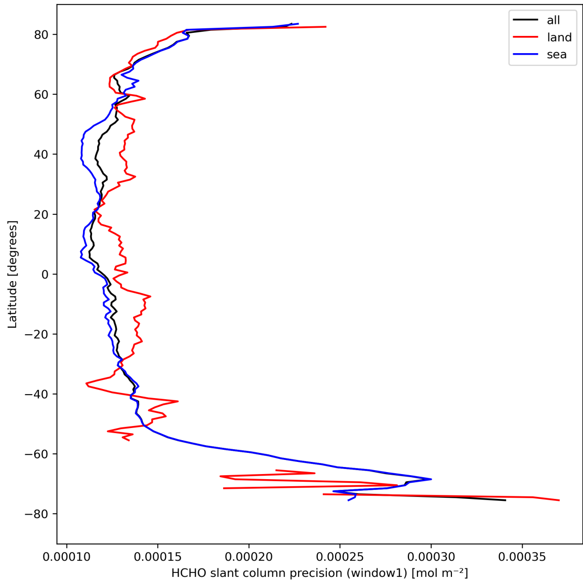
Figure 25: Zonal average of “HCHO slant column precision (window1)” for 2024-04-12 to 2024-04-14.
