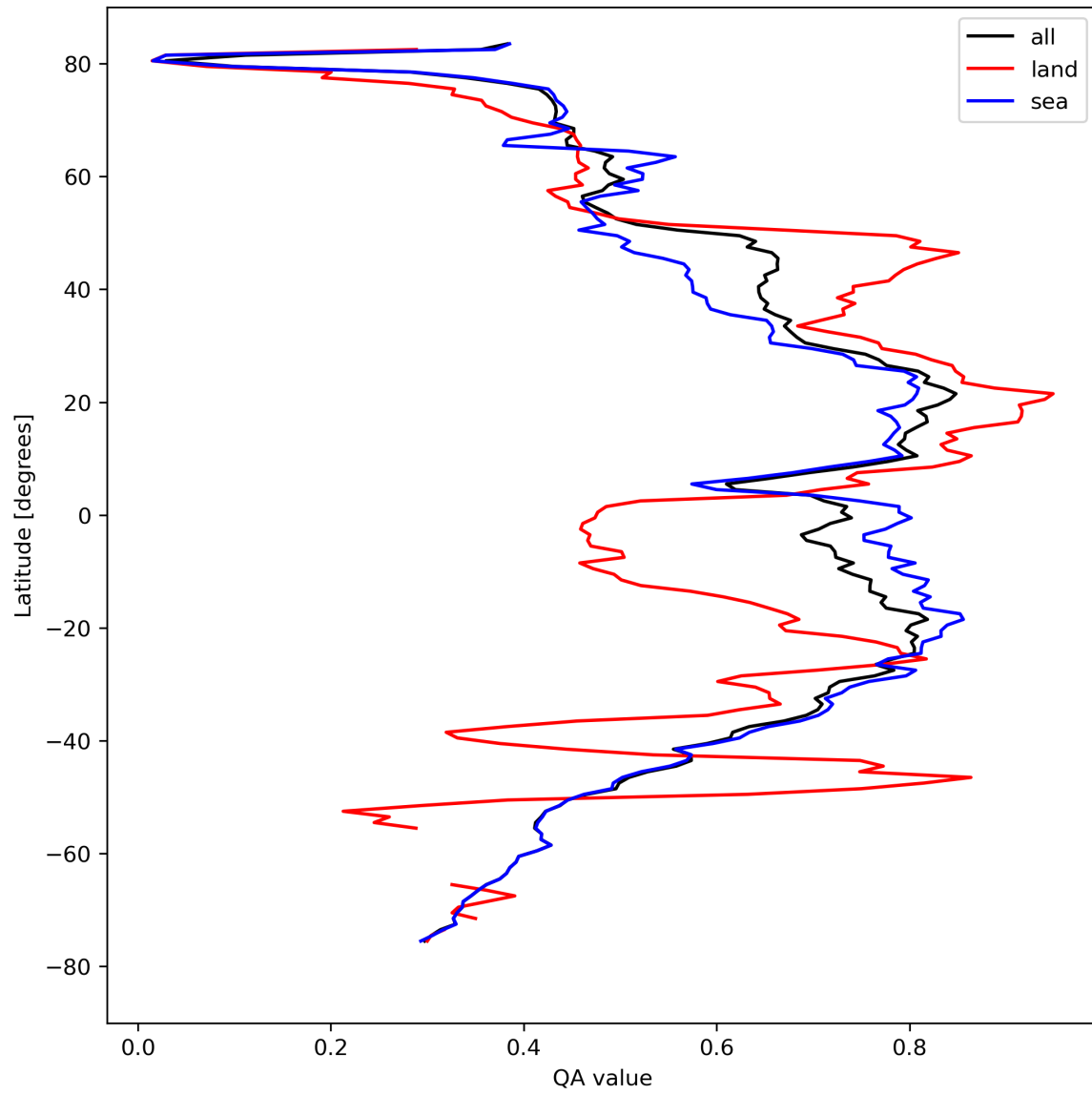
Figure 20: Zonal average of “QA value” for 2024-04-12 to 2024-04-14.
