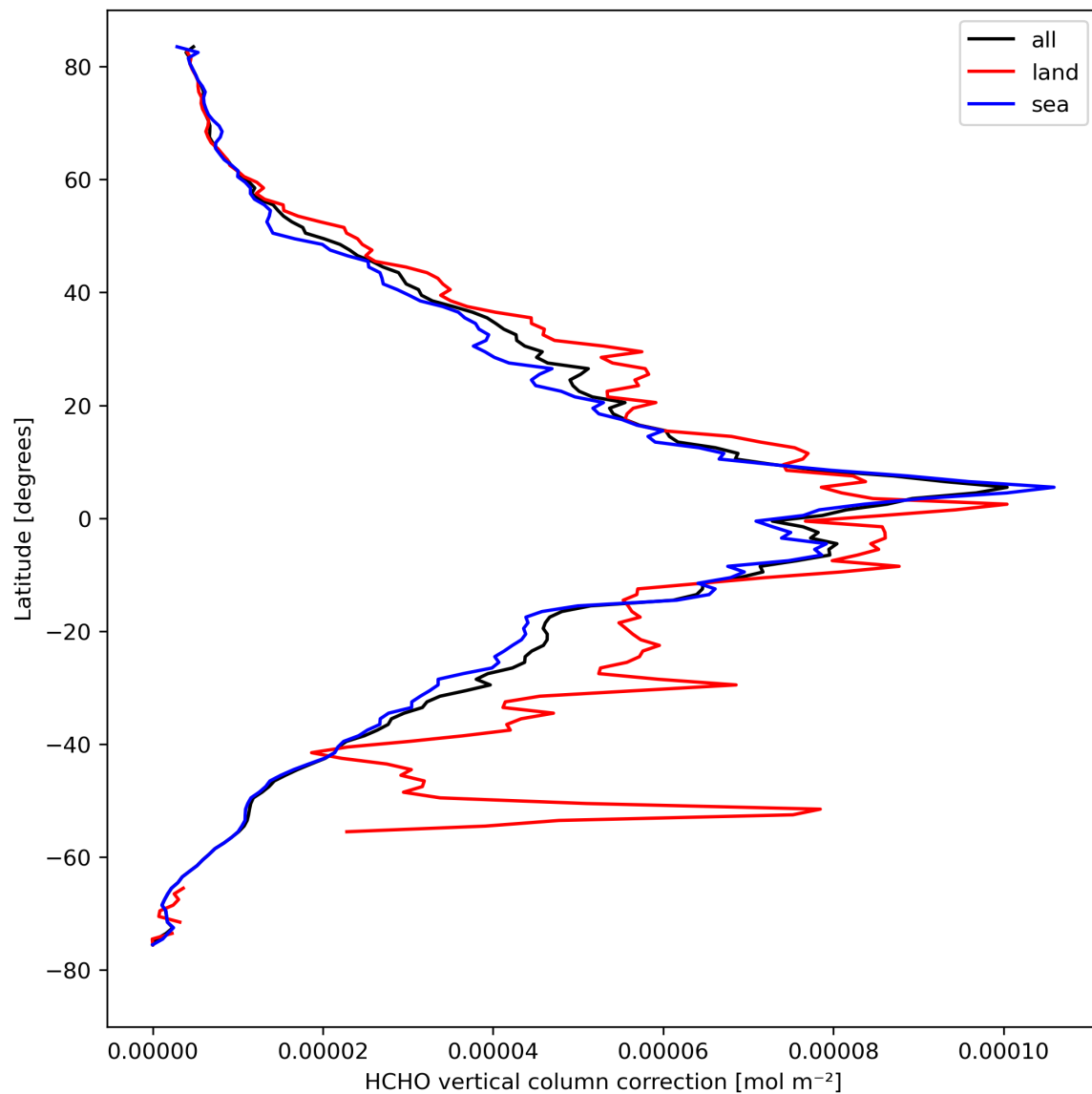
Figure 23: Zonal average of “HCHO vertical column correction” for 2024-04-12 to 2024-04-14.
