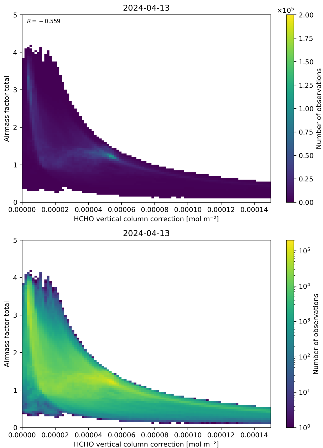
Figure 120: Scatter density plot of “HCHO vertical column correction” against “Airmass factor total” for 2024-04-12 to 2024-04-14.
