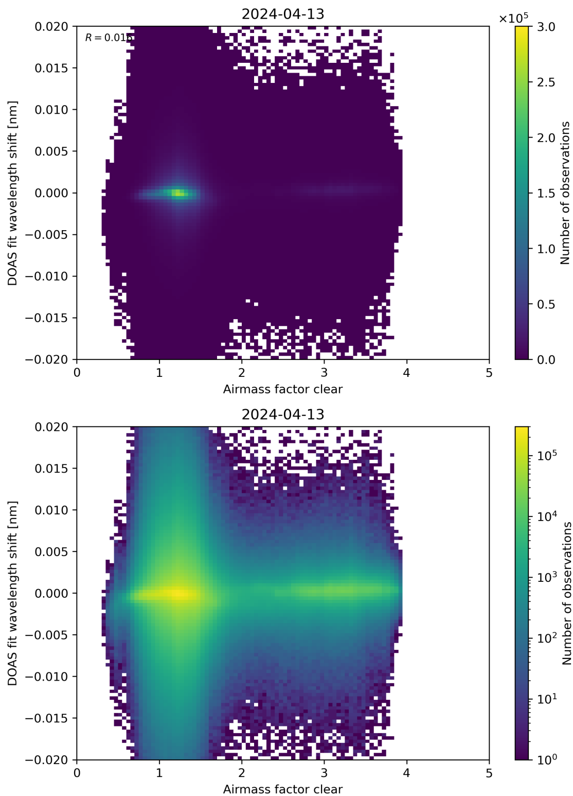
Figure 72: Scatter density plot of “Airmass factor clear” against “DOAS fit wavelength shift” for 2024-04-12 to 2024-04-14.
