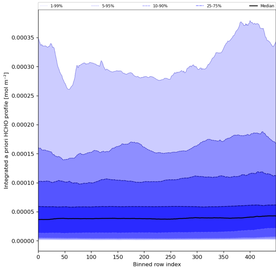
Figure 57: Along track statistics of “Integrated a priori HCHO profile” for 2024-04-12 to 2024-04-14
