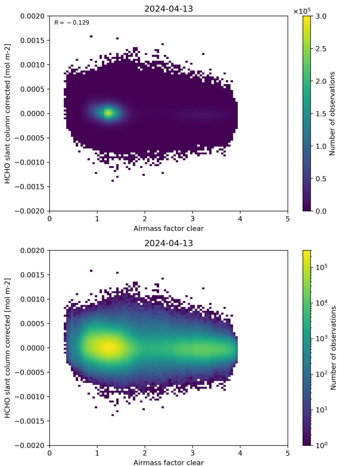
Figure 74: Scatter density plot of “Airmass factor clear” against “HCHO slant column corrected” for 2024-04-12 to 2024-04-14.
