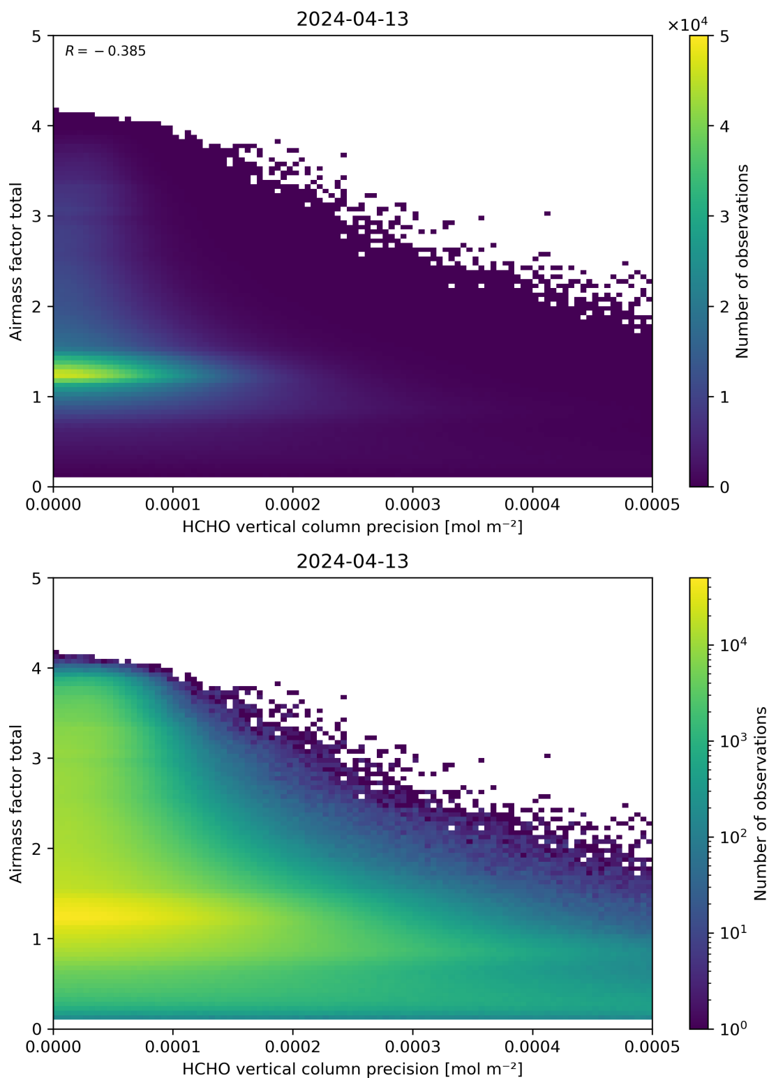
Figure 144: Scatter density plot of “HCHO vertical column precision” against “Airmass factor total” for 2024-04-12 to 2024-04-14.
