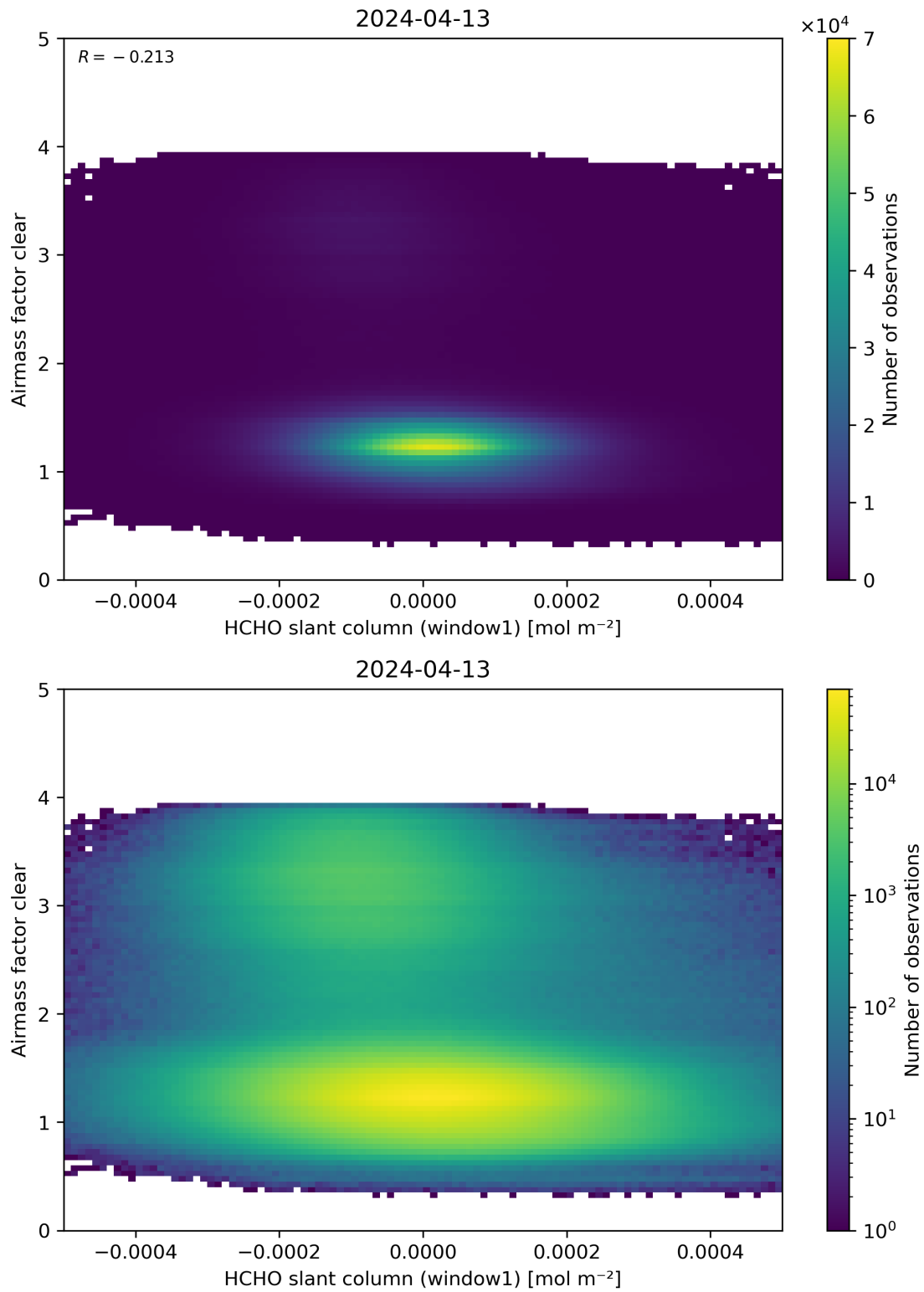
Figure 81: Scatter density plot of “HCHO slant column (window1)” against “Airmass factor clear” for 2024-04-12 to 2024-04-14.
