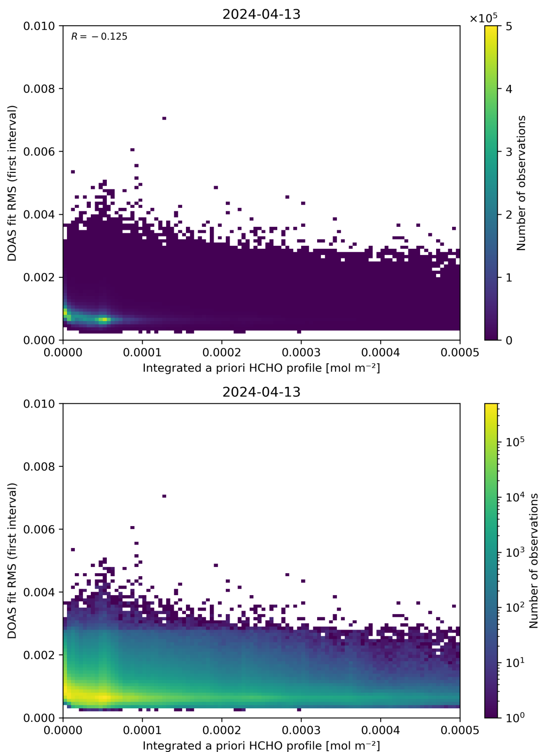
Figure 148: Scatter density plot of “Integrated a priori HCHO profile” against “DOAS fit RMS (first interval)” for 2024-04-12 to 2024-04-14.
