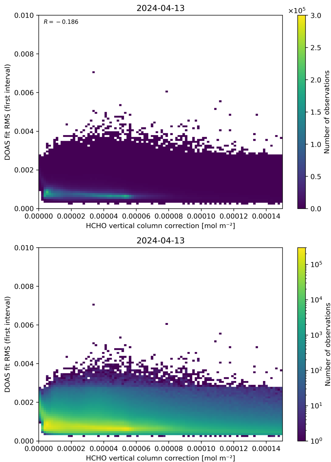
Figure 112: Scatter density plot of “HCHO vertical column correction” against “DOAS fit RMS (first interval)” for 2024-04-12 to 2024-04-14.
