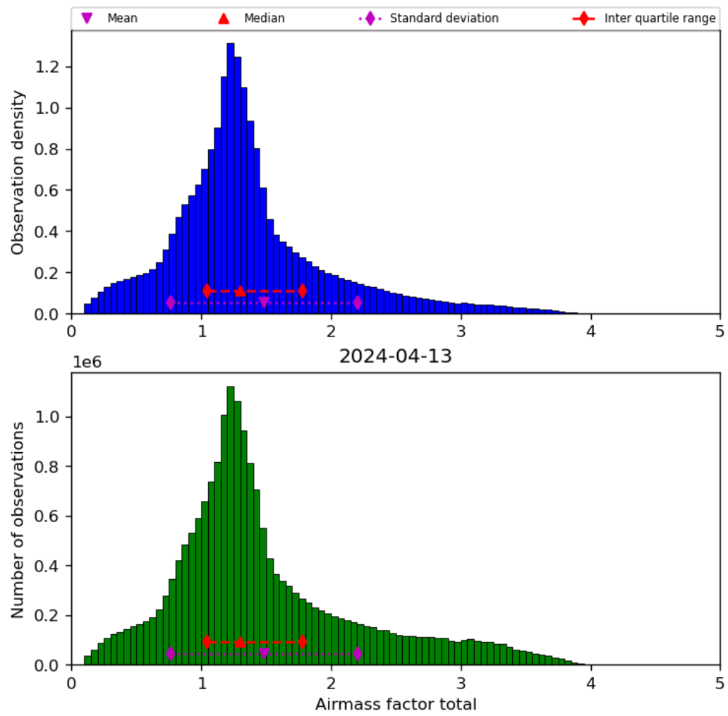
Figure 40: Histogram of “Airmass factor total” for 2024-04-12 to 2024-04-14
