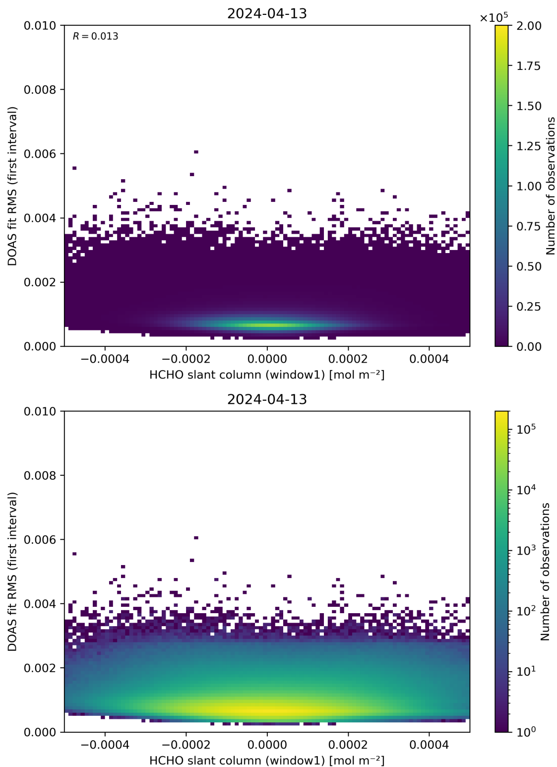
Figure 78: Scatter density plot of “HCHO slant column (window1)” against “DOAS fit RMS (first interval)” for 2024-04-12 to 2024-04-14.
