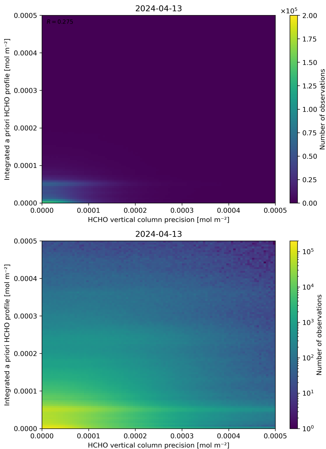
Figure 147: Scatter density plot of “HCHO vertical column precision” against “Integrated a priori HCHO profile” for 2024-04-12 to 2024-04-14.
