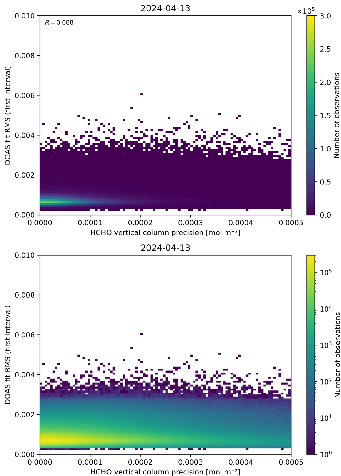
Figure 136: Scatter density plot of “HCHO vertical column precision” against “DOAS fit RMS (first interval)” for 2024-04-12 to 2024-04-14.
