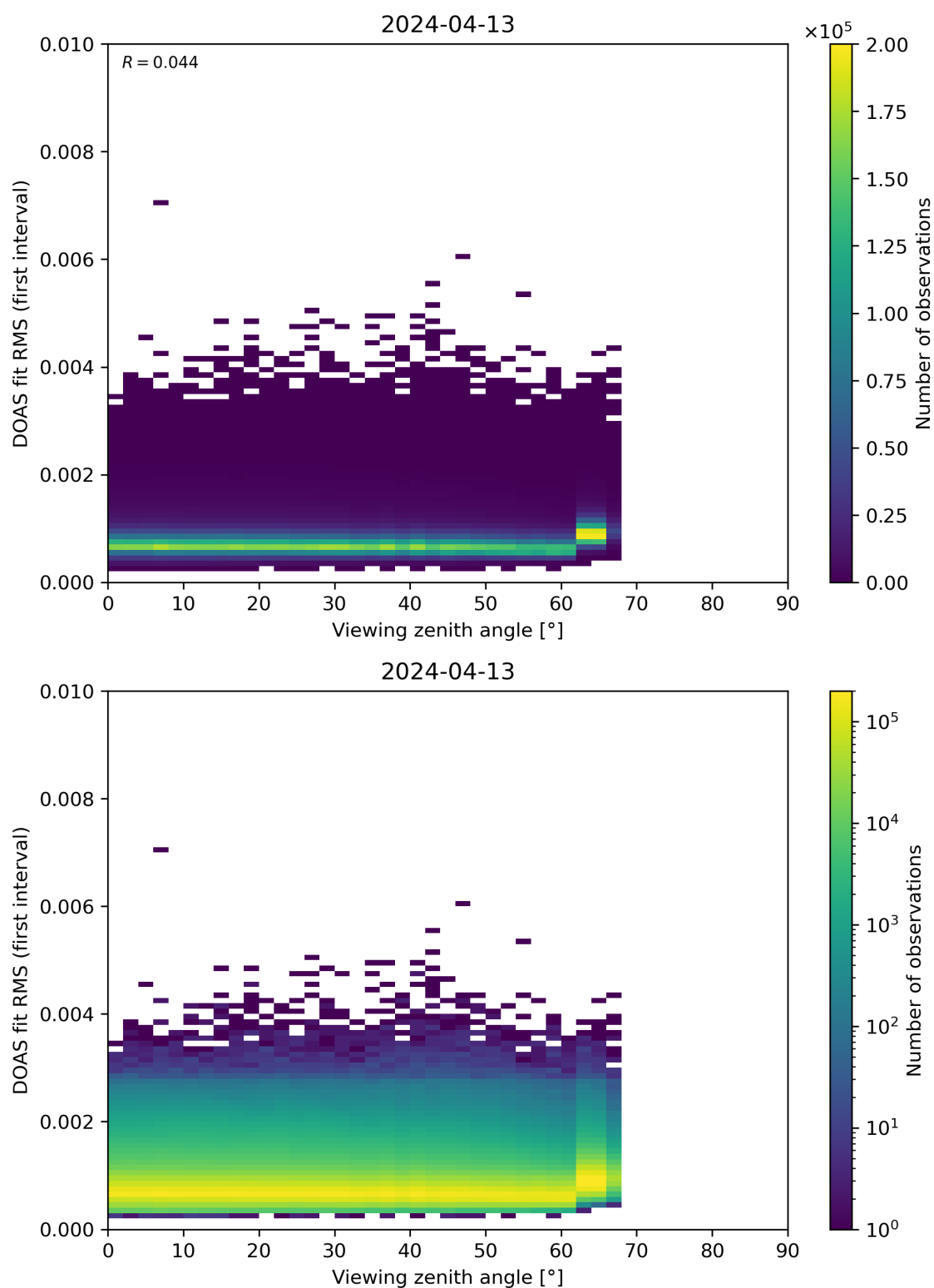
Figure 182: Scatter density plot of “Viewing zenith angle” against “DOAS fit RMS (first interval)” for 2024-04-12 to 2024-04-14.
