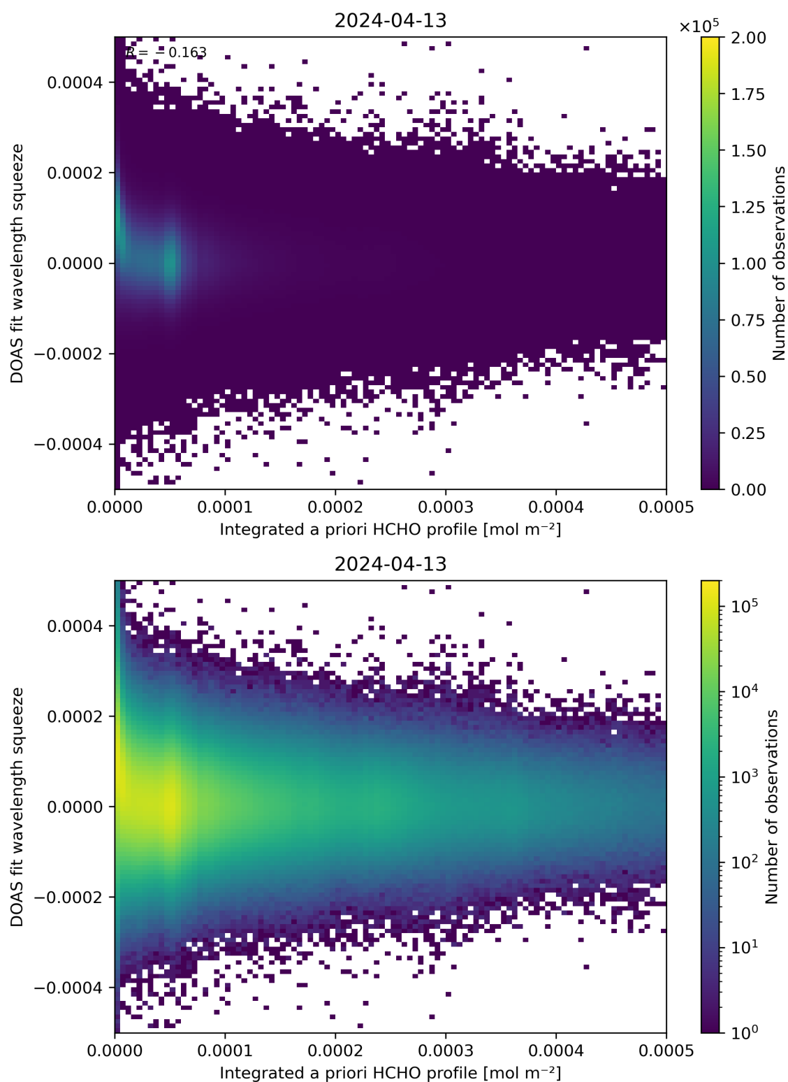
Figure 150: Scatter density plot of “Integrated a priori HCHO profile” against “DOAS fit wavelength squeeze” for 2024-04-12 to 2024-04-14.
