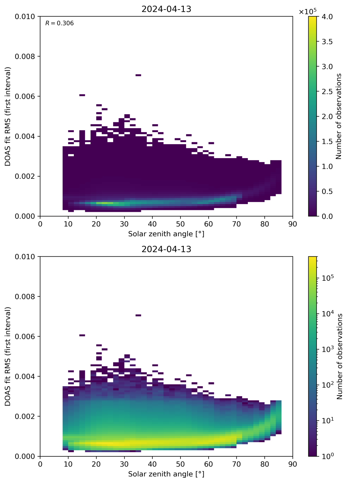
Figure 167: Scatter density plot of “Solar zenith angle” against “DOAS fit RMS (first interval)” for 2024-04-12 to 2024-04-14.
