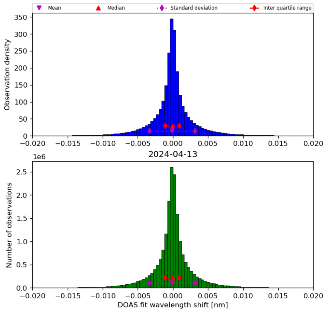
Figure 44: Histogram of “DOAS fit wavelength shift” for 2024-04-12 to 2024-04-14
