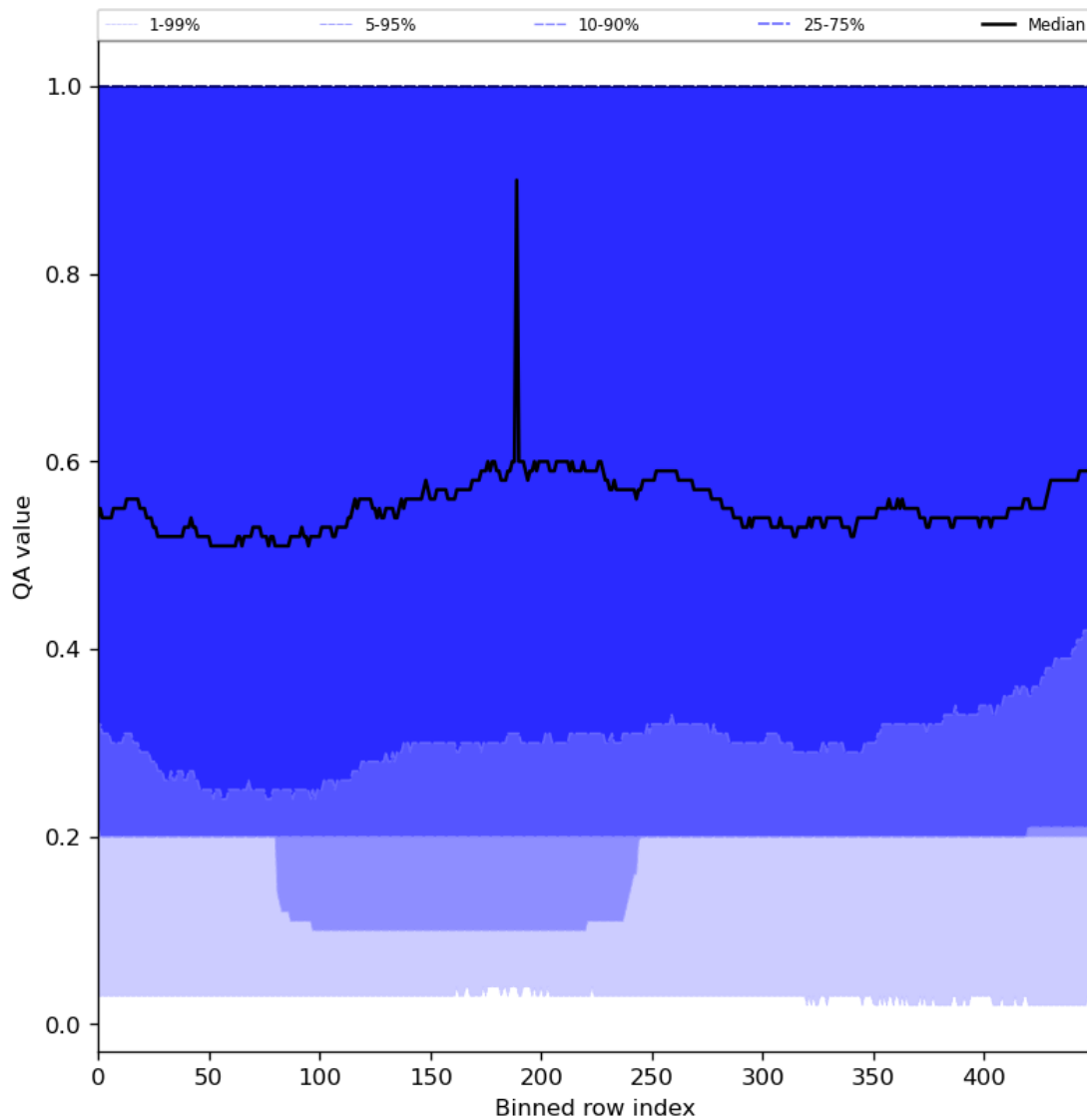
Figure 48: Along track statistics of “QA value” for 2024-04-12 to 2024-04-14
