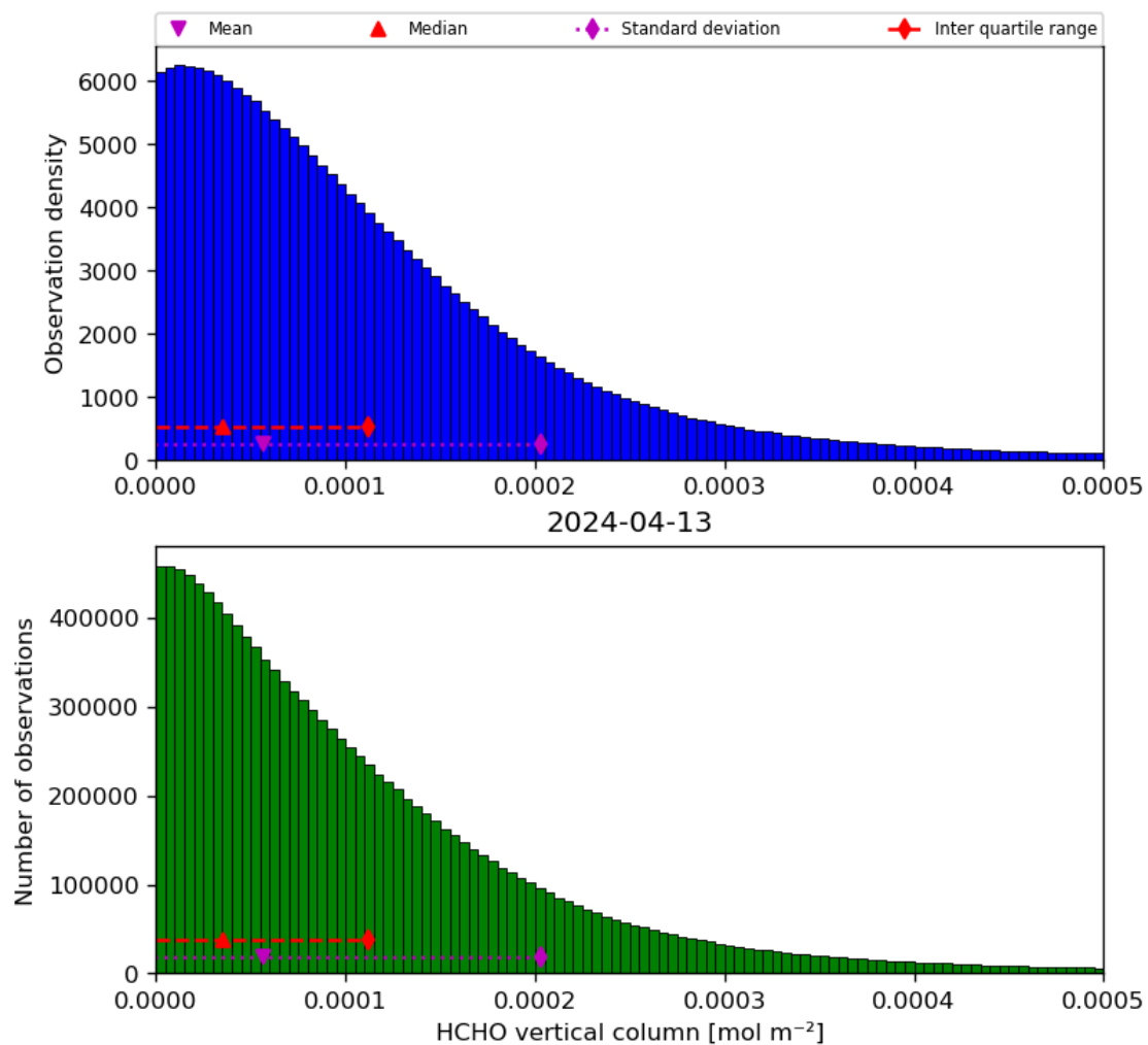
Figure 35: Histogram of “HCHO vertical column” for 2024-04-12 to 2024-04-14
