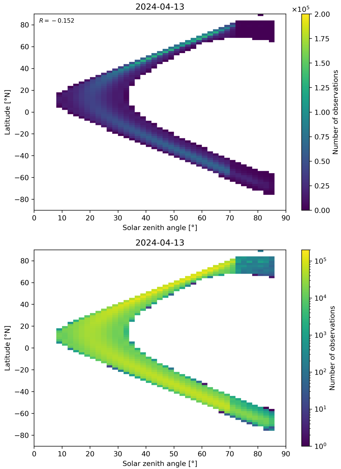
Figure 181: Scatter density plot of “Solar zenith angle” against “Latitude” for 2024-04-12 to 2024-04-14.
