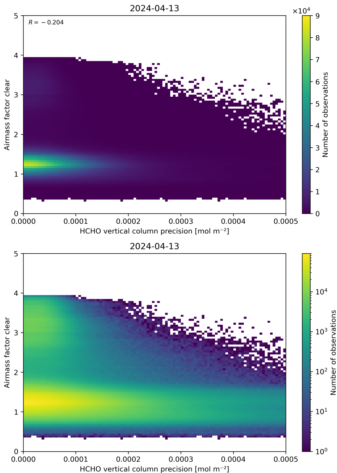
Figure 139: Scatter density plot of “HCHO vertical column precision” against “Airmass factor clear” for 2024-04-12 to 2024-04-14.
