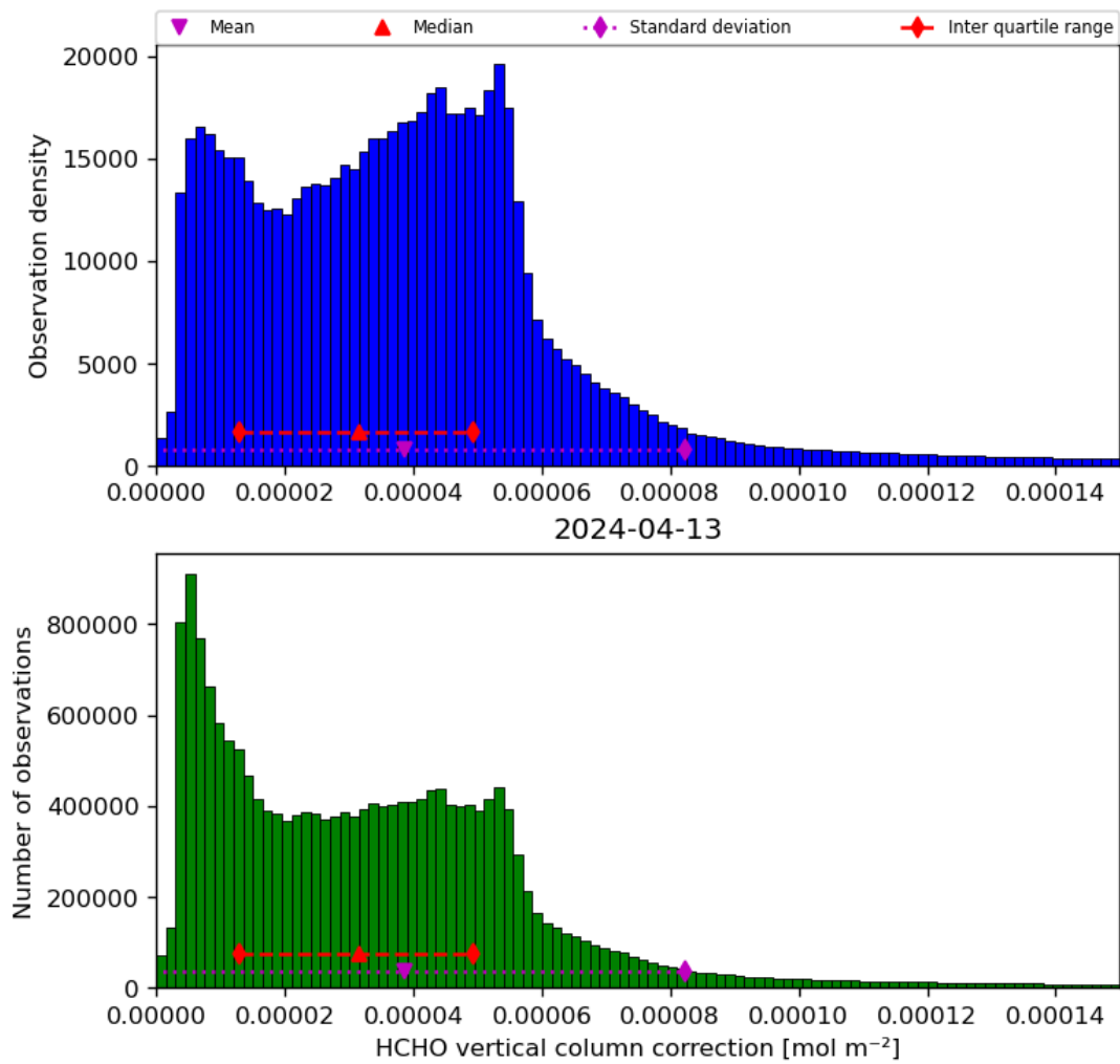
Figure 37: Histogram of “HCHO vertical column correction” for 2024-04-12 to 2024-04-14
