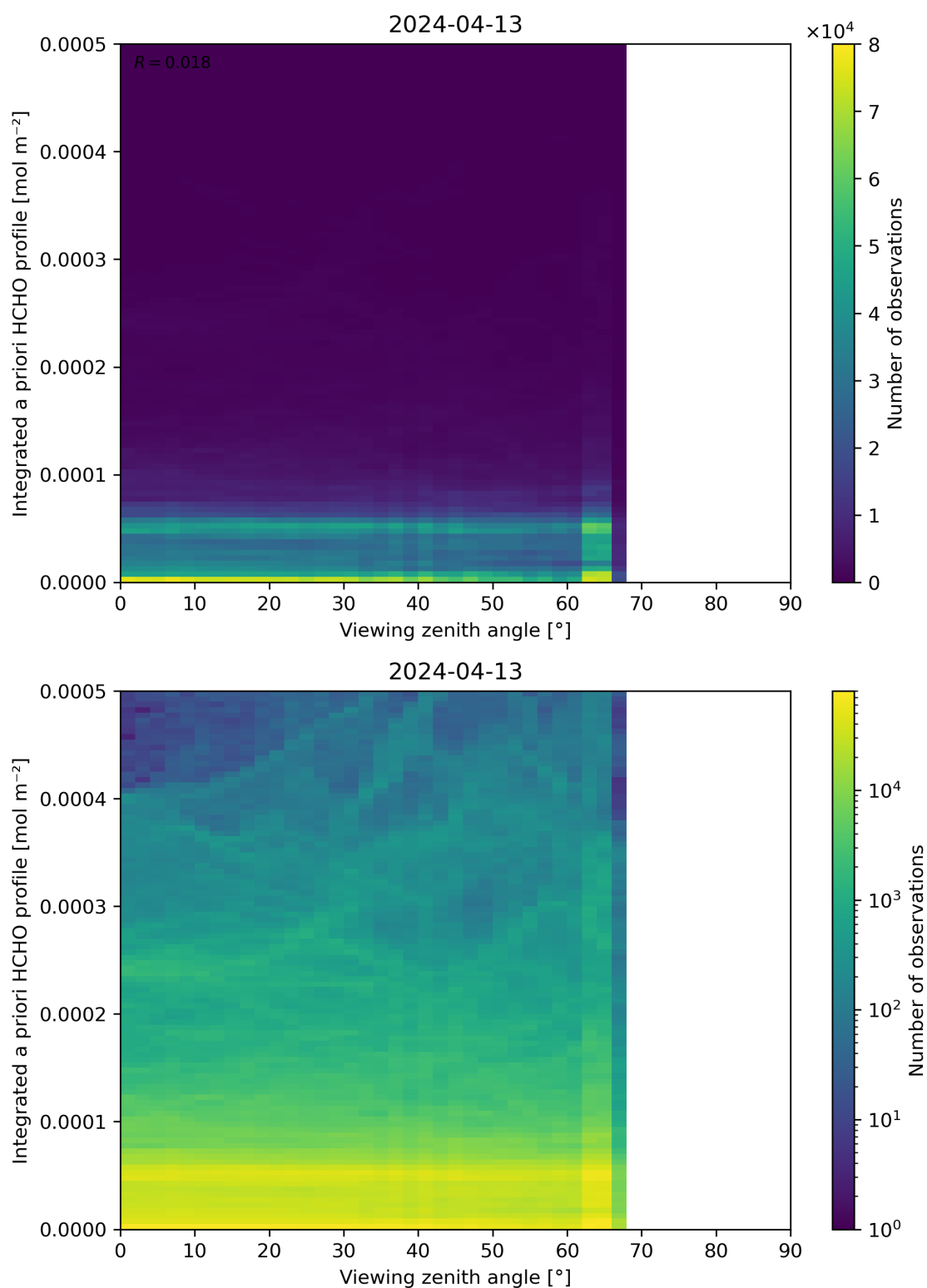
Figure 195: Scatter density plot of “Viewing zenith angle” against “Integrated a priori HCHO profile” for 2024-04-12 to 2024-04-14.
