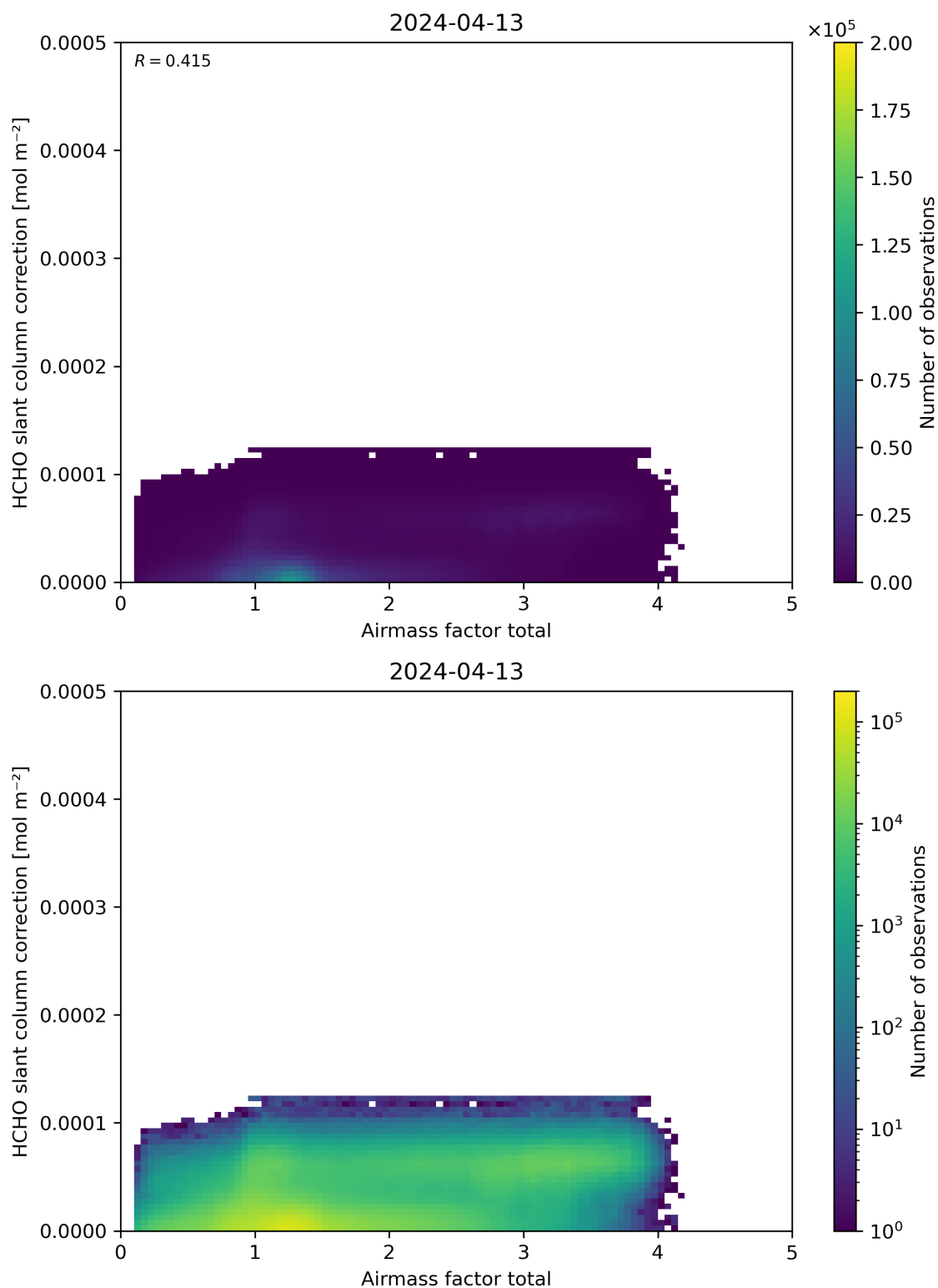
Figure 102: Scatter density plot of “Airmass factor total” against “HCHO slant column correction” for 2024-04-12 to 2024-04-14.
