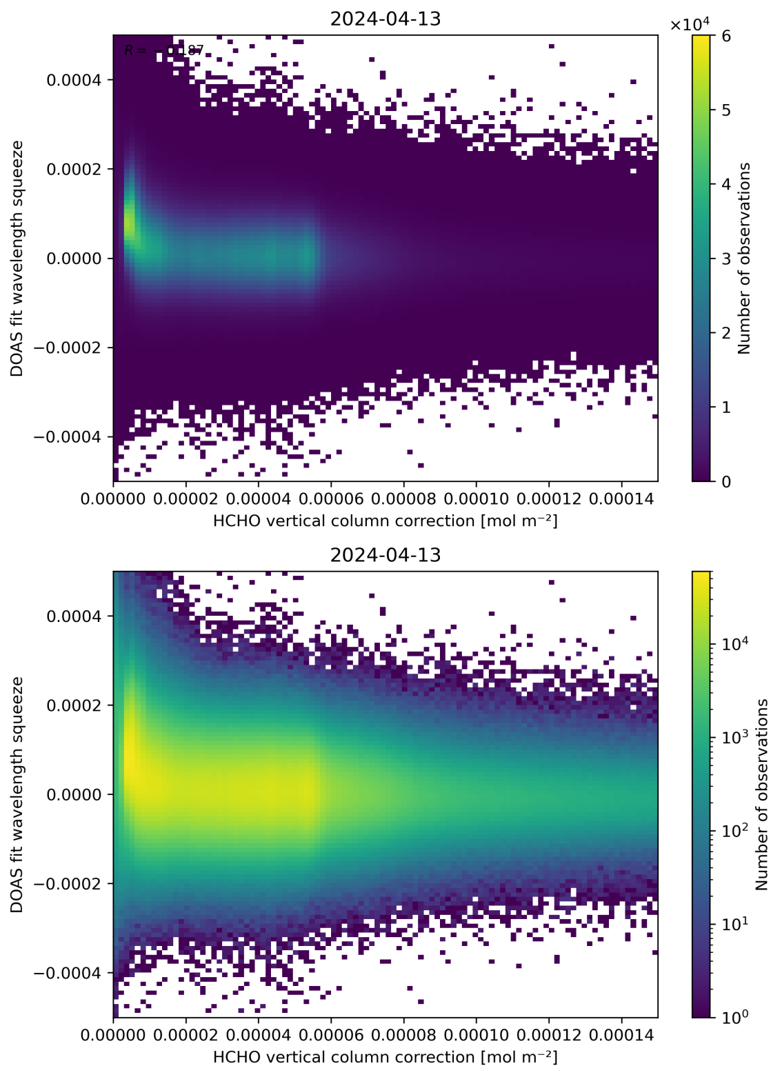
Figure 114: Scatter density plot of “HCHO vertical column correction” against “DOAS fit wavelength squeeze” for 2024-04-12 to 2024-04-14.
