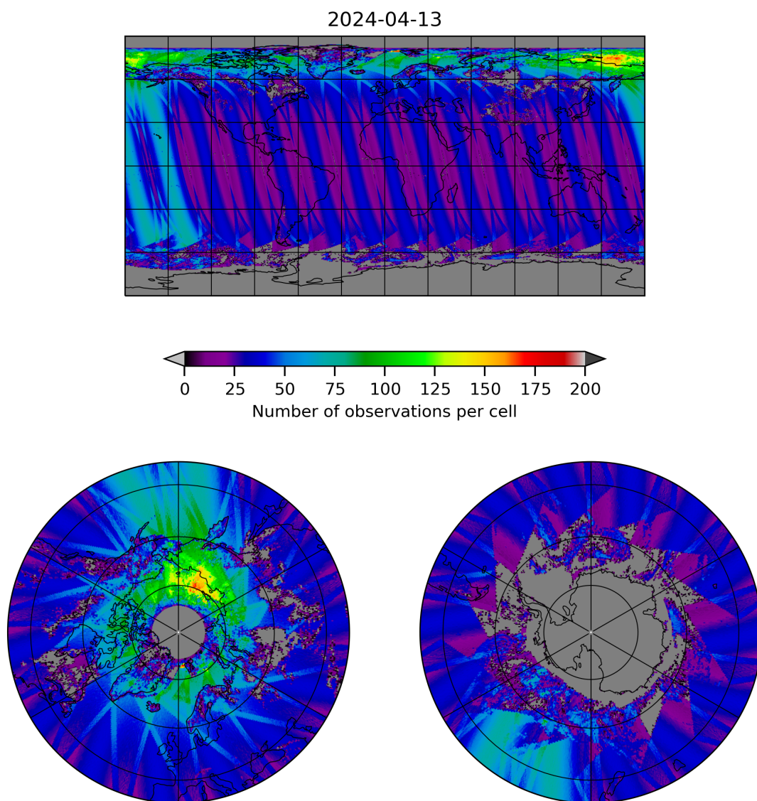
Figure 19: Map of the number of observations for 2024-04-12 to 2024-04-14
