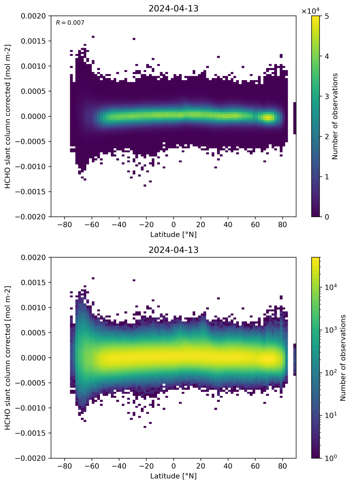
Figure 157: Scatter density plot of “Latitude” against “HCHO slant column corrected” for 2024-04-12 to 2024-04-14.
