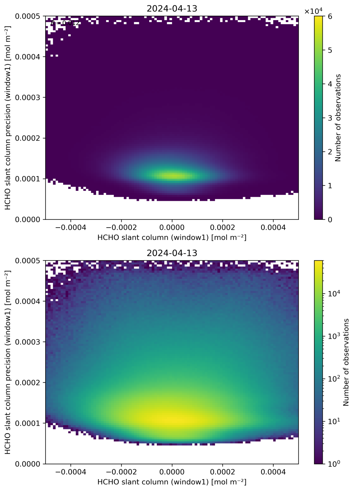
Figure 84: Scatter density plot of “HCHO slant column (window1)” against “HCHO slant column precision (window1)” for 2024-04-12 to 2024-04-14.
