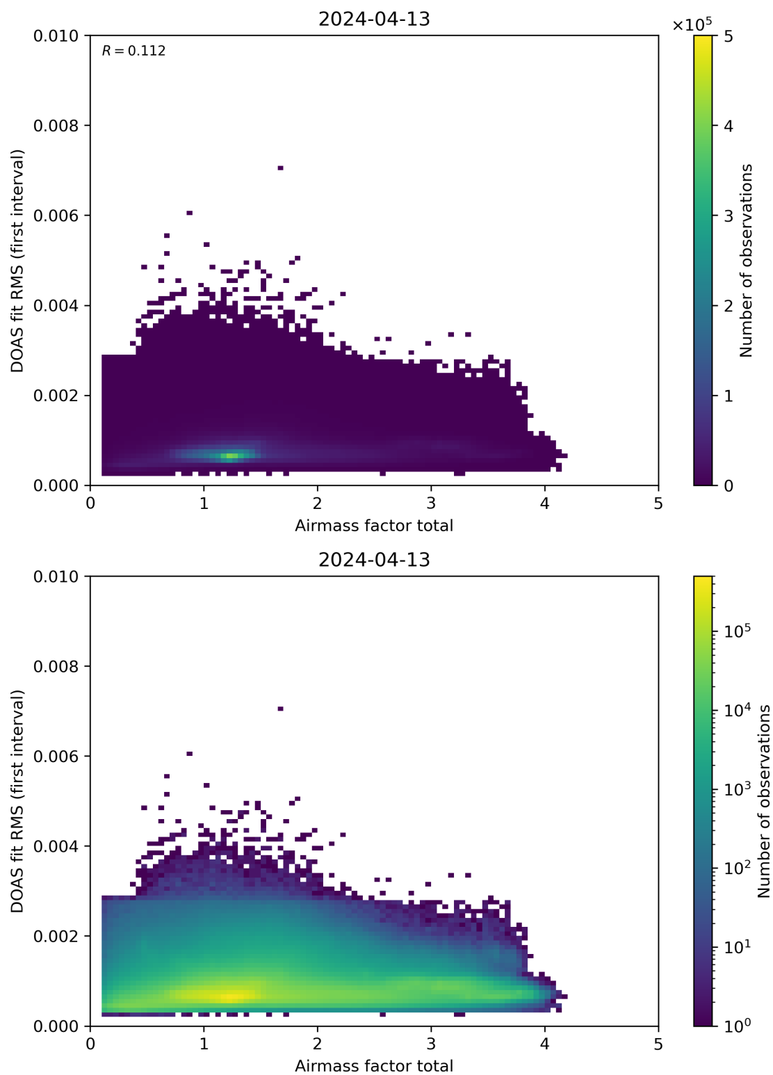
Figure 97: Scatter density plot of “Airmass factor total” against “DOAS fit RMS (first interval)” for 2024-04-12 to 2024-04-14.
