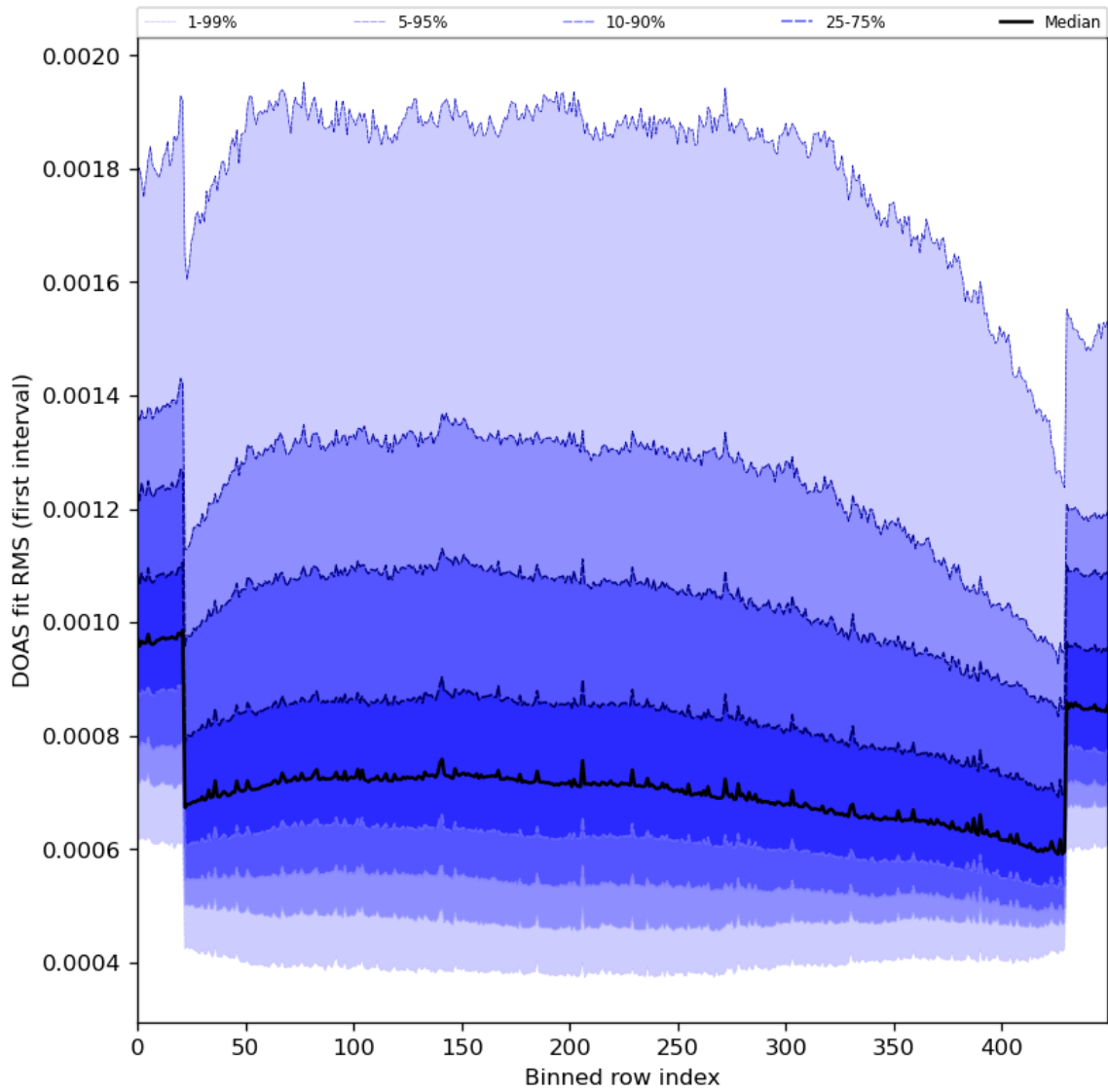
Figure 60: Along track statistics of “DOAS fit RMS (first interval)” for 2024-04-12 to 2024-04-14
