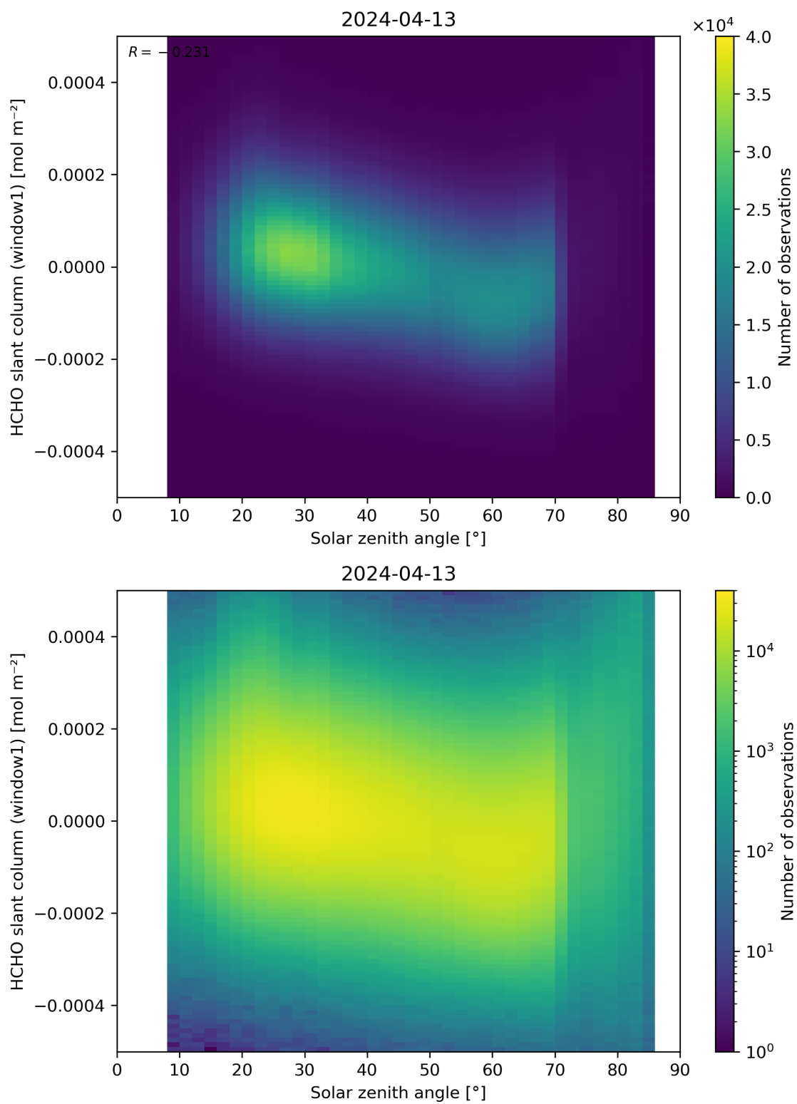
Figure 173: Scatter density plot of “Solar zenith angle” against “HCHO slant column (window1)” for 2024-04-12 to 2024-04-14.
