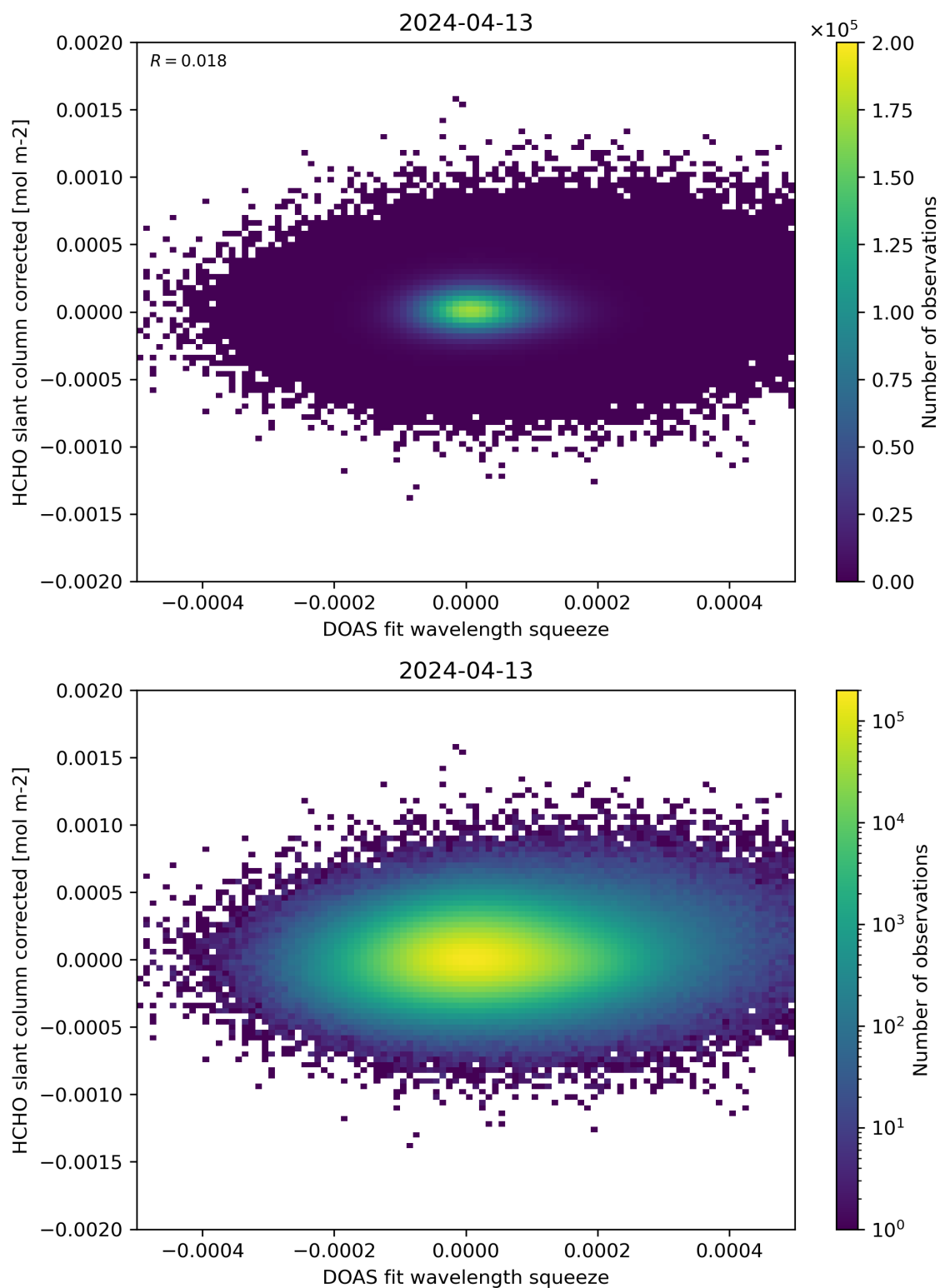
Figure 69: Scatter density plot of “DOAS fit wavelength squeeze” against “HCHO slant column corrected” for 2024-04-12 to 2024-04-14.
