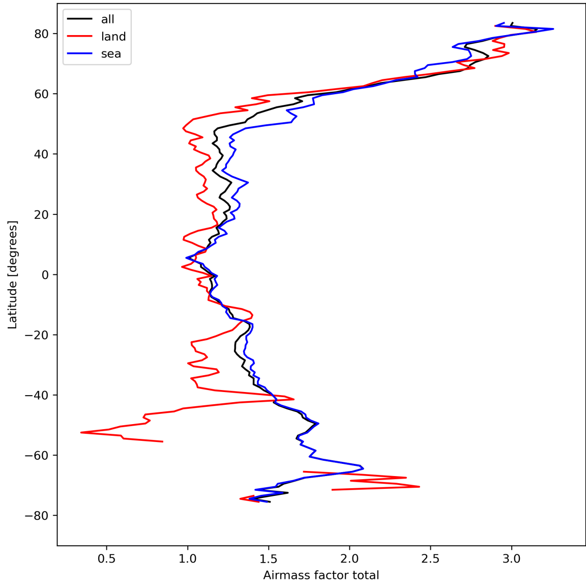
Figure 26: Zonal average of “Airmass factor total” for 2024-04-12 to 2024-04-14.
