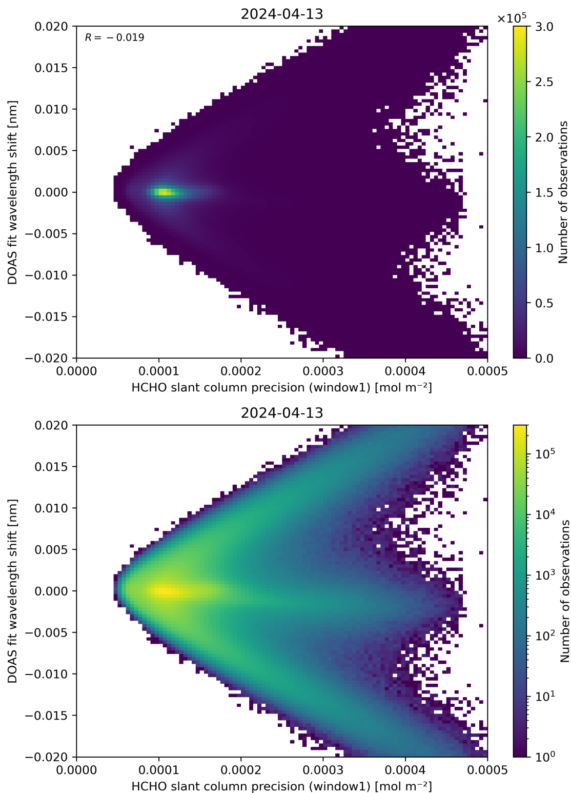
Figure 89: Scatter density plot of “HCHO slant column precision (window1)” against “DOAS fit wavelength shift” for 2024-04-12 to 2024-04-14.
