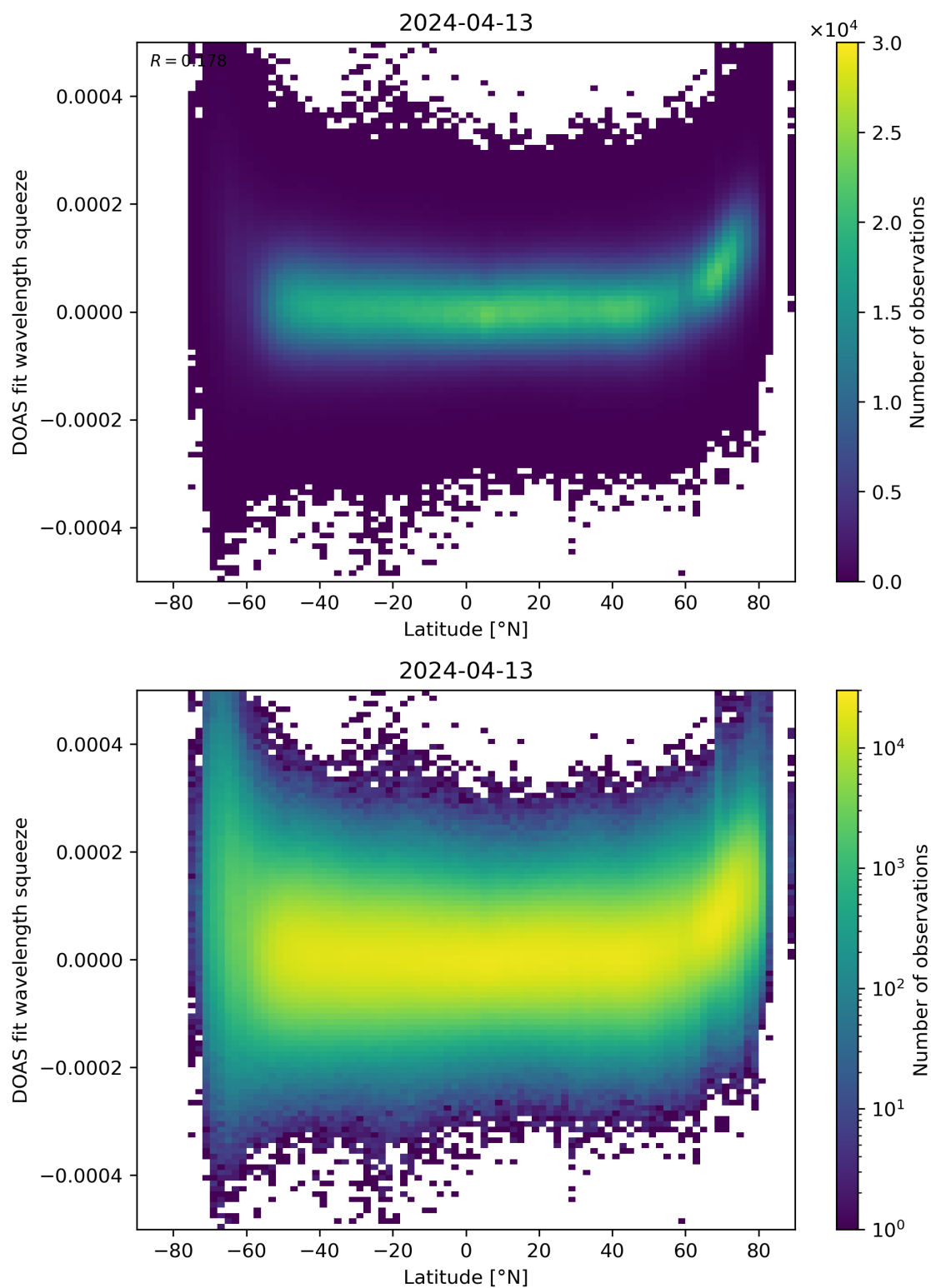
Figure 155: Scatter density plot of “Latitude” against “DOAS fit wavelength squeeze” for 2024-04-12 to 2024-04-14.
