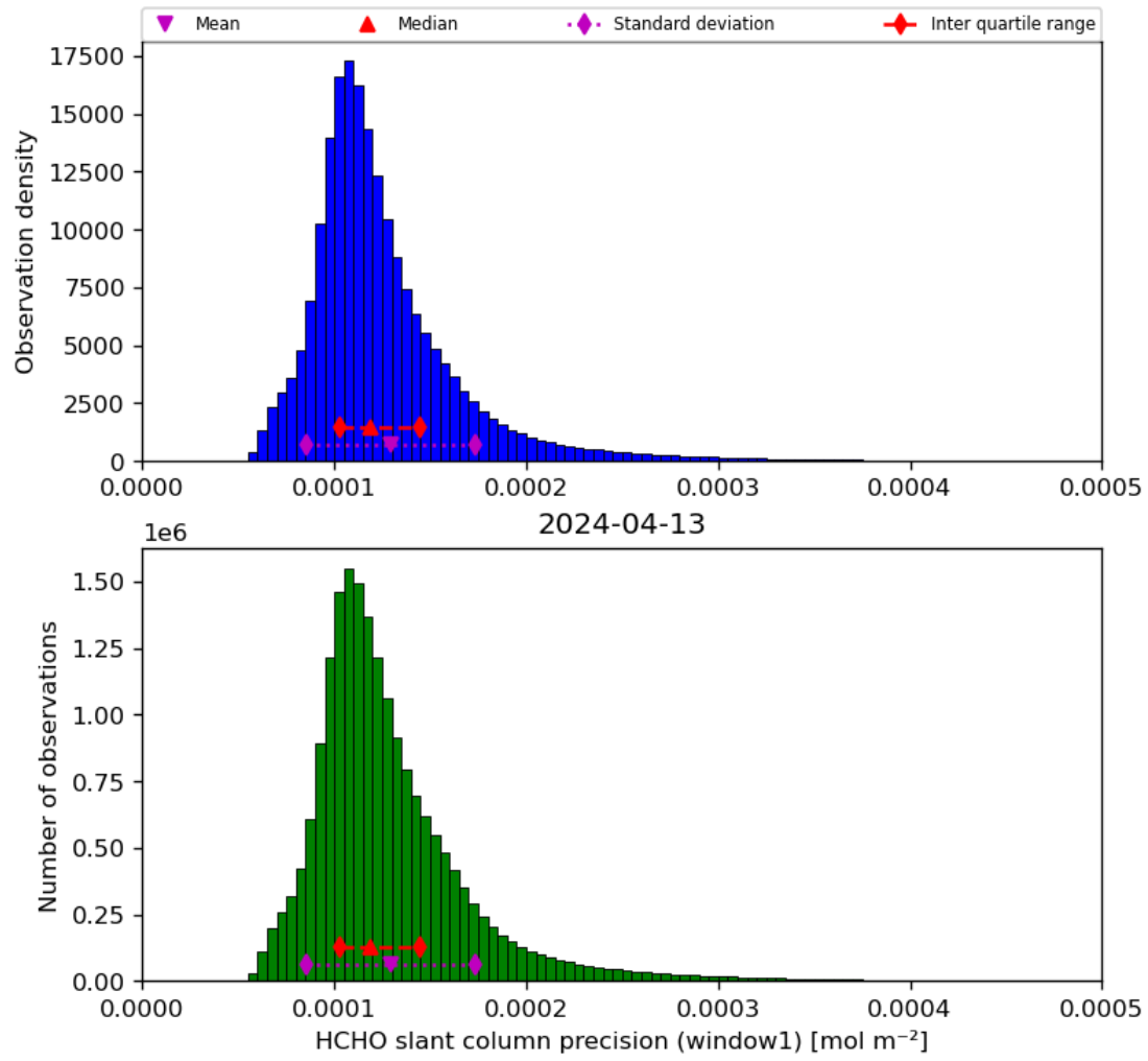
Figure 39: Histogram of “HCHO slant column precision (window1)” for 2024-04-12 to 2024-04-14
