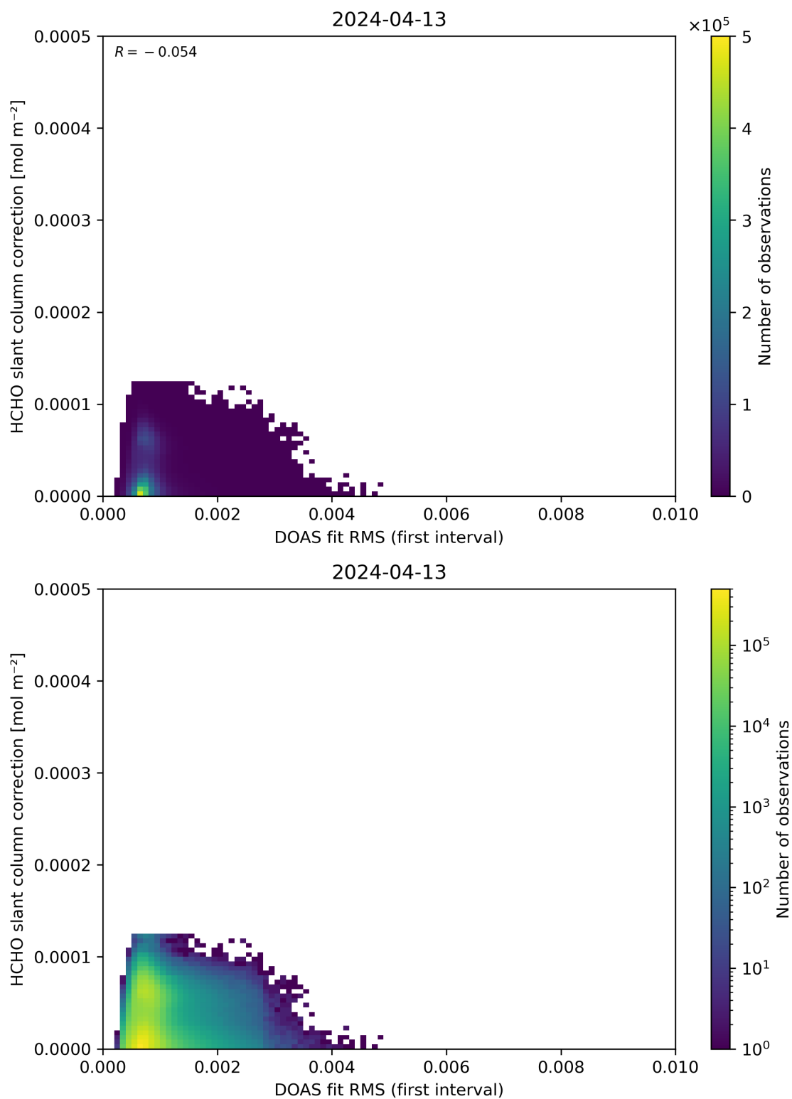
Figure 63: Scatter density plot of “DOAS fit RMS (first interval)” against “HCHO slant column correction” for 2024-04-12 to 2024-04-14.
