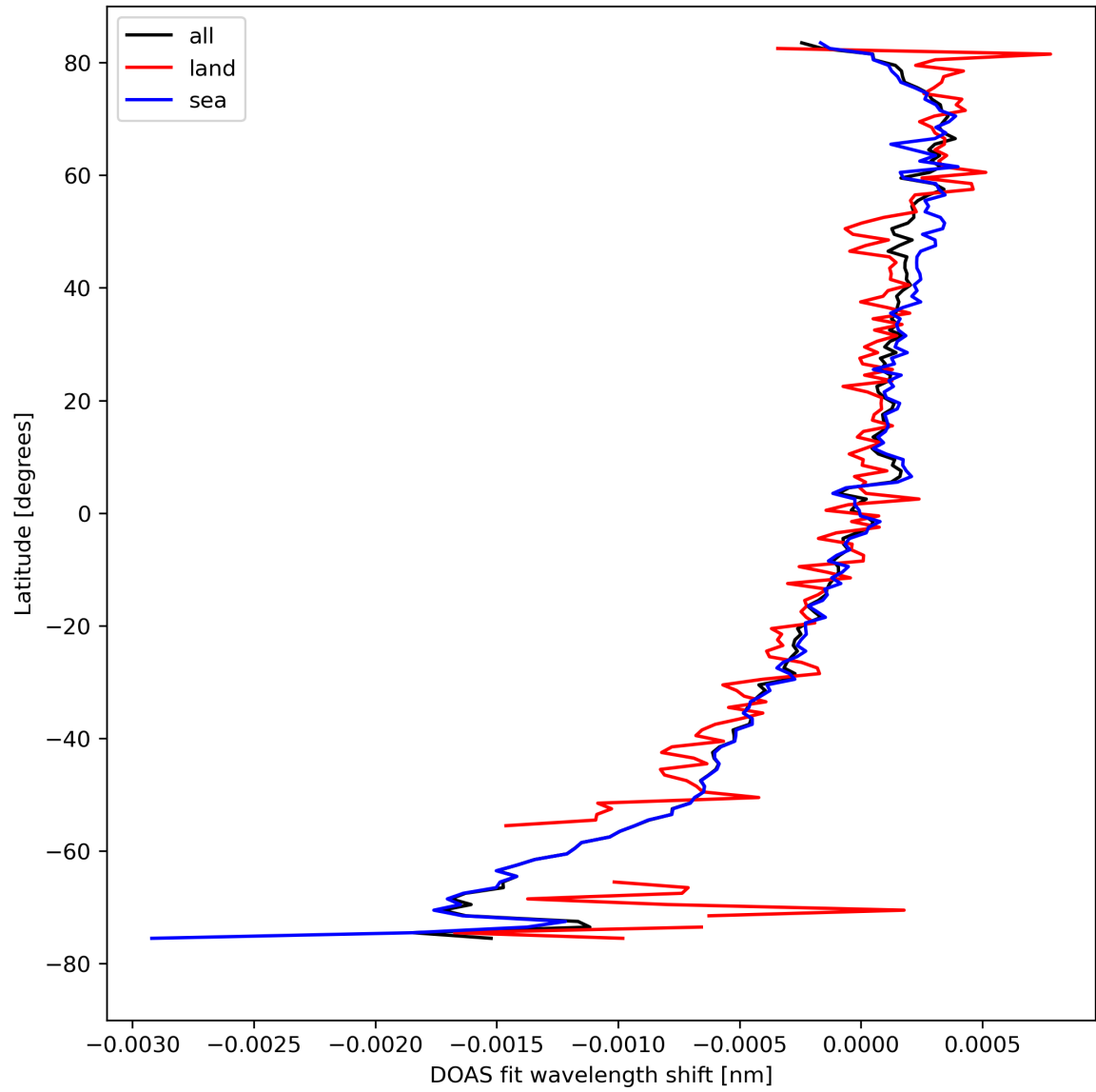
Figure 30: Zonal average of “DOAS fit wavelength shift” for 2024-04-12 to 2024-04-14.
