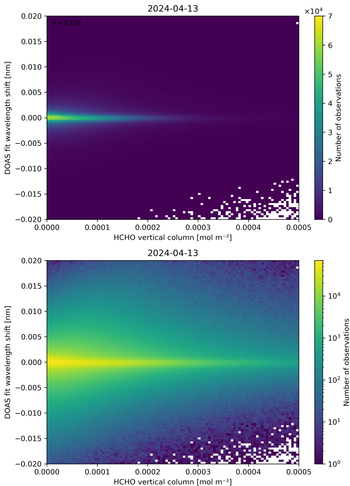
Figure 124: Scatter density plot of “HCHO vertical column” against “DOAS fit wavelength shift” for 2024-04-12 to 2024-04-14.
