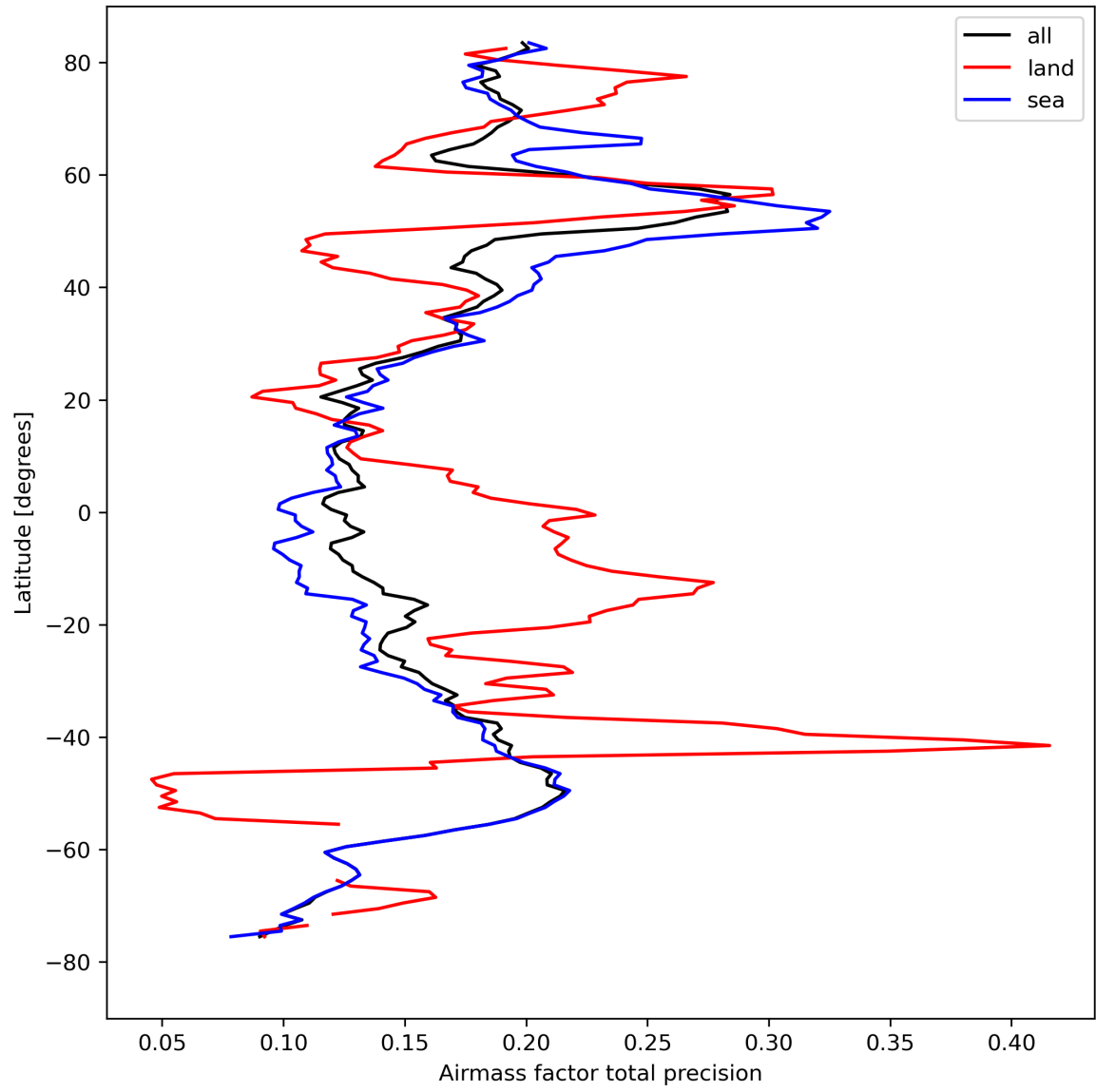
Figure 27: Zonal average of “Airmass factor total precision” for 2024-04-12 to 2024-04-14.
