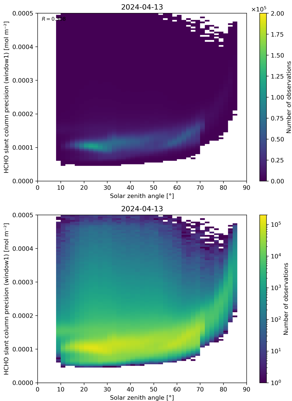
Figure 174: Scatter density plot of “Solar zenith angle” against “HCHO slant column precision (window1)” for 2024-04-12 to 2024-04-14.
