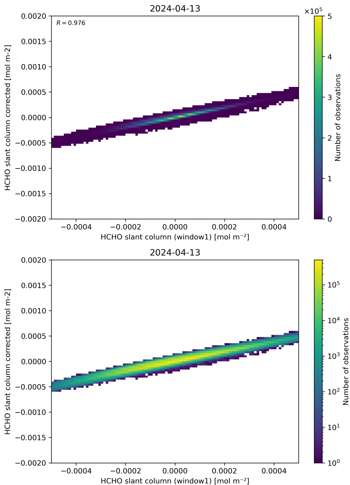
Figure 82: Scatter density plot of “HCHO slant column (window1)” against “HCHO slant column corrected” for 2024-04-12 to 2024-04-14.
