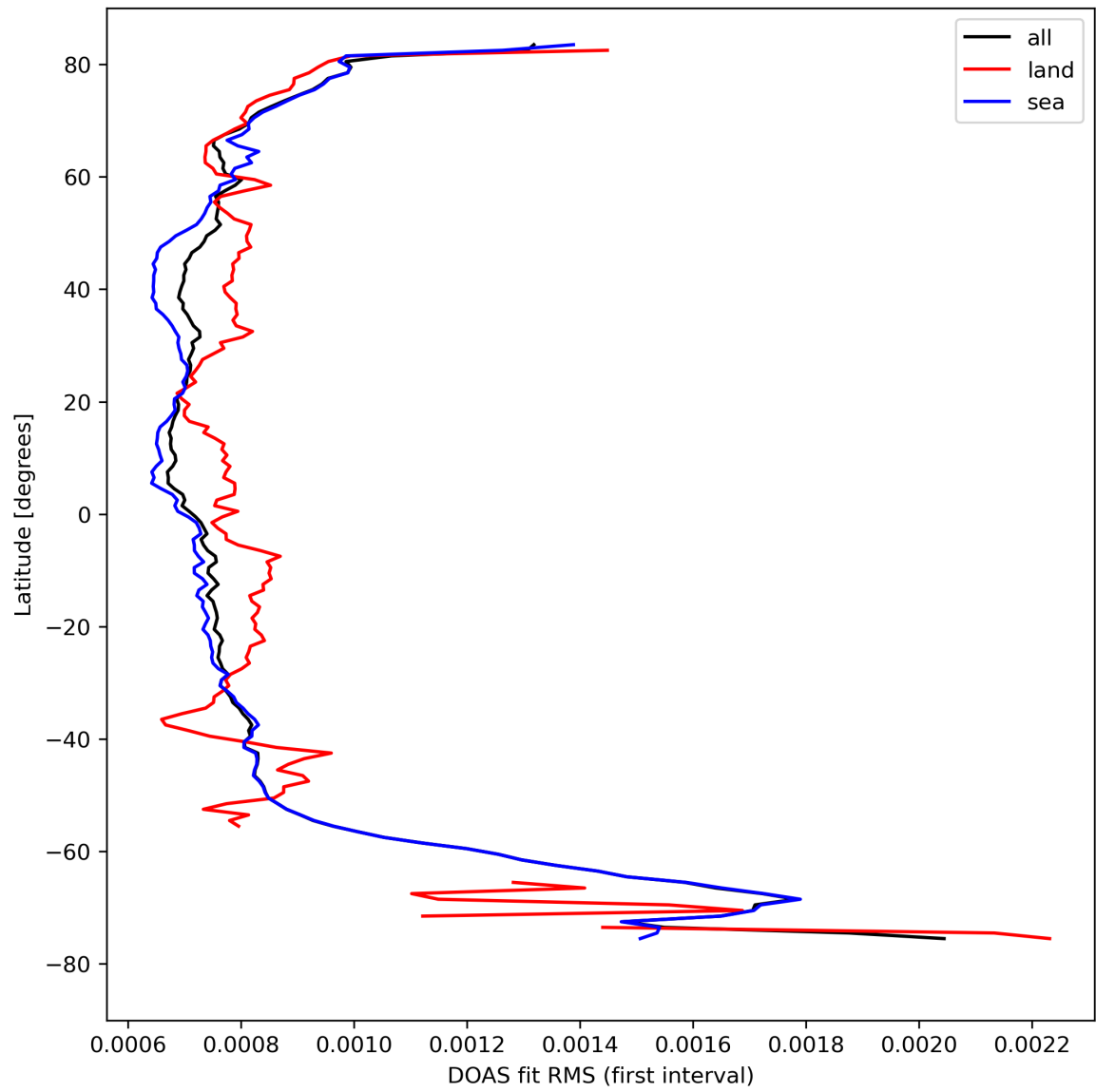
Figure 32: Zonal average of “DOAS fit RMS (first interval)” for 2024-04-12 to 2024-04-14.
