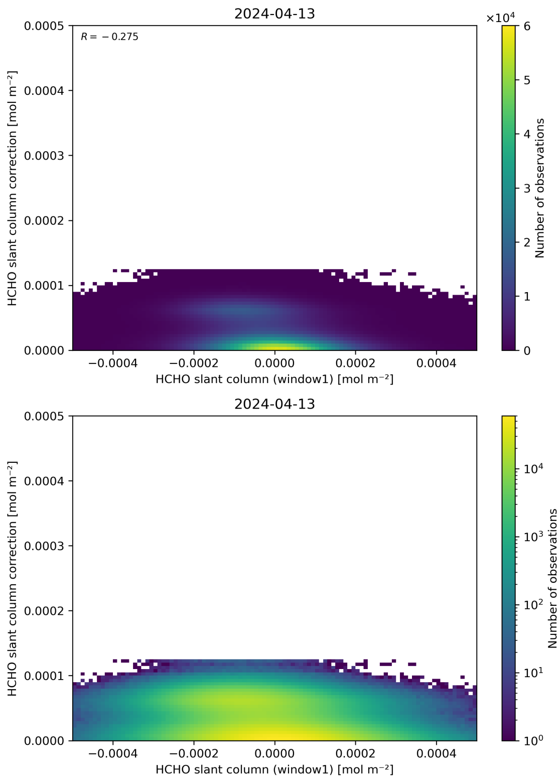
Figure 83: Scatter density plot of “HCHO slant column (window1)” against “HCHO slant column correction” for 2024-04-12 to 2024-04-14.
