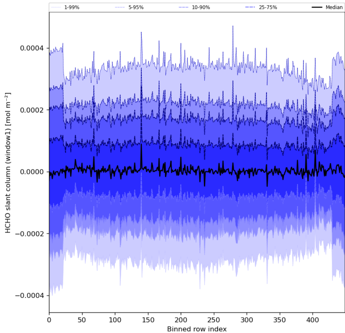
Figure 52: Along track statistics of “HCHO slant column (window1)” for 2024-04-12 to 2024-04-14
