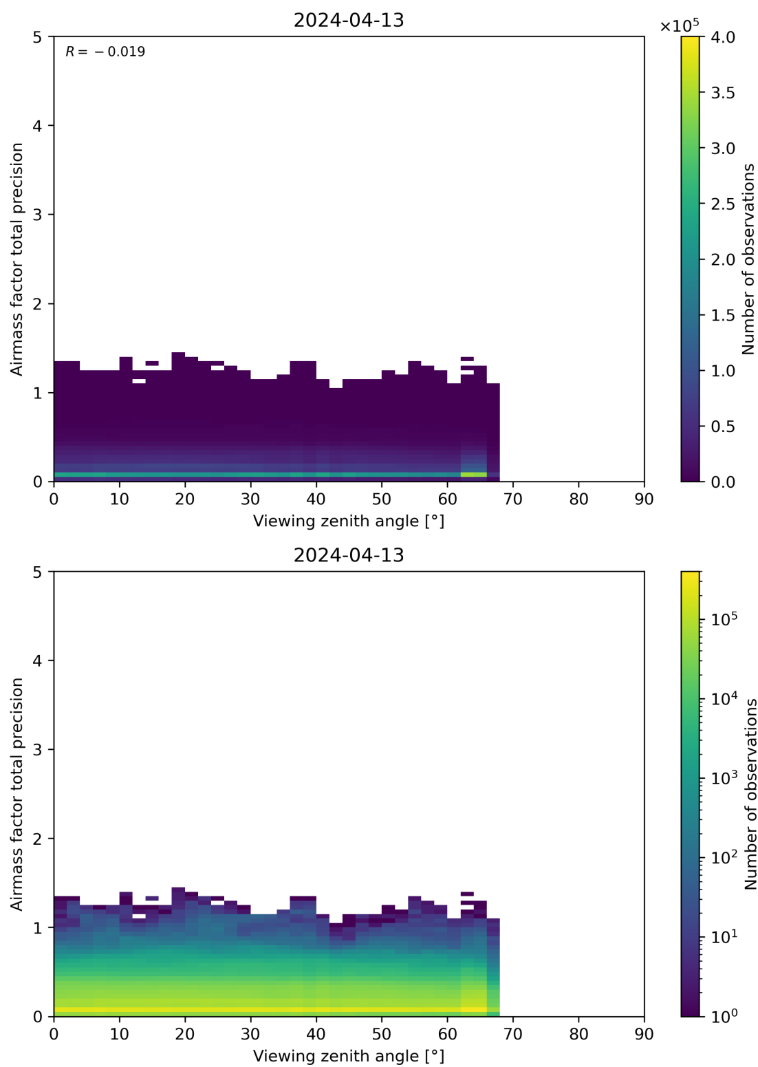
Figure 191: Scatter density plot of “Viewing zenith angle” against “Airmass factor total precision” for 2024-04-12 to 2024-04-14.
