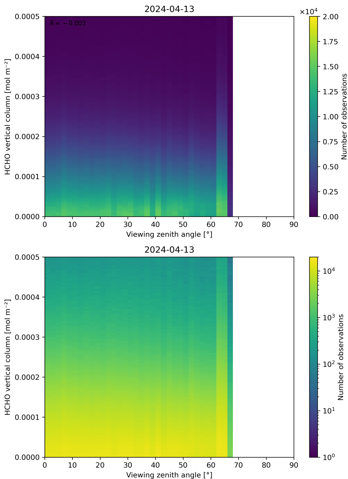
Figure 192: Scatter density plot of “Viewing zenith angle” against “HCHO vertical column” for 2024-04-12 to 2024-04-14.
