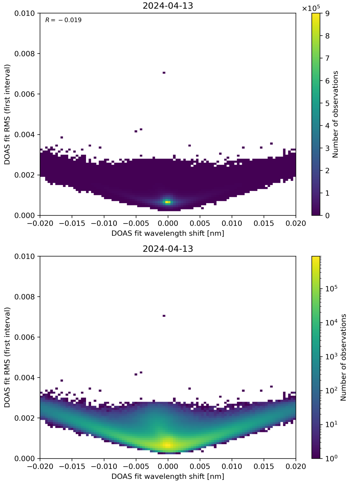
Figure 64: Scatter density plot of “DOAS fit wavelength shift” against “DOAS fit RMS (first interval)” for 2024-04-12 to 2024-04-14.
