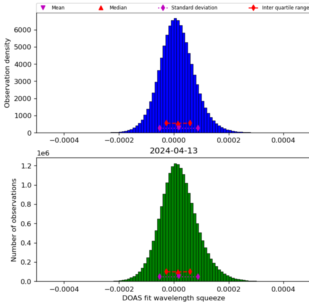
Figure 45: Histogram of “DOAS fit wavelength squeeze” for 2024-04-12 to 2024-04-14
