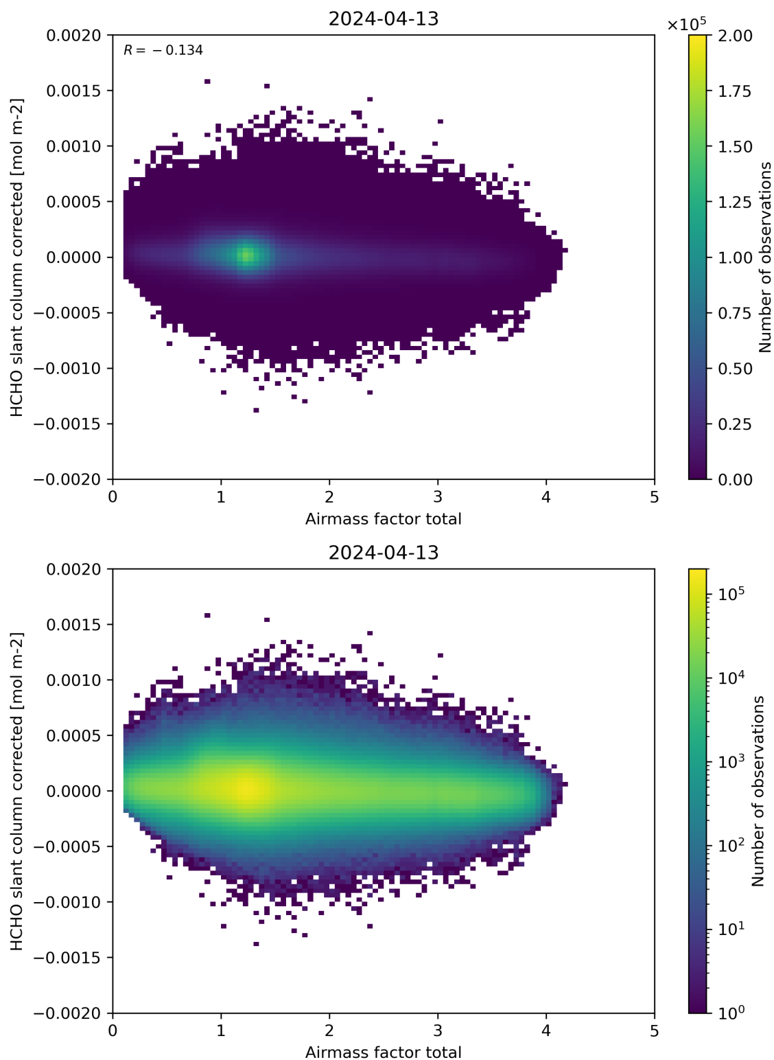
Figure 101: Scatter density plot of “Airmass factor total” against “HCHO slant column corrected” for 2024-04-12 to 2024-04-14.
