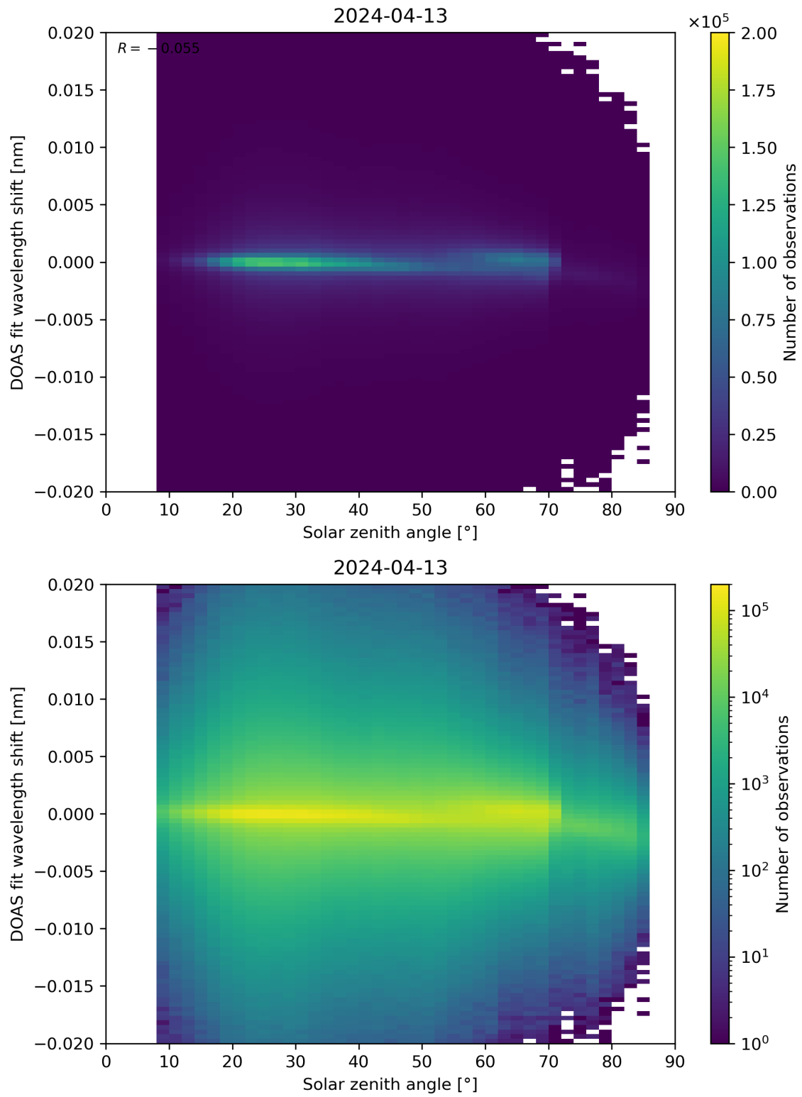
Figure 168: Scatter density plot of “Solar zenith angle” against “DOAS fit wavelength shift” for 2024-04-12 to 2024-04-14.
