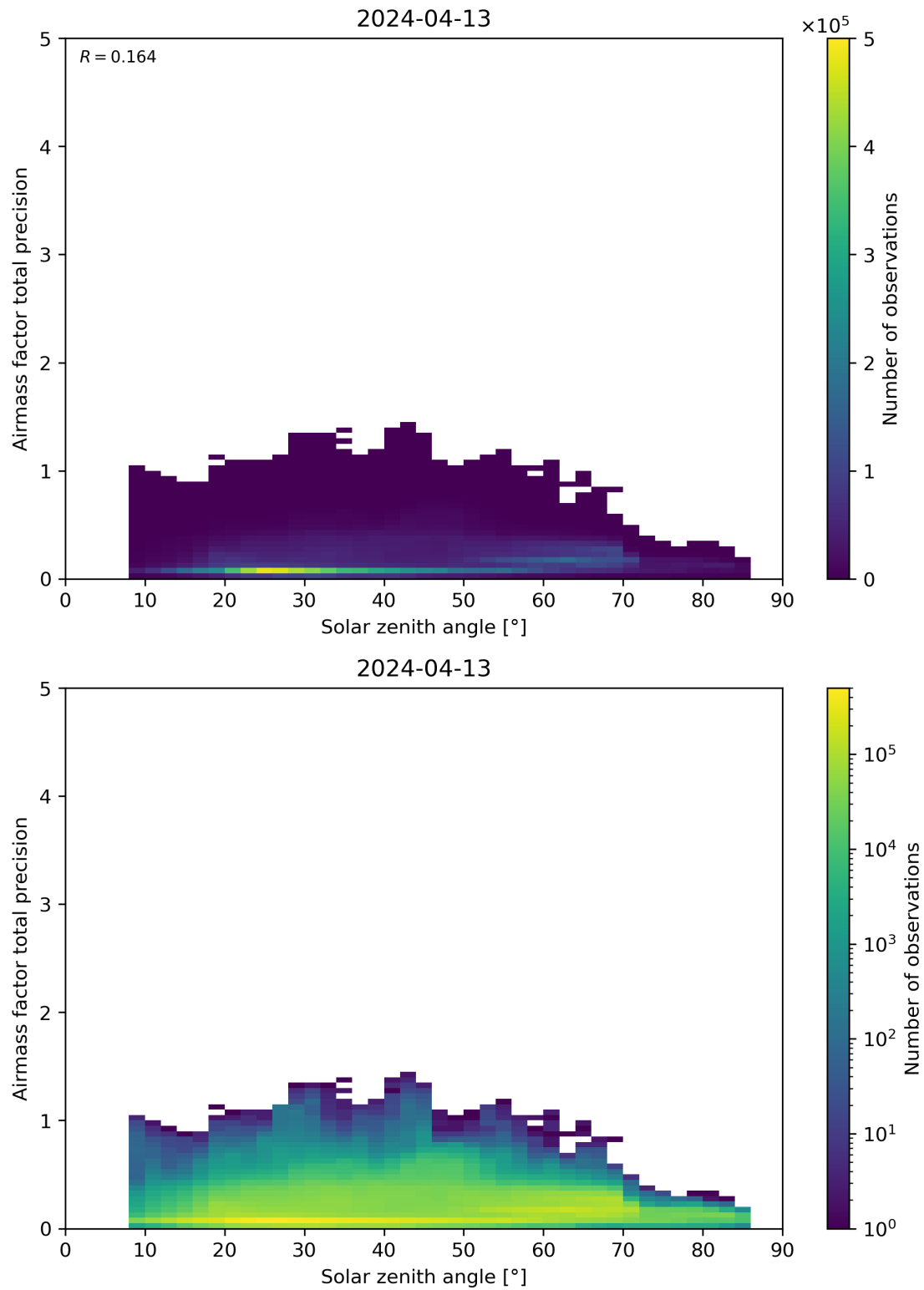
Figure 176: Scatter density plot of “Solar zenith angle” against “Airmass factor total precision” for 2024-04-12 to 2024-04-14.
