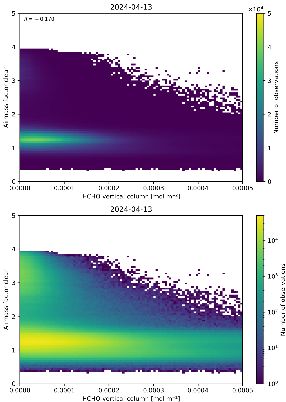
Figure 126: Scatter density plot of “HCHO vertical column” against “Airmass factor clear” for 2024-04-12 to 2024-04-14.
