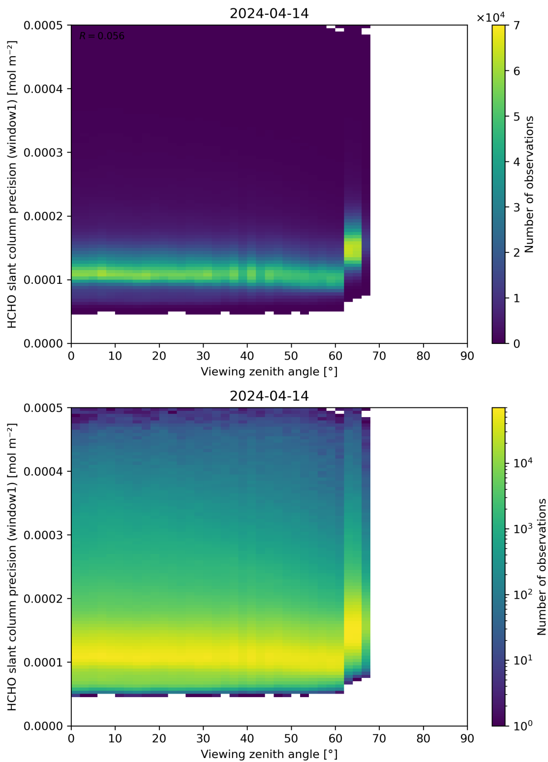
Figure 189: Scatter density plot of “Viewing zenith angle” against “HCHO slant column precision (window1)” for 2024-04-13 to 2024-04-15.
