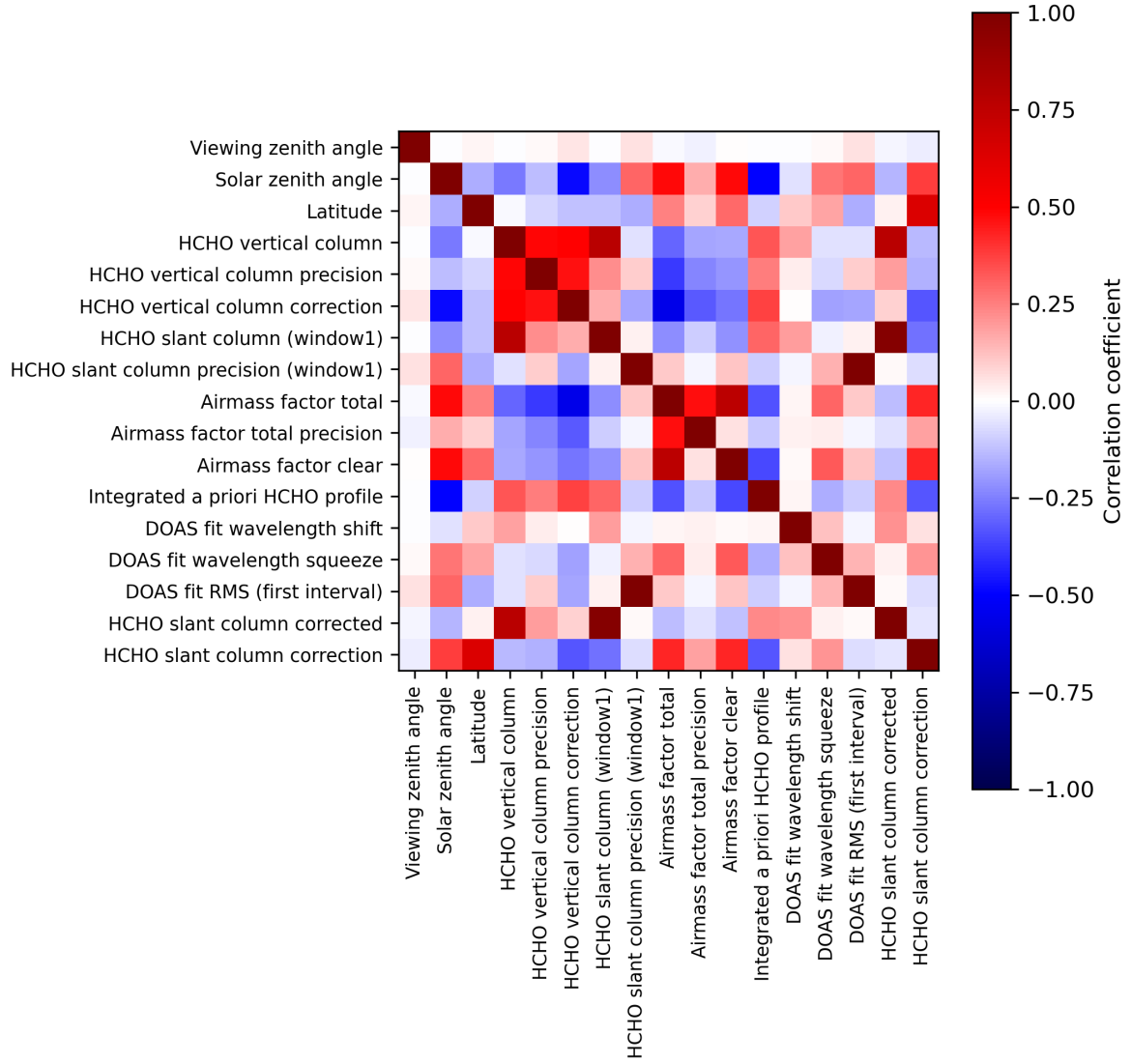
Figure 2: Map of correlation matrix for 2024-04-13 to 2024-04-15.
