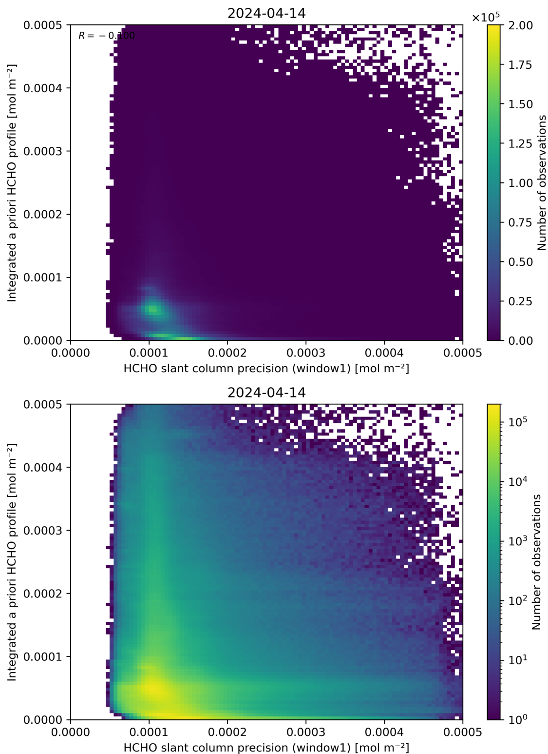
Figure 96: Scatter density plot of “HCHO slant column precision (window1)” against “Integrated a priori HCHO profile” for 2024-04-13 to 2024-04-15.
