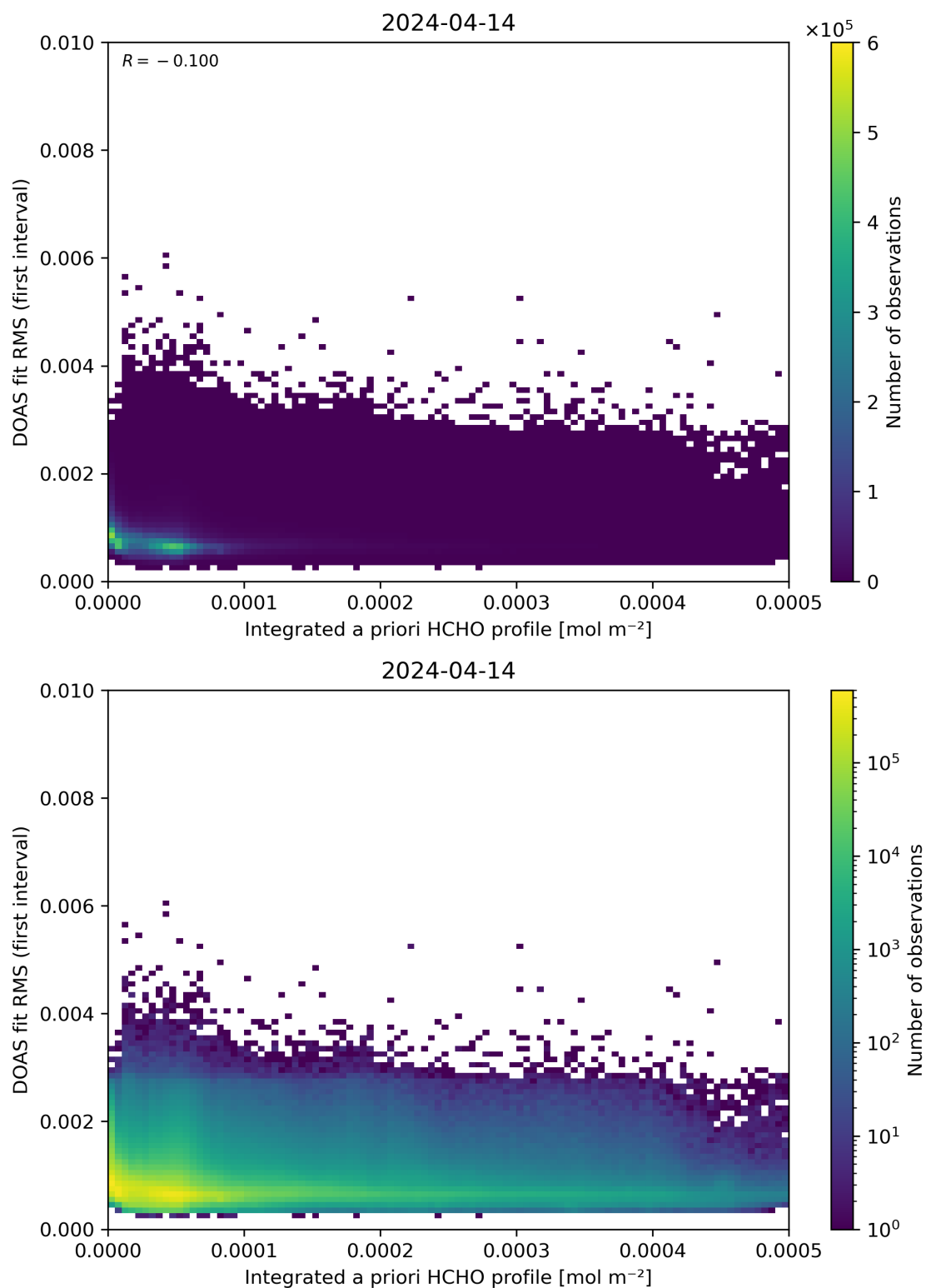
Figure 148: Scatter density plot of “Integrated a priori HCHO profile” against “DOAS fit RMS (first interval)” for 2024-04-13 to 2024-04-15.
