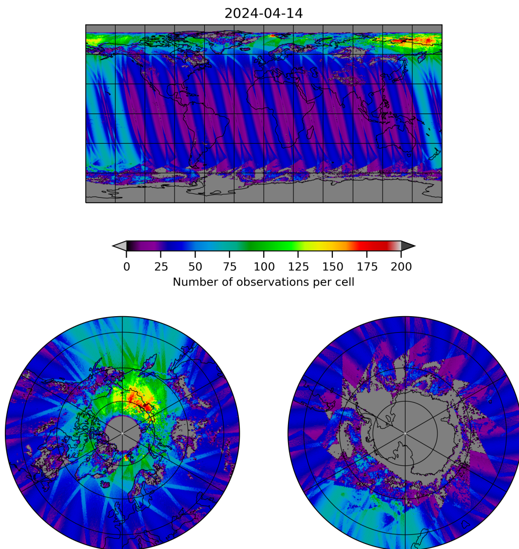
Figure 19: Map of the number of observations for 2024-04-13 to 2024-04-15
