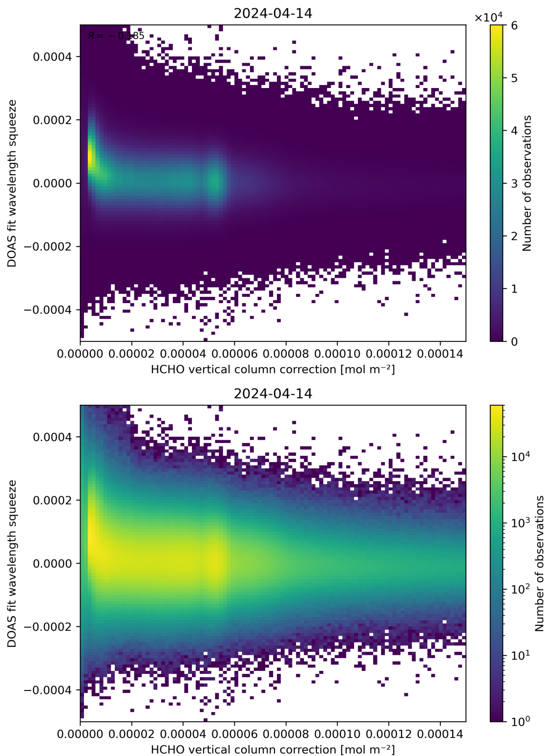
Figure 114: Scatter density plot of “HCHO vertical column correction” against “DOAS fit wavelength squeeze” for 2024-04-13 to 2024-04-15.
