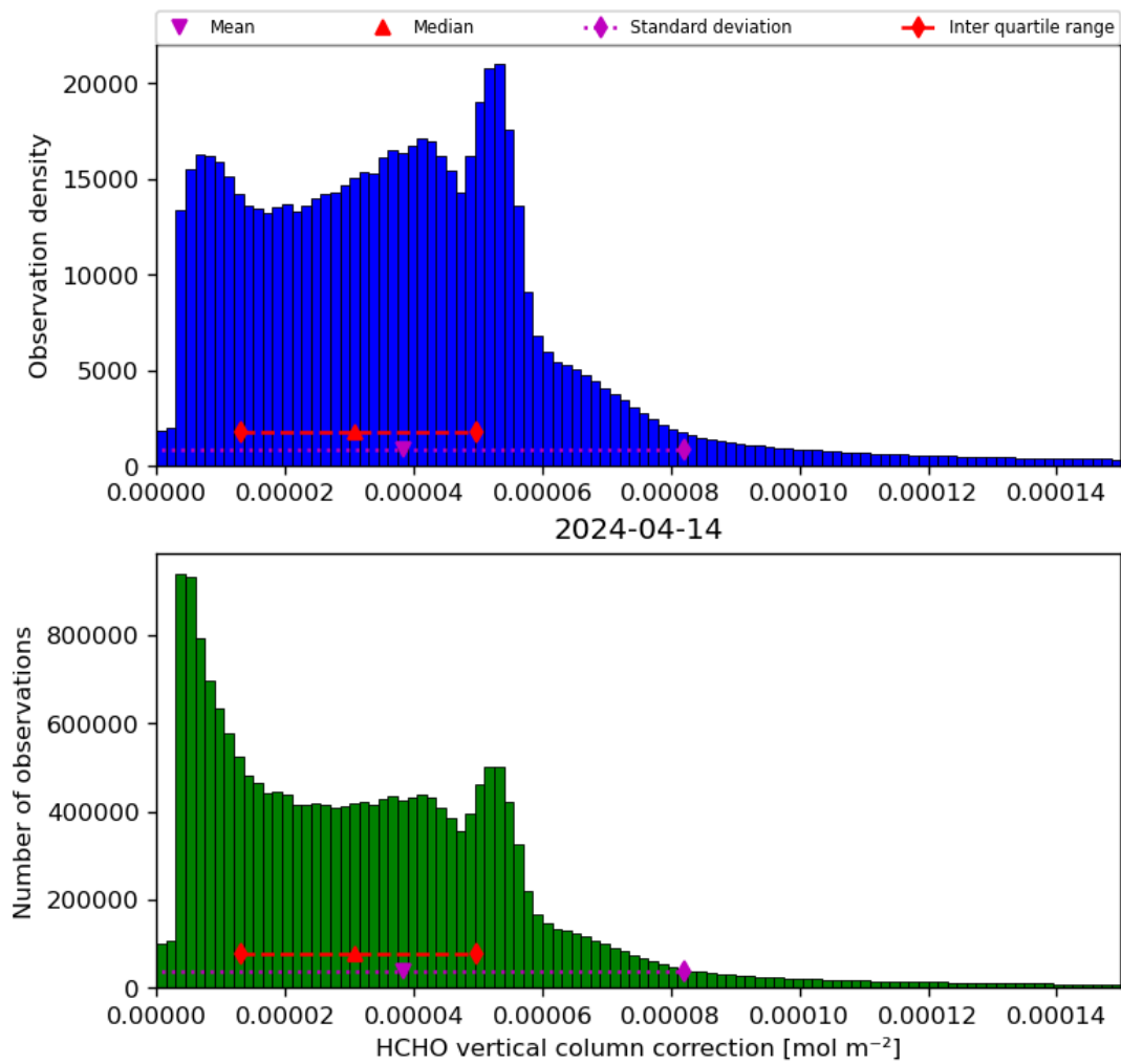
Figure 37: Histogram of “HCHO vertical column correction” for 2024-04-13 to 2024-04-15
