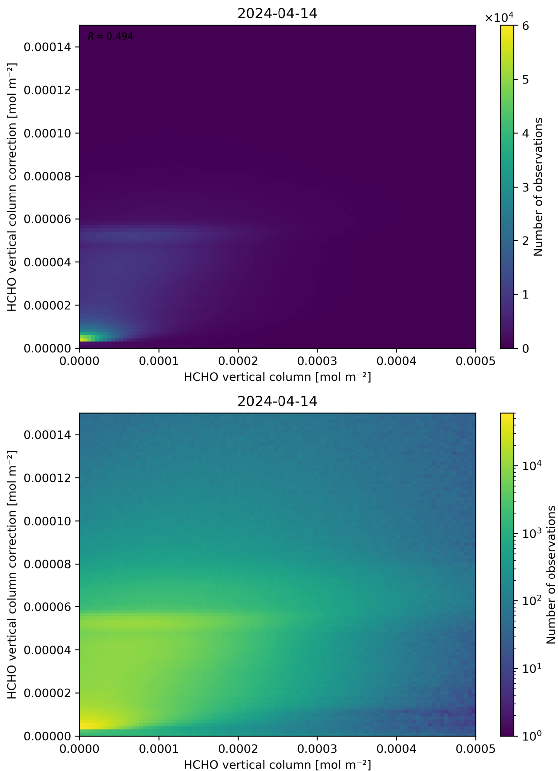
Figure 133: Scatter density plot of “HCHO vertical column” against “HCHO vertical column correction” for 2024-04-13 to 2024-04-15.
