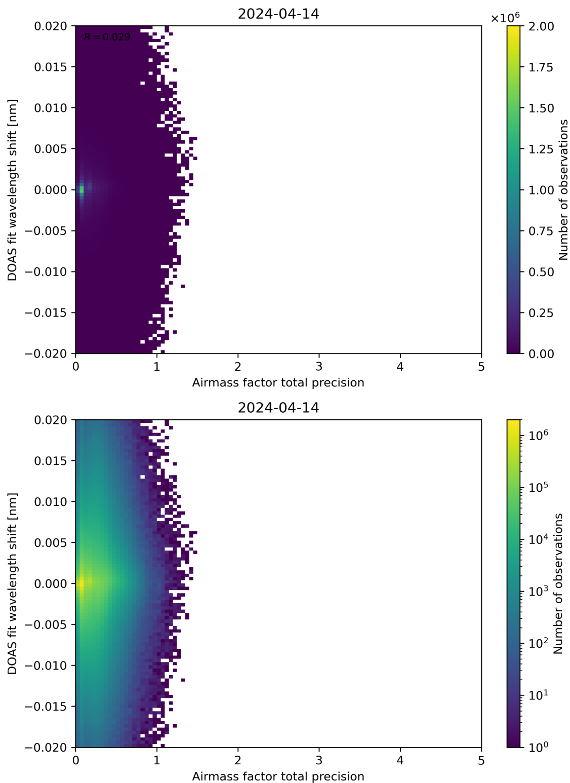
Figure 106: Scatter density plot of “Airmass factor total precision” against “DOAS fit wavelength shift” for 2024-04-13 to 2024-04-15.
