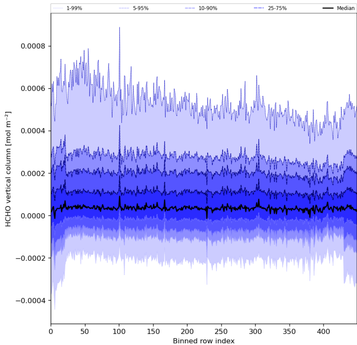
Figure 49: Along track statistics of “HCHO vertical column” for 2024-04-13 to 2024-04-15
