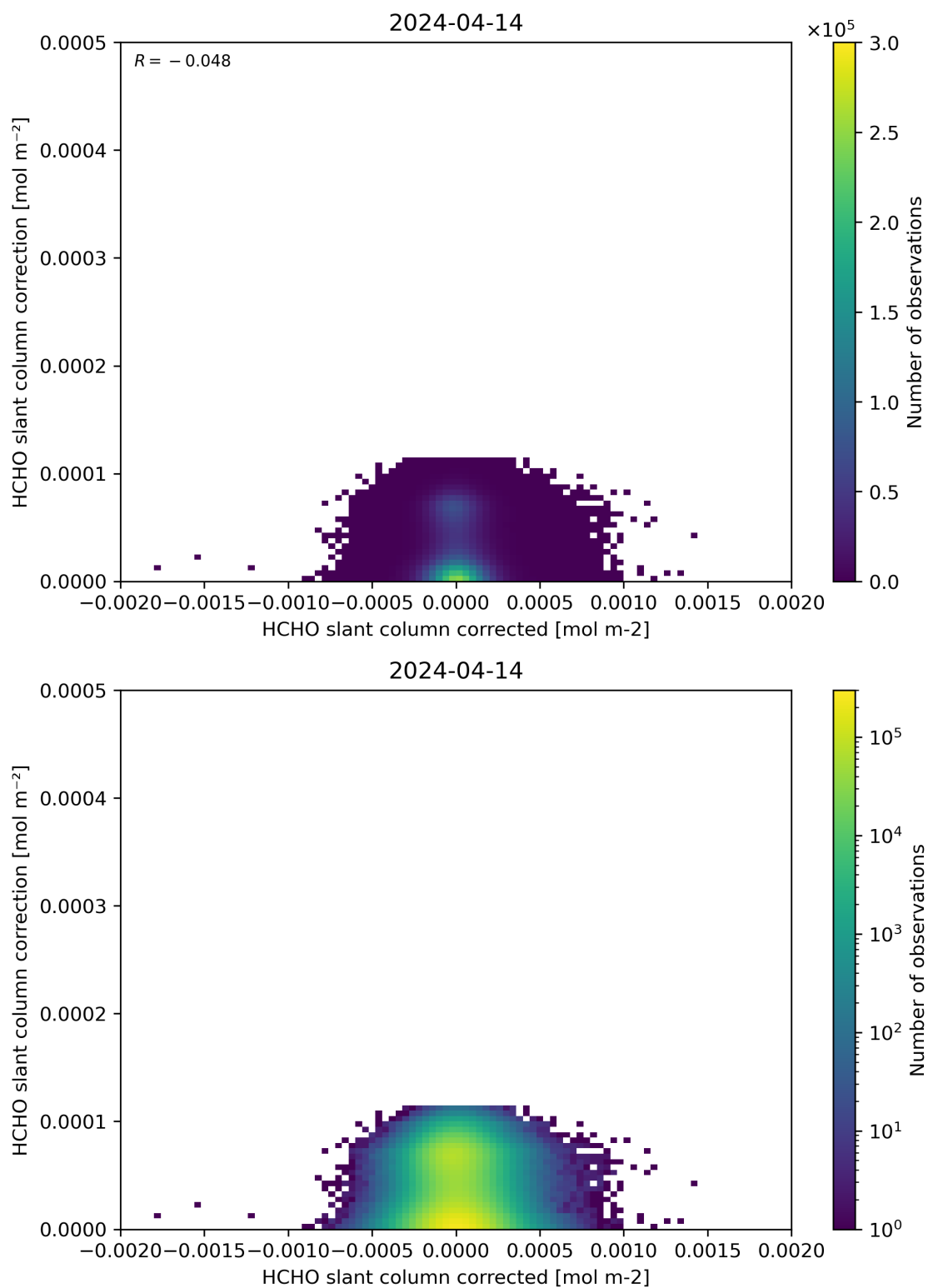
Figure 77: Scatter density plot of “HCHO slant column corrected” against “HCHO slant column correction” for 2024-04-13 to 2024-04-15.
