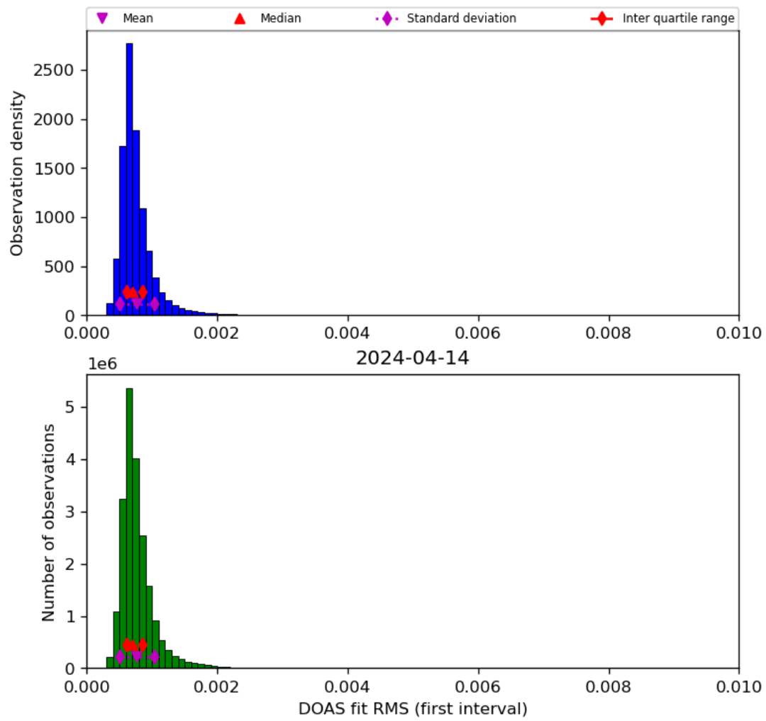
Figure 46: Histogram of “DOAS fit RMS (first interval)” for 2024-04-13 to 2024-04-15
