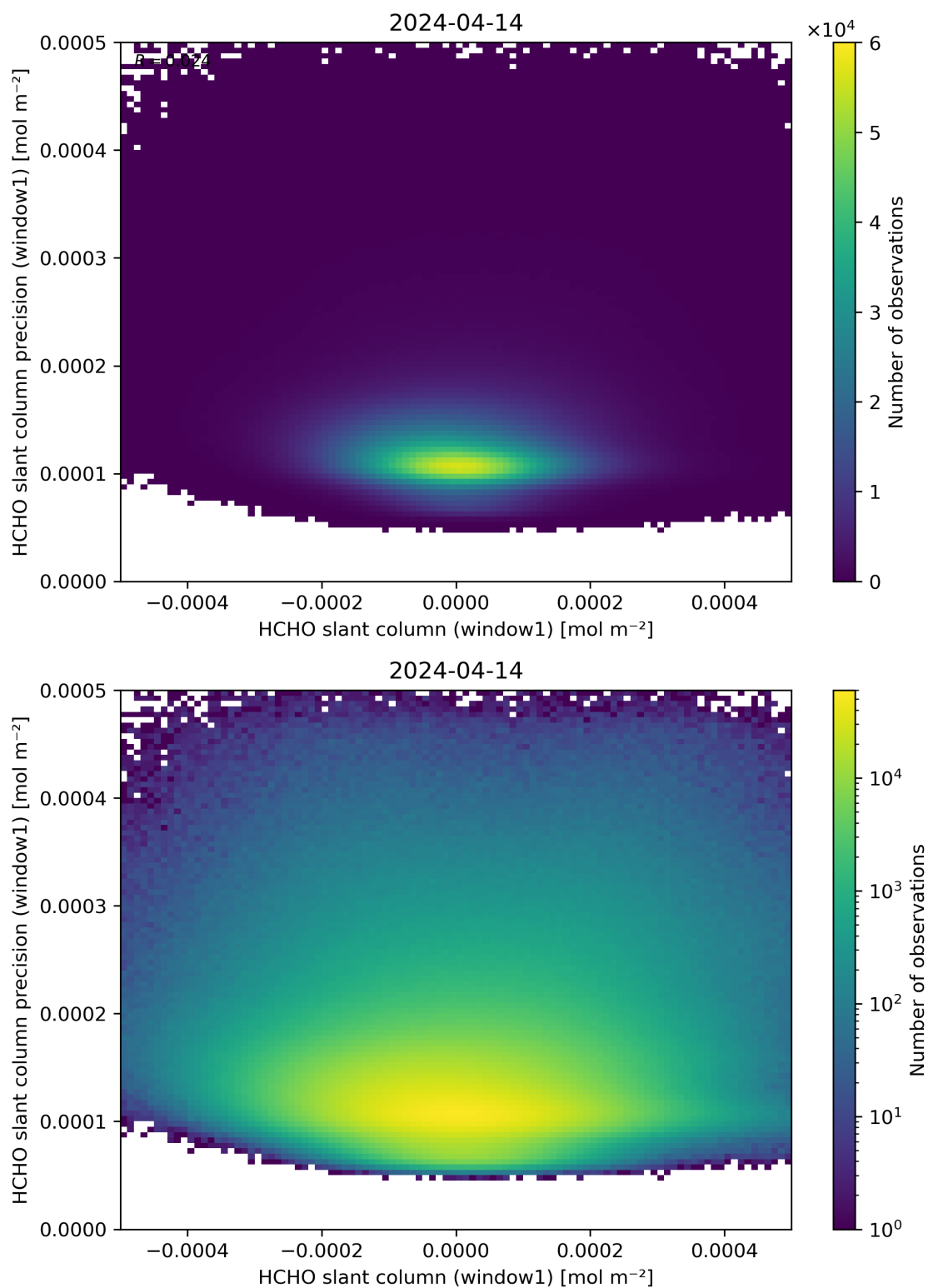
Figure 84: Scatter density plot of “HCHO slant column (window1)” against “HCHO slant column precision (window1)” for 2024-04-13 to 2024-04-15.
