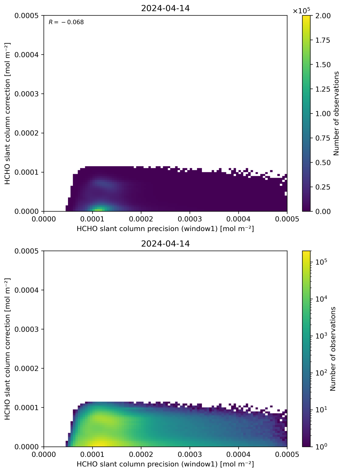
Figure 93: Scatter density plot of “HCHO slant column precision (window1)” against “HCHO slant column correction” for 2024-04-13 to 2024-04-15.
