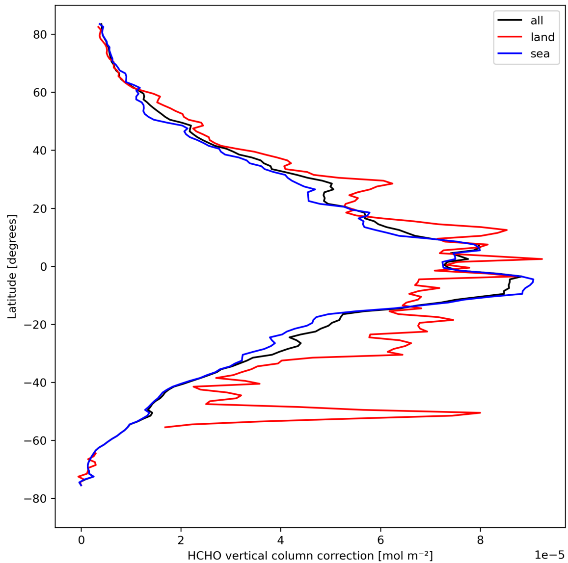
Figure 23: Zonal average of “HCHO vertical column correction” for 2024-04-13 to 2024-04-15.
