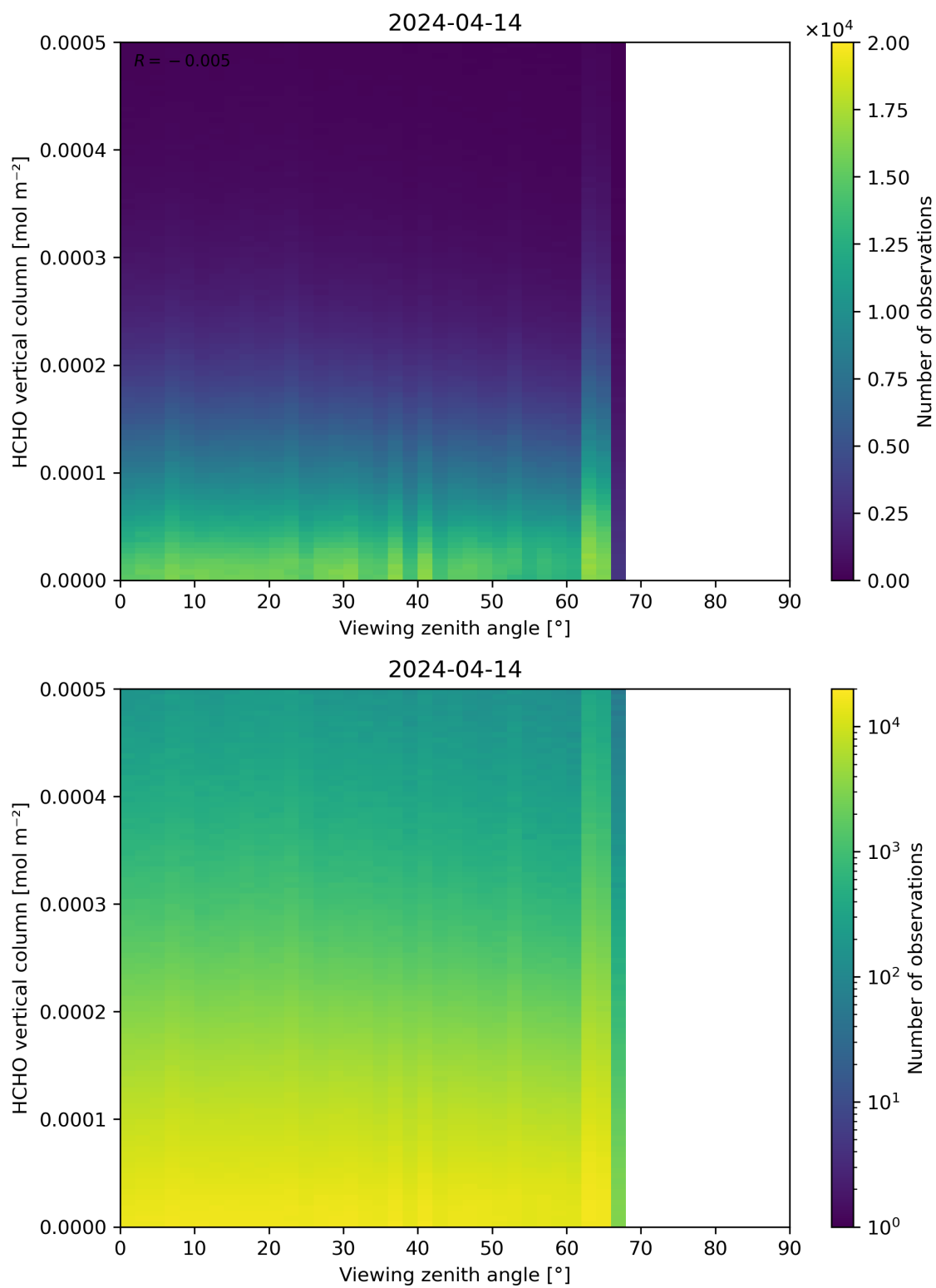
Figure 192: Scatter density plot of “Viewing zenith angle” against “HCHO vertical column” for 2024-04-13 to 2024-04-15.
