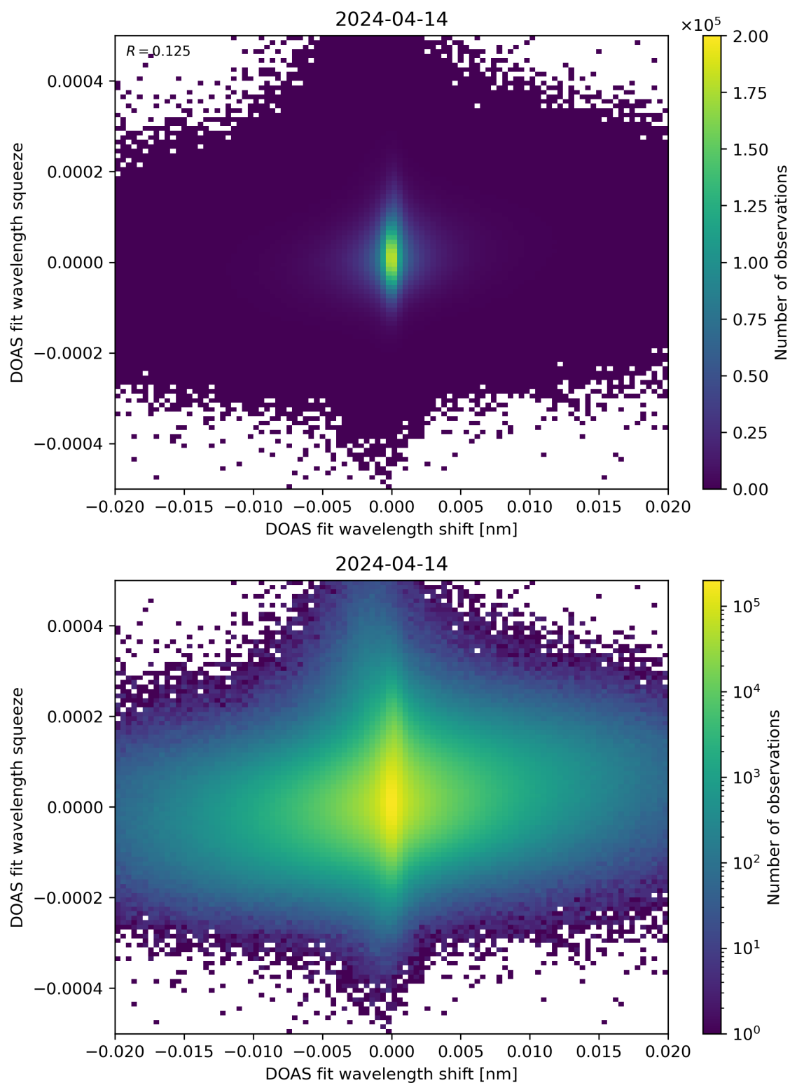
Figure 65: Scatter density plot of “DOAS fit wavelength shift” against “DOAS fit wavelength squeeze” for 2024-04-13 to 2024-04-15.
