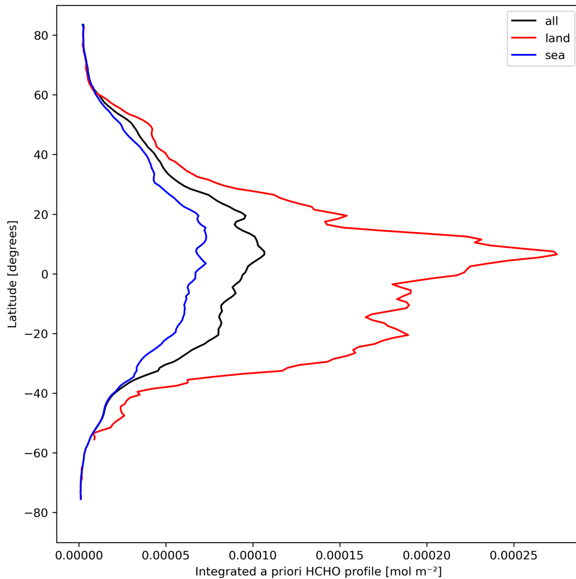
Figure 29: Zonal average of “Integrated a priori HCHO profile” for 2024-04-13 to 2024-04-15.
