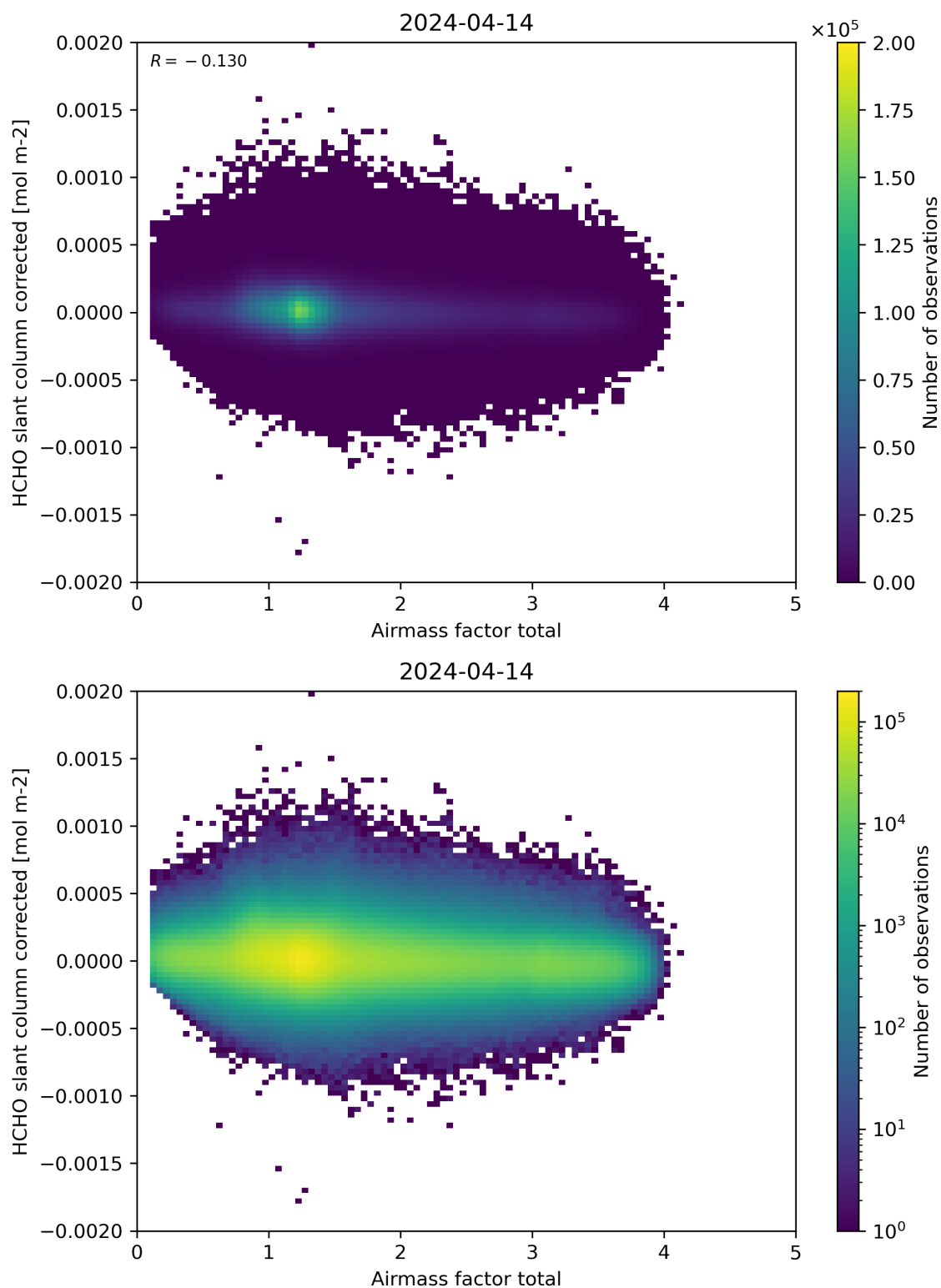
Figure 101: Scatter density plot of “Airmass factor total” against “HCHO slant column corrected” for 2024-04-13 to 2024-04-15.
