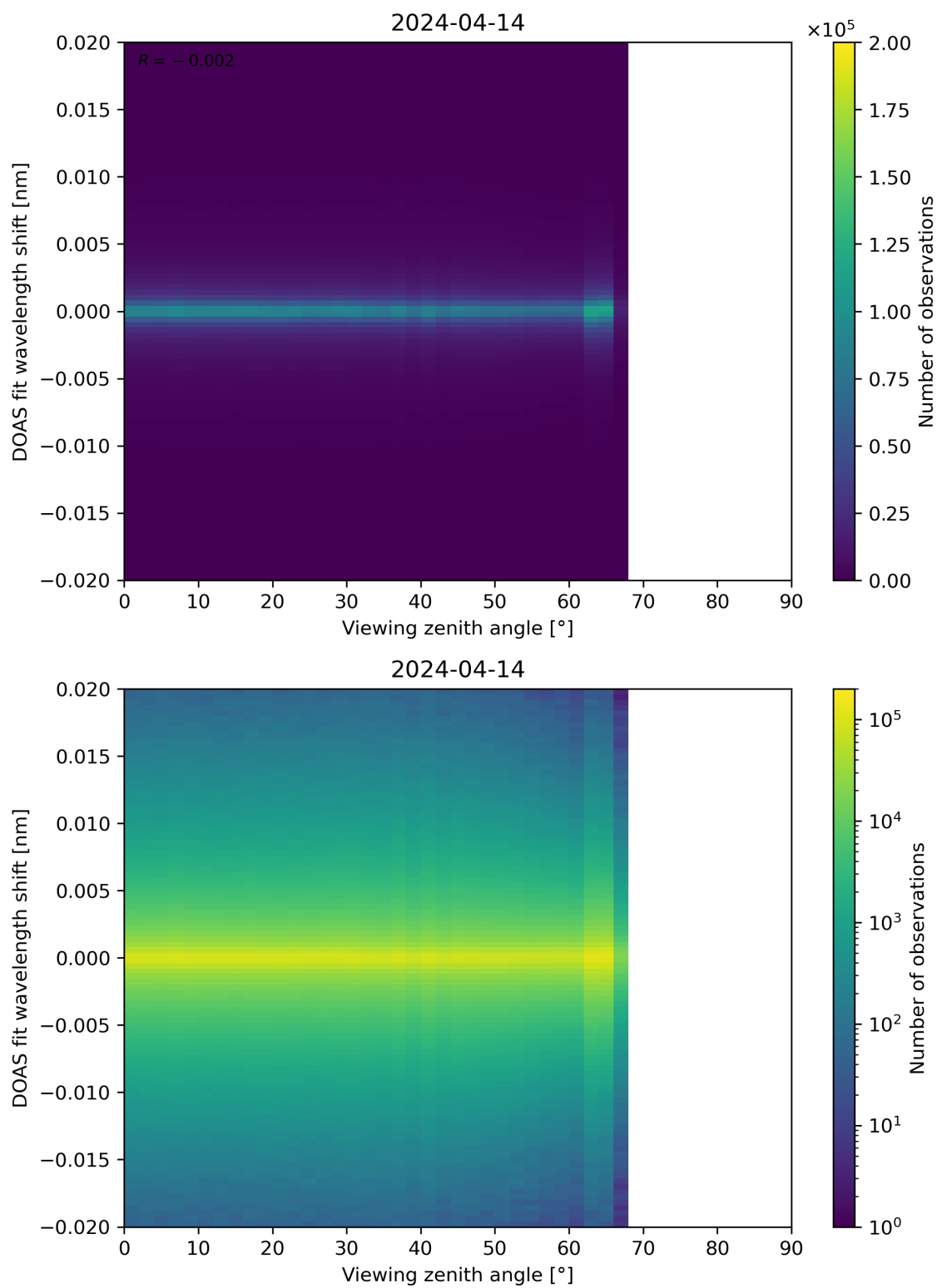
Figure 183: Scatter density plot of “Viewing zenith angle” against “DOAS fit wavelength shift” for 2024-04-13 to 2024-04-15.
