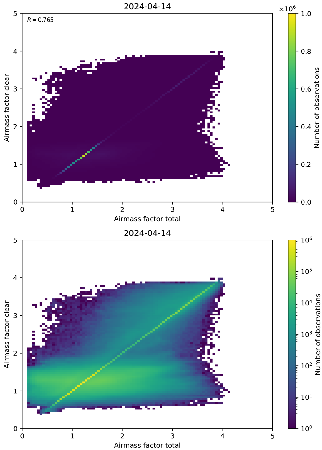
Figure 100: Scatter density plot of “Airmass factor total” against “Airmass factor clear” for 2024-04-13 to 2024-04-15.
