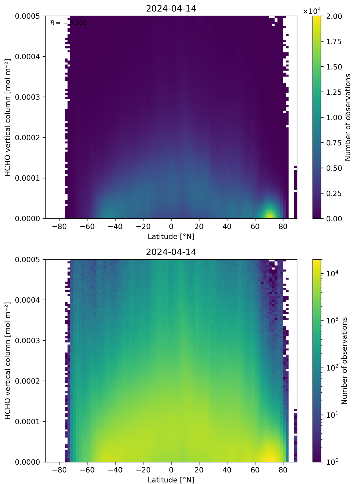
Figure 163: Scatter density plot of “Latitude” against “HCHO vertical column” for 2024-04-13 to 2024-04-15.
