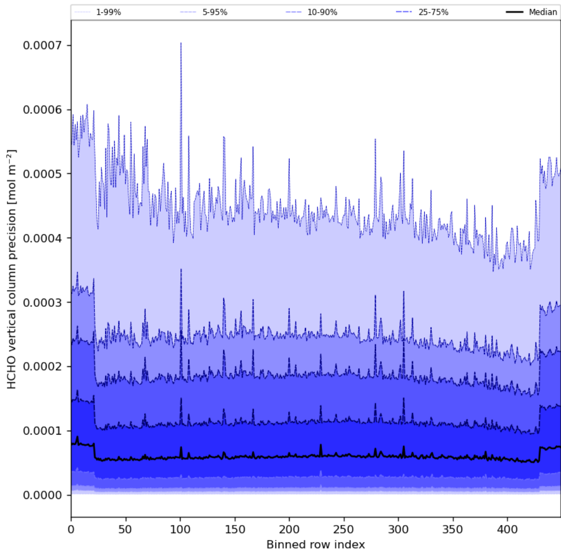
Figure 50: Along track statistics of “HCHO vertical column precision” for 2024-04-13 to 2024-04-15
