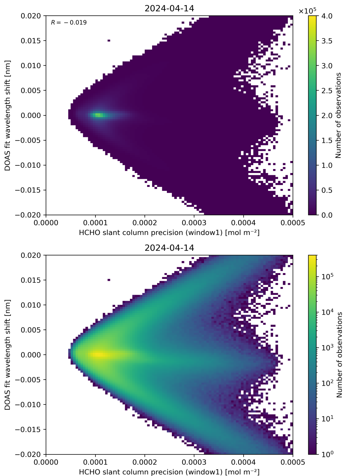
Figure 89: Scatter density plot of “HCHO slant column precision (window1)” against “DOAS fit wavelength shift” for 2024-04-13 to 2024-04-15.
