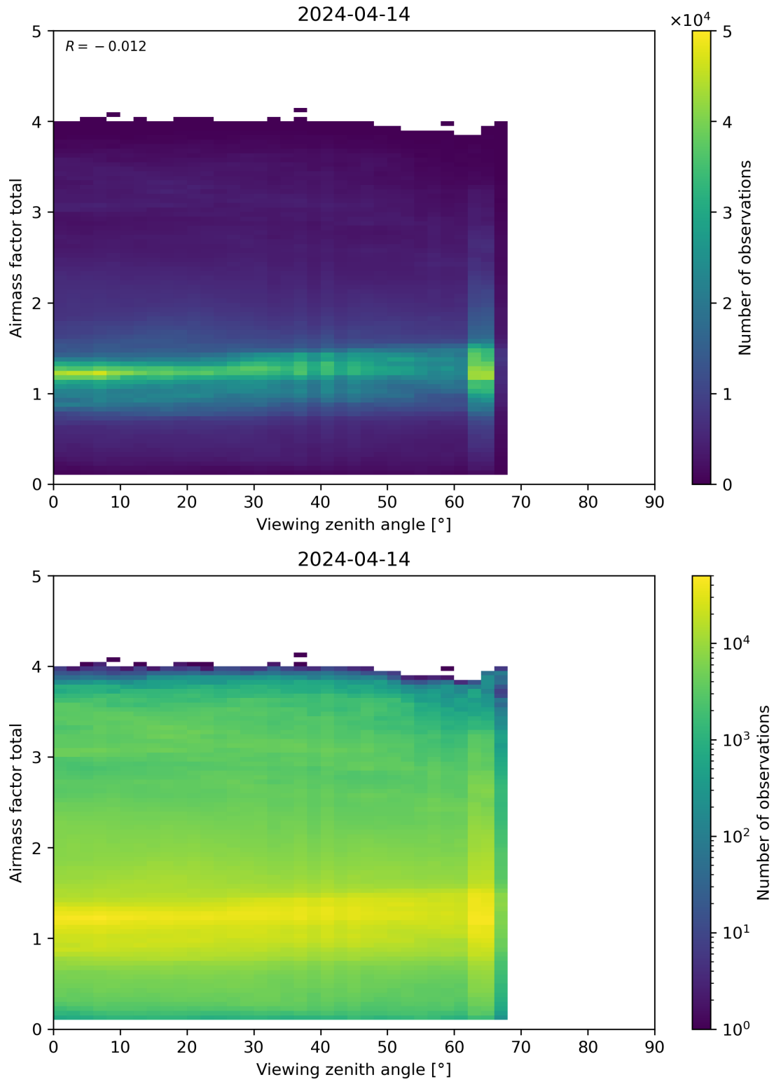
Figure 190: Scatter density plot of “Viewing zenith angle” against “Airmass factor total” for 2024-04-13 to 2024-04-15.
