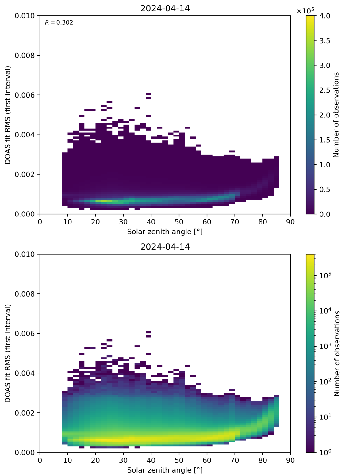
Figure 167: Scatter density plot of “Solar zenith angle” against “DOAS fit RMS (first interval)” for 2024-04-13 to 2024-04-15.
