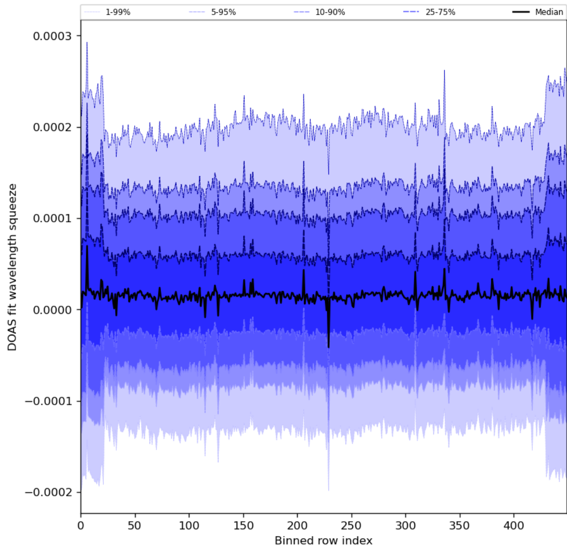
Figure 59: Along track statistics of “DOAS fit wavelength squeeze” for 2024-04-13 to 2024-04-15
