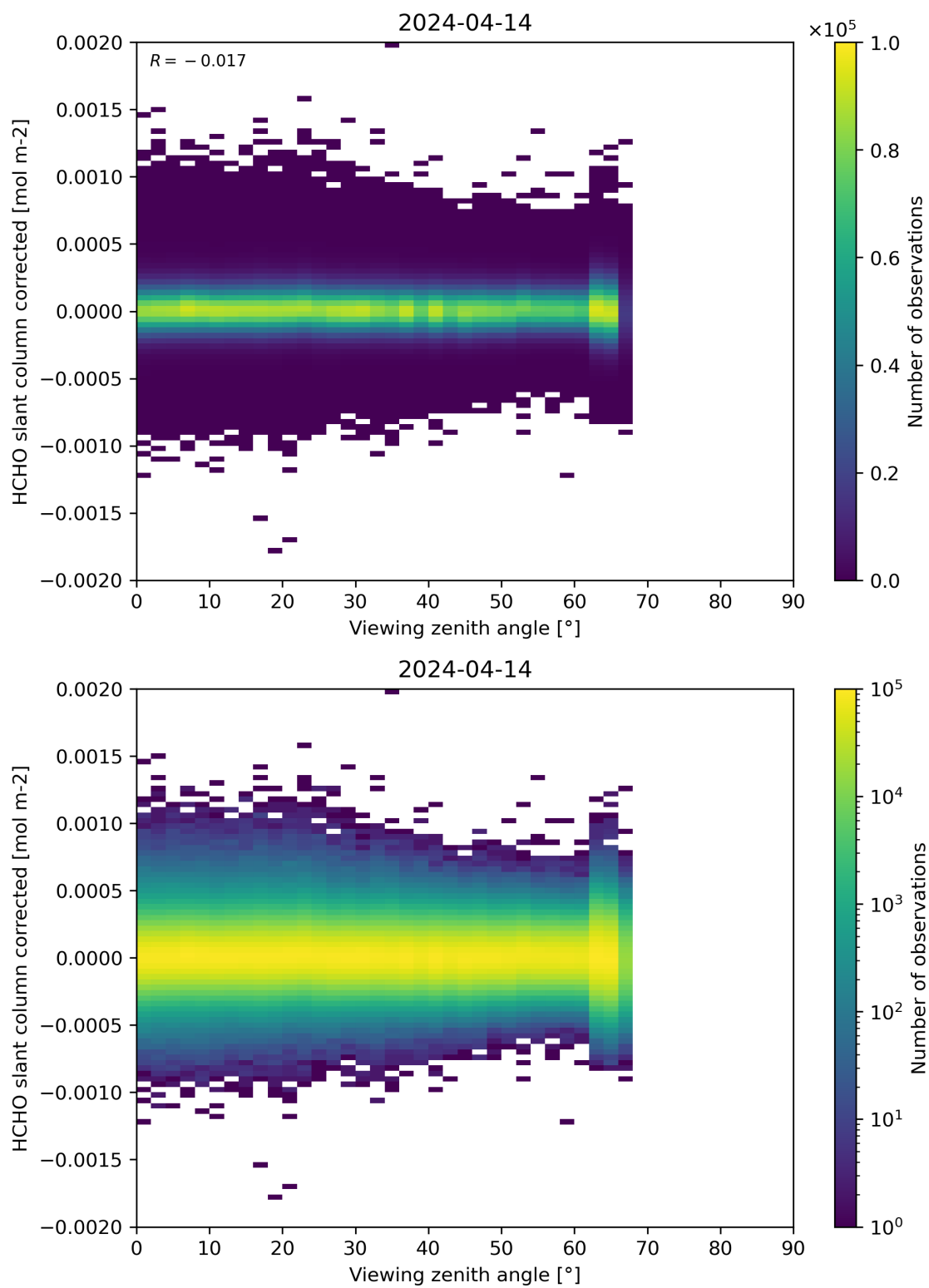
Figure 186: Scatter density plot of “Viewing zenith angle” against “HCHO slant column corrected” for 2024-04-13 to 2024-04-15.
