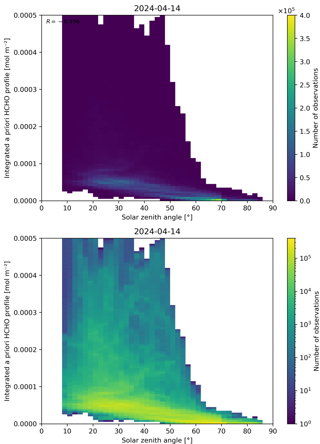
Figure 180: Scatter density plot of “Solar zenith angle” against “Integrated a priori HCHO profile” for 2024-04-13 to 2024-04-15.
