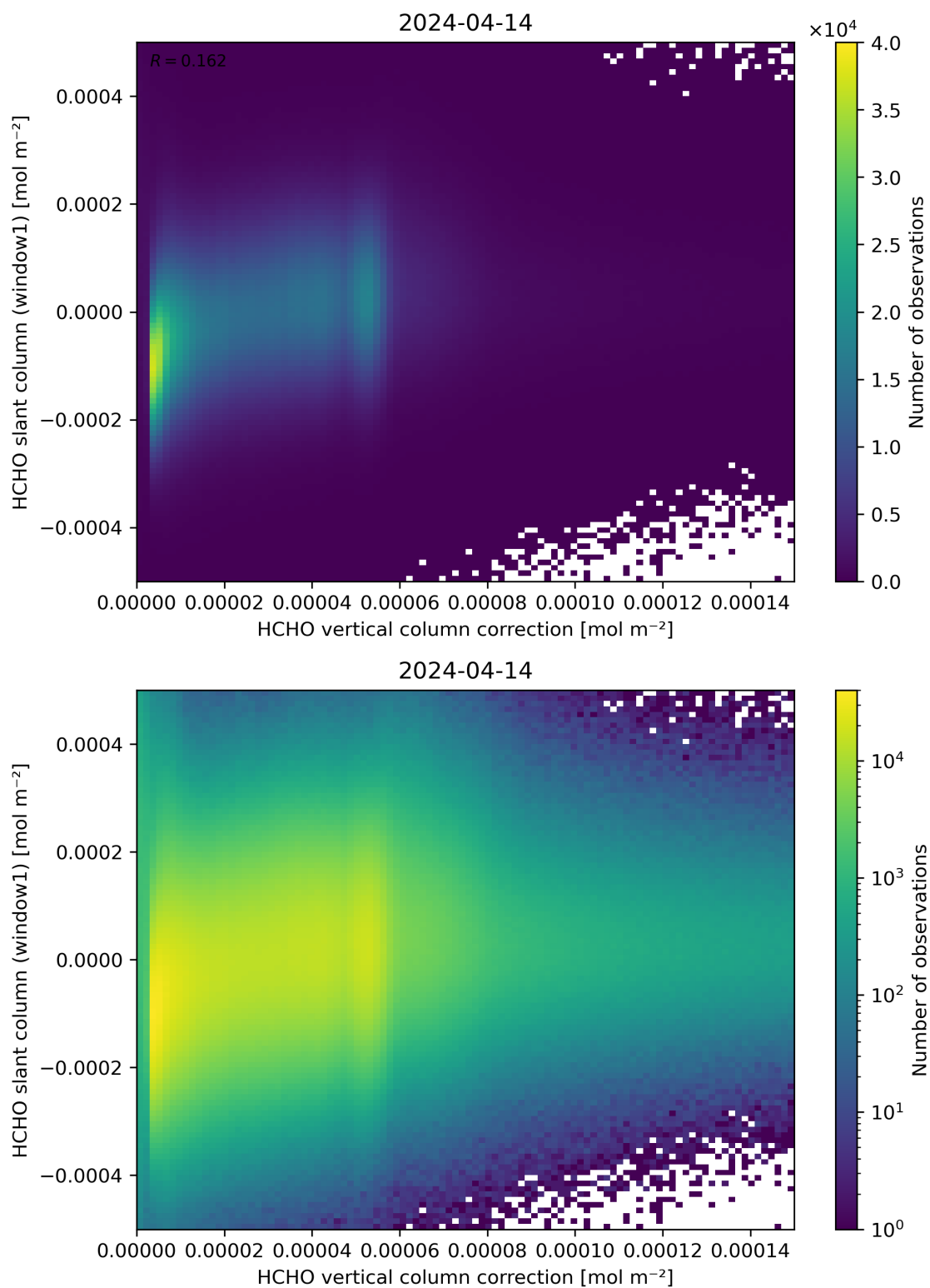
Figure 118: Scatter density plot of “HCHO vertical column correction” against “HCHO slant column (window1)” for 2024-04-13 to 2024-04-15.
