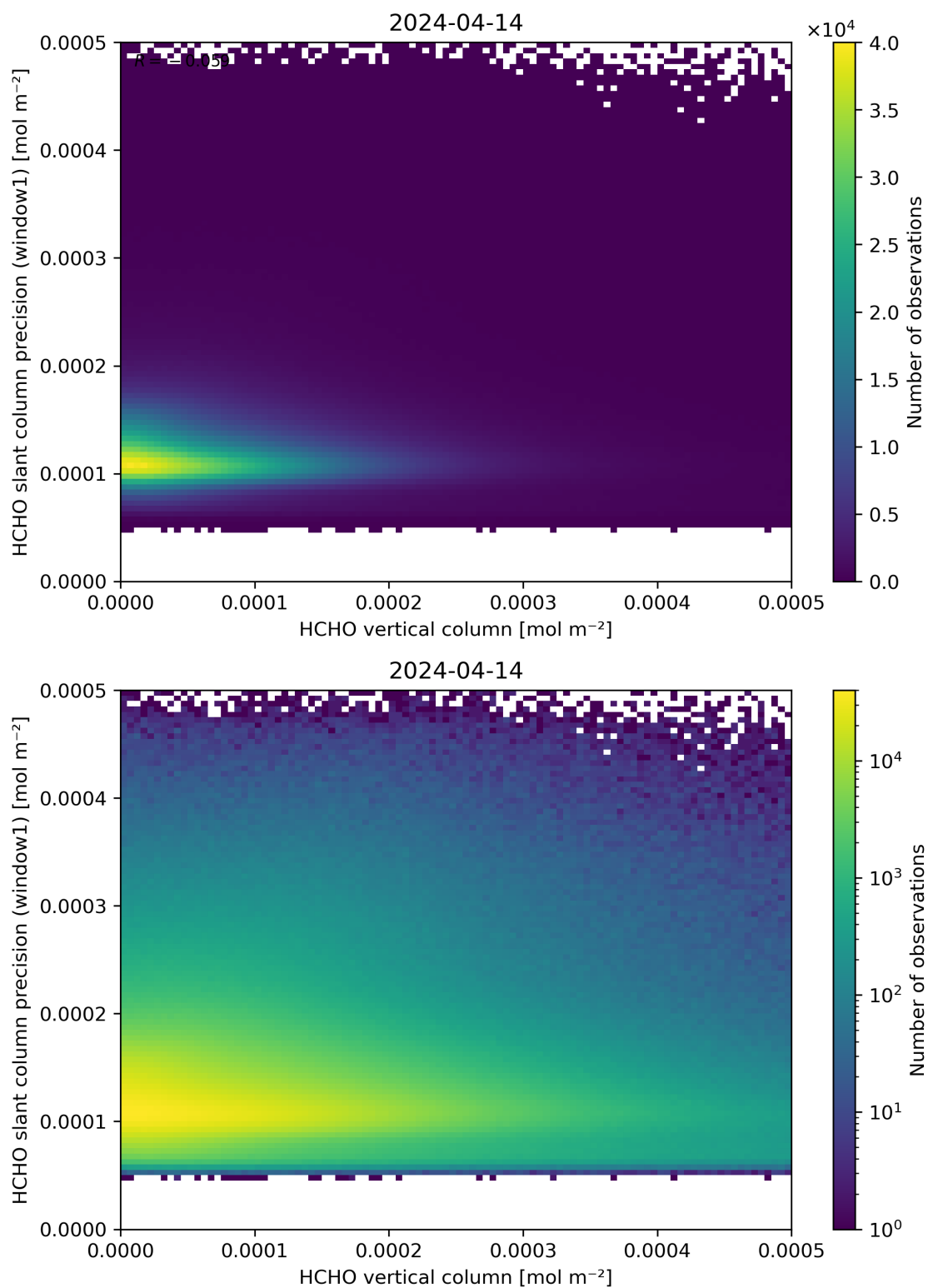
Figure 130: Scatter density plot of “HCHO vertical column” against “HCHO slant column precision (window1)” for 2024-04-13 to 2024-04-15.
