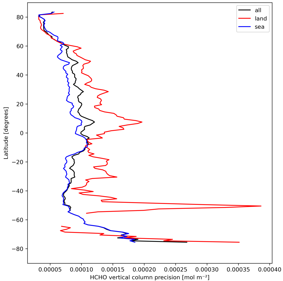
Figure 22: Zonal average of “HCHO vertical column precision” for 2024-04-13 to 2024-04-15.
