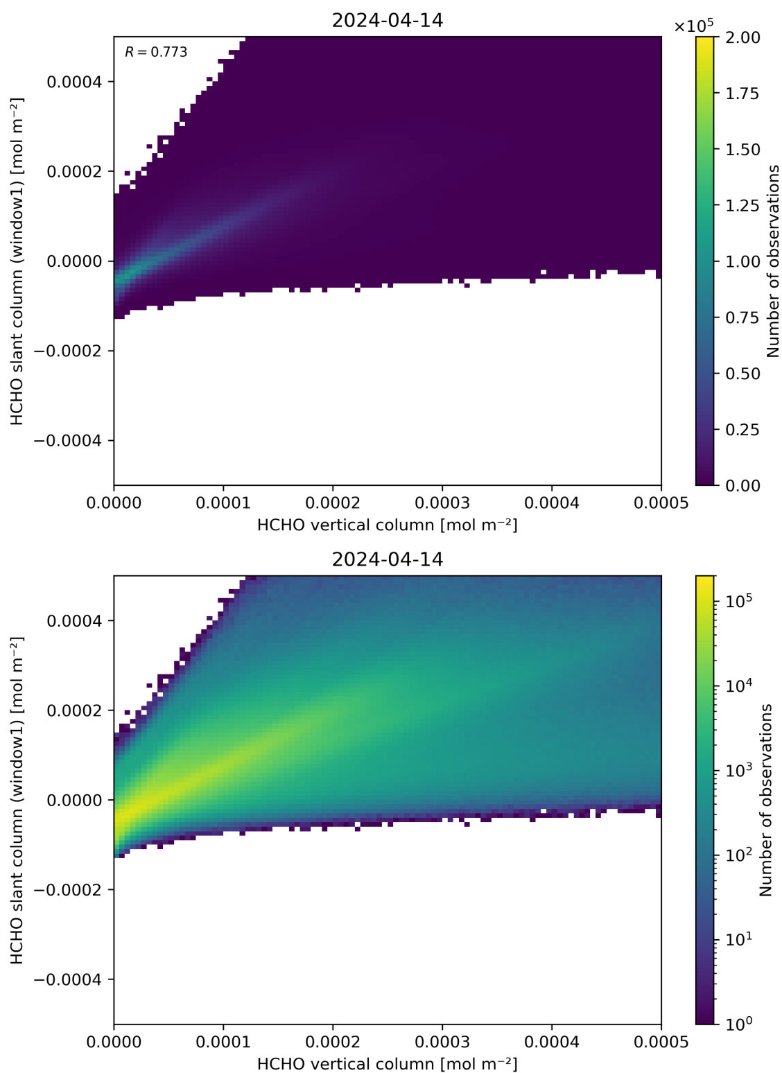
Figure 129: Scatter density plot of “HCHO vertical column” against “HCHO slant column (window1)” for 2024-04-13 to 2024-04-15.
