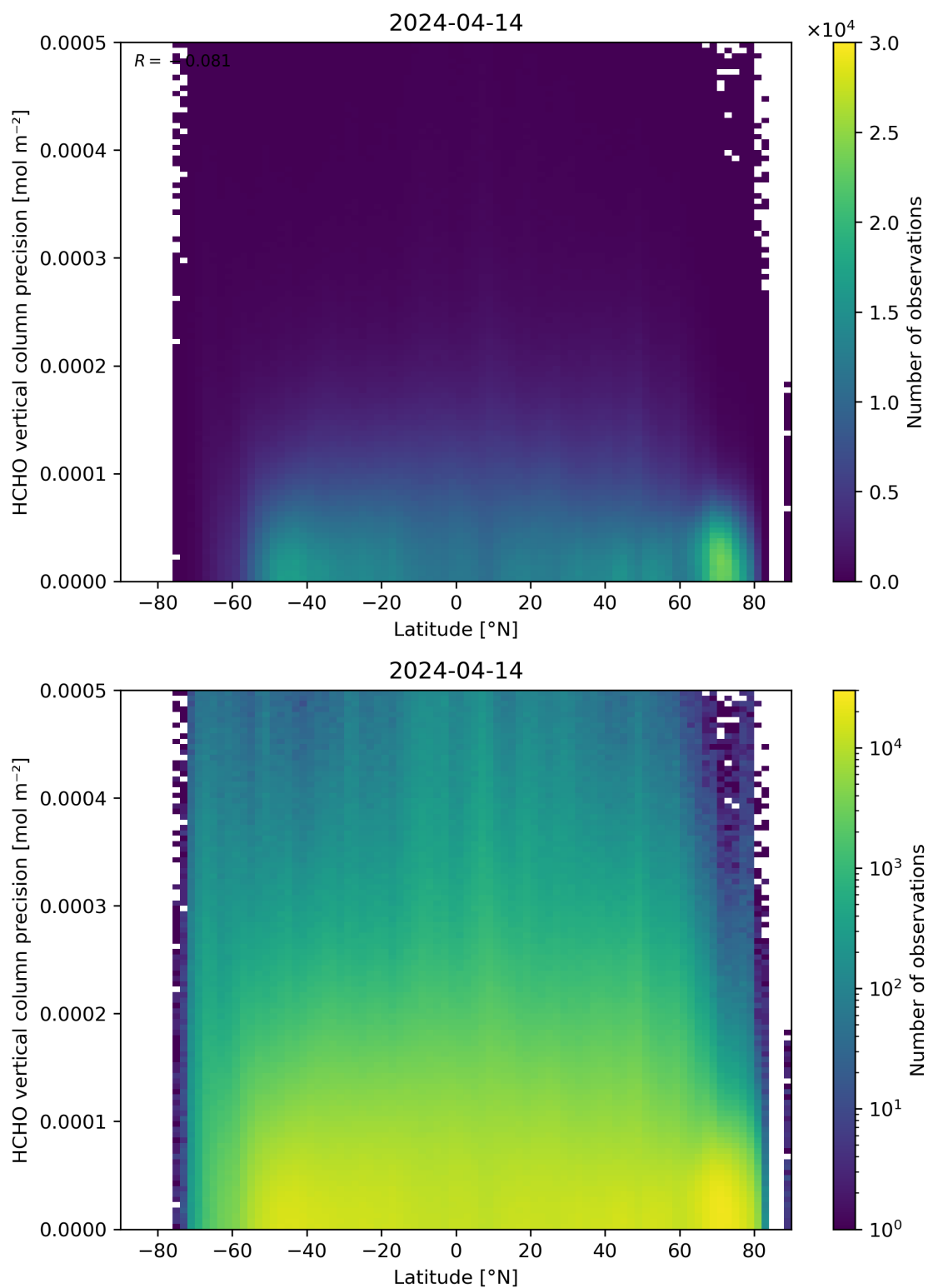
Figure 165: Scatter density plot of “Latitude” against “HCHO vertical column precision” for 2024-04-13 to 2024-04-15.
