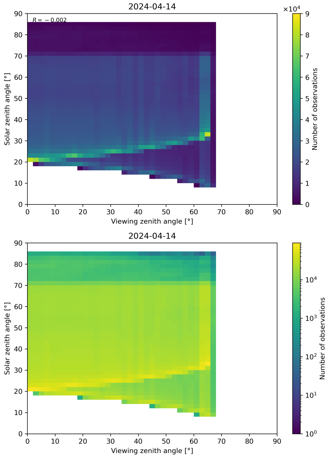
Figure 197: Scatter density plot of “Viewing zenith angle” against “Solar zenith angle” for 2024-04-13 to 2024-04-15.
