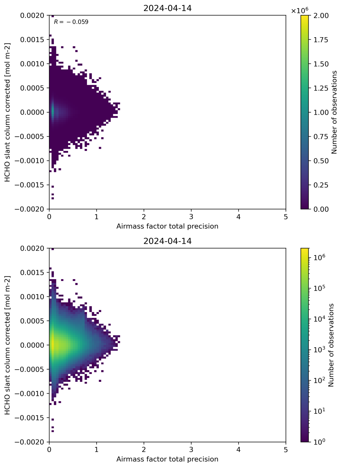
Figure 109: Scatter density plot of “Airmass factor total precision” against “HCHO slant column corrected” for 2024-04-13 to 2024-04-15.
