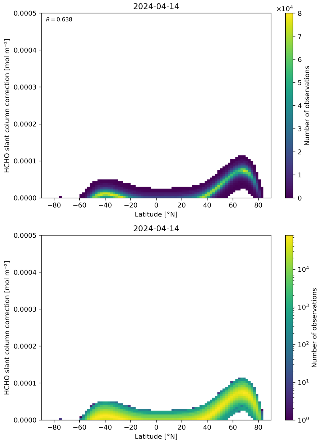
Figure 158: Scatter density plot of “Latitude” against “HCHO slant column correction” for 2024-04-13 to 2024-04-15.
