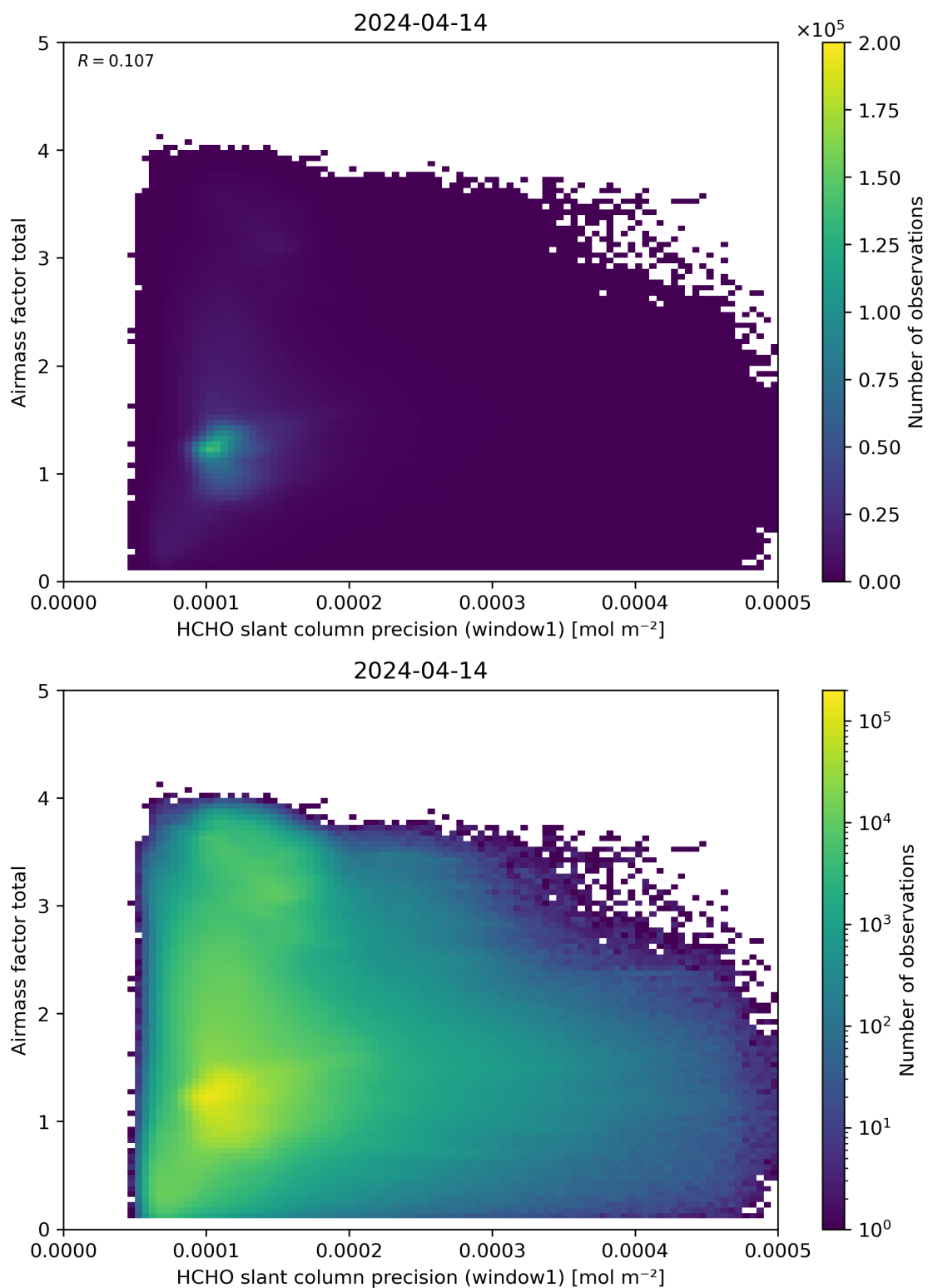
Figure 94: Scatter density plot of “HCHO slant column precision (window1)” against “Airmass factor total” for 2024-04-13 to 2024-04-15.
