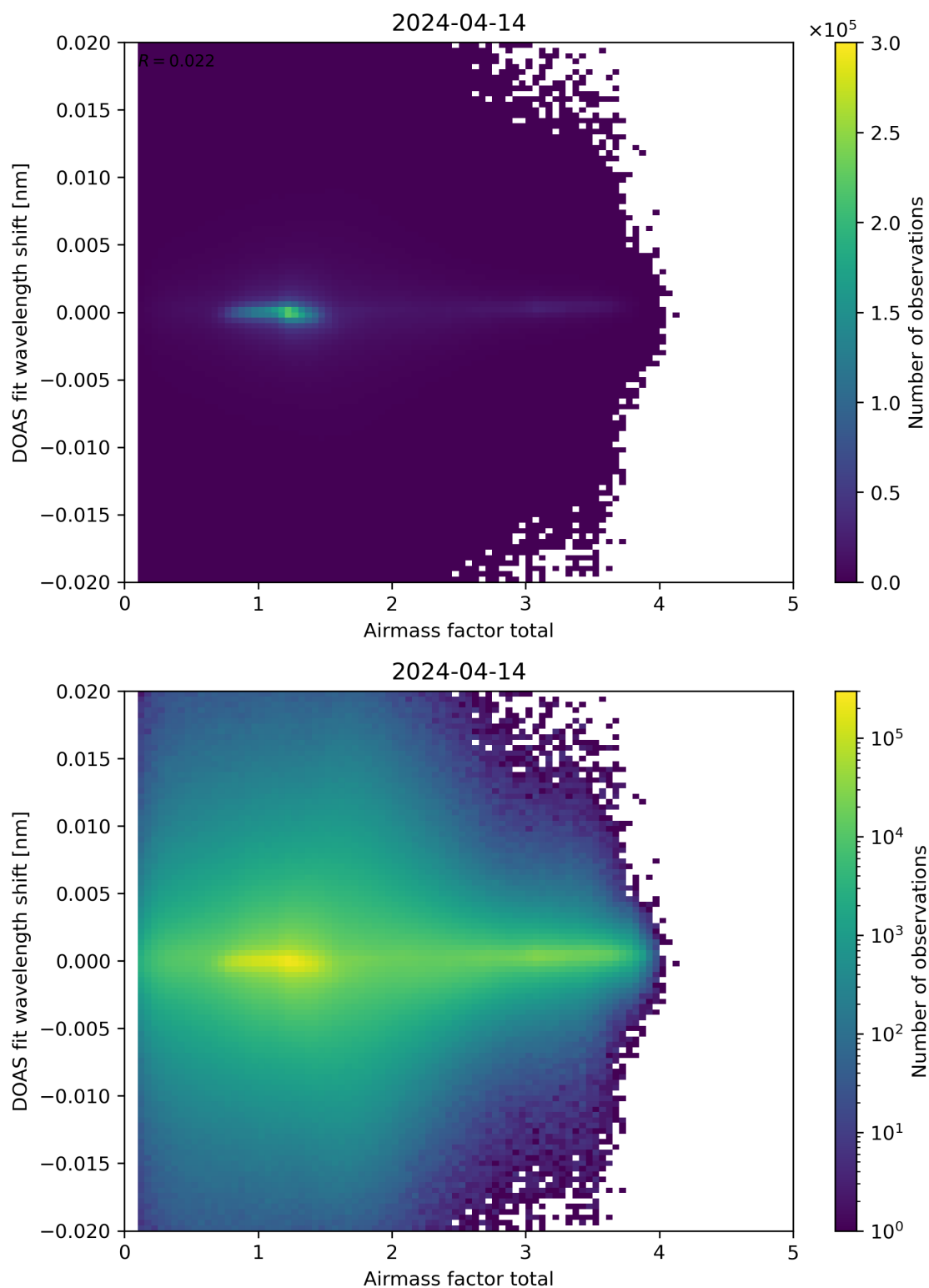
Figure 98: Scatter density plot of “Airmass factor total” against “DOAS fit wavelength shift” for 2024-04-13 to 2024-04-15.
