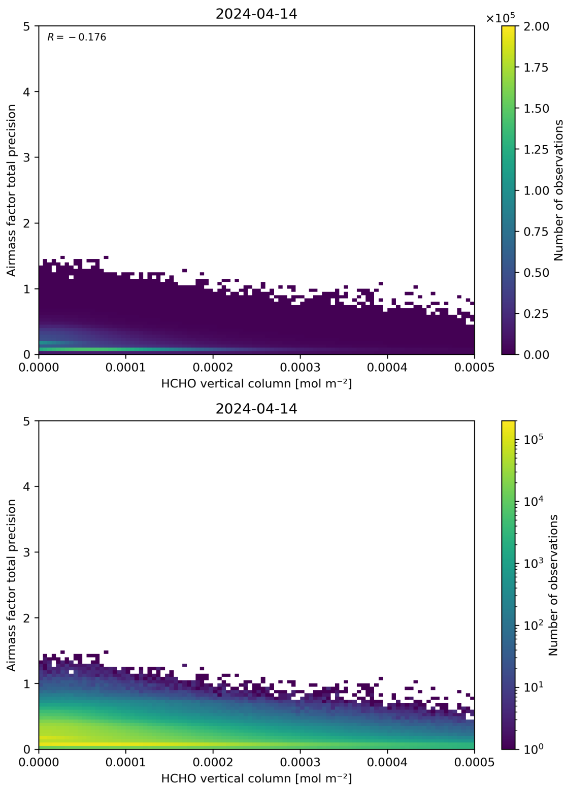
Figure 132: Scatter density plot of “HCHO vertical column” against “Airmass factor total precision” for 2024-04-13 to 2024-04-15.
