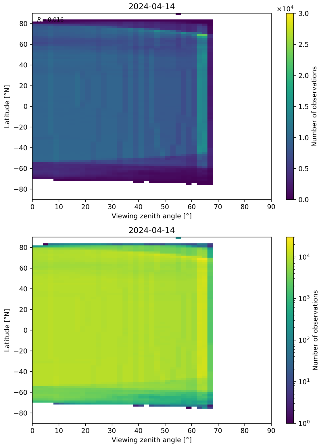
Figure 196: Scatter density plot of “Viewing zenith angle” against “Latitude” for 2024-04-13 to 2024-04-15.
