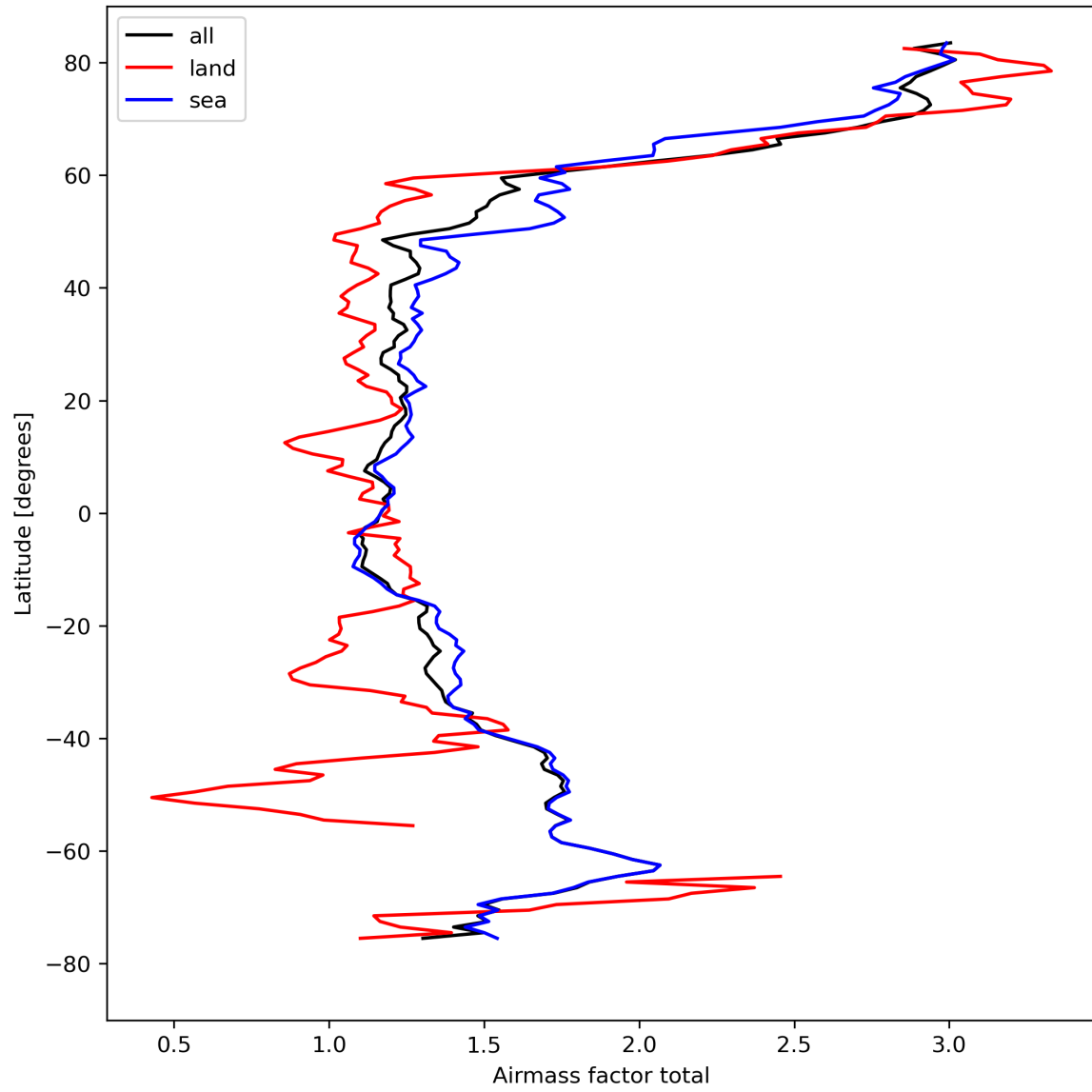
Figure 26: Zonal average of “Airmass factor total” for 2024-04-13 to 2024-04-15.
