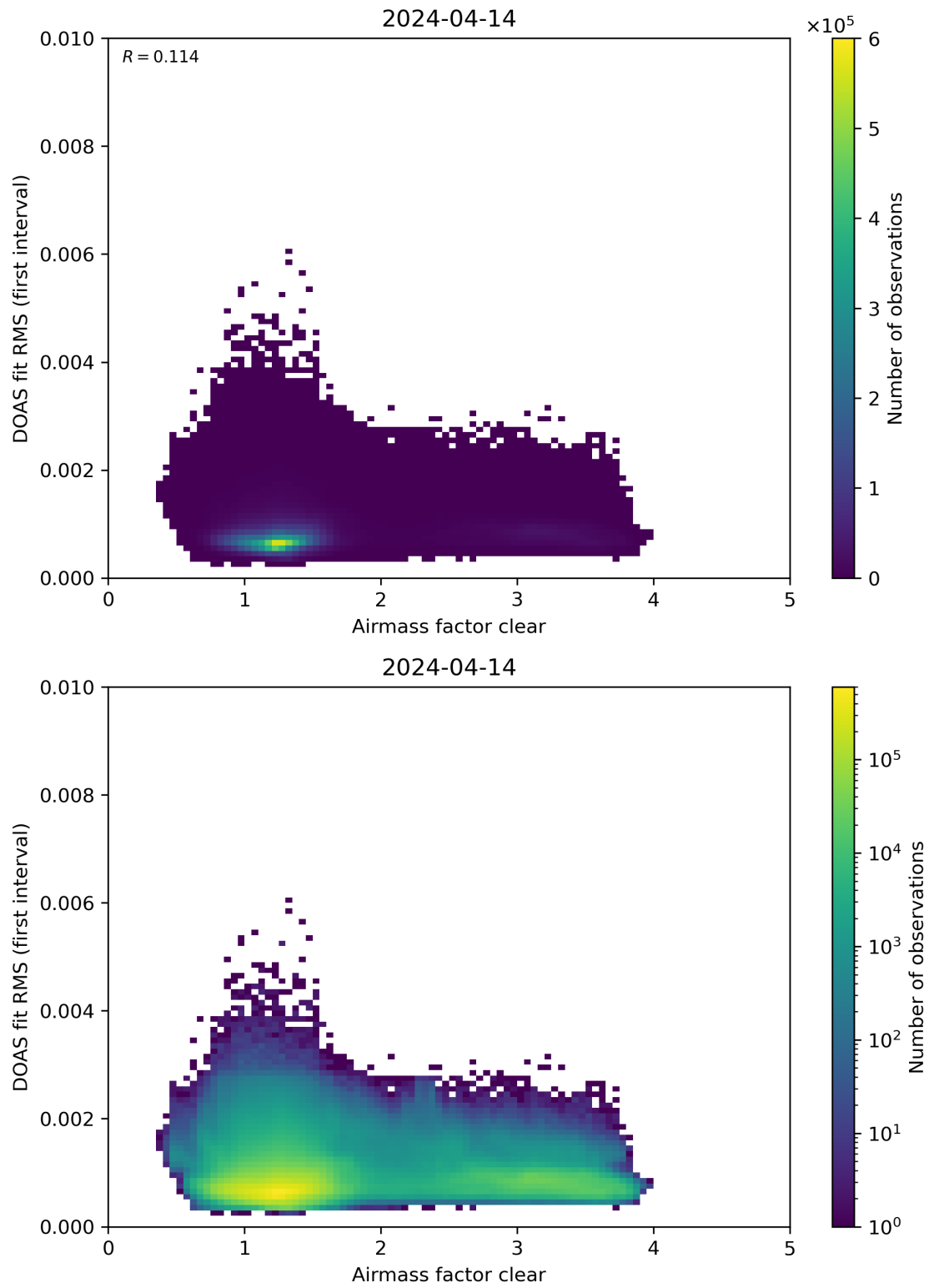
Figure 71: Scatter density plot of “Airmass factor clear” against “DOAS fit RMS (first interval)” for 2024-04-13 to 2024-04-15.
