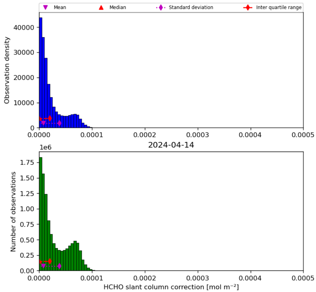
Figure 47: Histogram of “HCHO slant column correction” for 2024-04-13 to 2024-04-15
