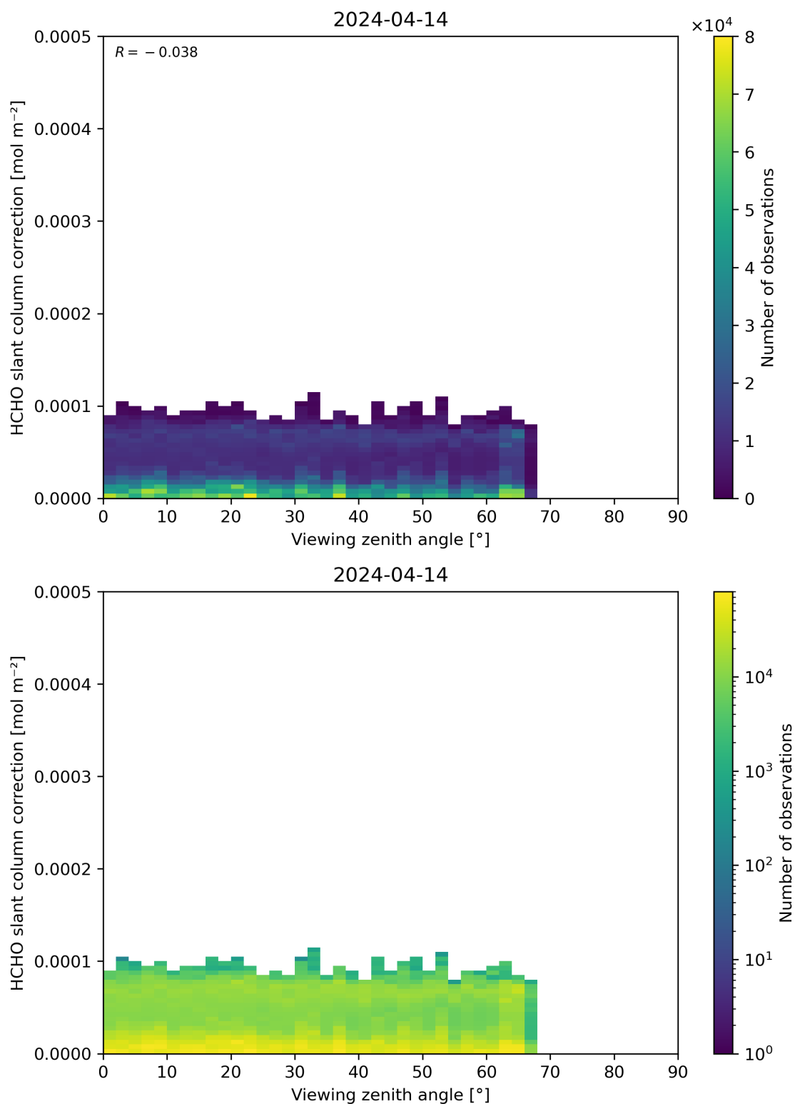
Figure 187: Scatter density plot of “Viewing zenith angle” against “HCHO slant column correction” for 2024-04-13 to 2024-04-15.
