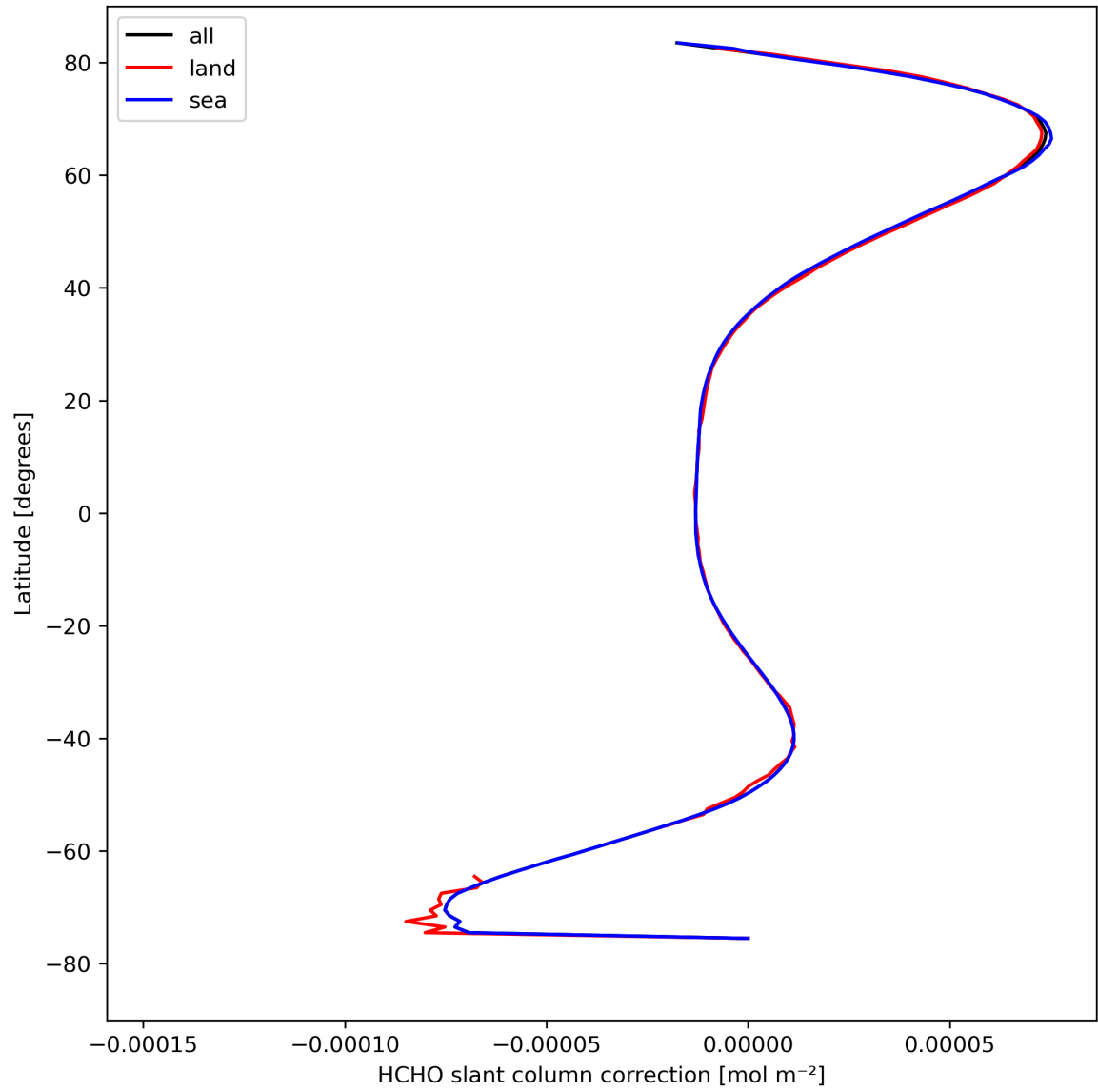
Figure 33: Zonal average of "HCHO slant column correction" for 2024-04-13 to 2024-04-15.
