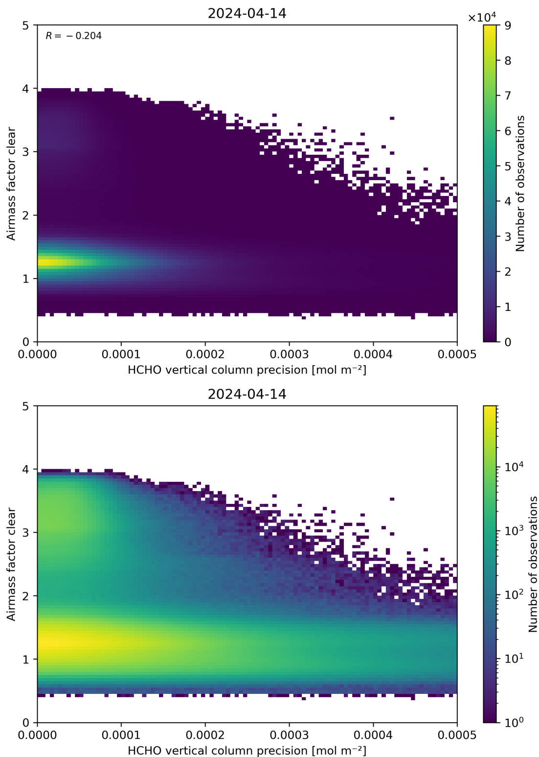
Figure 139: Scatter density plot of “HCHO vertical column precision” against “Airmass factor clear” for 2024-04-13 to 2024-04-15.
