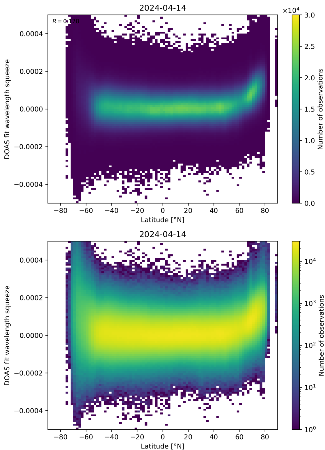
Figure 155: Scatter density plot of “Latitude” against “DOAS fit wavelength squeeze” for 2024-04-13 to 2024-04-15.
