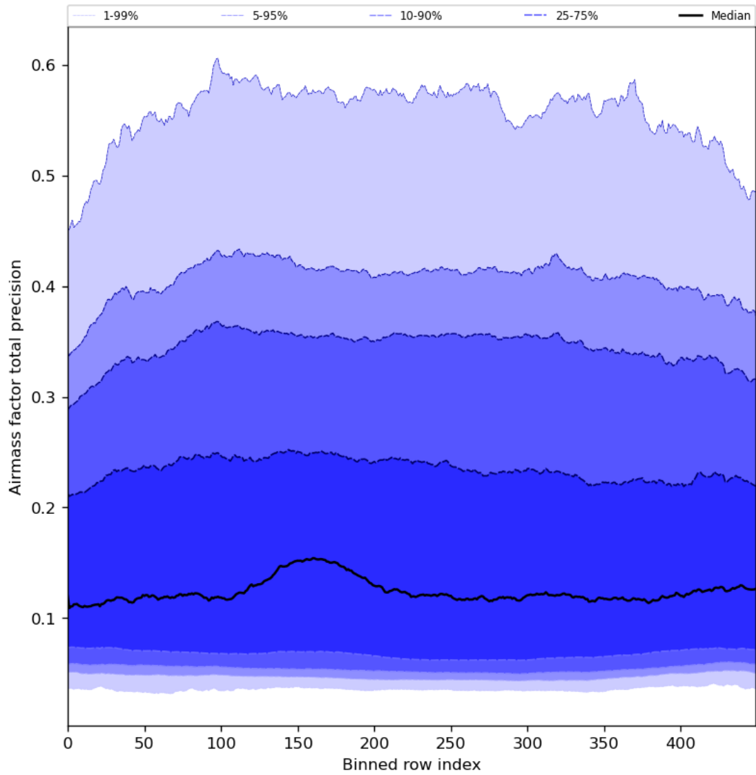
Figure 55: Along track statistics of “Airmass factor total precision” for 2024-04-13 to 2024-04-15
