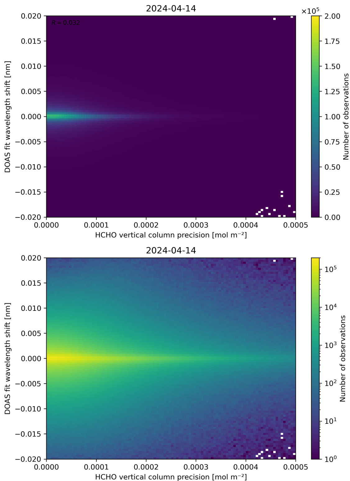
Figure 137: Scatter density plot of “HCHO vertical column precision” against “DOAS fit wavelength shift” for 2024-04-13 to 2024-04-15.
