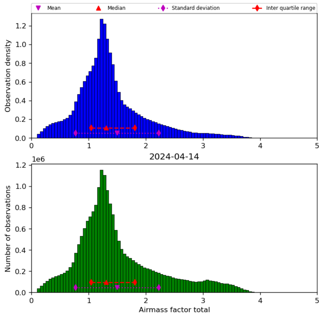
Figure 40: Histogram of “Airmass factor total” for 2024-04-13 to 2024-04-15
