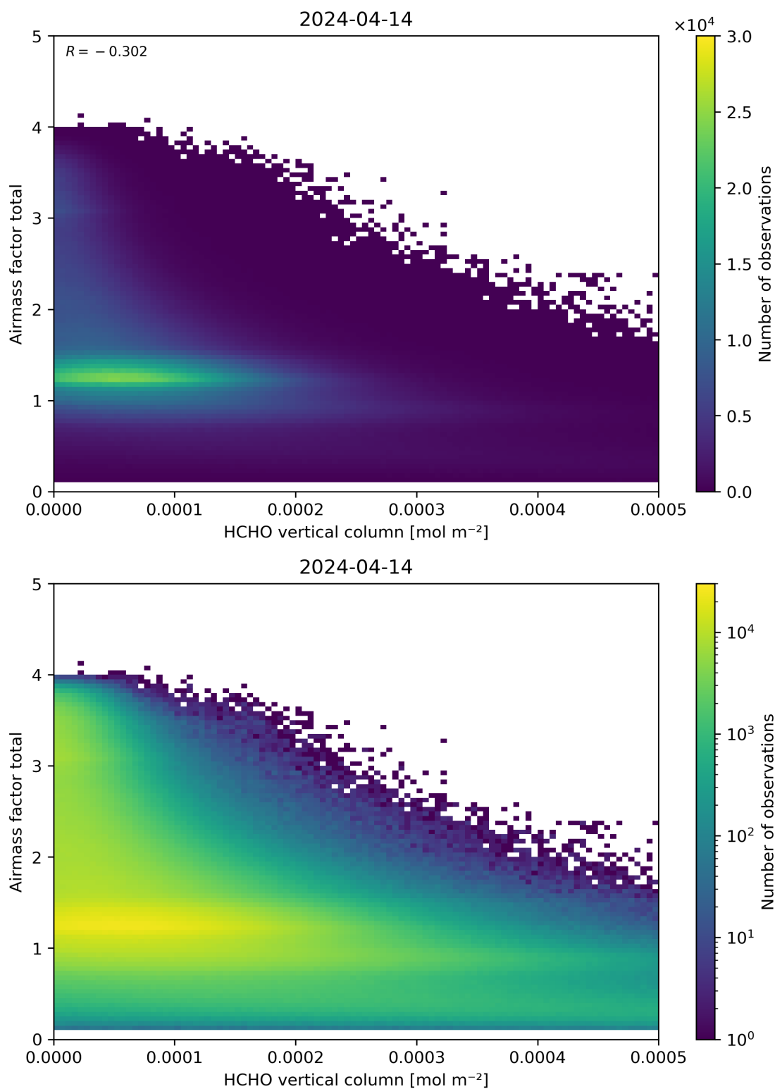
Figure 131: Scatter density plot of “HCHO vertical column” against “Airmass factor total” for 2024-04-13 to 2024-04-15.
