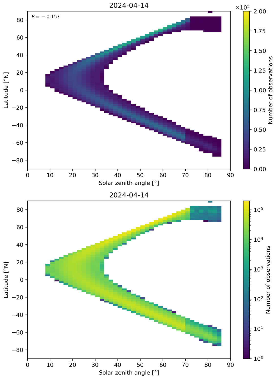
Figure 181: Scatter density plot of “Solar zenith angle” against “Latitude” for 2024-04-13 to 2024-04-15.
