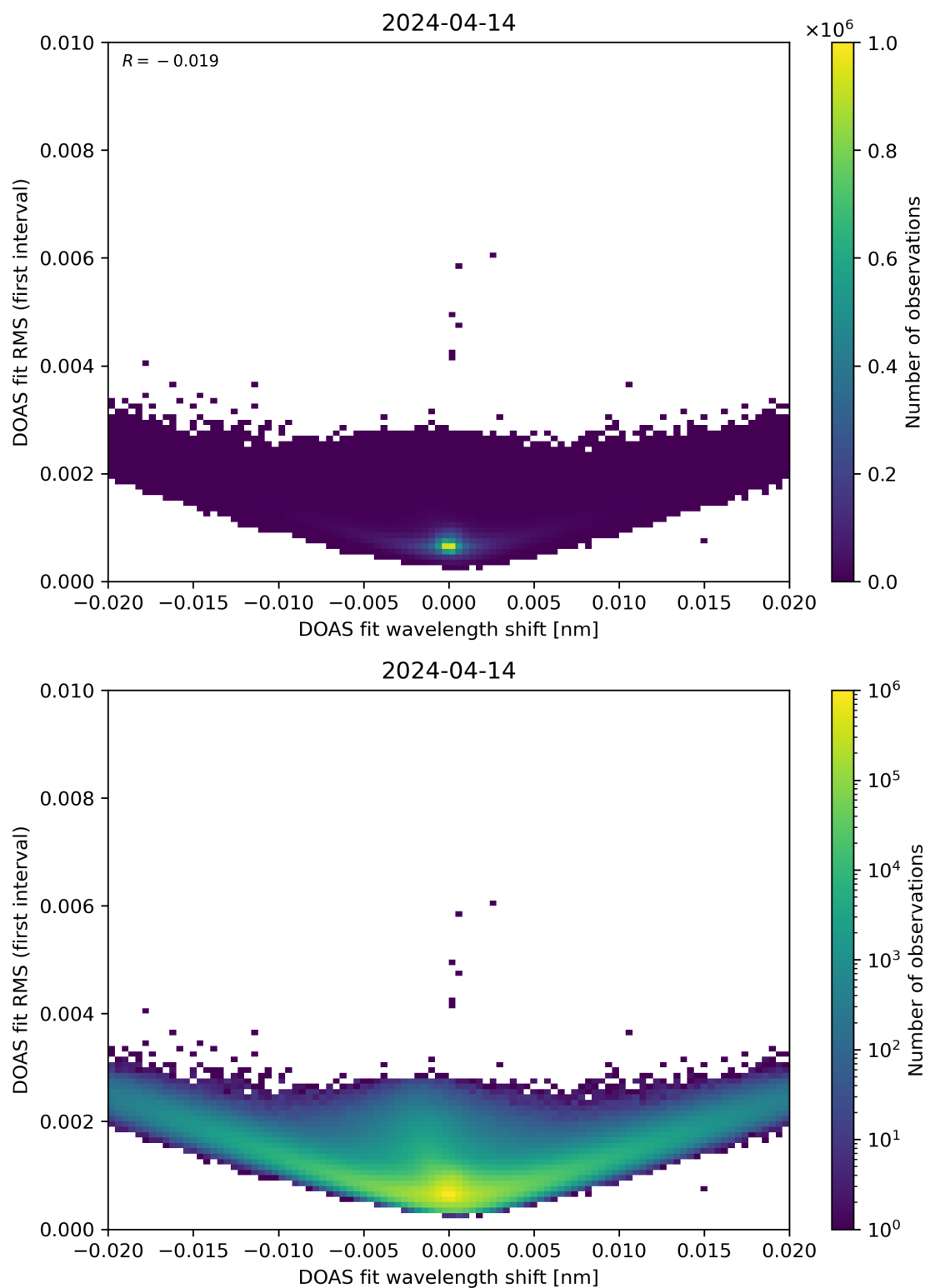
Figure 64: Scatter density plot of “DOAS fit wavelength shift” against “DOAS fit RMS (first interval)” for 2024-04-13 to 2024-04-15.
