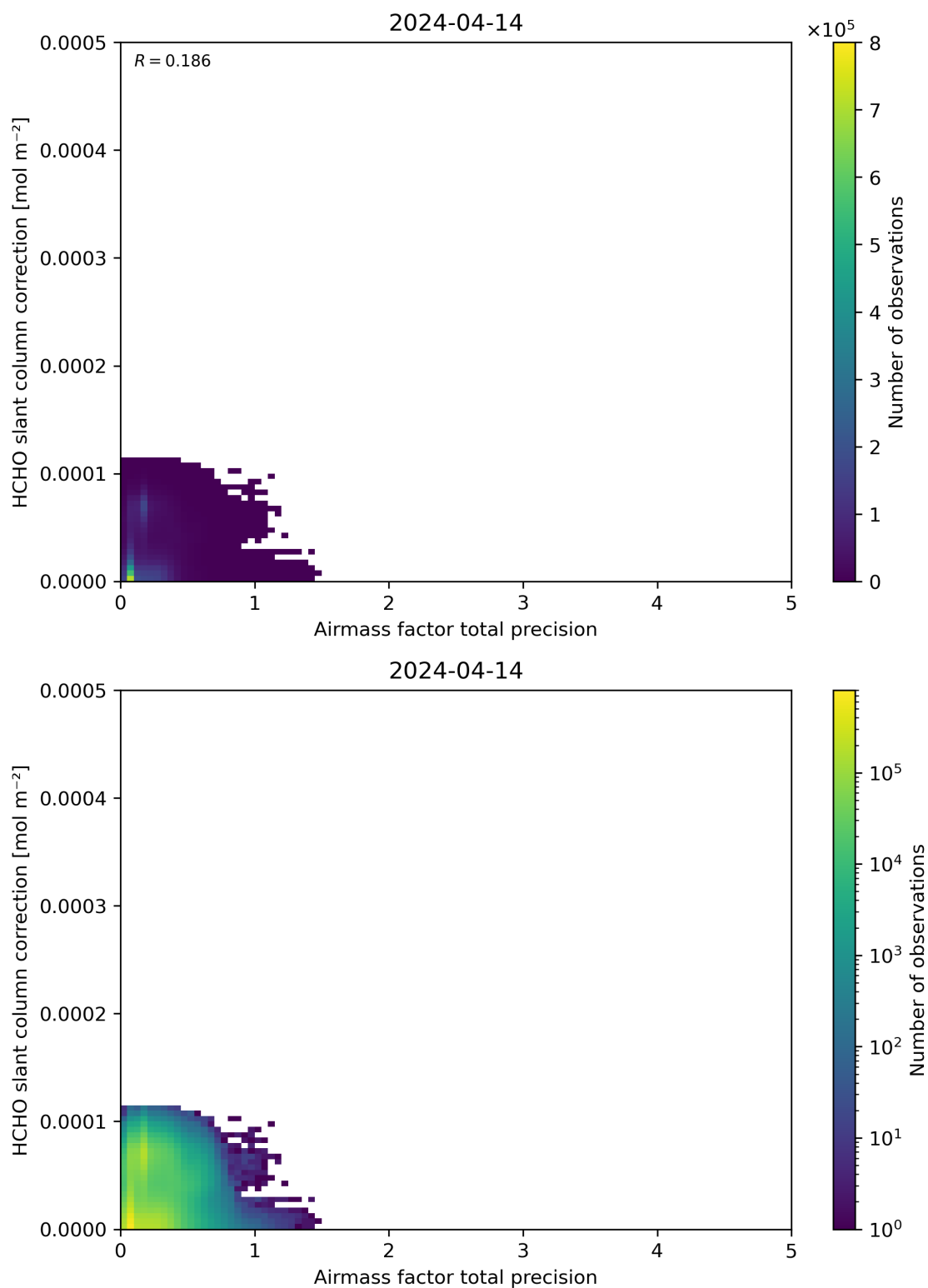
Figure 110: Scatter density plot of “Airmass factor total precision” against “HCHO slant column correction” for 2024-04-13 to 2024-04-15.
