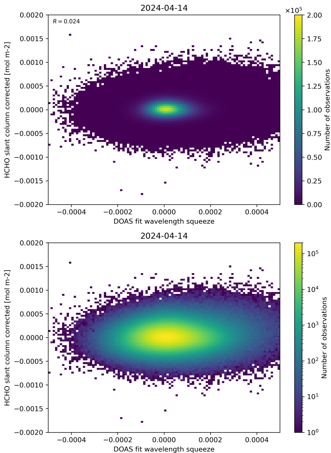
Figure 69: Scatter density plot of “DOAS fit wavelength squeeze” against “HCHO slant column corrected” for 2024-04-13 to 2024-04-15.
