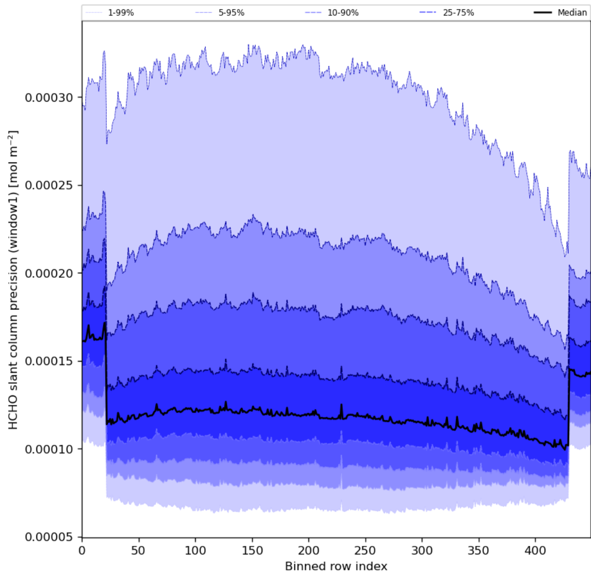
Figure 53: Along track statistics of “HCHO slant column precision (window1)” for 2024-04-13 to 2024-04-15
