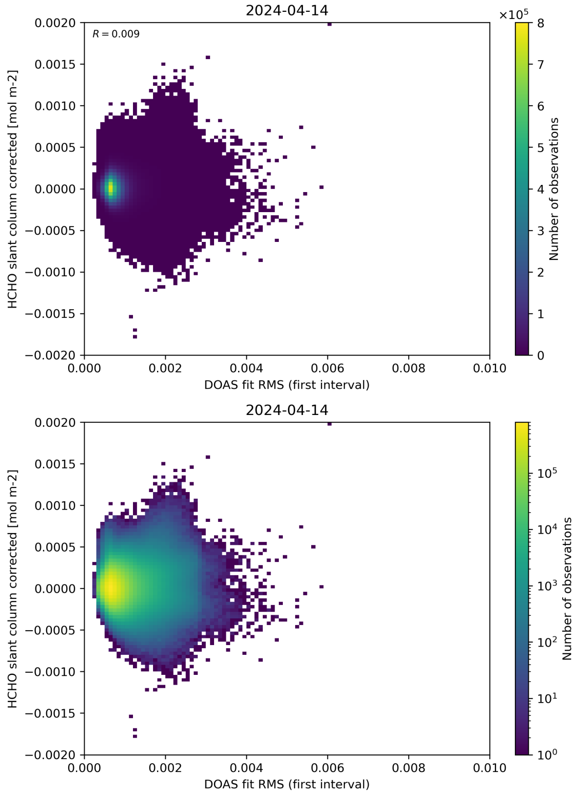
Figure 62: Scatter density plot of “DOAS fit RMS (first interval)” against “HCHO slant column corrected” for 2024-04-13 to 2024-04-15.
