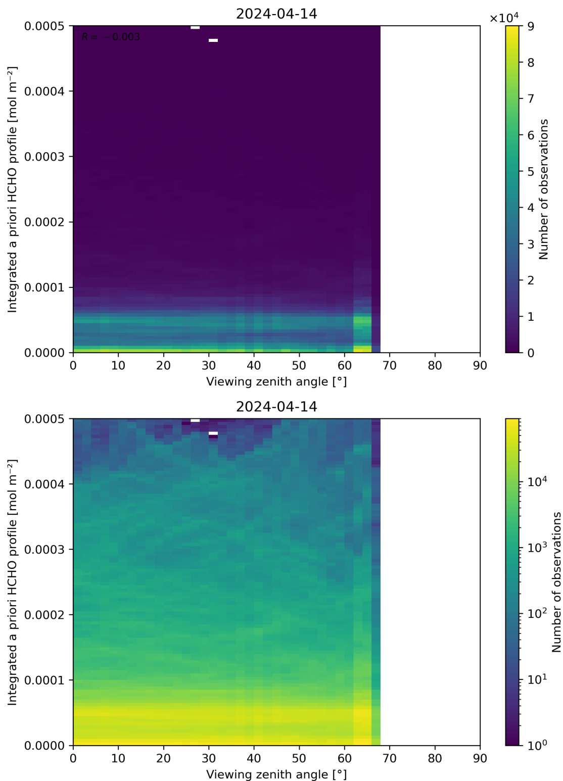
Figure 195: Scatter density plot of “Viewing zenith angle” against “Integrated a priori HCHO profile” for 2024-04-13 to 2024-04-15.
