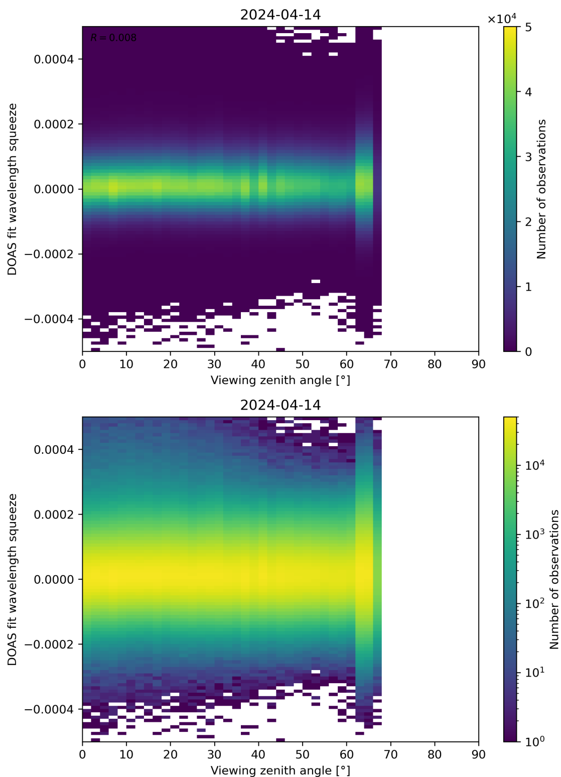
Figure 184: Scatter density plot of “Viewing zenith angle” against “DOAS fit wavelength squeeze” for 2024-04-13 to 2024-04-15.
