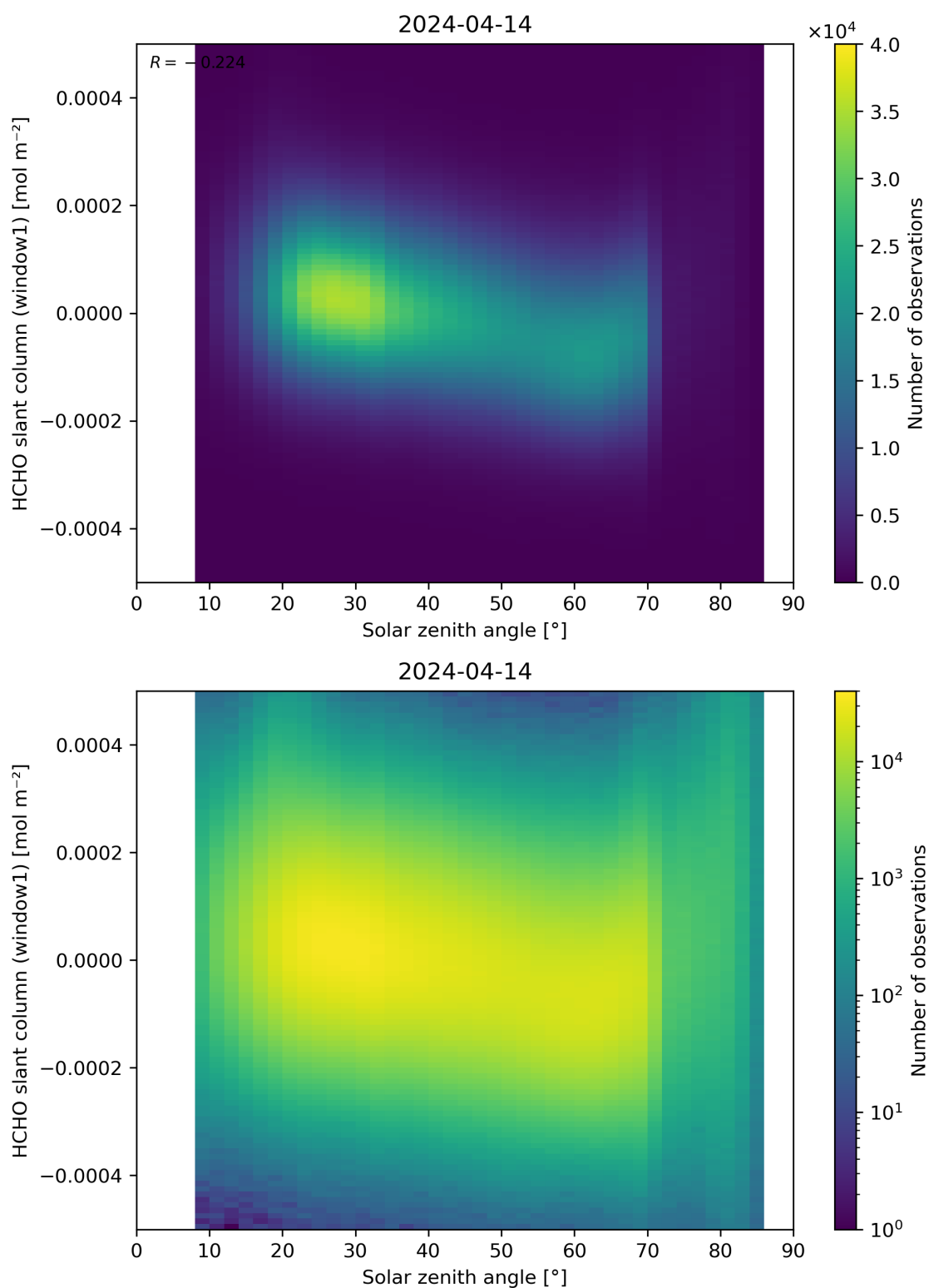
Figure 173: Scatter density plot of “Solar zenith angle” against “HCHO slant column (window1)” for 2024-04-13 to 2024-04-15.
