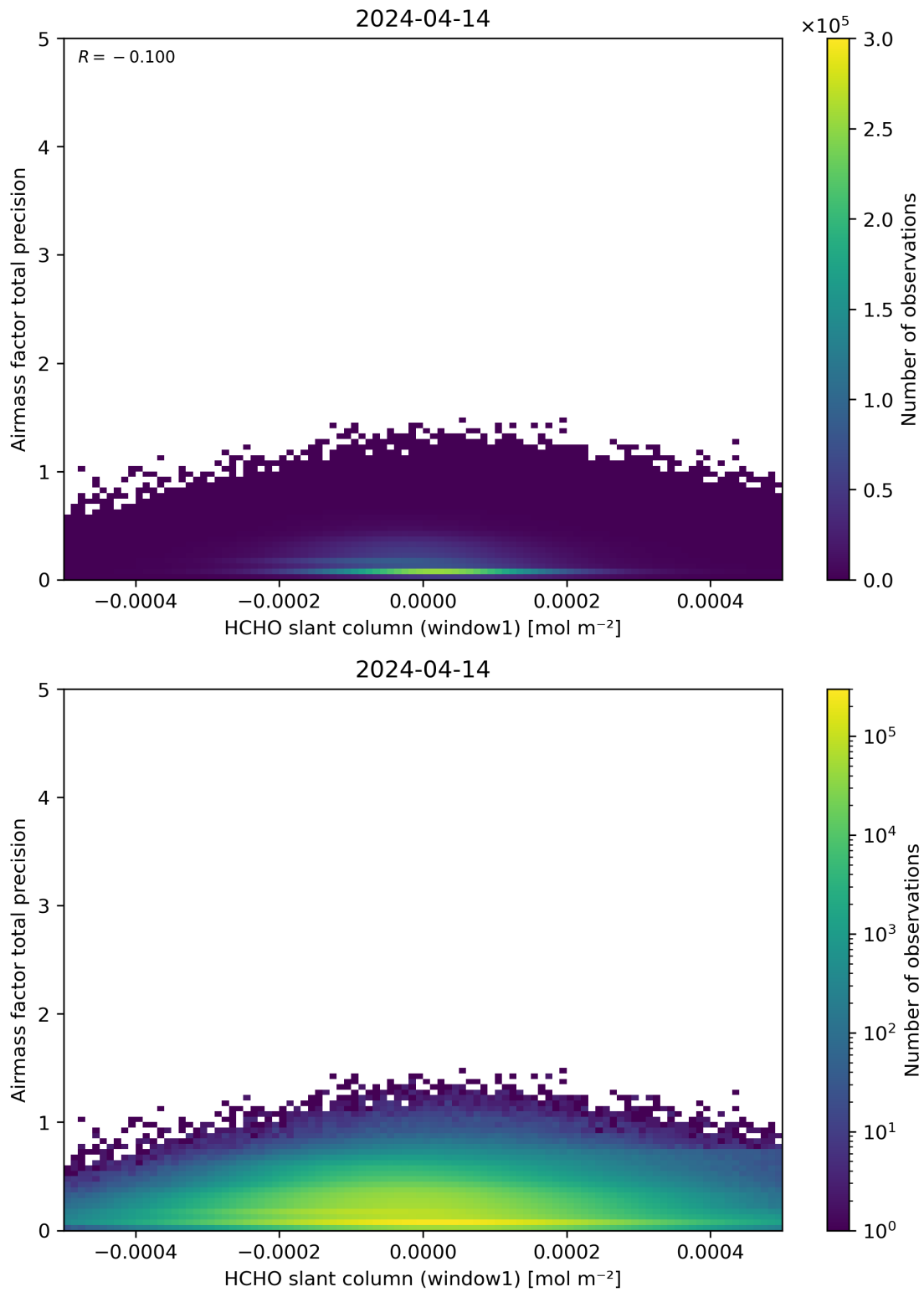
Figure 86: Scatter density plot of “HCHO slant column (window1)” against “Airmass factor total precision” for 2024-04-13 to 2024-04-15.
