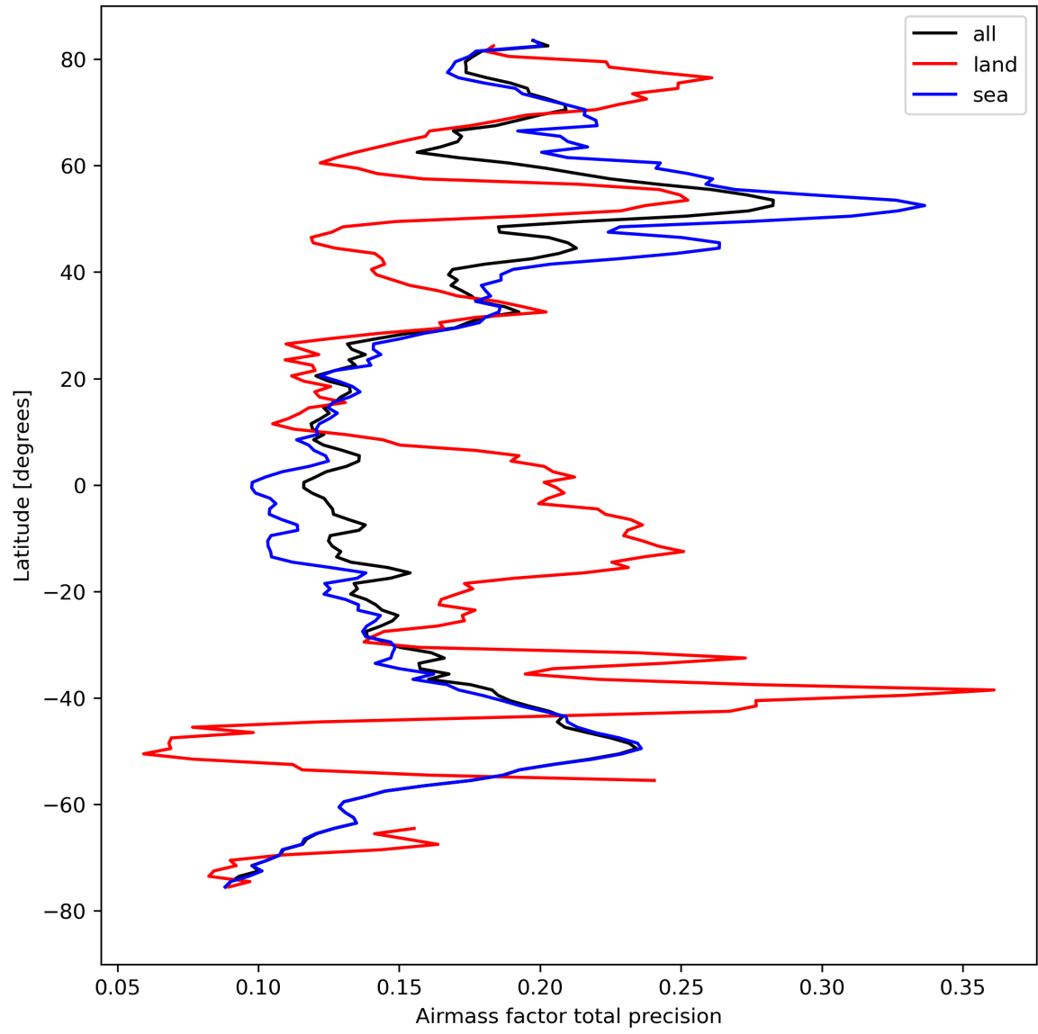
Figure 27: Zonal average of “Airmass factor total precision” for 2024-04-13 to 2024-04-15.
