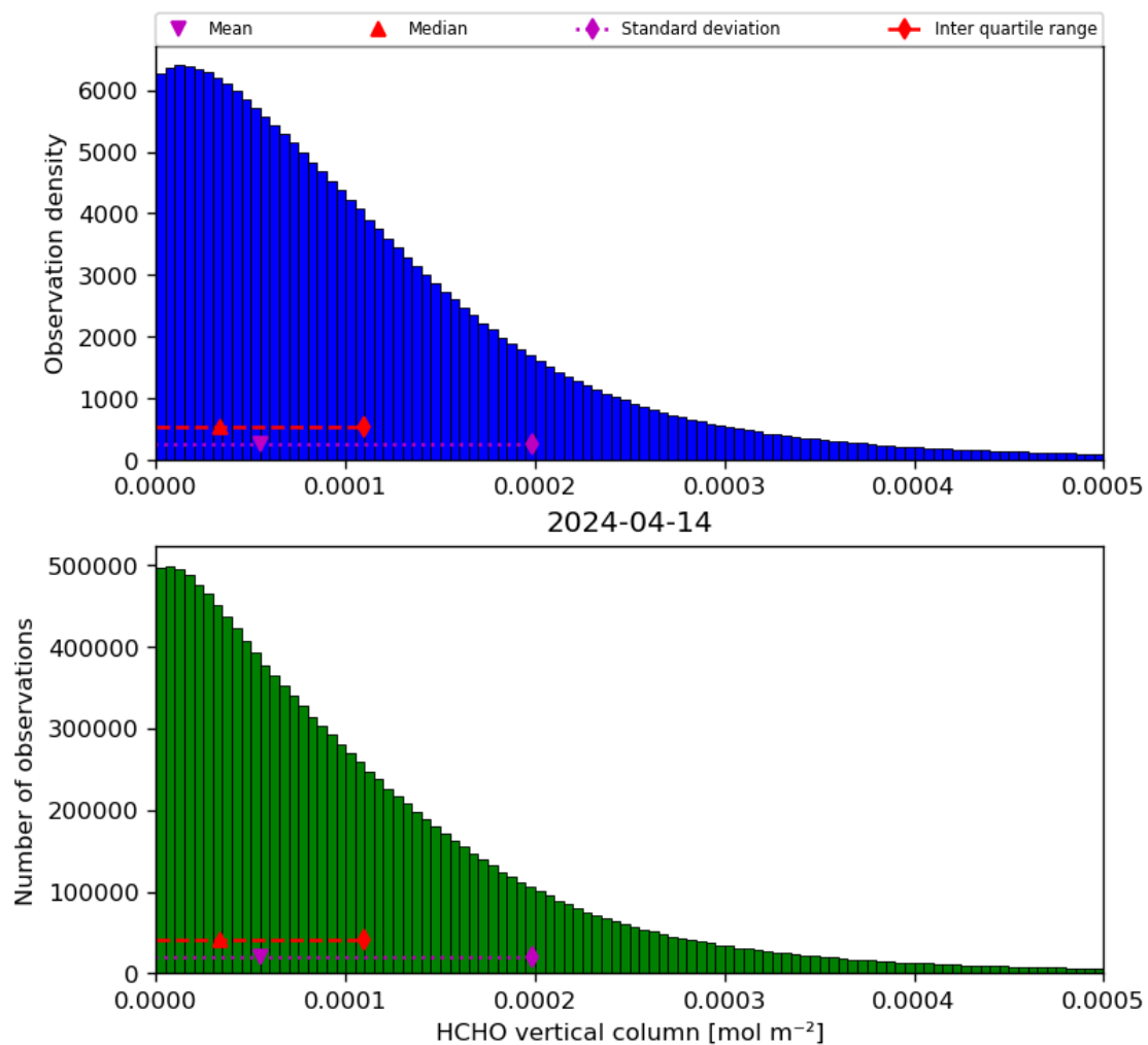
Figure 35: Histogram of “HCHO vertical column” for 2024-04-13 to 2024-04-15
