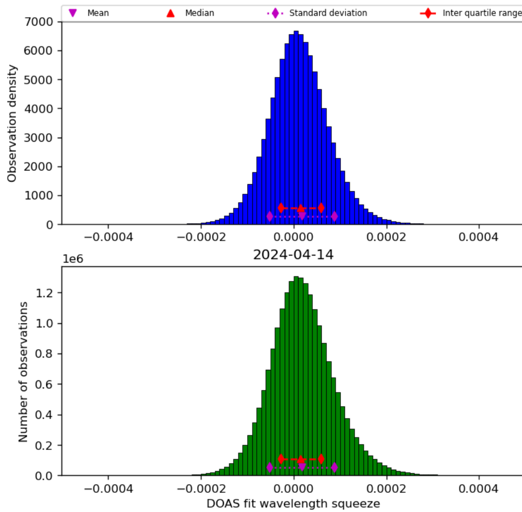
Figure 45: Histogram of “DOAS fit wavelength squeeze” for 2024-04-13 to 2024-04-15
