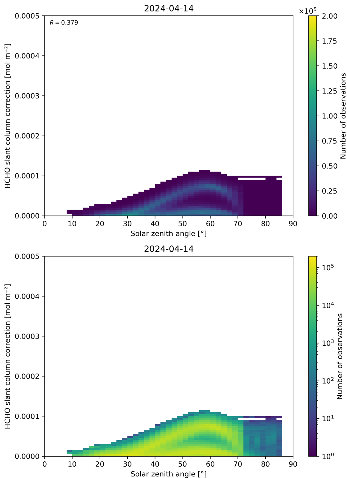
Figure 172: Scatter density plot of “Solar zenith angle” against “HCHO slant column correction” for 2024-04-13 to 2024-04-15.
