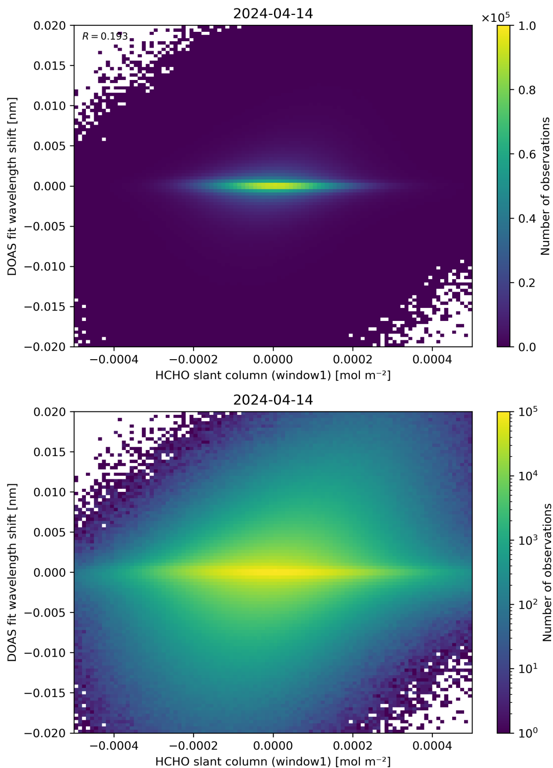
Figure 79: Scatter density plot of “HCHO slant column (window1)” against “DOAS fit wavelength shift” for 2024-04-13 to 2024-04-15.
