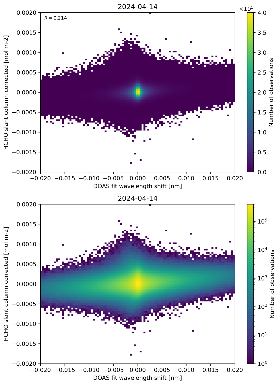
Figure 66: Scatter density plot of “DOAS fit wavelength shift” against “HCHO slant column corrected” for 2024-04-13 to 2024-04-15.
