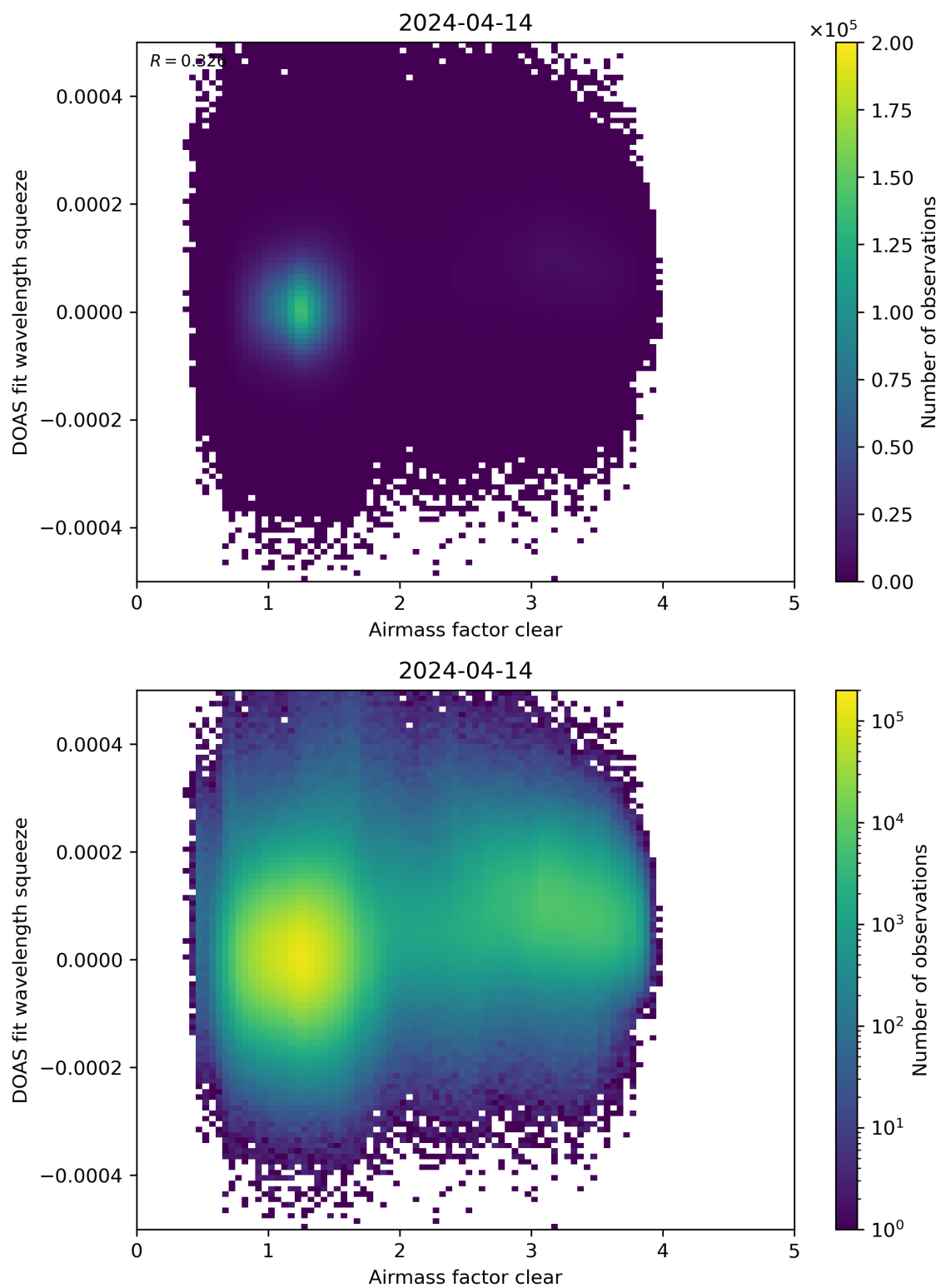
Figure 73: Scatter density plot of “Airmass factor clear” against “DOAS fit wavelength squeeze” for 2024-04-13 to 2024-04-15.
