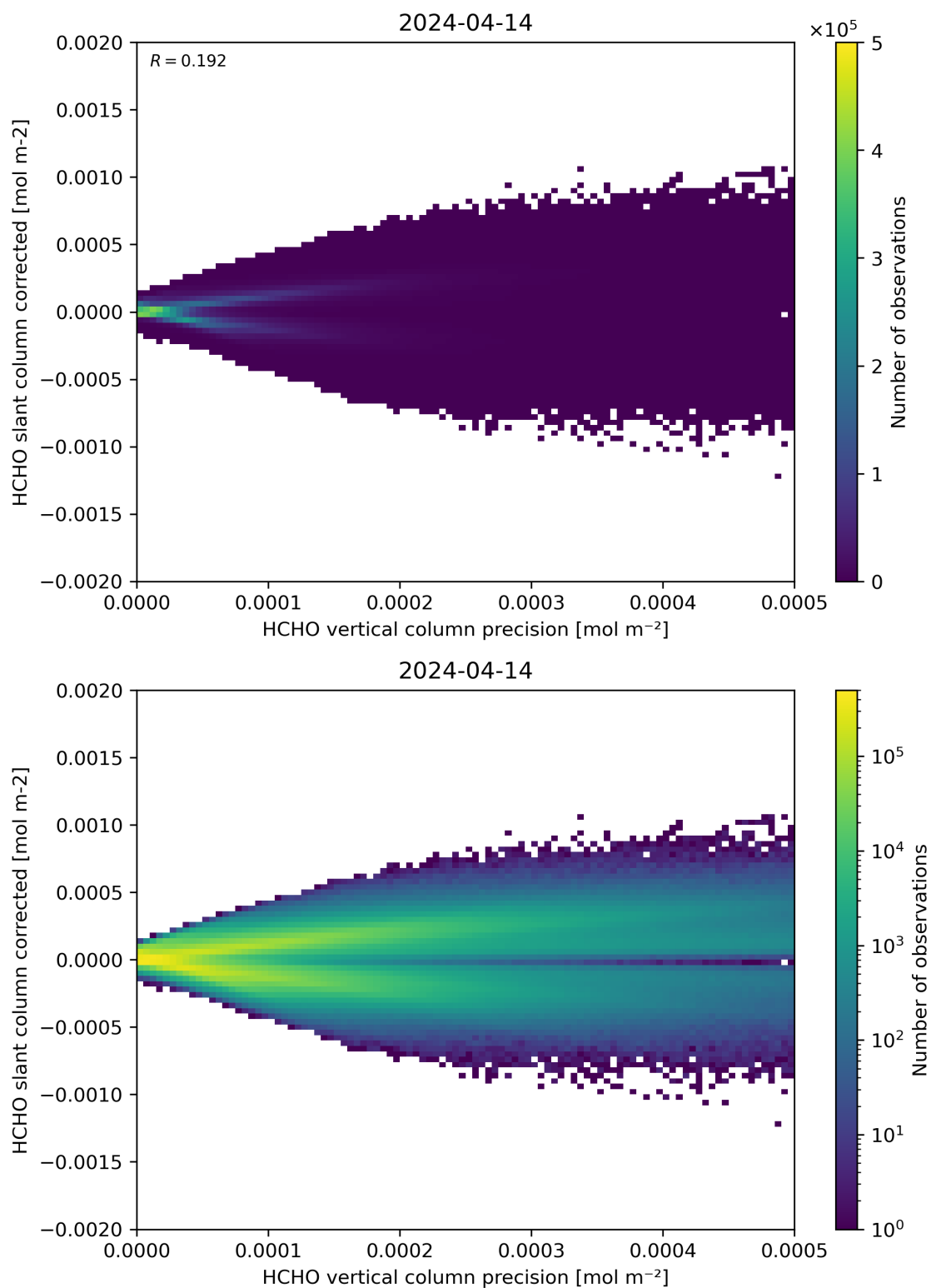
Figure 140: Scatter density plot of “HCHO vertical column precision” against “HCHO slant column corrected” for 2024-04-13 to 2024-04-15.
