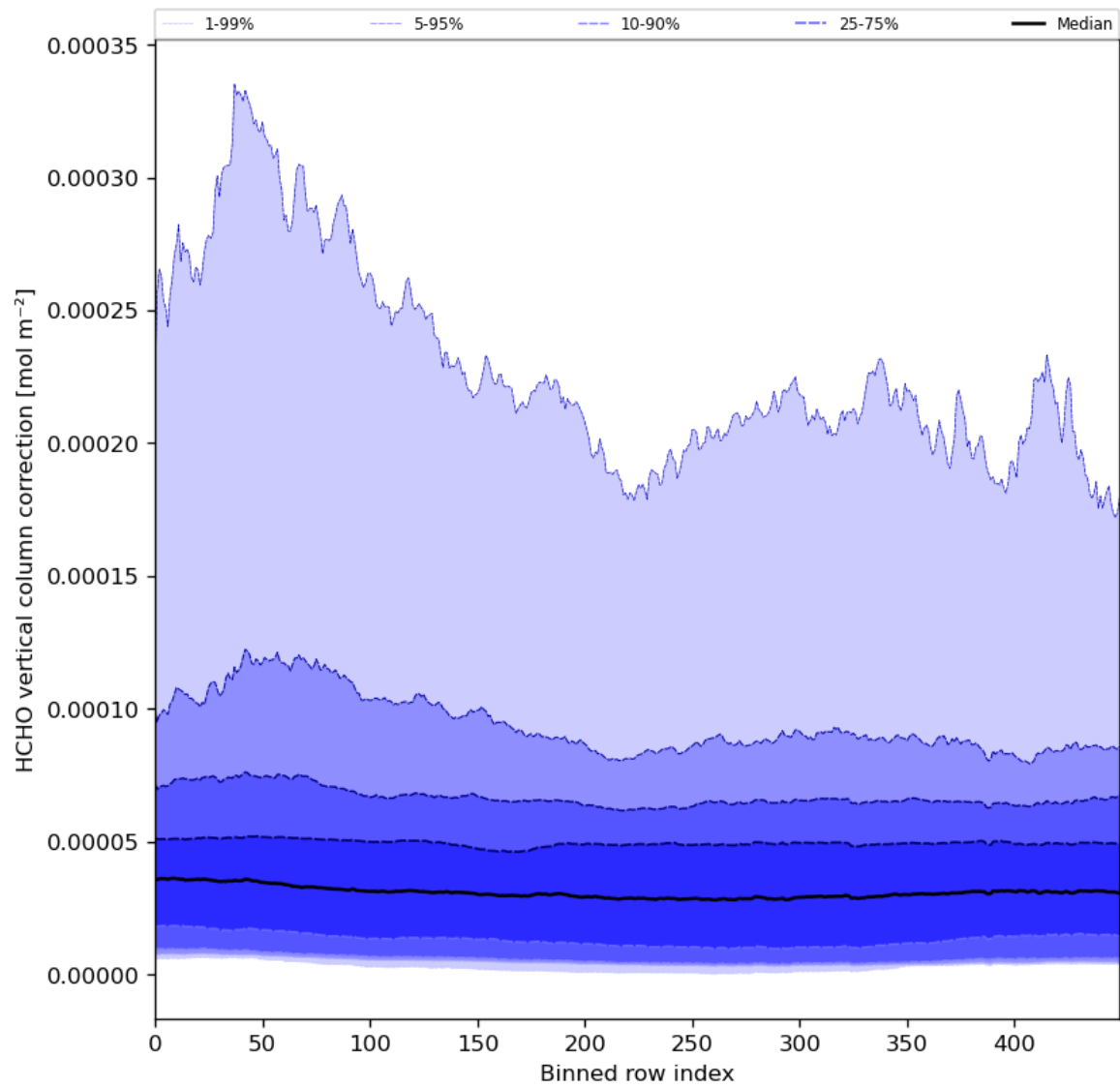
Figure 51: Along track statistics of “HCHO vertical column correction” for 2024-04-13 to 2024-04-15
