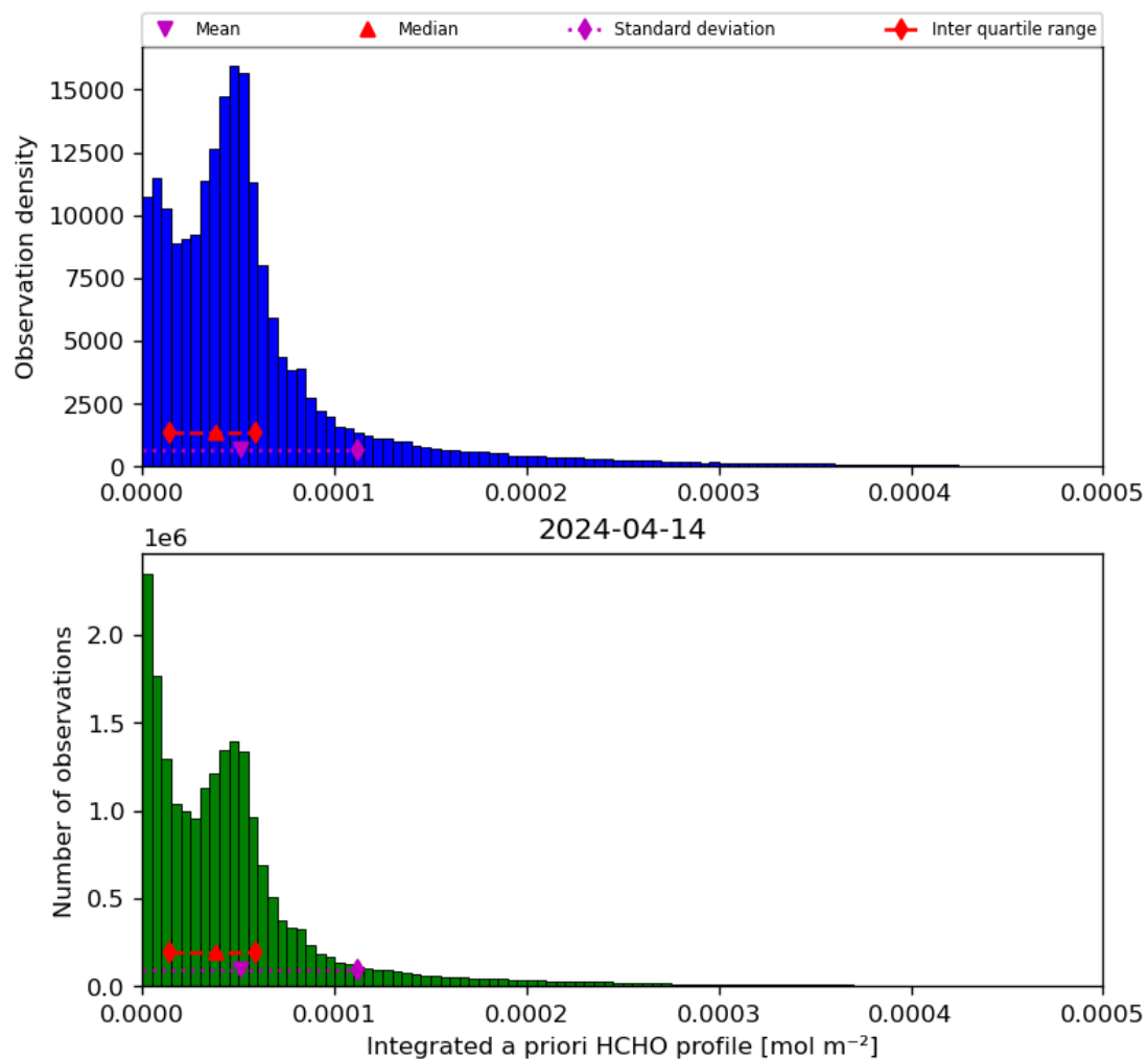
Figure 43: Histogram of “Integrated a priori HCHO profile” for 2024-04-13 to 2024-04-15
