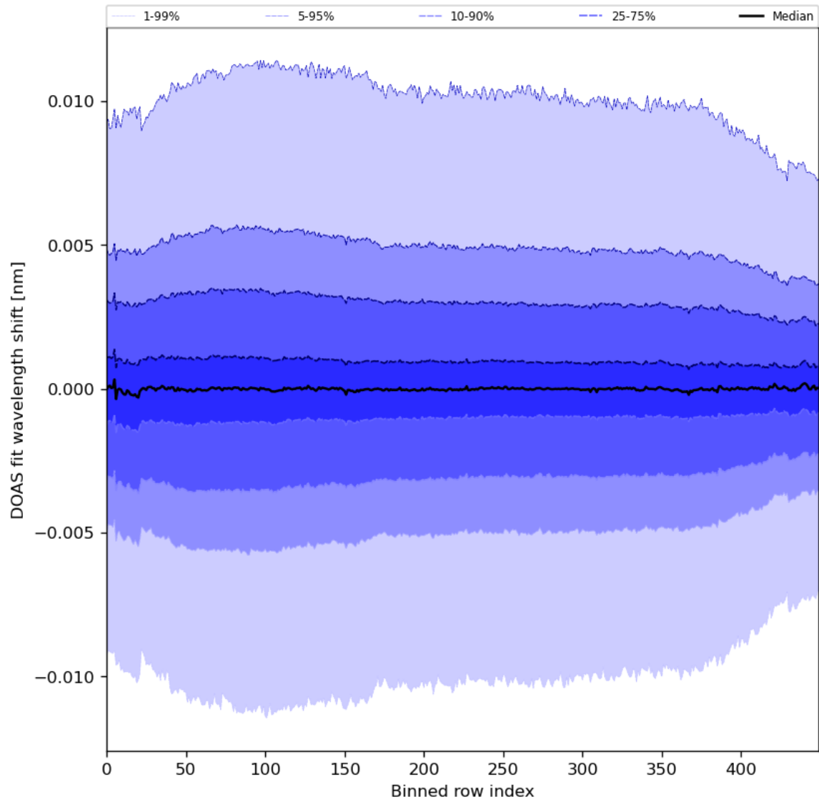
Figure 58: Along track statistics of “DOAS fit wavelength shift” for 2024-04-13 to 2024-04-15
