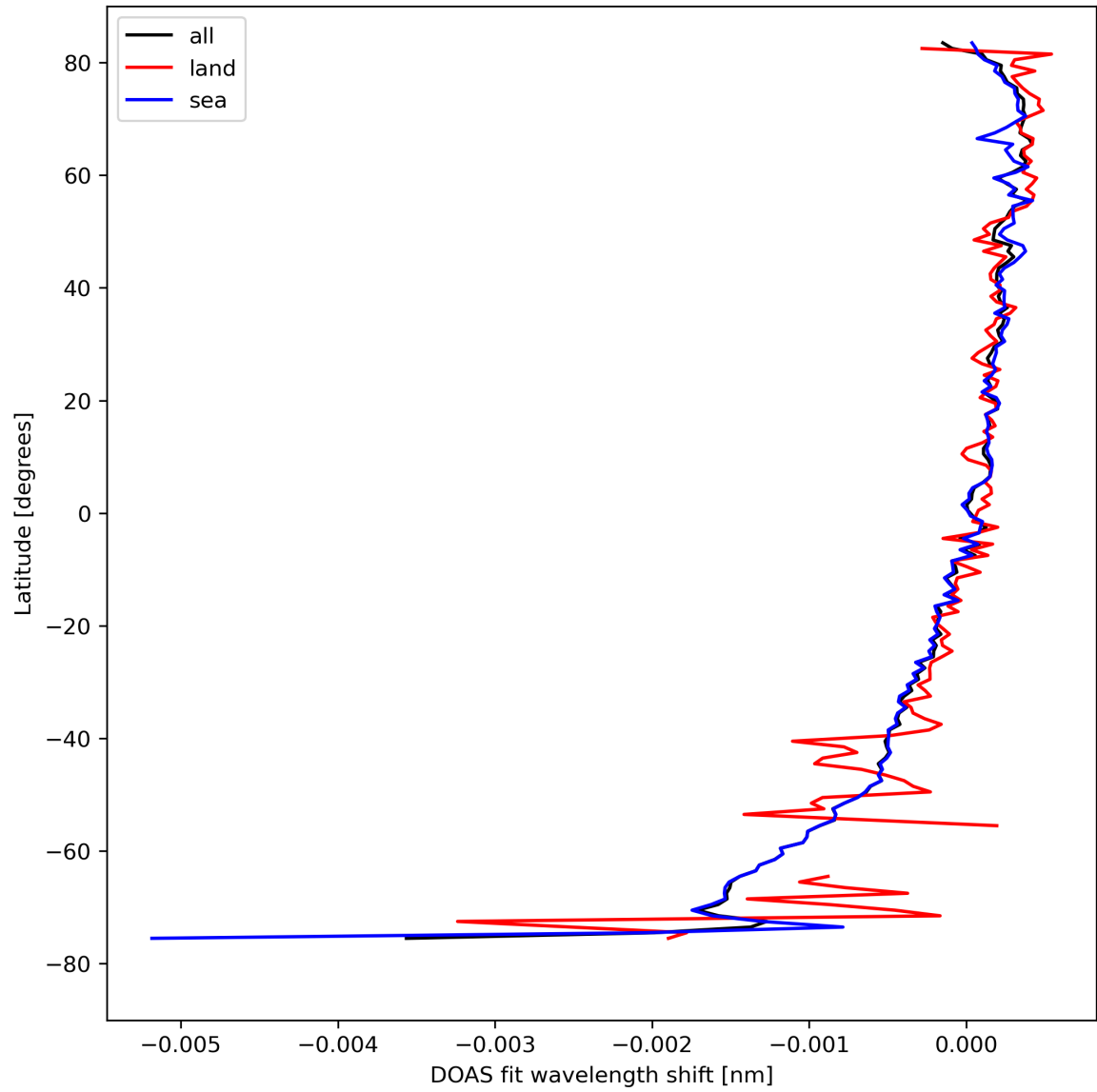
Figure 30: Zonal average of “DOAS fit wavelength shift” for 2024-04-13 to 2024-04-15.
