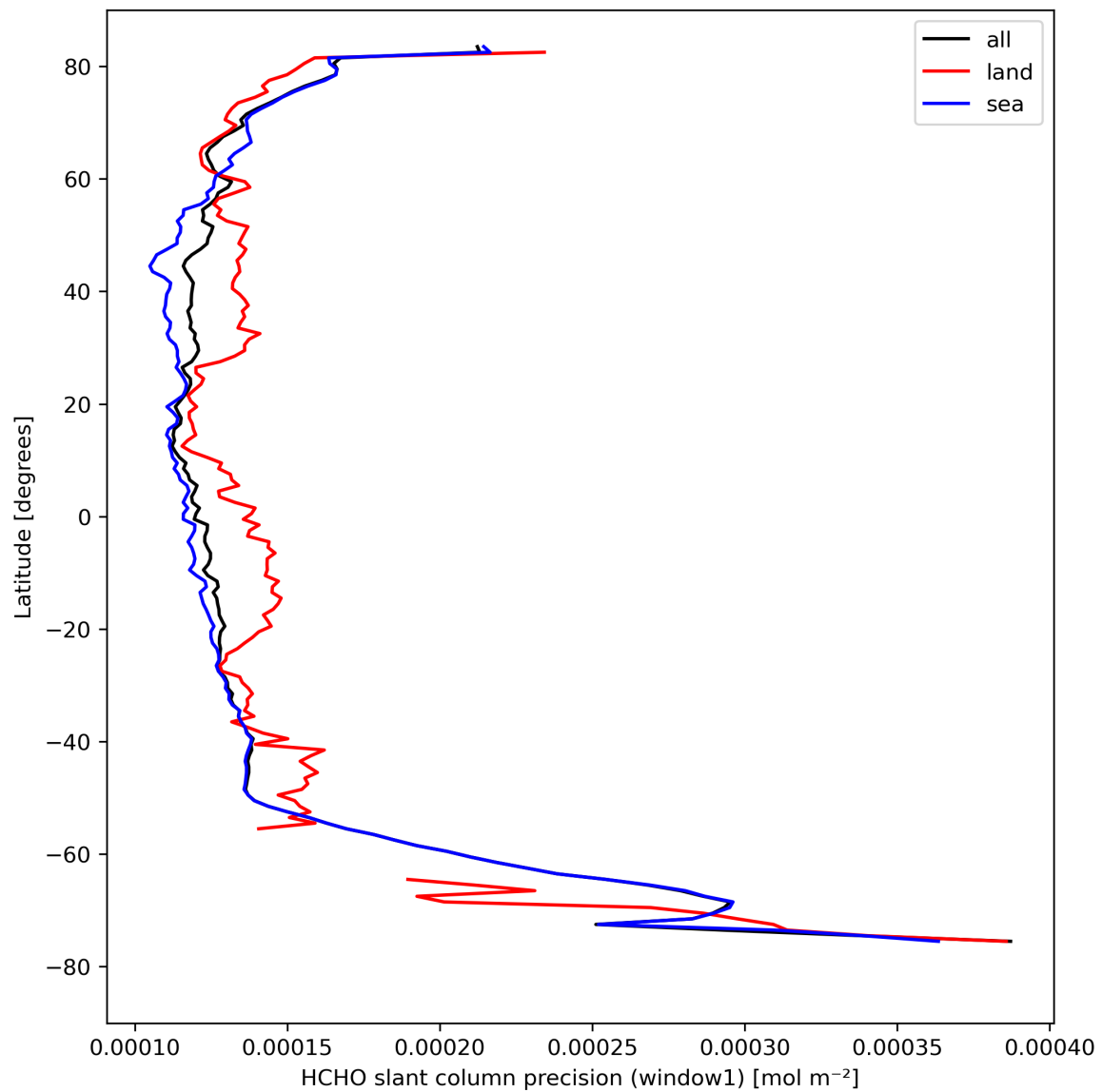
Figure 25: Zonal average of “HCHO slant column precision (window1)” for 2024-04-13 to 2024-04-15.
