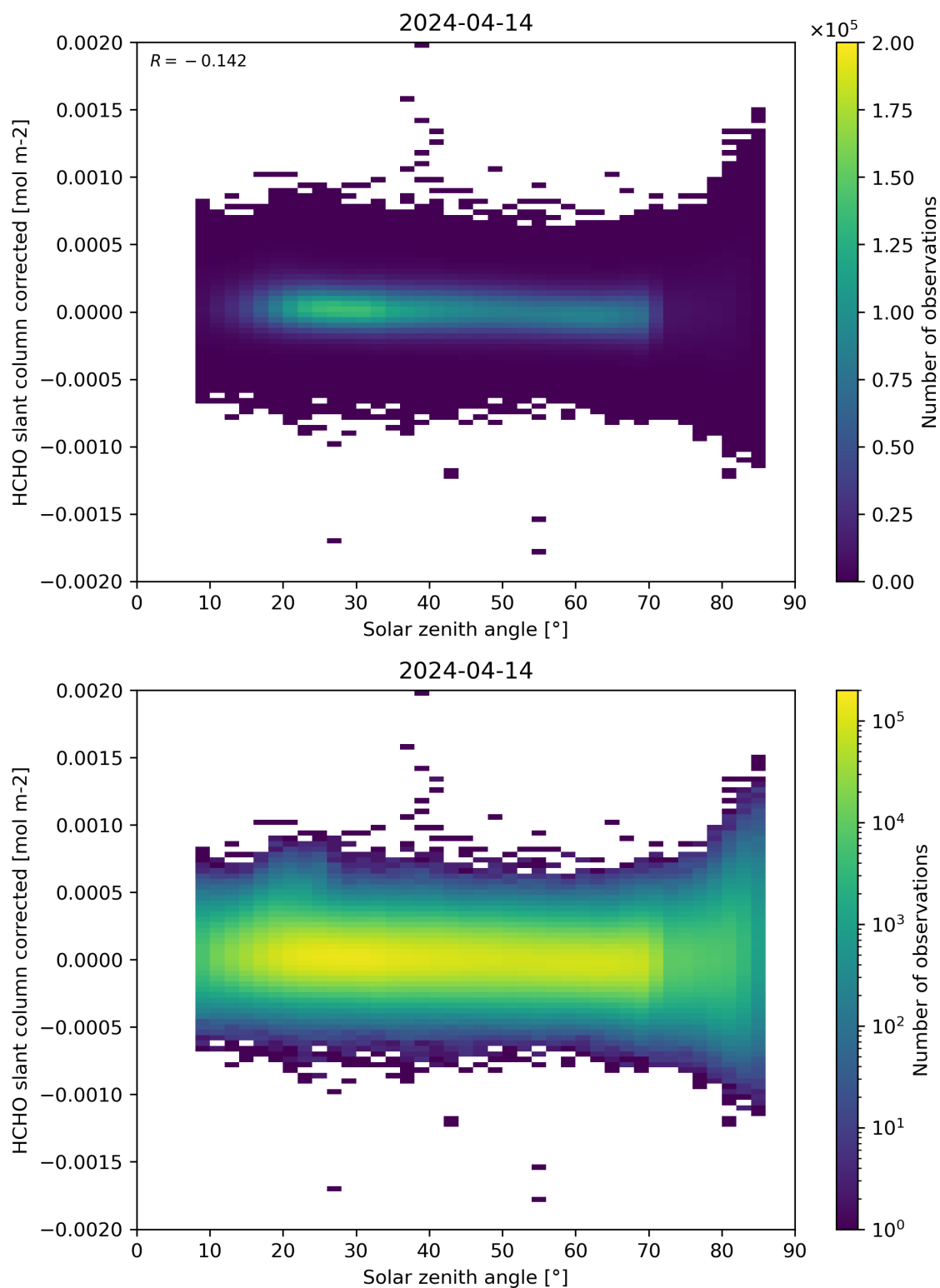
Figure 171: Scatter density plot of “Solar zenith angle” against “HCHO slant column corrected” for 2024-04-13 to 2024-04-15.
