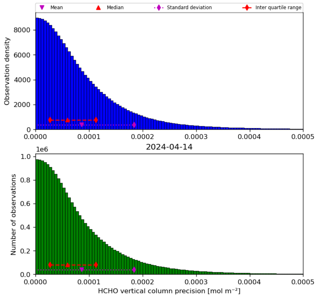
Figure 36: Histogram of “HCHO vertical column precision” for 2024-04-13 to 2024-04-15
