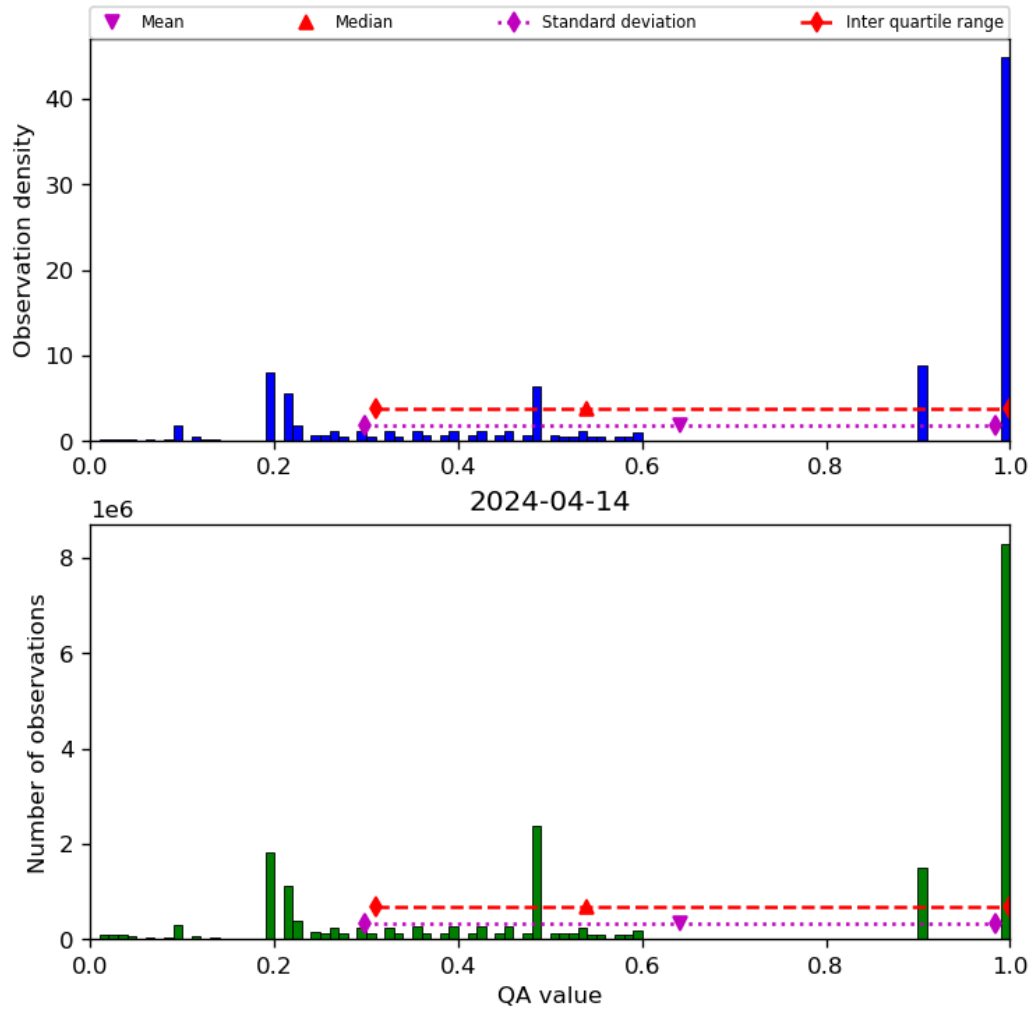
Figure 34: Histogram of “QA value” for 2024-04-13 to 2024-04-15
