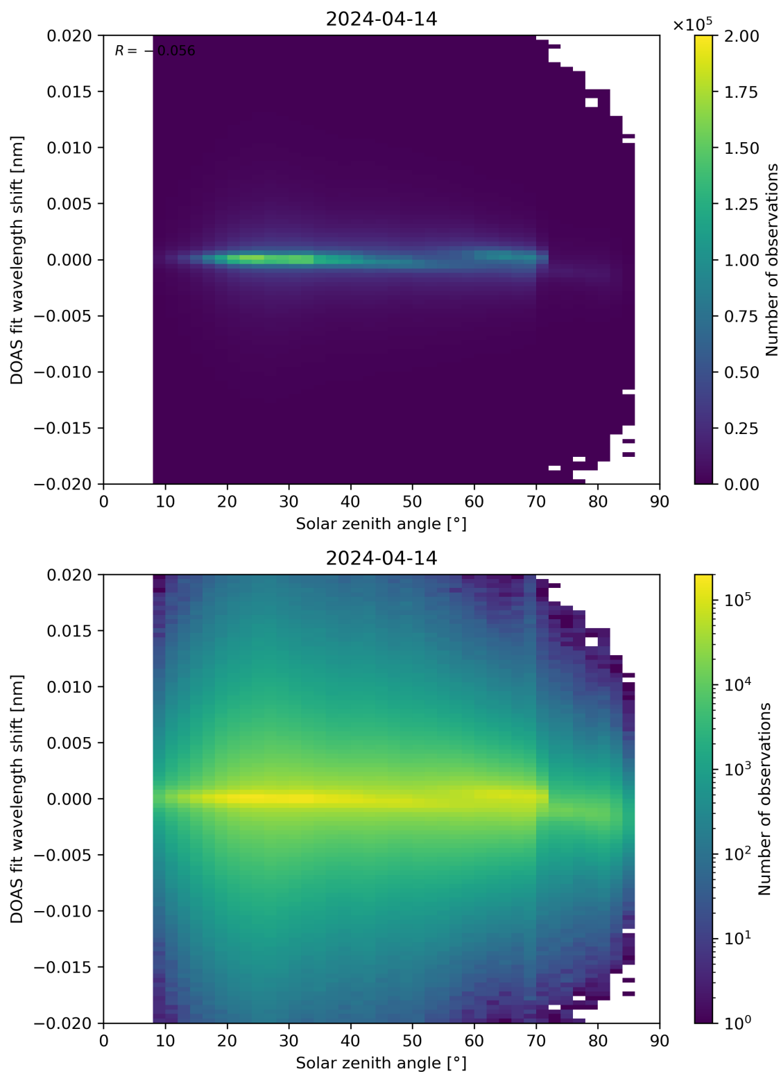
Figure 168: Scatter density plot of “Solar zenith angle” against “DOAS fit wavelength shift” for 2024-04-13 to 2024-04-15.
