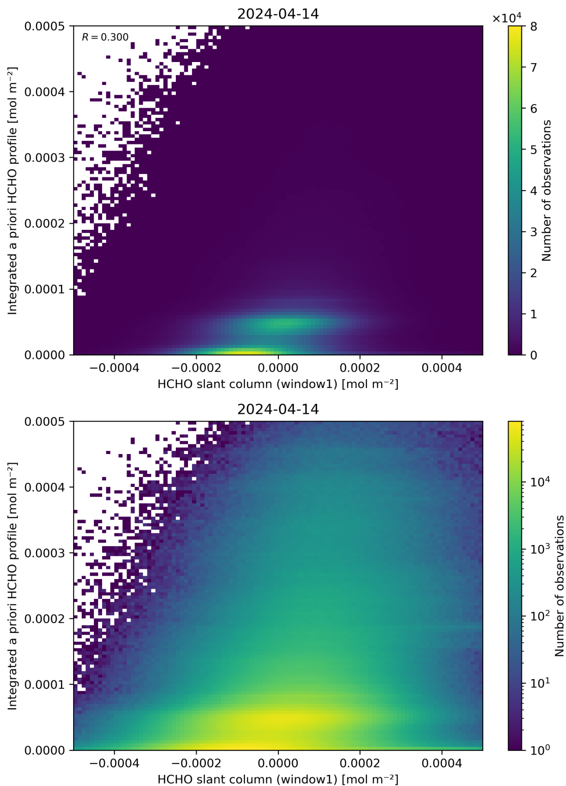
Figure 87: Scatter density plot of “HCHO slant column (window1)” against “Integrated a priori HCHO profile” for 2024-04-13 to 2024-04-15.
