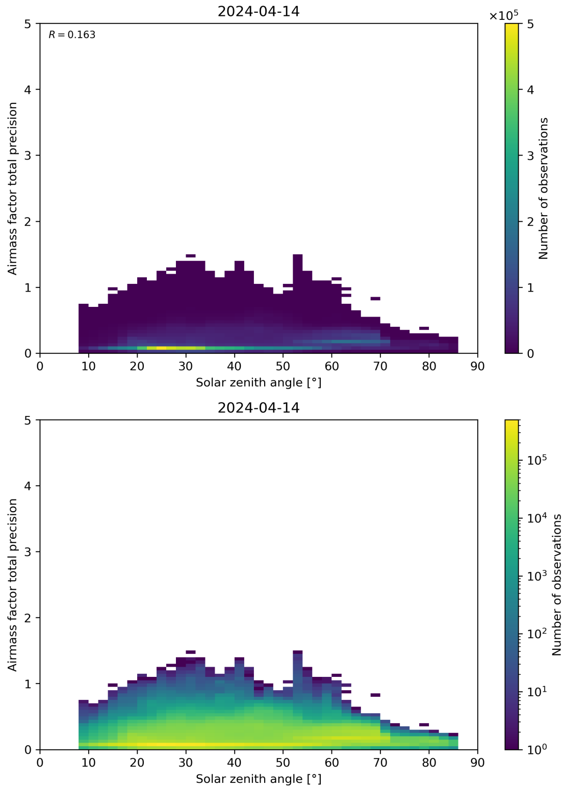
Figure 176: Scatter density plot of “Solar zenith angle” against “Airmass factor total precision” for 2024-04-13 to 2024-04-15.
