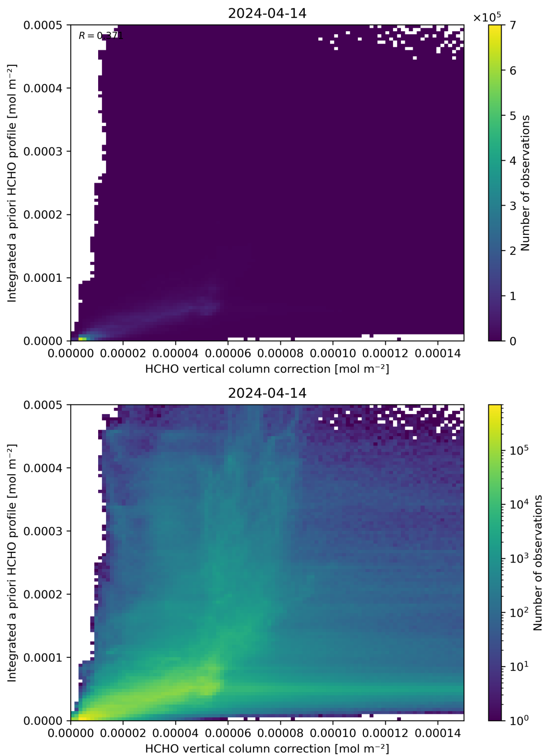
Figure 122: Scatter density plot of “HCHO vertical column correction” against “Integrated a priori HCHO profile” for 2024-04-13 to 2024-04-15.
