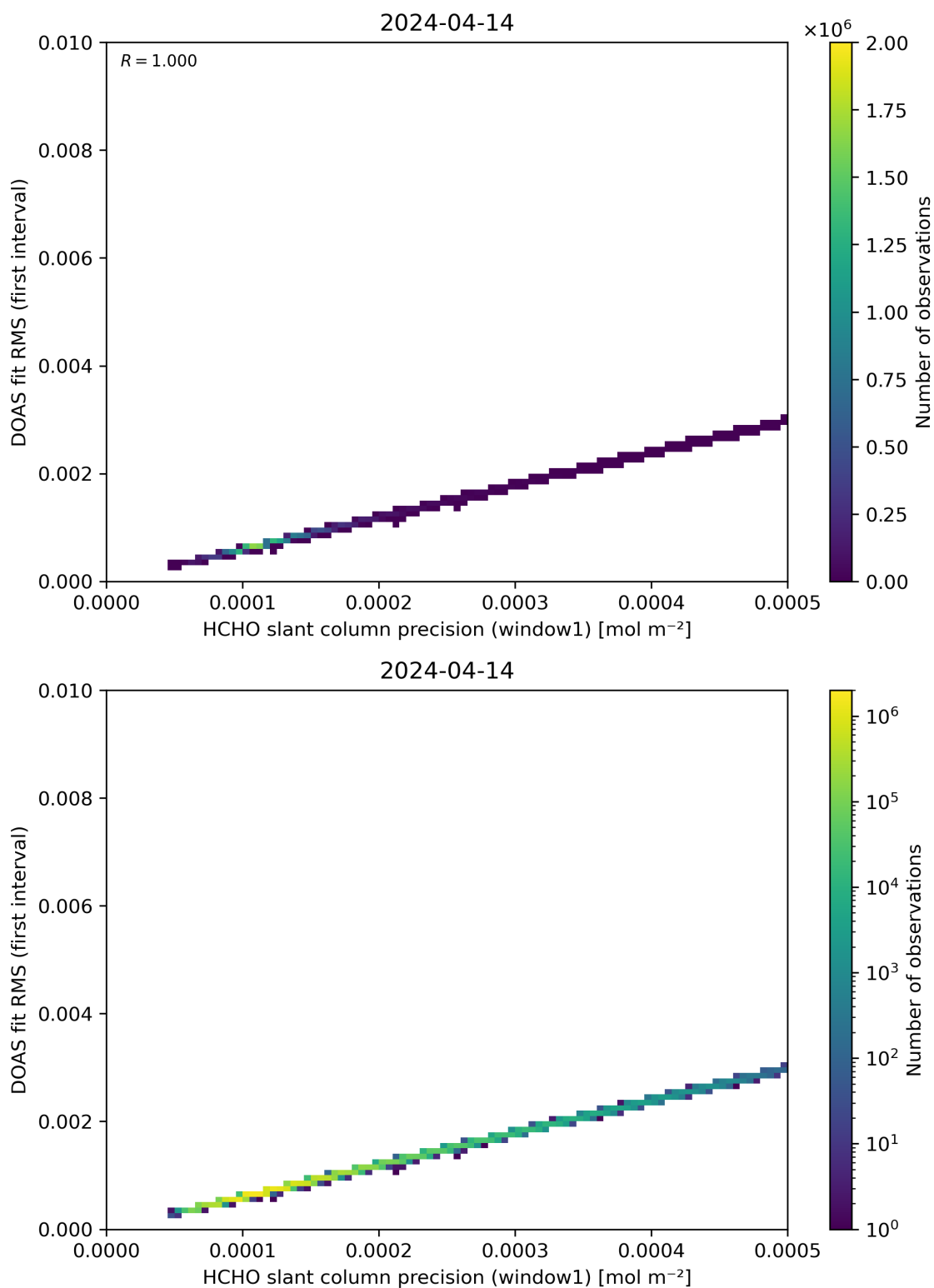
Figure 88: Scatter density plot of “HCHO slant column precision (window1)” against “DOAS fit RMS (first interval)” for 2024-04-13 to 2024-04-15.
