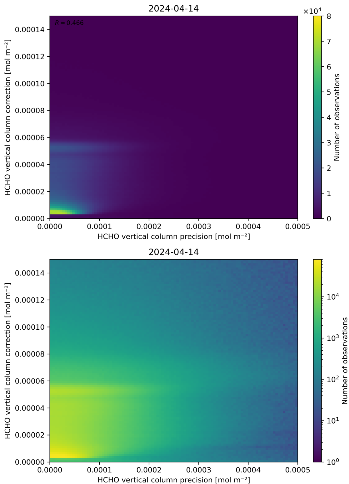
Figure 146: Scatter density plot of “HCHO vertical column precision” against “HCHO vertical column correction” for 2024-04-13 to 2024-04-15.
