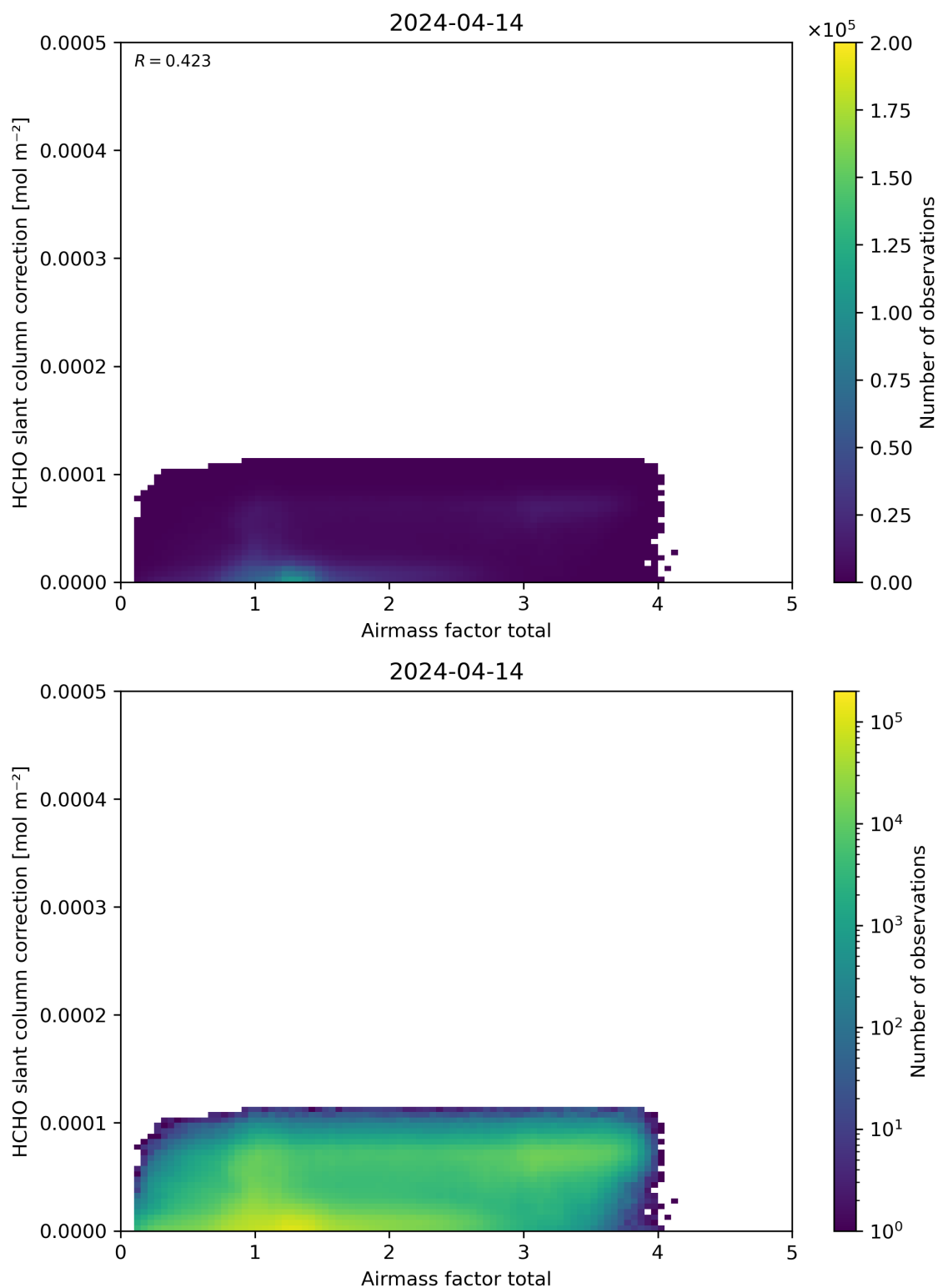
Figure 102: Scatter density plot of “Airmass factor total” against “HCHO slant column correction” for 2024-04-13 to 2024-04-15.
