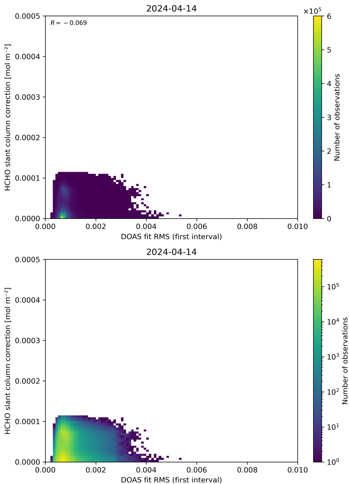
Figure 63: Scatter density plot of “DOAS fit RMS (first interval)” against “HCHO slant column correction” for 2024-04-13 to 2024-04-15.
