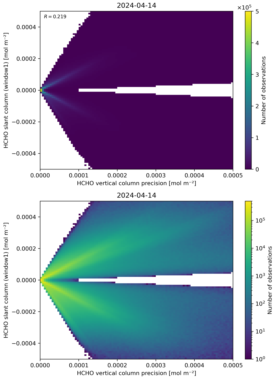
Figure 142: Scatter density plot of “HCHO vertical column precision” against “HCHO slant column (window1)” for 2024-04-13 to 2024-04-15.
