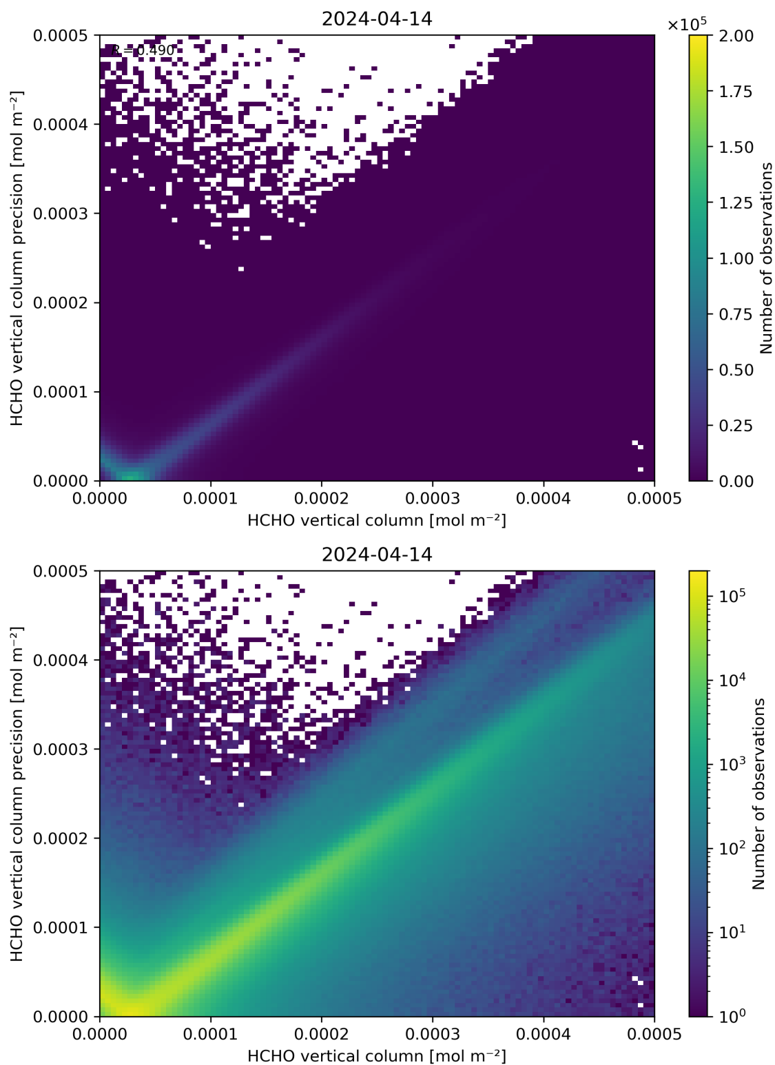
Figure 134: Scatter density plot of “HCHO vertical column” against “HCHO vertical column precision” for 2024-04-13 to 2024-04-15.
