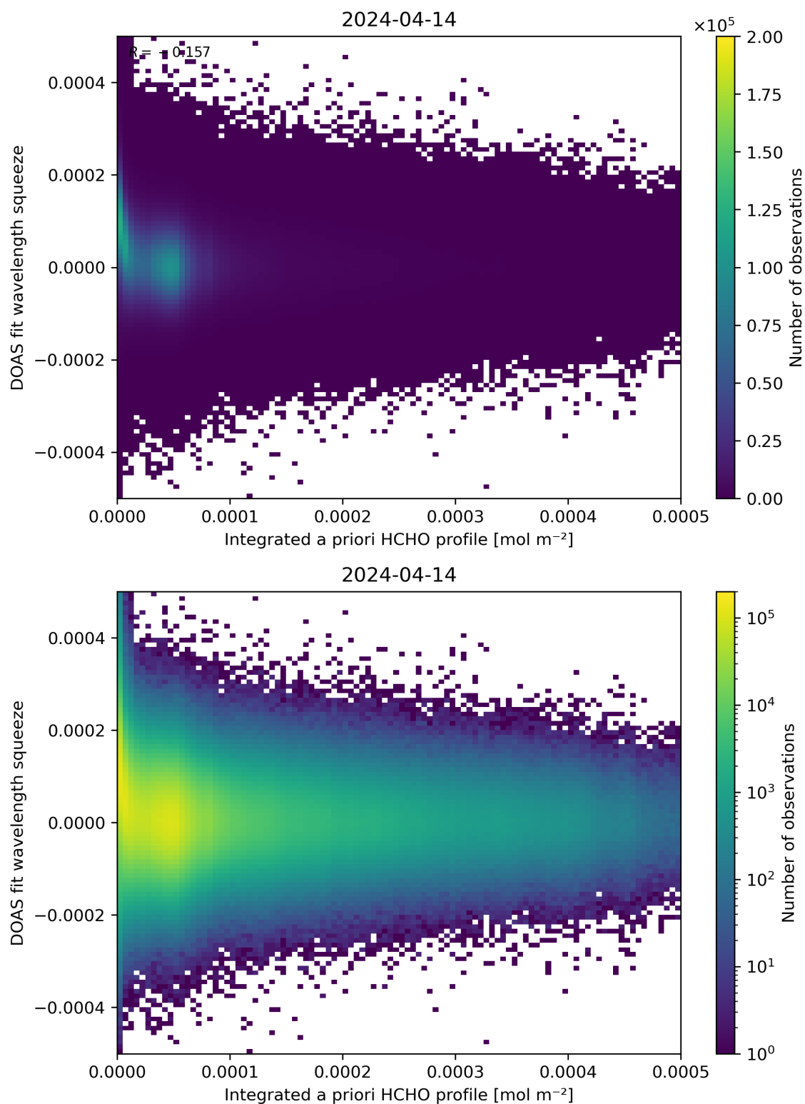
Figure 150: Scatter density plot of “Integrated a priori HCHO profile” against “DOAS fit wavelength squeeze” for 2024-04-13 to 2024-04-15.
