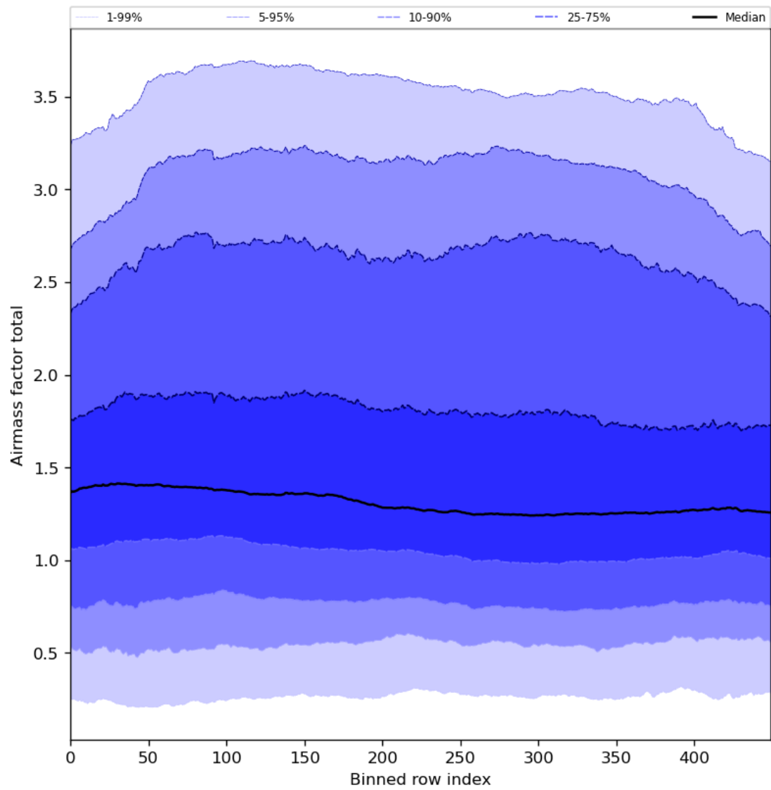
Figure 54: Along track statistics of “Airmass factor total” for 2024-04-13 to 2024-04-15
