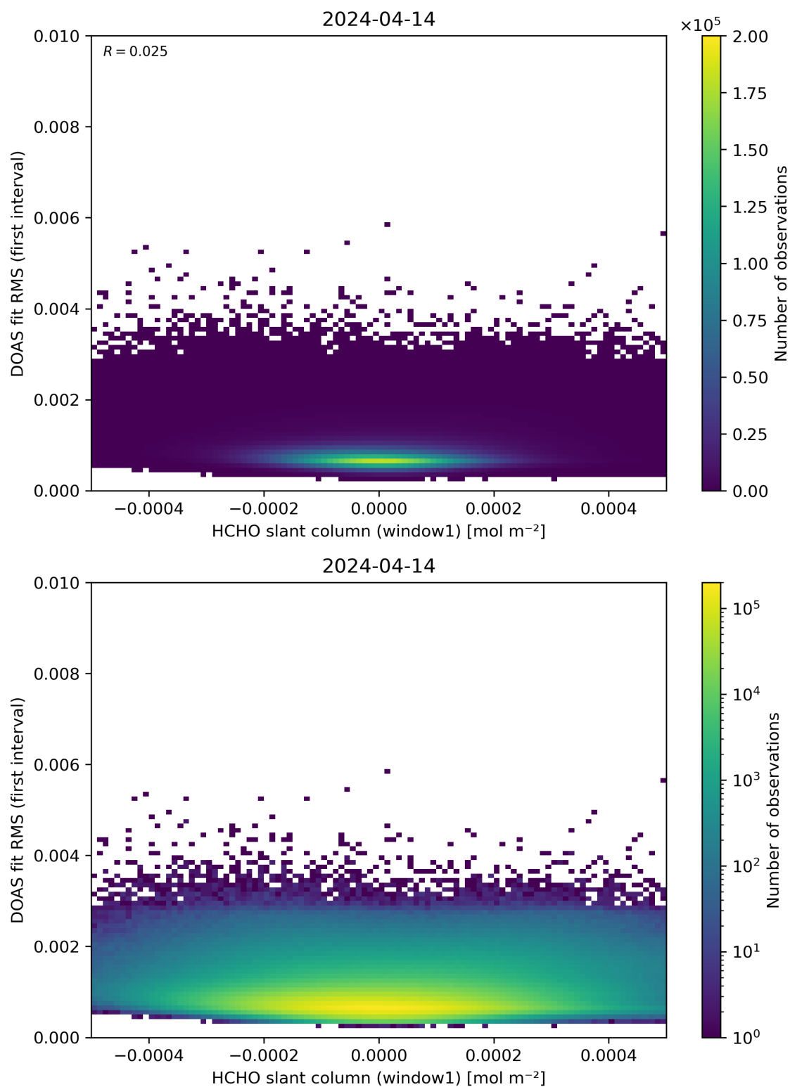
Figure 78: Scatter density plot of “HCHO slant column (window1)” against “DOAS fit RMS (first interval)” for 2024-04-13 to 2024-04-15.
