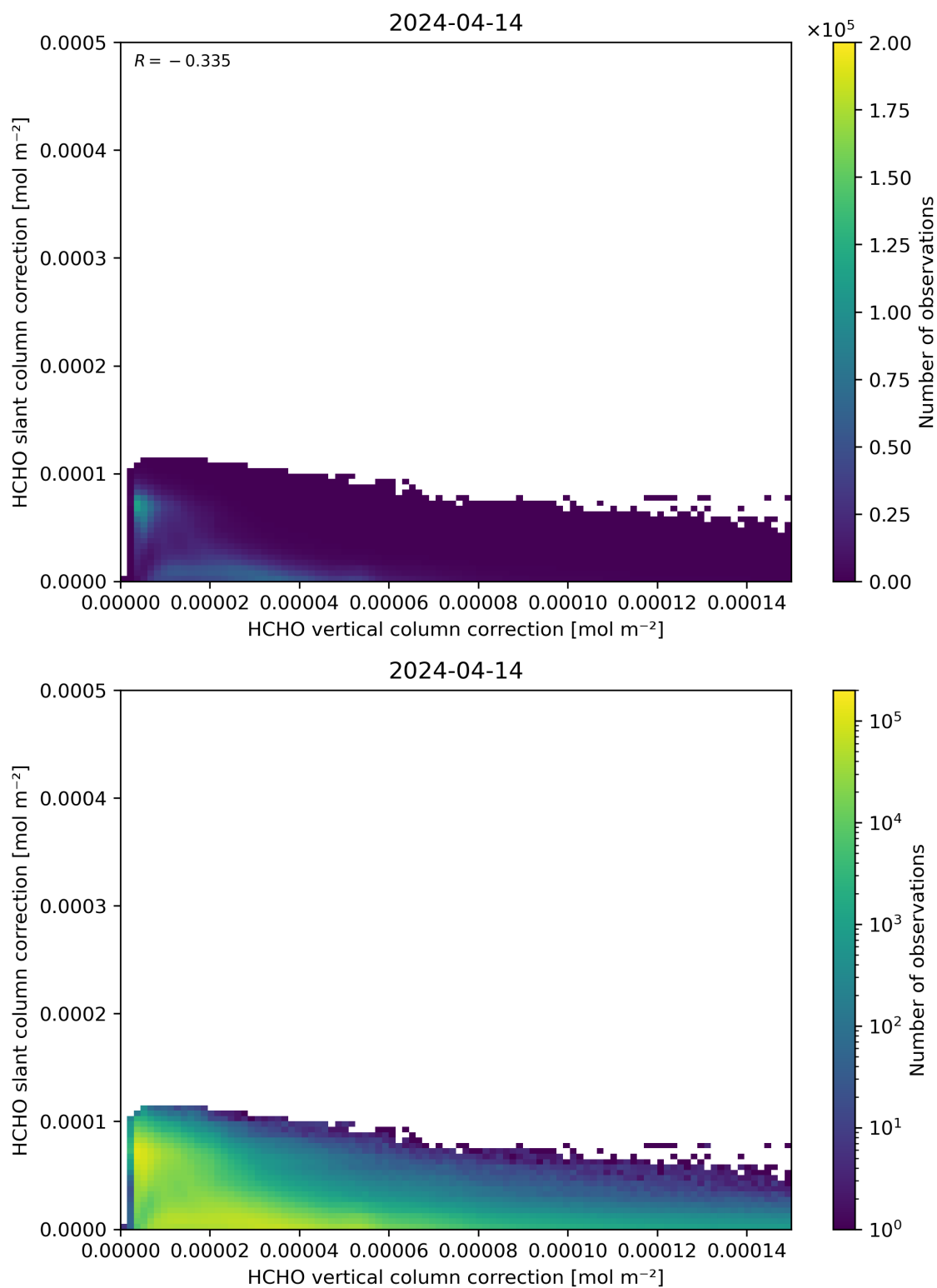
Figure 117: Scatter density plot of “HCHO vertical column correction” against “HCHO slant column correction” for 2024-04-13 to 2024-04-15.
