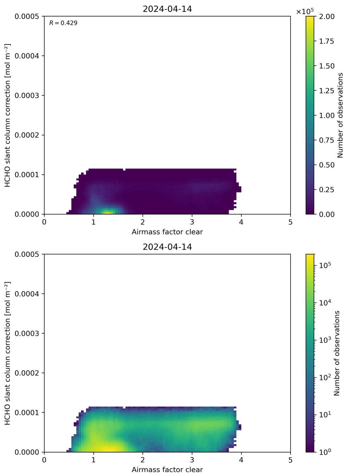
Figure 75: Scatter density plot of “Airmass factor clear” against “HCHO slant column correction” for 2024-04-13 to 2024-04-15.
