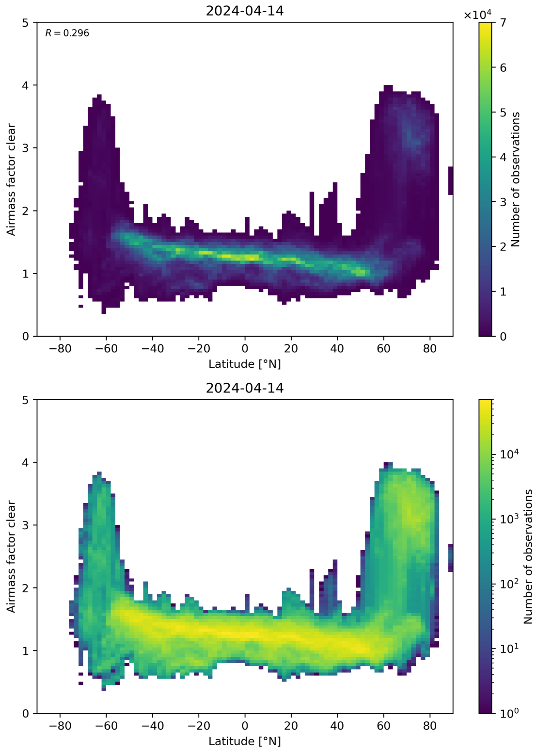
Figure 156: Scatter density plot of “Latitude” against “Airmass factor clear” for 2024-04-13 to 2024-04-15.
