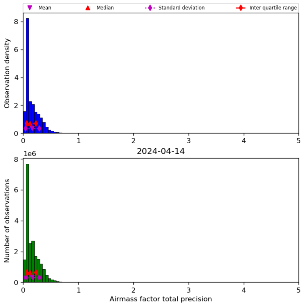
Figure 41: Histogram of “Airmass factor total precision” for 2024-04-13 to 2024-04-15
