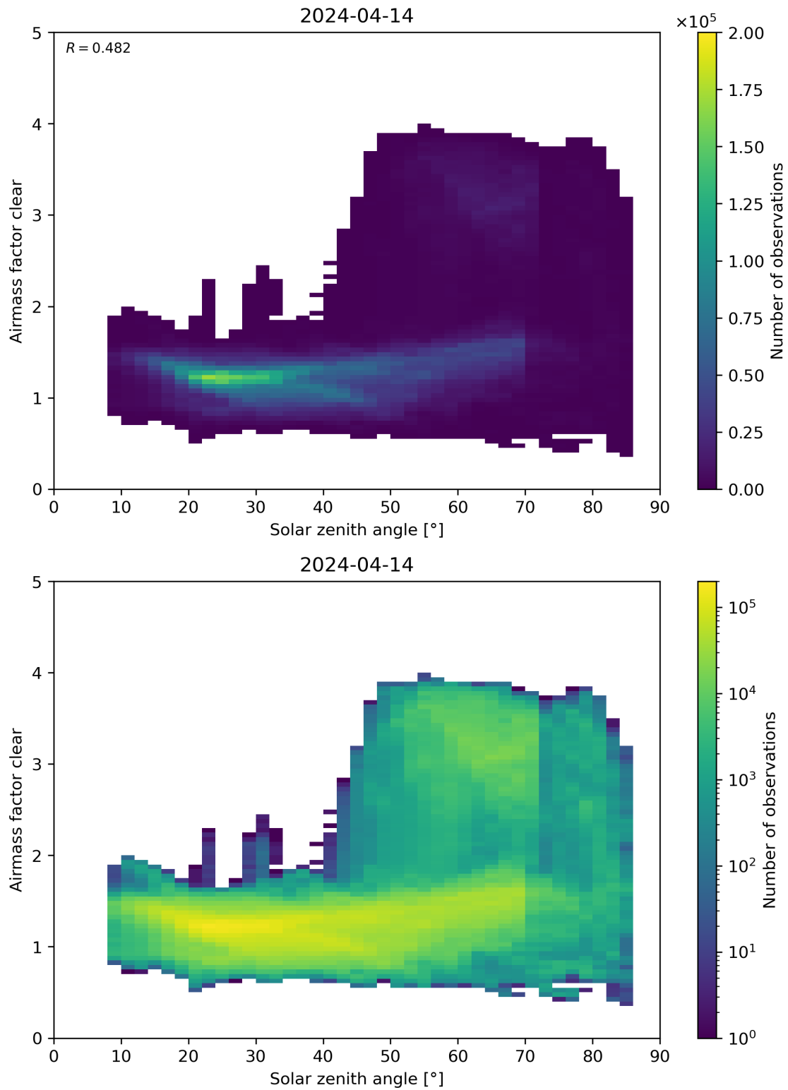
Figure 170: Scatter density plot of “Solar zenith angle” against “Airmass factor clear” for 2024-04-13 to 2024-04-15.
