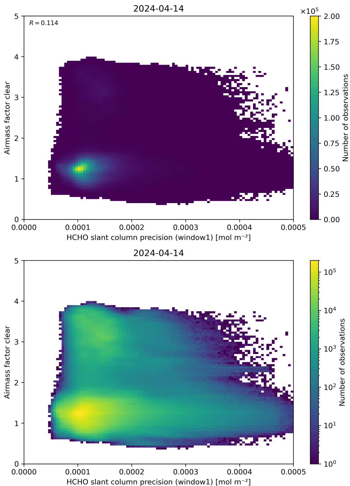
Figure 91: Scatter density plot of “HCHO slant column precision (window1)” against “Airmass factor clear” for 2024-04-13 to 2024-04-15.
