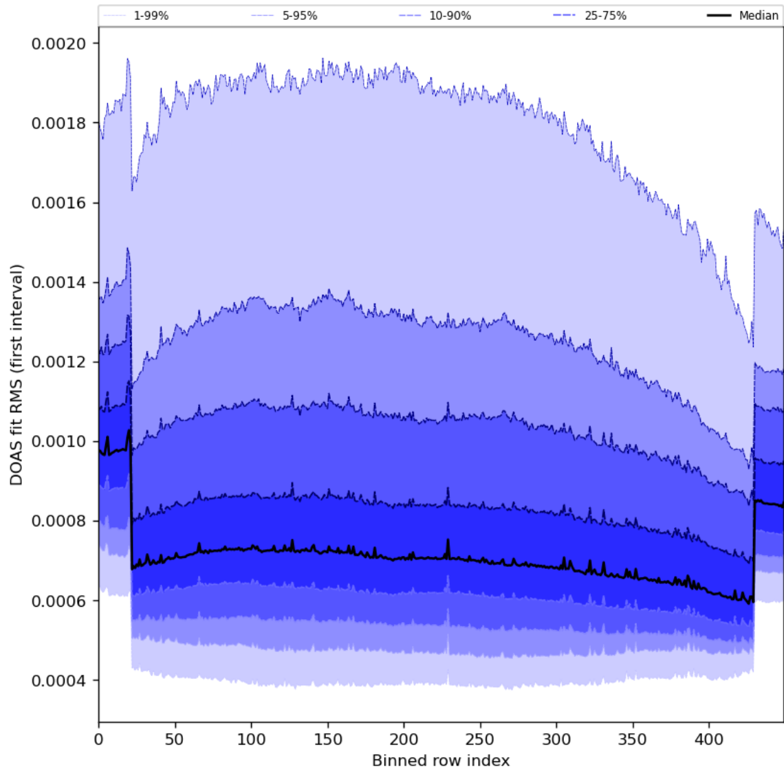
Figure 60: Along track statistics of “DOAS fit RMS (first interval)” for 2024-04-13 to 2024-04-15
