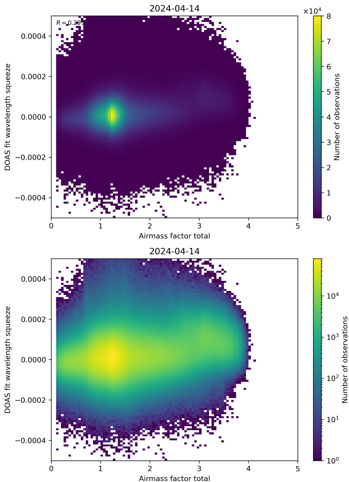
Figure 99: Scatter density plot of “Airmass factor total” against “DOAS fit wavelength squeeze” for 2024-04-13 to 2024-04-15.
