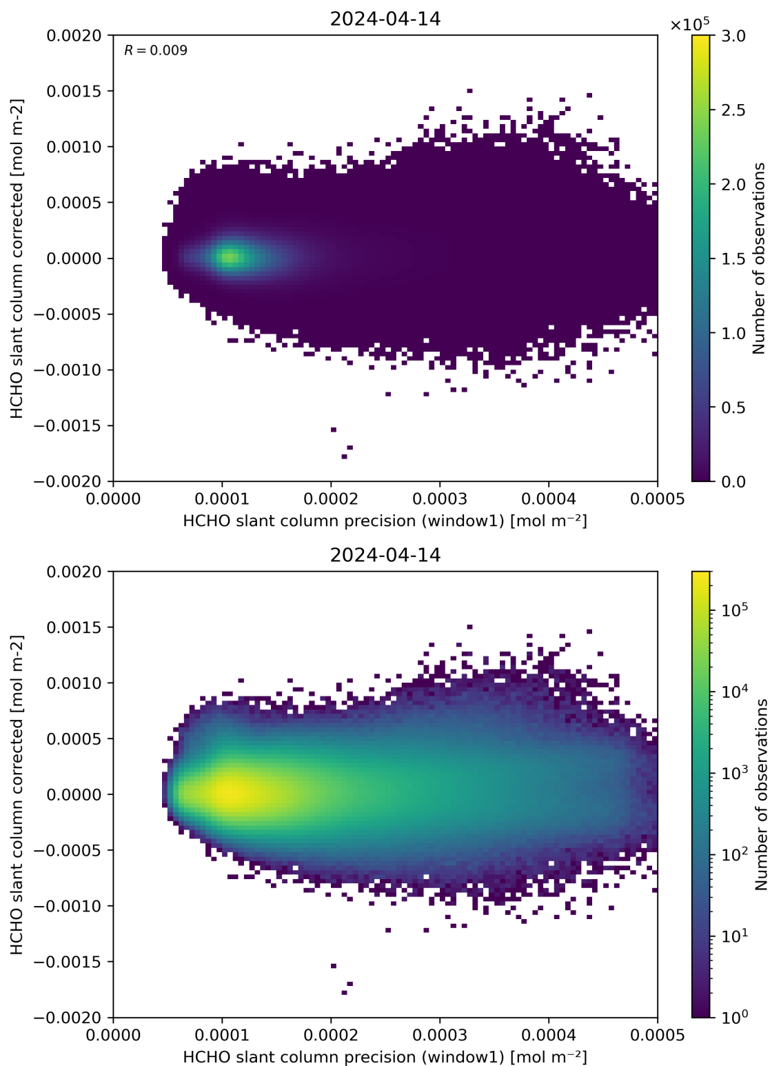
Figure 92: Scatter density plot of “HCHO slant column precision (window1)” against “HCHO slant column corrected” for 2024-04-13 to 2024-04-15.
