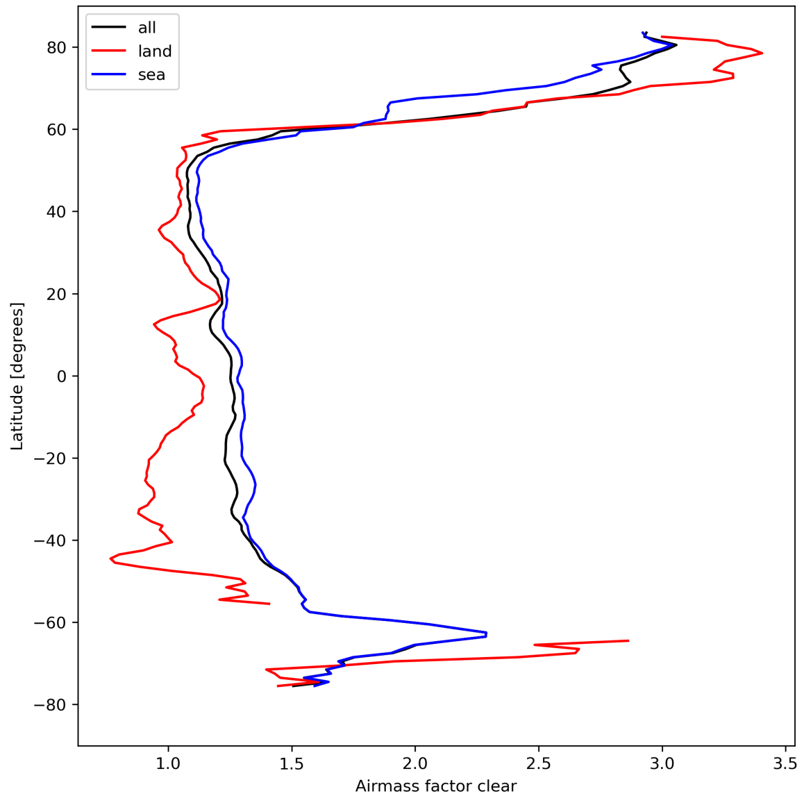
Figure 28: Zonal average of “Airmass factor clear” for 2024-04-13 to 2024-04-15.
