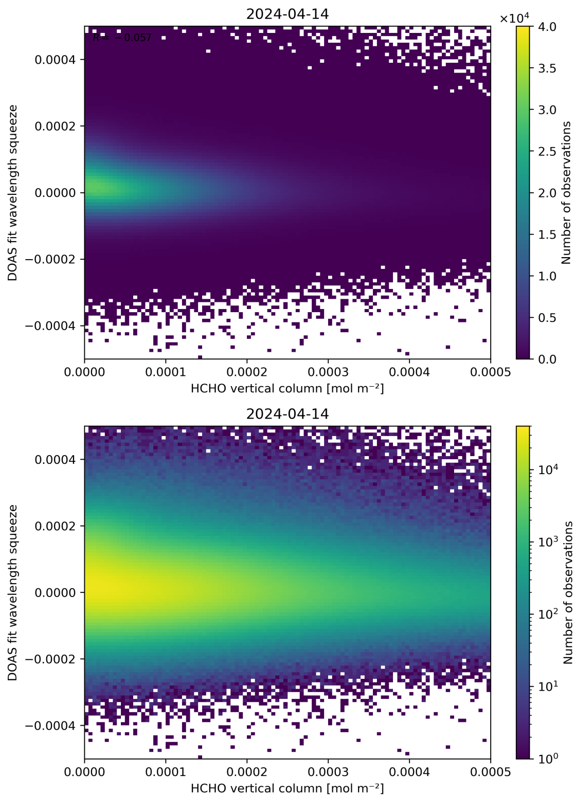
Figure 125: Scatter density plot of “HCHO vertical column” against “DOAS fit wavelength squeeze” for 2024-04-13 to 2024-04-15.
