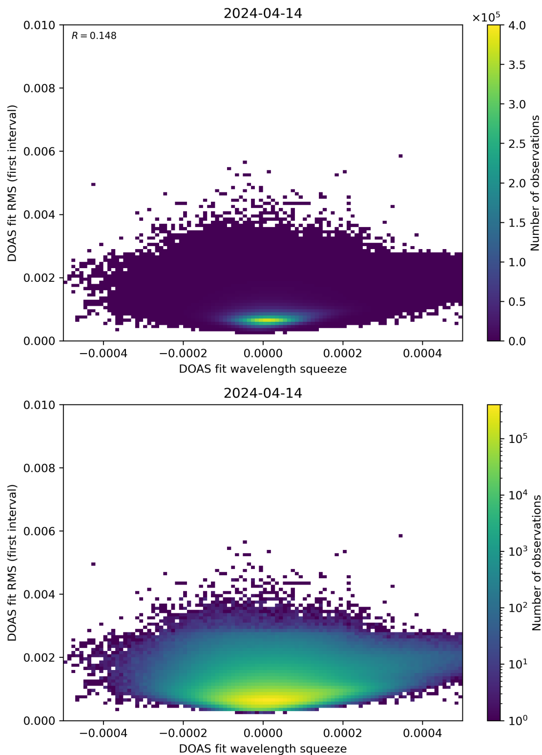
Figure 68: Scatter density plot of “DOAS fit wavelength squeeze” against “DOAS fit RMS (first interval)” for 2024-04-13 to 2024-04-15.
