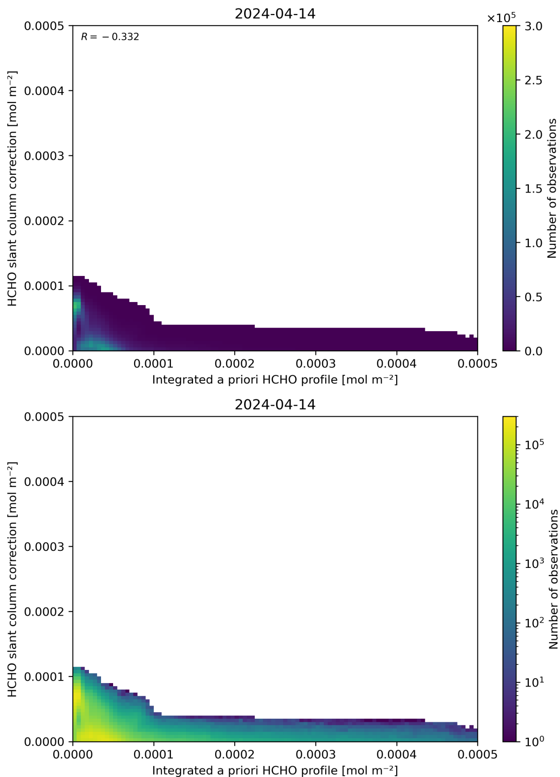
Figure 152: Scatter density plot of “Integrated a priori HCHO profile” against “HCHO slant column correction” for 2024-04-13 to 2024-04-15.
