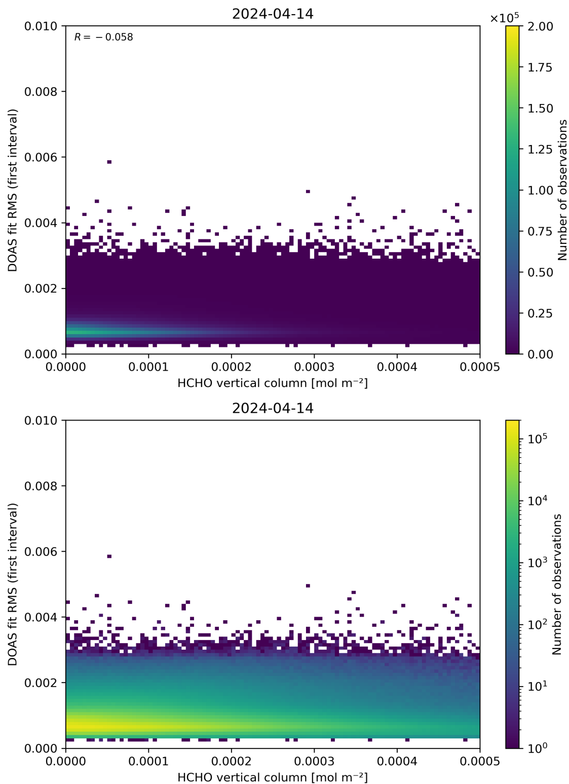
Figure 123: Scatter density plot of “HCHO vertical column” against “DOAS fit RMS (first interval)” for 2024-04-13 to 2024-04-15.
