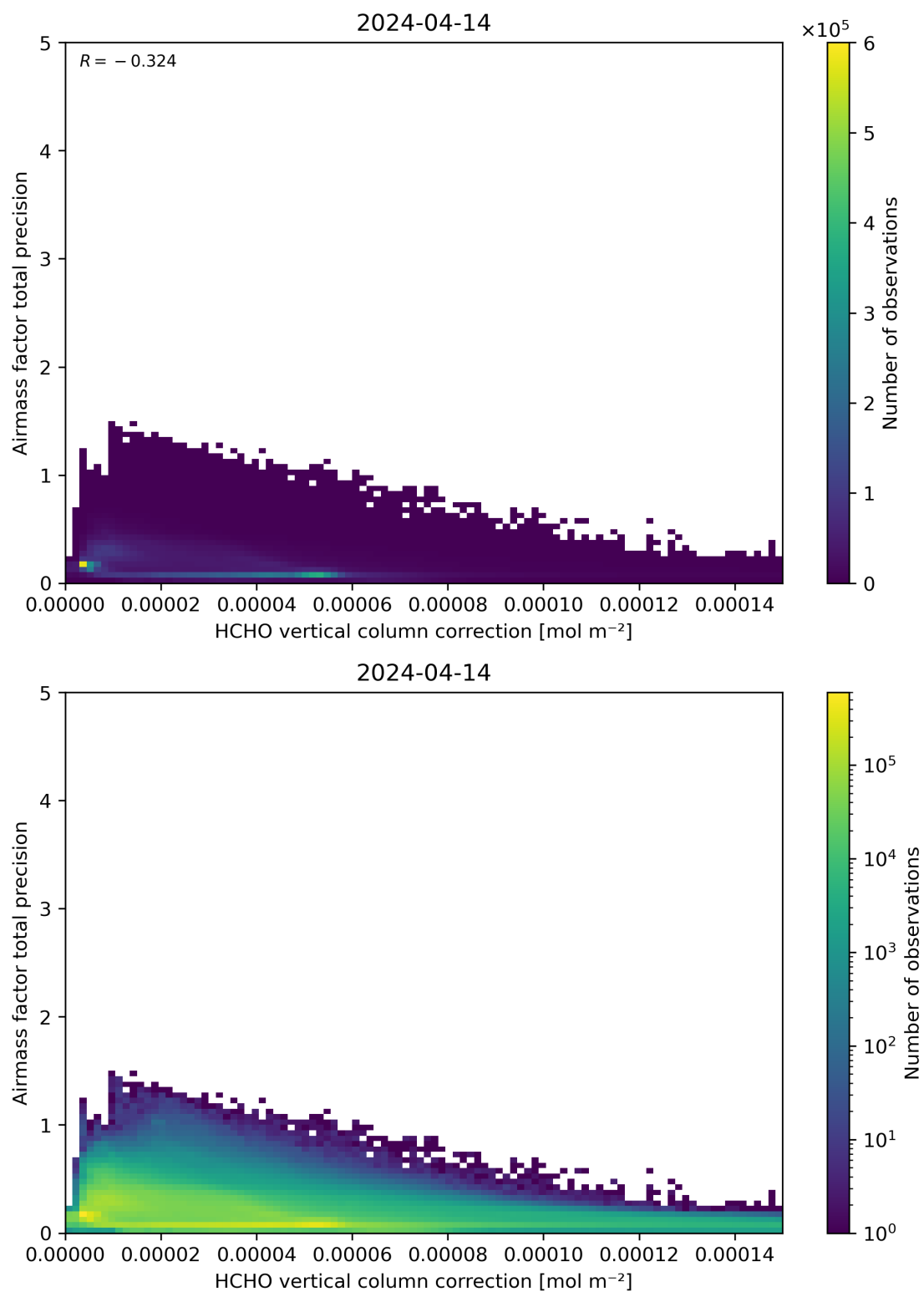
Figure 121: Scatter density plot of “HCHO vertical column correction” against “Airmass factor total precision” for 2024-04-13 to 2024-04-15.
