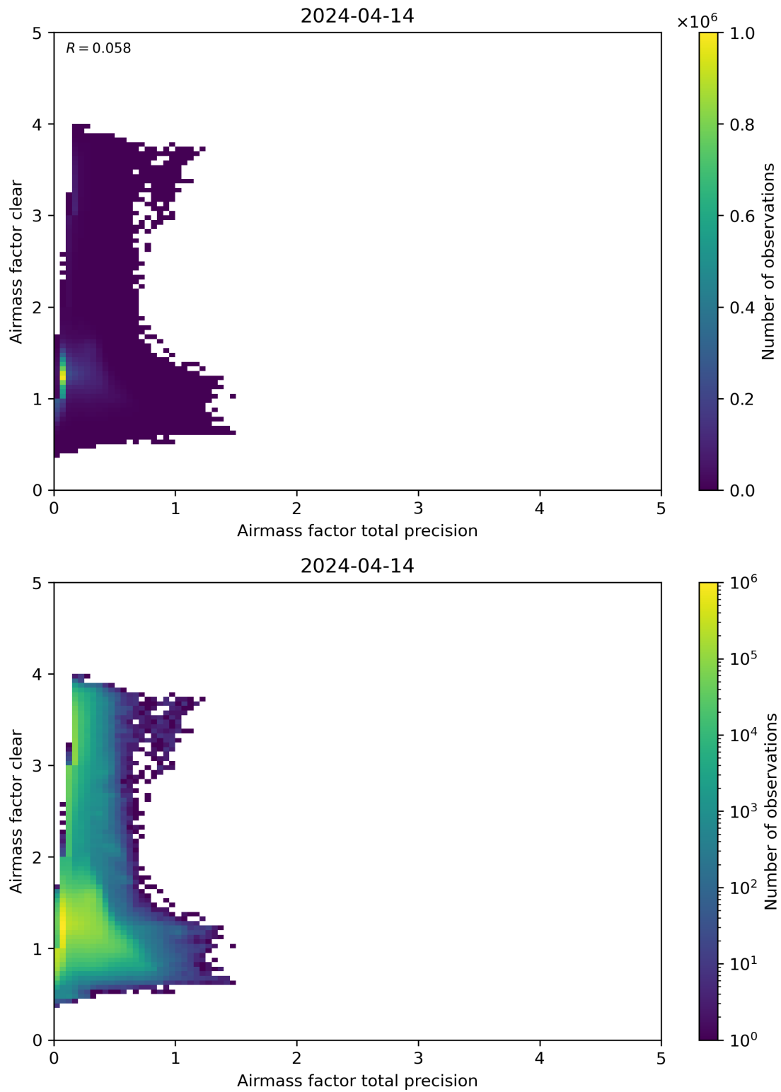
Figure 108: Scatter density plot of “Airmass factor total precision” against “Airmass factor clear” for 2024-04-13 to 2024-04-15.
