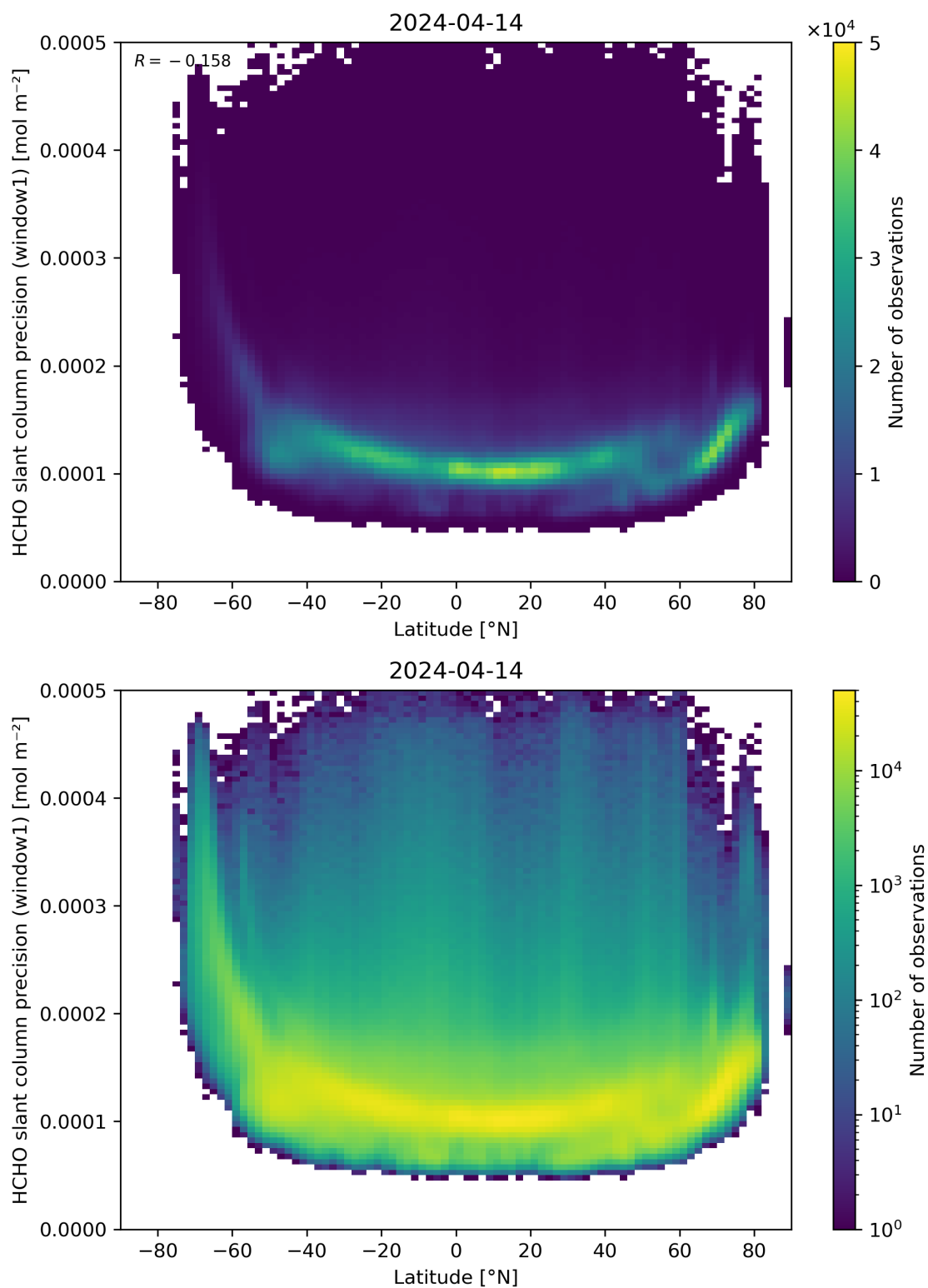
Figure 160: Scatter density plot of “Latitude” against “HCHO slant column precision (window1)” for 2024-04-13 to 2024-04-15.
