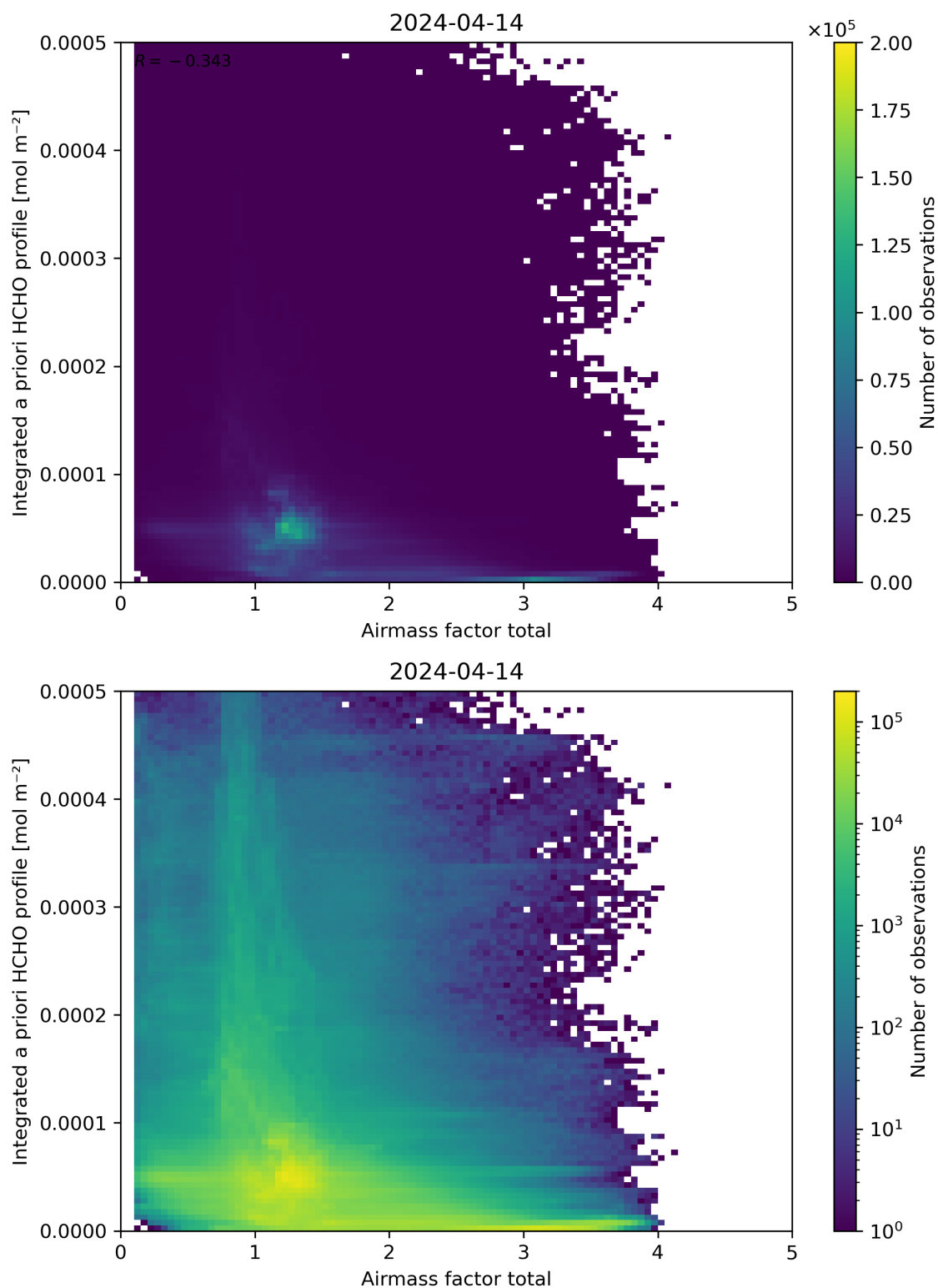
Figure 104: Scatter density plot of “Airmass factor total” against “Integrated a priori HCHO profile” for 2024-04-13 to 2024-04-15.
