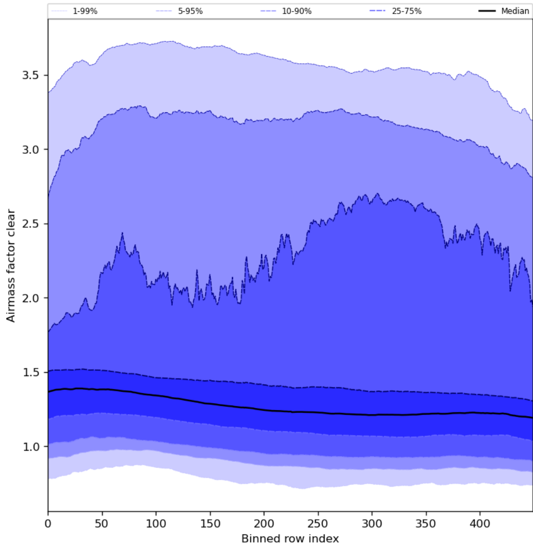
Figure 56: Along track statistics of “Airmass factor clear” for 2024-04-13 to 2024-04-15
