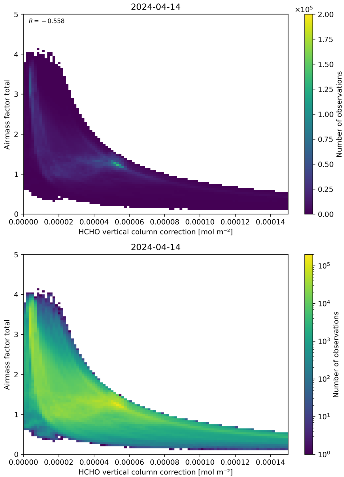
Figure 120: Scatter density plot of “HCHO vertical column correction” against “Airmass factor total” for 2024-04-13 to 2024-04-15.
