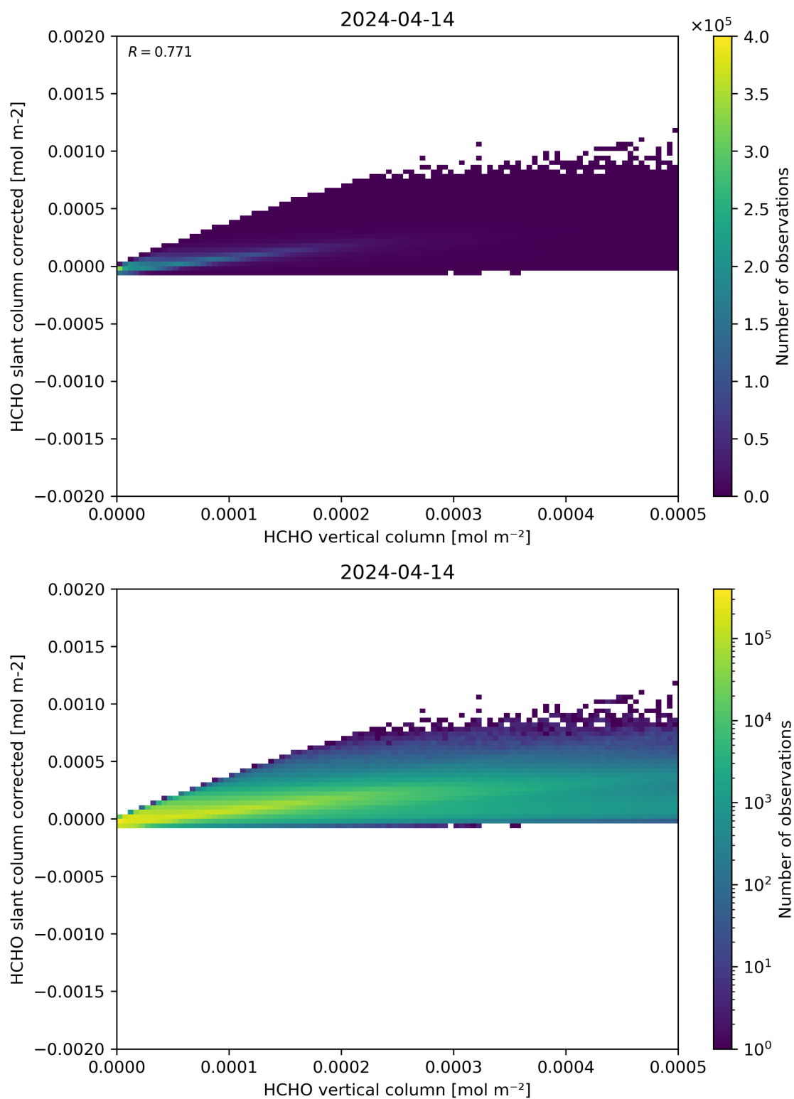
Figure 127: Scatter density plot of “HCHO vertical column” against “HCHO slant column corrected” for 2024-04-13 to 2024-04-15.
