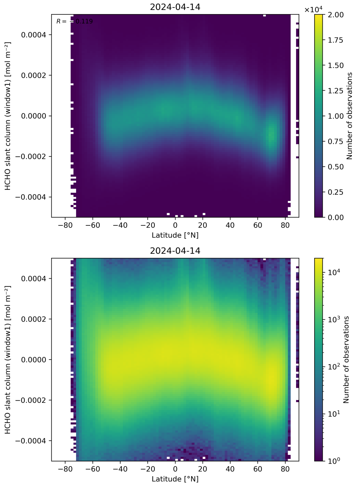
Figure 159: Scatter density plot of “Latitude” against “HCHO slant column (window1)” for 2024-04-13 to 2024-04-15.
