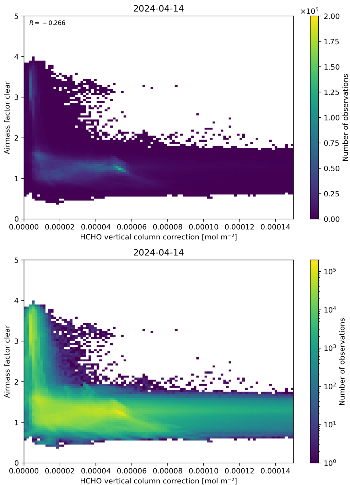
Figure 115: Scatter density plot of “HCHO vertical column correction” against “Airmass factor clear” for 2024-04-13 to 2024-04-15.
