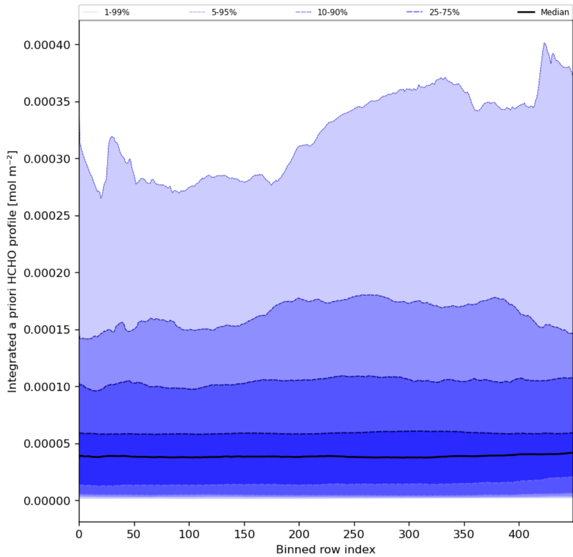
Figure 57: Along track statistics of "Integrated a priori HCHO profile" for 2024-04-13 to 2024-04-15
