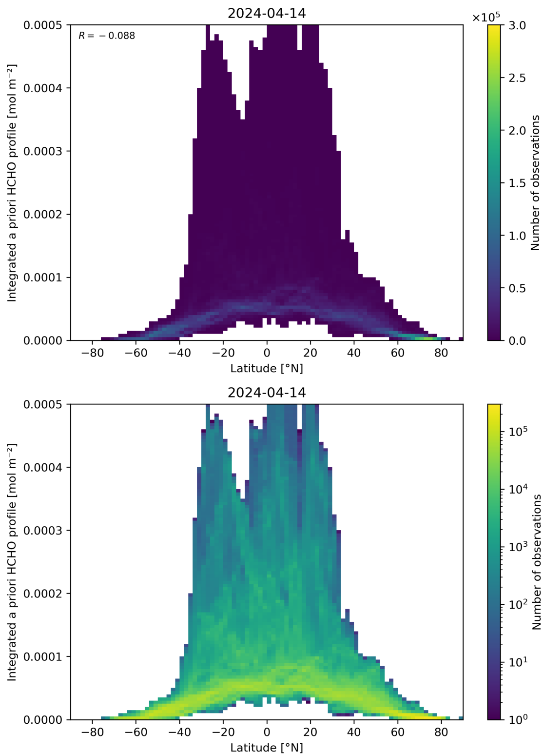
Figure 166: Scatter density plot of “Latitude” against “Integrated a priori HCHO profile” for 2024-04-13 to 2024-04-15.
