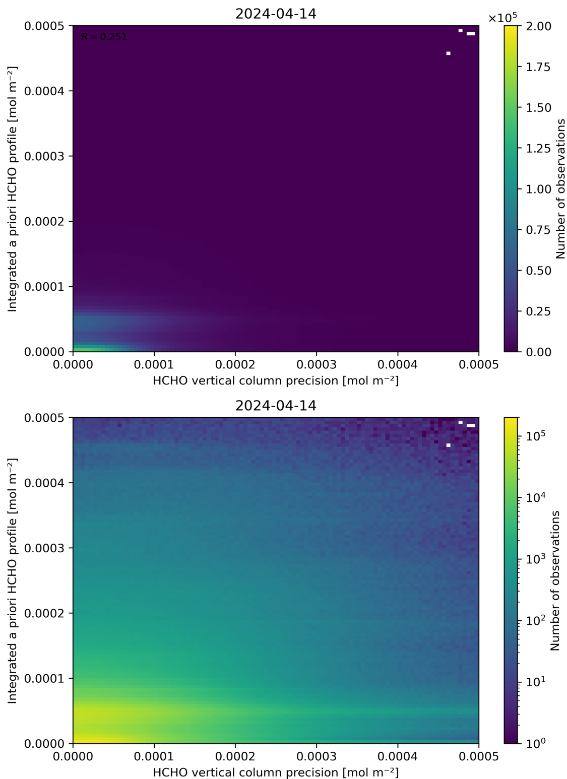
Figure 147: Scatter density plot of “HCHO vertical column precision” against “Integrated a priori HCHO profile” for 2024-04-13 to 2024-04-15.
