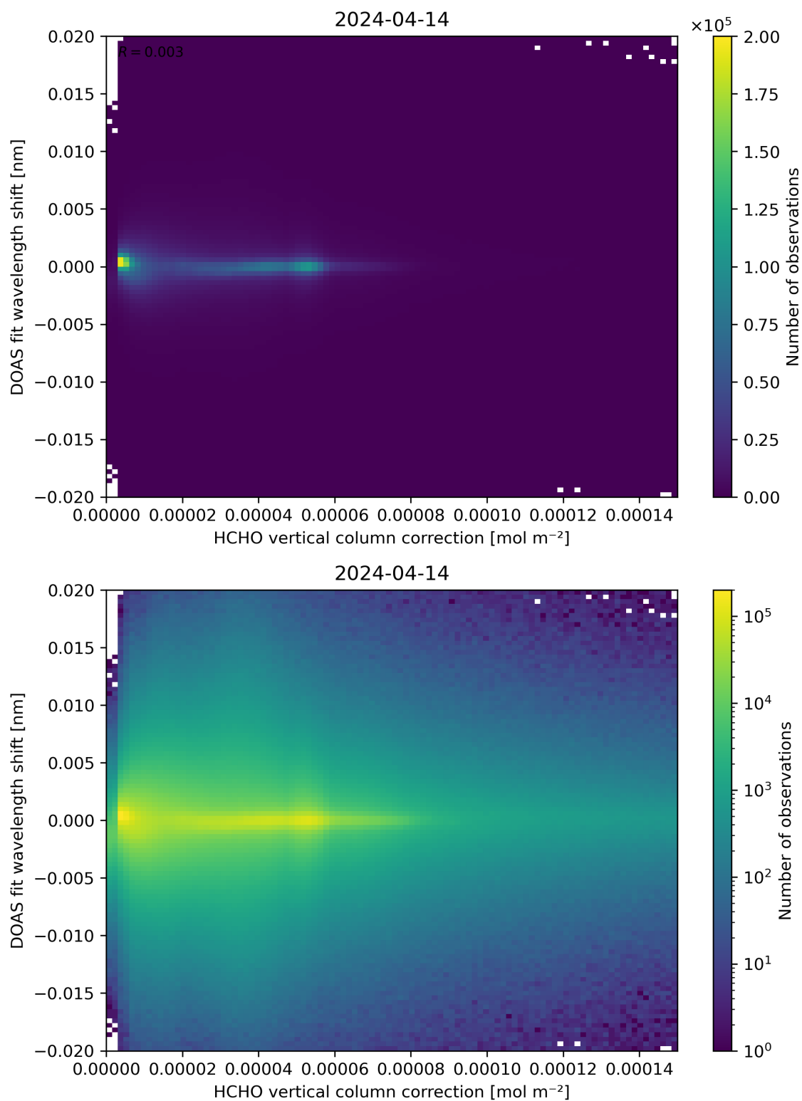
Figure 113: Scatter density plot of “HCHO vertical column correction” against “DOAS fit wavelength shift” for 2024-04-13 to 2024-04-15.
