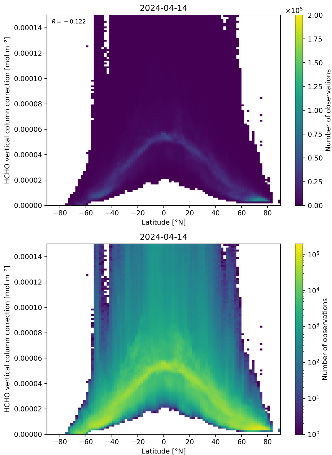
Figure 164: Scatter density plot of “Latitude” against “HCHO vertical column correction” for 2024-04-13 to 2024-04-15.
