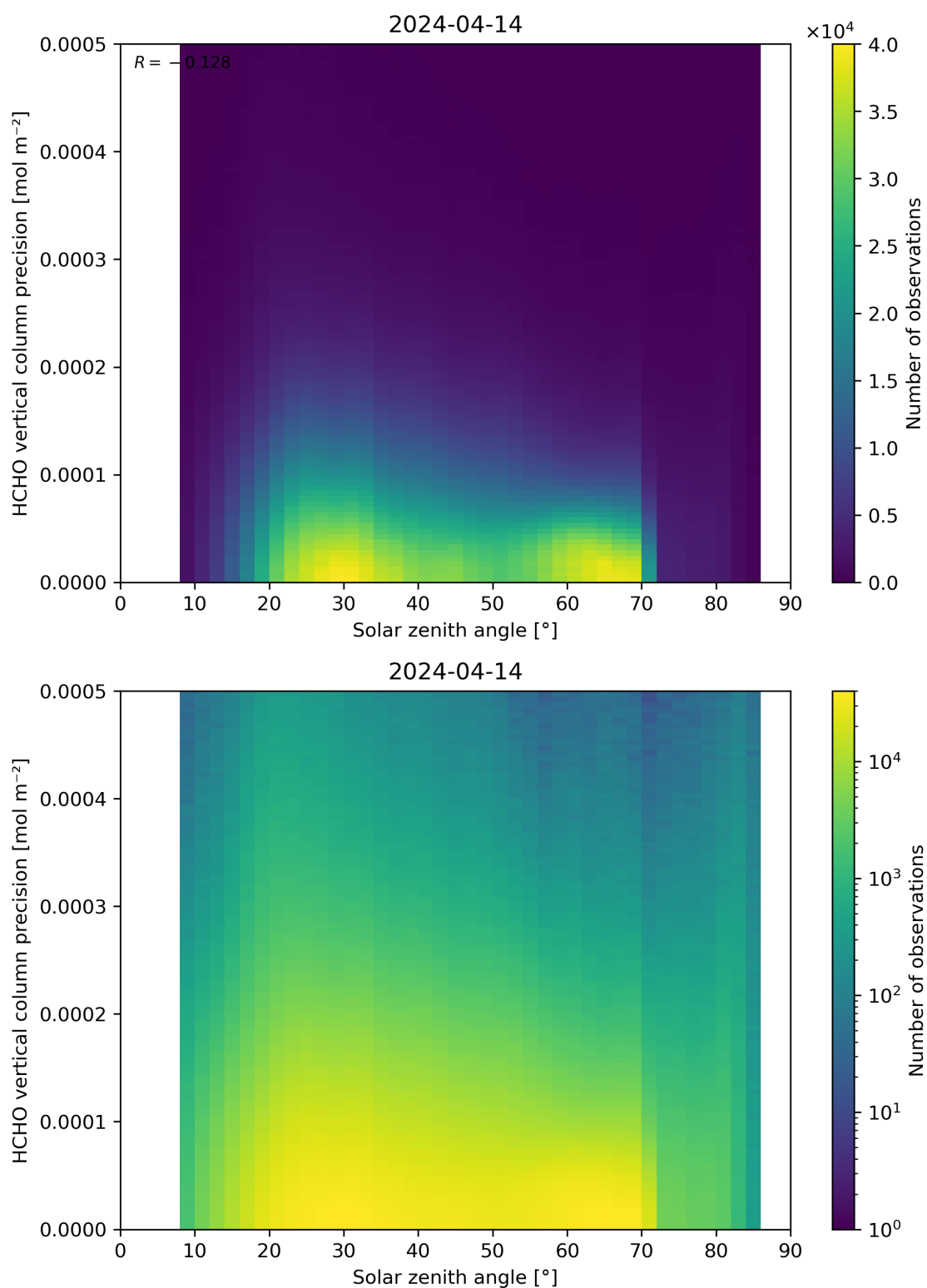
Figure 179: Scatter density plot of “Solar zenith angle” against “HCHO vertical column precision” for 2024-04-13 to 2024-04-15.
