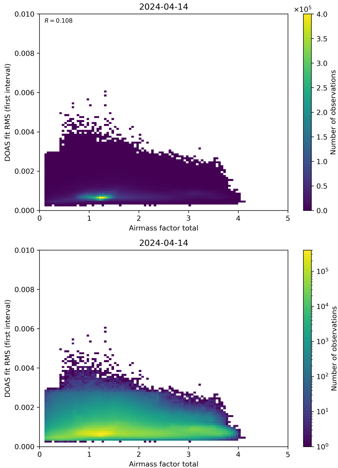
Figure 97: Scatter density plot of “Airmass factor total” against “DOAS fit RMS (first interval)” for 2024-04-13 to 2024-04-15.
