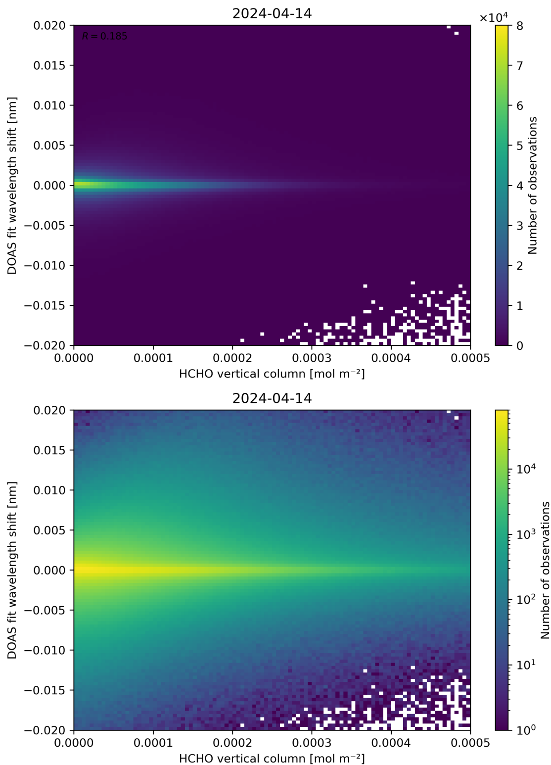
Figure 124: Scatter density plot of “HCHO vertical column” against “DOAS fit wavelength shift” for 2024-04-13 to 2024-04-15.
