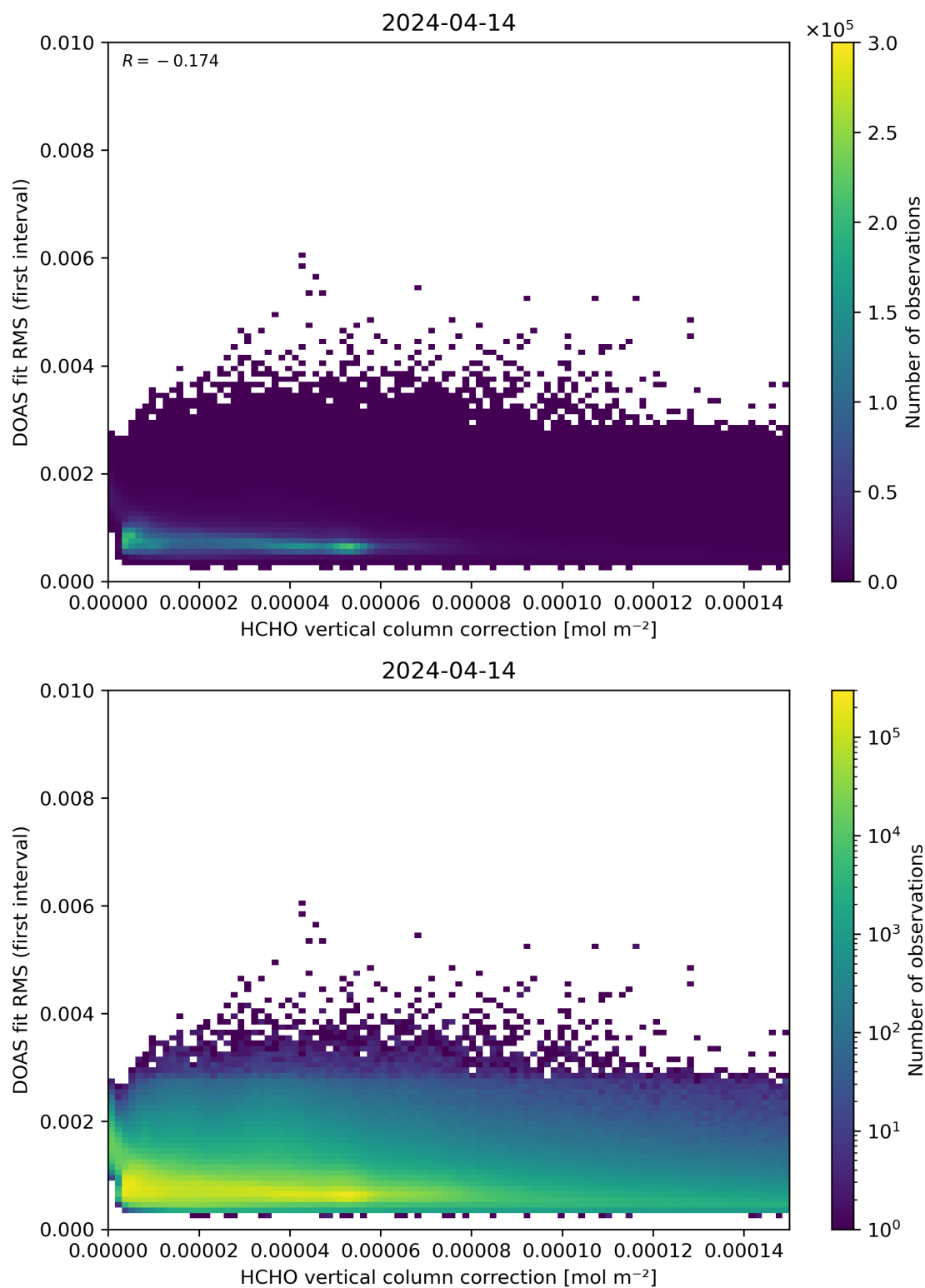
Figure 112: Scatter density plot of “HCHO vertical column correction” against “DOAS fit RMS (first interval)” for 2024-04-13 to 2024-04-15.
