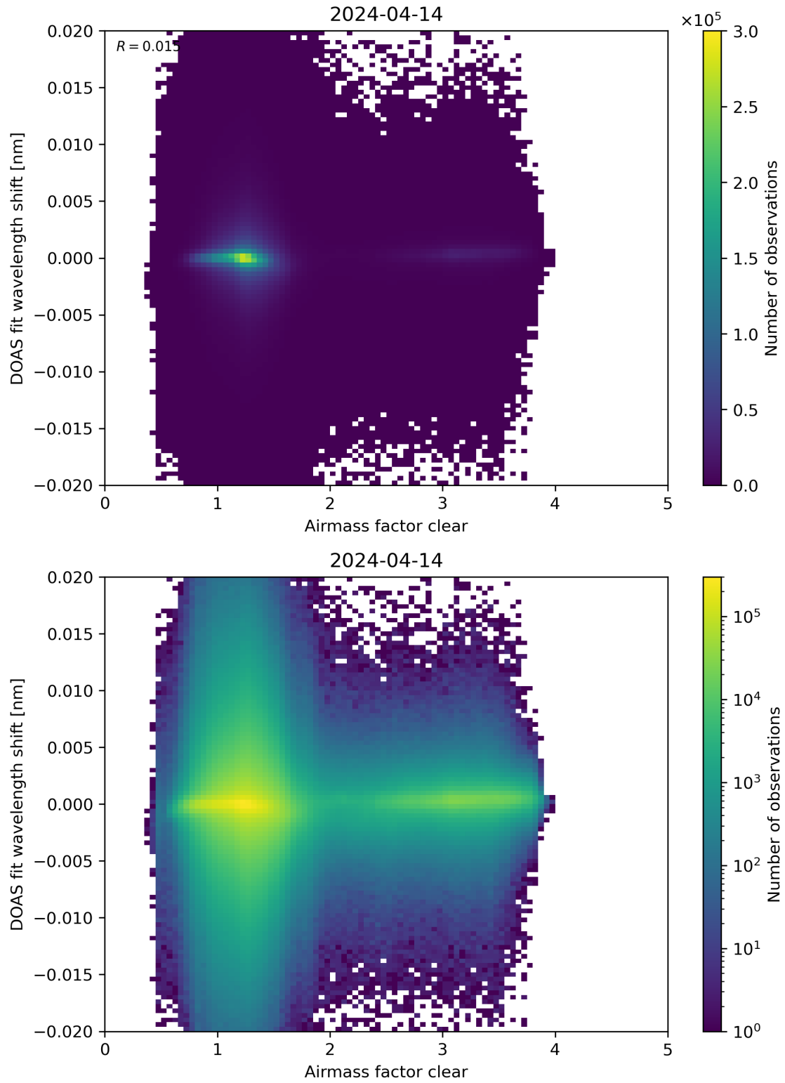
Figure 72: Scatter density plot of “Airmass factor clear” against “DOAS fit wavelength shift” for 2024-04-13 to 2024-04-15.
