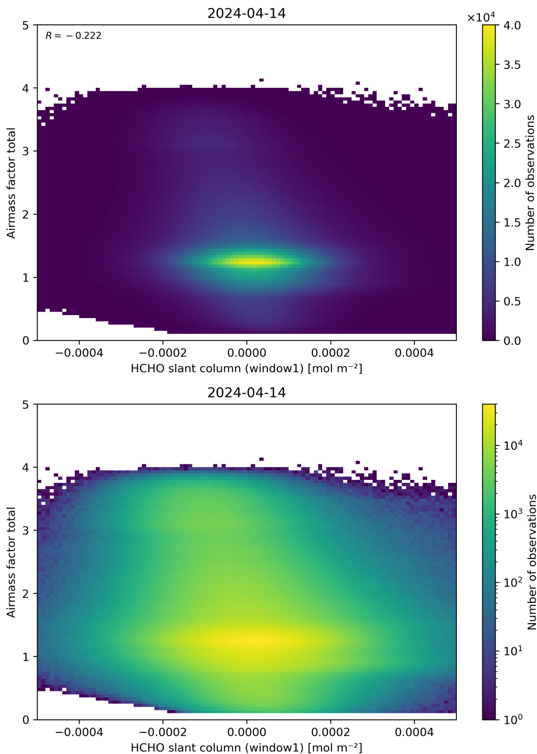
Figure 85: Scatter density plot of “HCHO slant column (window1)” against “Airmass factor total” for 2024-04-13 to 2024-04-15.
