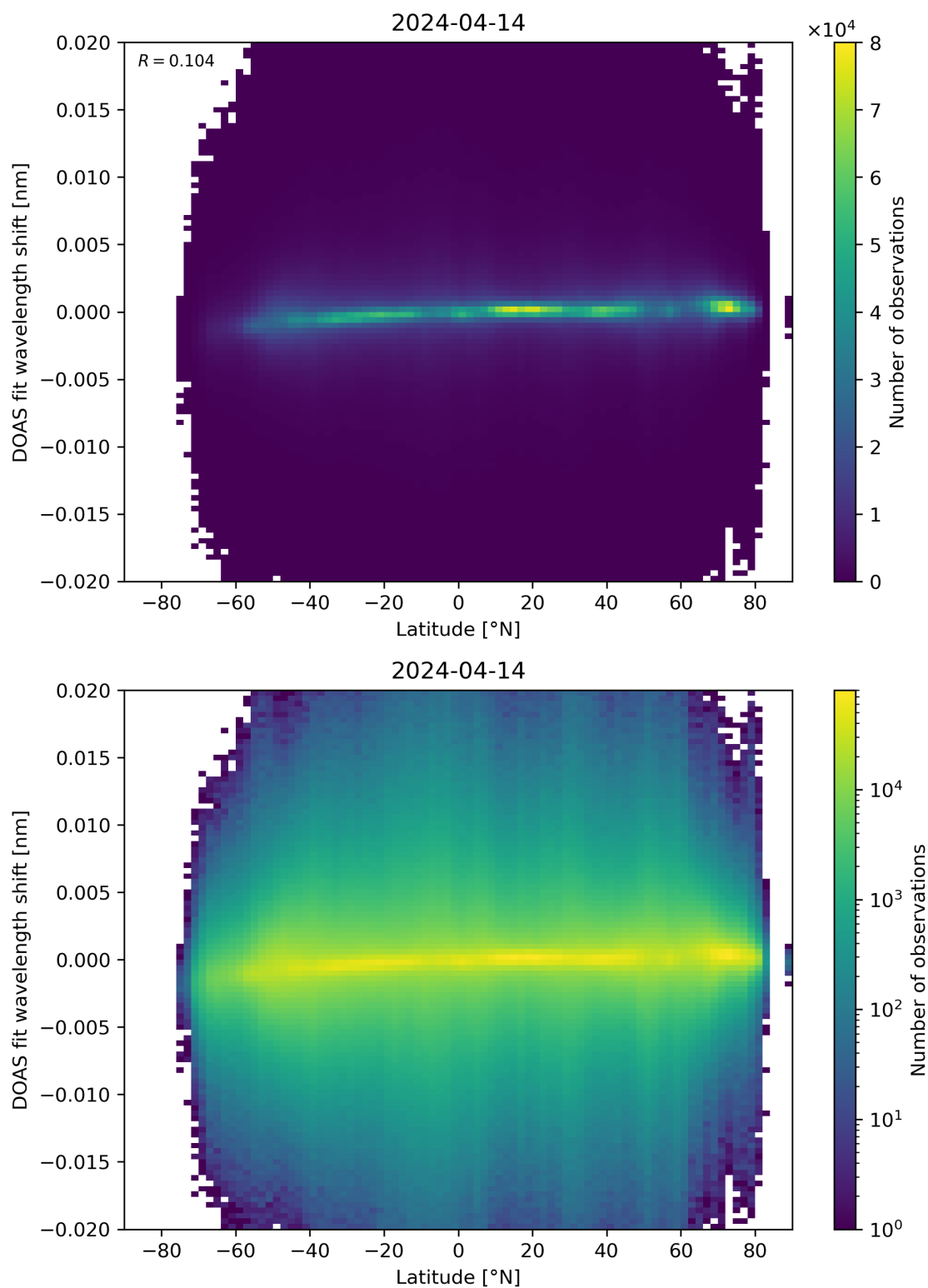
Figure 154: Scatter density plot of “Latitude” against “DOAS fit wavelength shift” for 2024-04-13 to 2024-04-15.
