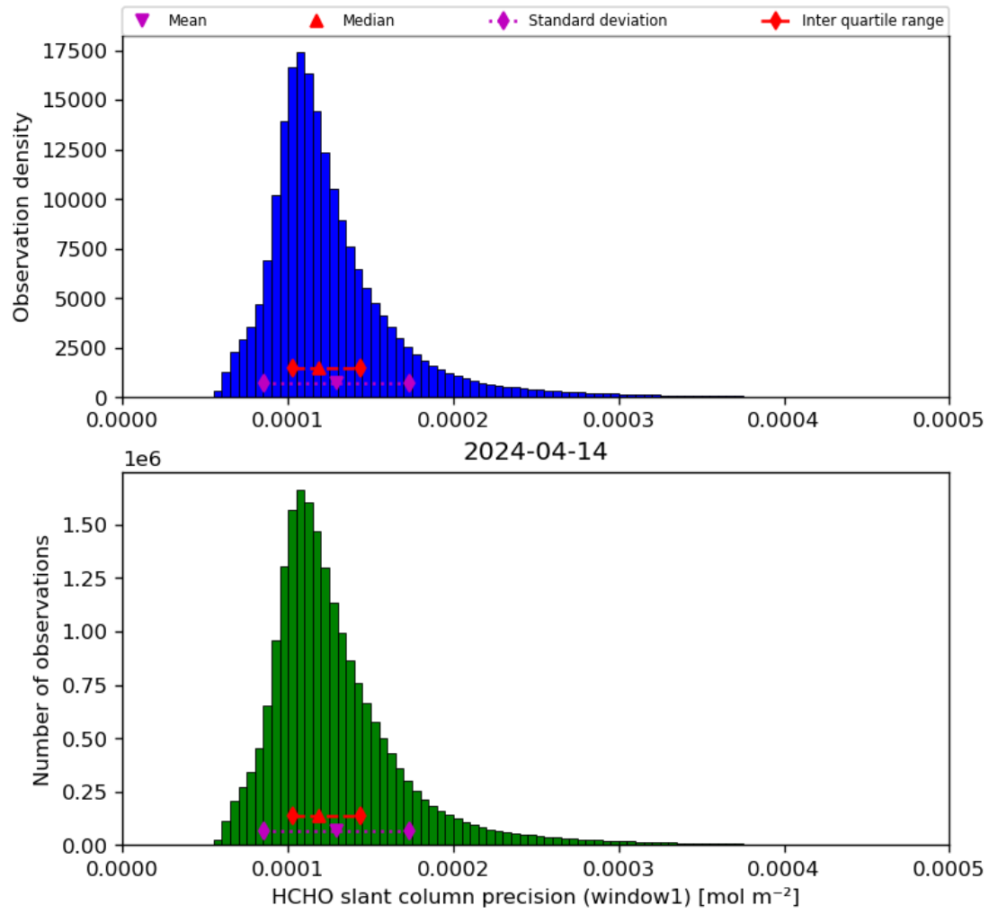
Figure 39: Histogram of “HCHO slant column precision (window1)” for 2024-04-13 to 2024-04-15
