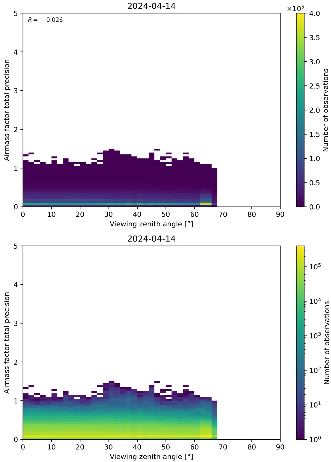
Figure 191: Scatter density plot of “Viewing zenith angle” against “Airmass factor total precision” for 2024-04-13 to 2024-04-15.
