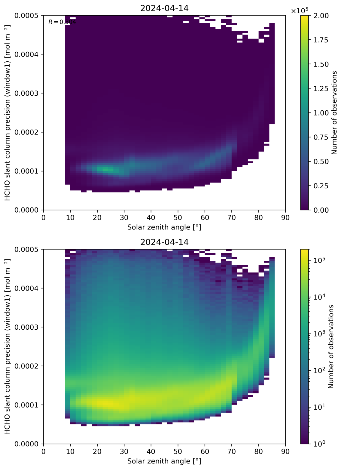
Figure 174: Scatter density plot of “Solar zenith angle” against “HCHO slant column precision (window1)” for 2024-04-13 to 2024-04-15.
