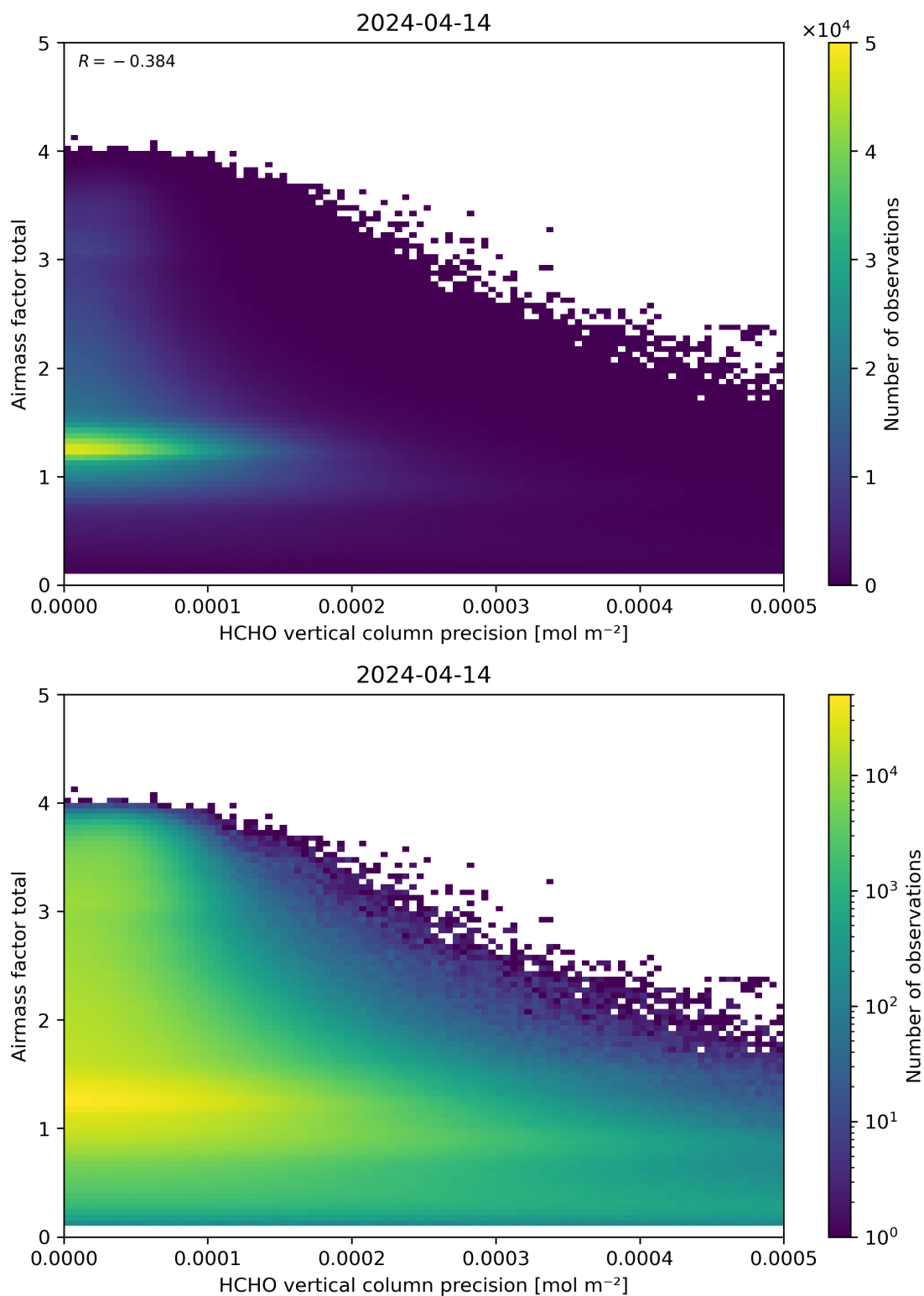
Figure 144: Scatter density plot of “HCHO vertical column precision” against “Airmass factor total” for 2024-04-13 to 2024-04-15.
