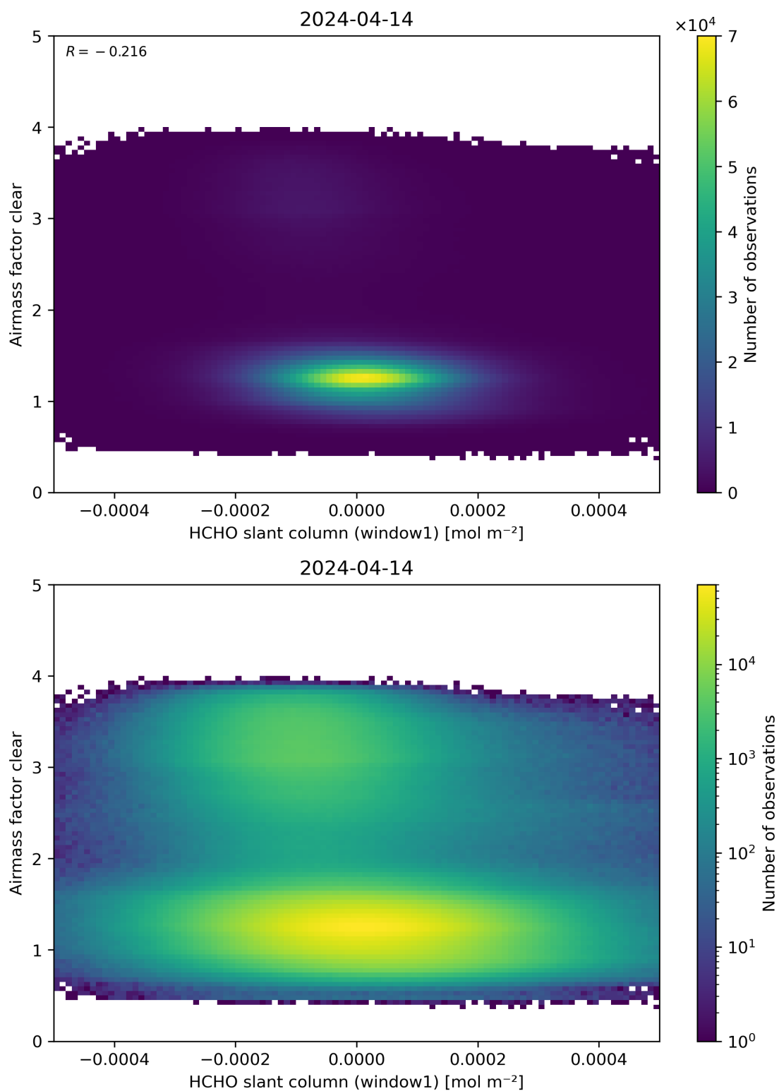
Figure 81: Scatter density plot of “HCHO slant column (window1)” against “Airmass factor clear” for 2024-04-13 to 2024-04-15.
