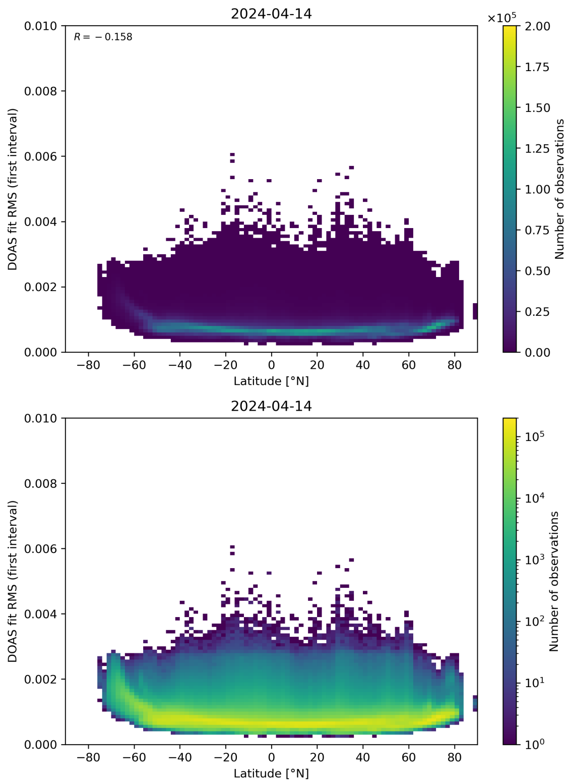
Figure 153: Scatter density plot of “Latitude” against “DOAS fit RMS (first interval)” for 2024-04-13 to 2024-04-15.
