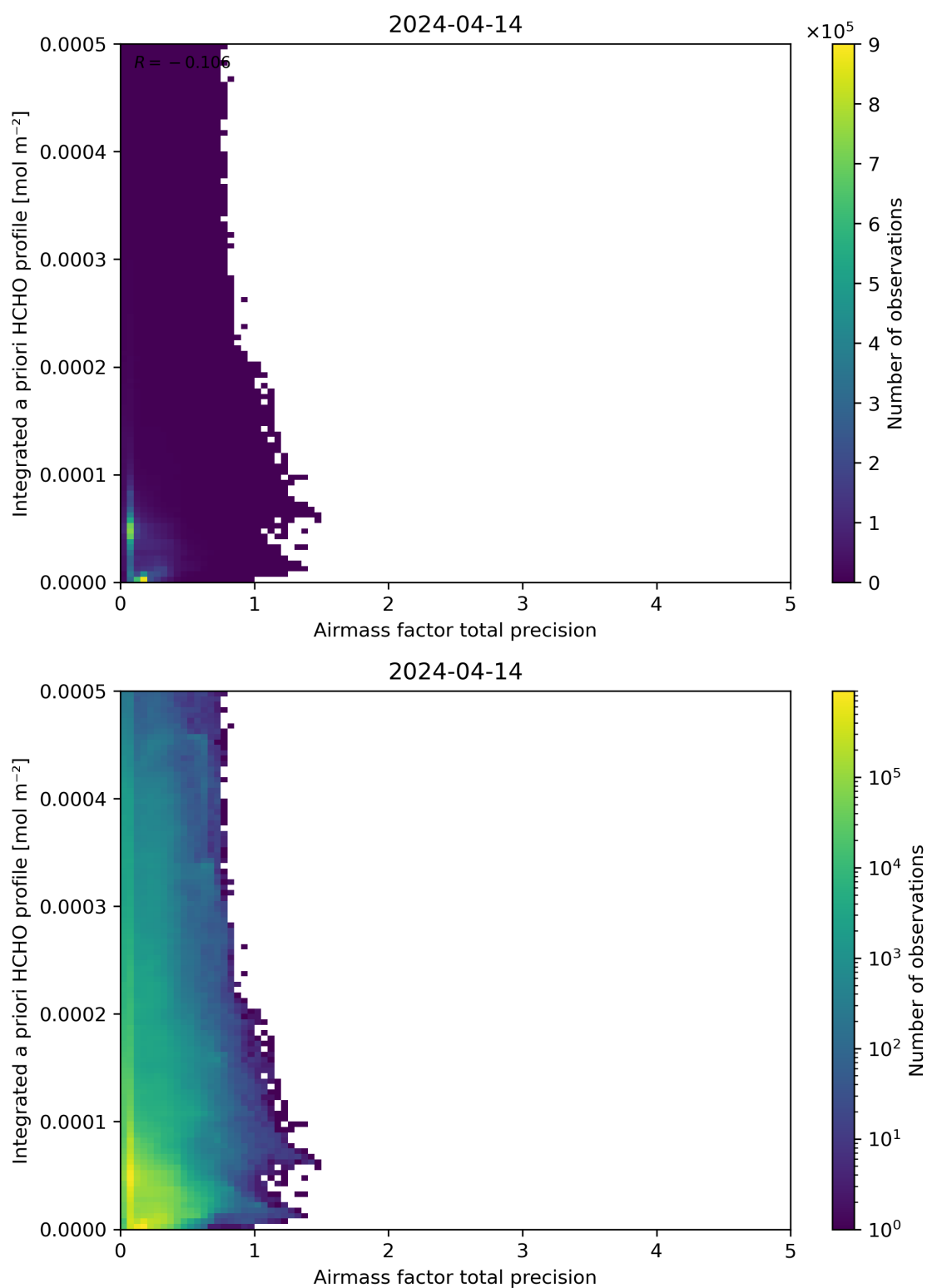
Figure 111: Scatter density plot of “Airmass factor total precision” against “Integrated a priori HCHO profile” for 2024-04-13 to 2024-04-15.
