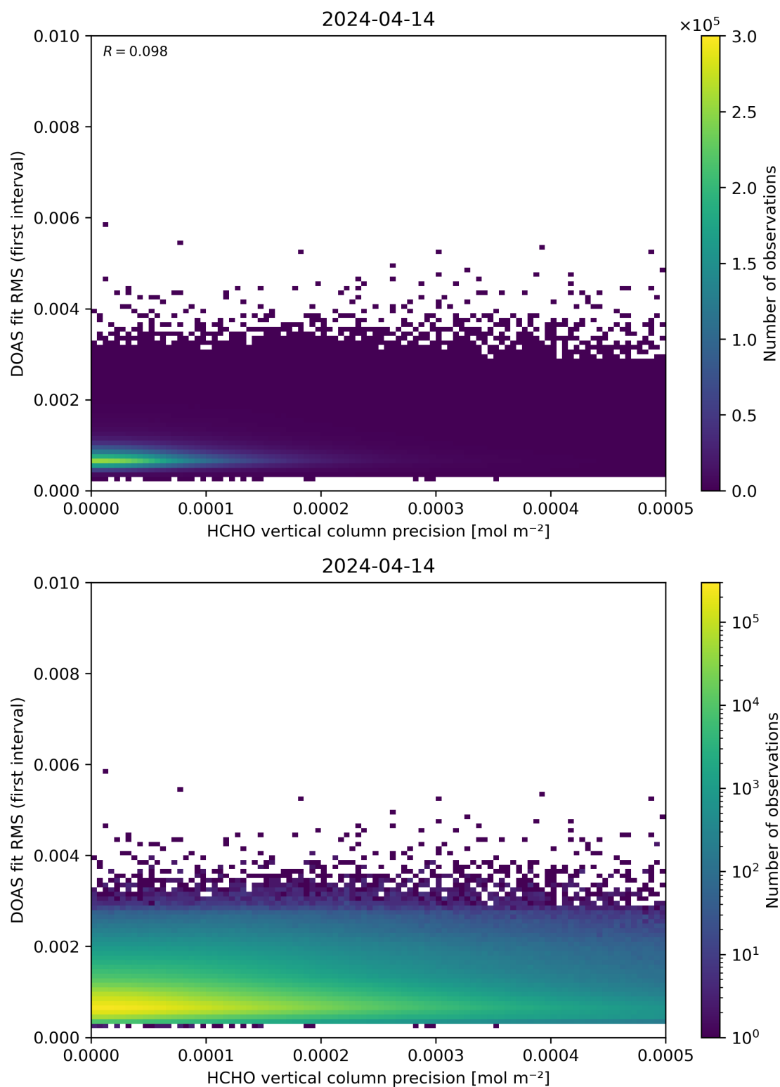
Figure 136: Scatter density plot of “HCHO vertical column precision” against “DOAS fit RMS (first interval)” for 2024-04-13 to 2024-04-15.
