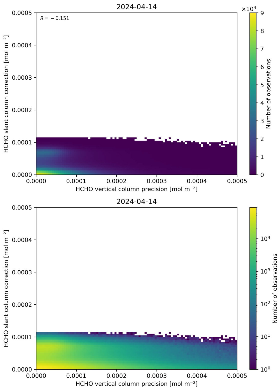
Figure 141: Scatter density plot of “HCHO vertical column precision” against “HCHO slant column correction” for 2024-04-13 to 2024-04-15.
