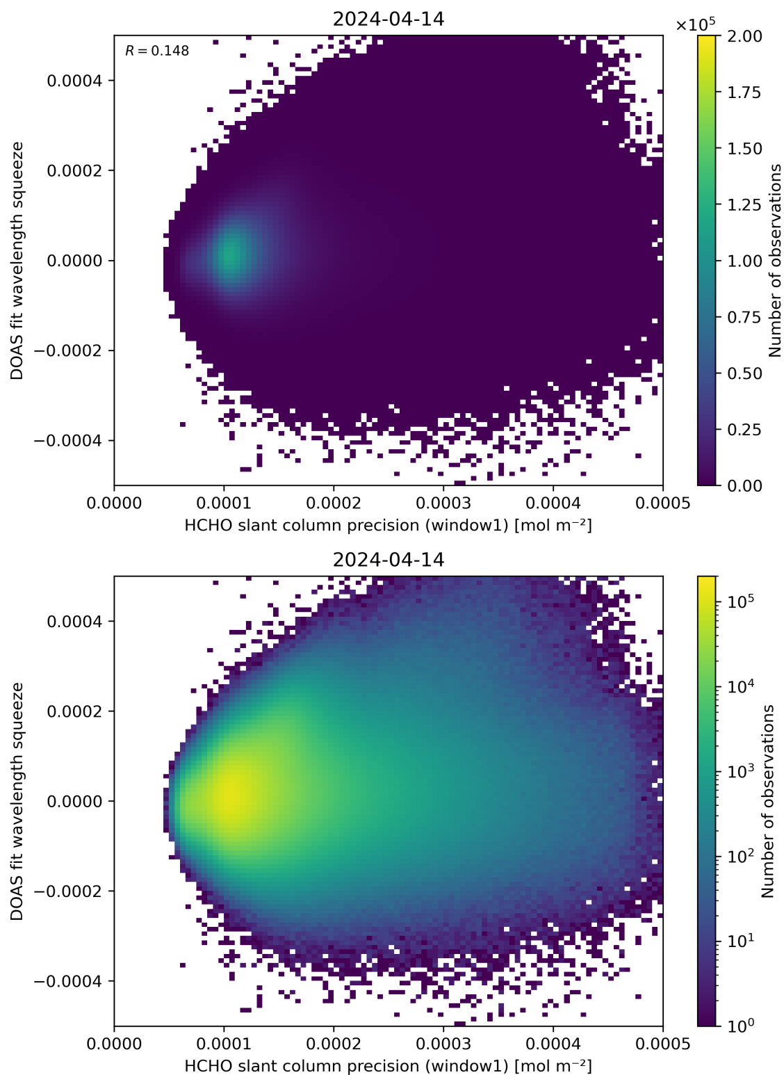
Figure 90: Scatter density plot of “HCHO slant column precision (window1)” against “DOAS fit wavelength squeeze” for 2024-04-13 to 2024-04-15.
