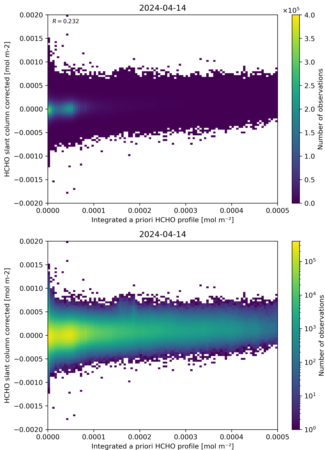
Figure 151: Scatter density plot of “Integrated a priori HCHO profile” against “HCHO slant column corrected” for 2024-04-13 to 2024-04-15.
