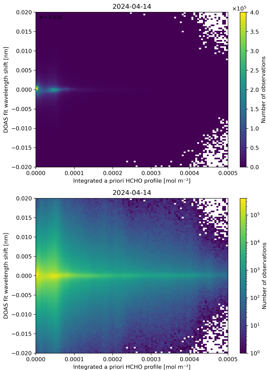
Figure 149: Scatter density plot of “Integrated a priori HCHO profile” against “DOAS fit wavelength shift” for 2024-04-13 to 2024-04-15.
