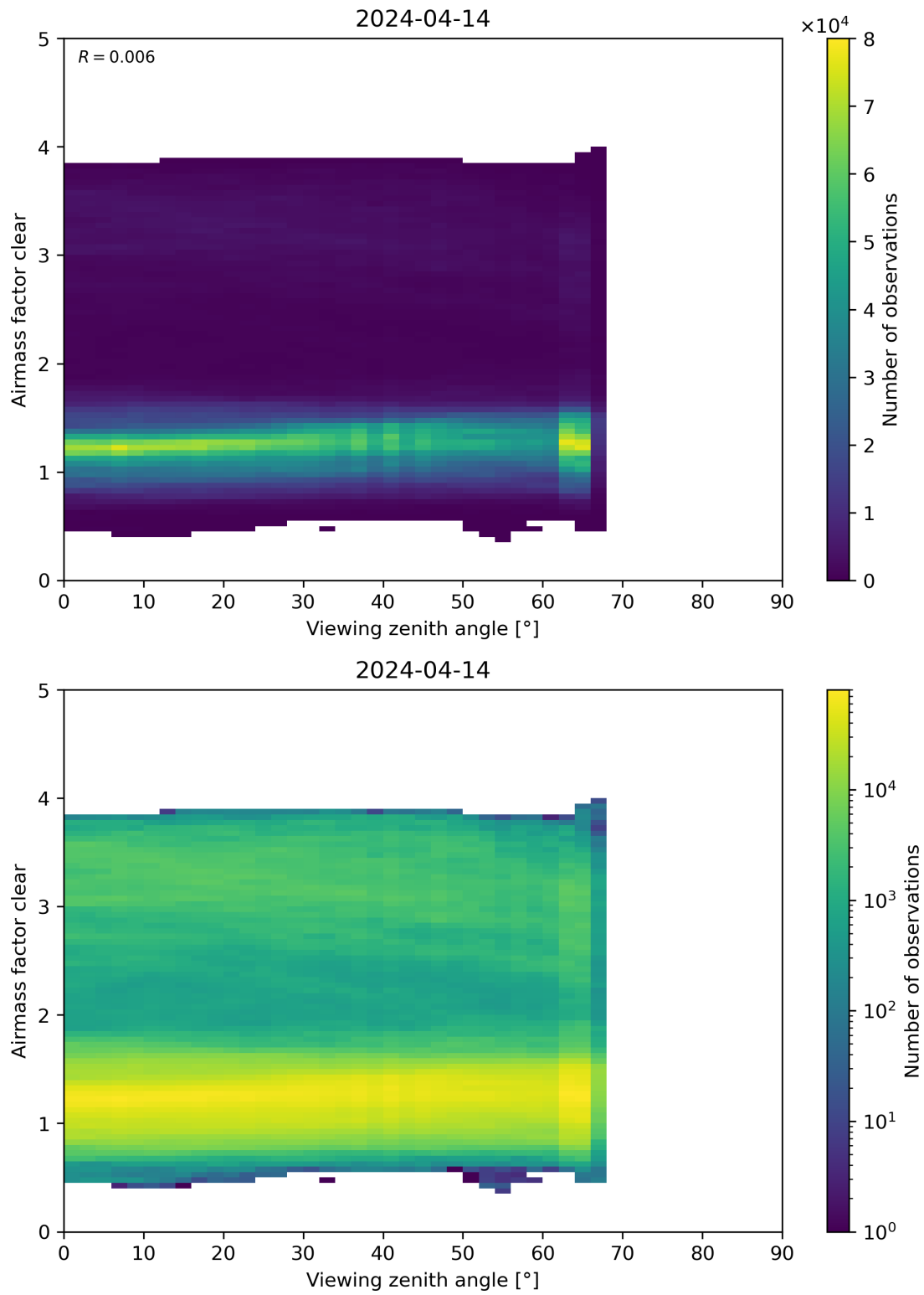
Figure 185: Scatter density plot of “Viewing zenith angle” against “Airmass factor clear” for 2024-04-13 to 2024-04-15.
