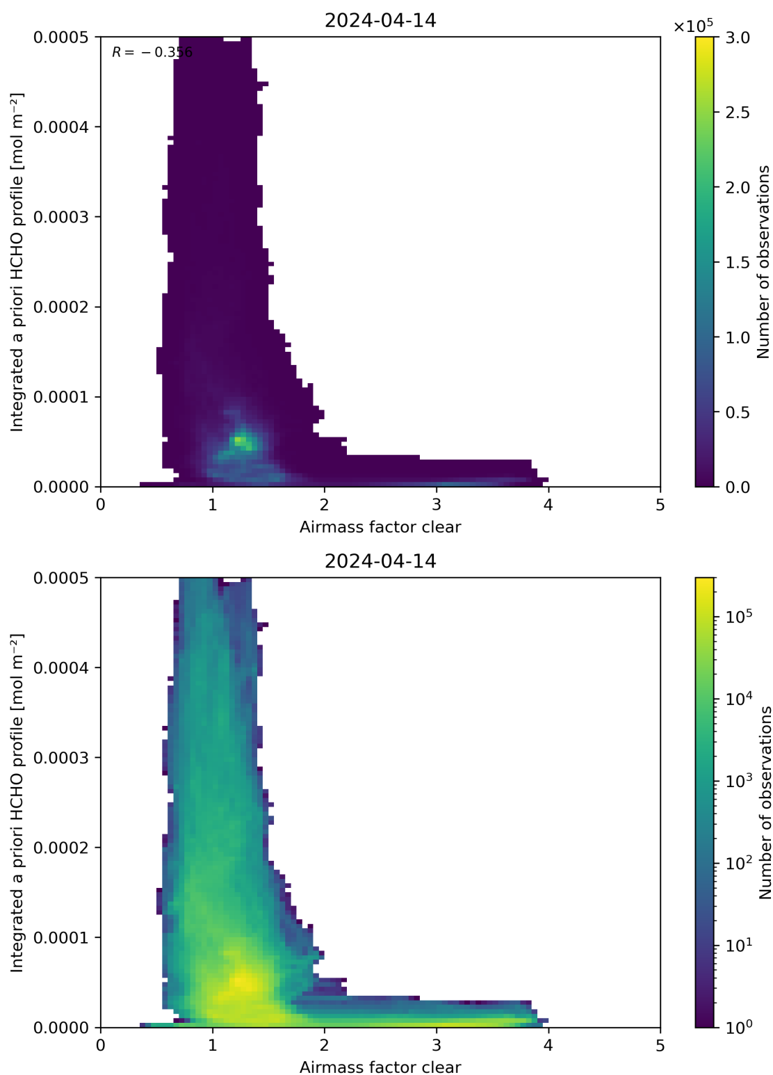
Figure 76: Scatter density plot of “Airmass factor clear” against “Integrated a priori HCHO profile” for 2024-04-13 to 2024-04-15.
