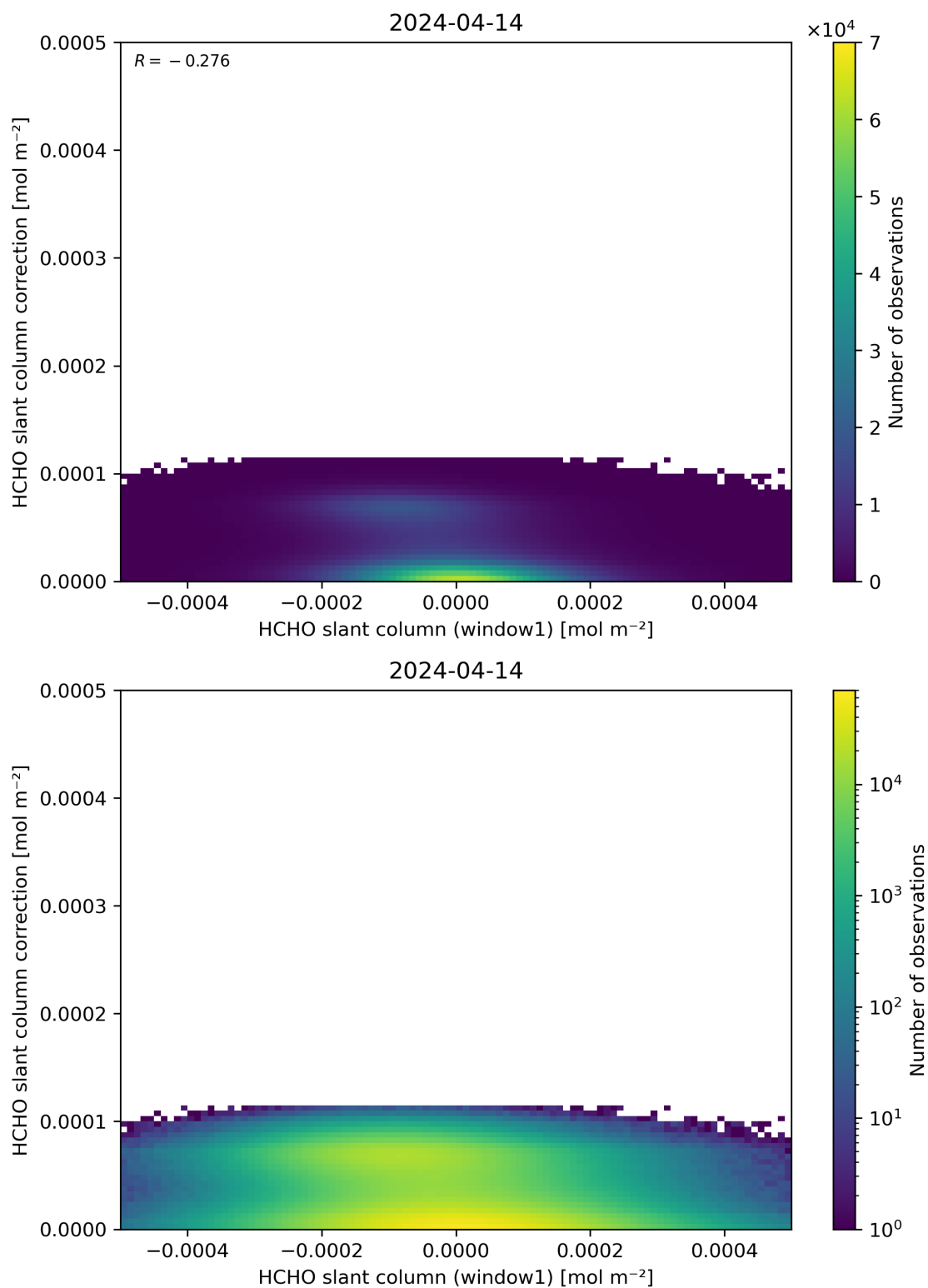
Figure 83: Scatter density plot of “HCHO slant column (window1)” against “HCHO slant column correction” for 2024-04-13 to 2024-04-15.
