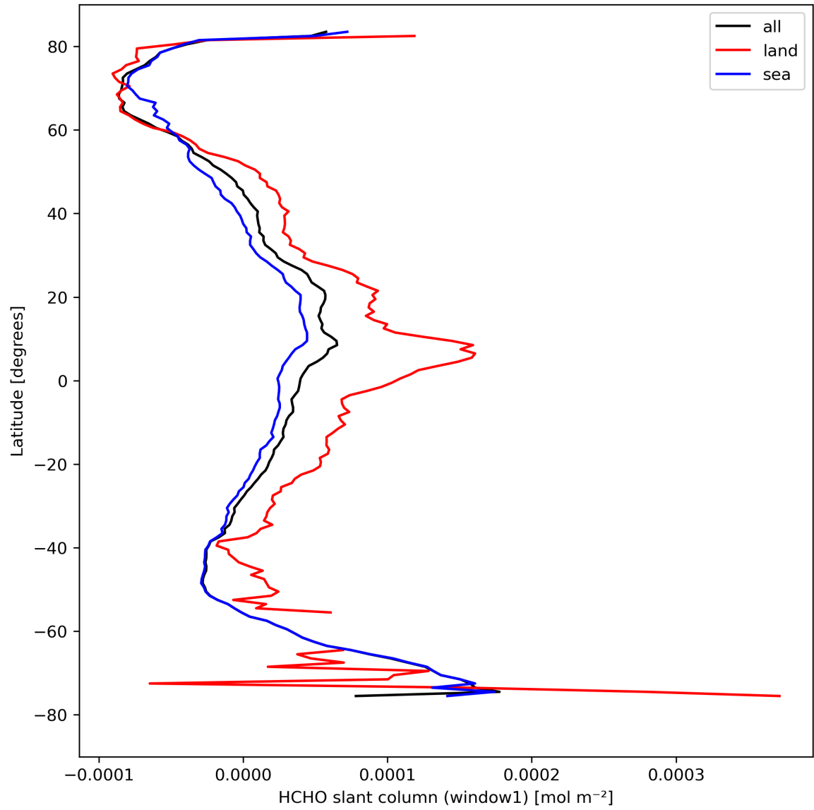
Figure 24: Zonal average of “HCHO slant column (window1)” for 2024-04-13 to 2024-04-15.
