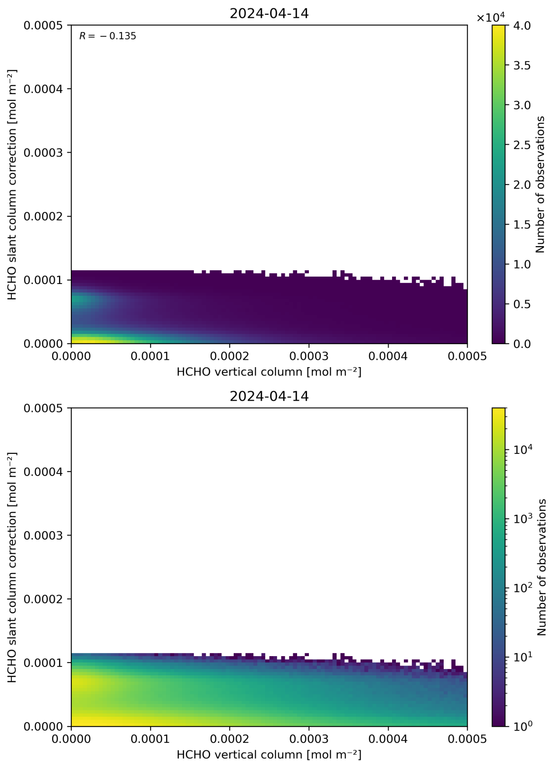
Figure 128: Scatter density plot of “HCHO vertical column” against “HCHO slant column correction” for 2024-04-13 to 2024-04-15.
