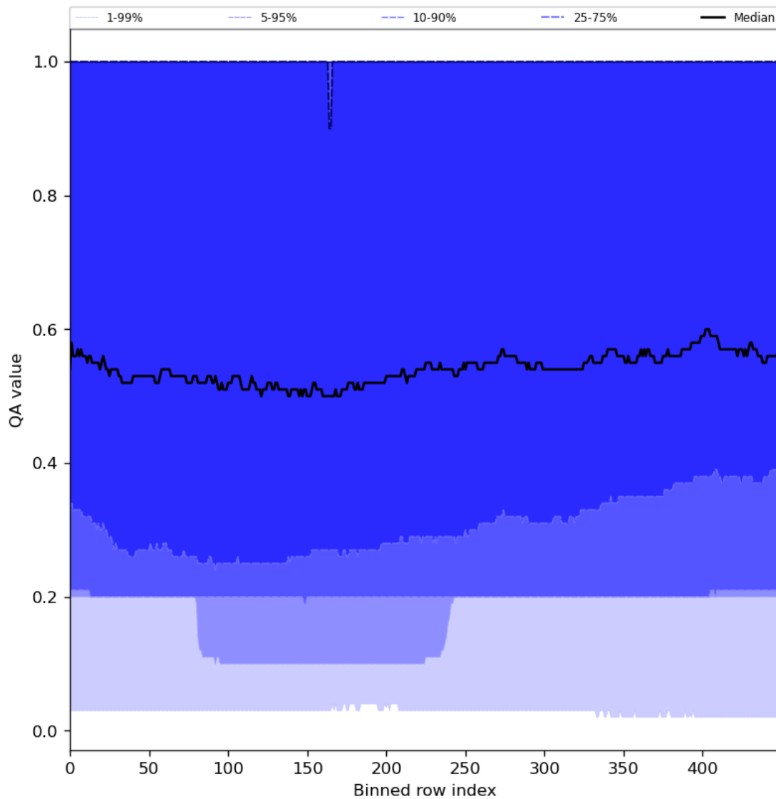
Figure 48: Along track statistics of “QA value” for 2024-04-13 to 2024-04-15
