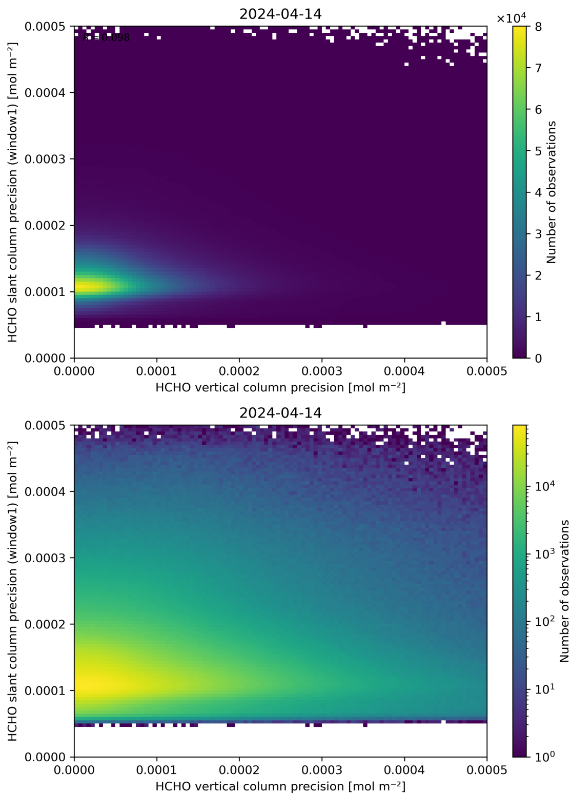
Figure 143: Scatter density plot of “HCHO vertical column precision” against “HCHO slant column precision (window1)” for 2024-04-13 to 2024-04-15.
