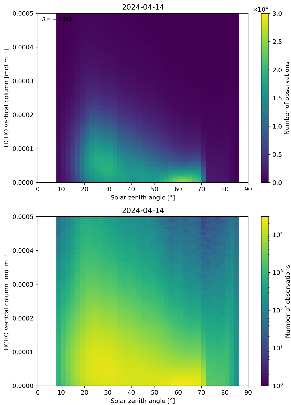
Figure 177: Scatter density plot of “Solar zenith angle” against “HCHO vertical column” for 2024-04-13 to 2024-04-15.
