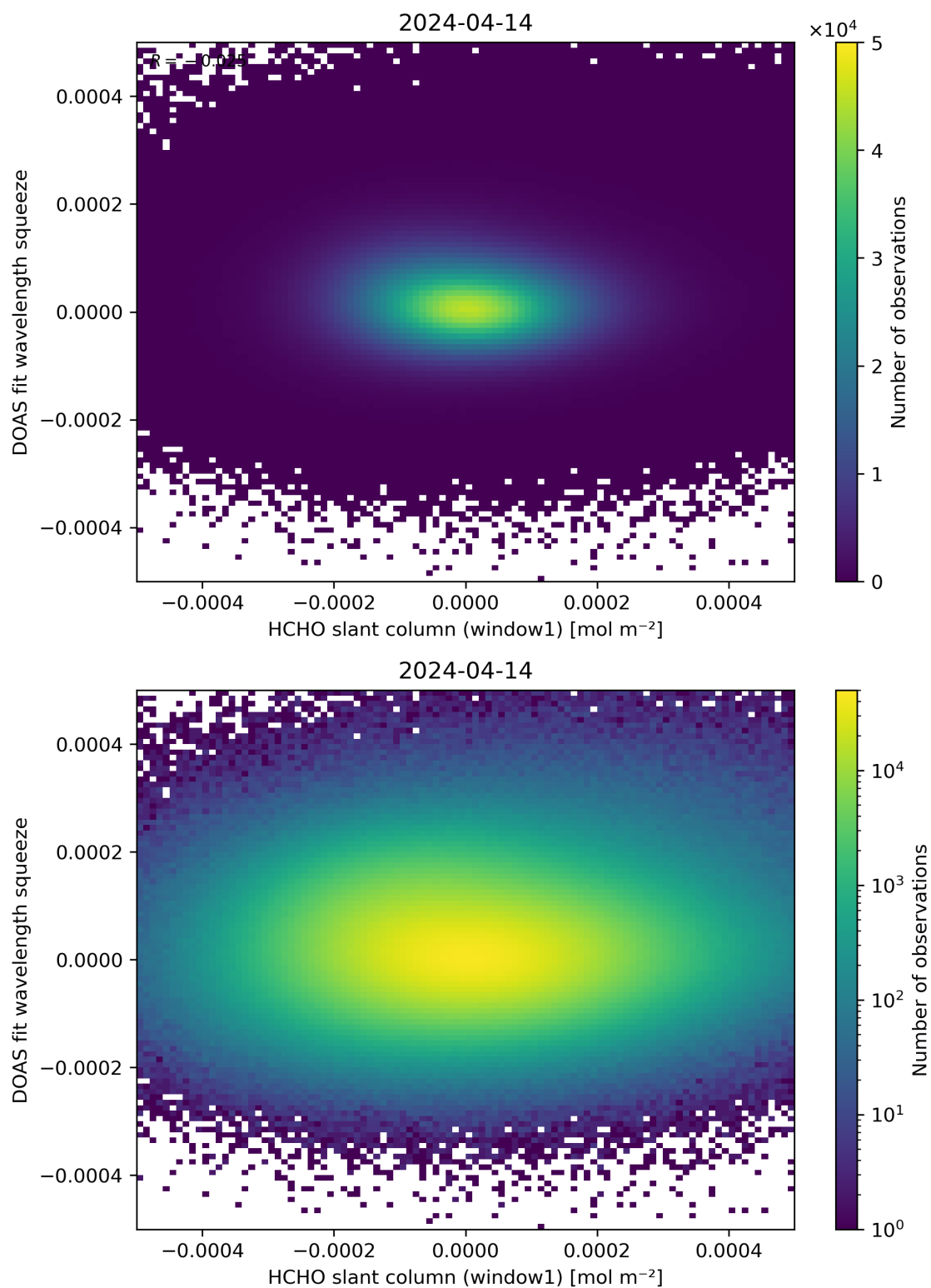
Figure 80: Scatter density plot of “HCHO slant column (window1)” against “DOAS fit wavelength squeeze” for 2024-04-13 to 2024-04-15.
