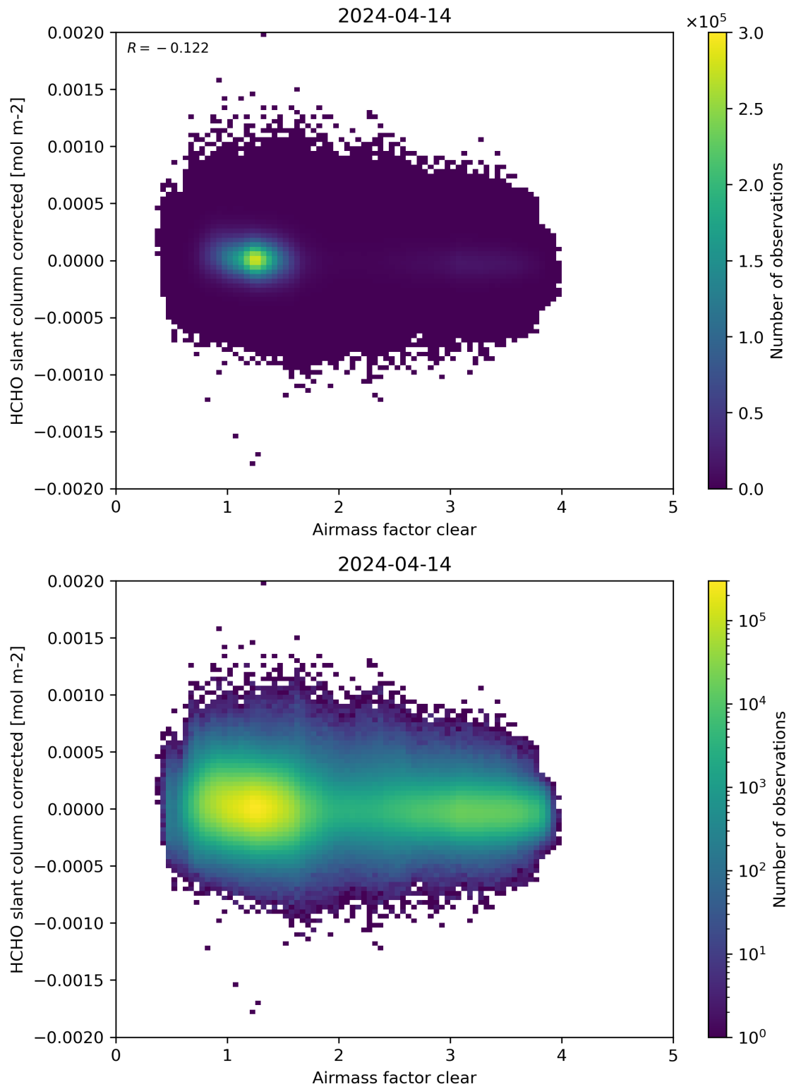
Figure 74: Scatter density plot of “Airmass factor clear” against “HCHO slant column corrected” for 2024-04-13 to 2024-04-15.
