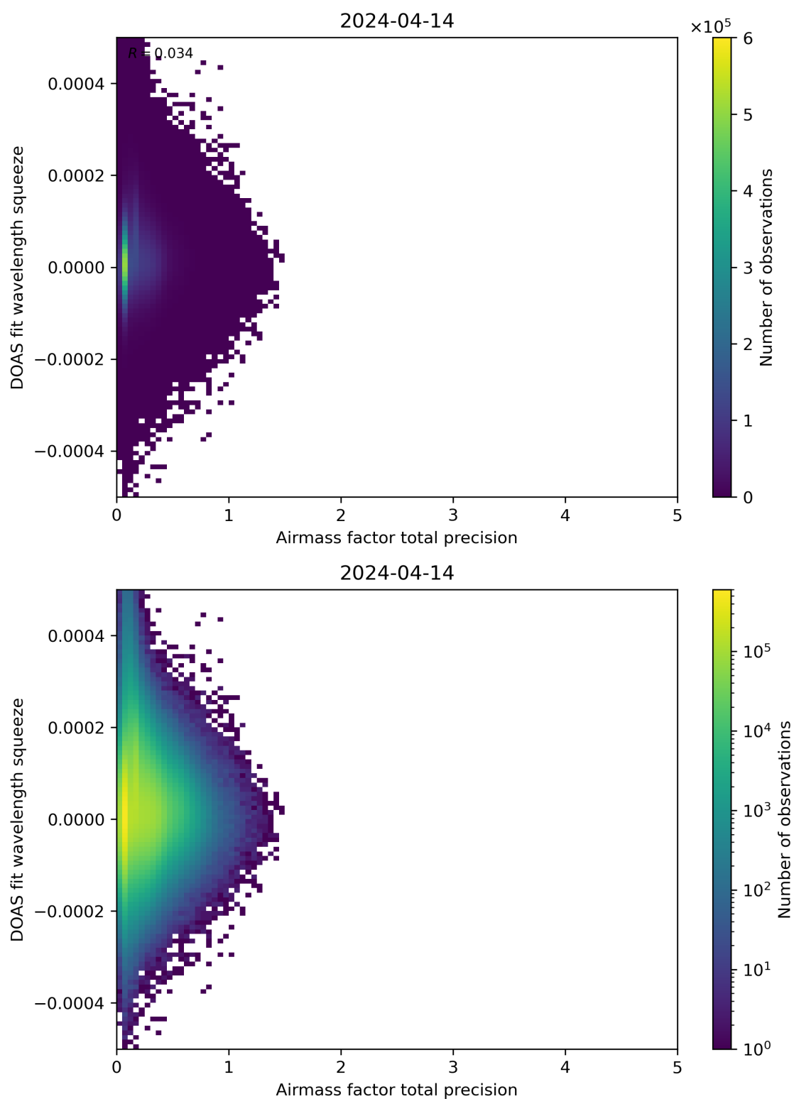
Figure 107: Scatter density plot of “Airmass factor total precision” against “DOAS fit wavelength squeeze” for 2024-04-13 to 2024-04-15.
