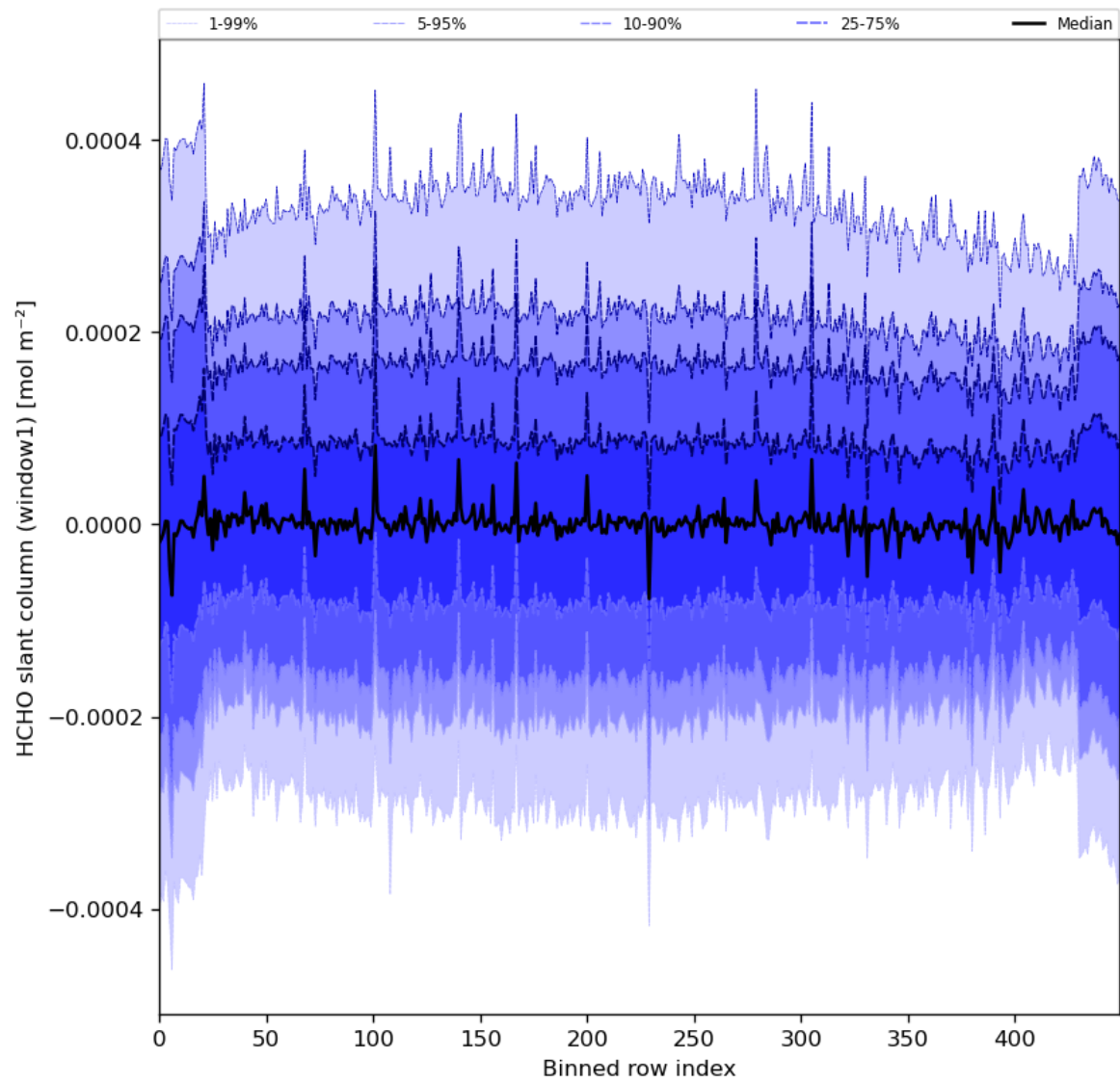
Figure 52: Along track statistics of “HCHO slant column (window1)” for 2024-04-13 to 2024-04-15
