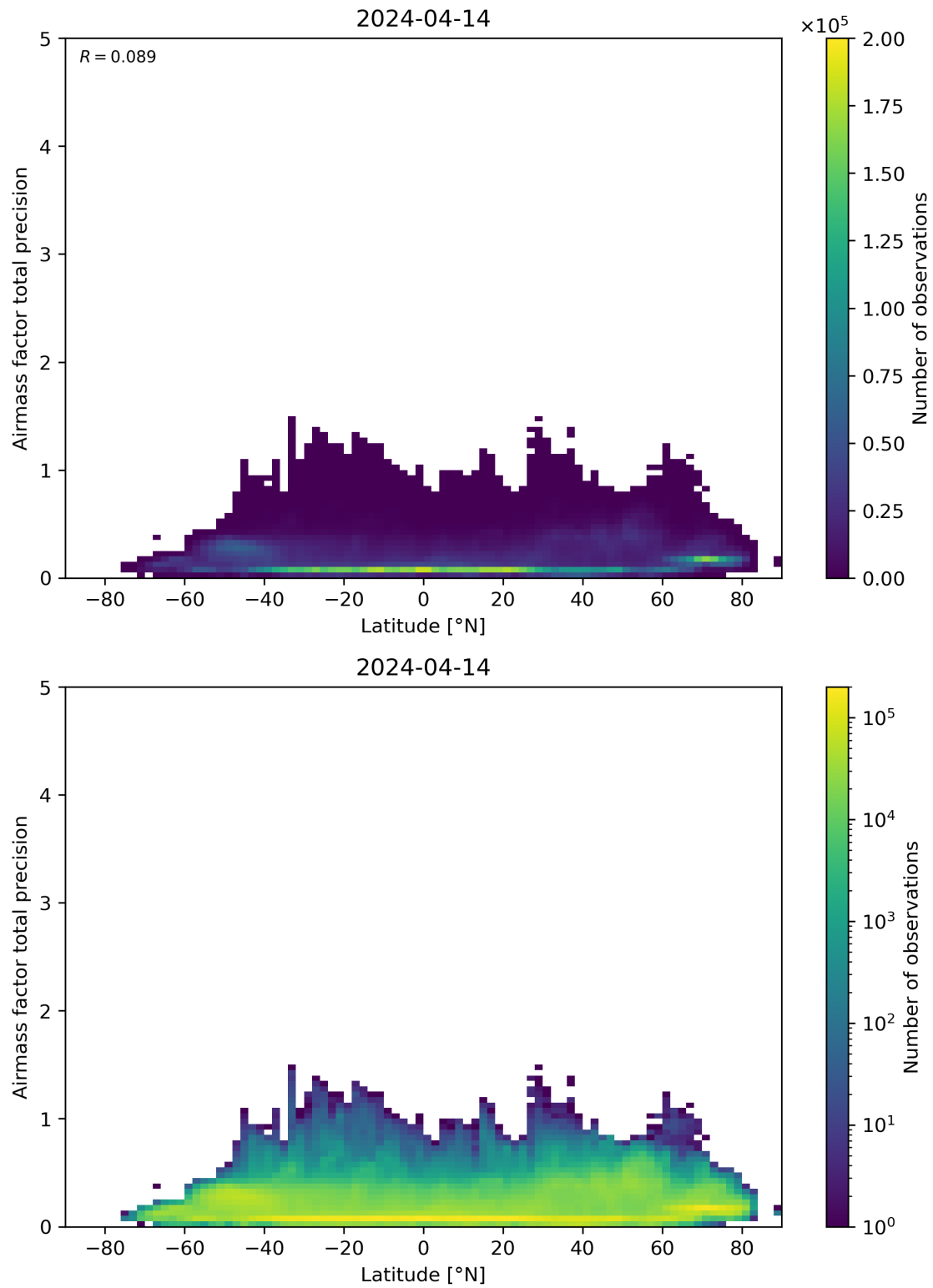
Figure 162: Scatter density plot of “Latitude” against “Airmass factor total precision” for 2024-04-13 to 2024-04-15.
