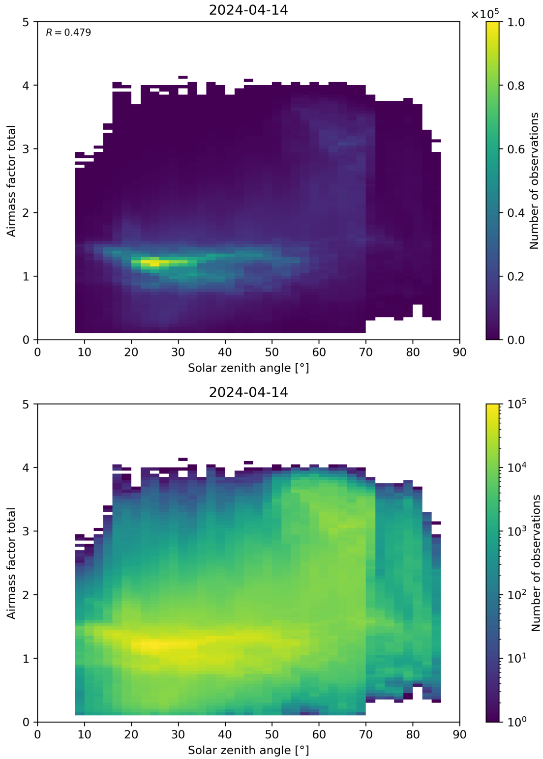
Figure 175: Scatter density plot of “Solar zenith angle” against “Airmass factor total” for 2024-04-13 to 2024-04-15.
