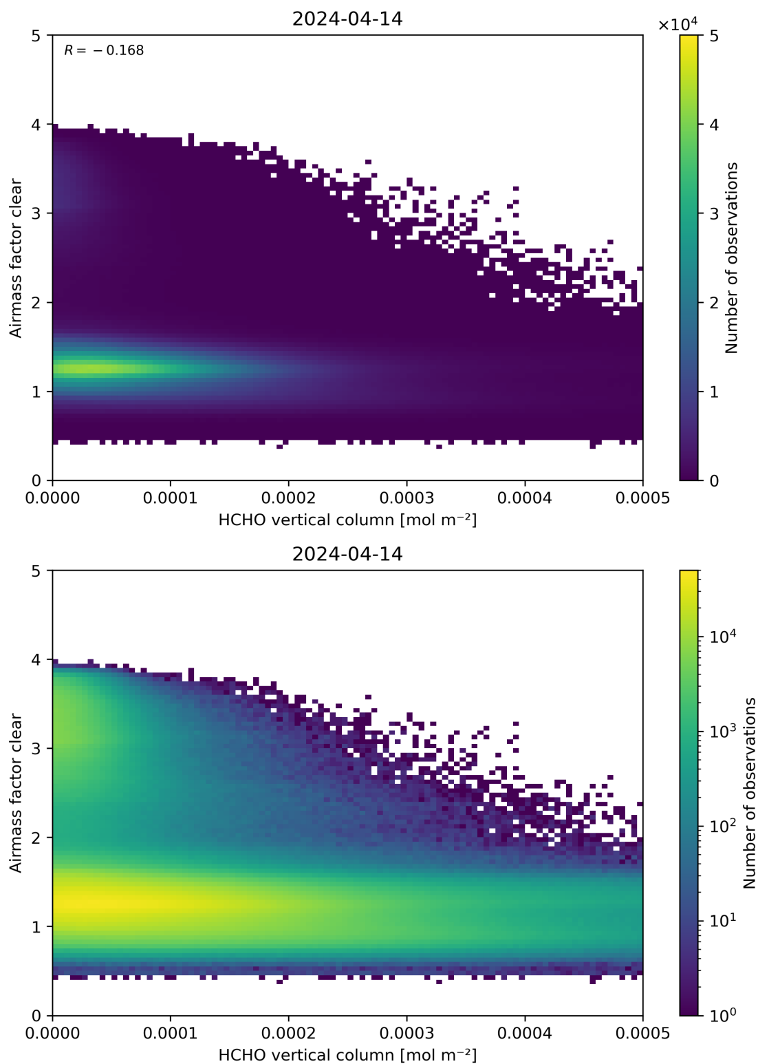
Figure 126: Scatter density plot of “HCHO vertical column” against “Airmass factor clear” for 2024-04-13 to 2024-04-15.
