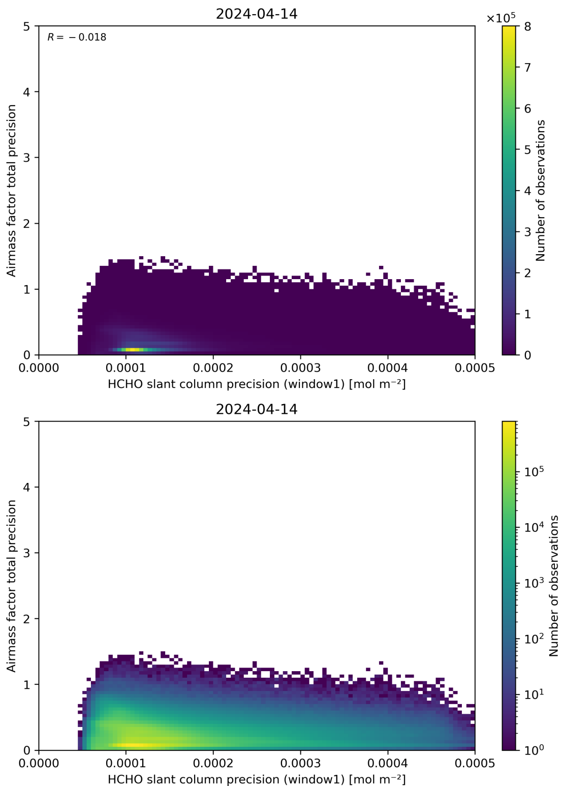
Figure 95: Scatter density plot of “HCHO slant column precision (window1)” against “Airmass factor total precision” for 2024-04-13 to 2024-04-15.
