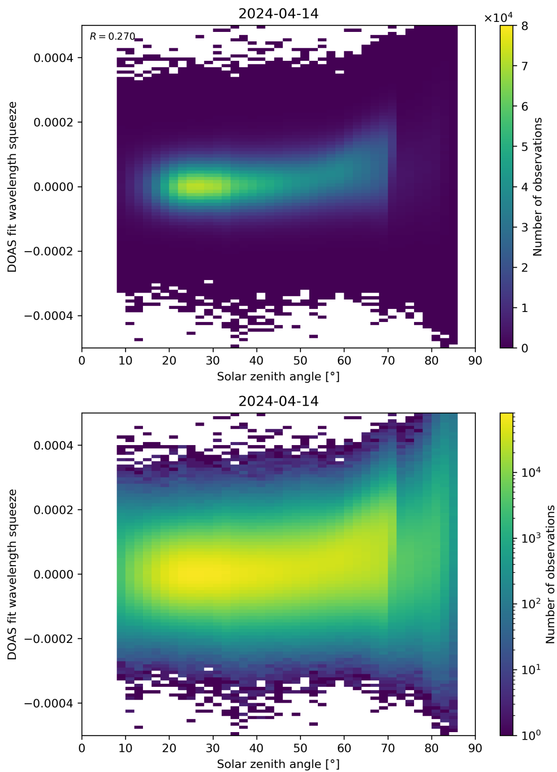
Figure 169: Scatter density plot of “Solar zenith angle” against “DOAS fit wavelength squeeze” for 2024-04-13 to 2024-04-15.
