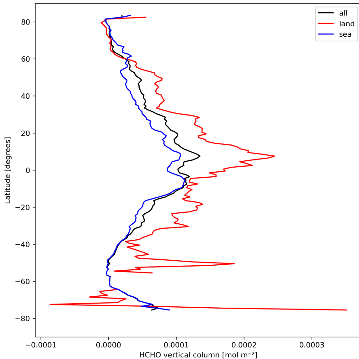
Figure 21: Zonal average of “HCHO vertical column” for 2024-04-13 to 2024-04-15.
