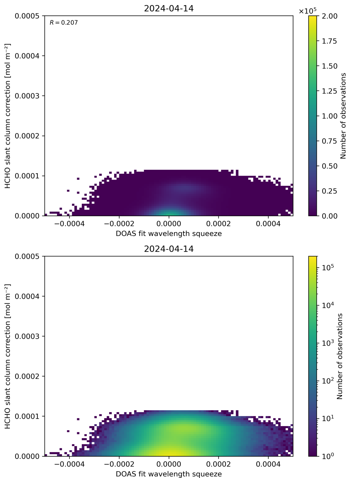
Figure 70: Scatter density plot of “DOAS fit wavelength squeeze” against “HCHO slant column correction” for 2024-04-13 to 2024-04-15.
