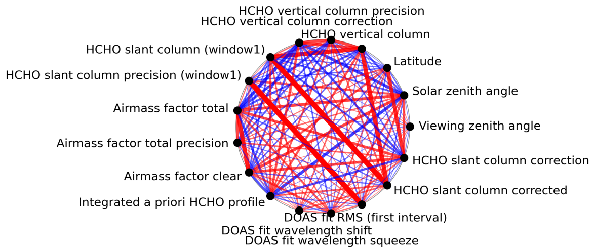
Figure 1: Map of correlation graph for 2024-04-13 to 2024-04-15.
