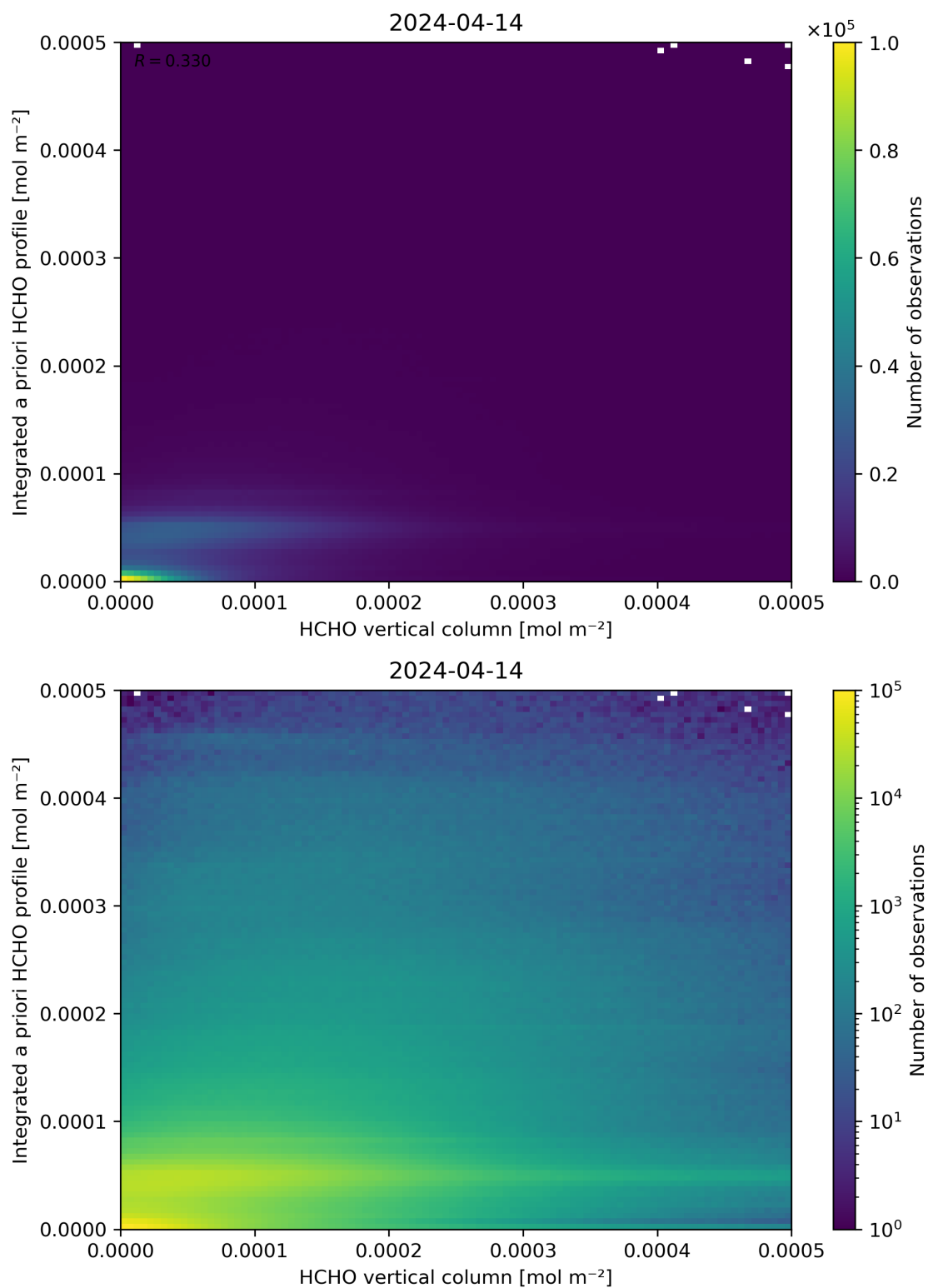
Figure 135: Scatter density plot of “HCHO vertical column” against “Integrated a priori HCHO profile” for 2024-04-13 to 2024-04-15.
