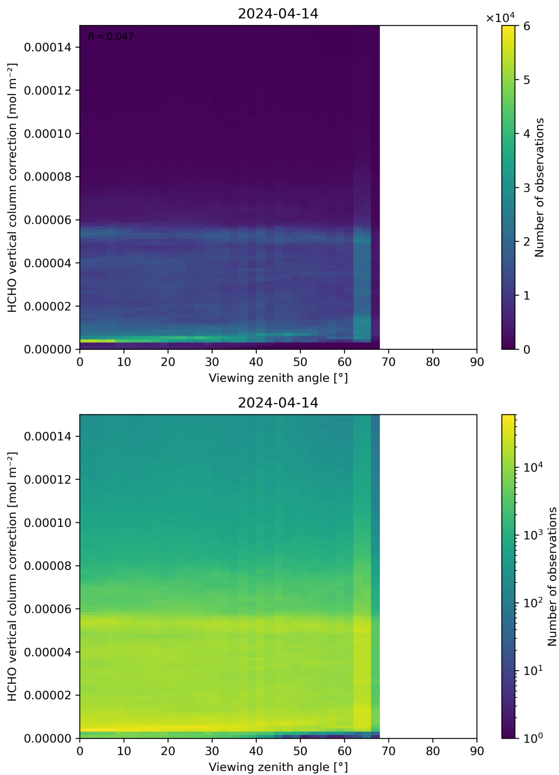
Figure 193: Scatter density plot of “Viewing zenith angle” against “HCHO vertical column correction” for 2024-04-13 to 2024-04-15.
