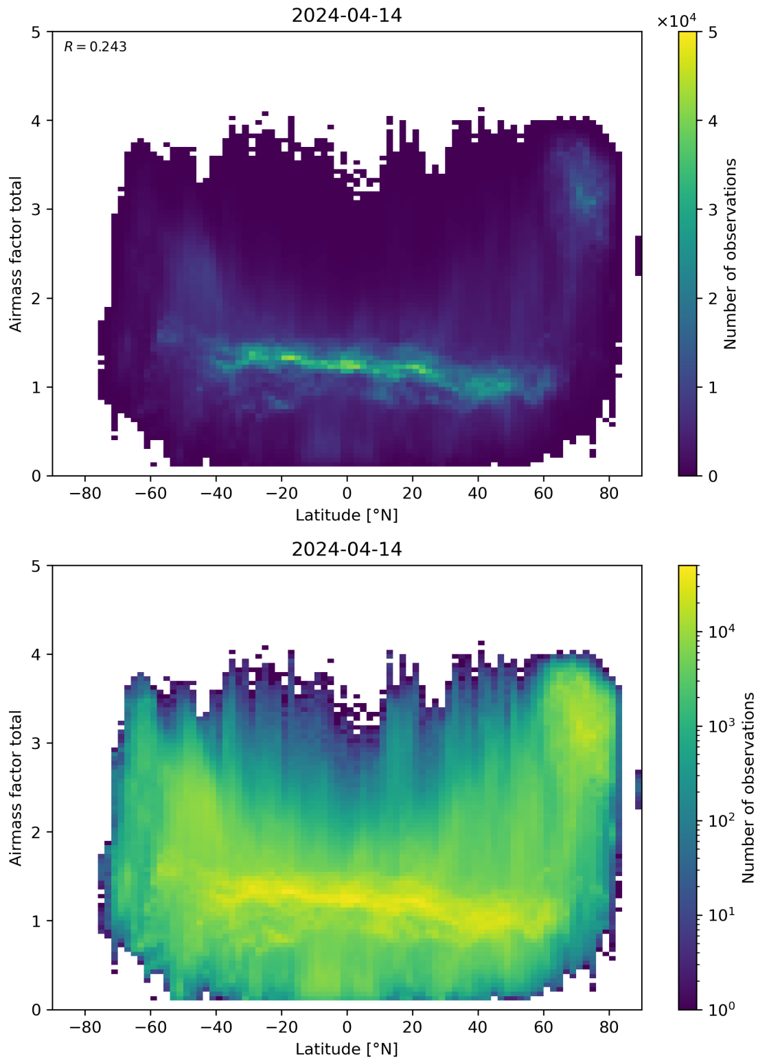
Figure 161: Scatter density plot of “Latitude” against “Airmass factor total” for 2024-04-13 to 2024-04-15.
