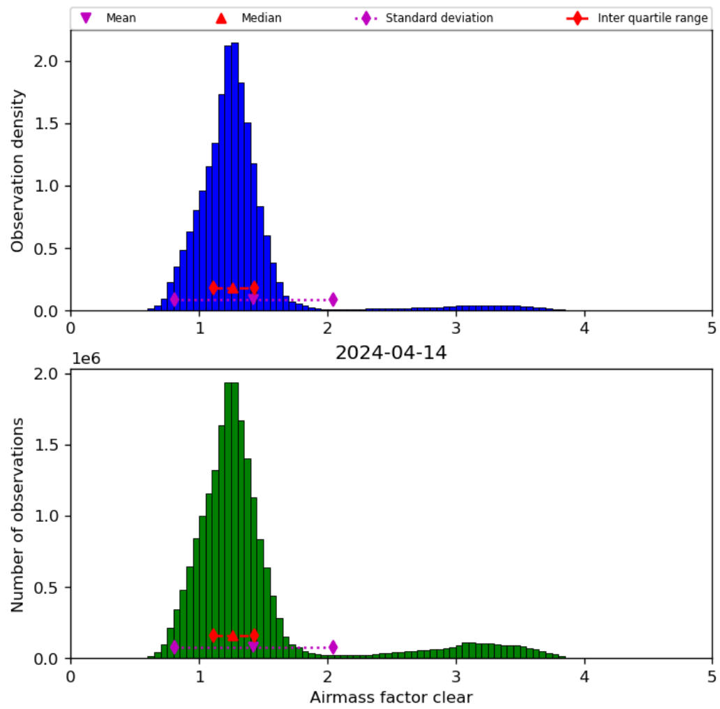
Figure 42: Histogram of “Airmass factor clear” for 2024-04-13 to 2024-04-15
