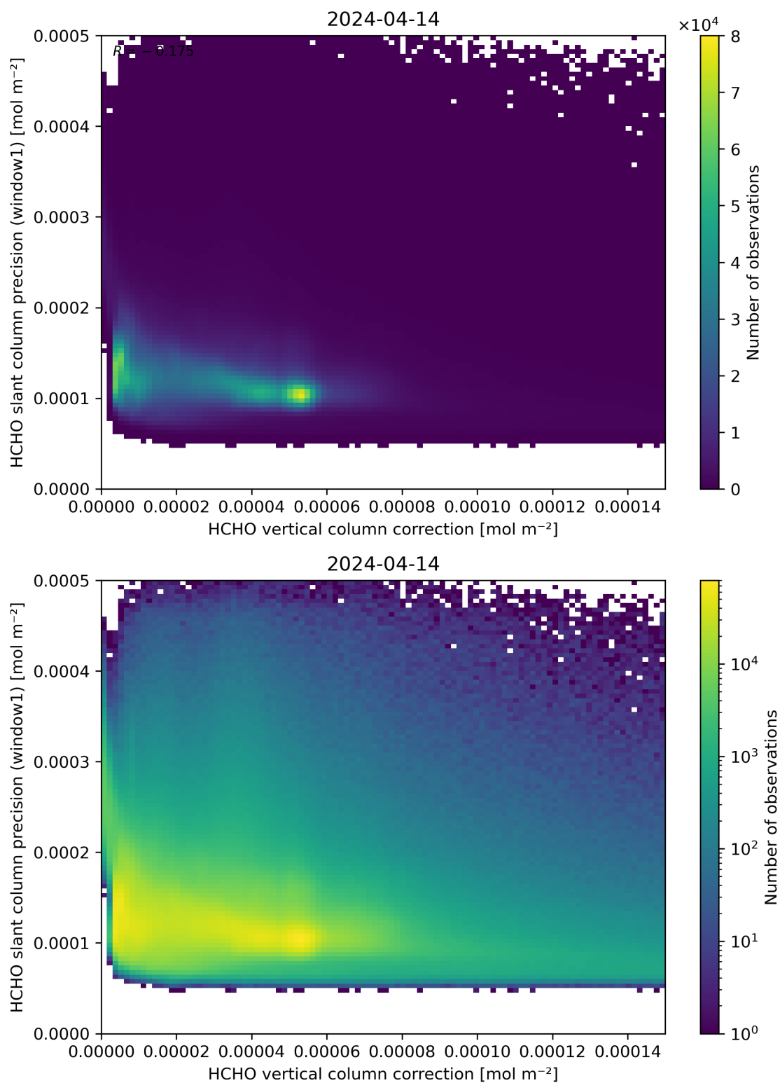
Figure 119: Scatter density plot of “HCHO vertical column correction” against “HCHO slant column precision (window1)” for 2024-04-13 to 2024-04-15.
