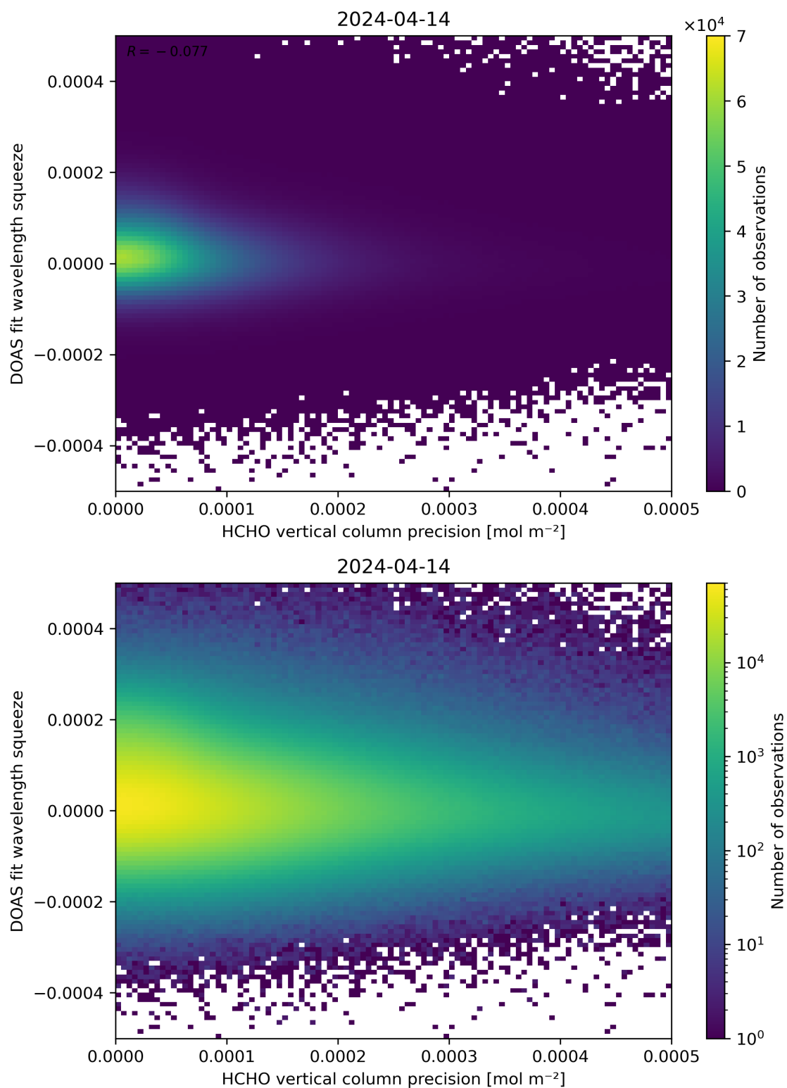
Figure 138: Scatter density plot of “HCHO vertical column precision” against “DOAS fit wavelength squeeze” for 2024-04-13 to 2024-04-15.
