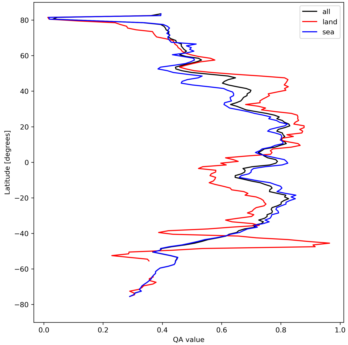
Figure 20: Zonal average of “QA value” for 2024-04-13 to 2024-04-15.
