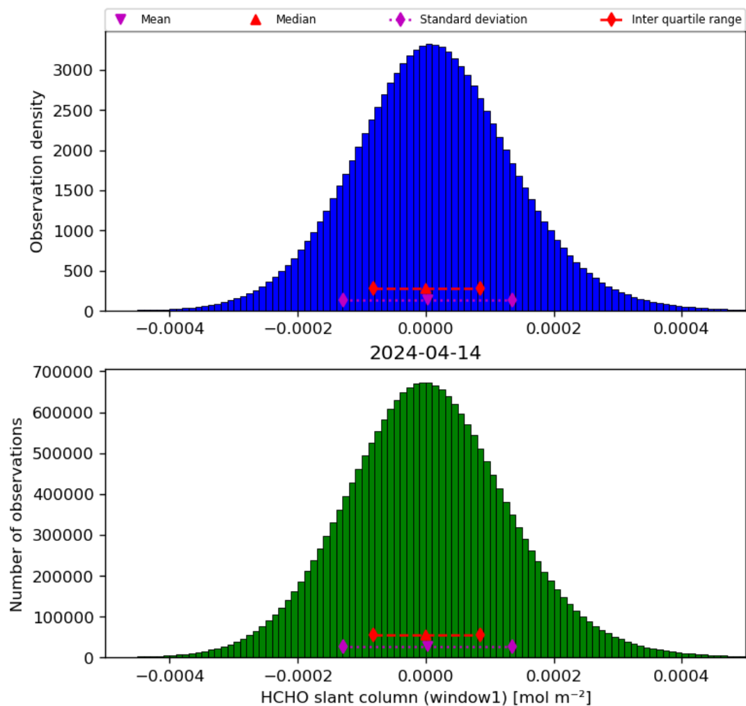
Figure 38: Histogram of “HCHO slant column (window1)” for 2024-04-13 to 2024-04-15
