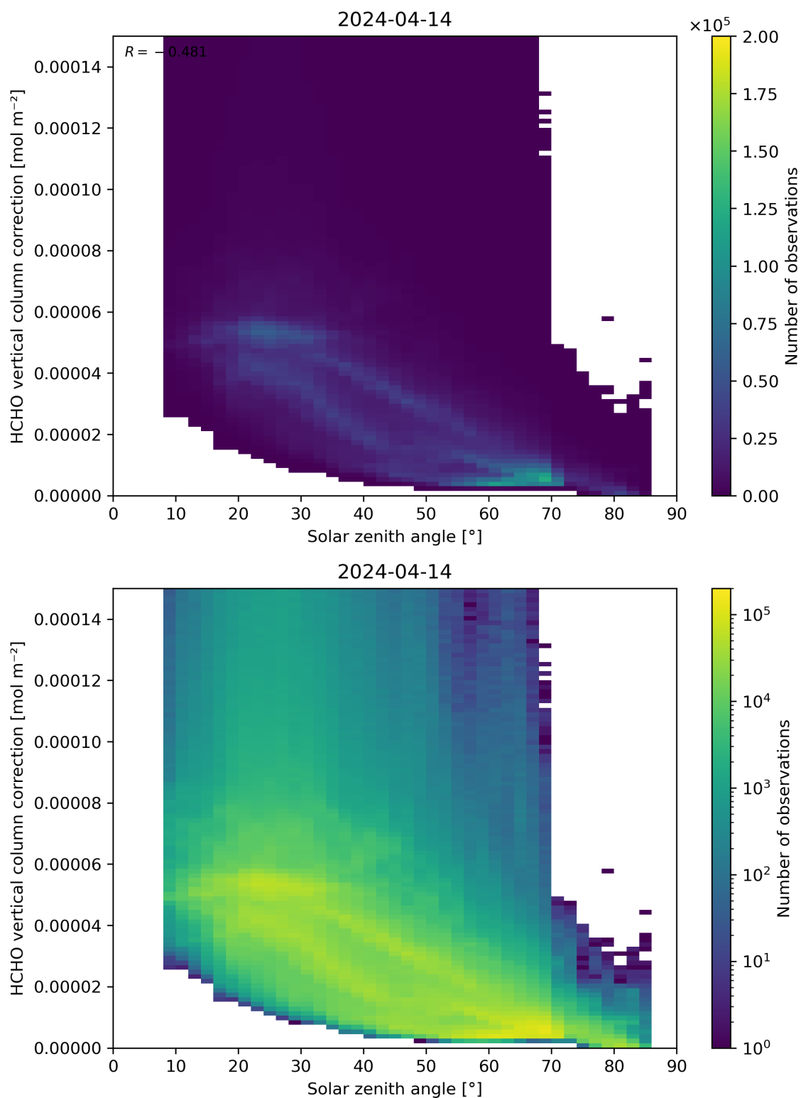
Figure 178: Scatter density plot of “Solar zenith angle” against “HCHO vertical column correction” for 2024-04-13 to 2024-04-15.
