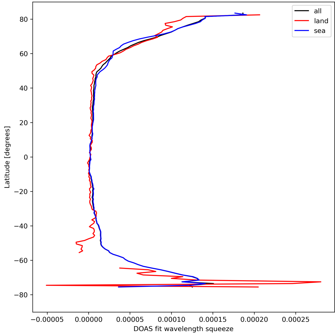
Figure 31: Zonal average of “DOAS fit wavelength squeeze” for 2024-04-13 to 2024-04-15.
