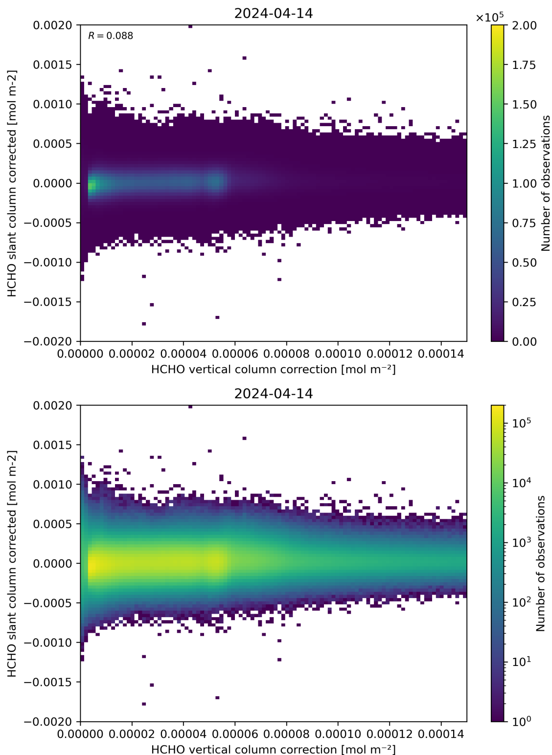
Figure 116: Scatter density plot of “HCHO vertical column correction” against “HCHO slant column corrected” for 2024-04-13 to 2024-04-15.
