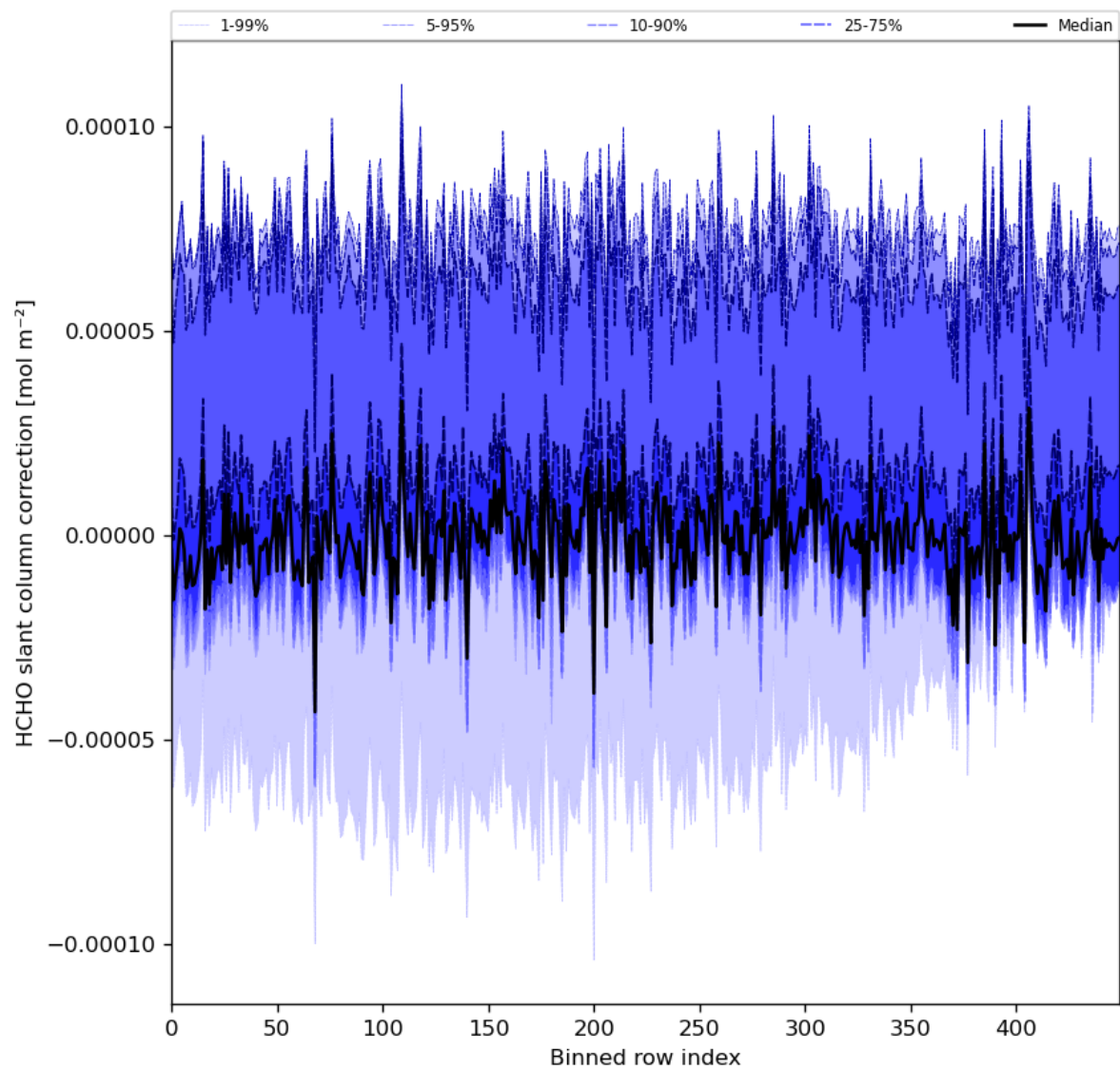
Figure 61: Along track statistics of “HCHO slant column correction” for 2024-04-13 to 2024-04-15
