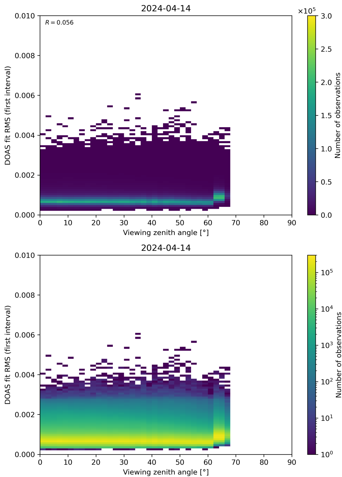
Figure 182: Scatter density plot of “Viewing zenith angle” against “DOAS fit RMS (first interval)” for 2024-04-13 to 2024-04-15.
