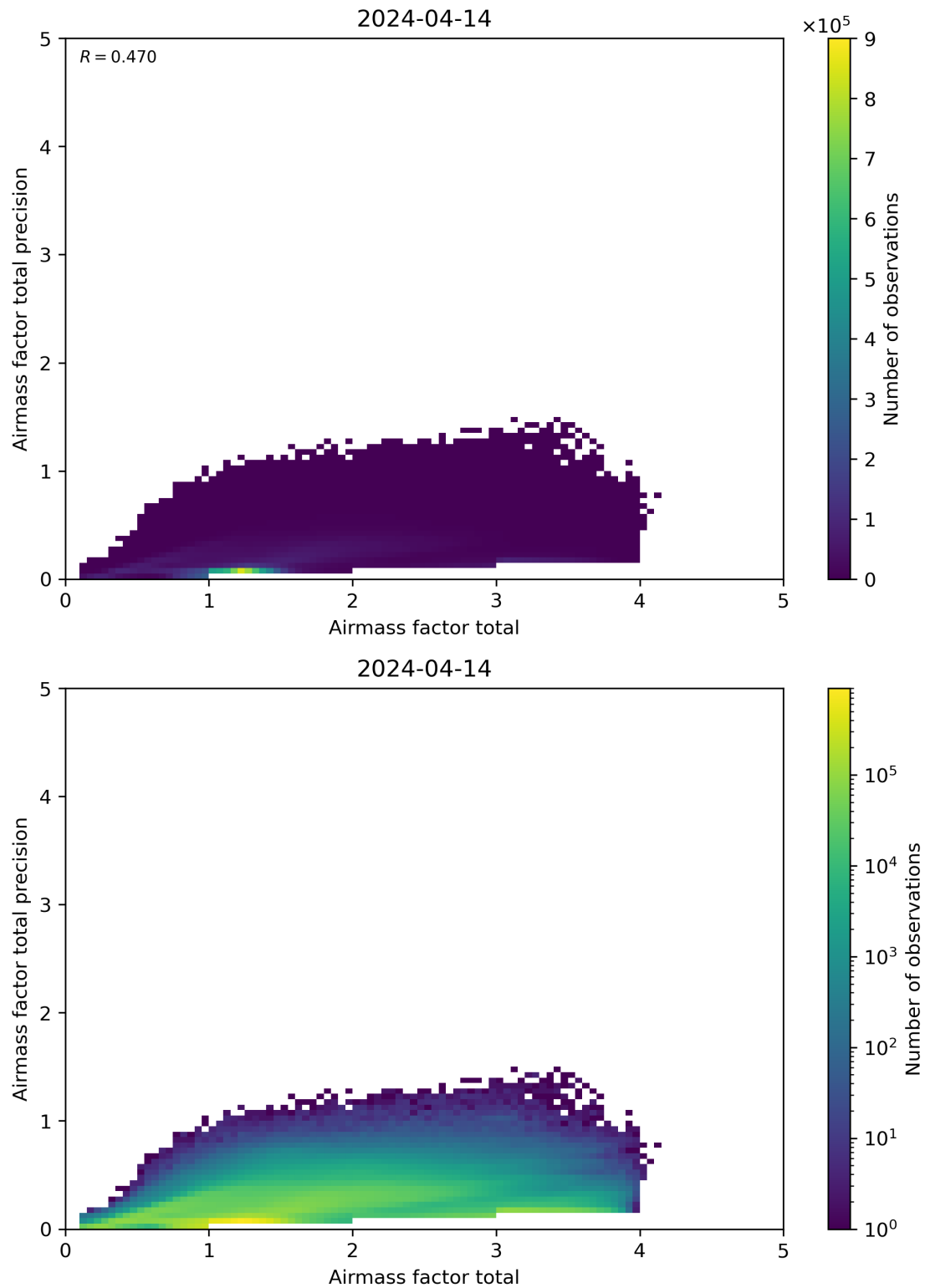
Figure 103: Scatter density plot of “Airmass factor total” against “Airmass factor total precision” for 2024-04-13 to 2024-04-15.
