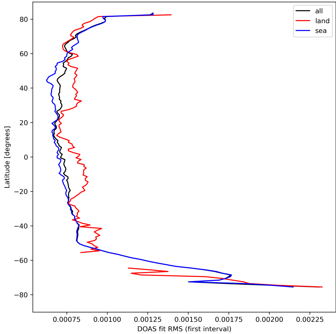
Figure 32: Zonal average of “DOAS fit RMS (first interval)” for 2024-04-13 to 2024-04-15.
