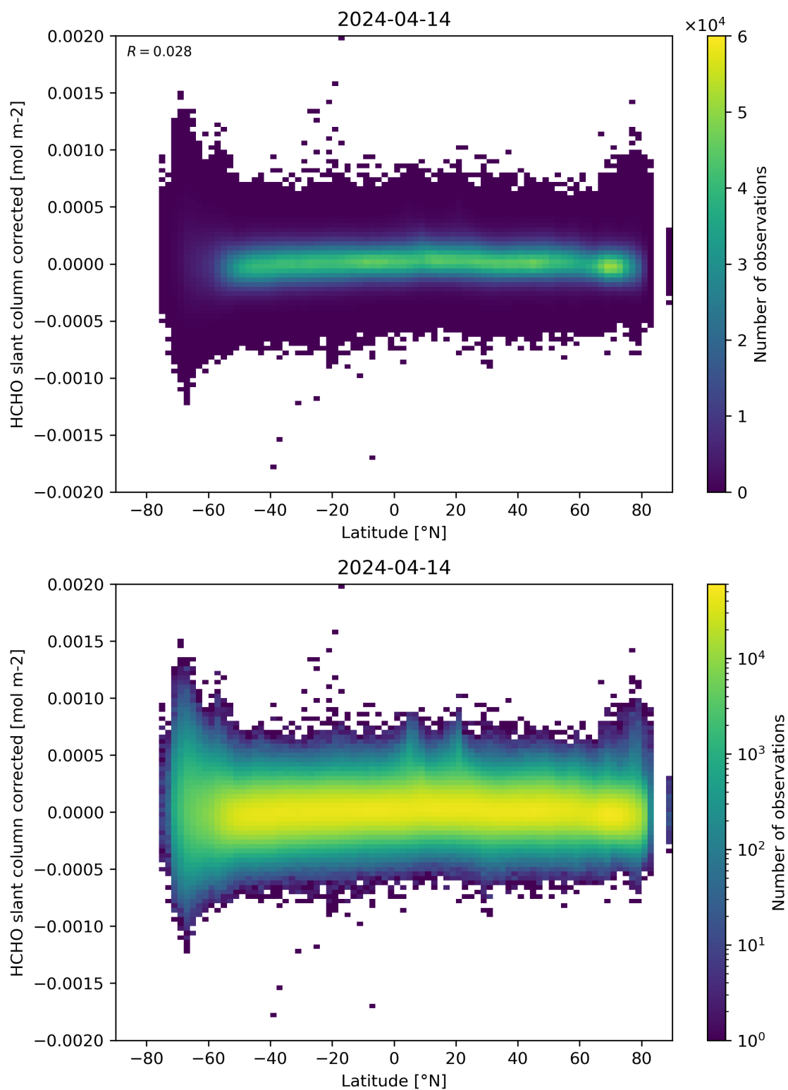
Figure 157: Scatter density plot of “Latitude” against “HCHO slant column corrected” for 2024-04-13 to 2024-04-15.
