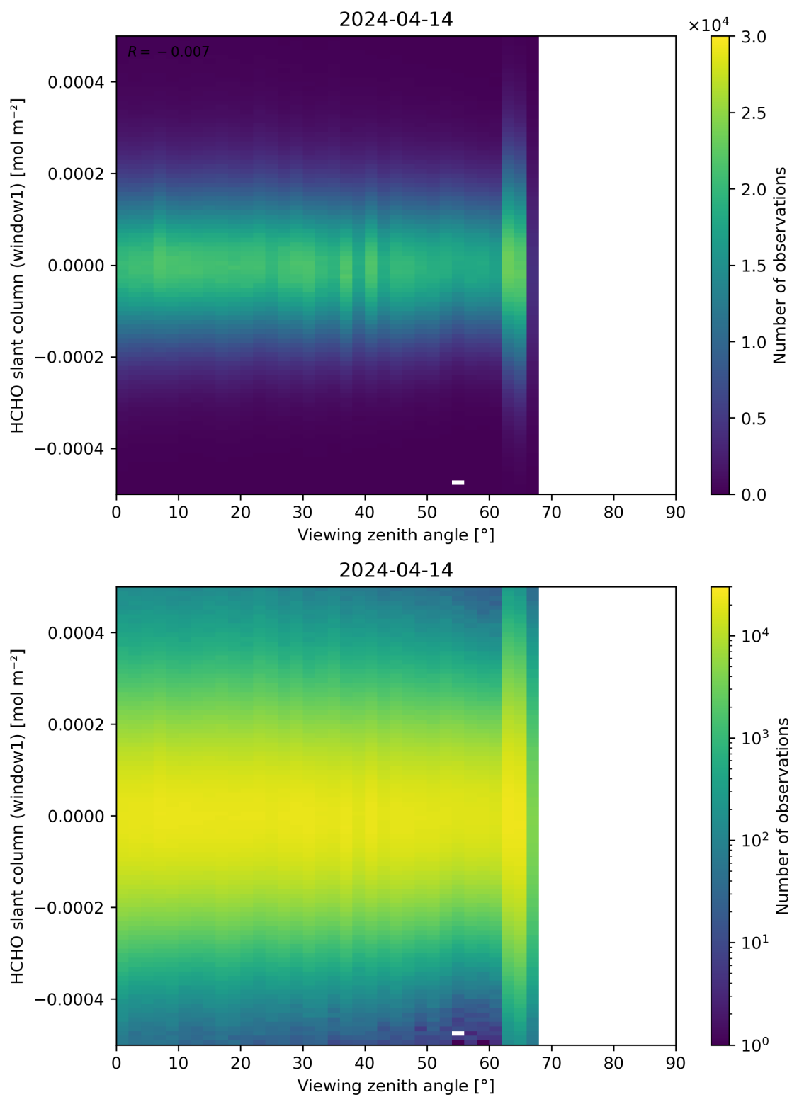
Figure 188: Scatter density plot of “Viewing zenith angle” against “HCHO slant column (window1)” for 2024-04-13 to 2024-04-15.
