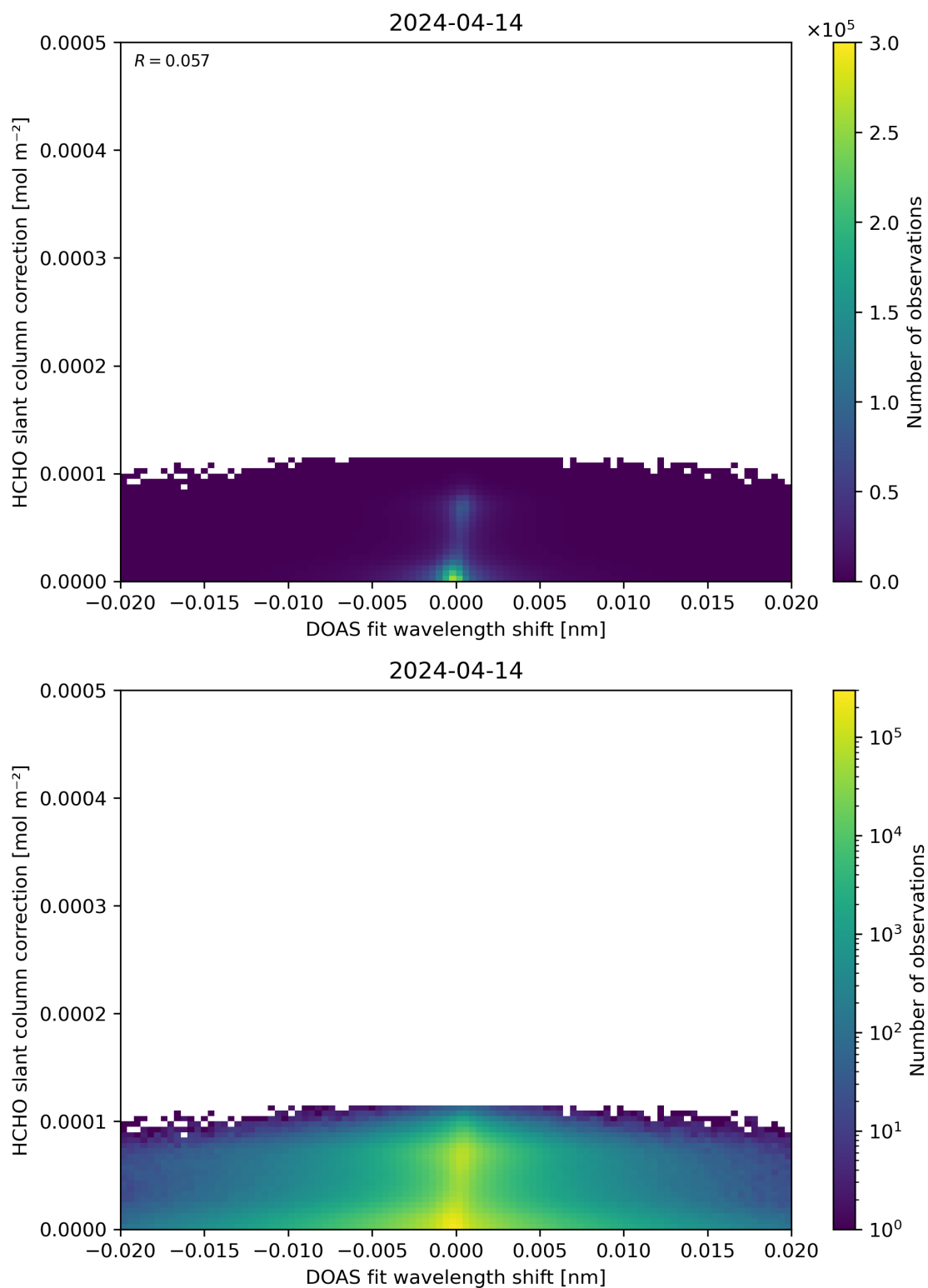
Figure 67: Scatter density plot of “DOAS fit wavelength shift” against “HCHO slant column correction” for 2024-04-13 to 2024-04-15.
