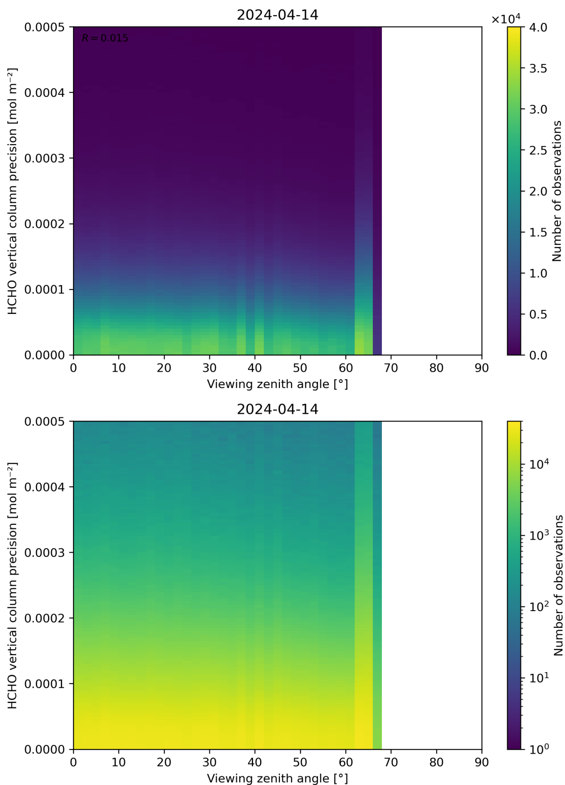
Figure 194: Scatter density plot of “Viewing zenith angle” against “HCHO vertical column precision” for 2024-04-13 to 2024-04-15.
