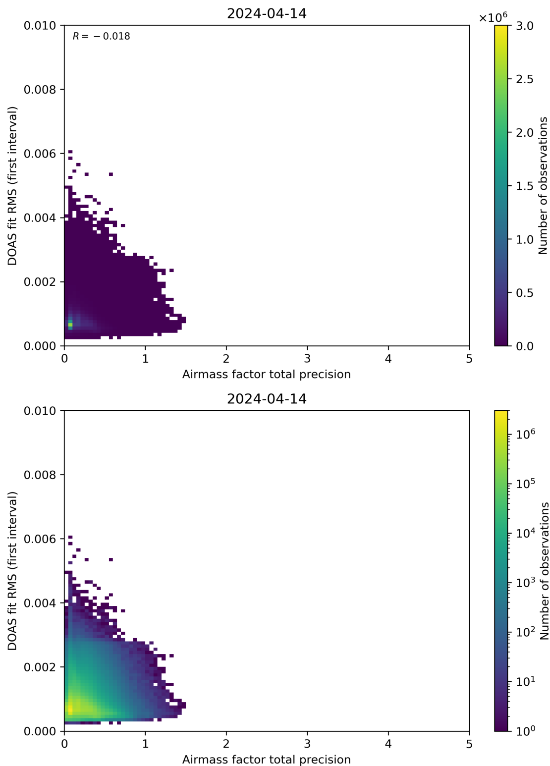
Figure 105: Scatter density plot of “Airmass factor total precision” against “DOAS fit RMS (first interval)” for 2024-04-13 to 2024-04-15.
