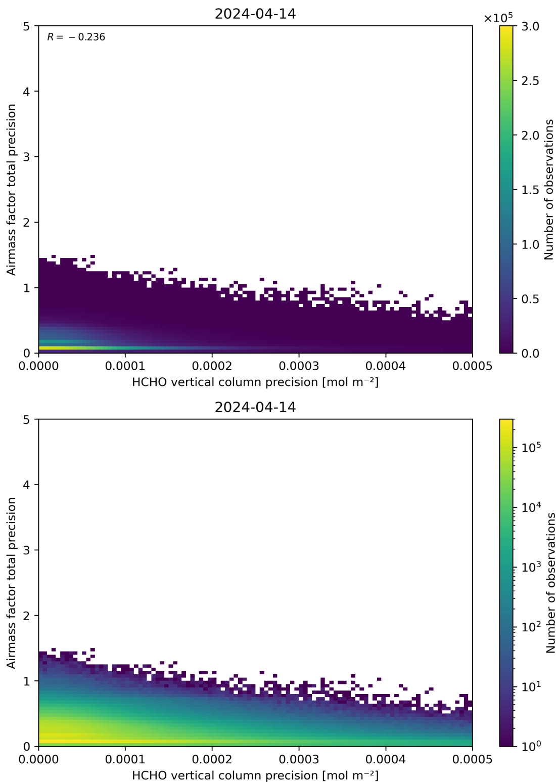
Figure 145: Scatter density plot of “HCHO vertical column precision” against “Airmass factor total precision” for 2024-04-13 to 2024-04-15.
