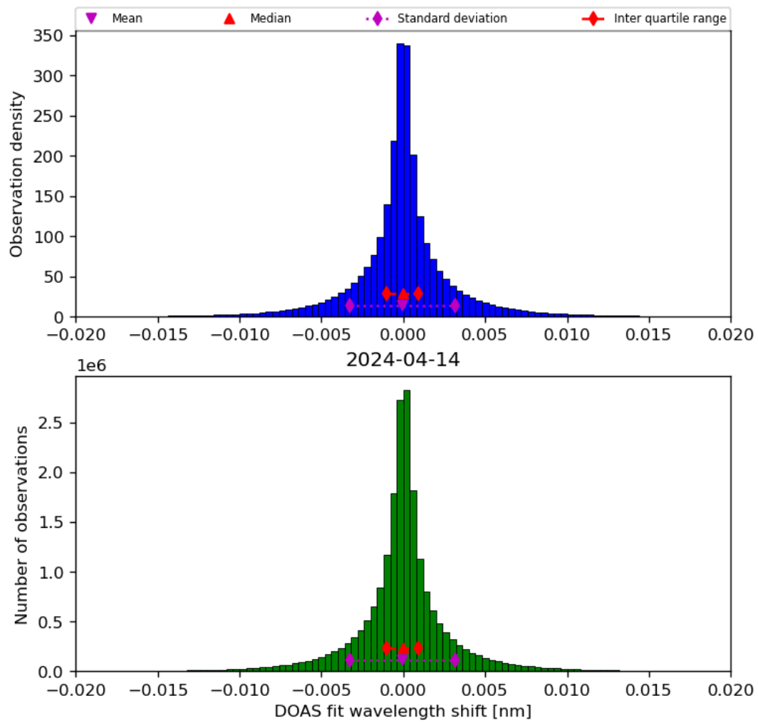
Figure 44: Histogram of “DOAS fit wavelength shift” for 2024-04-13 to 2024-04-15
