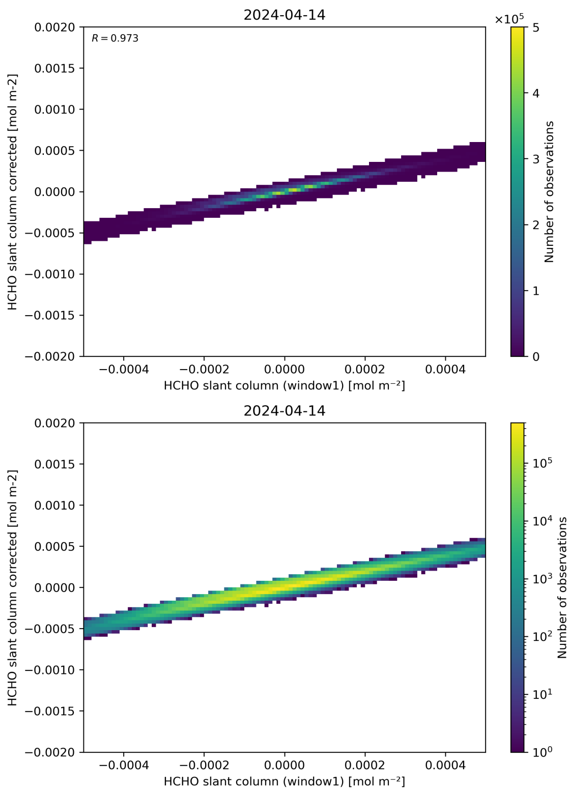
Figure 82: Scatter density plot of “HCHO slant column (window1)” against “HCHO slant column corrected” for 2024-04-13 to 2024-04-15.
